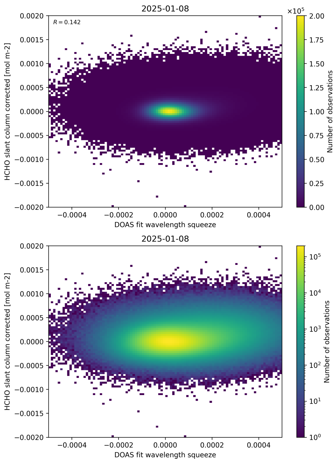
Figure 69: Scatter density plot of “DOAS fit wavelength squeeze” against “HCHO slant column corrected” for 2025-01-07 to 2025-01-09.
