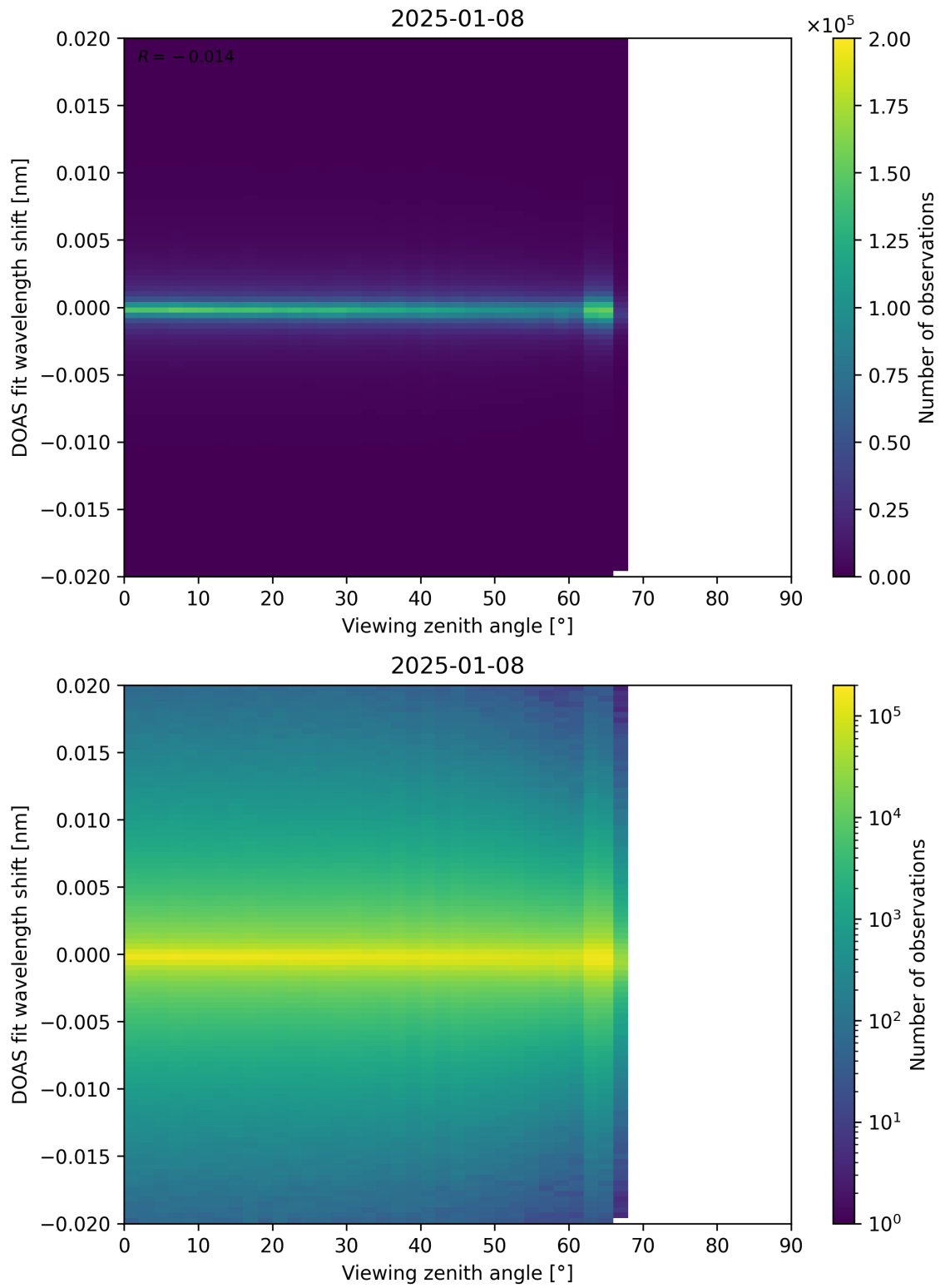
Figure 183: Scatter density plot of “Viewing zenith angle” against “DOAS fit wavelength shift” for 2025-01-07 to 2025-01-09.
