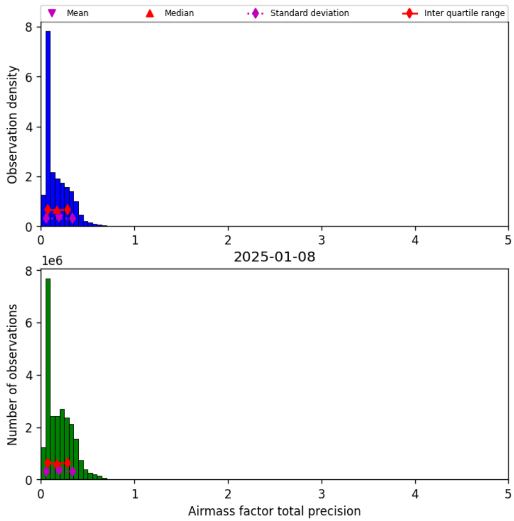
Figure 41: Histogram of “Airmass factor total precision” for 2025-01-07 to 2025-01-09
