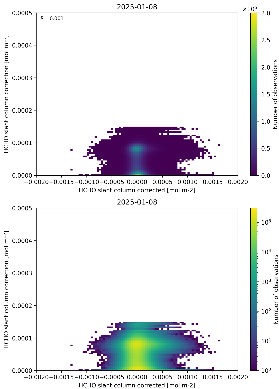
Figure 77: Scatter density plot of “HCHO slant column corrected” against “HCHO slant column correction” for 2025-01-07 to 2025-01-09.
