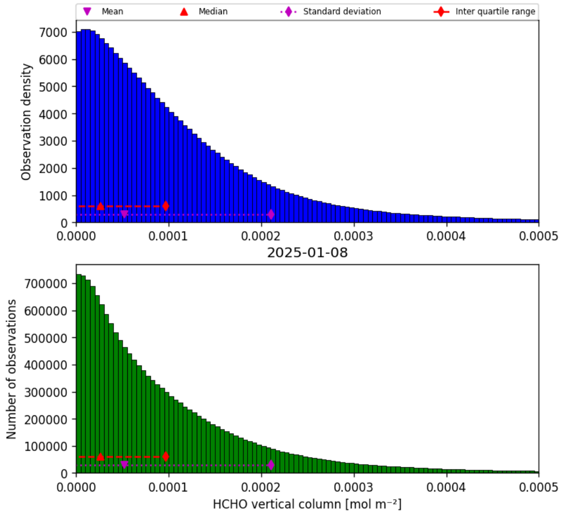
Figure 35: Histogram of “HCHO vertical column” for 2025-01-07 to 2025-01-09
