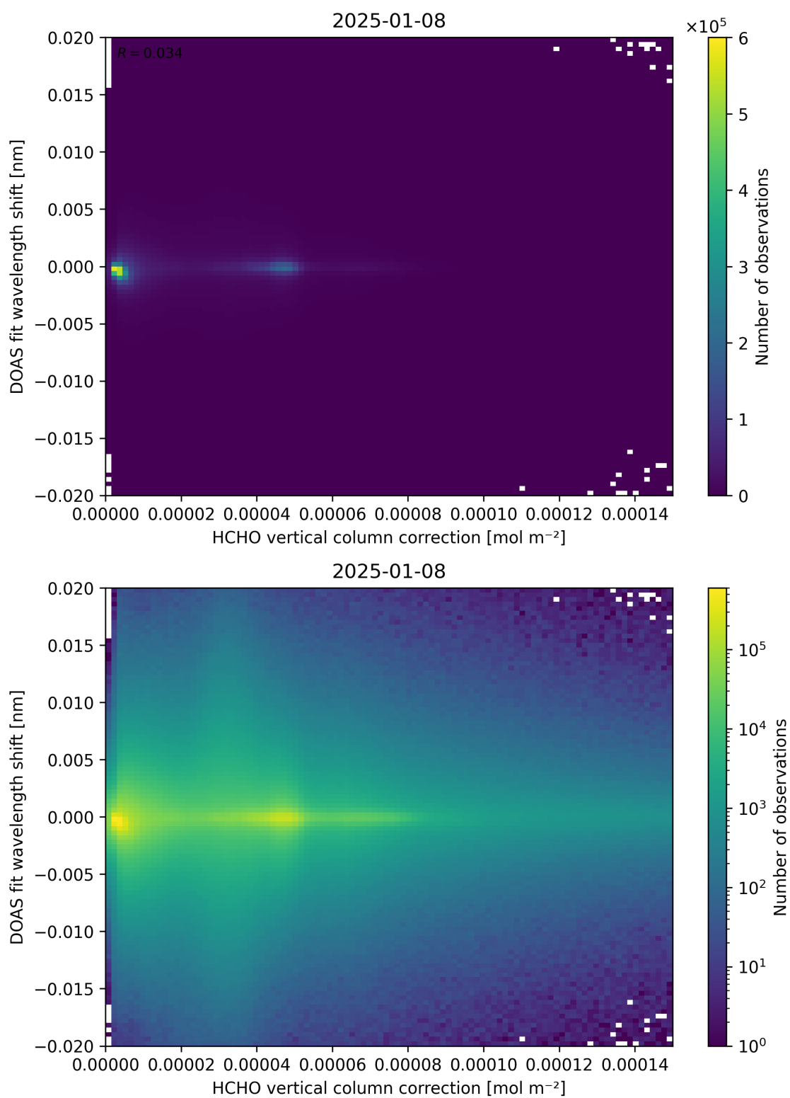
Figure 113: Scatter density plot of “HCHO vertical column correction” against “DOAS fit wavelength shift” for 2025-01-07 to 2025-01-09.
