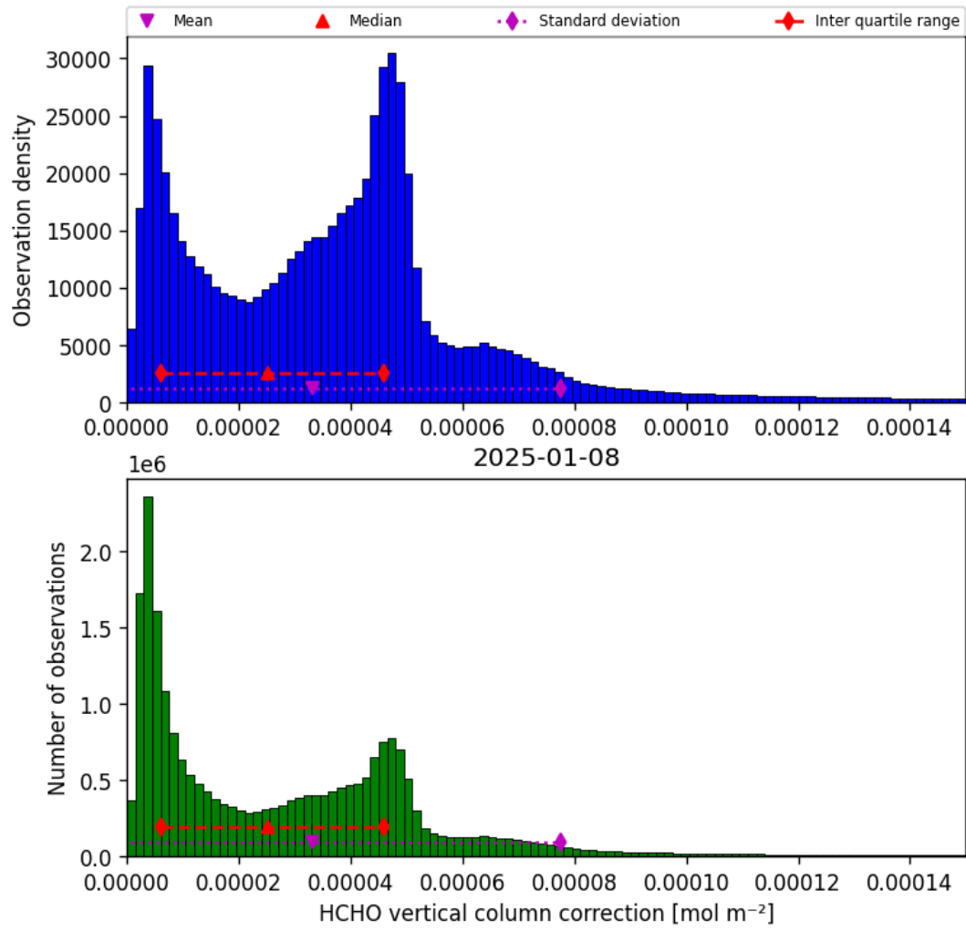
Figure 37: Histogram of “HCHO vertical column correction” for 2025-01-07 to 2025-01-09
