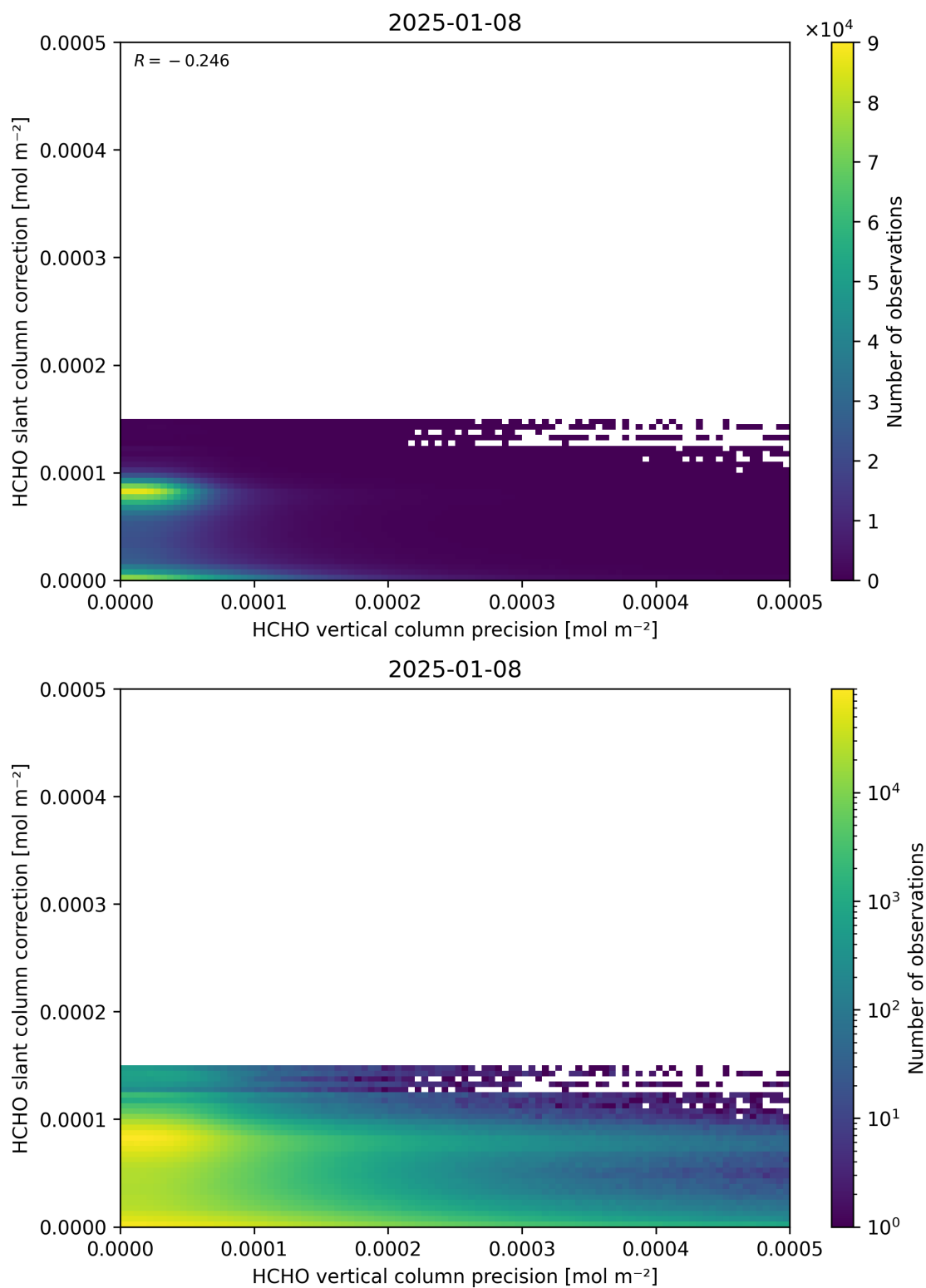
Figure 141: Scatter density plot of “HCHO vertical column precision” against “HCHO slant column correction” for 2025-01-07 to 2025-01-09.
