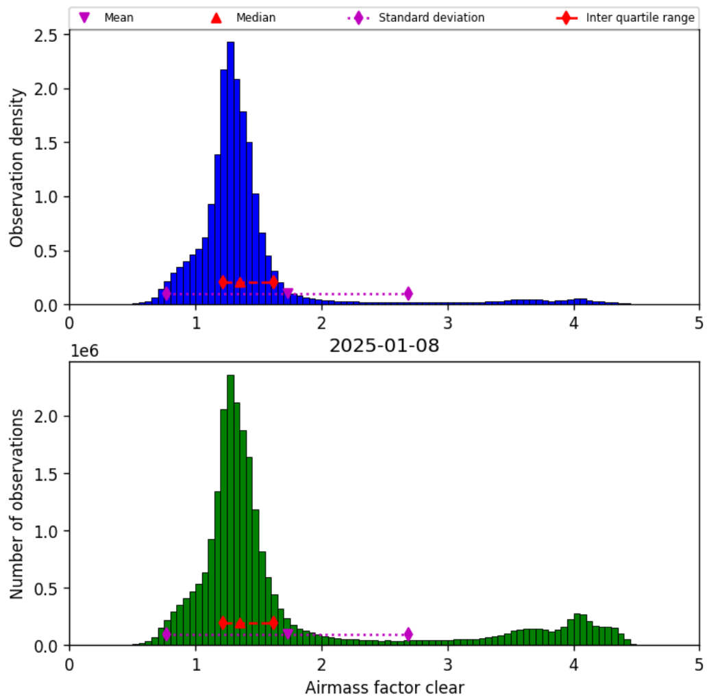
Figure 42: Histogram of “Airmass factor clear” for 2025-01-07 to 2025-01-09
