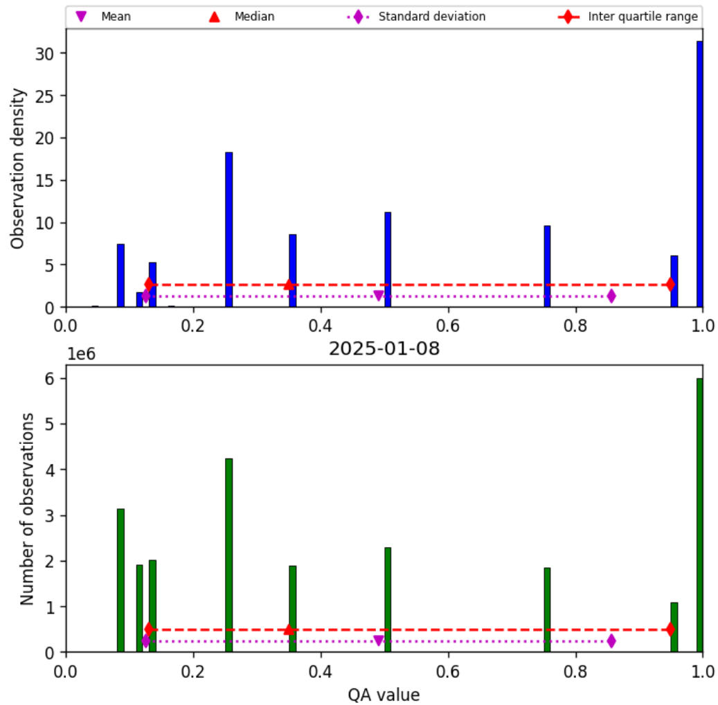
Figure 34: Histogram of “QA value” for 2025-01-07 to 2025-01-09
