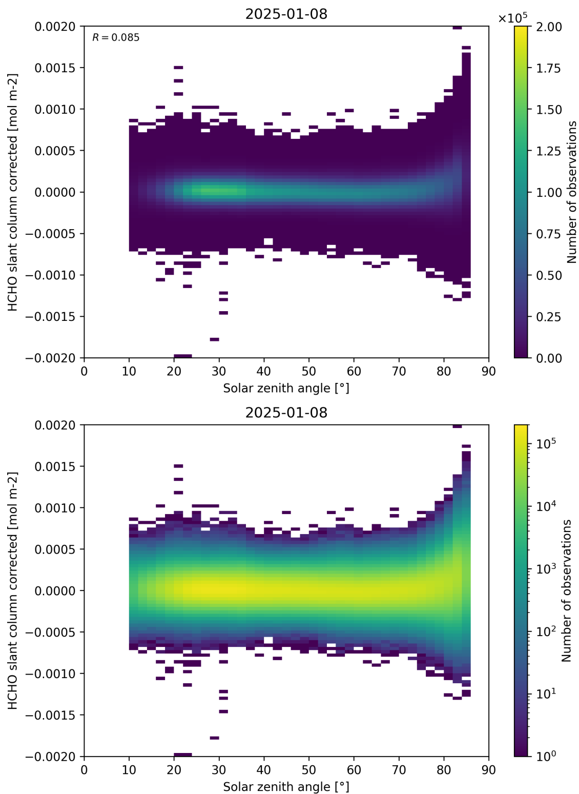
Figure 171: Scatter density plot of “Solar zenith angle” against “HCHO slant column corrected” for 2025-01-07 to 2025-01-09.
