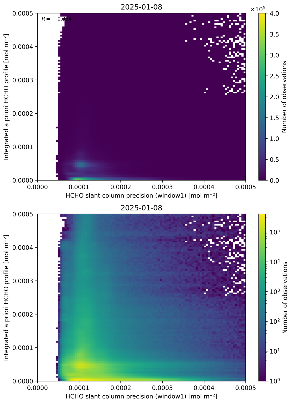
Figure 96: Scatter density plot of “HCHO slant column precision (window1)” against “Integrated a priori HCHO profile” for 2025-01-07 to 2025-01-09.
