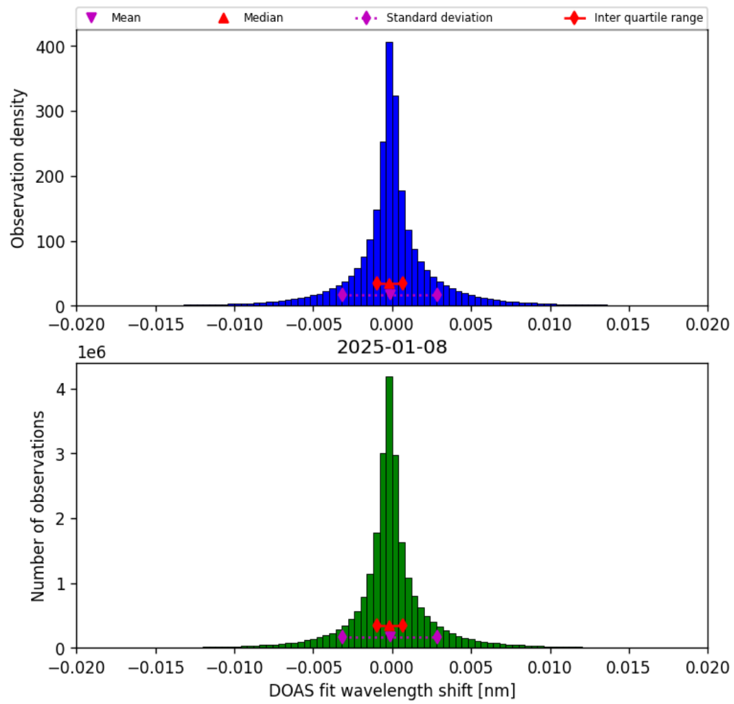
Figure 44: Histogram of “DOAS fit wavelength shift” for 2025-01-07 to 2025-01-09
