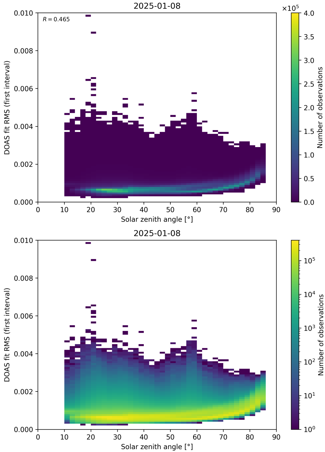
Figure 167: Scatter density plot of “Solar zenith angle” against “DOAS fit RMS (first interval)” for 2025-01-07 to 2025-01-09.
