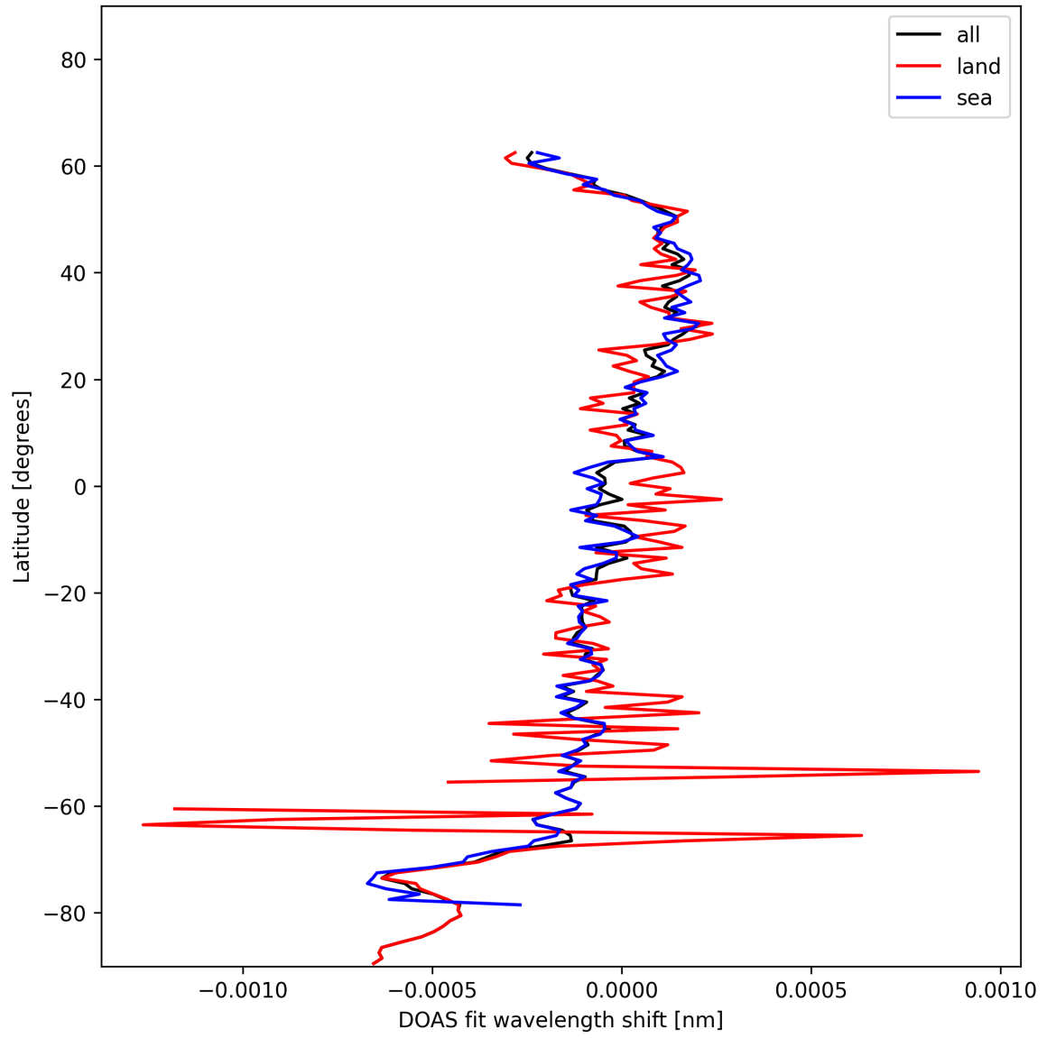
Figure 30: Zonal average of “DOAS fit wavelength shift” for 2025-01-07 to 2025-01-09.
