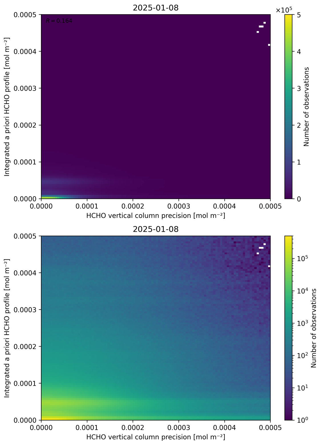
Figure 147: Scatter density plot of “HCHO vertical column precision” against “Integrated a priori HCHO profile” for 2025-01-07 to 2025-01-09.
