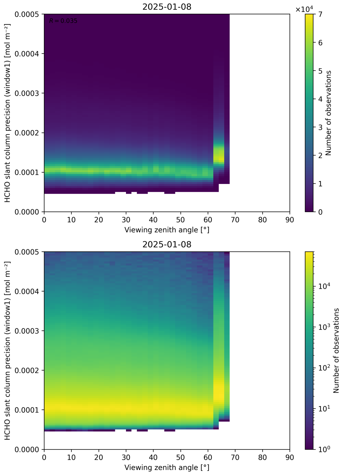
Figure 189: Scatter density plot of “Viewing zenith angle” against “HCHO slant column precision (window1)” for 2025-01-07 to 2025-01-09.
