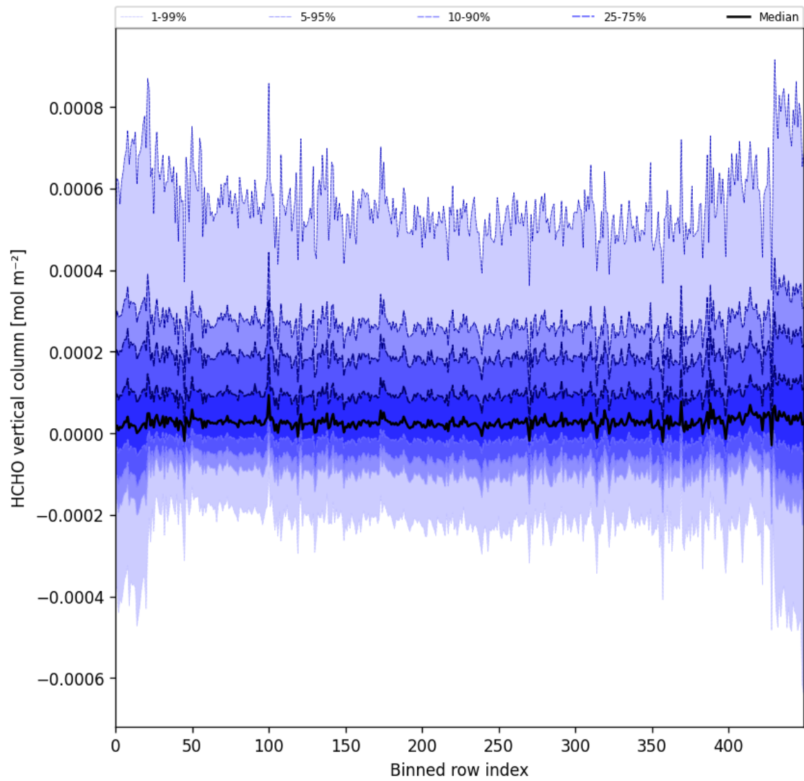
Figure 49: Along track statistics of “HCHO vertical column” for 2025-01-07 to 2025-01-09
