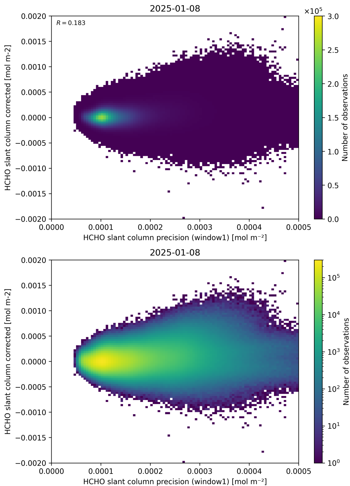
Figure 92: Scatter density plot of “HCHO slant column precision (window1)” against “HCHO slant column corrected” for 2025-01-07 to 2025-01-09.
