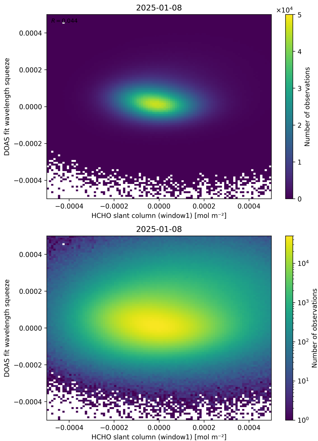
Figure 80: Scatter density plot of “HCHO slant column (window1)” against “DOAS fit wavelength squeeze” for 2025-01-07 to 2025-01-09.
