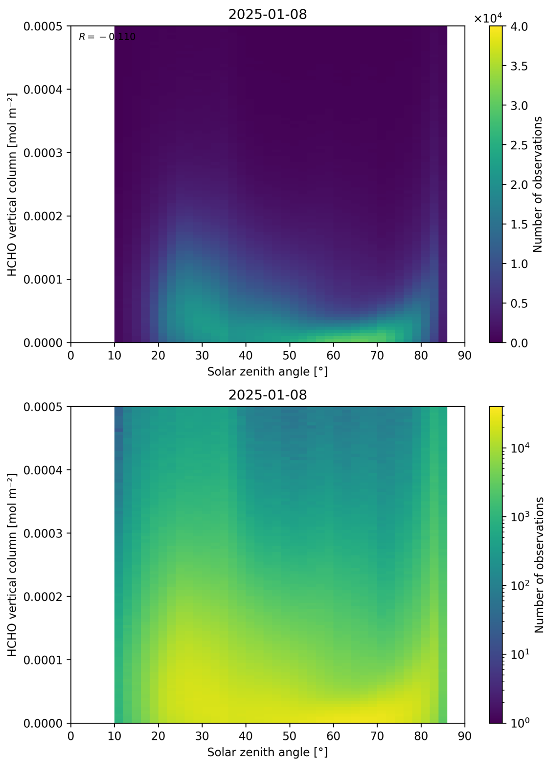
Figure 177: Scatter density plot of “Solar zenith angle” against “HCHO vertical column” for 2025-01-07 to 2025-01-09.
