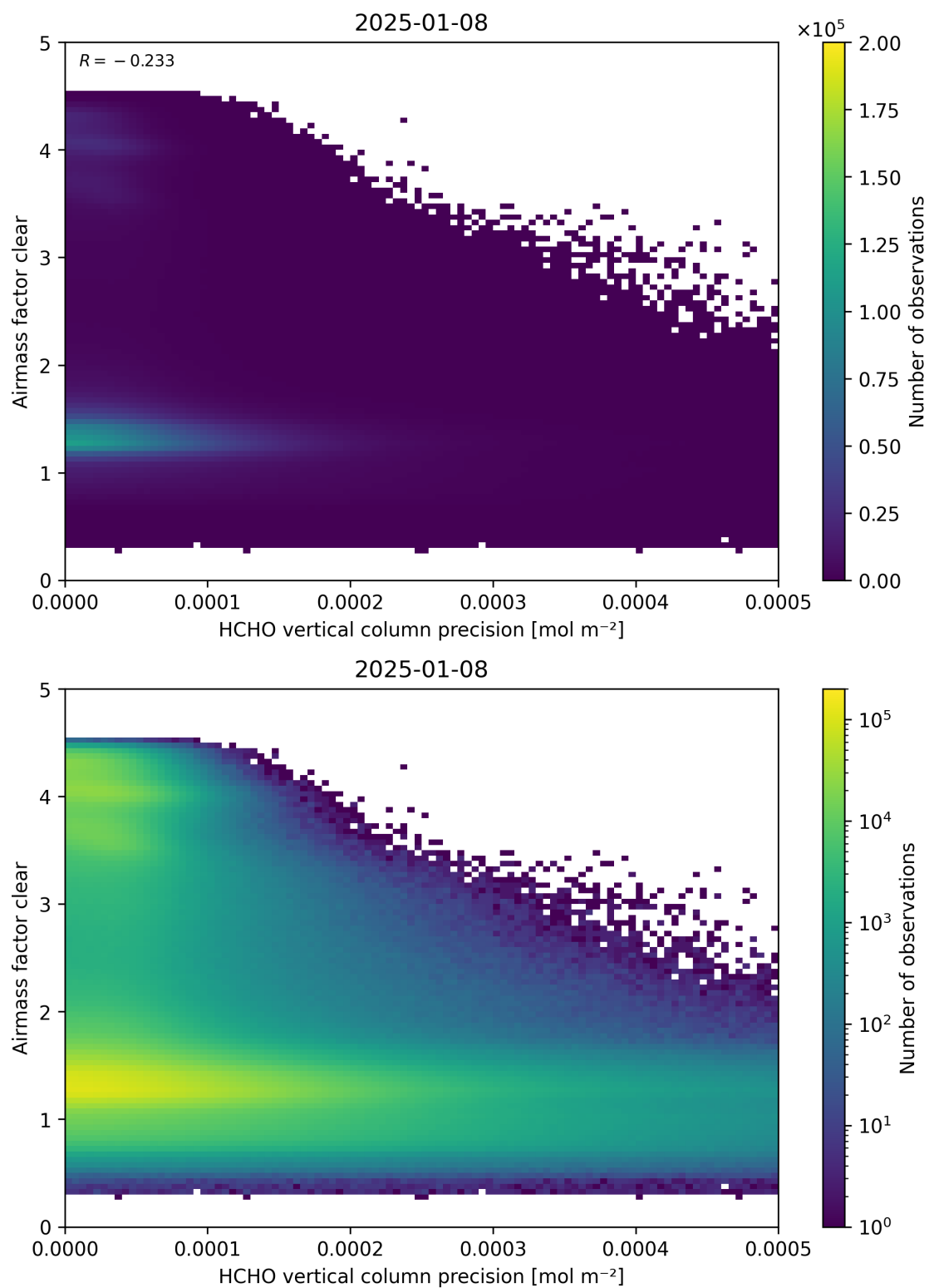
Figure 139: Scatter density plot of “HCHO vertical column precision” against “Airmass factor clear” for 2025-01-07 to 2025-01-09.
