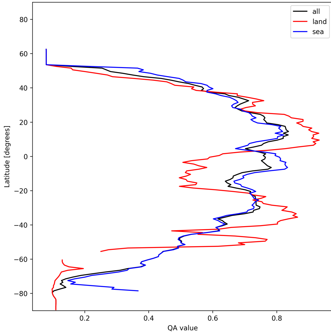
Figure 20: Zonal average of “QA value” for 2025-01-07 to 2025-01-09.
