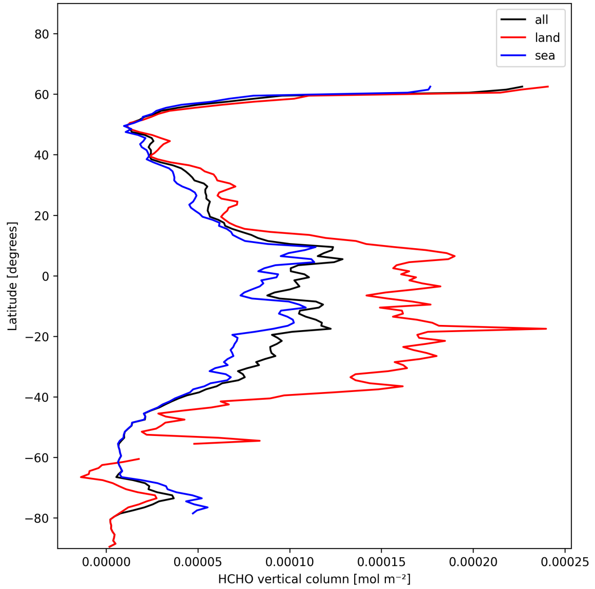
Figure 21: Zonal average of “HCHO vertical column” for 2025-01-07 to 2025-01-09.
