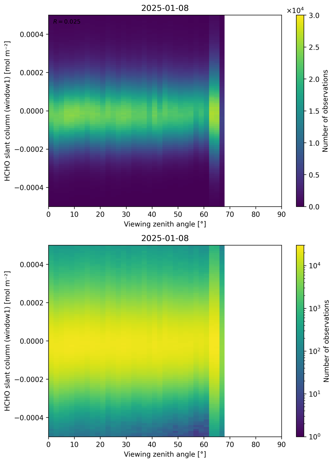
Figure 188: Scatter density plot of “Viewing zenith angle” against “HCHO slant column (window1)” for 2025-01-07 to 2025-01-09.
