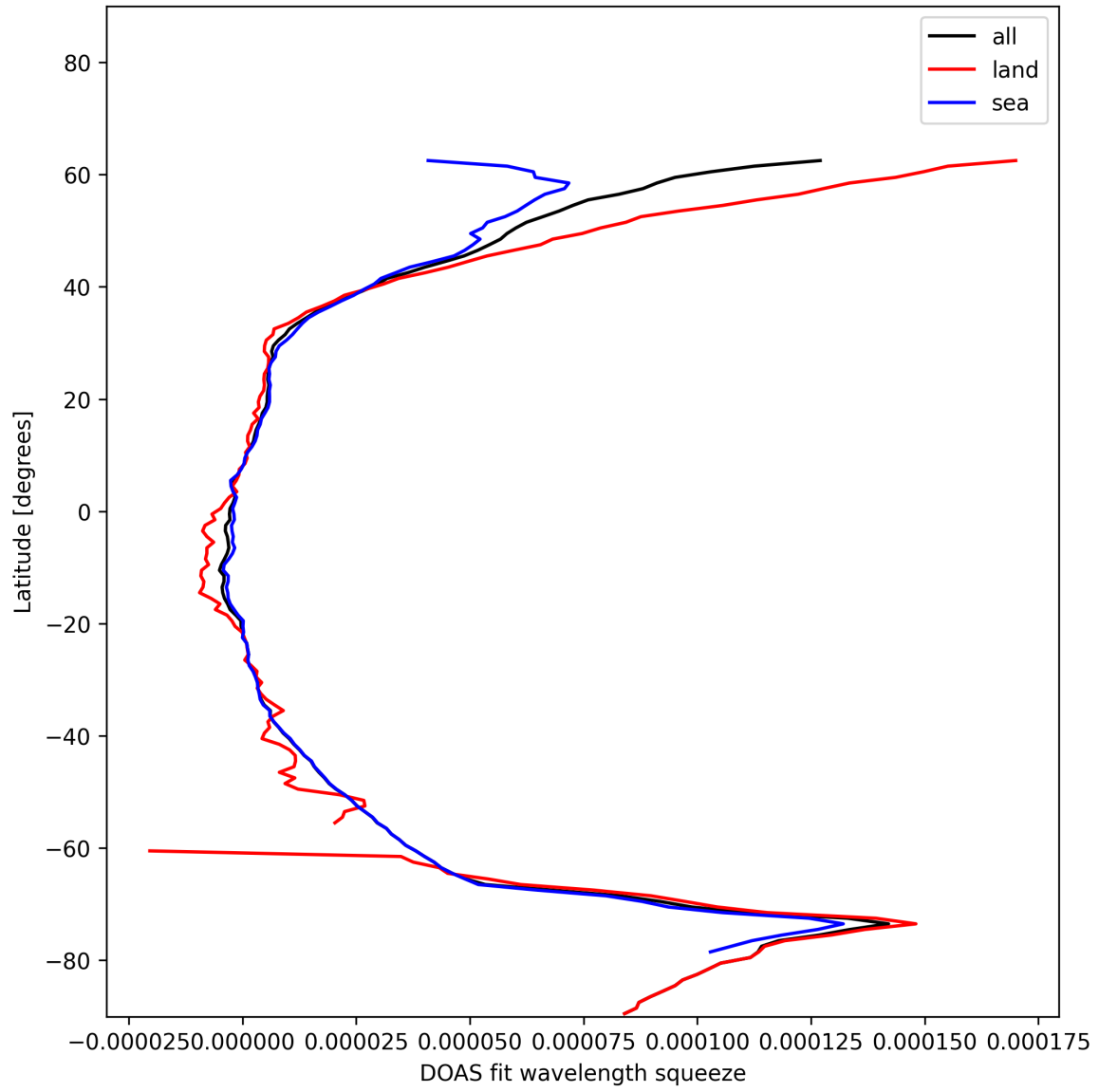
Figure 31: Zonal average of “DOAS fit wavelength squeeze” for 2025-01-07 to 2025-01-09.
