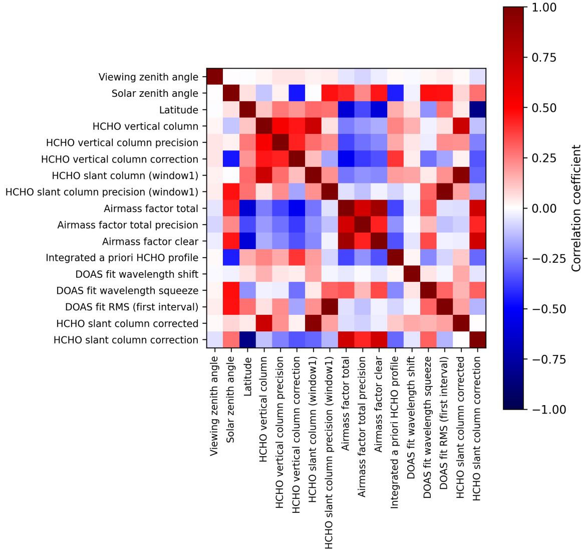
Figure 2: Map of correlation matrix for 2025-01-07 to 2025-01-09.
