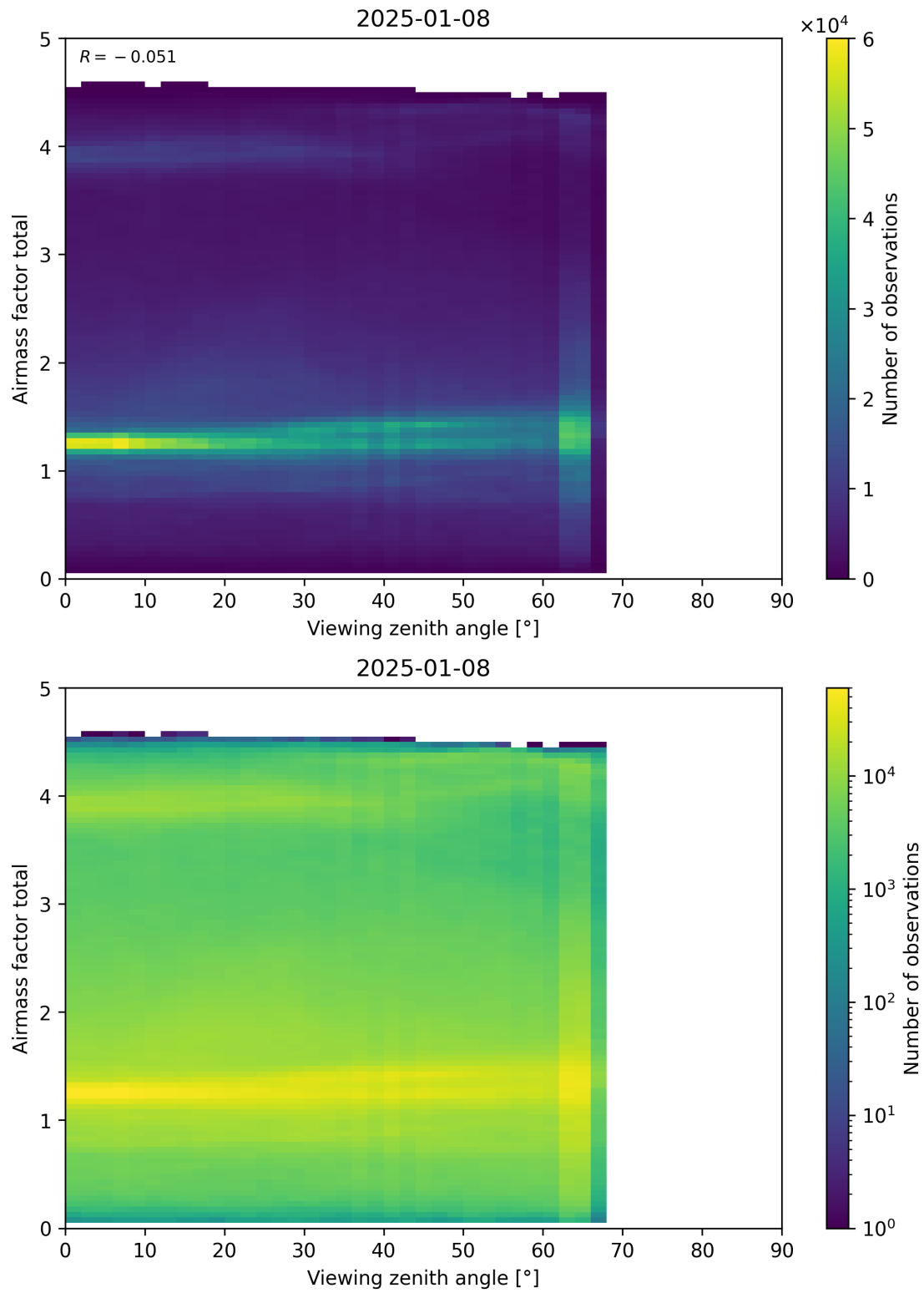
Figure 190: Scatter density plot of “Viewing zenith angle” against “Airmass factor total” for 2025-01-07 to 2025-01-09.
