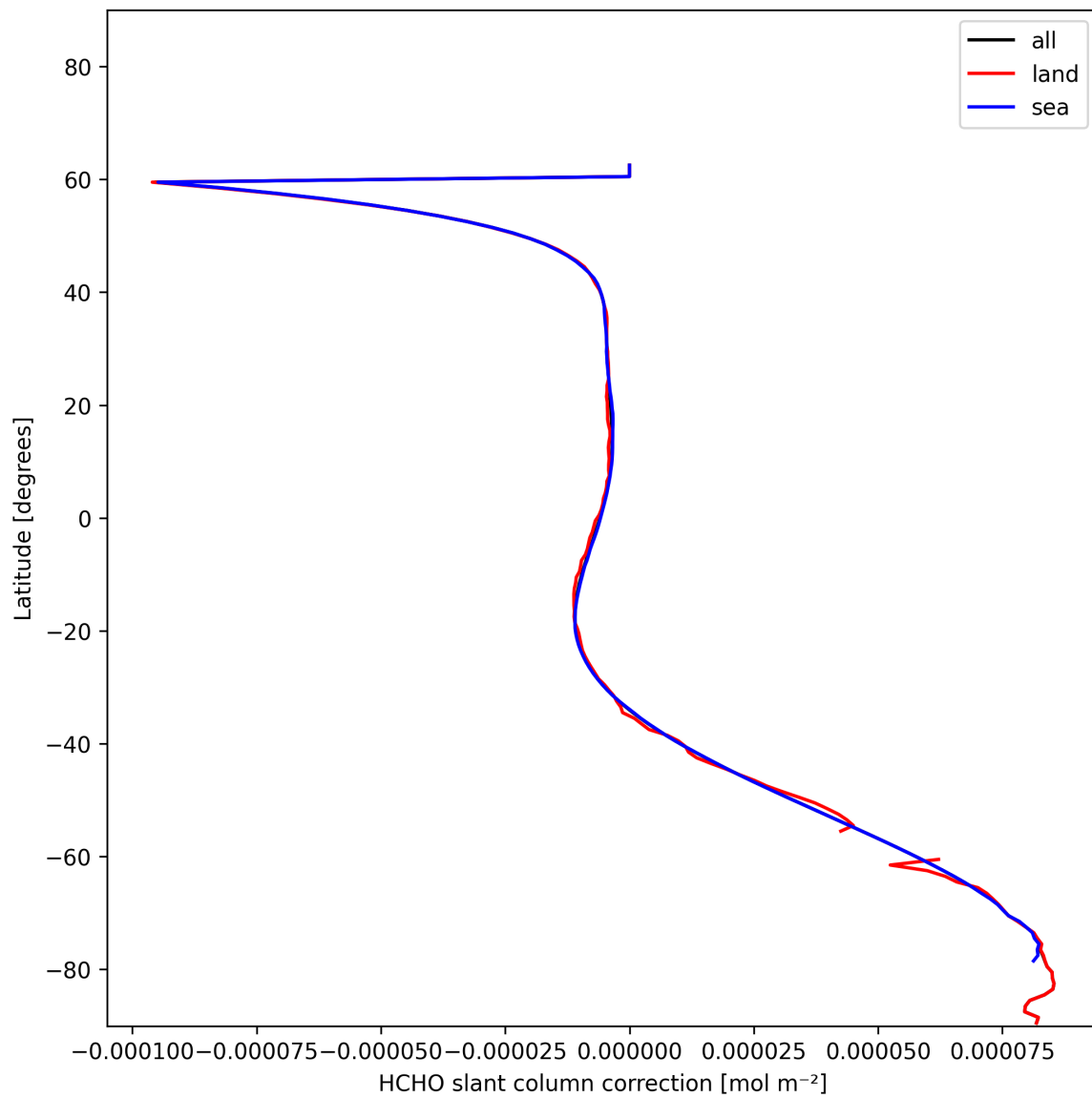
Figure 33: Zonal average of “HCHO slant column correction” for 2025-01-07 to 2025-01-09.
