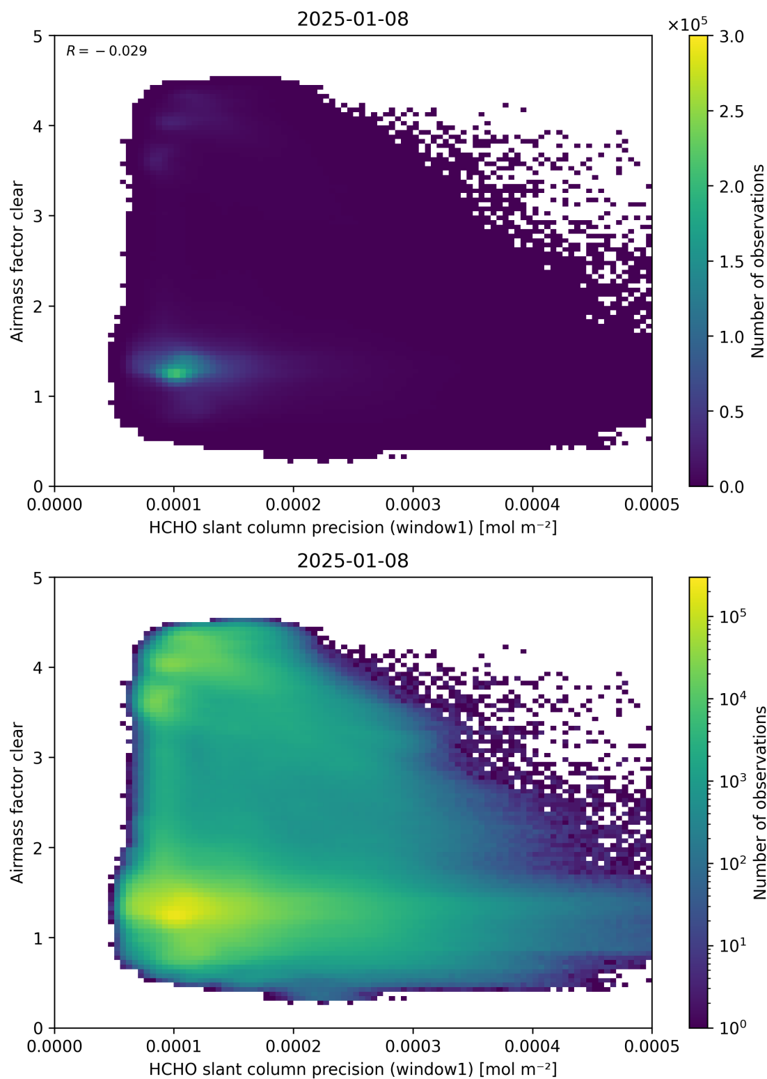
Figure 91: Scatter density plot of “HCHO slant column precision (window1)” against “Airmass factor clear” for 2025-01-07 to 2025-01-09.
