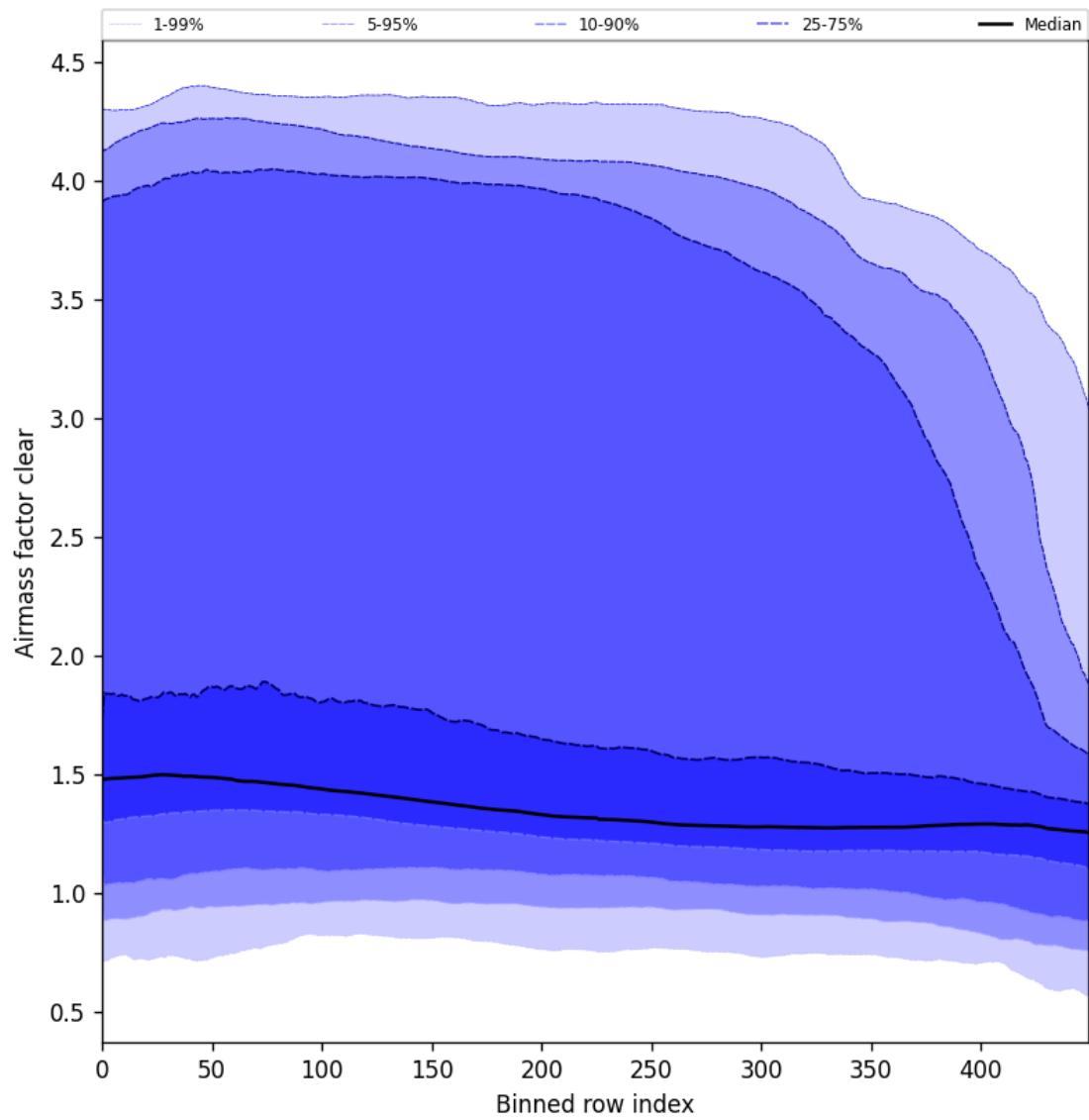
Figure 56: Along track statistics of “Air mass factor clear” for 2025-01-07 to 2025-01-09
