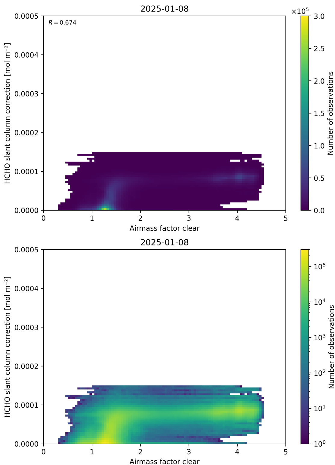
Figure 75: Scatter density plot of “Air mass factor clear” against “HCHO slant column correction” for 2025-01-07 to 2025-01-09.
