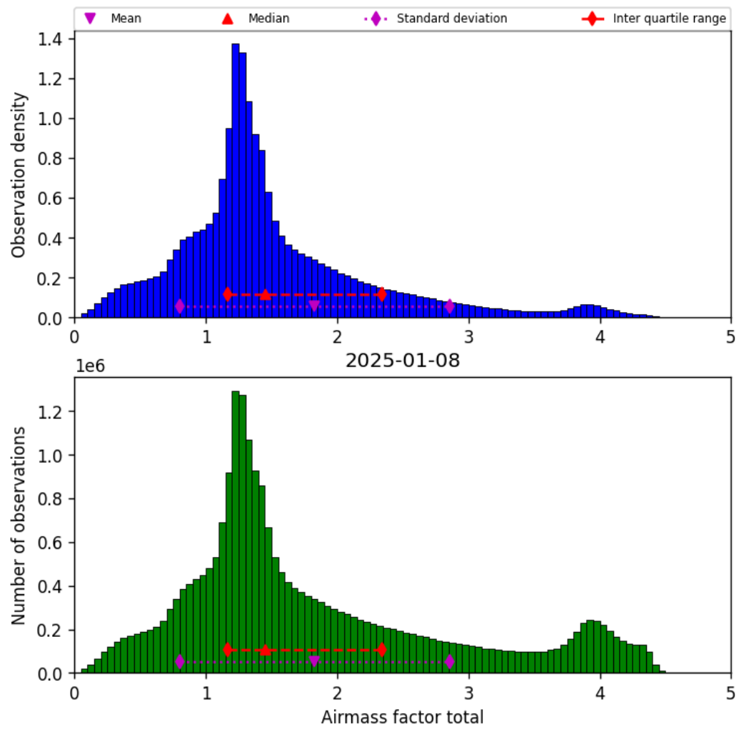
Figure 40: Histogram of “Airmass factor total” for 2025-01-07 to 2025-01-09
