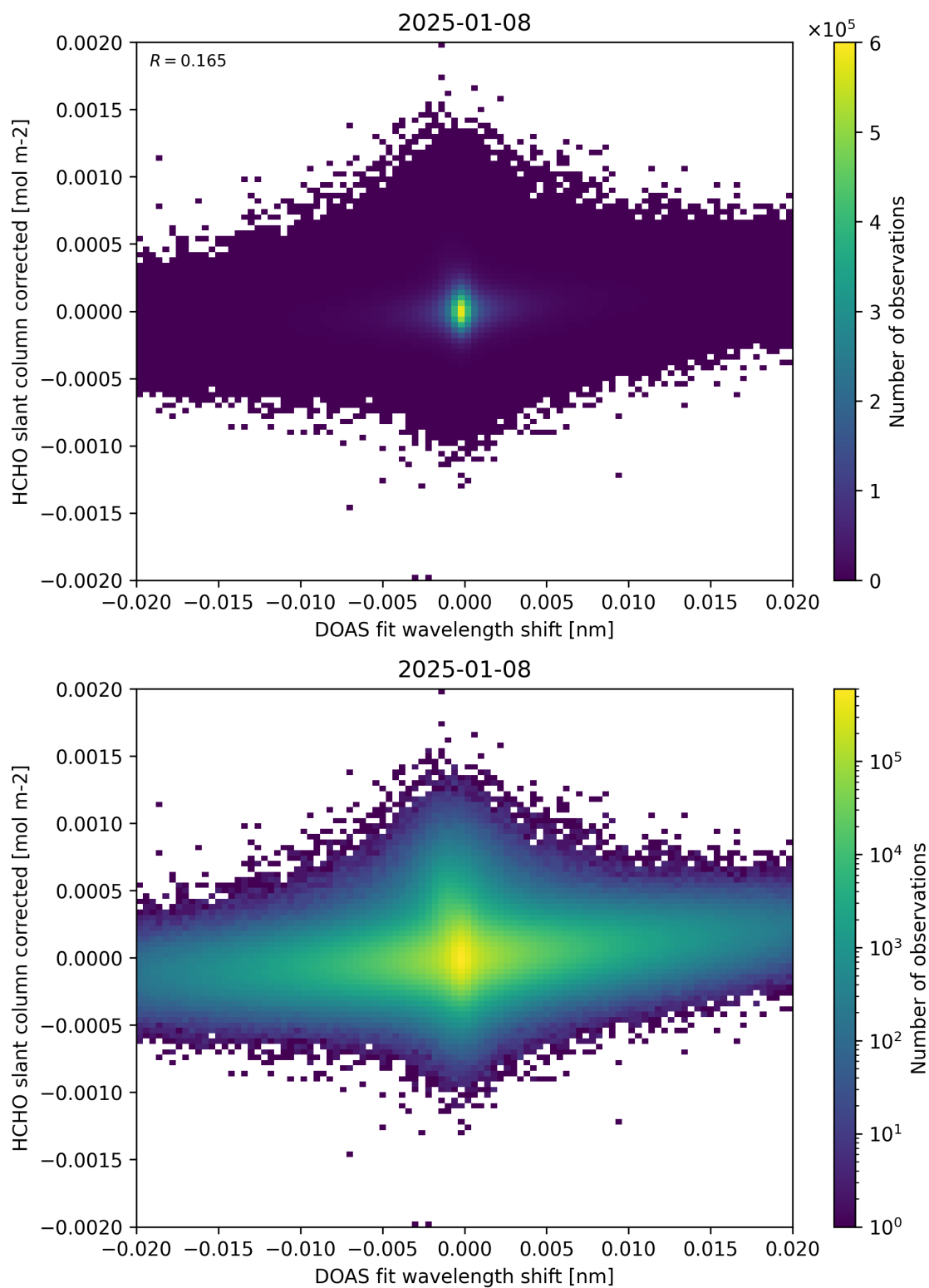
Figure 66: Scatter density plot of “DOAS fit wavelength shift” against “HCHO slant column corrected” for 2025-01-07 to 2025-01-09.
