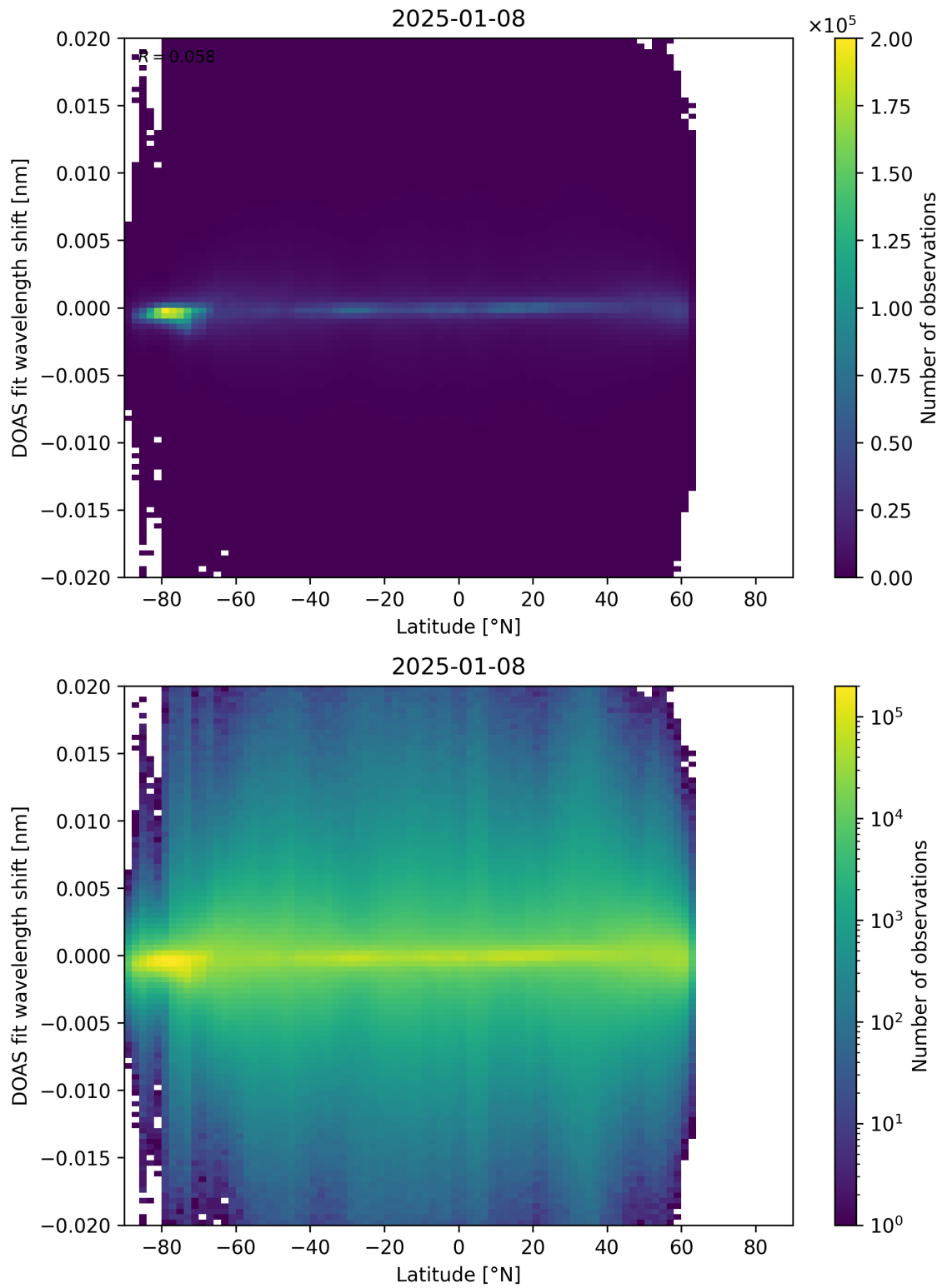
Figure 154: Scatter density plot of “Latitude” against “DOAS fit wavelength shift” for 2025-01-07 to 2025-01-09.
