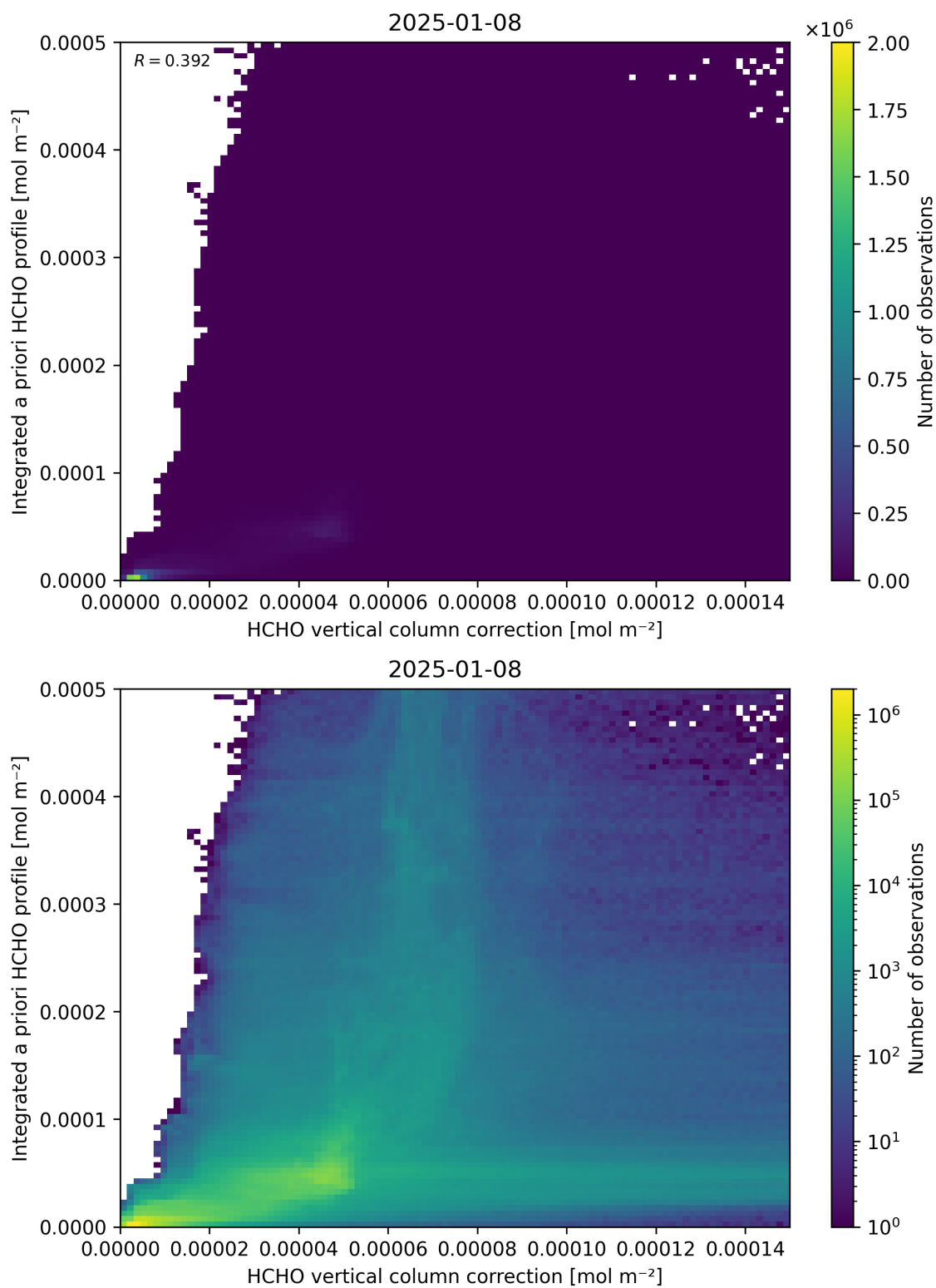
Figure 122: Scatter density plot of “HCHO vertical column correction” against “Integrated a priori HCHO profile” for 2025-01-07 to 2025-01-09.
