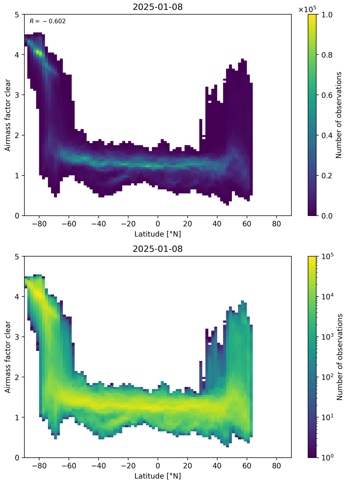
Figure 156: Scatter density plot of “Latitude” against “Airmass factor clear” for 2025-01-07 to 2025-01-09.
