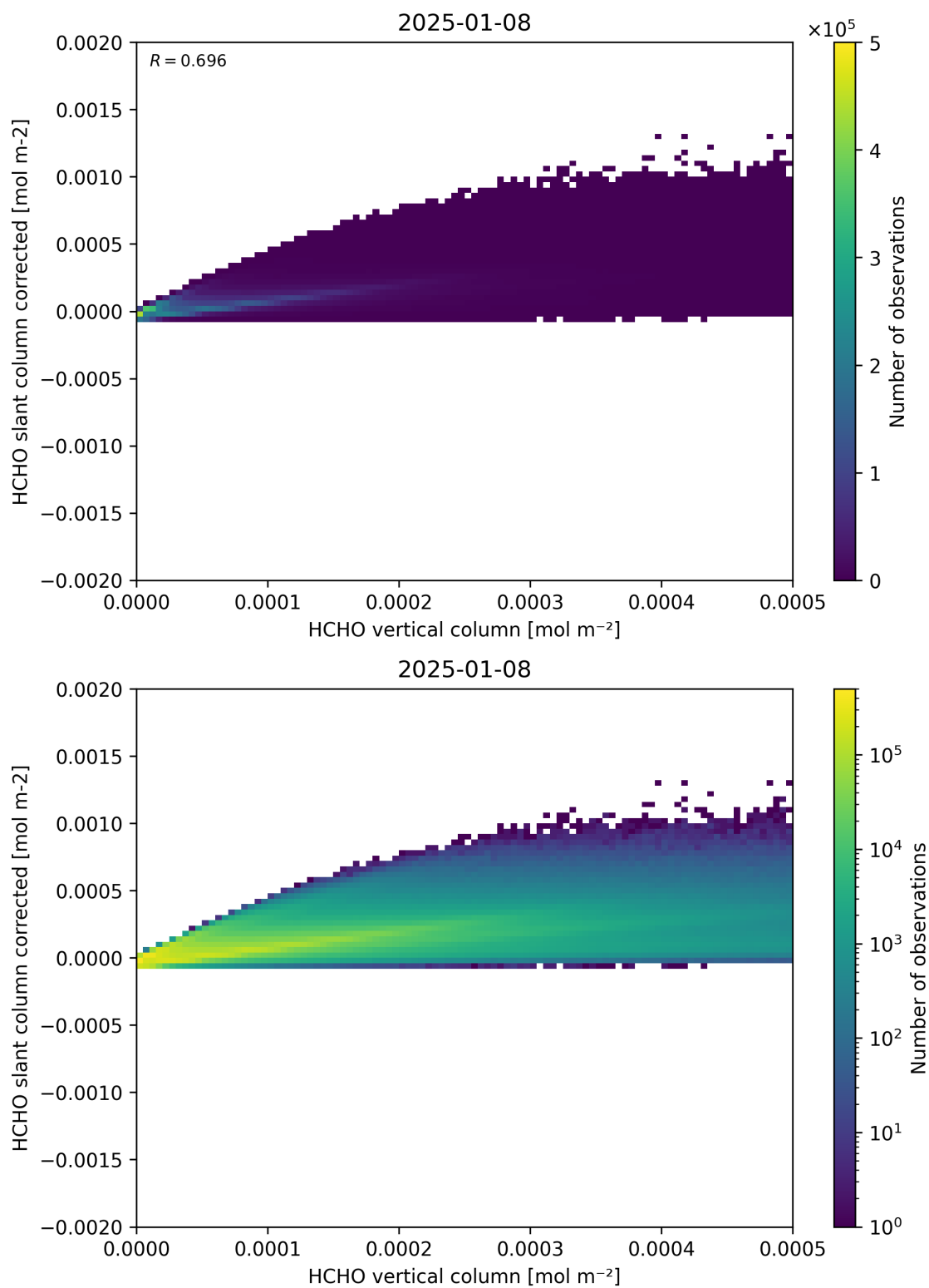
Figure 127: Scatter density plot of “HCHO vertical column” against “HCHO slant column corrected” for 2025-01-07 to 2025-01-09.
