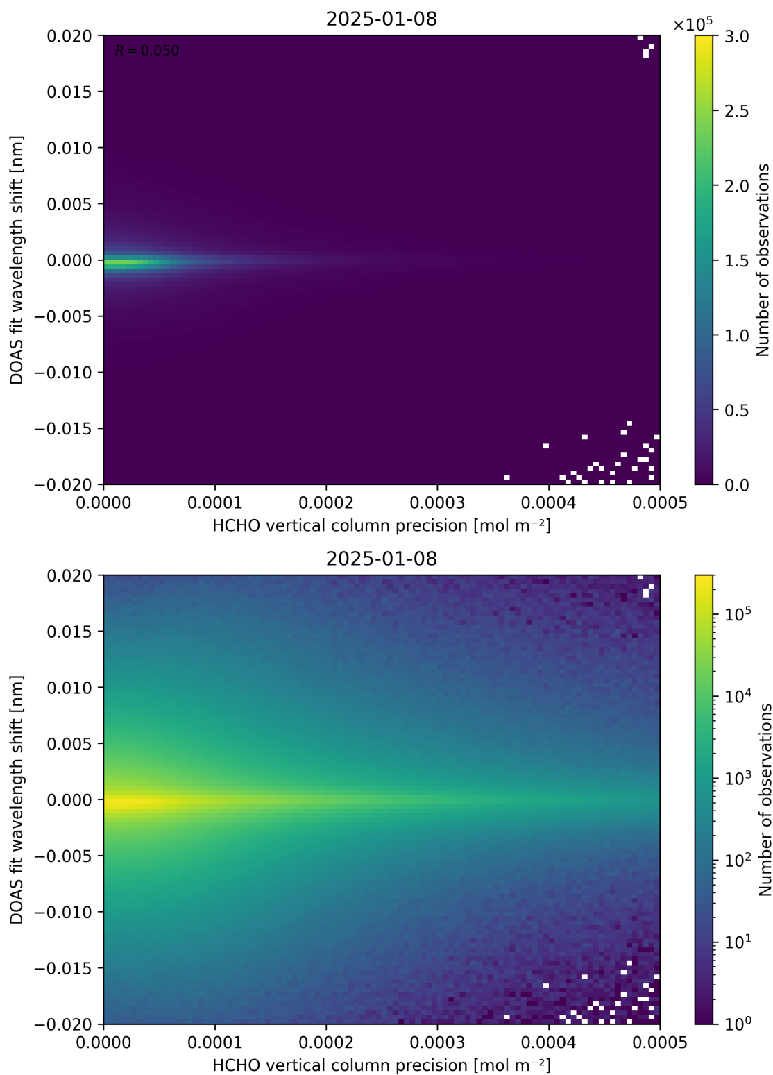
Figure 137: Scatter density plot of “HCHO vertical column precision” against “DOAS fit wavelength shift” for 2025-01-07 to 2025-01-09.
