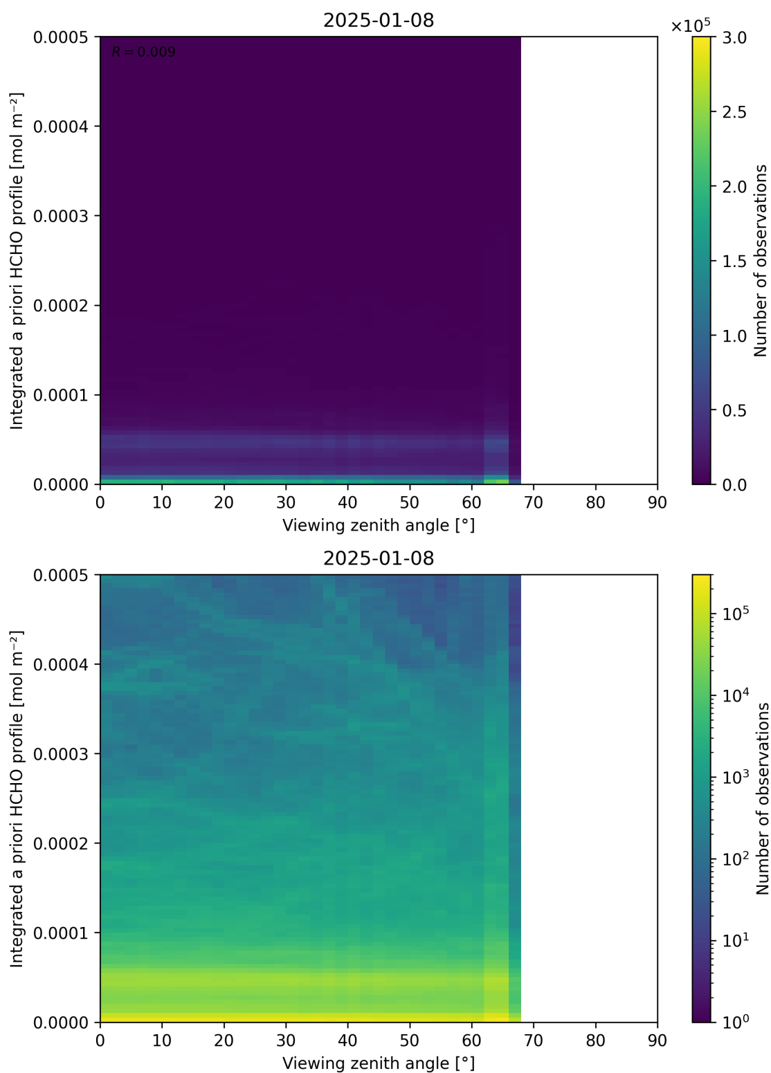
Figure 195: Scatter density plot of “Viewing zenith angle” against “Integrated a priori HCHO profile” for 2025-01-07 to 2025-01-09.
