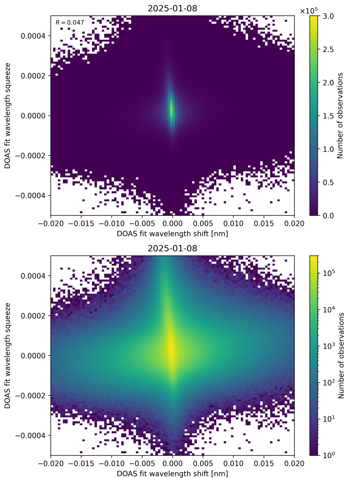
Figure 65: Scatter density plot of “DOAS fit wavelength shift” against “DOAS fit wavelength squeeze” for 2025-01-07 to 2025-01-09.
