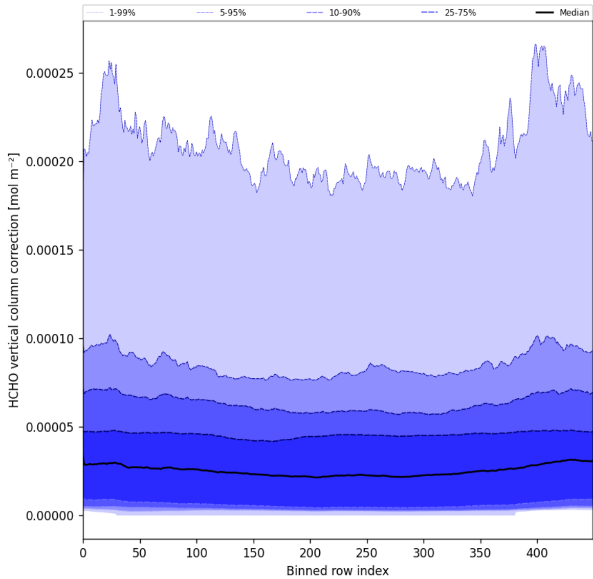
Figure 51: Along track statistics of “HCHO vertical column correction” for 2025-01-07 to 2025-01-09
