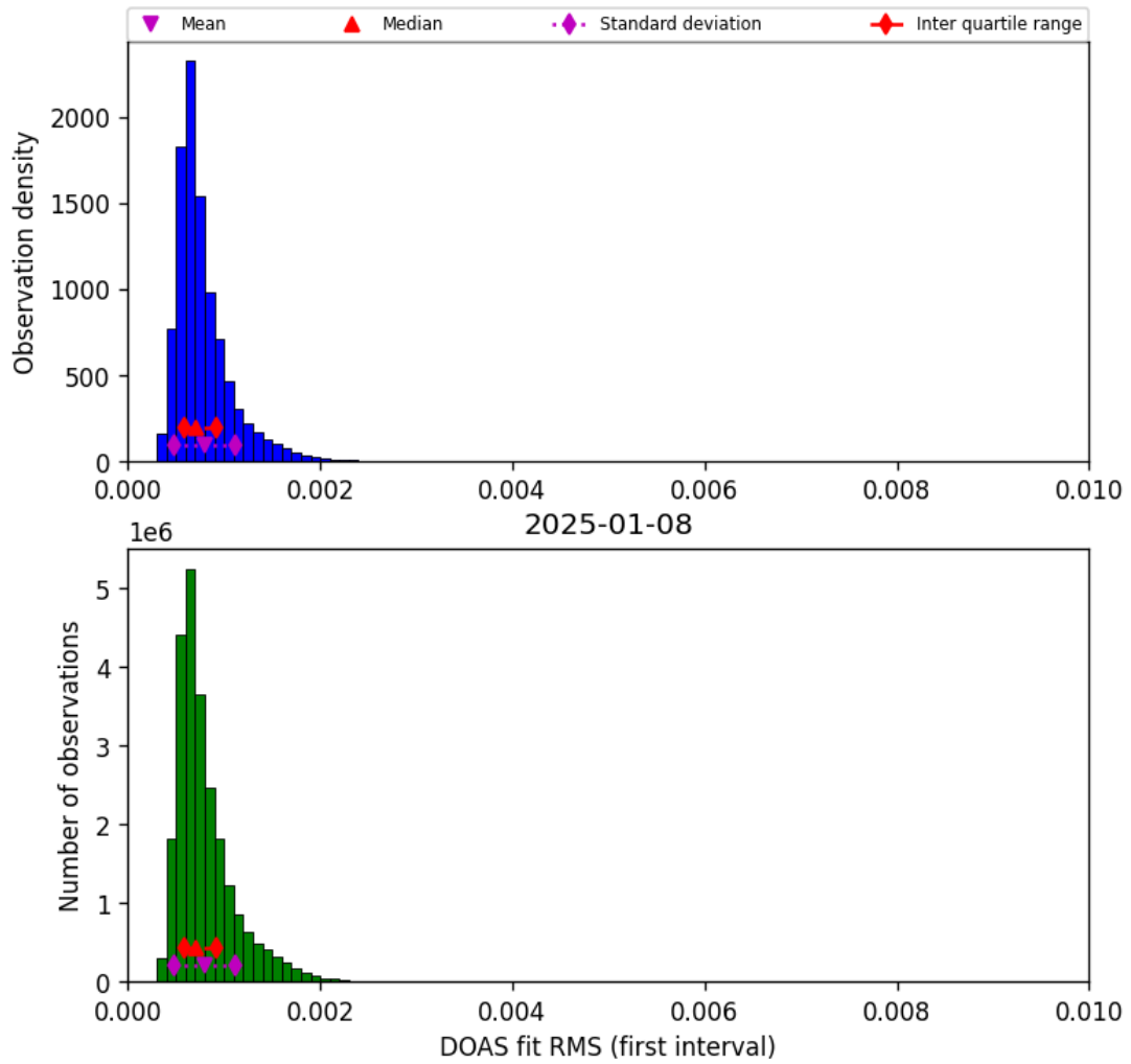
Figure 46: Histogram of “DOAS fit RMS (first interval)” for 2025-01-07 to 2025-01-09
