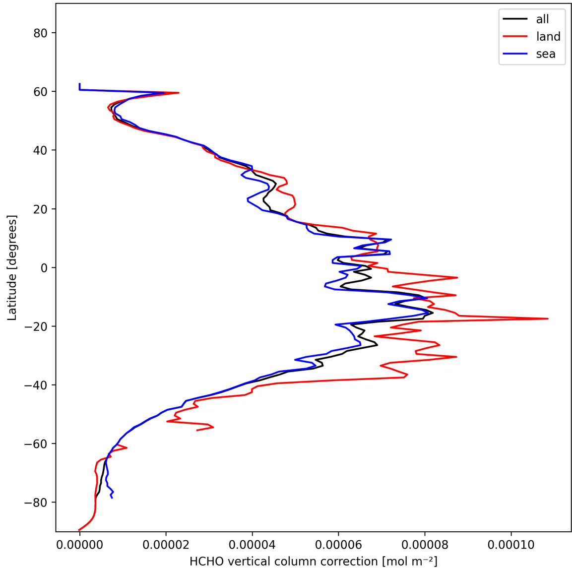
Figure 23: Zonal average of “HCHO vertical column correction” for 2025-01-07 to 2025-01-09.
