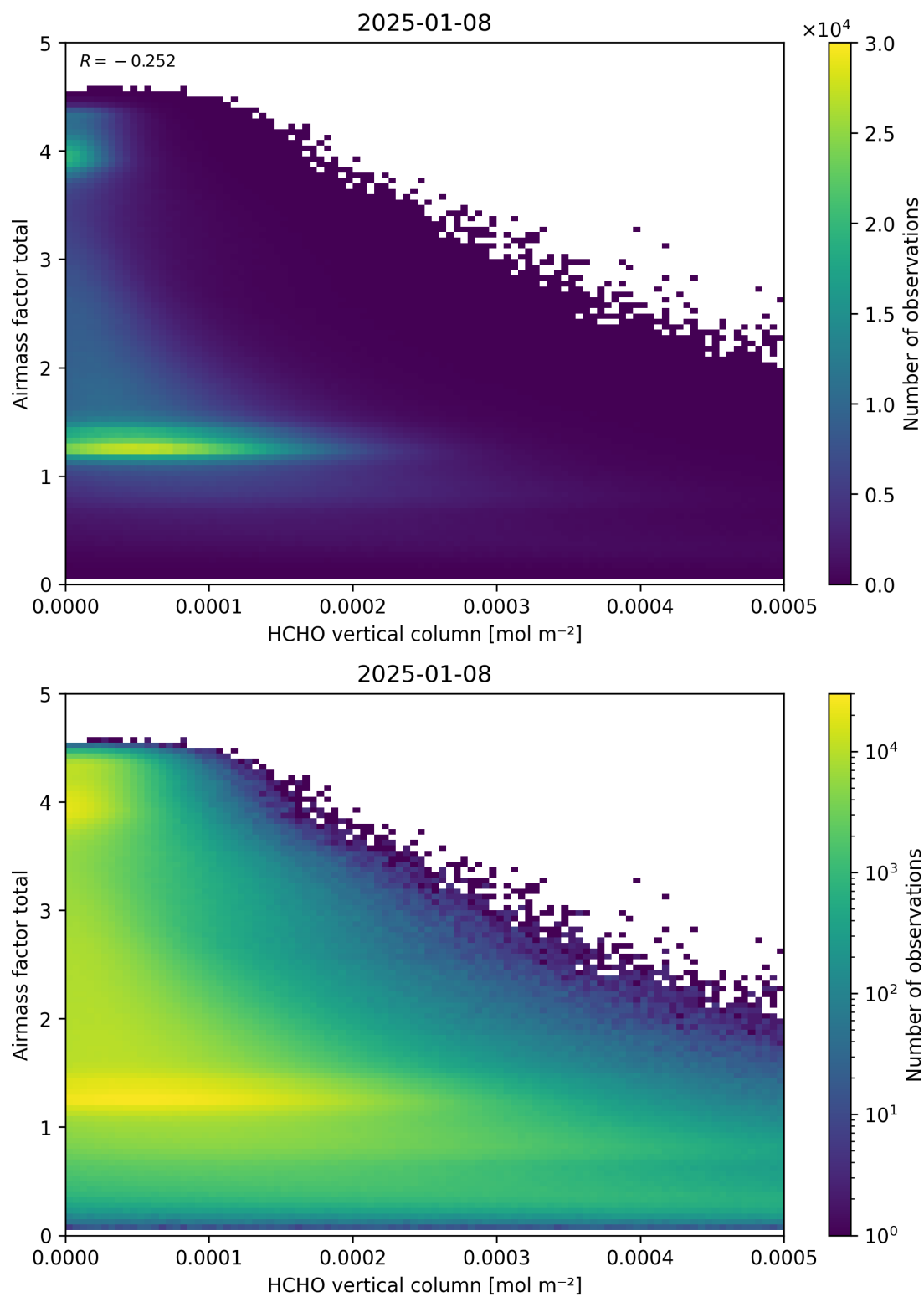
Figure 131: Scatter density plot of “HCHO vertical column” against “Airmass factor total” for 2025-01-07 to 2025-01-09.
