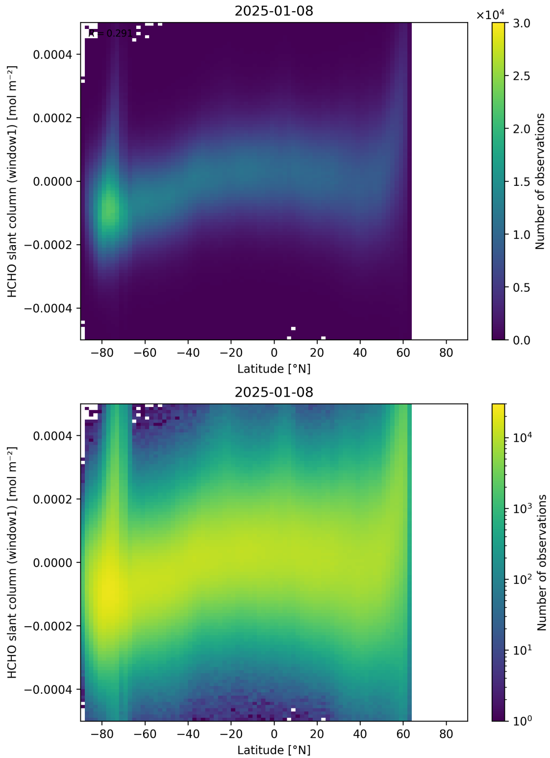
Figure 159: Scatter density plot of “Latitude” against “HCHO slant column (window1)” for 2025-01-07 to 2025-01-09.
