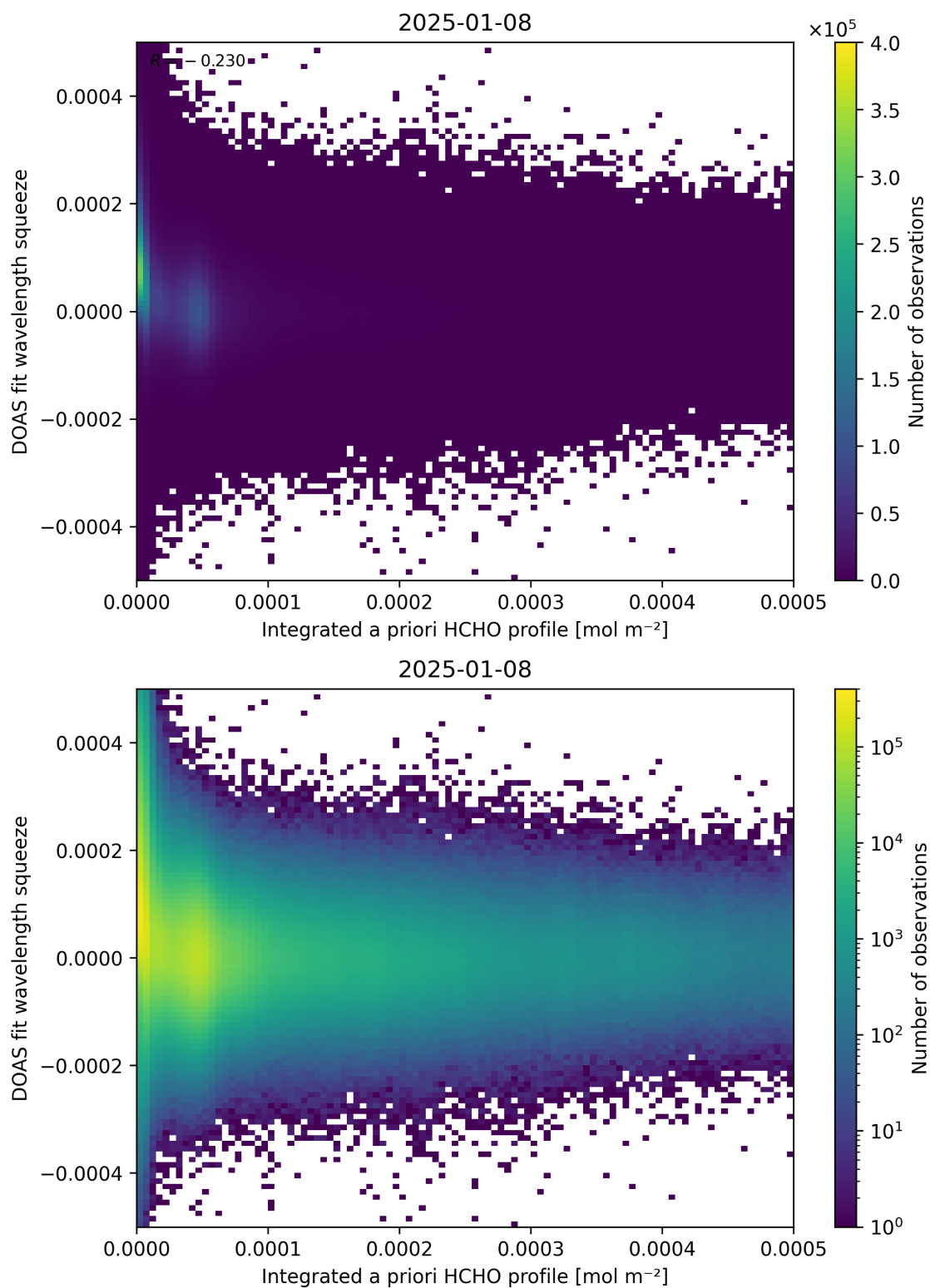
Figure 150: Scatter density plot of “Integrated a priori HCHO profile” against “DOAS fit wavelength squeeze” for 2025-01-07 to 2025-01-09.
