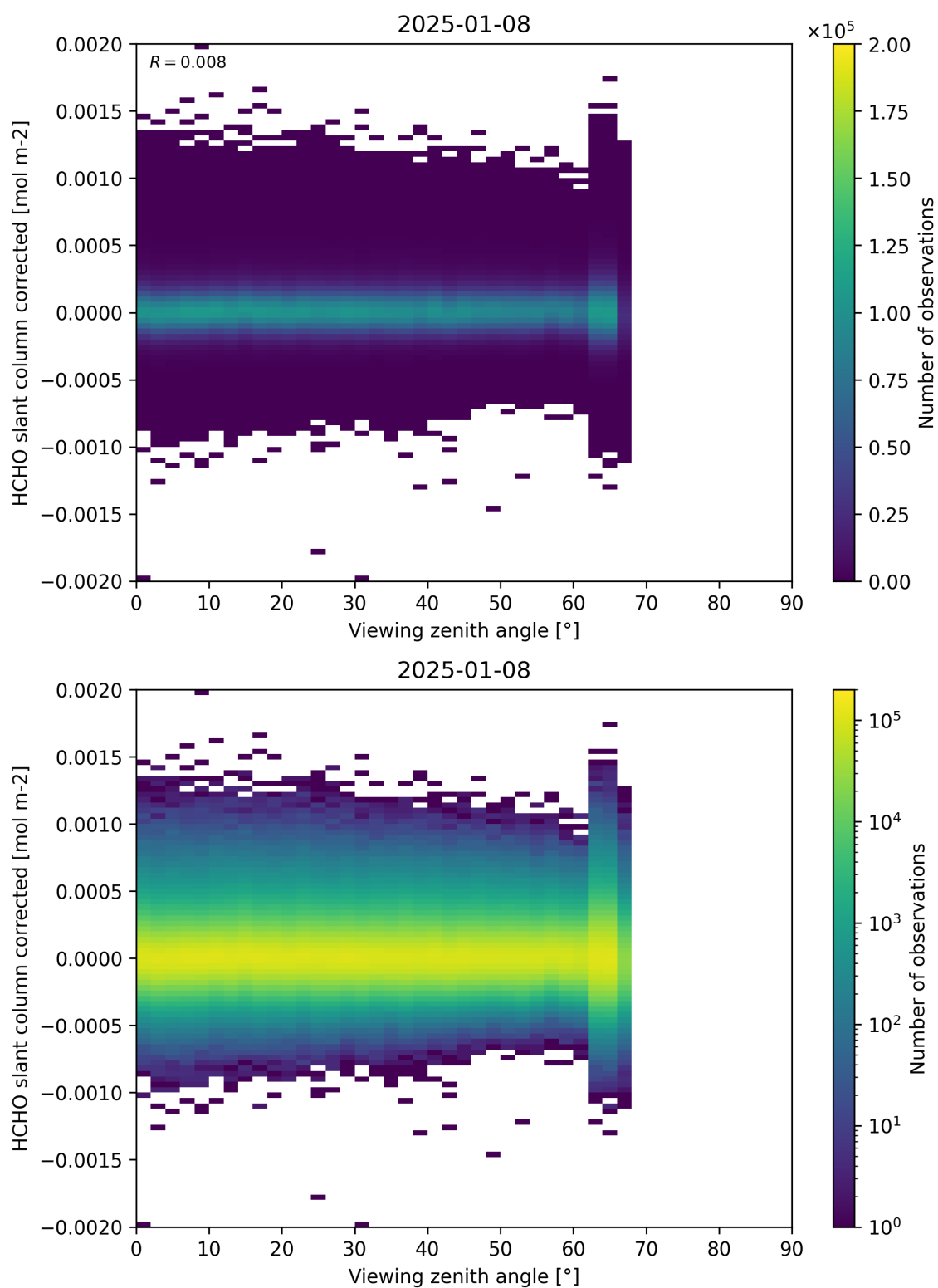
Figure 186: Scatter density plot of “Viewing zenith angle” against “HCHO slant column corrected” for 2025-01-07 to 2025-01-09.
