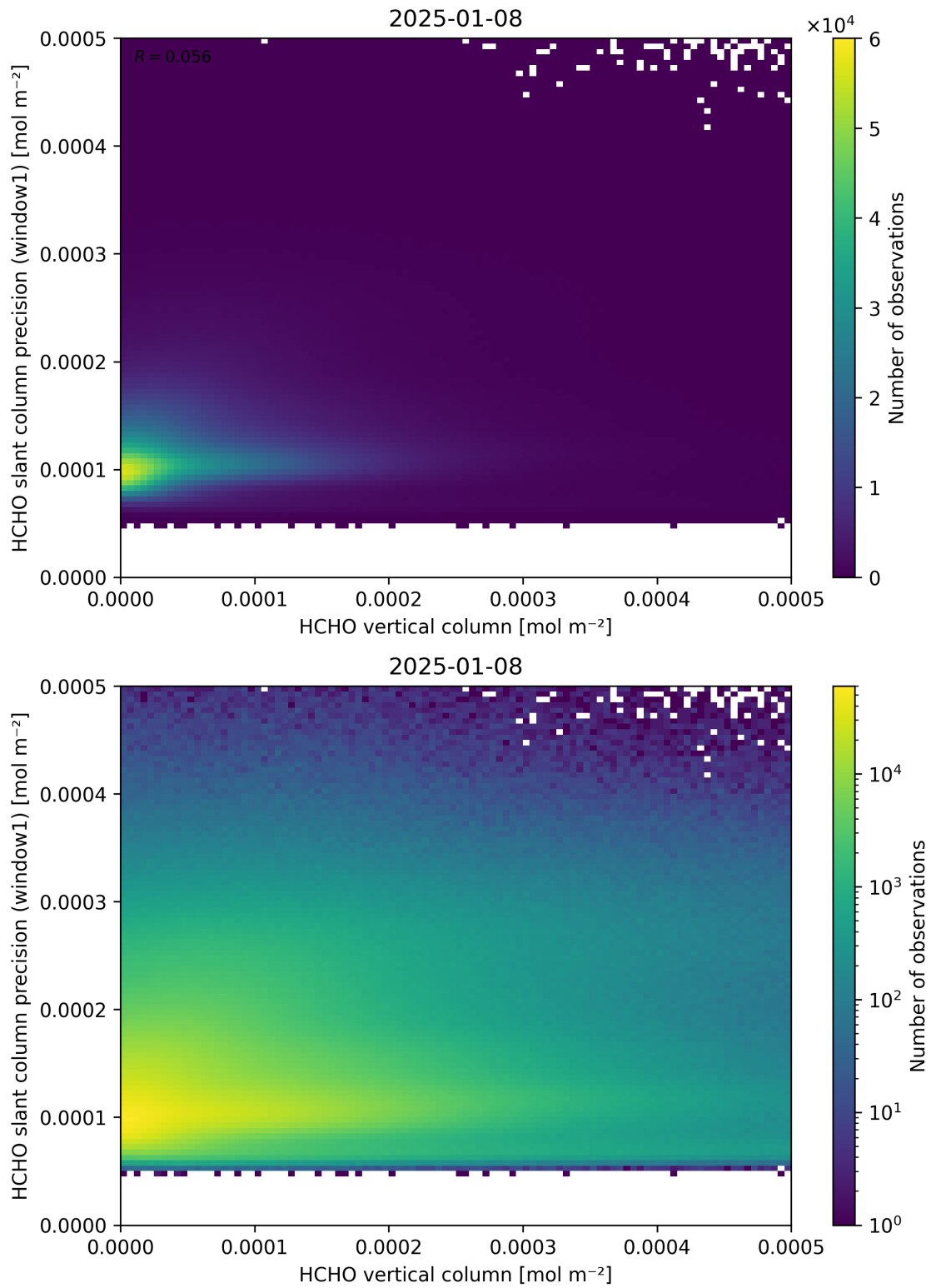
Figure 130: Scatter density plot of “HCHO vertical column” against “HCHO slant column precision (window1)” for 2025-01-07 to 2025-01-09.
