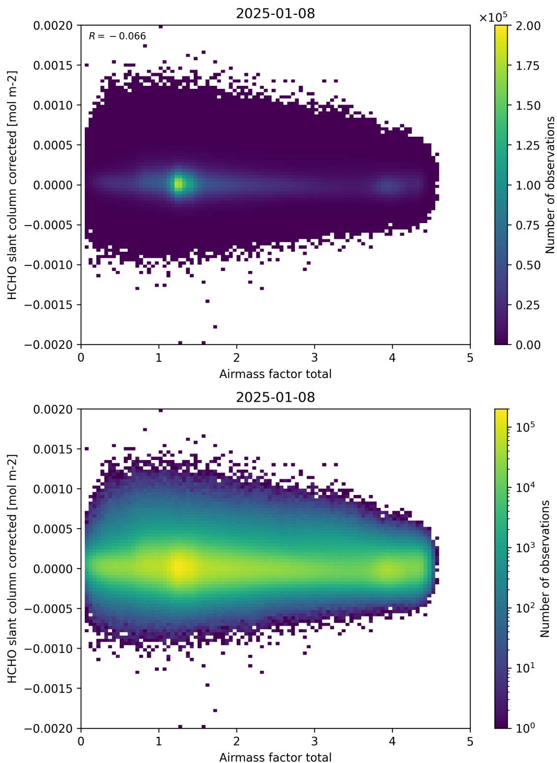
Figure 101: Scatter density plot of “Airmass factor total” against “HCHO slant column corrected” for 2025-01-07 to 2025-01-09.
