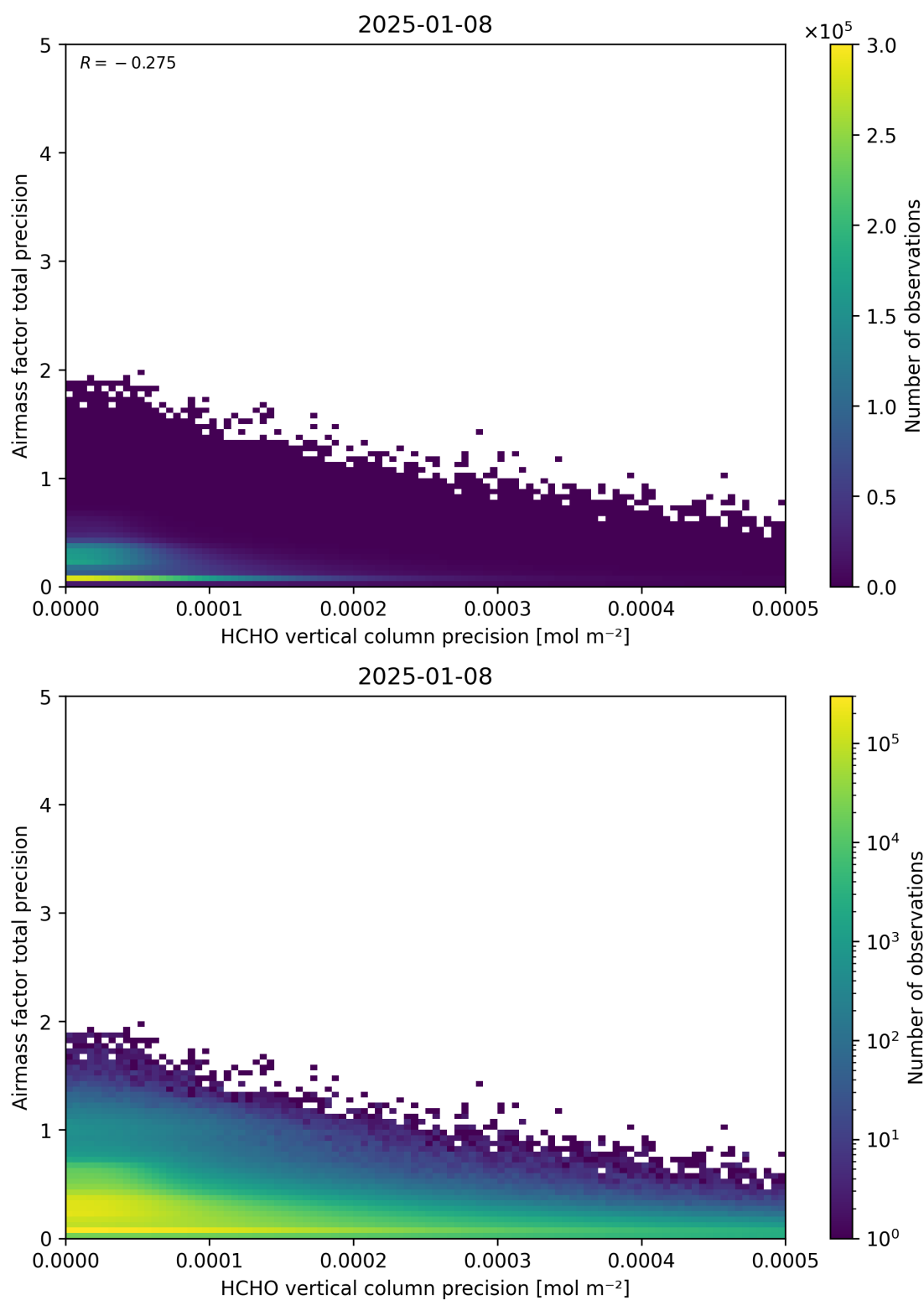
Figure 145: Scatter density plot of “HCHO vertical column precision” against “Airmass factor total precision” for 2025-01-07 to 2025-01-09.
