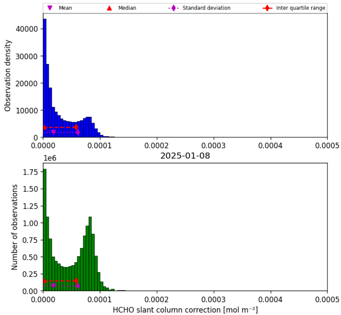
Figure 47: Histogram of “HCHO slant column correction” for 2025-01-07 to 2025-01-09
