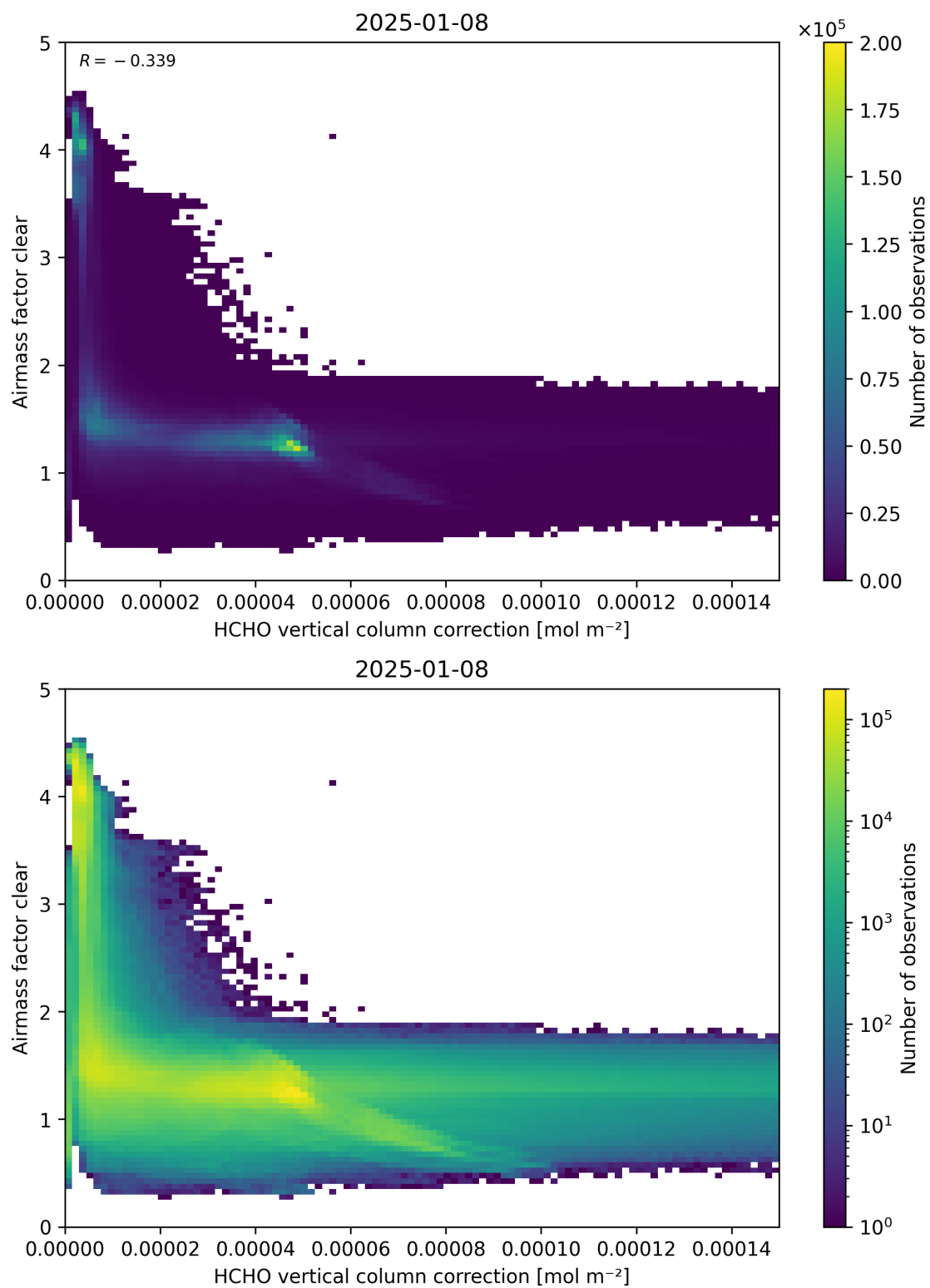
Figure 115: Scatter density plot of “HCHO vertical column correction” against “Airmass factor clear” for 2025-01-07 to 2025-01-09.
