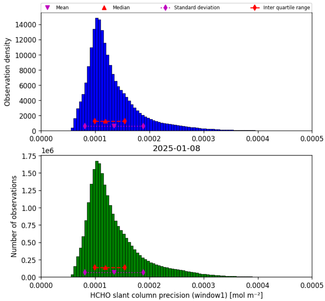
Figure 39: Histogram of “HCHO slant column precision (window1)” for 2025-01-07 to 2025-01-09
