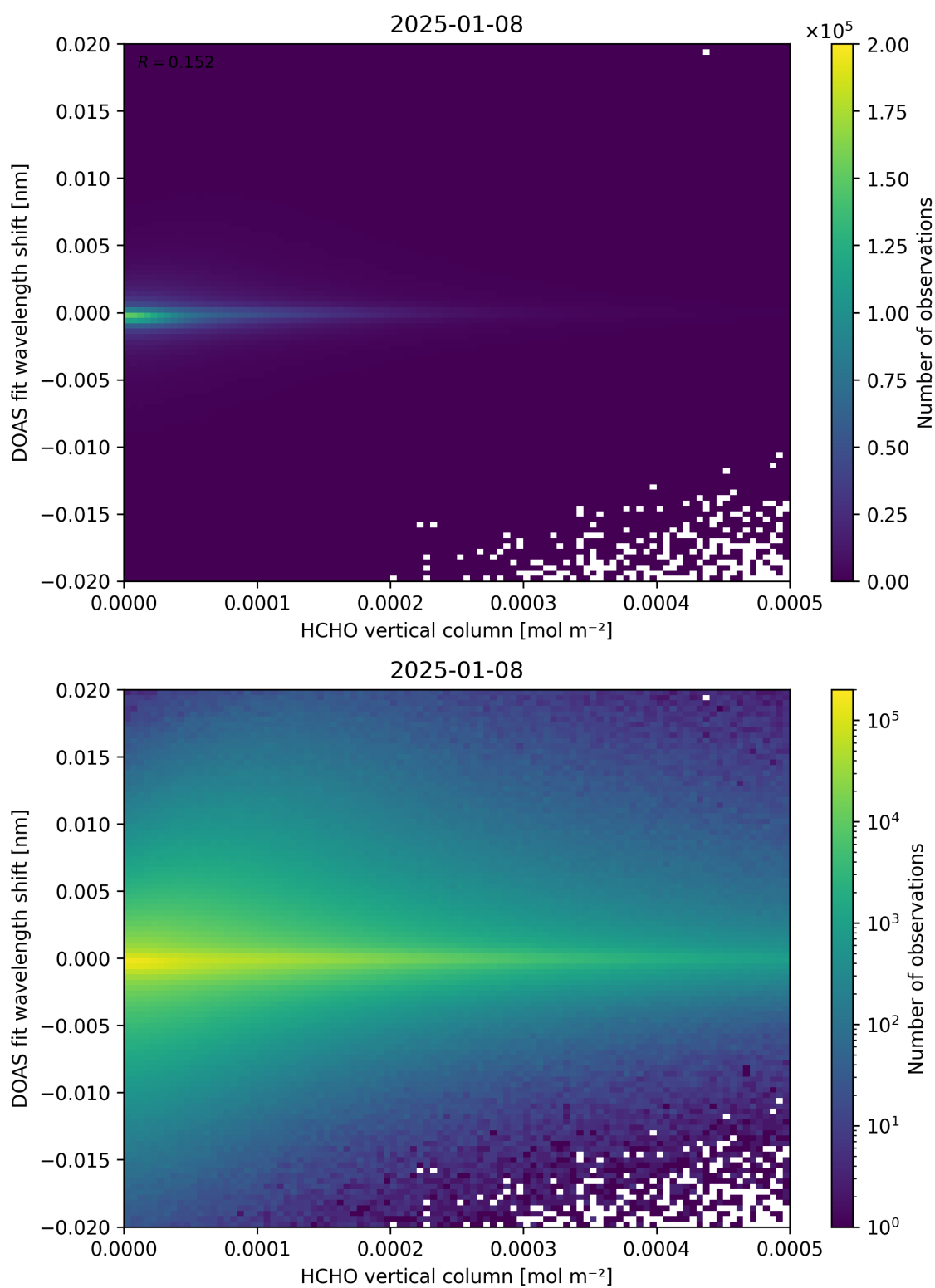
Figure 124: Scatter density plot of “HCHO vertical column” against “DOAS fit wavelength shift” for 2025-01-07 to 2025-01-09.
