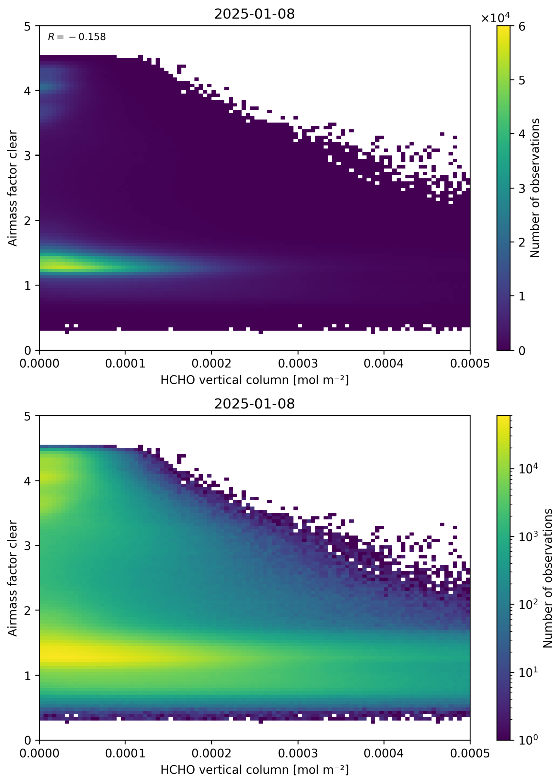
Figure 126: Scatter density plot of “HCHO vertical column” against “Airmass factor clear” for 2025-01-07 to 2025-01-09.
