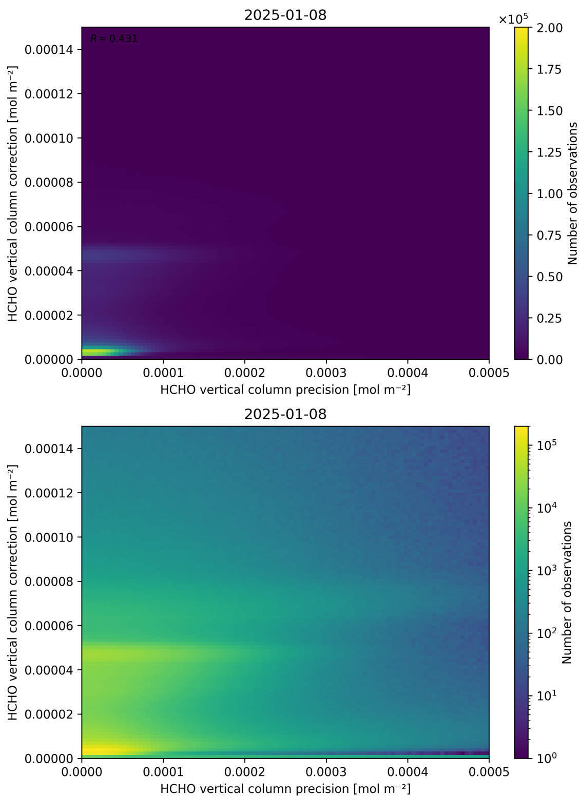
Figure 146: Scatter density plot of “HCHO vertical column precision” against “HCHO vertical column correction” for 2025-01-07 to 2025-01-09.
