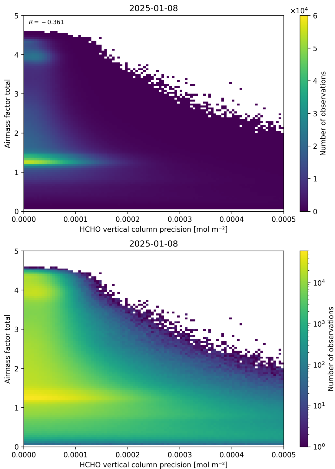
Figure 144: Scatter density plot of “HCHO vertical column precision” against “Airmass factor total” for 2025-01-07 to 2025-01-09.
