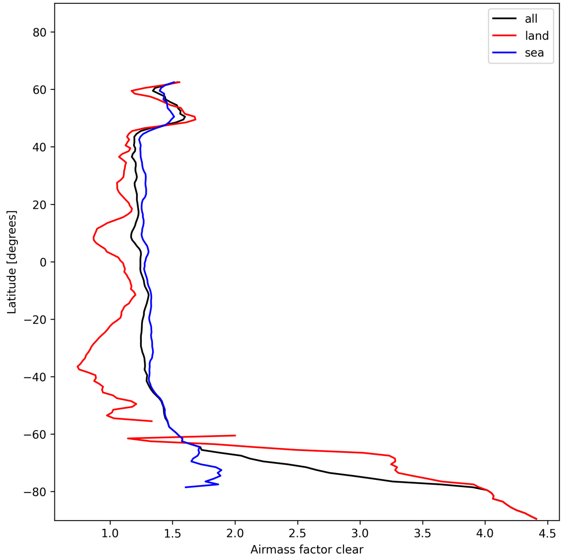
Figure 28: Zonal average of “Airmass factor clear” for 2025-01-07 to 2025-01-09.
