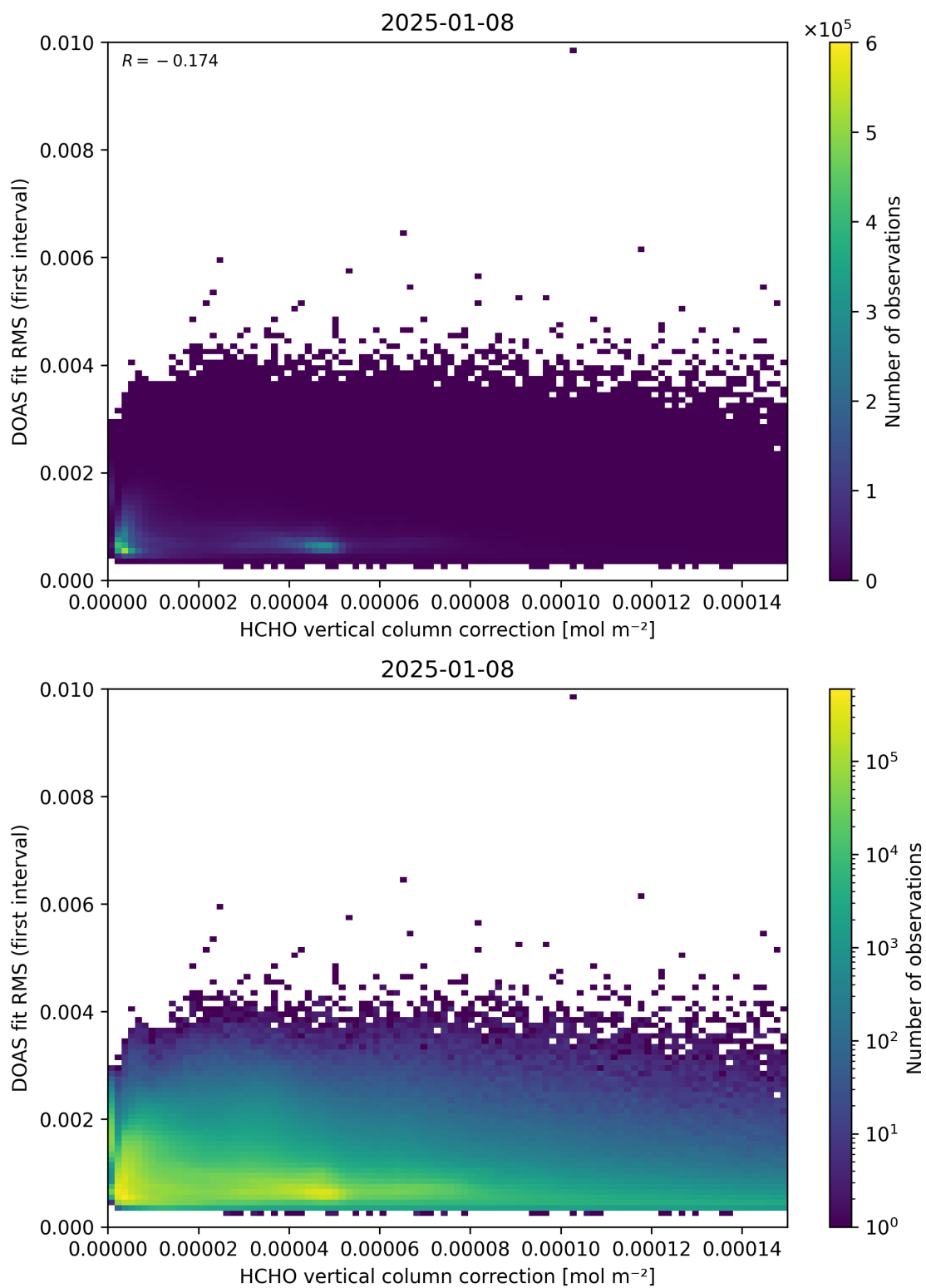
Figure 112: Scatter density plot of “HCHO vertical column correction” against “DOAS fit RMS (first interval)” for 2025-01-07 to 2025-01-09.
