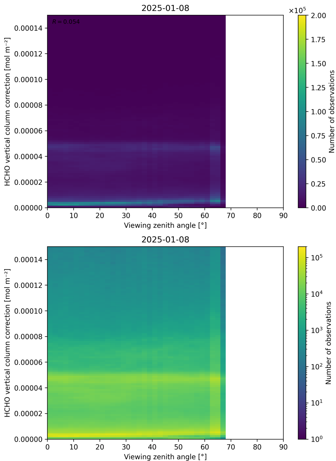
Figure 193: Scatter density plot of “Viewing zenith angle” against “HCHO vertical column correction” for 2025-01-07 to 2025-01-09.
