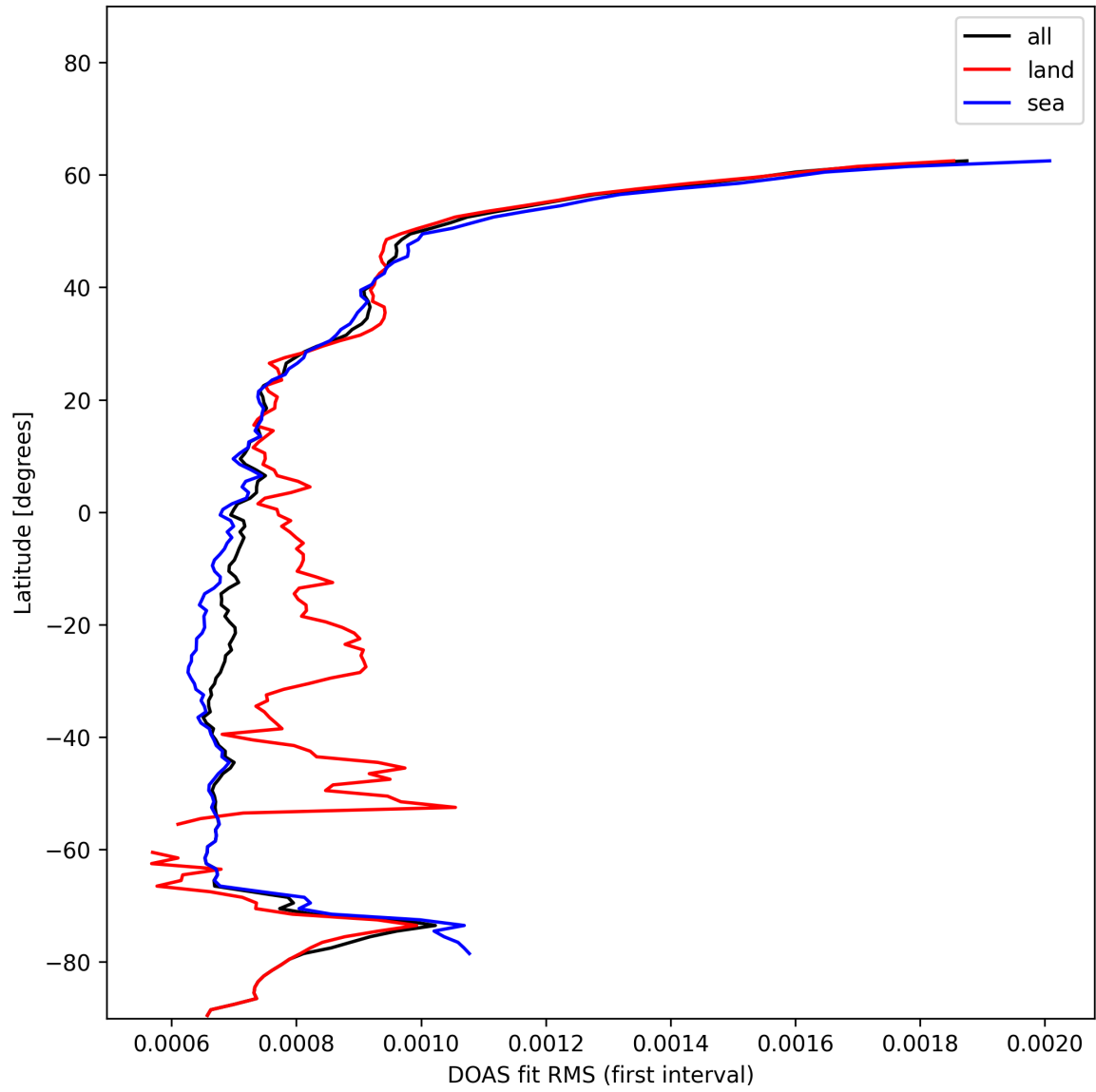
Figure 32: Zonal average of “DOAS fit RMS (first interval)” for 2025-01-07 to 2025-01-09.
