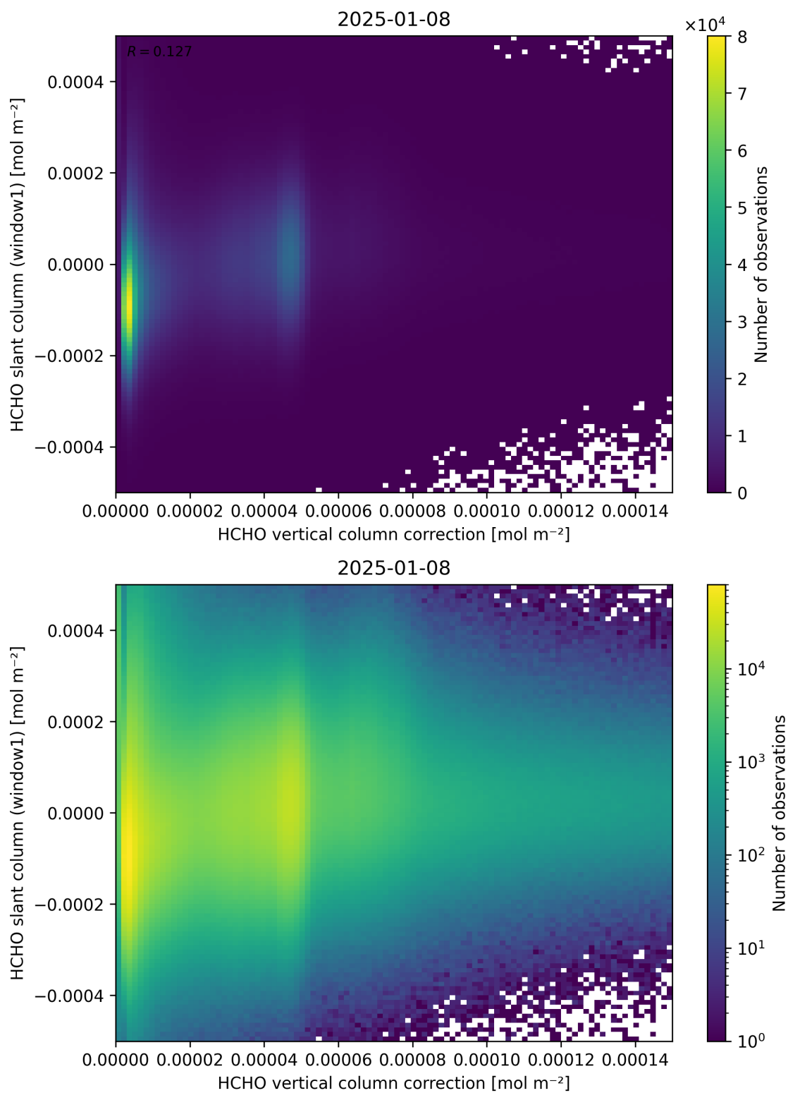
Figure 118: Scatter density plot of “HCHO vertical column correction” against “HCHO slant column (window1)” for 2025-01-07 to 2025-01-09.
