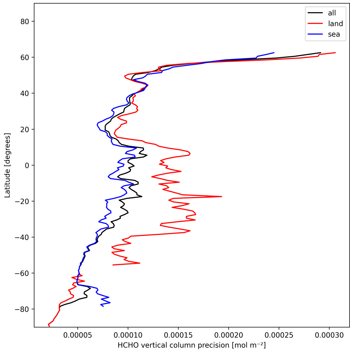
Figure 22: Zonal average of “HCHO vertical column precision” for 2025-01-07 to 2025-01-09.
