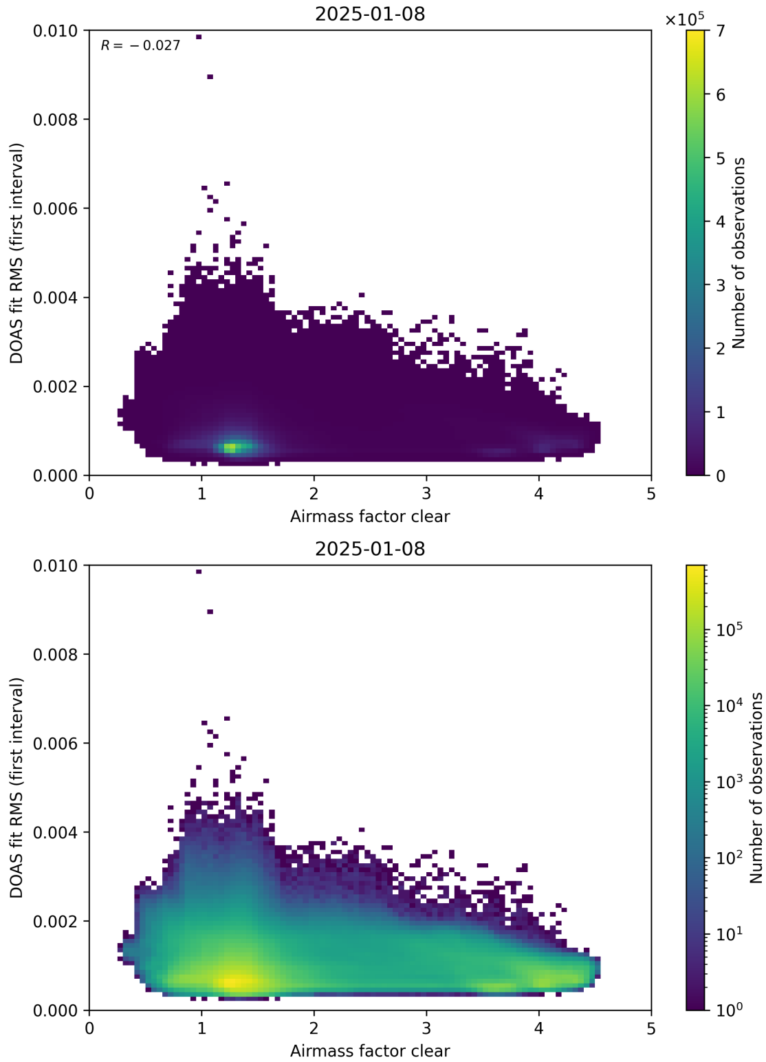
Figure 71: Scatter density plot of “Airmass factor clear” against “DOAS fit RMS (first interval)” for 2025-01-07 to 2025-01-09.
