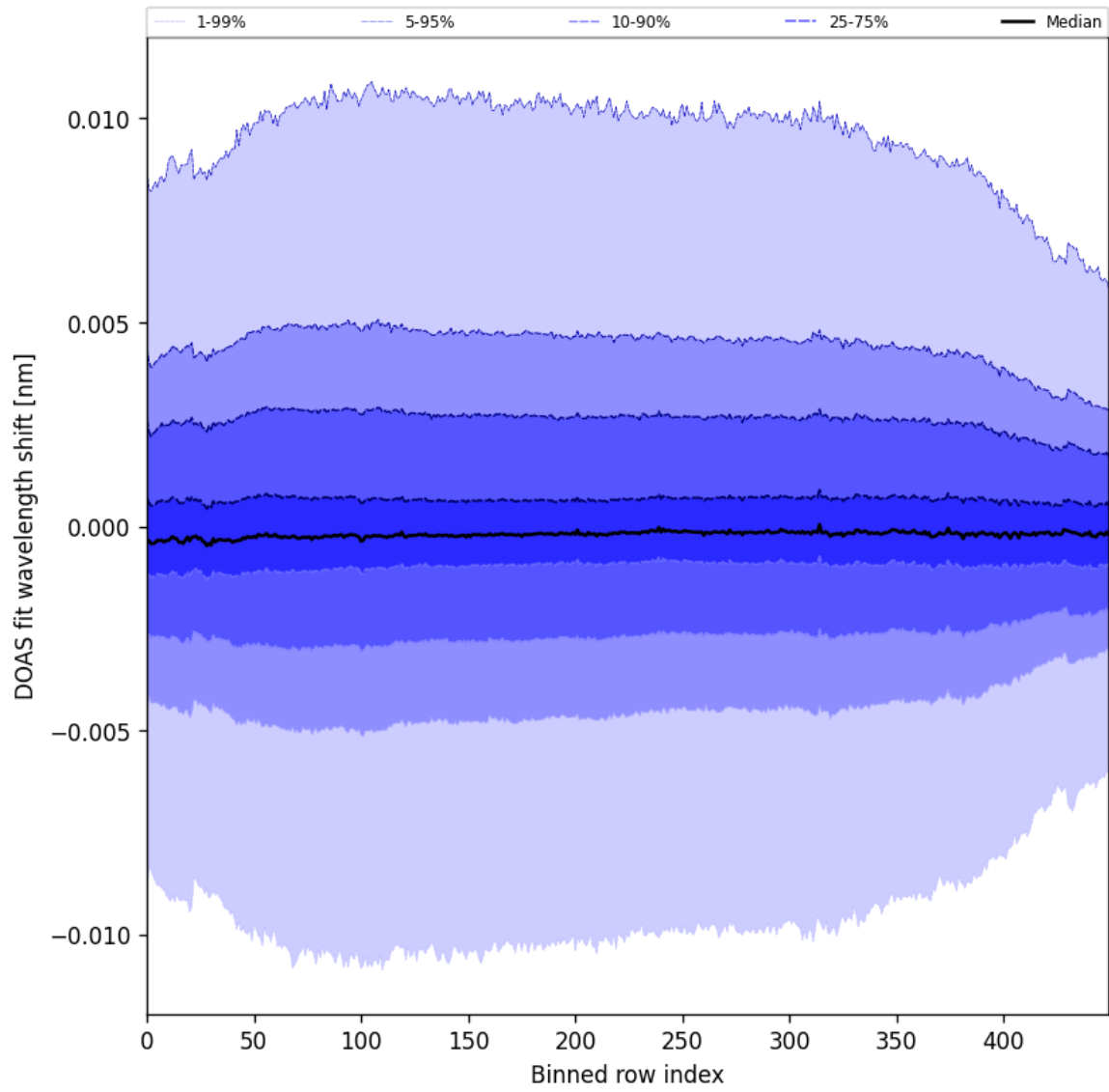
Figure 58: Along track statistics of “DOAS fit wavelength shift” for 2025-01-07 to 2025-01-09
