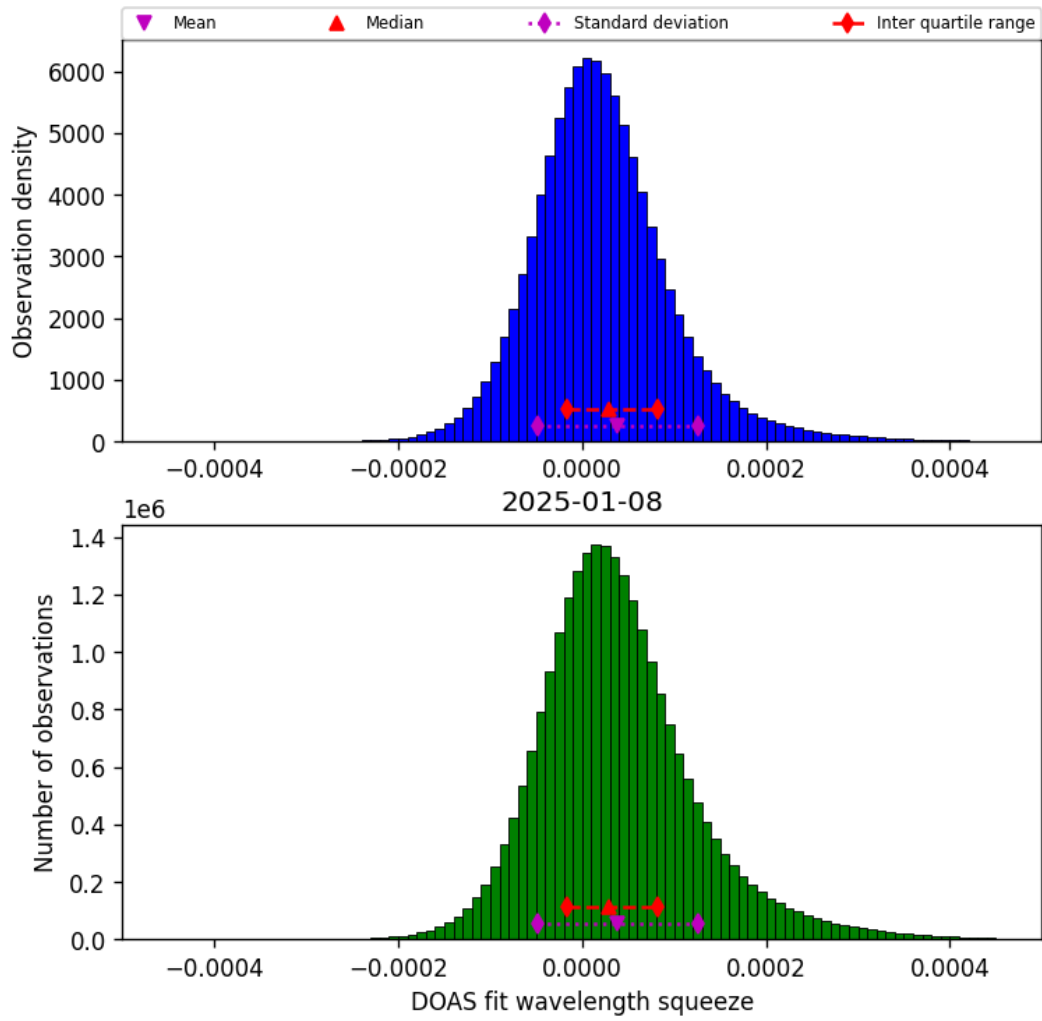
Figure 45: Histogram of “DOAS fit wavelength squeeze” for 2025-01-07 to 2025-01-09
