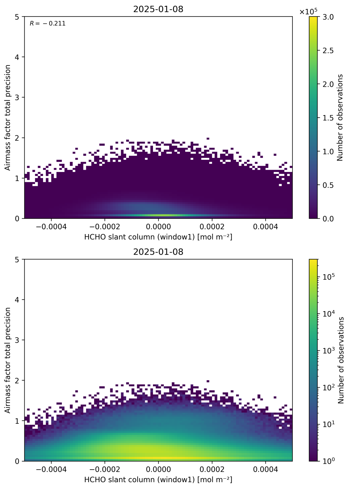
Figure 86: Scatter density plot of “HCHO slant column (window1)” against “Airmass factor total precision” for 2025-01-07 to 2025-01-09.
