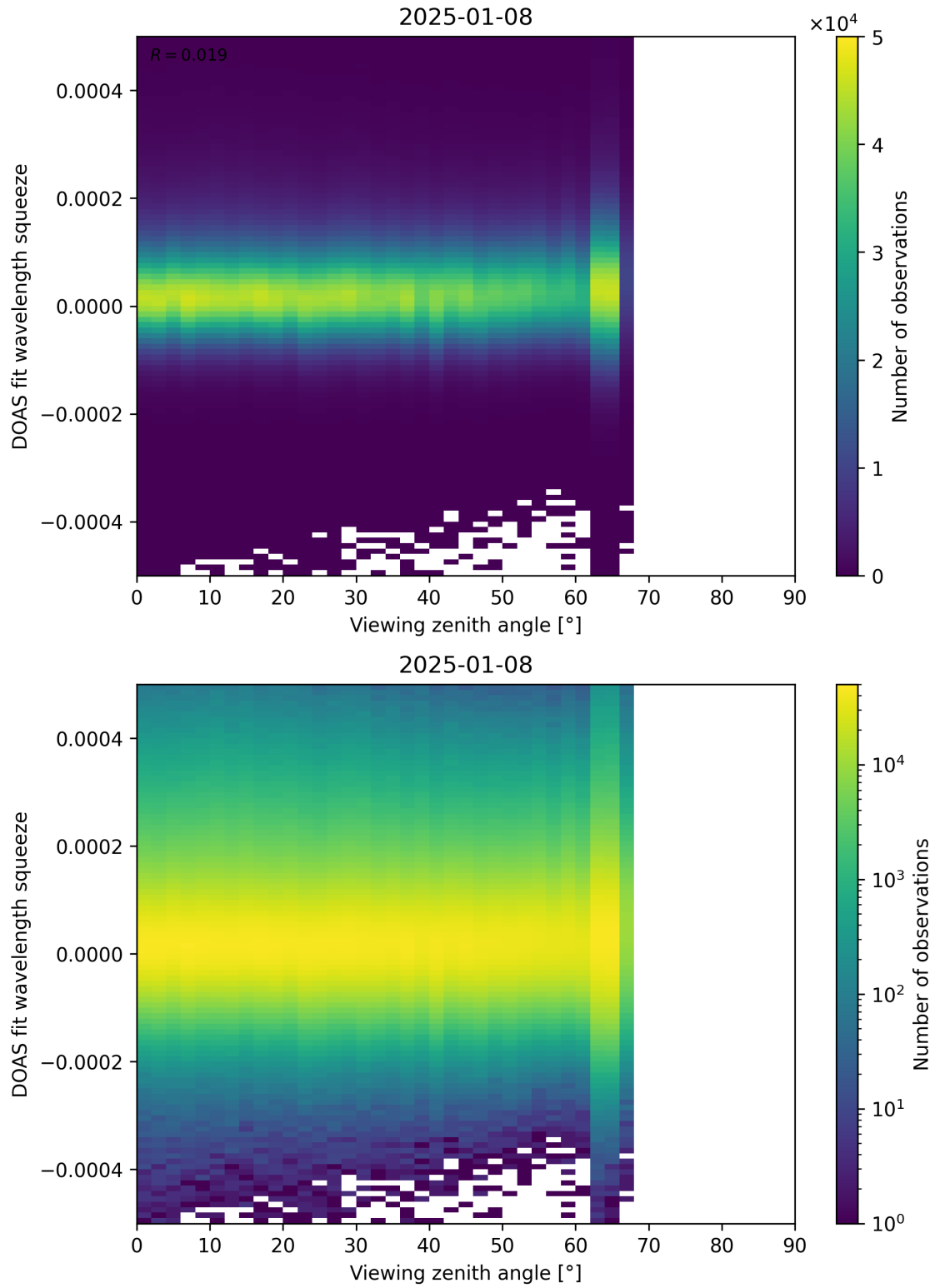
Figure 184: Scatter density plot of “Viewing zenith angle” against “DOAS fit wavelength squeeze” for 2025-01-07 to 2025-01-09.
