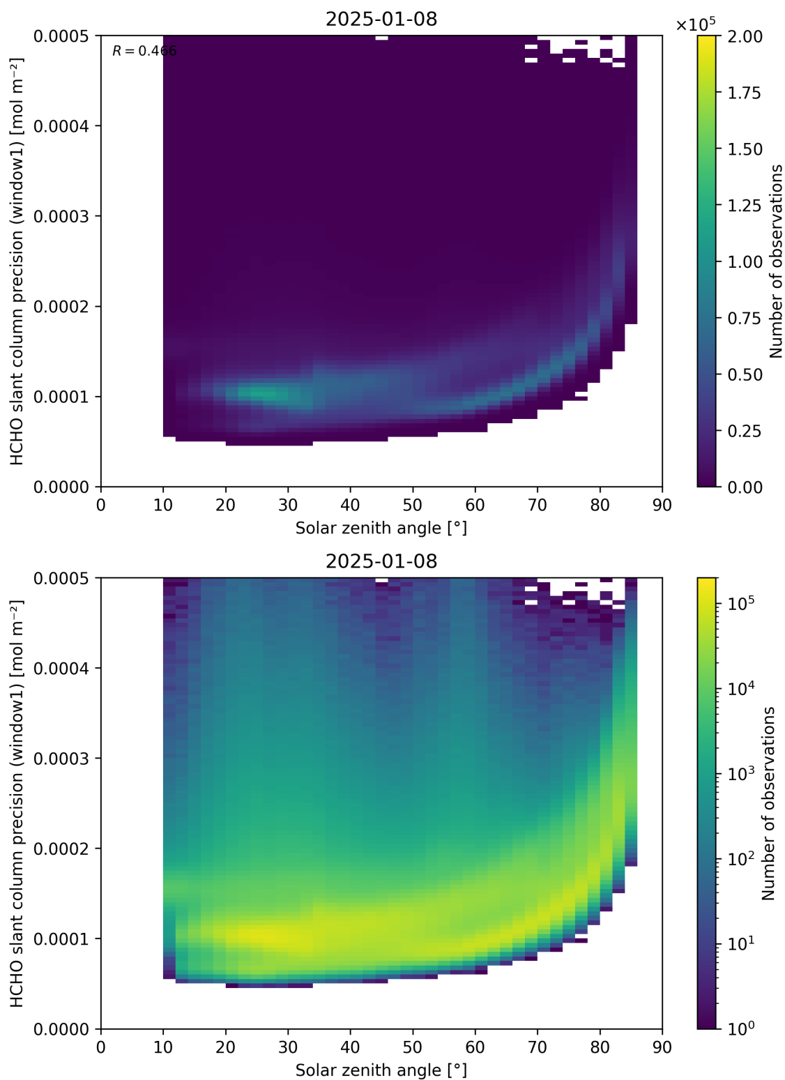
Figure 174: Scatter density plot of “Solar zenith angle” against “HCHO slant column precision (window1)” for 2025-01-07 to 2025-01-09.
