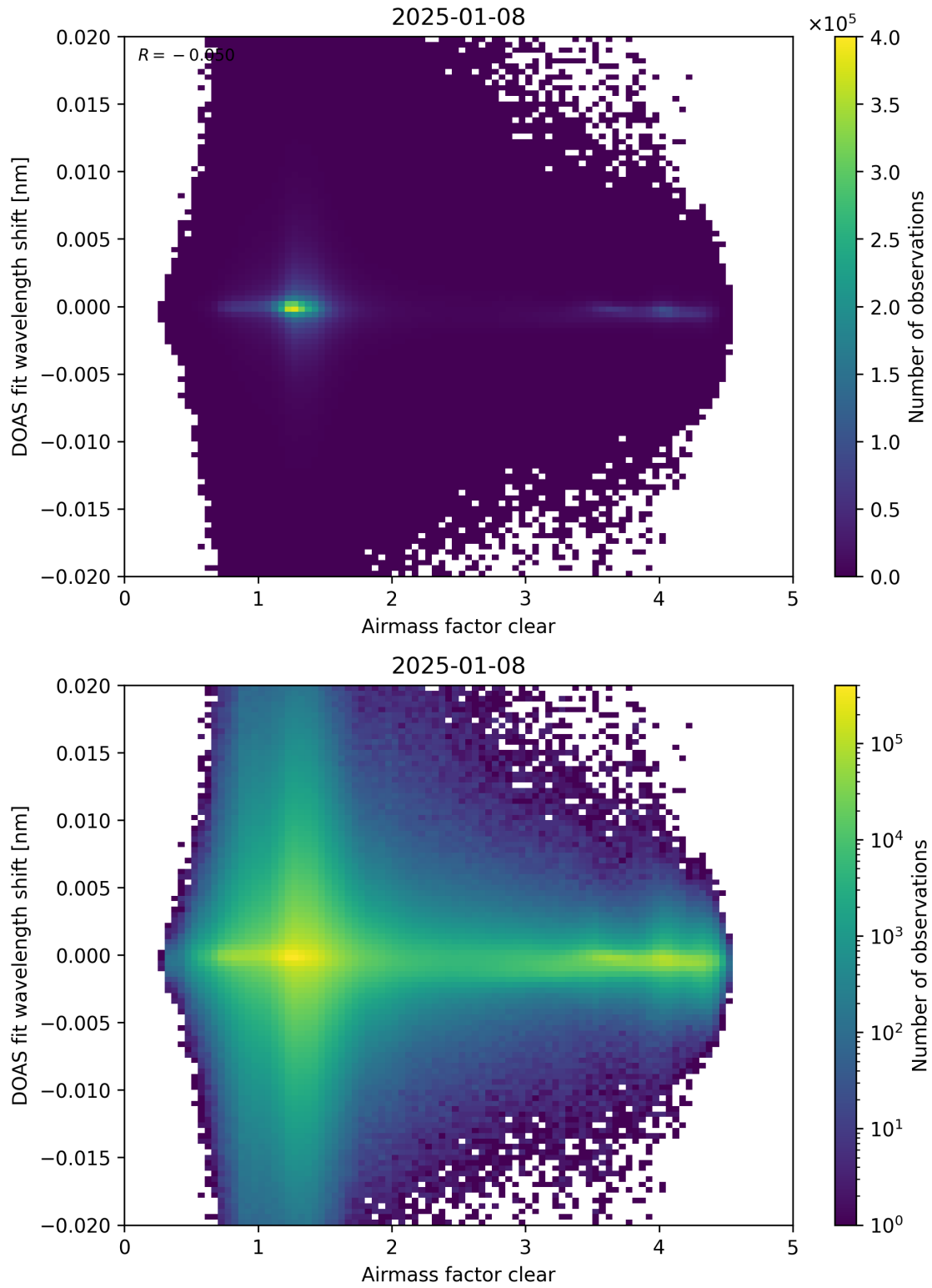
Figure 72: Scatter density plot of “Airmass factor clear” against “DOAS fit wavelength shift” for 2025-01-07 to 2025-01-09.
