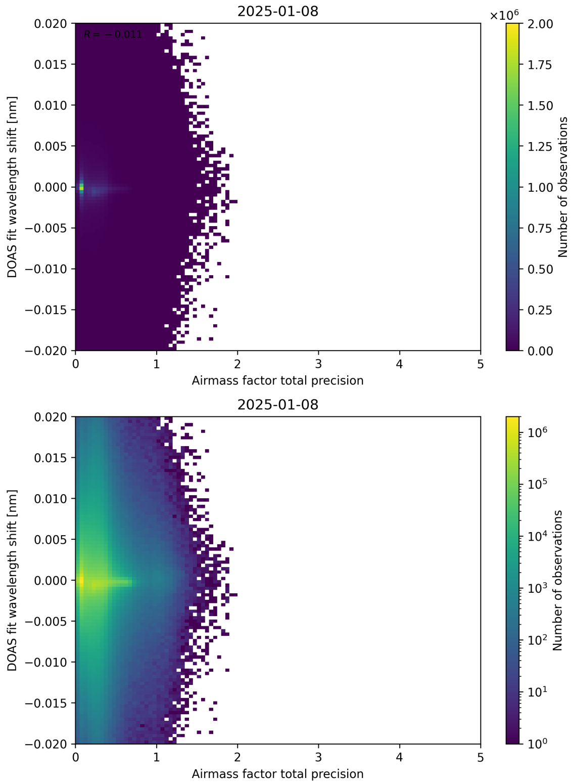
Figure 106: Scatter density plot of “Airmass factor total precision” against “DOAS fit wavelength shift” for 2025-01-07 to 2025-01-09.
