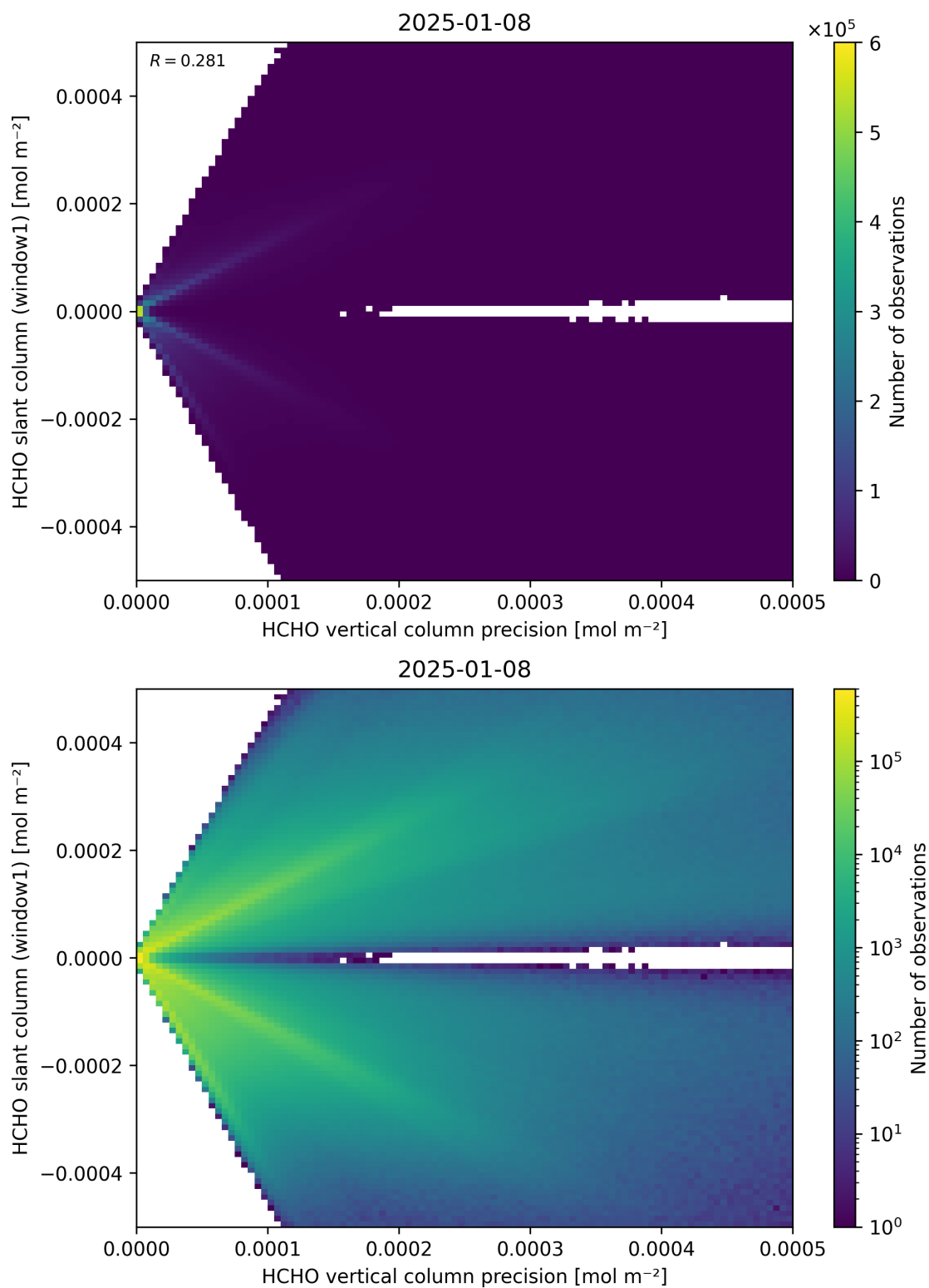
Figure 142: Scatter density plot of “HCHO vertical column precision” against “HCHO slant column (window1)” for 2025-01-07 to 2025-01-09.
