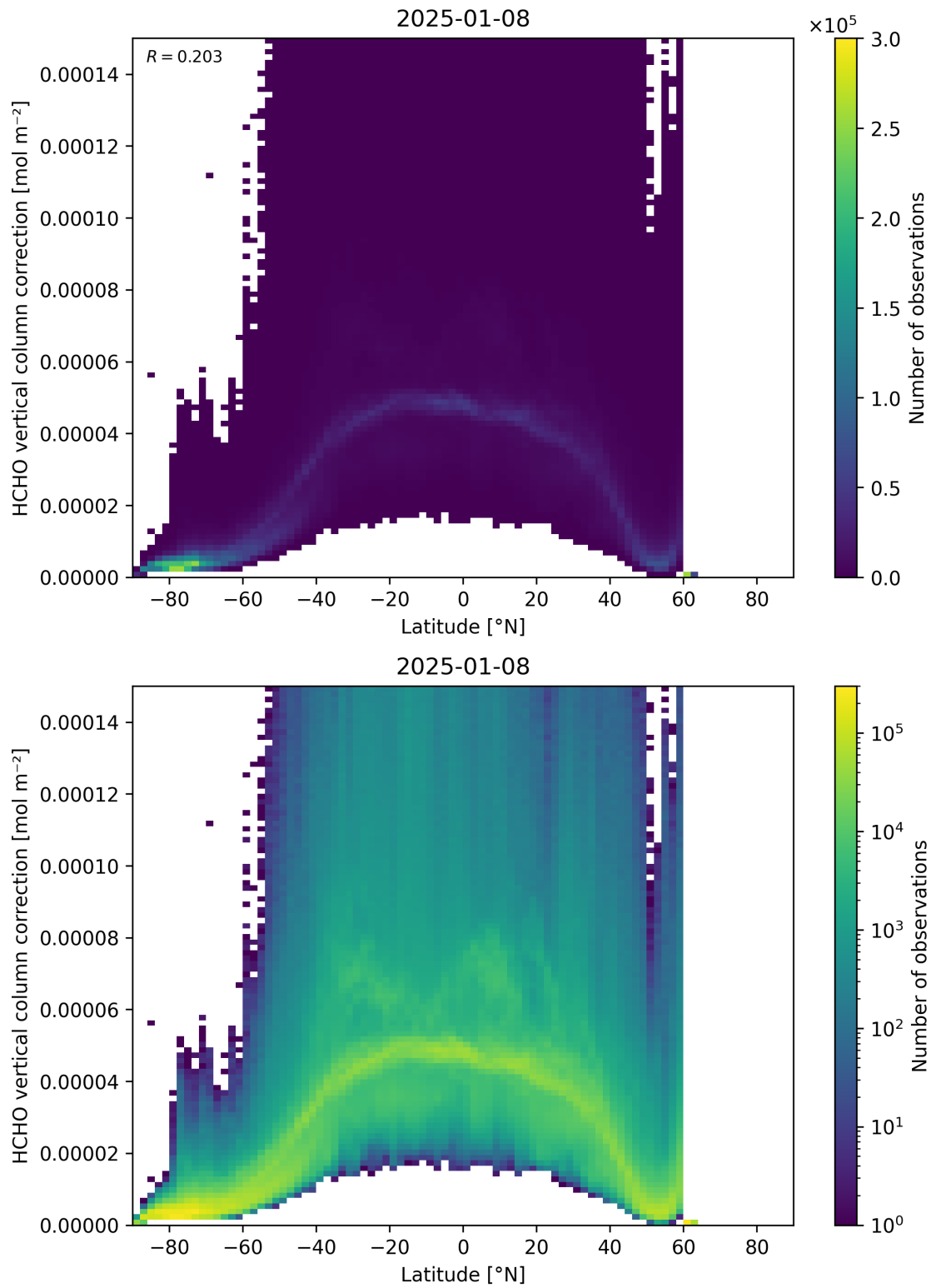
Figure 164: Scatter density plot of “Latitude” against “HCHO vertical column correction” for 2025-01-07 to 2025-01-09.
