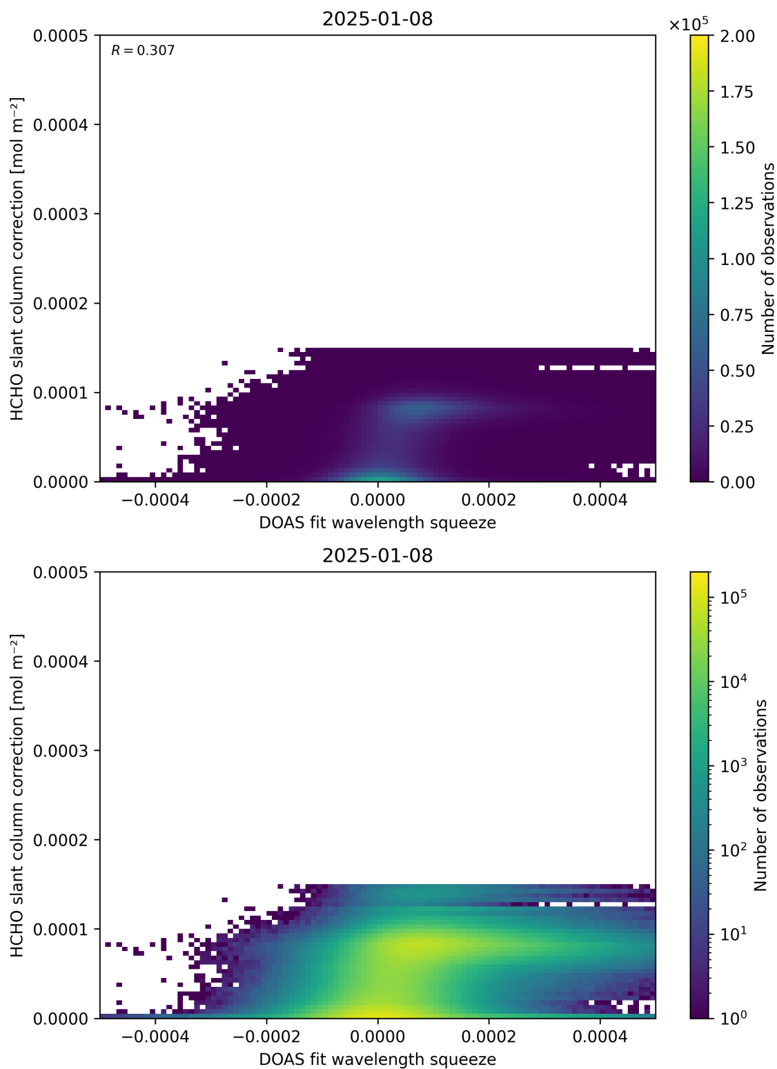
Figure 70: Scatter density plot of “DOAS fit wavelength squeeze” against “HCHO slant column correction” for 2025-01-07 to 2025-01-09.
