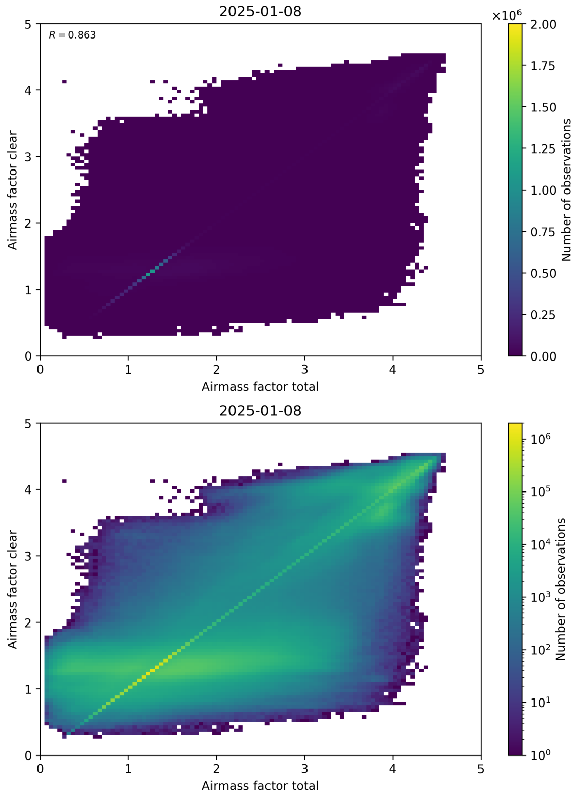
Figure 100: Scatter density plot of “Airmass factor total” against “Airmass factor clear” for 2025-01-07 to 2025-01-09.
