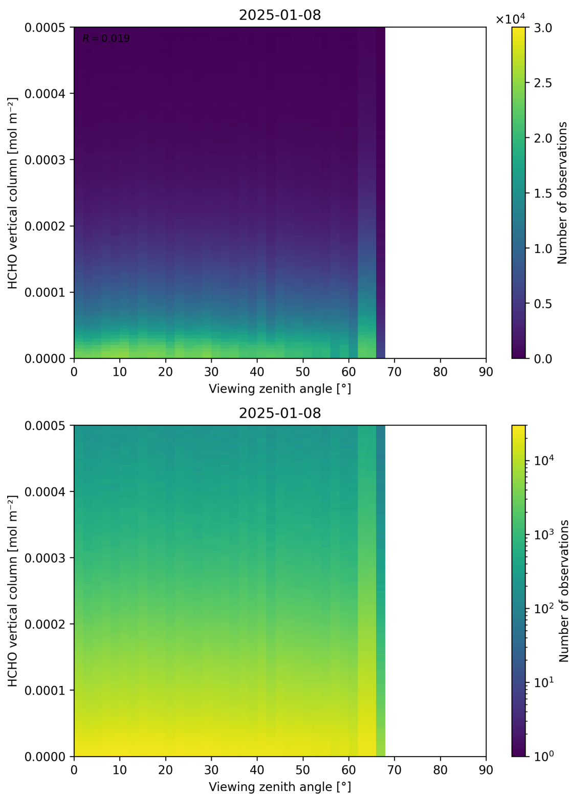
Figure 192: Scatter density plot of “Viewing zenith angle” against “HCHO vertical column” for 2025-01-07 to 2025-01-09.
