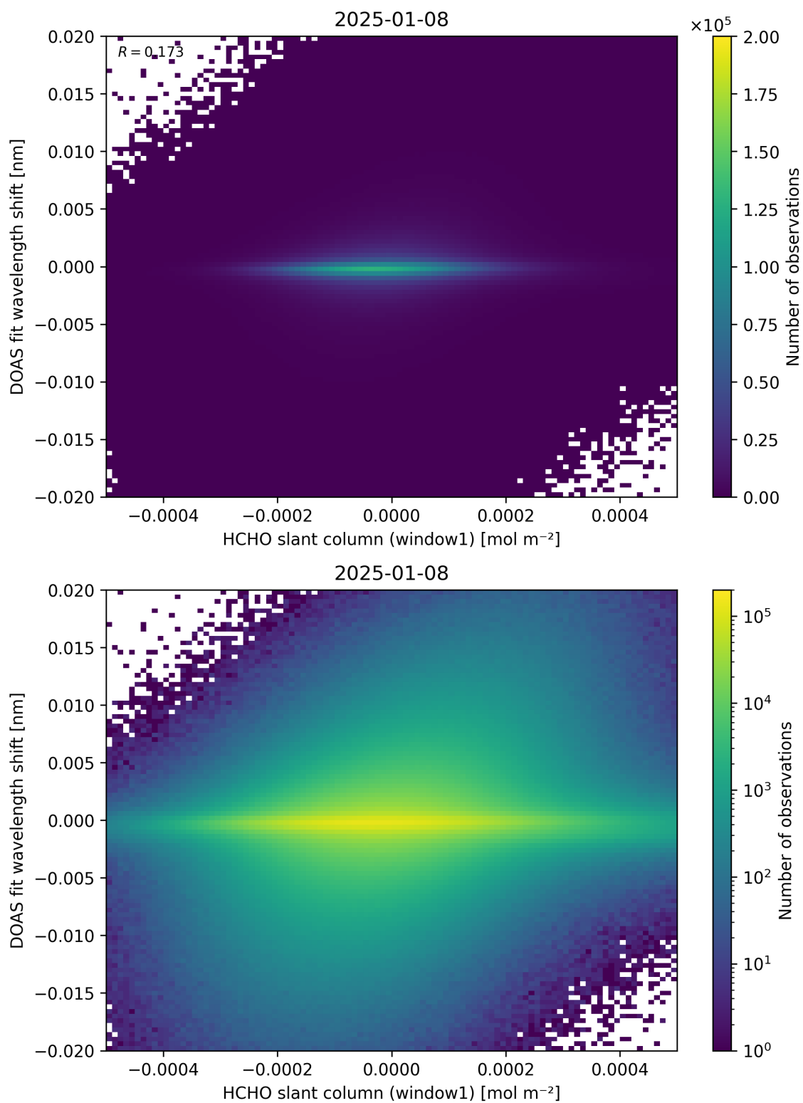
Figure 79: Scatter density plot of “HCHO slant column (window1)” against “DOAS fit wavelength shift” for 2025-01-07 to 2025-01-09.
