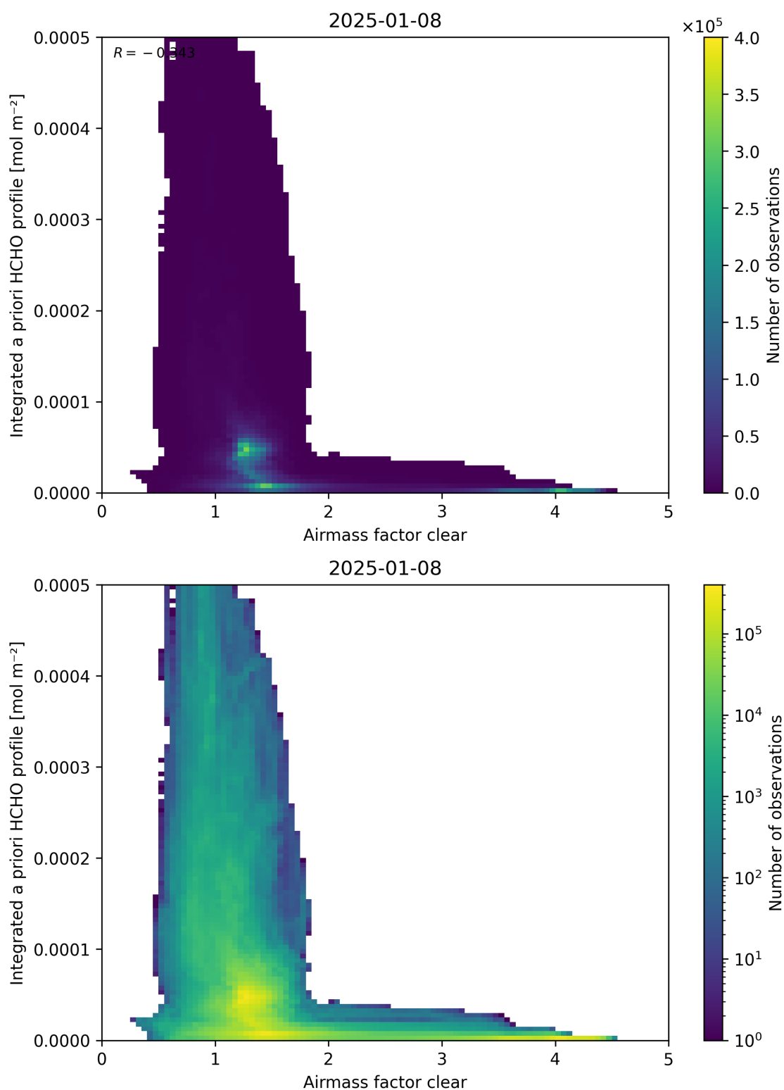
Figure 76: Scatter density plot of “Airmass factor clear” against “Integrated a priori HCHO profile” for 2025-01-07 to 2025-01-09.
