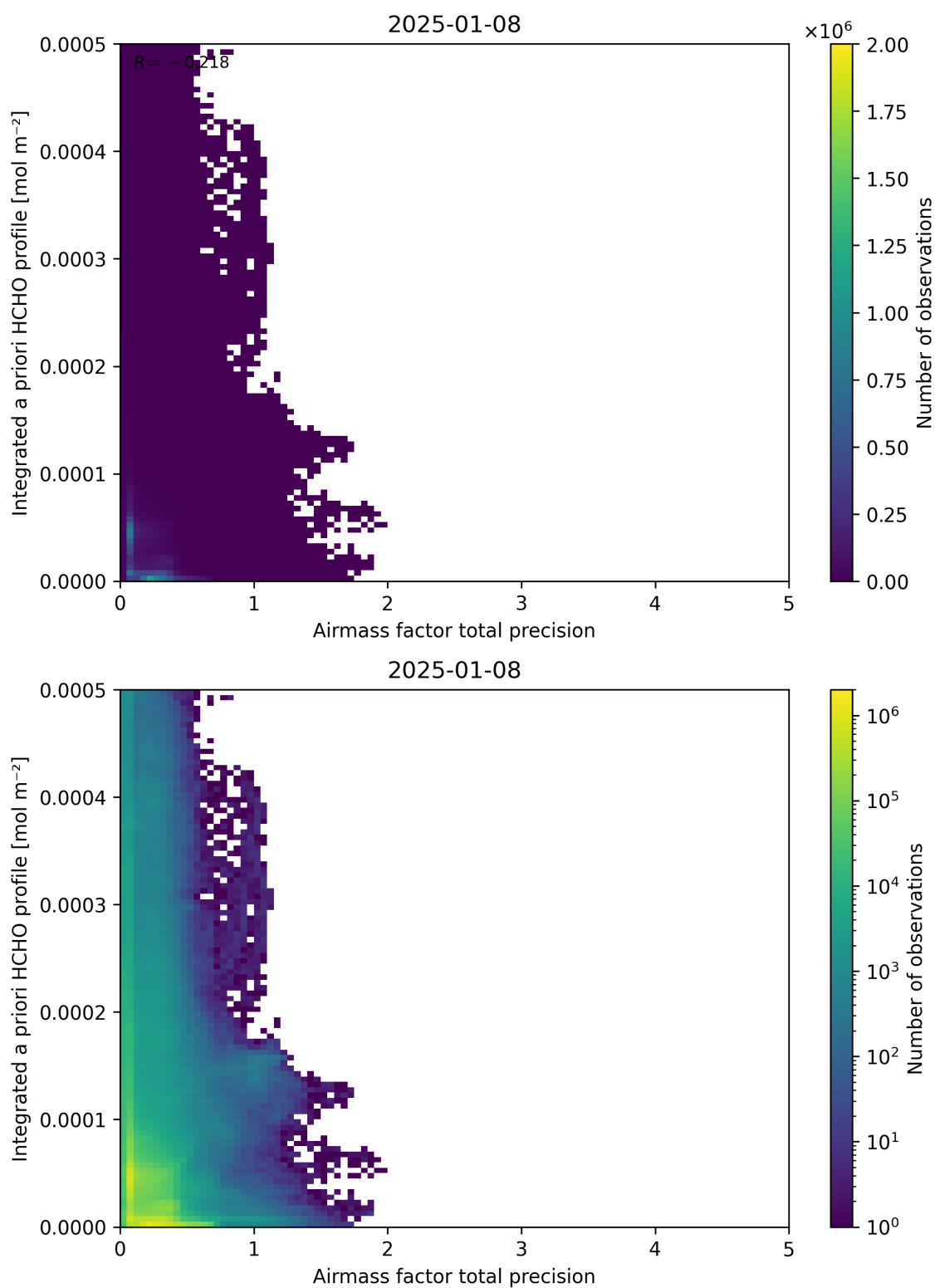
Figure 111: Scatter density plot of “Airmass factor total precision” against “Integrated a priori HCHO profile” for 2025-01-07 to 2025-01-09.
