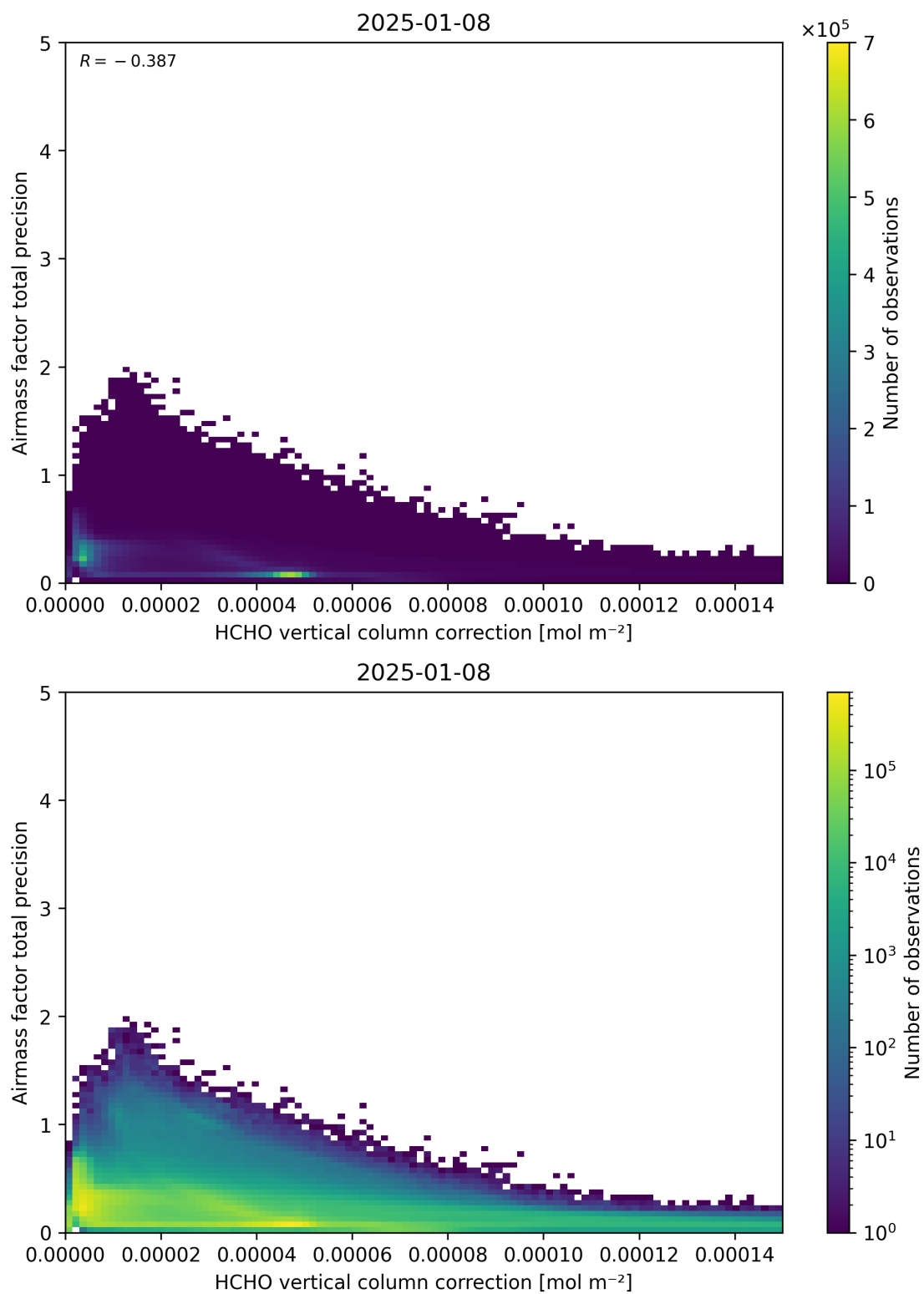
Figure 121: Scatter density plot of “HCHO vertical column correction” against “Airmass factor total precision” for 2025-01-07 to 2025-01-09.
