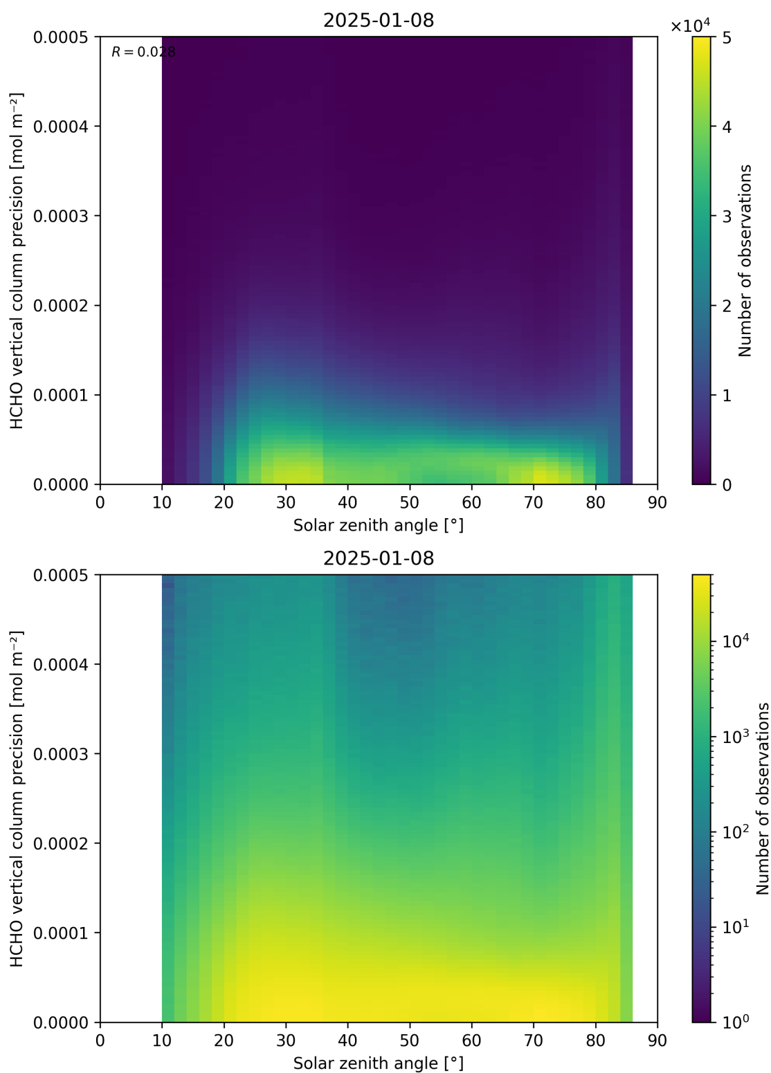
Figure 179: Scatter density plot of “Solar zenith angle” against “HCHO vertical column precision” for 2025-01-07 to 2025-01-09.
