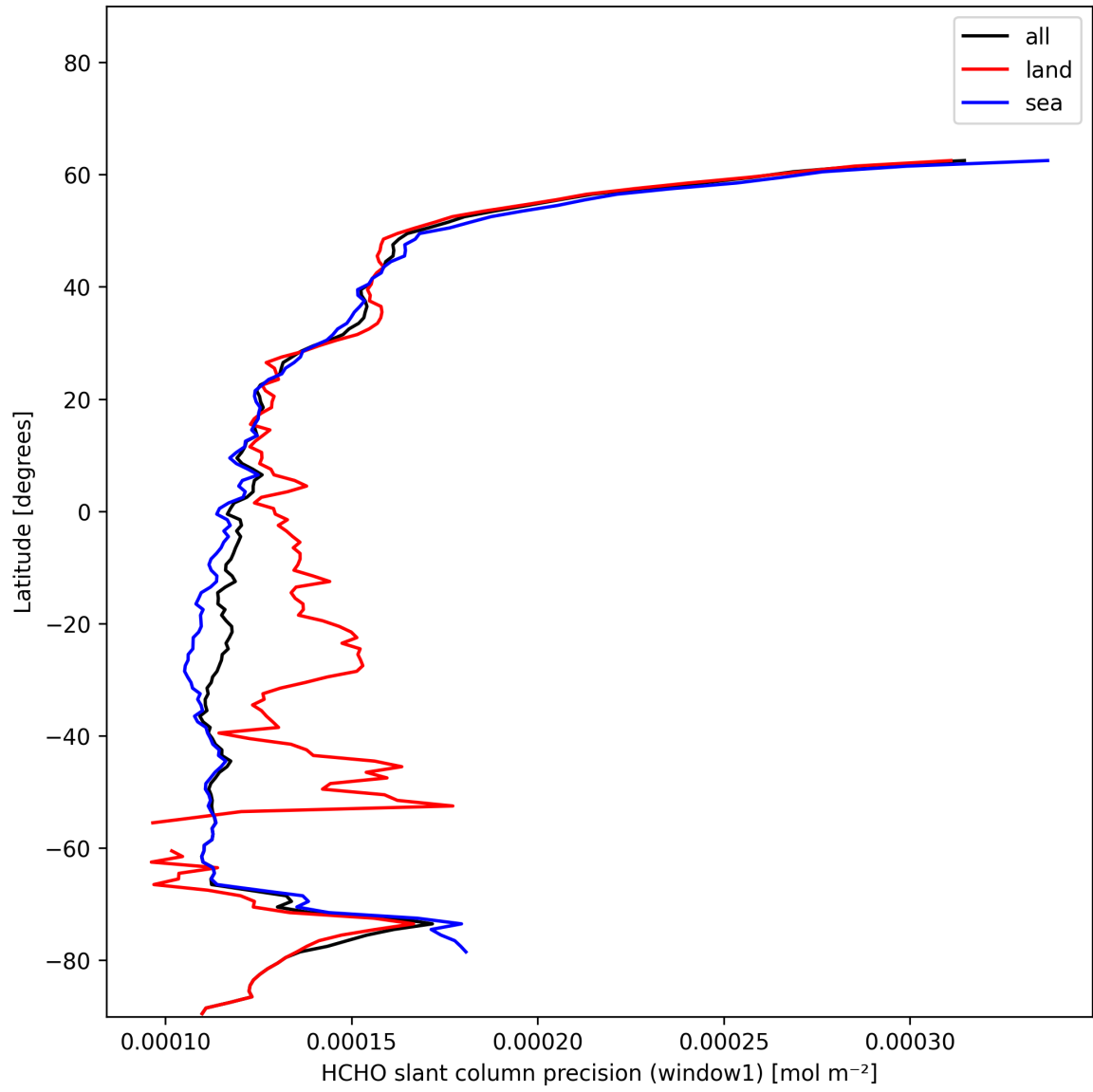
Figure 25: Zonal average of “HCHO slant column precision (window1)” for 2025-01-07 to 2025-01-09.
