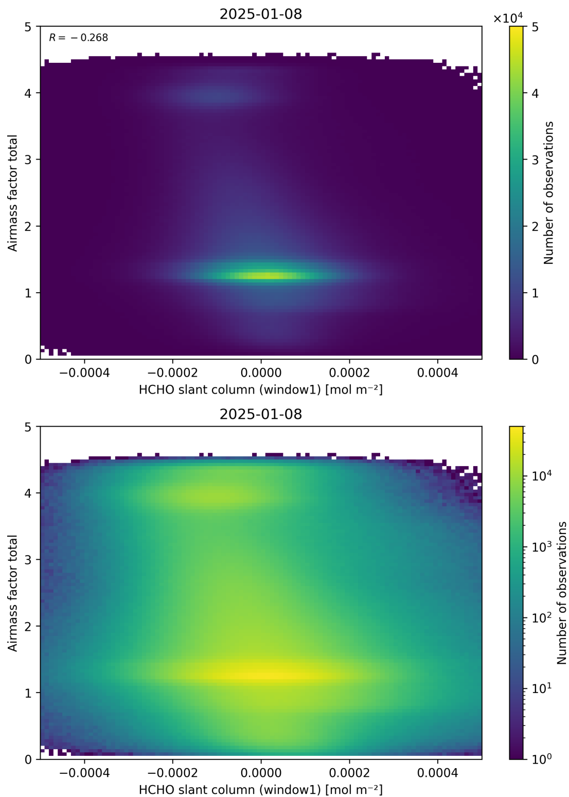
Figure 85: Scatter density plot of “HCHO slant column (window1)” against “Airmass factor total” for 2025-01-07 to 2025-01-09.
