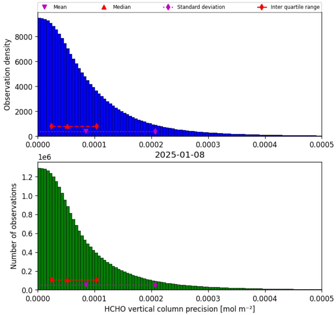
Figure 36: Histogram of “HCHO vertical column precision” for 2025-01-07 to 2025-01-09
