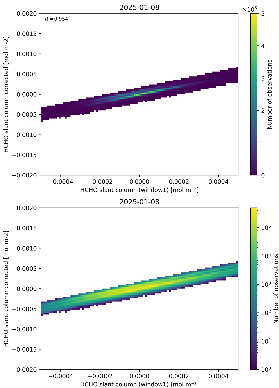
Figure 82: Scatter density plot of “HCHO slant column (window1)” against “HCHO slant column corrected” for 2025-01-07 to 2025-01-09.
