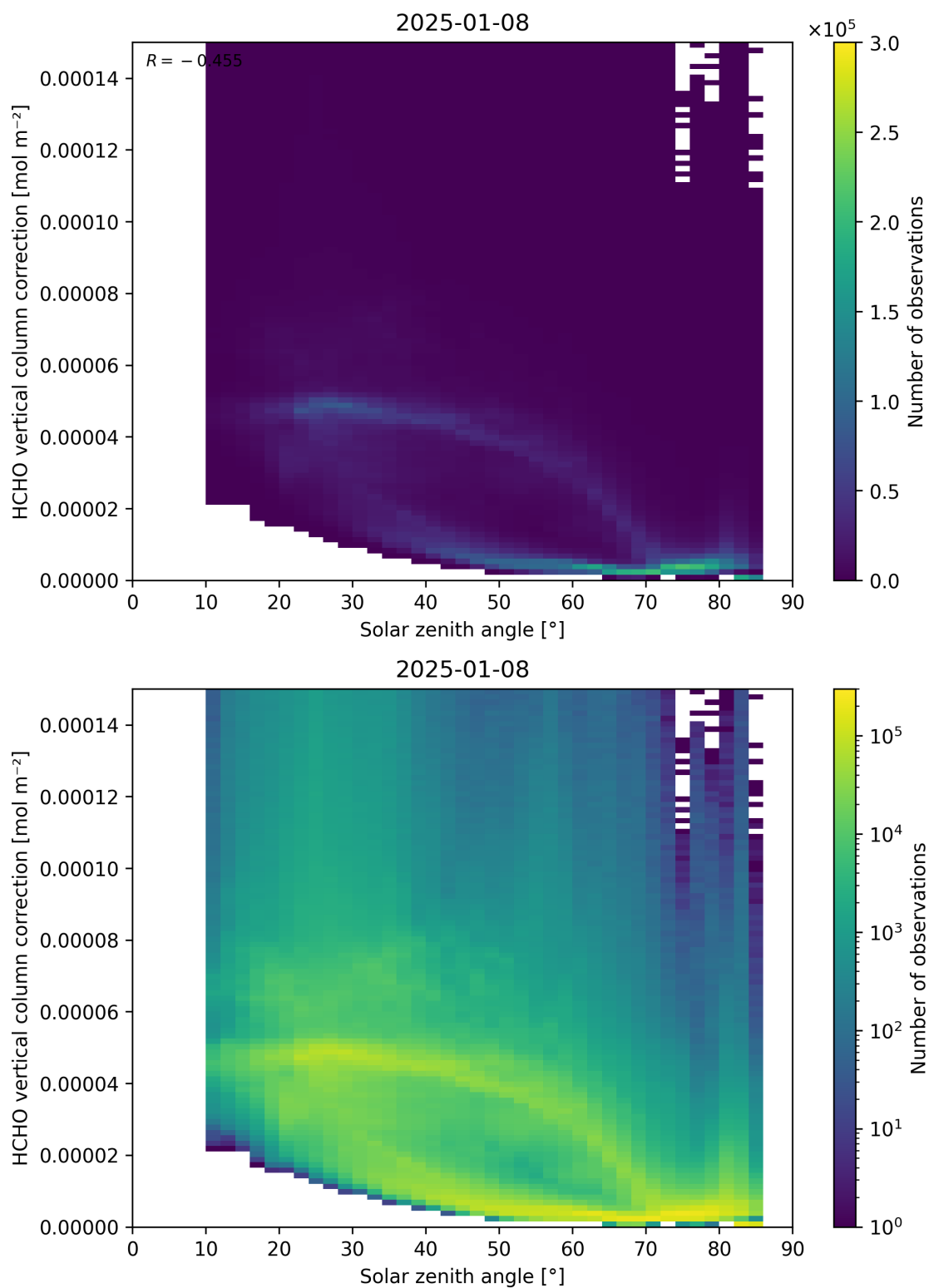
Figure 178: Scatter density plot of “Solar zenith angle” against “HCHO vertical column correction” for 2025-01-07 to 2025-01-09.
