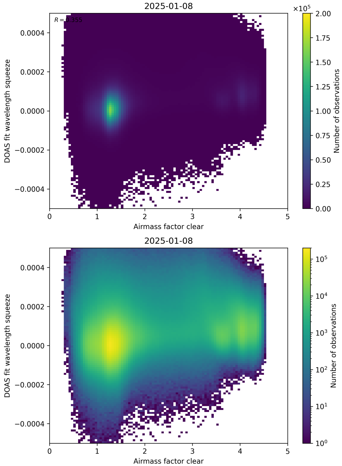
Figure 73: Scatter density plot of “Airmass factor clear” against “DOAS fit wavelength squeeze” for 2025-01-07 to 2025-01-09.
