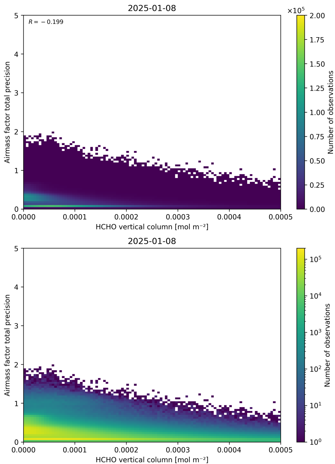
Figure 132: Scatter density plot of “HCHO vertical column” against “Airmass factor total precision” for 2025-01-07 to 2025-01-09.
