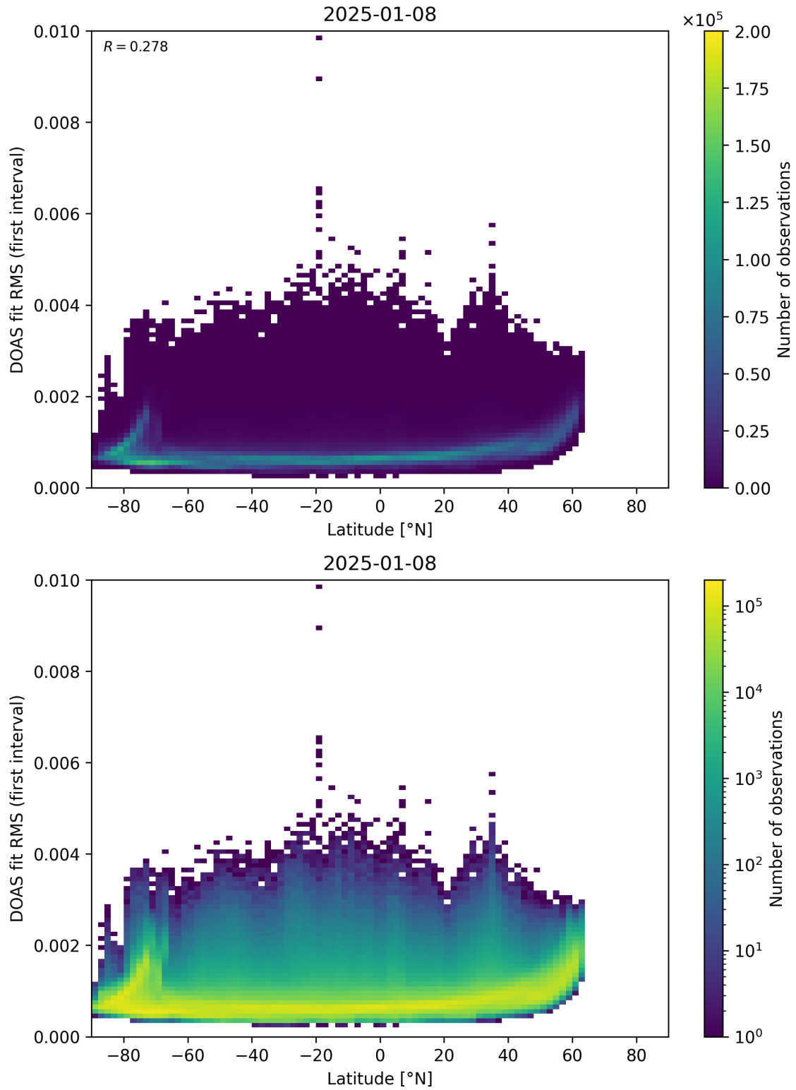
Figure 153: Scatter density plot of “Latitude” against “DOAS fit RMS (first interval)” for 2025-01-07 to 2025-01-09.
