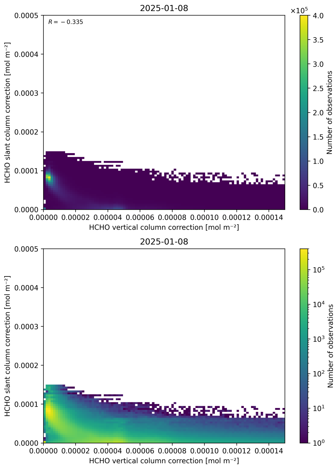
Figure 117: Scatter density plot of “HCHO vertical column correction” against “HCHO slant column correction” for 2025-01-07 to 2025-01-09.
