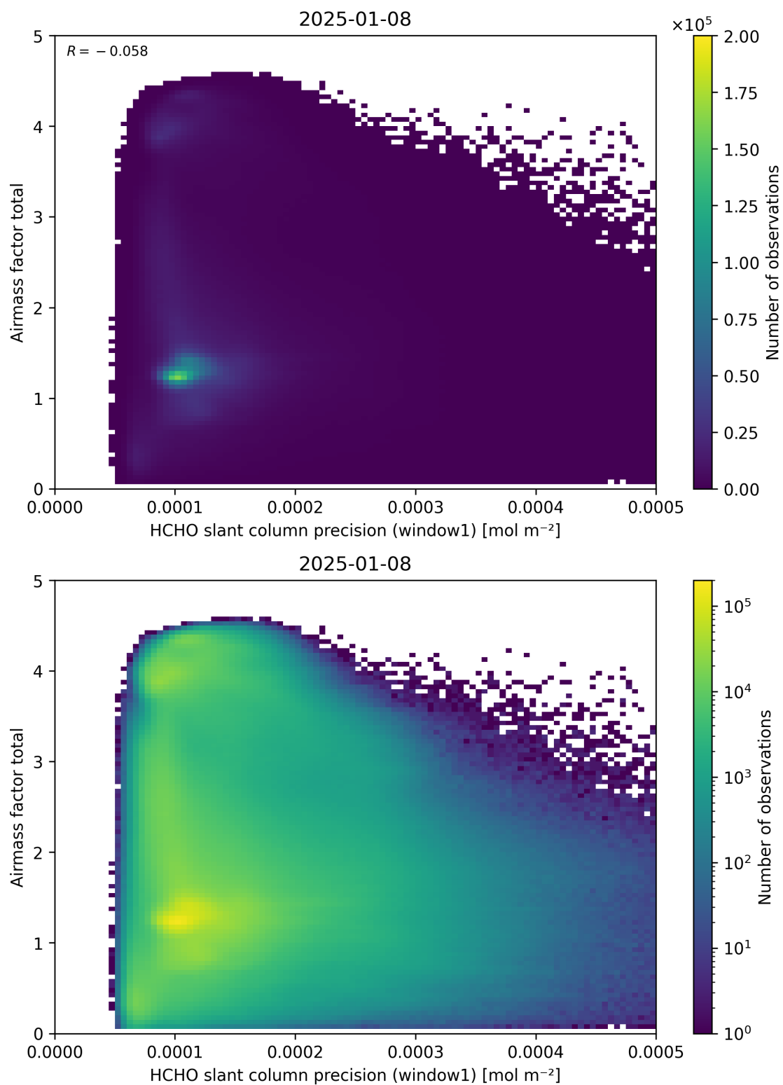
Figure 94: Scatter density plot of “HCHO slant column precision (window1)” against “Airmass factor total” for 2025-01-07 to 2025-01-09.
