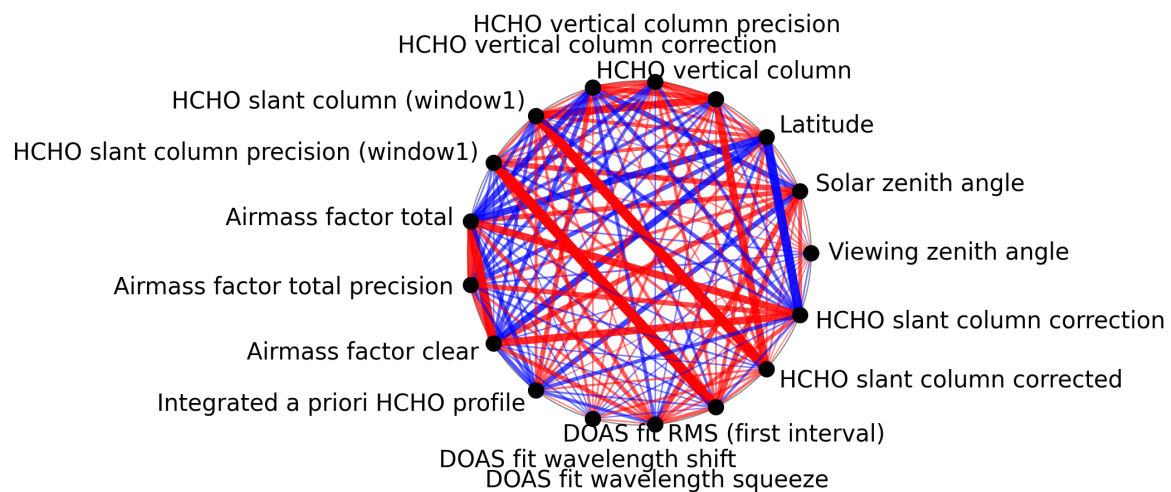
Figure 1: Map of correlation graph for 2025-01-07 to 2025-01-09.
