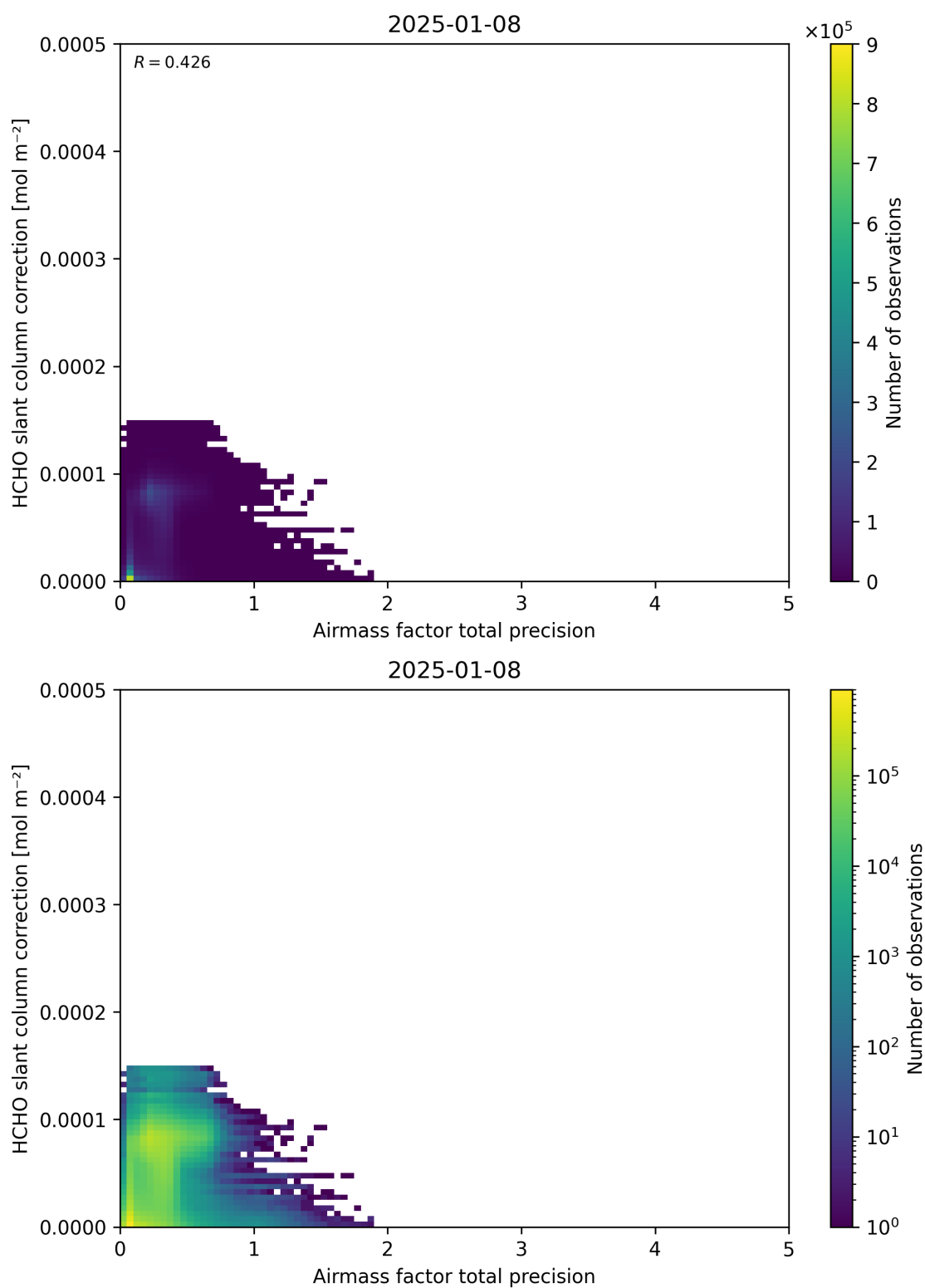
Figure 110: Scatter density plot of “Airmass factor total precision” against “HCHO slant column correction” for 2025-01-07 to 2025-01-09.
