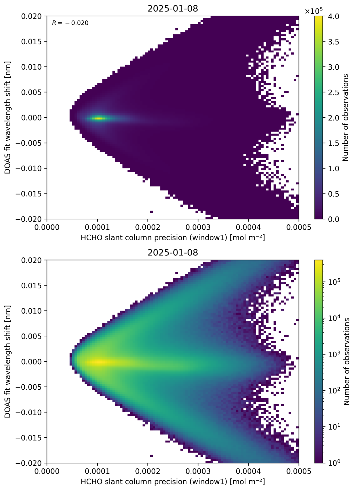
Figure 89: Scatter density plot of “HCHO slant column precision (window1)” against “DOAS fit wavelength shift” for 2025-01-07 to 2025-01-09.
