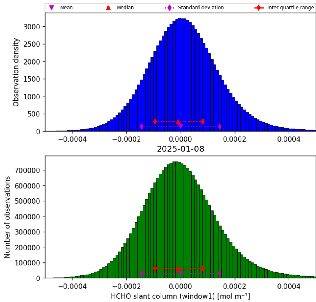
Figure 38: Histogram of “HCHO slant column (window1)” for 2025-01-07 to 2025-01-09
