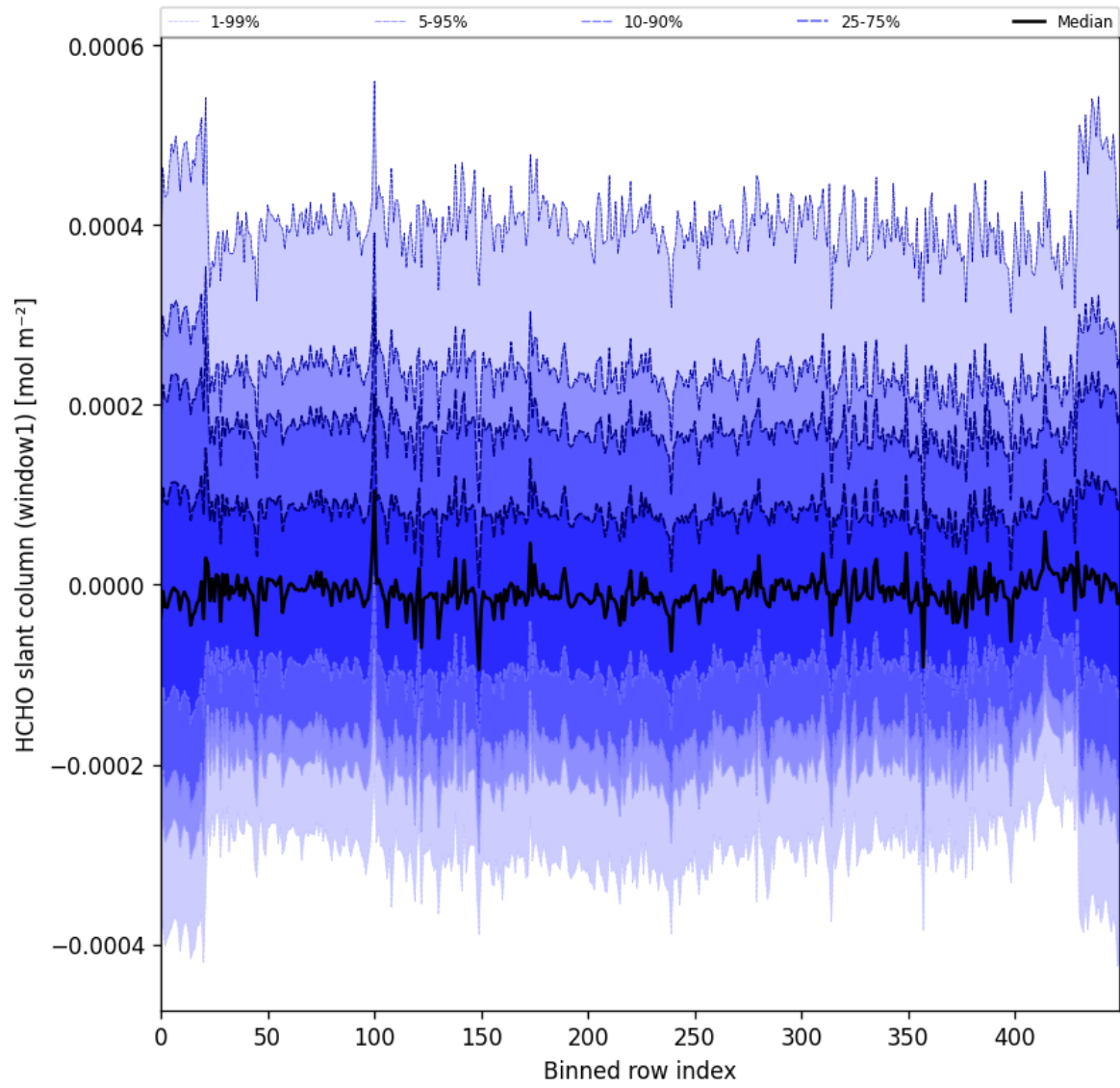
Figure 52: Along track statistics of “HCHO slant column (window1)” for 2025-01-07 to 2025-01-09
