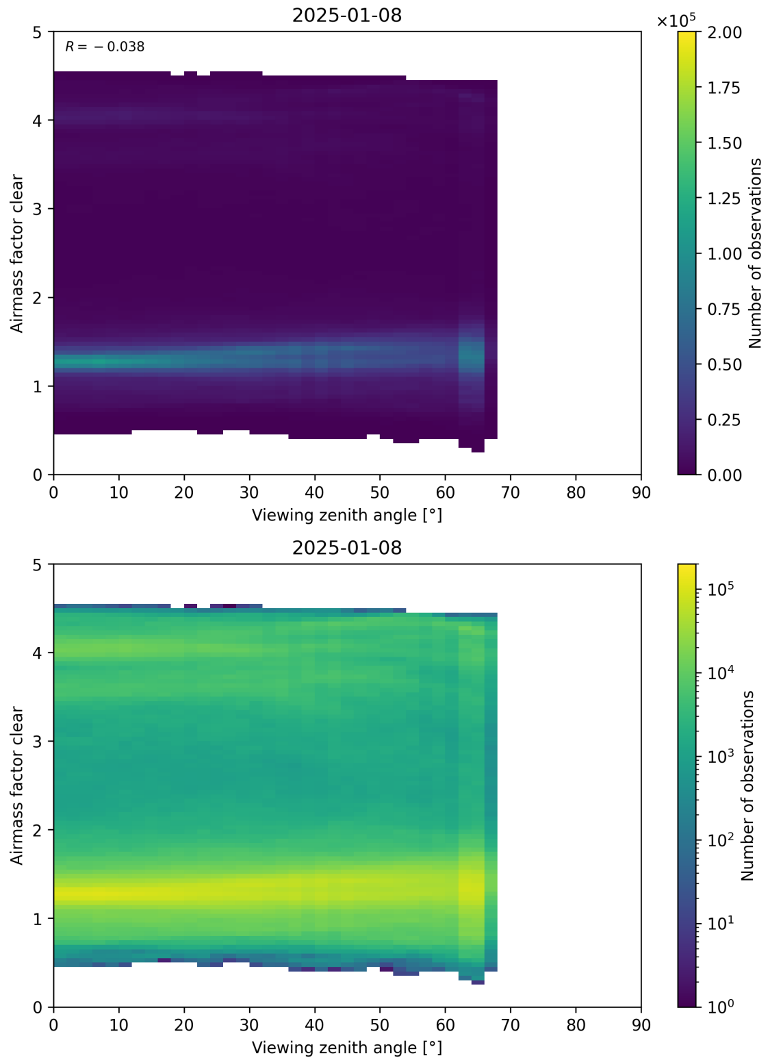
Figure 185: Scatter density plot of “Viewing zenith angle” against “Airmass factor clear” for 2025-01-07 to 2025-01-09.
