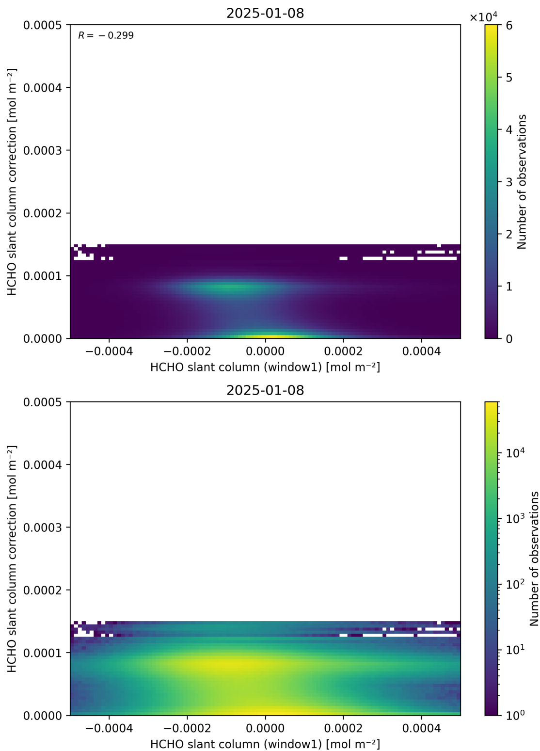
Figure 83: Scatter density plot of “HCHO slant column (window1)” against “HCHO slant column correction” for 2025-01-07 to 2025-01-09.
