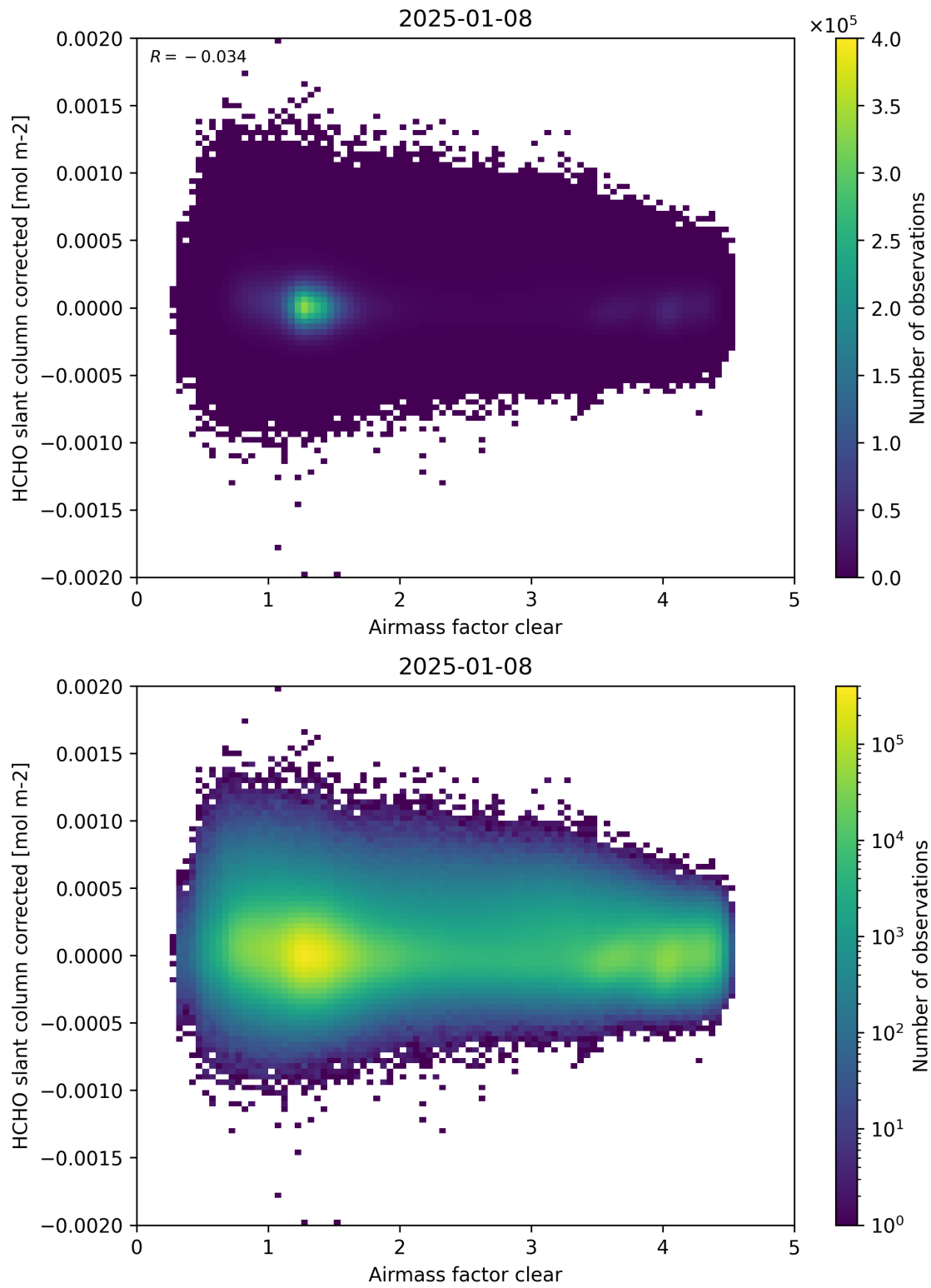
Figure 74: Scatter density plot of “Airmass factor clear” against “HCHO slant column corrected” for 2025-01-07 to 2025-01-09.
