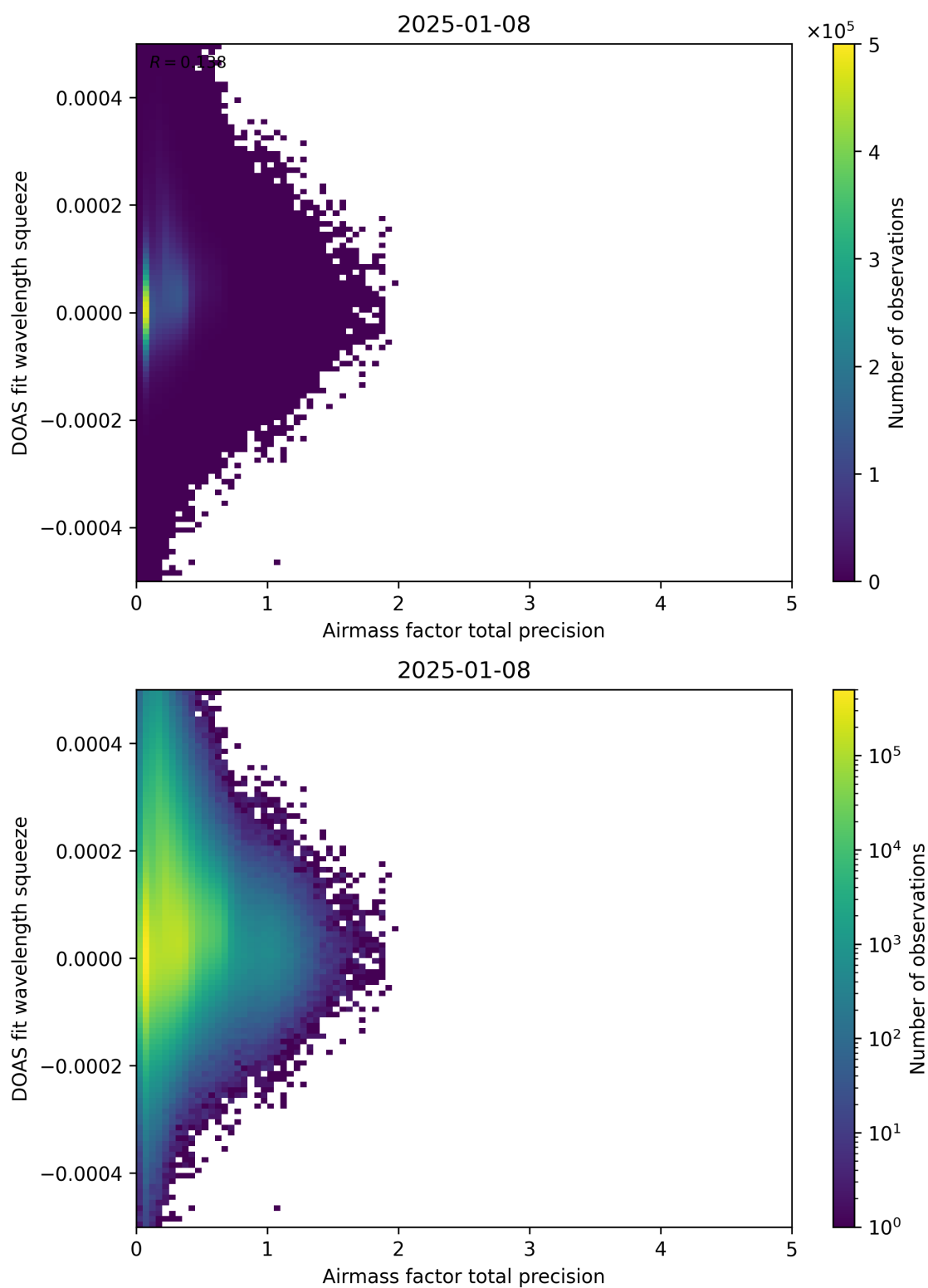
Figure 107: Scatter density plot of “Airmass factor total precision” against “DOAS fit wavelength squeeze” for 2025-01-07 to 2025-01-09.
