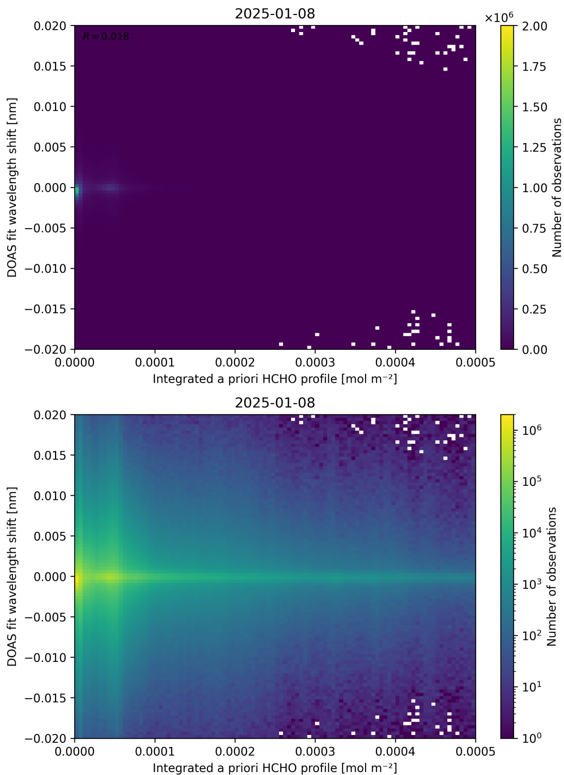
Figure 149: Scatter density plot of “Integrated a priori HCHO profile” against “DOAS fit wavelength shift” for 2025-01-07 to 2025-01-09.
