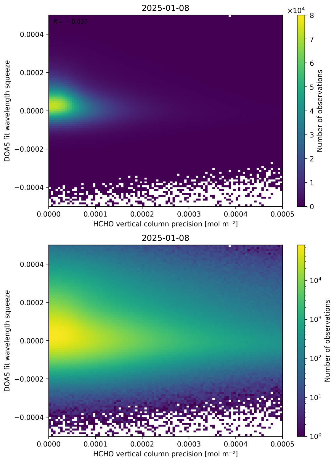
Figure 138: Scatter density plot of “HCHO vertical column precision” against “DOAS fit wavelength squeeze” for 2025-01-07 to 2025-01-09.
