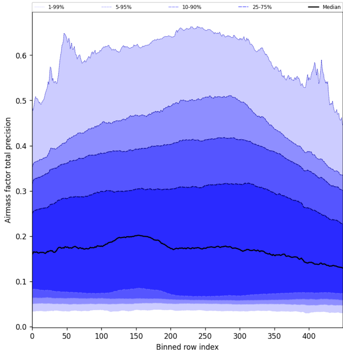
Figure 55: Along track statistics of “Airmass factor total precision” for 2025-01-07 to 2025-01-09
