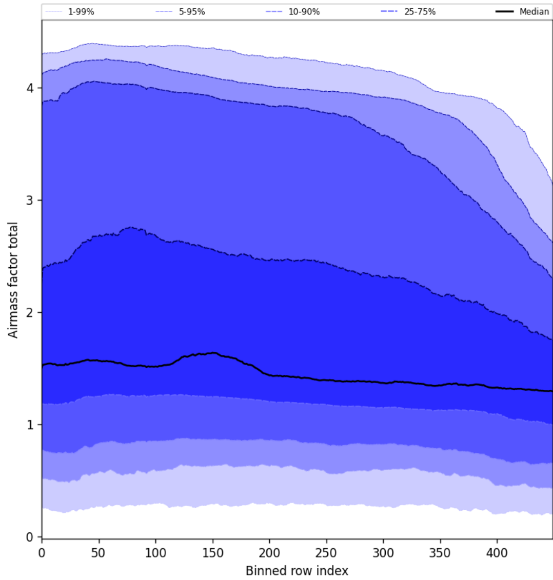
Figure 54: Along track statistics of “Airmass factor total” for 2025-01-07 to 2025-01-09
