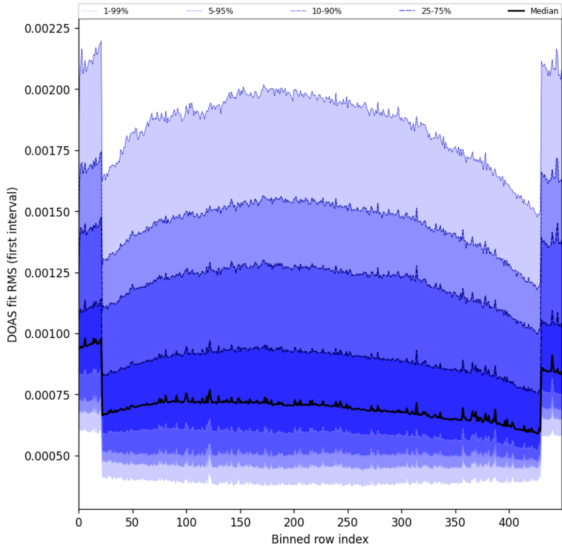
Figure 60: Along track statistics of “DOAS fit RMS (first interval)” for 2025-01-07 to 2025-01-09
