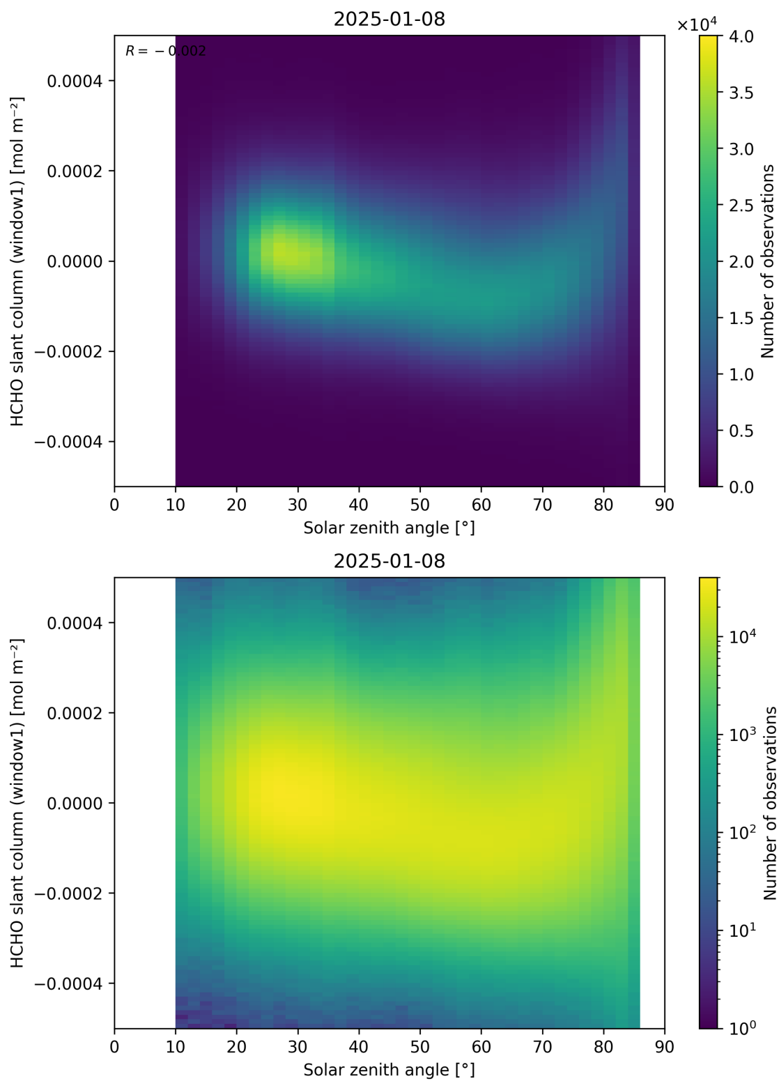
Figure 173: Scatter density plot of “Solar zenith angle” against “HCHO slant column (window1)” for 2025-01-07 to 2025-01-09.
