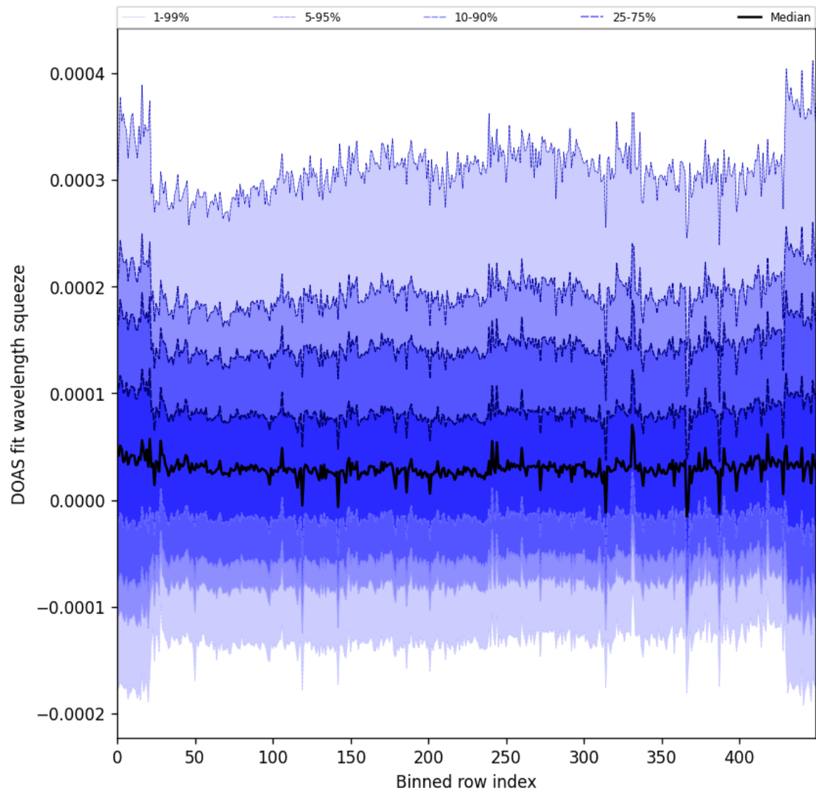
Figure 59: Along track statistics of “DOAS fit wavelength squeeze” for 2025-01-07 to 2025-01-09
