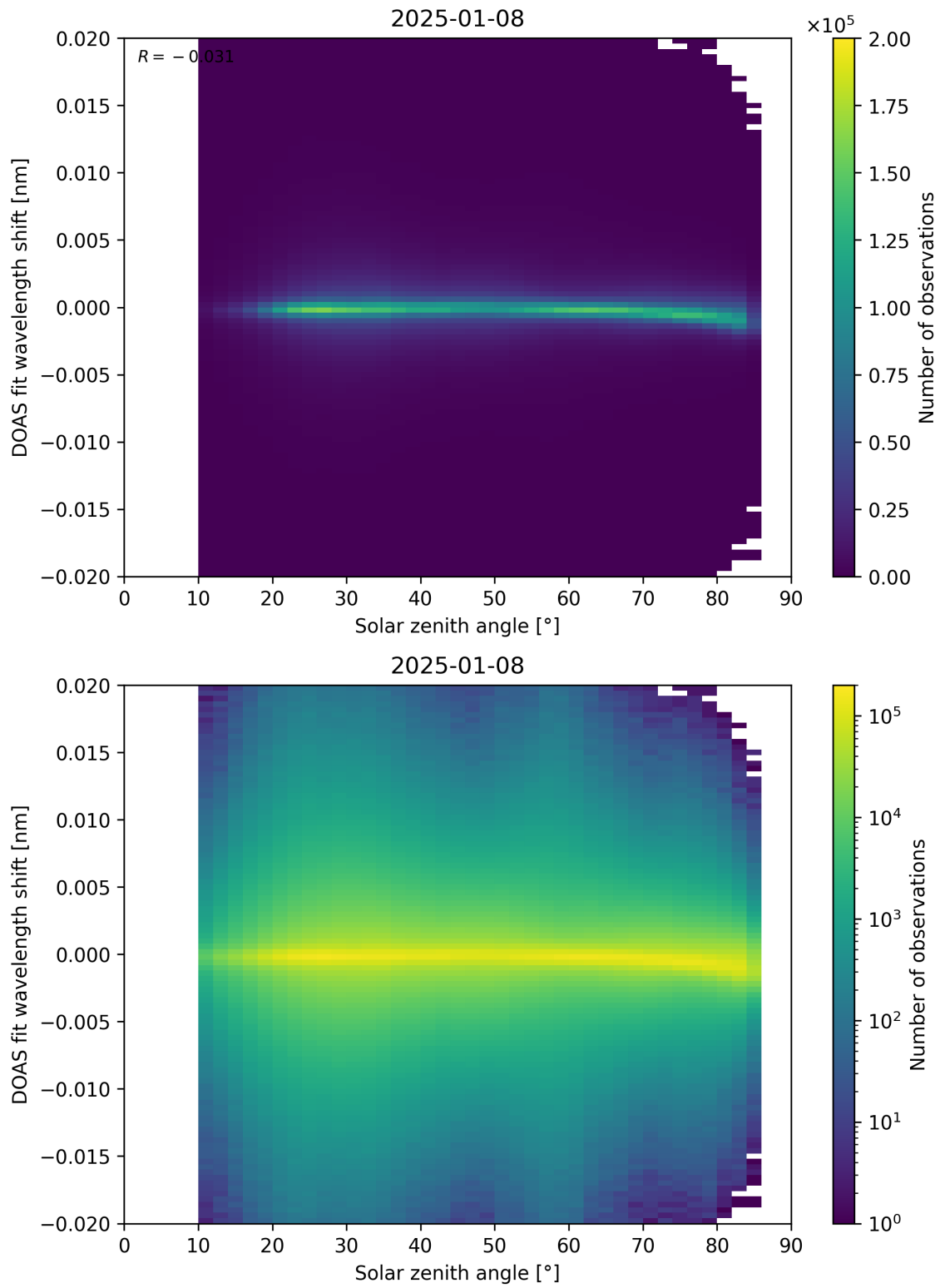
Figure 168: Scatter density plot of “Solar zenith angle” against “DOAS fit wavelength shift” for 2025-01-07 to 2025-01-09.
