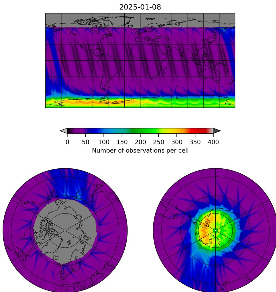
Figure 19: Map of the number of observations for 2025-01-07 to 2025-01-09
