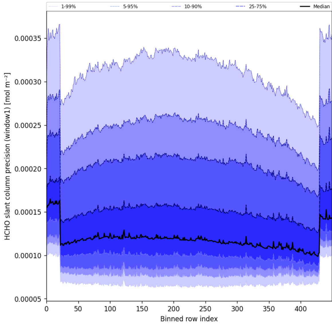
Figure 53: Along track statistics of "HCHO slant column precision (window1)" for 2025-01-07 to 2025-01-09
