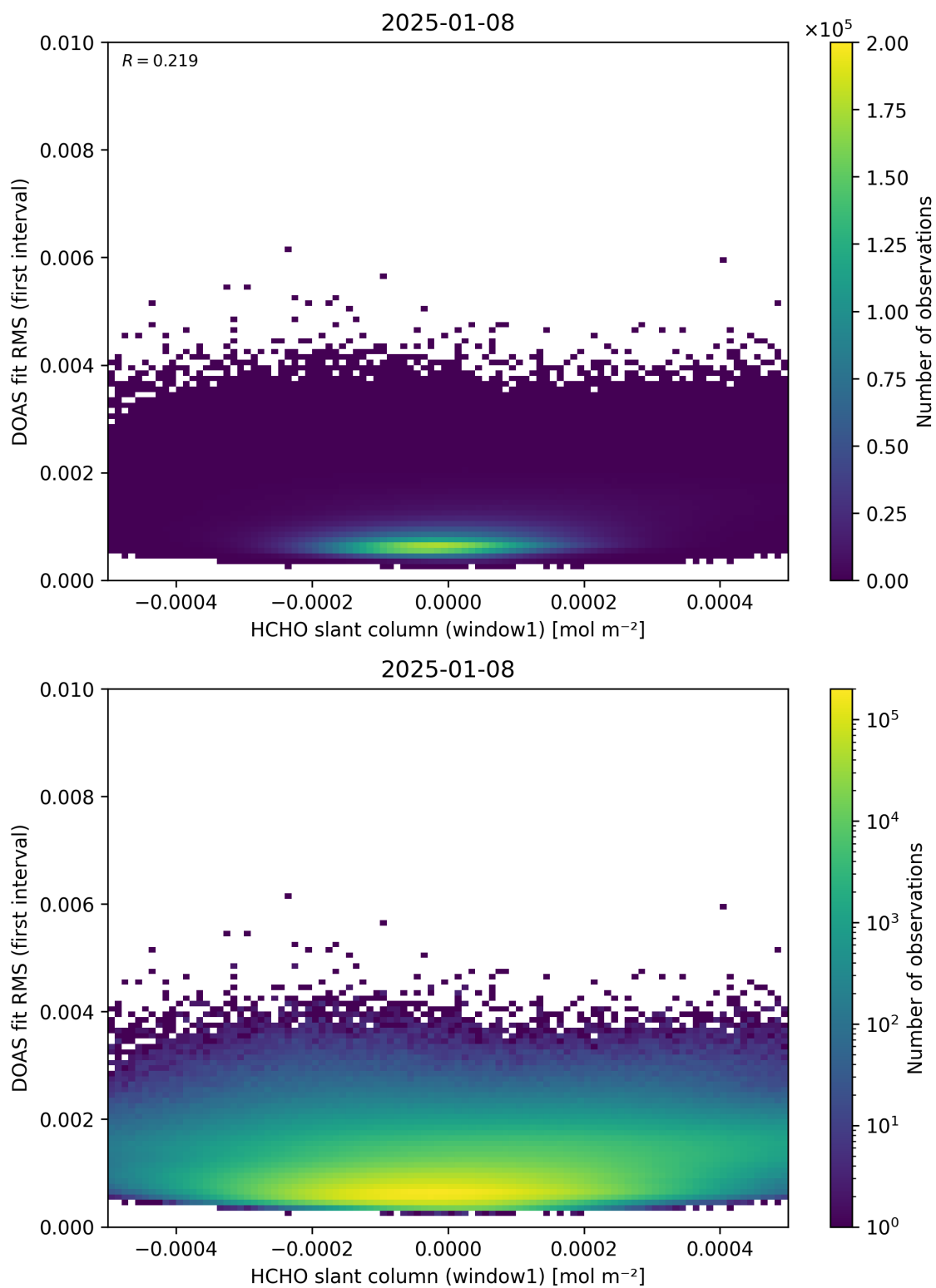
Figure 78: Scatter density plot of “HCHO slant column (window1)” against “DOAS fit RMS (first interval)” for 2025-01-07 to 2025-01-09.
