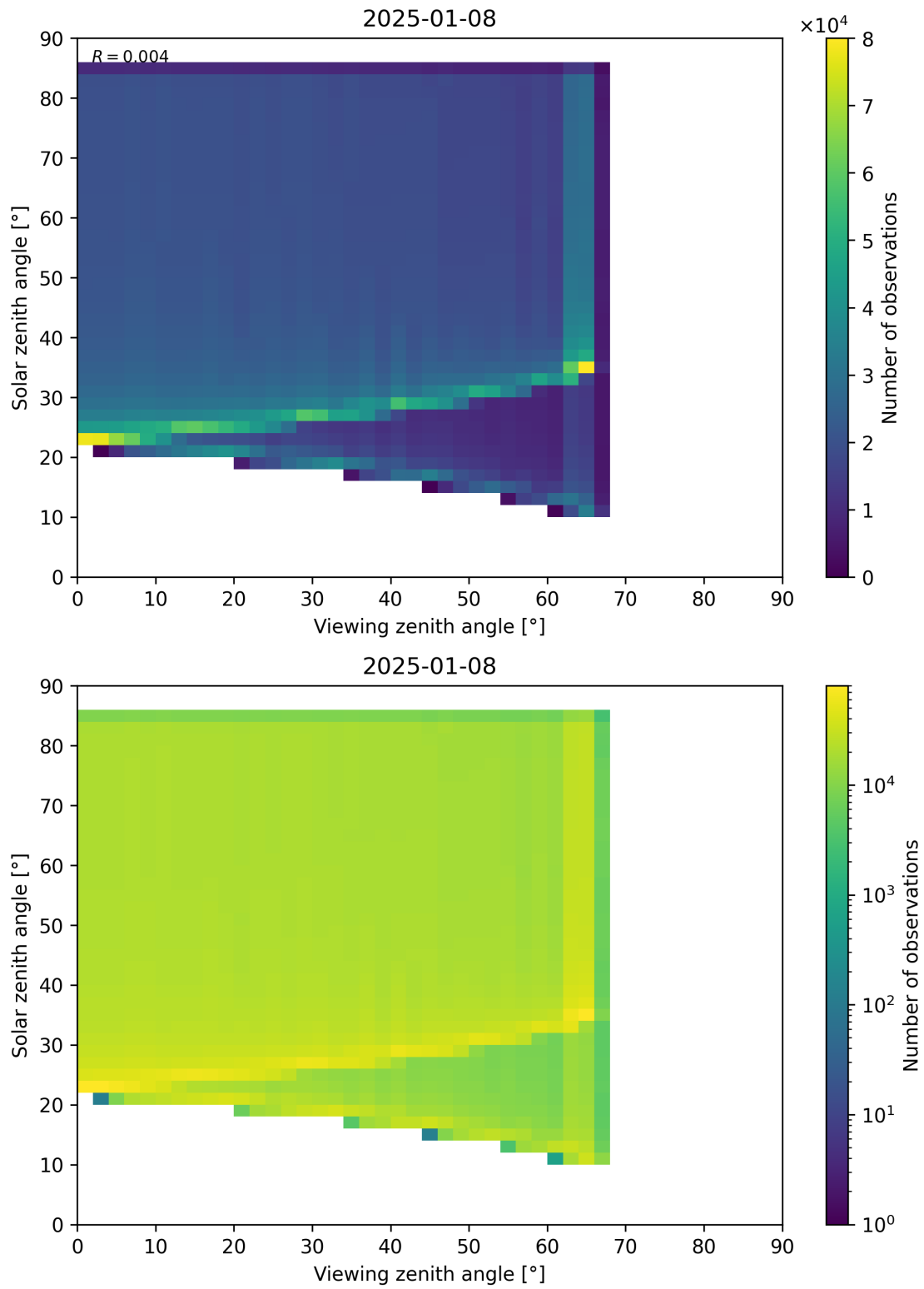
Figure 197: Scatter density plot of “Viewing zenith angle” against “Solar zenith angle” for 2025-01-07 to 2025-01-09.
