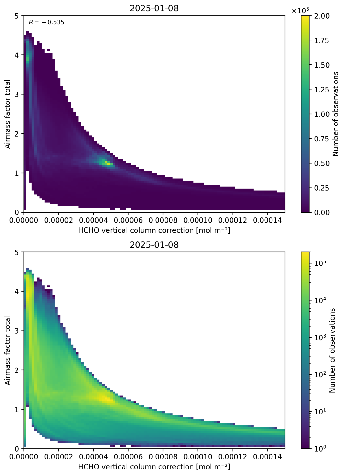
Figure 120: Scatter density plot of “HCHO vertical column correction” against “Airmass factor total” for 2025-01-07 to 2025-01-09.
