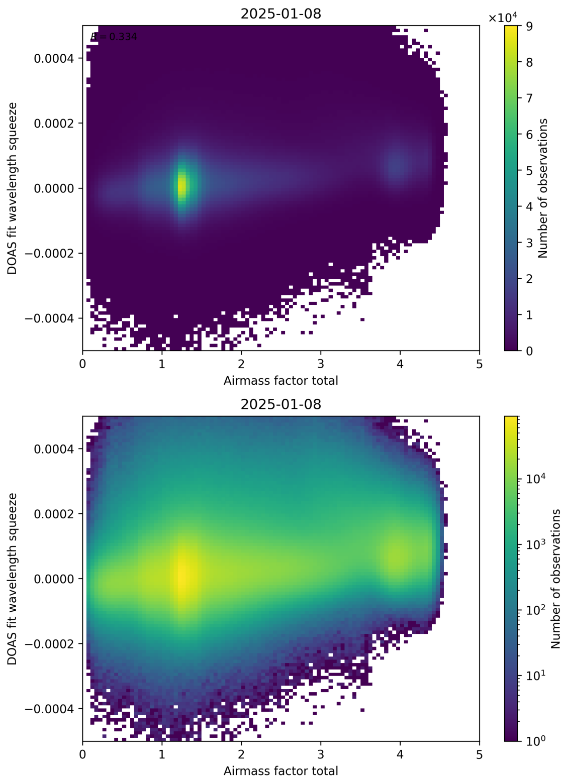
Figure 99: Scatter density plot of “Airmass factor total” against “DOAS fit wavelength squeeze” for 2025-01-07 to 2025-01-09.
