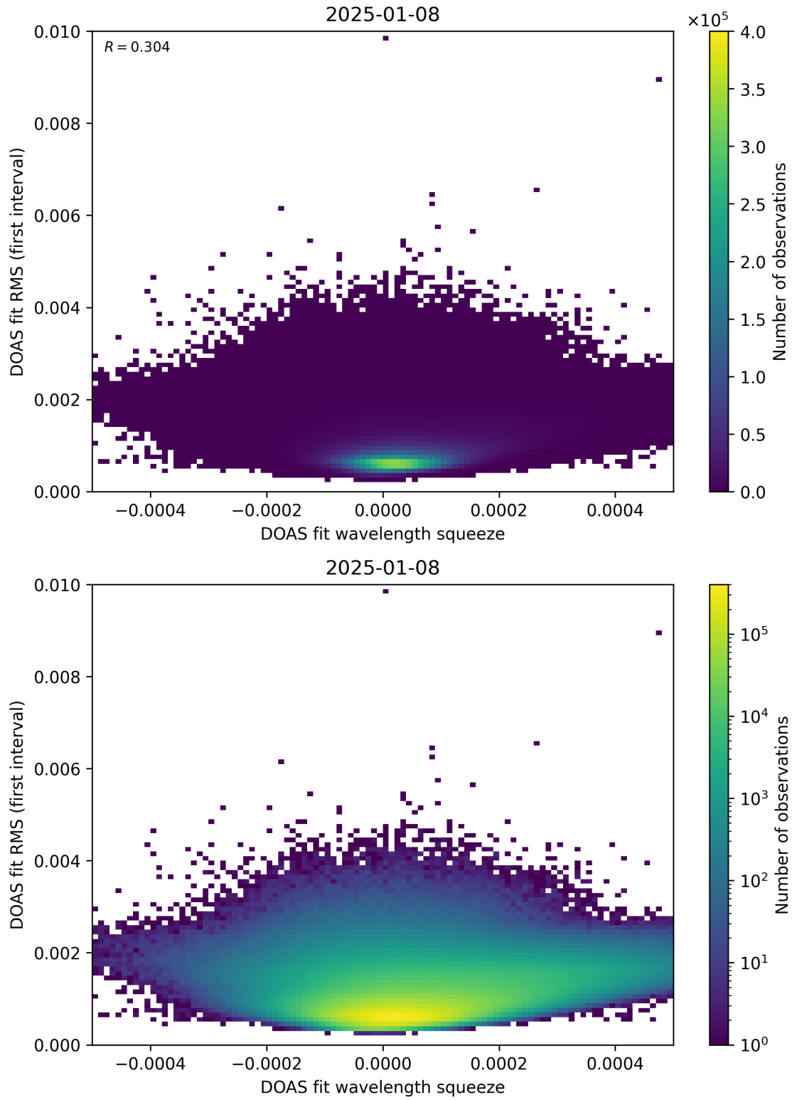
Figure 68: Scatter density plot of “DOAS fit wavelength squeeze” against “DOAS fit RMS (first interval)” for 2025-01-07 to 2025-01-09.
