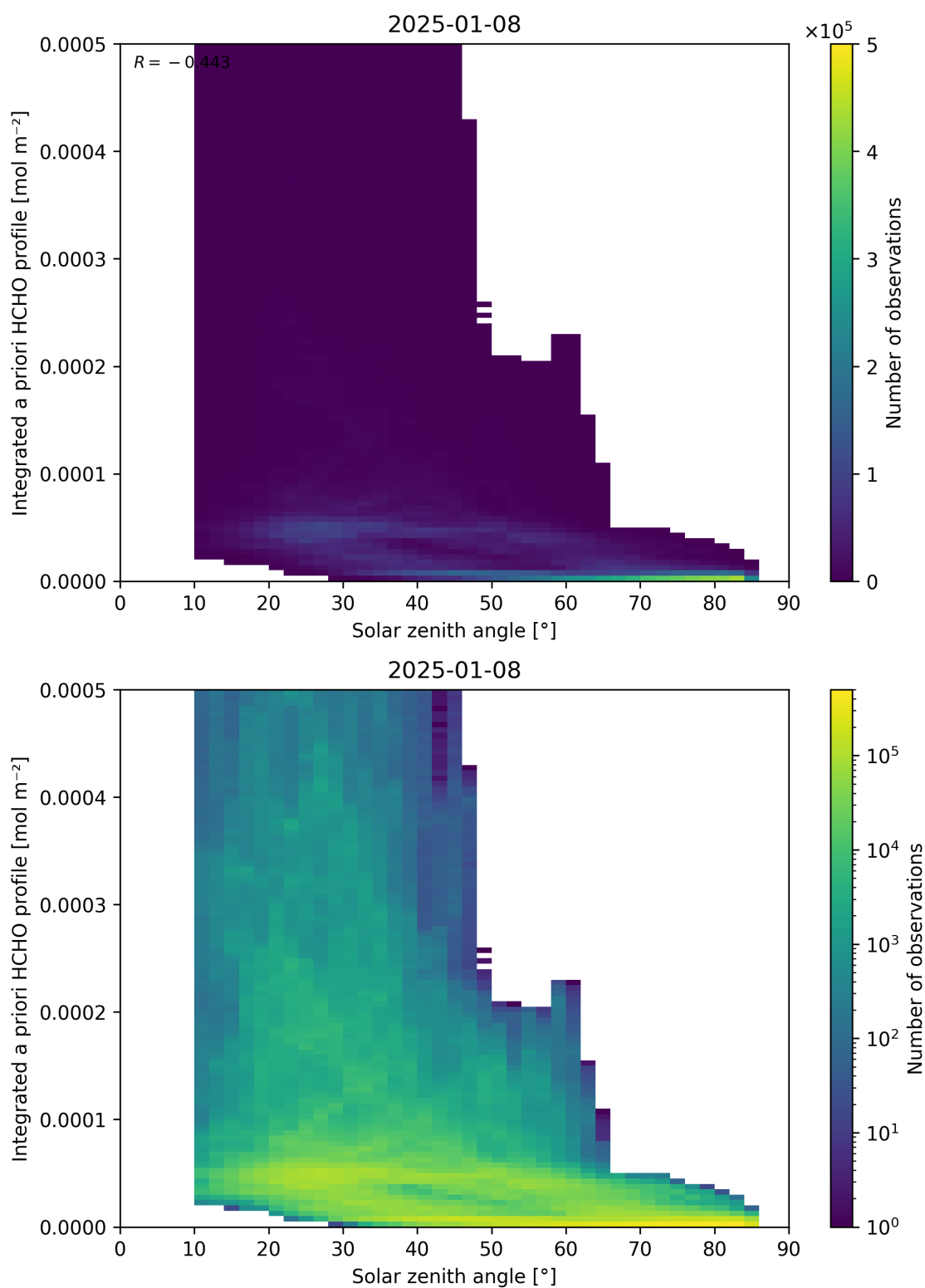
Figure 180: Scatter density plot of “Solar zenith angle” against “Integrated a priori HCHO profile” for 2025-01-07 to 2025-01-09.
