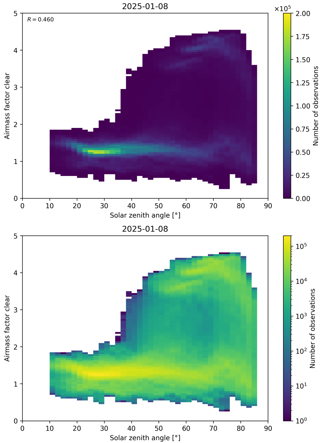
Figure 170: Scatter density plot of “Solar zenith angle” against “Airmass factor clear” for 2025-01-07 to 2025-01-09.
