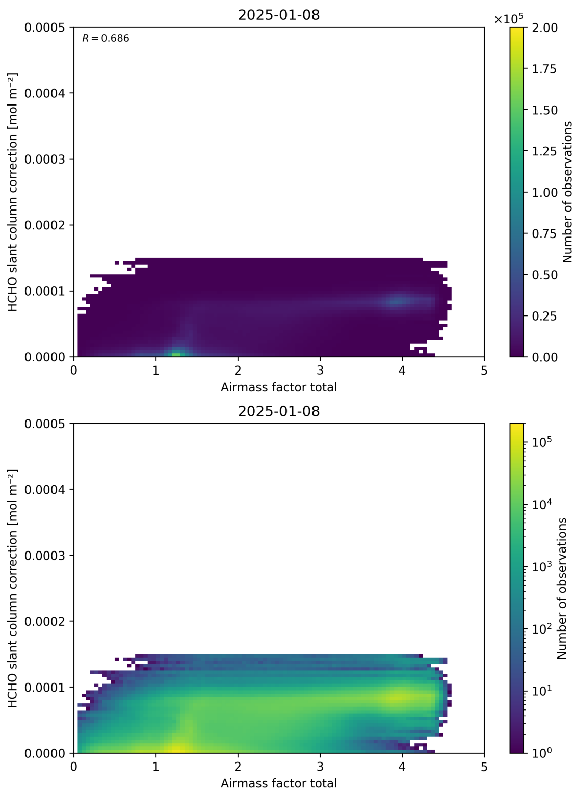
Figure 102: Scatter density plot of “Airmass factor total” against “HCHO slant column correction” for 2025-01-07 to 2025-01-09.
