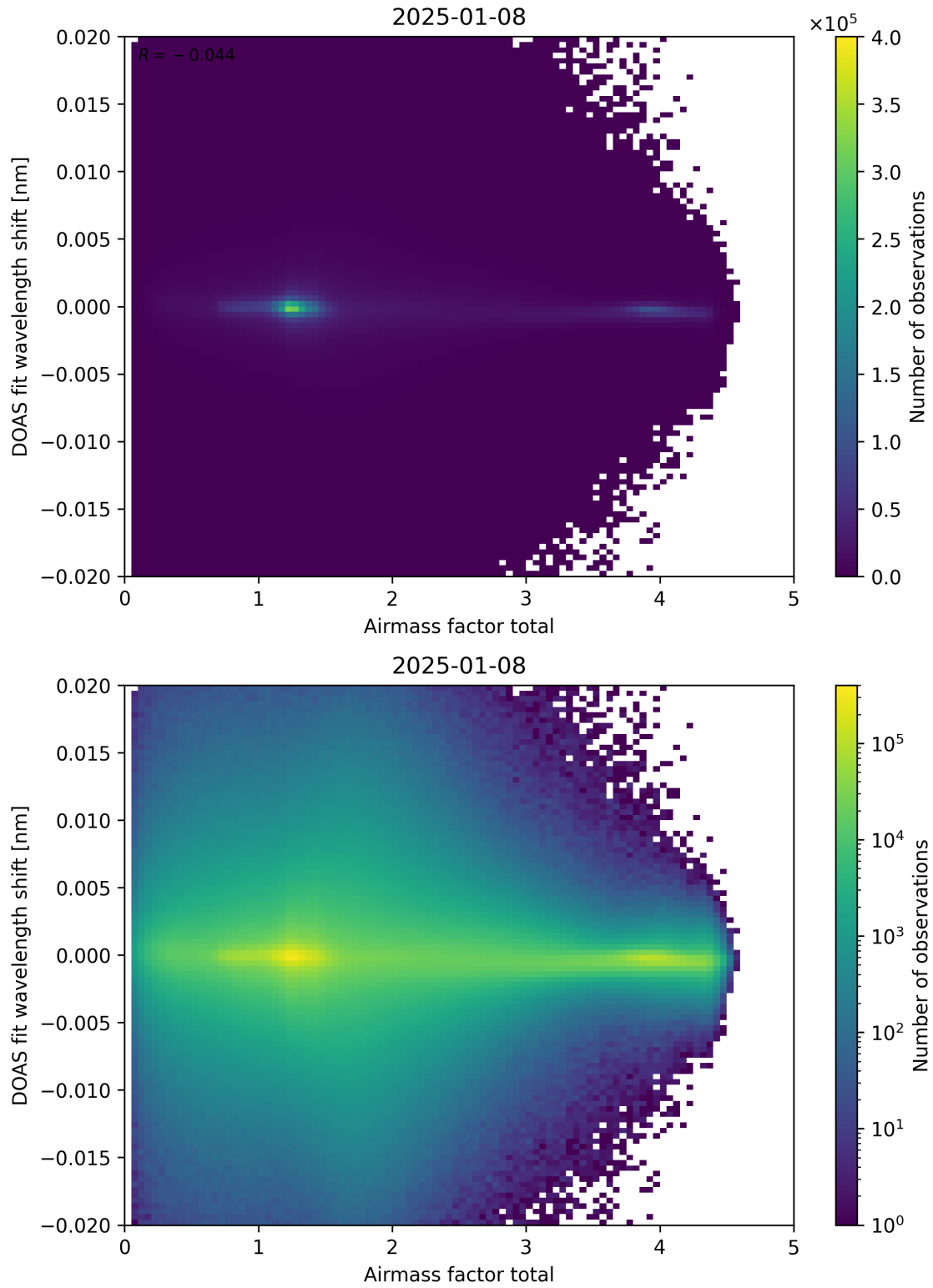
Figure 98: Scatter density plot of “Airmass factor total” against “DOAS fit wavelength shift” for 2025-01-07 to 2025-01-09.
