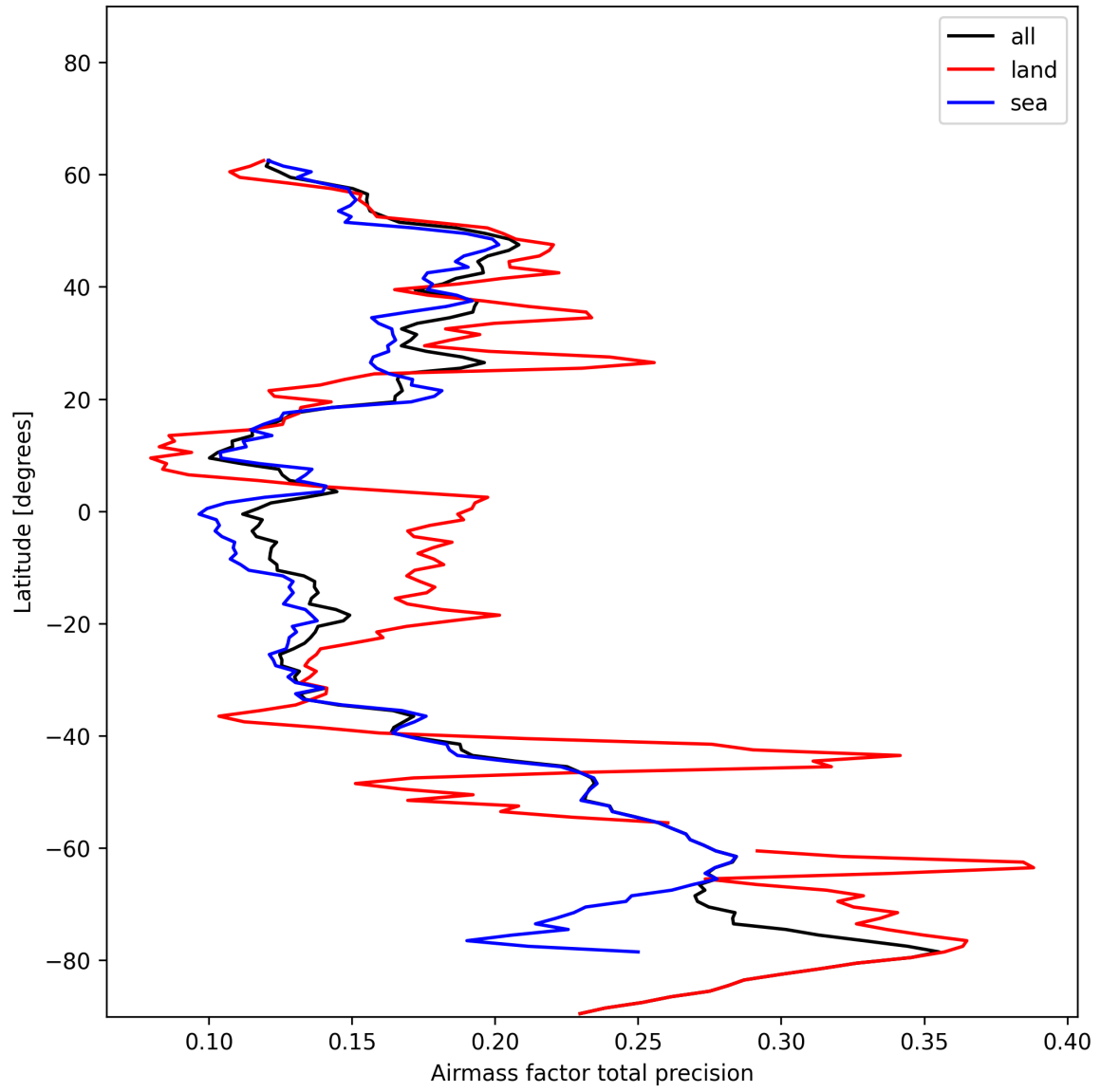
Figure 27: Zonal average of “Airmass factor total precision” for 2025-01-07 to 2025-01-09.
