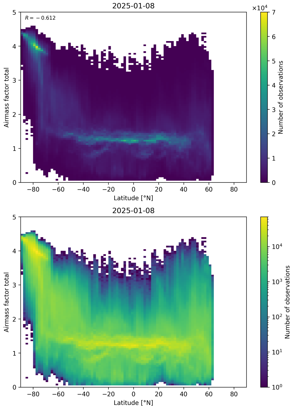
Figure 161: Scatter density plot of “Latitude” against “Airmass factor total” for 2025-01-07 to 2025-01-09.
