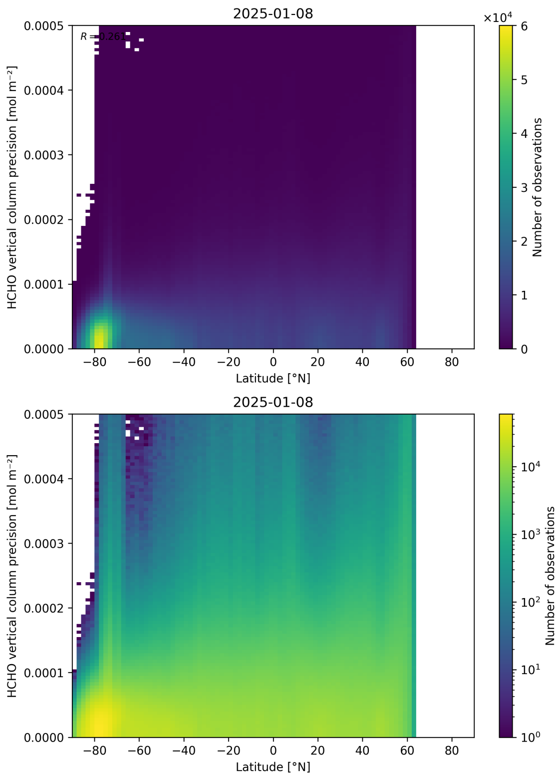
Figure 165: Scatter density plot of “Latitude” against “HCHO vertical column precision” for 2025-01-07 to 2025-01-09.
