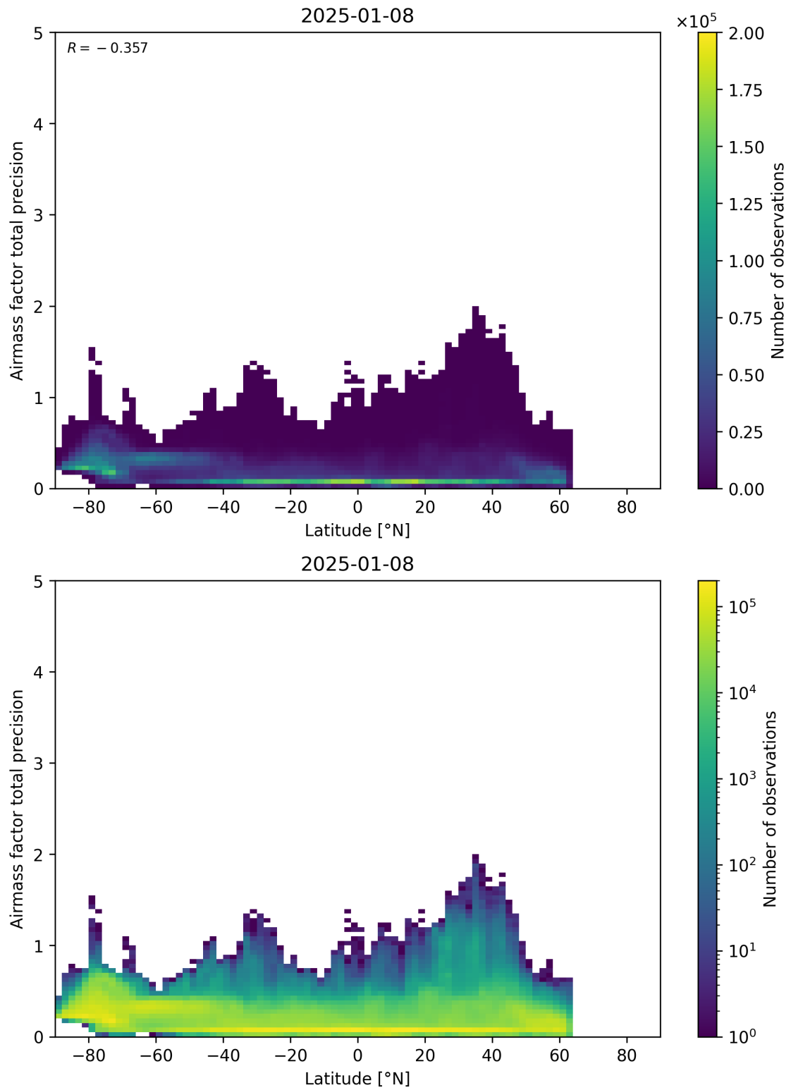
Figure 162: Scatter density plot of “Latitude” against “Airmass factor total precision” for 2025-01-07 to 2025-01-09.
