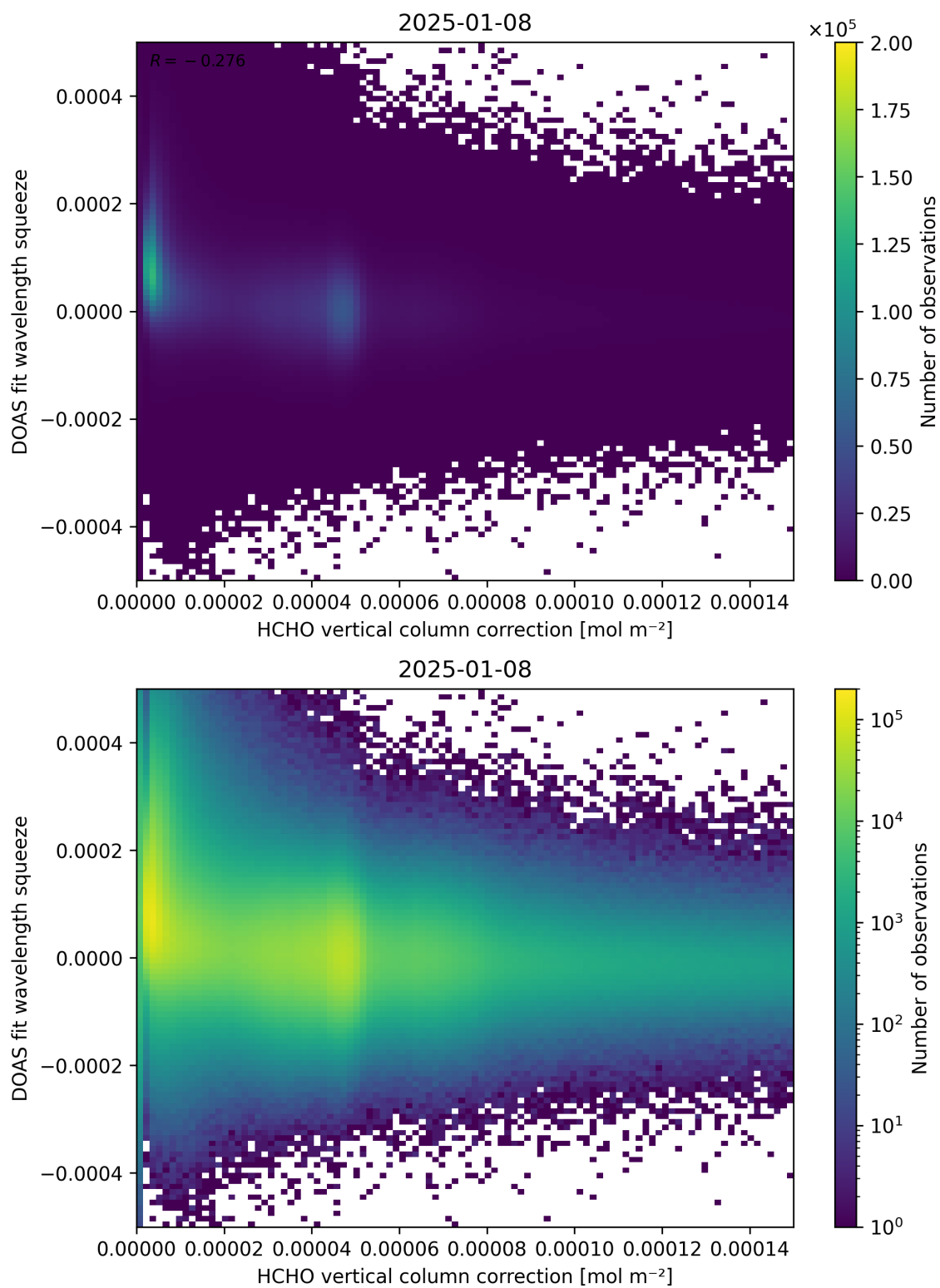
Figure 114: Scatter density plot of “HCHO vertical column correction” against “DOAS fit wavelength squeeze” for 2025-01-07 to 2025-01-09.
