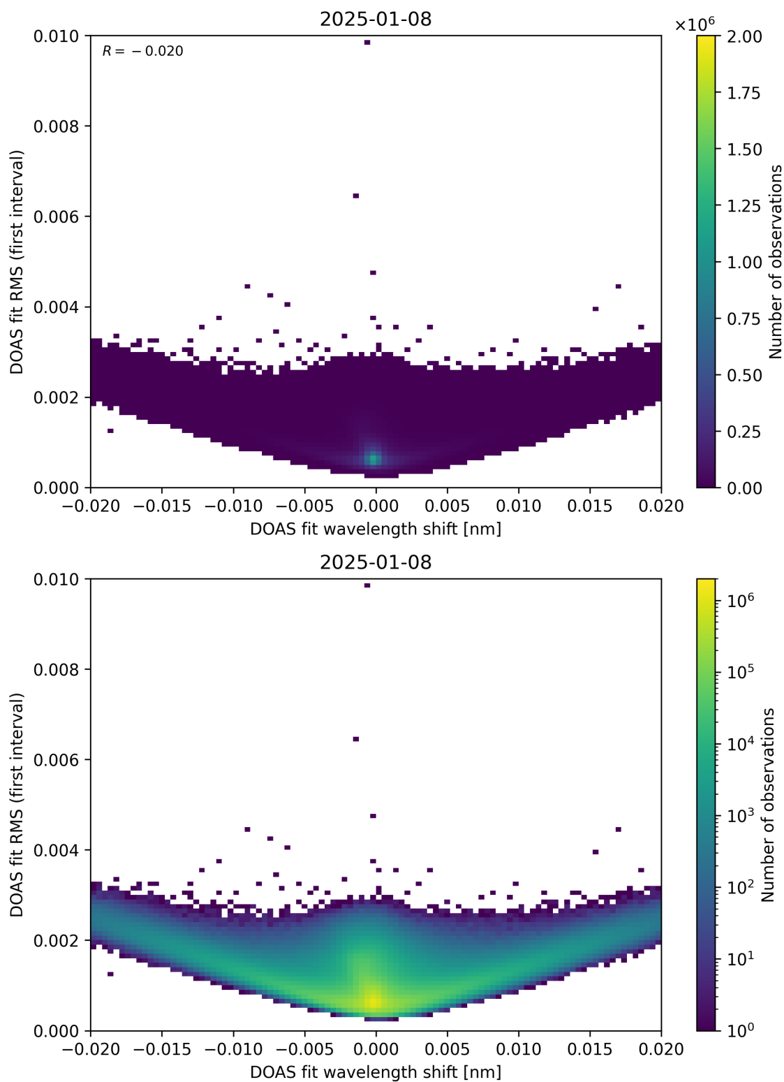
Figure 64: Scatter density plot of “DOAS fit wavelength shift” against “DOAS fit RMS (first interval)” for 2025-01-07 to 2025-01-09.
