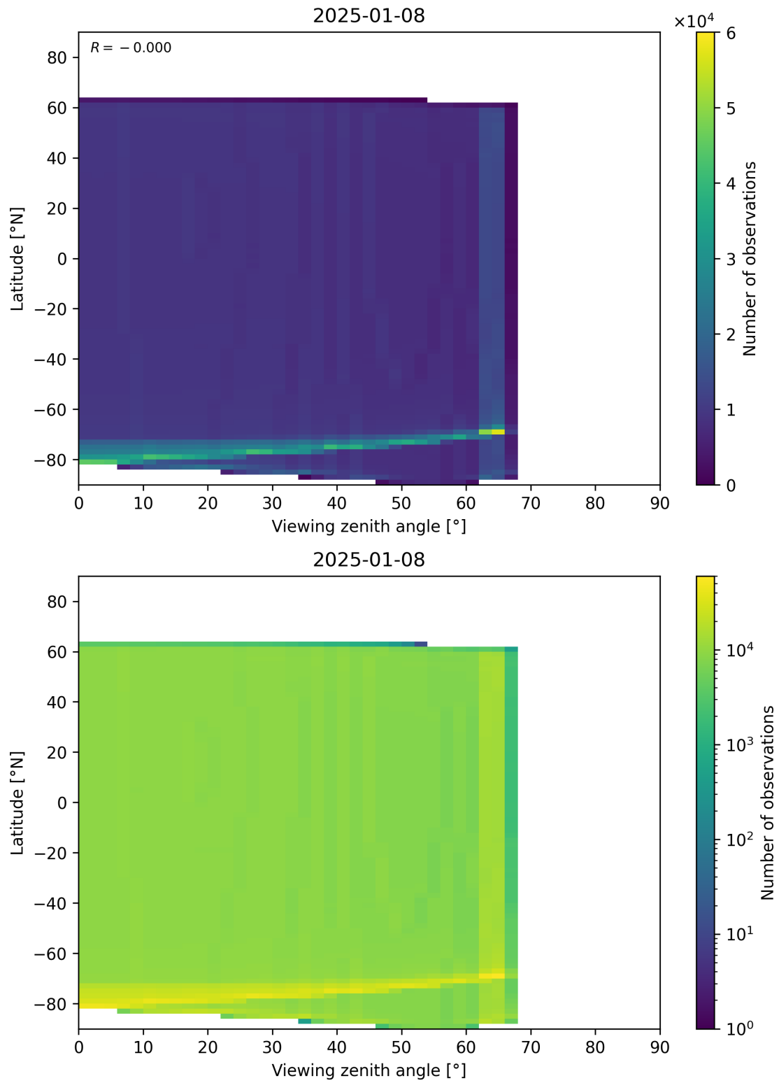
Figure 196: Scatter density plot of “Viewing zenith angle” against “Latitude” for 2025-01-07 to 2025-01-09.
