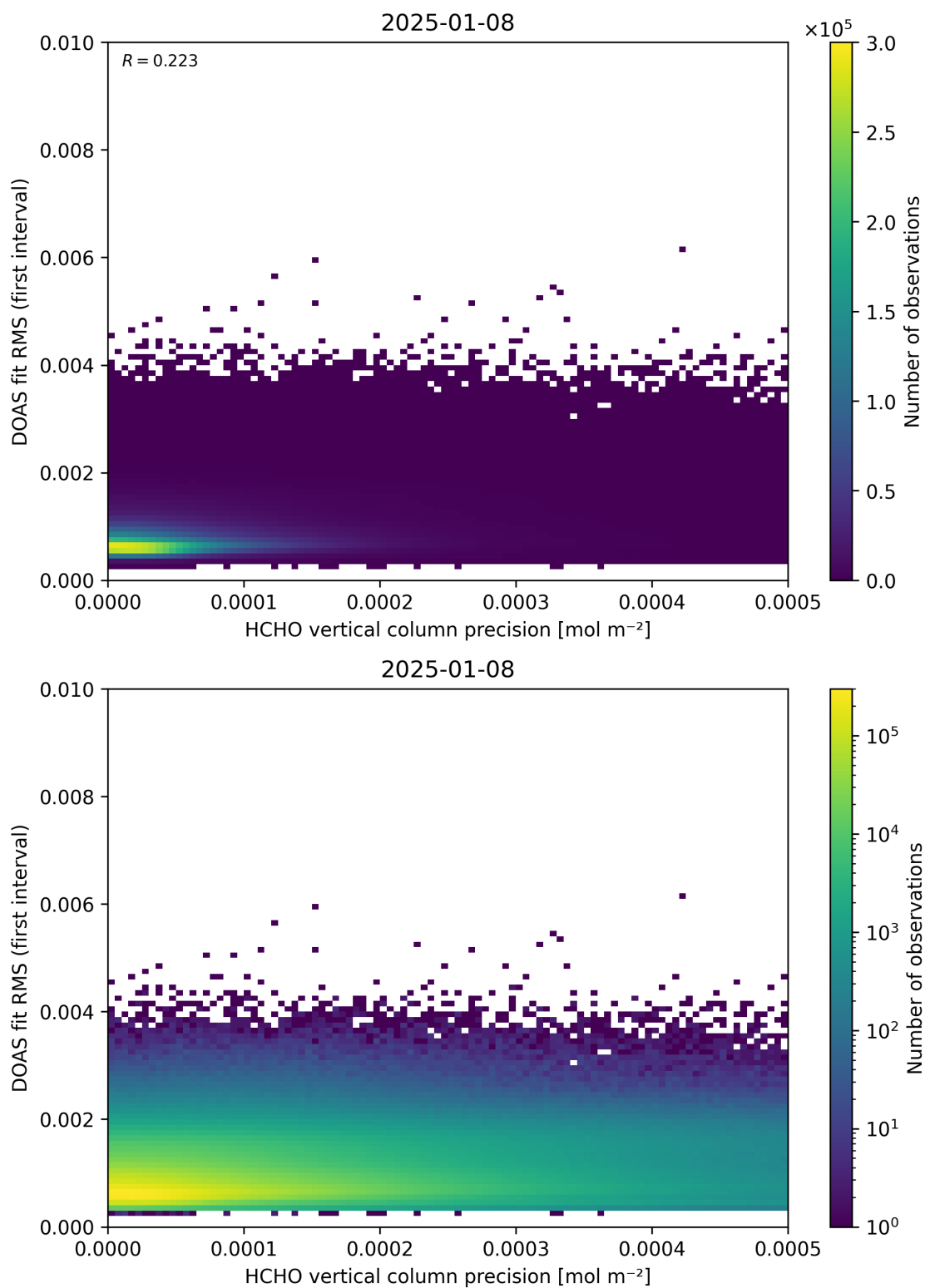
Figure 136: Scatter density plot of “HCHO vertical column precision” against “DOAS fit RMS (first interval)” for 2025-01-07 to 2025-01-09.
