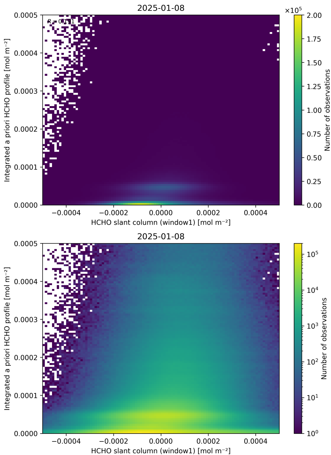
Figure 87: Scatter density plot of “HCHO slant column (window1)” against “Integrated a priori HCHO profile” for 2025-01-07 to 2025-01-09.
