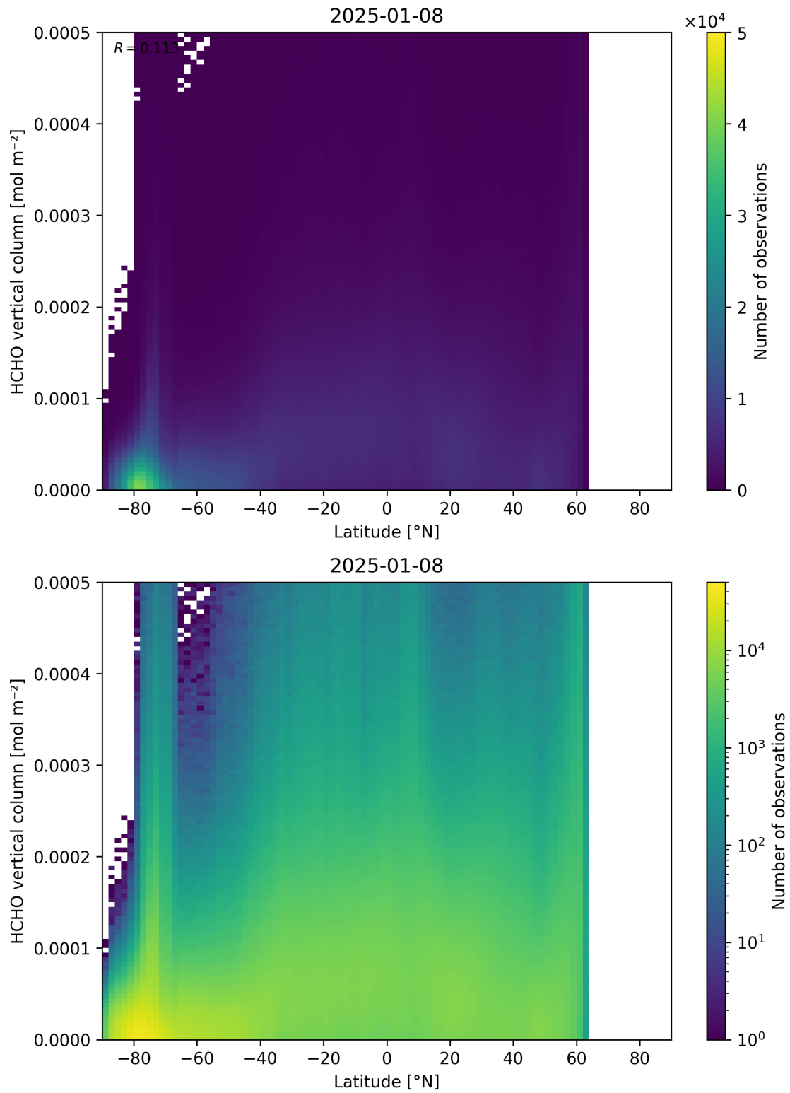
Figure 163: Scatter density plot of “Latitude” against “HCHO vertical column” for 2025-01-07 to 2025-01-09.
