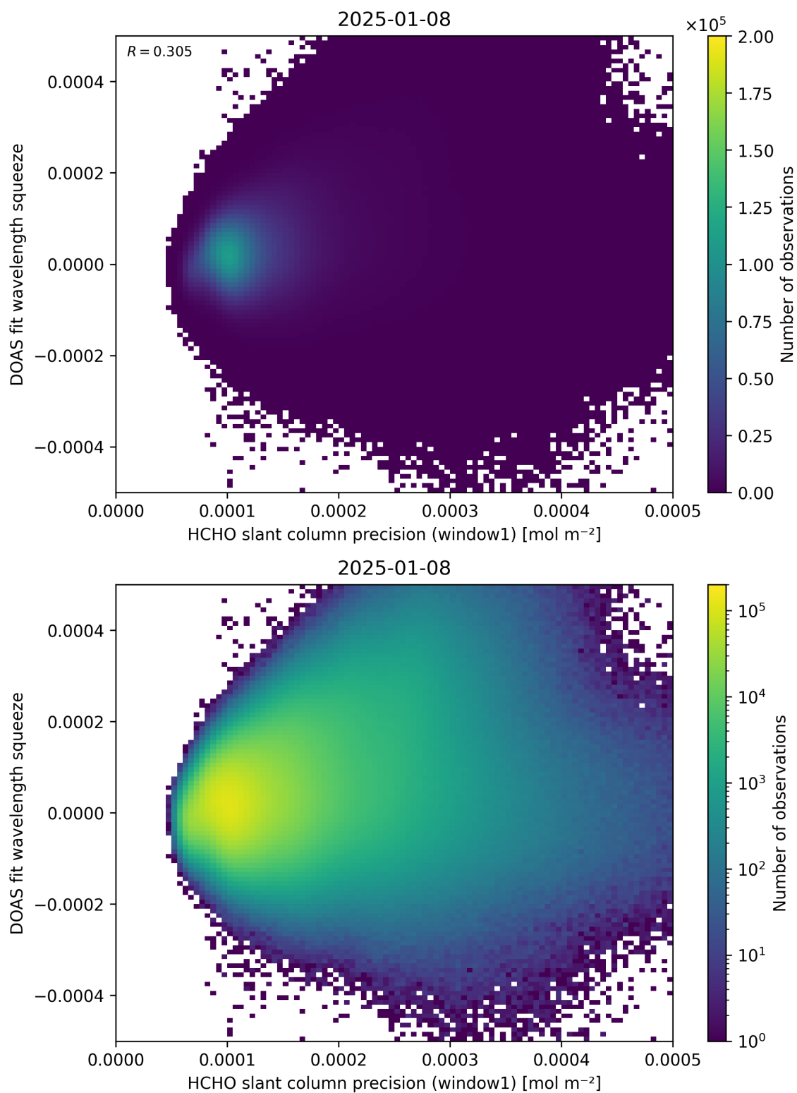
Figure 90: Scatter density plot of “HCHO slant column precision (window1)” against “DOAS fit wavelength squeeze” for 2025-01-07 to 2025-01-09.
