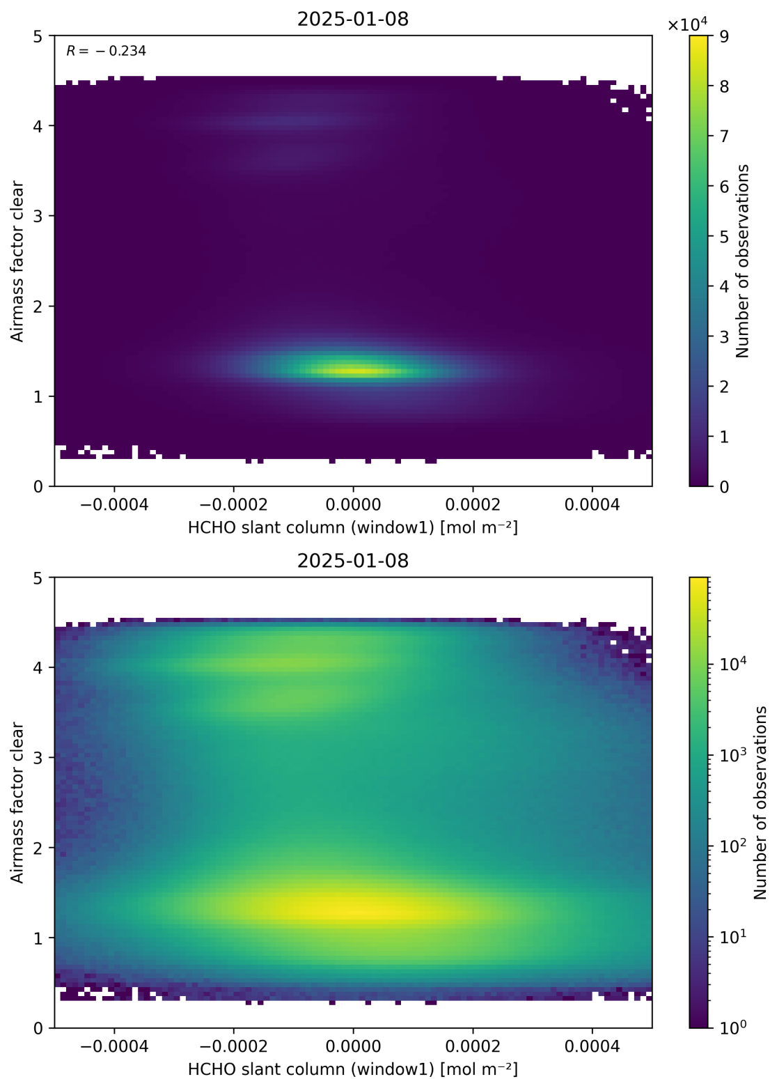
Figure 81: Scatter density plot of “HCHO slant column (window1)” against “Airmass factor clear” for 2025-01-07 to 2025-01-09.
