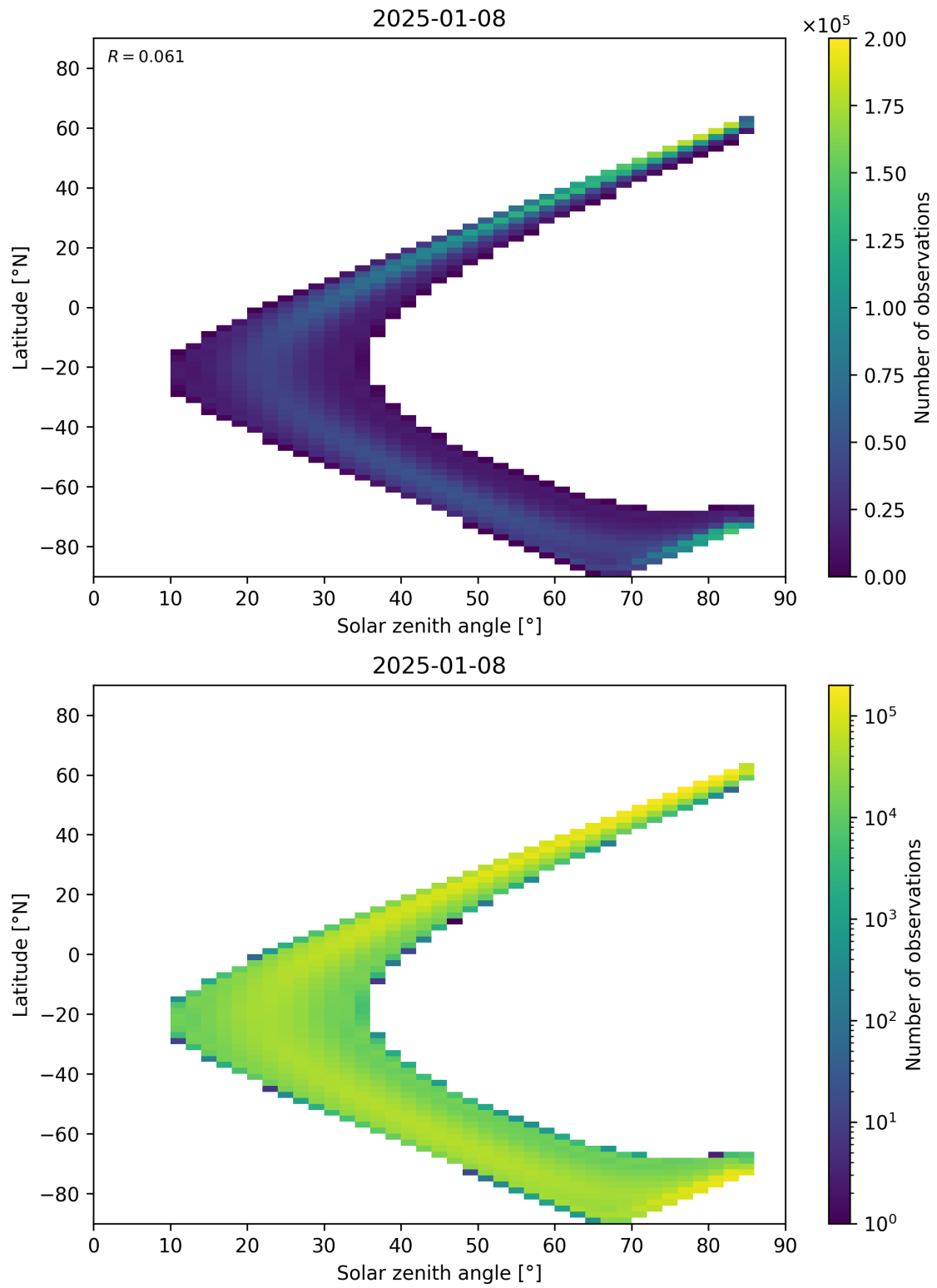
Figure 181: Scatter density plot of “Solar zenith angle” against “Latitude” for 2025-01-07 to 2025-01-09.
