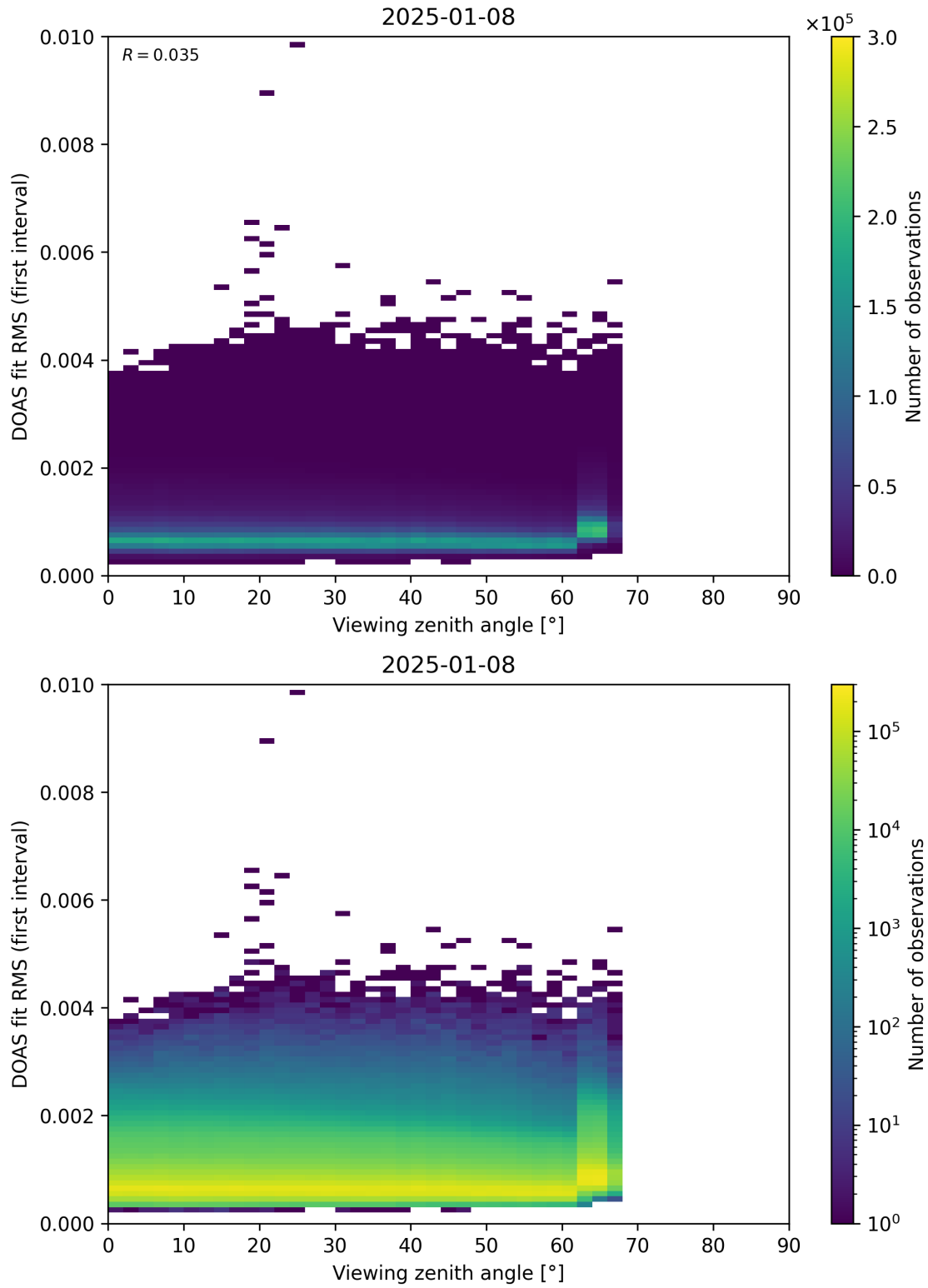
Figure 182: Scatter density plot of “Viewing zenith angle” against “DOAS fit RMS (first interval)” for 2025-01-07 to 2025-01-09.
