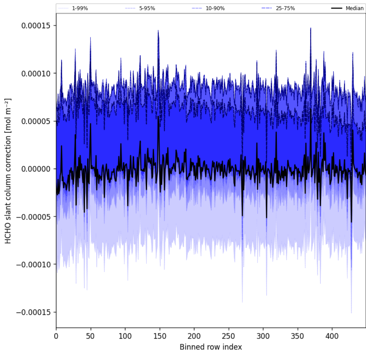
Figure 61: Along track statistics of “HCHO slant column correction” for 2025-01-07 to 2025-01-09
