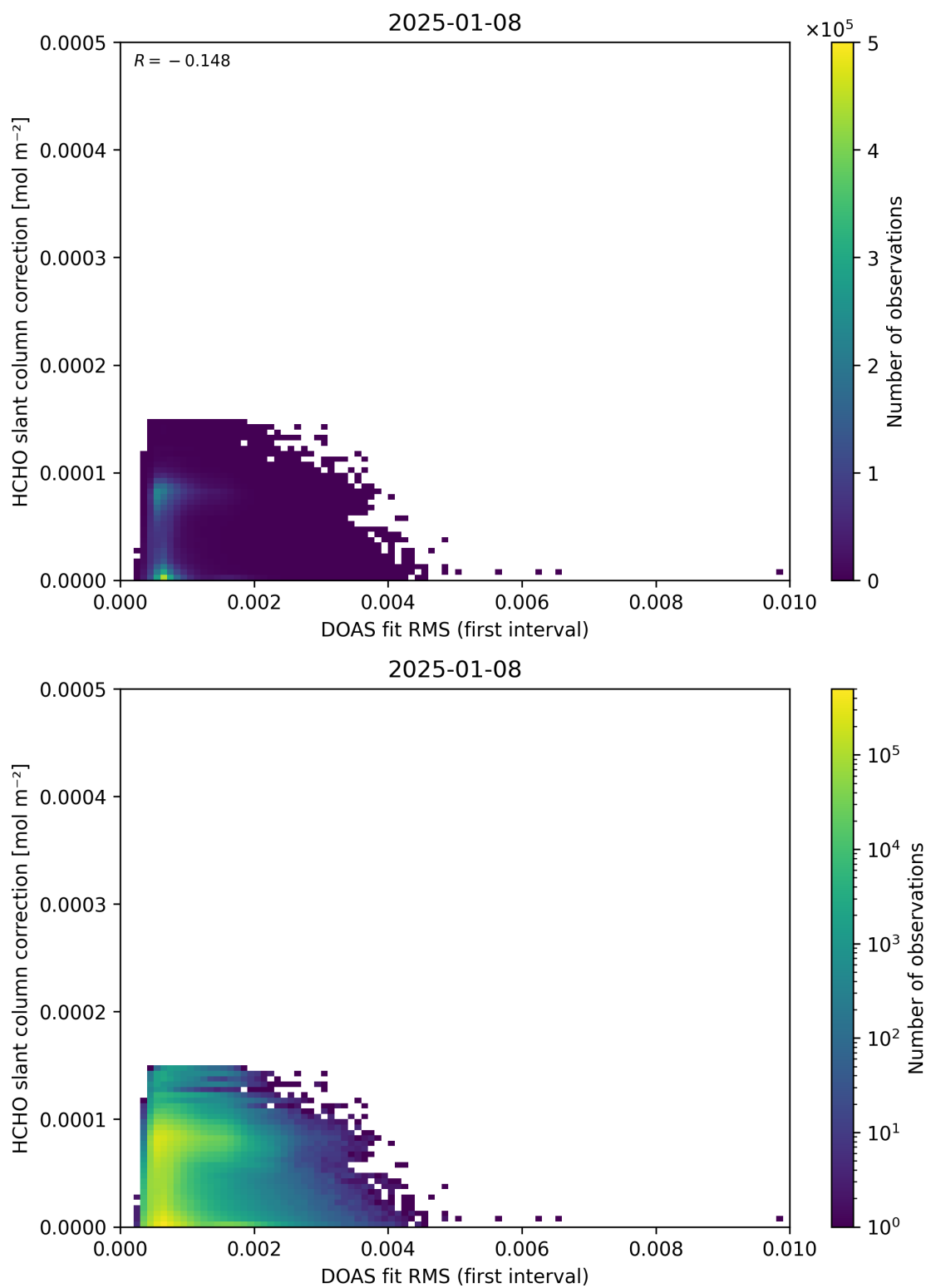
Figure 63: Scatter density plot of “DOAS fit RMS (first interval)” against “HCHO slant column correction” for 2025-01-07 to 2025-01-09.
