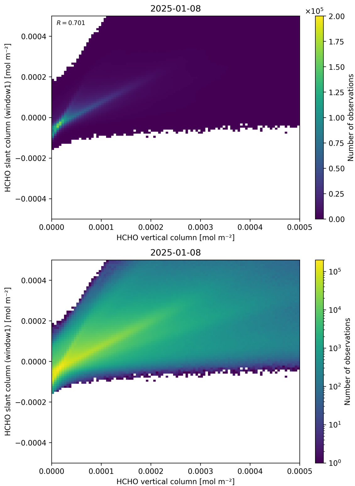
Figure 129: Scatter density plot of “HCHO vertical column” against “HCHO slant column (window1)” for 2025-01-07 to 2025-01-09.
