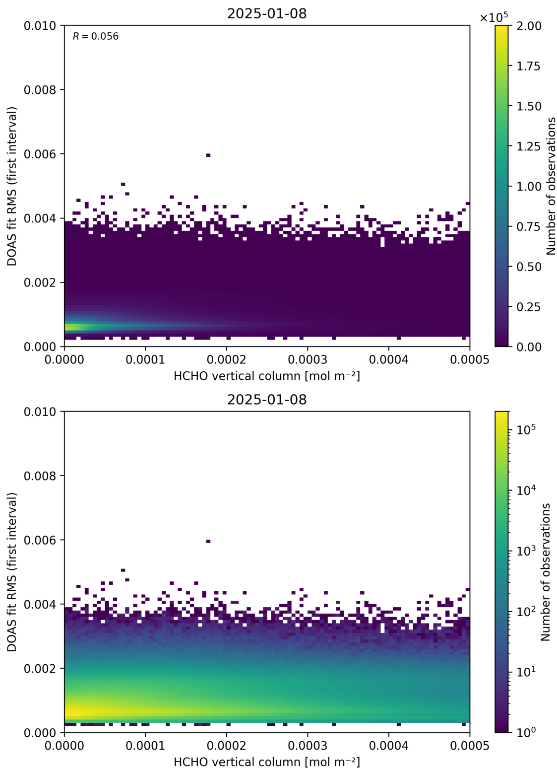
Figure 123: Scatter density plot of “HCHO vertical column” against “DOAS fit RMS (first interval)” for 2025-01-07 to 2025-01-09.
