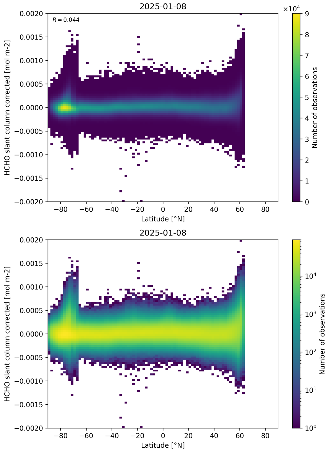
Figure 157: Scatter density plot of “Latitude” against “HCHO slant column corrected” for 2025-01-07 to 2025-01-09.
