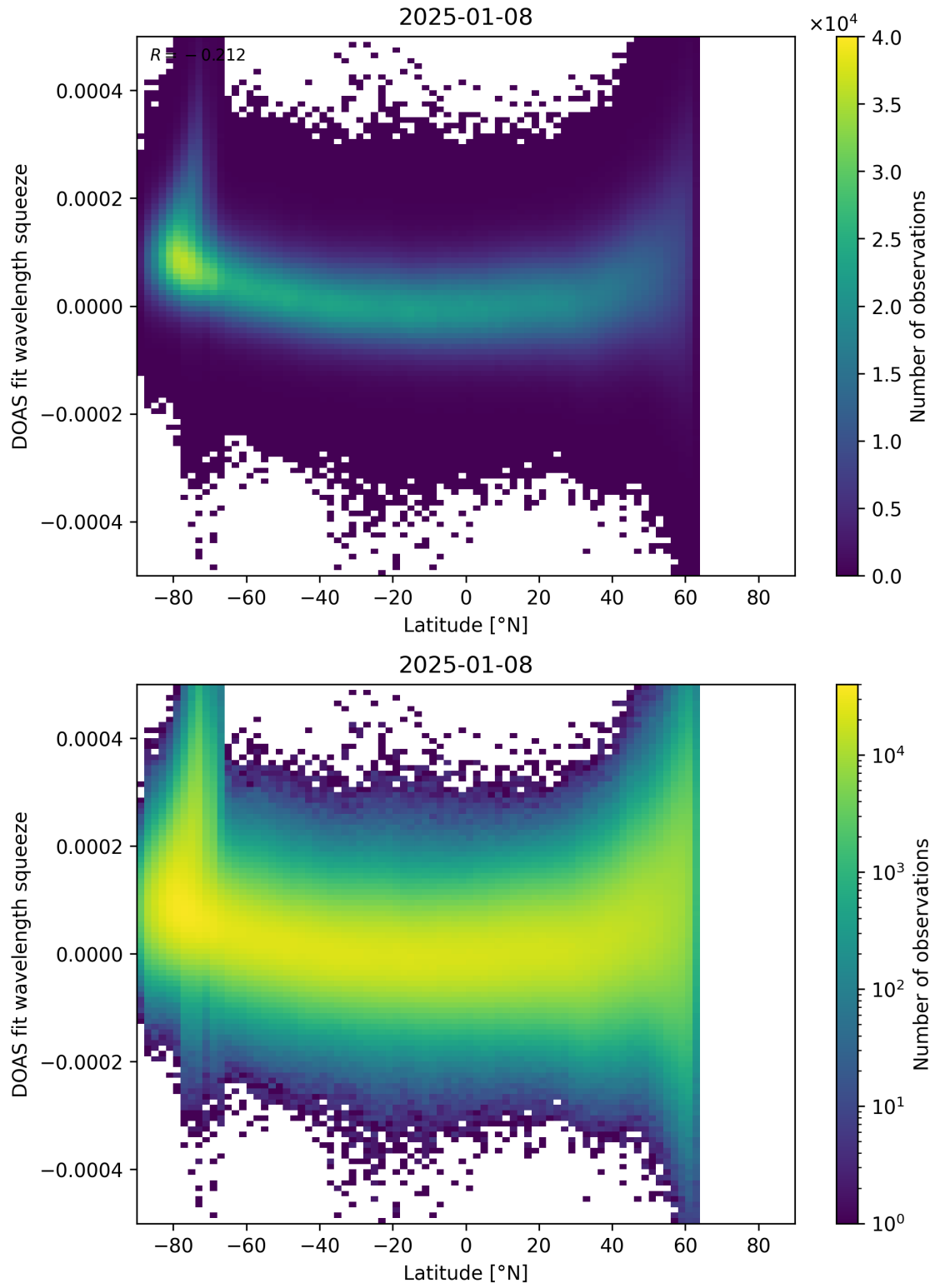
Figure 155: Scatter density plot of “Latitude” against “DOAS fit wavelength squeeze” for 2025-01-07 to 2025-01-09.
