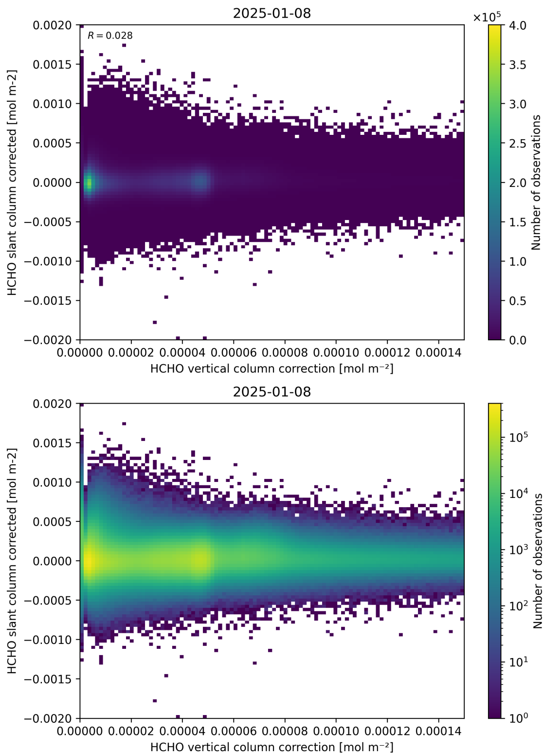
Figure 116: Scatter density plot of “HCHO vertical column correction” against “HCHO slant column corrected” for 2025-01-07 to 2025-01-09.
