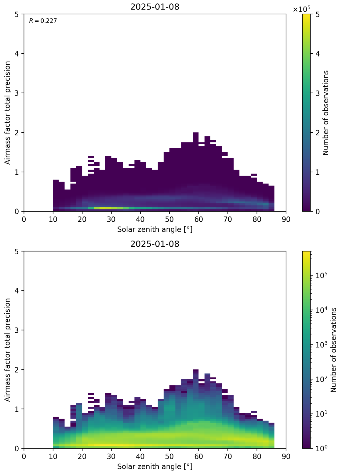
Figure 176: Scatter density plot of “Solar zenith angle” against “Airmass factor total precision” for 2025-01-07 to 2025-01-09.
