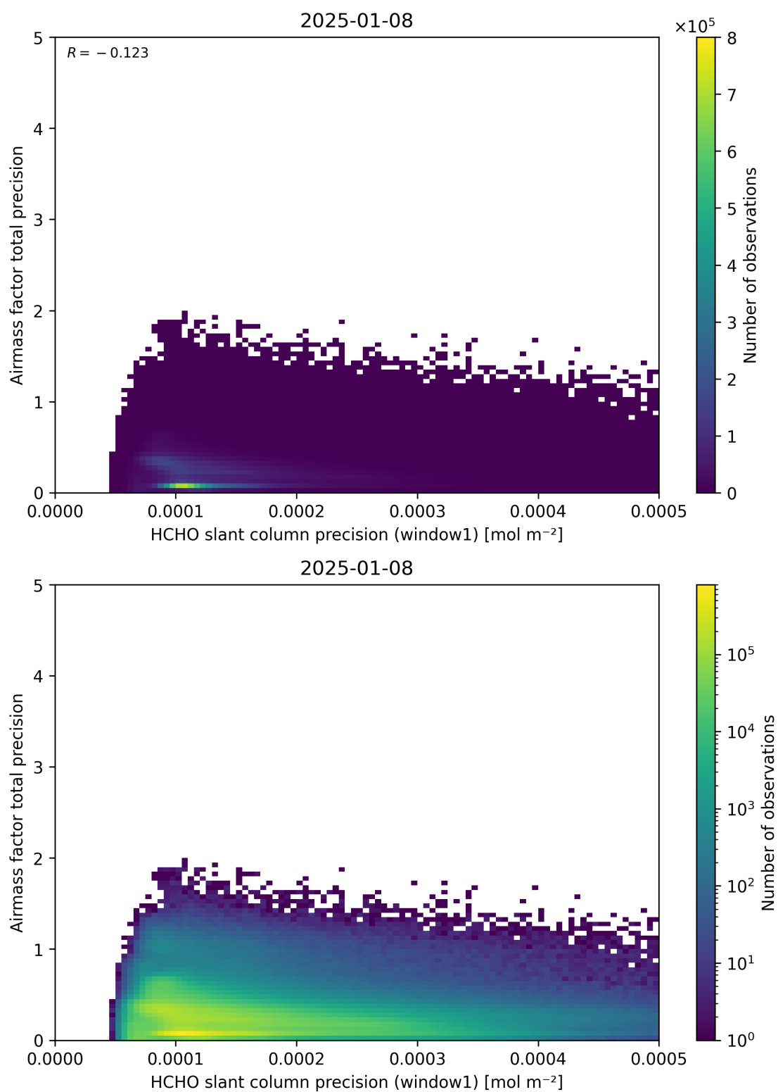
Figure 95: Scatter density plot of “HCHO slant column precision (window1)” against “Airmass factor total precision” for 2025-01-07 to 2025-01-09.
