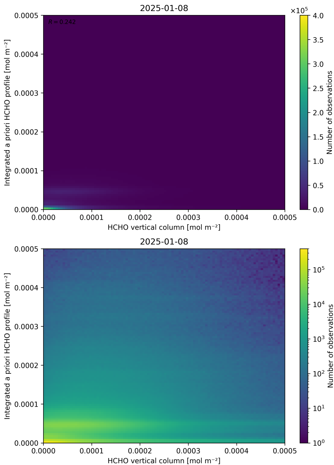
Figure 135: Scatter density plot of “HCHO vertical column” against “Integrated a priori HCHO profile” for 2025-01-07 to 2025-01-09.
