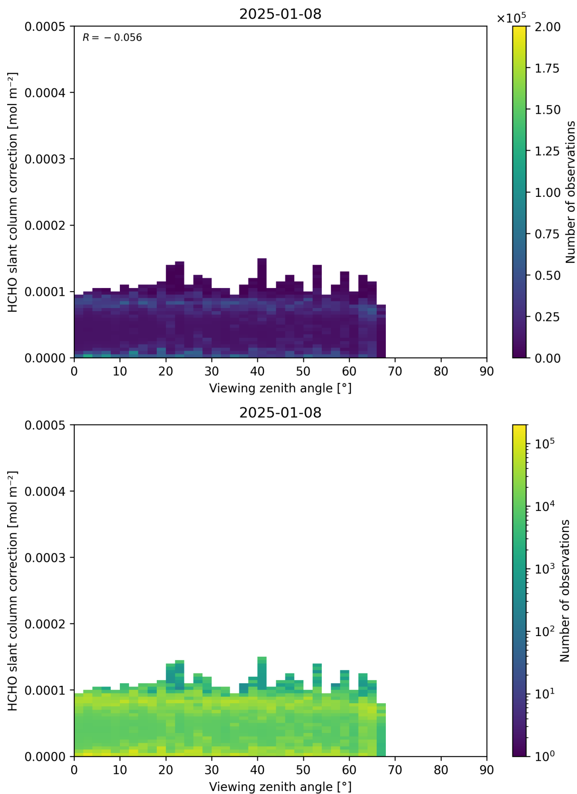
Figure 187: Scatter density plot of “Viewing zenith angle” against “HCHO slant column correction” for 2025-01-07 to 2025-01-09.
