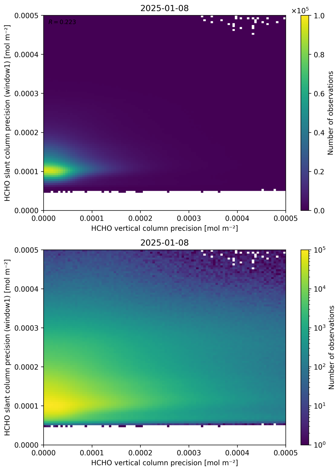
Figure 143: Scatter density plot of “HCHO vertical column precision” against “HCHO slant column precision (window1)” for 2025-01-07 to 2025-01-09.
