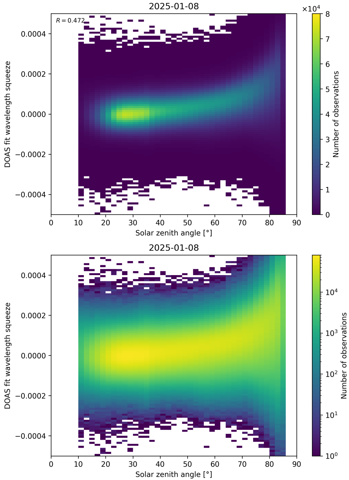
Figure 169: Scatter density plot of “Solar zenith angle” against “DOAS fit wavelength squeeze” for 2025-01-07 to 2025-01-09.
