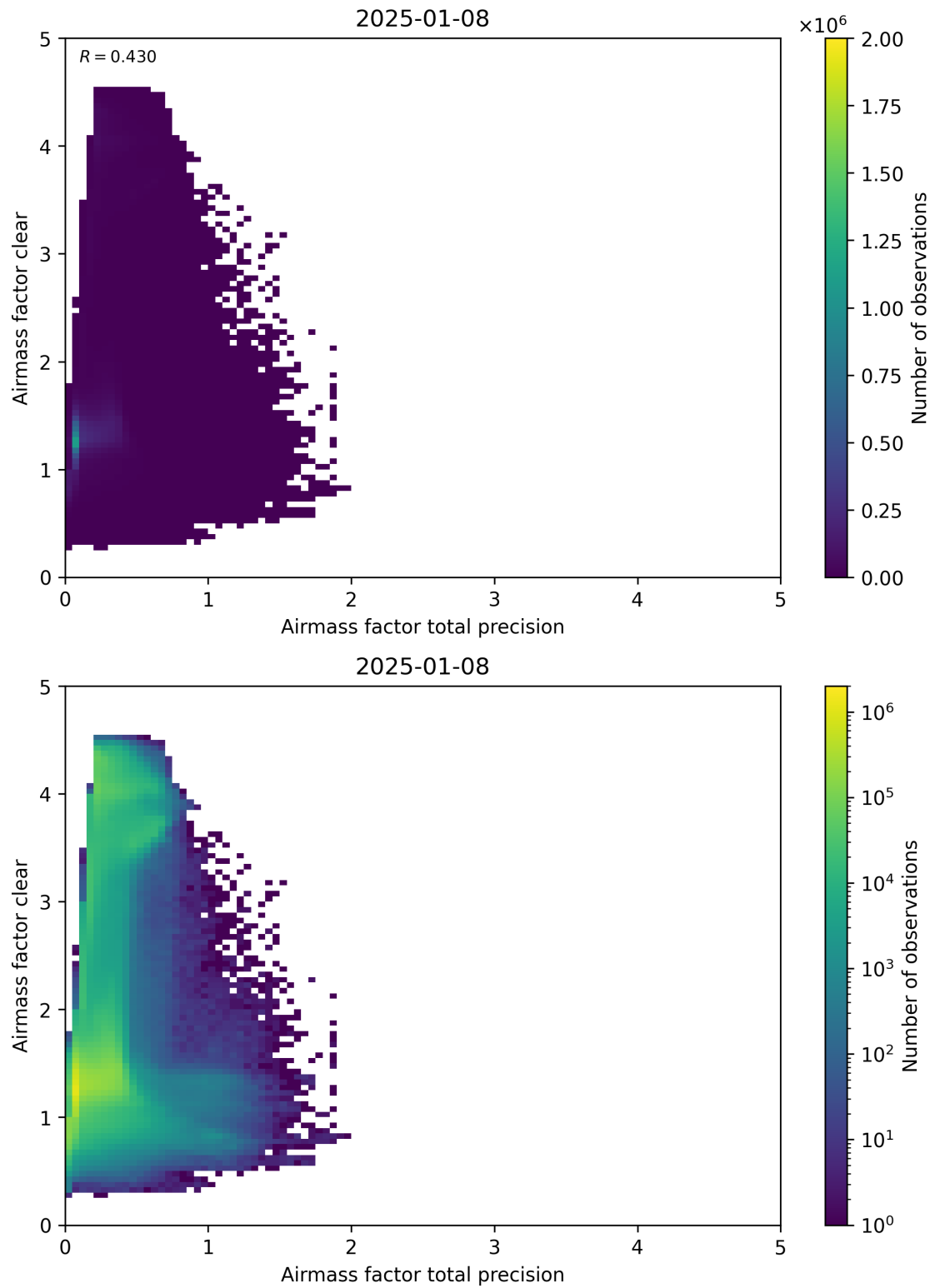
Figure 108: Scatter density plot of “Airmass factor total precision” against “Airmass factor clear” for 2025-01-07 to 2025-01-09.
