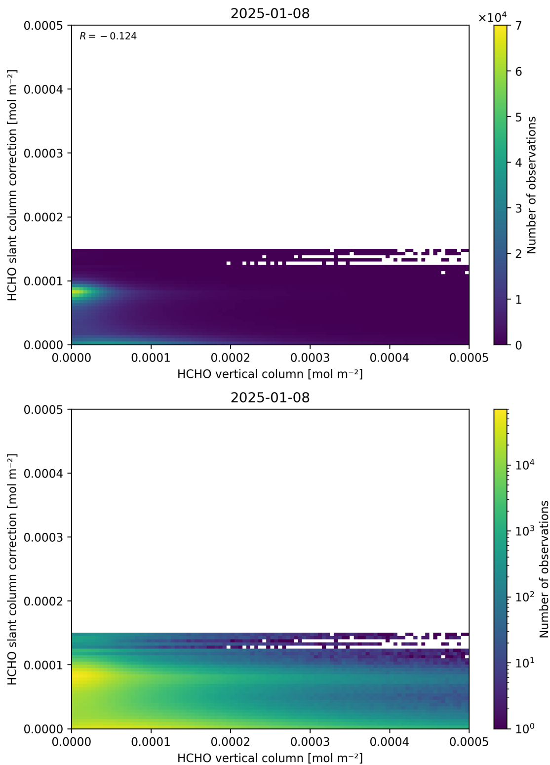
Figure 128: Scatter density plot of “HCHO vertical column” against “HCHO slant column correction” for 2025-01-07 to 2025-01-09.
