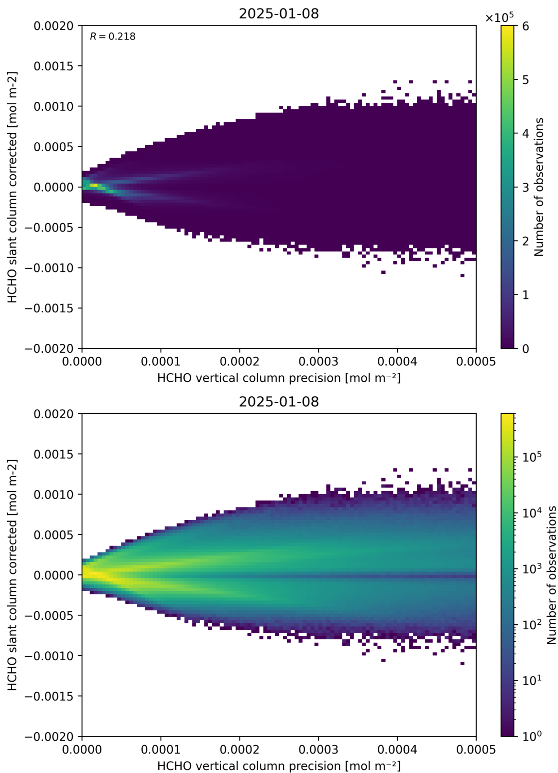
Figure 140: Scatter density plot of “HCHO vertical column precision” against “HCHO slant column corrected” for 2025-01-07 to 2025-01-09.
