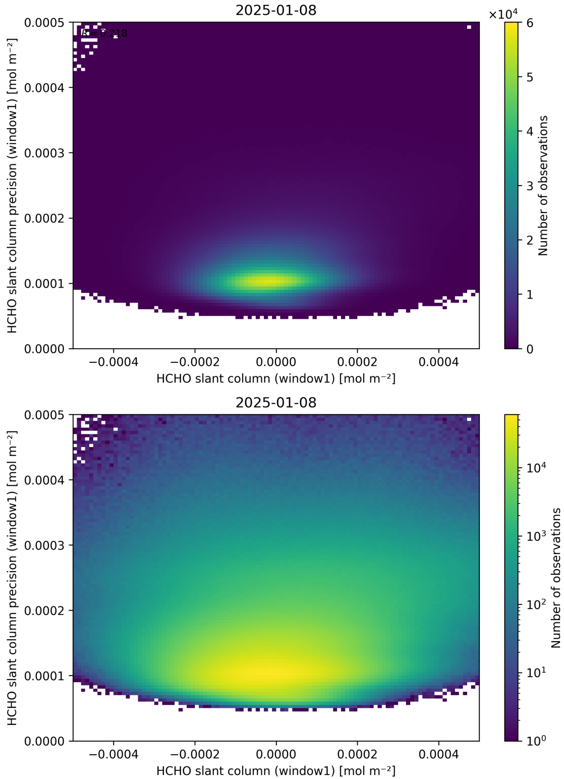
Figure 84: Scatter density plot of “HCHO slant column (window1)” against “HCHO slant column precision (window1)” for 2025-01-07 to 2025-01-09.
