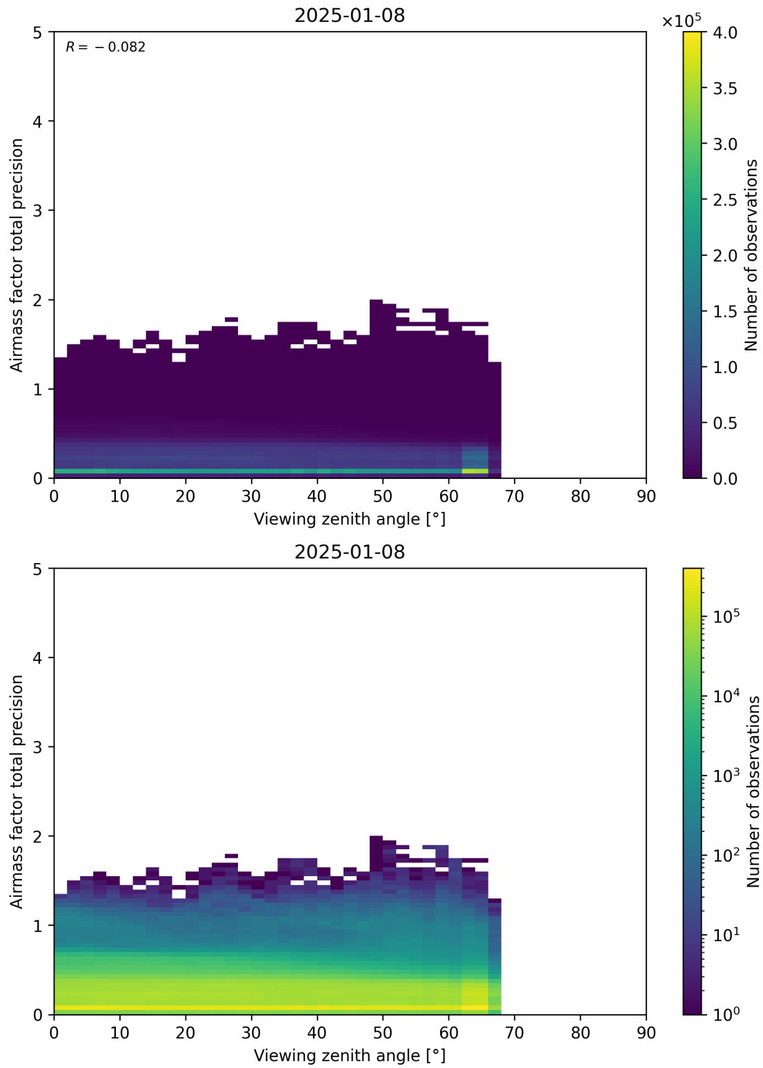
Figure 191: Scatter density plot of “Viewing zenith angle” against “Airmass factor total precision” for 2025-01-07 to 2025-01-09.
