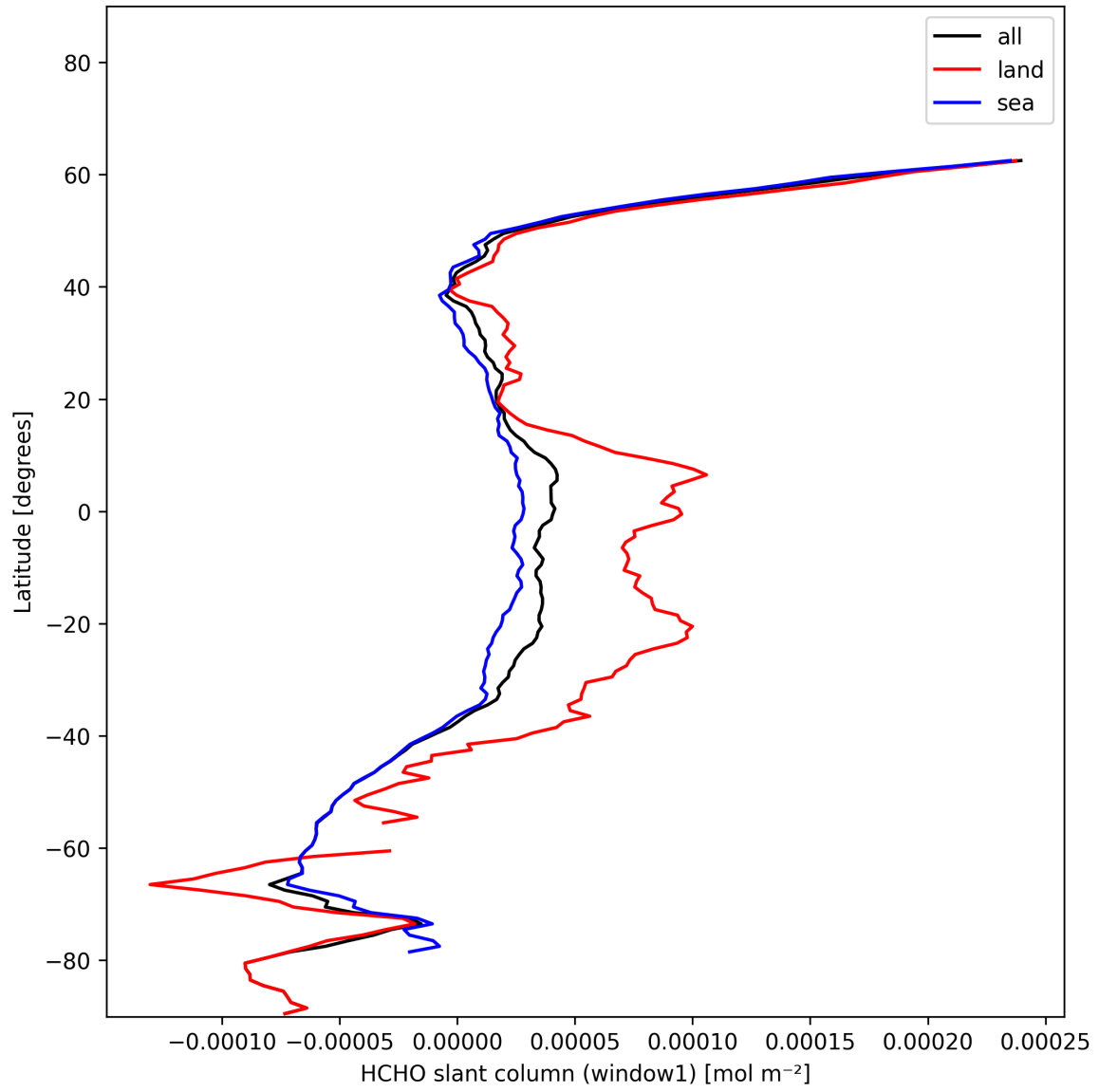
Figure 24: Zonal average of “HCHO slant column (window1)” for 2025-01-07 to 2025-01-09.
