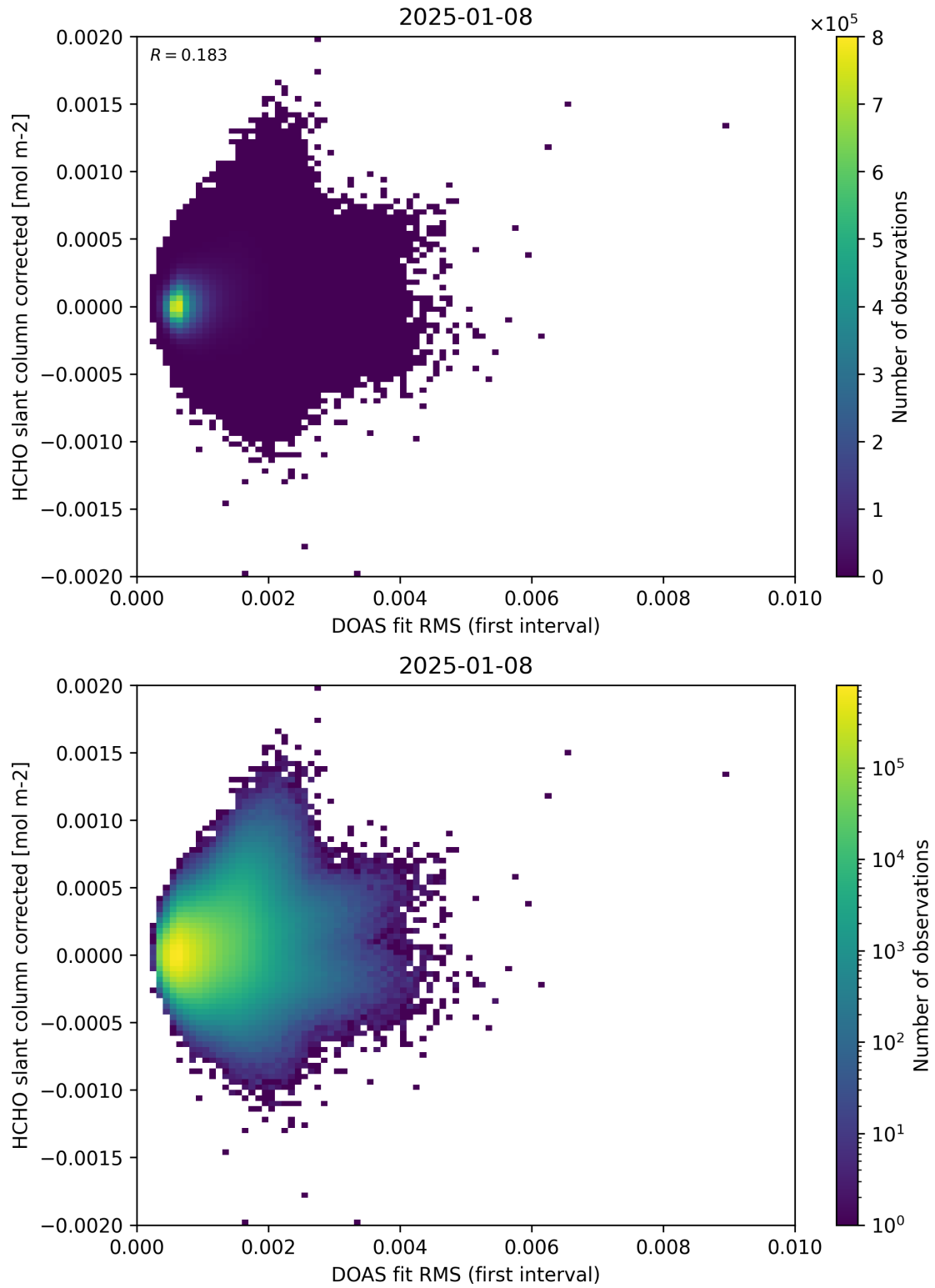
Figure 62: Scatter density plot of “DOAS fit RMS (first interval)” against “HCHO slant column corrected” for 2025-01-07 to 2025-01-09.
