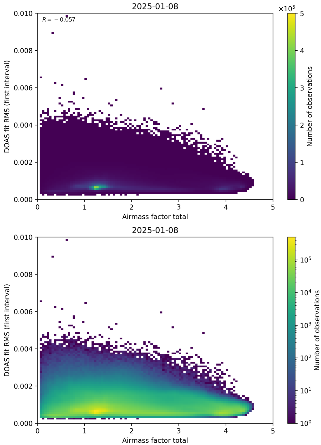
Figure 97: Scatter density plot of “Airmass factor total” against “DOAS fit RMS (first interval)” for 2025-01-07 to 2025-01-09.
