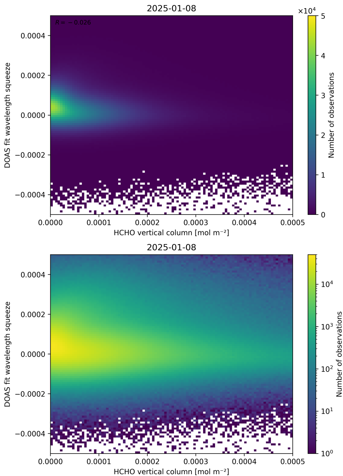
Figure 125: Scatter density plot of “HCHO vertical column” against “DOAS fit wavelength squeeze” for 2025-01-07 to 2025-01-09.
