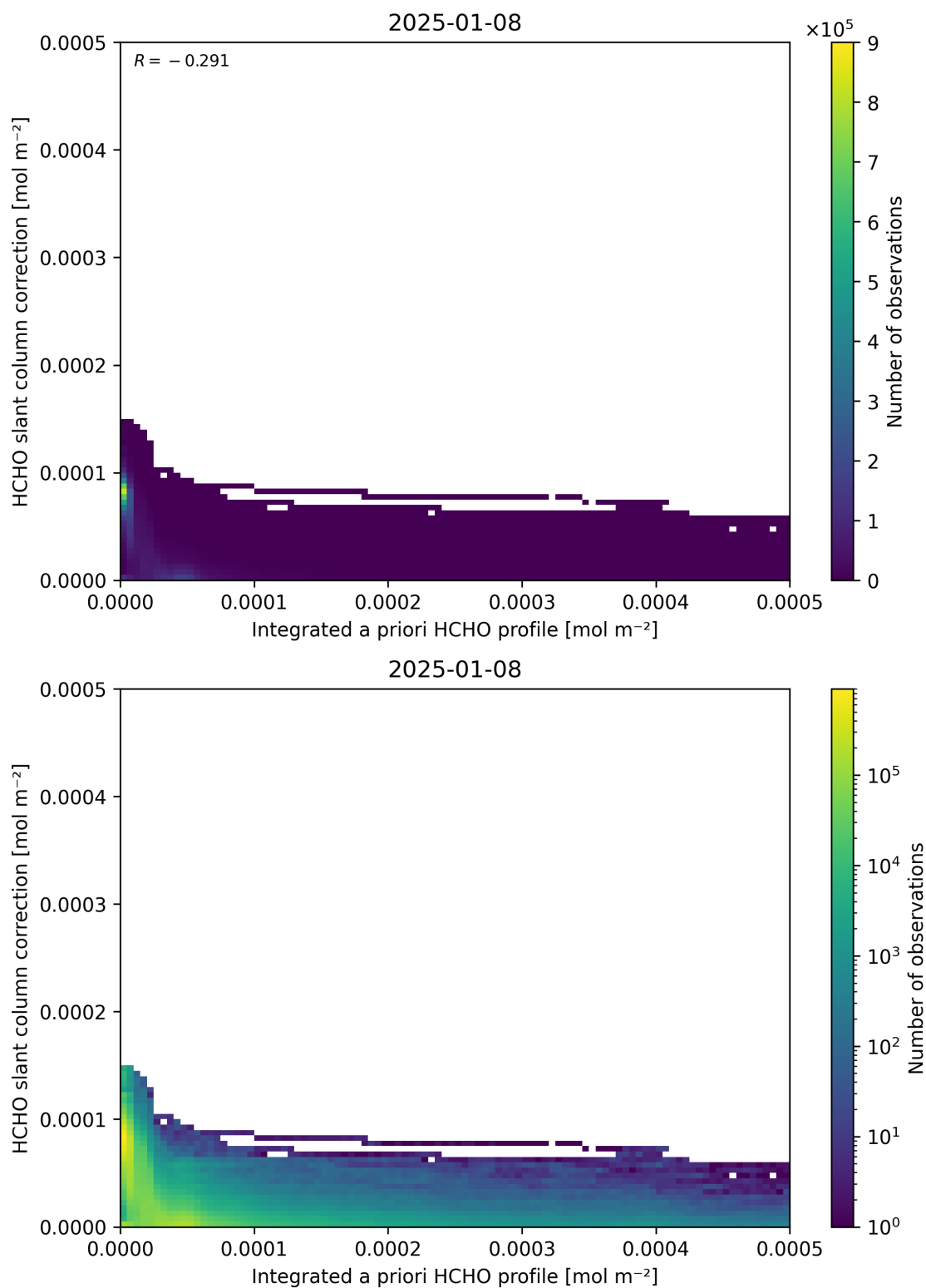
Figure 152: Scatter density plot of “Integrated a priori HCHO profile” against “HCHO slant column correction” for 2025-01-07 to 2025-01-09.
