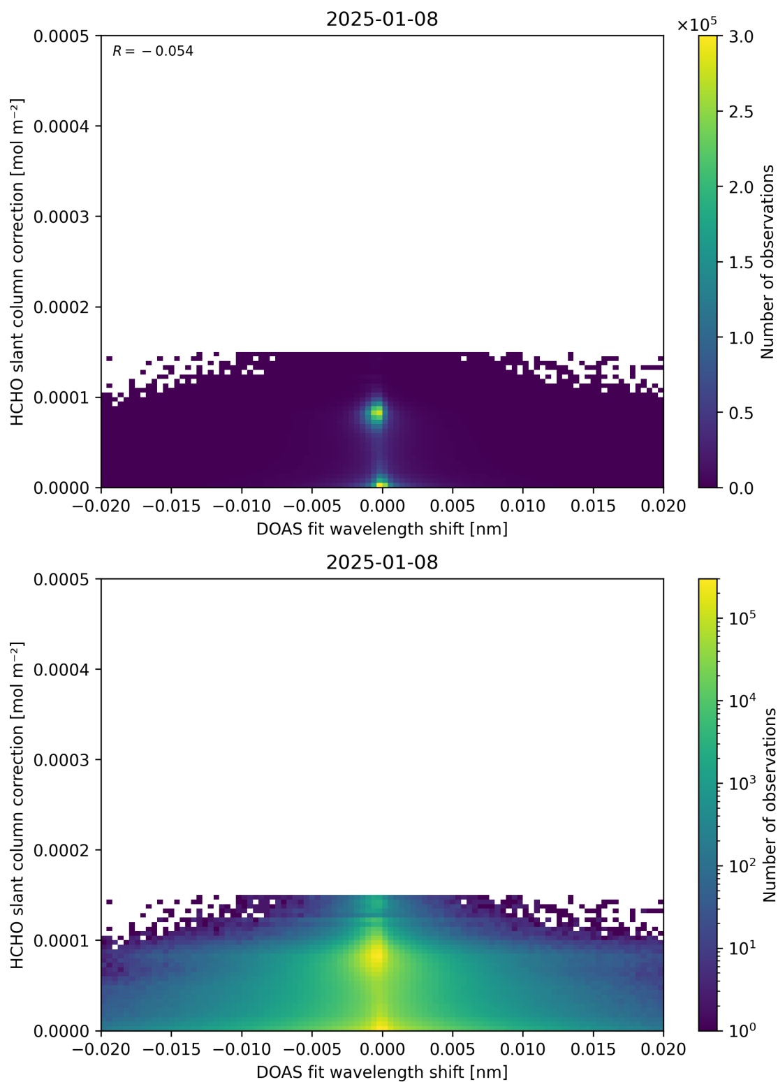
Figure 67: Scatter density plot of “DOAS fit wavelength shift” against “HCHO slant column correction” for 2025-01-07 to 2025-01-09.
