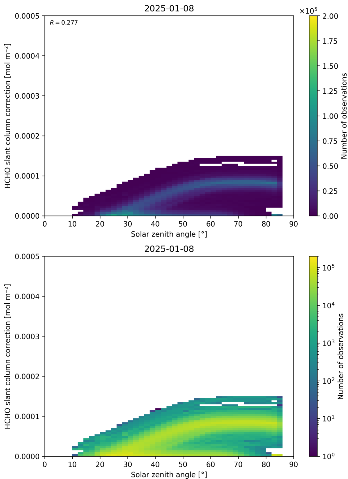
Figure 172: Scatter density plot of “Solar zenith angle” against “HCHO slant column correction” for 2025-01-07 to 2025-01-09.
