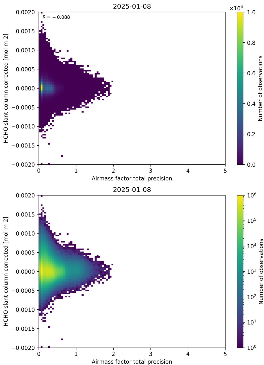
Figure 109: Scatter density plot of “Airmass factor total precision” against “HCHO slant column corrected” for 2025-01-07 to 2025-01-09.
