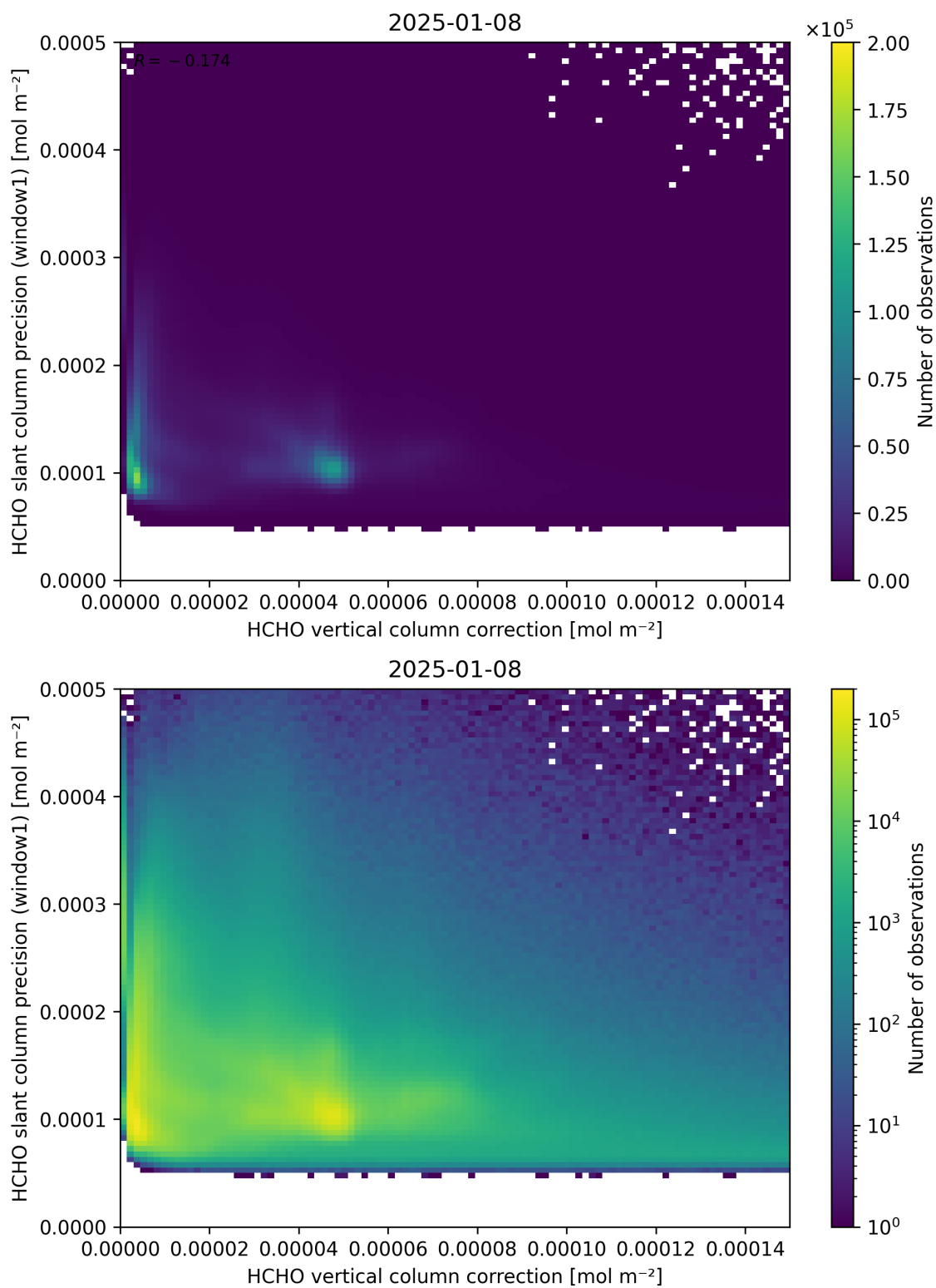
Figure 119: Scatter density plot of “HCHO vertical column correction” against “HCHO slant column precision (window1)” for 2025-01-07 to 2025-01-09.
