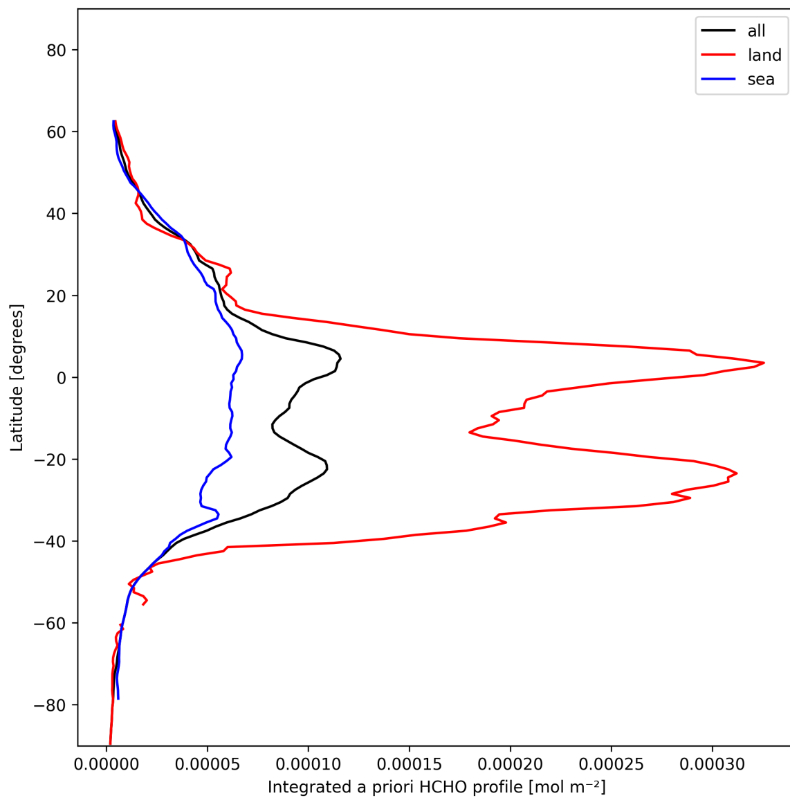
Figure 29: Zonal average of “Integrated a priori HCHO profile” for 2025-01-07 to 2025-01-09.
