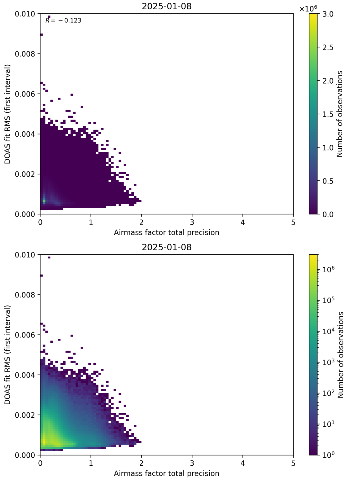
Figure 105: Scatter density plot of “Airmass factor total precision” against “DOAS fit RMS (first interval)” for 2025-01-07 to 2025-01-09.
