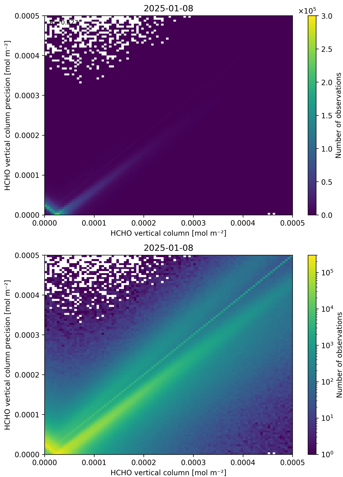
Figure 134: Scatter density plot of “HCHO vertical column” against “HCHO vertical column precision” for 2025-01-07 to 2025-01-09.
