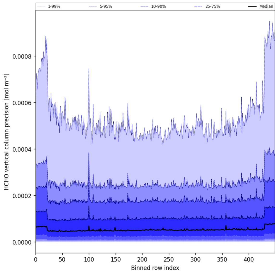
Figure 50: Along track statistics of “HCHO vertical column precision” for 2025-01-07 to 2025-01-09
