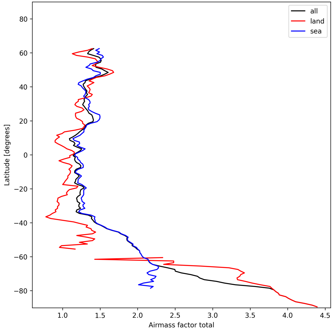
Figure 26: Zonal average of “Airmass factor total” for 2025-01-07 to 2025-01-09.
