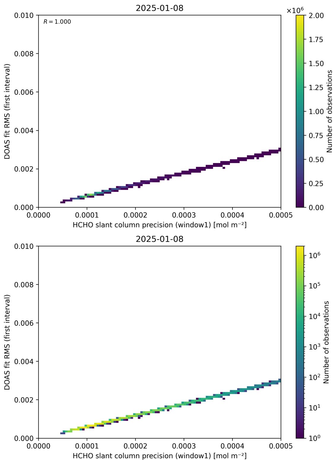
Figure 88: Scatter density plot of “HCHO slant column precision (window1)” against “DOAS fit RMS (first interval)” for 2025-01-07 to 2025-01-09.
