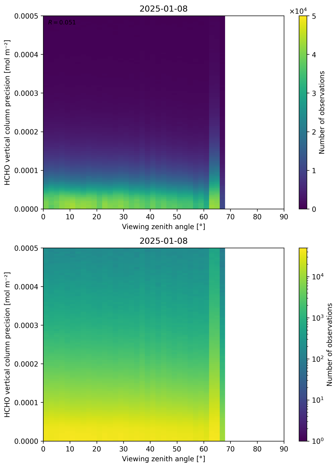
Figure 194: Scatter density plot of “Viewing zenith angle” against “HCHO vertical column precision” for 2025-01-07 to 2025-01-09.
