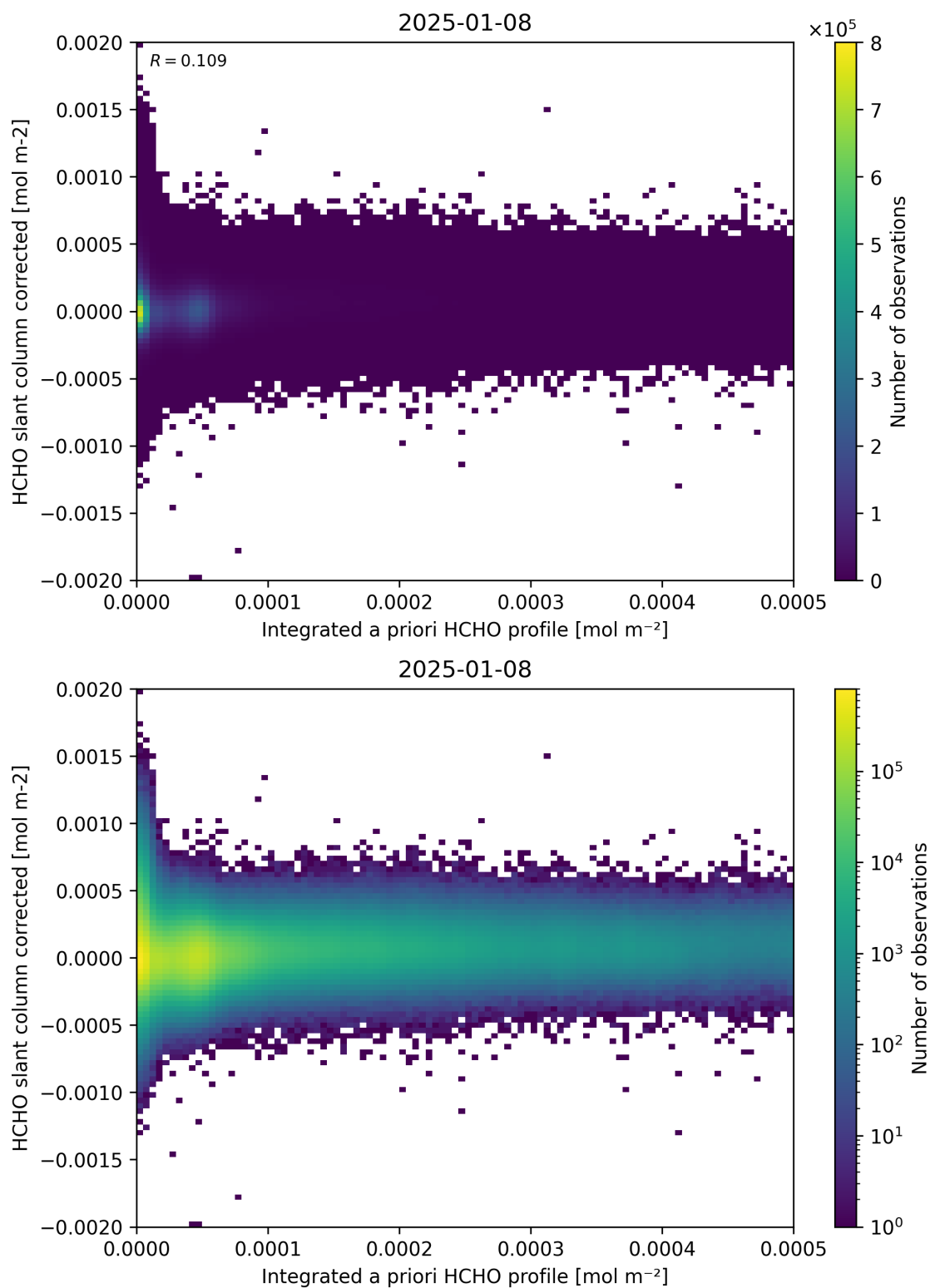
Figure 151: Scatter density plot of “Integrated a priori HCHO profile” against “HCHO slant column corrected” for 2025-01-07 to 2025-01-09.
