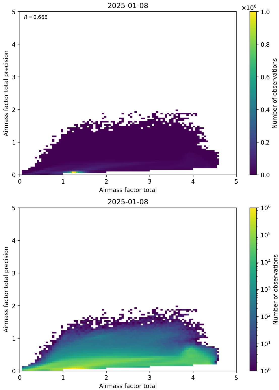
Figure 103: Scatter density plot of “Airmass factor total” against “Airmass factor total precision” for 2025-01-07 to 2025-01-09.
