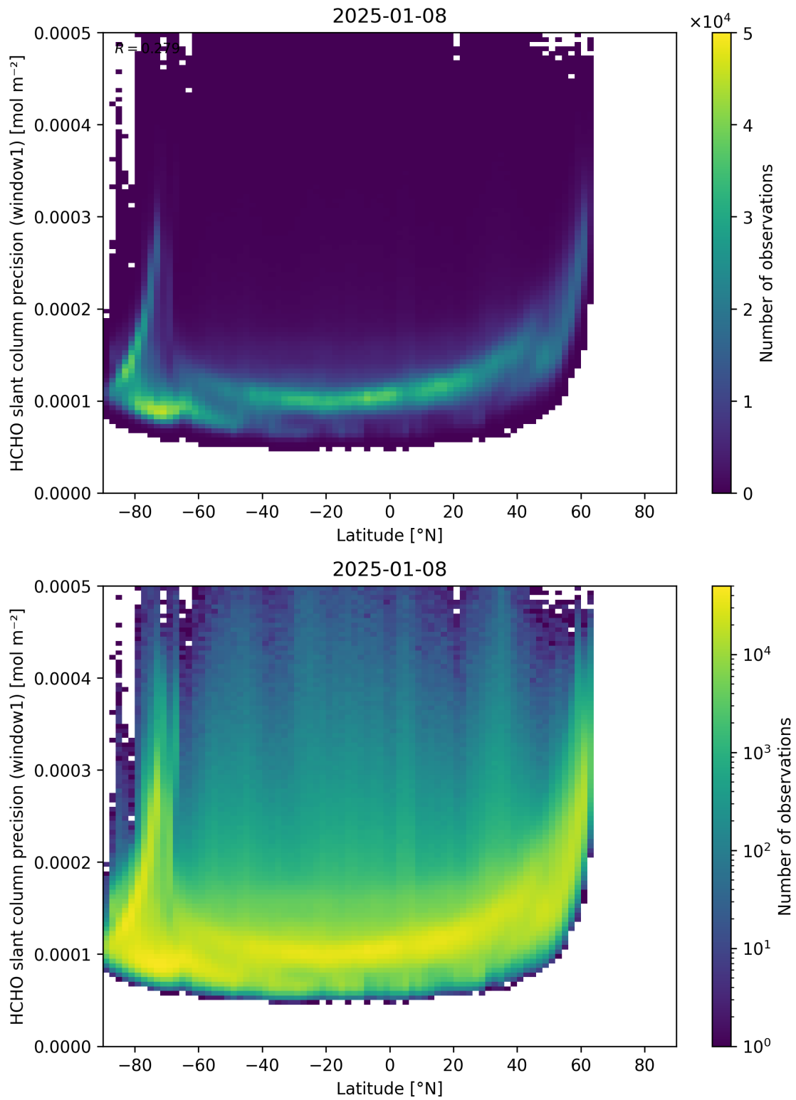
Figure 160: Scatter density plot of “Latitude” against “HCHO slant column precision (window1)” for 2025-01-07 to 2025-01-09.
