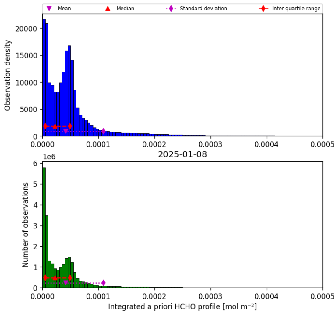
Figure 43: Histogram of “Integrated a priori HCHO profile” for 2025-01-07 to 2025-01-09
