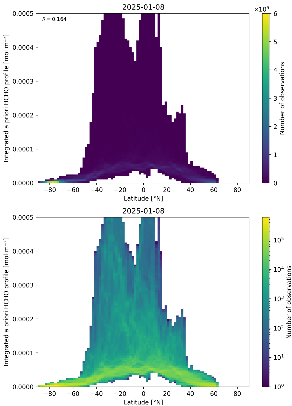
Figure 166: Scatter density plot of “Latitude” against “Integrated a priori HCHO profile” for 2025-01-07 to 2025-01-09.
