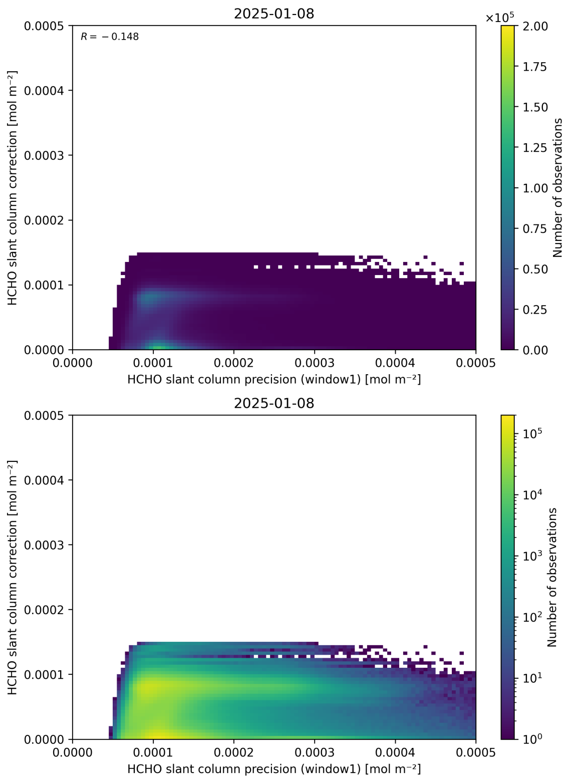
Figure 93: Scatter density plot of “HCHO slant column precision (window1)” against “HCHO slant column correction” for 2025-01-07 to 2025-01-09.
