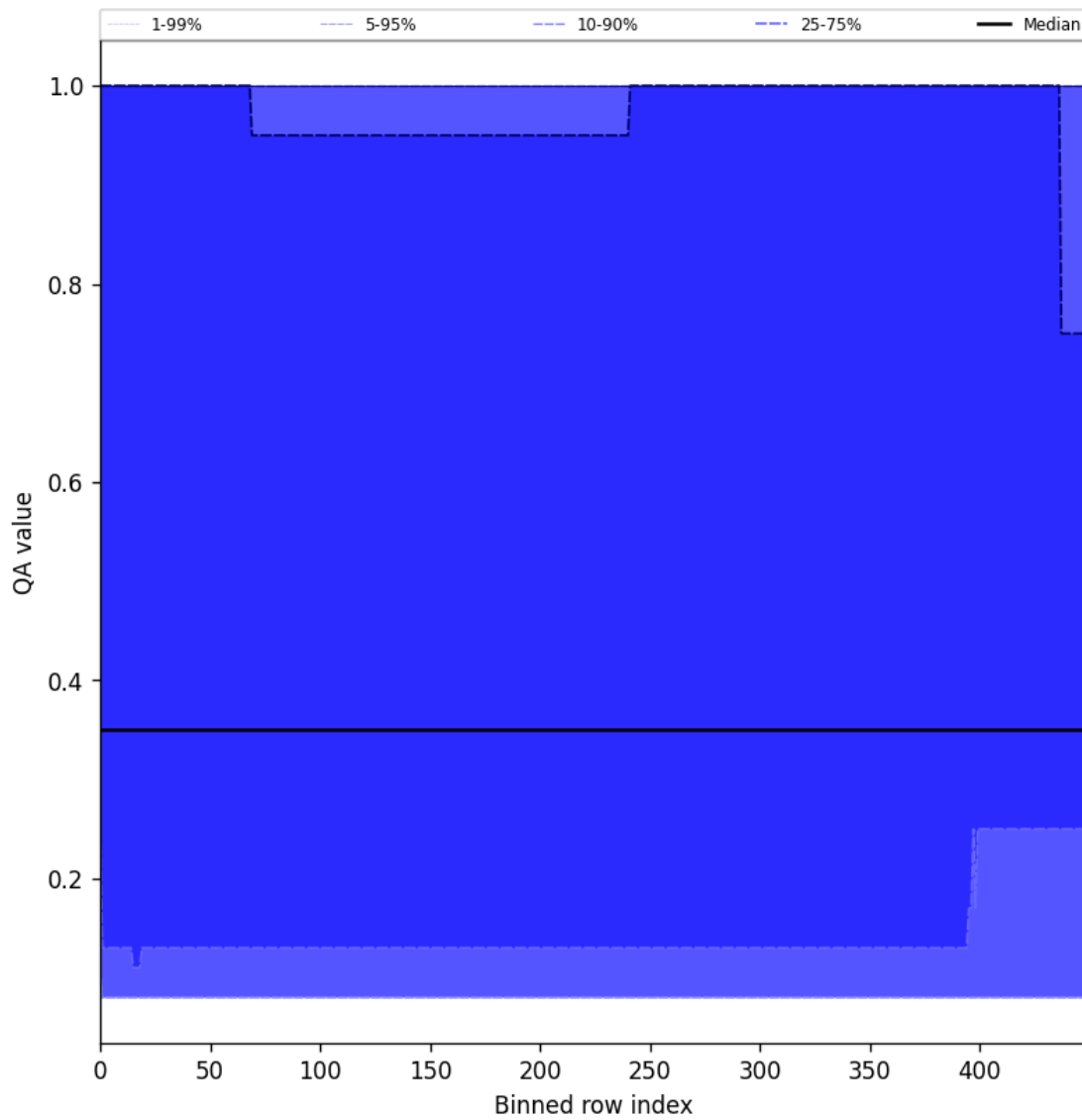
Figure 48: Along track statistics of “QA value” for 2025-01-07 to 2025-01-09
