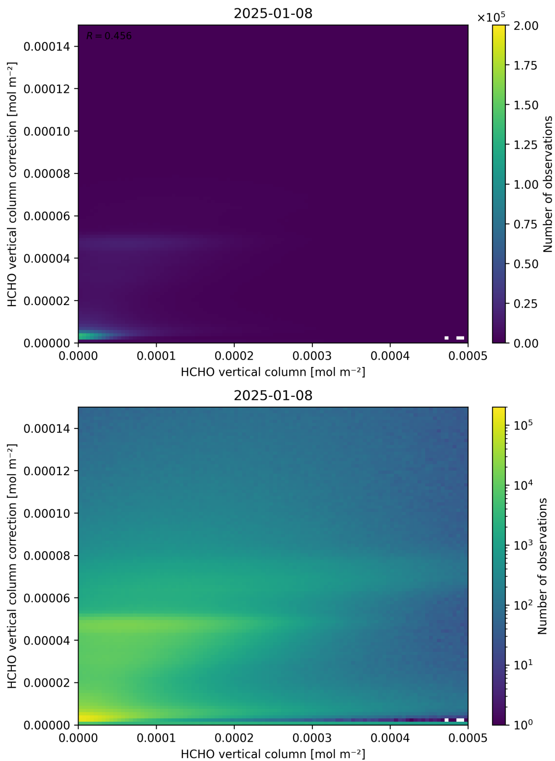
Figure 133: Scatter density plot of “HCHO vertical column” against “HCHO vertical column correction” for 2025-01-07 to 2025-01-09.
