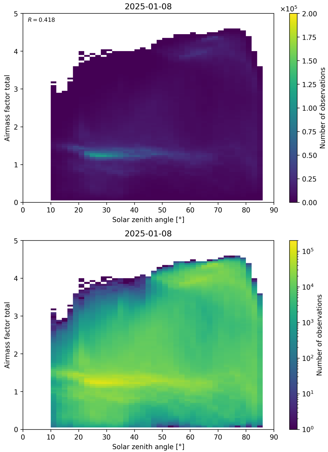
Figure 175: Scatter density plot of “Solar zenith angle” against “Airmass factor total” for 2025-01-07 to 2025-01-09.
