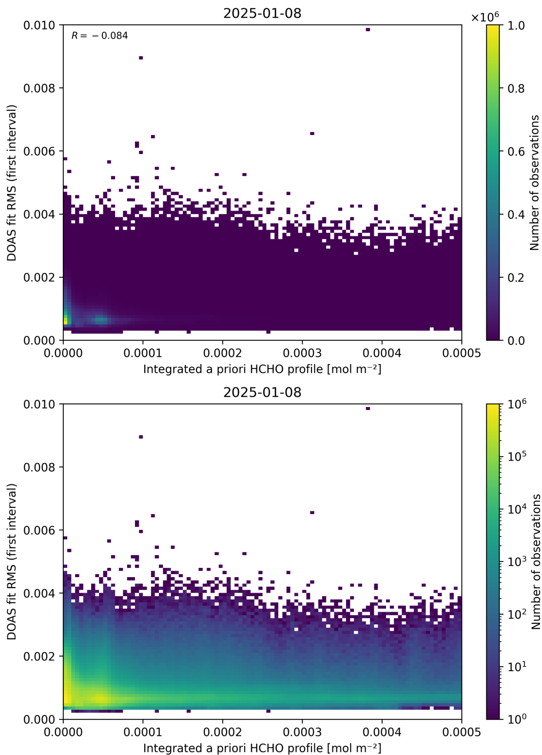
Figure 148: Scatter density plot of “Integrated a priori HCHO profile” against “DOAS fit RMS (first interval)” for 2025-01-07 to 2025-01-09.
