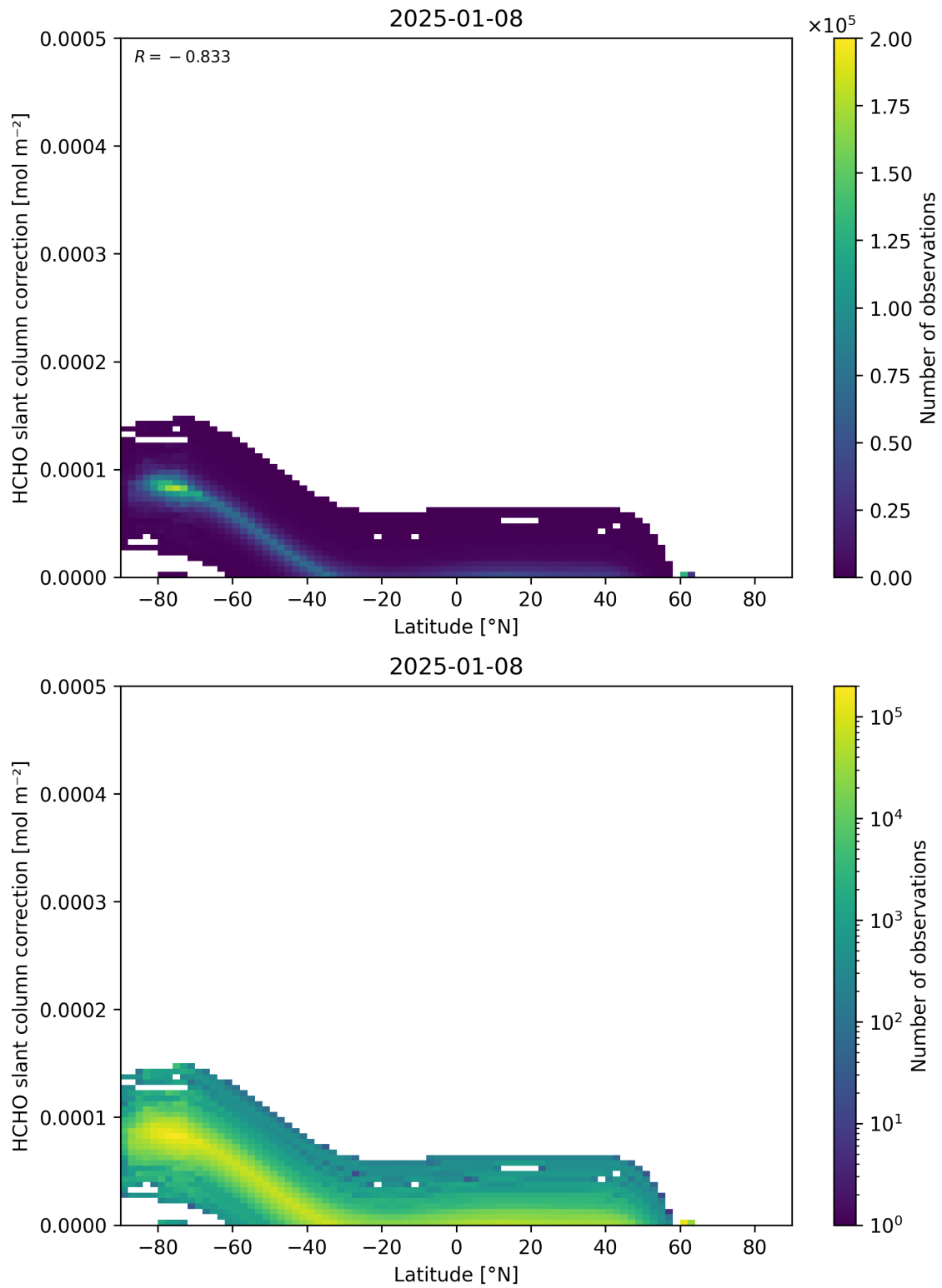
Figure 158: Scatter density plot of “Latitude” against “HCHO slant column correction” for 2025-01-07 to 2025-01-09.
