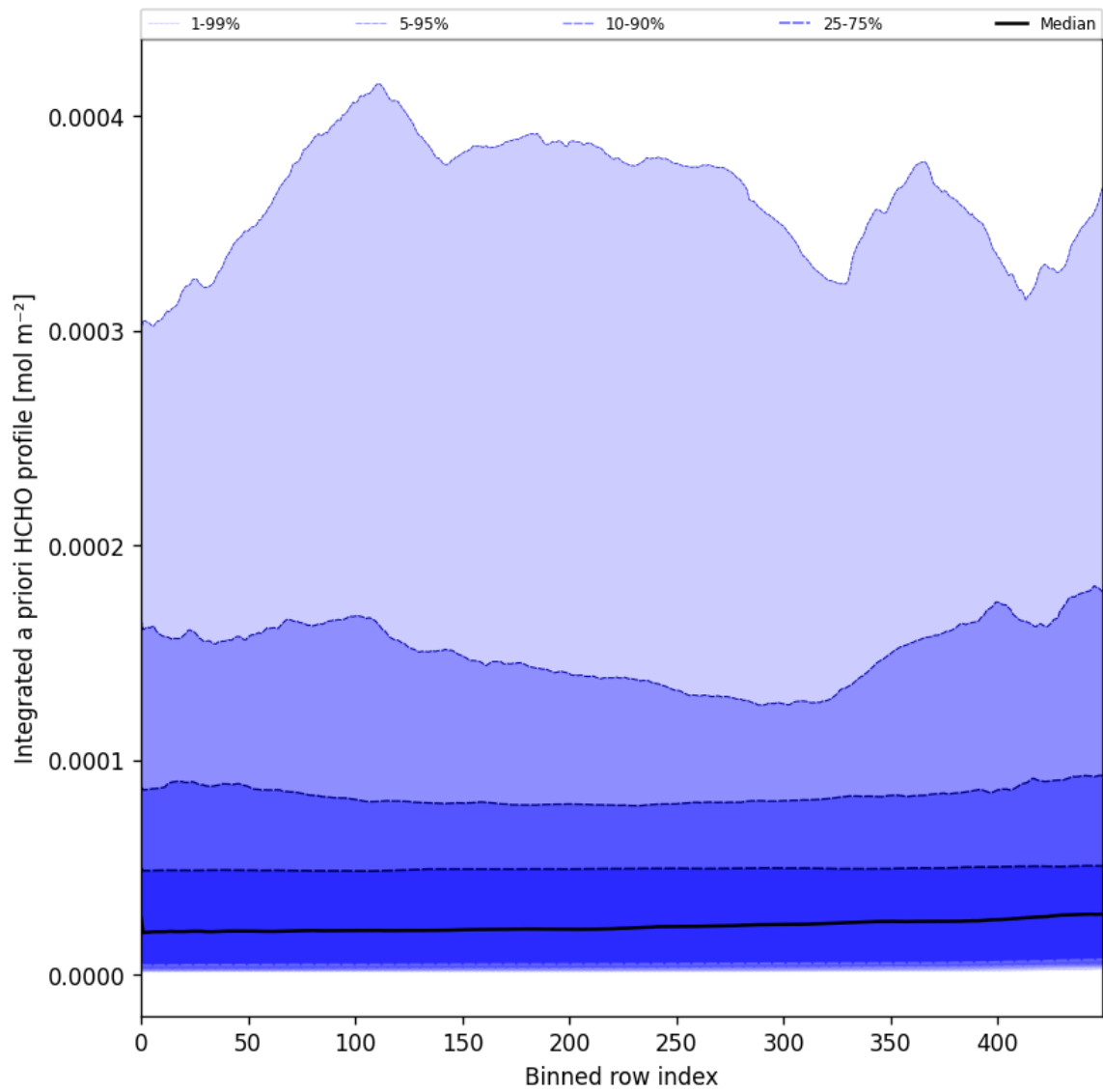
Figure 57: Along track statistics of "Integrated a priori HCHO profile" for 2025-01-07 to 2025-01-09
