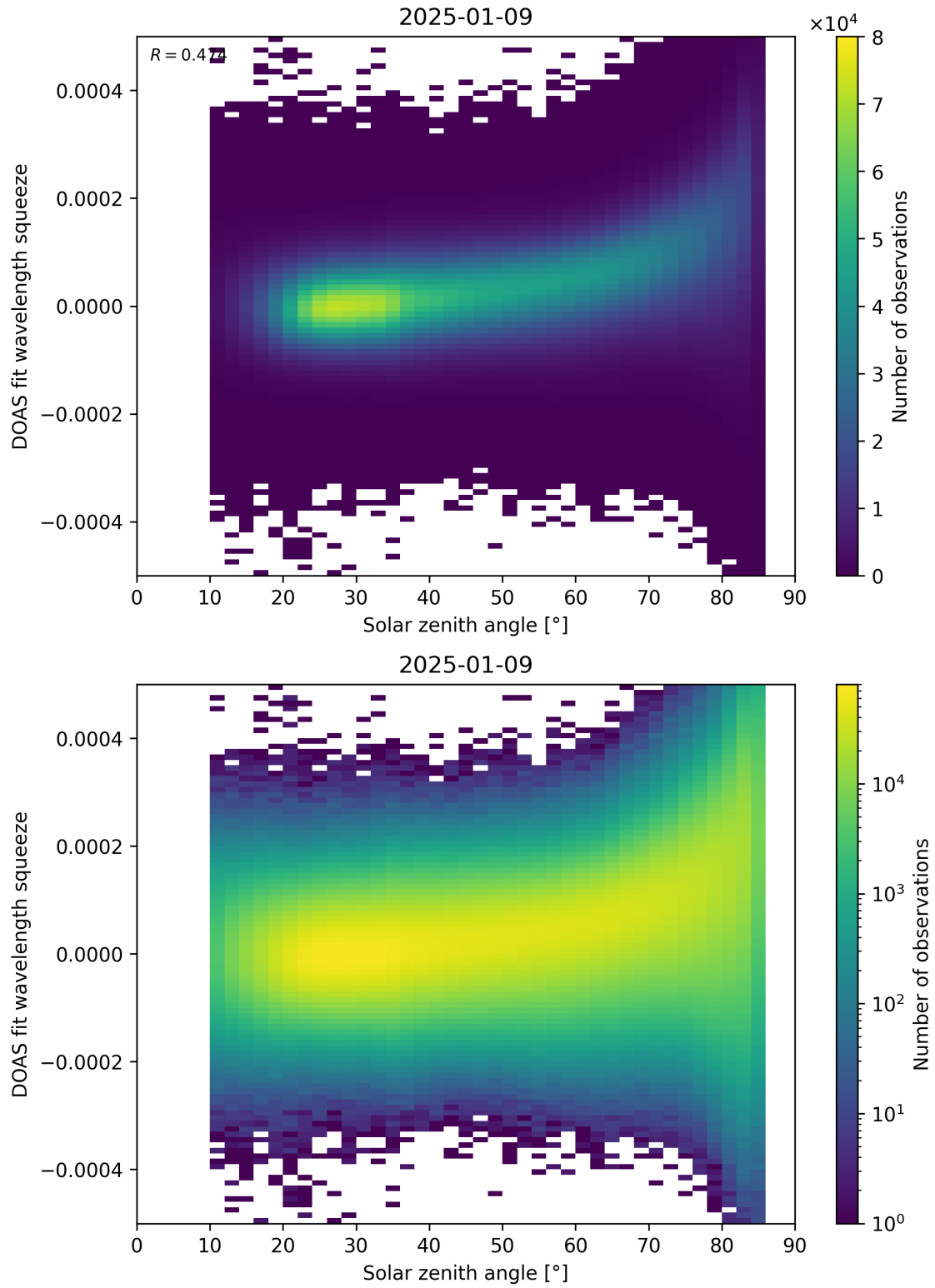
Figure 169: Scatter density plot of “Solar zenith angle” against “DOAS fit wavelength squeeze” for 2025-01-08 to 2025-01-10.
