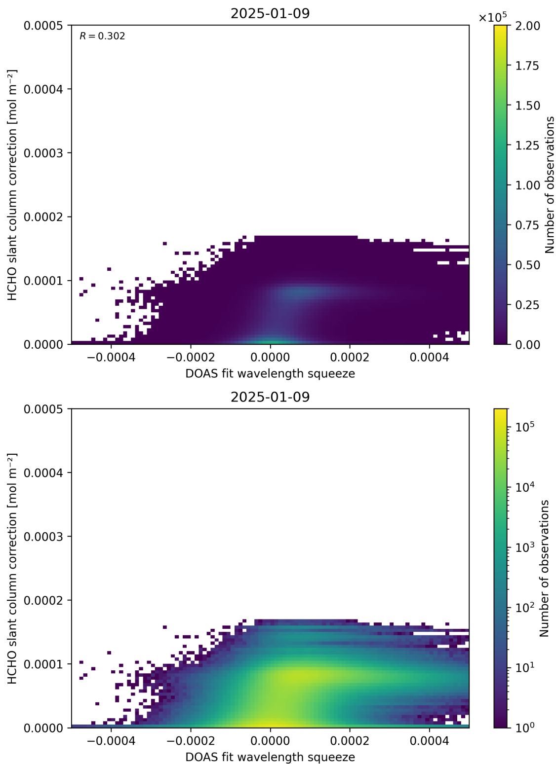
Figure 70: Scatter density plot of “DOAS fit wavelength squeeze” against “HCHO slant column correction” for 2025-01-08 to 2025-01-10.
