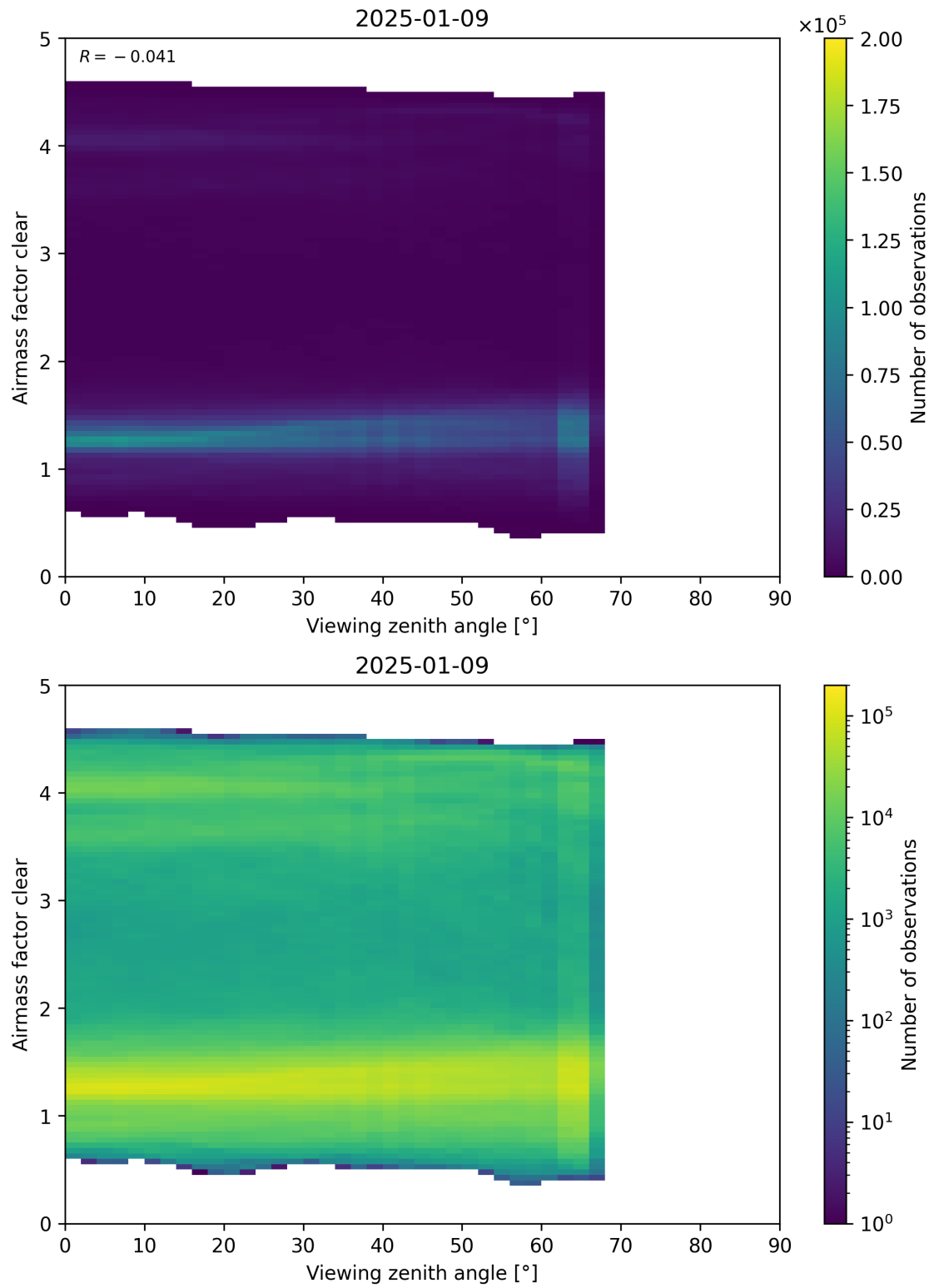
Figure 185: Scatter density plot of “Viewing zenith angle” against “Airmass factor clear” for 2025-01-08 to 2025-01-10.
