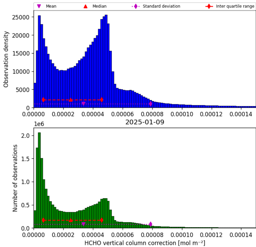
Figure 37: Histogram of “HCHO vertical column correction” for 2025-01-08 to 2025-01-10
