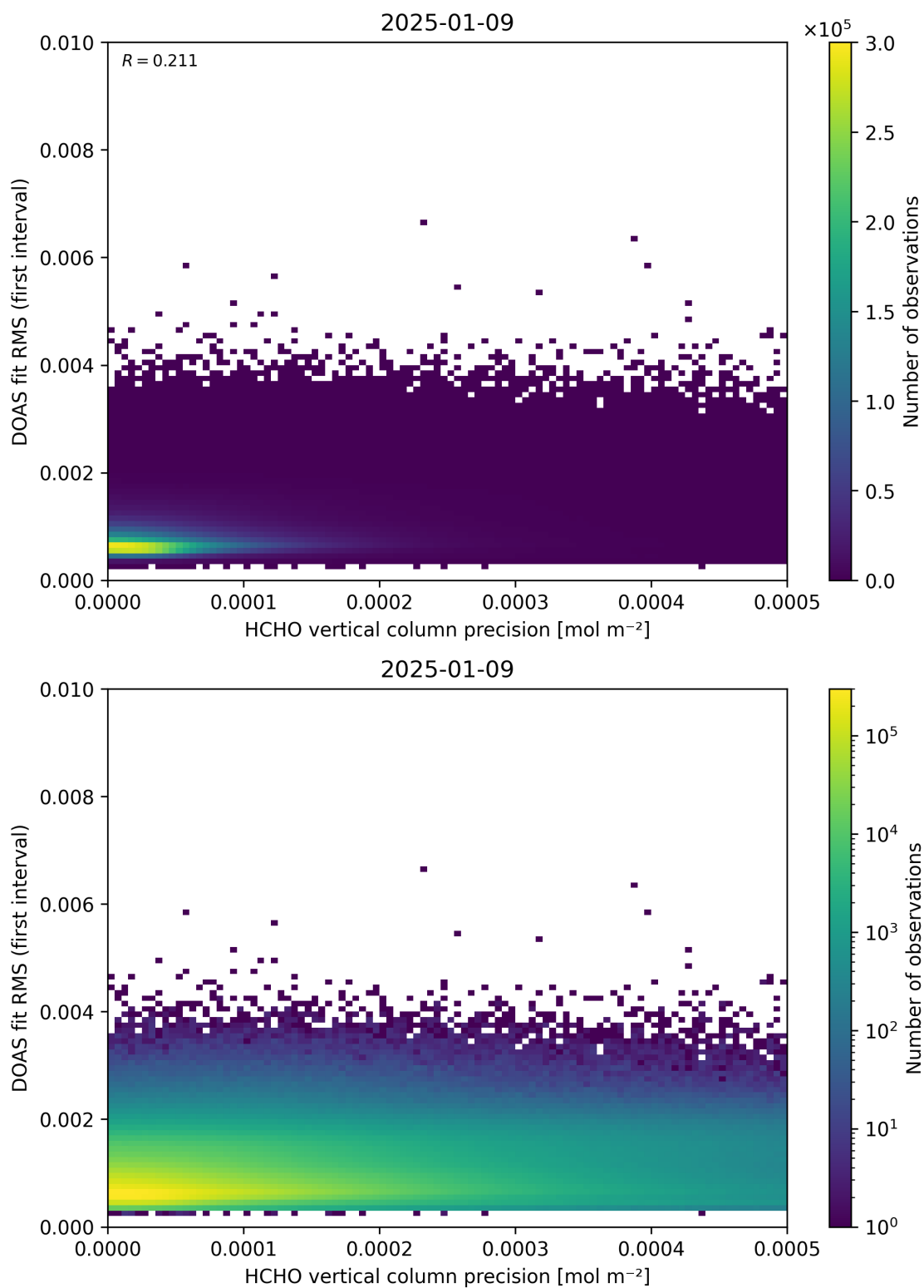
Figure 136: Scatter density plot of “HCHO vertical column precision” against “DOAS fit RMS (first interval)” for 2025-01-08 to 2025-01-10.
