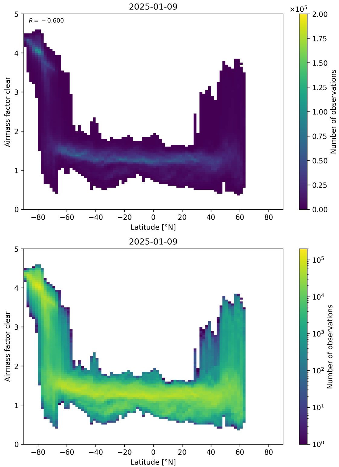
Figure 156: Scatter density plot of “Latitude” against “Airmass factor clear” for 2025-01-08 to 2025-01-10.
