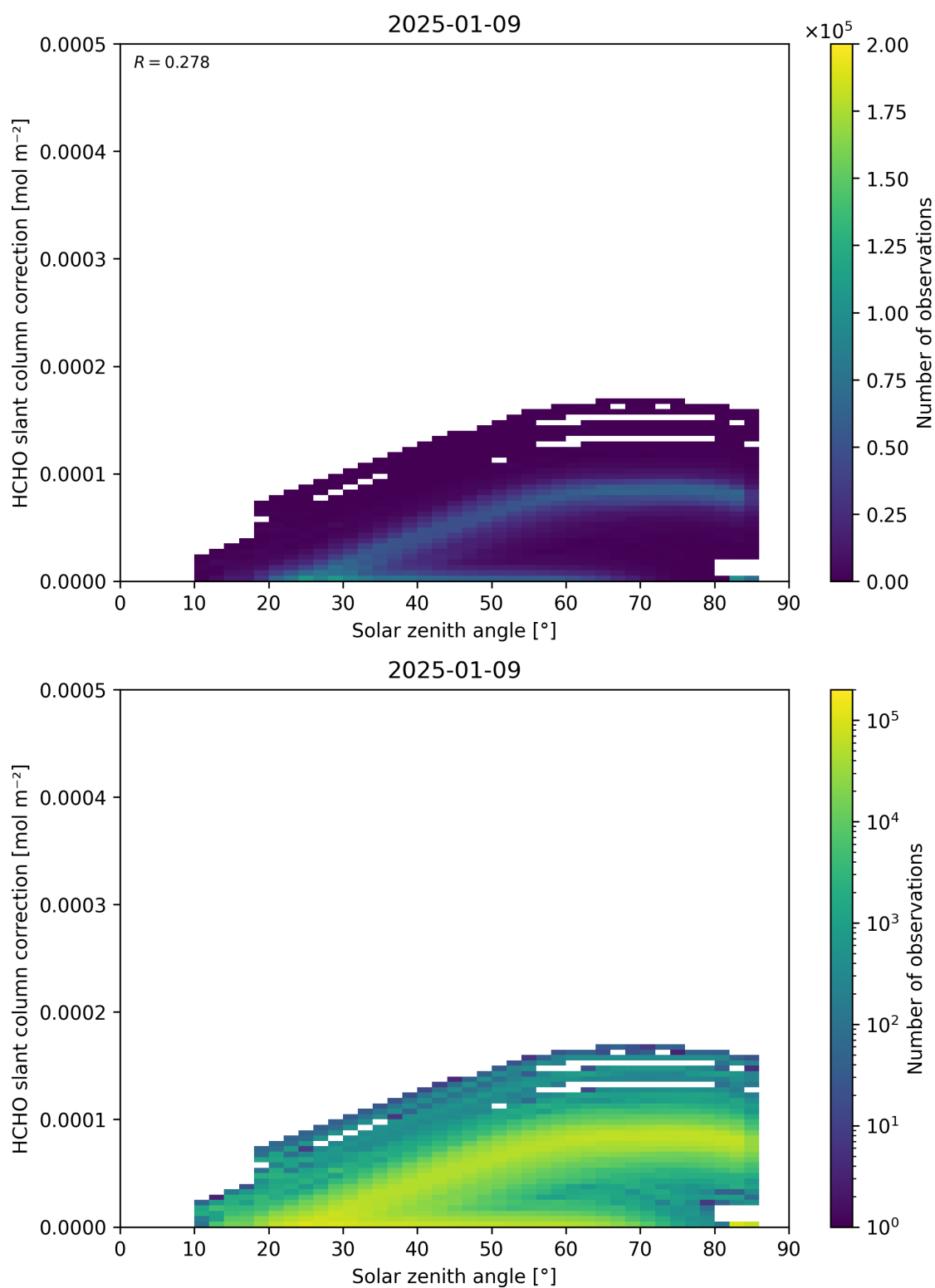
Figure 172: Scatter density plot of “Solar zenith angle” against “HCHO slant column correction” for 2025-01-08 to 2025-01-10.
