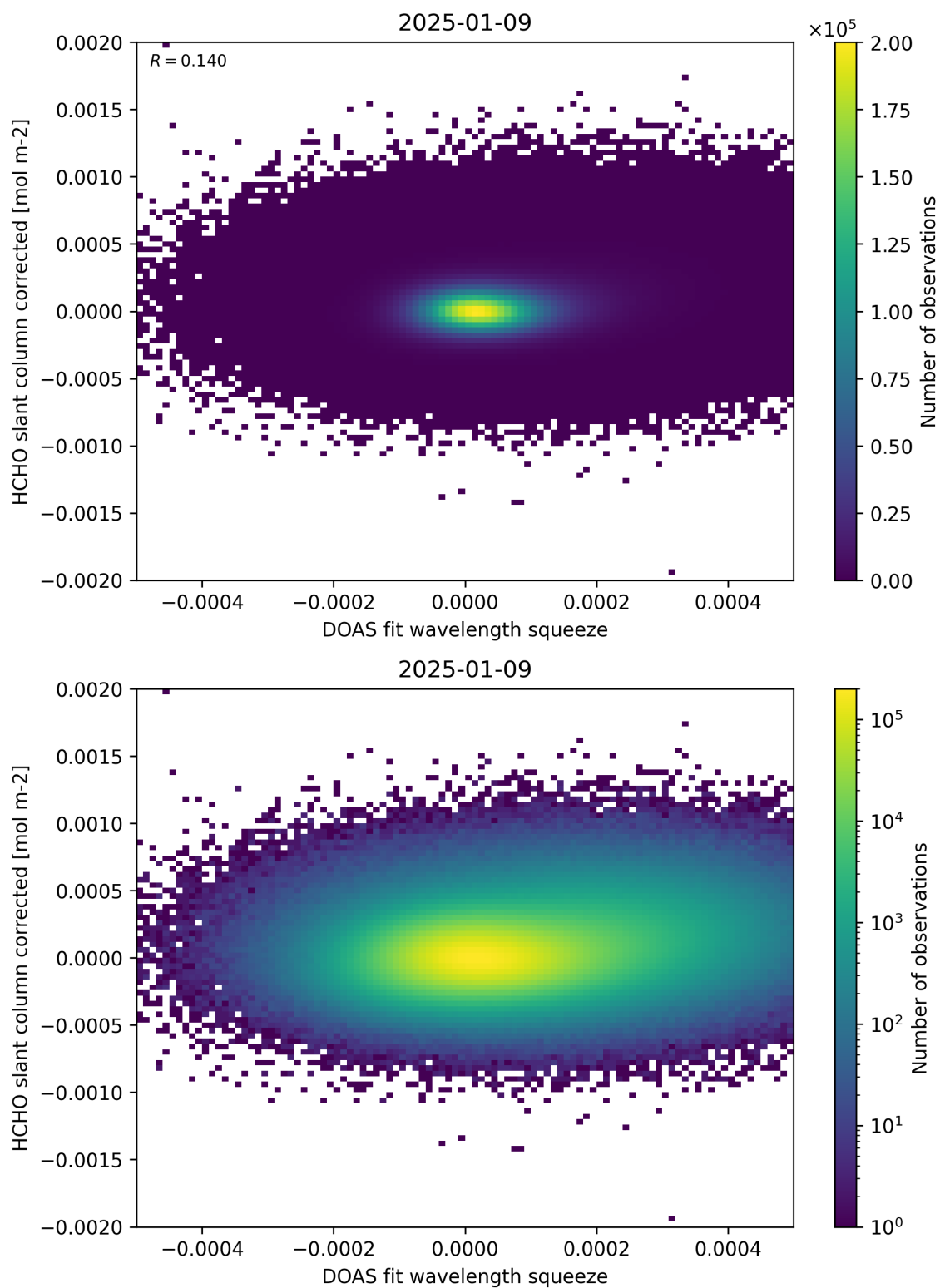
Figure 69: Scatter density plot of “DOAS fit wavelength squeeze” against “HCHO slant column corrected” for 2025-01-08 to 2025-01-10.
