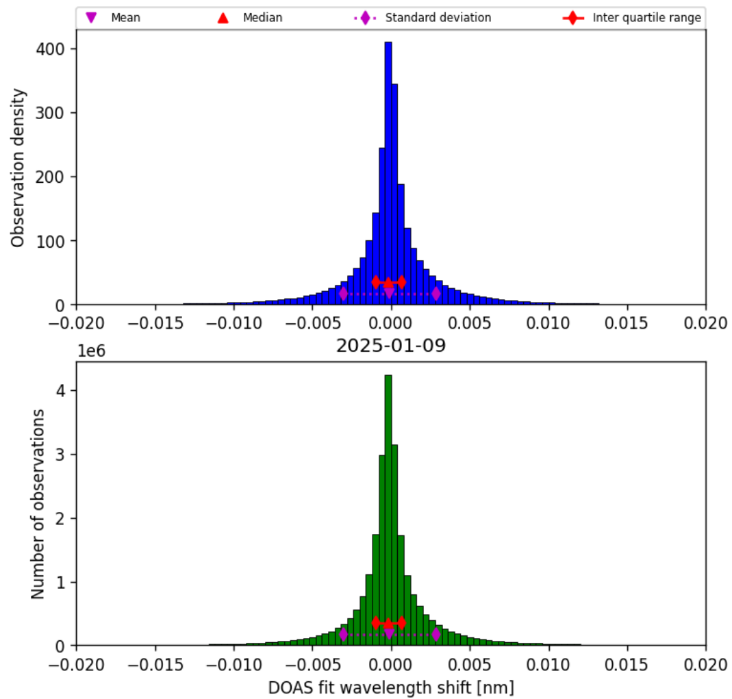
Figure 44: Histogram of “DOAS fit wavelength shift” for 2025-01-08 to 2025-01-10
