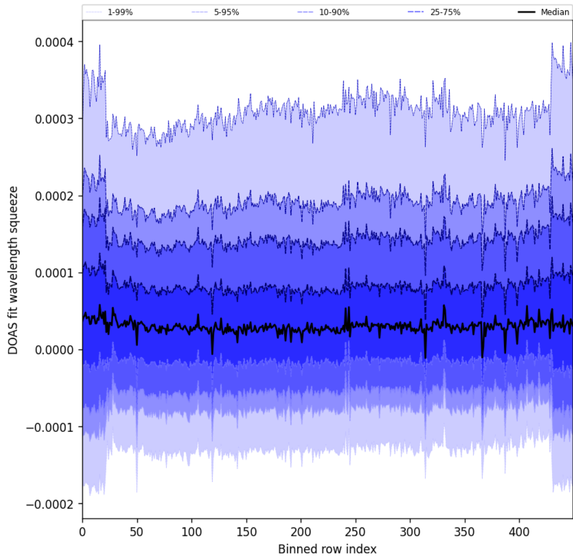
Figure 59: Along track statistics of “DOAS fit wavelength squeeze” for 2025-01-08 to 2025-01-10
