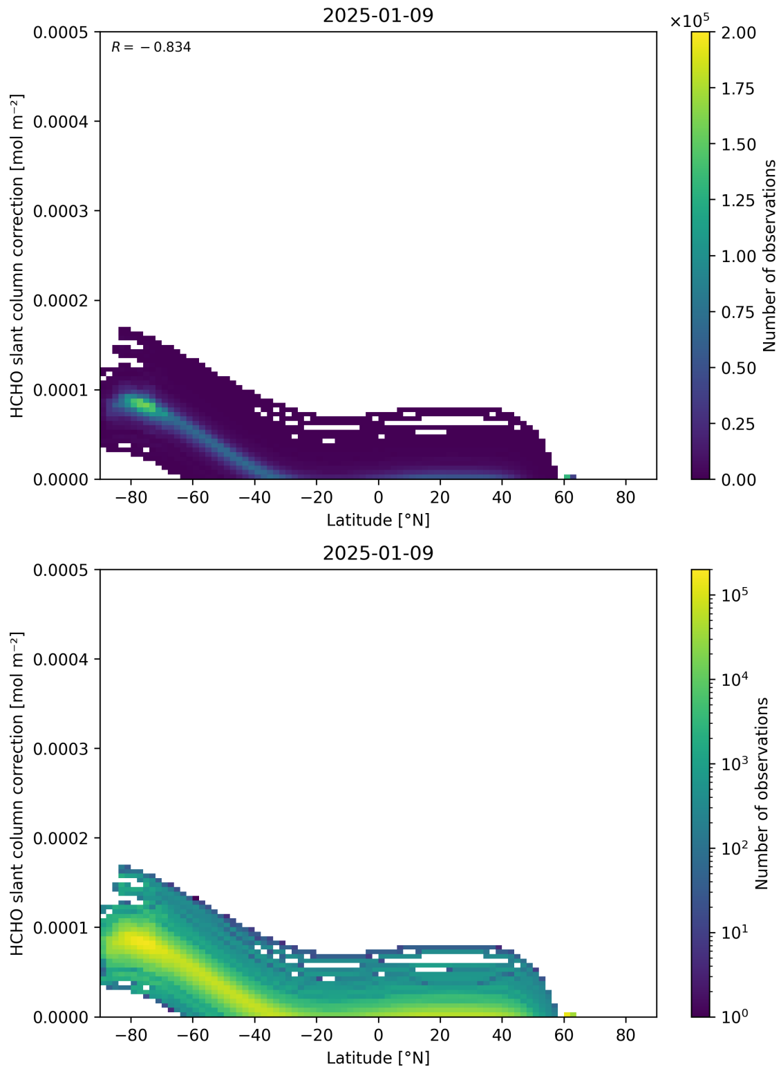
Figure 158: Scatter density plot of “Latitude” against “HCHO slant column correction” for 2025-01-08 to 2025-01-10.
