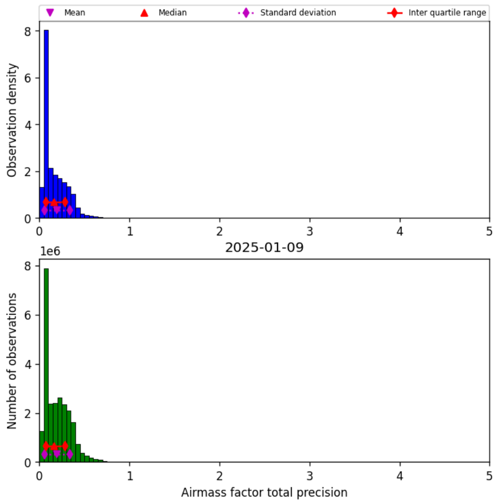
Figure 41: Histogram of “Airmass factor total precision” for 2025-01-08 to 2025-01-10
