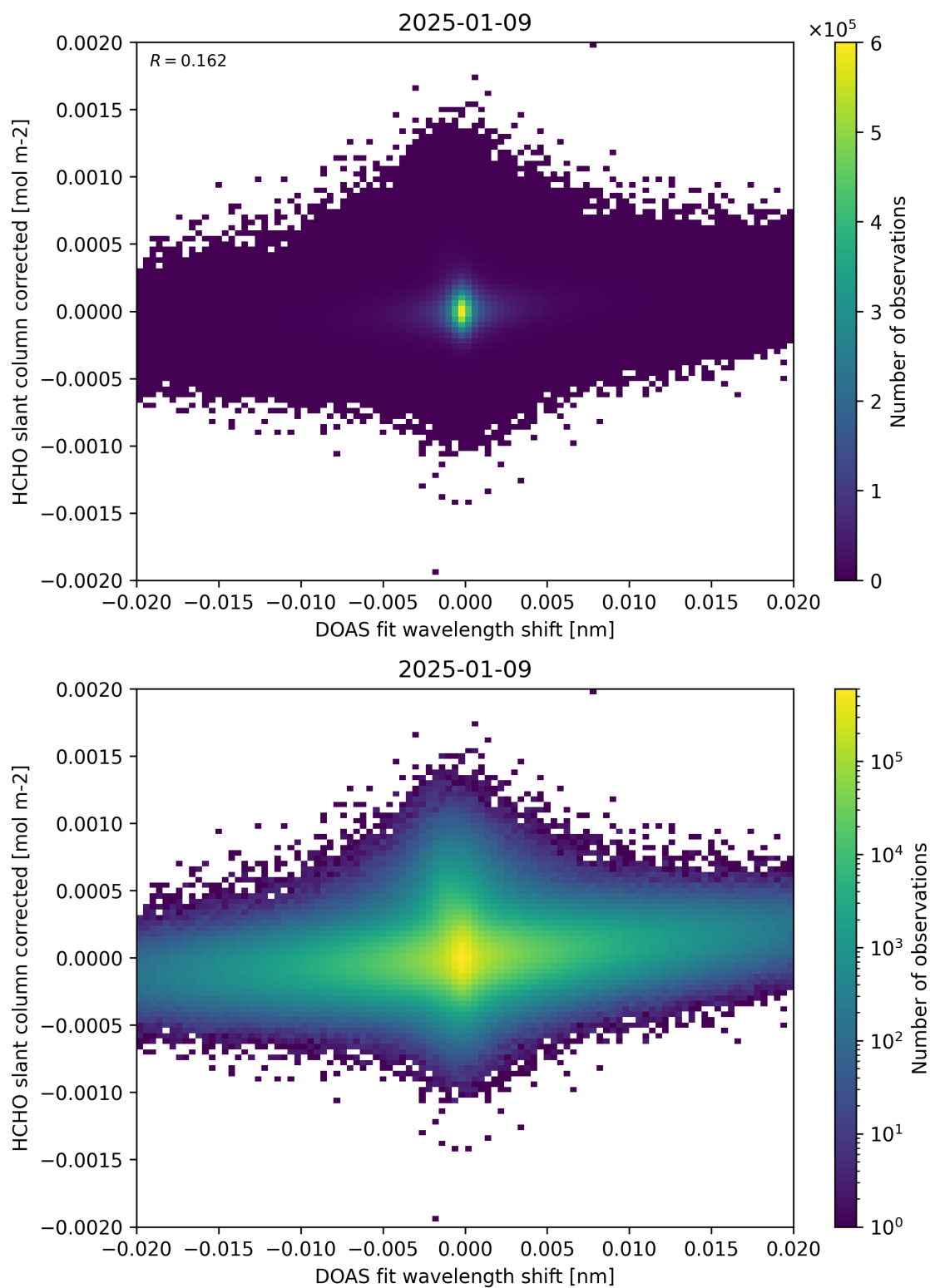
Figure 66: Scatter density plot of “DOAS fit wavelength shift” against “HCHO slant column corrected” for 2025-01-08 to 2025-01-10.
