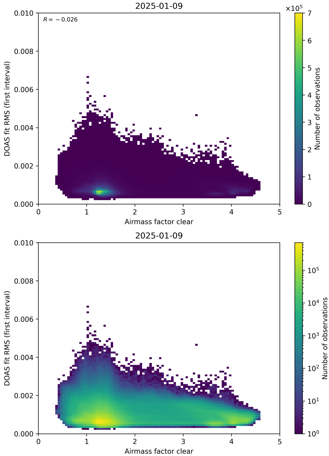
Figure 71: Scatter density plot of “Airmass factor clear” against “DOAS fit RMS (first interval)” for 2025-01-08 to 2025-01-10.
