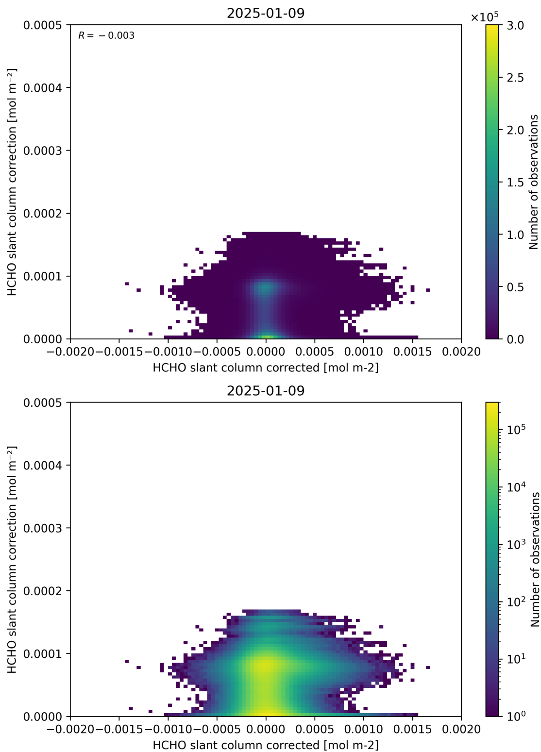
Figure 77: Scatter density plot of “HCHO slant column corrected” against “HCHO slant column correction” for 2025-01-08 to 2025-01-10.
