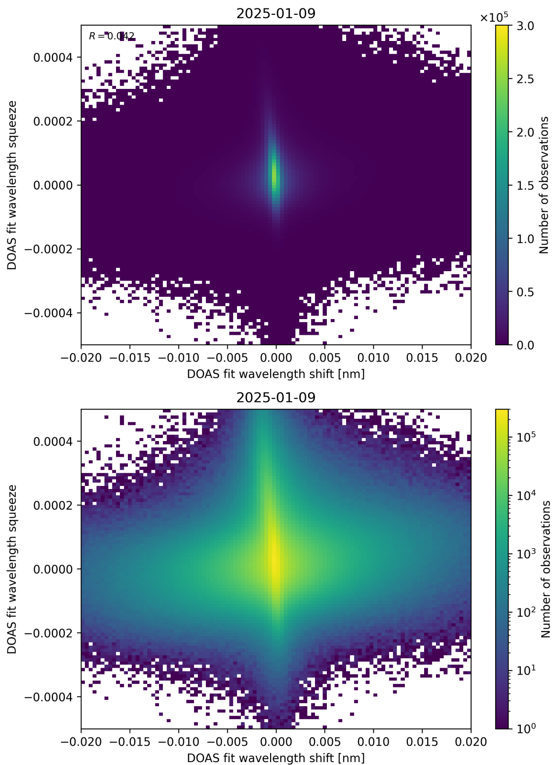
Figure 65: Scatter density plot of “DOAS fit wavelength shift” against “DOAS fit wavelength squeeze” for 2025-01-08 to 2025-01-10.
