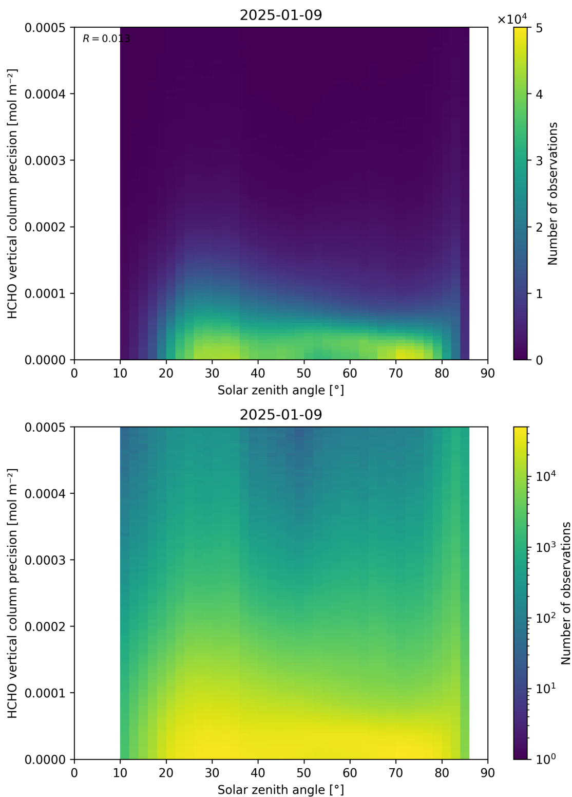
Figure 179: Scatter density plot of “Solar zenith angle” against “HCHO vertical column precision” for 2025-01-08 to 2025-01-10.
