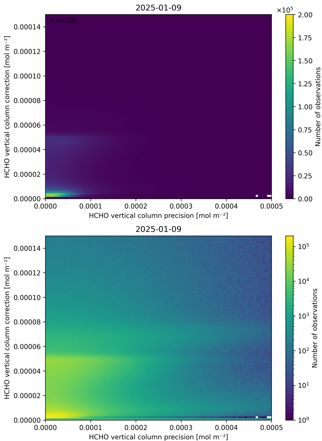
Figure 146: Scatter density plot of “HCHO vertical column precision” against “HCHO vertical column correction” for 2025-01-08 to 2025-01-10.
