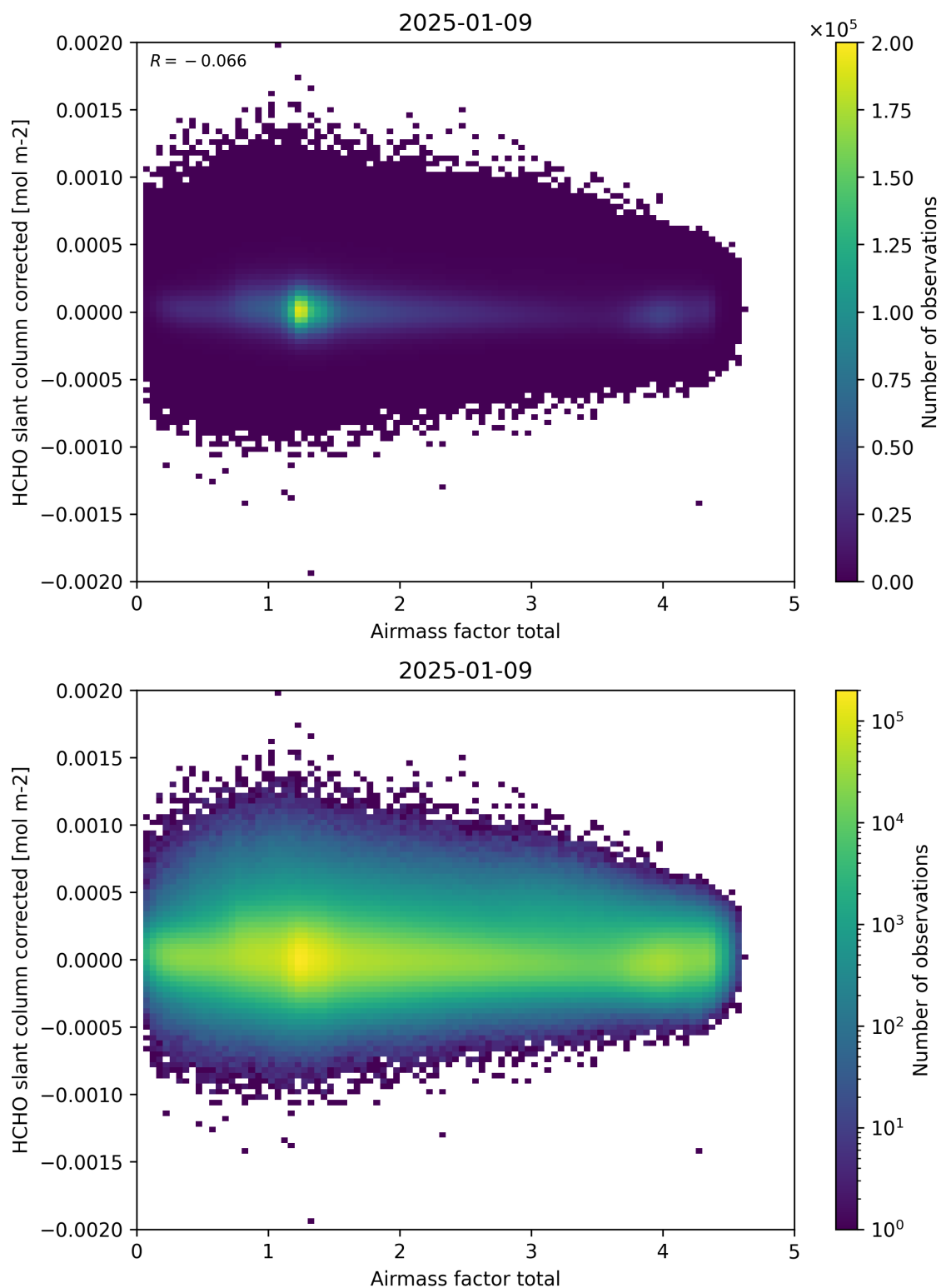
Figure 101: Scatter density plot of “Airmass factor total” against “HCHO slant column corrected” for 2025-01-08 to 2025-01-10.
