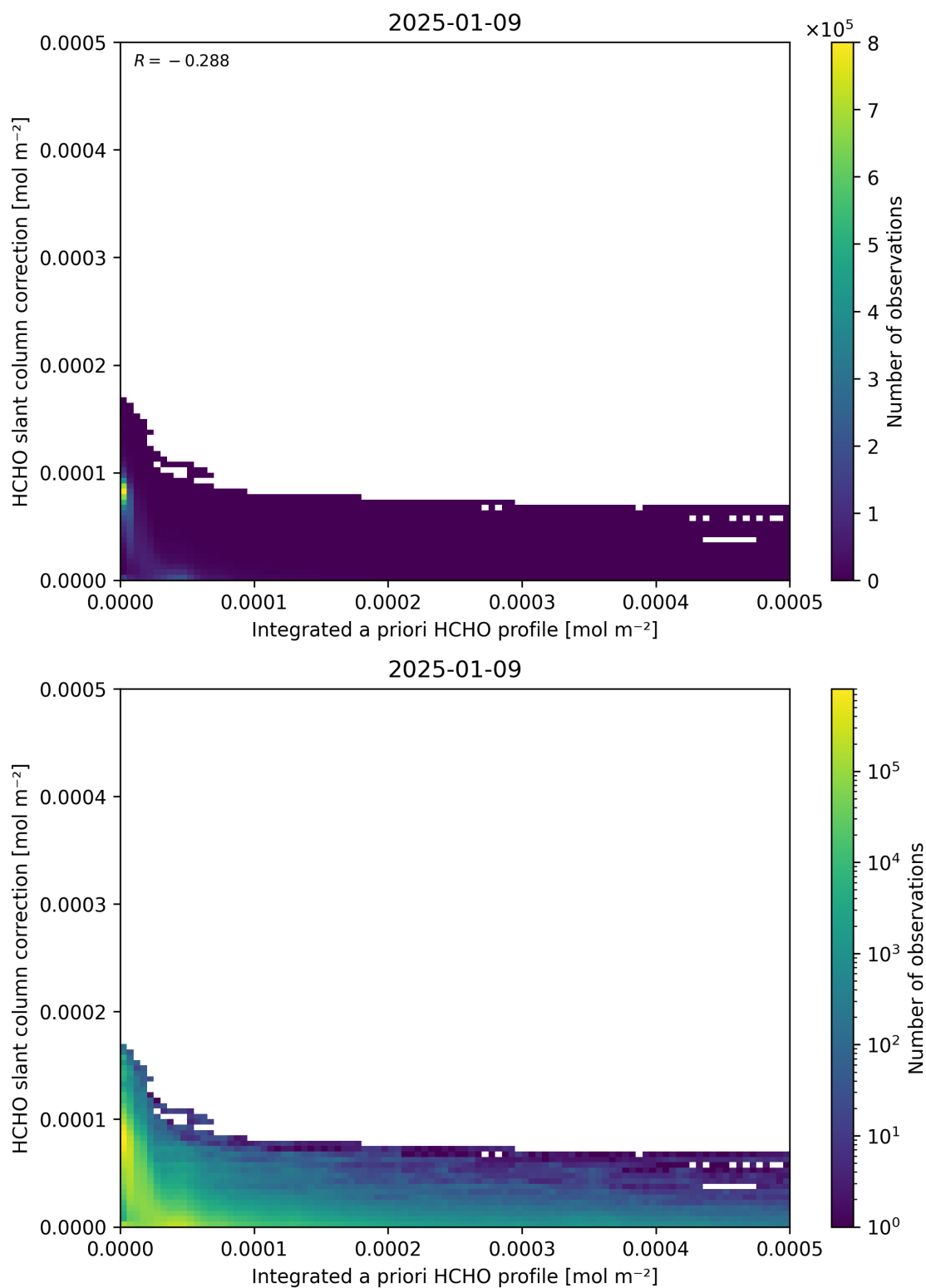
Figure 152: Scatter density plot of “Integrated a priori HCHO profile” against “HCHO slant column correction” for 2025-01-08 to 2025-01-10.
