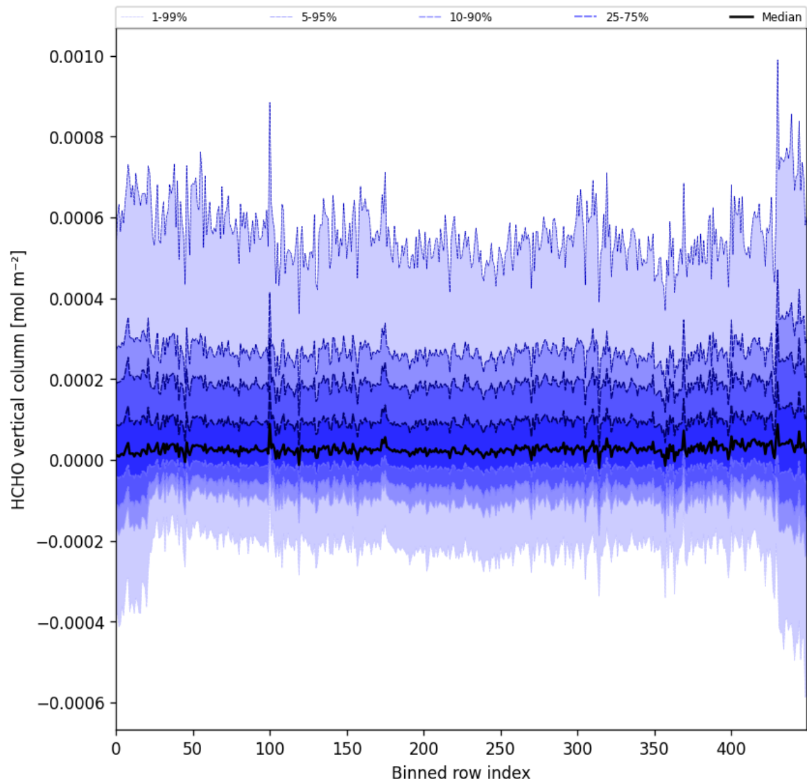
Figure 49: Along track statistics of “HCHO vertical column” for 2025-01-08 to 2025-01-10
