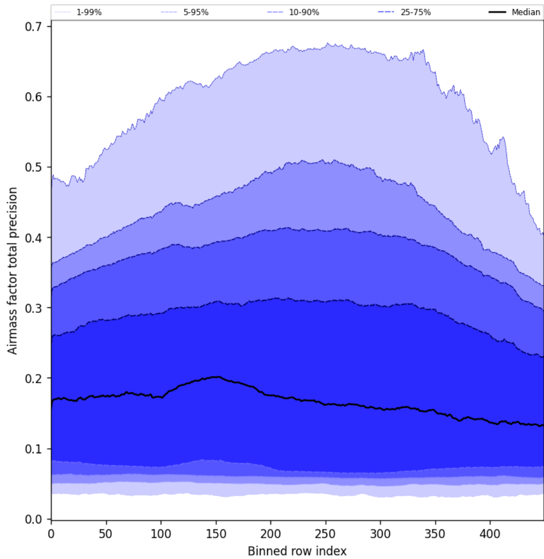
Figure 55: Along track statistics of “Airmass factor total precision” for 2025-01-08 to 2025-01-10
