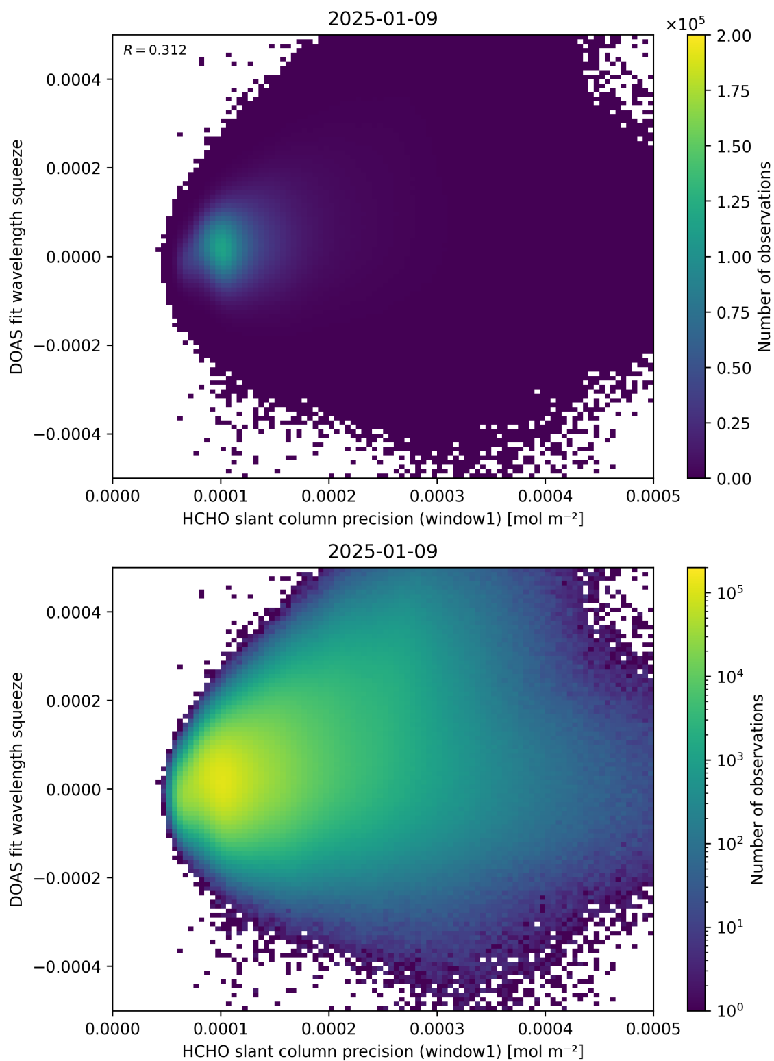
Figure 90: Scatter density plot of “HCHO slant column precision (window1)” against “DOAS fit wavelength squeeze” for 2025-01-08 to 2025-01-10.
