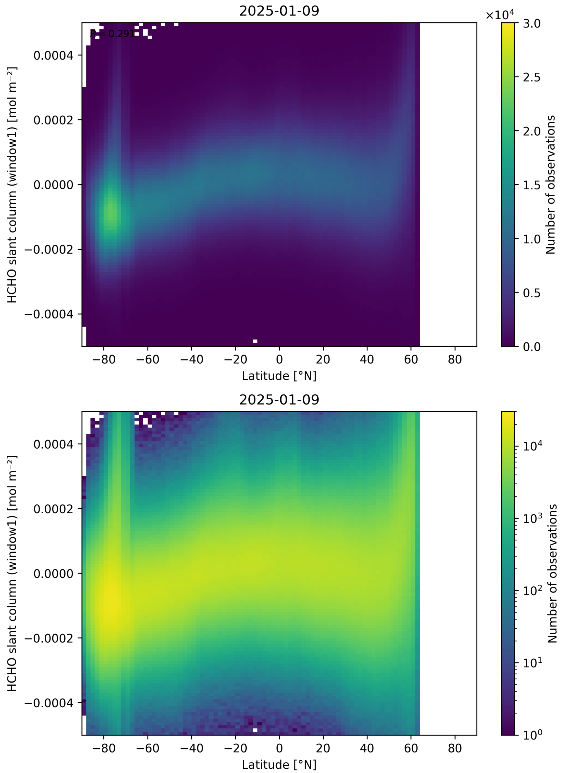
Figure 159: Scatter density plot of “Latitude” against “HCHO slant column (window1)” for 2025-01-08 to 2025-01-10.
