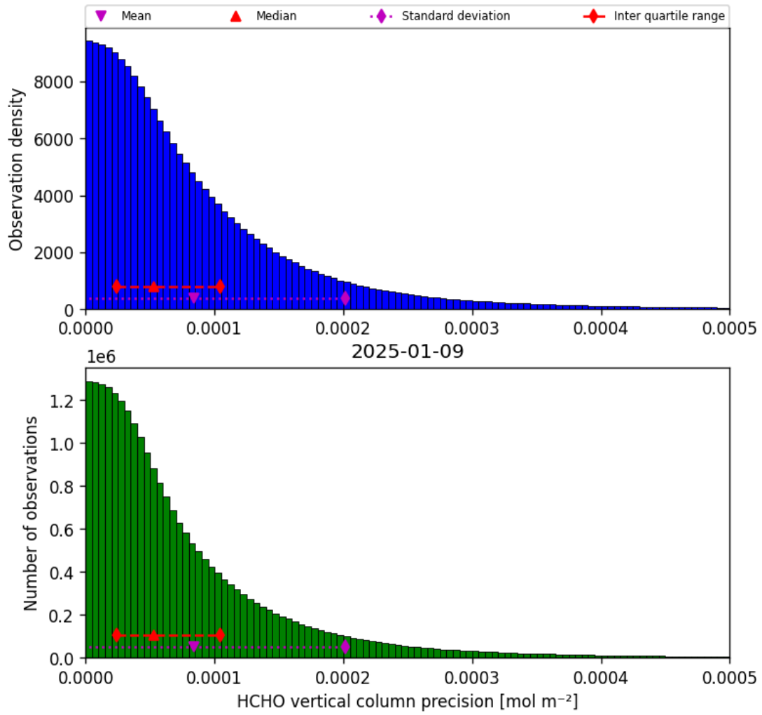
Figure 36: Histogram of “HCHO vertical column precision” for 2025-01-08 to 2025-01-10
