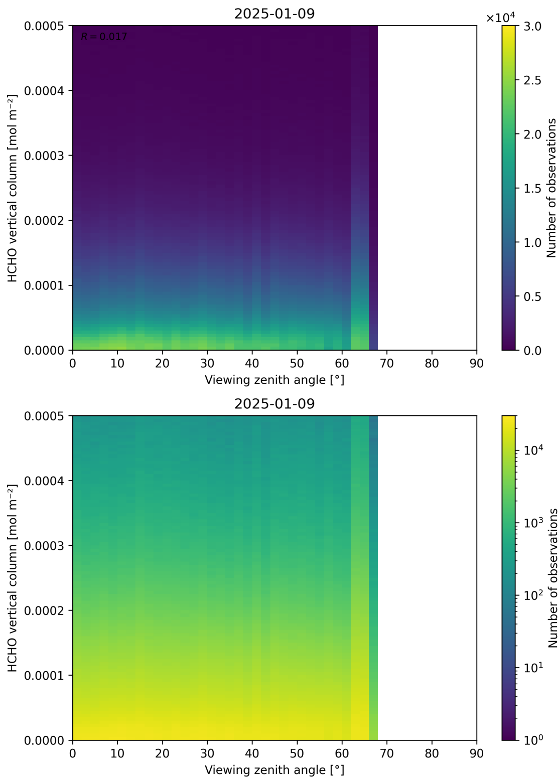
Figure 192: Scatter density plot of “Viewing zenith angle” against “HCHO vertical column” for 2025-01-08 to 2025-01-10.
