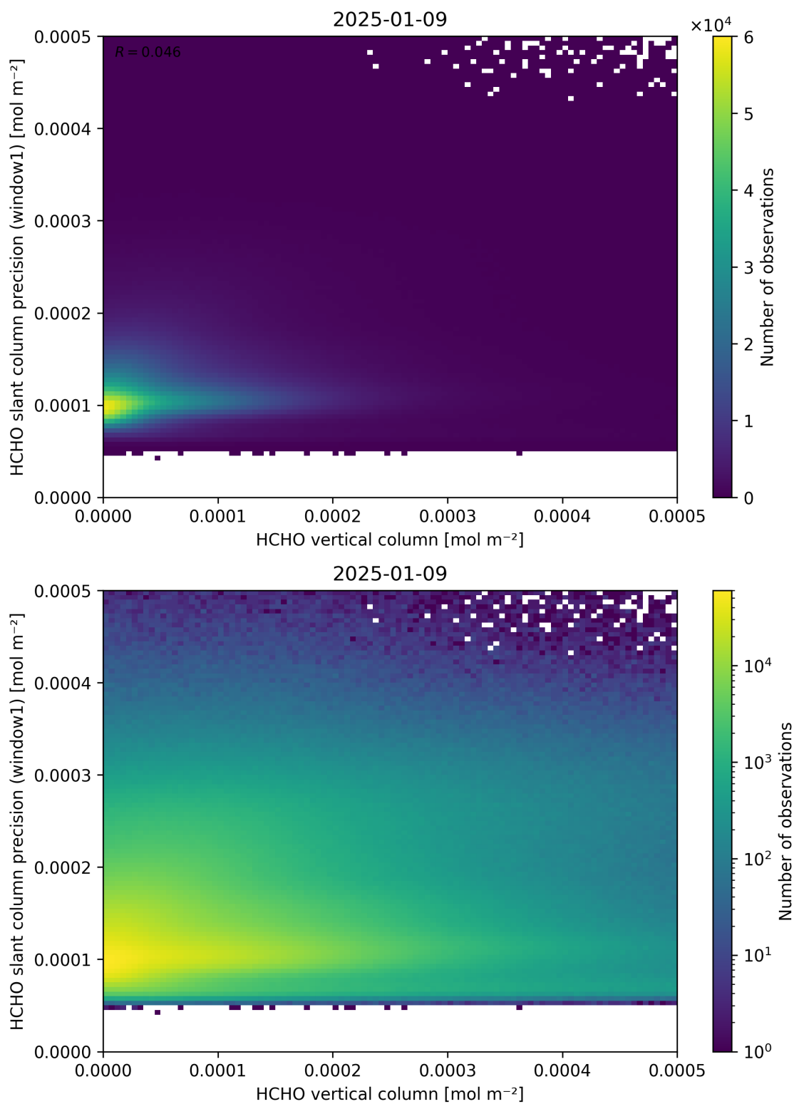
Figure 130: Scatter density plot of “HCHO vertical column” against “HCHO slant column precision (window1)” for 2025-01-08 to 2025-01-10.
