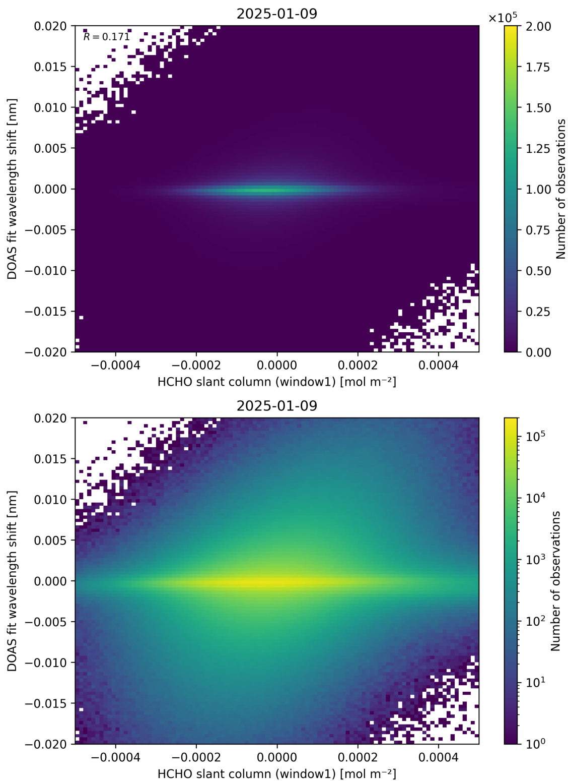
Figure 79: Scatter density plot of “HCHO slant column (window1)” against “DOAS fit wavelength shift” for 2025-01-08 to 2025-01-10.
