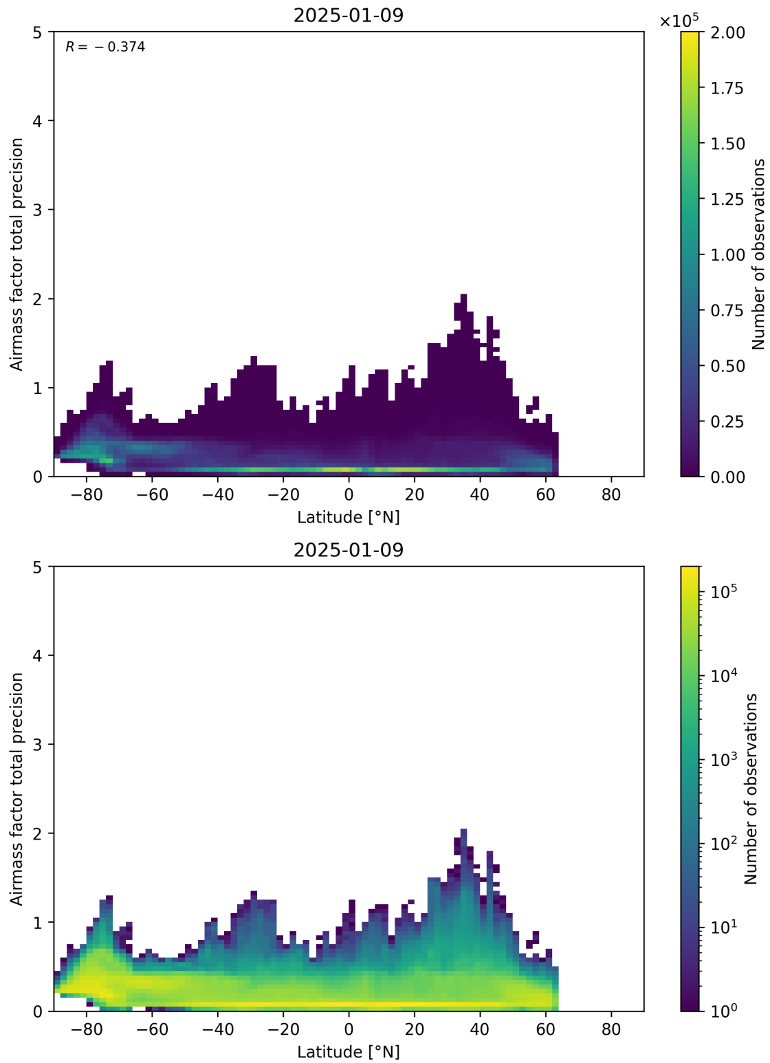
Figure 162: Scatter density plot of “Latitude” against “Airmass factor total precision” for 2025-01-08 to 2025-01-10.
