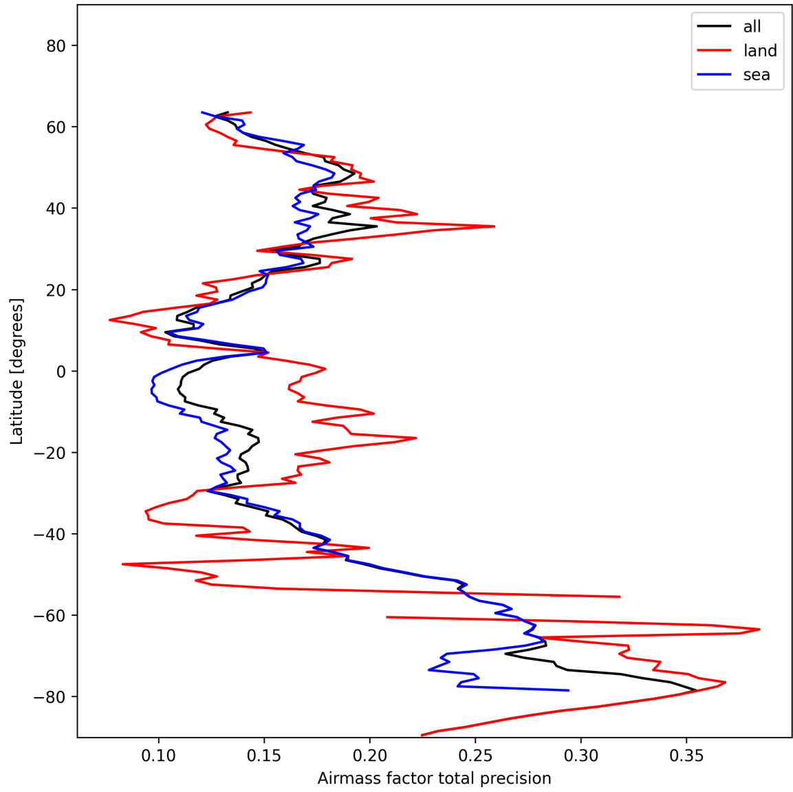
Figure 27: Zonal average of “Airmass factor total precision” for 2025-01-08 to 2025-01-10.
