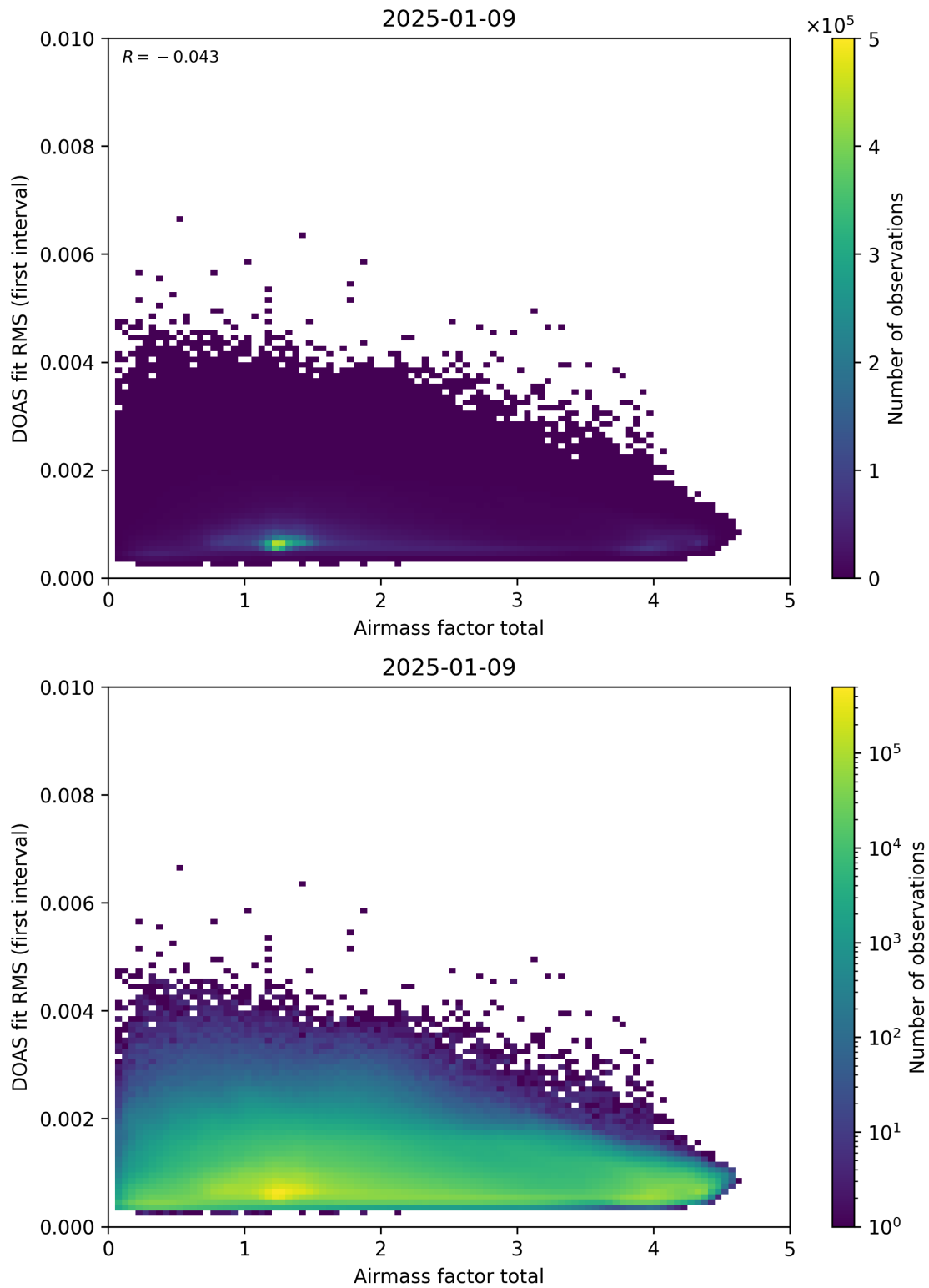
Figure 97: Scatter density plot of “Airmass factor total” against “DOAS fit RMS (first interval)” for 2025-01-08 to 2025-01-10.
