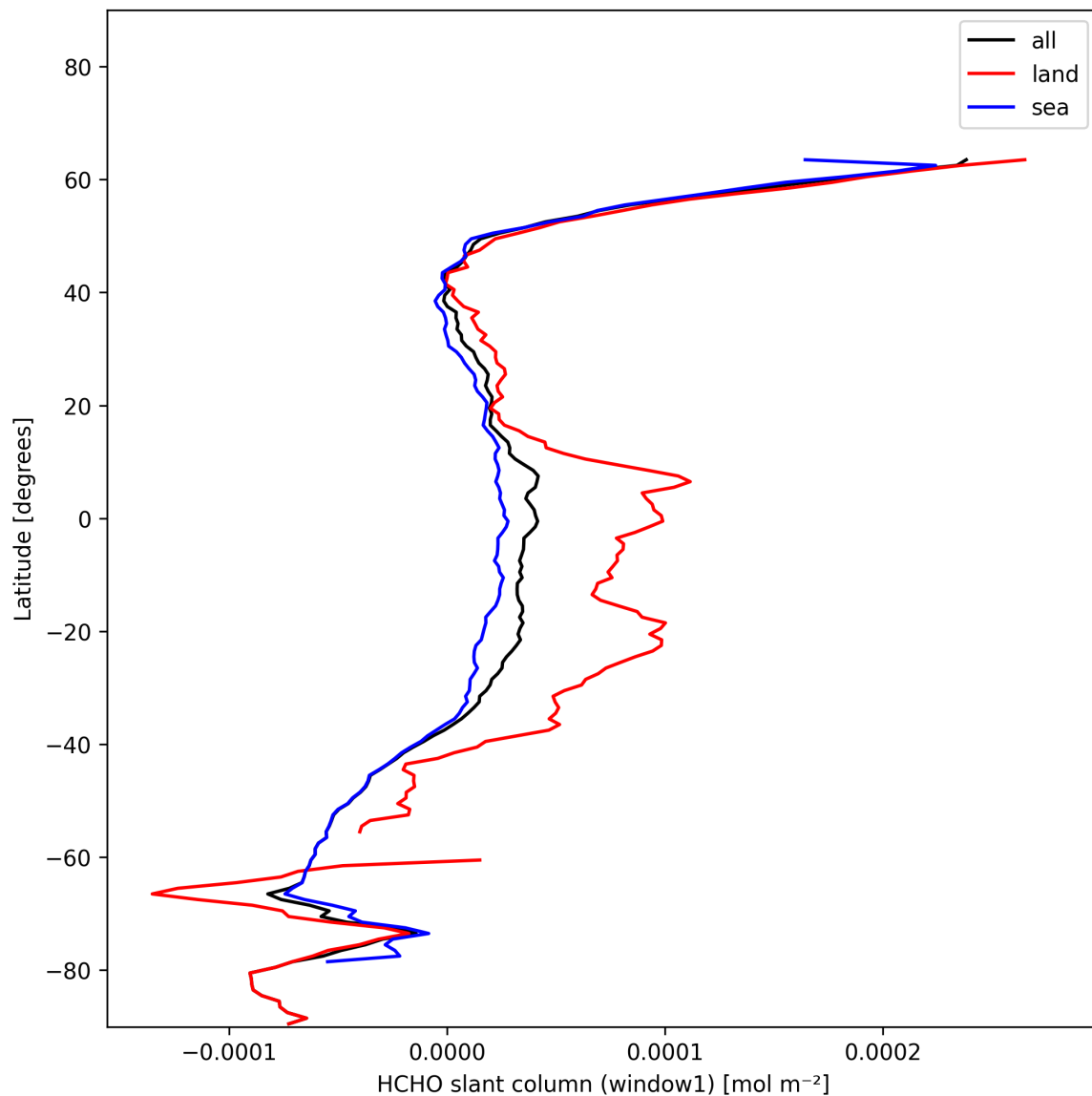
Figure 24: Zonal average of “HCHO slant column (window1)” for 2025-01-08 to 2025-01-10.
