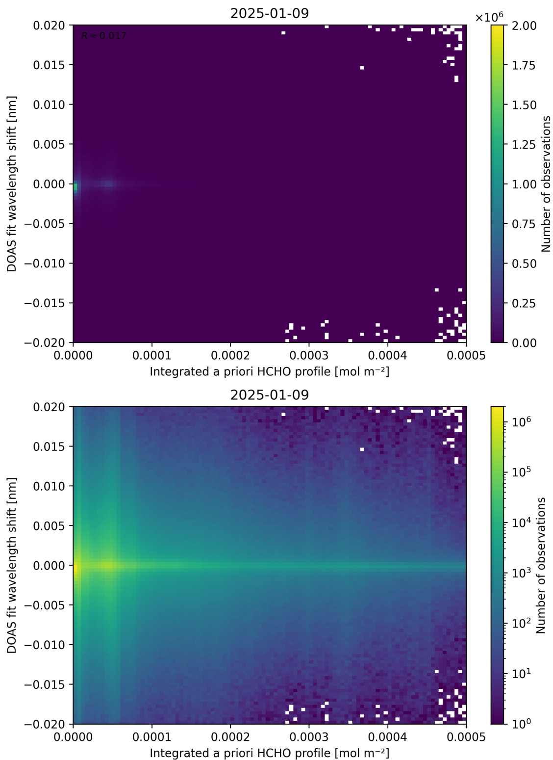
Figure 149: Scatter density plot of “Integrated a priori HCHO profile” against “DOAS fit wavelength shift” for 2025-01-08 to 2025-01-10.
