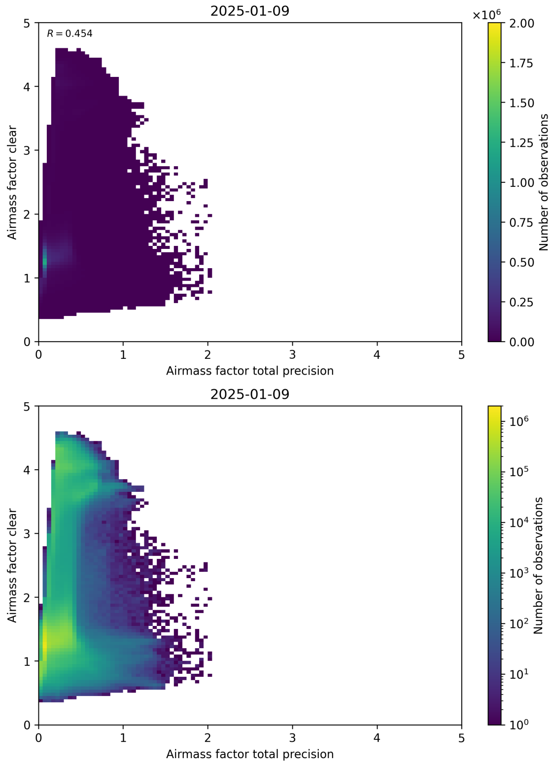
Figure 108: Scatter density plot of “Airmass factor total precision” against “Airmass factor clear” for 2025-01-08 to 2025-01-10.
