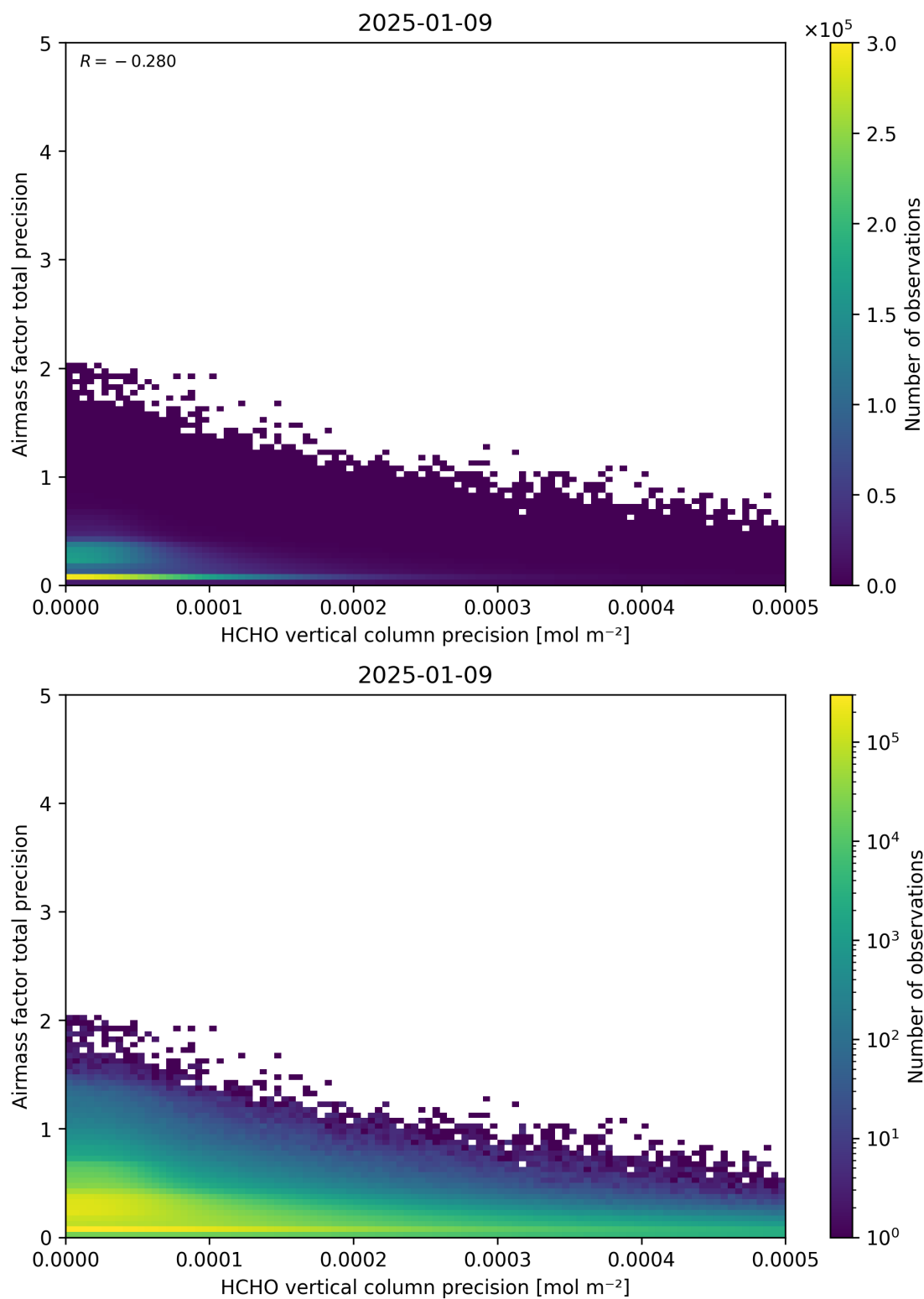
Figure 145: Scatter density plot of “HCHO vertical column precision” against “Airmass factor total precision” for 2025-01-08 to 2025-01-10.
