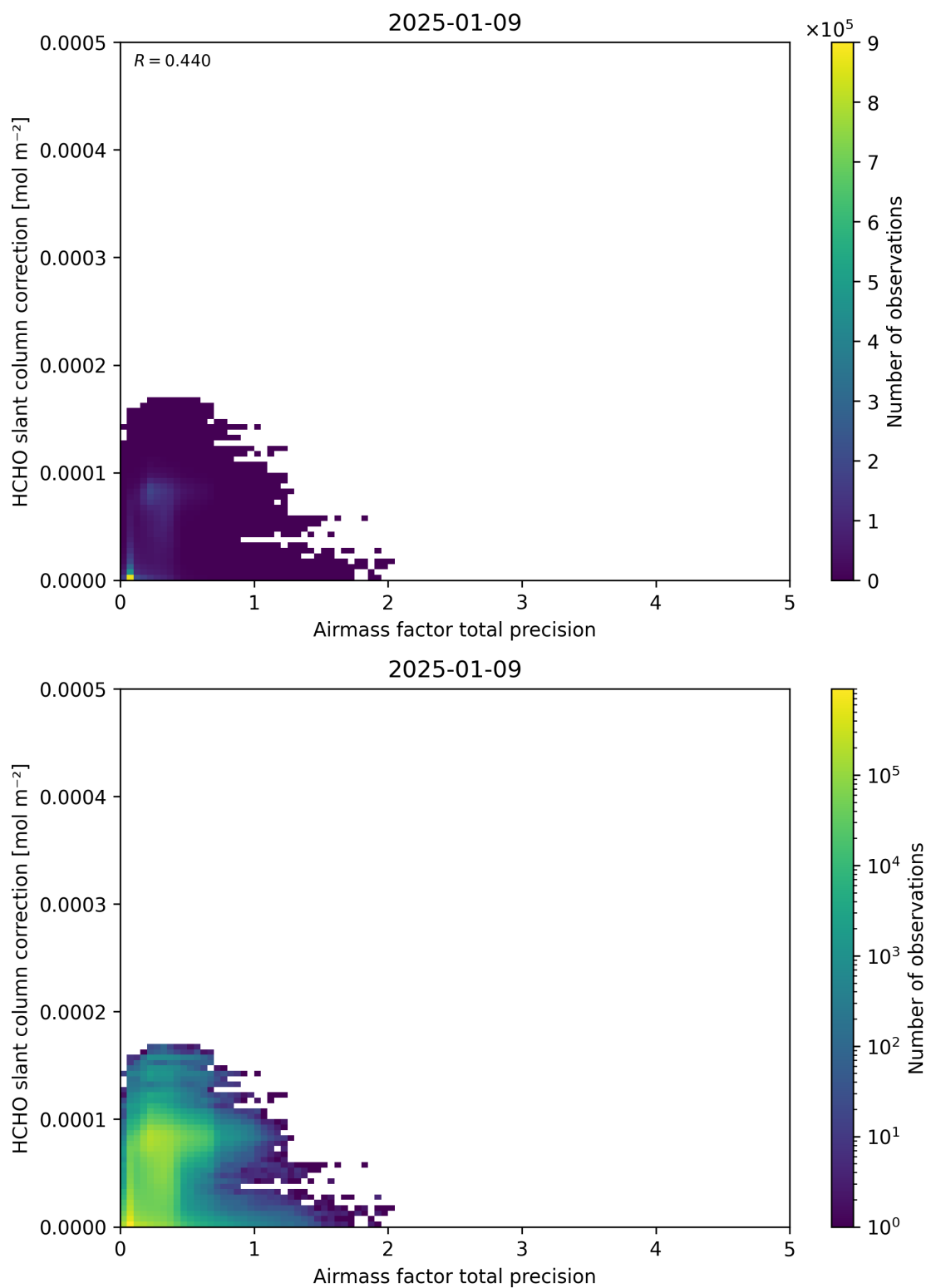
Figure 110: Scatter density plot of “Airmass factor total precision” against “HCHO slant column correction” for 2025-01-08 to 2025-01-10.
