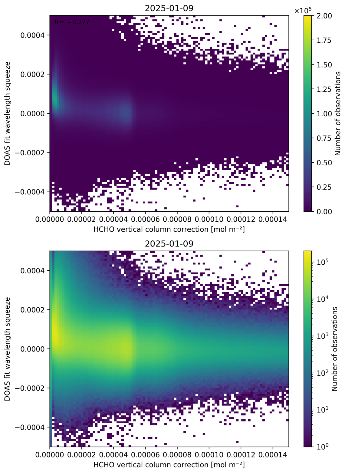
Figure 114: Scatter density plot of “HCHO vertical column correction” against “DOAS fit wavelength squeeze” for 2025-01-08 to 2025-01-10.
