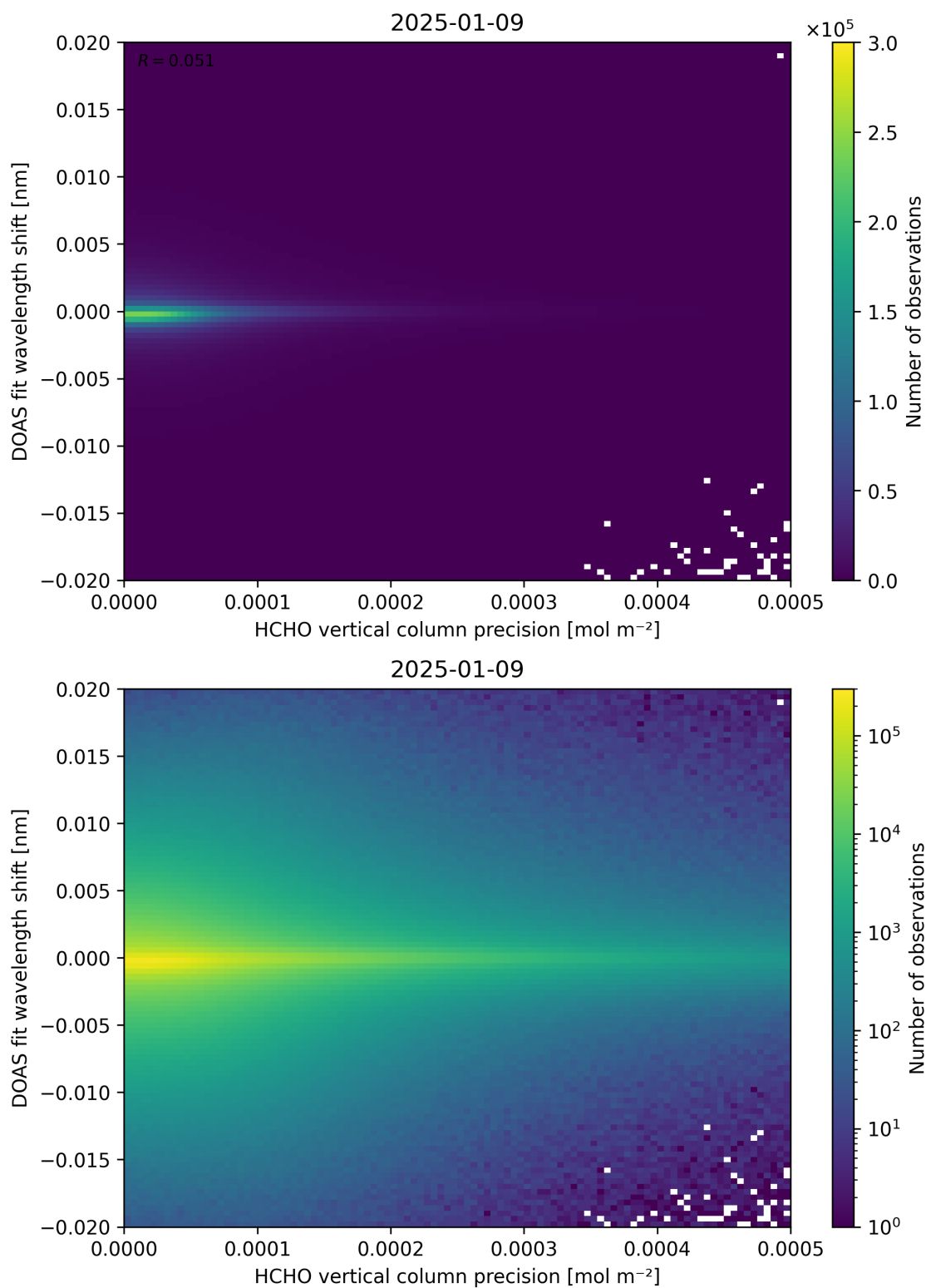
Figure 137: Scatter density plot of “HCHO vertical column precision” against “DOAS fit wavelength shift” for 2025-01-08 to 2025-01-10.
