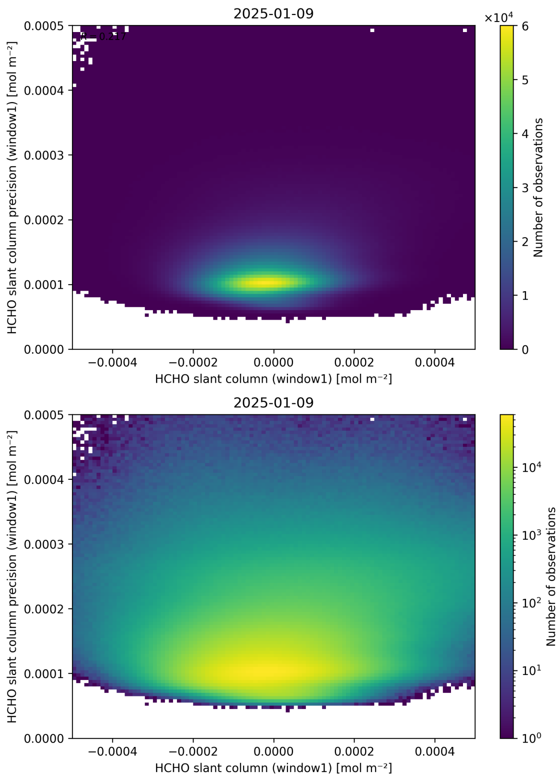
Figure 84: Scatter density plot of “HCHO slant column (window1)” against “HCHO slant column precision (window1)” for 2025-01-08 to 2025-01-10.
