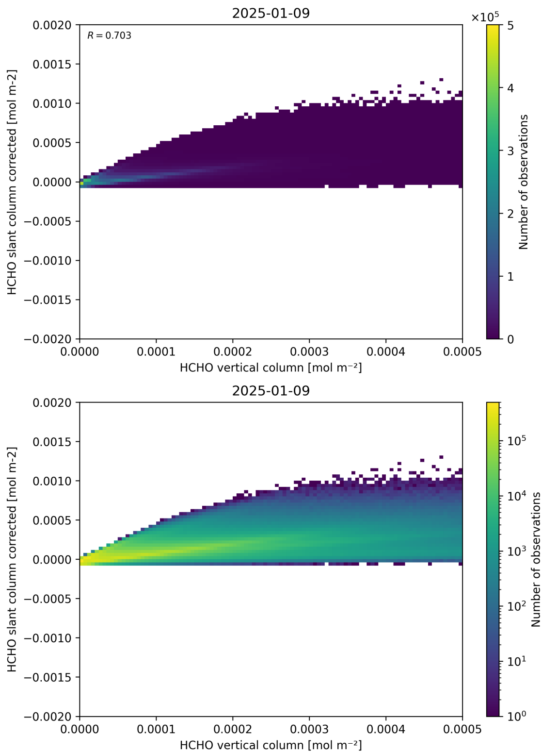
Figure 127: Scatter density plot of “HCHO vertical column” against “HCHO slant column corrected” for 2025-01-08 to 2025-01-10.
