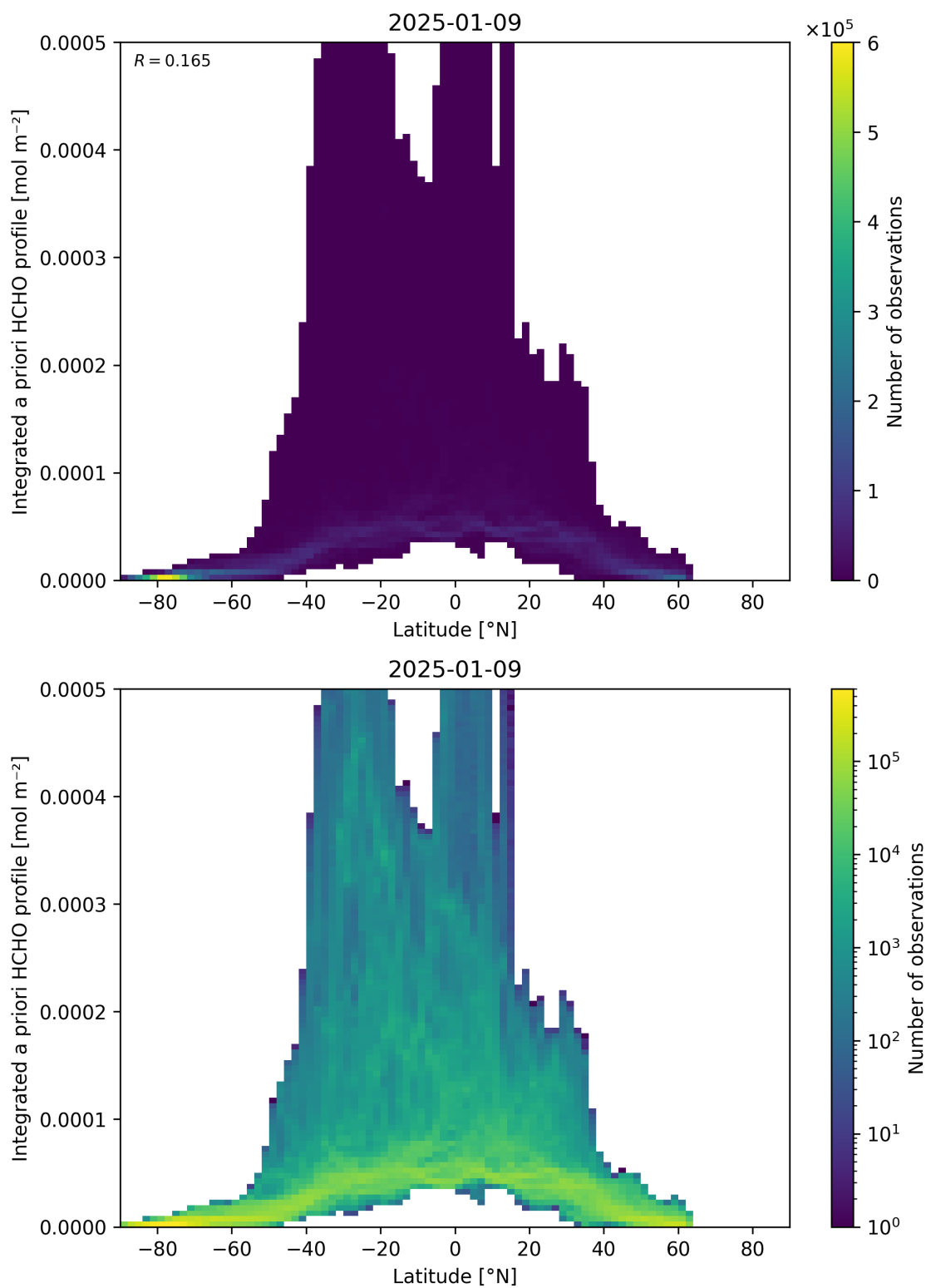
Figure 166: Scatter density plot of “Latitude” against “Integrated a priori HCHO profile” for 2025-01-08 to 2025-01-10.
