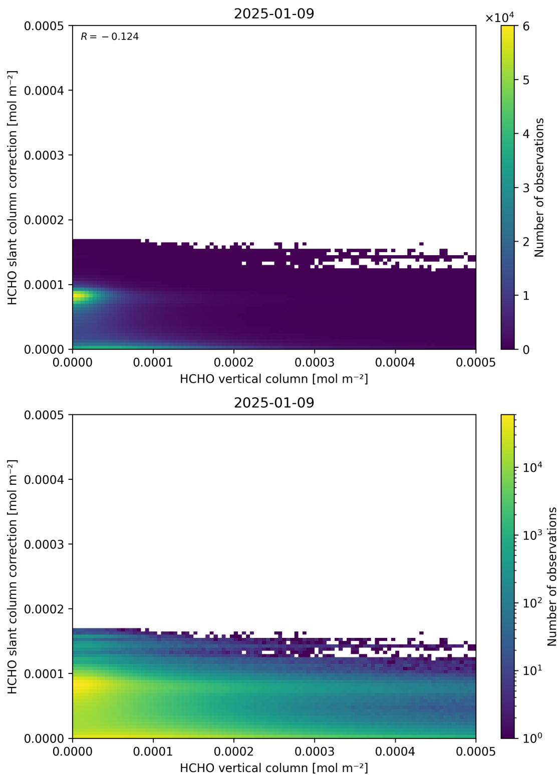
Figure 128: Scatter density plot of “HCHO vertical column” against “HCHO slant column correction” for 2025-01-08 to 2025-01-10.
