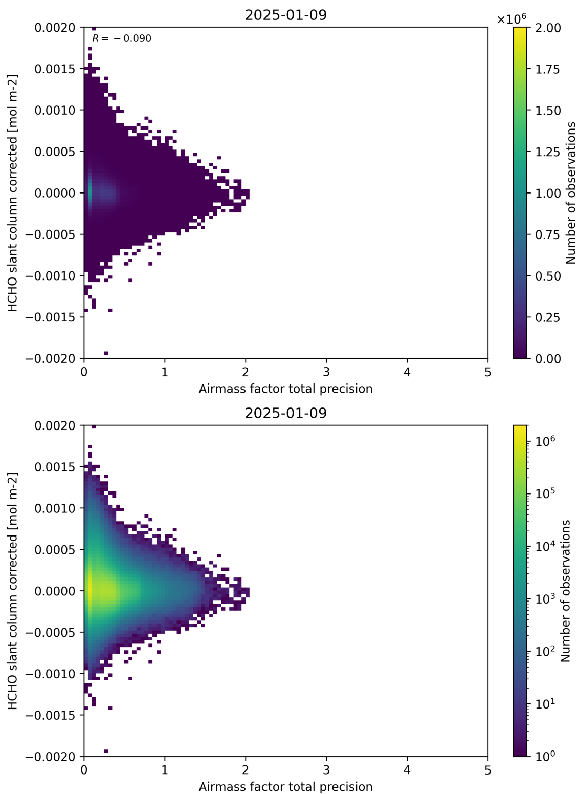
Figure 109: Scatter density plot of “Airmass factor total precision” against “HCHO slant column corrected” for 2025-01-08 to 2025-01-10.
