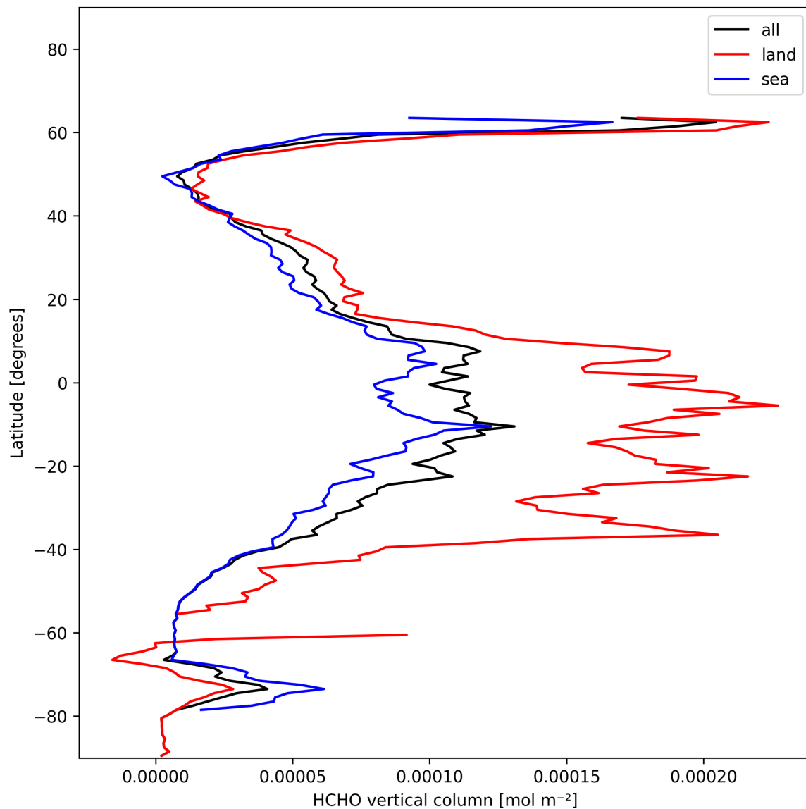
Figure 21: Zonal average of “HCHO vertical column” for 2025-01-08 to 2025-01-10.
