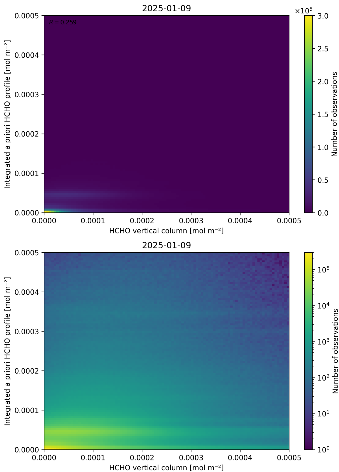
Figure 135: Scatter density plot of “HCHO vertical column” against “Integrated a priori HCHO profile” for 2025-01-08 to 2025-01-10.
