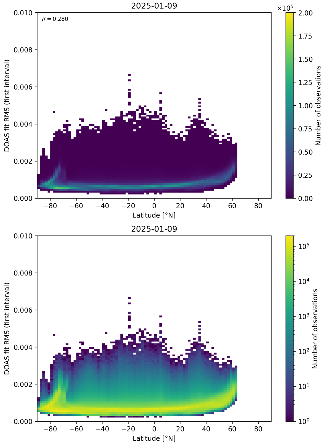
Figure 153: Scatter density plot of “Latitude” against “DOAS fit RMS (first interval)” for 2025-01-08 to 2025-01-10.
