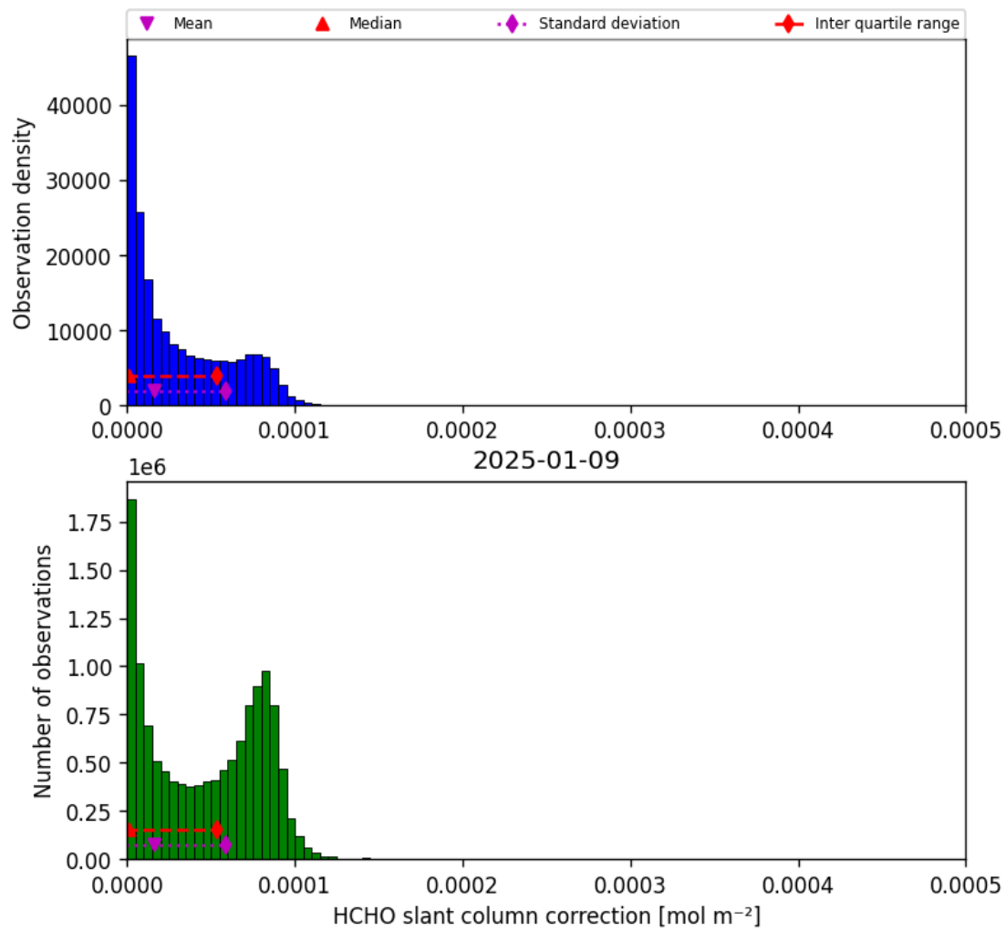
Figure 47: Histogram of “HCHO slant column correction” for 2025-01-08 to 2025-01-10
