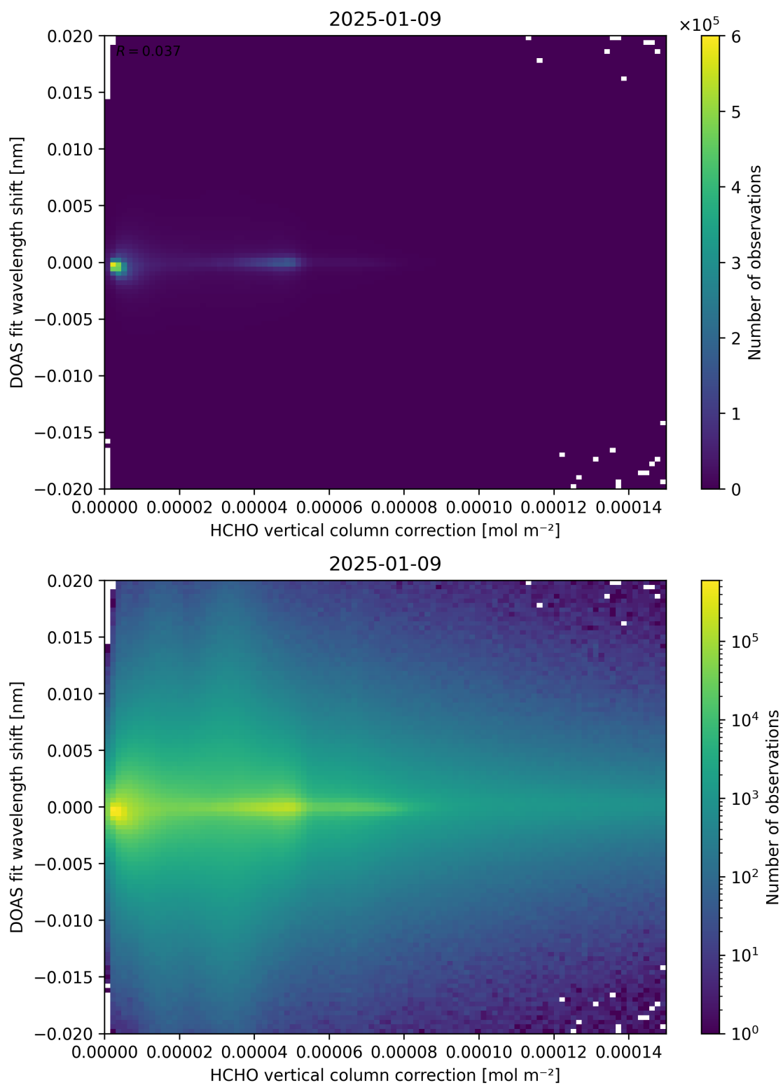
Figure 113: Scatter density plot of “HCHO vertical column correction” against “DOAS fit wavelength shift” for 2025-01-08 to 2025-01-10.
