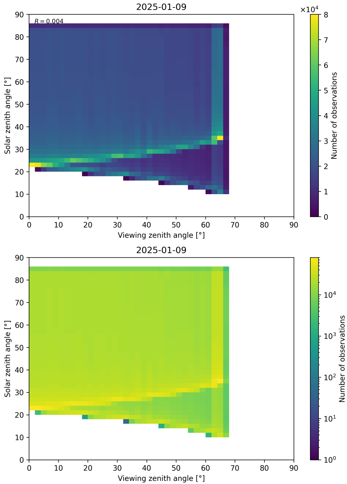
Figure 197: Scatter density plot of “Viewing zenith angle” against “Solar zenith angle” for 2025-01-08 to 2025-01-10.
