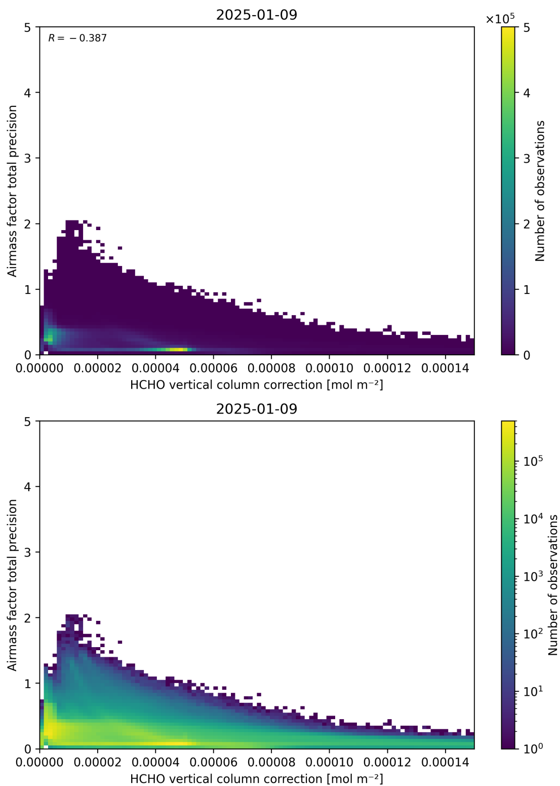
Figure 121: Scatter density plot of “HCHO vertical column correction” against “Airmass factor total precision” for 2025-01-08 to 2025-01-10.
