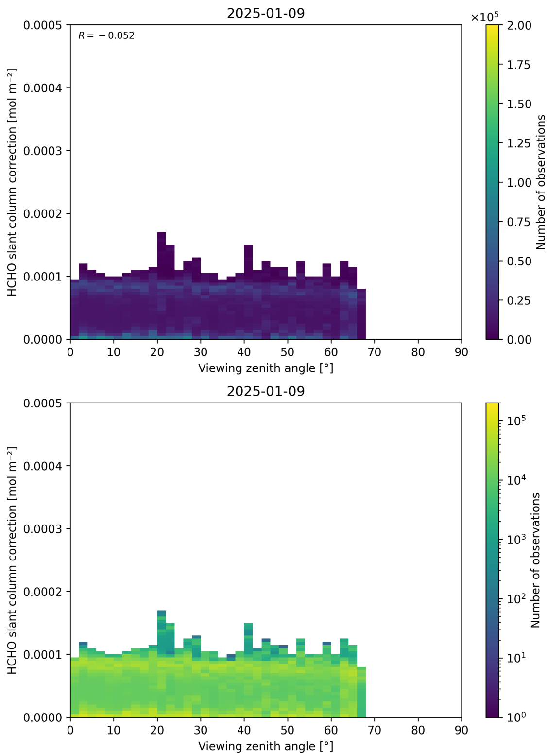
Figure 187: Scatter density plot of “Viewing zenith angle” against “HCHO slant column correction” for 2025-01-08 to 2025-01-10.
