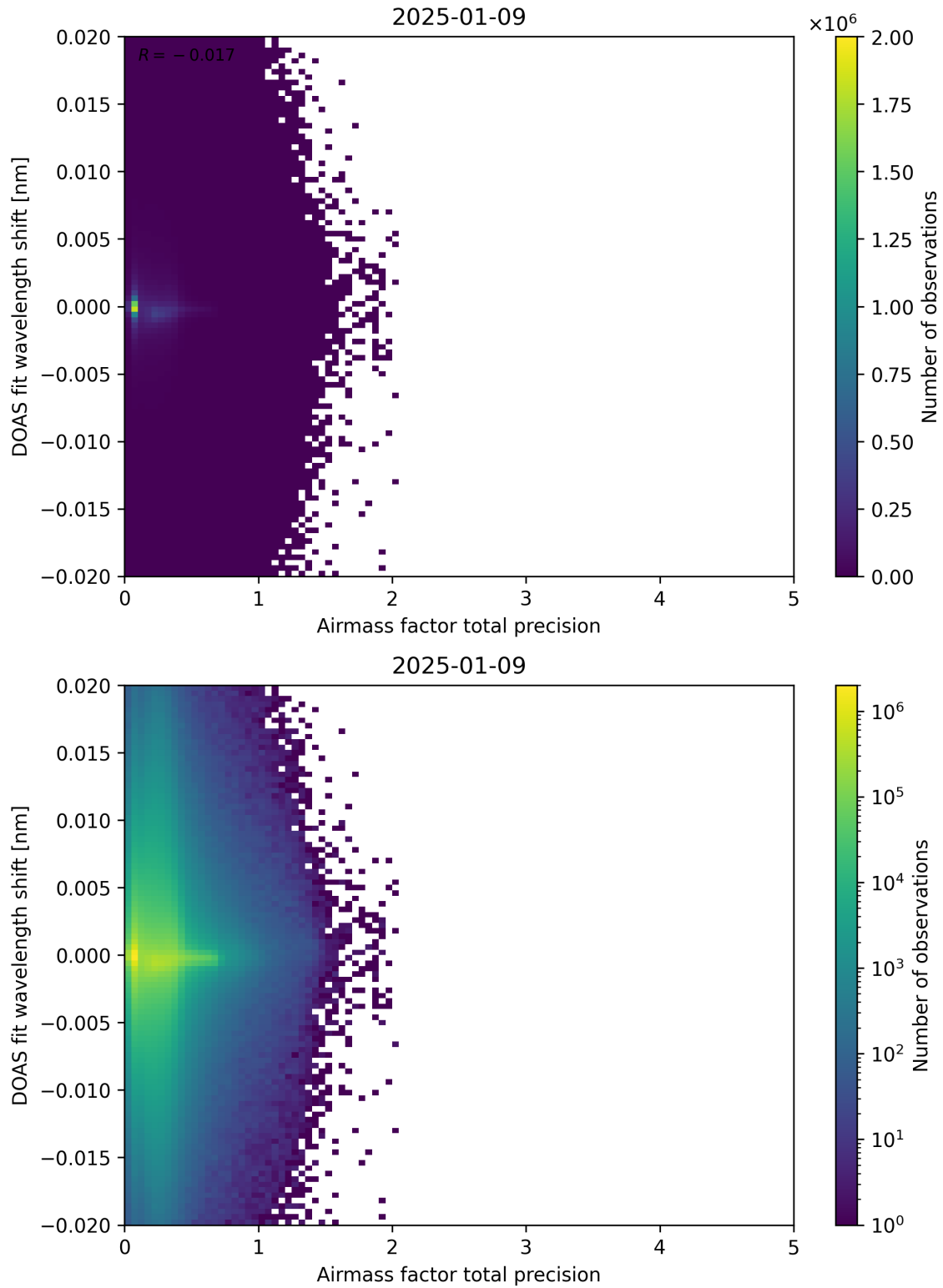
Figure 106: Scatter density plot of “Airmass factor total precision” against “DOAS fit wavelength shift” for 2025-01-08 to 2025-01-10.
