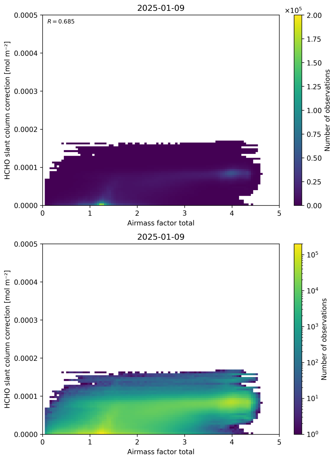
Figure 102: Scatter density plot of “Airmass factor total” against “HCHO slant column correction” for 2025-01-08 to 2025-01-10.
