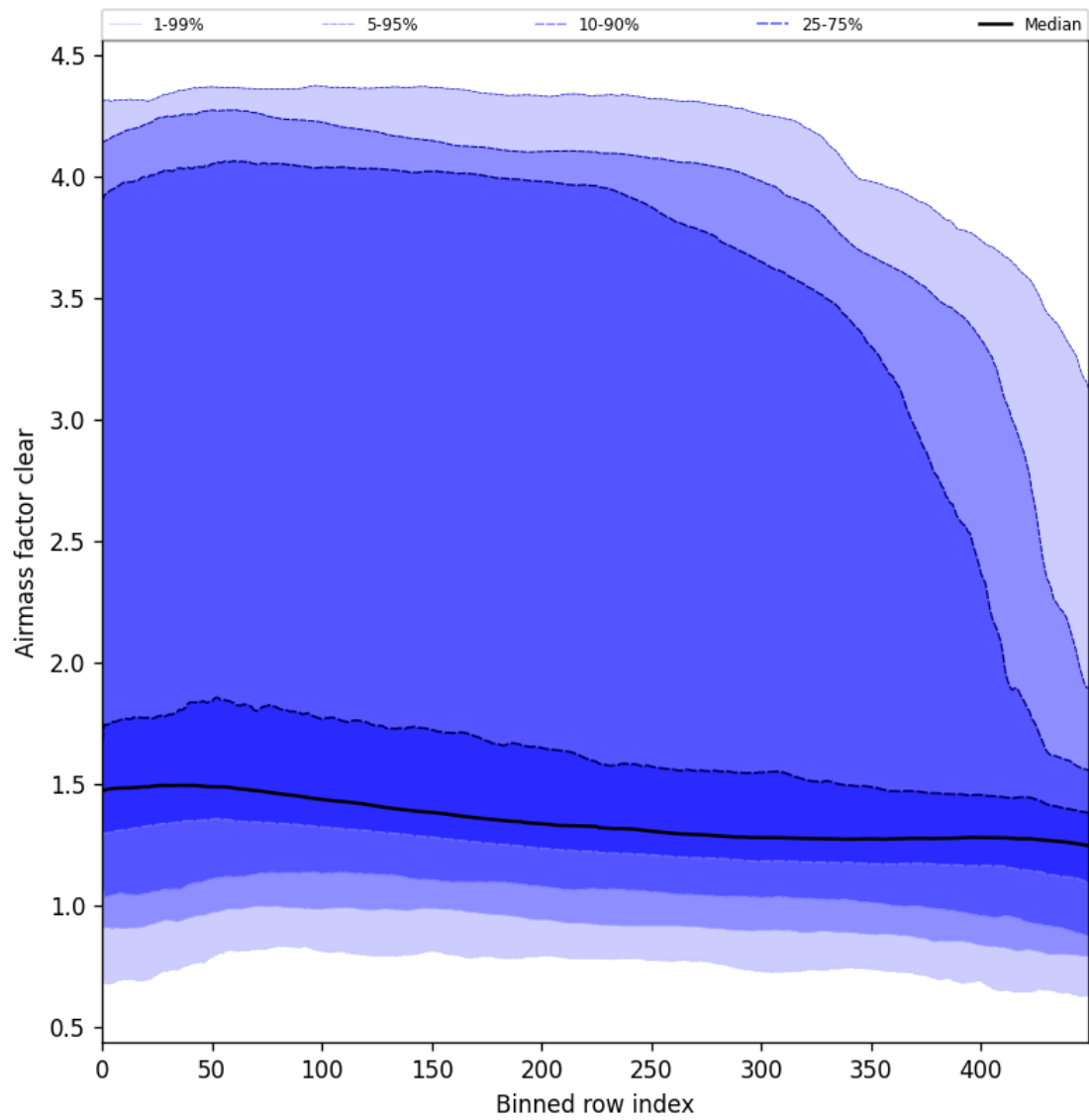
Figure 56: Along track statistics of “Airmass factor clear” for 2025-01-08 to 2025-01-10
