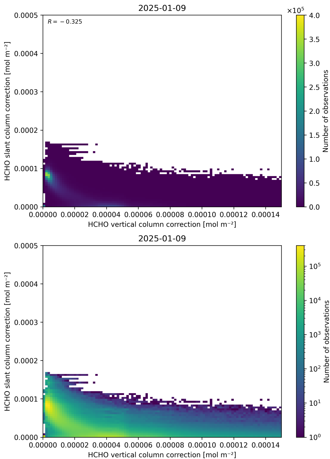
Figure 117: Scatter density plot of “HCHO vertical column correction” against “HCHO slant column correction” for 2025-01-08 to 2025-01-10.
