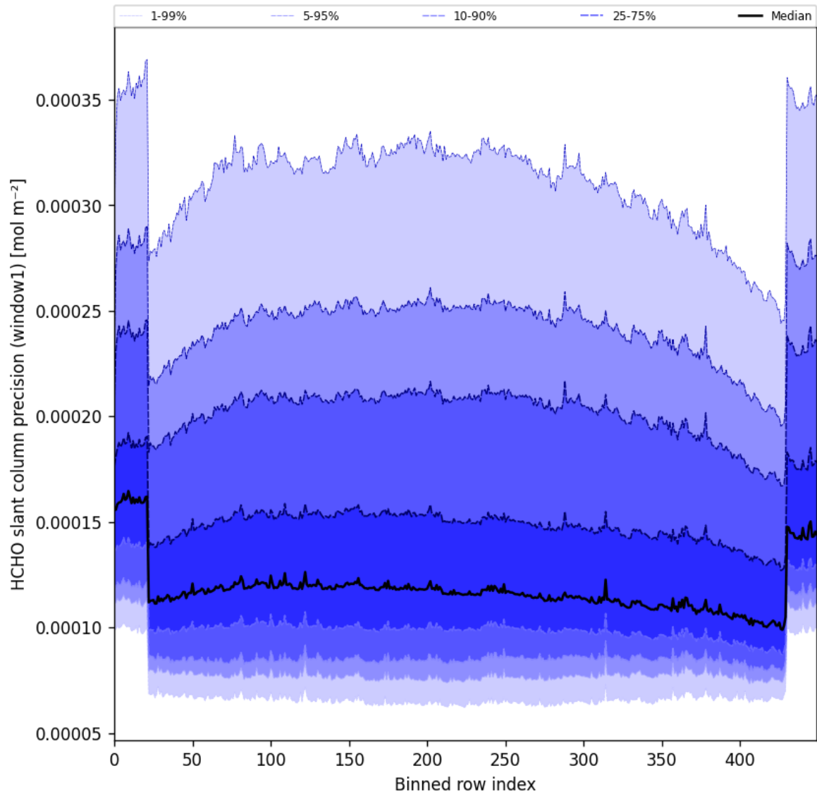
Figure 53: Along track statistics of “HCHO slant column precision (window1)” for 2025-01-08 to 2025-01-10
