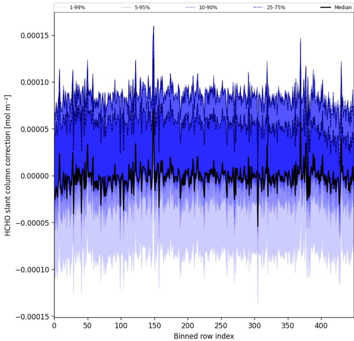
Figure 61: Along track statistics of “HCHO slant column correction” for 2025-01-08 to 2025-01-10
