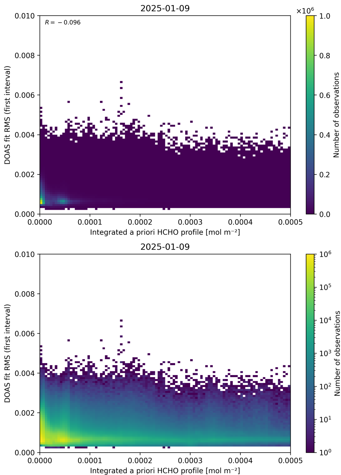
Figure 148: Scatter density plot of “Integrated a priori HCHO profile” against “DOAS fit RMS (first interval)” for 2025-01-08 to 2025-01-10.
