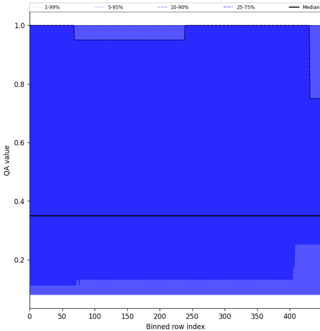
Figure 48: Along track statistics of “QA value” for 2025-01-08 to 2025-01-10
