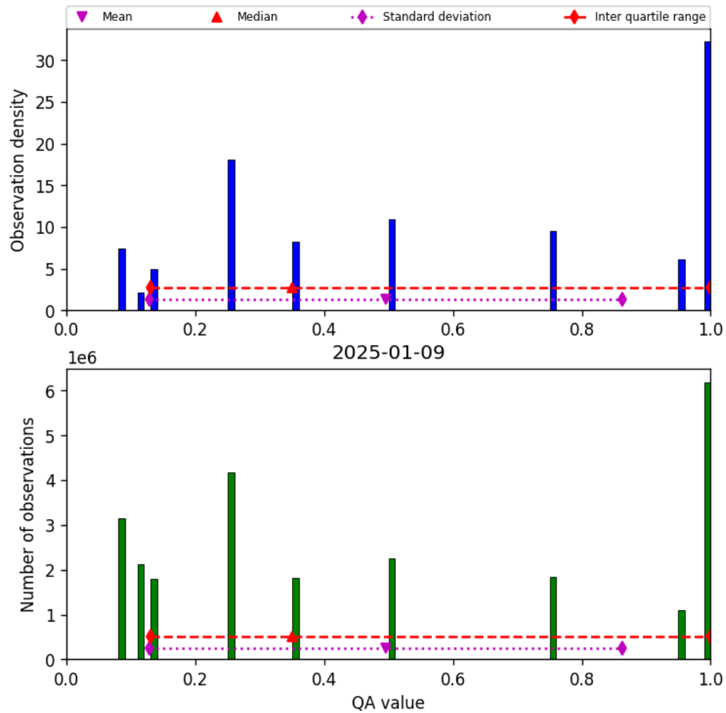
Figure 34: Histogram of “QA value” for 2025-01-08 to 2025-01-10
