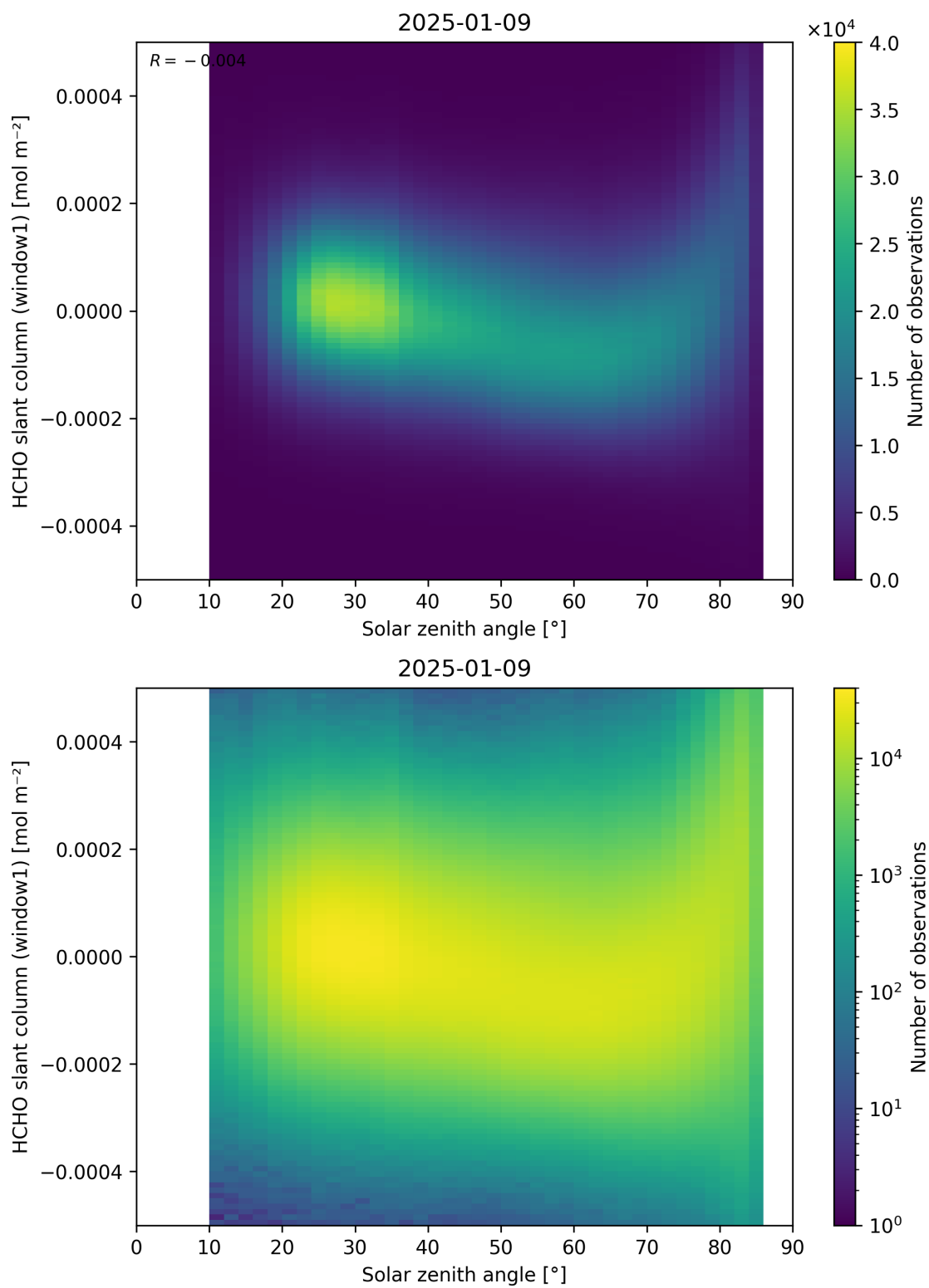
Figure 173: Scatter density plot of “Solar zenith angle” against “HCHO slant column (window1)” for 2025-01-08 to 2025-01-10.
