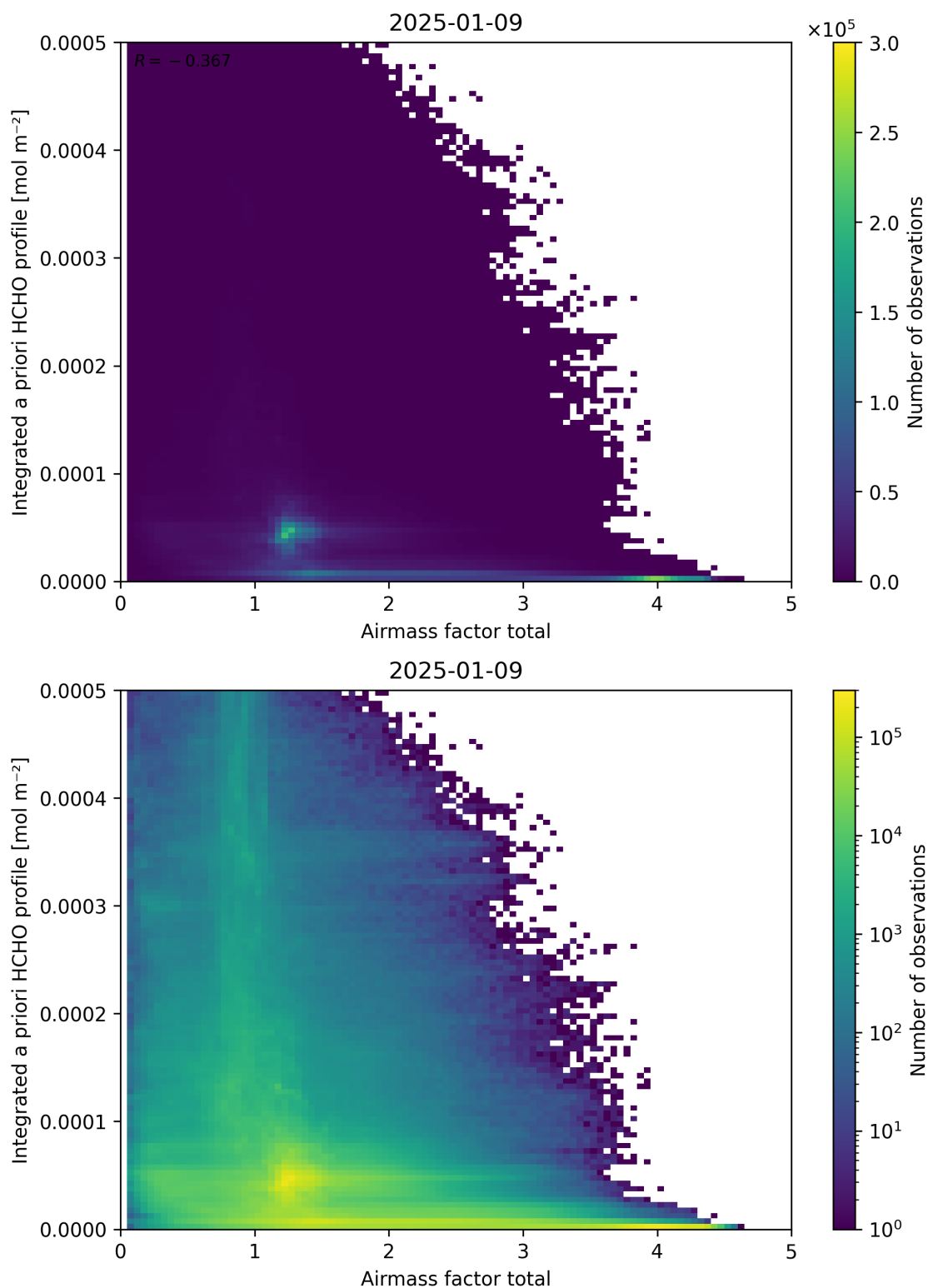
Figure 104: Scatter density plot of “Airmass factor total” against “Integrated a priori HCHO profile” for 2025-01-08 to 2025-01-10.
