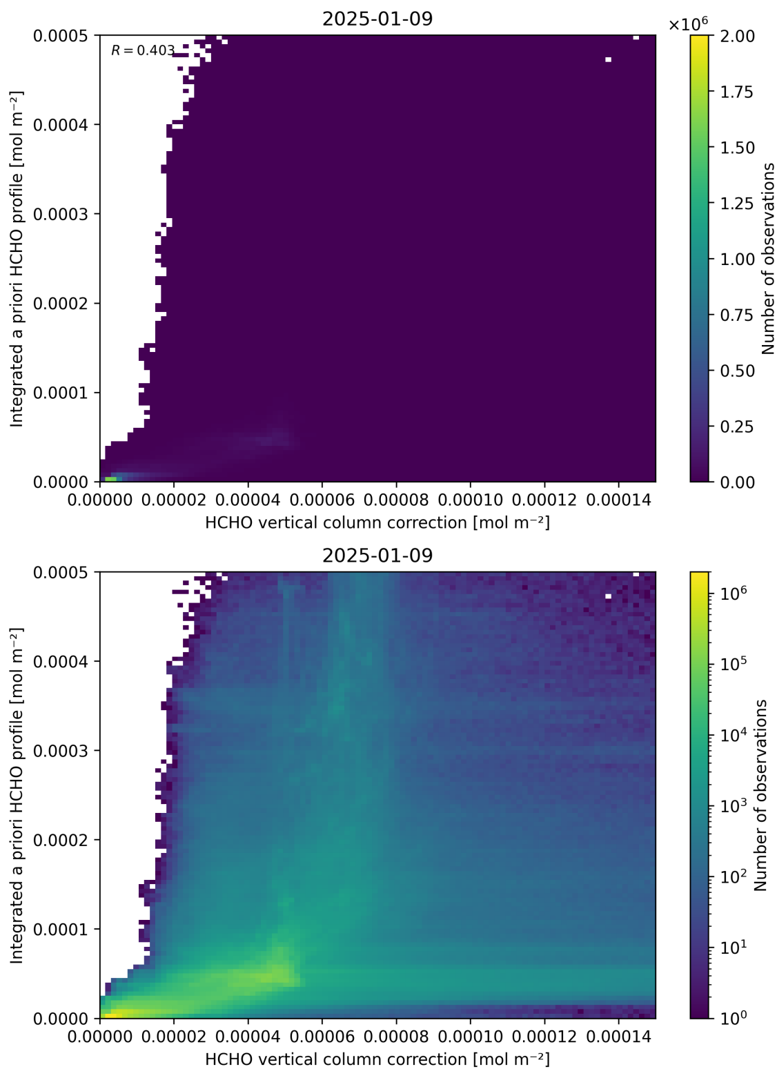
Figure 122: Scatter density plot of “HCHO vertical column correction” against “Integrated a priori HCHO profile” for 2025-01-08 to 2025-01-10.
