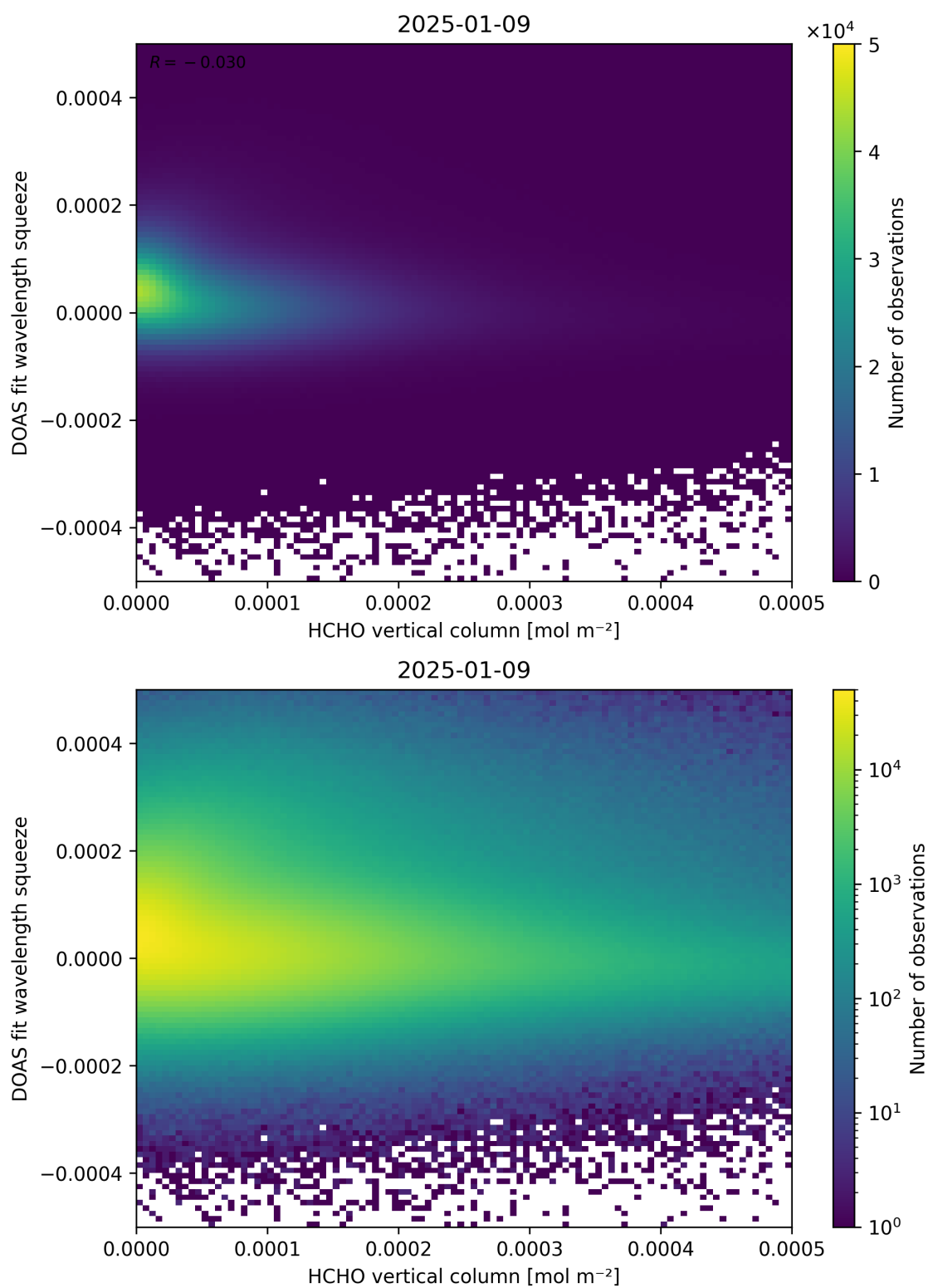
Figure 125: Scatter density plot of “HCHO vertical column” against “DOAS fit wavelength squeeze” for 2025-01-08 to 2025-01-10.
