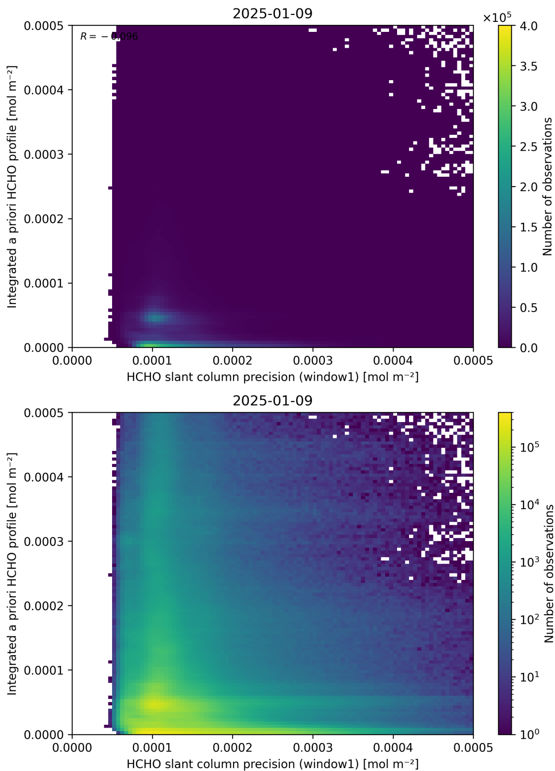
Figure 96: Scatter density plot of “HCHO slant column precision (window1)” against “Integrated a priori HCHO profile” for 2025-01-08 to 2025-01-10.
