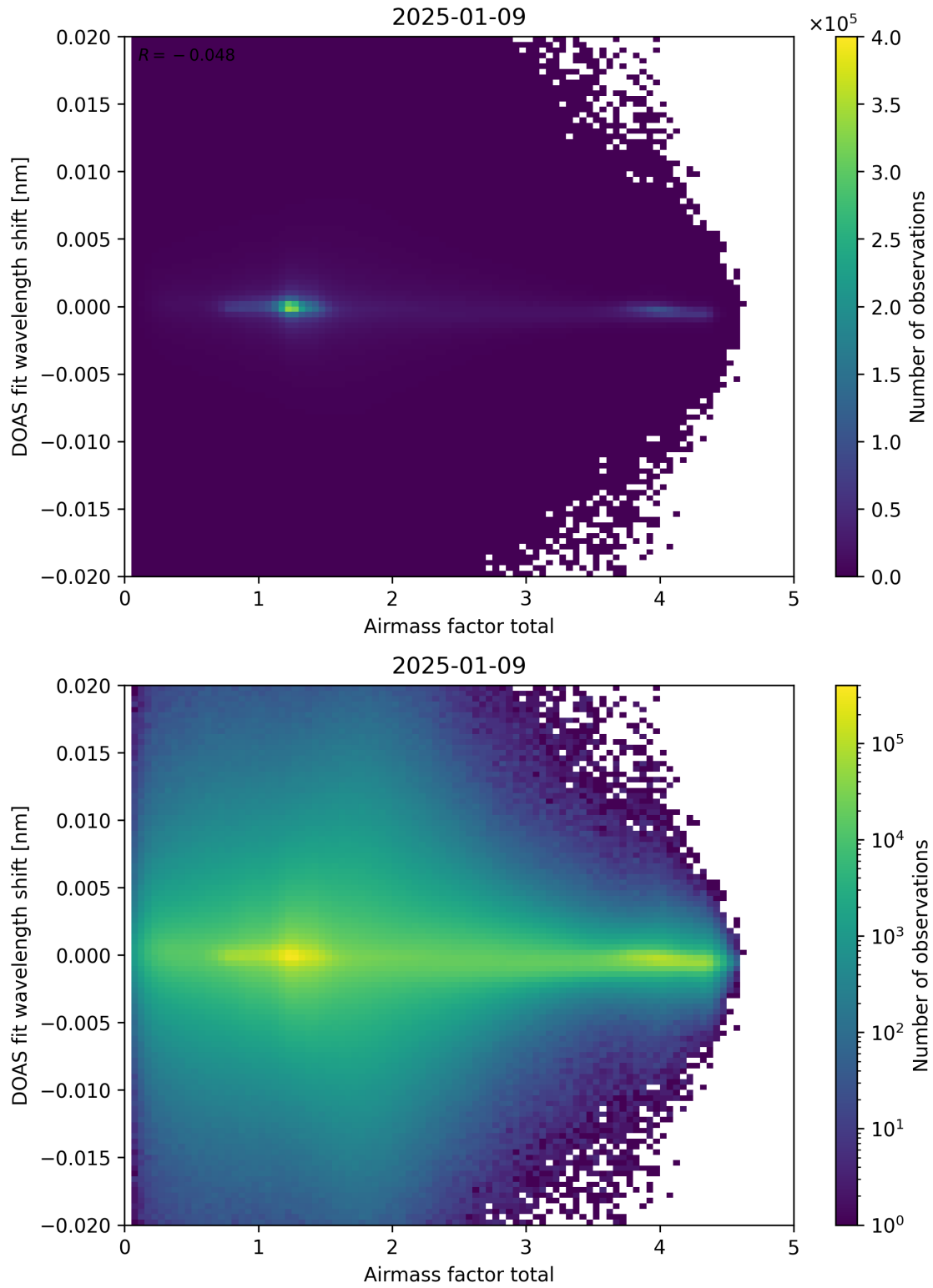
Figure 98: Scatter density plot of “Airmass factor total” against “DOAS fit wavelength shift” for 2025-01-08 to 2025-01-10.
