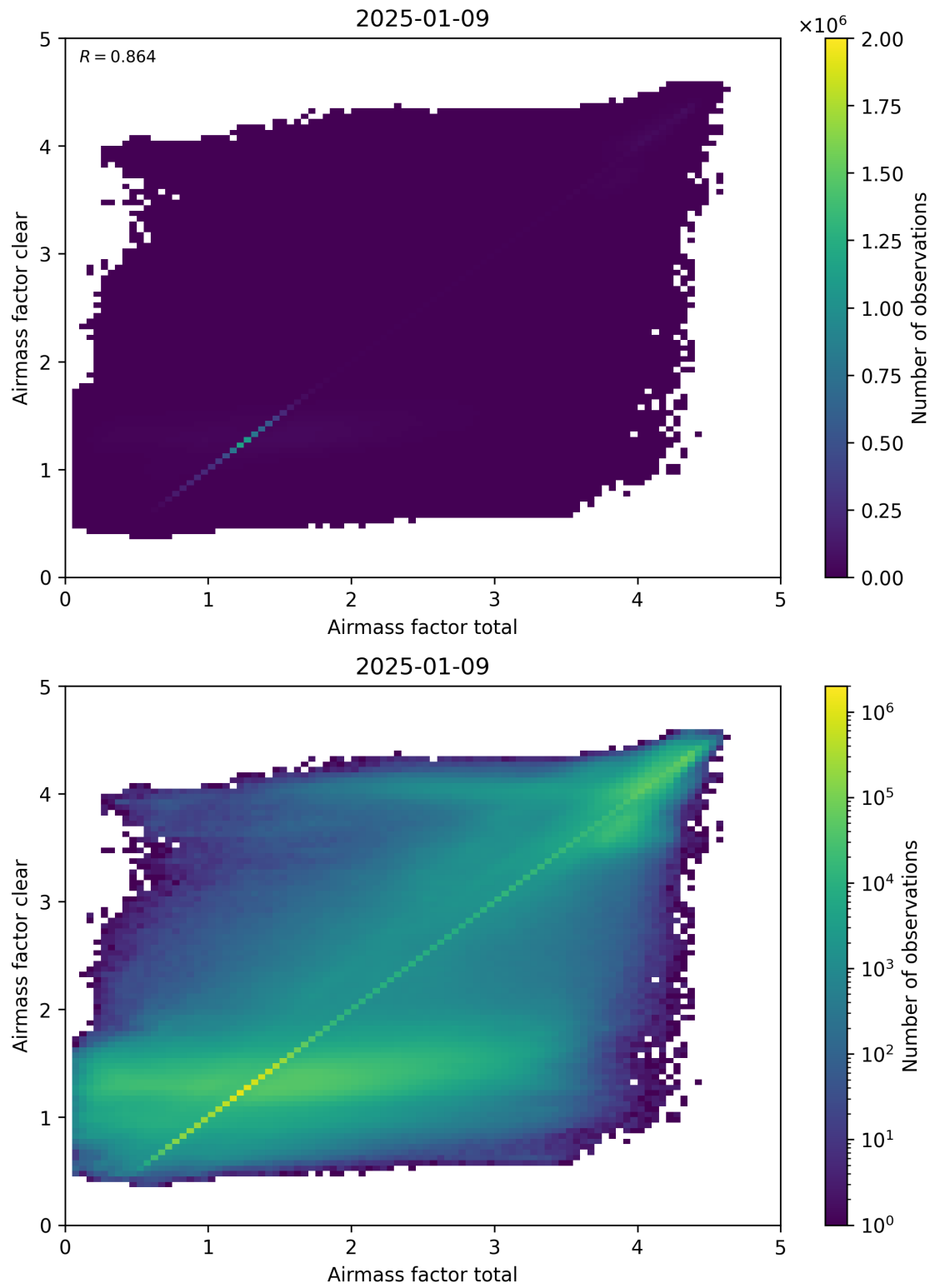
Figure 100: Scatter density plot of “Airmass factor total” against “Airmass factor clear” for 2025-01-08 to 2025-01-10.
