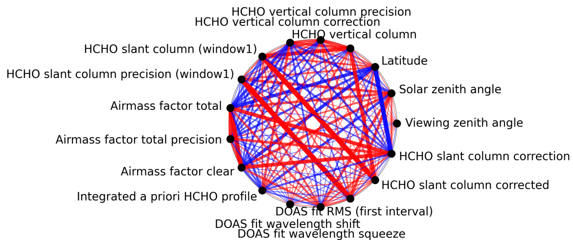
Figure 1: Map of correlation graph for 2025-01-08 to 2025-01-10.
