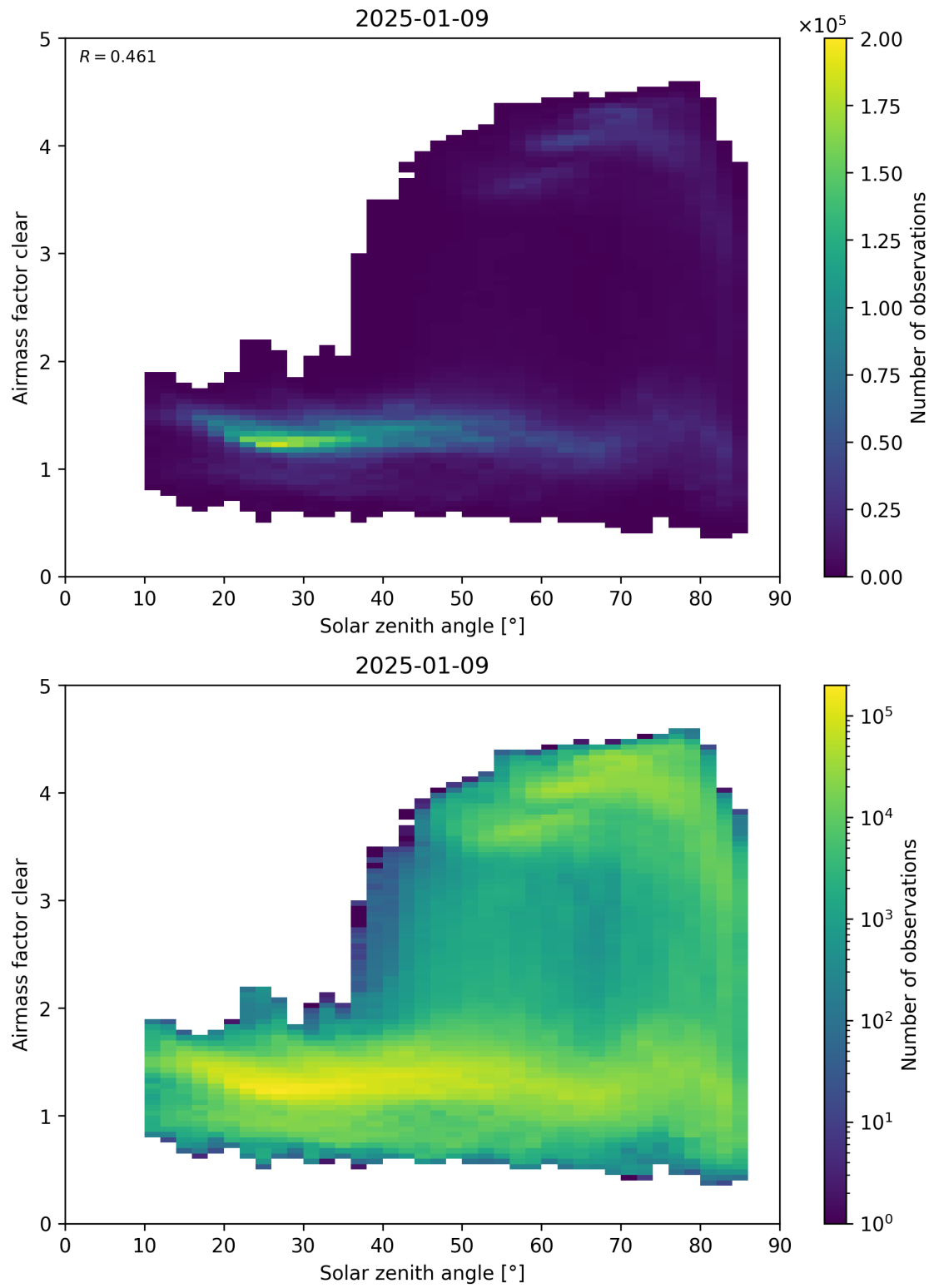
Figure 170: Scatter density plot of “Solar zenith angle” against “Airmass factor clear” for 2025-01-08 to 2025-01-10.
