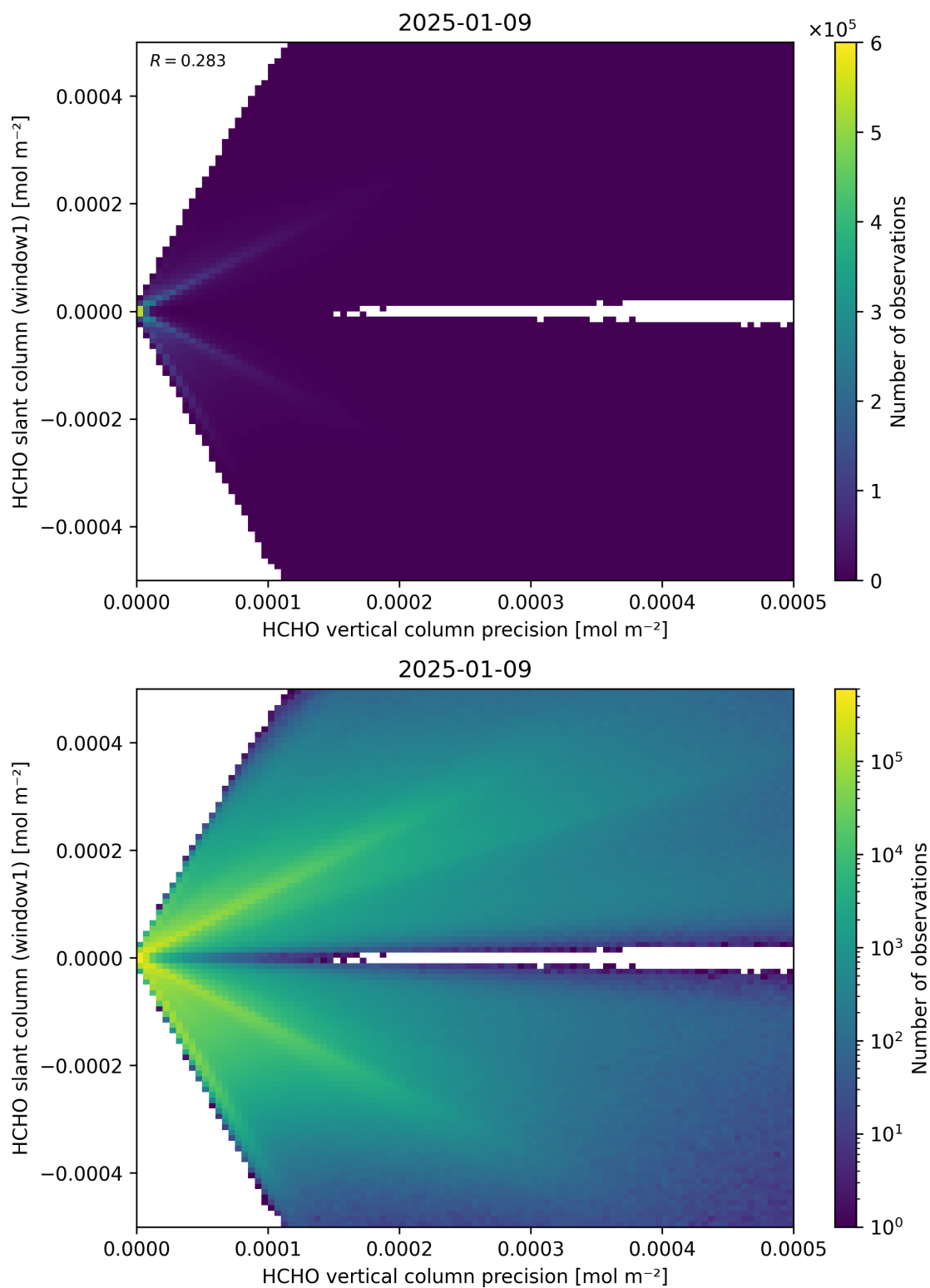
Figure 142: Scatter density plot of “HCHO vertical column precision” against “HCHO slant column (window1)” for 2025-01-08 to 2025-01-10.
