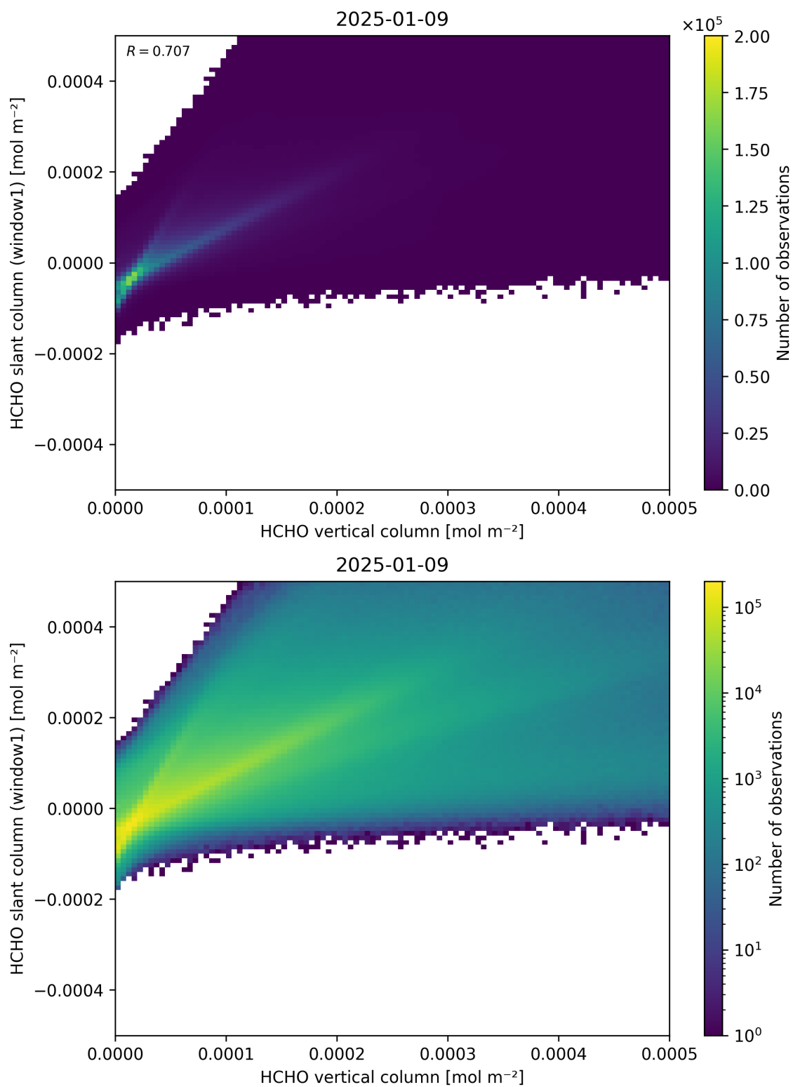
Figure 129: Scatter density plot of “HCHO vertical column” against “HCHO slant column (window1)” for 2025-01-08 to 2025-01-10.
