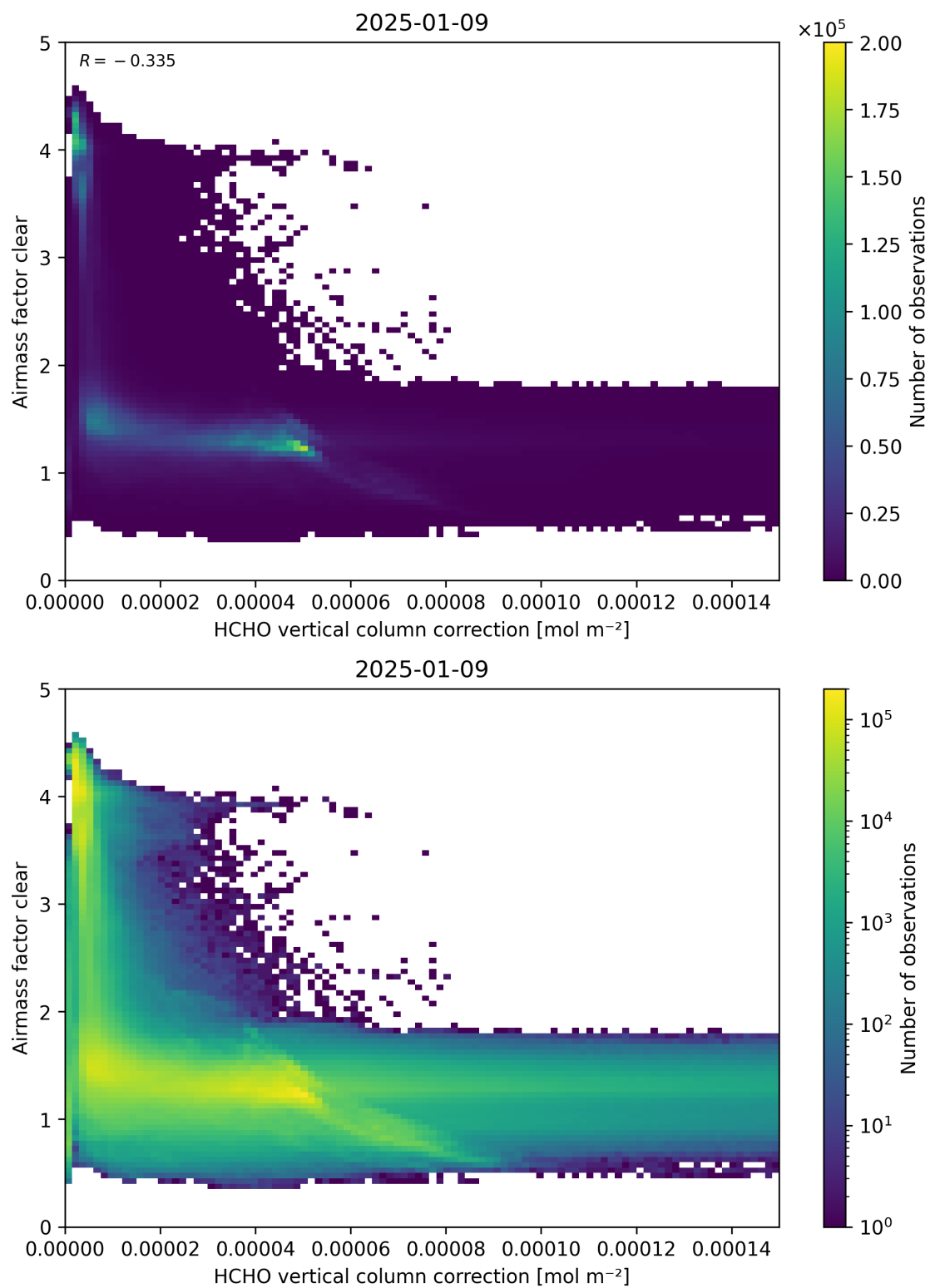
Figure 115: Scatter density plot of “HCHO vertical column correction” against “Airmass factor clear” for 2025-01-08 to 2025-01-10.
