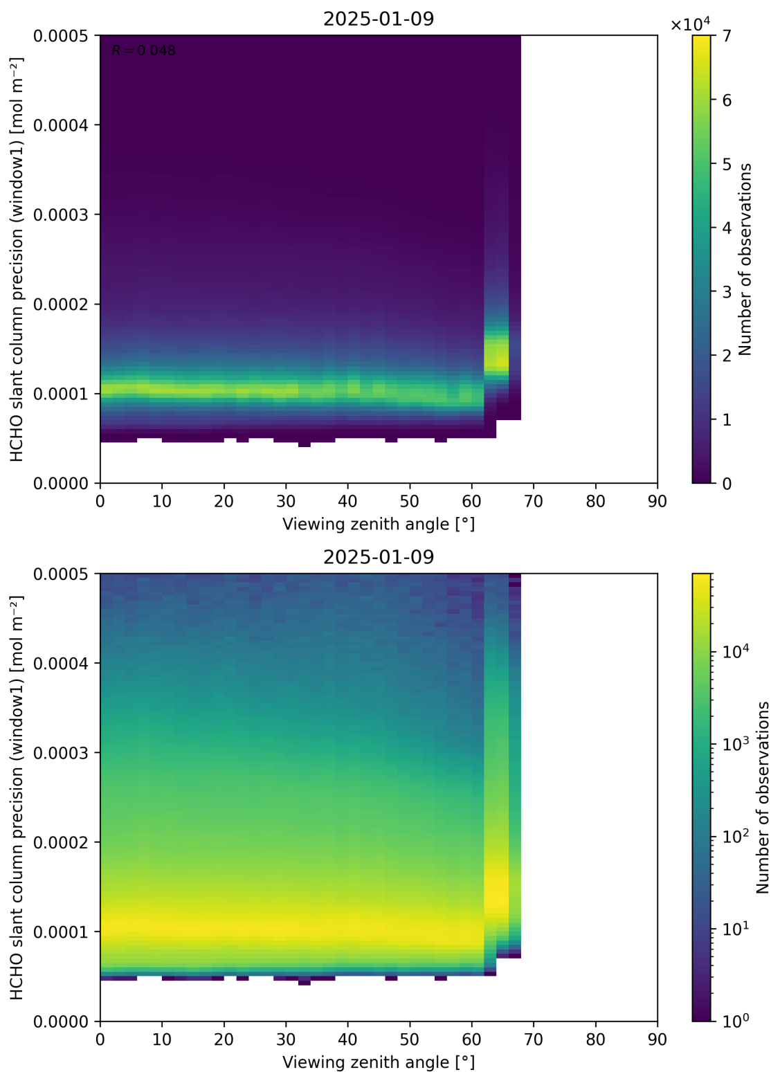
Figure 189: Scatter density plot of “Viewing zenith angle” against “HCHO slant column precision (window1)” for 2025-01-08 to 2025-01-10.
