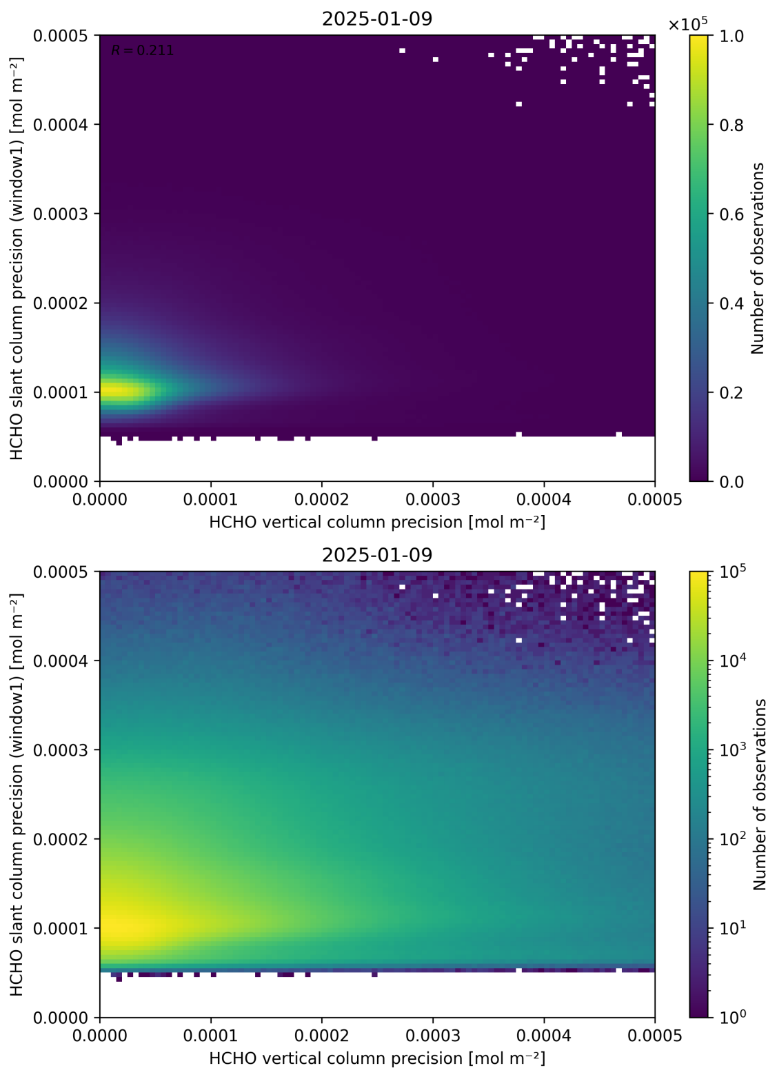
Figure 143: Scatter density plot of “HCHO vertical column precision” against “HCHO slant column precision (window1)” for 2025-01-08 to 2025-01-10.
