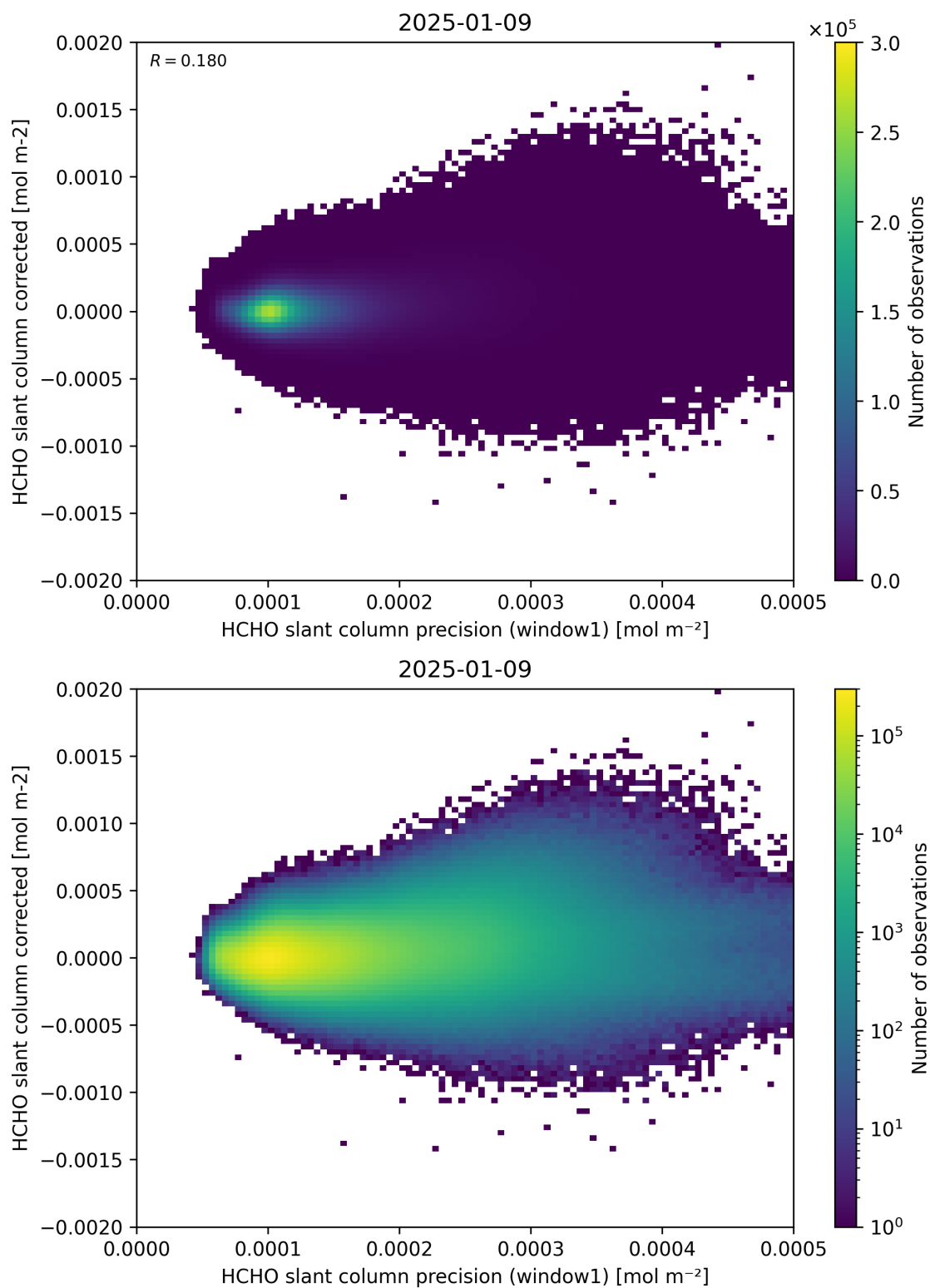
Figure 92: Scatter density plot of “HCHO slant column precision (window1)” against “HCHO slant column corrected” for 2025-01-08 to 2025-01-10.
