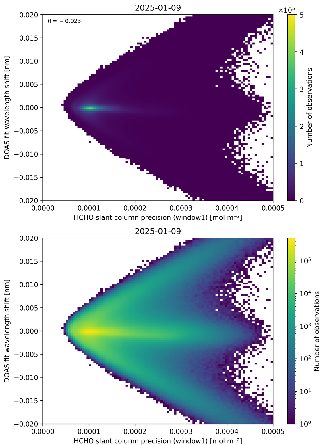
Figure 89: Scatter density plot of “HCHO slant column precision (window1)” against “DOAS fit wavelength shift” for 2025-01-08 to 2025-01-10.
