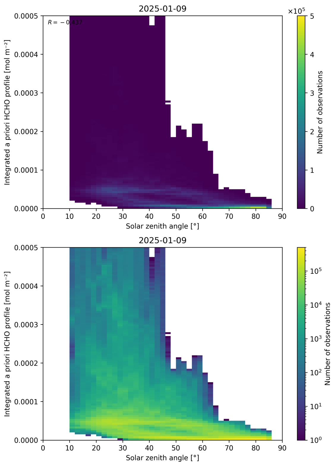
Figure 180: Scatter density plot of “Solar zenith angle” against “Integrated a priori HCHO profile” for 2025-01-08 to 2025-01-10.
