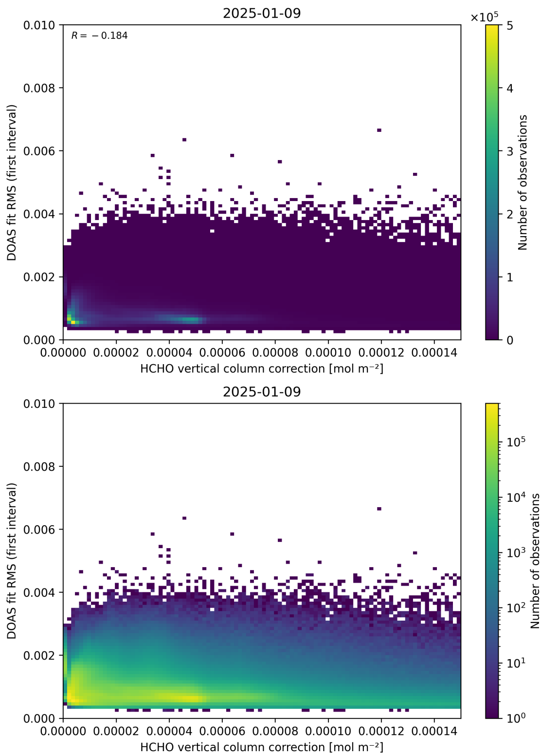
Figure 112: Scatter density plot of “HCHO vertical column correction” against “DOAS fit RMS (first interval)” for 2025-01-08 to 2025-01-10.
