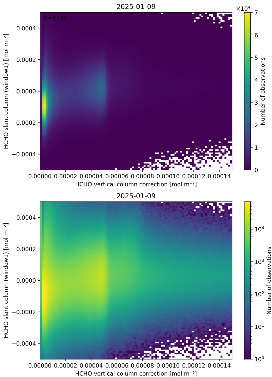
Figure 118: Scatter density plot of “HCHO vertical column correction” against “HCHO slant column (window1)” for 2025-01-08 to 2025-01-10.
