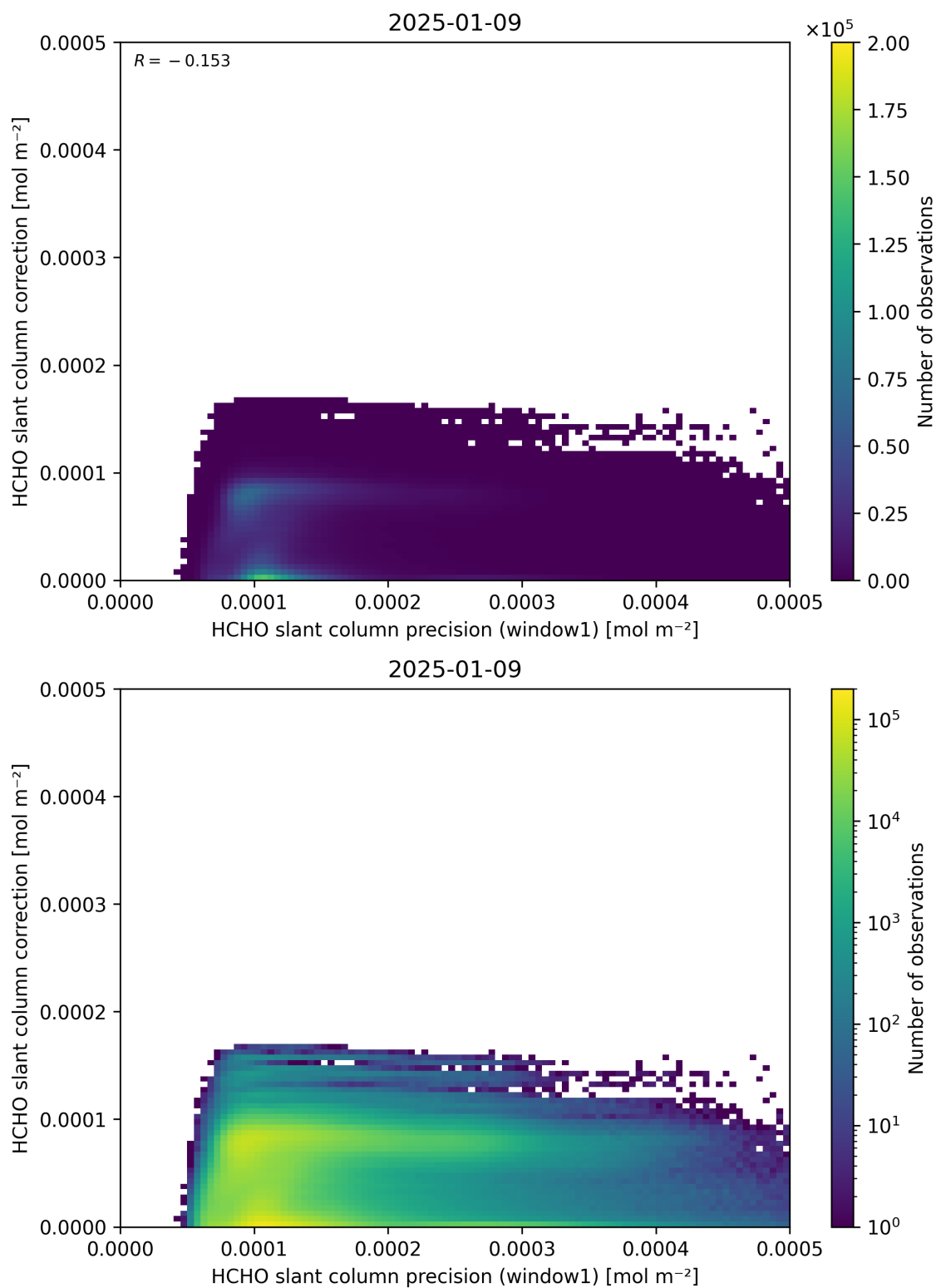
Figure 93: Scatter density plot of “HCHO slant column precision (window1)” against “HCHO slant column correction” for 2025-01-08 to 2025-01-10.
