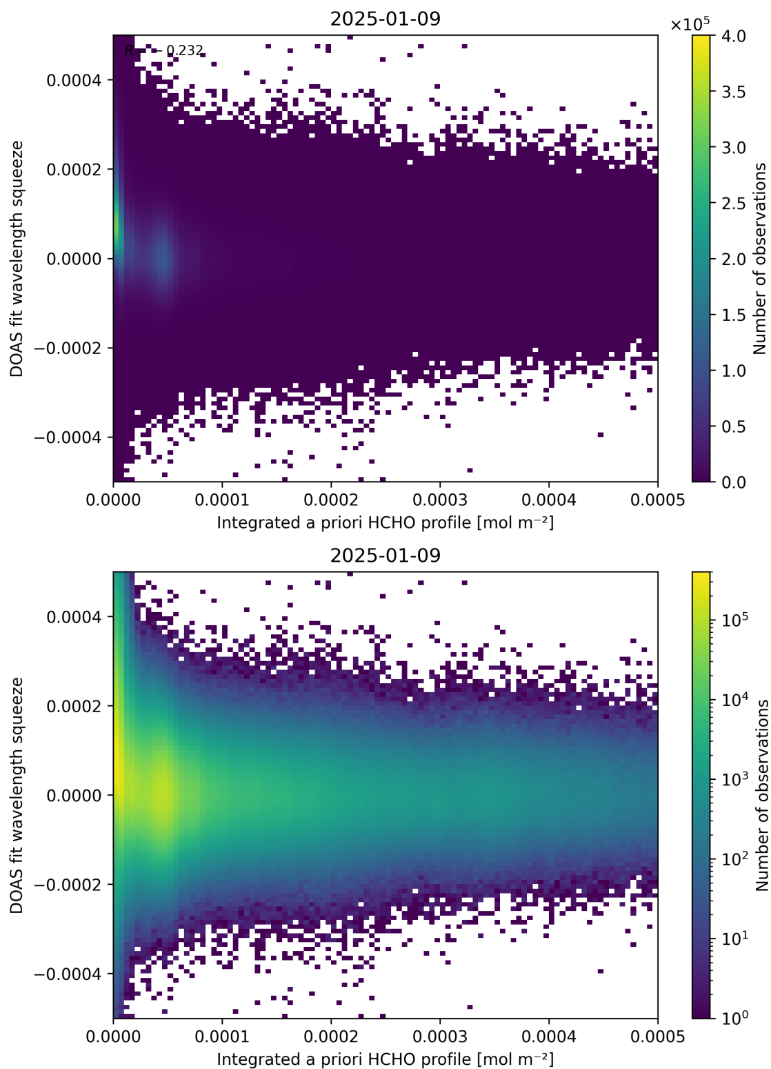
Figure 150: Scatter density plot of “Integrated a priori HCHO profile” against “DOAS fit wavelength squeeze” for 2025-01-08 to 2025-01-10.
