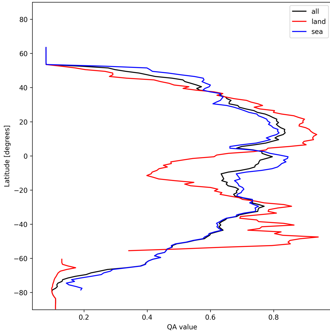
Figure 20: Zonal average of “QA value” for 2025-01-08 to 2025-01-10.
