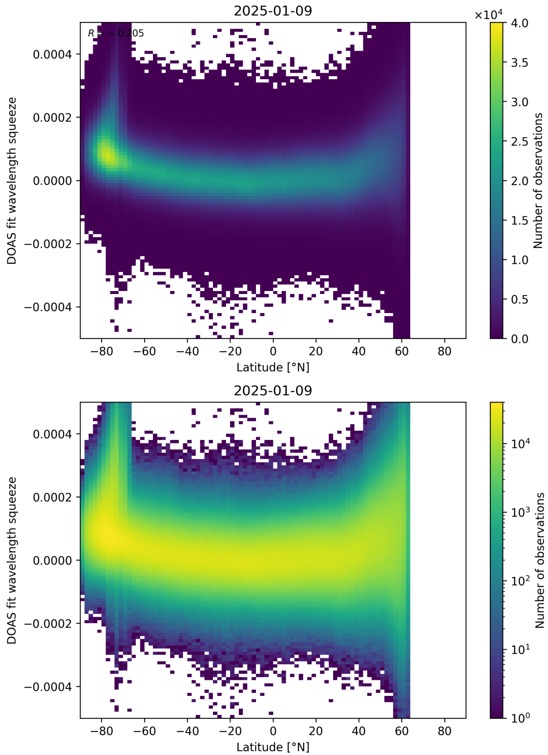
Figure 155: Scatter density plot of “Latitude” against “DOAS fit wavelength squeeze” for 2025-01-08 to 2025-01-10.
