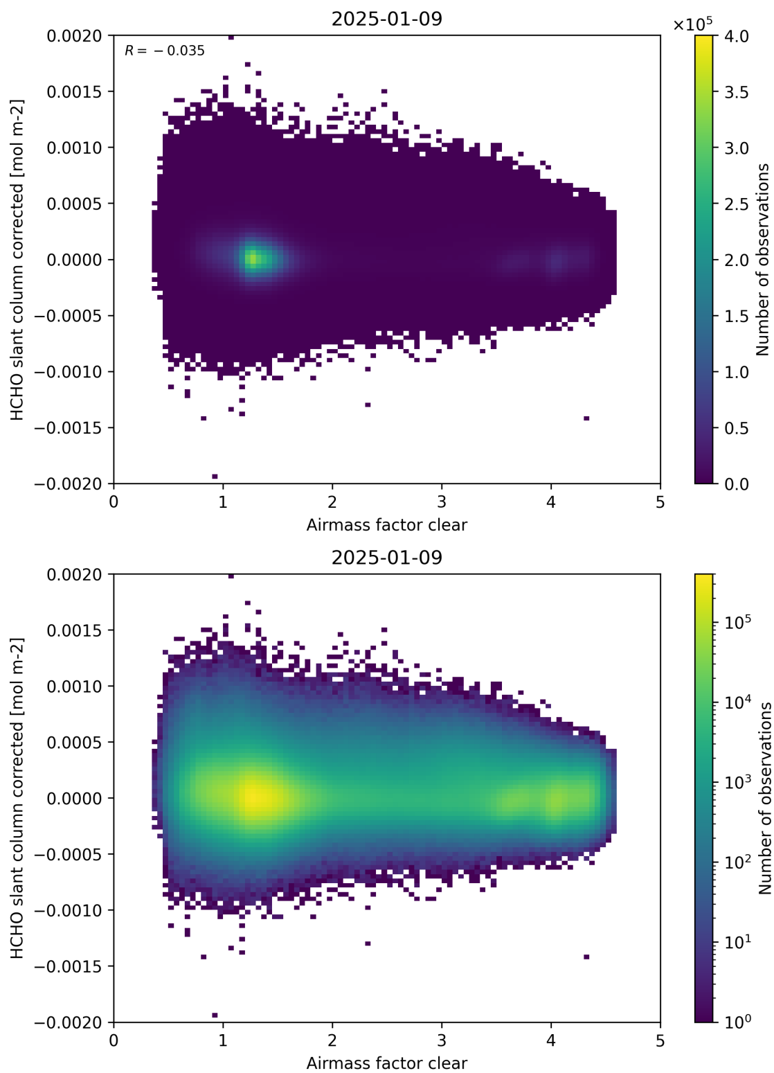
Figure 74: Scatter density plot of “Airmass factor clear” against “HCHO slant column corrected” for 2025-01-08 to 2025-01-10.
