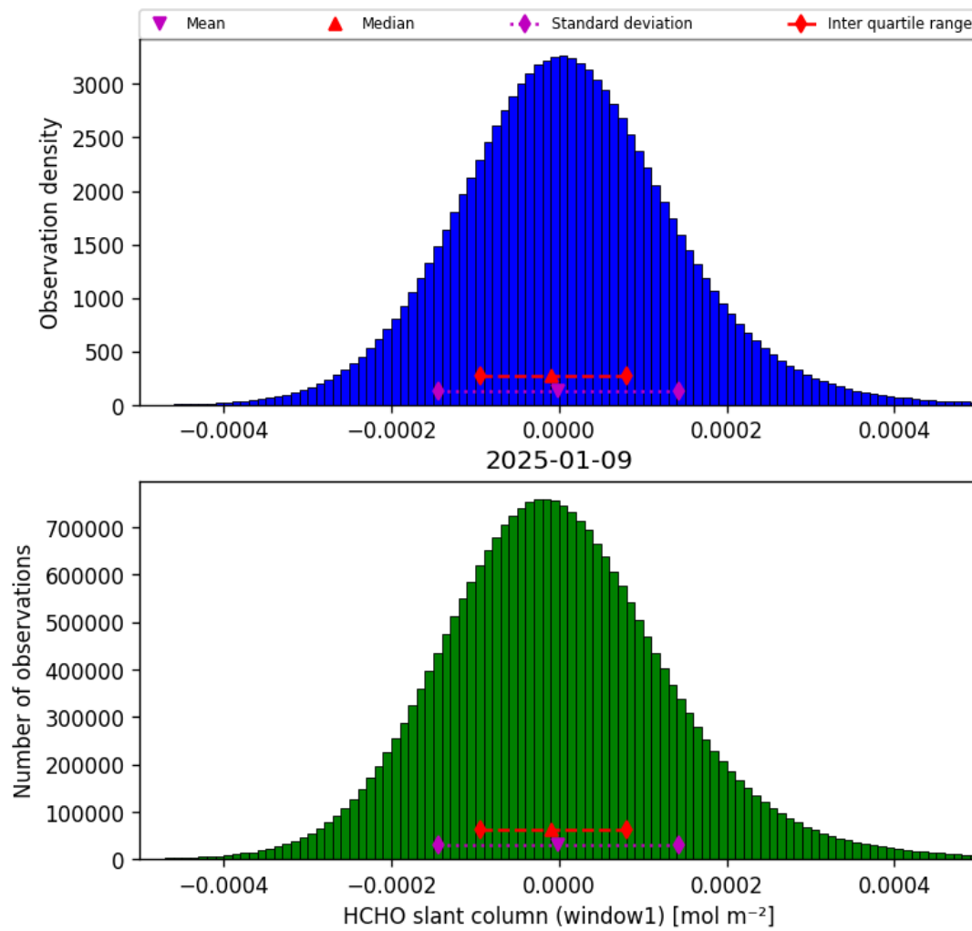
Figure 38: Histogram of “HCHO slant column (window1)” for 2025-01-08 to 2025-01-10
