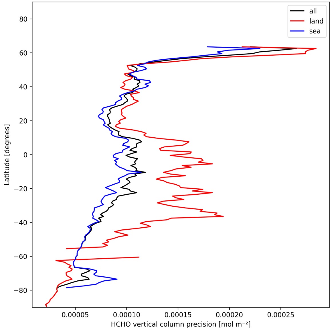
Figure 22: Zonal average of “HCHO vertical column precision” for 2025-01-08 to 2025-01-10.
