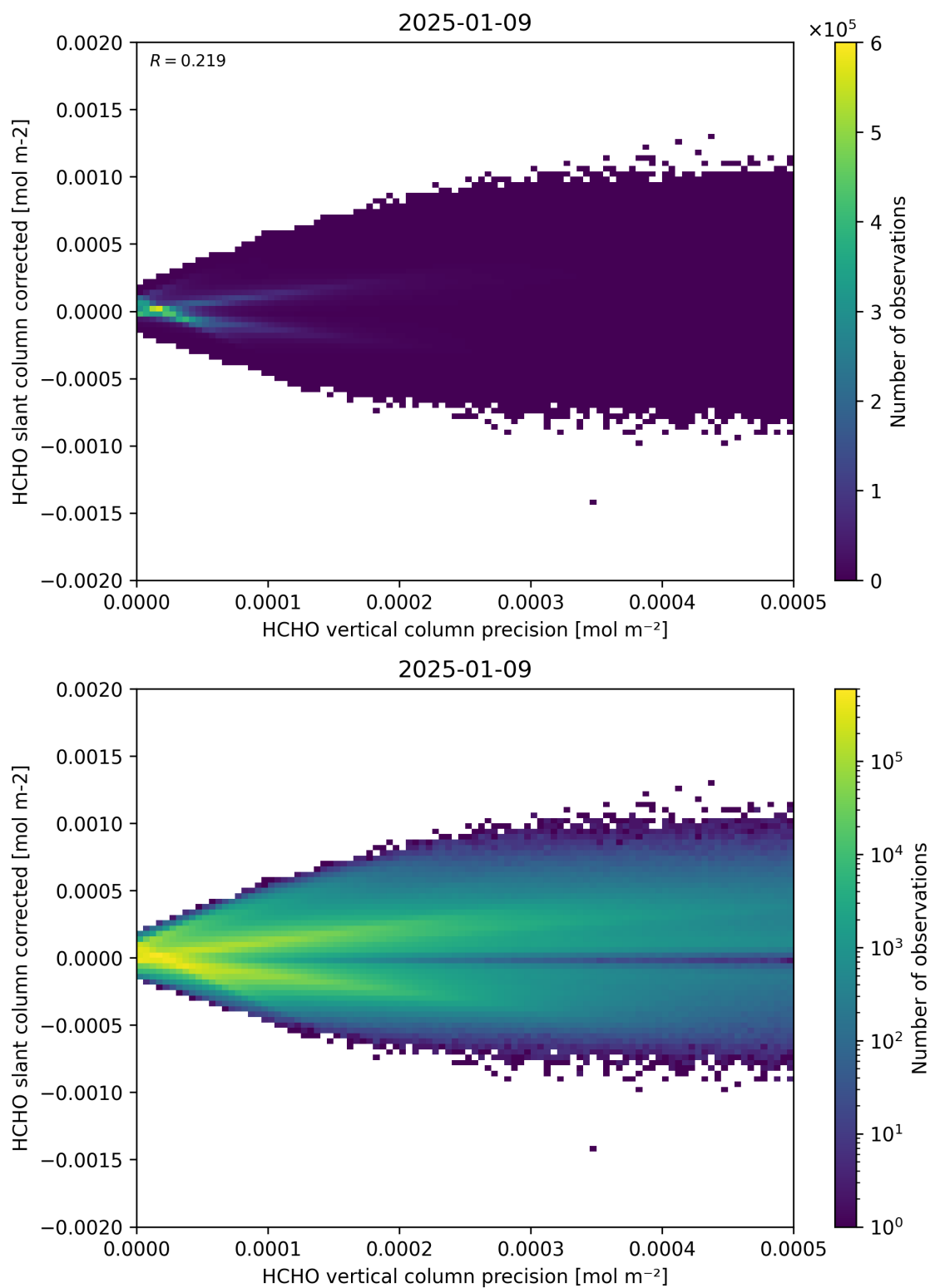
Figure 140: Scatter density plot of “HCHO vertical column precision” against “HCHO slant column corrected” for 2025-01-08 to 2025-01-10.
