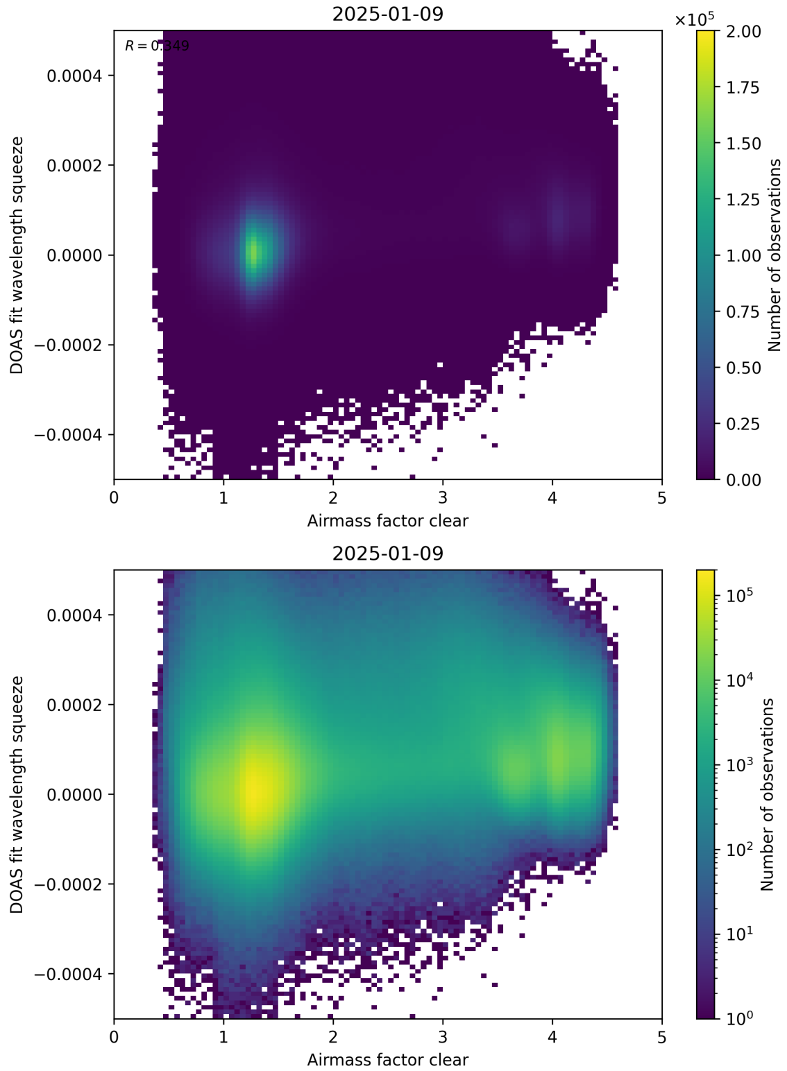
Figure 73: Scatter density plot of “Airmass factor clear” against “DOAS fit wavelength squeeze” for 2025-01-08 to 2025-01-10.
