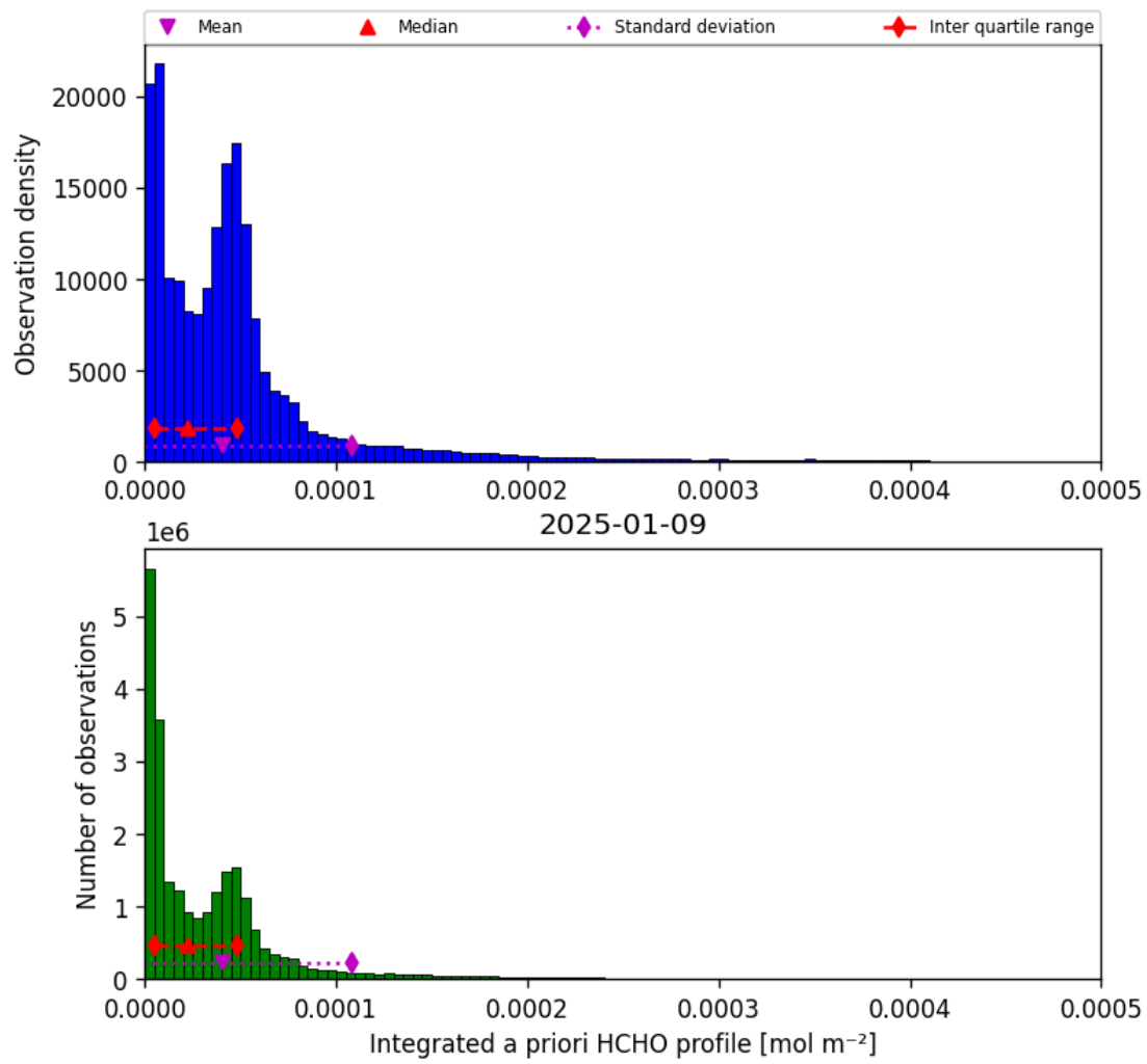
Figure 43: Histogram of “Integrated a priori HCHO profile” for 2025-01-08 to 2025-01-10
