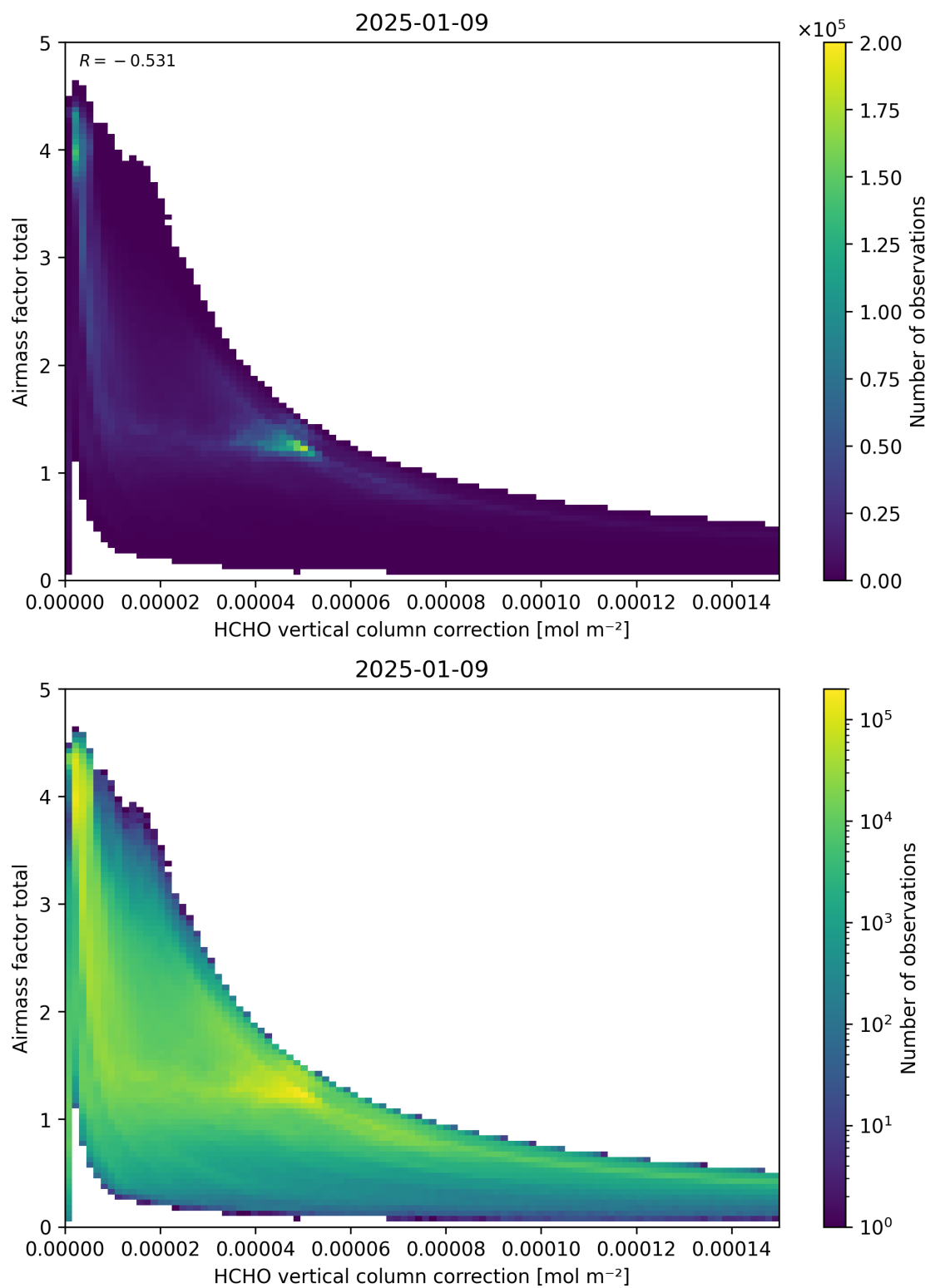
Figure 120: Scatter density plot of “HCHO vertical column correction” against “Airmass factor total” for 2025-01-08 to 2025-01-10.
