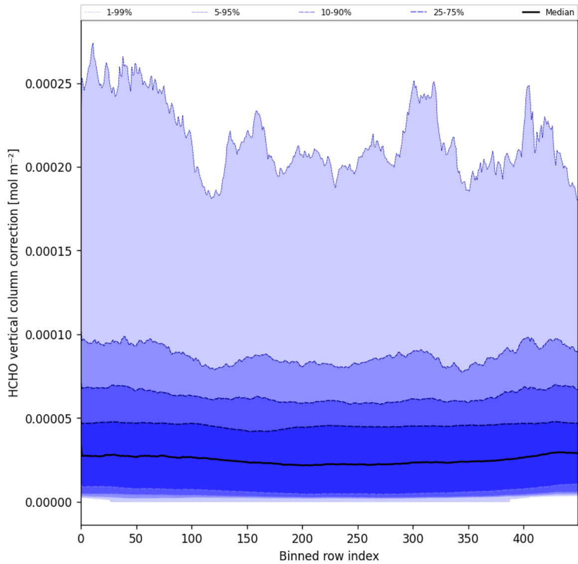
Figure 51: Along track statistics of “HCHO vertical column correction” for 2025-01-08 to 2025-01-10
