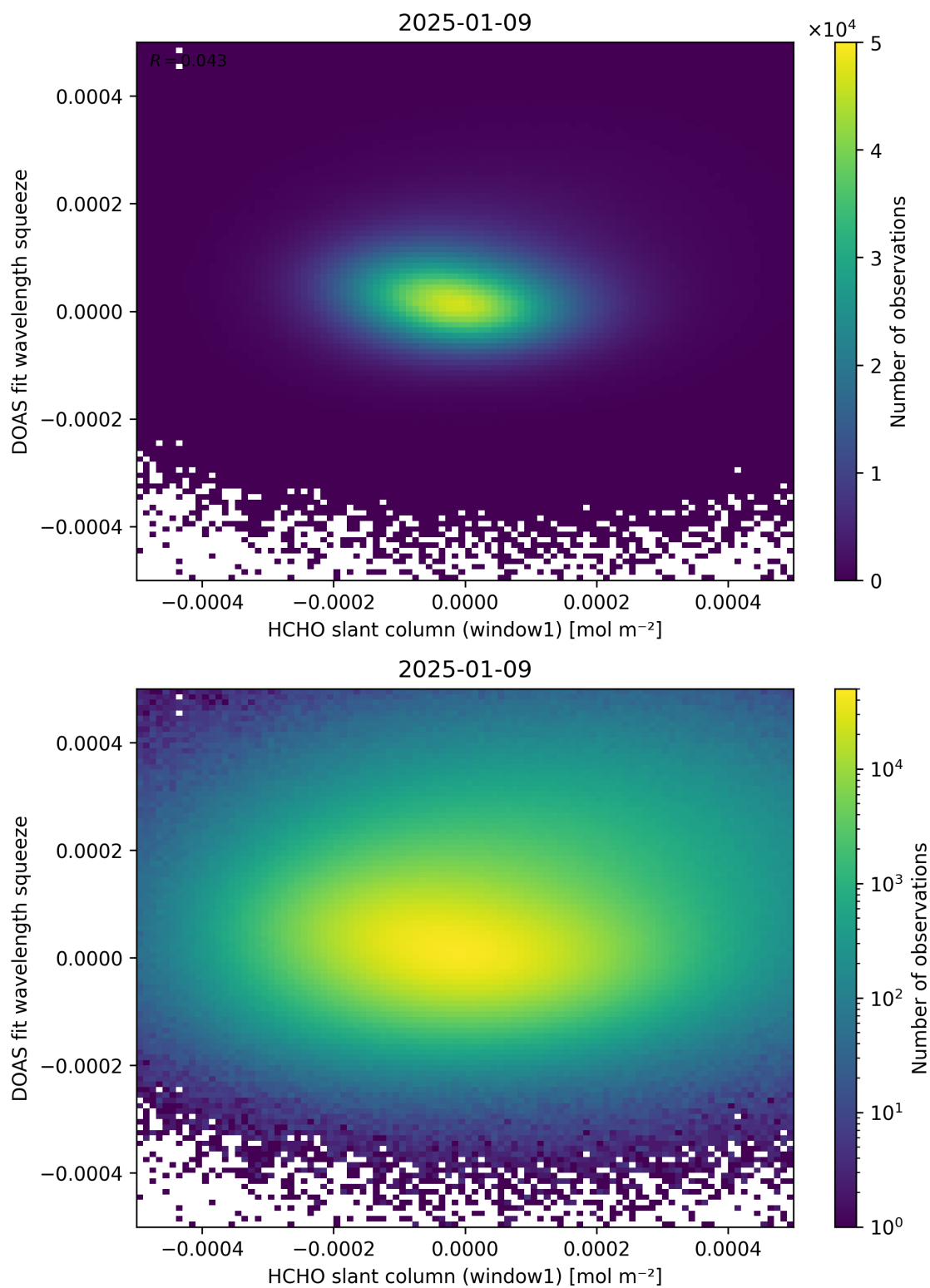
Figure 80: Scatter density plot of “HCHO slant column (window1)” against “DOAS fit wavelength squeeze” for 2025-01-08 to 2025-01-10.
