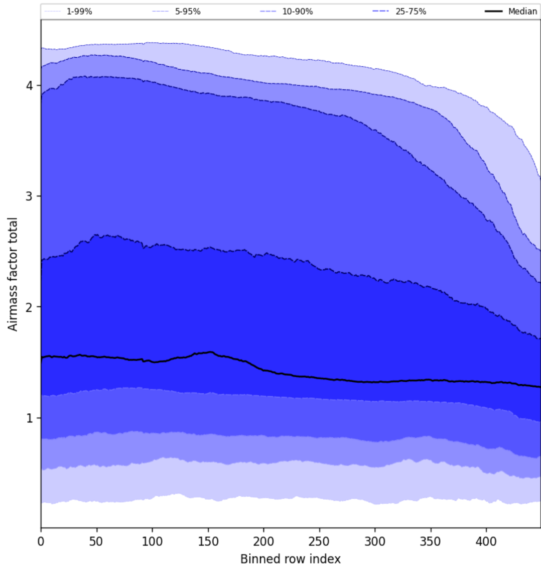
Figure 54: Along track statistics of “Airmass factor total” for 2025-01-08 to 2025-01-10
