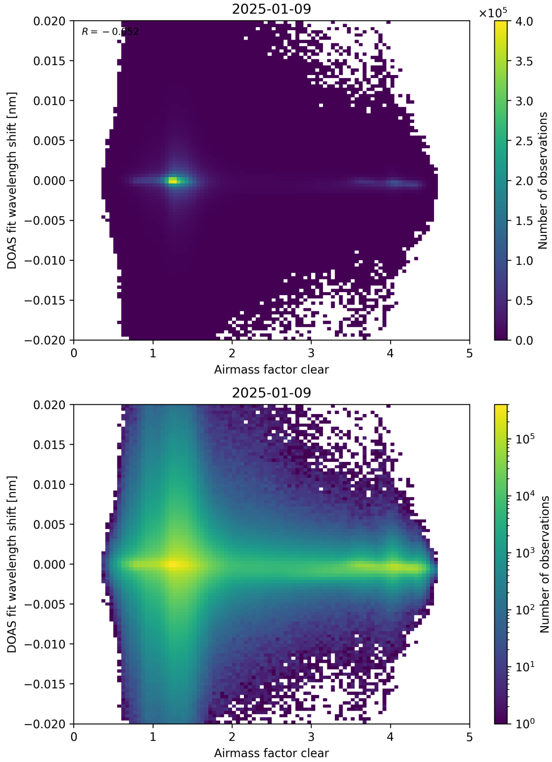
Figure 72: Scatter density plot of “Airmass factor clear” against “DOAS fit wavelength shift” for 2025-01-08 to 2025-01-10.
