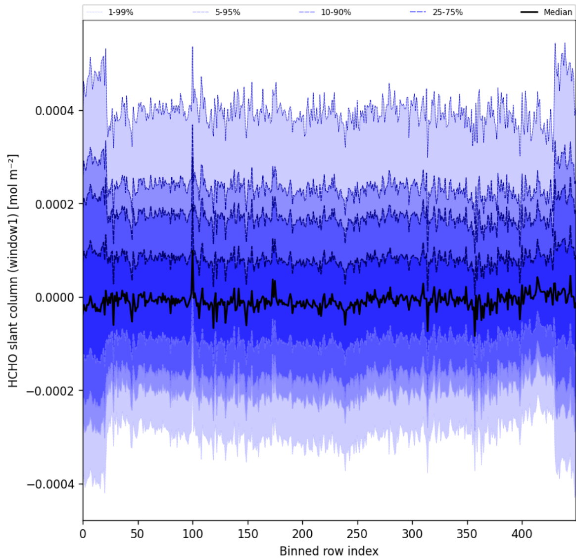
Figure 52: Along track statistics of “HCHO slant column (window1)” for 2025-01-08 to 2025-01-10
