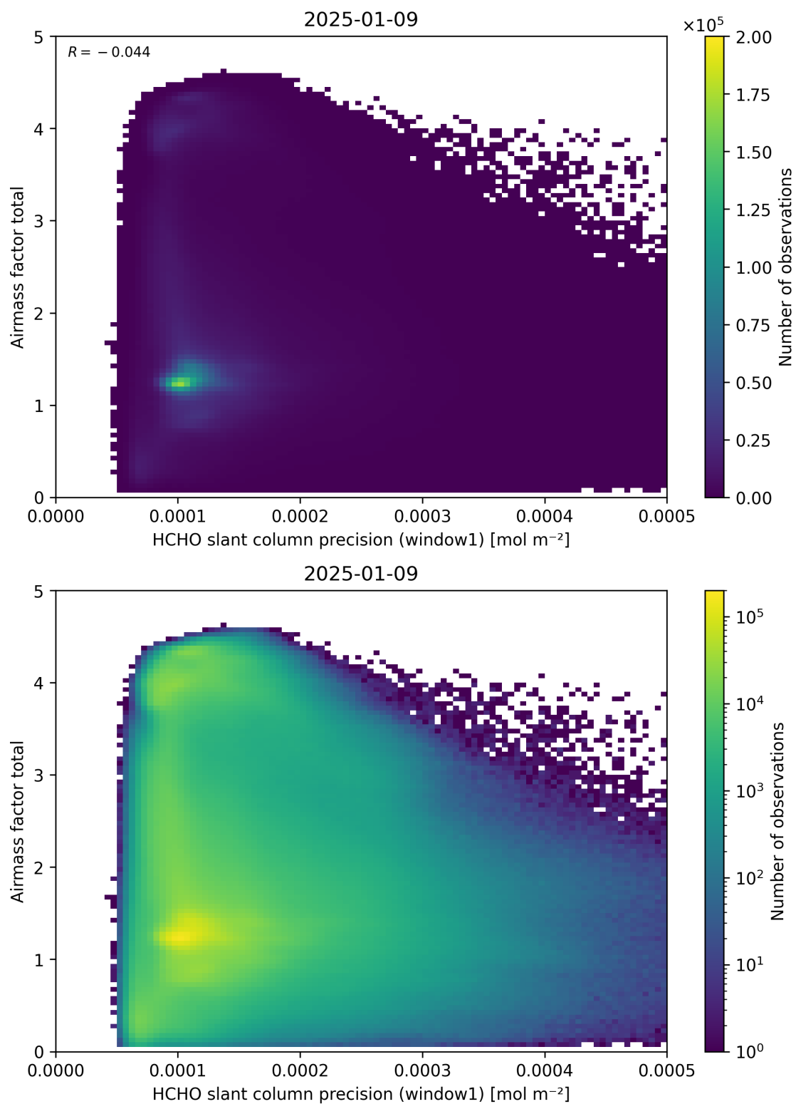
Figure 94: Scatter density plot of “HCHO slant column precision (window1)” against “Airmass factor total” for 2025-01-08 to 2025-01-10.
