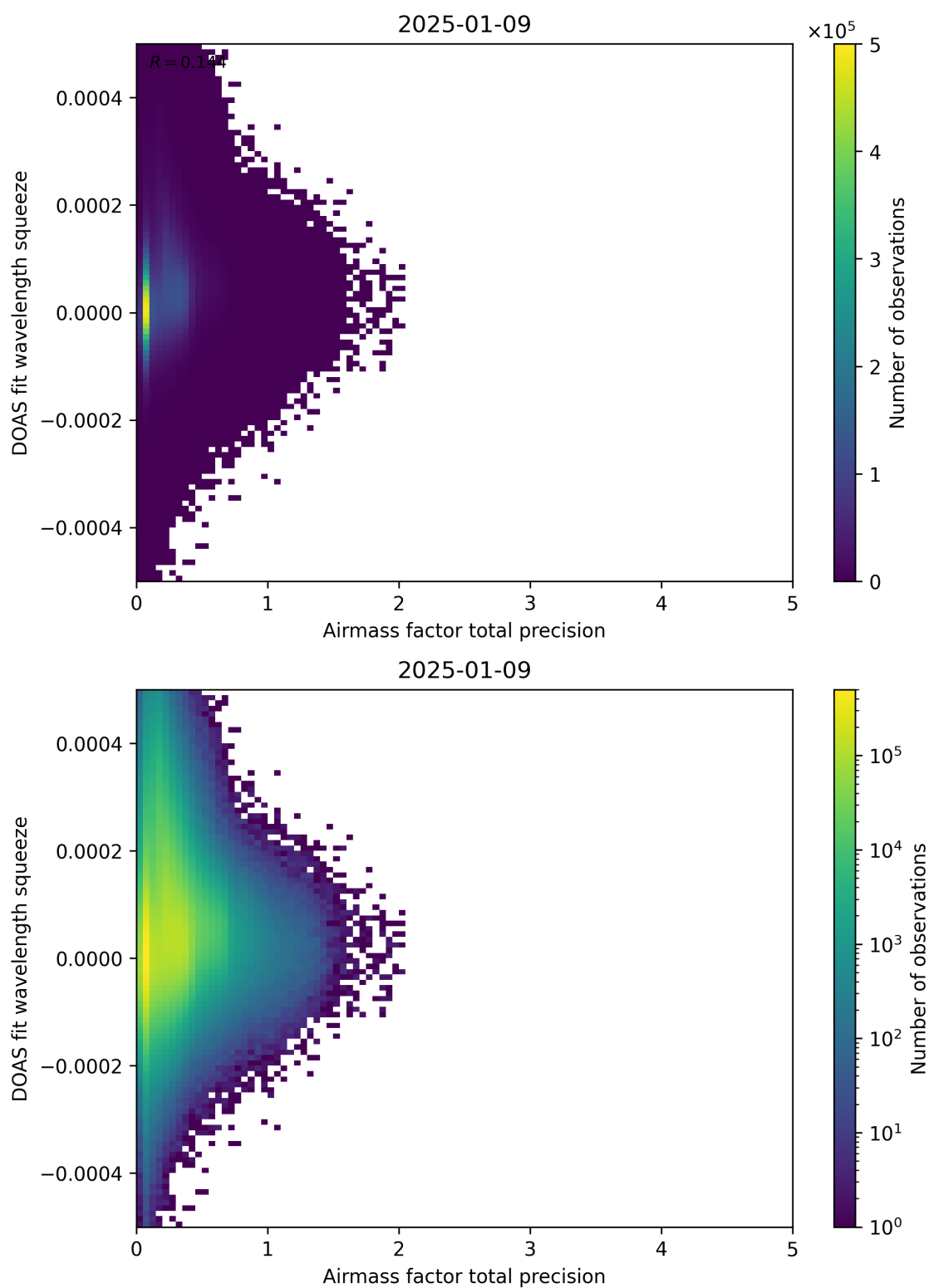
Figure 107: Scatter density plot of “Airmass factor total precision” against “DOAS fit wavelength squeeze” for 2025-01-08 to 2025-01-10.
