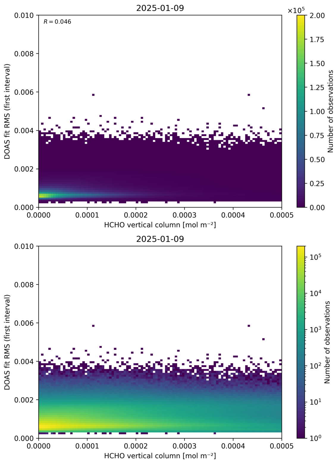
Figure 123: Scatter density plot of “HCHO vertical column” against “DOAS fit RMS (first interval)” for 2025-01-08 to 2025-01-10.
