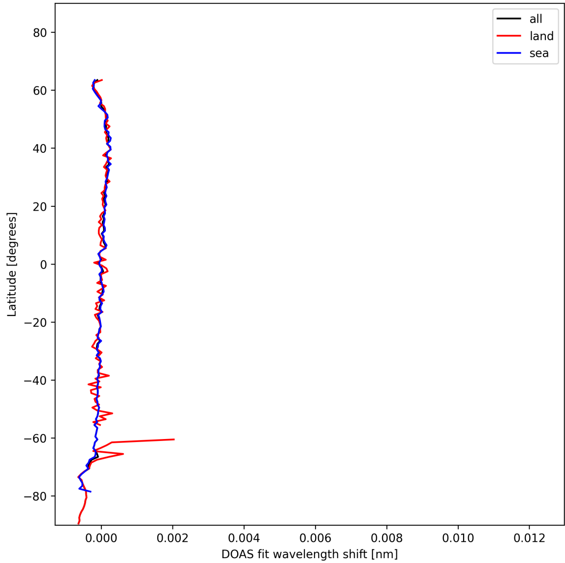
Figure 30: Zonal average of “DOAS fit wavelength shift” for 2025-01-08 to 2025-01-10.
