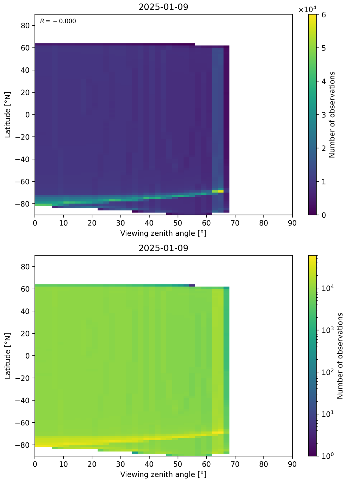
Figure 196: Scatter density plot of “Viewing zenith angle” against “Latitude” for 2025-01-08 to 2025-01-10.
