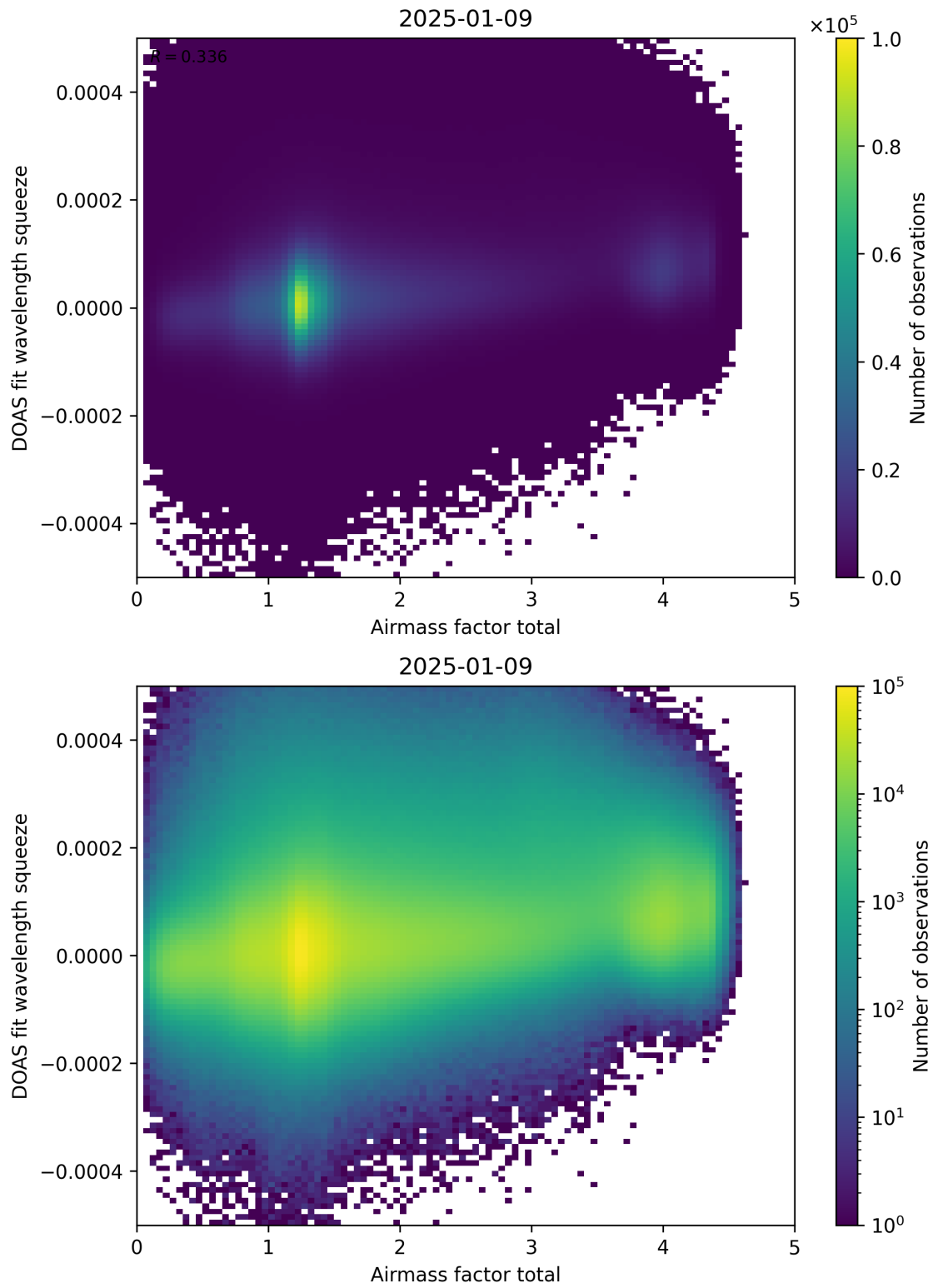
Figure 99: Scatter density plot of “Airmass factor total” against “DOAS fit wavelength squeeze” for 2025-01-08 to 2025-01-10.
