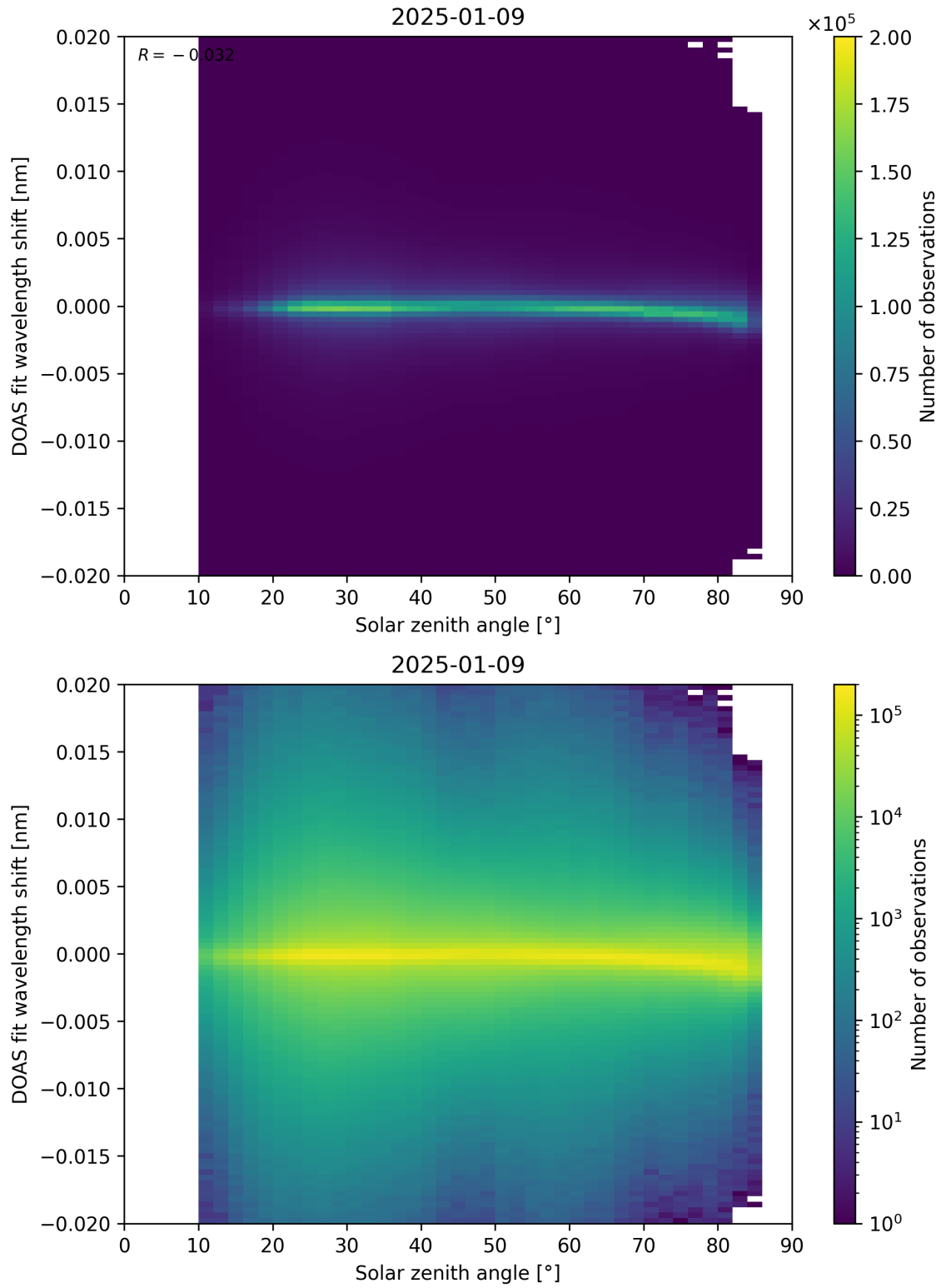
Figure 168: Scatter density plot of “Solar zenith angle” against “DOAS fit wavelength shift” for 2025-01-08 to 2025-01-10.
