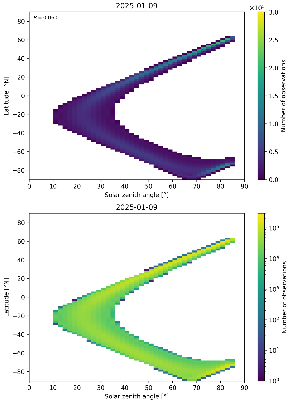
Figure 181: Scatter density plot of “Solar zenith angle” against “Latitude” for 2025-01-08 to 2025-01-10.
