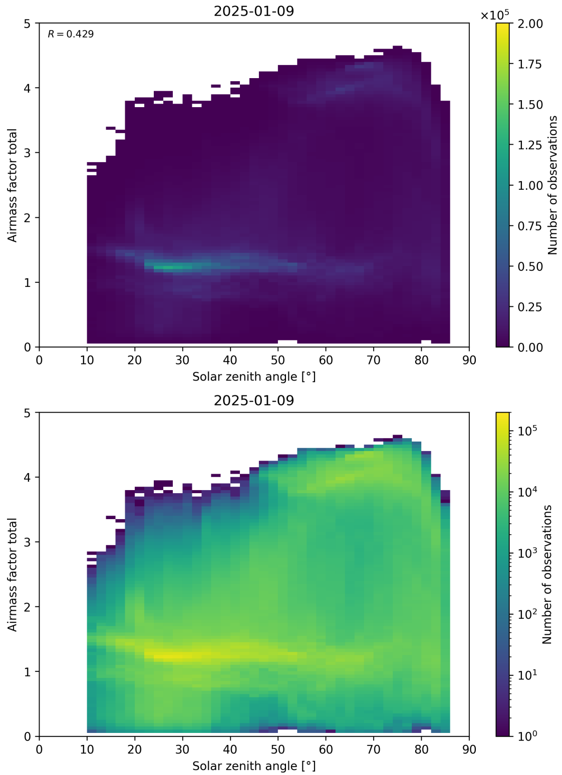
Figure 175: Scatter density plot of “Solar zenith angle” against “Airmass factor total” for 2025-01-08 to 2025-01-10.
