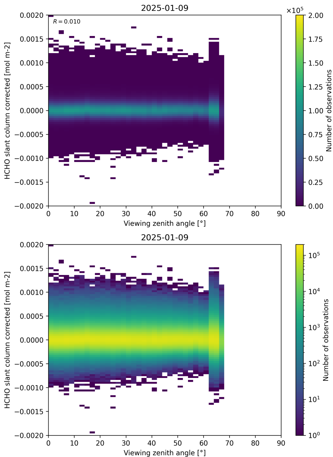
Figure 186: Scatter density plot of “Viewing zenith angle” against “HCHO slant column corrected” for 2025-01-08 to 2025-01-10.
