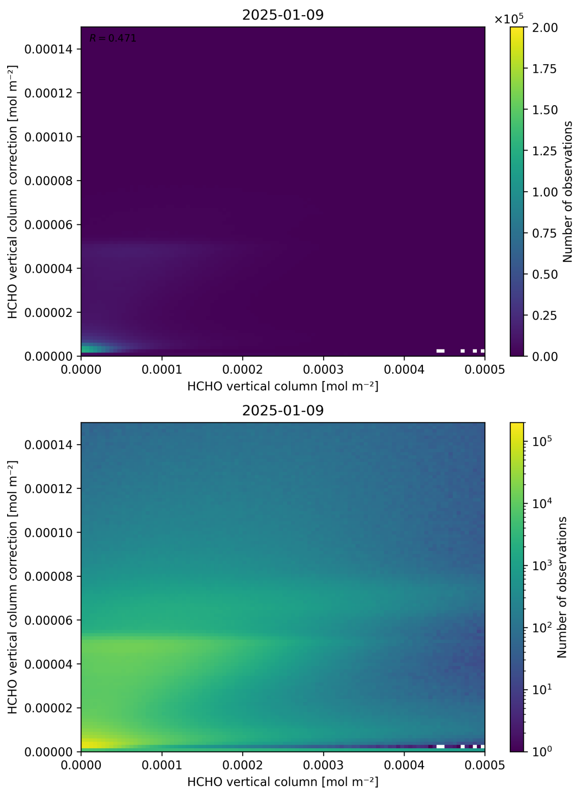
Figure 133: Scatter density plot of “HCHO vertical column” against “HCHO vertical column correction” for 2025-01-08 to 2025-01-10.
