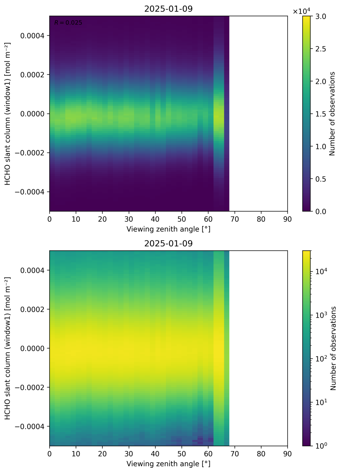
Figure 188: Scatter density plot of “Viewing zenith angle” against “HCHO slant column (window1)” for 2025-01-08 to 2025-01-10.
