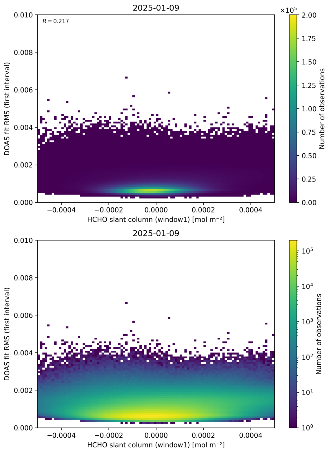
Figure 78: Scatter density plot of “HCHO slant column (window1)” against “DOAS fit RMS (first interval)” for 2025-01-08 to 2025-01-10.
