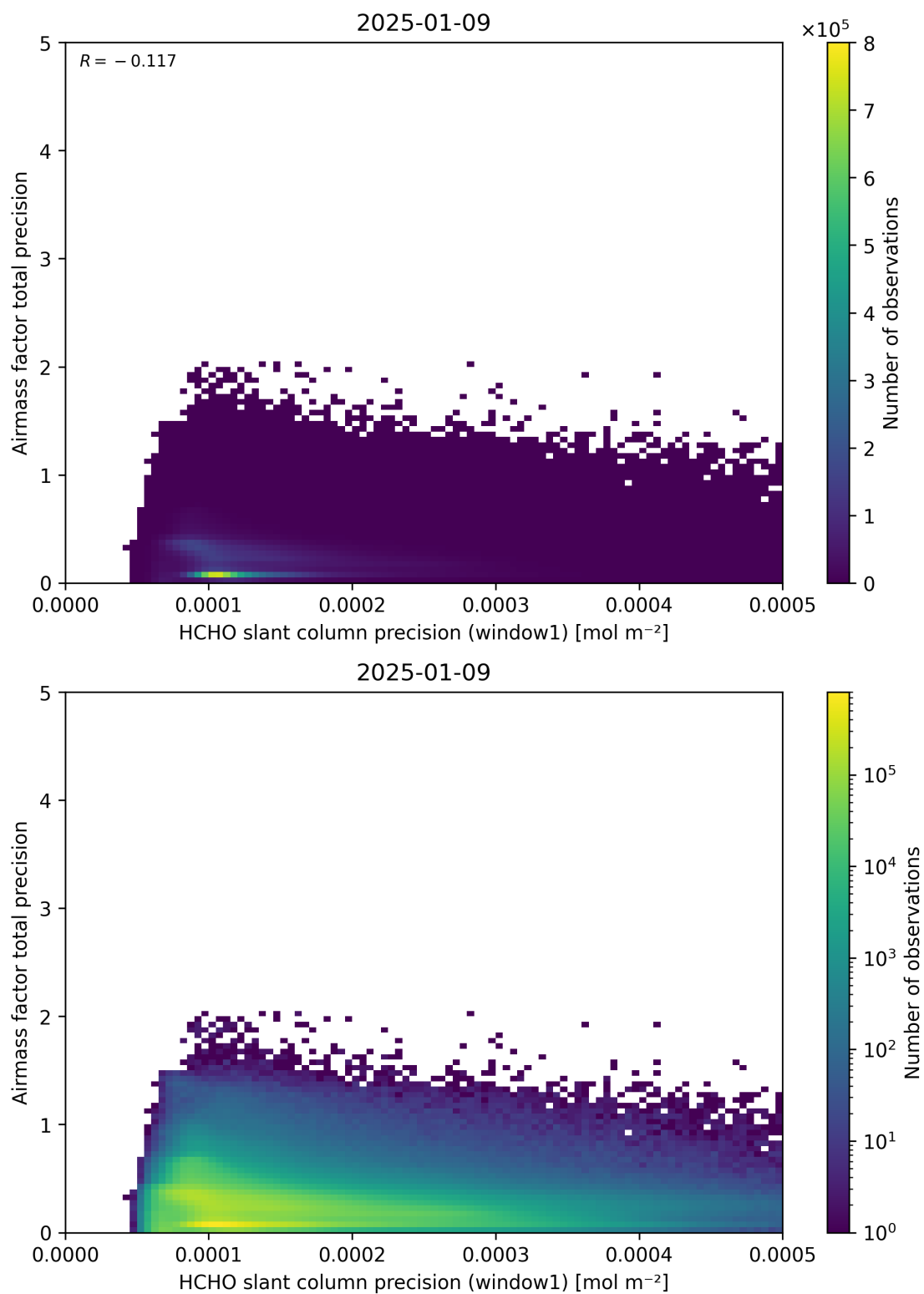
Figure 95: Scatter density plot of “HCHO slant column precision (window1)” against “Airmass factor total precision” for 2025-01-08 to 2025-01-10.
