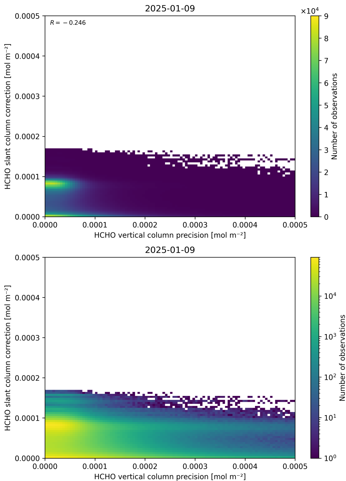
Figure 141: Scatter density plot of “HCHO vertical column precision” against “HCHO slant column correction” for 2025-01-08 to 2025-01-10.
