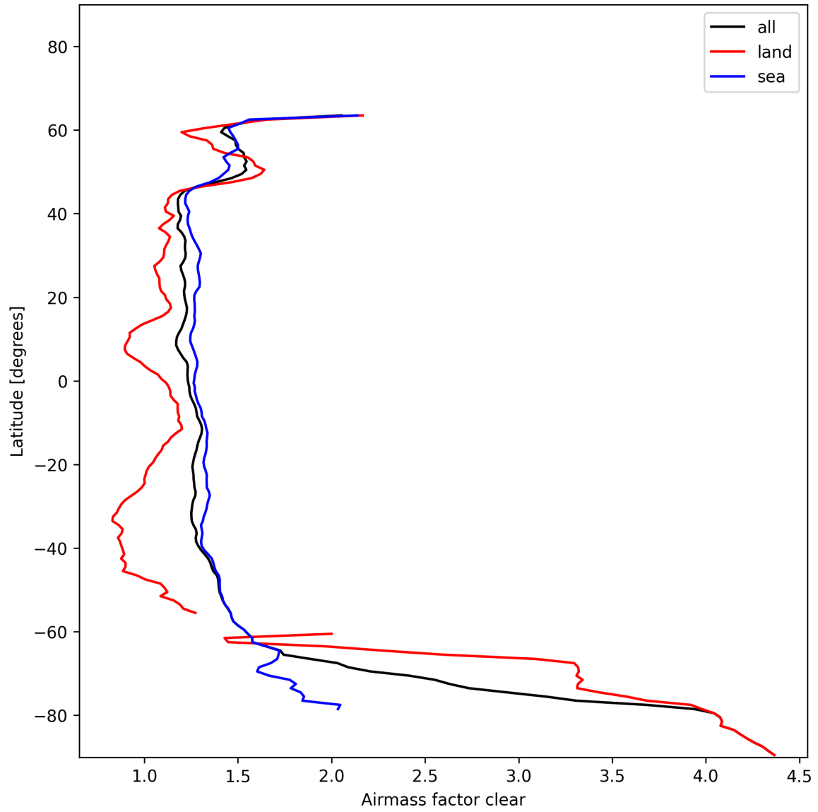
Figure 28: Zonal average of “Airmass factor clear” for 2025-01-08 to 2025-01-10.
