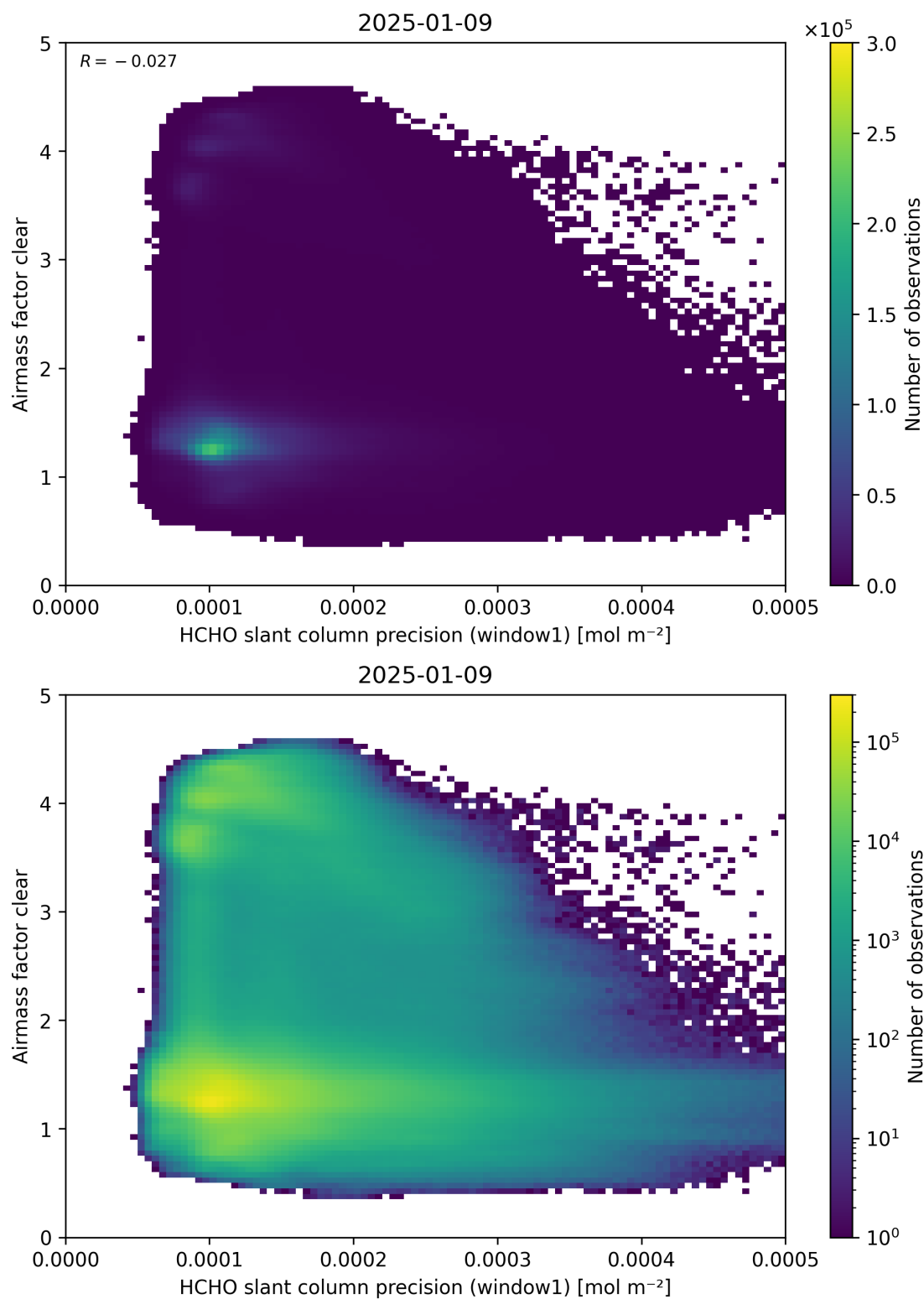
Figure 91: Scatter density plot of “HCHO slant column precision (window1)” against “Airmass factor clear” for 2025-01-08 to 2025-01-10.
