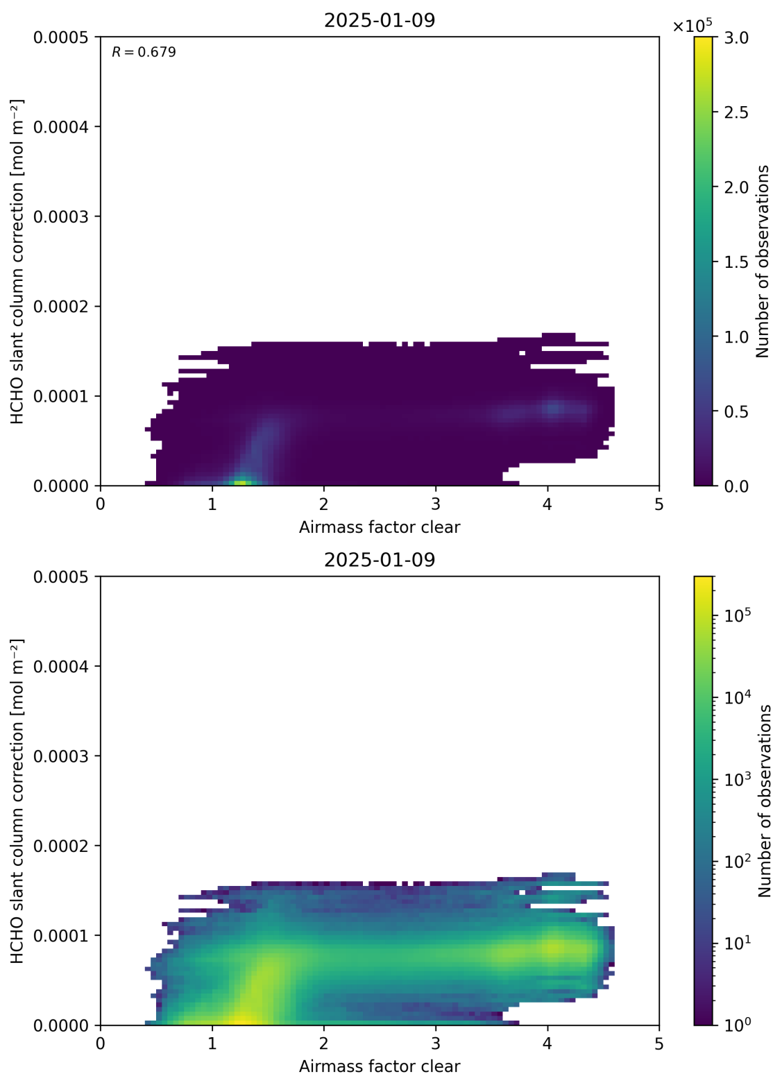
Figure 75: Scatter density plot of “Airmass factor clear” against “HCHO slant column correction” for 2025-01-08 to 2025-01-10.
