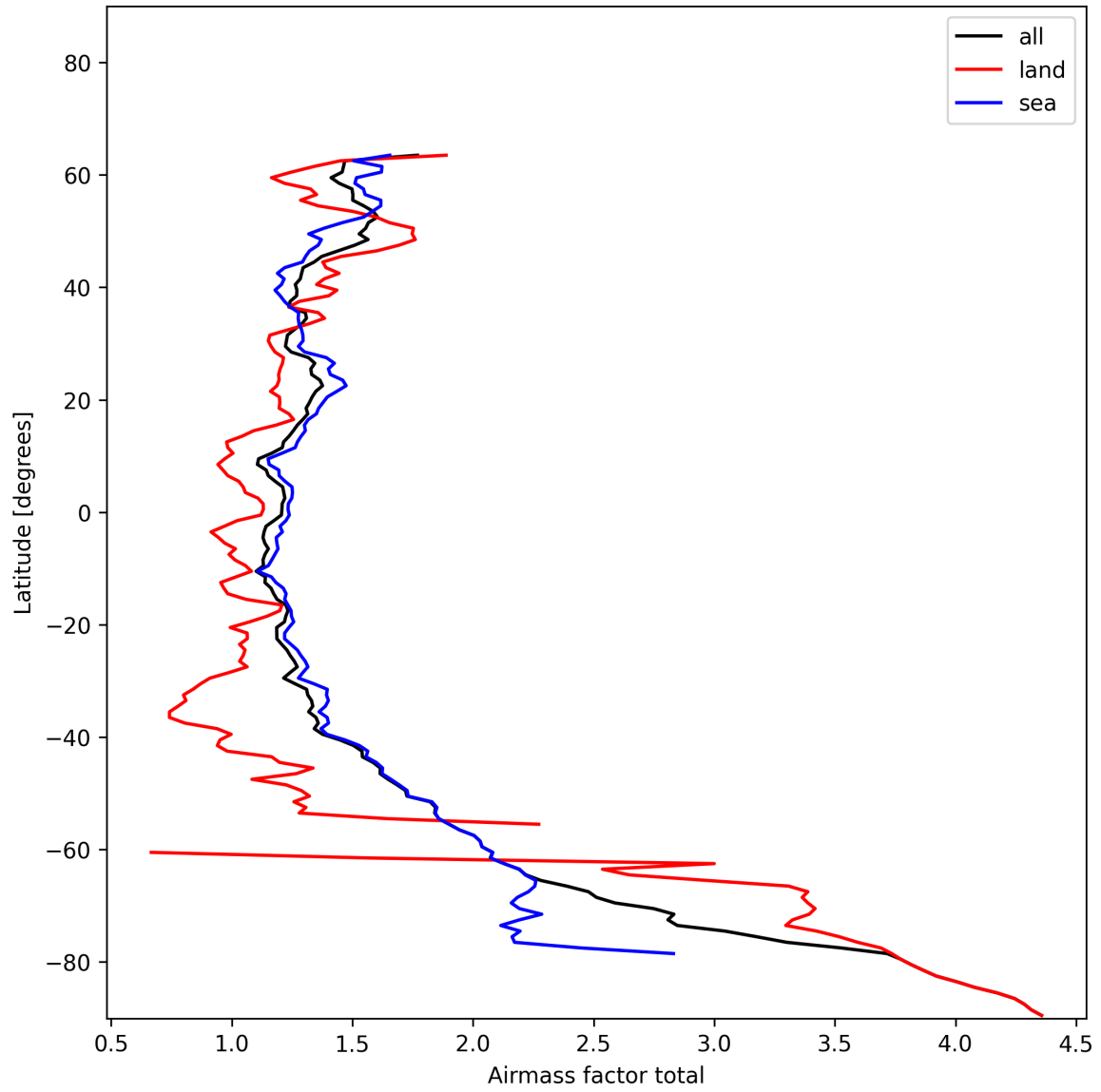
Figure 26: Zonal average of “Airmass factor total” for 2025-01-08 to 2025-01-10.
