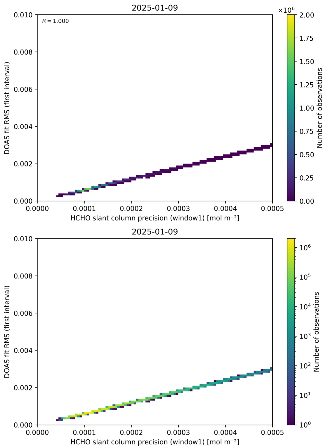
Figure 88: Scatter density plot of “HCHO slant column precision (window1)” against “DOAS fit RMS (first interval)” for 2025-01-08 to 2025-01-10.
