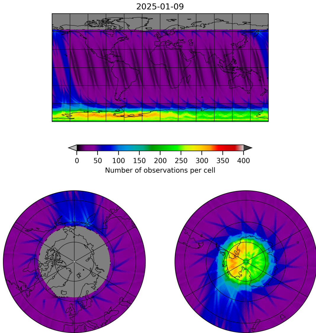
Figure 19: Map of the number of observations for 2025-01-08 to 2025-01-10
