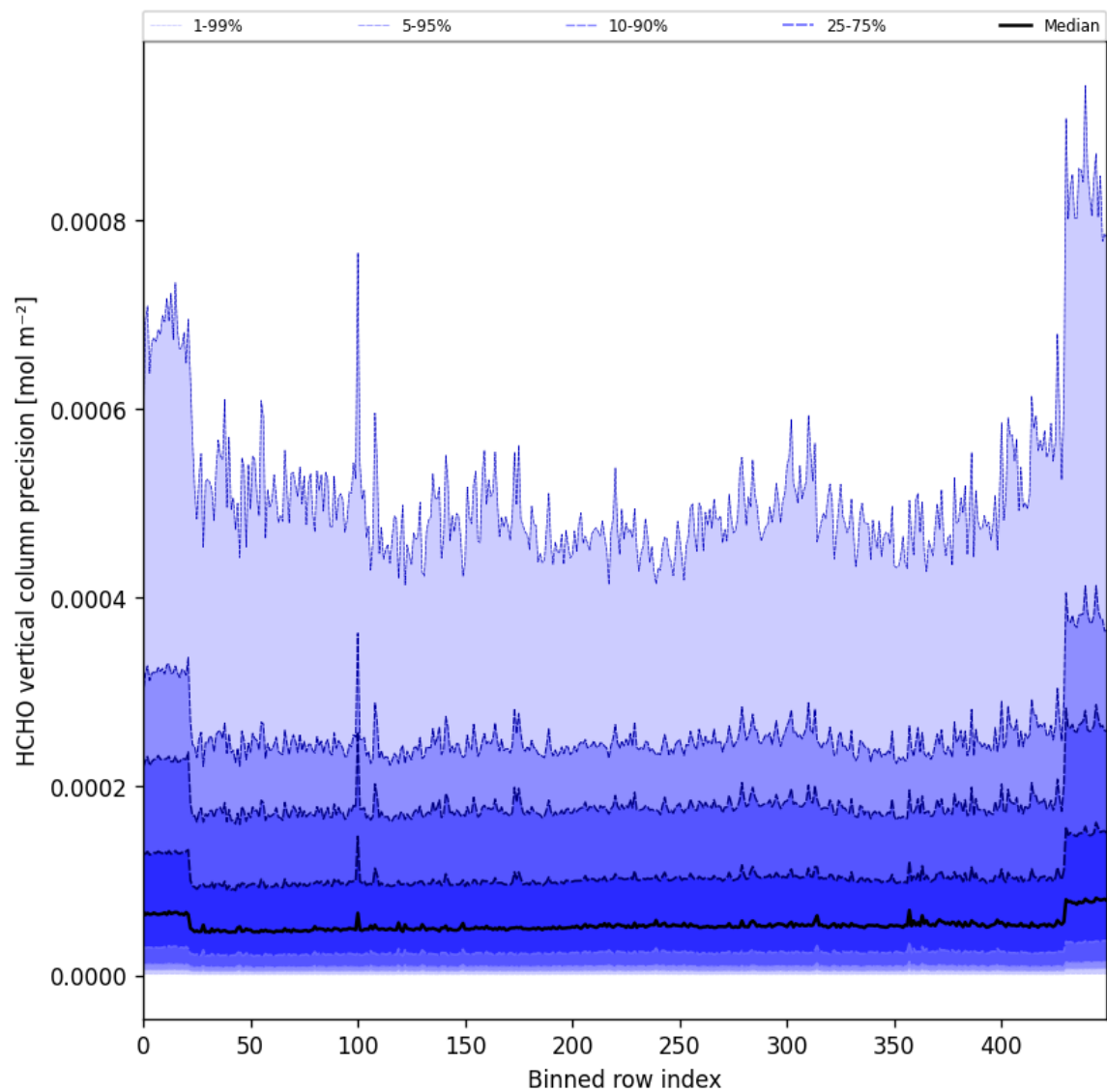
Figure 50: Along track statistics of “HCHO vertical column precision” for 2025-01-08 to 2025-01-10
