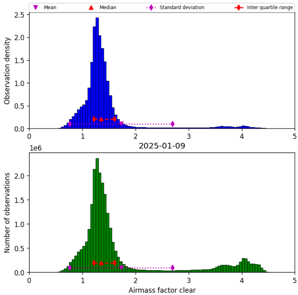
Figure 42: Histogram of “Airmass factor clear” for 2025-01-08 to 2025-01-10
