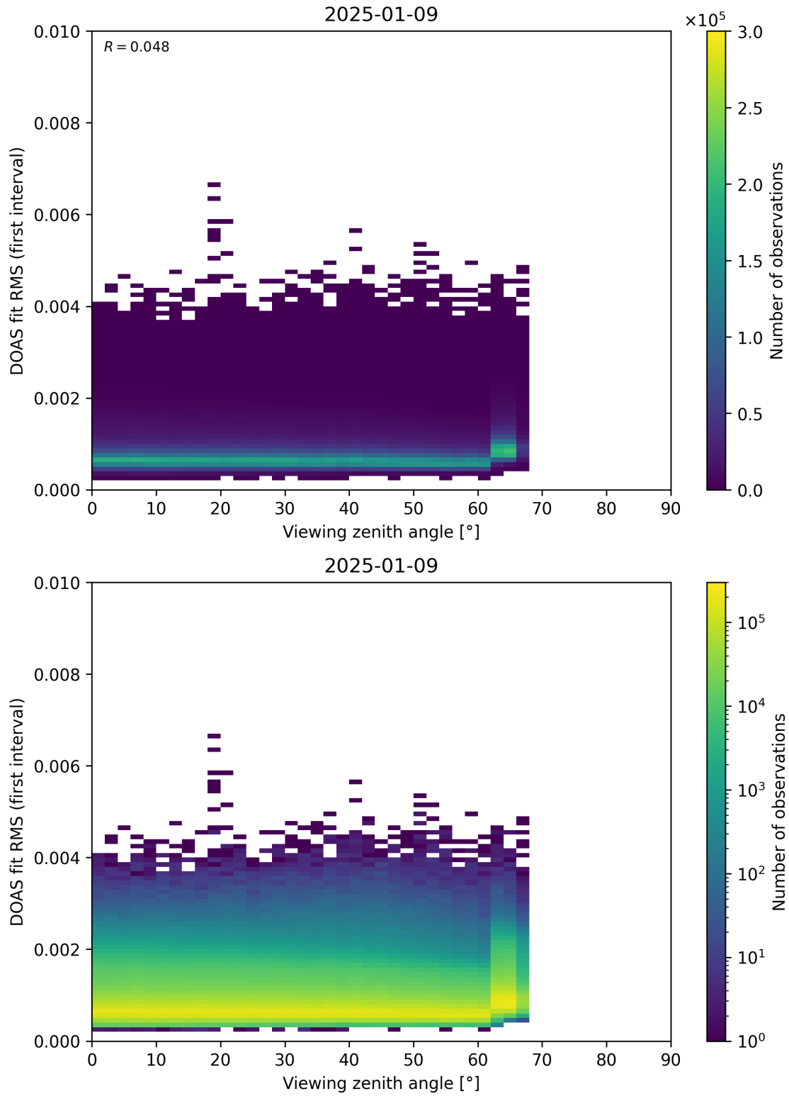
Figure 182: Scatter density plot of “Viewing zenith angle” against “DOAS fit RMS (first interval)” for 2025-01-08 to 2025-01-10.
