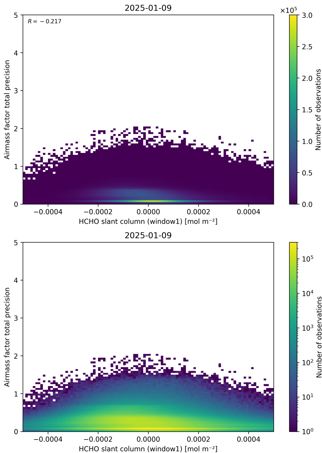
Figure 86: Scatter density plot of “HCHO slant column (window1)” against “Airmass factor total precision” for 2025-01-08 to 2025-01-10.
