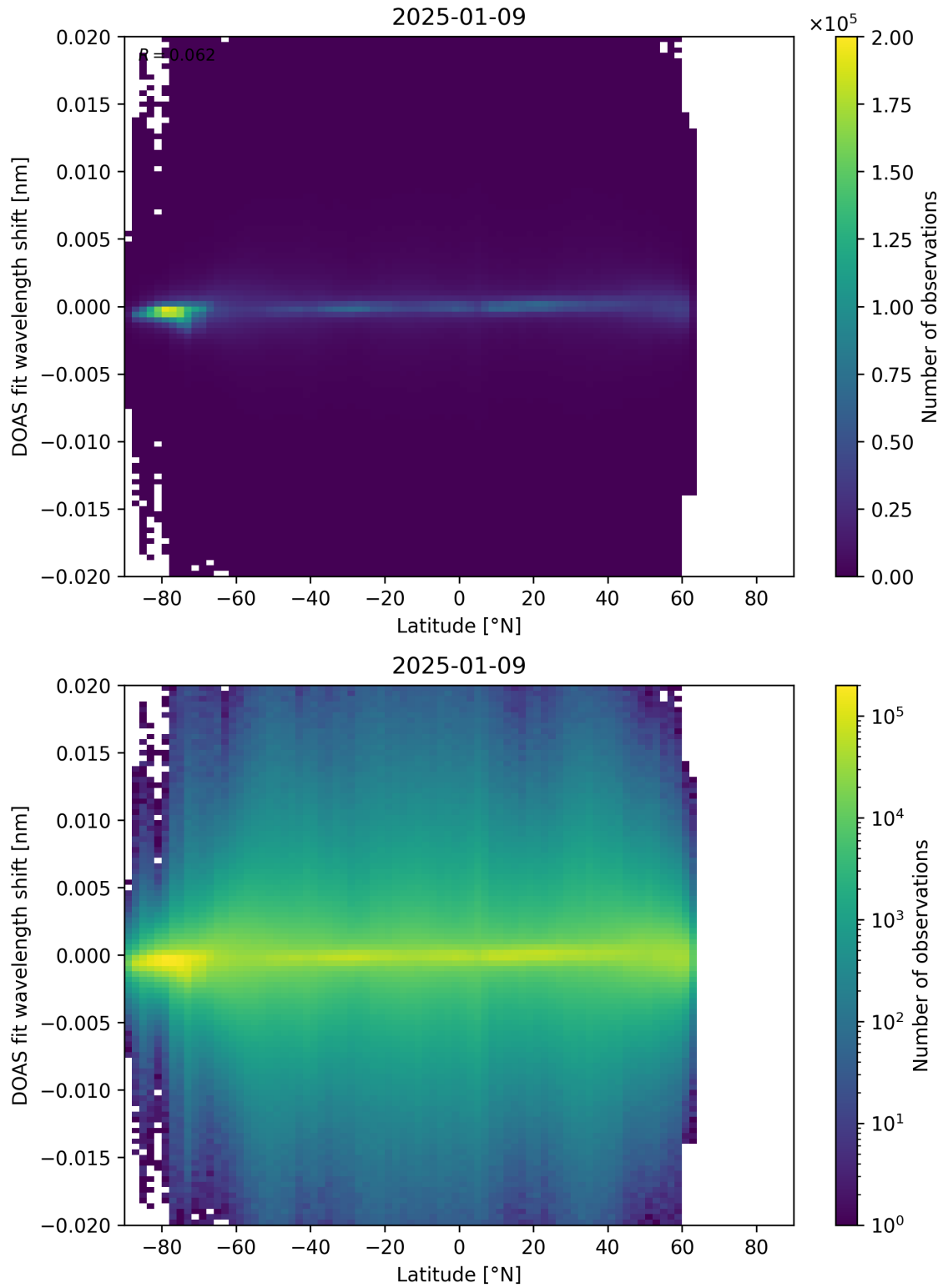
Figure 154: Scatter density plot of “Latitude” against “DOAS fit wavelength shift” for 2025-01-08 to 2025-01-10.
