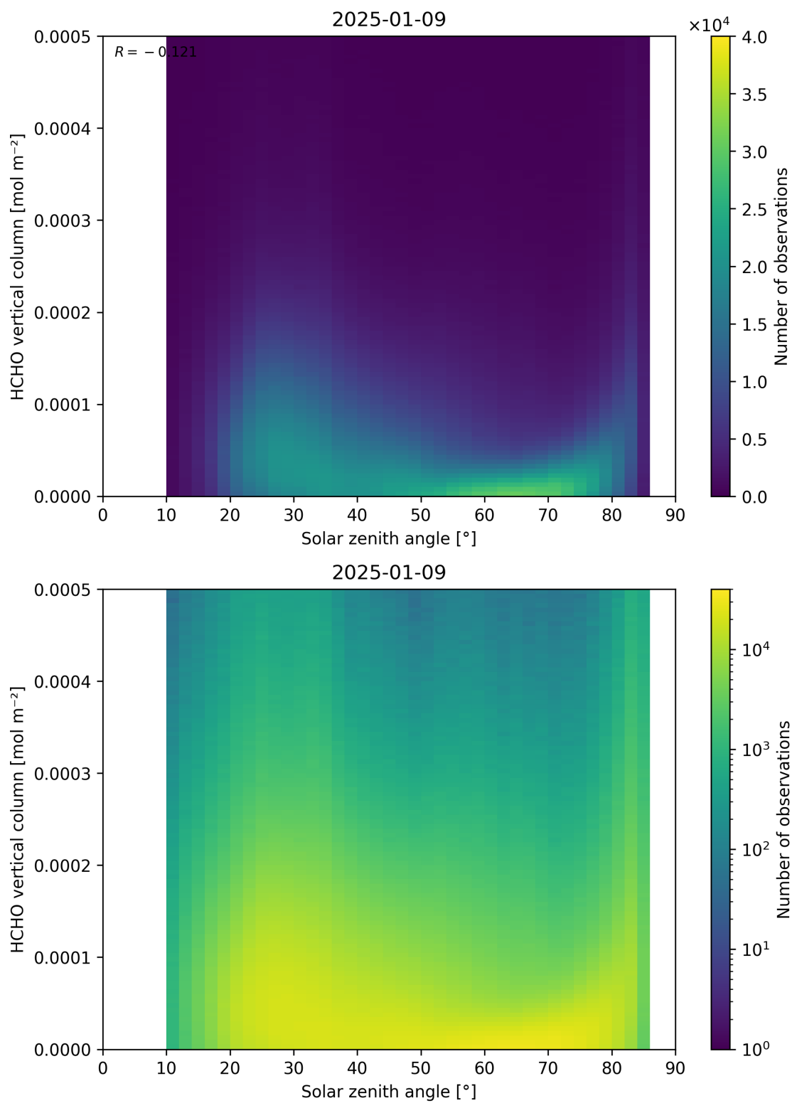
Figure 177: Scatter density plot of “Solar zenith angle” against “HCHO vertical column” for 2025-01-08 to 2025-01-10.
