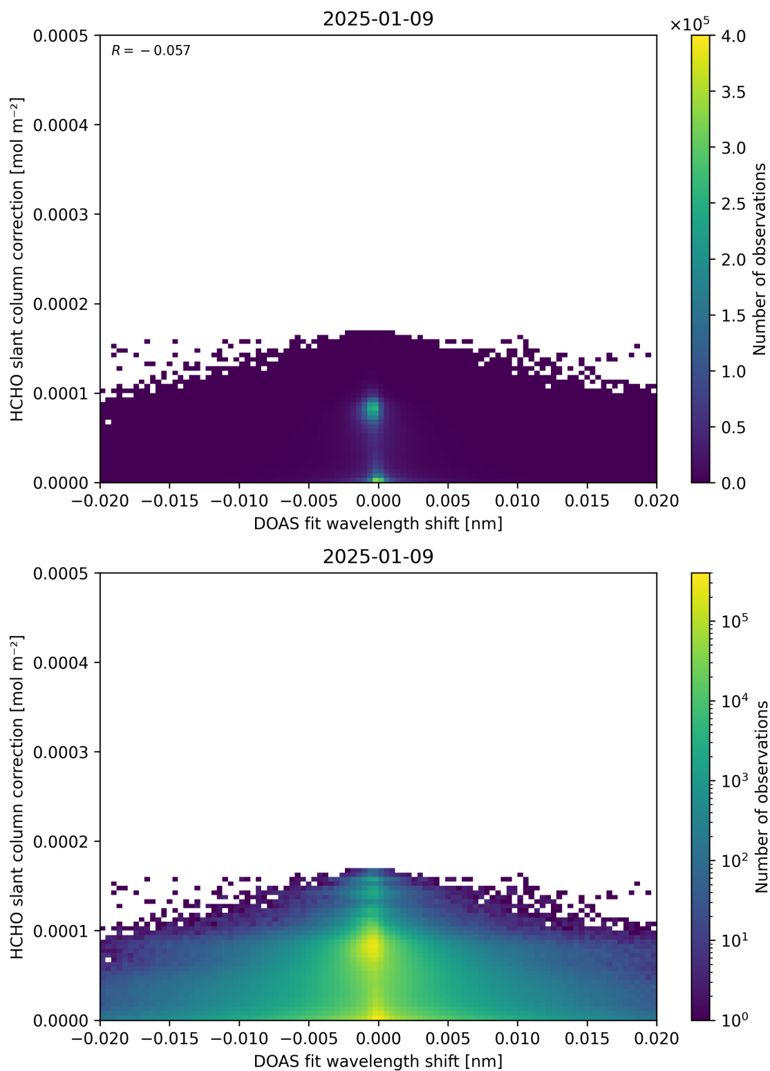
Figure 67: Scatter density plot of “DOAS fit wavelength shift” against “HCHO slant column correction” for 2025-01-08 to 2025-01-10.
