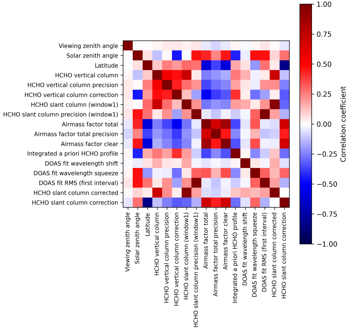
Figure 2: Map of correlation matrix for 2025-01-08 to 2025-01-10.
