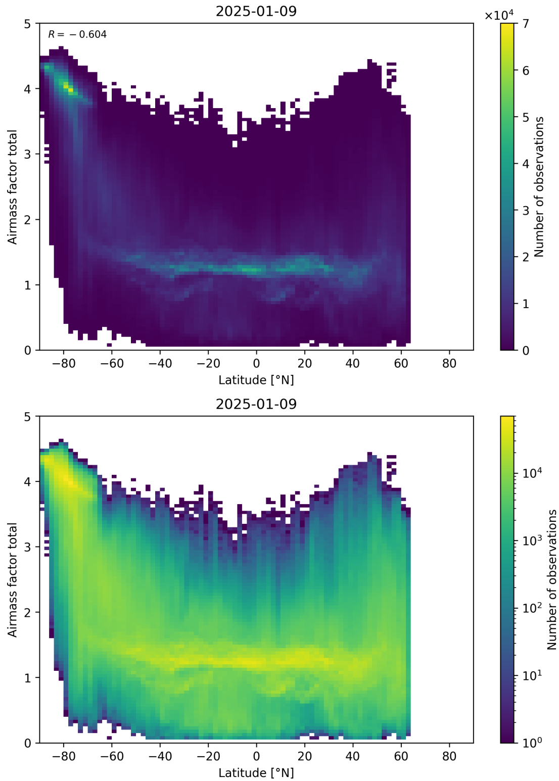
Figure 161: Scatter density plot of “Latitude” against “Airmass factor total” for 2025-01-08 to 2025-01-10.
