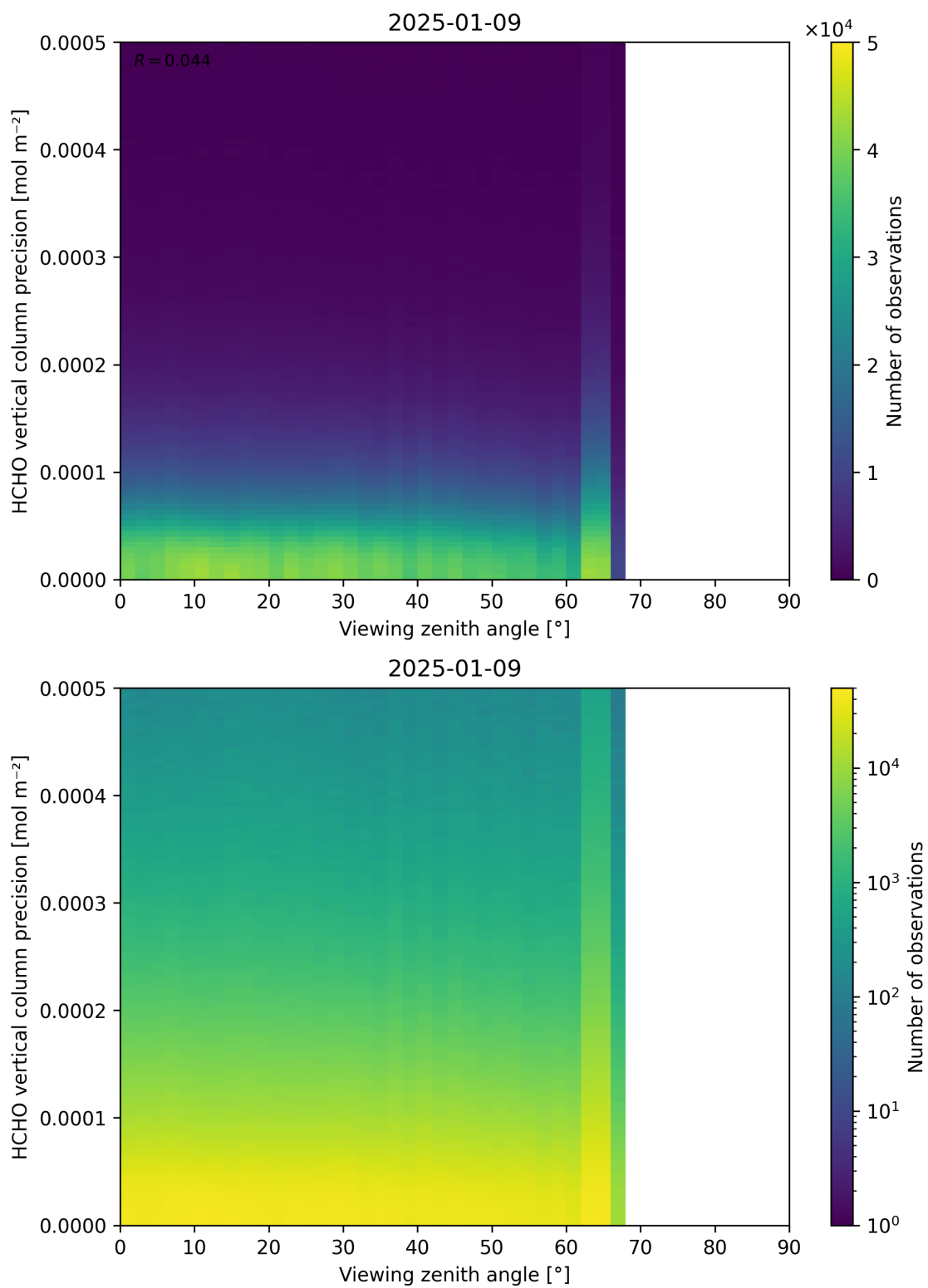
Figure 194: Scatter density plot of “Viewing zenith angle” against “HCHO vertical column precision” for 2025-01-08 to 2025-01-10.
