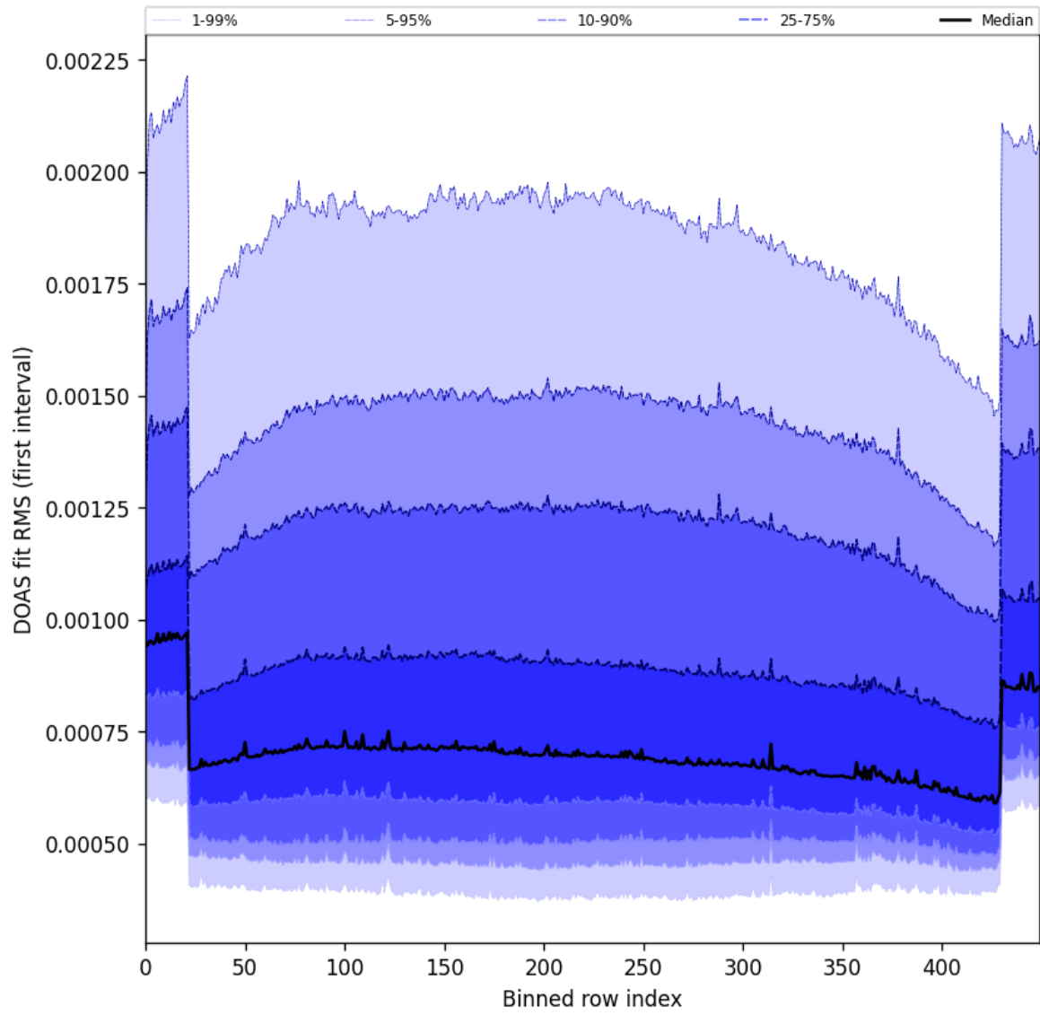
Figure 60: Along track statistics of “DOAS fit RMS (first interval)” for 2025-01-08 to 2025-01-10
