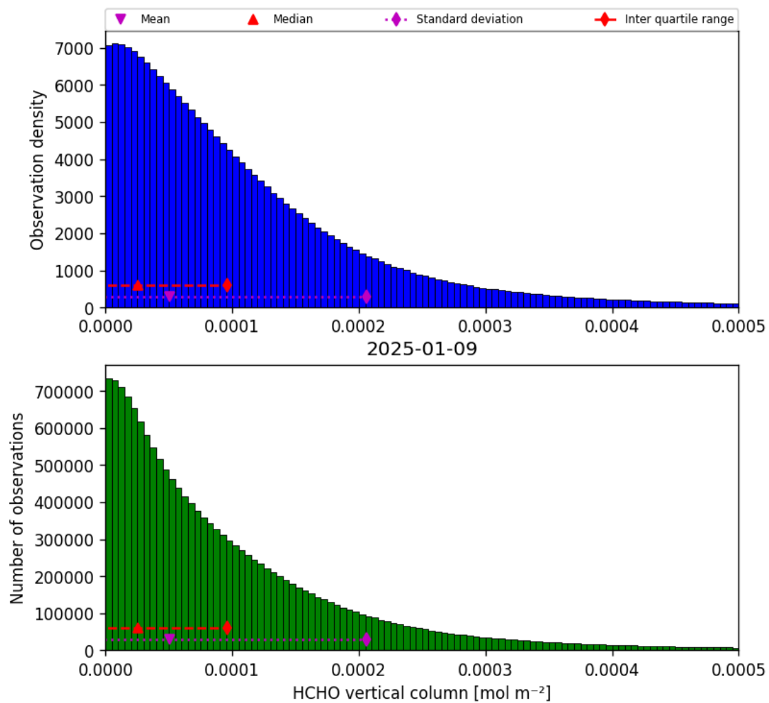
Figure 35: Histogram of “HCHO vertical column” for 2025-01-08 to 2025-01-10
