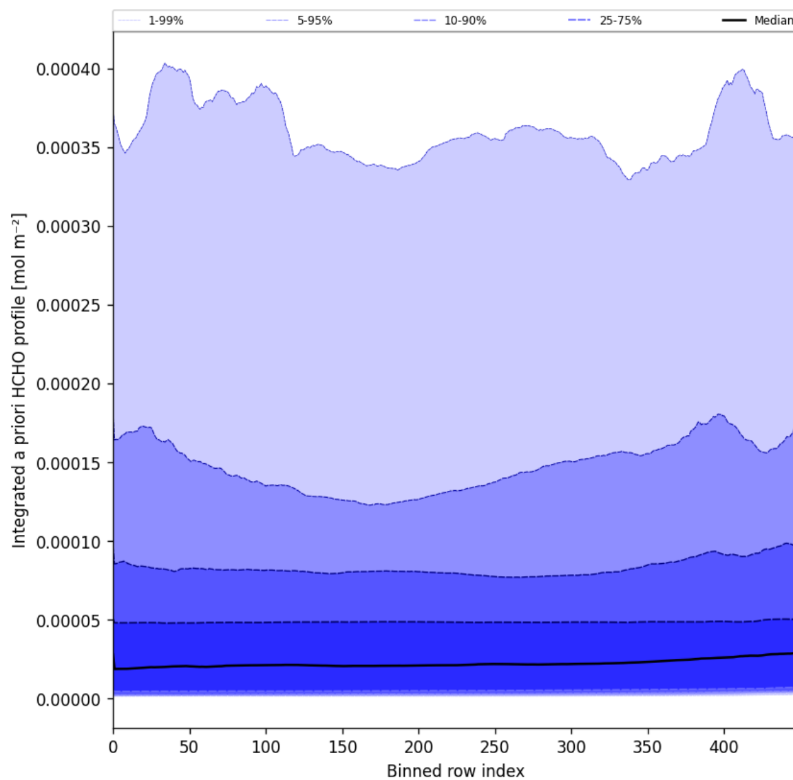
Figure 57: Along track statistics of "Integrated a priori HCHO profile" for 2025-01-08 to 2025-01-10
