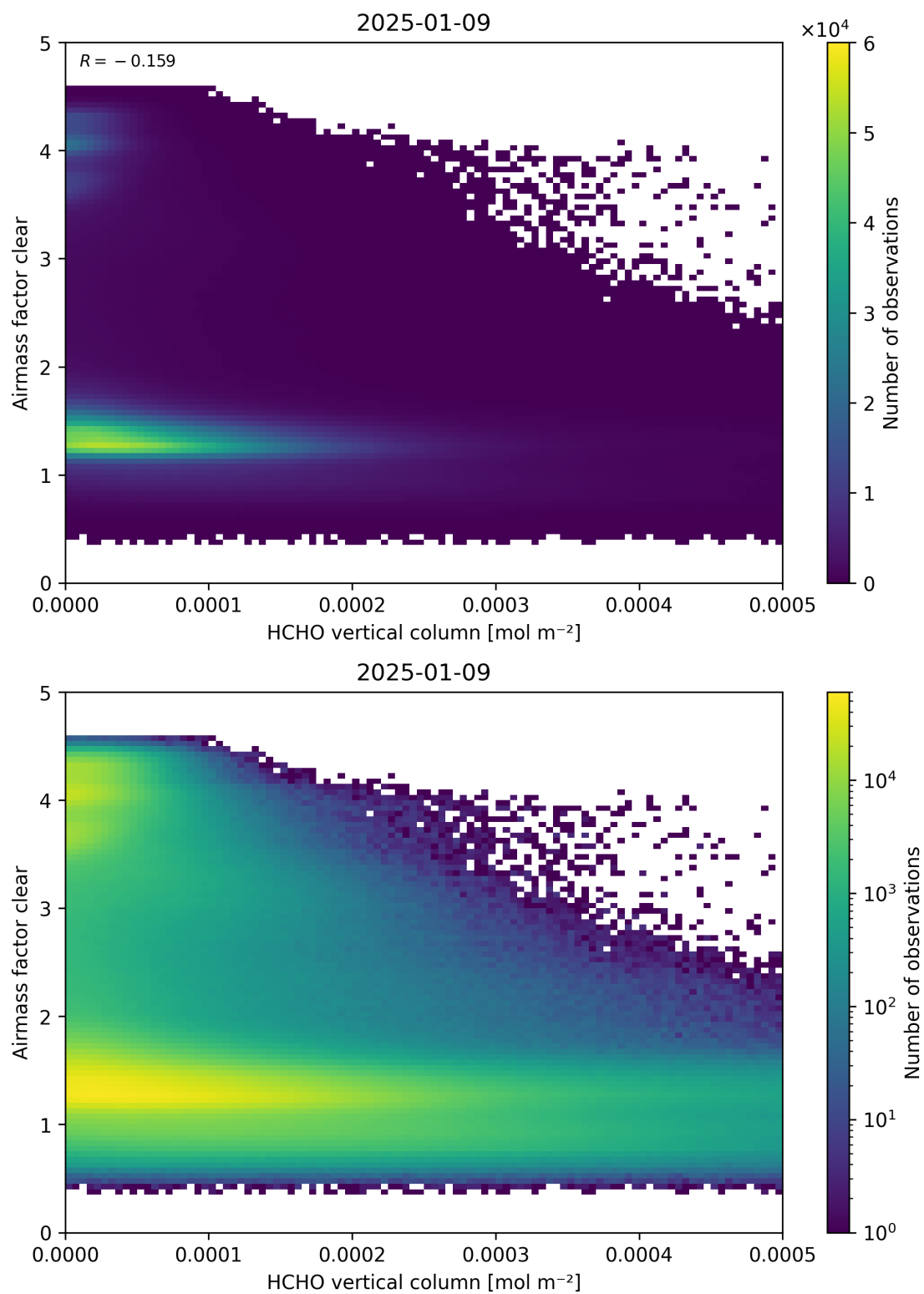
Figure 126: Scatter density plot of “HCHO vertical column” against “Airmass factor clear” for 2025-01-08 to 2025-01-10.
