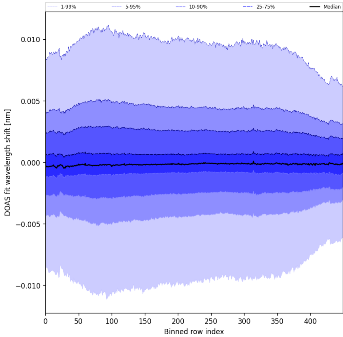
Figure 58: Along track statistics of “DOAS fit wavelength shift” for 2025-01-08 to 2025-01-10
