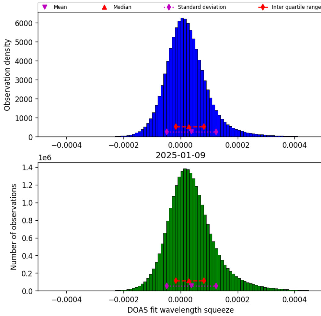
Figure 45: Histogram of “DOAS fit wavelength squeeze” for 2025-01-08 to 2025-01-10
