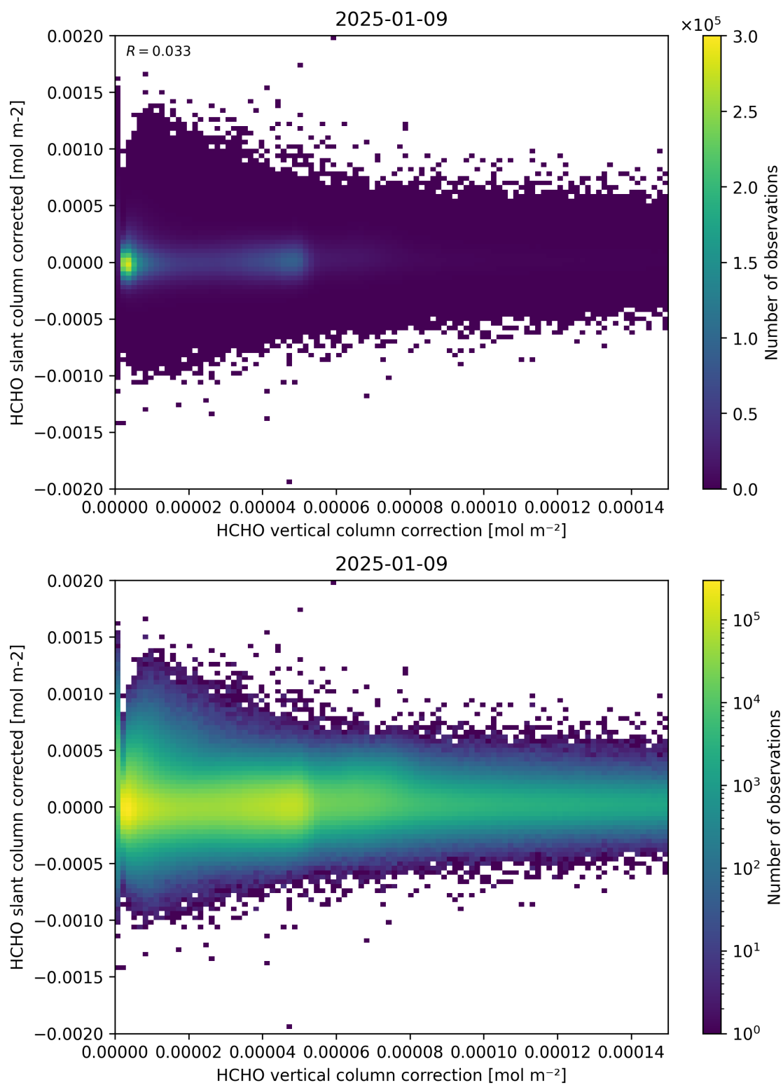
Figure 116: Scatter density plot of “HCHO vertical column correction” against “HCHO slant column corrected” for 2025-01-08 to 2025-01-10.
