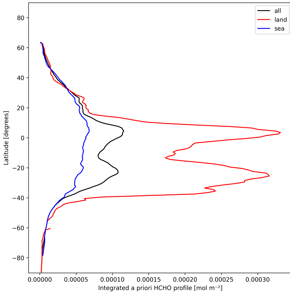
Figure 29: Zonal average of “Integrated a priori HCHO profile” for 2025-01-08 to 2025-01-10.
