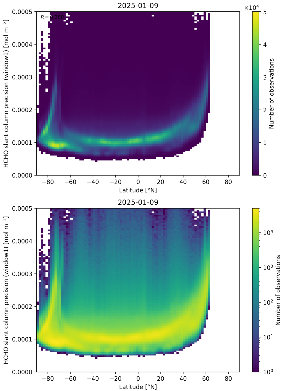
Figure 160: Scatter density plot of “Latitude” against “HCHO slant column precision (window1)” for 2025-01-08 to 2025-01-10.
