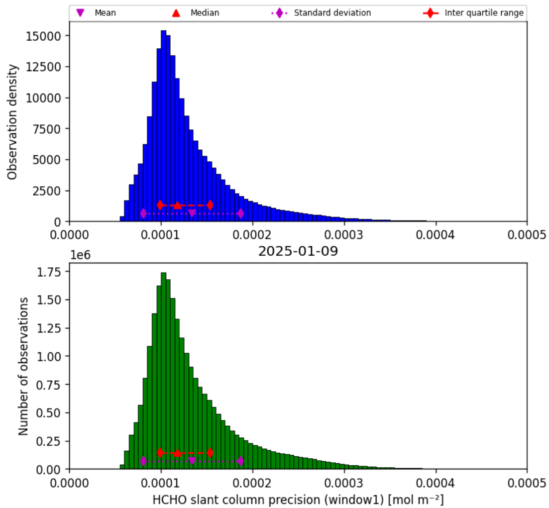
Figure 39: Histogram of “HCHO slant column precision (window1)” for 2025-01-08 to 2025-01-10
