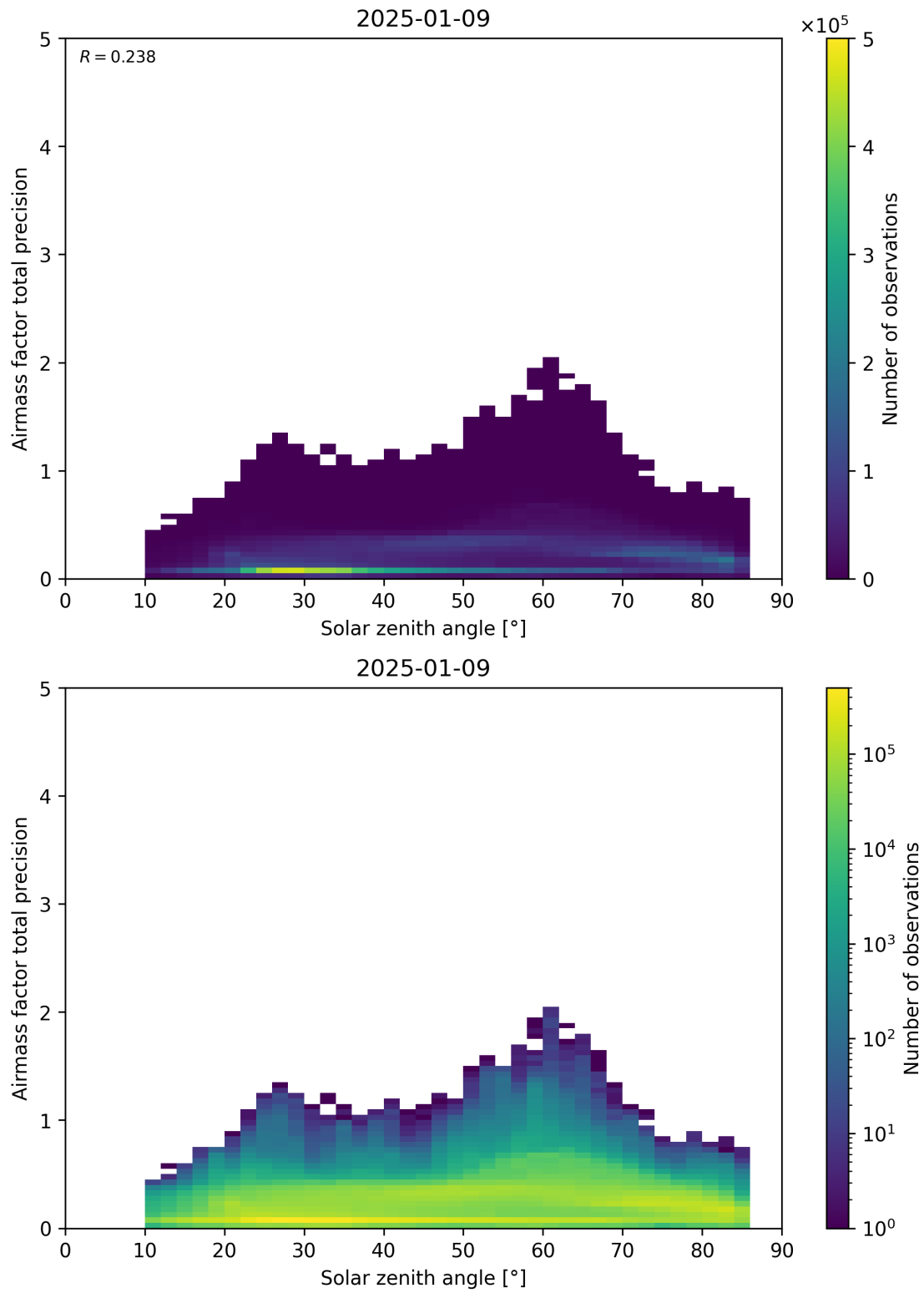
Figure 176: Scatter density plot of “Solar zenith angle” against “Airmass factor total precision” for 2025-01-08 to 2025-01-10.
