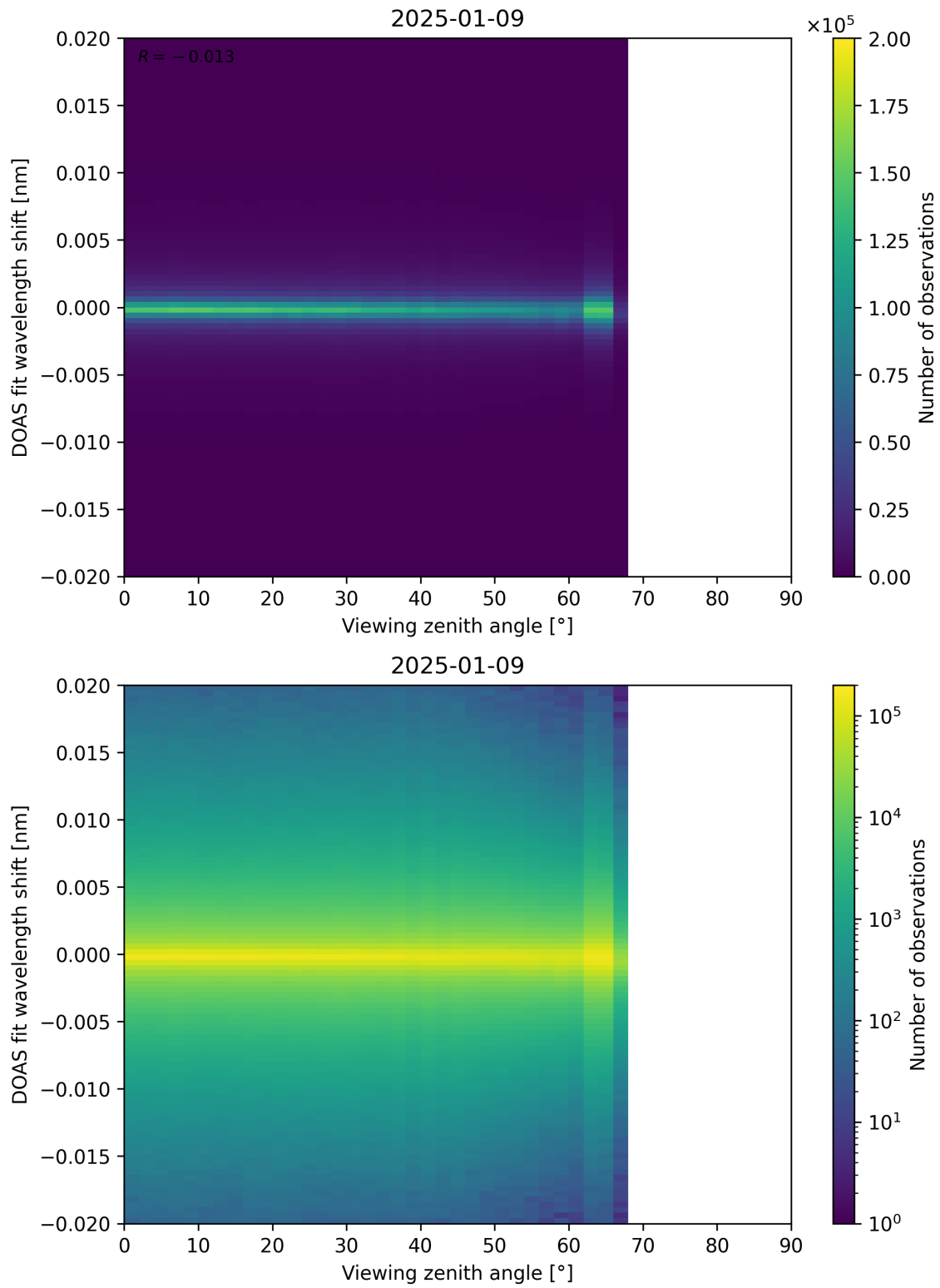
Figure 183: Scatter density plot of “Viewing zenith angle” against “DOAS fit wavelength shift” for 2025-01-08 to 2025-01-10.
