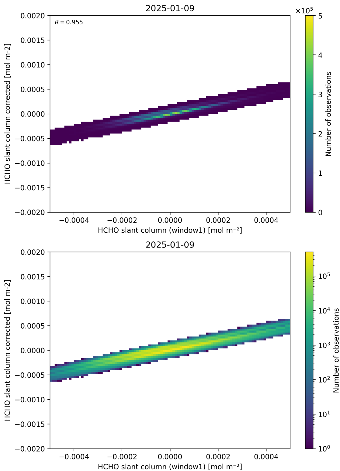
Figure 82: Scatter density plot of “HCHO slant column (window1)” against “HCHO slant column corrected” for 2025-01-08 to 2025-01-10.
