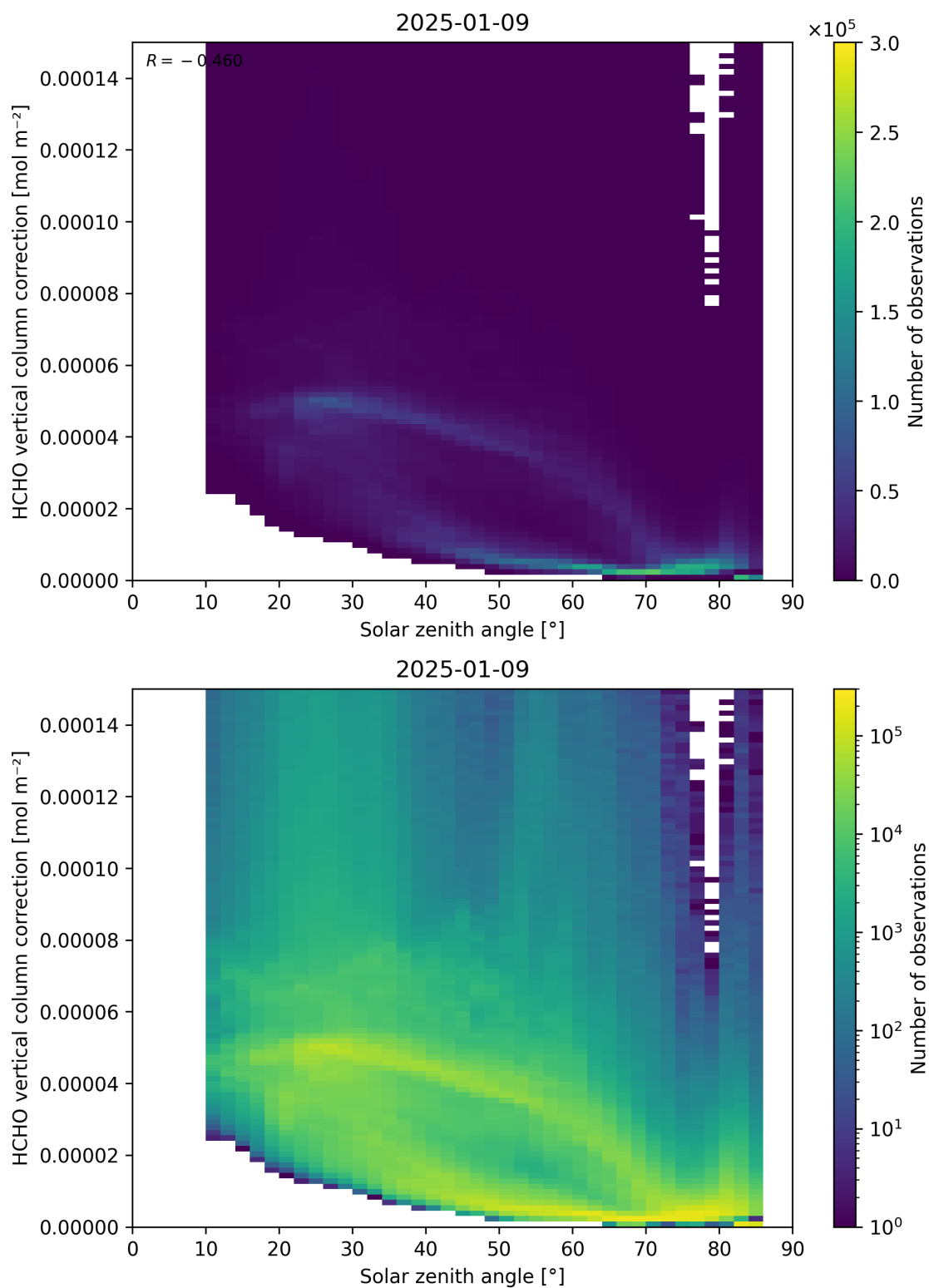
Figure 178: Scatter density plot of “Solar zenith angle” against “HCHO vertical column correction” for 2025-01-08 to 2025-01-10.
