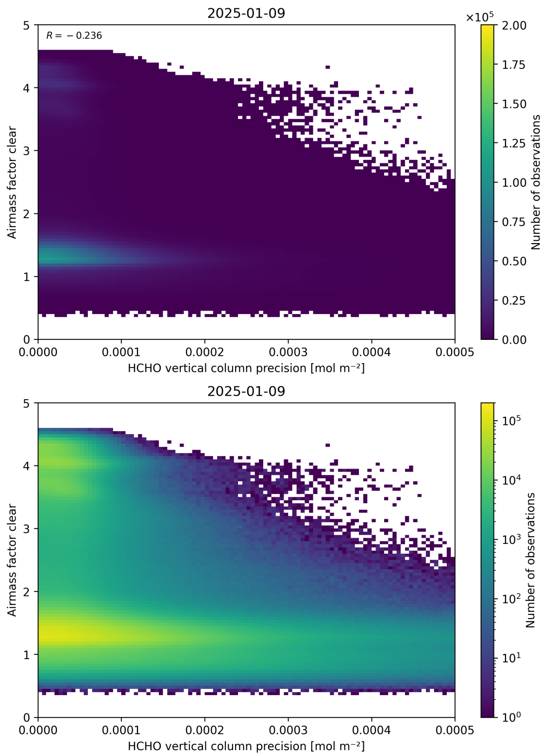
Figure 139: Scatter density plot of “HCHO vertical column precision” against “Airmass factor clear” for 2025-01-08 to 2025-01-10.
