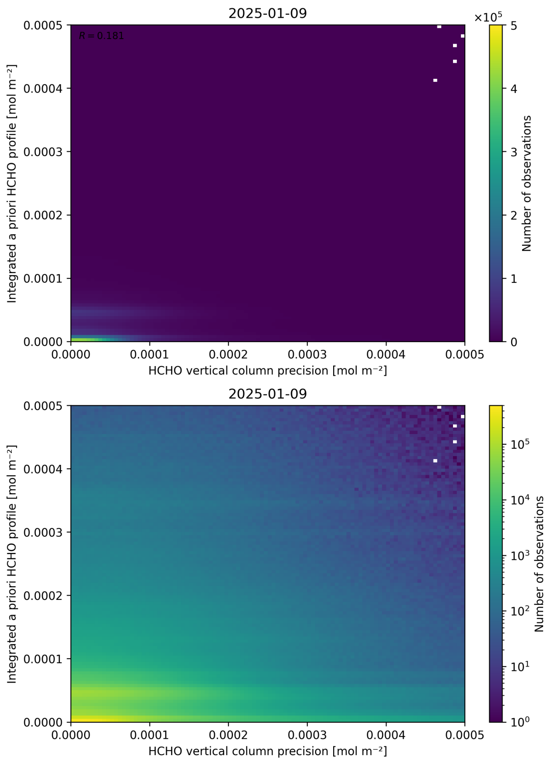
Figure 147: Scatter density plot of “HCHO vertical column precision” against “Integrated a priori HCHO profile” for 2025-01-08 to 2025-01-10.
