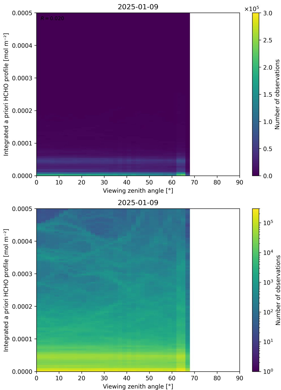
Figure 195: Scatter density plot of “Viewing zenith angle” against “Integrated a priori HCHO profile” for 2025-01-08 to 2025-01-10.
