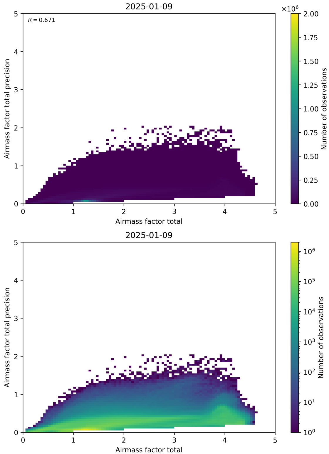
Figure 103: Scatter density plot of “Airmass factor total” against “Airmass factor total precision” for 2025-01-08 to 2025-01-10.
