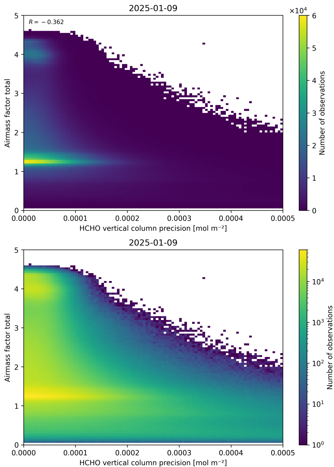
Figure 144: Scatter density plot of “HCHO vertical column precision” against “Airmass factor total” for 2025-01-08 to 2025-01-10.
