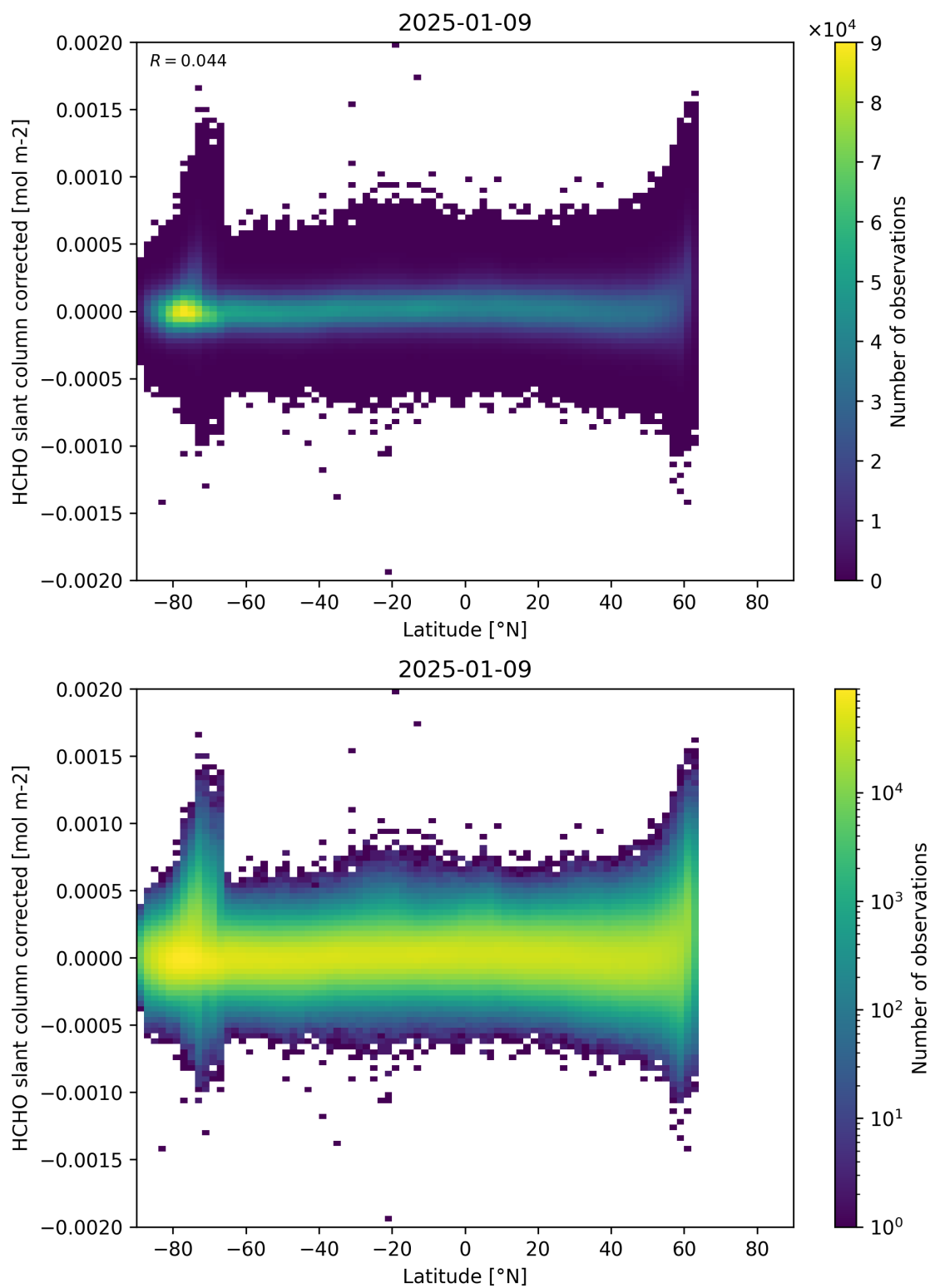
Figure 157: Scatter density plot of “Latitude” against “HCHO slant column corrected” for 2025-01-08 to 2025-01-10.
