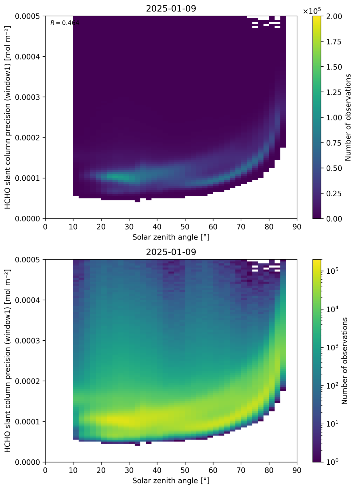
Figure 174: Scatter density plot of “Solar zenith angle” against “HCHO slant column precision (window1)” for 2025-01-08 to 2025-01-10.
