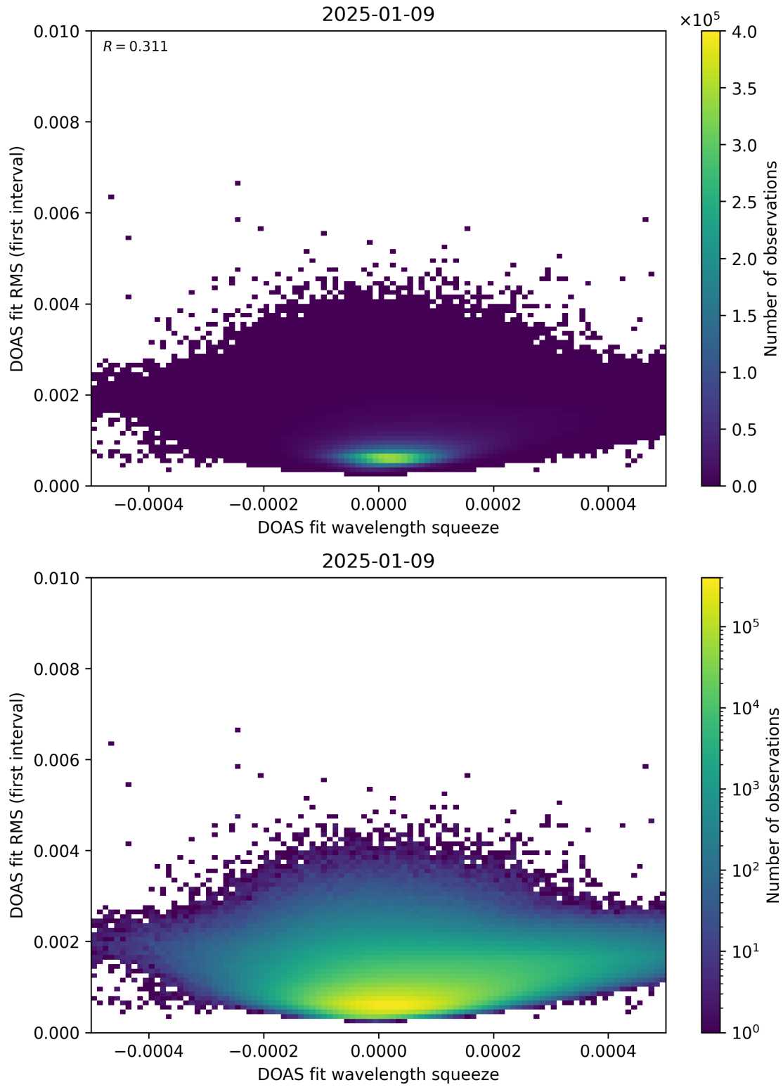
Figure 68: Scatter density plot of “DOAS fit wavelength squeeze” against “DOAS fit RMS (first interval)” for 2025-01-08 to 2025-01-10.
