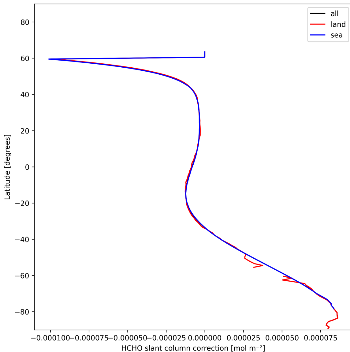
Figure 33: Zonal average of “HCHO slant column correction” for 2025-01-08 to 2025-01-10.
