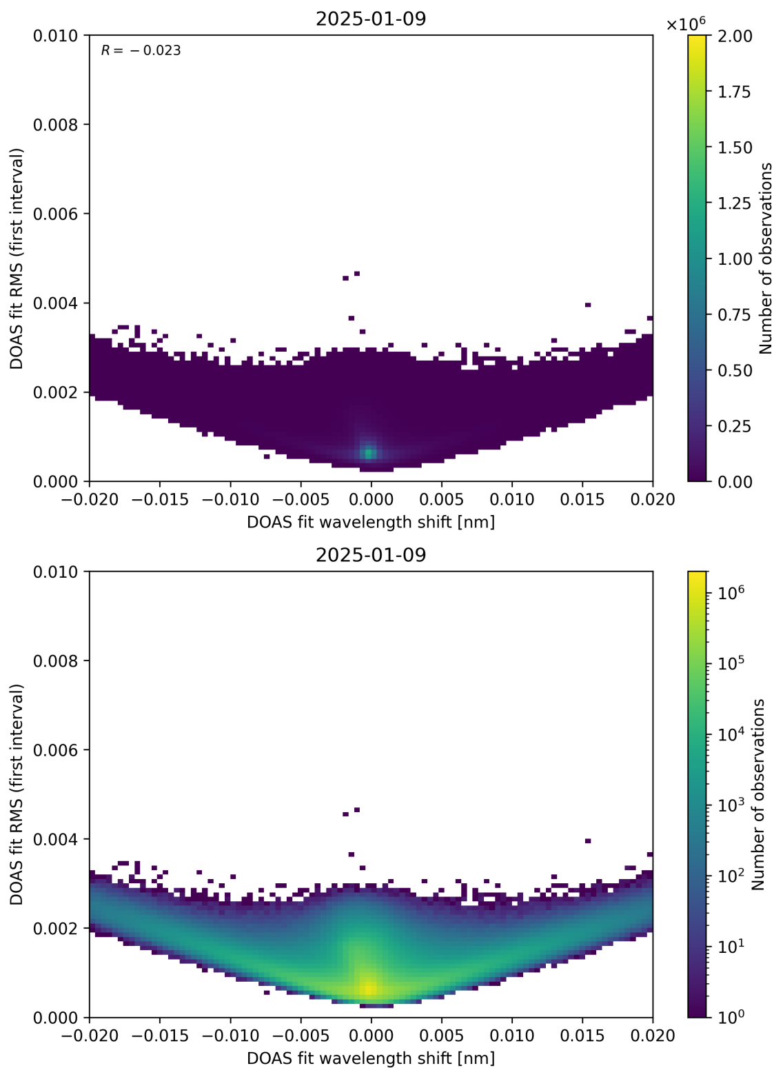
Figure 64: Scatter density plot of “DOAS fit wavelength shift” against “DOAS fit RMS (first interval)” for 2025-01-08 to 2025-01-10.
