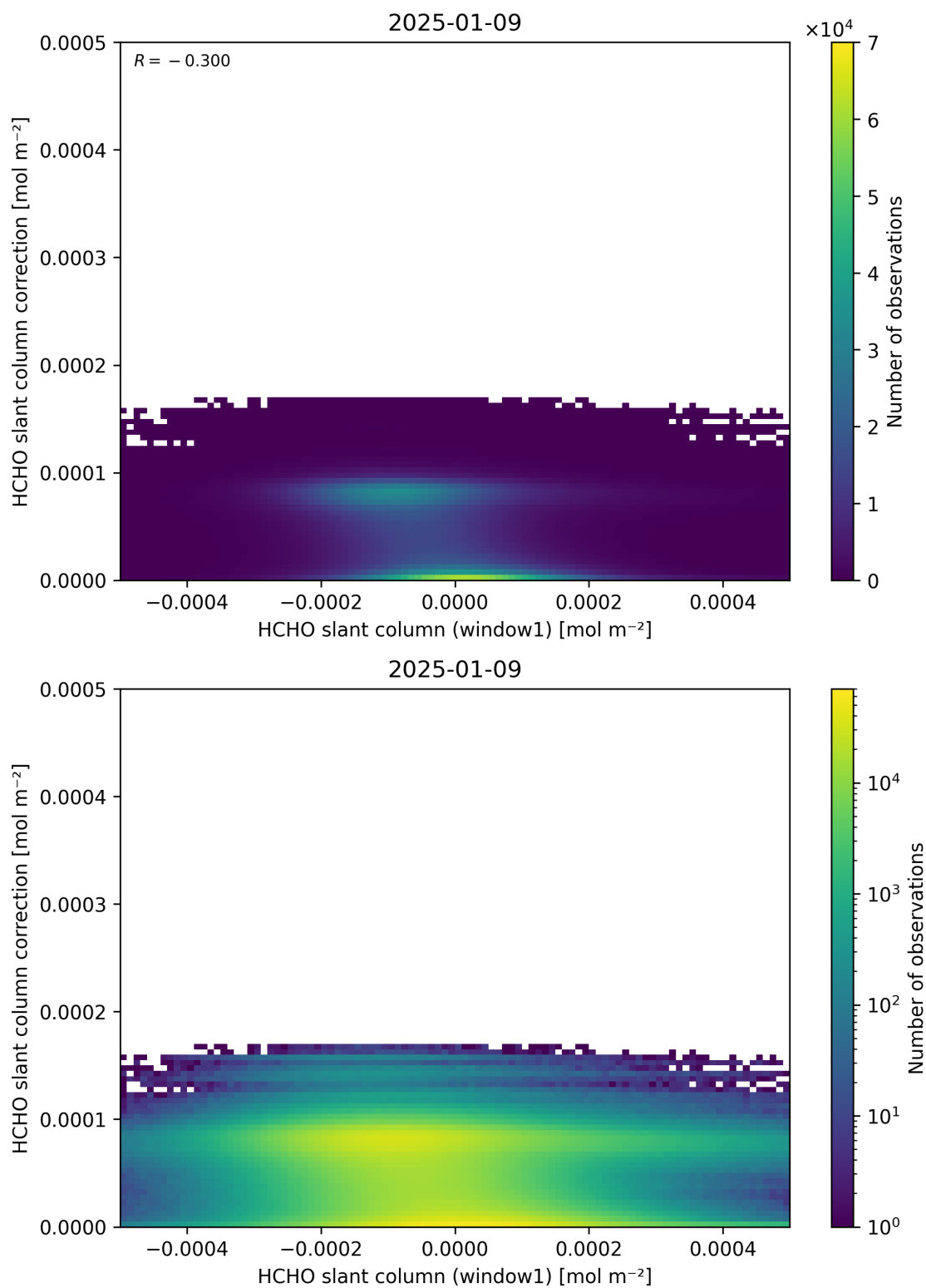
Figure 83: Scatter density plot of “HCHO slant column (window1)” against “HCHO slant column correction” for 2025-01-08 to 2025-01-10.
