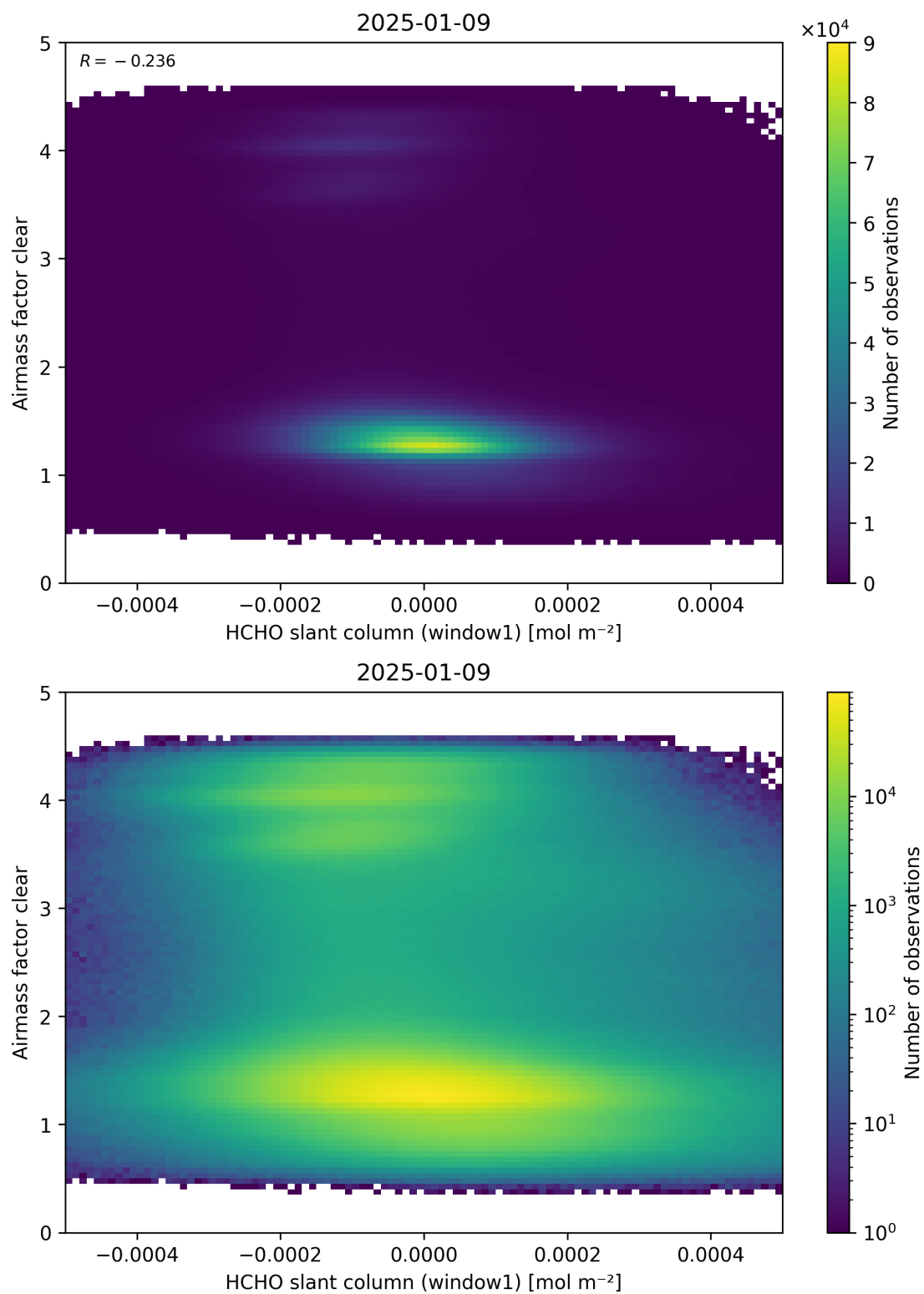
Figure 81: Scatter density plot of “HCHO slant column (window1)” against “Airmass factor clear” for 2025-01-08 to 2025-01-10.
