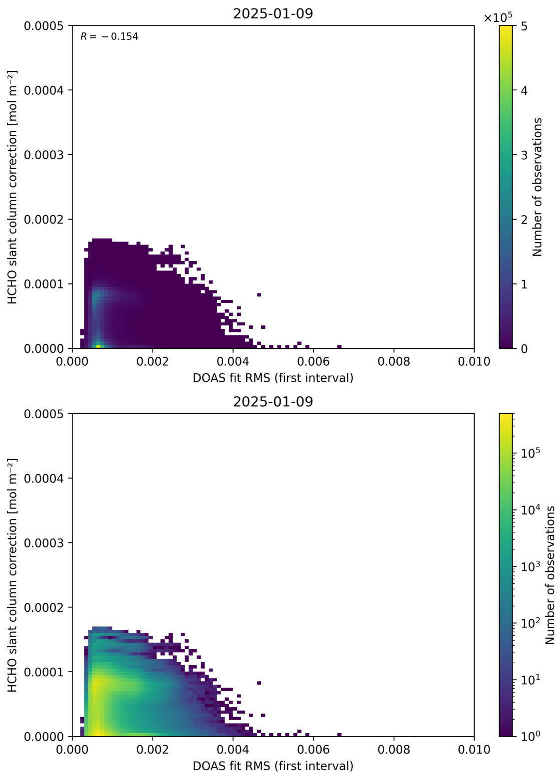
Figure 63: Scatter density plot of “DOAS fit RMS (first interval)” against “HCHO slant column correction” for 2025-01-08 to 2025-01-10.
