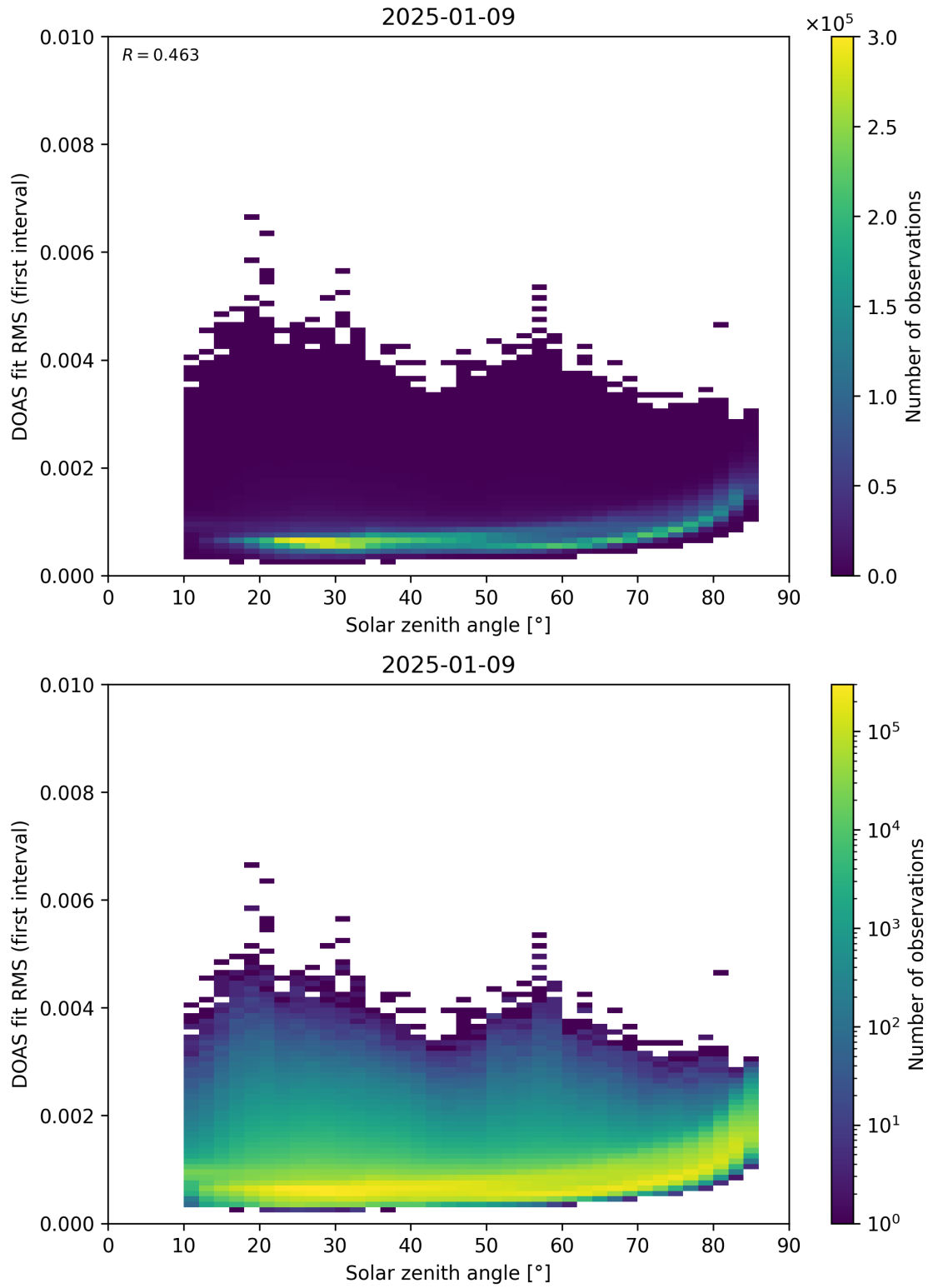
Figure 167: Scatter density plot of “Solar zenith angle” against “DOAS fit RMS (first interval)” for 2025-01-08 to 2025-01-10.
