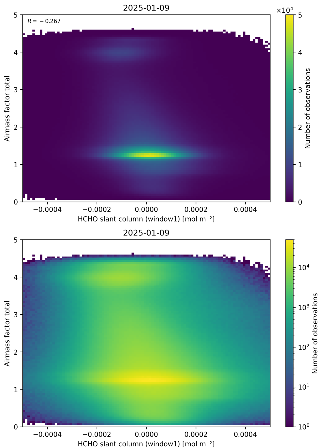
Figure 85: Scatter density plot of “HCHO slant column (window1)” against “Airmass factor total” for 2025-01-08 to 2025-01-10.
