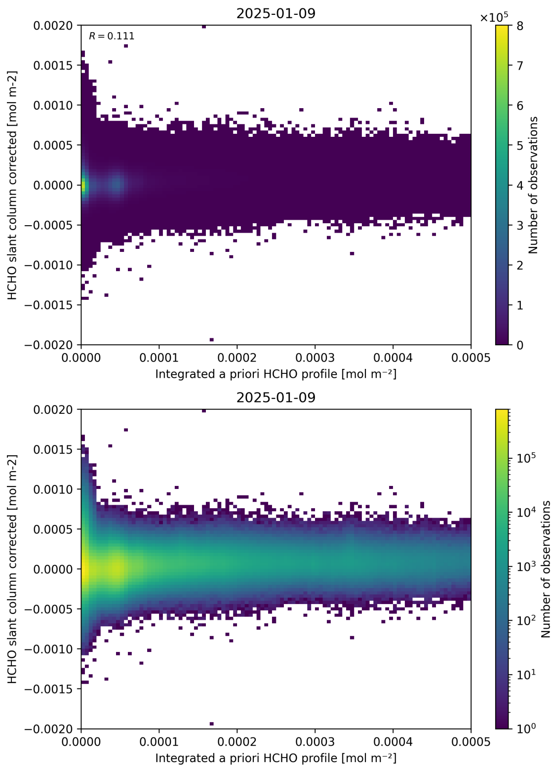
Figure 151: Scatter density plot of “Integrated a priori HCHO profile” against “HCHO slant column corrected” for 2025-01-08 to 2025-01-10.
