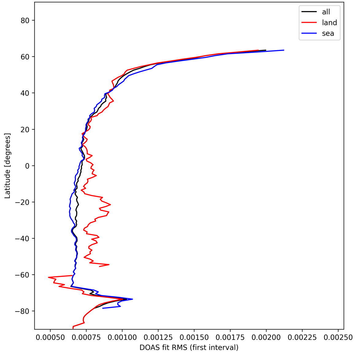
Figure 32: Zonal average of “DOAS fit RMS (first interval)” for 2025-01-08 to 2025-01-10.
