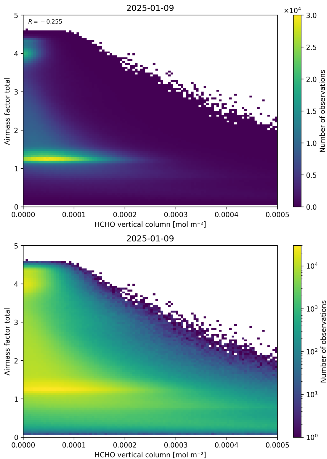
Figure 131: Scatter density plot of “HCHO vertical column” against “Airmass factor total” for 2025-01-08 to 2025-01-10.
