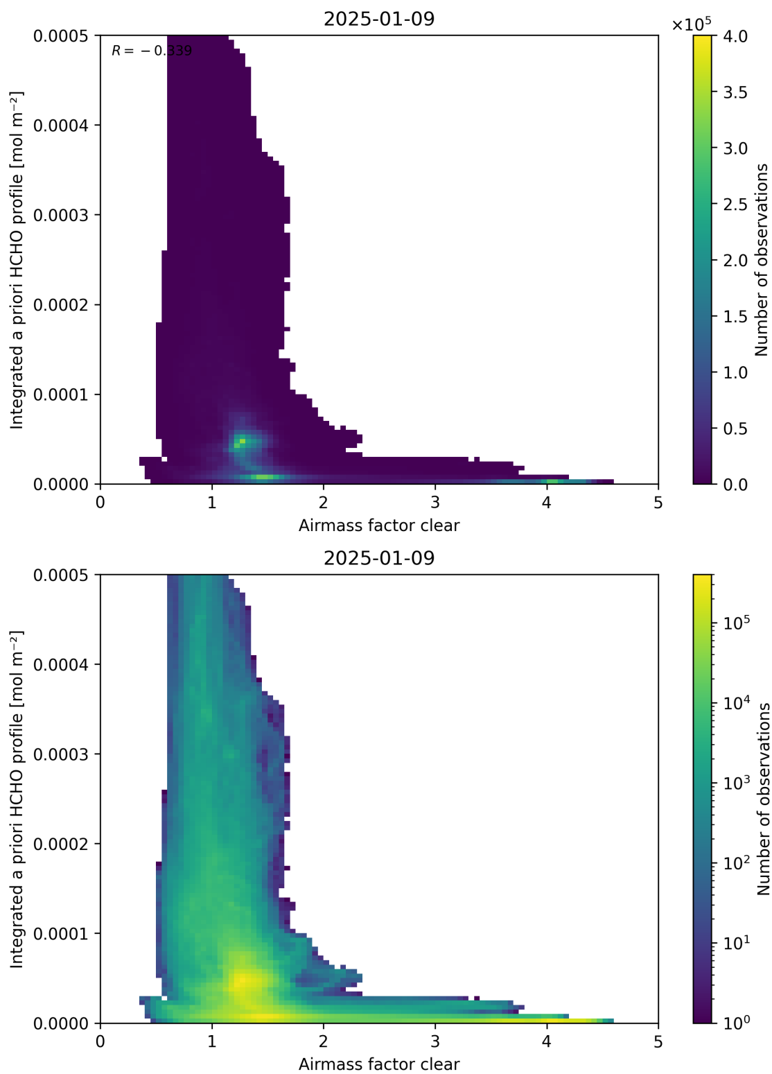
Figure 76: Scatter density plot of “Airmass factor clear” against “Integrated a priori HCHO profile” for 2025-01-08 to 2025-01-10.
