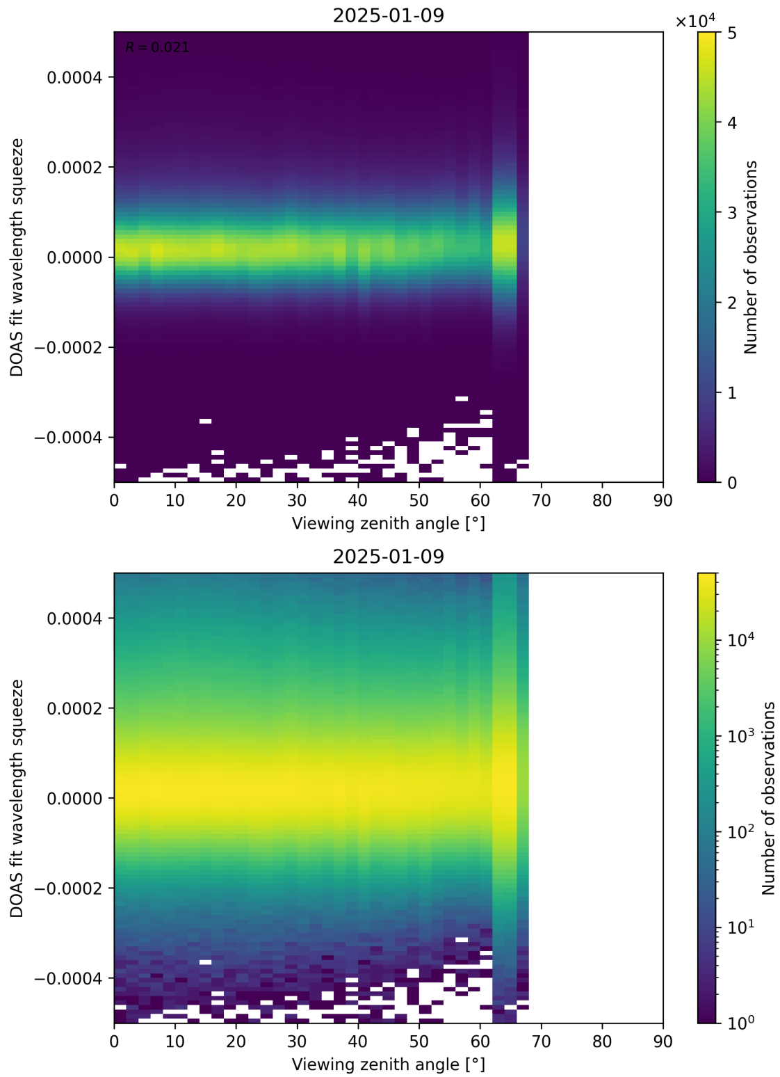
Figure 184: Scatter density plot of “Viewing zenith angle” against “DOAS fit wavelength squeeze” for 2025-01-08 to 2025-01-10.
