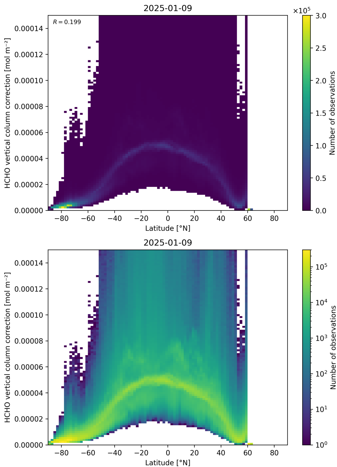
Figure 164: Scatter density plot of “Latitude” against “HCHO vertical column correction” for 2025-01-08 to 2025-01-10.
