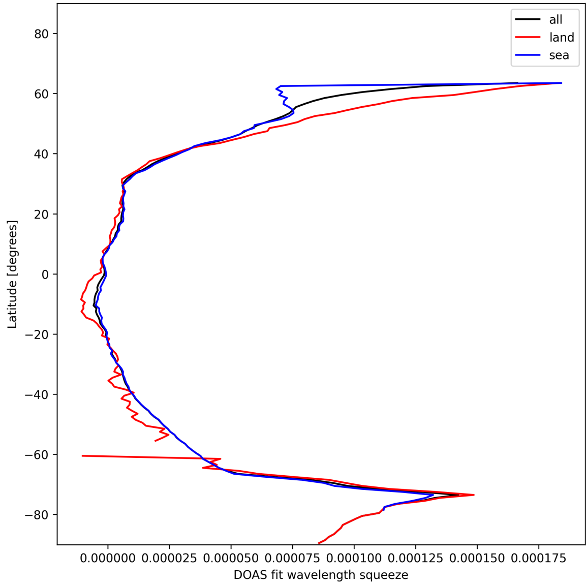
Figure 31: Zonal average of “DOAS fit wavelength squeeze” for 2025-01-08 to 2025-01-10.
