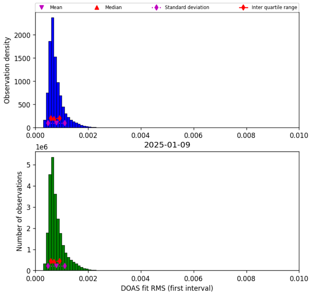
Figure 46: Histogram of “DOAS fit RMS (first interval)” for 2025-01-08 to 2025-01-10
