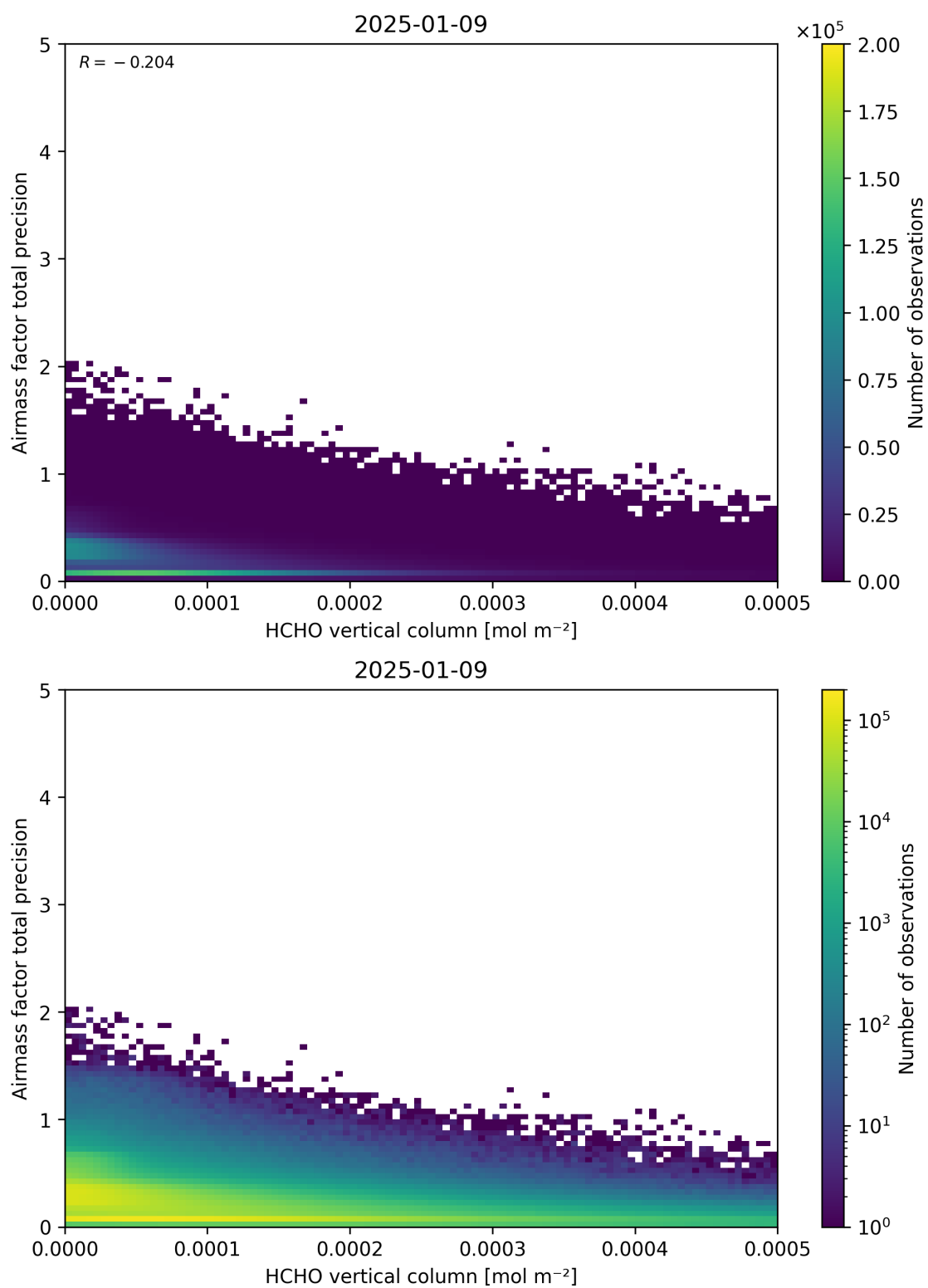
Figure 132: Scatter density plot of “HCHO vertical column” against “Airmass factor total precision” for 2025-01-08 to 2025-01-10.
