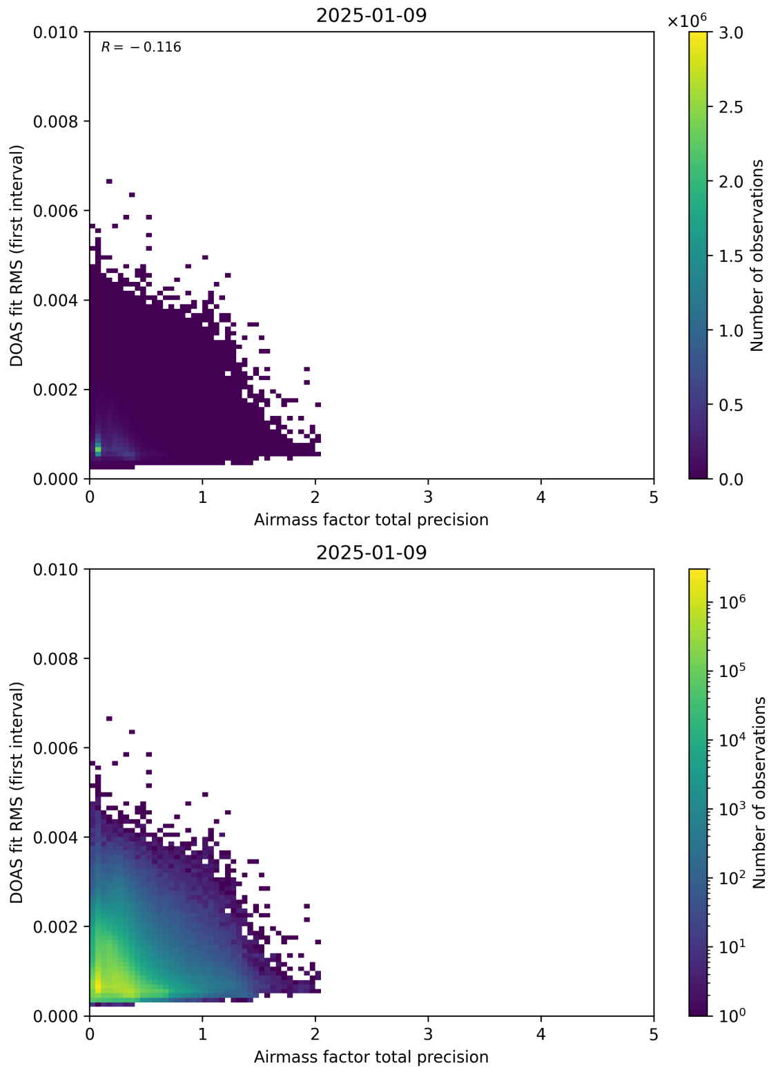
Figure 105: Scatter density plot of “Airmass factor total precision” against “DOAS fit RMS (first interval)” for 2025-01-08 to 2025-01-10.
