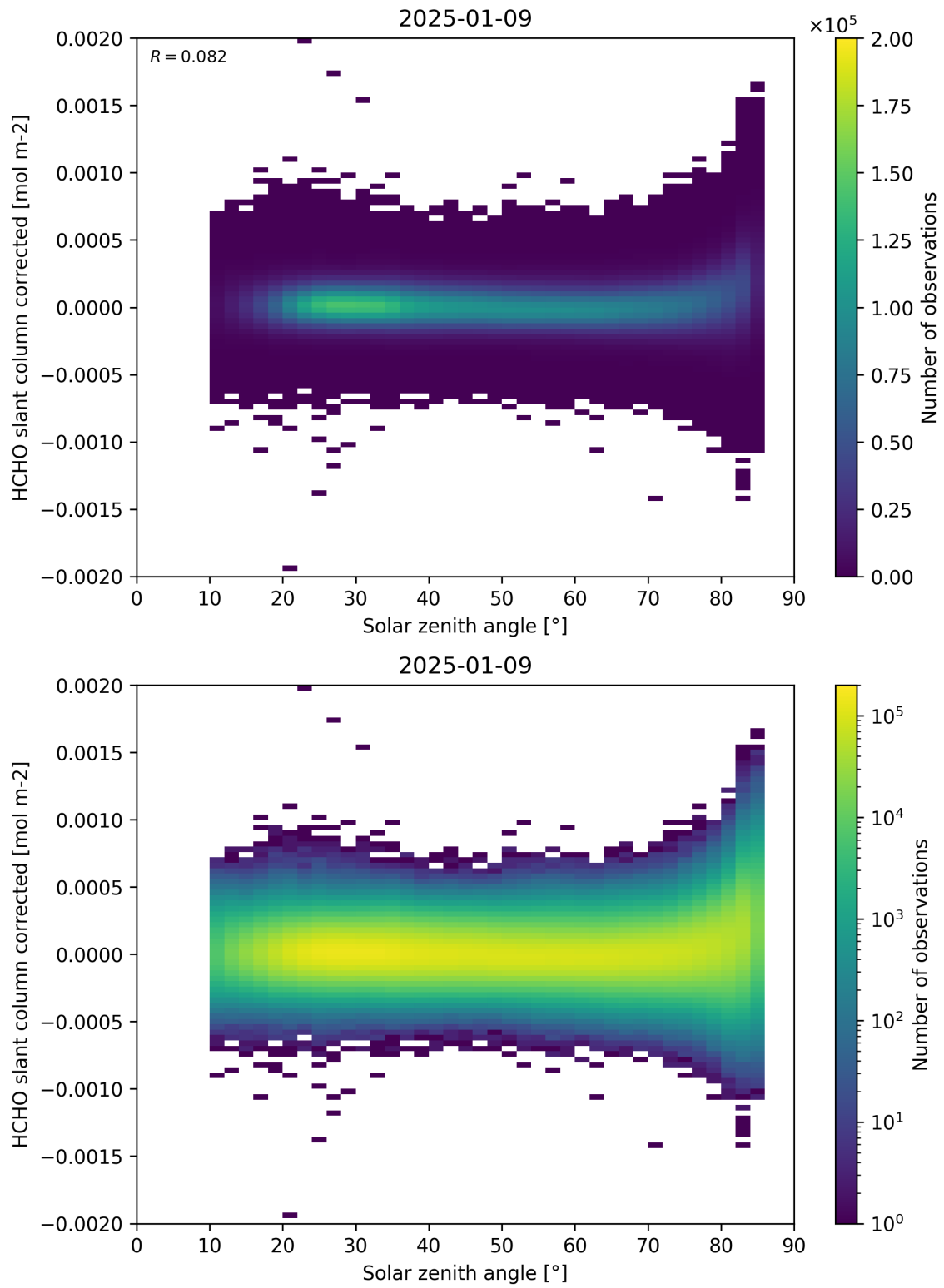
Figure 171: Scatter density plot of “Solar zenith angle” against “HCHO slant column corrected” for 2025-01-08 to 2025-01-10.
