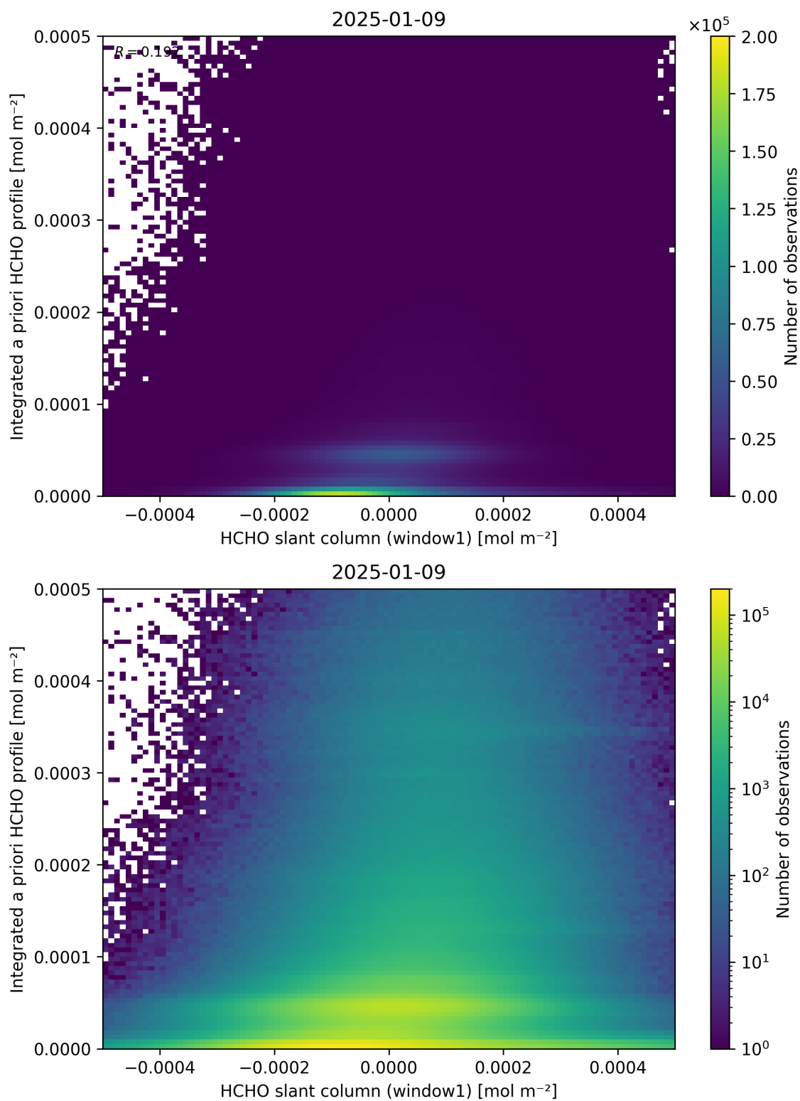
Figure 87: Scatter density plot of “HCHO slant column (window1)” against “Integrated a priori HCHO profile” for 2025-01-08 to 2025-01-10.
