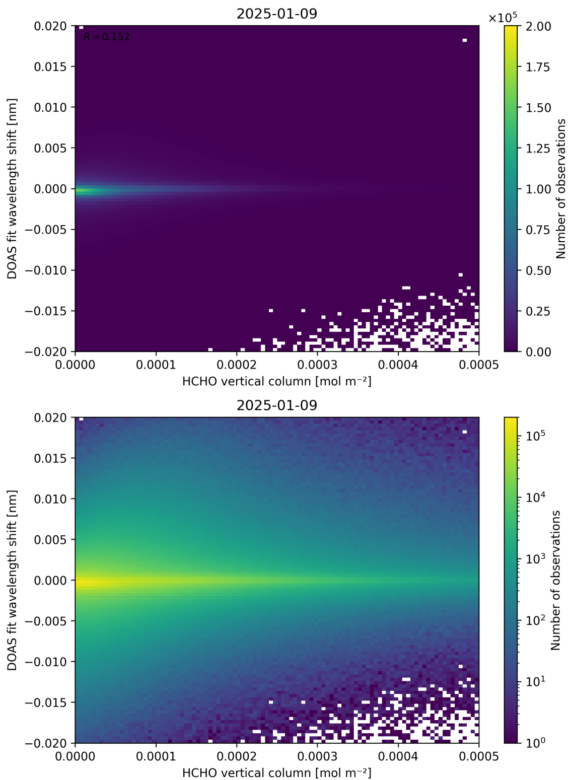
Figure 124: Scatter density plot of “HCHO vertical column” against “DOAS fit wavelength shift” for 2025-01-08 to 2025-01-10.
