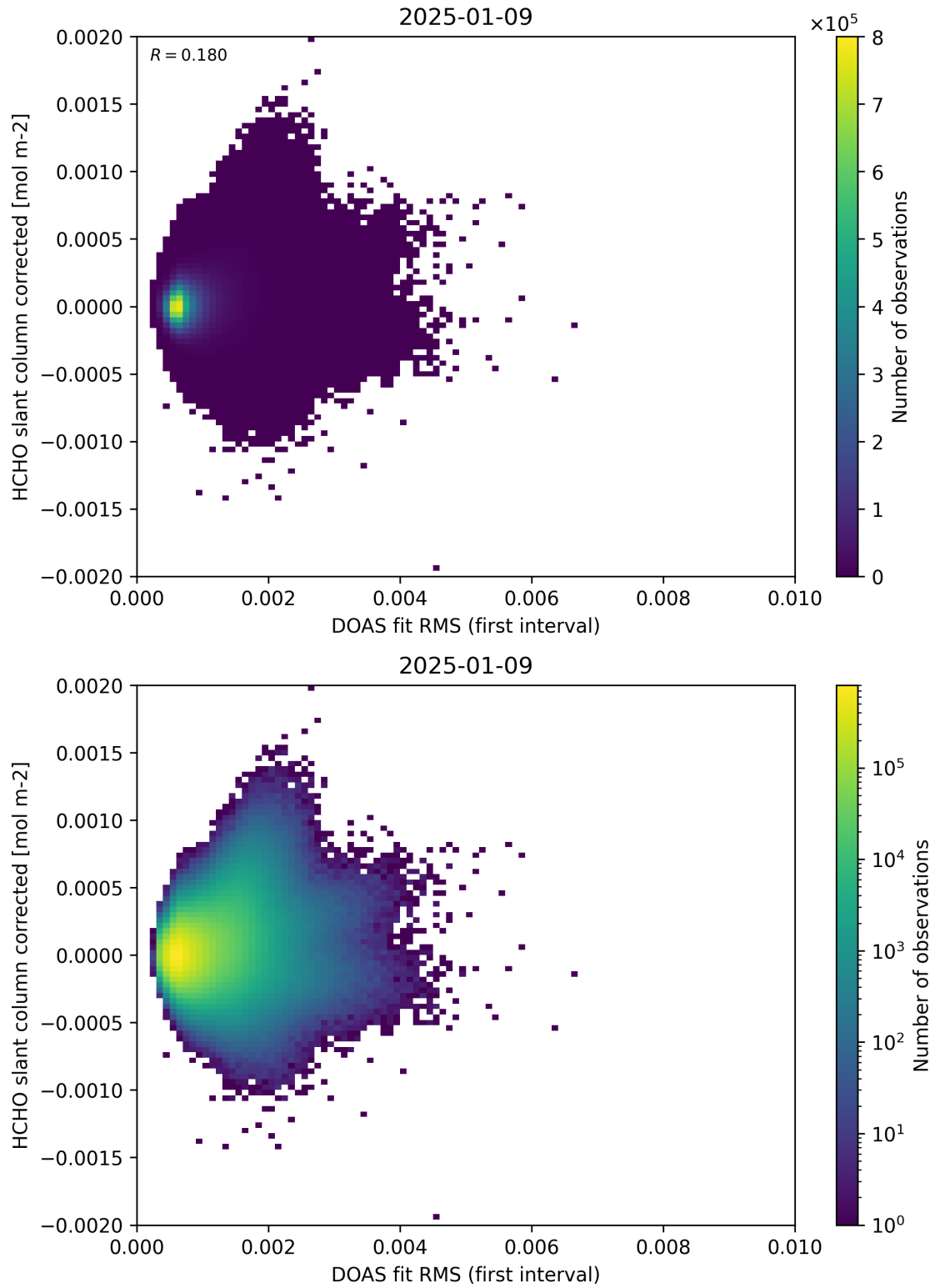
Figure 62: Scatter density plot of “DOAS fit RMS (first interval)” against “HCHO slant column corrected” for 2025-01-08 to 2025-01-10.
