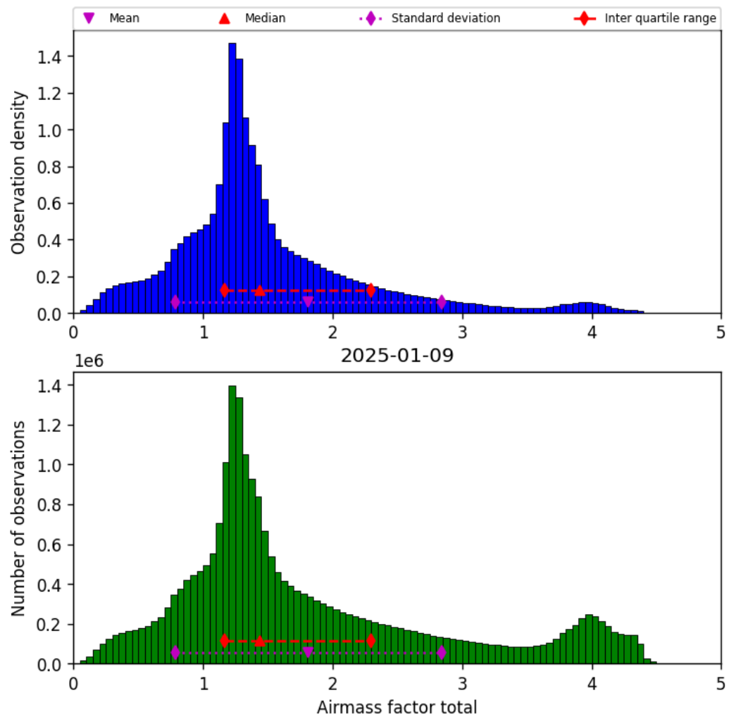
Figure 40: Histogram of “Airmass factor total” for 2025-01-08 to 2025-01-10
