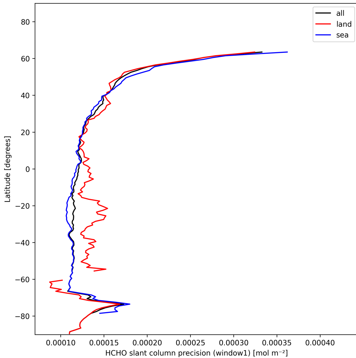
Figure 25: Zonal average of “HCHO slant column precision (window1)” for 2025-01-08 to 2025-01-10.
