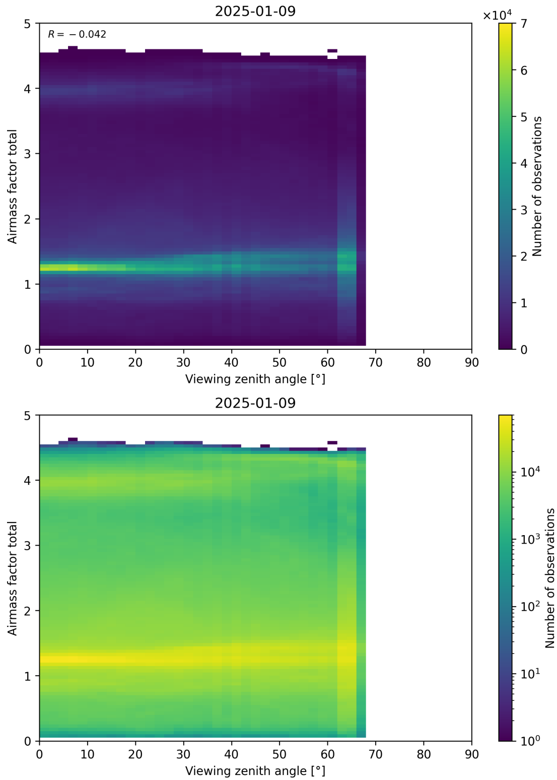
Figure 190: Scatter density plot of “Viewing zenith angle” against “Airmass factor total” for 2025-01-08 to 2025-01-10.
