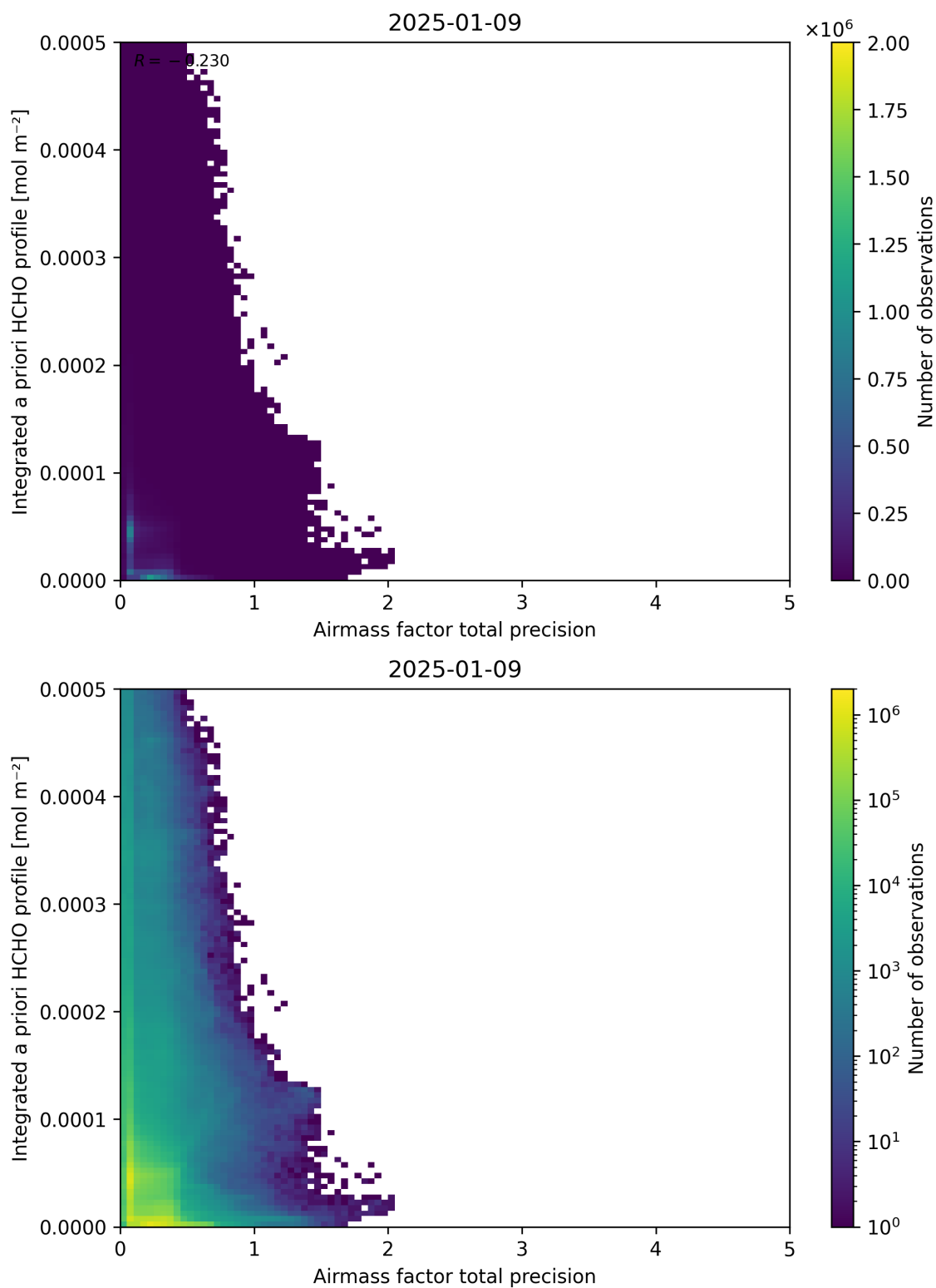
Figure 111: Scatter density plot of “Airmass factor total precision” against “Integrated a priori HCHO profile” for 2025-01-08 to 2025-01-10.
