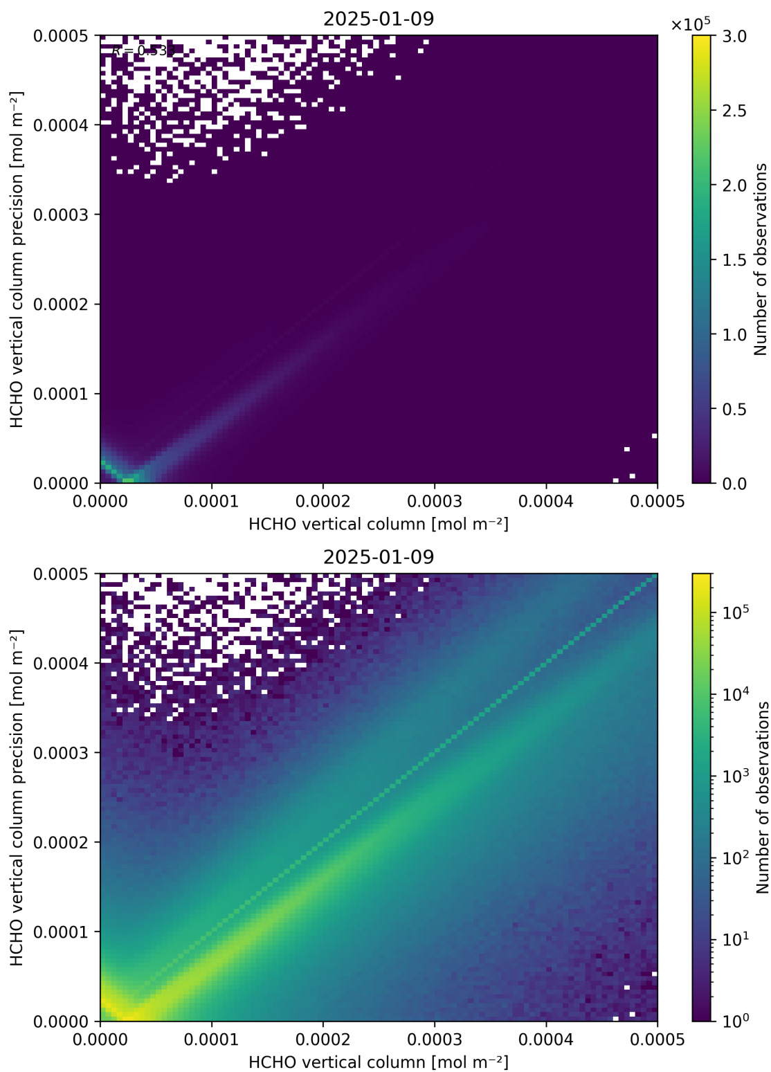
Figure 134: Scatter density plot of “HCHO vertical column” against “HCHO vertical column precision” for 2025-01-08 to 2025-01-10.
