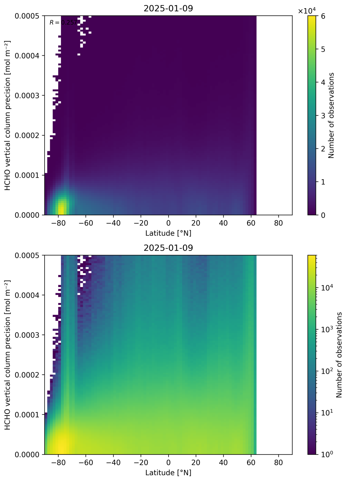
Figure 165: Scatter density plot of “Latitude” against “HCHO vertical column precision” for 2025-01-08 to 2025-01-10.
