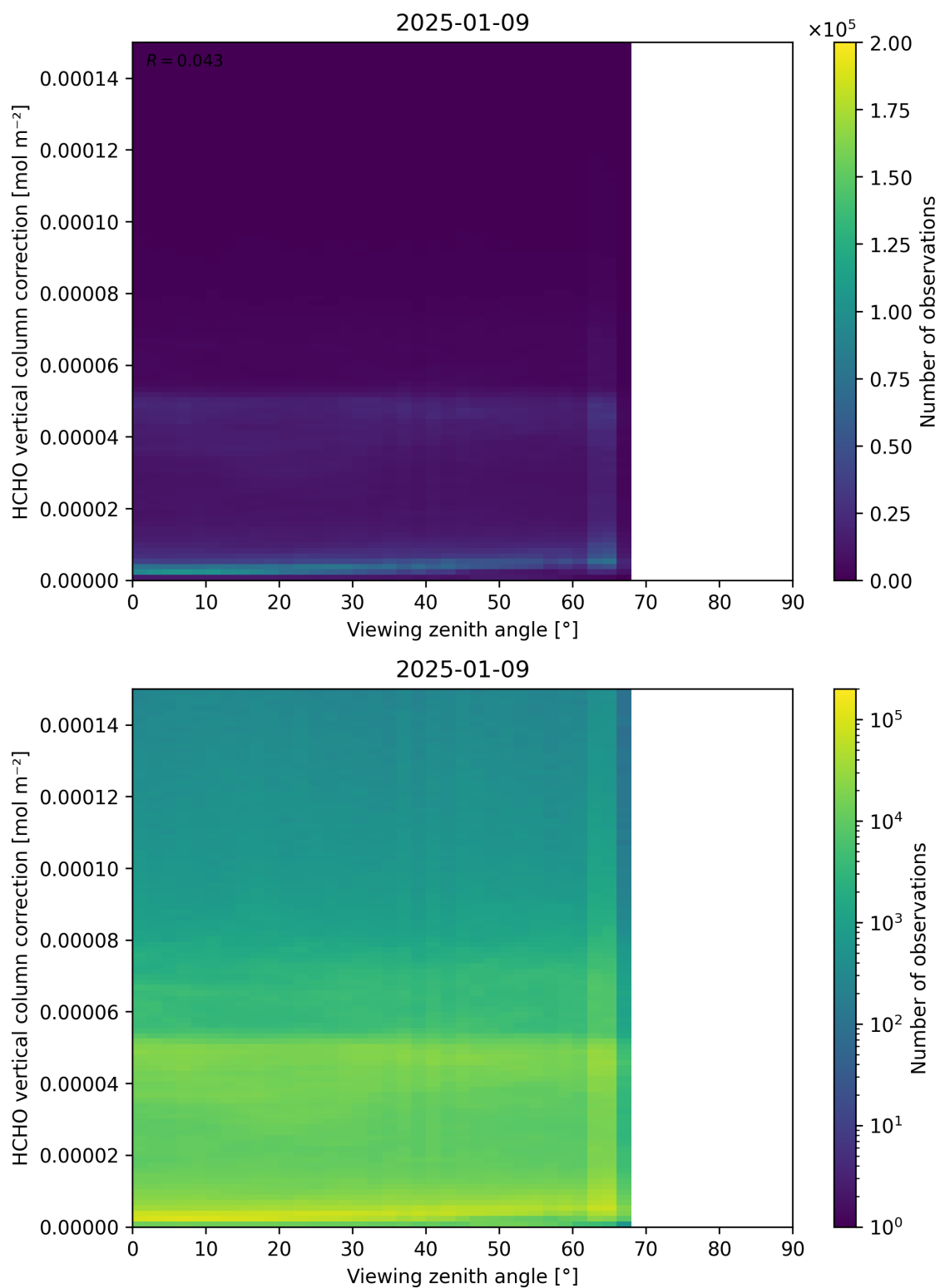
Figure 193: Scatter density plot of “Viewing zenith angle” against “HCHO vertical column correction” for 2025-01-08 to 2025-01-10.
