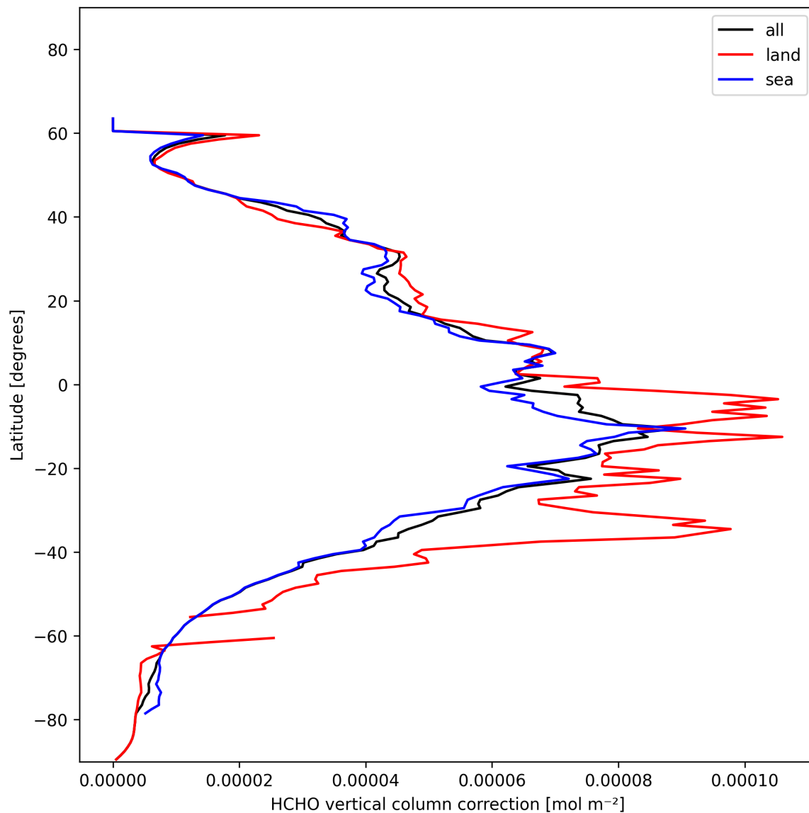
Figure 23: Zonal average of “HCHO vertical column correction” for 2025-01-08 to 2025-01-10.
