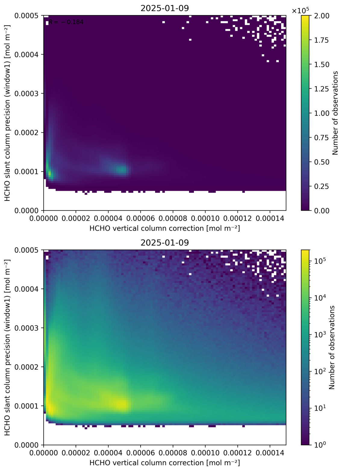
Figure 119: Scatter density plot of “HCHO vertical column correction” against “HCHO slant column precision (window1)” for 2025-01-08 to 2025-01-10.
