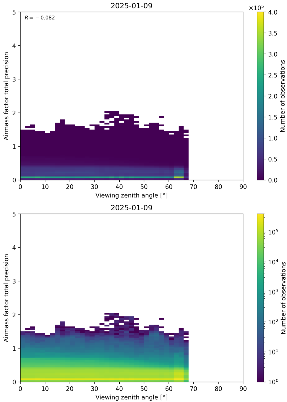
Figure 191: Scatter density plot of “Viewing zenith angle” against “Airmass factor total precision” for 2025-01-08 to 2025-01-10.
