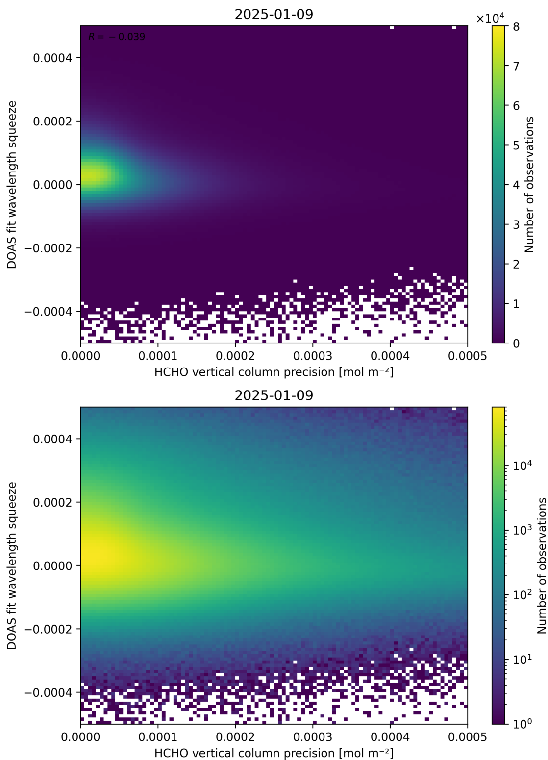
Figure 138: Scatter density plot of “HCHO vertical column precision” against “DOAS fit wavelength squeeze” for 2025-01-08 to 2025-01-10.
