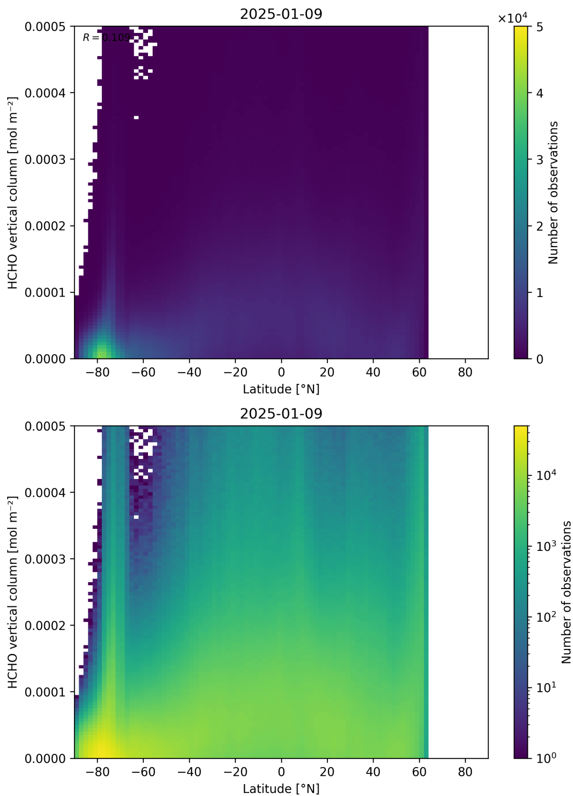
Figure 163: Scatter density plot of “Latitude” against “HCHO vertical column” for 2025-01-08 to 2025-01-10.
