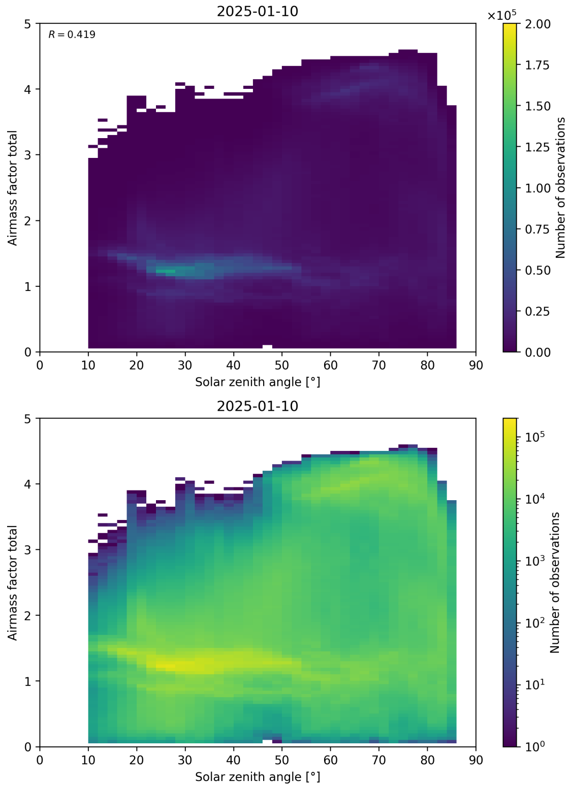
Figure 175: Scatter density plot of “Solar zenith angle” against “Airmass factor total” for 2025-01-09 to 2025-01-11.
