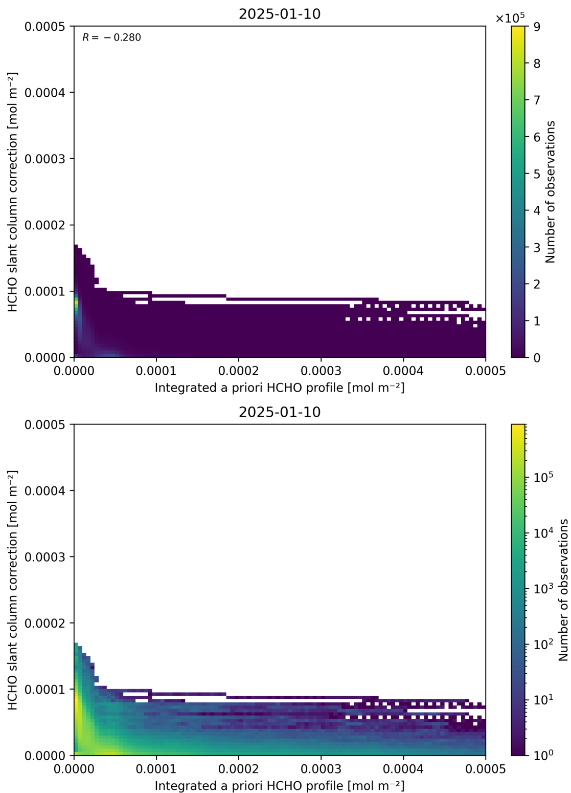
Figure 152: Scatter density plot of “Integrated a priori HCHO profile” against “HCHO slant column correction” for 2025-01-09 to 2025-01-11.
