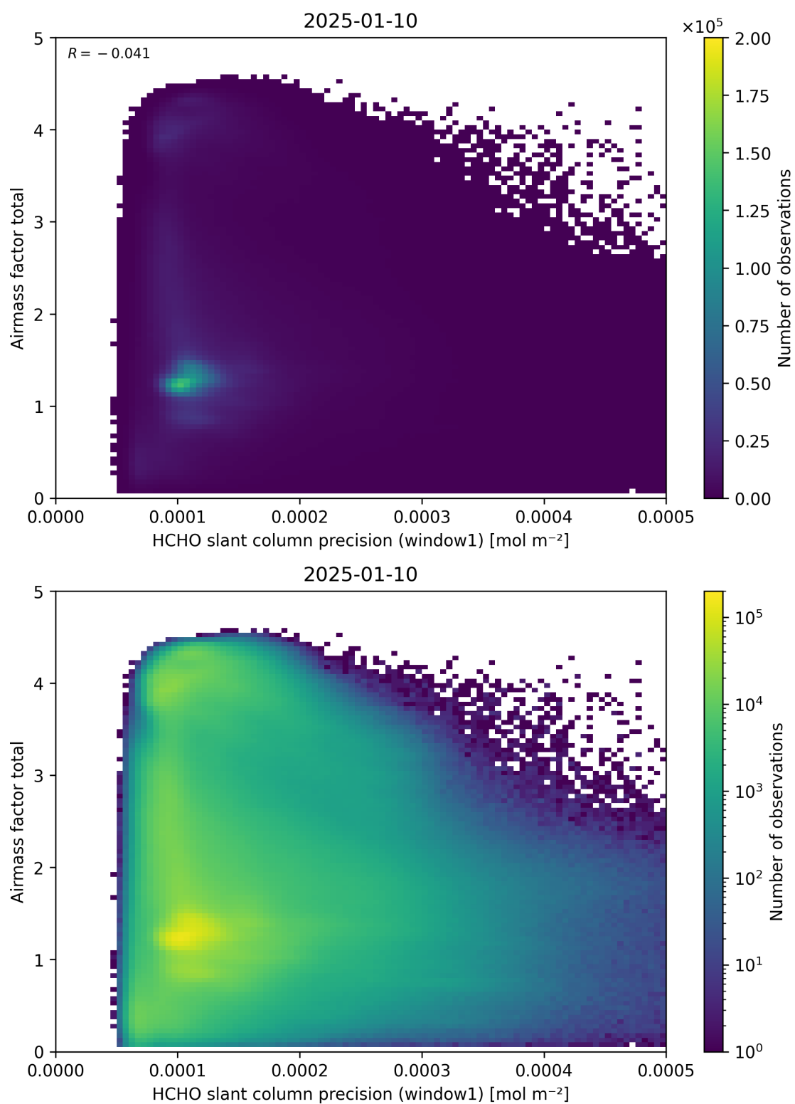
Figure 94: Scatter density plot of “HCHO slant column precision (window1)” against “Airmass factor total” for 2025-01-09 to 2025-01-11.
