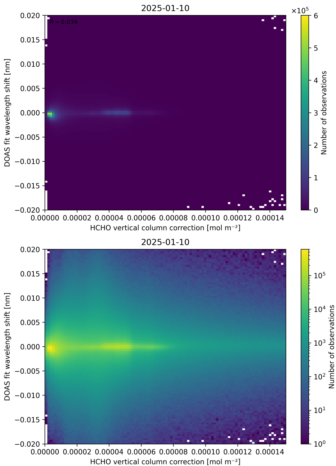
Figure 113: Scatter density plot of “HCHO vertical column correction” against “DOAS fit wavelength shift” for 2025-01-09 to 2025-01-11.
