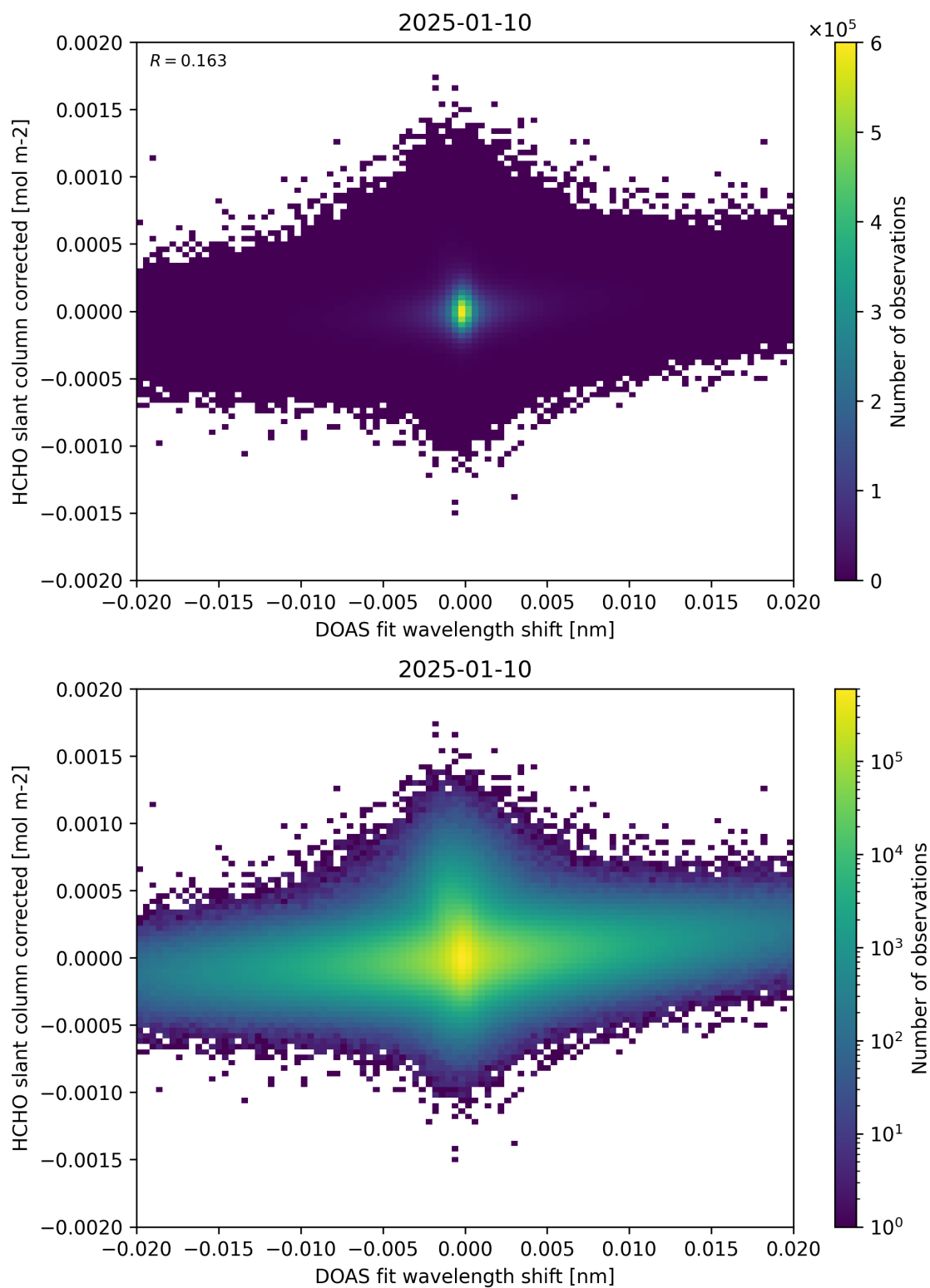
Figure 66: Scatter density plot of “DOAS fit wavelength shift” against “HCHO slant column corrected” for 2025-01-09 to 2025-01-11.
