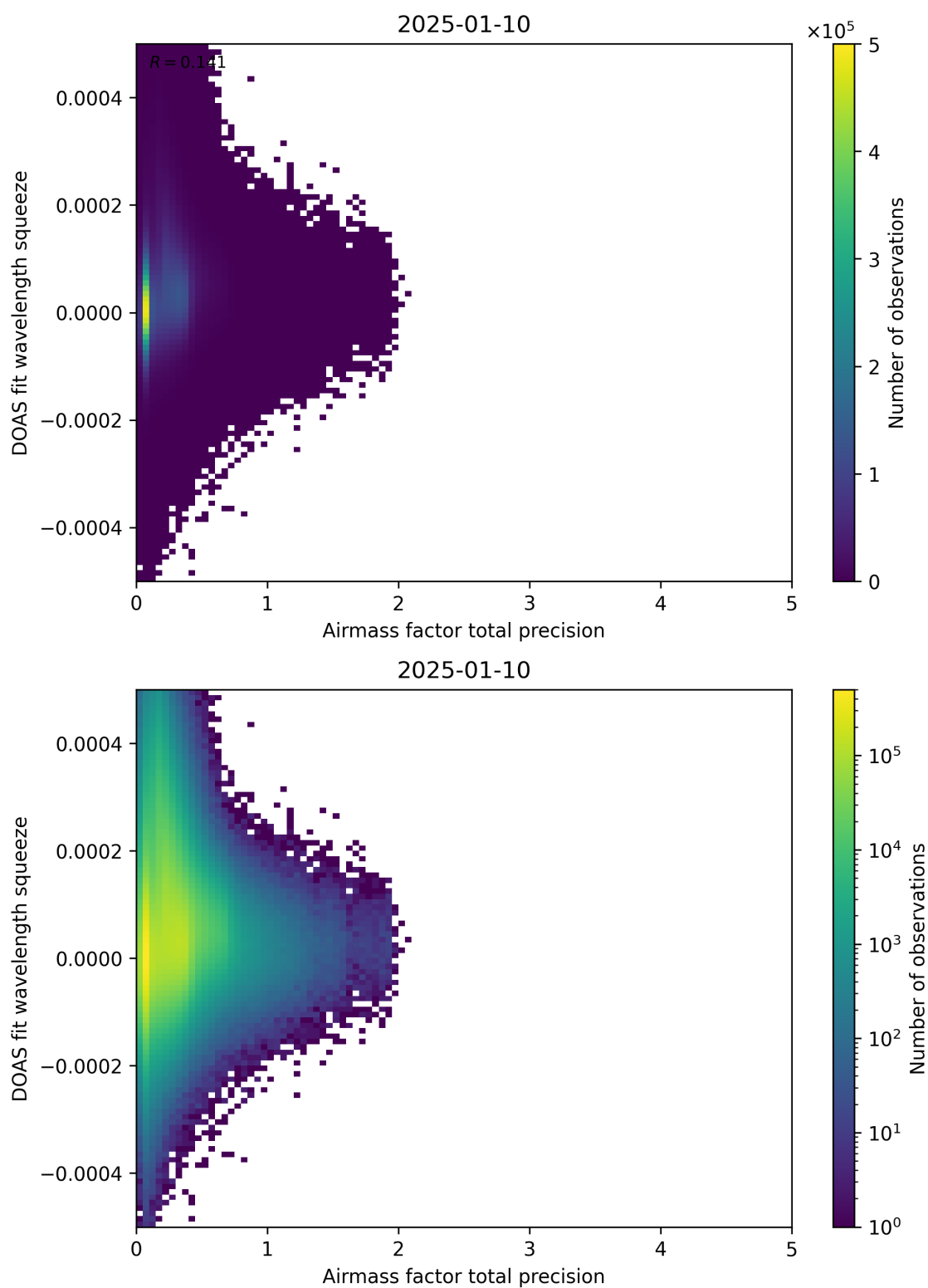
Figure 107: Scatter density plot of “Airmass factor total precision” against “DOAS fit wavelength squeeze” for 2025-01-09 to 2025-01-11.
