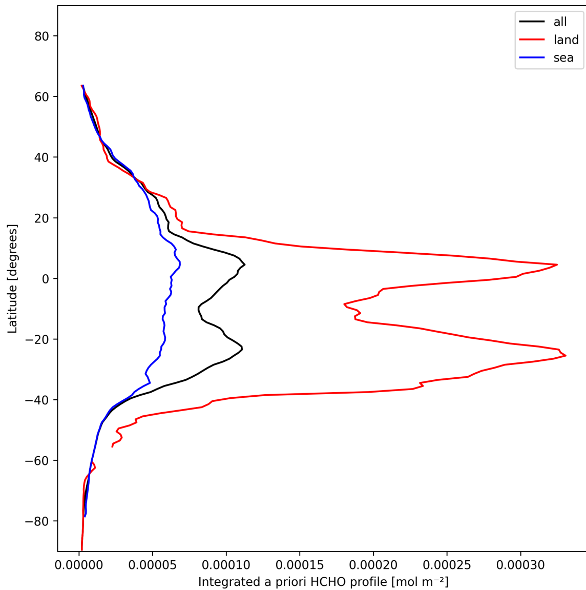
Figure 29: Zonal average of “Integrated a priori HCHO profile” for 2025-01-09 to 2025-01-11.
