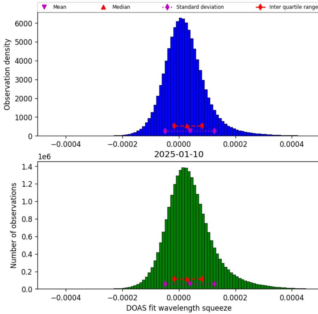
Figure 45: Histogram of “DOAS fit wavelength squeeze” for 2025-01-09 to 2025-01-11
