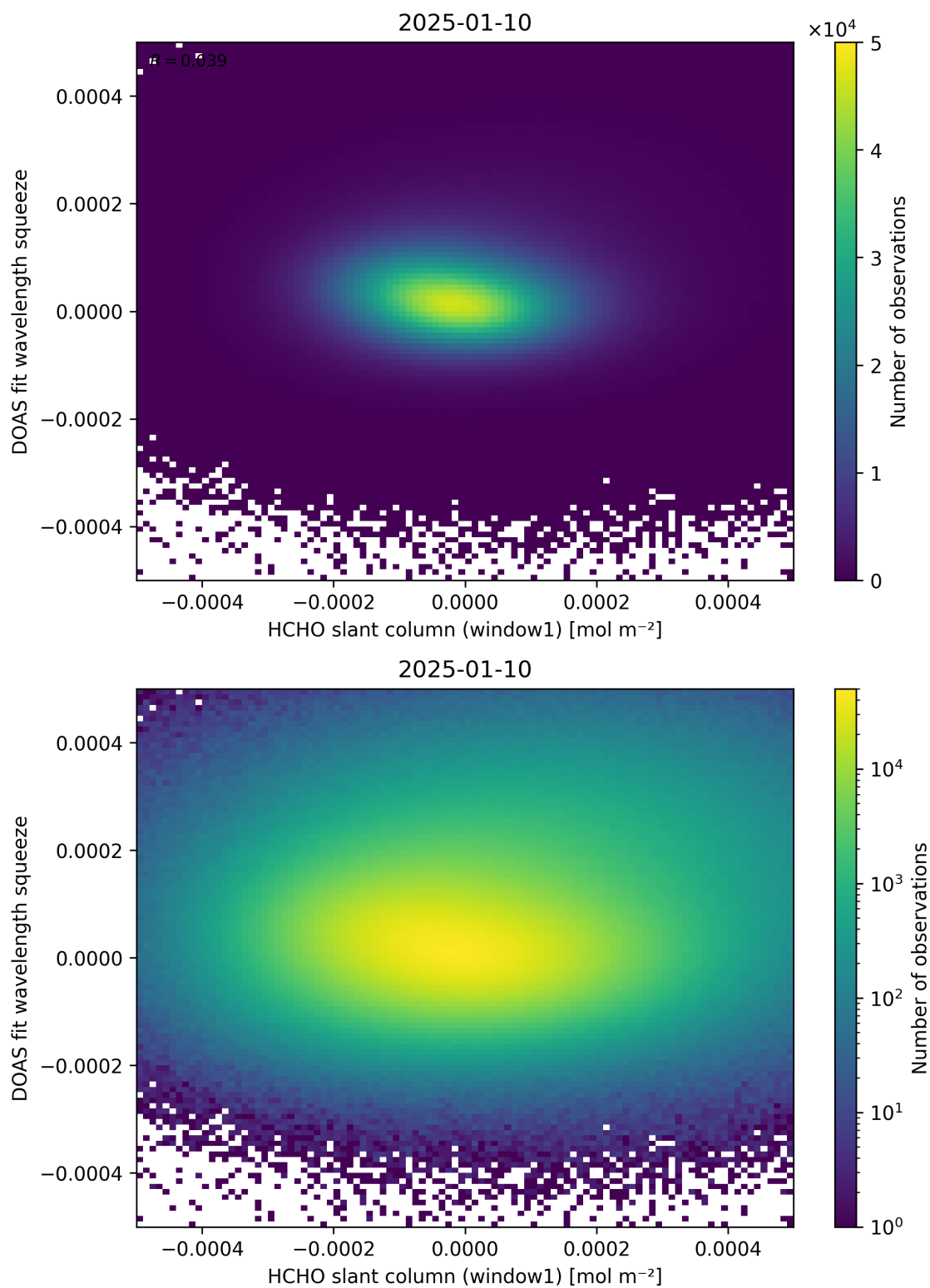
Figure 80: Scatter density plot of “HCHO slant column (window1)” against “DOAS fit wavelength squeeze” for 2025-01-09 to 2025-01-11.
