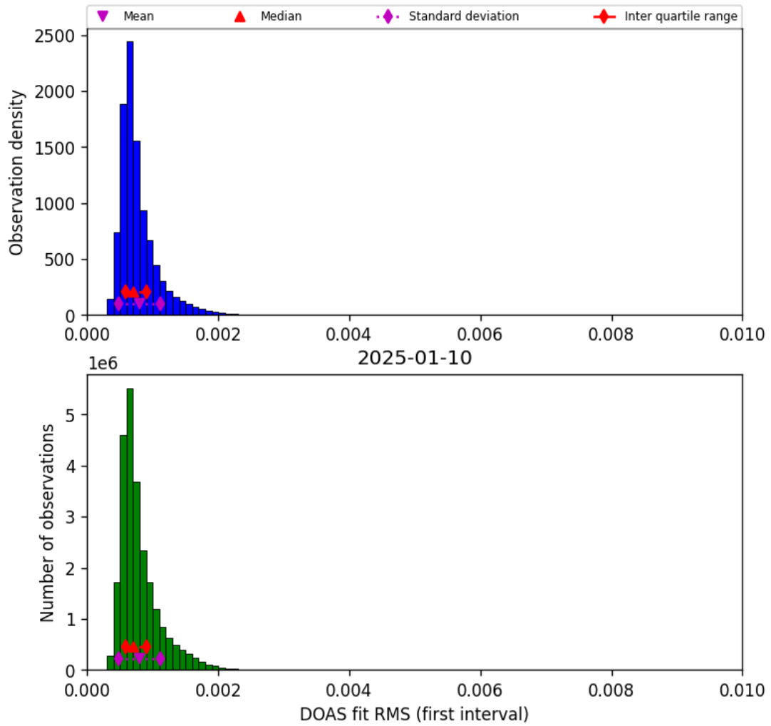
Figure 46: Histogram of “DOAS fit RMS (first interval)” for 2025-01-09 to 2025-01-11
