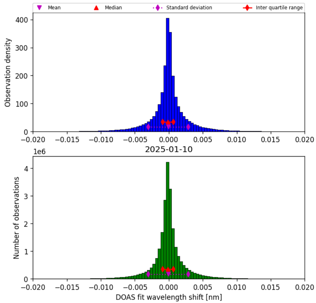
Figure 44: Histogram of “DOAS fit wavelength shift” for 2025-01-09 to 2025-01-11
