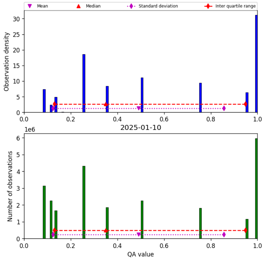
Figure 34: Histogram of “QA value” for 2025-01-09 to 2025-01-11
