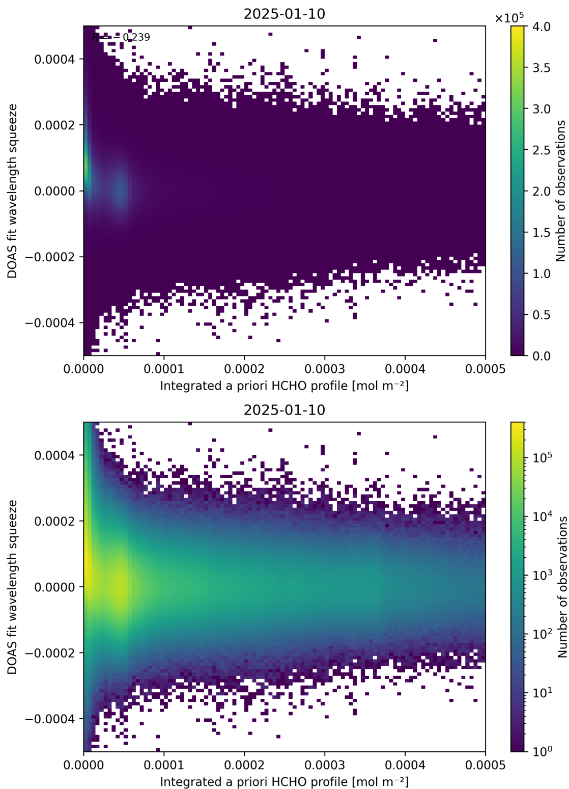
Figure 150: Scatter density plot of “Integrated a priori HCHO profile” against “DOAS fit wavelength squeeze” for 2025-01-09 to 2025-01-11.
