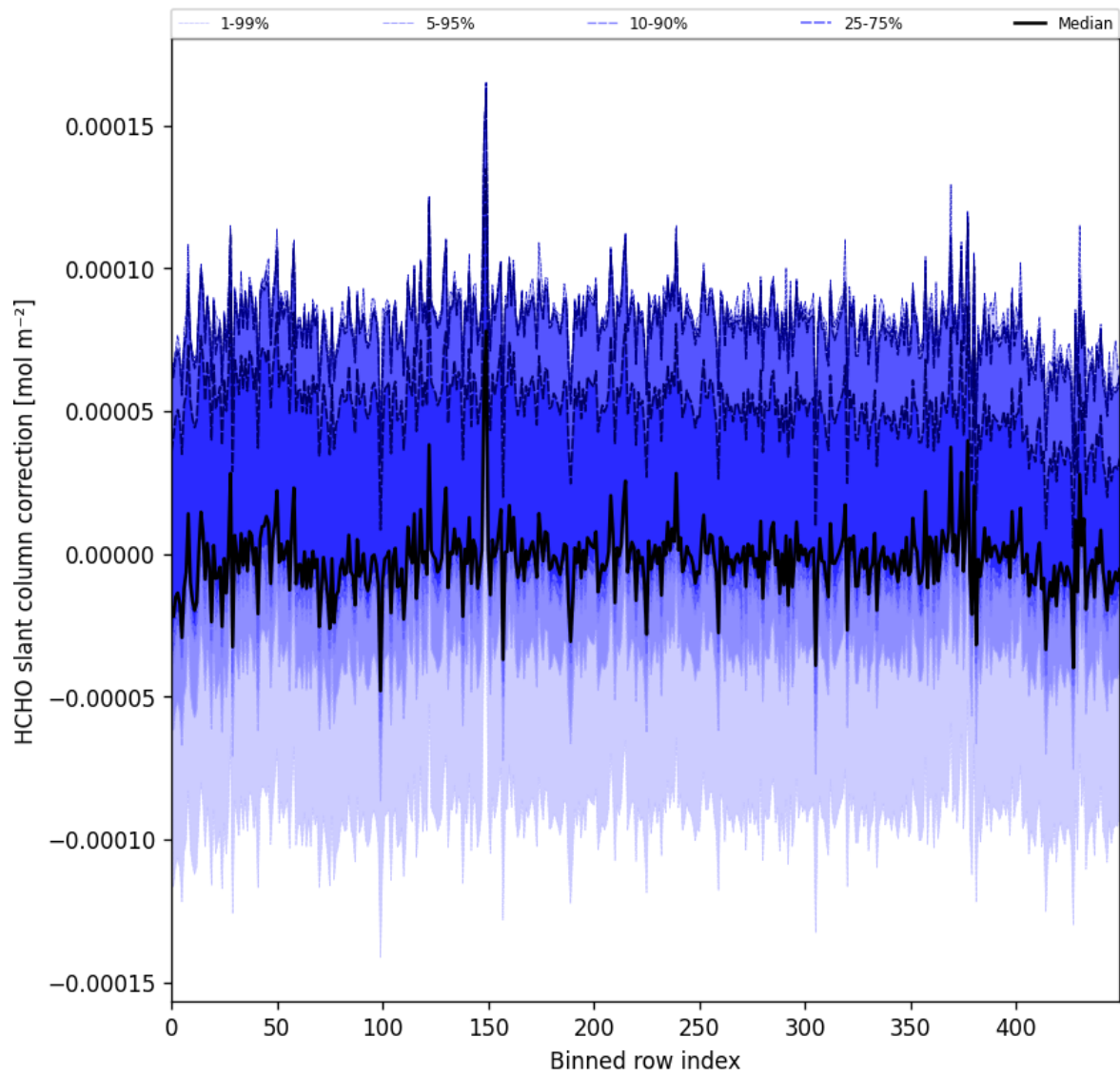
Figure 61: Along track statistics of “HCHO slant column correction” for 2025-01-09 to 2025-01-11
