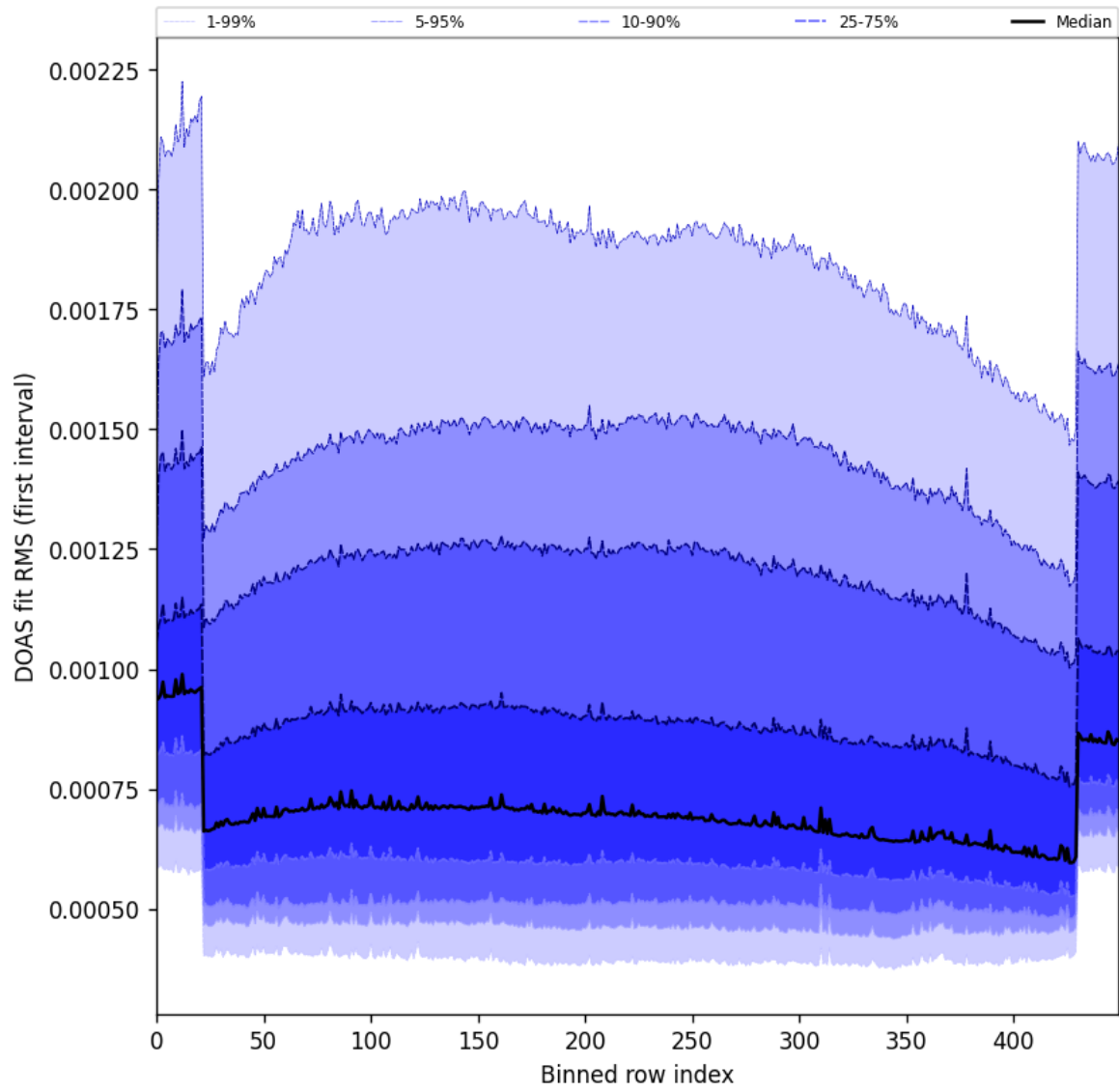
Figure 60: Along track statistics of “DOAS fit RMS (first interval)” for 2025-01-09 to 2025-01-11
