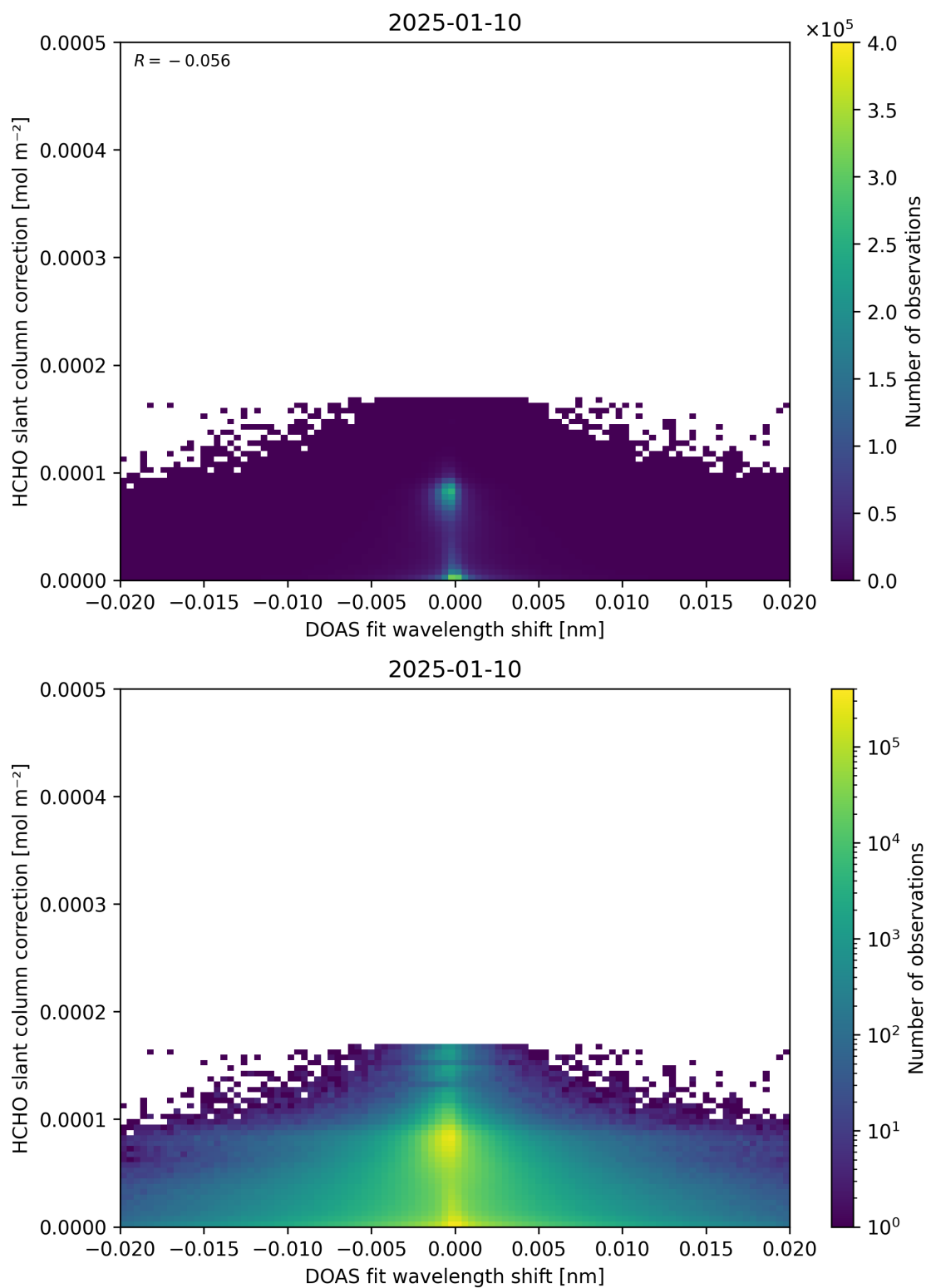
Figure 67: Scatter density plot of “DOAS fit wavelength shift” against “HCHO slant column correction” for 2025-01-09 to 2025-01-11.
