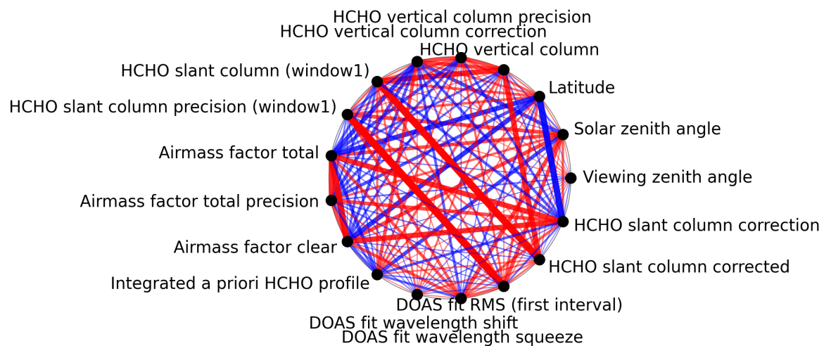
Figure 1: Map of correlation graph for 2025-01-09 to 2025-01-11.
