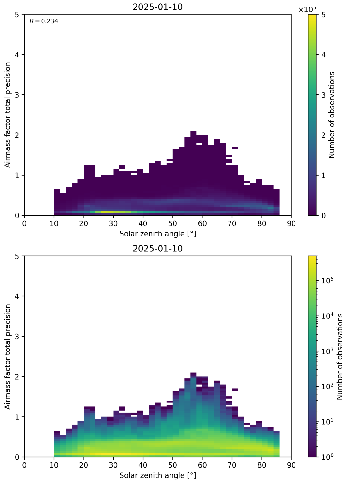
Figure 176: Scatter density plot of “Solar zenith angle” against “Airmass factor total precision” for 2025-01-09 to 2025-01-11.
