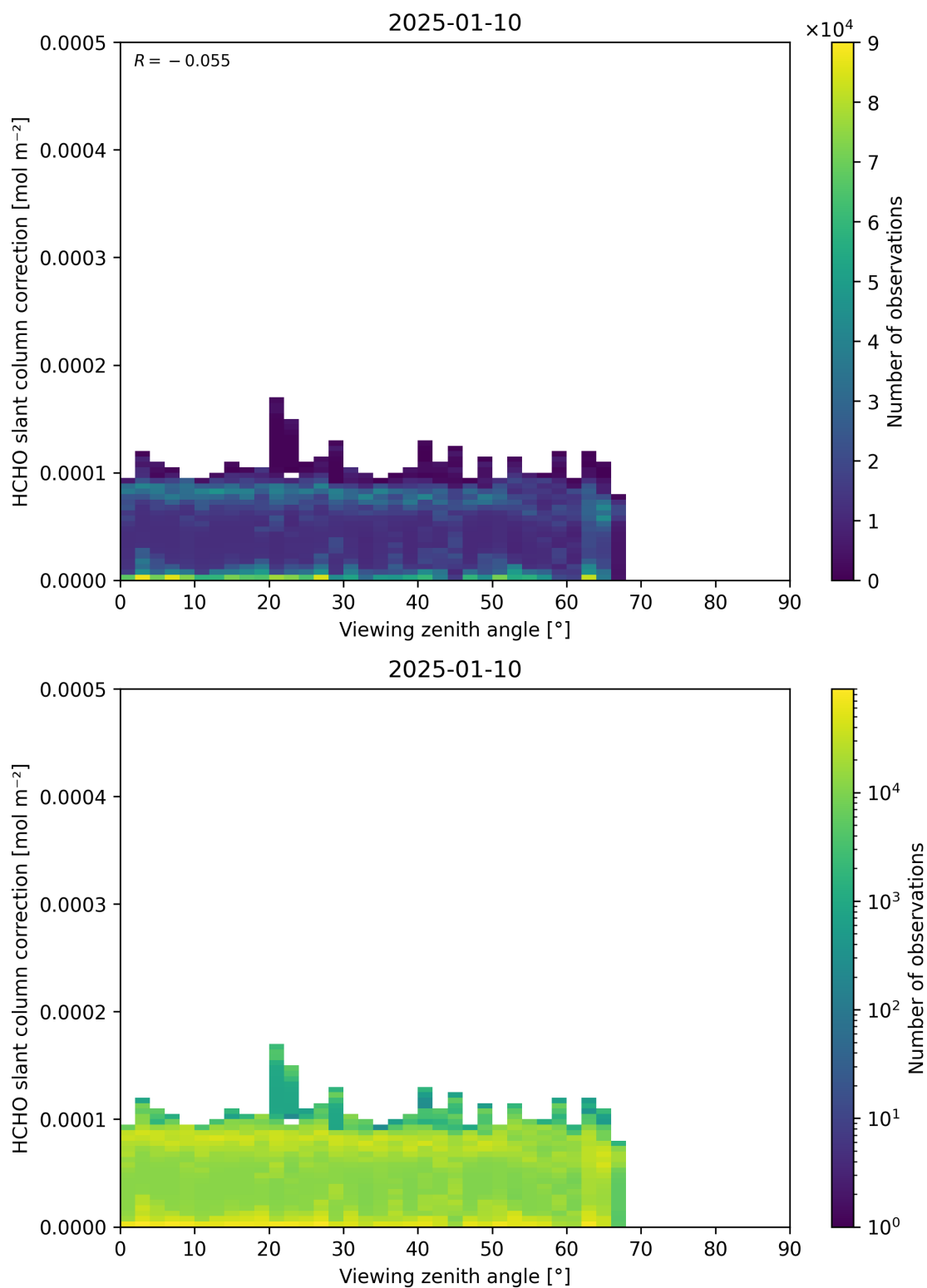
Figure 187: Scatter density plot of “Viewing zenith angle” against “HCHO slant column correction” for 2025-01-09 to 2025-01-11.
