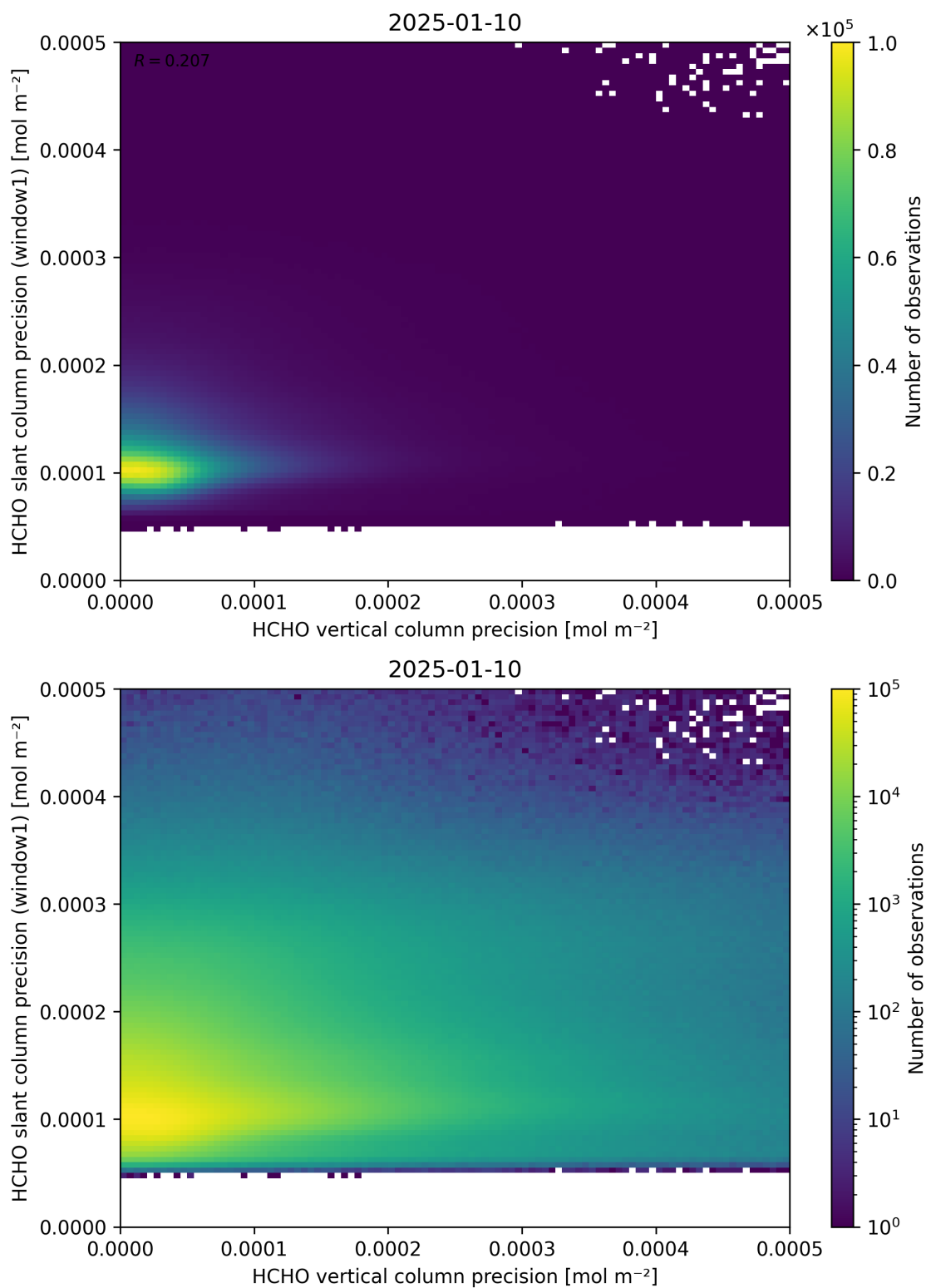
Figure 143: Scatter density plot of “HCHO vertical column precision” against “HCHO slant column precision (window1)” for 2025-01-09 to 2025-01-11.
