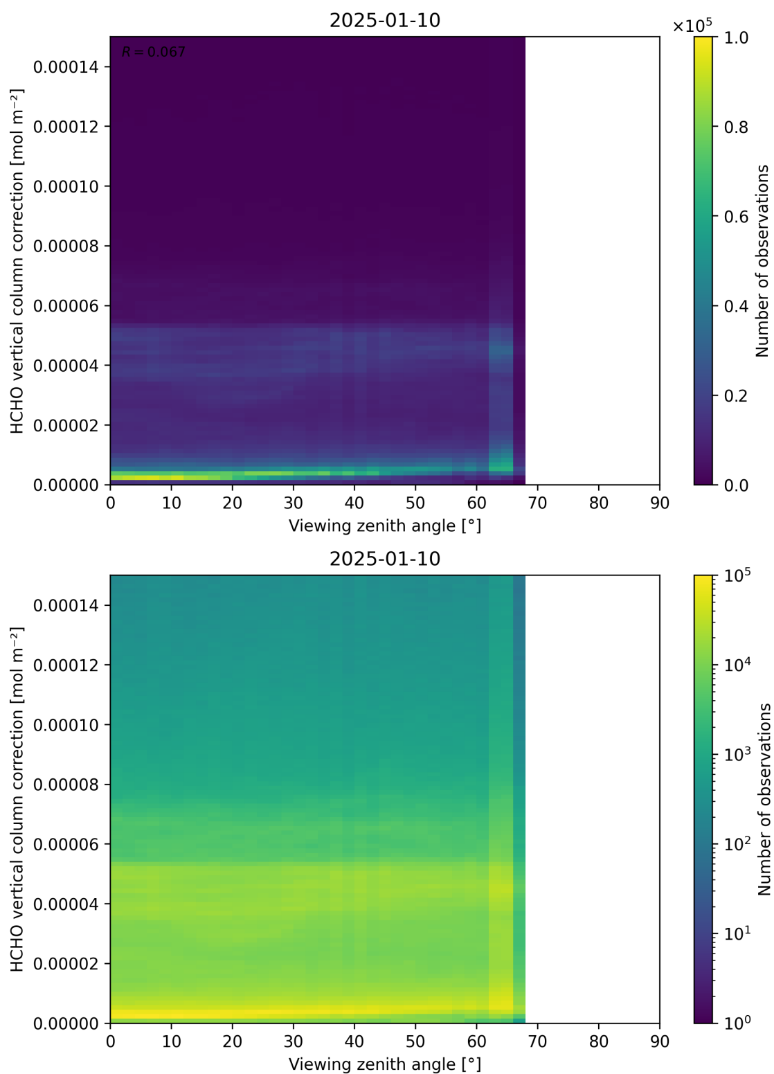
Figure 193: Scatter density plot of “Viewing zenith angle” against “HCHO vertical column correction” for 2025-01-09 to 2025-01-11.
