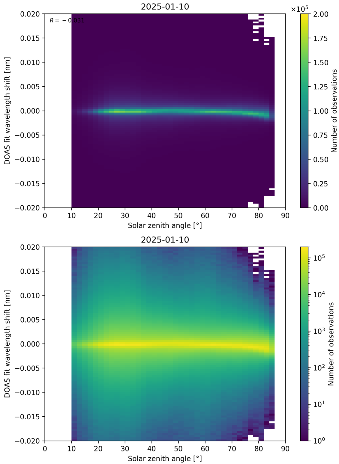
Figure 168: Scatter density plot of “Solar zenith angle” against “DOAS fit wavelength shift” for 2025-01-09 to 2025-01-11.
