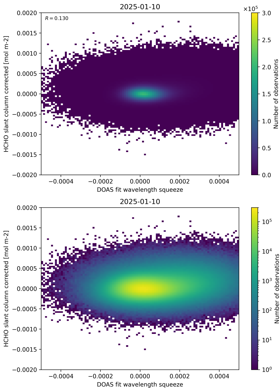
Figure 69: Scatter density plot of “DOAS fit wavelength squeeze” against “HCHO slant column corrected” for 2025-01-09 to 2025-01-11.
