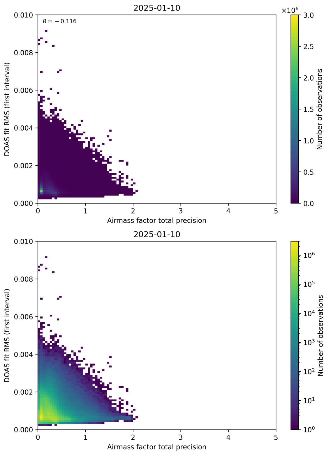
Figure 105: Scatter density plot of “Airmass factor total precision” against “DOAS fit RMS (first interval)” for 2025-01-09 to 2025-01-11.
