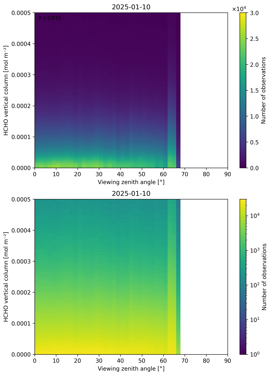
Figure 192: Scatter density plot of “Viewing zenith angle” against “HCHO vertical column” for 2025-01-09 to 2025-01-11.
