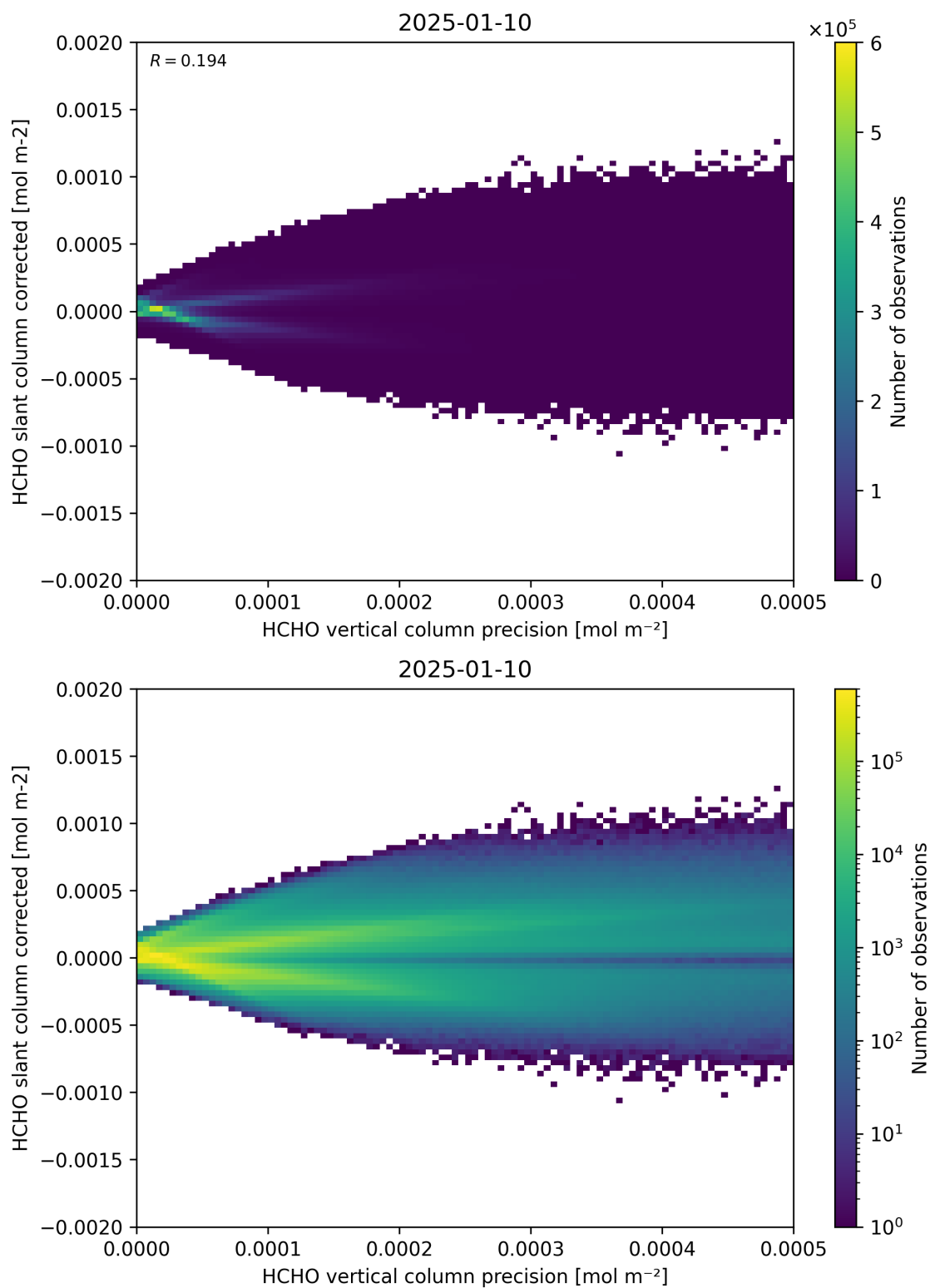
Figure 140: Scatter density plot of “HCHO vertical column precision” against “HCHO slant column corrected” for 2025-01-09 to 2025-01-11.
