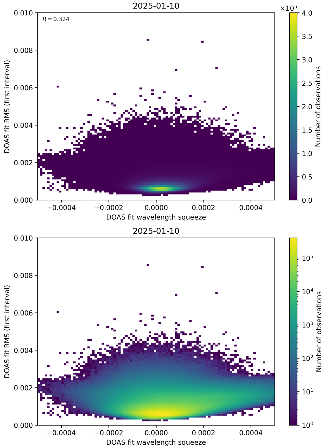
Figure 68: Scatter density plot of “DOAS fit wavelength squeeze” against “DOAS fit RMS (first interval)” for 2025-01-09 to 2025-01-11.
