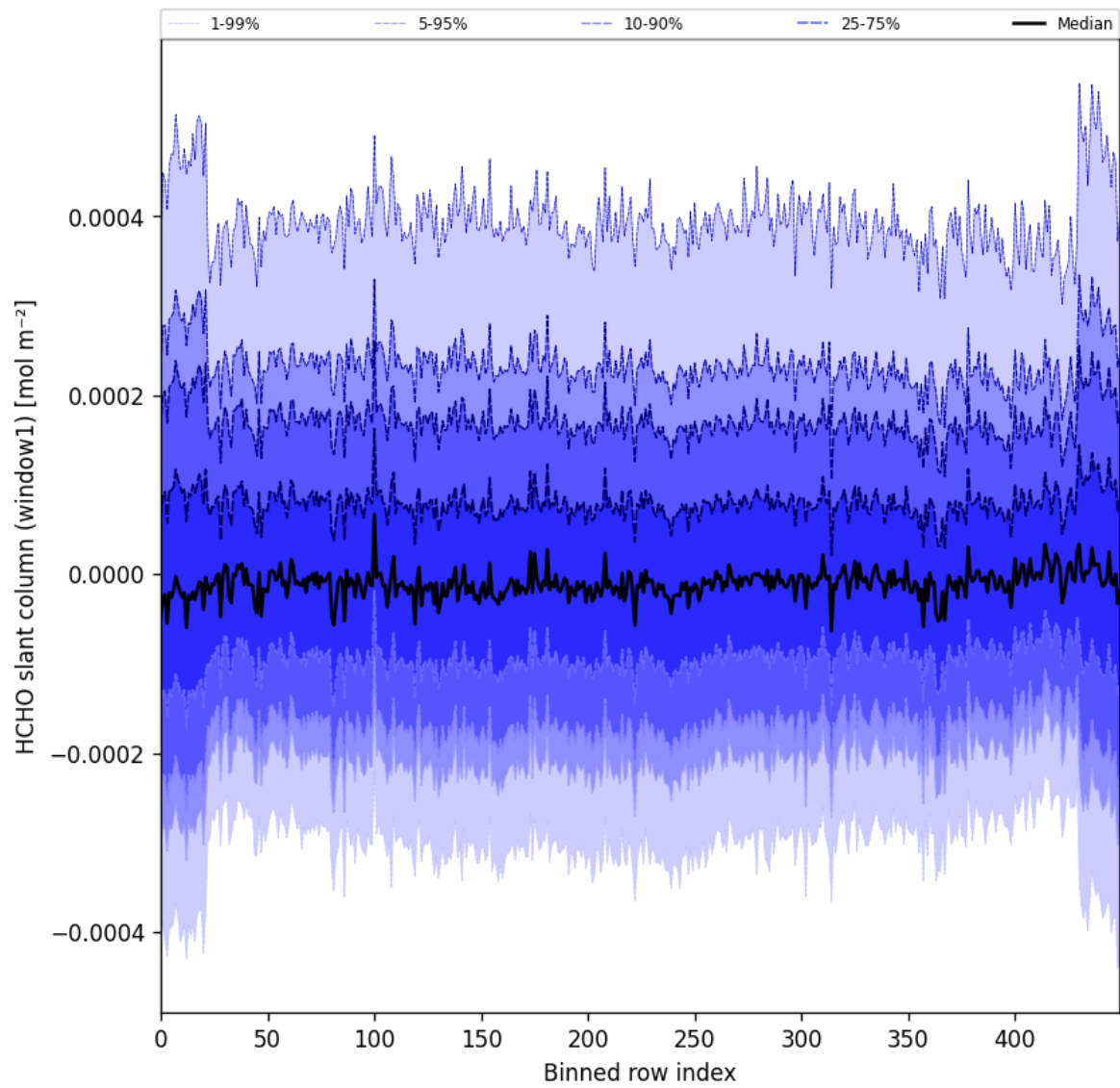
Figure 52: Along track statistics of “HCHO slant column (window1)” for 2025-01-09 to 2025-01-11
