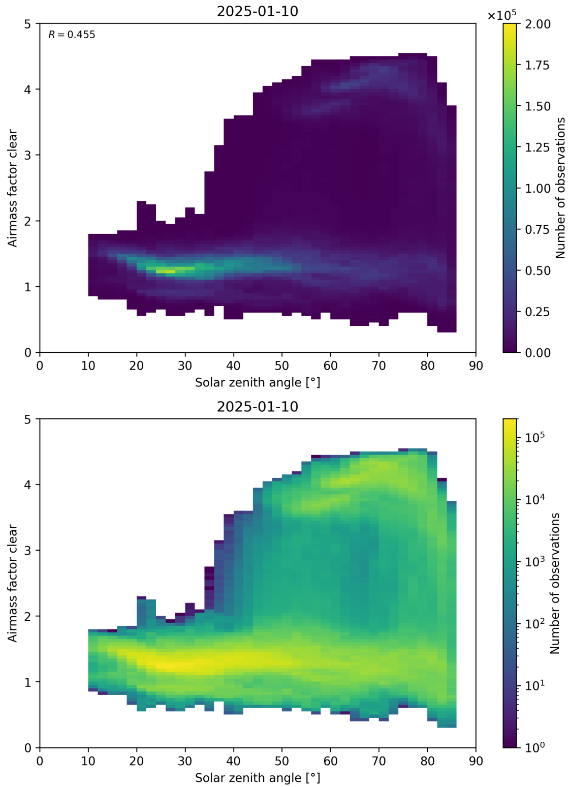
Figure 170: Scatter density plot of “Solar zenith angle” against “Airmass factor clear” for 2025-01-09 to 2025-01-11.
