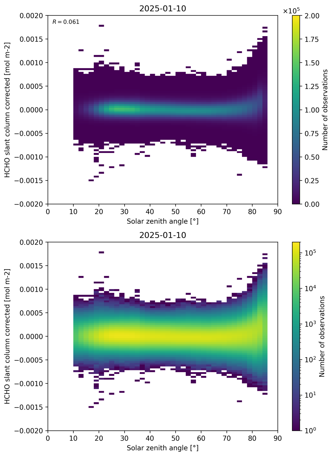
Figure 171: Scatter density plot of “Solar zenith angle” against “HCHO slant column corrected” for 2025-01-09 to 2025-01-11.
