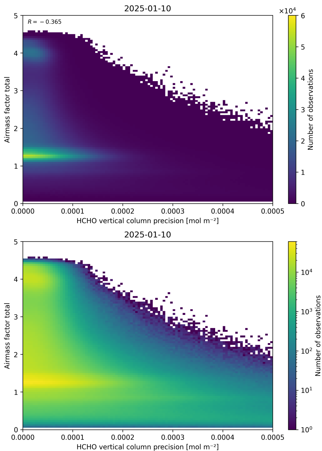
Figure 144: Scatter density plot of “HCHO vertical column precision” against “Airmass factor total” for 2025-01-09 to 2025-01-11.
