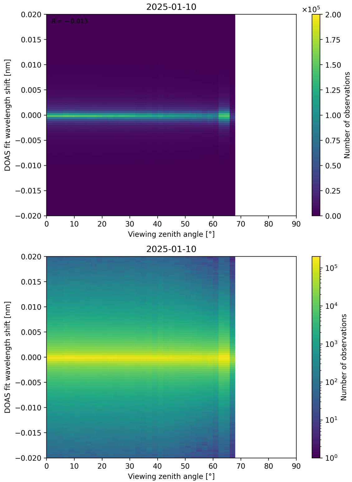
Figure 183: Scatter density plot of “Viewing zenith angle” against “DOAS fit wavelength shift” for 2025-01-09 to 2025-01-11.
