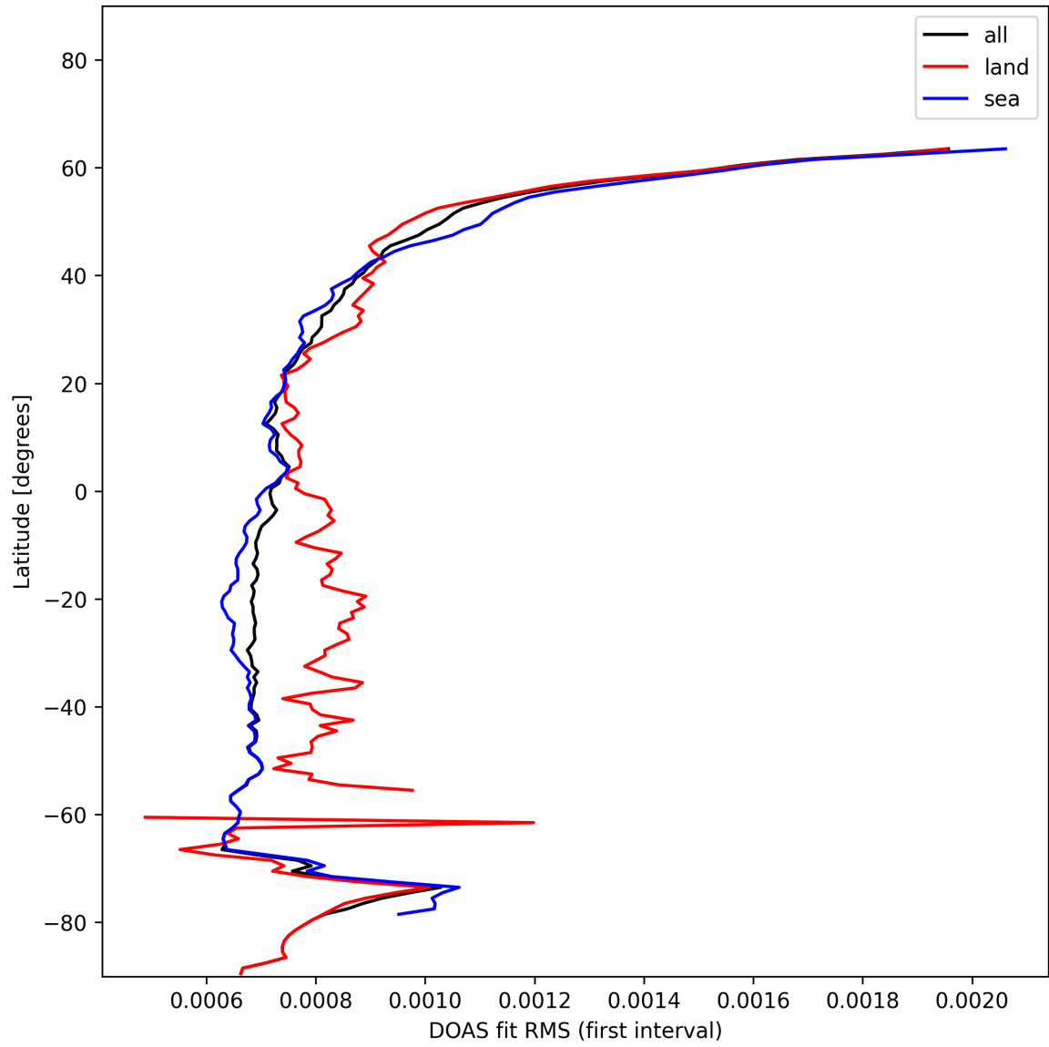
Figure 32: Zonal average of “DOAS fit RMS (first interval)” for 2025-01-09 to 2025-01-11.
