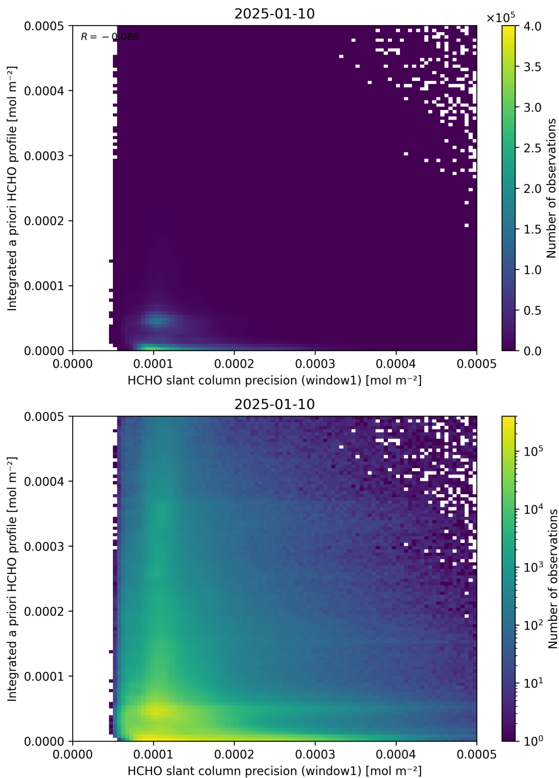
Figure 96: Scatter density plot of “HCHO slant column precision (window1)” against “Integrated a priori HCHO profile” for 2025-01-09 to 2025-01-11.
