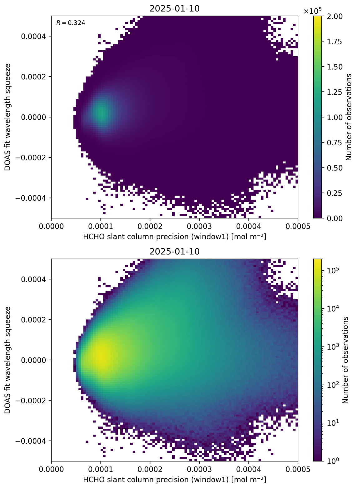
Figure 90: Scatter density plot of “HCHO slant column precision (window1)” against “DOAS fit wavelength squeeze” for 2025-01-09 to 2025-01-11.
