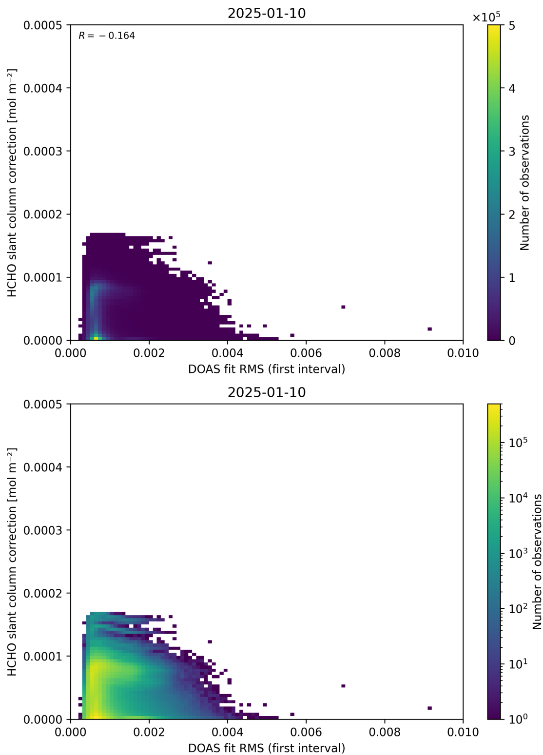
Figure 63: Scatter density plot of “DOAS fit RMS (first interval)” against “HCHO slant column correction” for 2025-01-09 to 2025-01-11.
