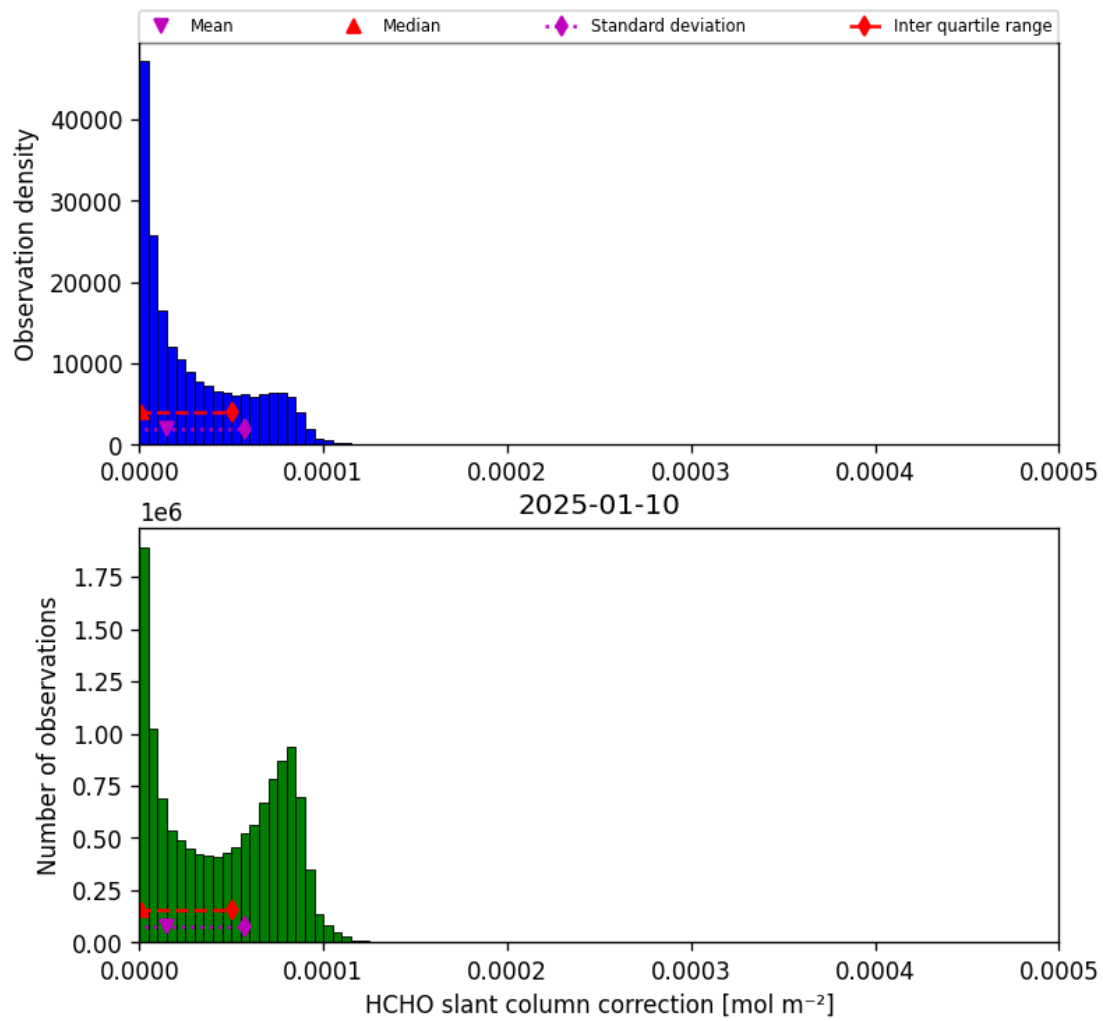
Figure 47: Histogram of "HCHO slant column correction" for 2025-01-09 to 2025-01-11
