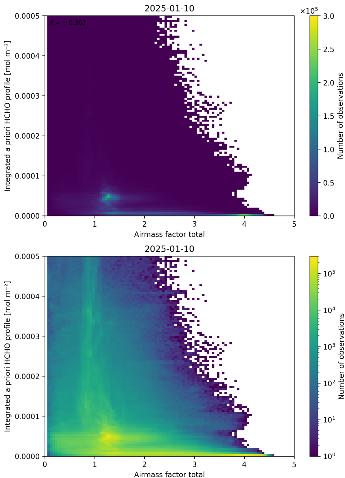
Figure 104: Scatter density plot of “Airmass factor total” against “Integrated a priori HCHO profile” for 2025-01-09 to 2025-01-11.
