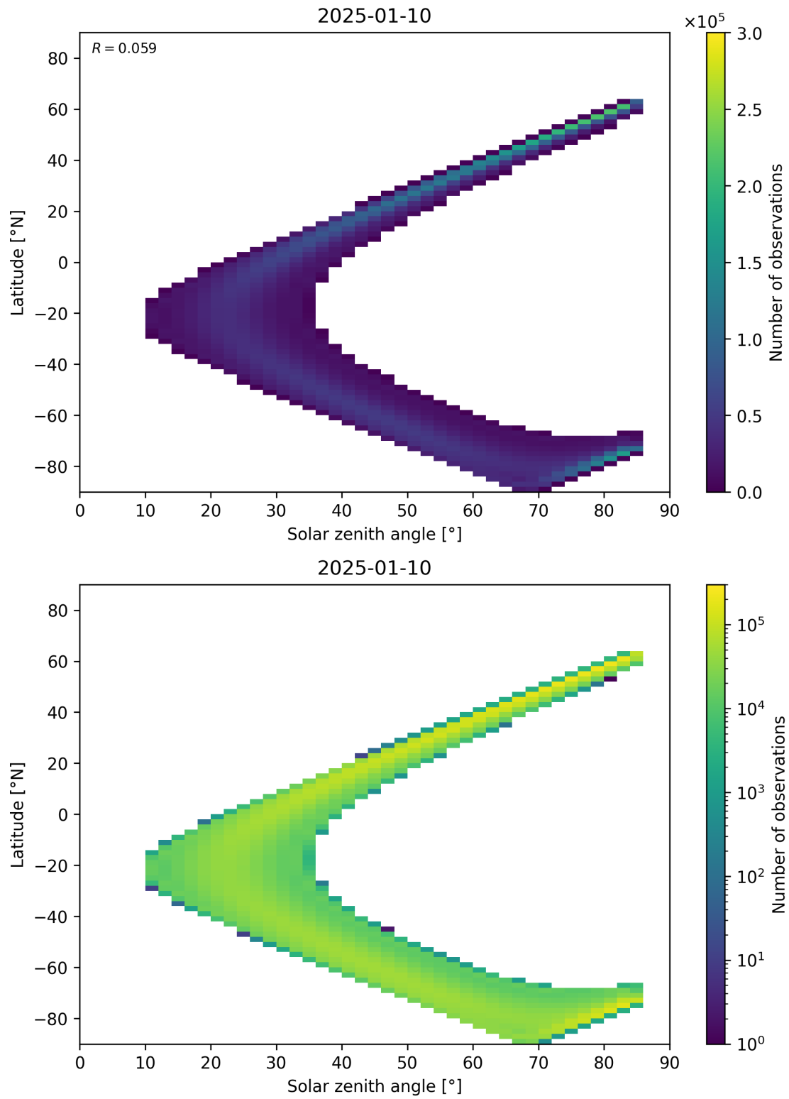
Figure 181: Scatter density plot of “Solar zenith angle” against “Latitude” for 2025-01-09 to 2025-01-11.
