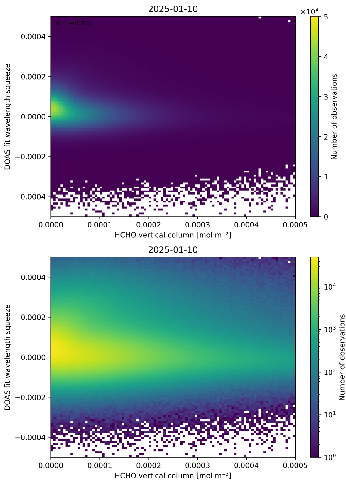
Figure 125: Scatter density plot of “HCHO vertical column” against “DOAS fit wavelength squeeze” for 2025-01-09 to 2025-01-11.
