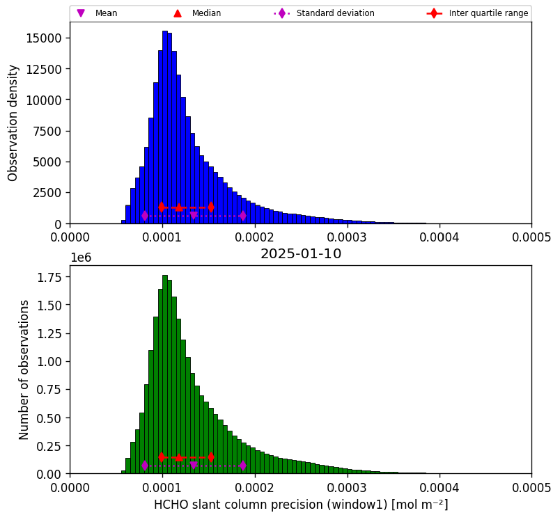
Figure 39: Histogram of “HCHO slant column precision (window1)” for 2025-01-09 to 2025-01-11
