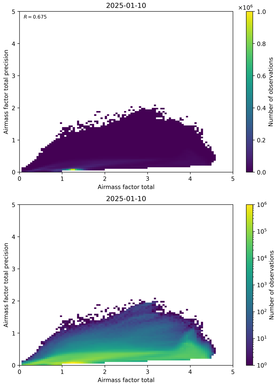
Figure 103: Scatter density plot of “Airmass factor total” against “Airmass factor total precision” for 2025-01-09 to 2025-01-11.
