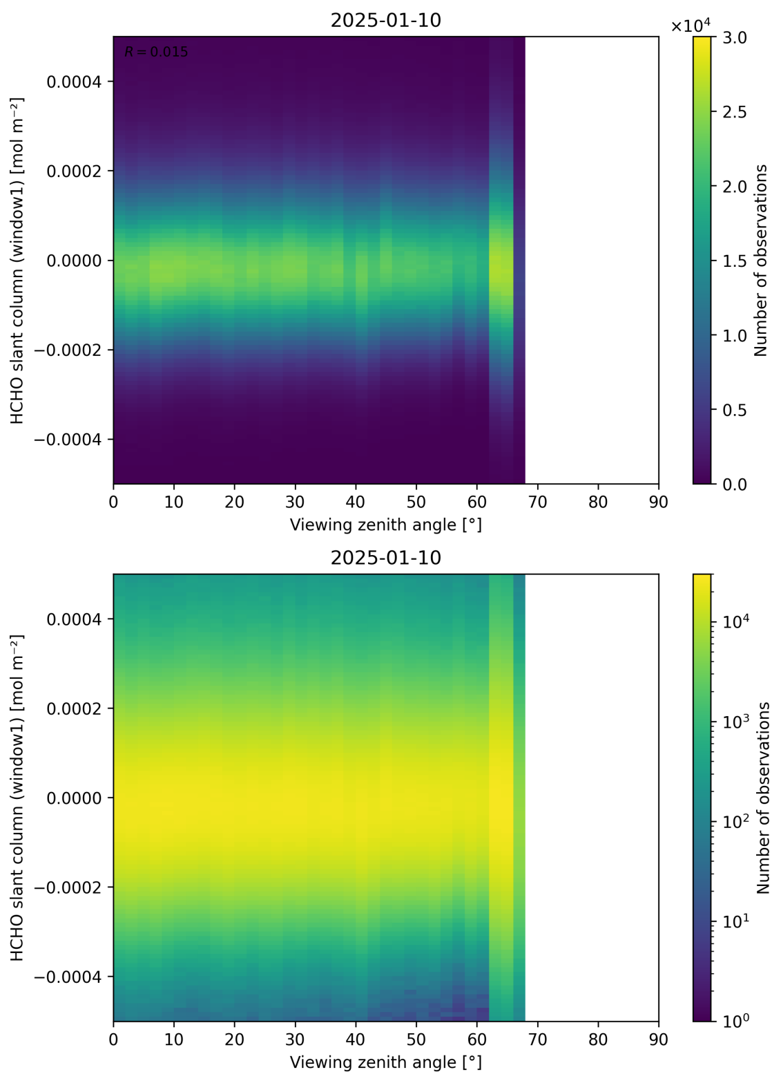
Figure 188: Scatter density plot of “Viewing zenith angle” against “HCHO slant column (window1)” for 2025-01-09 to 2025-01-11.
