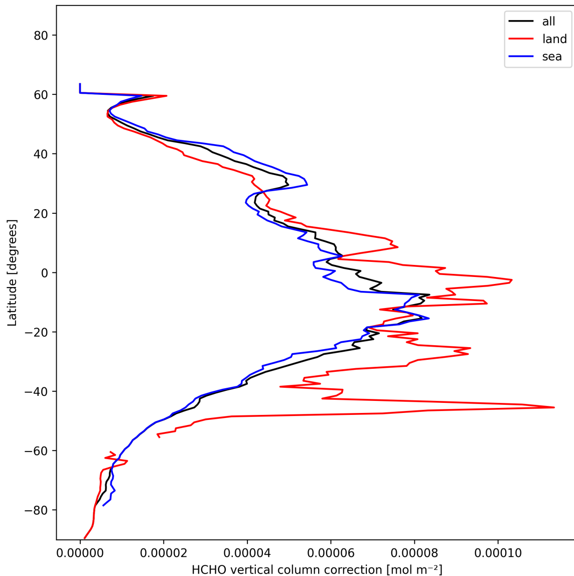
Figure 23: Zonal average of “HCHO vertical column correction” for 2025-01-09 to 2025-01-11.
