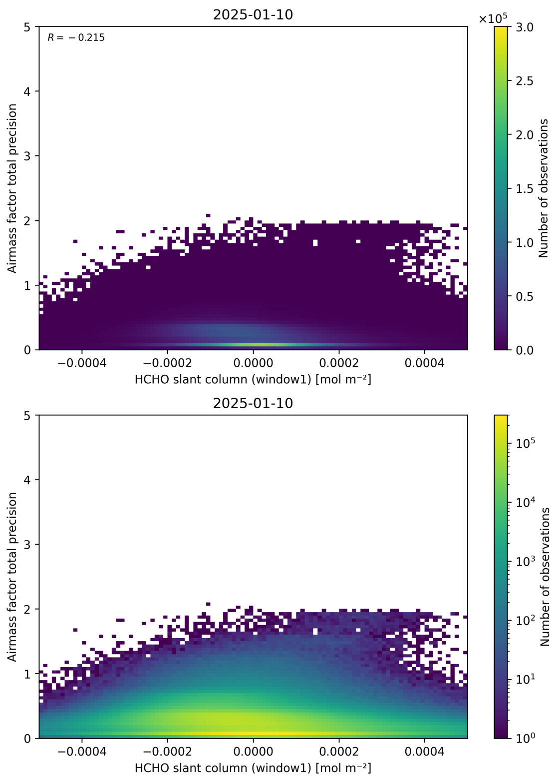
Figure 86: Scatter density plot of “HCHO slant column (window1)” against “Airmass factor total precision” for 2025-01-09 to 2025-01-11.
