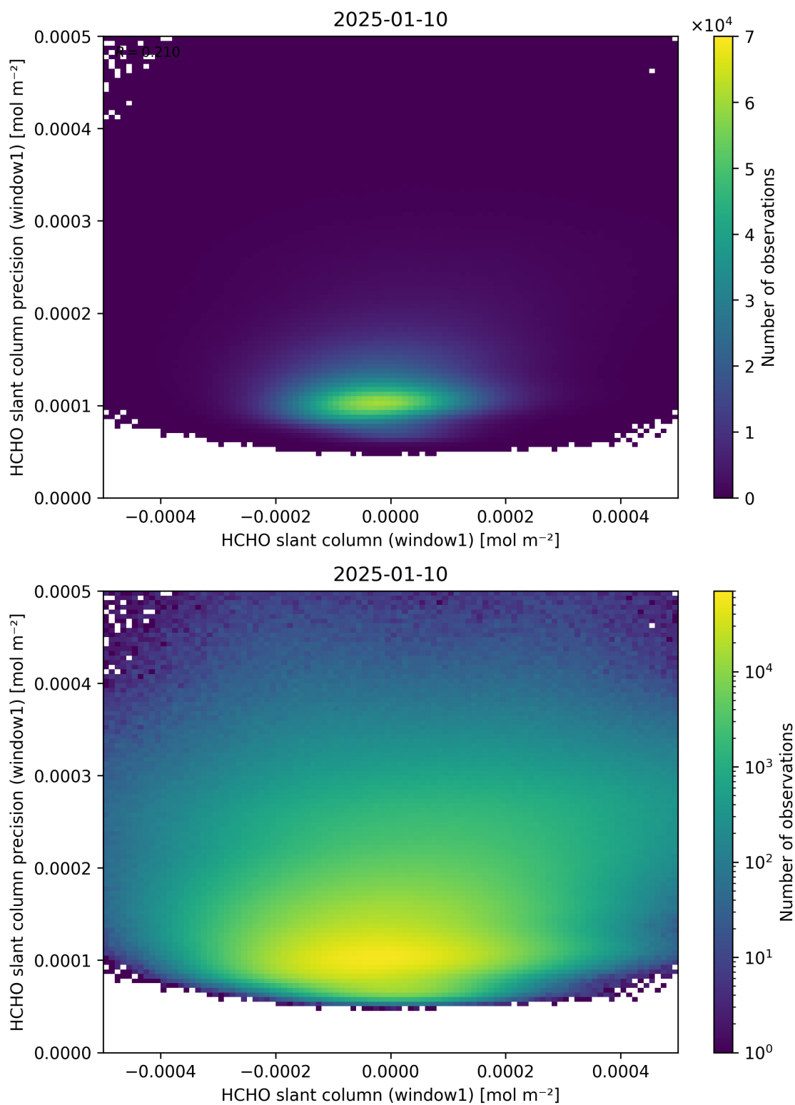
Figure 84: Scatter density plot of “HCHO slant column (window1)” against “HCHO slant column precision (window1)” for 2025-01-09 to 2025-01-11.
