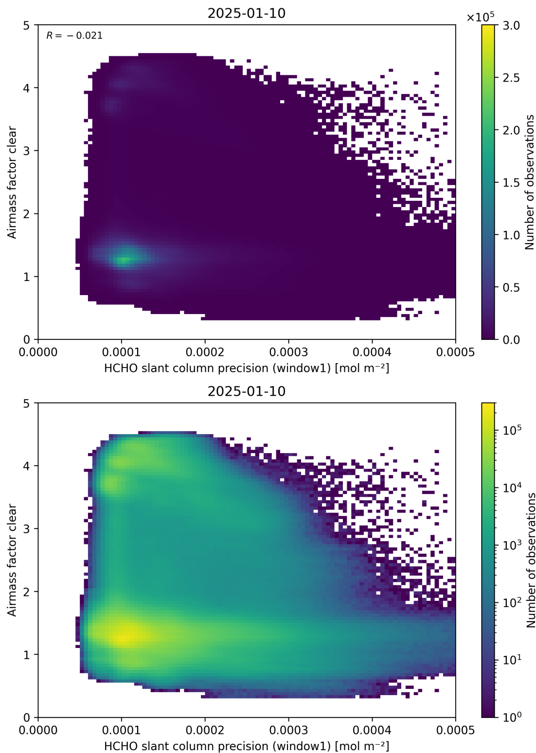
Figure 91: Scatter density plot of “HCHO slant column precision (window1)” against “Airmass factor clear” for 2025-01-09 to 2025-01-11.
