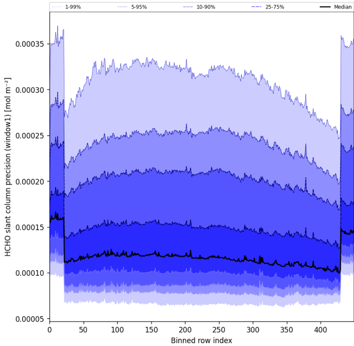
Figure 53: Along track statistics of “HCHO slant column precision (window1)” for 2025-01-09 to 2025-01-11
