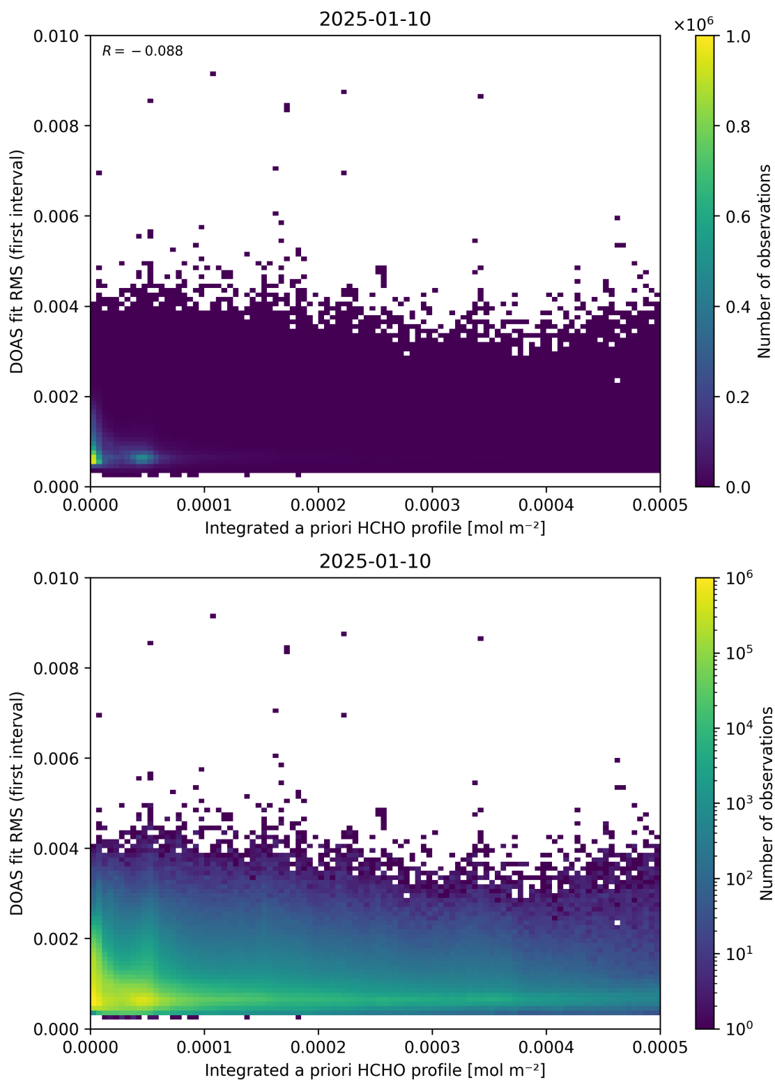
Figure 148: Scatter density plot of “Integrated a priori HCHO profile” against “DOAS fit RMS (first interval)” for 2025-01-09 to 2025-01-11.
