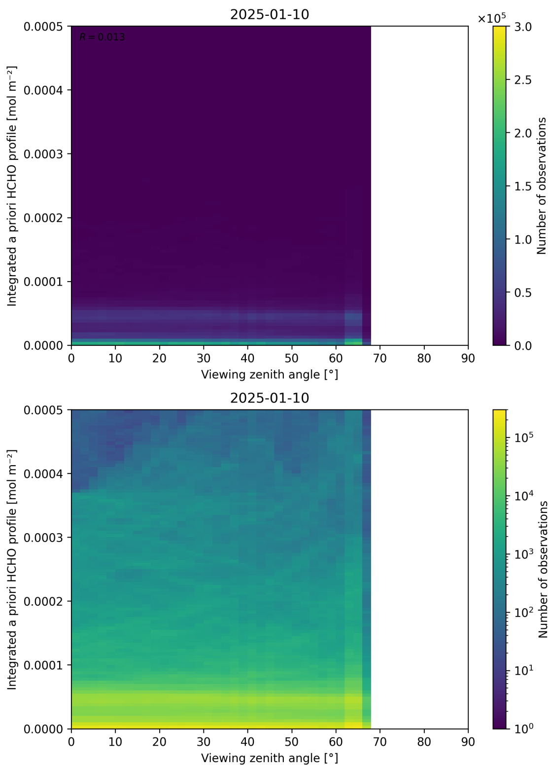
Figure 195: Scatter density plot of “Viewing zenith angle” against “Integrated a priori HCHO profile” for 2025-01-09 to 2025-01-11.
