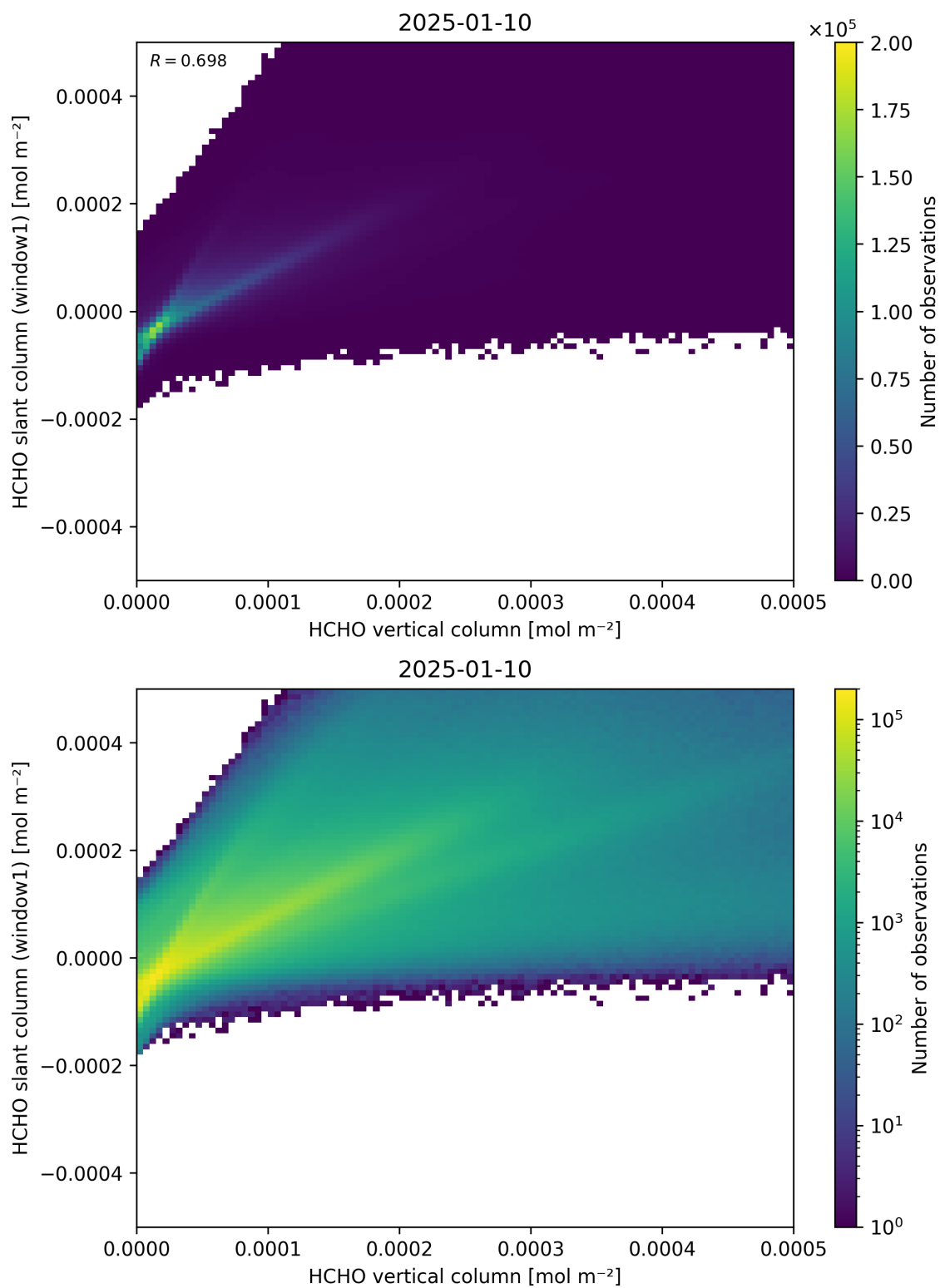
Figure 129: Scatter density plot of “HCHO vertical column” against “HCHO slant column (window1)” for 2025-01-09 to 2025-01-11.
