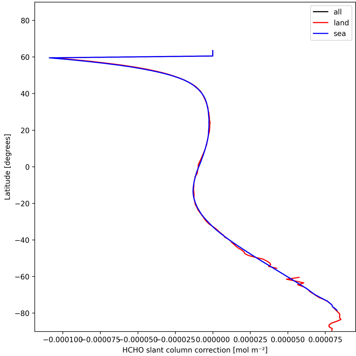
Figure 33: Zonal average of “HCHO slant column correction” for 2025-01-09 to 2025-01-11.
