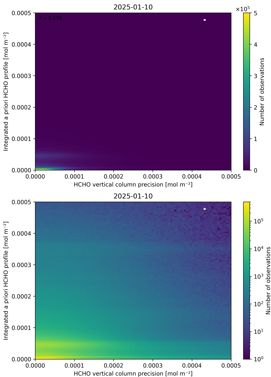
Figure 147: Scatter density plot of “HCHO vertical column precision” against “Integrated a priori HCHO profile” for 2025-01-09 to 2025-01-11.
