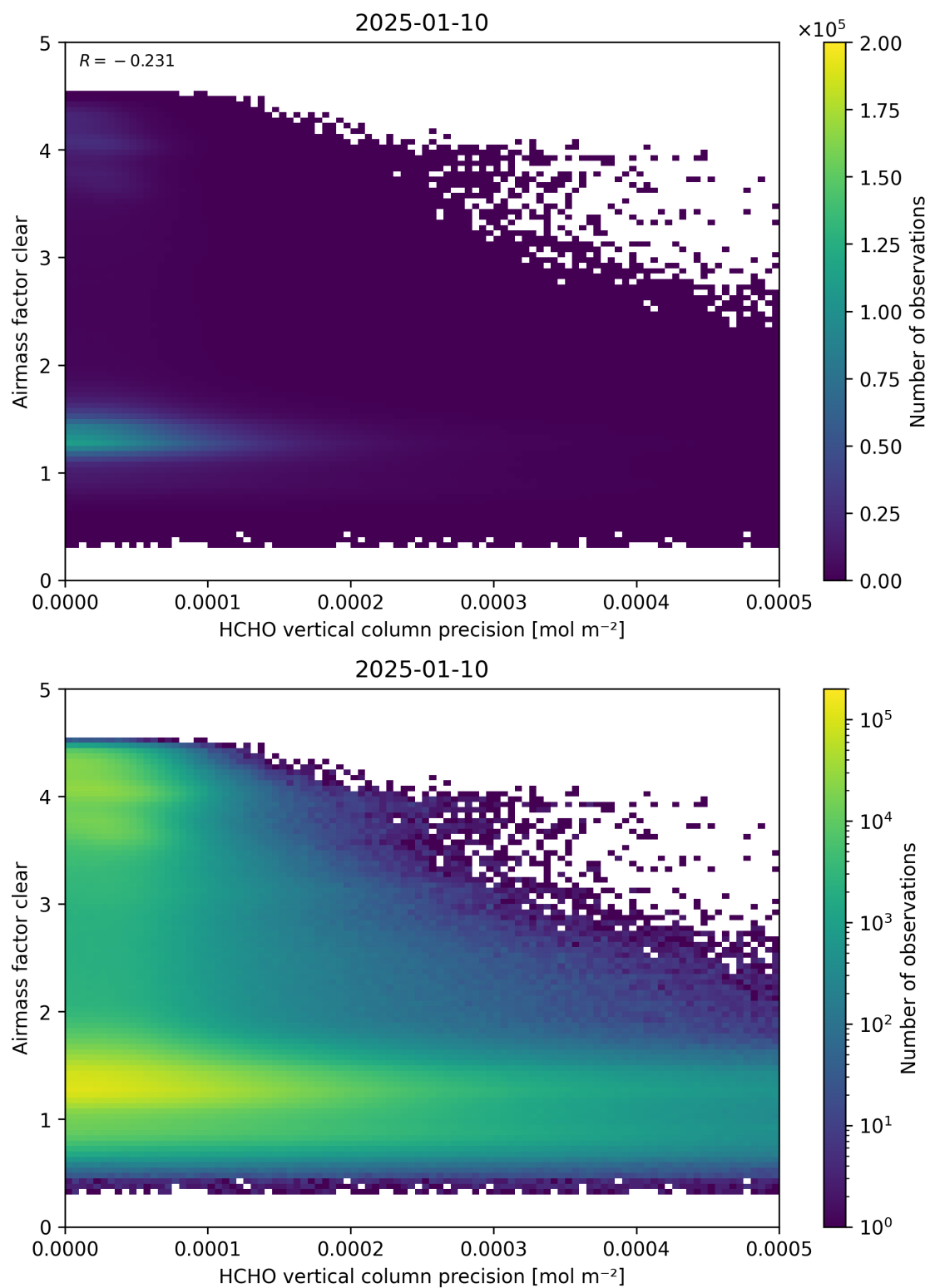
Figure 139: Scatter density plot of “HCHO vertical column precision” against “Airmass factor clear” for 2025-01-09 to 2025-01-11.
