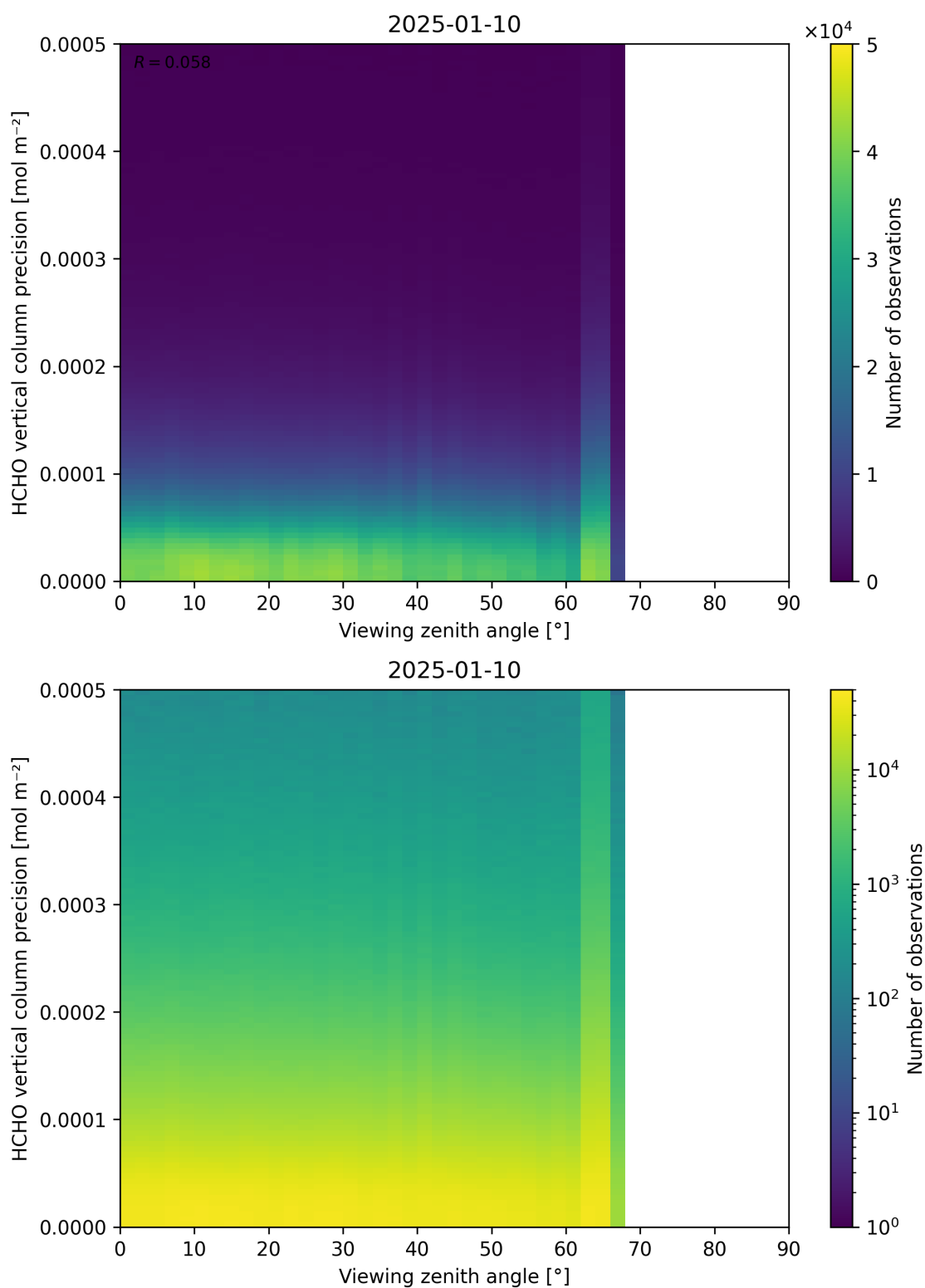
Figure 194: Scatter density plot of “Viewing zenith angle” against “HCHO vertical column precision” for 2025-01-09 to 2025-01-11.
