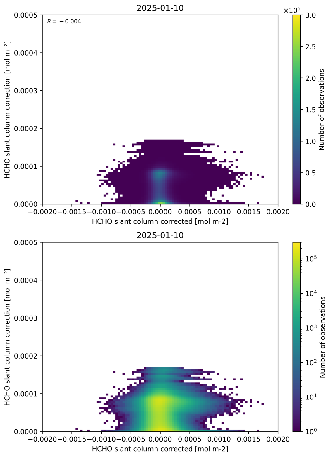
Figure 77: Scatter density plot of “HCHO slant column corrected” against “HCHO slant column correction” for 2025-01-09 to 2025-01-11.
