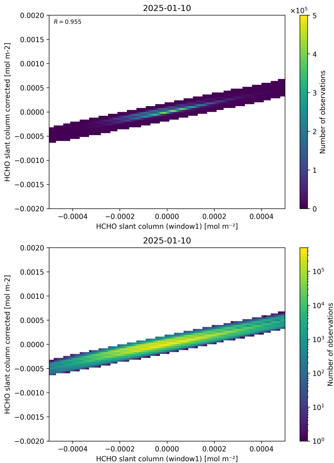
Figure 82: Scatter density plot of “HCHO slant column (window1)” against “HCHO slant column corrected” for 2025-01-09 to 2025-01-11.
