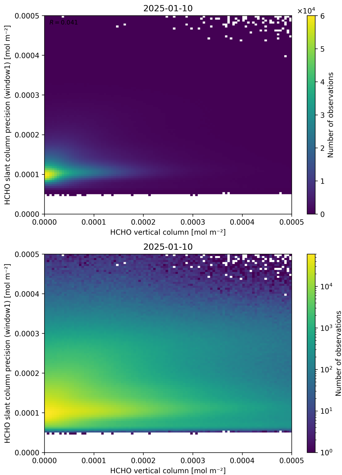
Figure 130: Scatter density plot of “HCHO vertical column” against “HCHO slant column precision (window1)” for 2025-01-09 to 2025-01-11.
