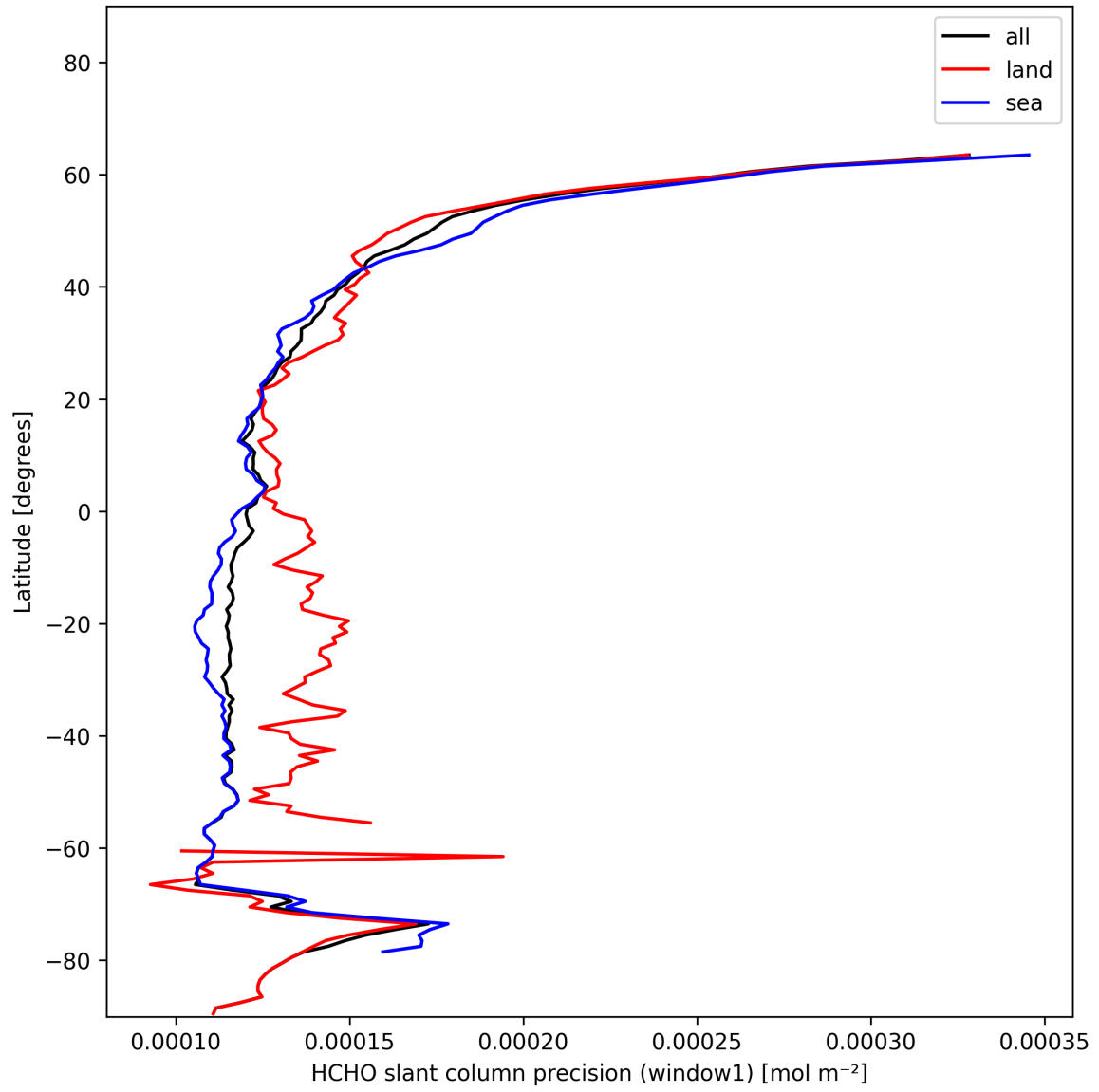
Figure 25: Zonal average of "HCHO slant column precision (window1)" for 2025-01-09 to 2025-01-11.
