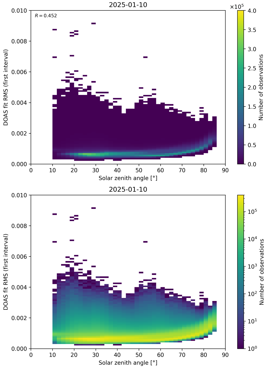
Figure 167: Scatter density plot of “Solar zenith angle” against “DOAS fit RMS (first interval)” for 2025-01-09 to 2025-01-11.
