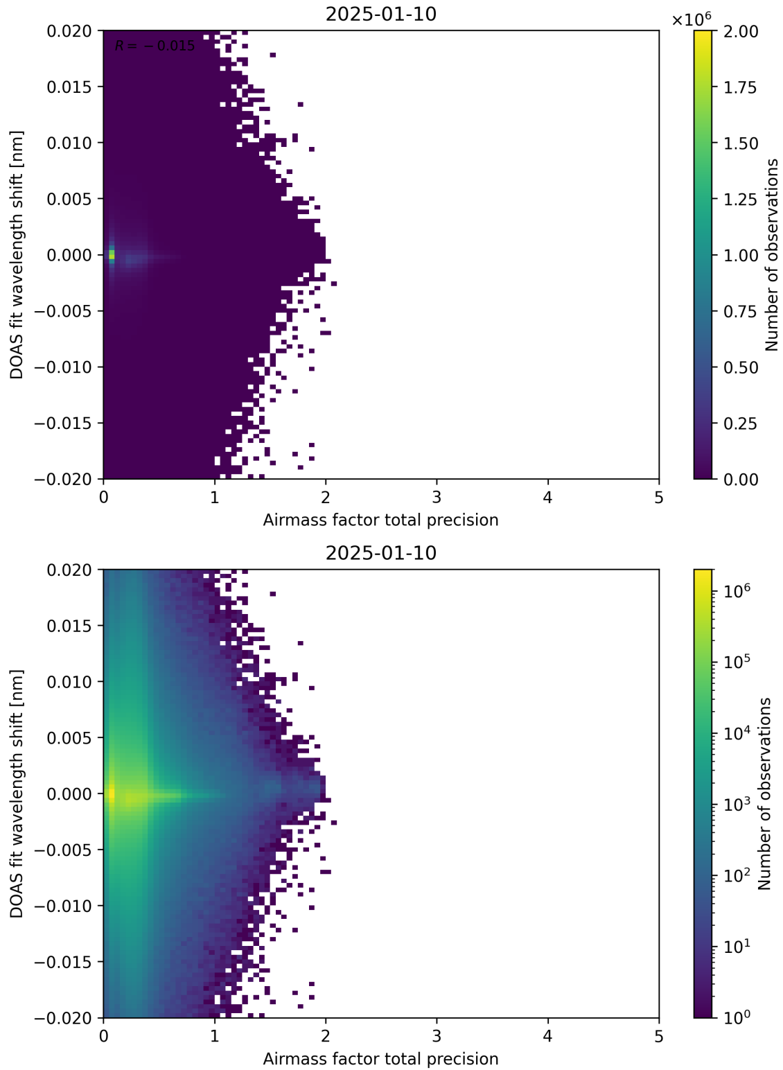
Figure 106: Scatter density plot of “Airmass factor total precision” against “DOAS fit wavelength shift” for 2025-01-09 to 2025-01-11.
