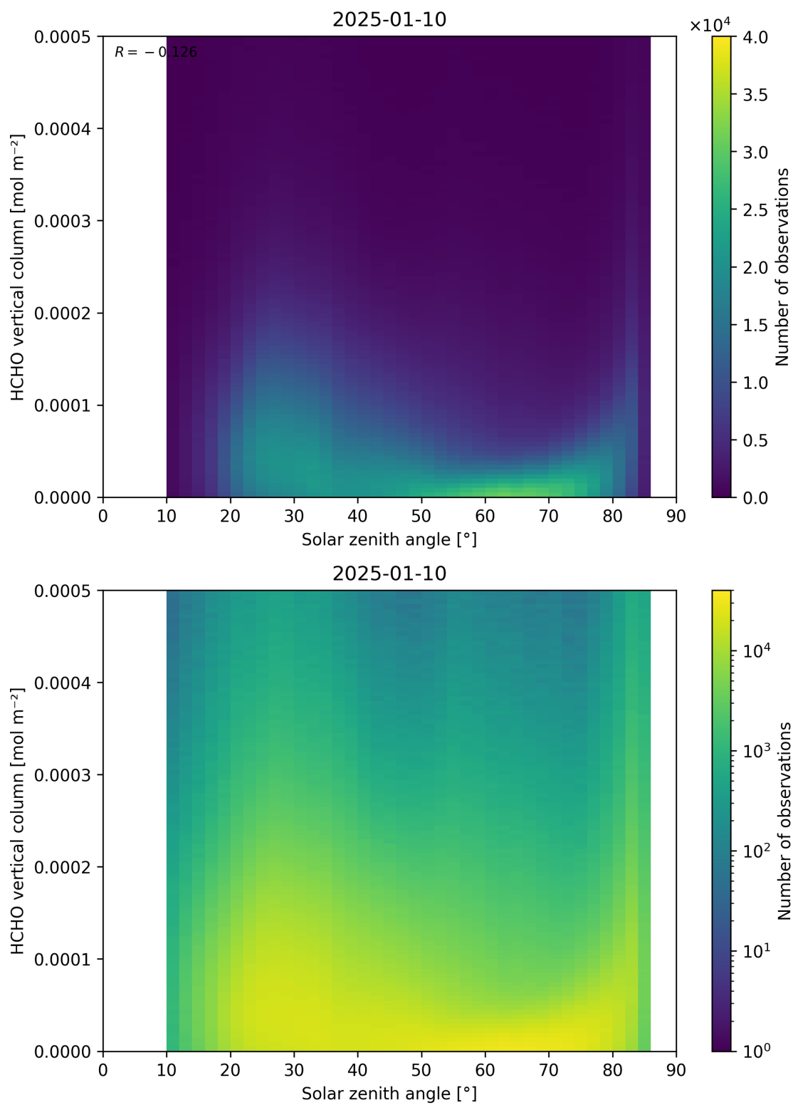
Figure 177: Scatter density plot of “Solar zenith angle” against “HCHO vertical column” for 2025-01-09 to 2025-01-11.
