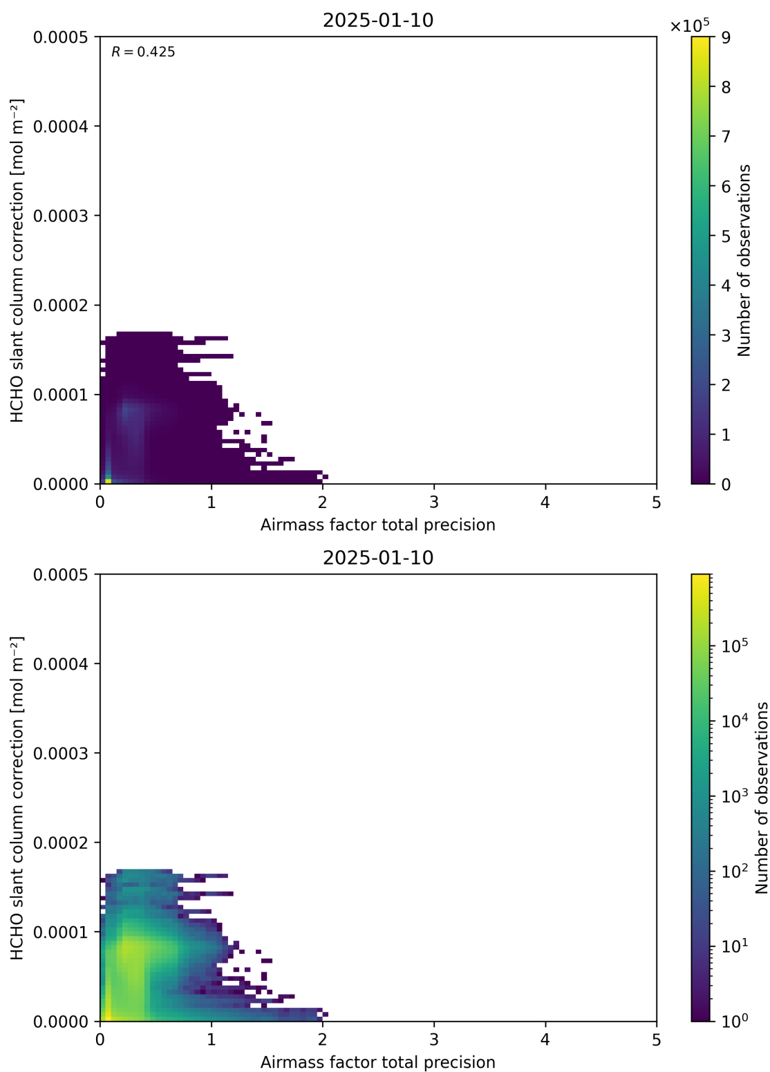
Figure 110: Scatter density plot of “Airmass factor total precision” against “HCHO slant column correction” for 2025-01-09 to 2025-01-11.
