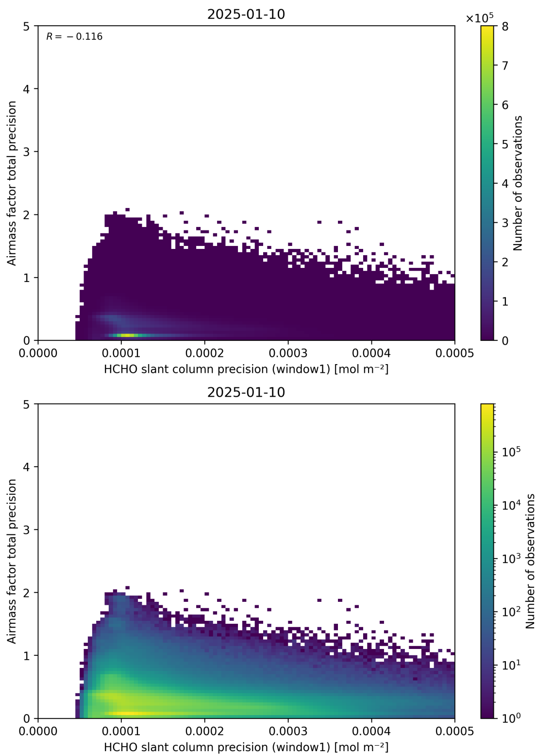
Figure 95: Scatter density plot of “HCHO slant column precision (window1)” against “Airmass factor total precision” for 2025-01-09 to 2025-01-11.
