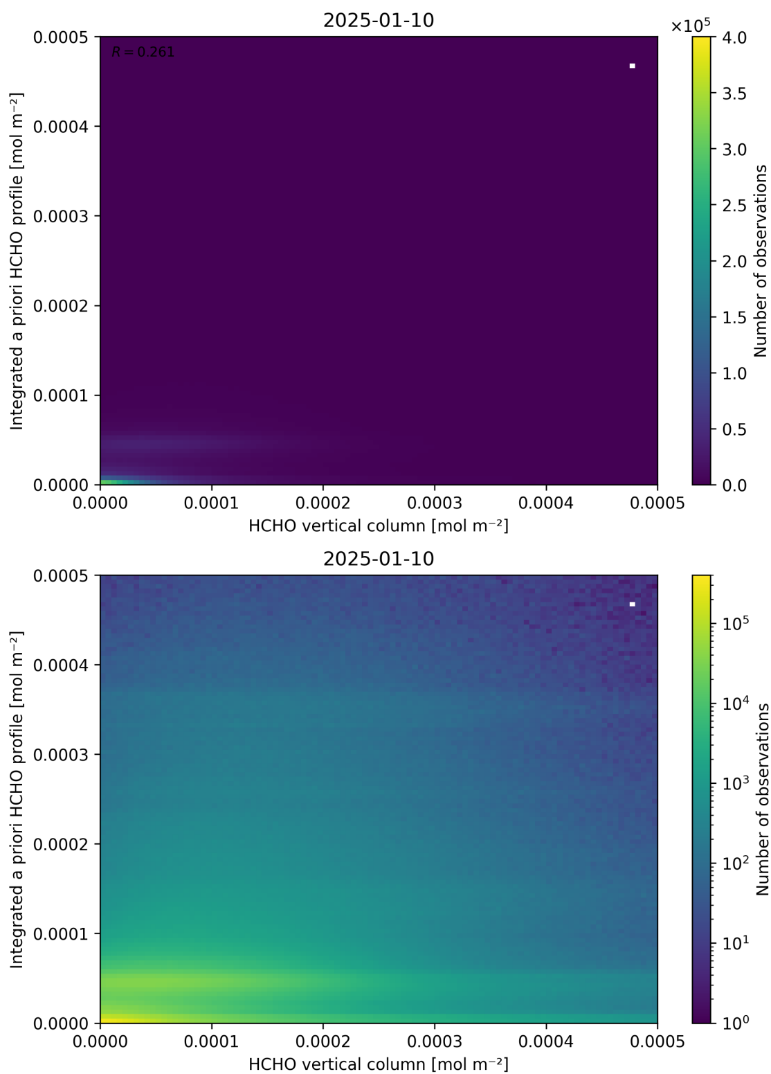
Figure 135: Scatter density plot of “HCHO vertical column” against “Integrated a priori HCHO profile” for 2025-01-09 to 2025-01-11.
