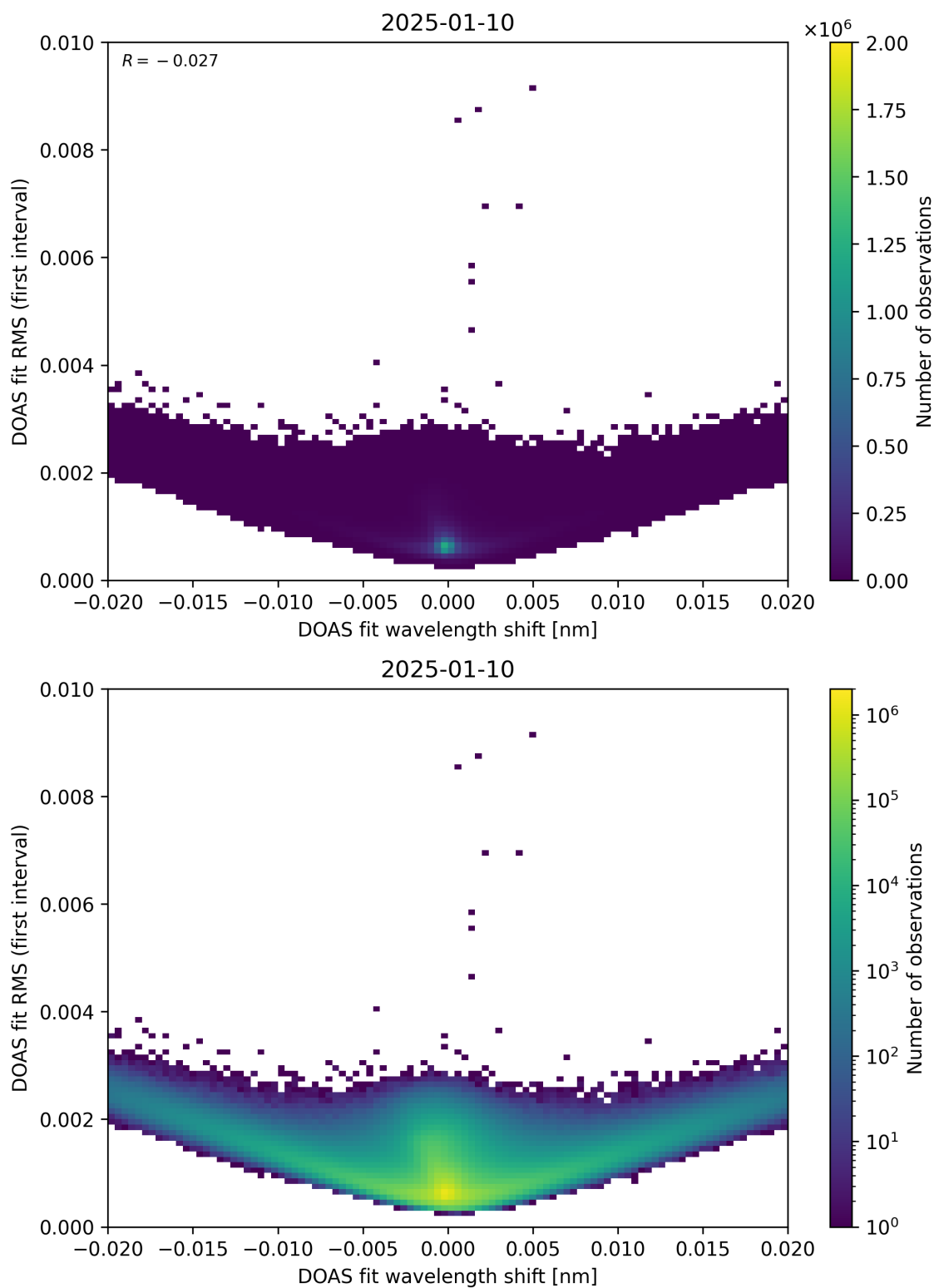
Figure 64: Scatter density plot of “DOAS fit wavelength shift” against “DOAS fit RMS (first interval)” for 2025-01-09 to 2025-01-11.
