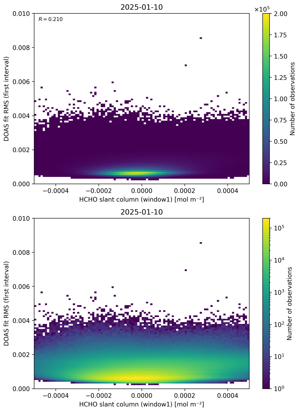
Figure 78: Scatter density plot of “HCHO slant column (window1)” against “DOAS fit RMS (first interval)” for 2025-01-09 to 2025-01-11.
