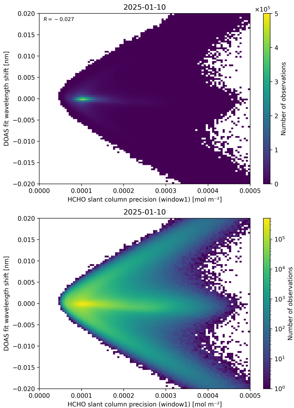
Figure 89: Scatter density plot of “HCHO slant column precision (window1)” against “DOAS fit wavelength shift” for 2025-01-09 to 2025-01-11.
