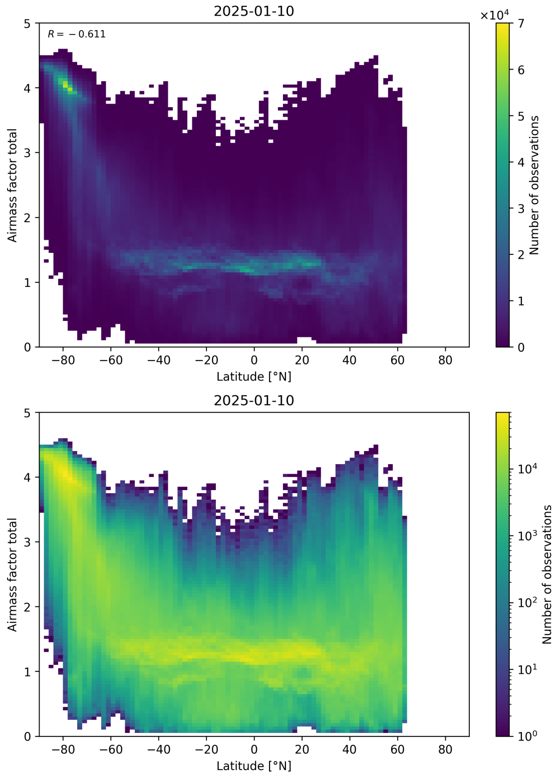
Figure 161: Scatter density plot of “Latitude” against “Airmass factor total” for 2025-01-09 to 2025-01-11.
