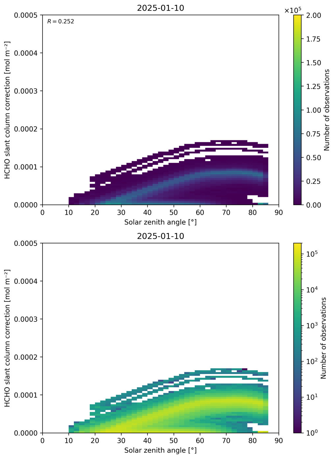
Figure 172: Scatter density plot of “Solar zenith angle” against “HCHO slant column correction” for 2025-01-09 to 2025-01-11.
