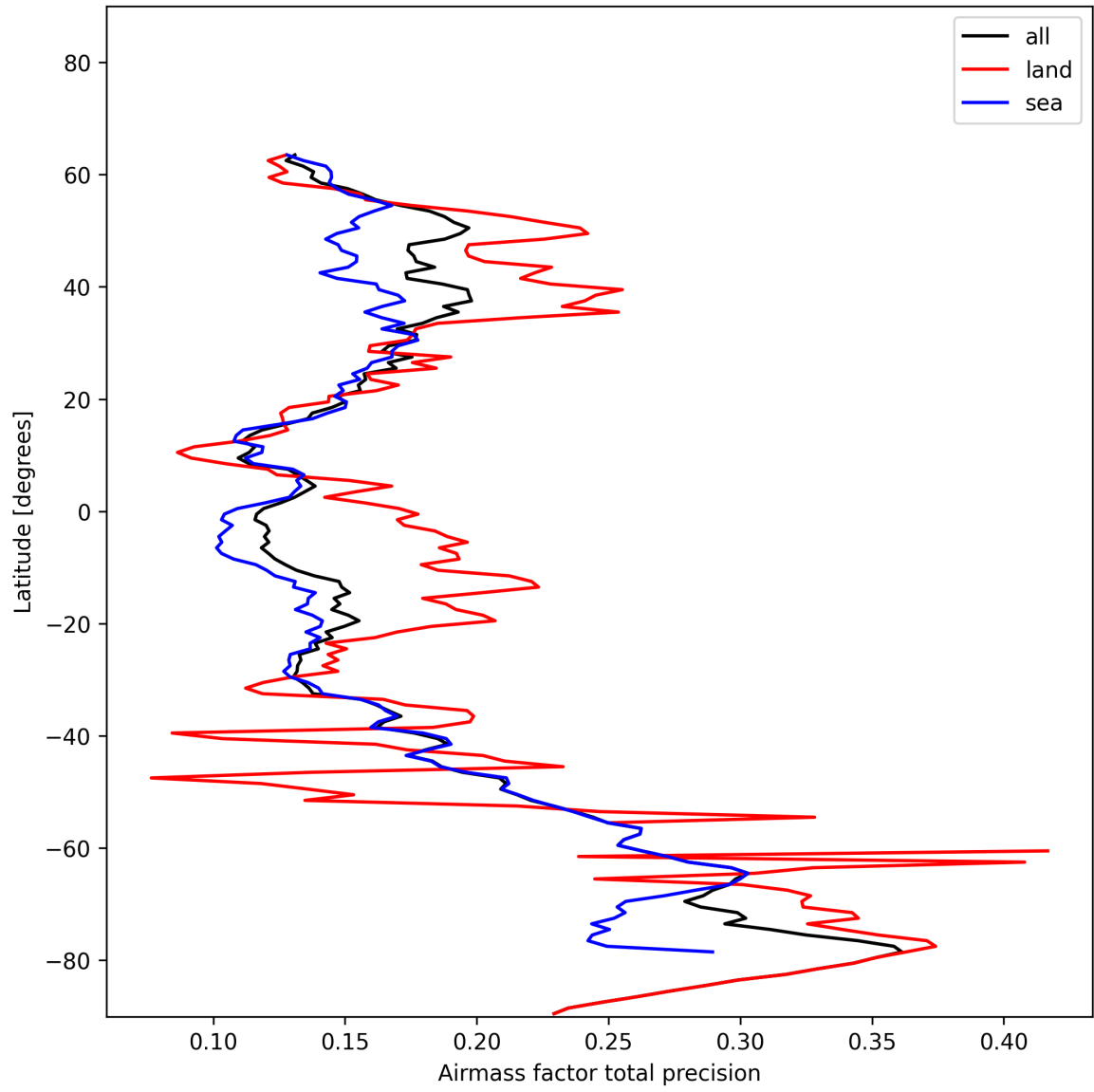
Figure 27: Zonal average of “Airmass factor total precision” for 2025-01-09 to 2025-01-11.
