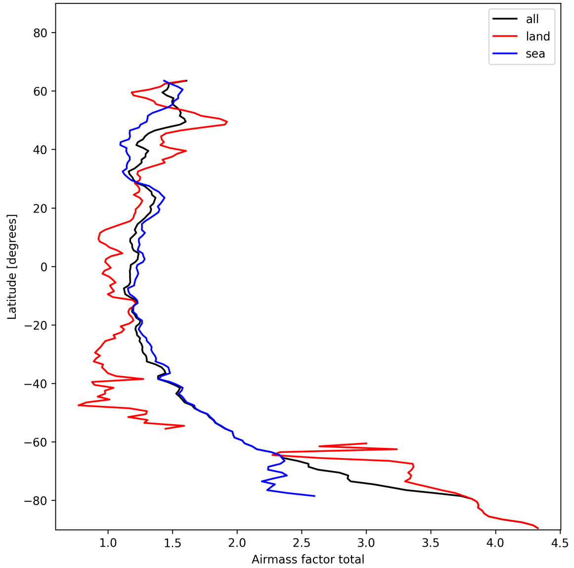
Figure 26: Zonal average of “Airmass factor total” for 2025-01-09 to 2025-01-11.
