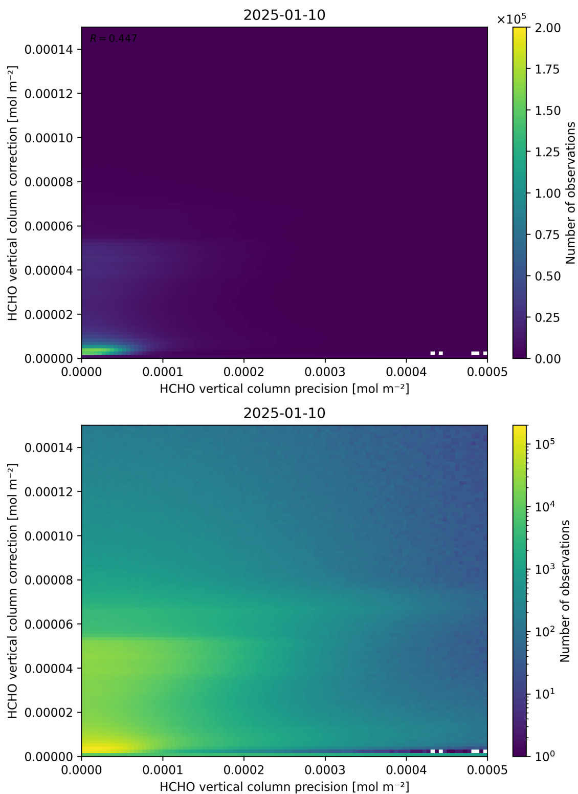
Figure 146: Scatter density plot of “HCHO vertical column precision” against “HCHO vertical column correction” for 2025-01-09 to 2025-01-11.
