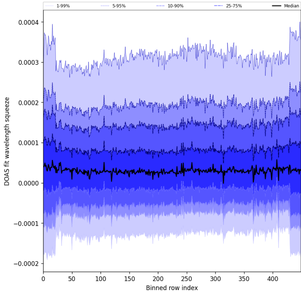
Figure 59: Along track statistics of “DOAS fit wavelength squeeze” for 2025-01-09 to 2025-01-11
