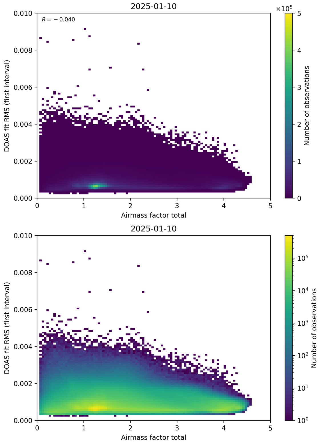
Figure 97: Scatter density plot of “Airmass factor total” against “DOAS fit RMS (first interval)” for 2025-01-09 to 2025-01-11.
