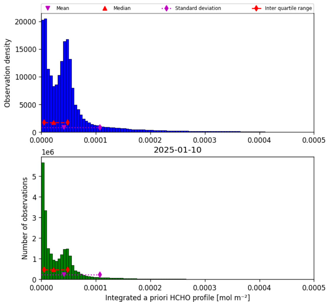
Figure 43: Histogram of “Integrated a priori HCHO profile” for 2025-01-09 to 2025-01-11
