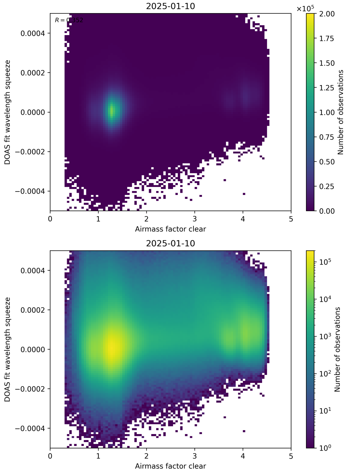
Figure 73: Scatter density plot of “Airmass factor clear” against “DOAS fit wavelength squeeze” for 2025-01-09 to 2025-01-11.
