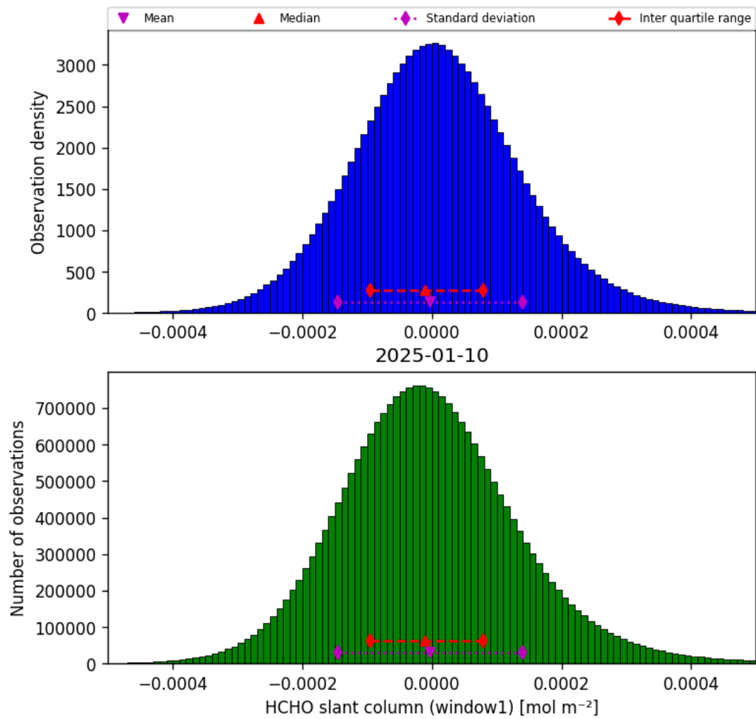
Figure 38: Histogram of “HCHO slant column (window1)” for 2025-01-09 to 2025-01-11
