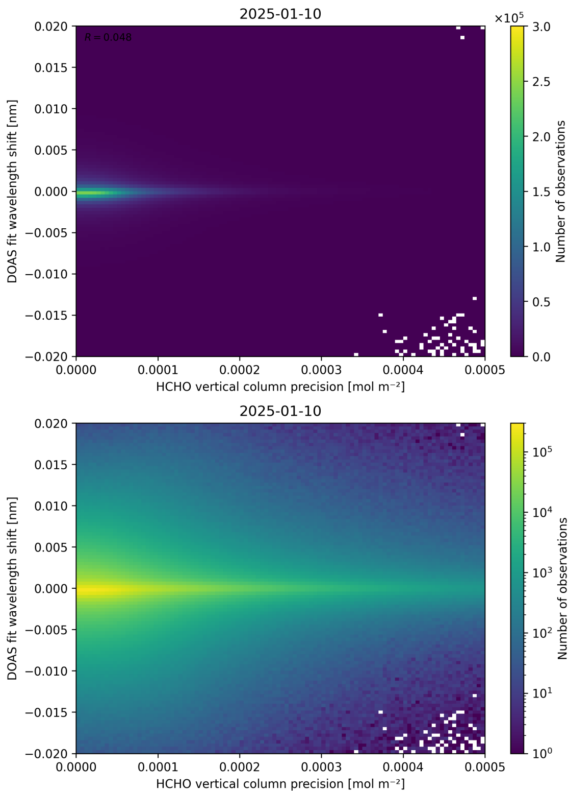
Figure 137: Scatter density plot of “HCHO vertical column precision” against “DOAS fit wavelength shift” for 2025-01-09 to 2025-01-11.
