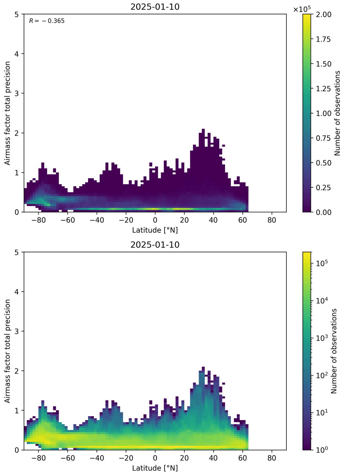
Figure 162: Scatter density plot of “Latitude” against “Airmass factor total precision” for 2025-01-09 to 2025-01-11.
