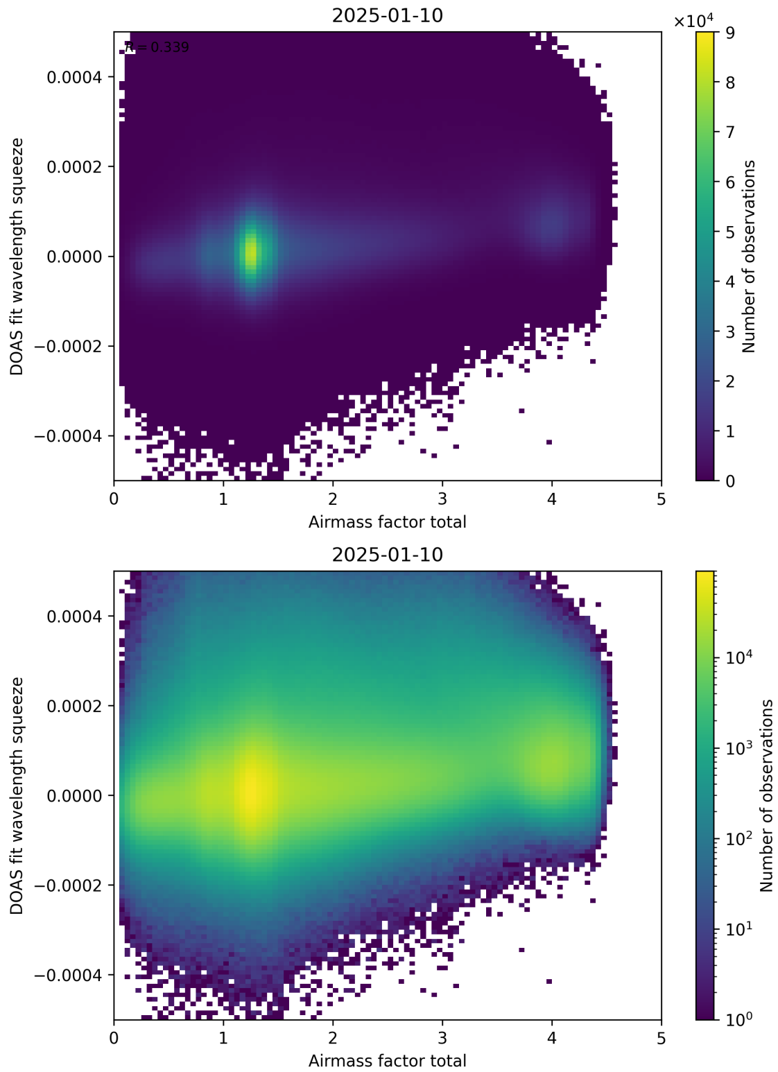
Figure 99: Scatter density plot of “Airmass factor total” against “DOAS fit wavelength squeeze” for 2025-01-09 to 2025-01-11.
