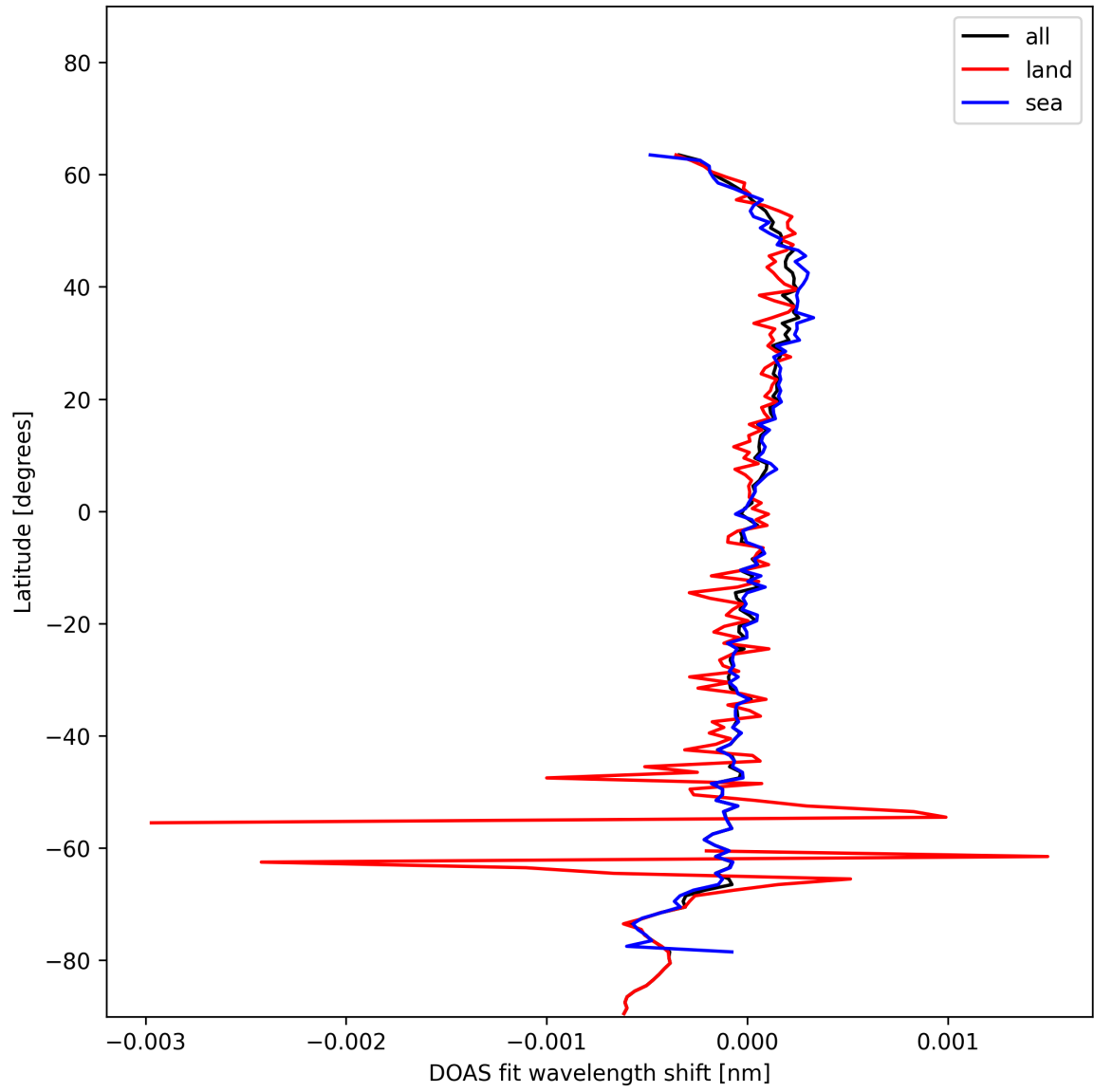
Figure 30: Zonal average of "DOAS fit wavelength shift" for 2025-01-09 to 2025-01-11.
