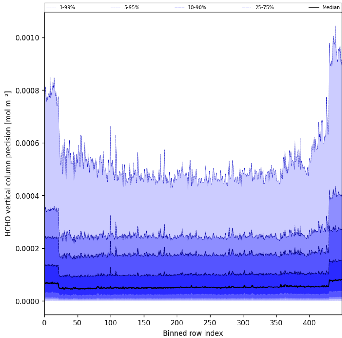
Figure 50: Along track statistics of “HCHO vertical column precision” for 2025-01-09 to 2025-01-11
