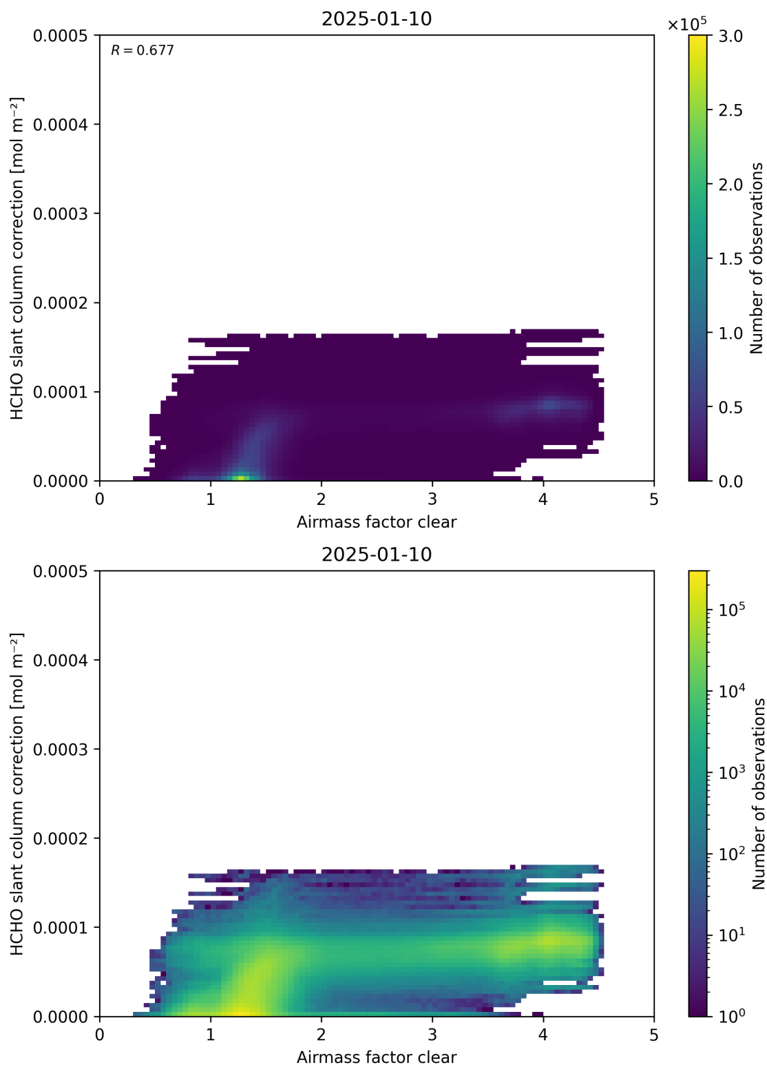
Figure 75: Scatter density plot of “Airmass factor clear” against “HCHO slant column correction” for 2025-01-09 to 2025-01-11.
