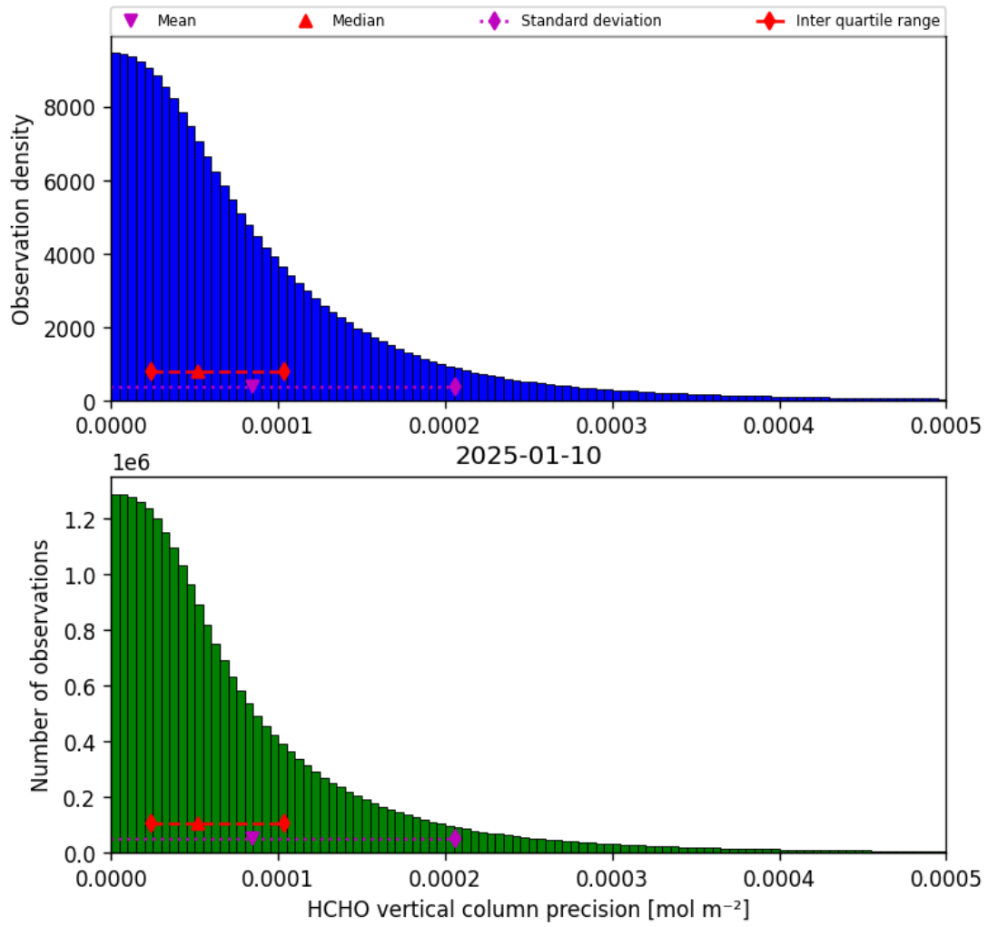
Figure 36: Histogram of “HCHO vertical column precision” for 2025-01-09 to 2025-01-11
