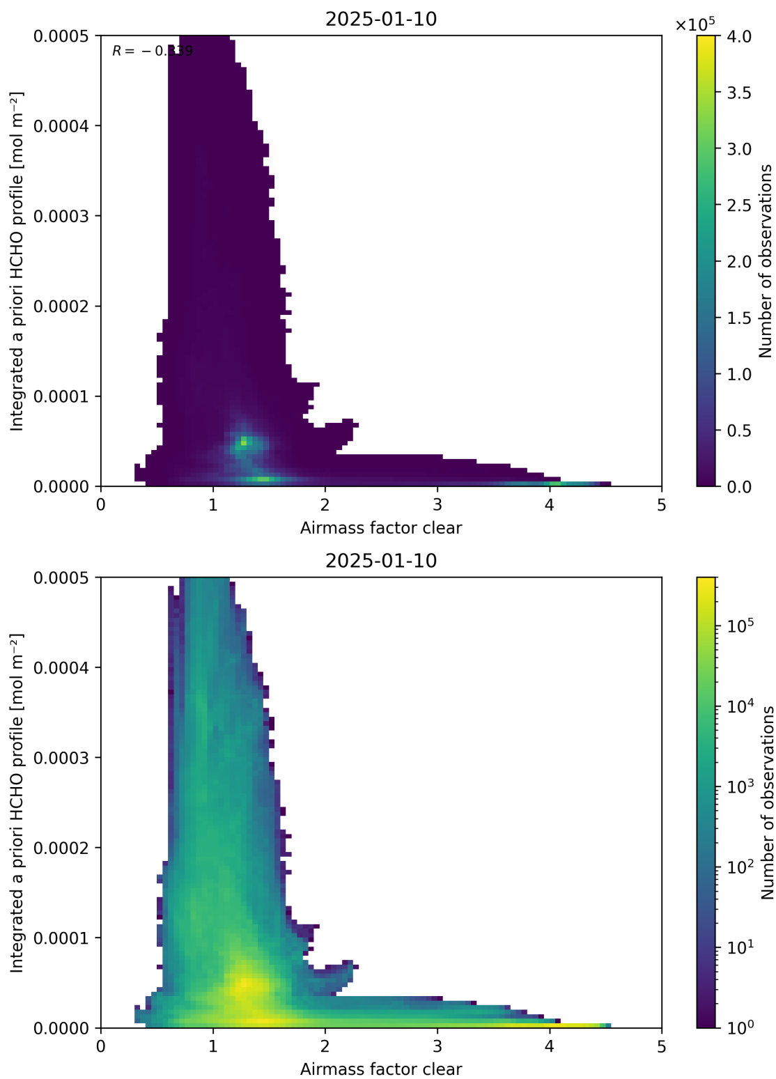
Figure 76: Scatter density plot of “Airmass factor clear” against “Integrated a priori HCHO profile” for 2025-01-09 to 2025-01-11.
