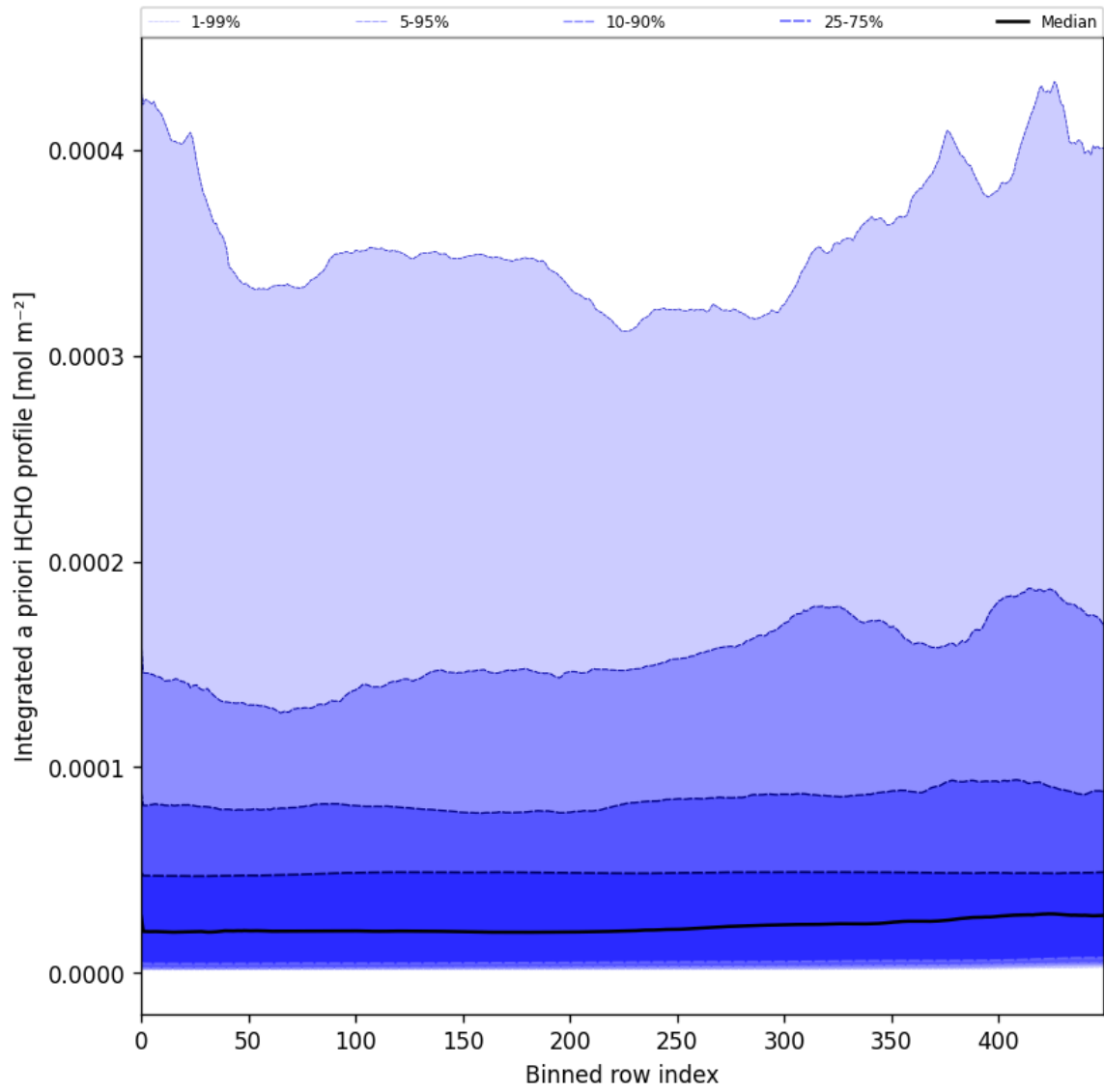
Figure 57: Along track statistics of “Integrated a priori HCHO profile” for 2025-01-09 to 2025-01-11
