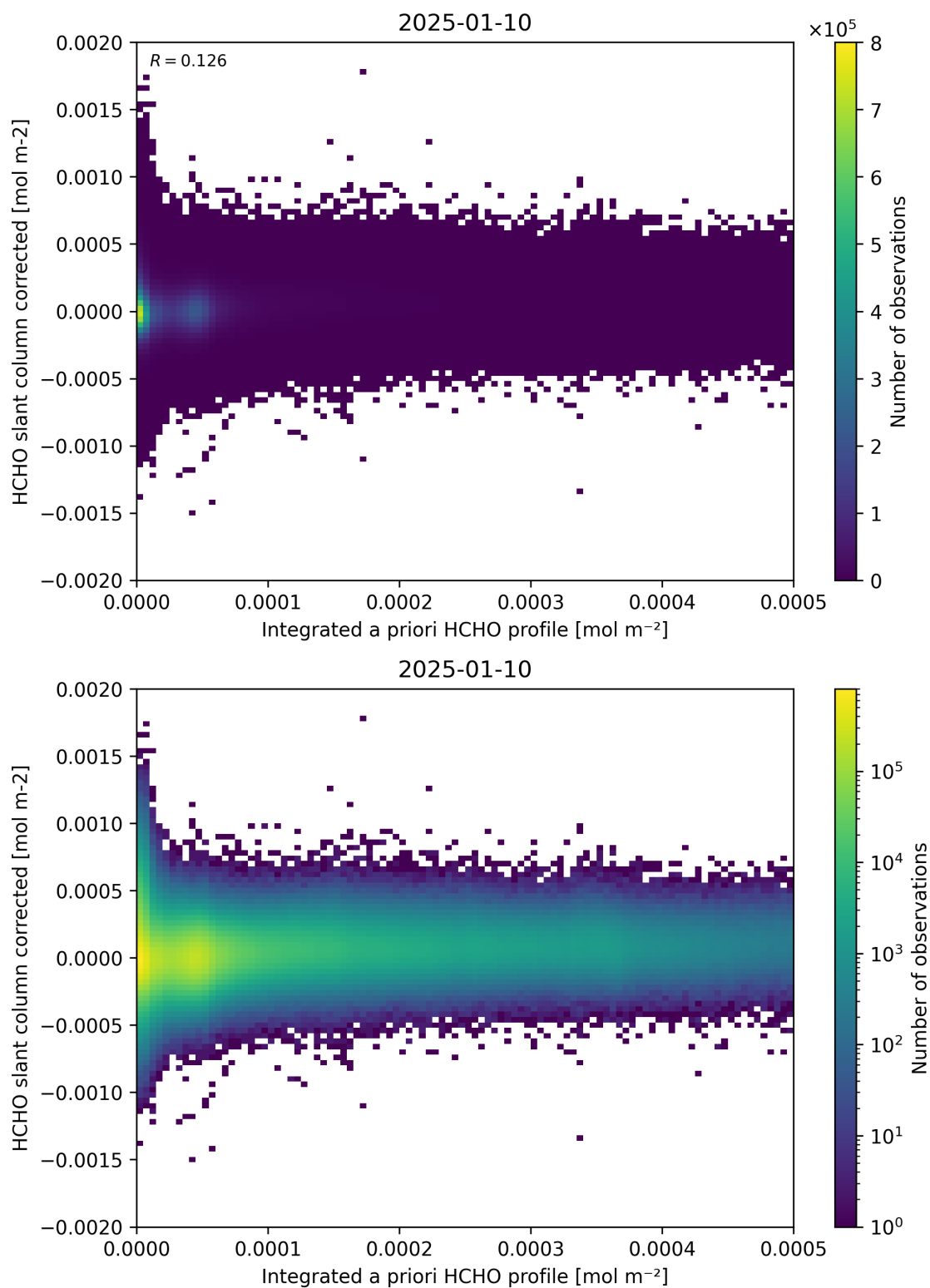
Figure 151: Scatter density plot of “Integrated a priori HCHO profile” against “HCHO slant column corrected” for 2025-01-09 to 2025-01-11.
