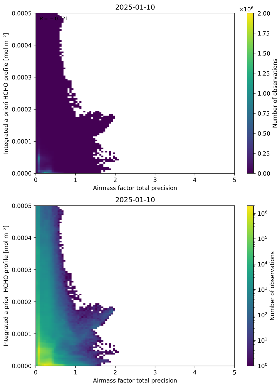
Figure 111: Scatter density plot of “Airmass factor total precision” against “Integrated a priori HCHO profile” for 2025-01-09 to 2025-01-11.
