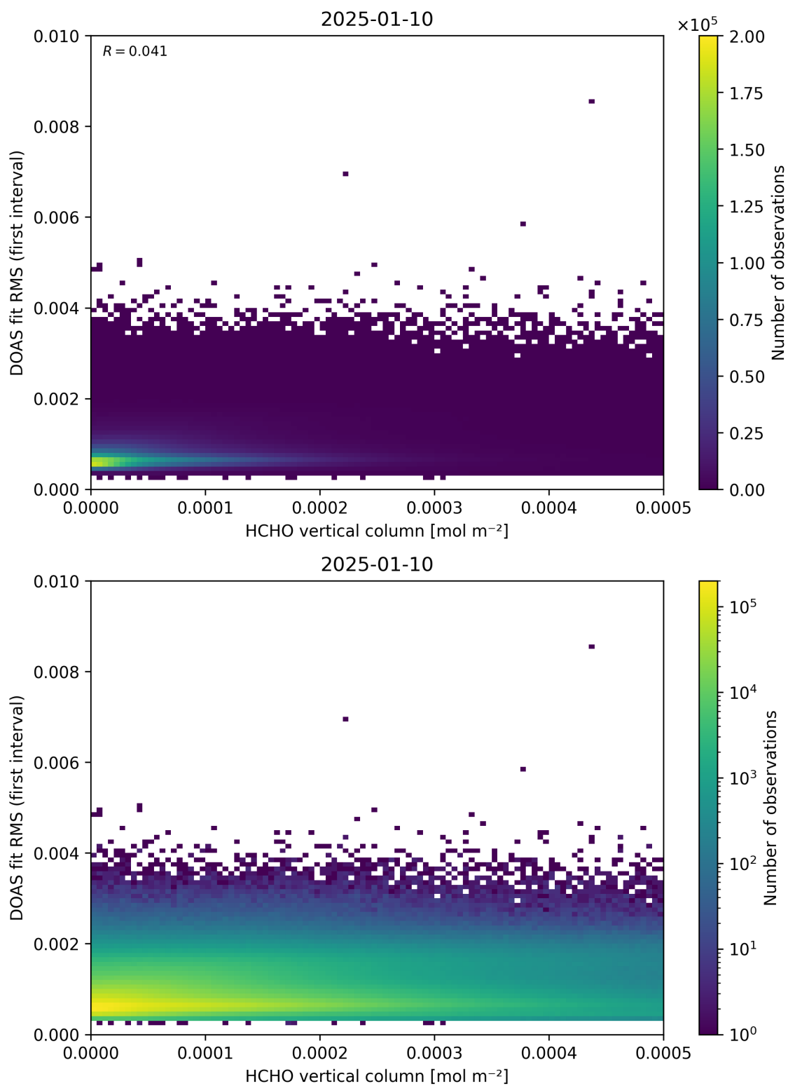
Figure 123: Scatter density plot of “HCHO vertical column” against “DOAS fit RMS (first interval)” for 2025-01-09 to 2025-01-11.
