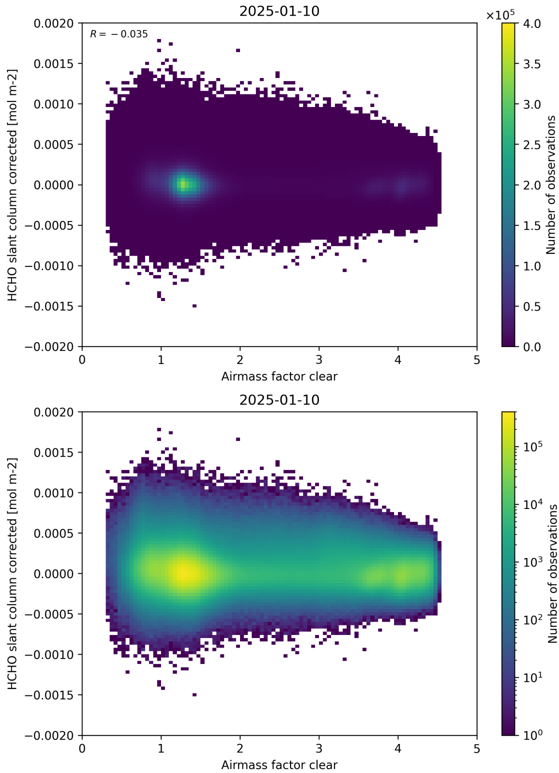
Figure 74: Scatter density plot of “Airmass factor clear” against “HCHO slant column corrected” for 2025-01-09 to 2025-01-11.
