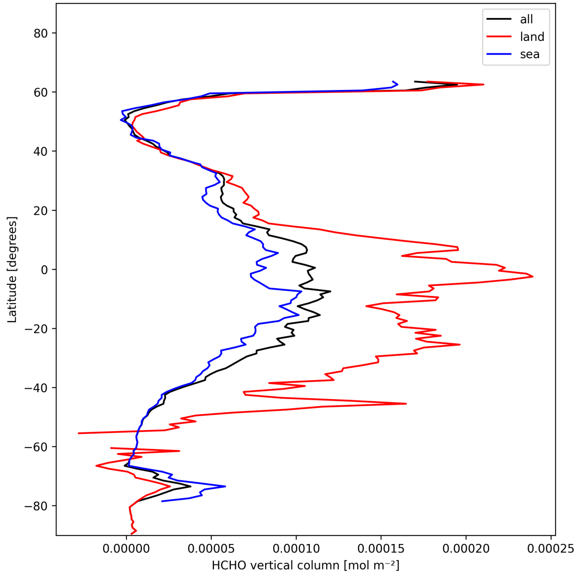
Figure 21: Zonal average of “HCHO vertical column” for 2025-01-09 to 2025-01-11.
