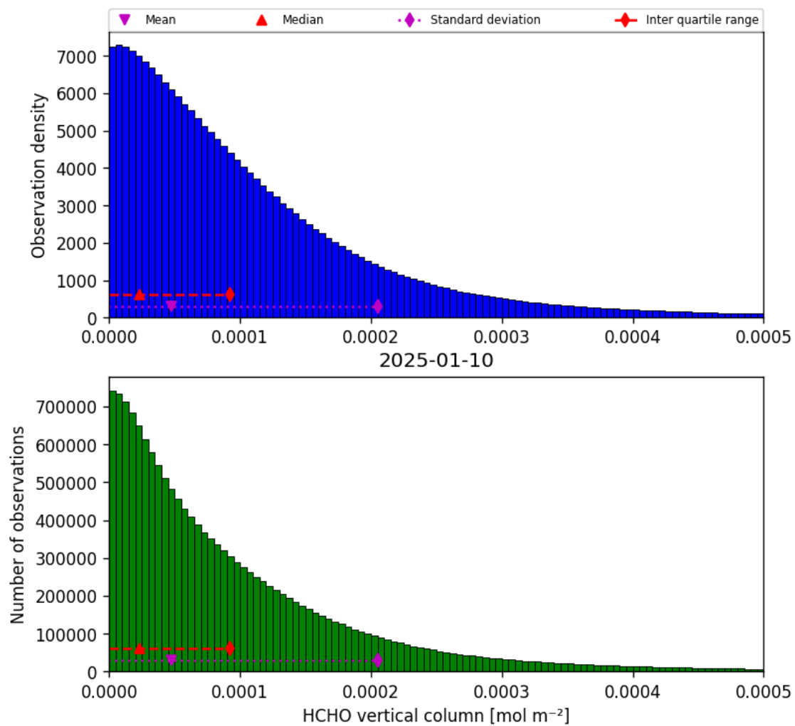
Figure 35: Histogram of “HCHO vertical column” for 2025-01-09 to 2025-01-11
