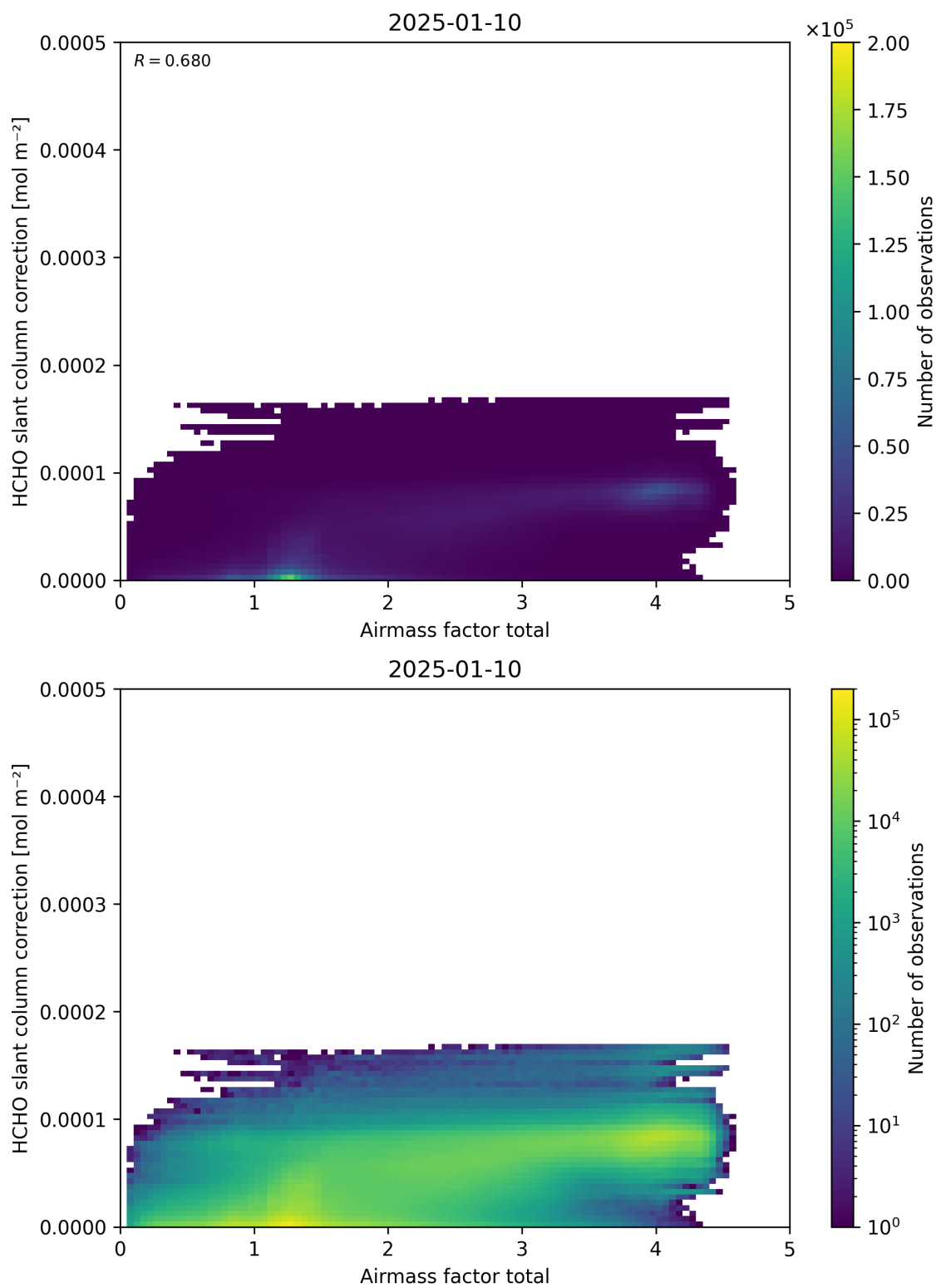
Figure 102: Scatter density plot of “Airmass factor total” against “HCHO slant column correction” for 2025-01-09 to 2025-01-11.
