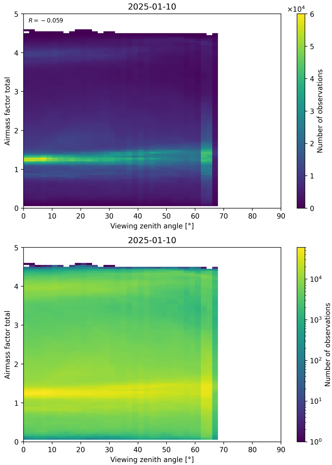
Figure 190: Scatter density plot of “Viewing zenith angle” against “Airmass factor total” for 2025-01-09 to 2025-01-11.
