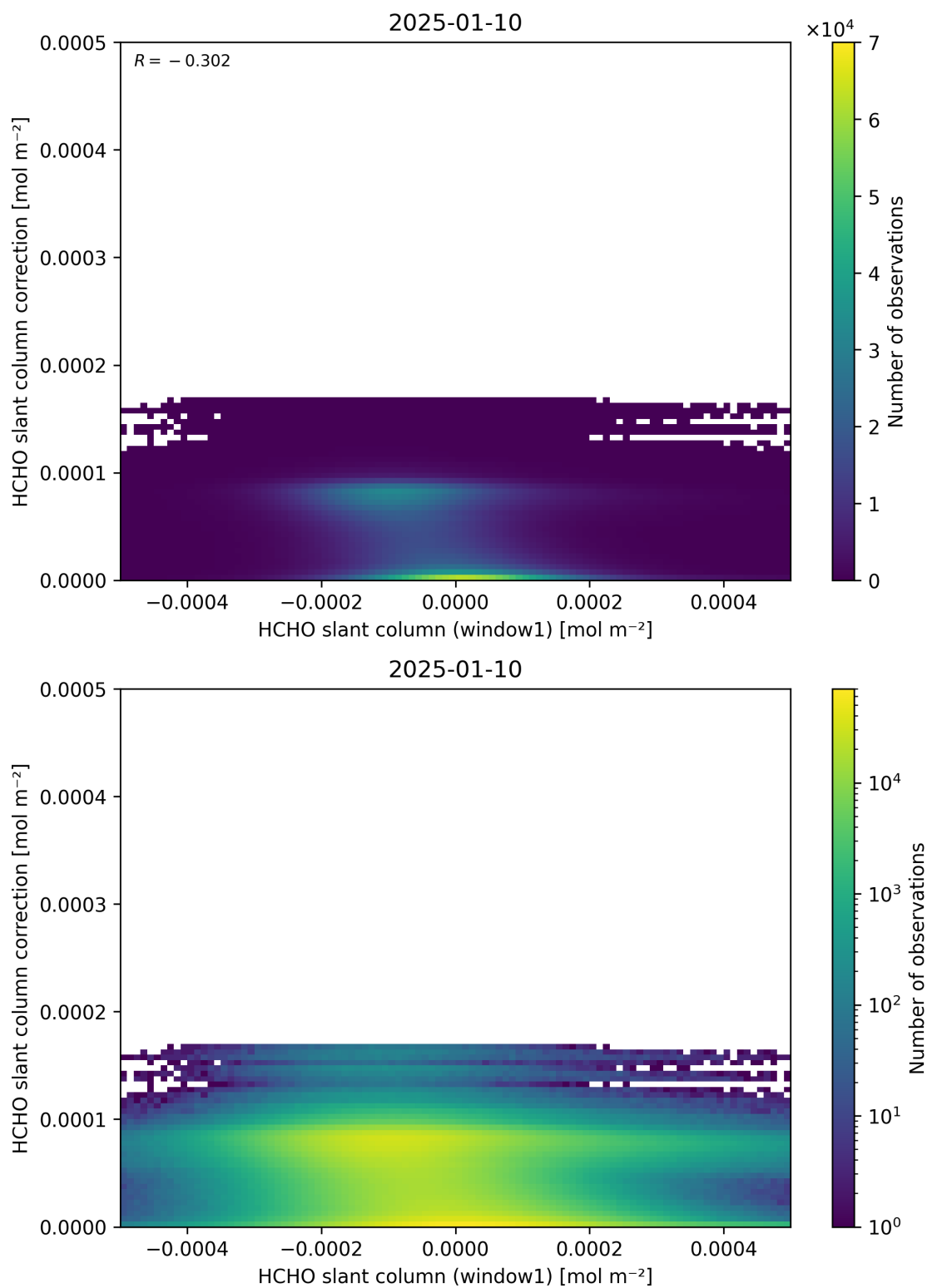
Figure 83: Scatter density plot of “HCHO slant column (window1)” against “HCHO slant column correction” for 2025-01-09 to 2025-01-11.
