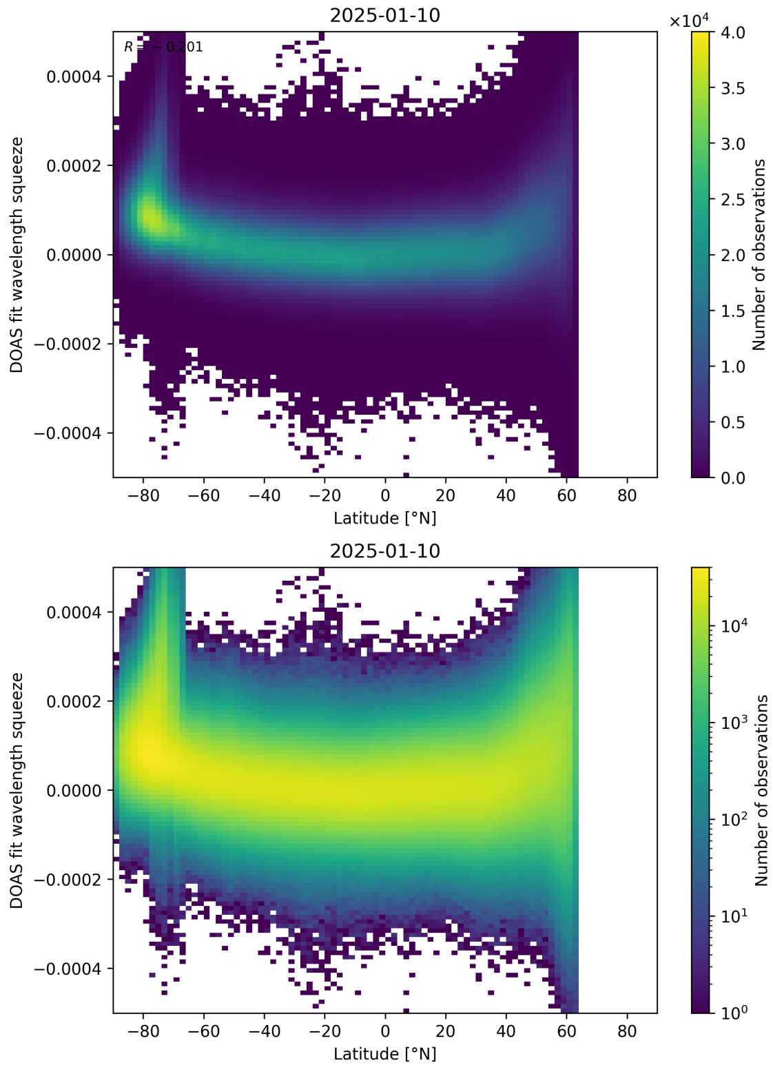
Figure 155: Scatter density plot of “Latitude” against “DOAS fit wavelength squeeze” for 2025-01-09 to 2025-01-11.
