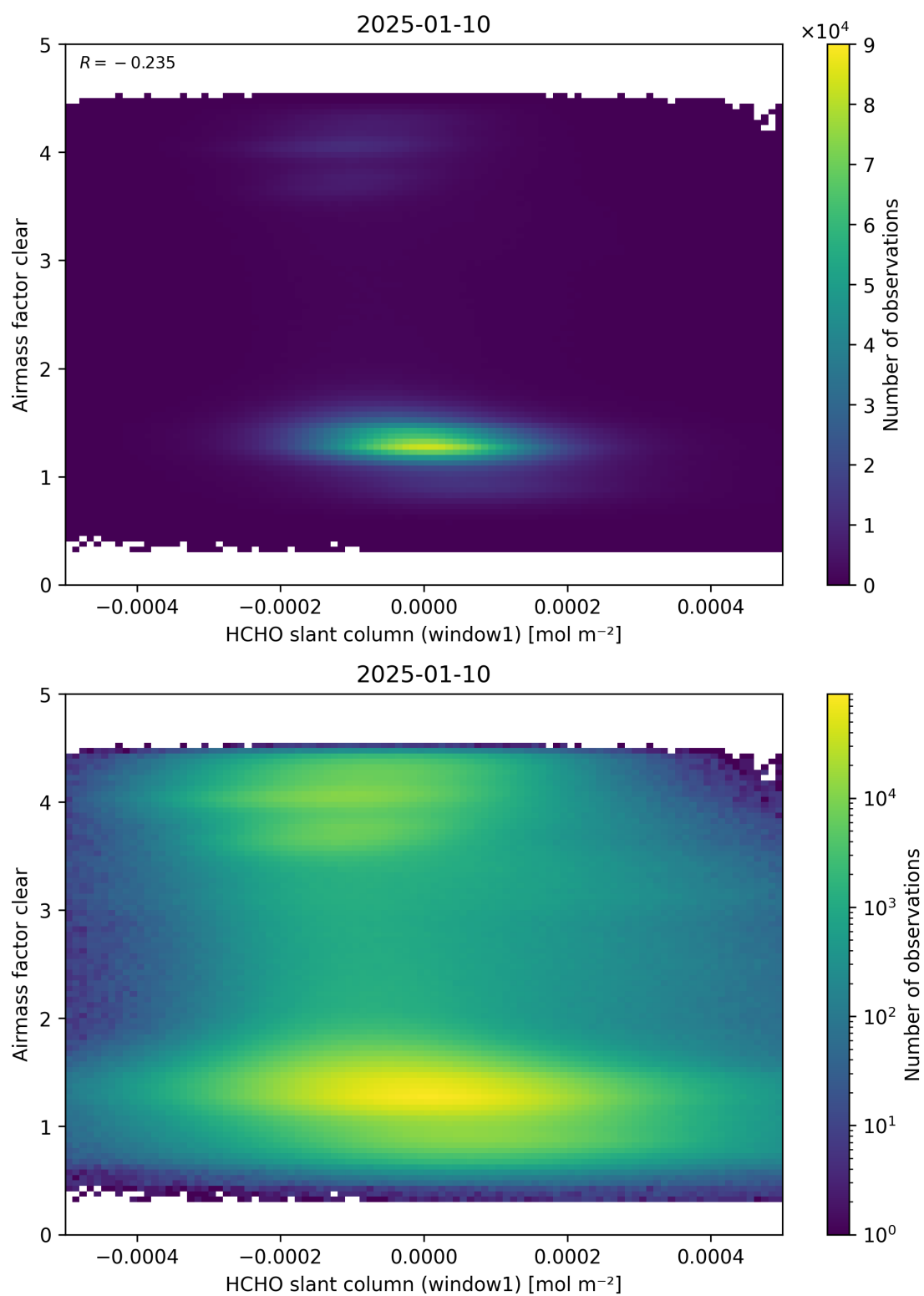
Figure 81: Scatter density plot of “HCHO slant column (window1)” against “Airmass factor clear” for 2025-01-09 to 2025-01-11.
