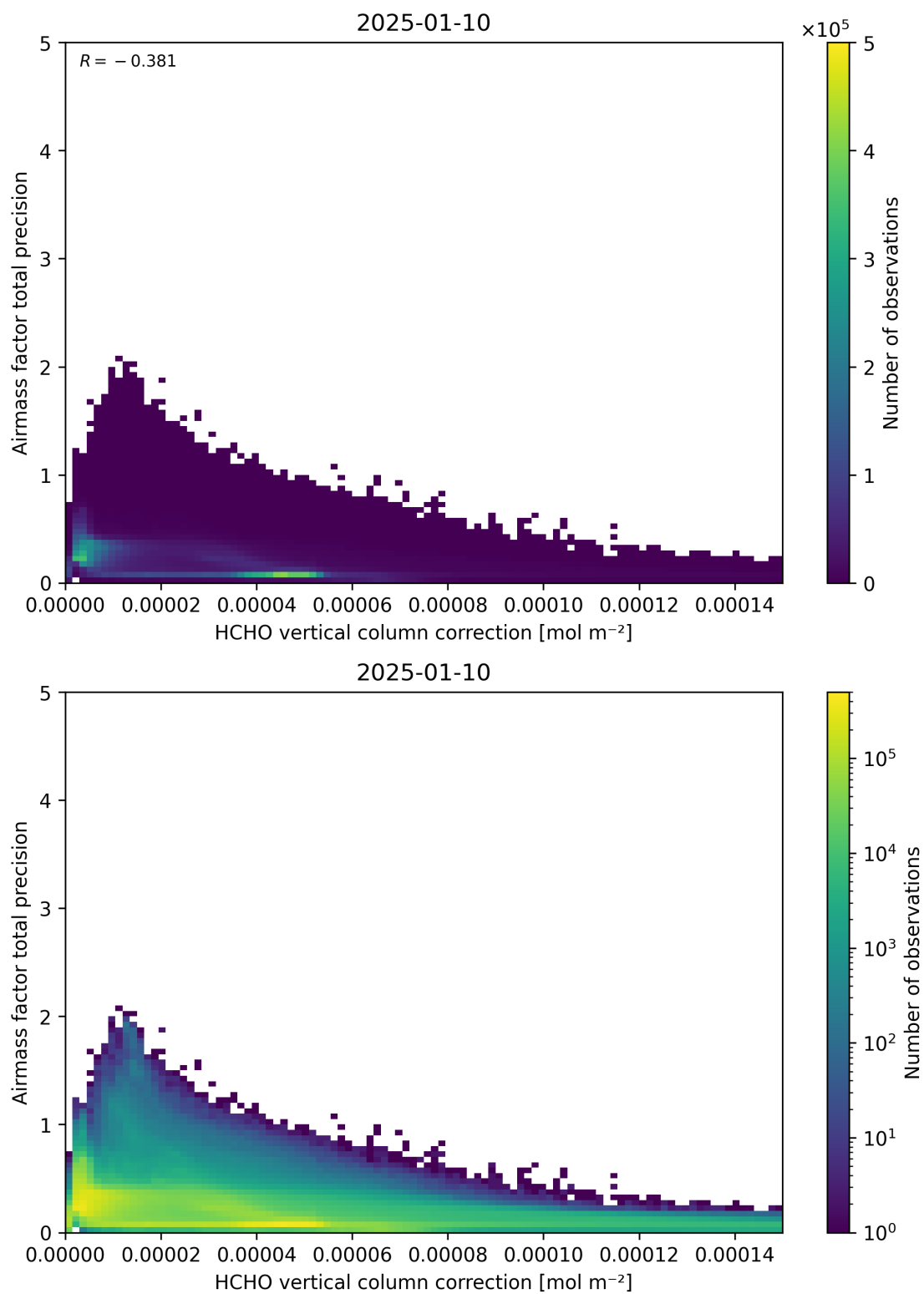
Figure 121: Scatter density plot of “HCHO vertical column correction” against “Airmass factor total precision” for 2025-01-09 to 2025-01-11.
