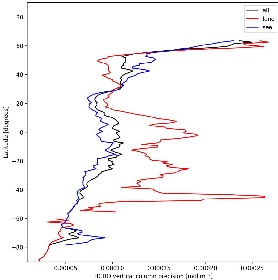
Figure 22: Zonal average of “HCHO vertical column precision” for 2025-01-09 to 2025-01-11.
