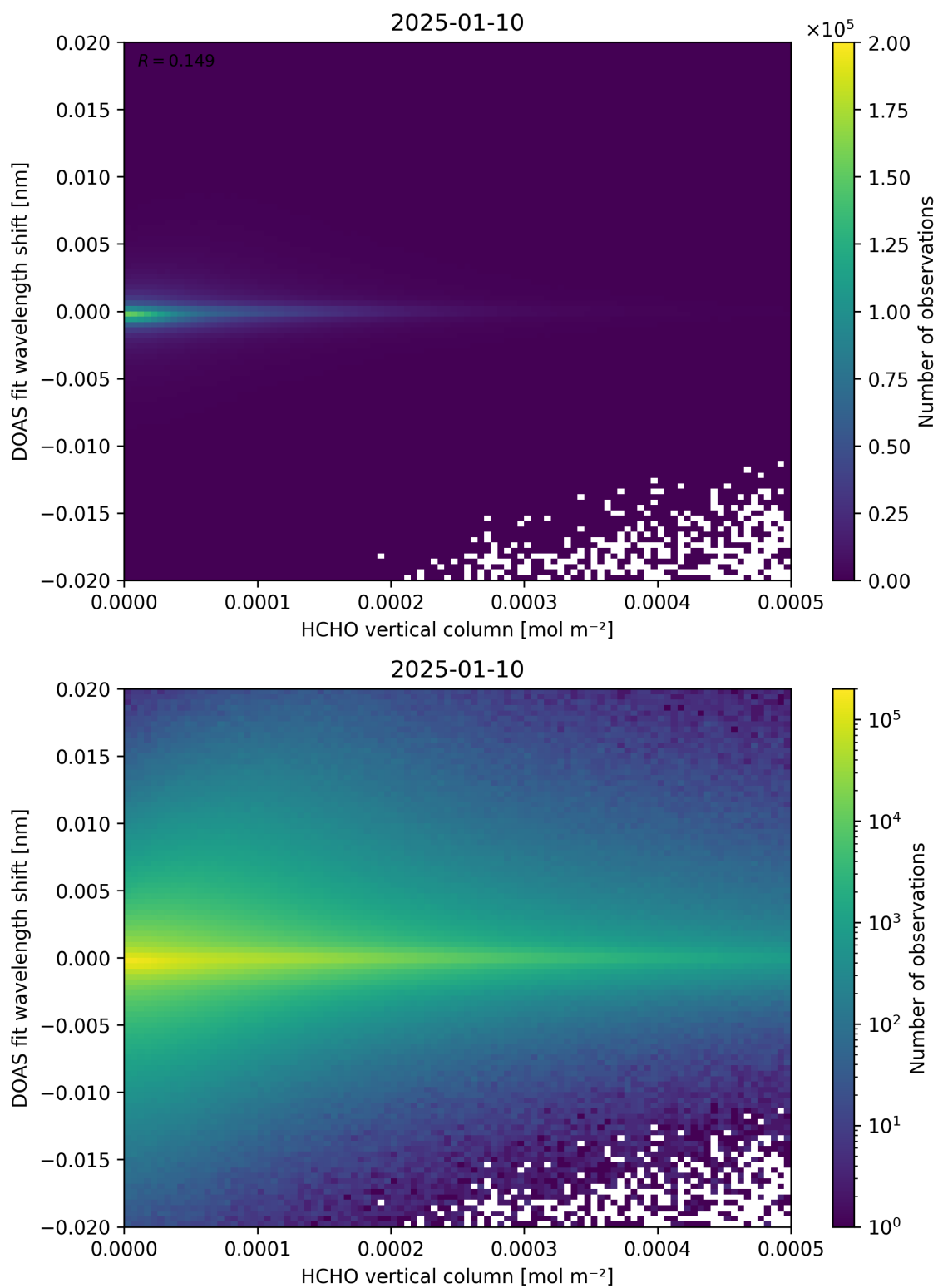
Figure 124: Scatter density plot of “HCHO vertical column” against “DOAS fit wavelength shift” for 2025-01-09 to 2025-01-11.
