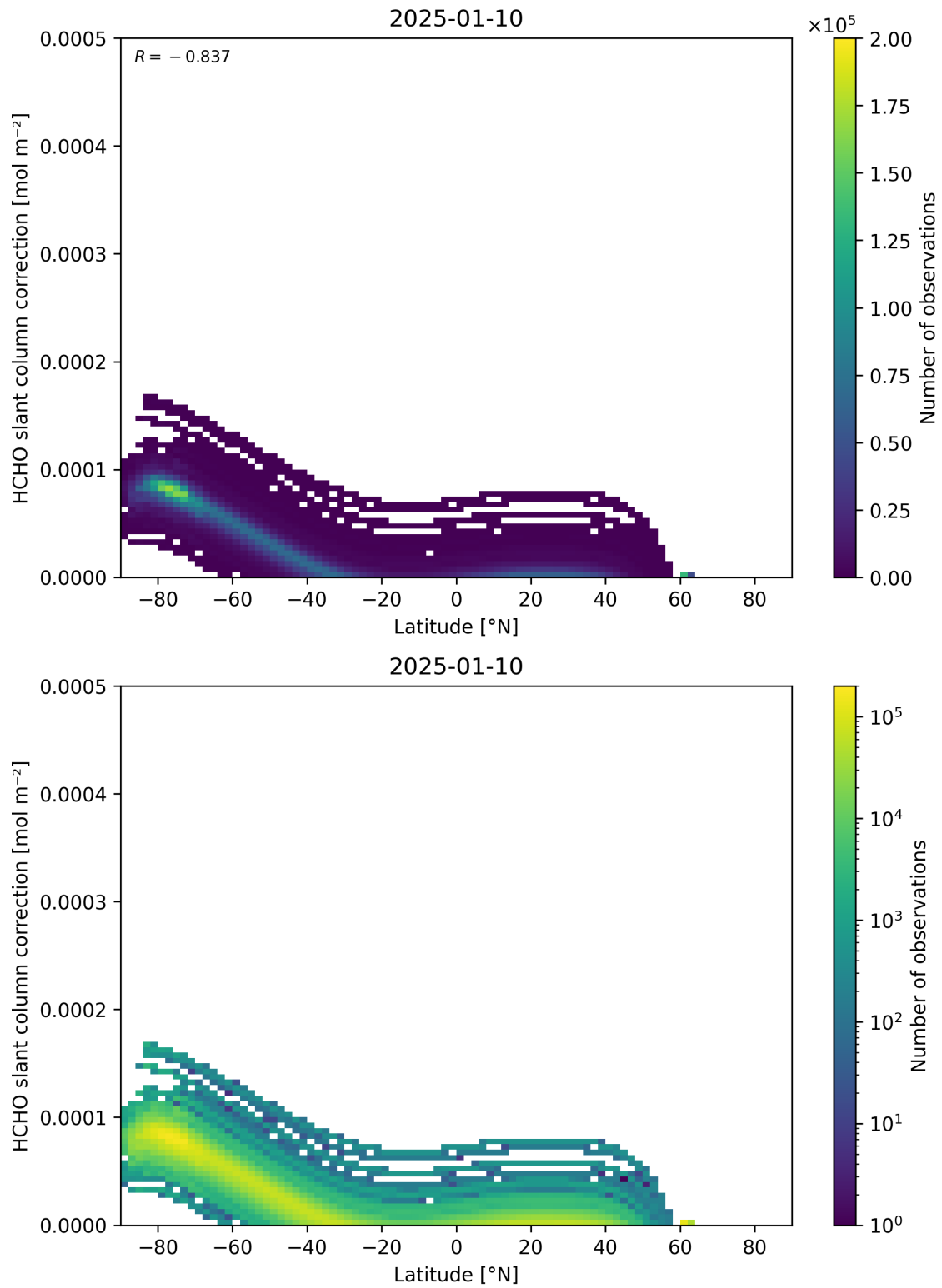
Figure 158: Scatter density plot of “Latitude” against “HCHO slant column correction” for 2025-01-09 to 2025-01-11.
