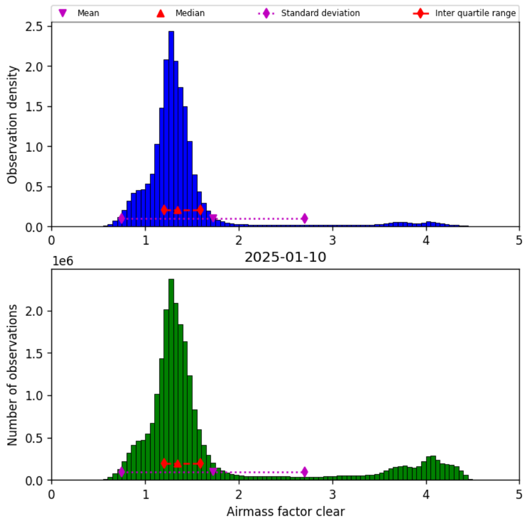
Figure 42: Histogram of “Airmass factor clear” for 2025-01-09 to 2025-01-11
