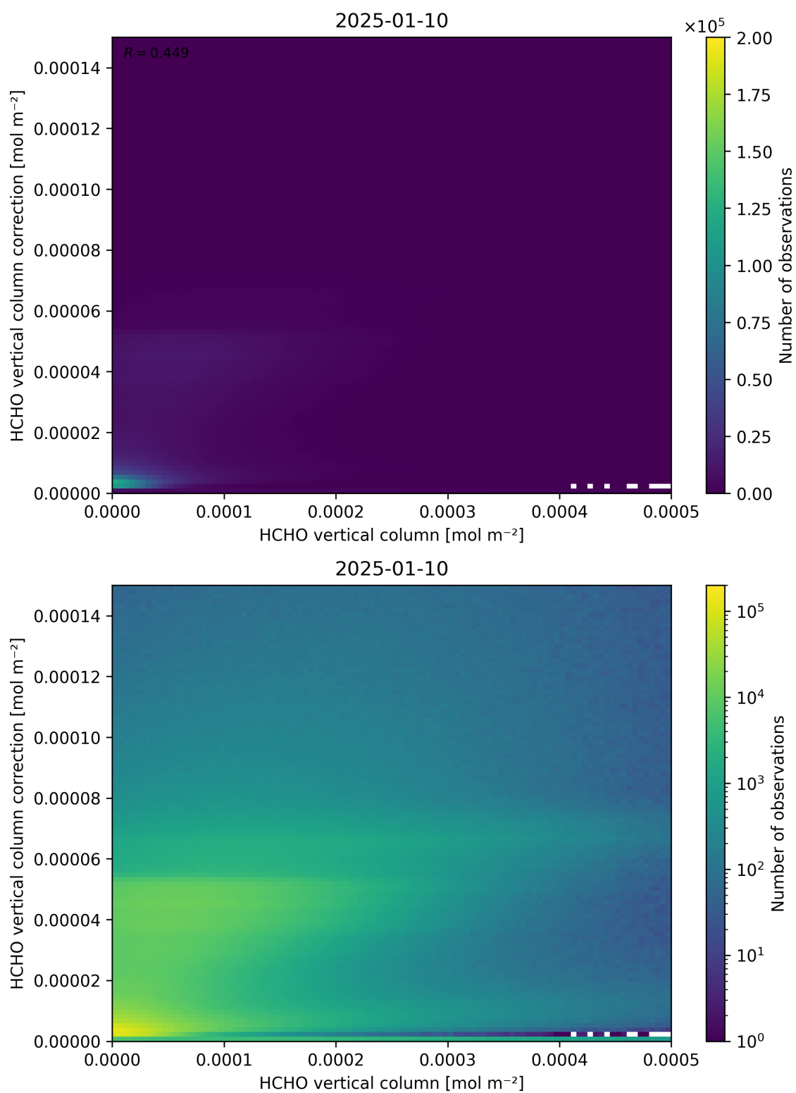
Figure 133: Scatter density plot of “HCHO vertical column” against “HCHO vertical column correction” for 2025-01-09 to 2025-01-11.
