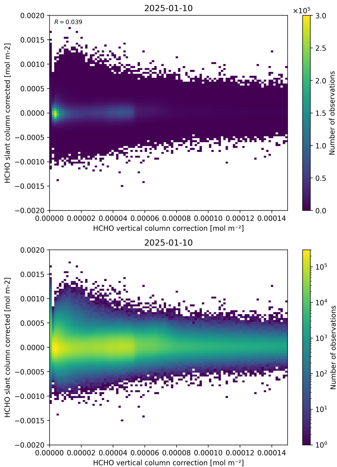
Figure 116: Scatter density plot of “HCHO vertical column correction” against “HCHO slant column corrected” for 2025-01-09 to 2025-01-11.
