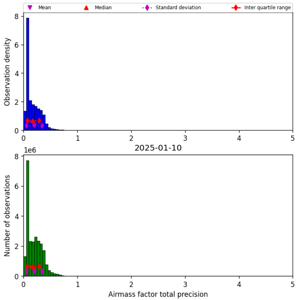
Figure 41: Histogram of “Airmass factor total precision” for 2025-01-09 to 2025-01-11
