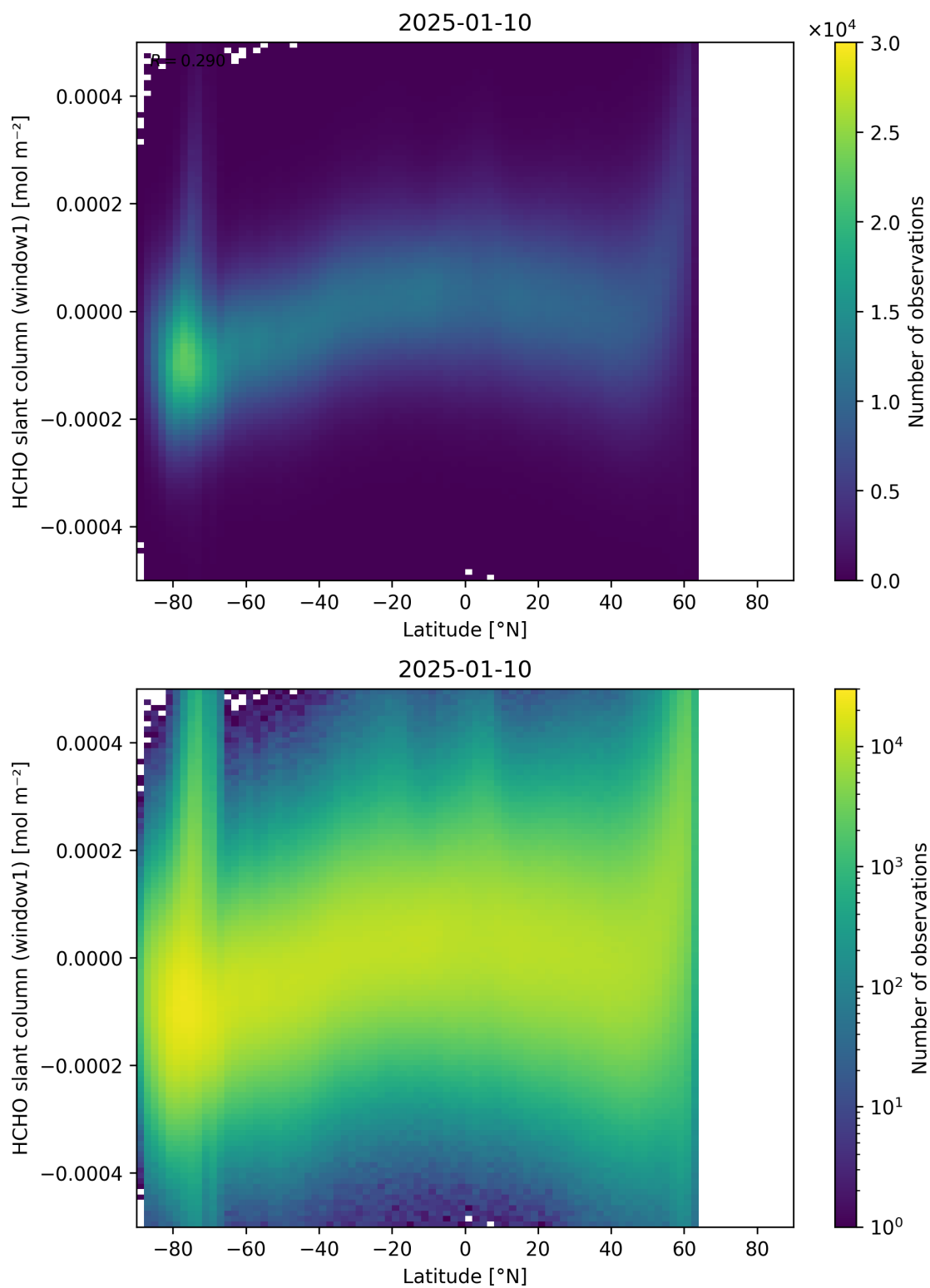
Figure 159: Scatter density plot of “Latitude” against “HCHO slant column (window1)” for 2025-01-09 to 2025-01-11.
