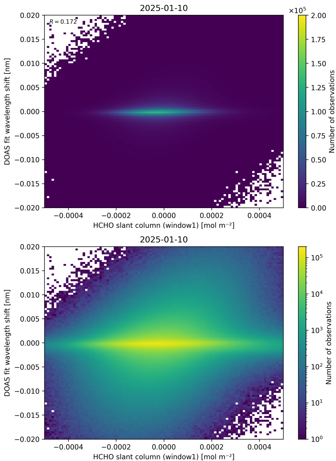
Figure 79: Scatter density plot of “HCHO slant column (window1)” against “DOAS fit wavelength shift” for 2025-01-09 to 2025-01-11.
