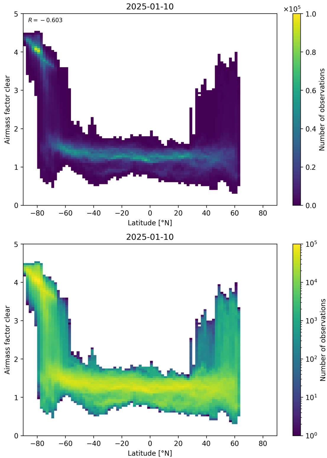
Figure 156: Scatter density plot of “Latitude” against “Airmass factor clear” for 2025-01-09 to 2025-01-11.
