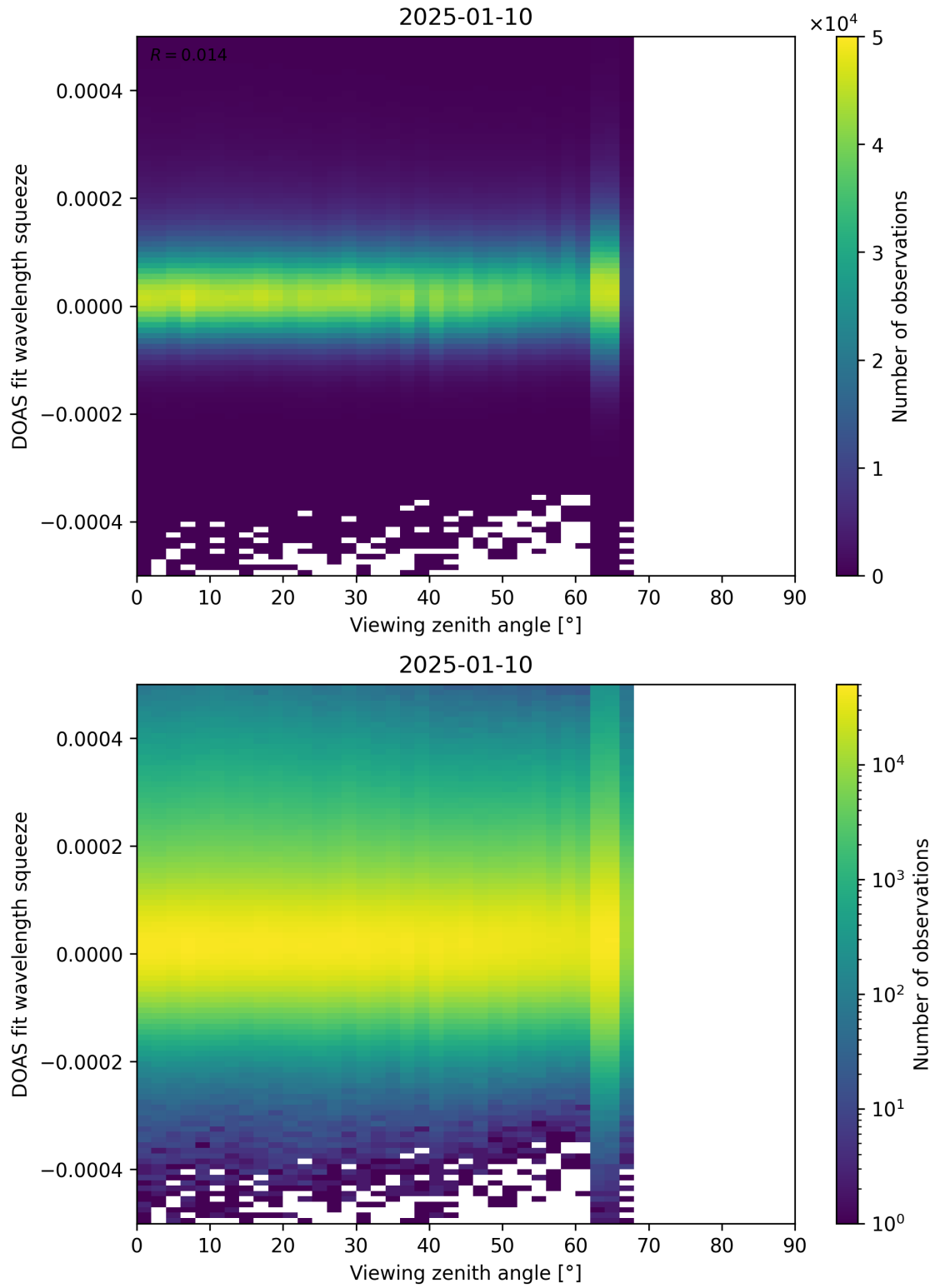
Figure 184: Scatter density plot of “Viewing zenith angle” against “DOAS fit wavelength squeeze” for 2025-01-09 to 2025-01-11.
