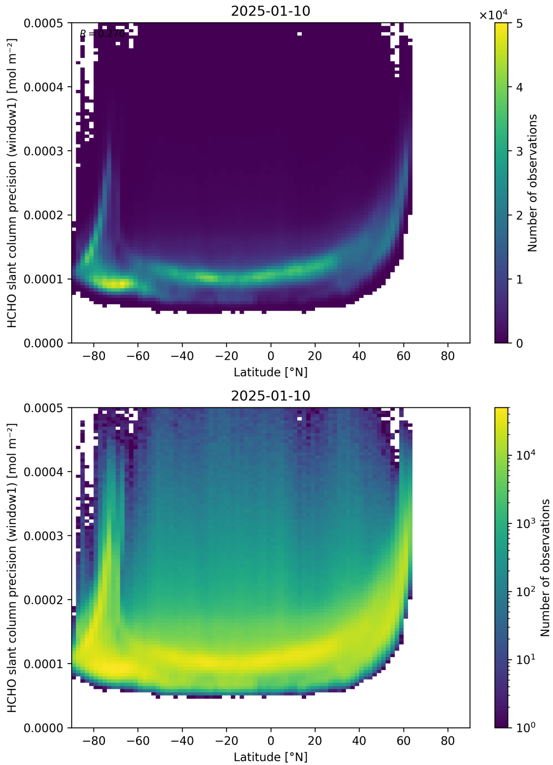
Figure 160: Scatter density plot of “Latitude” against “HCHO slant column precision (window1)” for 2025-01-09 to 2025-01-11.
