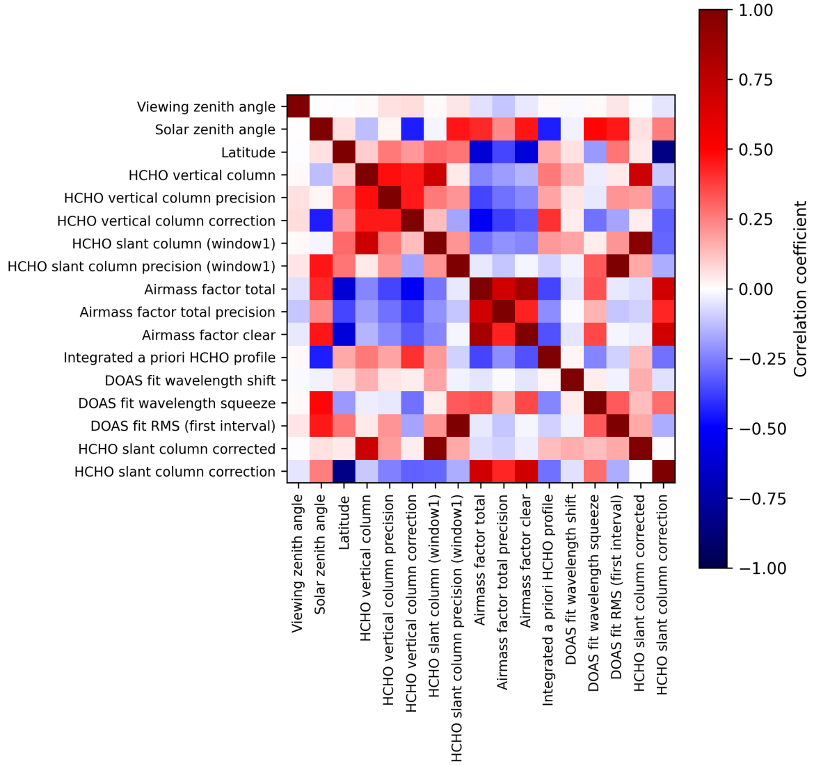
Figure 2: Map of correlation matrix for 2025-01-09 to 2025-01-11.
