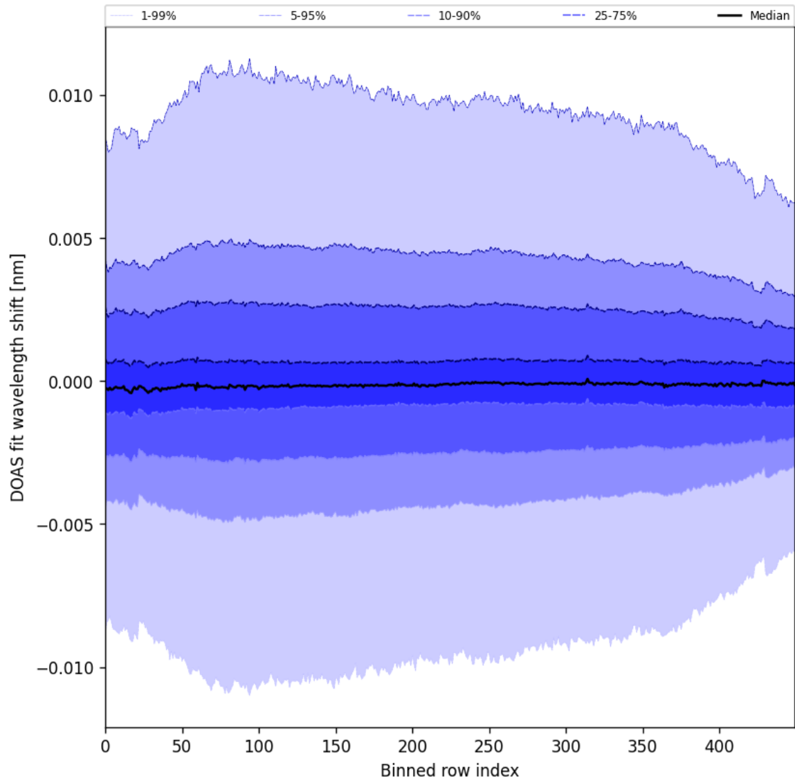
Figure 58: Along track statistics of “DOAS fit wavelength shift” for 2025-01-09 to 2025-01-11
