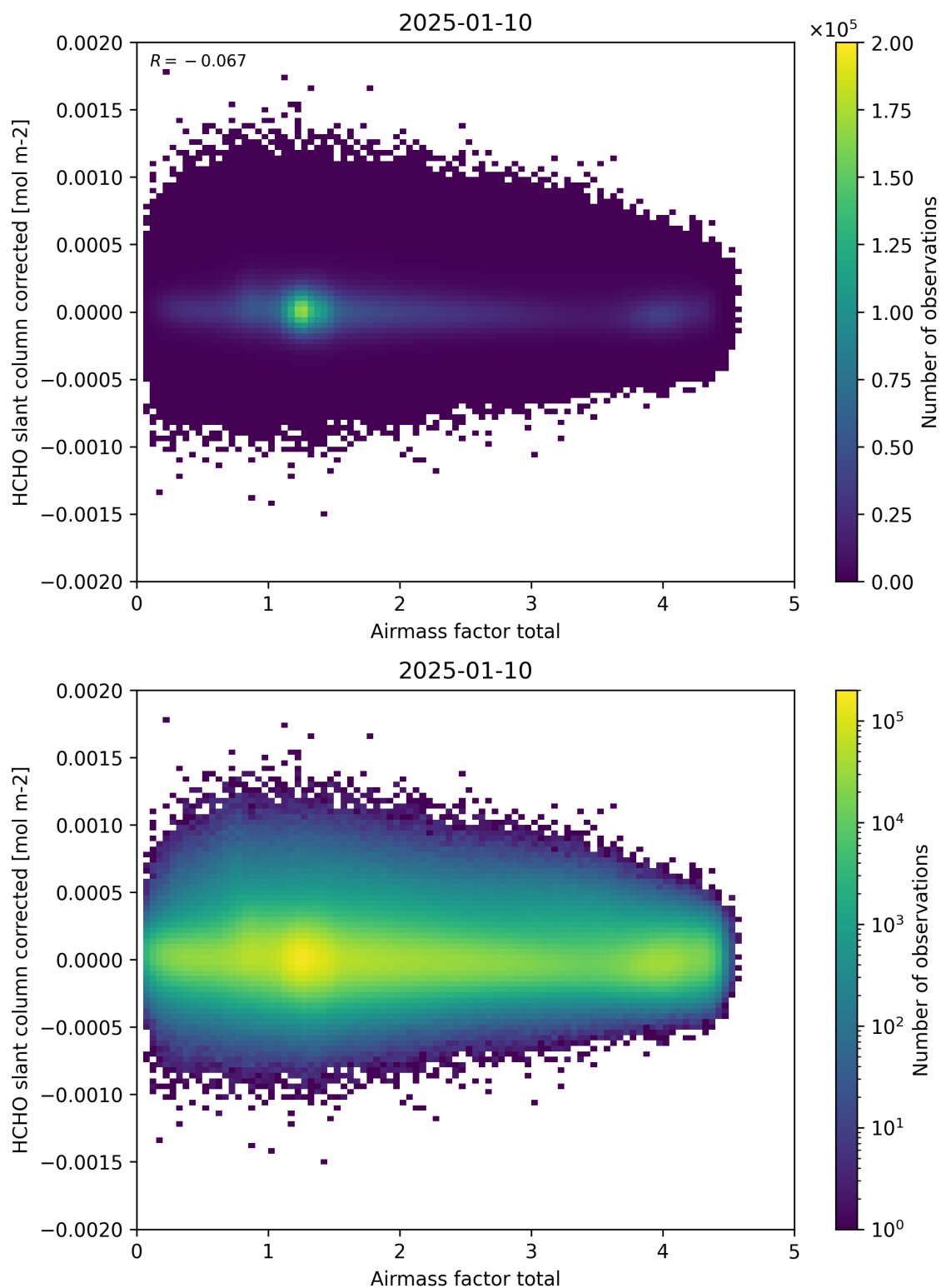
Figure 101: Scatter density plot of “Airmass factor total” against “HCHO slant column corrected” for 2025-01-09 to 2025-01-11.
