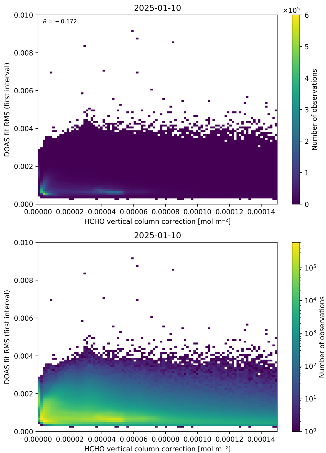
Figure 112: Scatter density plot of “HCHO vertical column correction” against “DOAS fit RMS (first interval)” for 2025-01-09 to 2025-01-11.
