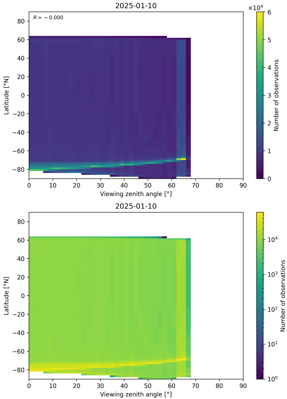
Figure 196: Scatter density plot of “Viewing zenith angle” against “Latitude” for 2025-01-09 to 2025-01-11.
