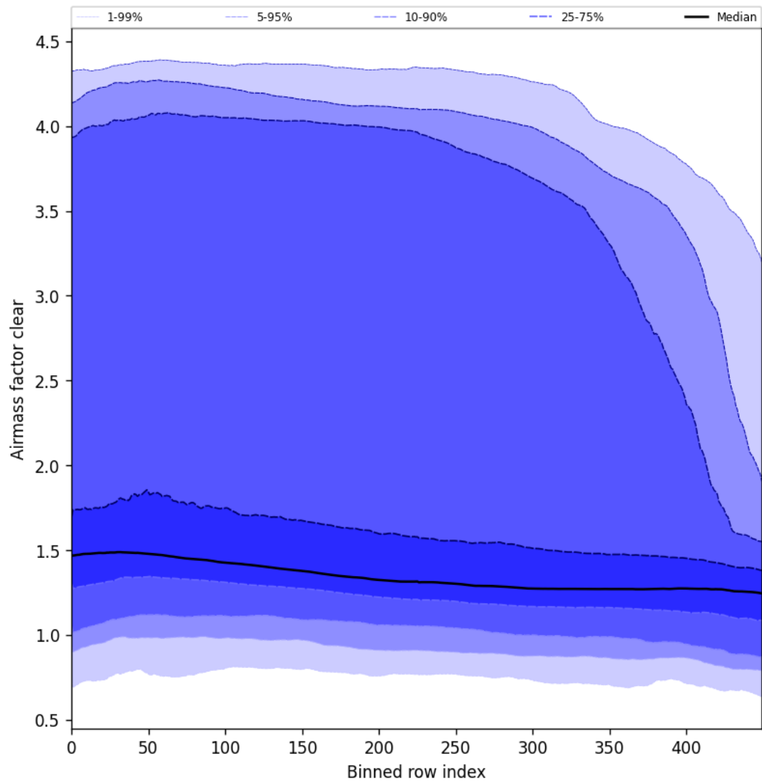
Figure 56: Along track statistics of “Airmass factor clear” for 2025-01-09 to 2025-01-11
