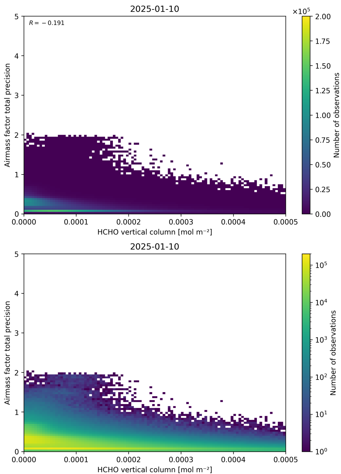
Figure 132: Scatter density plot of “HCHO vertical column” against “Airmass factor total precision” for 2025-01-09 to 2025-01-11.
