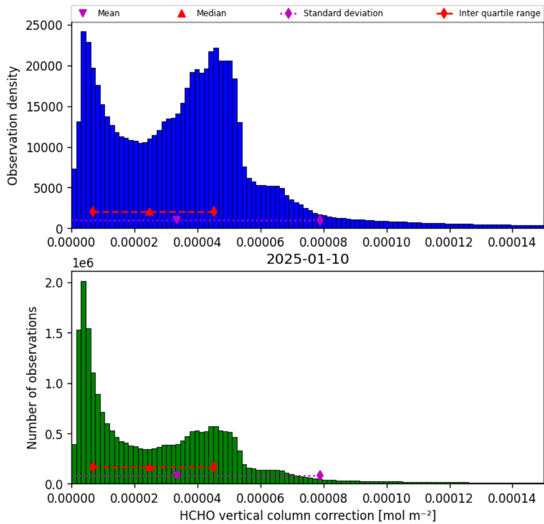
Figure 37: Histogram of “HCHO vertical column correction” for 2025-01-09 to 2025-01-11
