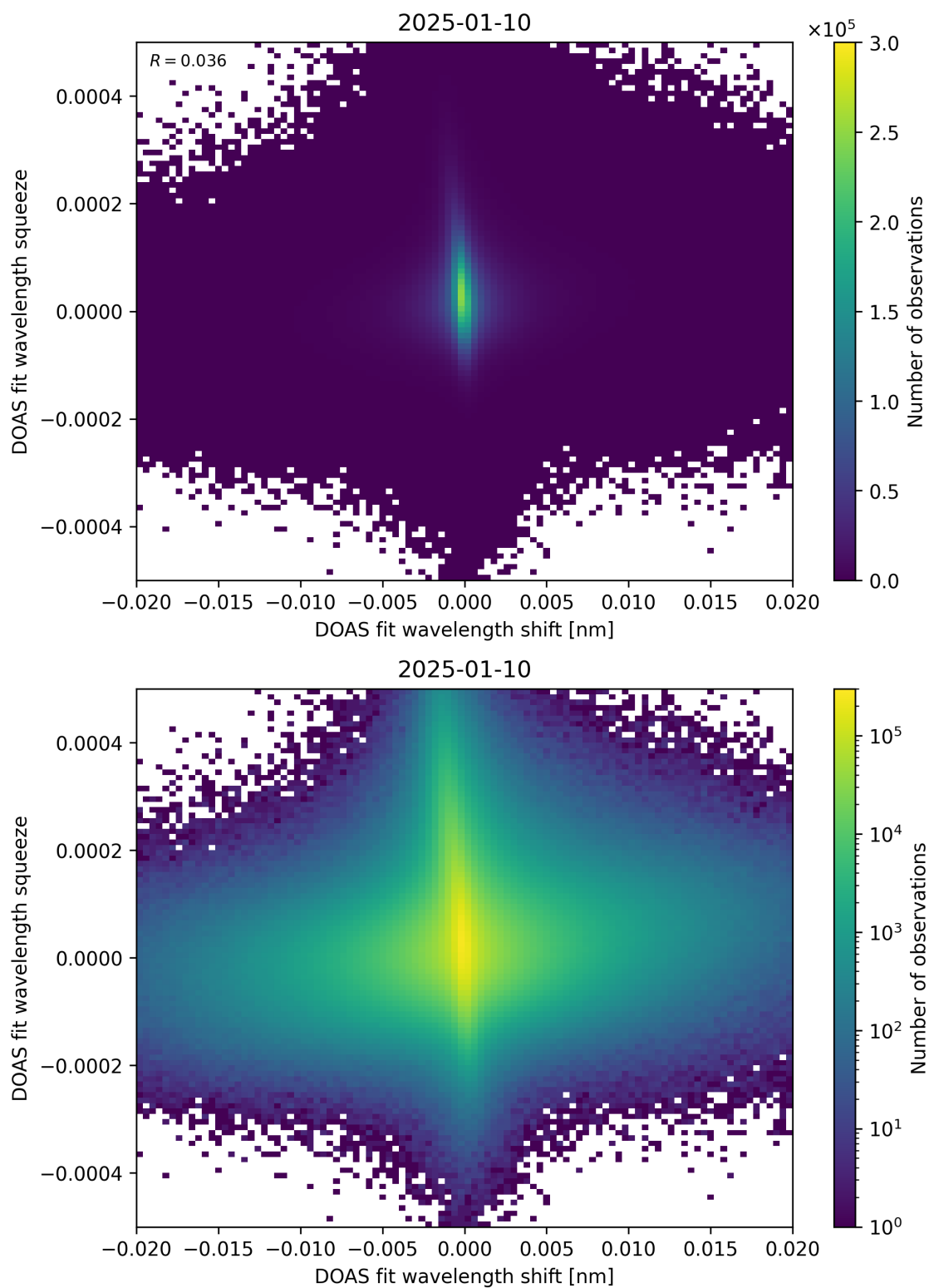
Figure 65: Scatter density plot of “DOAS fit wavelength shift” against “DOAS fit wavelength squeeze” for 2025-01-09 to 2025-01-11.
