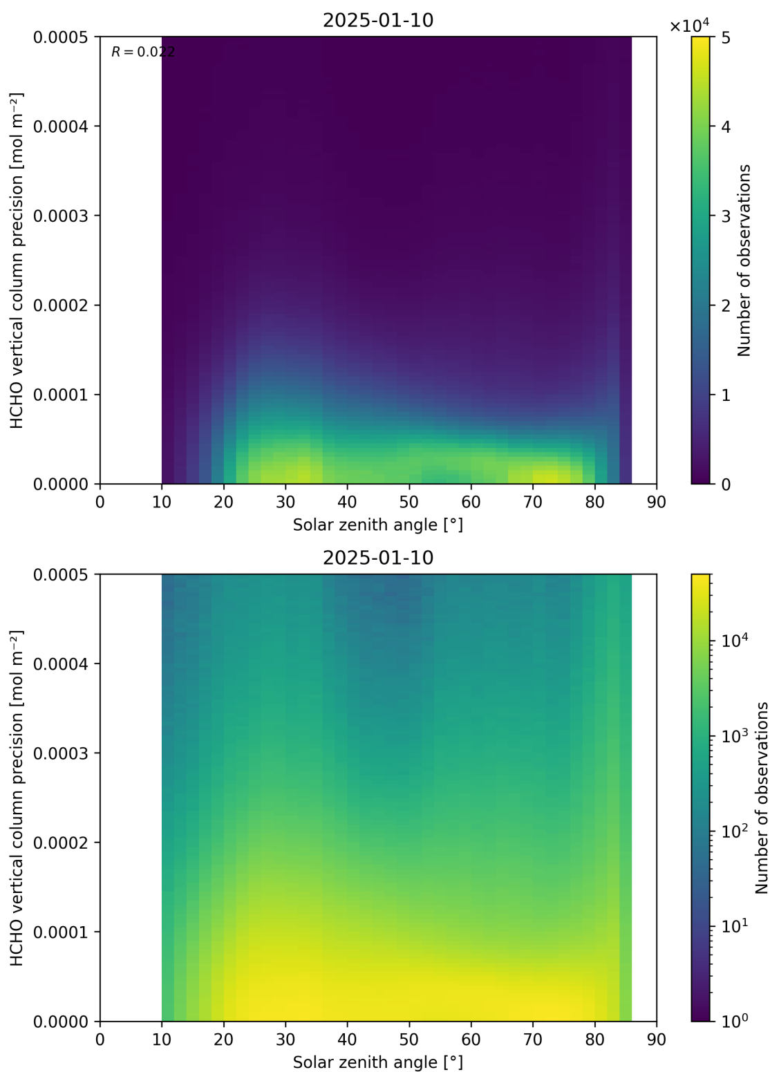
Figure 179: Scatter density plot of “Solar zenith angle” against “HCHO vertical column precision” for 2025-01-09 to 2025-01-11.
