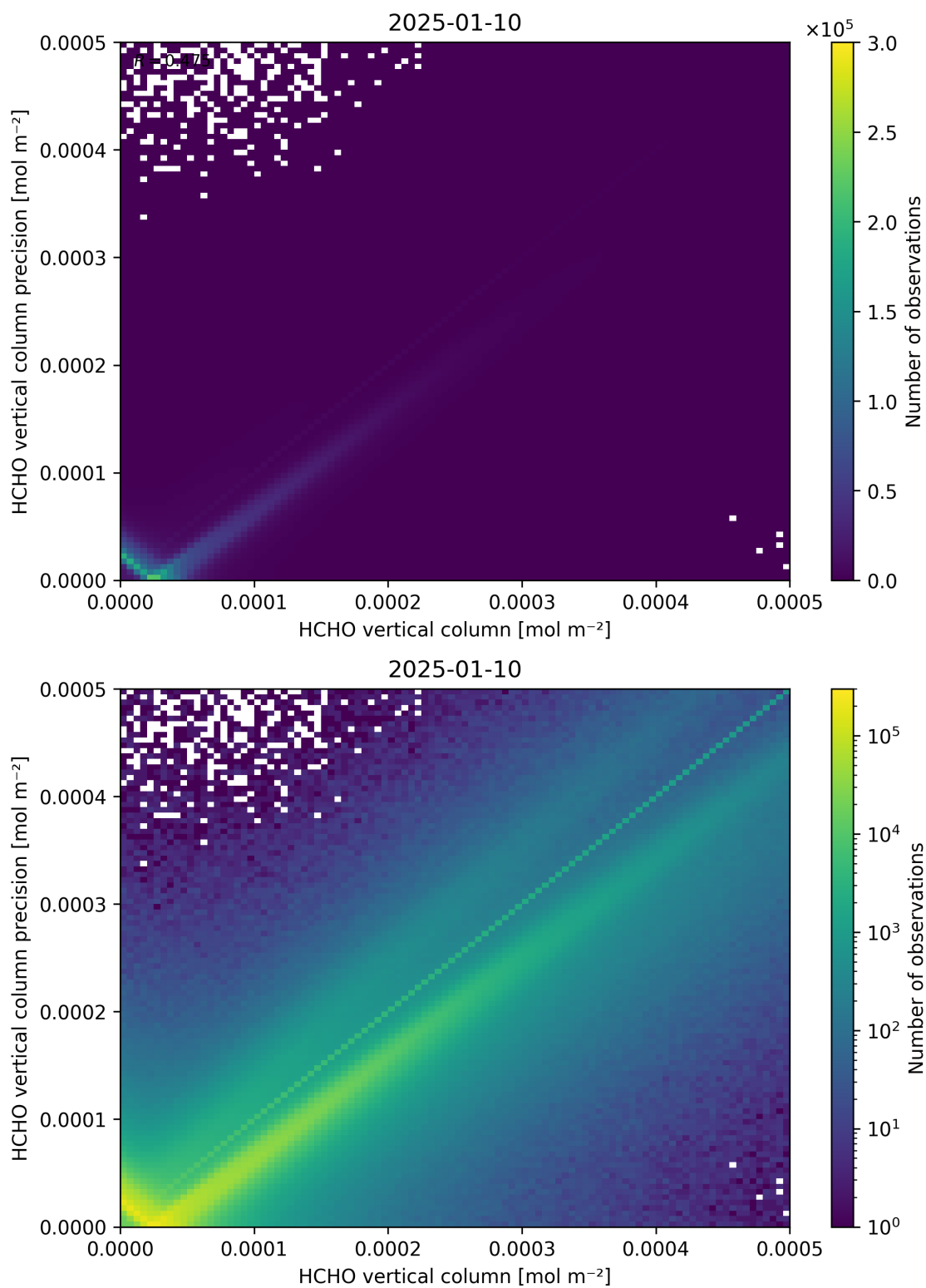
Figure 134: Scatter density plot of “HCHO vertical column” against “HCHO vertical column precision” for 2025-01-09 to 2025-01-11.
