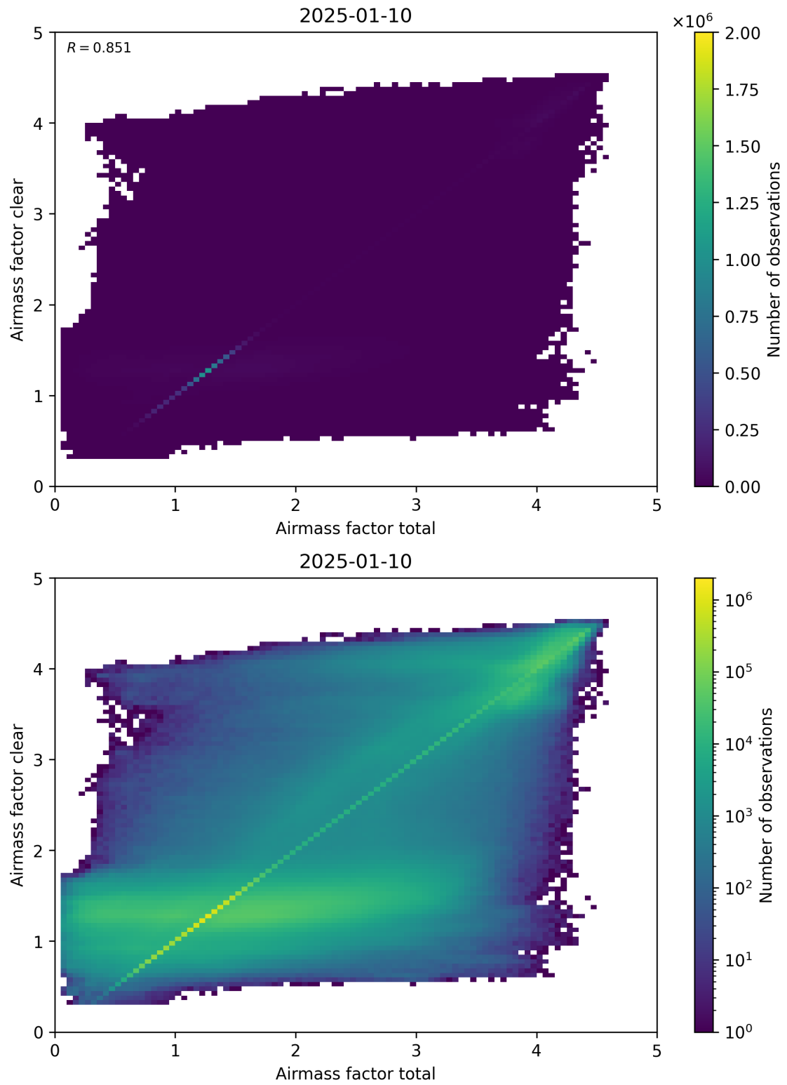
Figure 100: Scatter density plot of “Airmass factor total” against “Airmass factor clear” for 2025-01-09 to 2025-01-11.
