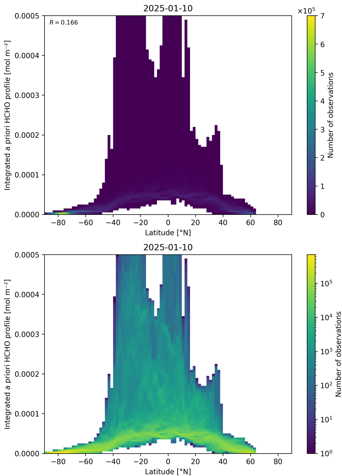
Figure 166: Scatter density plot of “Latitude” against “Integrated a priori HCHO profile” for 2025-01-09 to 2025-01-11.
