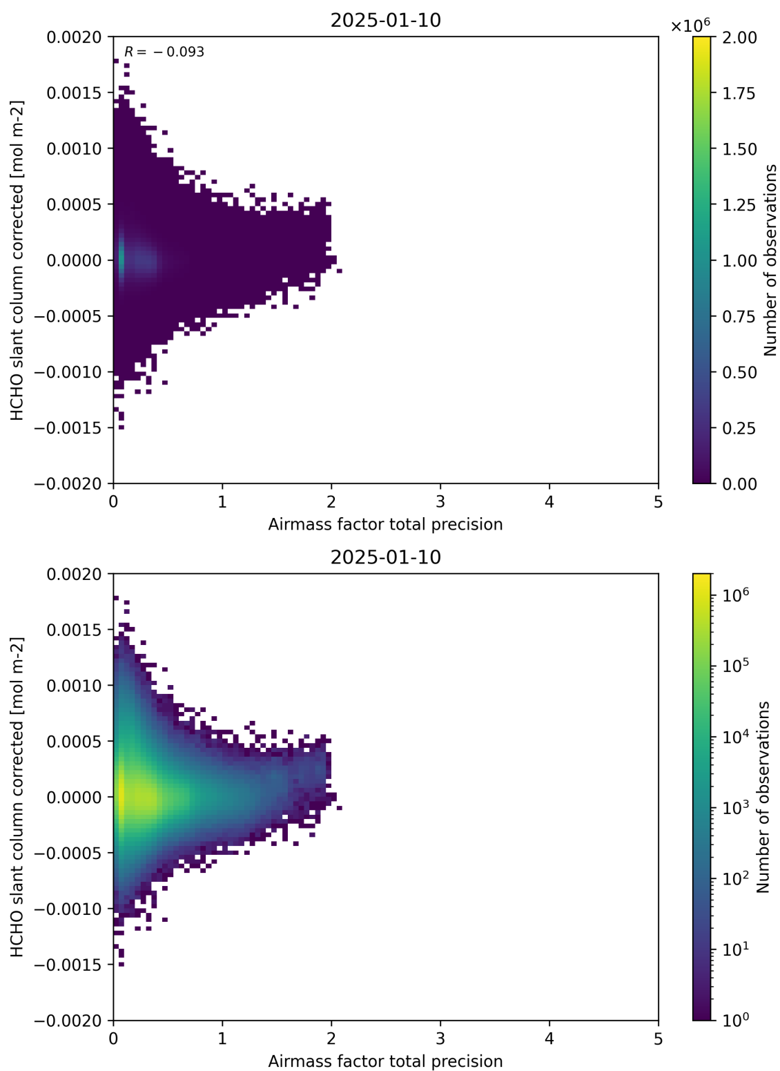
Figure 109: Scatter density plot of “Airmass factor total precision” against “HCHO slant column corrected” for 2025-01-09 to 2025-01-11.
