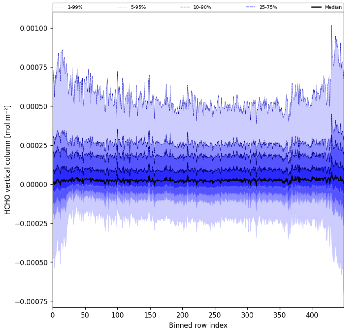
Figure 49: Along track statistics of “HCHO vertical column” for 2025-01-09 to 2025-01-11
