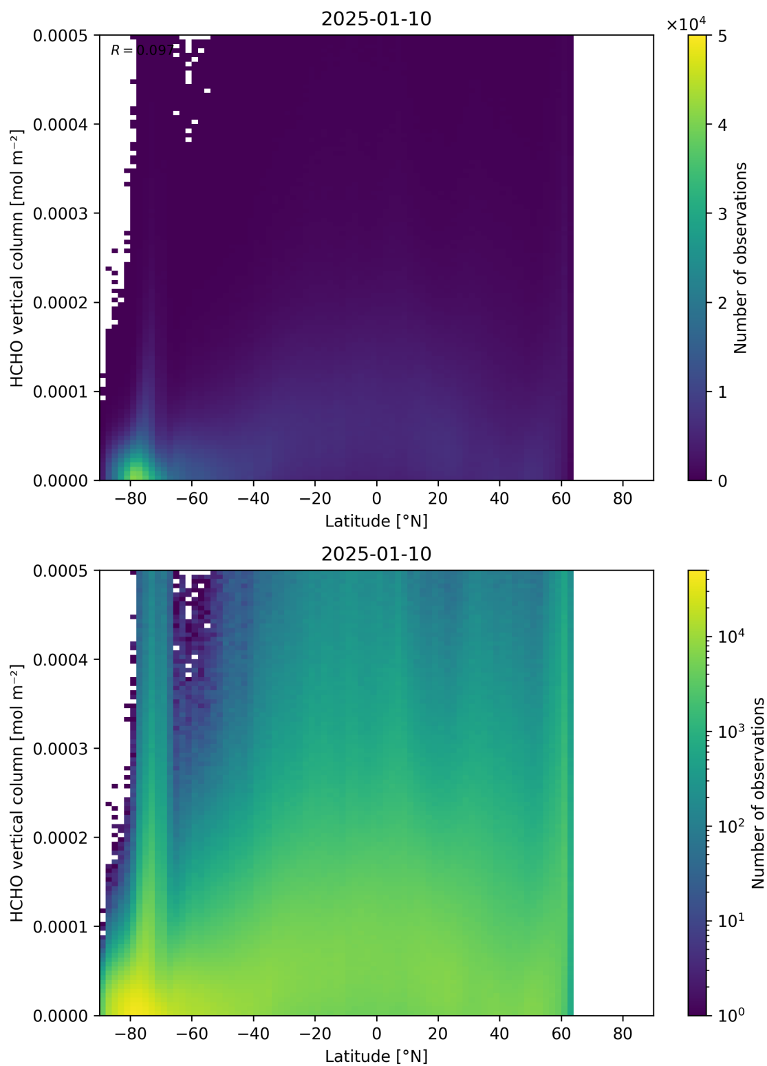
Figure 163: Scatter density plot of “Latitude” against “HCHO vertical column” for 2025-01-09 to 2025-01-11.
