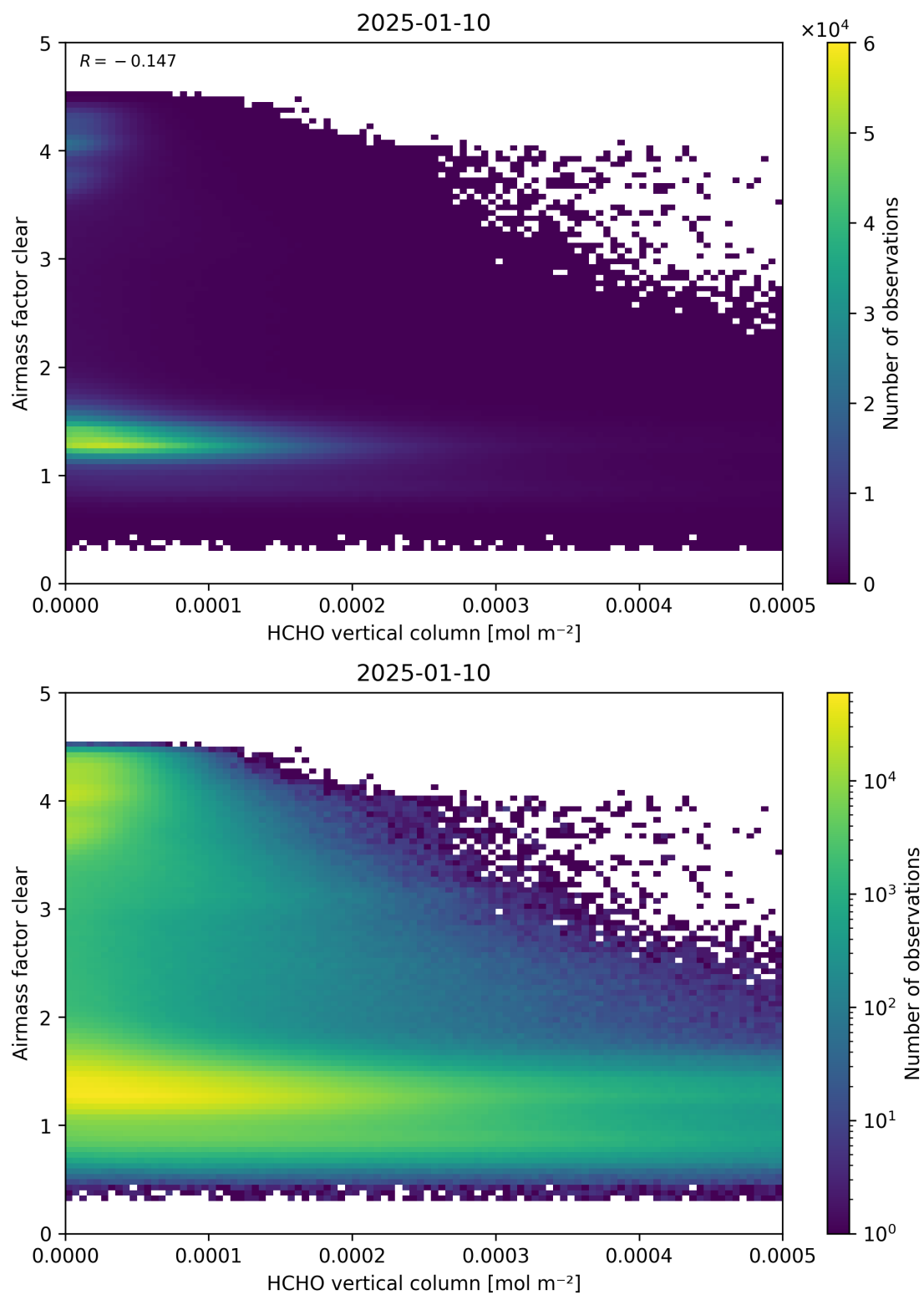
Figure 126: Scatter density plot of “HCHO vertical column” against “Airmass factor clear” for 2025-01-09 to 2025-01-11.
