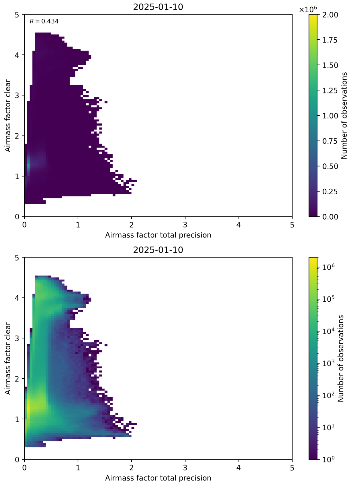
Figure 108: Scatter density plot of “Airmass factor total precision” against “Airmass factor clear” for 2025-01-09 to 2025-01-11.
