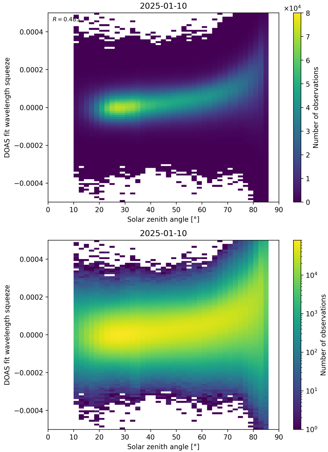
Figure 169: Scatter density plot of “Solar zenith angle” against “DOAS fit wavelength squeeze” for 2025-01-09 to 2025-01-11.
