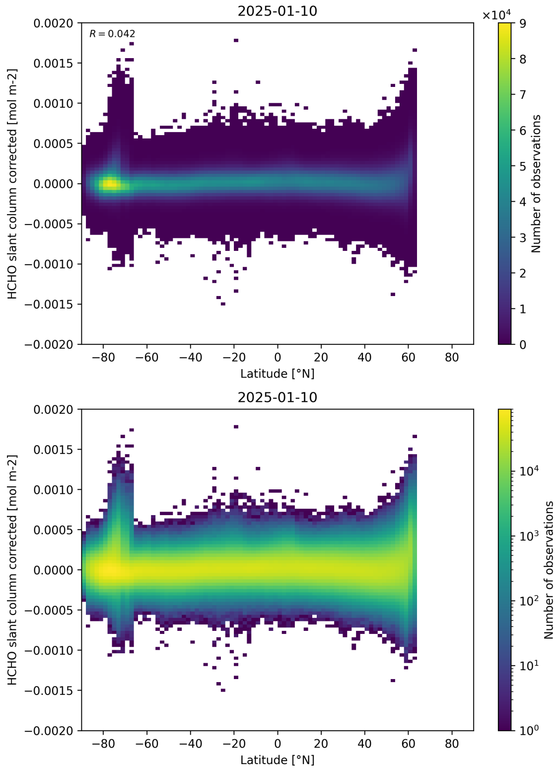
Figure 157: Scatter density plot of “Latitude” against “HCHO slant column corrected” for 2025-01-09 to 2025-01-11.
