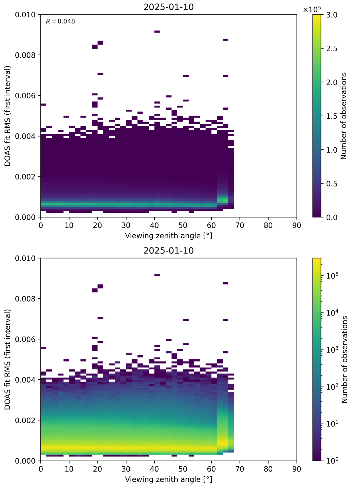
Figure 182: Scatter density plot of “Viewing zenith angle” against “DOAS fit RMS (first interval)” for 2025-01-09 to 2025-01-11.
