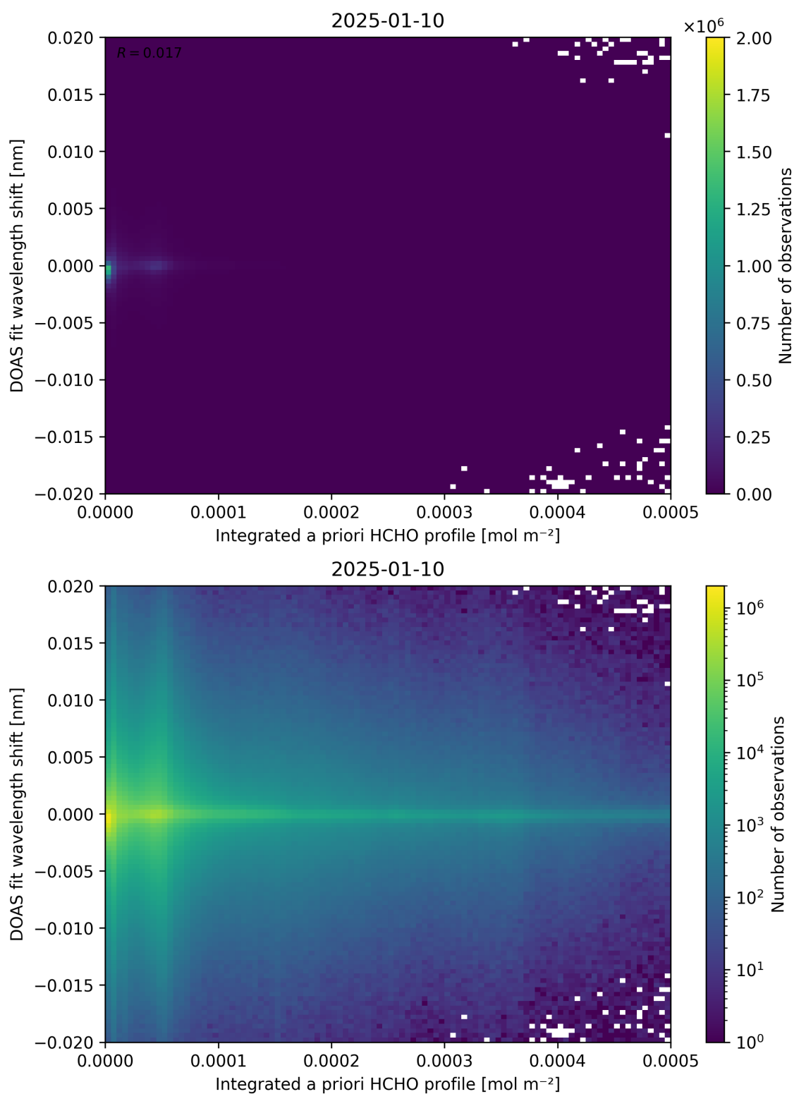
Figure 149: Scatter density plot of “Integrated a priori HCHO profile” against “DOAS fit wavelength shift” for 2025-01-09 to 2025-01-11.
