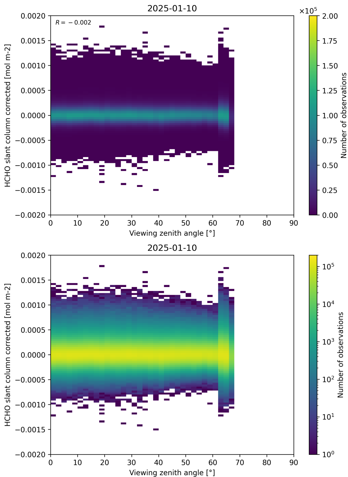
Figure 186: Scatter density plot of “Viewing zenith angle” against “HCHO slant column corrected” for 2025-01-09 to 2025-01-11.
