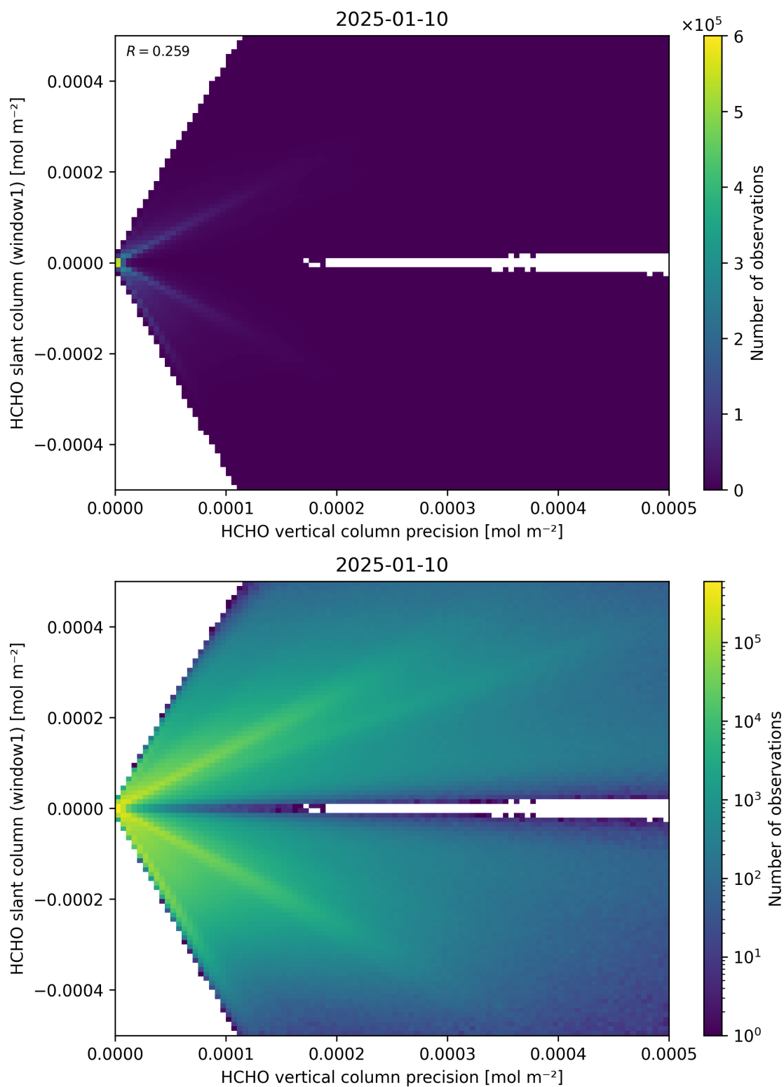
Figure 142: Scatter density plot of “HCHO vertical column precision” against “HCHO slant column (window1)” for 2025-01-09 to 2025-01-11.
