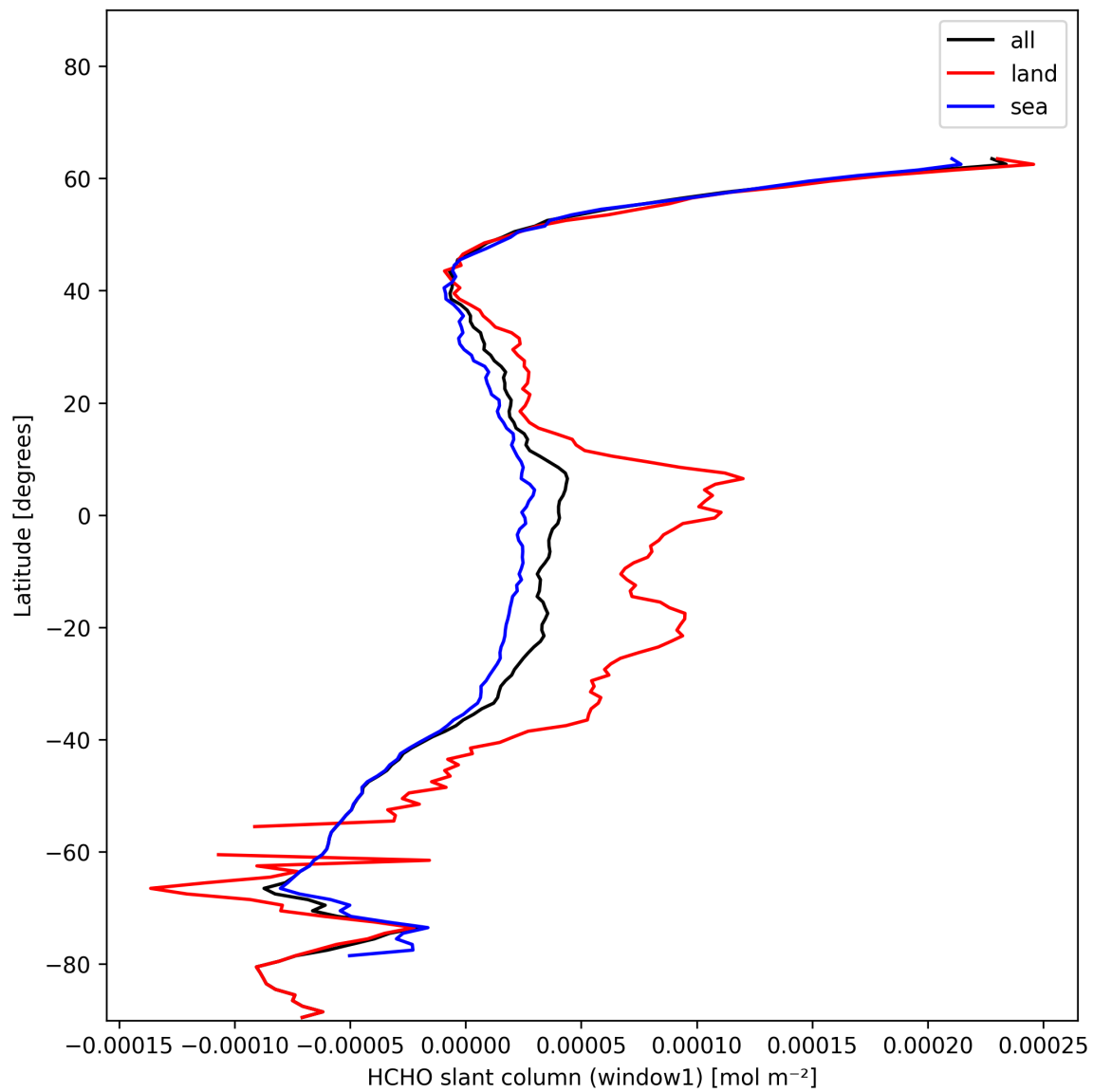
Figure 24: Zonal average of “HCHO slant column (window1)” for 2025-01-09 to 2025-01-11.
