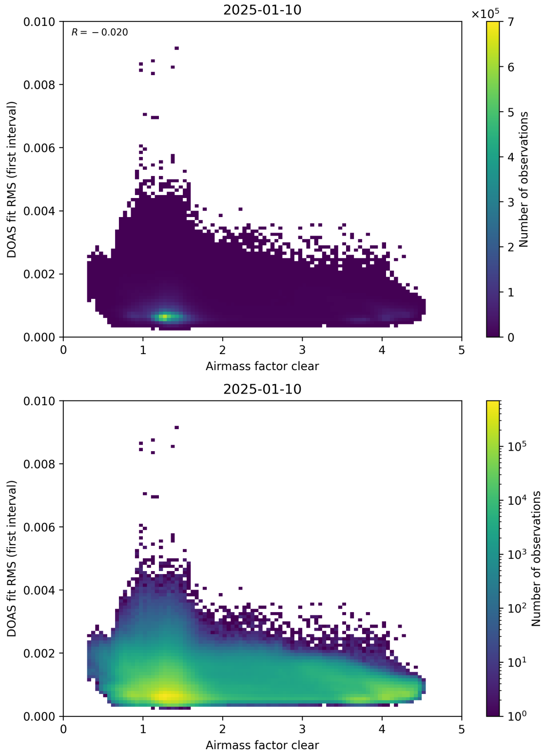
Figure 71: Scatter density plot of “Airmass factor clear” against “DOAS fit RMS (first interval)” for 2025-01-09 to 2025-01-11.
