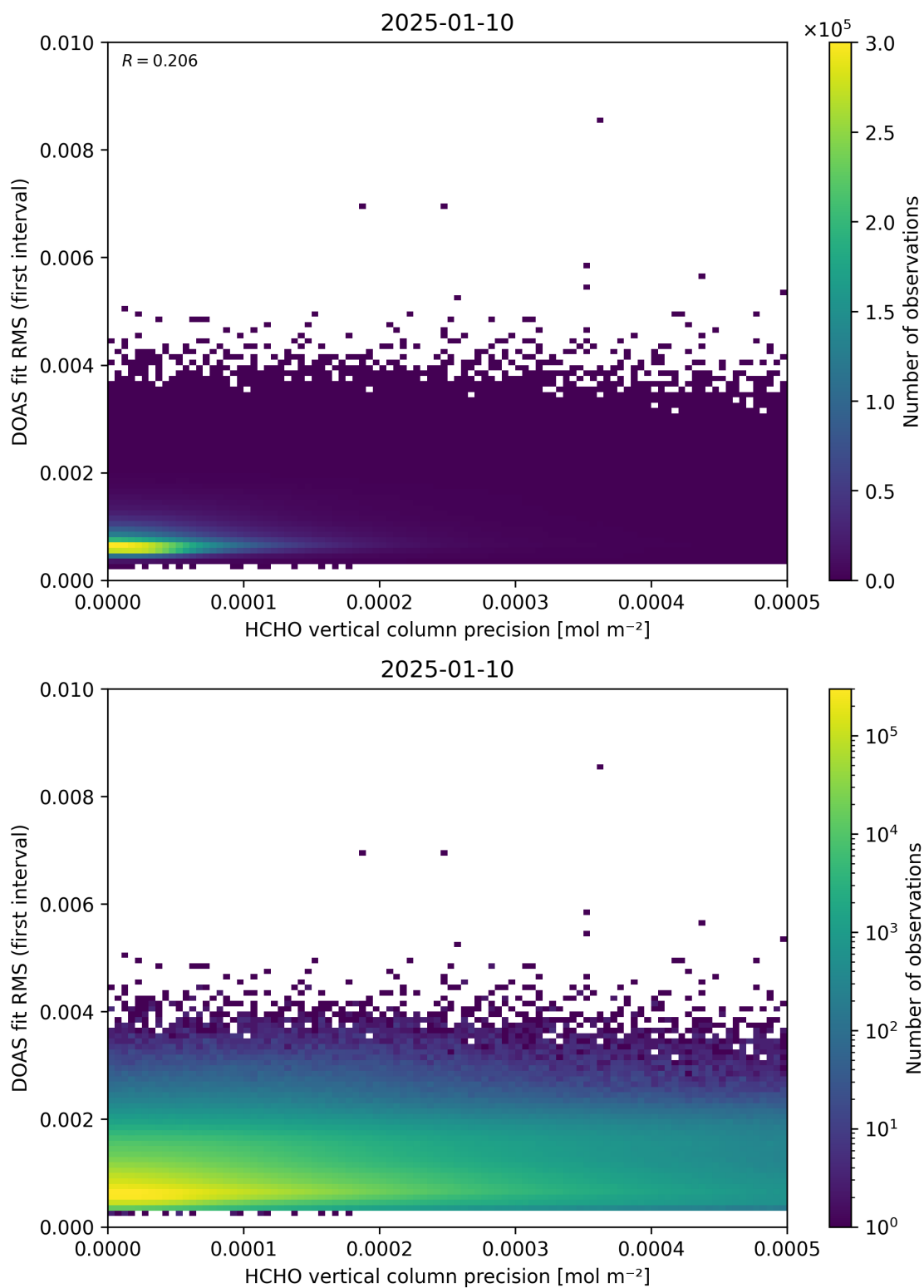
Figure 136: Scatter density plot of “HCHO vertical column precision” against “DOAS fit RMS (first interval)” for 2025-01-09 to 2025-01-11.
