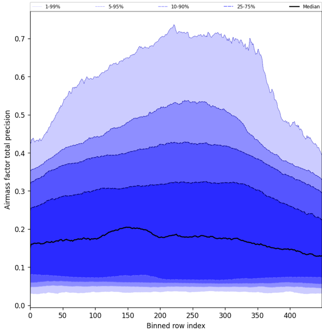
Figure 55: Along track statistics of “Airmass factor total precision” for 2025-01-09 to 2025-01-11
