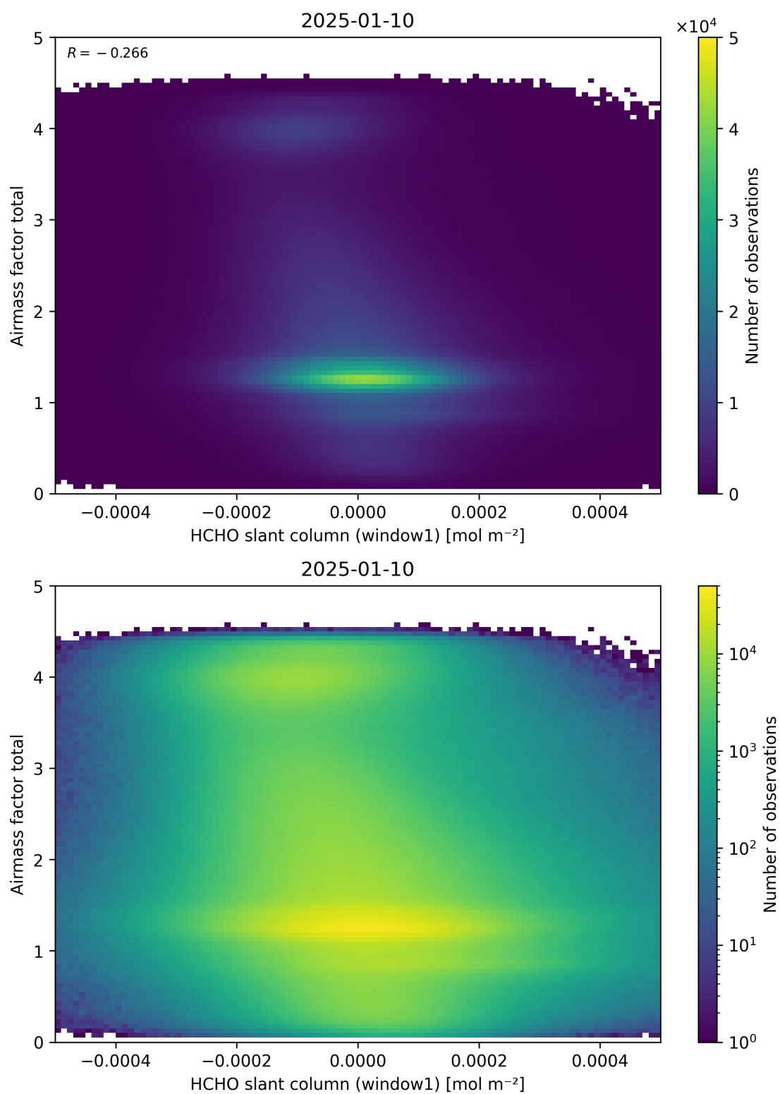
Figure 85: Scatter density plot of “HCHO slant column (window1)” against “Airmass factor total” for 2025-01-09 to 2025-01-11.
