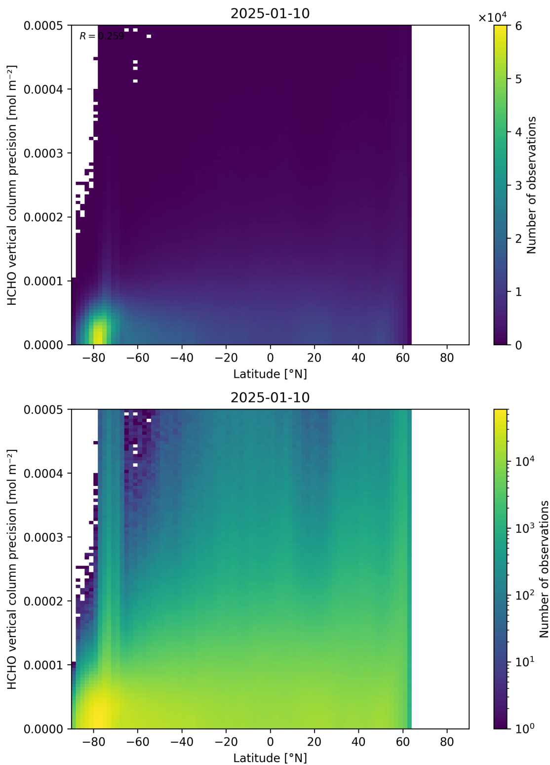
Figure 165: Scatter density plot of “Latitude” against “HCHO vertical column precision” for 2025-01-09 to 2025-01-11.
