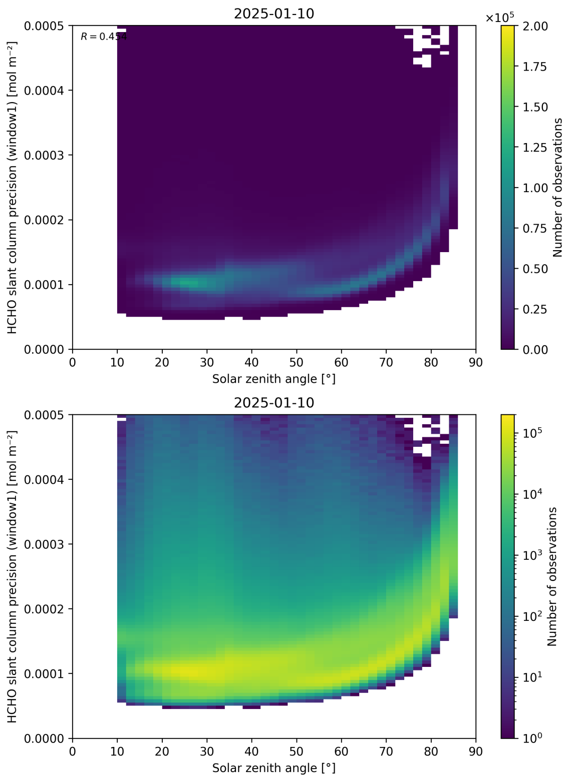
Figure 174: Scatter density plot of “Solar zenith angle” against “HCHO slant column precision (window1)” for 2025-01-09 to 2025-01-11.
