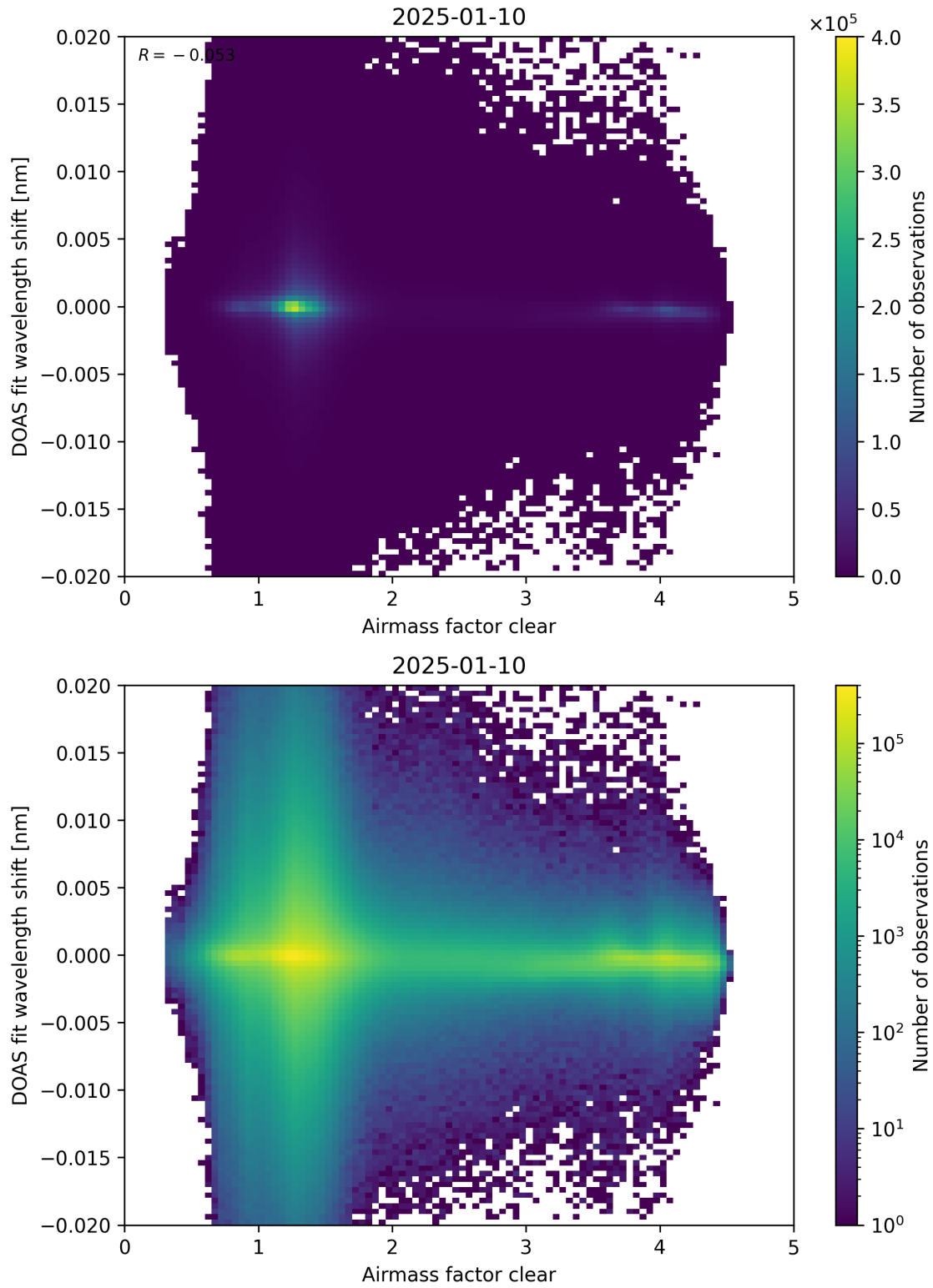
Figure 72: Scatter density plot of “Airmass factor clear” against “DOAS fit wavelength shift” for 2025-01-09 to 2025-01-11.
