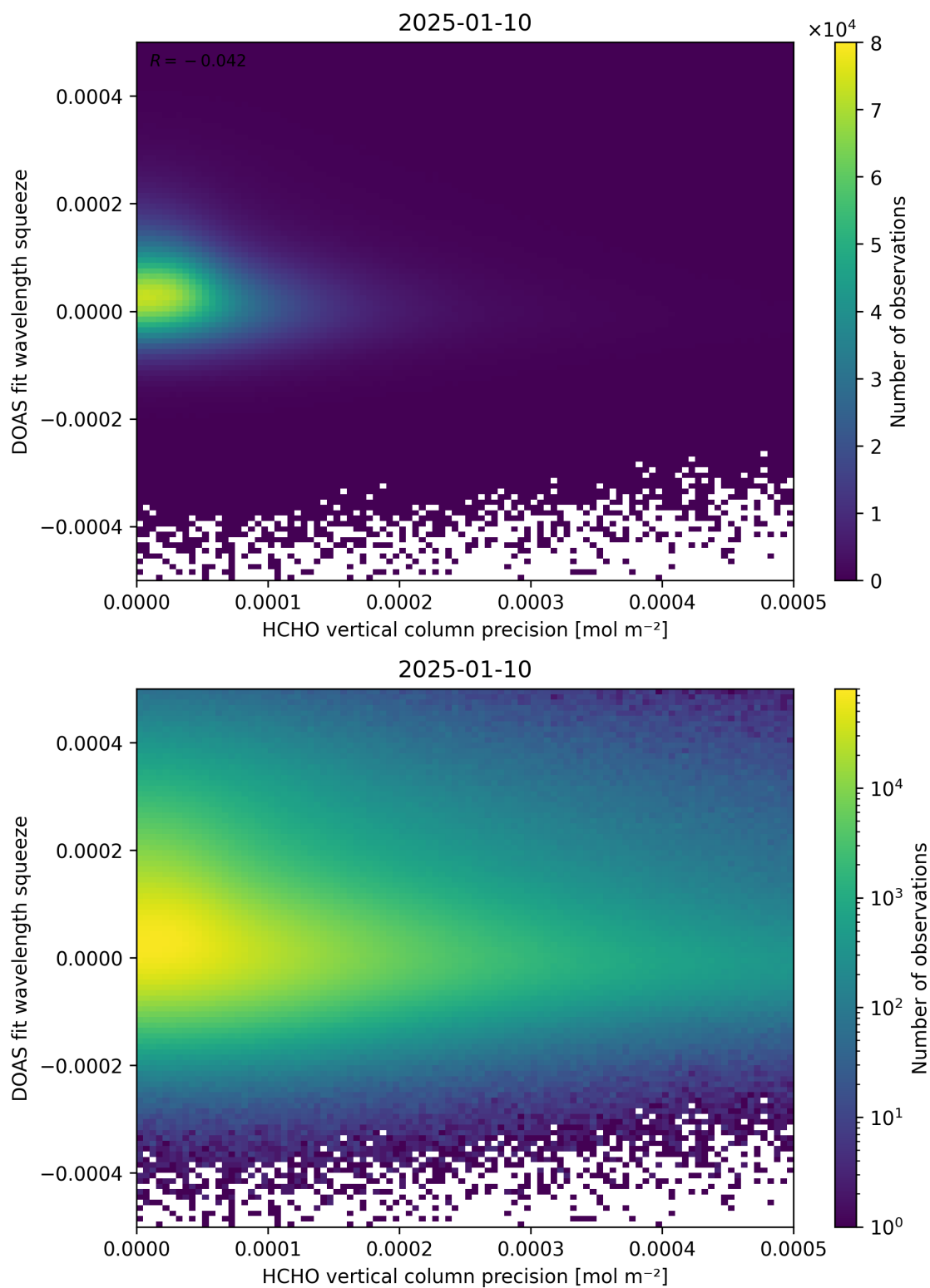
Figure 138: Scatter density plot of “HCHO vertical column precision” against “DOAS fit wavelength squeeze” for 2025-01-09 to 2025-01-11.
