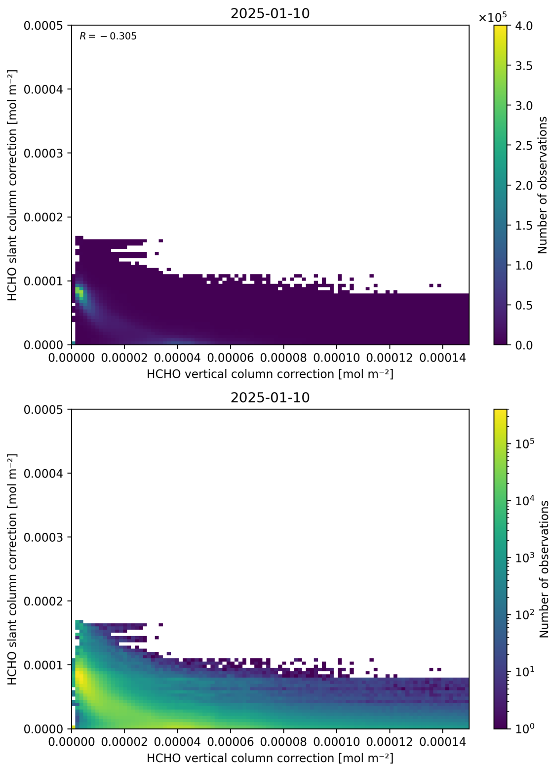
Figure 117: Scatter density plot of “HCHO vertical column correction” against “HCHO slant column correction” for 2025-01-09 to 2025-01-11.
