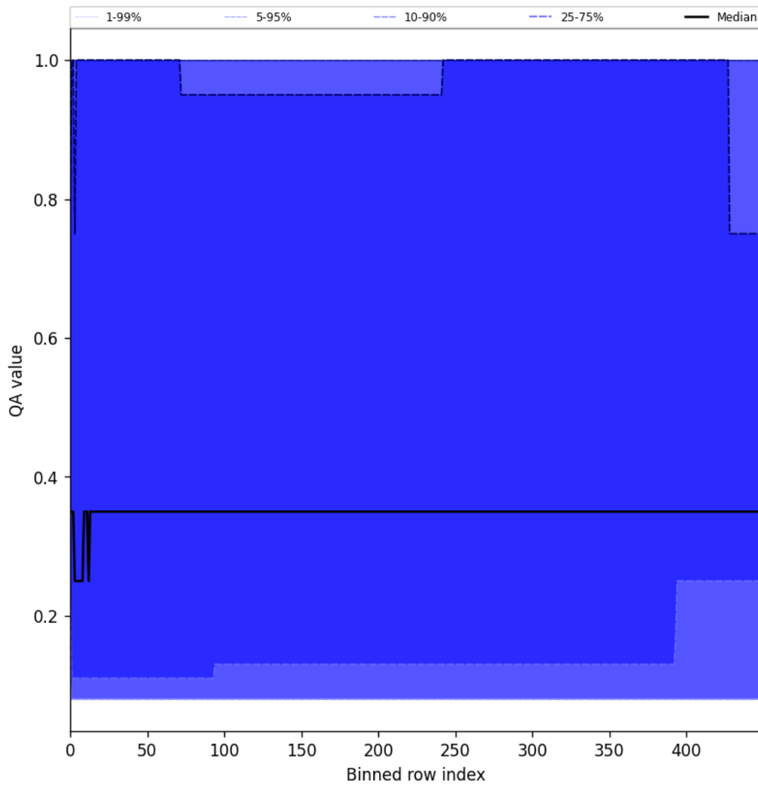
Figure 48: Along track statistics of “QA value” for 2025-01-09 to 2025-01-11
