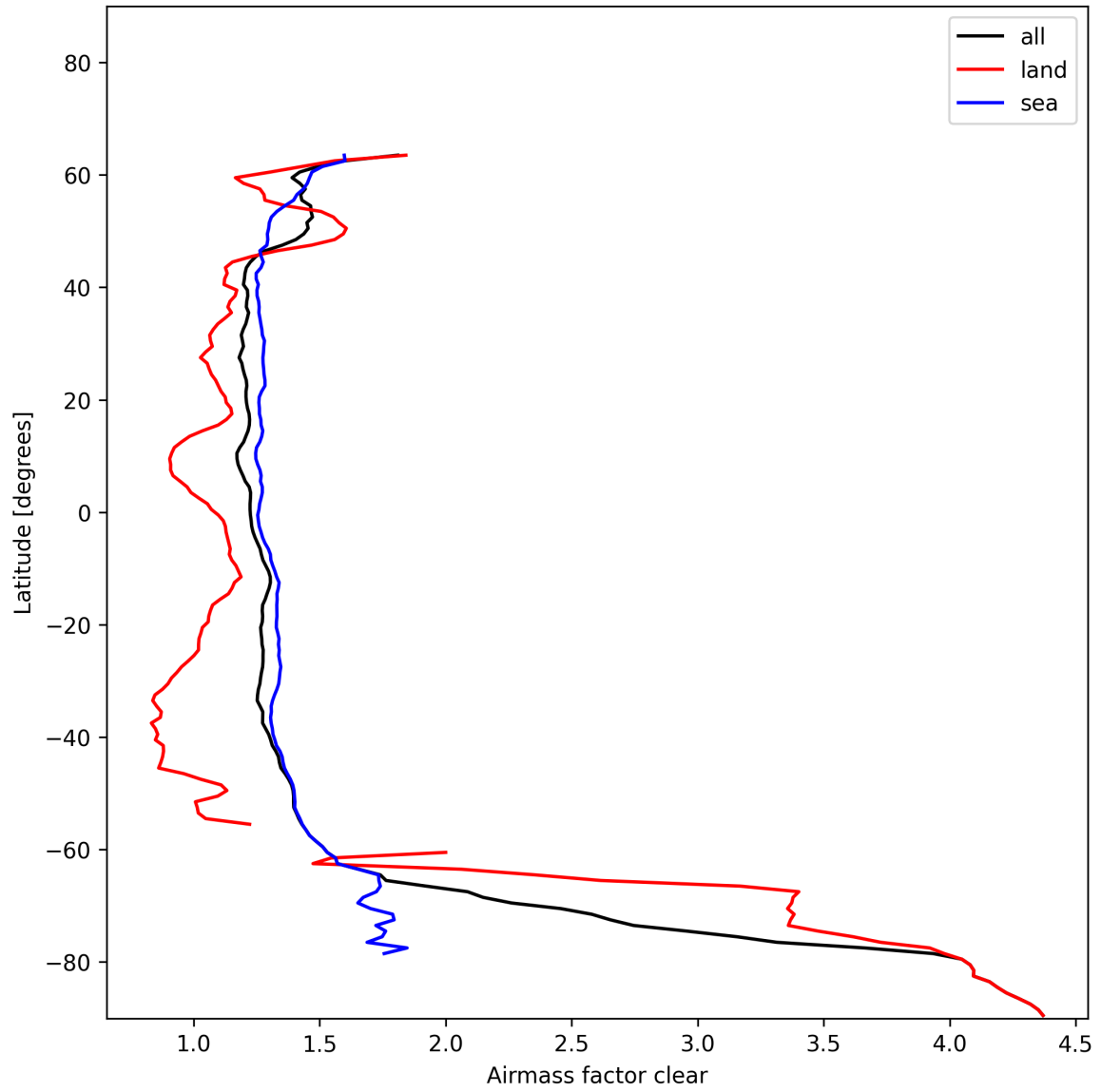
Figure 28: Zonal average of “Airmass factor clear” for 2025-01-09 to 2025-01-11.
