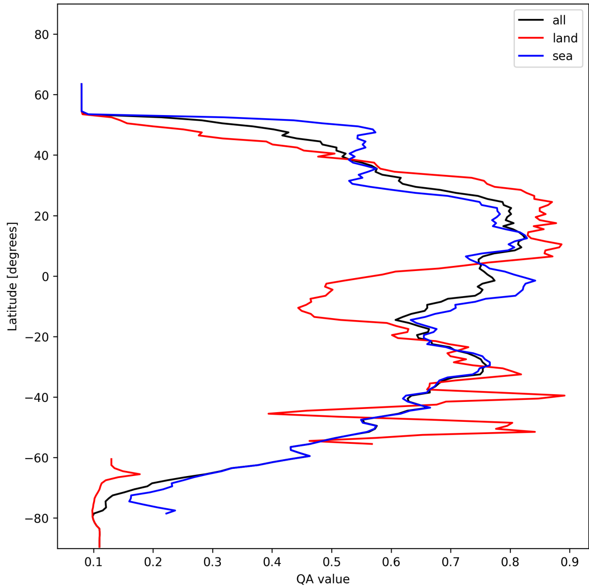
Figure 20: Zonal average of “QA value” for 2025-01-09 to 2025-01-11.
