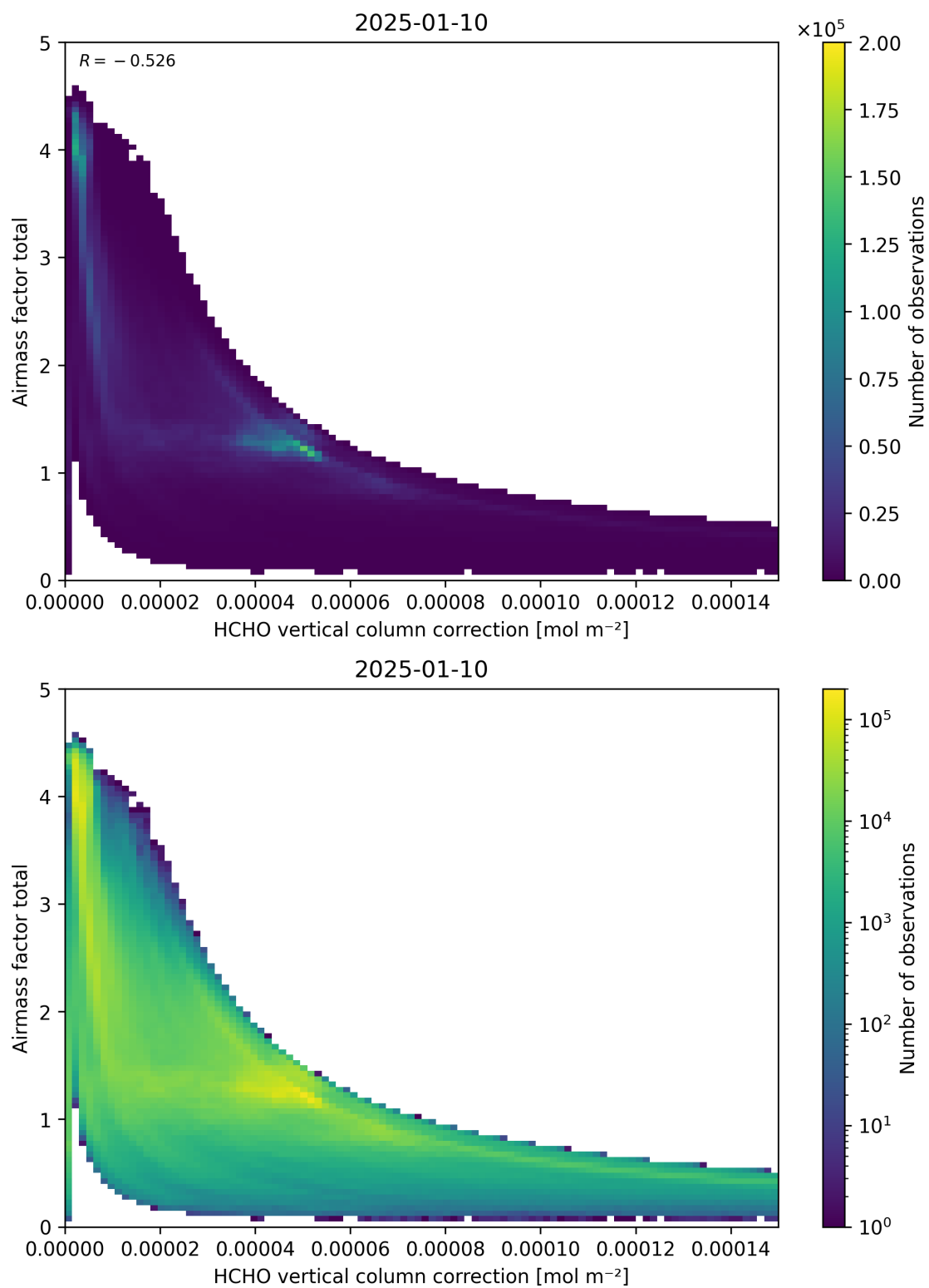
Figure 120: Scatter density plot of “HCHO vertical column correction” against “Airmass factor total” for 2025-01-09 to 2025-01-11.
