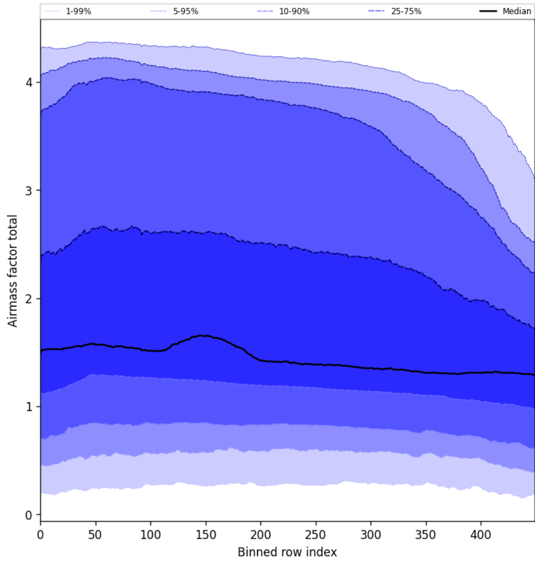
Figure 54: Along track statistics of “Airmass factor total” for 2025-01-09 to 2025-01-11
