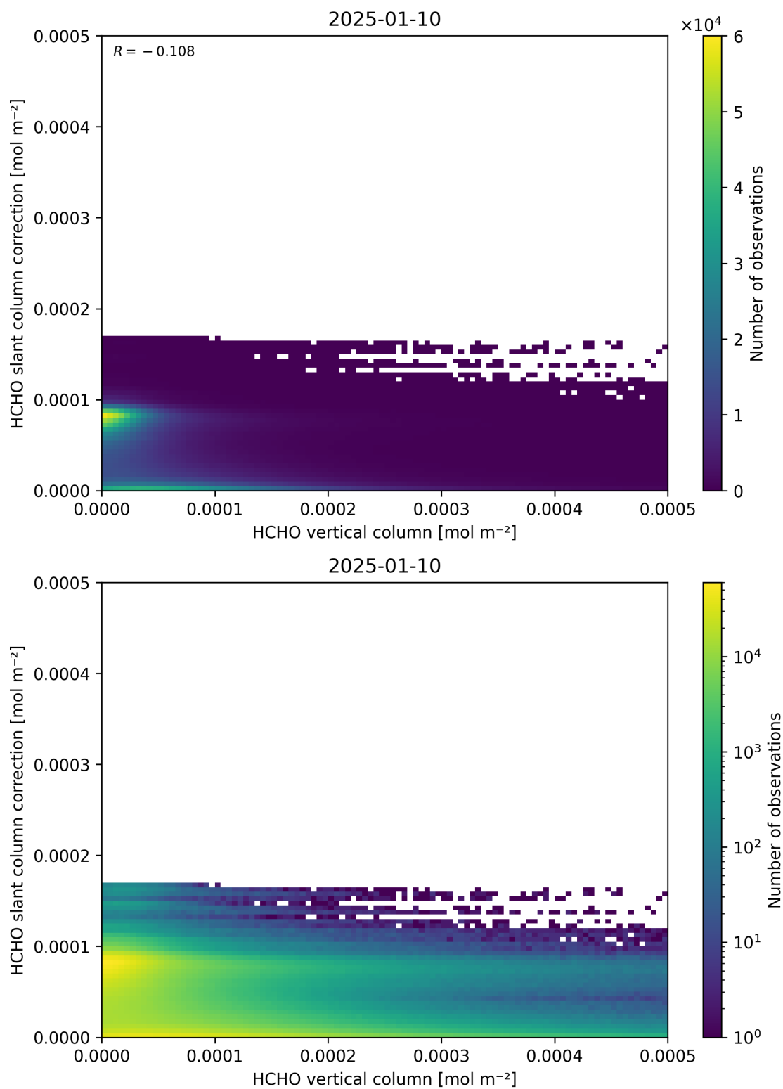
Figure 128: Scatter density plot of “HCHO vertical column” against “HCHO slant column correction” for 2025-01-09 to 2025-01-11.
