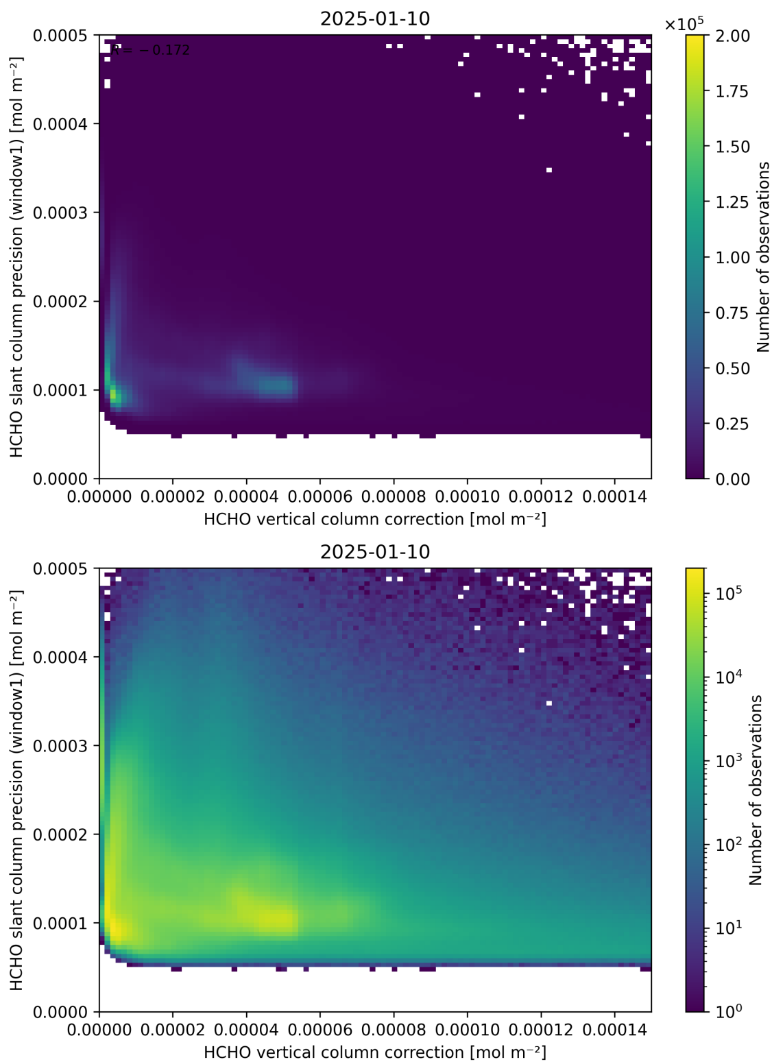
Figure 119: Scatter density plot of “HCHO vertical column correction” against “HCHO slant column precision (window1)” for 2025-01-09 to 2025-01-11.
