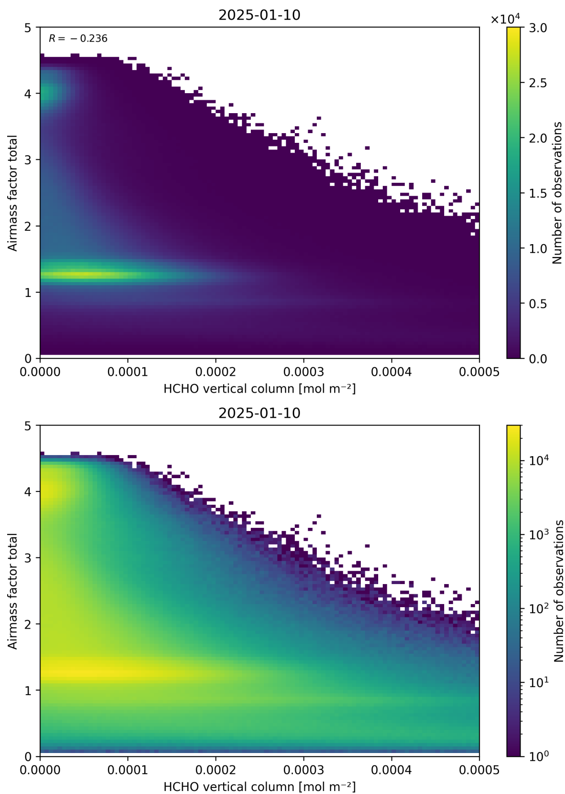
Figure 131: Scatter density plot of “HCHO vertical column” against “Airmass factor total” for 2025-01-09 to 2025-01-11.
