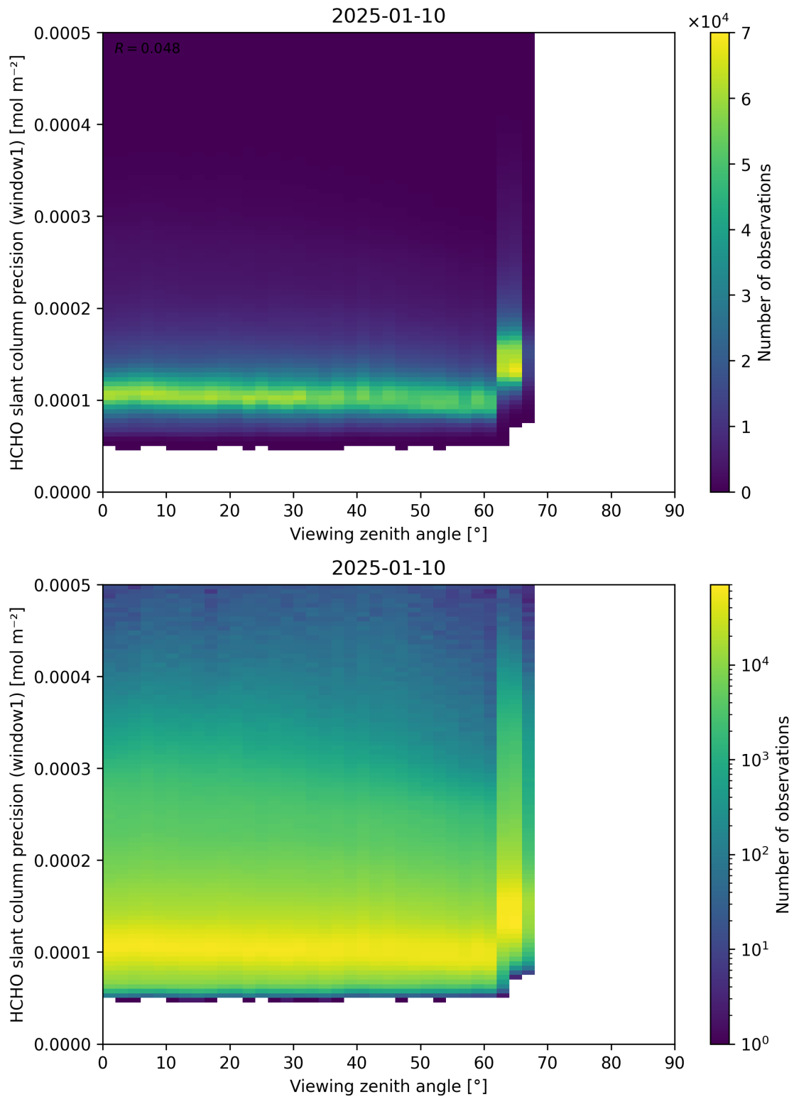
Figure 189: Scatter density plot of “Viewing zenith angle” against “HCHO slant column precision (window1)” for 2025-01-09 to 2025-01-11.
