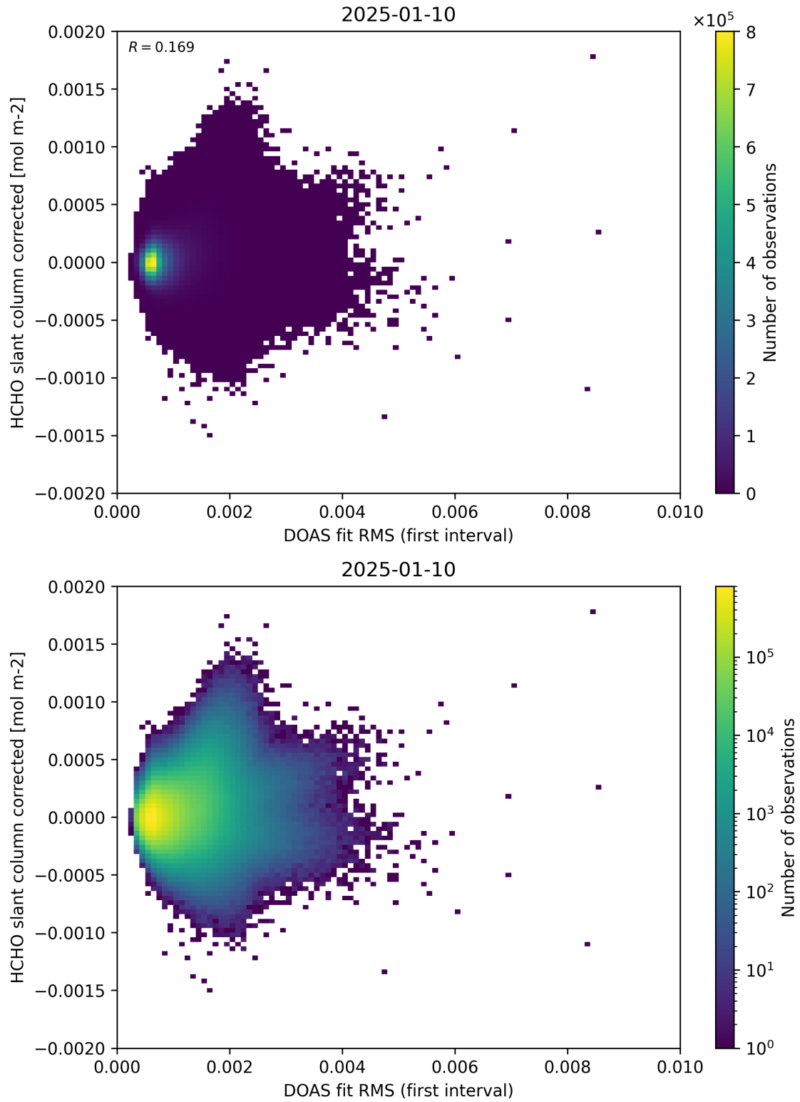
Figure 62: Scatter density plot of “DOAS fit RMS (first interval)” against “HCHO slant column corrected” for 2025-01-09 to 2025-01-11.
