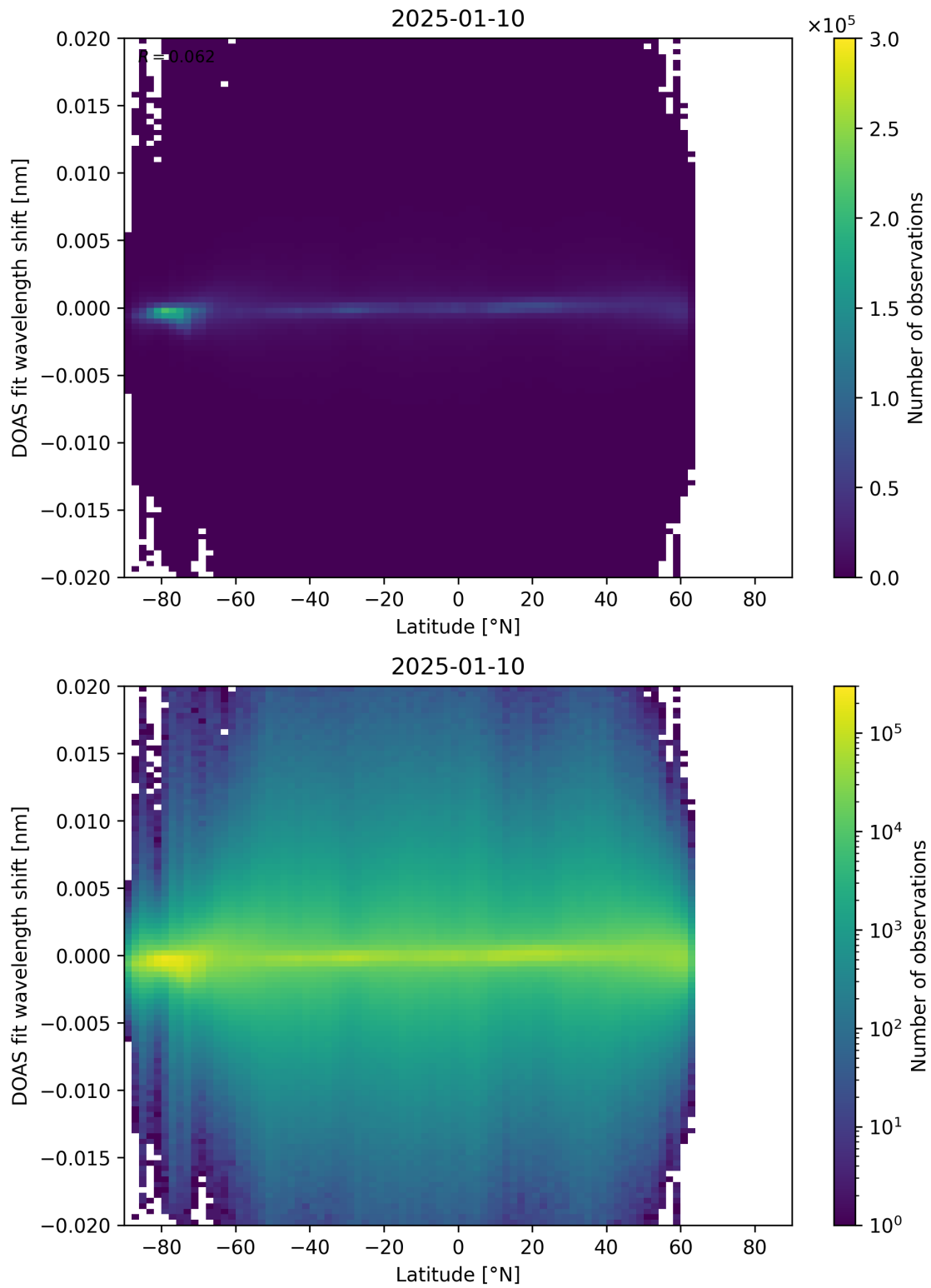
Figure 154: Scatter density plot of “Latitude” against “DOAS fit wavelength shift” for 2025-01-09 to 2025-01-11.
