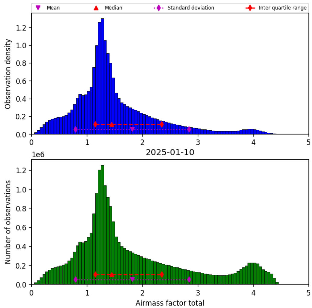
Figure 40: Histogram of “Airmass factor total” for 2025-01-09 to 2025-01-11
