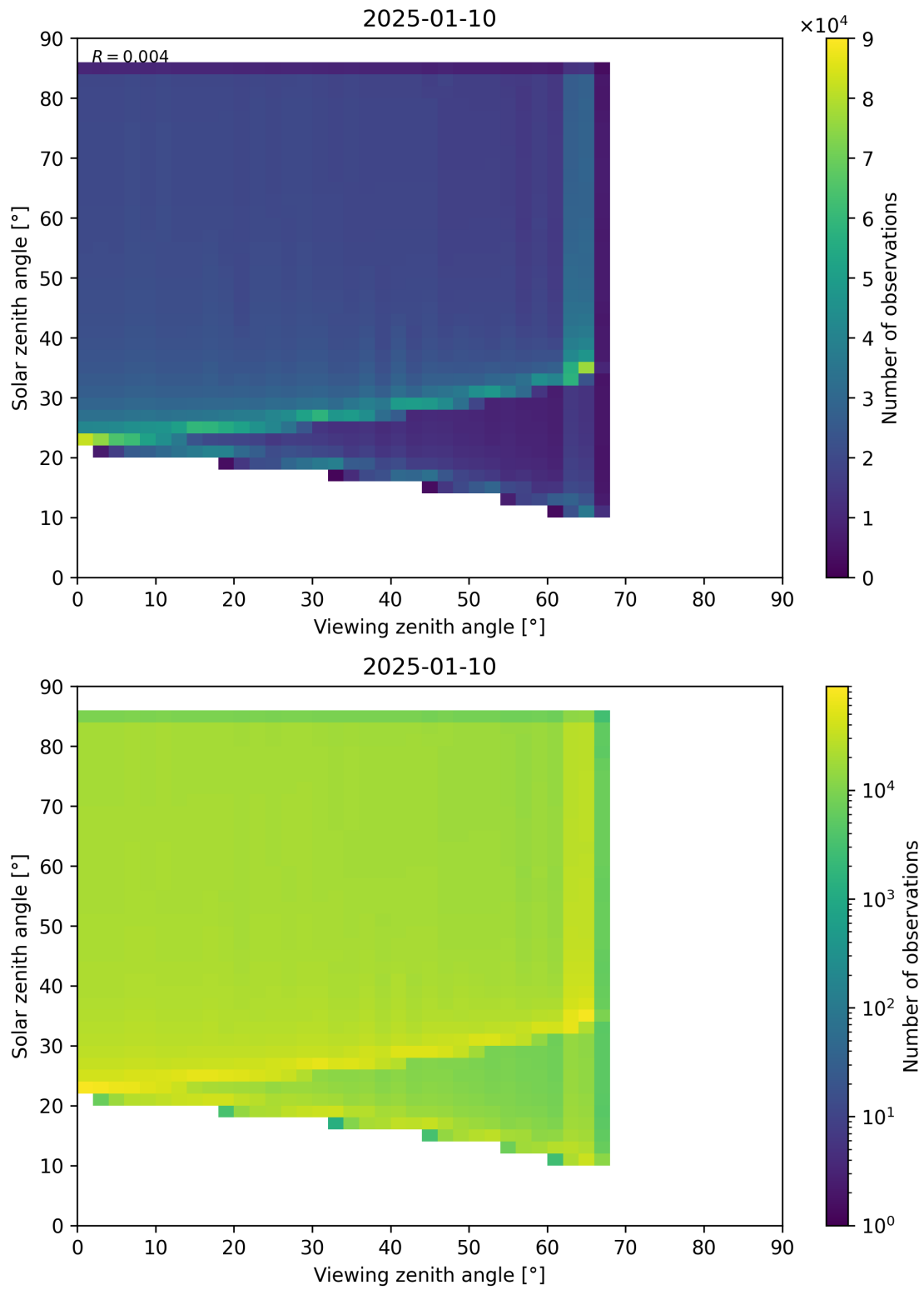
Figure 197: Scatter density plot of “Viewing zenith angle” against “Solar zenith angle” for 2025-01-09 to 2025-01-11.
