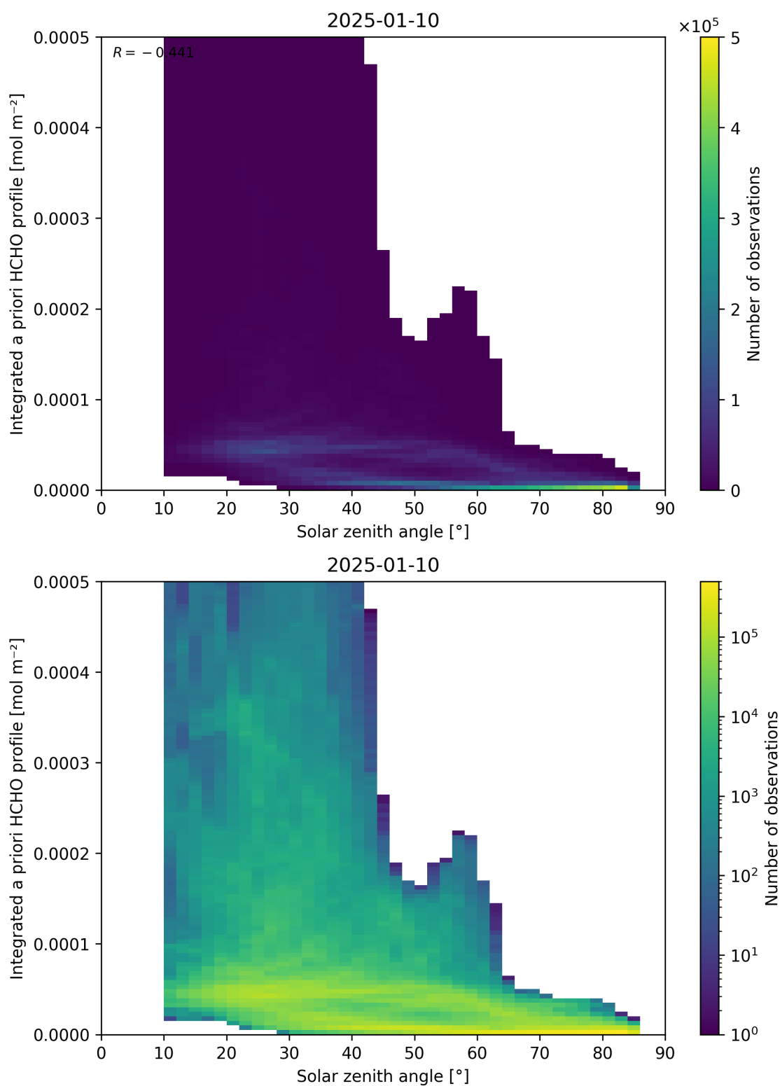
Figure 180: Scatter density plot of “Solar zenith angle” against “Integrated a priori HCHO profile” for 2025-01-09 to 2025-01-11.
