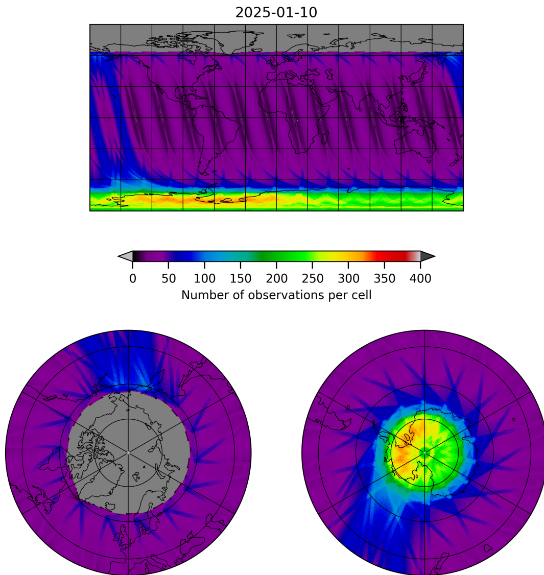
Figure 19: Map of the number of observations for 2025-01-09 to 2025-01-11
