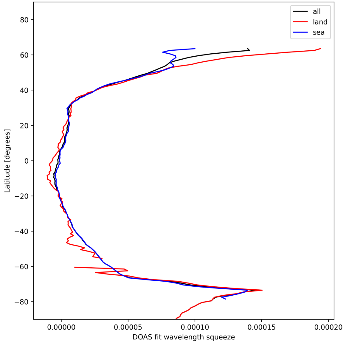
Figure 31: Zonal average of “DOAS fit wavelength squeeze” for 2025-01-09 to 2025-01-11.
