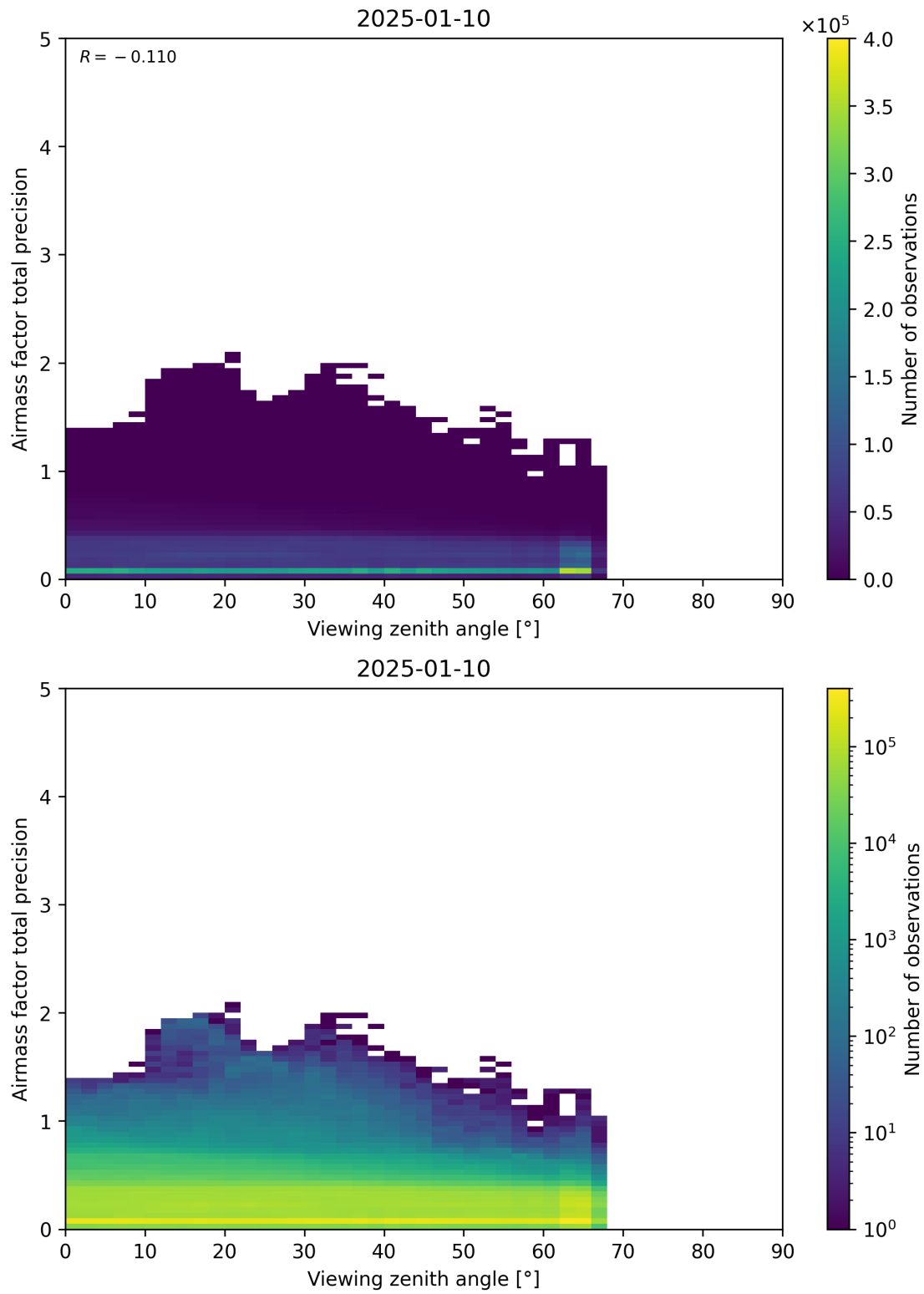
Figure 191: Scatter density plot of “Viewing zenith angle” against “Airmass factor total precision” for 2025-01-09 to 2025-01-11.
