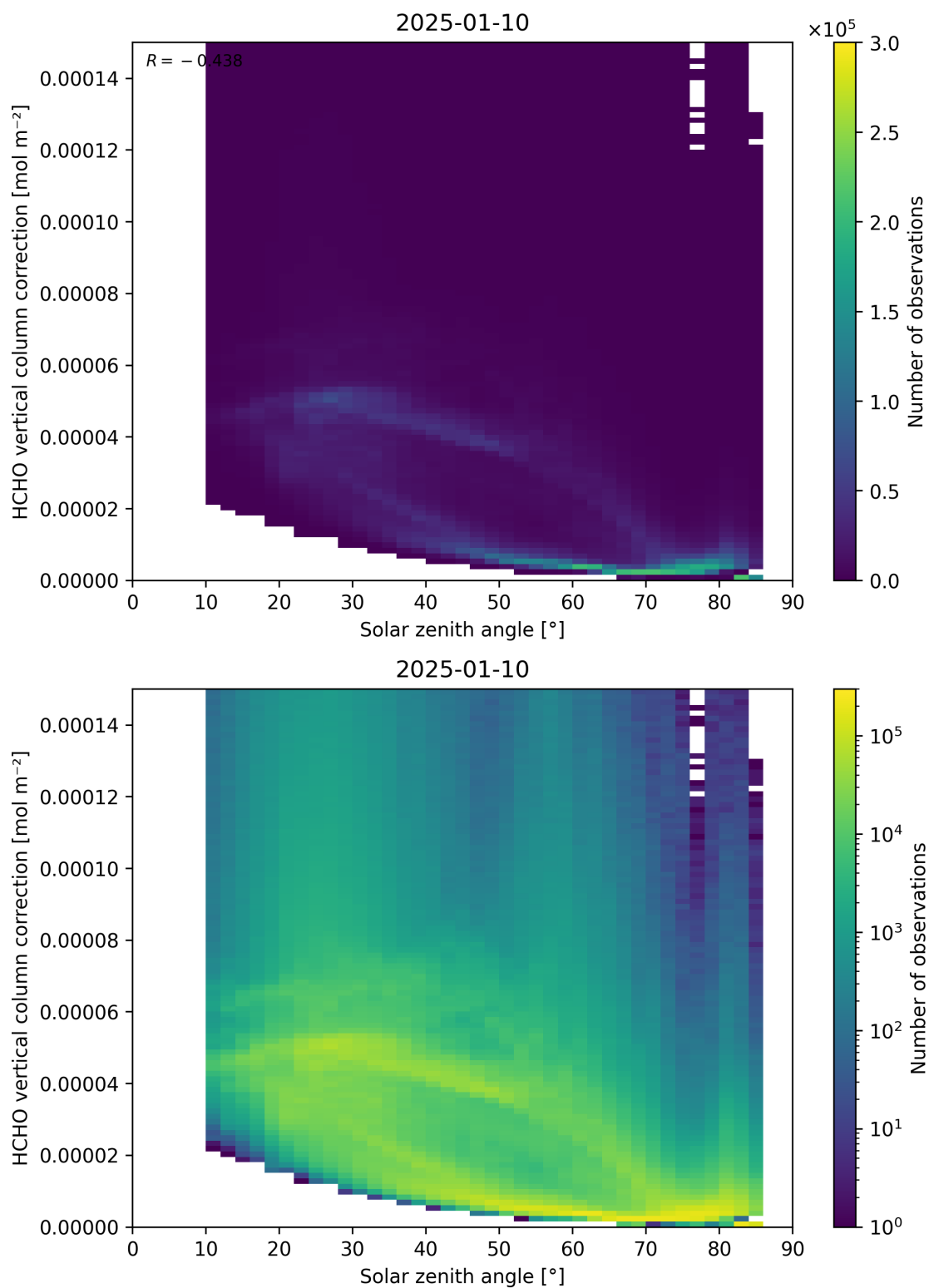
Figure 178: Scatter density plot of “Solar zenith angle” against “HCHO vertical column correction” for 2025-01-09 to 2025-01-11.
