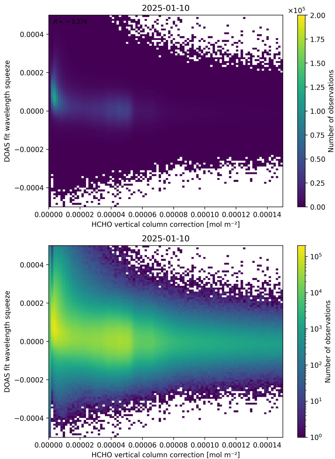
Figure 114: Scatter density plot of “HCHO vertical column correction” against “DOAS fit wavelength squeeze” for 2025-01-09 to 2025-01-11.
