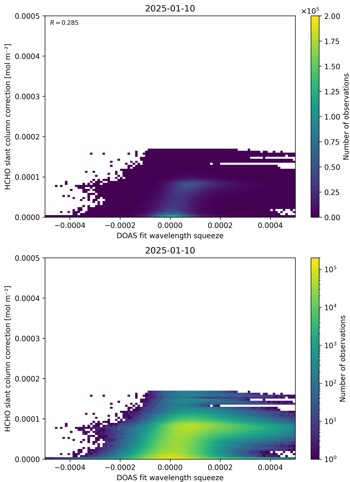
Figure 70: Scatter density plot of “DOAS fit wavelength squeeze” against “HCHO slant column correction” for 2025-01-09 to 2025-01-11.
