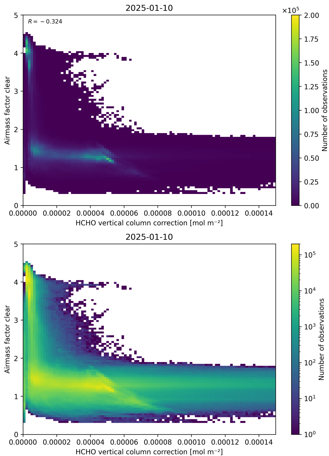
Figure 115: Scatter density plot of “HCHO vertical column correction” against “Airmass factor clear” for 2025-01-09 to 2025-01-11.
