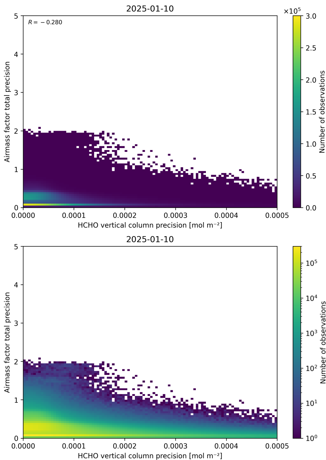
Figure 145: Scatter density plot of “HCHO vertical column precision” against “Airmass factor total precision” for 2025-01-09 to 2025-01-11.
