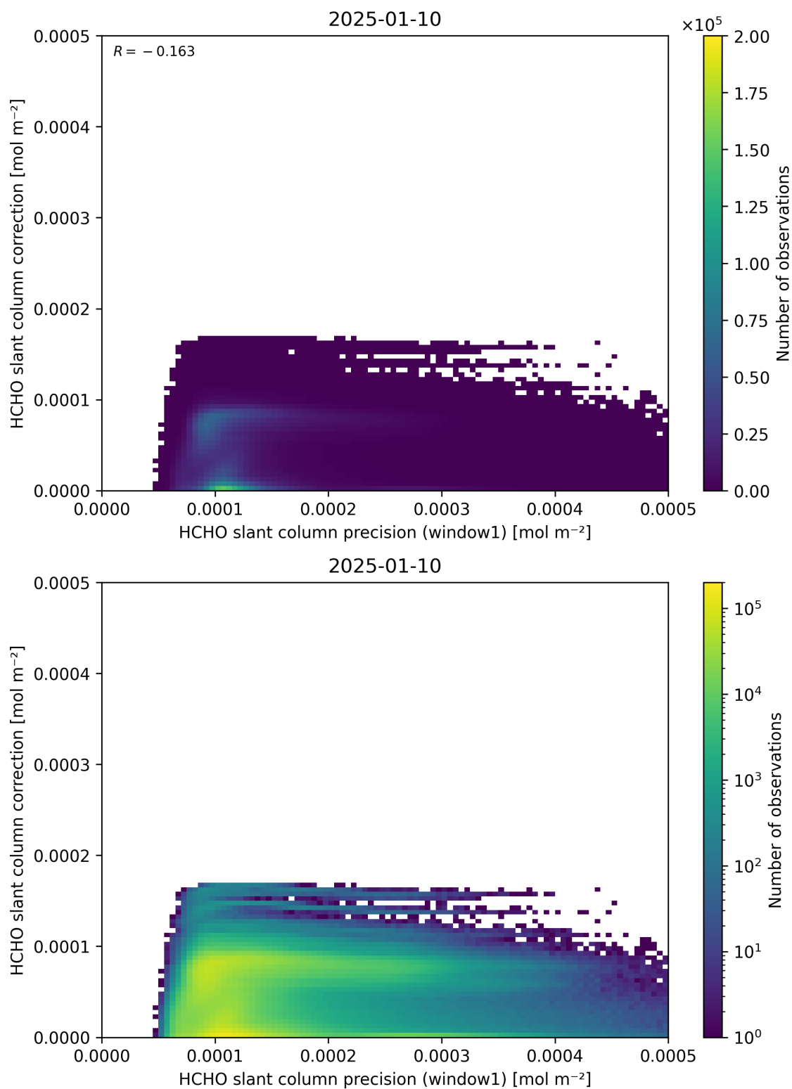
Figure 93: Scatter density plot of “HCHO slant column precision (window1)” against “HCHO slant column correction” for 2025-01-09 to 2025-01-11.
