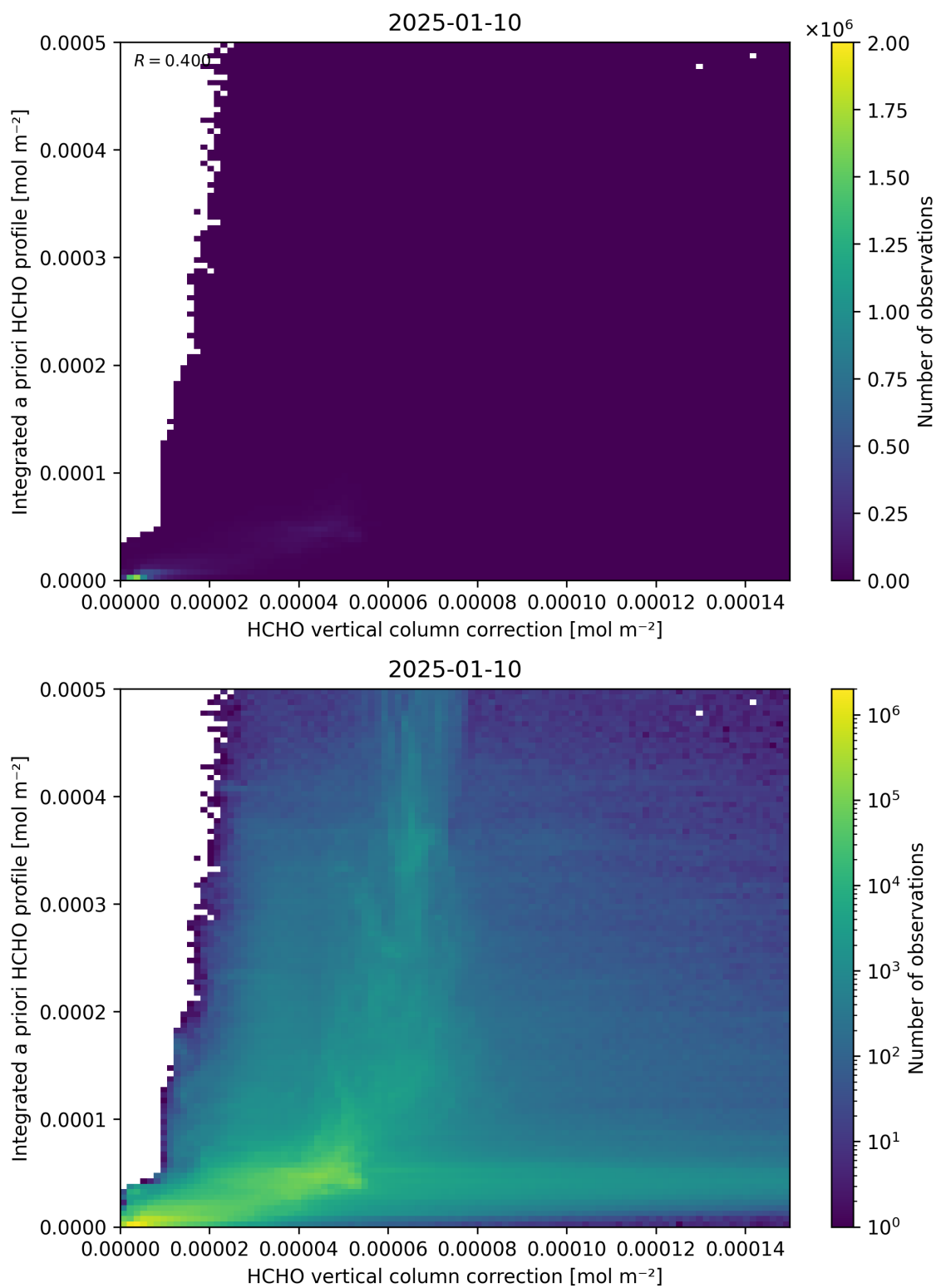
Figure 122: Scatter density plot of “HCHO vertical column correction” against “Integrated a priori HCHO profile” for 2025-01-09 to 2025-01-11.
