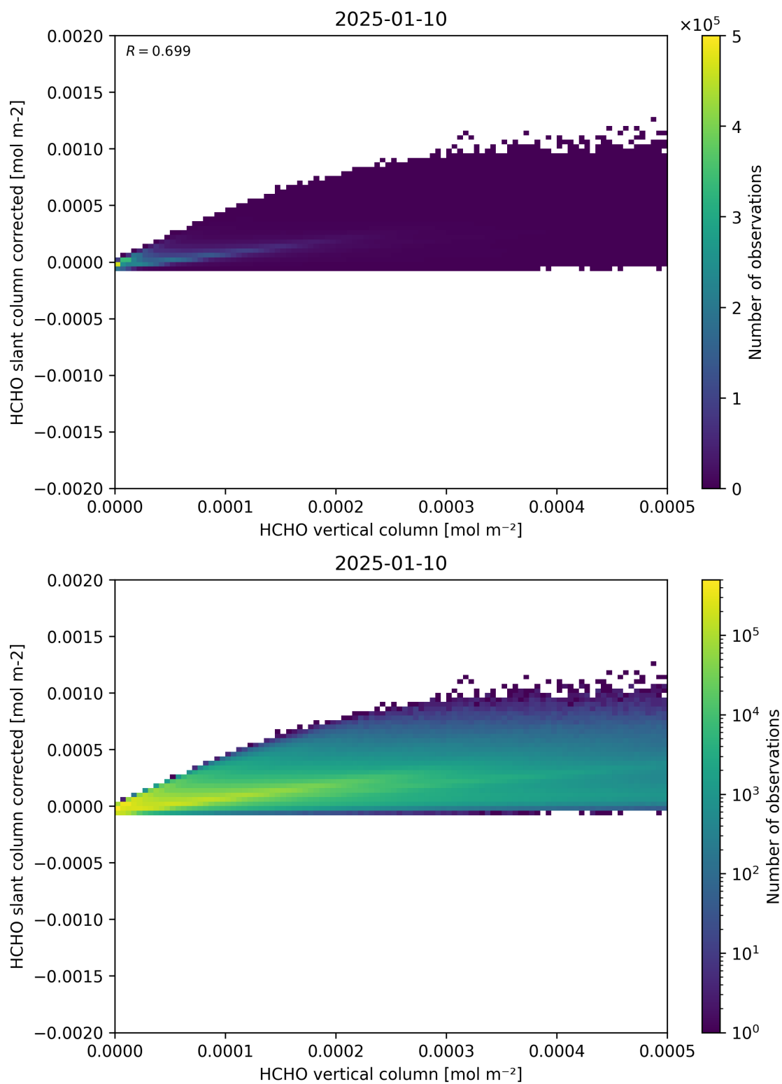
Figure 127: Scatter density plot of “HCHO vertical column” against “HCHO slant column corrected” for 2025-01-09 to 2025-01-11.
