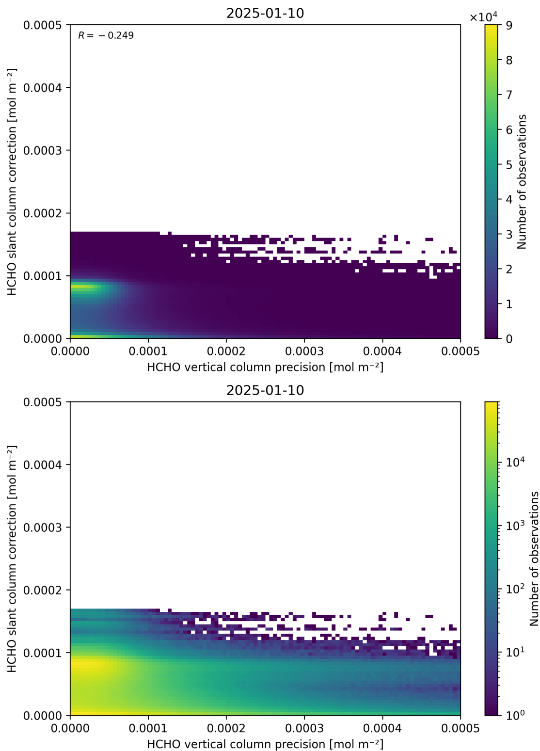
Figure 141: Scatter density plot of “HCHO vertical column precision” against “HCHO slant column correction” for 2025-01-09 to 2025-01-11.
