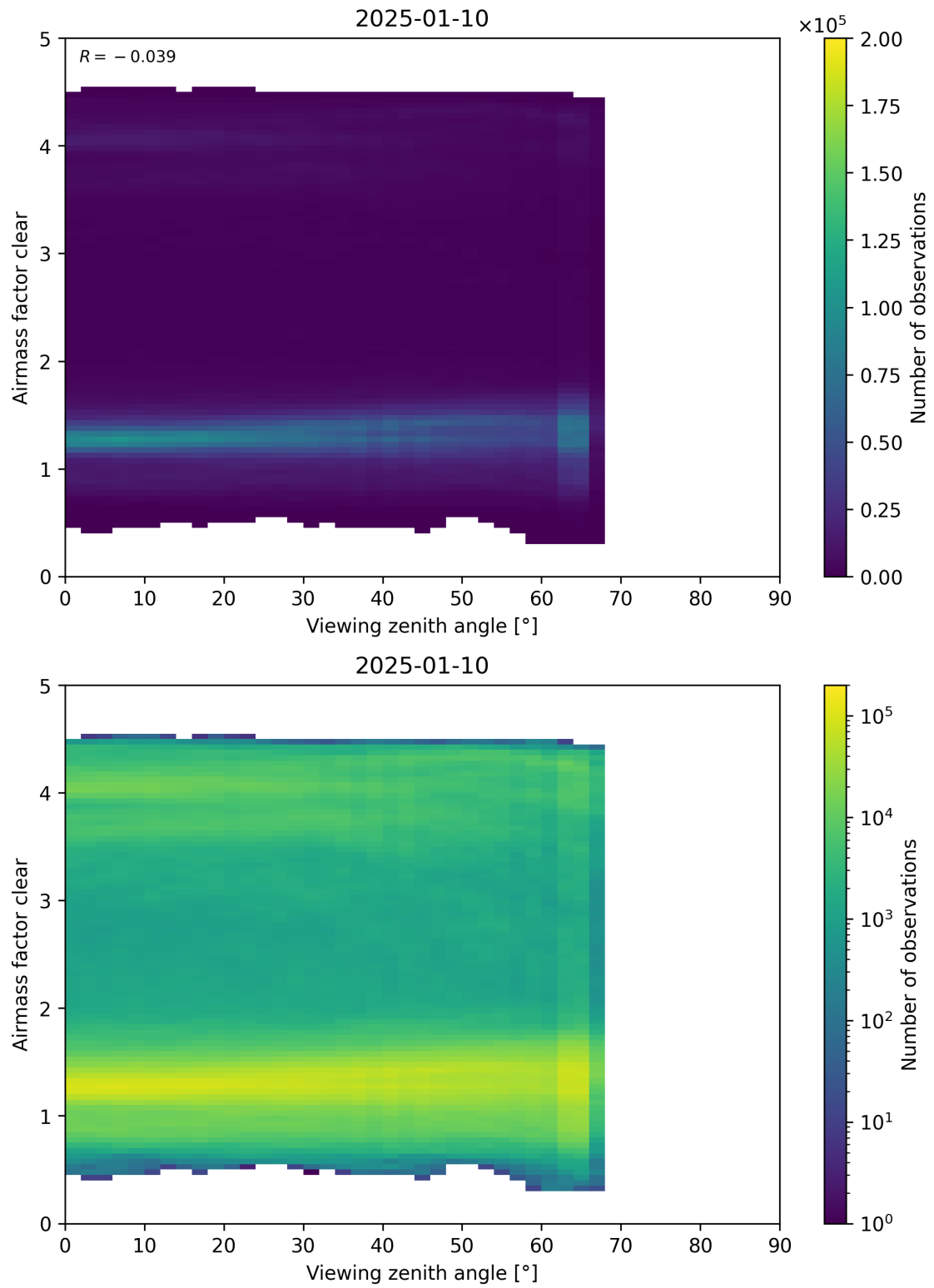
Figure 185: Scatter density plot of “Viewing zenith angle” against “Airmass factor clear” for 2025-01-09 to 2025-01-11.
