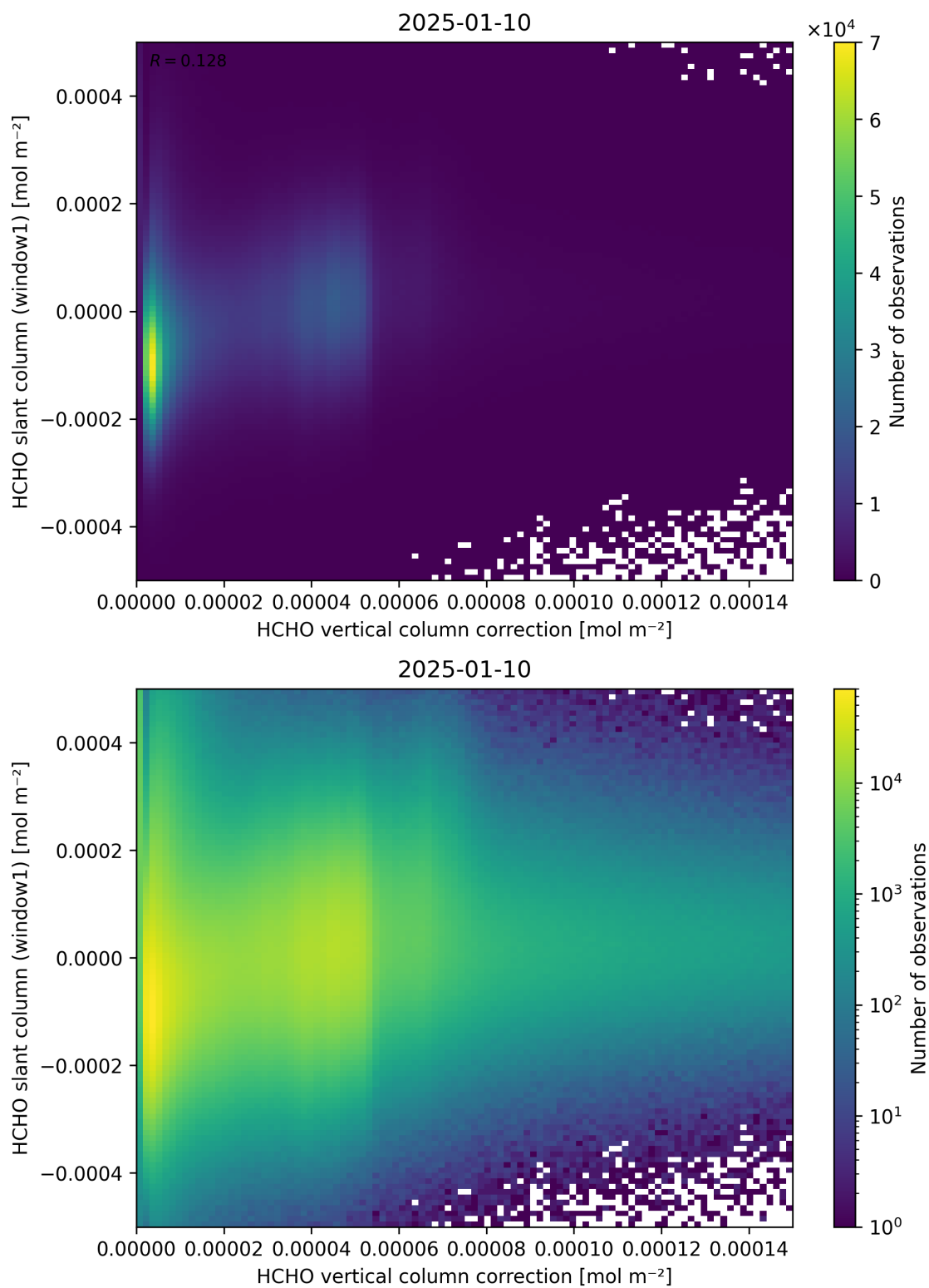
Figure 118: Scatter density plot of “HCHO vertical column correction” against “HCHO slant column (window1)” for 2025-01-09 to 2025-01-11.
