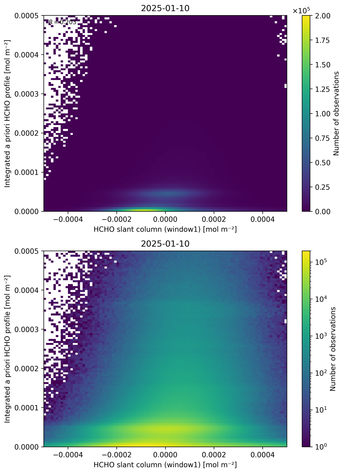
Figure 87: Scatter density plot of “HCHO slant column (window1)” against “Integrated a priori HCHO profile” for 2025-01-09 to 2025-01-11.
