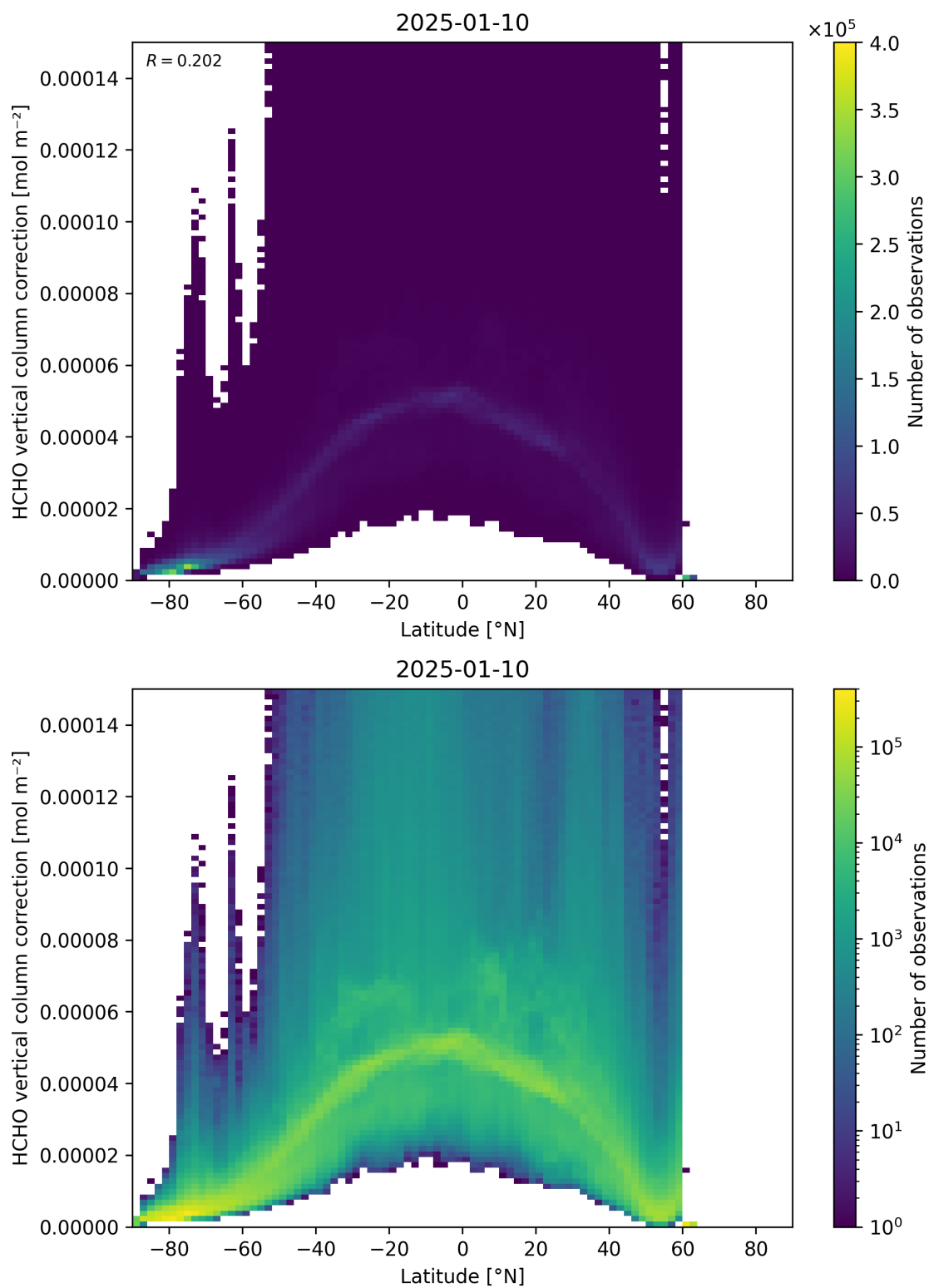
Figure 164: Scatter density plot of “Latitude” against “HCHO vertical column correction” for 2025-01-09 to 2025-01-11.
