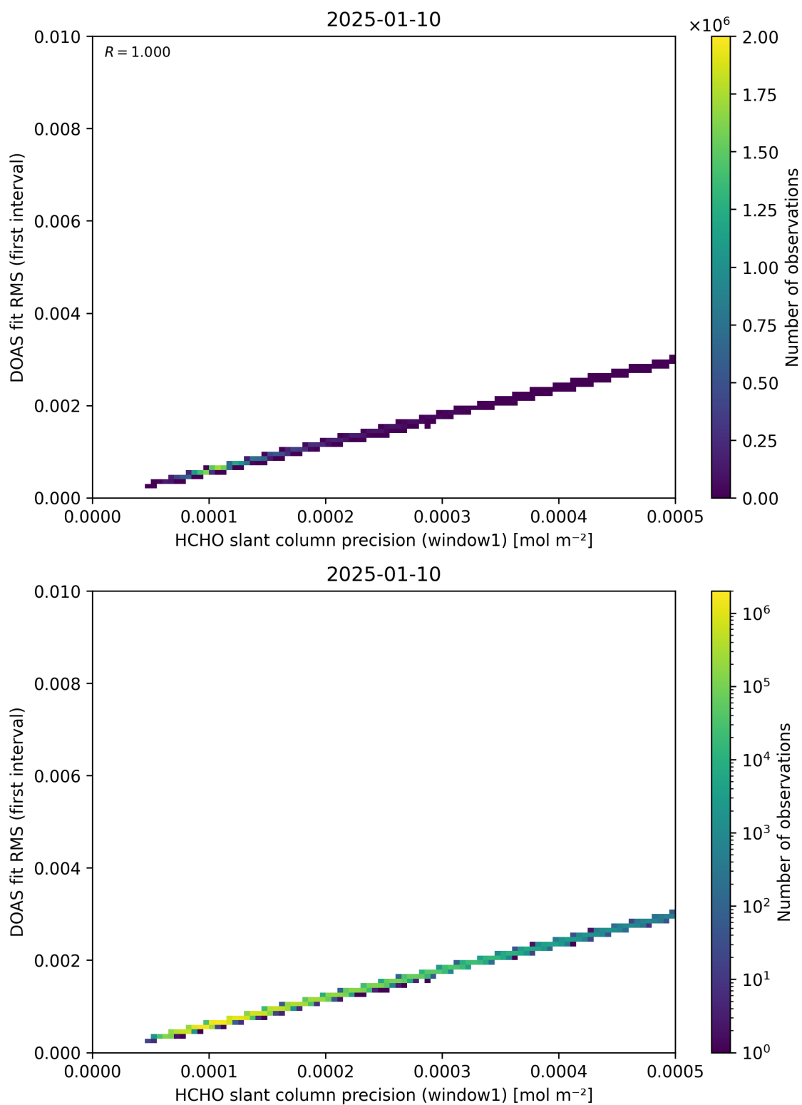
Figure 88: Scatter density plot of “HCHO slant column precision (window1)” against “DOAS fit RMS (first interval)” for 2025-01-09 to 2025-01-11.
