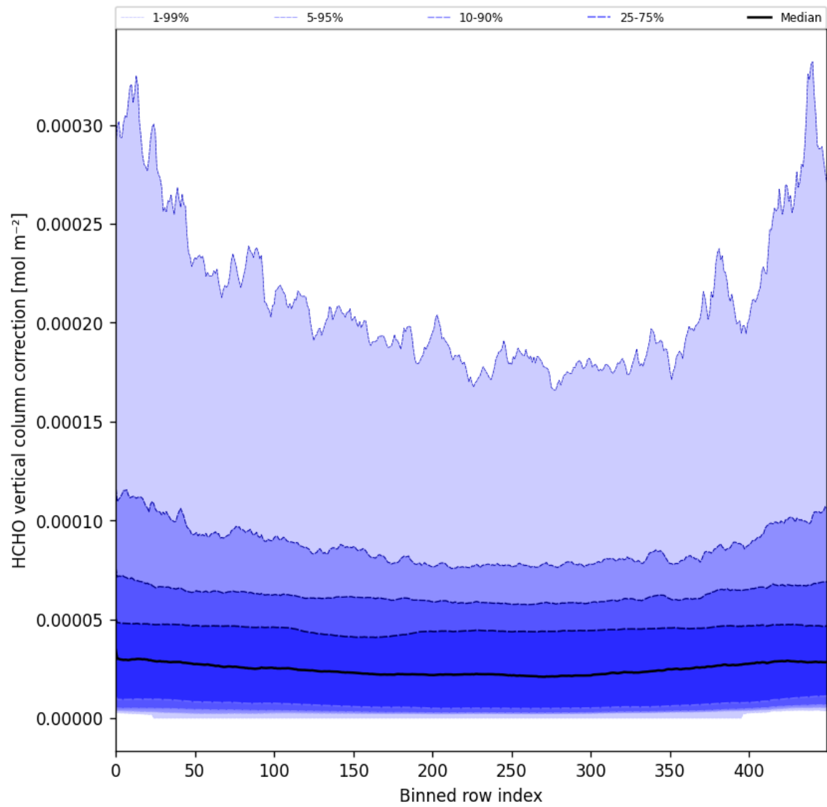
Figure 51: Along track statistics of “HCHO vertical column correction” for 2025-01-09 to 2025-01-11
