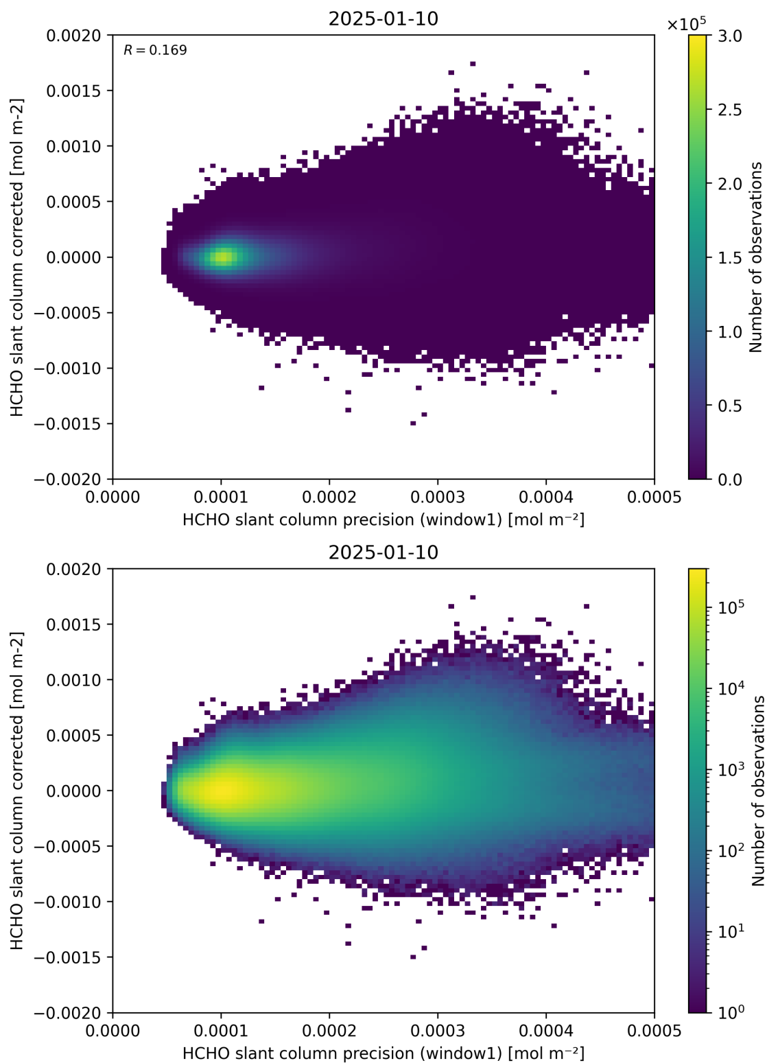
Figure 92: Scatter density plot of “HCHO slant column precision (window1)” against “HCHO slant column corrected” for 2025-01-09 to 2025-01-11.
