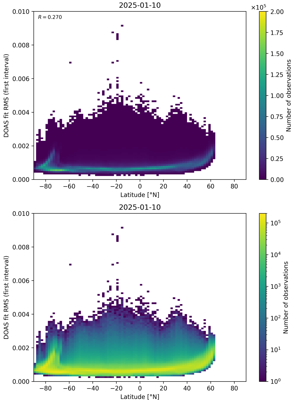
Figure 153: Scatter density plot of “Latitude” against “DOAS fit RMS (first interval)” for 2025-01-09 to 2025-01-11.
