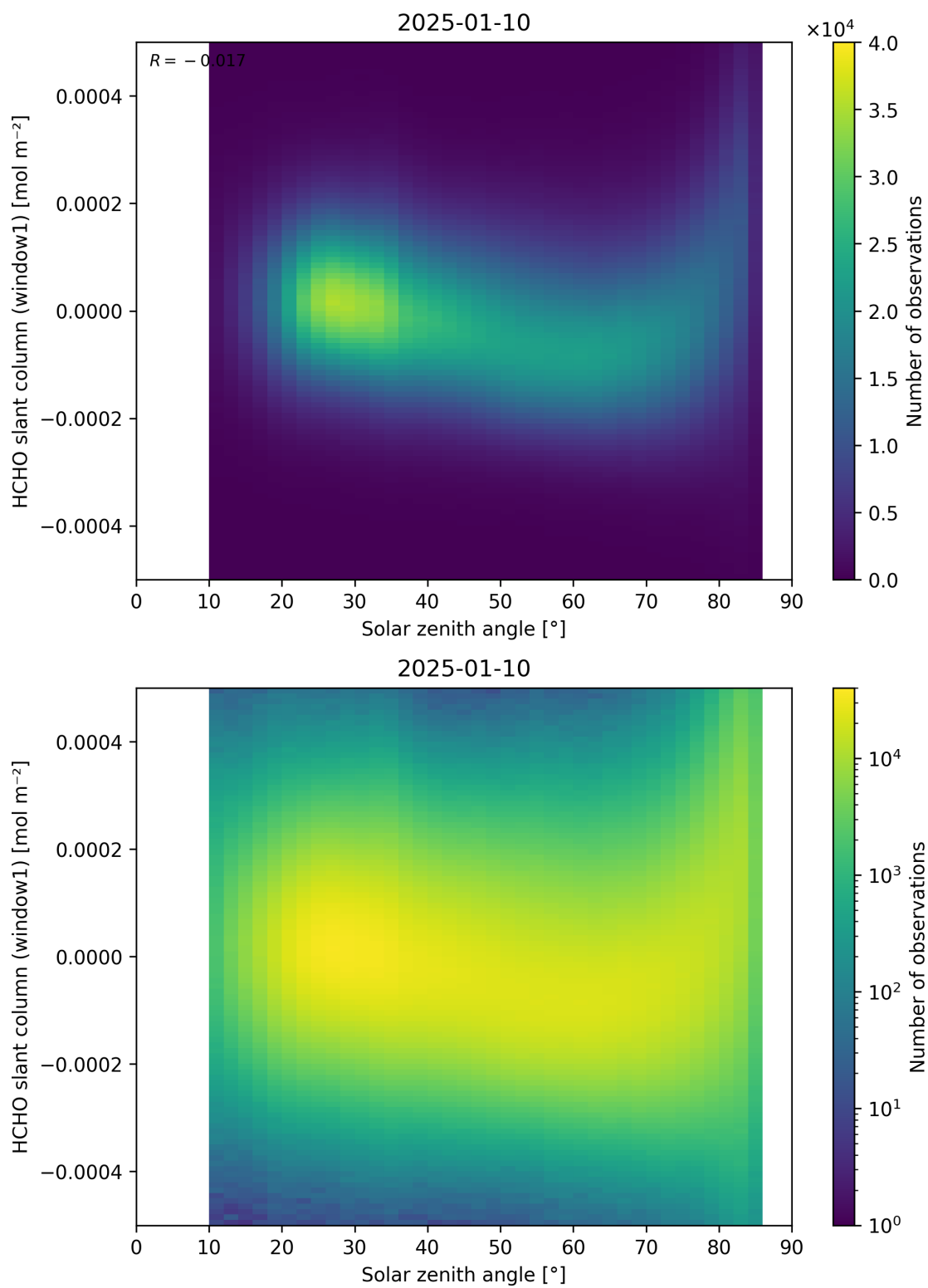
Figure 173: Scatter density plot of “Solar zenith angle” against “HCHO slant column (window1)” for 2025-01-09 to 2025-01-11.
