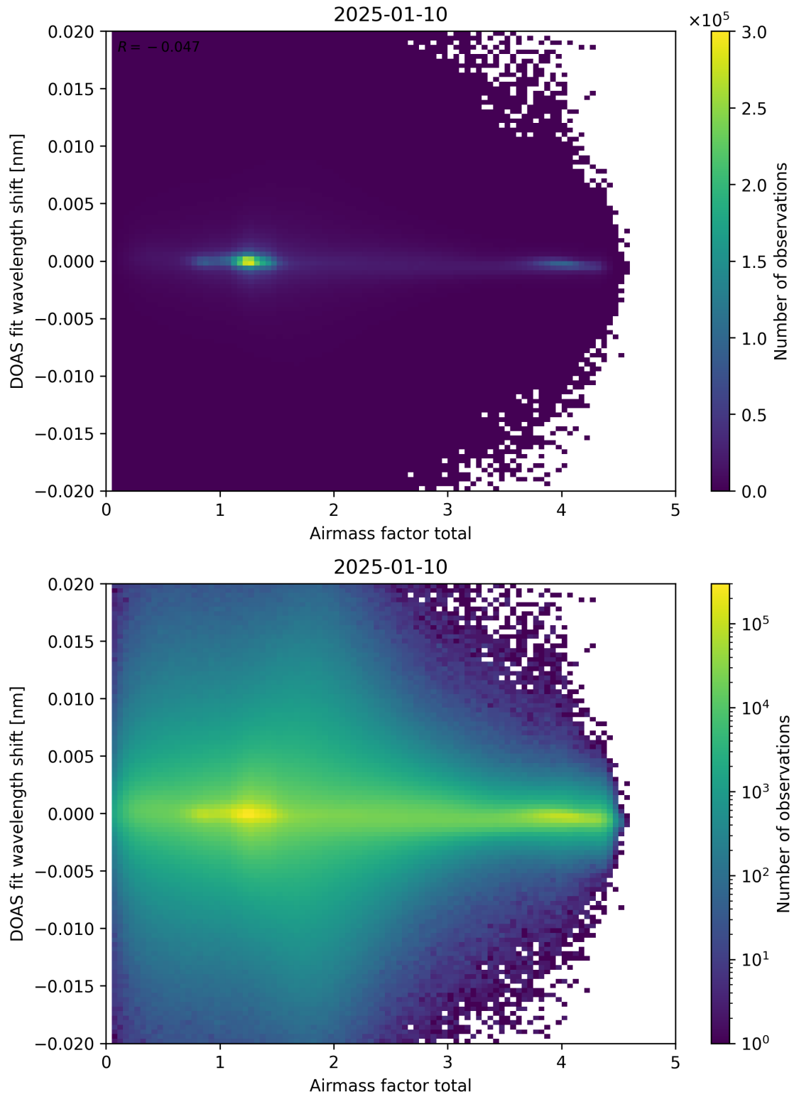
Figure 98: Scatter density plot of “Airmass factor total” against “DOAS fit wavelength shift” for 2025-01-09 to 2025-01-11.
