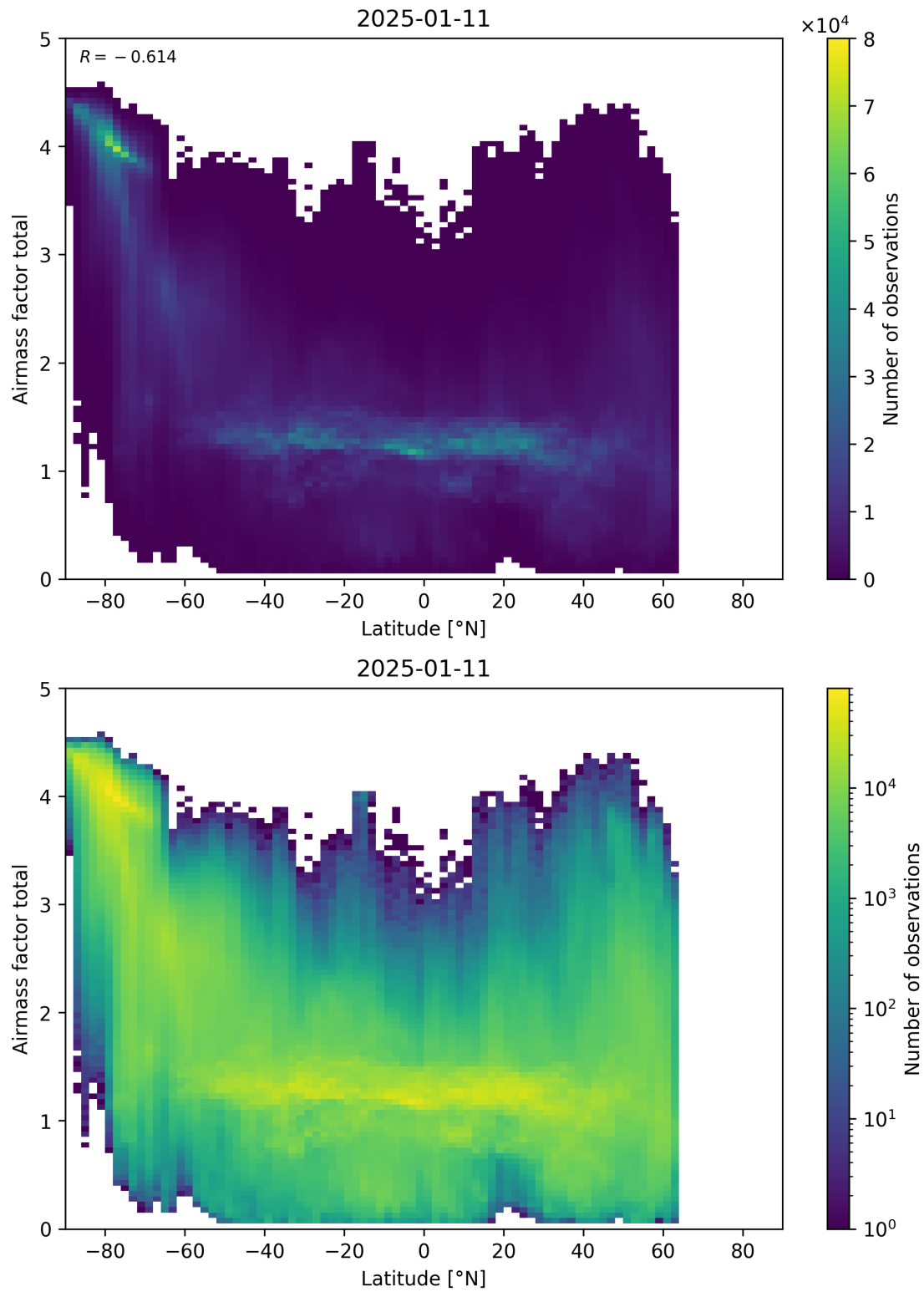
Figure 161: Scatter density plot of “Latitude” against “Airmass factor total” for 2025-01-10 to 2025-01-12.
