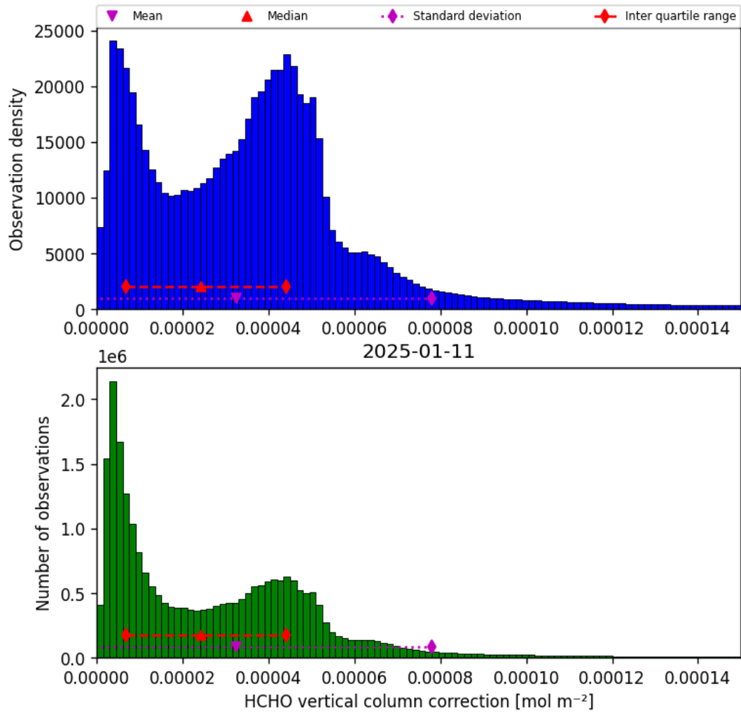
Figure 37: Histogram of “HCHO vertical column correction” for 2025-01-10 to 2025-01-12
