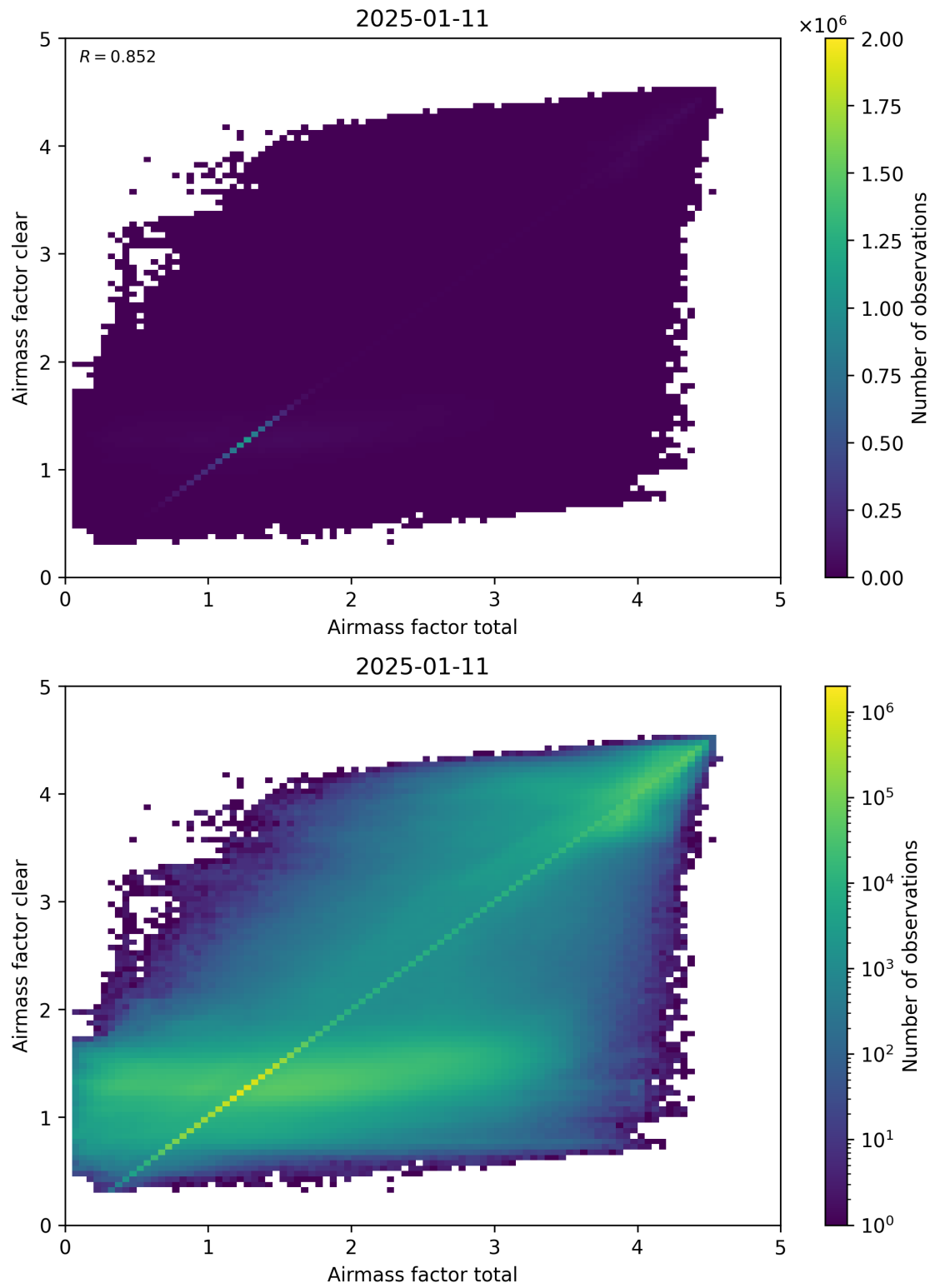
Figure 100: Scatter density plot of “Airmass factor total” against “Airmass factor clear” for 2025-01-10 to 2025-01-12.
