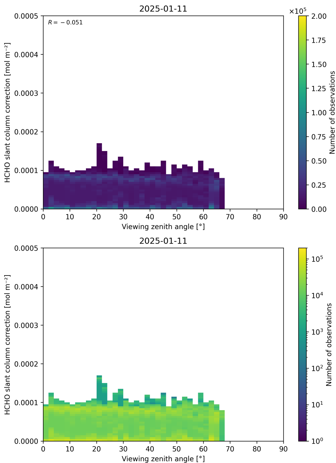
Figure 187: Scatter density plot of “Viewing zenith angle” against “HCHO slant column correction” for 2025-01-10 to 2025-01-12.
