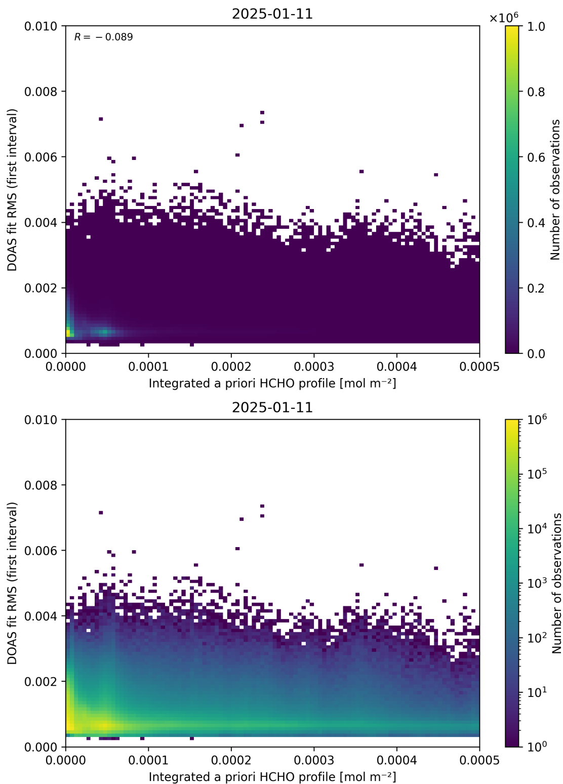
Figure 148: Scatter density plot of “Integrated a priori HCHO profile” against “DOAS fit RMS (first interval)” for 2025-01-10 to 2025-01-12.
