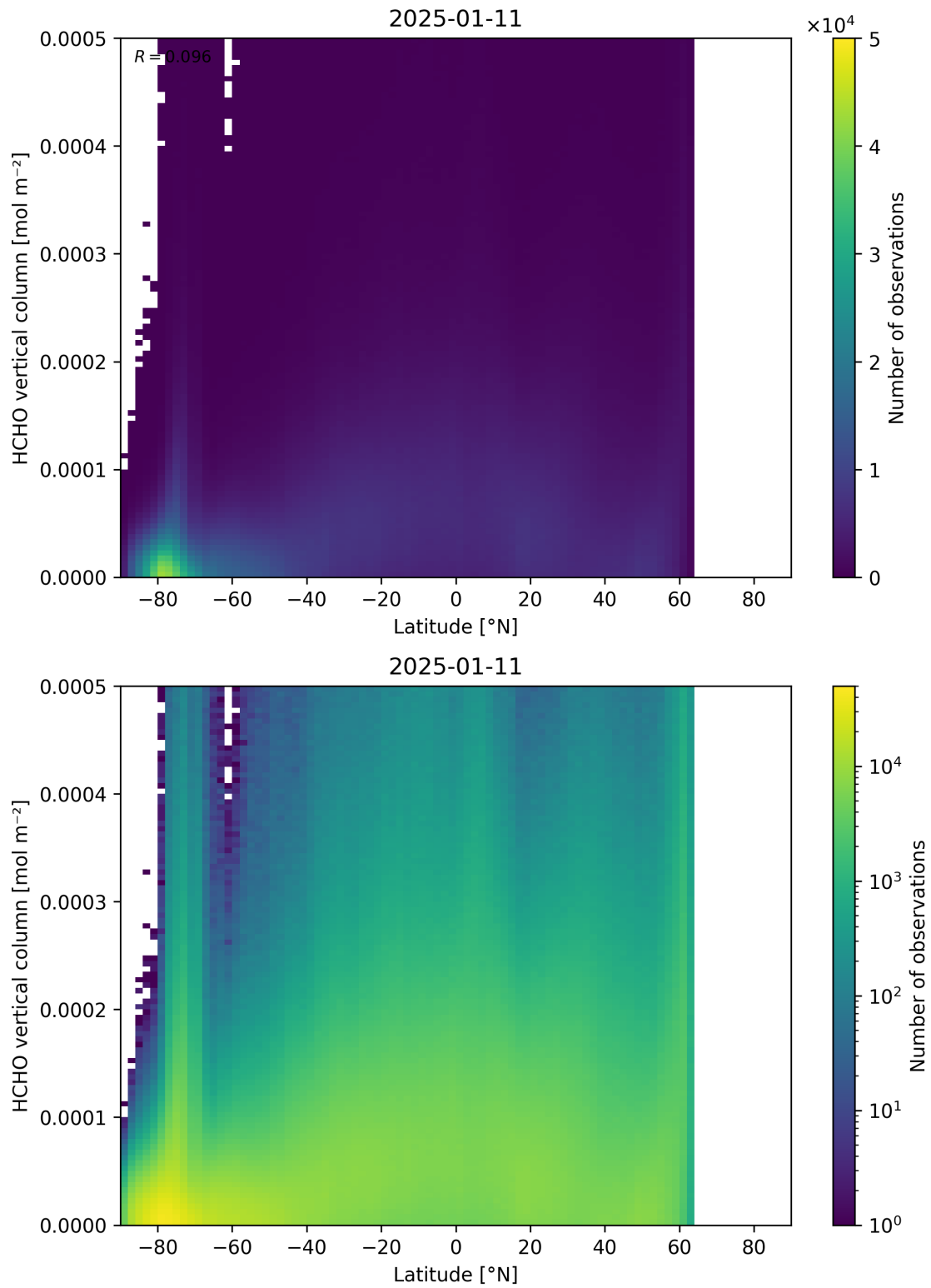
Figure 163: Scatter density plot of “Latitude” against “HCHO vertical column” for 2025-01-10 to 2025-01-12.
