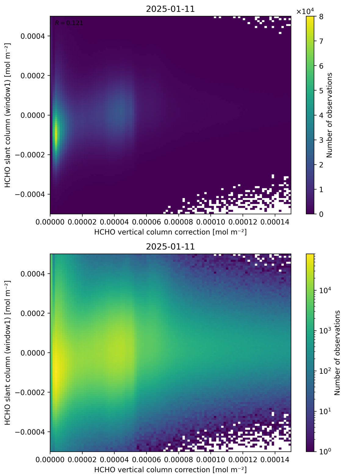
Figure 118: Scatter density plot of “HCHO vertical column correction” against “HCHO slant column (window1)” for 2025-01-10 to 2025-01-12.
