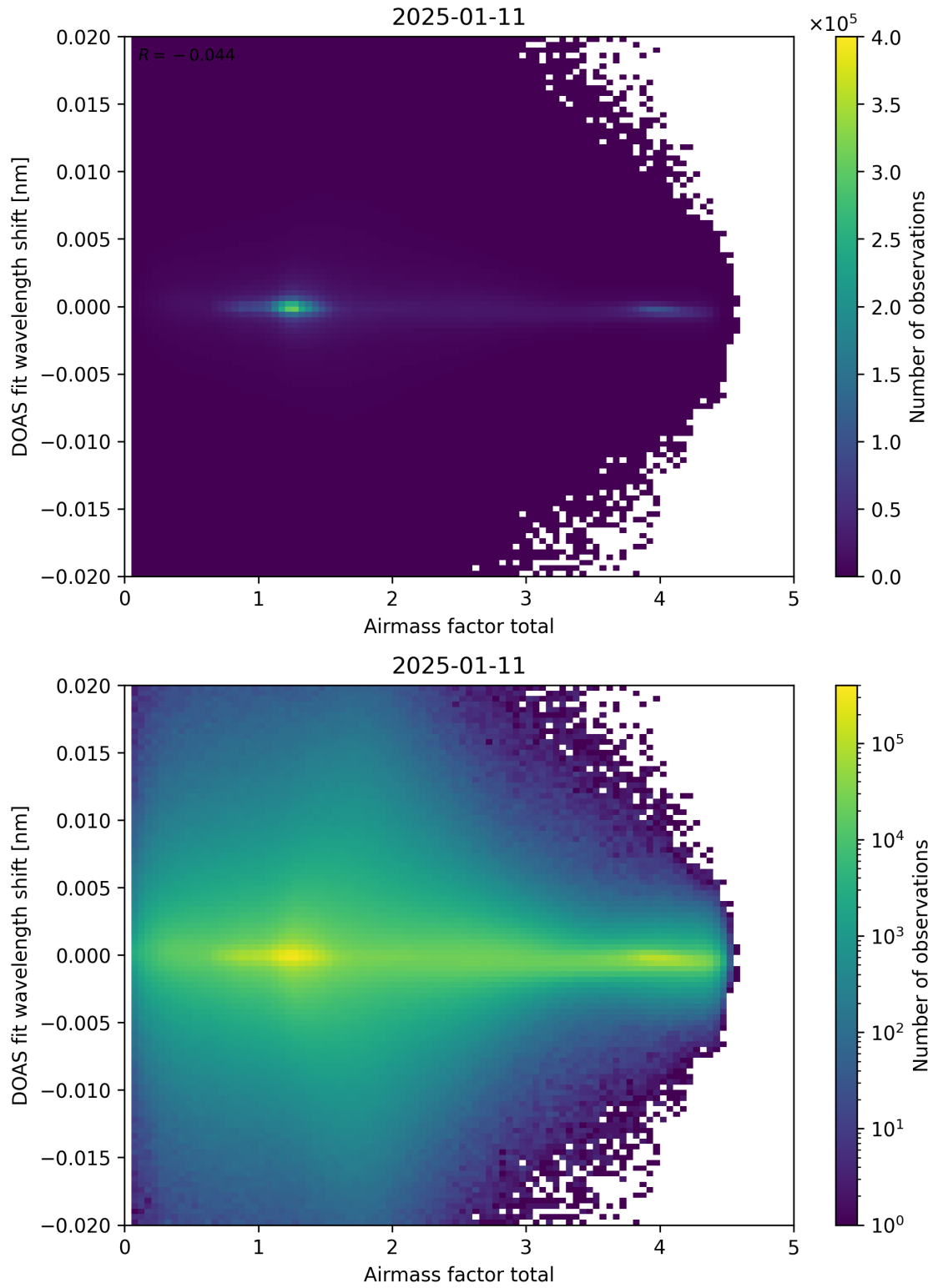
Figure 98: Scatter density plot of “Airmass factor total” against “DOAS fit wavelength shift” for 2025-01-10 to 2025-01-12.
