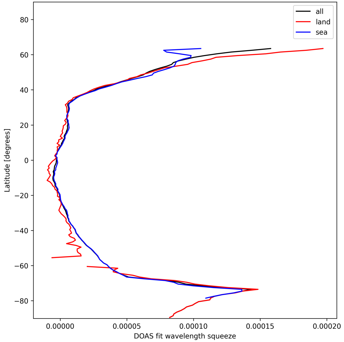
Figure 31: Zonal average of “DOAS fit wavelength squeeze” for 2025-01-10 to 2025-01-12.
