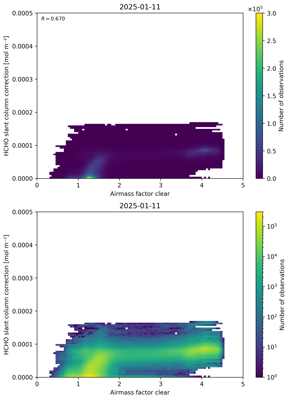
Figure 75: Scatter density plot of “Airmass factor clear” against “HCHO slant column correction” for 2025-01-10 to 2025-01-12.
