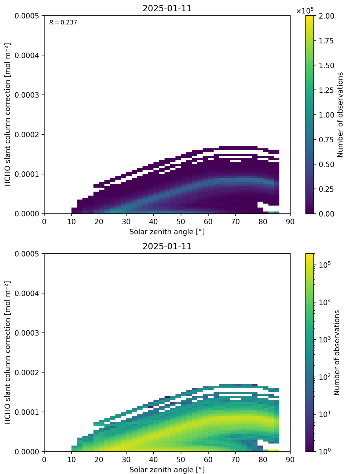
Figure 172: Scatter density plot of “Solar zenith angle” against “HCHO slant column correction” for 2025-01-10 to 2025-01-12.
