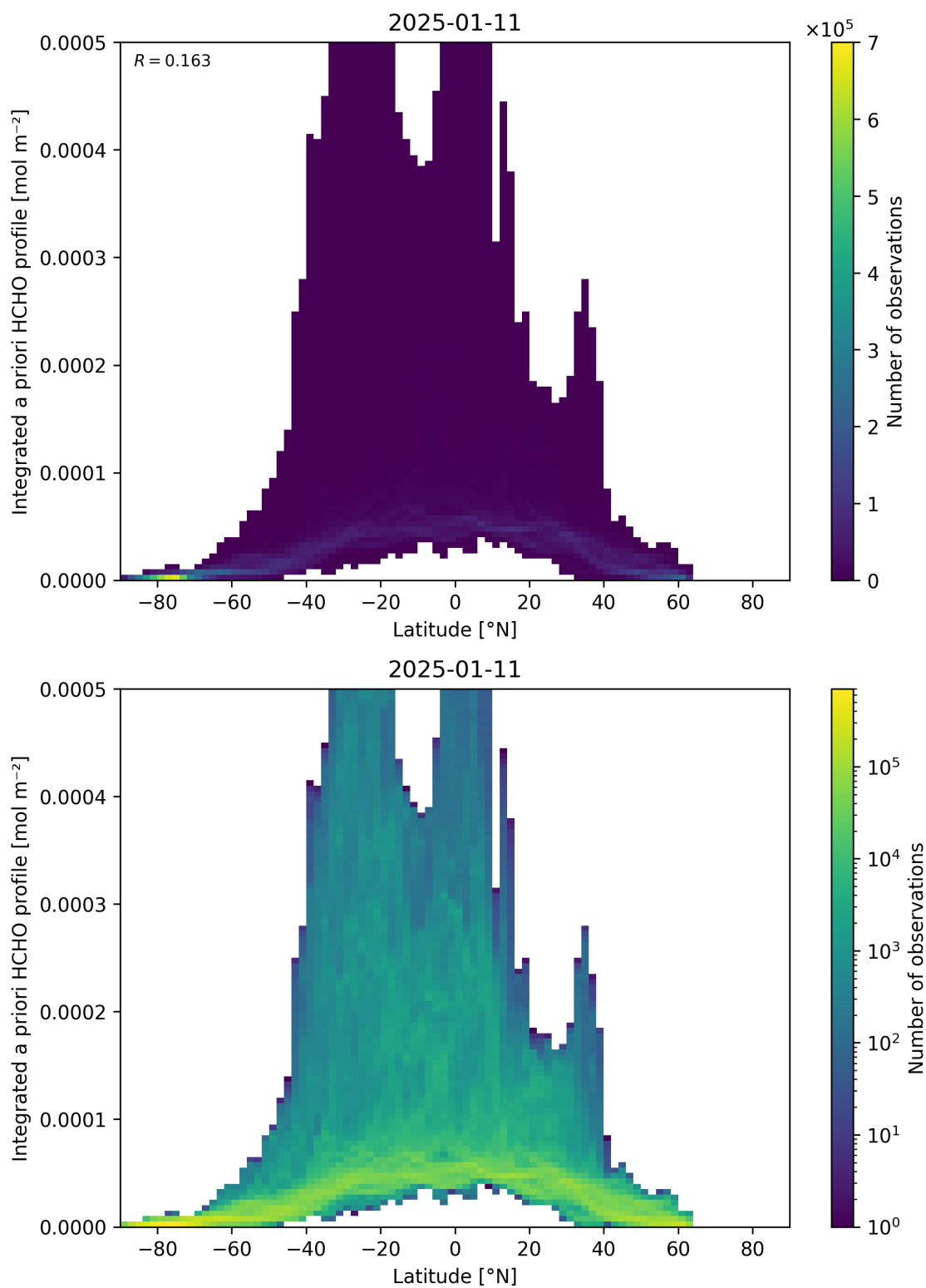
Figure 166: Scatter density plot of “Latitude” against “Integrated a priori HCHO profile” for 2025-01-10 to 2025-01-12.
