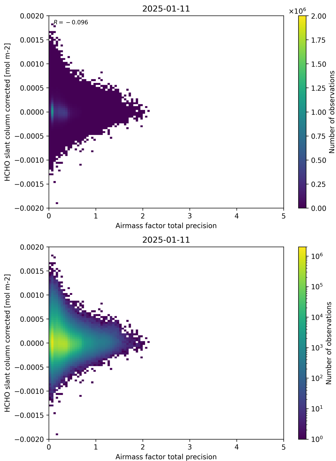
Figure 109: Scatter density plot of “Airmass factor total precision” against “HCHO slant column corrected” for 2025-01-10 to 2025-01-12.
