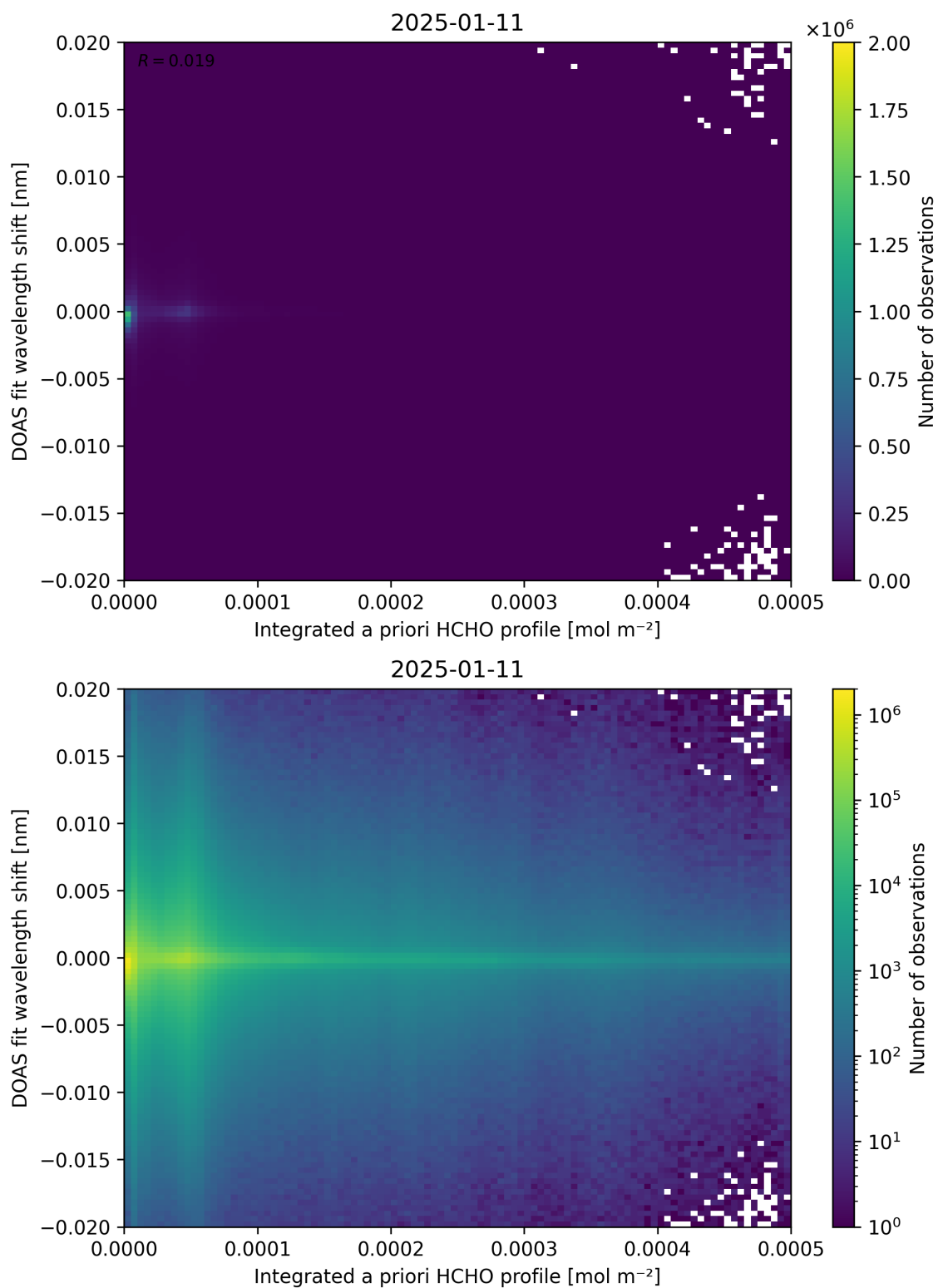
Figure 149: Scatter density plot of “Integrated a priori HCHO profile” against “DOAS fit wavelength shift” for 2025-01-10 to 2025-01-12.
