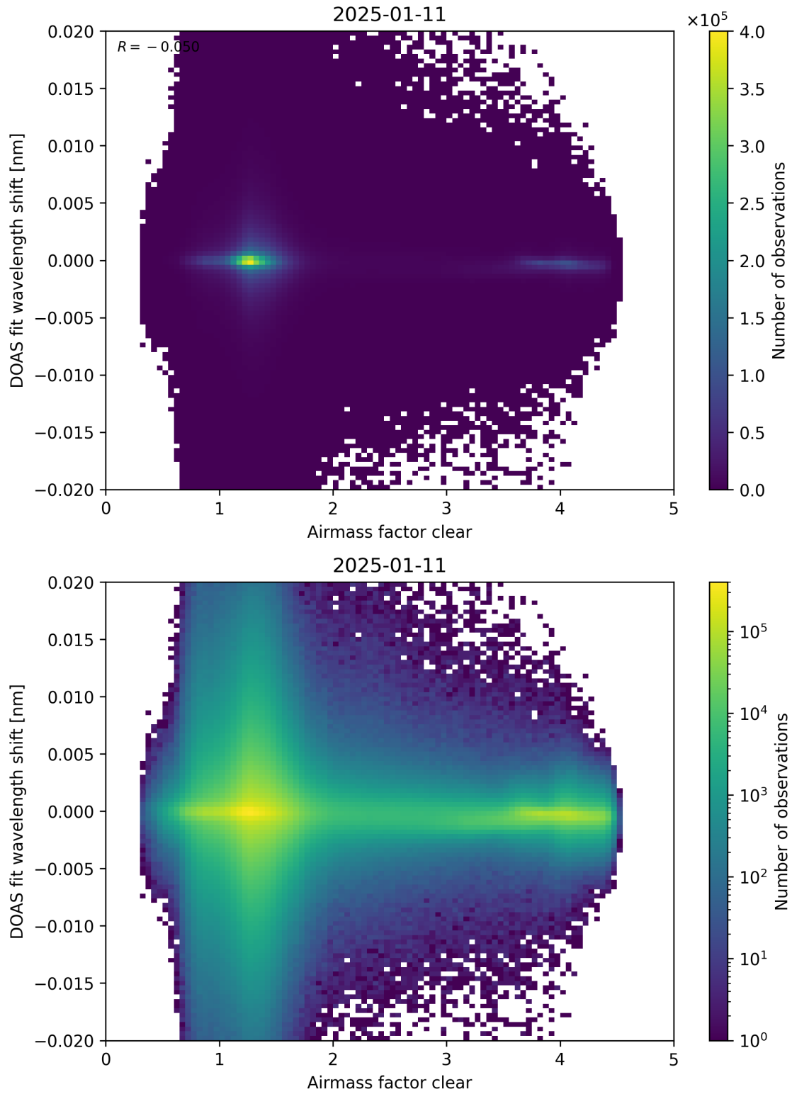
Figure 72: Scatter density plot of “Airmass factor clear” against “DOAS fit wavelength shift” for 2025-01-10 to 2025-01-12.
