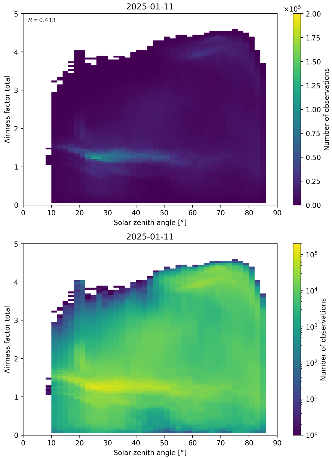
Figure 175: Scatter density plot of “Solar zenith angle” against “Airmass factor total” for 2025-01-10 to 2025-01-12.
