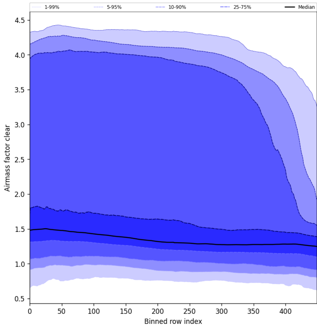
Figure 56: Along track statistics of “Airmass factor clear” for 2025-01-10 to 2025-01-12
