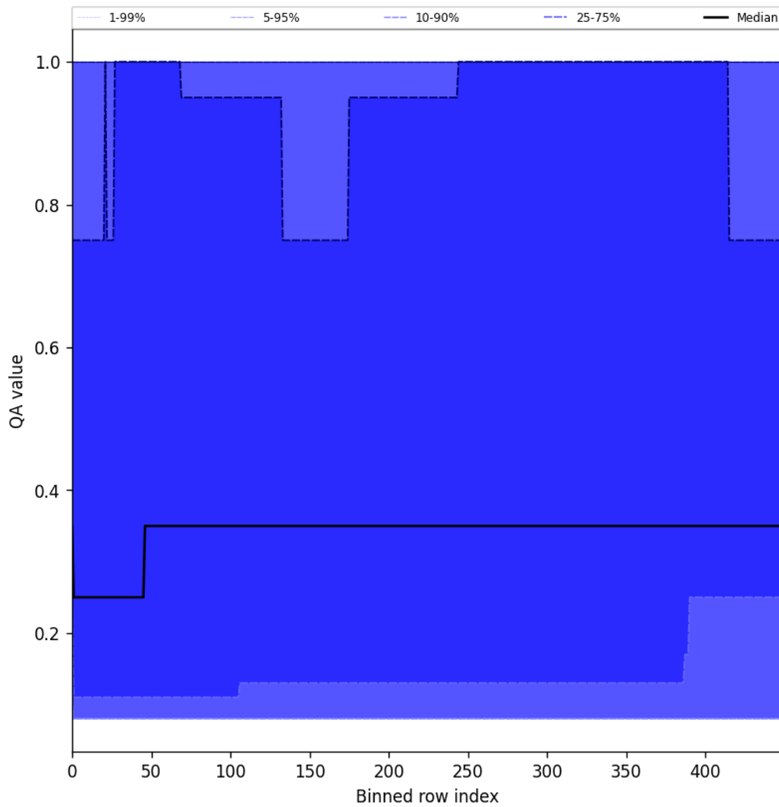
Figure 48: Along track statistics of “QA value” for 2025-01-10 to 2025-01-12
