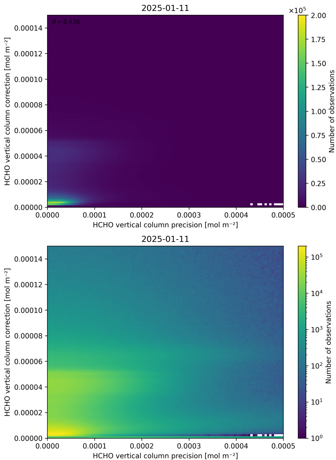
Figure 146: Scatter density plot of “HCHO vertical column precision” against “HCHO vertical column correction” for 2025-01-10 to 2025-01-12.
