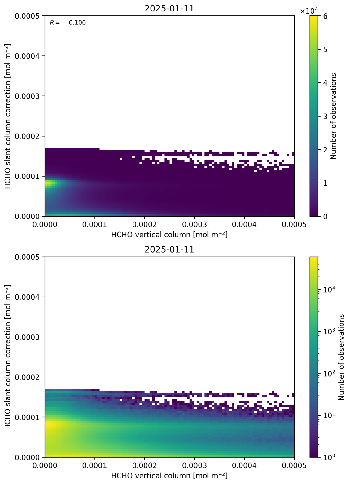
Figure 128: Scatter density plot of “HCHO vertical column” against “HCHO slant column correction” for 2025-01-10 to 2025-01-12.
