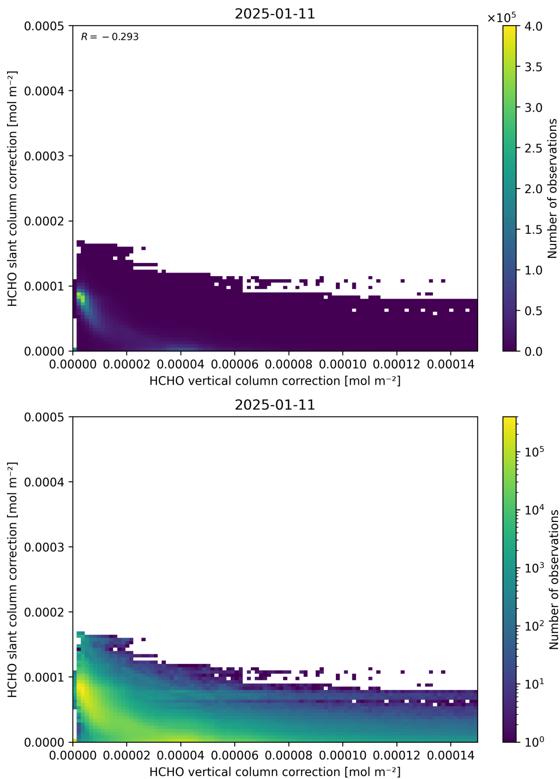
Figure 117: Scatter density plot of “HCHO vertical column correction” against “HCHO slant column correction” for 2025-01-10 to 2025-01-12.
