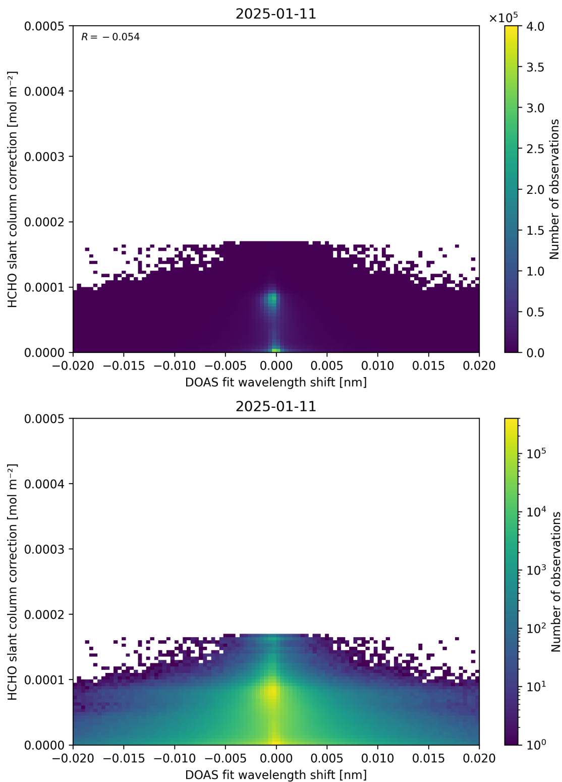
Figure 67: Scatter density plot of “DOAS fit wavelength shift” against “HCHO slant column correction” for 2025-01-10 to 2025-01-12.
