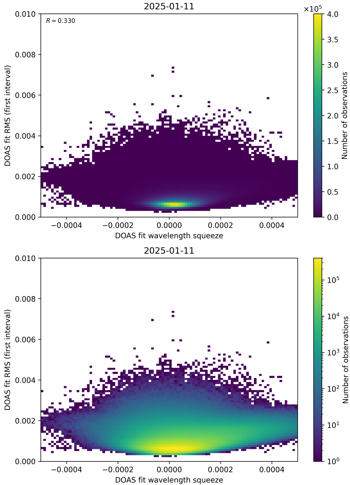
Figure 68: Scatter density plot of “DOAS fit wavelength squeeze” against “DOAS fit RMS (first interval)” for 2025-01-10 to 2025-01-12.
