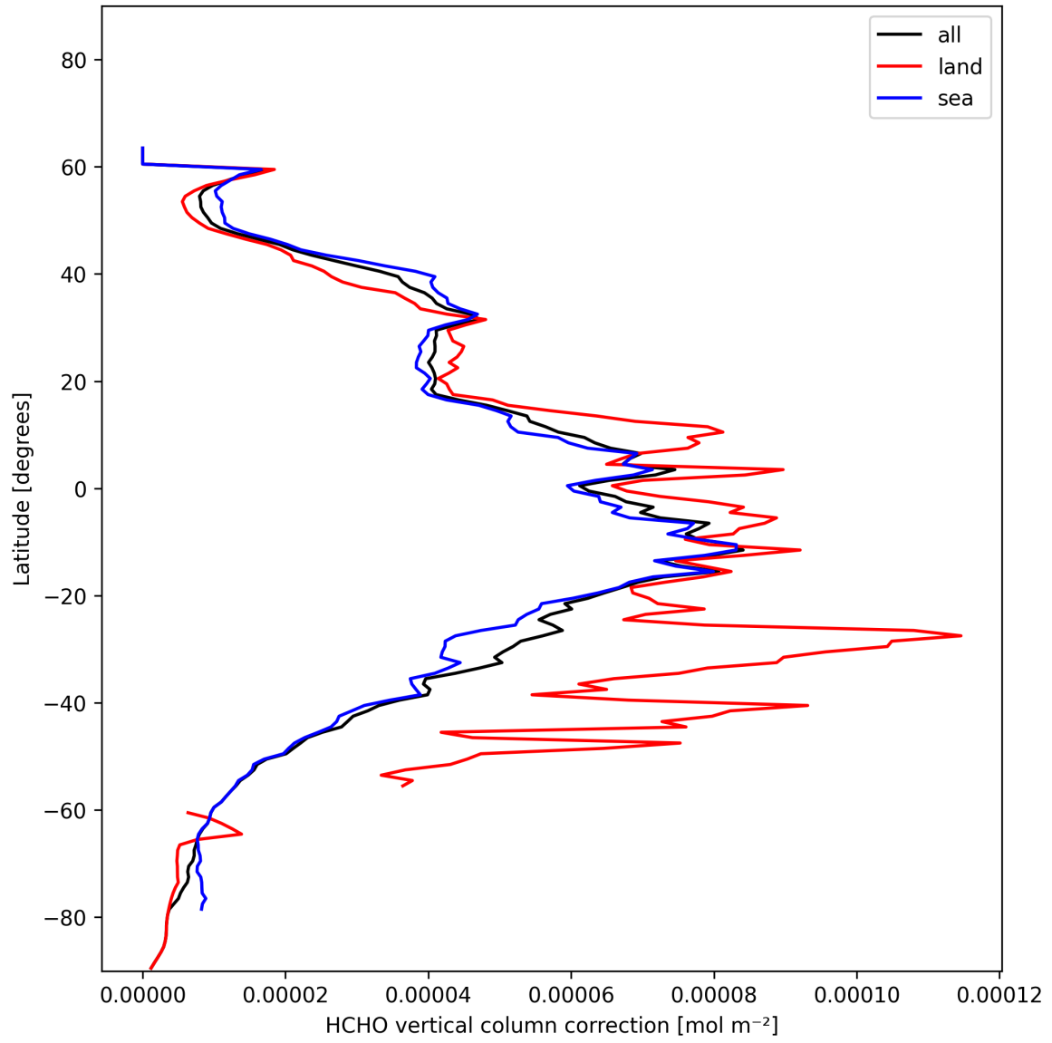
Figure 23: Zonal average of “HCHO vertical column correction” for 2025-01-10 to 2025-01-12.
