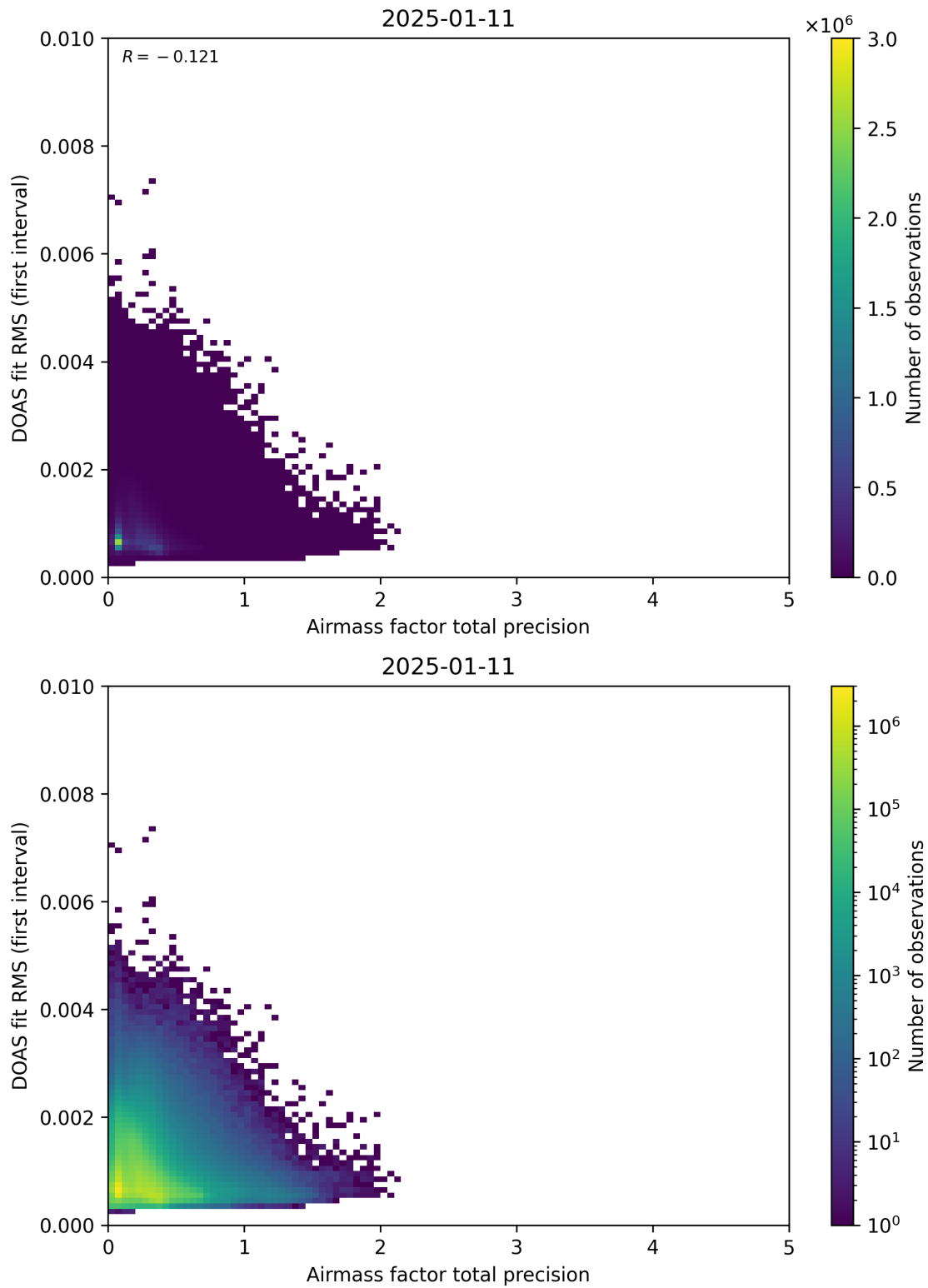
Figure 105: Scatter density plot of “Airmass factor total precision” against “DOAS fit RMS (first interval)” for 2025-01-10 to 2025-01-12.
