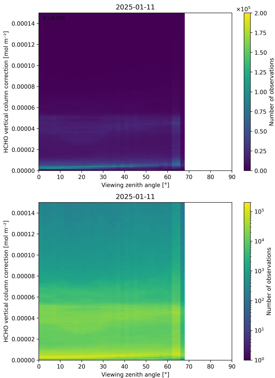
Figure 193: Scatter density plot of “Viewing zenith angle” against “HCHO vertical column correction” for 2025-01-10 to 2025-01-12.
