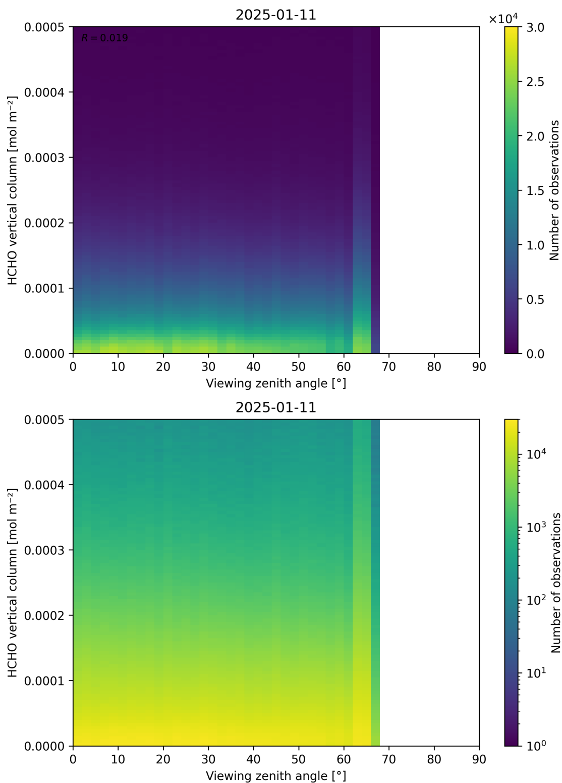
Figure 192: Scatter density plot of “Viewing zenith angle” against “HCHO vertical column” for 2025-01-10 to 2025-01-12.
