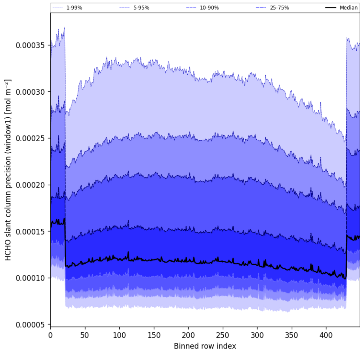
Figure 53: Along track statistics of “HCHO slant column precision (window1)” for 2025-01-10 to 2025-01-12
