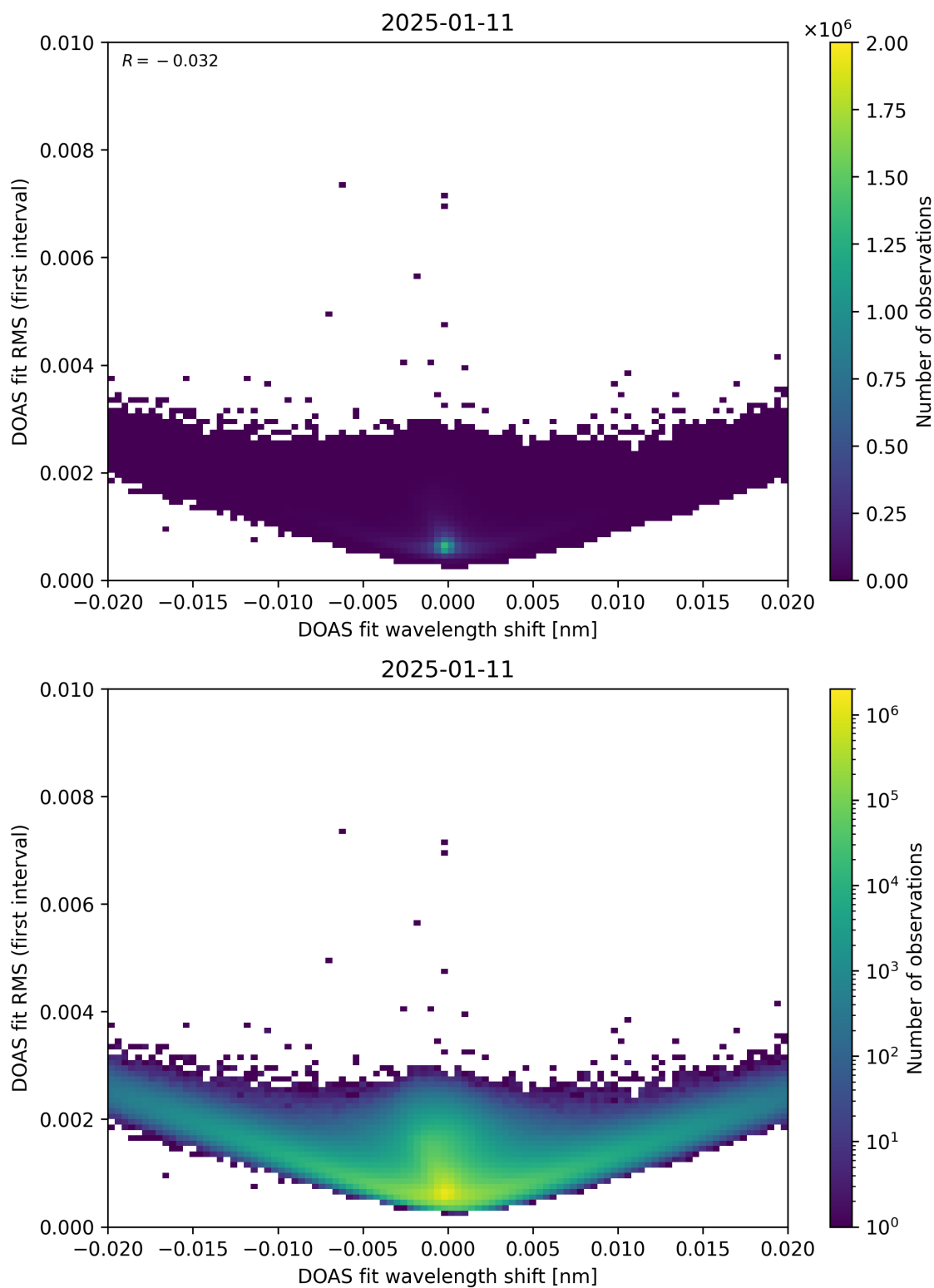
Figure 64: Scatter density plot of “DOAS fit wavelength shift” against “DOAS fit RMS (first interval)” for 2025-01-10 to 2025-01-12.
