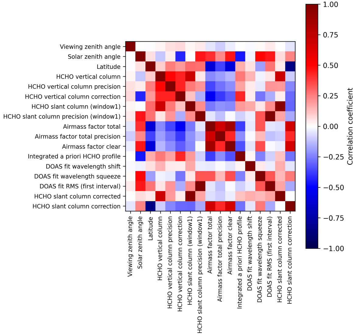
Figure 2: Map of correlation matrix for 2025-01-10 to 2025-01-12.
