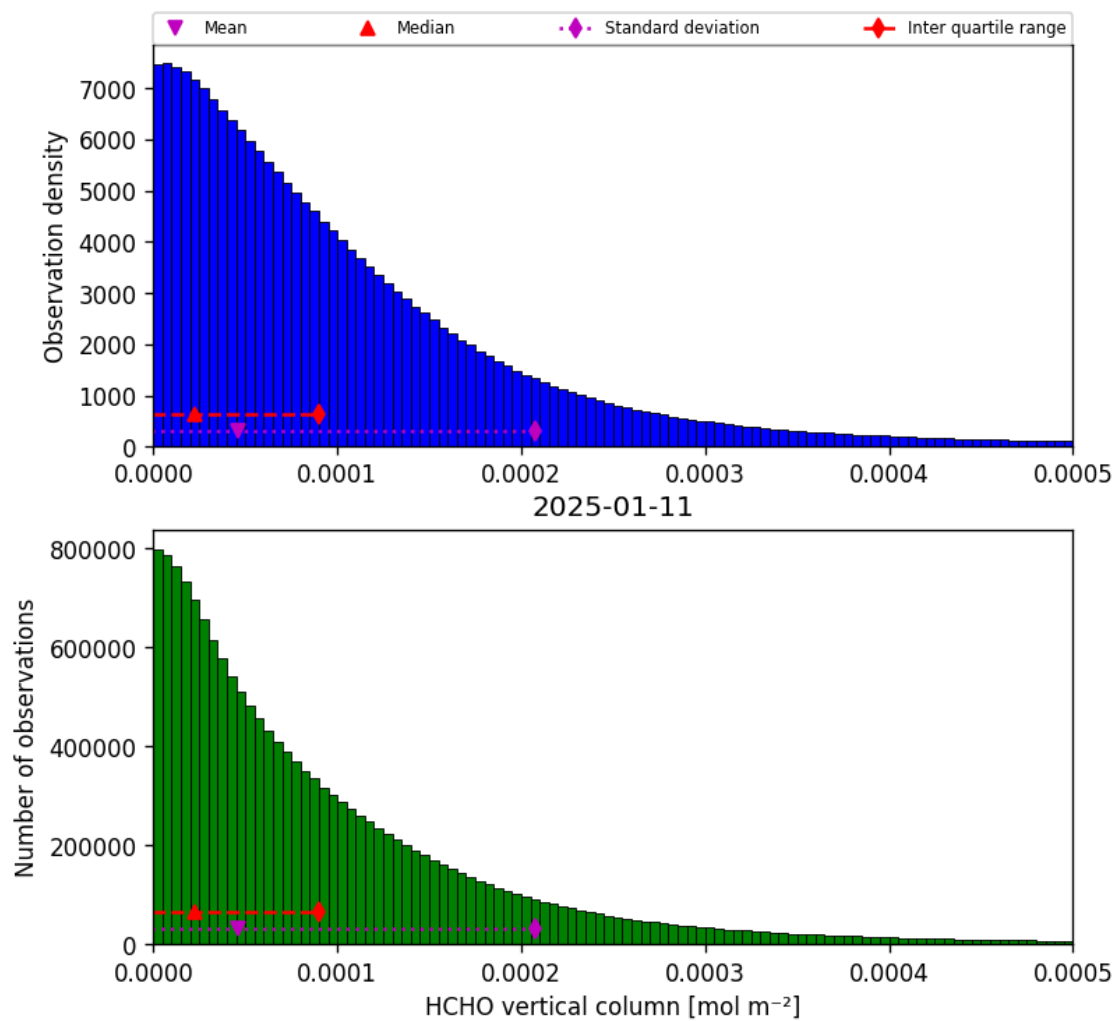
Figure 35: Histogram of “HCHO vertical column” for 2025-01-10 to 2025-01-12
