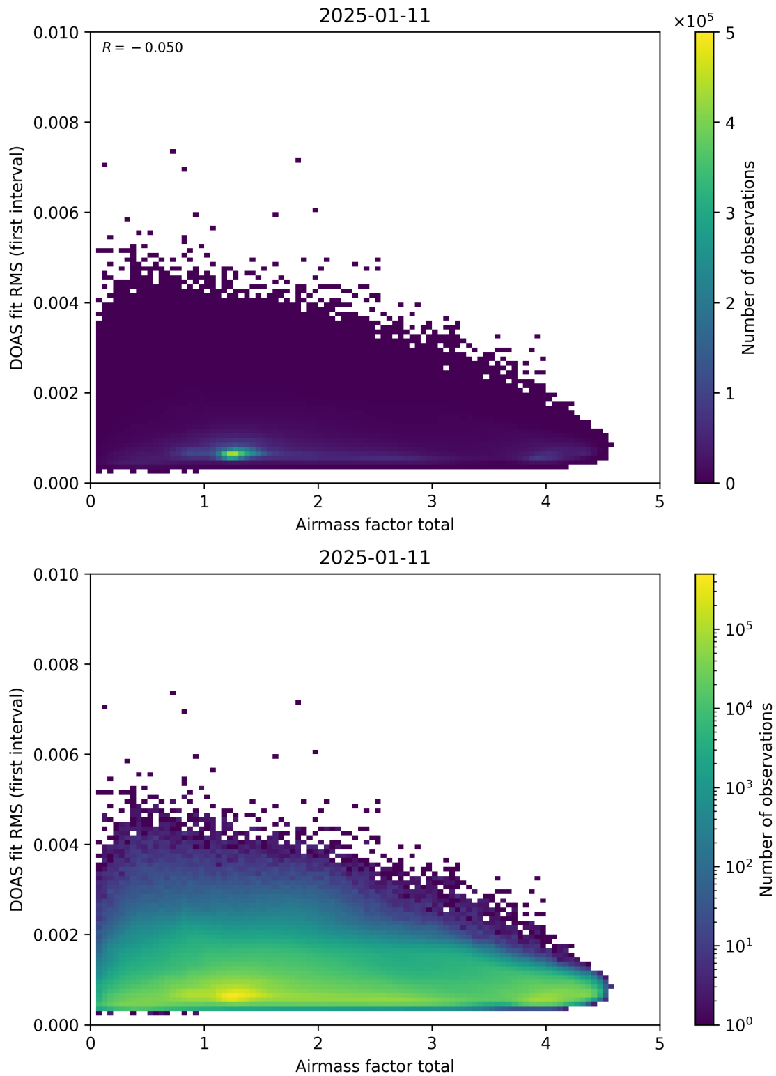
Figure 97: Scatter density plot of “Airmass factor total” against “DOAS fit RMS (first interval)” for 2025-01-10 to 2025-01-12.
