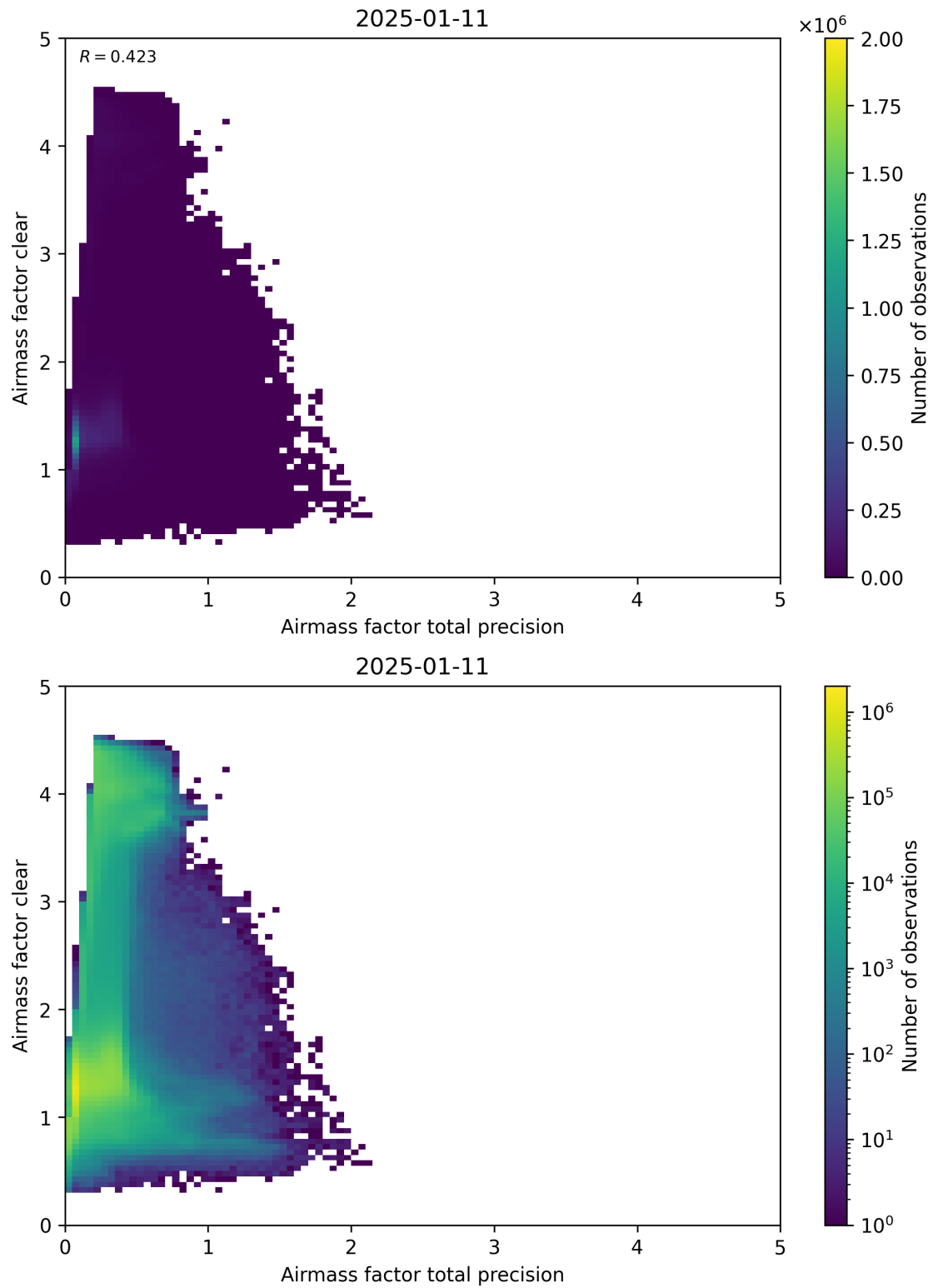
Figure 108: Scatter density plot of “Airmass factor total precision” against “Airmass factor clear” for 2025-01-10 to 2025-01-12.
