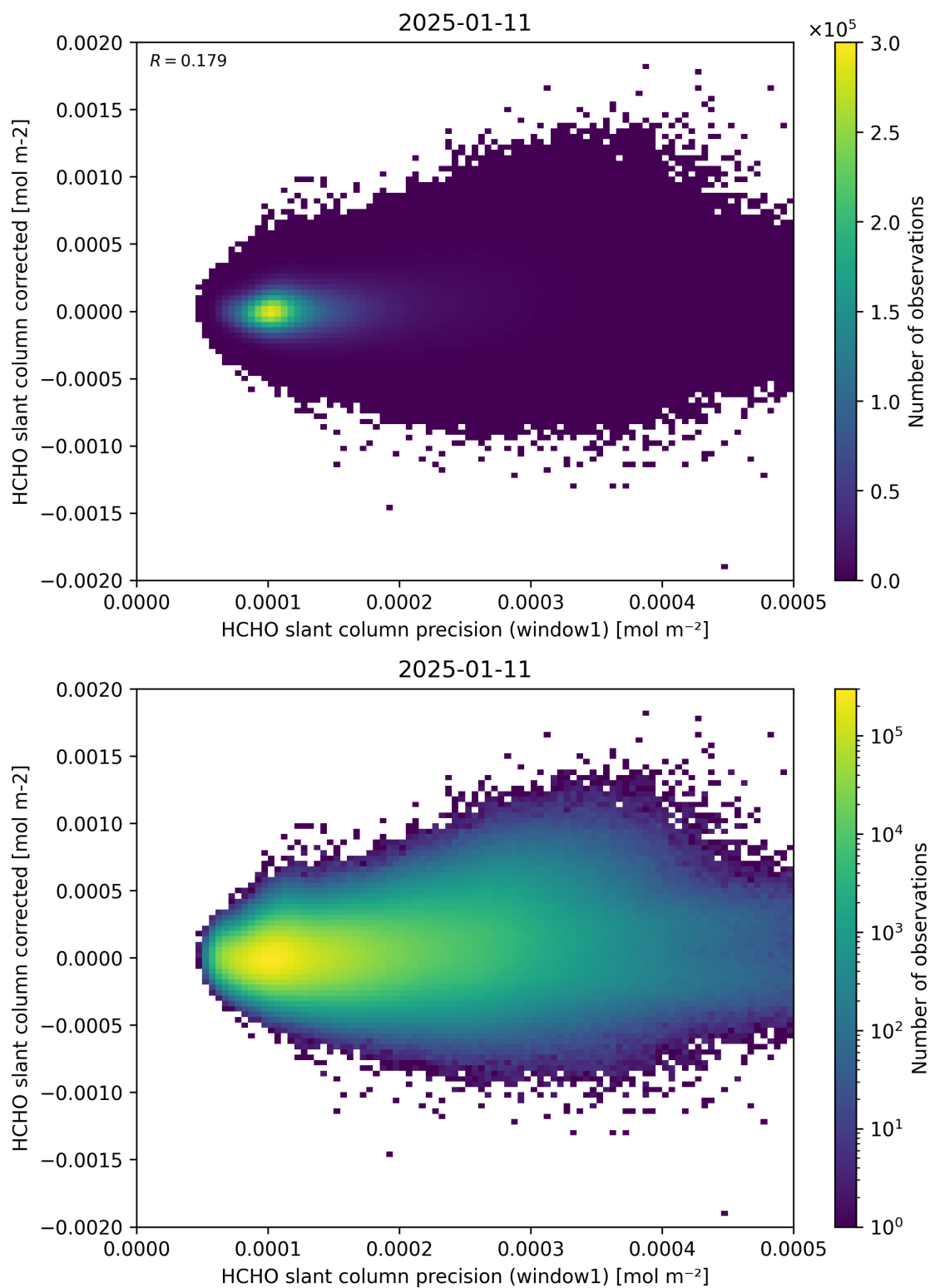
Figure 92: Scatter density plot of “HCHO slant column precision (window1)” against “HCHO slant column corrected” for 2025-01-10 to 2025-01-12.
