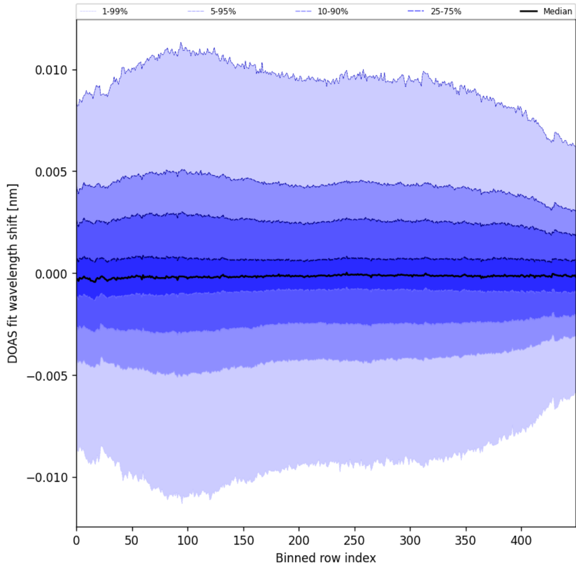
Figure 58: Along track statistics of “DOAS fit wavelength shift” for 2025-01-10 to 2025-01-12
