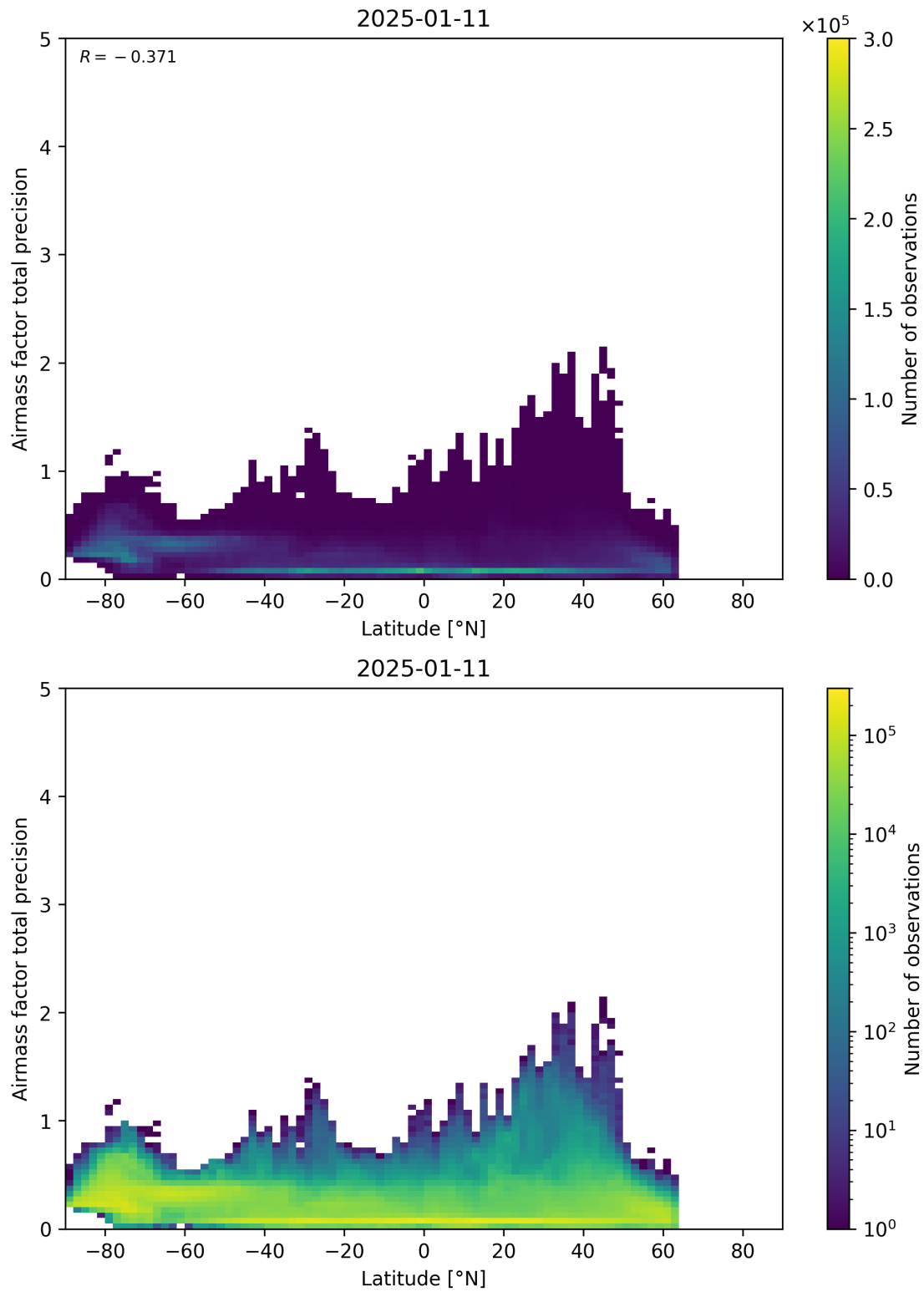
Figure 162: Scatter density plot of “Latitude” against “Airmass factor total precision” for 2025-01-10 to 2025-01-12.
