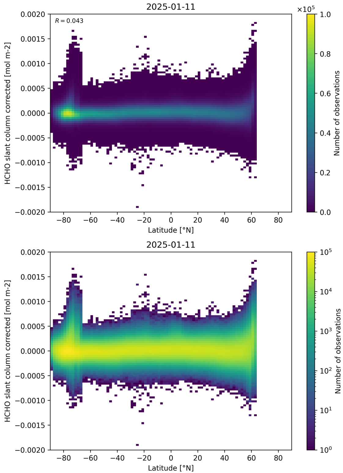
Figure 157: Scatter density plot of “Latitude” against “HCHO slant column corrected” for 2025-01-10 to 2025-01-12.
