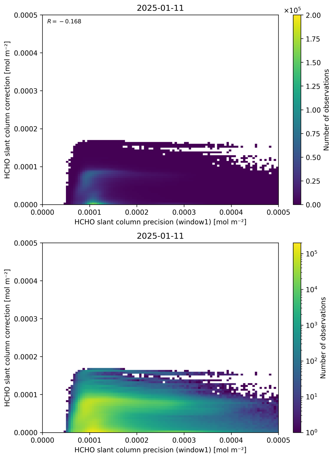
Figure 93: Scatter density plot of “HCHO slant column precision (window1)” against “HCHO slant column correction” for 2025-01-10 to 2025-01-12.
