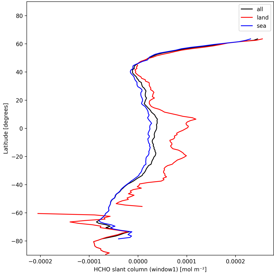
Figure 24: Zonal average of “HCHO slant column (window1)” for 2025-01-10 to 2025-01-12.
