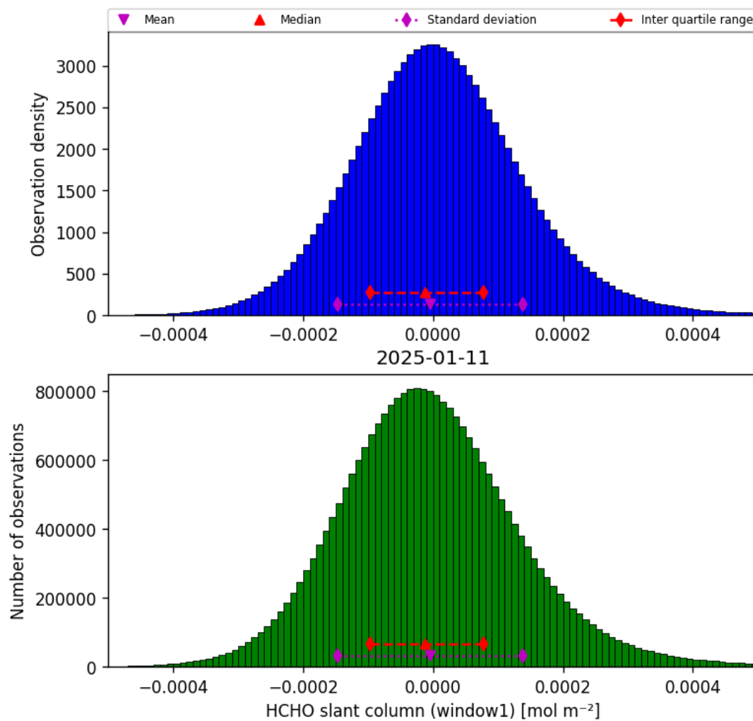
Figure 38: Histogram of “HCHO slant column (window1)” for 2025-01-10 to 2025-01-12
