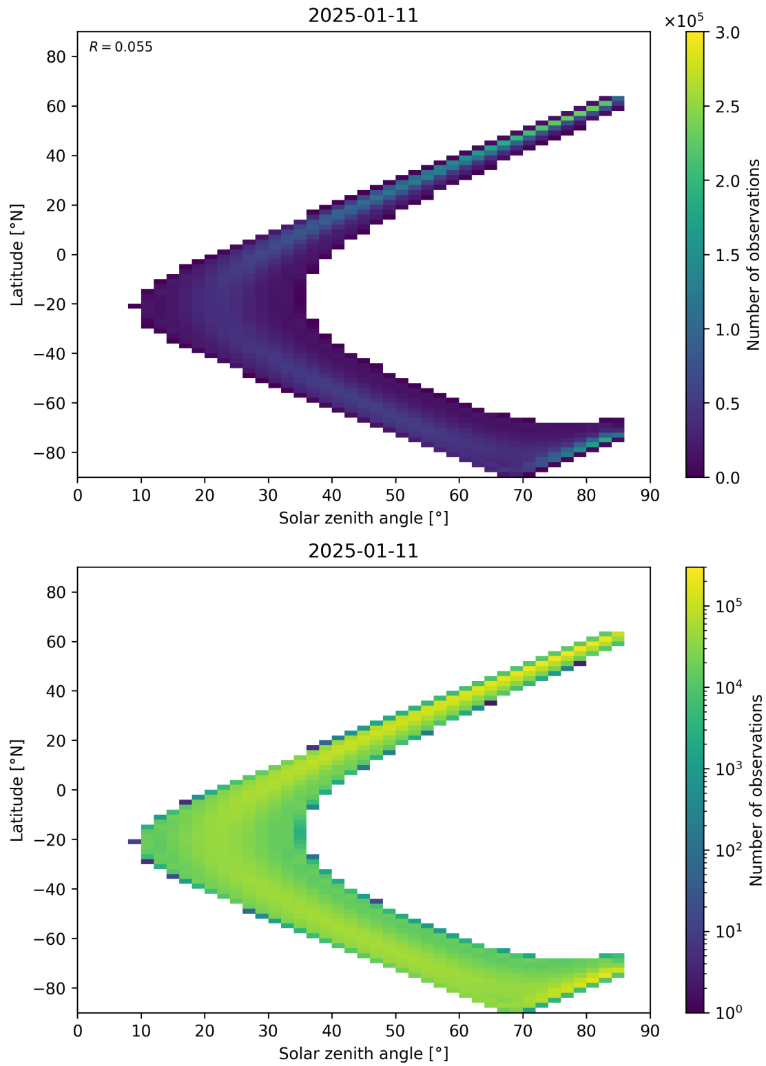
Figure 181: Scatter density plot of “Solar zenith angle” against “Latitude” for 2025-01-10 to 2025-01-12.
