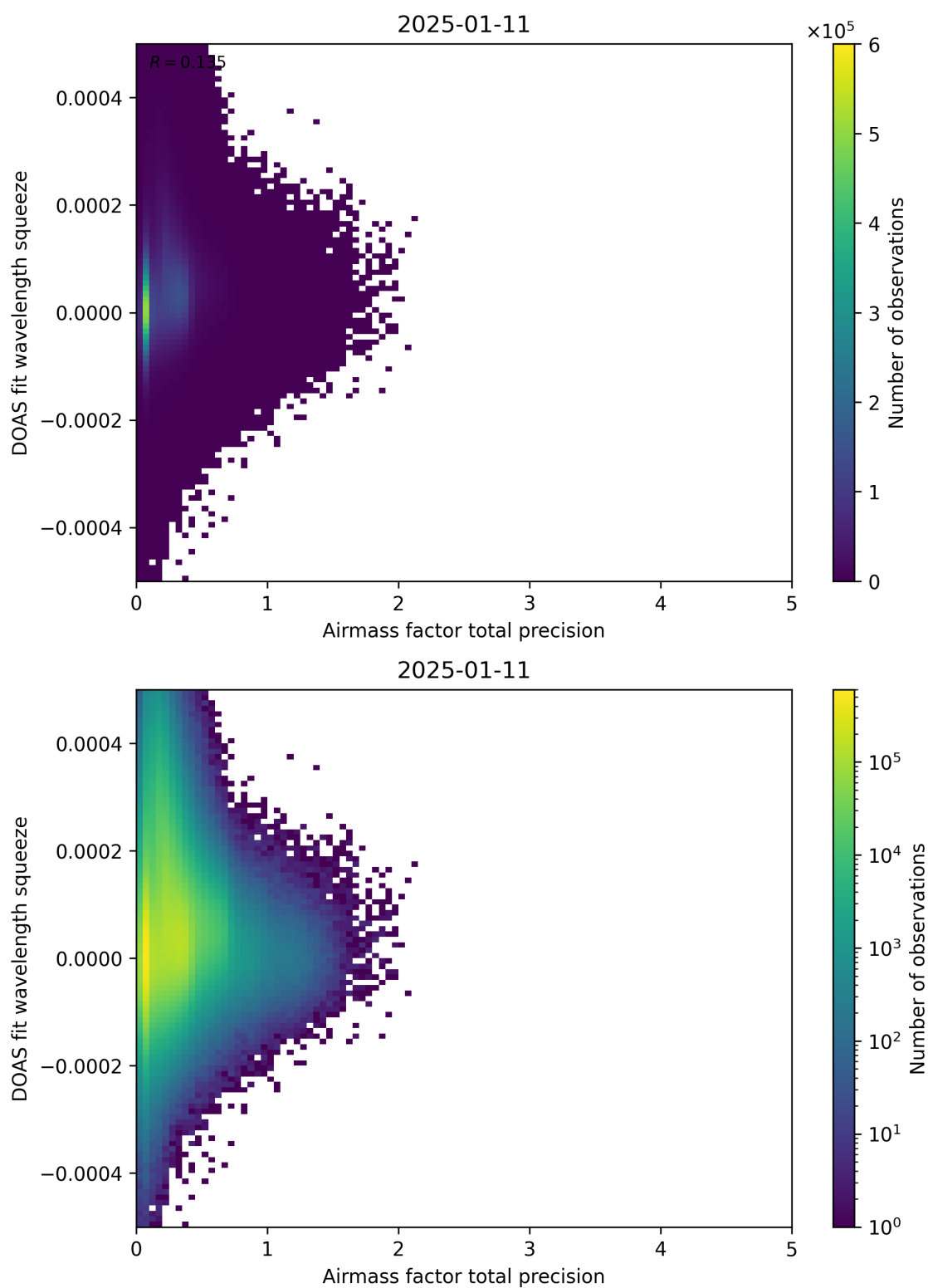
Figure 107: Scatter density plot of “Airmass factor total precision” against “DOAS fit wavelength squeeze” for 2025-01-10 to 2025-01-12.
