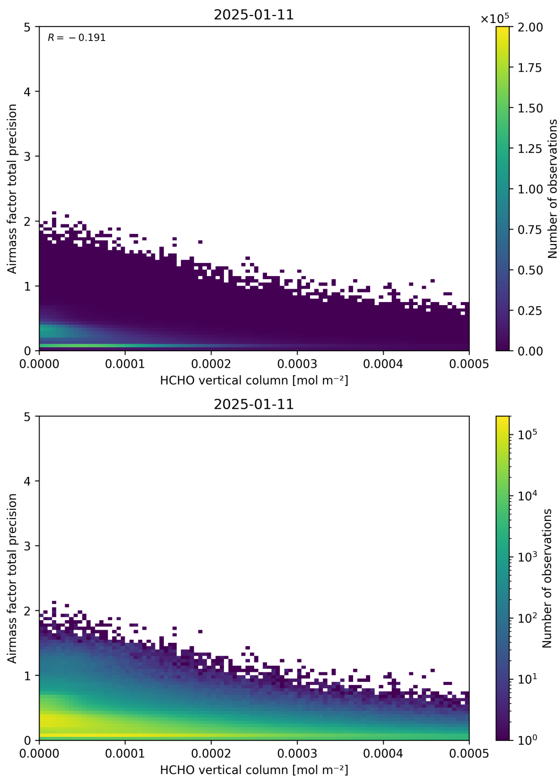
Figure 132: Scatter density plot of “HCHO vertical column” against “Airmass factor total precision” for 2025-01-10 to 2025-01-12.
