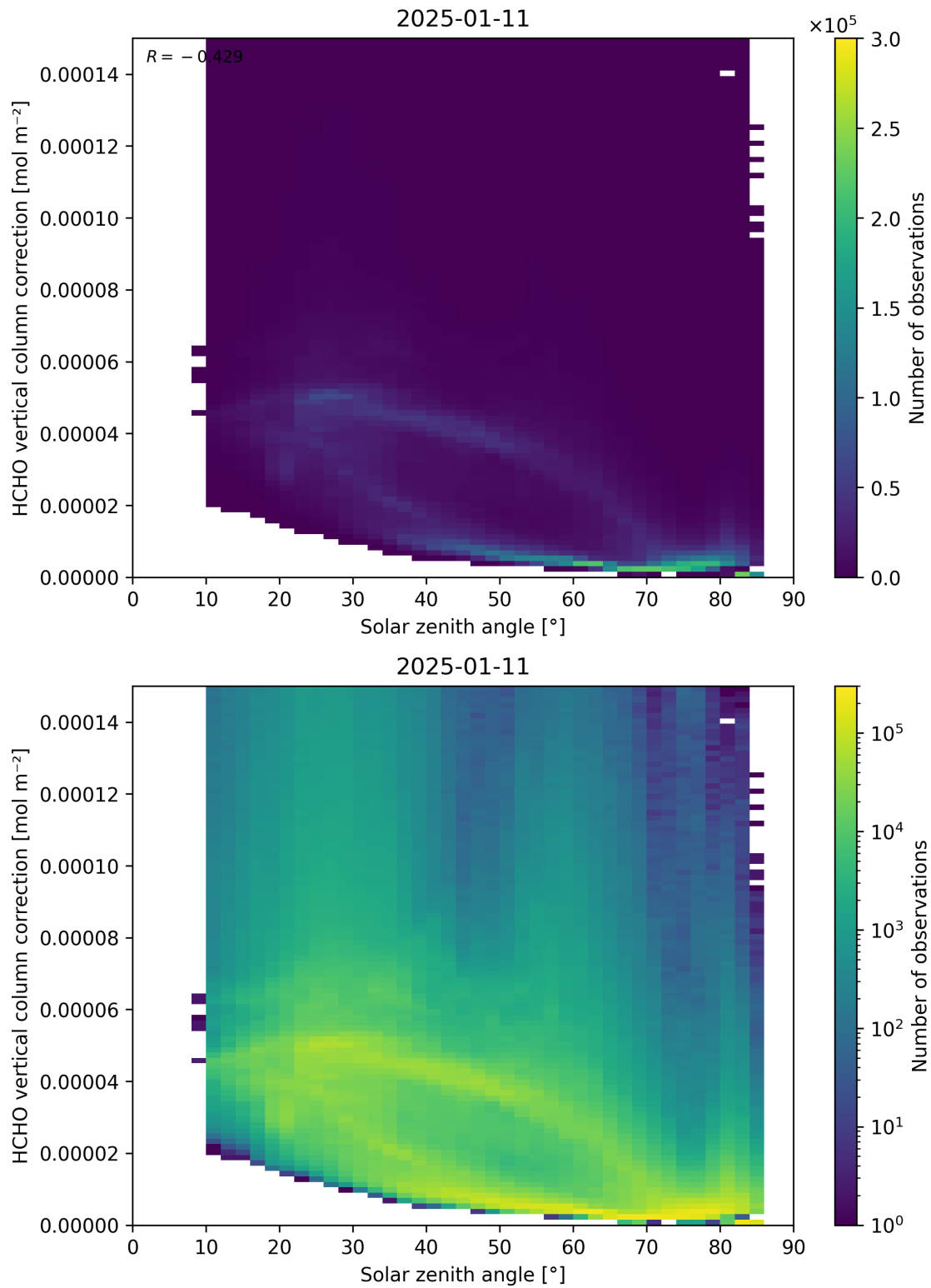
Figure 178: Scatter density plot of “Solar zenith angle” against “HCHO vertical column correction” for 2025-01-10 to 2025-01-12.
