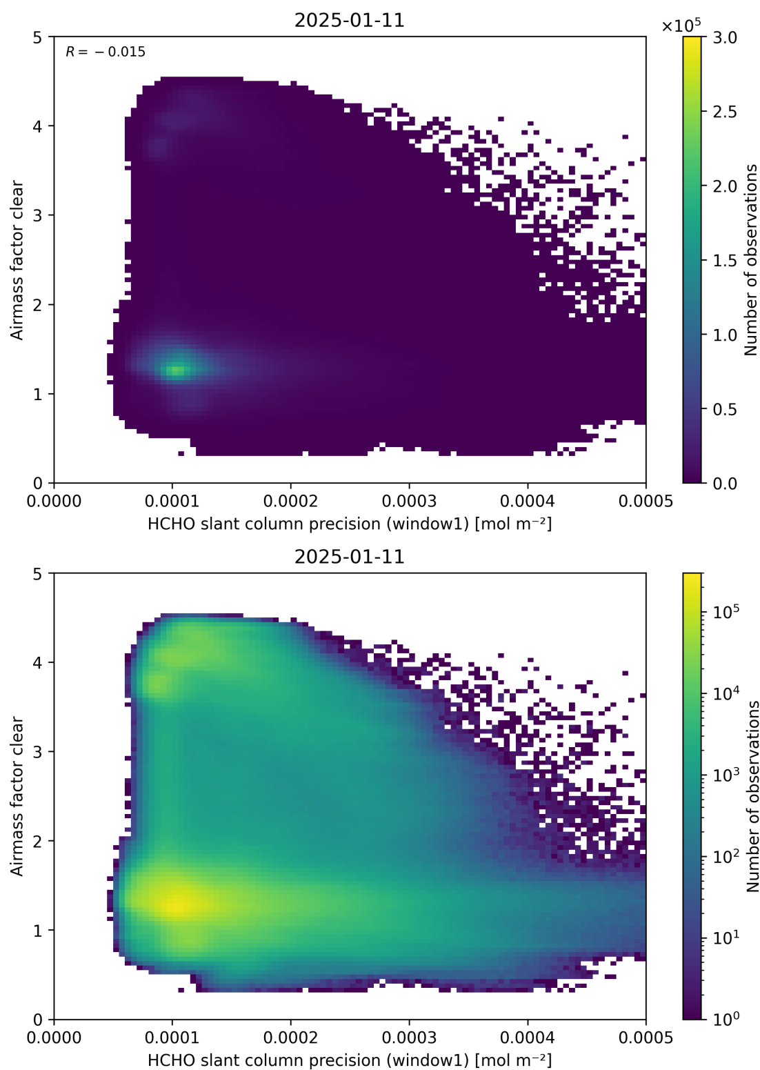
Figure 91: Scatter density plot of “HCHO slant column precision (window1)” against “Airmass factor clear” for 2025-01-10 to 2025-01-12.
