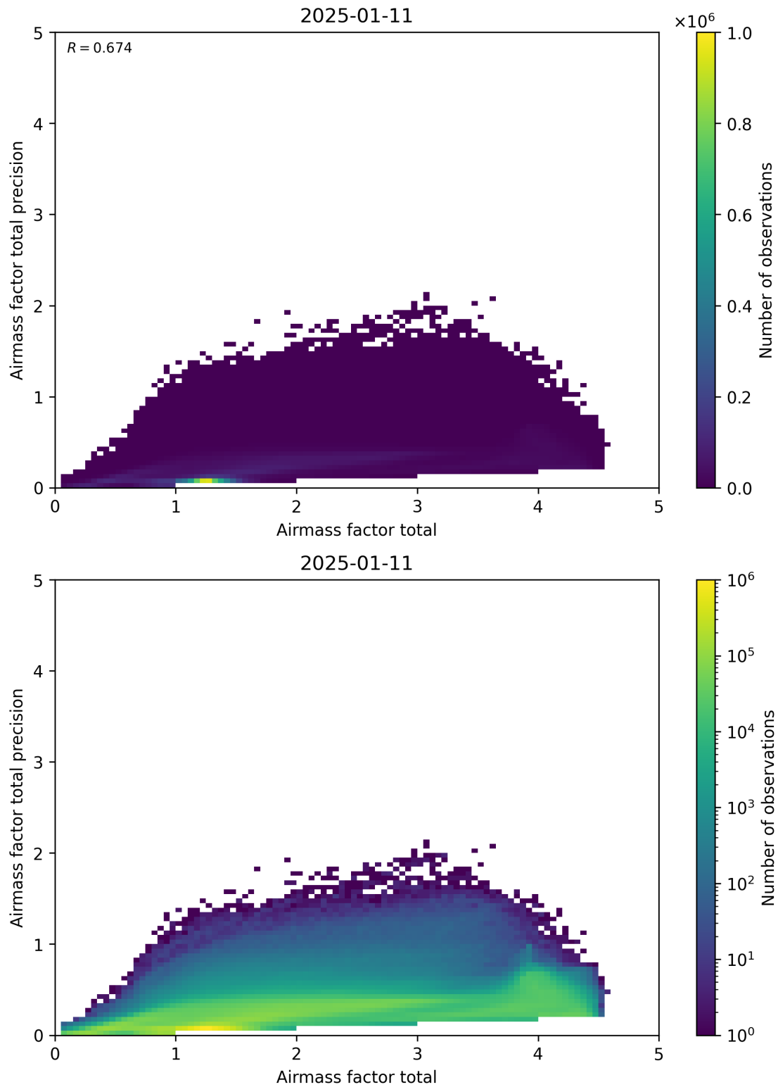
Figure 103: Scatter density plot of “Airmass factor total” against “Airmass factor total precision” for 2025-01-10 to 2025-01-12.
