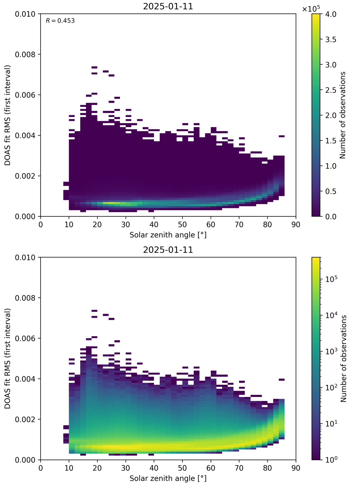
Figure 167: Scatter density plot of “Solar zenith angle” against “DOAS fit RMS (first interval)” for 2025-01-10 to 2025-01-12.
