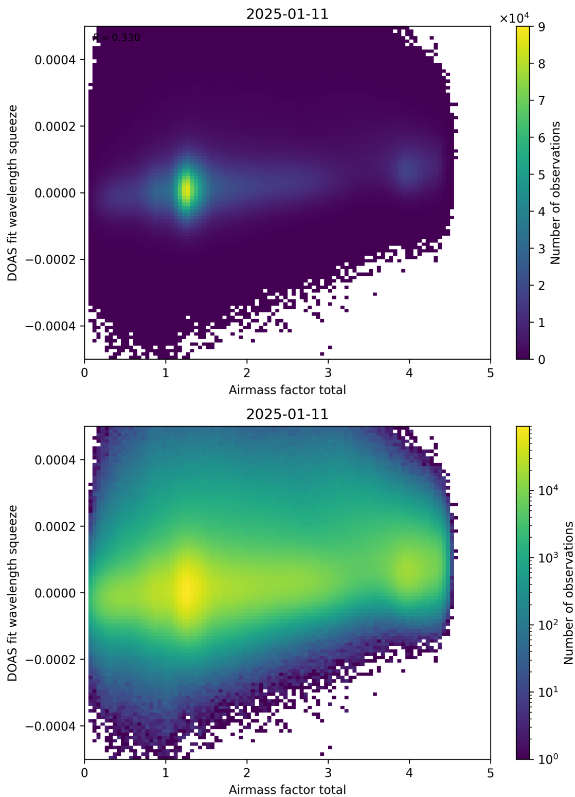
Figure 99: Scatter density plot of “Airmass factor total” against “DOAS fit wavelength squeeze” for 2025-01-10 to 2025-01-12.
