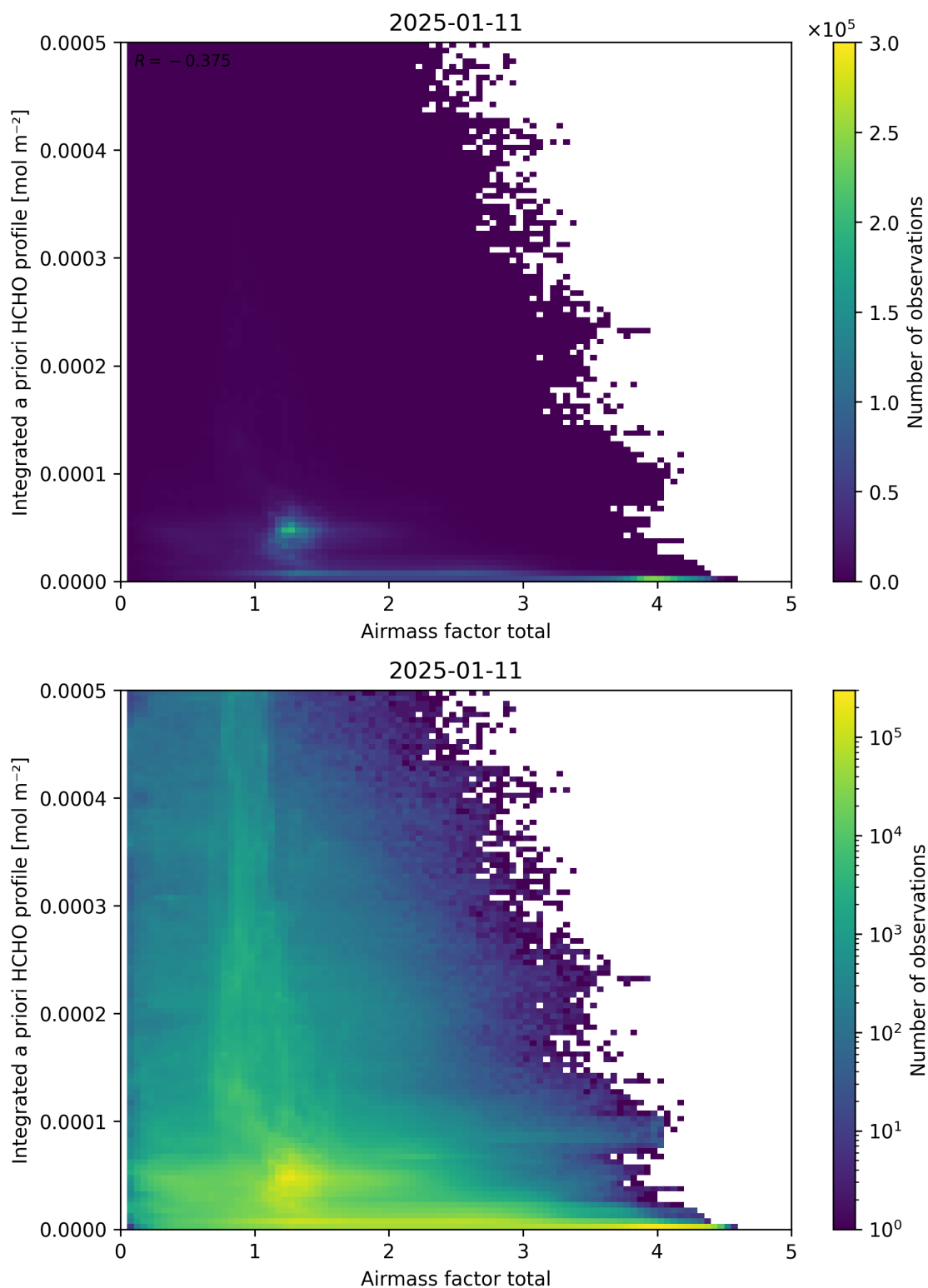
Figure 104: Scatter density plot of “Airmass factor total” against “Integrated a priori HCHO profile” for 2025-01-10 to 2025-01-12.
