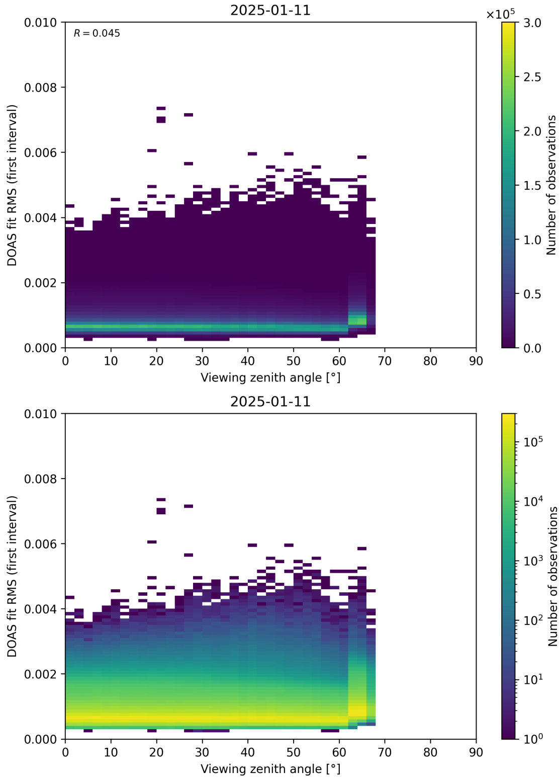
Figure 182: Scatter density plot of “Viewing zenith angle” against “DOAS fit RMS (first interval)” for 2025-01-10 to 2025-01-12.
