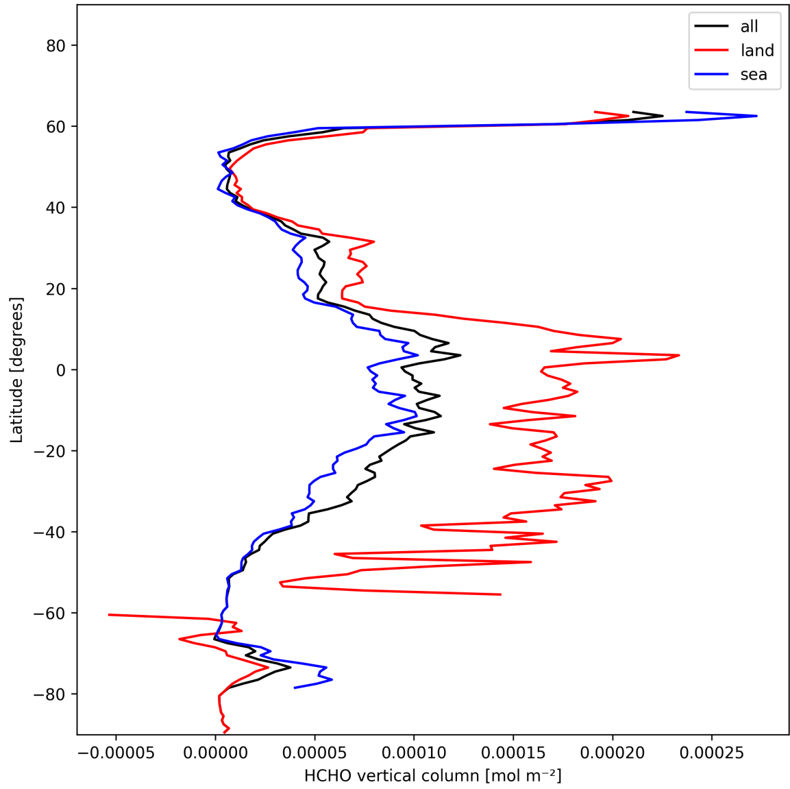
Figure 21: Zonal average of “HCHO vertical column” for 2025-01-10 to 2025-01-12.
