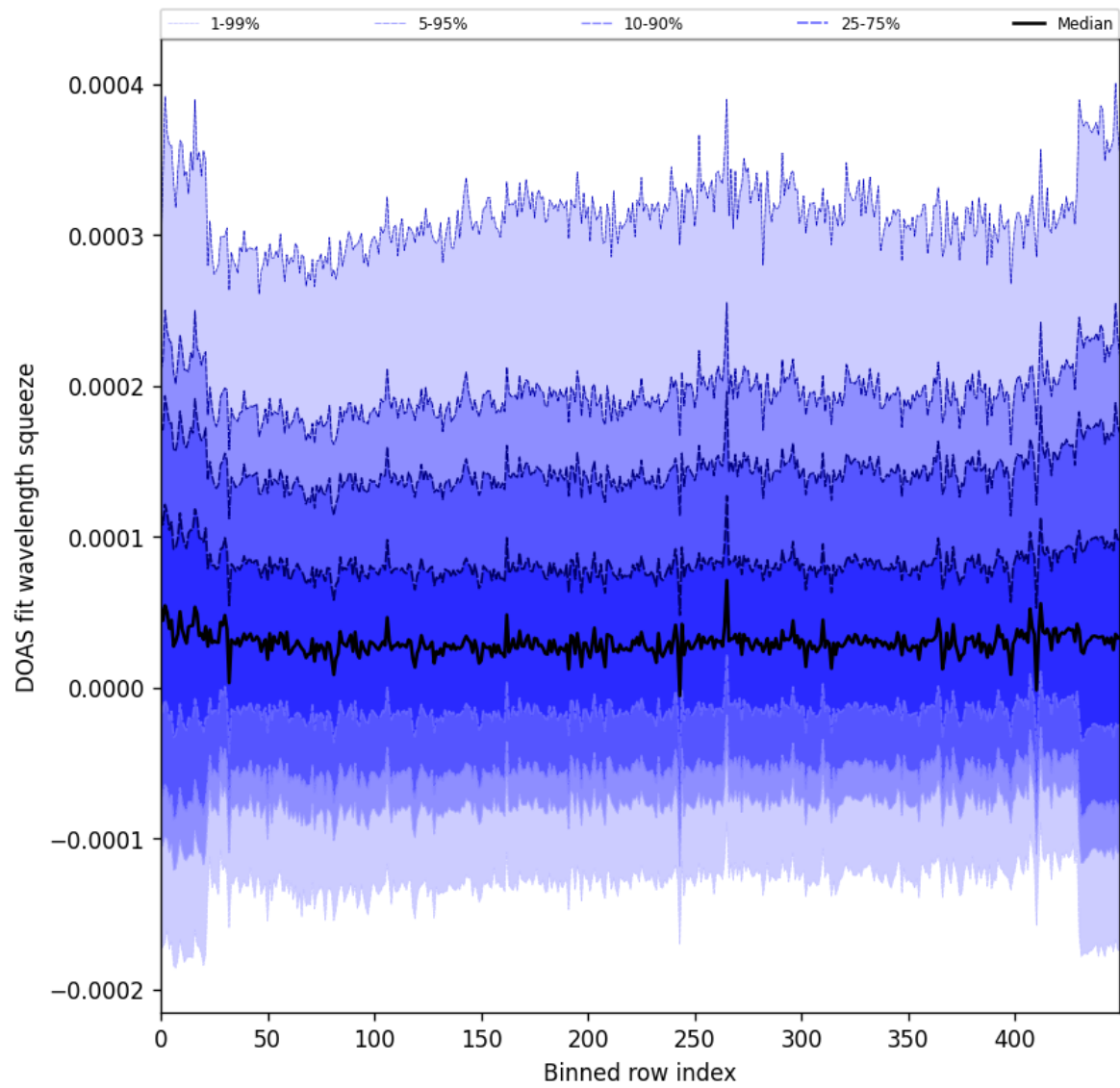
Figure 59: Along track statistics of “DOAS fit wavelength squeeze” for 2025-01-10 to 2025-01-12
