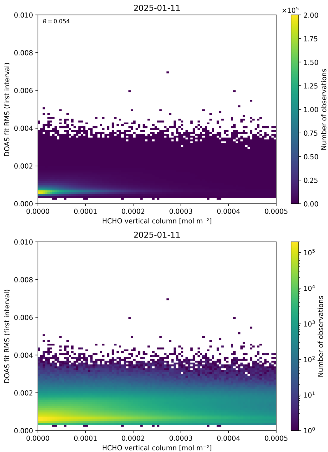
Figure 123: Scatter density plot of “HCHO vertical column” against “DOAS fit RMS (first interval)” for 2025-01-10 to 2025-01-12.
