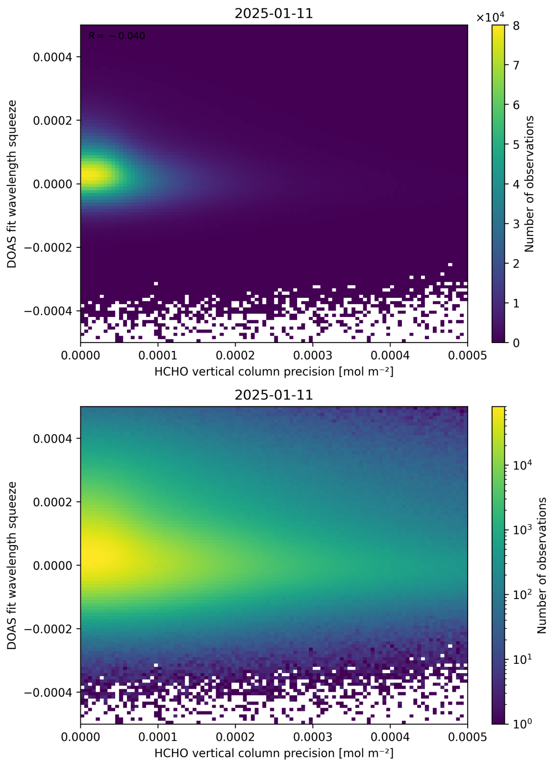
Figure 138: Scatter density plot of “HCHO vertical column precision” against “DOAS fit wavelength squeeze” for 2025-01-10 to 2025-01-12.
