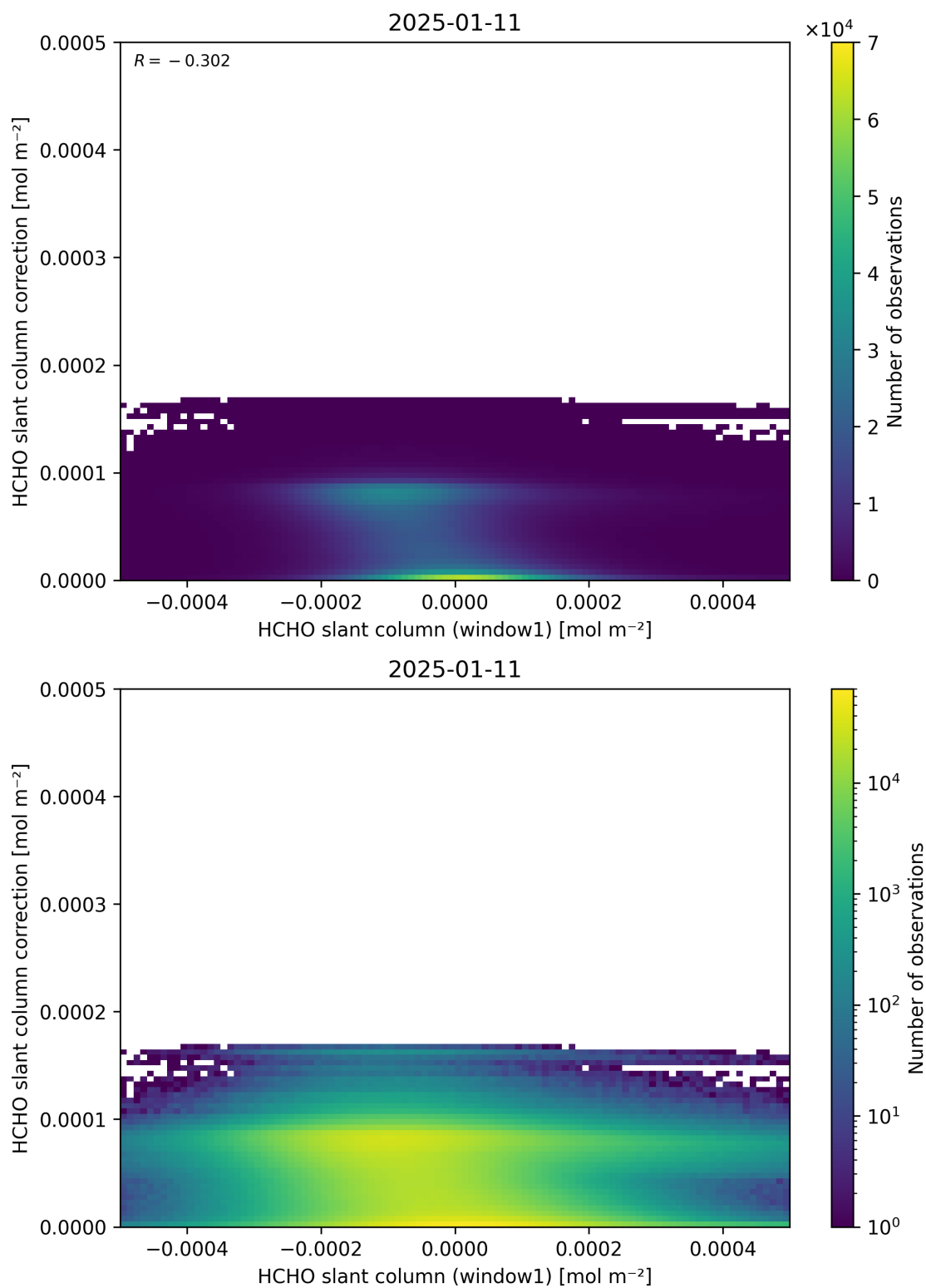
Figure 83: Scatter density plot of “HCHO slant column (window1)” against “HCHO slant column correction” for 2025-01-10 to 2025-01-12.
