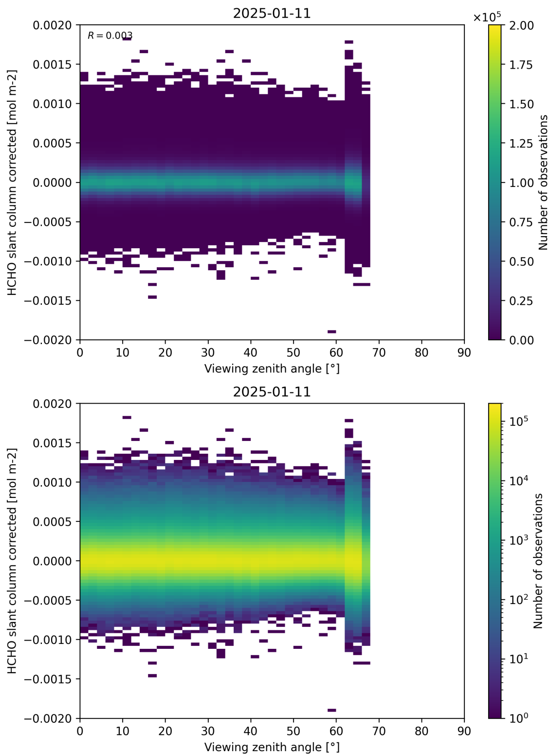
Figure 186: Scatter density plot of “Viewing zenith angle” against “HCHO slant column corrected” for 2025-01-10 to 2025-01-12.
