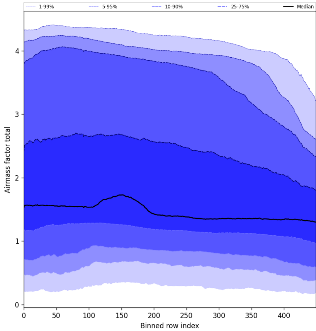
Figure 54: Along track statistics of “Airmass factor total” for 2025-01-10 to 2025-01-12
