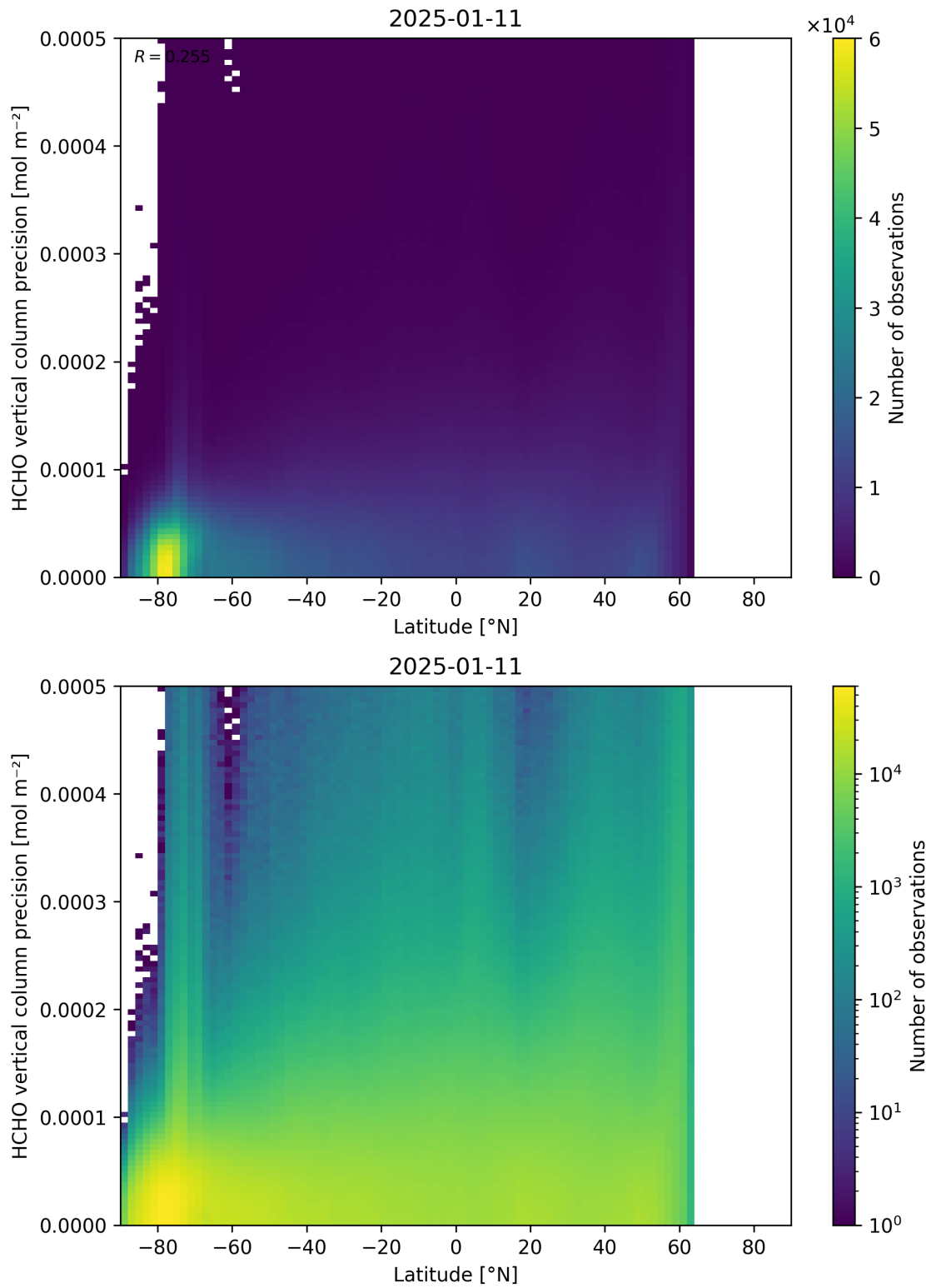
Figure 165: Scatter density plot of “Latitude” against “HCHO vertical column precision” for 2025-01-10 to 2025-01-12.
