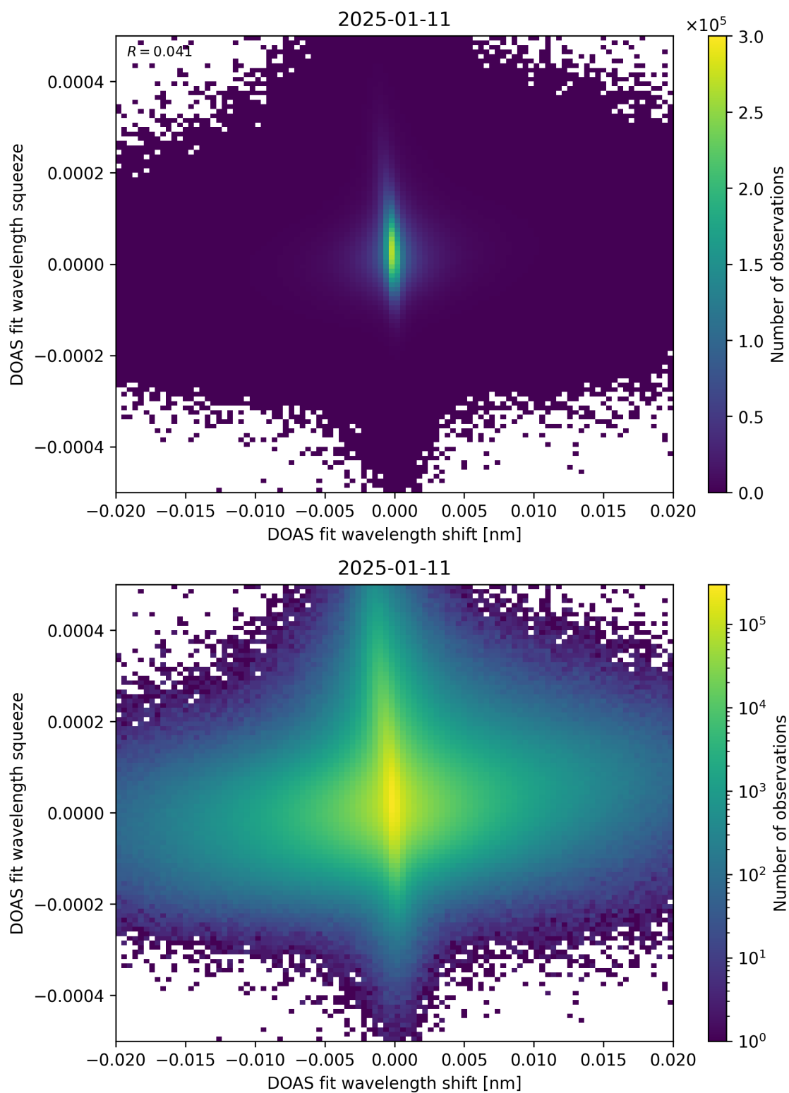
Figure 65: Scatter density plot of “DOAS fit wavelength shift” against “DOAS fit wavelength squeeze” for 2025-01-10 to 2025-01-12.
