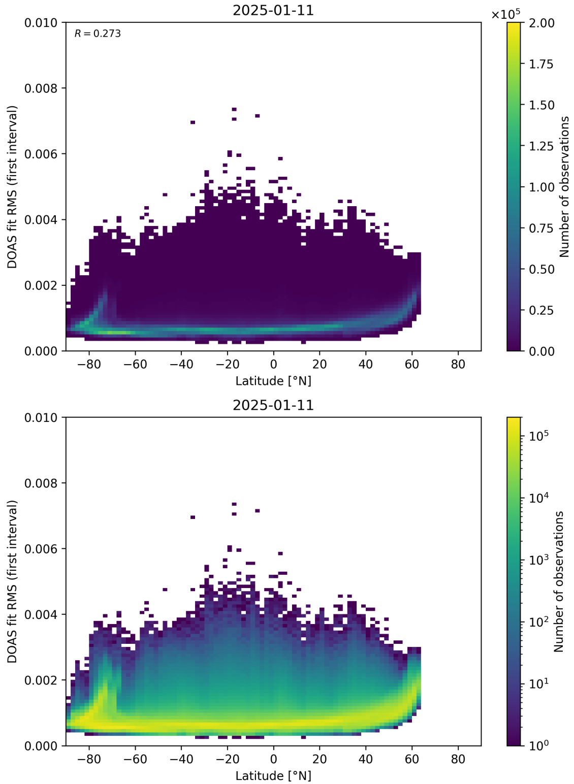
Figure 153: Scatter density plot of “Latitude” against “DOAS fit RMS (first interval)” for 2025-01-10 to 2025-01-12.
