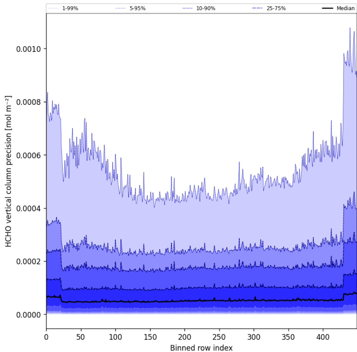
Figure 50: Along track statistics of “HCHO vertical column precision” for 2025-01-10 to 2025-01-12
