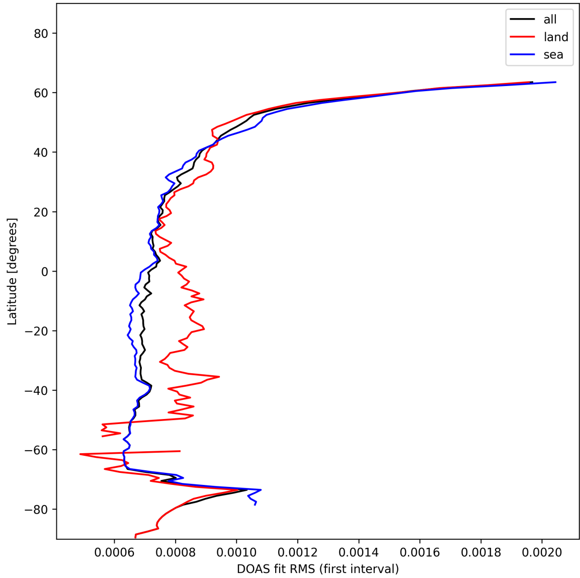
Figure 32: Zonal average of "DOAS fit RMS (first interval)" for 2025-01-10 to 2025-01-12.
