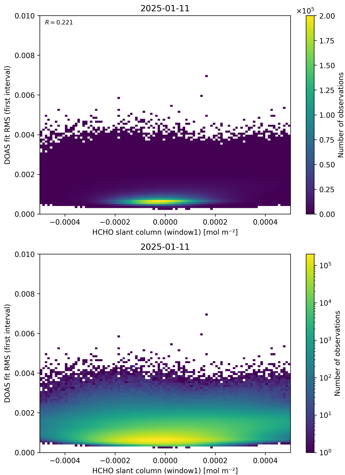
Figure 78: Scatter density plot of “HCHO slant column (window1)” against “DOAS fit RMS (first interval)” for 2025-01-10 to 2025-01-12.
