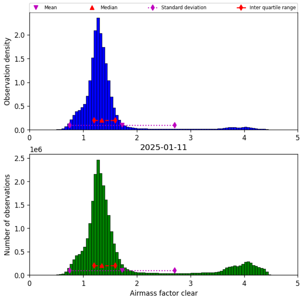
Figure 42: Histogram of “Airmass factor clear” for 2025-01-10 to 2025-01-12
