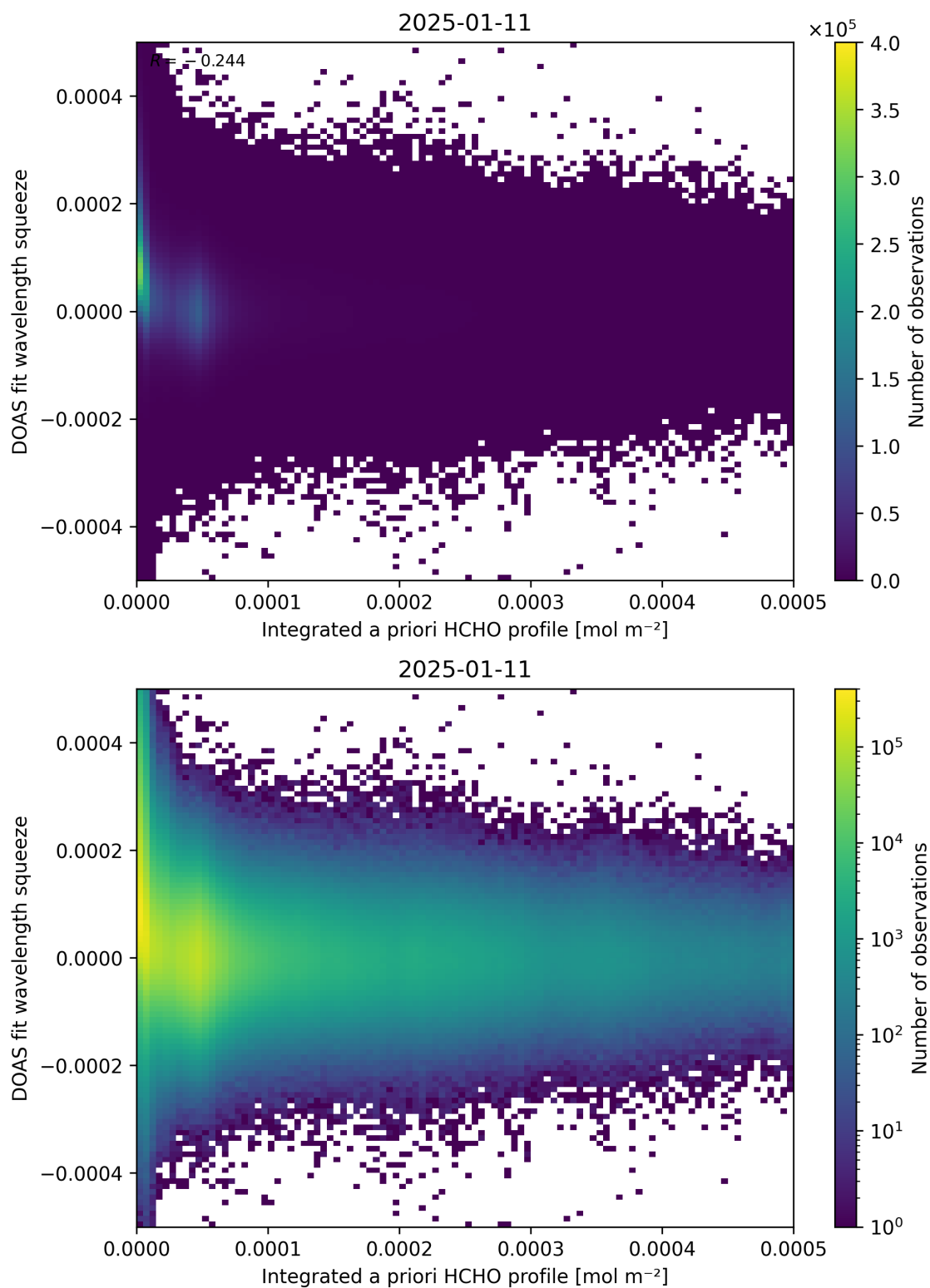
Figure 150: Scatter density plot of “Integrated a priori HCHO profile” against “DOAS fit wavelength squeeze” for 2025-01-10 to 2025-01-12.
