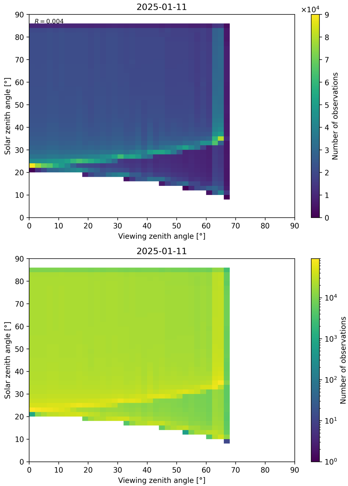
Figure 197: Scatter density plot of “Viewing zenith angle” against “Solar zenith angle” for 2025-01-10 to 2025-01-12.
