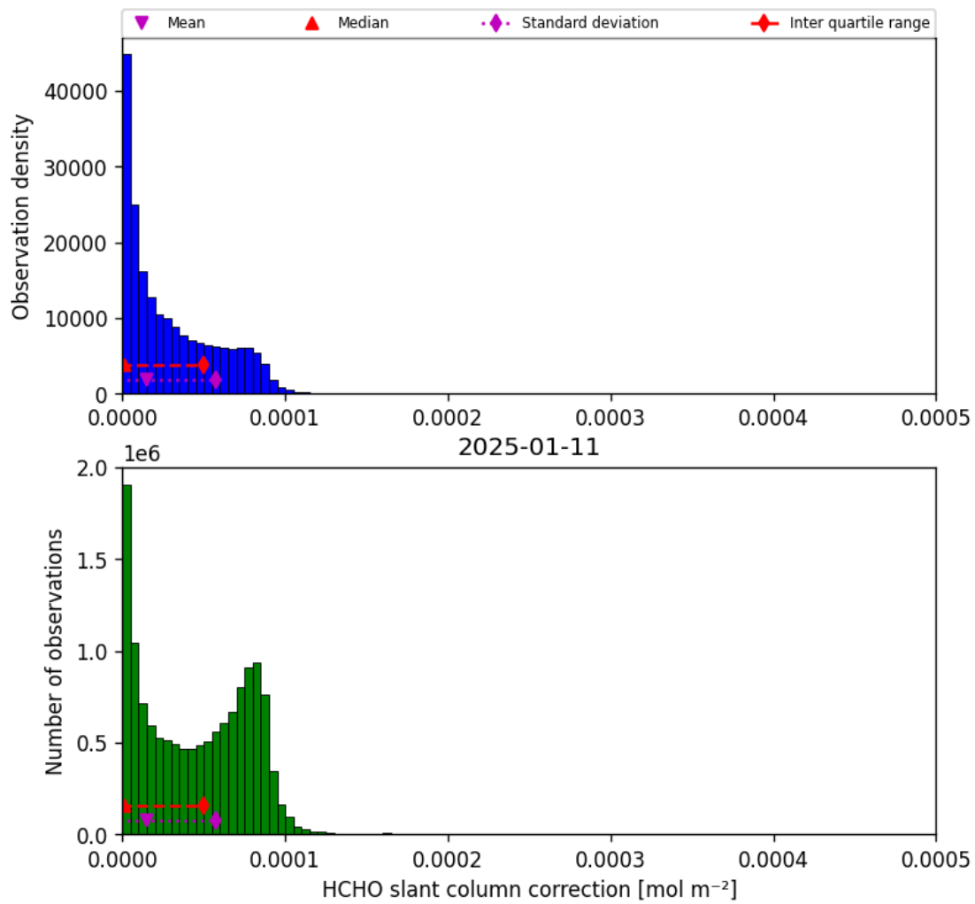
Figure 47: Histogram of “HCHO slant column correction” for 2025-01-10 to 2025-01-12
