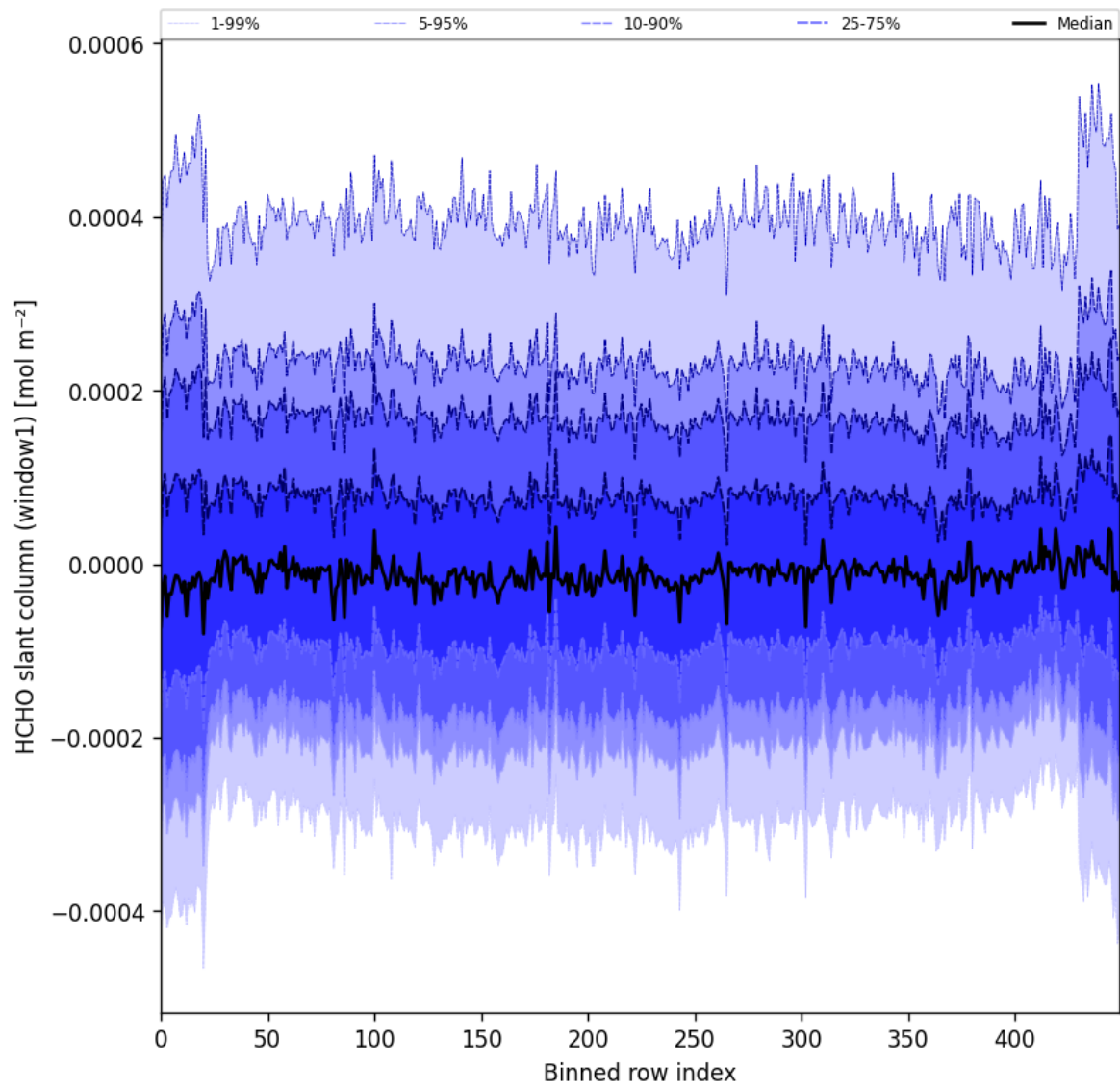
Figure 52: Along track statistics of “HCHO slant column (window1)” for 2025-01-10 to 2025-01-12
