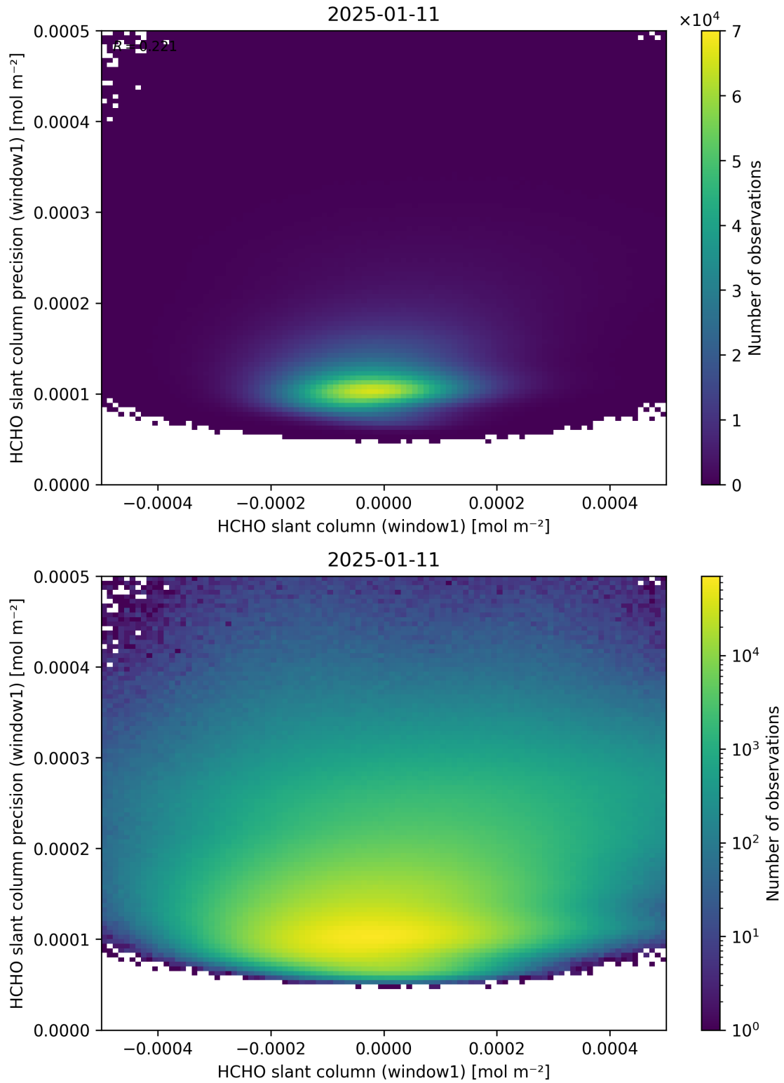
Figure 84: Scatter density plot of “HCHO slant column (window1)” against “HCHO slant column precision (window1)” for 2025-01-10 to 2025-01-12.
