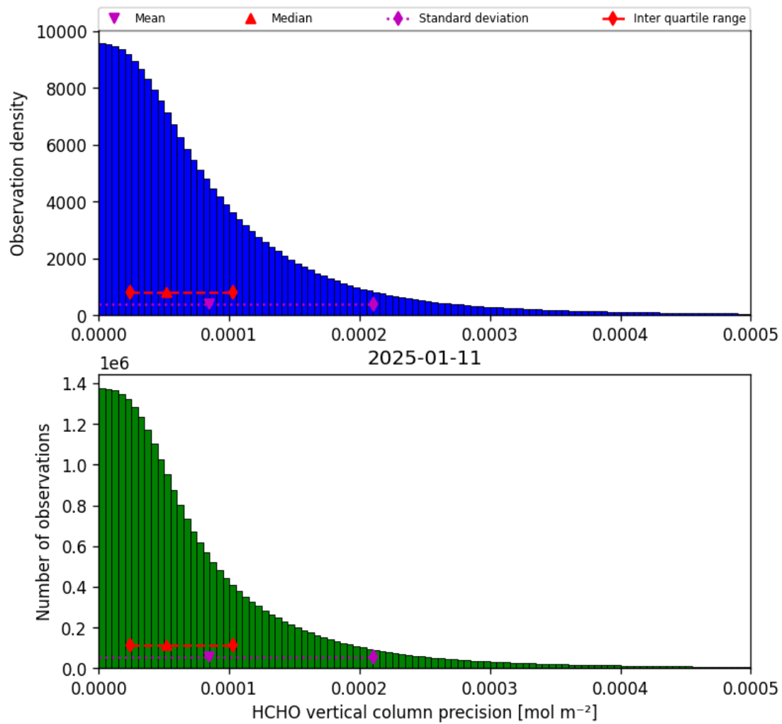
Figure 36: Histogram of “HCHO vertical column precision” for 2025-01-10 to 2025-01-12
