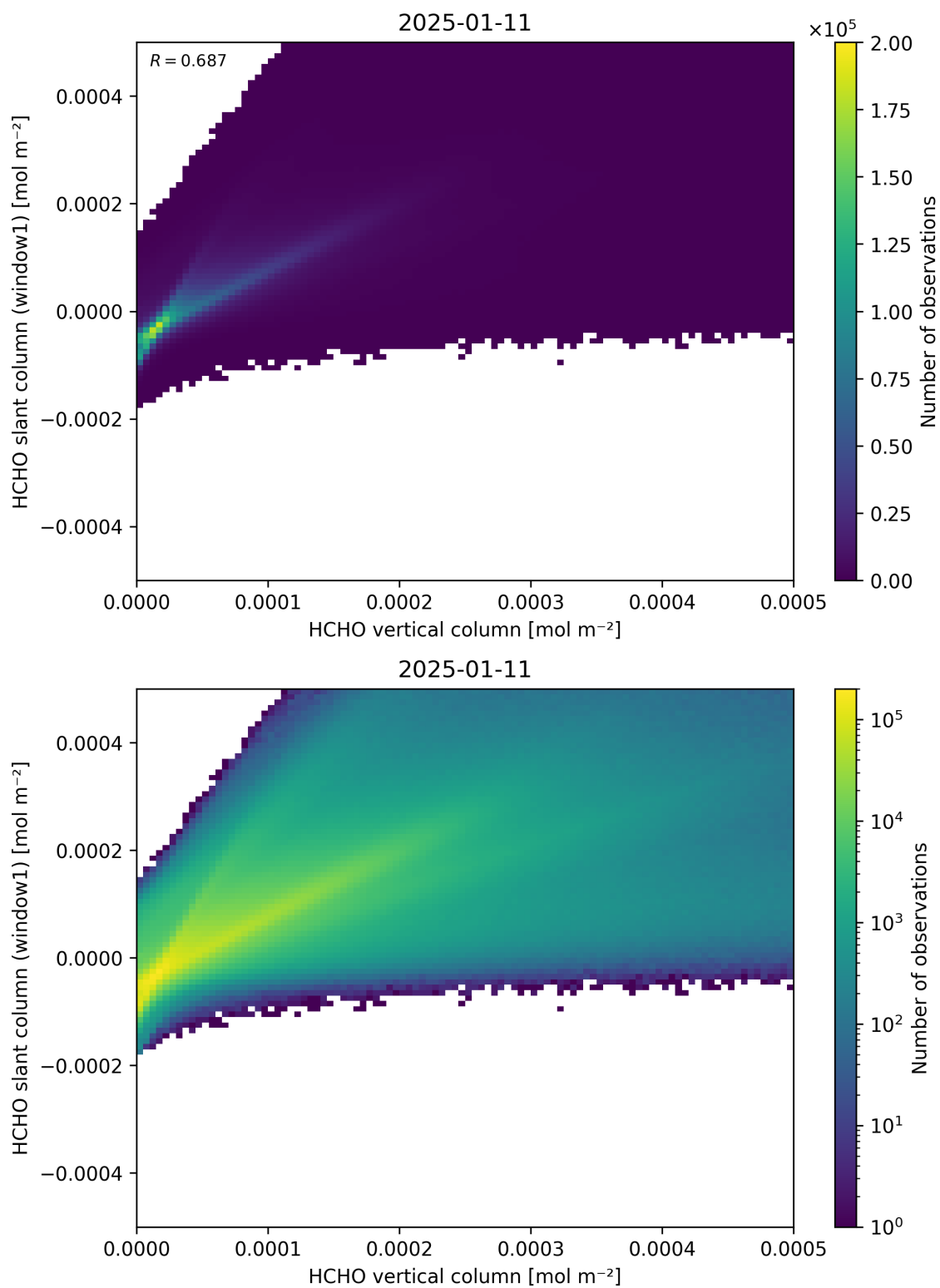
Figure 129: Scatter density plot of “HCHO vertical column” against “HCHO slant column (window1)” for 2025-01-10 to 2025-01-12.
