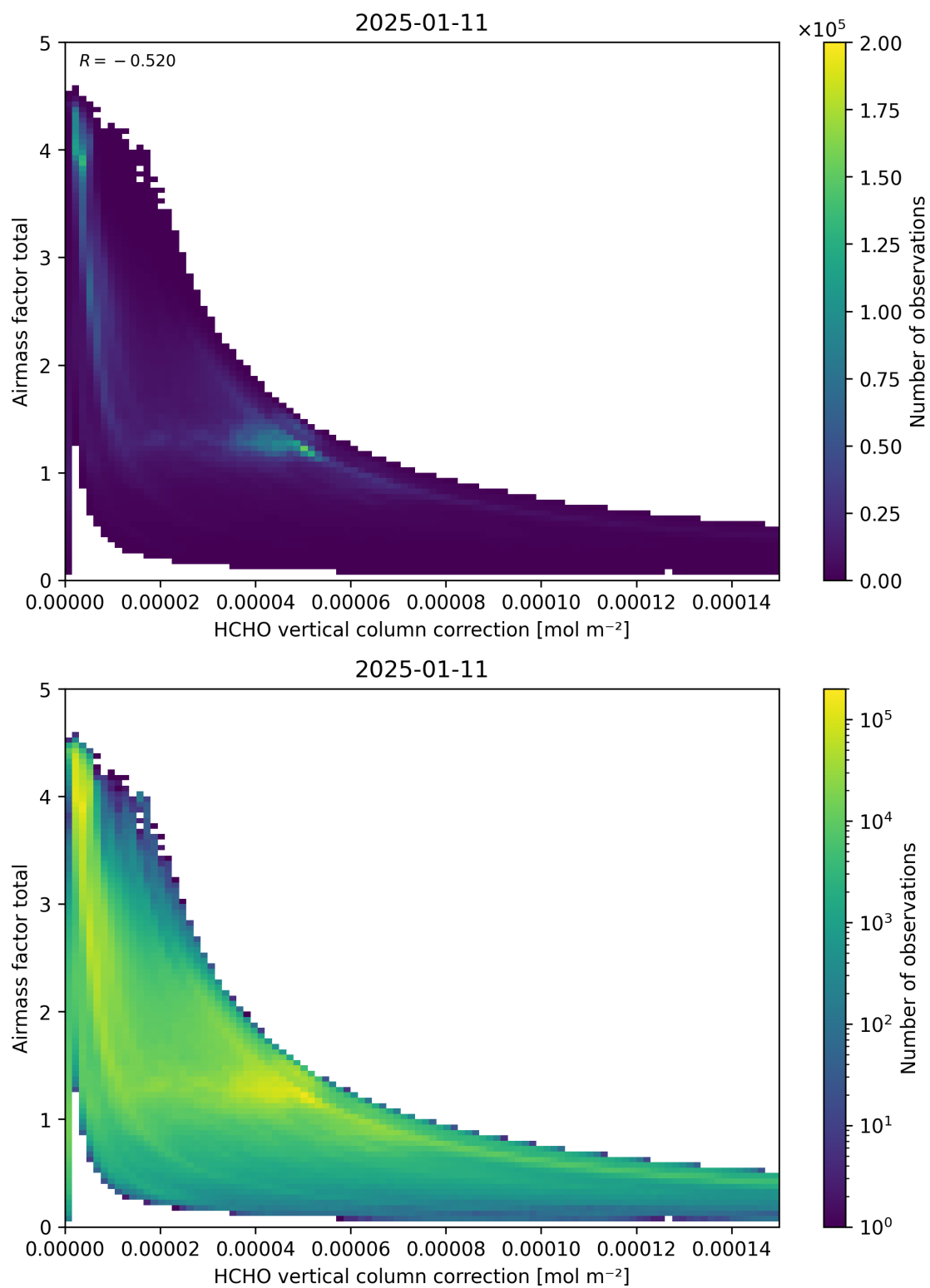
Figure 120: Scatter density plot of “HCHO vertical column correction” against “Airmass factor total” for 2025-01-10 to 2025-01-12.
