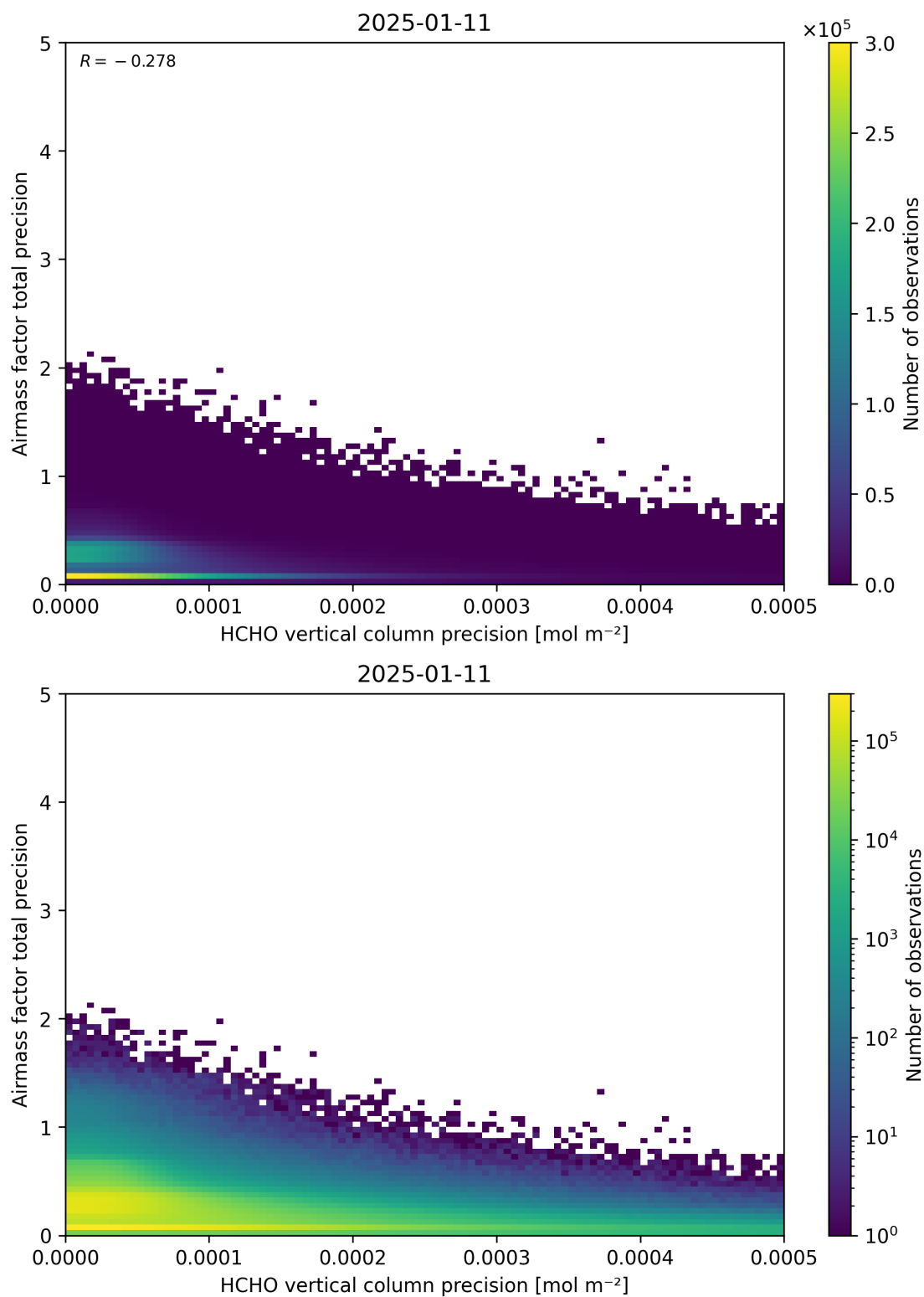
Figure 145: Scatter density plot of “HCHO vertical column precision” against “Airmass factor total precision” for 2025-01-10 to 2025-01-12.
