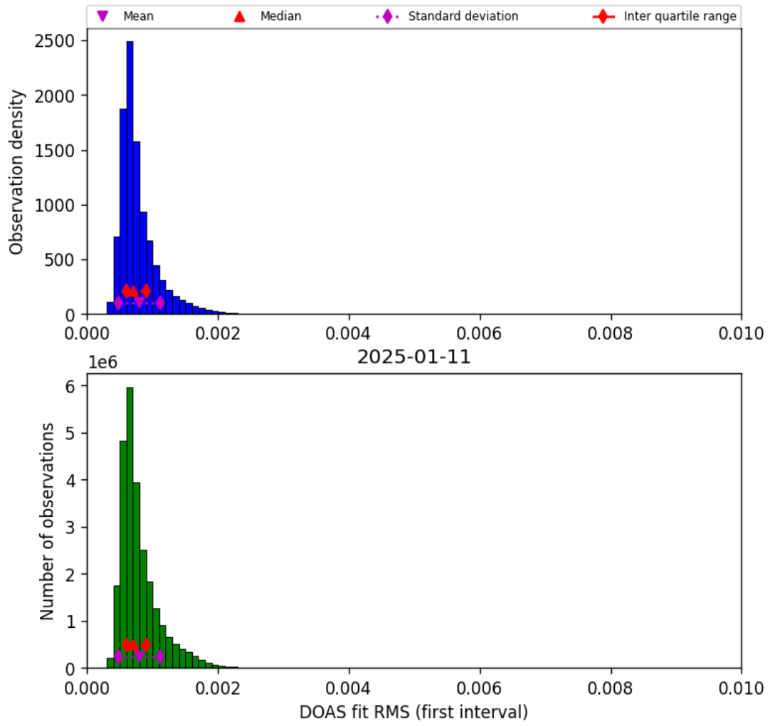
Figure 46: Histogram of “DOAS fit RMS (first interval)” for 2025-01-10 to 2025-01-12
