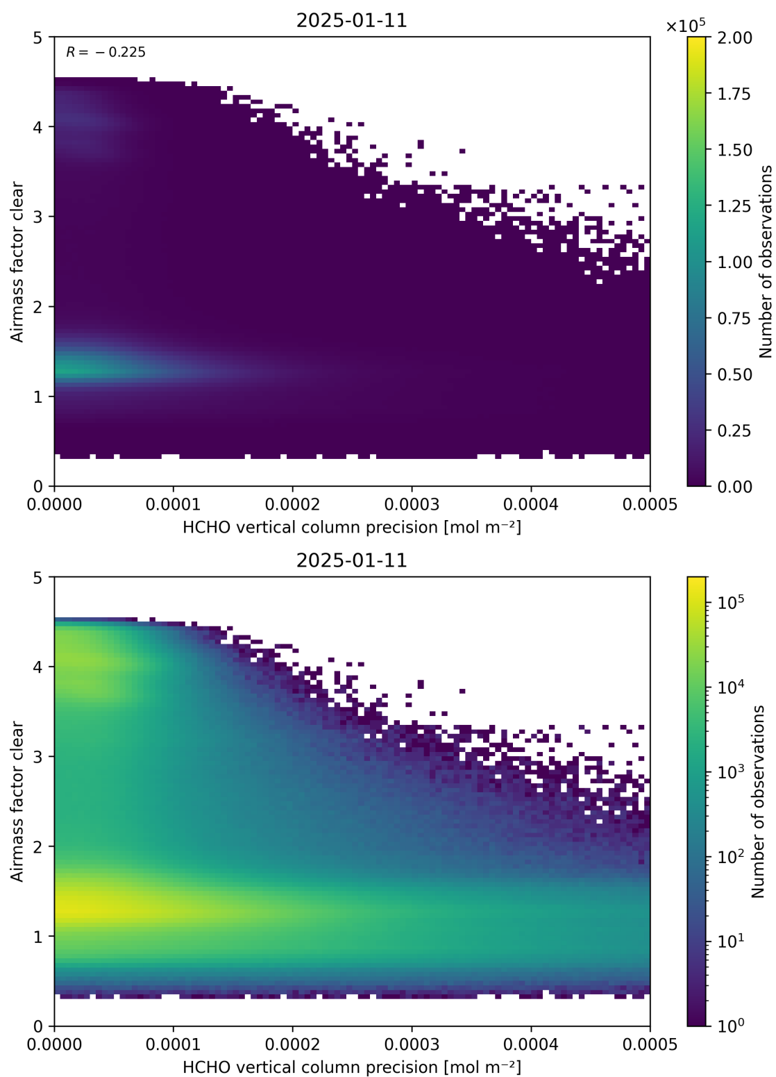
Figure 139: Scatter density plot of “HCHO vertical column precision” against “Airmass factor clear” for 2025-01-10 to 2025-01-12.
