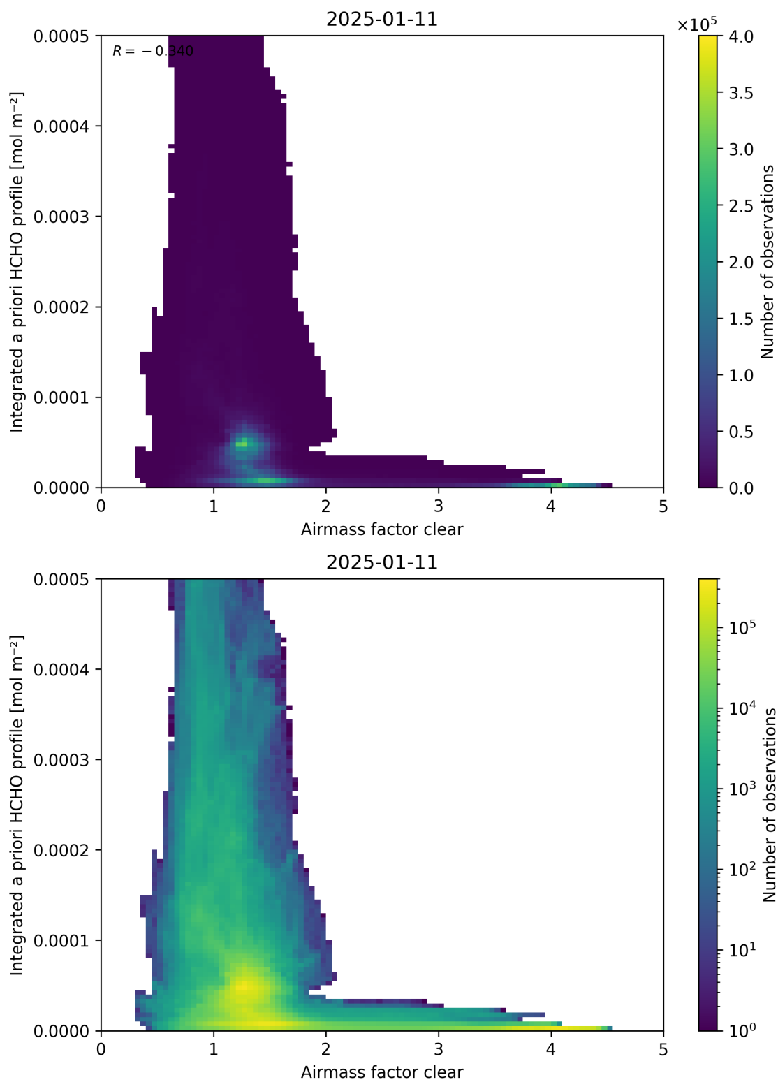
Figure 76: Scatter density plot of “Airmass factor clear” against “Integrated a priori HCHO profile” for 2025-01-10 to 2025-01-12.
