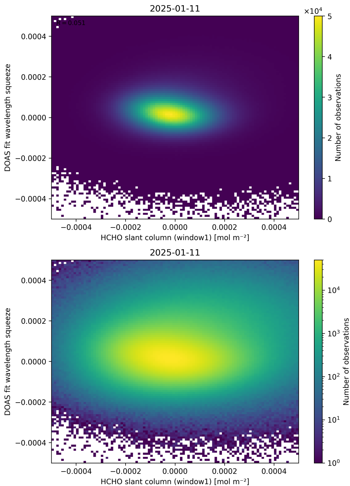
Figure 80: Scatter density plot of “HCHO slant column (window1)” against “DOAS fit wavelength squeeze” for 2025-01-10 to 2025-01-12.
