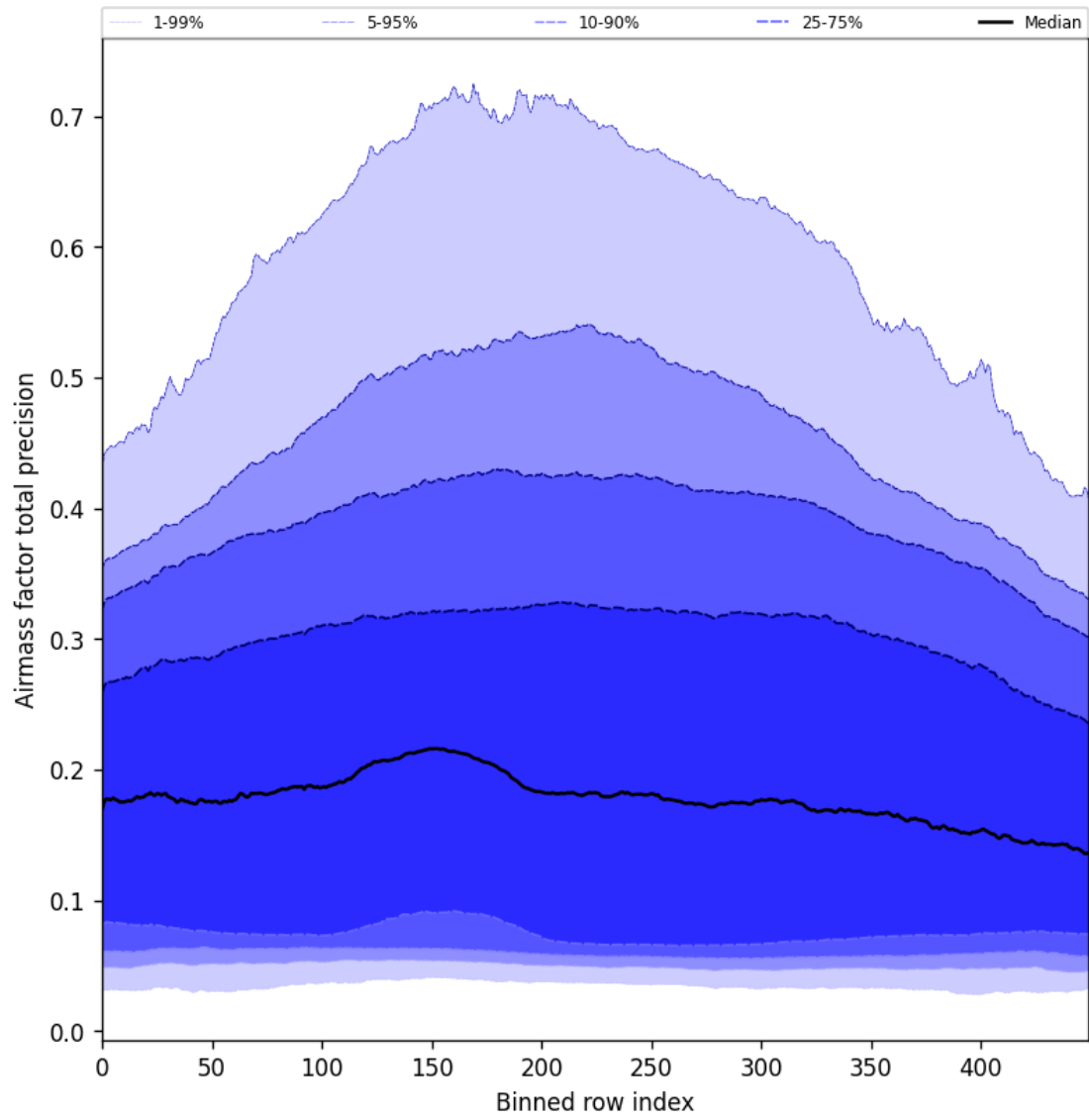
Figure 55: Along track statistics of “Airmass factor total precision” for 2025-01-10 to 2025-01-12
