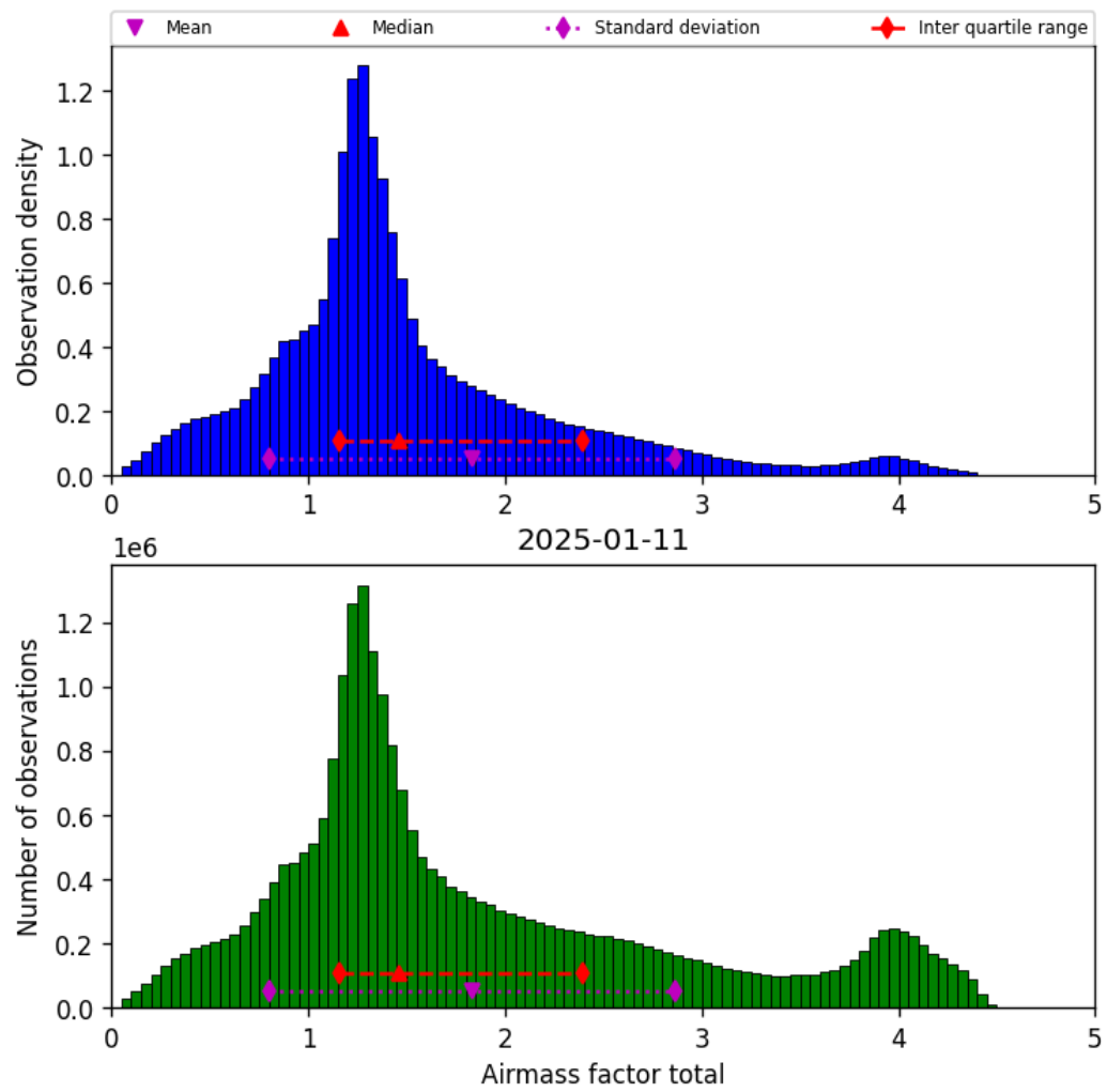
Figure 40: Histogram of “Airmass factor total” for 2025-01-10 to 2025-01-12
