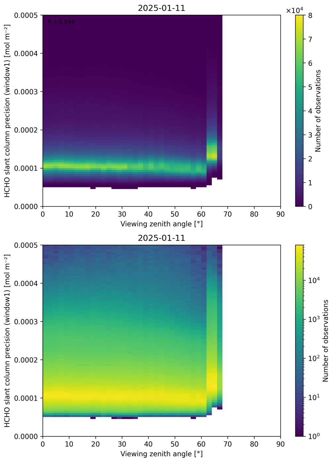
Figure 189: Scatter density plot of “Viewing zenith angle” against “HCHO slant column precision (window1)” for 2025-01-10 to 2025-01-12.
