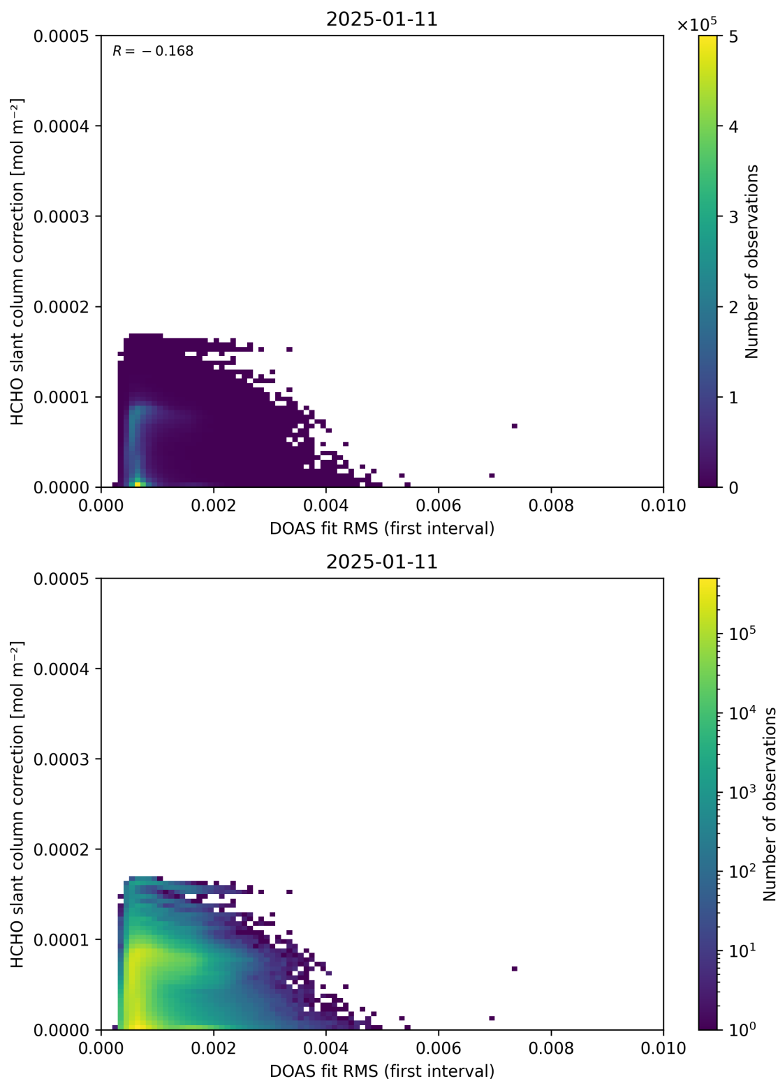
Figure 63: Scatter density plot of “DOAS fit RMS (first interval)” against “HCHO slant column correction” for 2025-01-10 to 2025-01-12.
