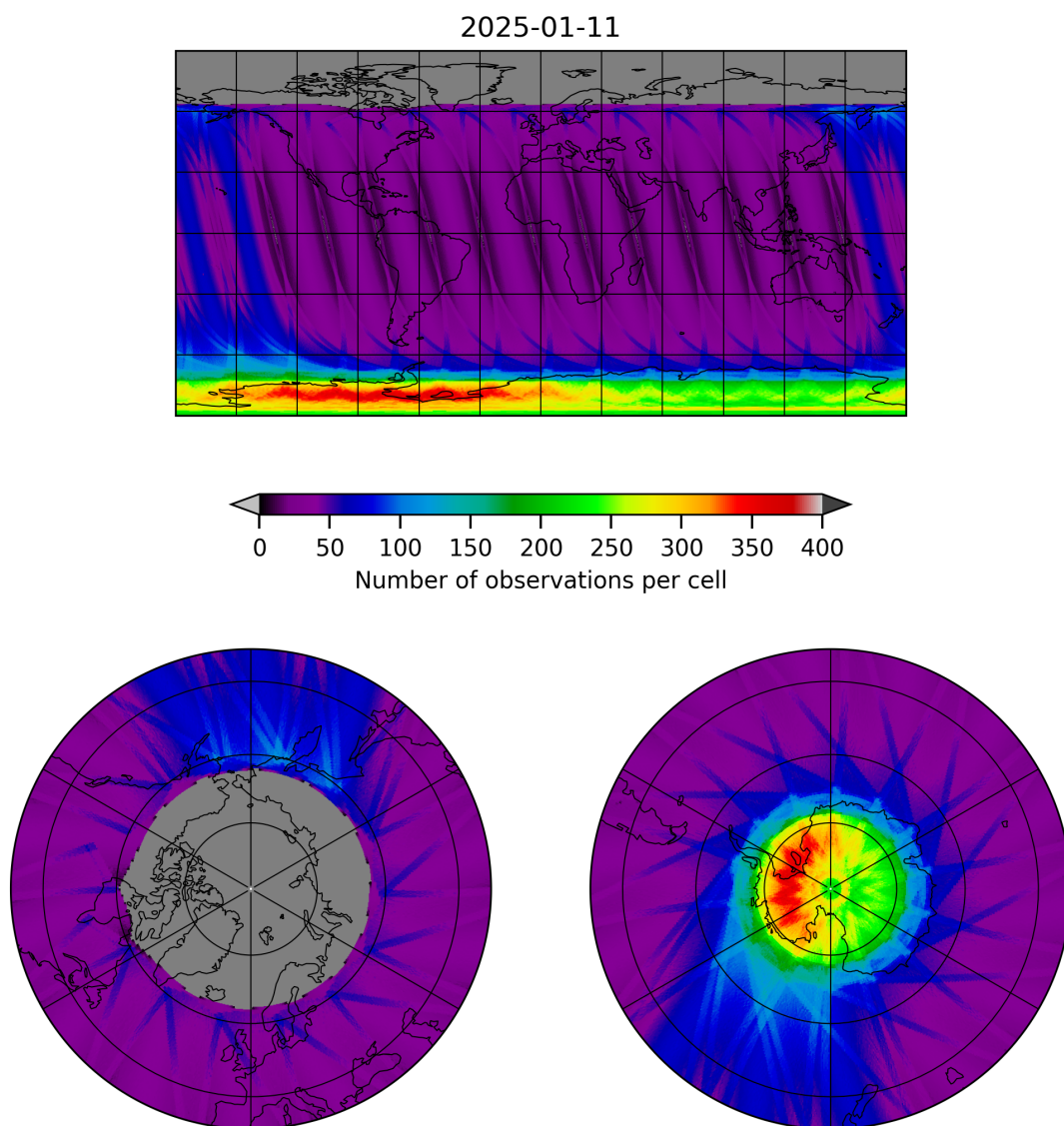
Figure 19: Map of the number of observations for 2025-01-10 to 2025-01-12
