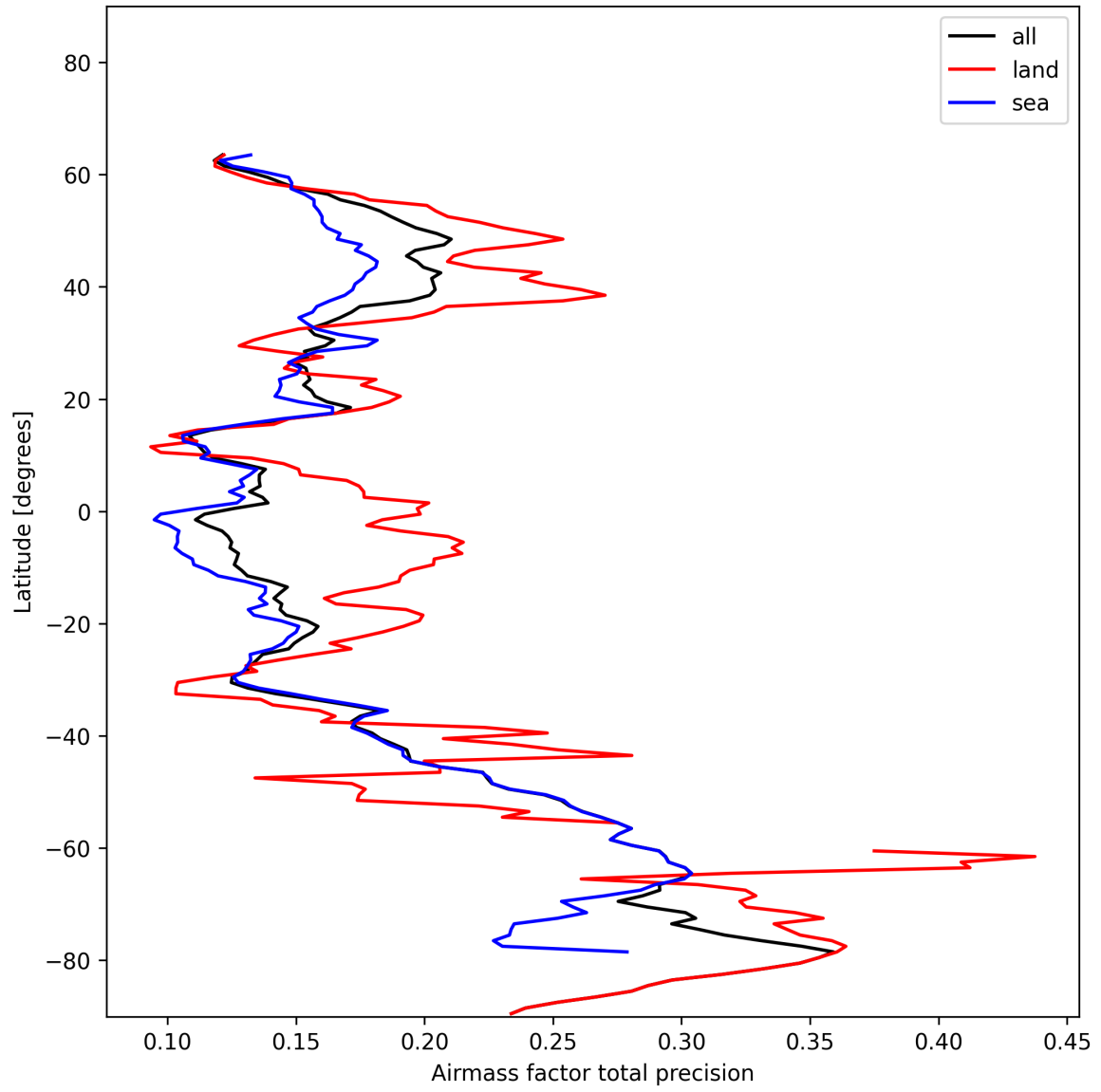
Figure 27: Zonal average of “Airmass factor total precision” for 2025-01-10 to 2025-01-12.
