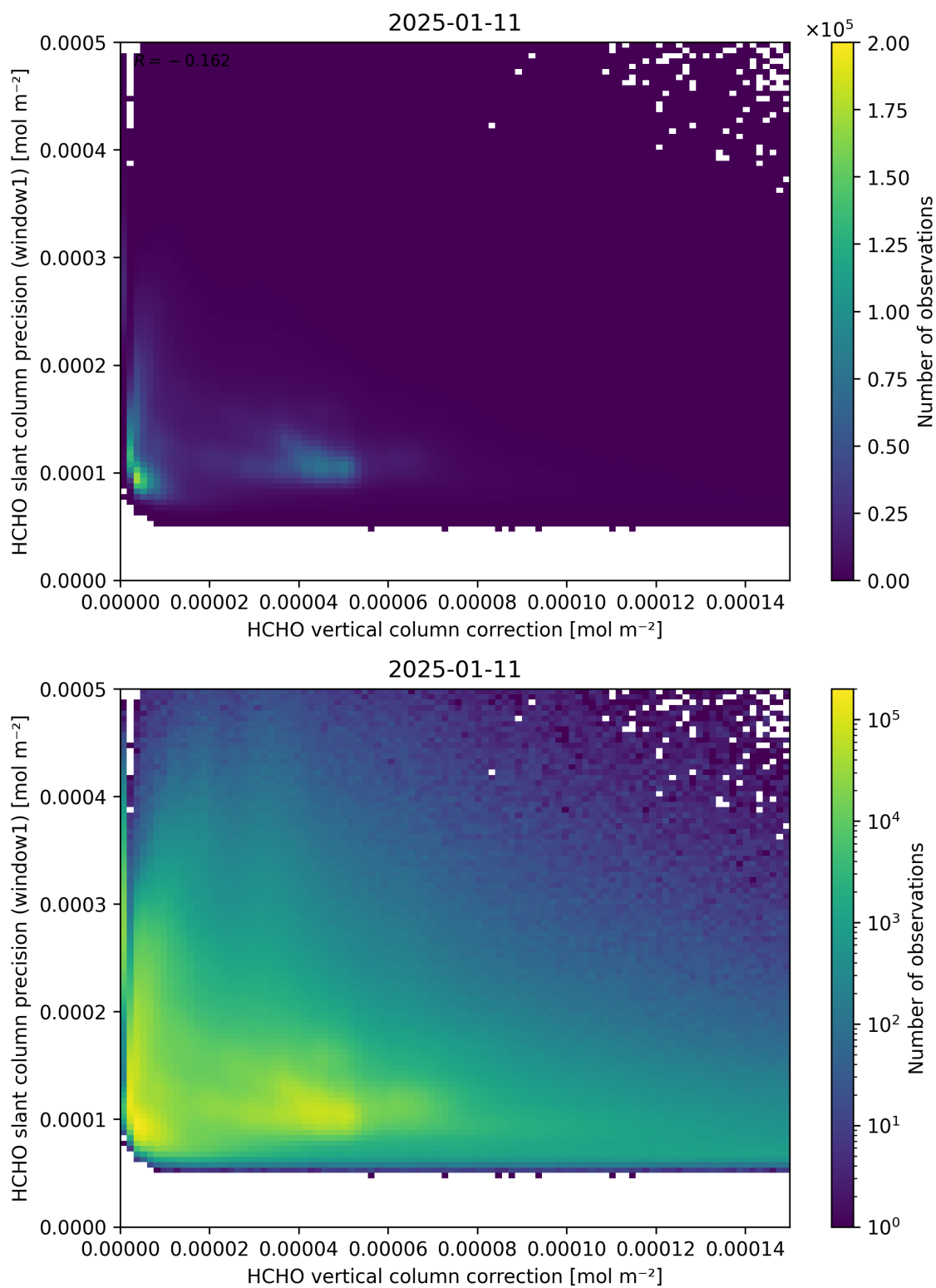
Figure 119: Scatter density plot of “HCHO vertical column correction” against “HCHO slant column precision (window1)” for 2025-01-10 to 2025-01-12.
