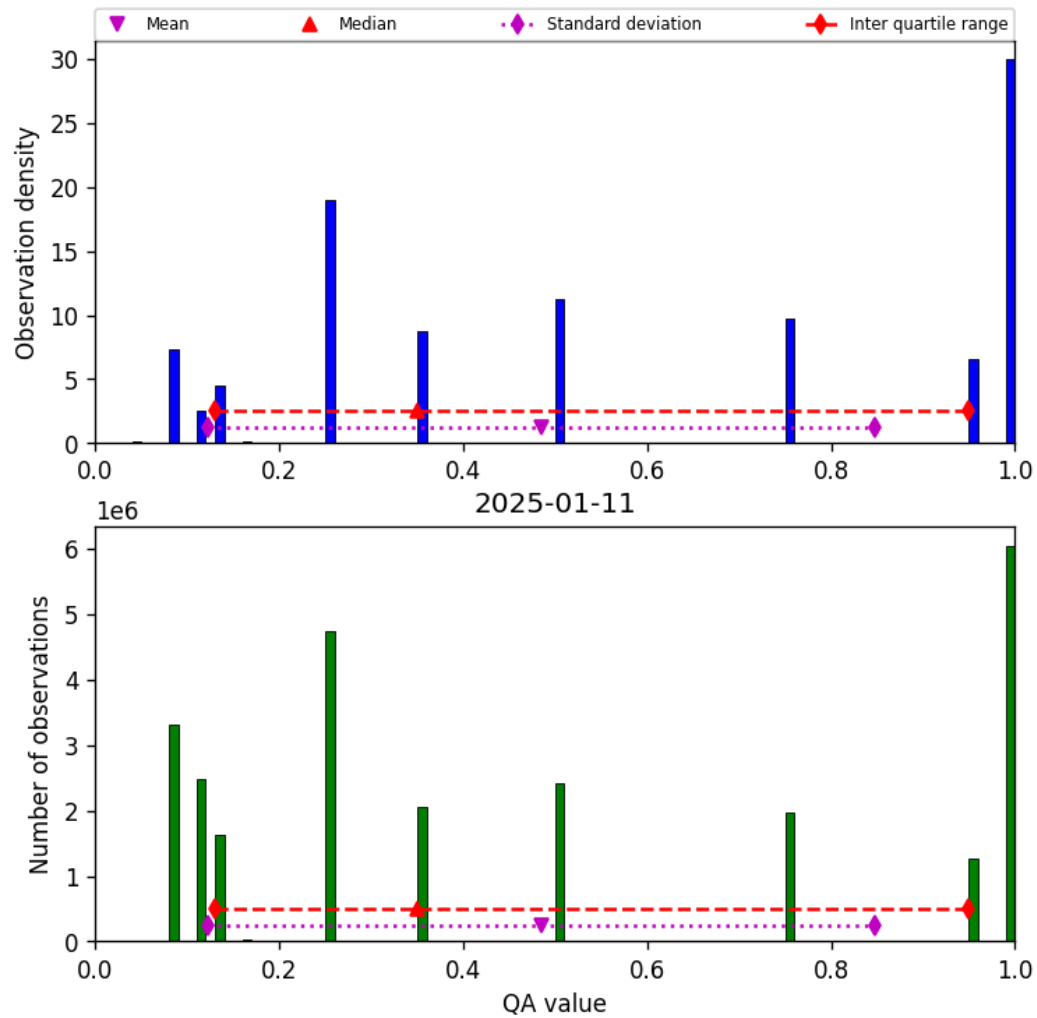
Figure 34: Histogram of “QA value” for 2025-01-10 to 2025-01-12
