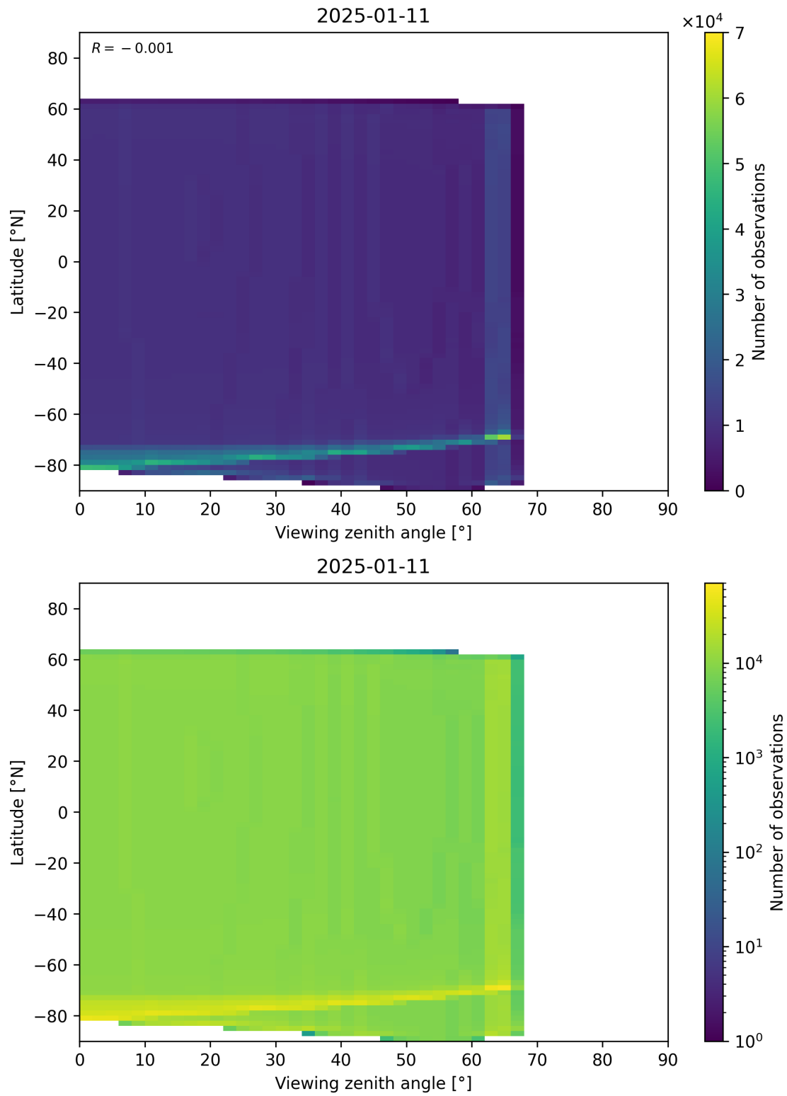
Figure 196: Scatter density plot of “Viewing zenith angle” against “Latitude” for 2025-01-10 to 2025-01-12.
