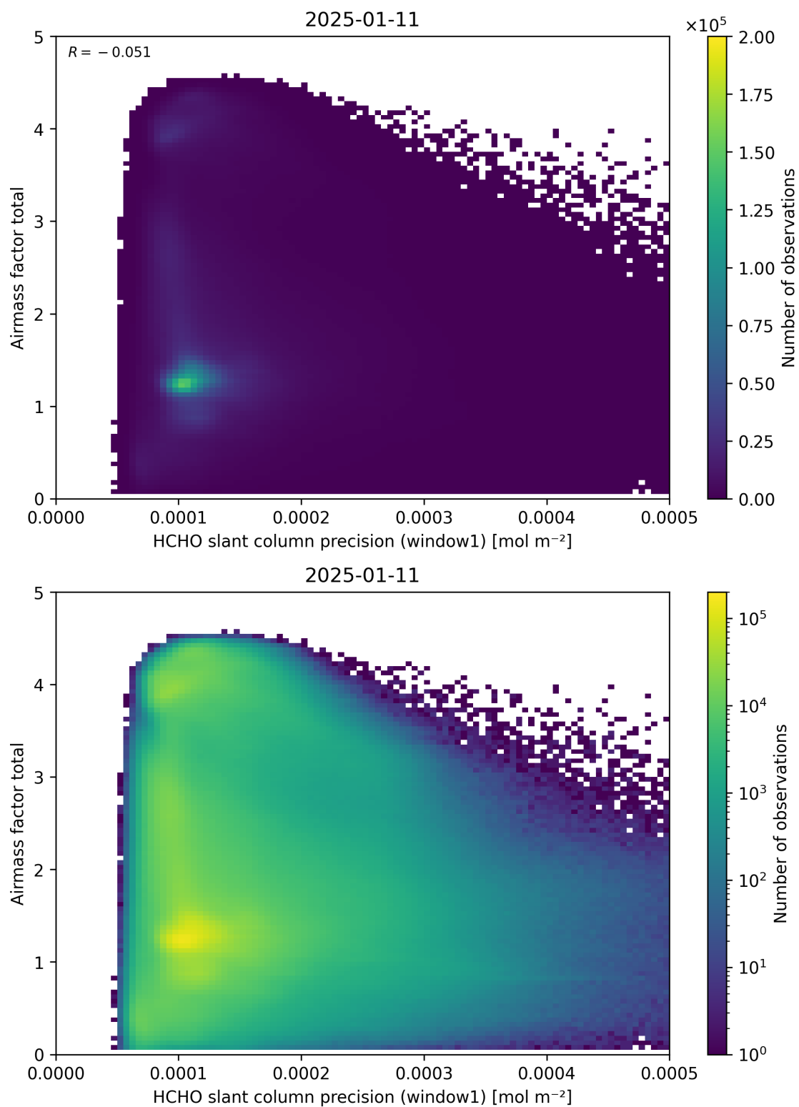
Figure 94: Scatter density plot of “HCHO slant column precision (window1)” against “Airmass factor total” for 2025-01-10 to 2025-01-12.
