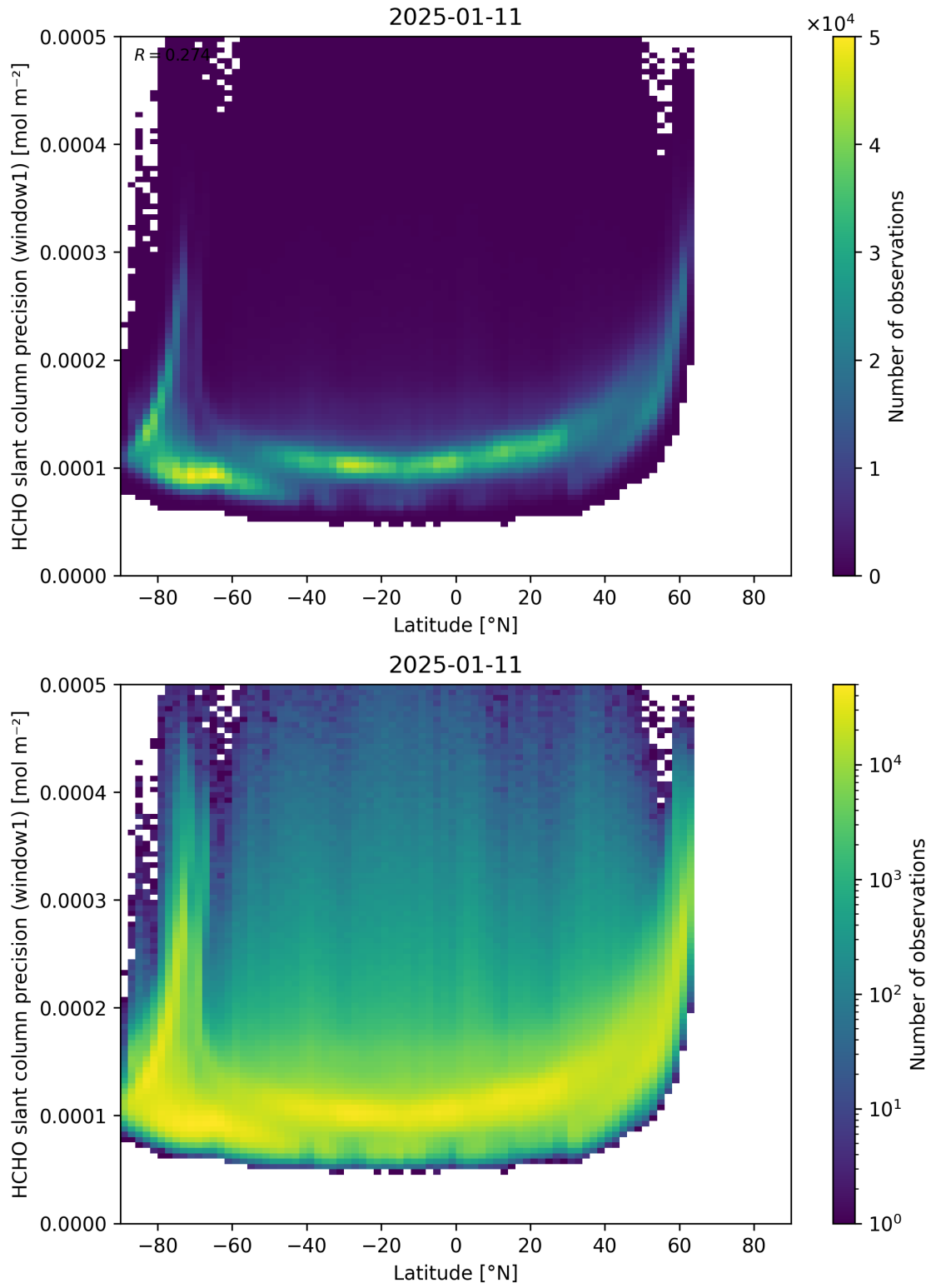
Figure 160: Scatter density plot of “Latitude” against “HCHO slant column precision (window1)” for 2025-01-10 to 2025-01-12.
