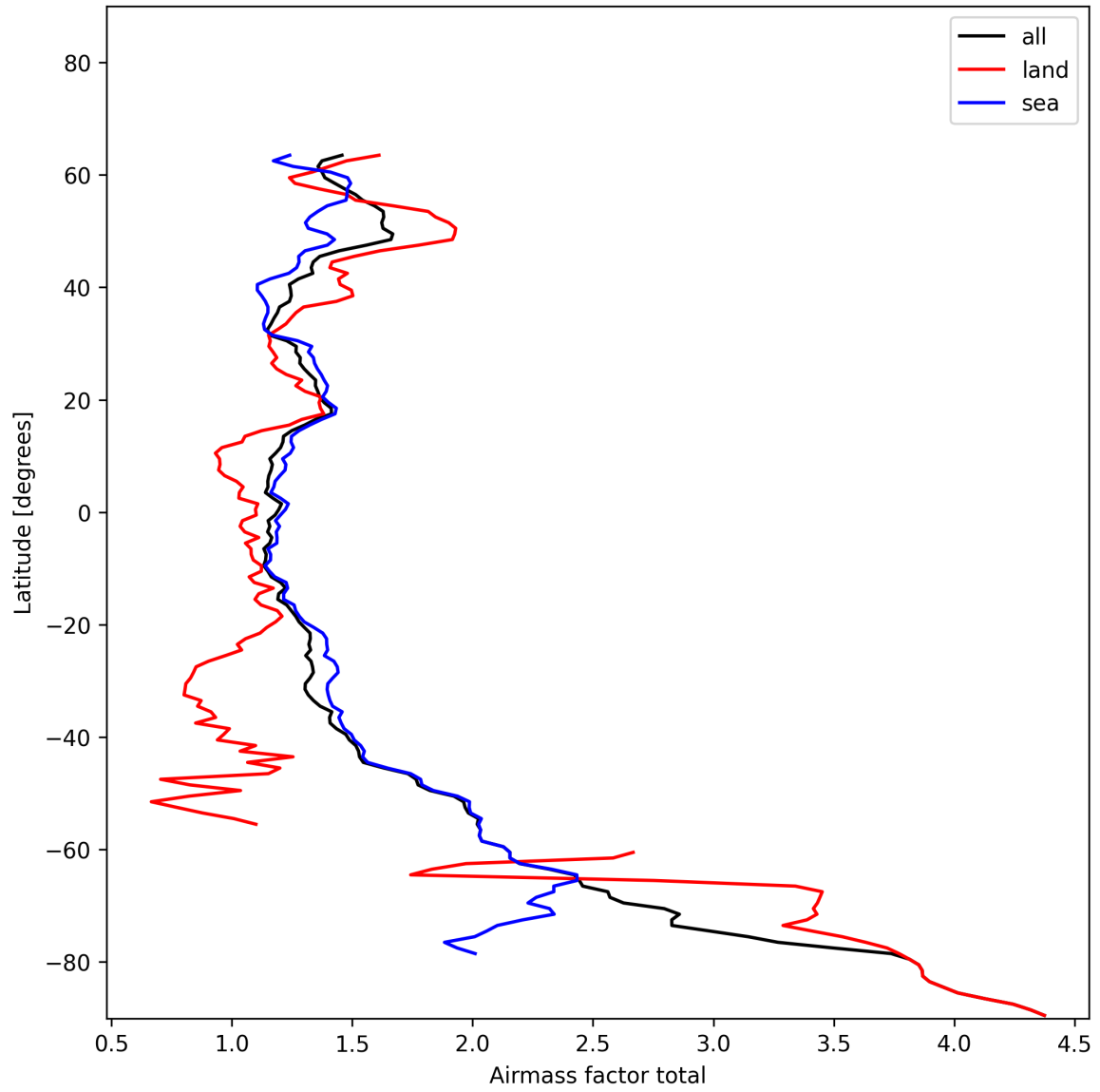
Figure 26: Zonal average of “Airmass factor total” for 2025-01-10 to 2025-01-12.
