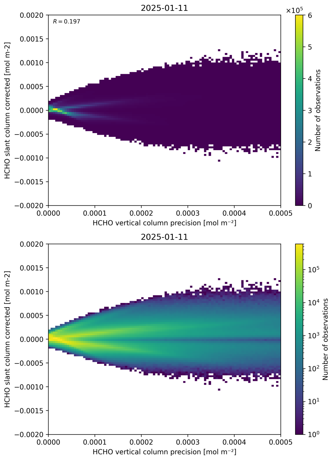
Figure 140: Scatter density plot of “HCHO vertical column precision” against “HCHO slant column corrected” for 2025-01-10 to 2025-01-12.
