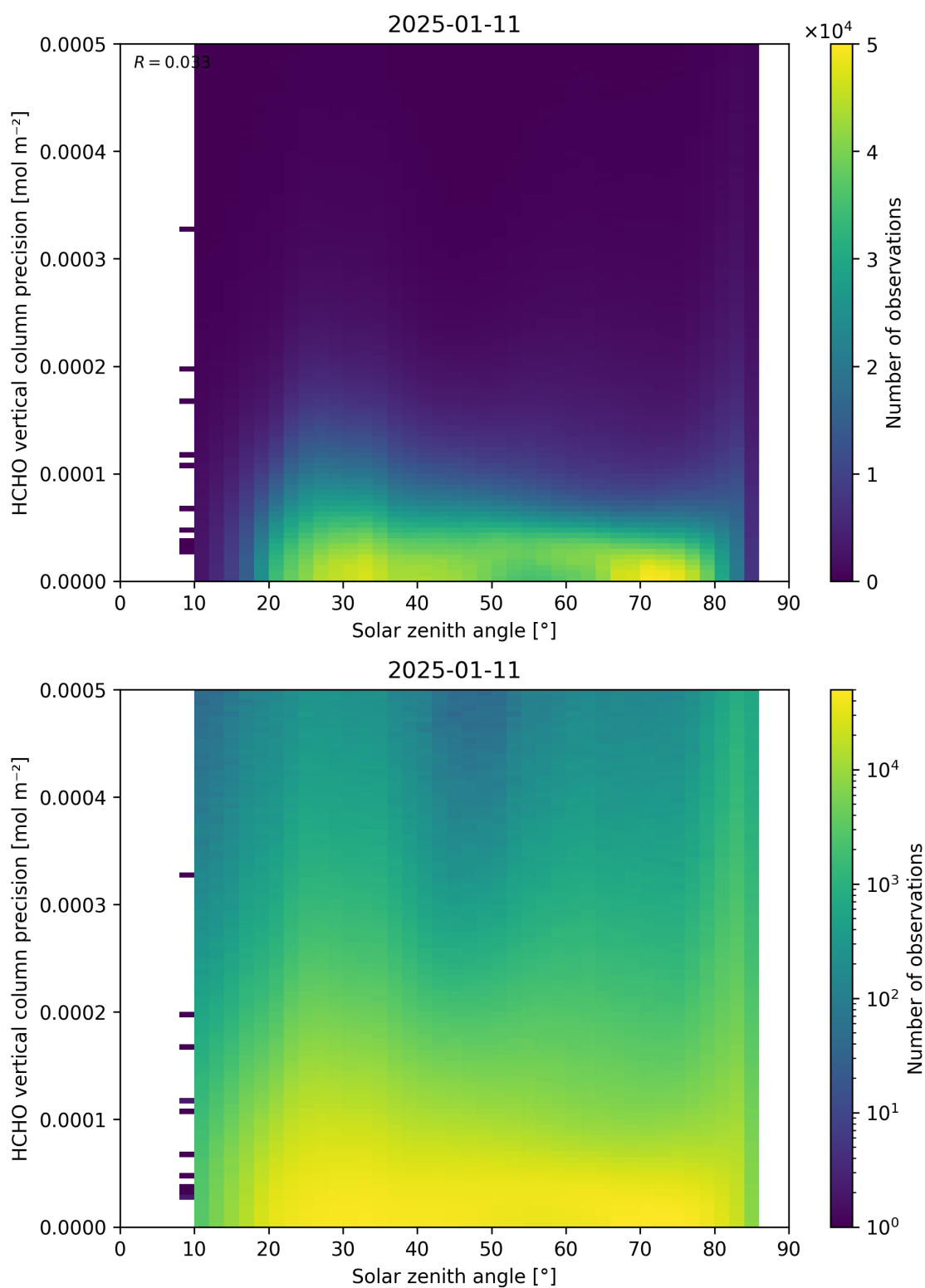
Figure 179: Scatter density plot of “Solar zenith angle” against “HCHO vertical column precision” for 2025-01-10 to 2025-01-12.
