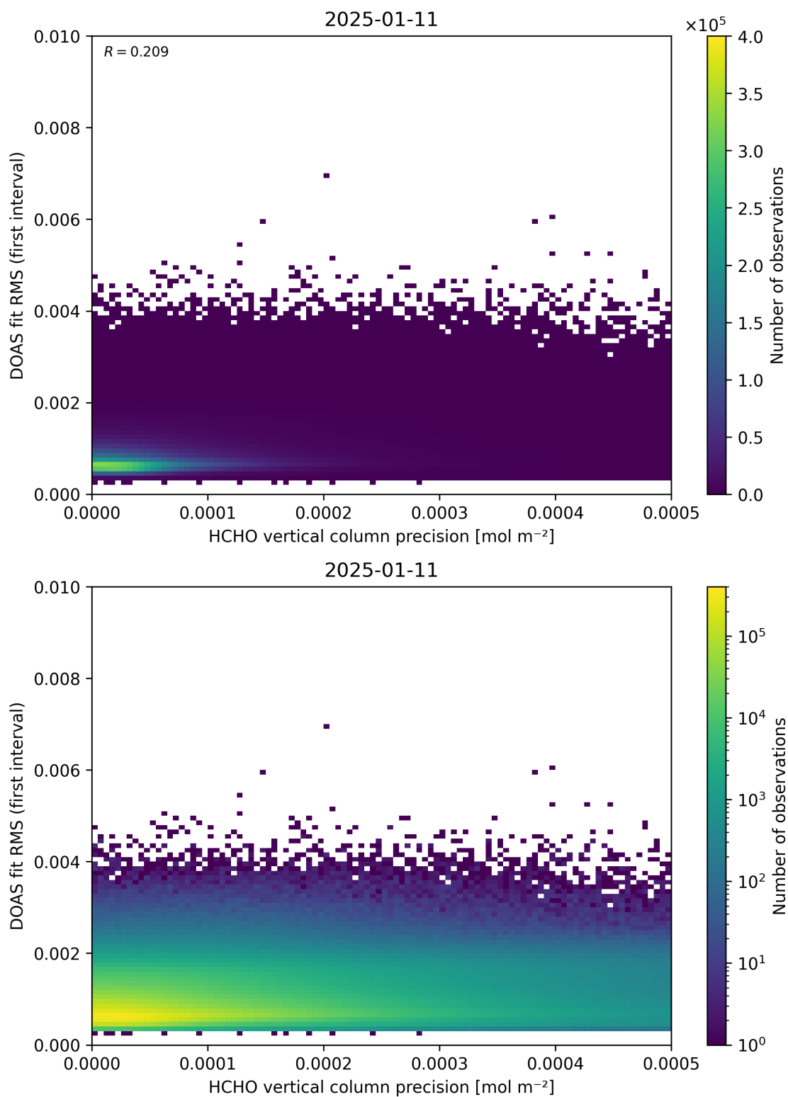
Figure 136: Scatter density plot of “HCHO vertical column precision” against “DOAS fit RMS (first interval)” for 2025-01-10 to 2025-01-12.
