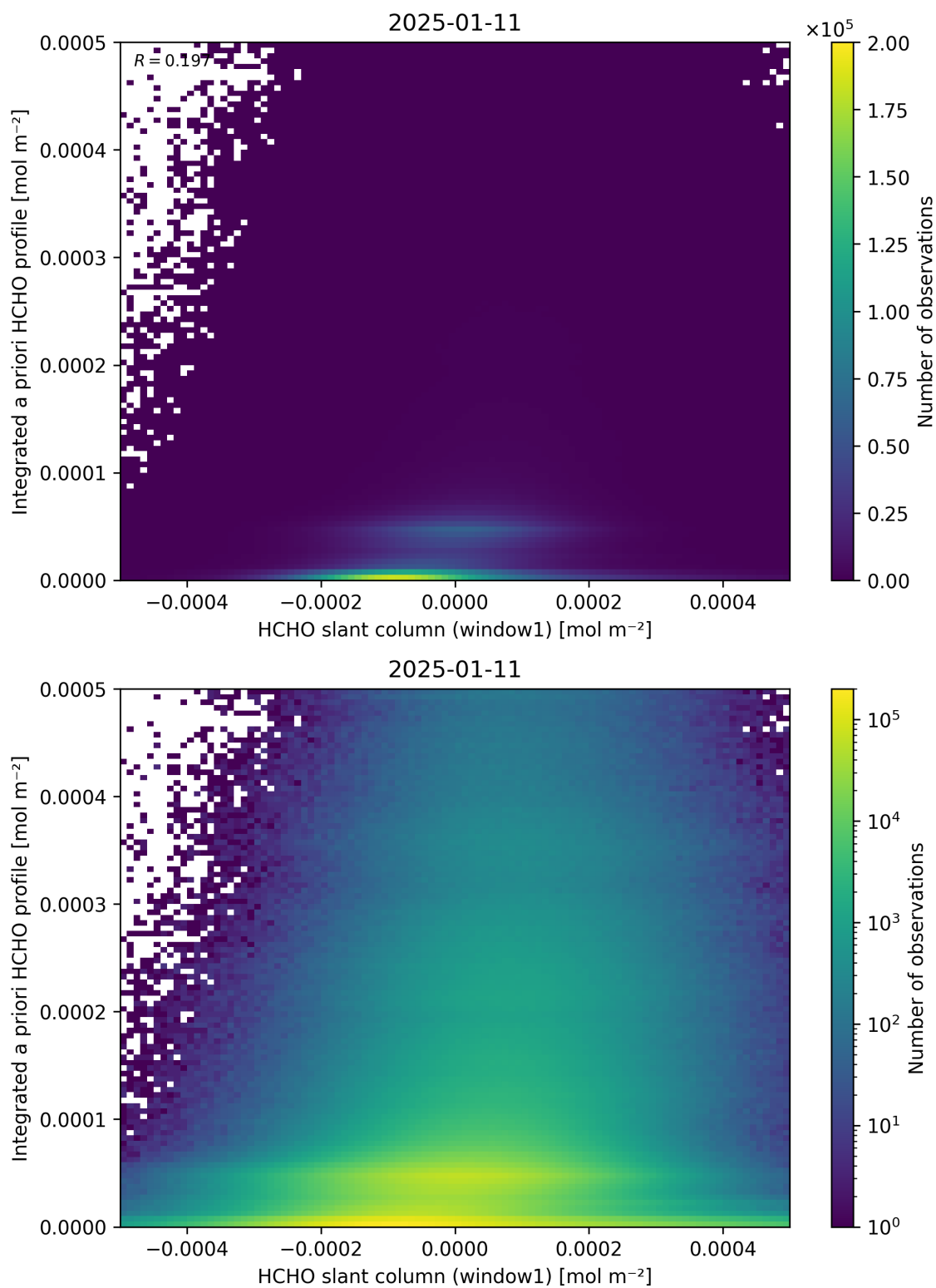
Figure 87: Scatter density plot of “HCHO slant column (window1)” against “Integrated a priori HCHO profile” for 2025-01-10 to 2025-01-12.
