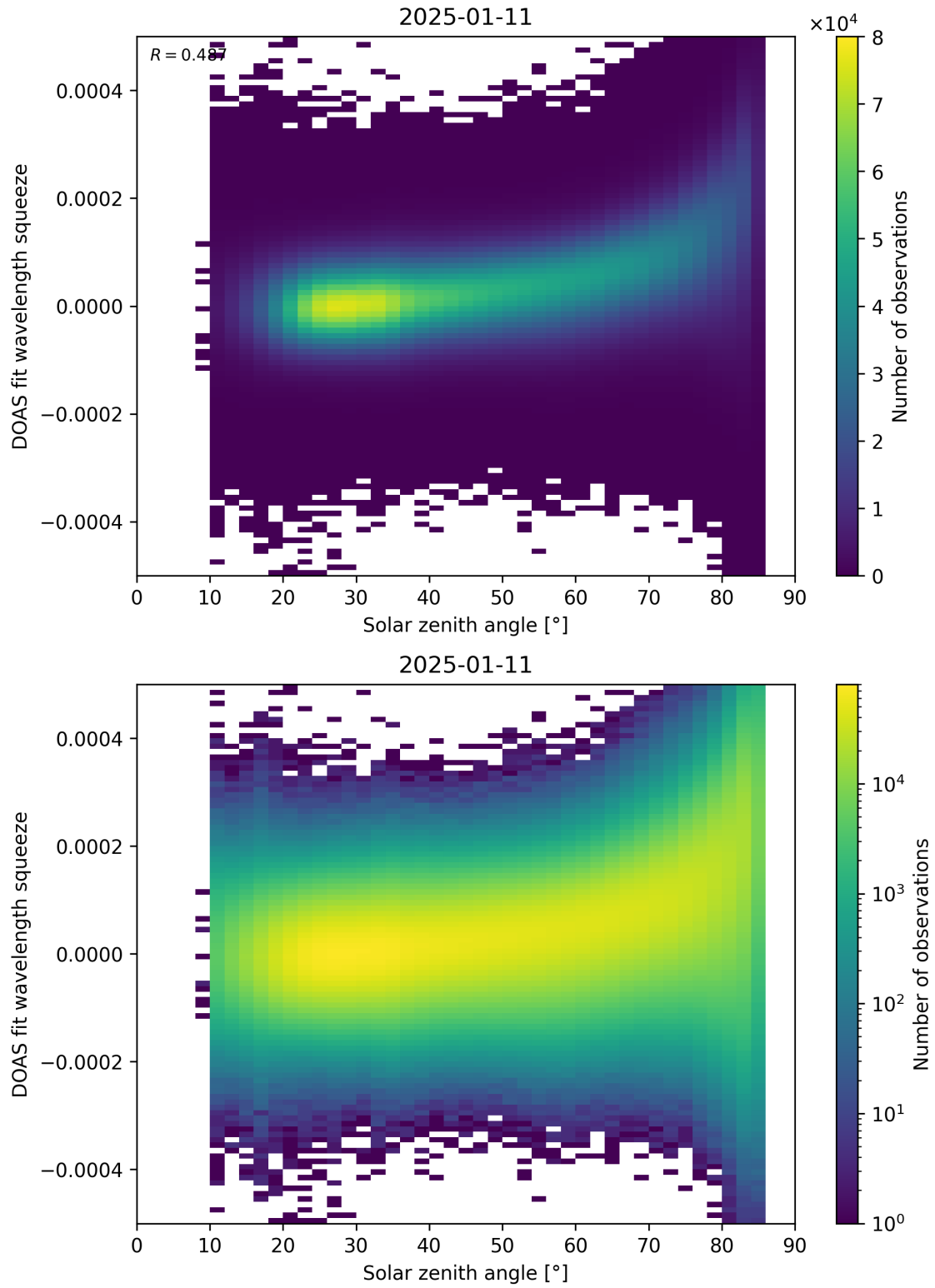
Figure 169: Scatter density plot of “Solar zenith angle” against “DOAS fit wavelength squeeze” for 2025-01-10 to 2025-01-12.
