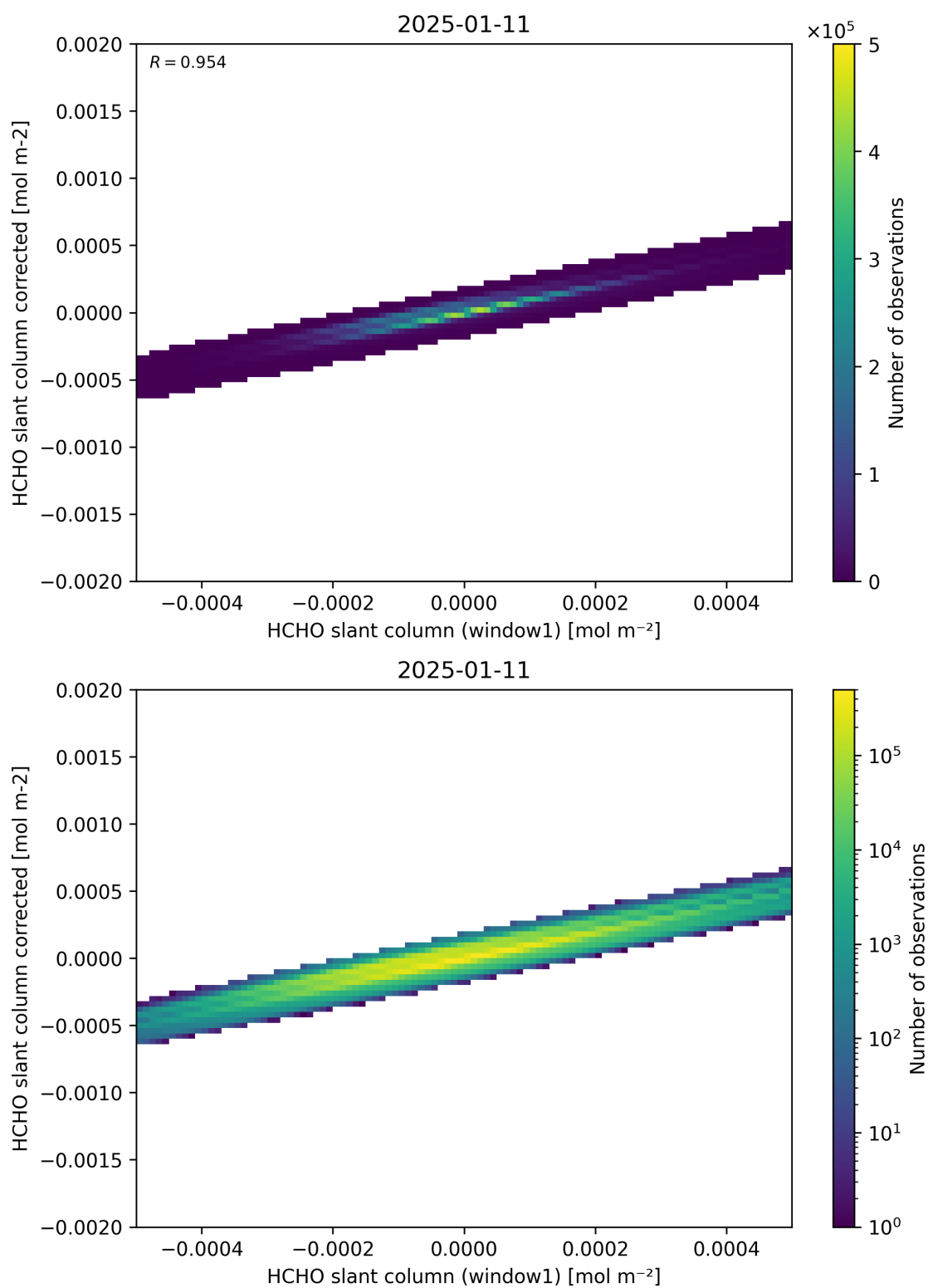
Figure 82: Scatter density plot of “HCHO slant column (window1)” against “HCHO slant column corrected” for 2025-01-10 to 2025-01-12.
