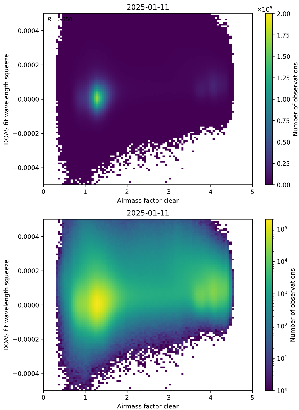
Figure 73: Scatter density plot of “Airmass factor clear” against “DOAS fit wavelength squeeze” for 2025-01-10 to 2025-01-12.
