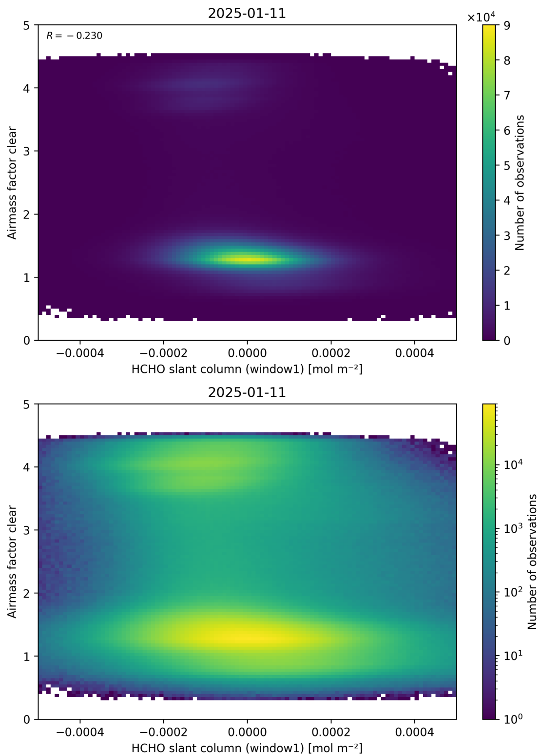
Figure 81: Scatter density plot of “HCHO slant column (window1)” against “Airmass factor clear” for 2025-01-10 to 2025-01-12.
