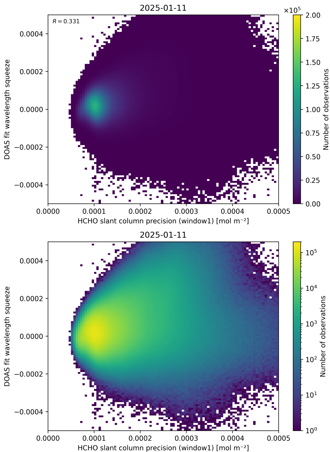
Figure 90: Scatter density plot of “HCHO slant column precision (window1)” against “DOAS fit wavelength squeeze” for 2025-01-10 to 2025-01-12.
