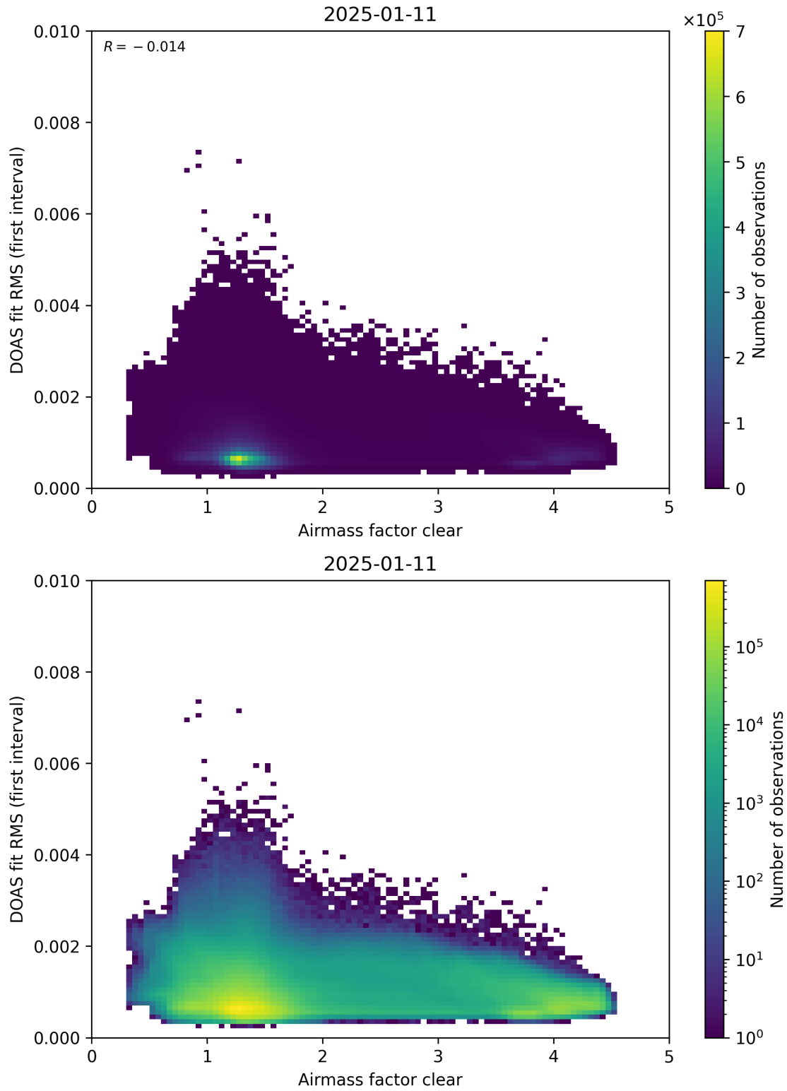
Figure 71: Scatter density plot of “Airmass factor clear” against “DOAS fit RMS (first interval)” for 2025-01-10 to 2025-01-12.
