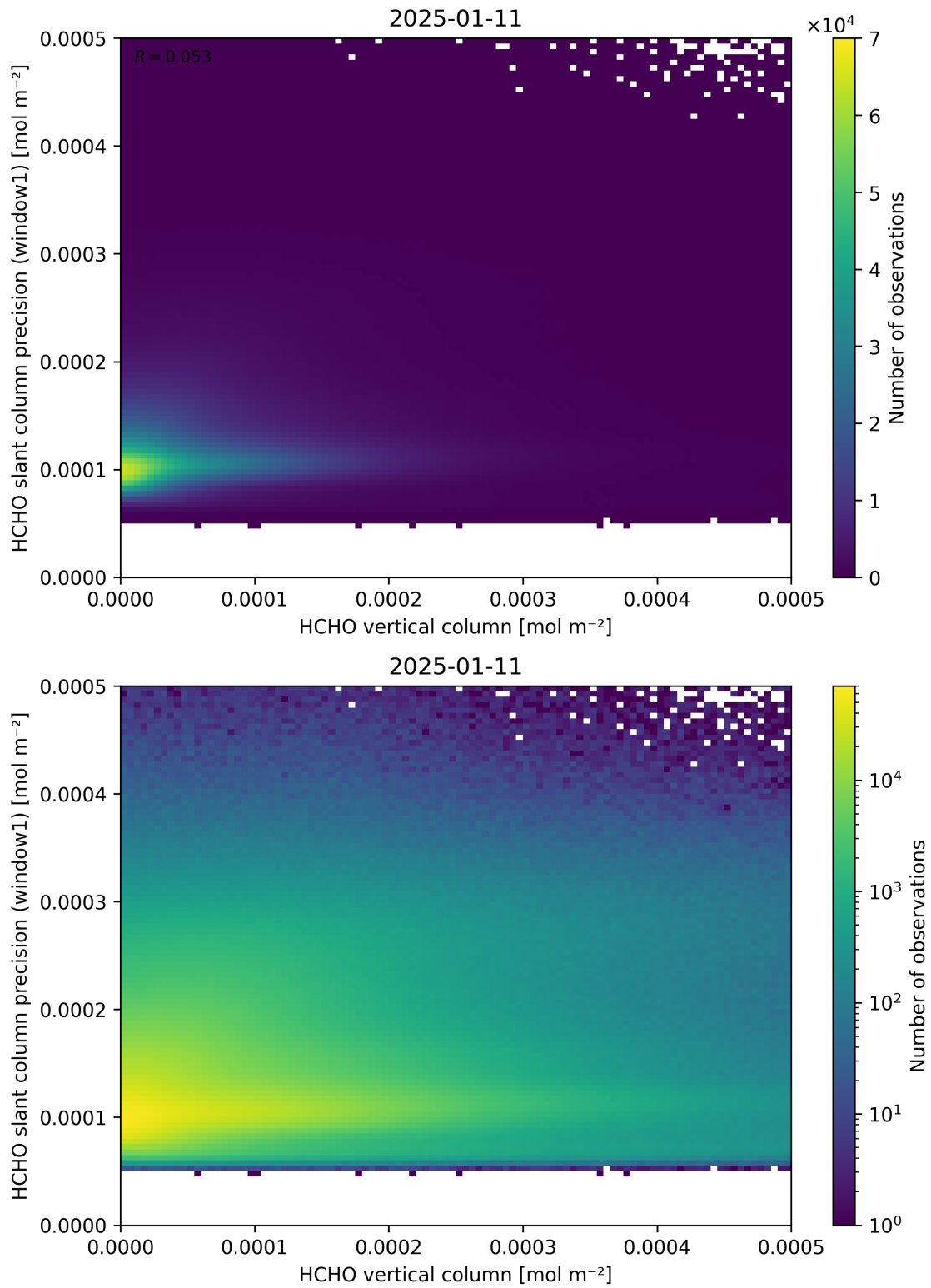
Figure 130: Scatter density plot of “HCHO vertical column” against “HCHO slant column precision (window1)” for 2025-01-10 to 2025-01-12.
