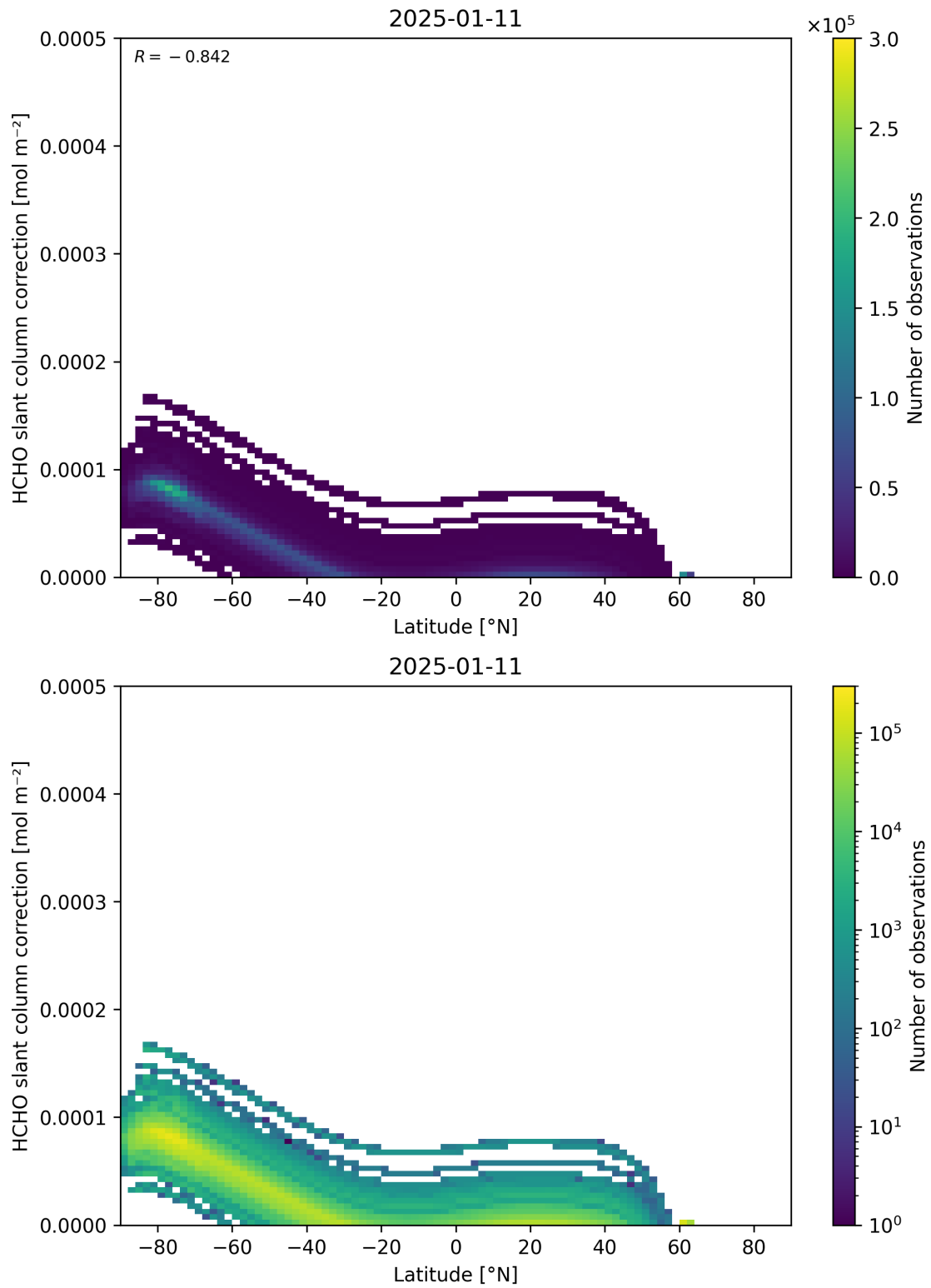
Figure 158: Scatter density plot of “Latitude” against “HCHO slant column correction” for 2025-01-10 to 2025-01-12.
