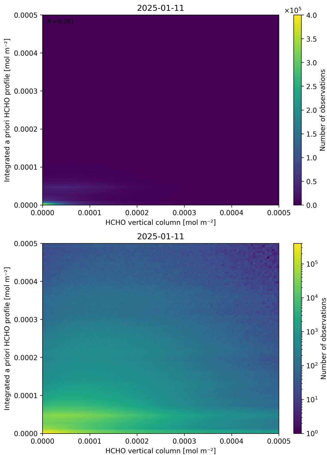
Figure 135: Scatter density plot of “HCHO vertical column” against “Integrated a priori HCHO profile” for 2025-01-10 to 2025-01-12.
