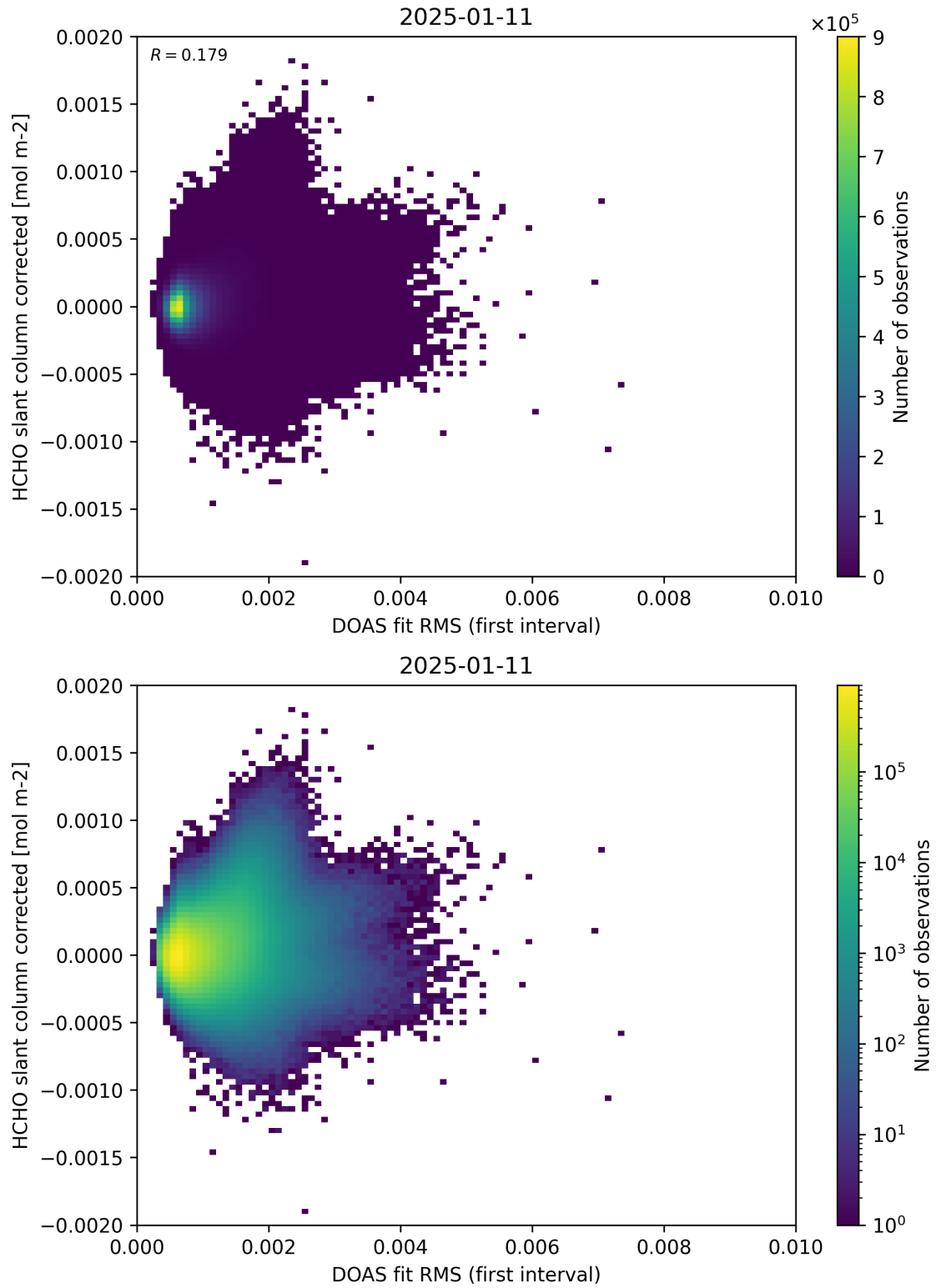
Figure 62: Scatter density plot of “DOAS fit RMS (first interval)” against “HCHO slant column corrected” for 2025-01-10 to 2025-01-12.
