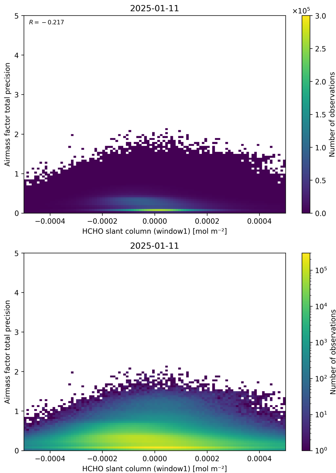
Figure 86: Scatter density plot of “HCHO slant column (window1)” against “Airmass factor total precision” for 2025-01-10 to 2025-01-12.
