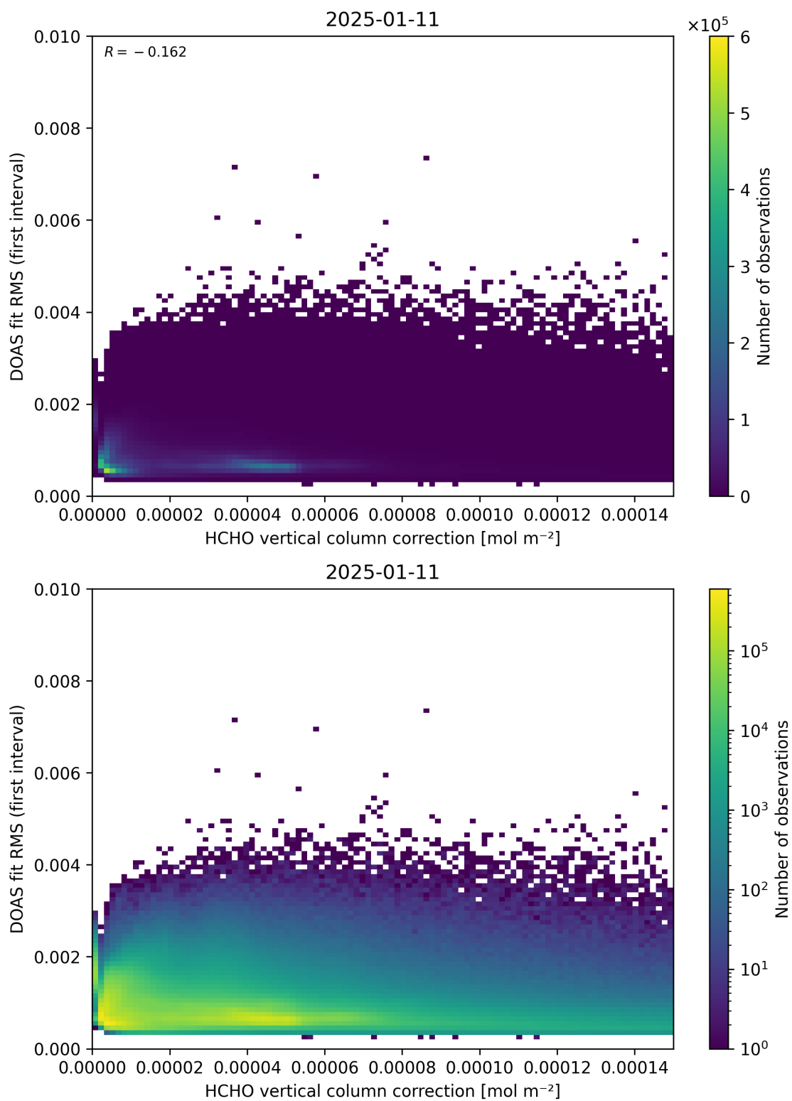
Figure 112: Scatter density plot of “HCHO vertical column correction” against “DOAS fit RMS (first interval)” for 2025-01-10 to 2025-01-12.
