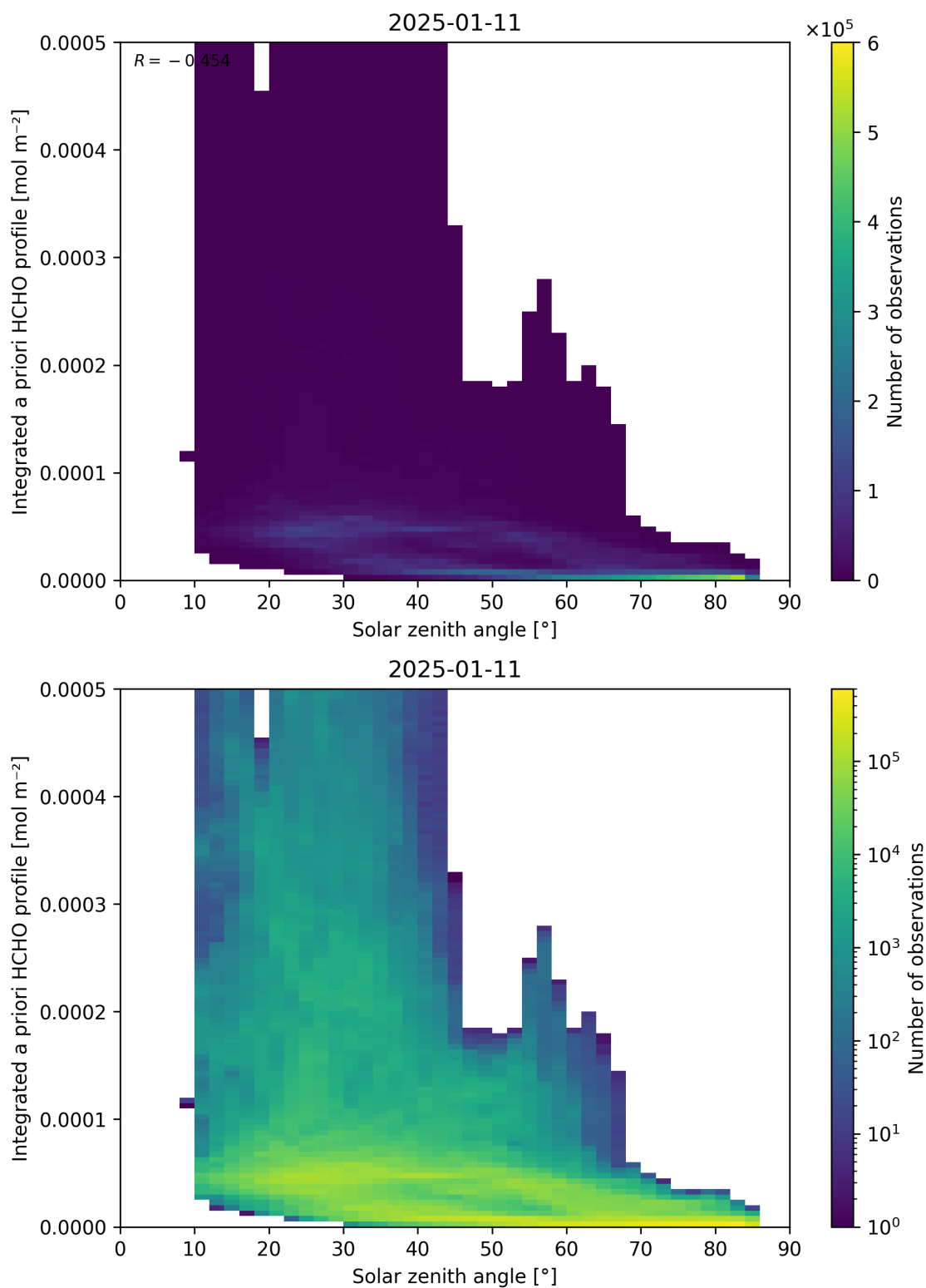
Figure 180: Scatter density plot of “Solar zenith angle” against “Integrated a priori HCHO profile” for 2025-01-10 to 2025-01-12.
