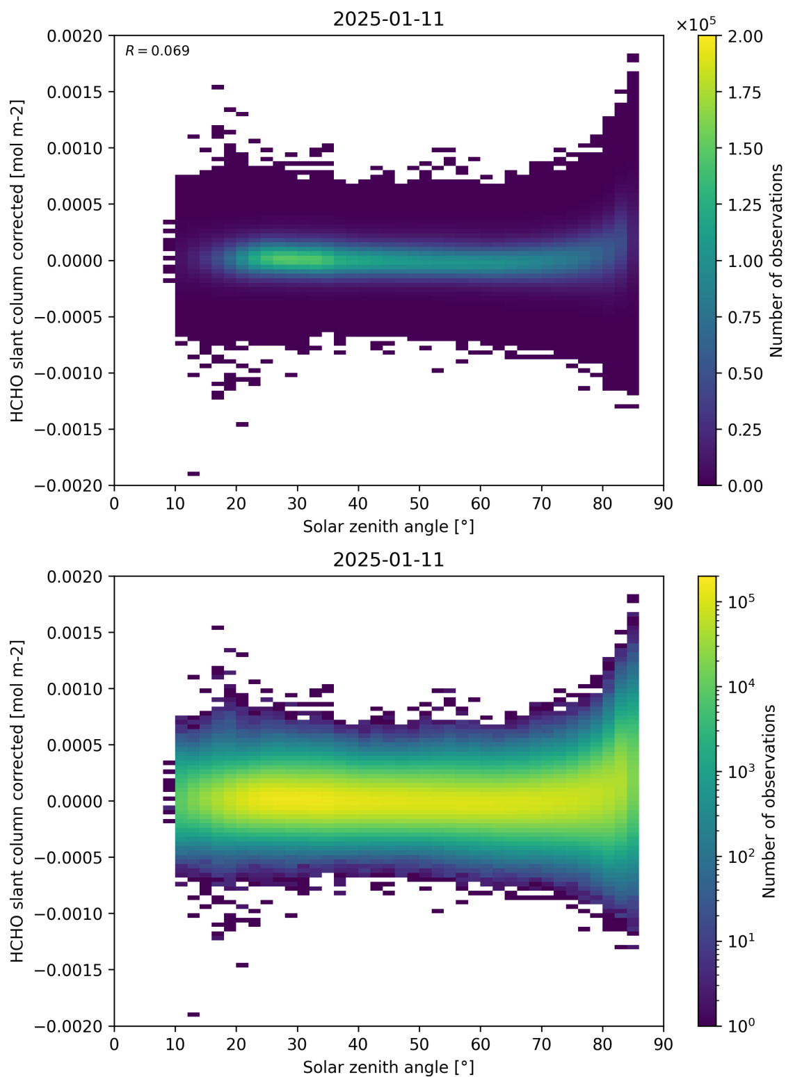
Figure 171: Scatter density plot of “Solar zenith angle” against “HCHO slant column corrected” for 2025-01-10 to 2025-01-12.
