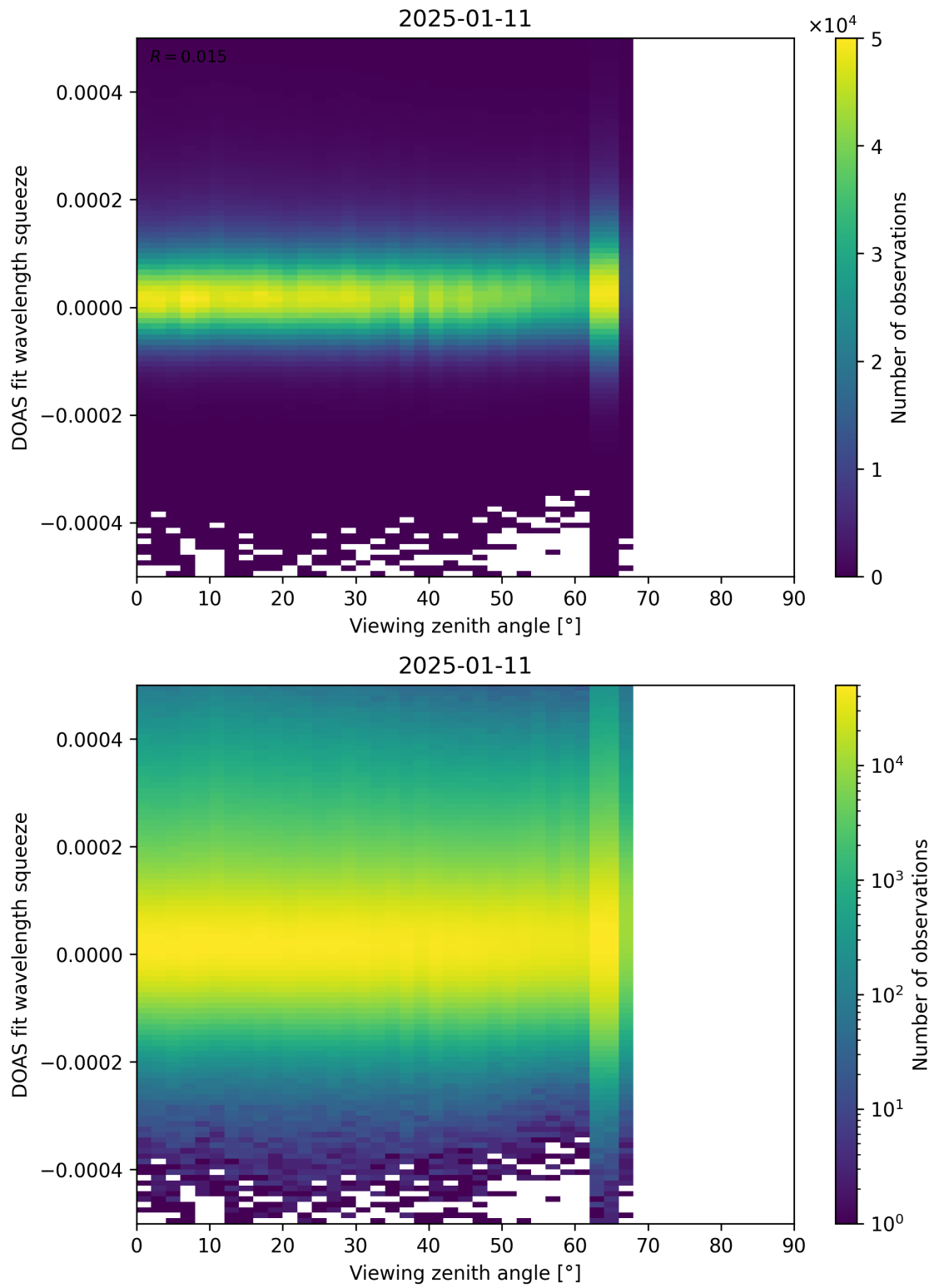
Figure 184: Scatter density plot of “Viewing zenith angle” against “DOAS fit wavelength squeeze” for 2025-01-10 to 2025-01-12.
