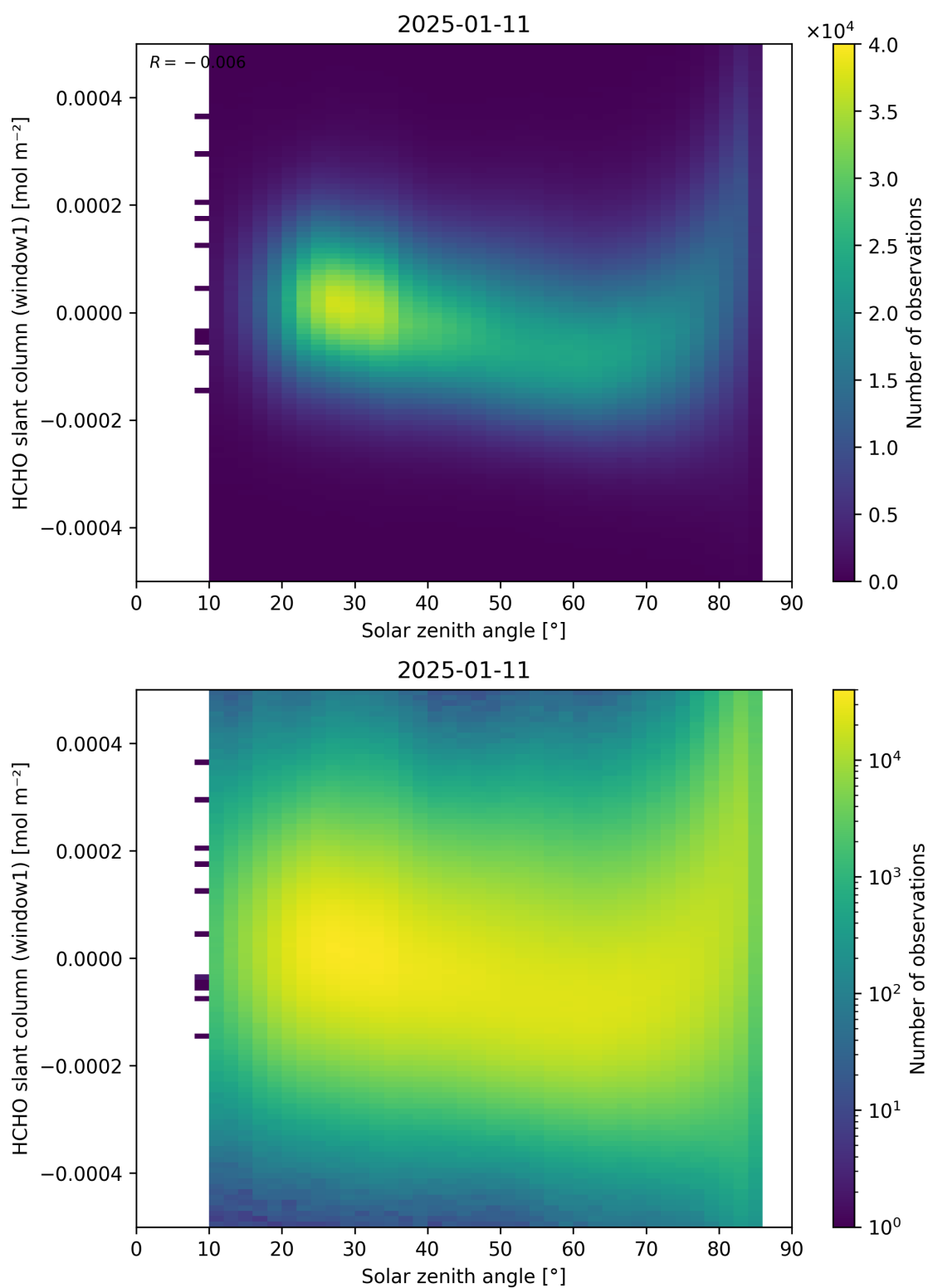
Figure 173: Scatter density plot of “Solar zenith angle” against “HCHO slant column (window1)” for 2025-01-10 to 2025-01-12.
