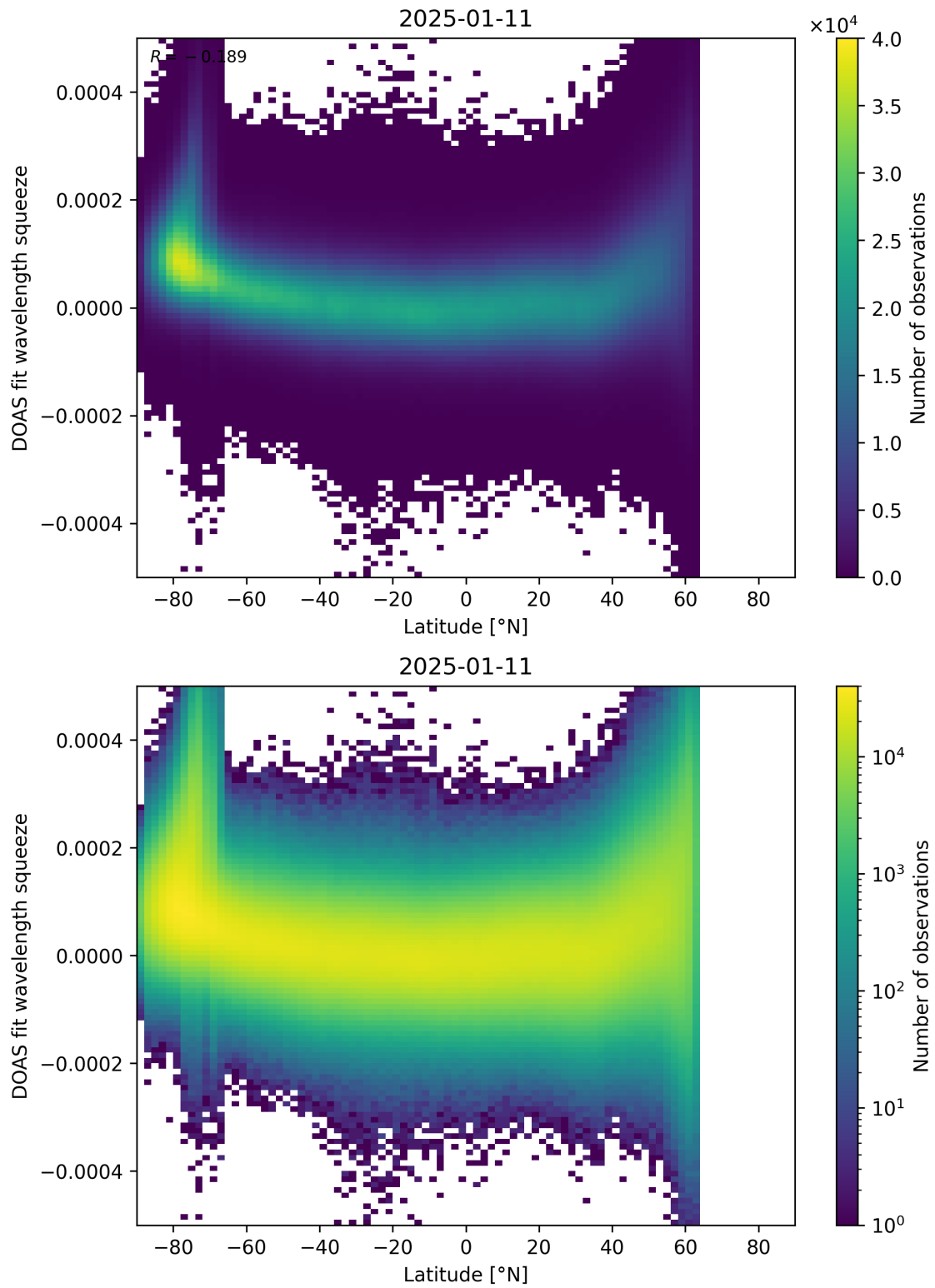
Figure 155: Scatter density plot of “Latitude” against “DOAS fit wavelength squeeze” for 2025-01-10 to 2025-01-12.
