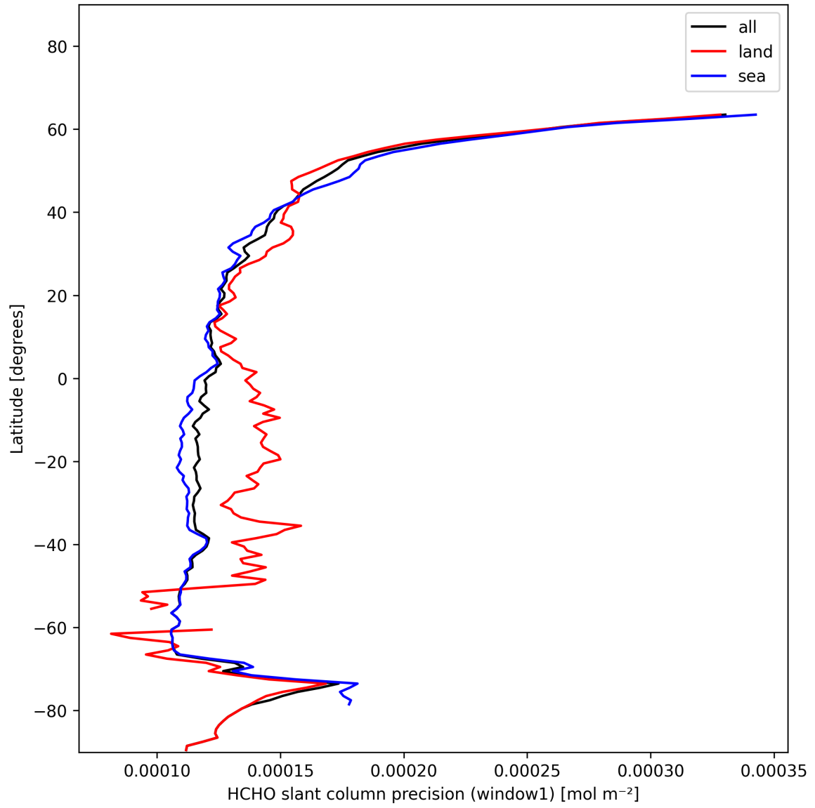
Figure 25: Zonal average of “HCHO slant column precision (window1)” for 2025-01-10 to 2025-01-12.
