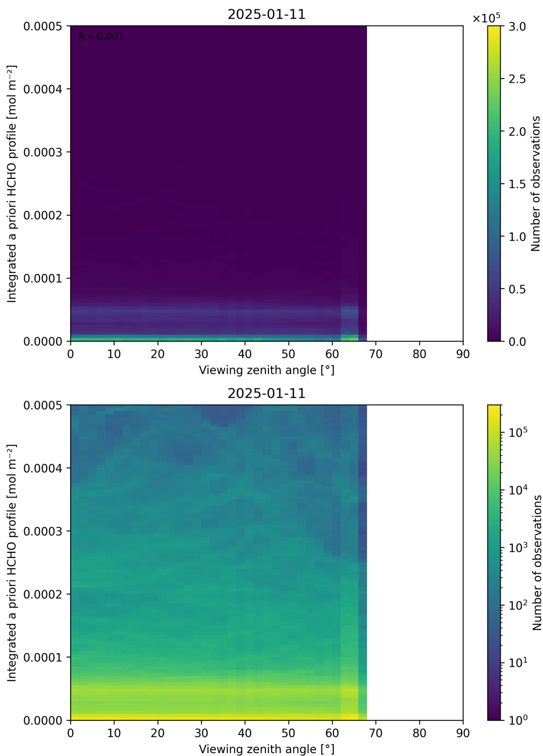
Figure 195: Scatter density plot of “Viewing zenith angle” against “Integrated a priori HCHO profile” for 2025-01-10 to 2025-01-12.
