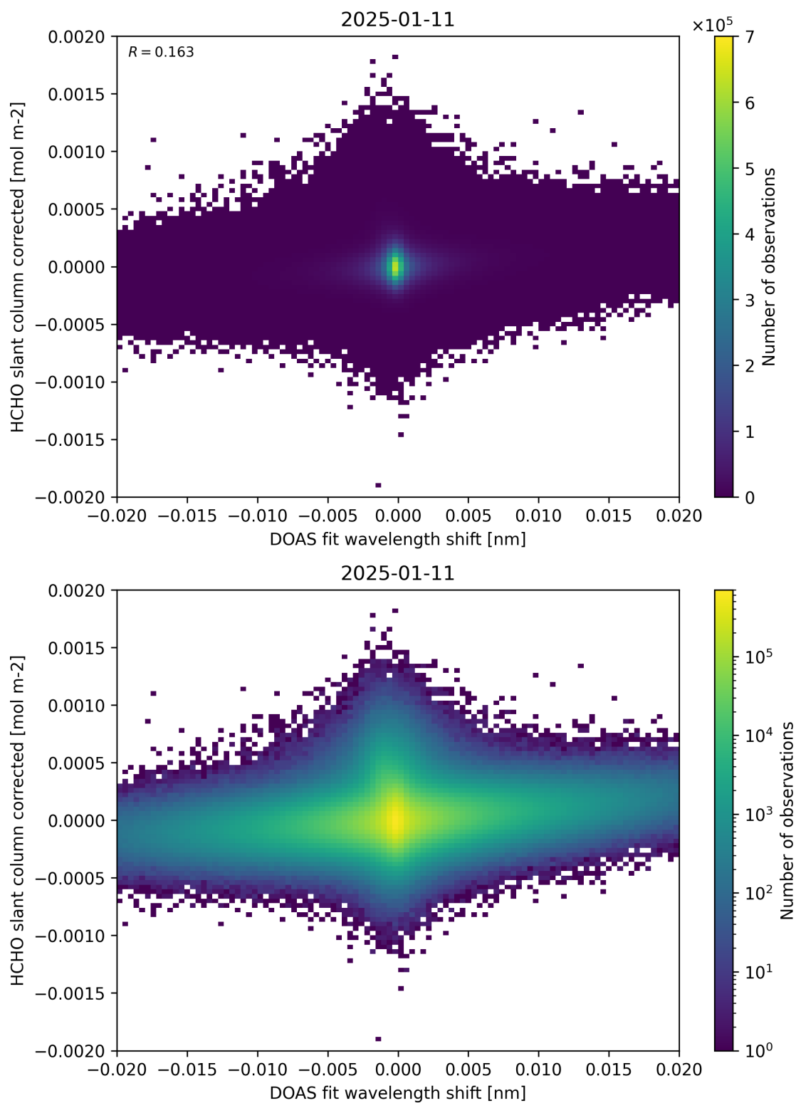
Figure 66: Scatter density plot of “DOAS fit wavelength shift” against “HCHO slant column corrected” for 2025-01-10 to 2025-01-12.
