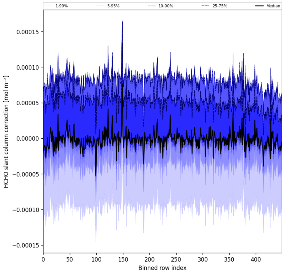
Figure 61: Along track statistics of “HCHO slant column correction” for 2025-01-10 to 2025-01-12
