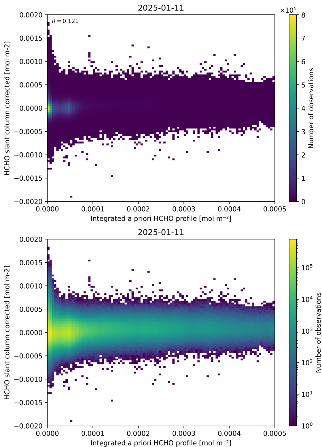
Figure 151: Scatter density plot of “Integrated a priori HCHO profile” against “HCHO slant column corrected” for 2025-01-10 to 2025-01-12.
