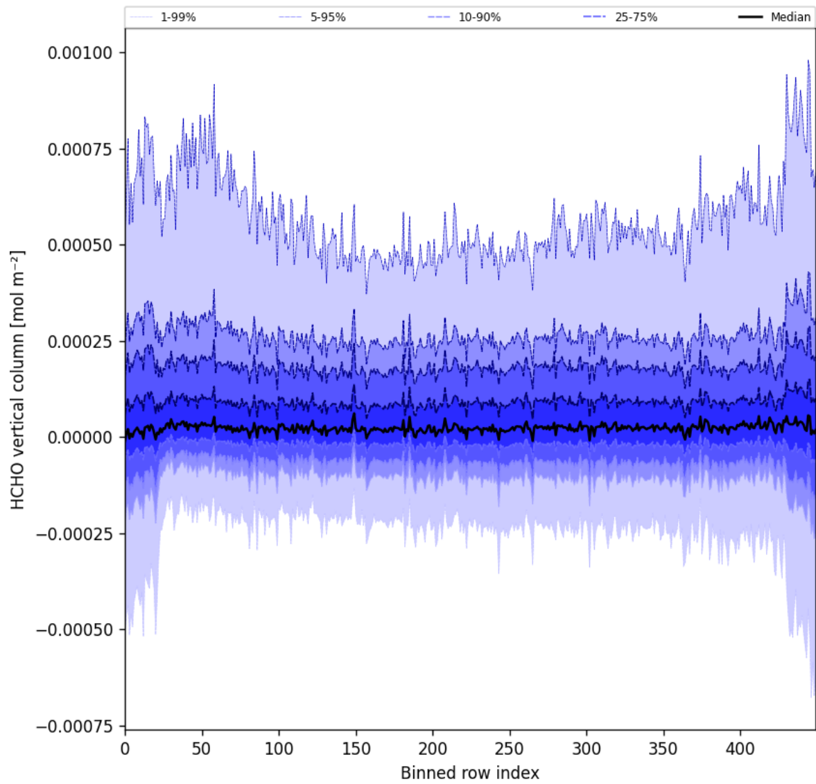
Figure 49: Along track statistics of “HCHO vertical column” for 2025-01-10 to 2025-01-12
