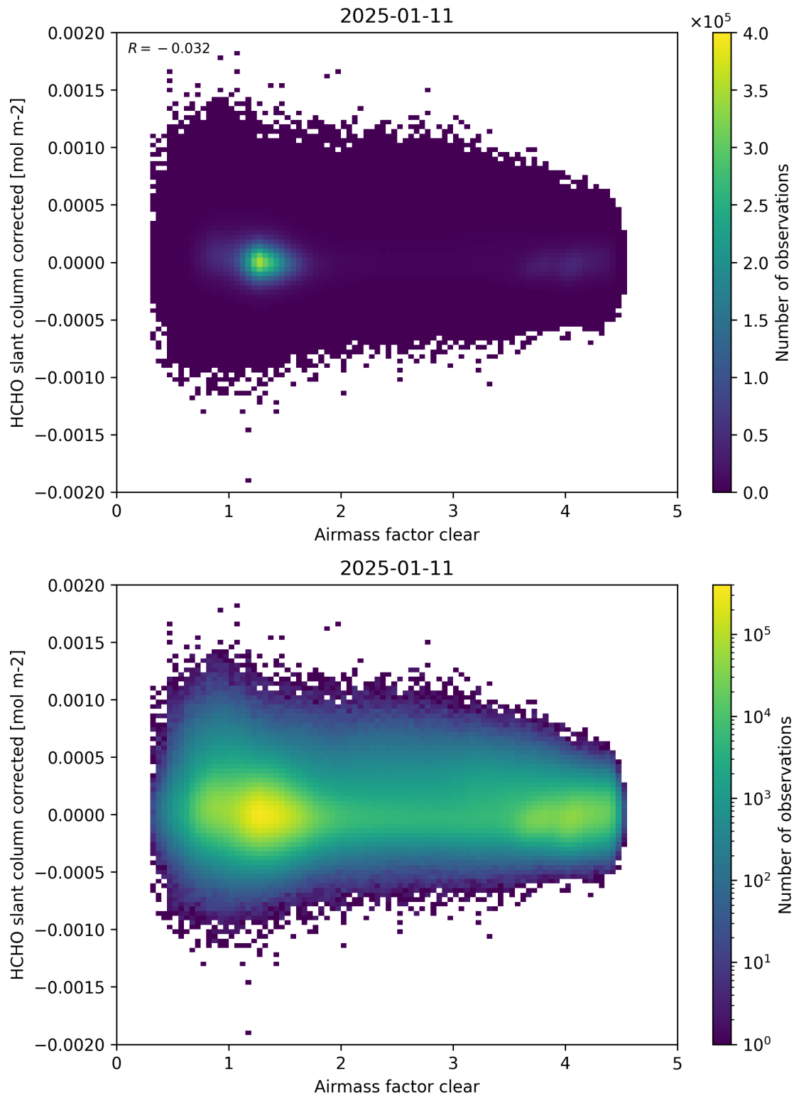
Figure 74: Scatter density plot of “Airmass factor clear” against “HCHO slant column corrected” for 2025-01-10 to 2025-01-12.
