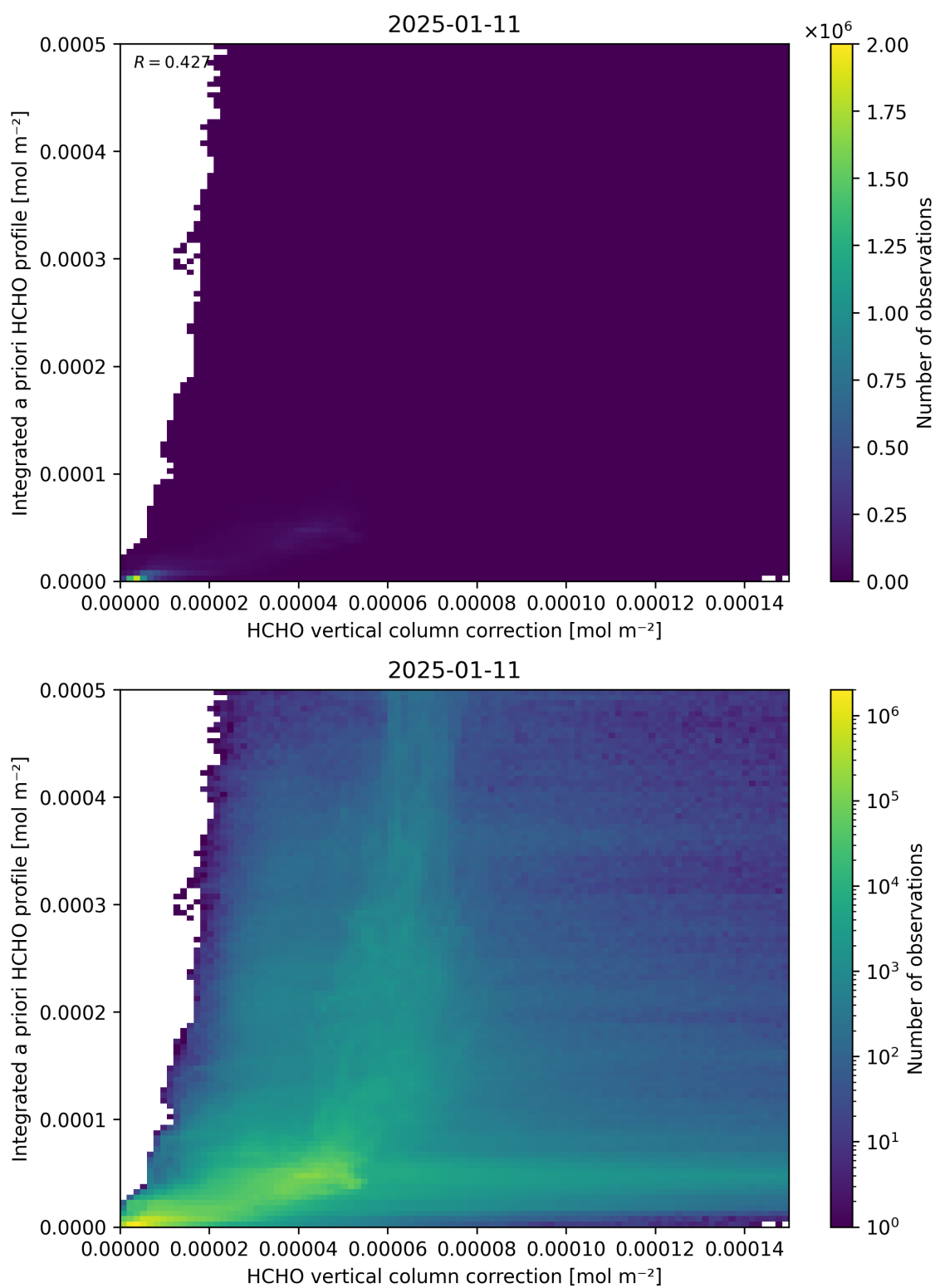
Figure 122: Scatter density plot of “HCHO vertical column correction” against “Integrated a priori HCHO profile” for 2025-01-10 to 2025-01-12.
