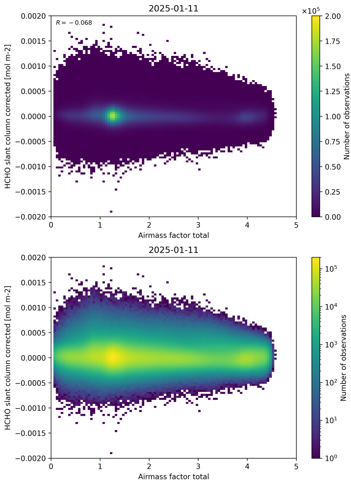
Figure 101: Scatter density plot of “Airmass factor total” against “HCHO slant column corrected” for 2025-01-10 to 2025-01-12.
