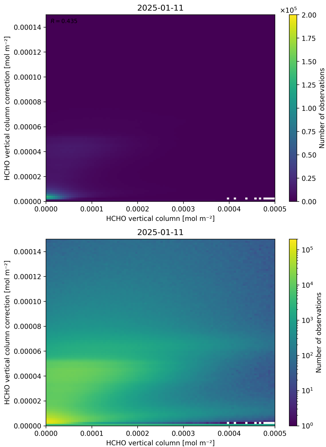
Figure 133: Scatter density plot of “HCHO vertical column” against “HCHO vertical column correction” for 2025-01-10 to 2025-01-12.
