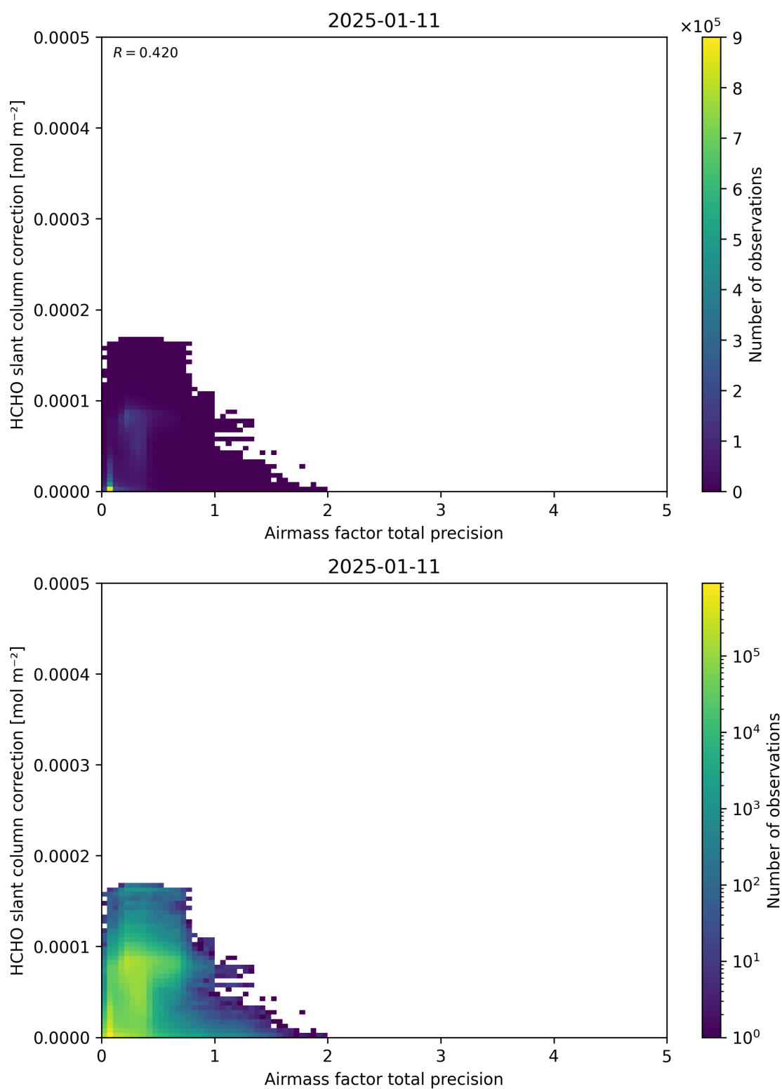
Figure 110: Scatter density plot of “Airmass factor total precision” against “HCHO slant column correction” for 2025-01-10 to 2025-01-12.
