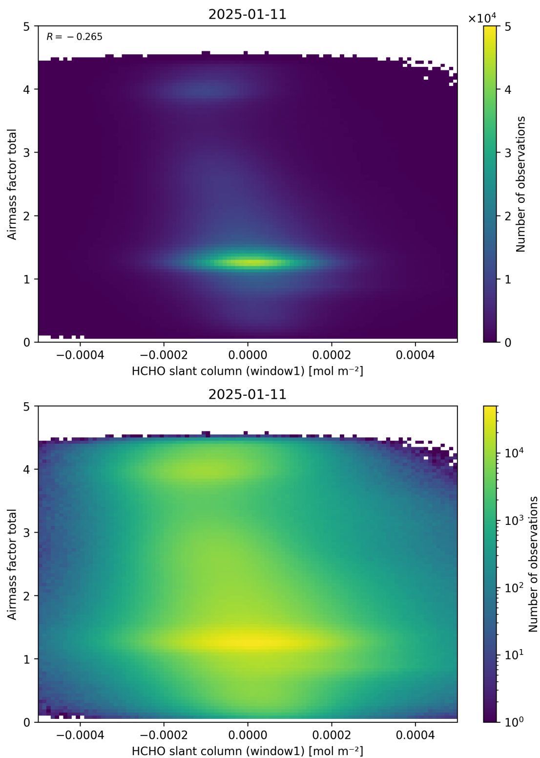
Figure 85: Scatter density plot of “HCHO slant column (window1)” against “Airmass factor total” for 2025-01-10 to 2025-01-12.
