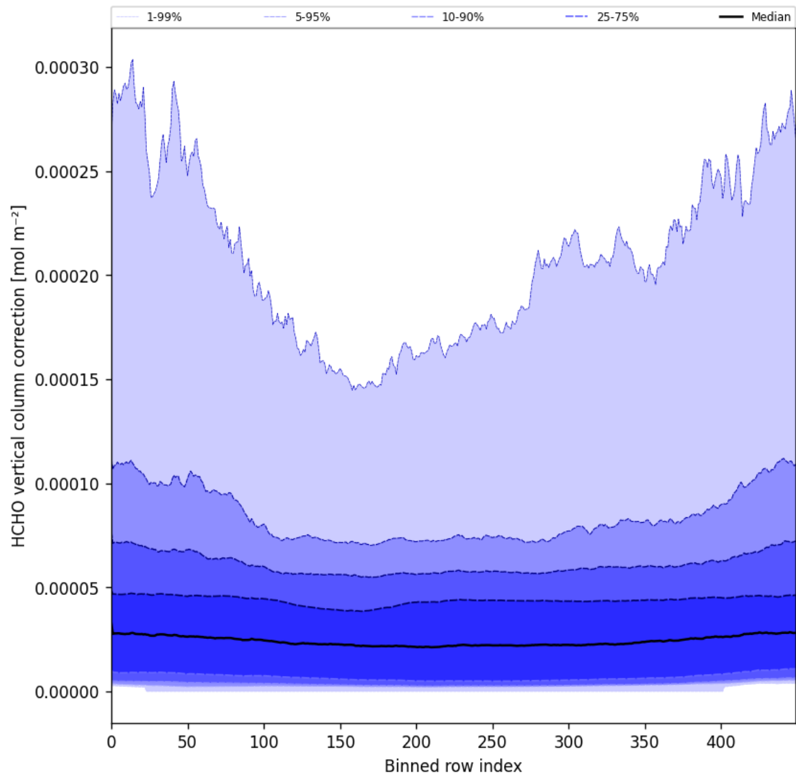
Figure 51: Along track statistics of “HCHO vertical column correction” for 2025-01-10 to 2025-01-12
