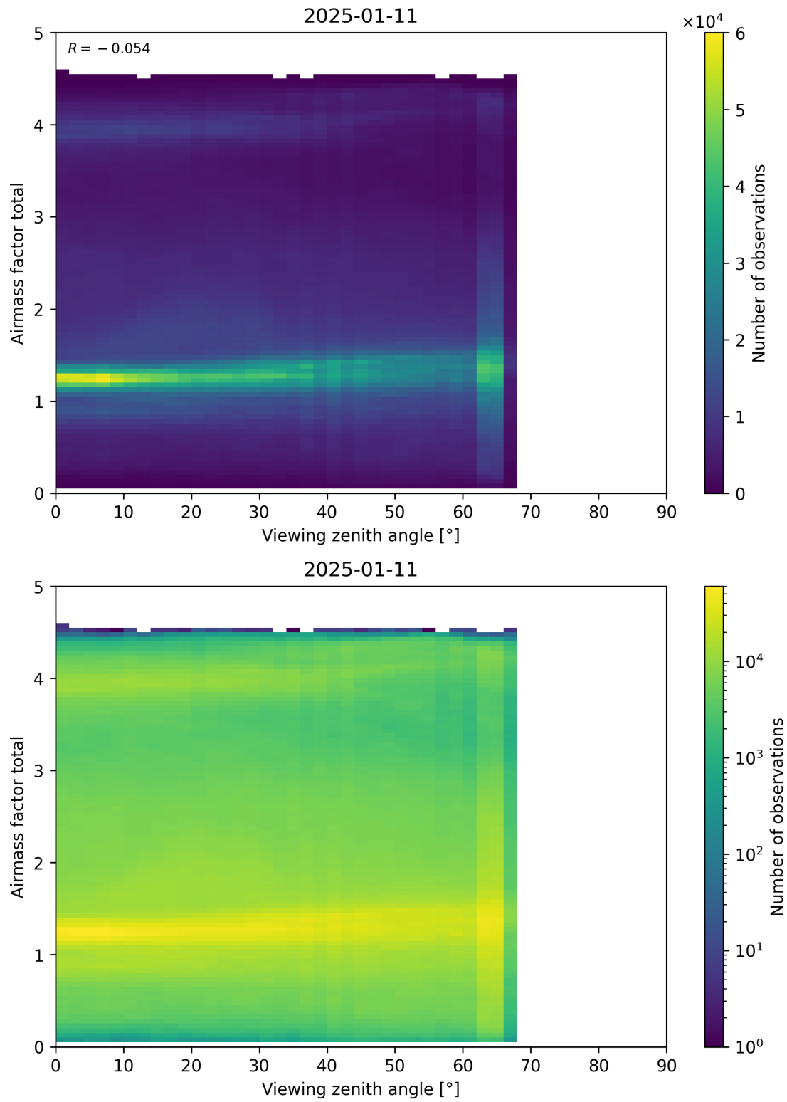
Figure 190: Scatter density plot of “Viewing zenith angle” against “Airmass factor total” for 2025-01-10 to 2025-01-12.
