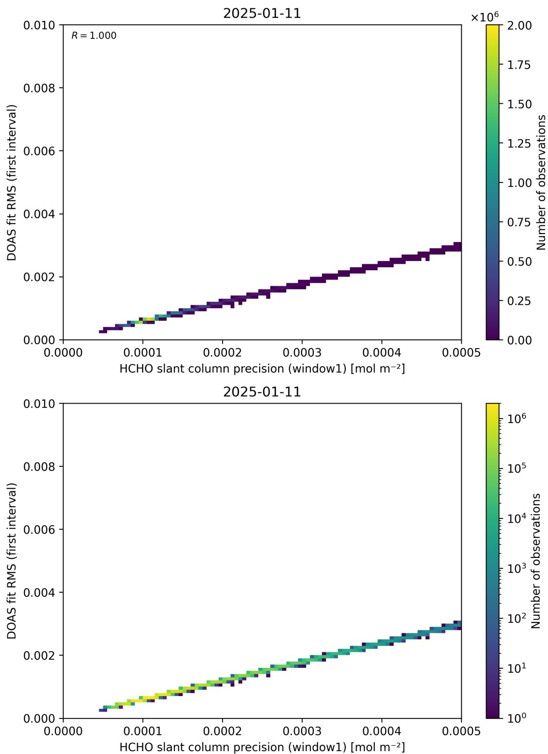
Figure 88: Scatter density plot of “HCHO slant column precision (window1)” against “DOAS fit RMS (first interval)” for 2025-01-10 to 2025-01-12.
