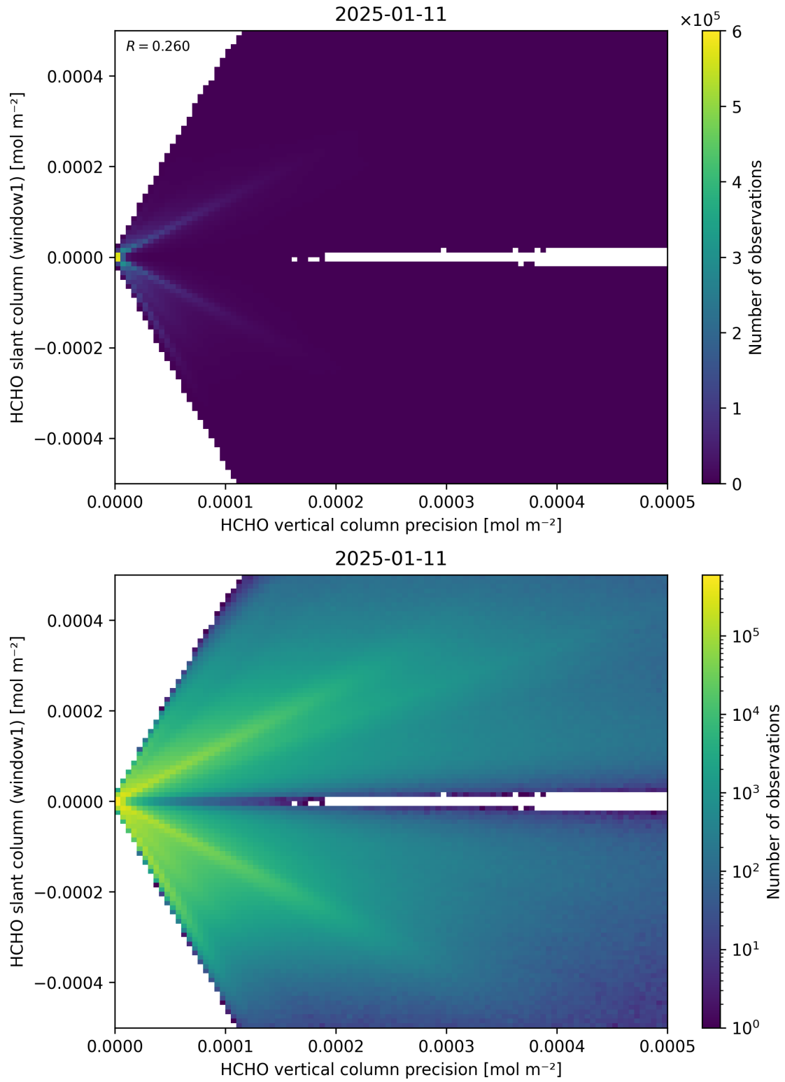
Figure 142: Scatter density plot of “HCHO vertical column precision” against “HCHO slant column (window1)” for 2025-01-10 to 2025-01-12.
