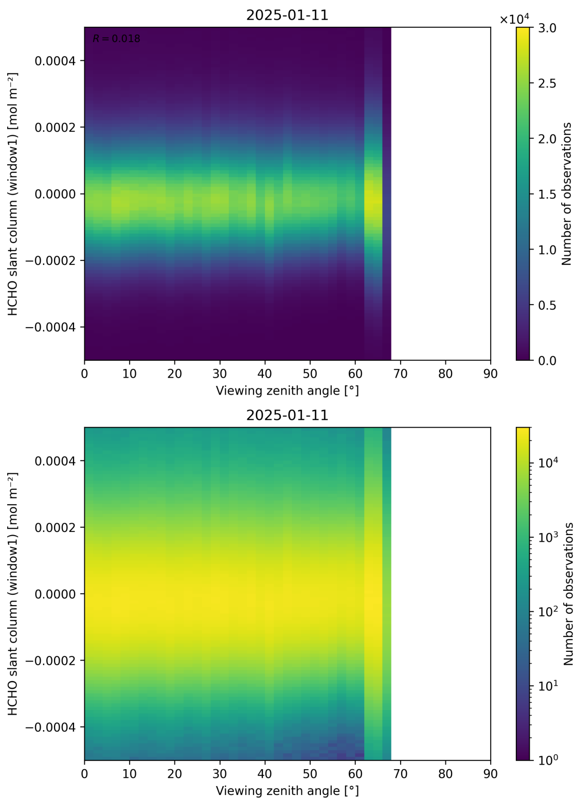
Figure 188: Scatter density plot of “Viewing zenith angle” against “HCHO slant column (window1)” for 2025-01-10 to 2025-01-12.
