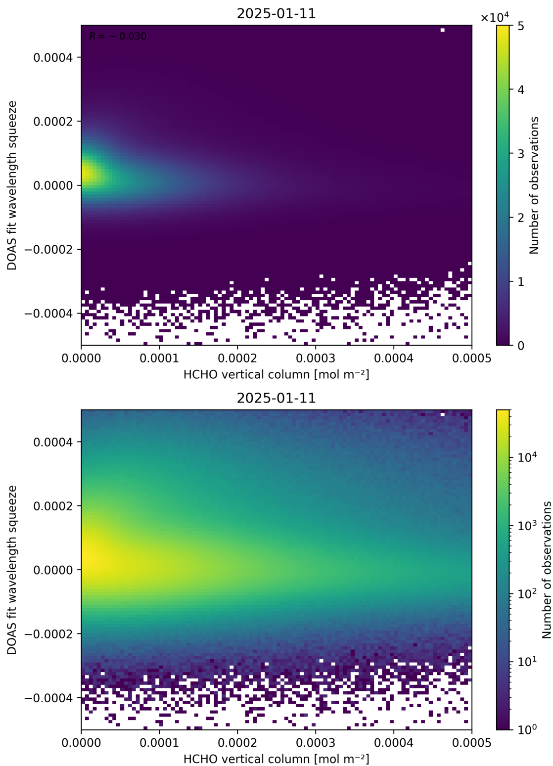
Figure 125: Scatter density plot of “HCHO vertical column” against “DOAS fit wavelength squeeze” for 2025-01-10 to 2025-01-12.
