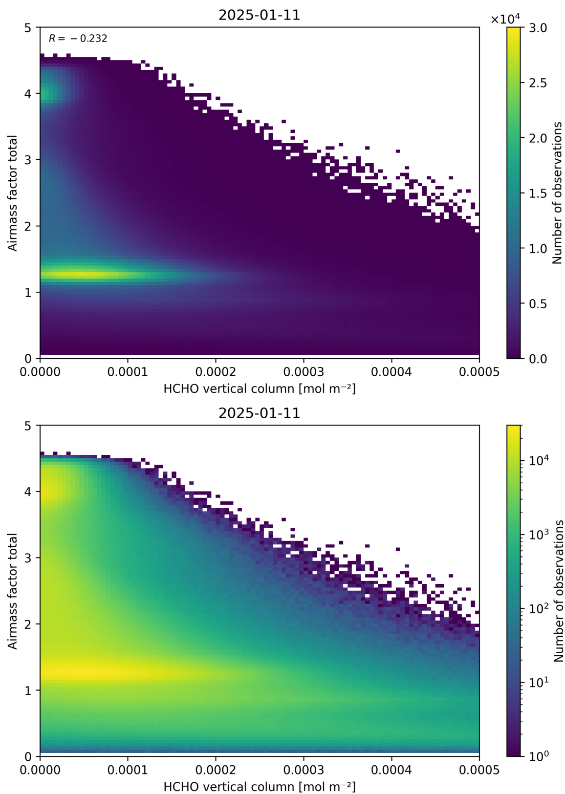
Figure 131: Scatter density plot of “HCHO vertical column” against “Airmass factor total” for 2025-01-10 to 2025-01-12.
