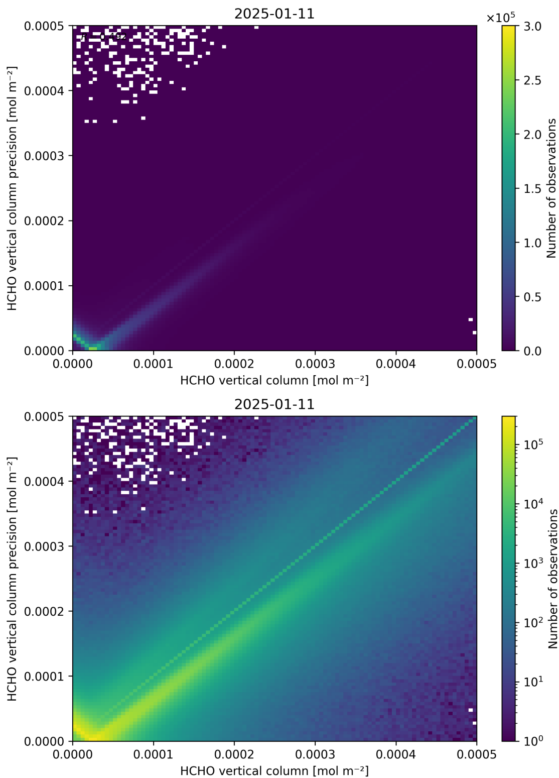
Figure 134: Scatter density plot of “HCHO vertical column” against “HCHO vertical column precision” for 2025-01-10 to 2025-01-12.
