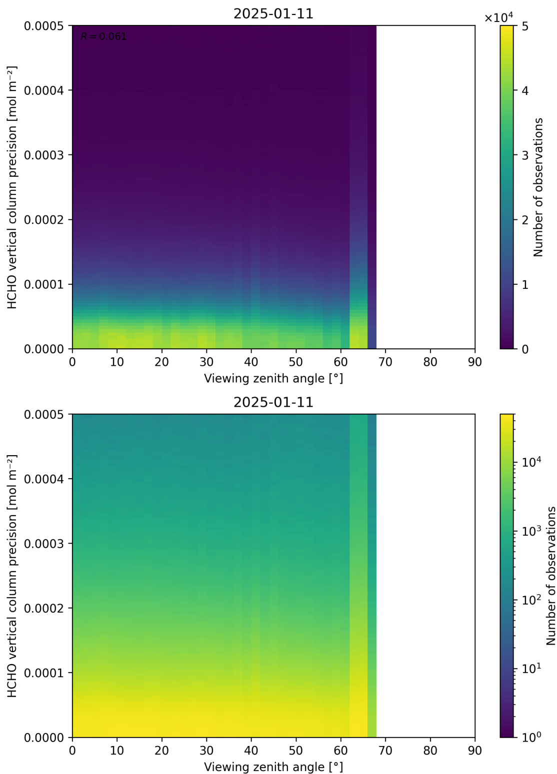
Figure 194: Scatter density plot of “Viewing zenith angle” against “HCHO vertical column precision” for 2025-01-10 to 2025-01-12.
