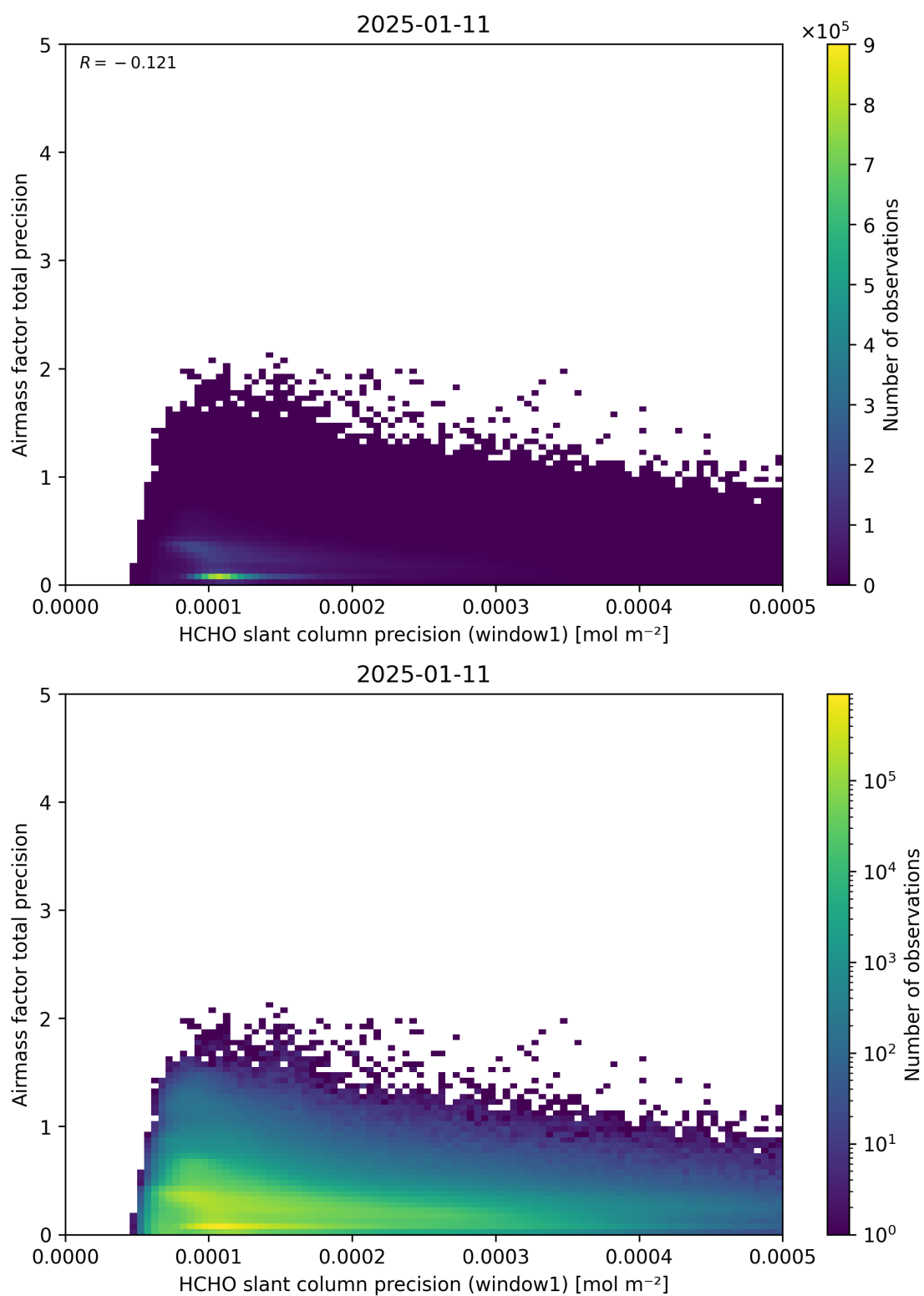
Figure 95: Scatter density plot of “HCHO slant column precision (window1)” against “Airmass factor total precision” for 2025-01-10 to 2025-01-12.
