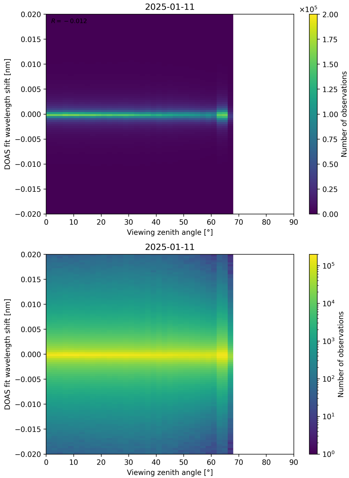
Figure 183: Scatter density plot of “Viewing zenith angle” against “DOAS fit wavelength shift” for 2025-01-10 to 2025-01-12.
