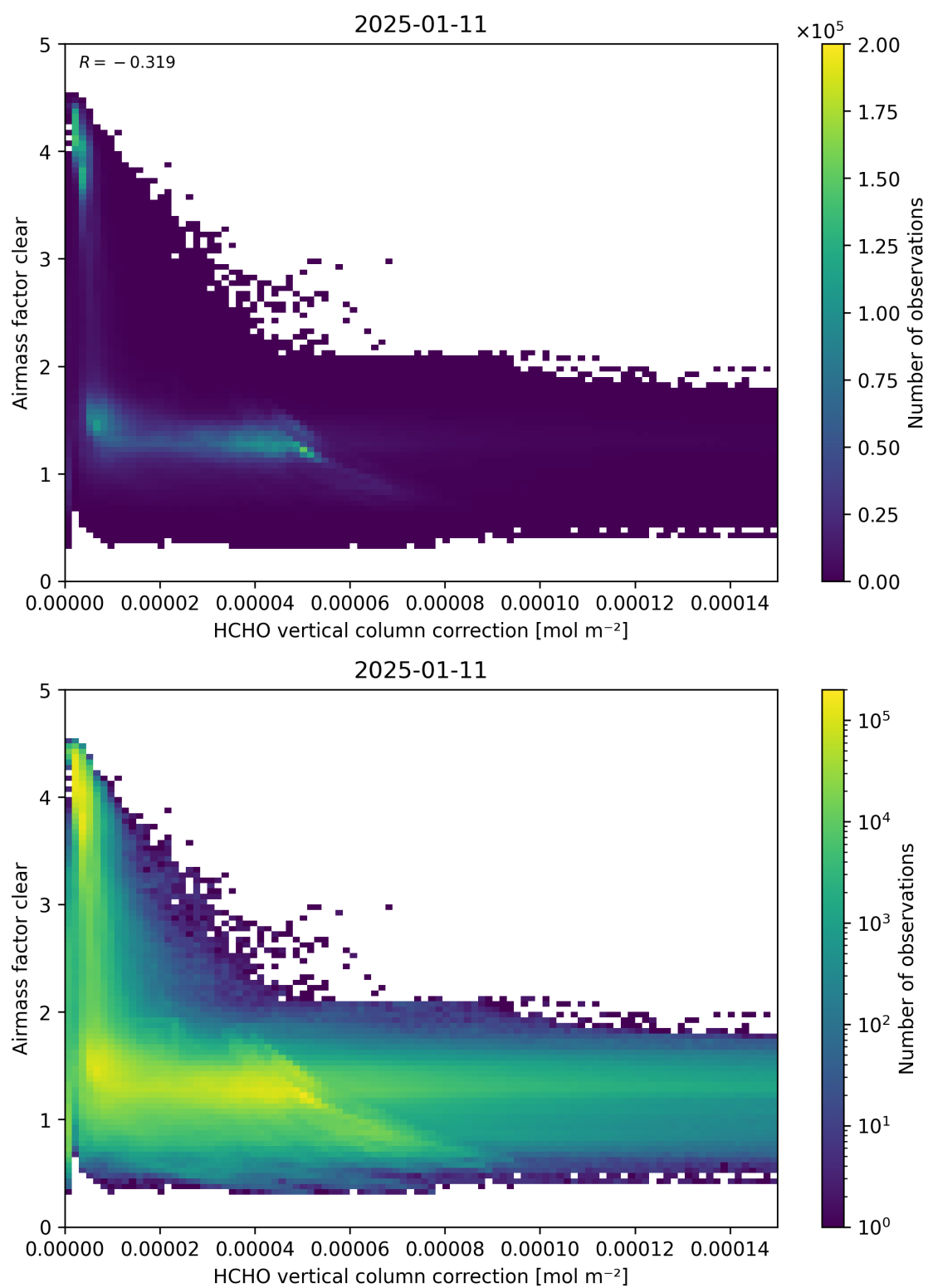
Figure 115: Scatter density plot of “HCHO vertical column correction” against “Airmass factor clear” for 2025-01-10 to 2025-01-12.
