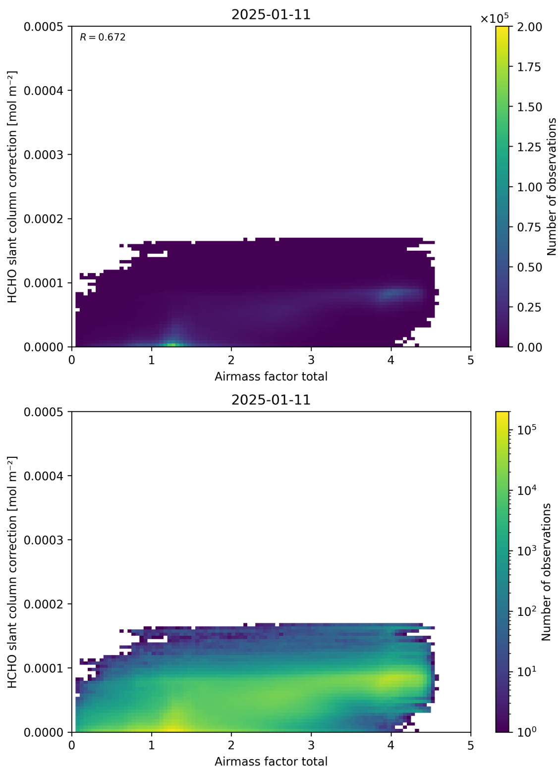
Figure 102: Scatter density plot of “Airmass factor total” against “HCHO slant column correction” for 2025-01-10 to 2025-01-12.
