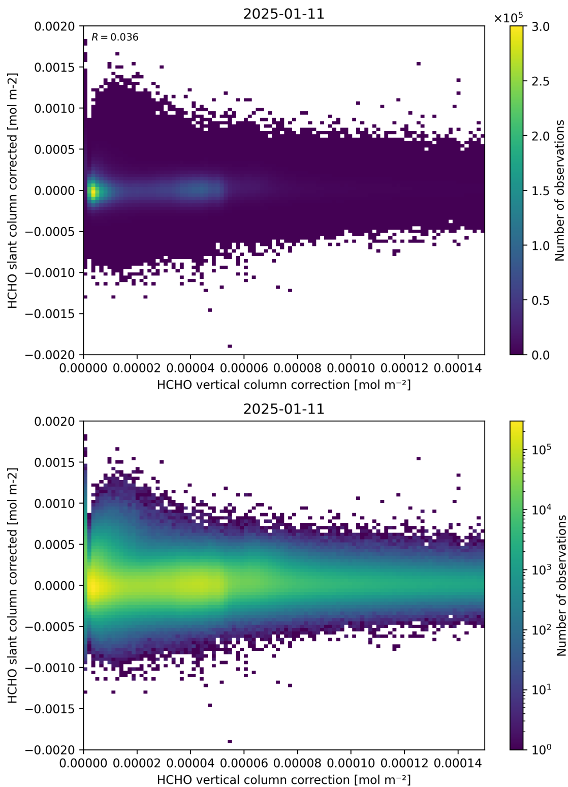
Figure 116: Scatter density plot of “HCHO vertical column correction” against “HCHO slant column corrected” for 2025-01-10 to 2025-01-12.
