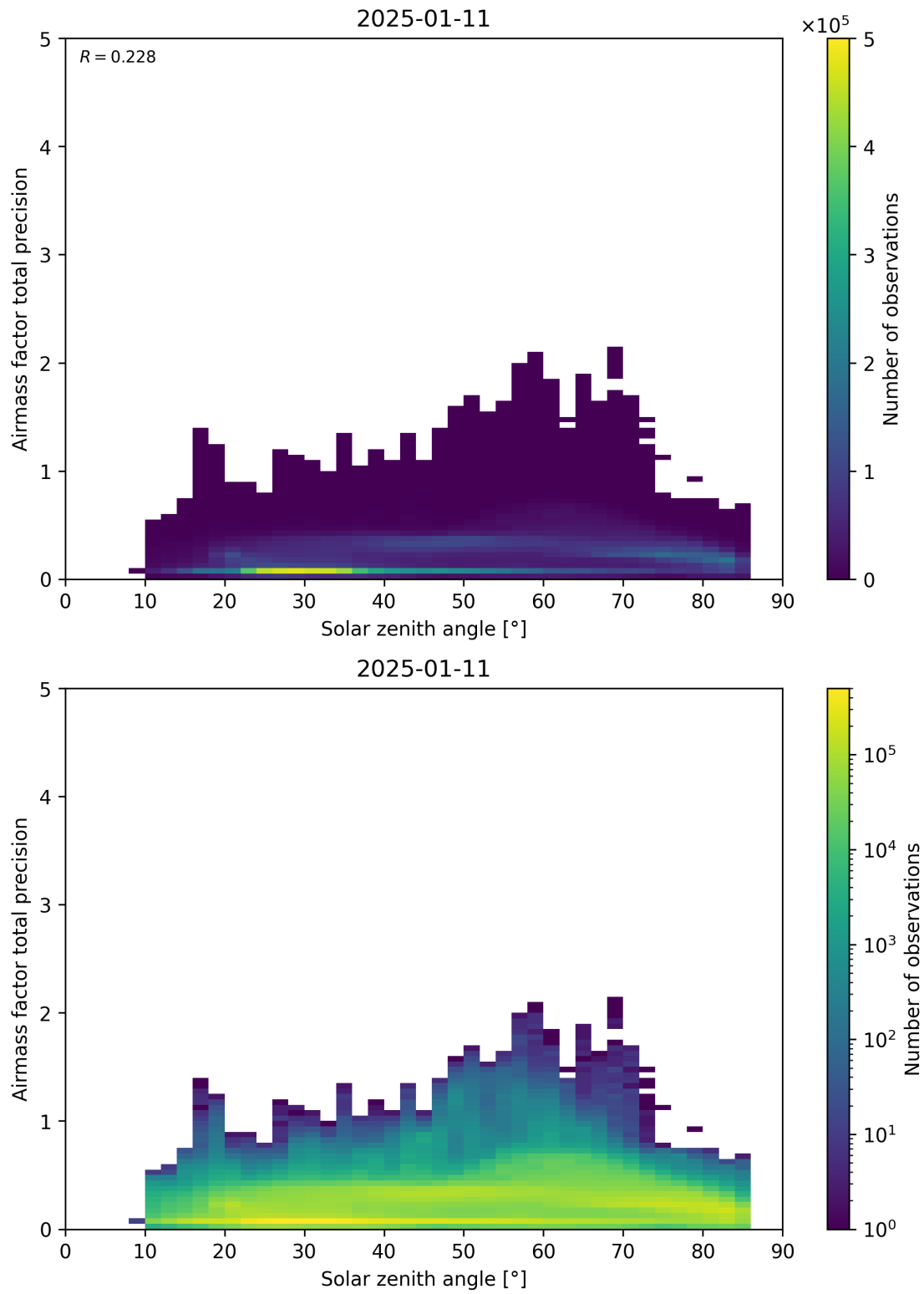
Figure 176: Scatter density plot of “Solar zenith angle” against “Airmass factor total precision” for 2025-01-10 to 2025-01-12.
