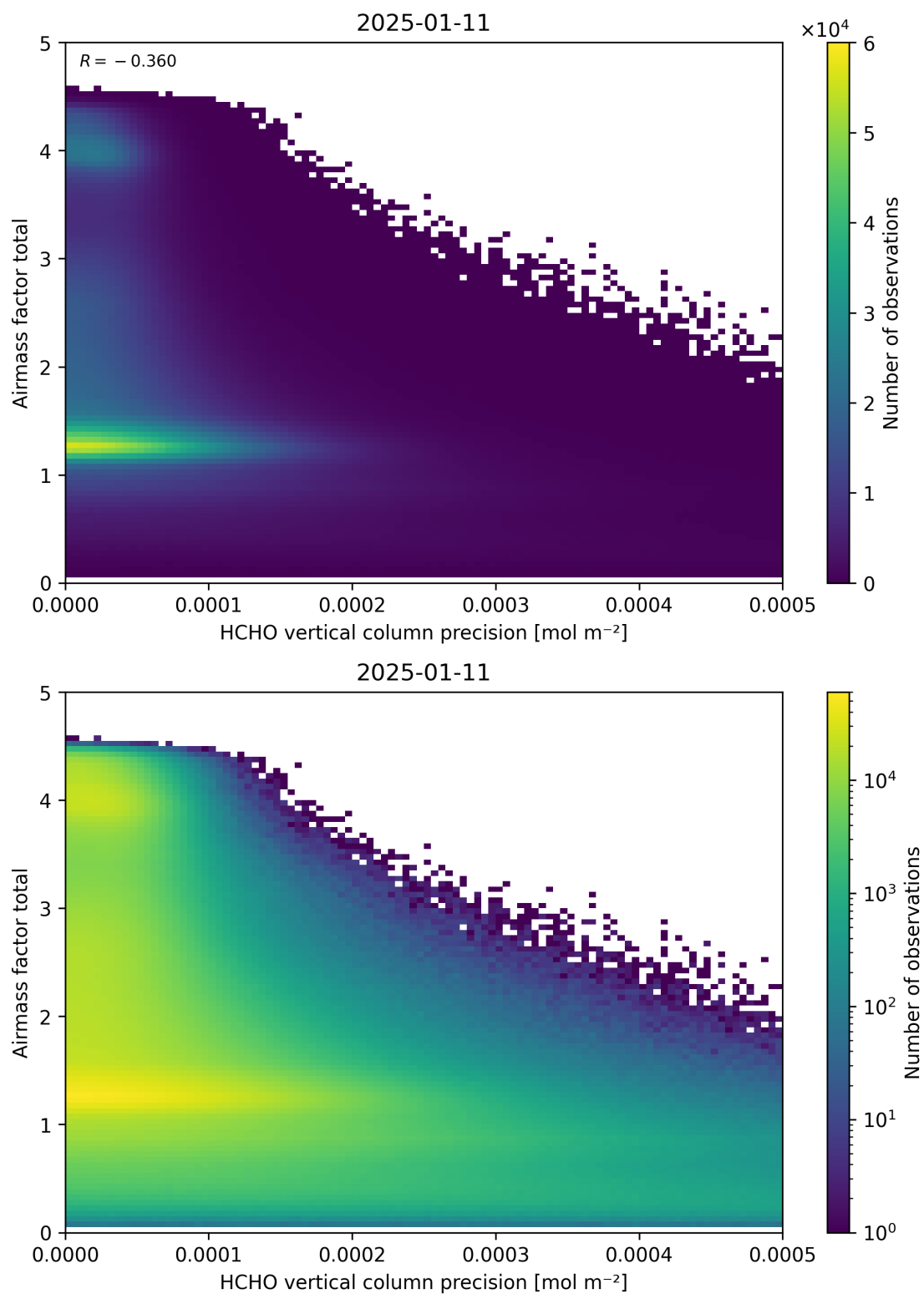
Figure 144: Scatter density plot of “HCHO vertical column precision” against “Airmass factor total” for 2025-01-10 to 2025-01-12.
