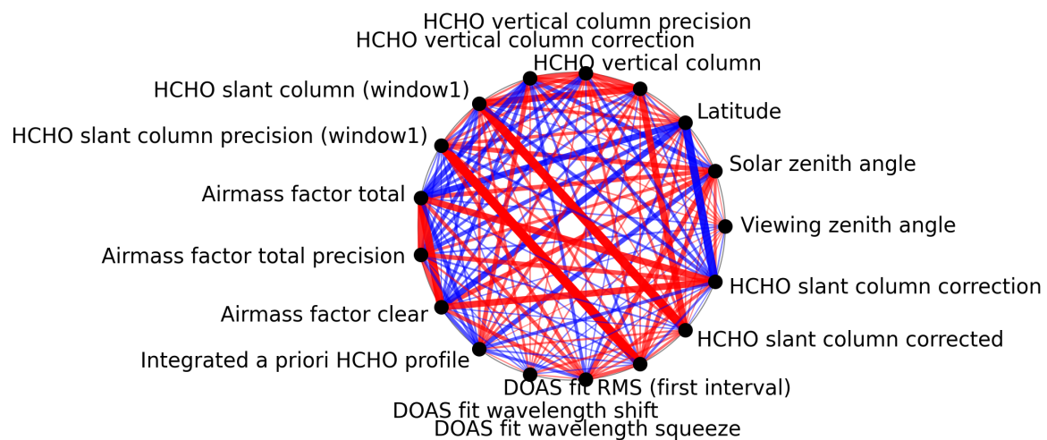
Figure 1: Map of correlation graph for 2025-01-10 to 2025-01-12.
