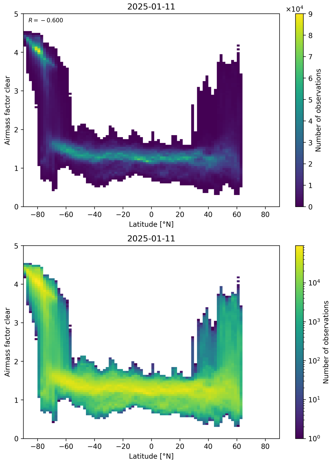
Figure 156: Scatter density plot of “Latitude” against “Airmass factor clear” for 2025-01-10 to 2025-01-12.
