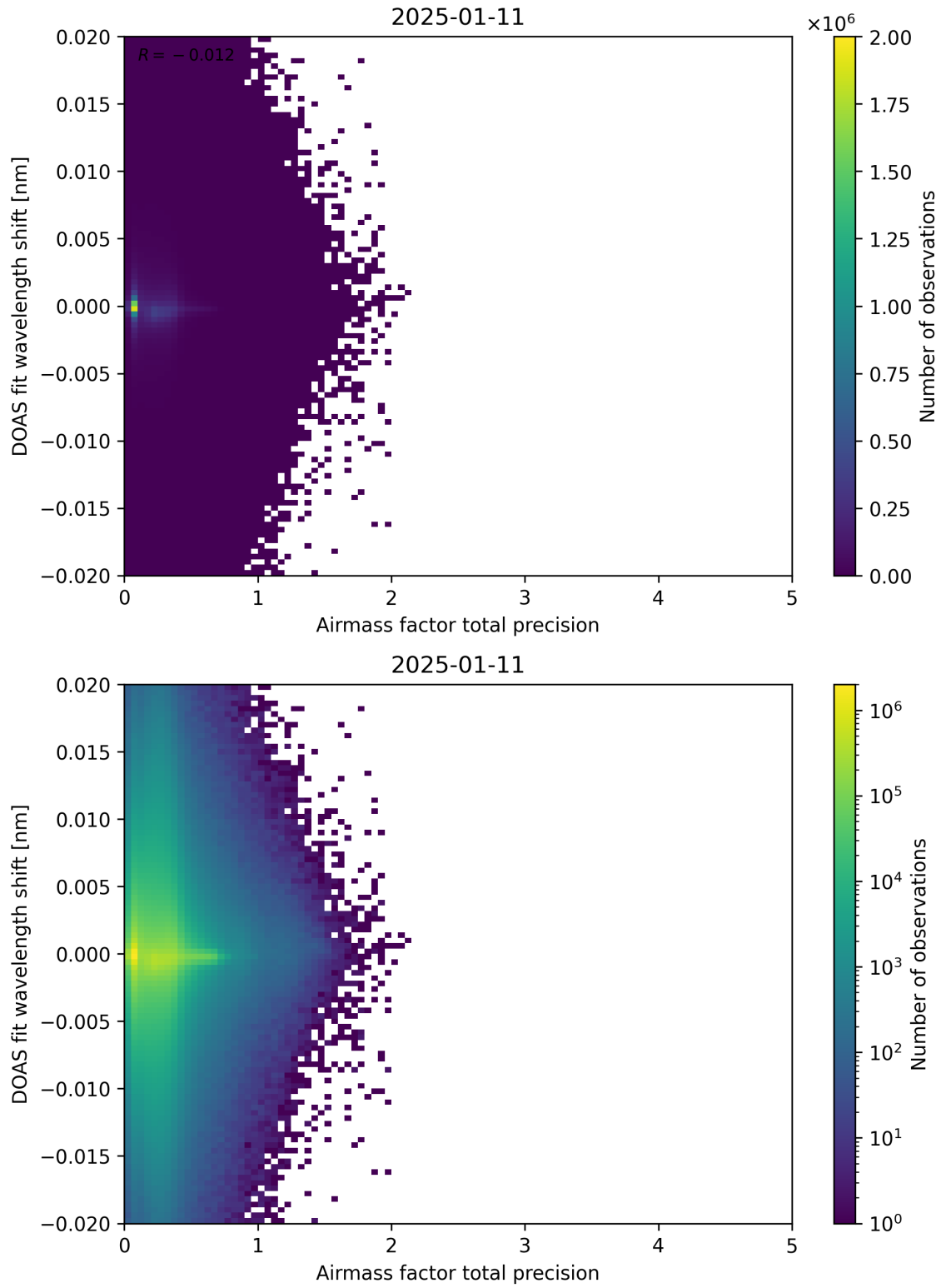
Figure 106: Scatter density plot of “Airmass factor total precision” against “DOAS fit wavelength shift” for 2025-01-10 to 2025-01-12.
