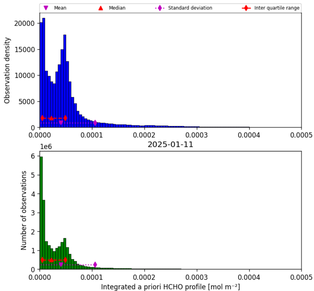
Figure 43: Histogram of “Integrated a priori HCHO profile” for 2025-01-10 to 2025-01-12
