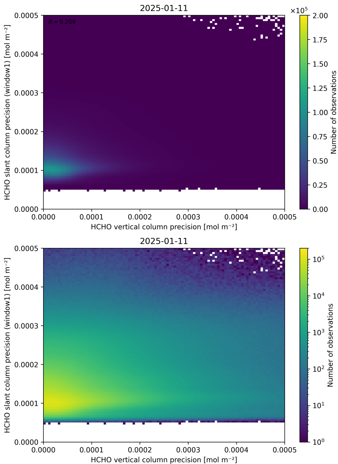
Figure 143: Scatter density plot of “HCHO vertical column precision” against “HCHO slant column precision (window1)” for 2025-01-10 to 2025-01-12.
