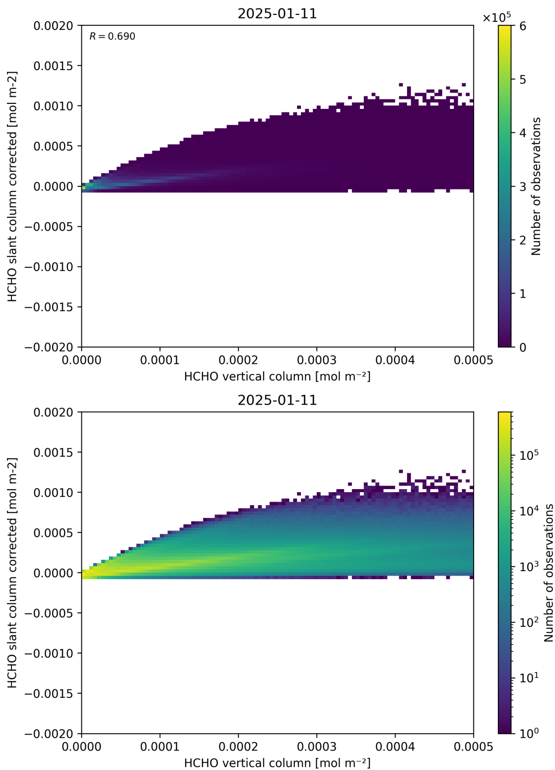
Figure 127: Scatter density plot of “HCHO vertical column” against “HCHO slant column corrected” for 2025-01-10 to 2025-01-12.
