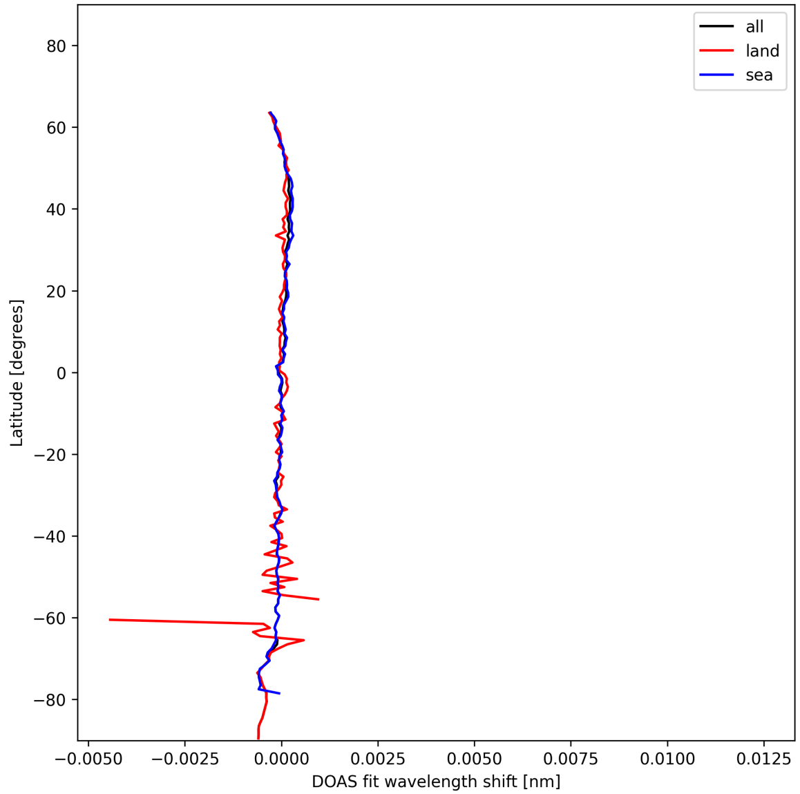
Figure 30: Zonal average of “DOAS fit wavelength shift” for 2025-01-10 to 2025-01-12.
