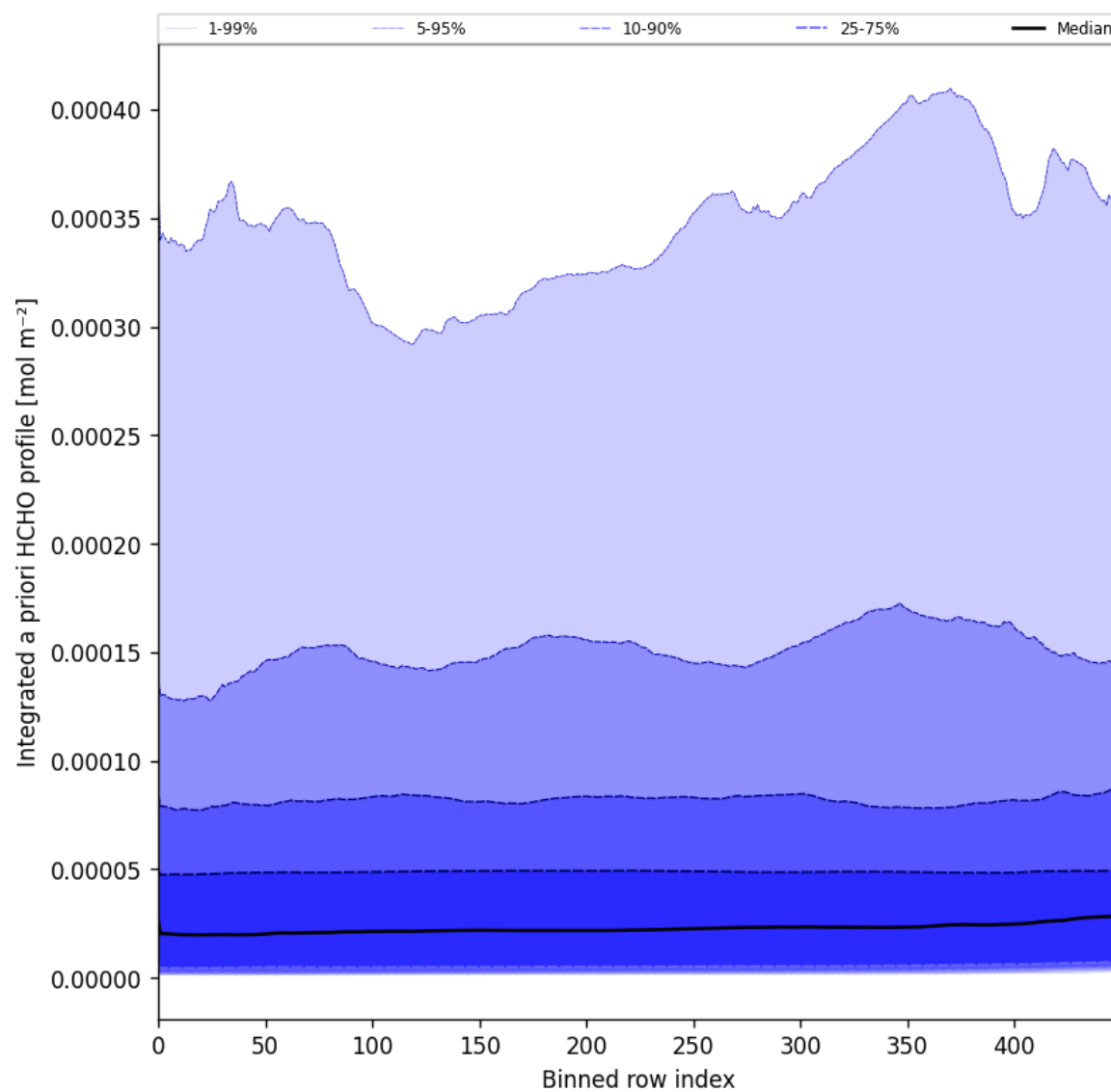
Figure 57: Along track statistics of "Integrated a priori HCHO profile" for 2025-01-10 to 2025-01-12
