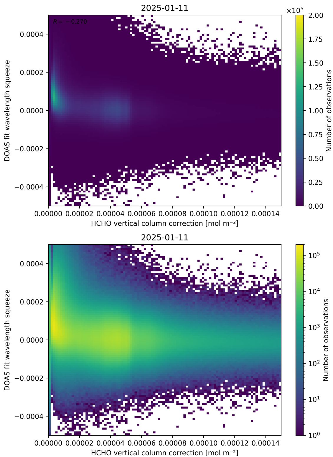
Figure 114: Scatter density plot of “HCHO vertical column correction” against “DOAS fit wavelength squeeze” for 2025-01-10 to 2025-01-12.
