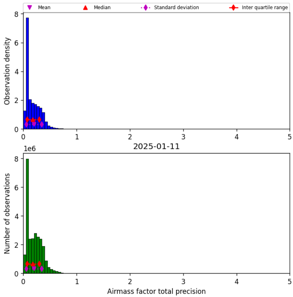
Figure 41: Histogram of “Airmass factor total precision” for 2025-01-10 to 2025-01-12
