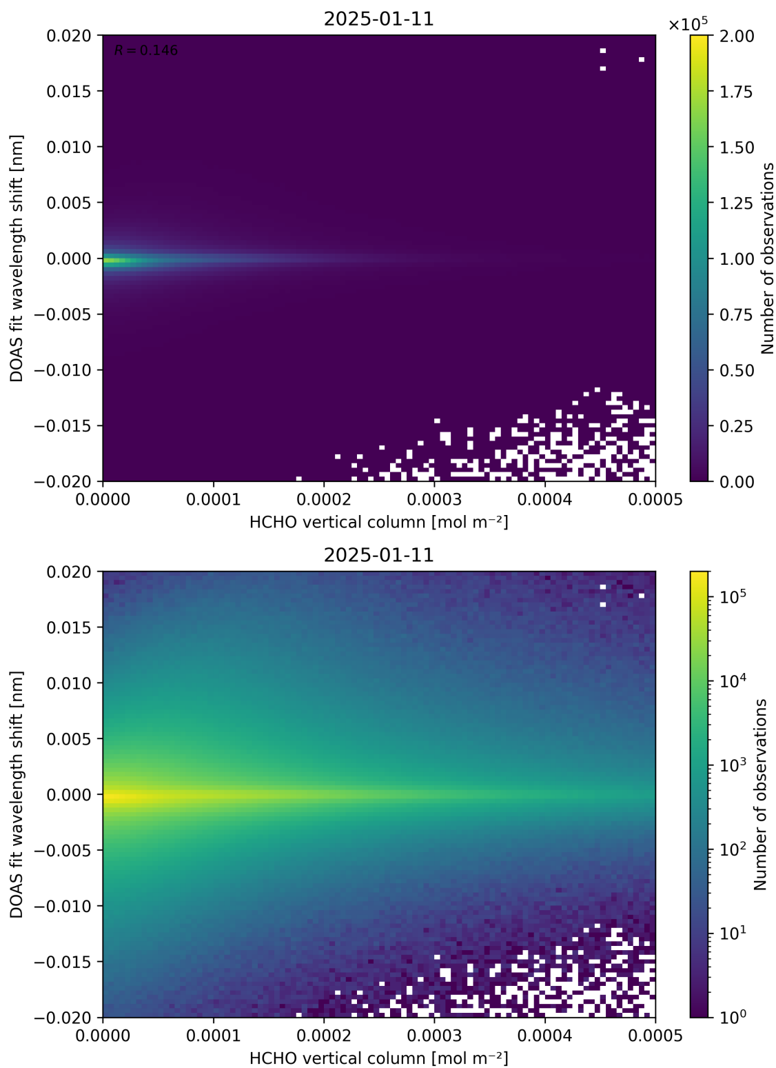
Figure 124: Scatter density plot of “HCHO vertical column” against “DOAS fit wavelength shift” for 2025-01-10 to 2025-01-12.
