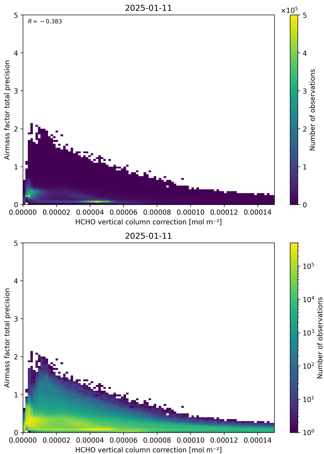
Figure 121: Scatter density plot of “HCHO vertical column correction” against “Airmass factor total precision” for 2025-01-10 to 2025-01-12.
