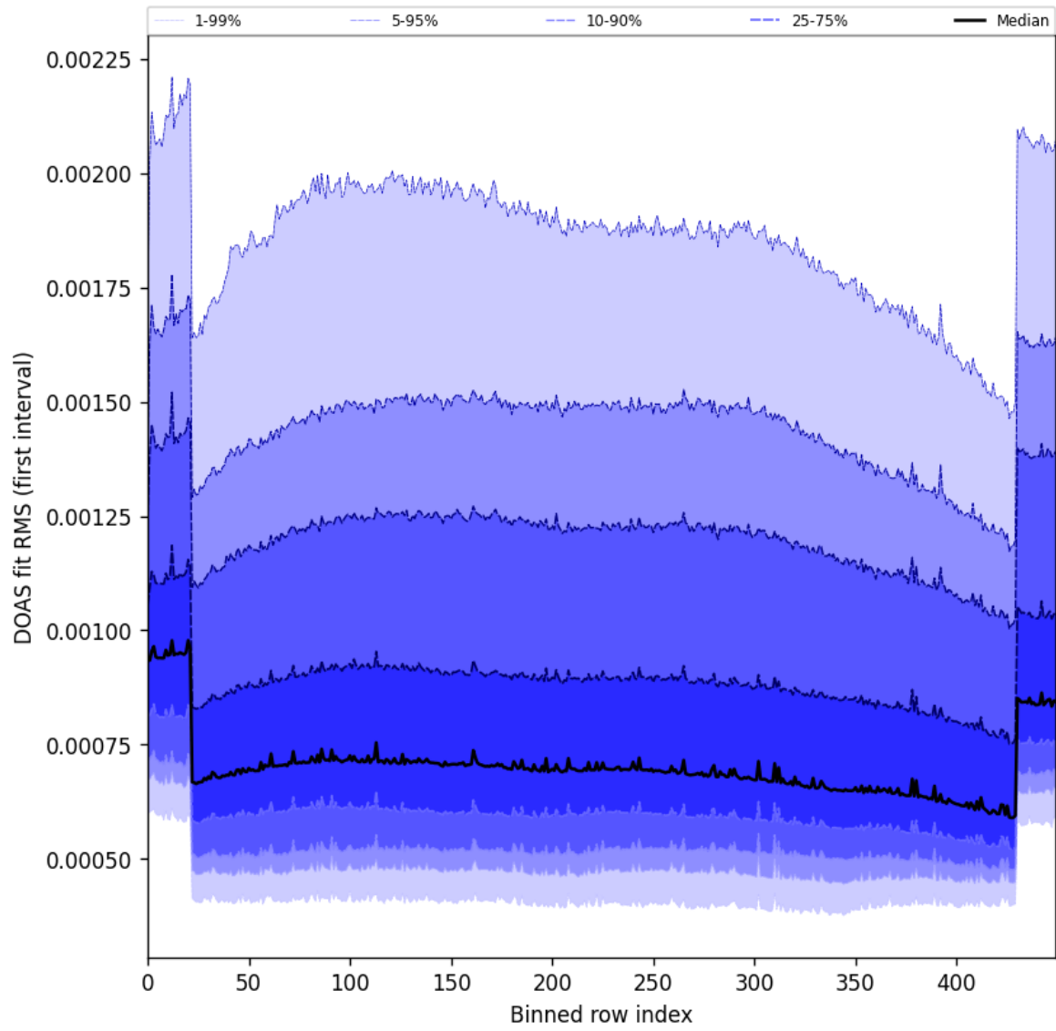
Figure 60: Along track statistics of “DOAS fit RMS (first interval)” for 2025-01-10 to 2025-01-12
