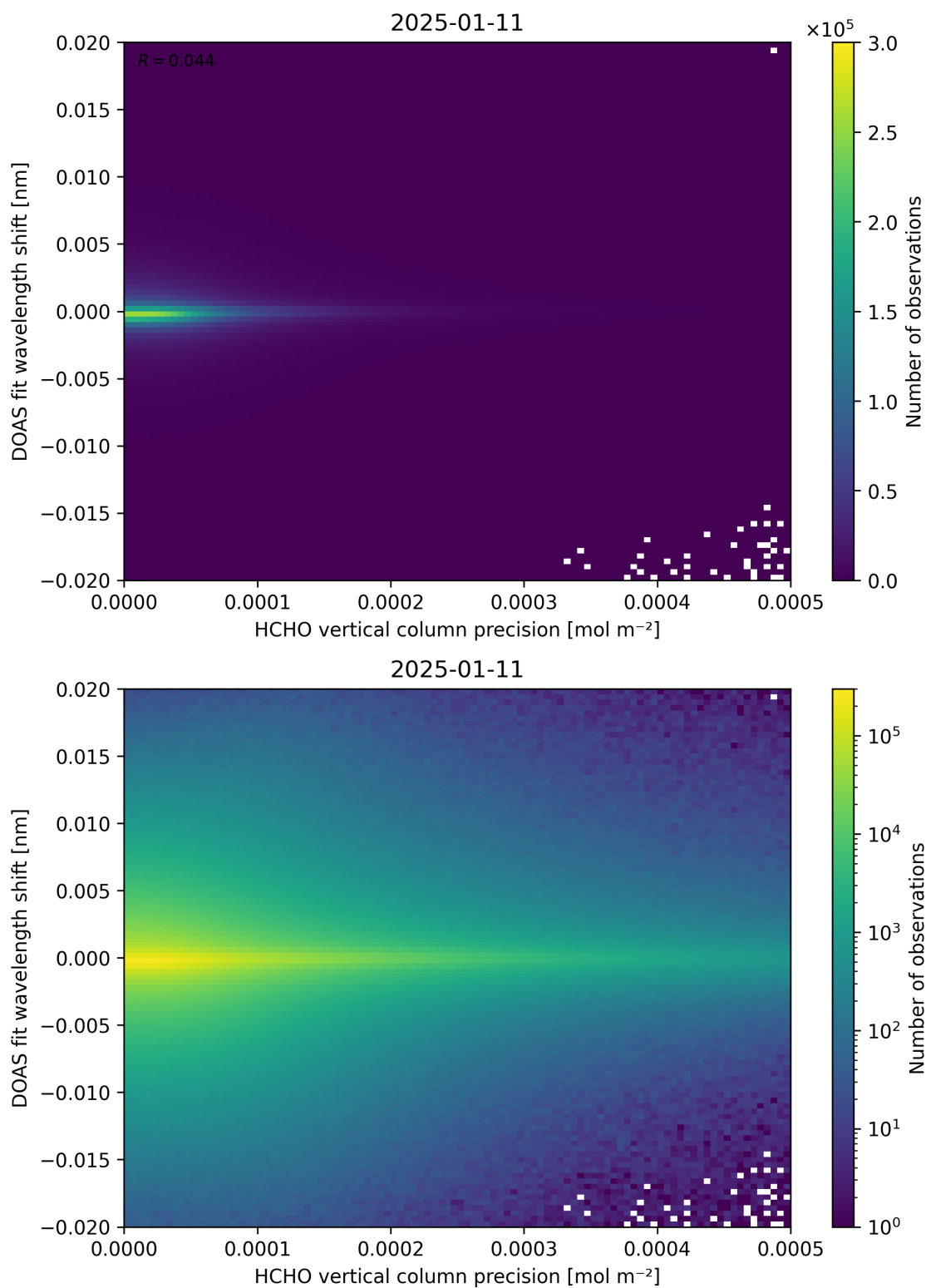
Figure 137: Scatter density plot of “HCHO vertical column precision” against “DOAS fit wavelength shift” for 2025-01-10 to 2025-01-12.
