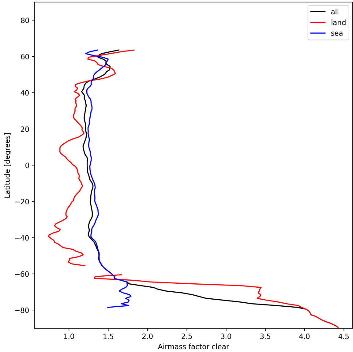
Figure 28: Zonal average of “Airmass factor clear” for 2025-01-10 to 2025-01-12.
