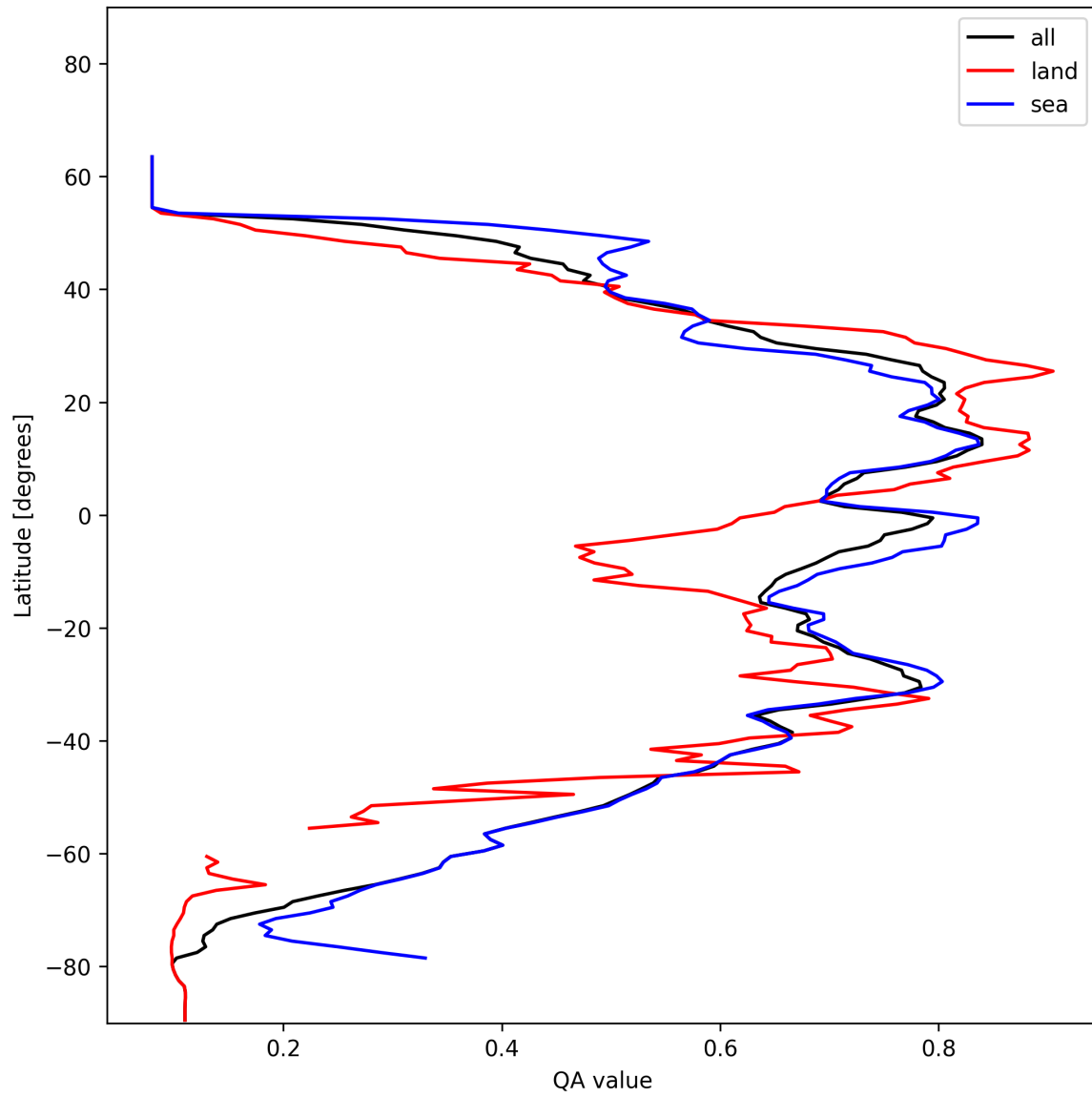
Figure 20: Zonal average of “QA value” for 2025-01-10 to 2025-01-12.
