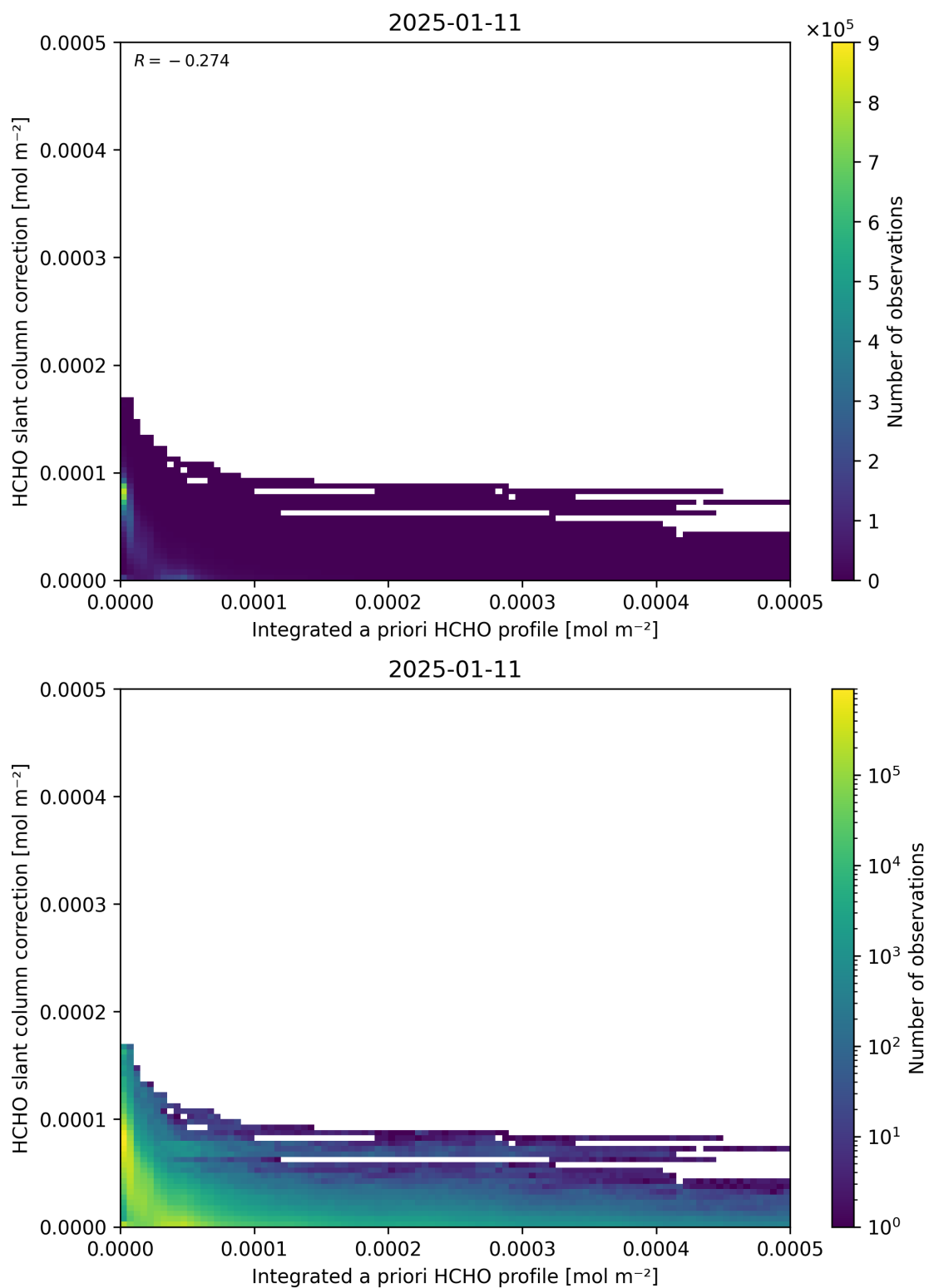
Figure 152: Scatter density plot of “Integrated a priori HCHO profile” against “HCHO slant column correction” for 2025-01-10 to 2025-01-12.
