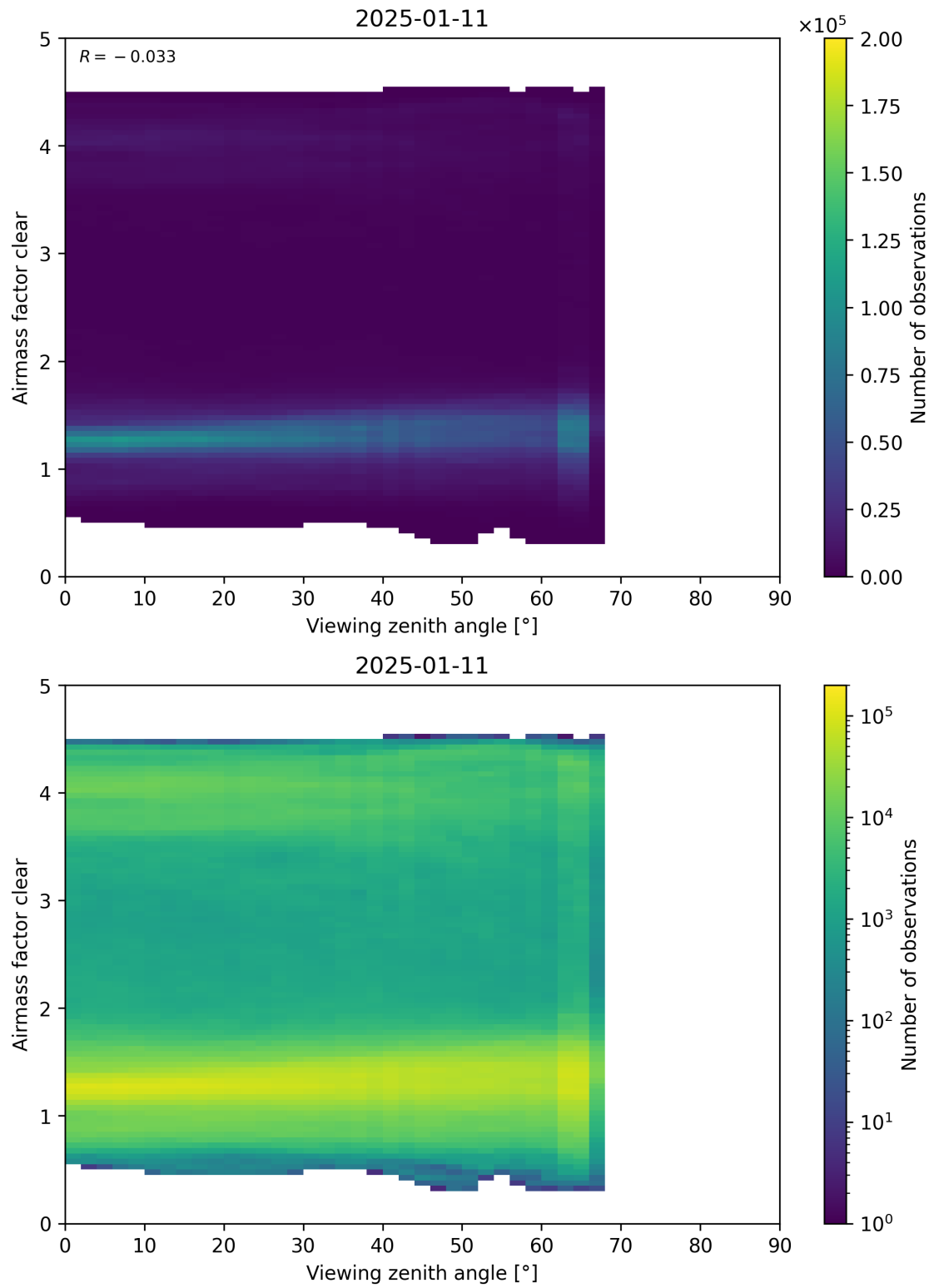
Figure 185: Scatter density plot of “Viewing zenith angle” against “Airmass factor clear” for 2025-01-10 to 2025-01-12.
