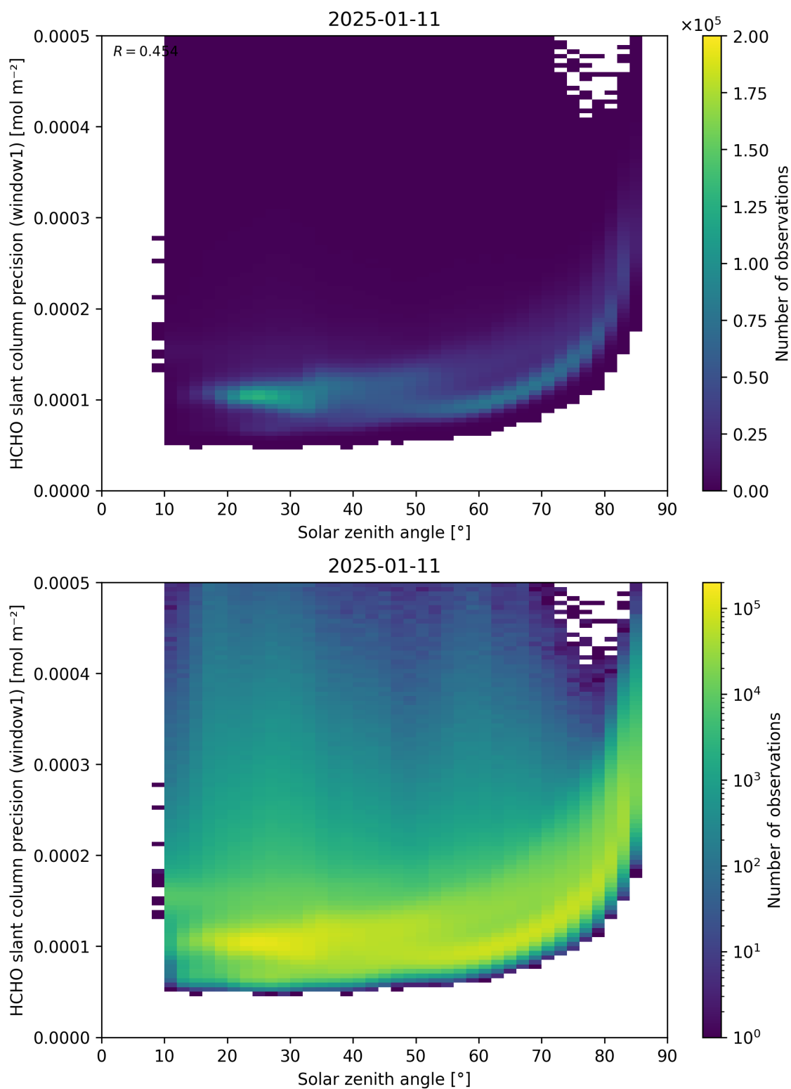
Figure 174: Scatter density plot of “Solar zenith angle” against “HCHO slant column precision (window1)” for 2025-01-10 to 2025-01-12.
