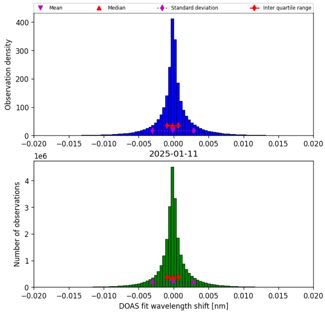
Figure 44: Histogram of “DOAS fit wavelength shift” for 2025-01-10 to 2025-01-12
