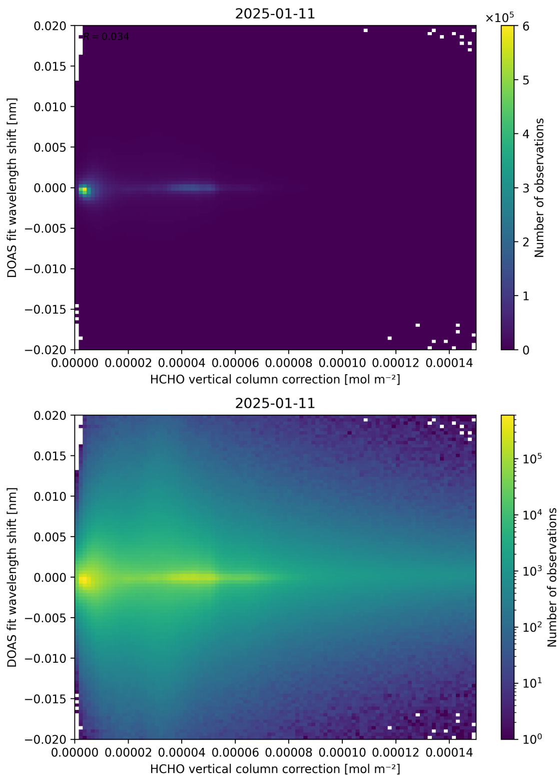
Figure 113: Scatter density plot of “HCHO vertical column correction” against “DOAS fit wavelength shift” for 2025-01-10 to 2025-01-12.
