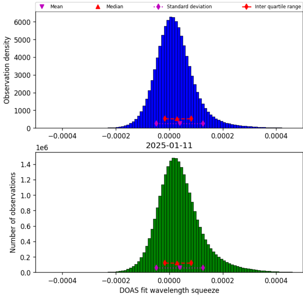
Figure 45: Histogram of “DOAS fit wavelength squeeze” for 2025-01-10 to 2025-01-12
