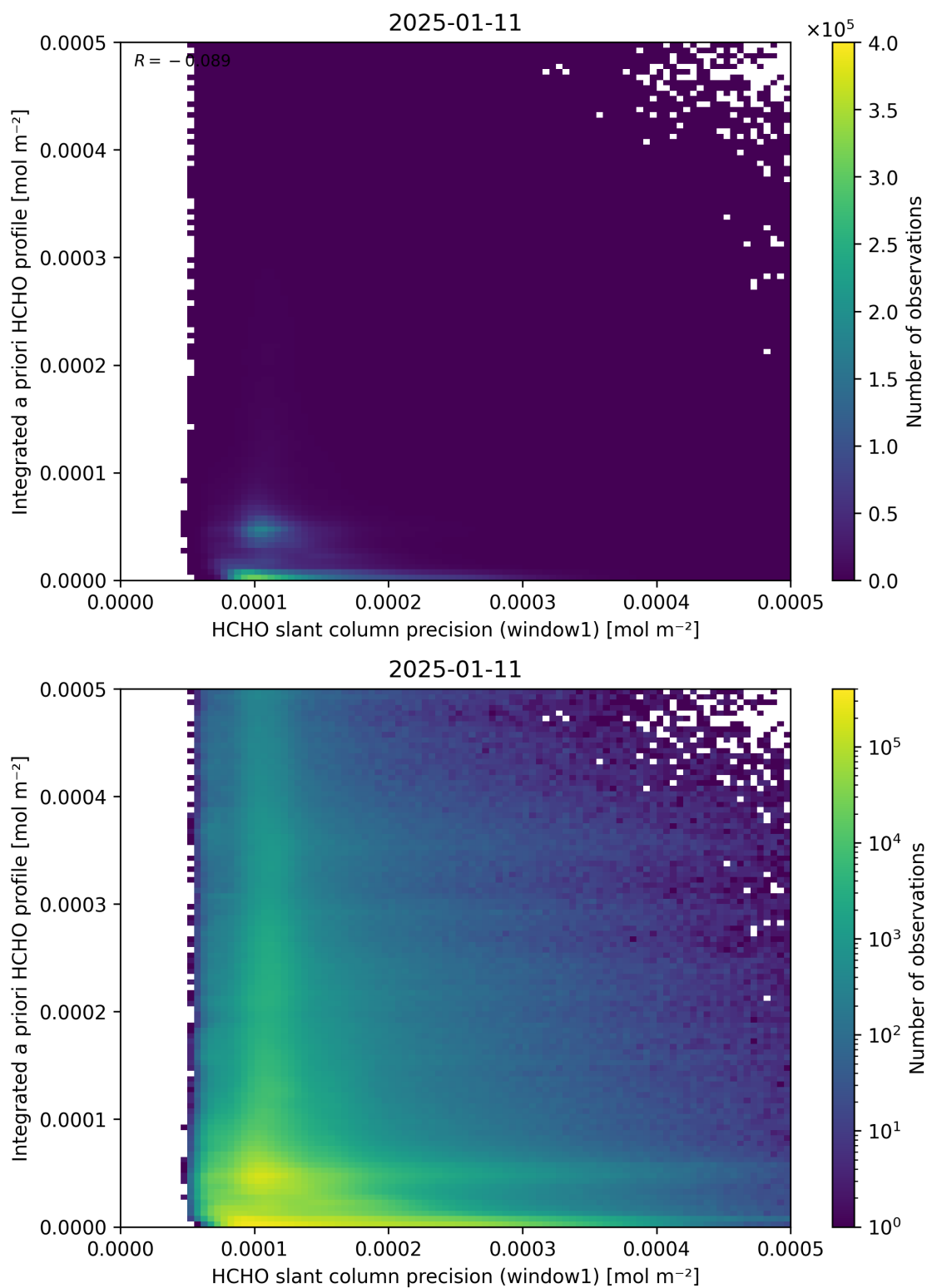
Figure 96: Scatter density plot of “HCHO slant column precision (window1)” against “Integrated a priori HCHO profile” for 2025-01-10 to 2025-01-12.
