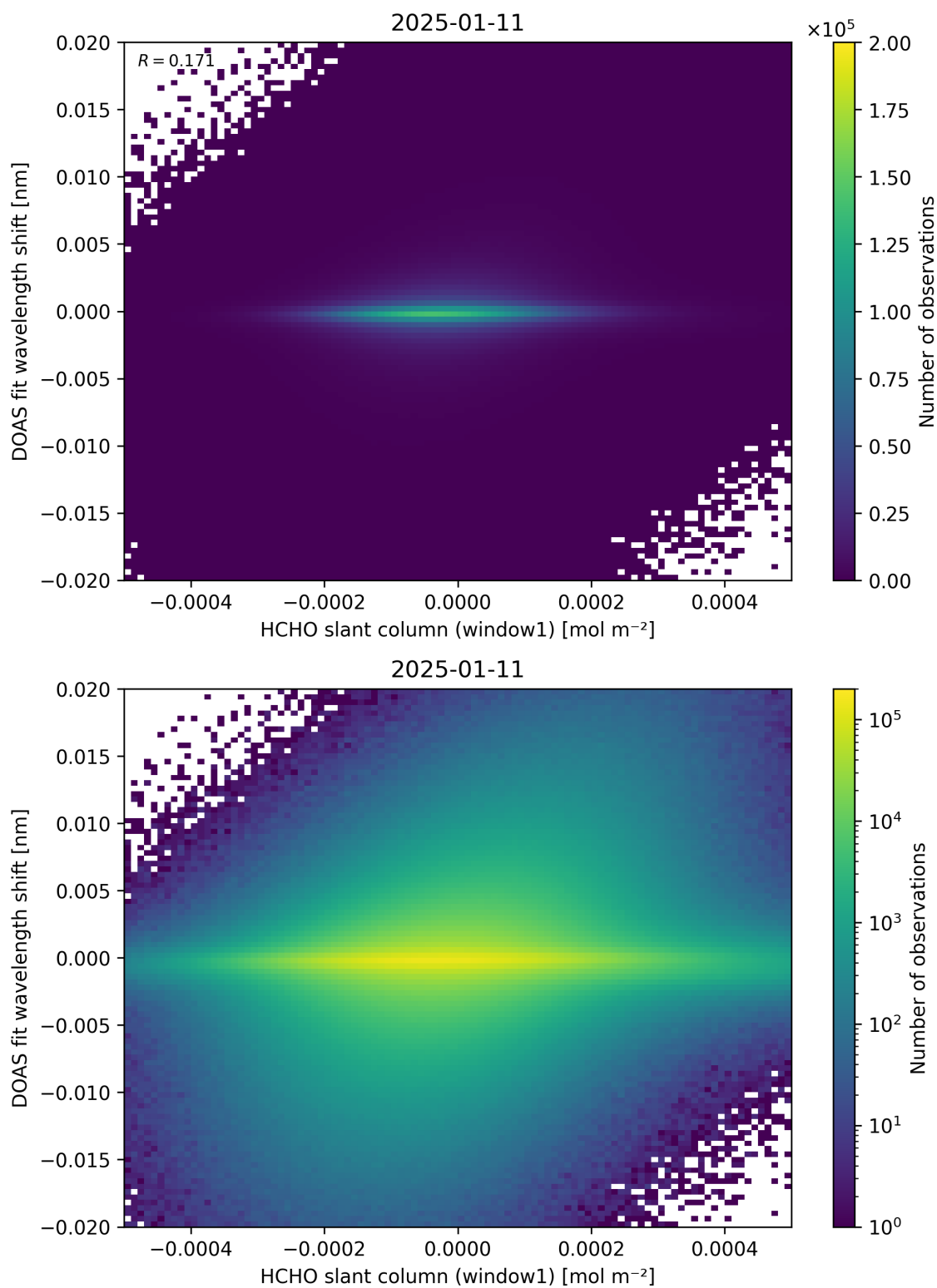
Figure 79: Scatter density plot of “HCHO slant column (window1)” against “DOAS fit wavelength shift” for 2025-01-10 to 2025-01-12.
