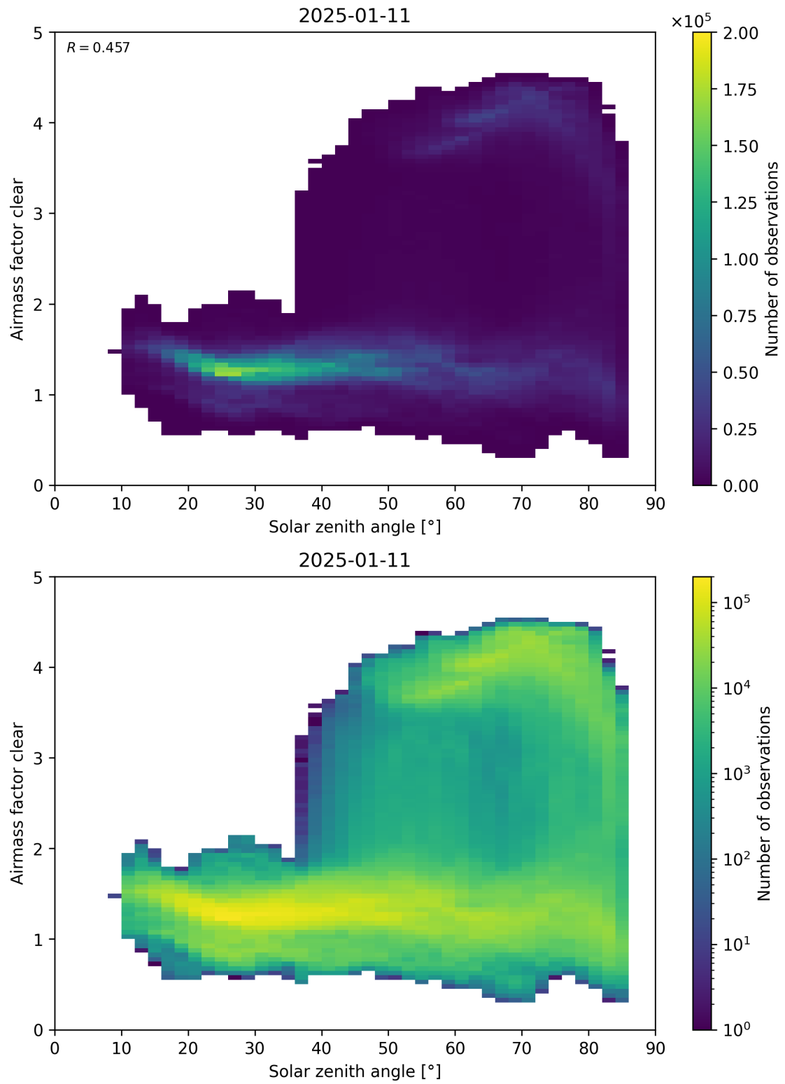
Figure 170: Scatter density plot of “Solar zenith angle” against “Airmass factor clear” for 2025-01-10 to 2025-01-12.
