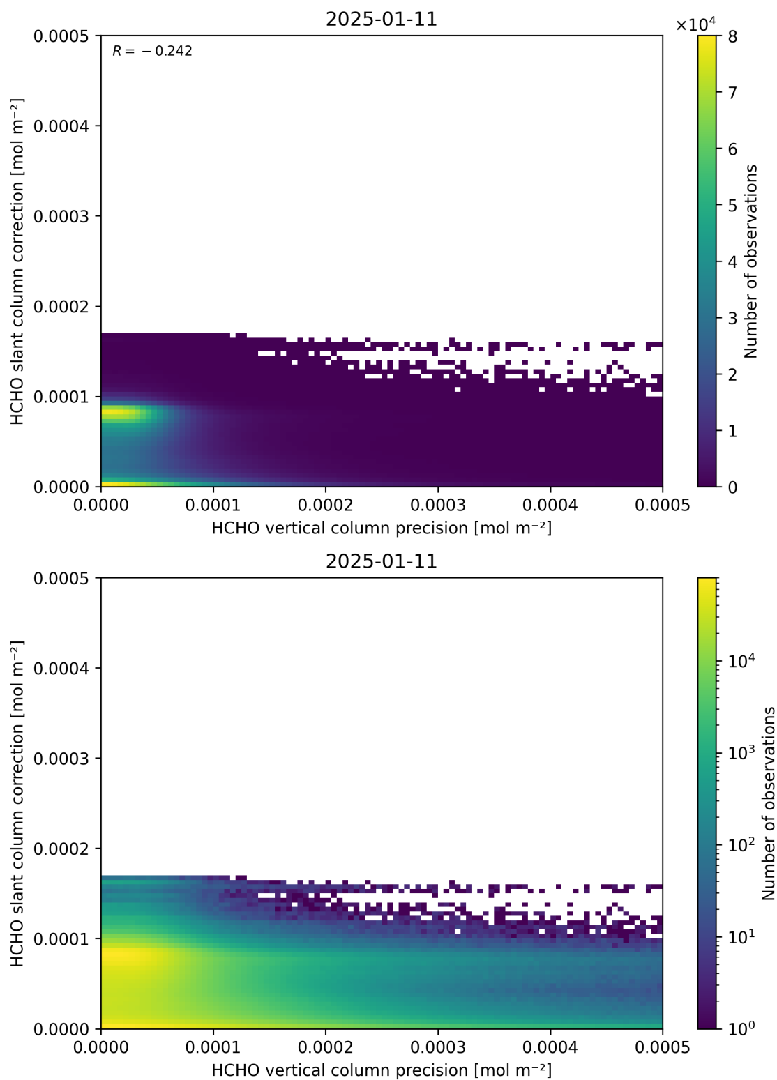
Figure 141: Scatter density plot of “HCHO vertical column precision” against “HCHO slant column correction” for 2025-01-10 to 2025-01-12.
