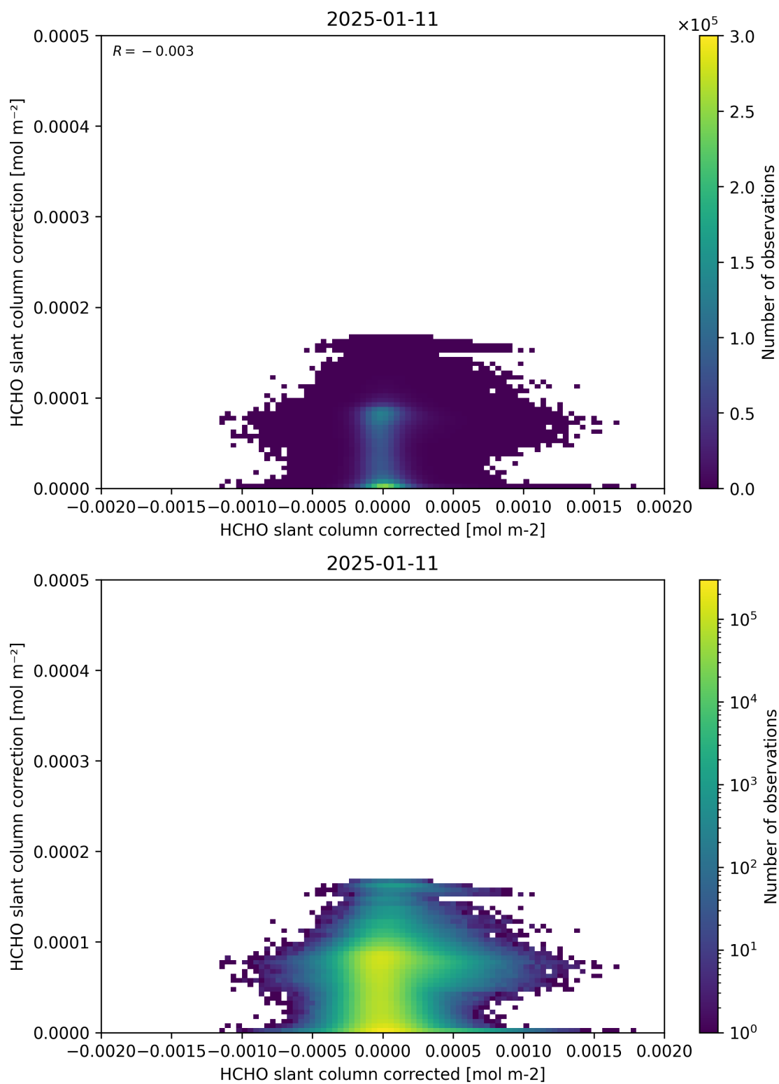
Figure 77: Scatter density plot of “HCHO slant column corrected” against “HCHO slant column correction” for 2025-01-10 to 2025-01-12.
