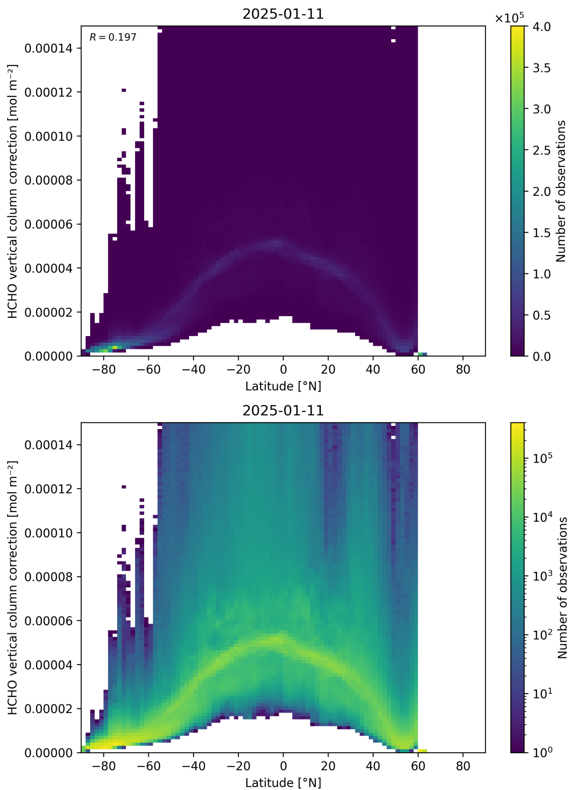
Figure 164: Scatter density plot of “Latitude” against “HCHO vertical column correction” for 2025-01-10 to 2025-01-12.
