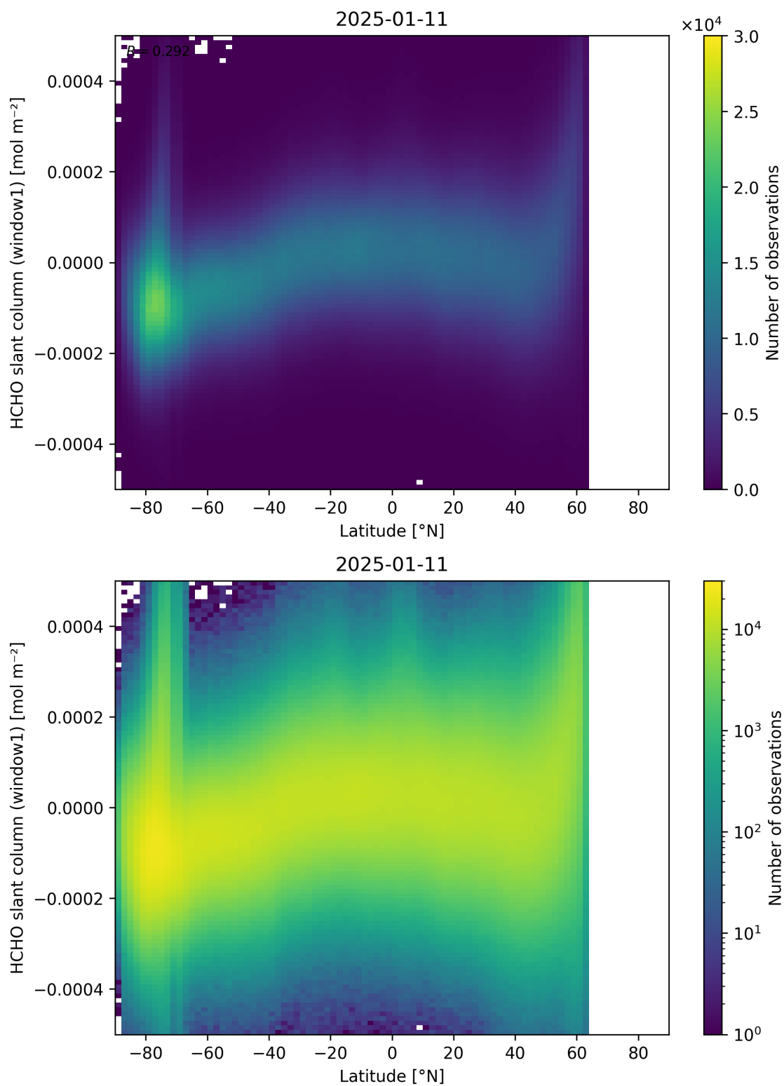
Figure 159: Scatter density plot of “Latitude” against “HCHO slant column (window1)” for 2025-01-10 to 2025-01-12.
