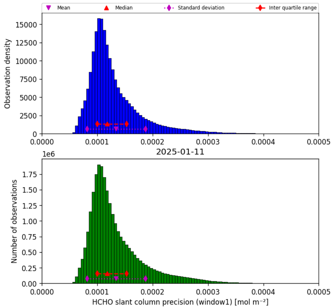
Figure 39: Histogram of “HCHO slant column precision (window1)” for 2025-01-10 to 2025-01-12
