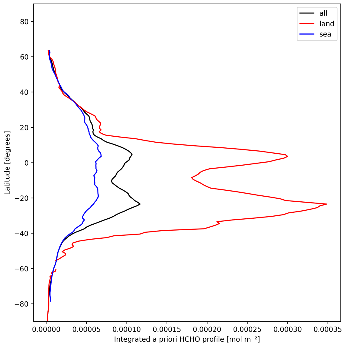
Figure 29: Zonal average of “Integrated a priori HCHO profile” for 2025-01-10 to 2025-01-12.
