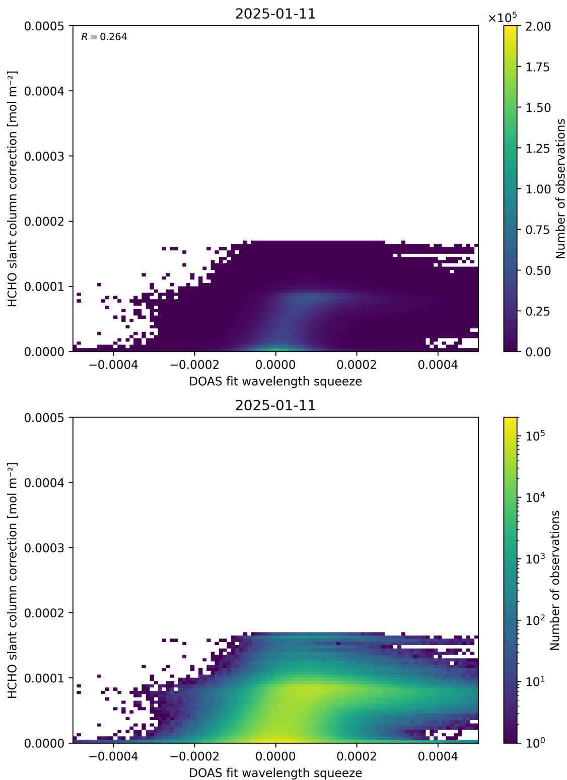
Figure 70: Scatter density plot of “DOAS fit wavelength squeeze” against “HCHO slant column correction” for 2025-01-10 to 2025-01-12.
