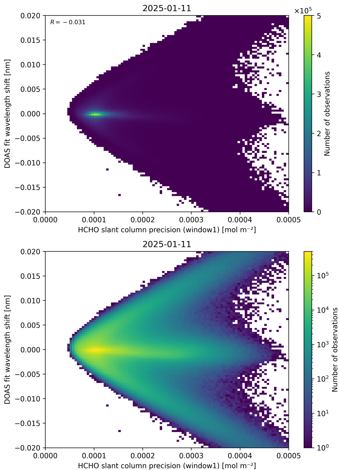
Figure 89: Scatter density plot of “HCHO slant column precision (window1)” against “DOAS fit wavelength shift” for 2025-01-10 to 2025-01-12.
