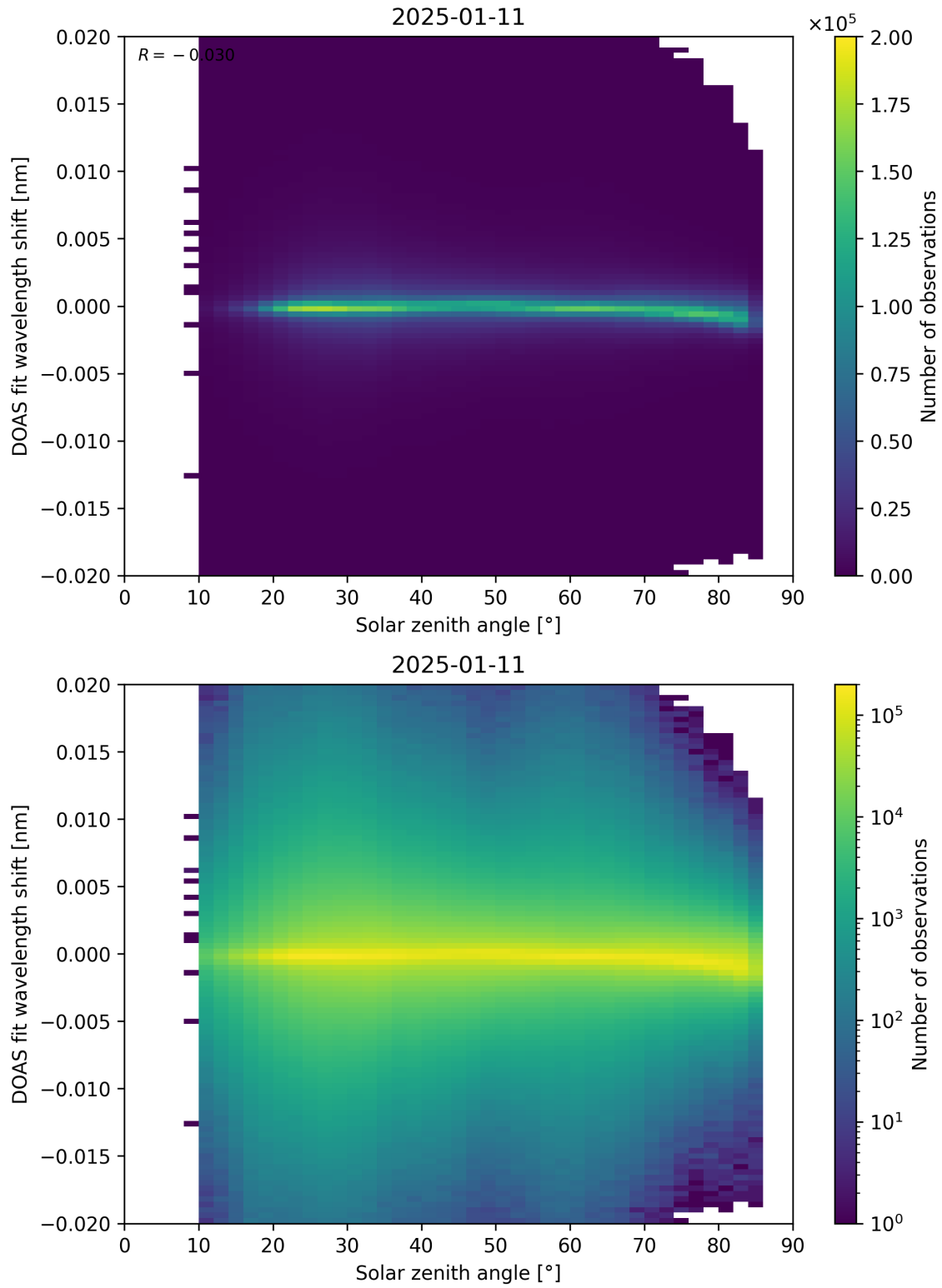
Figure 168: Scatter density plot of “Solar zenith angle” against “DOAS fit wavelength shift” for 2025-01-10 to 2025-01-12.
