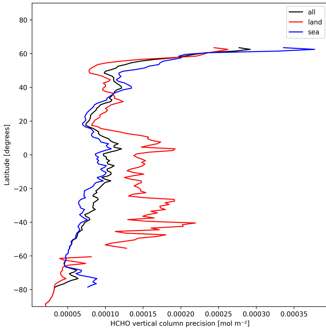
Figure 22: Zonal average of “HCHO vertical column precision” for 2025-01-10 to 2025-01-12.
