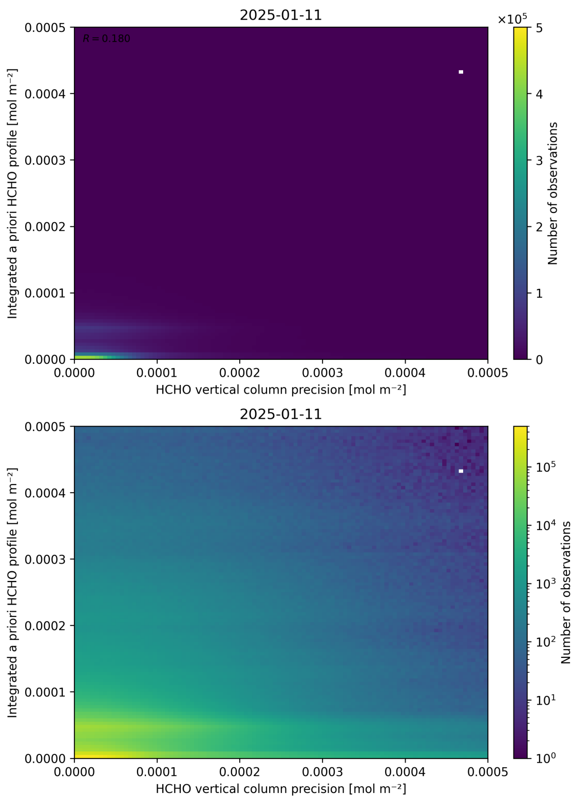
Figure 147: Scatter density plot of “HCHO vertical column precision” against “Integrated a priori HCHO profile” for 2025-01-10 to 2025-01-12.
