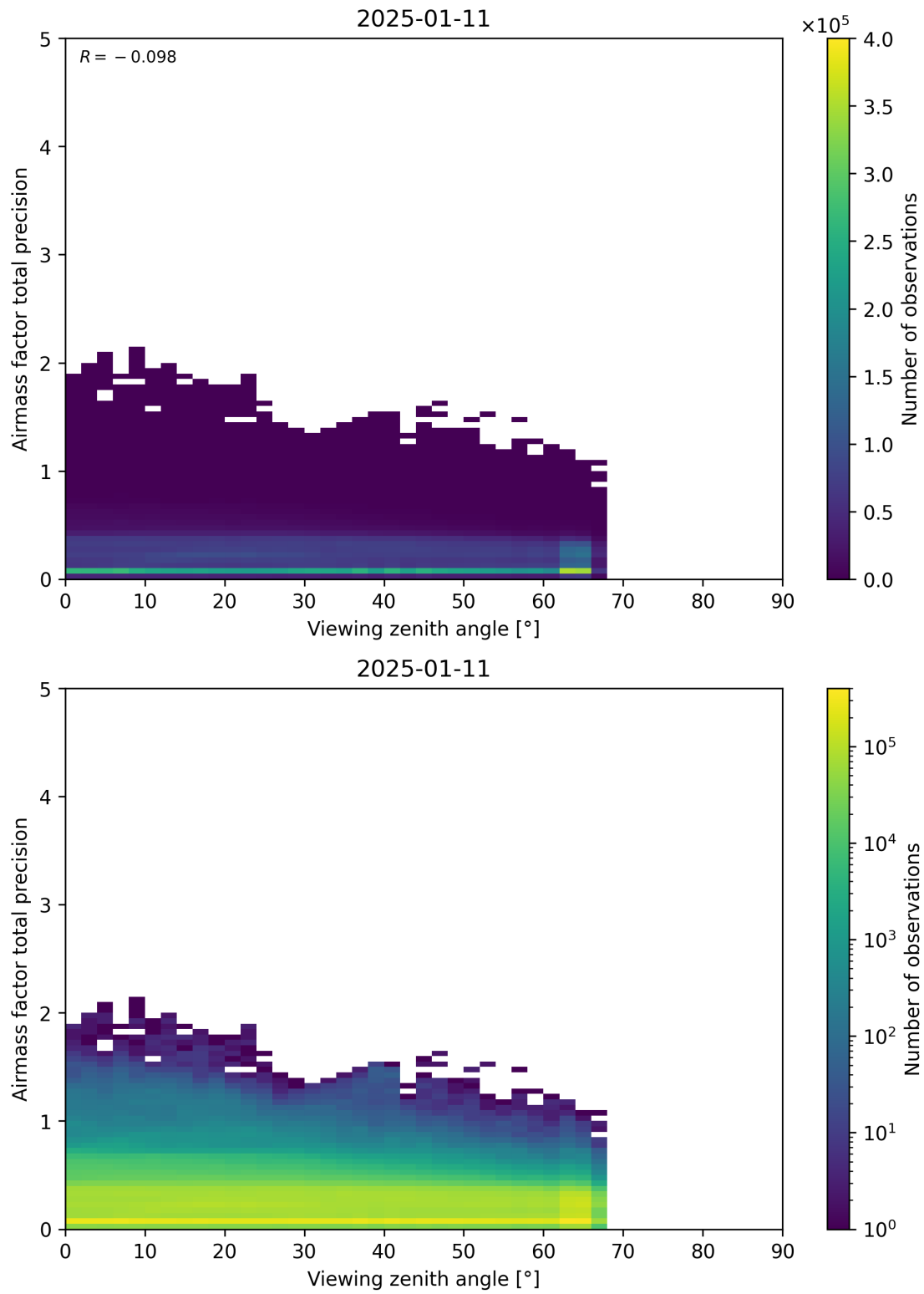
Figure 191: Scatter density plot of “Viewing zenith angle” against “Airmass factor total precision” for 2025-01-10 to 2025-01-12.
