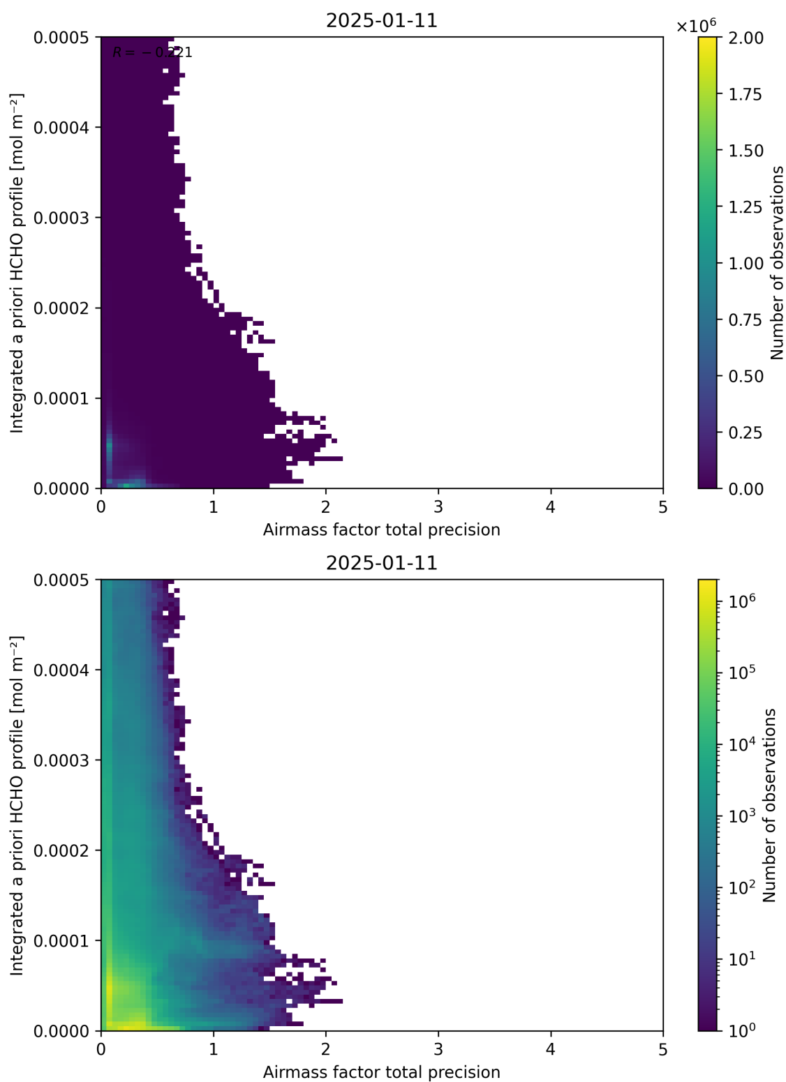
Figure 111: Scatter density plot of “Airmass factor total precision” against “Integrated a priori HCHO profile” for 2025-01-10 to 2025-01-12.
