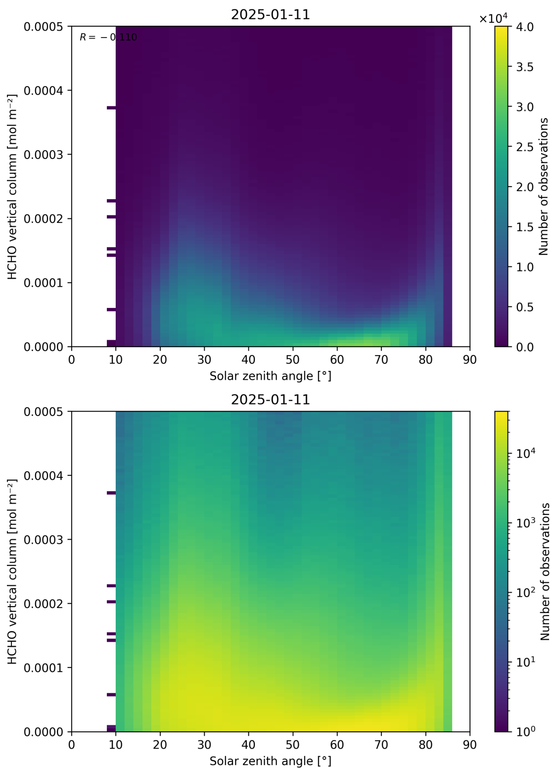
Figure 177: Scatter density plot of “Solar zenith angle” against “HCHO vertical column” for 2025-01-10 to 2025-01-12.
