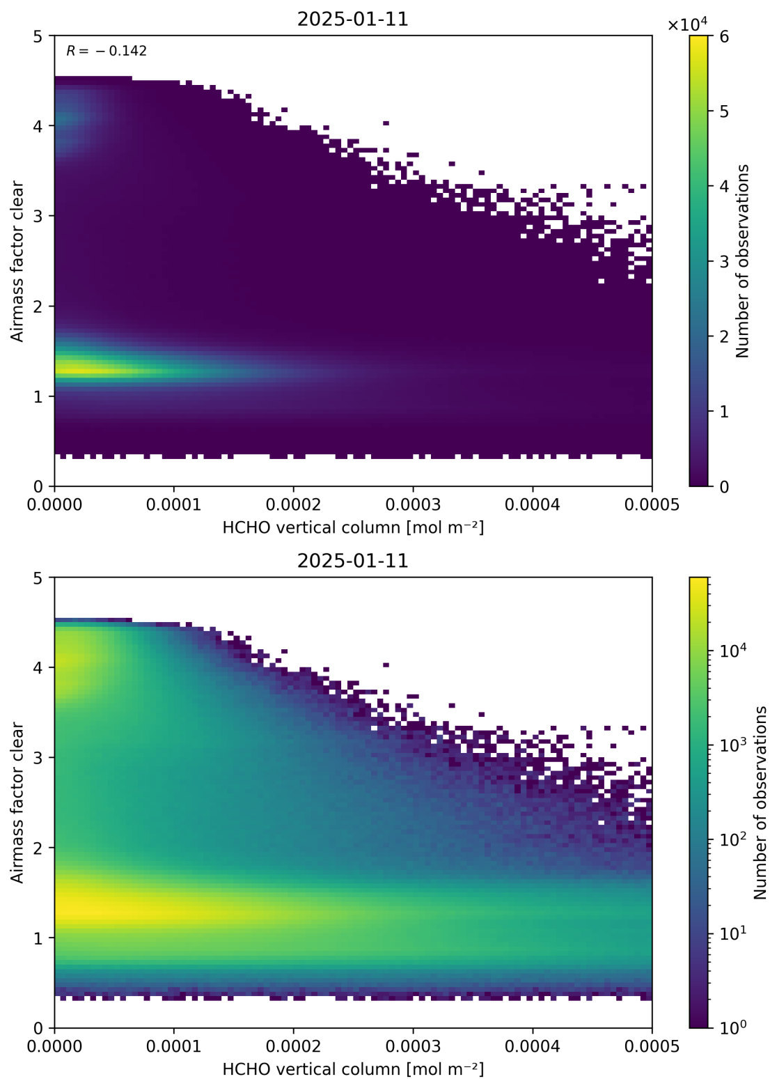
Figure 126: Scatter density plot of “HCHO vertical column” against “Airmass factor clear” for 2025-01-10 to 2025-01-12.
