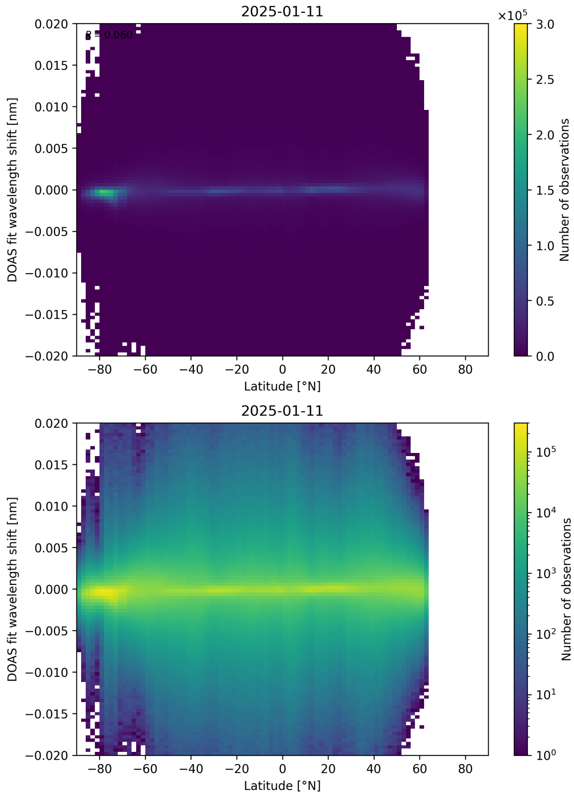
Figure 154: Scatter density plot of “Latitude” against “DOAS fit wavelength shift” for 2025-01-10 to 2025-01-12.
