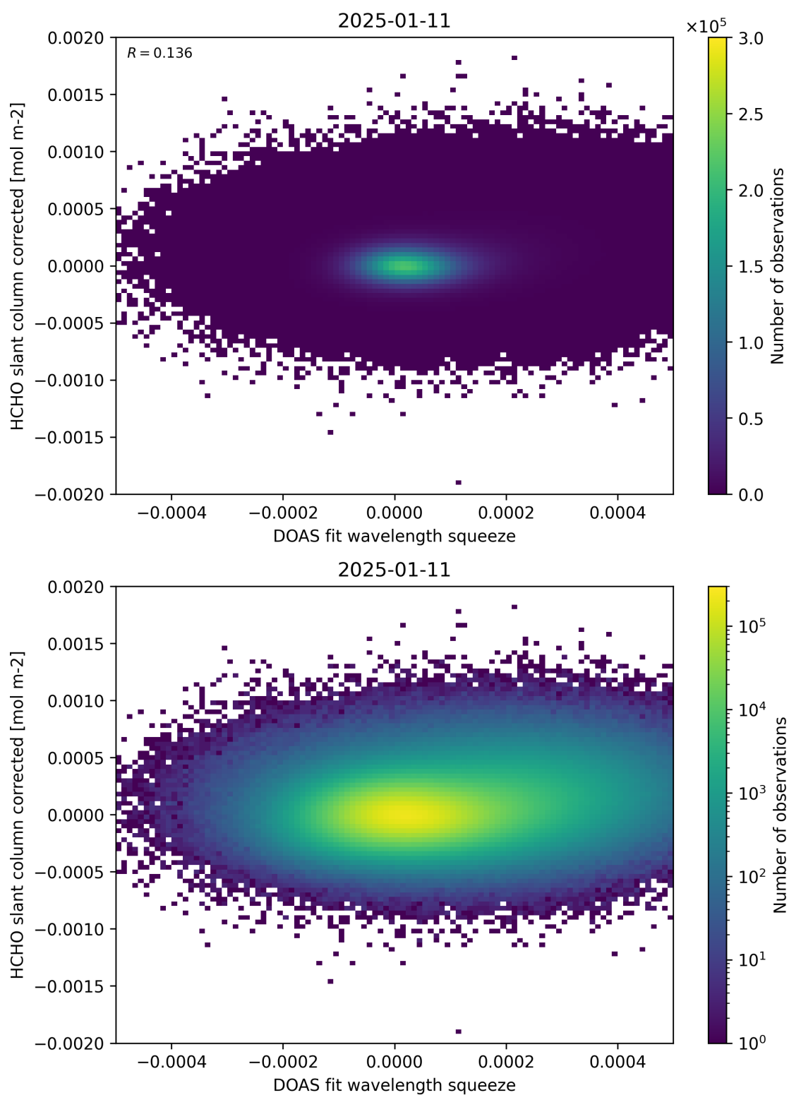
Figure 69: Scatter density plot of “DOAS fit wavelength squeeze” against “HCHO slant column corrected” for 2025-01-10 to 2025-01-12.
