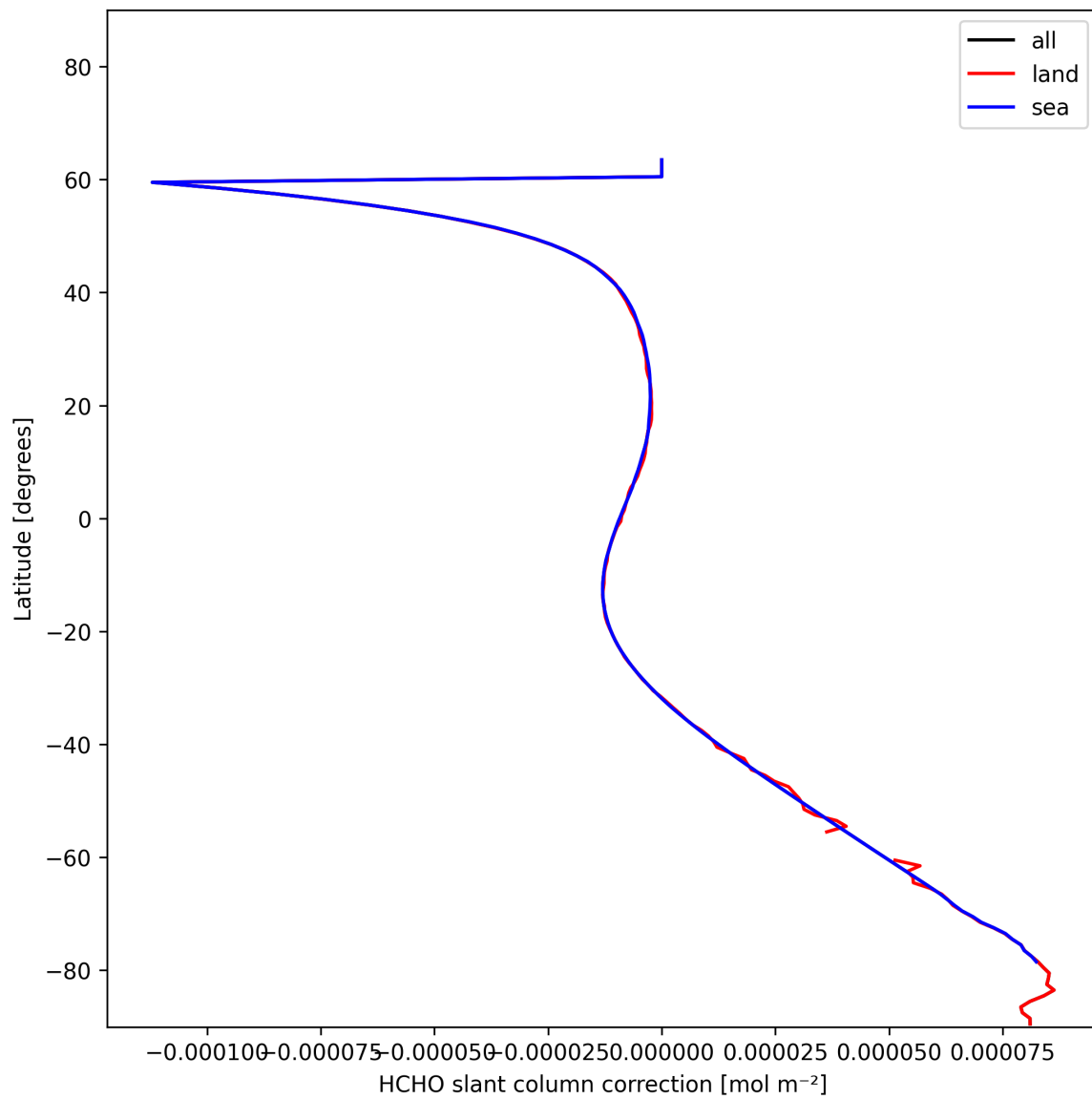
Figure 33: Zonal average of “HCHO slant column correction” for 2025-01-10 to 2025-01-12.
