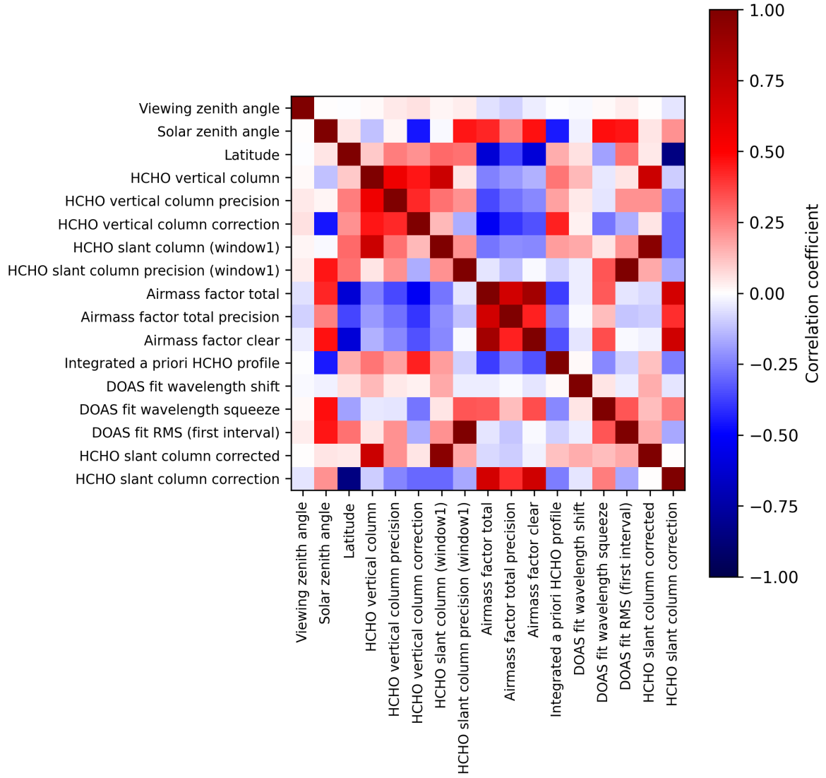
Figure 2: Map of correlation matrix for 2025-01-12 to 2025-01-14.
