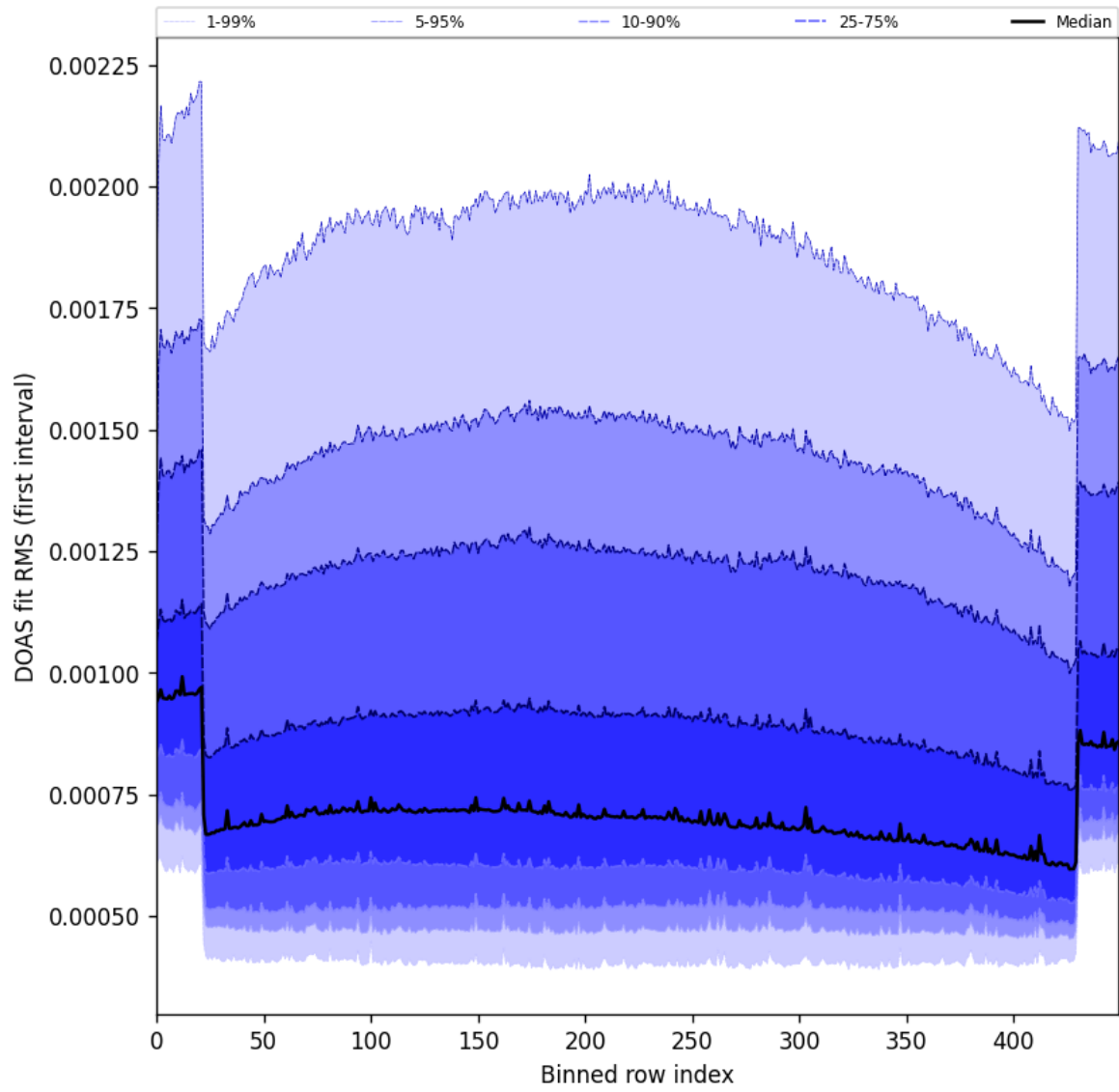
Figure 60: Along track statistics of “DOAS fit RMS (first interval)” for 2025-01-12 to 2025-01-14
