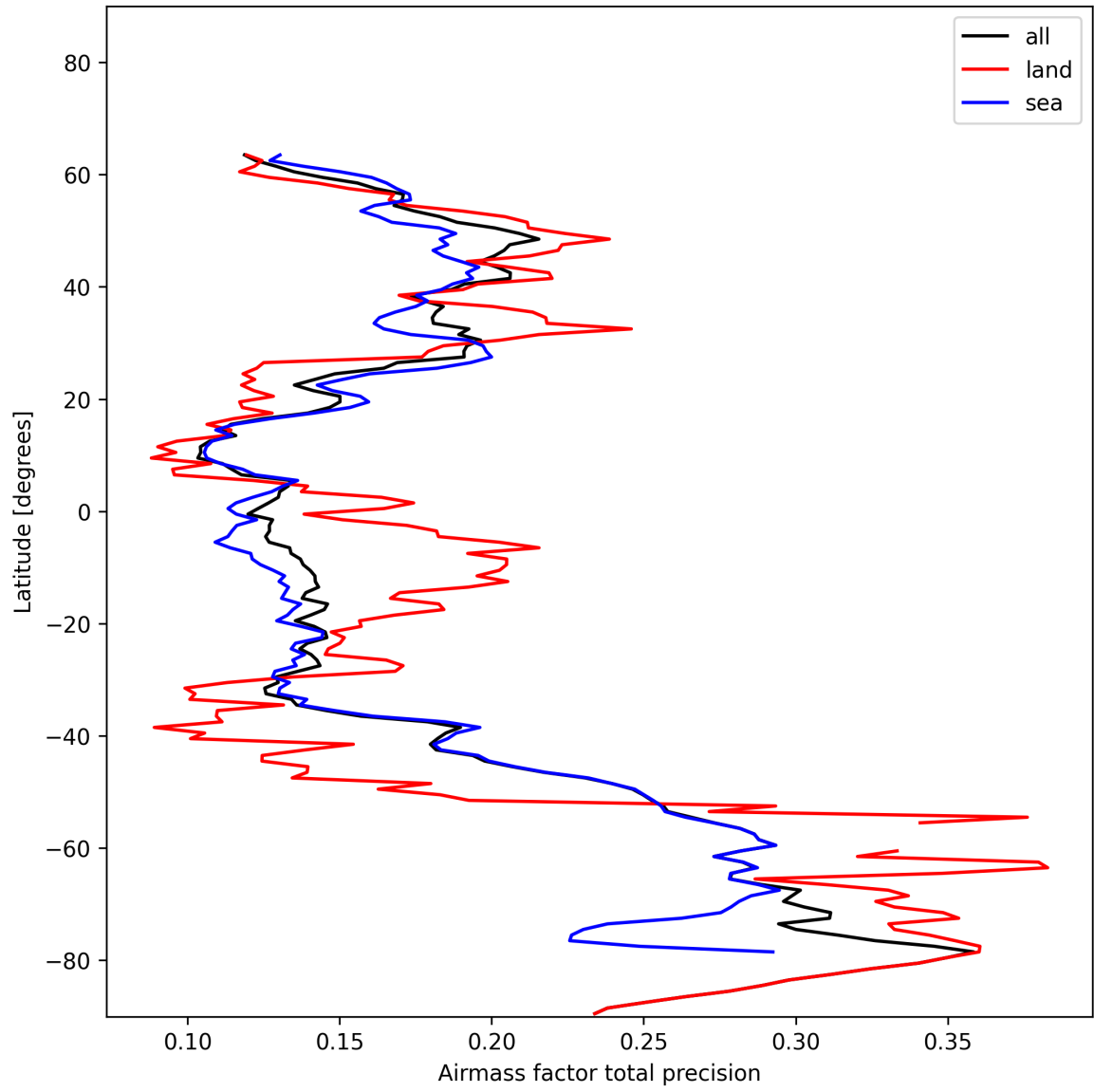
Figure 27: Zonal average of “Airmass factor total precision” for 2025-01-12 to 2025-01-14.
