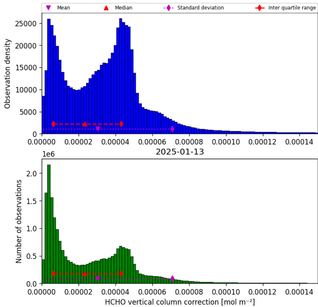
Figure 37: Histogram of “HCHO vertical column correction” for 2025-01-12 to 2025-01-14
