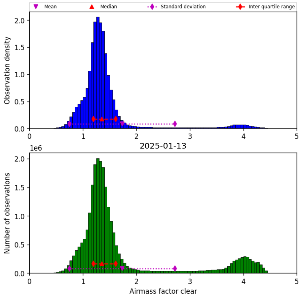
Figure 42: Histogram of “Airmass factor clear” for 2025-01-12 to 2025-01-14
