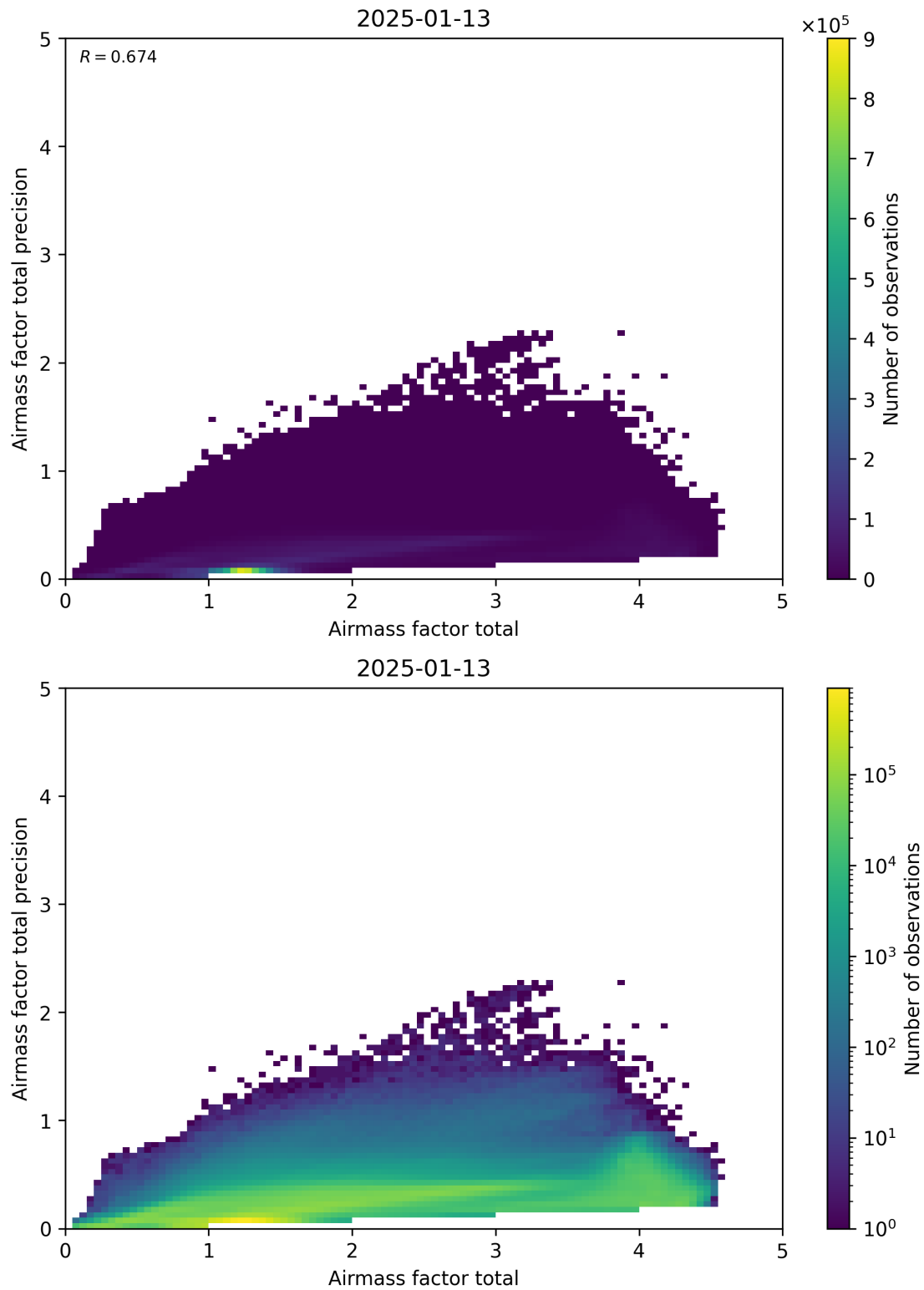
Figure 103: Scatter density plot of “Airmass factor total” against “Airmass factor total precision” for 2025-01-12 to 2025-01-14.
