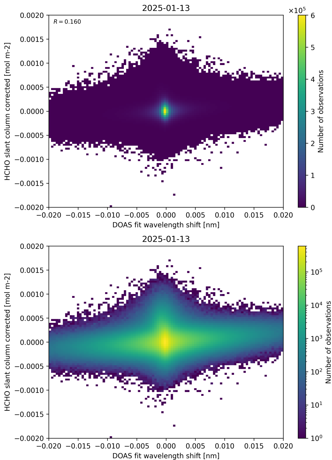
Figure 66: Scatter density plot of “DOAS fit wavelength shift” against “HCHO slant column corrected” for 2025-01-12 to 2025-01-14.
