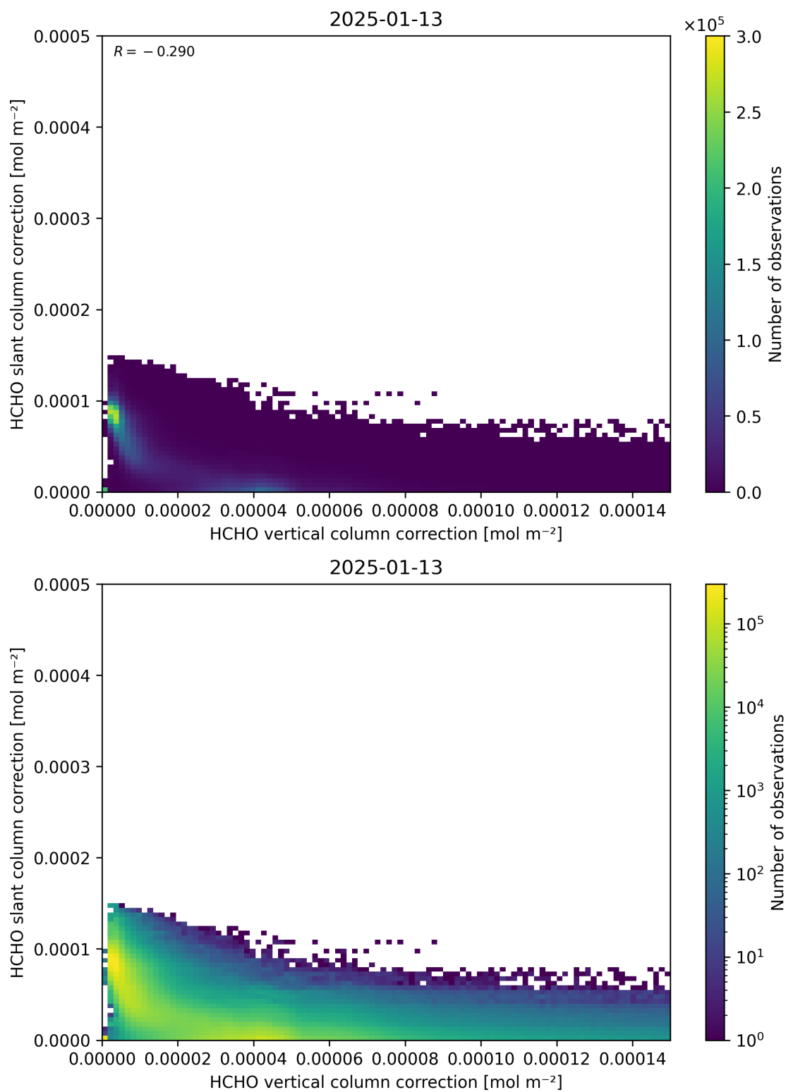
Figure 117: Scatter density plot of “HCHO vertical column correction” against “HCHO slant column correction” for 2025-01-12 to 2025-01-14.
