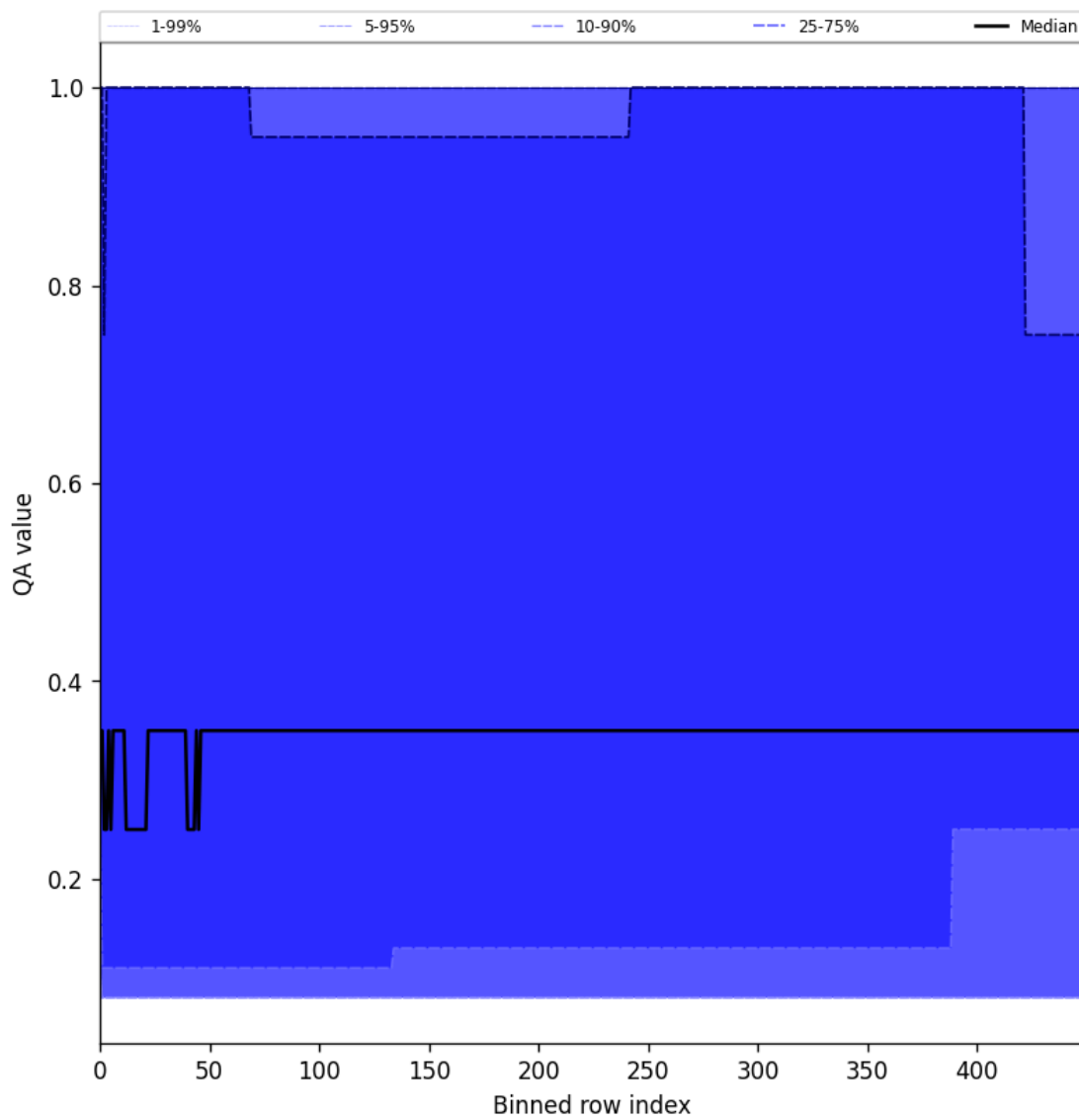
Figure 48: Along track statistics of “QA value” for 2025-01-12 to 2025-01-14
