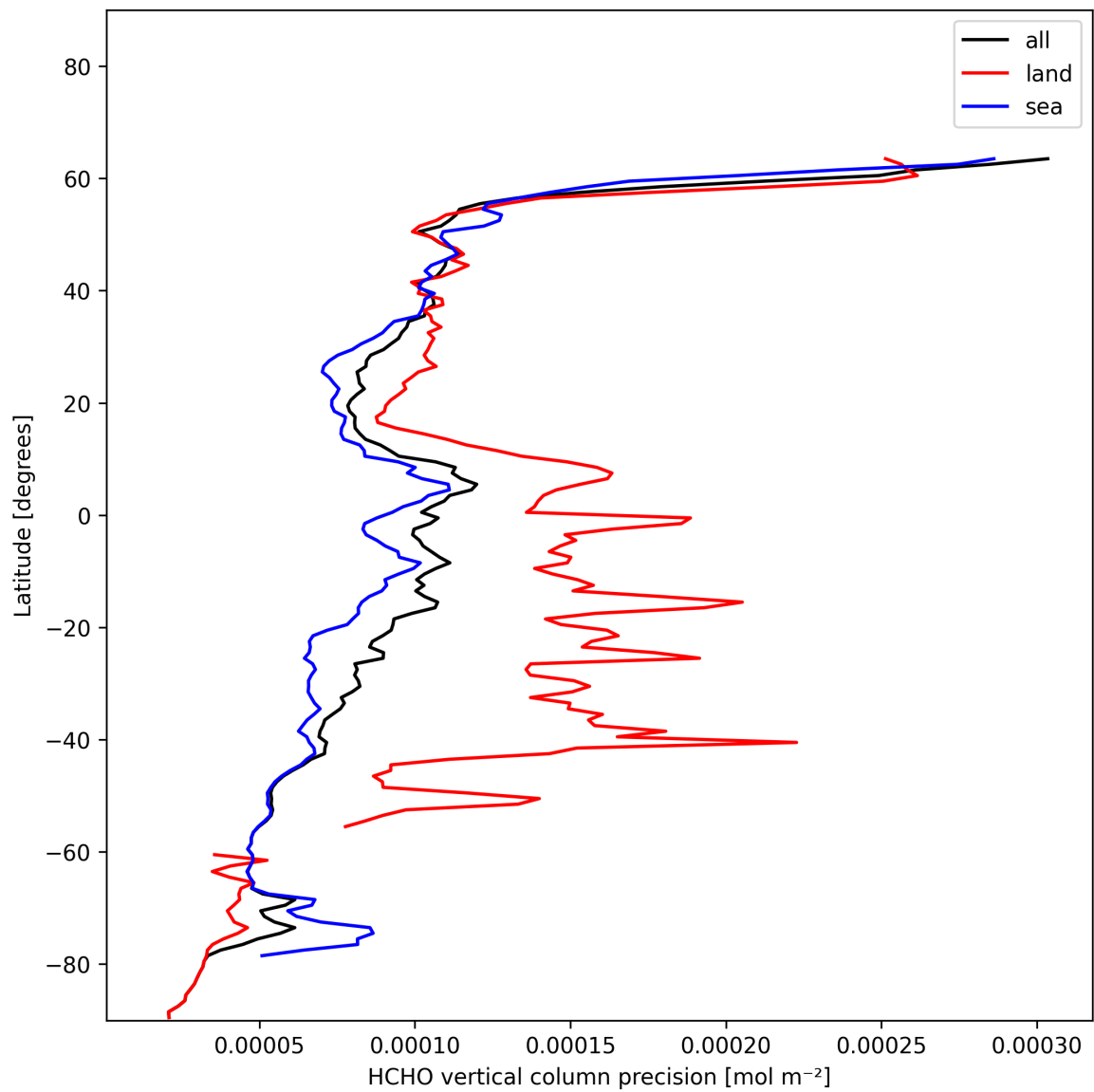
Figure 22: Zonal average of “HCHO vertical column precision” for 2025-01-12 to 2025-01-14.
