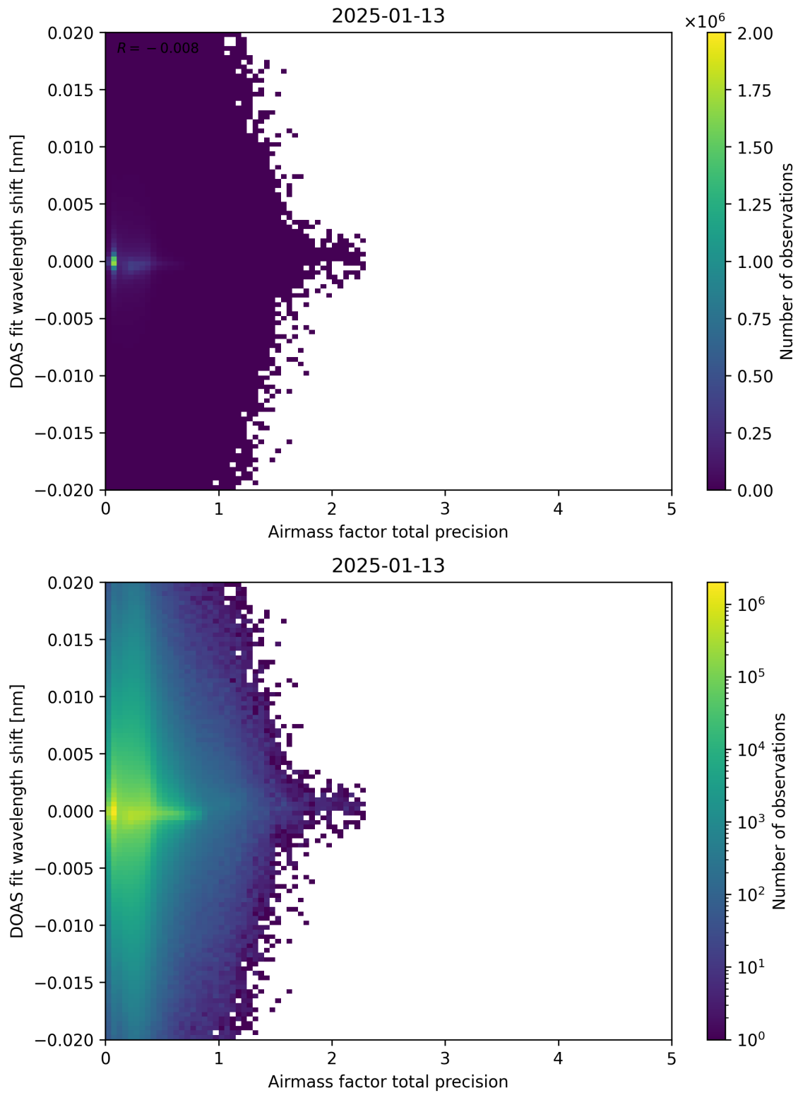
Figure 106: Scatter density plot of “Airmass factor total precision” against “DOAS fit wavelength shift” for 2025-01-12 to 2025-01-14.
