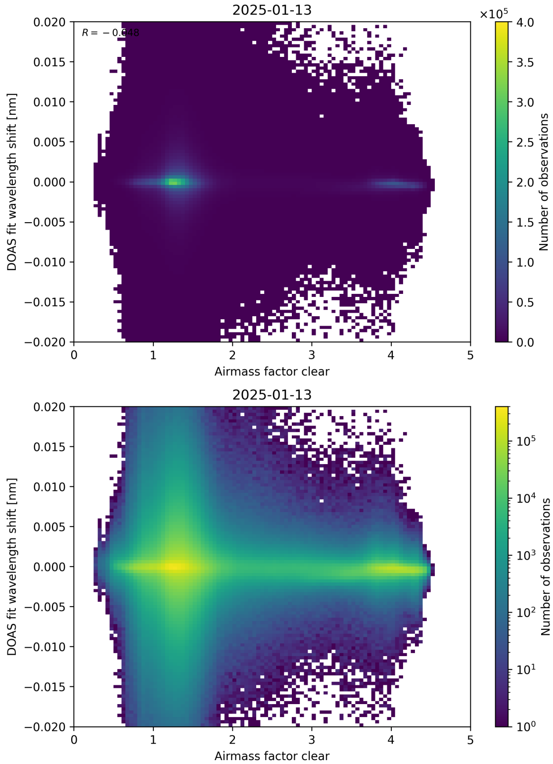
Figure 72: Scatter density plot of “Airmass factor clear” against “DOAS fit wavelength shift” for 2025-01-12 to 2025-01-14.
