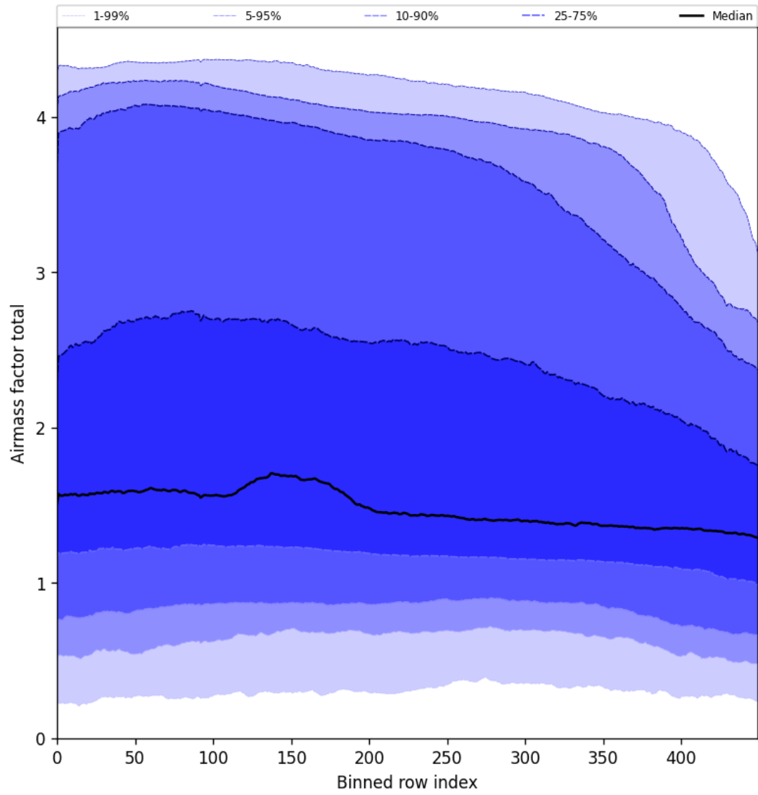
Figure 54: Along track statistics of “Airmass factor total” for 2025-01-12 to 2025-01-14
