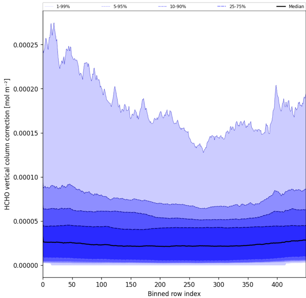
Figure 51: Along track statistics of “HCHO vertical column correction” for 2025-01-12 to 2025-01-14
