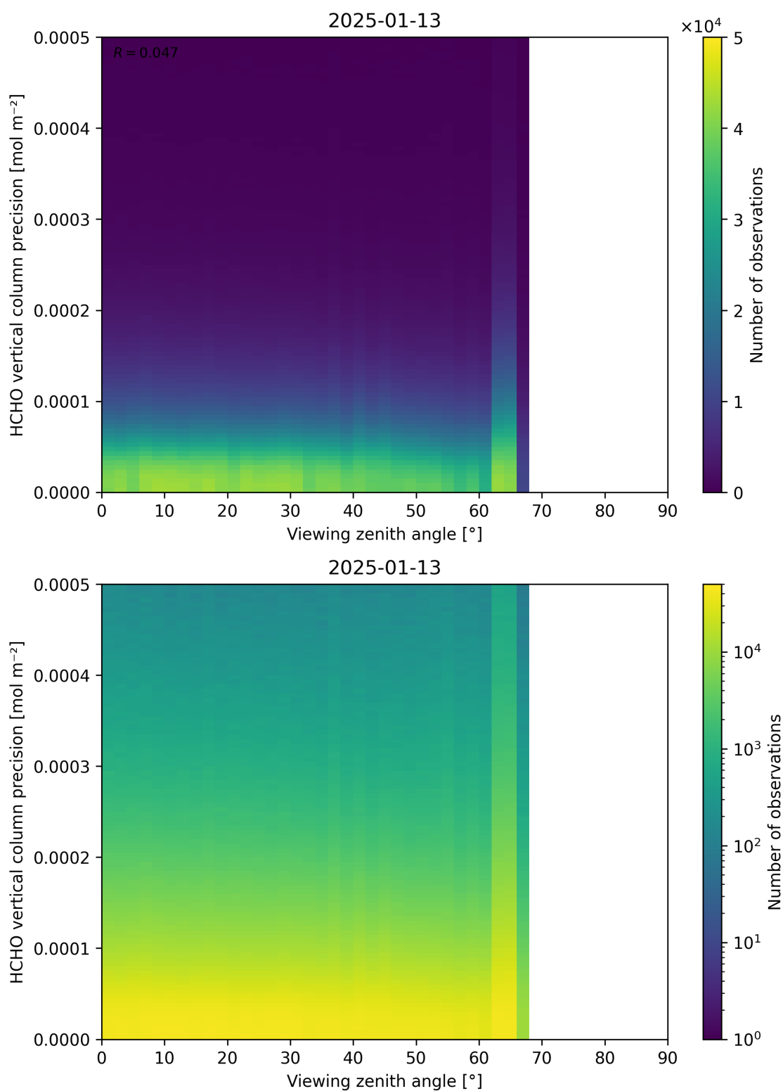
Figure 194: Scatter density plot of “Viewing zenith angle” against “HCHO vertical column precision” for 2025-01-12 to 2025-01-14.
