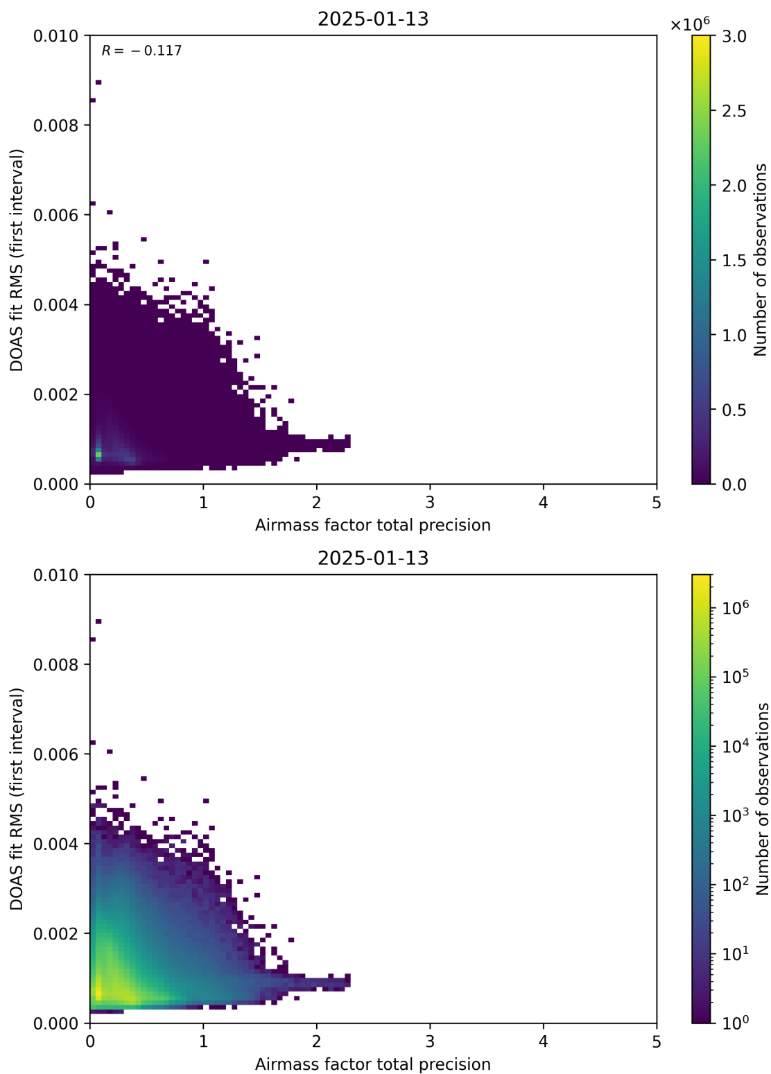
Figure 105: Scatter density plot of “Airmass factor total precision” against “DOAS fit RMS (first interval)” for 2025-01-12 to 2025-01-14.
