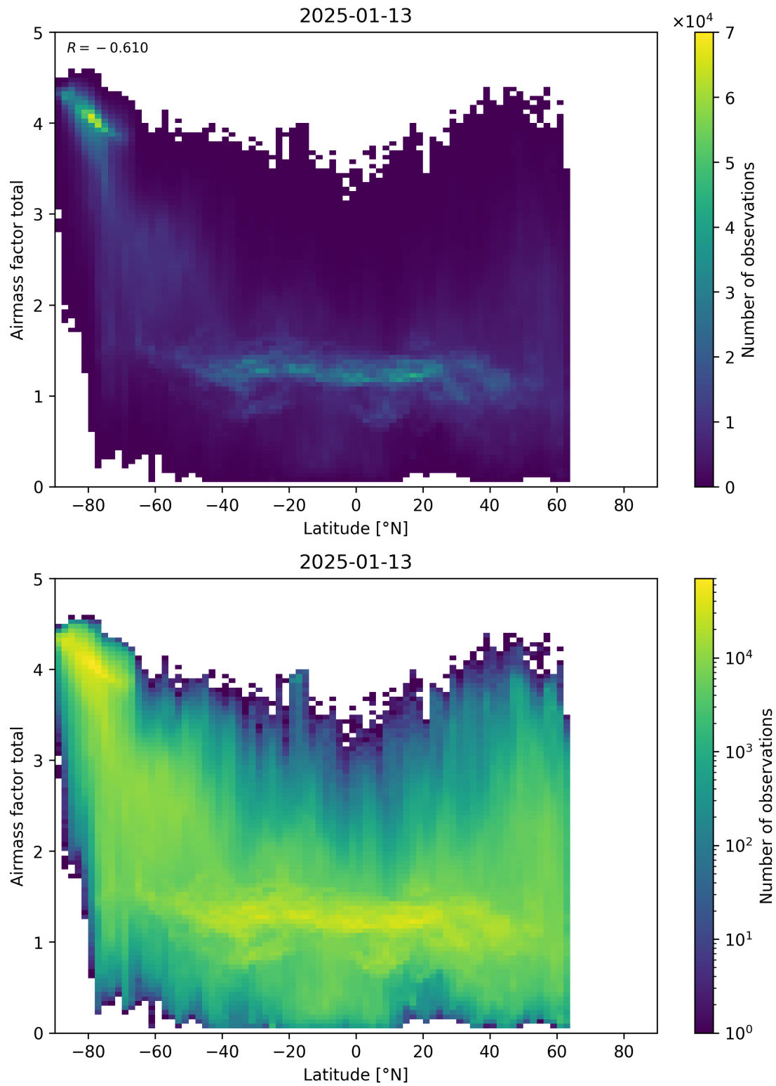
Figure 161: Scatter density plot of “Latitude” against “Airmass factor total” for 2025-01-12 to 2025-01-14.
