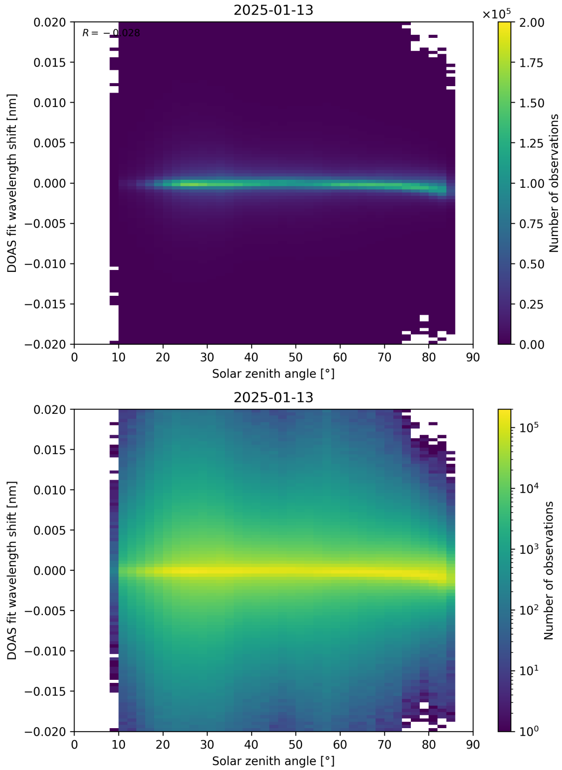
Figure 168: Scatter density plot of “Solar zenith angle” against “DOAS fit wavelength shift” for 2025-01-12 to 2025-01-14.
