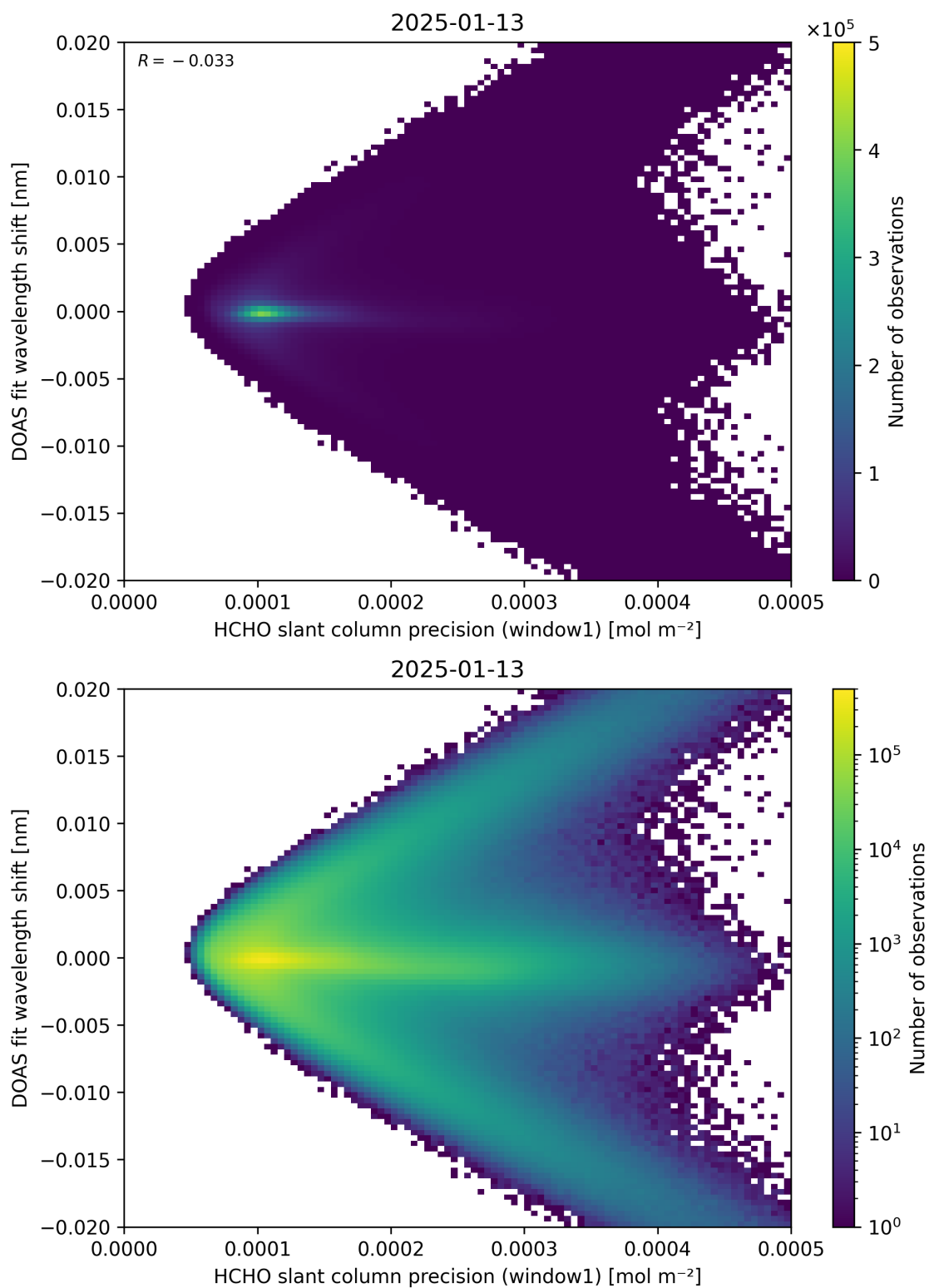
Figure 89: Scatter density plot of “HCHO slant column precision (window1)” against “DOAS fit wavelength shift” for 2025-01-12 to 2025-01-14.
