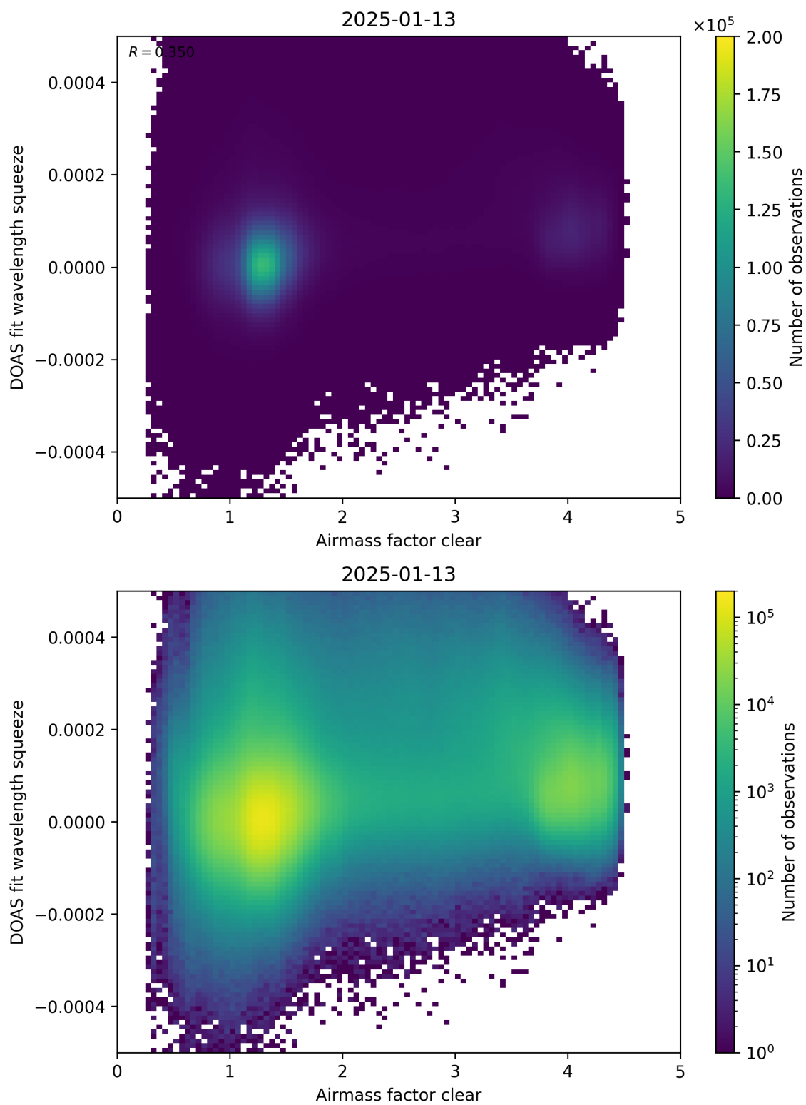
Figure 73: Scatter density plot of “Airmass factor clear” against “DOAS fit wavelength squeeze” for 2025-01-12 to 2025-01-14.
