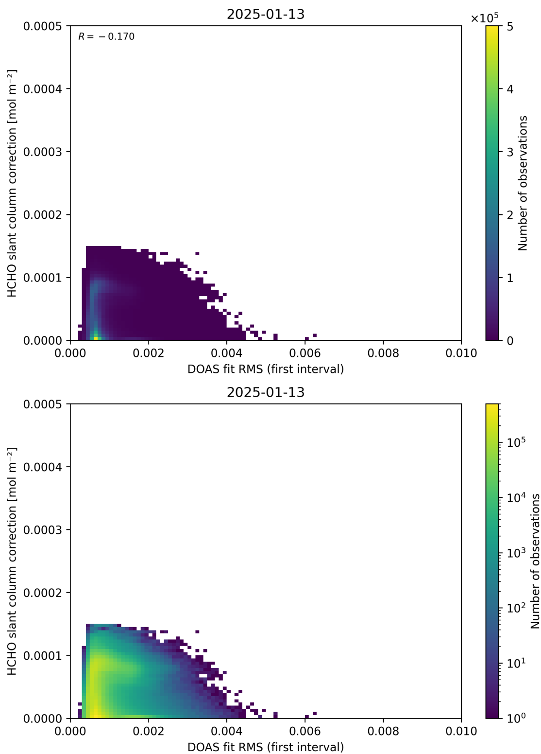
Figure 63: Scatter density plot of “DOAS fit RMS (first interval)” against “HCHO slant column correction” for 2025-01-12 to 2025-01-14.
