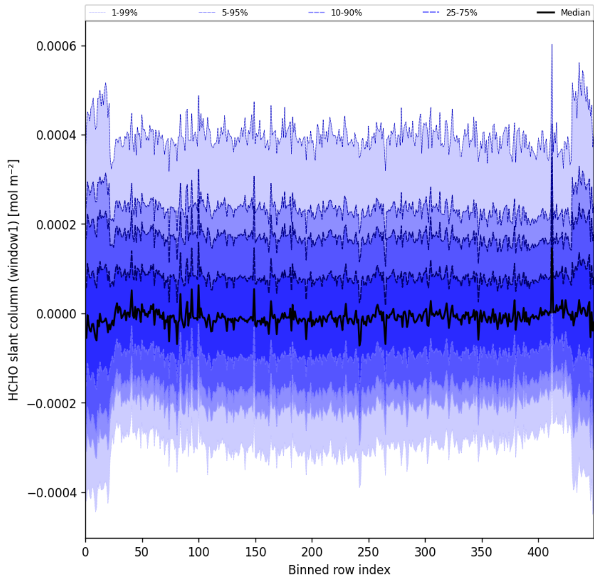
Figure 52: Along track statistics of “HCHO slant column (window1)” for 2025-01-12 to 2025-01-14
