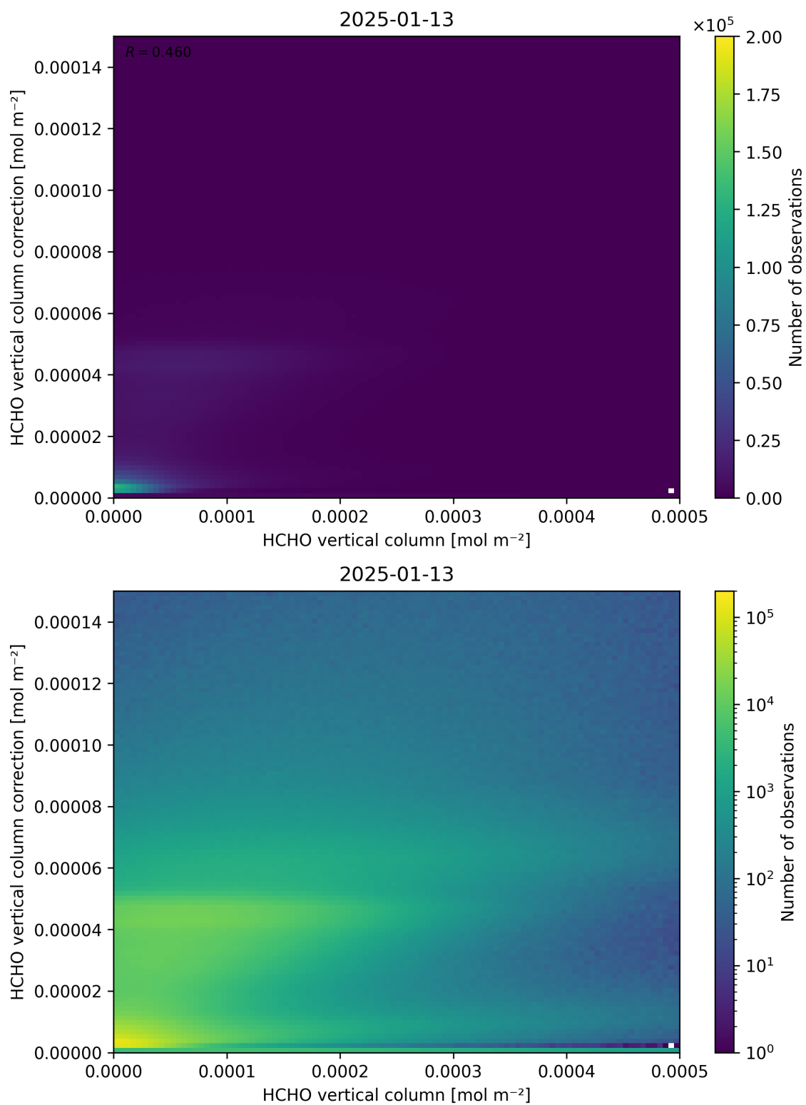
Figure 133: Scatter density plot of “HCHO vertical column” against “HCHO vertical column correction” for 2025-01-12 to 2025-01-14.
