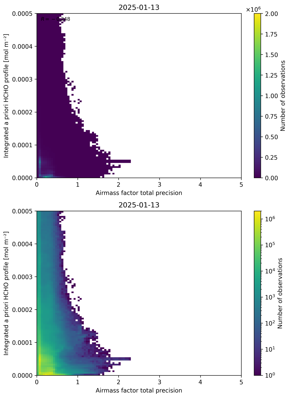
Figure 111: Scatter density plot of “Airmass factor total precision” against “Integrated a priori HCHO profile” for 2025-01-12 to 2025-01-14.
