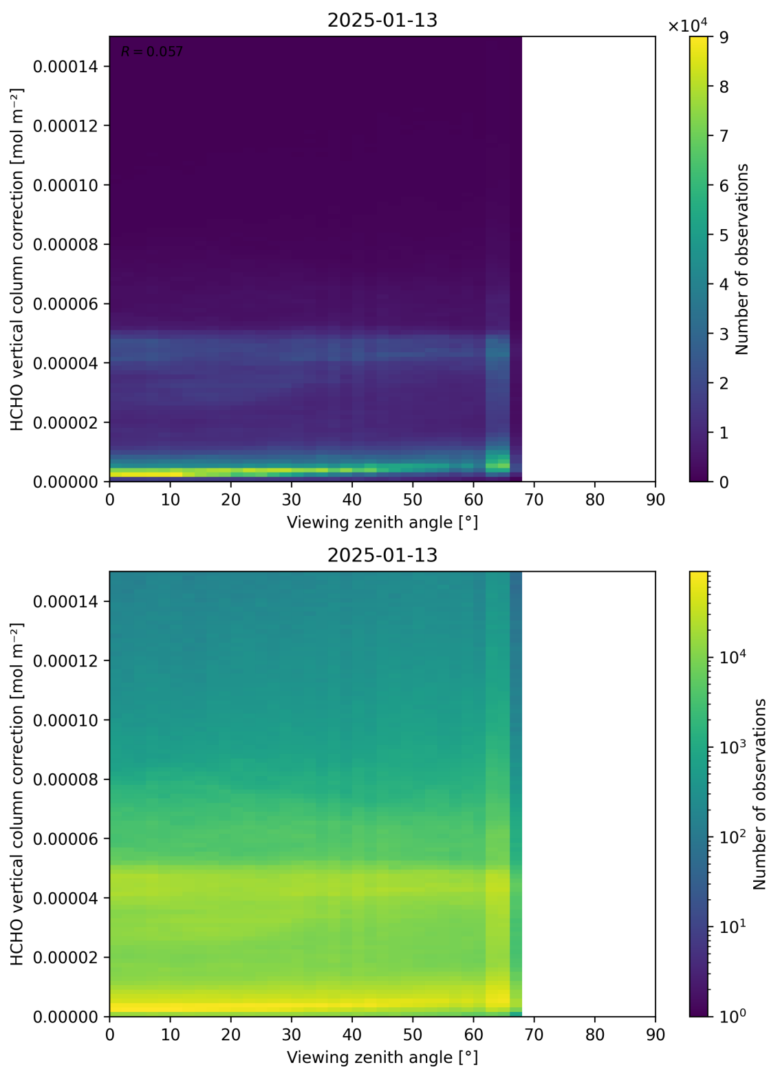
Figure 193: Scatter density plot of “Viewing zenith angle” against “HCHO vertical column correction” for 2025-01-12 to 2025-01-14.
