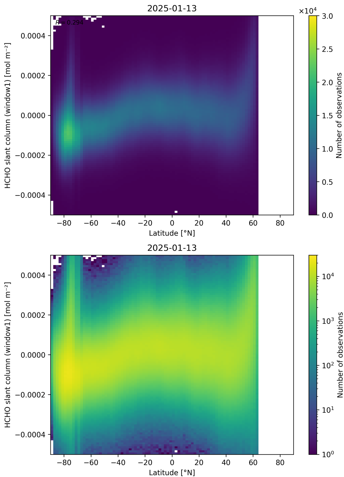
Figure 159: Scatter density plot of “Latitude” against “HCHO slant column (window1)” for 2025-01-12 to 2025-01-14.
