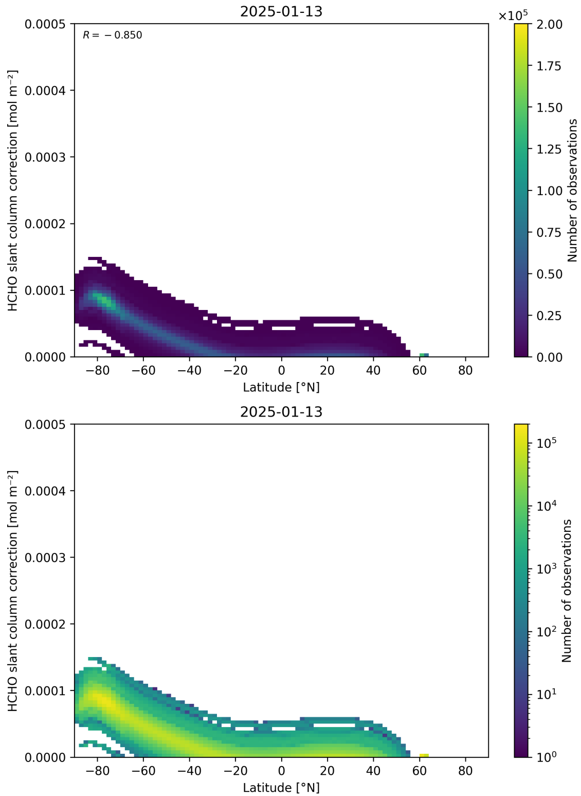
Figure 158: Scatter density plot of “Latitude” against “HCHO slant column correction” for 2025-01-12 to 2025-01-14.
