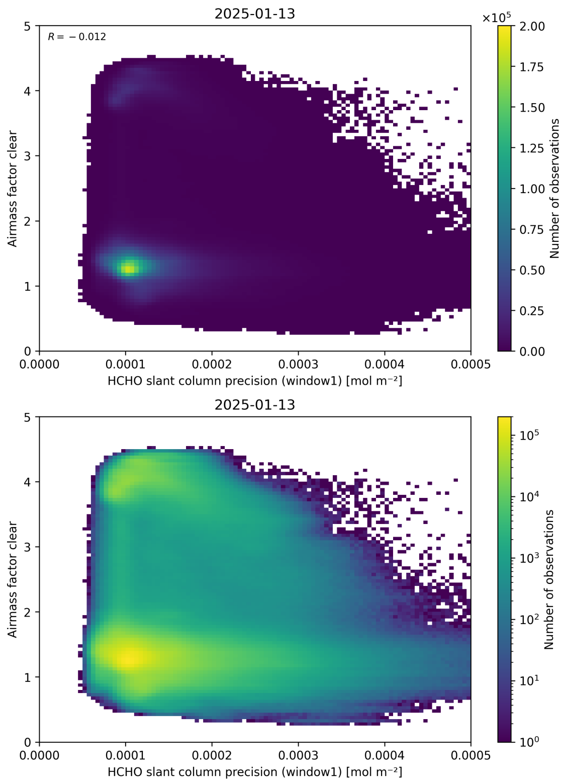
Figure 91: Scatter density plot of “HCHO slant column precision (window1)” against “Airmass factor clear” for 2025-01-12 to 2025-01-14.
