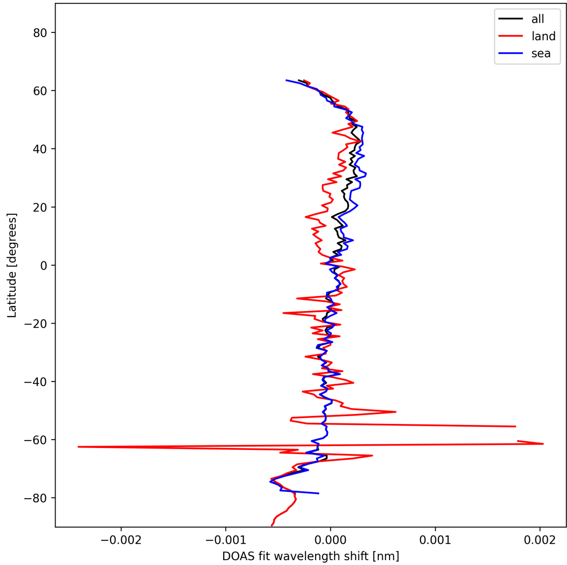
Figure 30: Zonal average of “DOAS fit wavelength shift” for 2025-01-12 to 2025-01-14.
