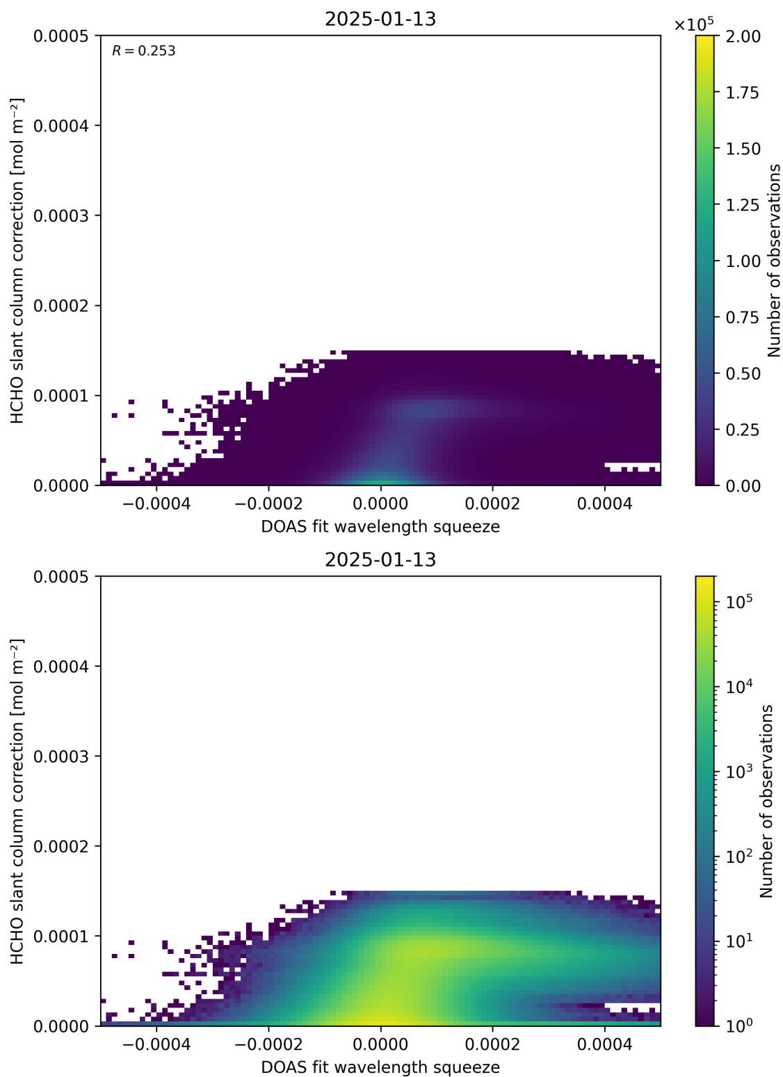
Figure 70: Scatter density plot of “DOAS fit wavelength squeeze” against “HCHO slant column correction” for 2025-01-12 to 2025-01-14.
