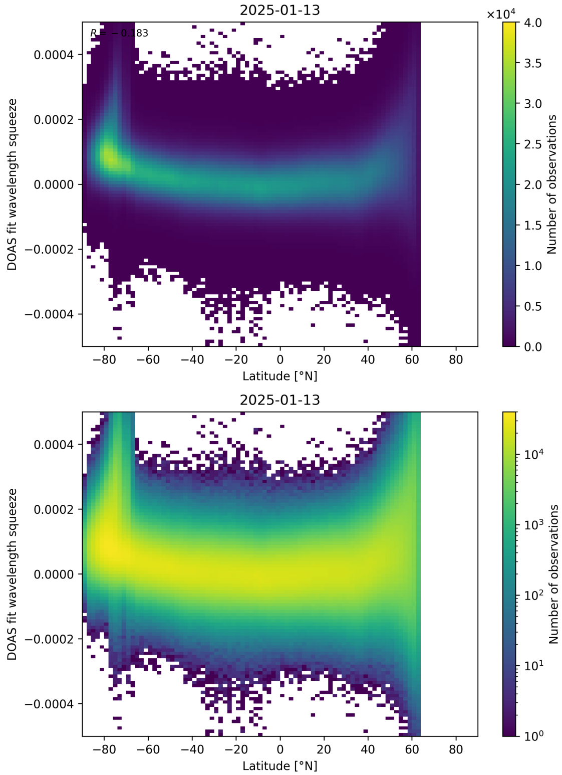
Figure 155: Scatter density plot of “Latitude” against “DOAS fit wavelength squeeze” for 2025-01-12 to 2025-01-14.
