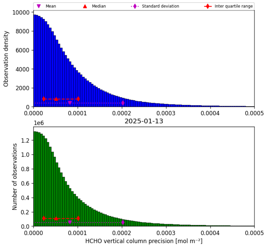
Figure 36: Histogram of “HCHO vertical column precision” for 2025-01-12 to 2025-01-14
