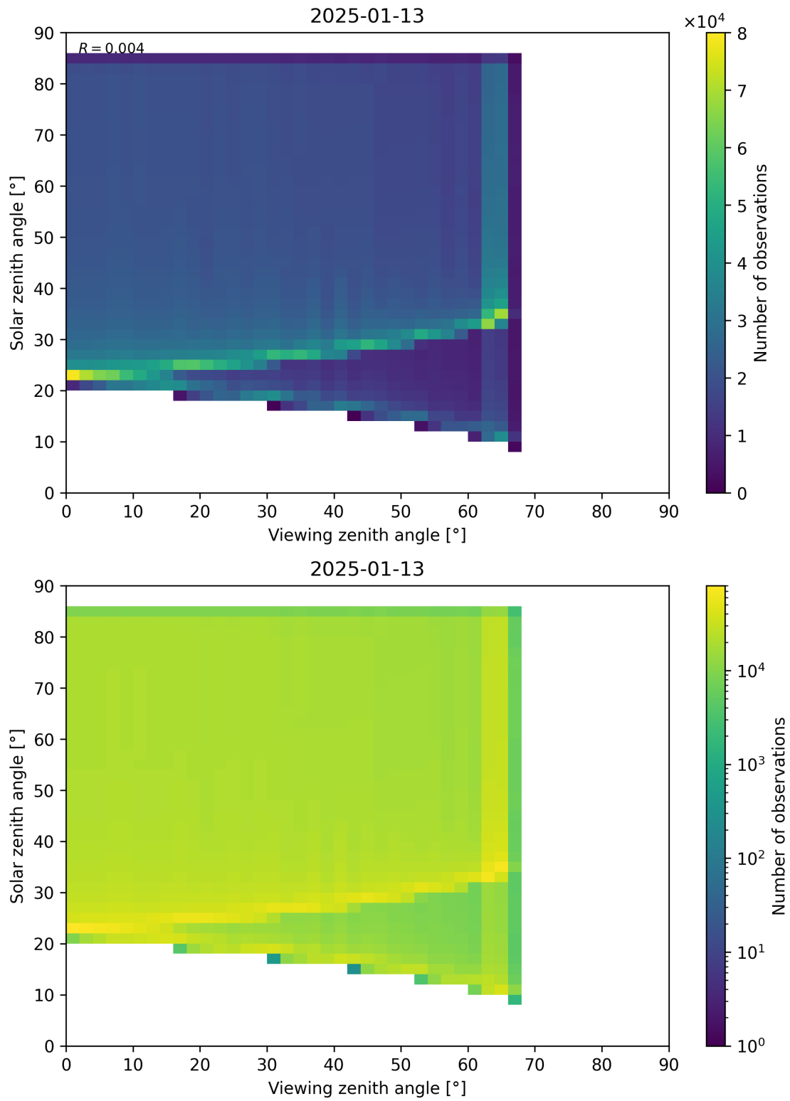
Figure 197: Scatter density plot of “Viewing zenith angle” against “Solar zenith angle” for 2025-01-12 to 2025-01-14.
