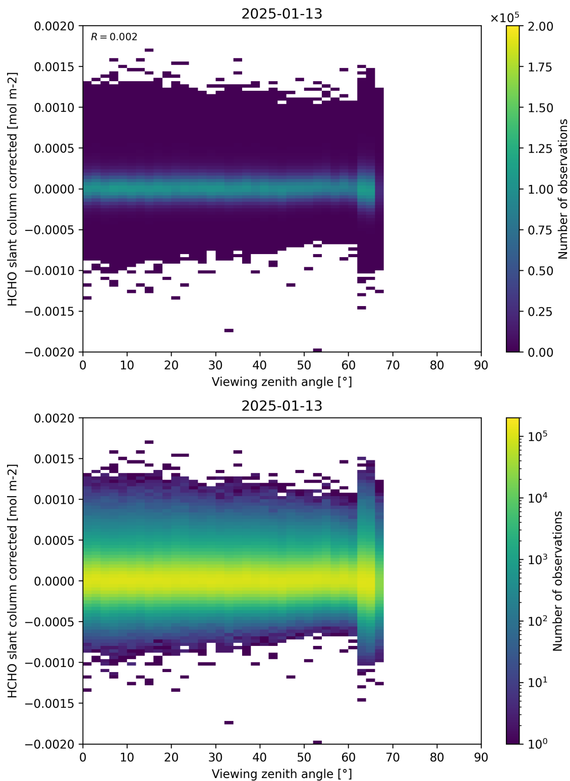
Figure 186: Scatter density plot of “Viewing zenith angle” against “HCHO slant column corrected” for 2025-01-12 to 2025-01-14.
