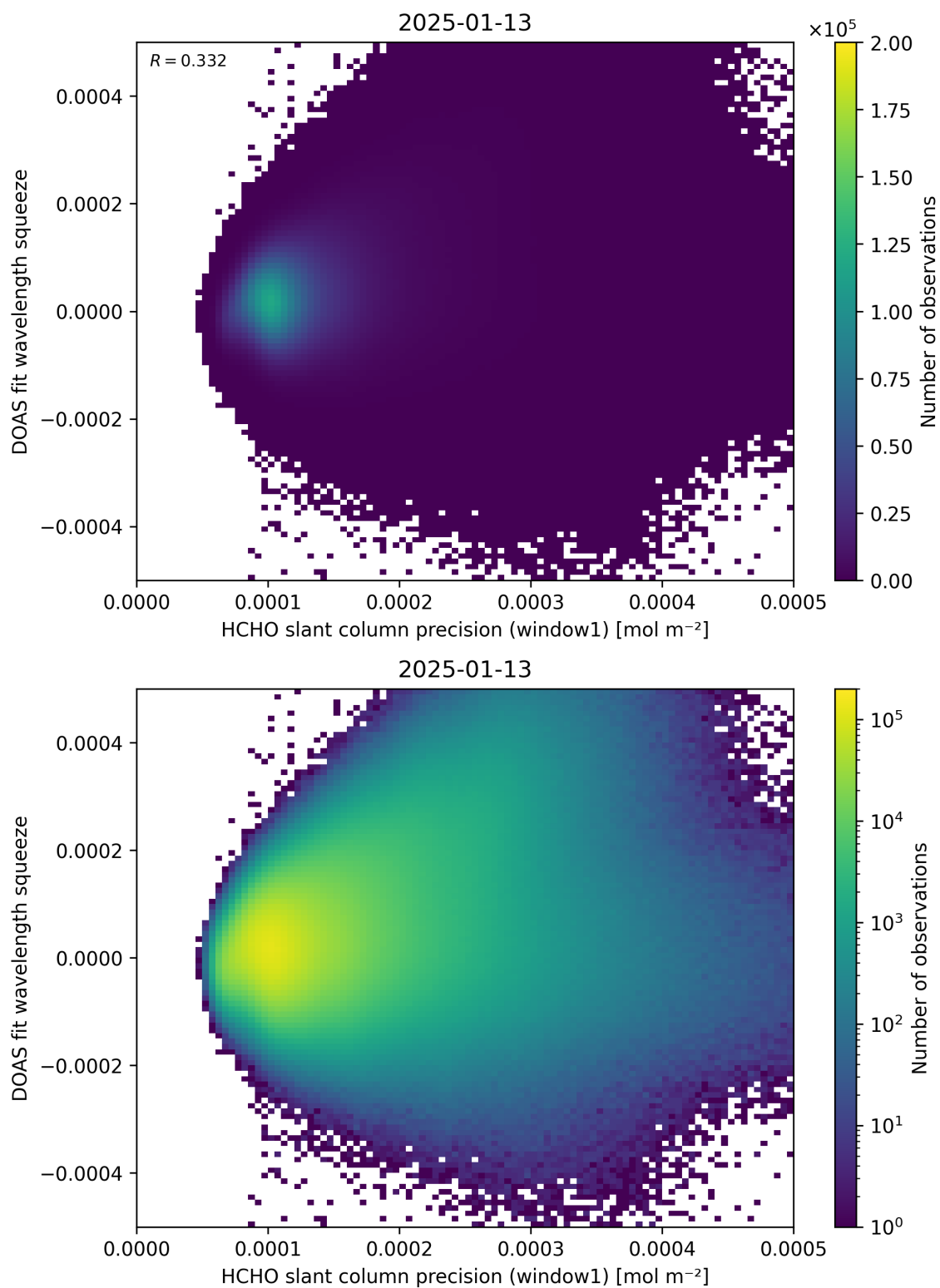
Figure 90: Scatter density plot of “HCHO slant column precision (window1)” against “DOAS fit wavelength squeeze” for 2025-01-12 to 2025-01-14.
