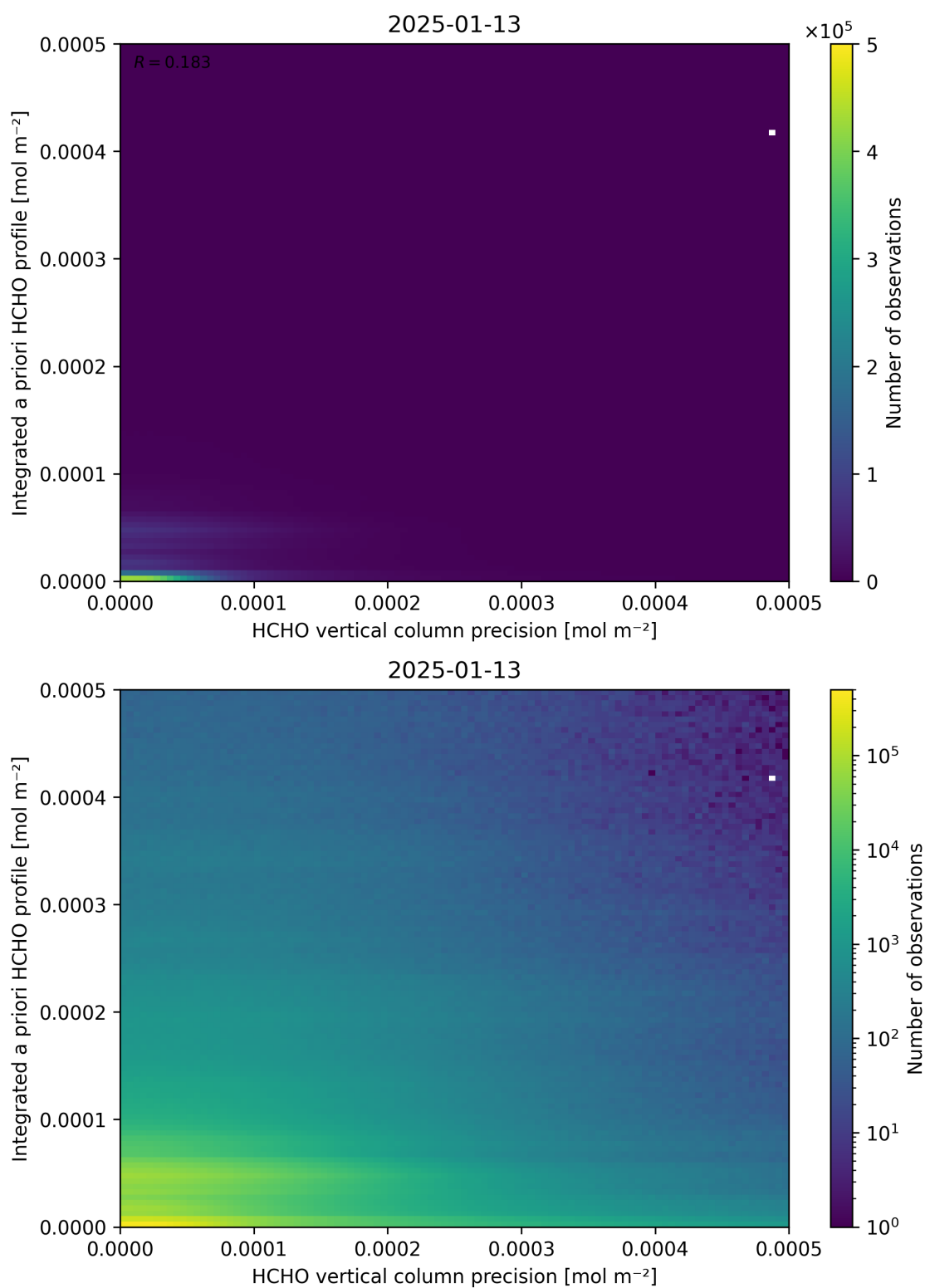
Figure 147: Scatter density plot of “HCHO vertical column precision” against “Integrated a priori HCHO profile” for 2025-01-12 to 2025-01-14.
