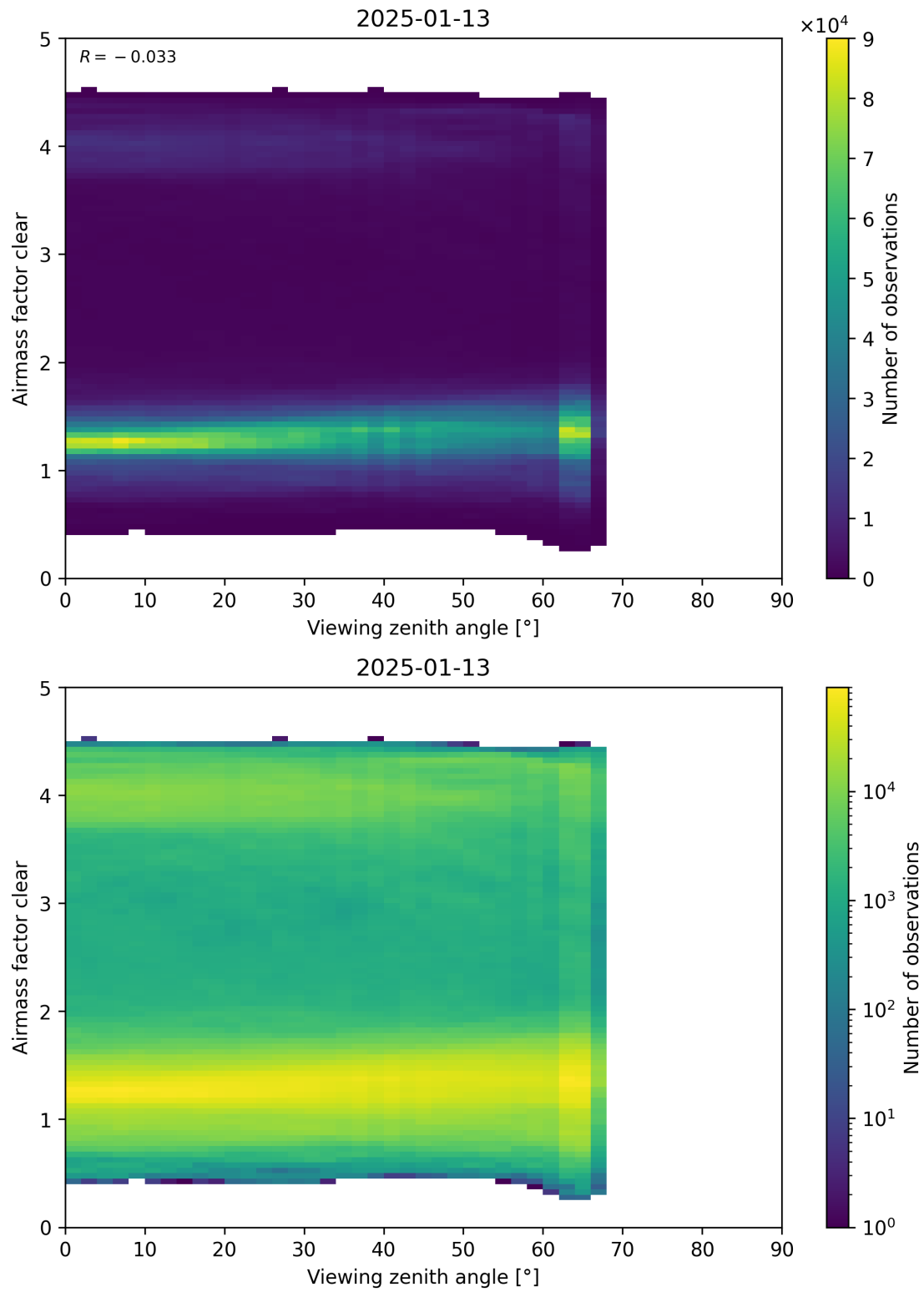
Figure 185: Scatter density plot of “Viewing zenith angle” against “Airmass factor clear” for 2025-01-12 to 2025-01-14.
