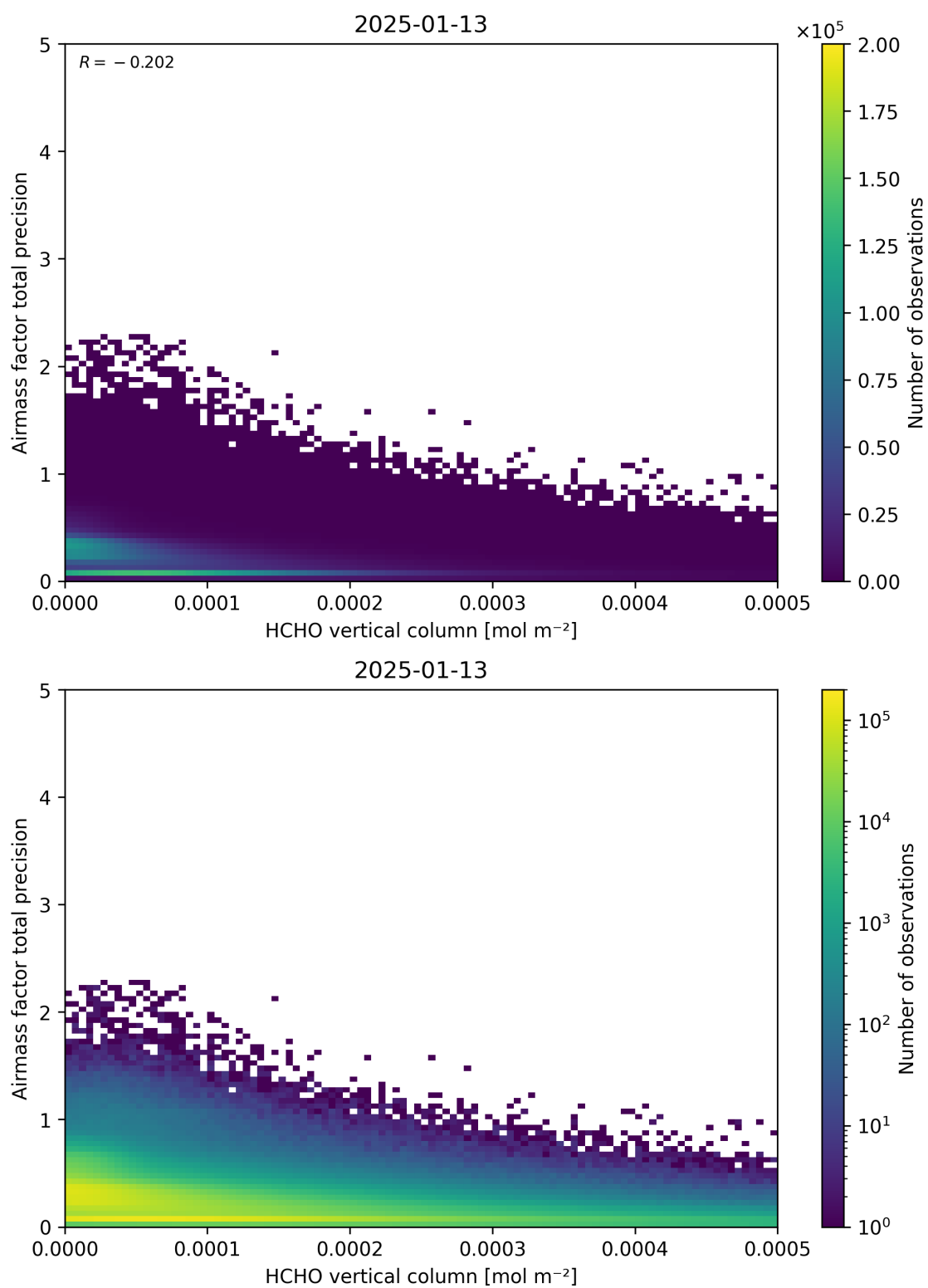
Figure 132: Scatter density plot of “HCHO vertical column” against “Airmass factor total precision” for 2025-01-12 to 2025-01-14.
