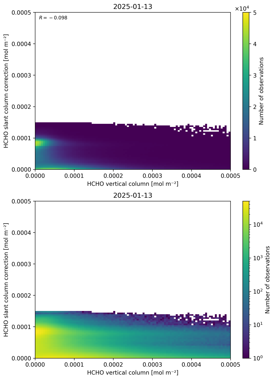
Figure 128: Scatter density plot of “HCHO vertical column” against “HCHO slant column correction” for 2025-01-12 to 2025-01-14.
