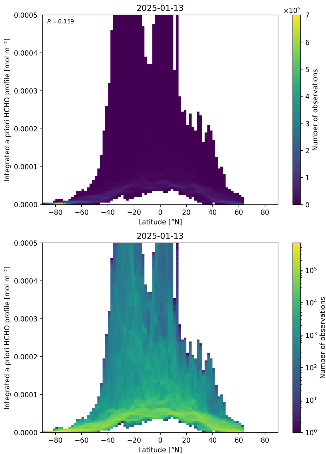
Figure 166: Scatter density plot of “Latitude” against “Integrated a priori HCHO profile” for 2025-01-12 to 2025-01-14.
