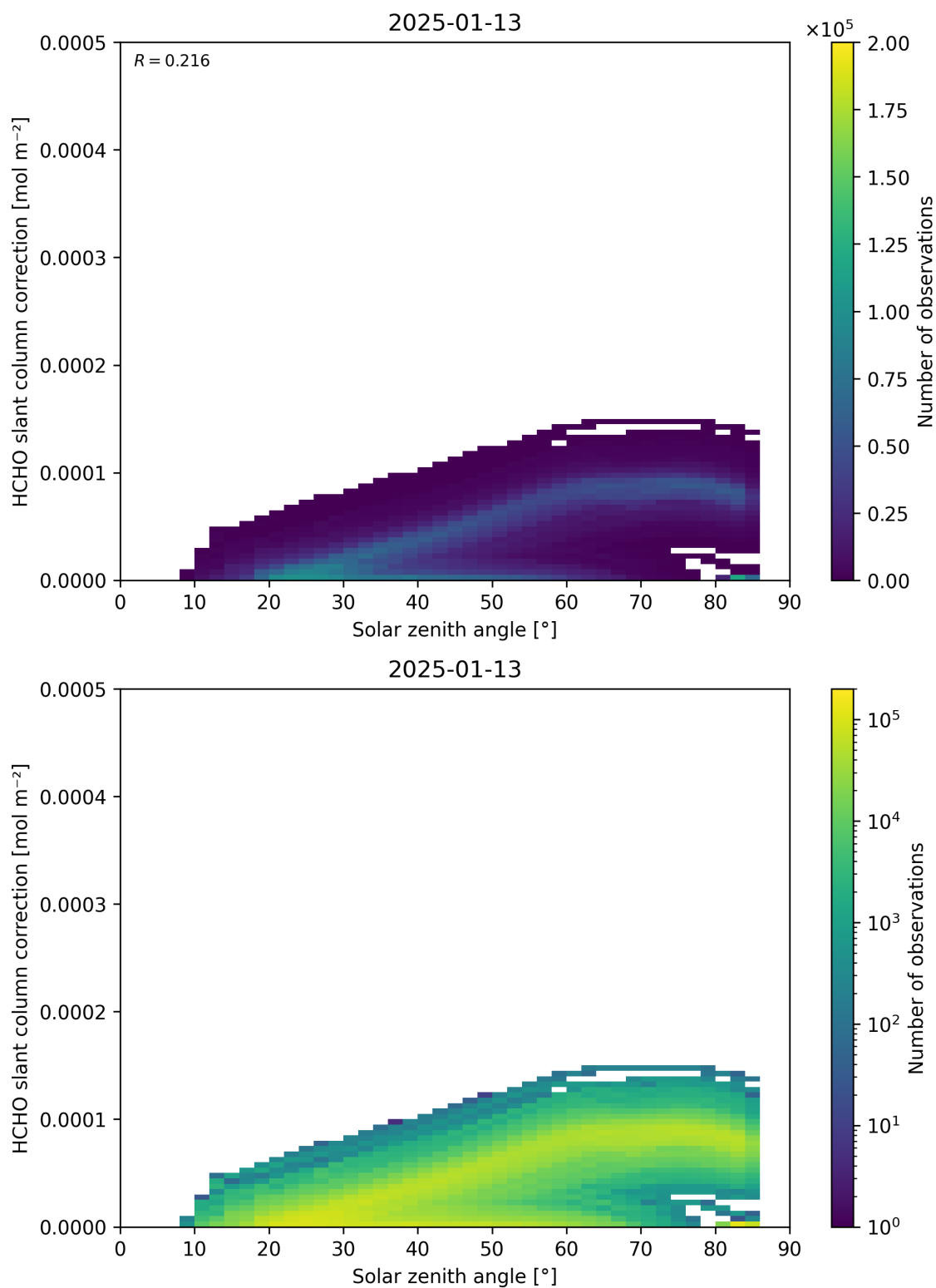
Figure 172: Scatter density plot of “Solar zenith angle” against “HCHO slant column correction” for 2025-01-12 to 2025-01-14.
