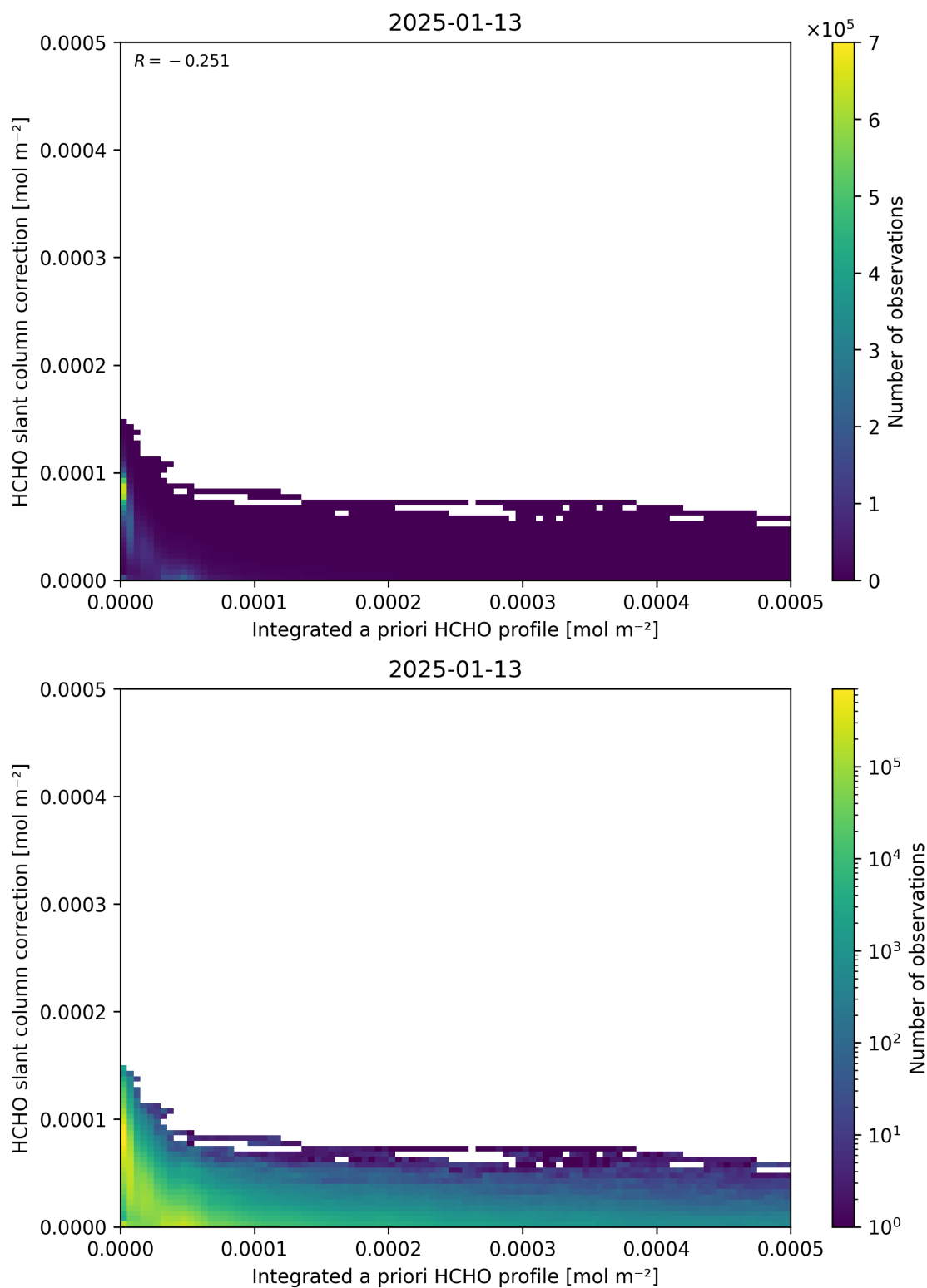
Figure 152: Scatter density plot of “Integrated a priori HCHO profile” against “HCHO slant column correction” for 2025-01-12 to 2025-01-14.
