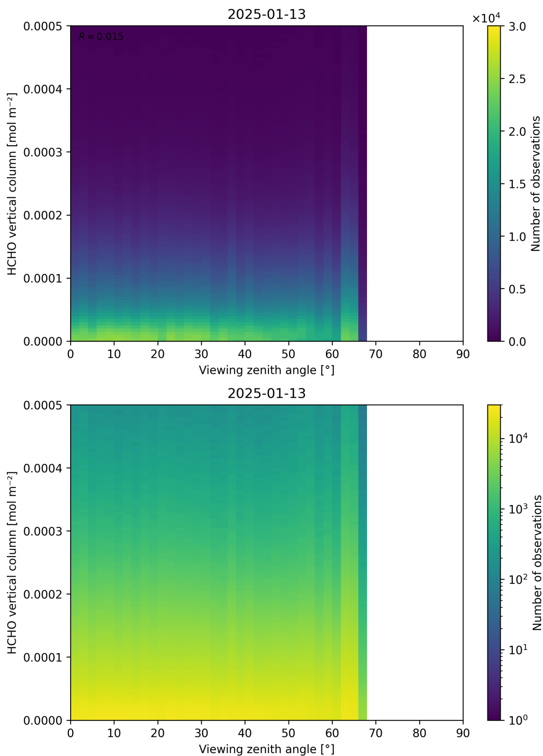
Figure 192: Scatter density plot of “Viewing zenith angle” against “HCHO vertical column” for 2025-01-12 to 2025-01-14.
