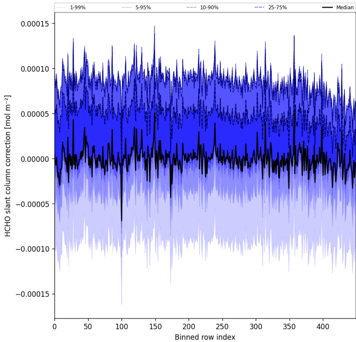
Figure 61: Along track statistics of “HCHO slant column correction” for 2025-01-12 to 2025-01-14
