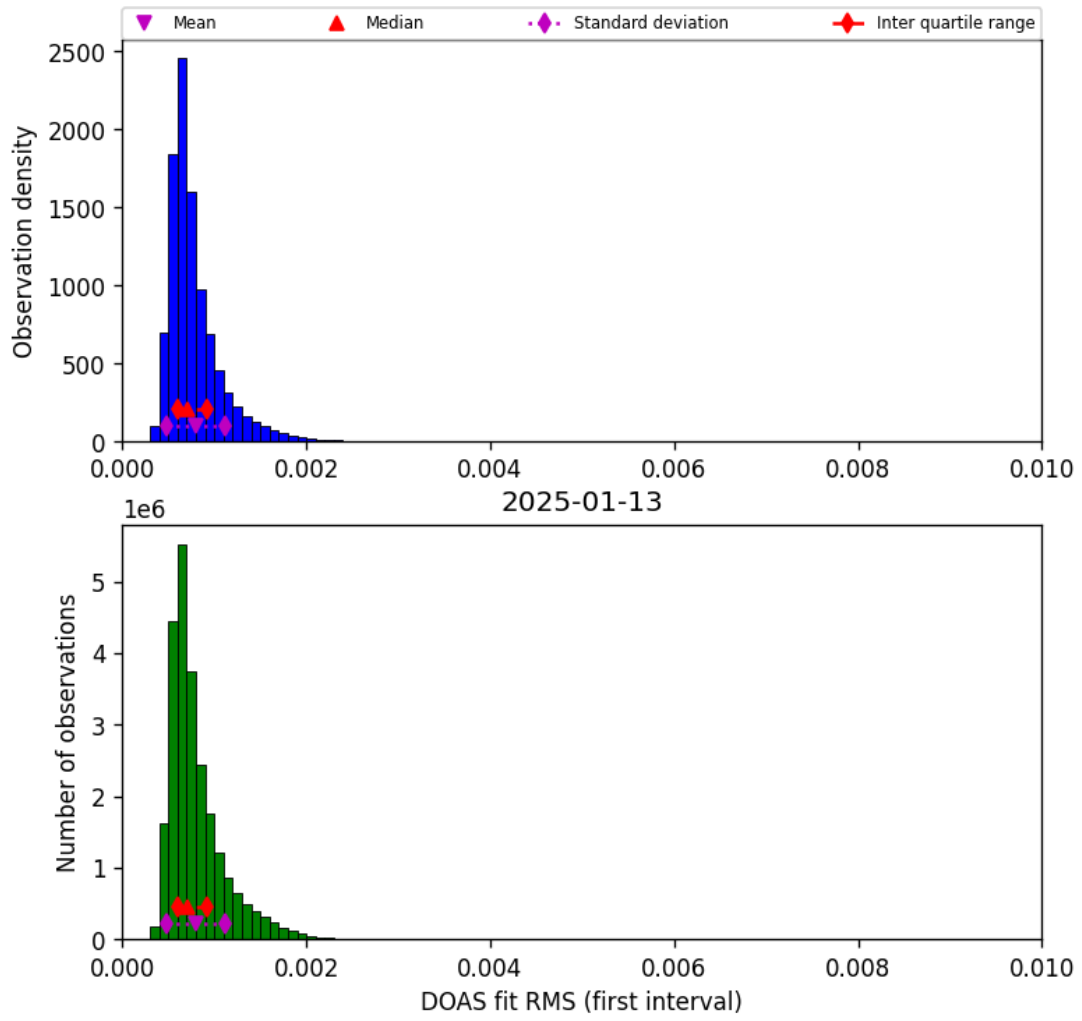
Figure 46: Histogram of “DOAS fit RMS (first interval)” for 2025-01-12 to 2025-01-14
