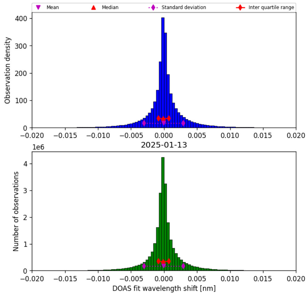
Figure 44: Histogram of “DOAS fit wavelength shift” for 2025-01-12 to 2025-01-14
