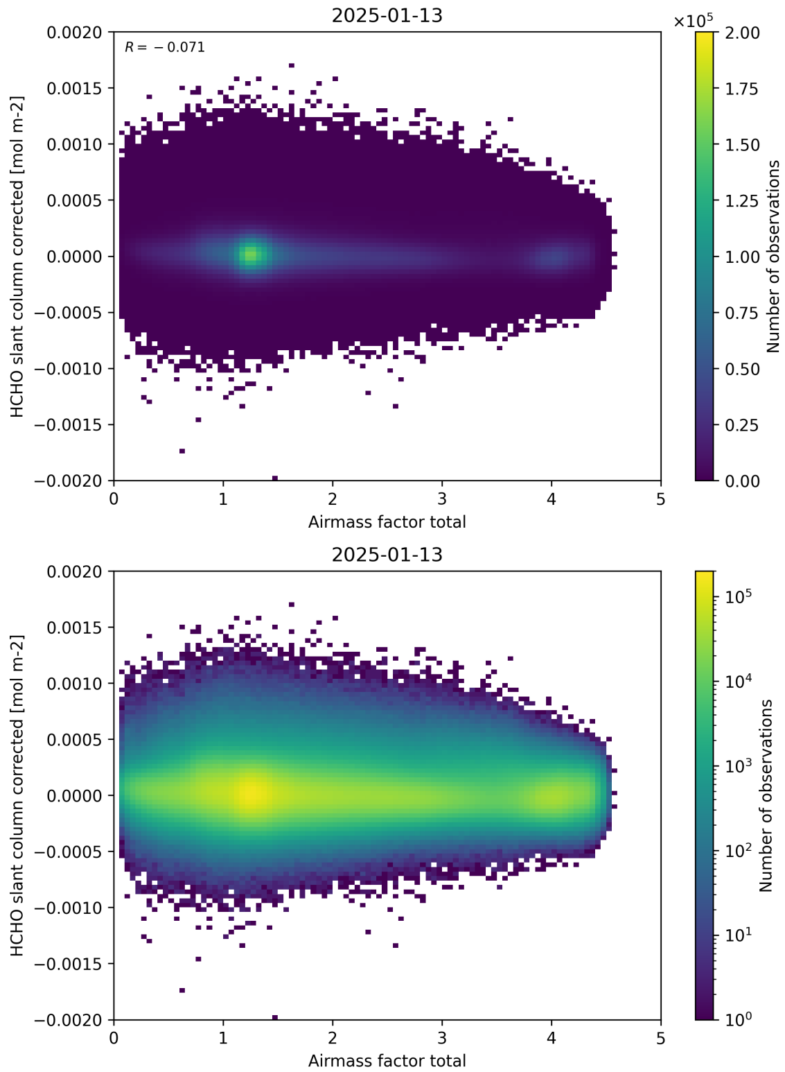
Figure 101: Scatter density plot of “Airmass factor total” against “HCHO slant column corrected” for 2025-01-12 to 2025-01-14.
