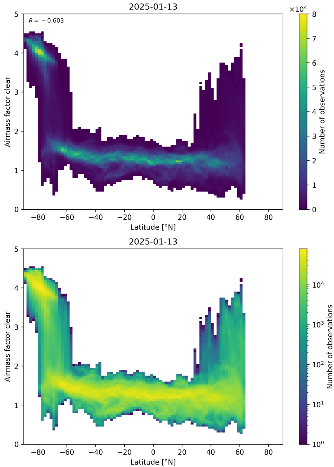
Figure 156: Scatter density plot of “Latitude” against “Airmass factor clear” for 2025-01-12 to 2025-01-14.
