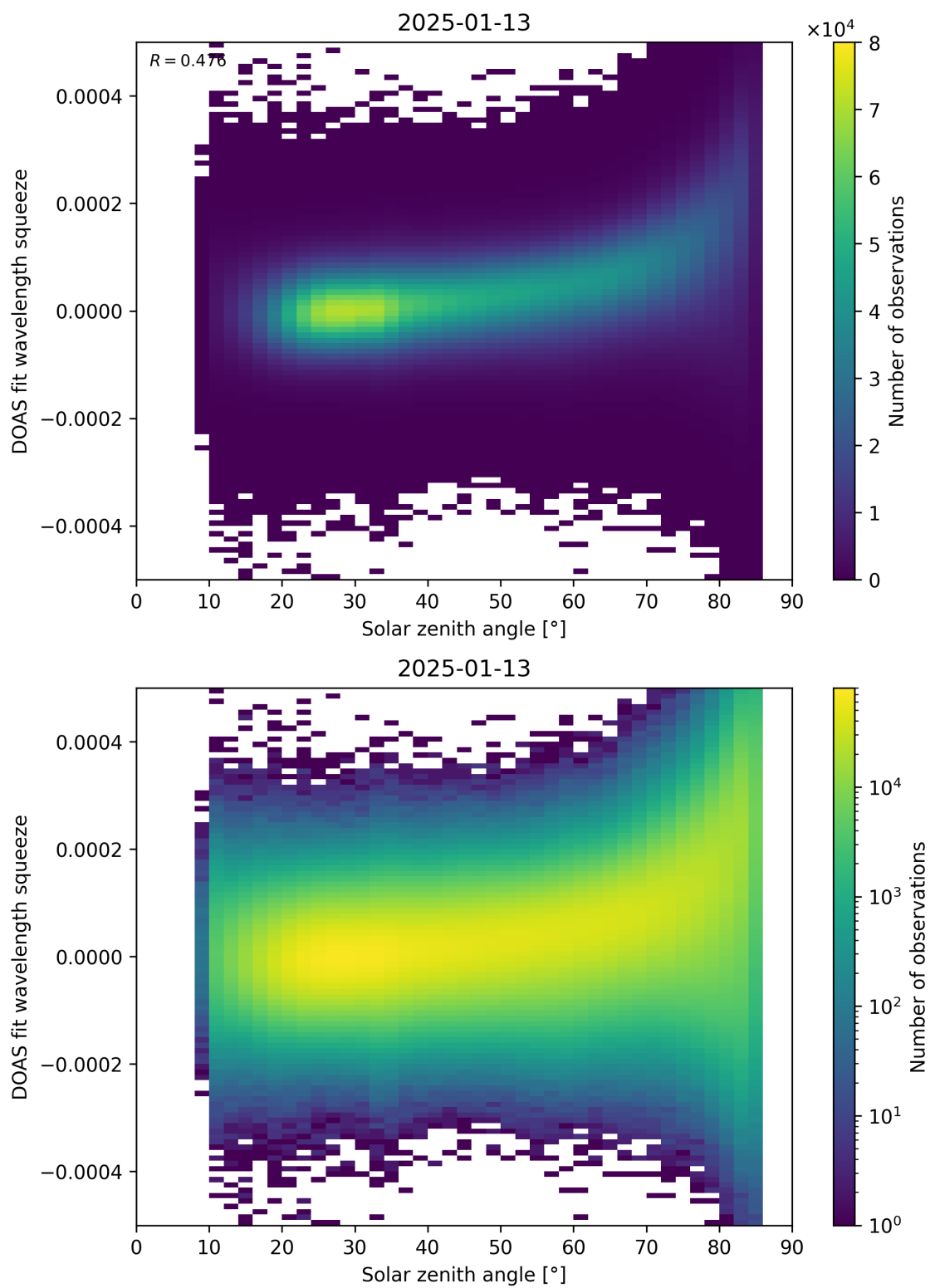
Figure 169: Scatter density plot of “Solar zenith angle” against “DOAS fit wavelength squeeze” for 2025-01-12 to 2025-01-14.
