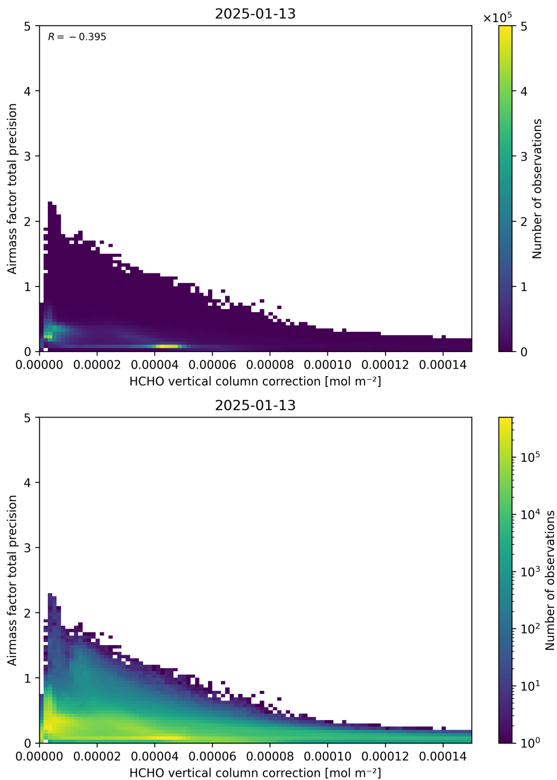
Figure 121: Scatter density plot of “HCHO vertical column correction” against “Airmass factor total precision” for 2025-01-12 to 2025-01-14.
