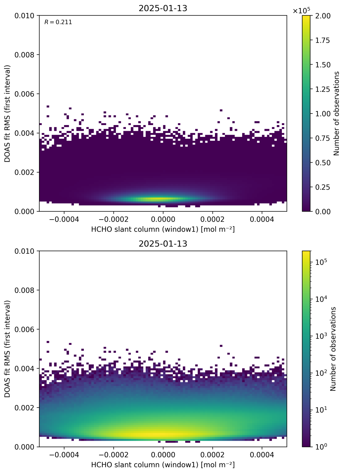
Figure 78: Scatter density plot of “HCHO slant column (window1)” against “DOAS fit RMS (first interval)” for 2025-01-12 to 2025-01-14.
