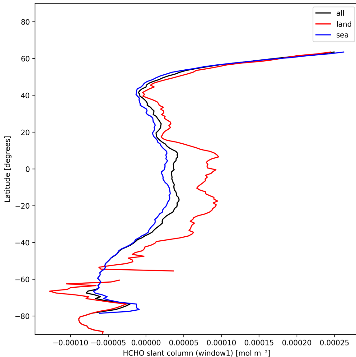
Figure 24: Zonal average of “HCHO slant column (window1)” for 2025-01-12 to 2025-01-14.
