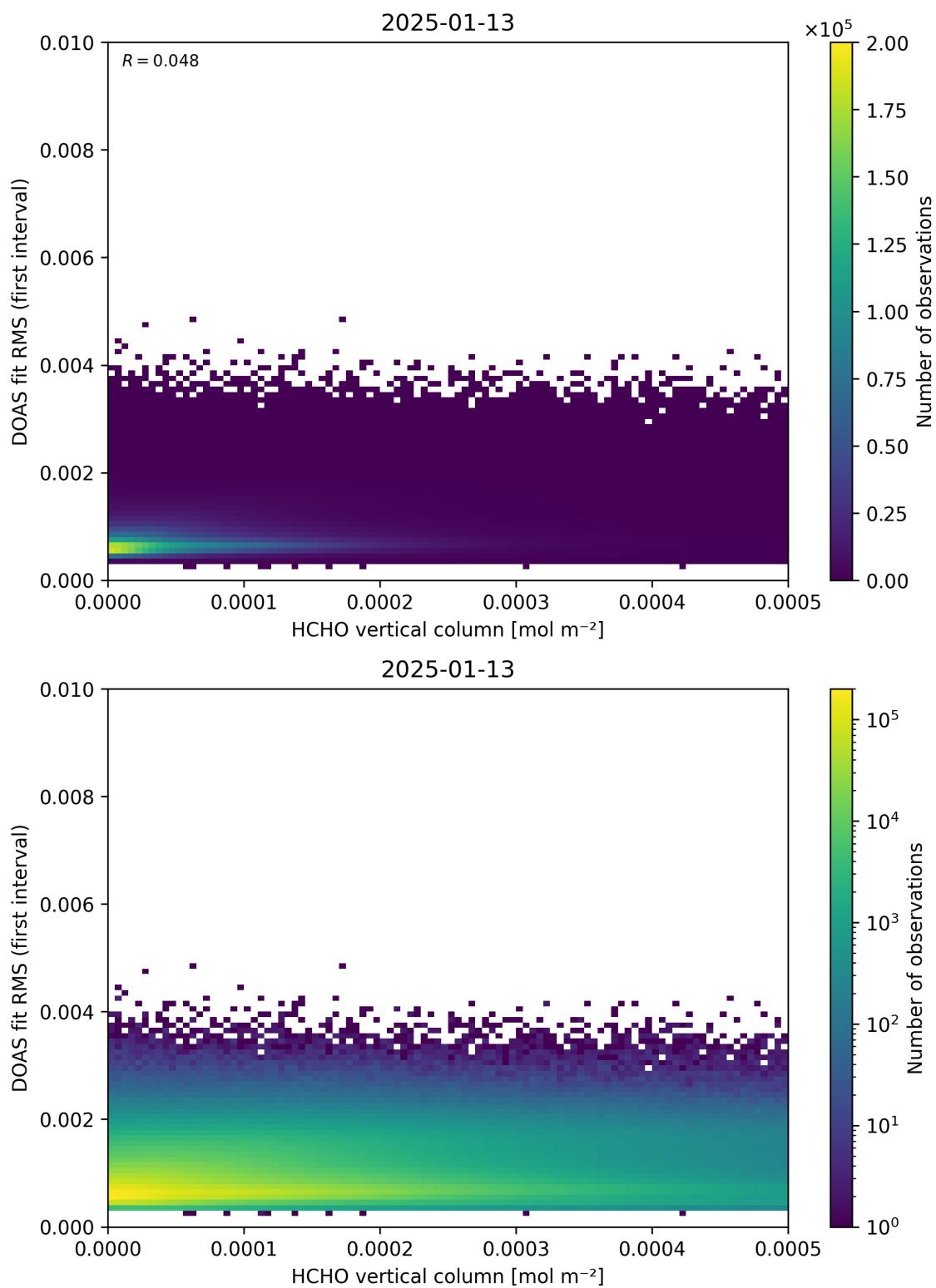
Figure 123: Scatter density plot of “HCHO vertical column” against “DOAS fit RMS (first interval)” for 2025-01-12 to 2025-01-14.
