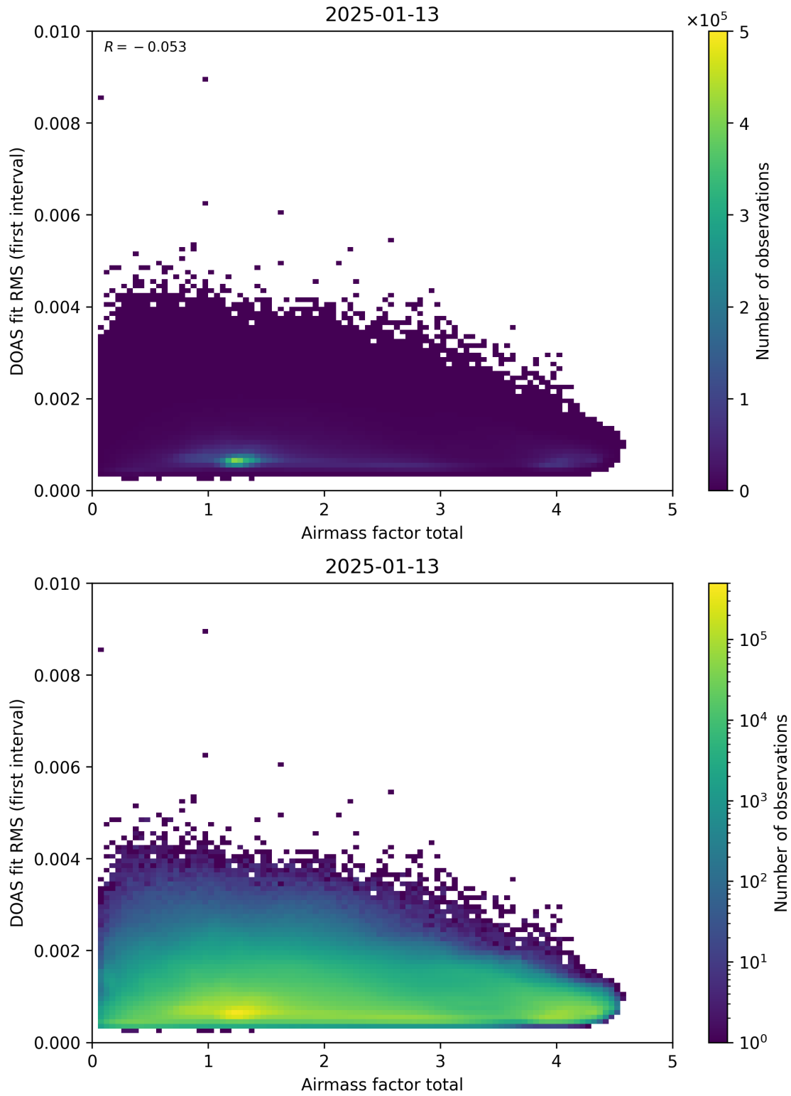
Figure 97: Scatter density plot of “Airmass factor total” against “DOAS fit RMS (first interval)” for 2025-01-12 to 2025-01-14.
