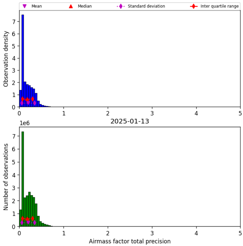
Figure 41: Histogram of “Airmass factor total precision” for 2025-01-12 to 2025-01-14
