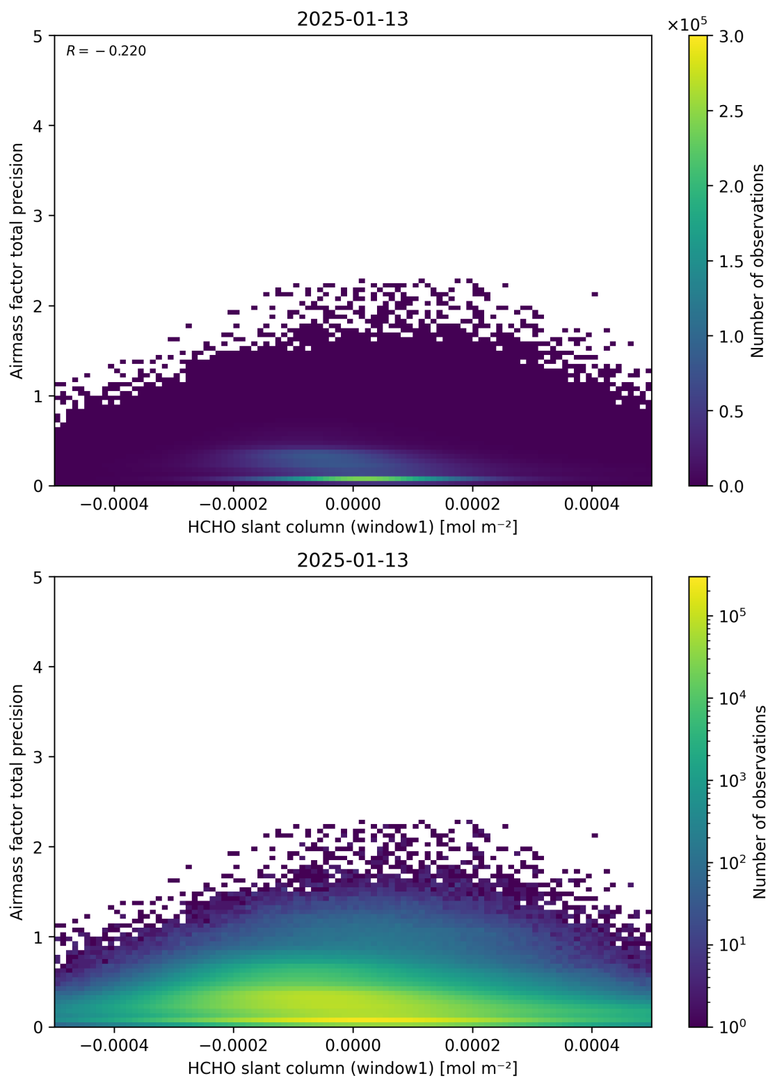
Figure 86: Scatter density plot of “HCHO slant column (window1)” against “Airmass factor total precision” for 2025-01-12 to 2025-01-14.
