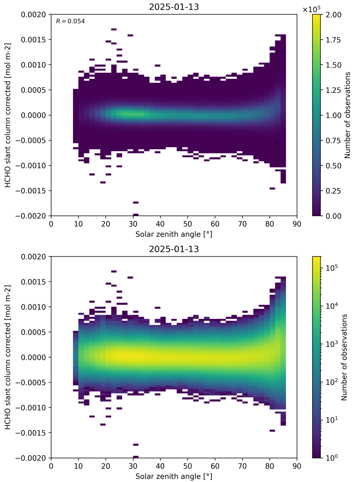
Figure 171: Scatter density plot of “Solar zenith angle” against “HCHO slant column corrected” for 2025-01-12 to 2025-01-14.
