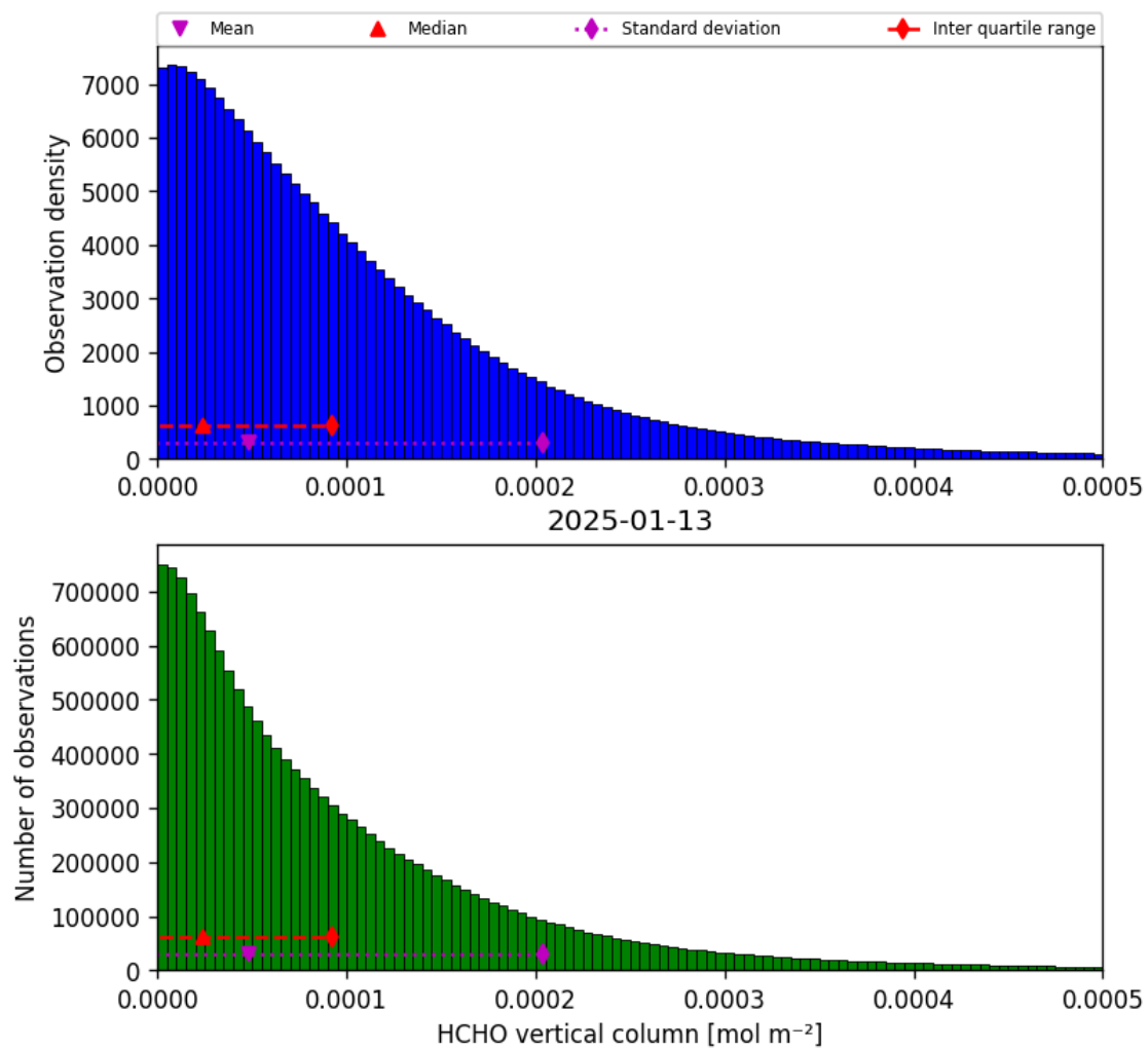
Figure 35: Histogram of “HCHO vertical column” for 2025-01-12 to 2025-01-14
