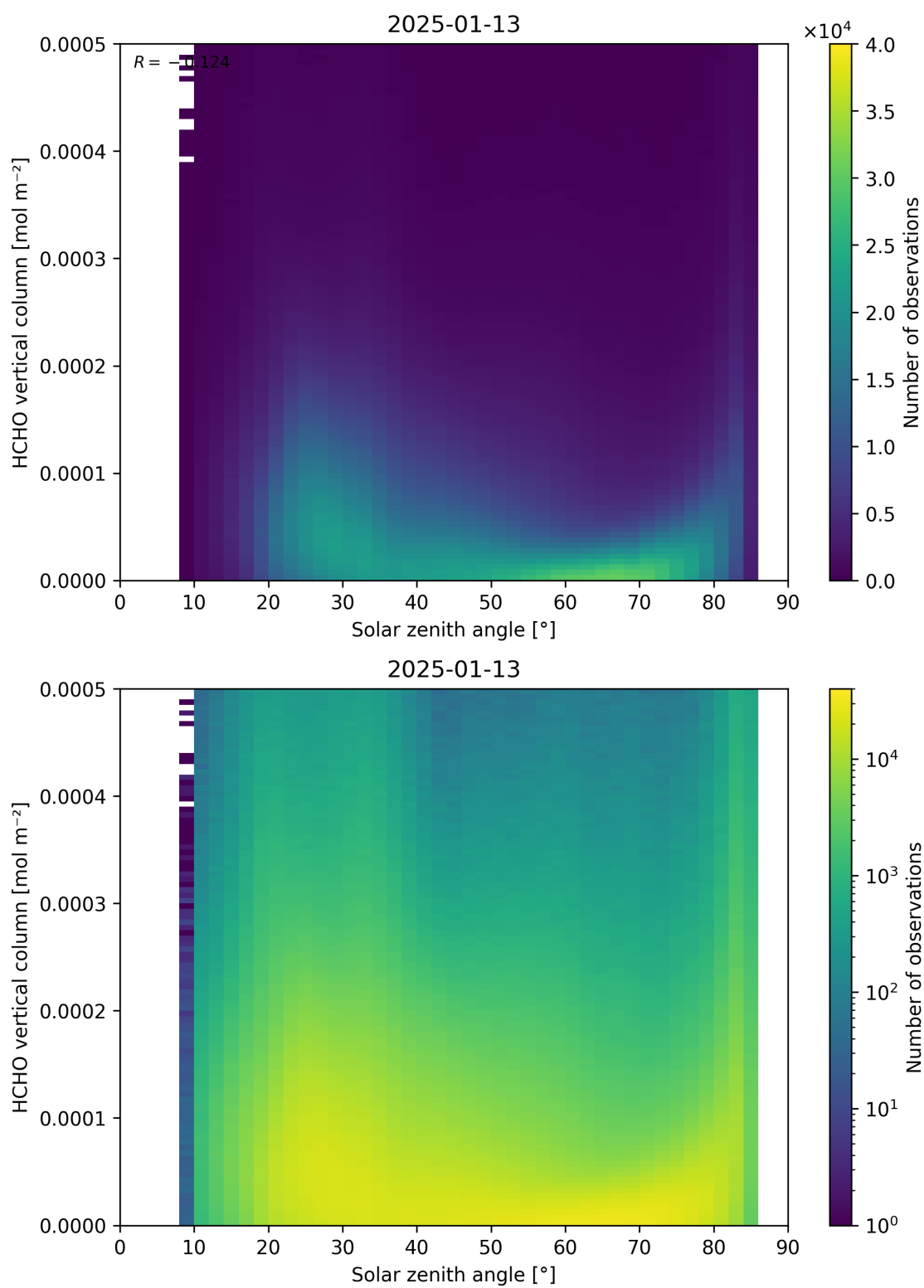
Figure 177: Scatter density plot of “Solar zenith angle” against “HCHO vertical column” for 2025-01-12 to 2025-01-14.
