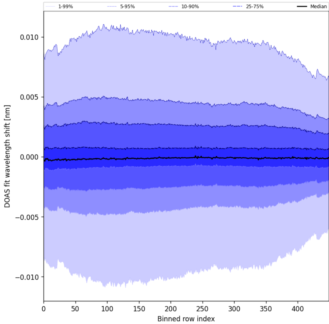
Figure 58: Along track statistics of “DOAS fit wavelength shift” for 2025-01-12 to 2025-01-14
