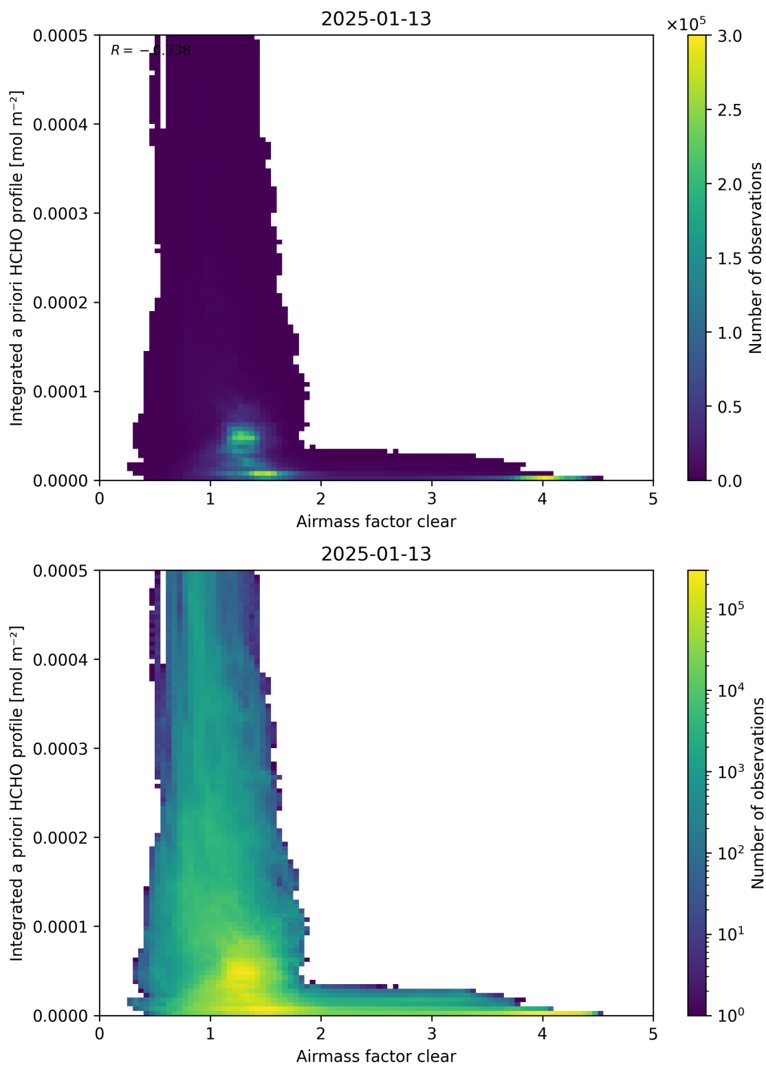
Figure 76: Scatter density plot of “Airmass factor clear” against “Integrated a priori HCHO profile” for 2025-01-12 to 2025-01-14.
