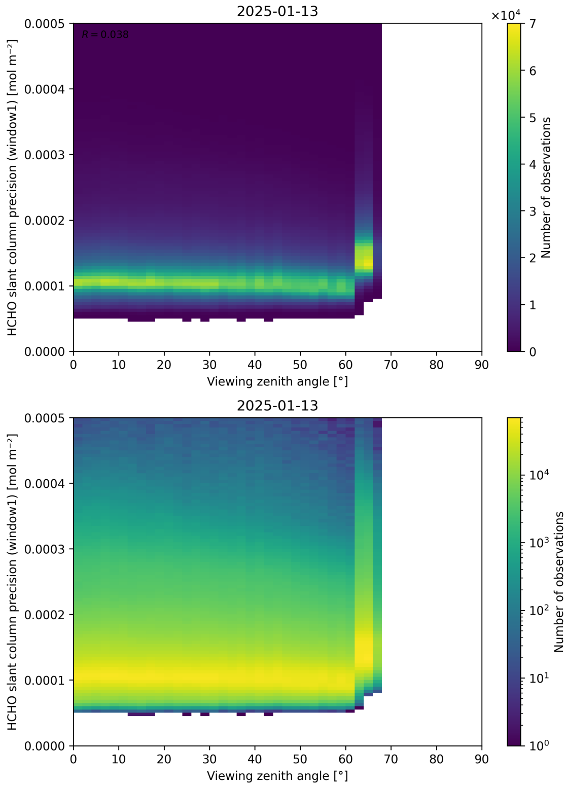
Figure 189: Scatter density plot of “Viewing zenith angle” against “HCHO slant column precision (window1)” for 2025-01-12 to 2025-01-14.
