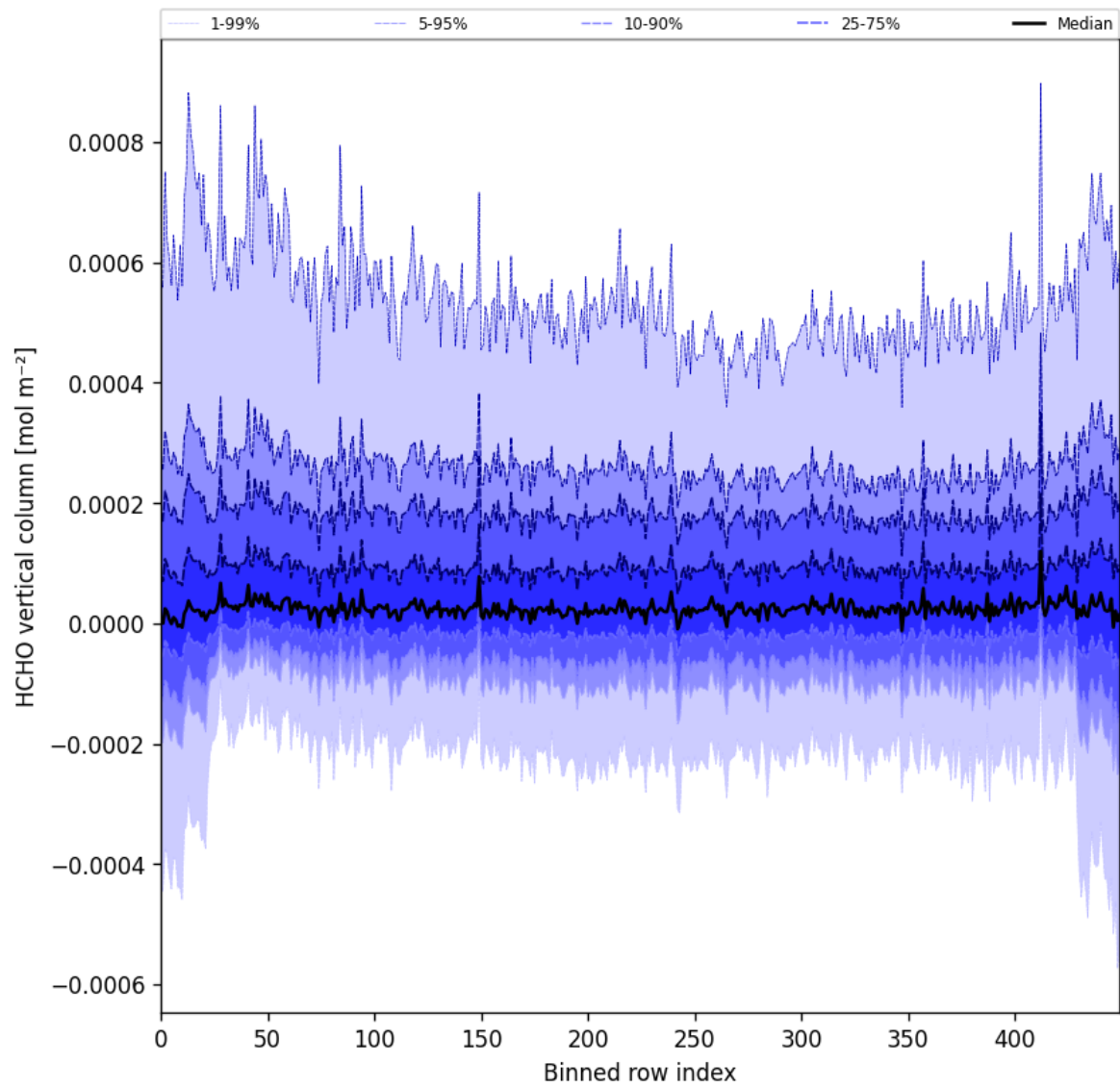
Figure 49: Along track statistics of “HCHO vertical column” for 2025-01-12 to 2025-01-14
