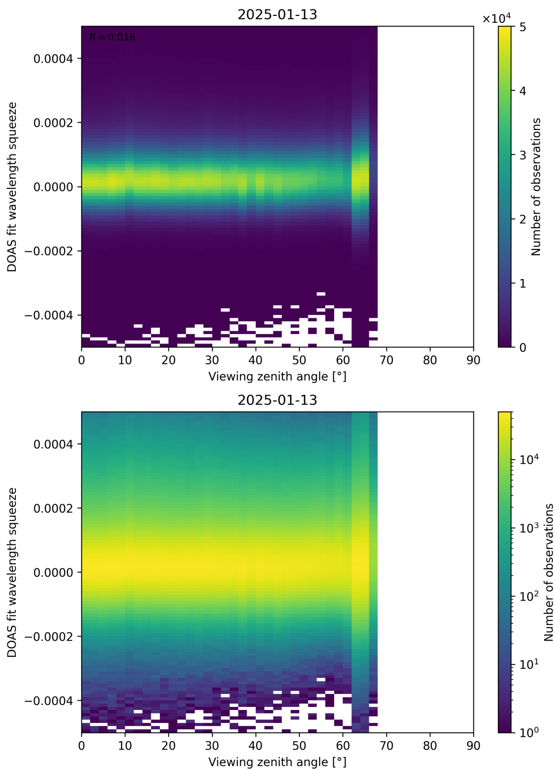
Figure 184: Scatter density plot of “Viewing zenith angle” against “DOAS fit wavelength squeeze” for 2025-01-12 to 2025-01-14.
