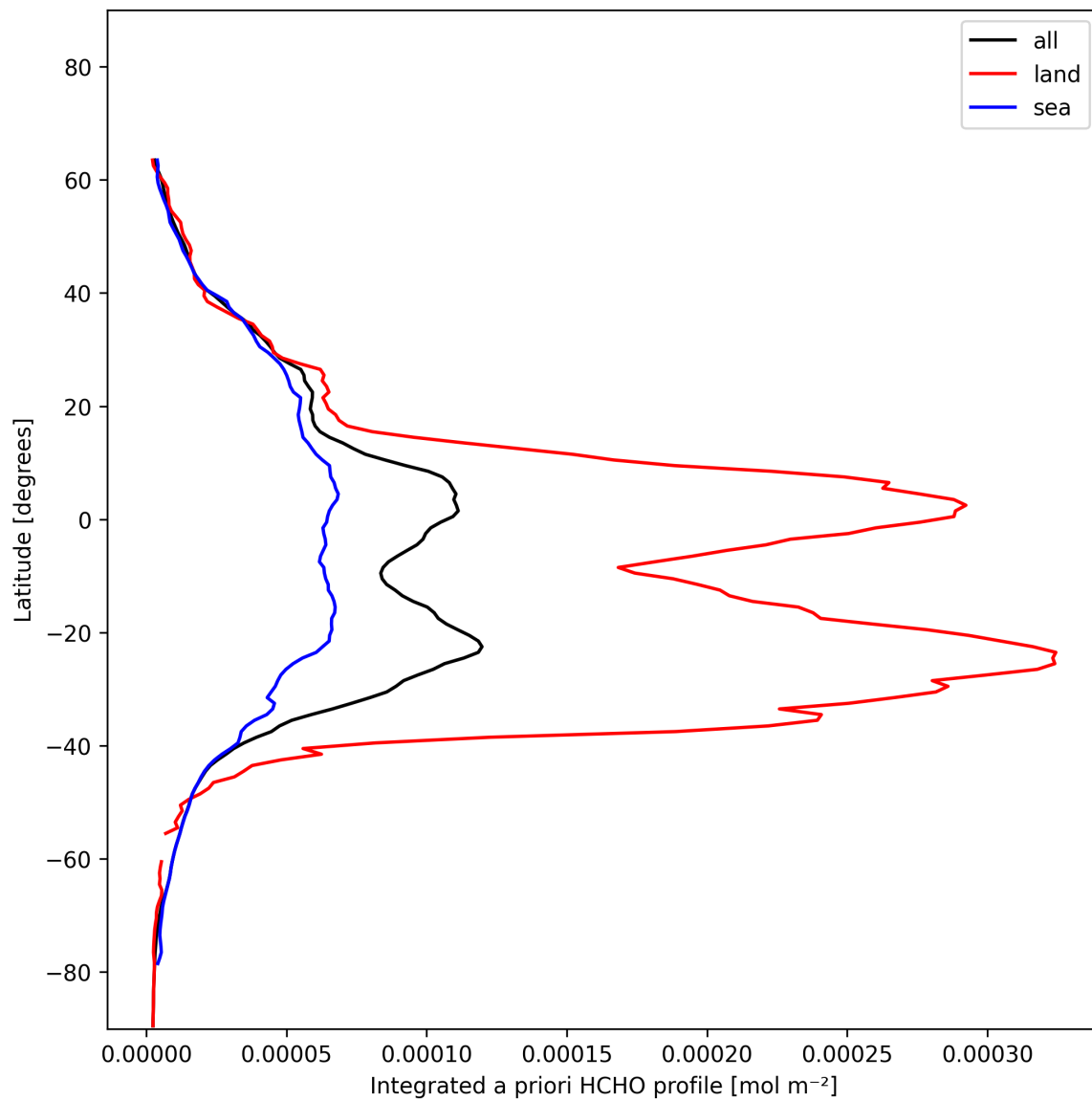
Figure 29: Zonal average of “Integrated a priori HCHO profile” for 2025-01-12 to 2025-01-14.
