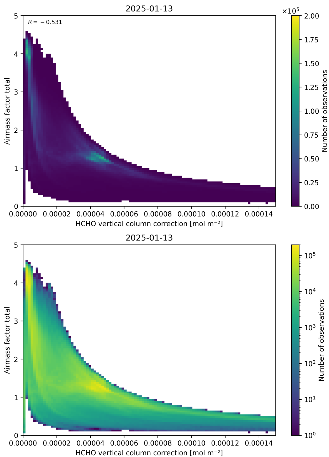
Figure 120: Scatter density plot of “HCHO vertical column correction” against “Airmass factor total” for 2025-01-12 to 2025-01-14.
