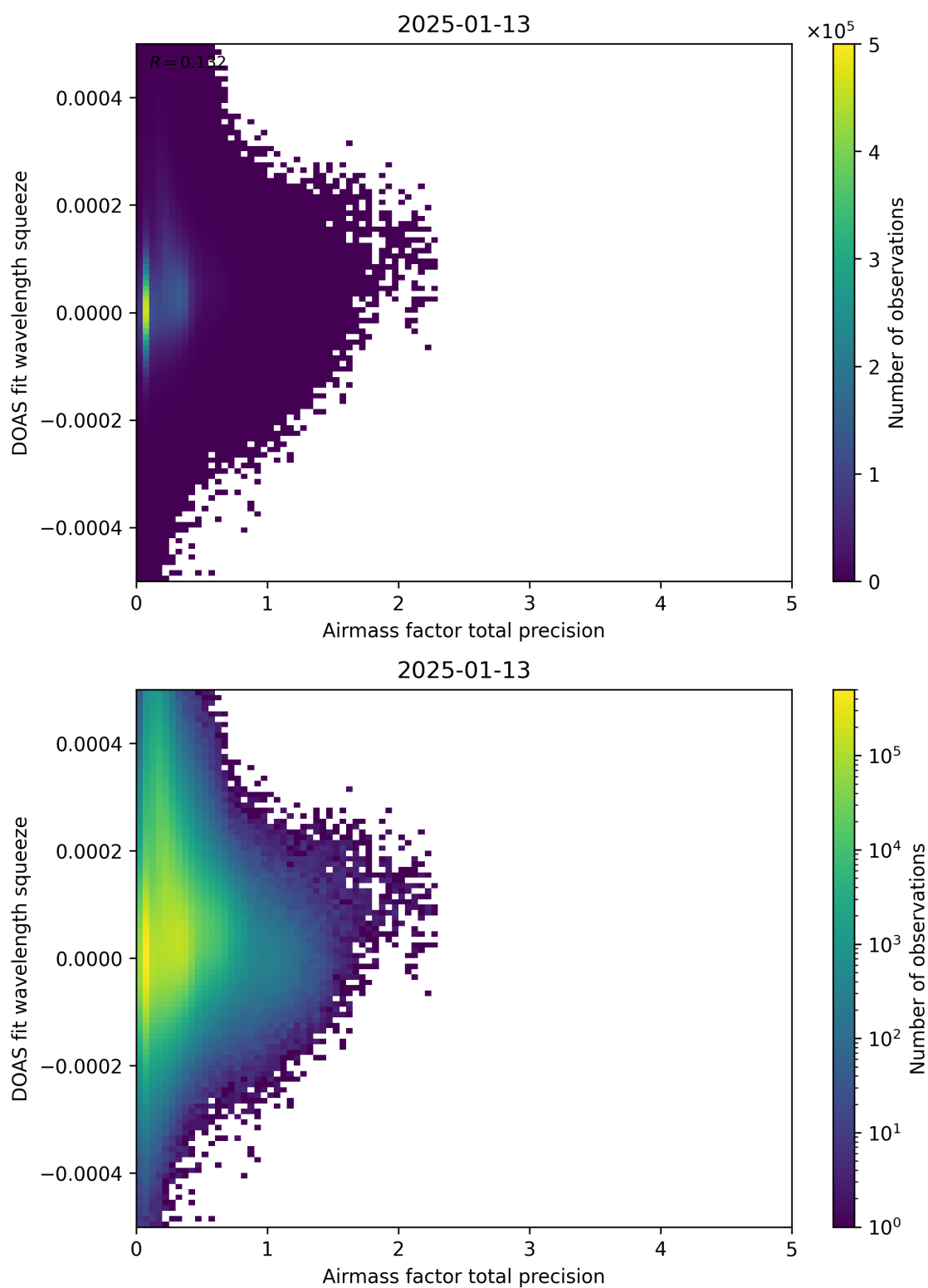
Figure 107: Scatter density plot of “Airmass factor total precision” against “DOAS fit wavelength squeeze” for 2025-01-12 to 2025-01-14.
