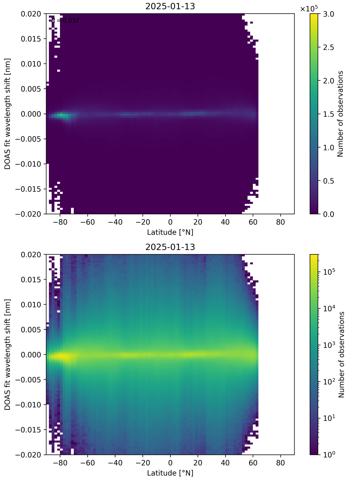
Figure 154: Scatter density plot of “Latitude” against “DOAS fit wavelength shift” for 2025-01-12 to 2025-01-14.
