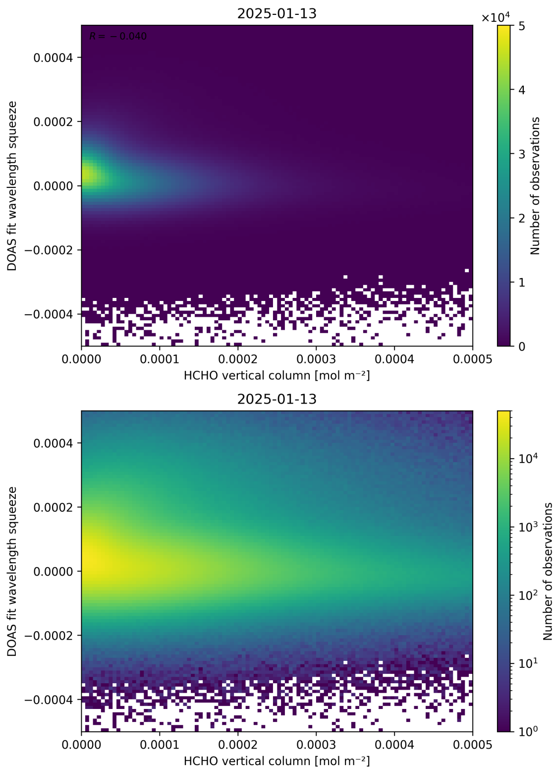
Figure 125: Scatter density plot of “HCHO vertical column” against “DOAS fit wavelength squeeze” for 2025-01-12 to 2025-01-14.
