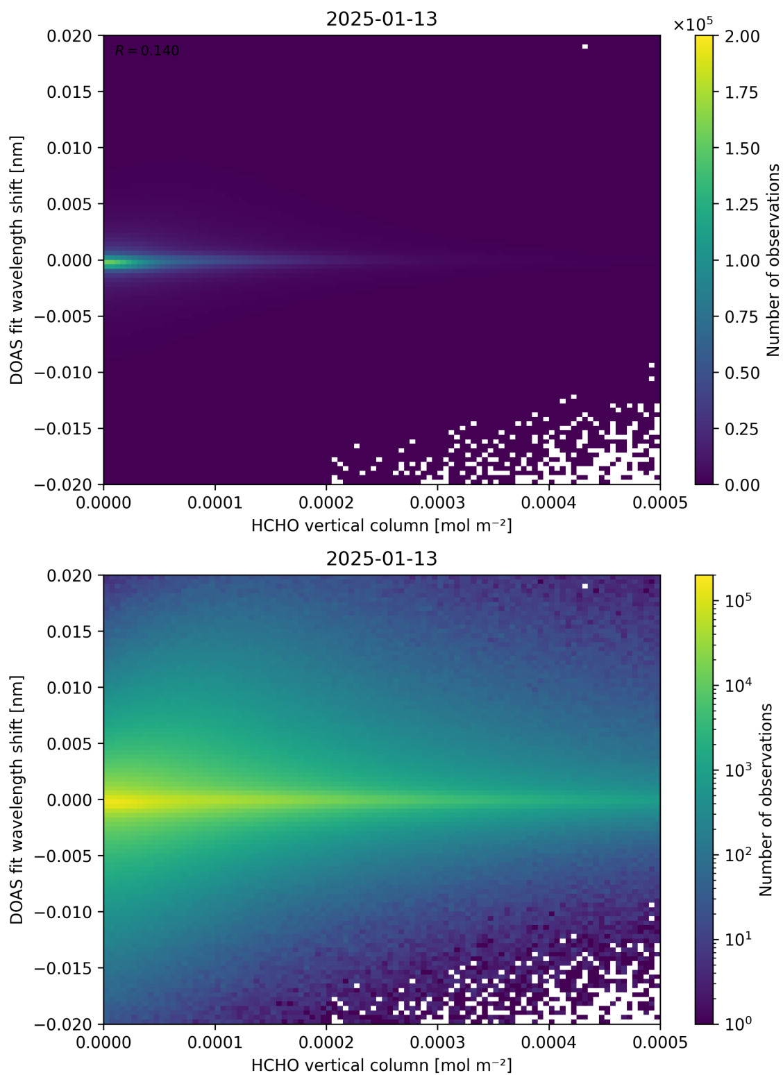
Figure 124: Scatter density plot of “HCHO vertical column” against “DOAS fit wavelength shift” for 2025-01-12 to 2025-01-14.
