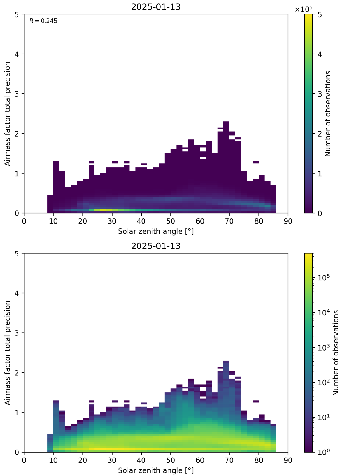
Figure 176: Scatter density plot of “Solar zenith angle” against “Airmass factor total precision” for 2025-01-12 to 2025-01-14.
