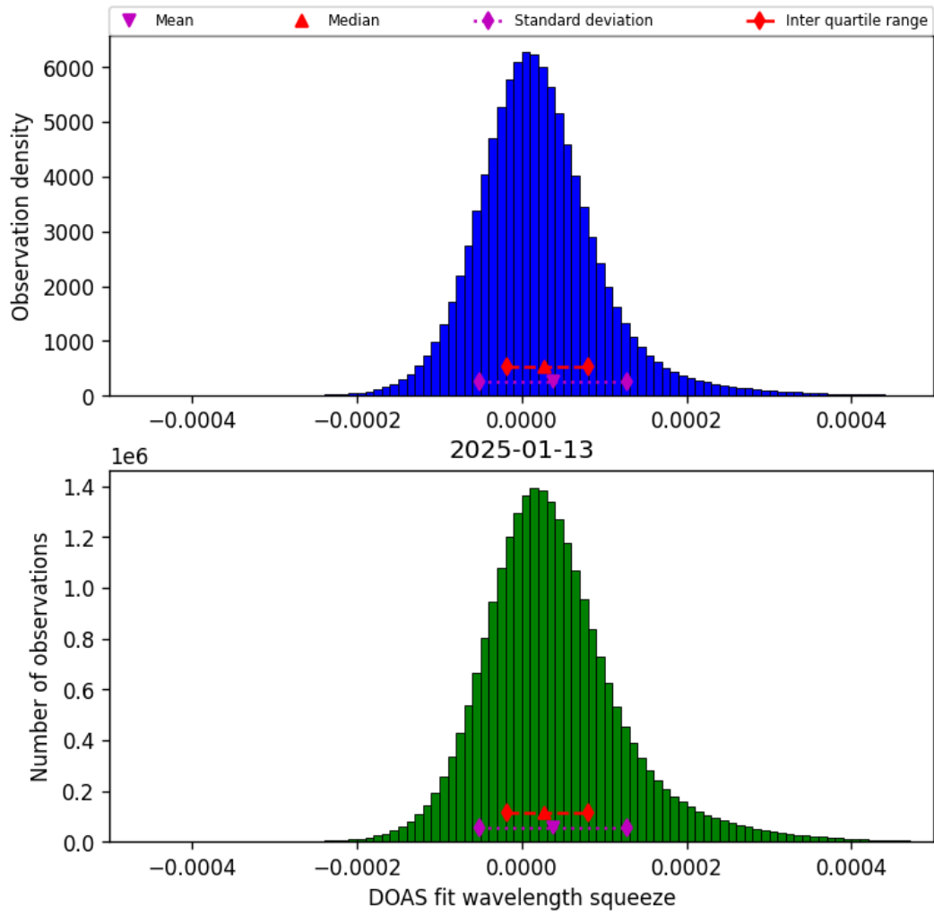
Figure 45: Histogram of “DOAS fit wavelength squeeze” for 2025-01-12 to 2025-01-14
