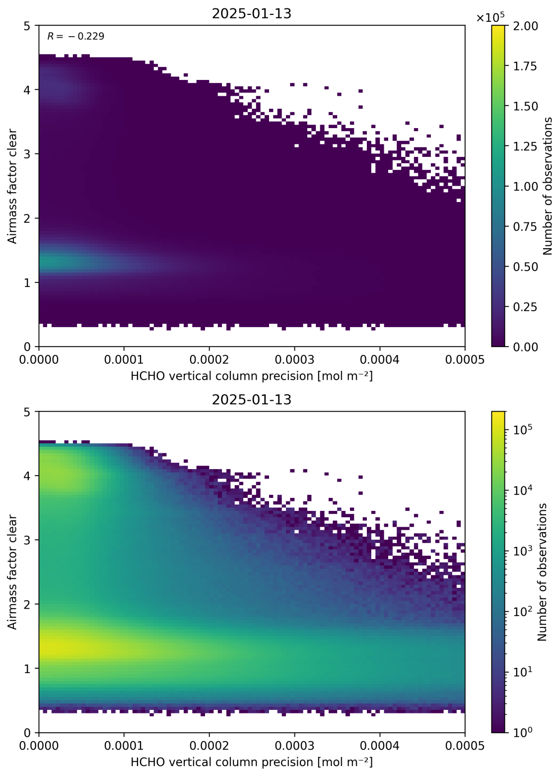
Figure 139: Scatter density plot of “HCHO vertical column precision” against “Airmass factor clear” for 2025-01-12 to 2025-01-14.
