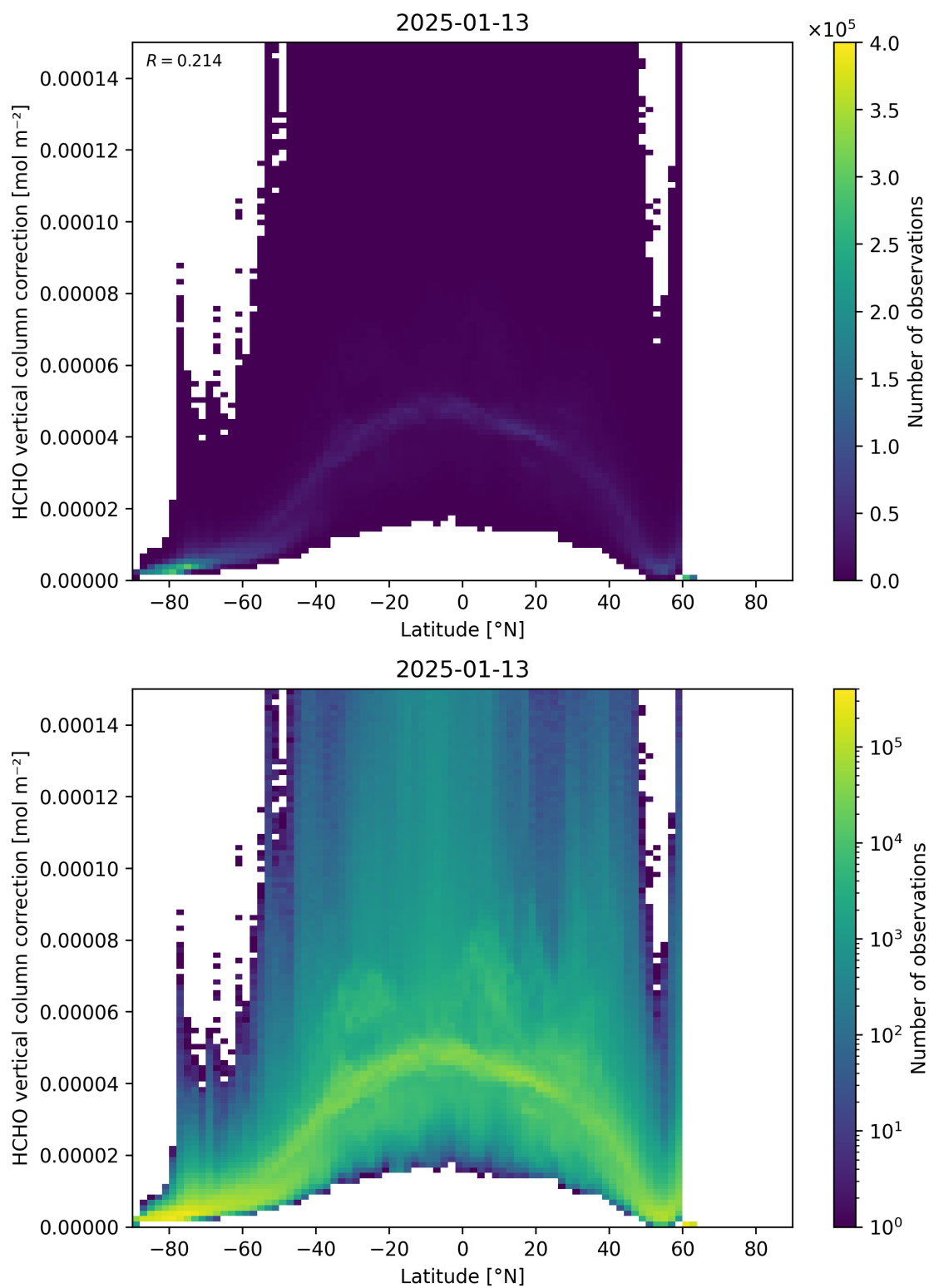
Figure 164: Scatter density plot of “Latitude” against “HCHO vertical column correction” for 2025-01-12 to 2025-01-14.
