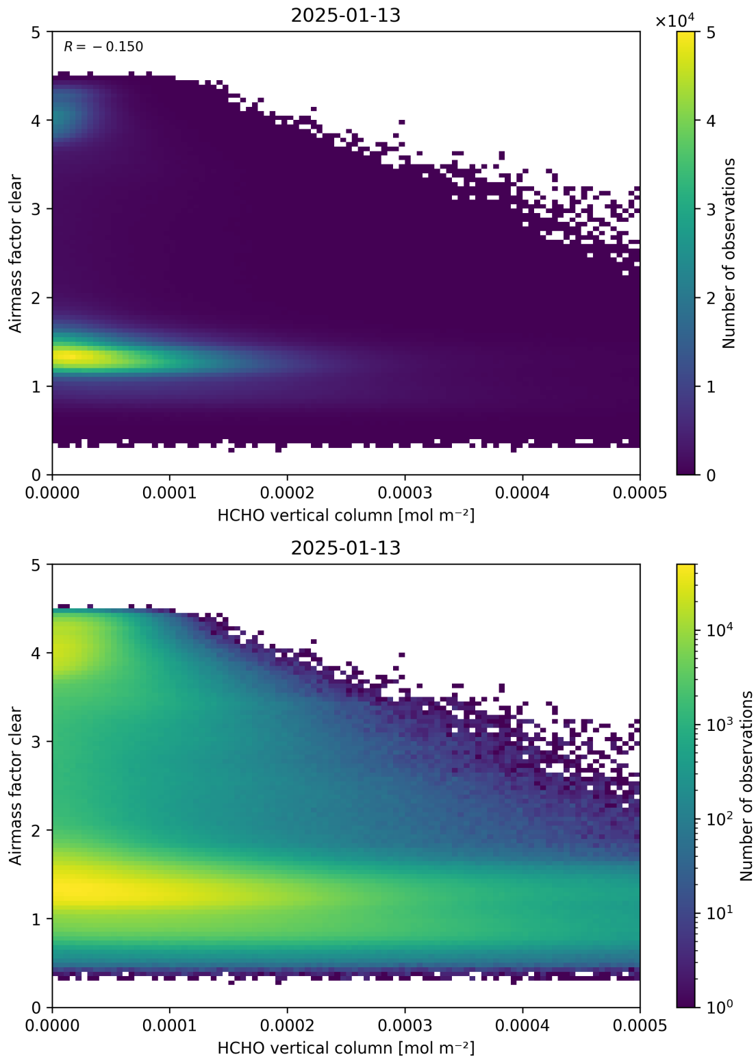
Figure 126: Scatter density plot of “HCHO vertical column” against “Airmass factor clear” for 2025-01-12 to 2025-01-14.
