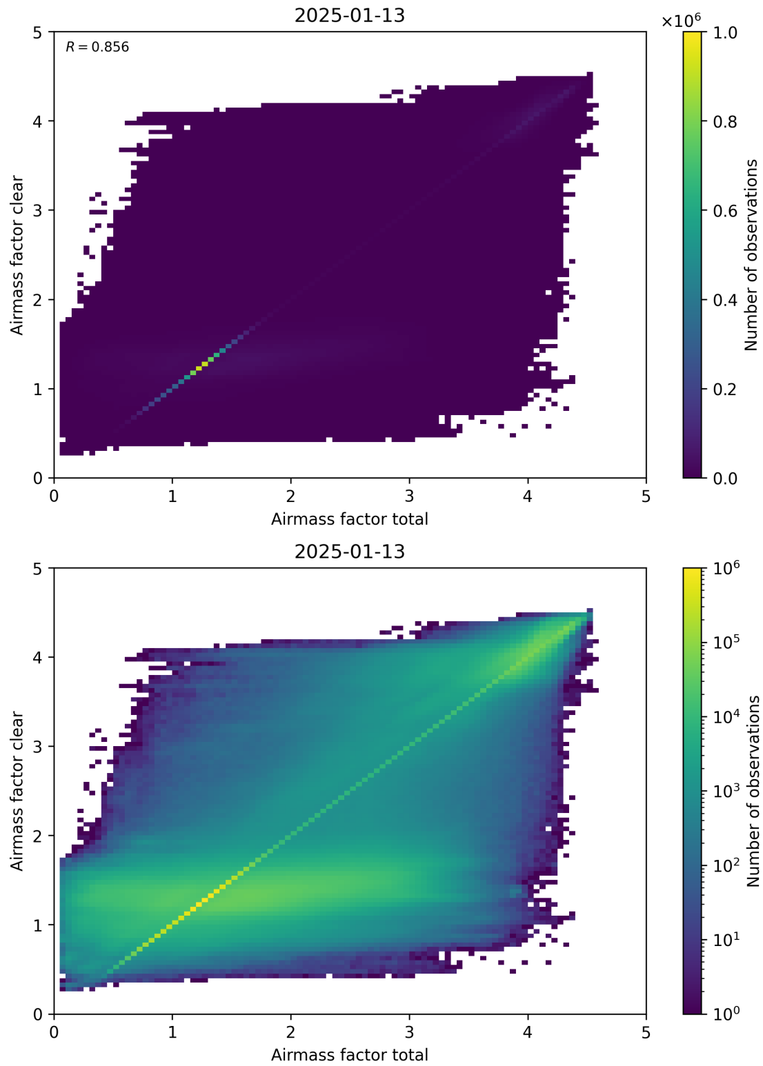
Figure 100: Scatter density plot of “Airmass factor total” against “Airmass factor clear” for 2025-01-12 to 2025-01-14.
