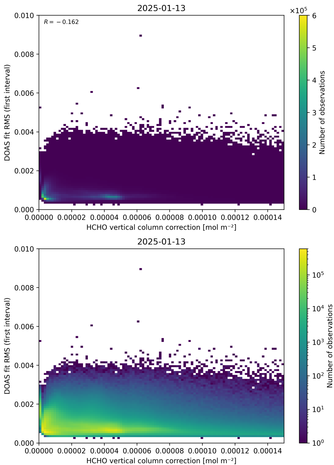
Figure 112: Scatter density plot of “HCHO vertical column correction” against “DOAS fit RMS (first interval)” for 2025-01-12 to 2025-01-14.
