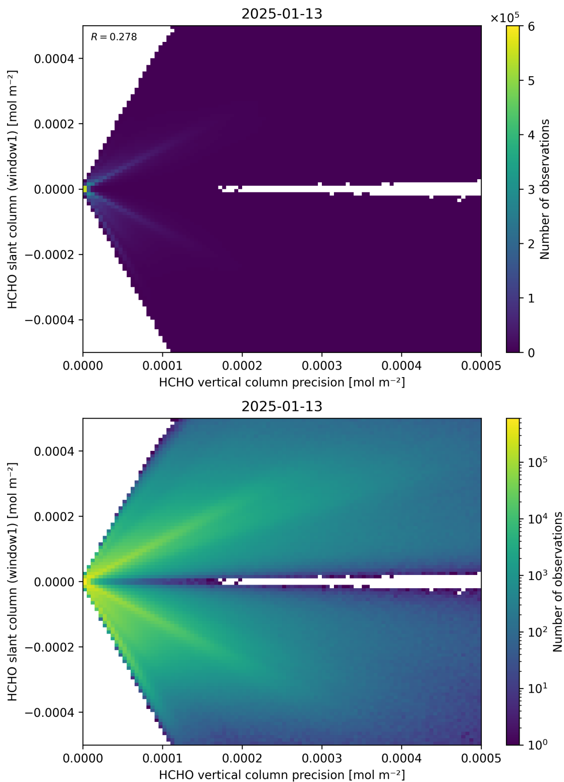
Figure 142: Scatter density plot of “HCHO vertical column precision” against “HCHO slant column (window1)” for 2025-01-12 to 2025-01-14.
