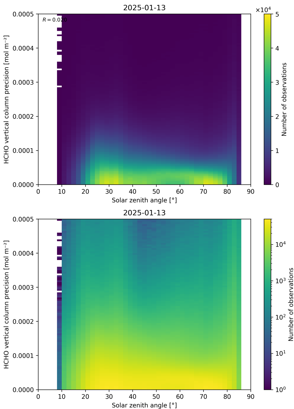
Figure 179: Scatter density plot of “Solar zenith angle” against “HCHO vertical column precision” for 2025-01-12 to 2025-01-14.
