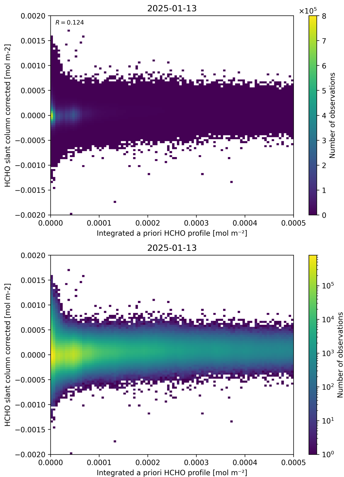
Figure 151: Scatter density plot of “Integrated a priori HCHO profile” against “HCHO slant column corrected” for 2025-01-12 to 2025-01-14.
