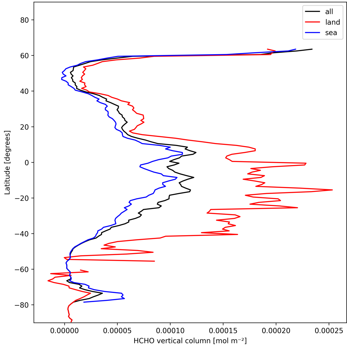
Figure 21: Zonal average of “HCHO vertical column” for 2025-01-12 to 2025-01-14.
