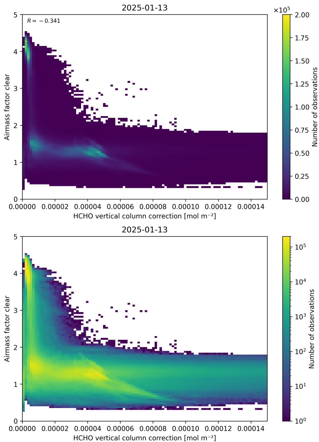
Figure 115: Scatter density plot of “HCHO vertical column correction” against “Airmass factor clear” for 2025-01-12 to 2025-01-14.
