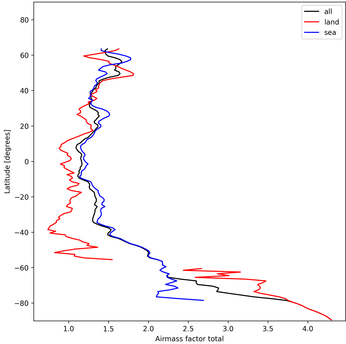
Figure 26: Zonal average of “Airmass factor total” for 2025-01-12 to 2025-01-14.
