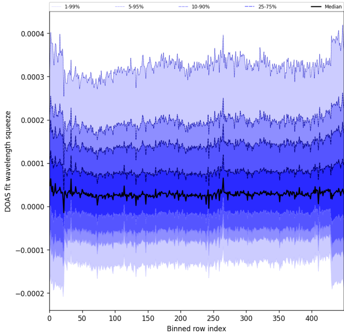
Figure 59: Along track statistics of “DOAS fit wavelength squeeze” for 2025-01-12 to 2025-01-14
