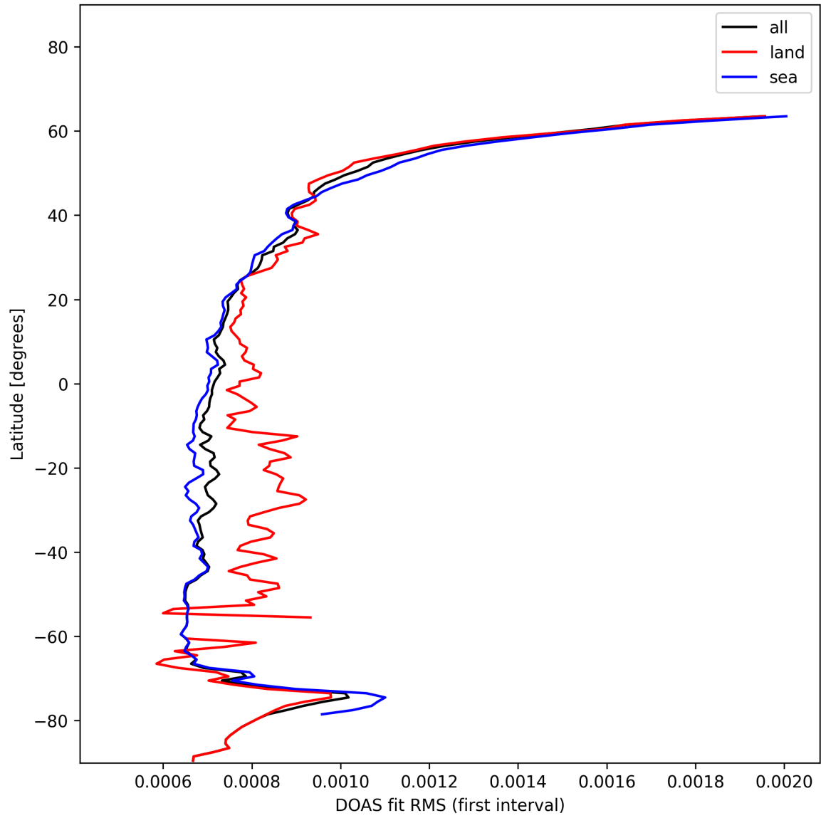
Figure 32: Zonal average of “DOAS fit RMS (first interval)” for 2025-01-12 to 2025-01-14.
