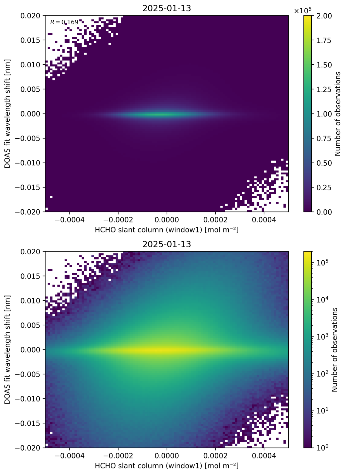
Figure 79: Scatter density plot of “HCHO slant column (window1)” against “DOAS fit wavelength shift” for 2025-01-12 to 2025-01-14.
