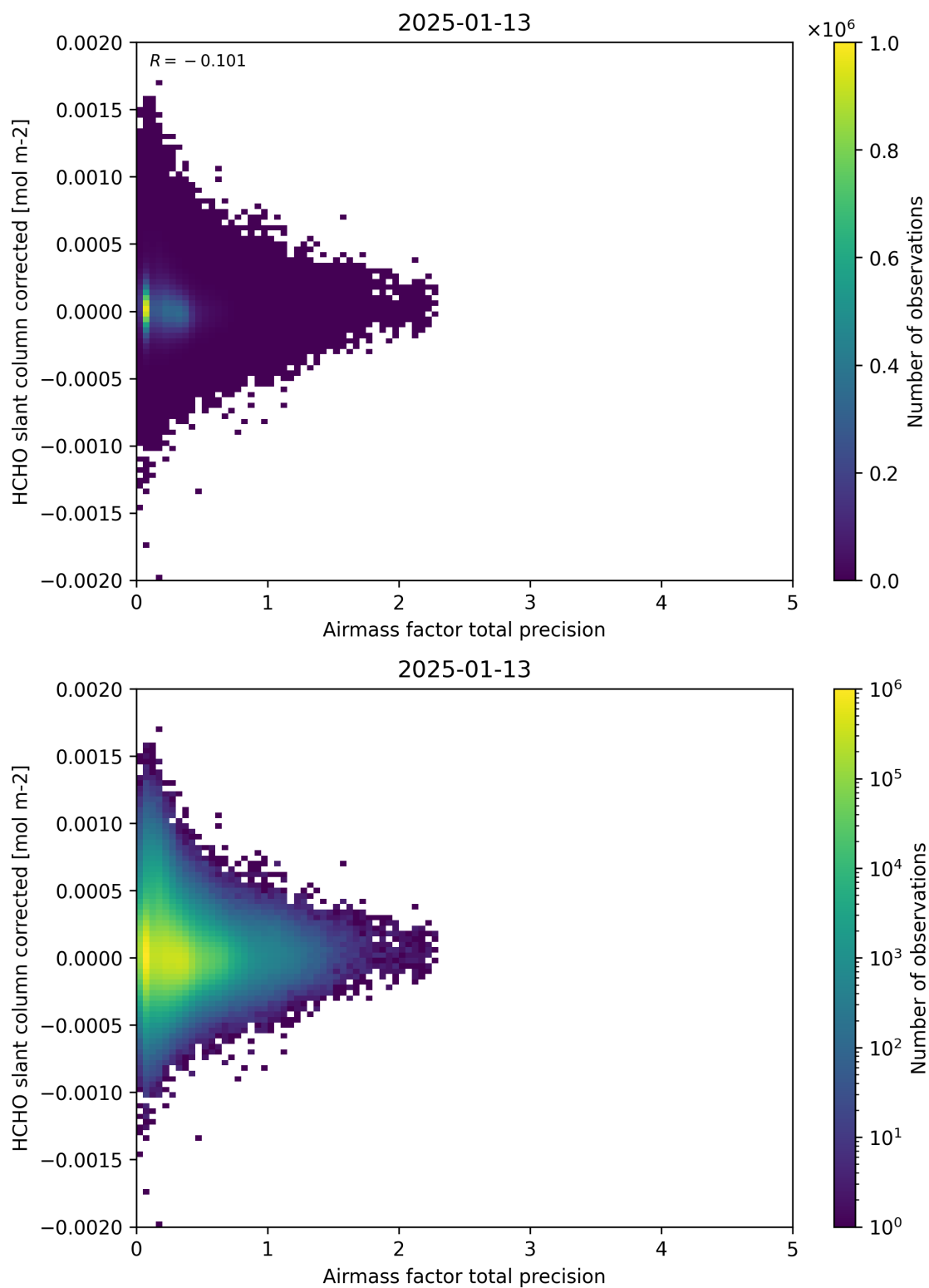
Figure 109: Scatter density plot of “Airmass factor total precision” against “HCHO slant column corrected” for 2025-01-12 to 2025-01-14.
