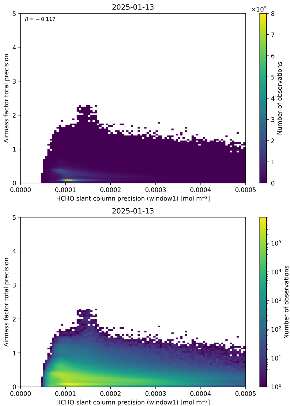
Figure 95: Scatter density plot of “HCHO slant column precision (window1)” against “Airmass factor total precision” for 2025-01-12 to 2025-01-14.
