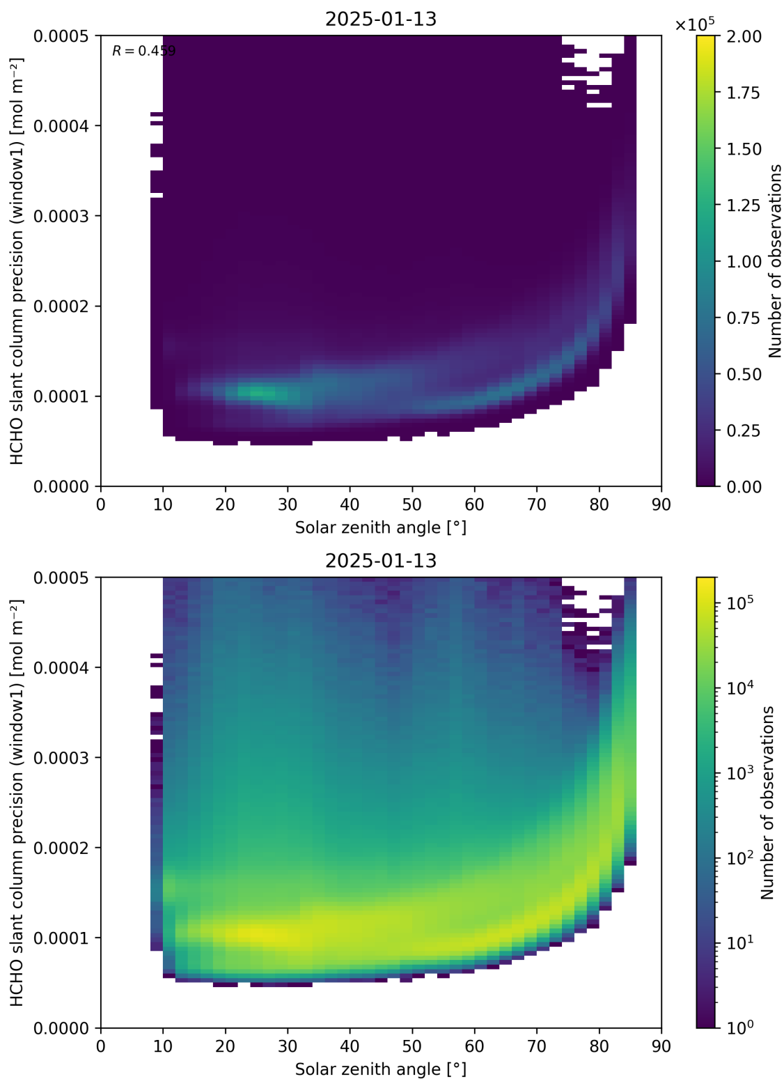
Figure 174: Scatter density plot of “Solar zenith angle” against “HCHO slant column precision (window1)” for 2025-01-12 to 2025-01-14.
