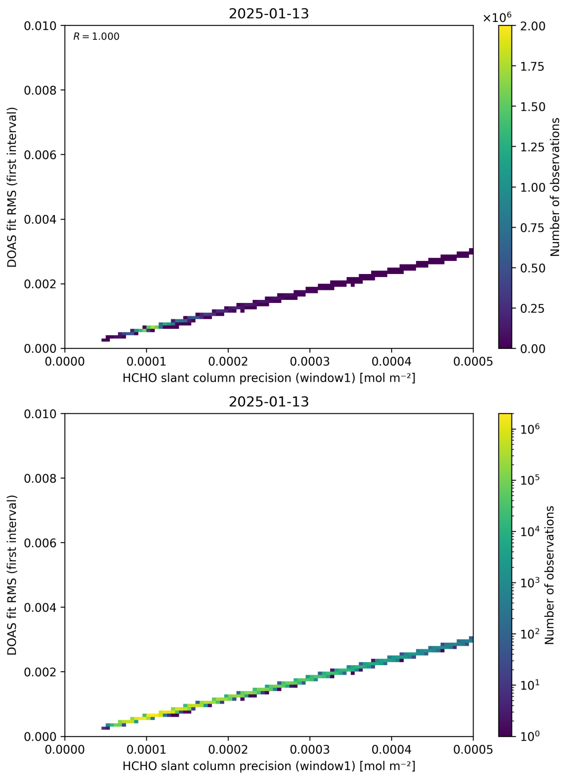
Figure 88: Scatter density plot of “HCHO slant column precision (window1)” against “DOAS fit RMS (first interval)” for 2025-01-12 to 2025-01-14.
