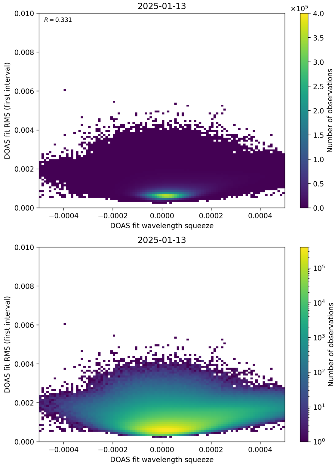
Figure 68: Scatter density plot of “DOAS fit wavelength squeeze” against “DOAS fit RMS (first interval)” for 2025-01-12 to 2025-01-14.
