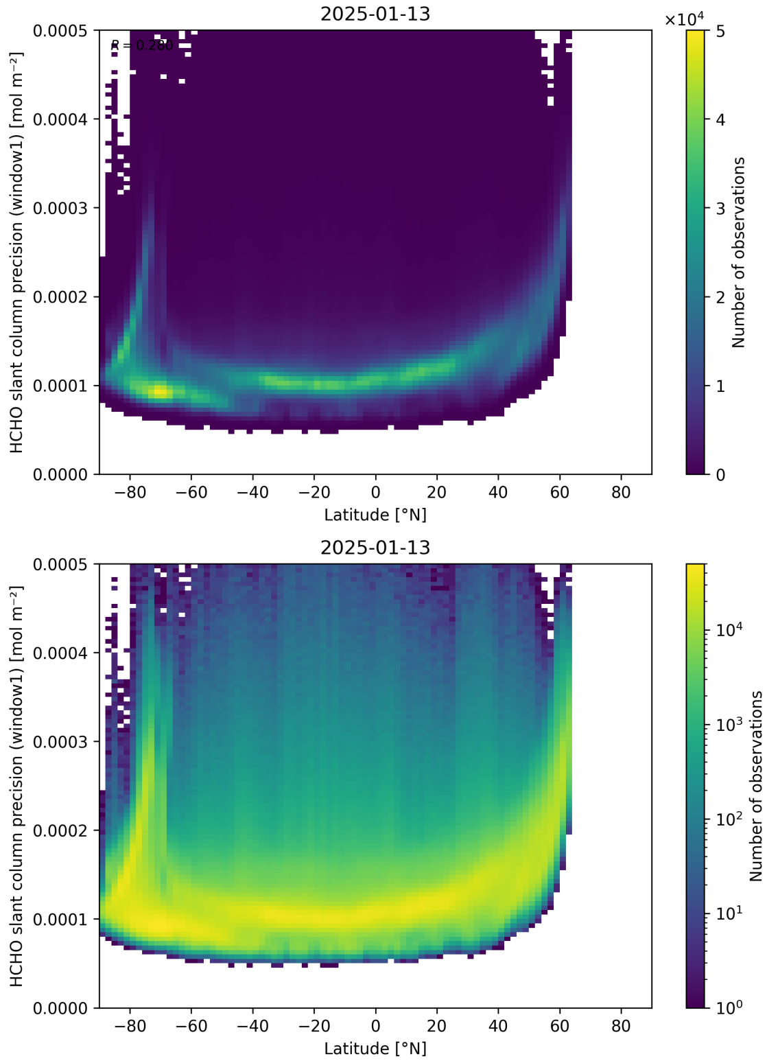
Figure 160: Scatter density plot of “Latitude” against “HCHO slant column precision (window1)” for 2025-01-12 to 2025-01-14.
