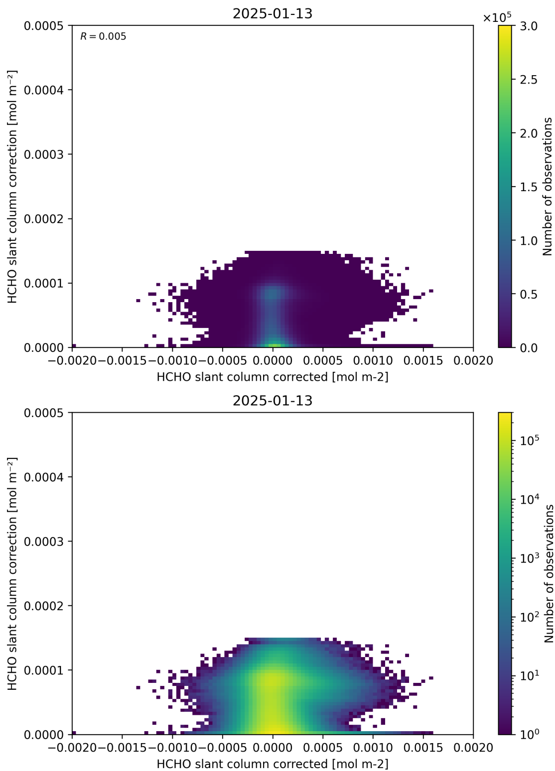
Figure 77: Scatter density plot of “HCHO slant column corrected” against “HCHO slant column correction” for 2025-01-12 to 2025-01-14.
