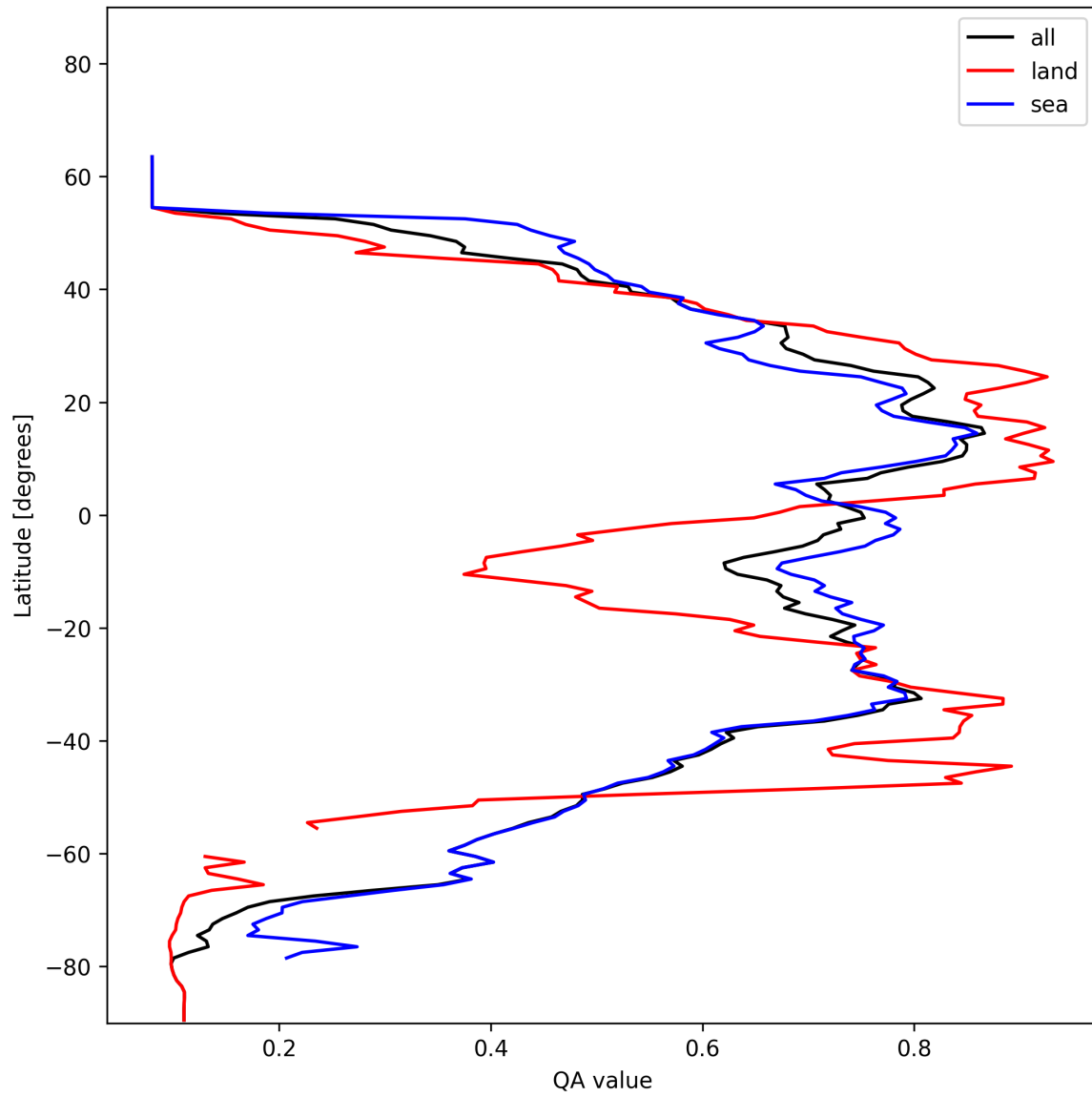
Figure 20: Zonal average of “QA value” for 2025-01-12 to 2025-01-14.
