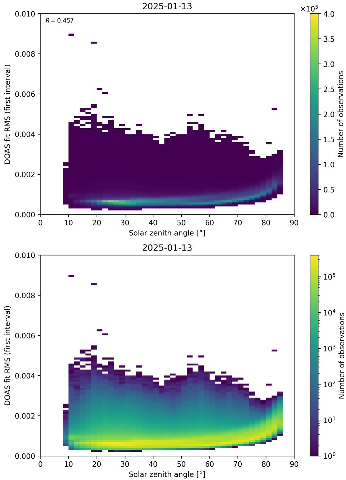
Figure 167: Scatter density plot of “Solar zenith angle” against “DOAS fit RMS (first interval)” for 2025-01-12 to 2025-01-14.
