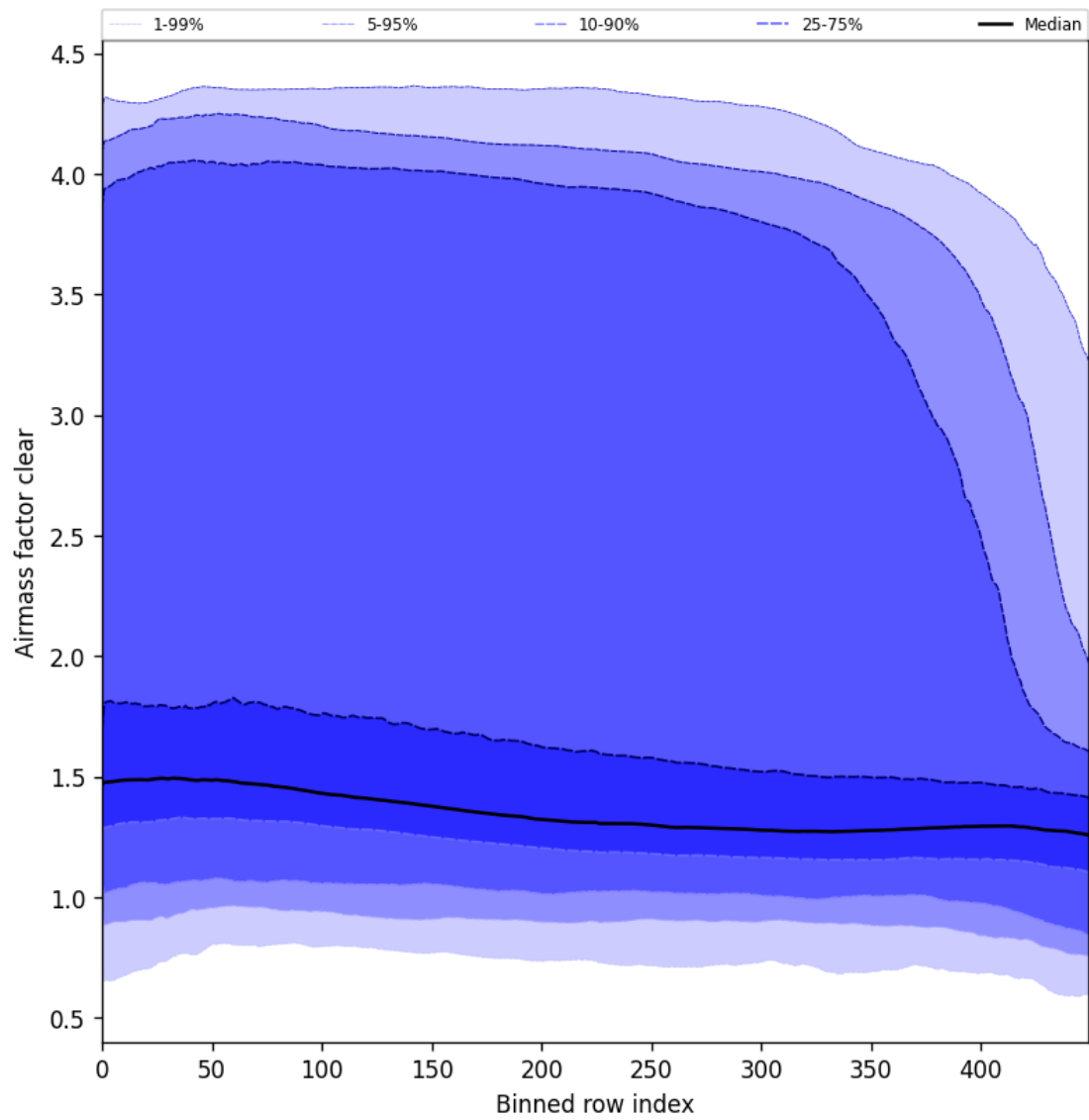
Figure 56: Along track statistics of “Airmass factor clear” for 2025-01-12 to 2025-01-14
