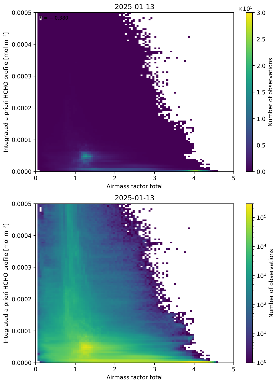
Figure 104: Scatter density plot of “Airmass factor total” against “Integrated a priori HCHO profile” for 2025-01-12 to 2025-01-14.
