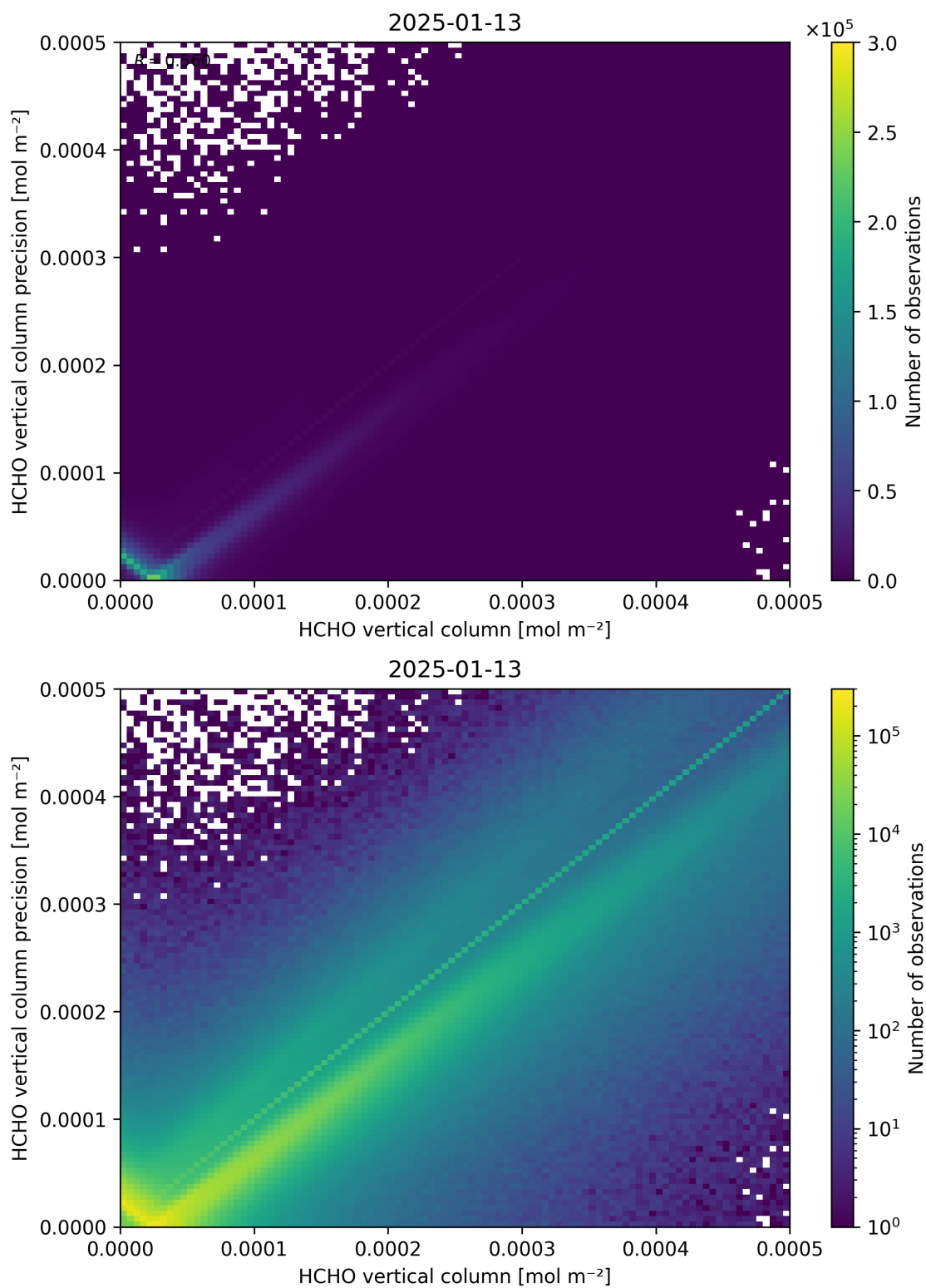
Figure 134: Scatter density plot of “HCHO vertical column” against “HCHO vertical column precision” for 2025-01-12 to 2025-01-14.
