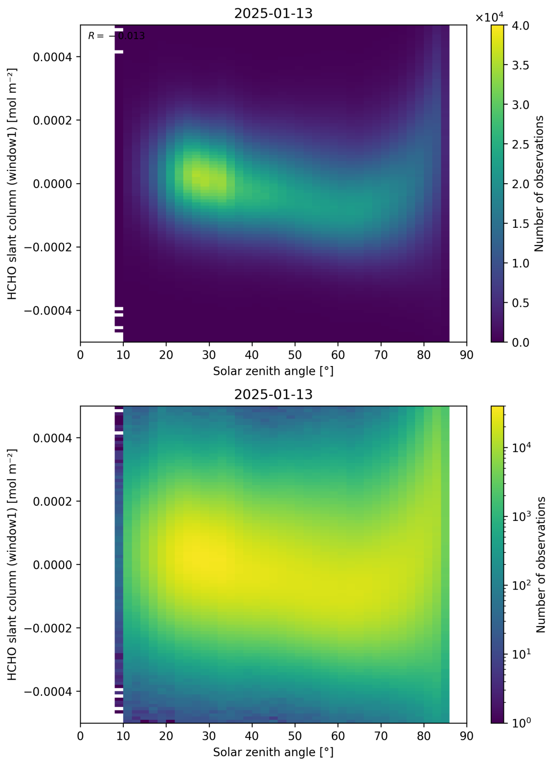
Figure 173: Scatter density plot of “Solar zenith angle” against “HCHO slant column (window1)” for 2025-01-12 to 2025-01-14.
