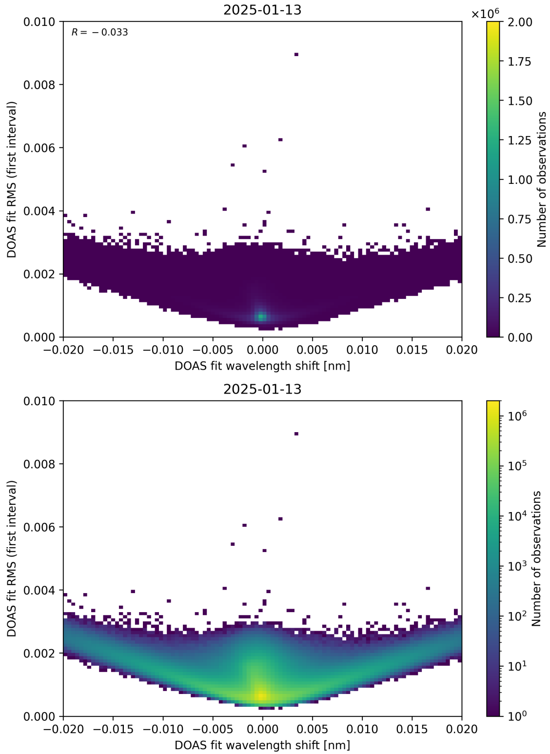
Figure 64: Scatter density plot of “DOAS fit wavelength shift” against “DOAS fit RMS (first interval)” for 2025-01-12 to 2025-01-14.
