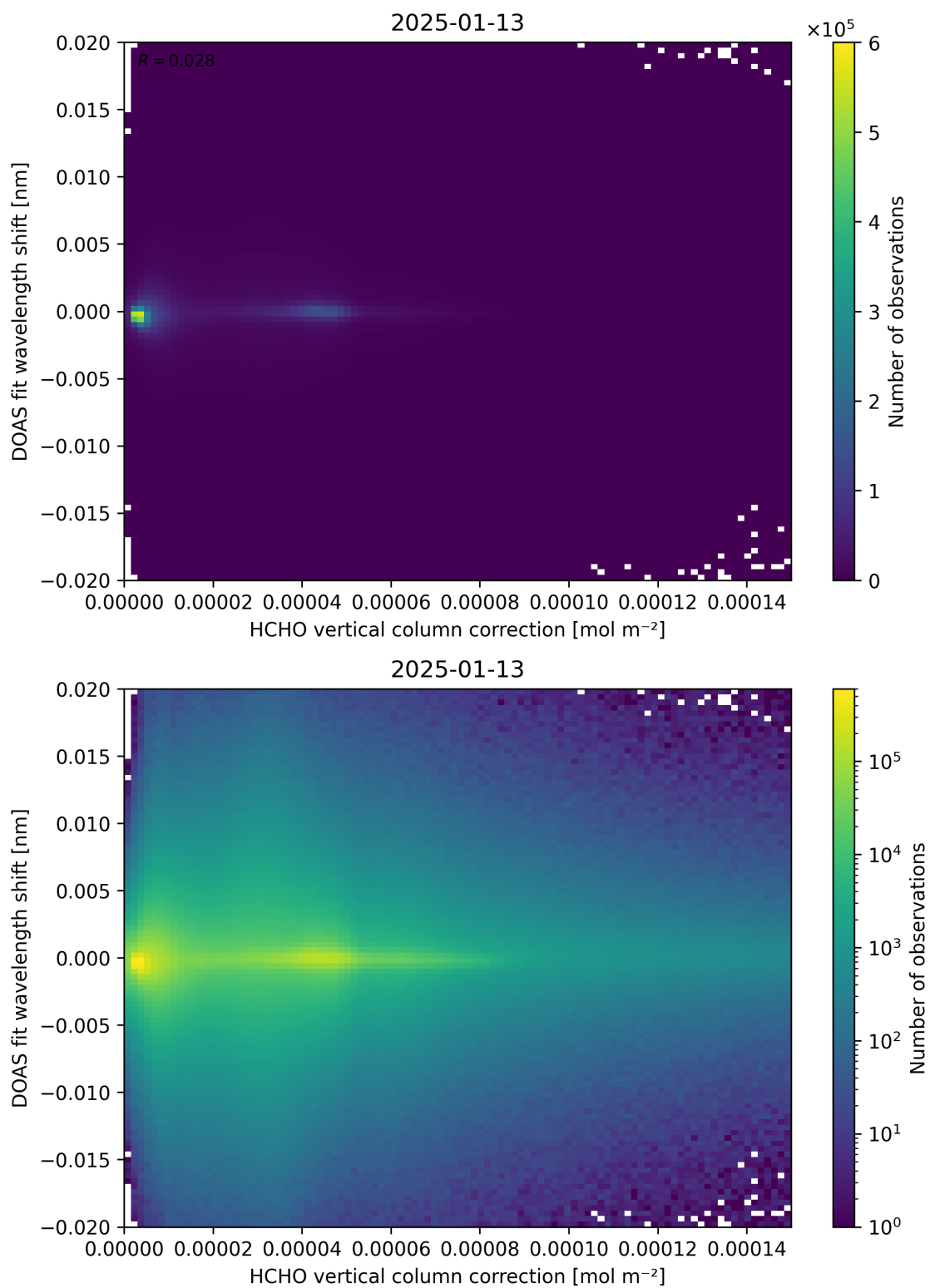
Figure 113: Scatter density plot of “HCHO vertical column correction” against “DOAS fit wavelength shift” for 2025-01-12 to 2025-01-14.
