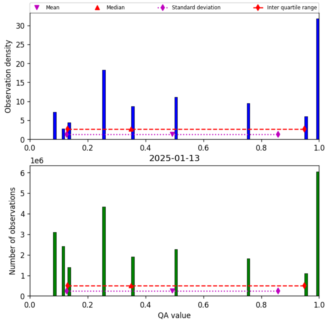
Figure 34: Histogram of “QA value” for 2025-01-12 to 2025-01-14
