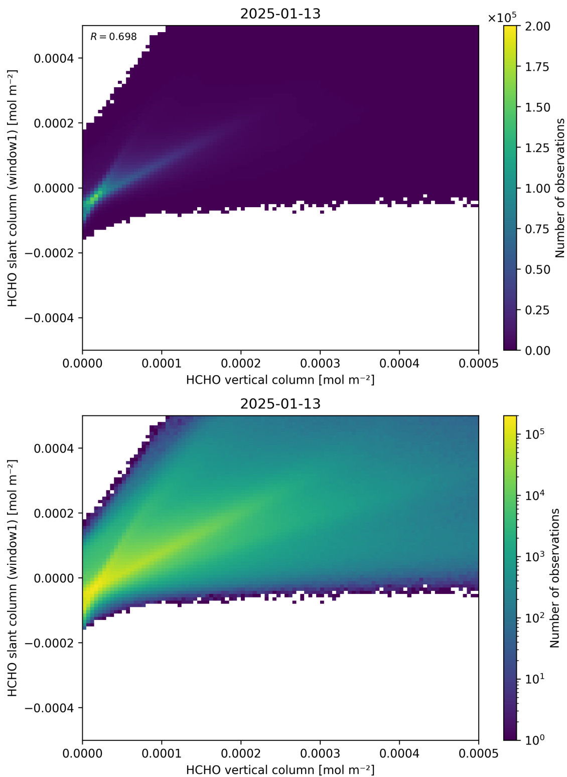
Figure 129: Scatter density plot of “HCHO vertical column” against “HCHO slant column (window1)” for 2025-01-12 to 2025-01-14.
