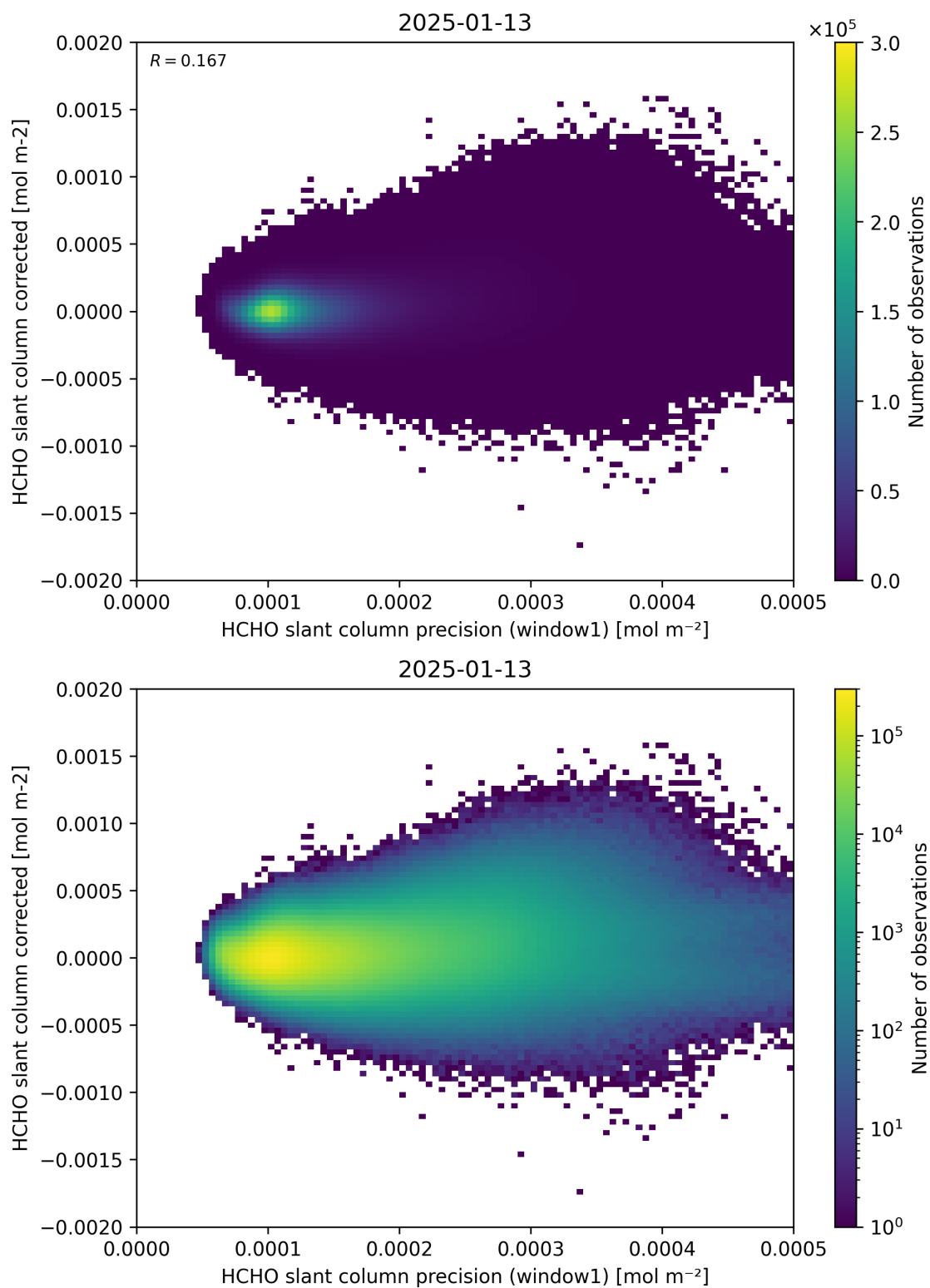
Figure 92: Scatter density plot of “HCHO slant column precision (window1)” against “HCHO slant column corrected” for 2025-01-12 to 2025-01-14.
