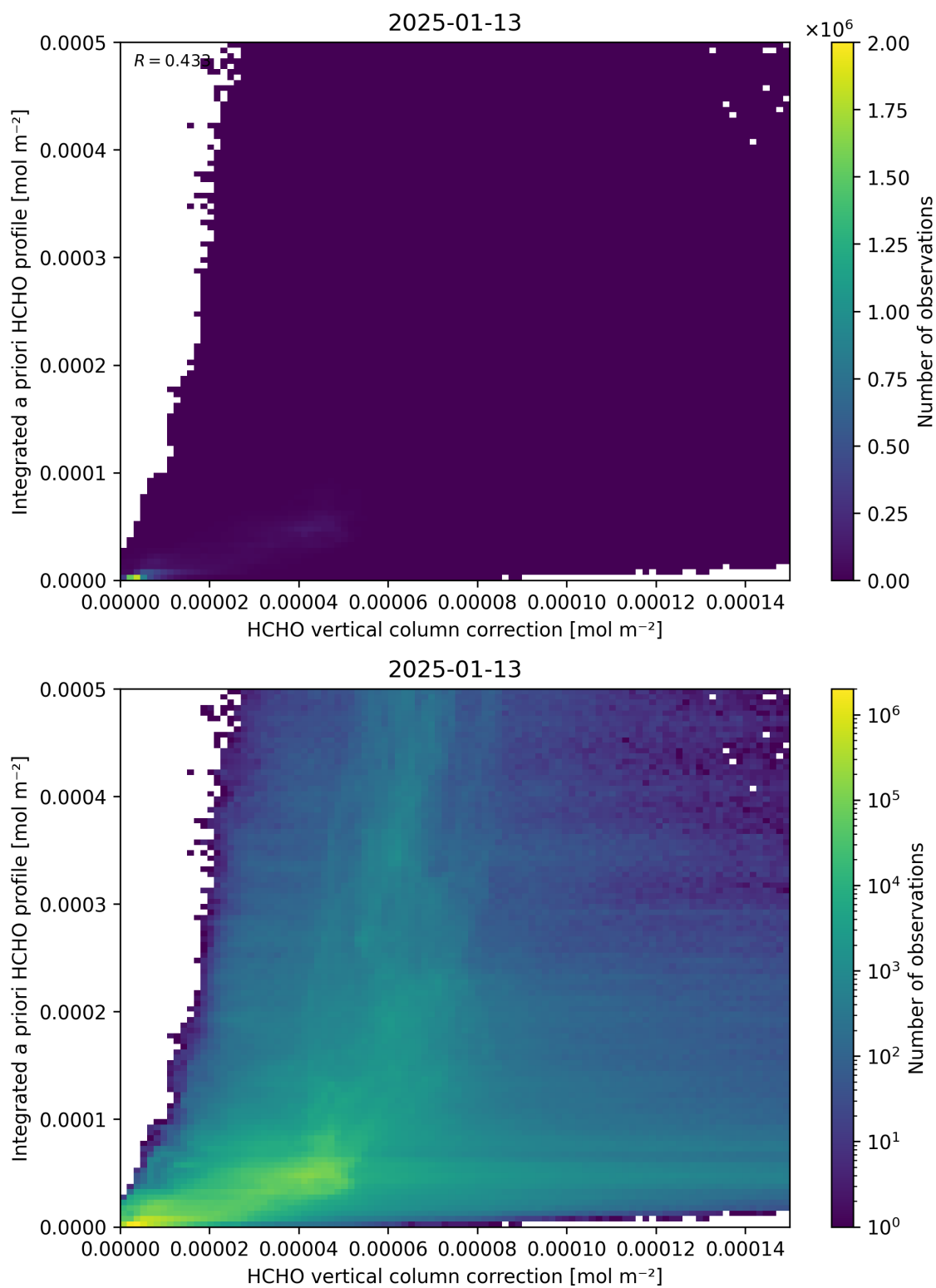
Figure 122: Scatter density plot of “HCHO vertical column correction” against “Integrated a priori HCHO profile” for 2025-01-12 to 2025-01-14.
