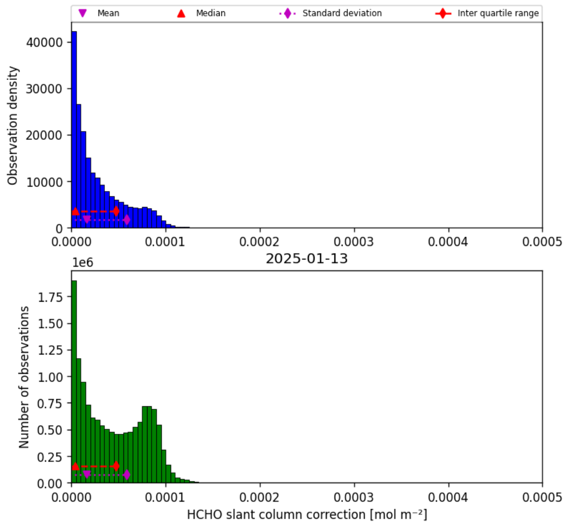
Figure 47: Histogram of “HCHO slant column correction” for 2025-01-12 to 2025-01-14
