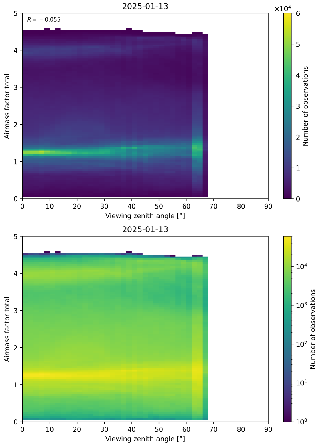
Figure 190: Scatter density plot of “Viewing zenith angle” against “Airmass factor total” for 2025-01-12 to 2025-01-14.
