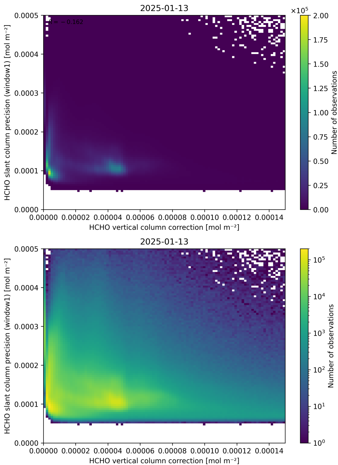
Figure 119: Scatter density plot of “HCHO vertical column correction” against “HCHO slant column precision (window1)” for 2025-01-12 to 2025-01-14.
