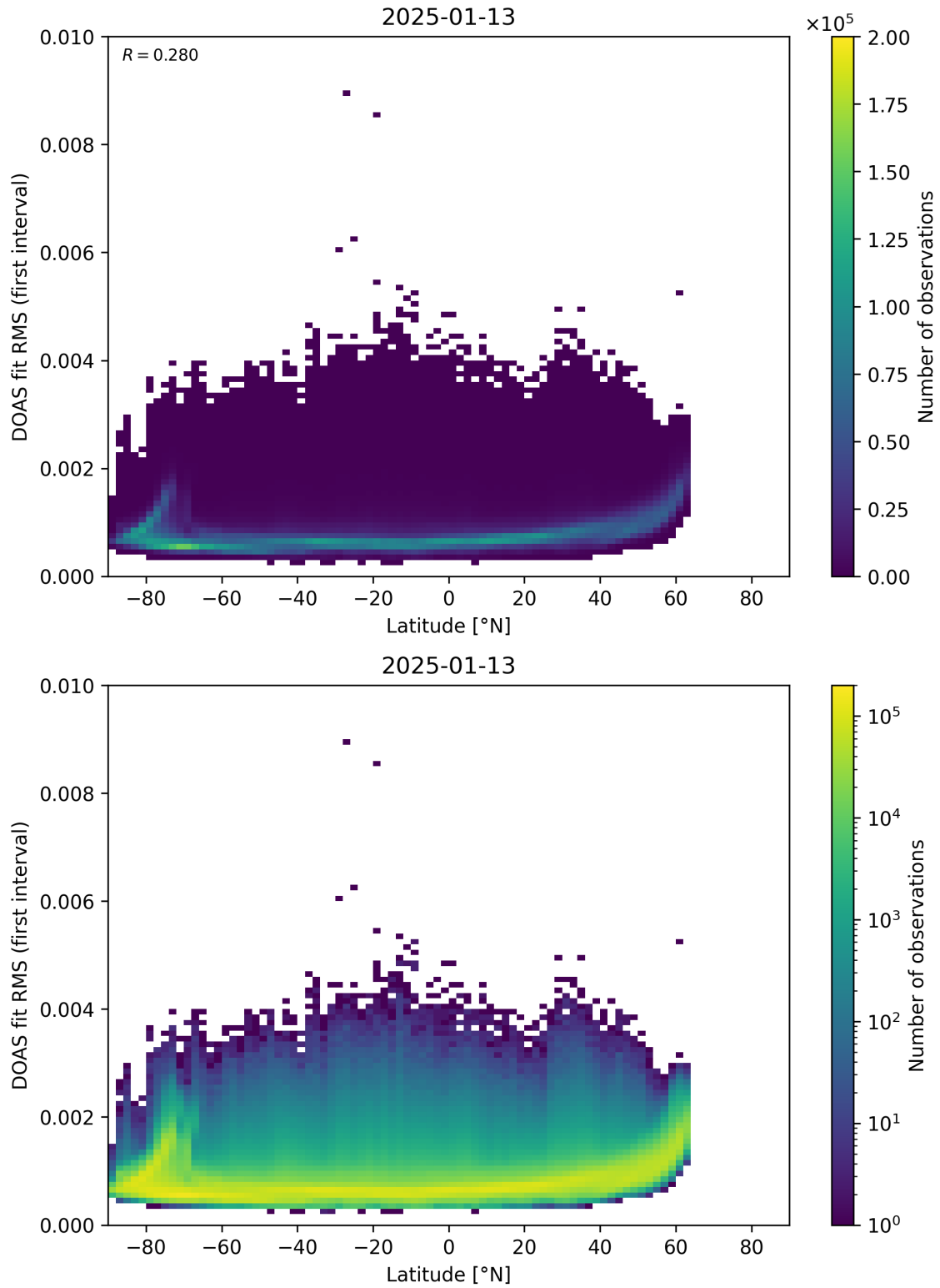
Figure 153: Scatter density plot of “Latitude” against “DOAS fit RMS (first interval)” for 2025-01-12 to 2025-01-14.
