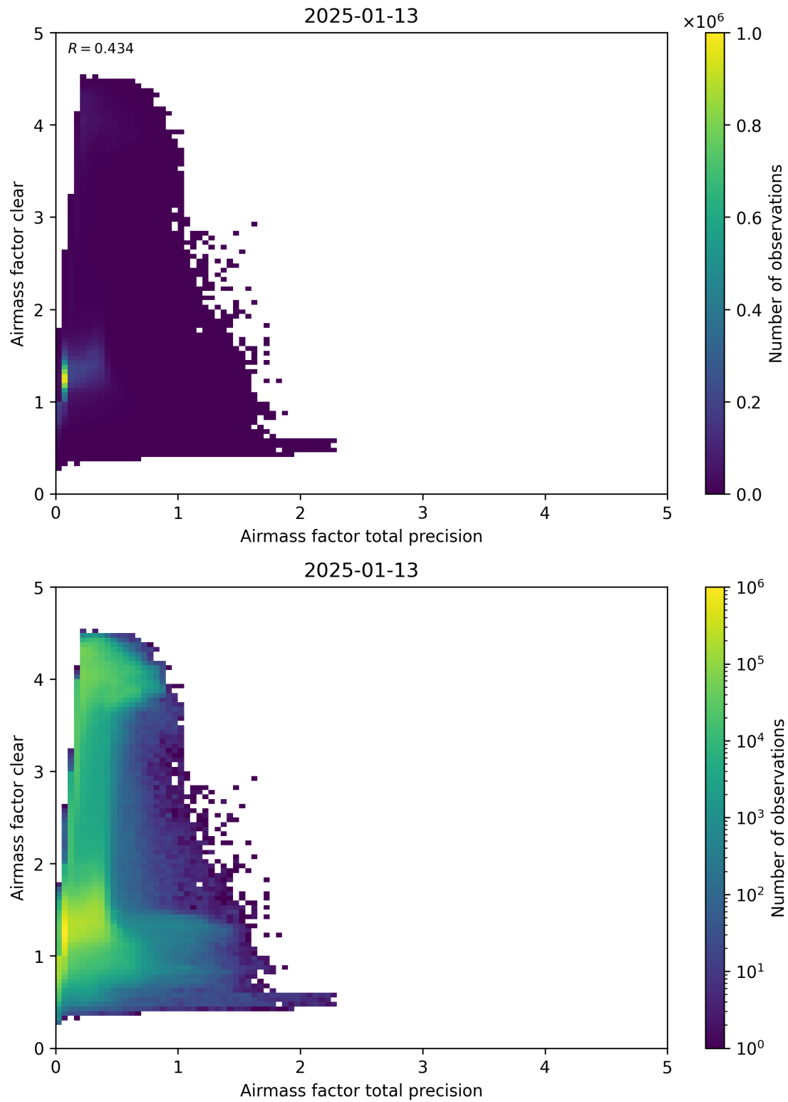
Figure 108: Scatter density plot of “Airmass factor total precision” against “Airmass factor clear” for 2025-01-12 to 2025-01-14.
