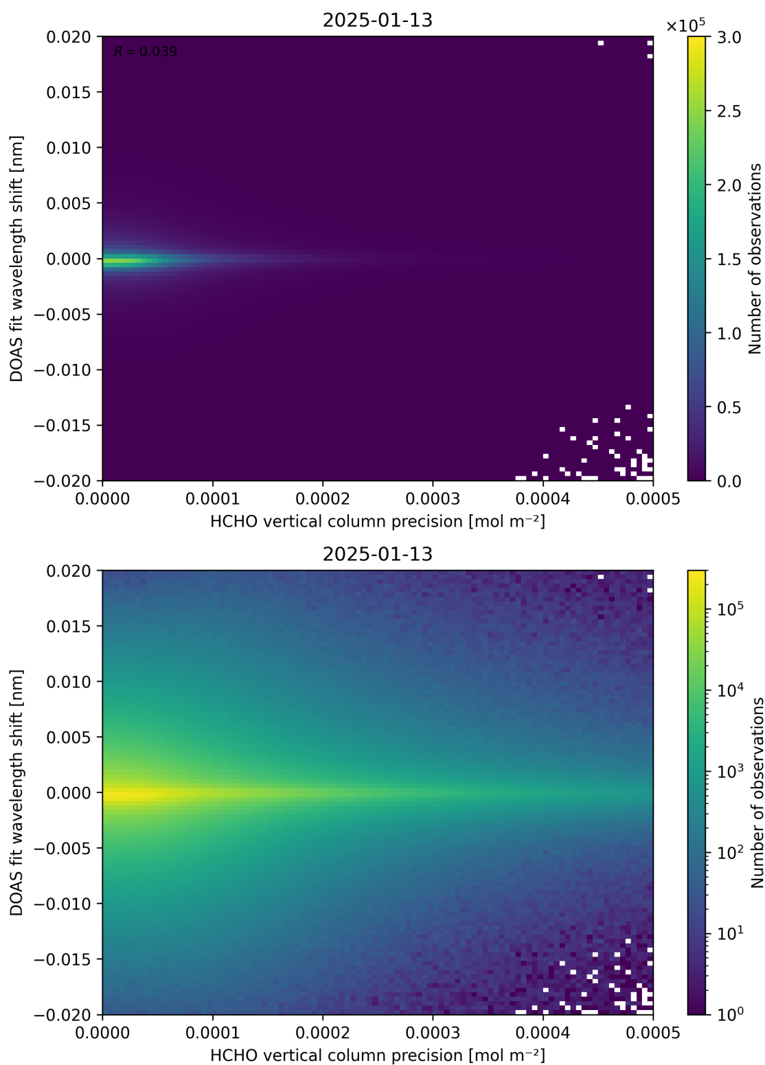
Figure 137: Scatter density plot of “HCHO vertical column precision” against “DOAS fit wavelength shift” for 2025-01-12 to 2025-01-14.
