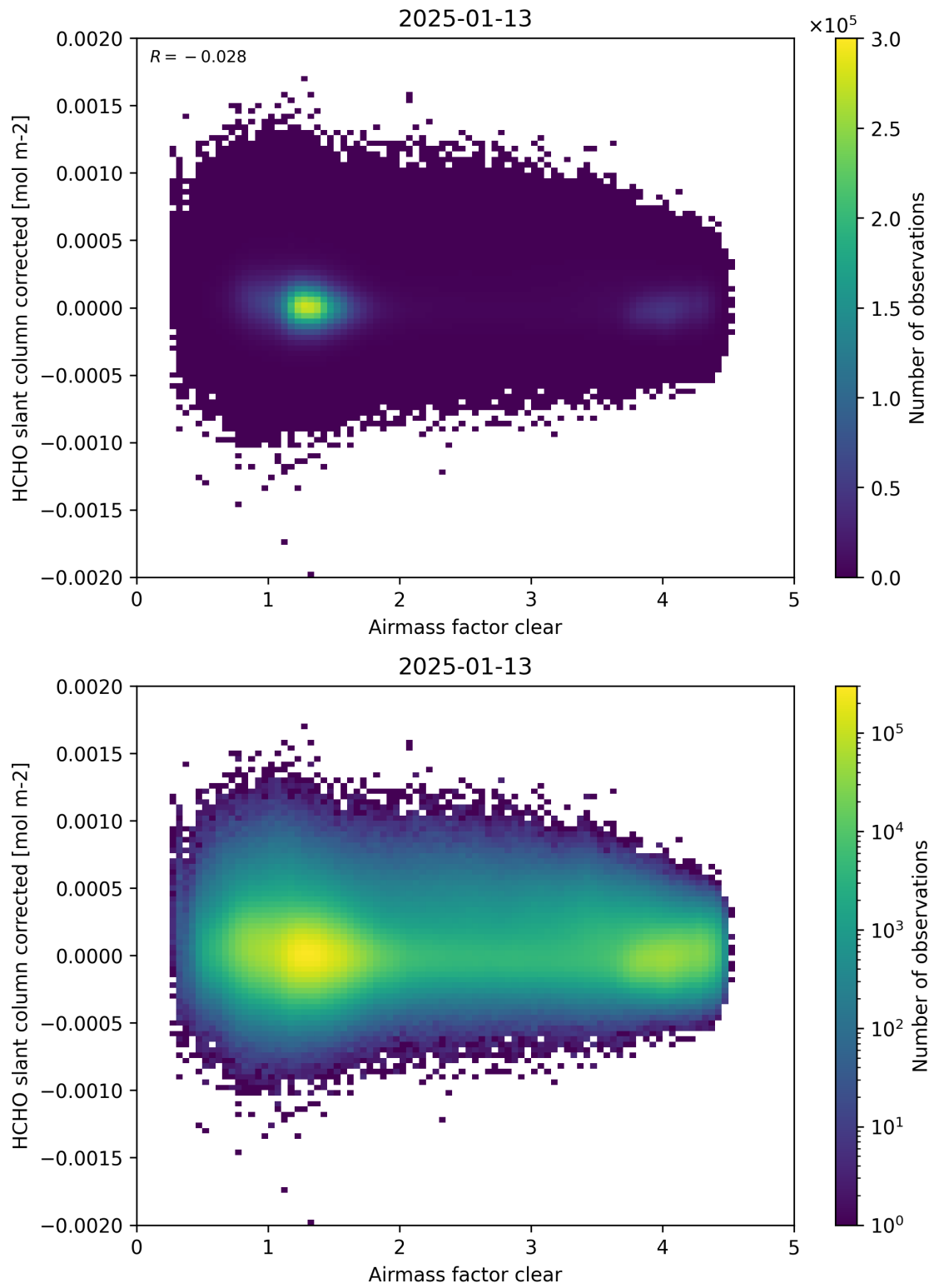
Figure 74: Scatter density plot of “Airmass factor clear” against “HCHO slant column corrected” for 2025-01-12 to 2025-01-14.
