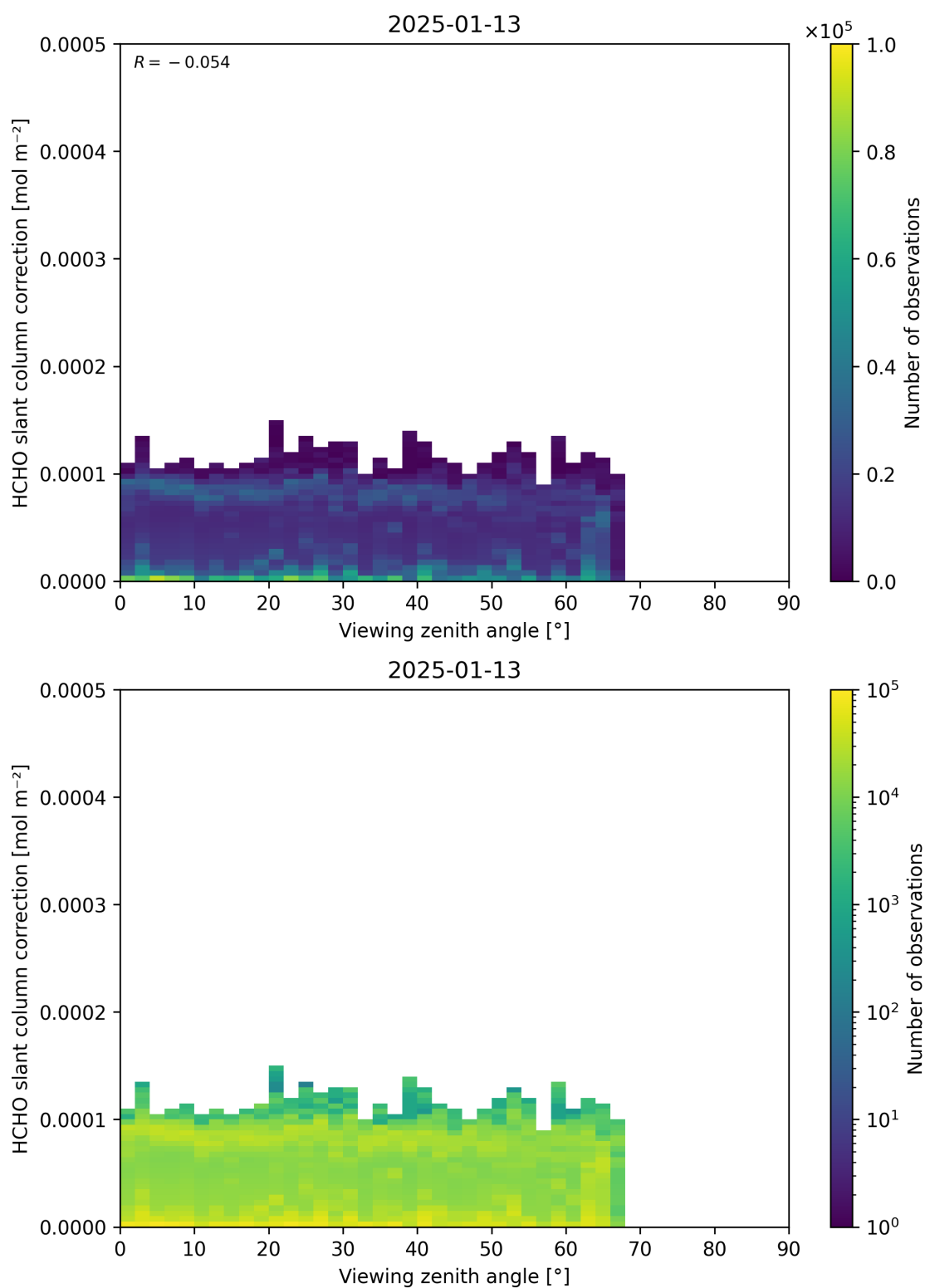
Figure 187: Scatter density plot of “Viewing zenith angle” against “HCHO slant column correction” for 2025-01-12 to 2025-01-14.
