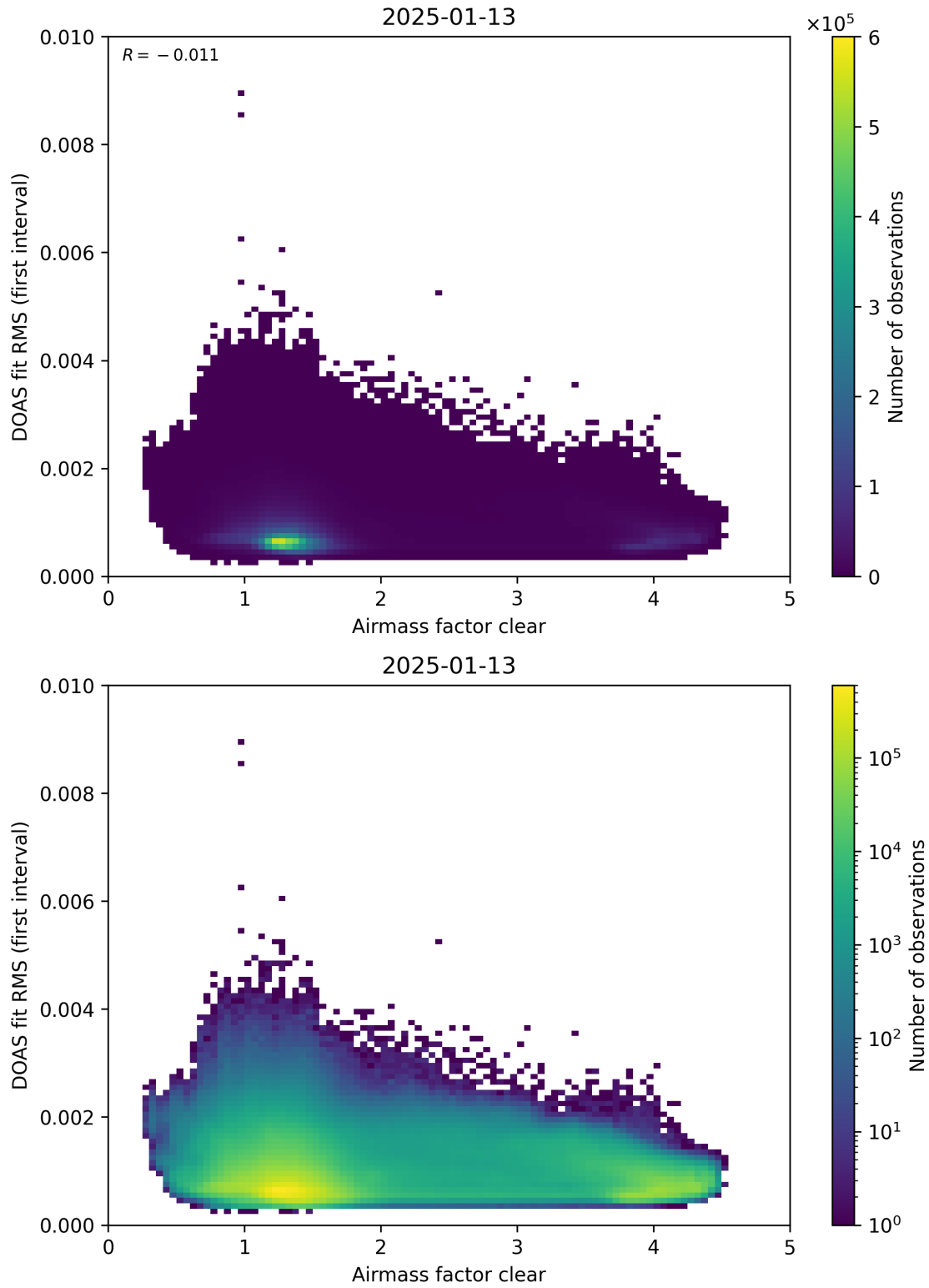
Figure 71: Scatter density plot of “Airmass factor clear” against “DOAS fit RMS (first interval)” for 2025-01-12 to 2025-01-14.
