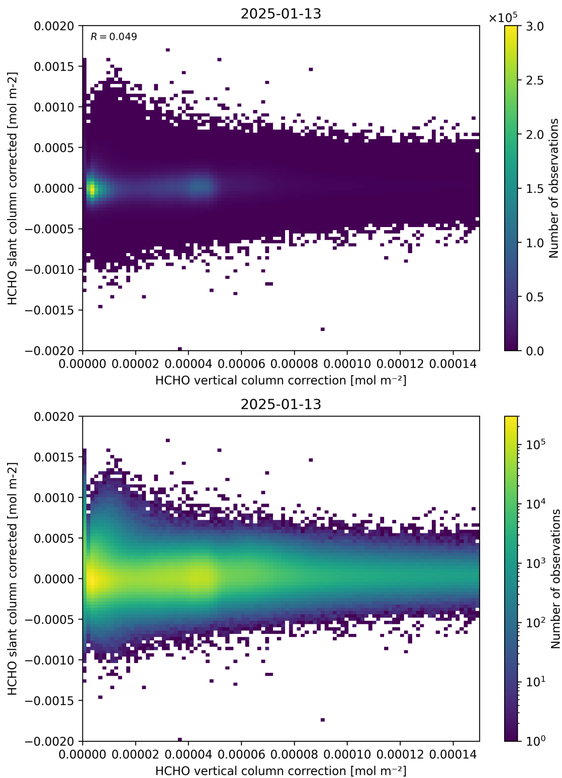
Figure 116: Scatter density plot of “HCHO vertical column correction” against “HCHO slant column corrected” for 2025-01-12 to 2025-01-14.
