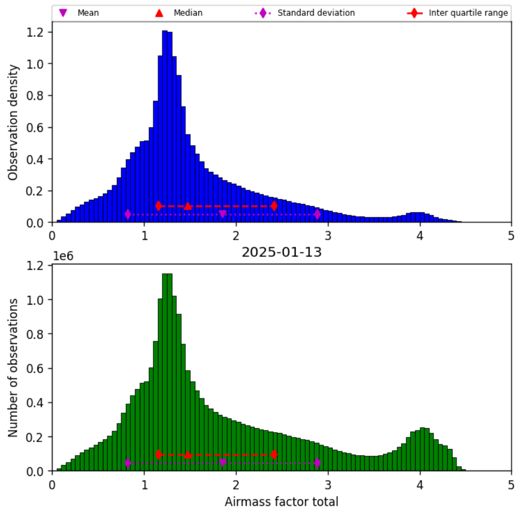
Figure 40: Histogram of “Airmass factor total” for 2025-01-12 to 2025-01-14
