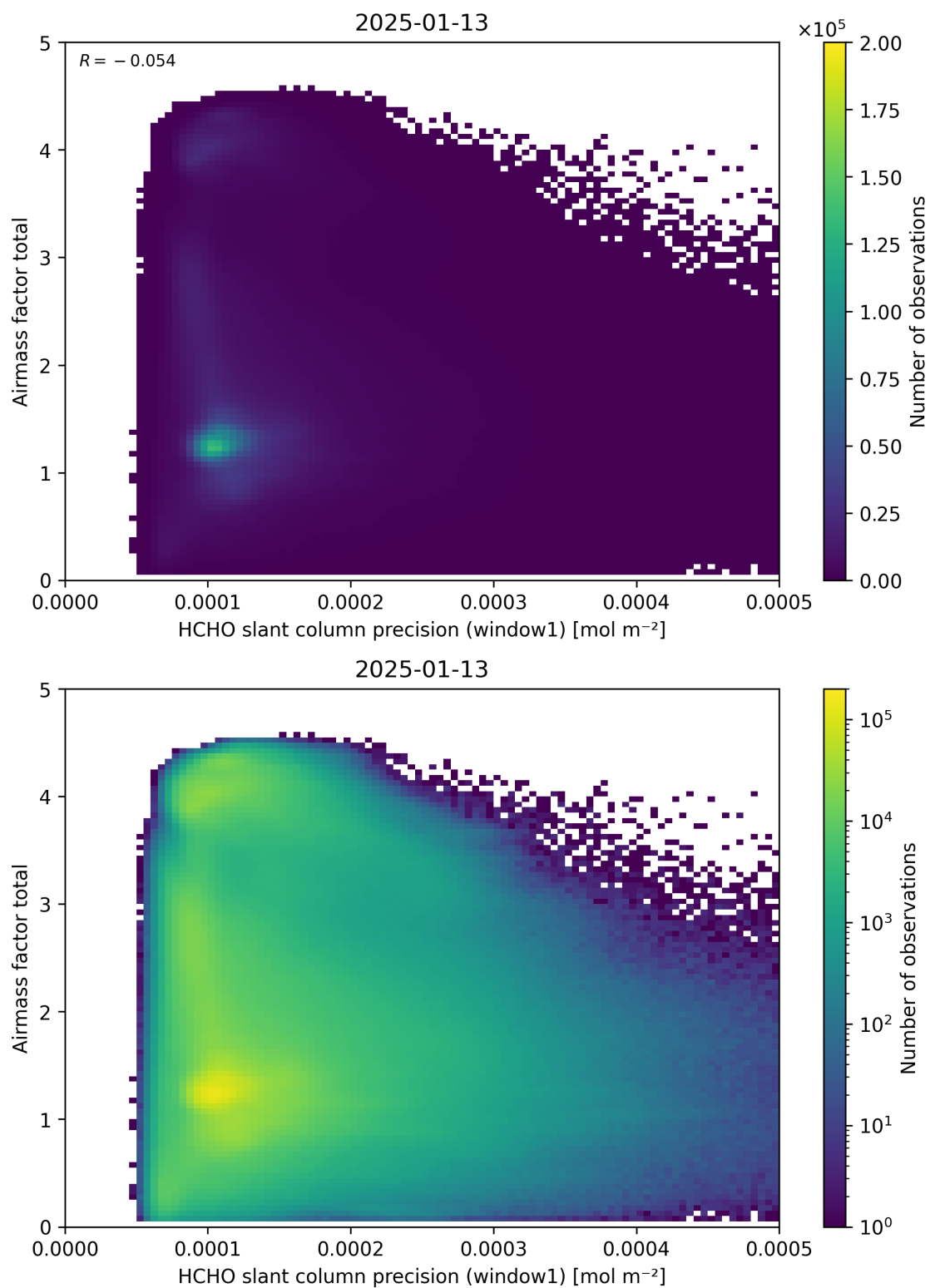
Figure 94: Scatter density plot of “HCHO slant column precision (window1)” against “Airmass factor total” for 2025-01-12 to 2025-01-14.
