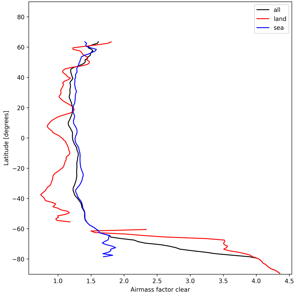
Figure 28: Zonal average of “Airmass factor clear” for 2025-01-12 to 2025-01-14.
