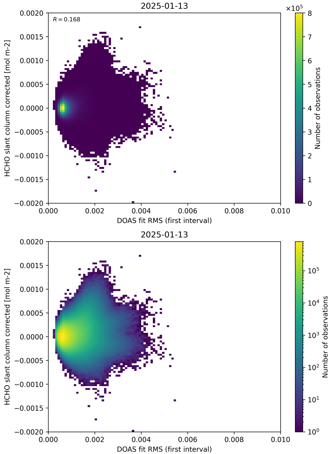
Figure 62: Scatter density plot of “DOAS fit RMS (first interval)” against “HCHO slant column corrected” for 2025-01-12 to 2025-01-14.
