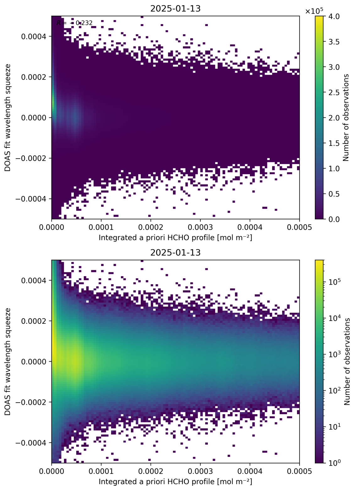
Figure 150: Scatter density plot of “Integrated a priori HCHO profile” against “DOAS fit wavelength squeeze” for 2025-01-12 to 2025-01-14.
