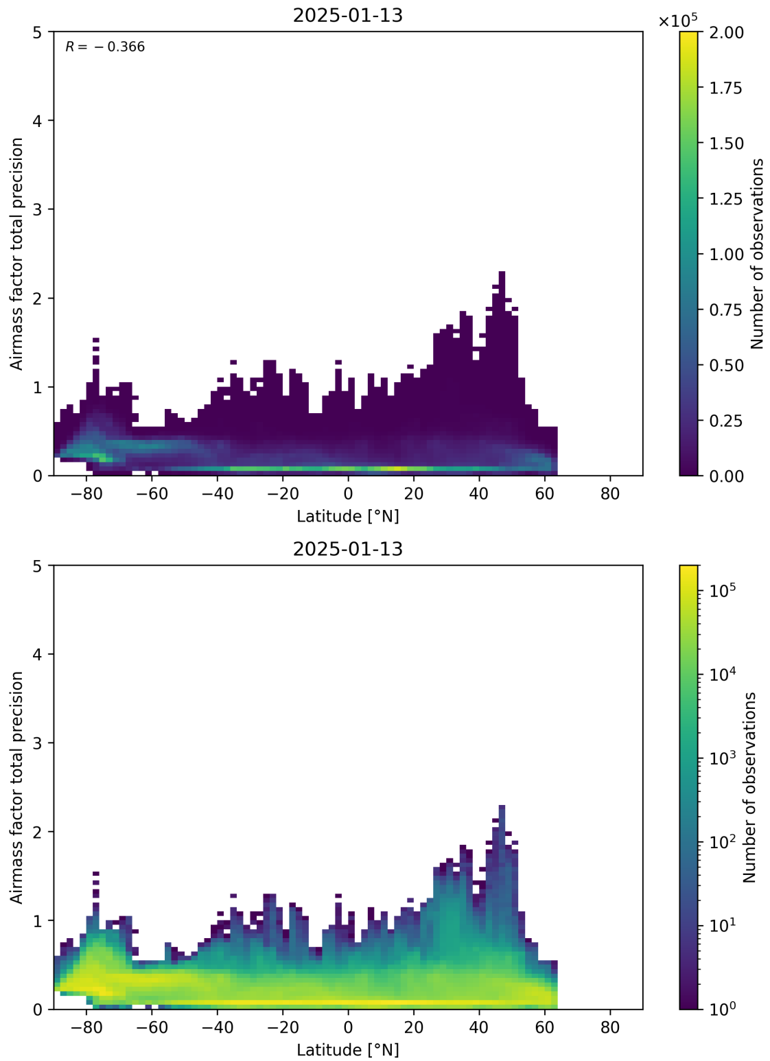
Figure 162: Scatter density plot of “Latitude” against “Airmass factor total precision” for 2025-01-12 to 2025-01-14.
