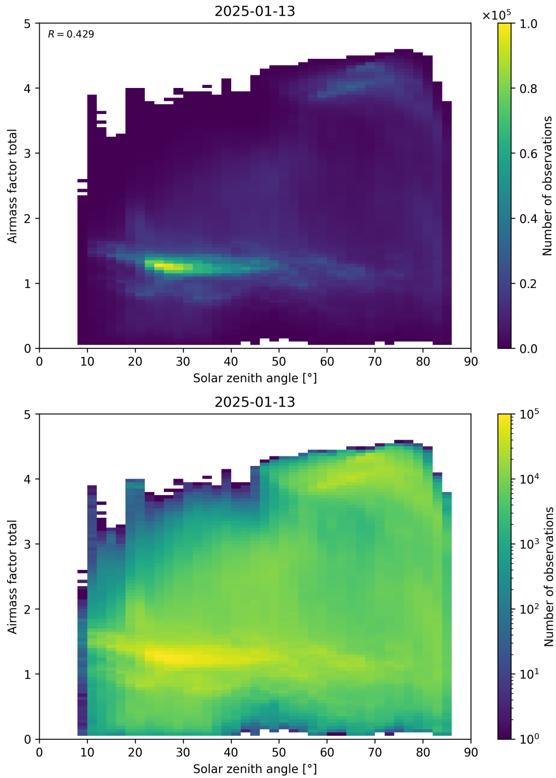
Figure 175: Scatter density plot of “Solar zenith angle” against “Airmass factor total” for 2025-01-12 to 2025-01-14.
