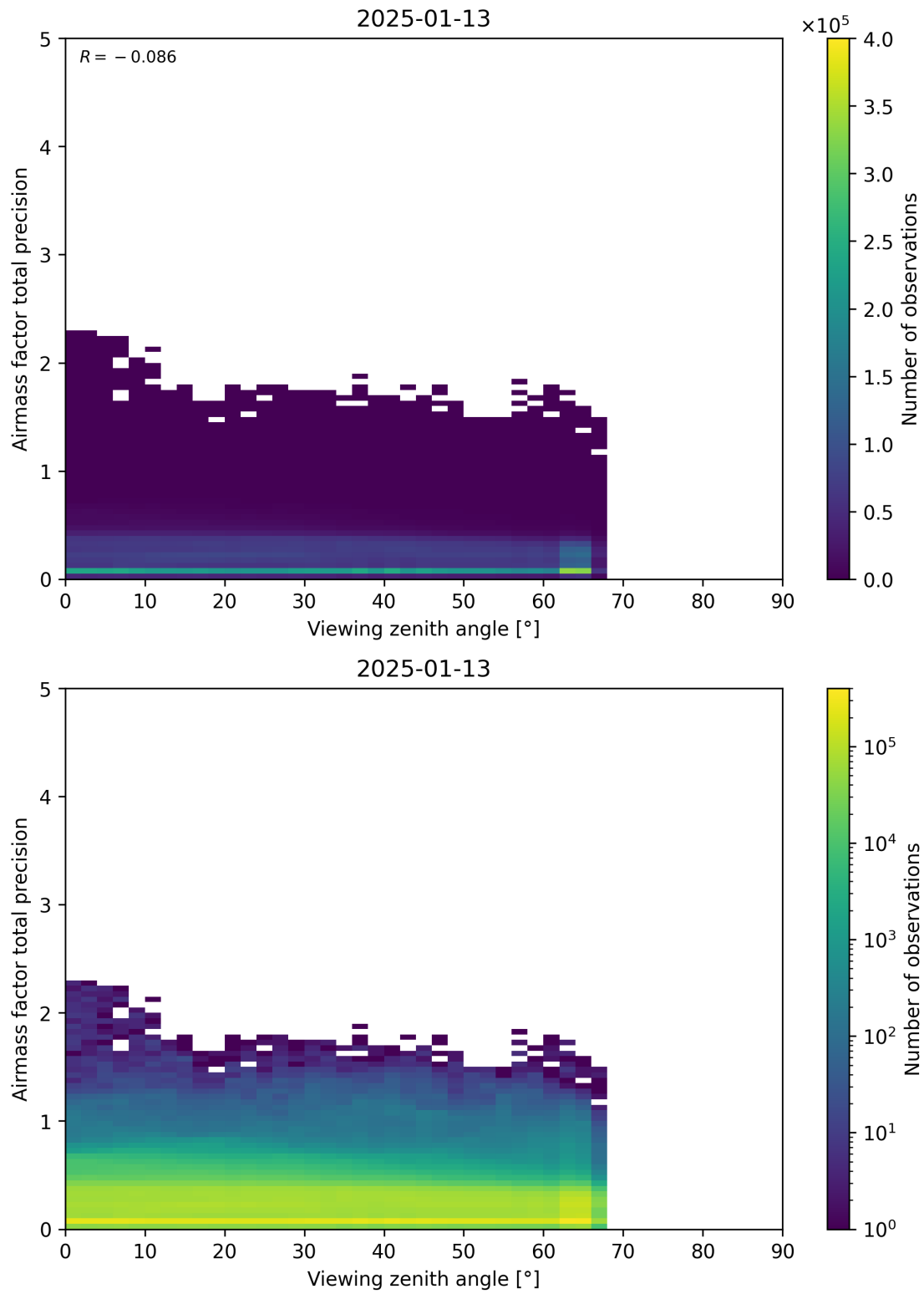
Figure 191: Scatter density plot of “Viewing zenith angle” against “Airmass factor total precision” for 2025-01-12 to 2025-01-14.
