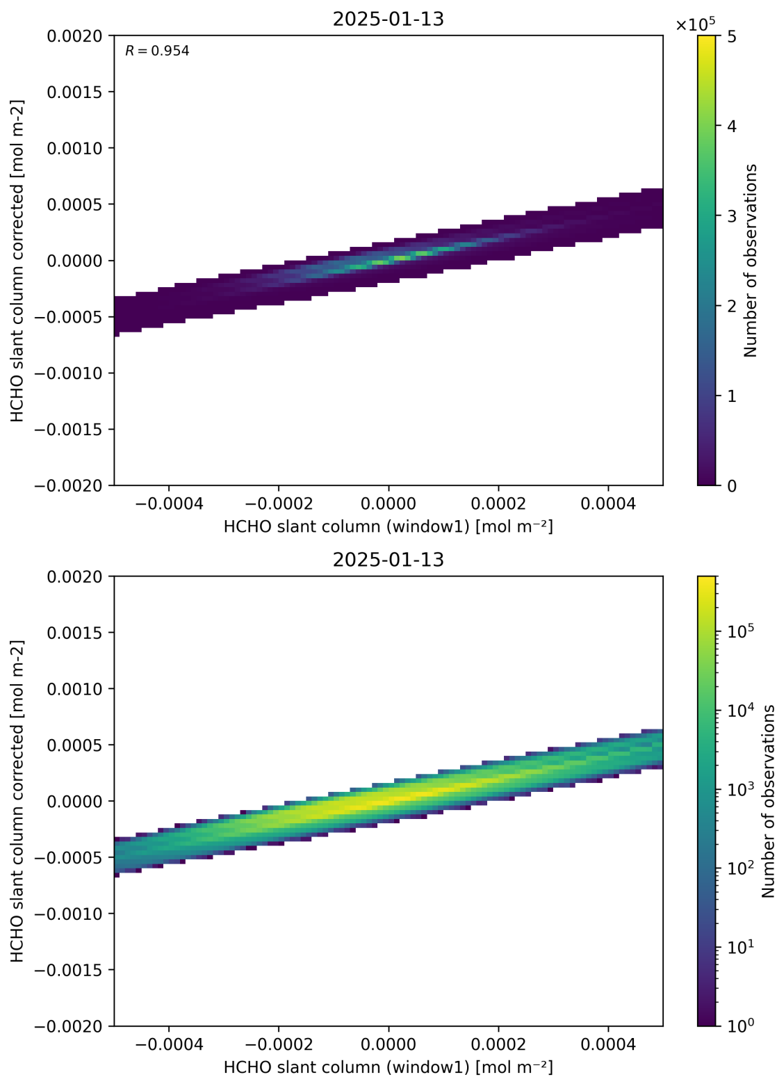
Figure 82: Scatter density plot of “HCHO slant column (window1)” against “HCHO slant column corrected” for 2025-01-12 to 2025-01-14.
