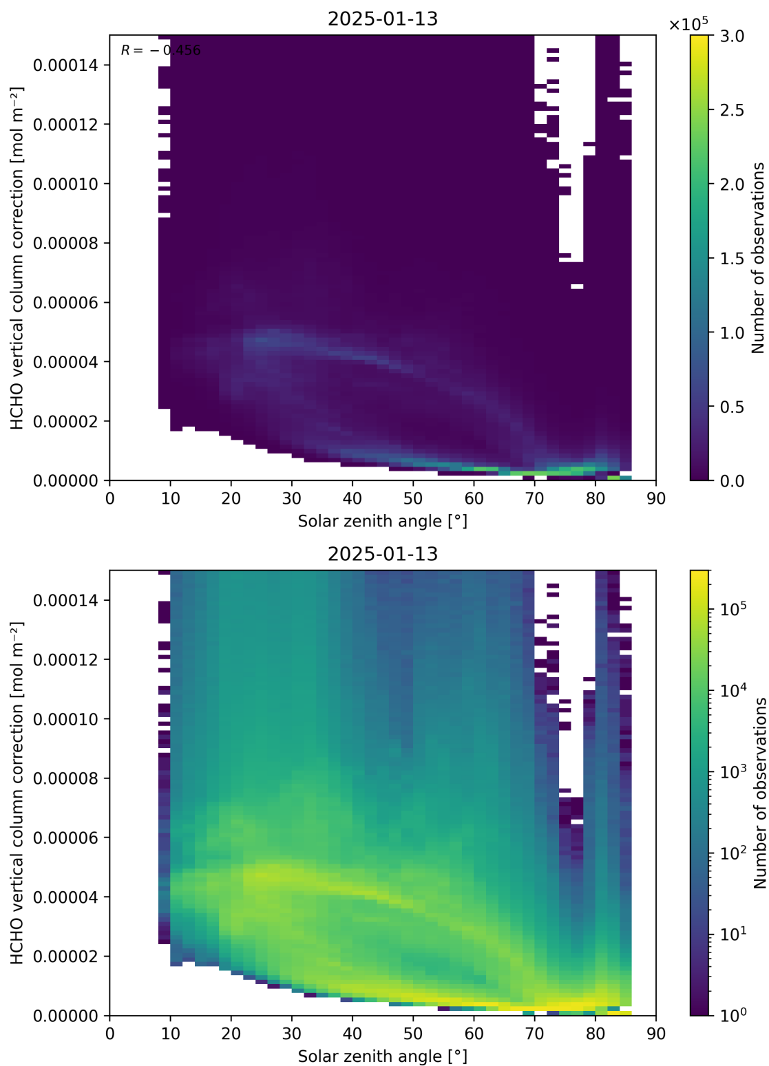
Figure 178: Scatter density plot of “Solar zenith angle” against “HCHO vertical column correction” for 2025-01-12 to 2025-01-14.
