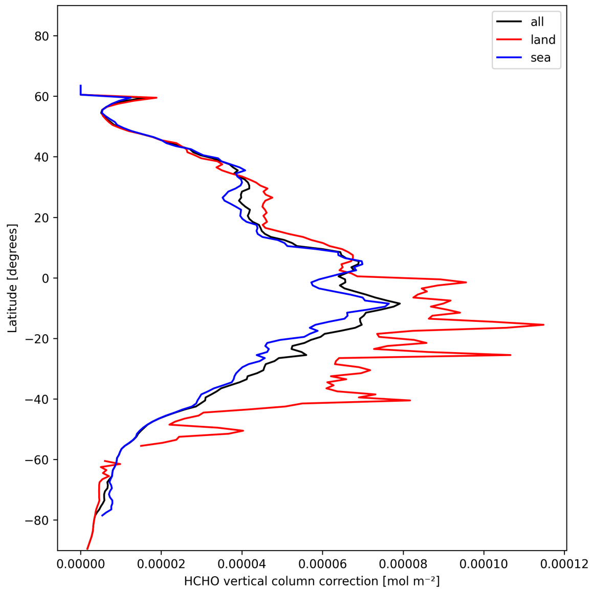
Figure 23: Zonal average of “HCHO vertical column correction” for 2025-01-12 to 2025-01-14.
