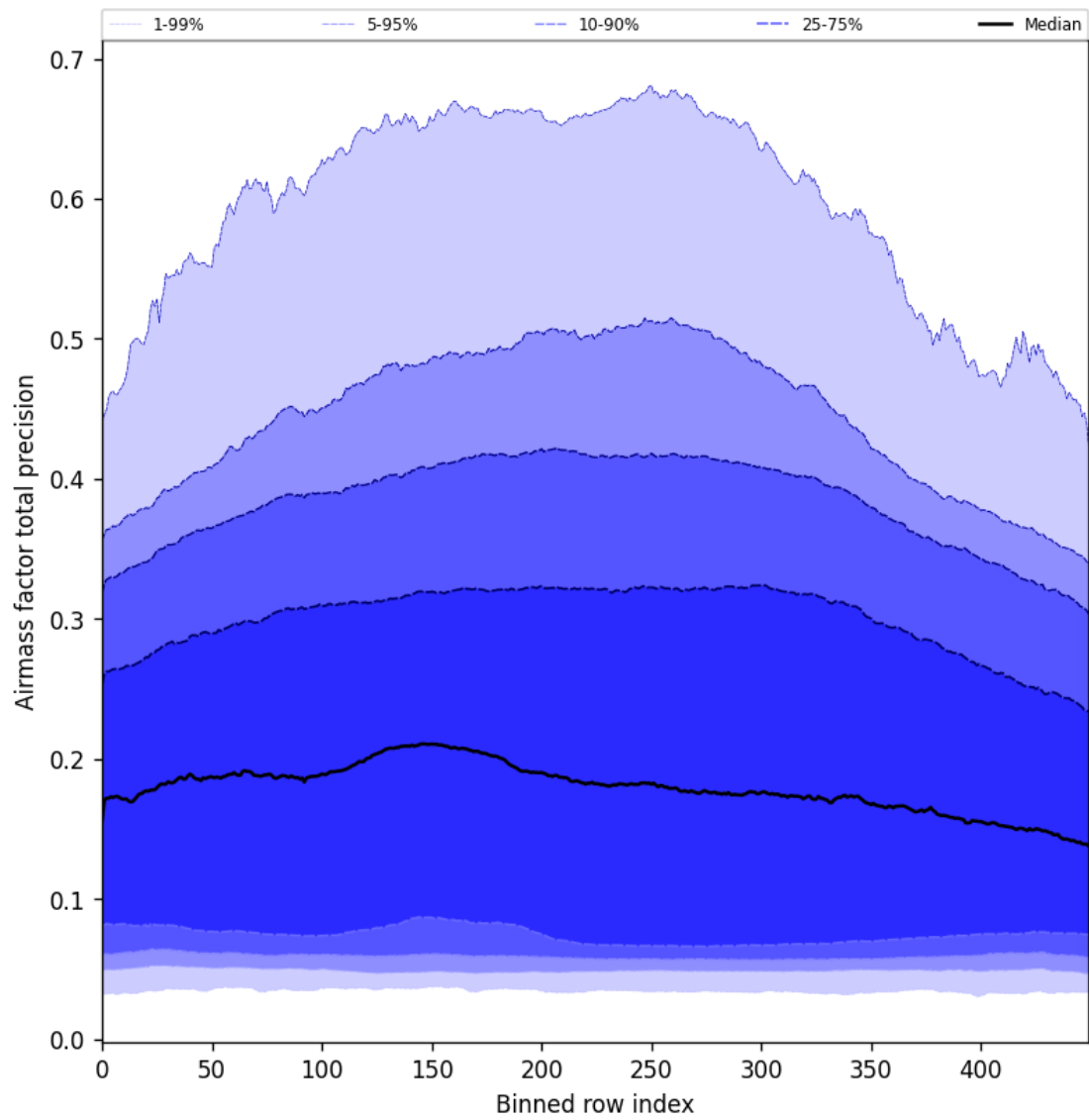
Figure 55: Along track statistics of “Airmass factor total precision” for 2025-01-12 to 2025-01-14
