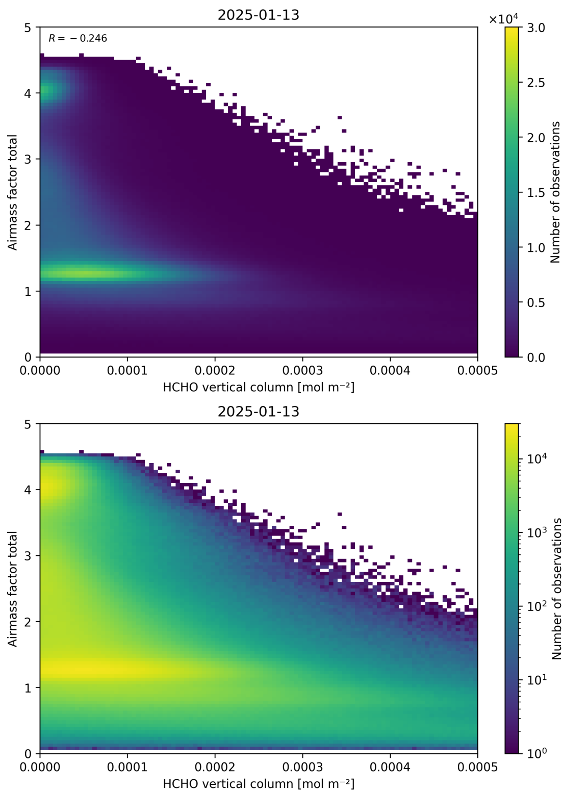
Figure 131: Scatter density plot of “HCHO vertical column” against “Airmass factor total” for 2025-01-12 to 2025-01-14.
