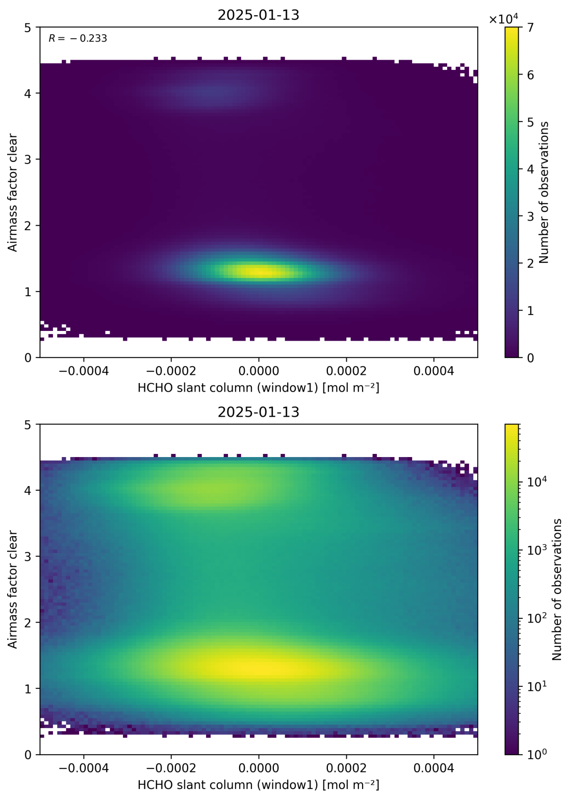
Figure 81: Scatter density plot of “HCHO slant column (window1)” against “Airmass factor clear” for 2025-01-12 to 2025-01-14.
