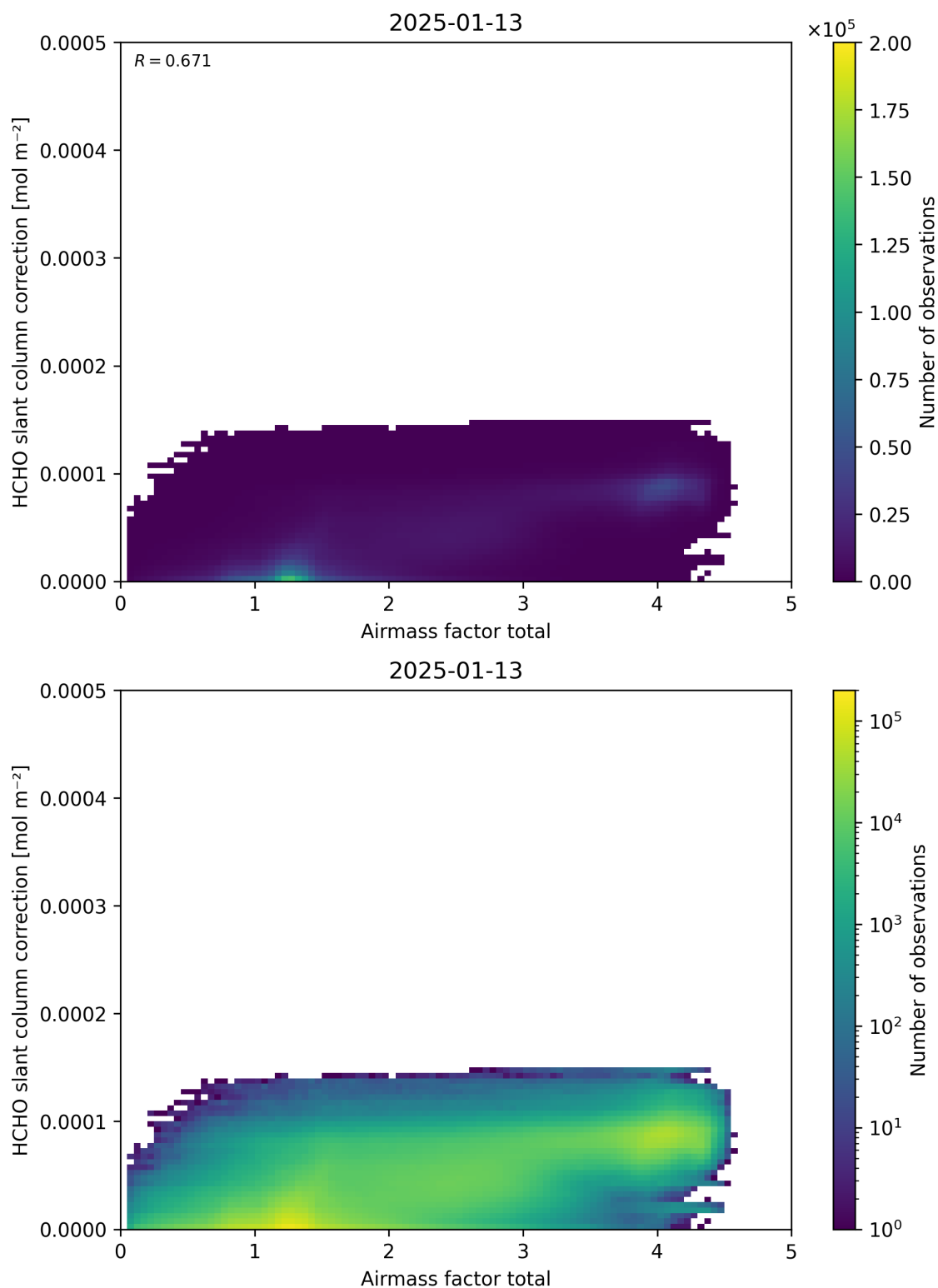
Figure 102: Scatter density plot of “Airmass factor total” against “HCHO slant column correction” for 2025-01-12 to 2025-01-14.
