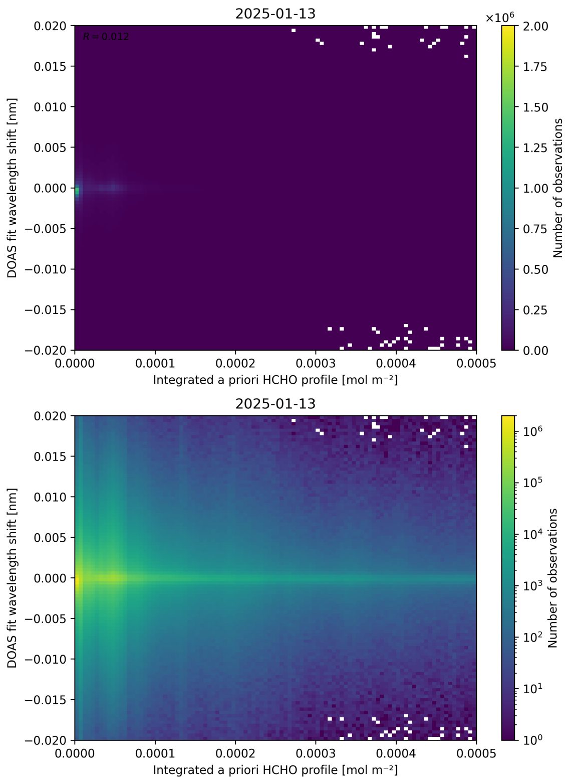
Figure 149: Scatter density plot of “Integrated a priori HCHO profile” against “DOAS fit wavelength shift” for 2025-01-12 to 2025-01-14.
