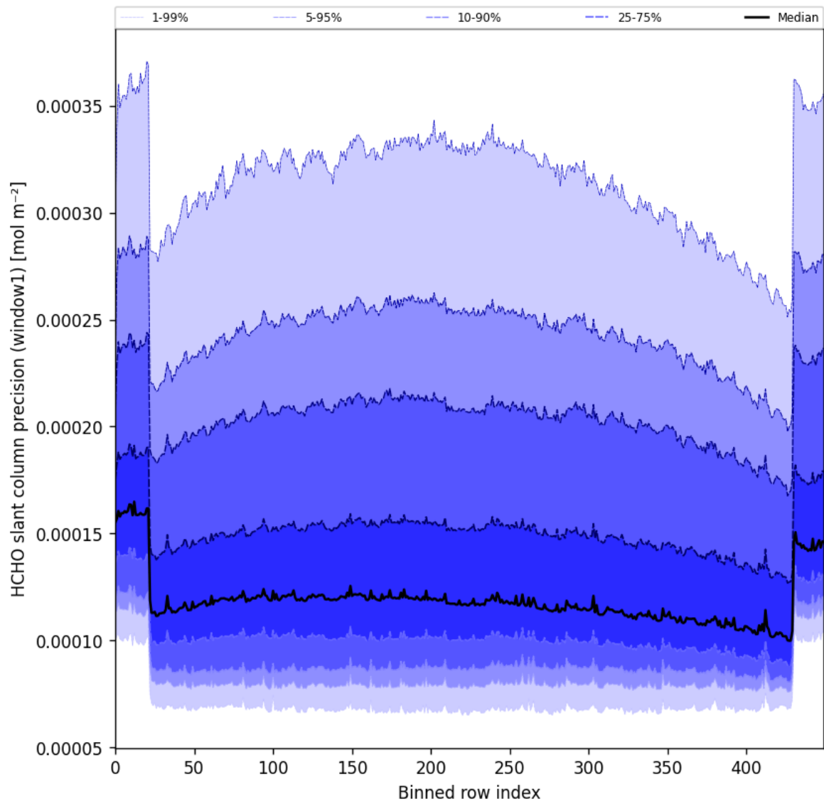
Figure 53: Along track statistics of “HCHO slant column precision (window1)” for 2025-01-12 to 2025-01-14
