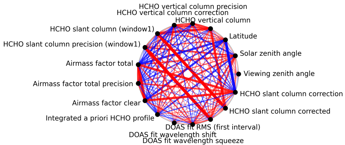
Figure 1: Map of correlation graph for 2025-01-12 to 2025-01-14.
