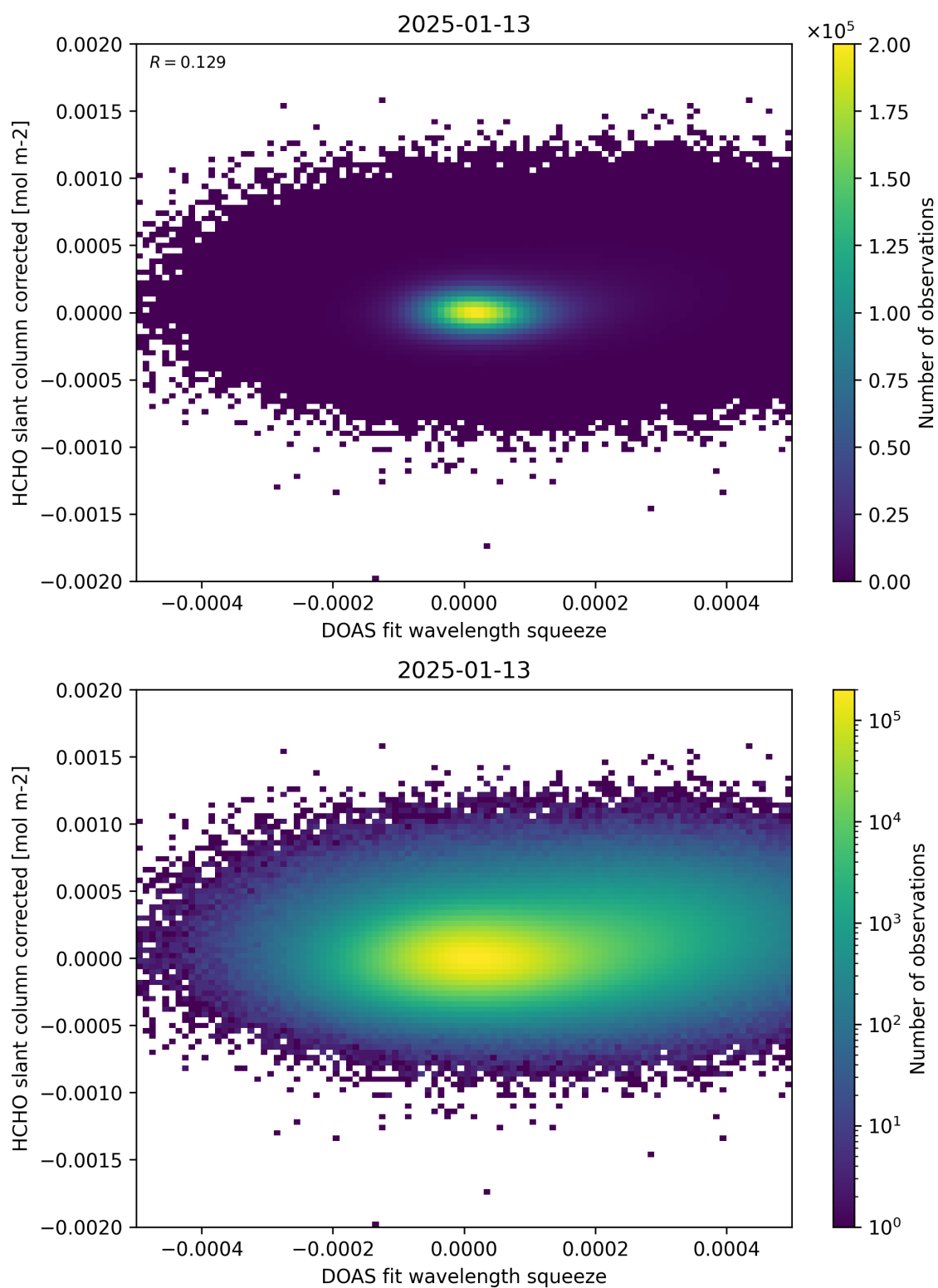
Figure 69: Scatter density plot of “DOAS fit wavelength squeeze” against “HCHO slant column corrected” for 2025-01-12 to 2025-01-14.
