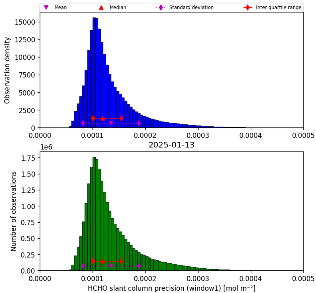
Figure 39: Histogram of “HCHO slant column precision (window1)” for 2025-01-12 to 2025-01-14
