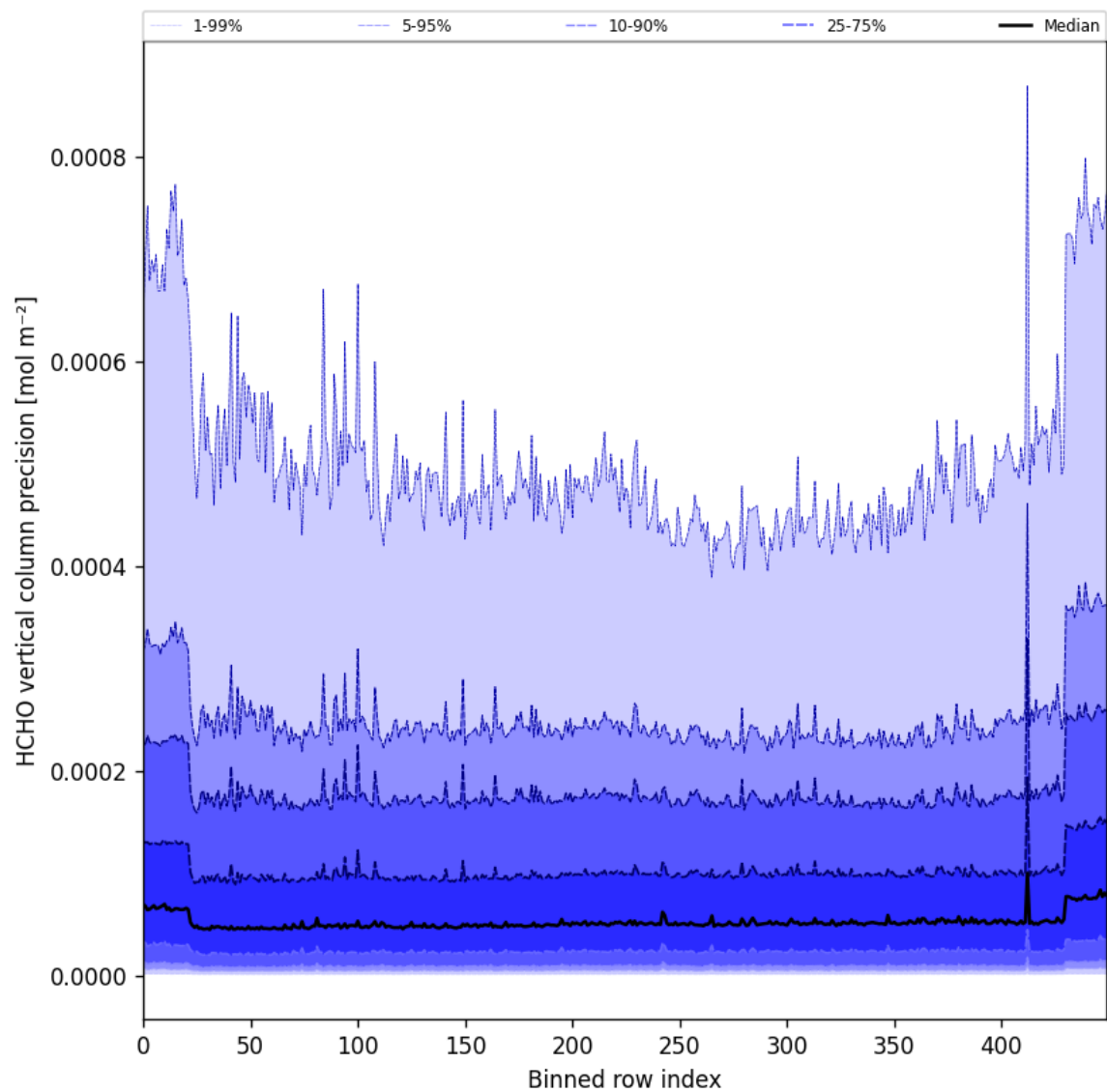
Figure 50: Along track statistics of “HCHO vertical column precision” for 2025-01-12 to 2025-01-14
