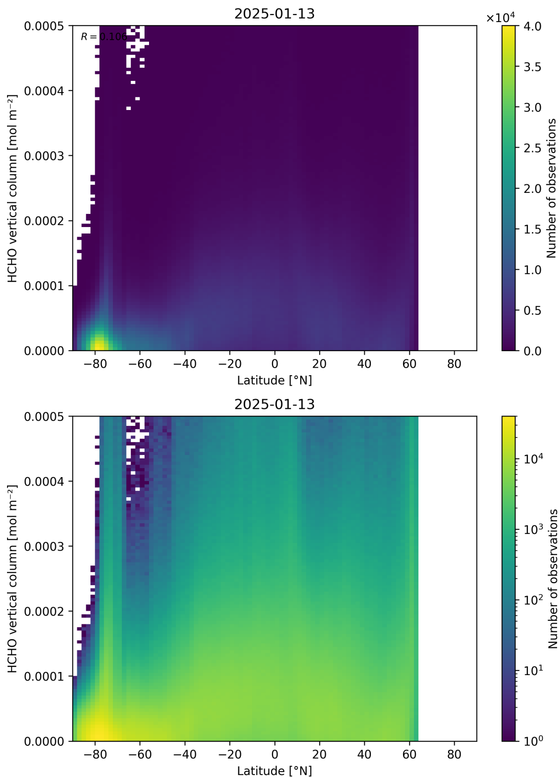
Figure 163: Scatter density plot of “Latitude” against “HCHO vertical column” for 2025-01-12 to 2025-01-14.
