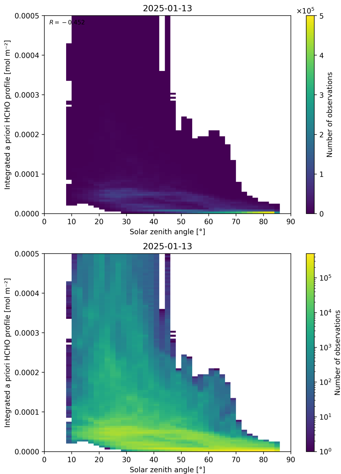
Figure 180: Scatter density plot of “Solar zenith angle” against “Integrated a priori HCHO profile” for 2025-01-12 to 2025-01-14.
