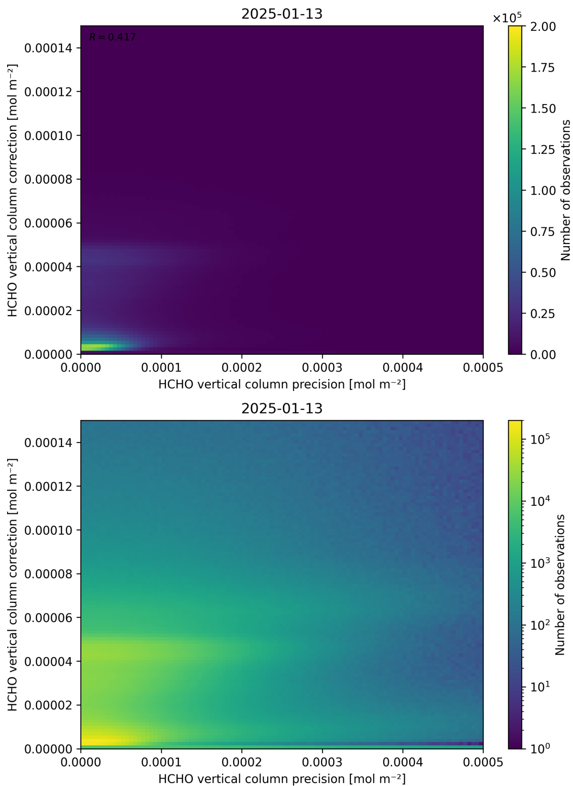
Figure 146: Scatter density plot of “HCHO vertical column precision” against “HCHO vertical column correction” for 2025-01-12 to 2025-01-14.
