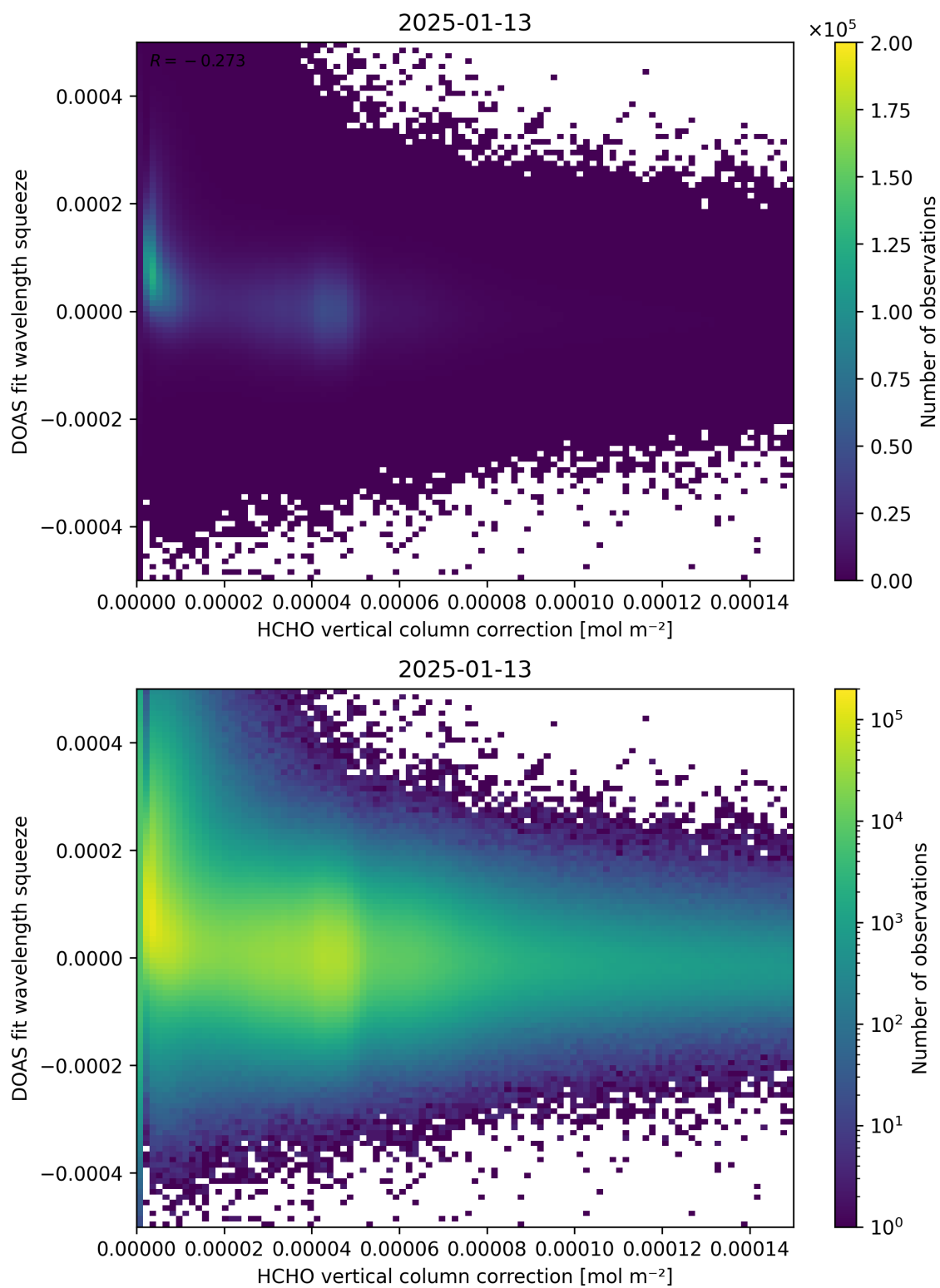
Figure 114: Scatter density plot of “HCHO vertical column correction” against “DOAS fit wavelength squeeze” for 2025-01-12 to 2025-01-14.
