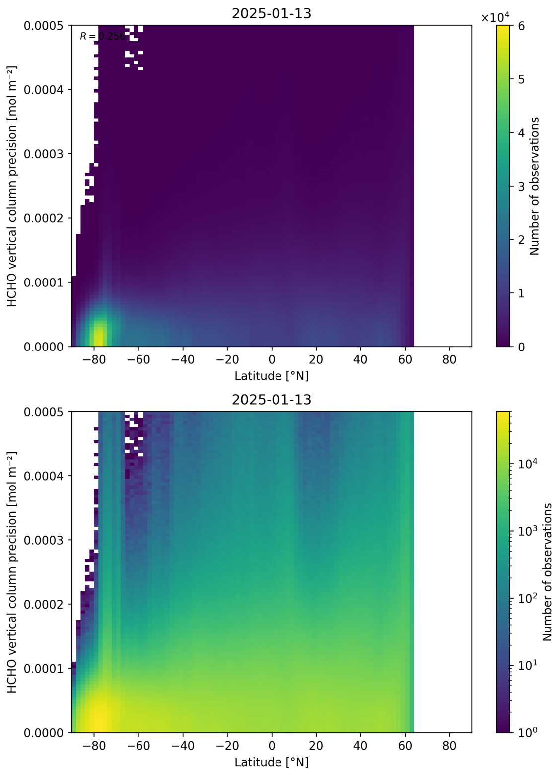
Figure 165: Scatter density plot of “Latitude” against “HCHO vertical column precision” for 2025-01-12 to 2025-01-14.
