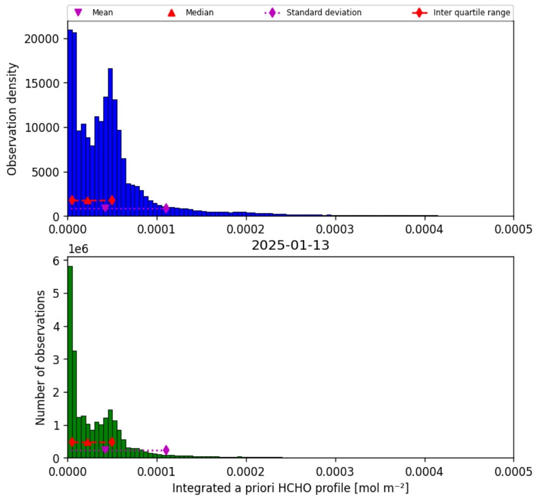
Figure 43: Histogram of “Integrated a priori HCHO profile” for 2025-01-12 to 2025-01-14
