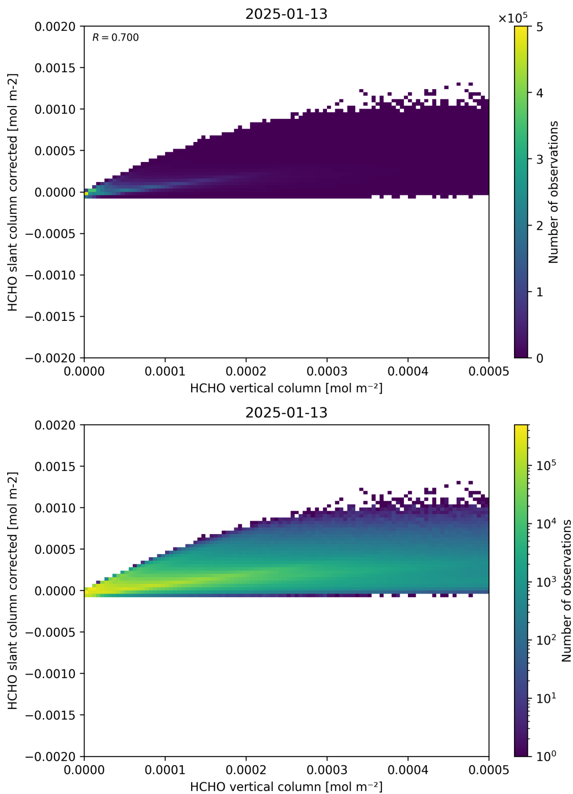
Figure 127: Scatter density plot of “HCHO vertical column” against “HCHO slant column corrected” for 2025-01-12 to 2025-01-14.
