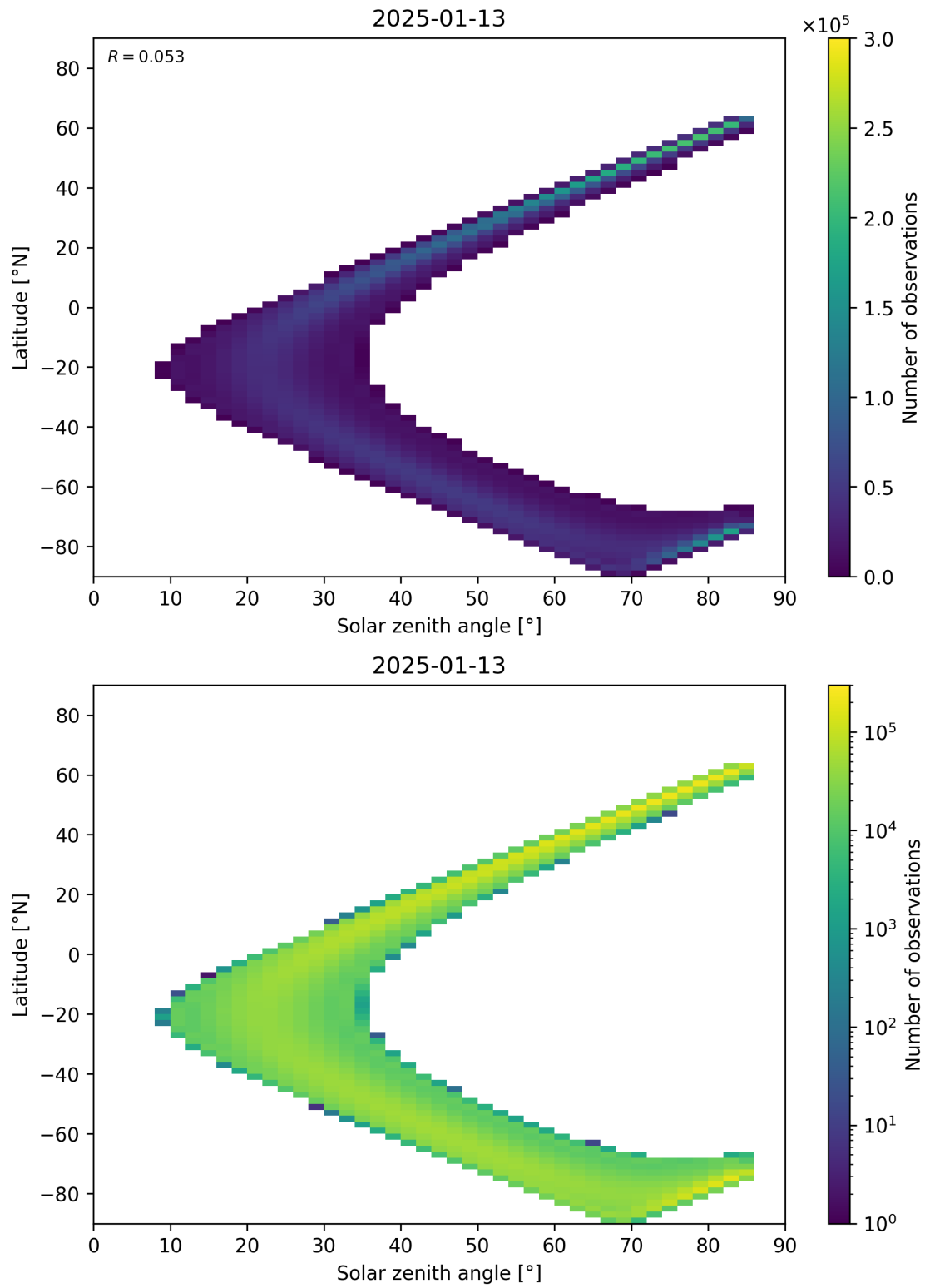
Figure 181: Scatter density plot of “Solar zenith angle” against “Latitude” for 2025-01-12 to 2025-01-14.
