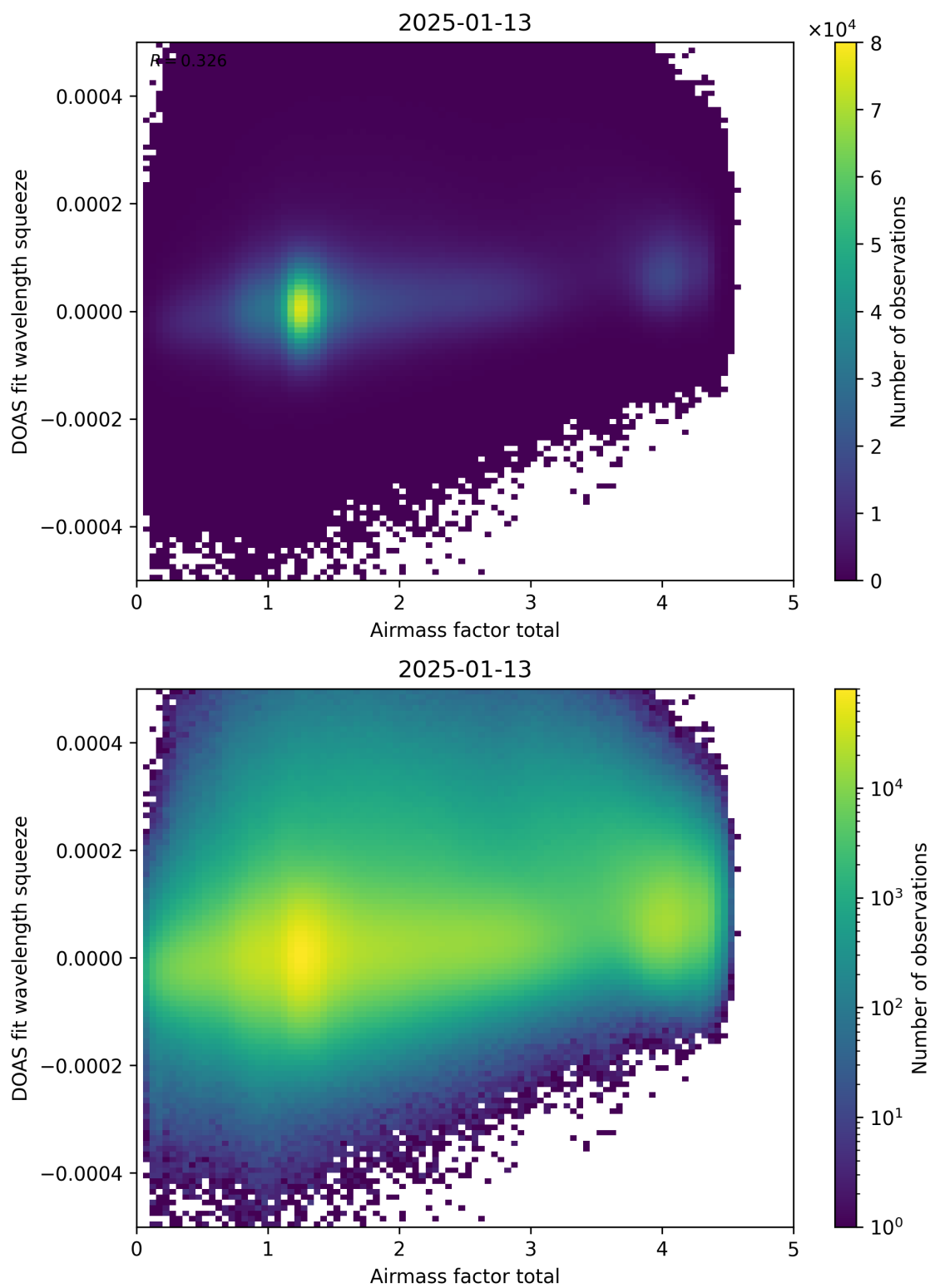
Figure 99: Scatter density plot of “Airmass factor total” against “DOAS fit wavelength squeeze” for 2025-01-12 to 2025-01-14.
