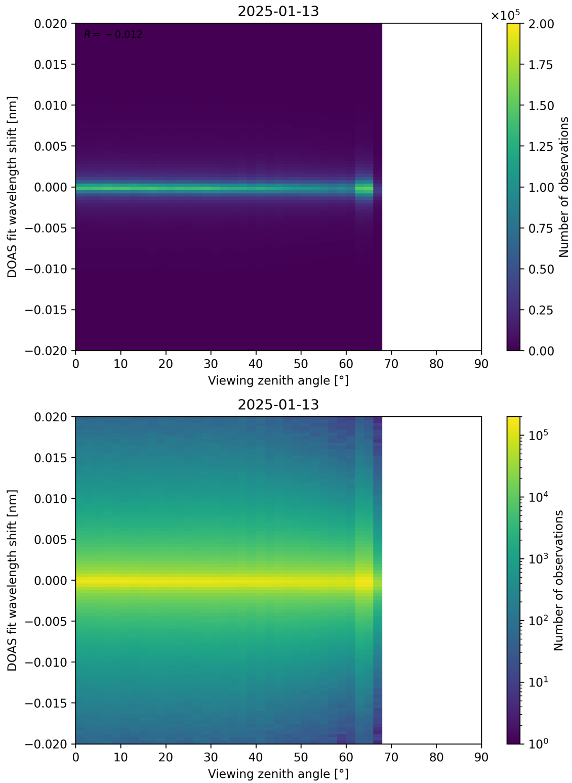
Figure 183: Scatter density plot of “Viewing zenith angle” against “DOAS fit wavelength shift” for 2025-01-12 to 2025-01-14.
