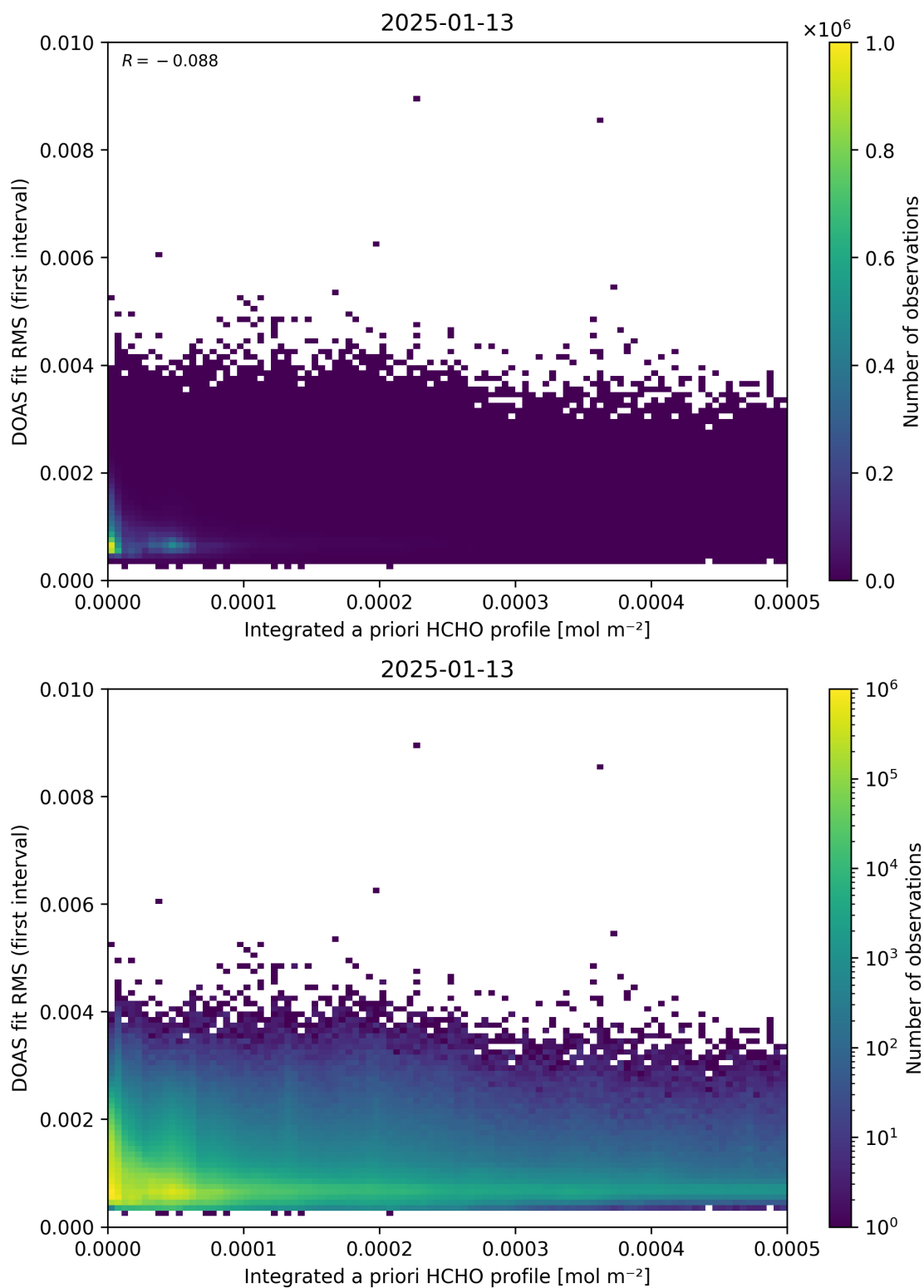
Figure 148: Scatter density plot of “Integrated a priori HCHO profile” against “DOAS fit RMS (first interval)” for 2025-01-12 to 2025-01-14.
