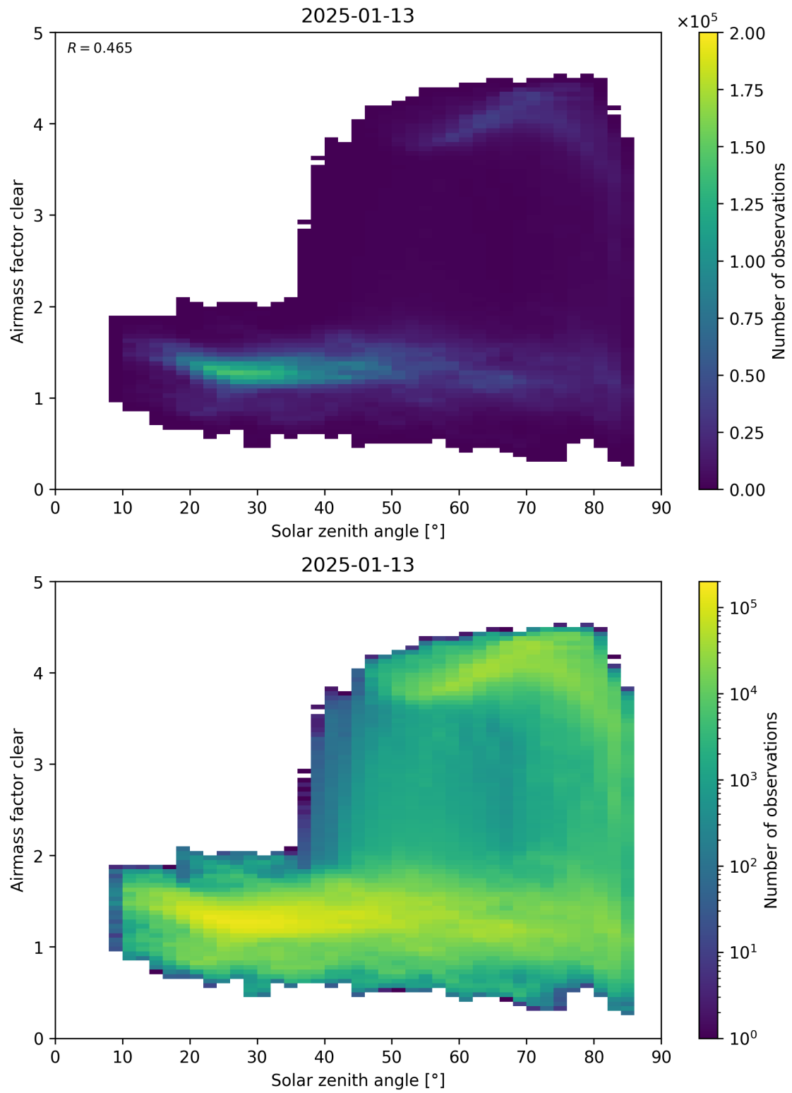
Figure 170: Scatter density plot of “Solar zenith angle” against “Airmass factor clear” for 2025-01-12 to 2025-01-14.
