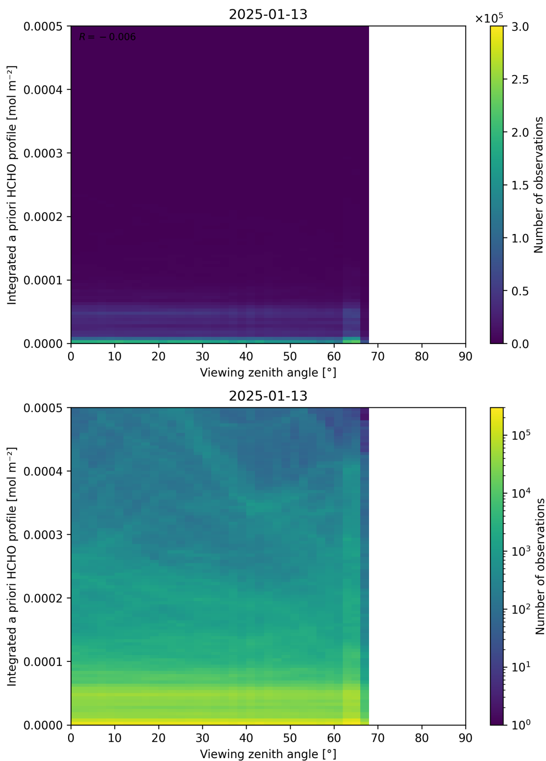
Figure 195: Scatter density plot of “Viewing zenith angle” against “Integrated a priori HCHO profile” for 2025-01-12 to 2025-01-14.
