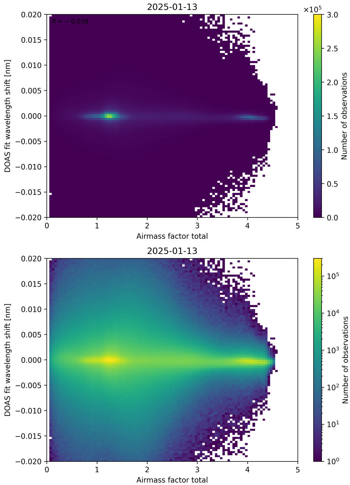
Figure 98: Scatter density plot of “Airmass factor total” against “DOAS fit wavelength shift” for 2025-01-12 to 2025-01-14.
