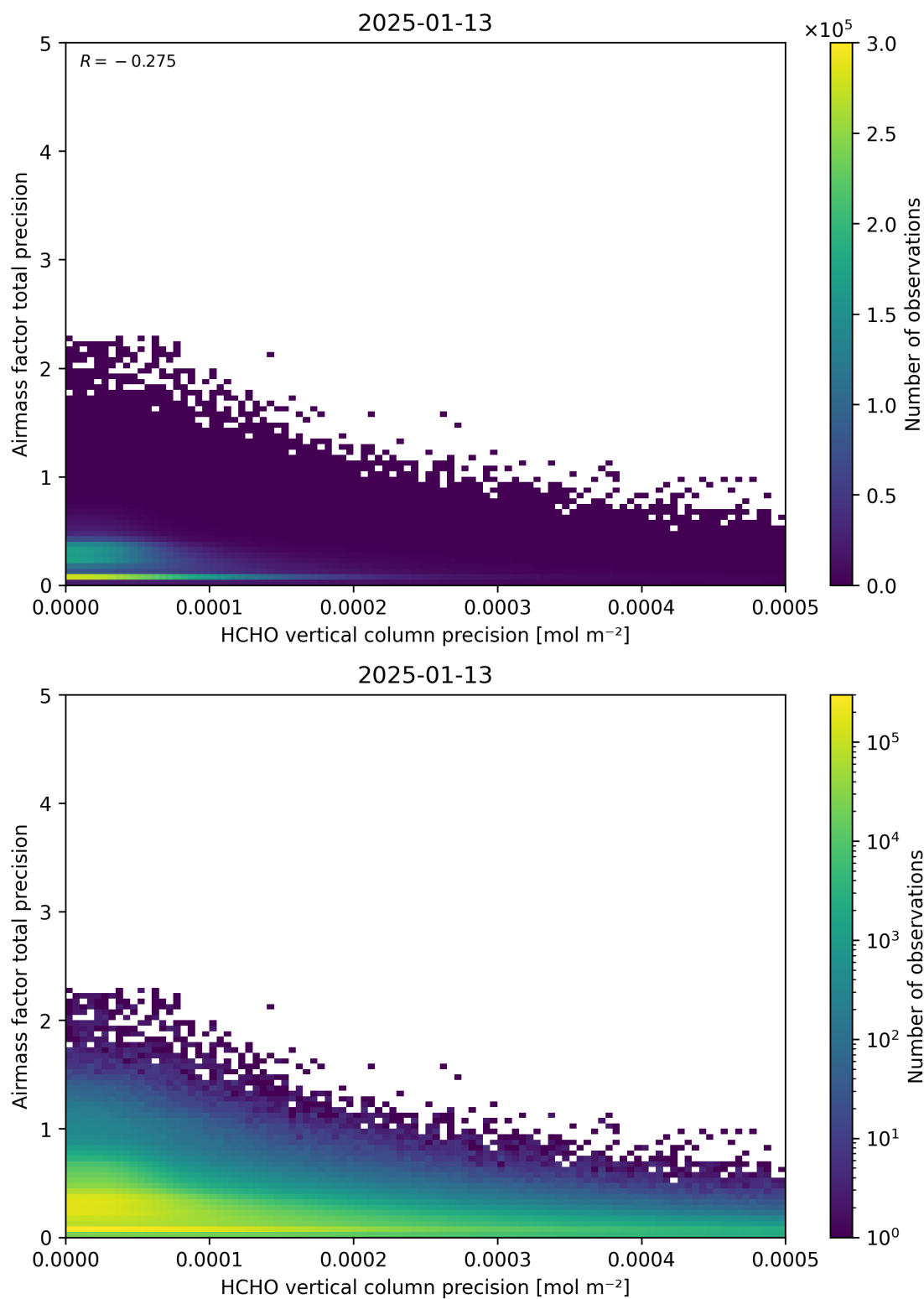
Figure 145: Scatter density plot of “HCHO vertical column precision” against “Airmass factor total precision” for 2025-01-12 to 2025-01-14.
