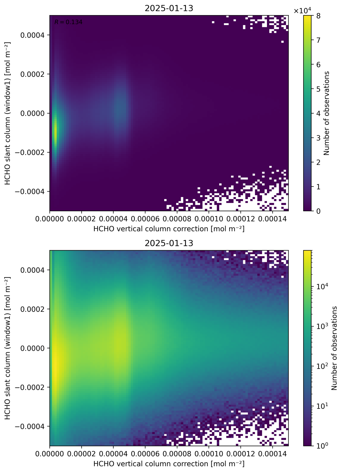
Figure 118: Scatter density plot of “HCHO vertical column correction” against “HCHO slant column (window1)” for 2025-01-12 to 2025-01-14.
