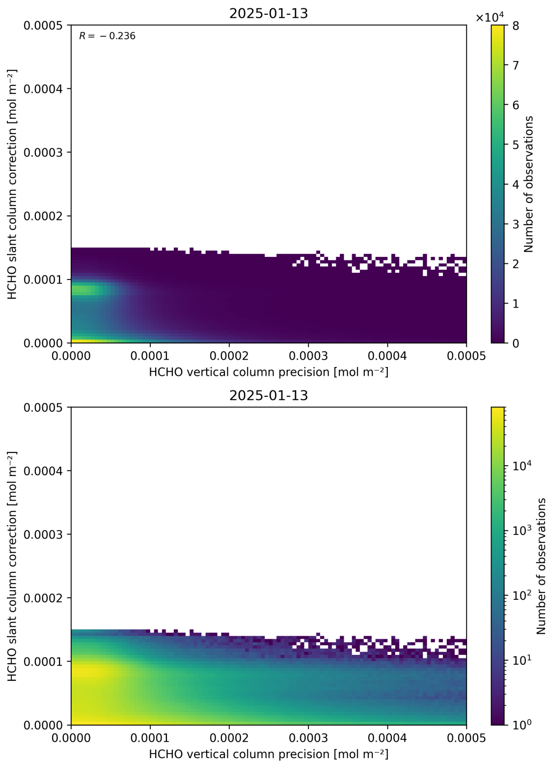
Figure 141: Scatter density plot of “HCHO vertical column precision” against “HCHO slant column correction” for 2025-01-12 to 2025-01-14.
