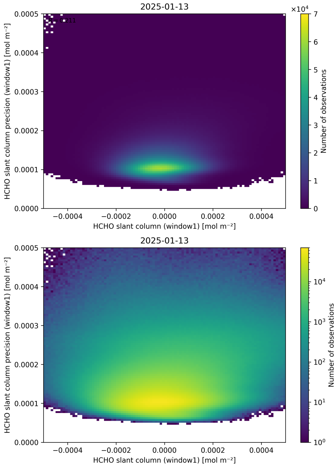
Figure 84: Scatter density plot of “HCHO slant column (window1)” against “HCHO slant column precision (window1)” for 2025-01-12 to 2025-01-14.
