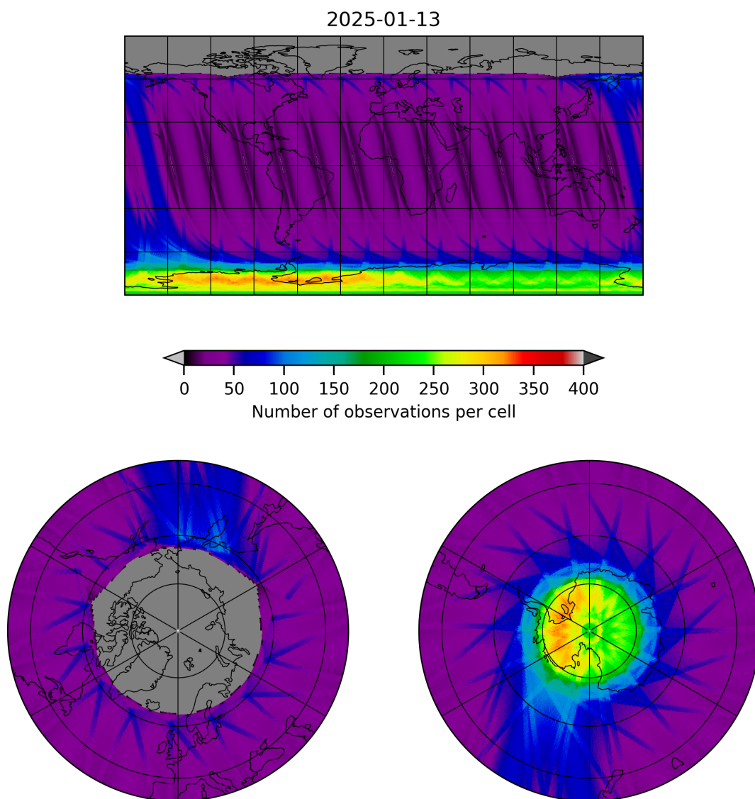
Figure 19: Map of the number of observations for 2025-01-12 to 2025-01-14
