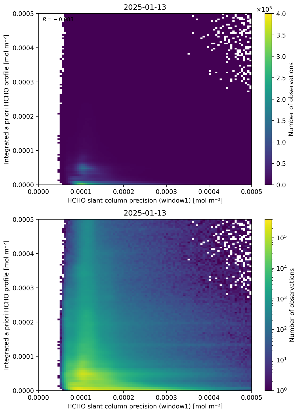
Figure 96: Scatter density plot of “HCHO slant column precision (window1)” against “Integrated a priori HCHO profile” for 2025-01-12 to 2025-01-14.
