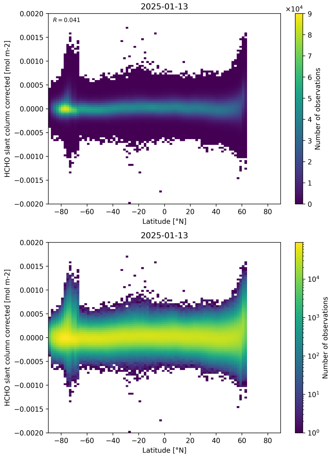
Figure 157: Scatter density plot of “Latitude” against “HCHO slant column corrected” for 2025-01-12 to 2025-01-14.
