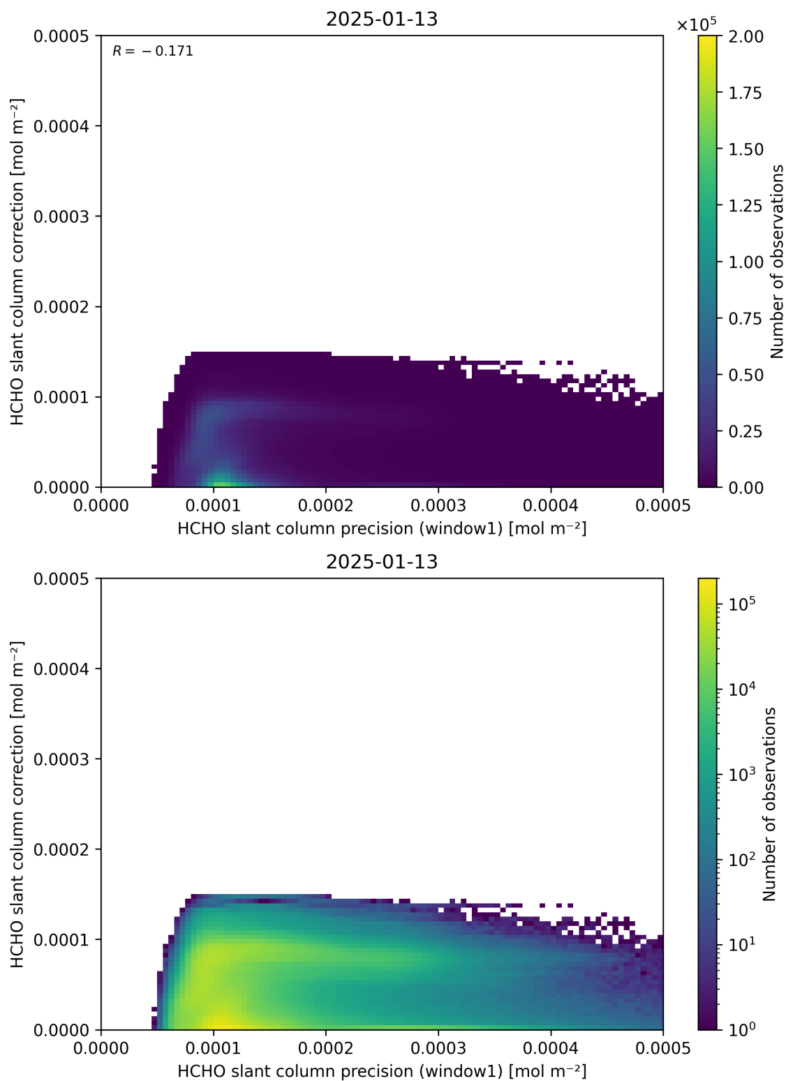
Figure 93: Scatter density plot of “HCHO slant column precision (window1)” against “HCHO slant column correction” for 2025-01-12 to 2025-01-14.
