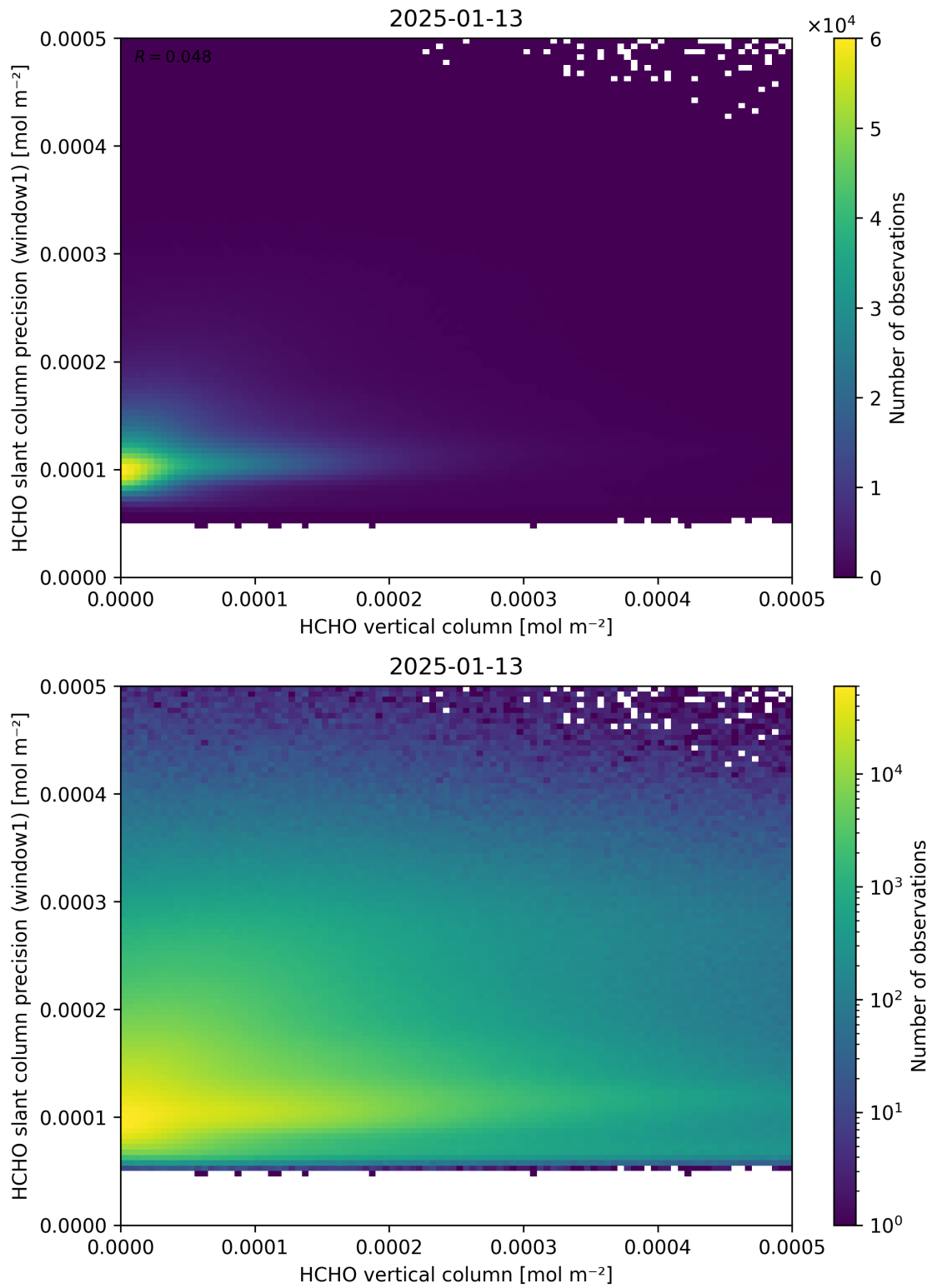
Figure 130: Scatter density plot of “HCHO vertical column” against “HCHO slant column precision (window1)” for 2025-01-12 to 2025-01-14.
