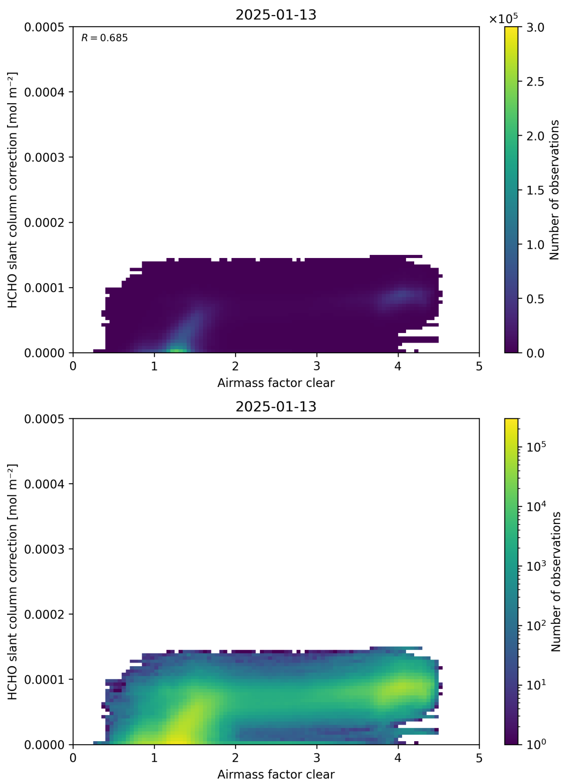
Figure 75: Scatter density plot of “Airmass factor clear” against “HCHO slant column correction” for 2025-01-12 to 2025-01-14.
