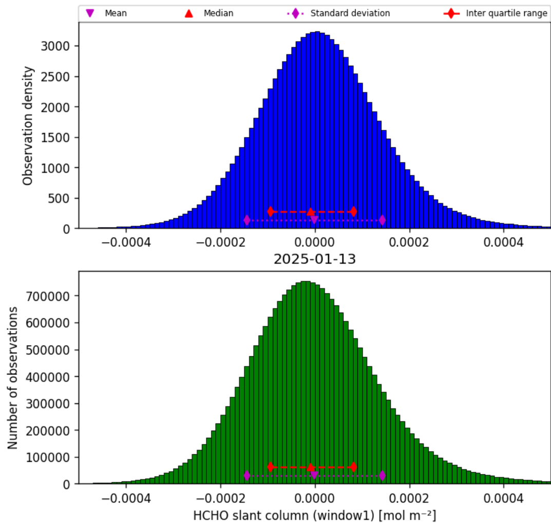
Figure 38: Histogram of “HCHO slant column (window1)” for 2025-01-12 to 2025-01-14
