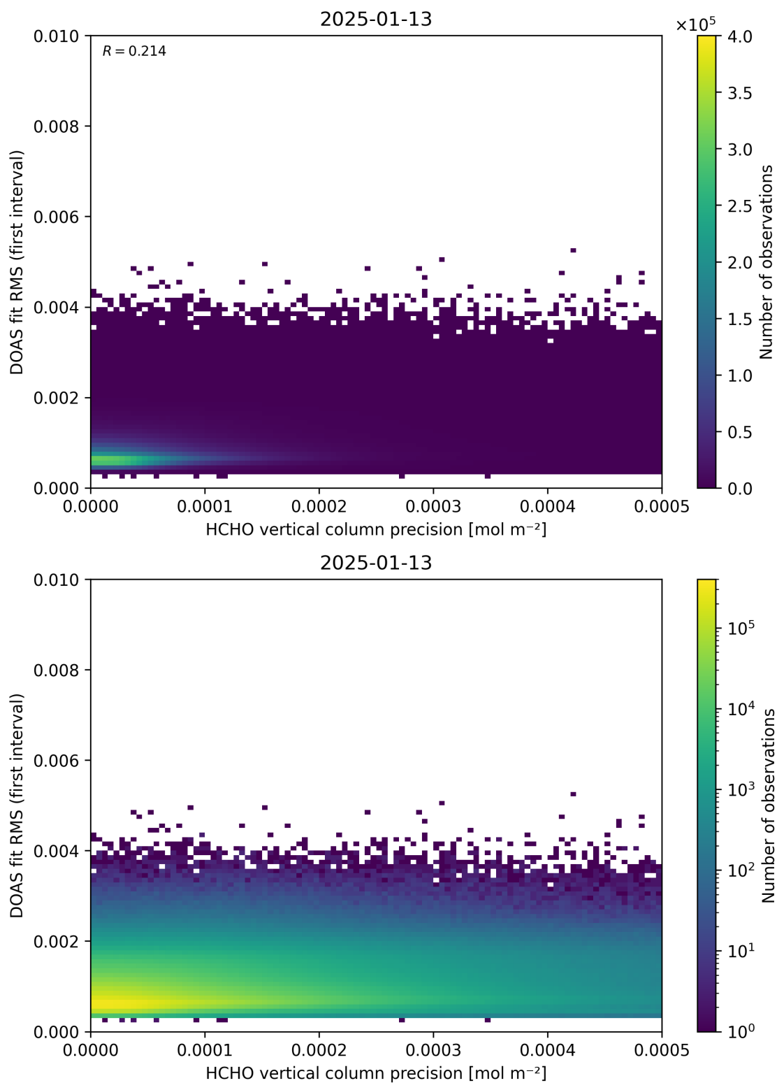
Figure 136: Scatter density plot of “HCHO vertical column precision” against “DOAS fit RMS (first interval)” for 2025-01-12 to 2025-01-14.
