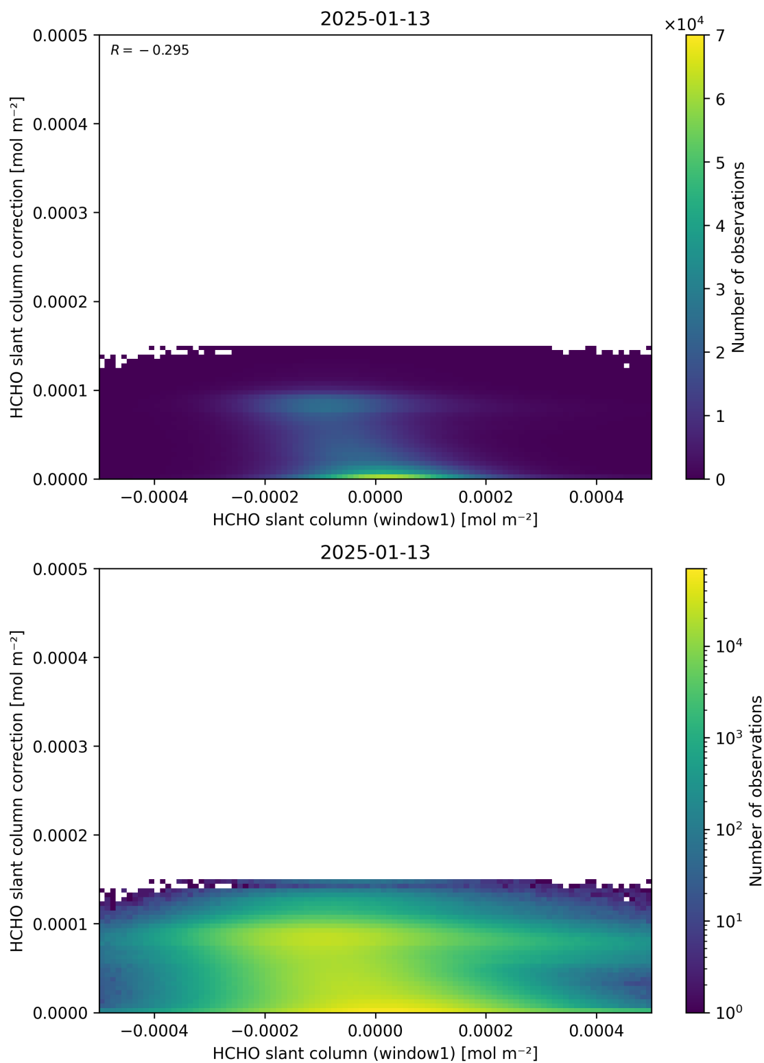
Figure 83: Scatter density plot of “HCHO slant column (window1)” against “HCHO slant column correction” for 2025-01-12 to 2025-01-14.
