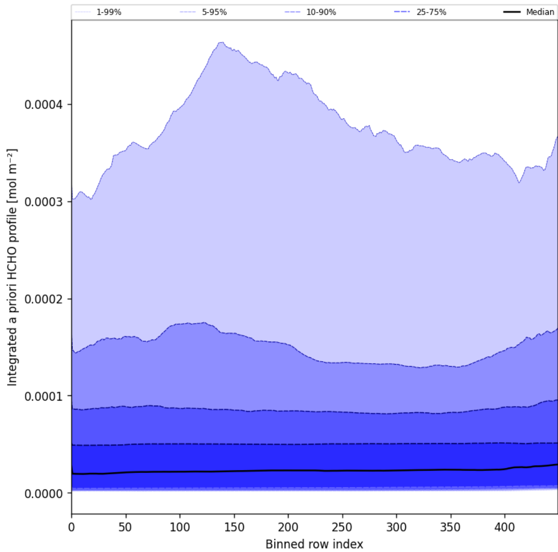
Figure 57: Along track statistics of “Integrated a priori HCHO profile” for 2025-01-12 to 2025-01-14
