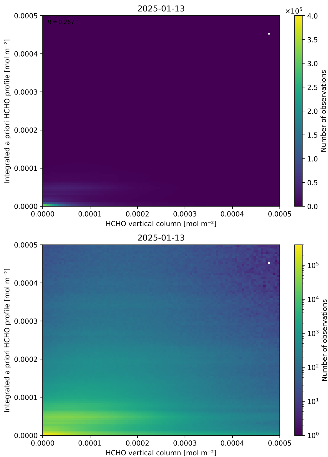
Figure 135: Scatter density plot of “HCHO vertical column” against “Integrated a priori HCHO profile” for 2025-01-12 to 2025-01-14.
