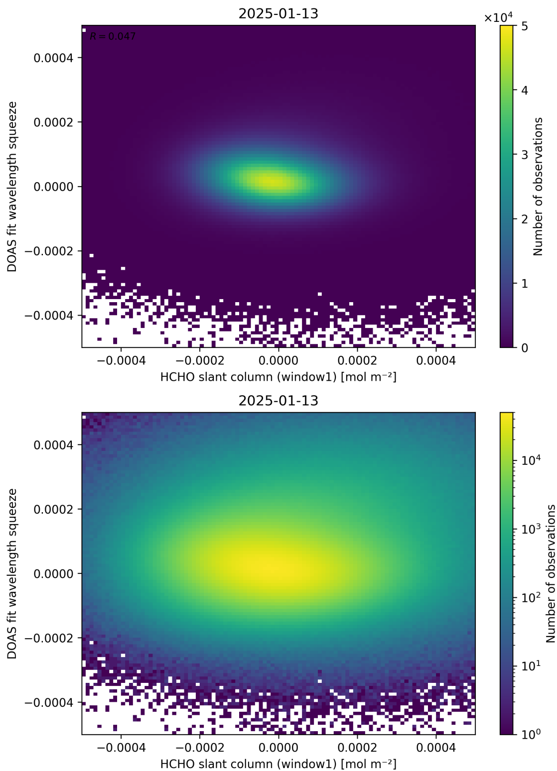
Figure 80: Scatter density plot of “HCHO slant column (window1)” against “DOAS fit wavelength squeeze” for 2025-01-12 to 2025-01-14.
