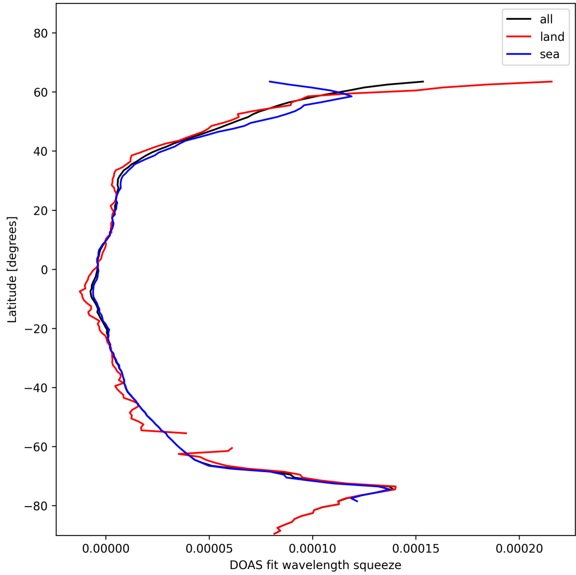
Figure 31: Zonal average of “DOAS fit wavelength squeeze” for 2025-01-12 to 2025-01-14.
