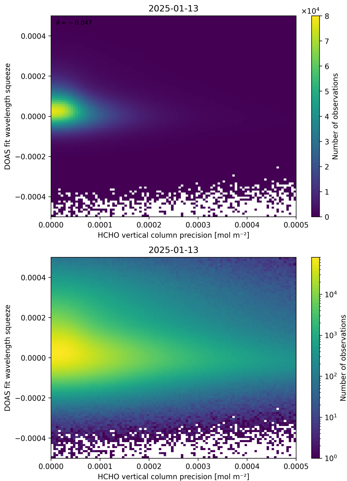
Figure 138: Scatter density plot of “HCHO vertical column precision” against “DOAS fit wavelength squeeze” for 2025-01-12 to 2025-01-14.
