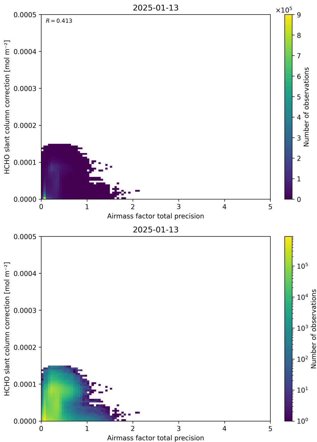
Figure 110: Scatter density plot of “Airmass factor total precision” against “HCHO slant column correction” for 2025-01-12 to 2025-01-14.
