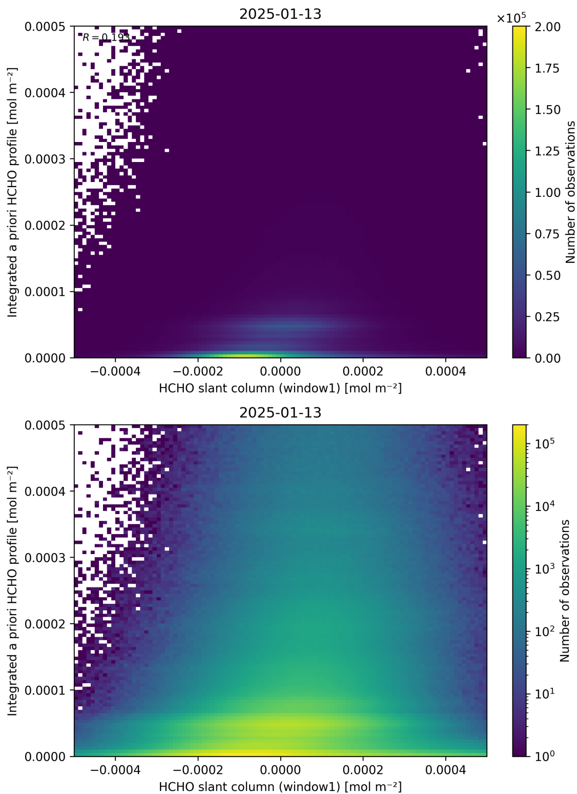
Figure 87: Scatter density plot of “HCHO slant column (window1)” against “Integrated a priori HCHO profile” for 2025-01-12 to 2025-01-14.
