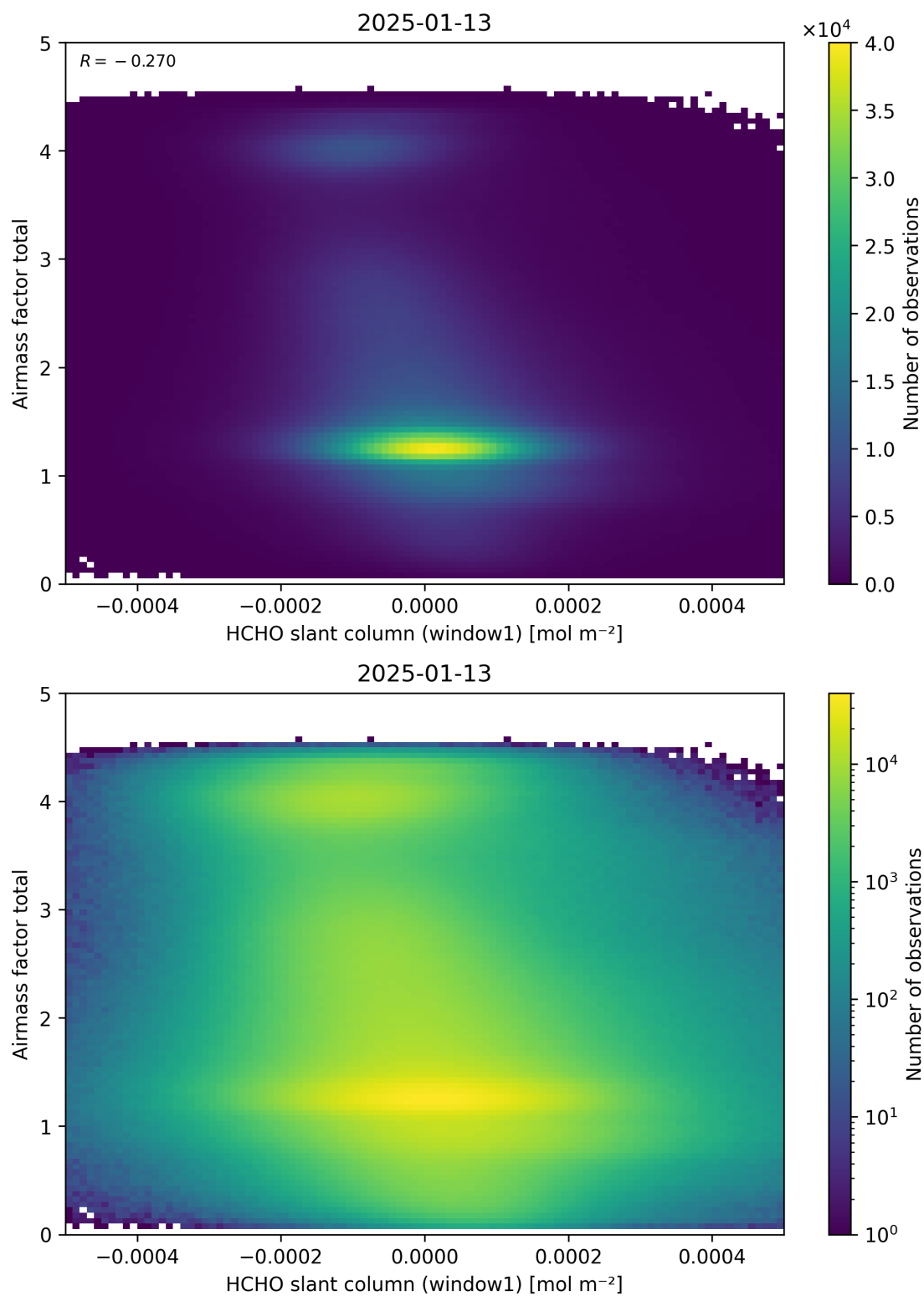
Figure 85: Scatter density plot of “HCHO slant column (window1)” against “Airmass factor total” for 2025-01-12 to 2025-01-14.
