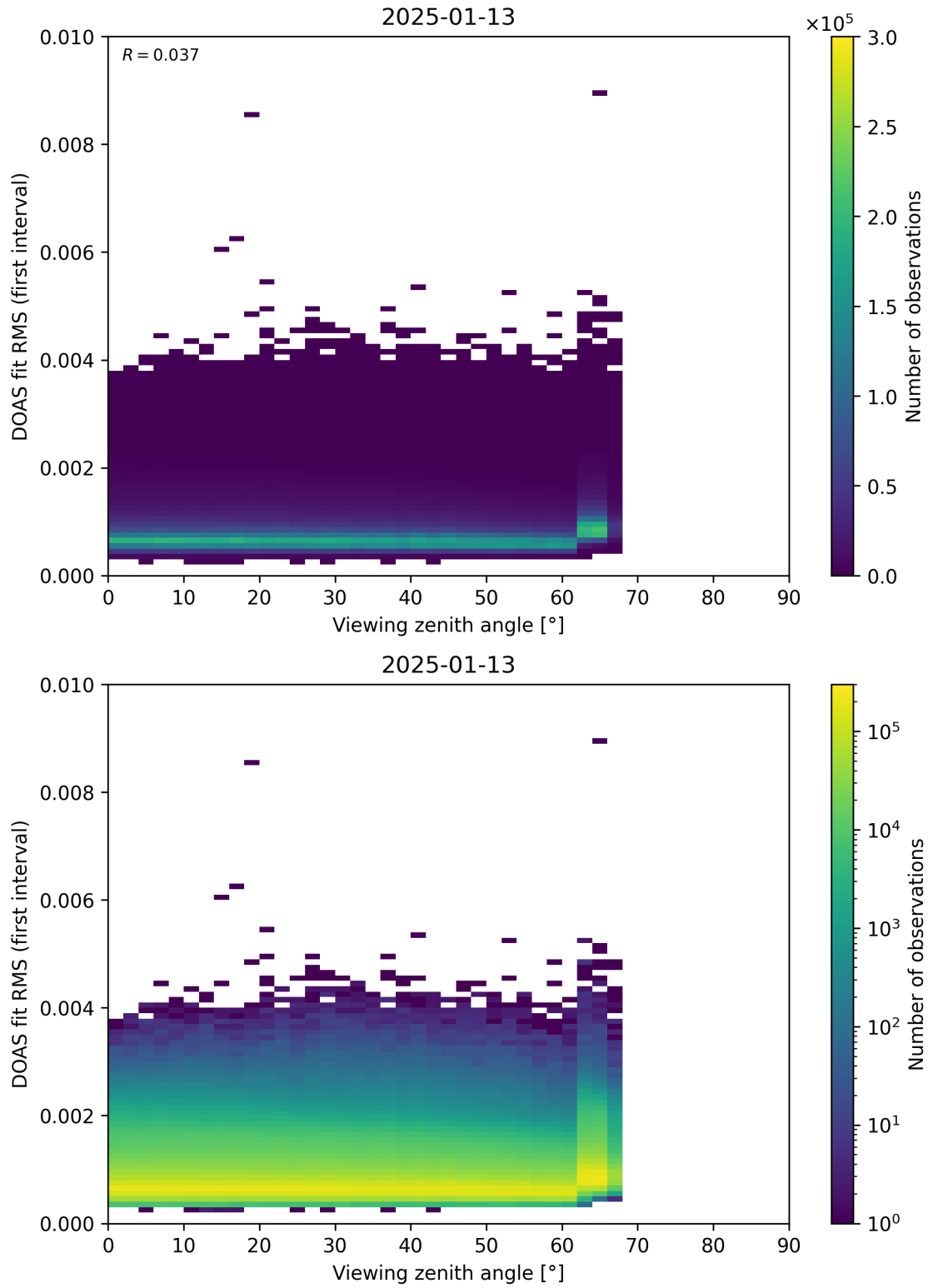
Figure 182: Scatter density plot of “Viewing zenith angle” against “DOAS fit RMS (first interval)” for 2025-01-12 to 2025-01-14.
