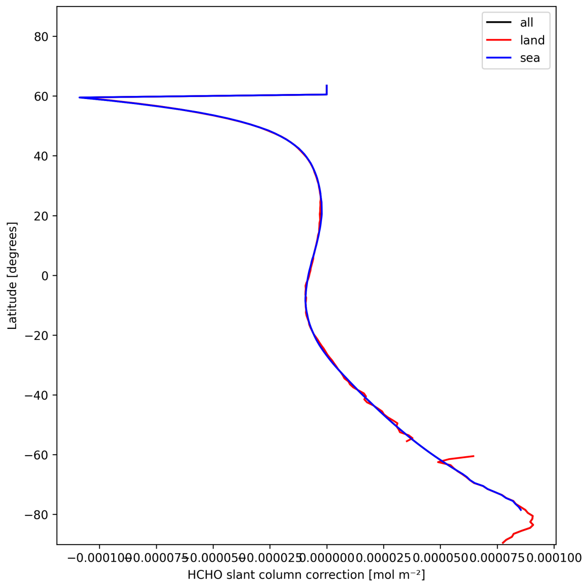
Figure 33: Zonal average of “HCHO slant column correction” for 2025-01-12 to 2025-01-14.
