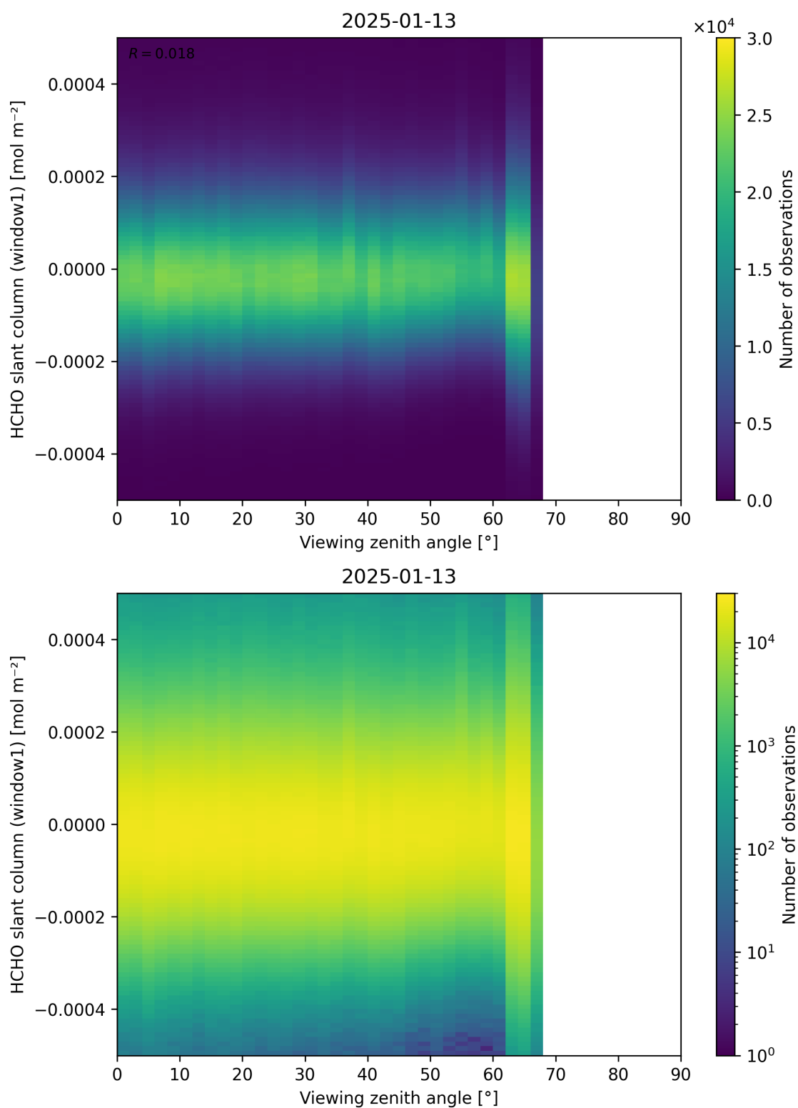
Figure 188: Scatter density plot of “Viewing zenith angle” against “HCHO slant column (window1)” for 2025-01-12 to 2025-01-14.
