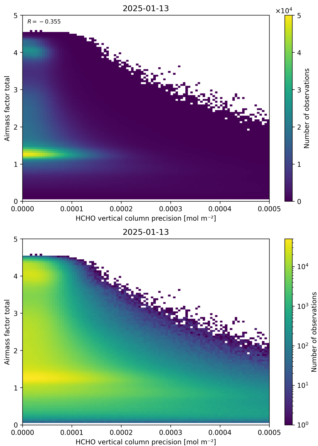
Figure 144: Scatter density plot of “HCHO vertical column precision” against “Airmass factor total” for 2025-01-12 to 2025-01-14.
