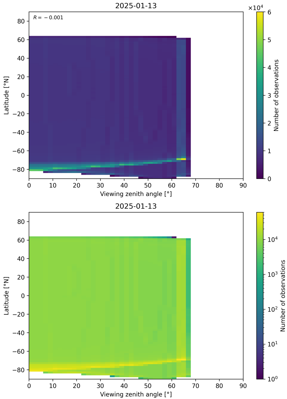
Figure 196: Scatter density plot of “Viewing zenith angle” against “Latitude” for 2025-01-12 to 2025-01-14.
