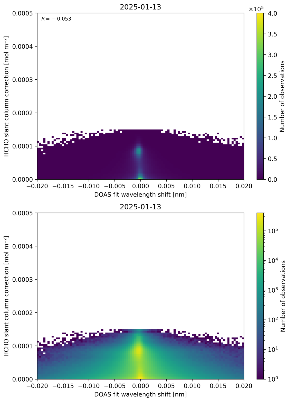
Figure 67: Scatter density plot of “DOAS fit wavelength shift” against “HCHO slant column correction” for 2025-01-12 to 2025-01-14.
