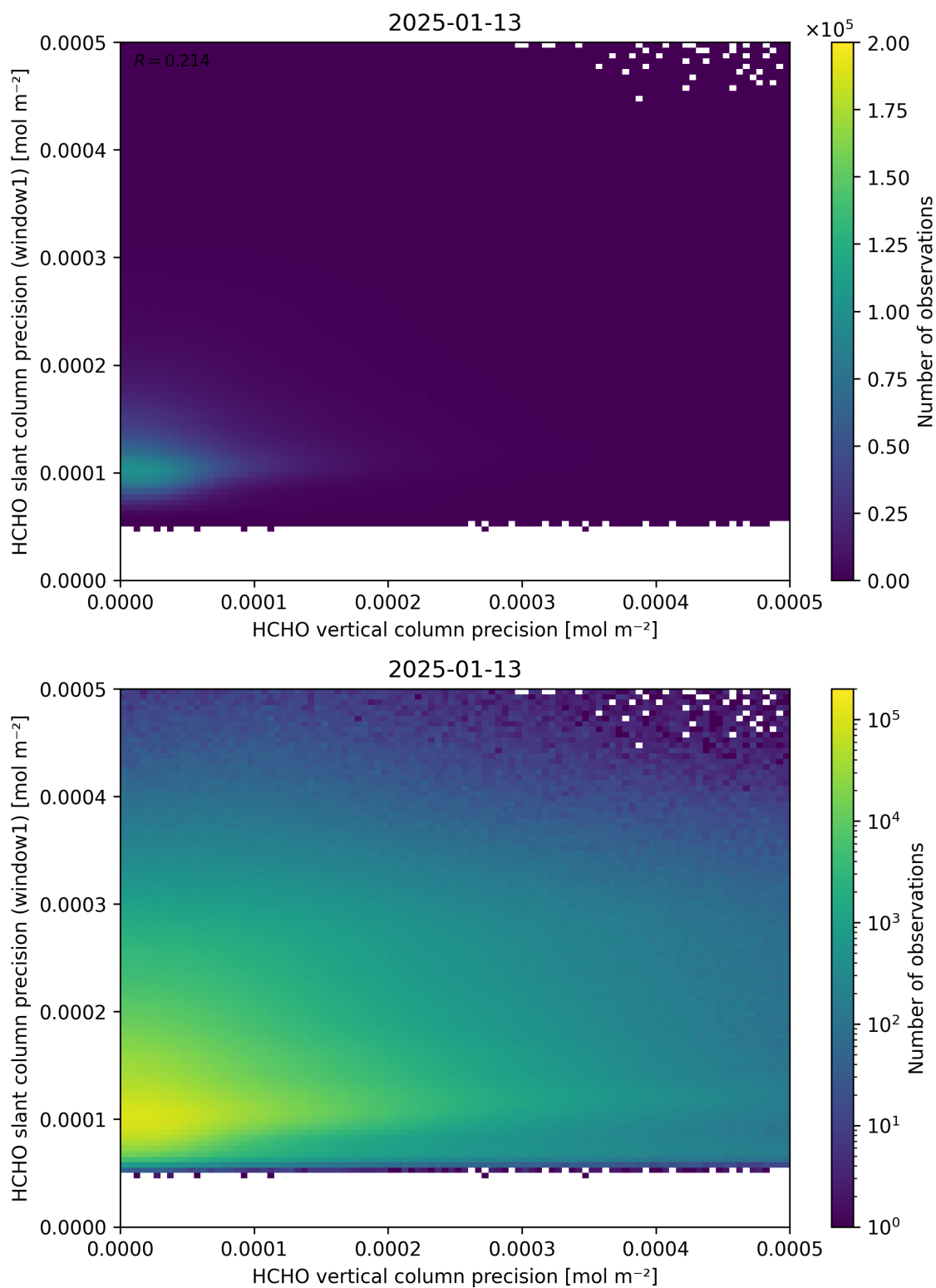
Figure 143: Scatter density plot of “HCHO vertical column precision” against “HCHO slant column precision (window1)” for 2025-01-12 to 2025-01-14.
