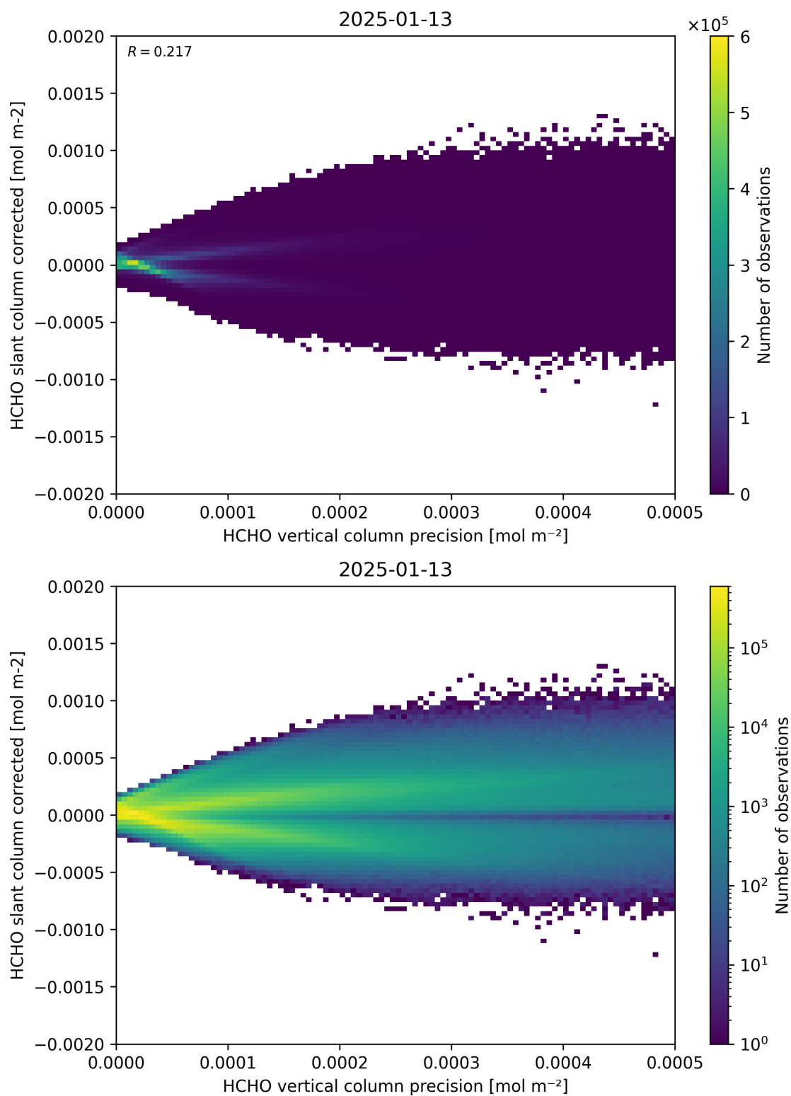
Figure 140: Scatter density plot of “HCHO vertical column precision” against “HCHO slant column corrected” for 2025-01-12 to 2025-01-14.
