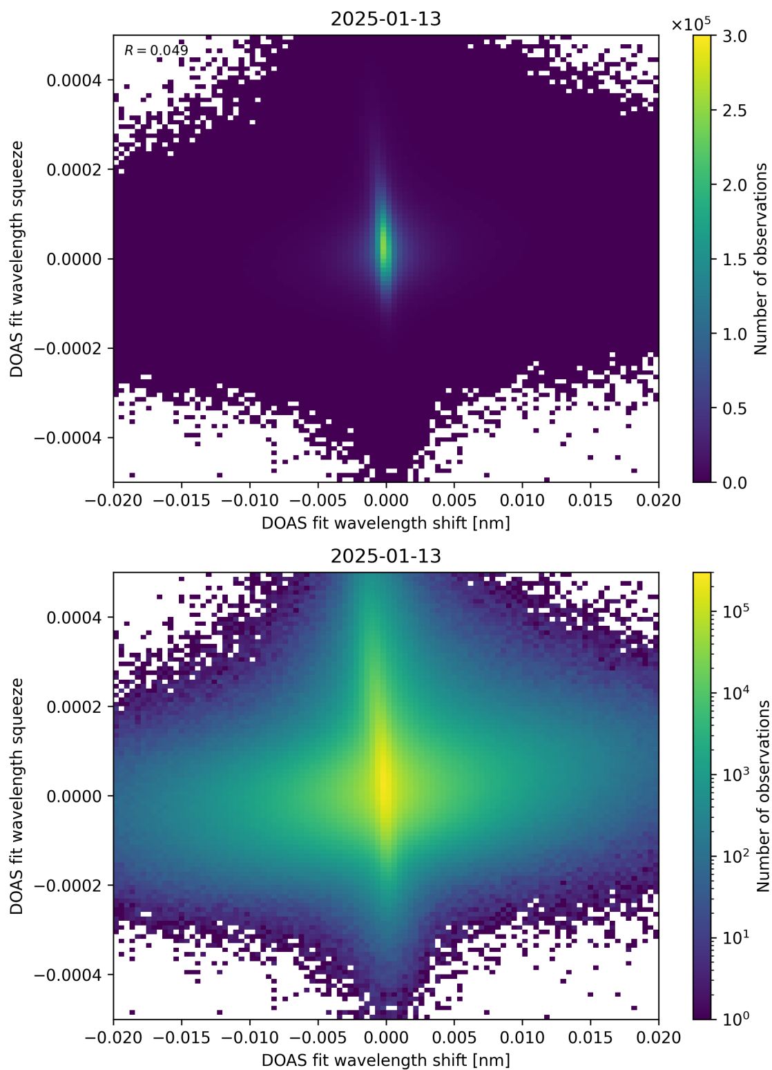
Figure 65: Scatter density plot of “DOAS fit wavelength shift” against “DOAS fit wavelength squeeze” for 2025-01-12 to 2025-01-14.
