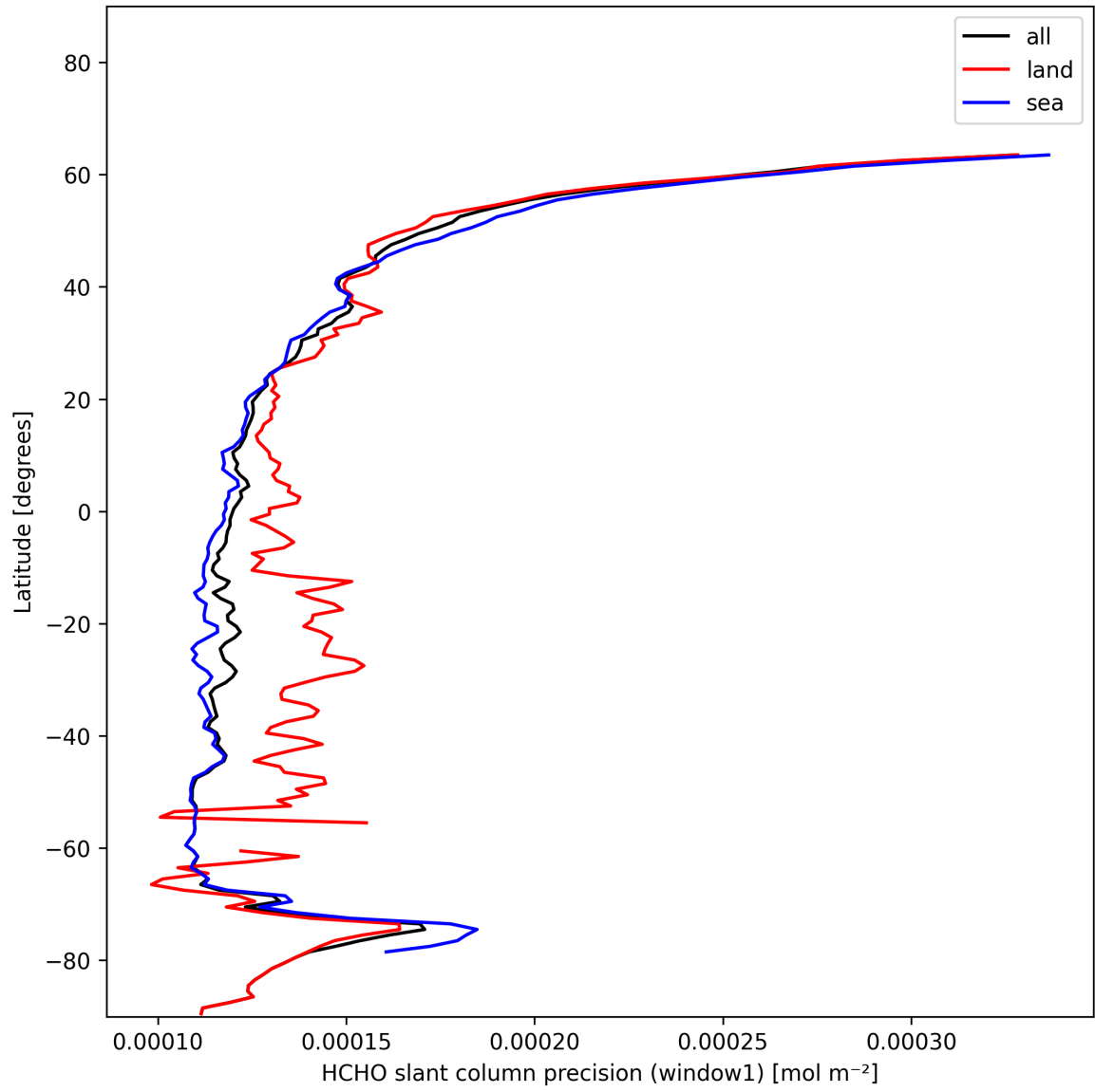
Figure 25: Zonal average of “HCHO slant column precision (window1)” for 2025-01-12 to 2025-01-14.
