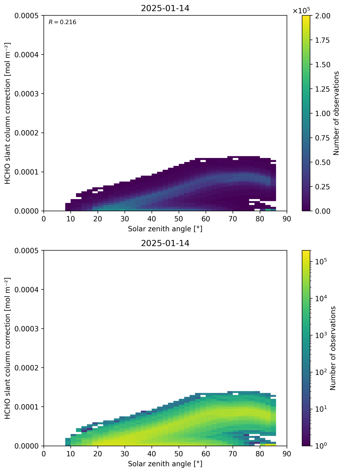
Figure 172: Scatter density plot of “Solar zenith angle” against “HCHO slant column correction” for 2025-01-13 to 2025-01-15.
