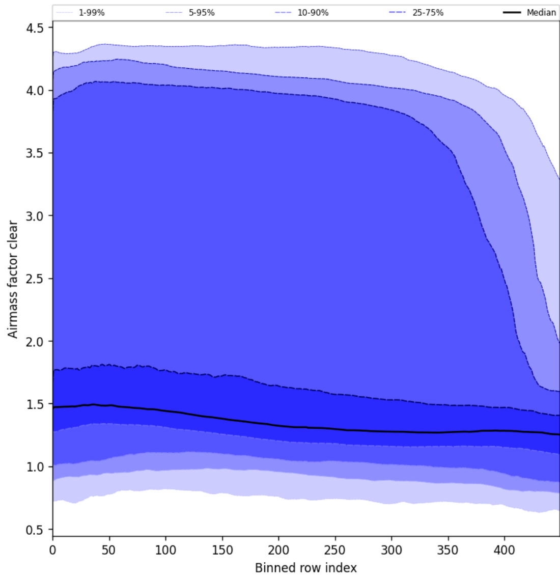
Figure 56: Along track statistics of “Airmass factor clear” for 2025-01-13 to 2025-01-15
