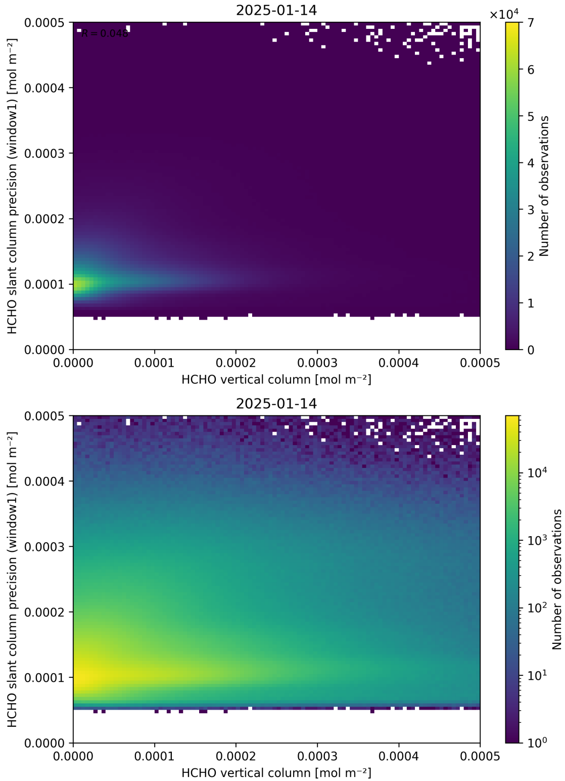
Figure 130: Scatter density plot of “HCHO vertical column” against “HCHO slant column precision (window1)” for 2025-01-13 to 2025-01-15.
