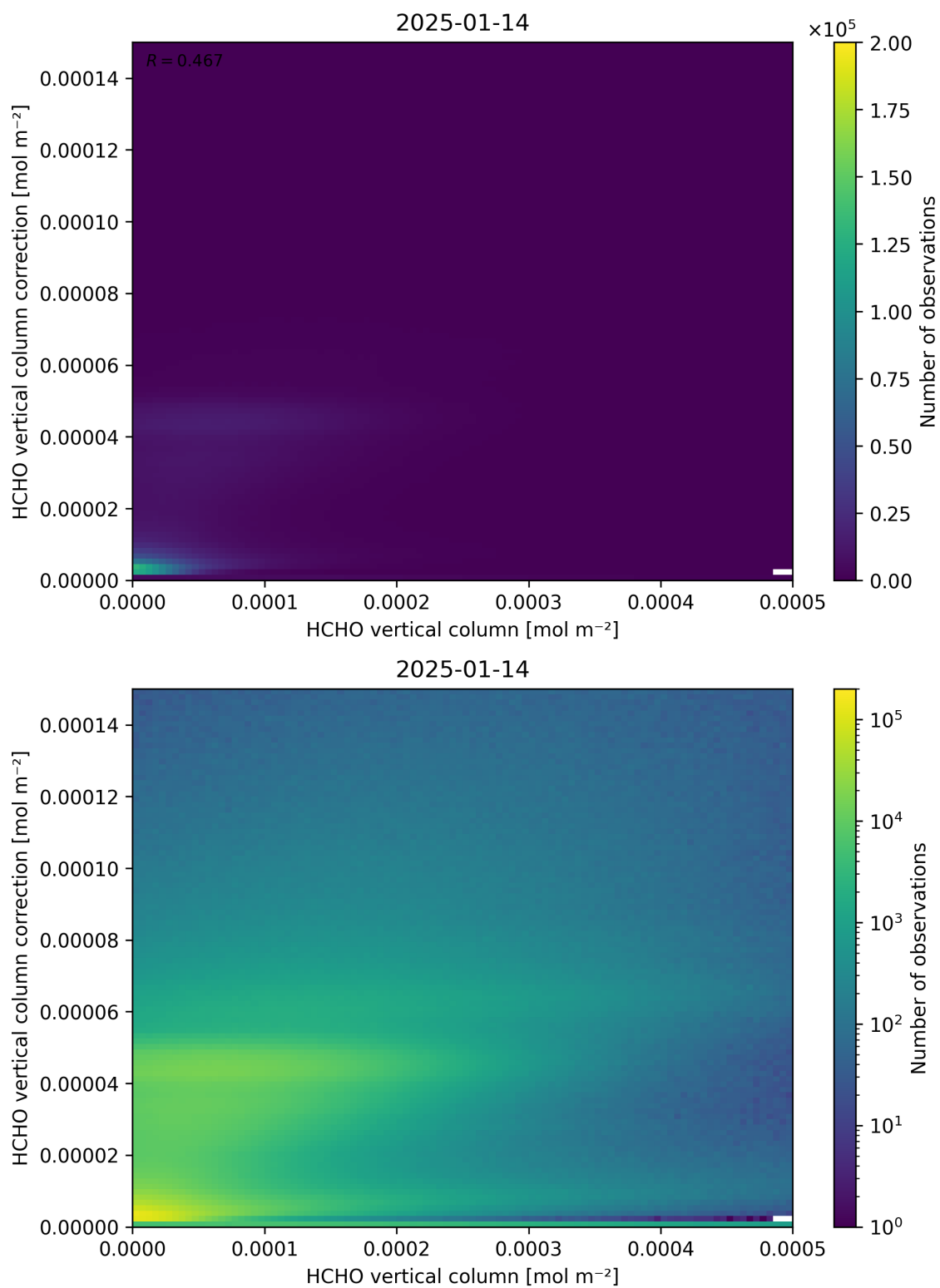
Figure 133: Scatter density plot of “HCHO vertical column” against “HCHO vertical column correction” for 2025-01-13 to 2025-01-15.
