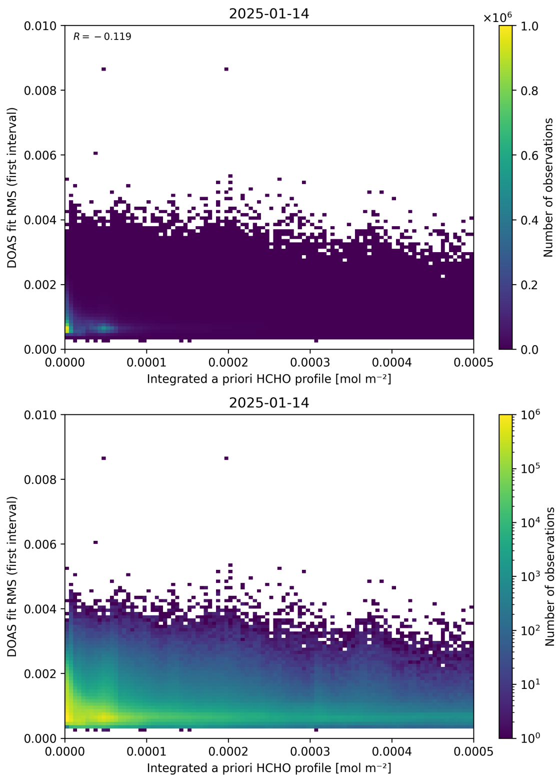
Figure 148: Scatter density plot of “Integrated a priori HCHO profile” against “DOAS fit RMS (first interval)” for 2025-01-13 to 2025-01-15.
