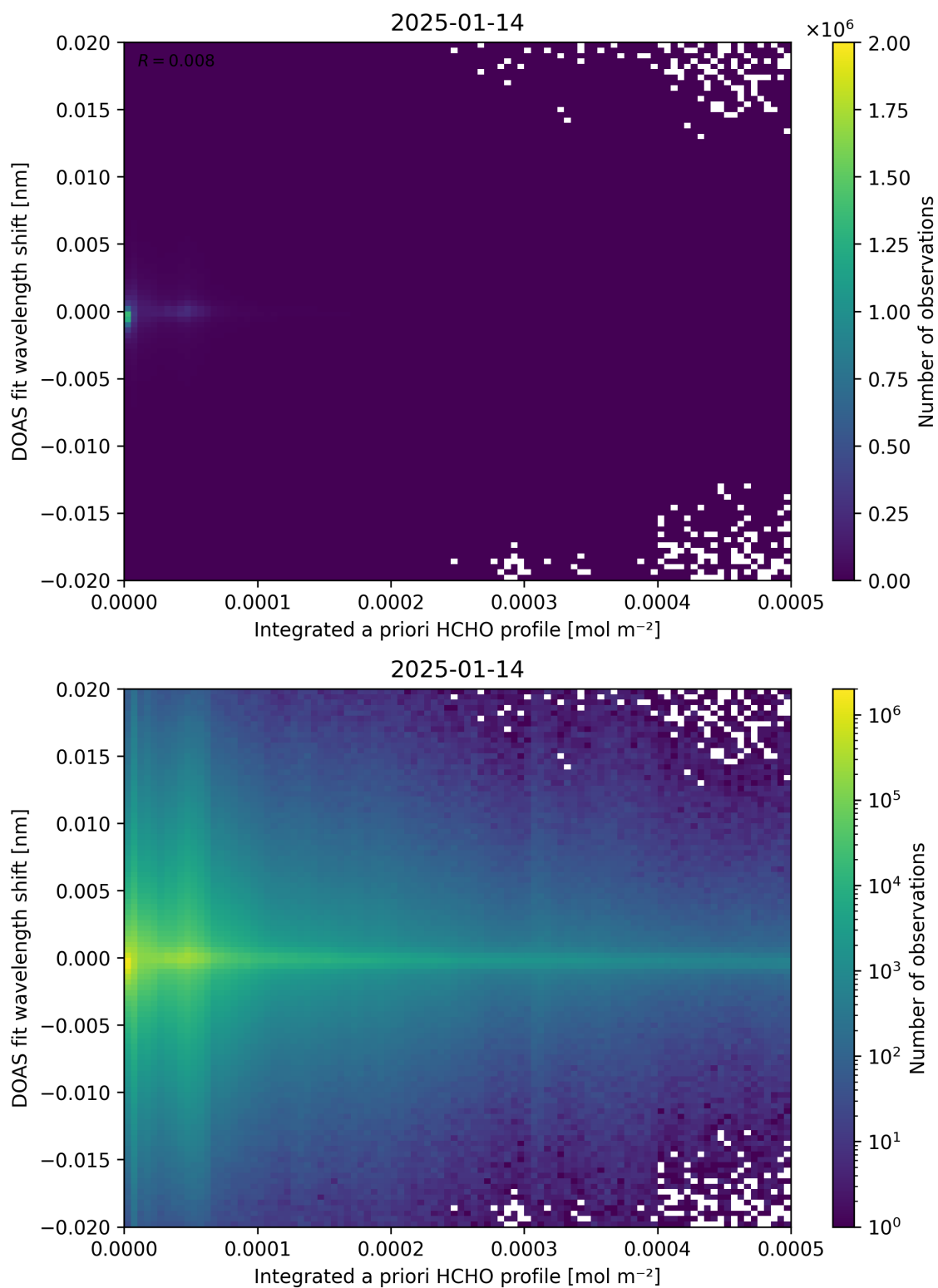
Figure 149: Scatter density plot of “Integrated a priori HCHO profile” against “DOAS fit wavelength shift” for 2025-01-13 to 2025-01-15.
