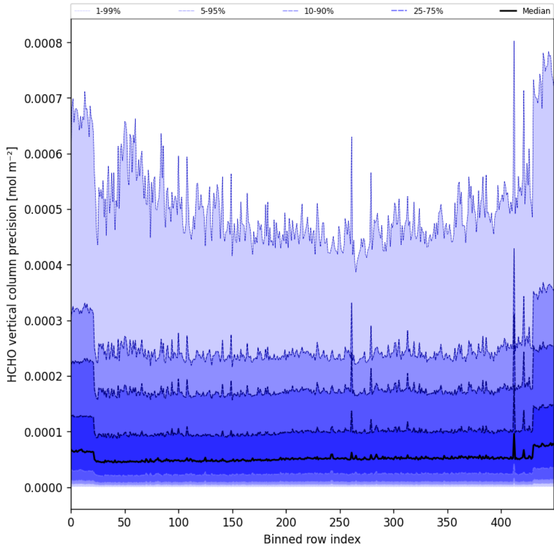
Figure 50: Along track statistics of “HCHO vertical column precision” for 2025-01-13 to 2025-01-15
