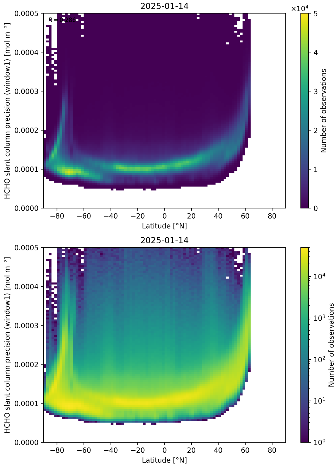
Figure 160: Scatter density plot of “Latitude” against “HCHO slant column precision (window1)” for 2025-01-13 to 2025-01-15.
