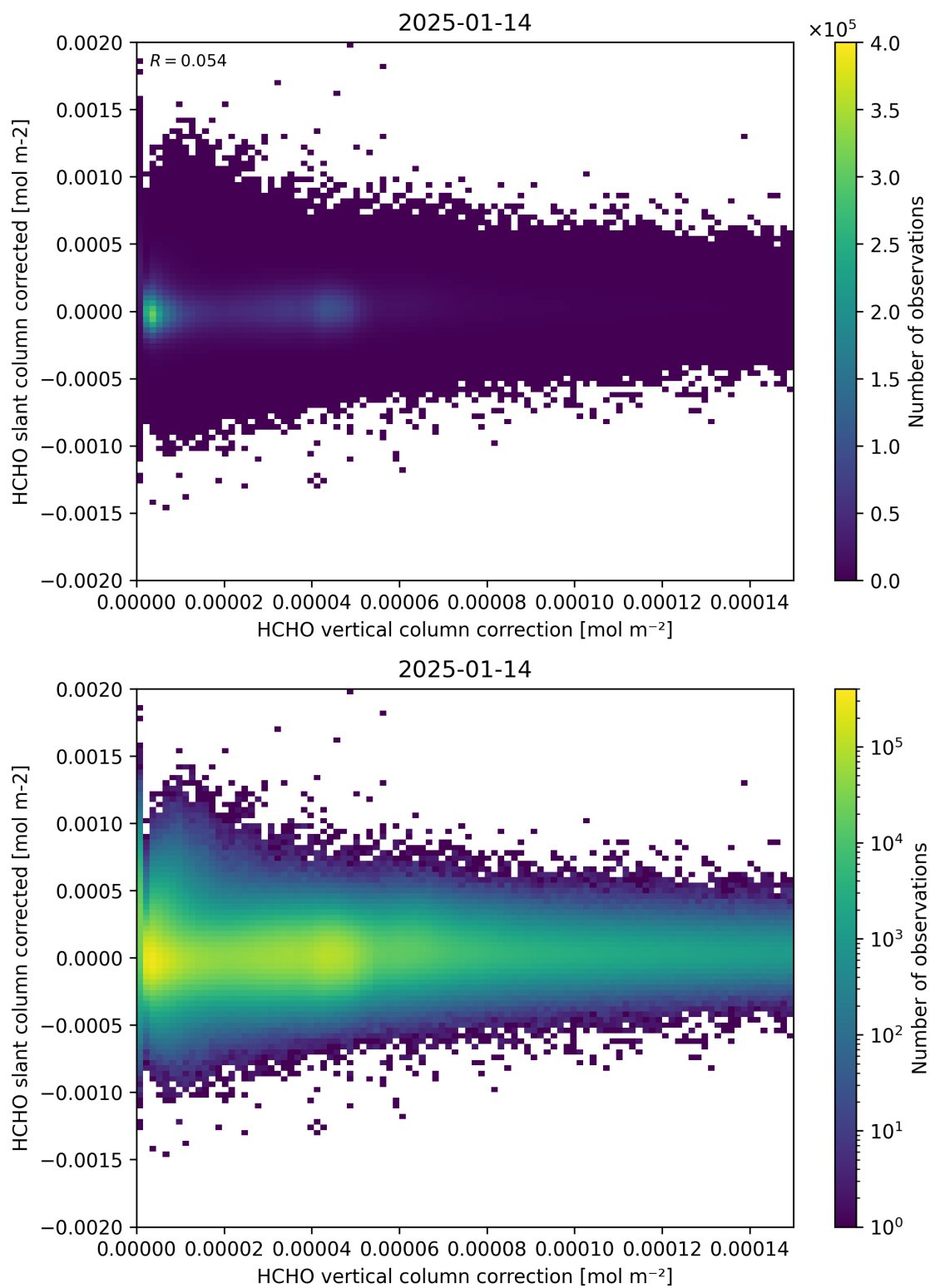
Figure 116: Scatter density plot of “HCHO vertical column correction” against “HCHO slant column corrected” for 2025-01-13 to 2025-01-15.
