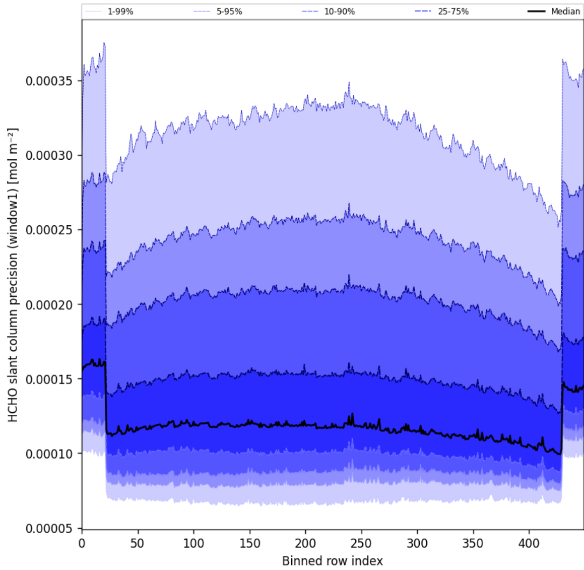
Figure 53: Along track statistics of “HCHO slant column precision (window1)” for 2025-01-13 to 2025-01-15
