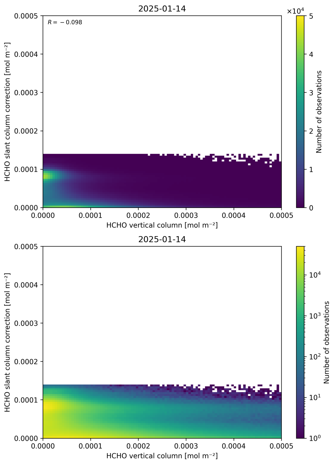
Figure 128: Scatter density plot of “HCHO vertical column” against “HCHO slant column correction” for 2025-01-13 to 2025-01-15.
