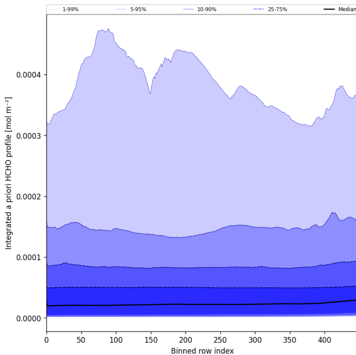
Figure 57: Along track statistics of “Integrated a priori HCHO profile” for 2025-01-13 to 2025-01-15
