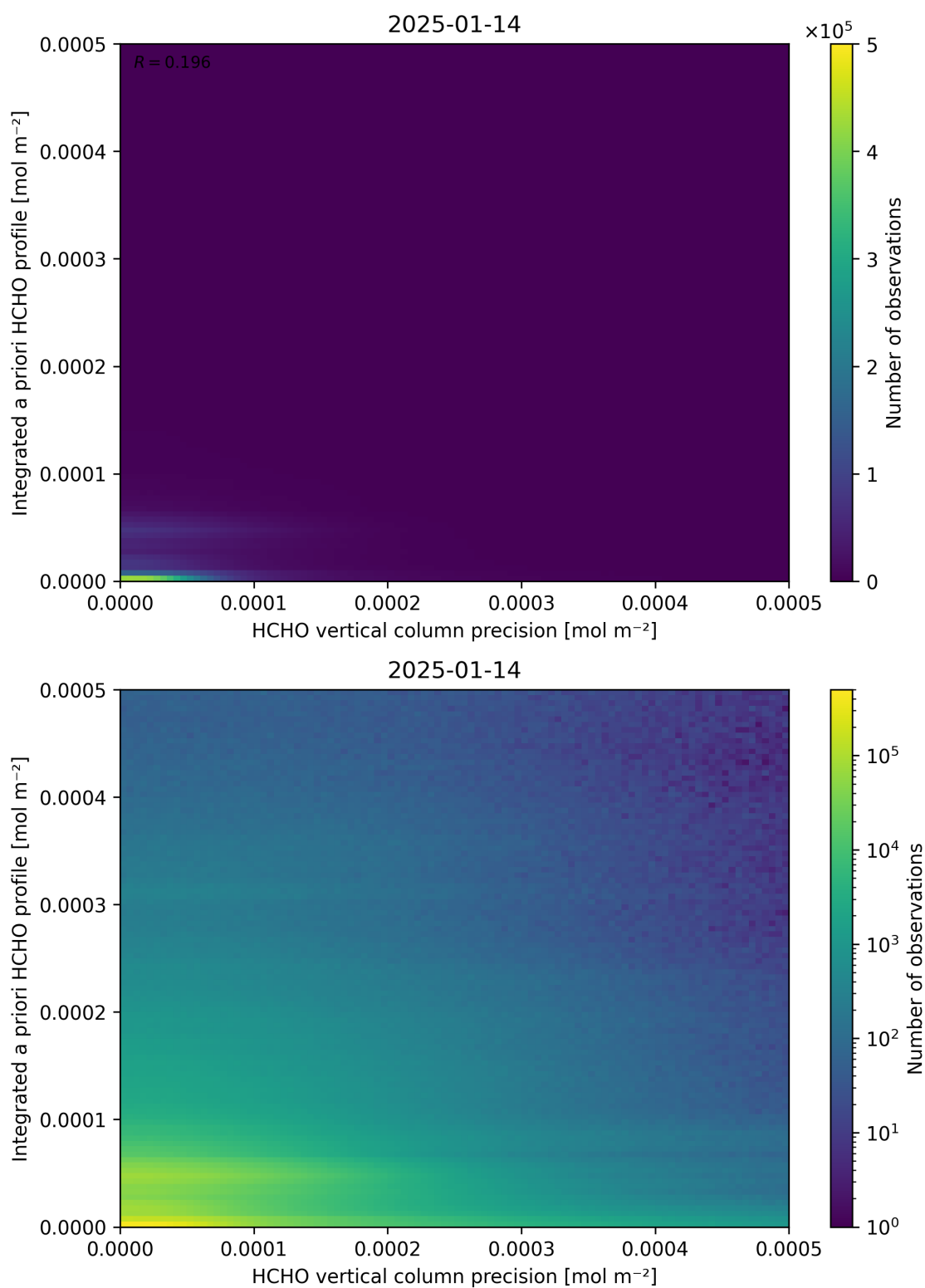
Figure 147: Scatter density plot of “HCHO vertical column precision” against “Integrated a priori HCHO profile” for 2025-01-13 to 2025-01-15.
