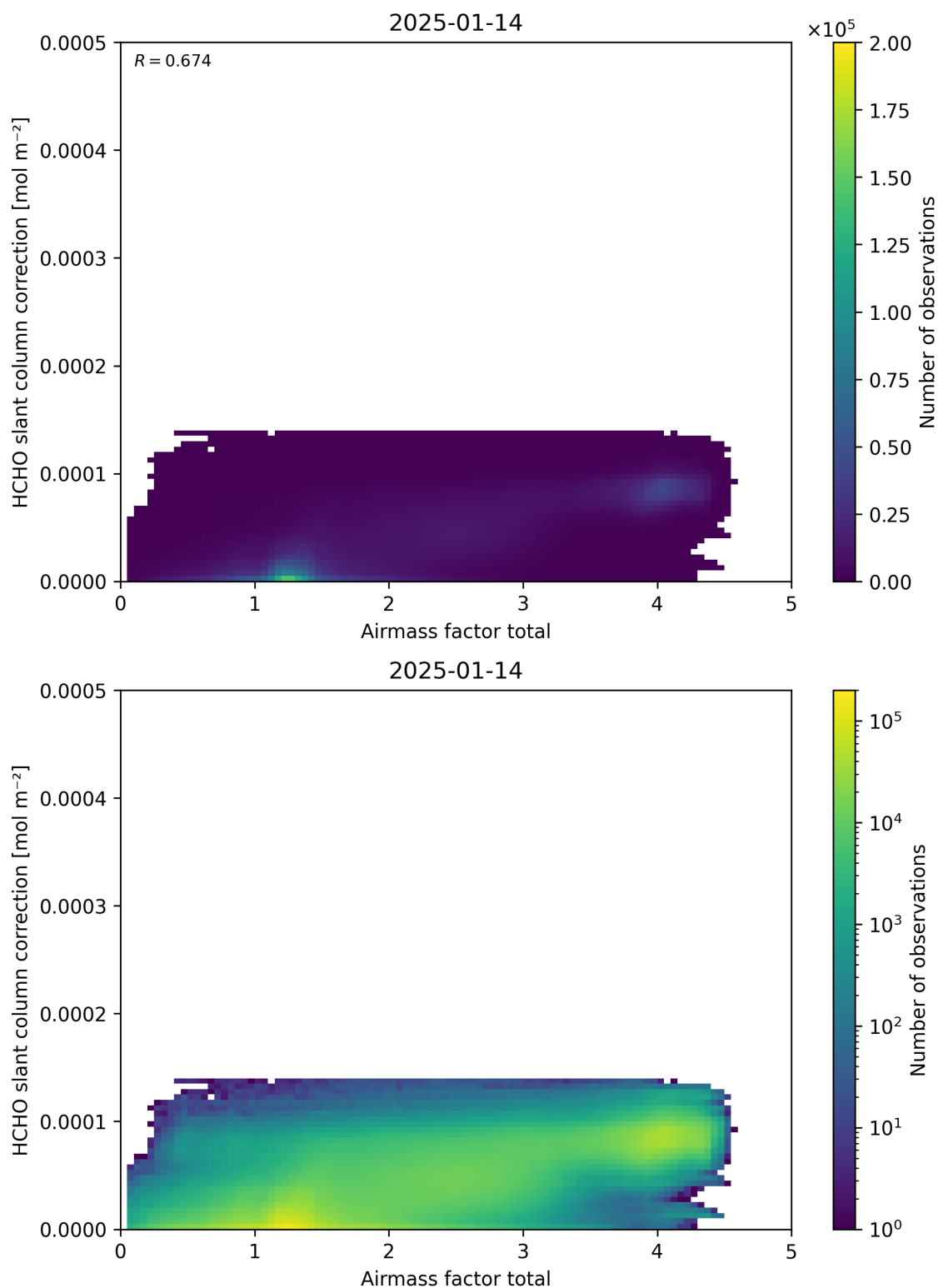
Figure 102: Scatter density plot of “Airmass factor total” against “HCHO slant column correction” for 2025-01-13 to 2025-01-15.
