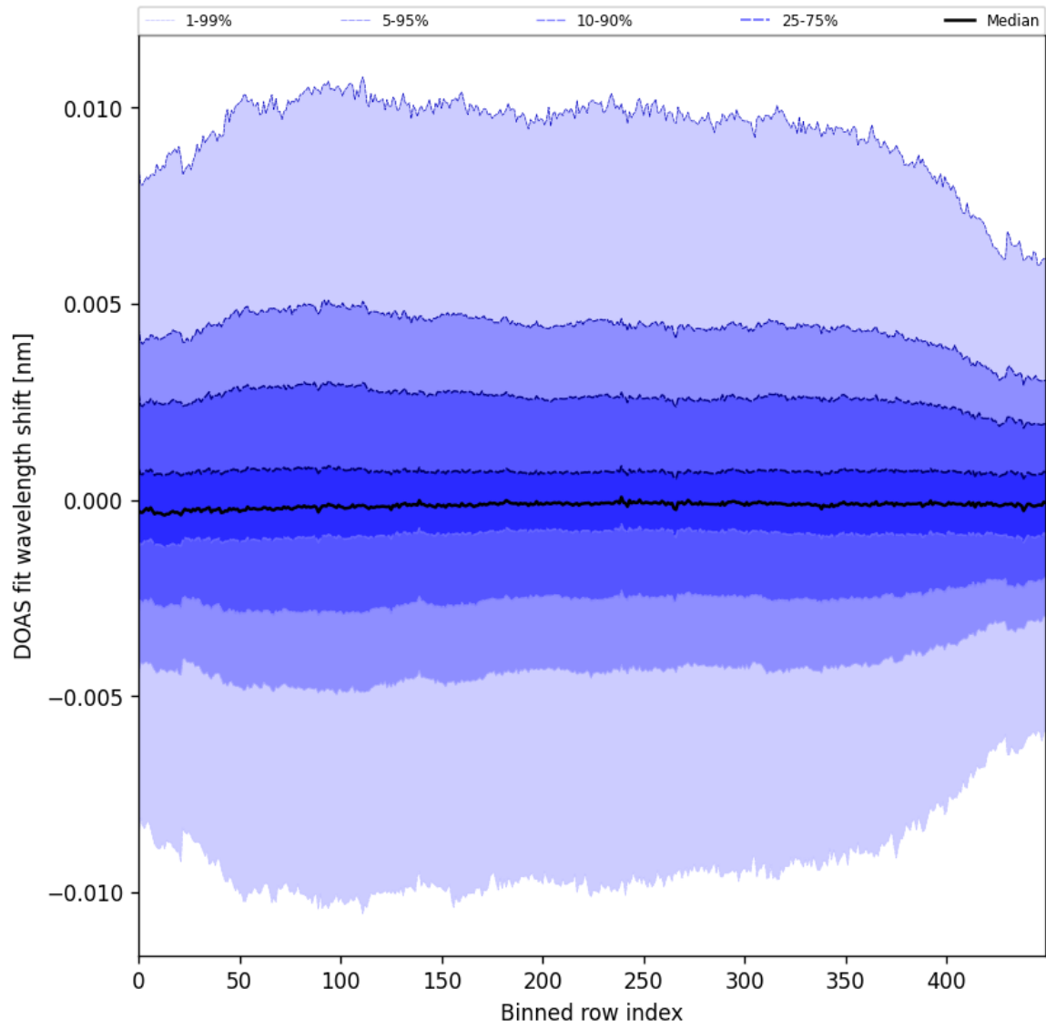
Figure 58: Along track statistics of “DOAS fit wavelength shift” for 2025-01-13 to 2025-01-15
