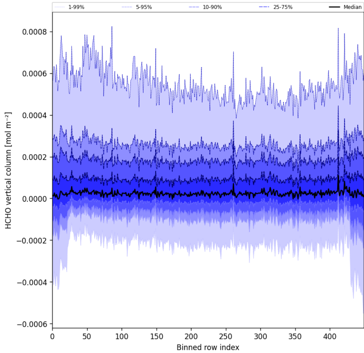
Figure 49: Along track statistics of “HCHO vertical column” for 2025-01-13 to 2025-01-15
