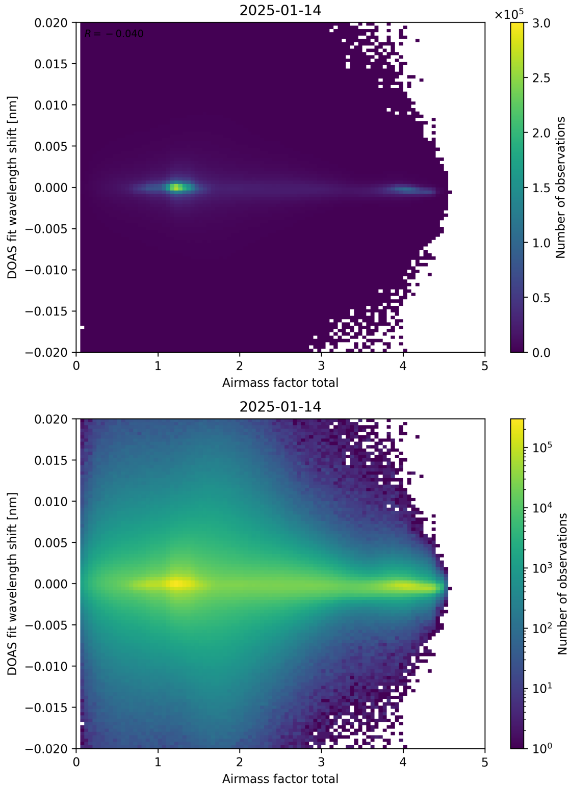
Figure 98: Scatter density plot of “Airmass factor total” against “DOAS fit wavelength shift” for 2025-01-13 to 2025-01-15.
