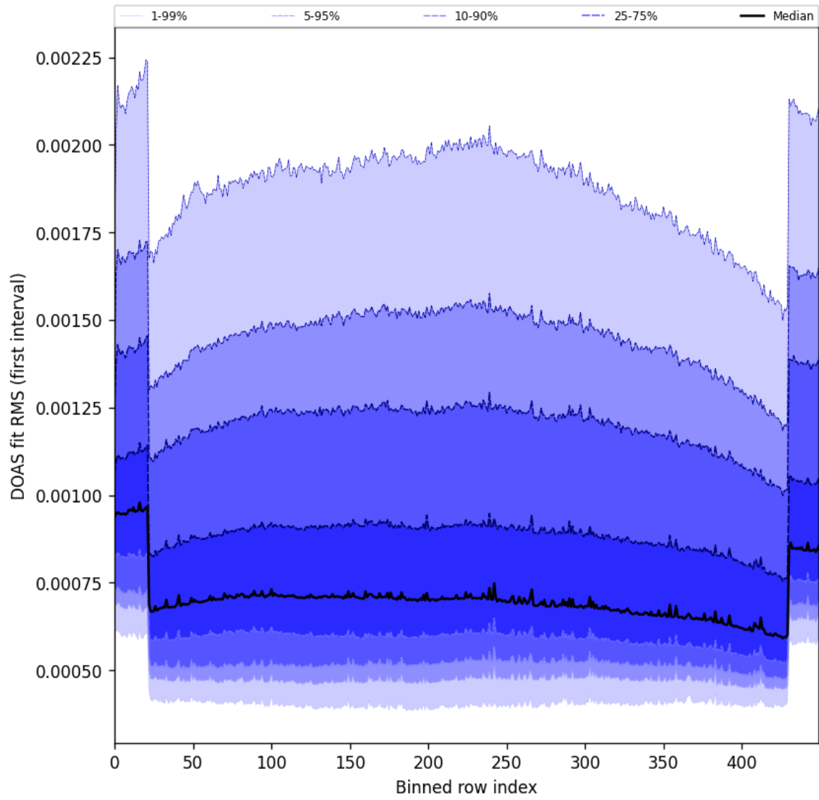
Figure 60: Along track statistics of “DOAS fit RMS (first interval)” for 2025-01-13 to 2025-01-15
