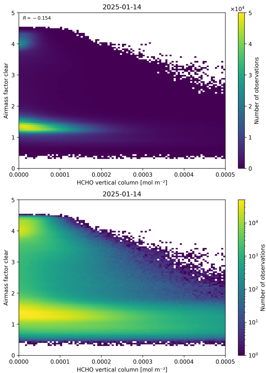
Figure 126: Scatter density plot of “HCHO vertical column” against “Airmass factor clear” for 2025-01-13 to 2025-01-15.
