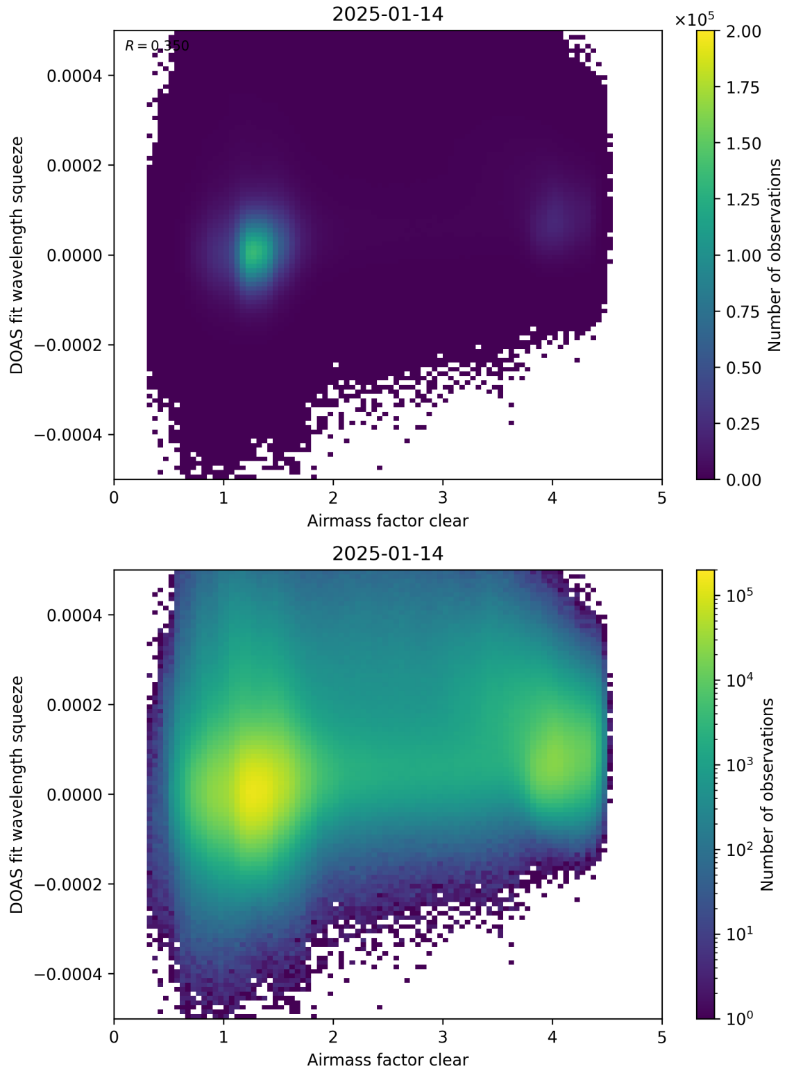
Figure 73: Scatter density plot of “Airmass factor clear” against “DOAS fit wavelength squeeze” for 2025-01-13 to 2025-01-15.
