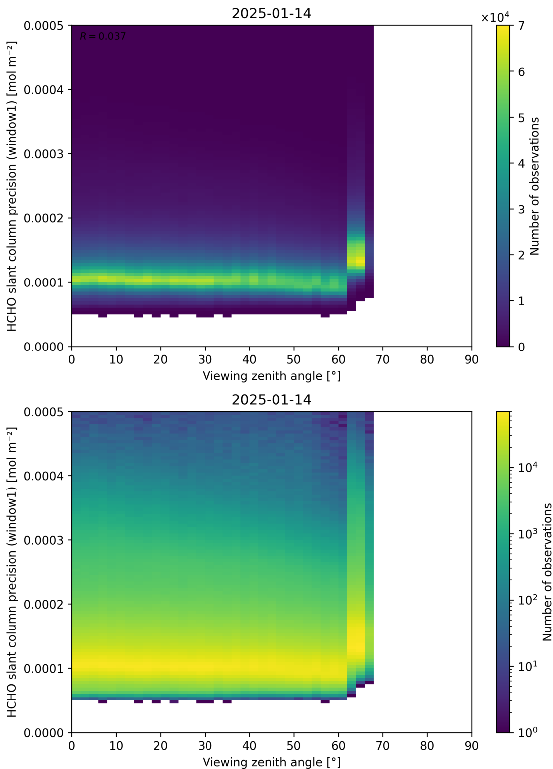
Figure 189: Scatter density plot of “Viewing zenith angle” against “HCHO slant column precision (window1)” for 2025-01-13 to 2025-01-15.
