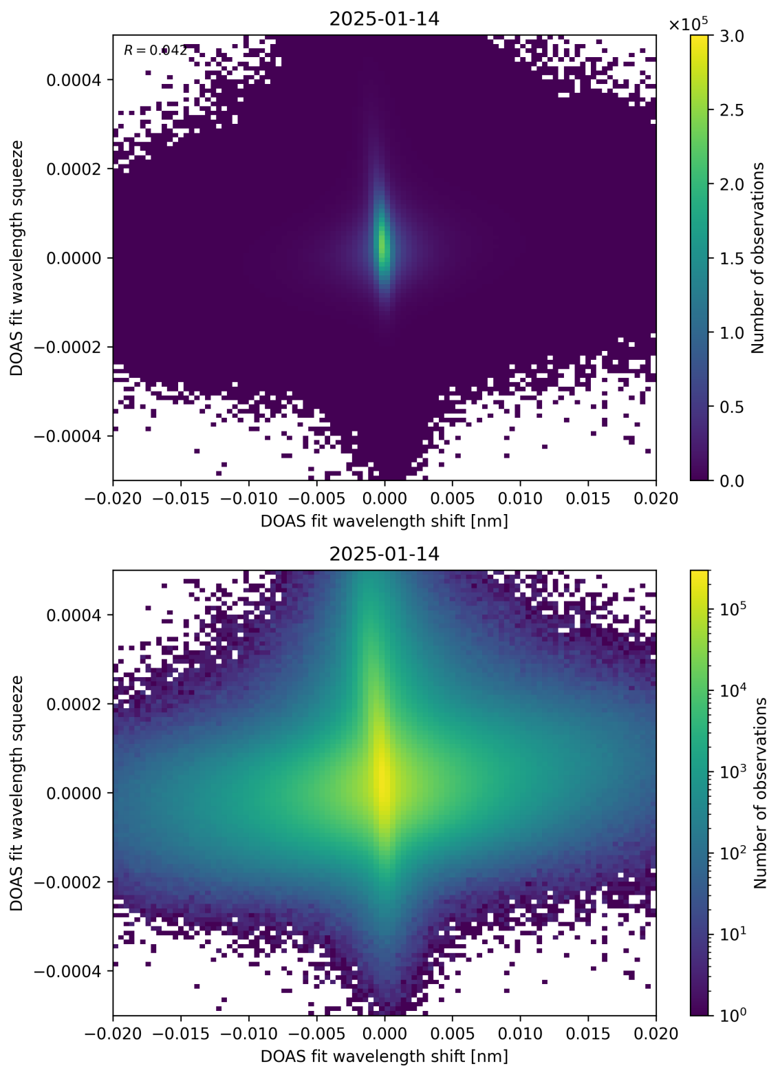
Figure 65: Scatter density plot of “DOAS fit wavelength shift” against “DOAS fit wavelength squeeze” for 2025-01-13 to 2025-01-15.
