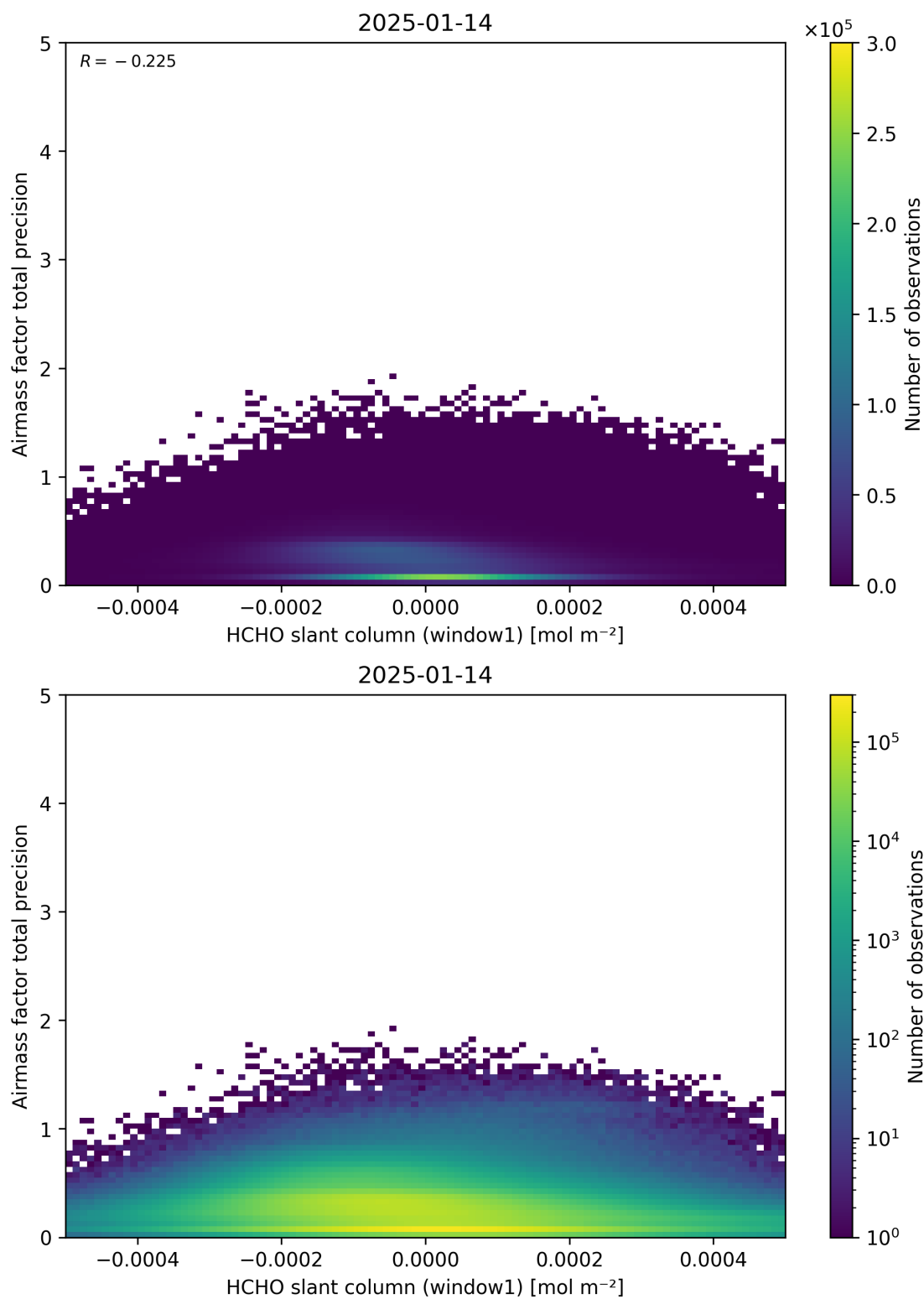
Figure 86: Scatter density plot of “HCHO slant column (window1)” against “Airmass factor total precision” for 2025-01-13 to 2025-01-15.
