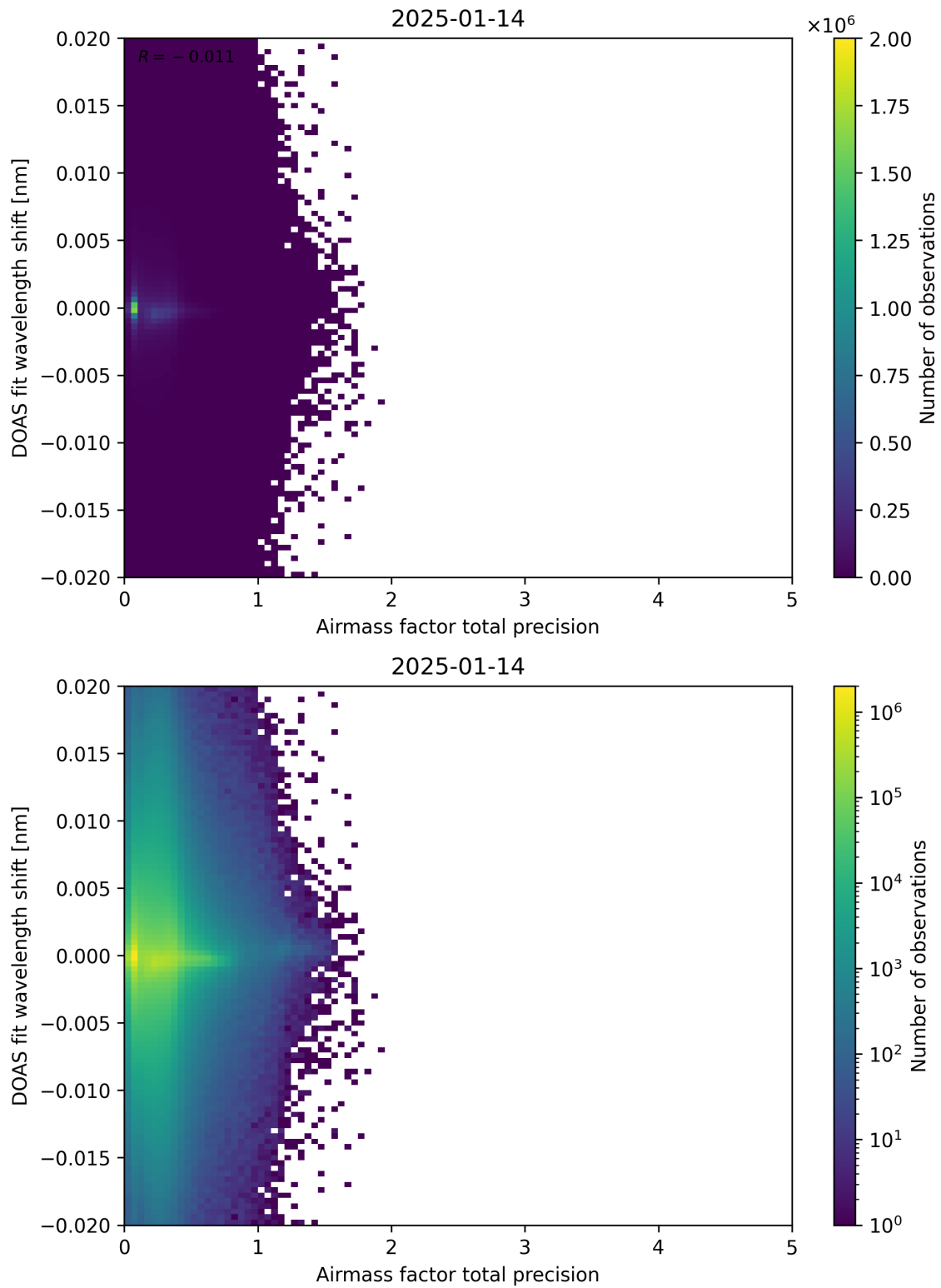
Figure 106: Scatter density plot of “Airmass factor total precision” against “DOAS fit wavelength shift” for 2025-01-13 to 2025-01-15.
