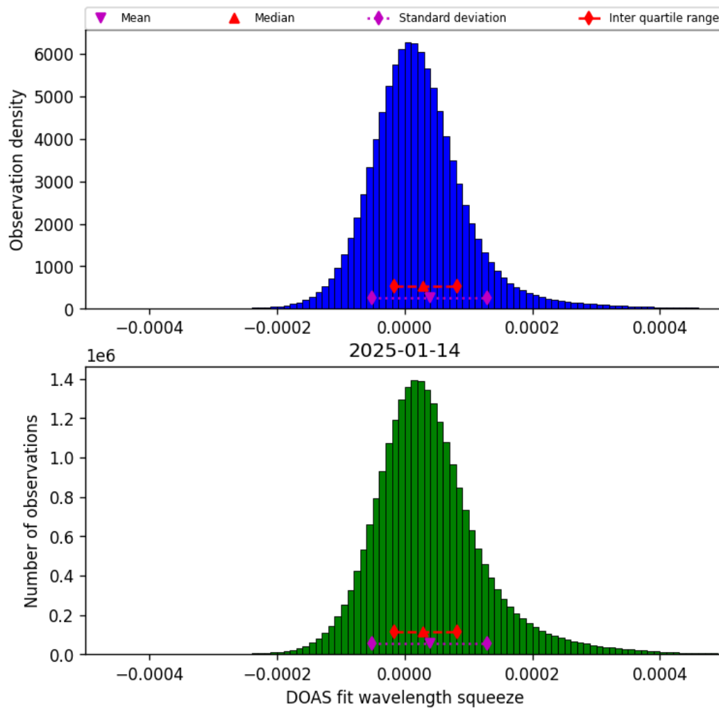
Figure 45: Histogram of “DOAS fit wavelength squeeze” for 2025-01-13 to 2025-01-15
