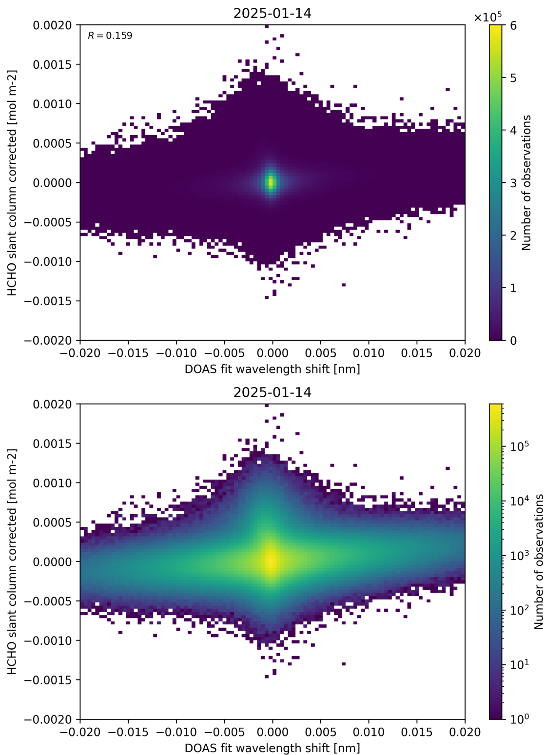
Figure 66: Scatter density plot of “DOAS fit wavelength shift” against “HCHO slant column corrected” for 2025-01-13 to 2025-01-15.
