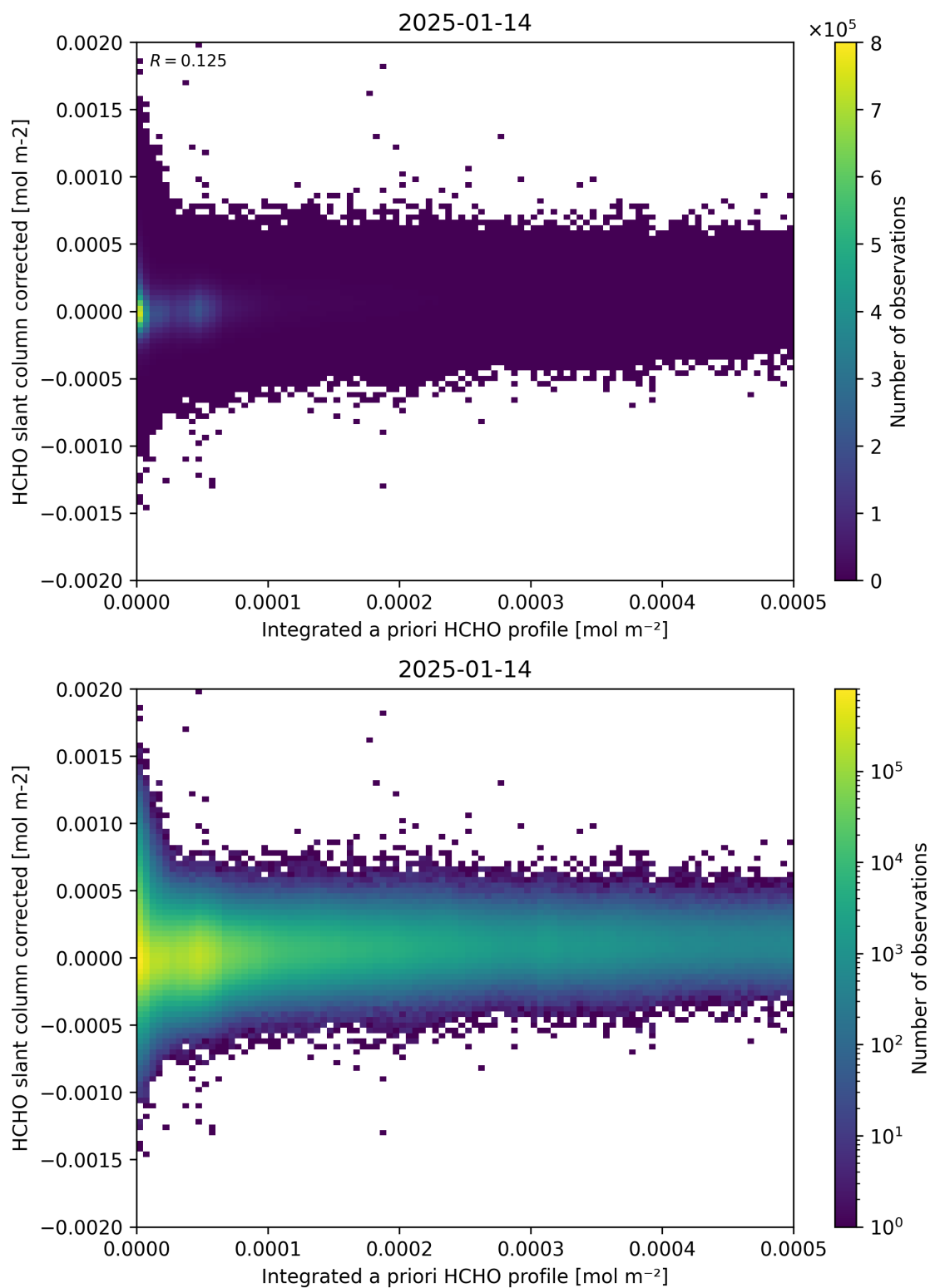
Figure 151: Scatter density plot of “Integrated a priori HCHO profile” against “HCHO slant column corrected” for 2025-01-13 to 2025-01-15.
