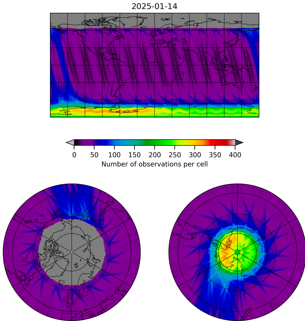
Figure 19: Map of the number of observations for 2025-01-13 to 2025-01-15
