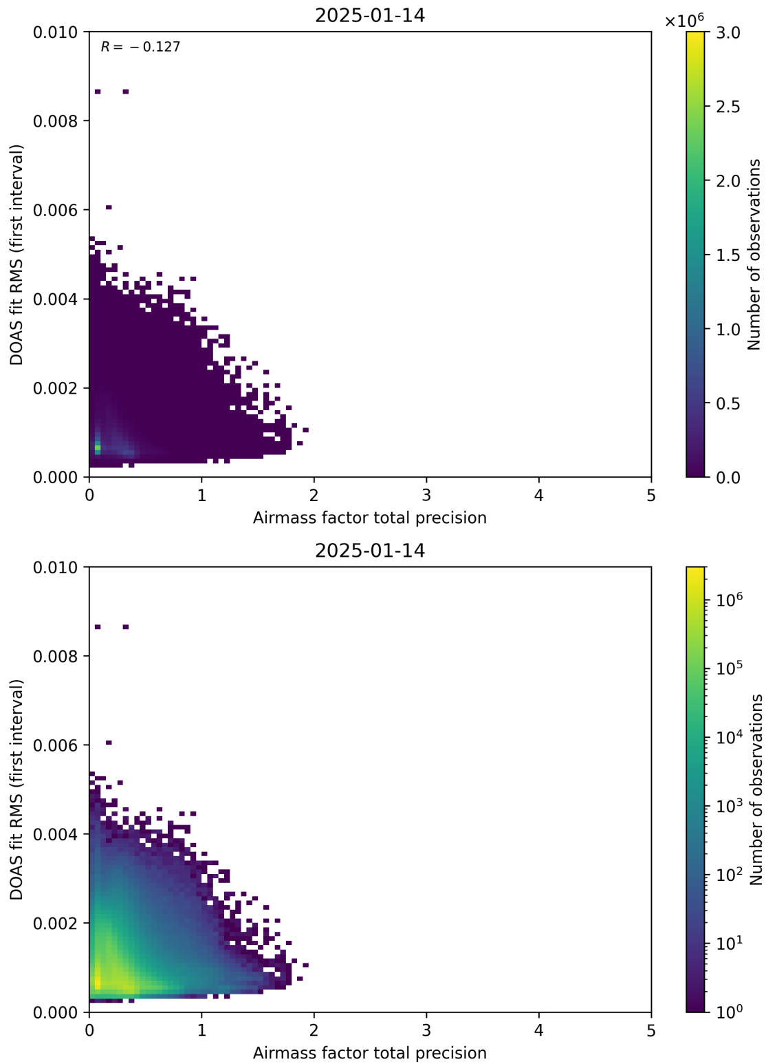
Figure 105: Scatter density plot of “Airmass factor total precision” against “DOAS fit RMS (first interval)” for 2025-01-13 to 2025-01-15.
