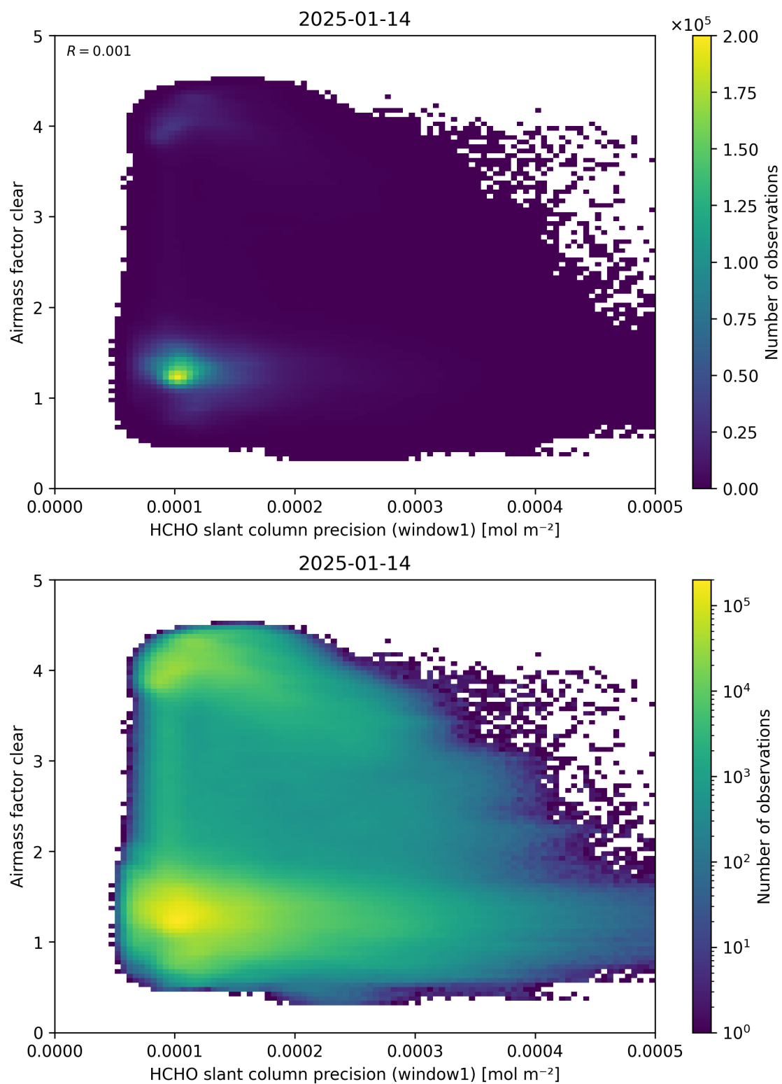
Figure 91: Scatter density plot of “HCHO slant column precision (window1)” against “Airmass factor clear” for 2025-01-13 to 2025-01-15.
