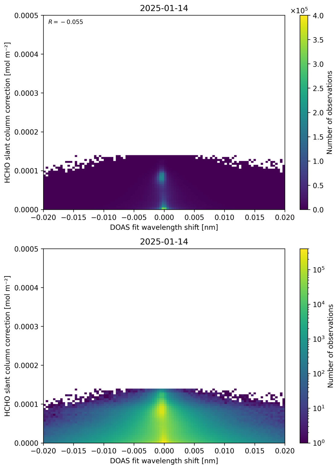
Figure 67: Scatter density plot of “DOAS fit wavelength shift” against “HCHO slant column correction” for 2025-01-13 to 2025-01-15.
