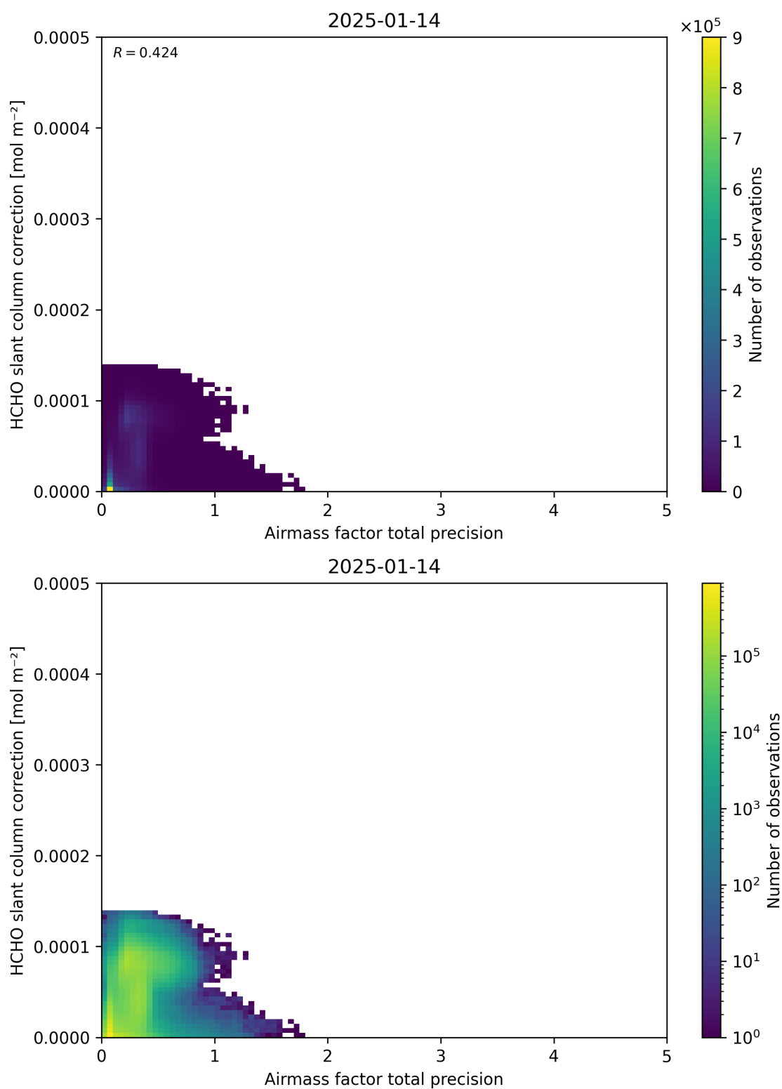
Figure 110: Scatter density plot of “Airmass factor total precision” against “HCHO slant column correction” for 2025-01-13 to 2025-01-15.
