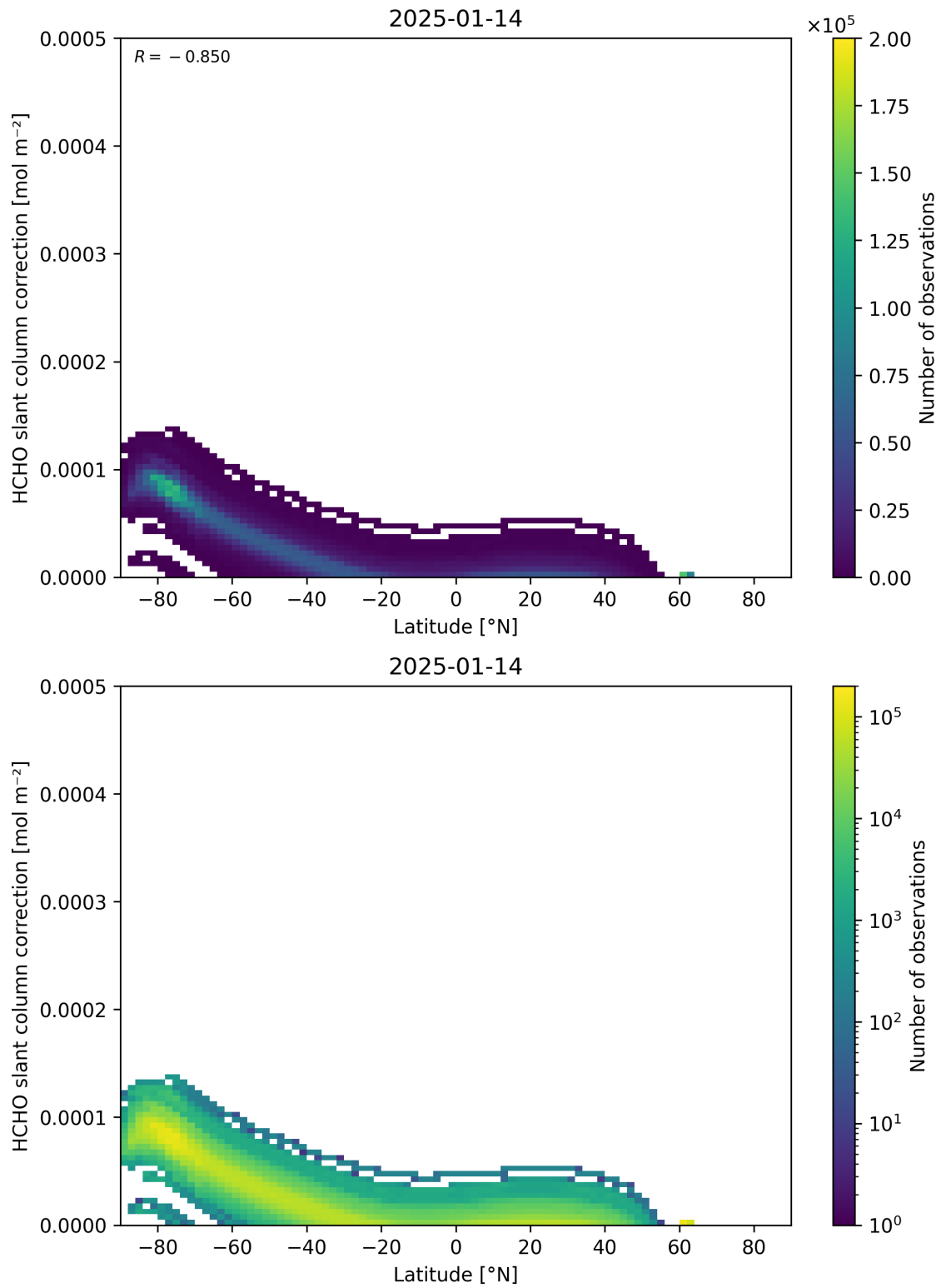
Figure 158: Scatter density plot of “Latitude” against “HCHO slant column correction” for 2025-01-13 to 2025-01-15.
