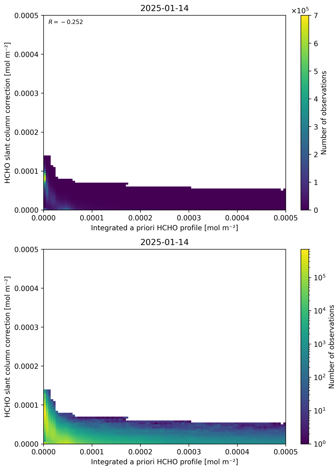
Figure 152: Scatter density plot of “Integrated a priori HCHO profile” against “HCHO slant column correction” for 2025-01-13 to 2025-01-15.
