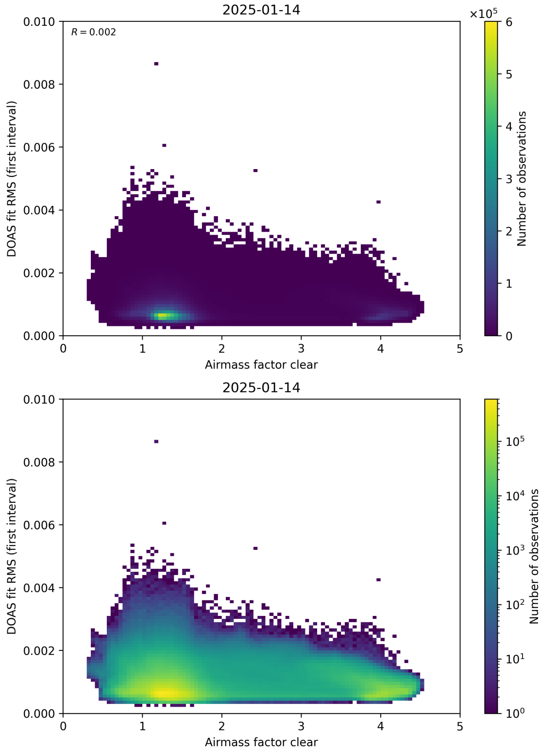
Figure 71: Scatter density plot of “Airmass factor clear” against “DOAS fit RMS (first interval)” for 2025-01-13 to 2025-01-15.
