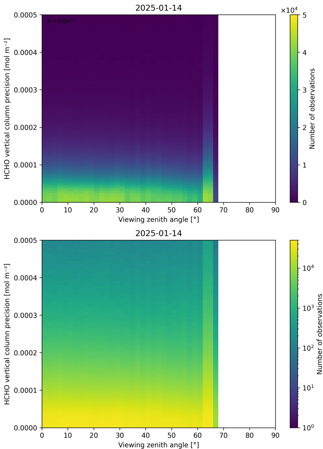
Figure 194: Scatter density plot of “Viewing zenith angle” against “HCHO vertical column precision” for 2025-01-13 to 2025-01-15.
