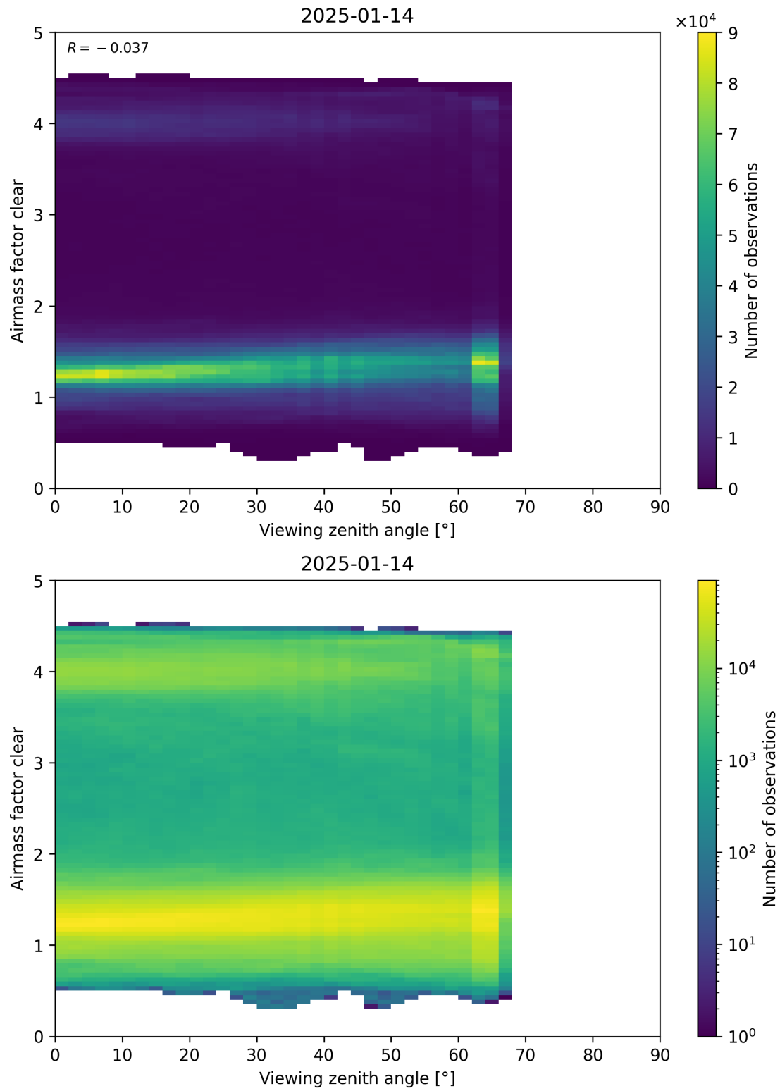
Figure 185: Scatter density plot of “Viewing zenith angle” against “Airmass factor clear” for 2025-01-13 to 2025-01-15.
