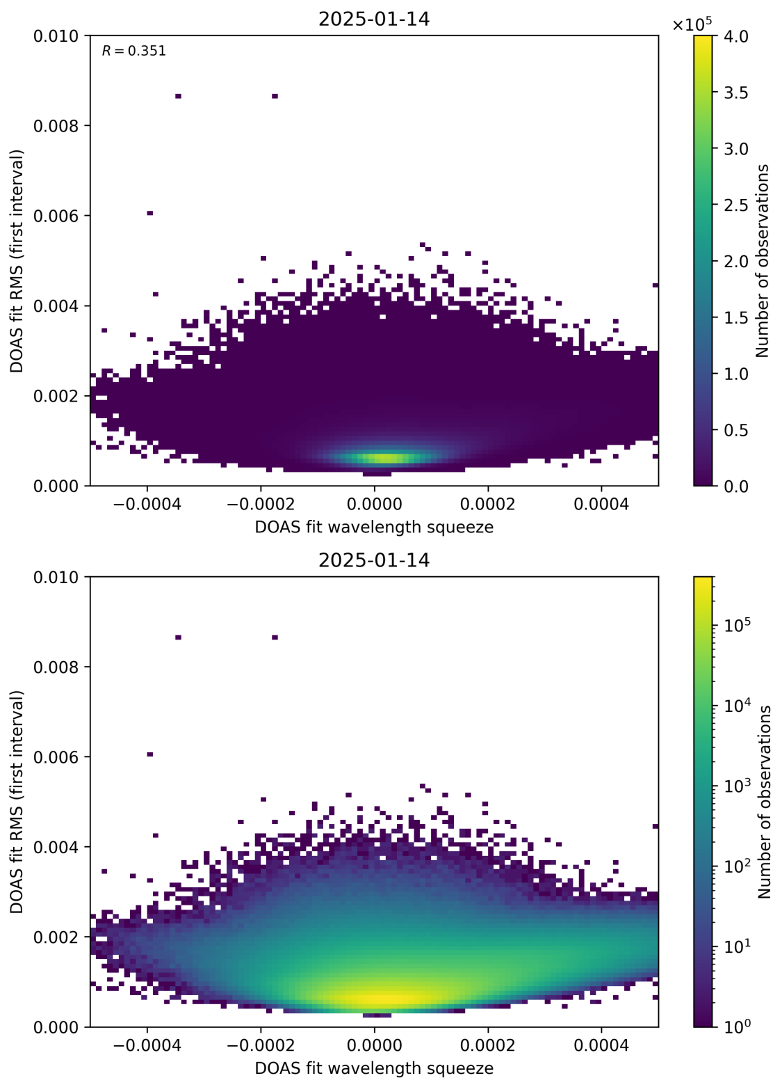
Figure 68: Scatter density plot of “DOAS fit wavelength squeeze” against “DOAS fit RMS (first interval)” for 2025-01-13 to 2025-01-15.
