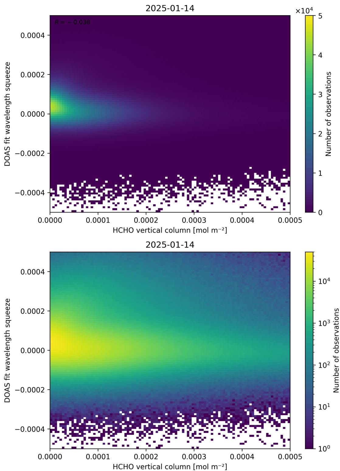
Figure 125: Scatter density plot of “HCHO vertical column” against “DOAS fit wavelength squeeze” for 2025-01-13 to 2025-01-15.
