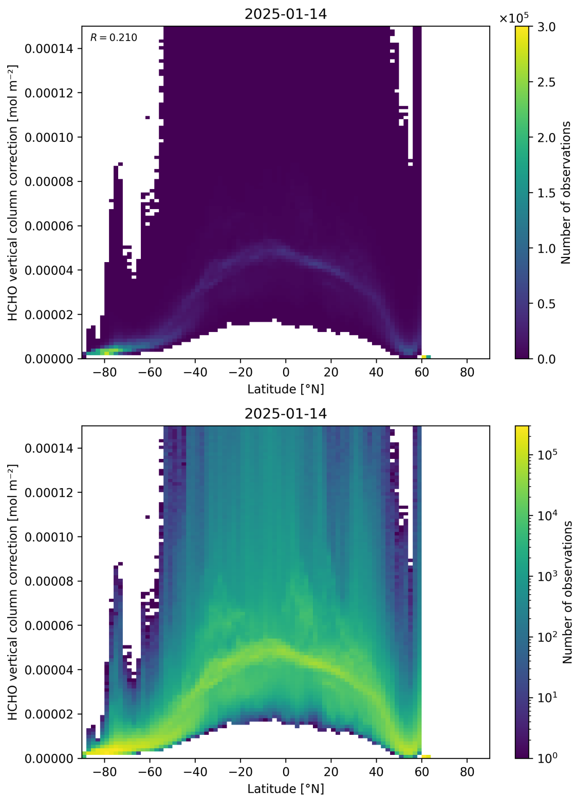
Figure 164: Scatter density plot of “Latitude” against “HCHO vertical column correction” for 2025-01-13 to 2025-01-15.
