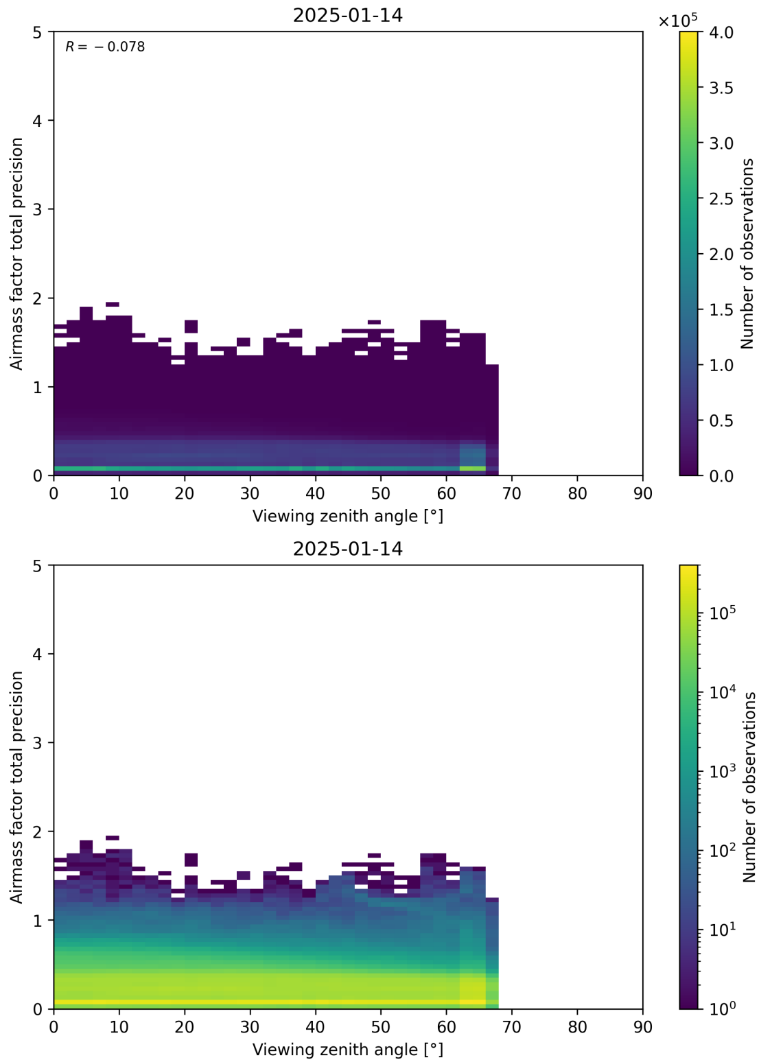
Figure 191: Scatter density plot of “Viewing zenith angle” against “Airmass factor total precision” for 2025-01-13 to 2025-01-15.
