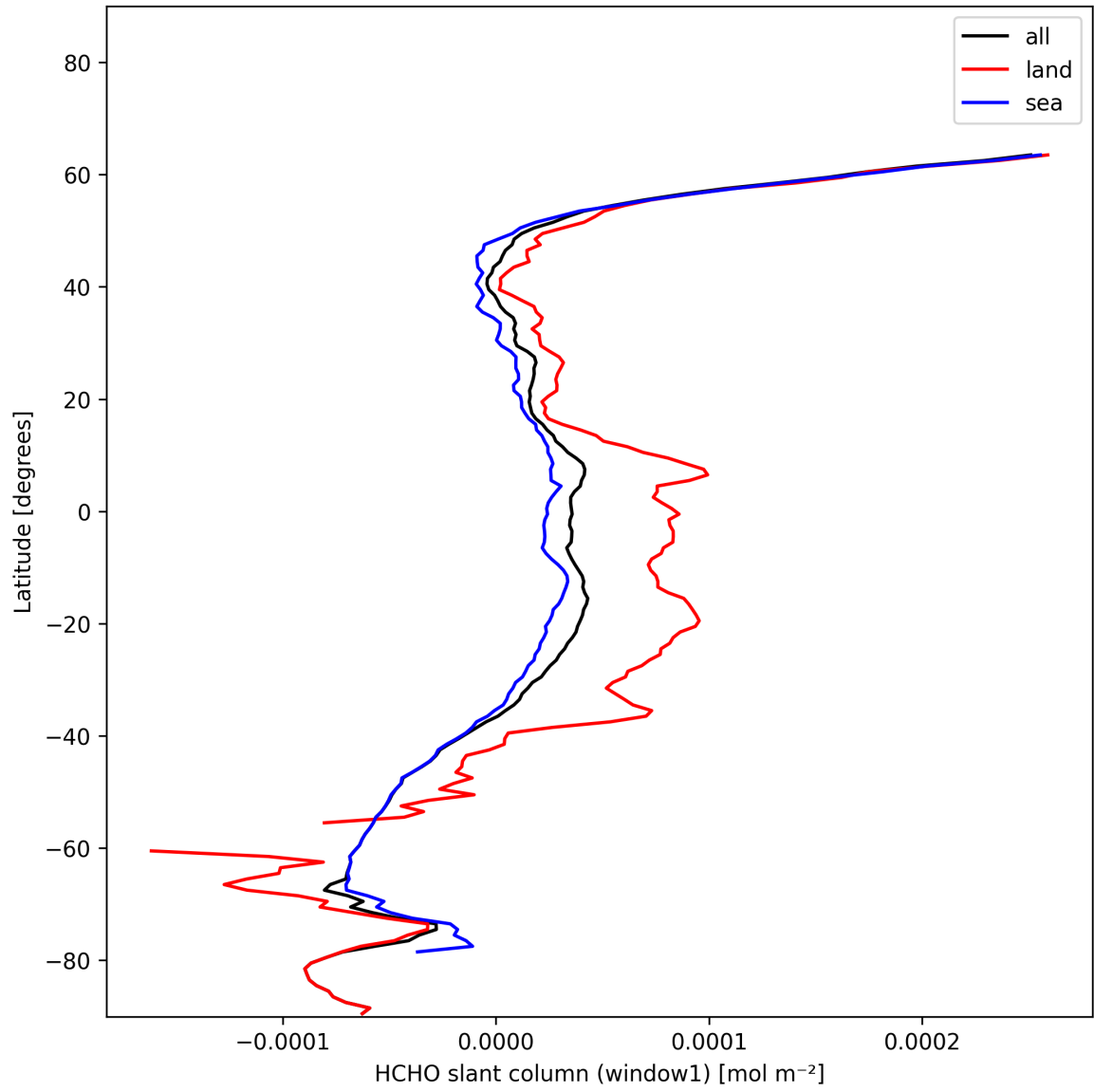
Figure 24: Zonal average of “HCHO slant column (window1)” for 2025-01-13 to 2025-01-15.
