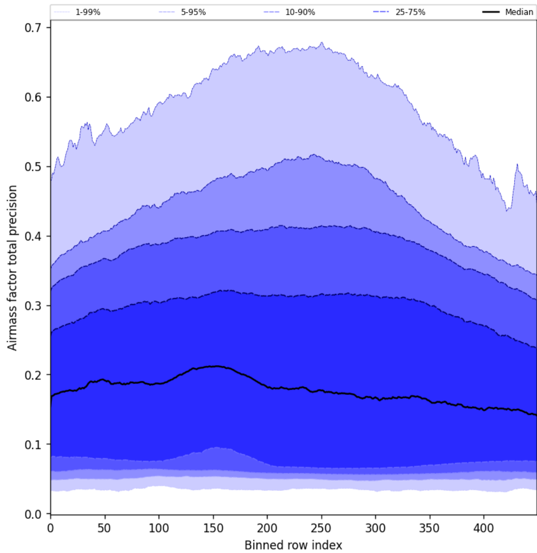
Figure 55: Along track statistics of “Airmass factor total precision” for 2025-01-13 to 2025-01-15
