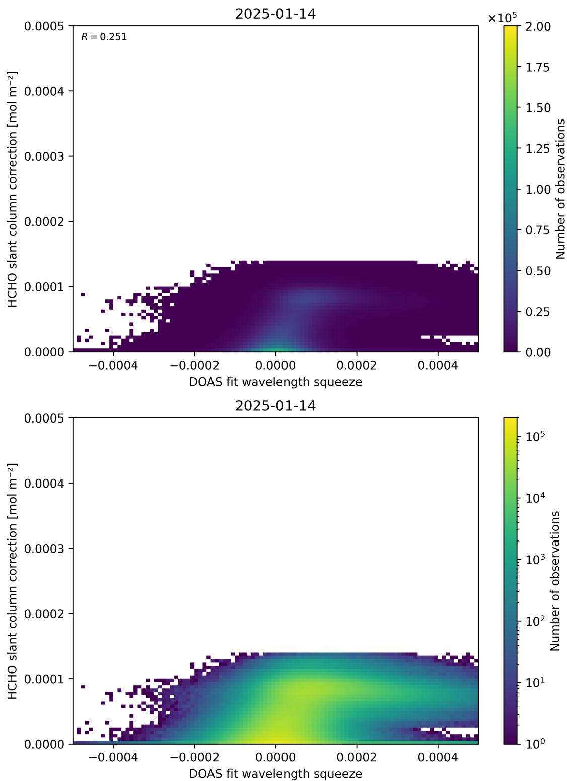
Figure 70: Scatter density plot of “DOAS fit wavelength squeeze” against “HCHO slant column correction” for 2025-01-13 to 2025-01-15.
