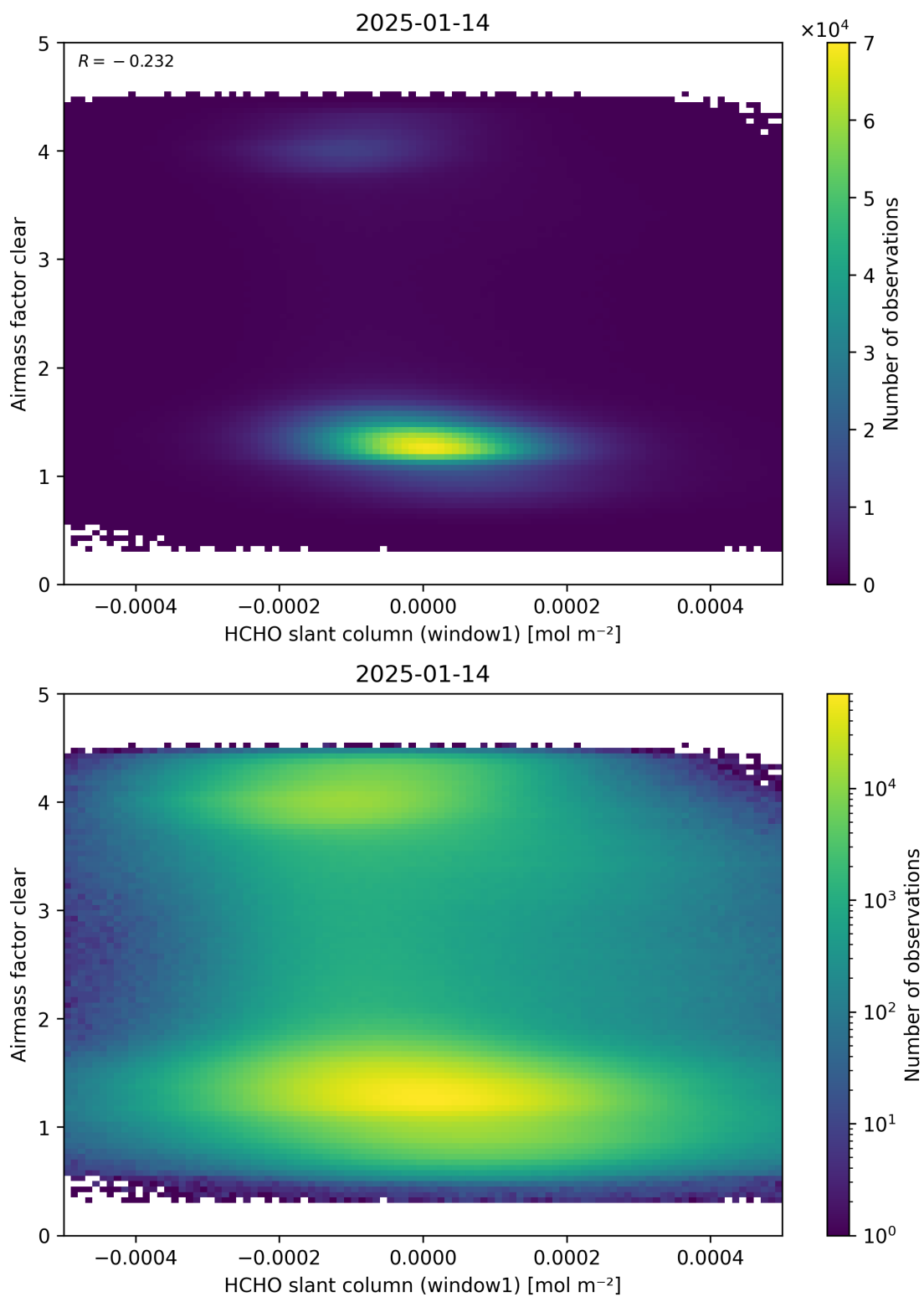
Figure 81: Scatter density plot of “HCHO slant column (window1)” against “Airmass factor clear” for 2025-01-13 to 2025-01-15.
