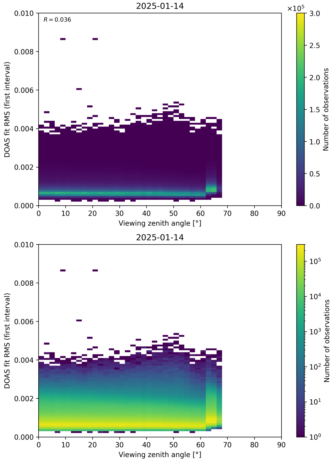
Figure 182: Scatter density plot of “Viewing zenith angle” against “DOAS fit RMS (first interval)” for 2025-01-13 to 2025-01-15.
