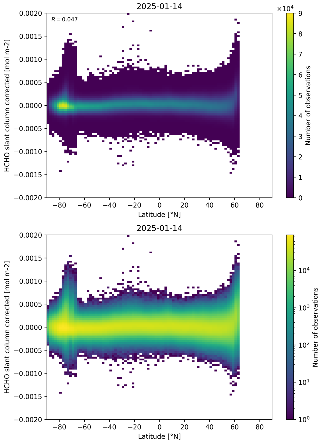
Figure 157: Scatter density plot of “Latitude” against “HCHO slant column corrected” for 2025-01-13 to 2025-01-15.
