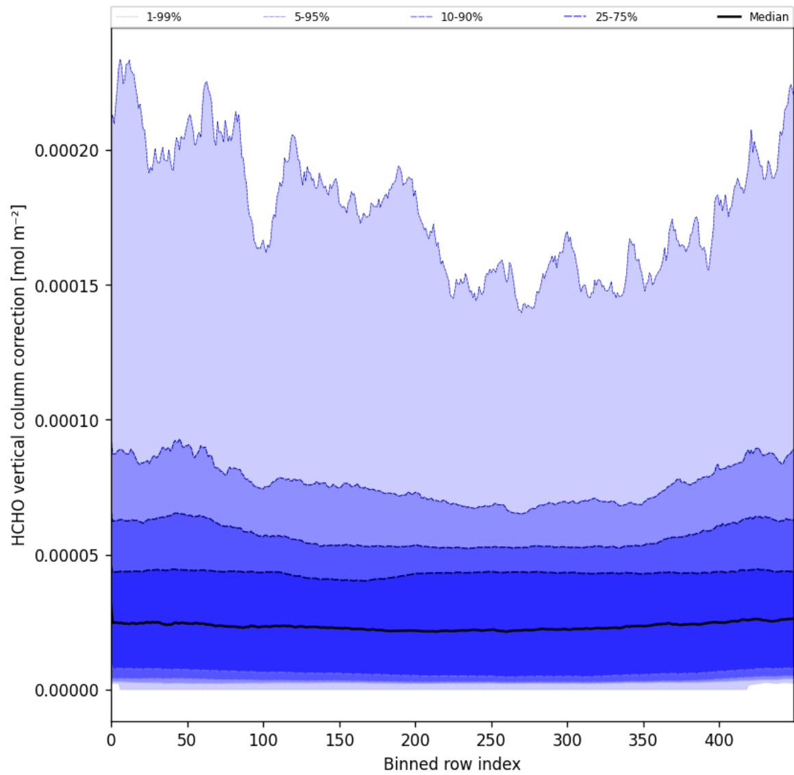
Figure 51: Along track statistics of “HCHO vertical column correction” for 2025-01-13 to 2025-01-15
