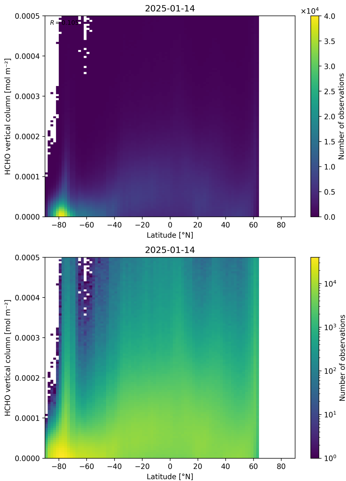
Figure 163: Scatter density plot of “Latitude” against “HCHO vertical column” for 2025-01-13 to 2025-01-15.
