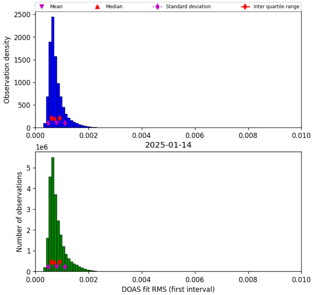
Figure 46: Histogram of “DOAS fit RMS (first interval)” for 2025-01-13 to 2025-01-15
