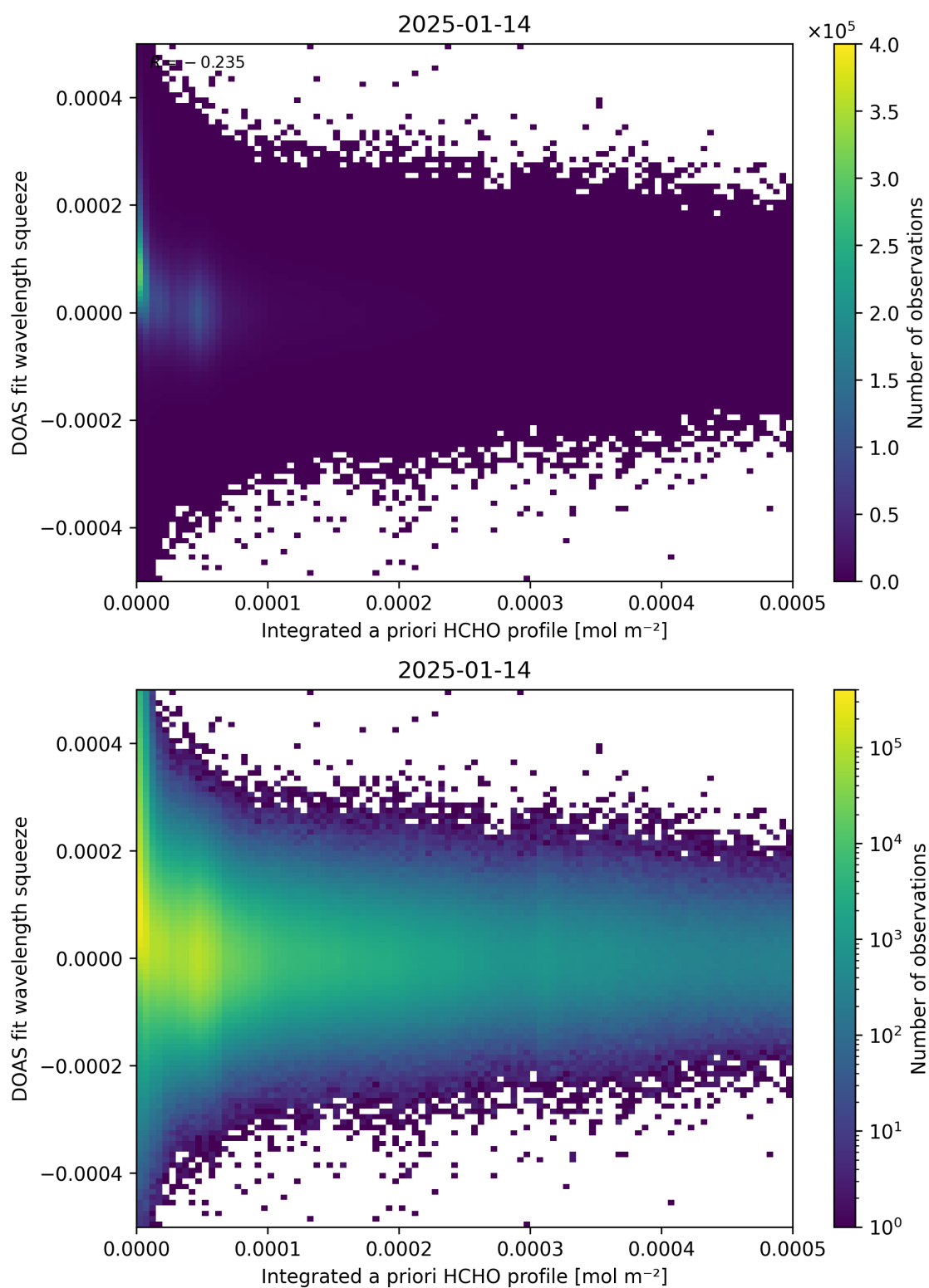
Figure 150: Scatter density plot of “Integrated a priori HCHO profile” against “DOAS fit wavelength squeeze” for 2025-01-13 to 2025-01-15.
