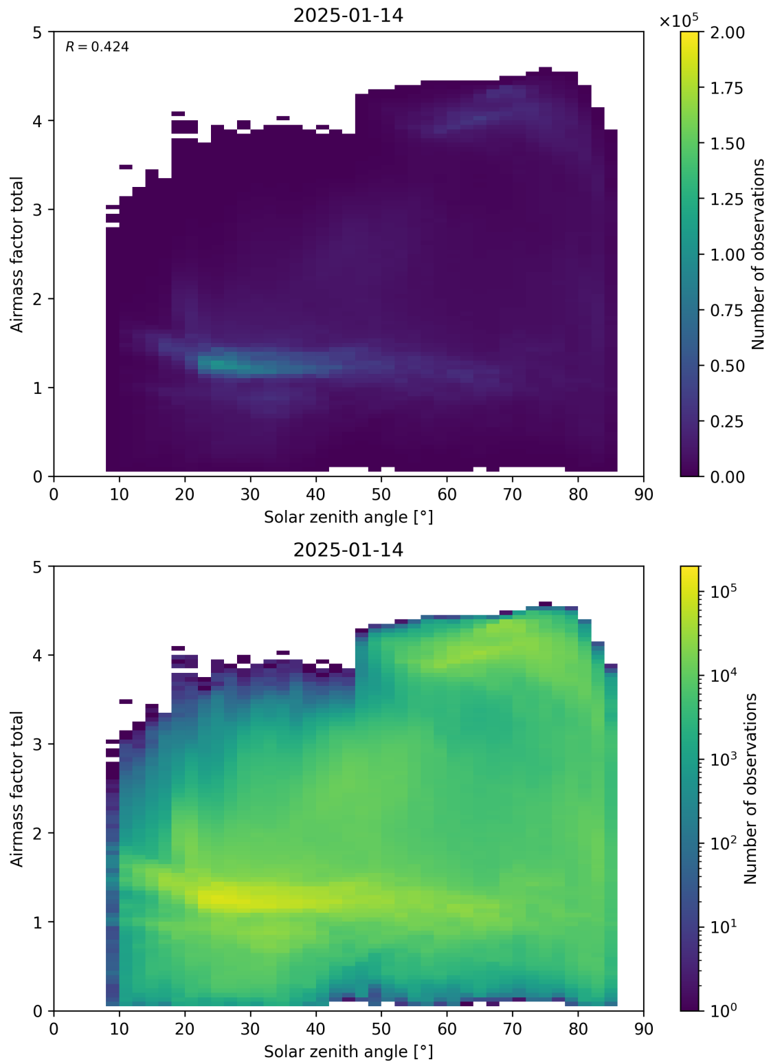
Figure 175: Scatter density plot of “Solar zenith angle” against “Airmass factor total” for 2025-01-13 to 2025-01-15.
