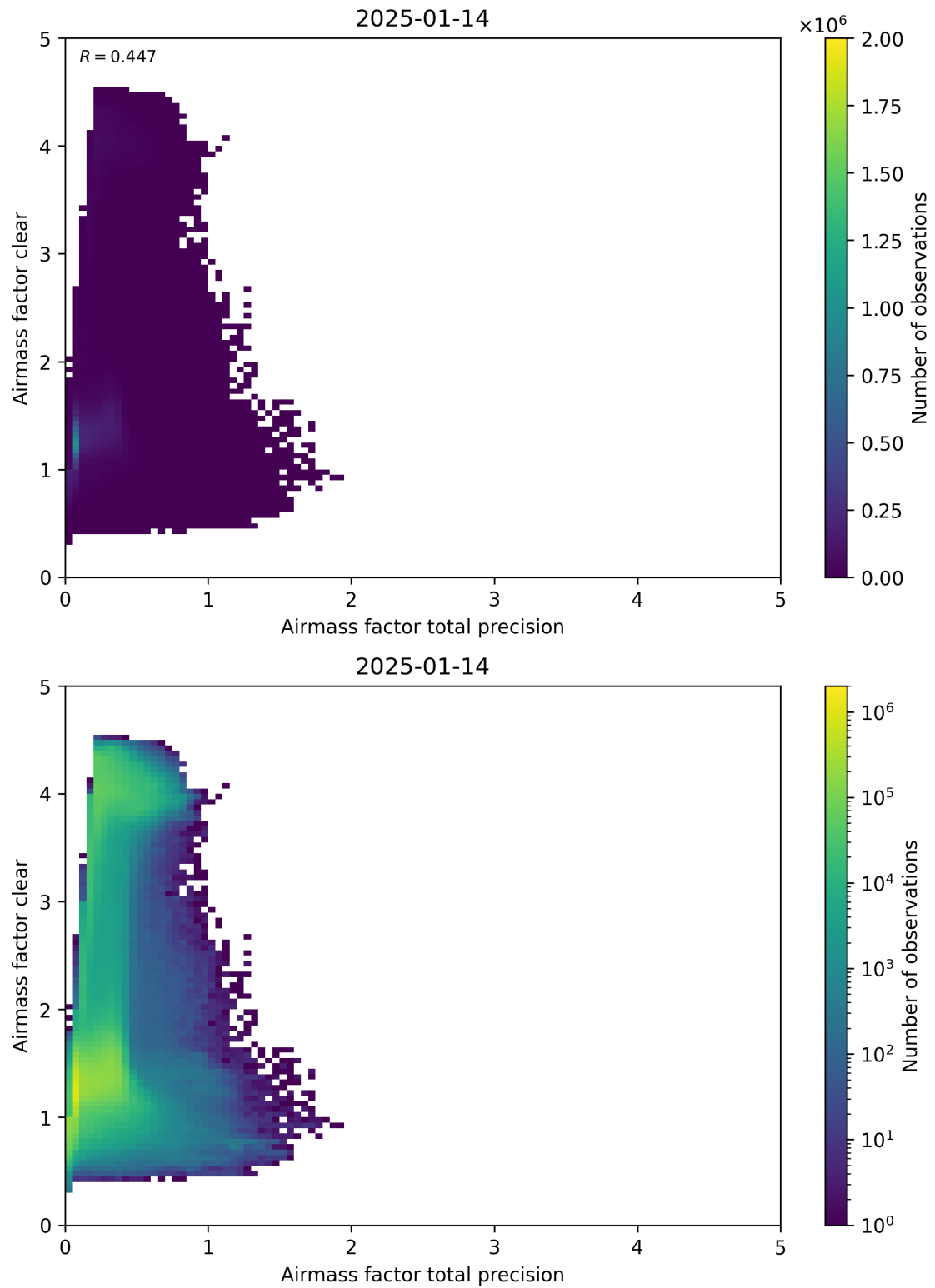
Figure 108: Scatter density plot of “Airmass factor total precision” against “Airmass factor clear” for 2025-01-13 to 2025-01-15.
