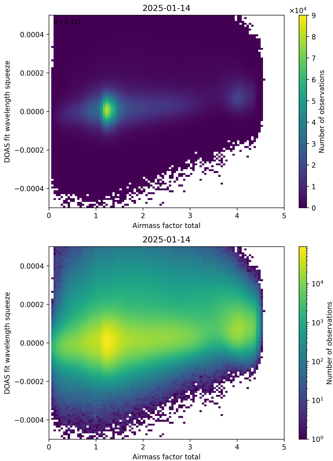
Figure 99: Scatter density plot of “Airmass factor total” against “DOAS fit wavelength squeeze” for 2025-01-13 to 2025-01-15.
