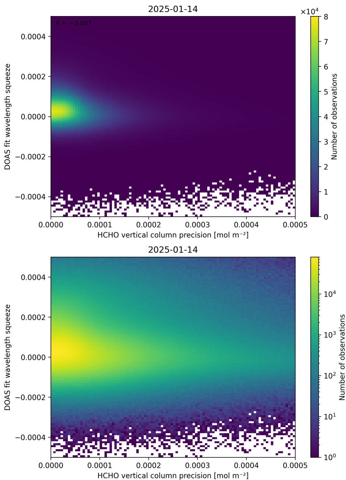
Figure 138: Scatter density plot of “HCHO vertical column precision” against “DOAS fit wavelength squeeze” for 2025-01-13 to 2025-01-15.
