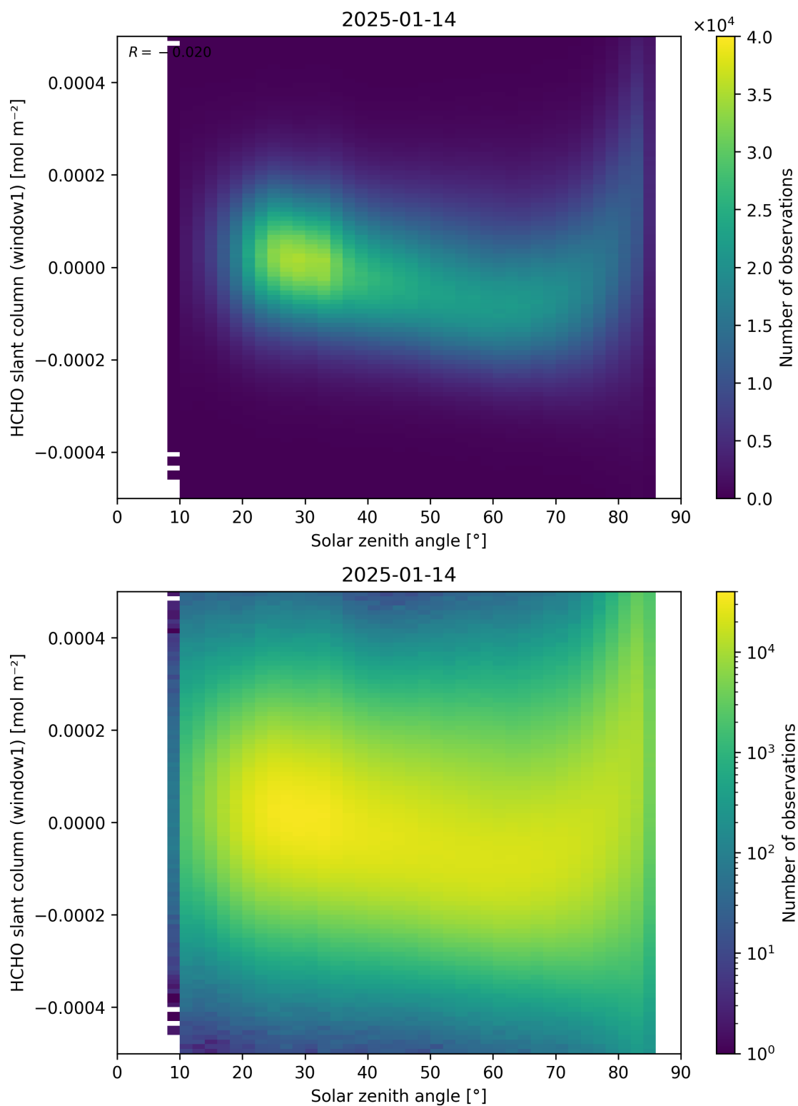
Figure 173: Scatter density plot of “Solar zenith angle” against “HCHO slant column (window1)” for 2025-01-13 to 2025-01-15.
