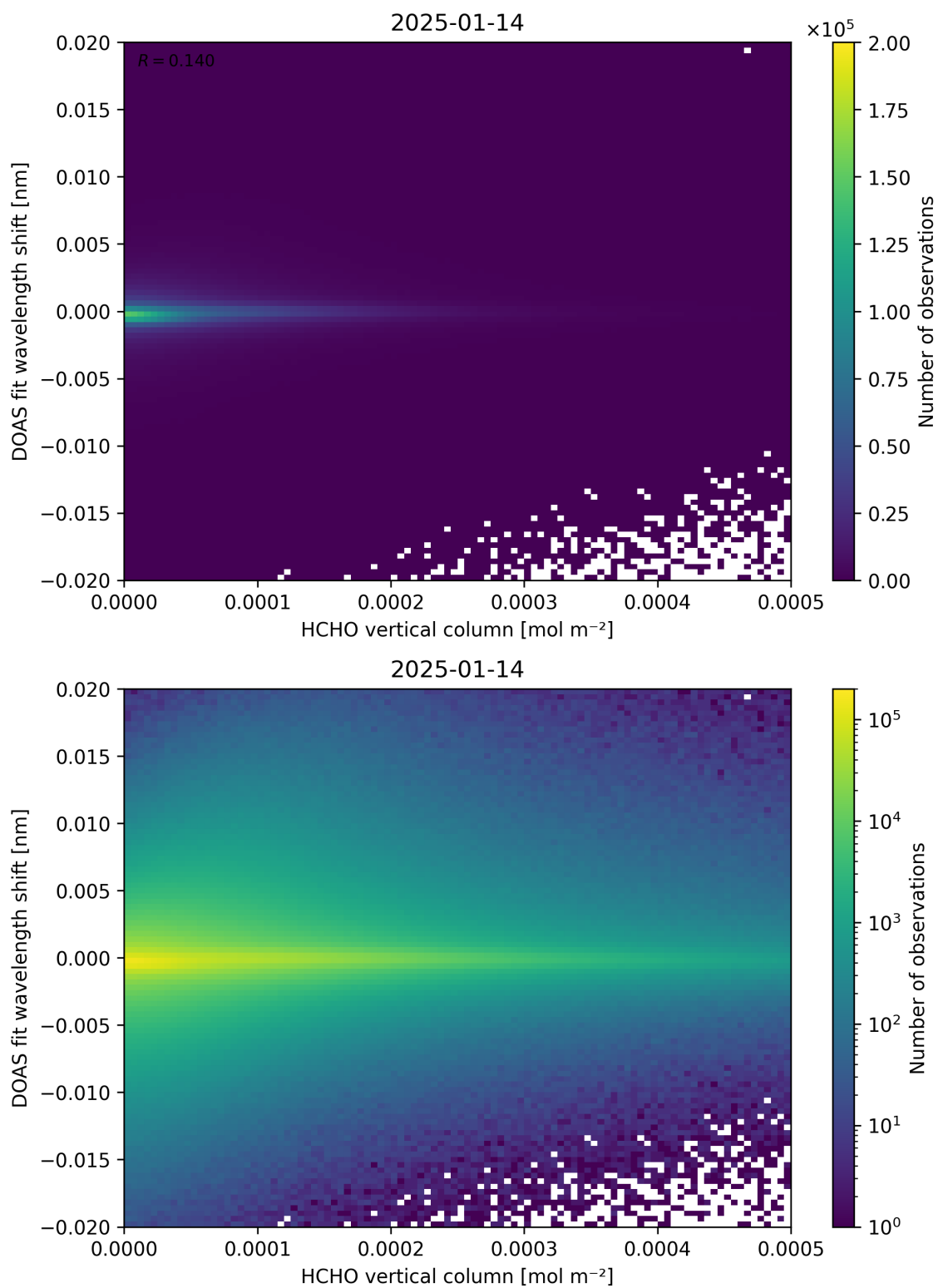
Figure 124: Scatter density plot of “HCHO vertical column” against “DOAS fit wavelength shift” for 2025-01-13 to 2025-01-15.
