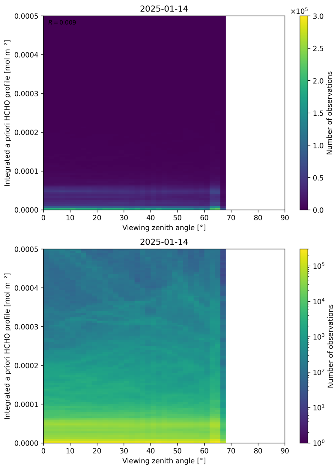
Figure 195: Scatter density plot of “Viewing zenith angle” against “Integrated a priori HCHO profile” for 2025-01-13 to 2025-01-15.
