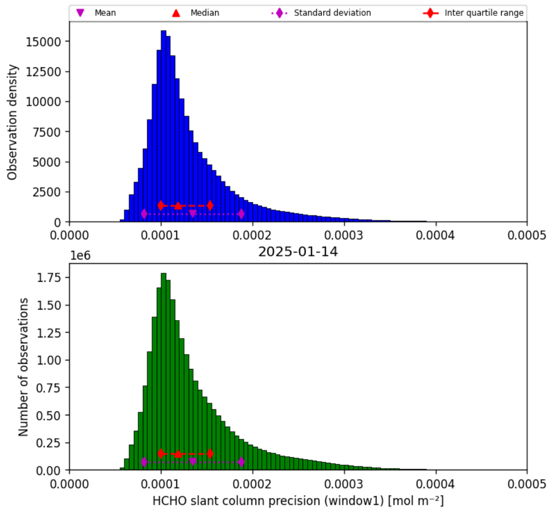
Figure 39: Histogram of “HCHO slant column precision (window1)” for 2025-01-13 to 2025-01-15
