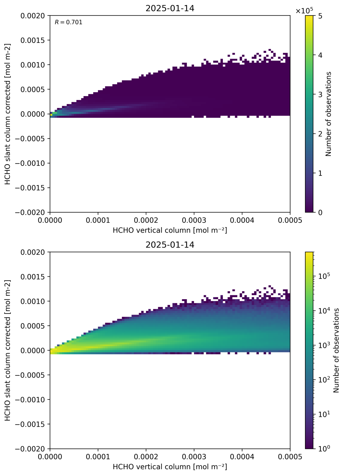
Figure 127: Scatter density plot of “HCHO vertical column” against “HCHO slant column corrected” for 2025-01-13 to 2025-01-15.
