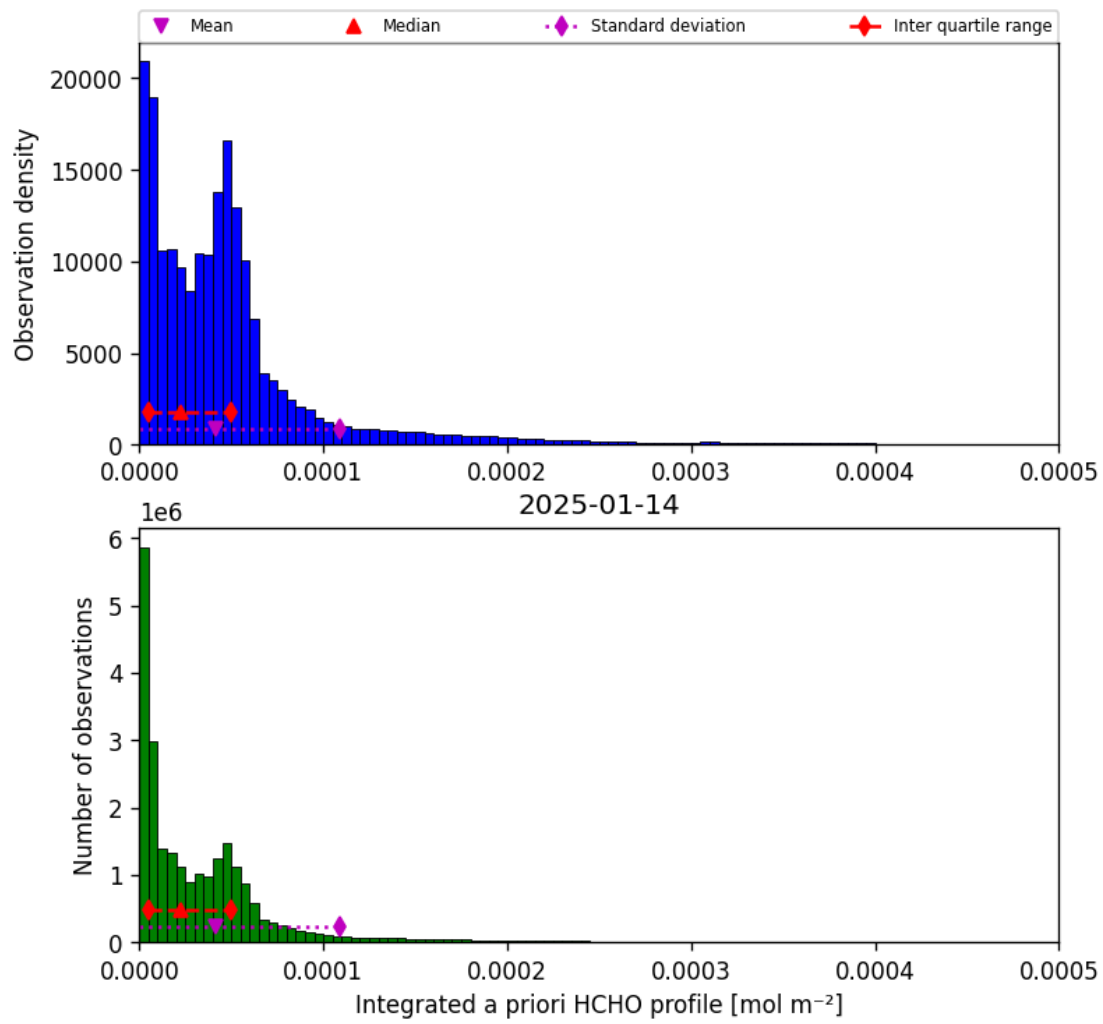
Figure 43: Histogram of “Integrated a priori HCHO profile” for 2025-01-13 to 2025-01-15
