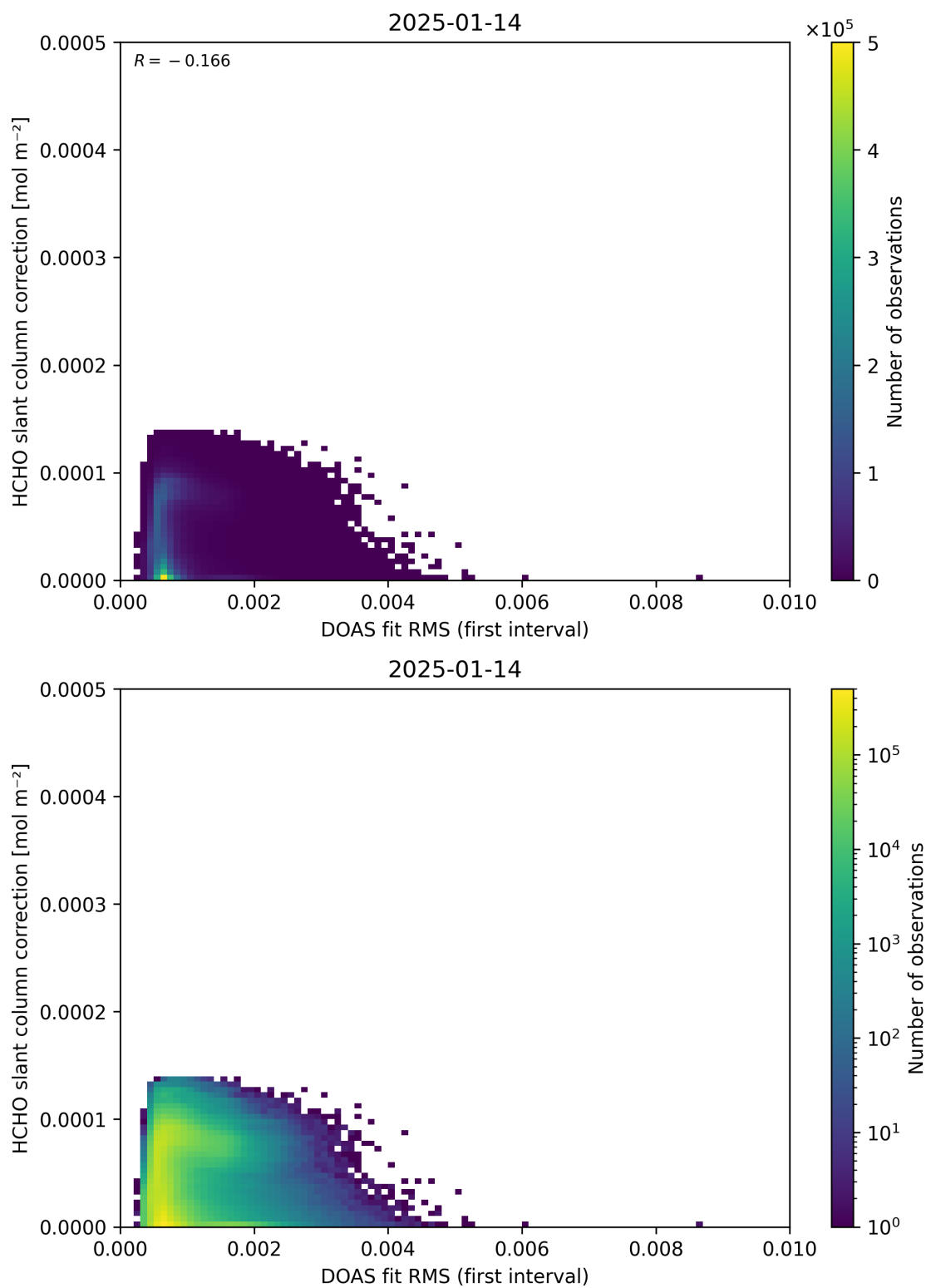
Figure 63: Scatter density plot of “DOAS fit RMS (first interval)” against “HCHO slant column correction” for 2025-01-13 to 2025-01-15.
