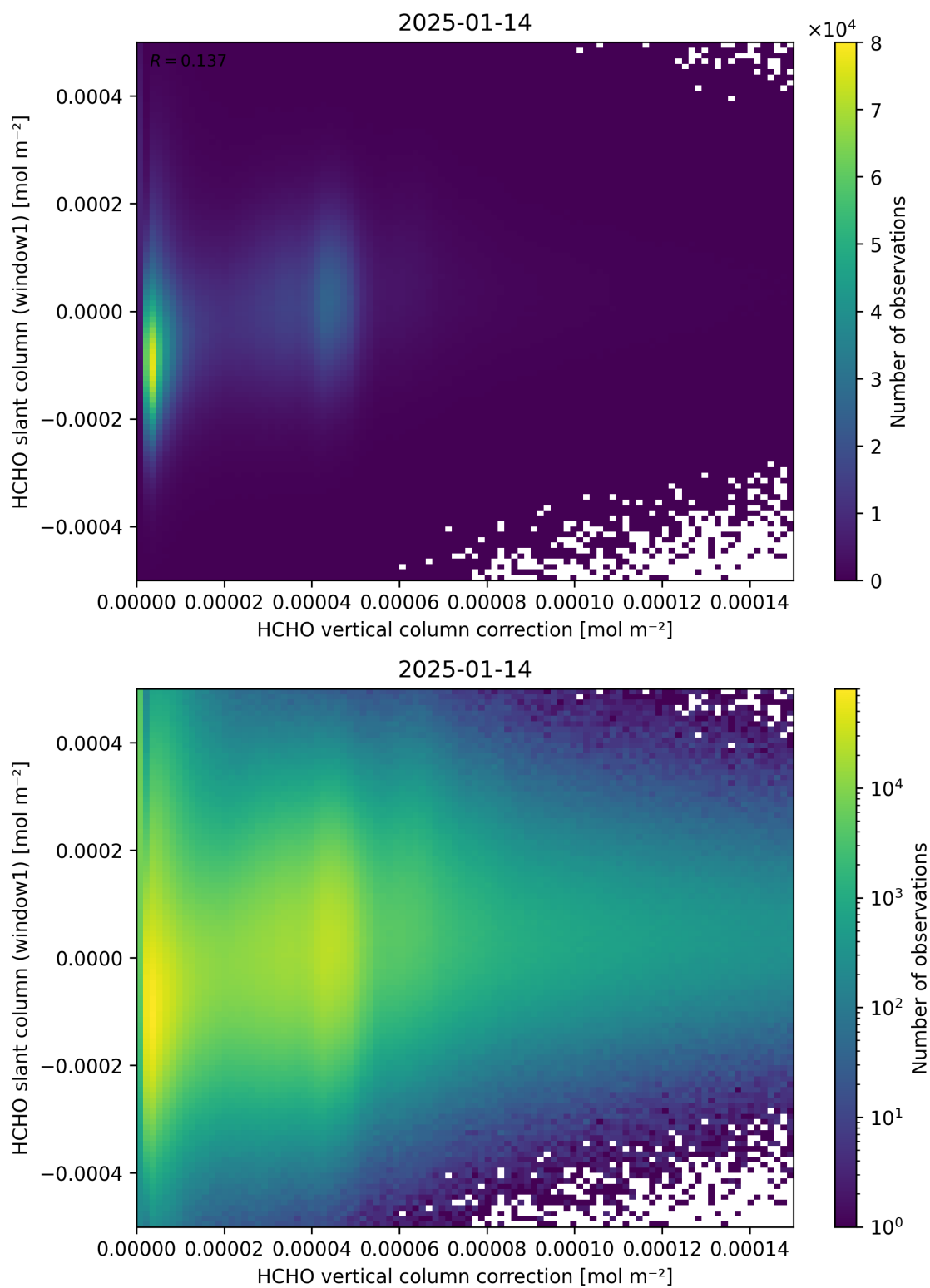
Figure 118: Scatter density plot of “HCHO vertical column correction” against “HCHO slant column (window1)” for 2025-01-13 to 2025-01-15.
