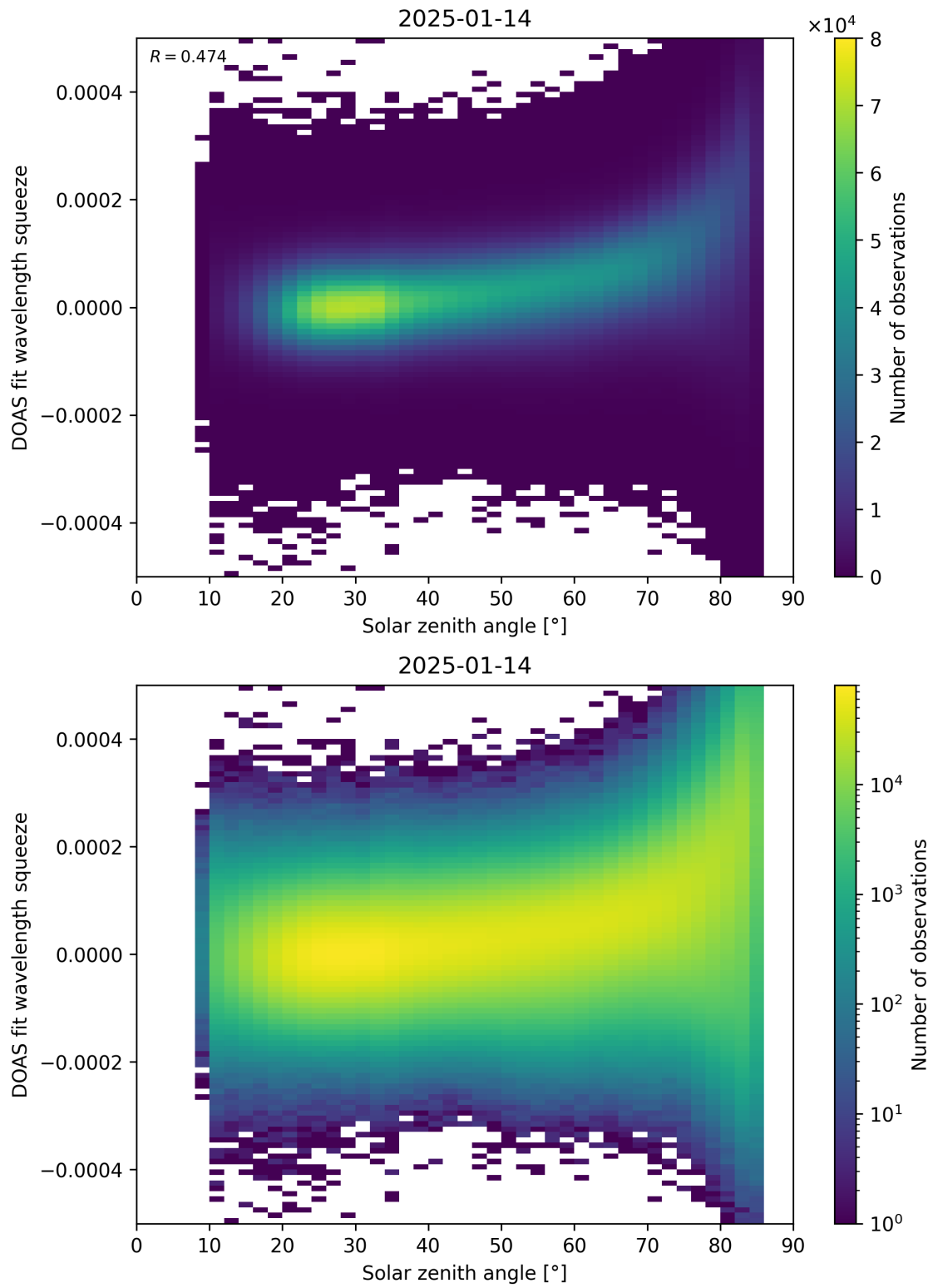
Figure 169: Scatter density plot of “Solar zenith angle” against “DOAS fit wavelength squeeze” for 2025-01-13 to 2025-01-15.
