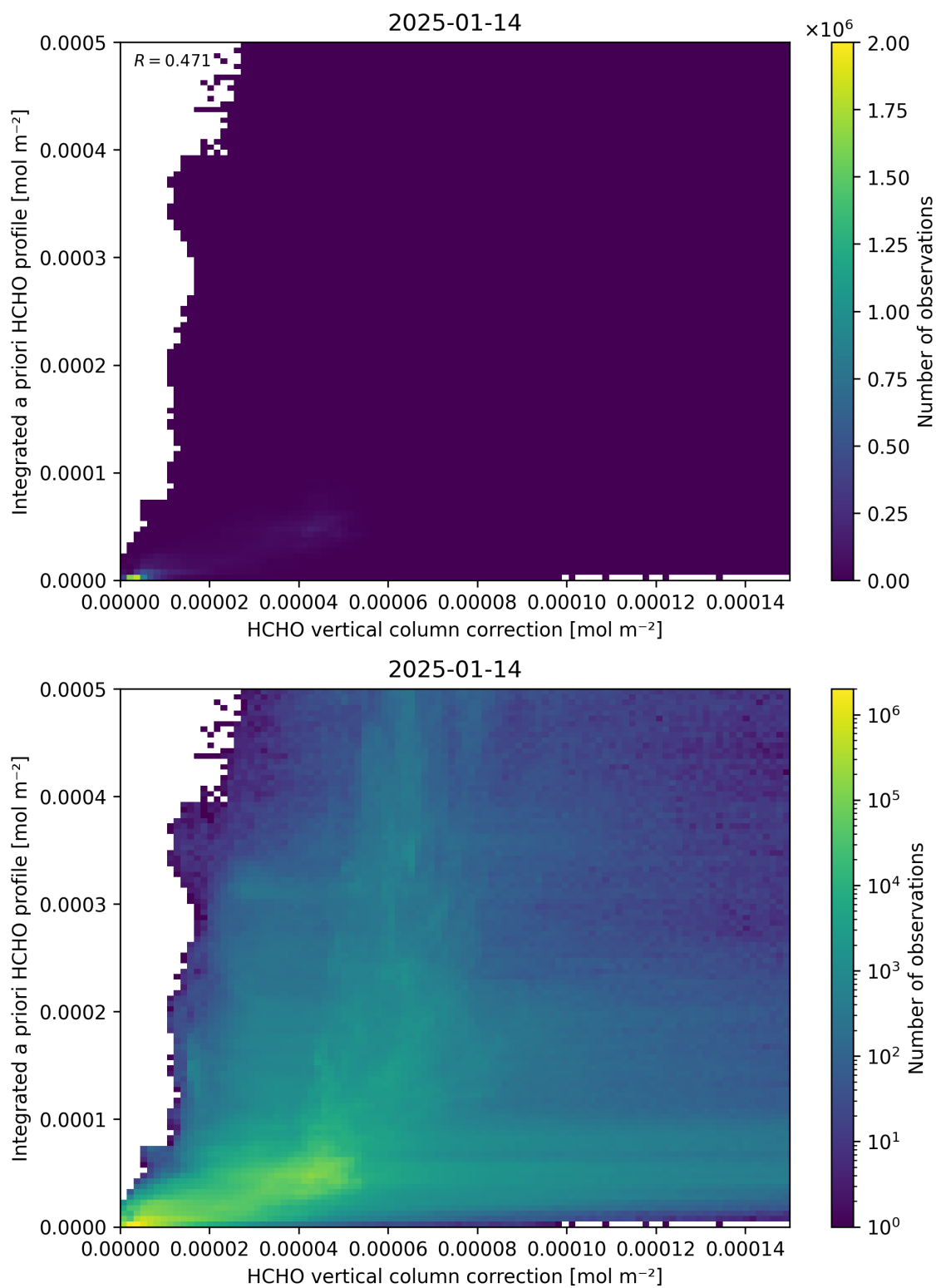
Figure 122: Scatter density plot of “HCHO vertical column correction” against “Integrated a priori HCHO profile” for 2025-01-13 to 2025-01-15.
