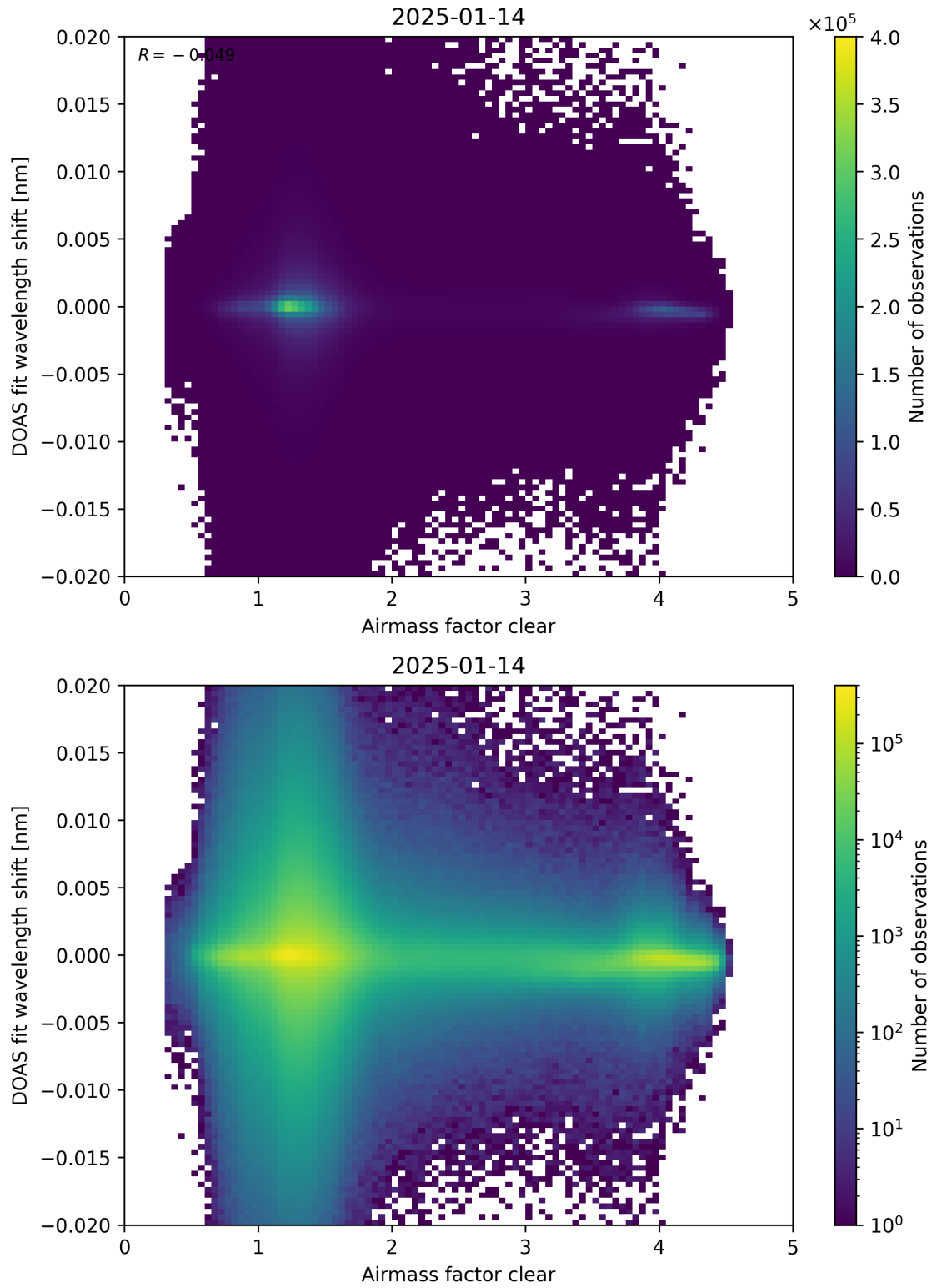
Figure 72: Scatter density plot of “Airmass factor clear” against “DOAS fit wavelength shift” for 2025-01-13 to 2025-01-15.
