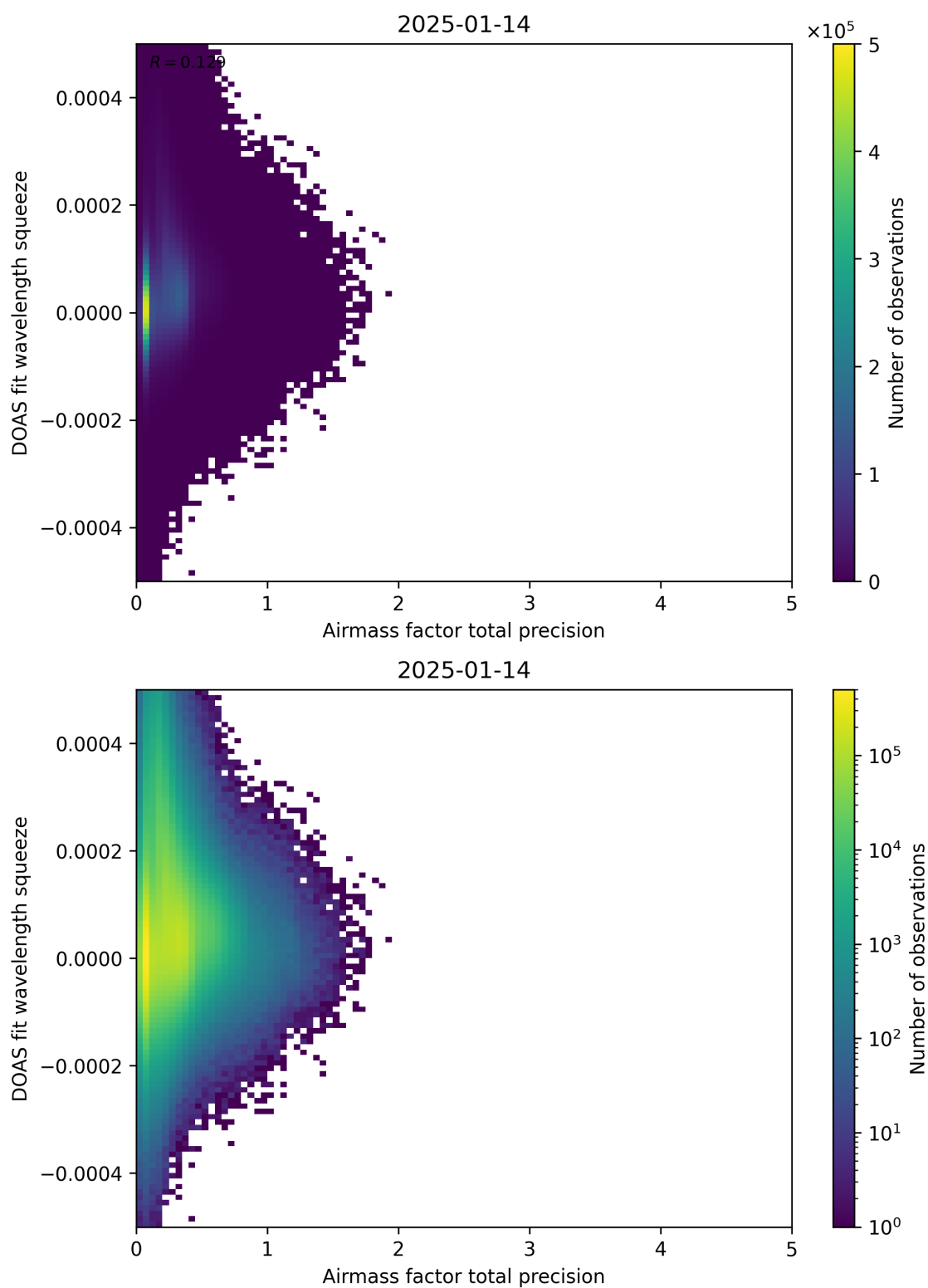
Figure 107: Scatter density plot of “Airmass factor total precision” against “DOAS fit wavelength squeeze” for 2025-01-13 to 2025-01-15.
