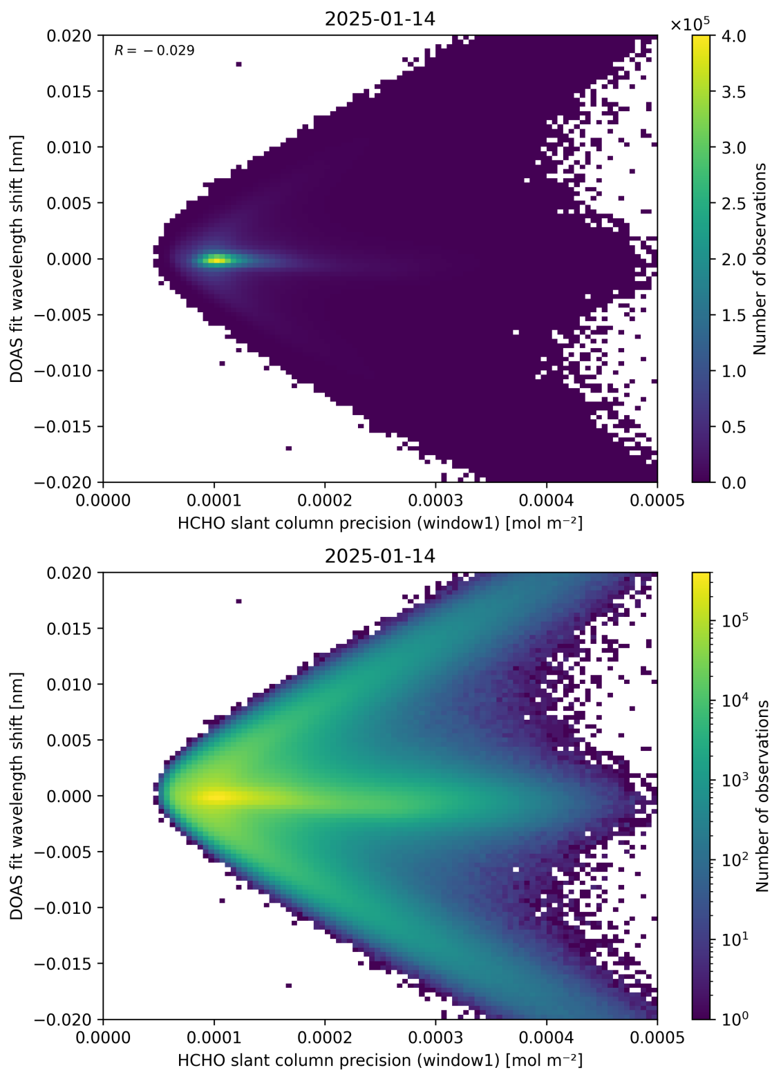
Figure 89: Scatter density plot of “HCHO slant column precision (window1)” against “DOAS fit wavelength shift” for 2025-01-13 to 2025-01-15.
