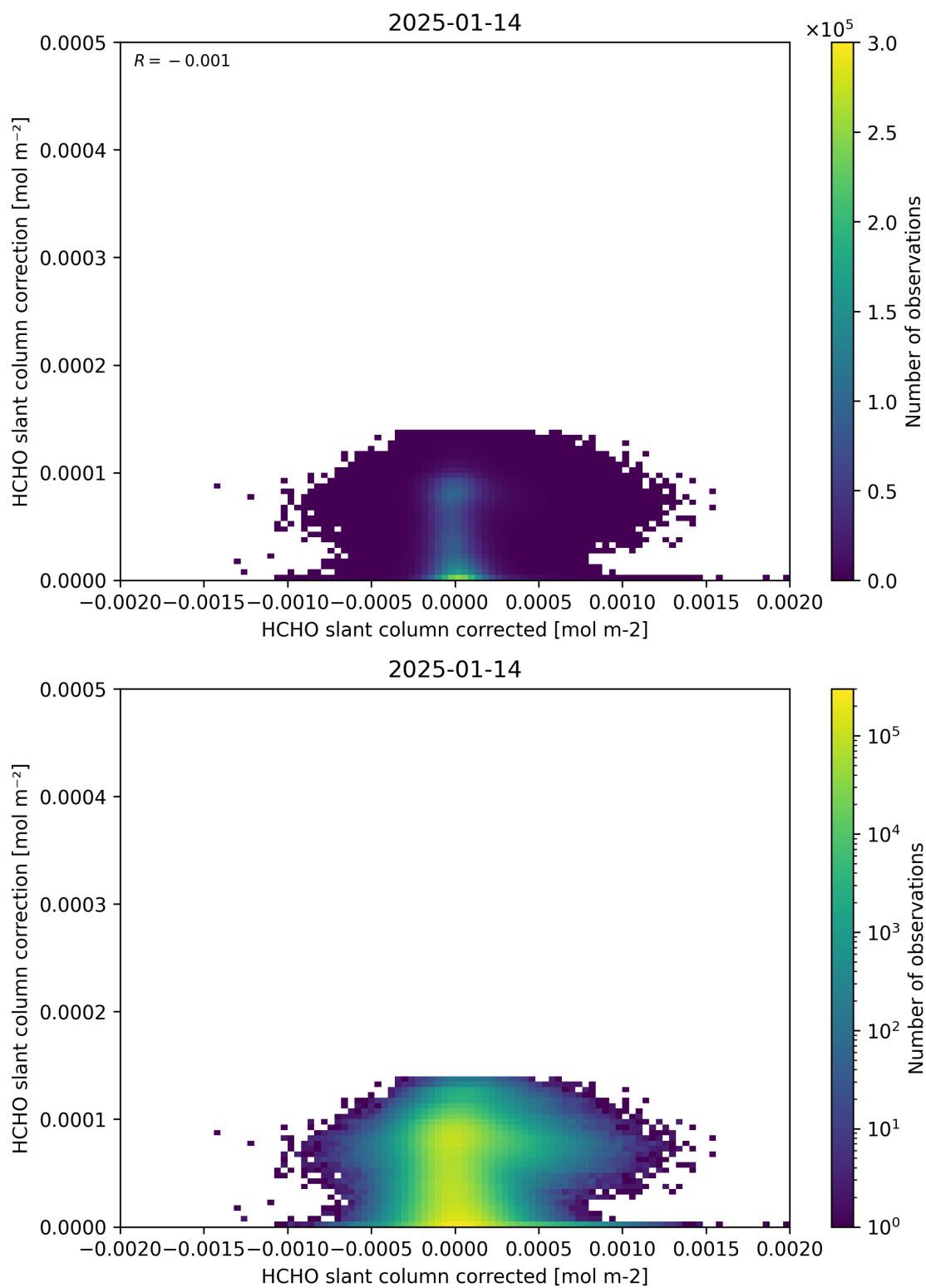
Figure 77: Scatter density plot of “HCHO slant column corrected” against “HCHO slant column correction” for 2025-01-13 to 2025-01-15.
