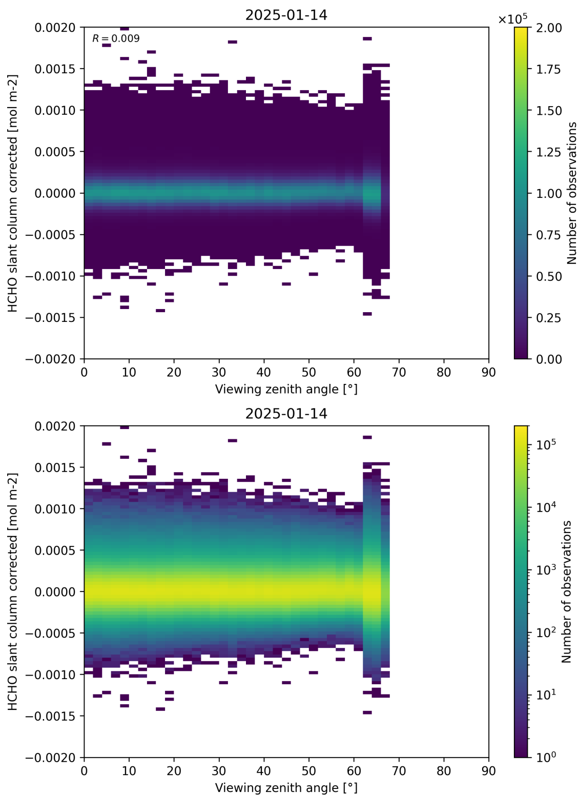
Figure 186: Scatter density plot of “Viewing zenith angle” against “HCHO slant column corrected” for 2025-01-13 to 2025-01-15.
