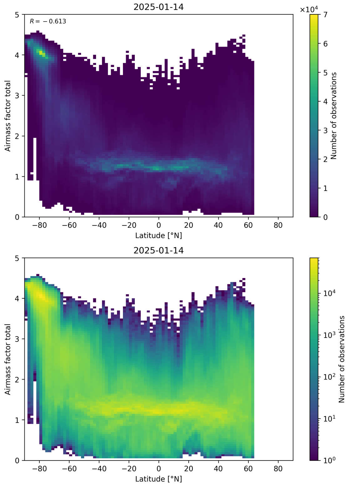
Figure 161: Scatter density plot of “Latitude” against “Airmass factor total” for 2025-01-13 to 2025-01-15.
