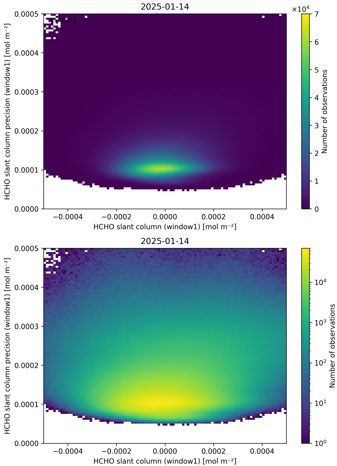
Figure 84: Scatter density plot of “HCHO slant column (window1)” against “HCHO slant column precision (window1)” for 2025-01-13 to 2025-01-15.
