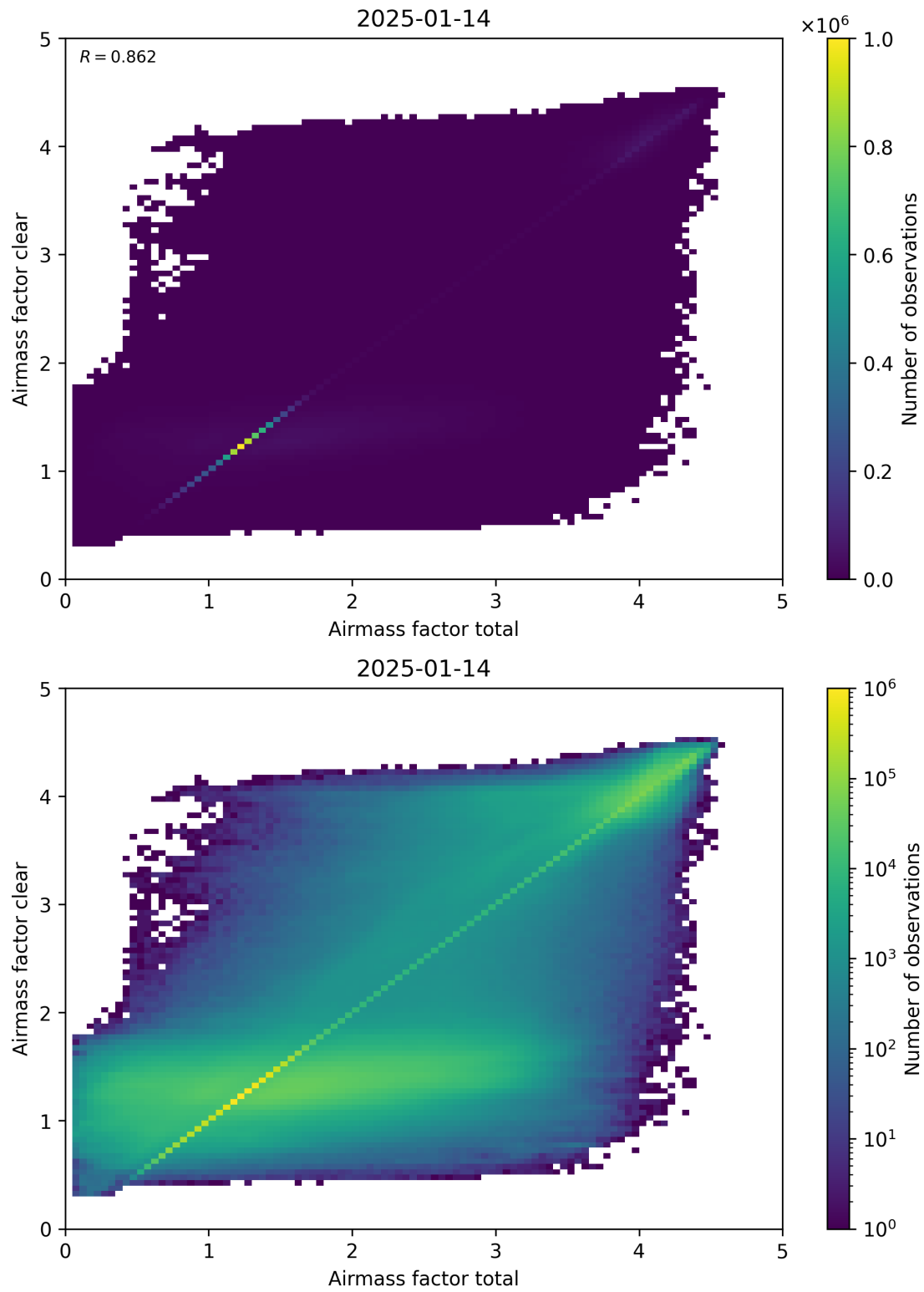
Figure 100: Scatter density plot of “Airmass factor total” against “Airmass factor clear” for 2025-01-13 to 2025-01-15.
