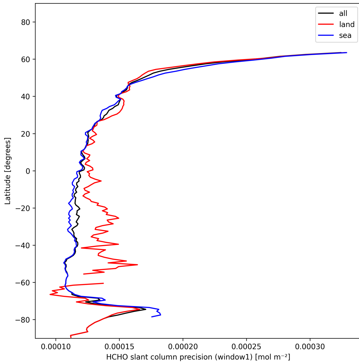
Figure 25: Zonal average of “HCHO slant column precision (window1)” for 2025-01-13 to 2025-01-15.
