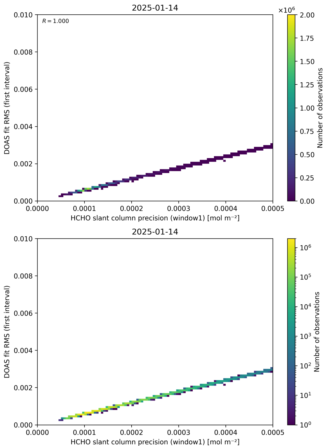
Figure 88: Scatter density plot of “HCHO slant column precision (window1)” against “DOAS fit RMS (first interval)” for 2025-01-13 to 2025-01-15.
