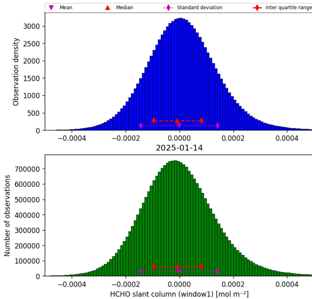
Figure 38: Histogram of “HCHO slant column (window1)” for 2025-01-13 to 2025-01-15
