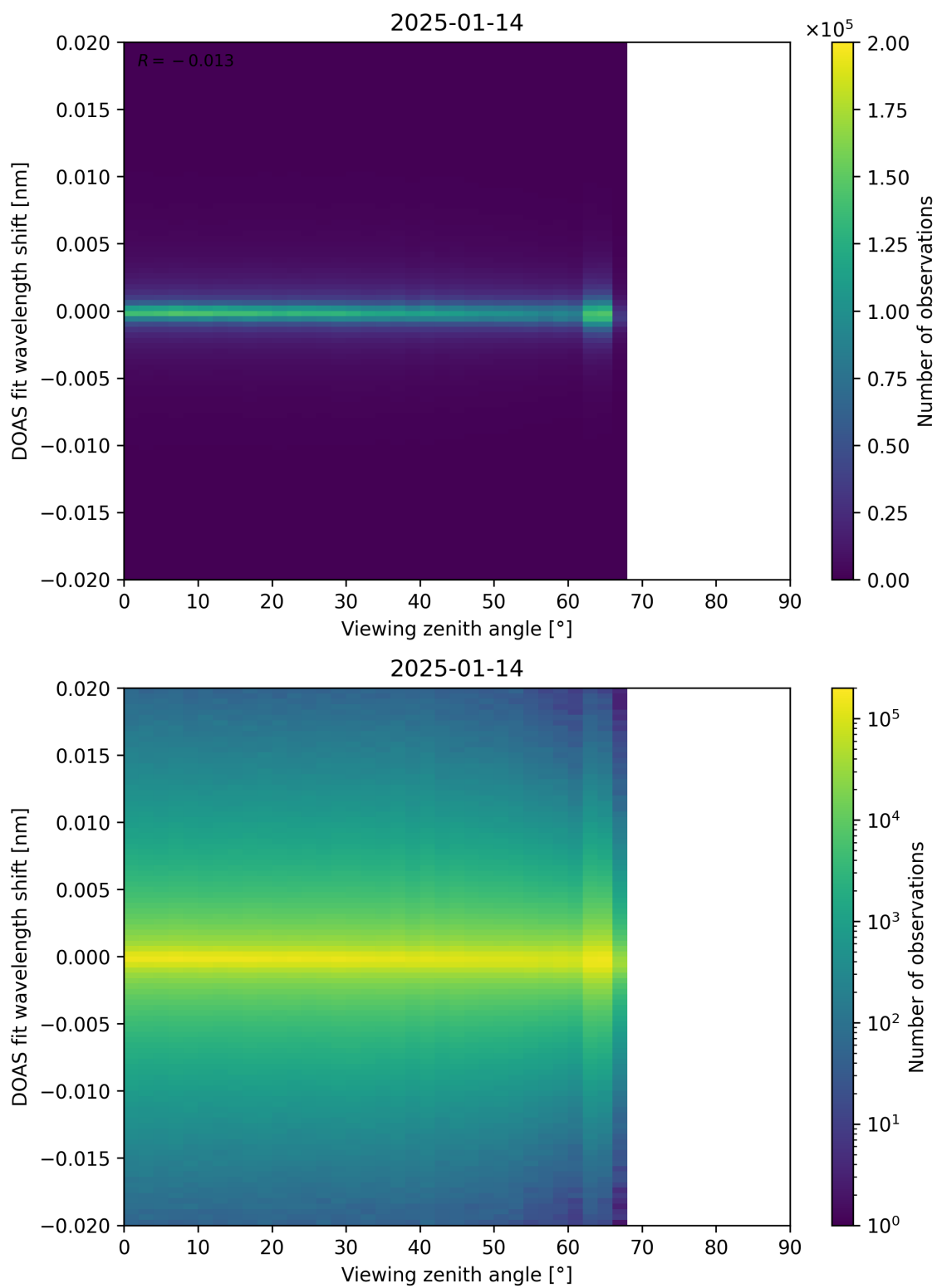
Figure 183: Scatter density plot of “Viewing zenith angle” against “DOAS fit wavelength shift” for 2025-01-13 to 2025-01-15.
