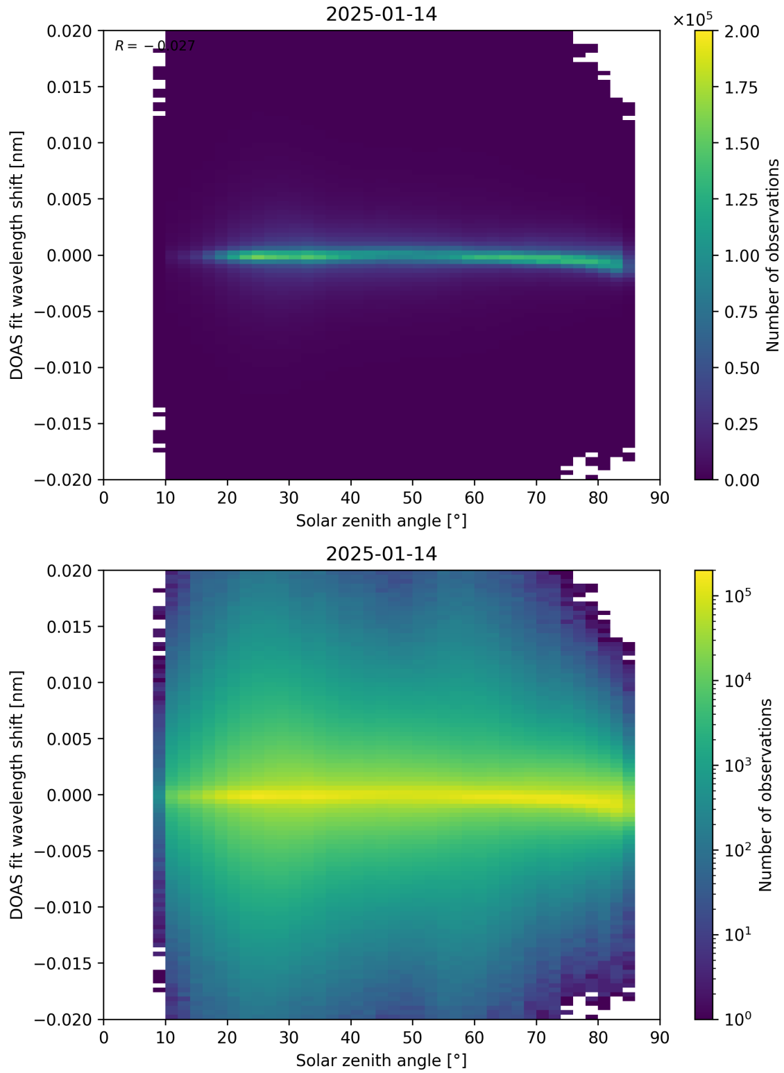
Figure 168: Scatter density plot of “Solar zenith angle” against “DOAS fit wavelength shift” for 2025-01-13 to 2025-01-15.
