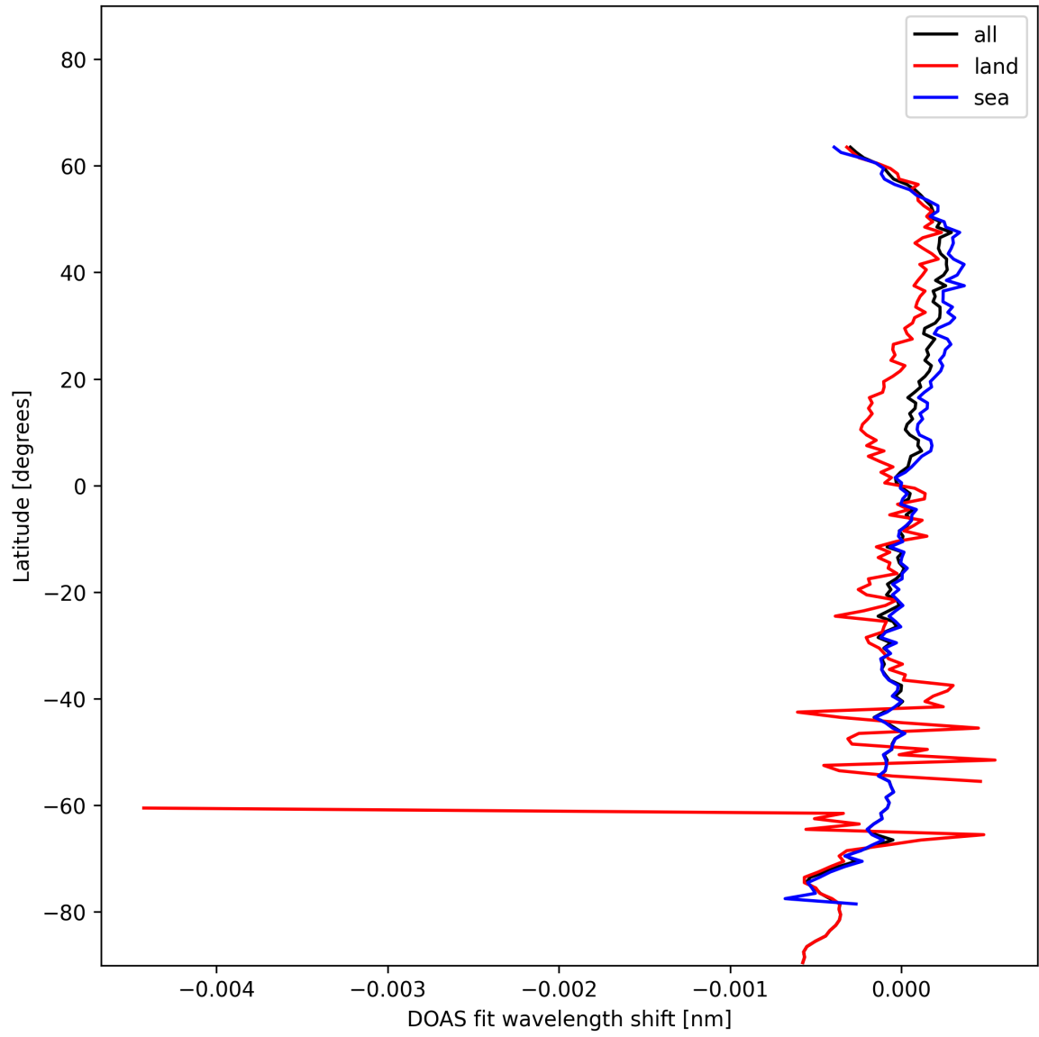
Figure 30: Zonal average of “DOAS fit wavelength shift” for 2025-01-13 to 2025-01-15.
