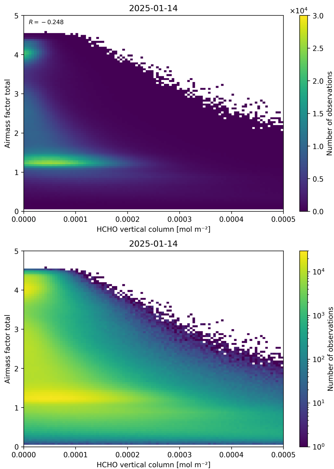
Figure 131: Scatter density plot of “HCHO vertical column” against “Airmass factor total” for 2025-01-13 to 2025-01-15.
