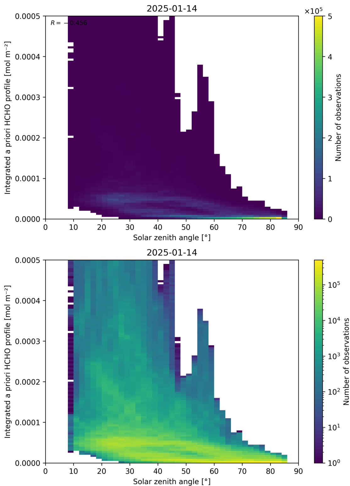
Figure 180: Scatter density plot of “Solar zenith angle” against “Integrated a priori HCHO profile” for 2025-01-13 to 2025-01-15.
