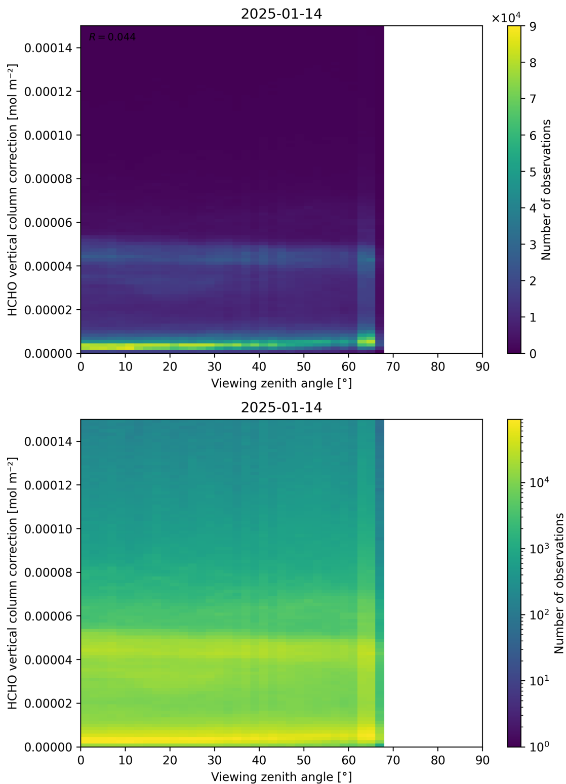
Figure 193: Scatter density plot of “Viewing zenith angle” against “HCHO vertical column correction” for 2025-01-13 to 2025-01-15.
