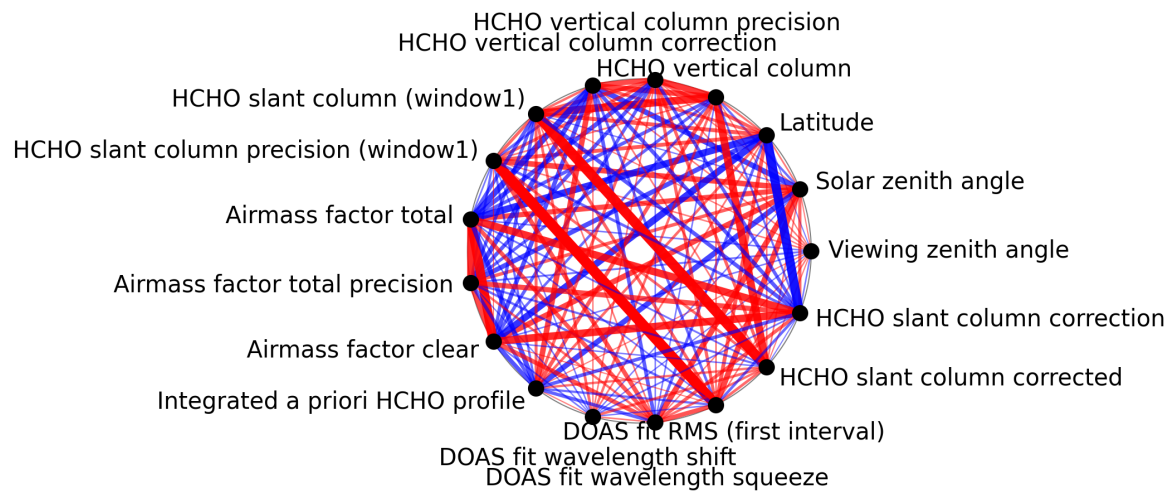
Figure 1: Map of correlation graph for 2025-01-13 to 2025-01-15.
