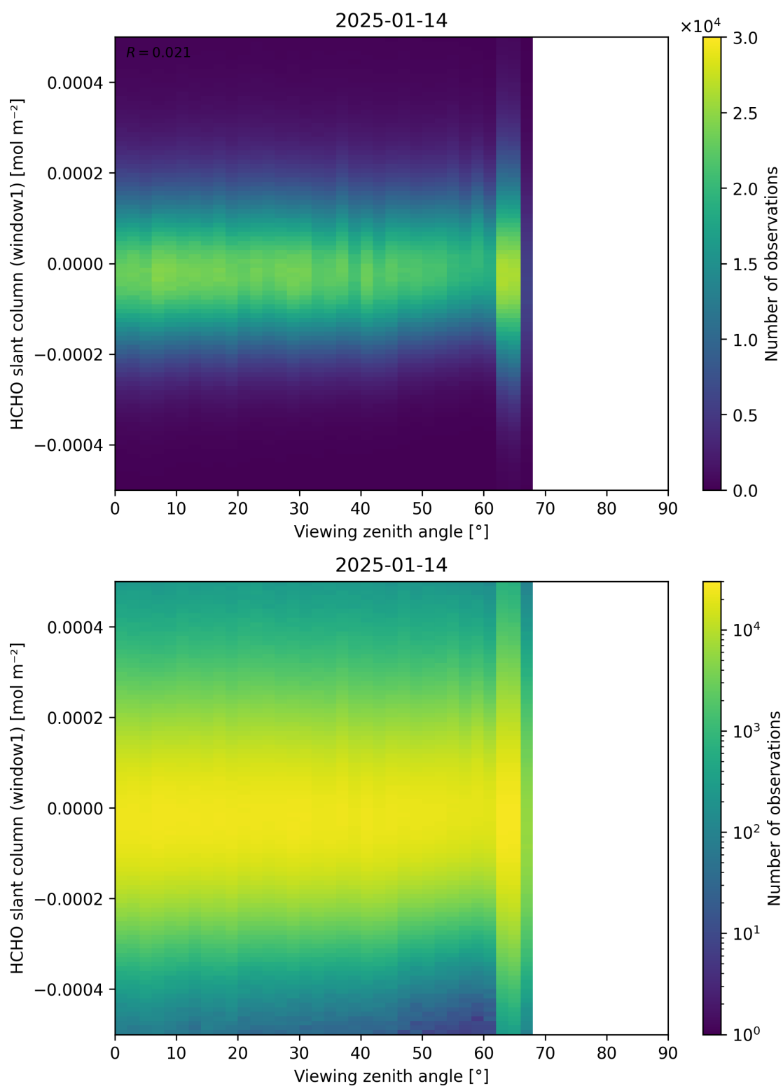
Figure 188: Scatter density plot of “Viewing zenith angle” against “HCHO slant column (window1)” for 2025-01-13 to 2025-01-15.
