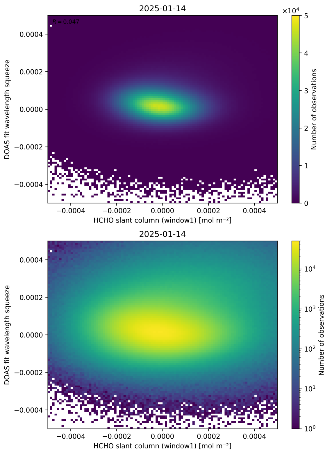
Figure 80: Scatter density plot of “HCHO slant column (window1)” against “DOAS fit wavelength squeeze” for 2025-01-13 to 2025-01-15.
