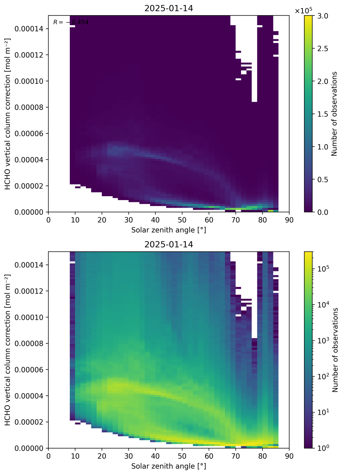
Figure 178: Scatter density plot of “Solar zenith angle” against “HCHO vertical column correction” for 2025-01-13 to 2025-01-15.
