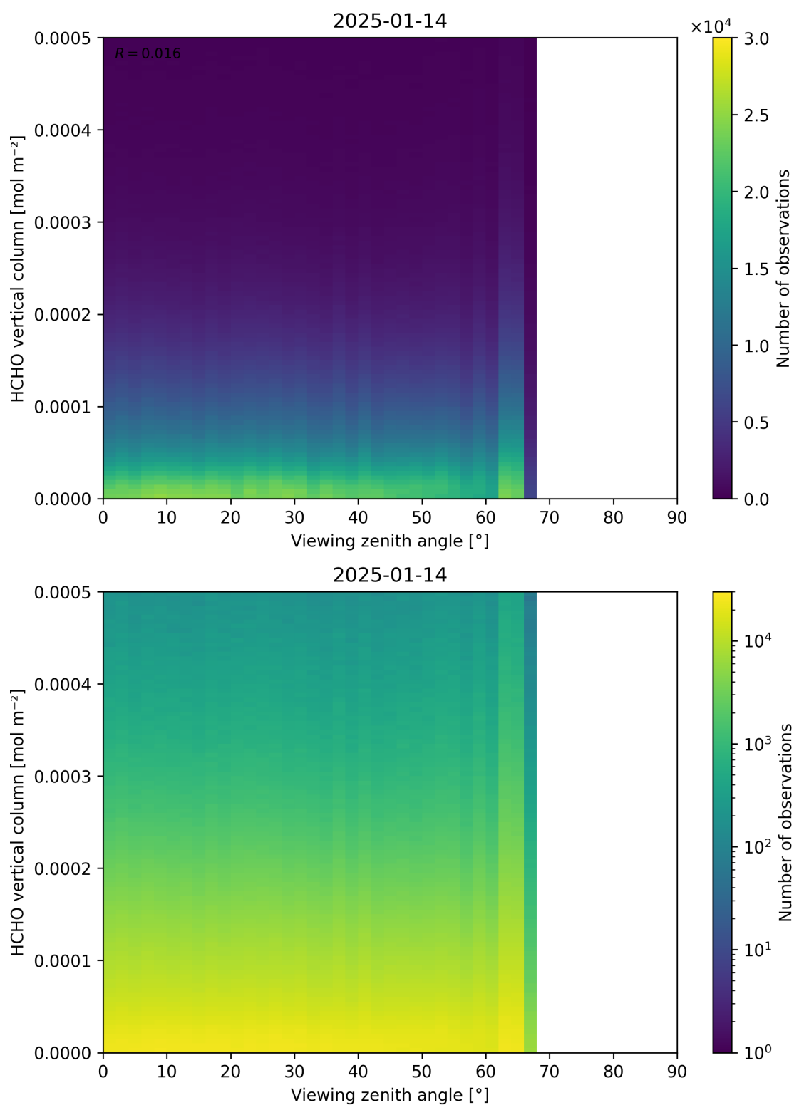
Figure 192: Scatter density plot of “Viewing zenith angle” against “HCHO vertical column” for 2025-01-13 to 2025-01-15.
