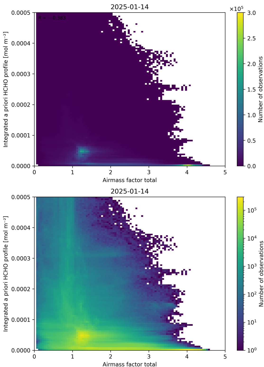
Figure 104: Scatter density plot of “Airmass factor total” against “Integrated a priori HCHO profile” for 2025-01-13 to 2025-01-15.
