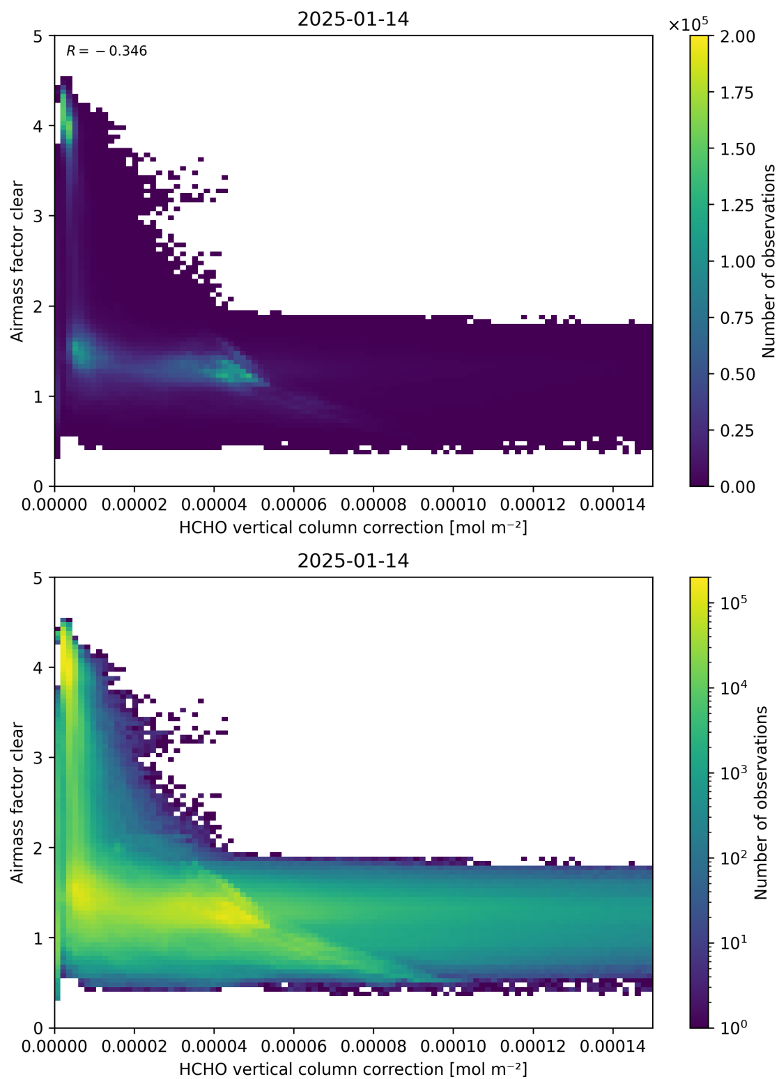
Figure 115: Scatter density plot of “HCHO vertical column correction” against “Airmass factor clear” for 2025-01-13 to 2025-01-15.
