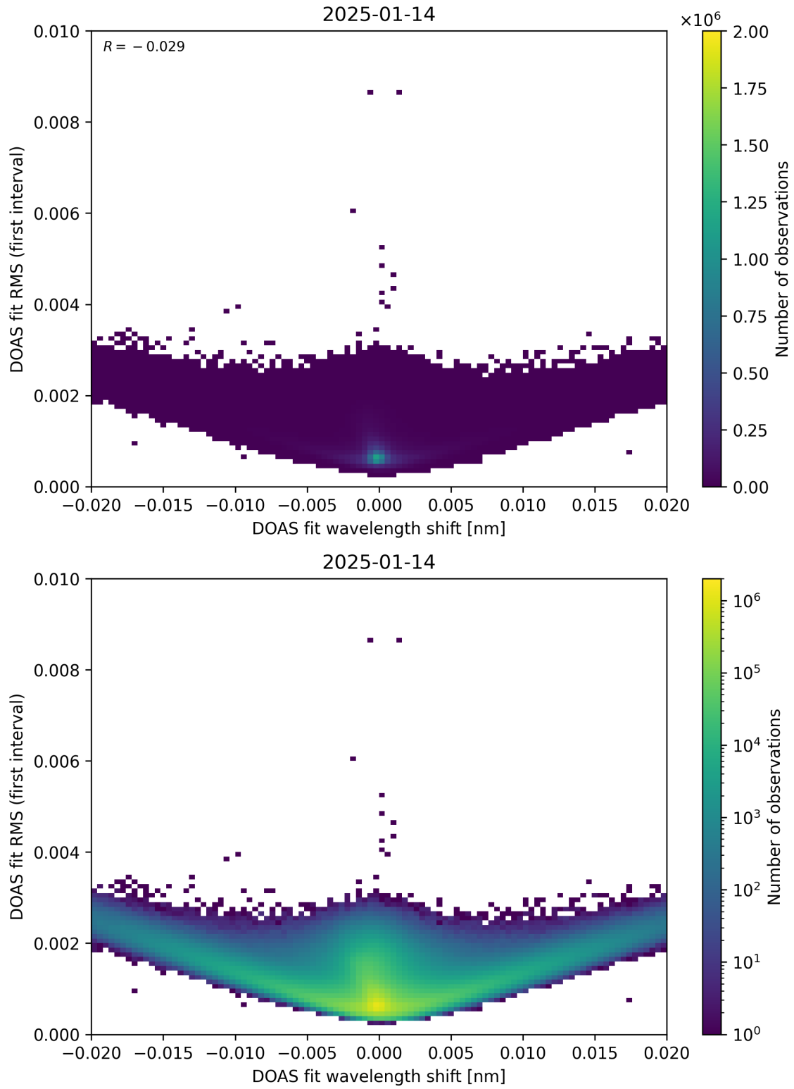
Figure 64: Scatter density plot of “DOAS fit wavelength shift” against “DOAS fit RMS (first interval)” for 2025-01-13 to 2025-01-15.
