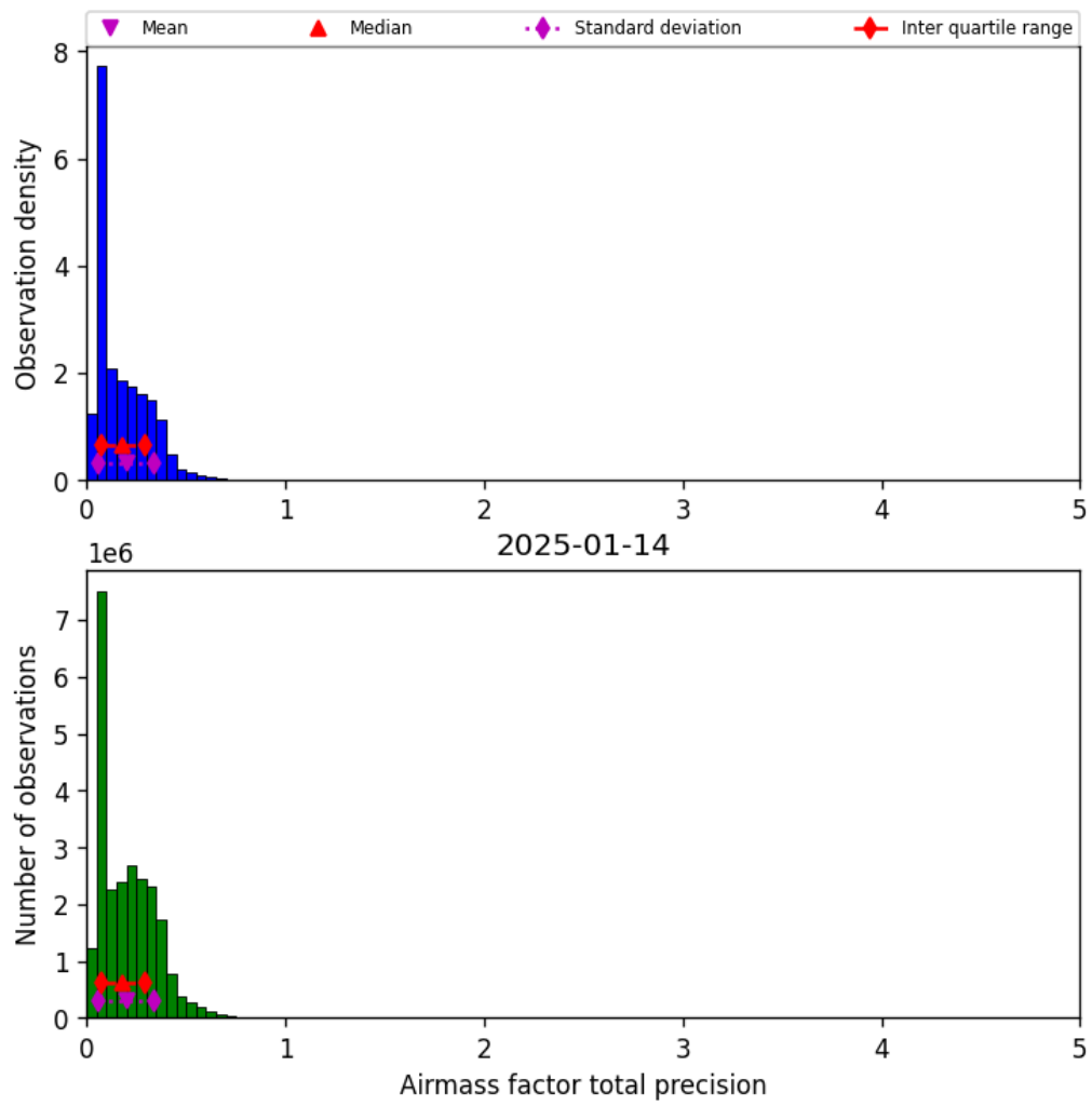
Figure 41: Histogram of “Airmass factor total precision” for 2025-01-13 to 2025-01-15
