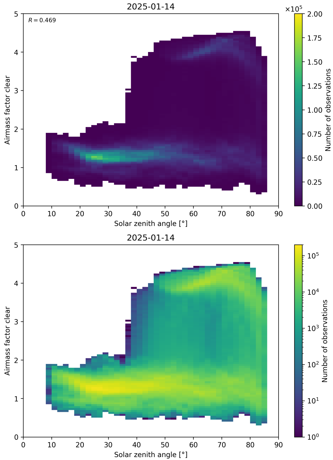
Figure 170: Scatter density plot of “Solar zenith angle” against “Airmass factor clear” for 2025-01-13 to 2025-01-15.
