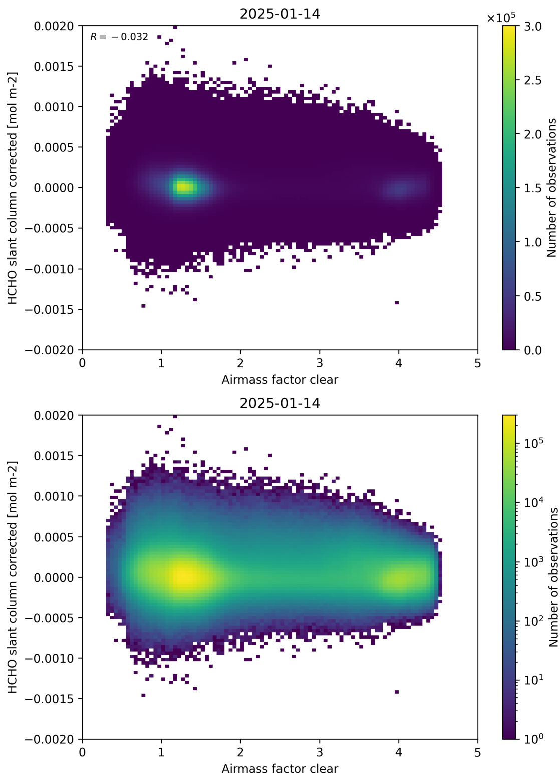
Figure 74: Scatter density plot of “Airmass factor clear” against “HCHO slant column corrected” for 2025-01-13 to 2025-01-15.
