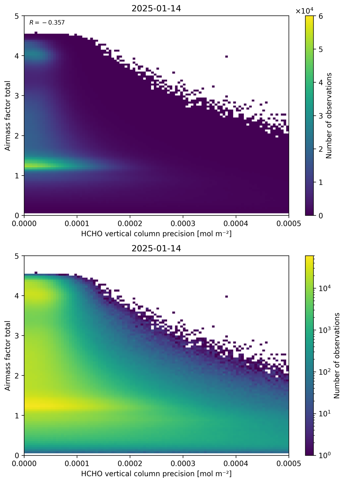
Figure 144: Scatter density plot of “HCHO vertical column precision” against “Airmass factor total” for 2025-01-13 to 2025-01-15.
