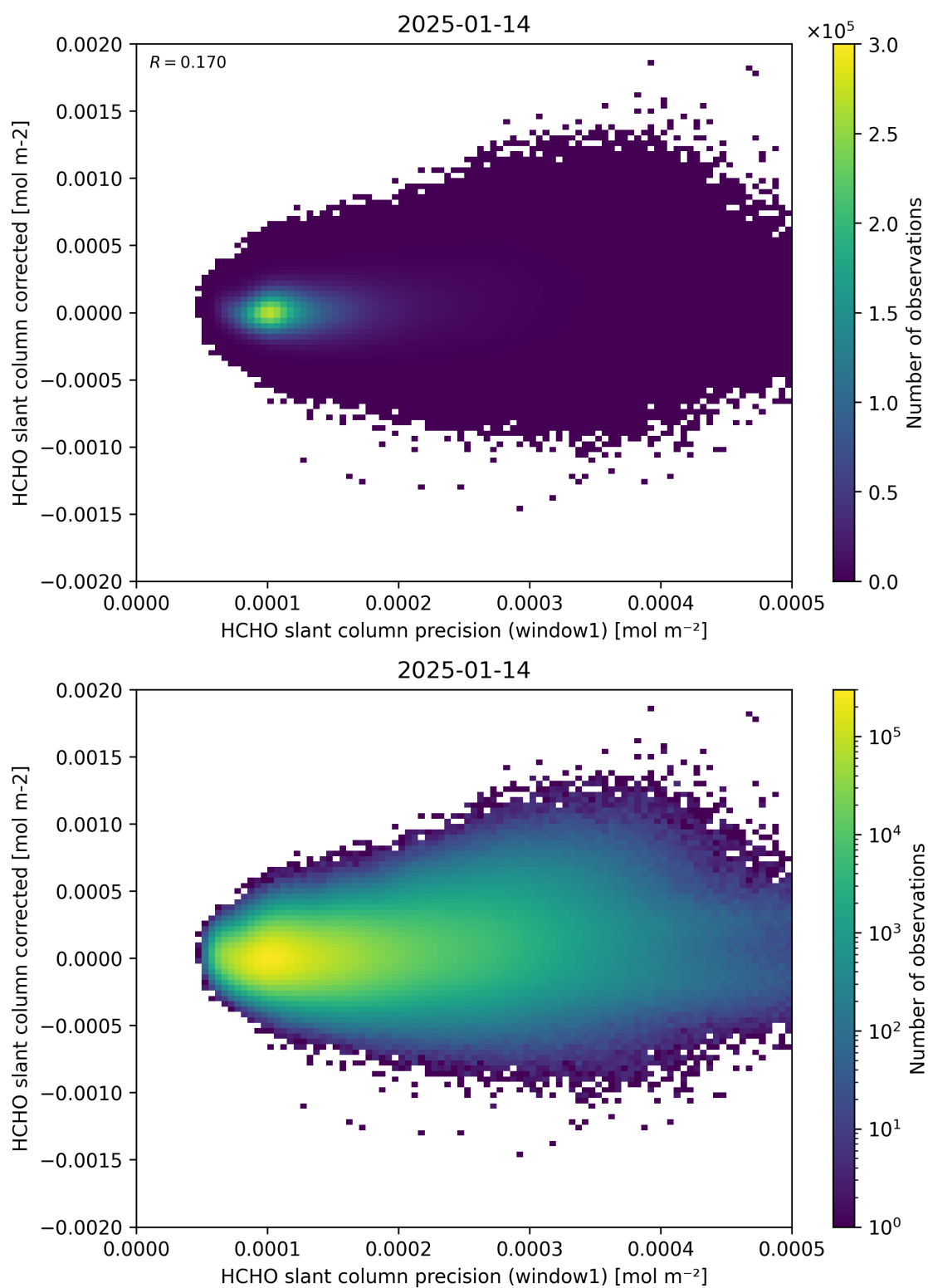
Figure 92: Scatter density plot of “HCHO slant column precision (window1)” against “HCHO slant column corrected” for 2025-01-13 to 2025-01-15.
