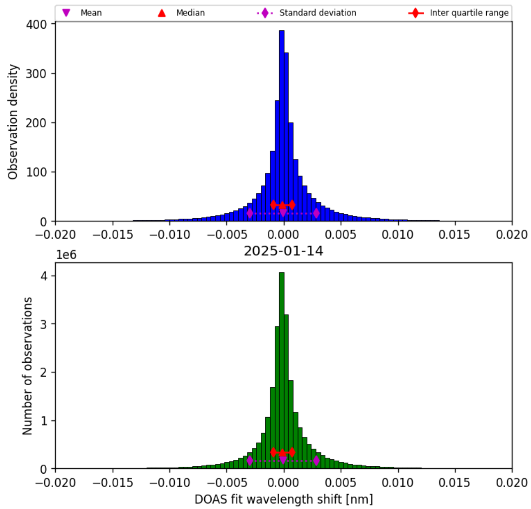
Figure 44: Histogram of “DOAS fit wavelength shift” for 2025-01-13 to 2025-01-15
