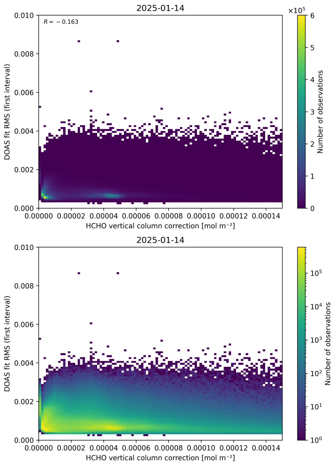
Figure 112: Scatter density plot of “HCHO vertical column correction” against “DOAS fit RMS (first interval)” for 2025-01-13 to 2025-01-15.
