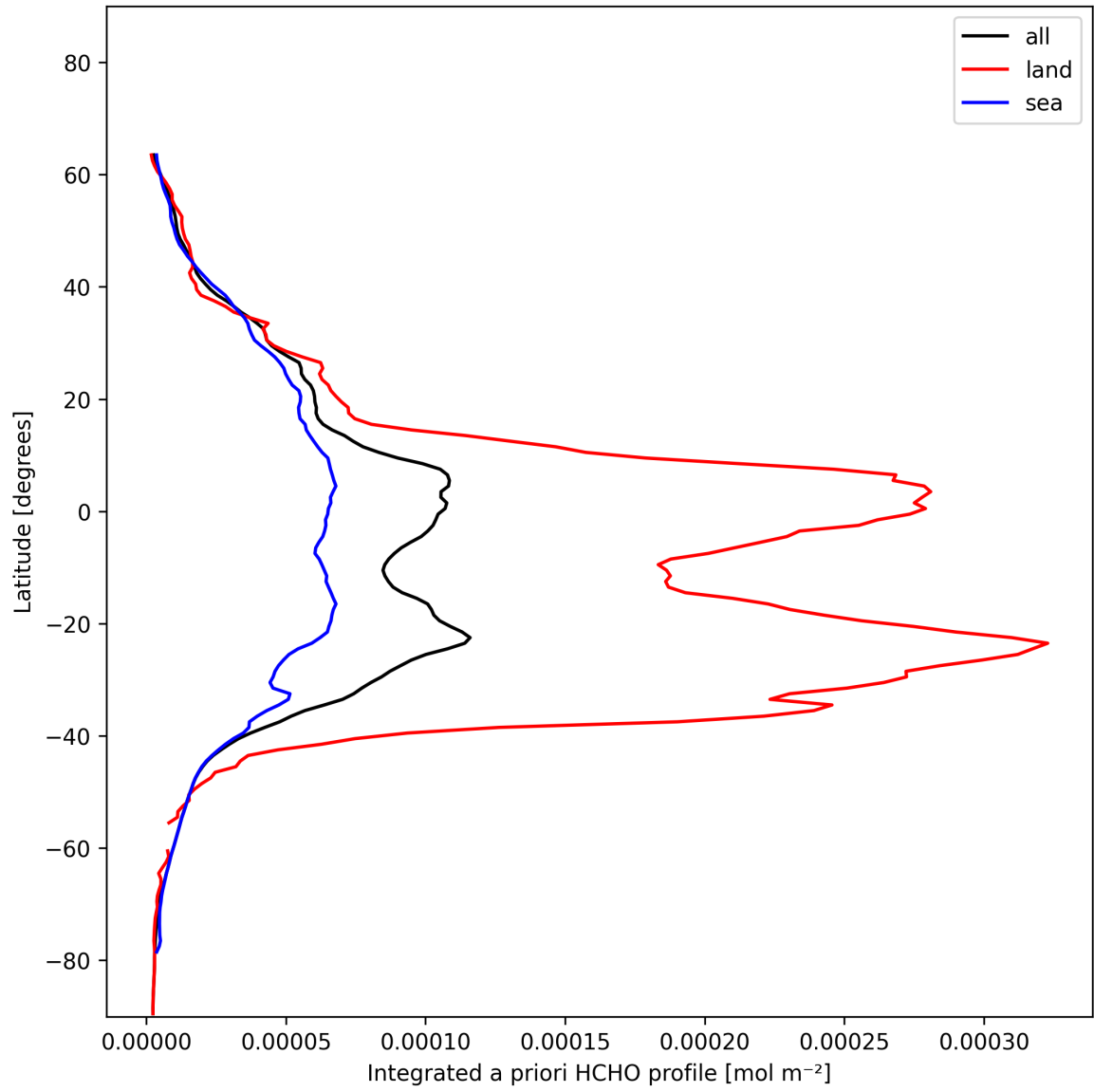
Figure 29: Zonal average of “Integrated a priori HCHO profile” for 2025-01-13 to 2025-01-15.
