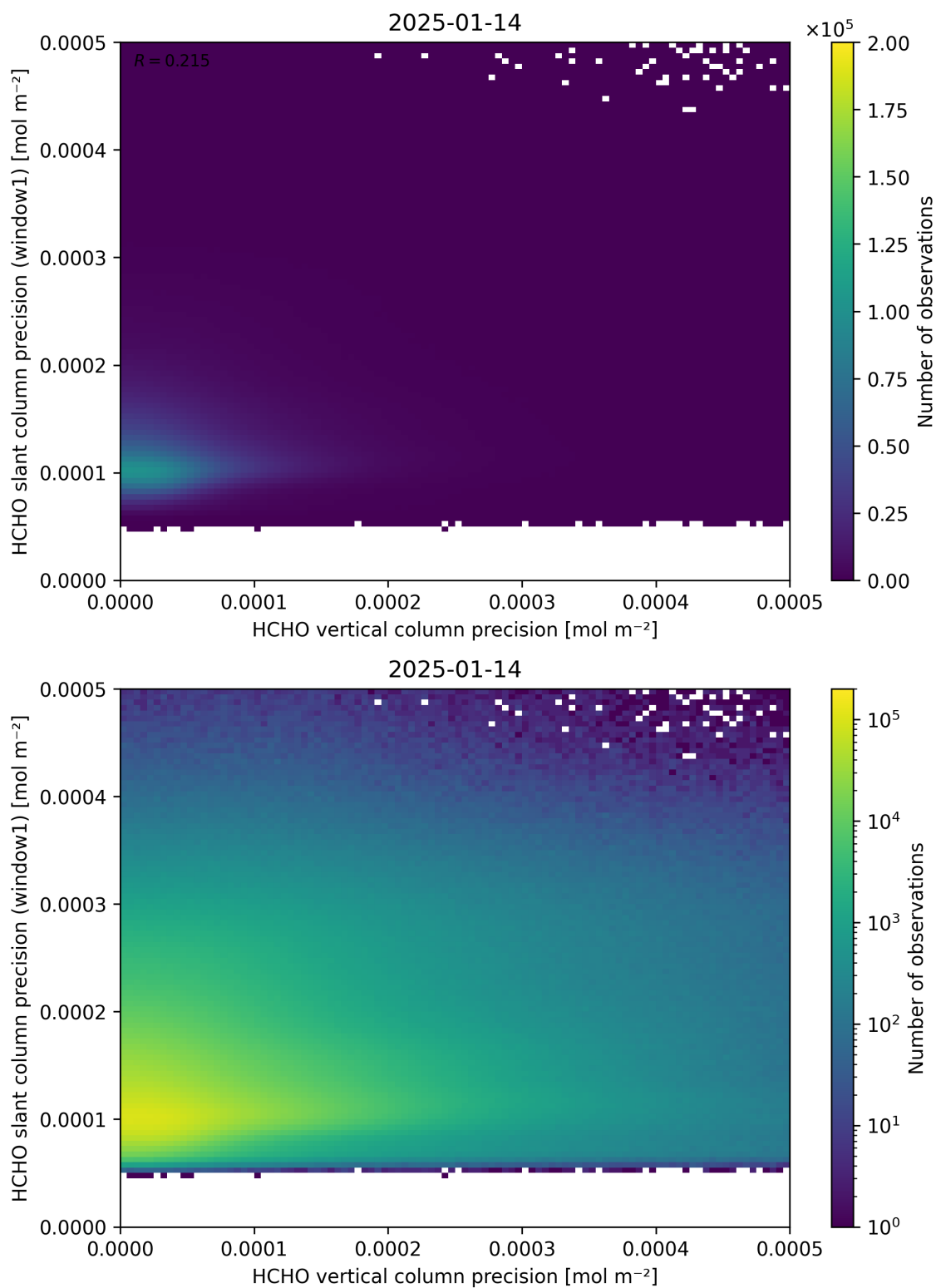
Figure 143: Scatter density plot of “HCHO vertical column precision” against “HCHO slant column precision (window1)” for 2025-01-13 to 2025-01-15.
