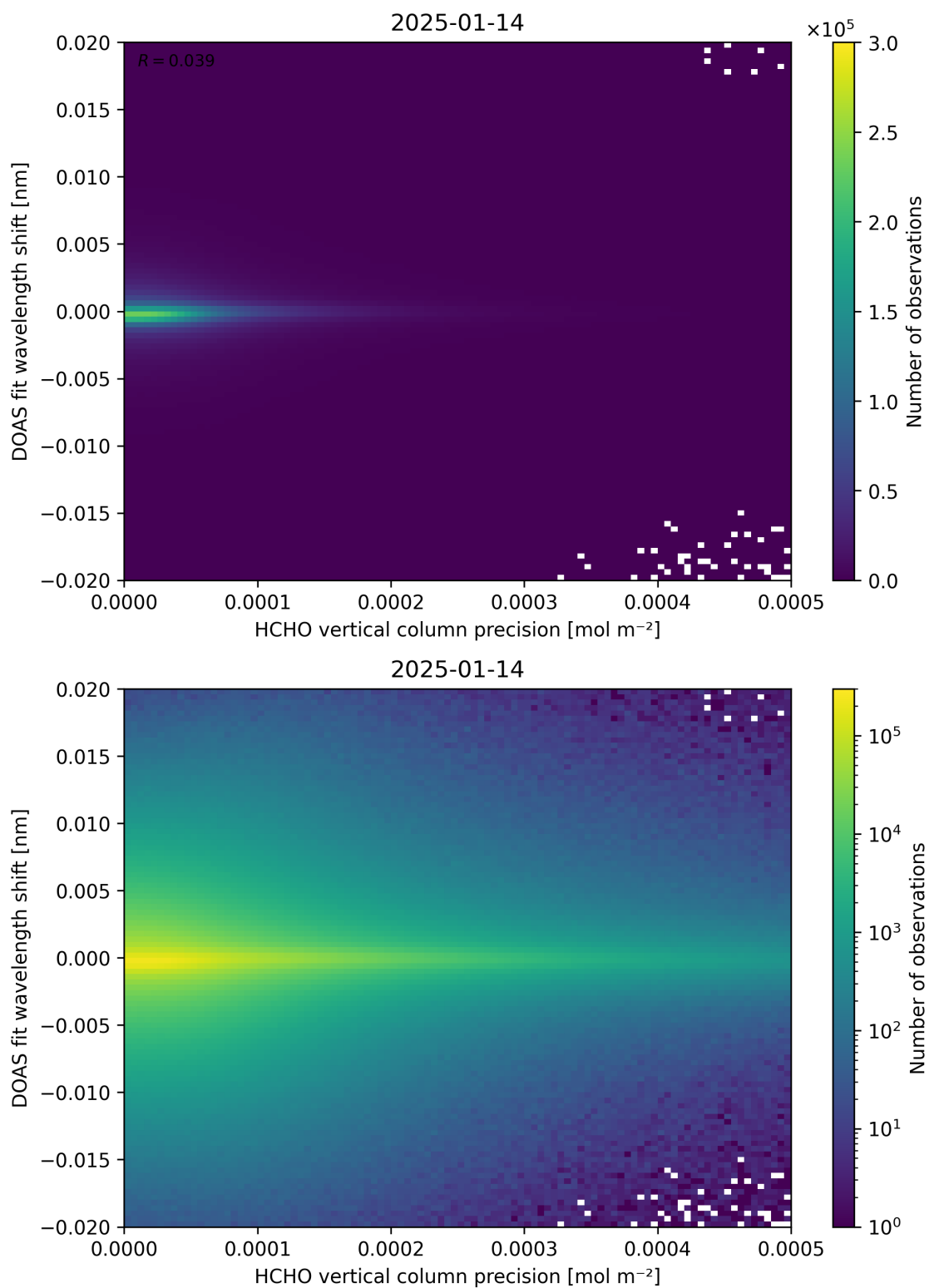
Figure 137: Scatter density plot of “HCHO vertical column precision” against “DOAS fit wavelength shift” for 2025-01-13 to 2025-01-15.
