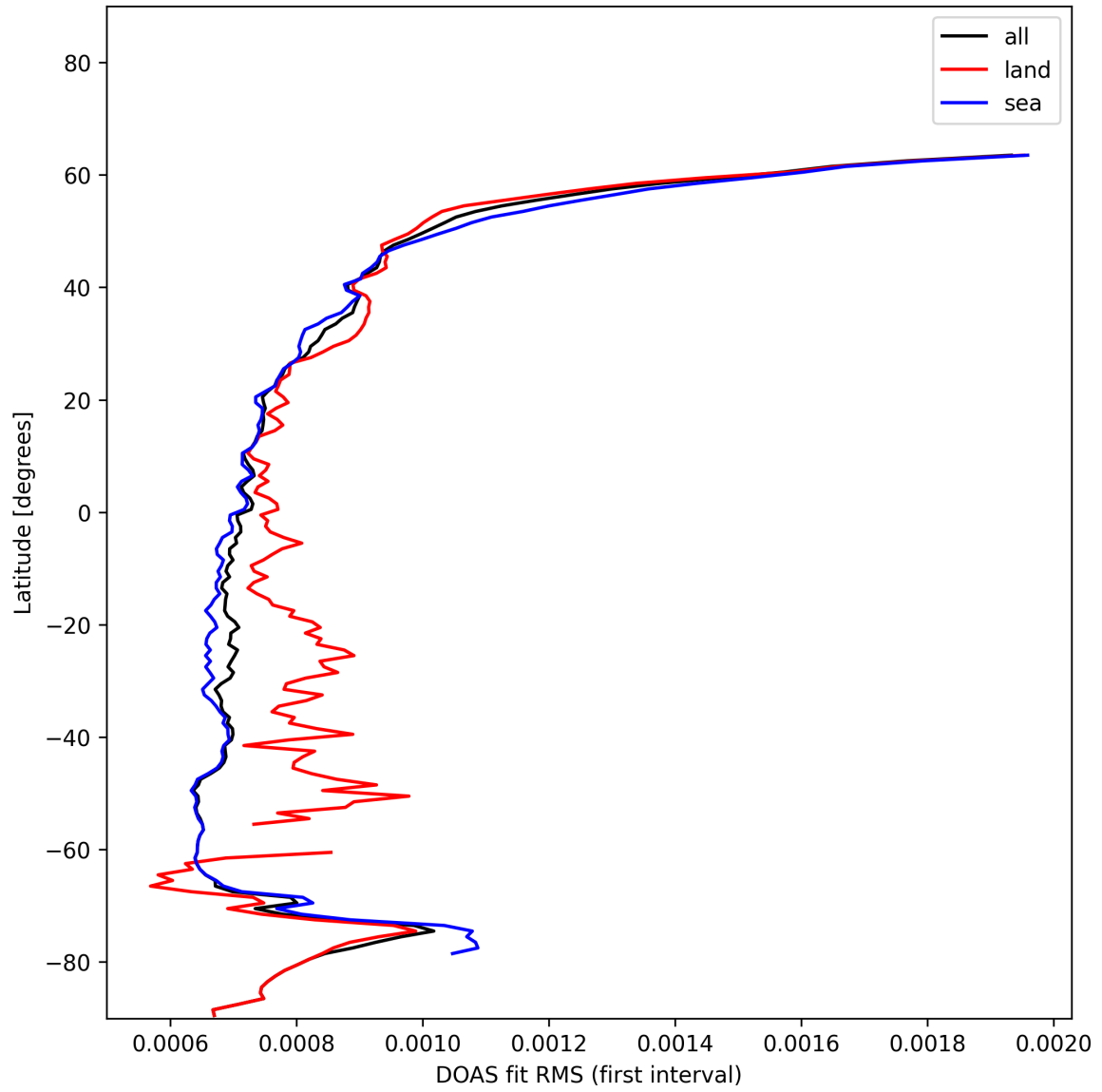
Figure 32: Zonal average of “DOAS fit RMS (first interval)” for 2025-01-13 to 2025-01-15.
