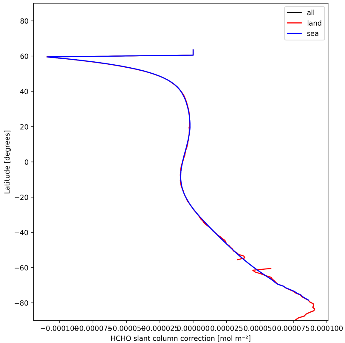
Figure 33: Zonal average of “HCHO slant column correction” for 2025-01-13 to 2025-01-15.
