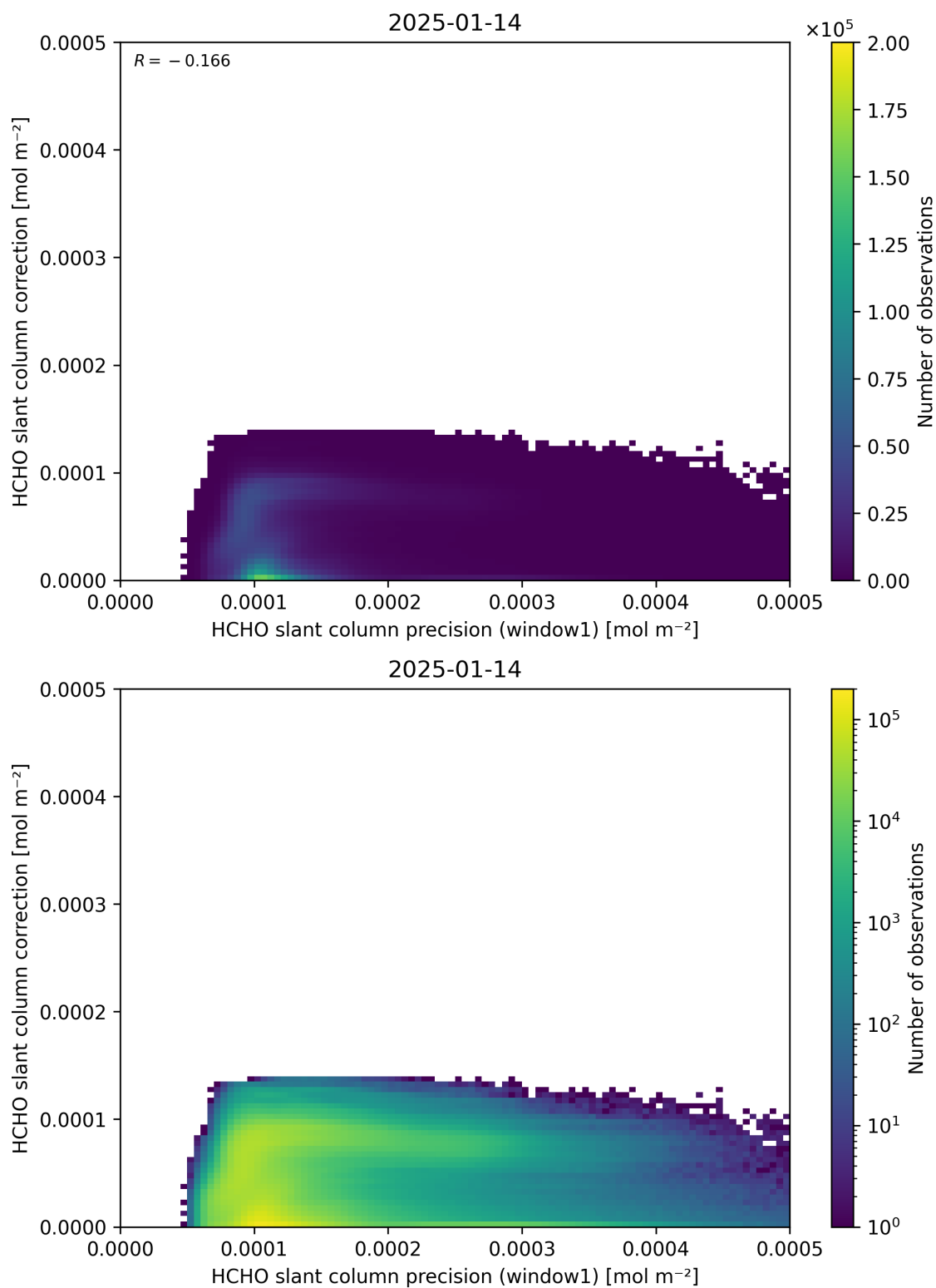
Figure 93: Scatter density plot of “HCHO slant column precision (window1)” against “HCHO slant column correction” for 2025-01-13 to 2025-01-15.
