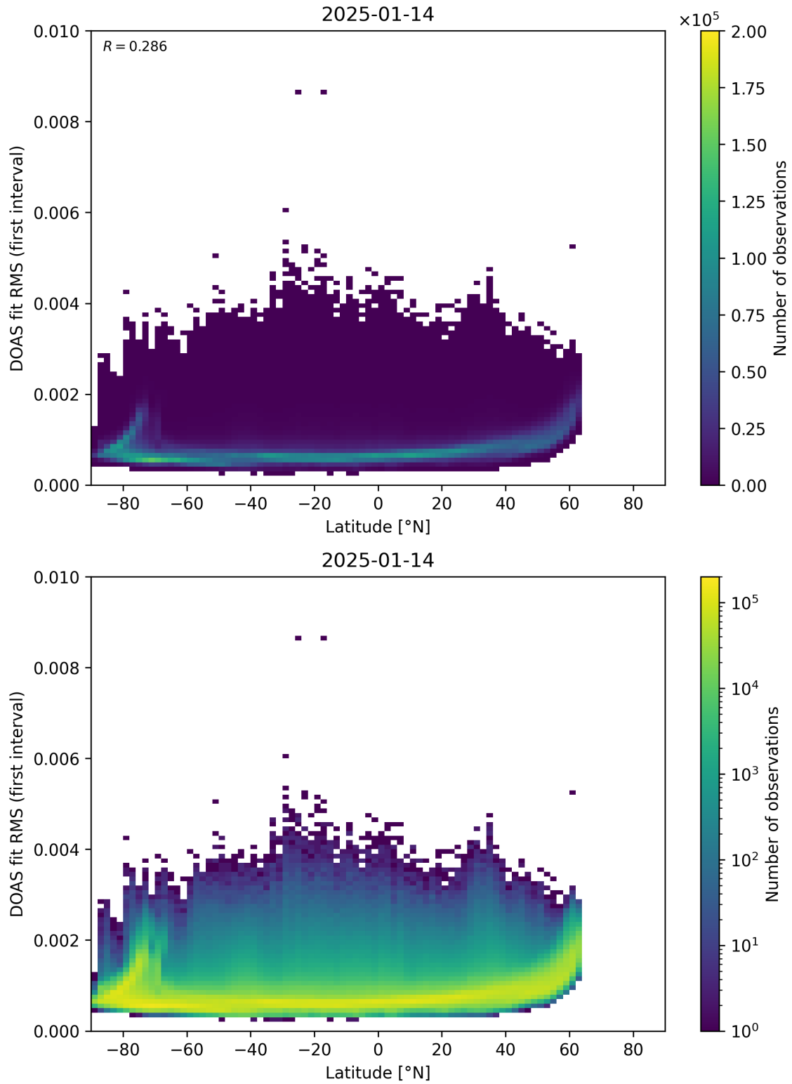
Figure 153: Scatter density plot of “Latitude” against “DOAS fit RMS (first interval)” for 2025-01-13 to 2025-01-15.
