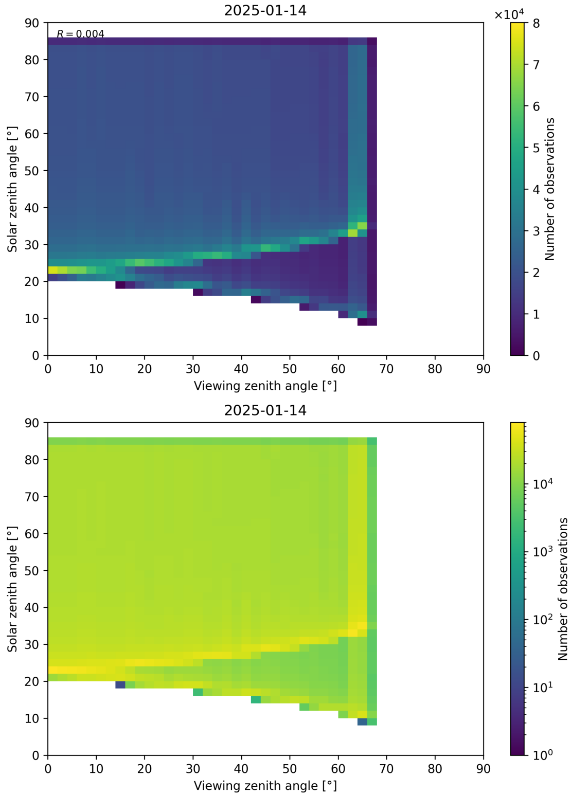
Figure 197: Scatter density plot of “Viewing zenith angle” against “Solar zenith angle” for 2025-01-13 to 2025-01-15.
