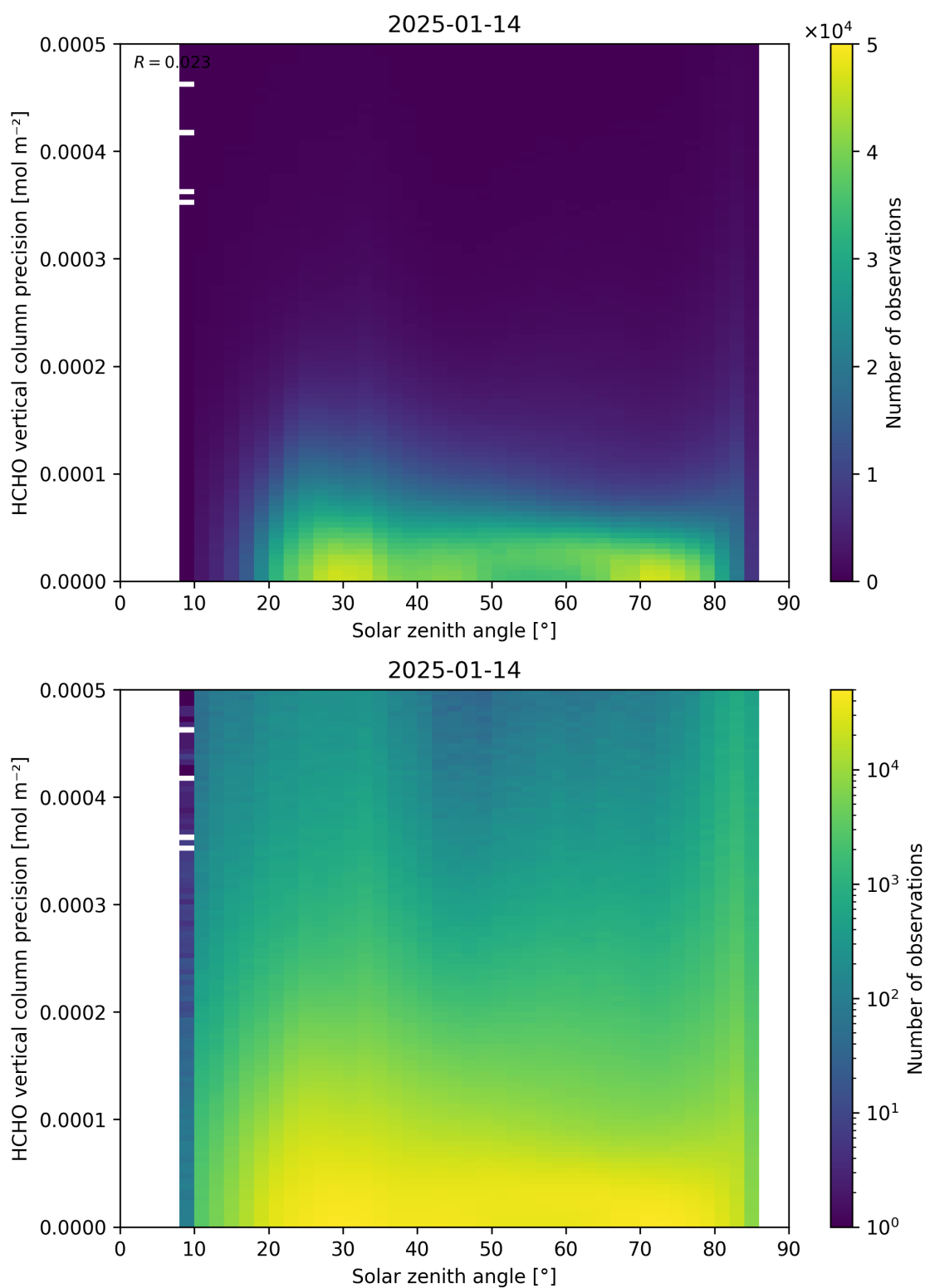
Figure 179: Scatter density plot of “Solar zenith angle” against “HCHO vertical column precision” for 2025-01-13 to 2025-01-15.
