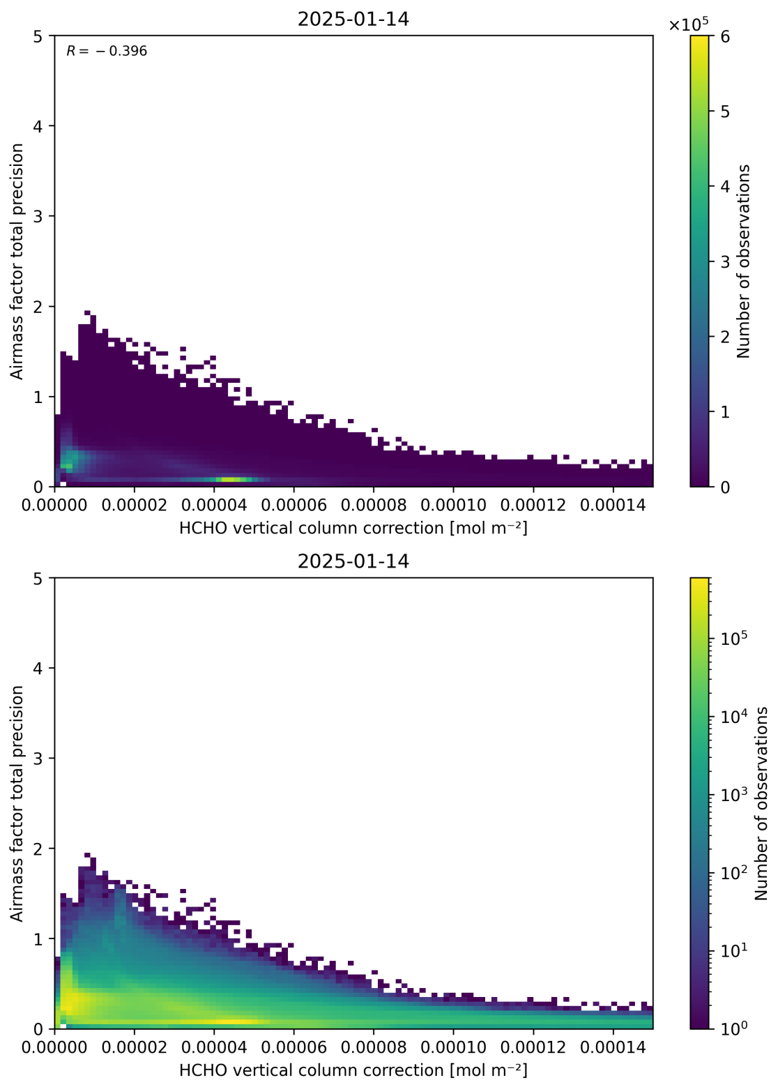
Figure 121: Scatter density plot of “HCHO vertical column correction” against “Airmass factor total precision” for 2025-01-13 to 2025-01-15.
