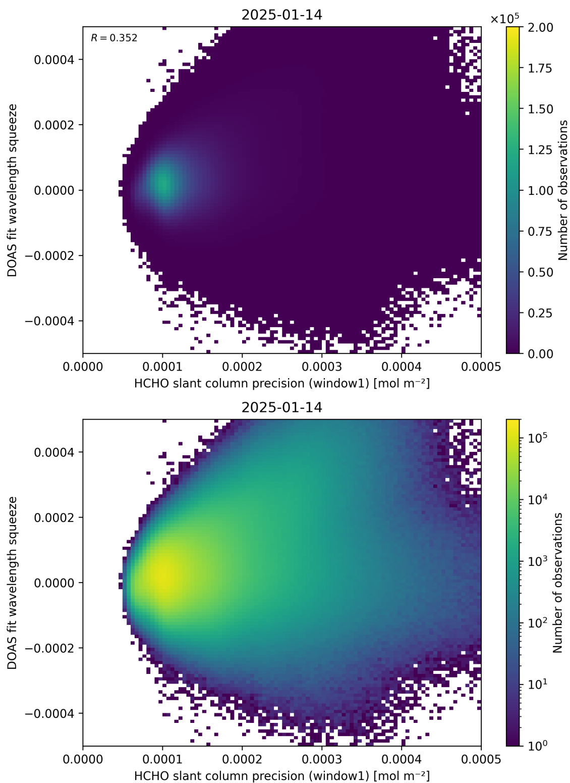
Figure 90: Scatter density plot of “HCHO slant column precision (window1)” against “DOAS fit wavelength squeeze” for 2025-01-13 to 2025-01-15.
