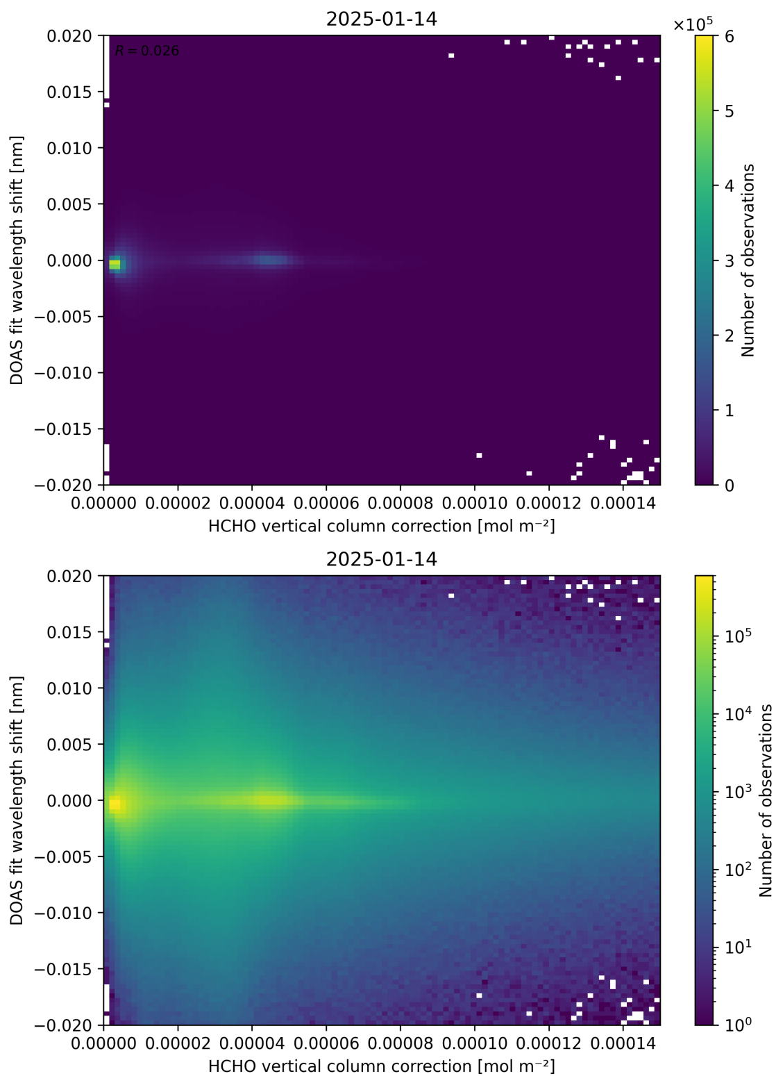
Figure 113: Scatter density plot of “HCHO vertical column correction” against “DOAS fit wavelength shift” for 2025-01-13 to 2025-01-15.
