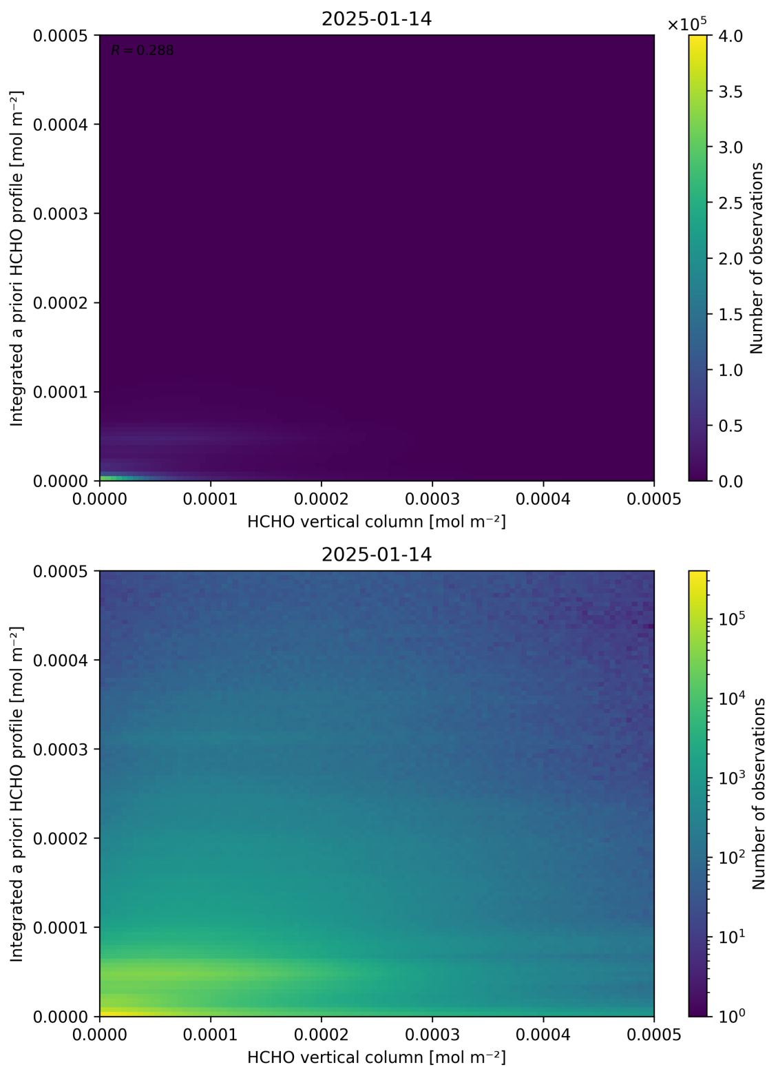
Figure 135: Scatter density plot of “HCHO vertical column” against “Integrated a priori HCHO profile” for 2025-01-13 to 2025-01-15.
