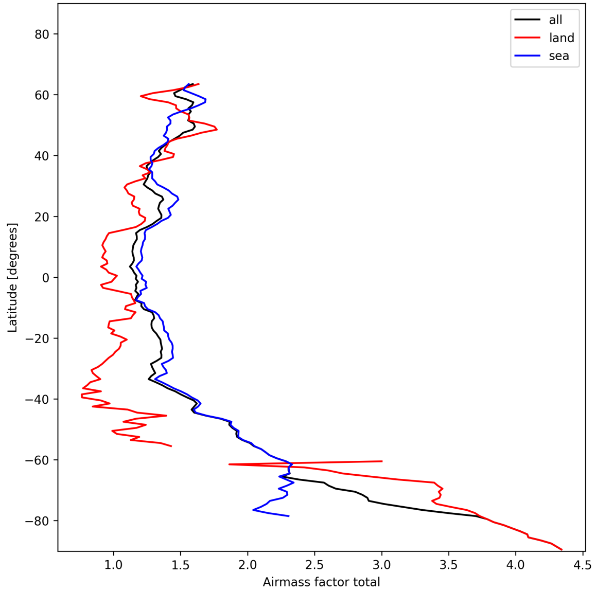
Figure 26: Zonal average of “Airmass factor total” for 2025-01-13 to 2025-01-15.
