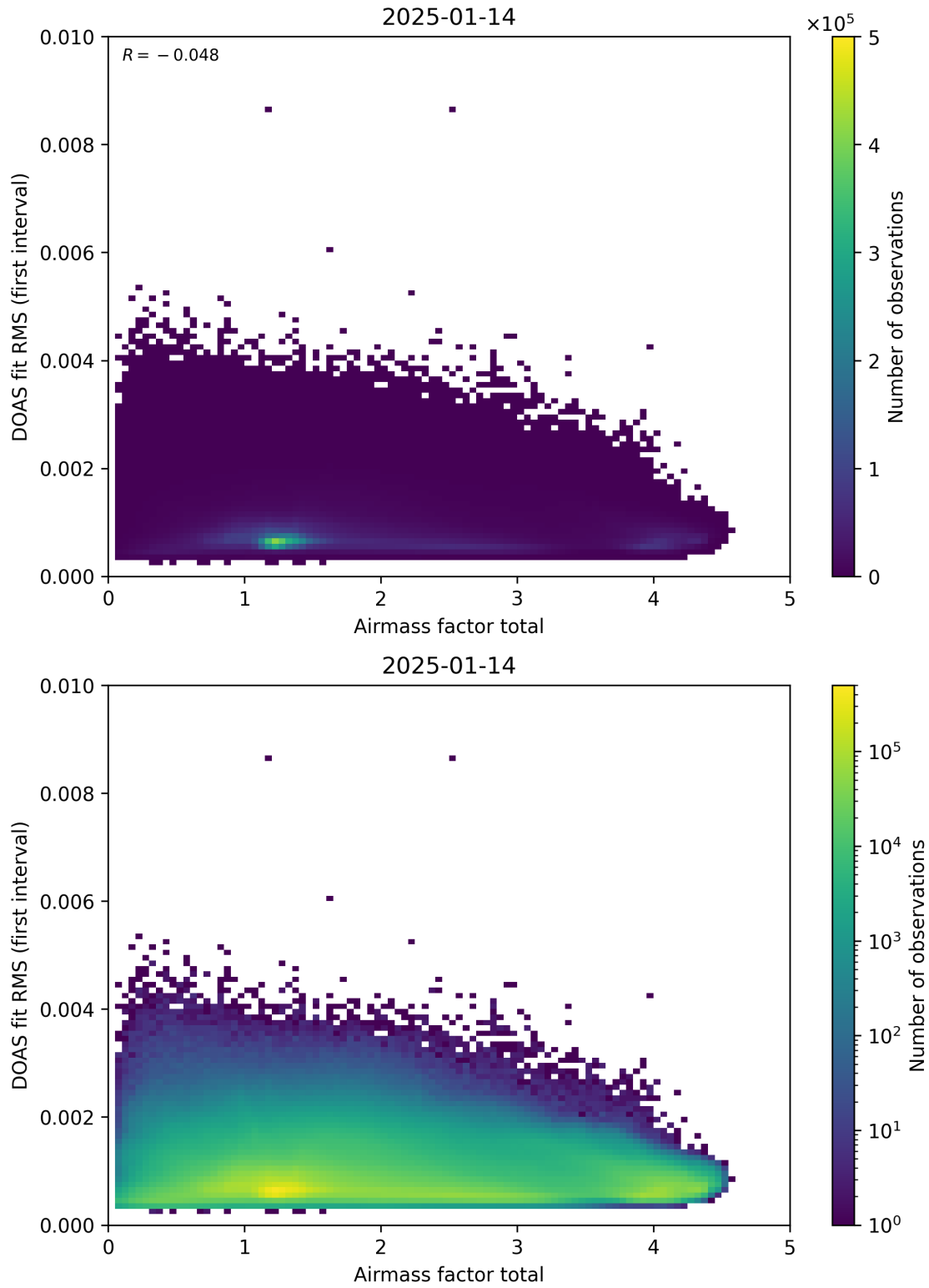
Figure 97: Scatter density plot of “Airmass factor total” against “DOAS fit RMS (first interval)” for 2025-01-13 to 2025-01-15.
