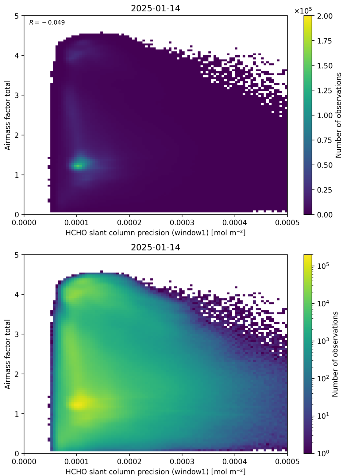
Figure 94: Scatter density plot of “HCHO slant column precision (window1)” against “Airmass factor total” for 2025-01-13 to 2025-01-15.
