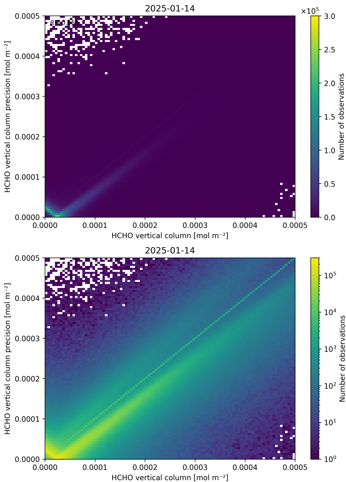
Figure 134: Scatter density plot of “HCHO vertical column” against “HCHO vertical column precision” for 2025-01-13 to 2025-01-15.
