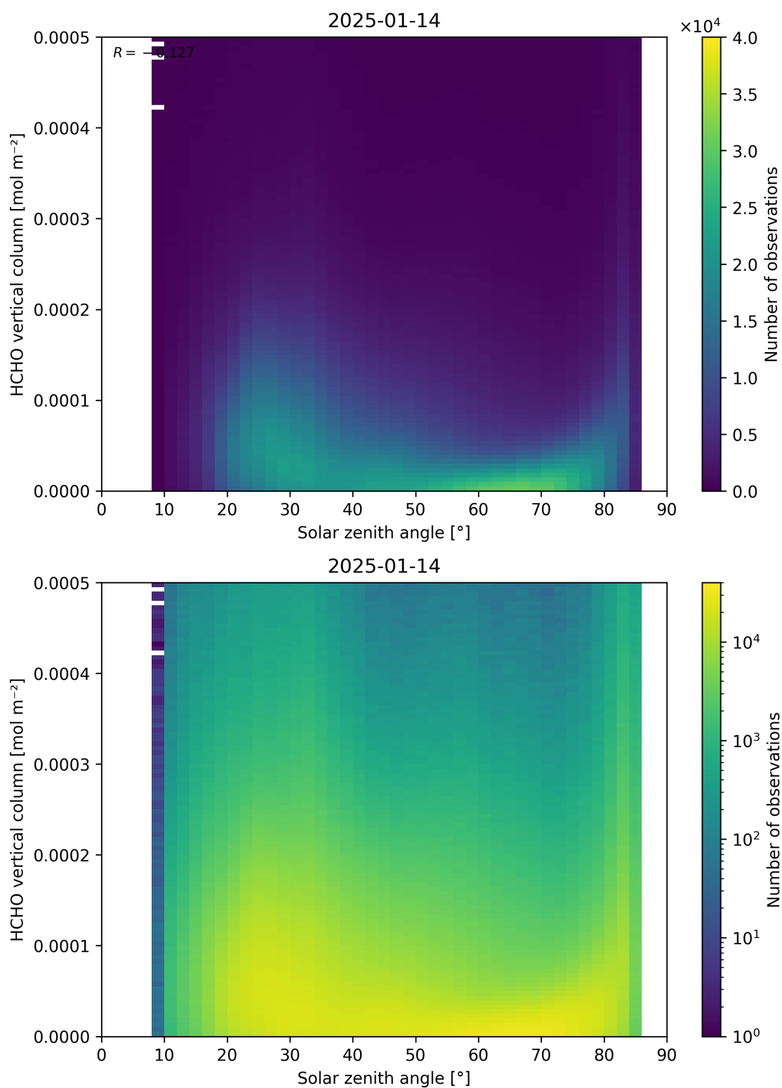
Figure 177: Scatter density plot of “Solar zenith angle” against “HCHO vertical column” for 2025-01-13 to 2025-01-15.
