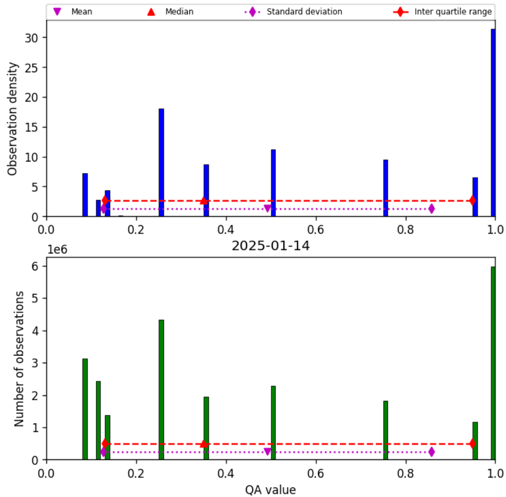
Figure 34: Histogram of “QA value” for 2025-01-13 to 2025-01-15
