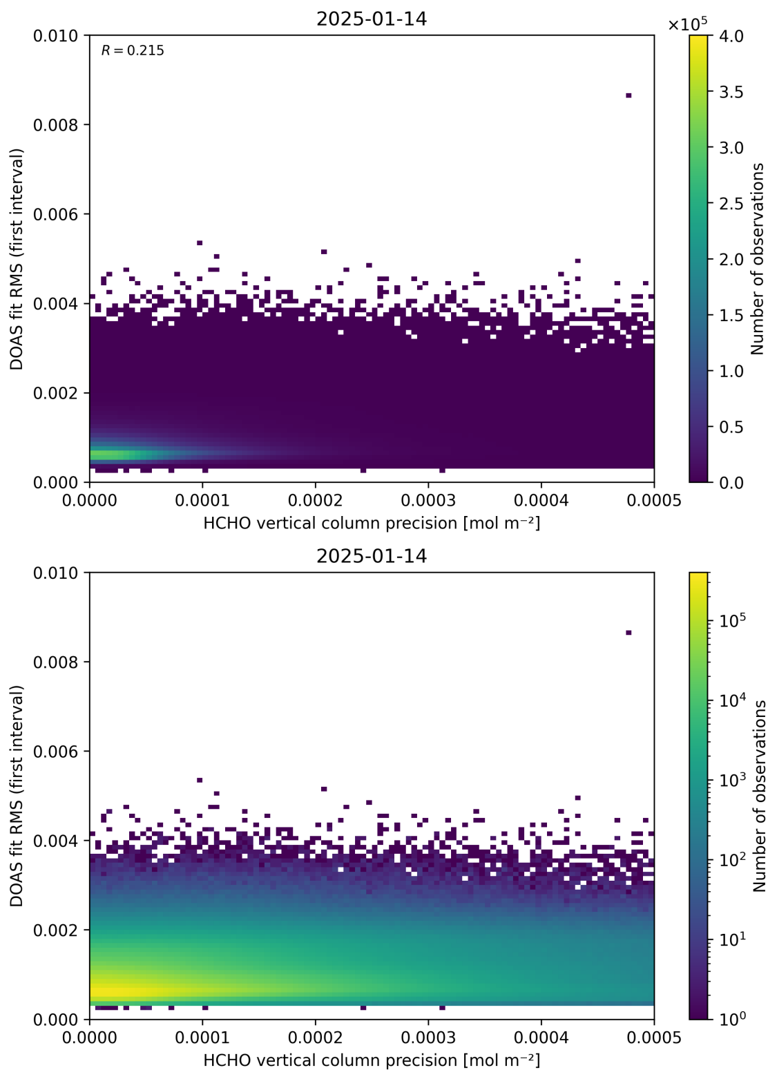
Figure 136: Scatter density plot of “HCHO vertical column precision” against “DOAS fit RMS (first interval)” for 2025-01-13 to 2025-01-15.
