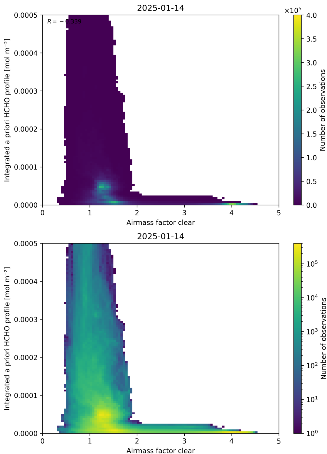
Figure 76: Scatter density plot of “Airmass factor clear” against “Integrated a priori HCHO profile” for 2025-01-13 to 2025-01-15.
