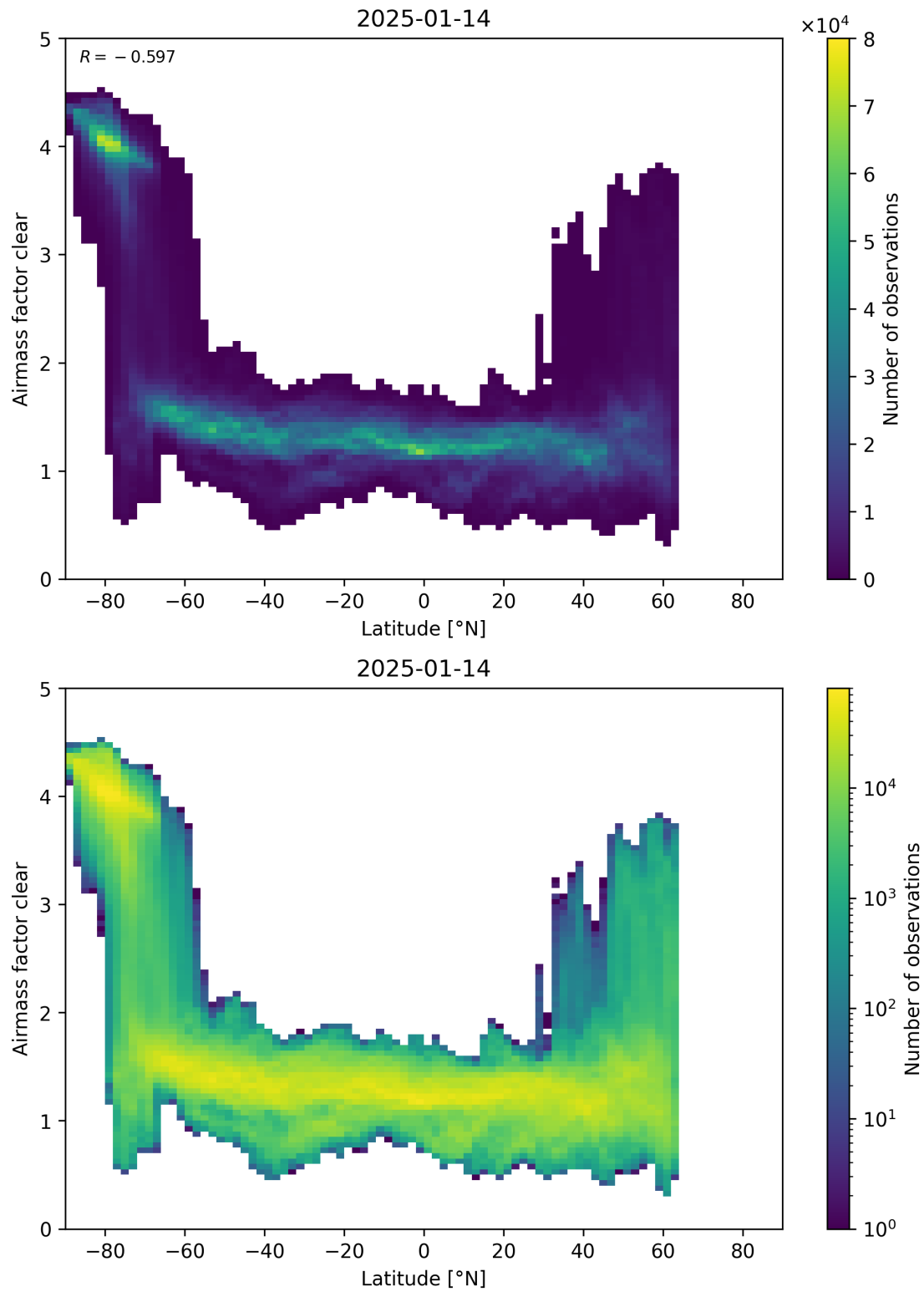
Figure 156: Scatter density plot of “Latitude” against “Airmass factor clear” for 2025-01-13 to 2025-01-15.
