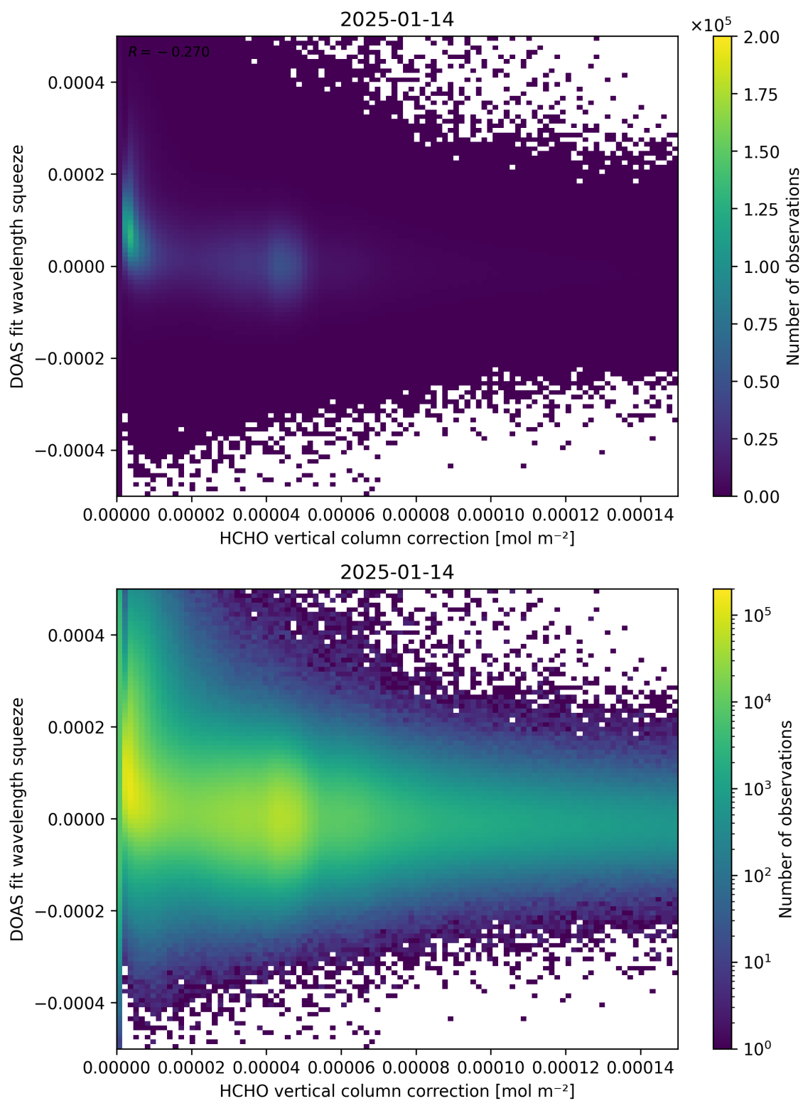
Figure 114: Scatter density plot of “HCHO vertical column correction” against “DOAS fit wavelength squeeze” for 2025-01-13 to 2025-01-15.
