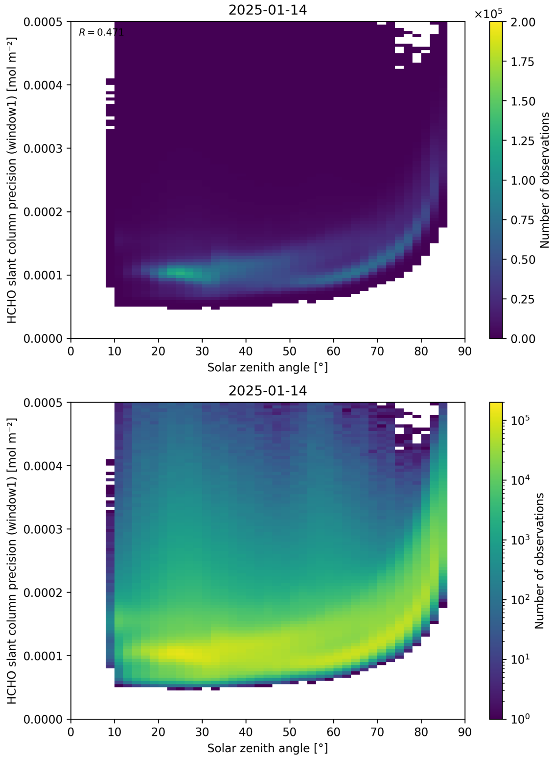
Figure 174: Scatter density plot of “Solar zenith angle” against “HCHO slant column precision (window1)” for 2025-01-13 to 2025-01-15.
