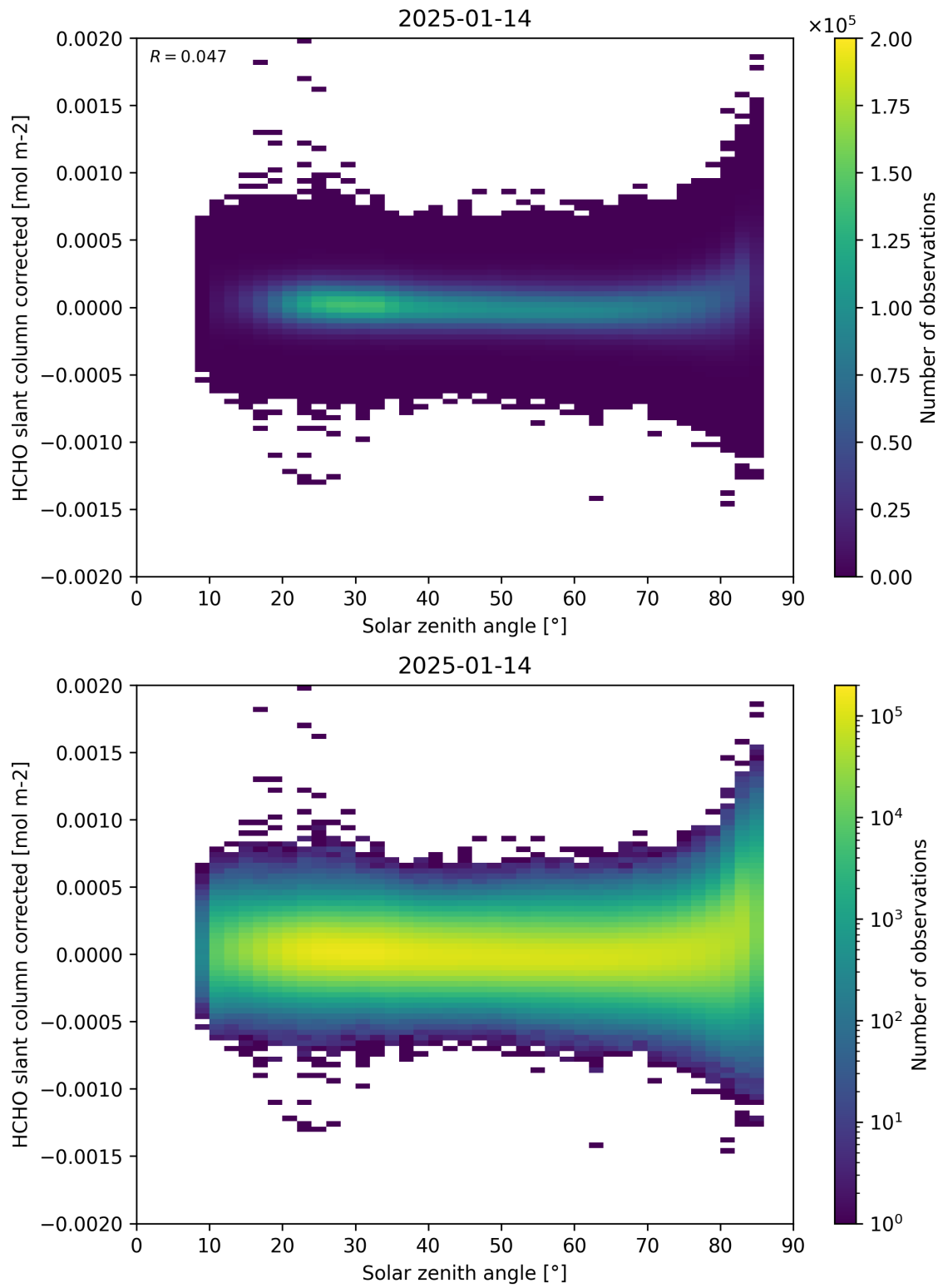
Figure 171: Scatter density plot of “Solar zenith angle” against “HCHO slant column corrected” for 2025-01-13 to 2025-01-15.
