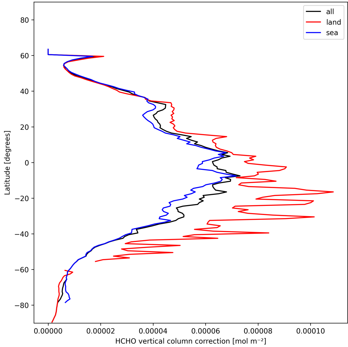
Figure 23: Zonal average of “HCHO vertical column correction” for 2025-01-13 to 2025-01-15.
