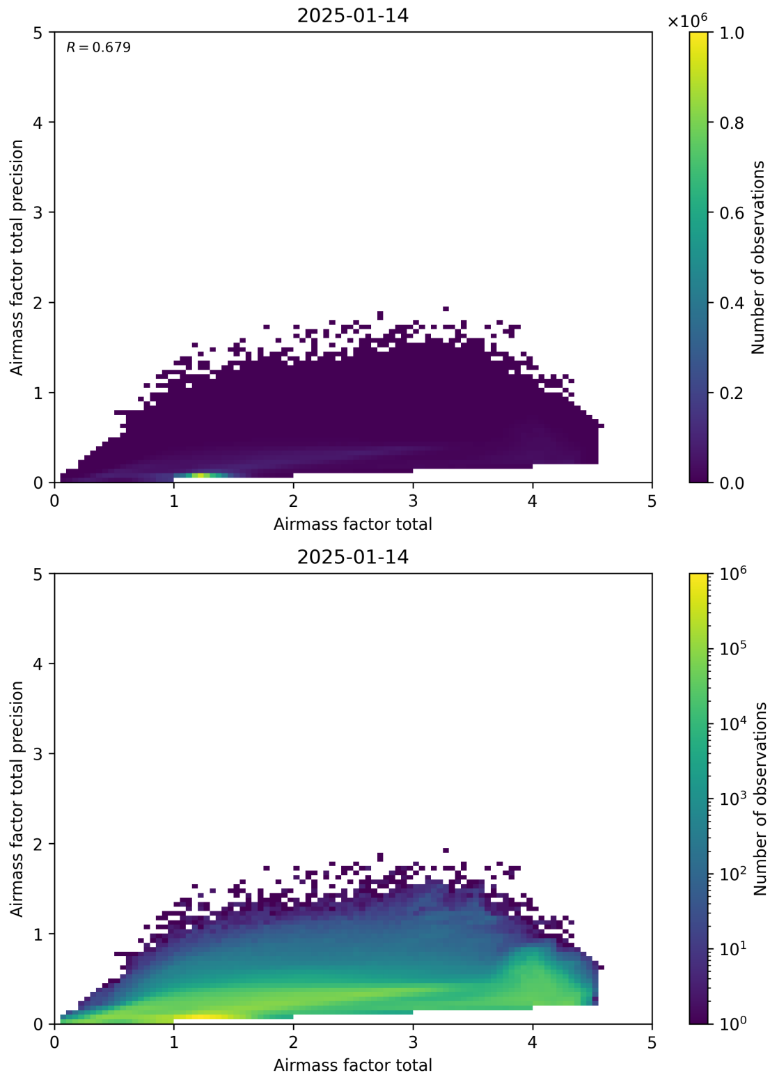
Figure 103: Scatter density plot of “Airmass factor total” against “Airmass factor total precision” for 2025-01-13 to 2025-01-15.
