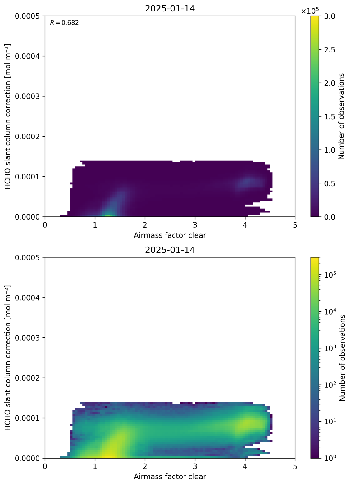
Figure 75: Scatter density plot of “Airmass factor clear” against “HCHO slant column correction” for 2025-01-13 to 2025-01-15.
