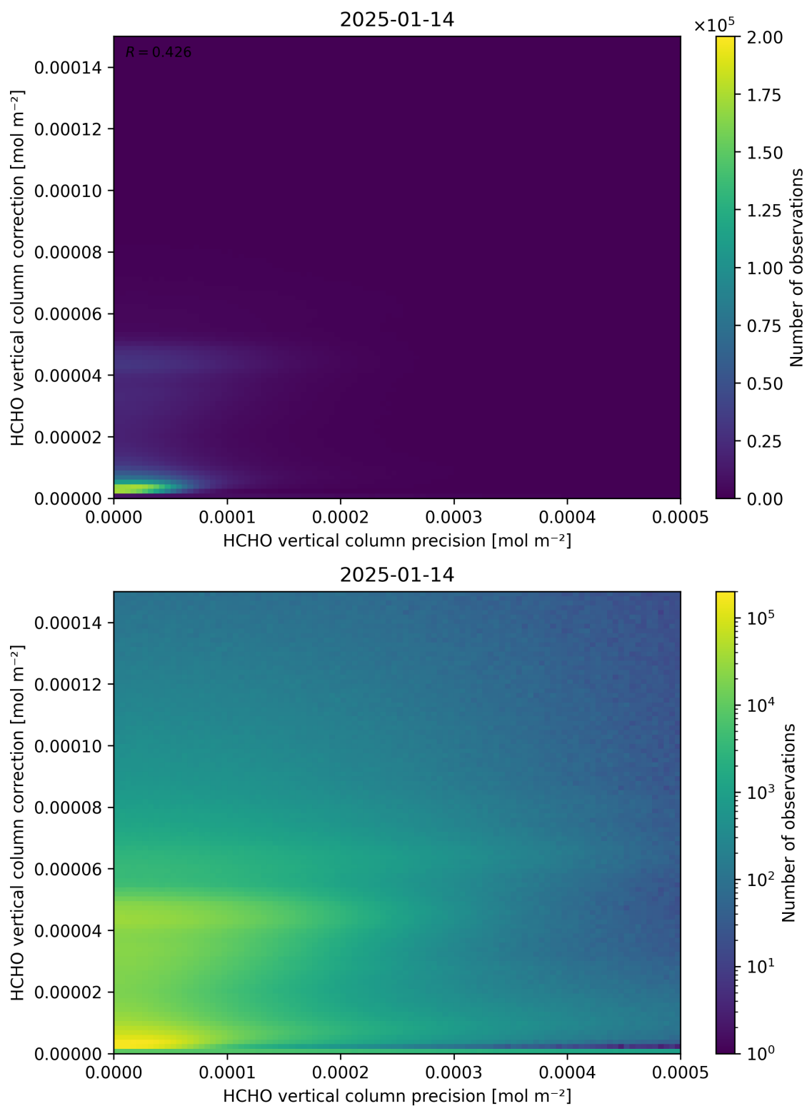
Figure 146: Scatter density plot of “HCHO vertical column precision” against “HCHO vertical column correction” for 2025-01-13 to 2025-01-15.
