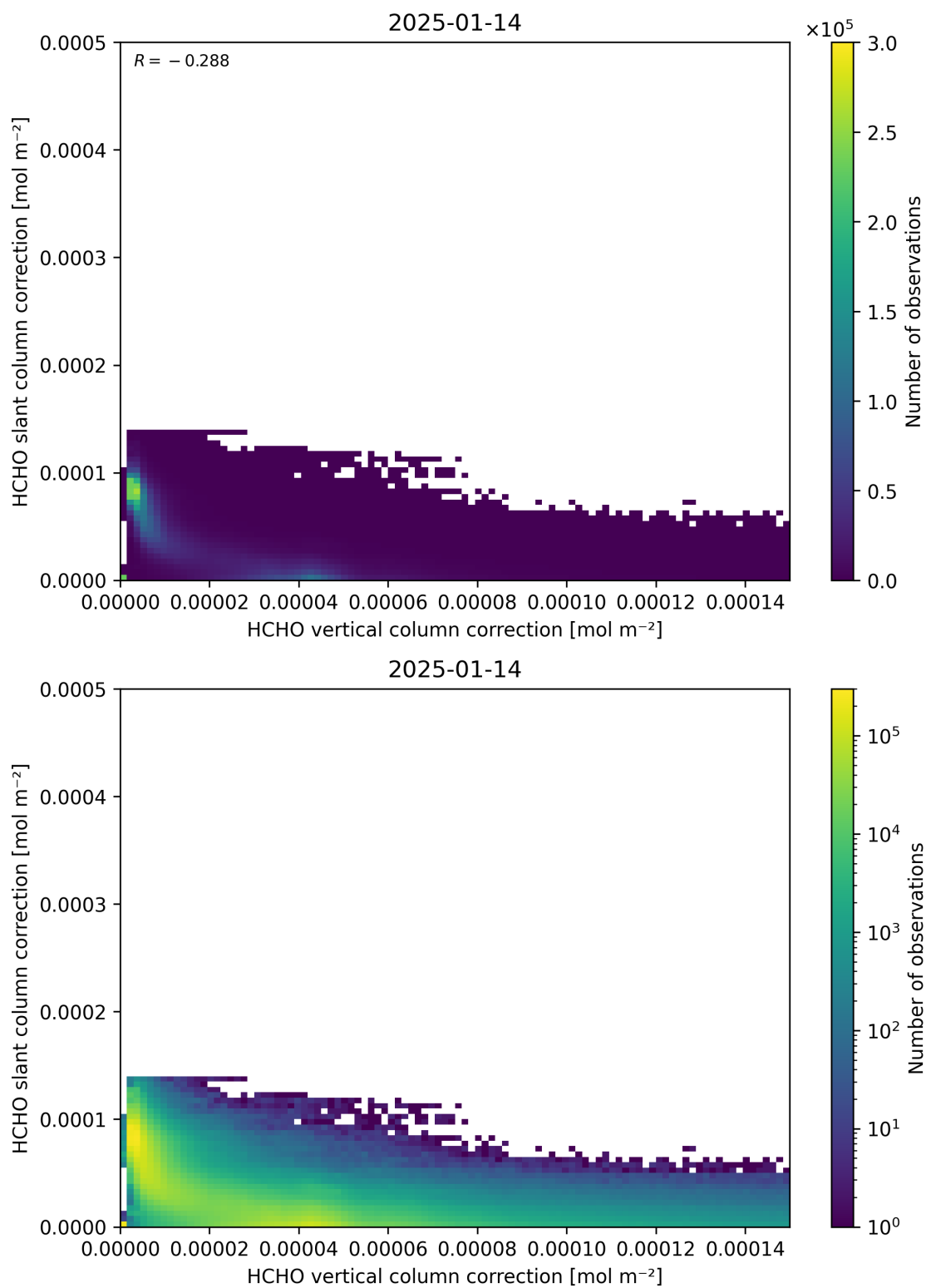
Figure 117: Scatter density plot of “HCHO vertical column correction” against “HCHO slant column correction” for 2025-01-13 to 2025-01-15.
