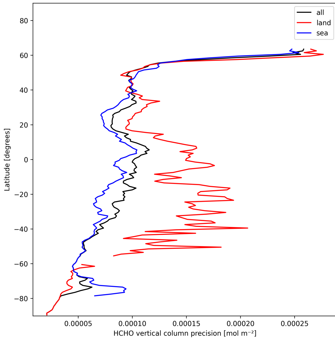
Figure 22: Zonal average of “HCHO vertical column precision” for 2025-01-13 to 2025-01-15.
