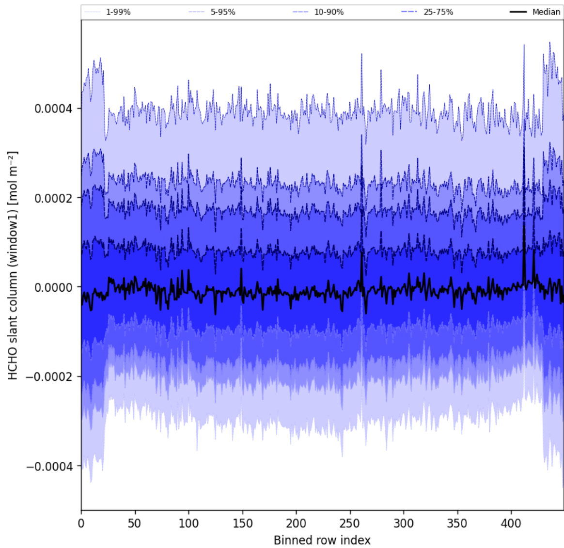
Figure 52: Along track statistics of “HCHO slant column (window1)” for 2025-01-13 to 2025-01-15
