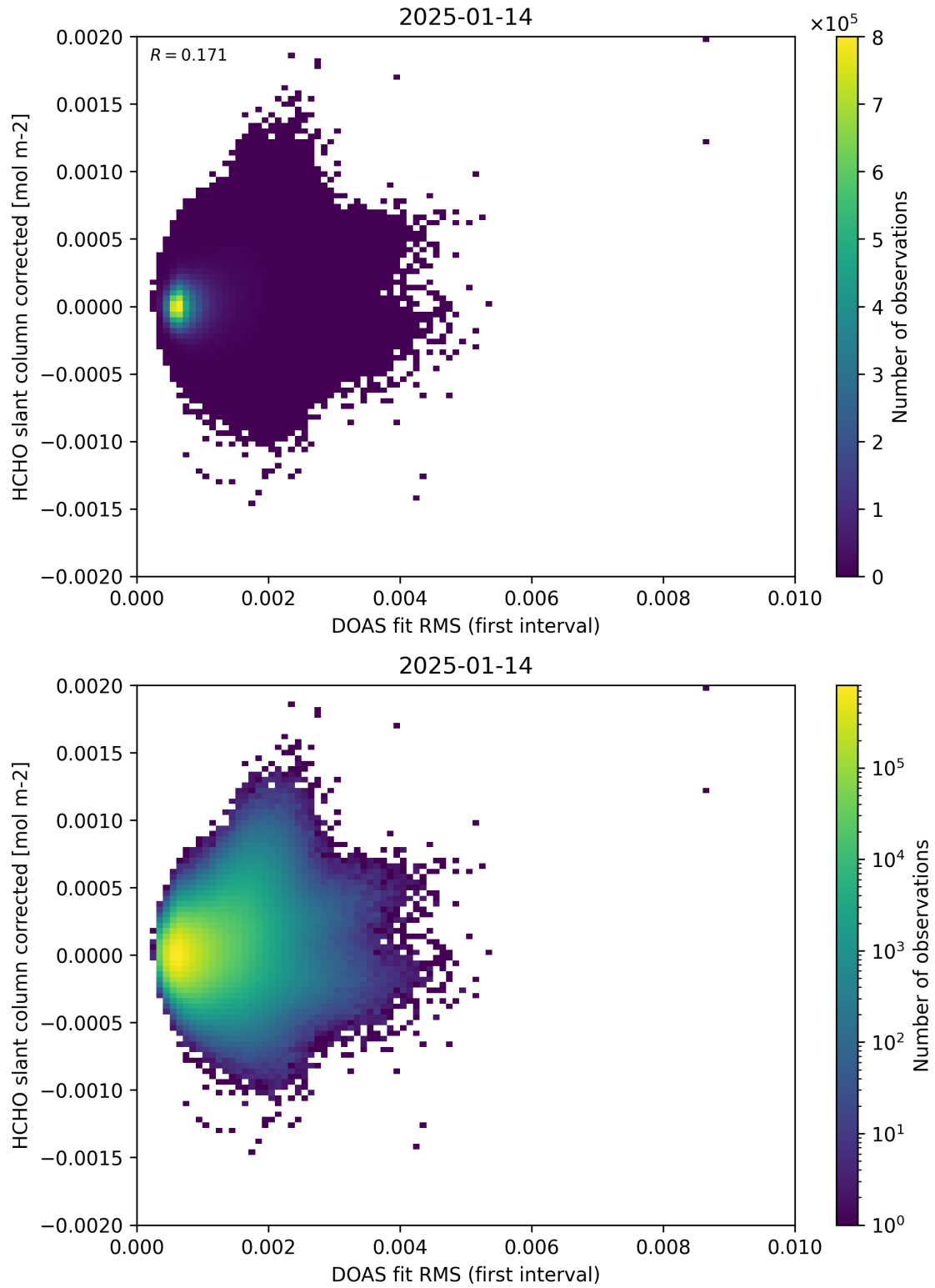
Figure 62: Scatter density plot of “DOAS fit RMS (first interval)” against “HCHO slant column corrected” for 2025-01-13 to 2025-01-15.
