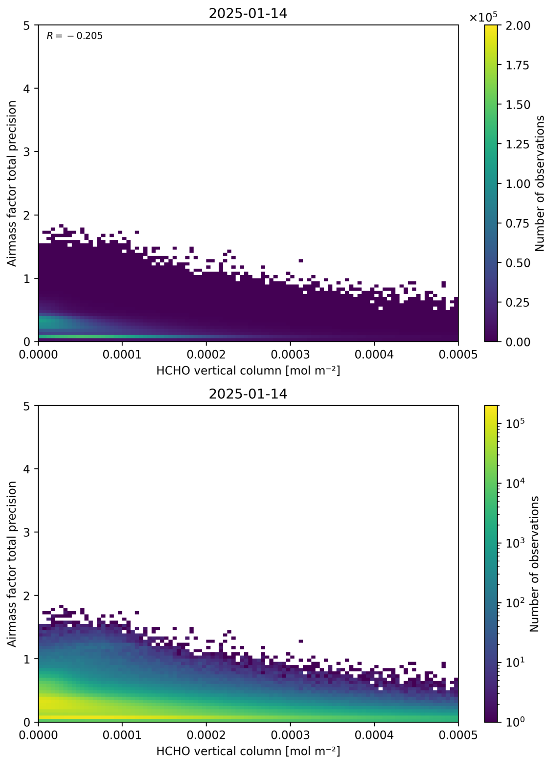
Figure 132: Scatter density plot of “HCHO vertical column” against “Airmass factor total precision” for 2025-01-13 to 2025-01-15.
