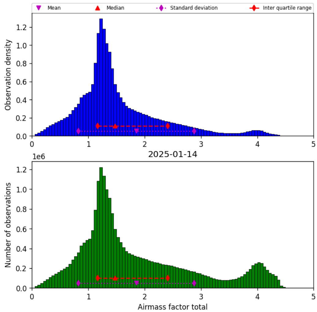
Figure 40: Histogram of “Airmass factor total” for 2025-01-13 to 2025-01-15
