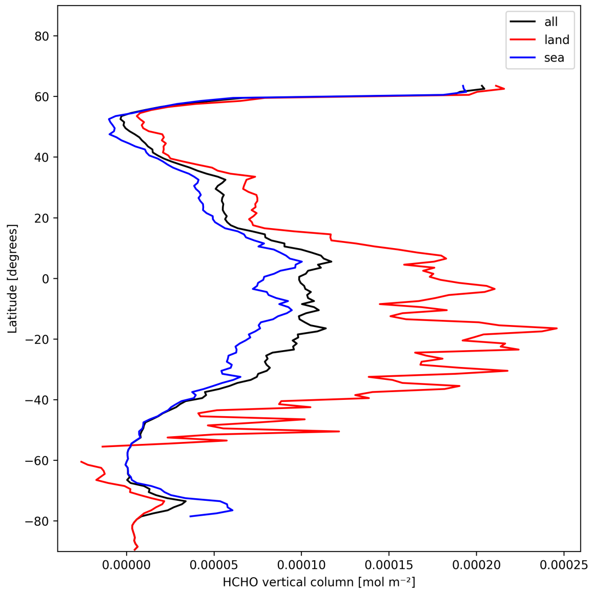
Figure 21: Zonal average of “HCHO vertical column” for 2025-01-13 to 2025-01-15.
