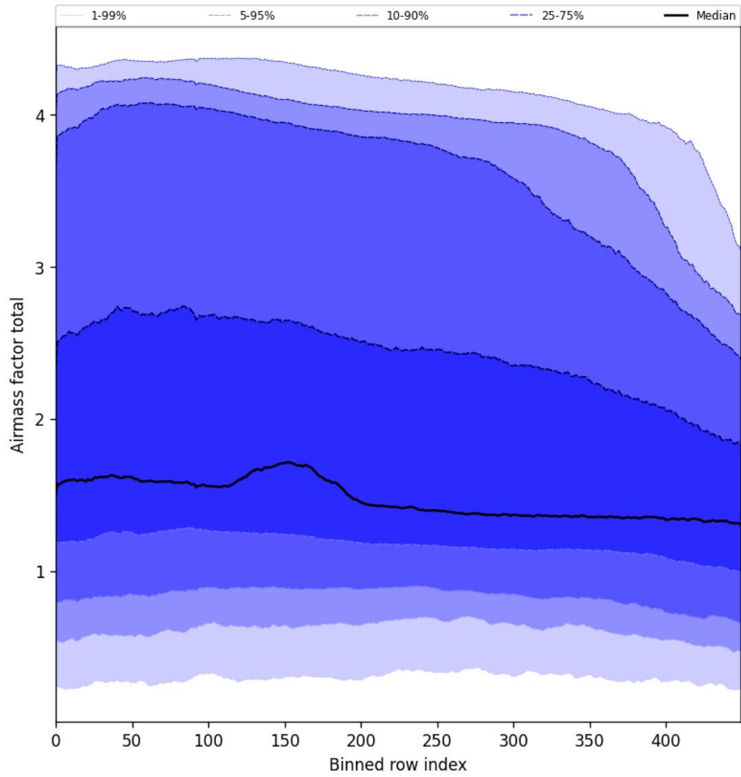
Figure 54: Along track statistics of “Airmass factor total” for 2025-01-13 to 2025-01-15
