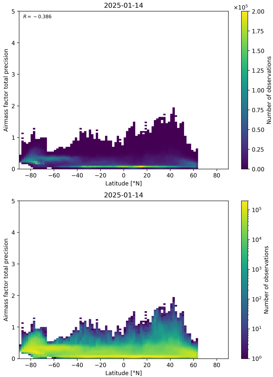
Figure 162: Scatter density plot of “Latitude” against “Airmass factor total precision” for 2025-01-13 to 2025-01-15.
