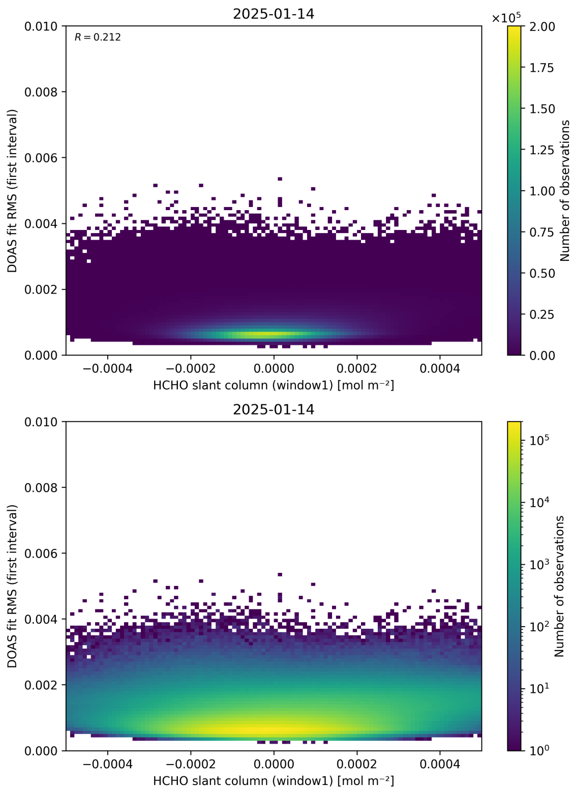
Figure 78: Scatter density plot of “HCHO slant column (window1)” against “DOAS fit RMS (first interval)” for 2025-01-13 to 2025-01-15.
