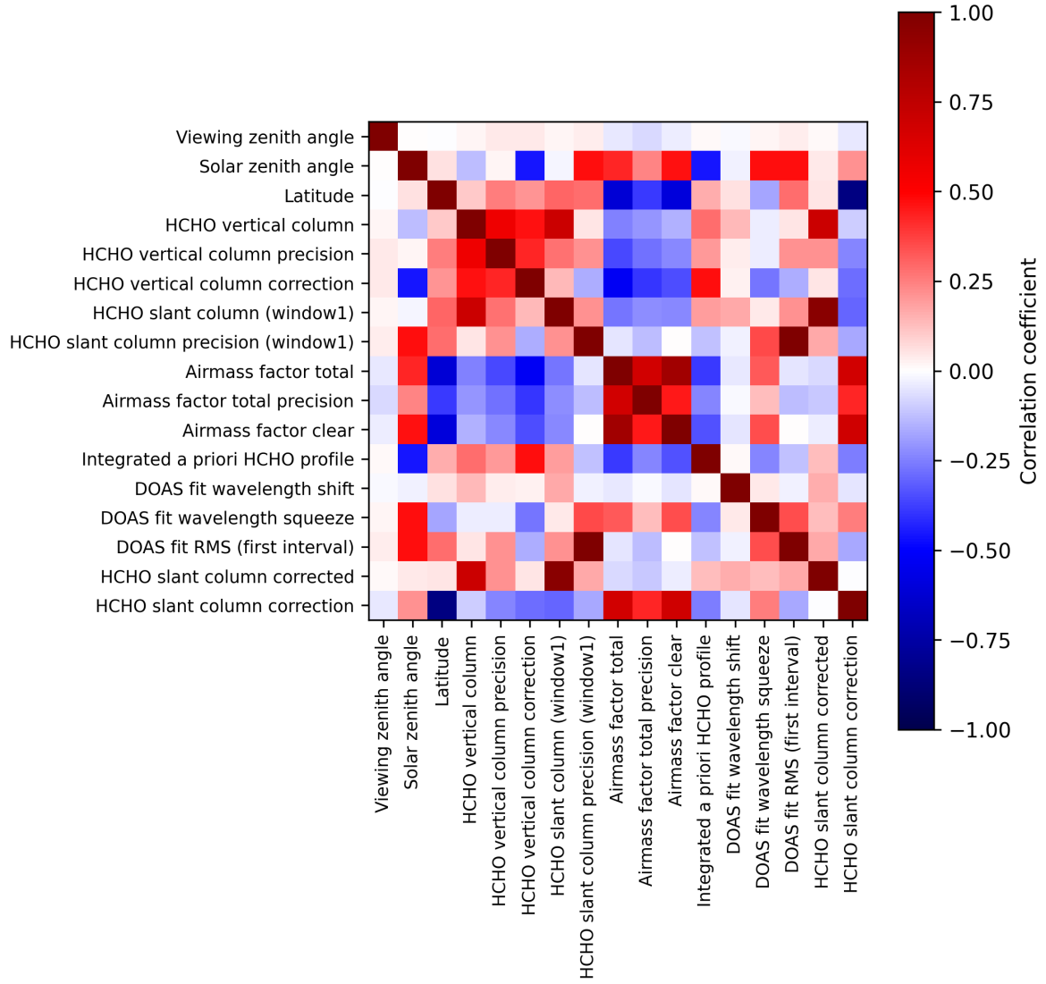
Figure 2: Map of correlation matrix for 2025-01-13 to 2025-01-15.
