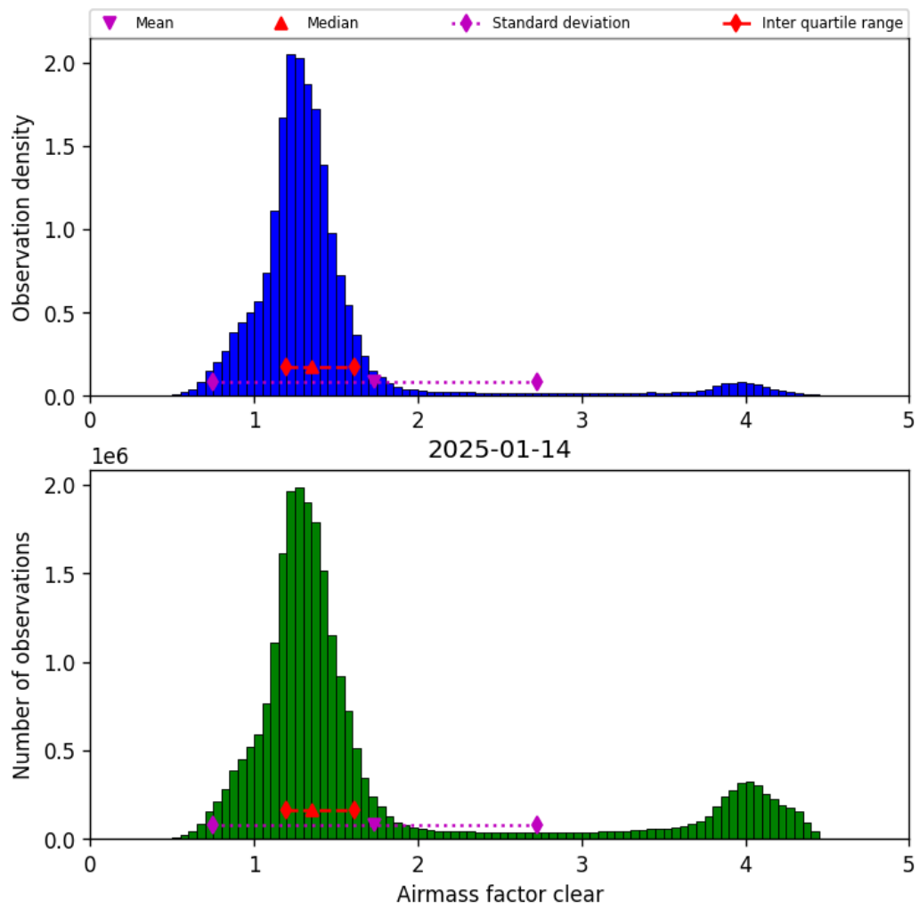
Figure 42: Histogram of “Airmass factor clear” for 2025-01-13 to 2025-01-15
