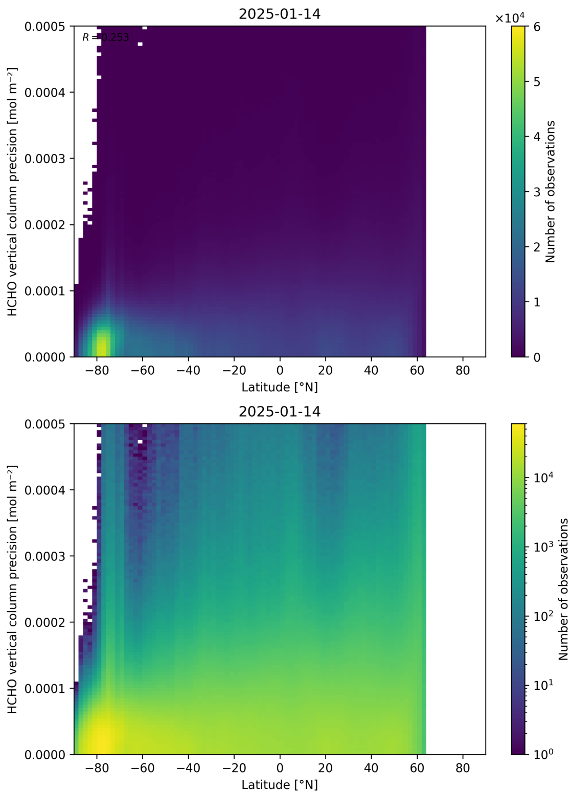
Figure 165: Scatter density plot of “Latitude” against “HCHO vertical column precision” for 2025-01-13 to 2025-01-15.
