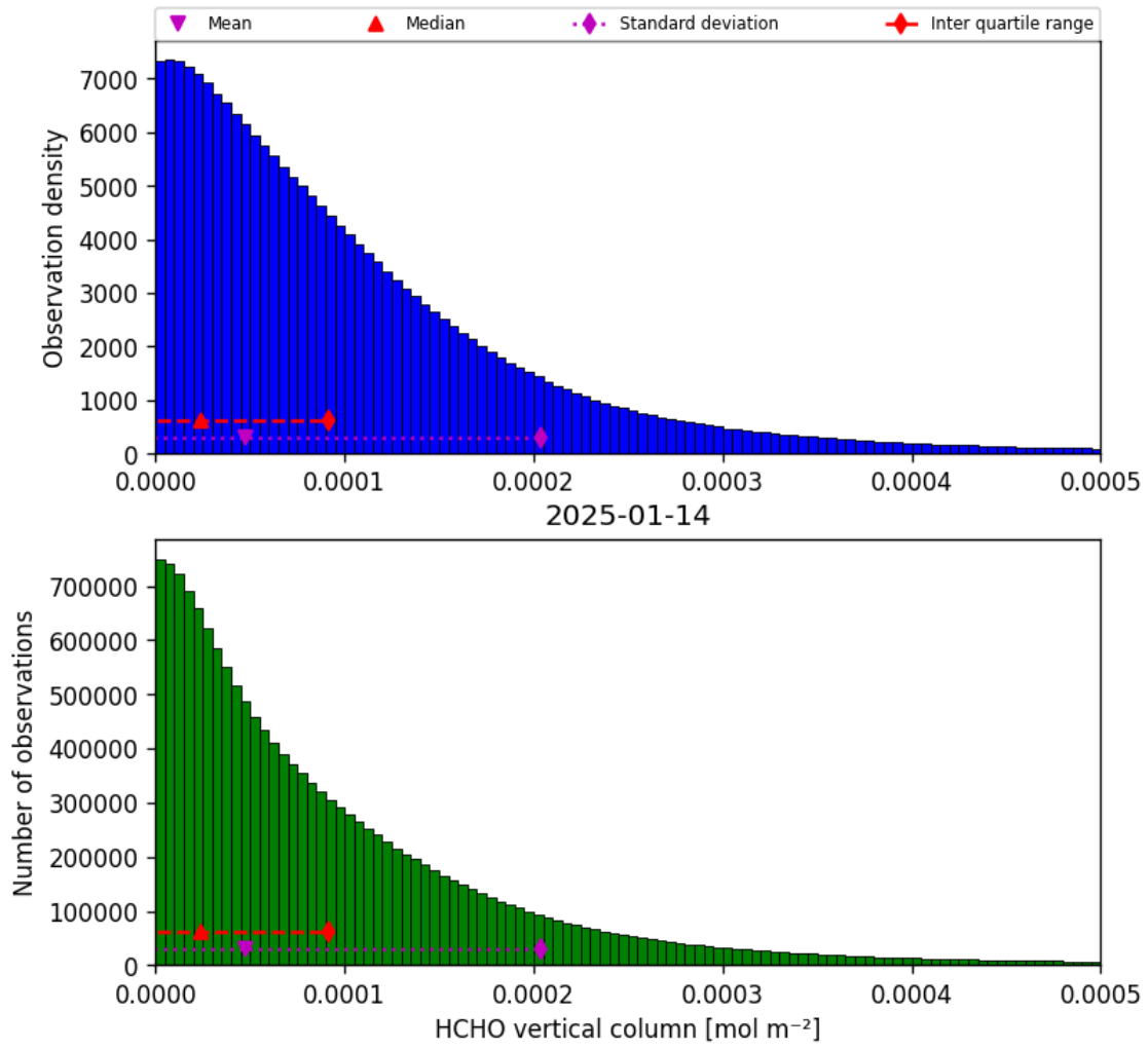
Figure 35: Histogram of “HCHO vertical column” for 2025-01-13 to 2025-01-15
