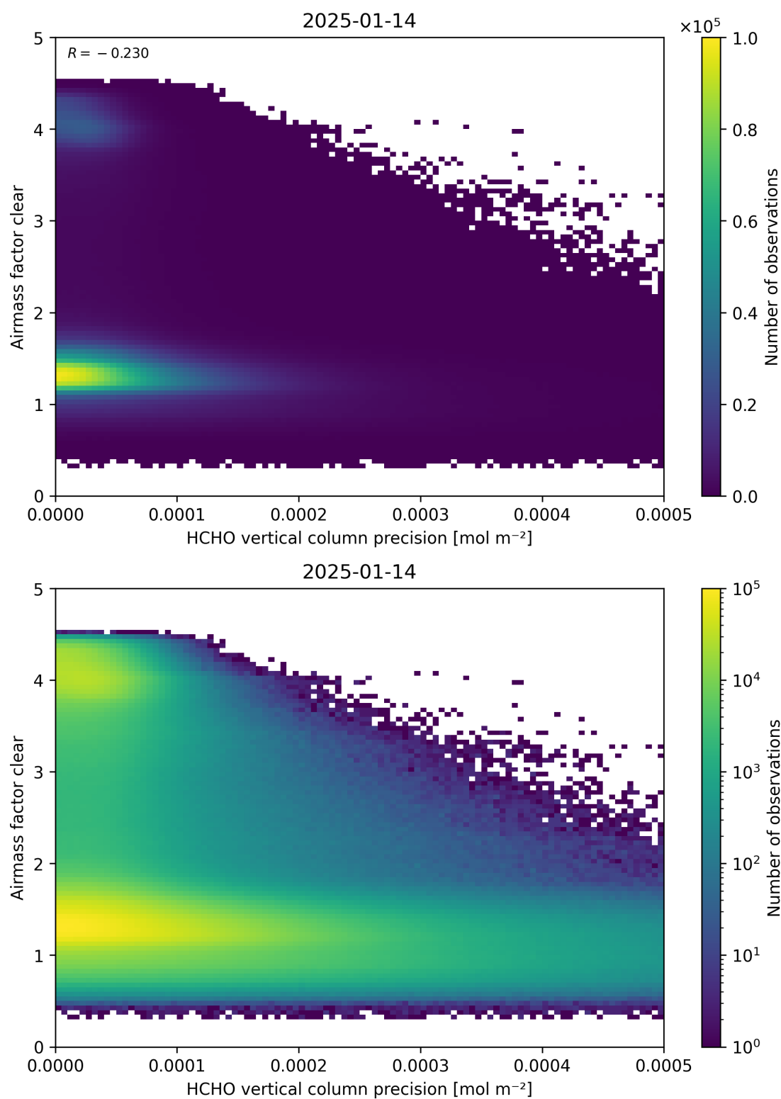
Figure 139: Scatter density plot of “HCHO vertical column precision” against “Airmass factor clear” for 2025-01-13 to 2025-01-15.
