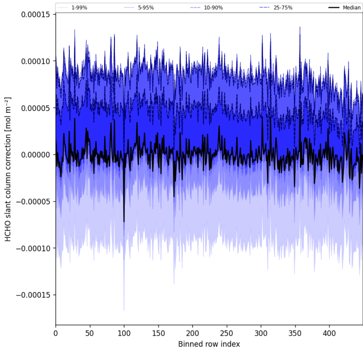
Figure 61: Along track statistics of “HCHO slant column correction” for 2025-01-13 to 2025-01-15
