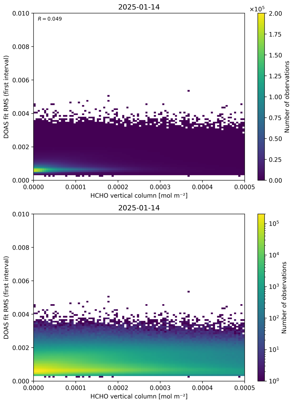
Figure 123: Scatter density plot of “HCHO vertical column” against “DOAS fit RMS (first interval)” for 2025-01-13 to 2025-01-15.
