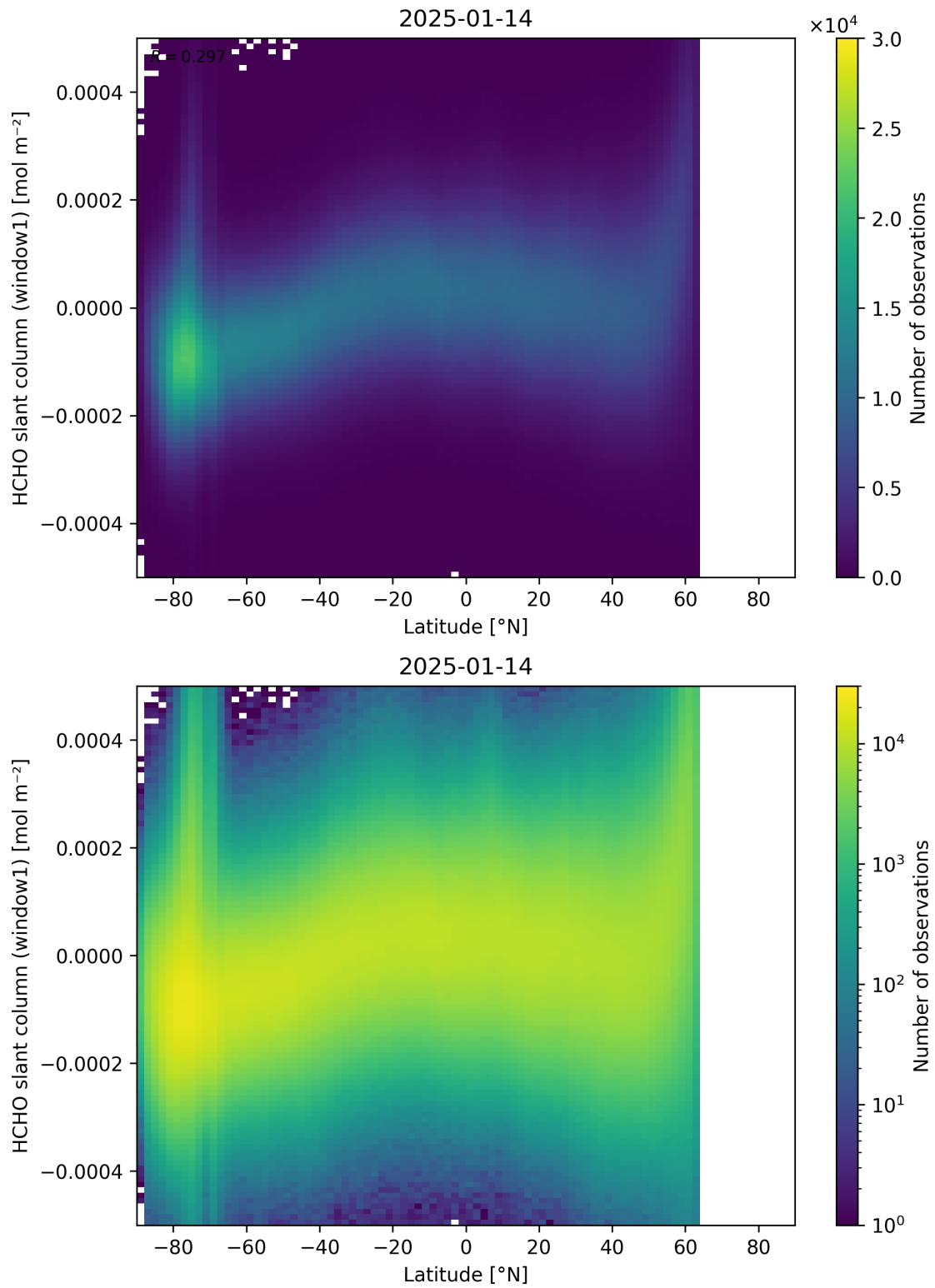
Figure 159: Scatter density plot of “Latitude” against “HCHO slant column (window1)” for 2025-01-13 to 2025-01-15.
