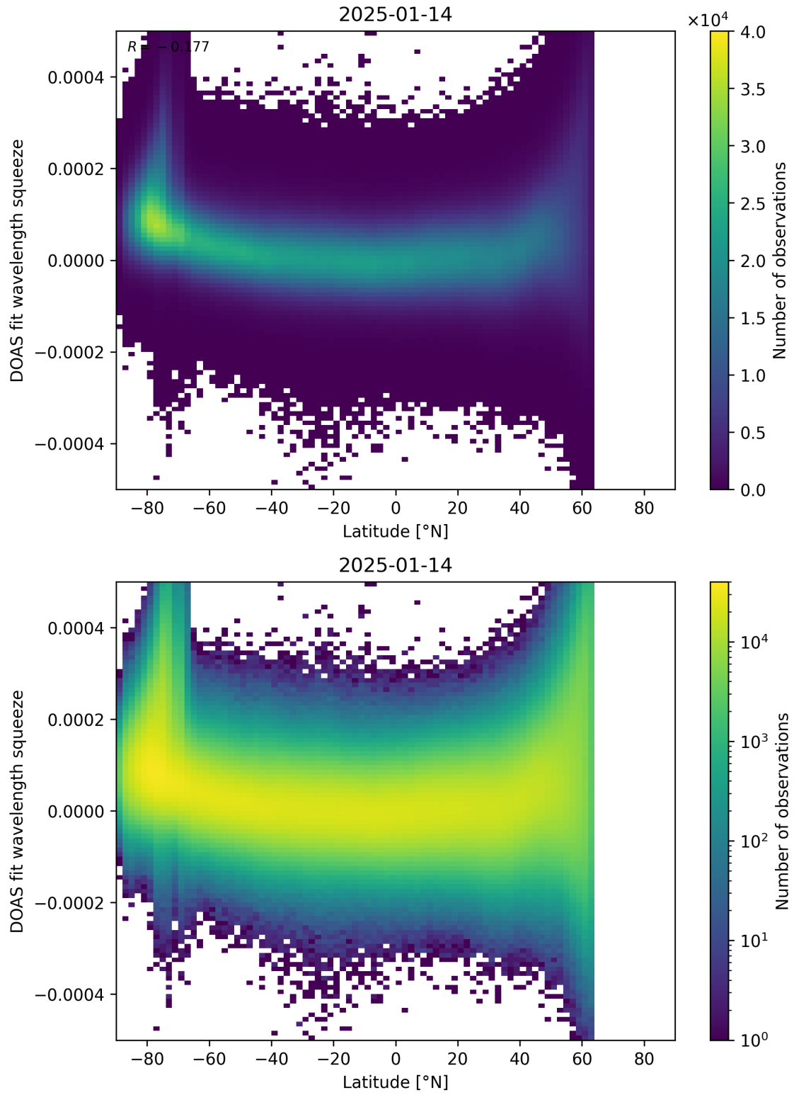
Figure 155: Scatter density plot of “Latitude” against “DOAS fit wavelength squeeze” for 2025-01-13 to 2025-01-15.
