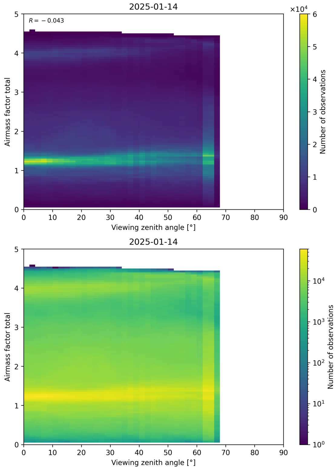
Figure 190: Scatter density plot of “Viewing zenith angle” against “Airmass factor total” for 2025-01-13 to 2025-01-15.
