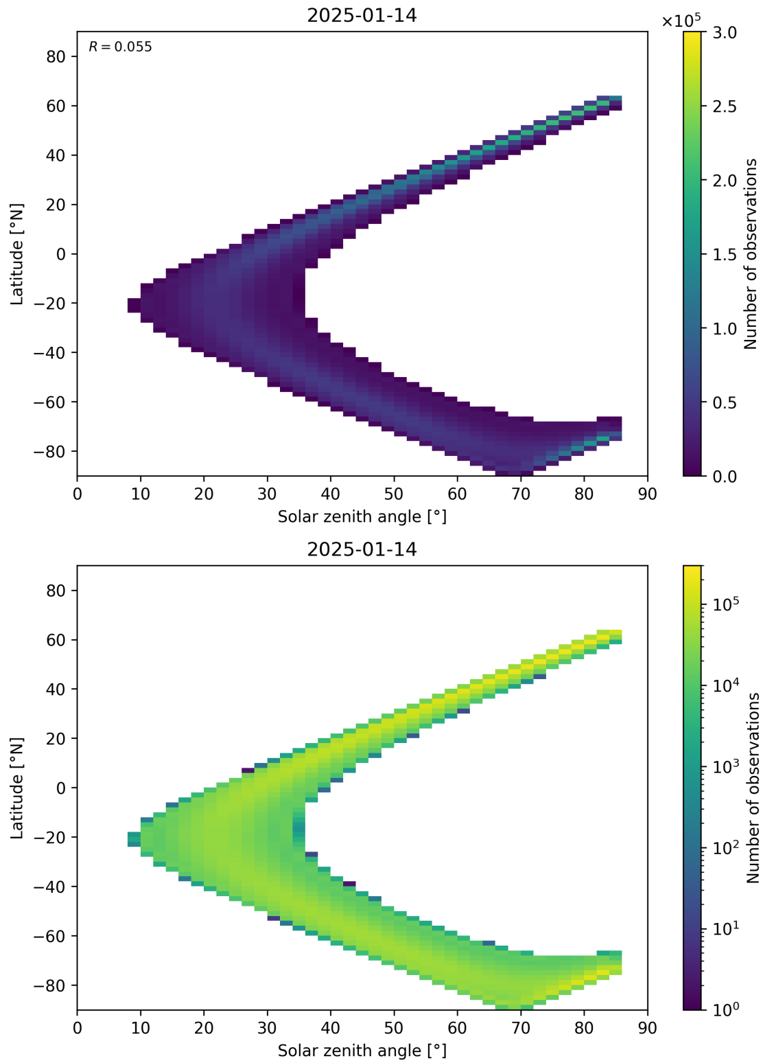
Figure 181: Scatter density plot of “Solar zenith angle” against “Latitude” for 2025-01-13 to 2025-01-15.
