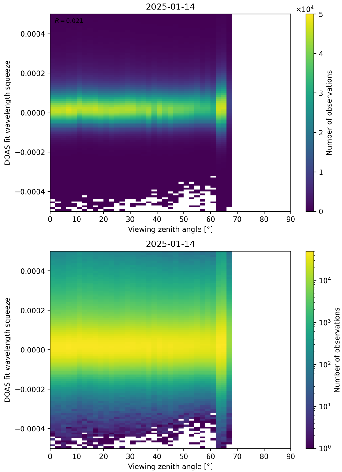
Figure 184: Scatter density plot of “Viewing zenith angle” against “DOAS fit wavelength squeeze” for 2025-01-13 to 2025-01-15.
