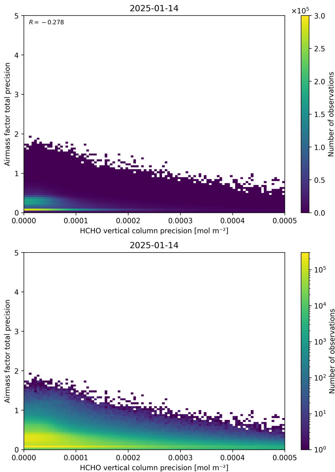
Figure 145: Scatter density plot of “HCHO vertical column precision” against “Airmass factor total precision” for 2025-01-13 to 2025-01-15.
