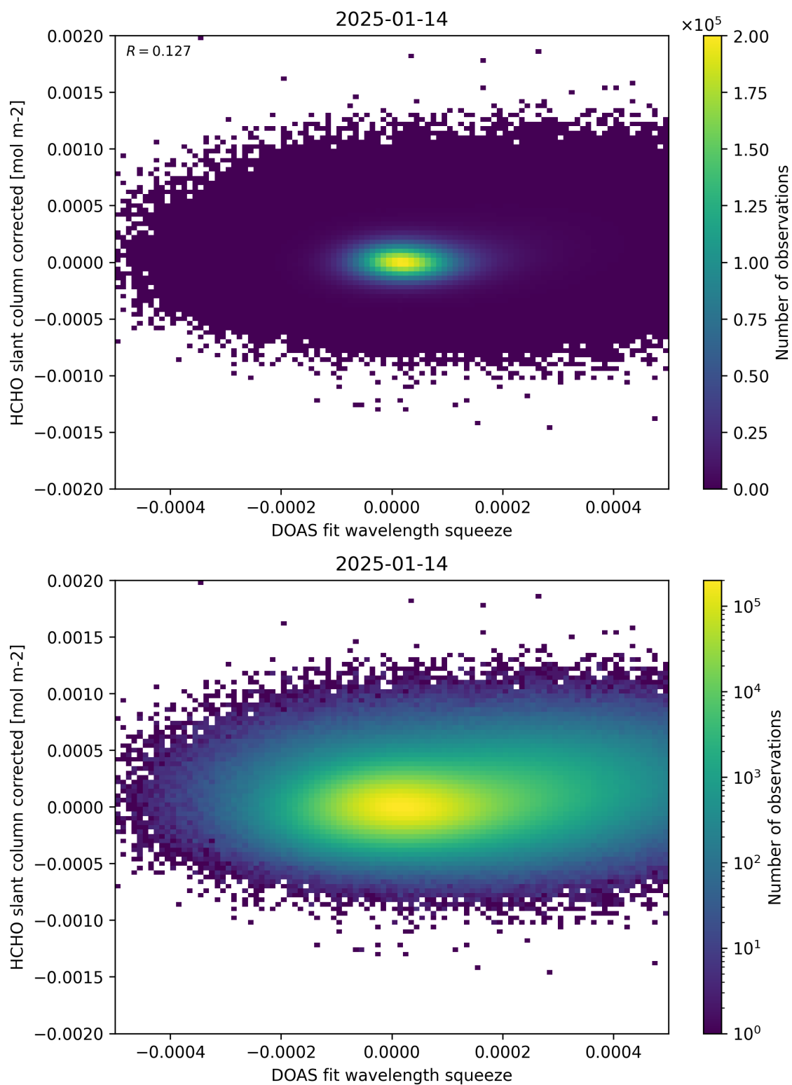
Figure 69: Scatter density plot of “DOAS fit wavelength squeeze” against “HCHO slant column corrected” for 2025-01-13 to 2025-01-15.
