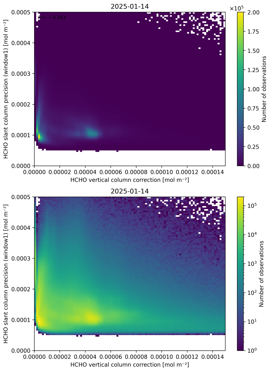
Figure 119: Scatter density plot of “HCHO vertical column correction” against “HCHO slant column precision (window1)” for 2025-01-13 to 2025-01-15.
