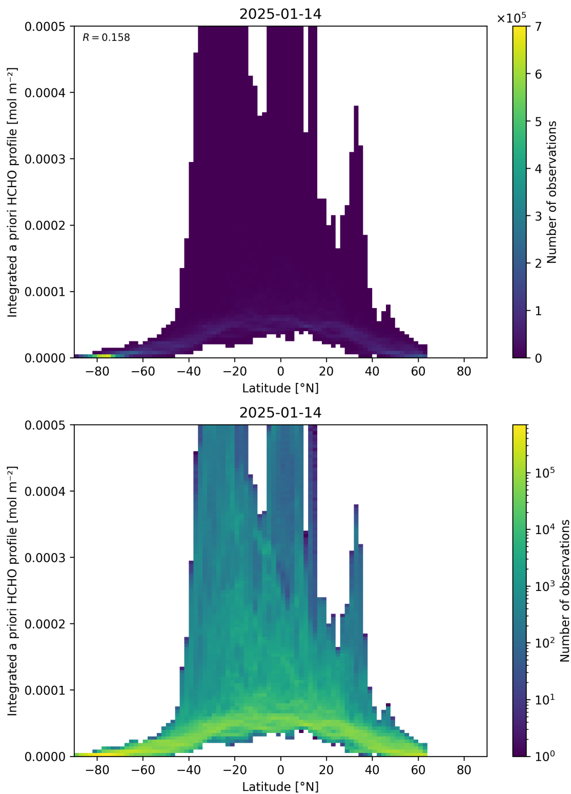
Figure 166: Scatter density plot of “Latitude” against “Integrated a priori HCHO profile” for 2025-01-13 to 2025-01-15.
