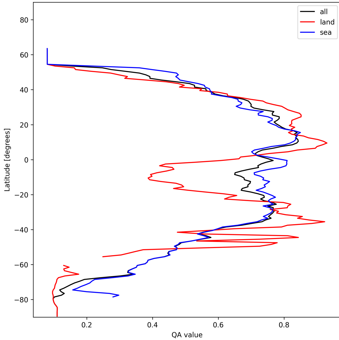
Figure 20: Zonal average of “QA value” for 2025-01-13 to 2025-01-15.
