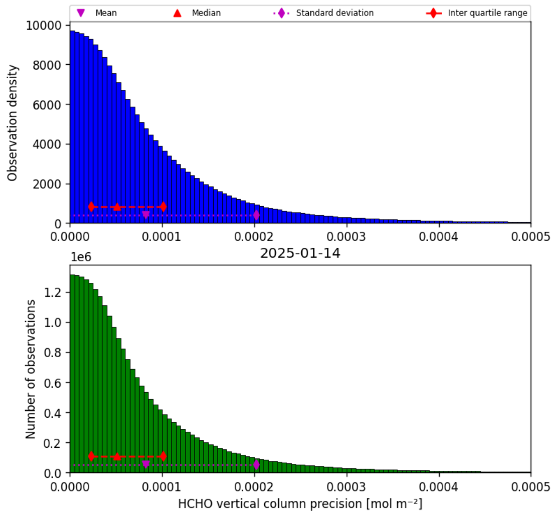
Figure 36: Histogram of “HCHO vertical column precision” for 2025-01-13 to 2025-01-15
