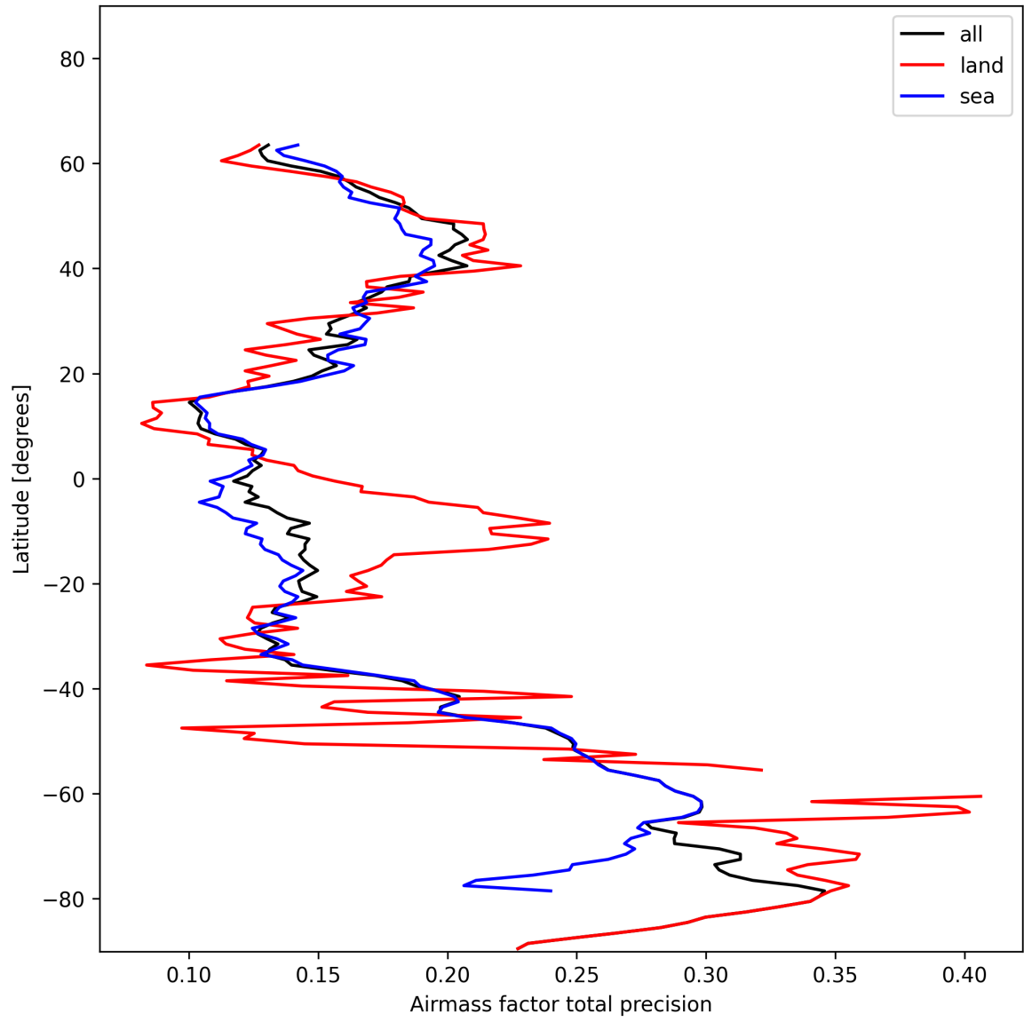
Figure 27: Zonal average of “Airmass factor total precision” for 2025-01-13 to 2025-01-15.
