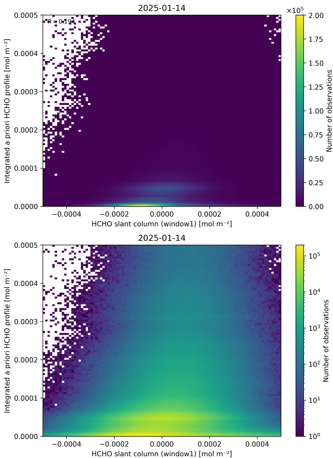
Figure 87: Scatter density plot of “HCHO slant column (window1)” against “Integrated a priori HCHO profile” for 2025-01-13 to 2025-01-15.
