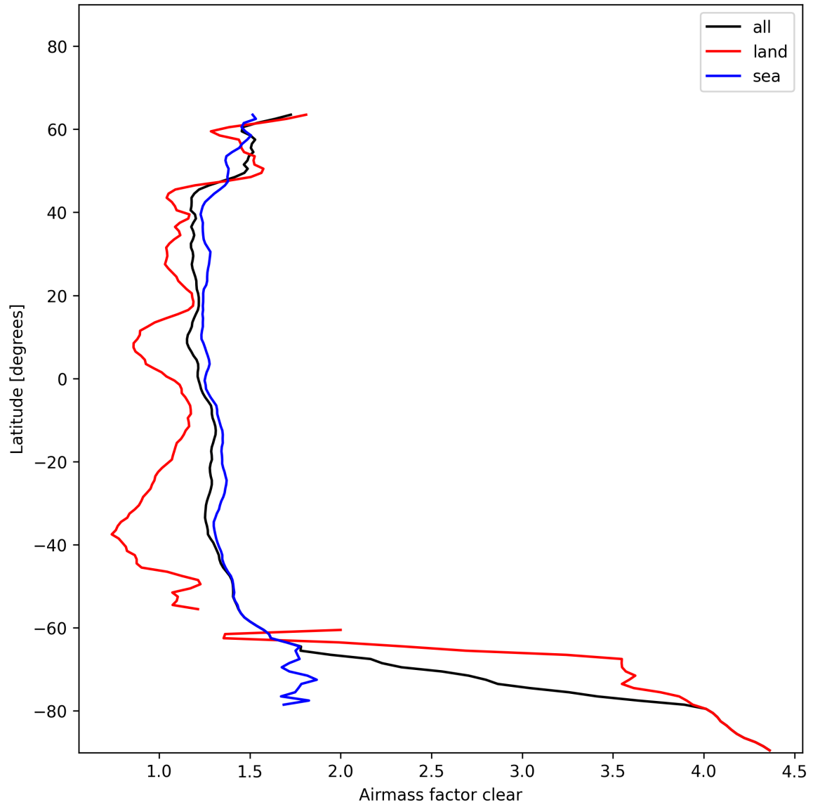
Figure 28: Zonal average of “Airmass factor clear” for 2025-01-13 to 2025-01-15.
