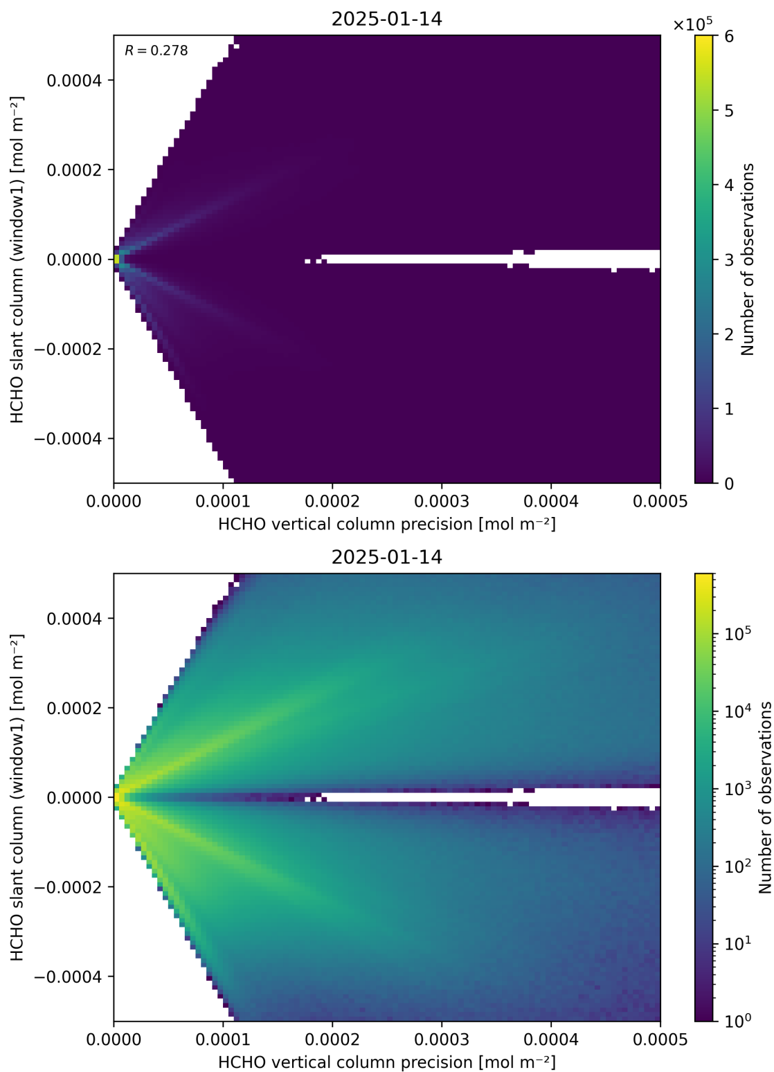
Figure 142: Scatter density plot of “HCHO vertical column precision” against “HCHO slant column (window1)” for 2025-01-13 to 2025-01-15.
