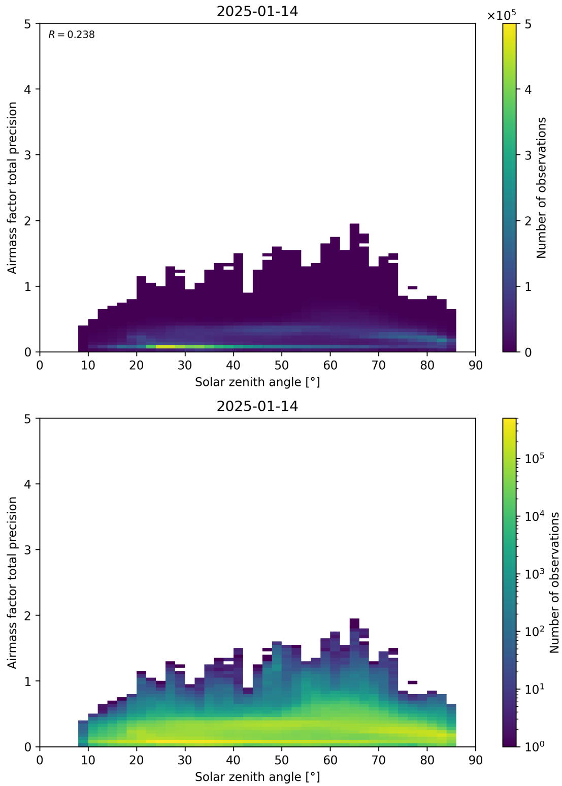
Figure 176: Scatter density plot of “Solar zenith angle” against “Airmass factor total precision” for 2025-01-13 to 2025-01-15.
