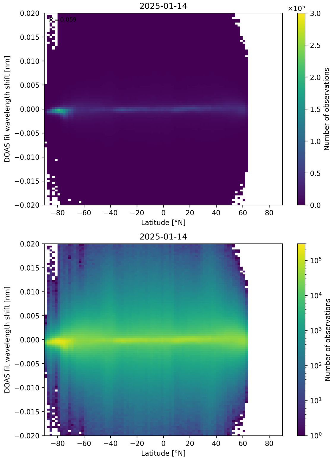
Figure 154: Scatter density plot of “Latitude” against “DOAS fit wavelength shift” for 2025-01-13 to 2025-01-15.
