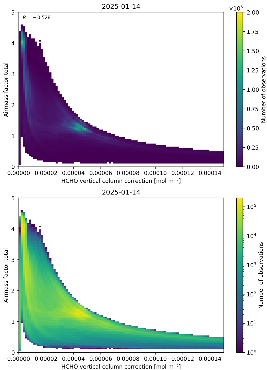
Figure 120: Scatter density plot of “HCHO vertical column correction” against “Airmass factor total” for 2025-01-13 to 2025-01-15.
