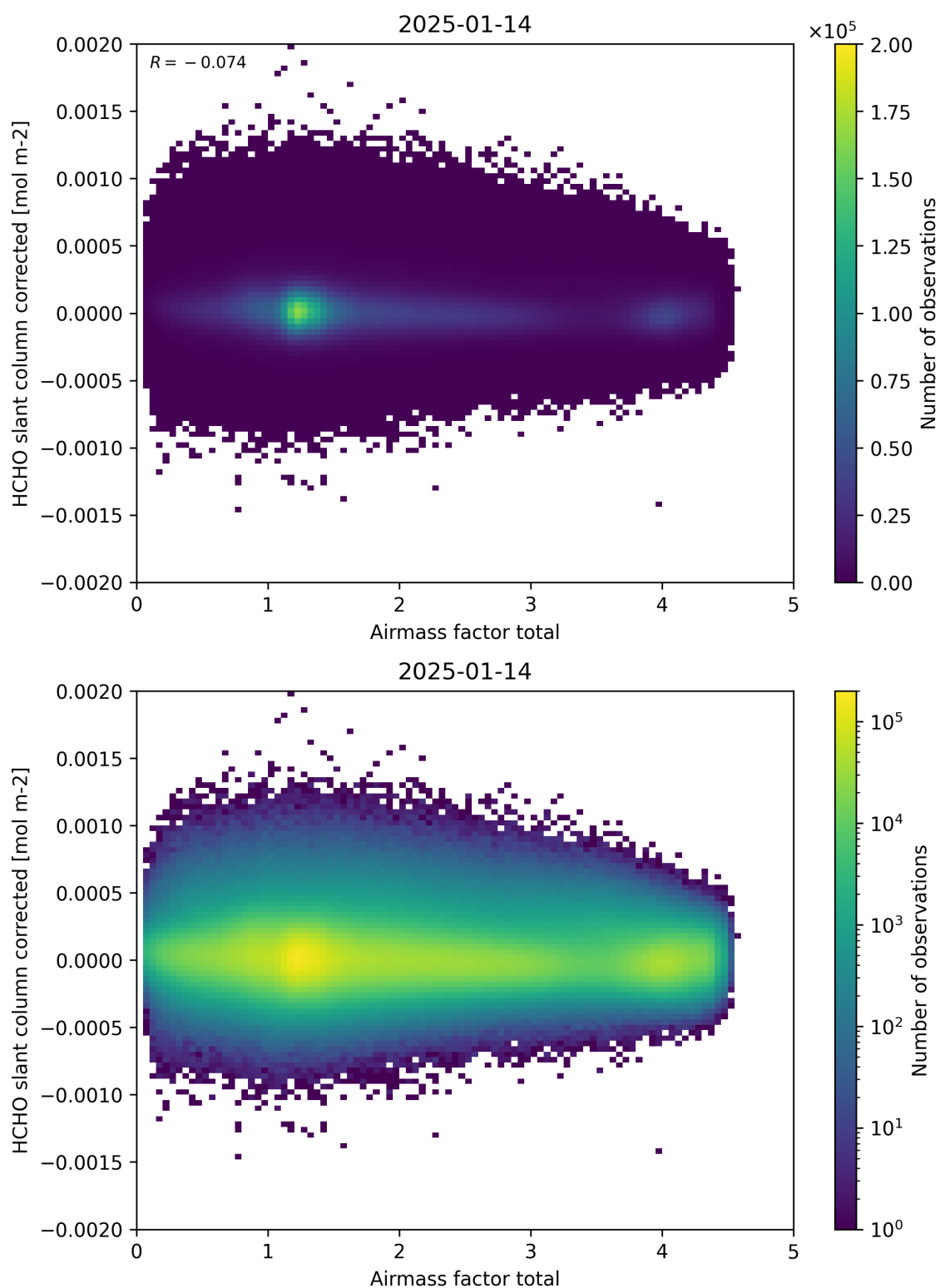
Figure 101: Scatter density plot of “Airmass factor total” against “HCHO slant column corrected” for 2025-01-13 to 2025-01-15.
