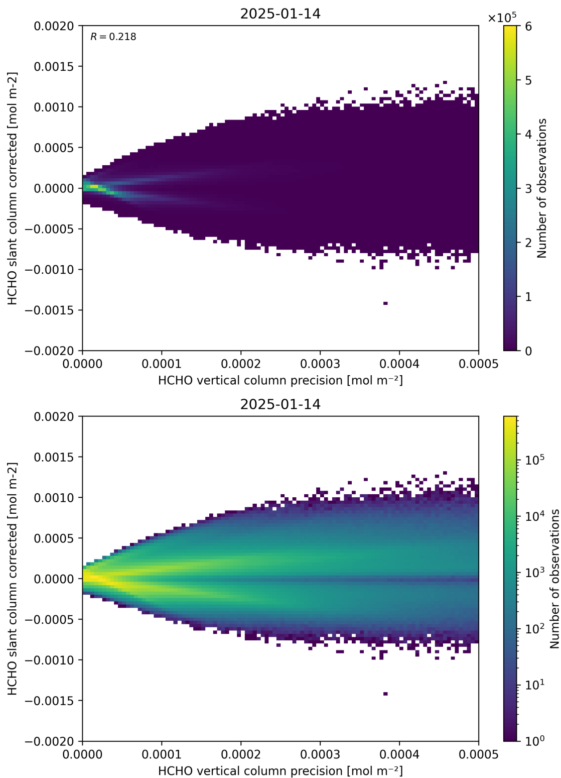
Figure 140: Scatter density plot of “HCHO vertical column precision” against “HCHO slant column corrected” for 2025-01-13 to 2025-01-15.
