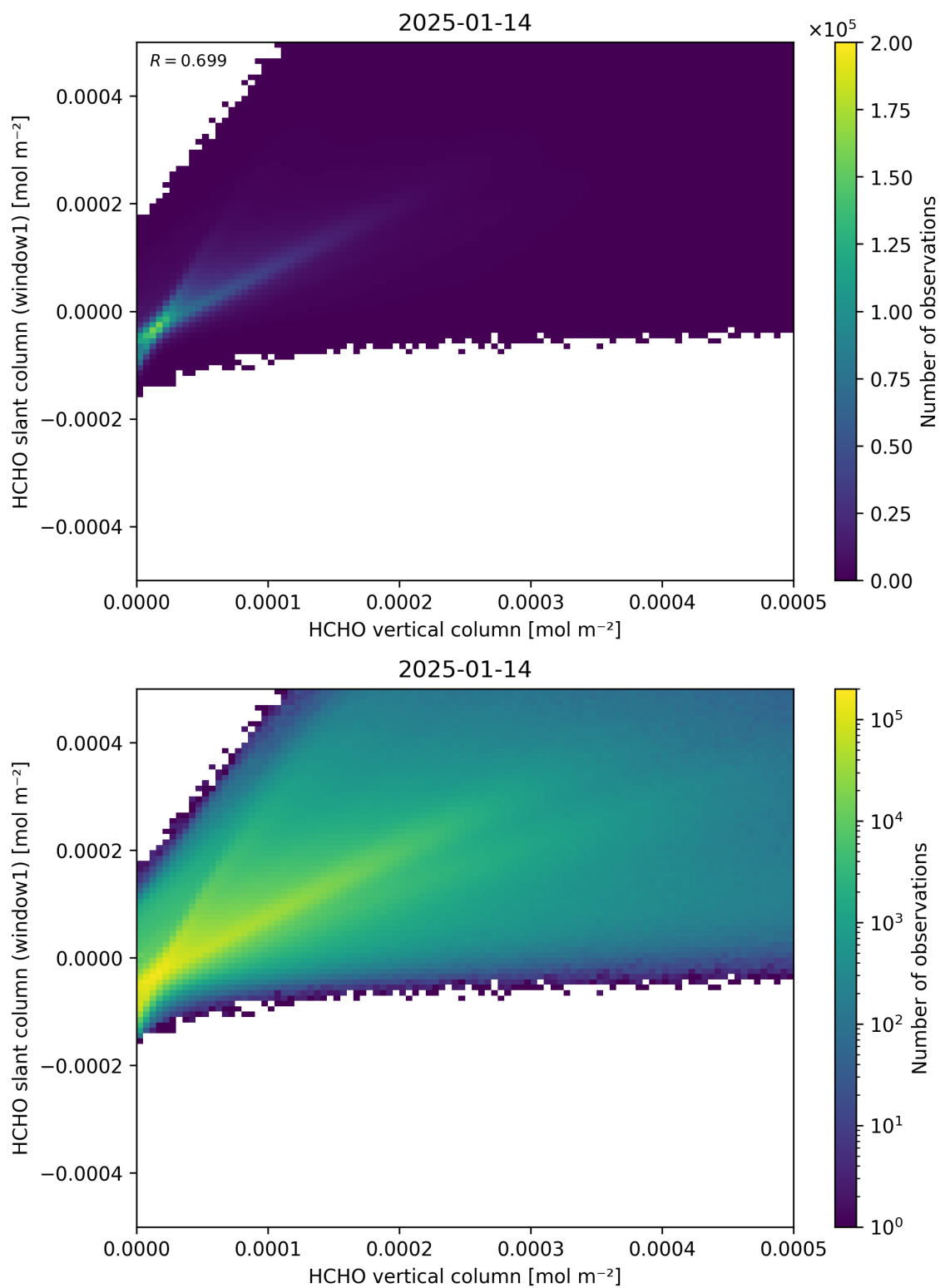
Figure 129: Scatter density plot of “HCHO vertical column” against “HCHO slant column (window1)” for 2025-01-13 to 2025-01-15.
