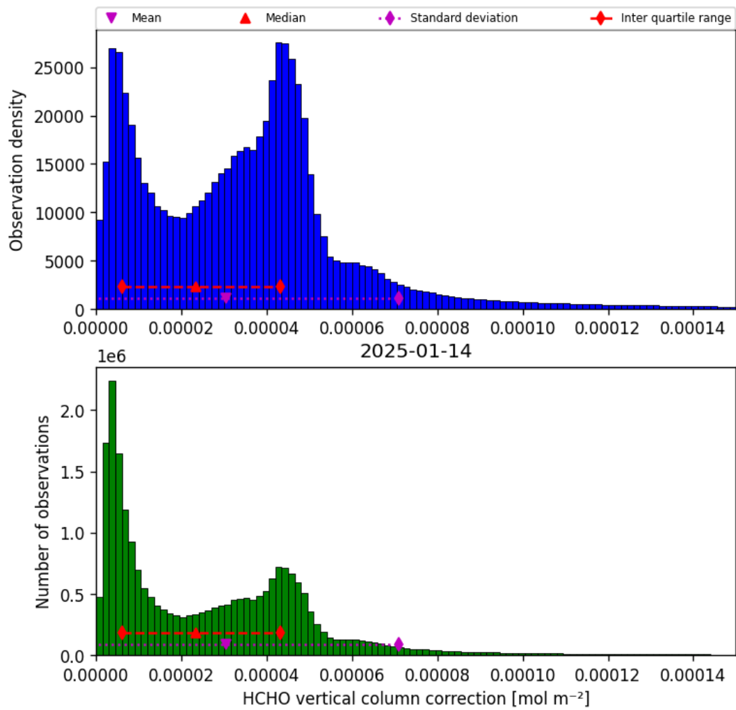
Figure 37: Histogram of “HCHO vertical column correction” for 2025-01-13 to 2025-01-15
