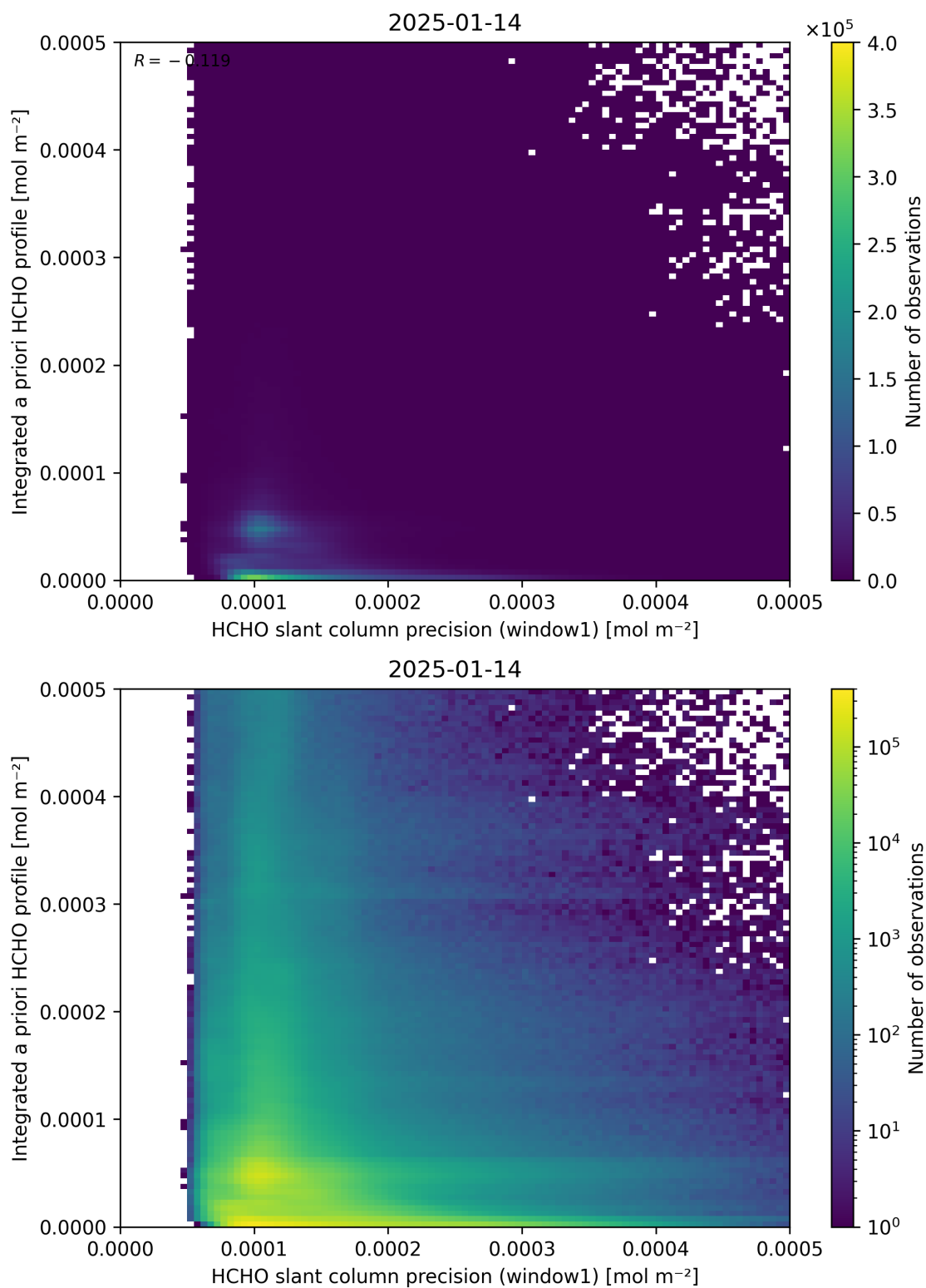
Figure 96: Scatter density plot of “HCHO slant column precision (window1)” against “Integrated a priori HCHO profile” for 2025-01-13 to 2025-01-15.
