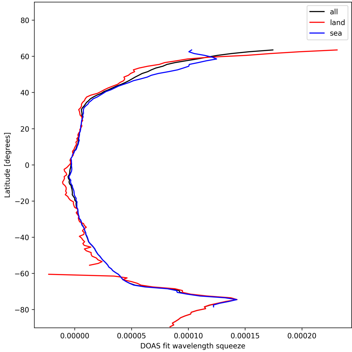
Figure 31: Zonal average of “DOAS fit wavelength squeeze” for 2025-01-13 to 2025-01-15.
