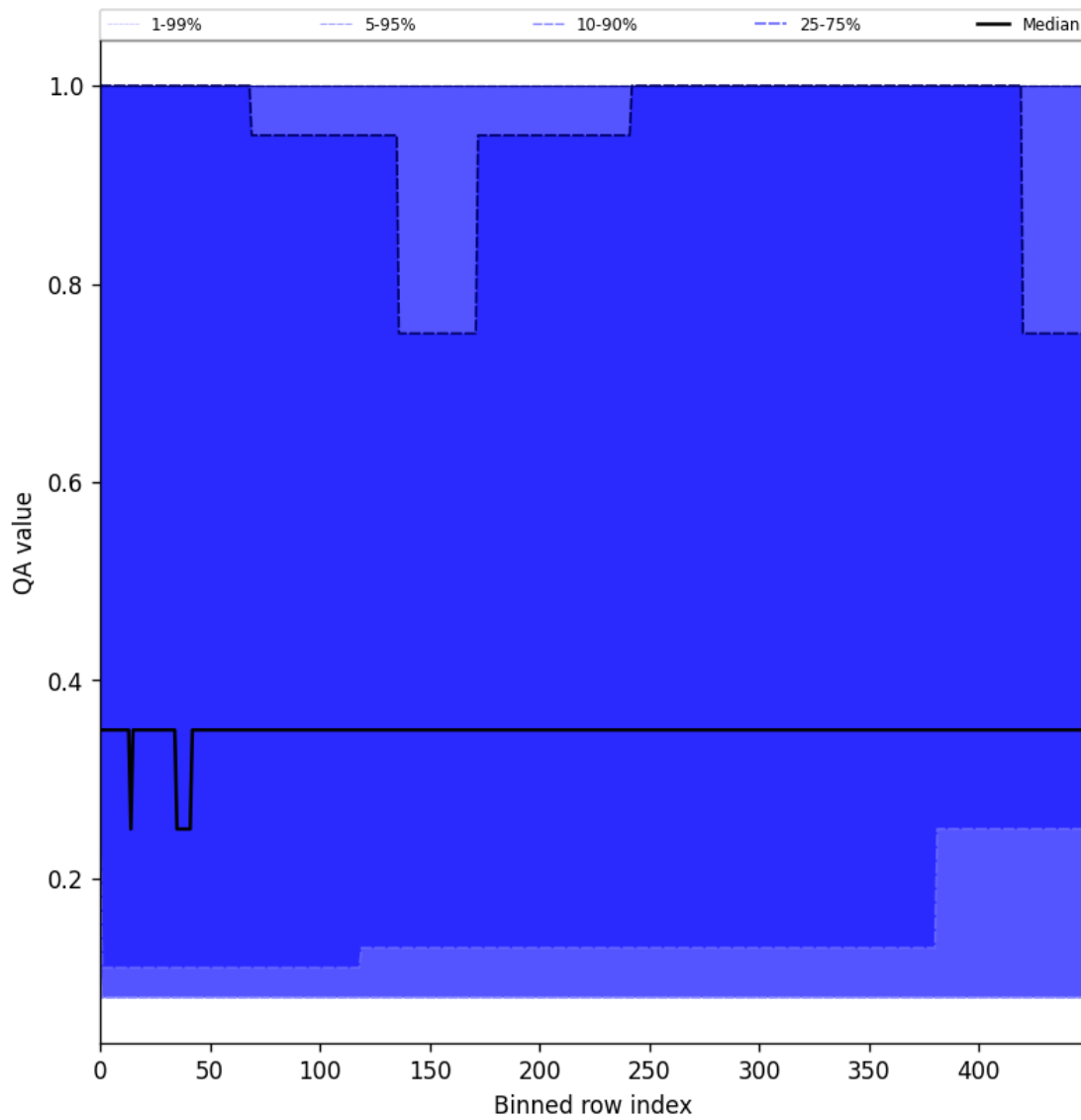
Figure 48: Along track statistics of “QA value” for 2025-01-13 to 2025-01-15
