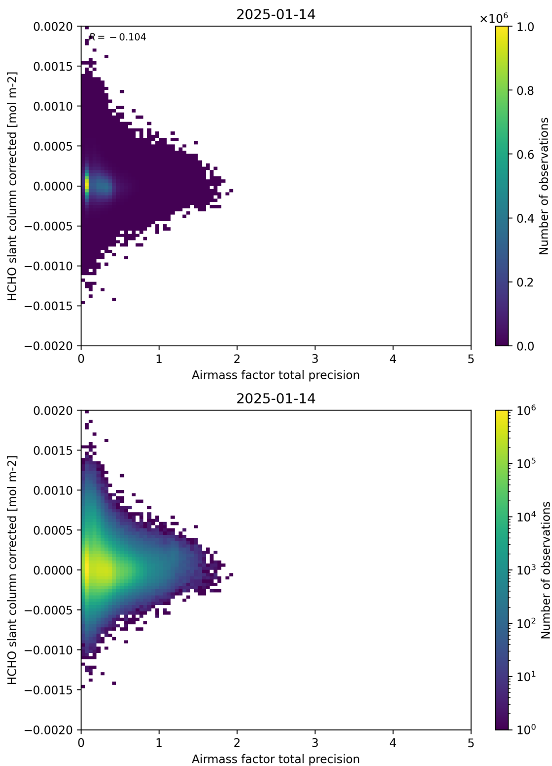
Figure 109: Scatter density plot of “Airmass factor total precision” against “HCHO slant column corrected” for 2025-01-13 to 2025-01-15.
