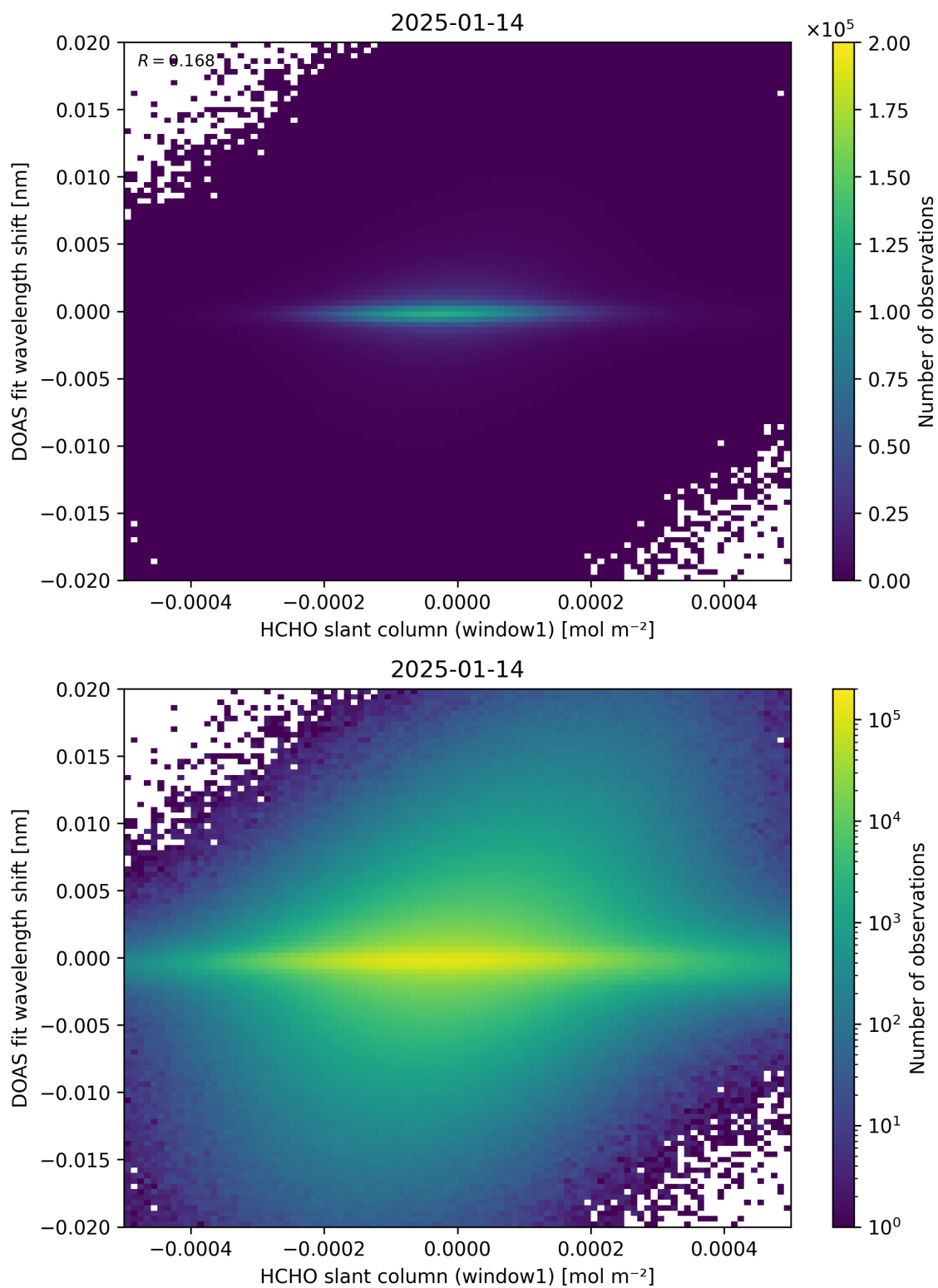
Figure 79: Scatter density plot of “HCHO slant column (window1)” against “DOAS fit wavelength shift” for 2025-01-13 to 2025-01-15.
