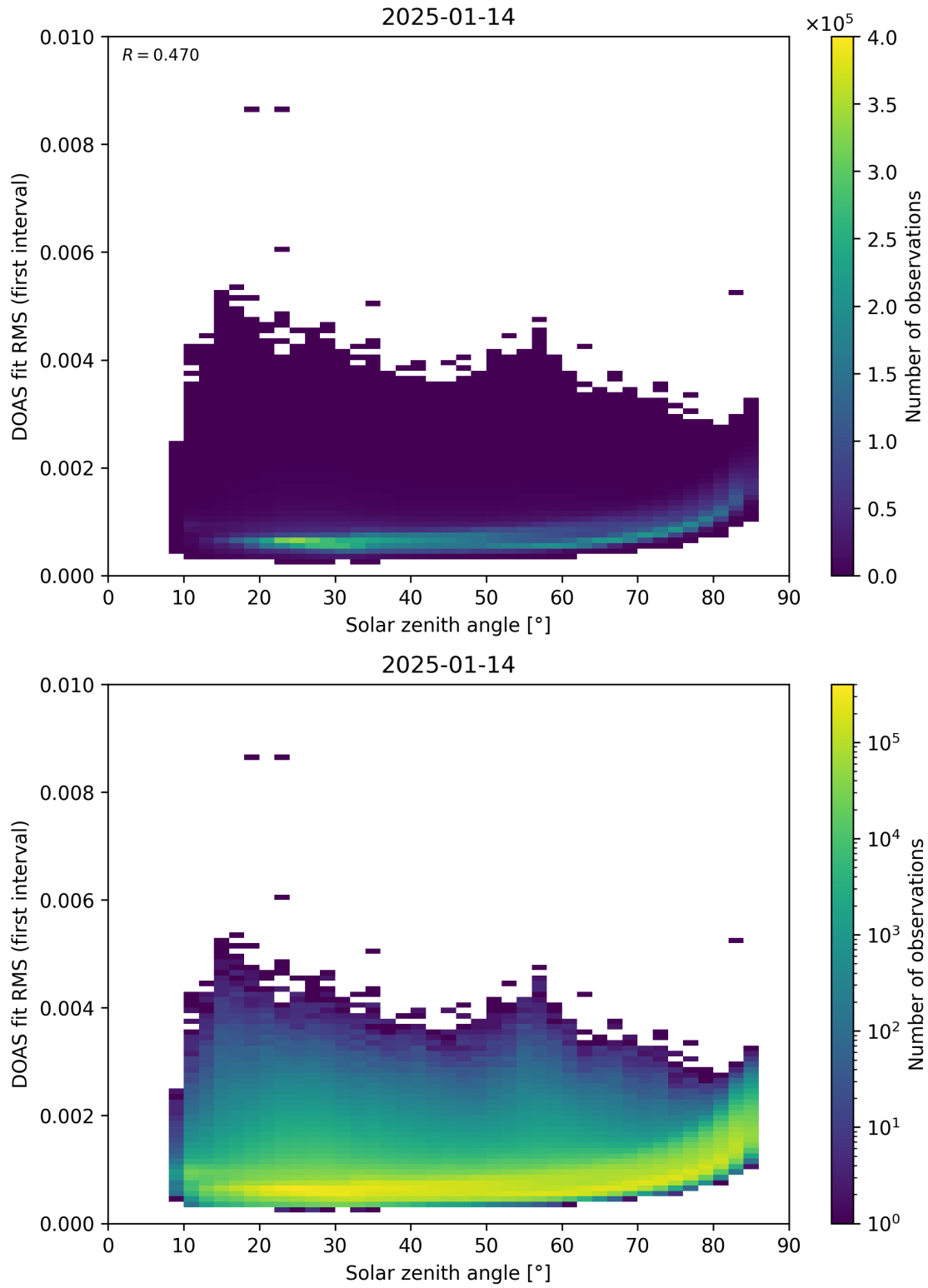
Figure 167: Scatter density plot of “Solar zenith angle” against “DOAS fit RMS (first interval)” for 2025-01-13 to 2025-01-15.
