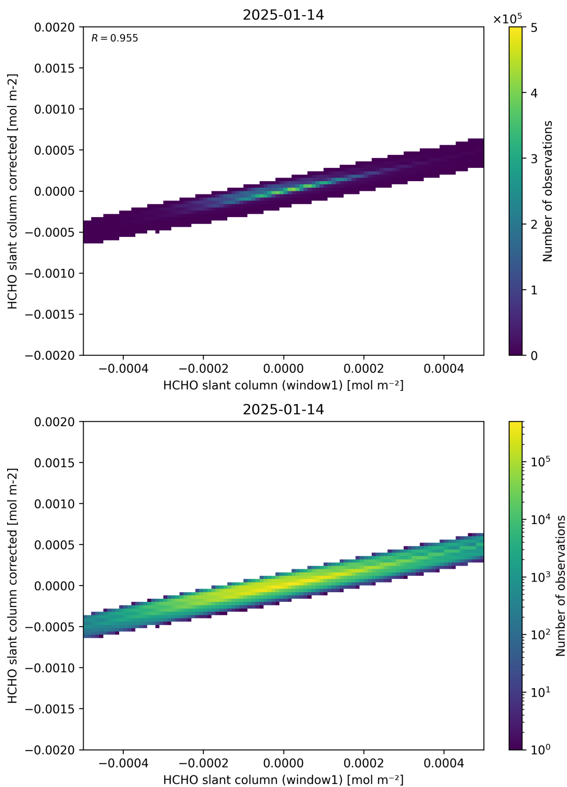
Figure 82: Scatter density plot of “HCHO slant column (window1)” against “HCHO slant column corrected” for 2025-01-13 to 2025-01-15.
