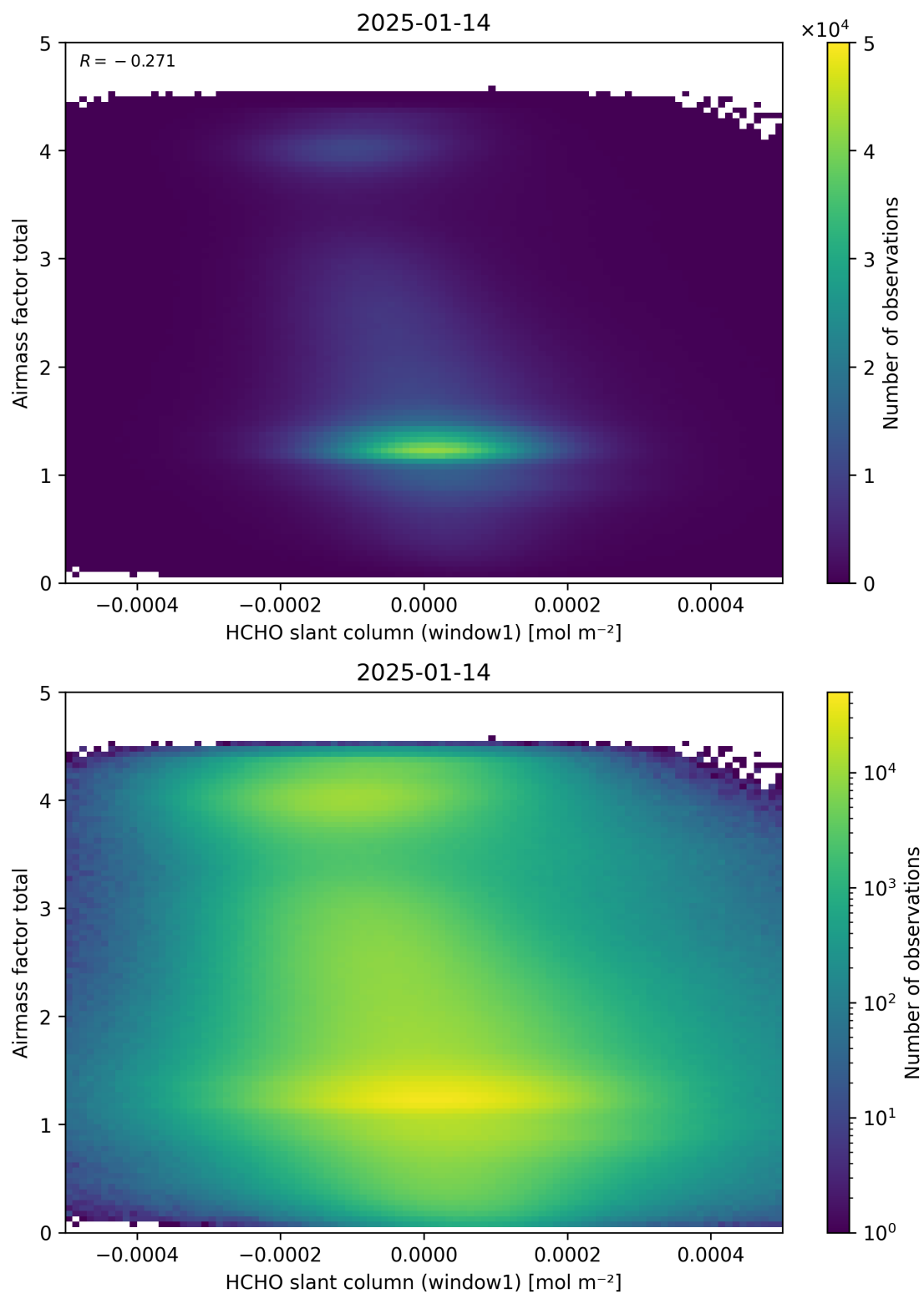
Figure 85: Scatter density plot of “HCHO slant column (window1)” against “Airmass factor total” for 2025-01-13 to 2025-01-15.
