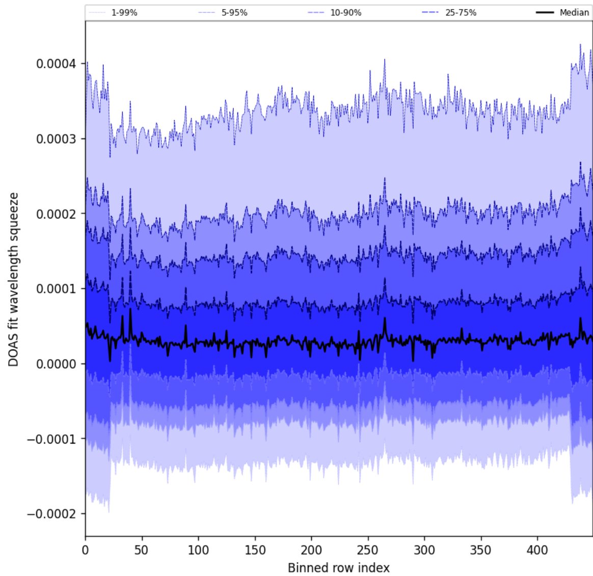
Figure 59: Along track statistics of “DOAS fit wavelength squeeze” for 2025-01-13 to 2025-01-15
