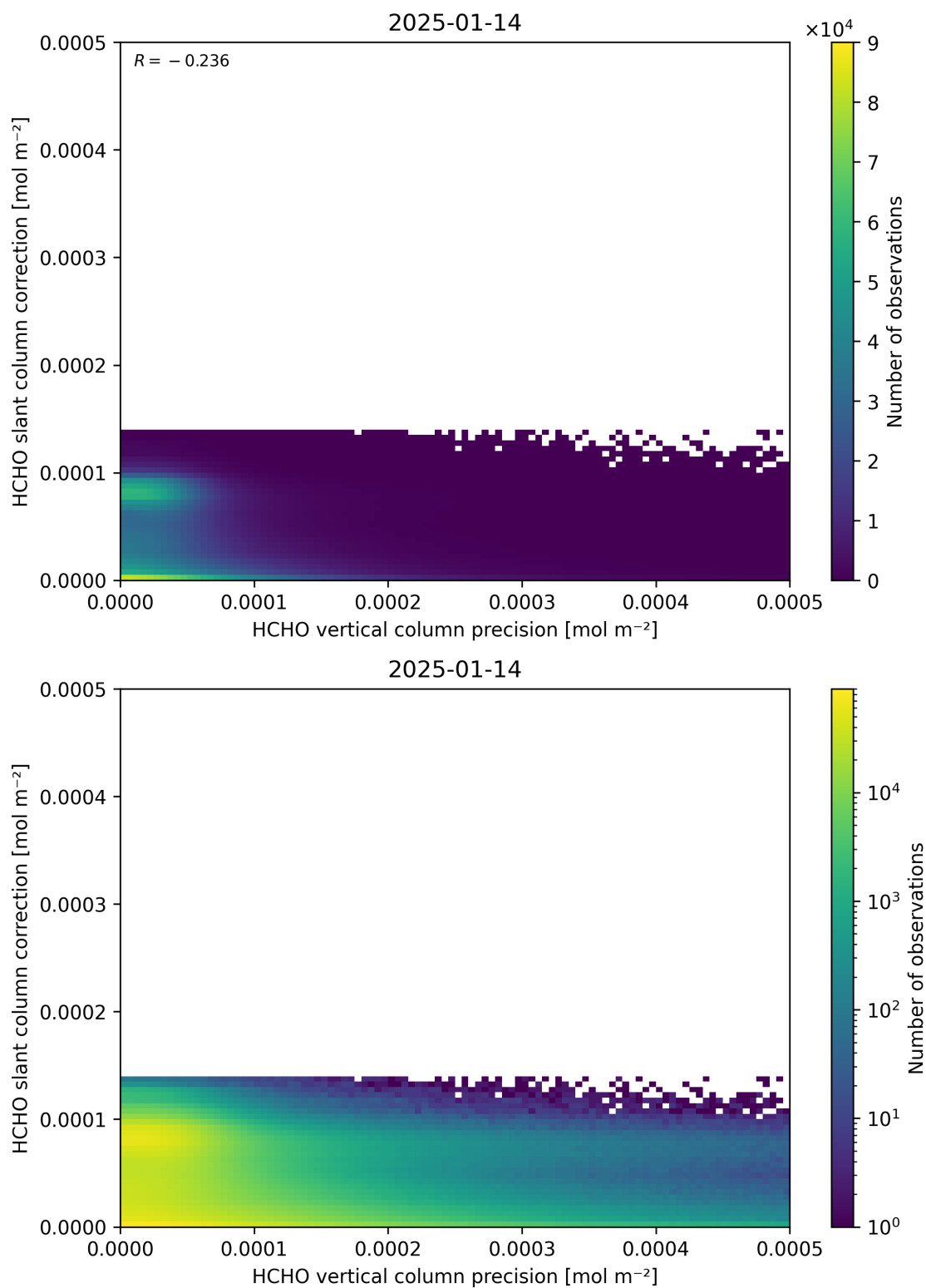
Figure 141: Scatter density plot of “HCHO vertical column precision” against “HCHO slant column correction” for 2025-01-13 to 2025-01-15.
