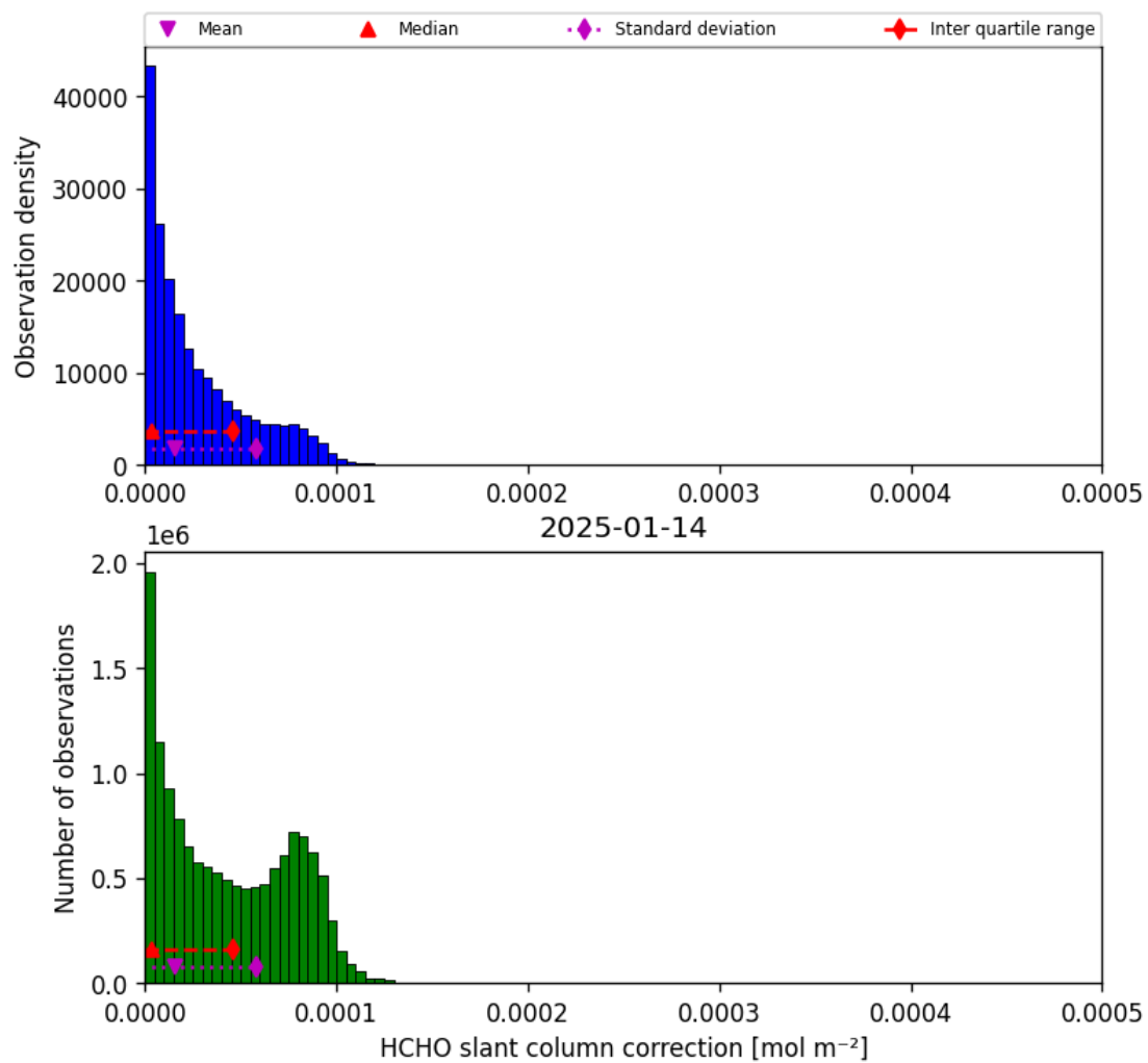
Figure 47: Histogram of “HCHO slant column correction” for 2025-01-13 to 2025-01-15
