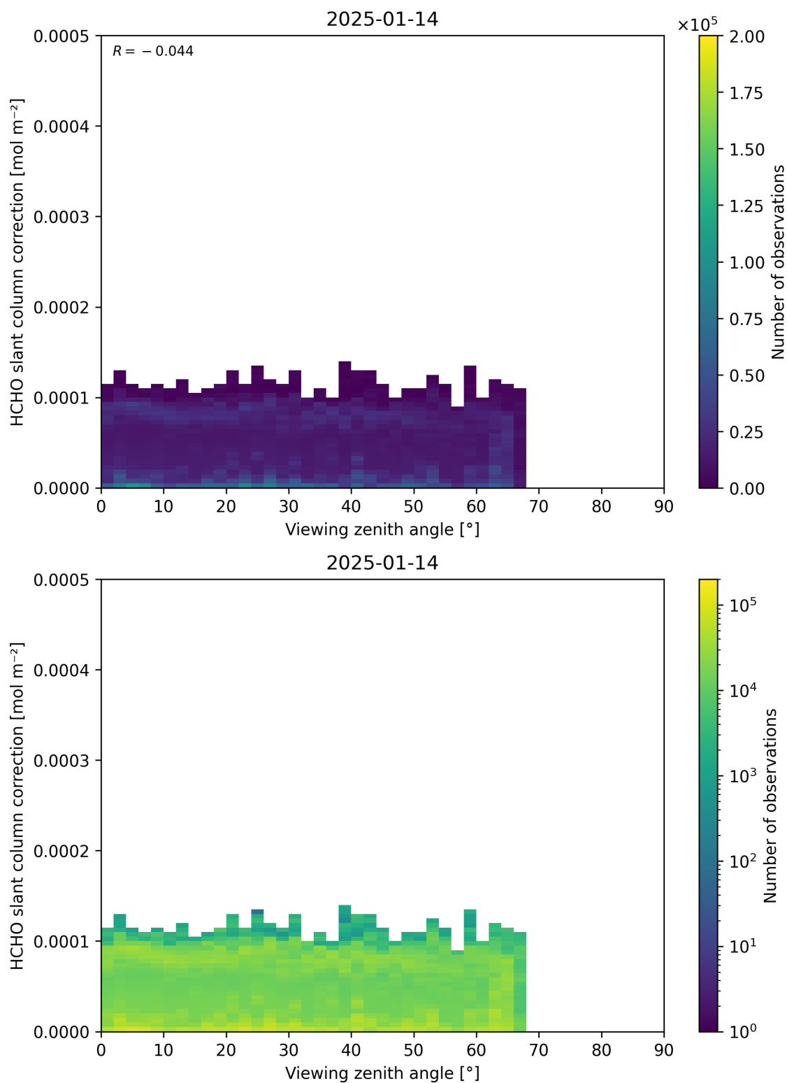
Figure 187: Scatter density plot of “Viewing zenith angle” against “HCHO slant column correction” for 2025-01-13 to 2025-01-15.
