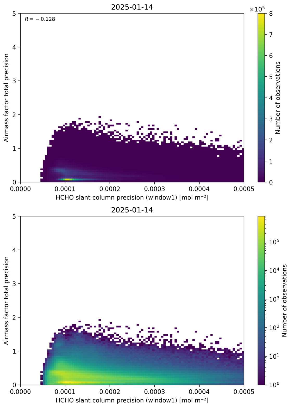
Figure 95: Scatter density plot of “HCHO slant column precision (window1)” against “Airmass factor total precision” for 2025-01-13 to 2025-01-15.
