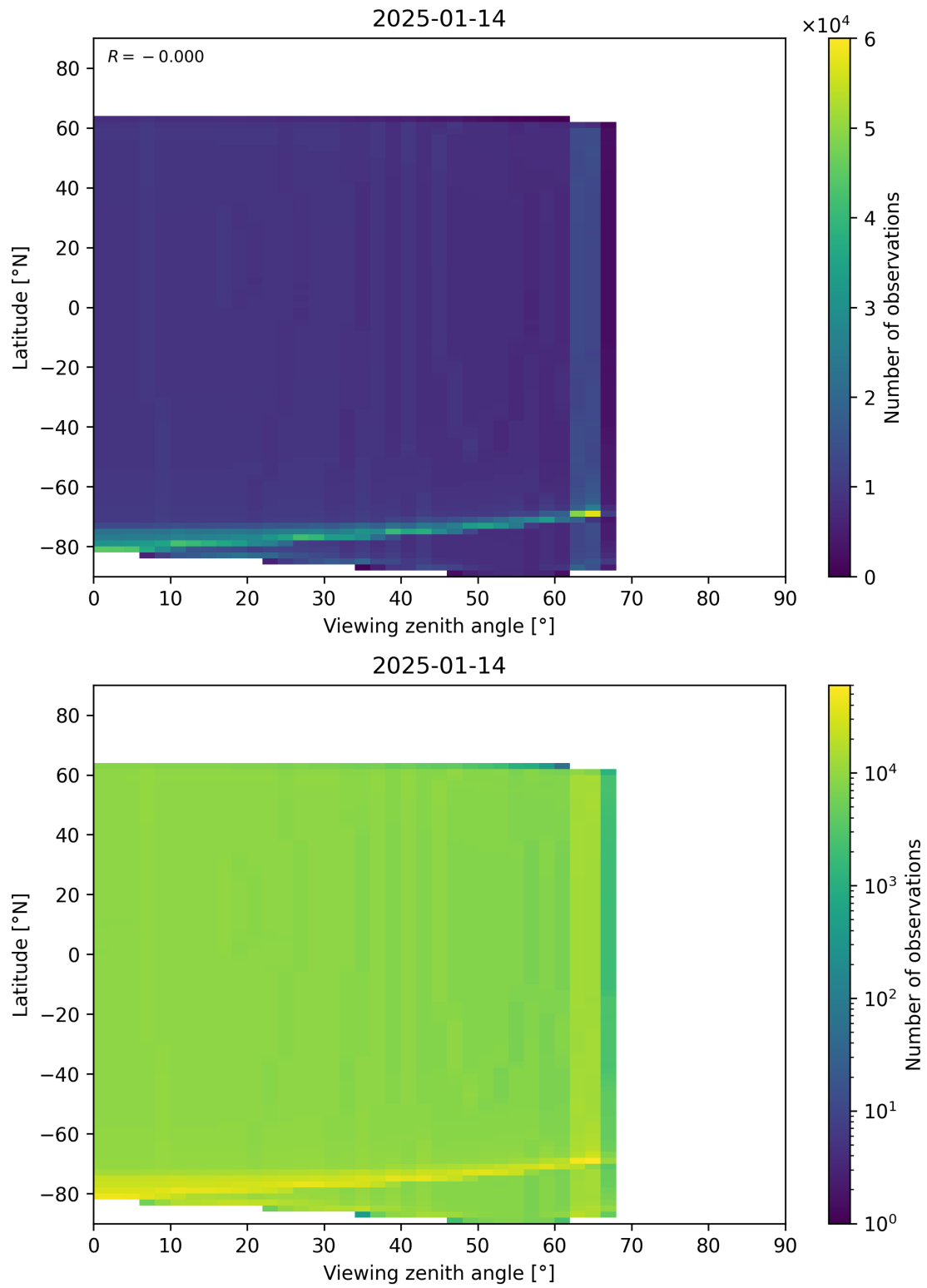
Figure 196: Scatter density plot of “Viewing zenith angle” against “Latitude” for 2025-01-13 to 2025-01-15.
