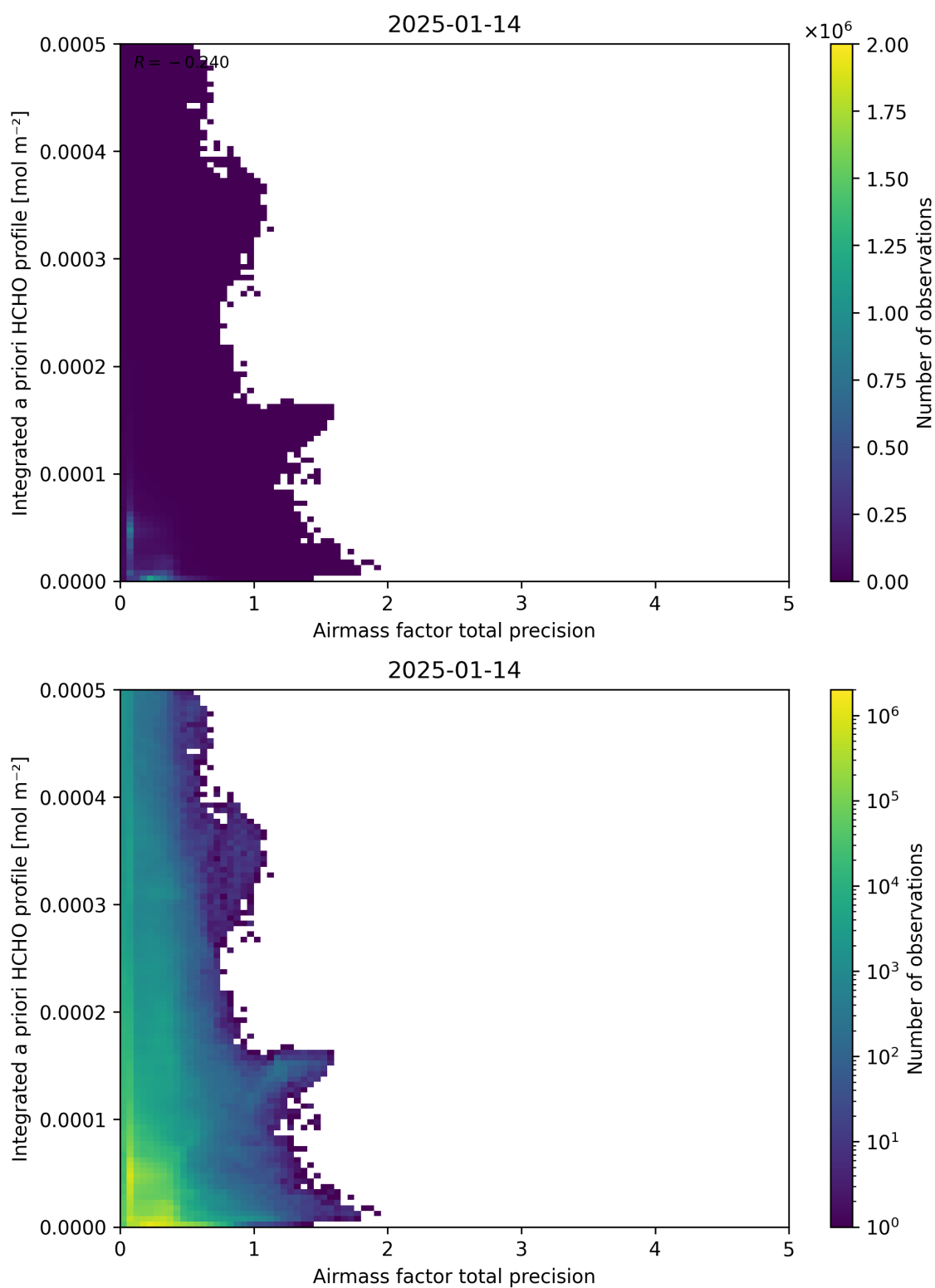
Figure 111: Scatter density plot of “Airmass factor total precision” against “Integrated a priori HCHO profile” for 2025-01-13 to 2025-01-15.
