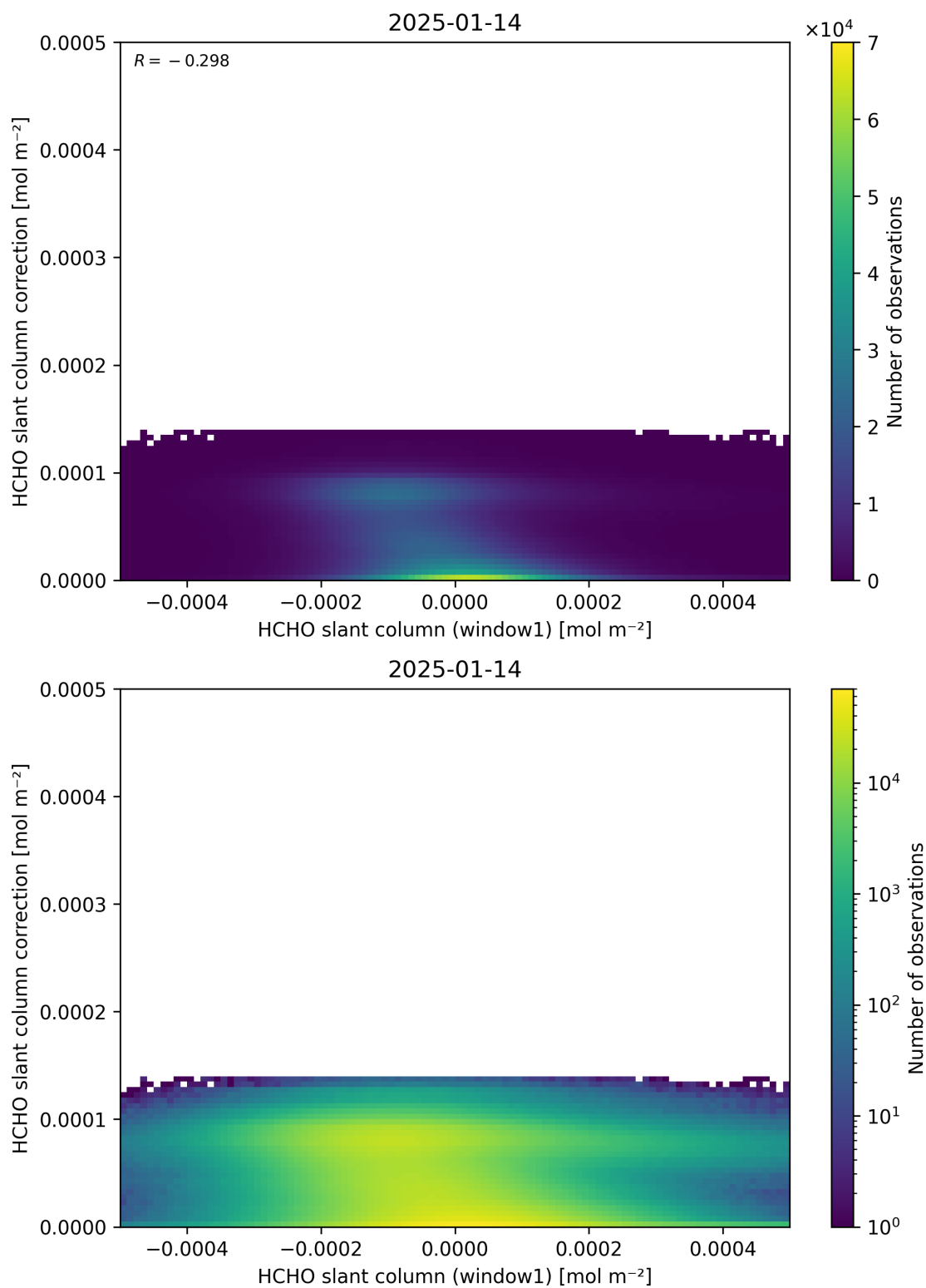
Figure 83: Scatter density plot of “HCHO slant column (window1)” against “HCHO slant column correction” for 2025-01-13 to 2025-01-15.
