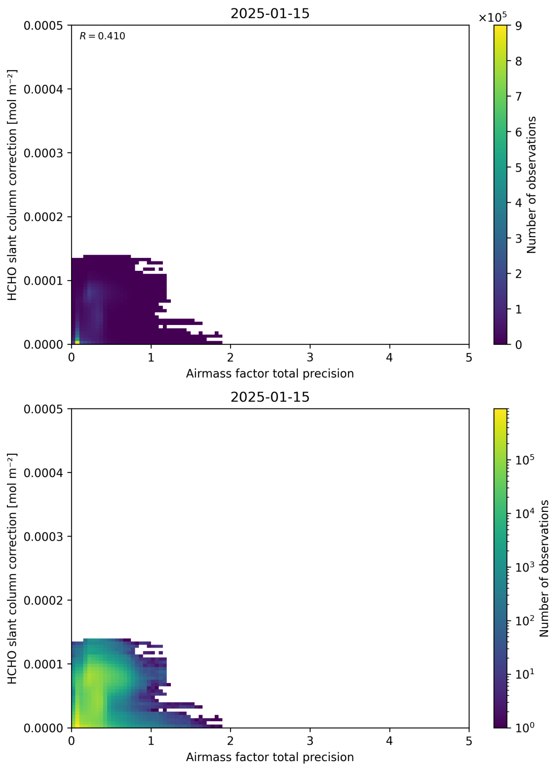
Figure 110: Scatter density plot of “Airmass factor total precision” against “HCHO slant column correction” for 2025-01-14 to 2025-01-16.
