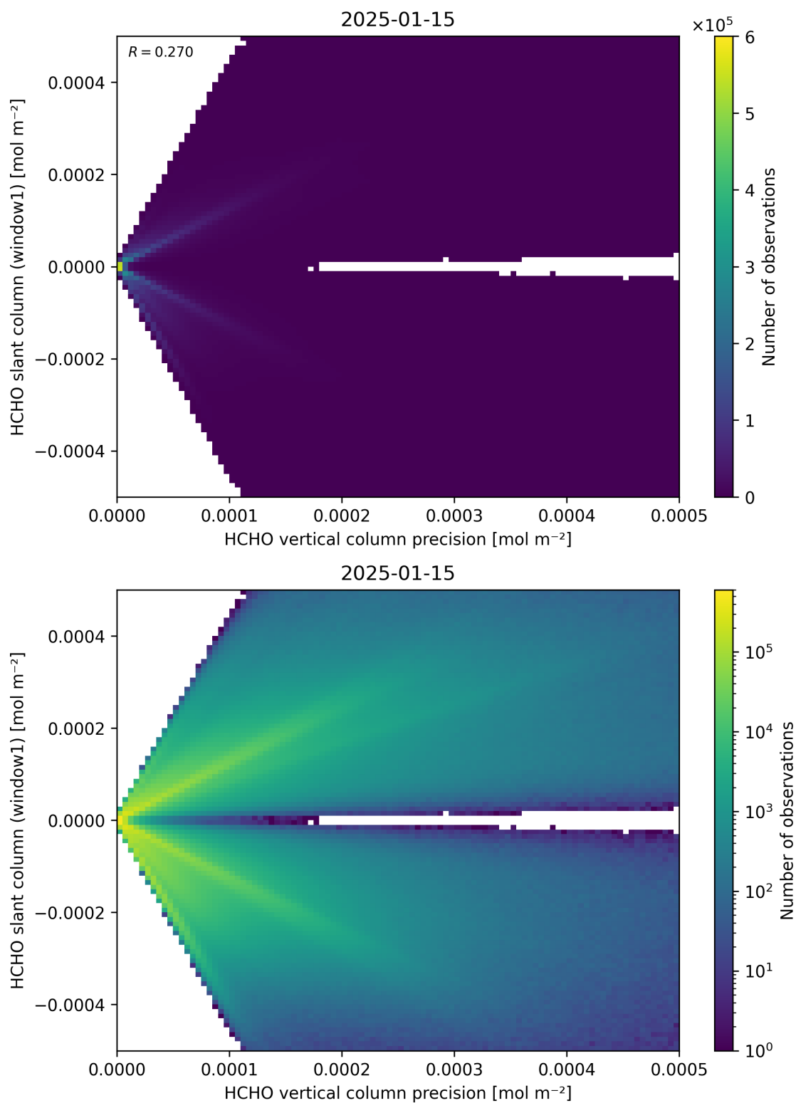
Figure 142: Scatter density plot of “HCHO vertical column precision” against “HCHO slant column (window1)” for 2025-01-14 to 2025-01-16.
