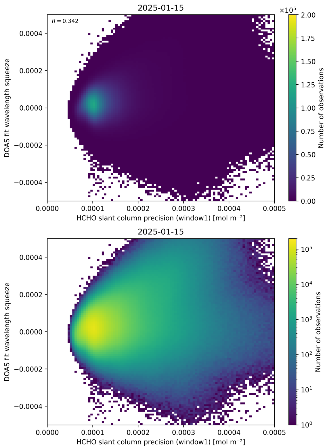
Figure 90: Scatter density plot of “HCHO slant column precision (window1)” against “DOAS fit wavelength squeeze” for 2025-01-14 to 2025-01-16.
