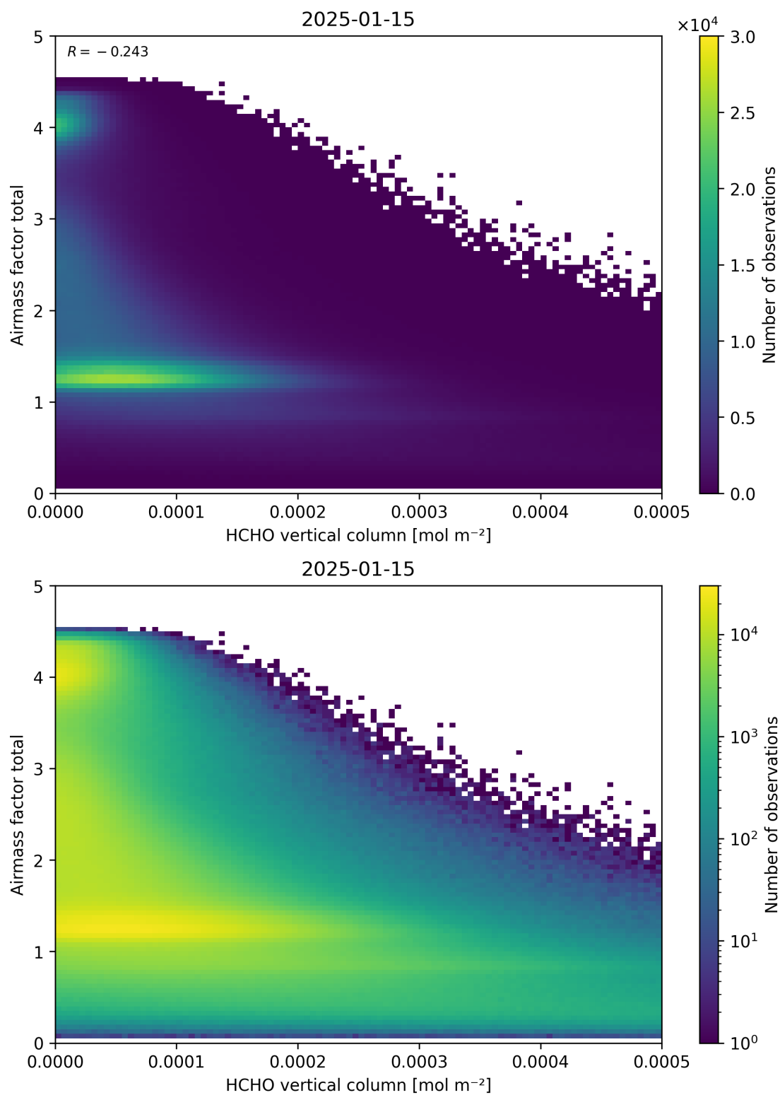
Figure 131: Scatter density plot of “HCHO vertical column” against “Airmass factor total” for 2025-01-14 to 2025-01-16.
