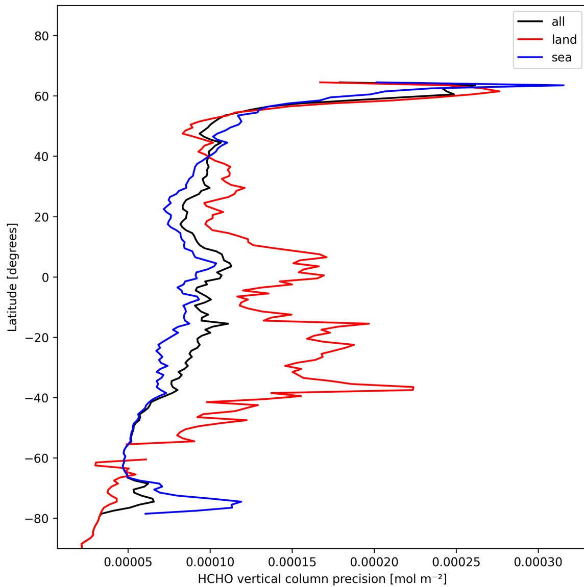
Figure 22: Zonal average of “HCHO vertical column precision” for 2025-01-14 to 2025-01-16.
