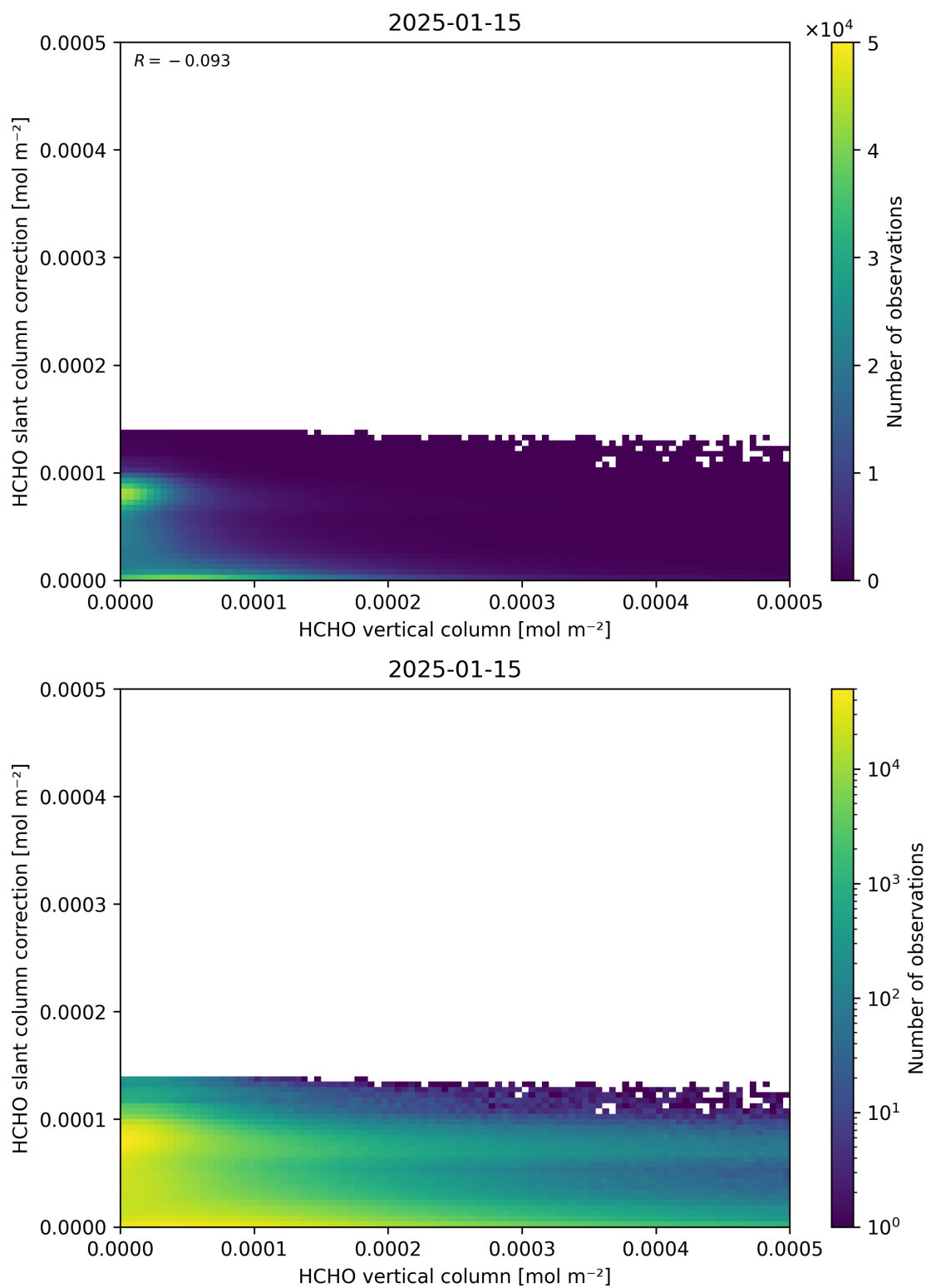
Figure 128: Scatter density plot of “HCHO vertical column” against “HCHO slant column correction” for 2025-01-14 to 2025-01-16.
