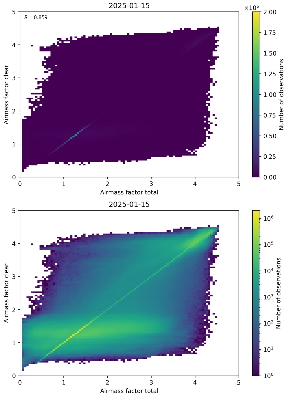
Figure 100: Scatter density plot of “Airmass factor total” against “Airmass factor clear” for 2025-01-14 to 2025-01-16.
