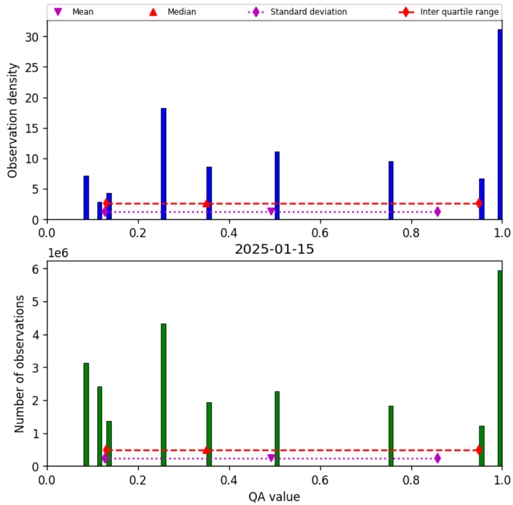
Figure 34: Histogram of “QA value” for 2025-01-14 to 2025-01-16
