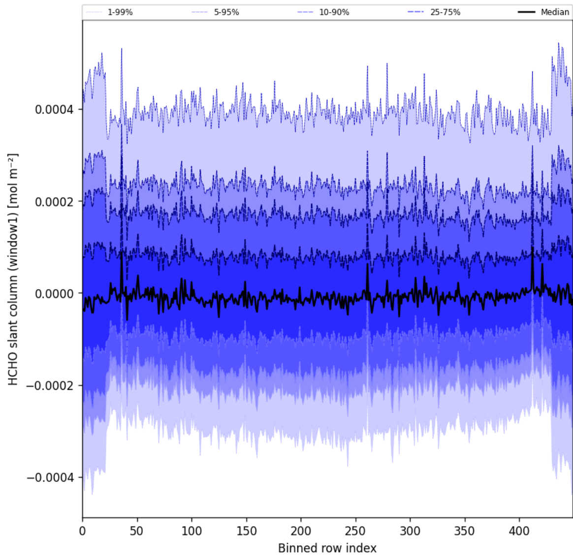
Figure 52: Along track statistics of “HCHO slant column (window1)” for 2025-01-14 to 2025-01-16
