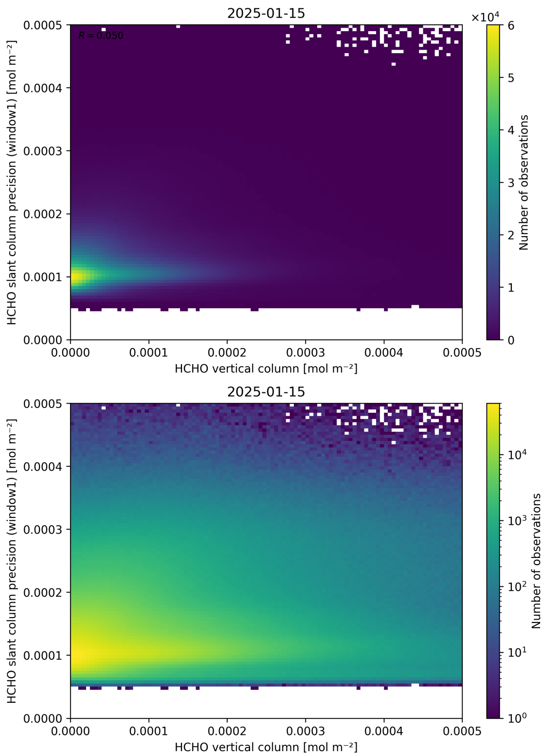
Figure 130: Scatter density plot of “HCHO vertical column” against “HCHO slant column precision (window1)” for 2025-01-14 to 2025-01-16.
