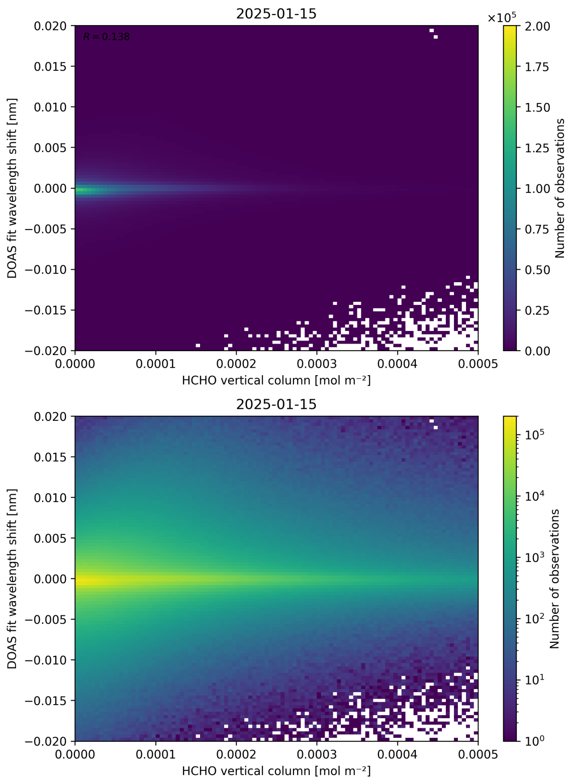
Figure 124: Scatter density plot of “HCHO vertical column” against “DOAS fit wavelength shift” for 2025-01-14 to 2025-01-16.
