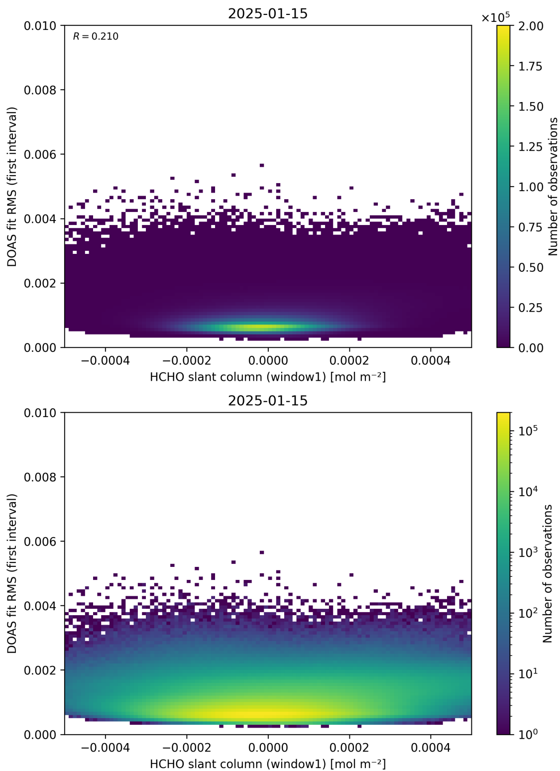
Figure 78: Scatter density plot of “HCHO slant column (window1)” against “DOAS fit RMS (first interval)” for 2025-01-14 to 2025-01-16.
