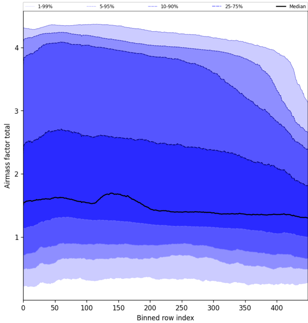
Figure 54: Along track statistics of “Airmass factor total” for 2025-01-14 to 2025-01-16
