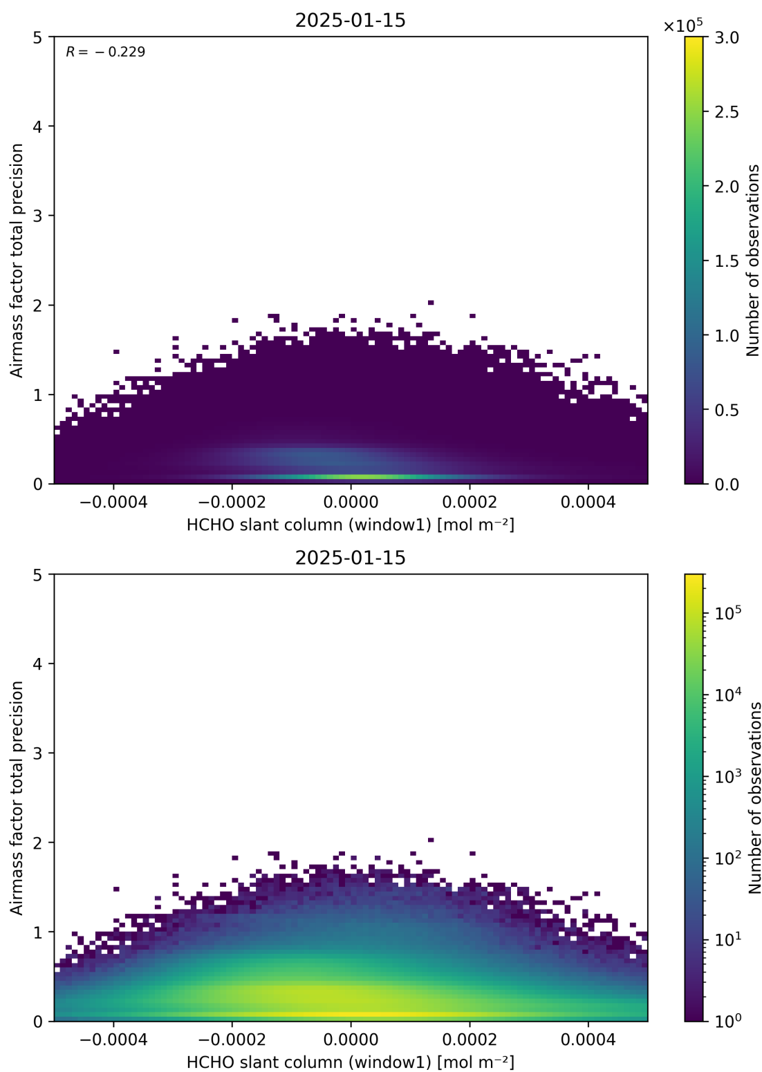
Figure 86: Scatter density plot of “HCHO slant column (window1)” against “Airmass factor total precision” for 2025-01-14 to 2025-01-16.
