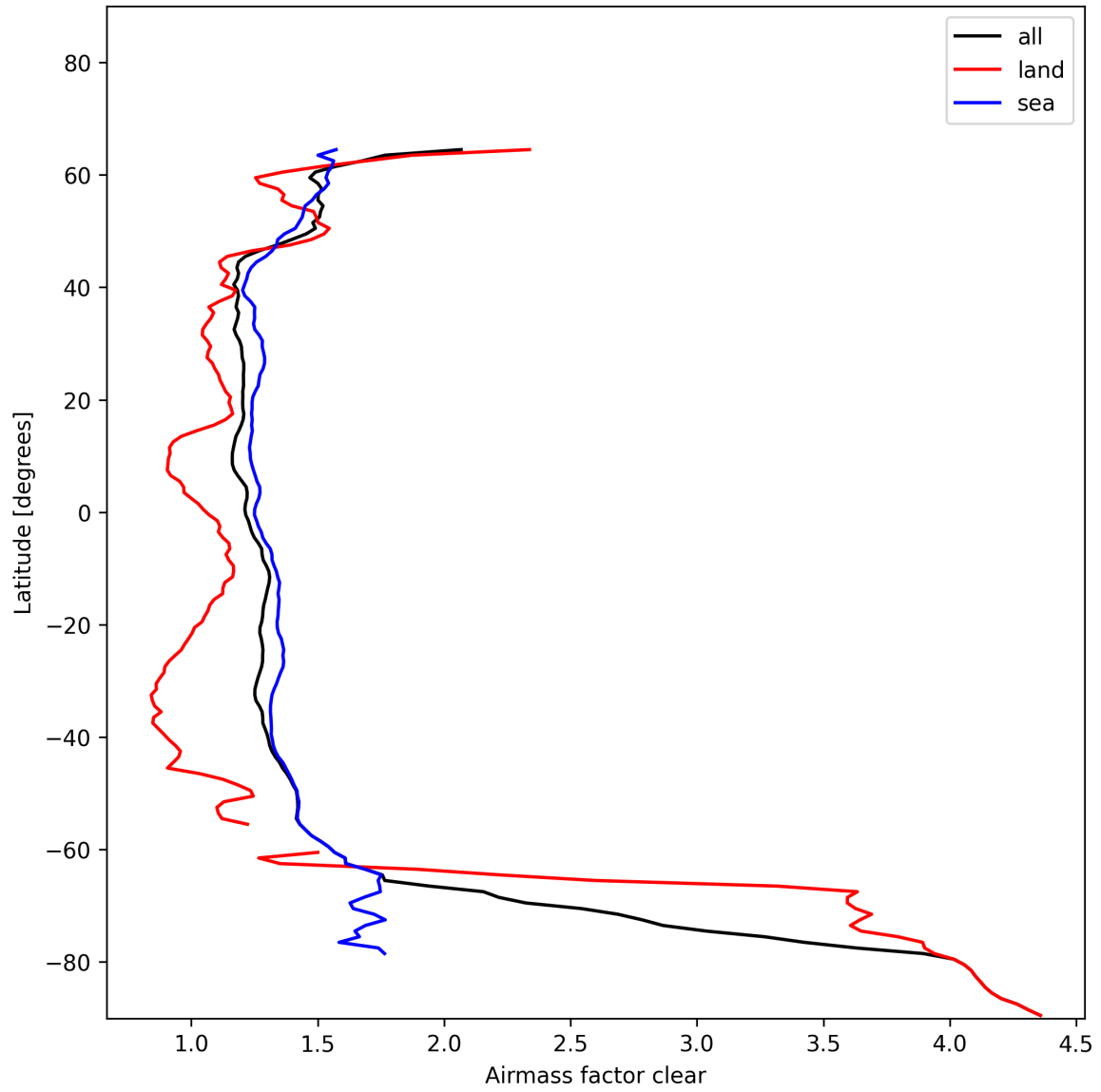
Figure 28: Zonal average of “Airmass factor clear” for 2025-01-14 to 2025-01-16.
