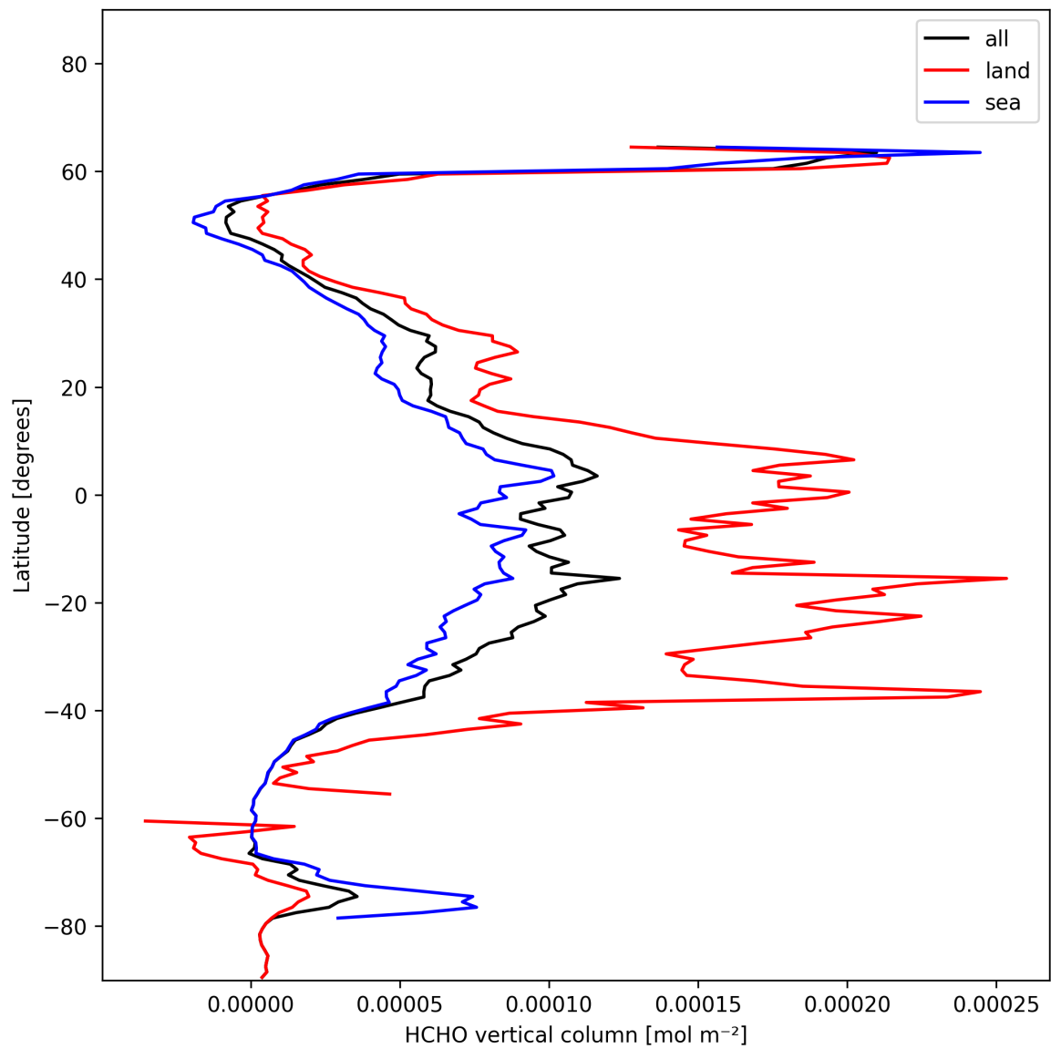
Figure 21: Zonal average of “HCHO vertical column” for 2025-01-14 to 2025-01-16.
