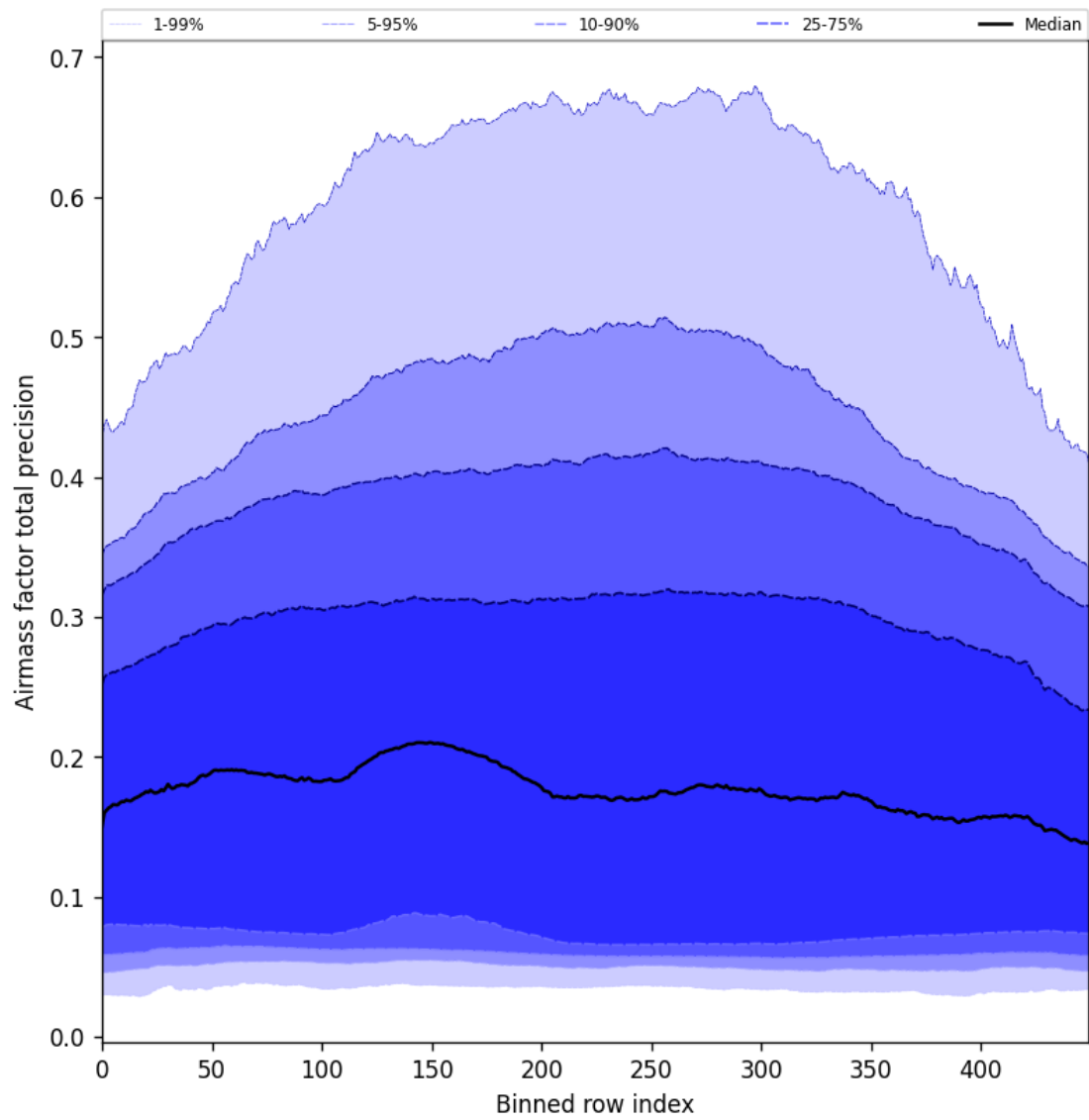
Figure 55: Along track statistics of “Airmass factor total precision” for 2025-01-14 to 2025-01-16
