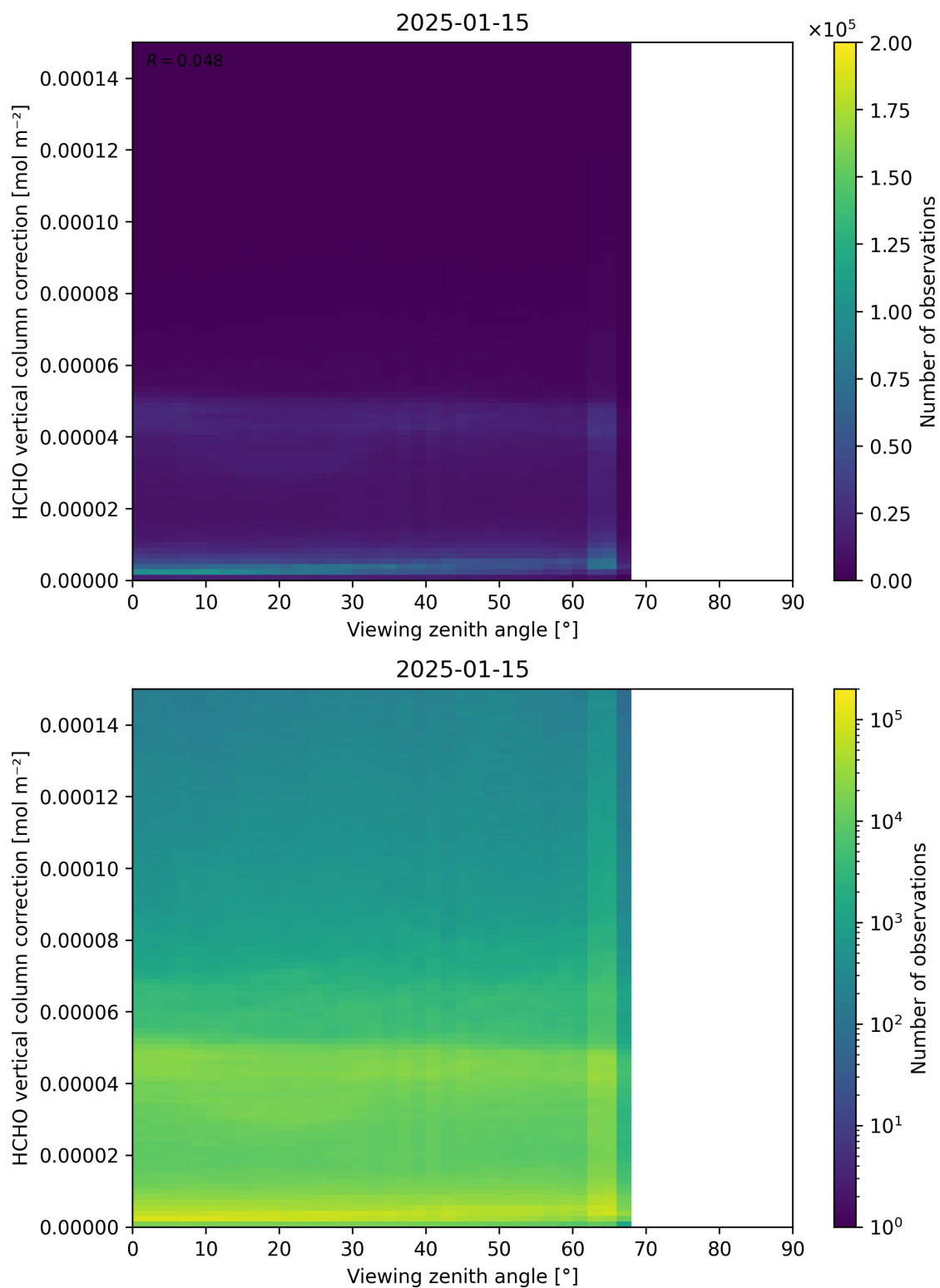
Figure 193: Scatter density plot of “Viewing zenith angle” against “HCHO vertical column correction” for 2025-01-14 to 2025-01-16.
