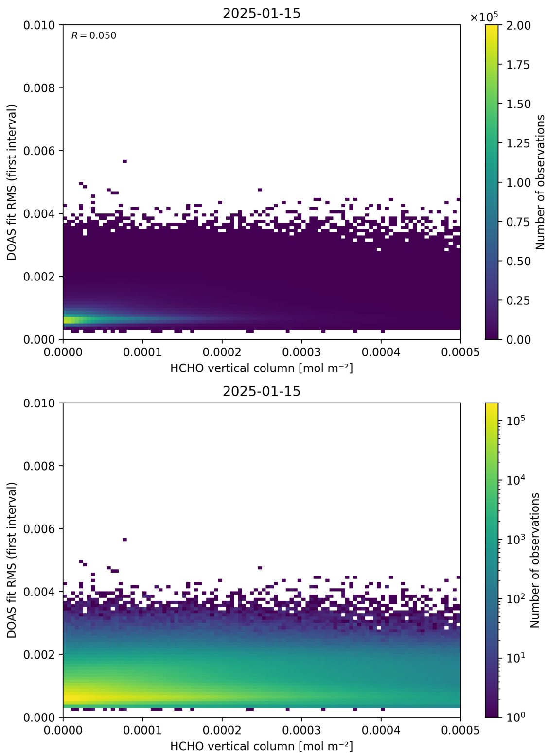
Figure 123: Scatter density plot of “HCHO vertical column” against “DOAS fit RMS (first interval)” for 2025-01-14 to 2025-01-16.
