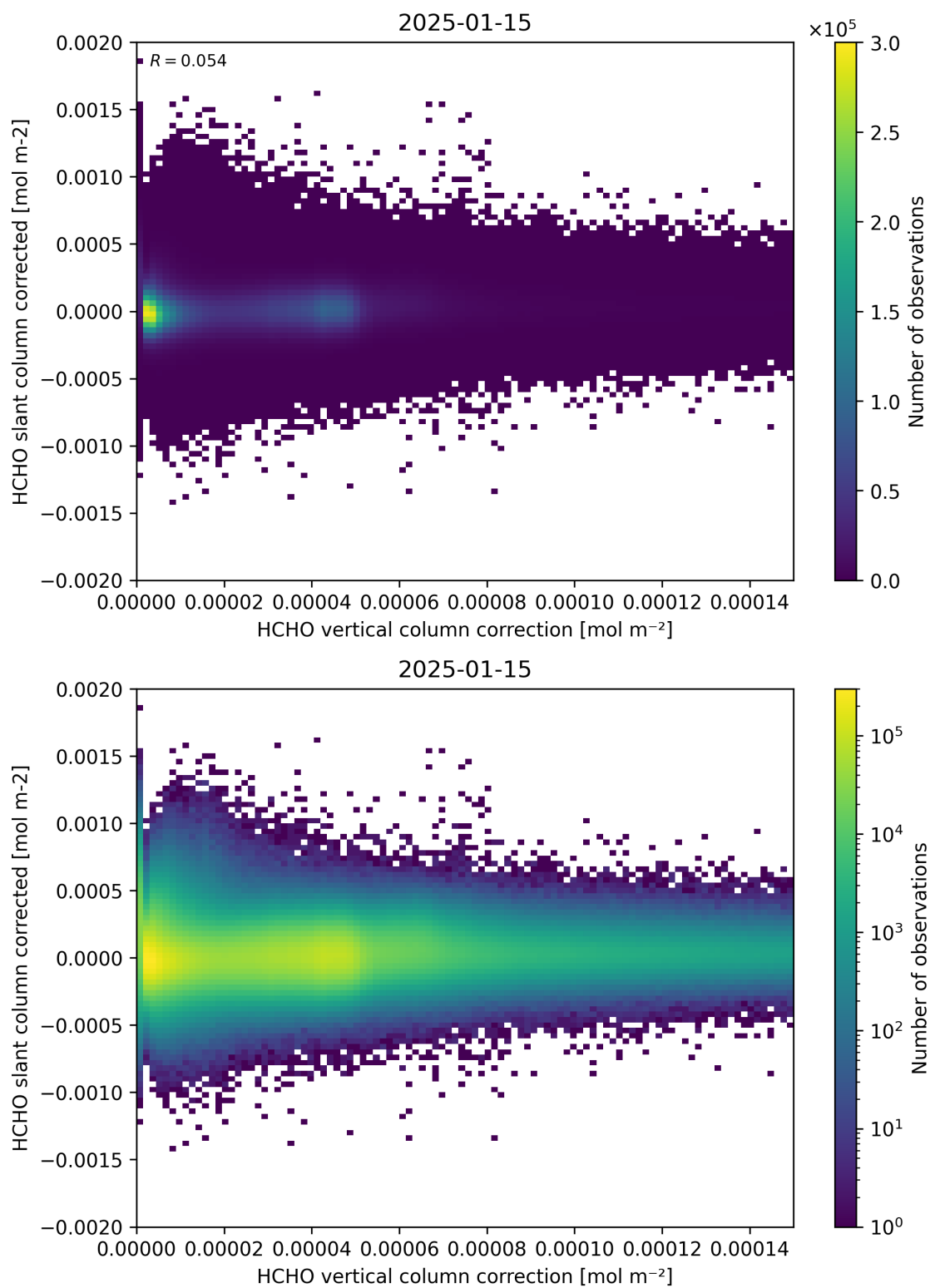
Figure 116: Scatter density plot of “HCHO vertical column correction” against “HCHO slant column corrected” for 2025-01-14 to 2025-01-16.
