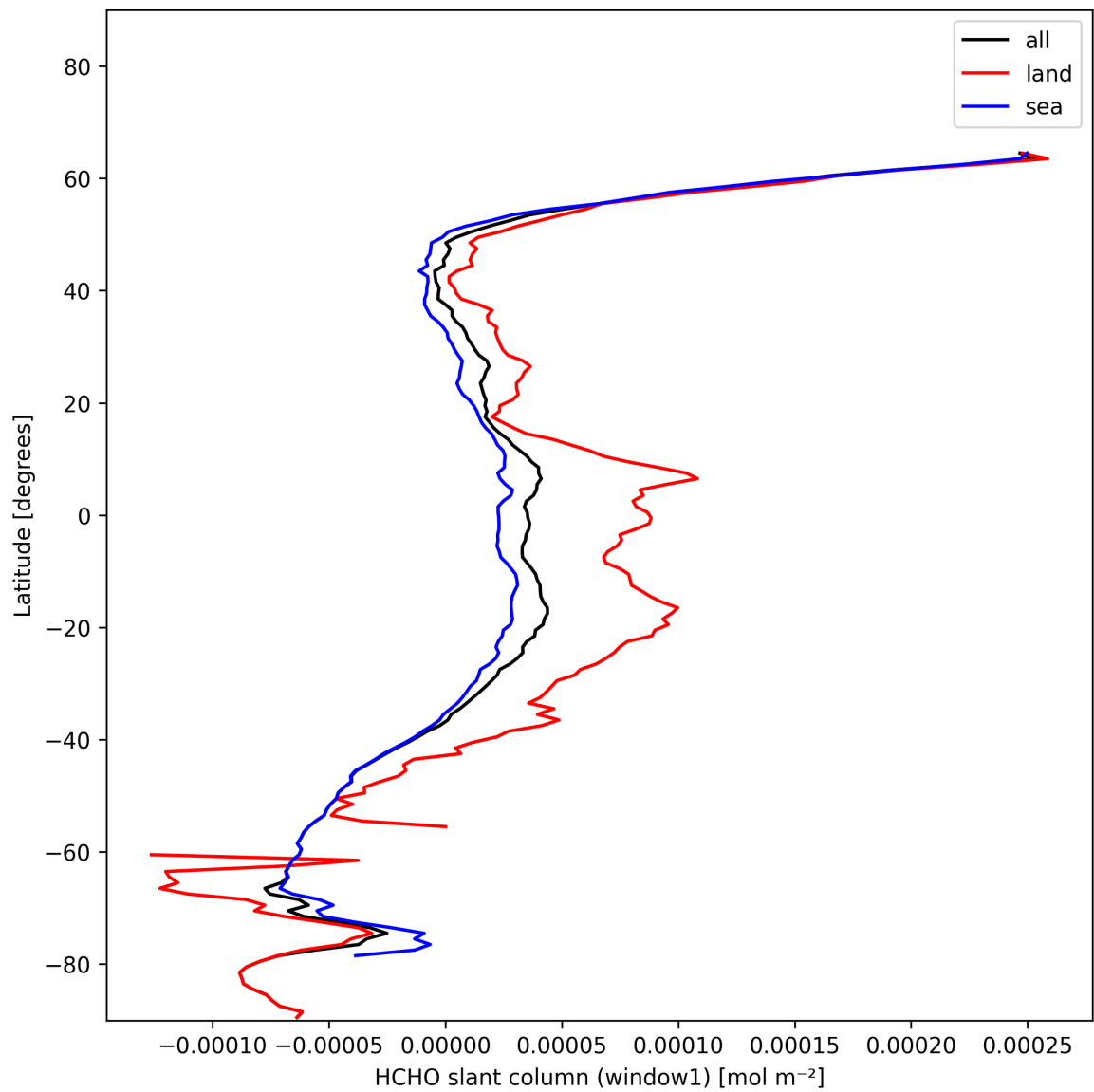
Figure 24: Zonal average of “HCHO slant column (window1)” for 2025-01-14 to 2025-01-16.
