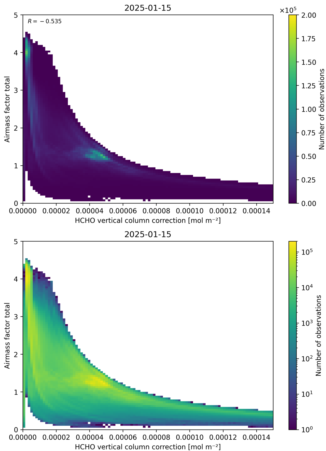
Figure 120: Scatter density plot of “HCHO vertical column correction” against “Airmass factor total” for 2025-01-14 to 2025-01-16.
