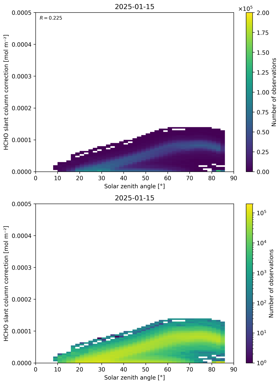
Figure 172: Scatter density plot of “Solar zenith angle” against “HCHO slant column correction” for 2025-01-14 to 2025-01-16.
