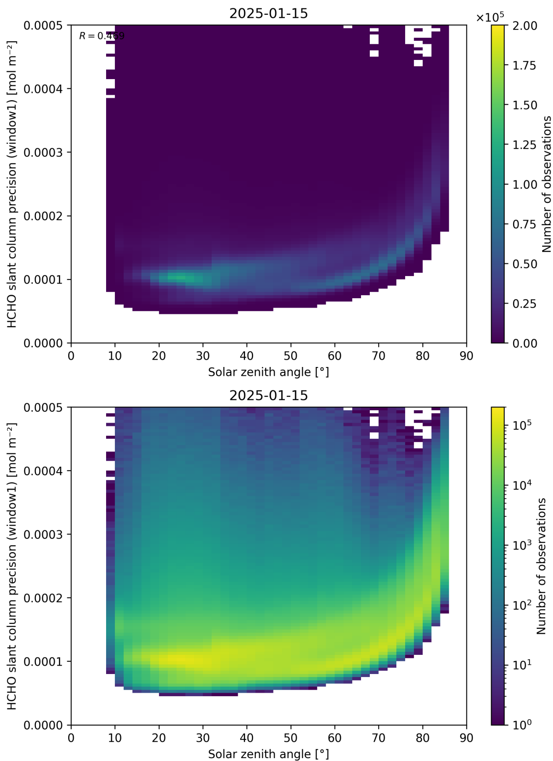
Figure 174: Scatter density plot of “Solar zenith angle” against “HCHO slant column precision (window1)” for 2025-01-14 to 2025-01-16.
