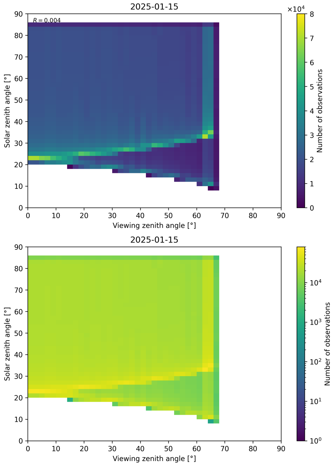
Figure 197: Scatter density plot of “Viewing zenith angle” against “Solar zenith angle” for 2025-01-14 to 2025-01-16.
