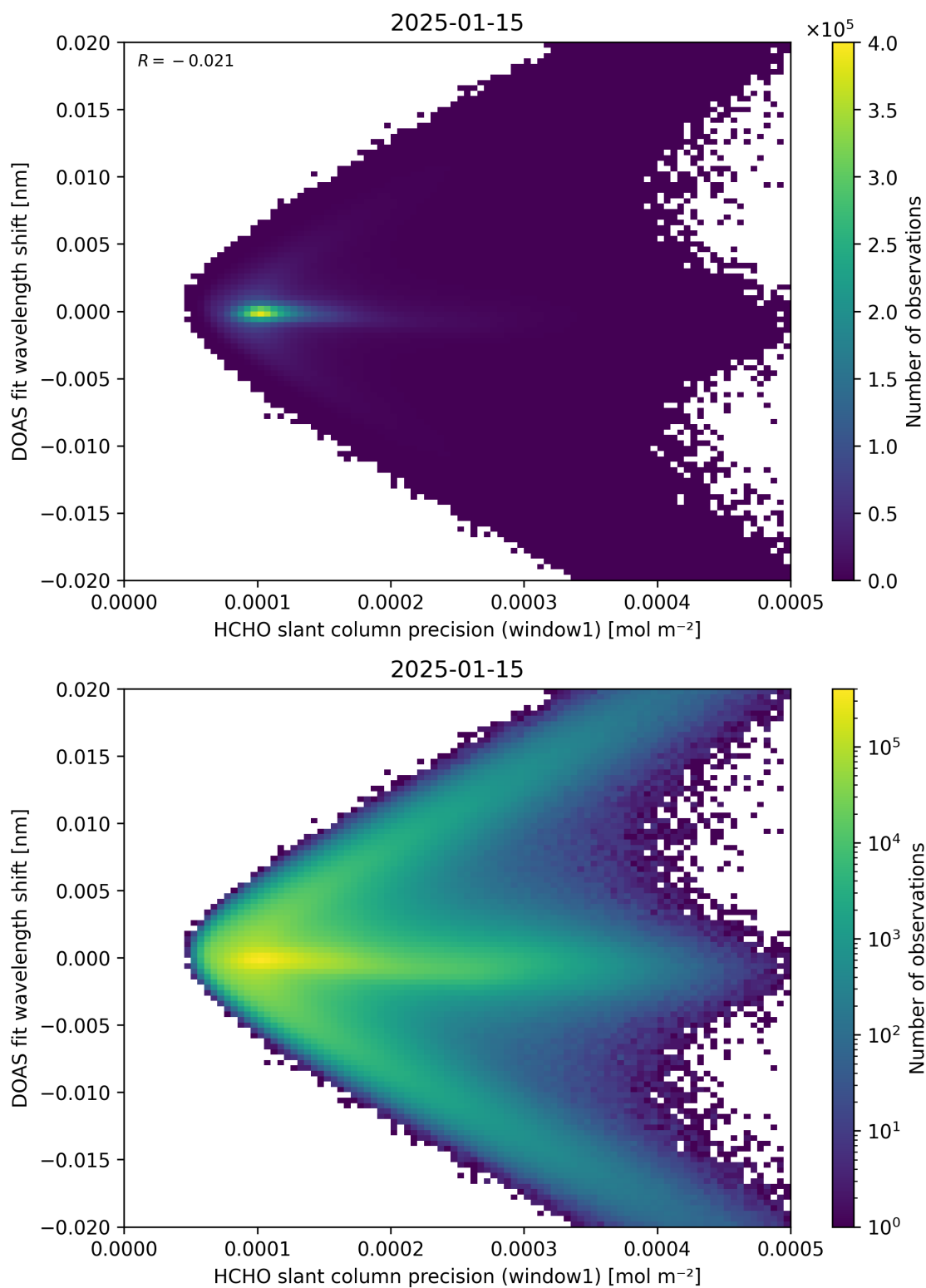
Figure 89: Scatter density plot of “HCHO slant column precision (window1)” against “DOAS fit wavelength shift” for 2025-01-14 to 2025-01-16.
