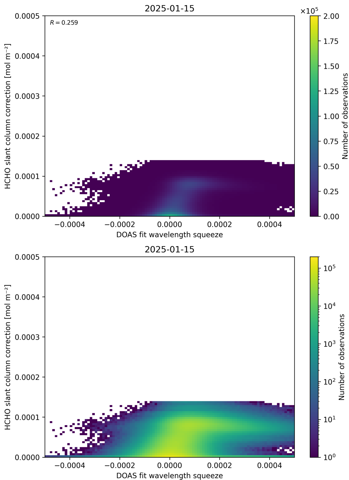
Figure 70: Scatter density plot of “DOAS fit wavelength squeeze” against “HCHO slant column correction” for 2025-01-14 to 2025-01-16.
