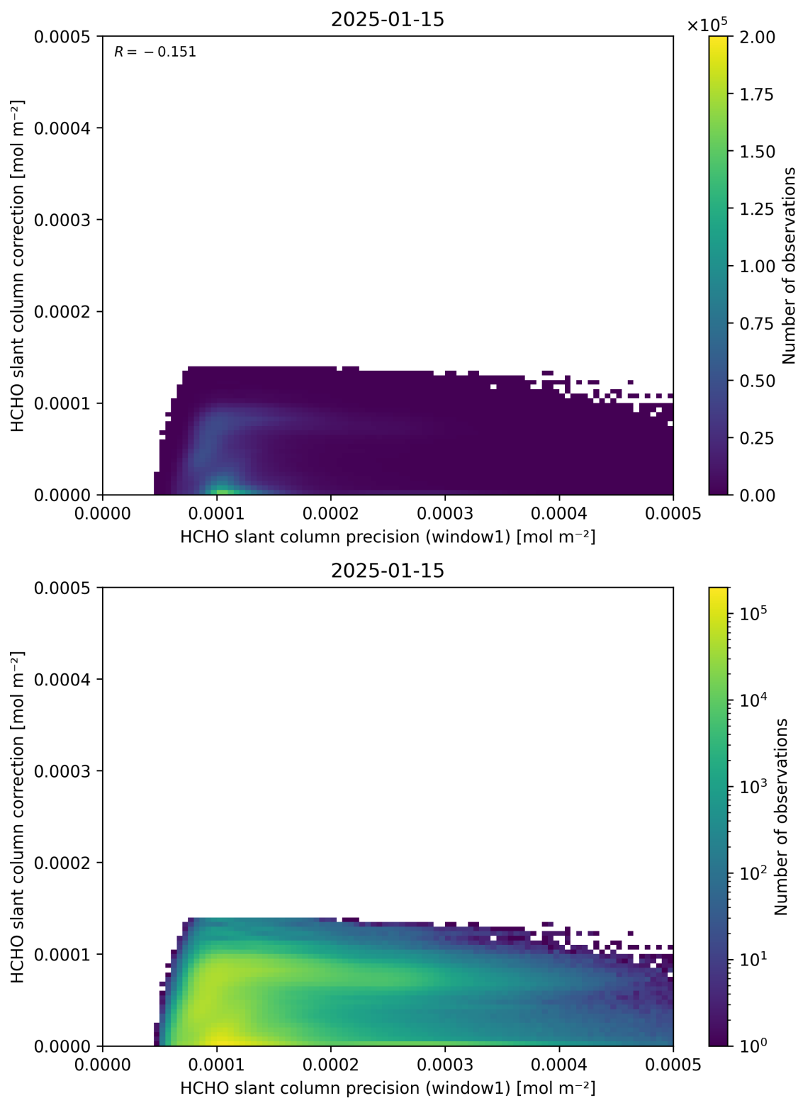
Figure 93: Scatter density plot of “HCHO slant column precision (window1)” against “HCHO slant column correction” for 2025-01-14 to 2025-01-16.
