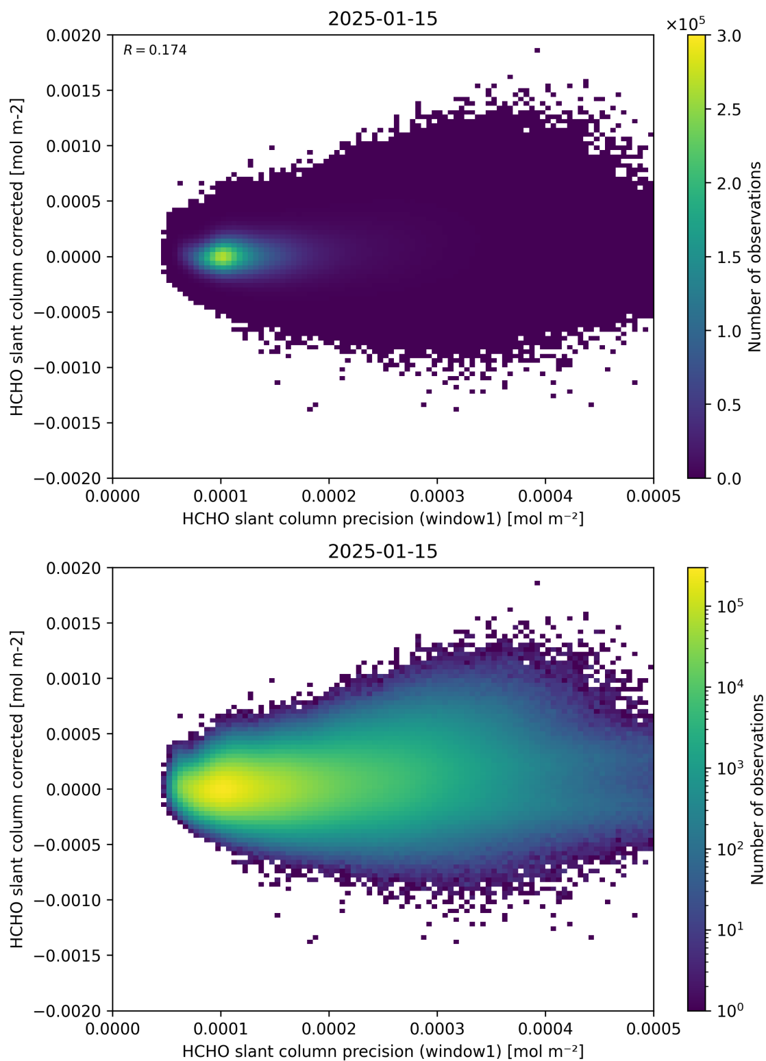
Figure 92: Scatter density plot of “HCHO slant column precision (window1)” against “HCHO slant column corrected” for 2025-01-14 to 2025-01-16.
