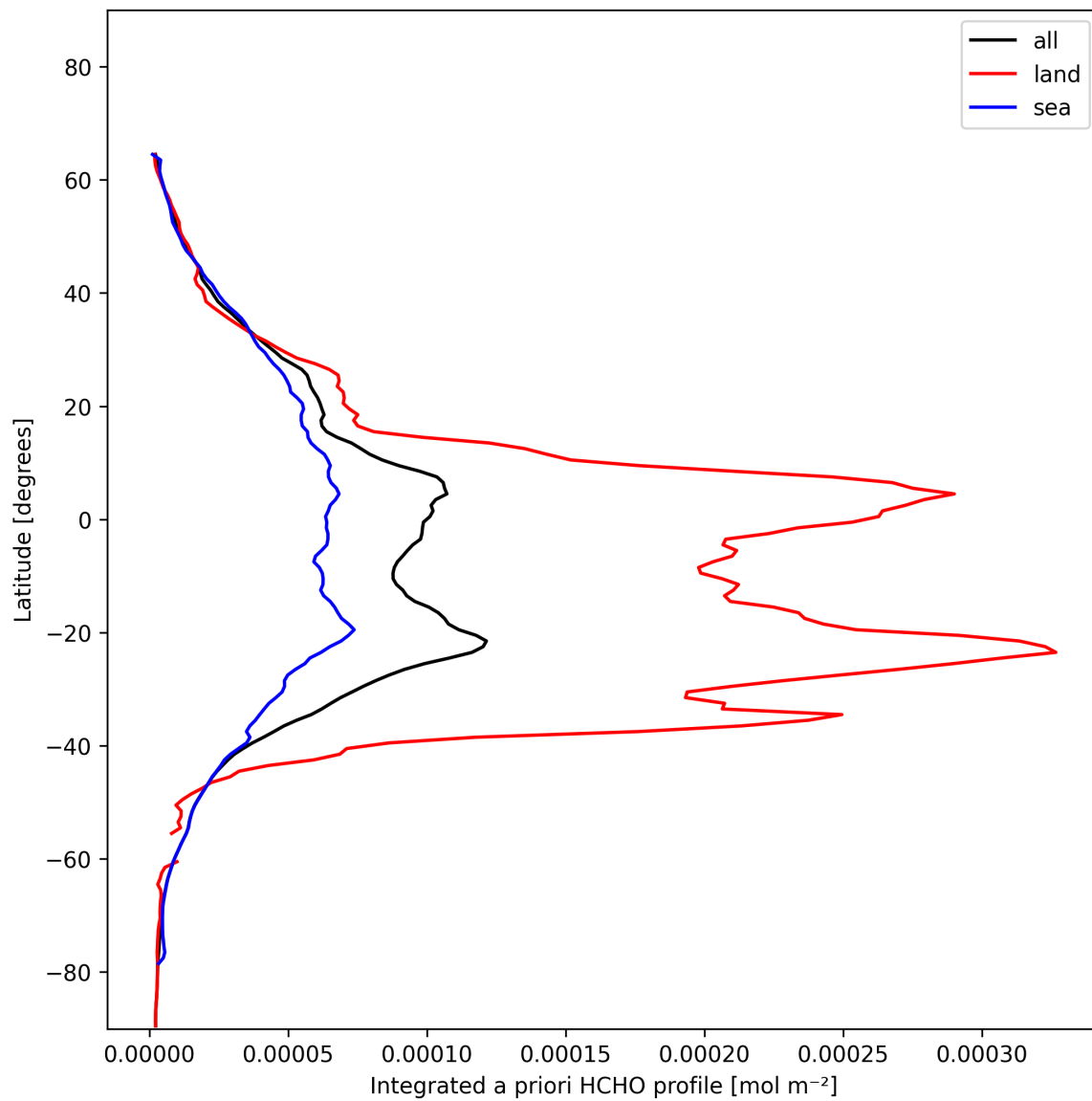
Figure 29: Zonal average of “Integrated a priori HCHO profile” for 2025-01-14 to 2025-01-16.
