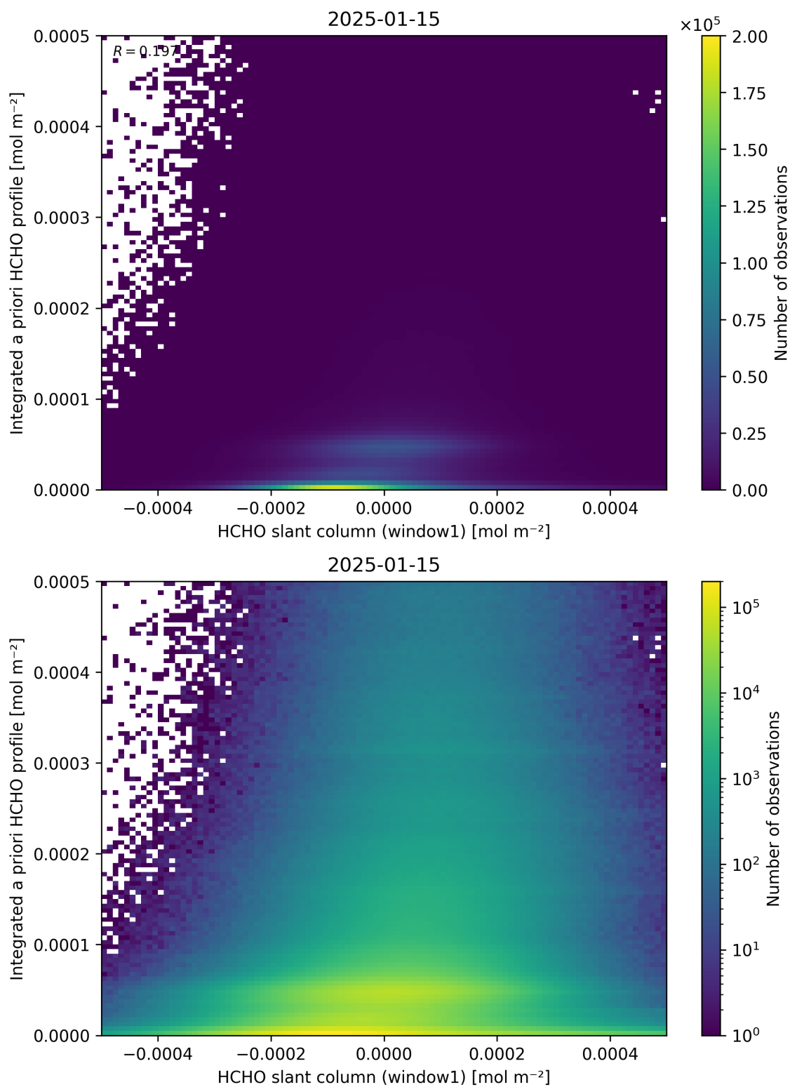
Figure 87: Scatter density plot of “HCHO slant column (window1)” against “Integrated a priori HCHO profile” for 2025-01-14 to 2025-01-16.
