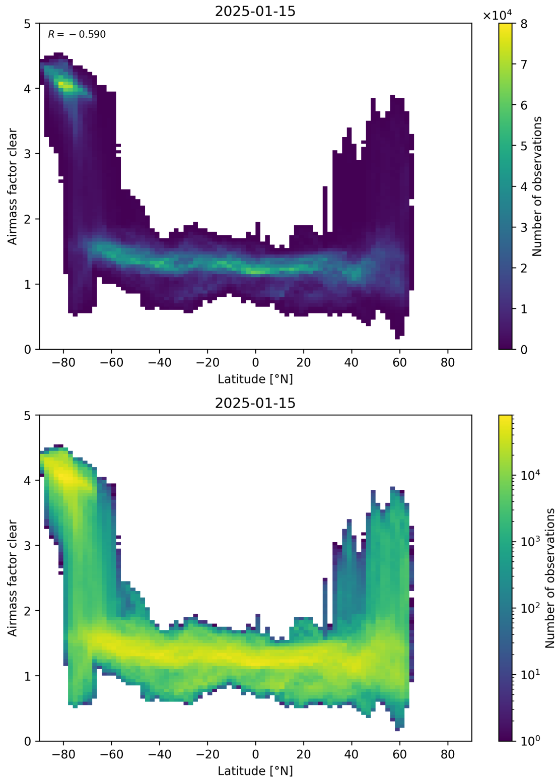
Figure 156: Scatter density plot of “Latitude” against “Airmass factor clear” for 2025-01-14 to 2025-01-16.
