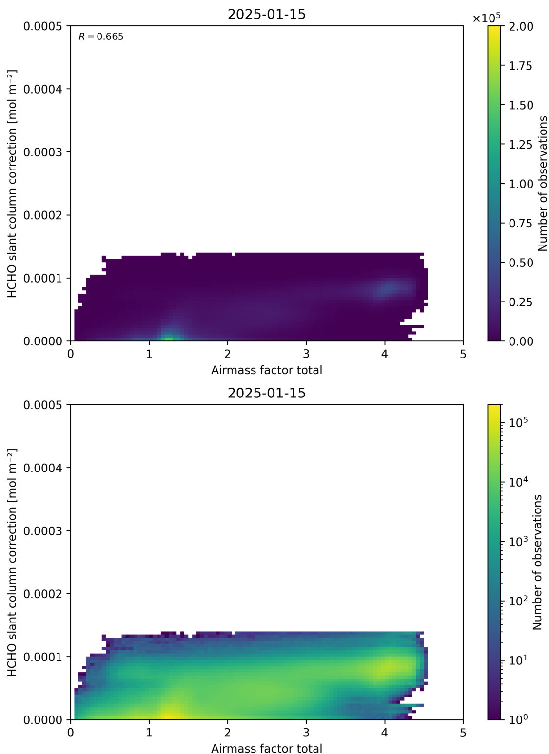
Figure 102: Scatter density plot of “Airmass factor total” against “HCHO slant column correction” for 2025-01-14 to 2025-01-16.
