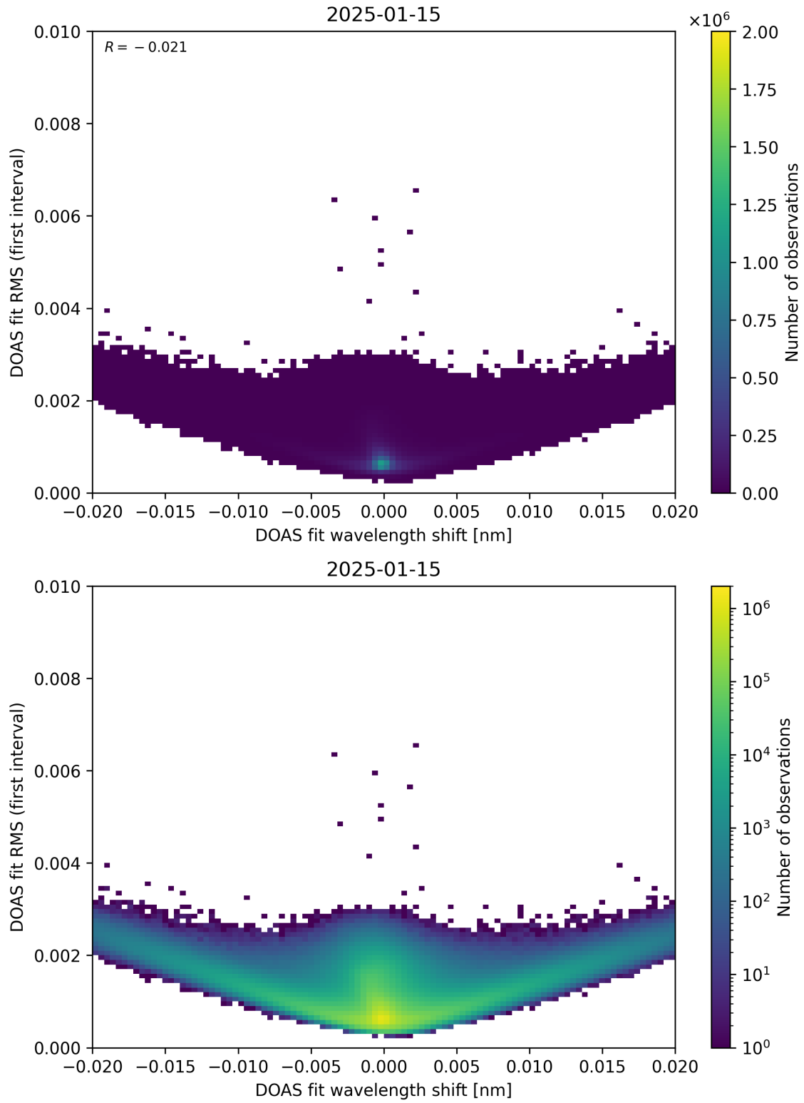
Figure 64: Scatter density plot of “DOAS fit wavelength shift” against “DOAS fit RMS (first interval)” for 2025-01-14 to 2025-01-16.
