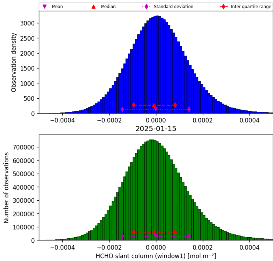
Figure 38: Histogram of “HCHO slant column (window1)” for 2025-01-14 to 2025-01-16
