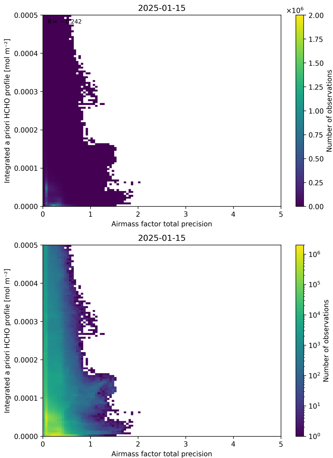
Figure 111: Scatter density plot of “Airmass factor total precision” against “Integrated a priori HCHO profile” for 2025-01-14 to 2025-01-16.
