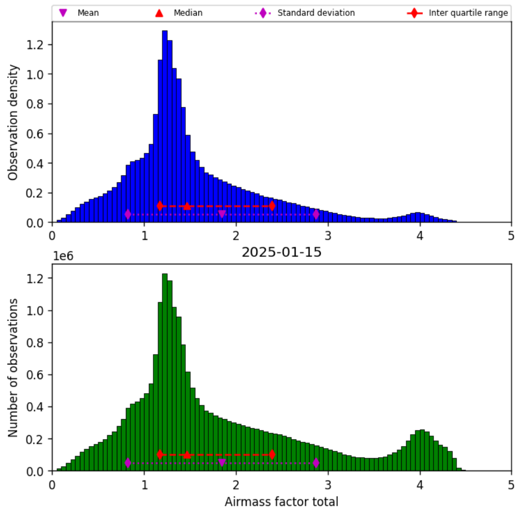
Figure 40: Histogram of “Airmass factor total” for 2025-01-14 to 2025-01-16
