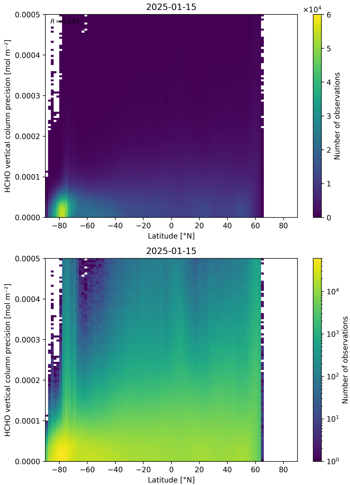
Figure 165: Scatter density plot of “Latitude” against “HCHO vertical column precision” for 2025-01-14 to 2025-01-16.
