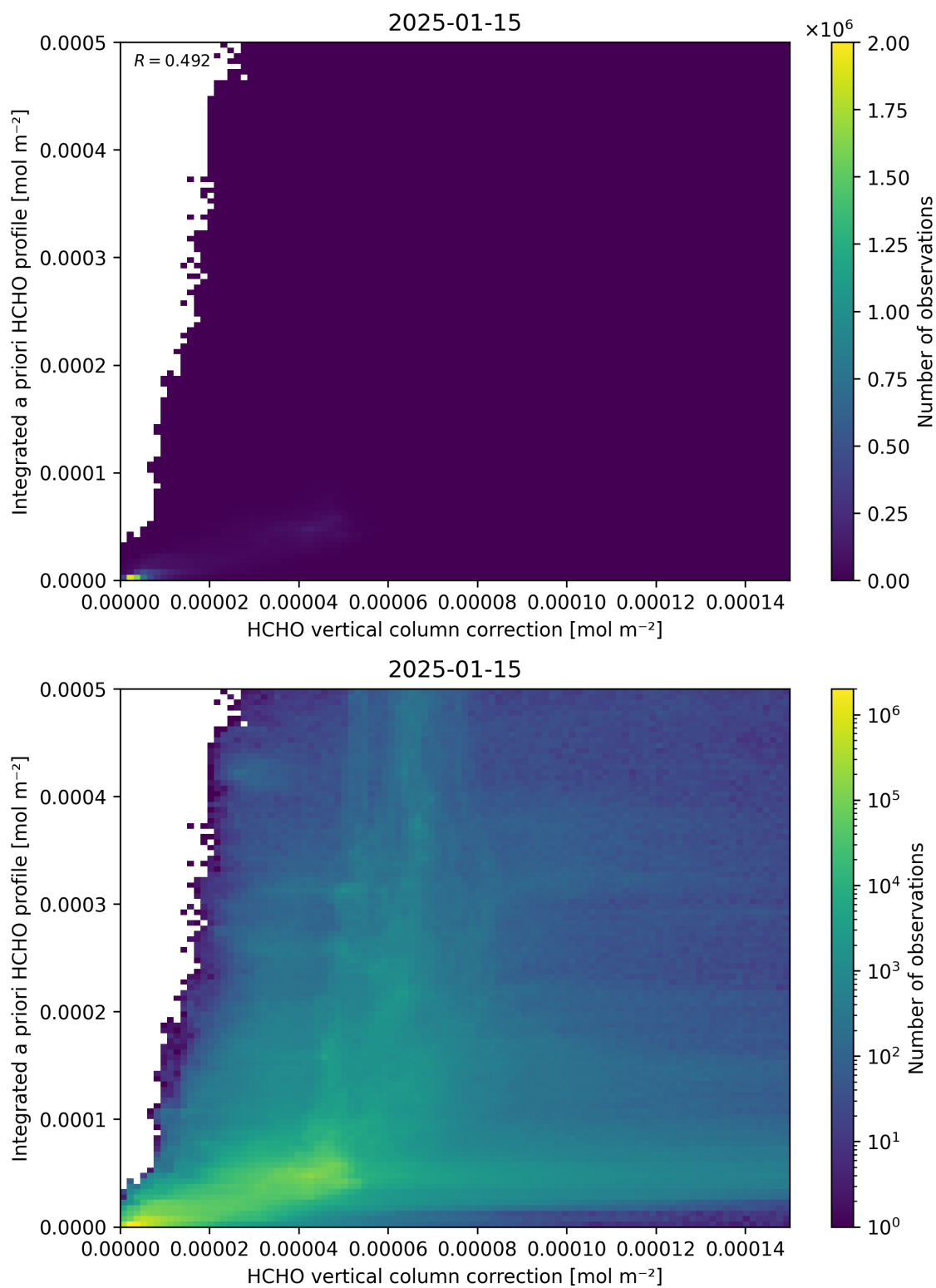
Figure 122: Scatter density plot of “HCHO vertical column correction” against “Integrated a priori HCHO profile” for 2025-01-14 to 2025-01-16.
