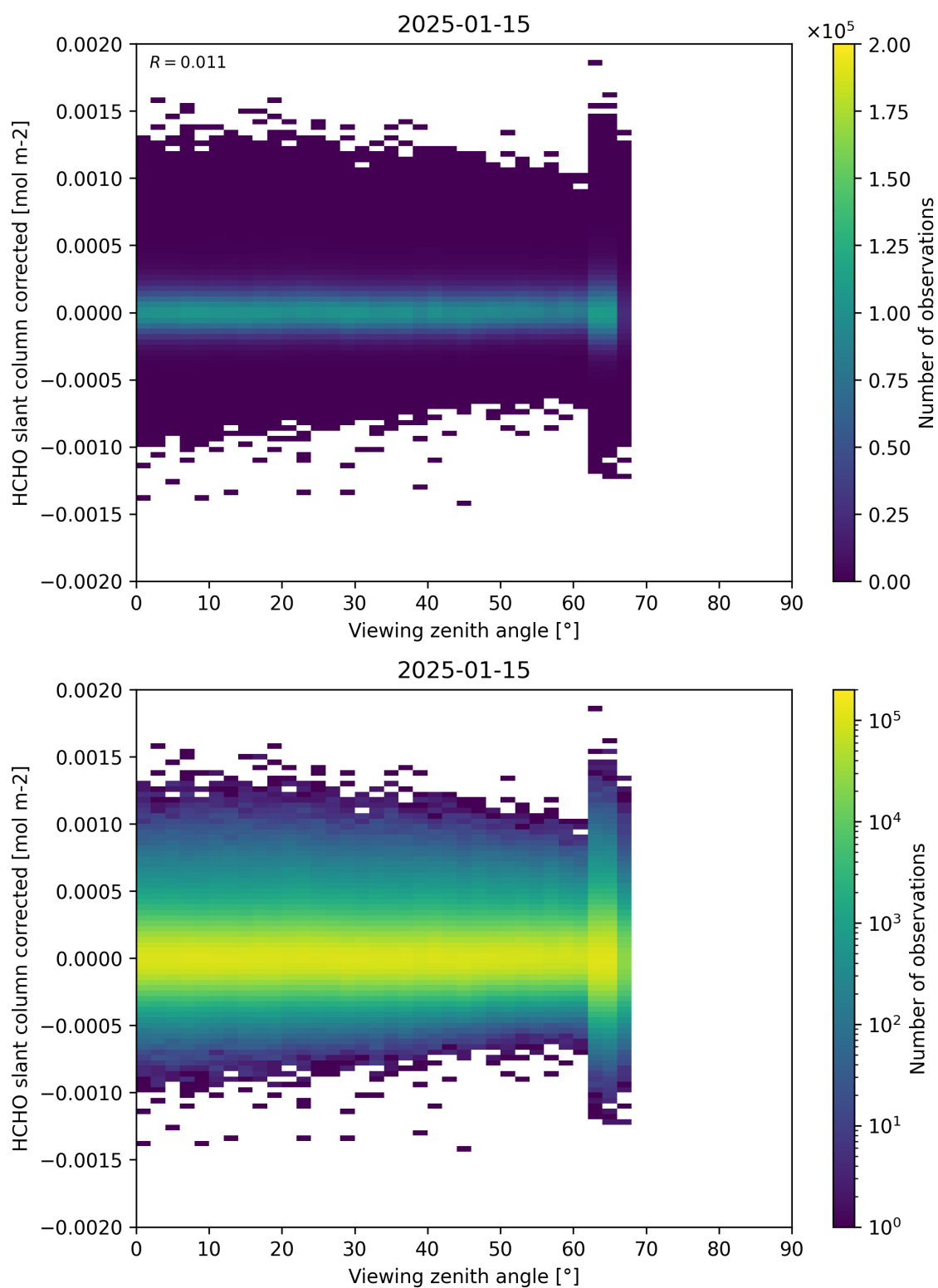
Figure 186: Scatter density plot of “Viewing zenith angle” against “HCHO slant column corrected” for 2025-01-14 to 2025-01-16.
