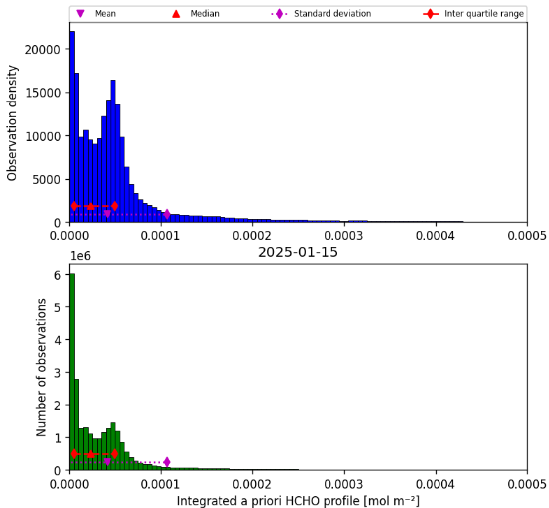
Figure 43: Histogram of “Integrated a priori HCHO profile” for 2025-01-14 to 2025-01-16
