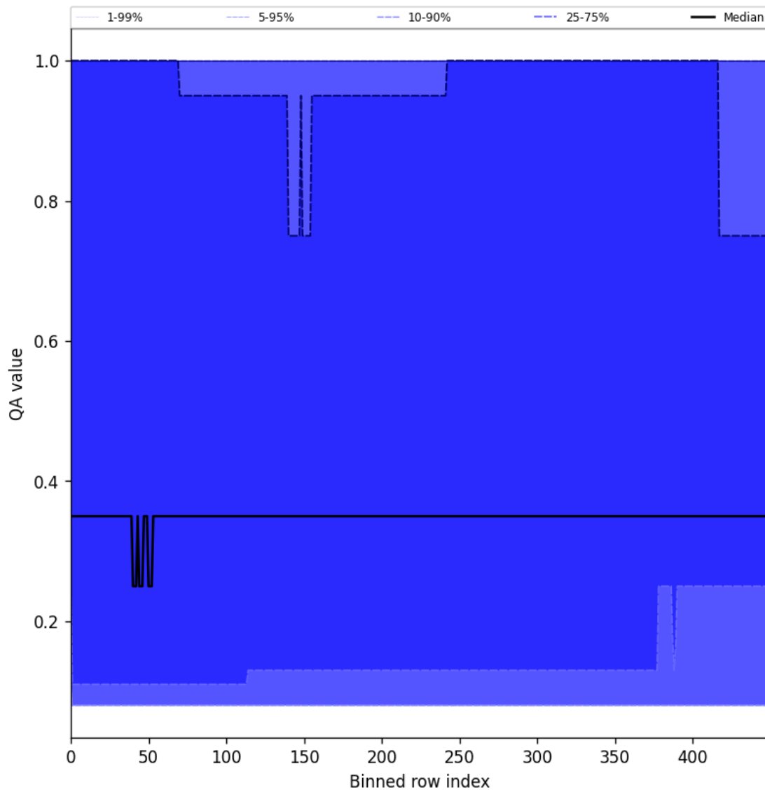
Figure 48: Along track statistics of “QA value” for 2025-01-14 to 2025-01-16
