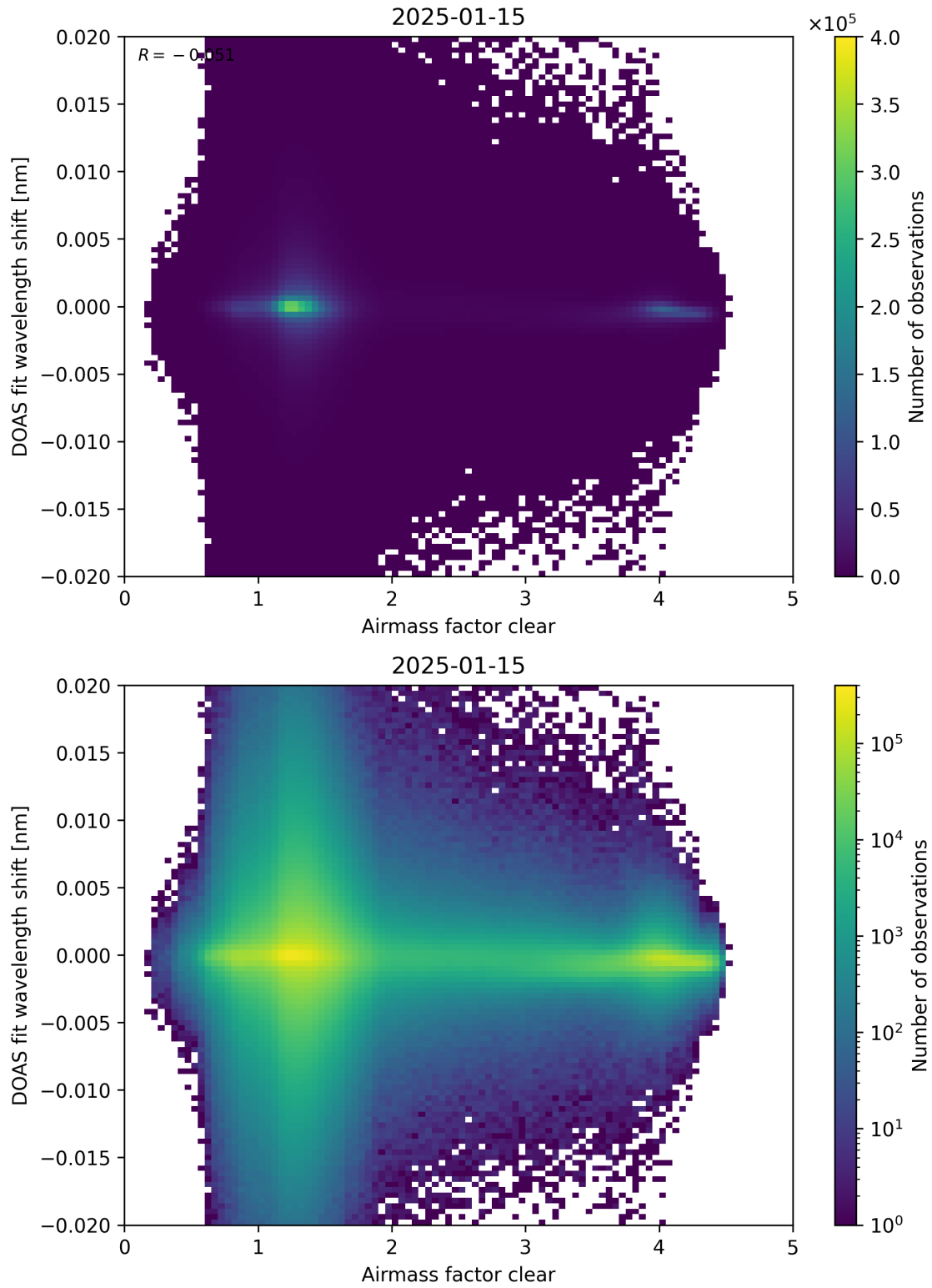
Figure 72: Scatter density plot of “Airmass factor clear” against “DOAS fit wavelength shift” for 2025-01-14 to 2025-01-16.
