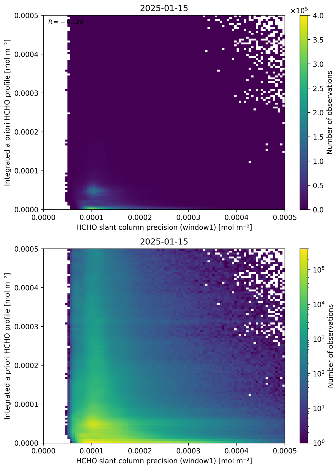
Figure 96: Scatter density plot of “HCHO slant column precision (window1)” against “Integrated a priori HCHO profile” for 2025-01-14 to 2025-01-16.
