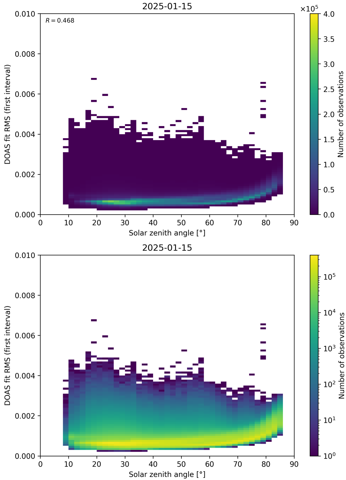
Figure 167: Scatter density plot of “Solar zenith angle” against “DOAS fit RMS (first interval)” for 2025-01-14 to 2025-01-16.
