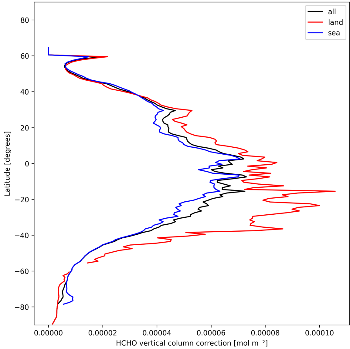
Figure 23: Zonal average of “HCHO vertical column correction” for 2025-01-14 to 2025-01-16.
