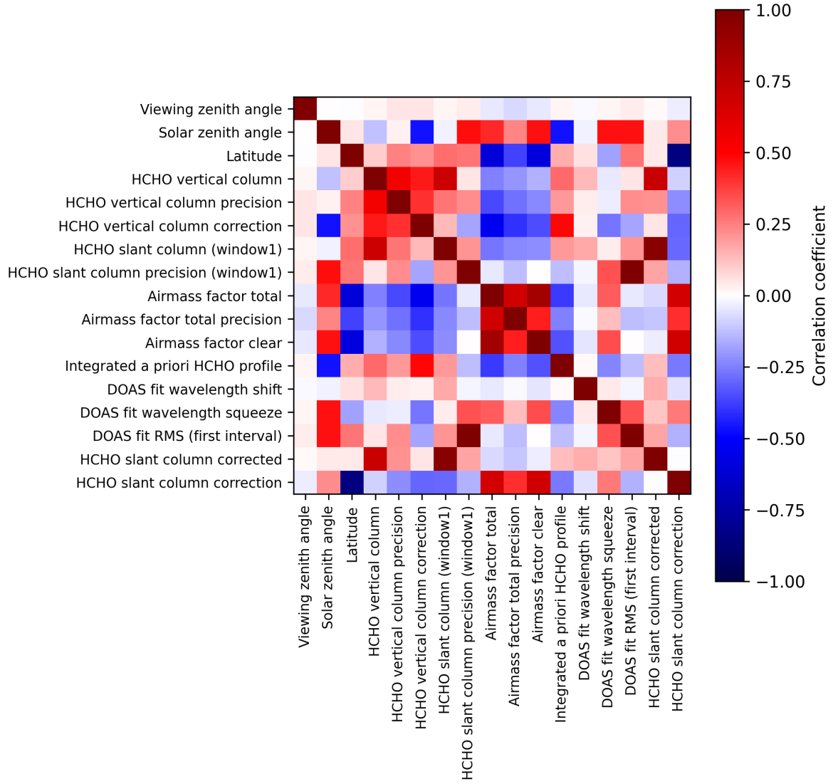
Figure 2: Map of correlation matrix for 2025-01-14 to 2025-01-16.
