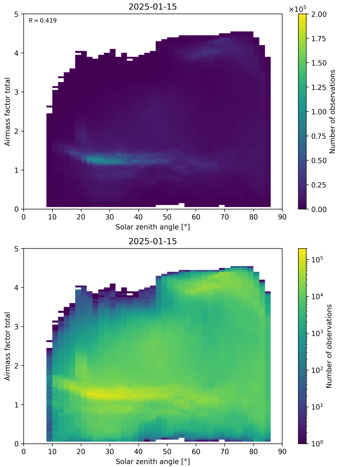
Figure 175: Scatter density plot of “Solar zenith angle” against “Airmass factor total” for 2025-01-14 to 2025-01-16.
