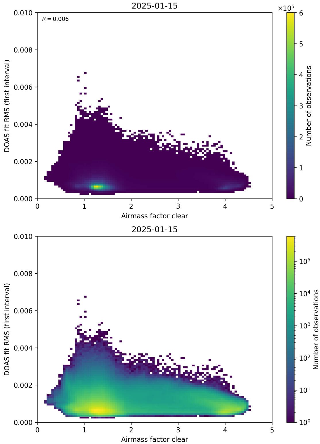
Figure 71: Scatter density plot of “Airmass factor clear” against “DOAS fit RMS (first interval)” for 2025-01-14 to 2025-01-16.
