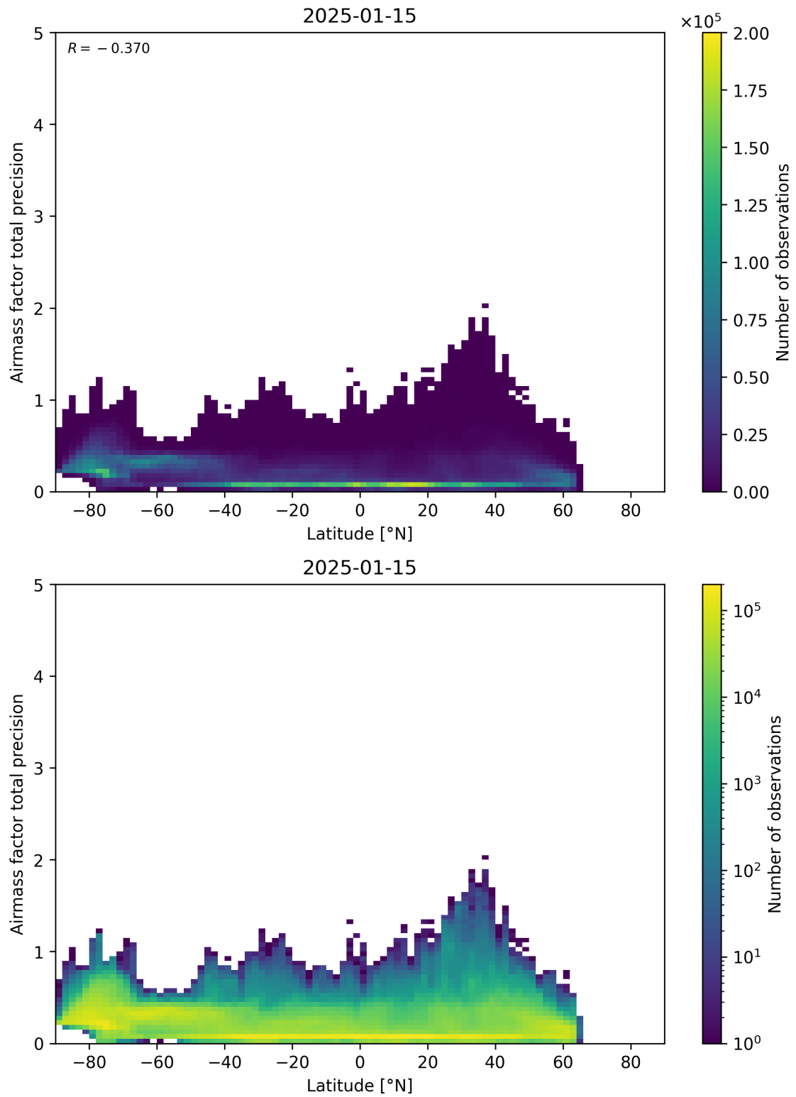
Figure 162: Scatter density plot of “Latitude” against “Airmass factor total precision” for 2025-01-14 to 2025-01-16.
