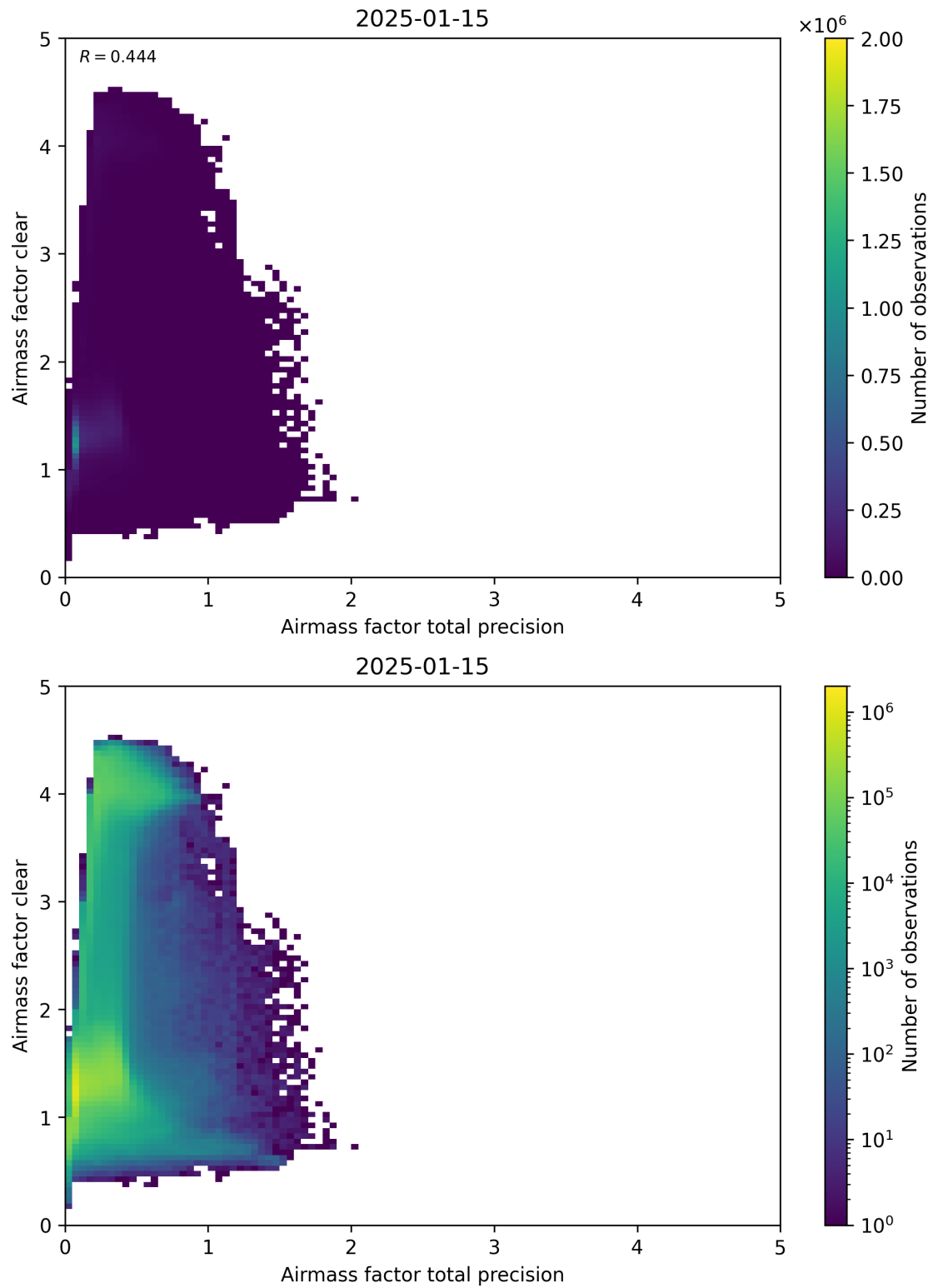
Figure 108: Scatter density plot of “Airmass factor total precision” against “Airmass factor clear” for 2025-01-14 to 2025-01-16.
