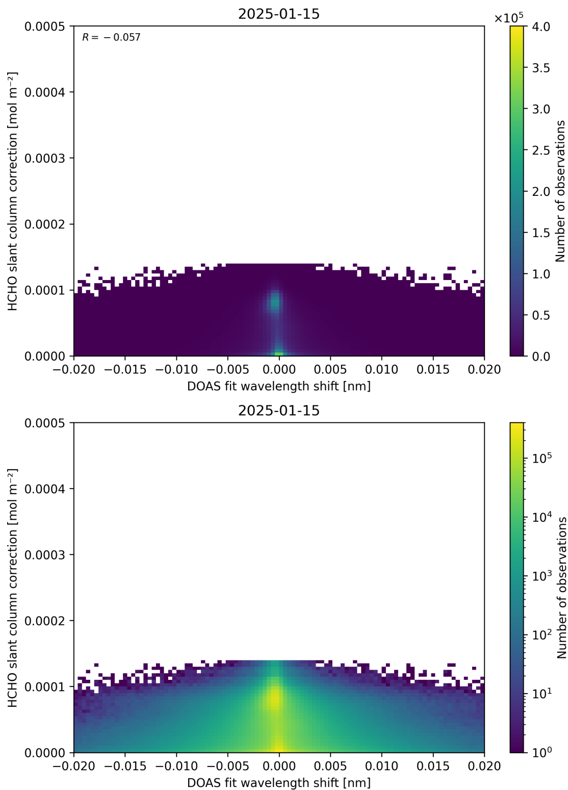
Figure 67: Scatter density plot of “DOAS fit wavelength shift” against “HCHO slant column correction” for 2025-01-14 to 2025-01-16.
