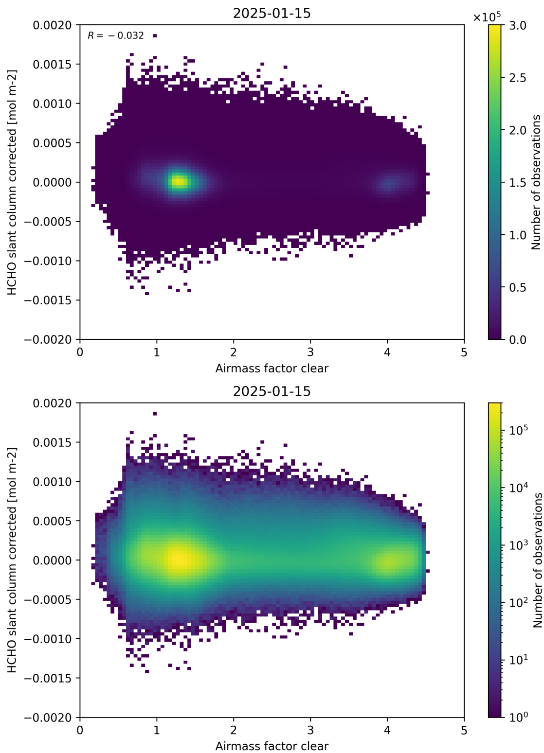
Figure 74: Scatter density plot of “Airmass factor clear” against “HCHO slant column corrected” for 2025-01-14 to 2025-01-16.
