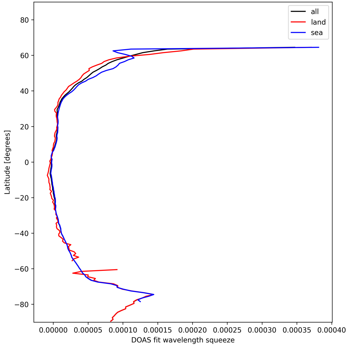
Figure 31: Zonal average of “DOAS fit wavelength squeeze” for 2025-01-14 to 2025-01-16.
