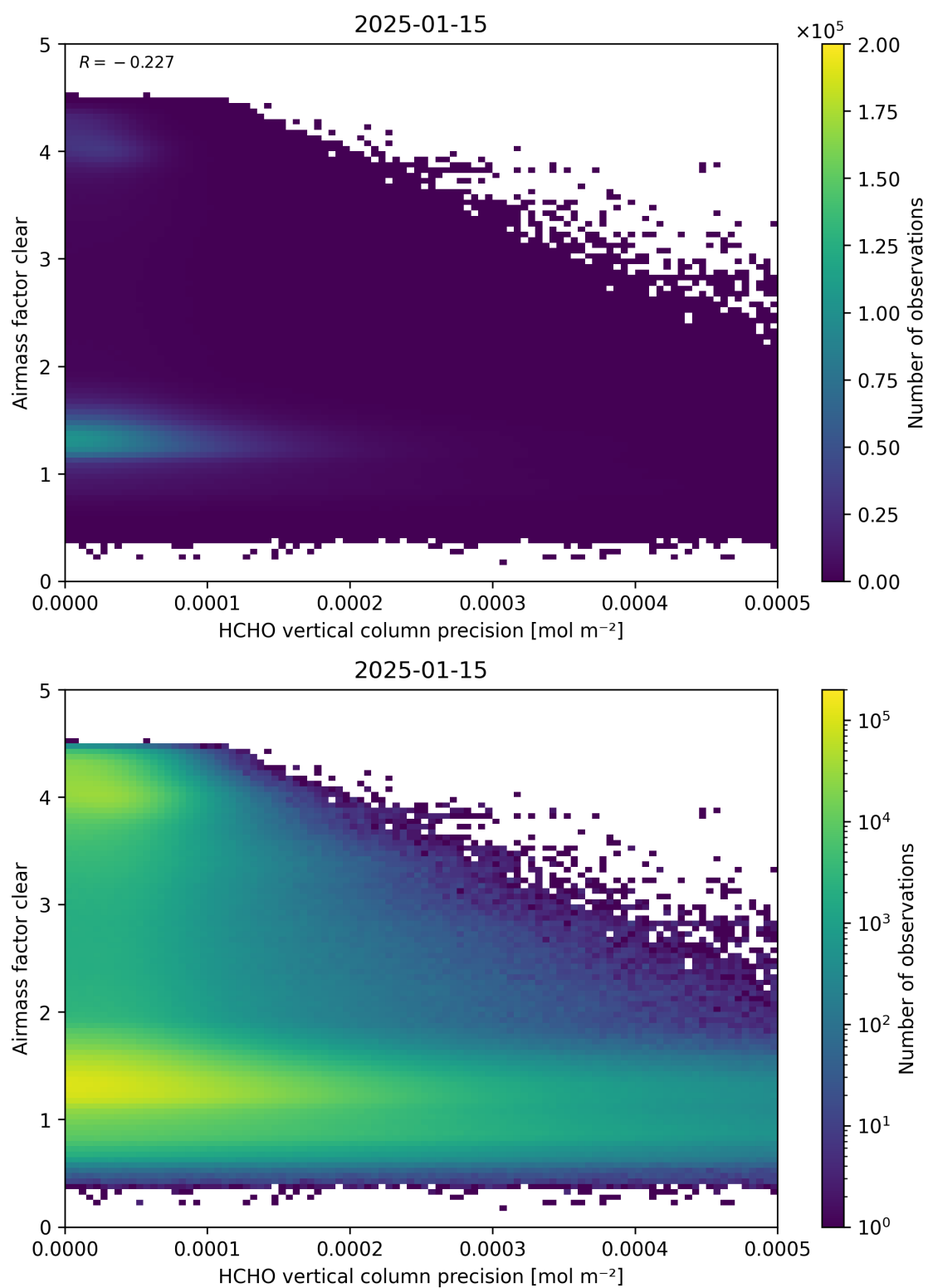
Figure 139: Scatter density plot of “HCHO vertical column precision” against “Airmass factor clear” for 2025-01-14 to 2025-01-16.
