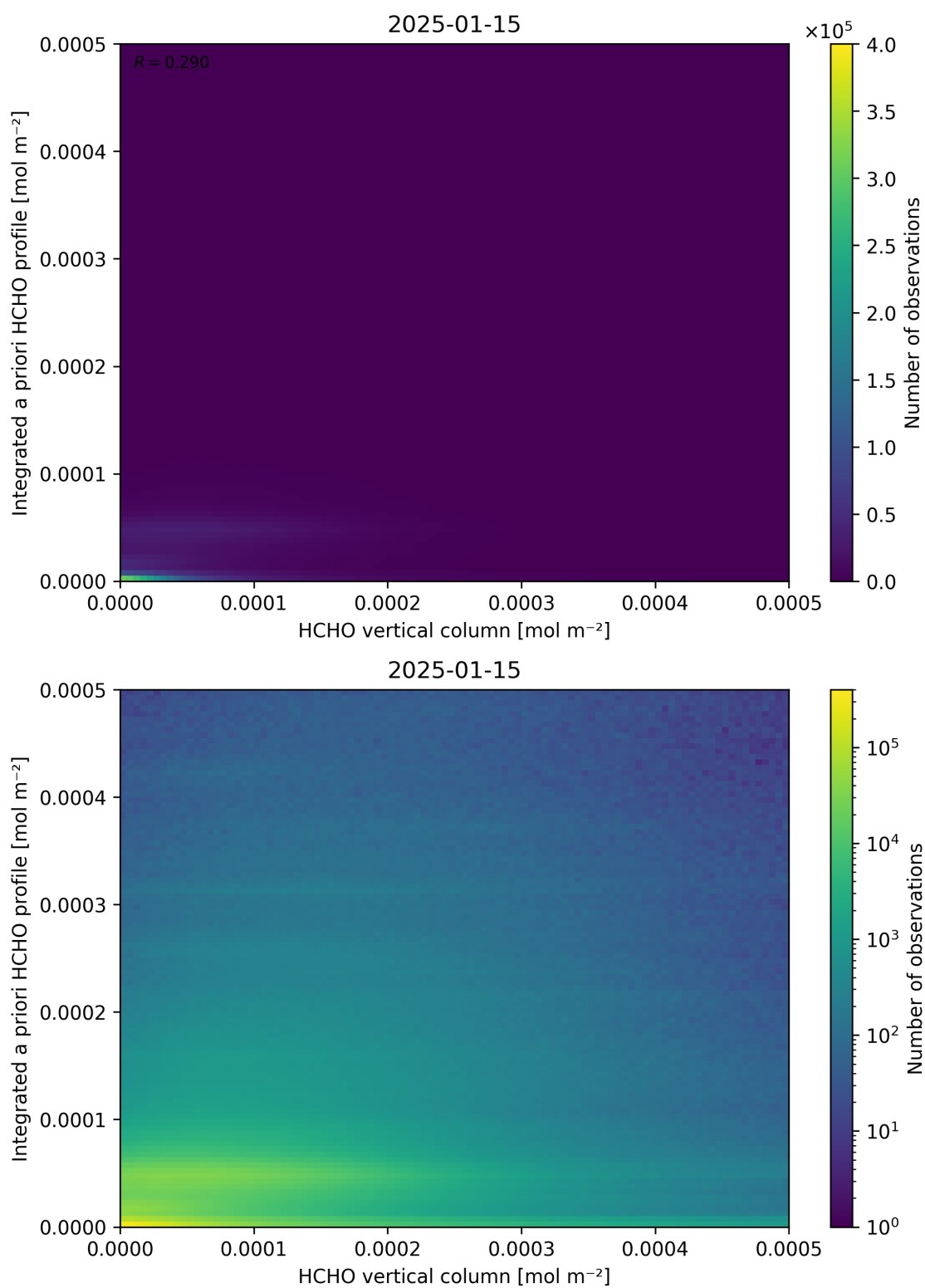
Figure 135: Scatter density plot of “HCHO vertical column” against “Integrated a priori HCHO profile” for 2025-01-14 to 2025-01-16.
