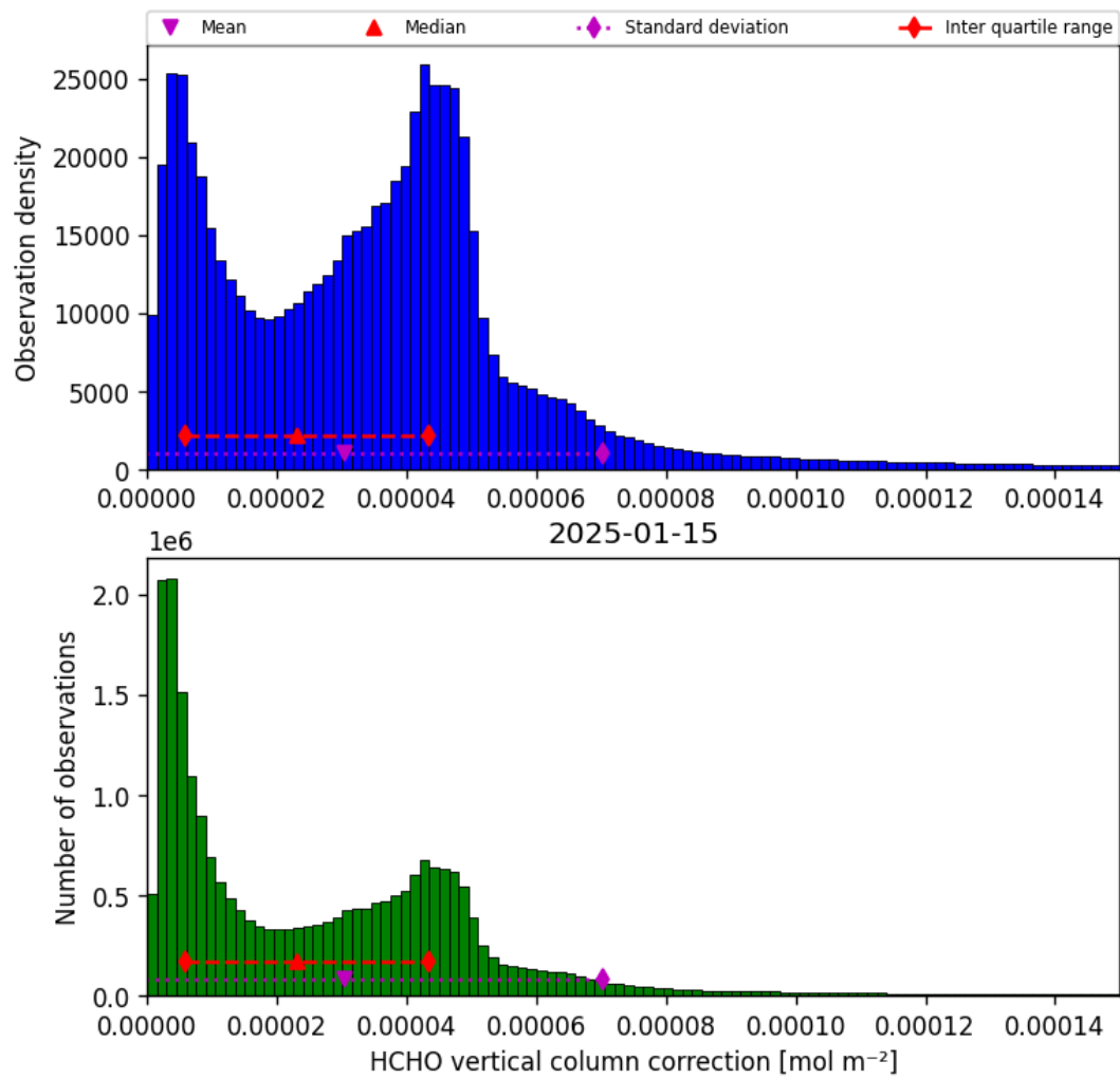
Figure 37: Histogram of “HCHO vertical column correction” for 2025-01-14 to 2025-01-16
