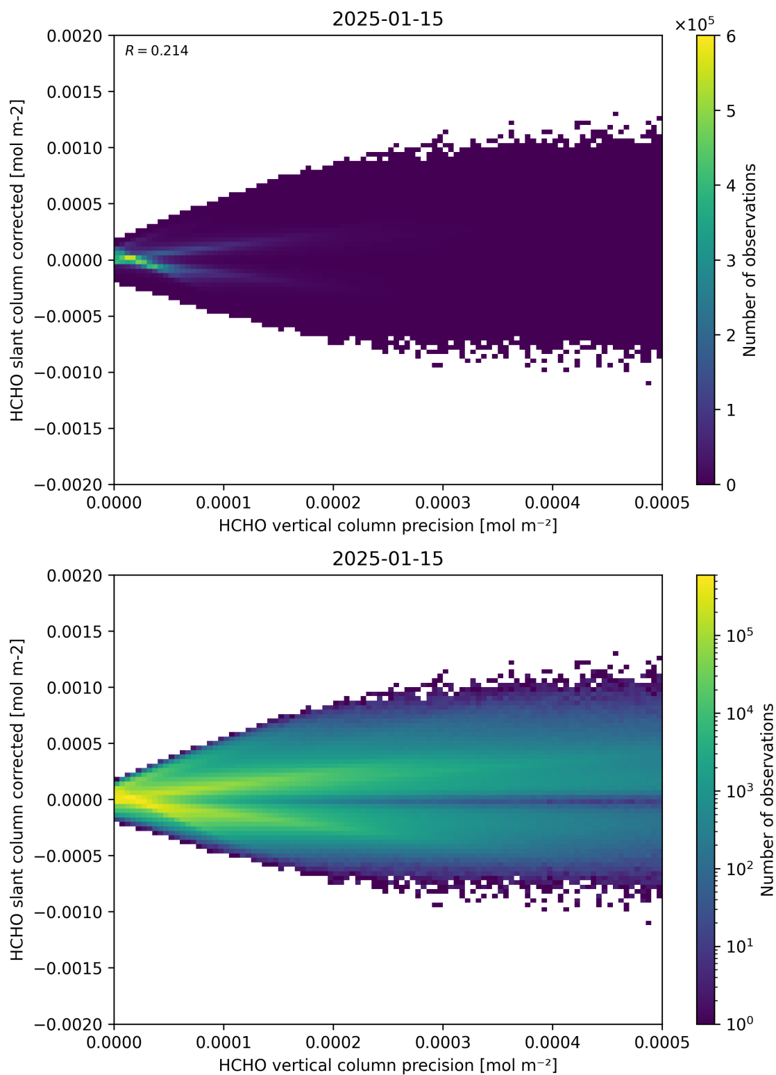
Figure 140: Scatter density plot of “HCHO vertical column precision” against “HCHO slant column corrected” for 2025-01-14 to 2025-01-16.
