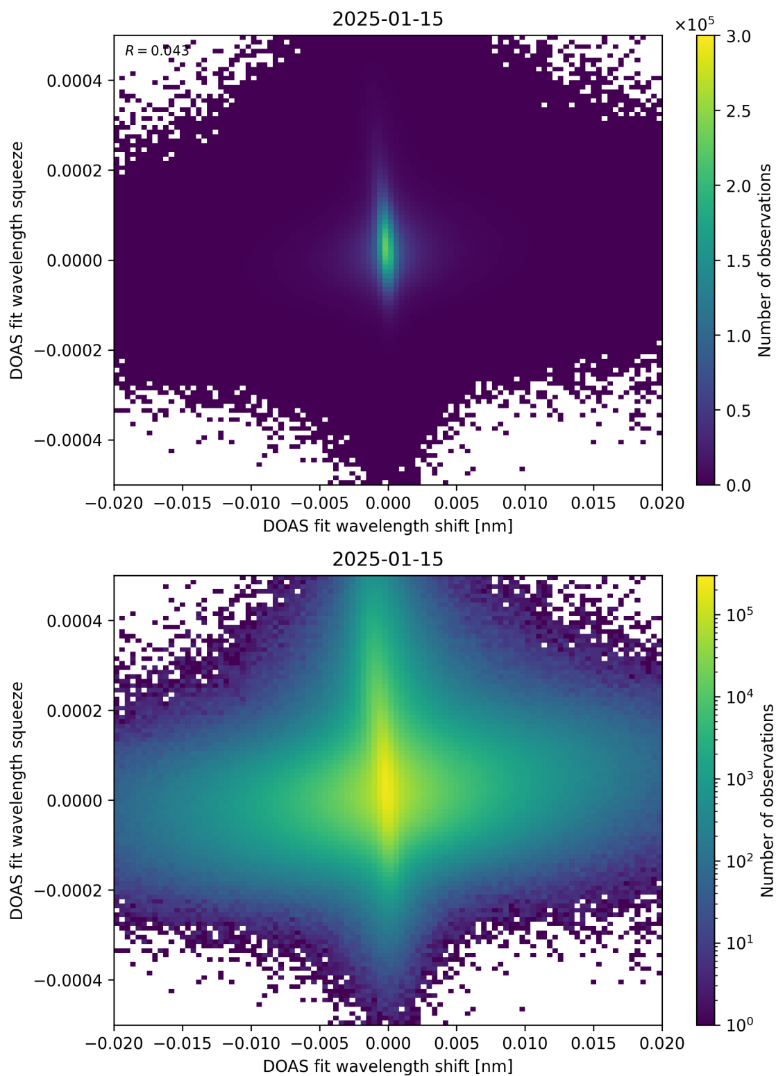
Figure 65: Scatter density plot of “DOAS fit wavelength shift” against “DOAS fit wavelength squeeze” for 2025-01-14 to 2025-01-16.
