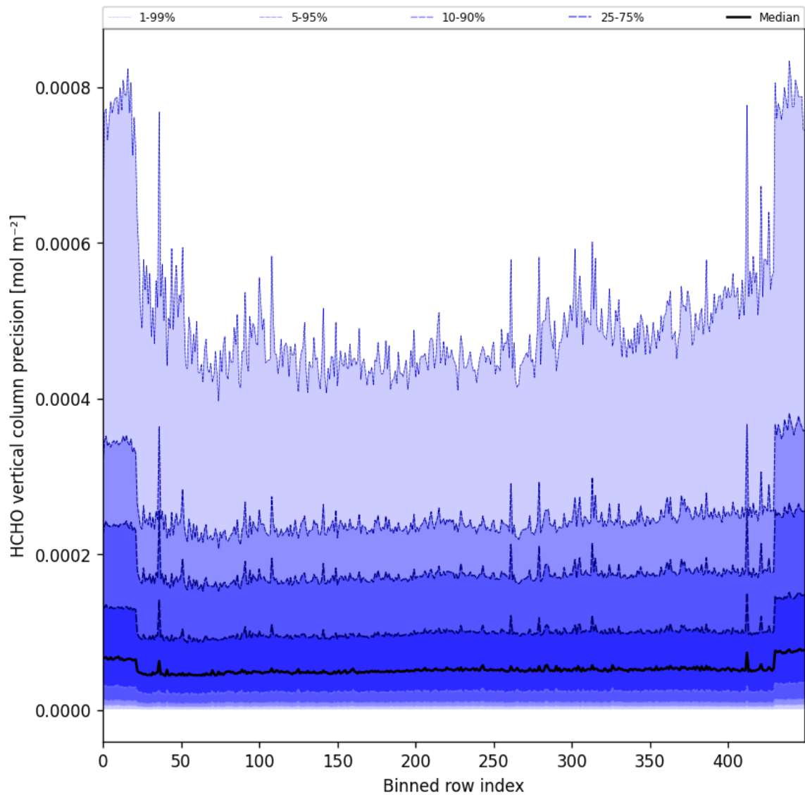
Figure 50: Along track statistics of “HCHO vertical column precision” for 2025-01-14 to 2025-01-16
