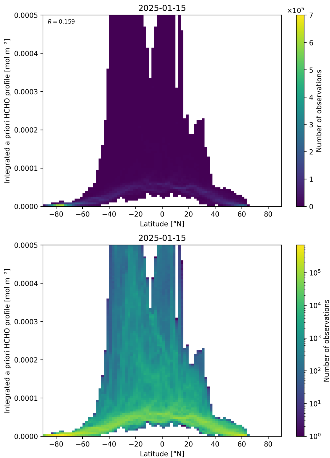
Figure 166: Scatter density plot of “Latitude” against “Integrated a priori HCHO profile” for 2025-01-14 to 2025-01-16.
