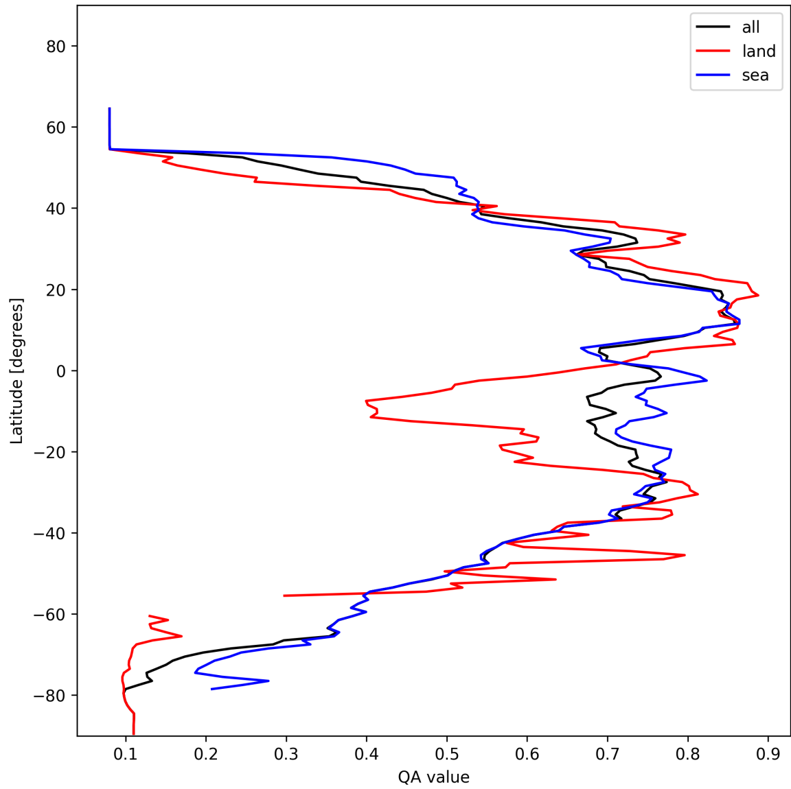
Figure 20: Zonal average of “QA value” for 2025-01-14 to 2025-01-16.
