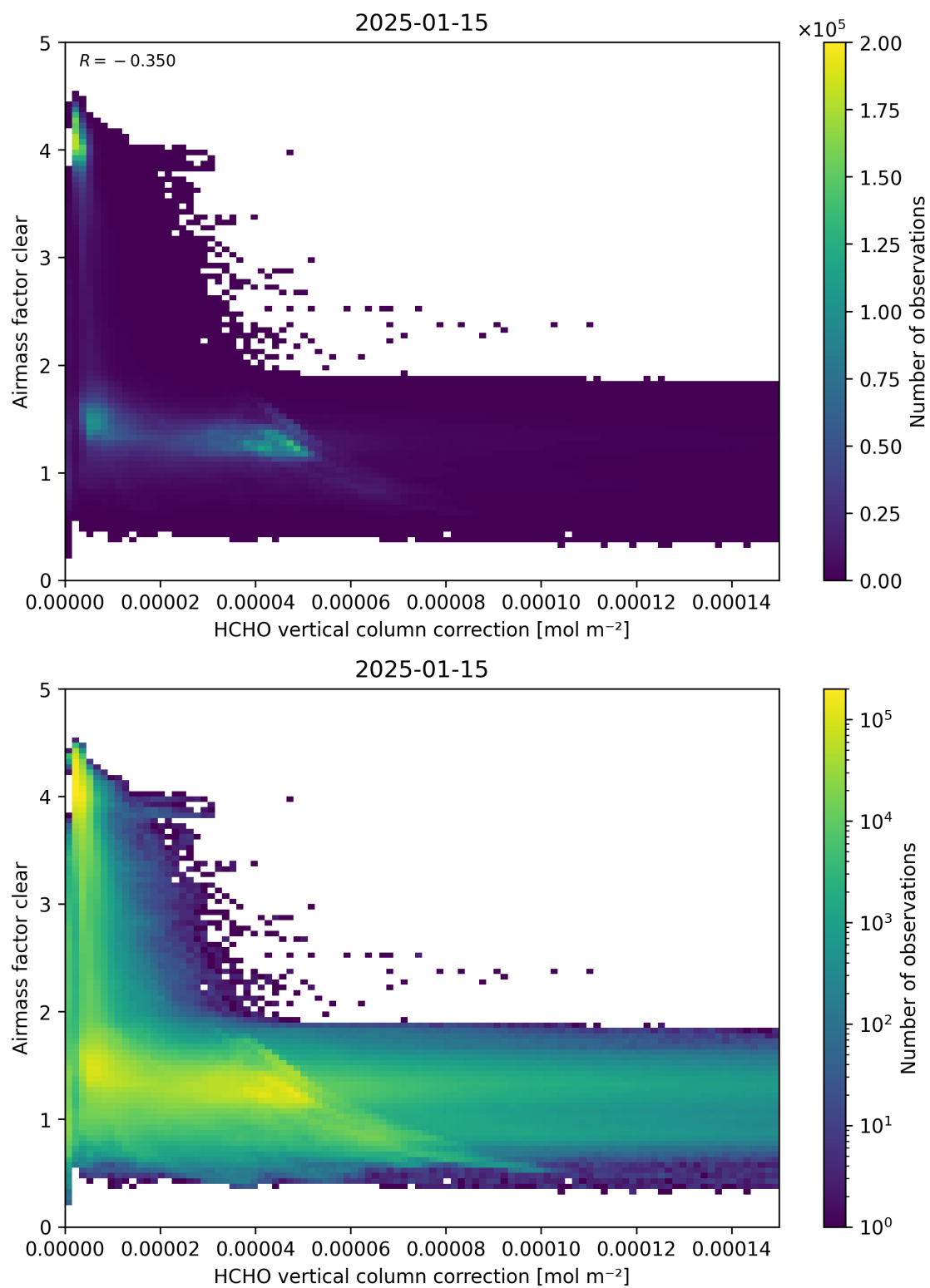
Figure 115: Scatter density plot of “HCHO vertical column correction” against “Airmass factor clear” for 2025-01-14 to 2025-01-16.
