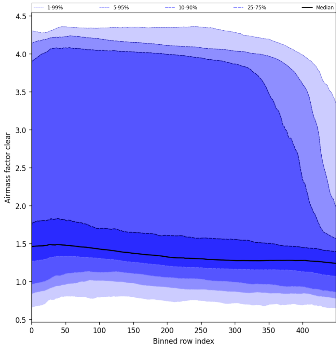
Figure 56: Along track statistics of “Airmass factor clear” for 2025-01-14 to 2025-01-16
