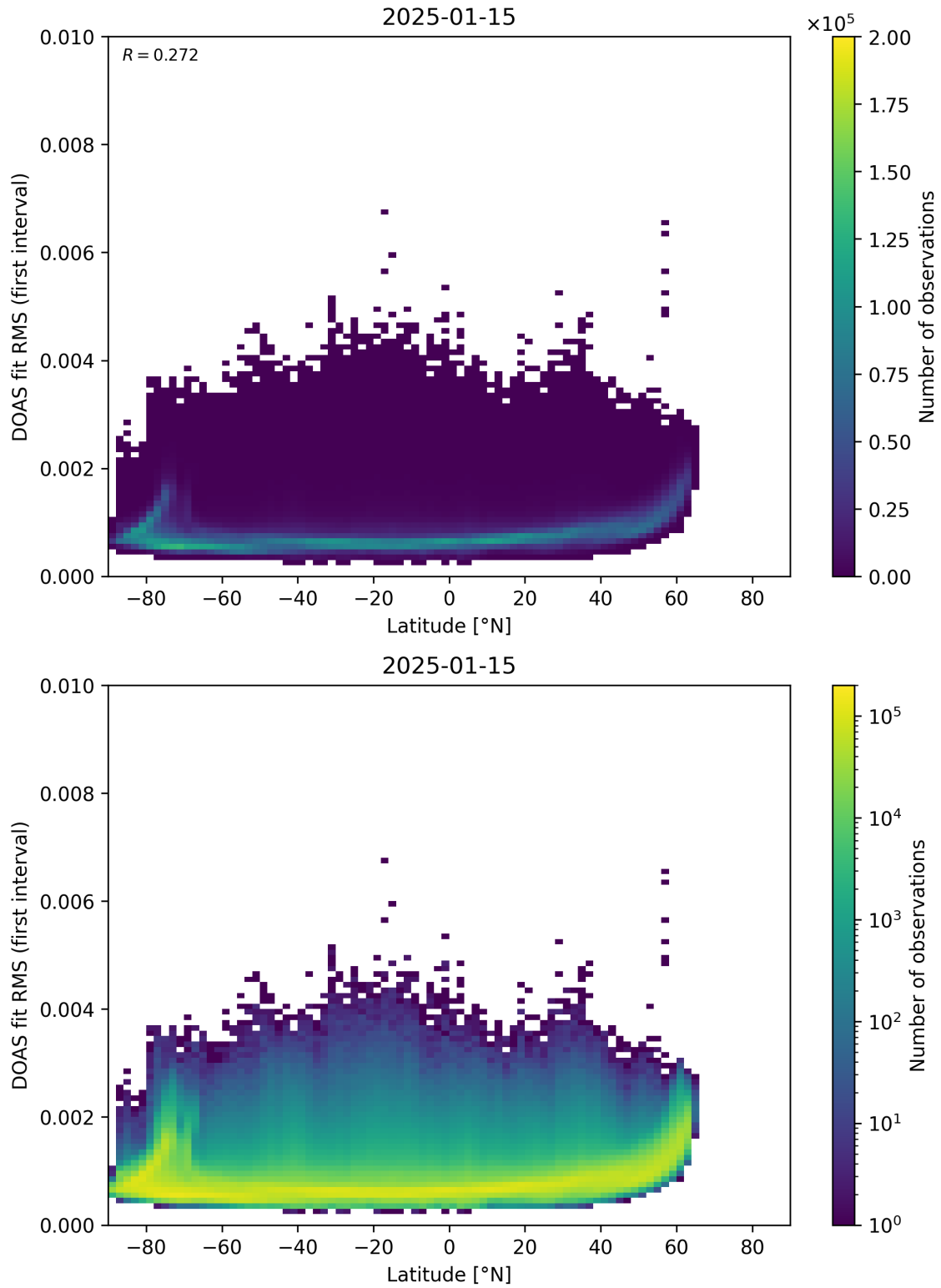
Figure 153: Scatter density plot of “Latitude” against “DOAS fit RMS (first interval)” for 2025-01-14 to 2025-01-16.
