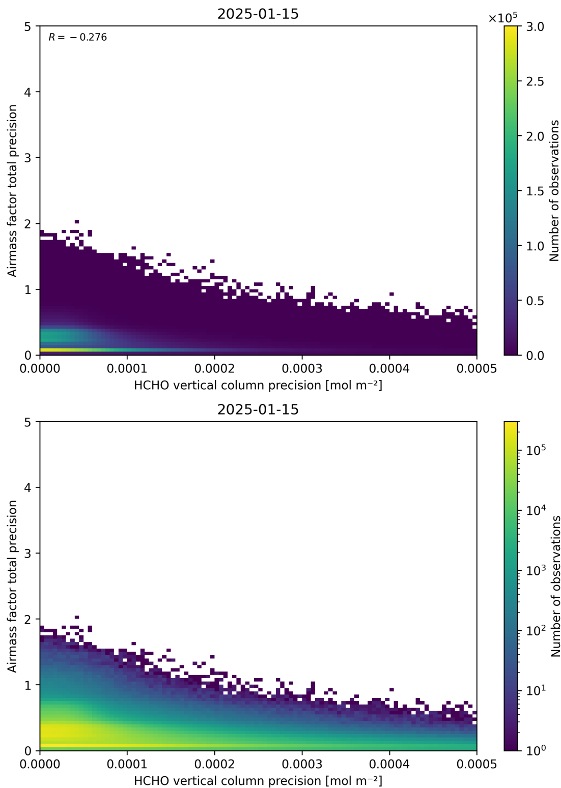
Figure 145: Scatter density plot of “HCHO vertical column precision” against “Airmass factor total precision” for 2025-01-14 to 2025-01-16.
