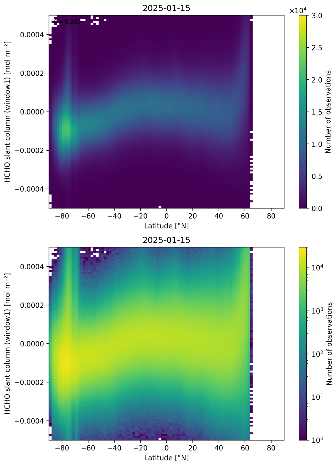
Figure 159: Scatter density plot of “Latitude” against “HCHO slant column (window1)” for 2025-01-14 to 2025-01-16.
