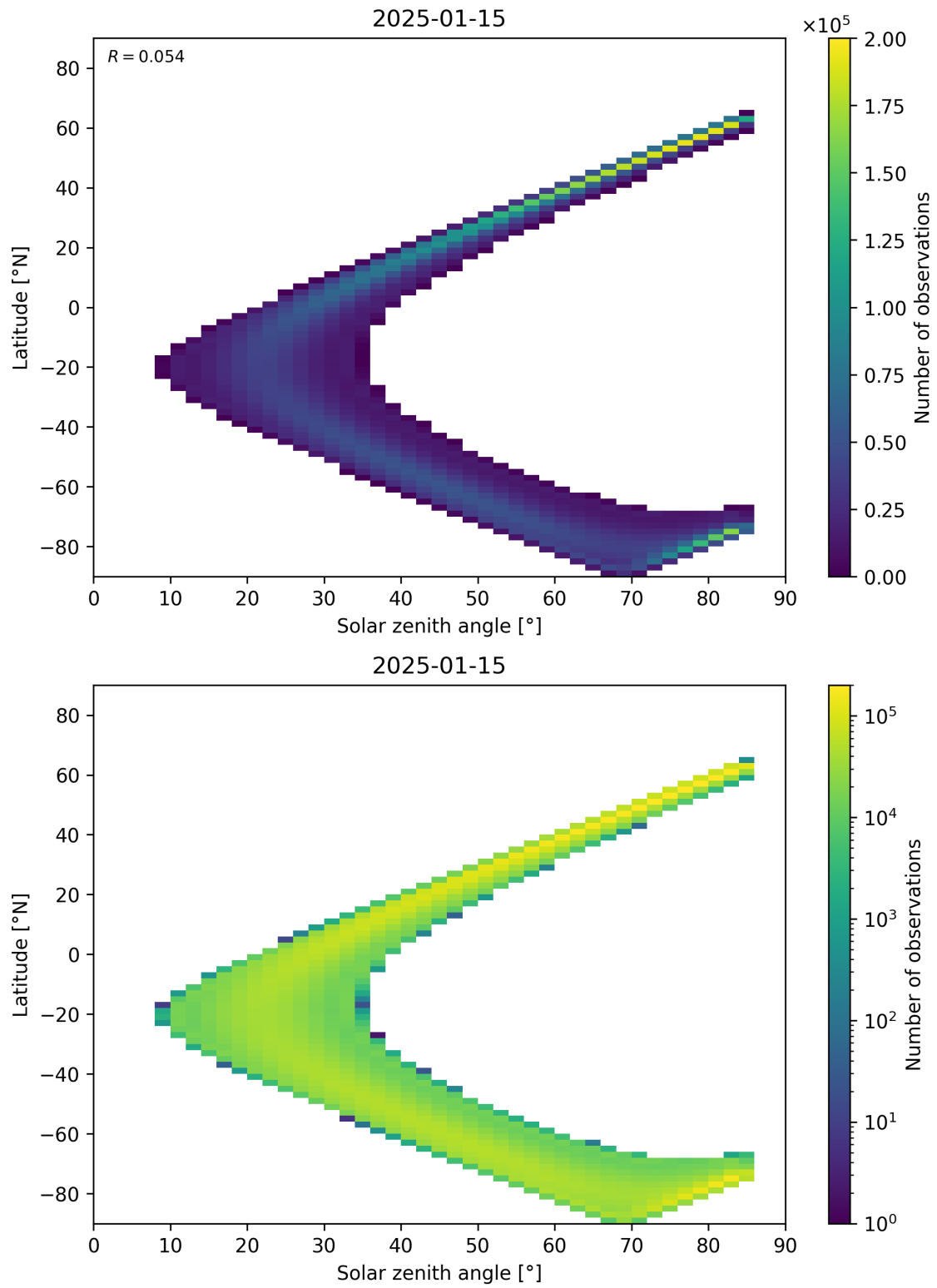
Figure 181: Scatter density plot of “Solar zenith angle” against “Latitude” for 2025-01-14 to 2025-01-16.
