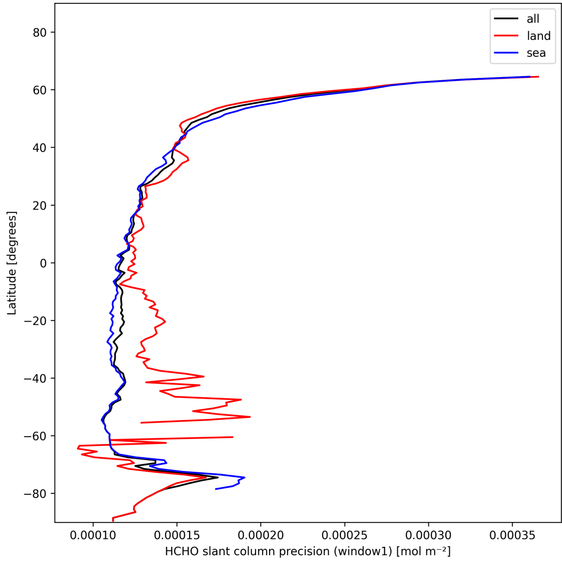
Figure 25: Zonal average of “HCHO slant column precision (window1)” for 2025-01-14 to 2025-01-16.
