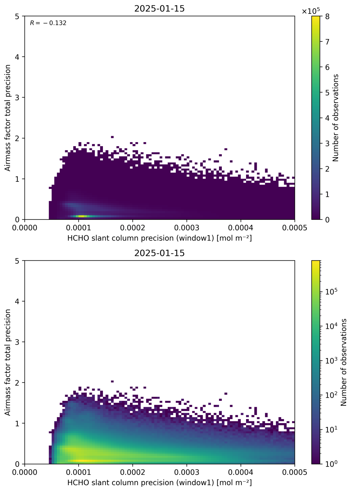
Figure 95: Scatter density plot of “HCHO slant column precision (window1)” against “Airmass factor total precision” for 2025-01-14 to 2025-01-16.
