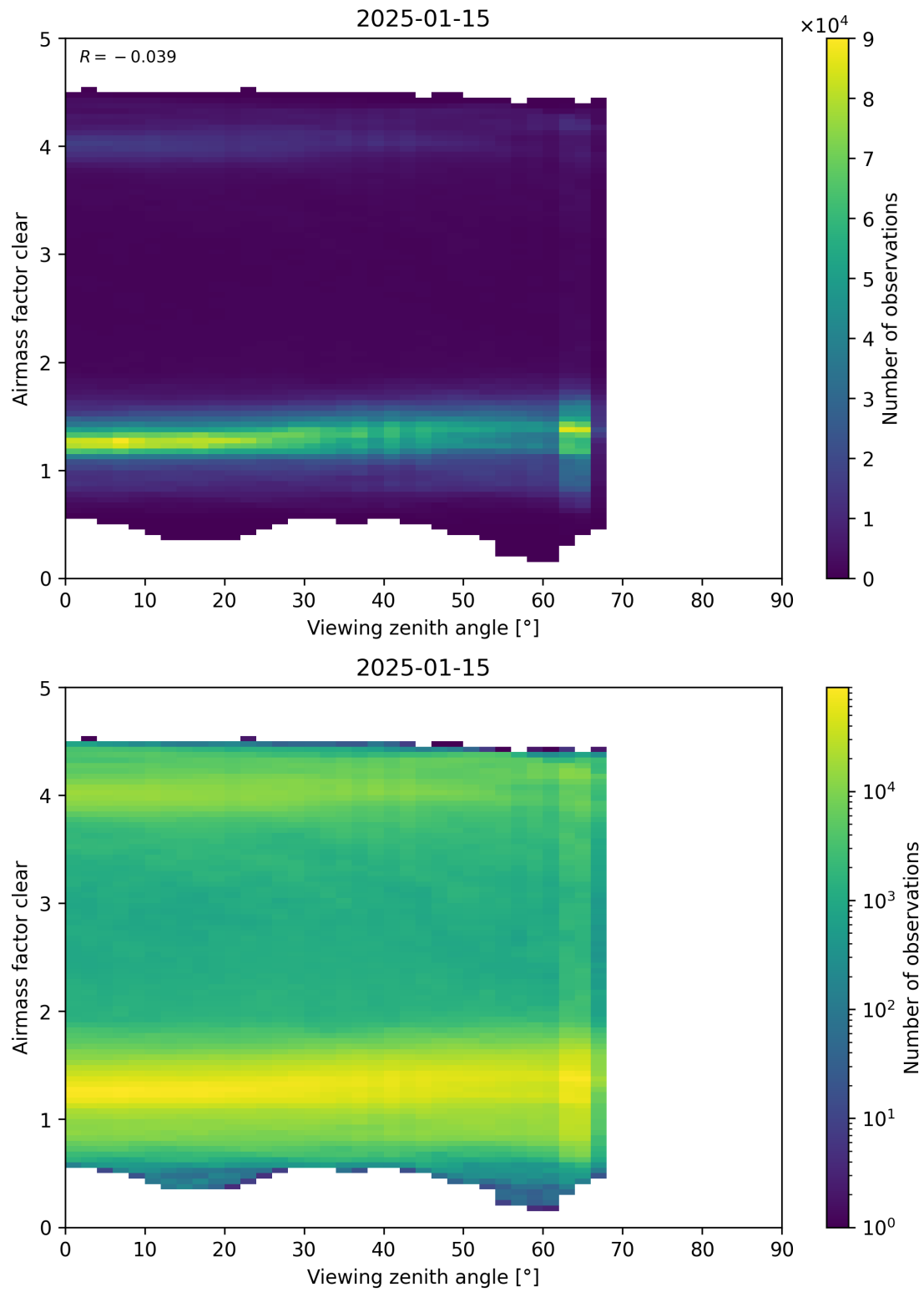
Figure 185: Scatter density plot of “Viewing zenith angle” against “Airmass factor clear” for 2025-01-14 to 2025-01-16.
