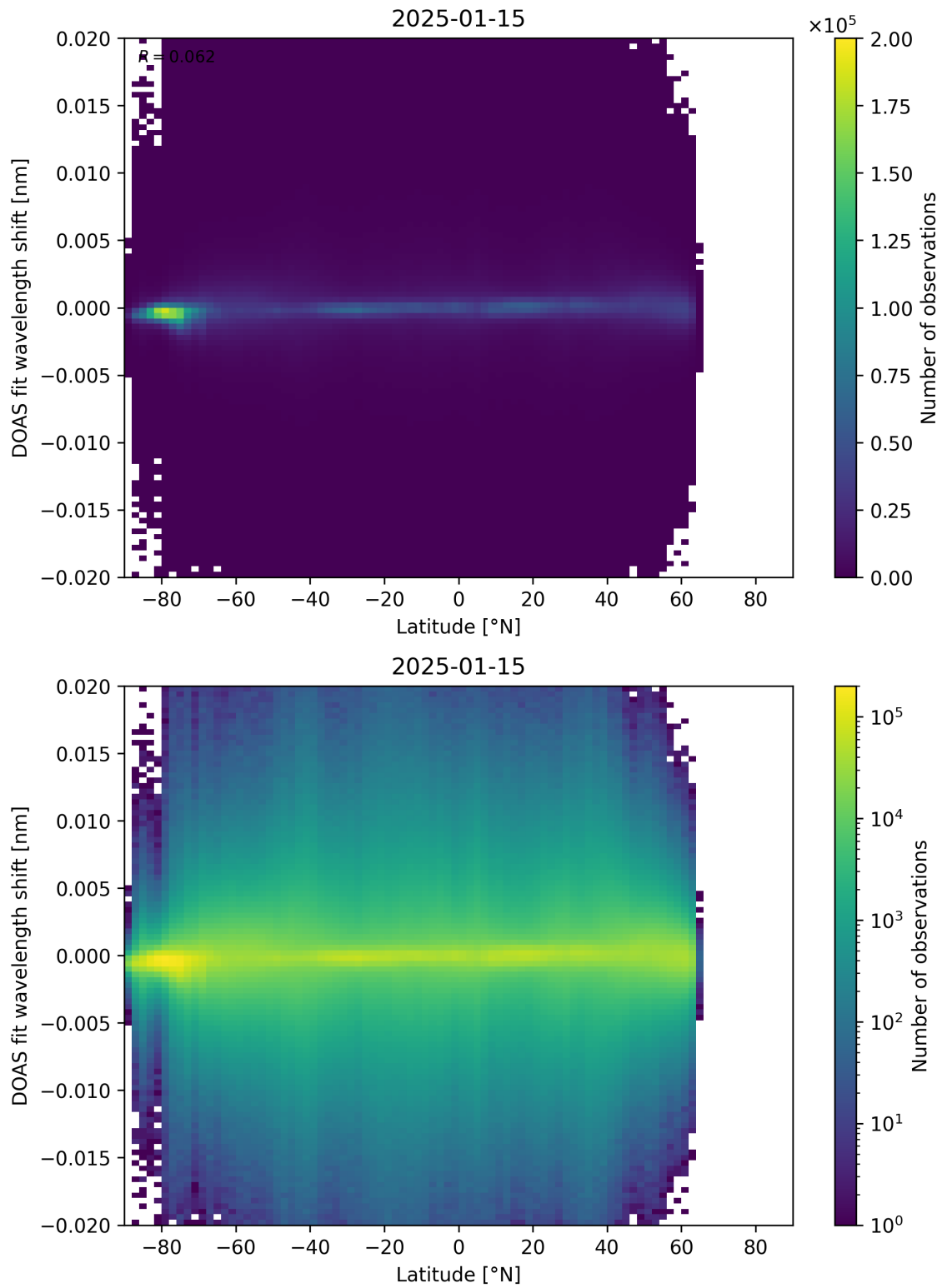
Figure 154: Scatter density plot of “Latitude” against “DOAS fit wavelength shift” for 2025-01-14 to 2025-01-16.
