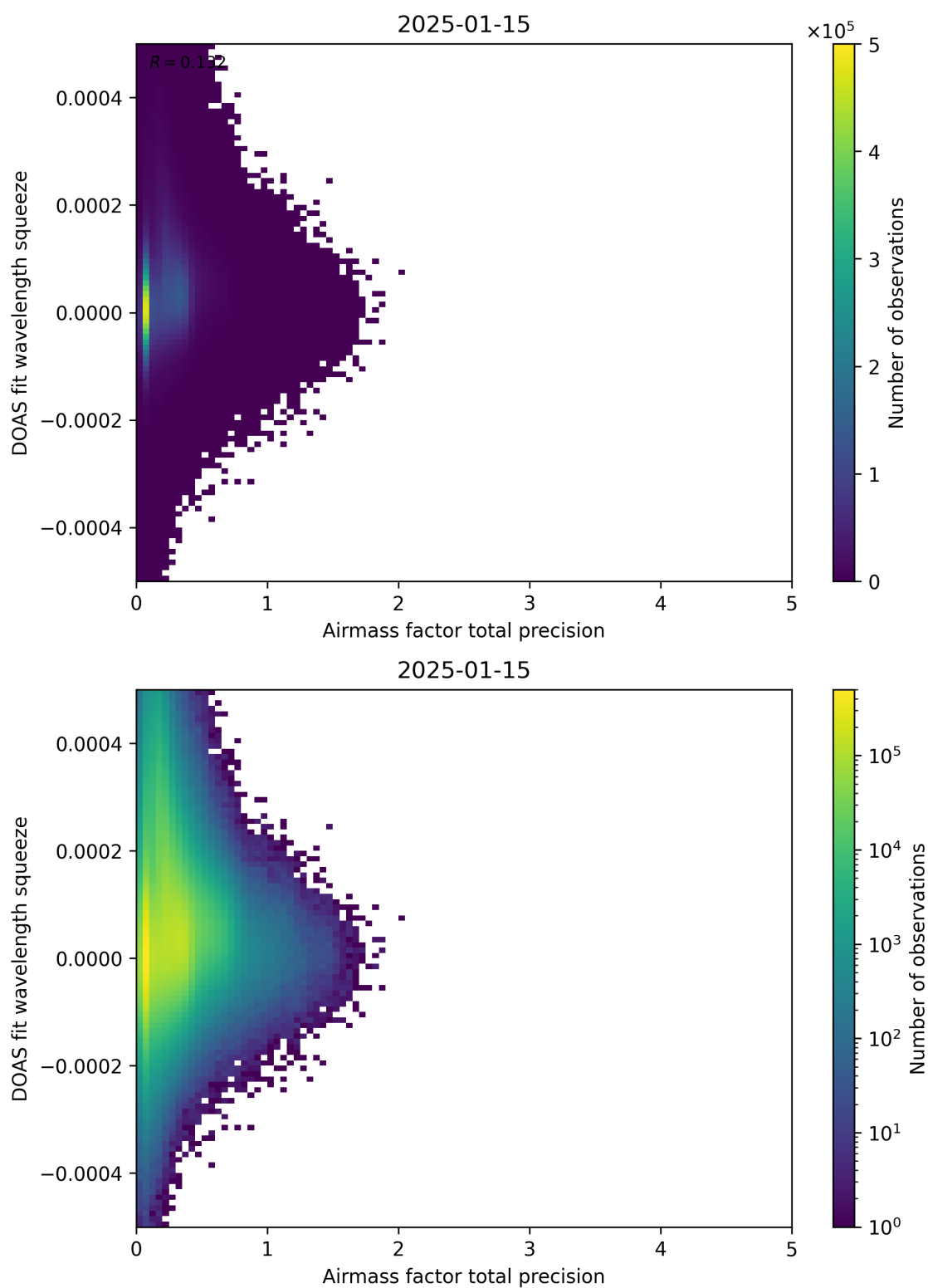
Figure 107: Scatter density plot of “Airmass factor total precision” against “DOAS fit wavelength squeeze” for 2025-01-14 to 2025-01-16.
