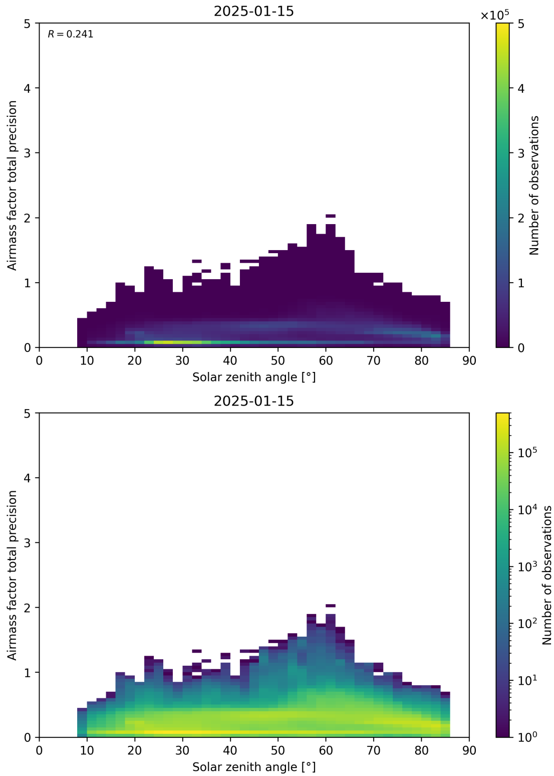
Figure 176: Scatter density plot of “Solar zenith angle” against “Airmass factor total precision” for 2025-01-14 to 2025-01-16.
