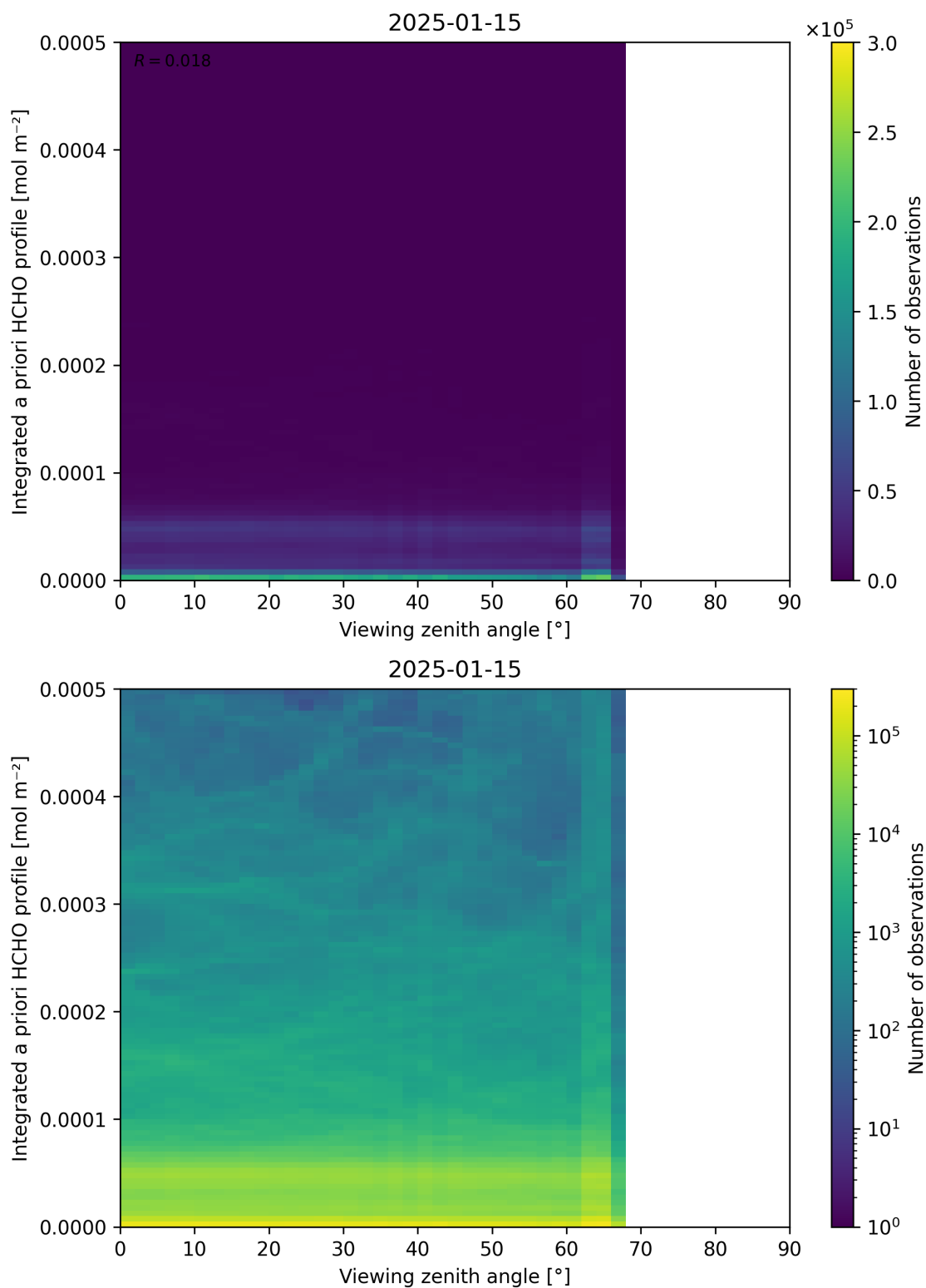
Figure 195: Scatter density plot of “Viewing zenith angle” against “Integrated a priori HCHO profile” for 2025-01-14 to 2025-01-16.
