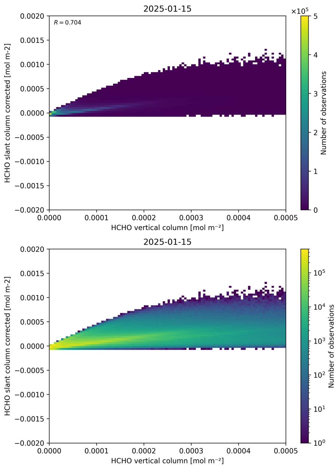
Figure 127: Scatter density plot of “HCHO vertical column” against “HCHO slant column corrected” for 2025-01-14 to 2025-01-16.
