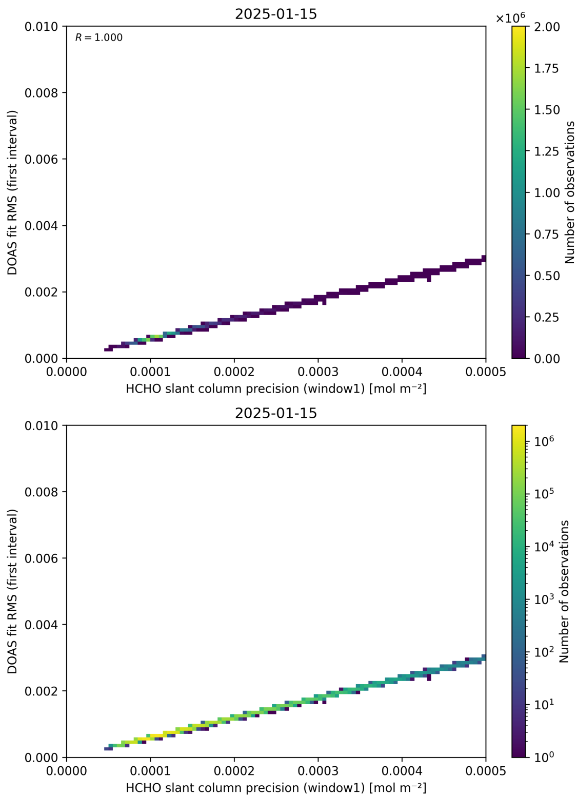
Figure 88: Scatter density plot of “HCHO slant column precision (window1)” against “DOAS fit RMS (first interval)” for 2025-01-14 to 2025-01-16.
