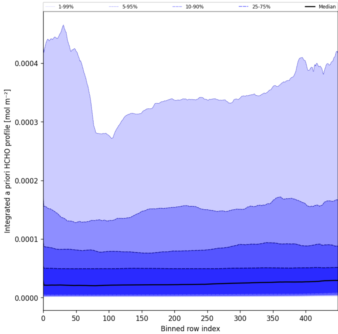
Figure 57: Along track statistics of “Integrated a priori HCHO profile” for 2025-01-14 to 2025-01-16
