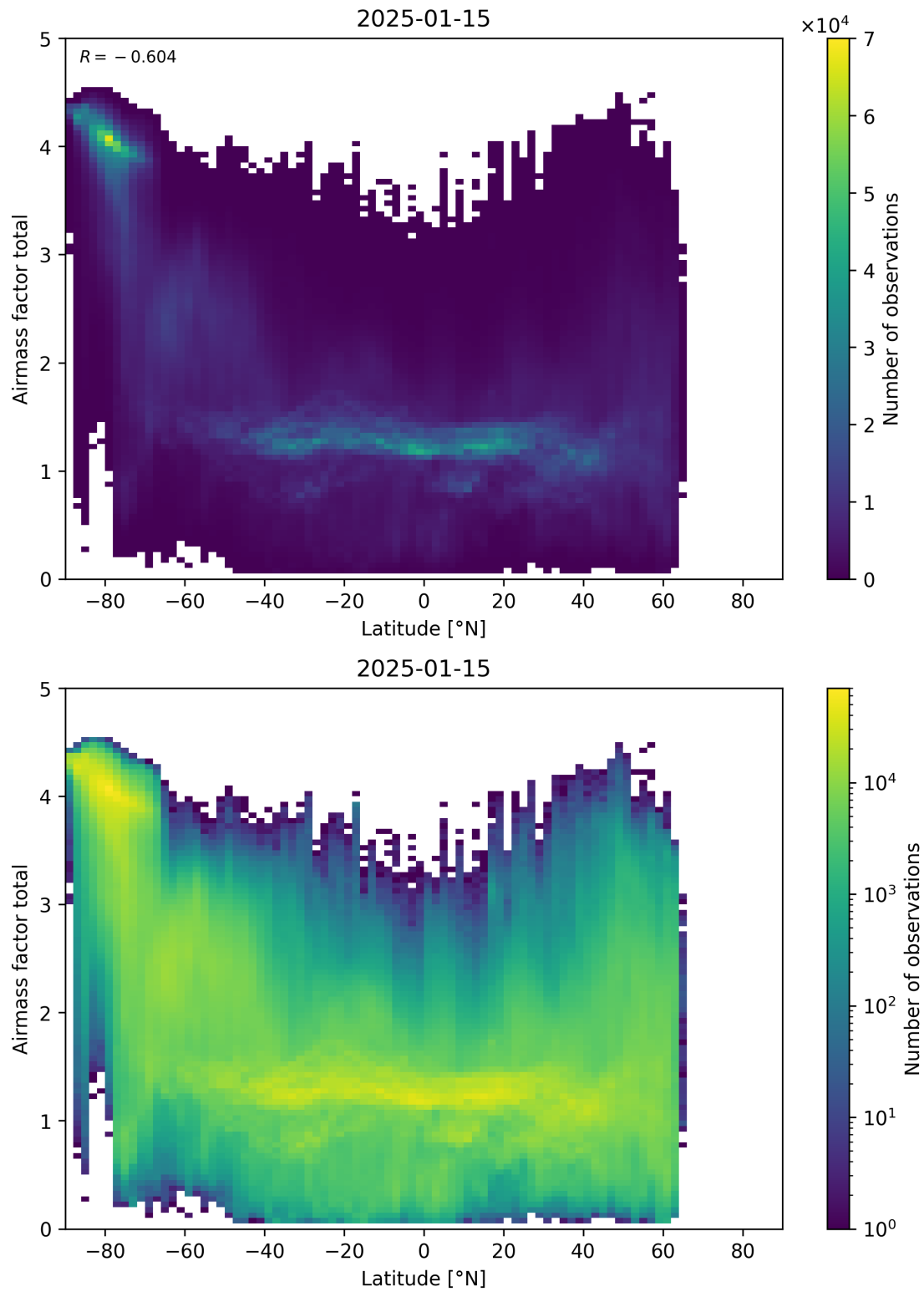
Figure 161: Scatter density plot of “Latitude” against “Airmass factor total” for 2025-01-14 to 2025-01-16.
