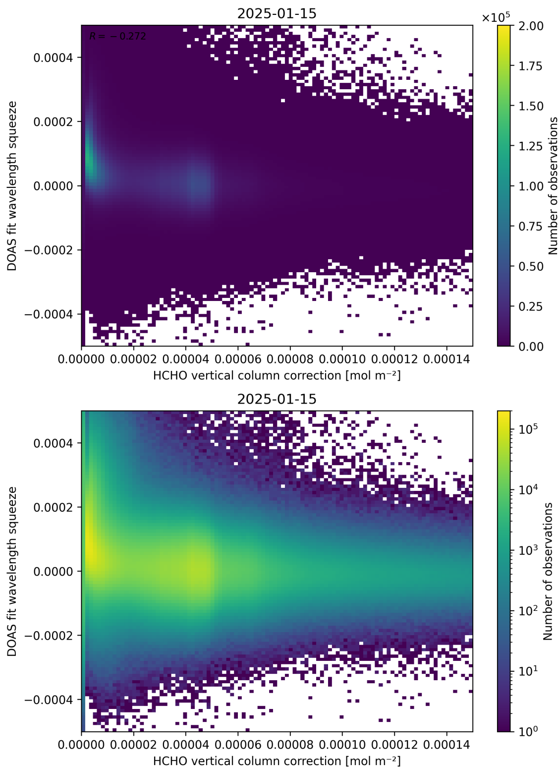
Figure 114: Scatter density plot of “HCHO vertical column correction” against “DOAS fit wavelength squeeze” for 2025-01-14 to 2025-01-16.
