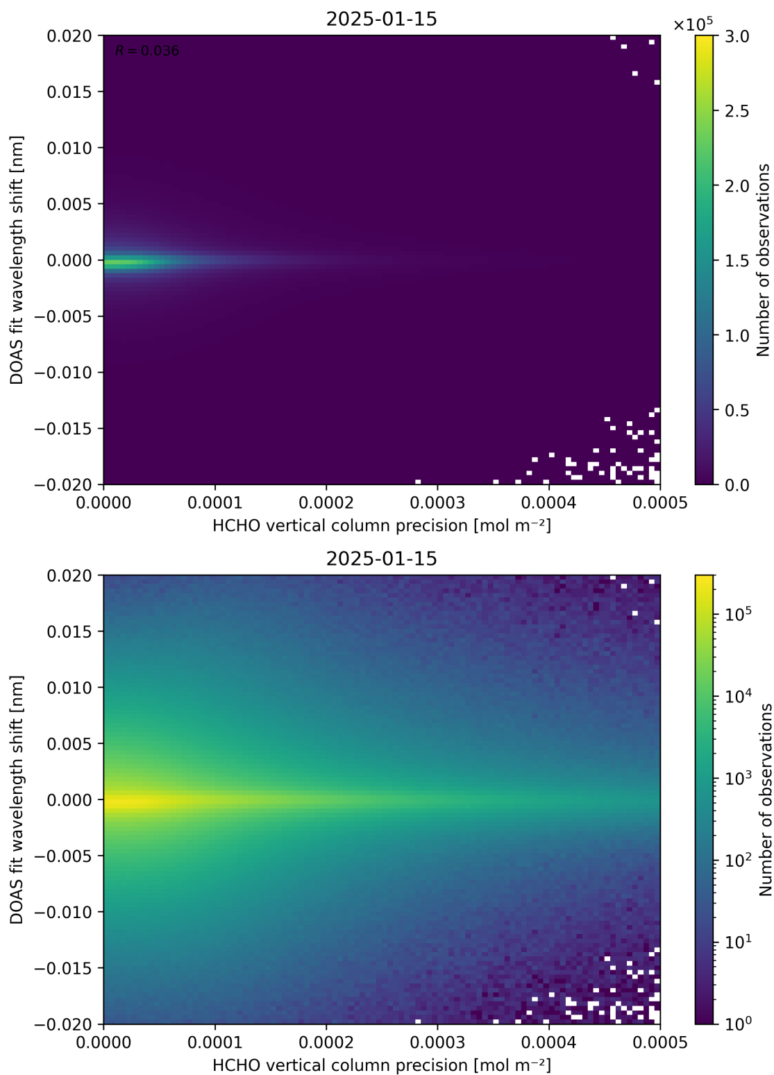
Figure 137: Scatter density plot of “HCHO vertical column precision” against “DOAS fit wavelength shift” for 2025-01-14 to 2025-01-16.
