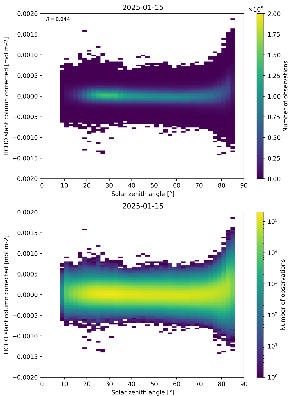
Figure 171: Scatter density plot of “Solar zenith angle” against “HCHO slant column corrected” for 2025-01-14 to 2025-01-16.
