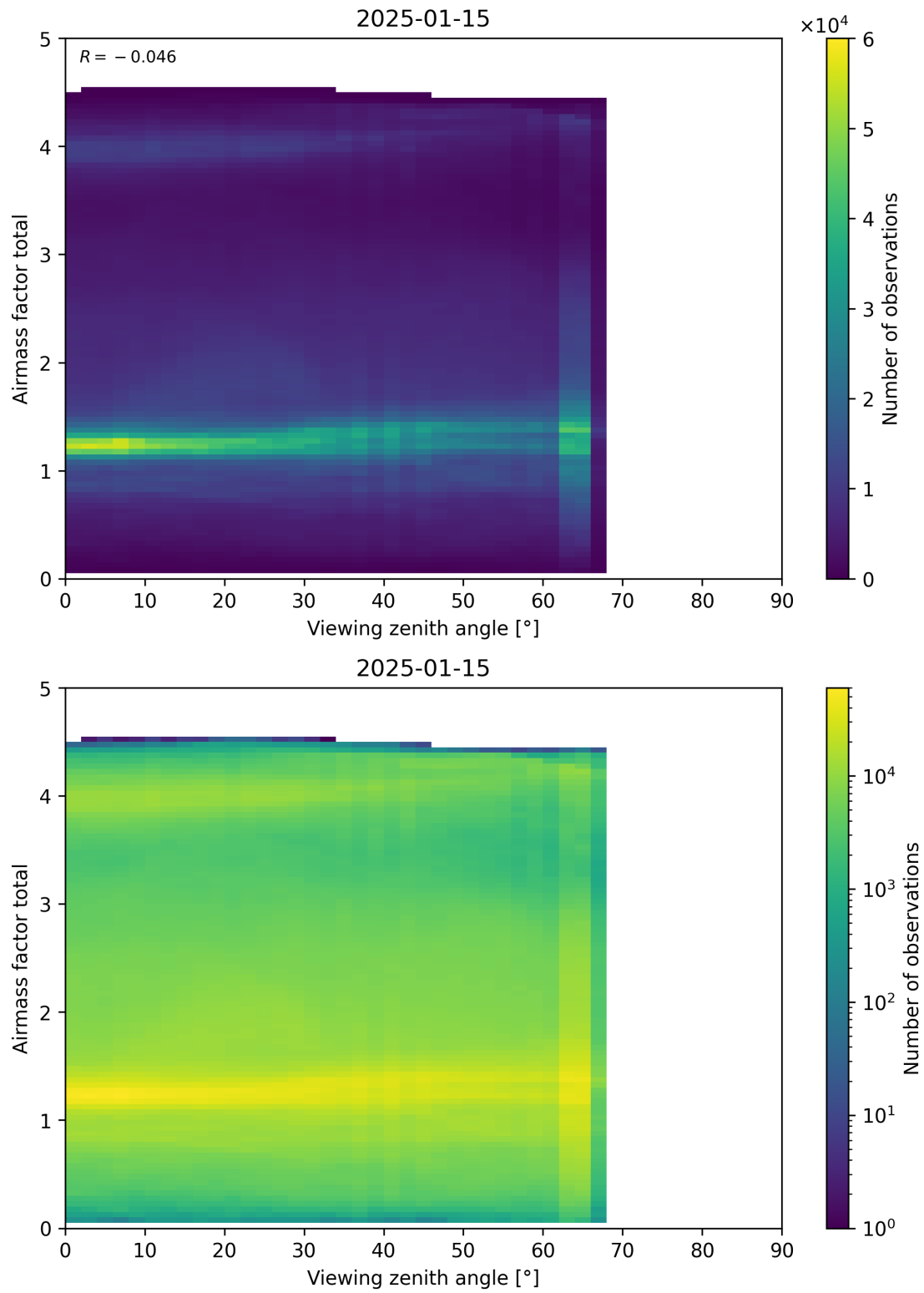
Figure 190: Scatter density plot of “Viewing zenith angle” against “Airmass factor total” for 2025-01-14 to 2025-01-16.
