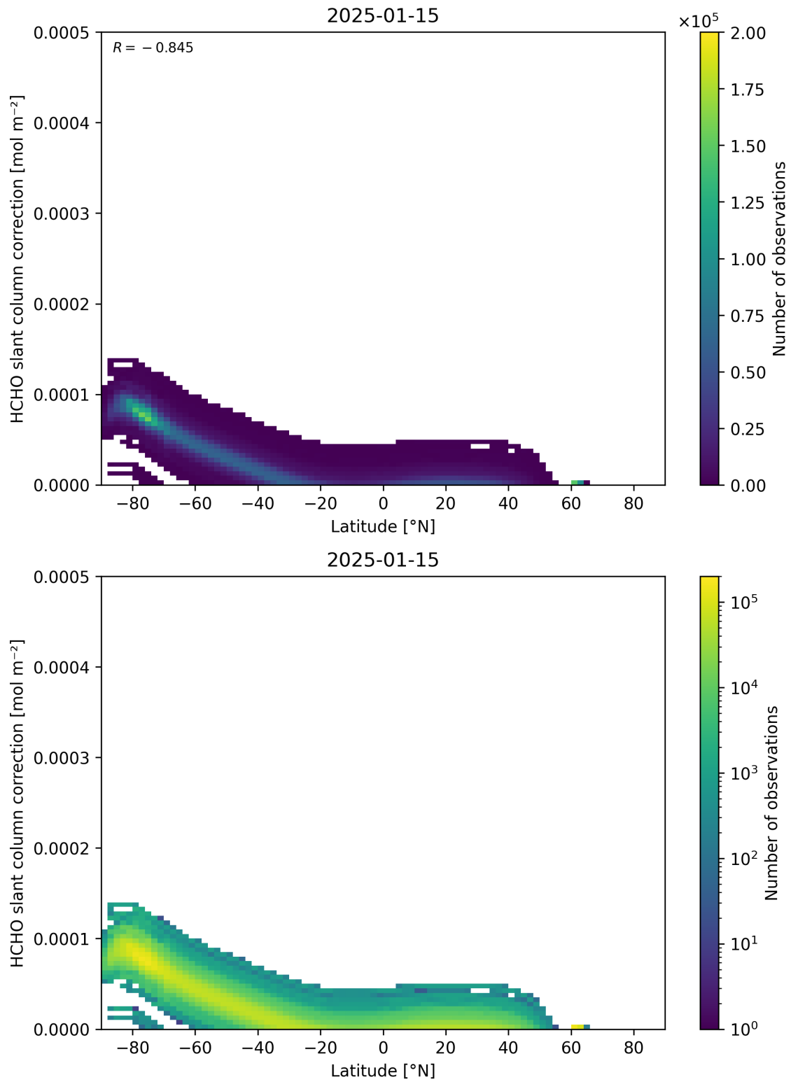
Figure 158: Scatter density plot of “Latitude” against “HCHO slant column correction” for 2025-01-14 to 2025-01-16.
