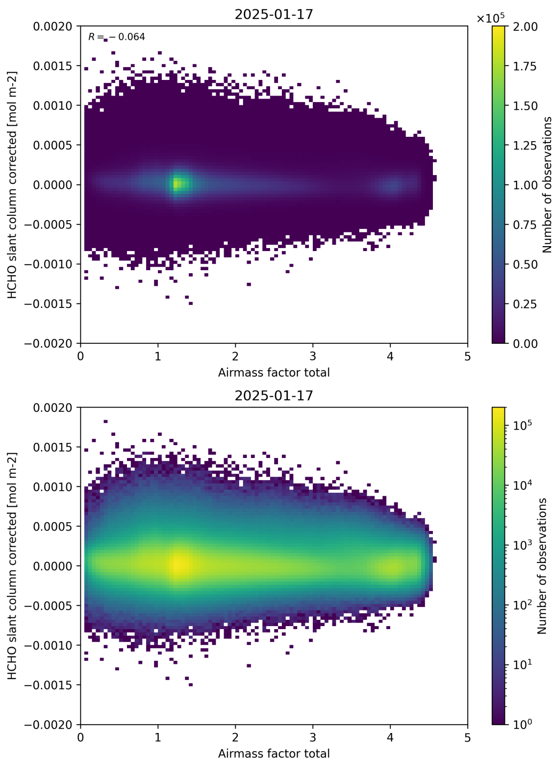
Figure 101: Scatter density plot of “Airmass factor total” against “HCHO slant column corrected” for 2025-01-17 to 2025-01-18.
