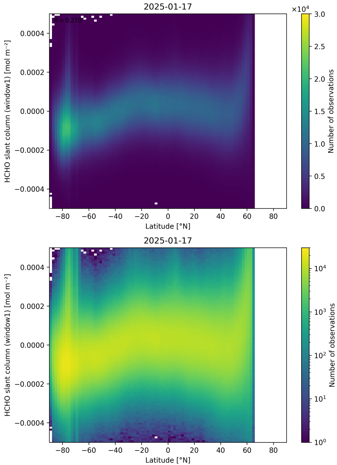
Figure 159: Scatter density plot of “Latitude” against “HCHO slant column (window1)” for 2025-01-17 to 2025-01-18.
