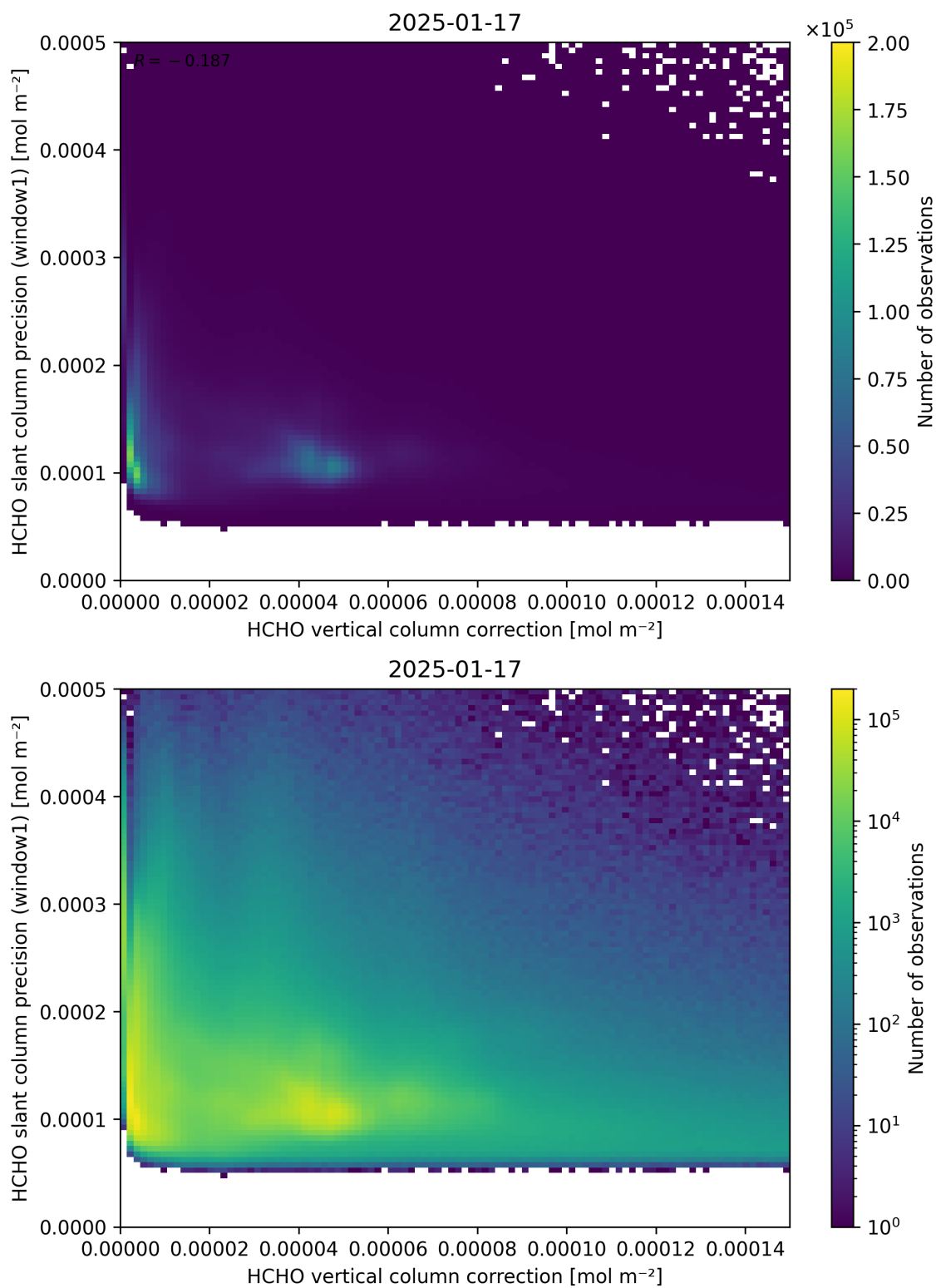
Figure 119: Scatter density plot of “HCHO vertical column correction” against “HCHO slant column precision (window1)” for 2025-01-17 to 2025-01-18.
