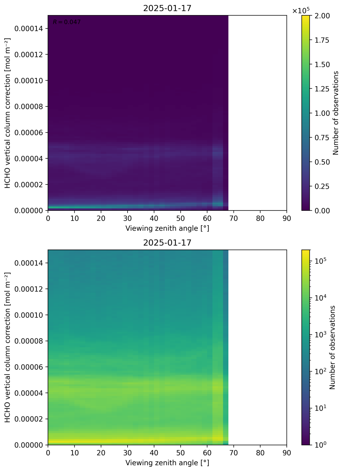
Figure 193: Scatter density plot of “Viewing zenith angle” against “HCHO vertical column correction” for 2025-01-17 to 2025-01-18.
