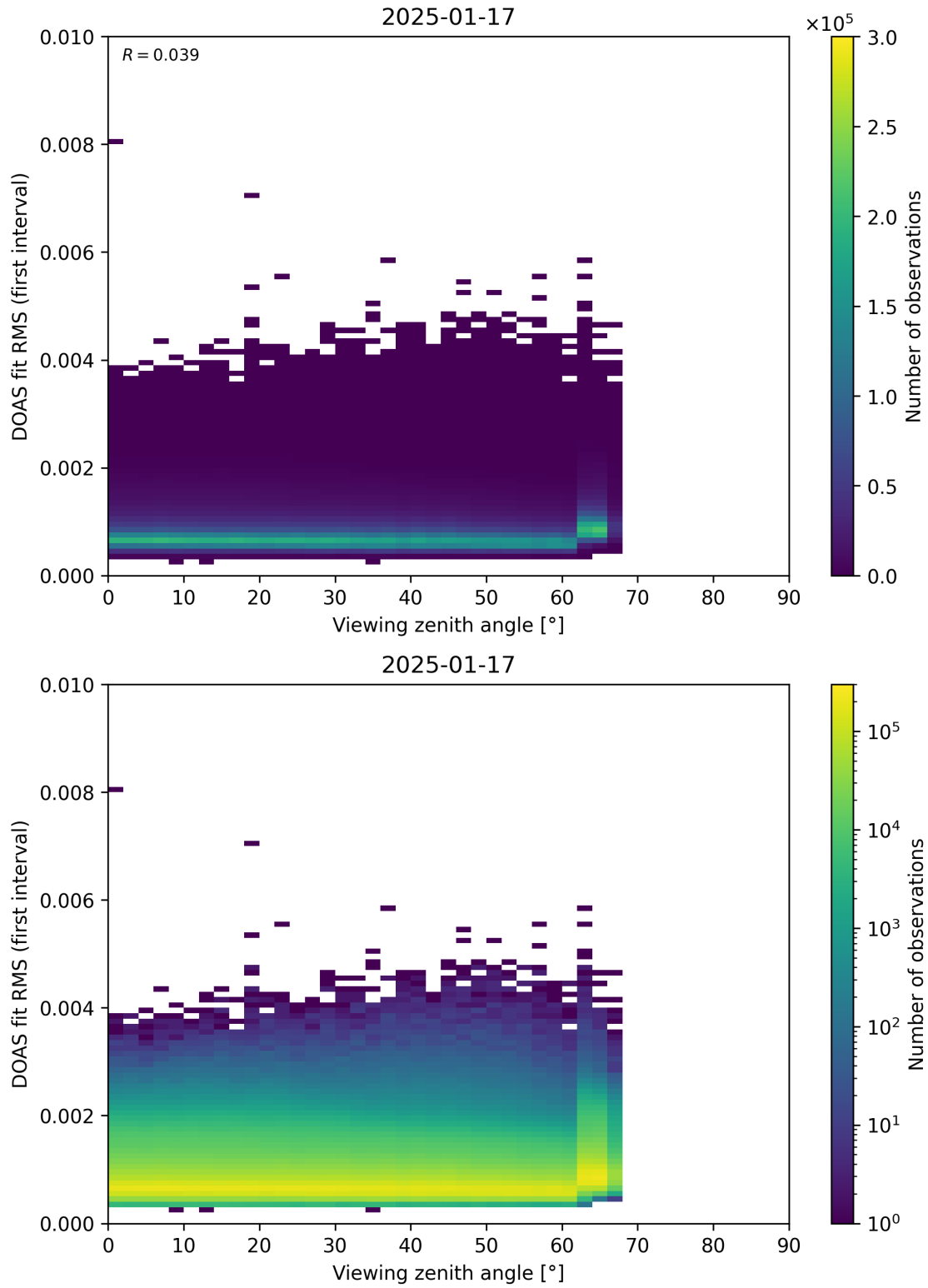
Figure 182: Scatter density plot of “Viewing zenith angle” against “DOAS fit RMS (first interval)” for 2025-01-17 to 2025-01-18.
