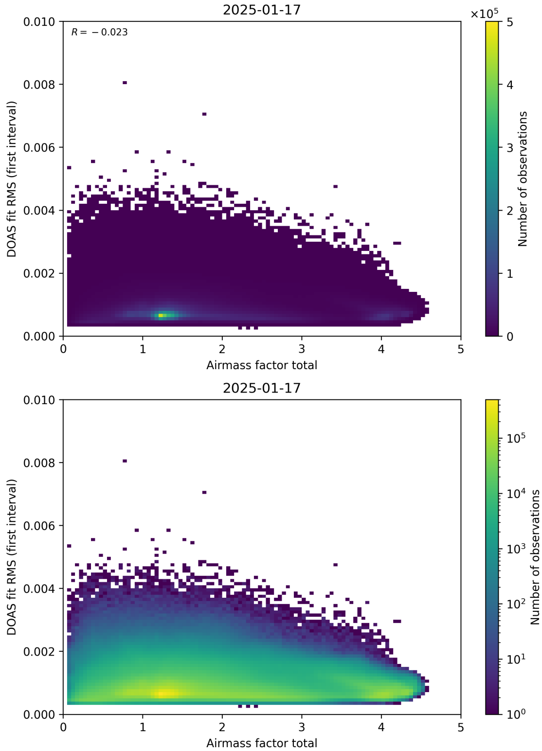
Figure 97: Scatter density plot of “Airmass factor total” against “DOAS fit RMS (first interval)” for 2025-01-17 to 2025-01-18.
