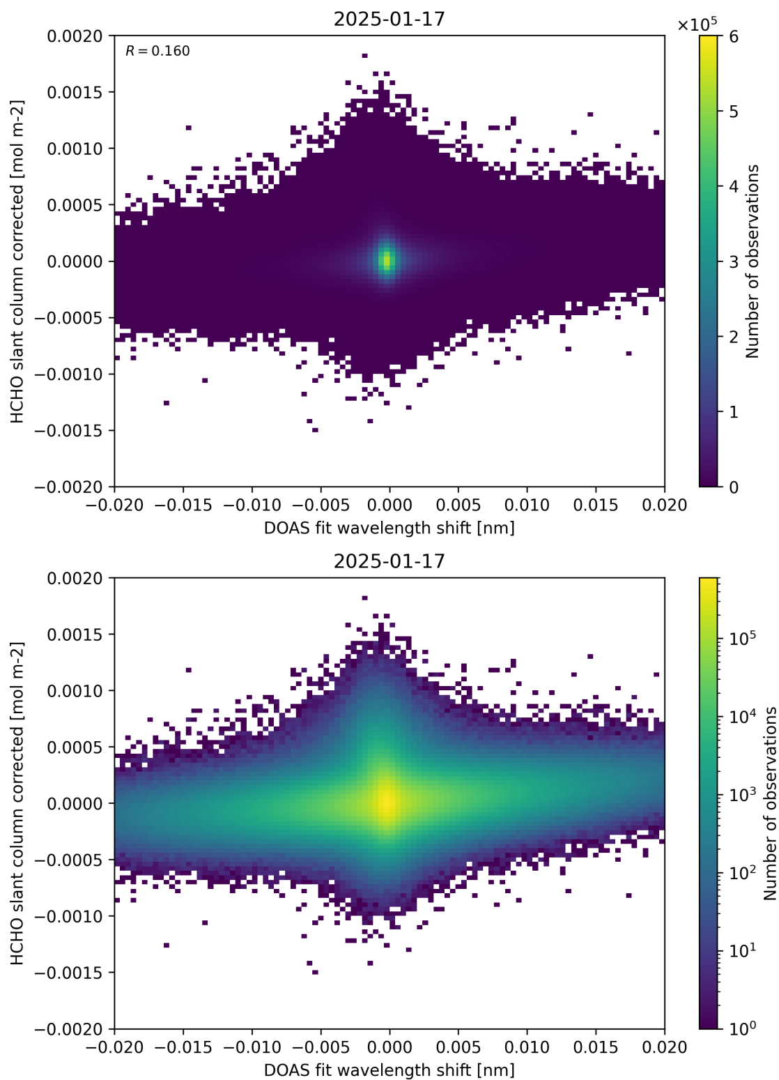
Figure 66: Scatter density plot of “DOAS fit wavelength shift” against “HCHO slant column corrected” for 2025-01-17 to 2025-01-18.
