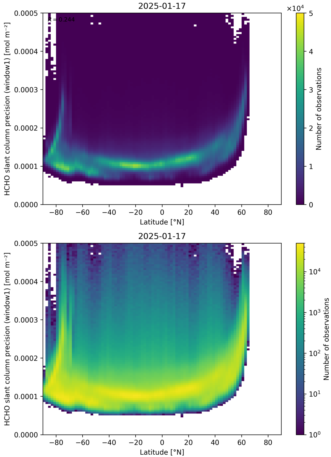
Figure 160: Scatter density plot of “Latitude” against “HCHO slant column precision (window1)” for 2025-01-17 to 2025-01-18.
