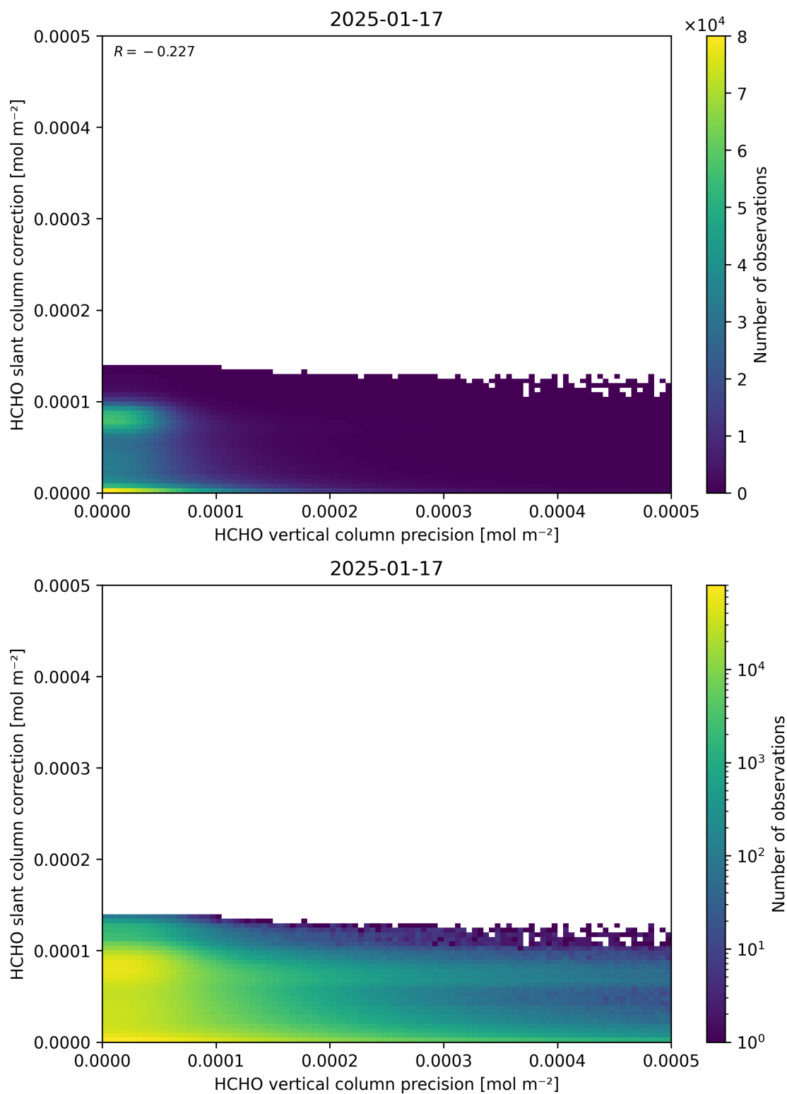
Figure 141: Scatter density plot of “HCHO vertical column precision” against “HCHO slant column correction” for 2025-01-17 to 2025-01-18.
