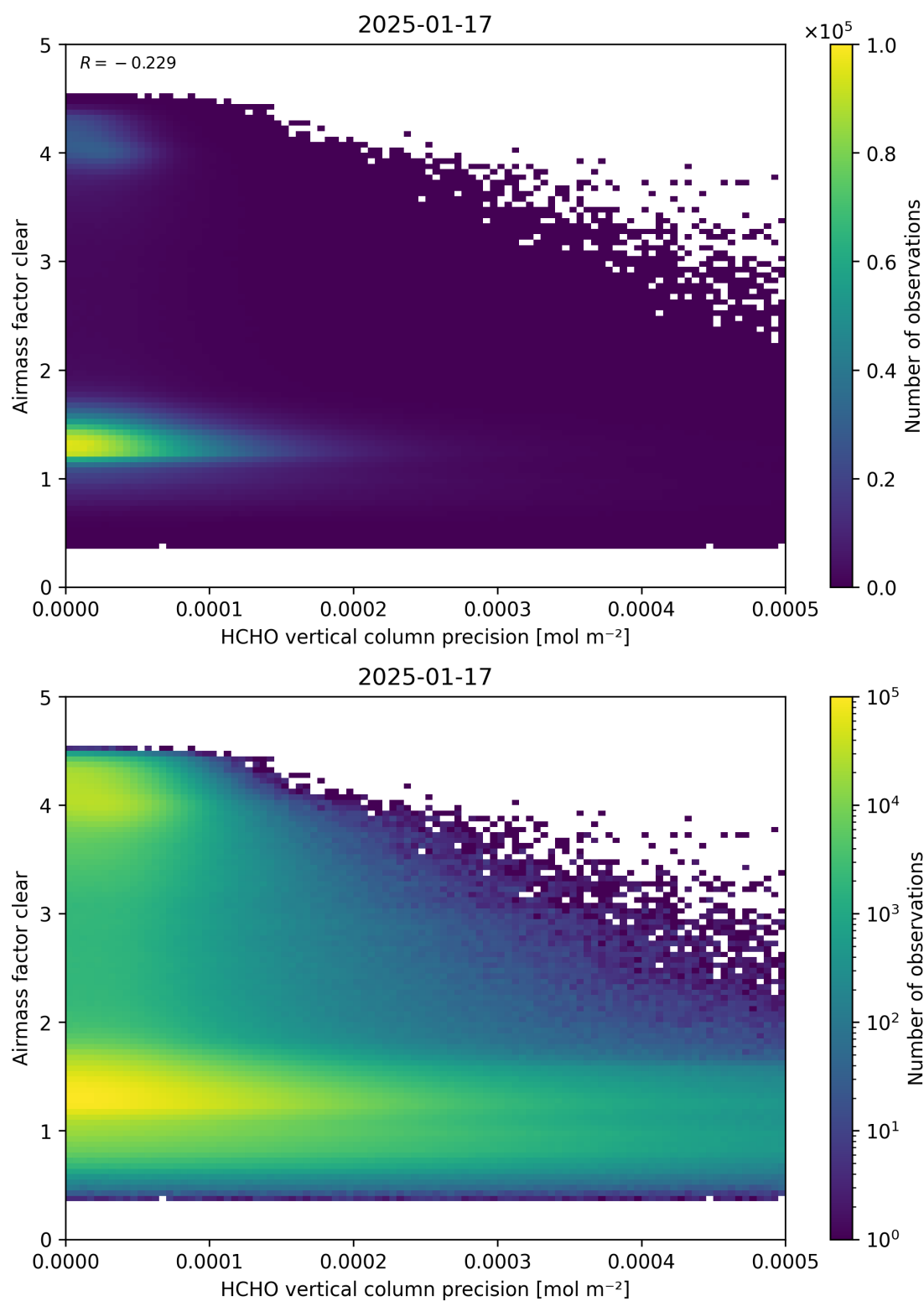
Figure 139: Scatter density plot of “HCHO vertical column precision” against “Airmass factor clear” for 2025-01-17 to 2025-01-18.
