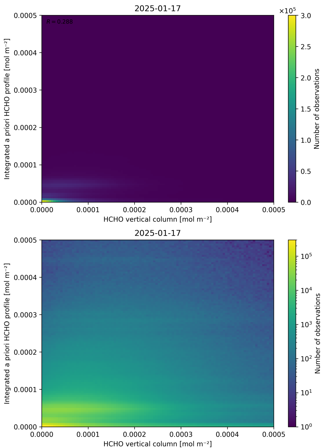
Figure 135: Scatter density plot of “HCHO vertical column” against “Integrated a priori HCHO profile” for 2025-01-17 to 2025-01-18.
