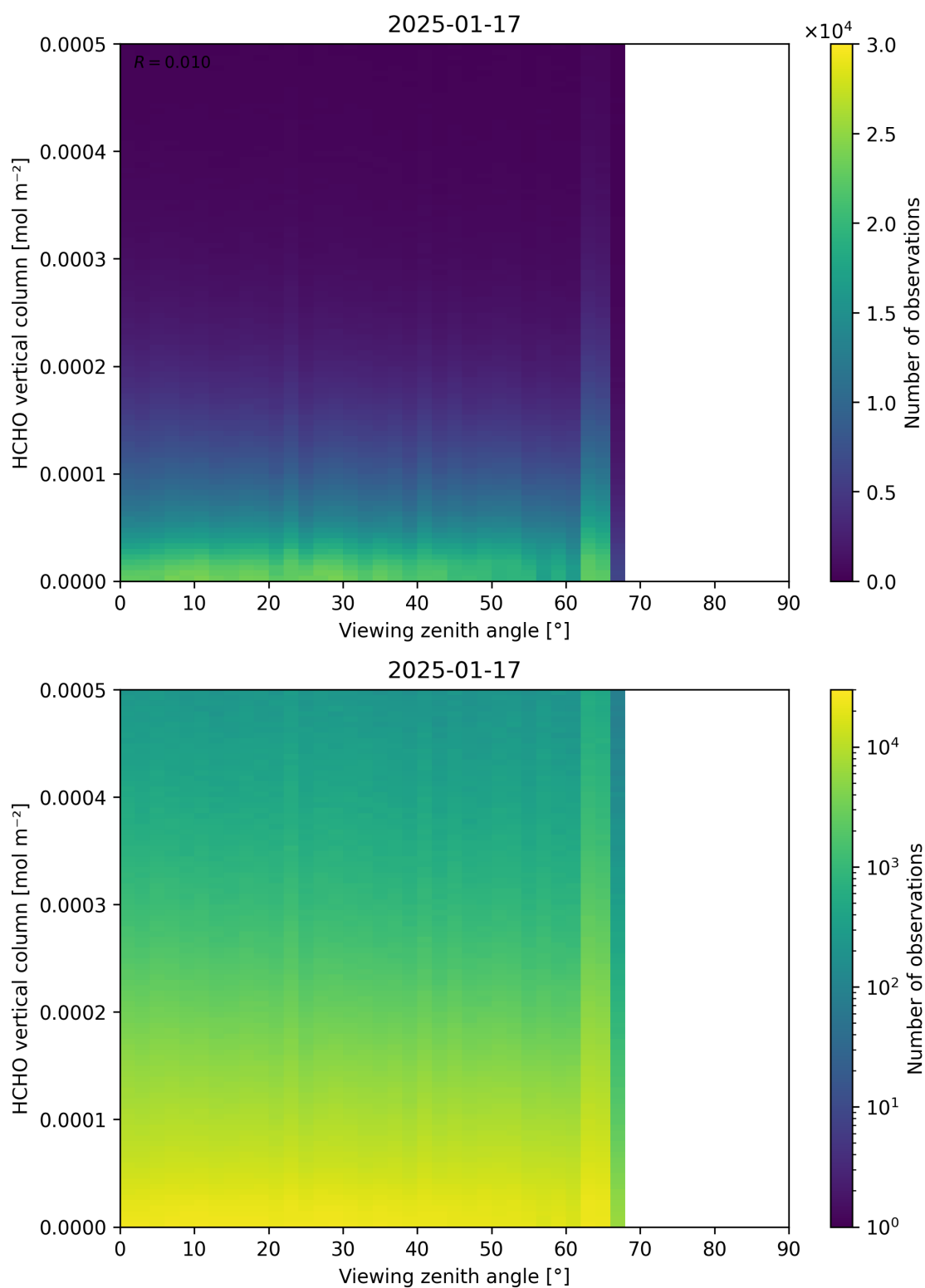
Figure 192: Scatter density plot of “Viewing zenith angle” against “HCHO vertical column” for 2025-01-17 to 2025-01-18.
