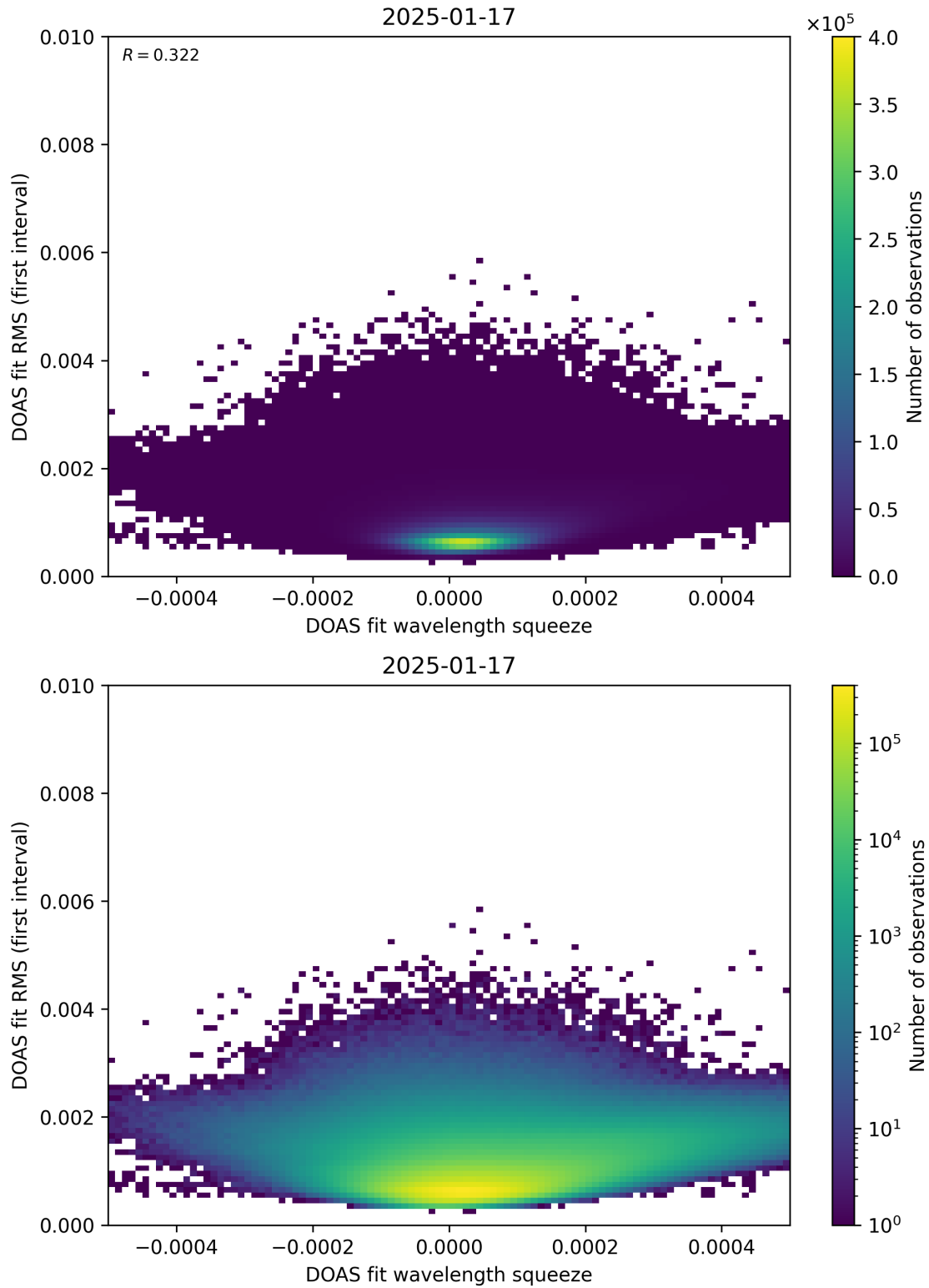
Figure 68: Scatter density plot of “DOAS fit wavelength squeeze” against “DOAS fit RMS (first interval)” for 2025-01-17 to 2025-01-18.
