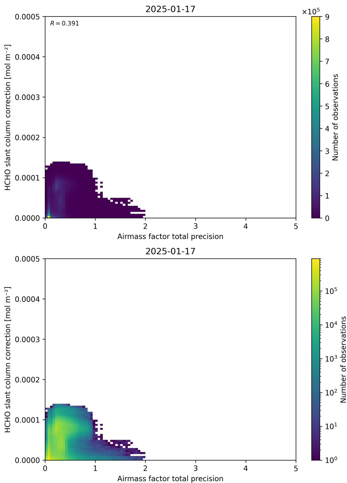
Figure 110: Scatter density plot of “Airmass factor total precision” against “HCHO slant column correction” for 2025-01-17 to 2025-01-18.
