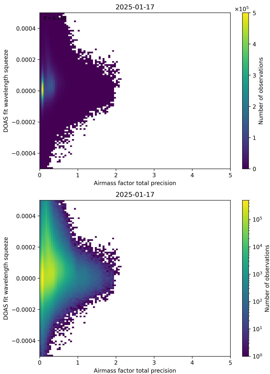
Figure 107: Scatter density plot of “Airmass factor total precision” against “DOAS fit wavelength squeeze” for 2025-01-17 to 2025-01-18.
