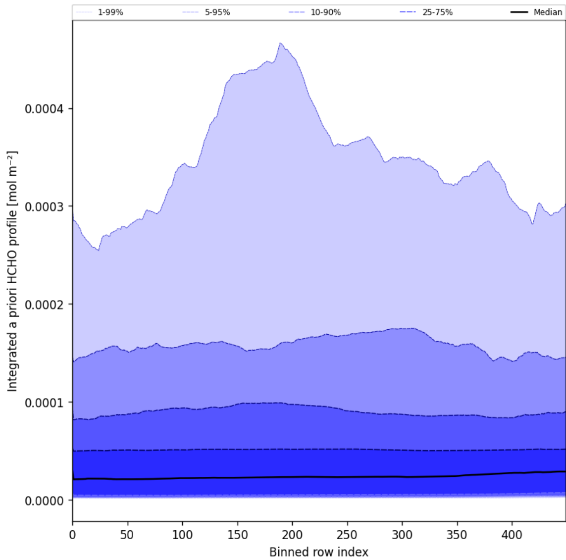
Figure 57: Along track statistics of “Integrated a priori HCHO profile” for 2025-01-17 to 2025-01-18
