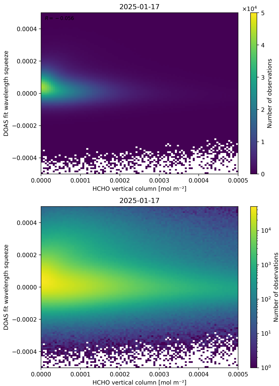
Figure 125: Scatter density plot of “HCHO vertical column” against “DOAS fit wavelength squeeze” for 2025-01-17 to 2025-01-18.
