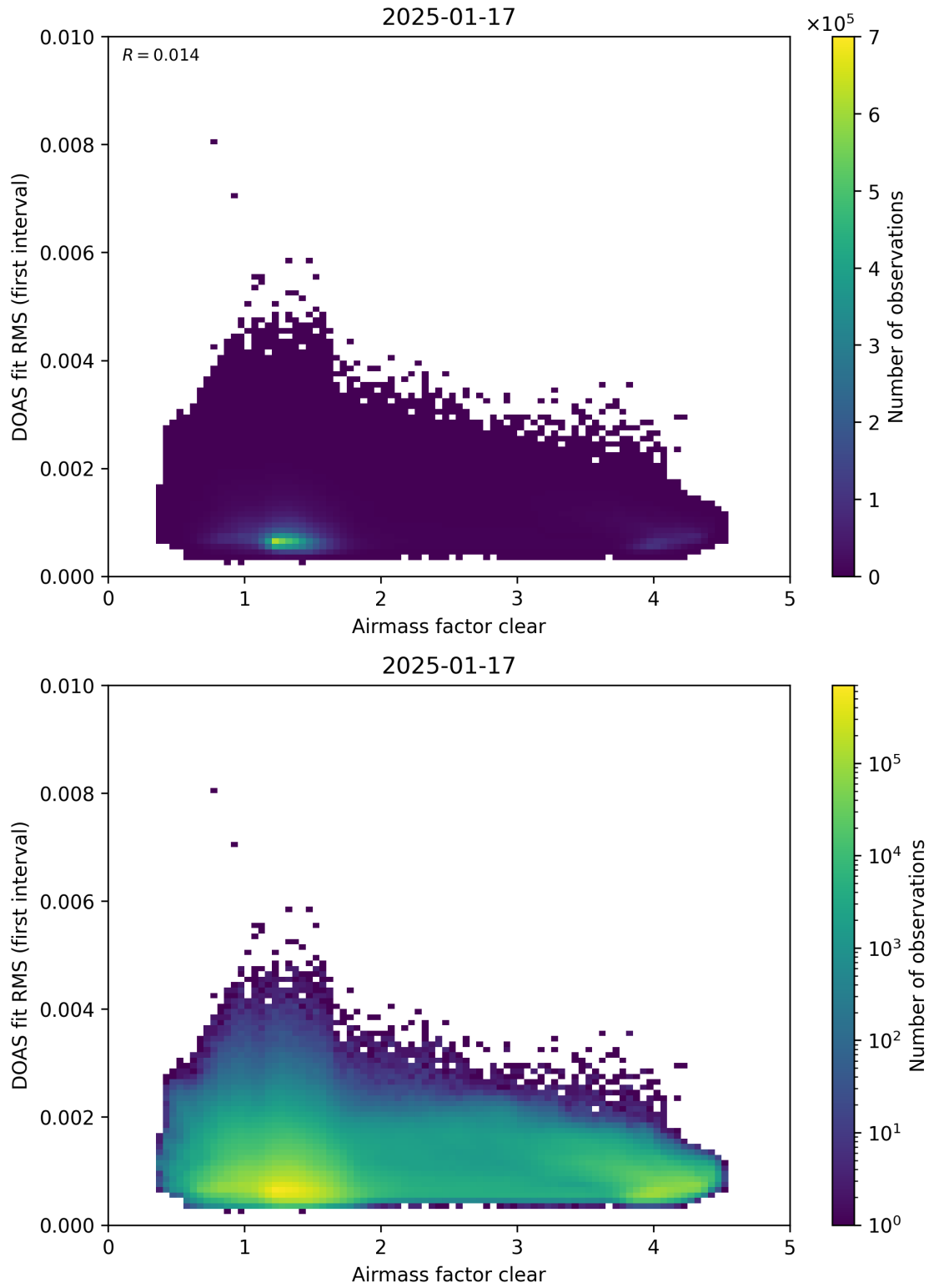
Figure 71: Scatter density plot of “Airmass factor clear” against “DOAS fit RMS (first interval)” for 2025-01-17 to 2025-01-18.
