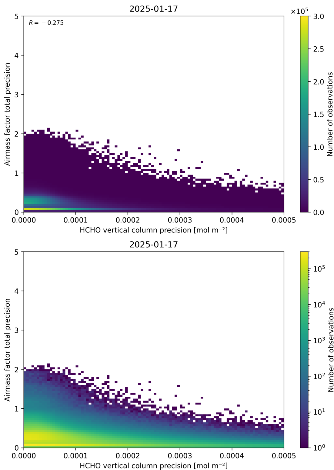
Figure 145: Scatter density plot of “HCHO vertical column precision” against “Airmass factor total precision” for 2025-01-17 to 2025-01-18.
