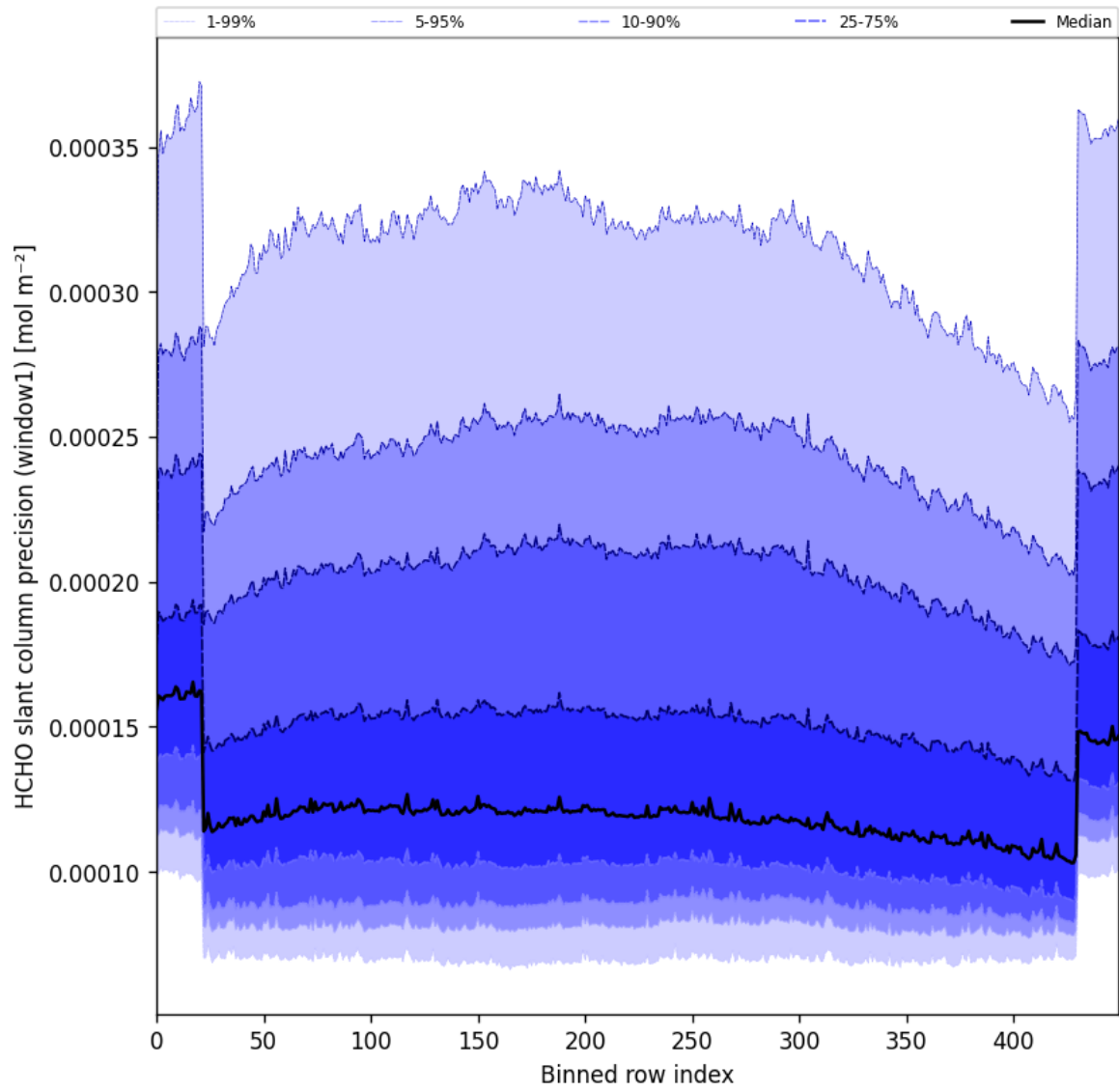
Figure 53: Along track statistics of “HCHO slant column precision (window1)” for 2025-01-17 to 2025-01-18
