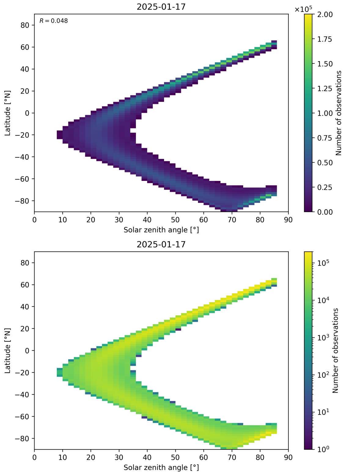
Figure 181: Scatter density plot of “Solar zenith angle” against “Latitude” for 2025-01-17 to 2025-01-18.
