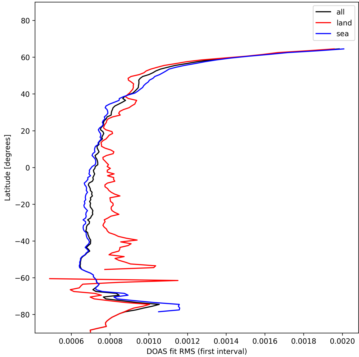
Figure 32: Zonal average of “DOAS fit RMS (first interval)” for 2025-01-17 to 2025-01-18.
