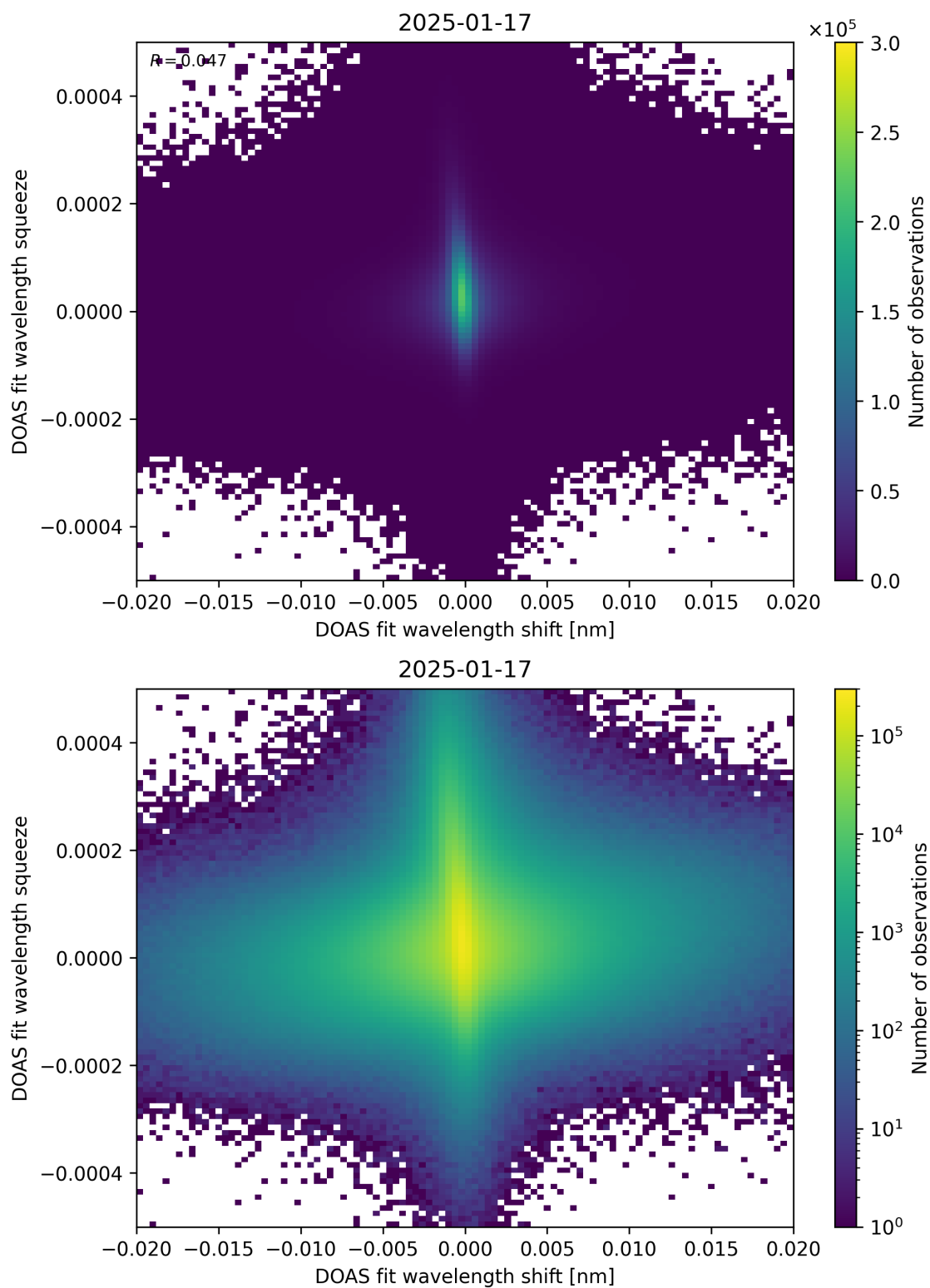
Figure 65: Scatter density plot of “DOAS fit wavelength shift” against “DOAS fit wavelength squeeze” for 2025-01-17 to 2025-01-18.
