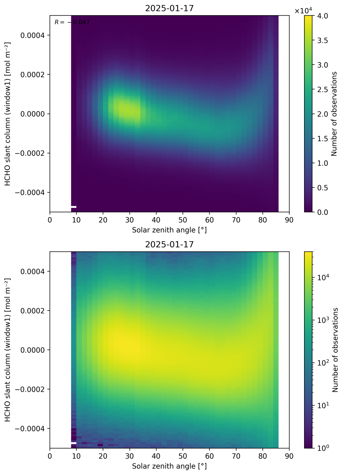
Figure 173: Scatter density plot of “Solar zenith angle” against “HCHO slant column (window1)” for 2025-01-17 to 2025-01-18.
