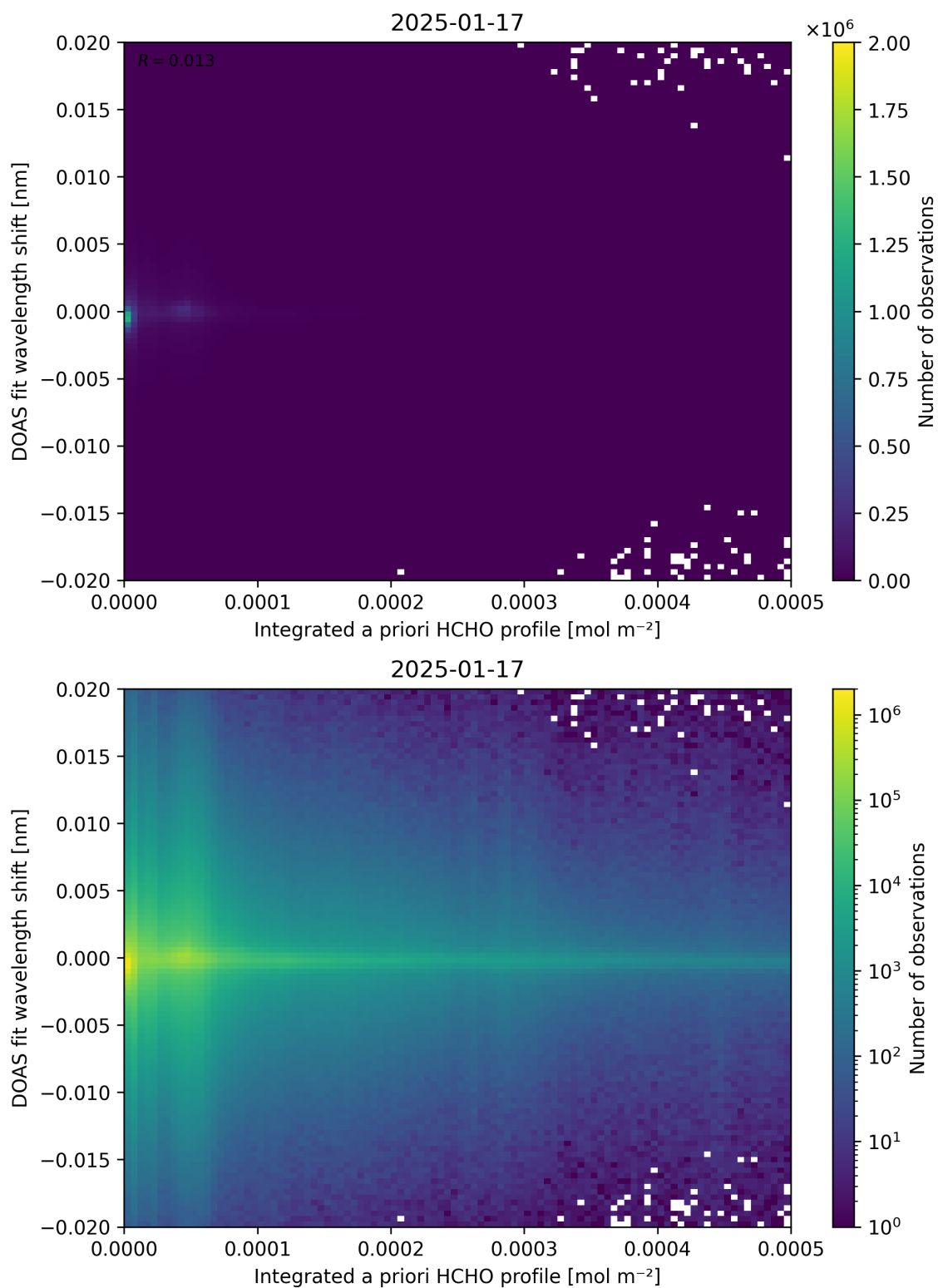
Figure 149: Scatter density plot of “Integrated a priori HCHO profile” against “DOAS fit wavelength shift” for 2025-01-17 to 2025-01-18.
