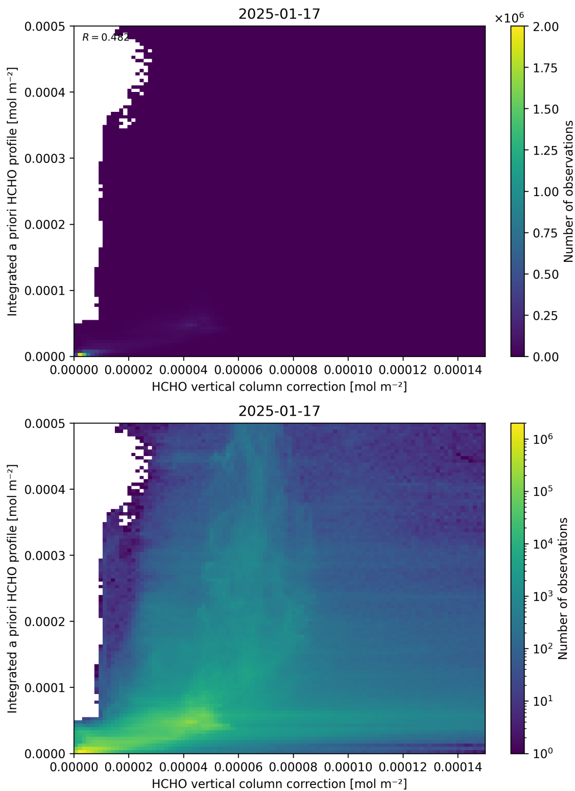
Figure 122: Scatter density plot of “HCHO vertical column correction” against “Integrated a priori HCHO profile” for 2025-01-17 to 2025-01-18.
