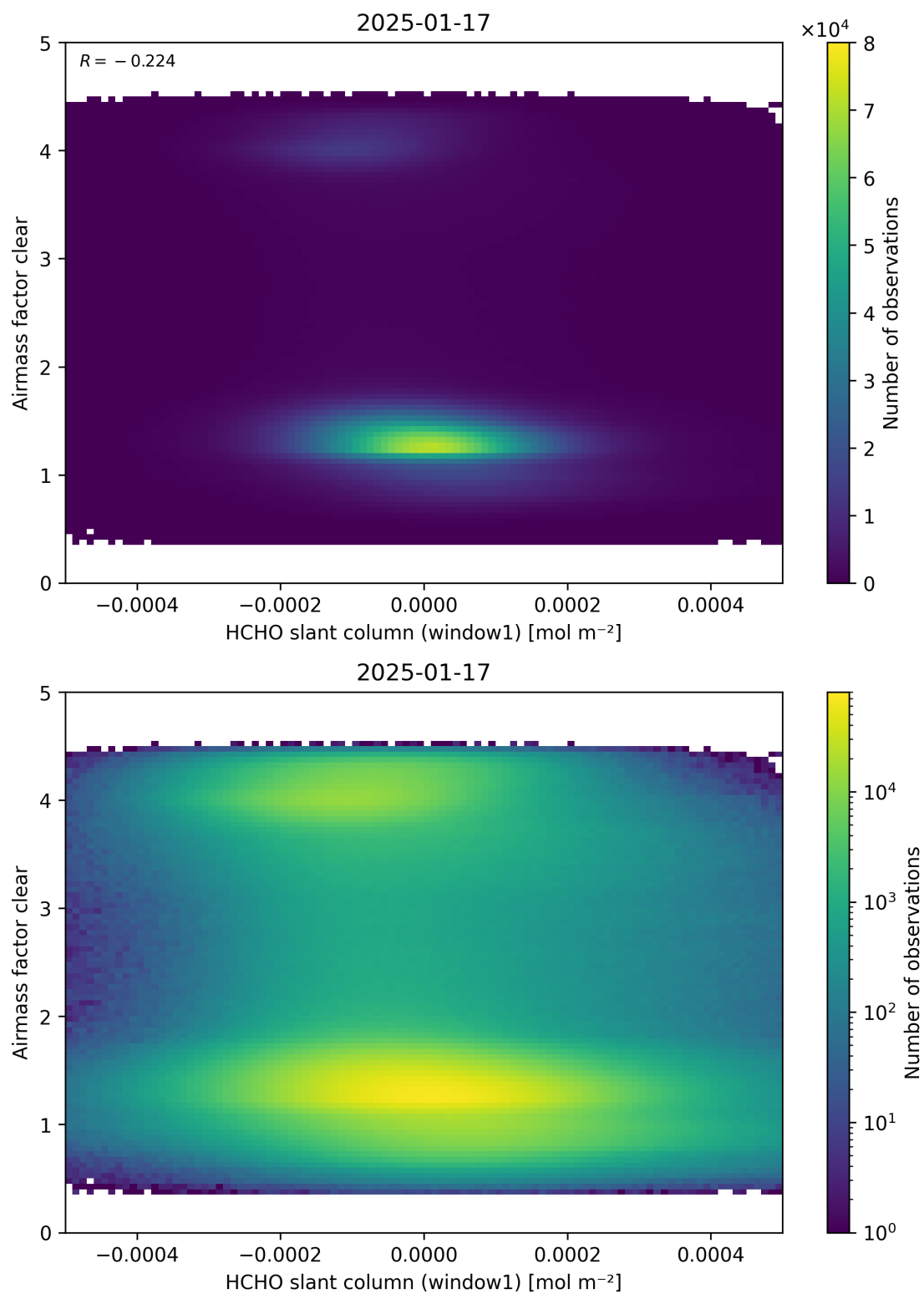
Figure 81: Scatter density plot of “HCHO slant column (window1)” against “Airmass factor clear” for 2025-01-17 to 2025-01-18.
