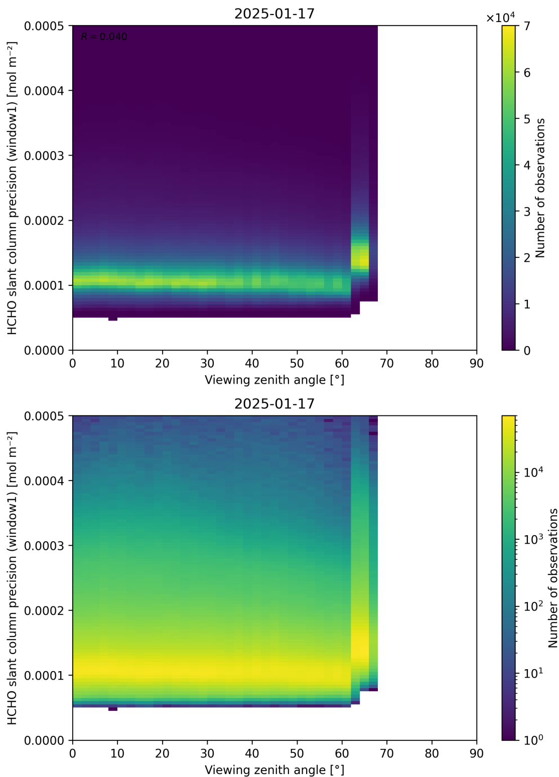
Figure 189: Scatter density plot of “Viewing zenith angle” against “HCHO slant column precision (window1)” for 2025-01-17 to 2025-01-18.
