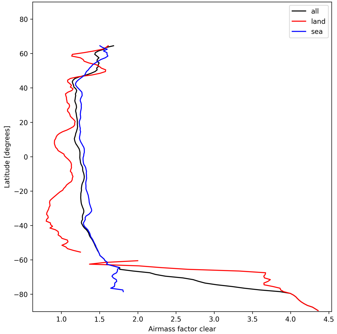
Figure 28: Zonal average of “Airmass factor clear” for 2025-01-17 to 2025-01-18.
