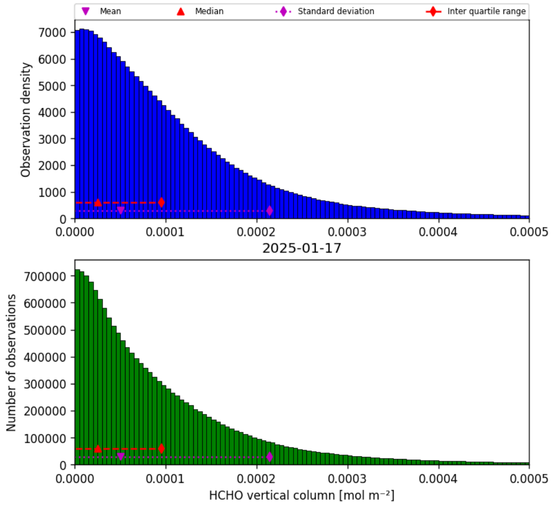
Figure 35: Histogram of “HCHO vertical column” for 2025-01-17 to 2025-01-18
