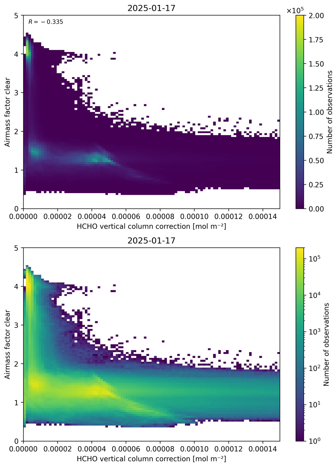
Figure 115: Scatter density plot of “HCHO vertical column correction” against “Airmass factor clear” for 2025-01-17 to 2025-01-18.
