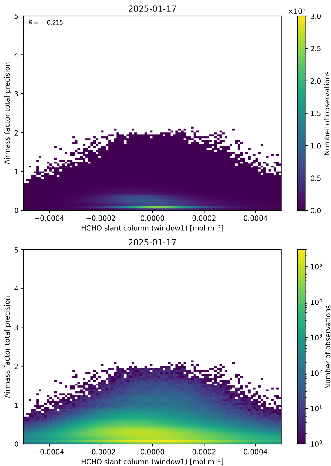
Figure 86: Scatter density plot of “HCHO slant column (window1)” against “Airmass factor total precision” for 2025-01-17 to 2025-01-18.
