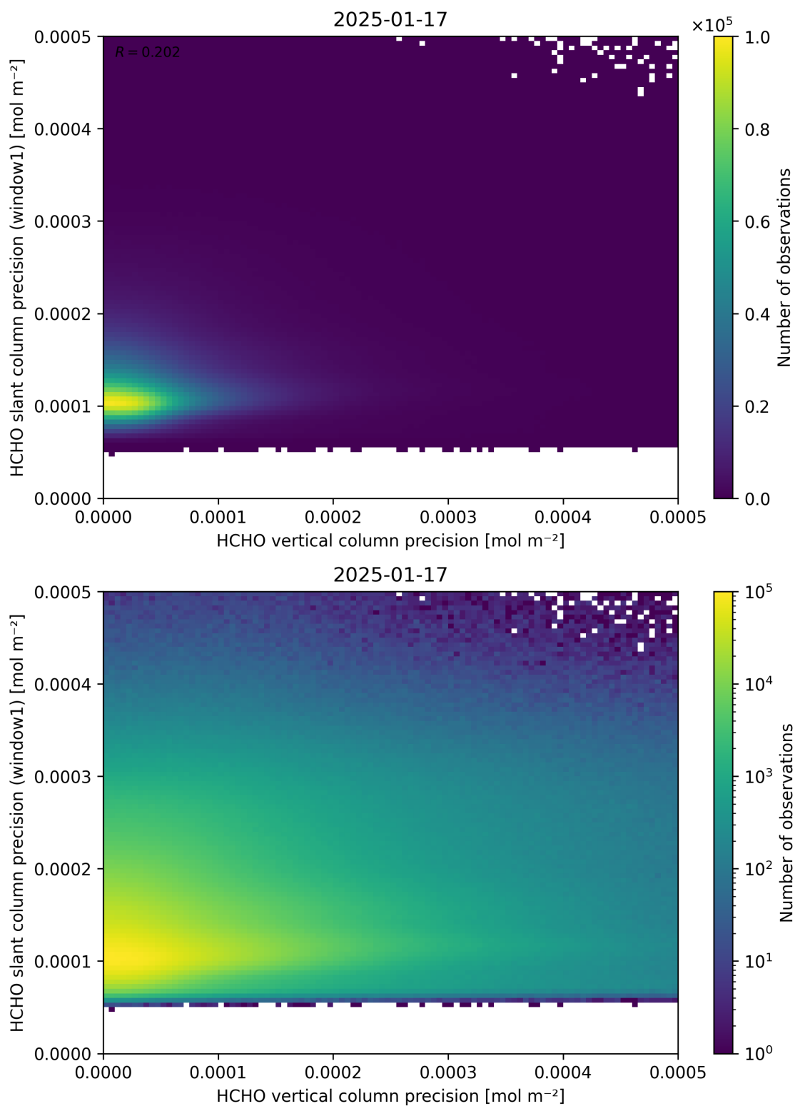
Figure 143: Scatter density plot of “HCHO vertical column precision” against “HCHO slant column precision (window1)” for 2025-01-17 to 2025-01-18.
