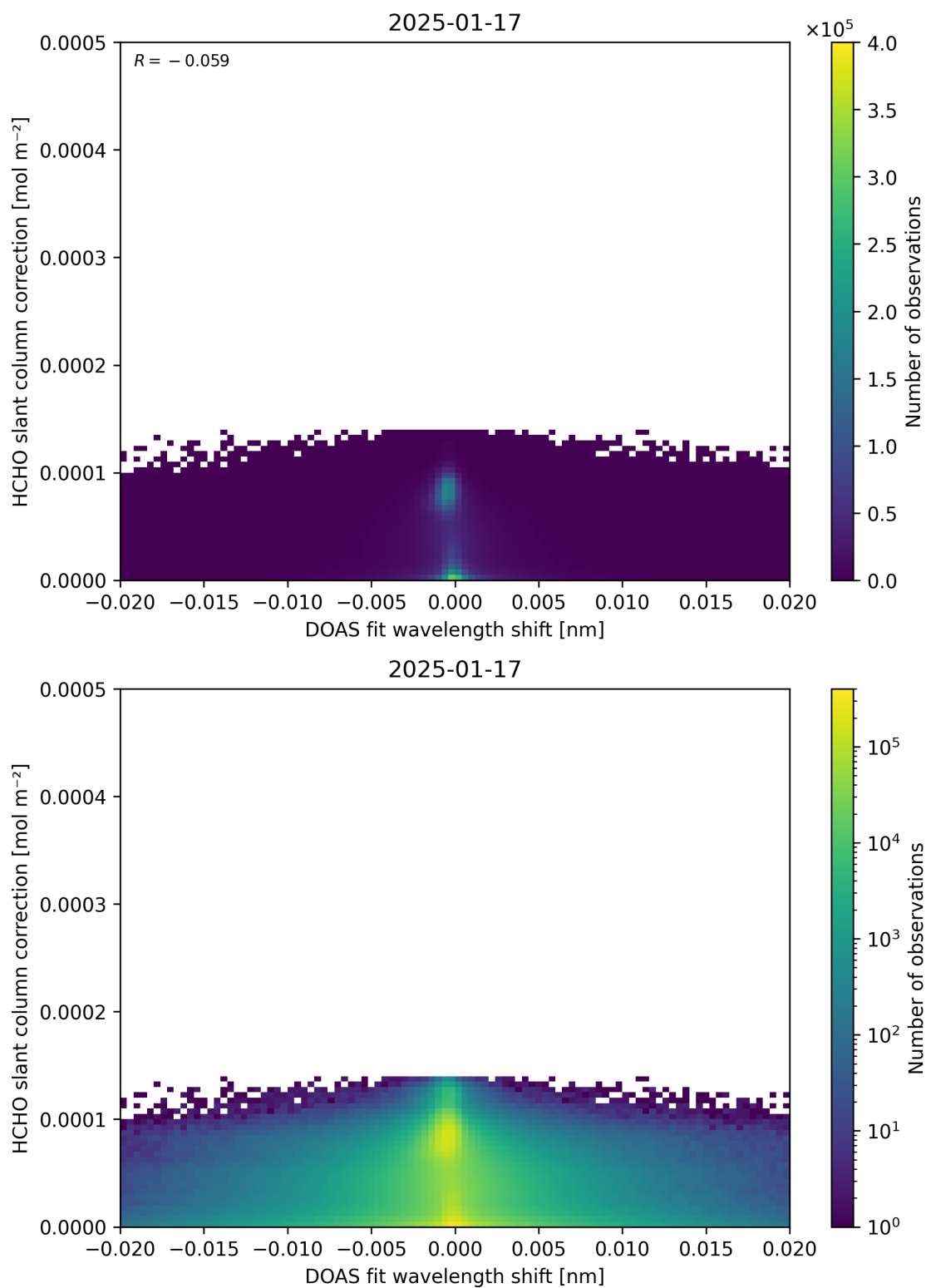
Figure 67: Scatter density plot of “DOAS fit wavelength shift” against “HCHO slant column correction” for 2025-01-17 to 2025-01-18.
