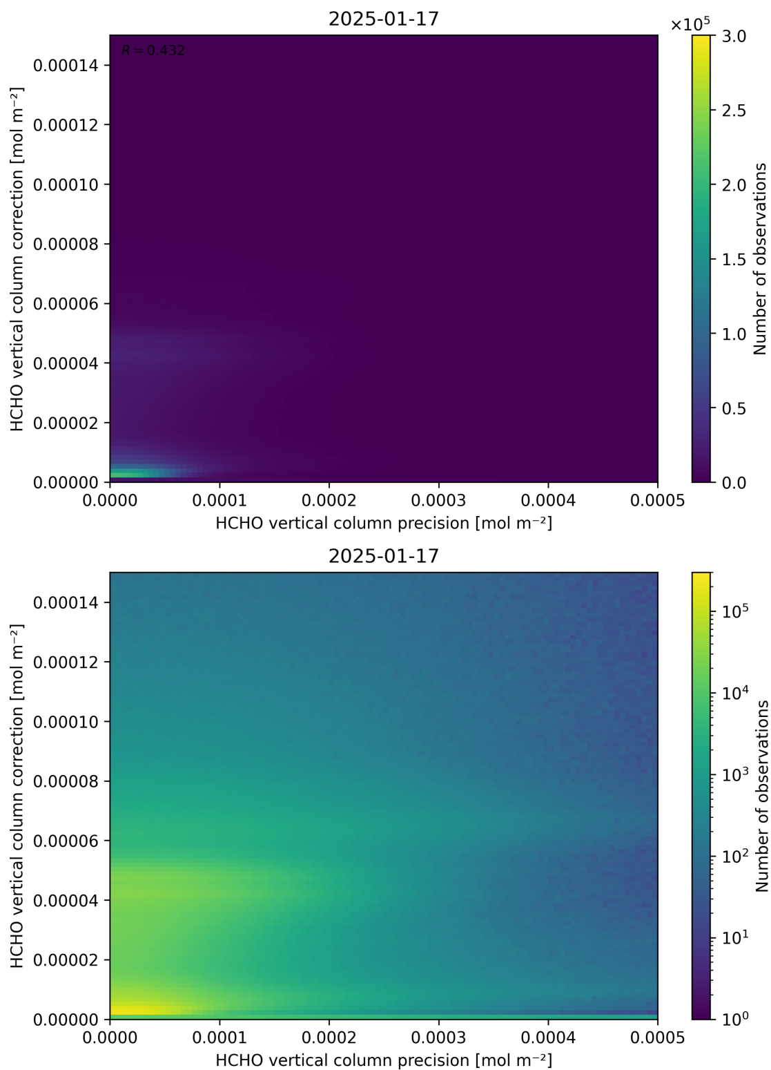
Figure 146: Scatter density plot of “HCHO vertical column precision” against “HCHO vertical column correction” for 2025-01-17 to 2025-01-18.
