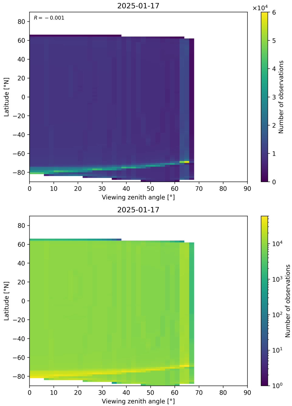
Figure 196: Scatter density plot of “Viewing zenith angle” against “Latitude” for 2025-01-17 to 2025-01-18.
