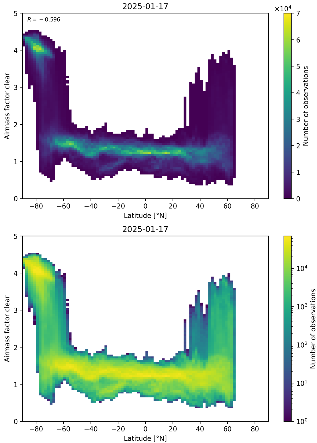
Figure 156: Scatter density plot of “Latitude” against “Airmass factor clear” for 2025-01-17 to 2025-01-18.
