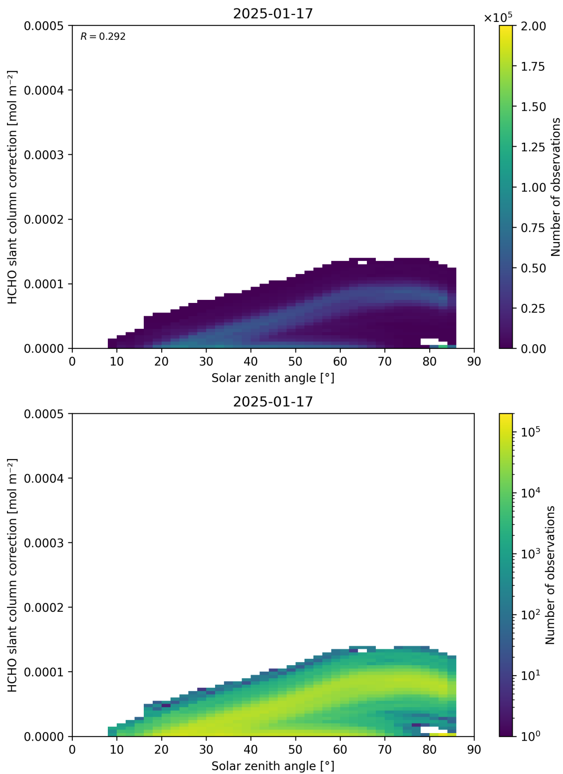
Figure 172: Scatter density plot of “Solar zenith angle” against “HCHO slant column correction” for 2025-01-17 to 2025-01-18.
