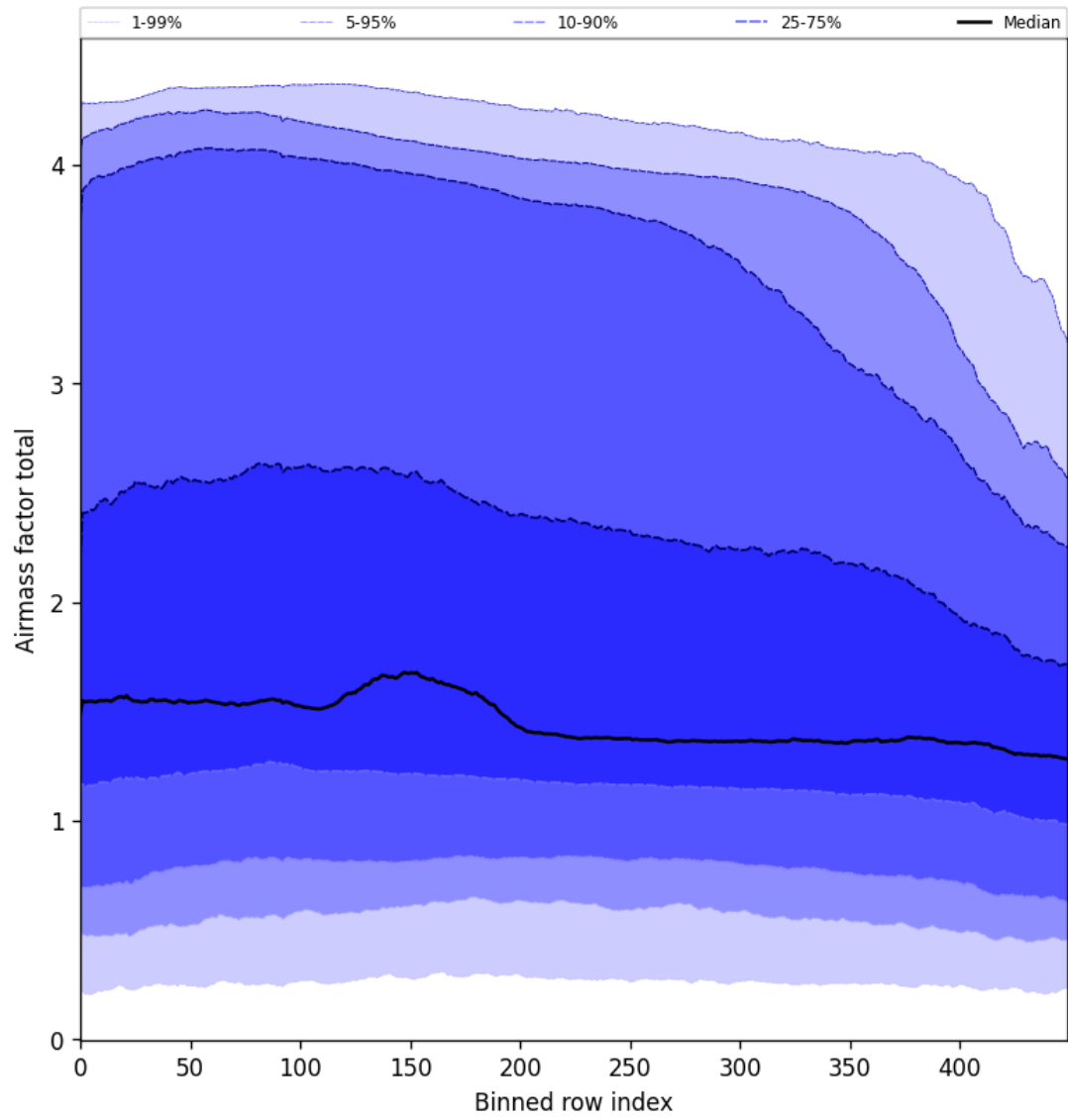
Figure 54: Along track statistics of “Airmass factor total” for 2025-01-17 to 2025-01-18
