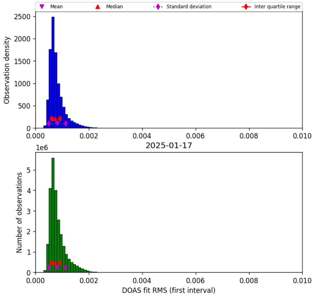
Figure 46: Histogram of “DOAS fit RMS (first interval)” for 2025-01-17 to 2025-01-18
