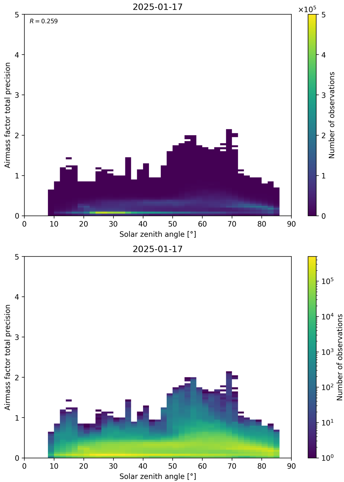
Figure 176: Scatter density plot of “Solar zenith angle” against “Airmass factor total precision” for 2025-01-17 to 2025-01-18.
