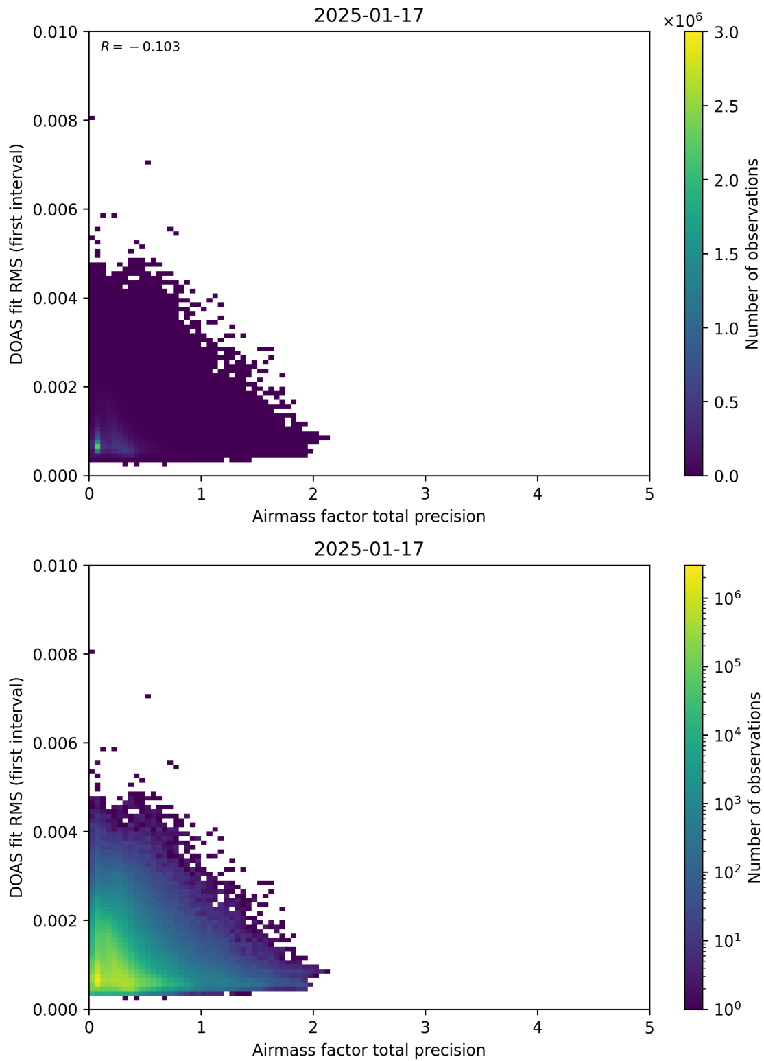
Figure 105: Scatter density plot of “Airmass factor total precision” against “DOAS fit RMS (first interval)” for 2025-01-17 to 2025-01-18.
