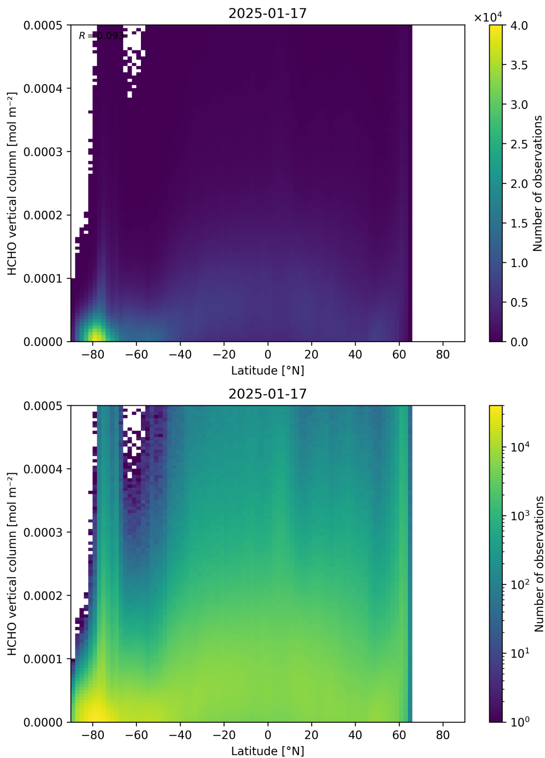
Figure 163: Scatter density plot of “Latitude” against “HCHO vertical column” for 2025-01-17 to 2025-01-18.
