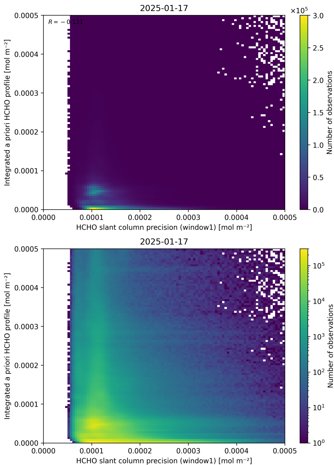
Figure 96: Scatter density plot of “HCHO slant column precision (window1)” against “Integrated a priori HCHO profile” for 2025-01-17 to 2025-01-18.
