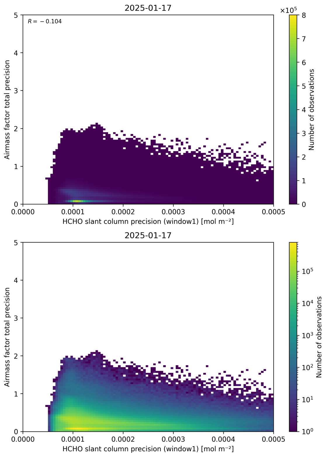
Figure 95: Scatter density plot of “HCHO slant column precision (window1)” against “Airmass factor total precision” for 2025-01-17 to 2025-01-18.
