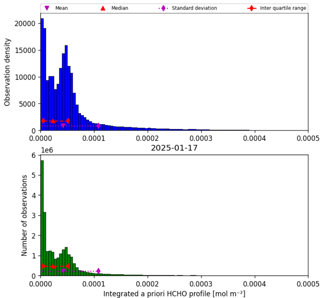
Figure 43: Histogram of “Integrated a priori HCHO profile” for 2025-01-17 to 2025-01-18
