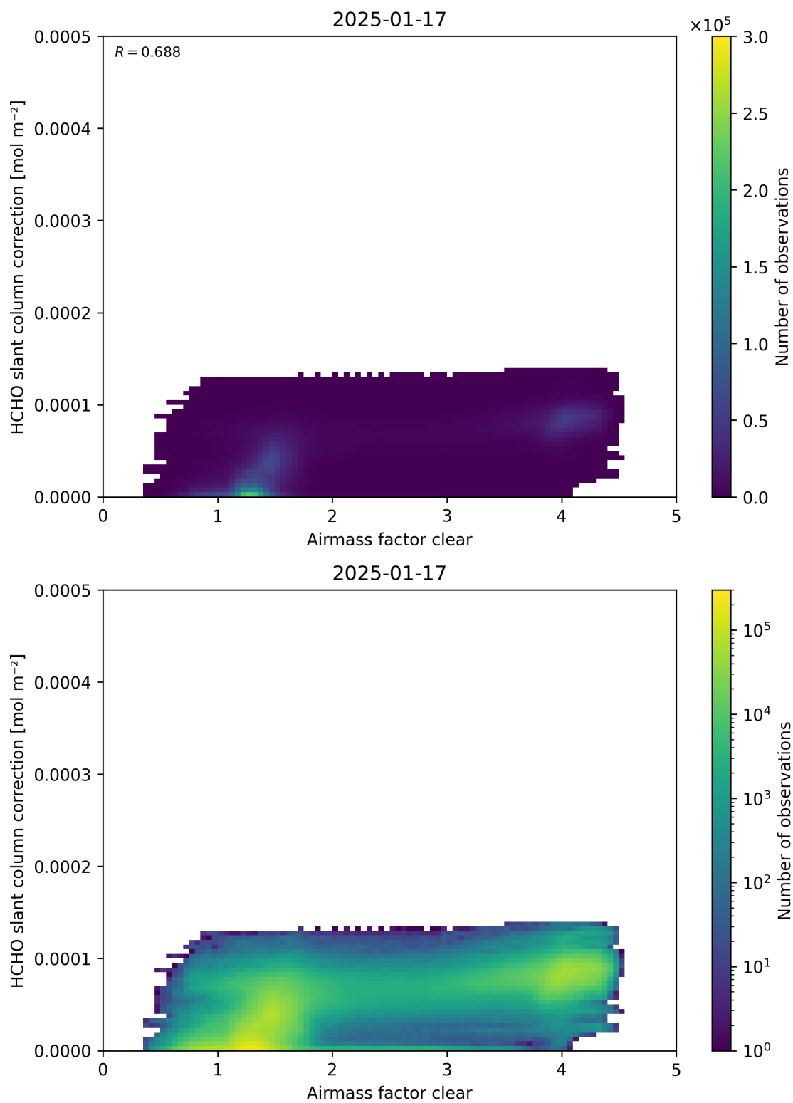
Figure 75: Scatter density plot of “Air mass factor clear” against “HCHO slant column correction” for 2025-01-17 to 2025-01-18.
