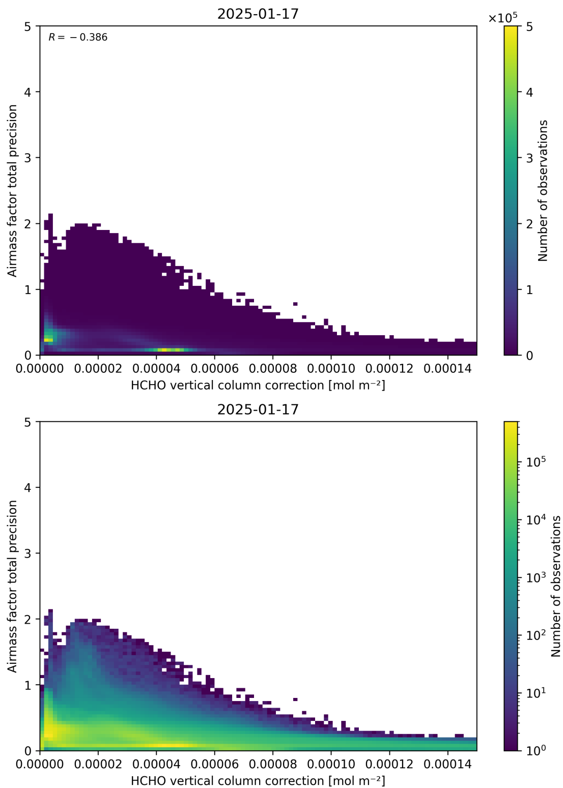
Figure 121: Scatter density plot of “HCHO vertical column correction” against “Airmass factor total precision” for 2025-01-17 to 2025-01-18.
