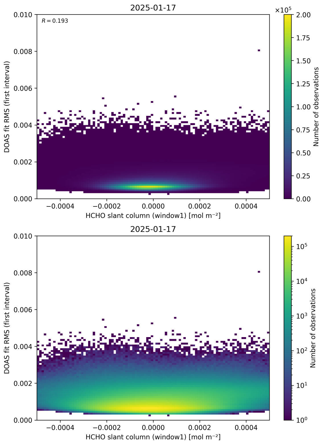
Figure 78: Scatter density plot of “HCHO slant column (window1)” against “DOAS fit RMS (first interval)” for 2025-01-17 to 2025-01-18.
