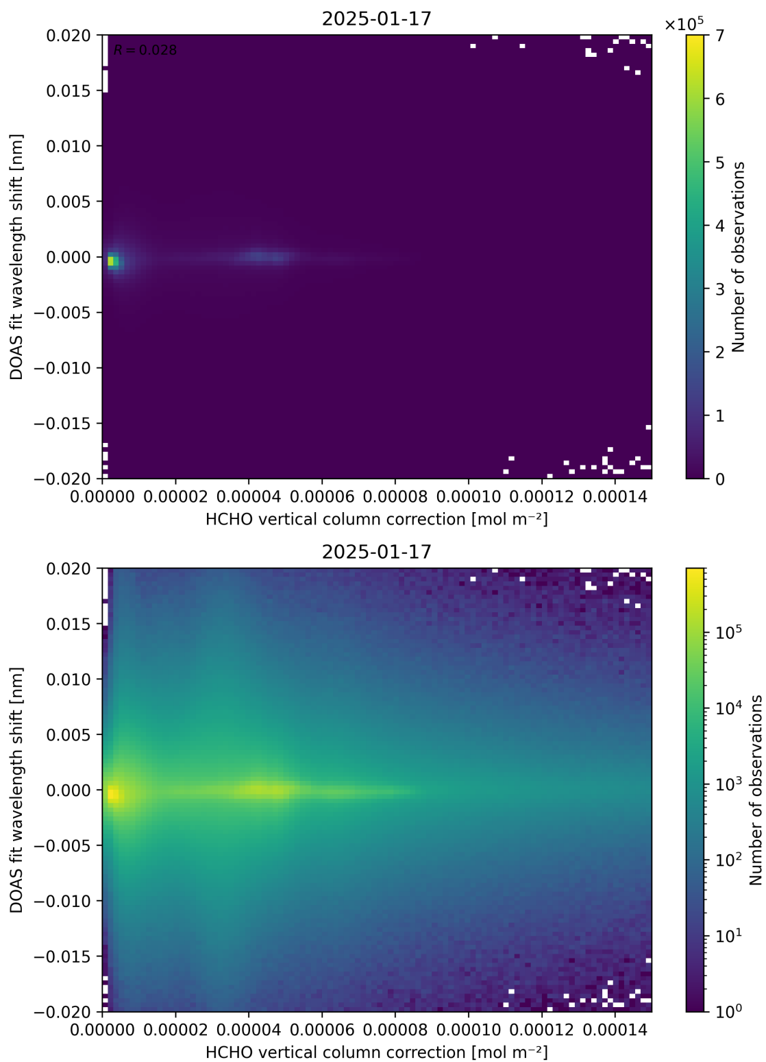
Figure 113: Scatter density plot of “HCHO vertical column correction” against “DOAS fit wavelength shift” for 2025-01-17 to 2025-01-18.
