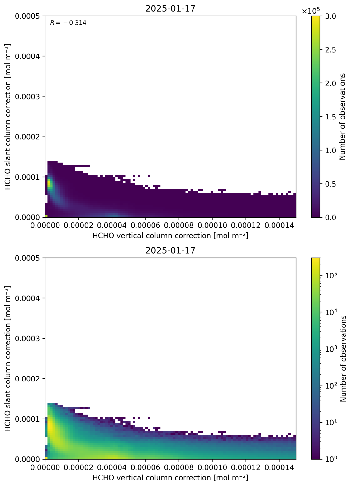
Figure 117: Scatter density plot of “HCHO vertical column correction” against “HCHO slant column correction” for 2025-01-17 to 2025-01-18.
