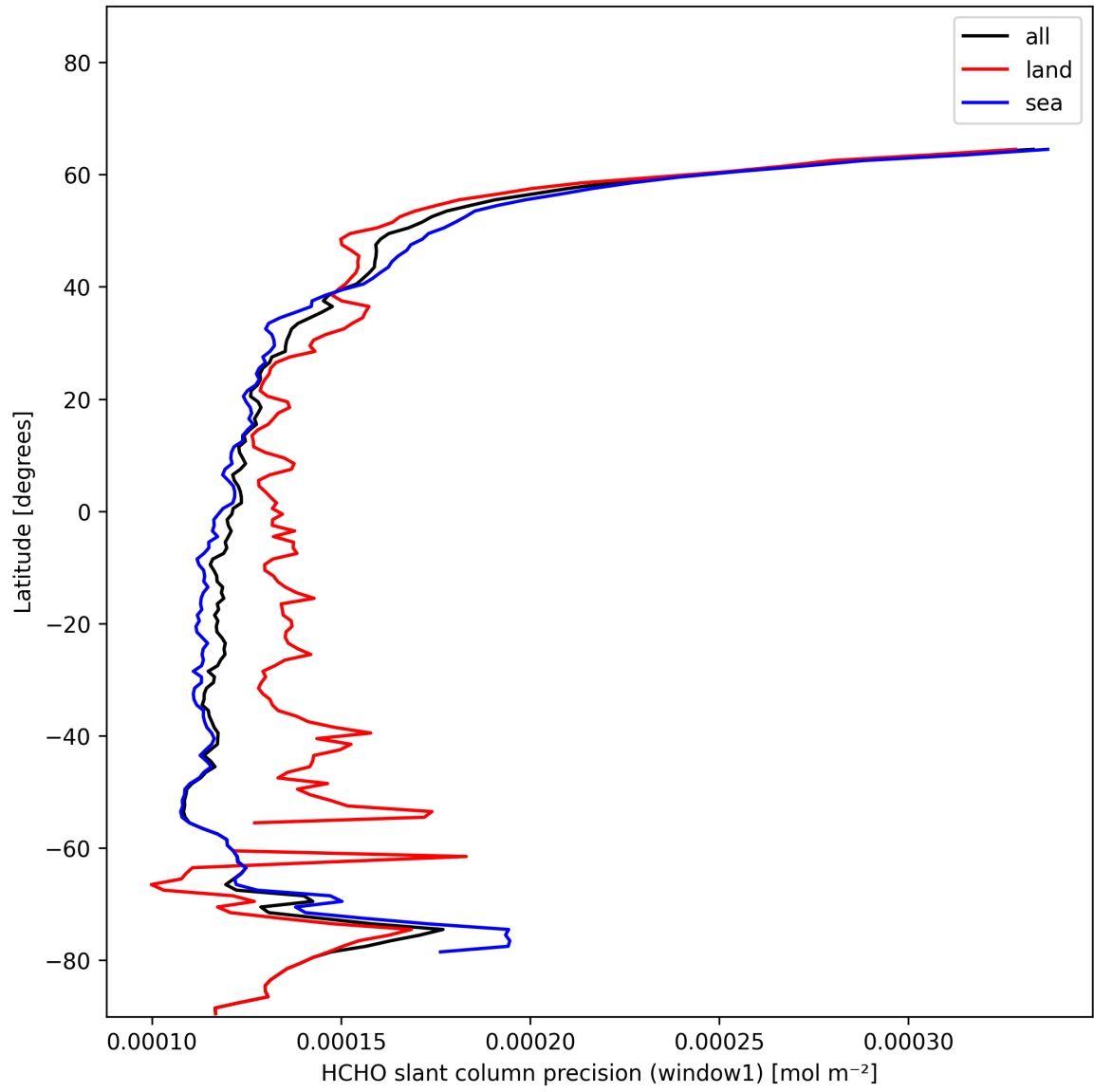
Figure 25: Zonal average of “HCHO slant column precision (window1)” for 2025-01-17 to 2025-01-18.
