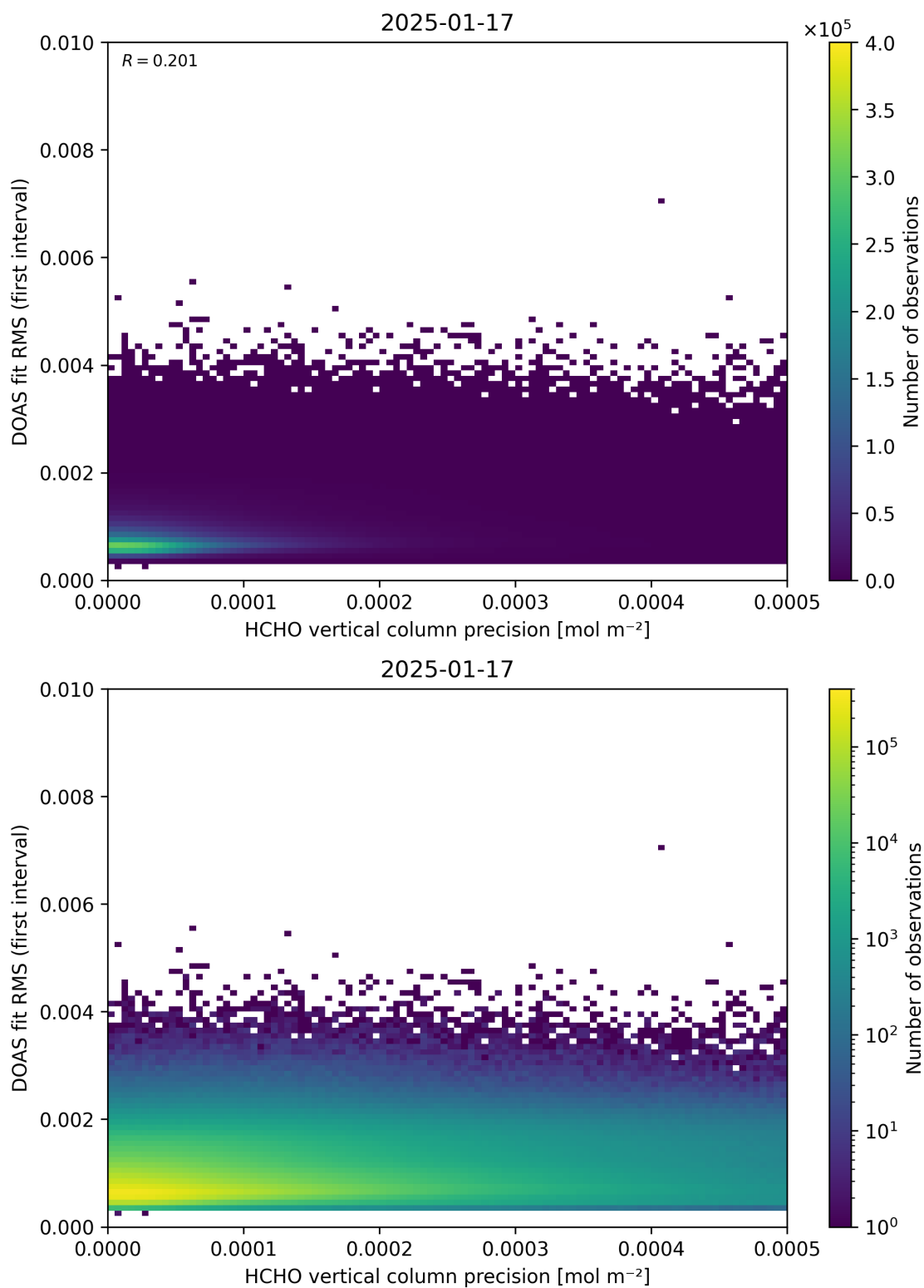
Figure 136: Scatter density plot of “HCHO vertical column precision” against “DOAS fit RMS (first interval)” for 2025-01-17 to 2025-01-18.
