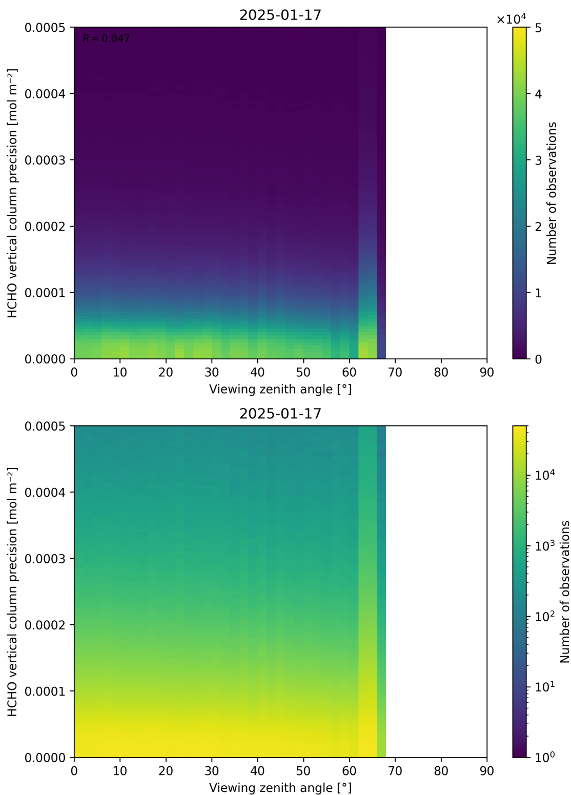
Figure 194: Scatter density plot of “Viewing zenith angle” against “HCHO vertical column precision” for 2025-01-17 to 2025-01-18.
