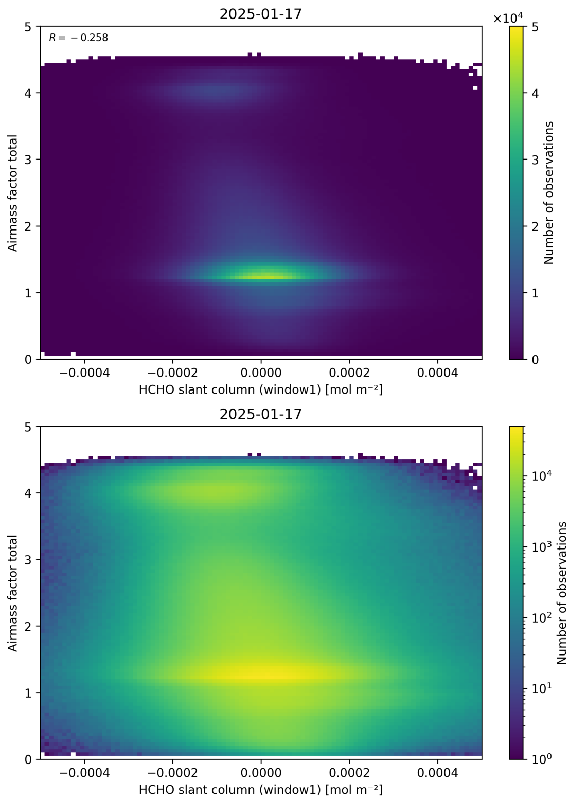
Figure 85: Scatter density plot of “HCHO slant column (window1)” against “Airmass factor total” for 2025-01-17 to 2025-01-18.
