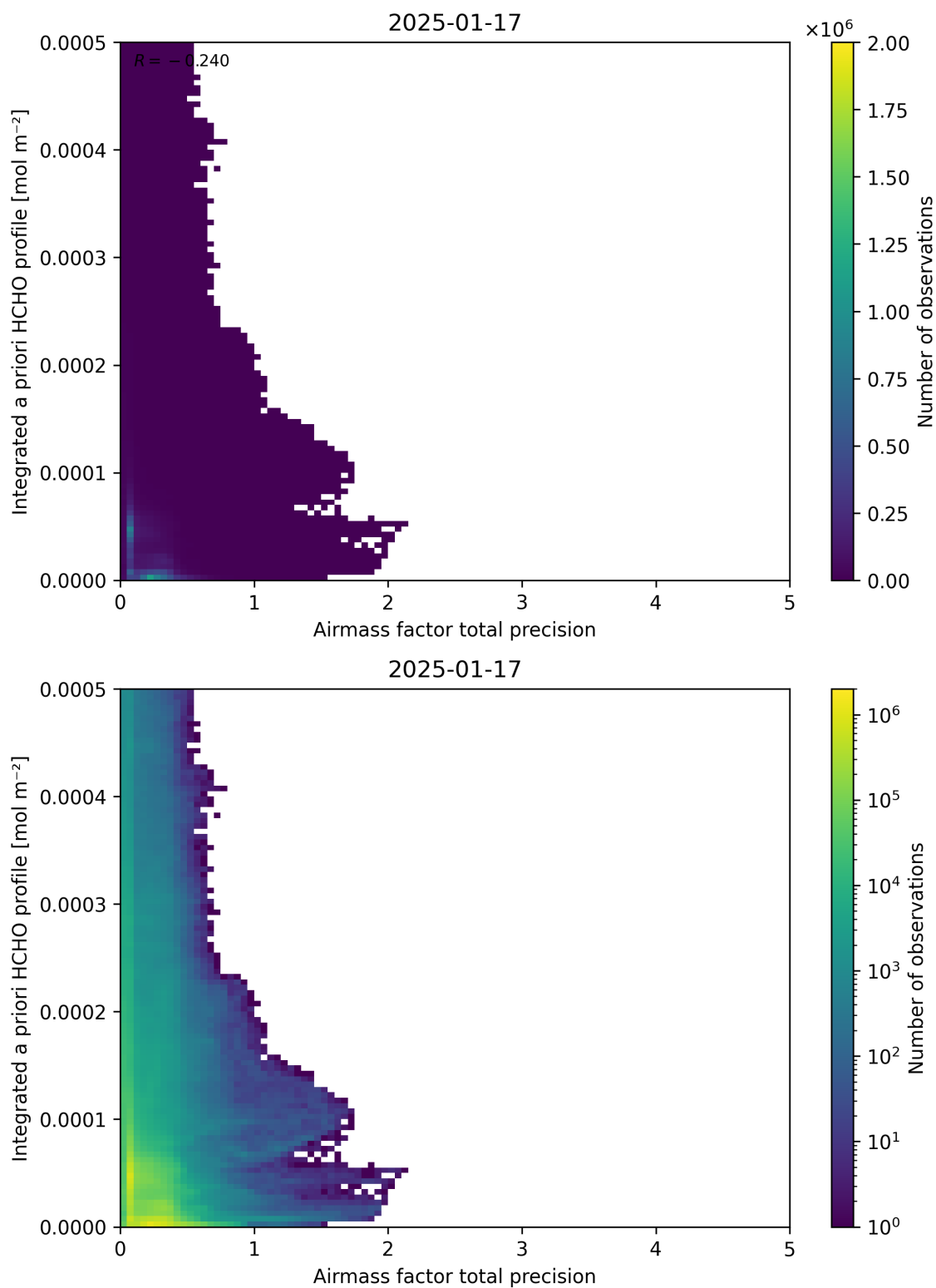
Figure 111: Scatter density plot of “Airmass factor total precision” against “Integrated a priori HCHO profile” for 2025-01-17 to 2025-01-18.
