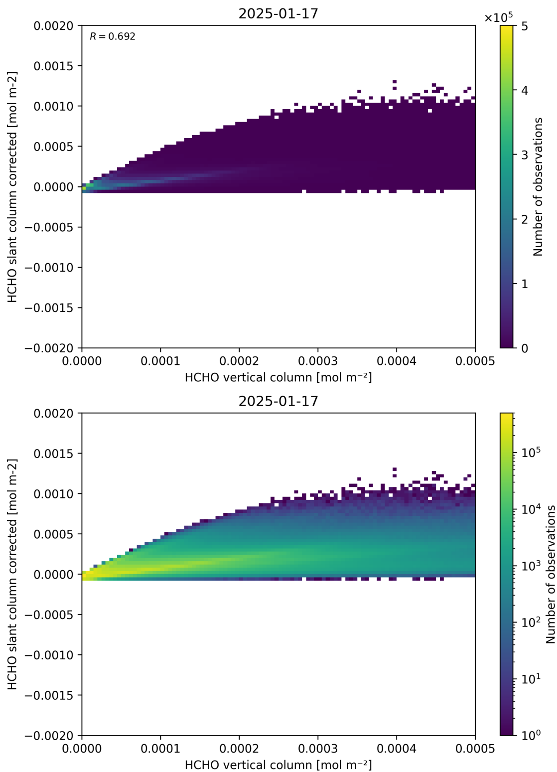
Figure 127: Scatter density plot of “HCHO vertical column” against “HCHO slant column corrected” for 2025-01-17 to 2025-01-18.
