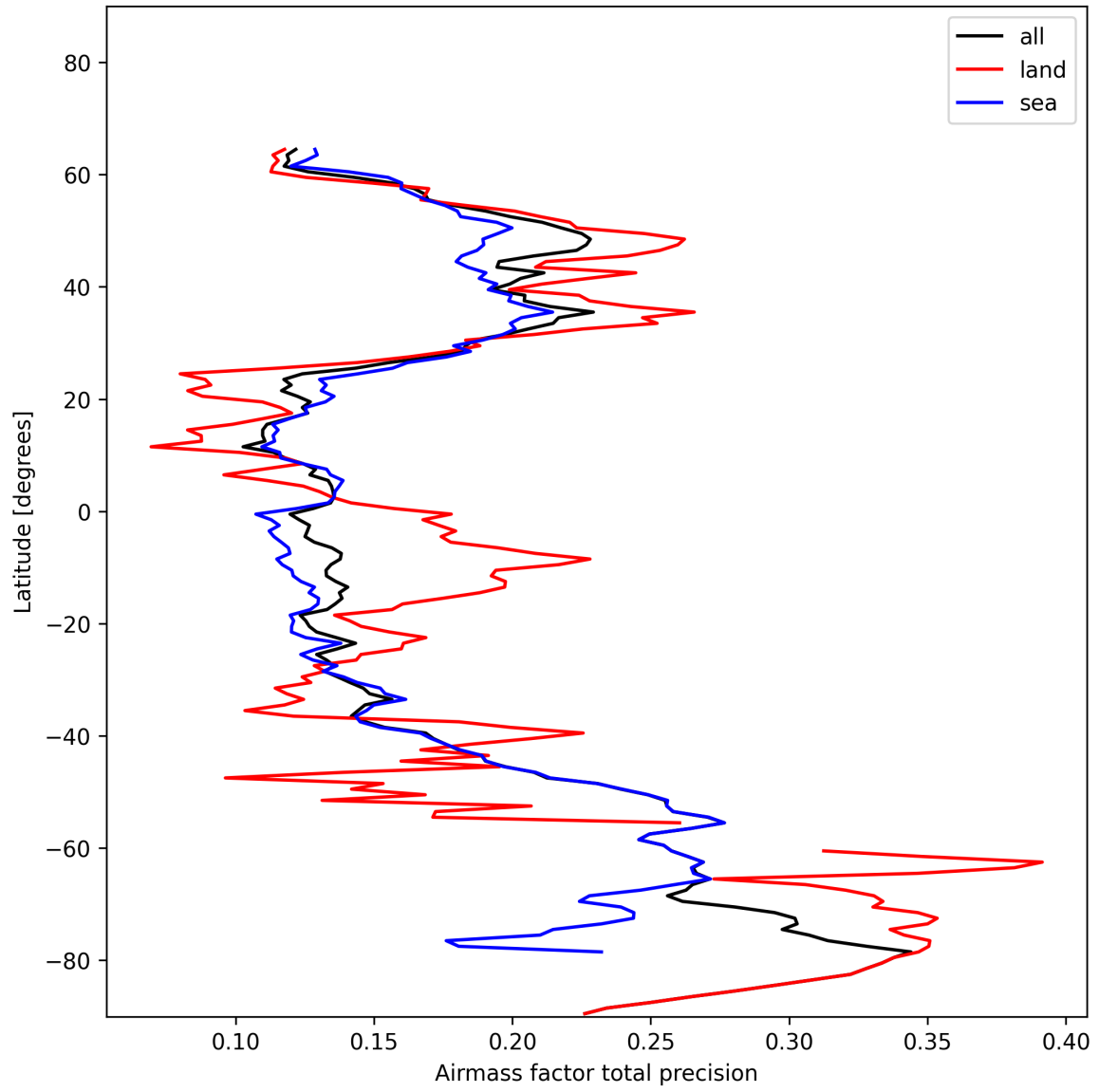
Figure 27: Zonal average of “Airmass factor total precision” for 2025-01-17 to 2025-01-18.
