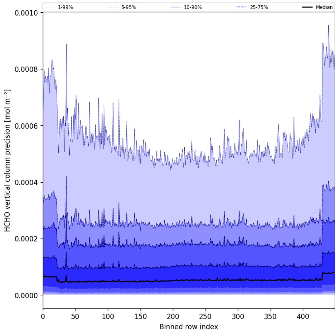
Figure 50: Along track statistics of “HCHO vertical column precision” for 2025-01-17 to 2025-01-18
