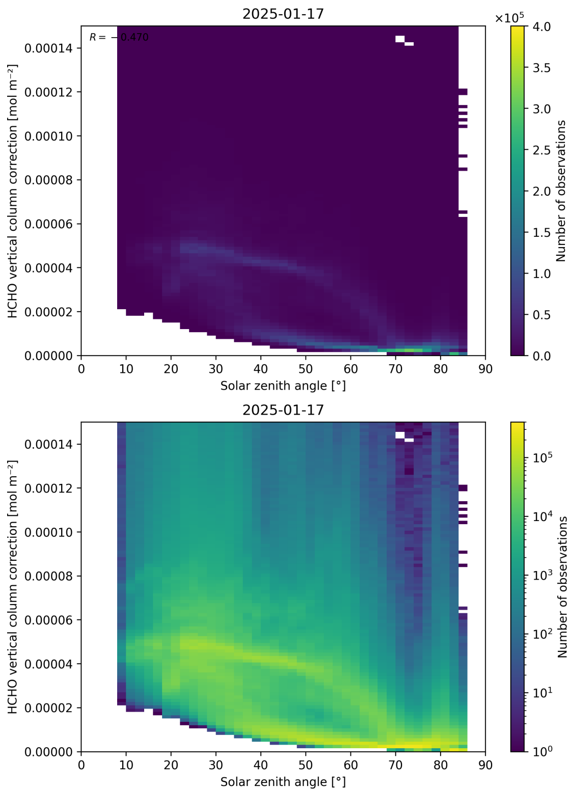
Figure 178: Scatter density plot of “Solar zenith angle” against “HCHO vertical column correction” for 2025-01-17 to 2025-01-18.
