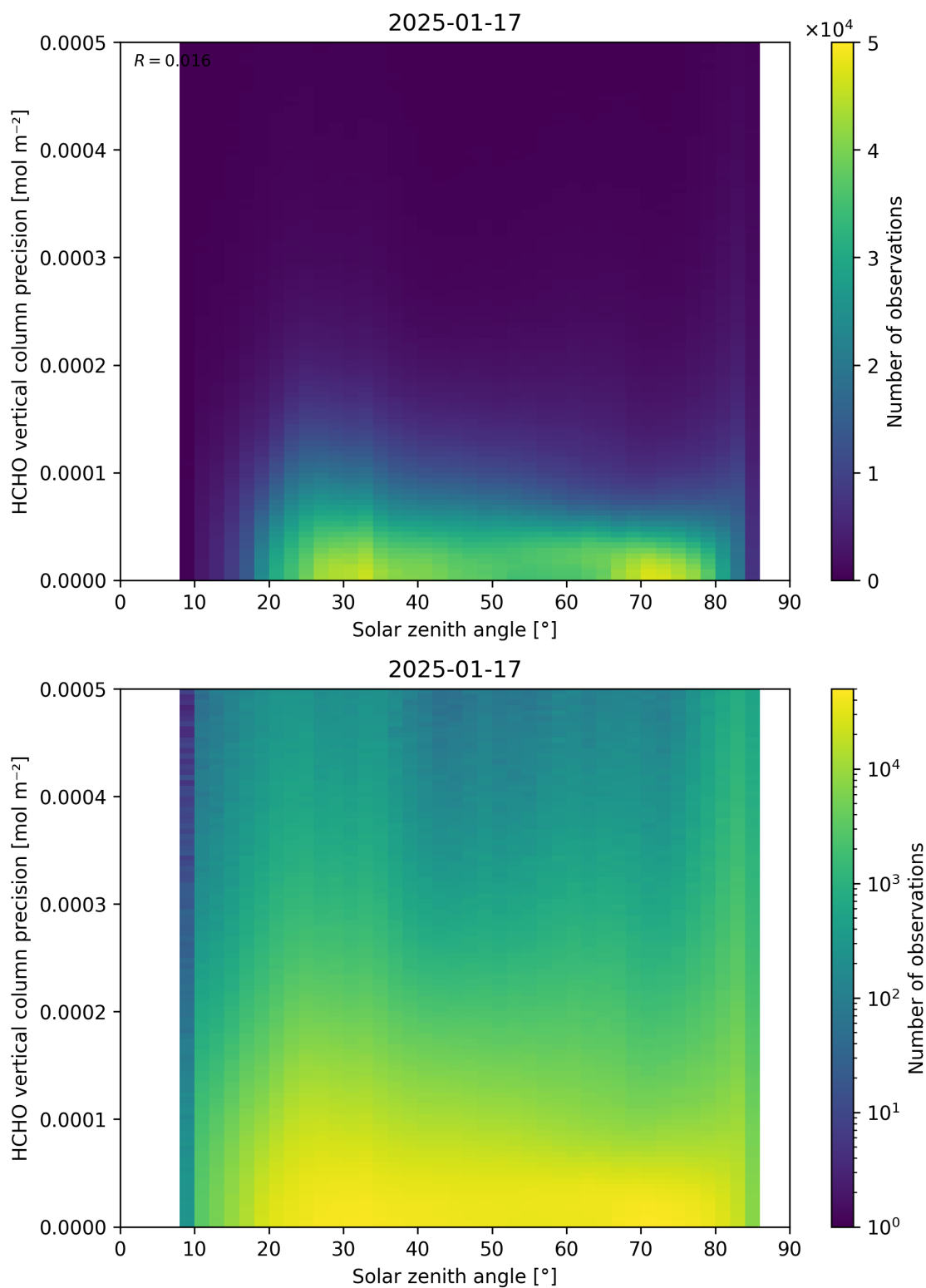
Figure 179: Scatter density plot of “Solar zenith angle” against “HCHO vertical column precision” for 2025-01-17 to 2025-01-18.
