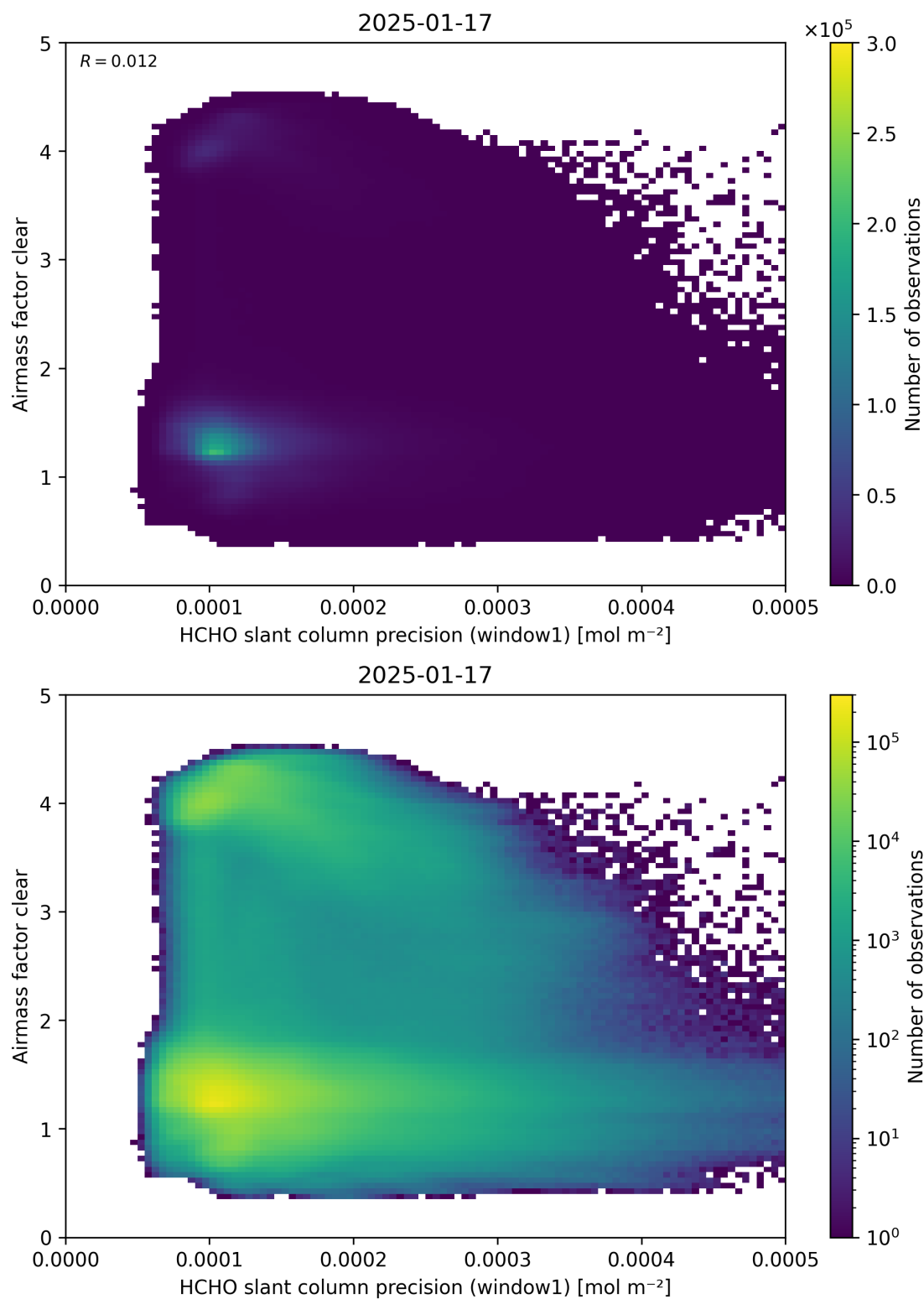
Figure 91: Scatter density plot of “HCHO slant column precision (window1)” against “Airmass factor clear” for 2025-01-17 to 2025-01-18.
