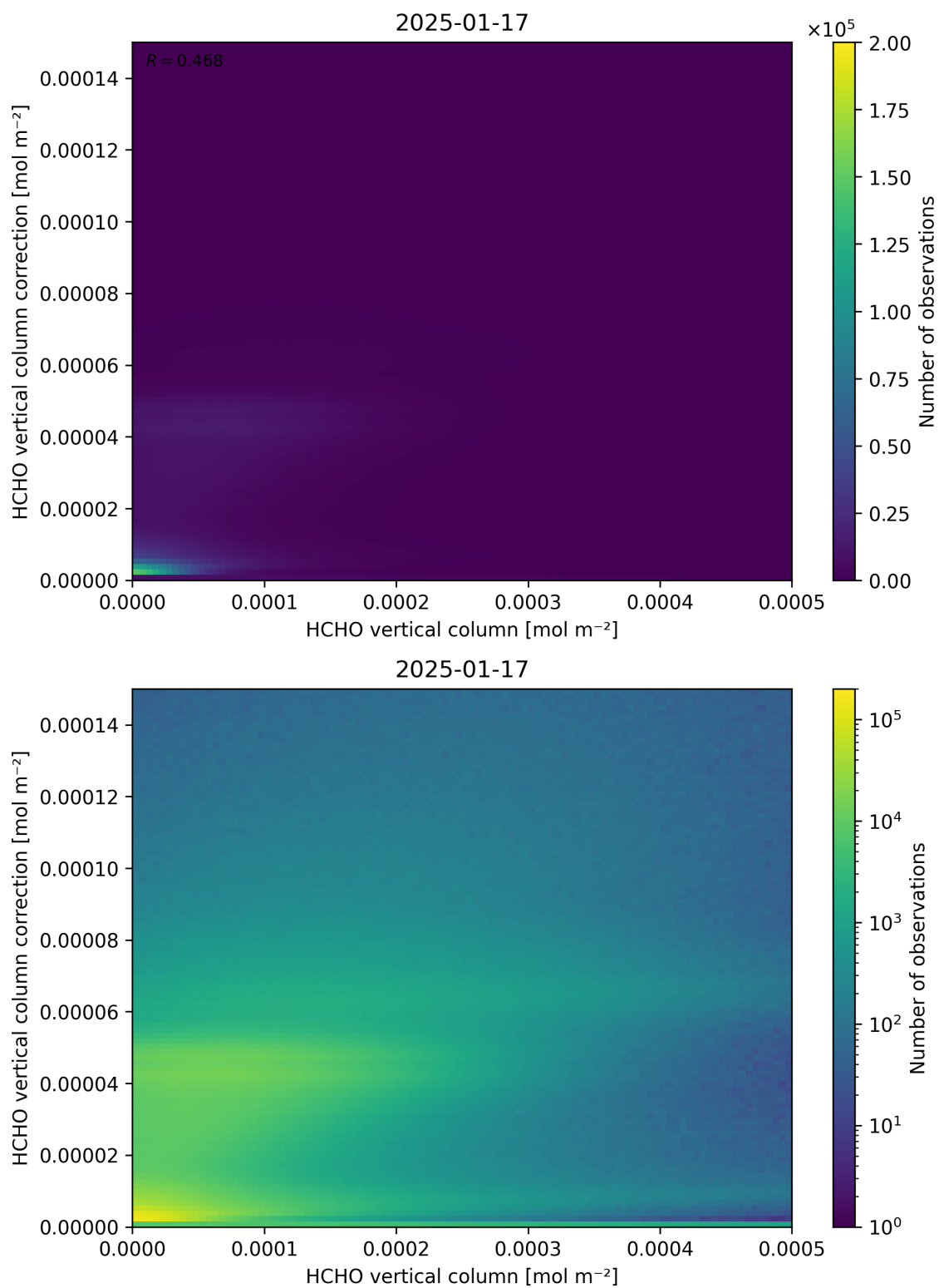
Figure 133: Scatter density plot of “HCHO vertical column” against “HCHO vertical column correction” for 2025-01-17 to 2025-01-18.
