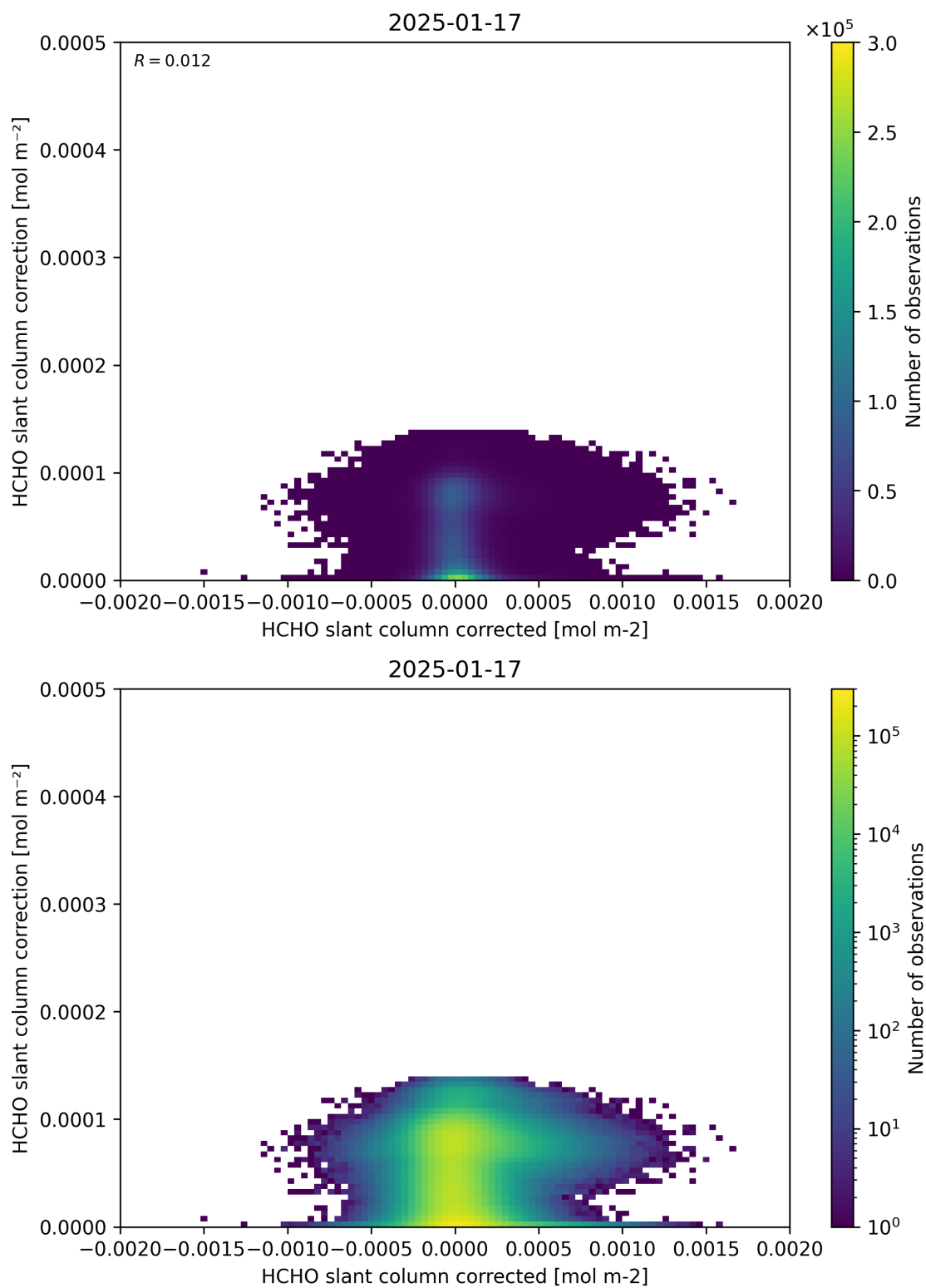
Figure 77: Scatter density plot of “HCHO slant column corrected” against “HCHO slant column correction” for 2025-01-17 to 2025-01-18.
