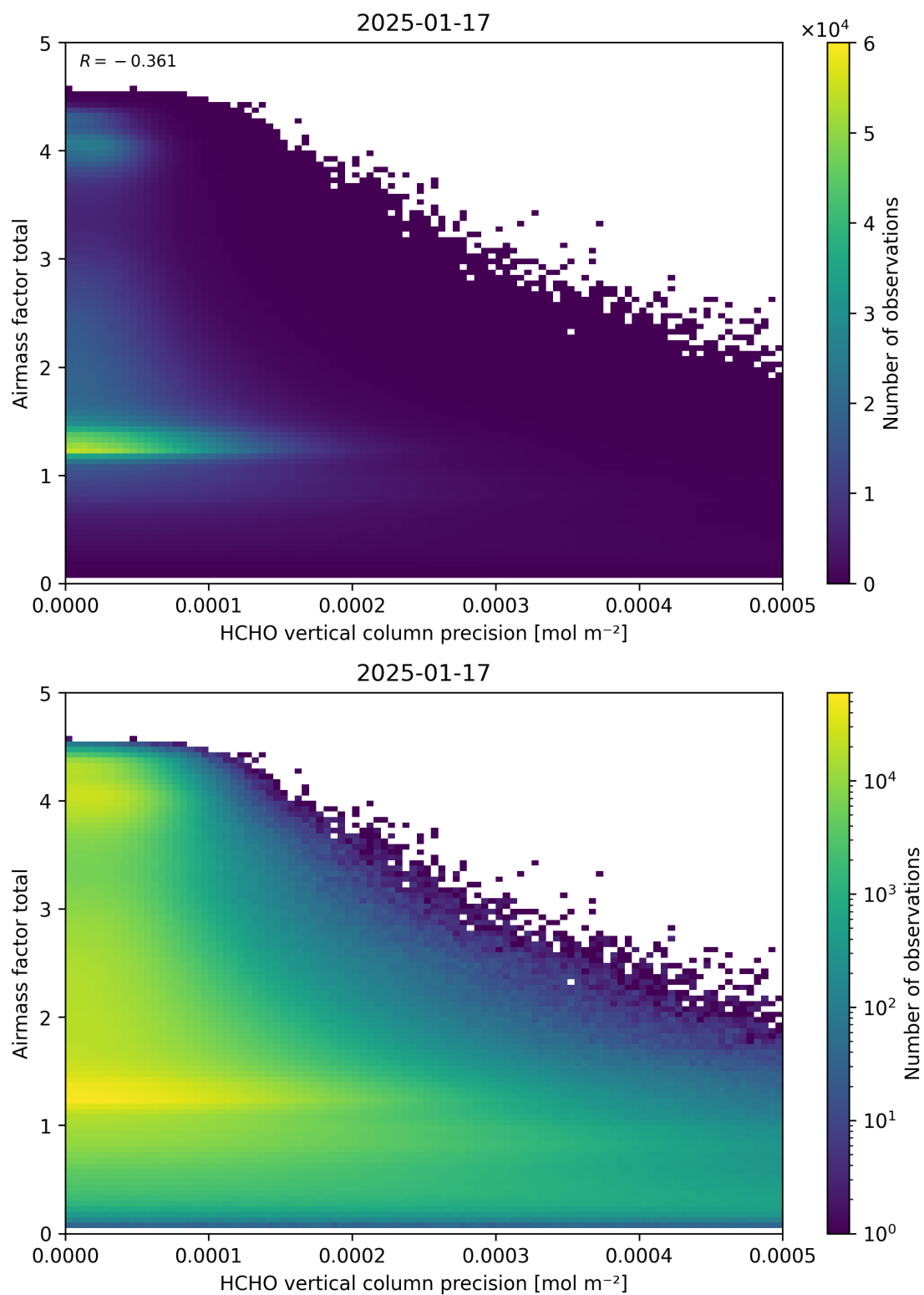
Figure 144: Scatter density plot of “HCHO vertical column precision” against “Airmass factor total” for 2025-01-17 to 2025-01-18.
