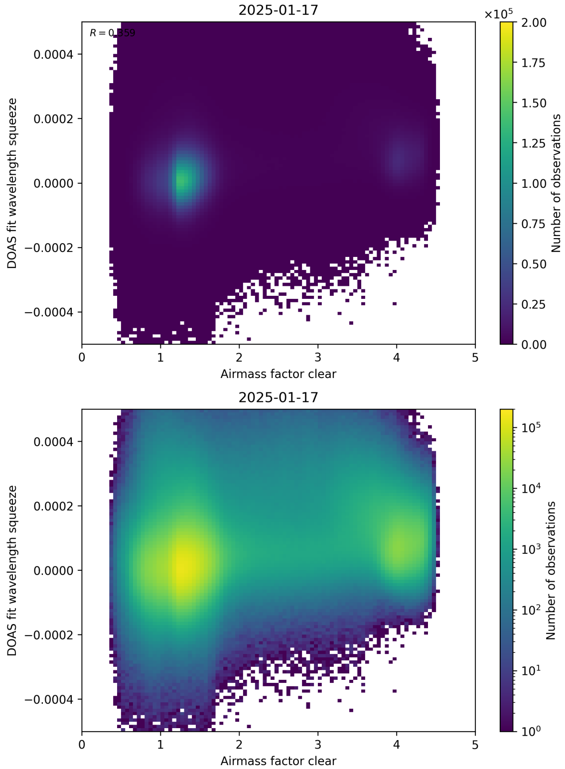
Figure 73: Scatter density plot of “Airmass factor clear” against “DOAS fit wavelength squeeze” for 2025-01-17 to 2025-01-18.
