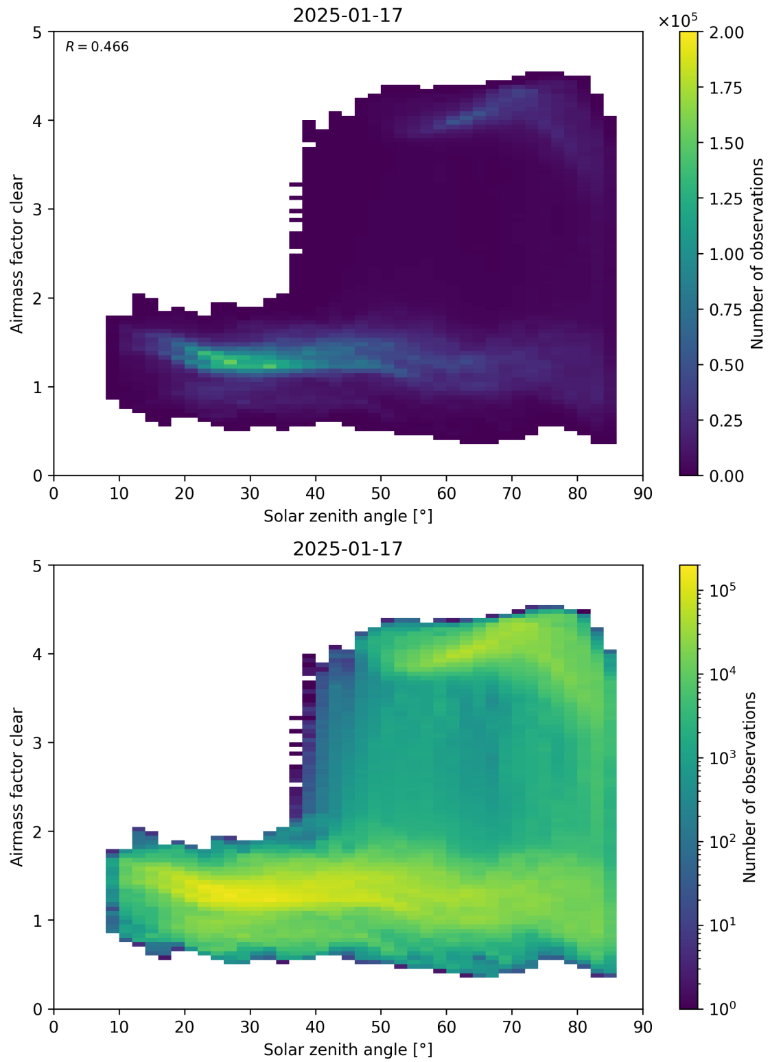
Figure 170: Scatter density plot of “Solar zenith angle” against “Airmass factor clear” for 2025-01-17 to 2025-01-18.
