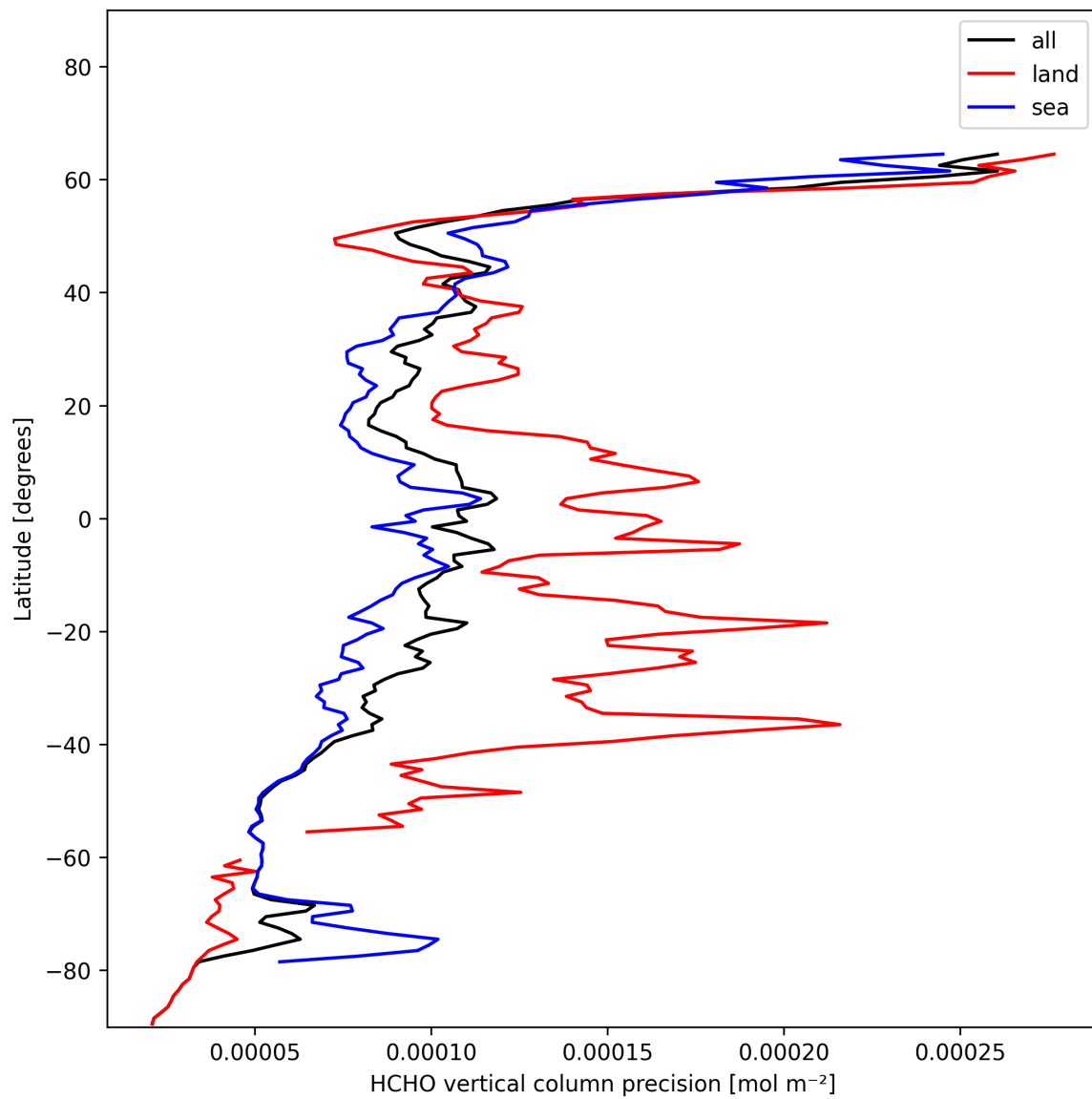
Figure 22: Zonal average of “HCHO vertical column precision” for 2025-01-17 to 2025-01-18.
