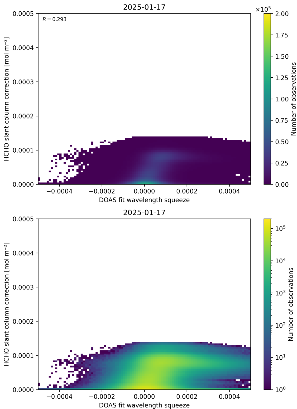
Figure 70: Scatter density plot of “DOAS fit wavelength squeeze” against “HCHO slant column correction” for 2025-01-17 to 2025-01-18.
