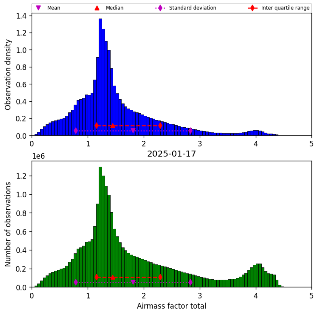
Figure 40: Histogram of “Airmass factor total” for 2025-01-17 to 2025-01-18
