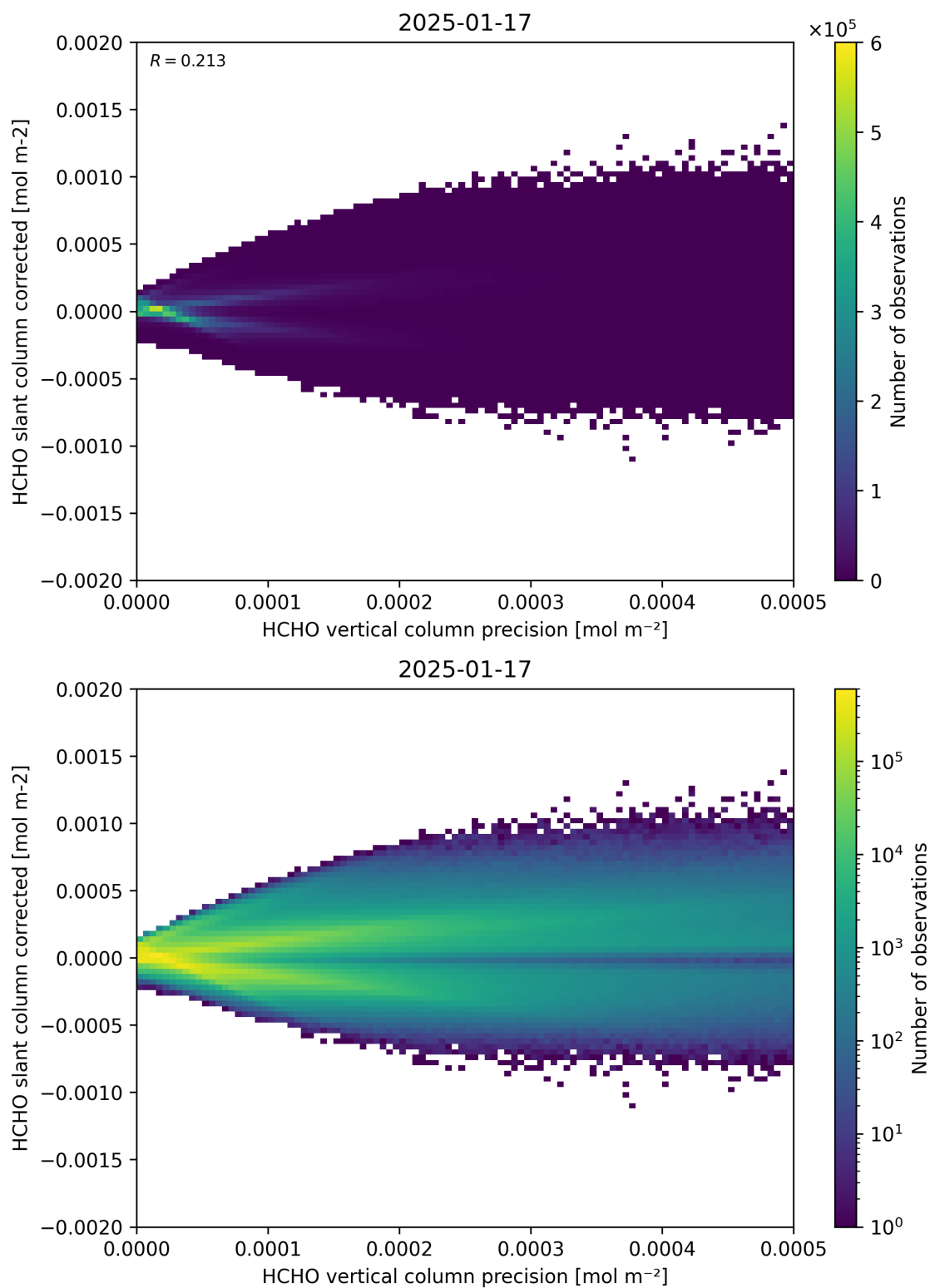
Figure 140: Scatter density plot of “HCHO vertical column precision” against “HCHO slant column corrected” for 2025-01-17 to 2025-01-18.
