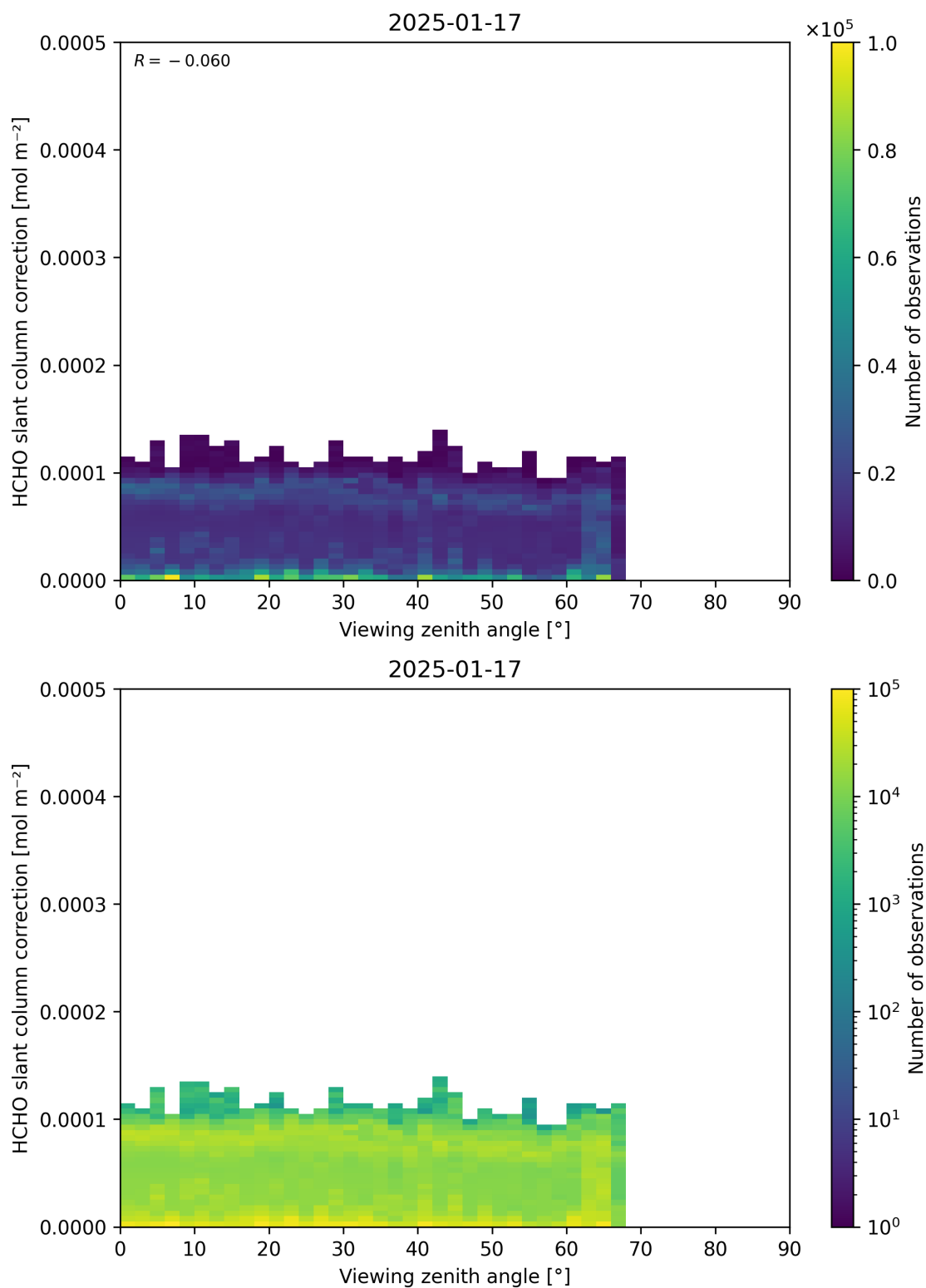
Figure 187: Scatter density plot of “Viewing zenith angle” against “HCHO slant column correction” for 2025-01-17 to 2025-01-18.
