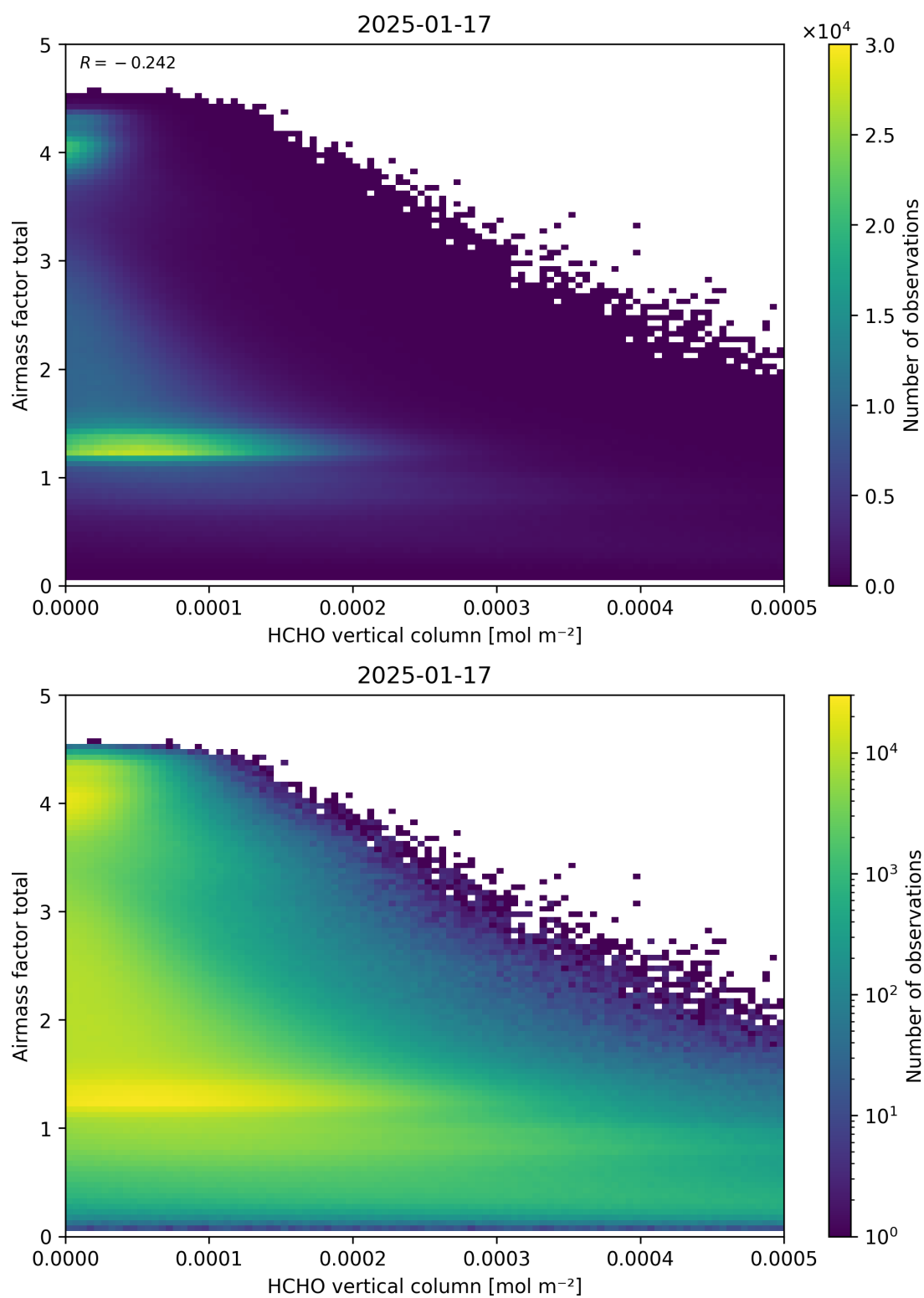
Figure 131: Scatter density plot of “HCHO vertical column” against “Airmass factor total” for 2025-01-17 to 2025-01-18.
