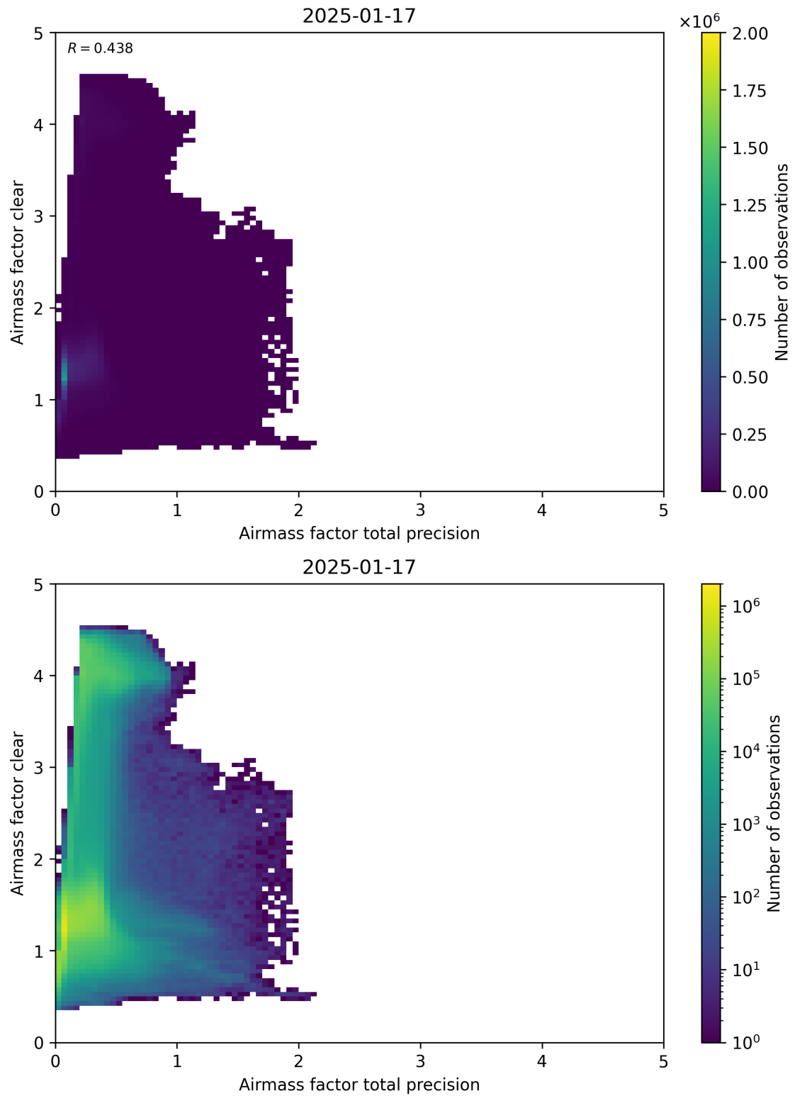
Figure 108: Scatter density plot of “Airmass factor total precision” against “Airmass factor clear” for 2025-01-17 to 2025-01-18.
