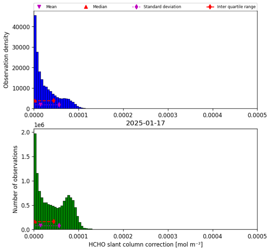
Figure 47: Histogram of “HCHO slant column correction” for 2025-01-17 to 2025-01-18
