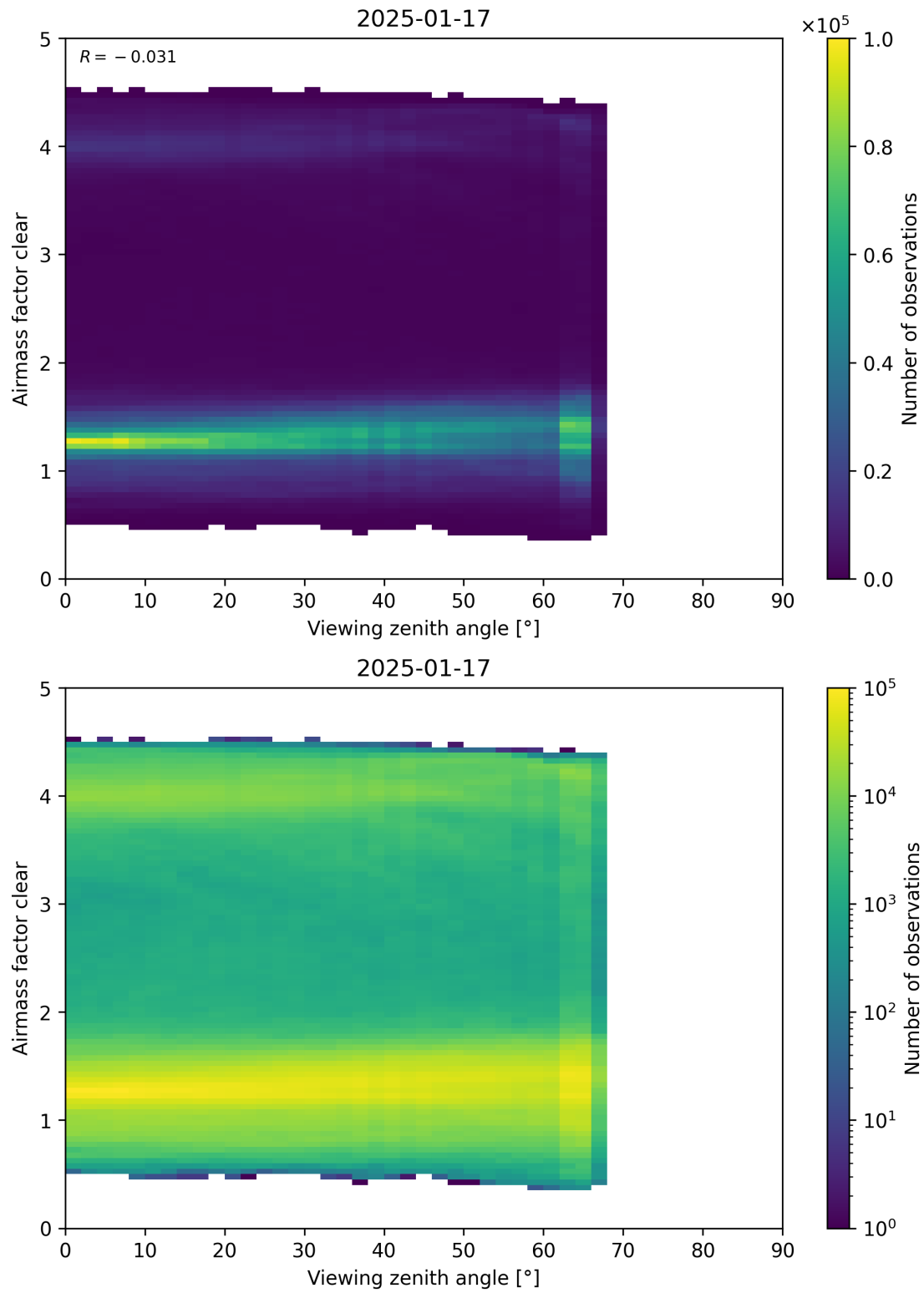
Figure 185: Scatter density plot of “Viewing zenith angle” against “Airmass factor clear” for 2025-01-17 to 2025-01-18.
