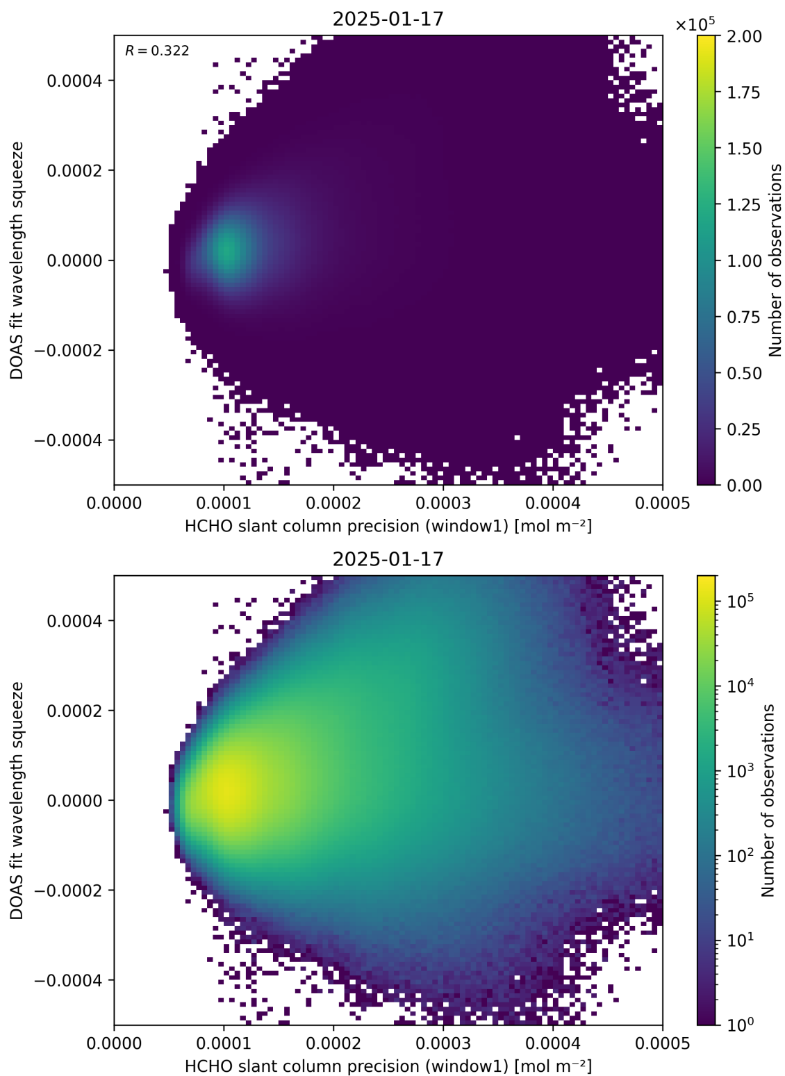
Figure 90: Scatter density plot of “HCHO slant column precision (window1)” against “DOAS fit wavelength squeeze” for 2025-01-17 to 2025-01-18.
