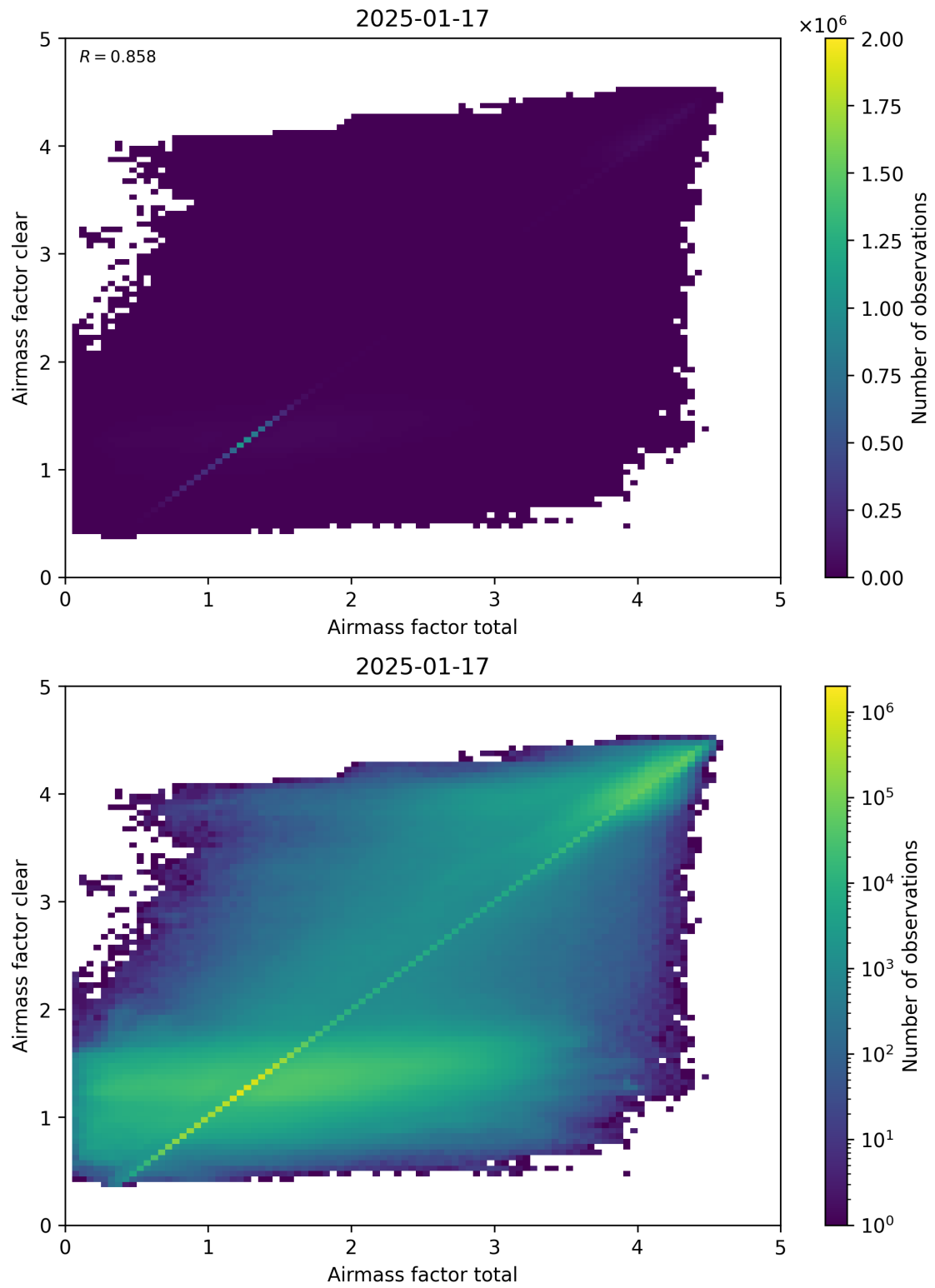
Figure 100: Scatter density plot of “Airmass factor total” against “Airmass factor clear” for 2025-01-17 to 2025-01-18.
