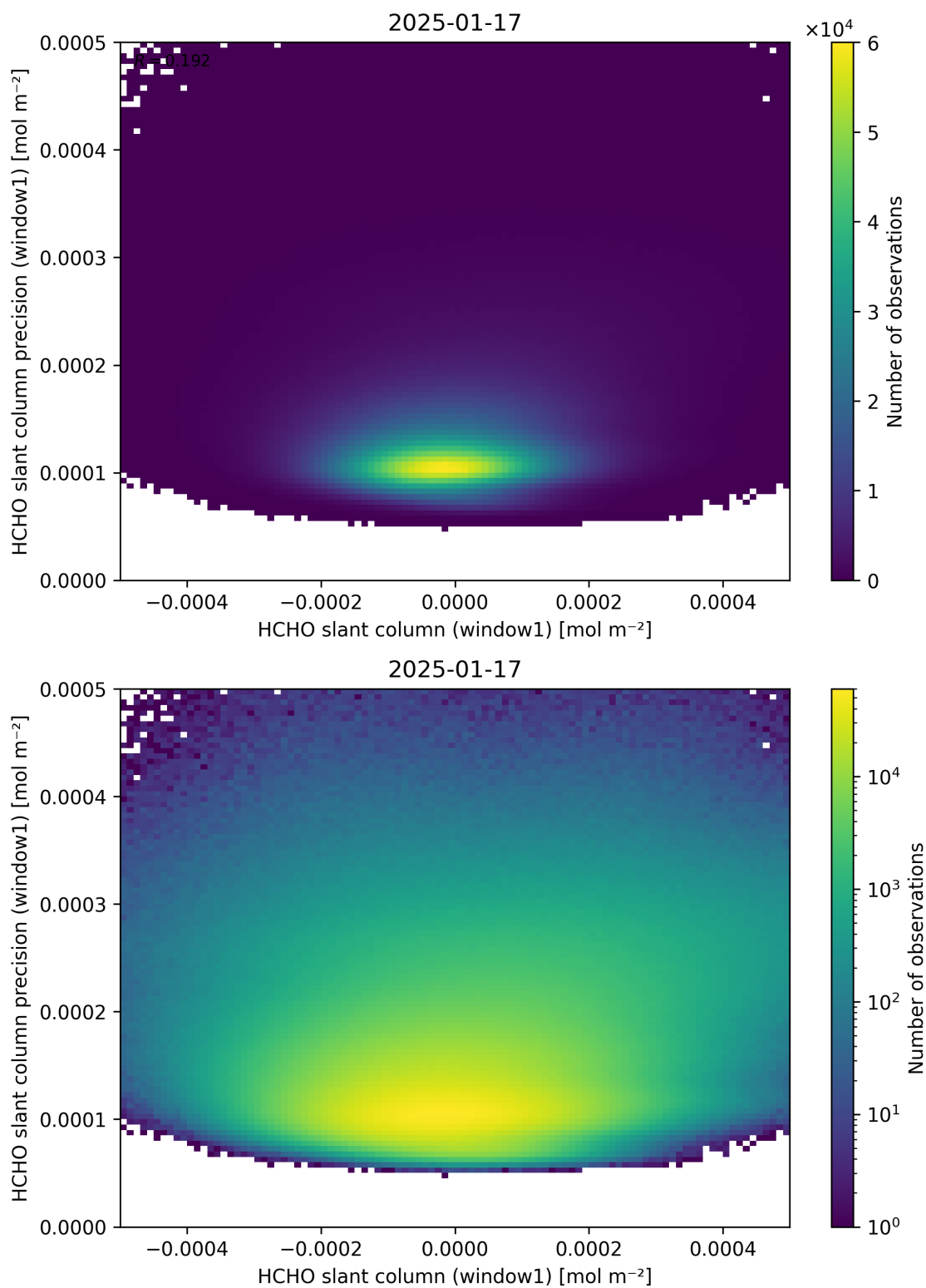
Figure 84: Scatter density plot of “HCHO slant column (window1)” against “HCHO slant column precision (window1)” for 2025-01-17 to 2025-01-18.
