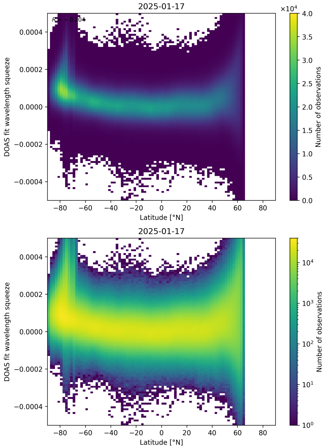
Figure 155: Scatter density plot of “Latitude” against “DOAS fit wavelength squeeze” for 2025-01-17 to 2025-01-18.
