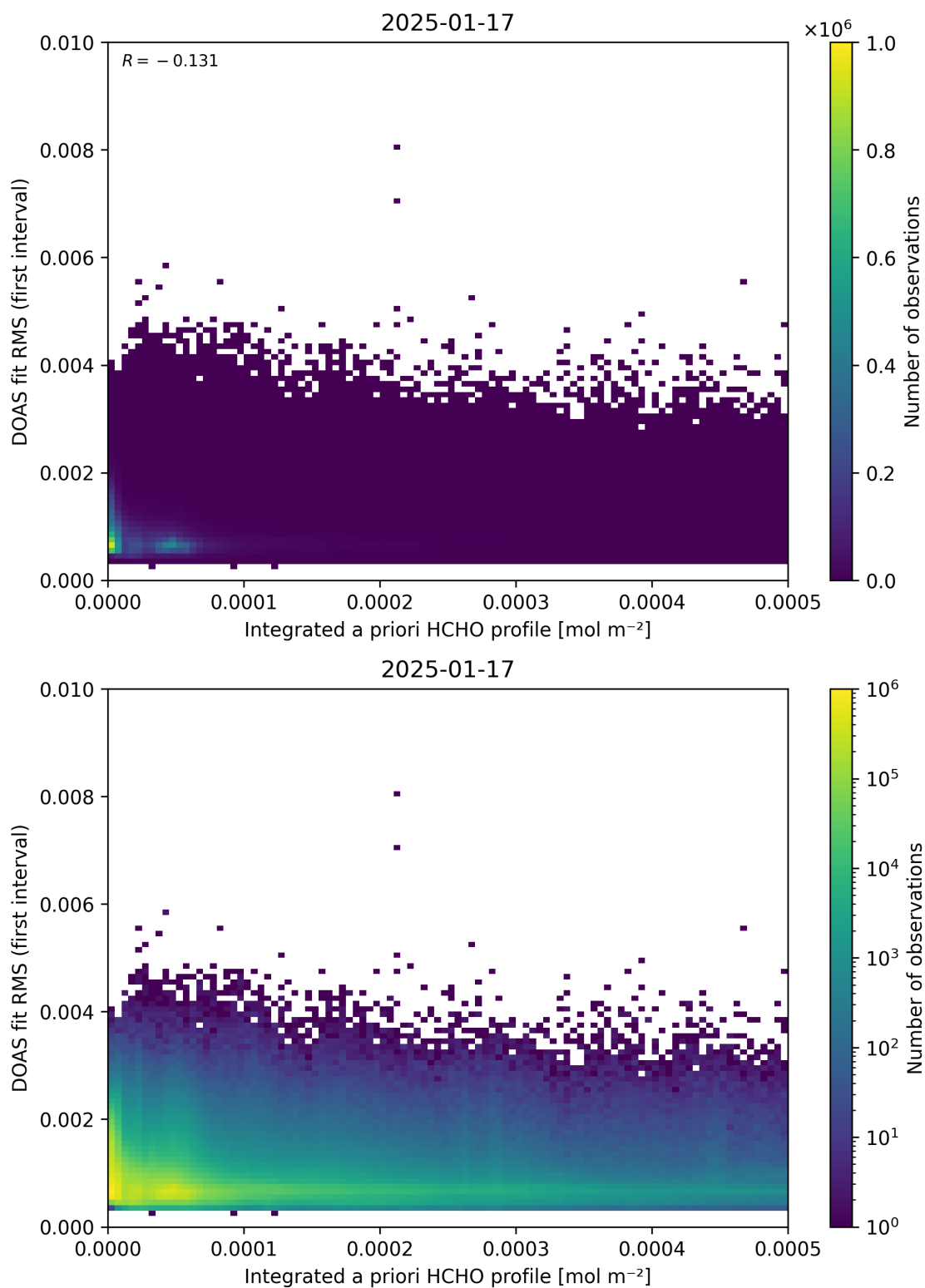
Figure 148: Scatter density plot of “Integrated a priori HCHO profile” against “DOAS fit RMS (first interval)” for 2025-01-17 to 2025-01-18.
