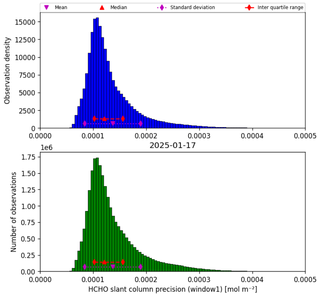
Figure 39: Histogram of “HCHO slant column precision (window1)” for 2025-01-17 to 2025-01-18
