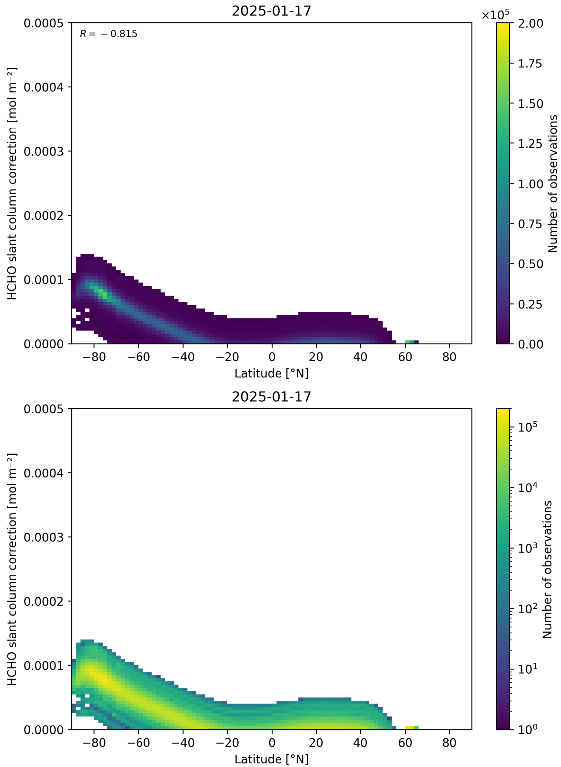
Figure 158: Scatter density plot of “Latitude” against “HCHO slant column correction” for 2025-01-17 to 2025-01-18.
