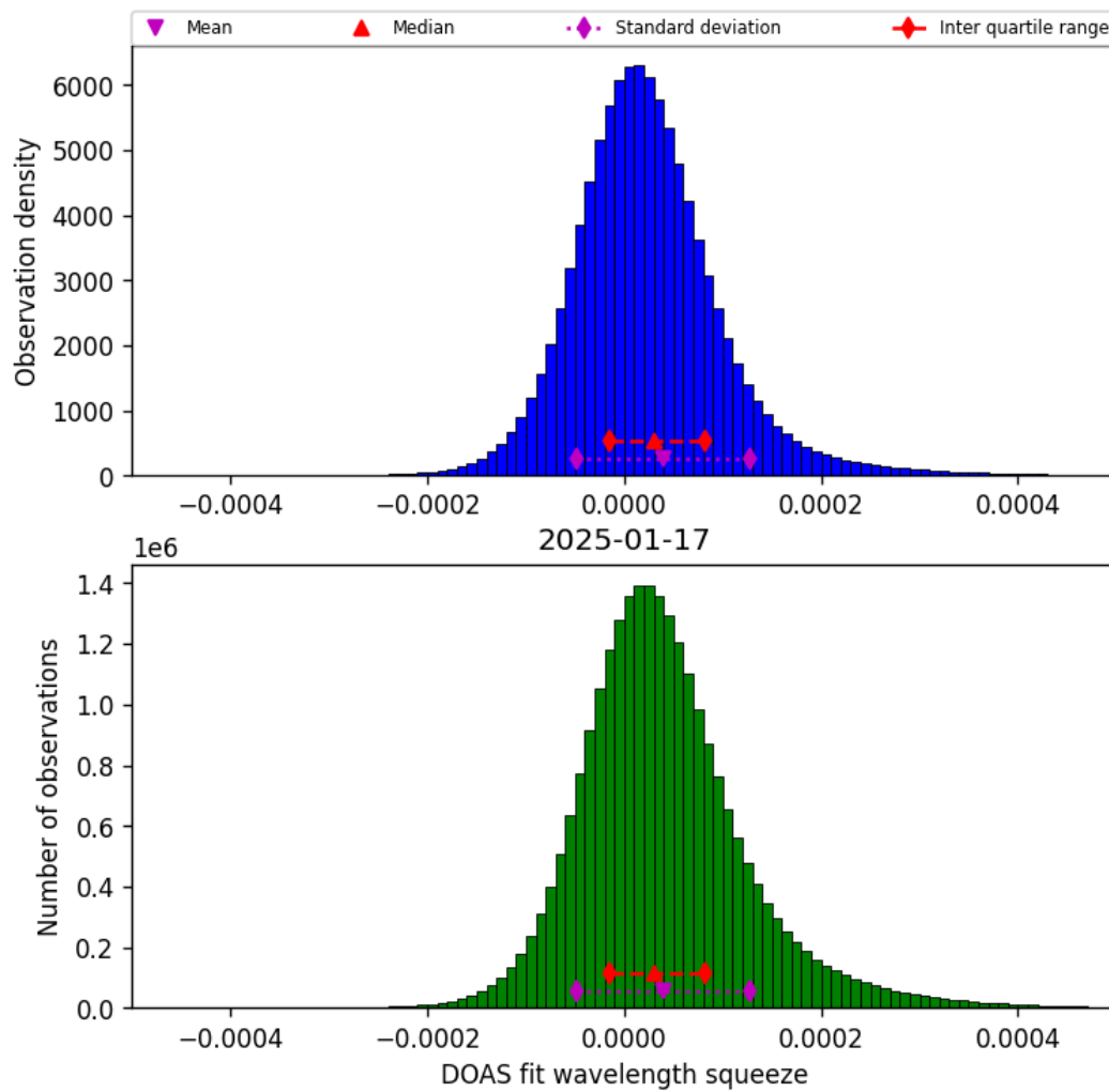
Figure 45: Histogram of "DOAS fit wavelength squeeze" for 2025-01-17 to 2025-01-18
