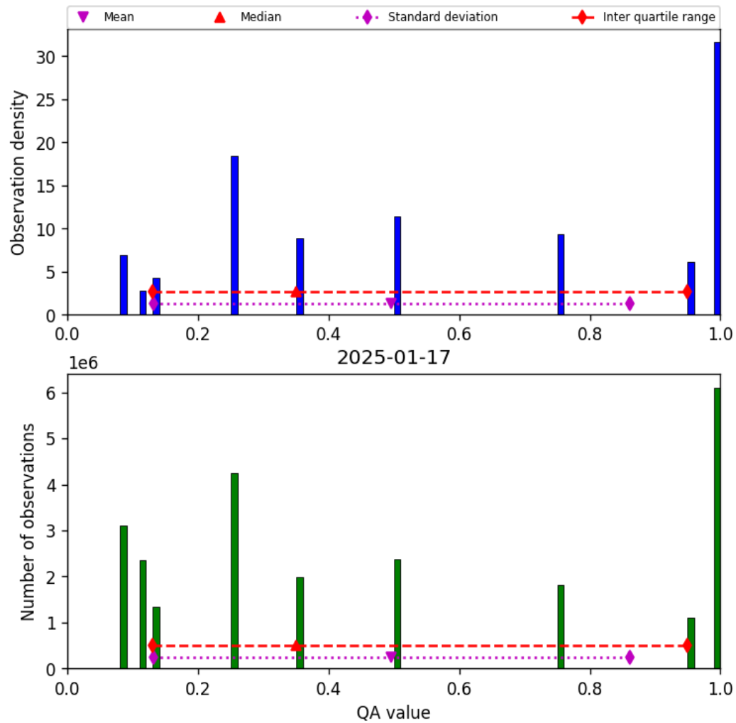
Figure 34: Histogram of “QA value” for 2025-01-17 to 2025-01-18
