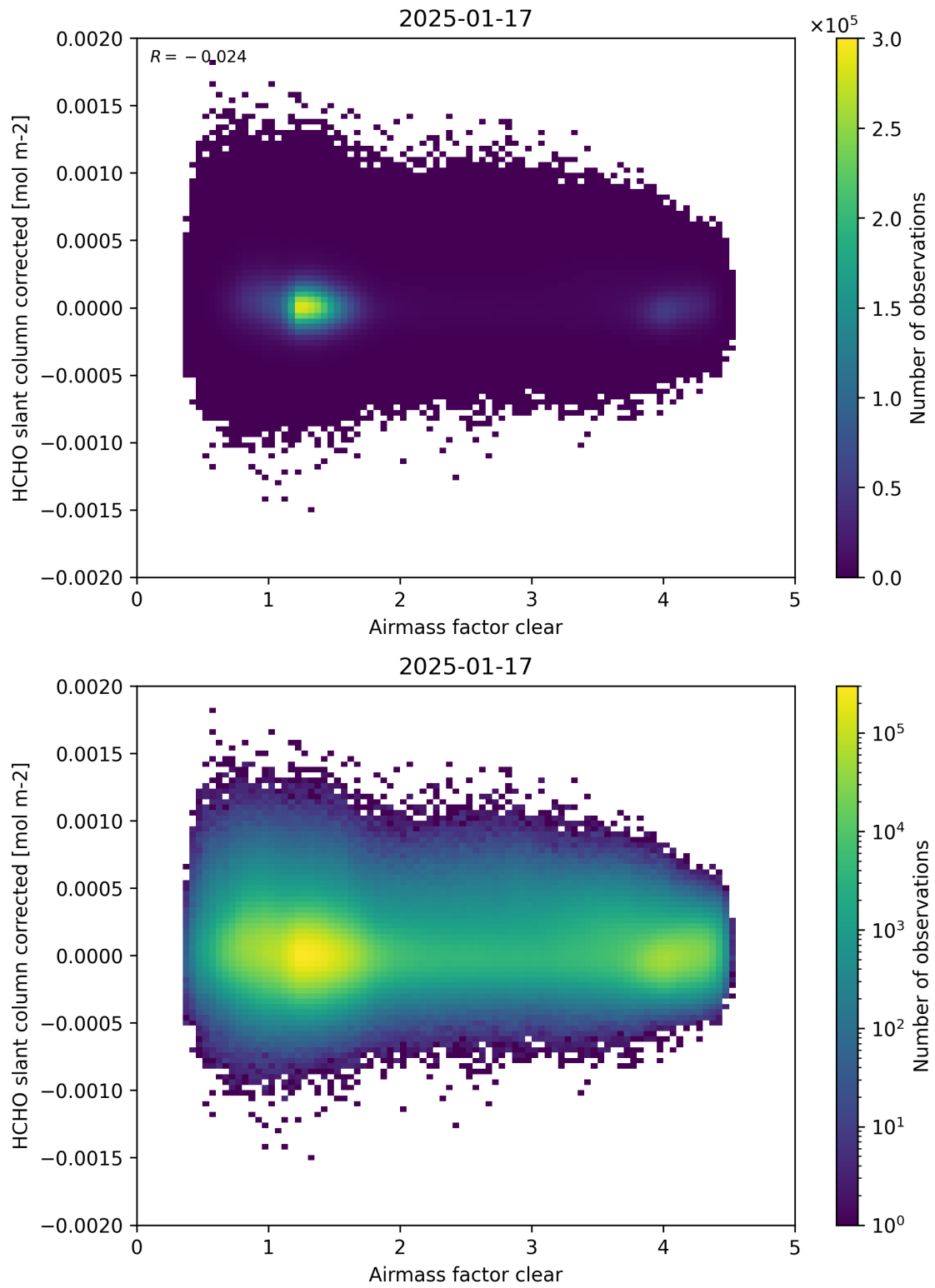
Figure 74: Scatter density plot of “Airmass factor clear” against “HCHO slant column corrected” for 2025-01-17 to 2025-01-18.
