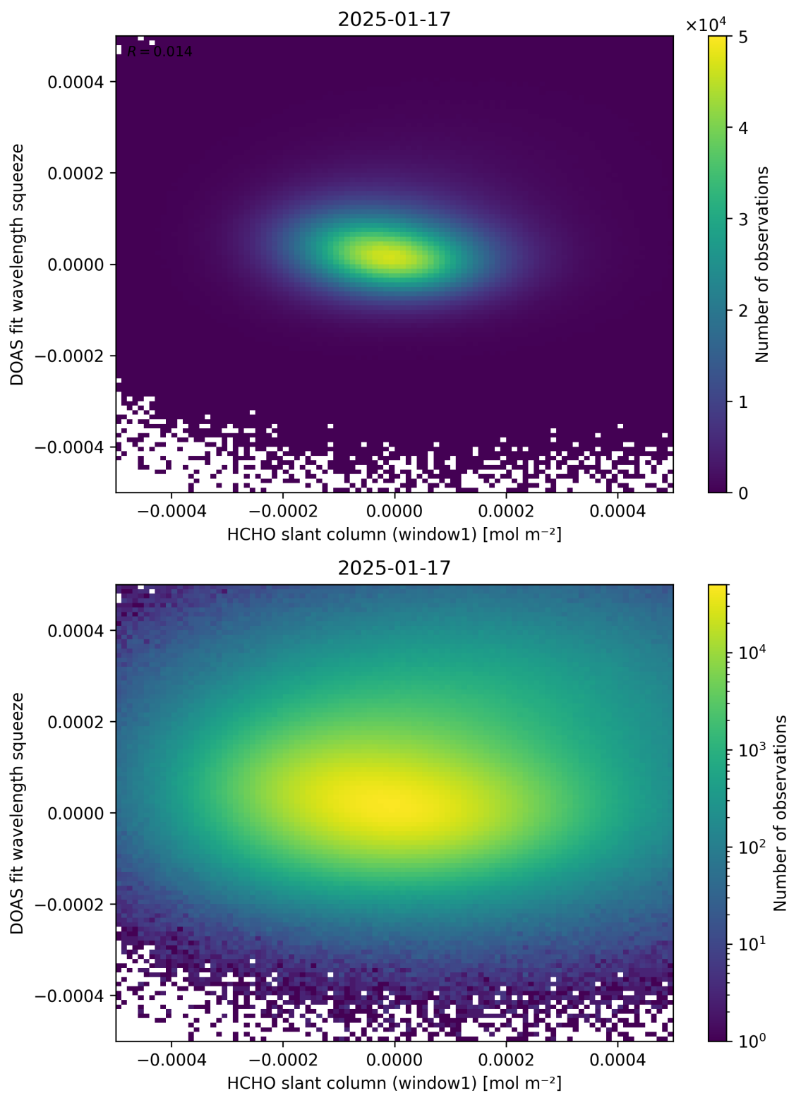
Figure 80: Scatter density plot of “HCHO slant column (window1)” against “DOAS fit wavelength squeeze” for 2025-01-17 to 2025-01-18.
