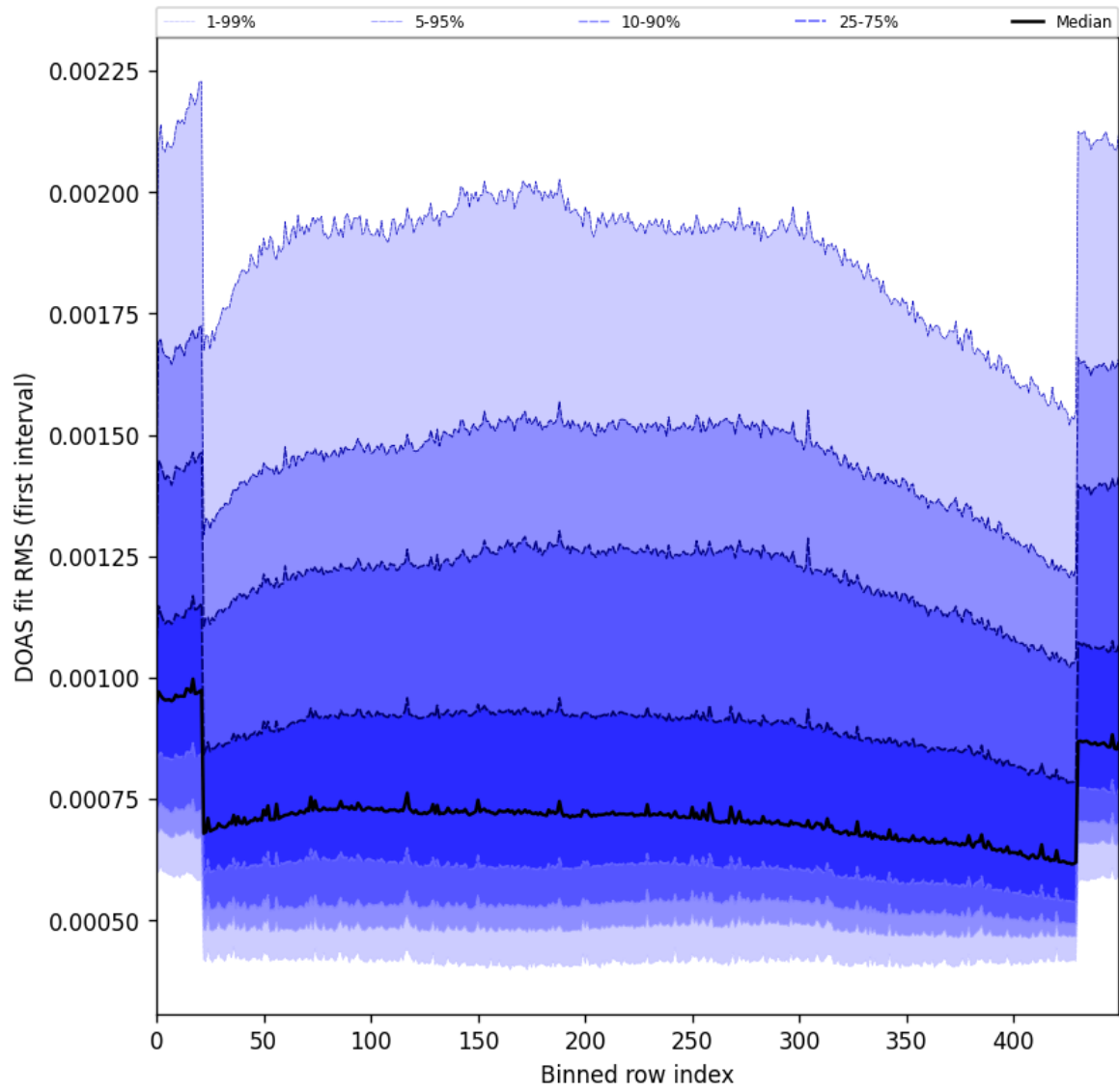
Figure 60: Along track statistics of “DOAS fit RMS (first interval)” for 2025-01-17 to 2025-01-18
