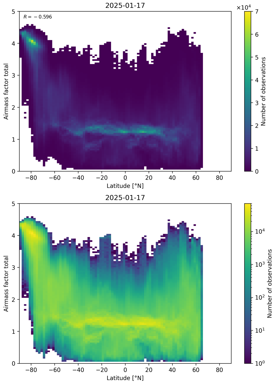
Figure 161: Scatter density plot of “Latitude” against “Airmass factor total” for 2025-01-17 to 2025-01-18.
