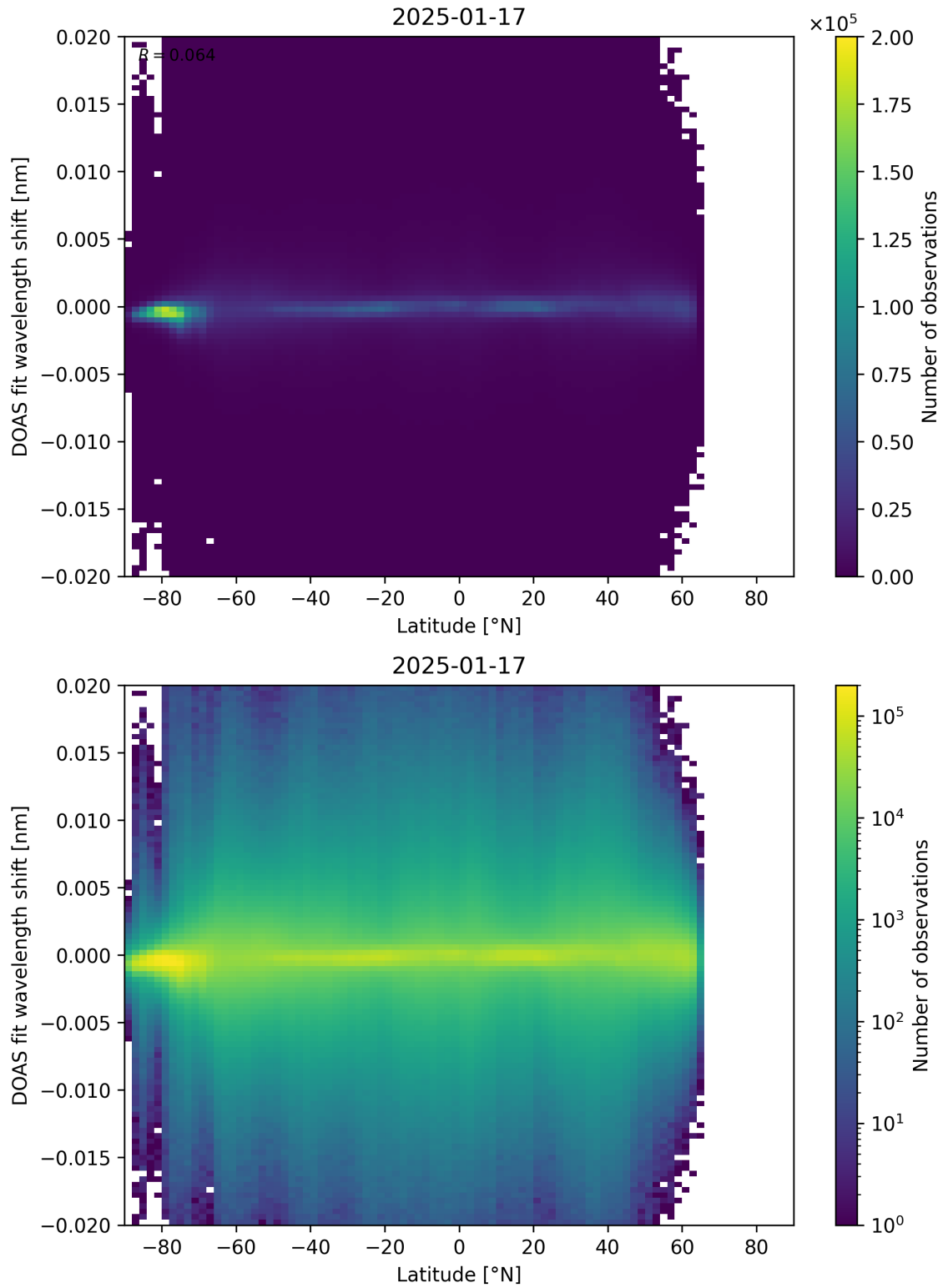
Figure 154: Scatter density plot of “Latitude” against “DOAS fit wavelength shift” for 2025-01-17 to 2025-01-18.
