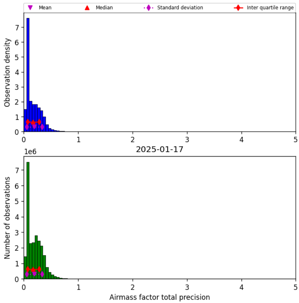
Figure 41: Histogram of “Airmass factor total precision” for 2025-01-17 to 2025-01-18
