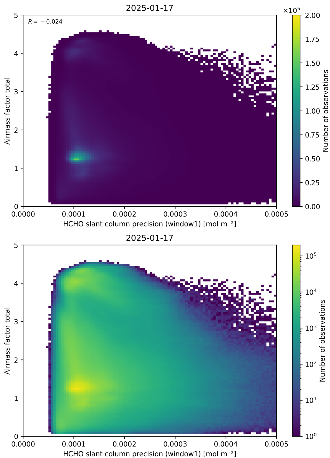
Figure 94: Scatter density plot of “HCHO slant column precision (window1)” against “Airmass factor total” for 2025-01-17 to 2025-01-18.
