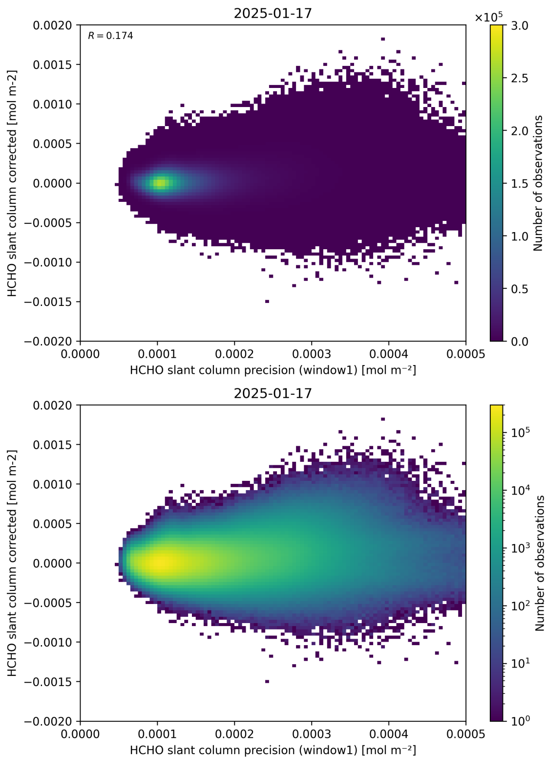
Figure 92: Scatter density plot of “HCHO slant column precision (window1)” against “HCHO slant column corrected” for 2025-01-17 to 2025-01-18.
