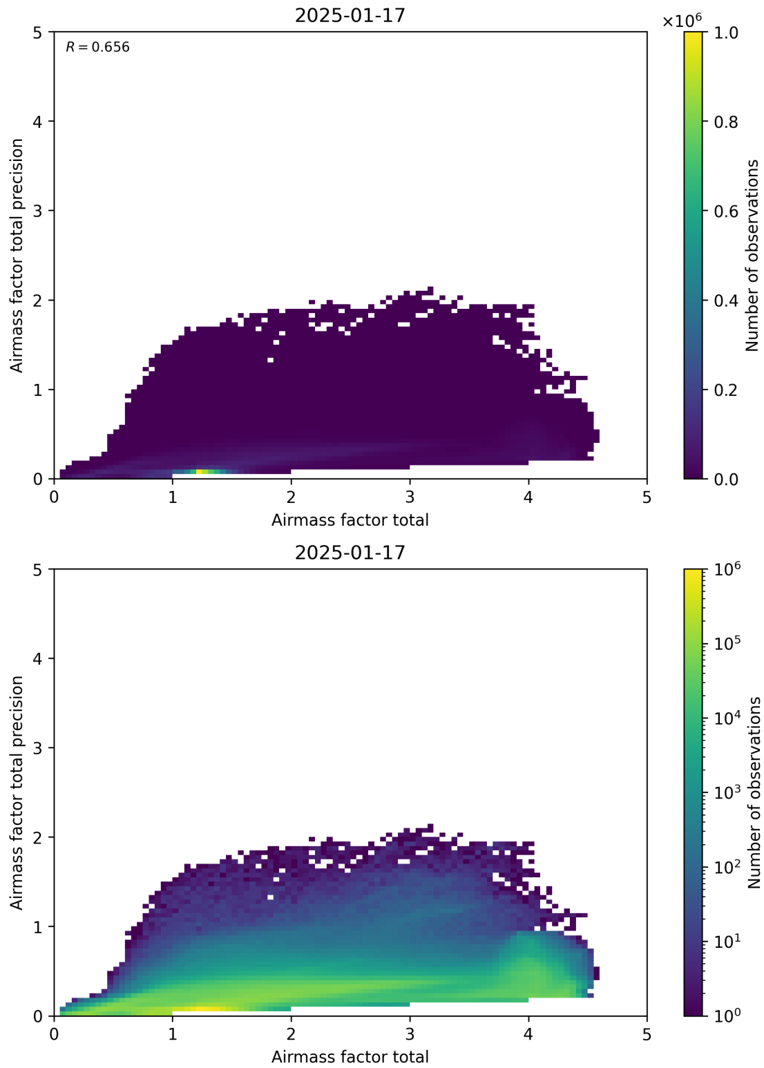
Figure 103: Scatter density plot of “Airmass factor total” against “Airmass factor total precision” for 2025-01-17 to 2025-01-18.
