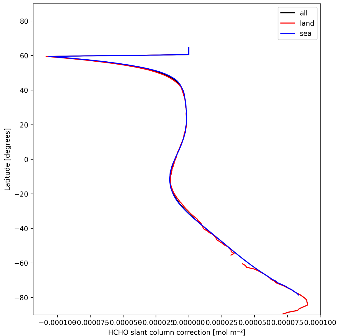
Figure 33: Zonal average of “HCHO slant column correction” for 2025-01-17 to 2025-01-18.
