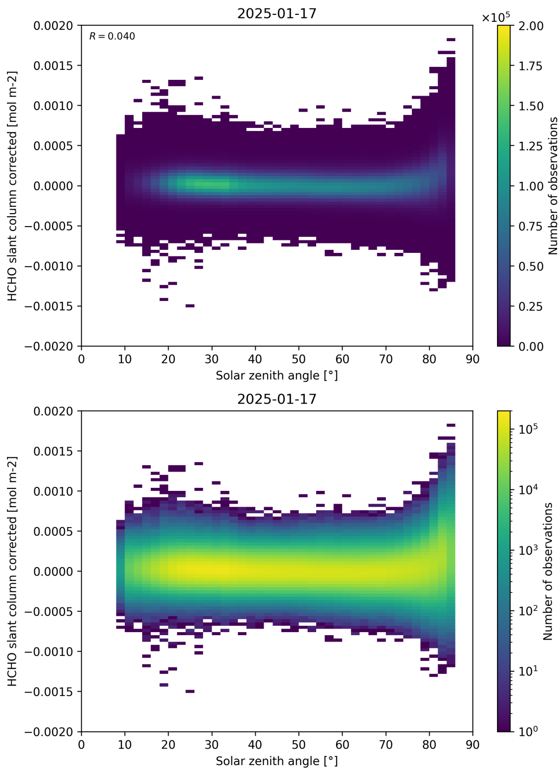
Figure 171: Scatter density plot of “Solar zenith angle” against “HCHO slant column corrected” for 2025-01-17 to 2025-01-18.
