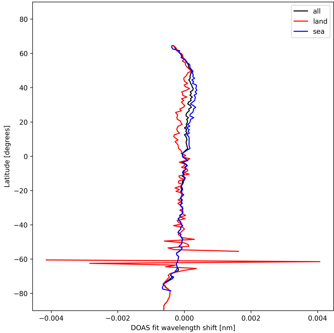
Figure 30: Zonal average of “DOAS fit wavelength shift” for 2025-01-17 to 2025-01-18.
