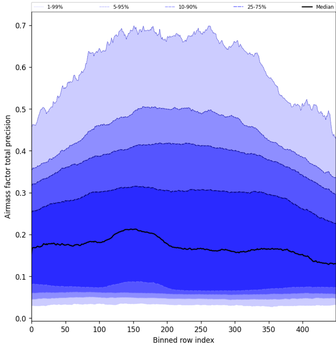
Figure 55: Along track statistics of “Airmass factor total precision” for 2025-01-17 to 2025-01-18
