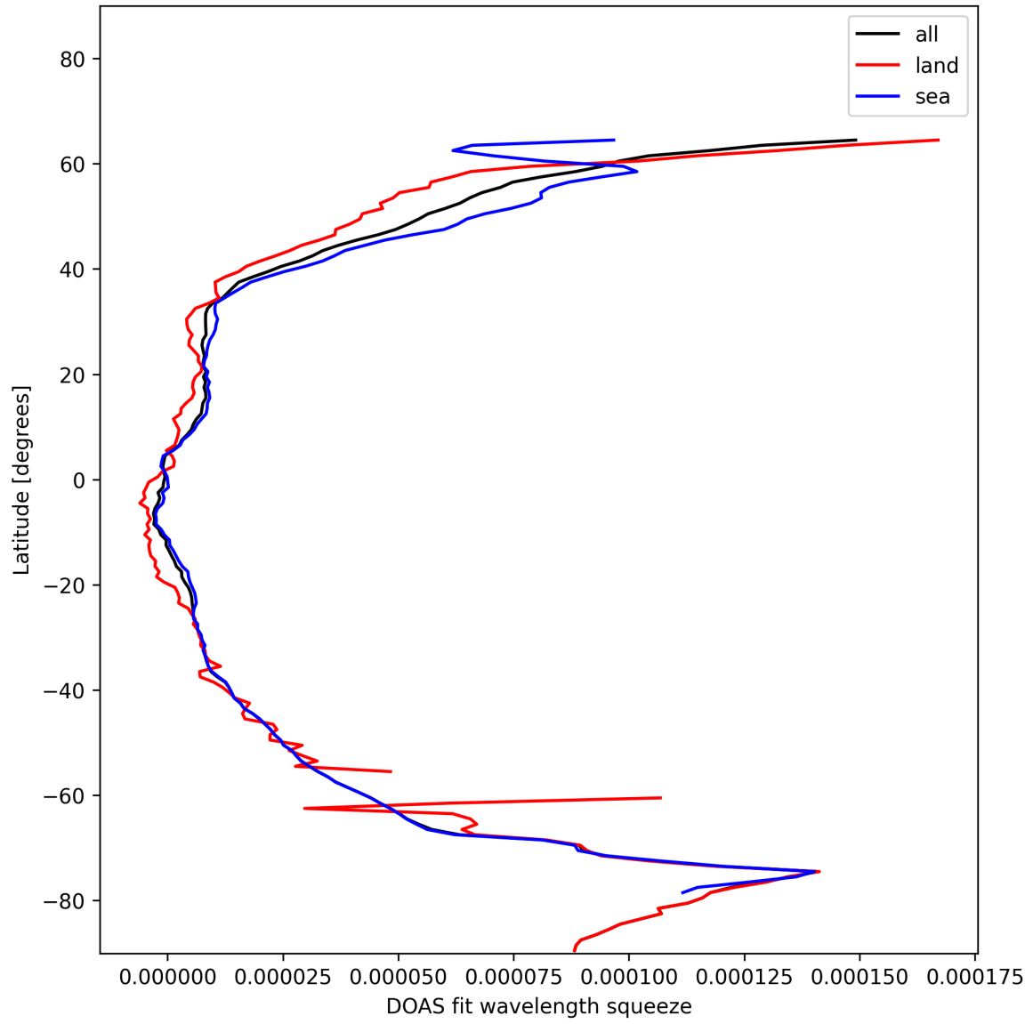
Figure 31: Zonal average of “DOAS fit wavelength squeeze” for 2025-01-17 to 2025-01-18.
