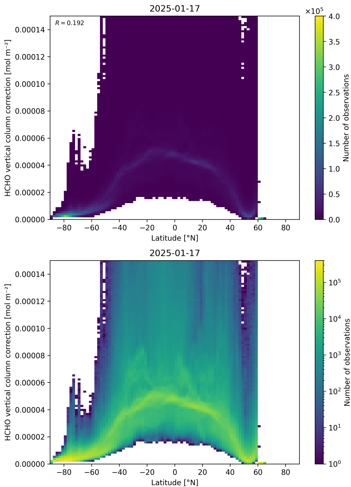
Figure 164: Scatter density plot of “Latitude” against “HCHO vertical column correction” for 2025-01-17 to 2025-01-18.
