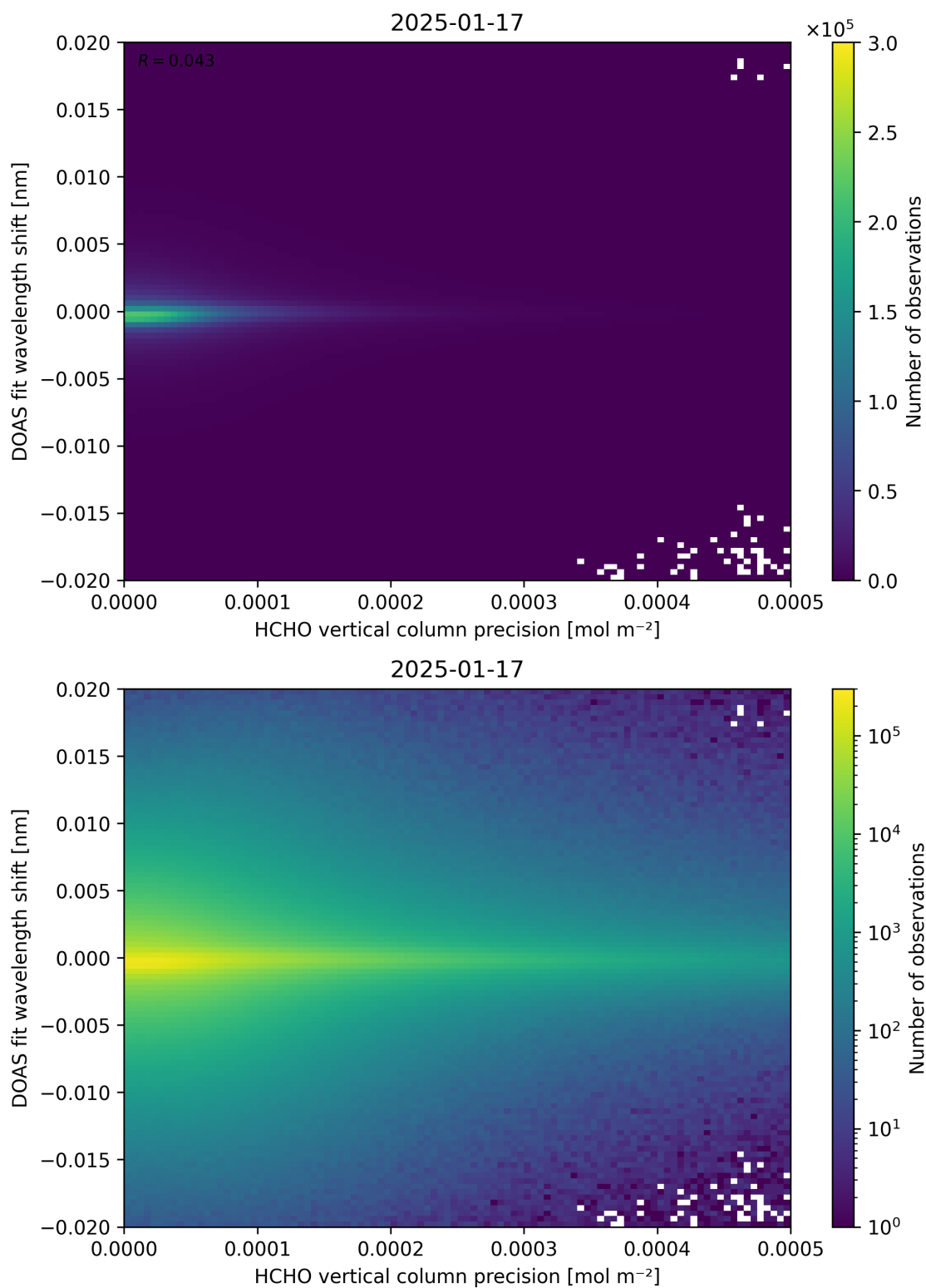
Figure 137: Scatter density plot of “HCHO vertical column precision” against “DOAS fit wavelength shift” for 2025-01-17 to 2025-01-18.
