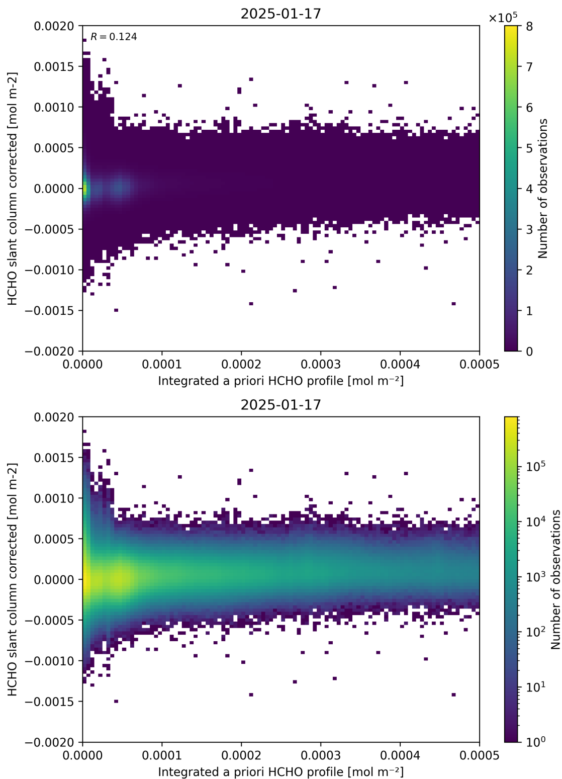
Figure 151: Scatter density plot of “Integrated a priori HCHO profile” against “HCHO slant column corrected” for 2025-01-17 to 2025-01-18.
