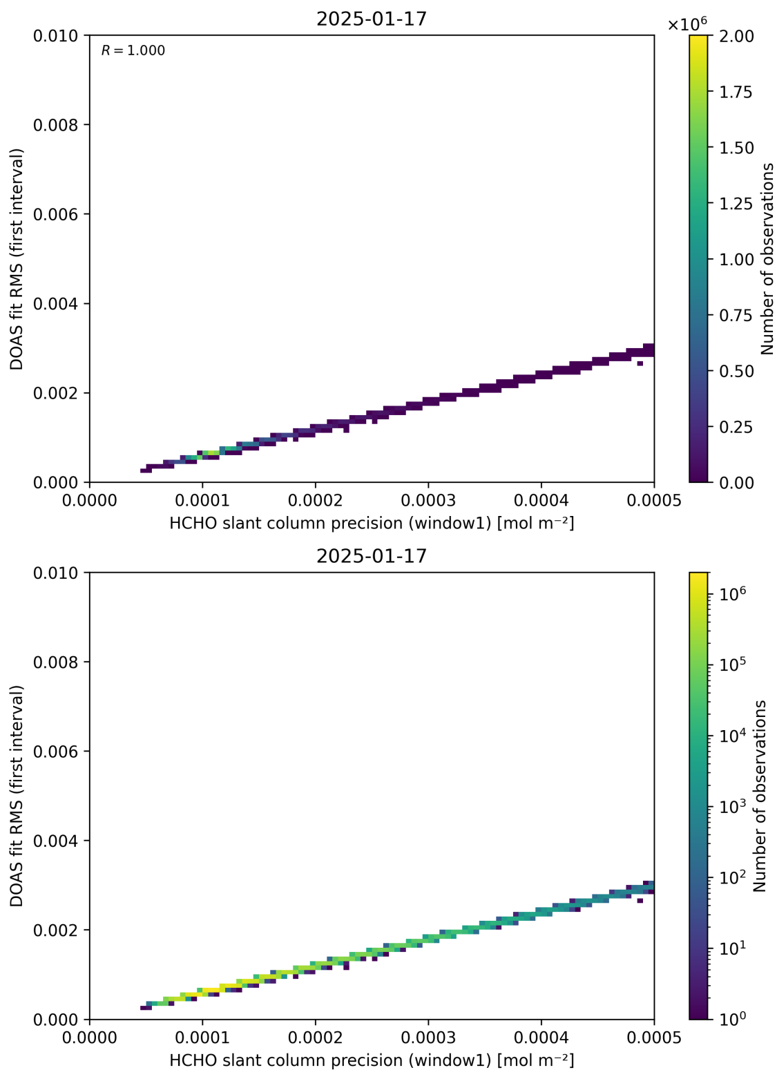
Figure 88: Scatter density plot of “HCHO slant column precision (window1)” against “DOAS fit RMS (first interval)” for 2025-01-17 to 2025-01-18.
