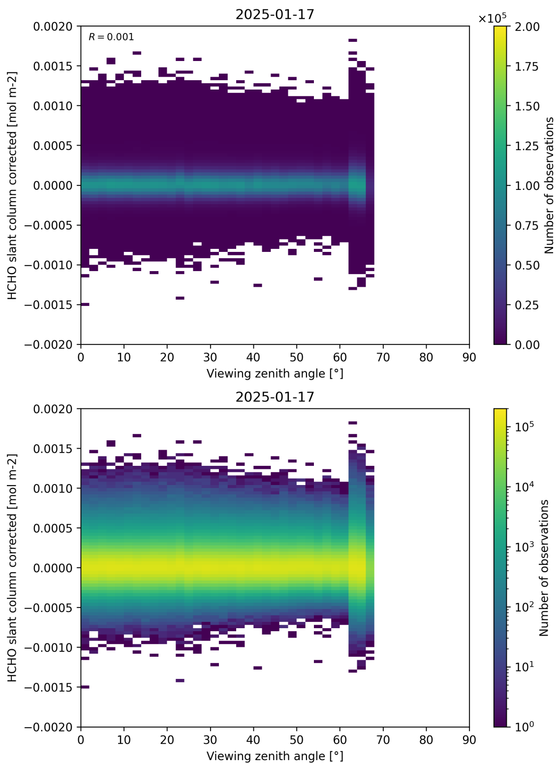
Figure 186: Scatter density plot of “Viewing zenith angle” against “HCHO slant column corrected” for 2025-01-17 to 2025-01-18.
