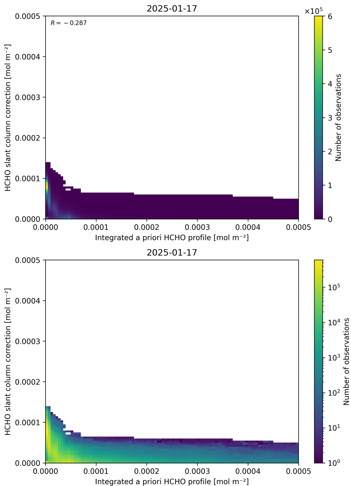
Figure 152: Scatter density plot of “Integrated a priori HCHO profile” against “HCHO slant column correction” for 2025-01-17 to 2025-01-18.
