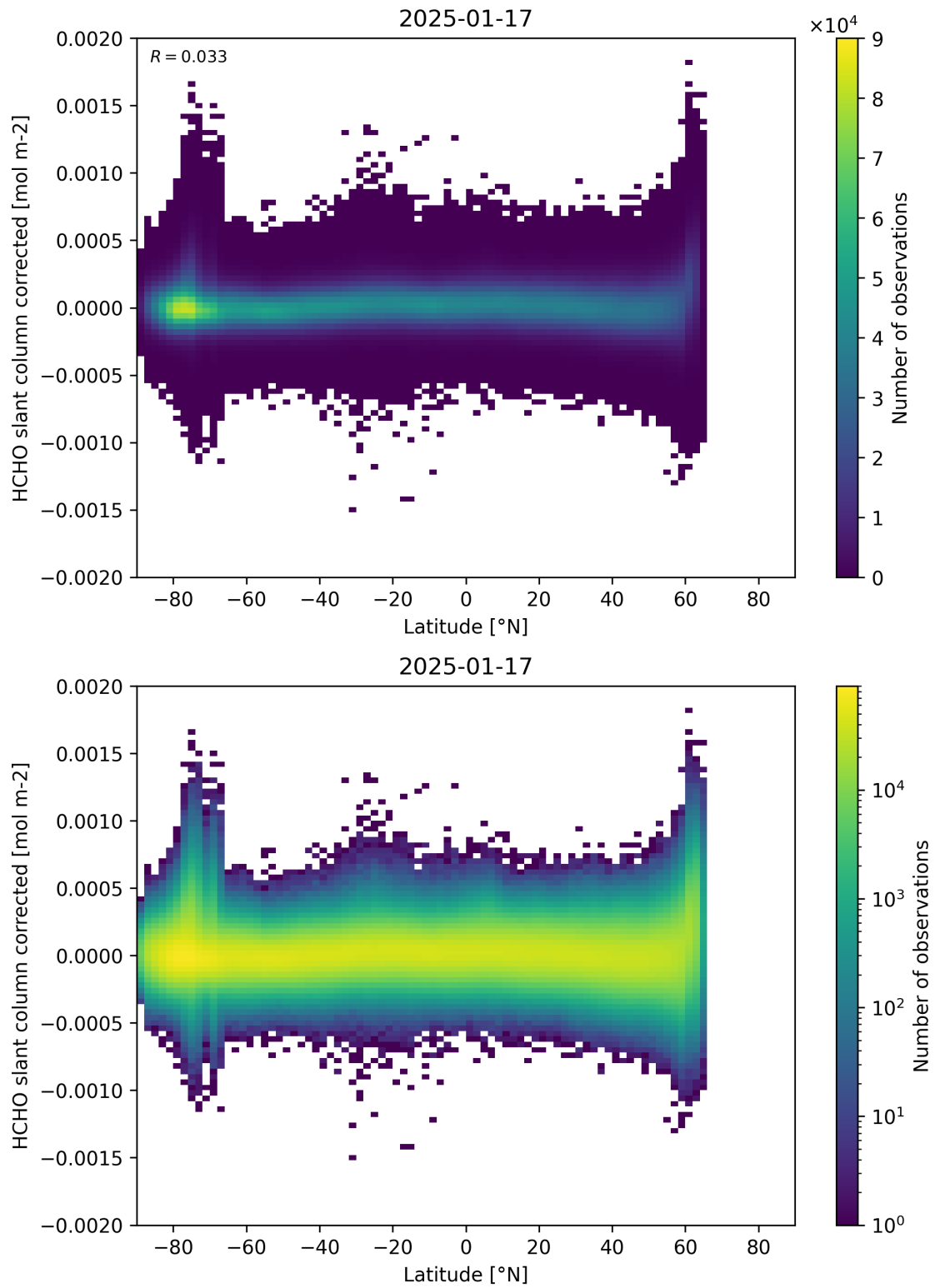
Figure 157: Scatter density plot of “Latitude” against “HCHO slant column corrected” for 2025-01-17 to 2025-01-18.
