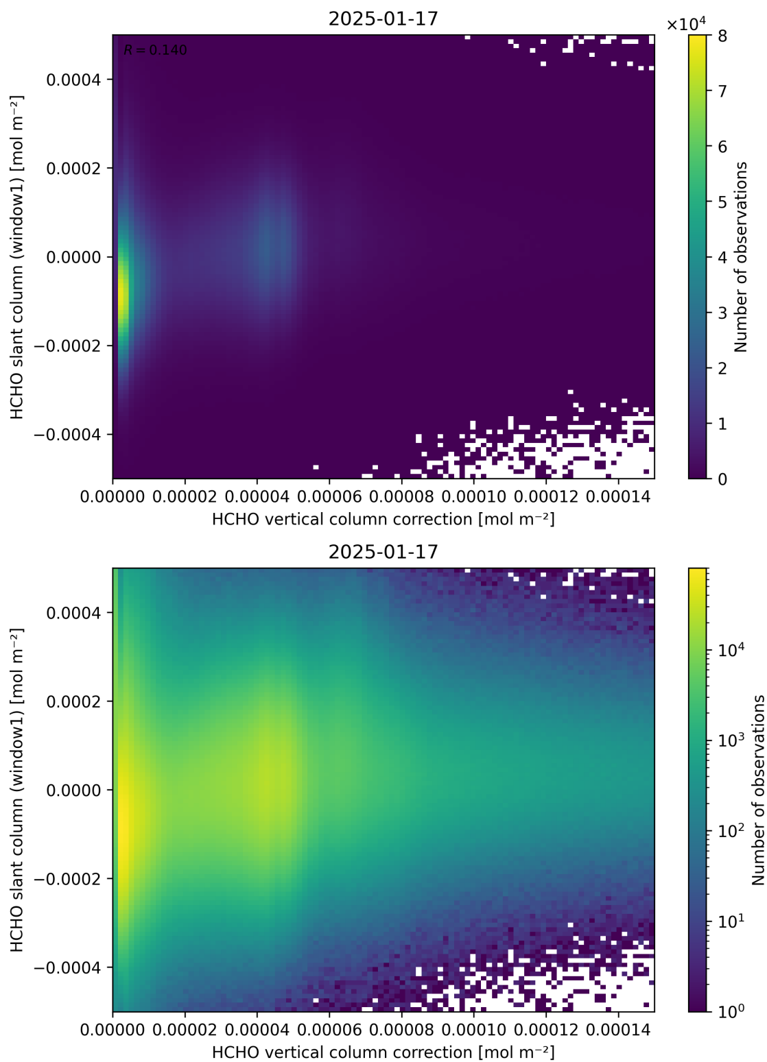
Figure 118: Scatter density plot of “HCHO vertical column correction” against “HCHO slant column (window1)” for 2025-01-17 to 2025-01-18.
