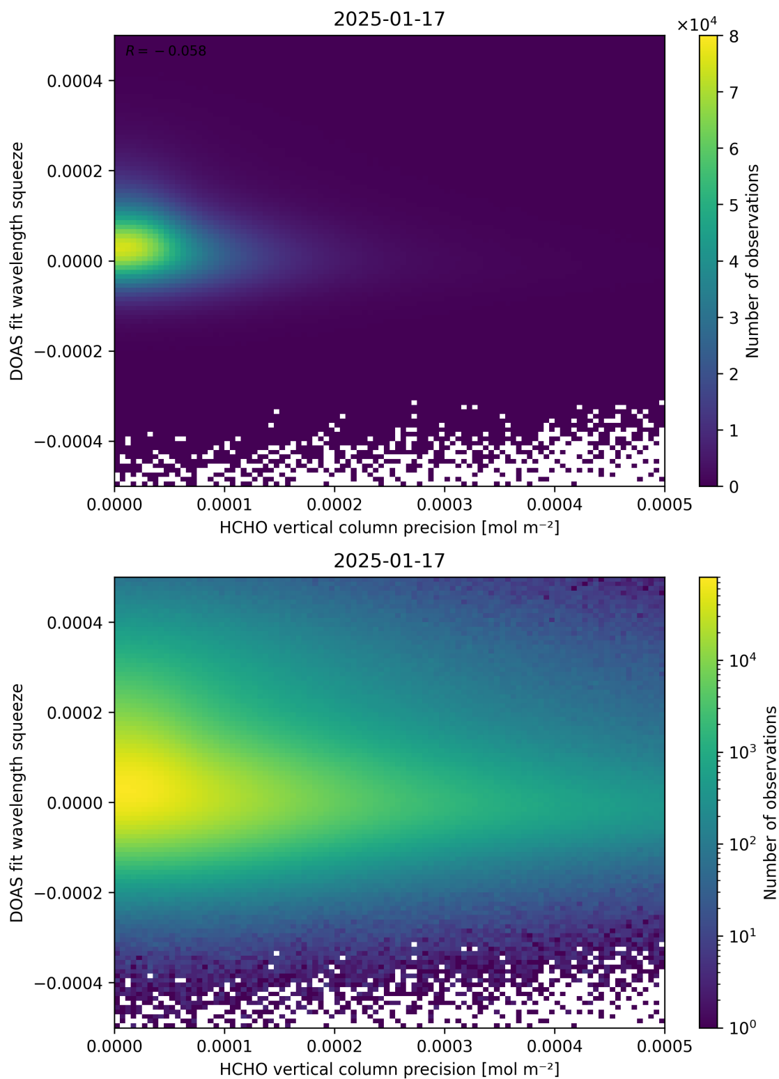
Figure 138: Scatter density plot of “HCHO vertical column precision” against “DOAS fit wavelength squeeze” for 2025-01-17 to 2025-01-18.
