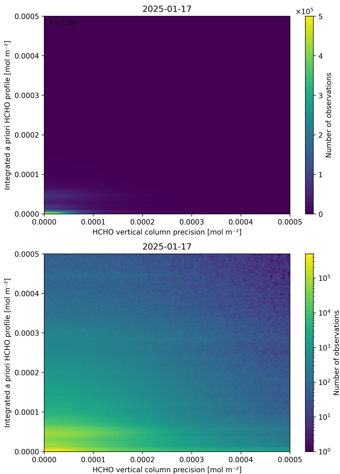
Figure 147: Scatter density plot of “HCHO vertical column precision” against “Integrated a priori HCHO profile” for 2025-01-17 to 2025-01-18.
