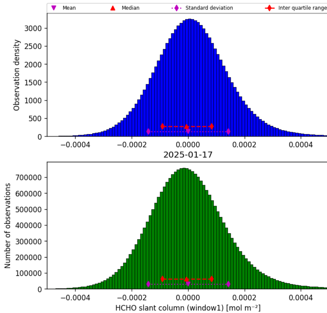
Figure 38: Histogram of “HCHO slant column (window1)” for 2025-01-17 to 2025-01-18
