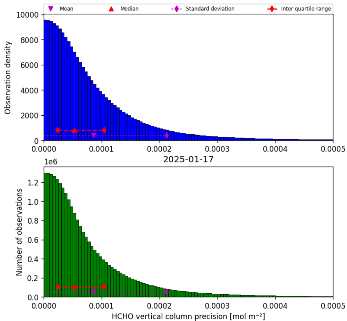
Figure 36: Histogram of “HCHO vertical column precision” for 2025-01-17 to 2025-01-18
