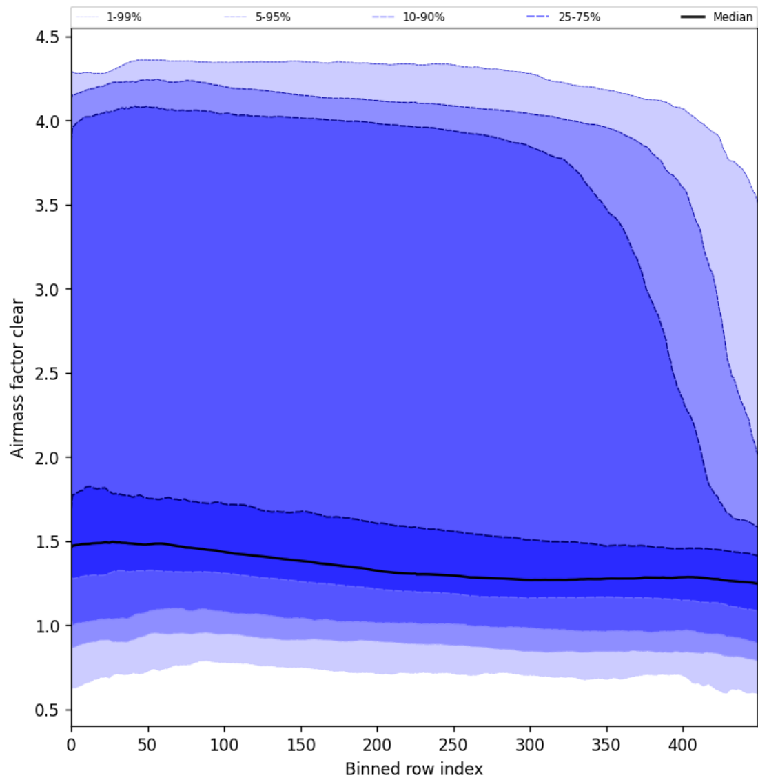
Figure 56: Along track statistics of “Airmass factor clear” for 2025-01-17 to 2025-01-18
