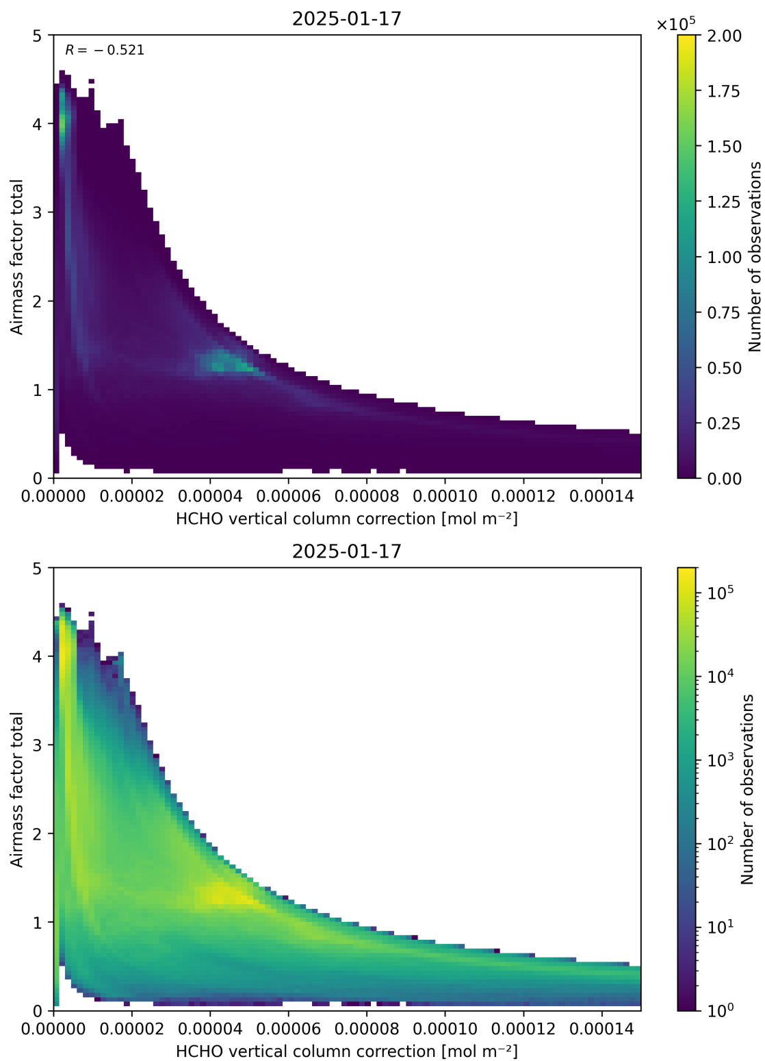
Figure 120: Scatter density plot of “HCHO vertical column correction” against “Airmass factor total” for 2025-01-17 to 2025-01-18.
