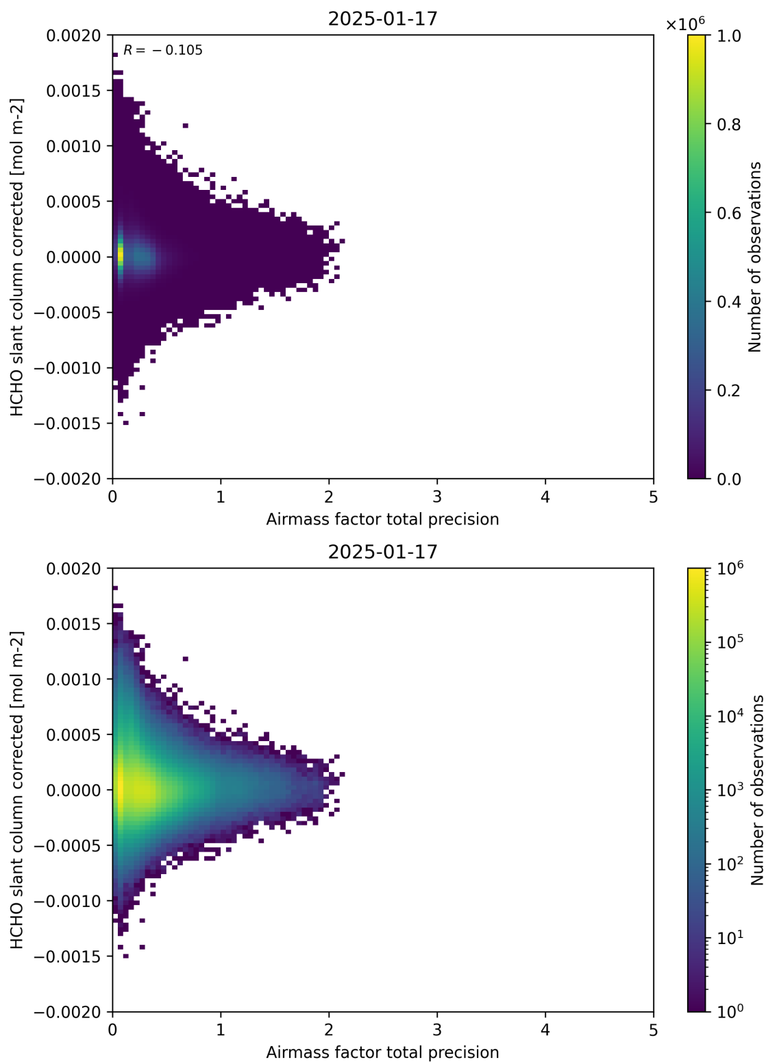
Figure 109: Scatter density plot of “Airmass factor total precision” against “HCHO slant column corrected” for 2025-01-17 to 2025-01-18.
