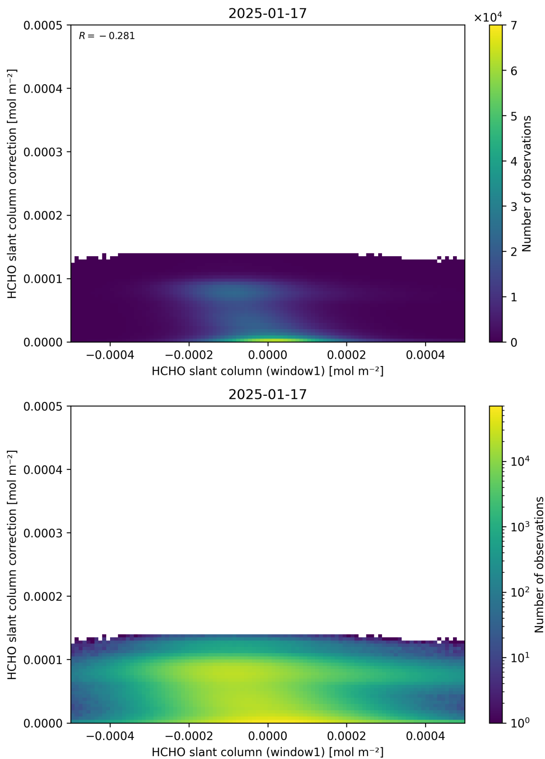
Figure 83: Scatter density plot of “HCHO slant column (window1)” against “HCHO slant column correction” for 2025-01-17 to 2025-01-18.
