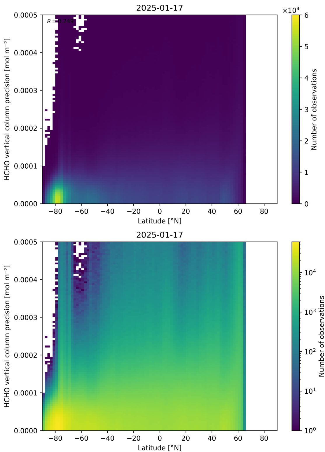
Figure 165: Scatter density plot of “Latitude” against “HCHO vertical column precision” for 2025-01-17 to 2025-01-18.
