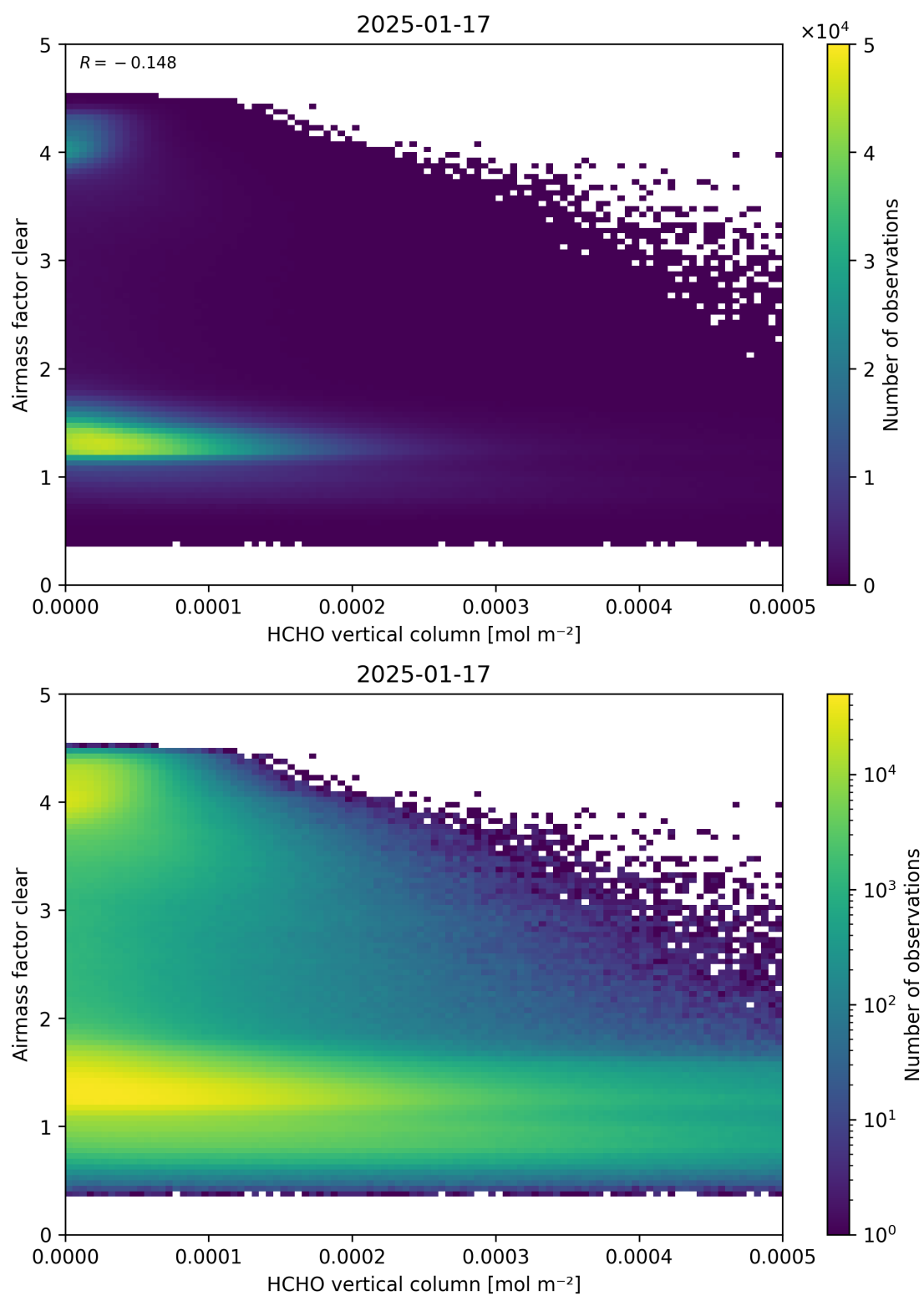
Figure 126: Scatter density plot of “HCHO vertical column” against “Airmass factor clear” for 2025-01-17 to 2025-01-18.
