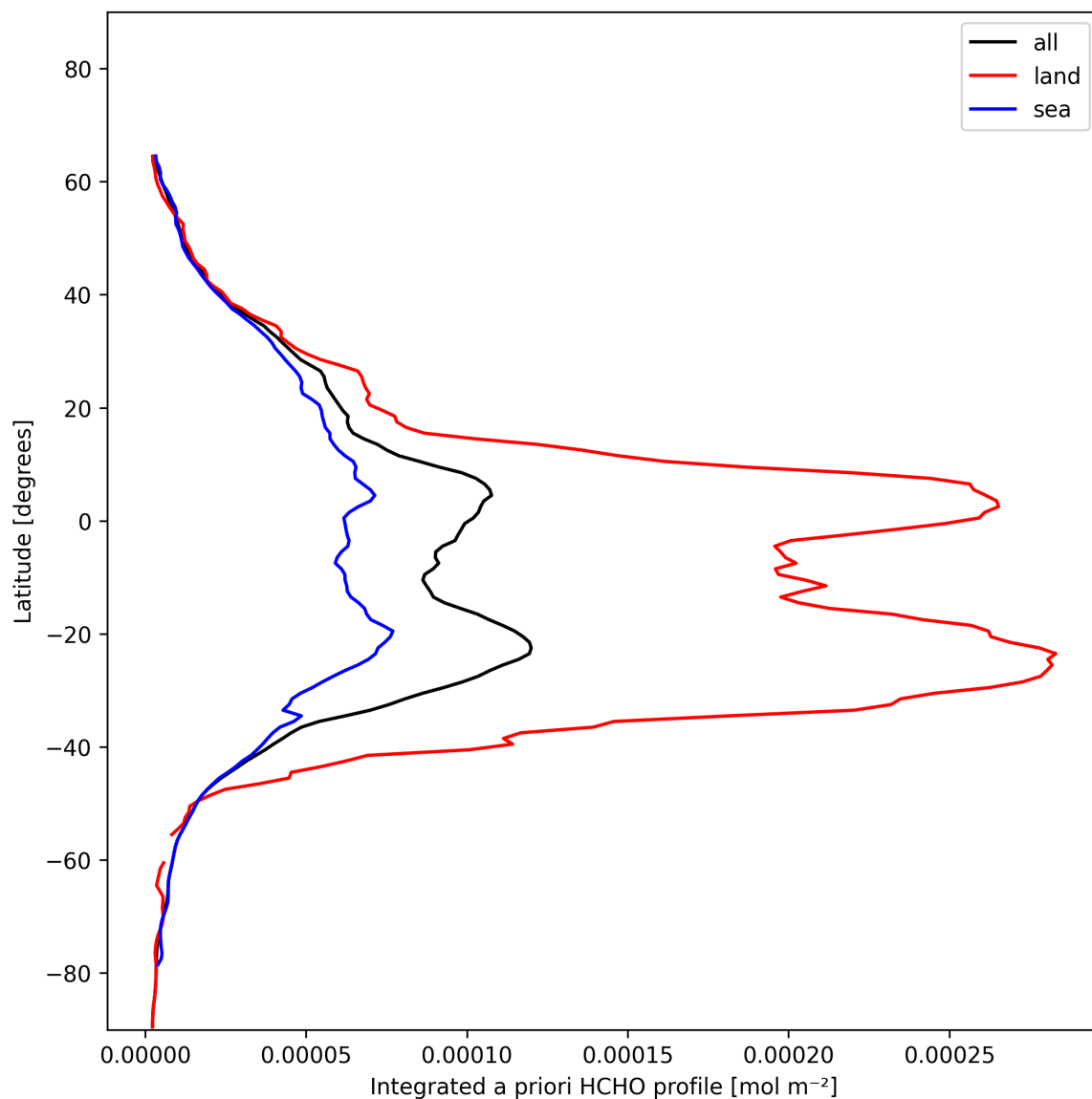
Figure 29: Zonal average of “Integrated a priori HCHO profile” for 2025-01-17 to 2025-01-18.
