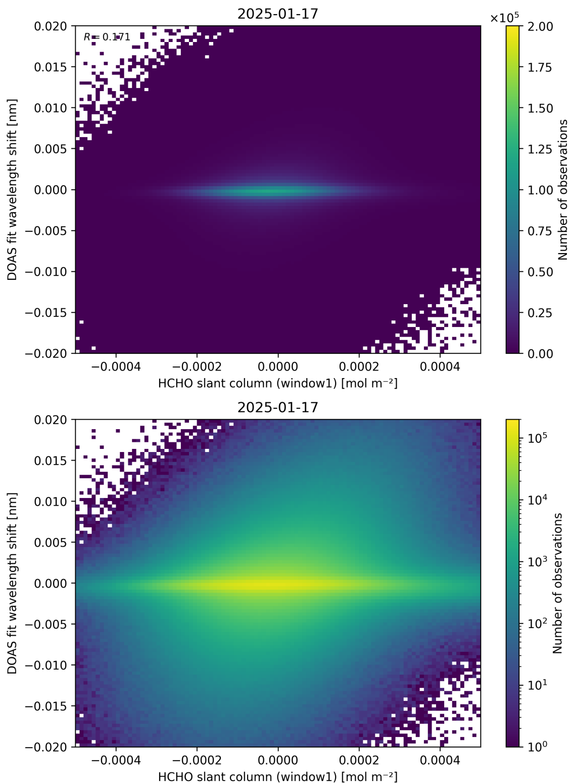
Figure 79: Scatter density plot of “HCHO slant column (window1)” against “DOAS fit wavelength shift” for 2025-01-17 to 2025-01-18.
