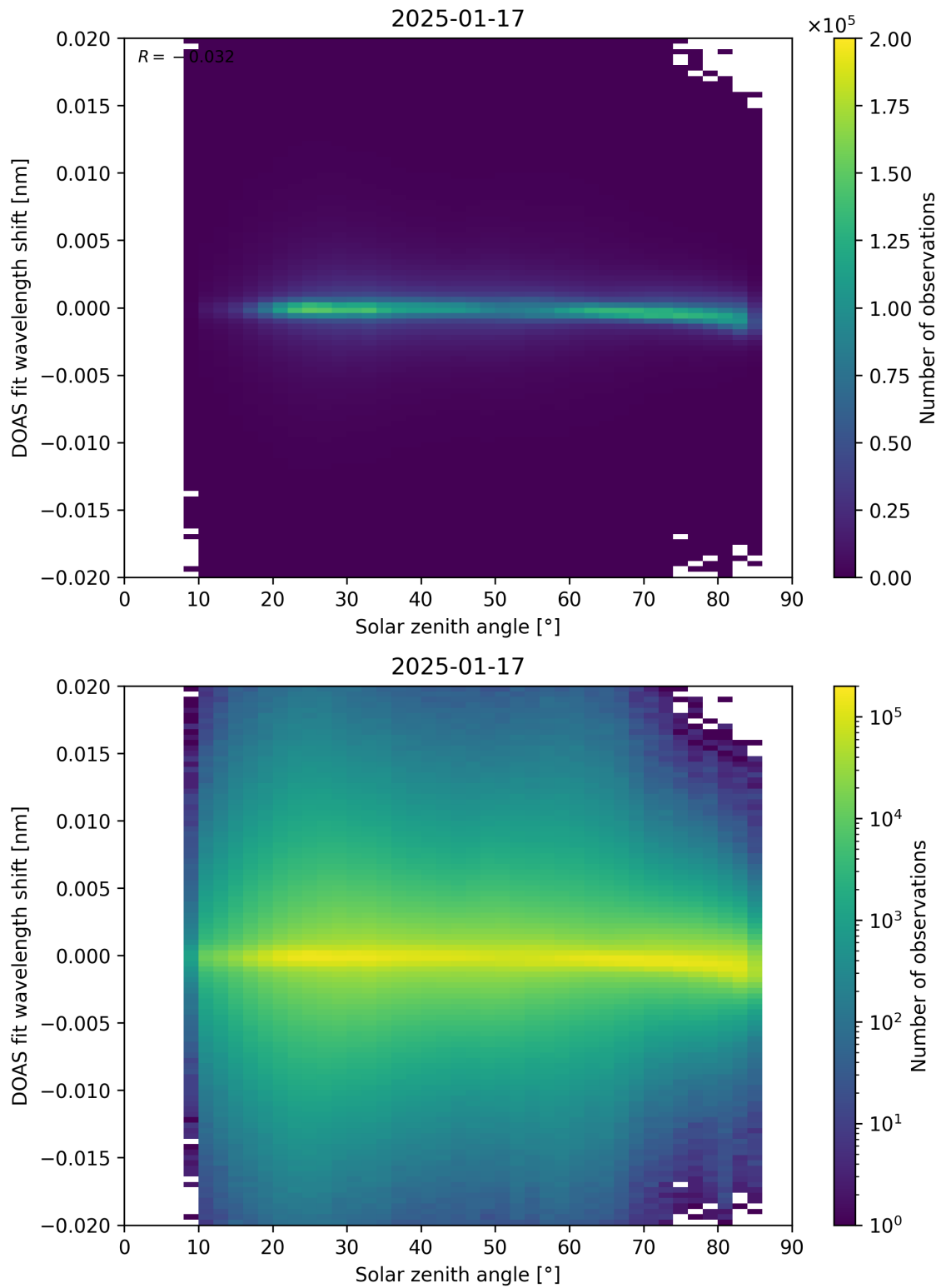
Figure 168: Scatter density plot of “Solar zenith angle” against “DOAS fit wavelength shift” for 2025-01-17 to 2025-01-18.
