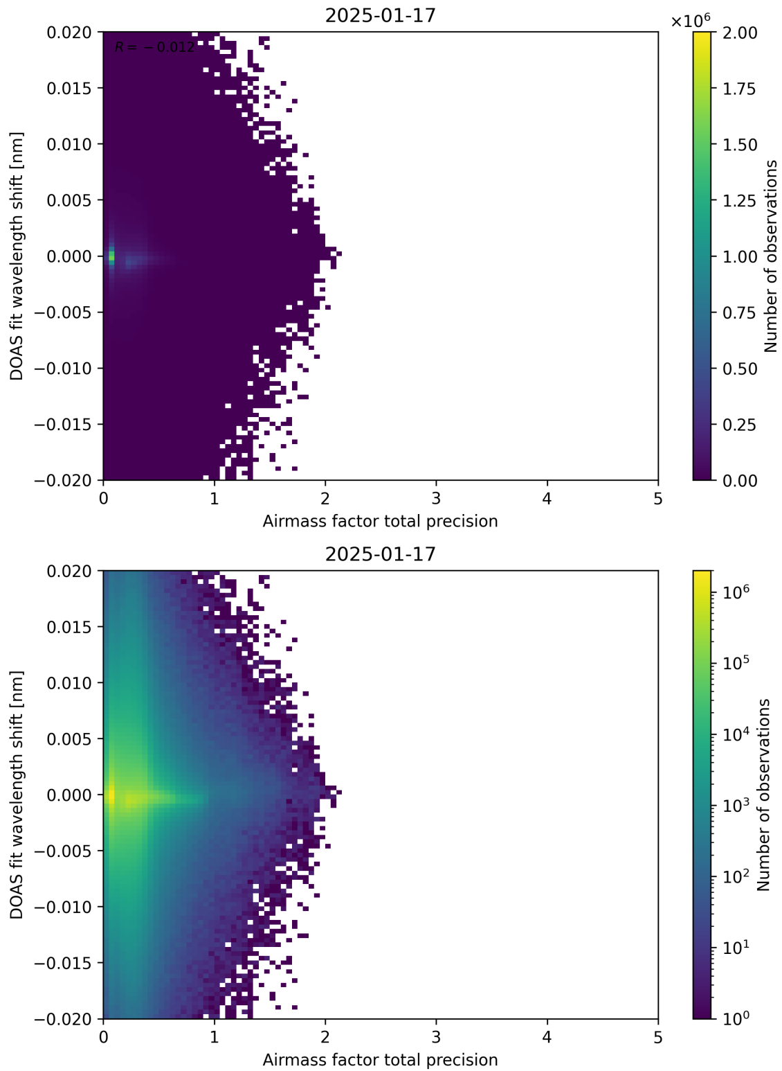
Figure 106: Scatter density plot of “Airmass factor total precision” against “DOAS fit wavelength shift” for 2025-01-17 to 2025-01-18.
