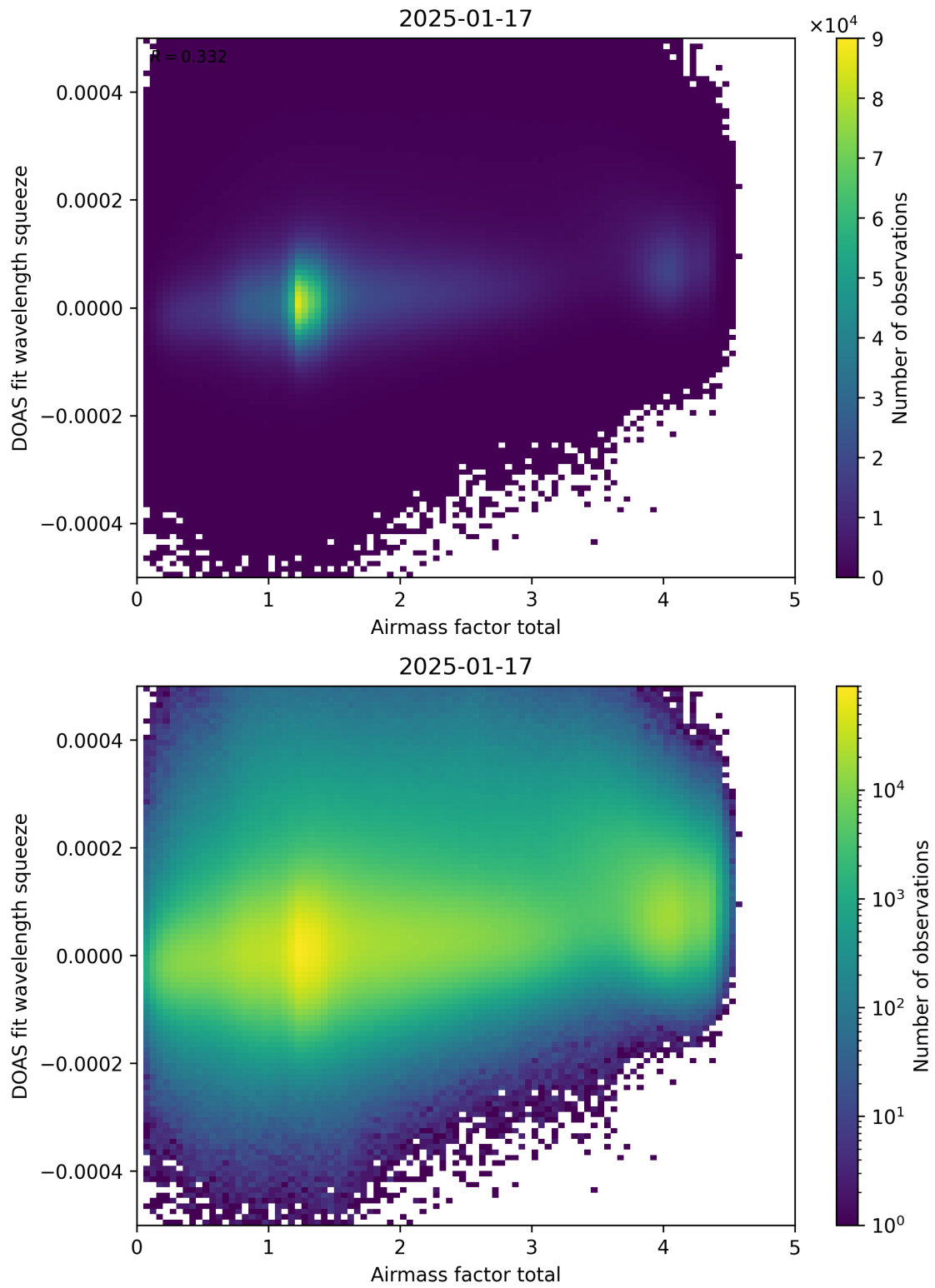
Figure 99: Scatter density plot of “Airmass factor total” against “DOAS fit wavelength squeeze” for 2025-01-17 to 2025-01-18.
