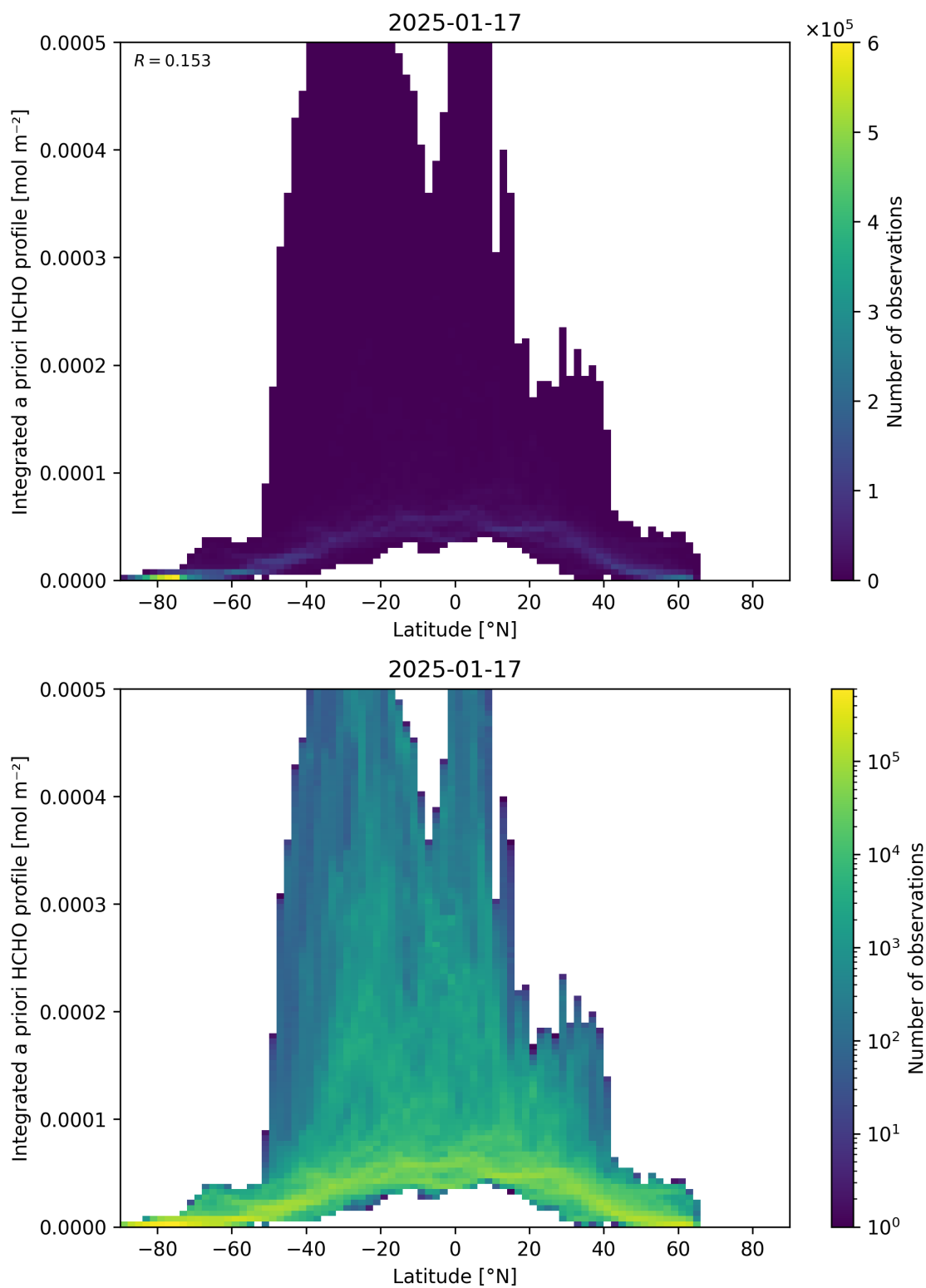
Figure 166: Scatter density plot of “Latitude” against “Integrated a priori HCHO profile” for 2025-01-17 to 2025-01-18.
