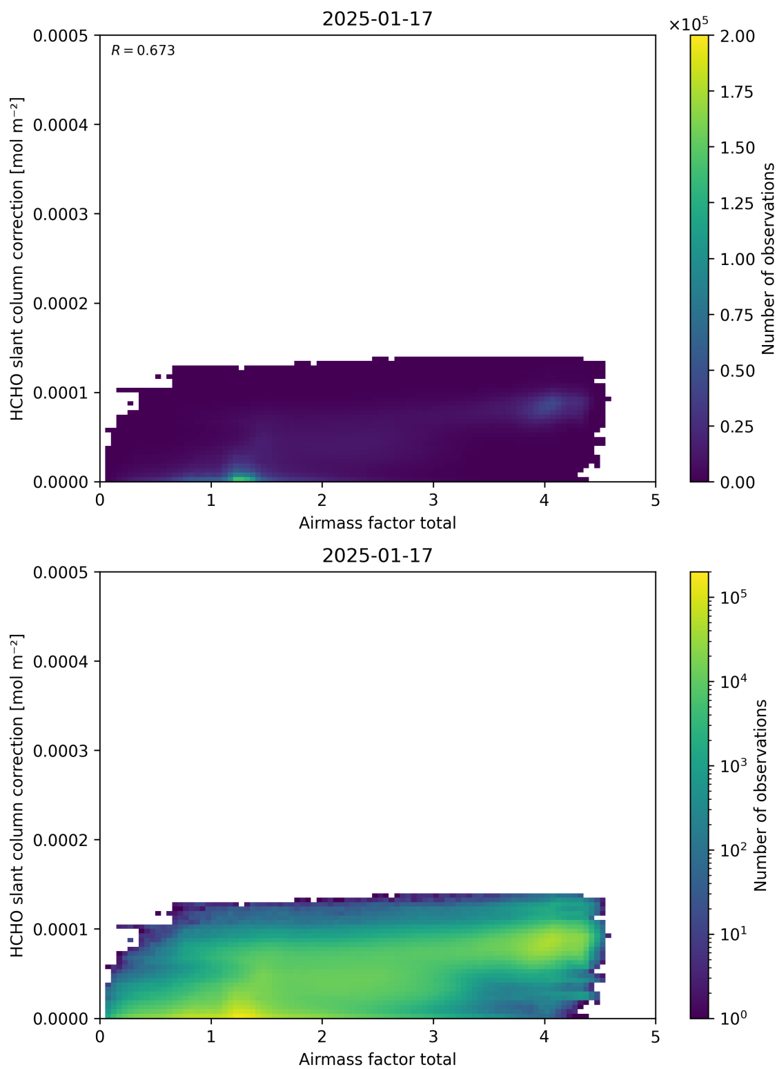
Figure 102: Scatter density plot of “Airmass factor total” against “HCHO slant column correction” for 2025-01-17 to 2025-01-18.
