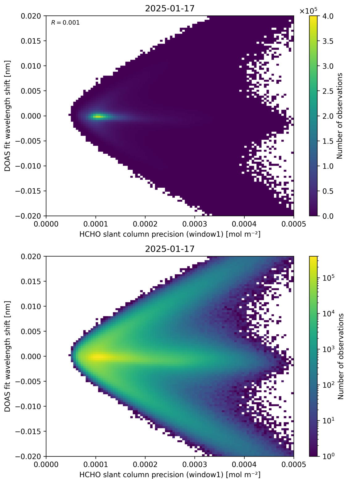
Figure 89: Scatter density plot of “HCHO slant column precision (window1)” against “DOAS fit wavelength shift” for 2025-01-17 to 2025-01-18.
