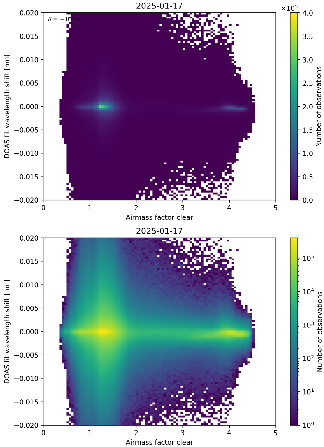
Figure 72: Scatter density plot of “Airmass factor clear” against “DOAS fit wavelength shift” for 2025-01-17 to 2025-01-18.
