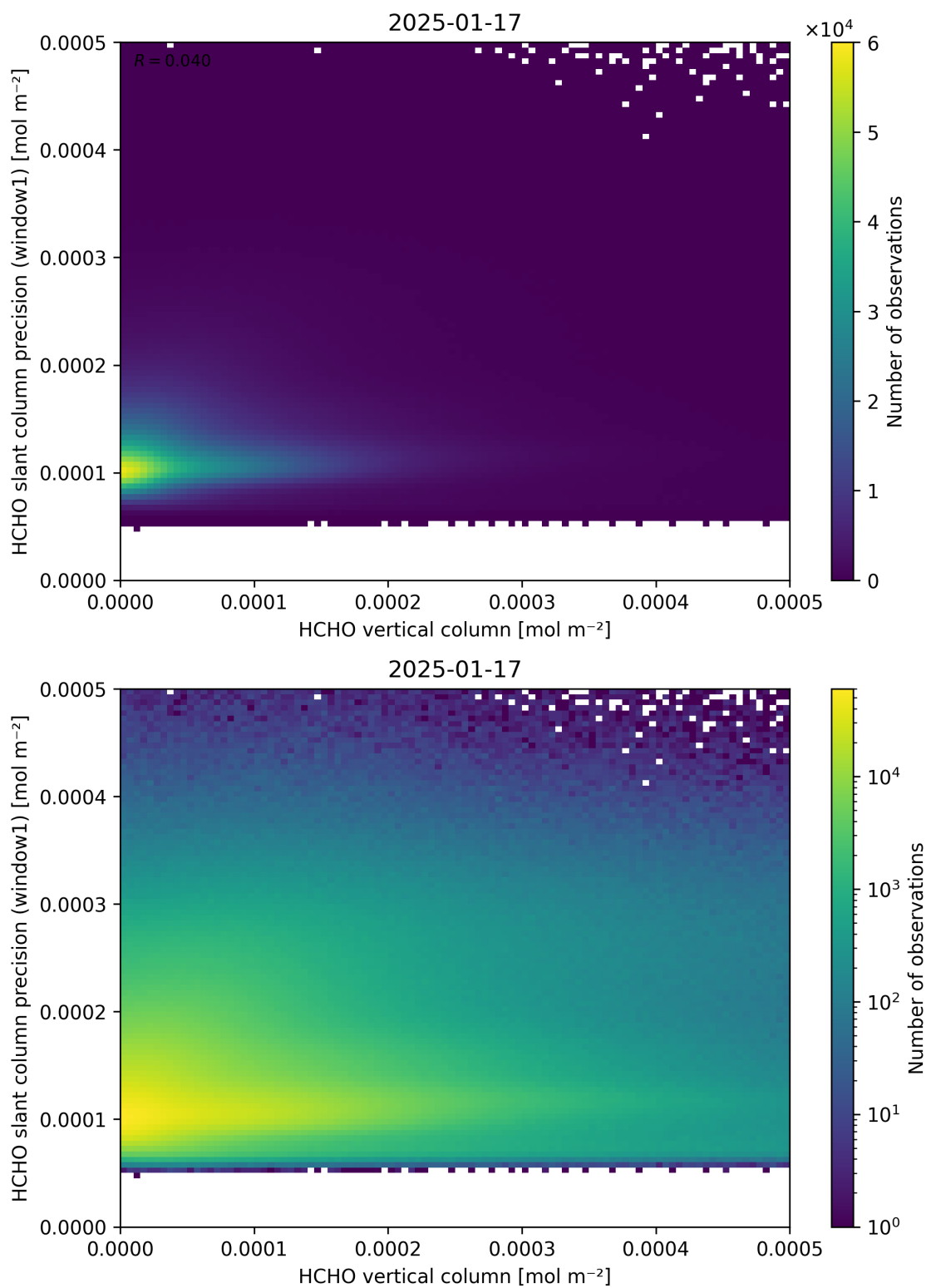
Figure 130: Scatter density plot of “HCHO vertical column” against “HCHO slant column precision (window1)” for 2025-01-17 to 2025-01-18.
