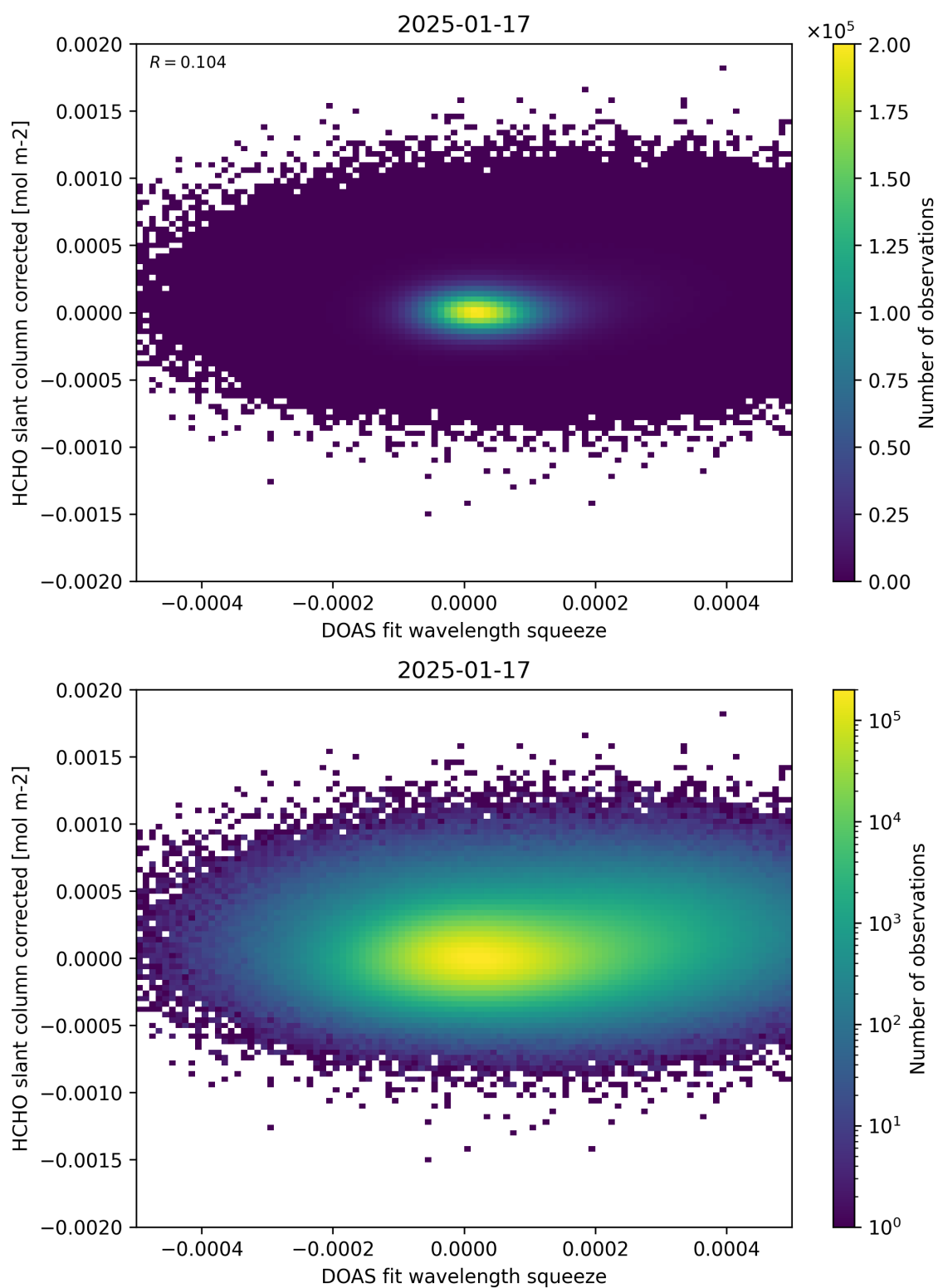
Figure 69: Scatter density plot of “DOAS fit wavelength squeeze” against “HCHO slant column corrected” for 2025-01-17 to 2025-01-18.
