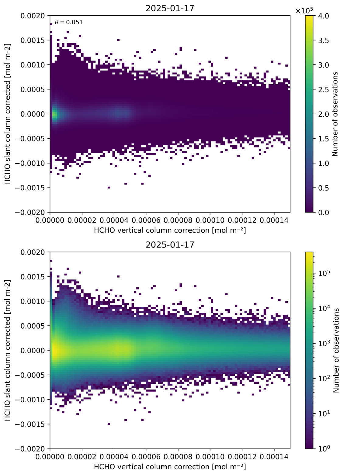
Figure 116: Scatter density plot of “HCHO vertical column correction” against “HCHO slant column corrected” for 2025-01-17 to 2025-01-18.
