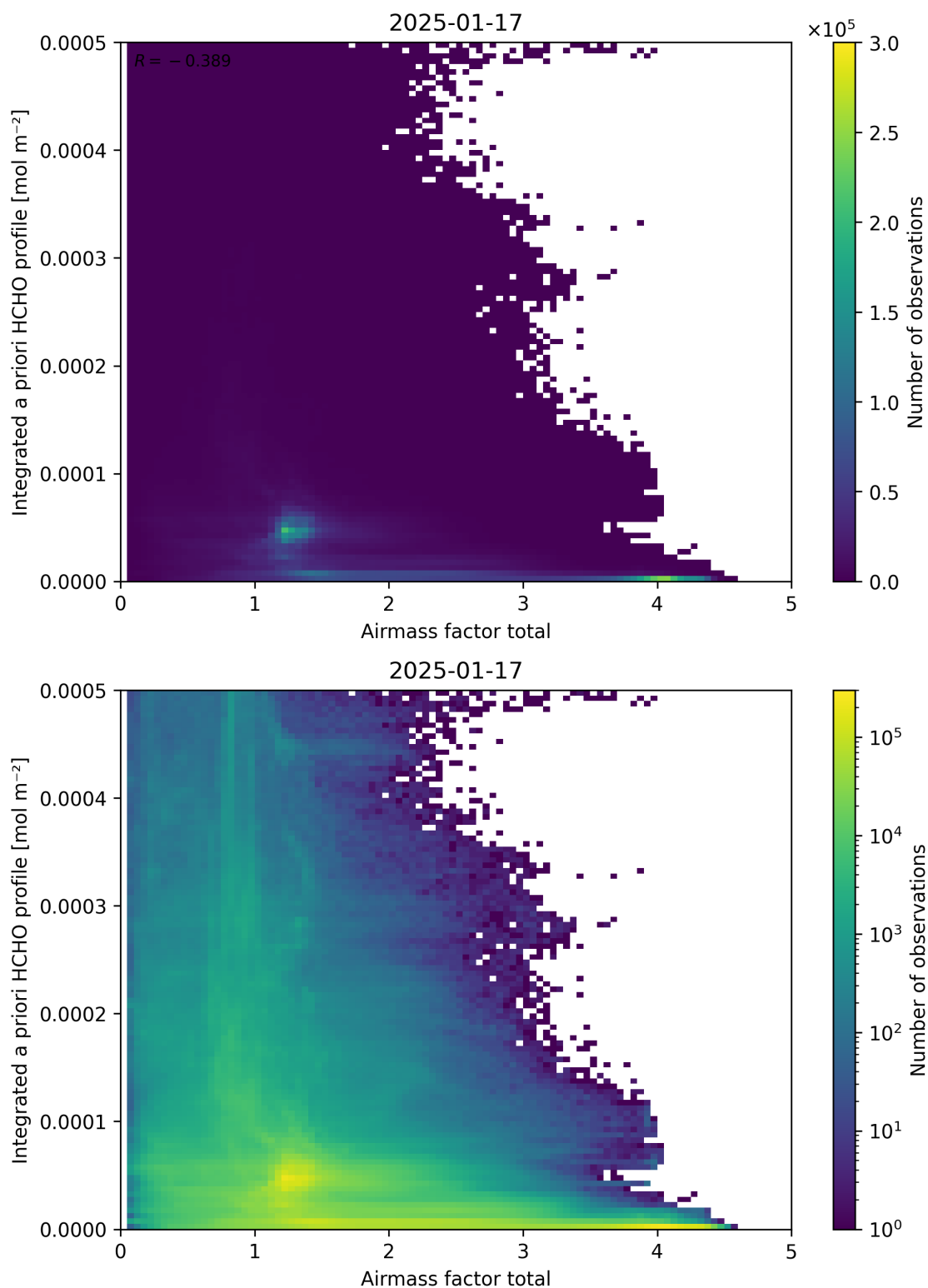
Figure 104: Scatter density plot of “Airmass factor total” against “Integrated a priori HCHO profile” for 2025-01-17 to 2025-01-18.
