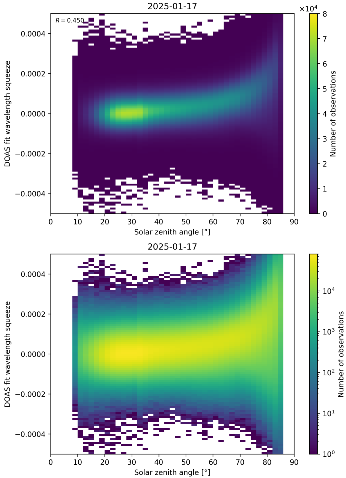
Figure 169: Scatter density plot of “Solar zenith angle” against “DOAS fit wavelength squeeze” for 2025-01-17 to 2025-01-18.
