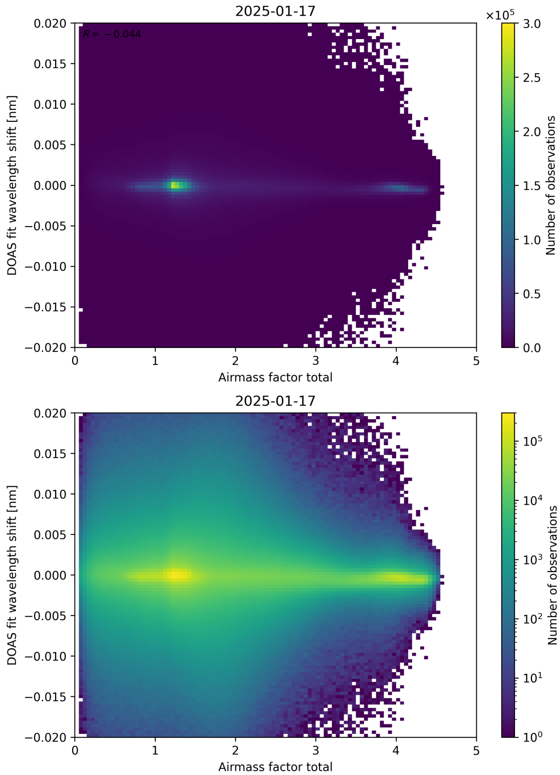
Figure 98: Scatter density plot of “Airmass factor total” against “DOAS fit wavelength shift” for 2025-01-17 to 2025-01-18.
