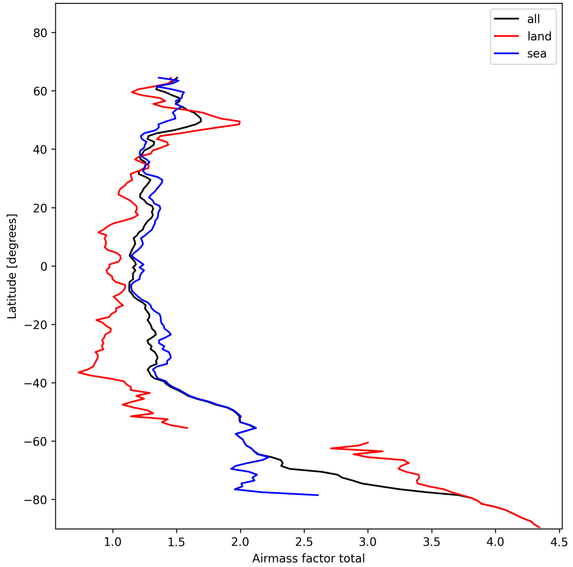
Figure 26: Zonal average of “Airmass factor total” for 2025-01-17 to 2025-01-18.
