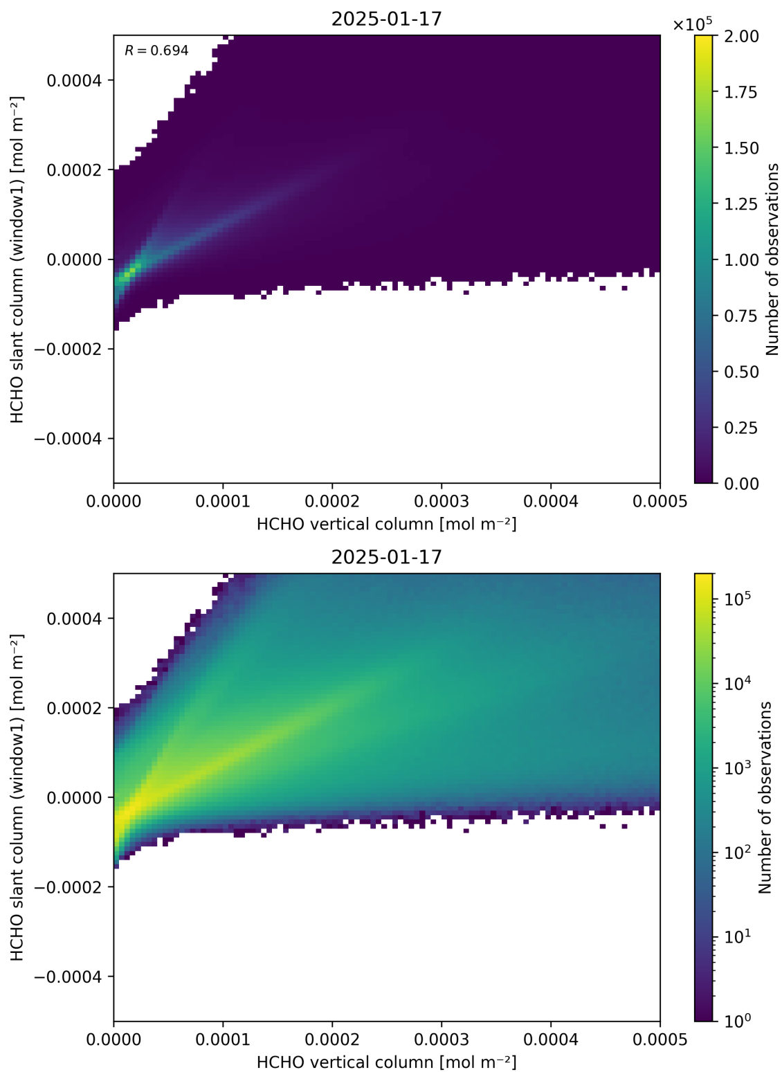
Figure 129: Scatter density plot of “HCHO vertical column” against “HCHO slant column (window1)” for 2025-01-17 to 2025-01-18.
