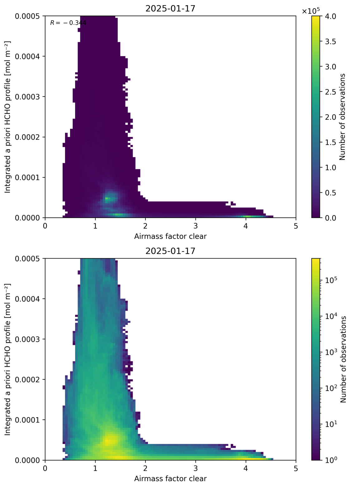
Figure 76: Scatter density plot of “Airmass factor clear” against “Integrated a priori HCHO profile” for 2025-01-17 to 2025-01-18.
