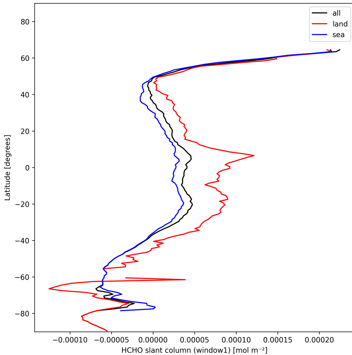
Figure 24: Zonal average of “HCHO slant column (window1)” for 2025-01-17 to 2025-01-18.
