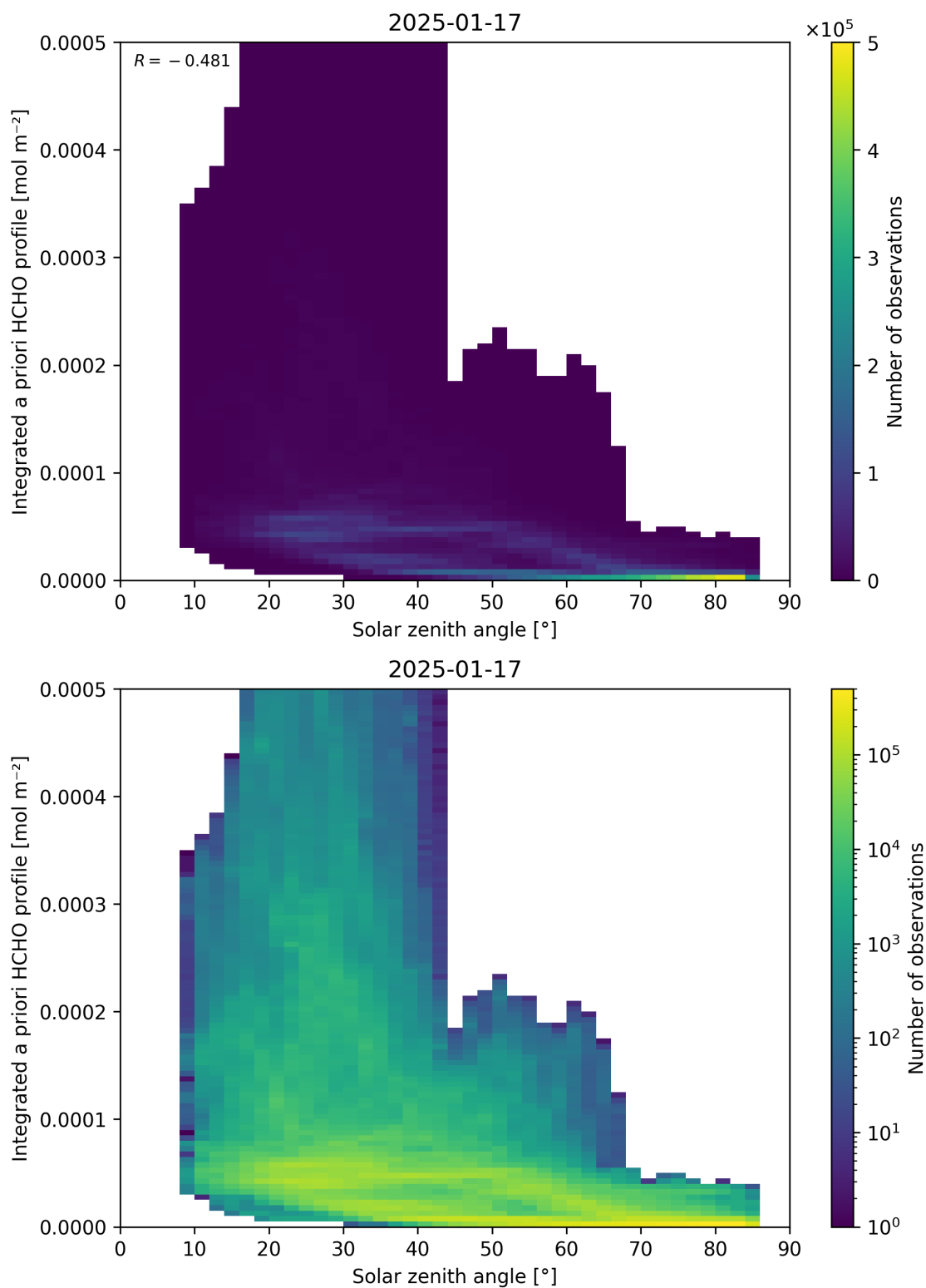
Figure 180: Scatter density plot of “Solar zenith angle” against “Integrated a priori HCHO profile” for 2025-01-17 to 2025-01-18.
