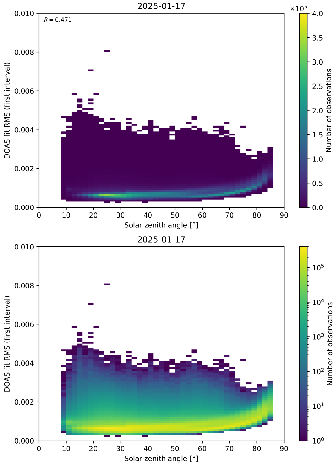
Figure 167: Scatter density plot of “Solar zenith angle” against “DOAS fit RMS (first interval)” for 2025-01-17 to 2025-01-18.
