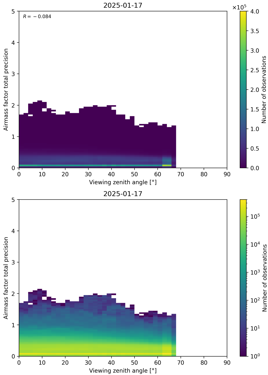
Figure 191: Scatter density plot of “Viewing zenith angle” against “Airmass factor total precision” for 2025-01-17 to 2025-01-18.
