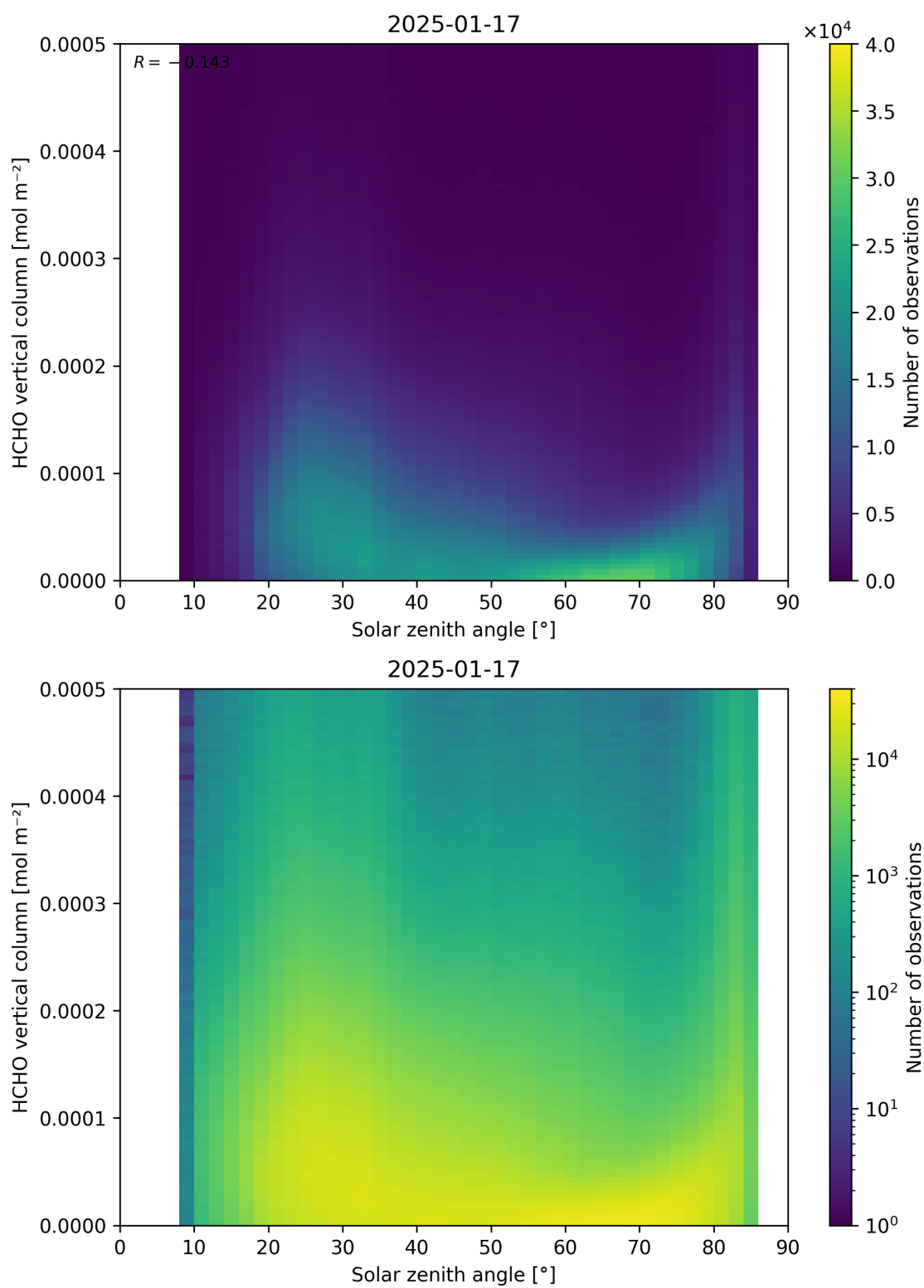
Figure 177: Scatter density plot of “Solar zenith angle” against “HCHO vertical column” for 2025-01-17 to 2025-01-18.
