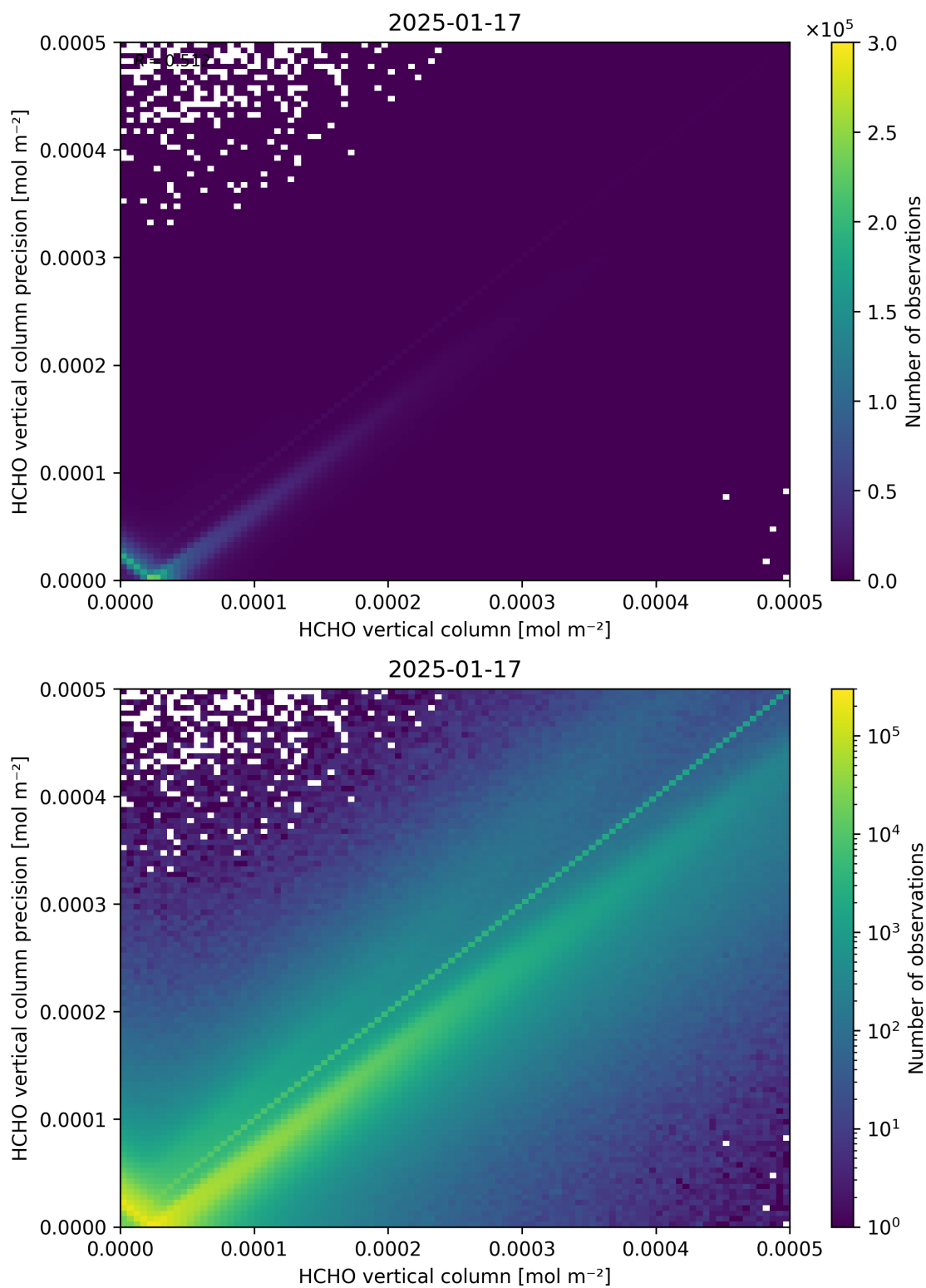
Figure 134: Scatter density plot of “HCHO vertical column” against “HCHO vertical column precision” for 2025-01-17 to 2025-01-18.
