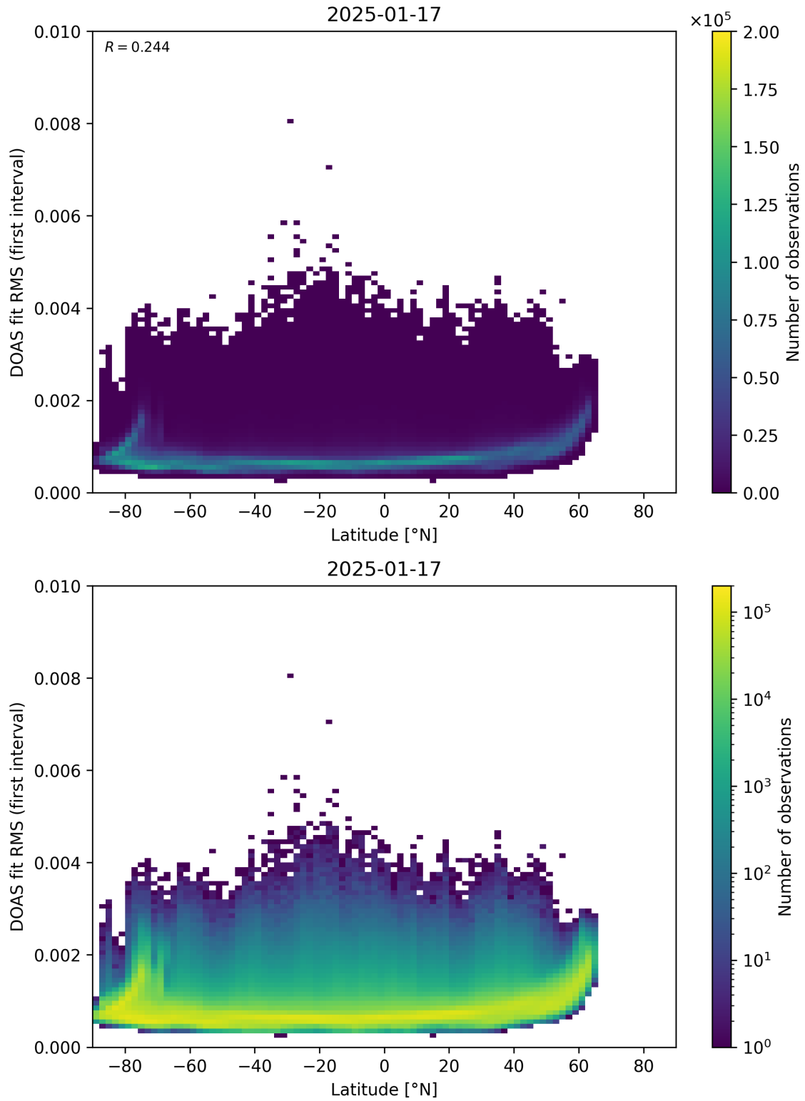
Figure 153: Scatter density plot of “Latitude” against “DOAS fit RMS (first interval)” for 2025-01-17 to 2025-01-18.
