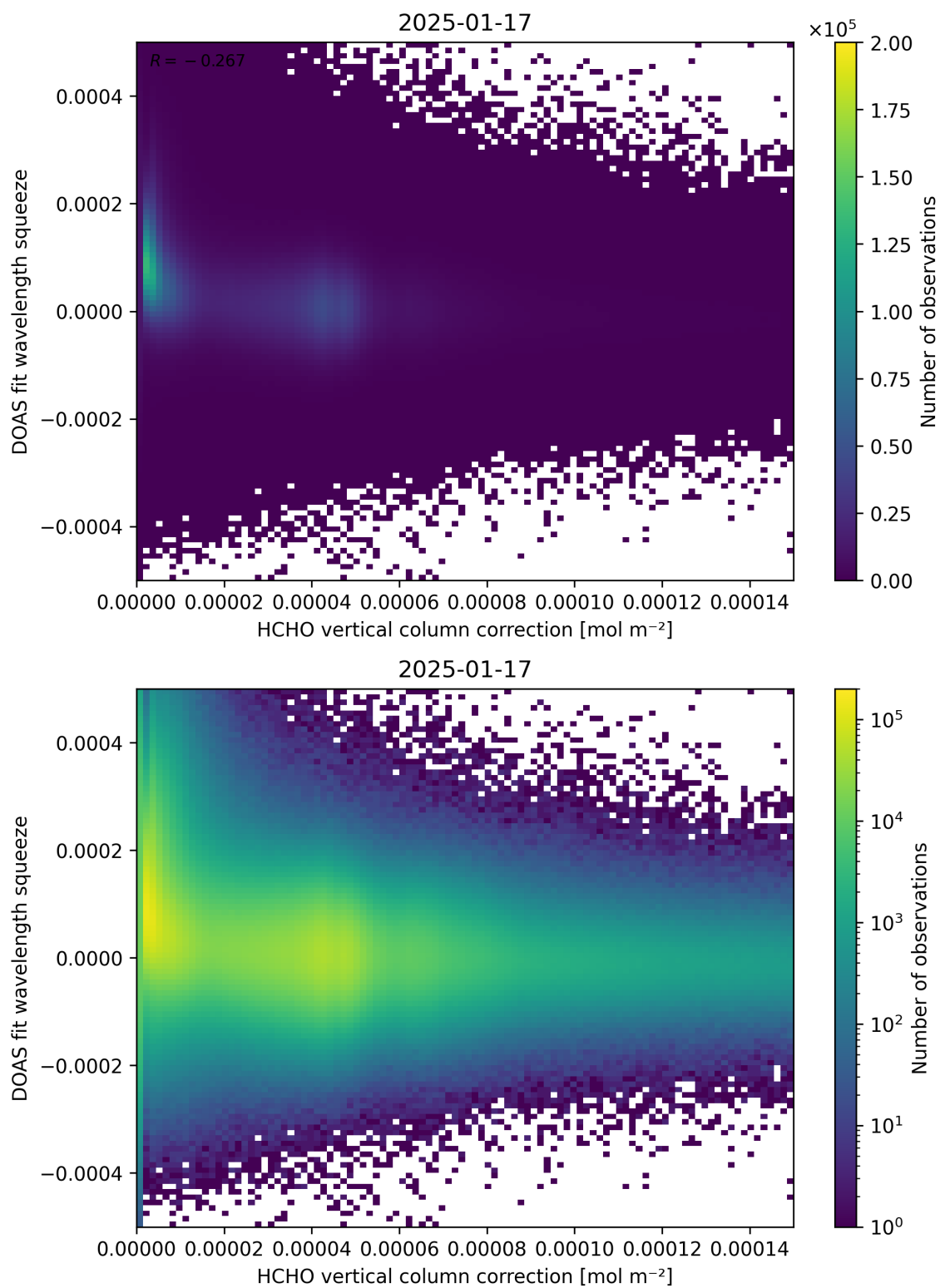
Figure 114: Scatter density plot of “HCHO vertical column correction” against “DOAS fit wavelength squeeze” for 2025-01-17 to 2025-01-18.
