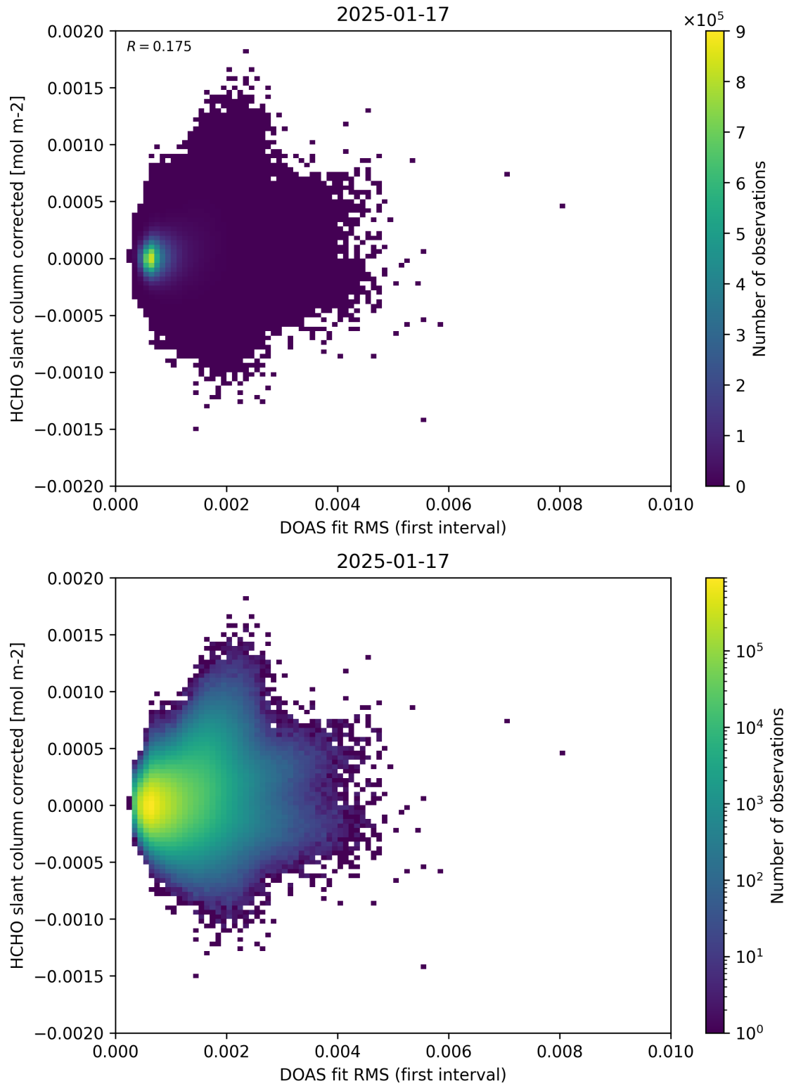
Figure 62: Scatter density plot of “DOAS fit RMS (first interval)” against “HCHO slant column corrected” for 2025-01-17 to 2025-01-18.
