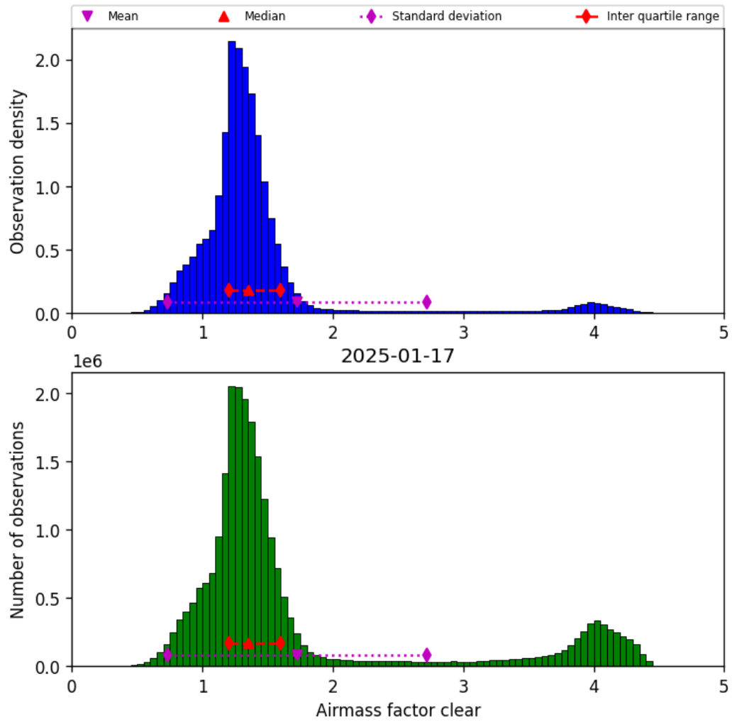
Figure 42: Histogram of “Airmass factor clear” for 2025-01-17 to 2025-01-18
