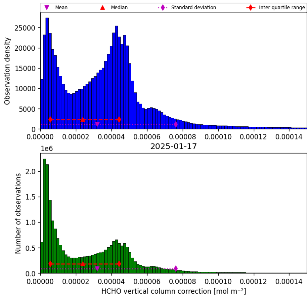
Figure 37: Histogram of “HCHO vertical column correction” for 2025-01-17 to 2025-01-18
