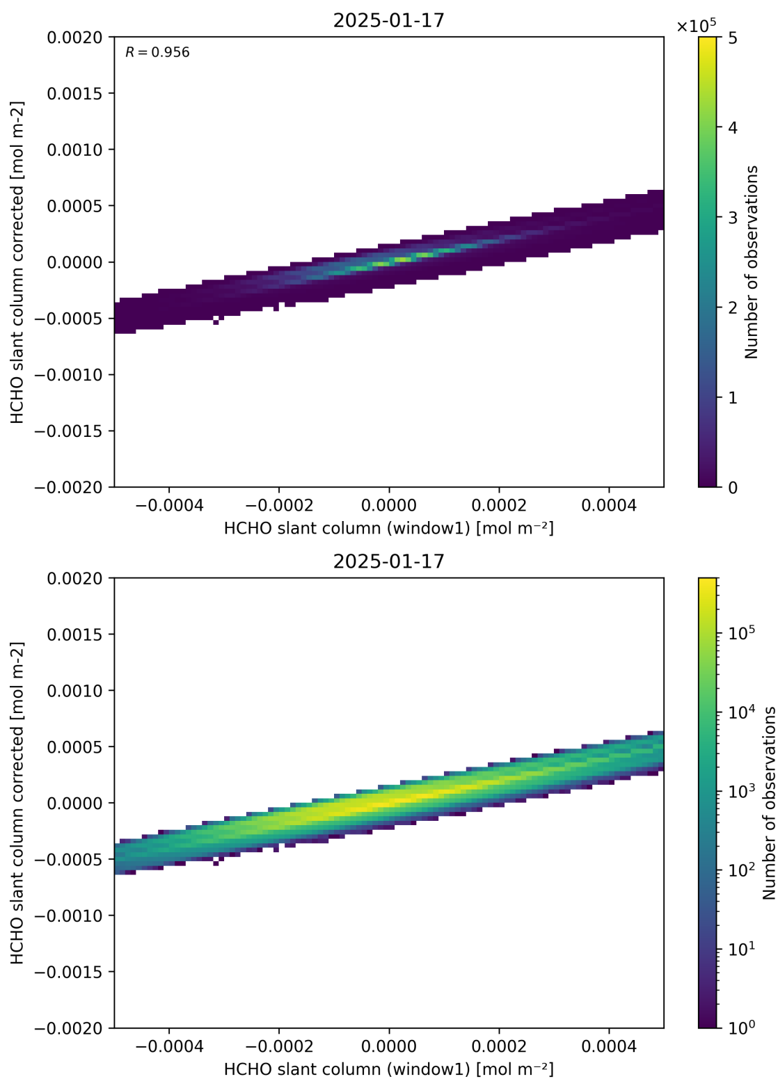
Figure 82: Scatter density plot of “HCHO slant column (window1)” against “HCHO slant column corrected” for 2025-01-17 to 2025-01-18.
