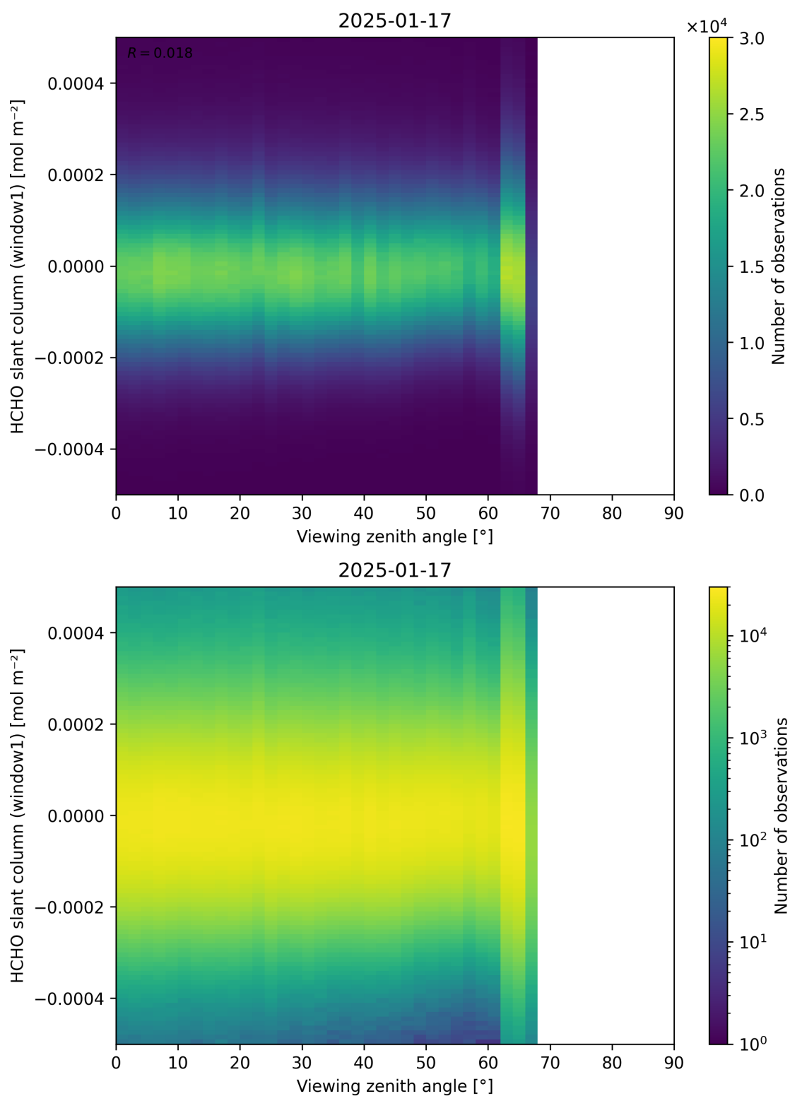
Figure 188: Scatter density plot of “Viewing zenith angle” against “HCHO slant column (window1)” for 2025-01-17 to 2025-01-18.
