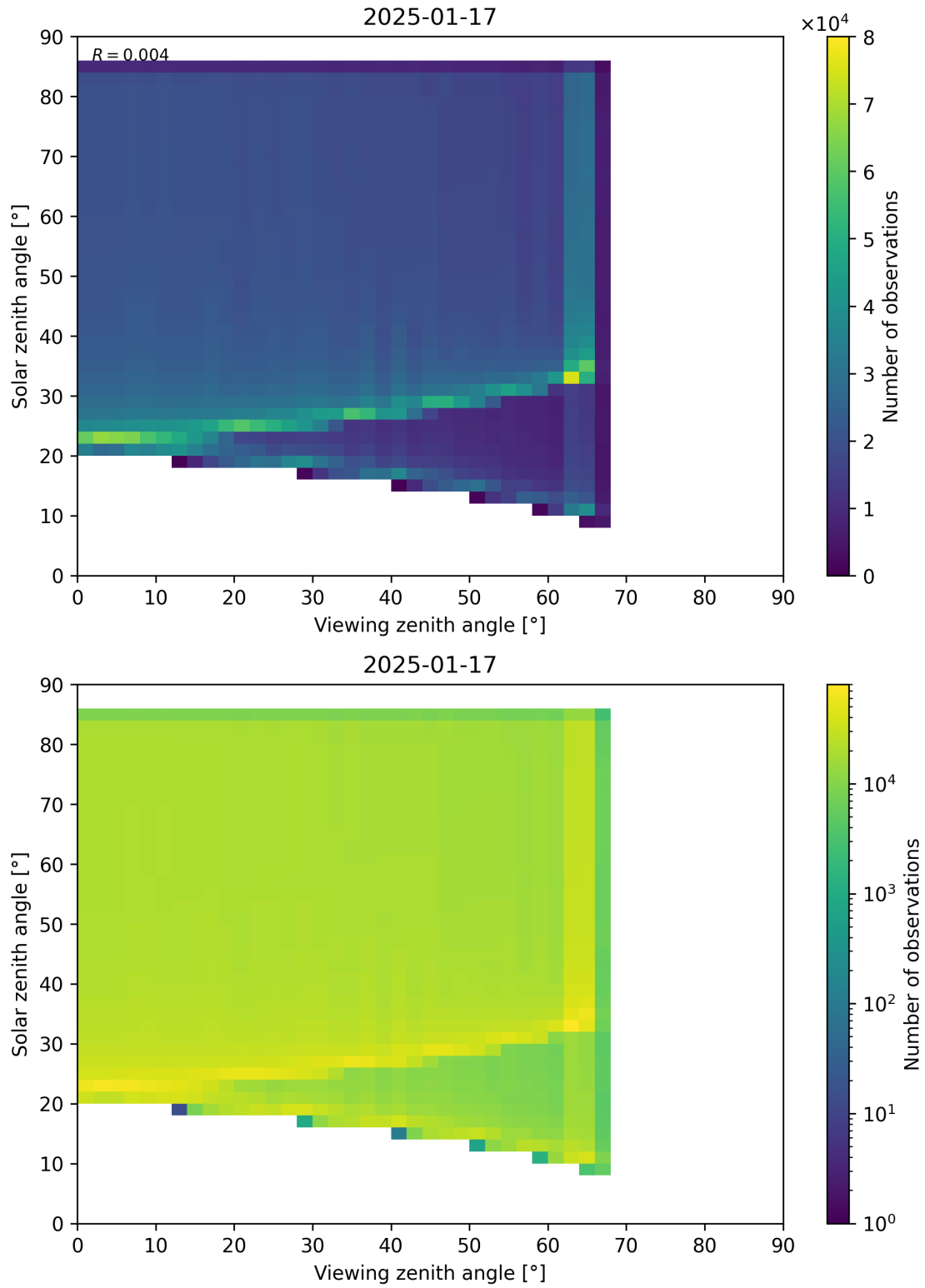
Figure 197: Scatter density plot of “Viewing zenith angle” against “Solar zenith angle” for 2025-01-17 to 2025-01-18.
