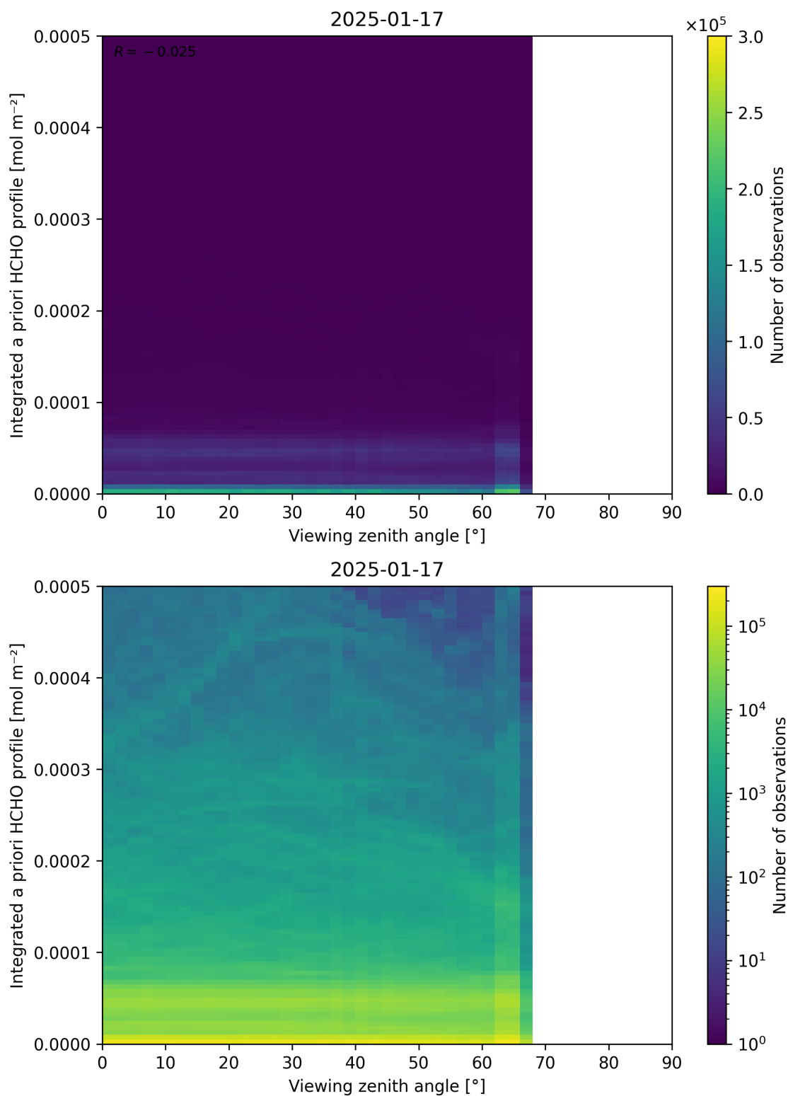
Figure 195: Scatter density plot of “Viewing zenith angle” against “Integrated a priori HCHO profile” for 2025-01-17 to 2025-01-18.
