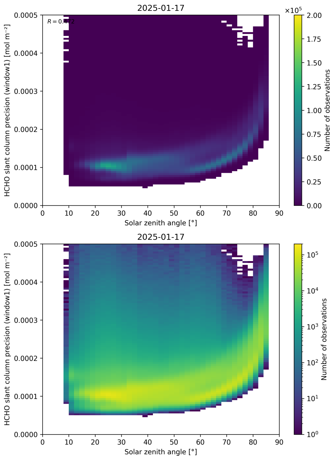
Figure 174: Scatter density plot of “Solar zenith angle” against “HCHO slant column precision (window1)” for 2025-01-17 to 2025-01-18.
