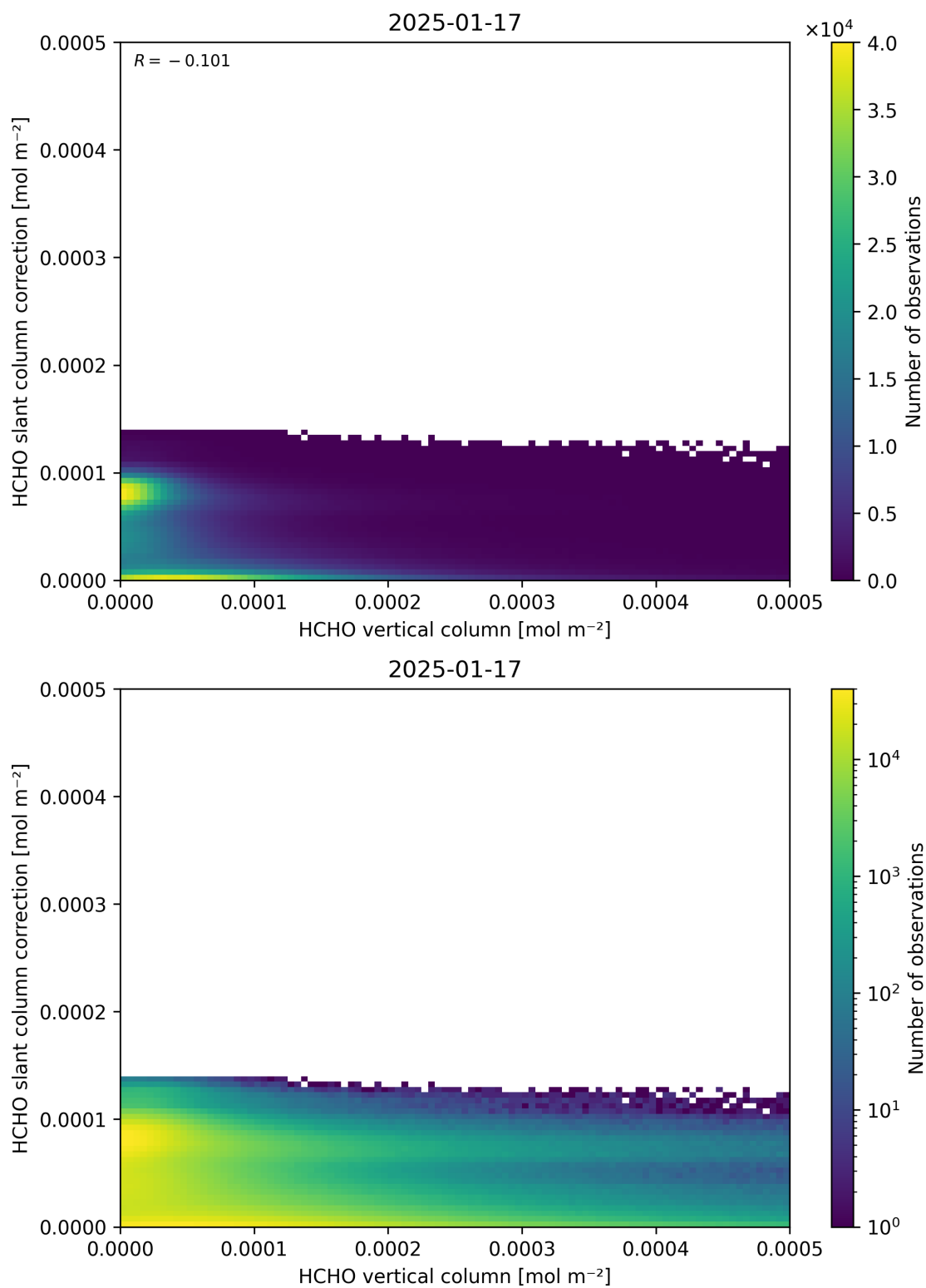
Figure 128: Scatter density plot of “HCHO vertical column” against “HCHO slant column correction” for 2025-01-17 to 2025-01-18.
