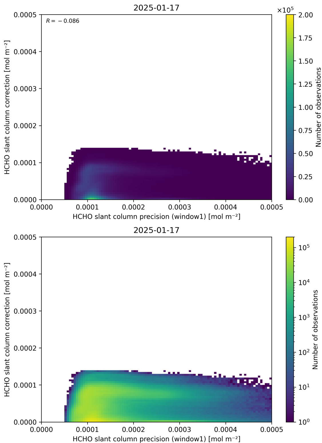
Figure 93: Scatter density plot of “HCHO slant column precision (window1)” against “HCHO slant column correction” for 2025-01-17 to 2025-01-18.
