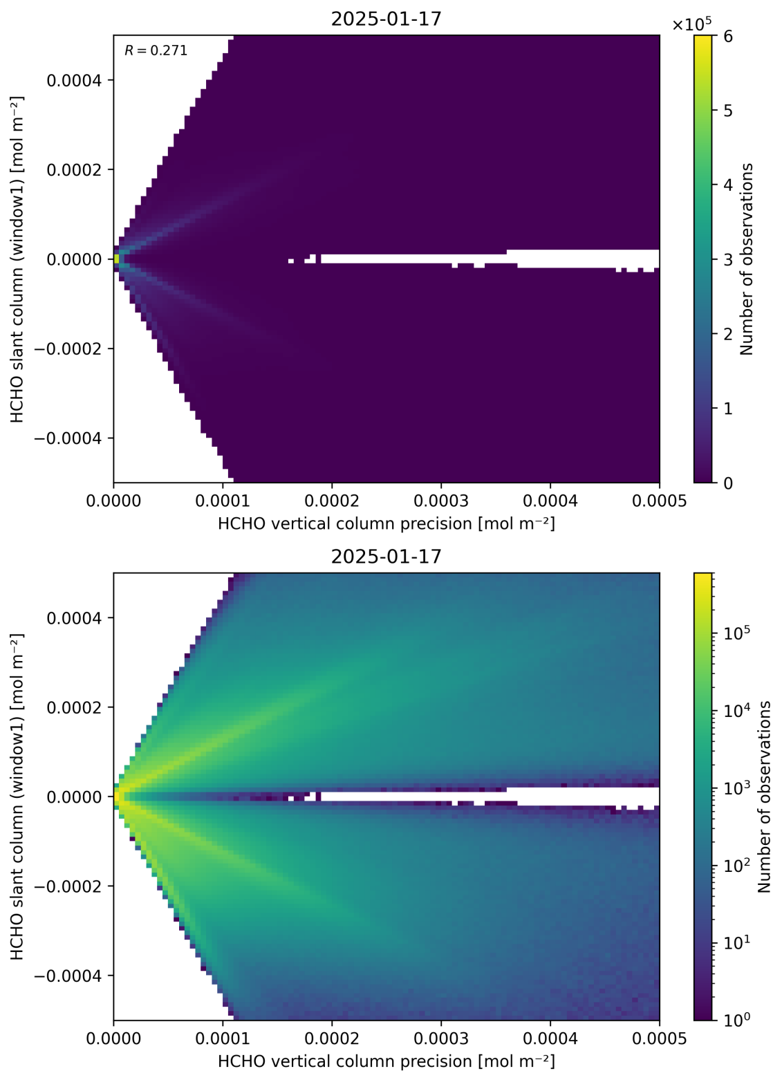
Figure 142: Scatter density plot of “HCHO vertical column precision” against “HCHO slant column (window1)” for 2025-01-17 to 2025-01-18.
