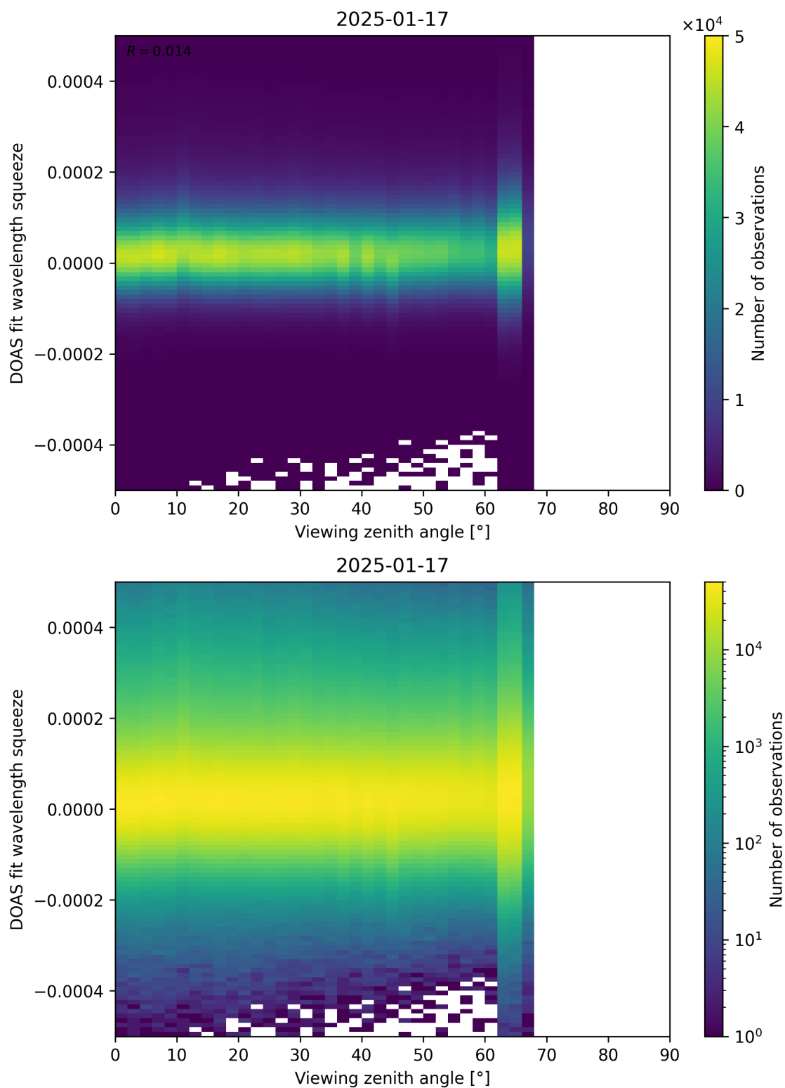
Figure 184: Scatter density plot of “Viewing zenith angle” against “DOAS fit wavelength squeeze” for 2025-01-17 to 2025-01-18.
