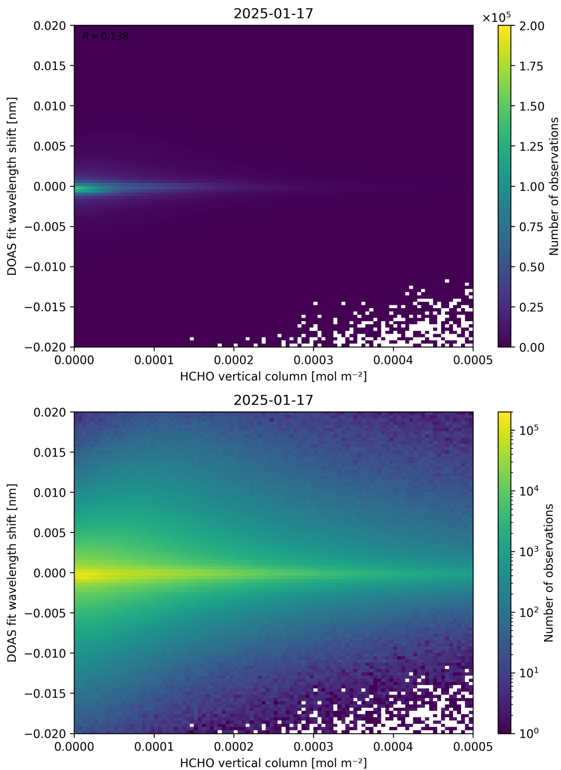
Figure 124: Scatter density plot of “HCHO vertical column” against “DOAS fit wavelength shift” for 2025-01-17 to 2025-01-18.
