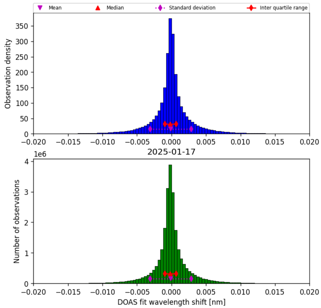
Figure 44: Histogram of “DOAS fit wavelength shift” for 2025-01-17 to 2025-01-18
