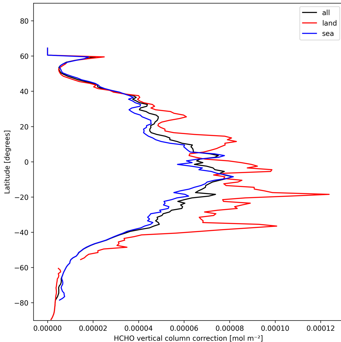
Figure 23: Zonal average of “HCHO vertical column correction” for 2025-01-17 to 2025-01-18.
