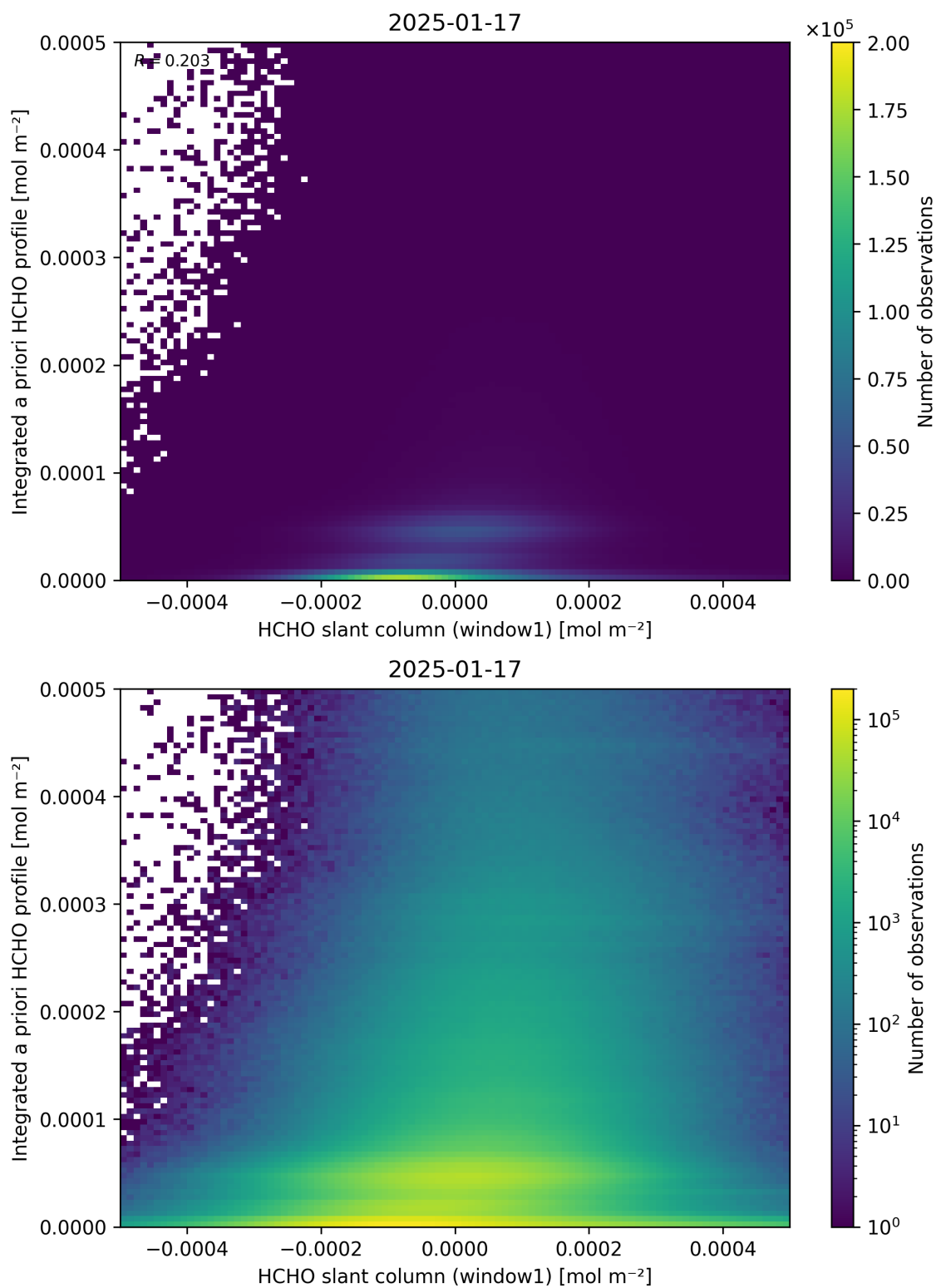
Figure 87: Scatter density plot of “HCHO slant column (window1)” against “Integrated a priori HCHO profile” for 2025-01-17 to 2025-01-18.
