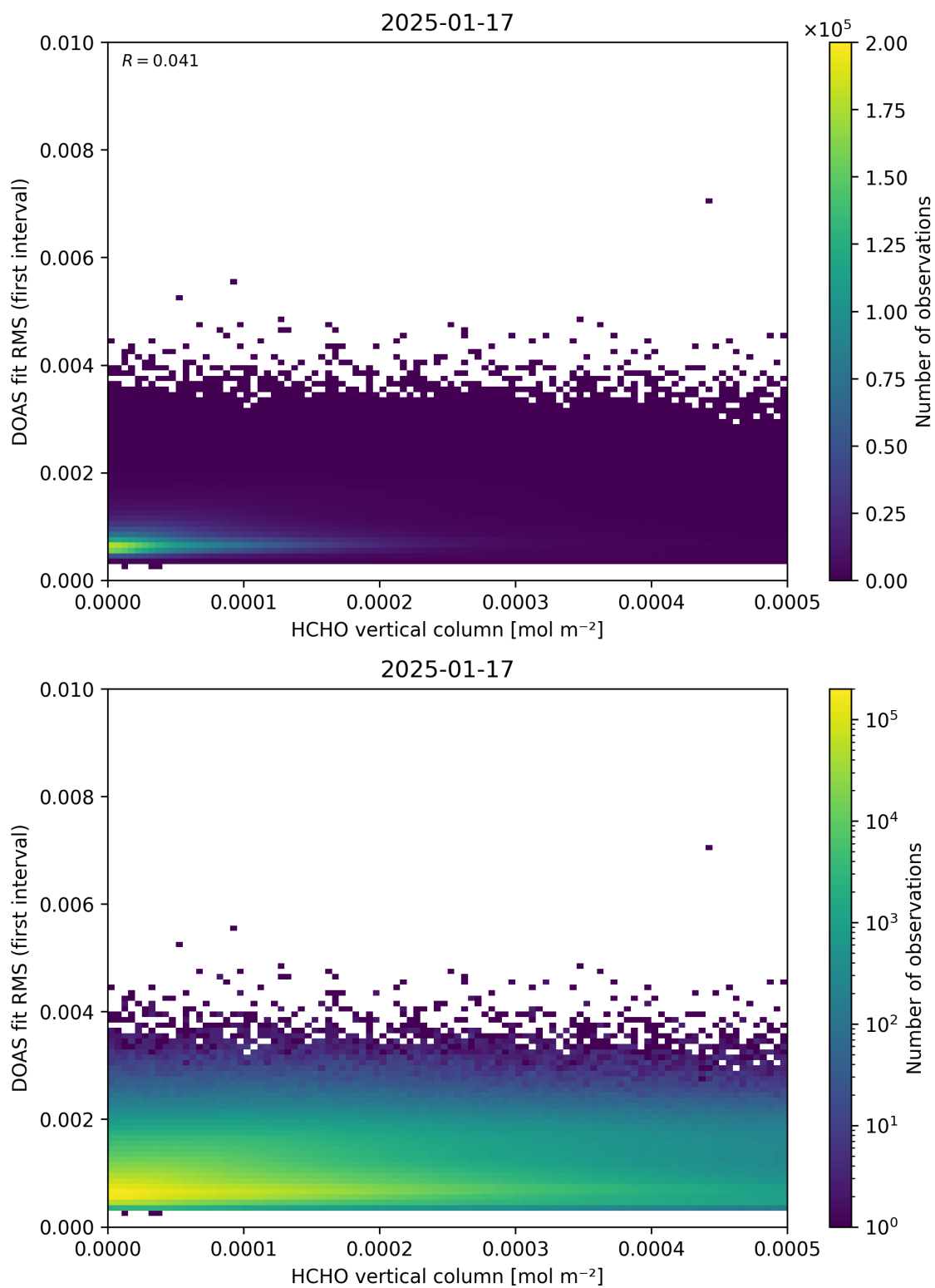
Figure 123: Scatter density plot of “HCHO vertical column” against “DOAS fit RMS (first interval)” for 2025-01-17 to 2025-01-18.
