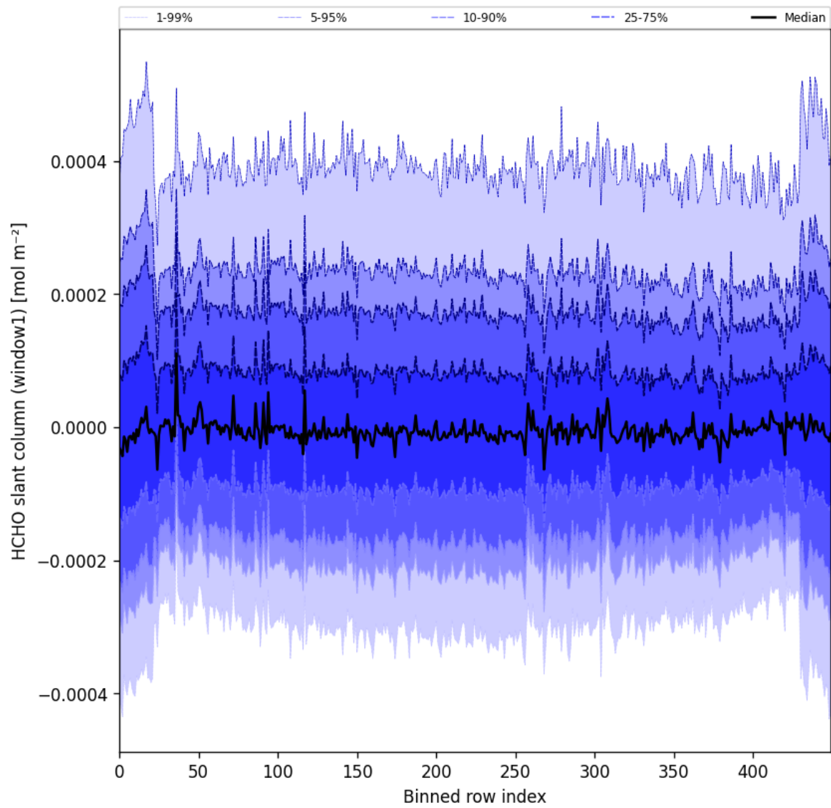
Figure 52: Along track statistics of “HCHO slant column (window1)” for 2025-01-17 to 2025-01-18
