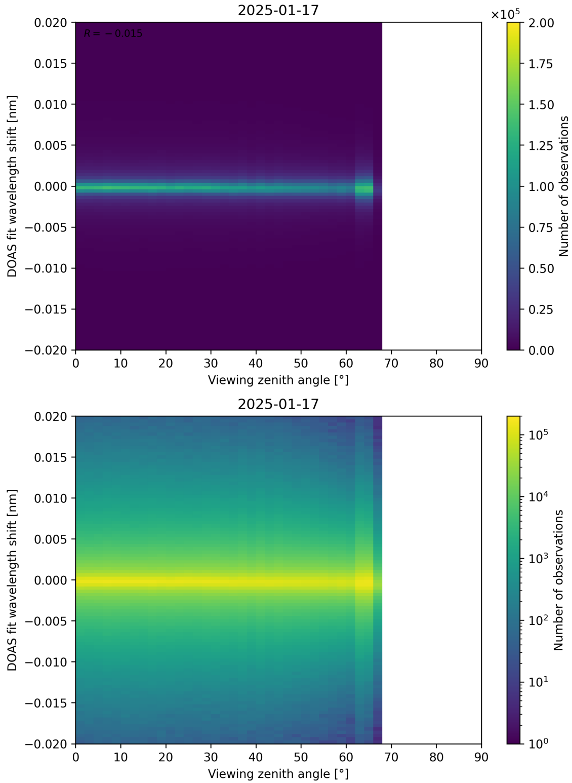
Figure 183: Scatter density plot of “Viewing zenith angle” against “DOAS fit wavelength shift” for 2025-01-17 to 2025-01-18.
