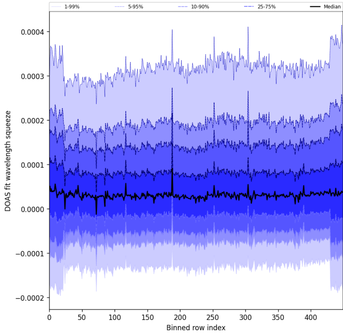
Figure 59: Along track statistics of “DOAS fit wavelength squeeze” for 2025-01-17 to 2025-01-18
