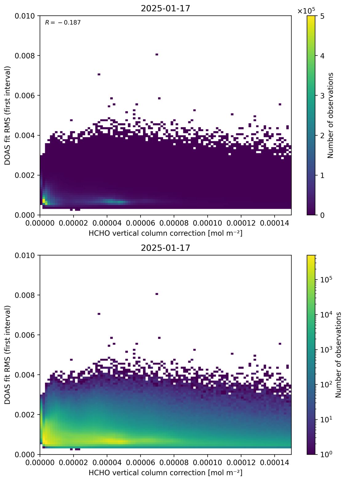
Figure 112: Scatter density plot of “HCHO vertical column correction” against “DOAS fit RMS (first interval)” for 2025-01-17 to 2025-01-18.
