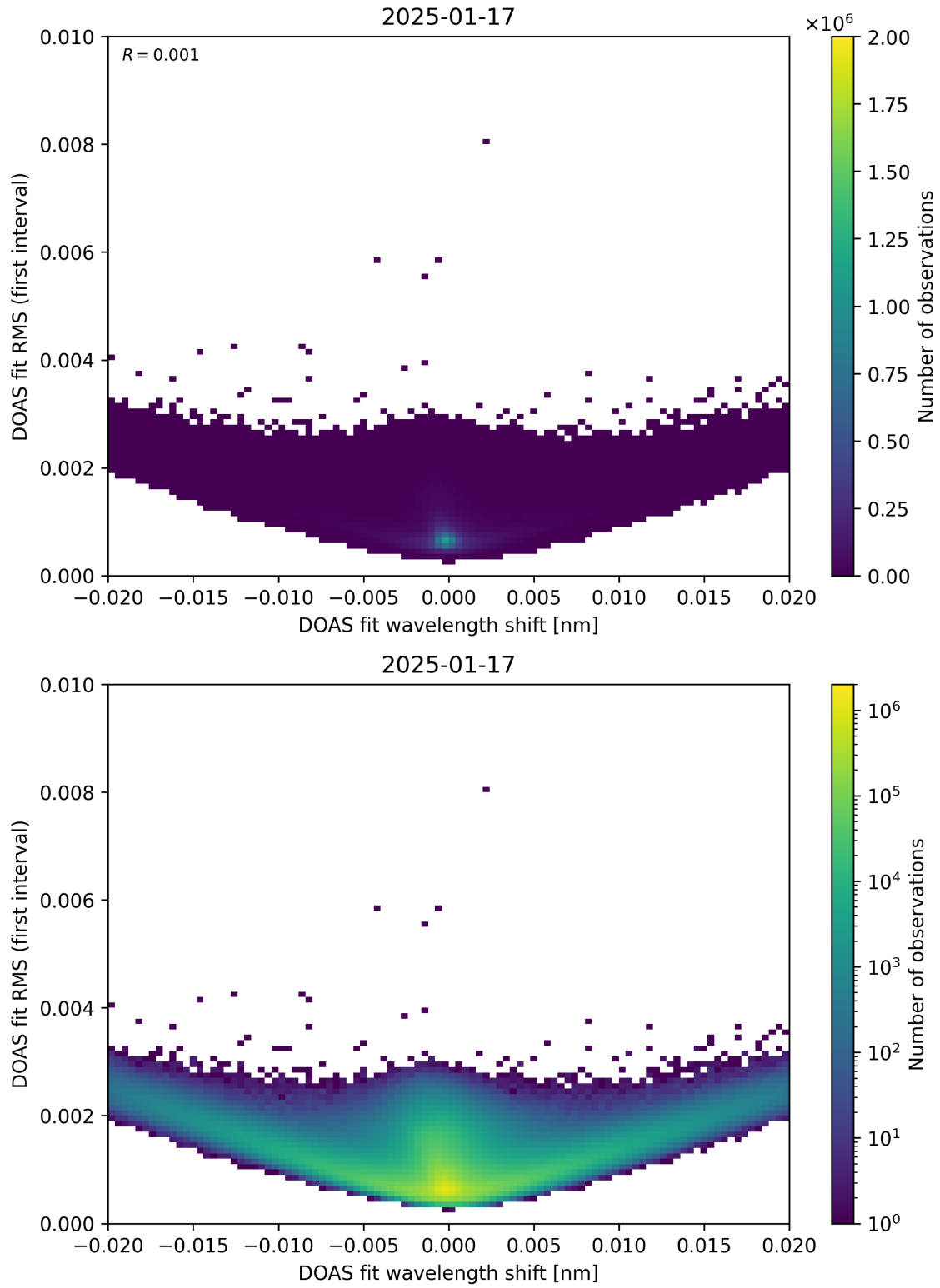
Figure 64: Scatter density plot of “DOAS fit wavelength shift” against “DOAS fit RMS (first interval)” for 2025-01-17 to 2025-01-18.
