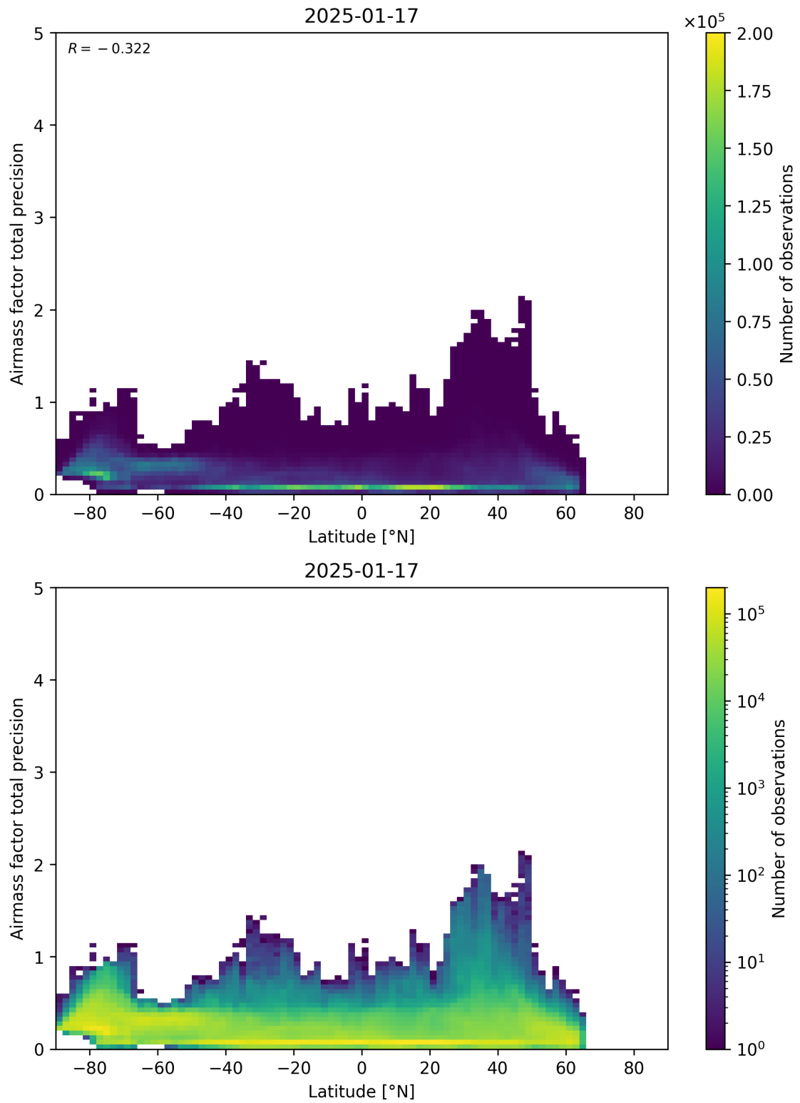
Figure 162: Scatter density plot of “Latitude” against “Airmass factor total precision” for 2025-01-17 to 2025-01-18.
