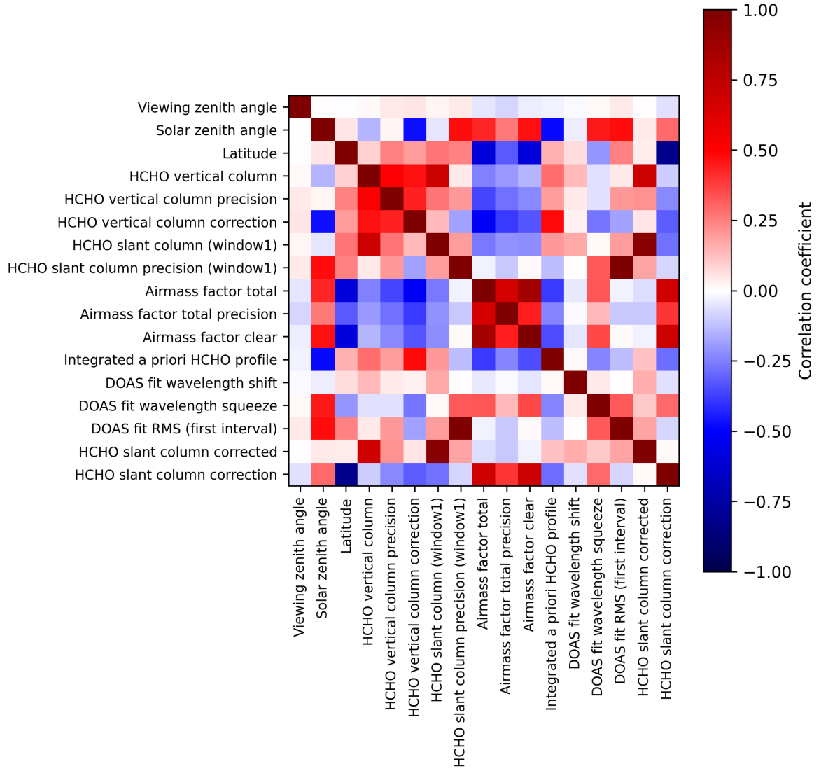
Figure 2: Map of correlation matrix for 2025-01-17 to 2025-01-18.
