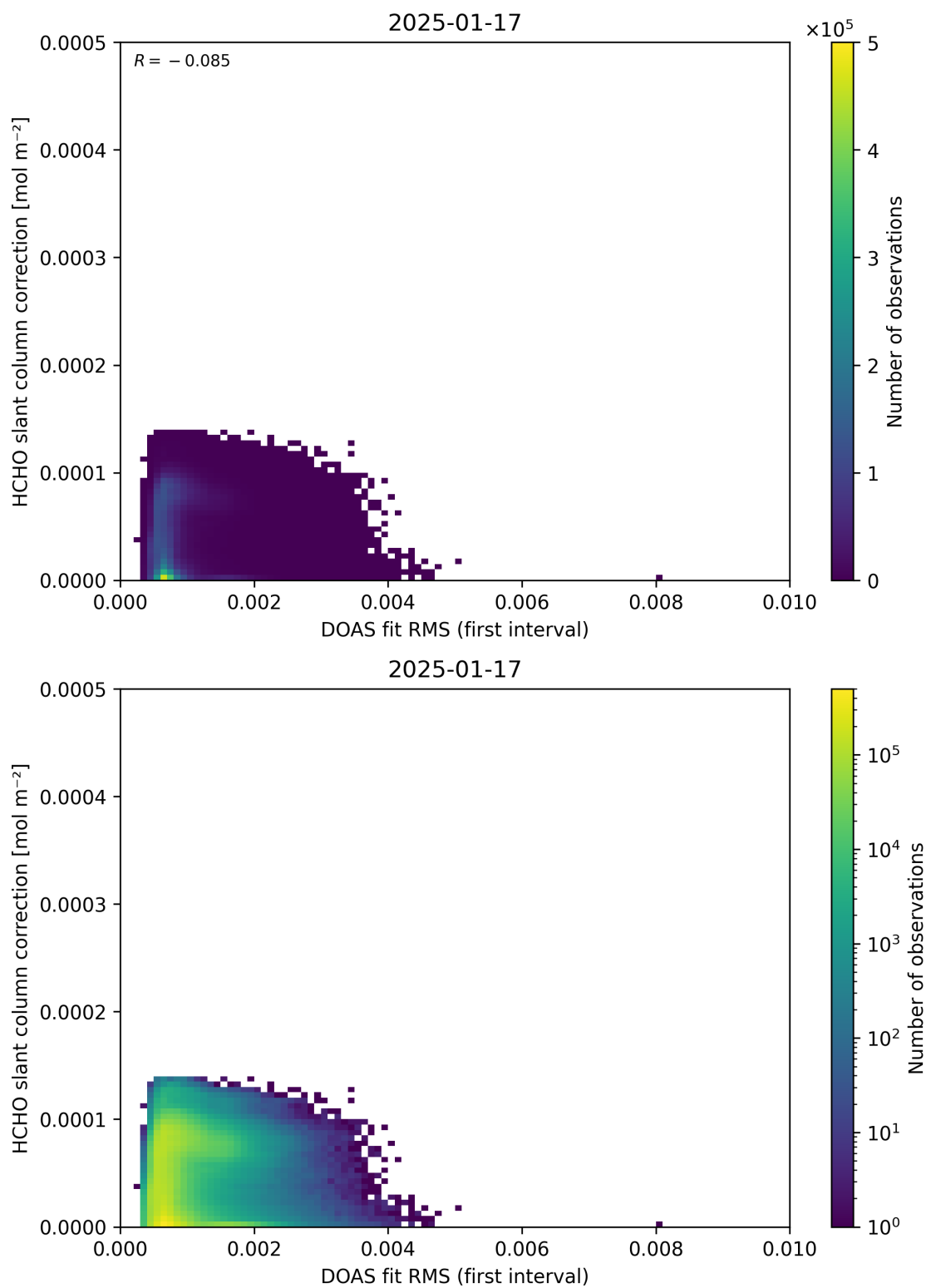
Figure 63: Scatter density plot of “DOAS fit RMS (first interval)” against “HCHO slant column correction” for 2025-01-17 to 2025-01-18.
