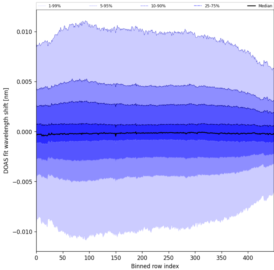
Figure 58: Along track statistics of “DOAS fit wavelength shift” for 2025-01-17 to 2025-01-18
