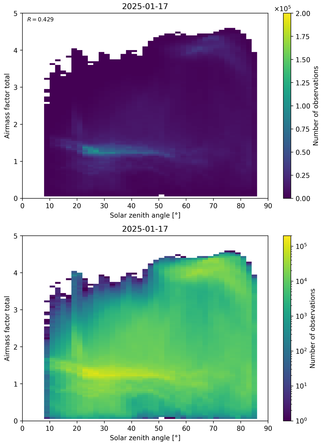
Figure 175: Scatter density plot of “Solar zenith angle” against “Airmass factor total” for 2025-01-17 to 2025-01-18.
