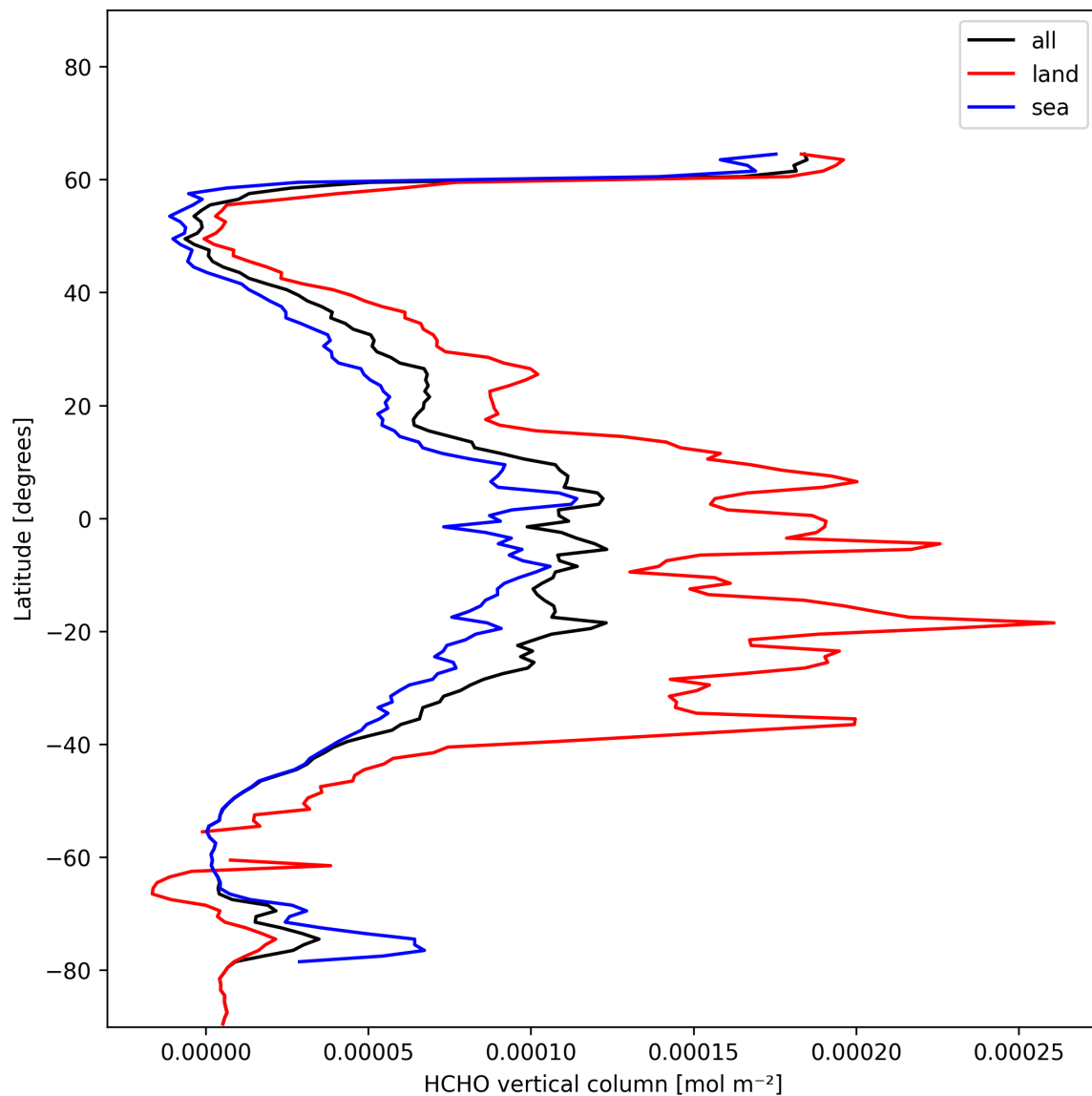
Figure 21: Zonal average of “HCHO vertical column” for 2025-01-17 to 2025-01-18.
