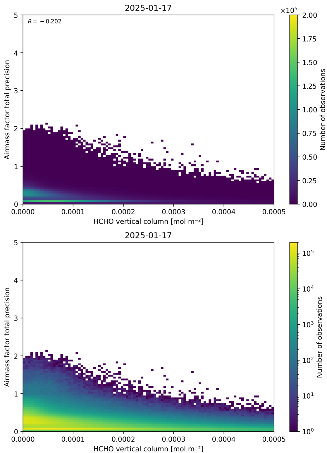
Figure 132: Scatter density plot of “HCHO vertical column” against “Airmass factor total precision” for 2025-01-17 to 2025-01-18.
