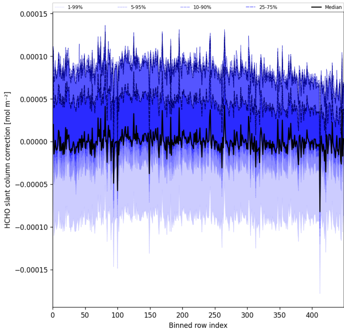
Figure 61: Along track statistics of “HCHO slant column correction” for 2025-01-17 to 2025-01-18
