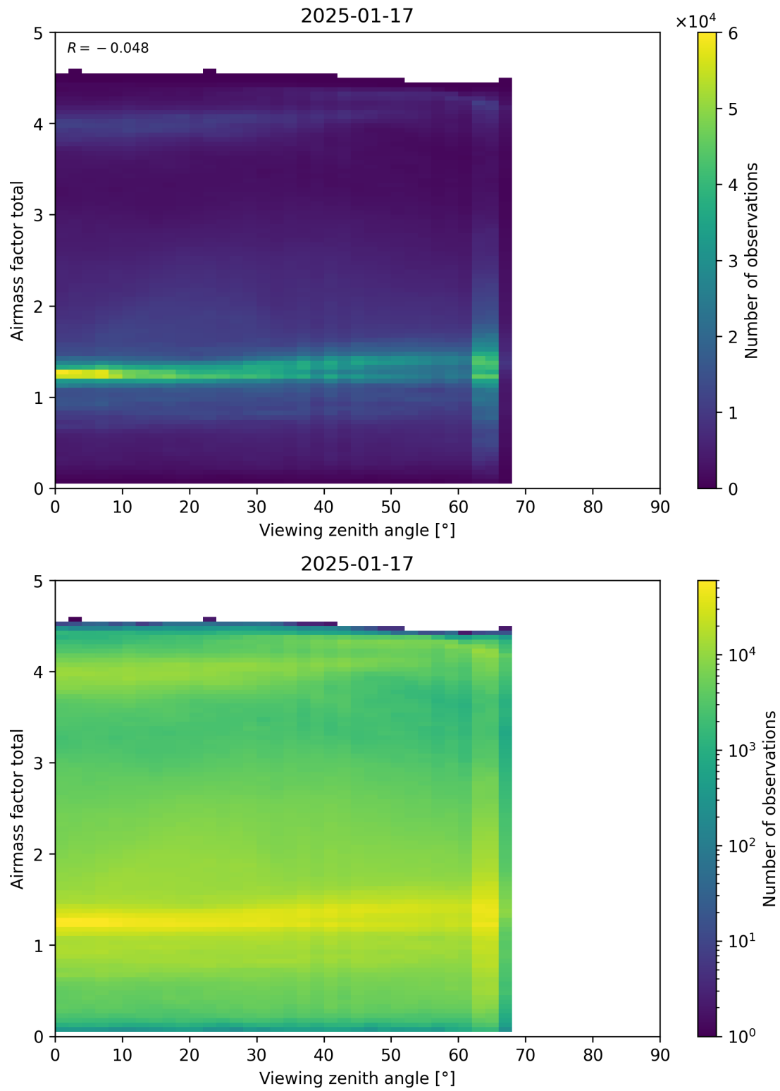
Figure 190: Scatter density plot of “Viewing zenith angle” against “Airmass factor total” for 2025-01-17 to 2025-01-18.
