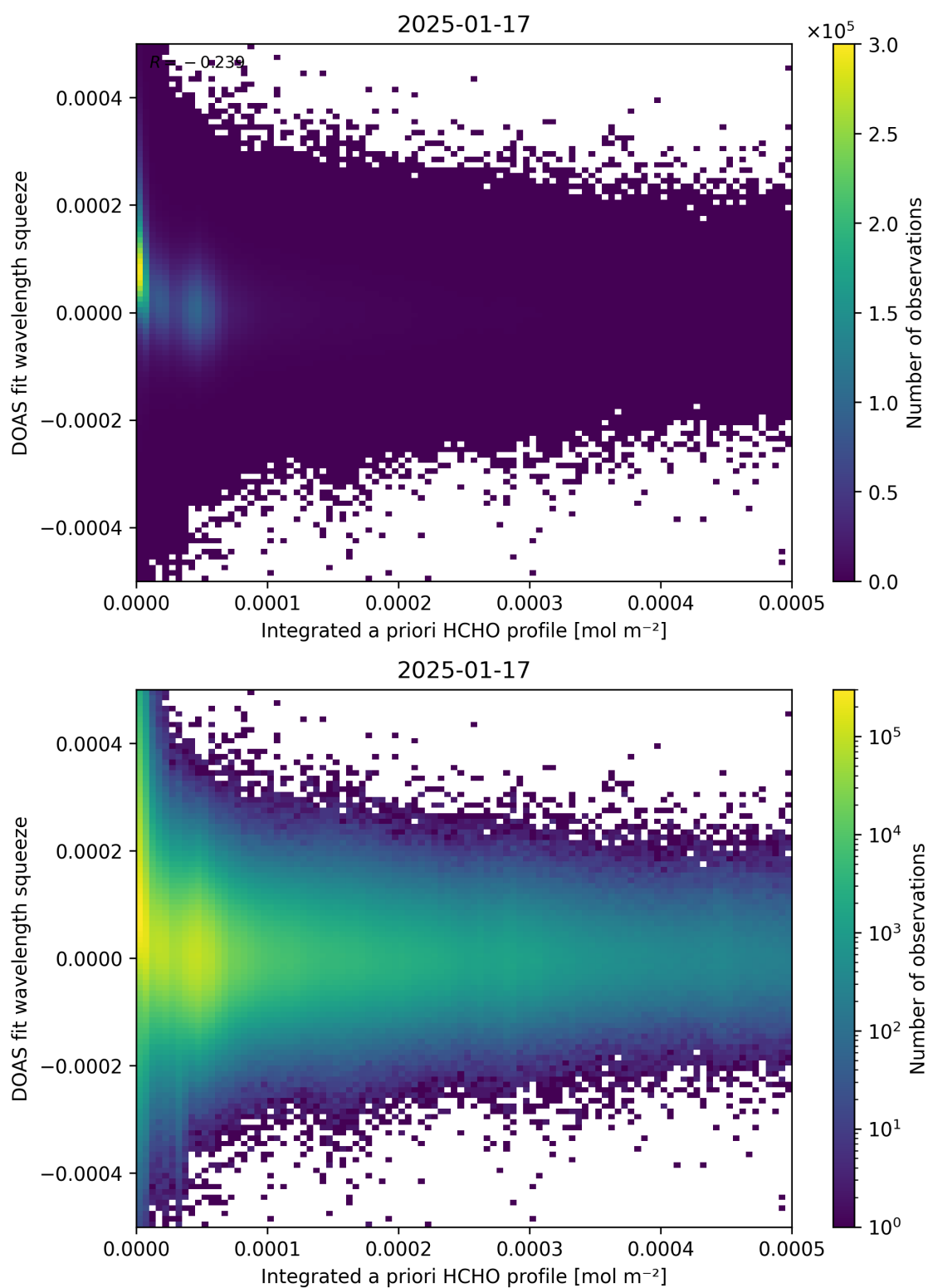
Figure 150: Scatter density plot of “Integrated a priori HCHO profile” against “DOAS fit wavelength squeeze” for 2025-01-17 to 2025-01-18.
