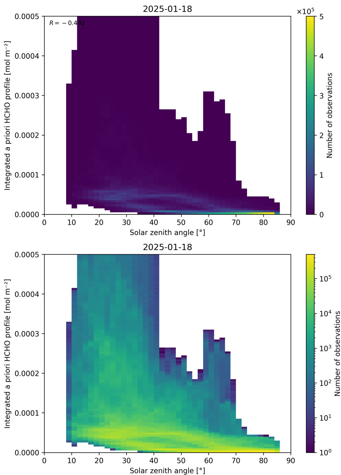
Figure 180: Scatter density plot of “Solar zenith angle” against “Integrated a priori HCHO profile” for 2025-01-17 to 2025-01-19.
