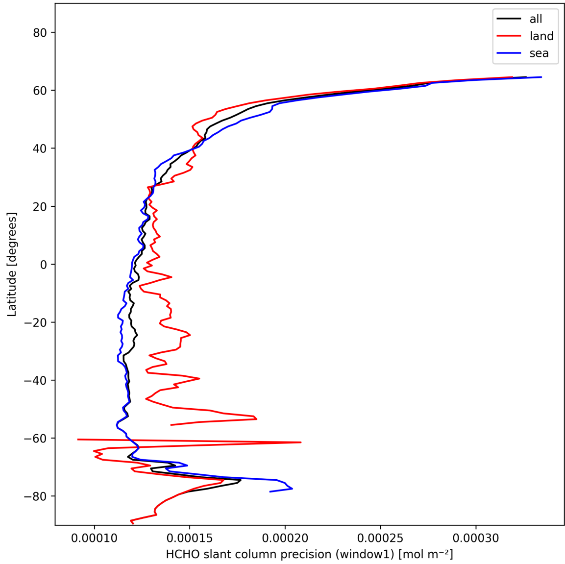
Figure 25: Zonal average of “HCHO slant column precision (window1)” for 2025-01-17 to 2025-01-19.
