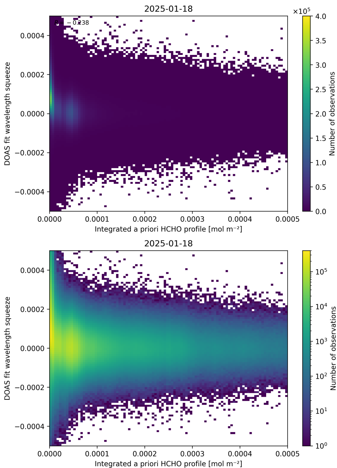
Figure 150: Scatter density plot of “Integrated a priori HCHO profile” against “DOAS fit wavelength squeeze” for 2025-01-17 to 2025-01-19.
