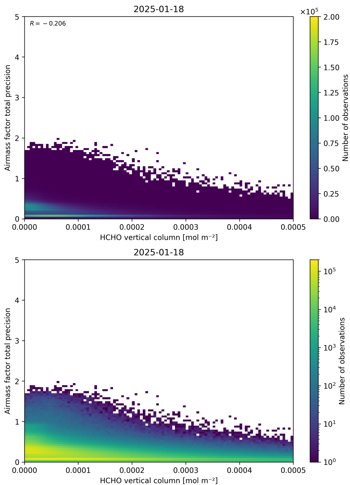
Figure 132: Scatter density plot of “HCHO vertical column” against “Airmass factor total precision” for 2025-01-17 to 2025-01-19.
