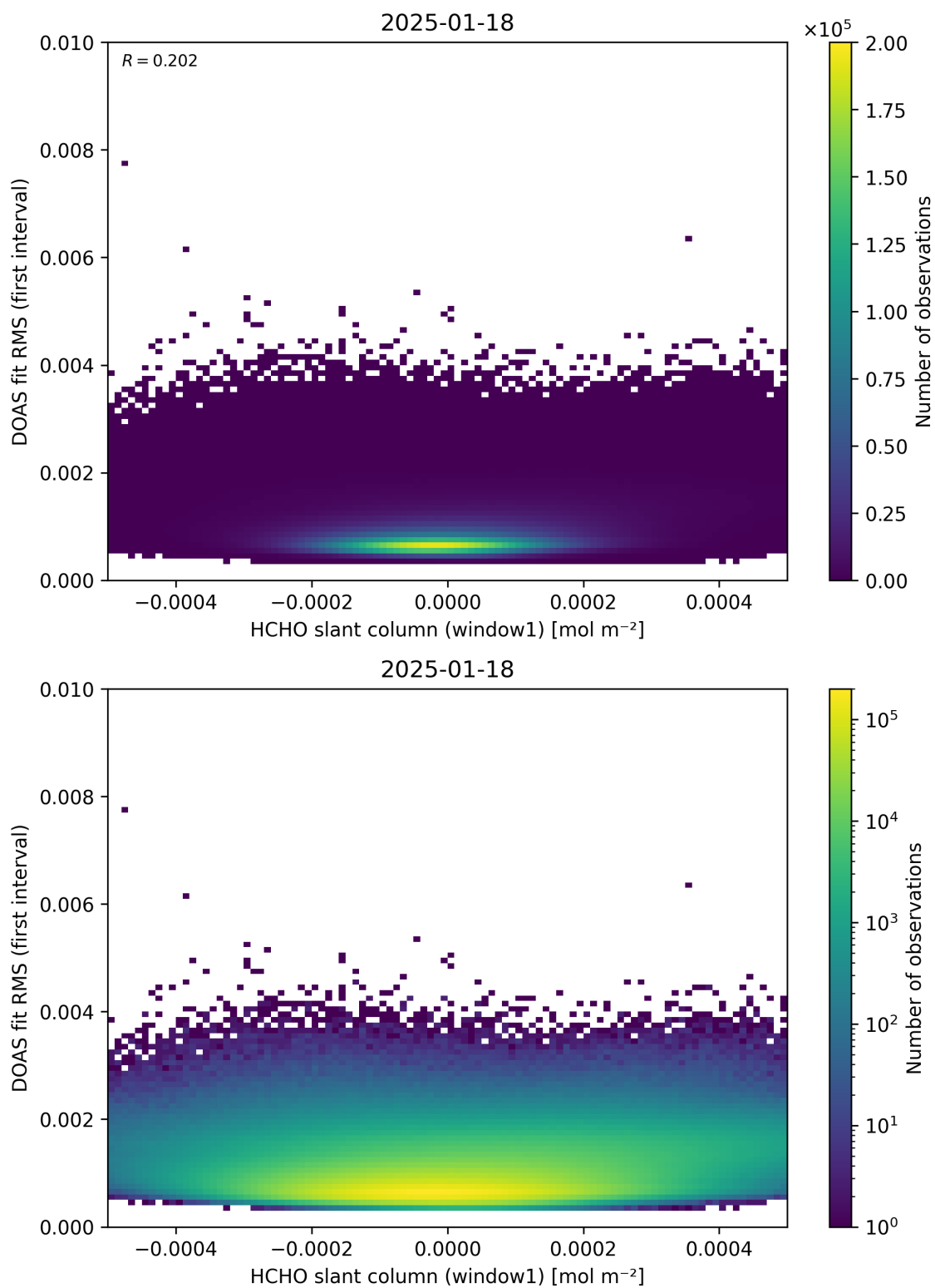
Figure 78: Scatter density plot of “HCHO slant column (window1)” against “DOAS fit RMS (first interval)” for 2025-01-17 to 2025-01-19.
