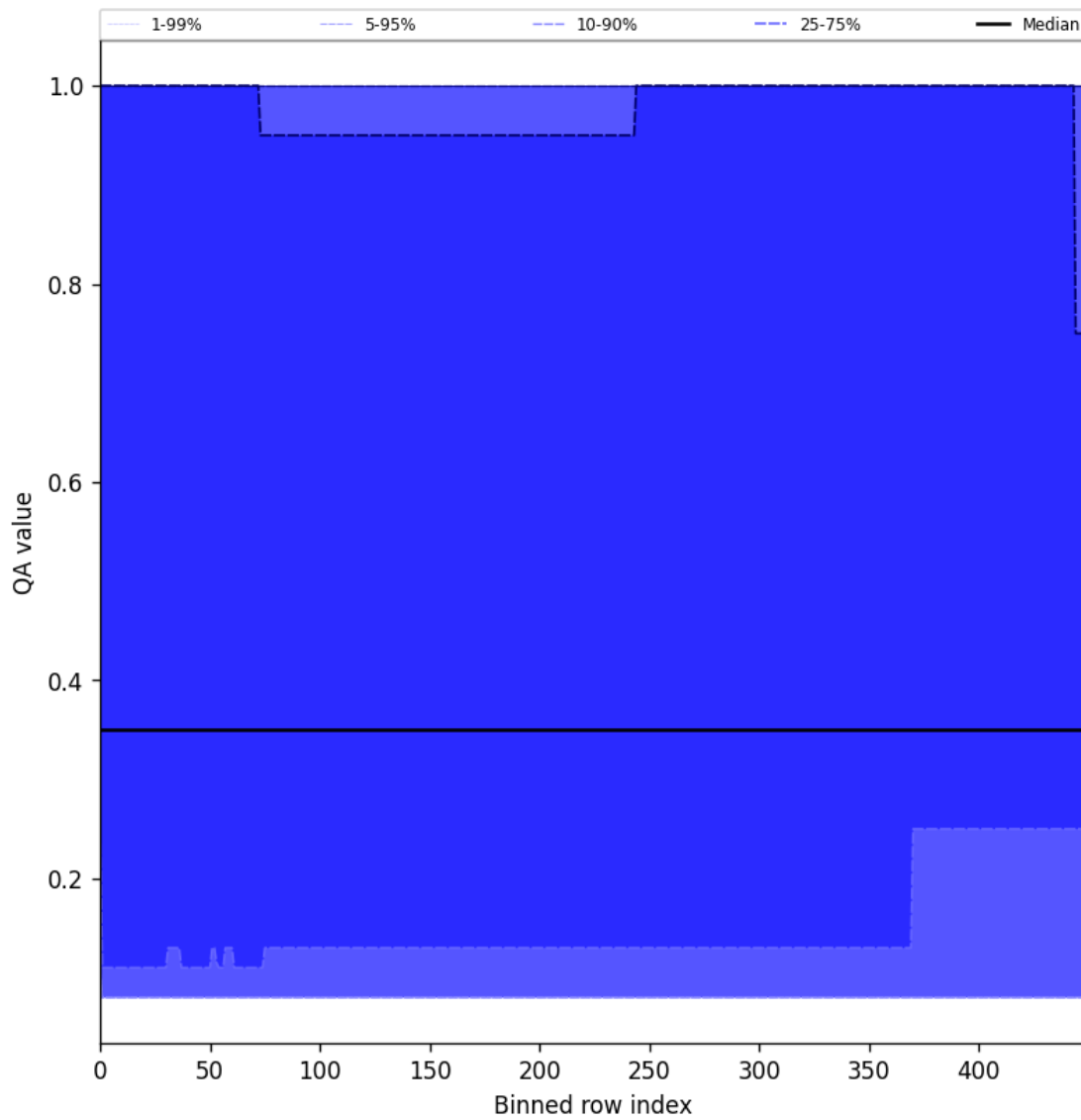
Figure 48: Along track statistics of “QA value” for 2025-01-17 to 2025-01-19
