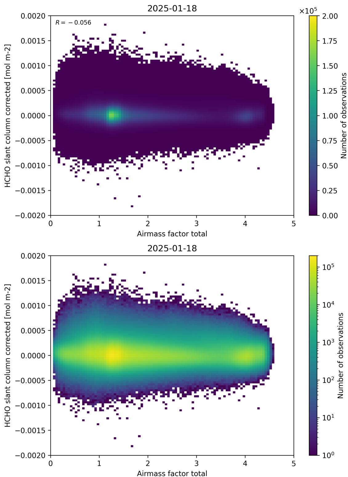
Figure 101: Scatter density plot of “Airmass factor total” against “HCHO slant column corrected” for 2025-01-17 to 2025-01-19.
