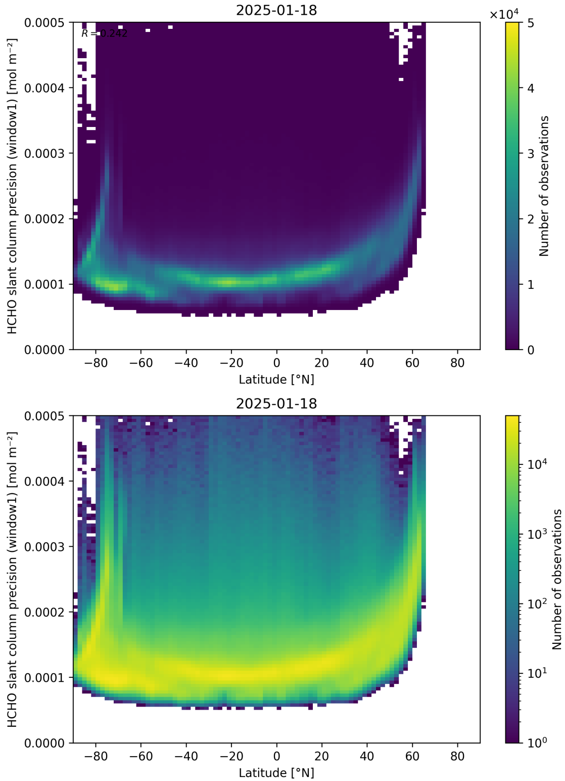
Figure 160: Scatter density plot of “Latitude” against “HCHO slant column precision (window1)” for 2025-01-17 to 2025-01-19.
