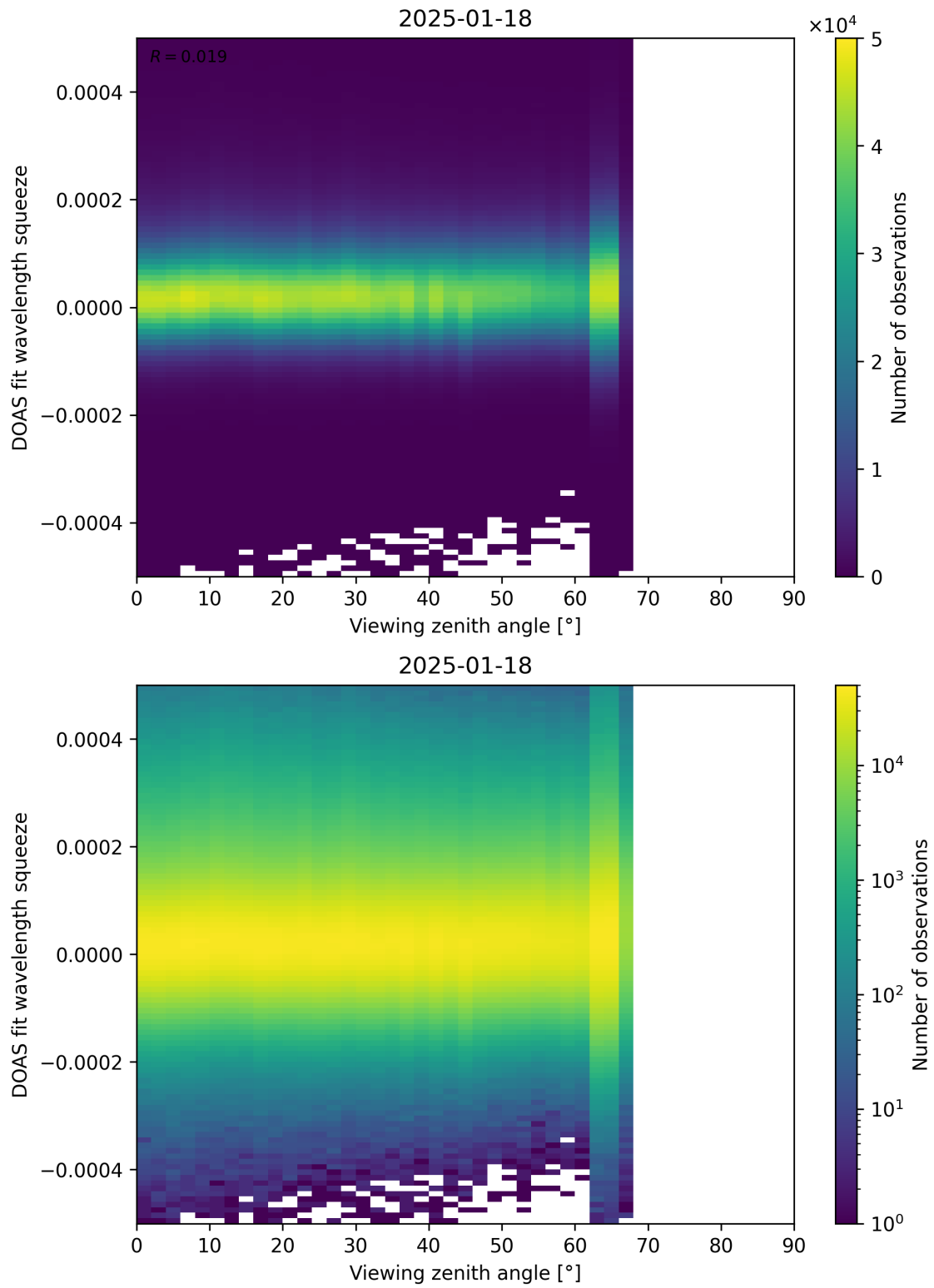
Figure 184: Scatter density plot of “Viewing zenith angle” against “DOAS fit wavelength squeeze” for 2025-01-17 to 2025-01-19.
