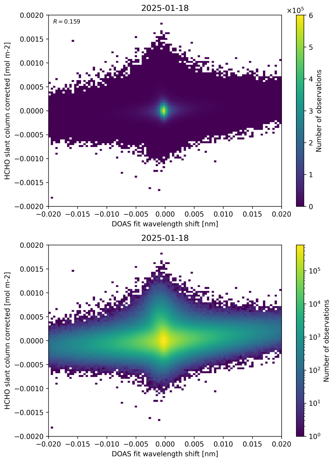
Figure 66: Scatter density plot of “DOAS fit wavelength shift” against “HCHO slant column corrected” for 2025-01-17 to 2025-01-19.
