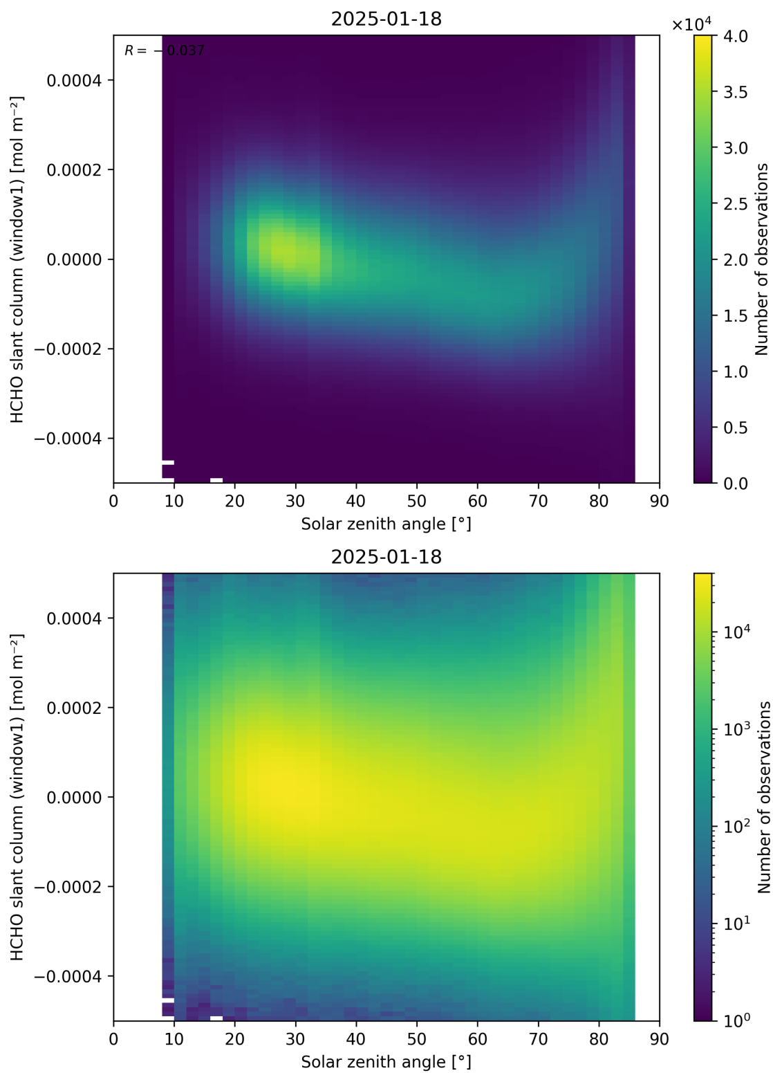
Figure 173: Scatter density plot of “Solar zenith angle” against “HCHO slant column (window1)” for 2025-01-17 to 2025-01-19.
