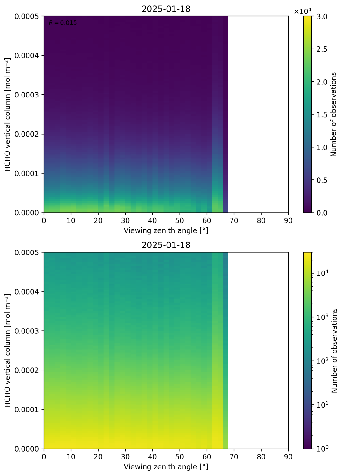
Figure 192: Scatter density plot of “Viewing zenith angle” against “HCHO vertical column” for 2025-01-17 to 2025-01-19.
