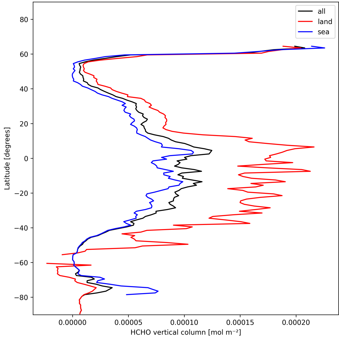
Figure 21: Zonal average of “HCHO vertical column” for 2025-01-17 to 2025-01-19.
