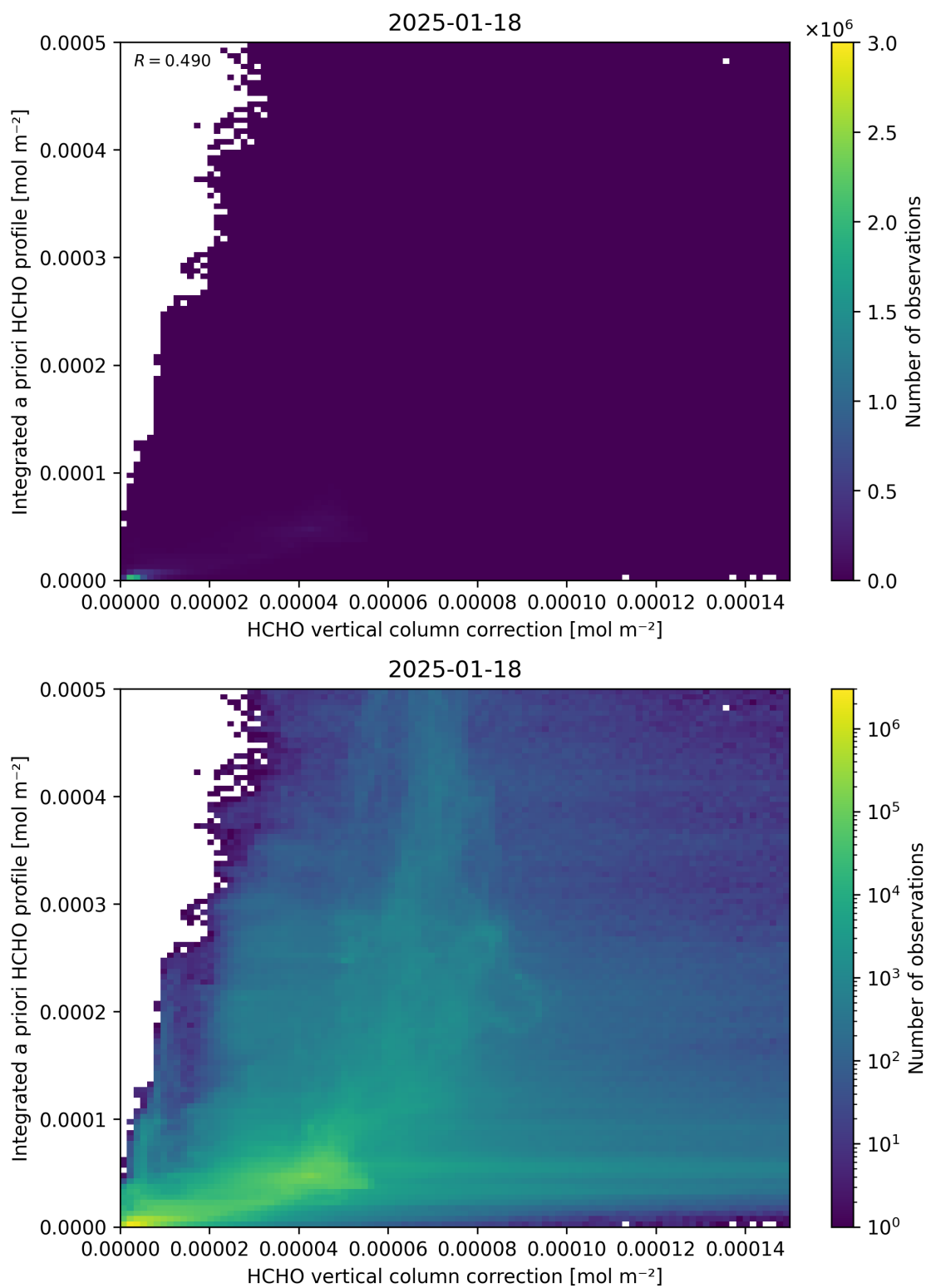
Figure 122: Scatter density plot of “HCHO vertical column correction” against “Integrated a priori HCHO profile” for 2025-01-17 to 2025-01-19.
