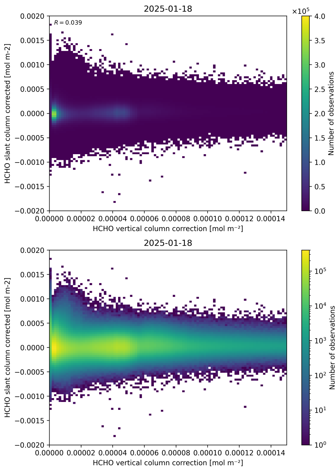
Figure 116: Scatter density plot of “HCHO vertical column correction” against “HCHO slant column corrected” for 2025-01-17 to 2025-01-19.
