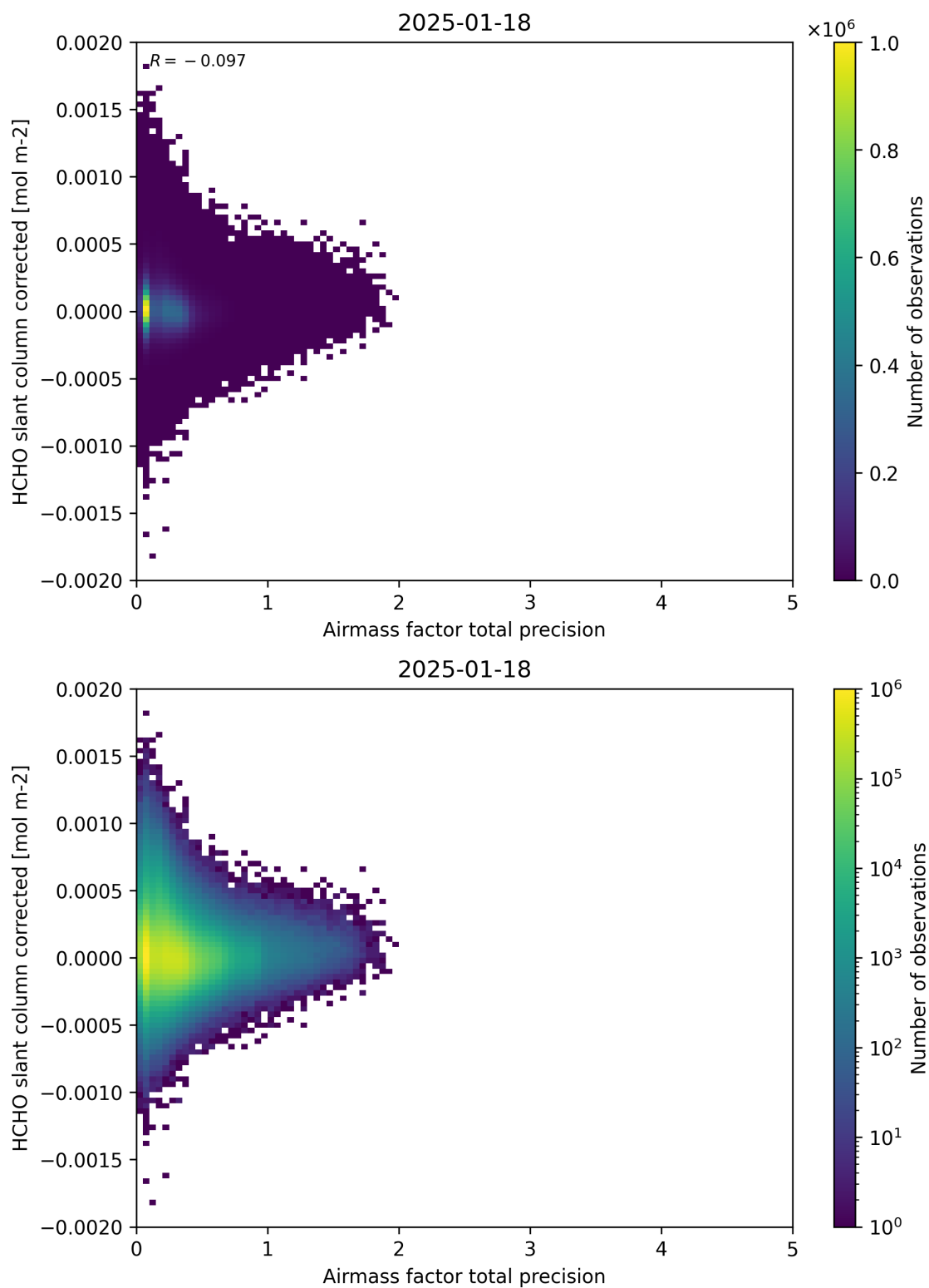
Figure 109: Scatter density plot of “Airmass factor total precision” against “HCHO slant column corrected” for 2025-01-17 to 2025-01-19.
