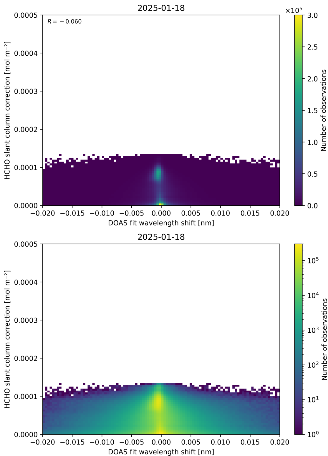
Figure 67: Scatter density plot of “DOAS fit wavelength shift” against “HCHO slant column correction” for 2025-01-17 to 2025-01-19.
