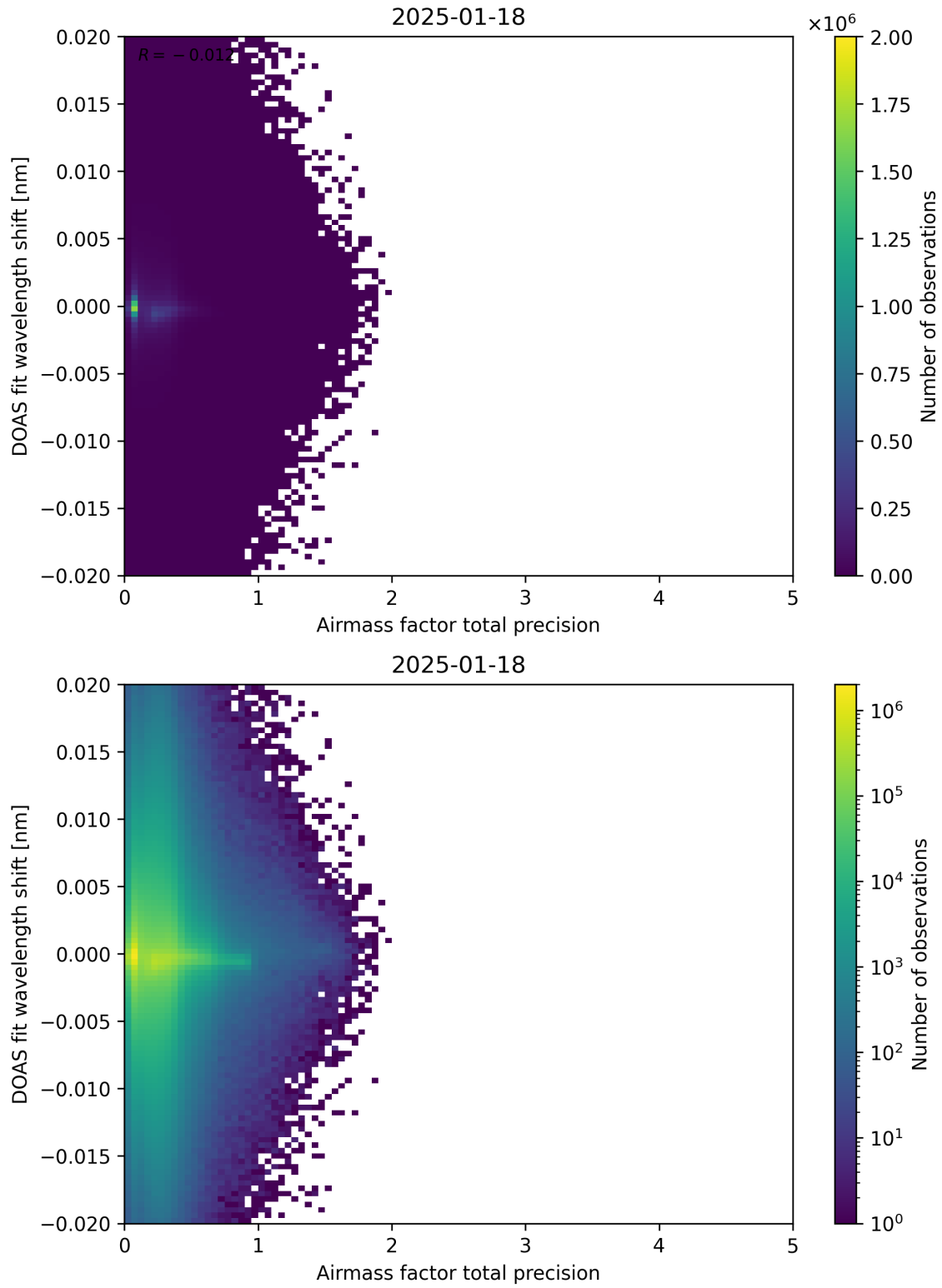
Figure 106: Scatter density plot of “Airmass factor total precision” against “DOAS fit wavelength shift” for 2025-01-17 to 2025-01-19.
