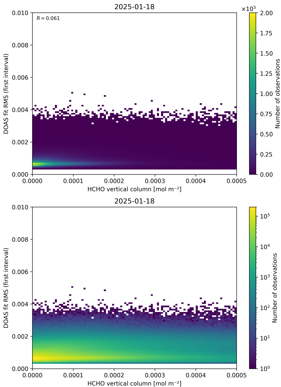
Figure 123: Scatter density plot of “HCHO vertical column” against “DOAS fit RMS (first interval)” for 2025-01-17 to 2025-01-19.
