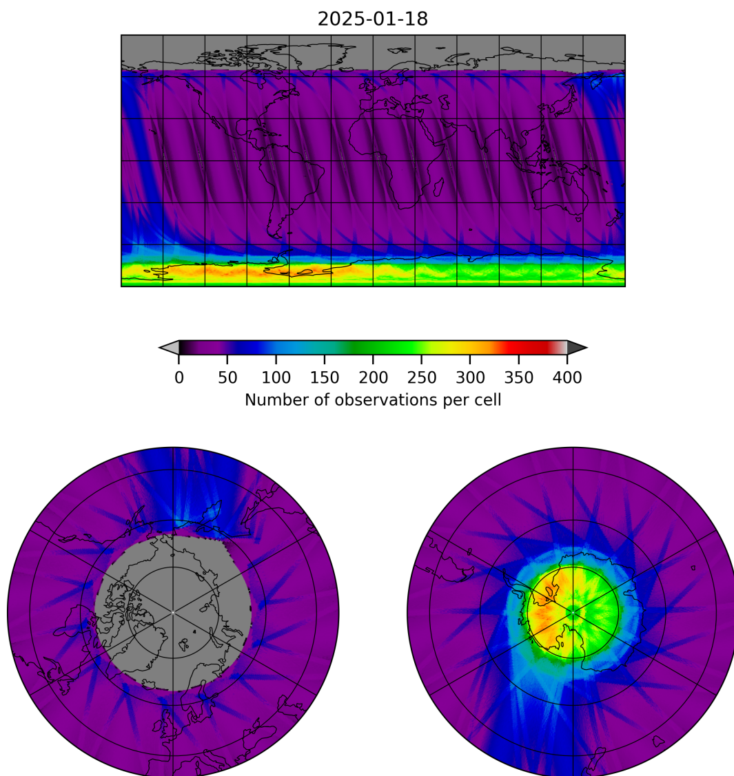
Figure 19: Map of the number of observations for 2025-01-17 to 2025-01-19
