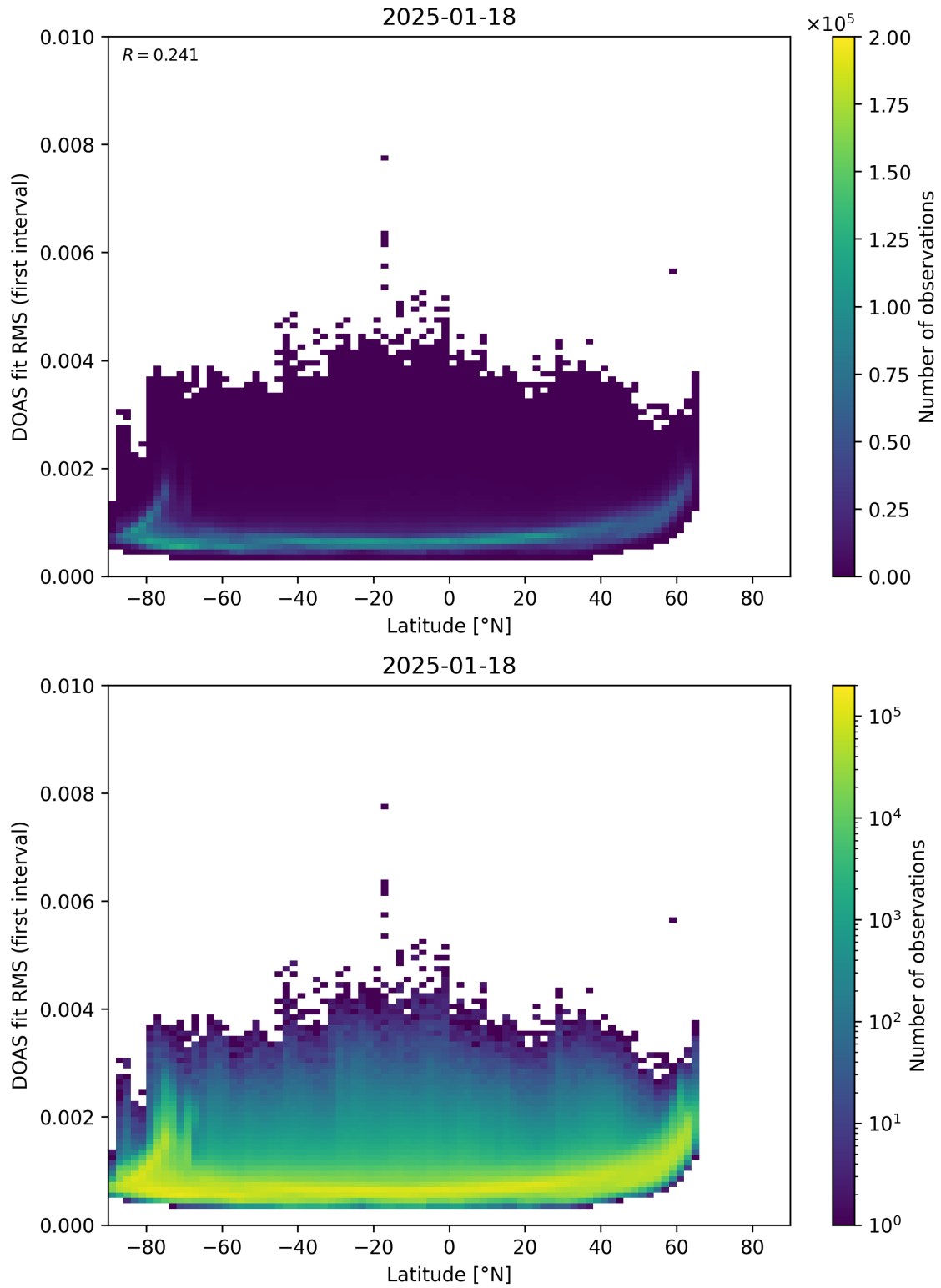
Figure 153: Scatter density plot of “Latitude” against “DOAS fit RMS (first interval)” for 2025-01-17 to 2025-01-19.
