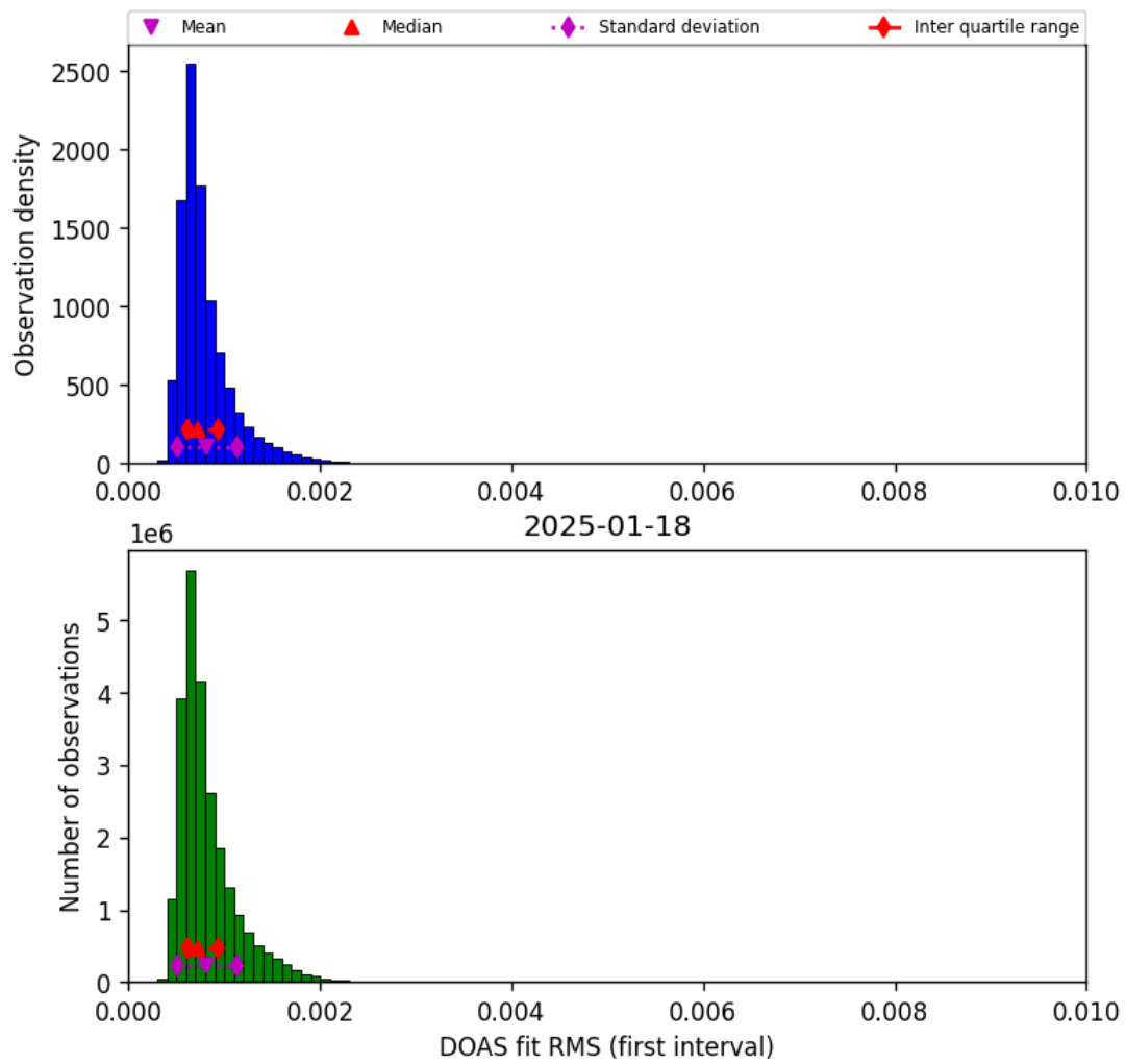
Figure 46: Histogram of “DOAS fit RMS (first interval)” for 2025-01-17 to 2025-01-19
