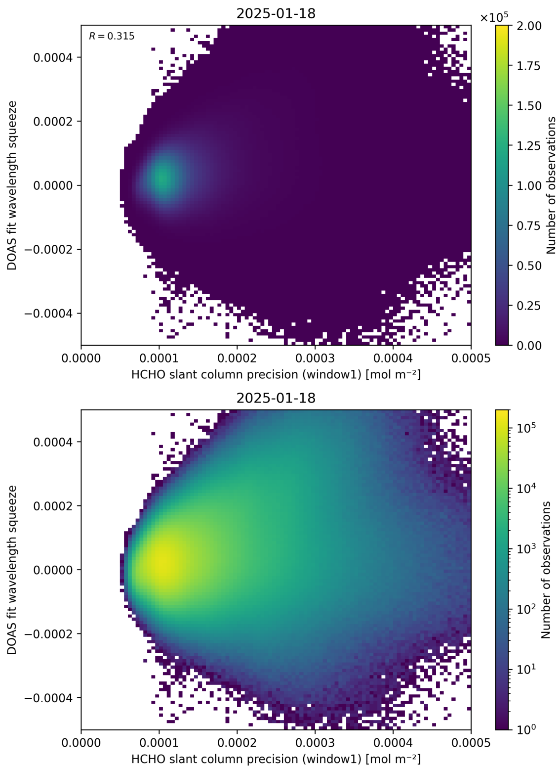
Figure 90: Scatter density plot of “HCHO slant column precision (window1)” against “DOAS fit wavelength squeeze” for 2025-01-17 to 2025-01-19.
