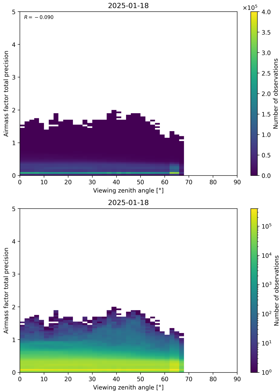
Figure 191: Scatter density plot of “Viewing zenith angle” against “Airmass factor total precision” for 2025-01-17 to 2025-01-19.
