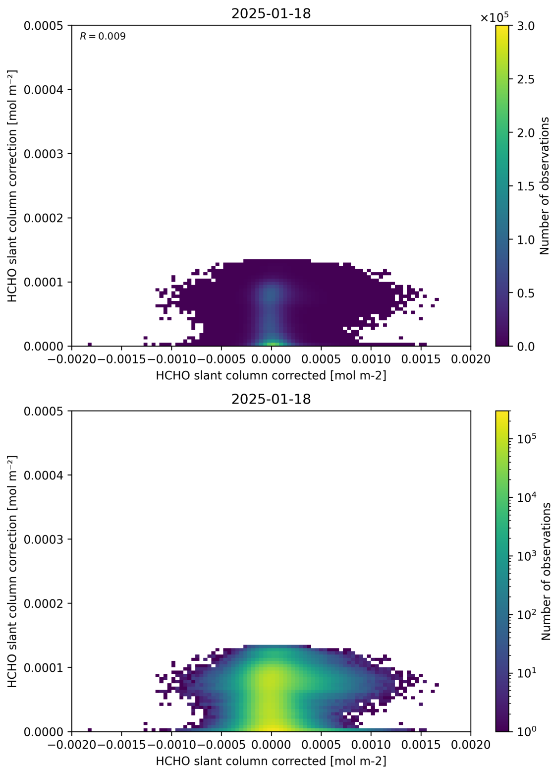
Figure 77: Scatter density plot of “HCHO slant column corrected” against “HCHO slant column correction” for 2025-01-17 to 2025-01-19.
