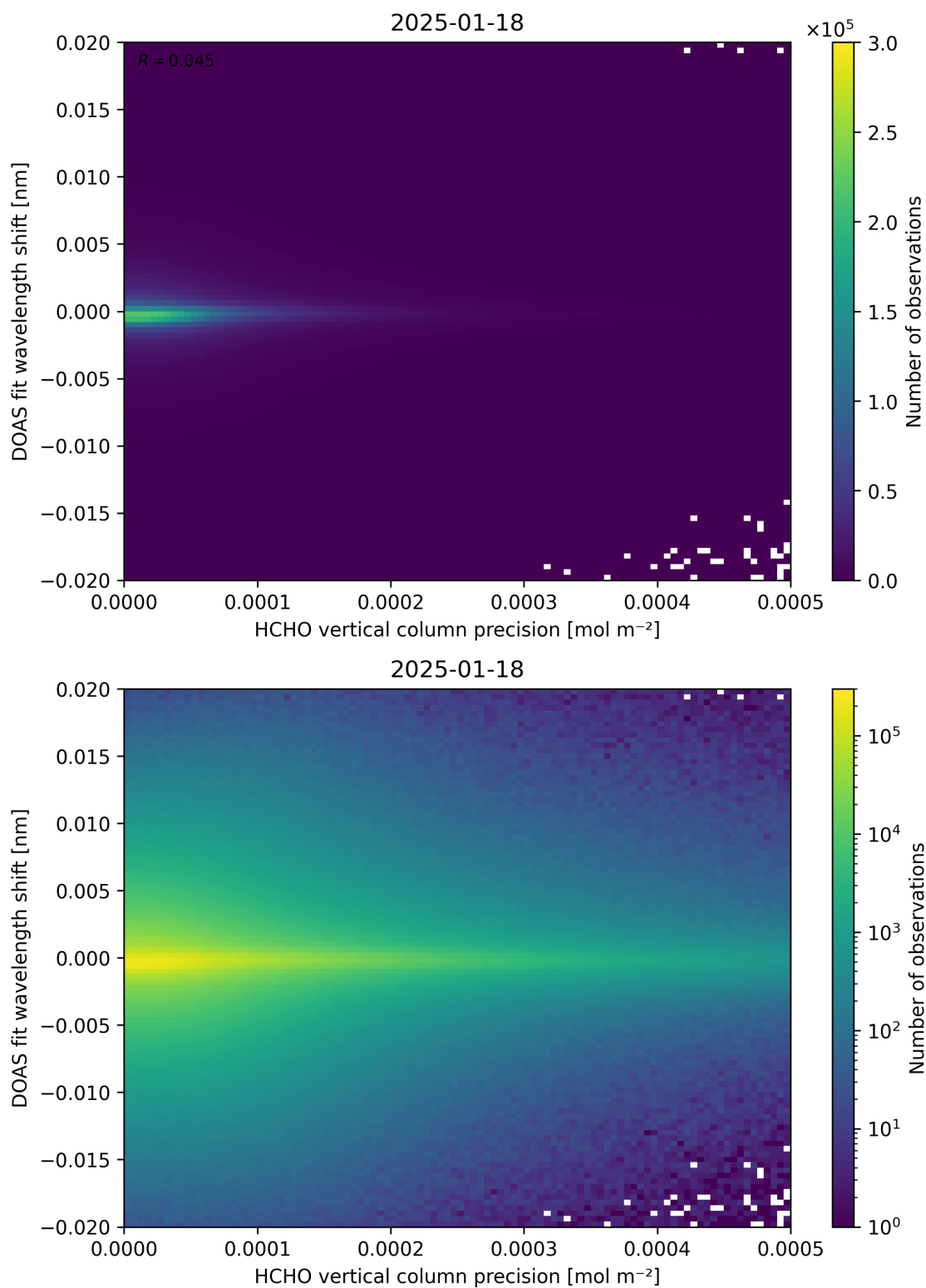
Figure 137: Scatter density plot of “HCHO vertical column precision” against “DOAS fit wavelength shift” for 2025-01-17 to 2025-01-19.
