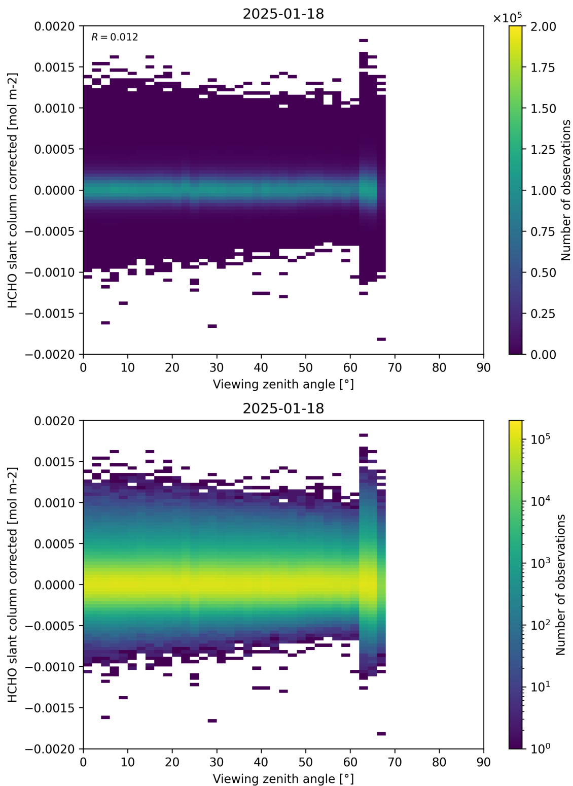
Figure 186: Scatter density plot of “Viewing zenith angle” against “HCHO slant column corrected” for 2025-01-17 to 2025-01-19.
