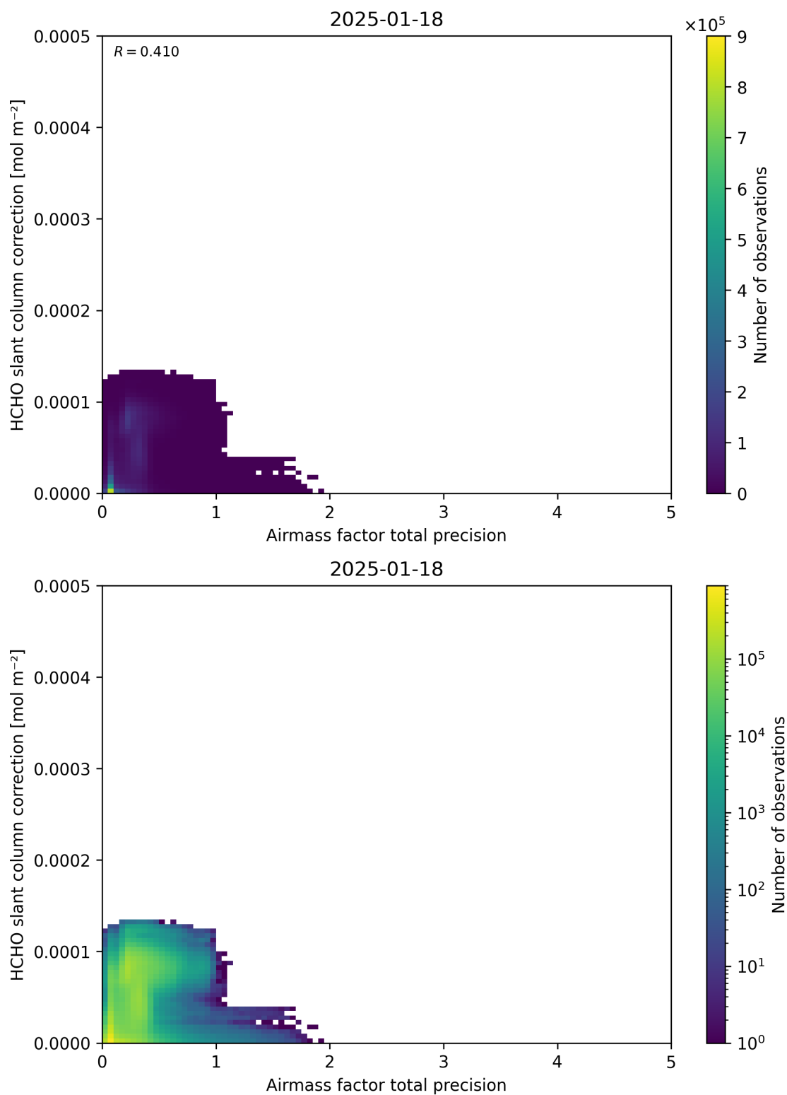
Figure 110: Scatter density plot of “Airmass factor total precision” against “HCHO slant column correction” for 2025-01-17 to 2025-01-19.
