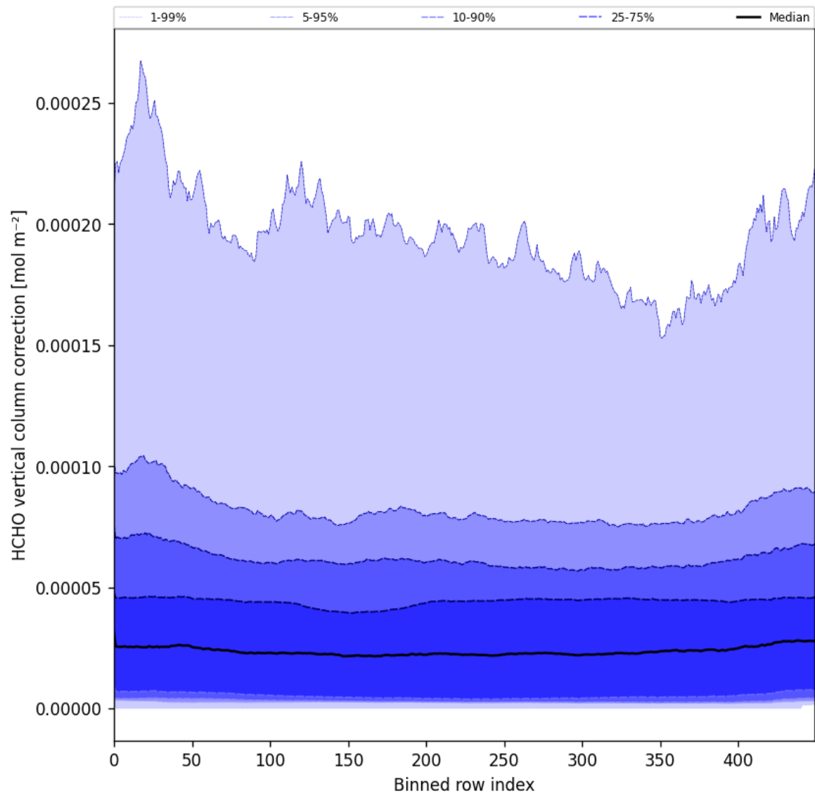
Figure 51: Along track statistics of “HCHO vertical column correction” for 2025-01-17 to 2025-01-19
