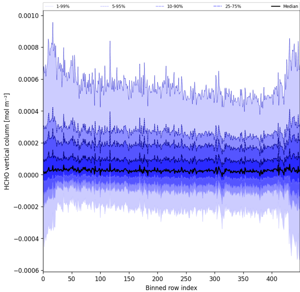
Figure 49: Along track statistics of “HCHO vertical column” for 2025-01-17 to 2025-01-19
