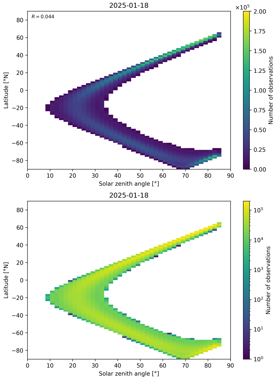
Figure 181: Scatter density plot of “Solar zenith angle” against “Latitude” for 2025-01-17 to 2025-01-19.
