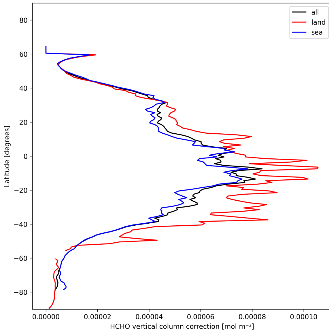
Figure 23: Zonal average of “HCHO vertical column correction” for 2025-01-17 to 2025-01-19.
