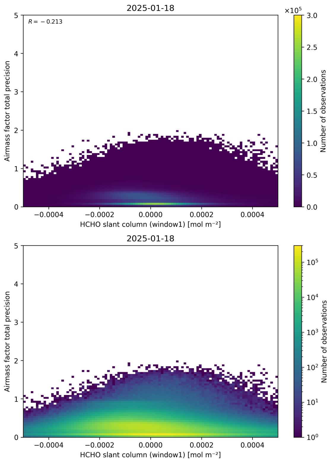
Figure 86: Scatter density plot of “HCHO slant column (window1)” against “Airmass factor total precision” for 2025-01-17 to 2025-01-19.
