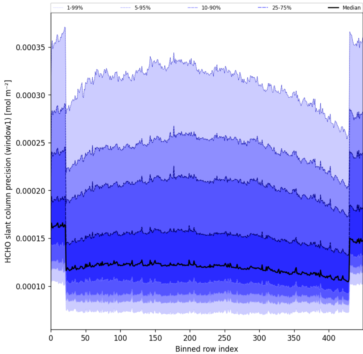
Figure 53: Along track statistics of “HCHO slant column precision (window1)” for 2025-01-17 to 2025-01-19
