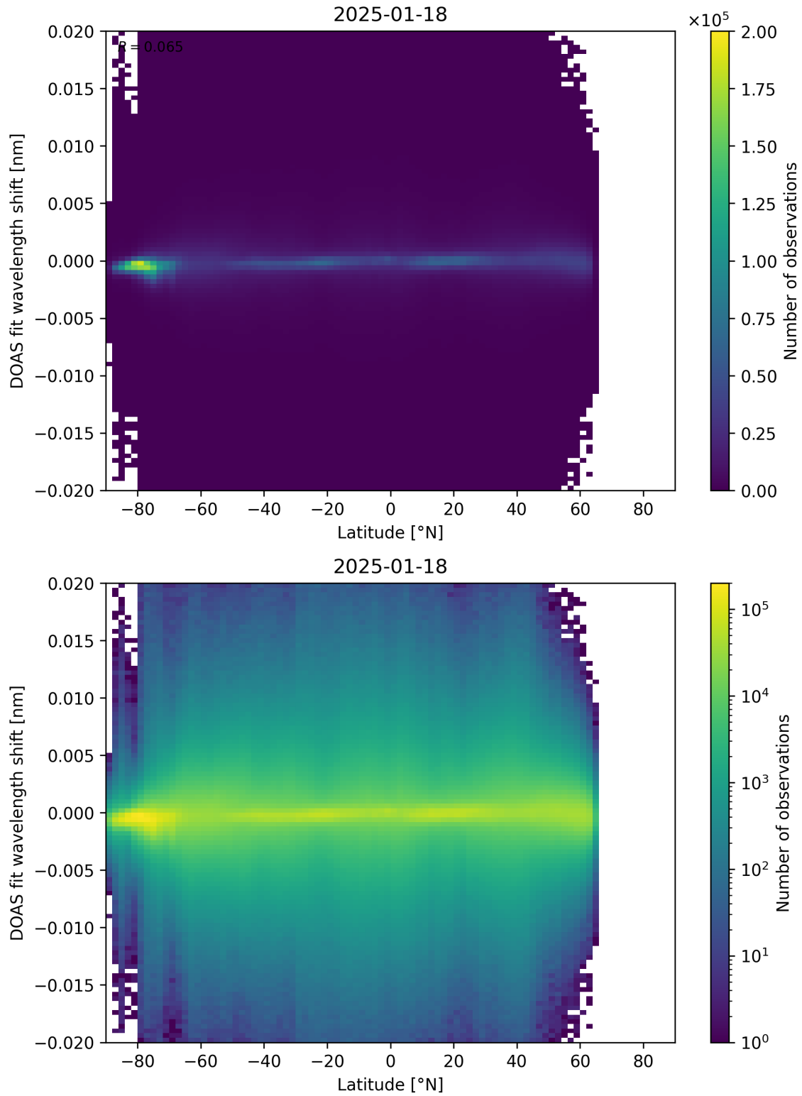
Figure 154: Scatter density plot of “Latitude” against “DOAS fit wavelength shift” for 2025-01-17 to 2025-01-19.
