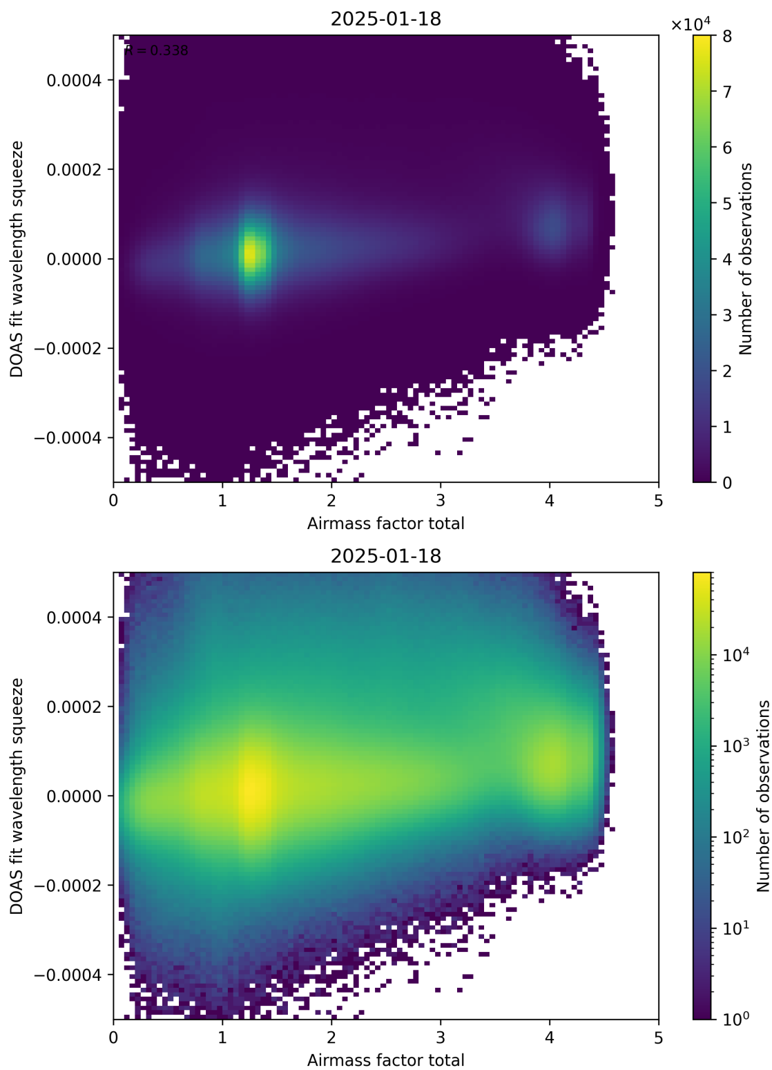
Figure 99: Scatter density plot of “Airmass factor total” against “DOAS fit wavelength squeeze” for 2025-01-17 to 2025-01-19.
