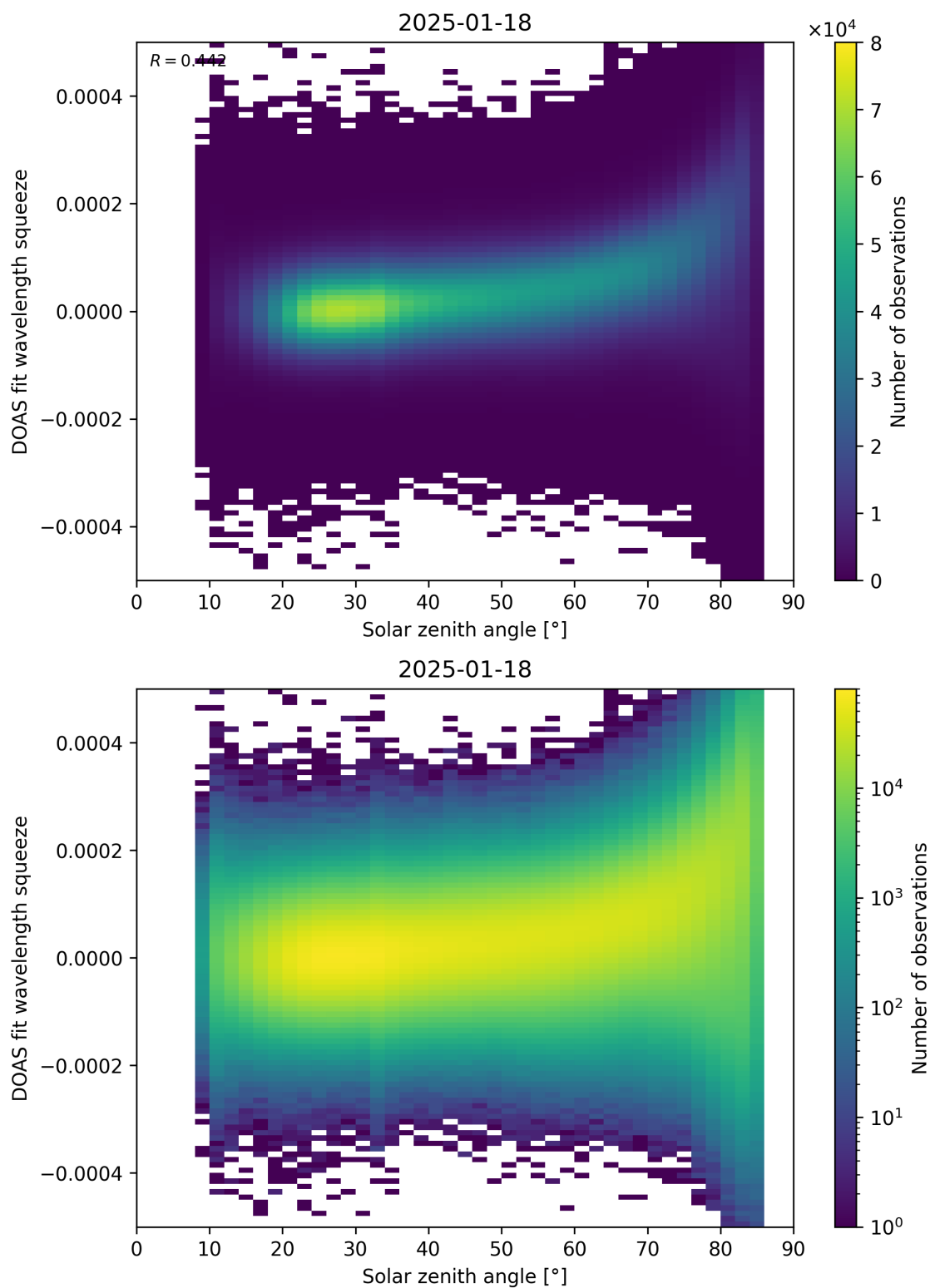
Figure 169: Scatter density plot of “Solar zenith angle” against “DOAS fit wavelength squeeze” for 2025-01-17 to 2025-01-19.
