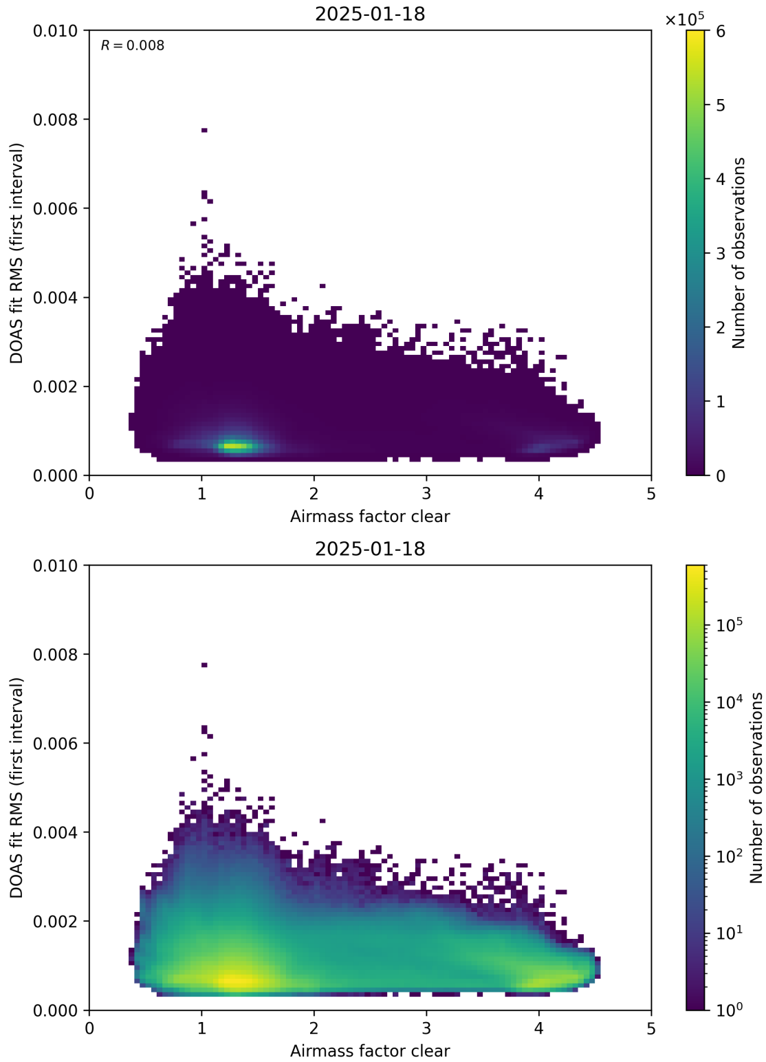
Figure 71: Scatter density plot of “Airmass factor clear” against “DOAS fit RMS (first interval)” for 2025-01-17 to 2025-01-19.
