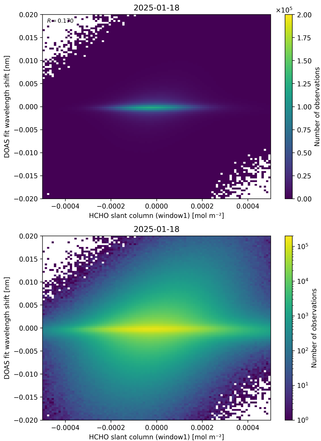
Figure 79: Scatter density plot of “HCHO slant column (window1)” against “DOAS fit wavelength shift” for 2025-01-17 to 2025-01-19.
