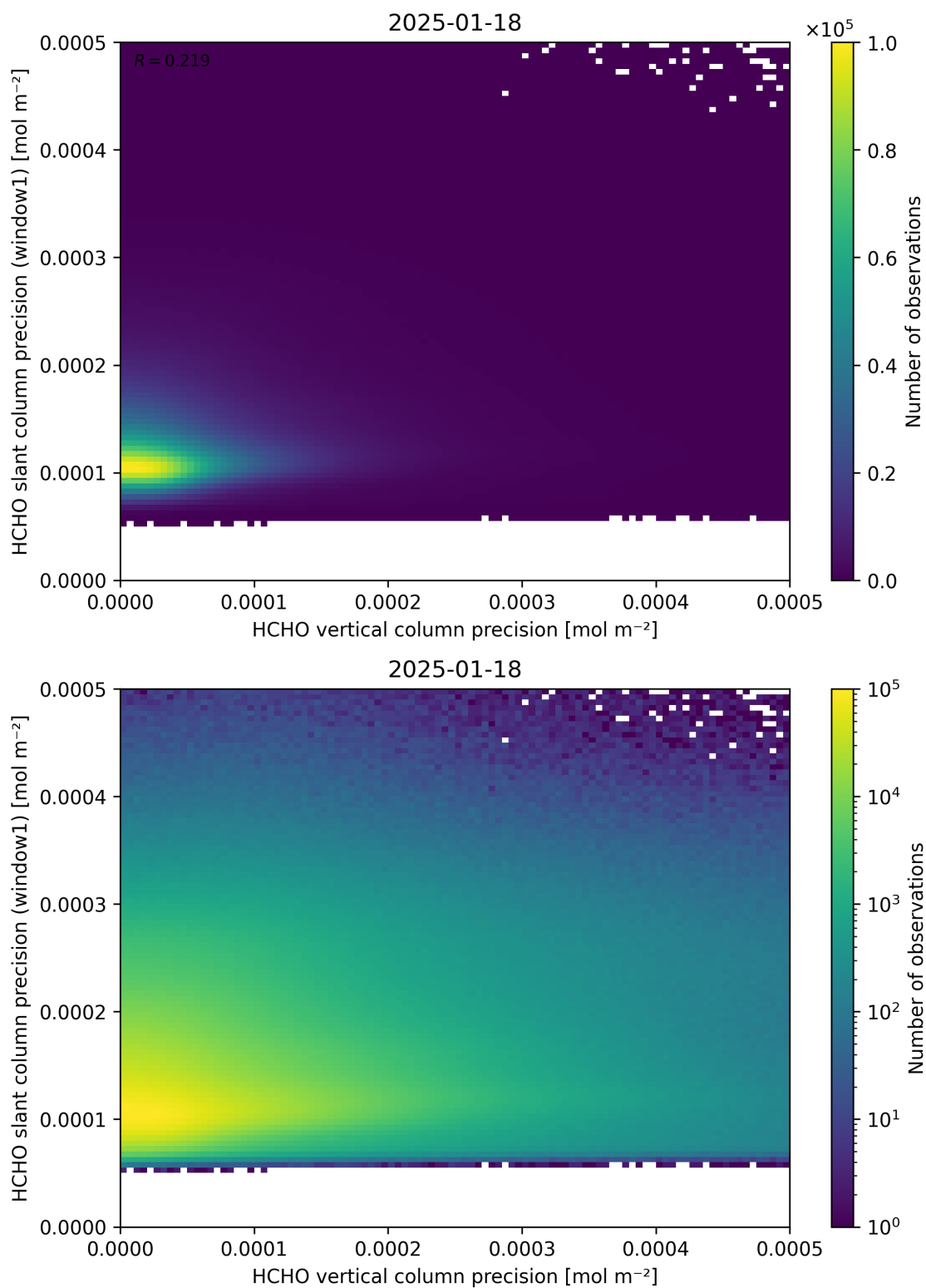
Figure 143: Scatter density plot of “HCHO vertical column precision” against “HCHO slant column precision (window1)” for 2025-01-17 to 2025-01-19.
