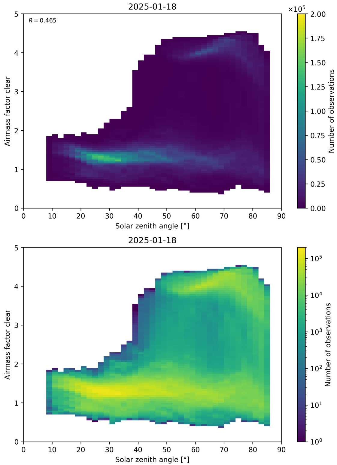
Figure 170: Scatter density plot of “Solar zenith angle” against “Airmass factor clear” for 2025-01-17 to 2025-01-19.
