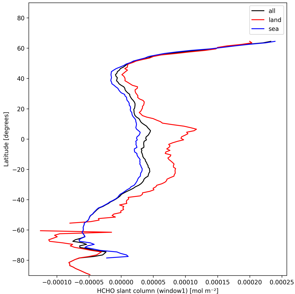
Figure 24: Zonal average of “HCHO slant column (window1)” for 2025-01-17 to 2025-01-19.
