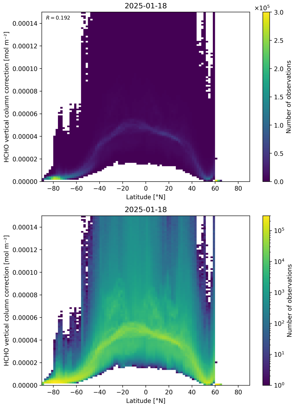
Figure 164: Scatter density plot of “Latitude” against “HCHO vertical column correction” for 2025-01-17 to 2025-01-19.
