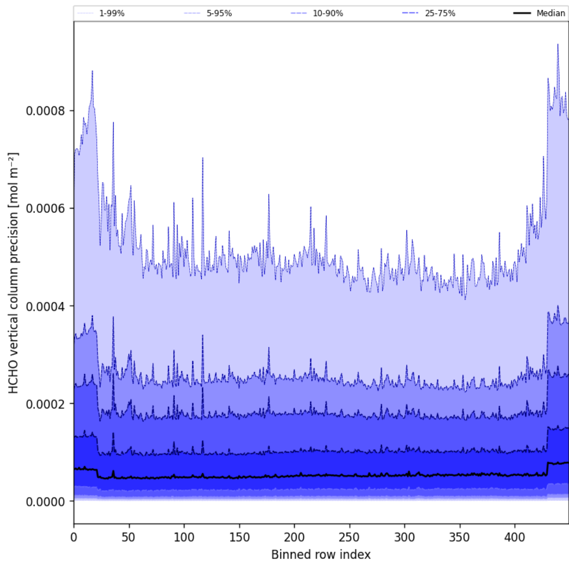
Figure 50: Along track statistics of “HCHO vertical column precision” for 2025-01-17 to 2025-01-19
