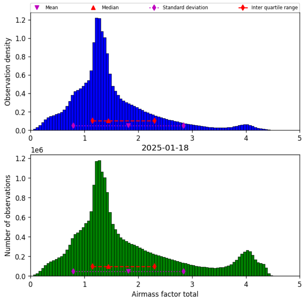
Figure 40: Histogram of “Airmass factor total” for 2025-01-17 to 2025-01-19
