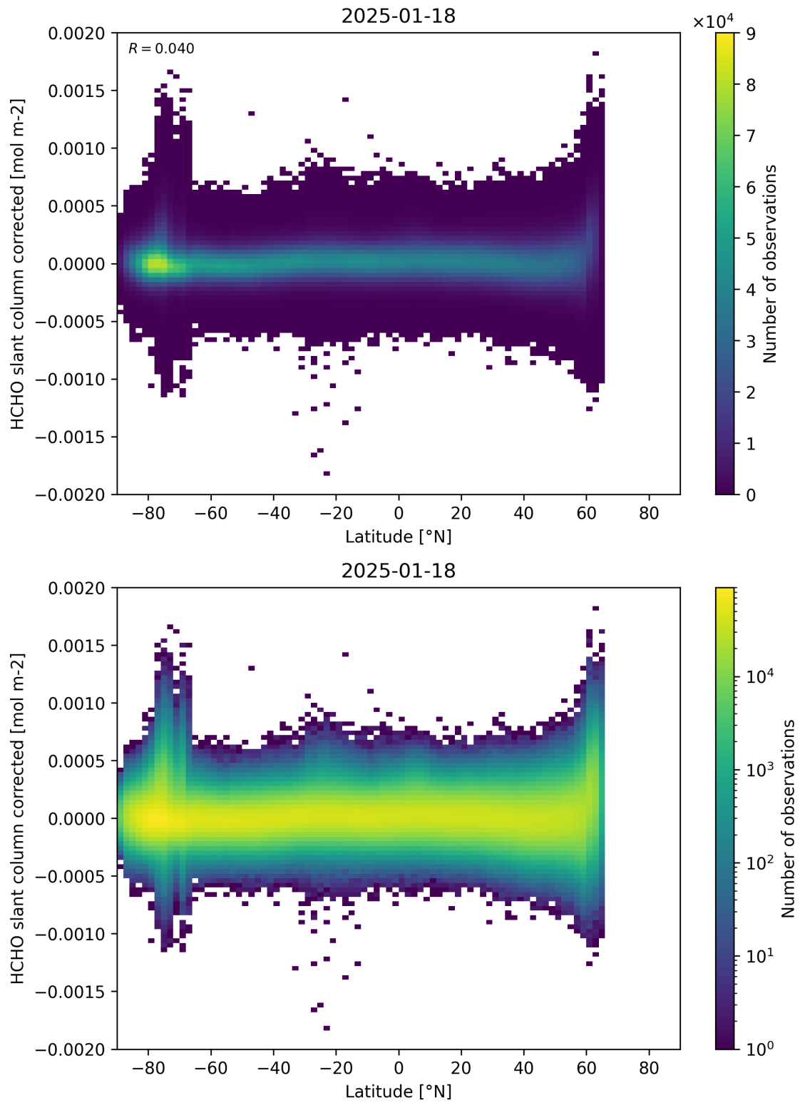
Figure 157: Scatter density plot of “Latitude” against “HCHO slant column corrected” for 2025-01-17 to 2025-01-19.
