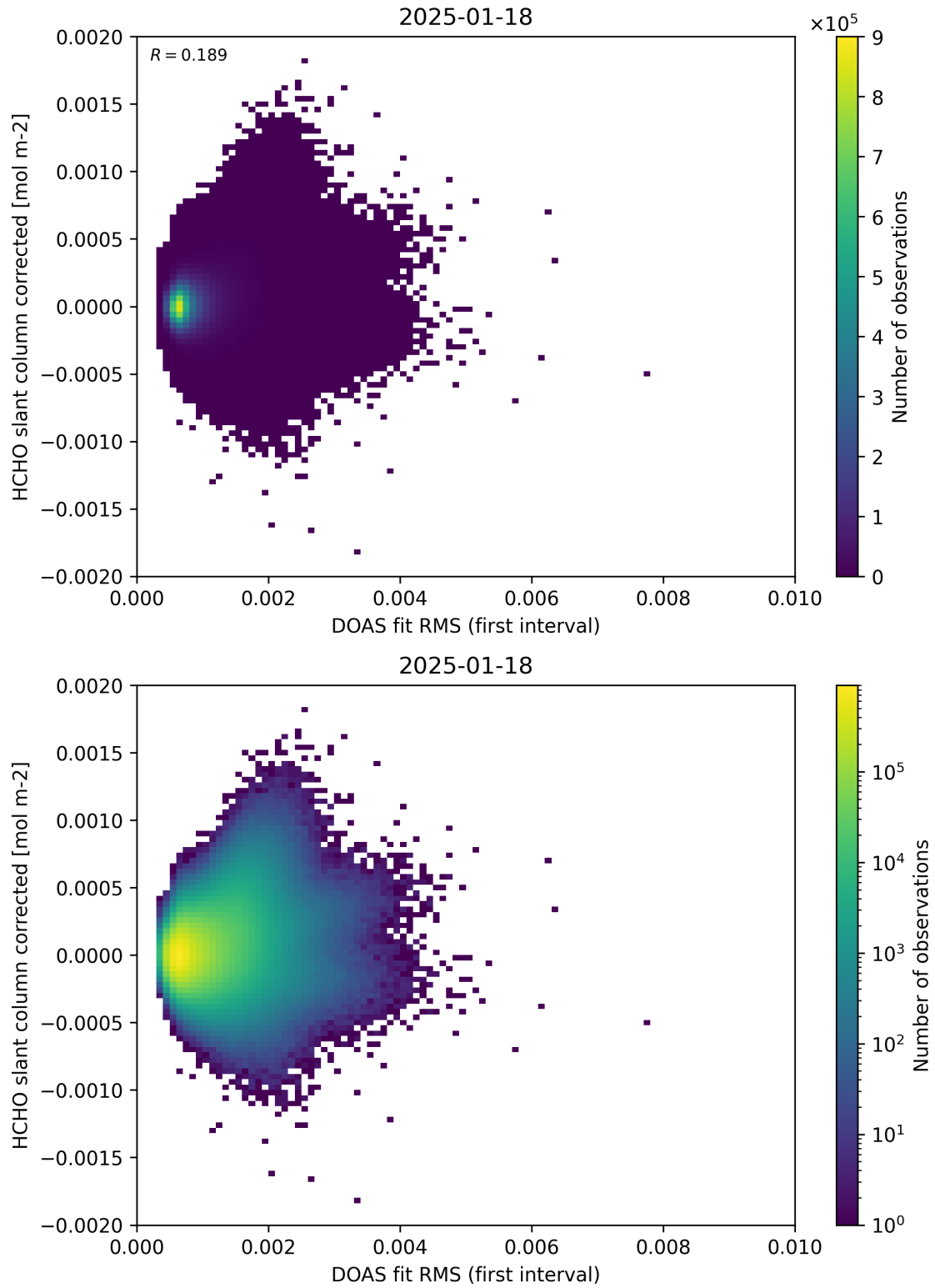
Figure 62: Scatter density plot of “DOAS fit RMS (first interval)” against “HCHO slant column corrected” for 2025-01-17 to 2025-01-19.
