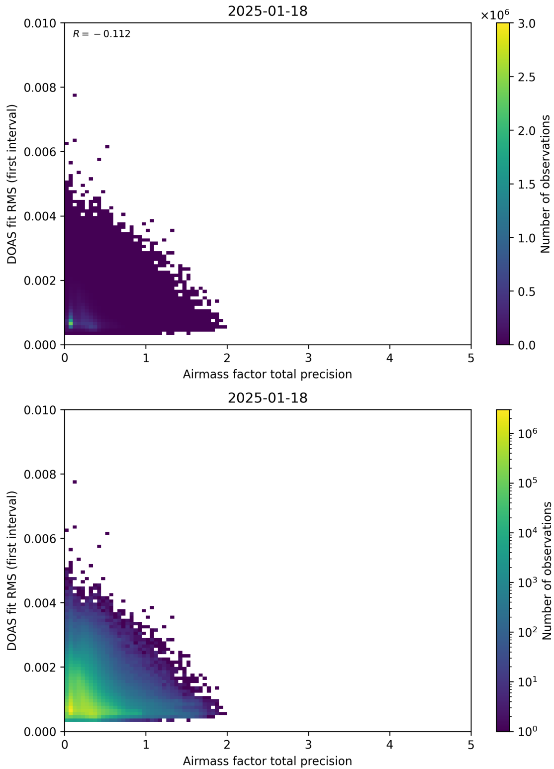
Figure 105: Scatter density plot of “Airmass factor total precision” against “DOAS fit RMS (first interval)” for 2025-01-17 to 2025-01-19.
