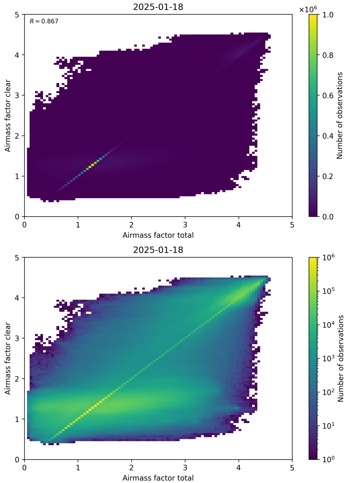
Figure 100: Scatter density plot of “Airmass factor total” against “Airmass factor clear” for 2025-01-17 to 2025-01-19.
