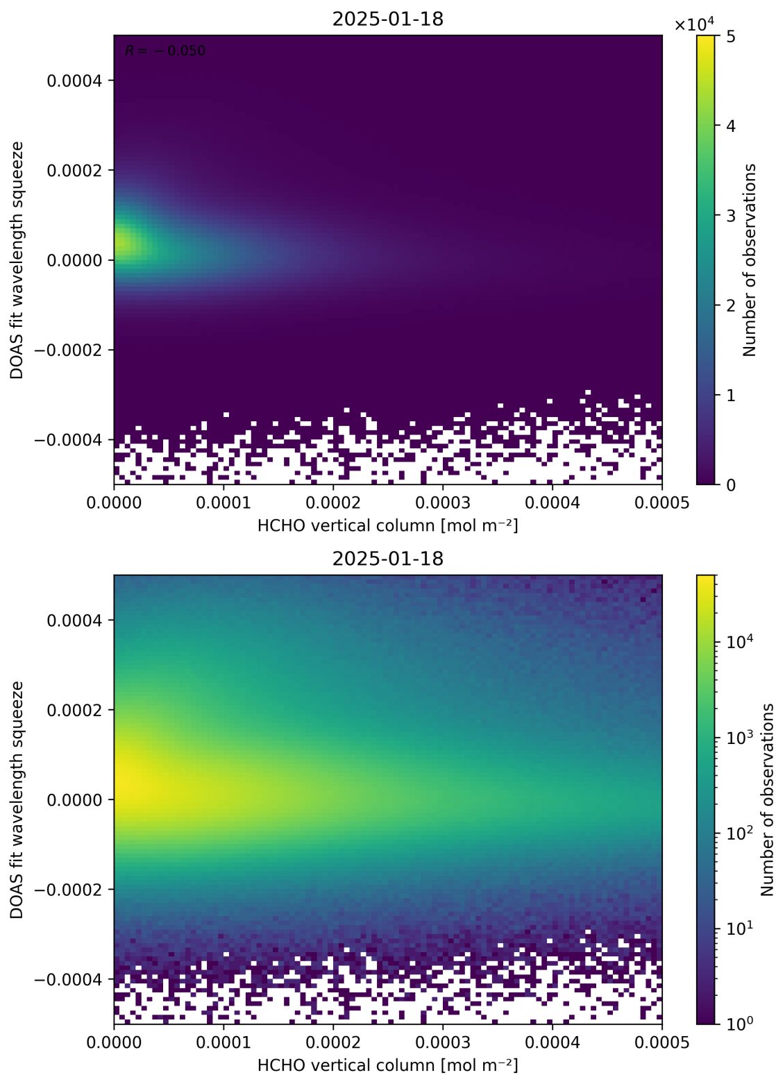
Figure 125: Scatter density plot of “HCHO vertical column” against “DOAS fit wavelength squeeze” for 2025-01-17 to 2025-01-19.
