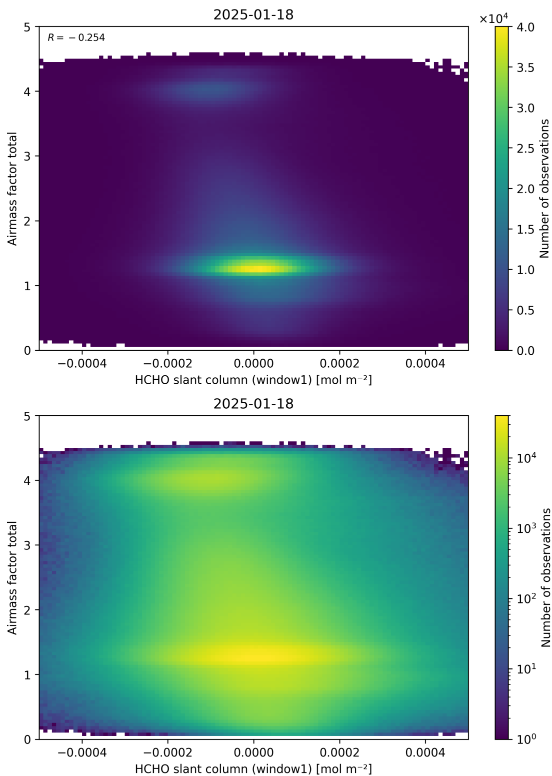
Figure 85: Scatter density plot of “HCHO slant column (window1)” against “Airmass factor total” for 2025-01-17 to 2025-01-19.
