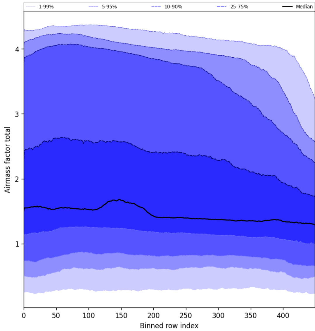
Figure 54: Along track statistics of “Airmass factor total” for 2025-01-17 to 2025-01-19
