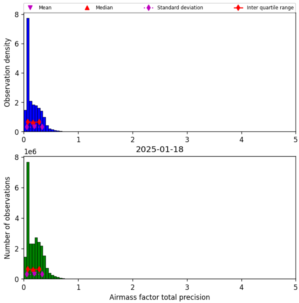
Figure 41: Histogram of “Airmass factor total precision” for 2025-01-17 to 2025-01-19
