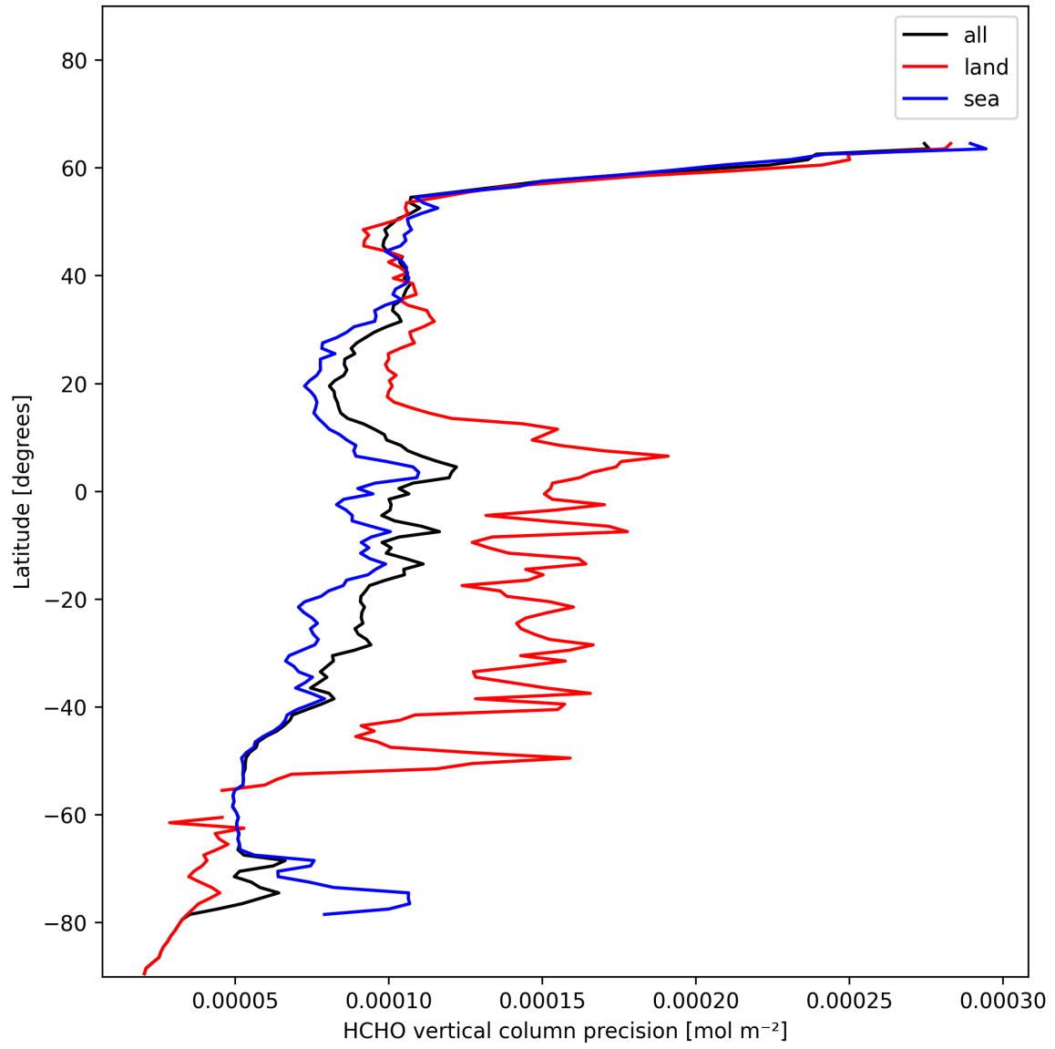
Figure 22: Zonal average of “HCHO vertical column precision” for 2025-01-17 to 2025-01-19.
