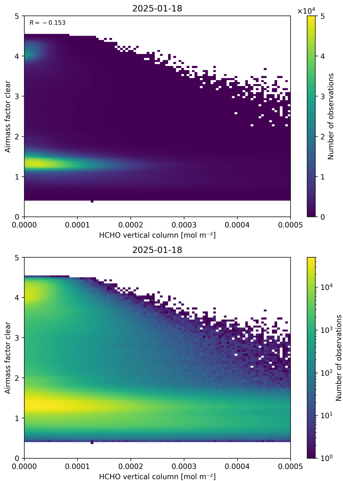
Figure 126: Scatter density plot of “HCHO vertical column” against “Airmass factor clear” for 2025-01-17 to 2025-01-19.
