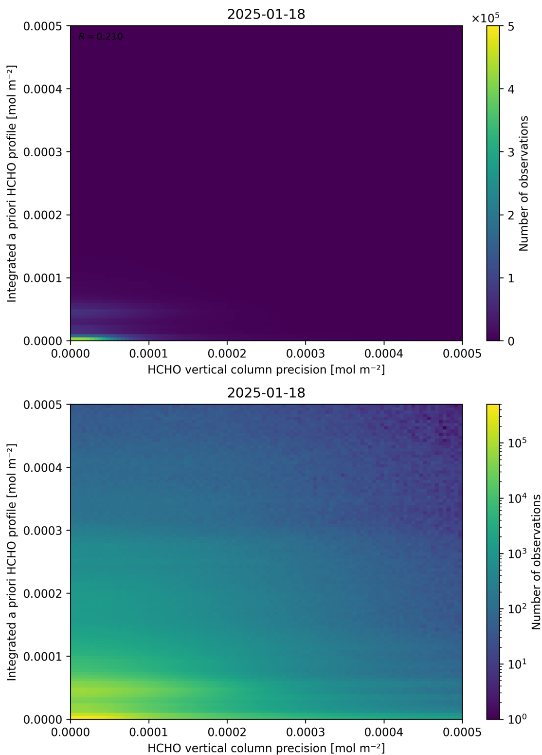
Figure 147: Scatter density plot of “HCHO vertical column precision” against “Integrated a priori HCHO profile” for 2025-01-17 to 2025-01-19.
