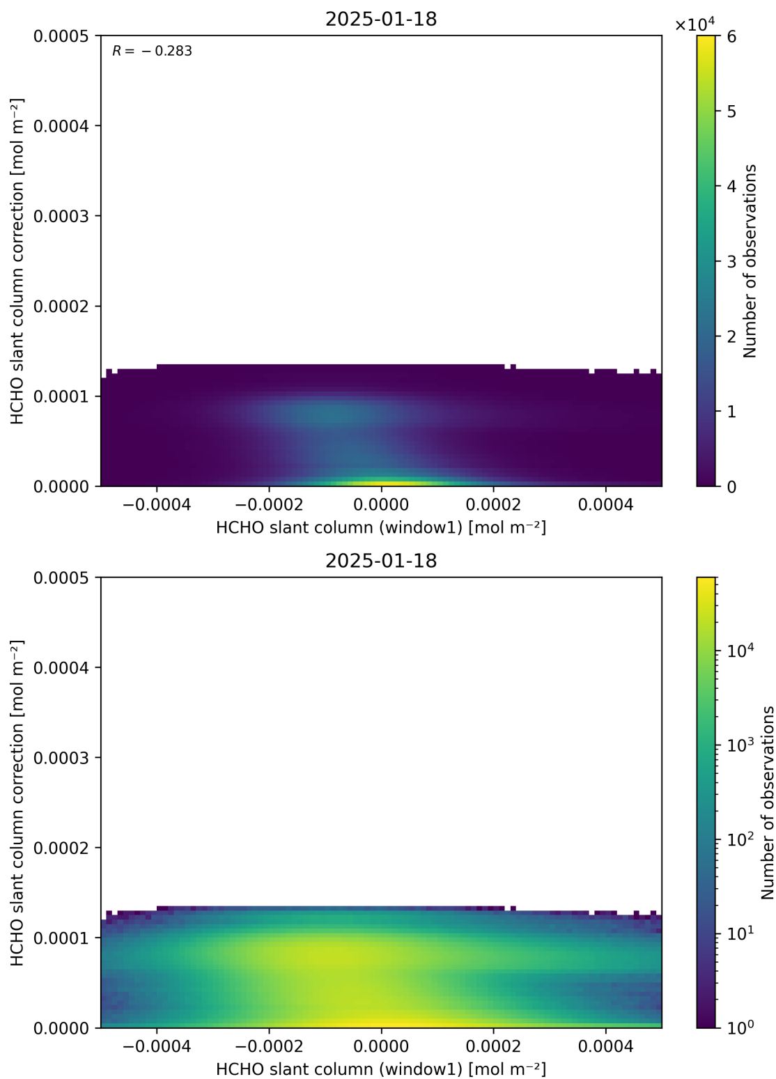
Figure 83: Scatter density plot of “HCHO slant column (window1)” against “HCHO slant column correction” for 2025-01-17 to 2025-01-19.
