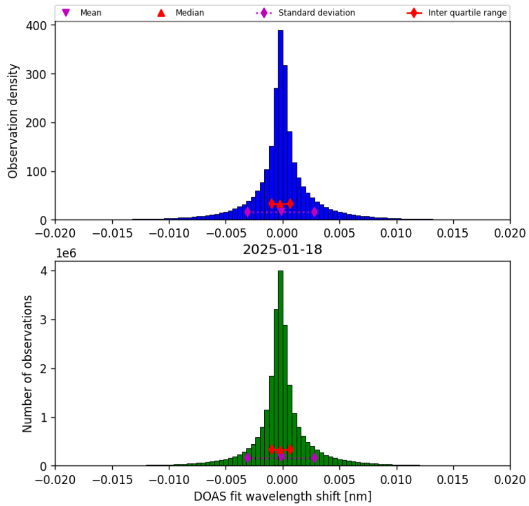
Figure 44: Histogram of “DOAS fit wavelength shift” for 2025-01-17 to 2025-01-19
