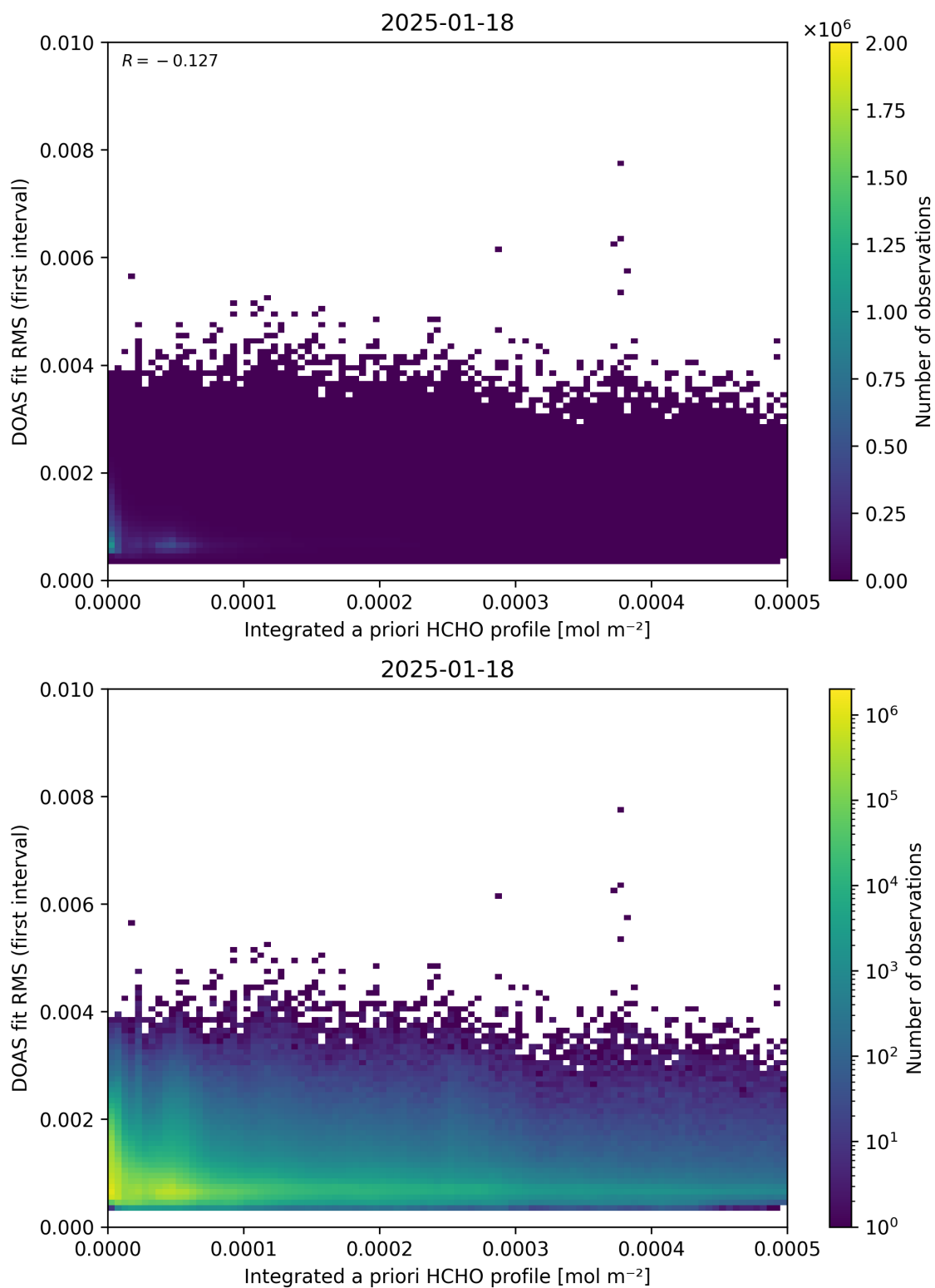
Figure 148: Scatter density plot of “Integrated a priori HCHO profile” against “DOAS fit RMS (first interval)” for 2025-01-17 to 2025-01-19.
