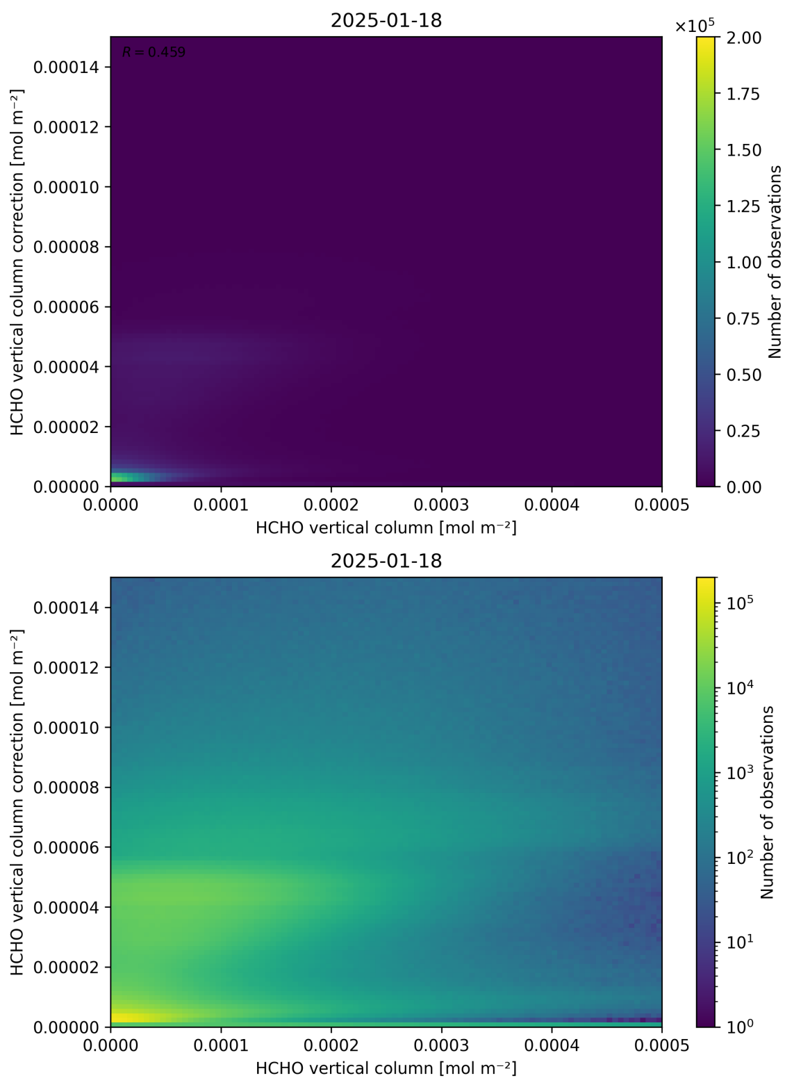
Figure 133: Scatter density plot of “HCHO vertical column” against “HCHO vertical column correction” for 2025-01-17 to 2025-01-19.
