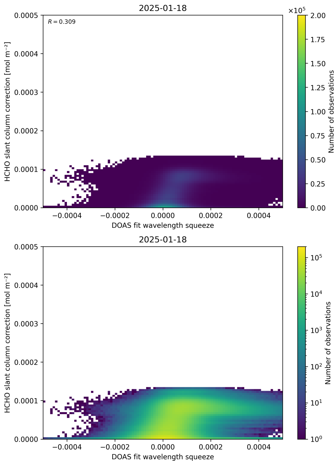
Figure 70: Scatter density plot of “DOAS fit wavelength squeeze” against “HCHO slant column correction” for 2025-01-17 to 2025-01-19.
