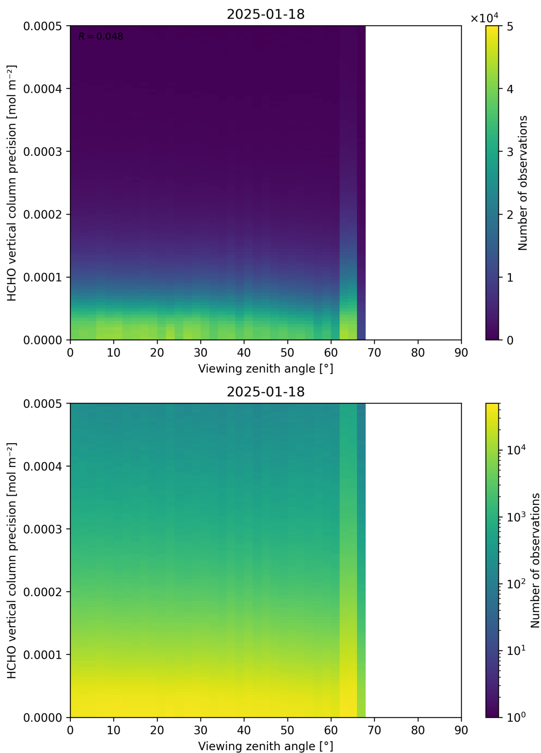
Figure 194: Scatter density plot of “Viewing zenith angle” against “HCHO vertical column precision” for 2025-01-17 to 2025-01-19.
