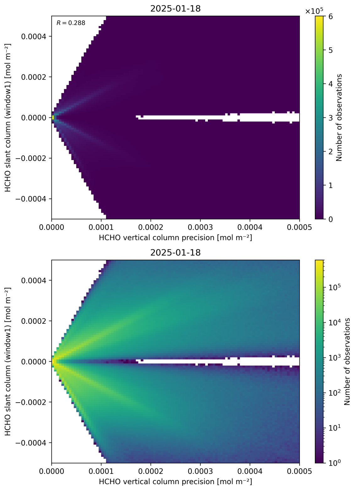
Figure 142: Scatter density plot of “HCHO vertical column precision” against “HCHO slant column (window1)” for 2025-01-17 to 2025-01-19.
