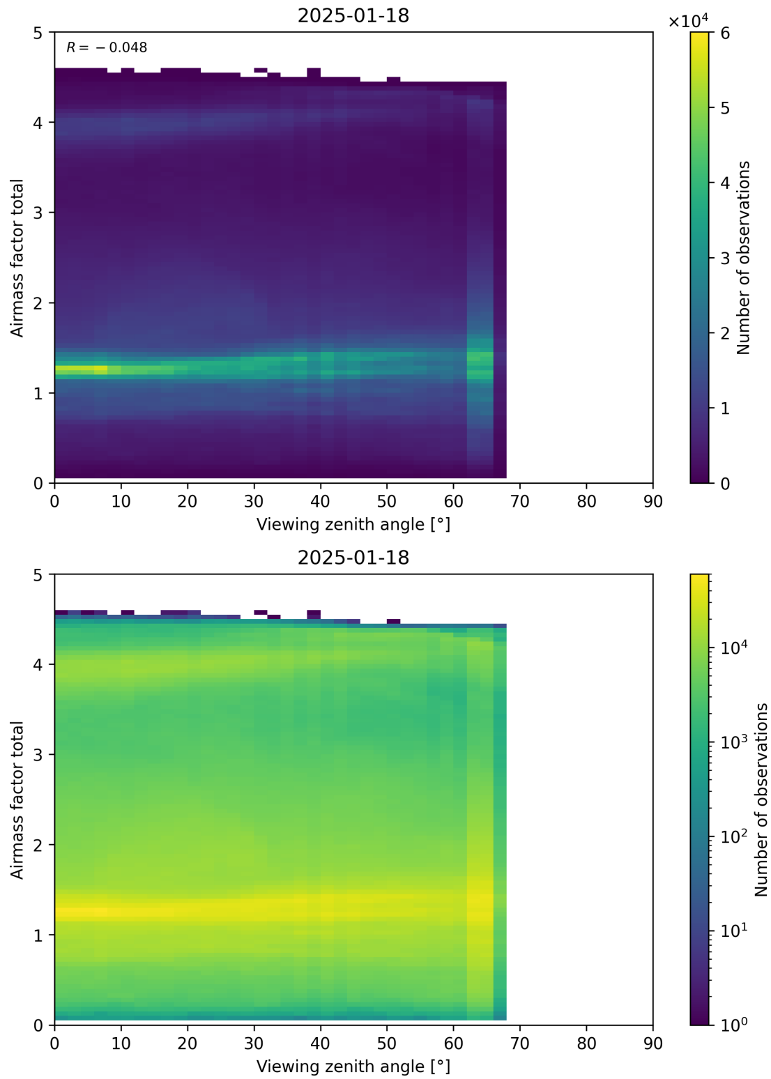
Figure 190: Scatter density plot of “Viewing zenith angle” against “Airmass factor total” for 2025-01-17 to 2025-01-19.
