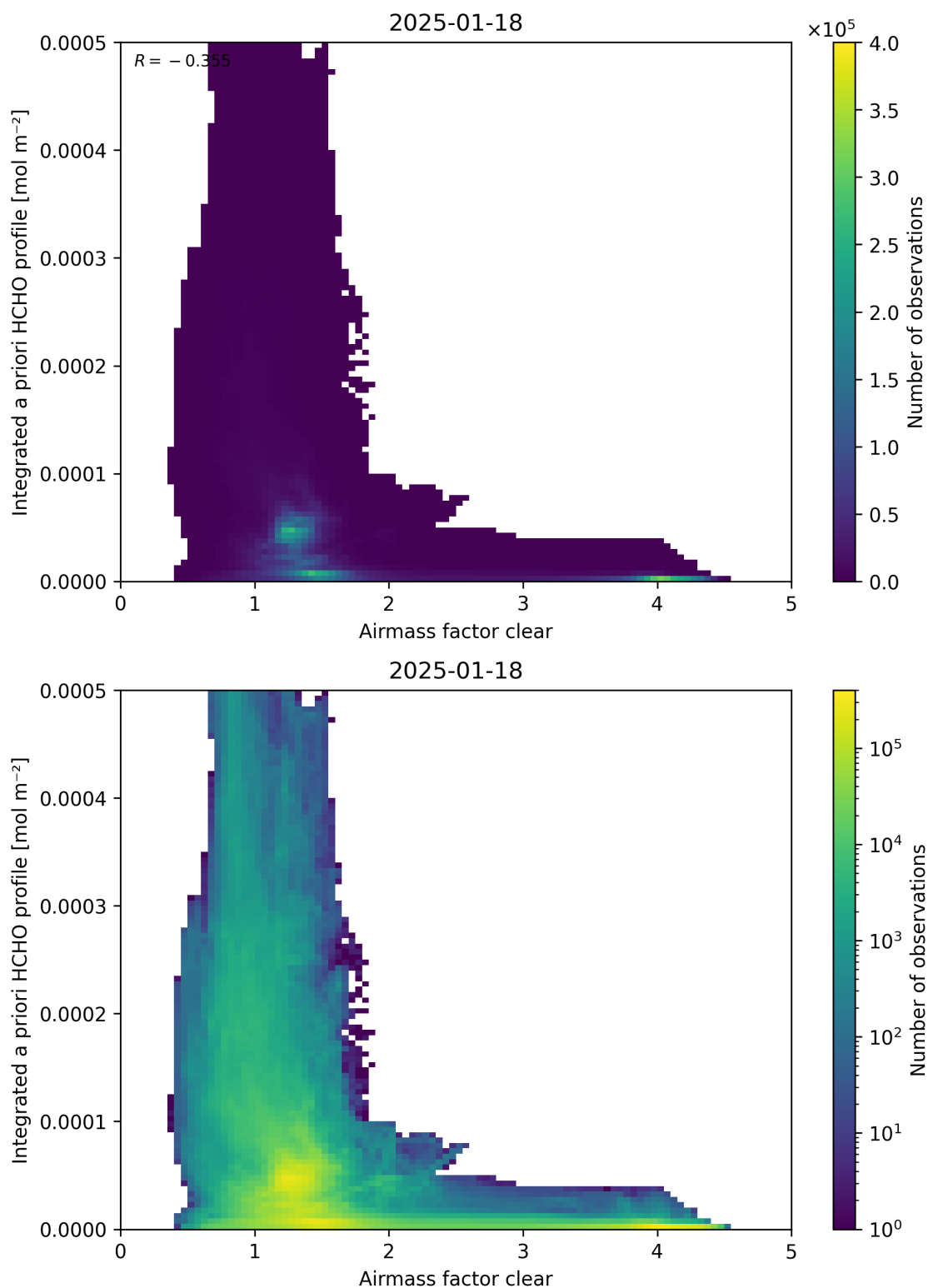
Figure 76: Scatter density plot of “Airmass factor clear” against “Integrated a priori HCHO profile” for 2025-01-17 to 2025-01-19.
