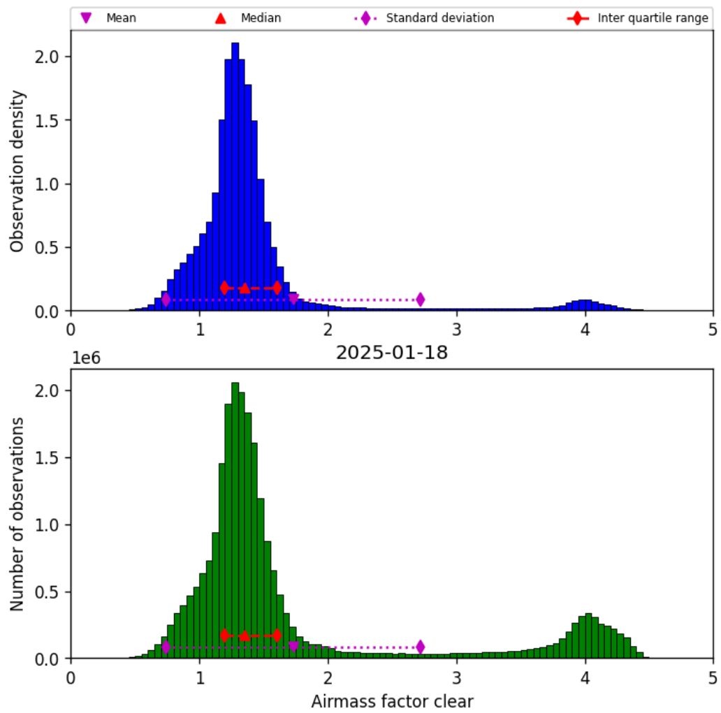
Figure 42: Histogram of “Airmass factor clear” for 2025-01-17 to 2025-01-19
