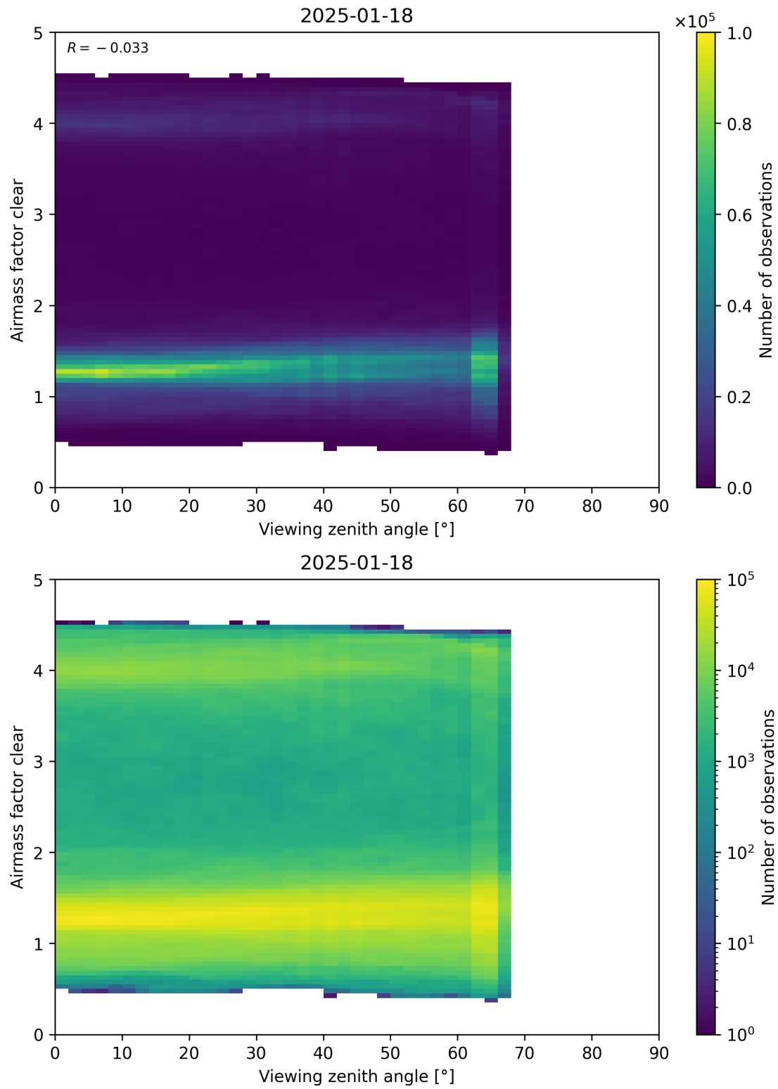
Figure 185: Scatter density plot of “Viewing zenith angle” against “Airmass factor clear” for 2025-01-17 to 2025-01-19.
