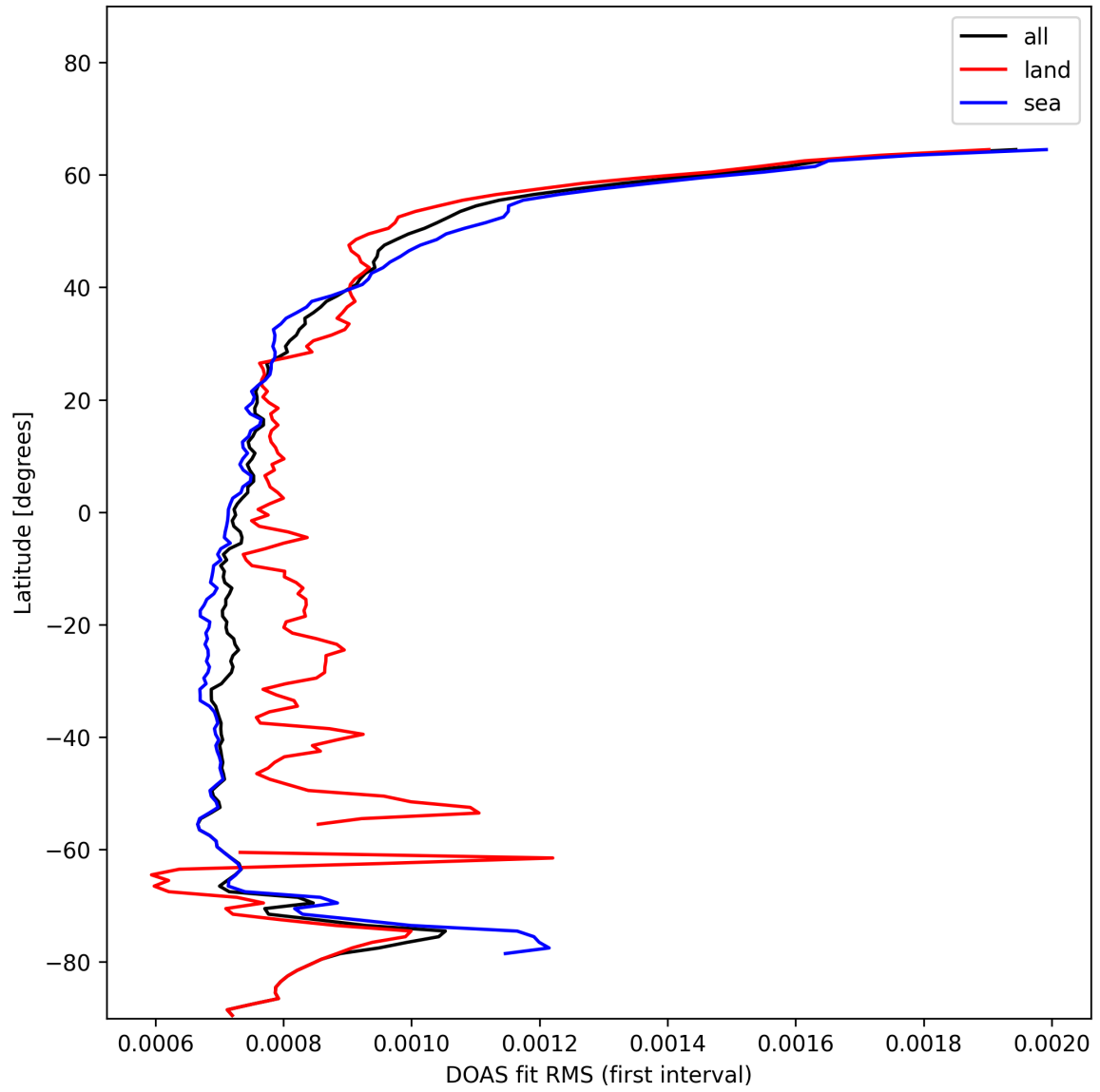
Figure 32: Zonal average of “DOAS fit RMS (first interval)” for 2025-01-17 to 2025-01-19.
