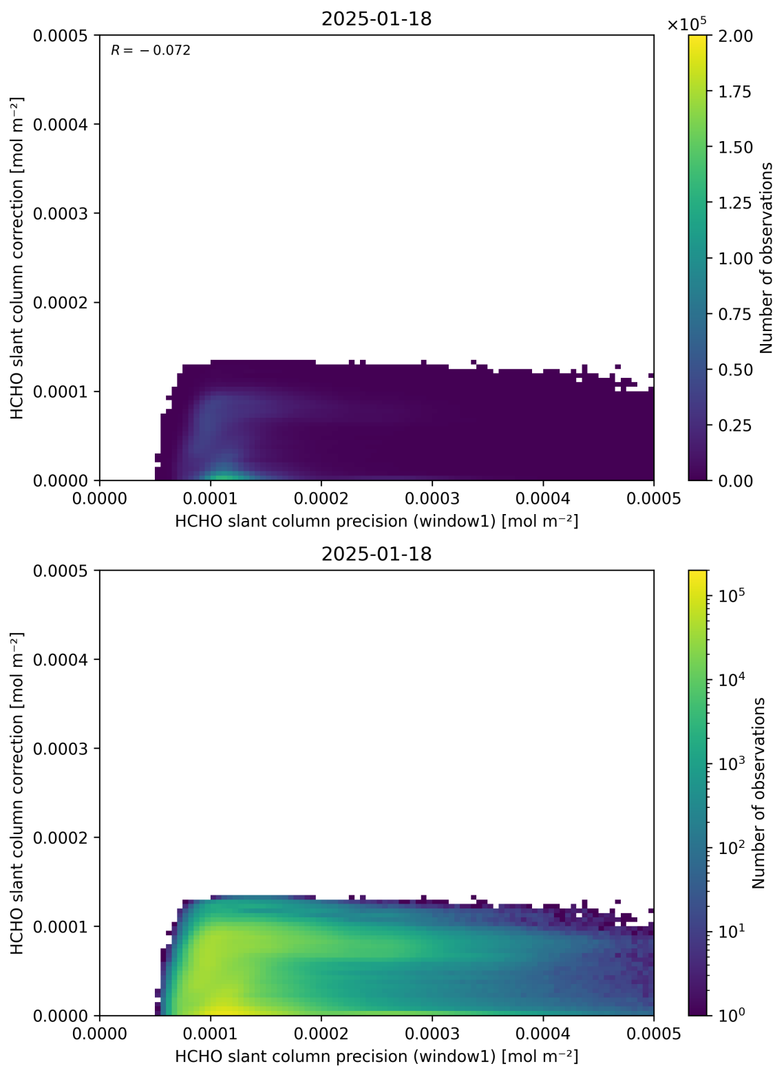
Figure 93: Scatter density plot of “HCHO slant column precision (window1)” against “HCHO slant column correction” for 2025-01-17 to 2025-01-19.
