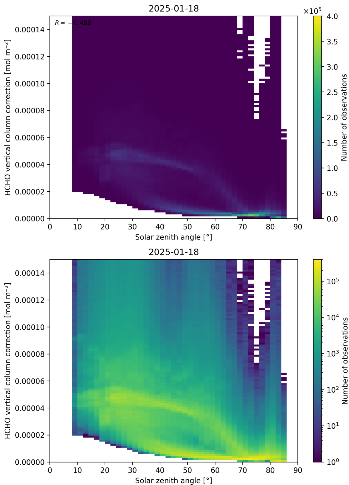
Figure 178: Scatter density plot of “Solar zenith angle” against “HCHO vertical column correction” for 2025-01-17 to 2025-01-19.
