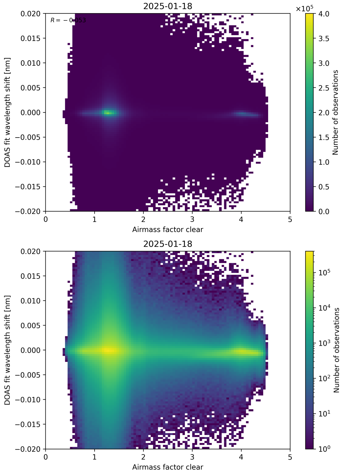
Figure 72: Scatter density plot of “Airmass factor clear” against “DOAS fit wavelength shift” for 2025-01-17 to 2025-01-19.
