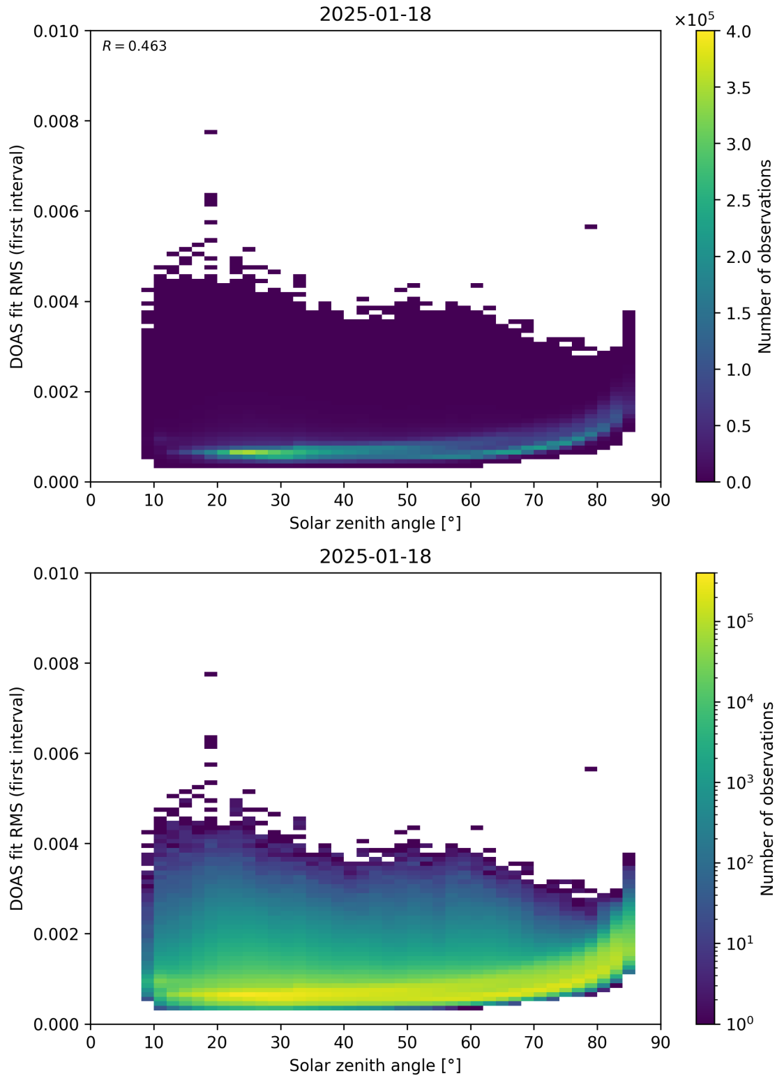
Figure 167: Scatter density plot of “Solar zenith angle” against “DOAS fit RMS (first interval)” for 2025-01-17 to 2025-01-19.
