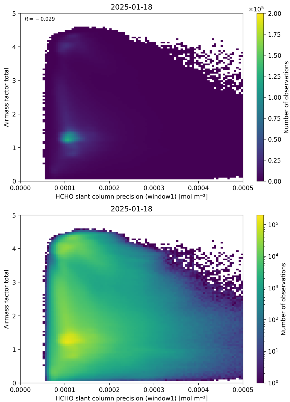
Figure 94: Scatter density plot of “HCHO slant column precision (window1)” against “Airmass factor total” for 2025-01-17 to 2025-01-19.
