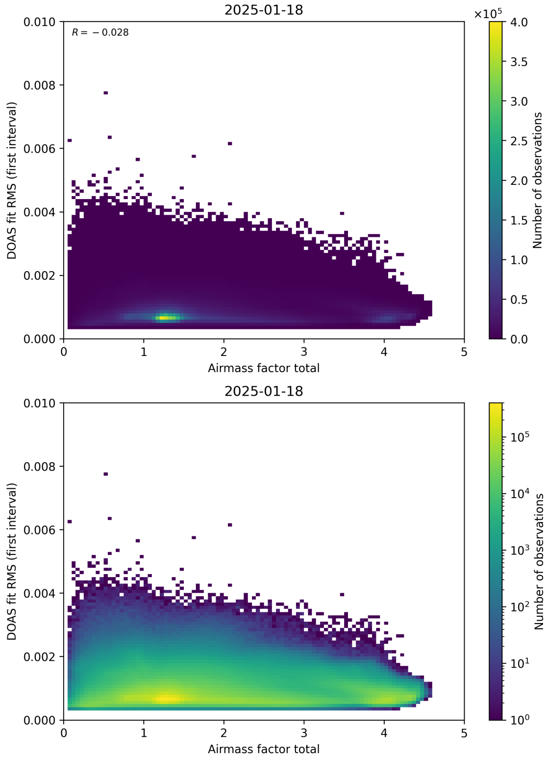
Figure 97: Scatter density plot of “Airmass factor total” against “DOAS fit RMS (first interval)” for 2025-01-17 to 2025-01-19.
