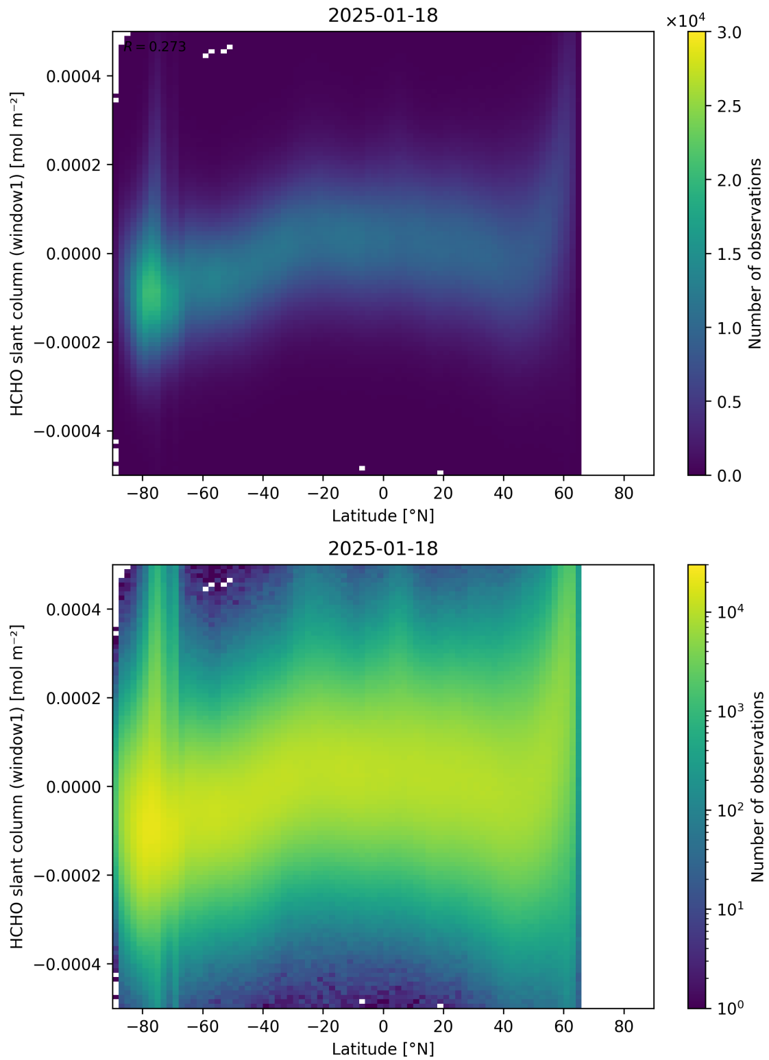
Figure 159: Scatter density plot of “Latitude” against “HCHO slant column (window1)” for 2025-01-17 to 2025-01-19.
