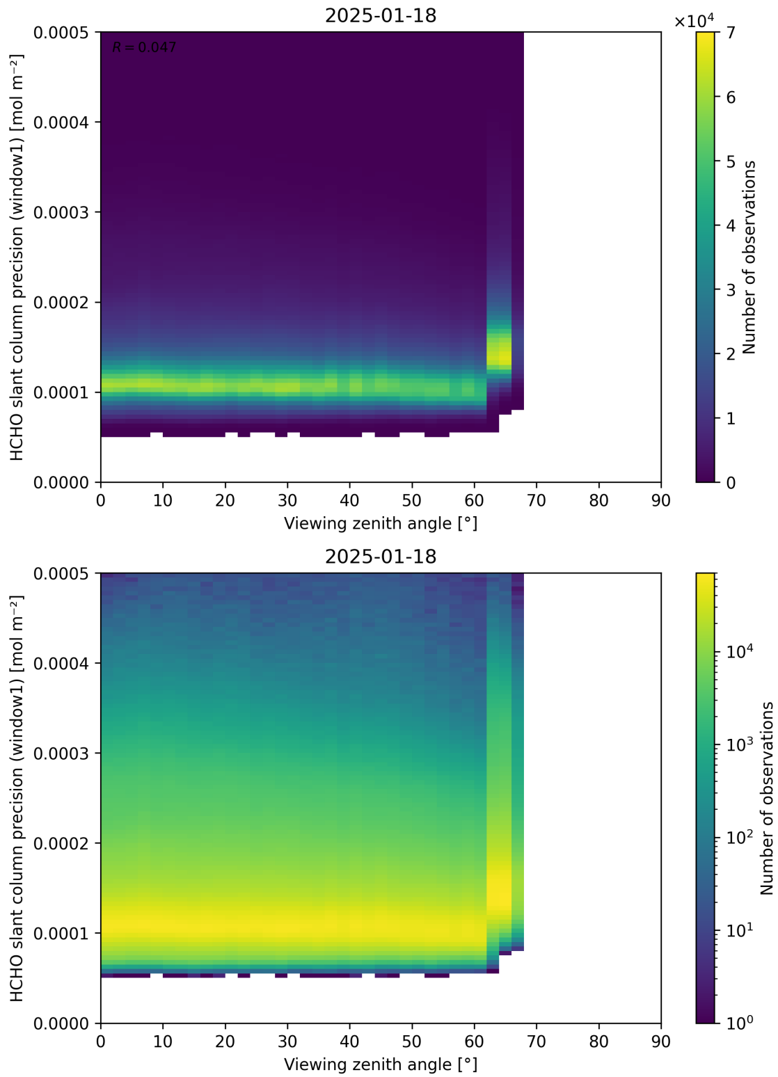
Figure 189: Scatter density plot of “Viewing zenith angle” against “HCHO slant column precision (window1)” for 2025-01-17 to 2025-01-19.
