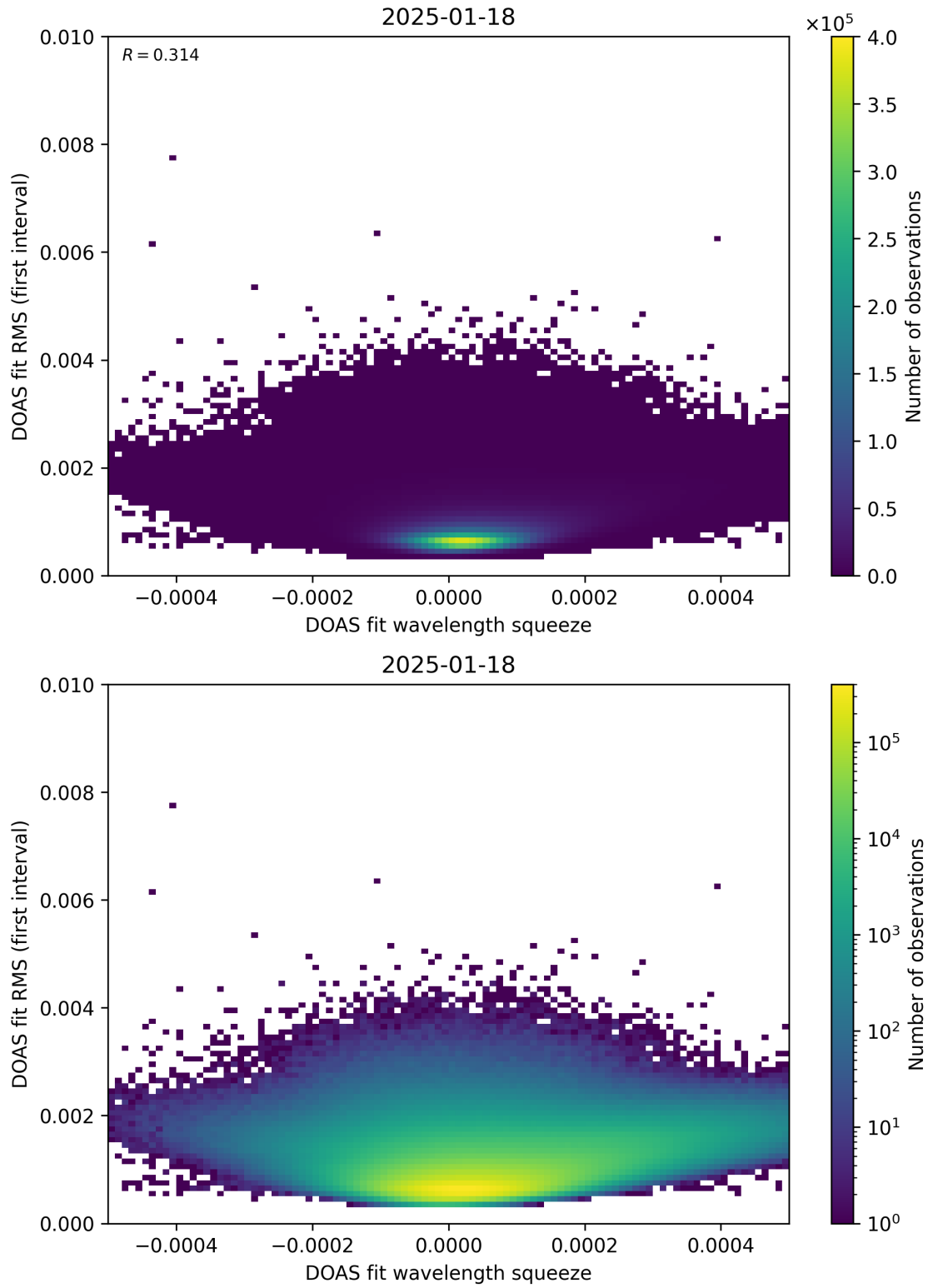
Figure 68: Scatter density plot of “DOAS fit wavelength squeeze” against “DOAS fit RMS (first interval)” for 2025-01-17 to 2025-01-19.
