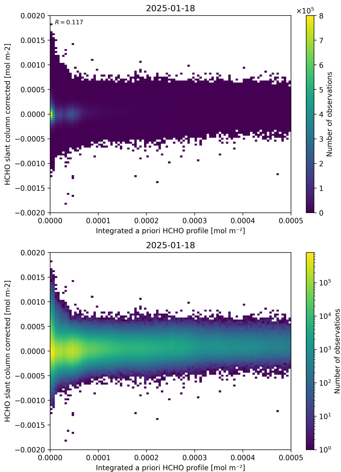
Figure 151: Scatter density plot of “Integrated a priori HCHO profile” against “HCHO slant column corrected” for 2025-01-17 to 2025-01-19.
