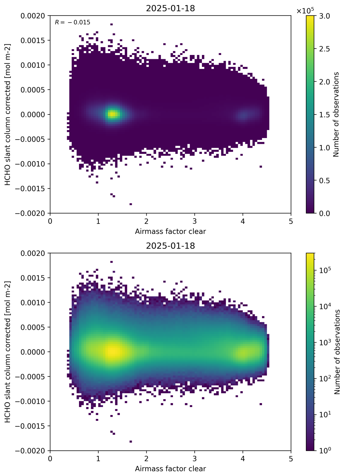
Figure 74: Scatter density plot of “Airmass factor clear” against “HCHO slant column corrected” for 2025-01-17 to 2025-01-19.
