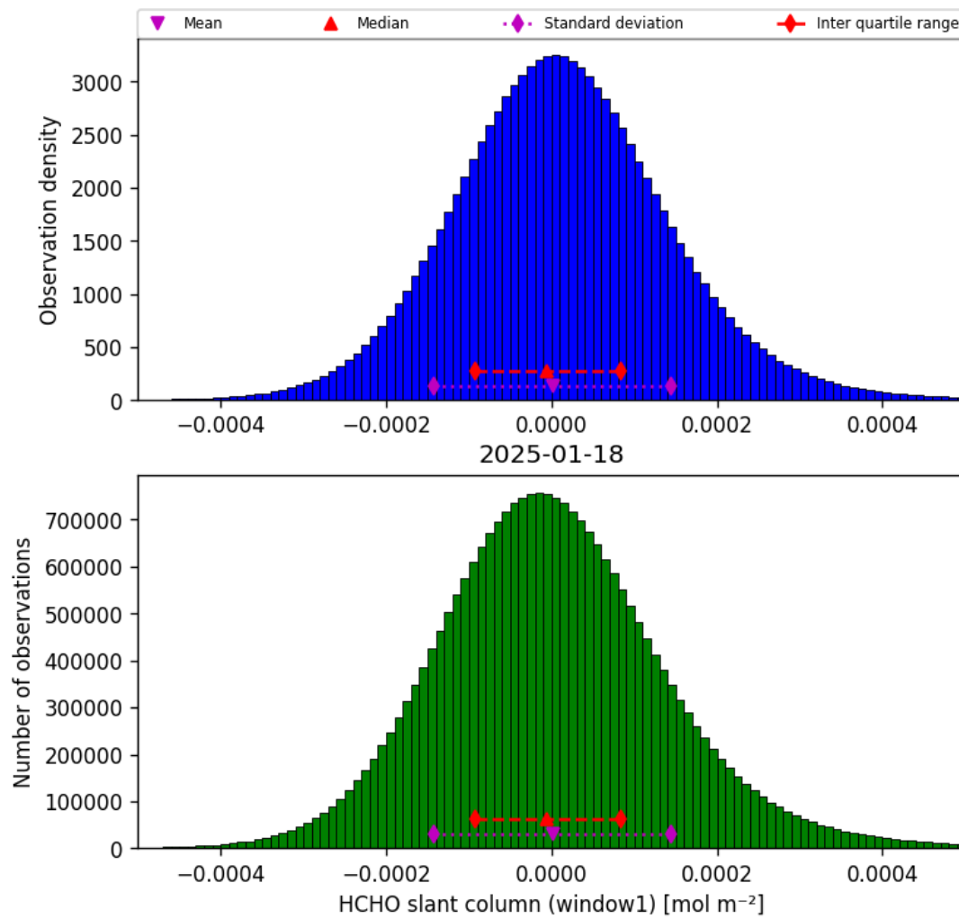
Figure 38: Histogram of “HCHO slant column (window1)” for 2025-01-17 to 2025-01-19
