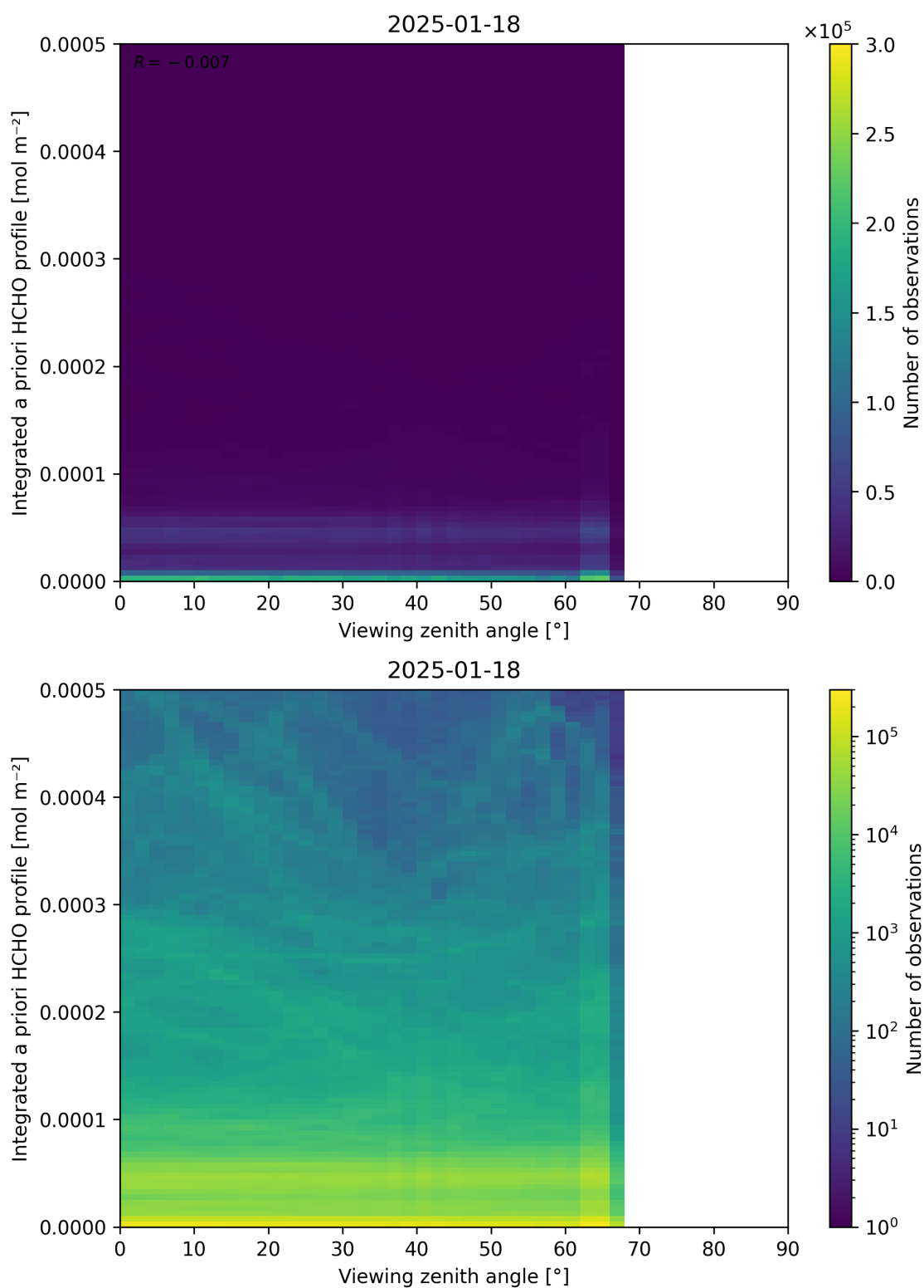
Figure 195: Scatter density plot of “Viewing zenith angle” against “Integrated a priori HCHO profile” for 2025-01-17 to 2025-01-19.
