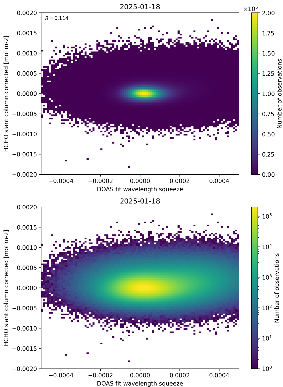
Figure 69: Scatter density plot of “DOAS fit wavelength squeeze” against “HCHO slant column corrected” for 2025-01-17 to 2025-01-19.
