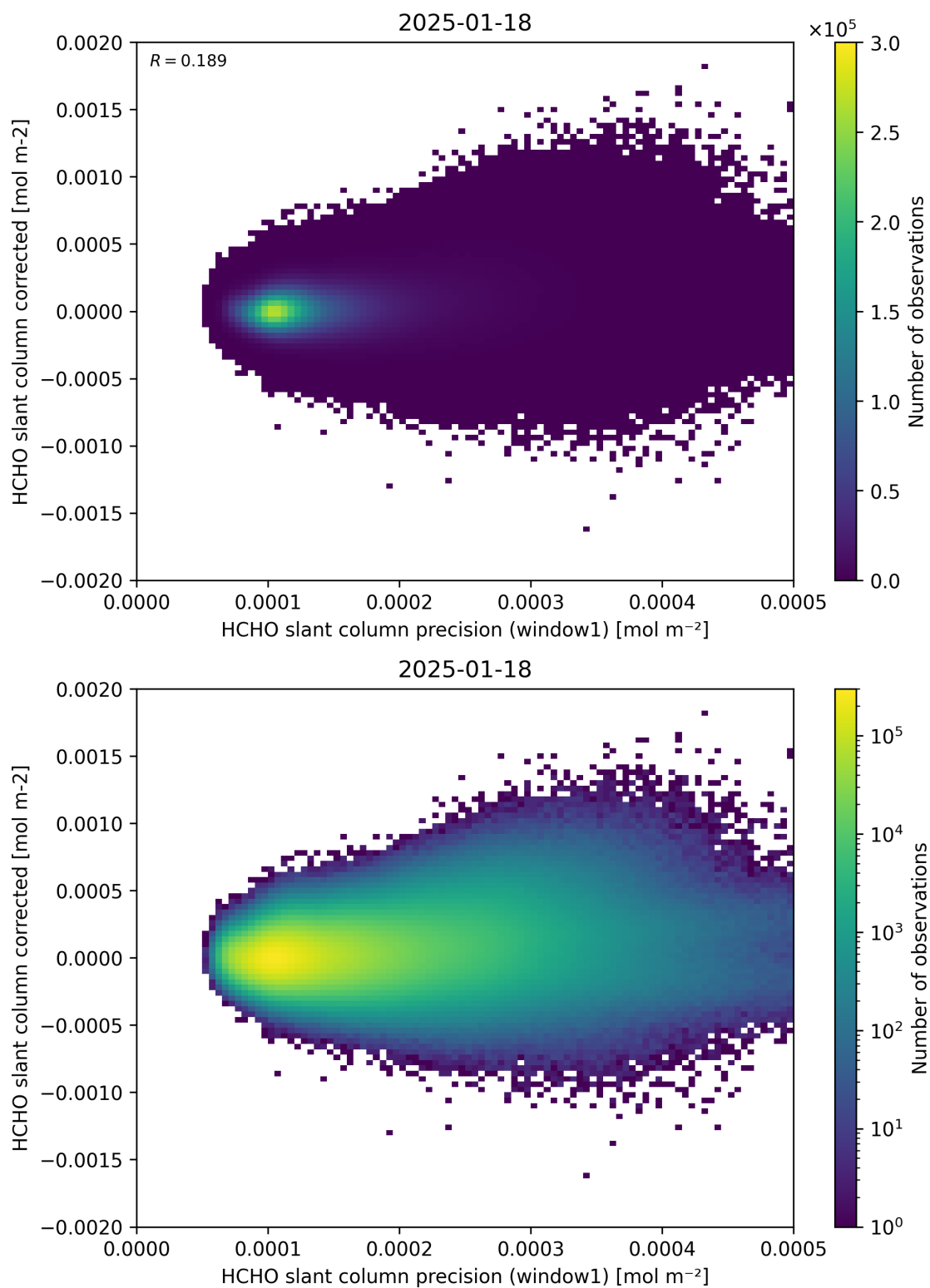
Figure 92: Scatter density plot of “HCHO slant column precision (window1)” against “HCHO slant column corrected” for 2025-01-17 to 2025-01-19.
