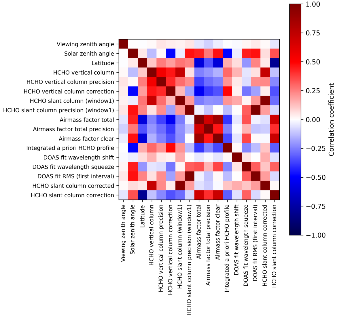
Figure 2: Map of correlation matrix for 2025-01-17 to 2025-01-19.
