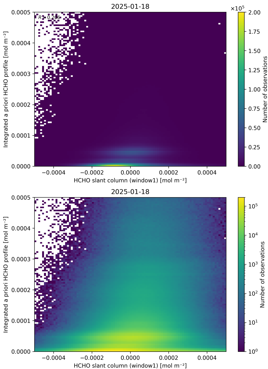
Figure 87: Scatter density plot of “HCHO slant column (window1)” against “Integrated a priori HCHO profile” for 2025-01-17 to 2025-01-19.
