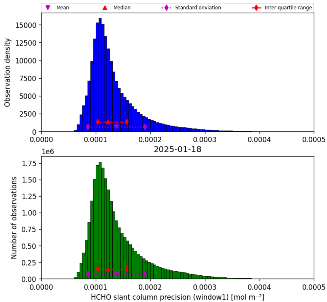
Figure 39: Histogram of “HCHO slant column precision (window1)” for 2025-01-17 to 2025-01-19
