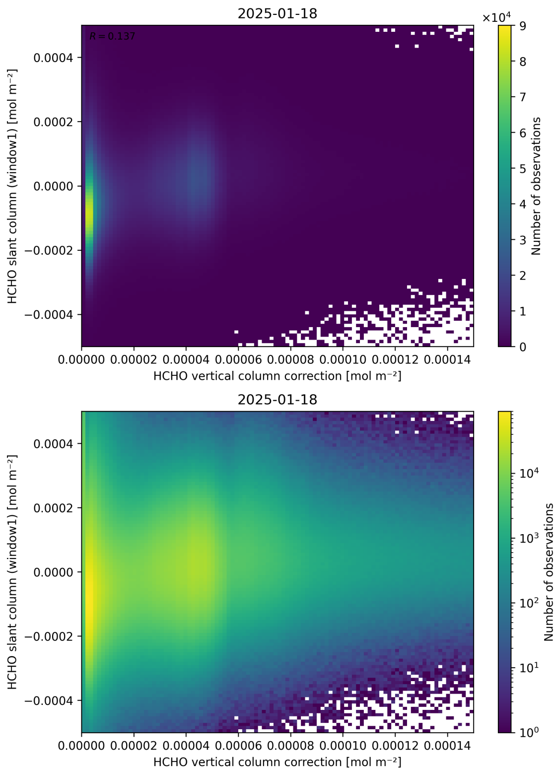
Figure 118: Scatter density plot of “HCHO vertical column correction” against “HCHO slant column (window1)” for 2025-01-17 to 2025-01-19.
