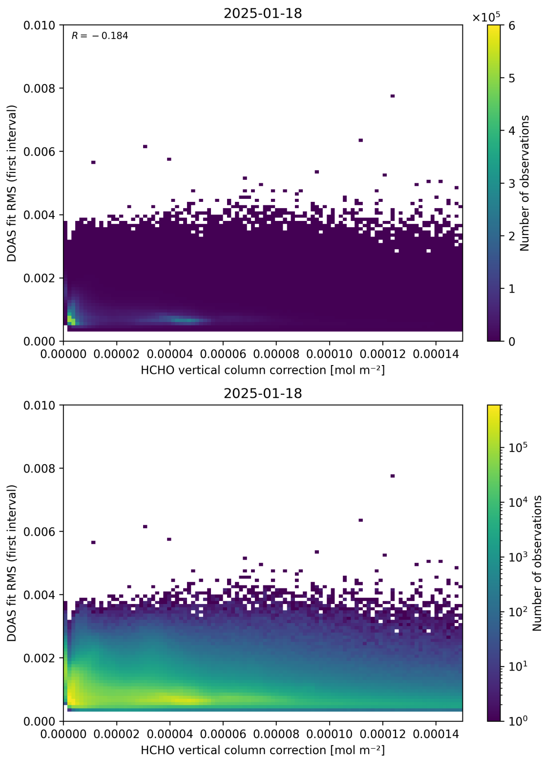
Figure 112: Scatter density plot of “HCHO vertical column correction” against “DOAS fit RMS (first interval)” for 2025-01-17 to 2025-01-19.
