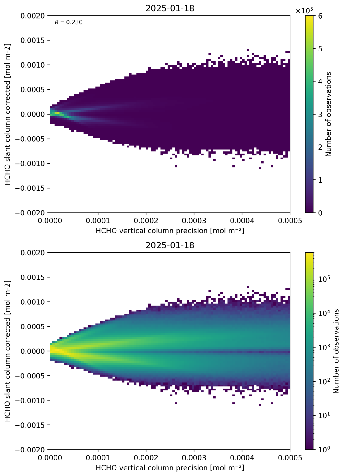
Figure 140: Scatter density plot of “HCHO vertical column precision” against “HCHO slant column corrected” for 2025-01-17 to 2025-01-19.
