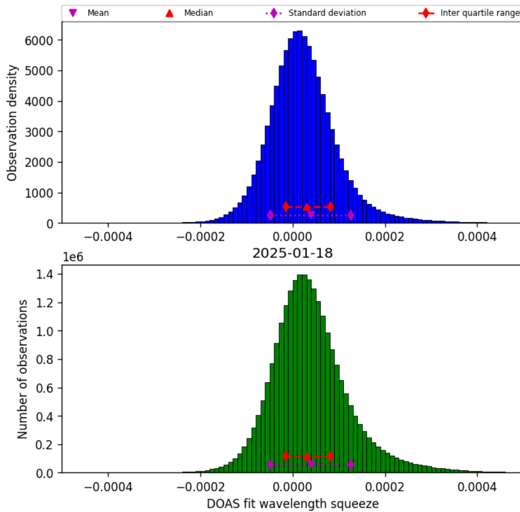
Figure 45: Histogram of “DOAS fit wavelength squeeze” for 2025-01-17 to 2025-01-19
