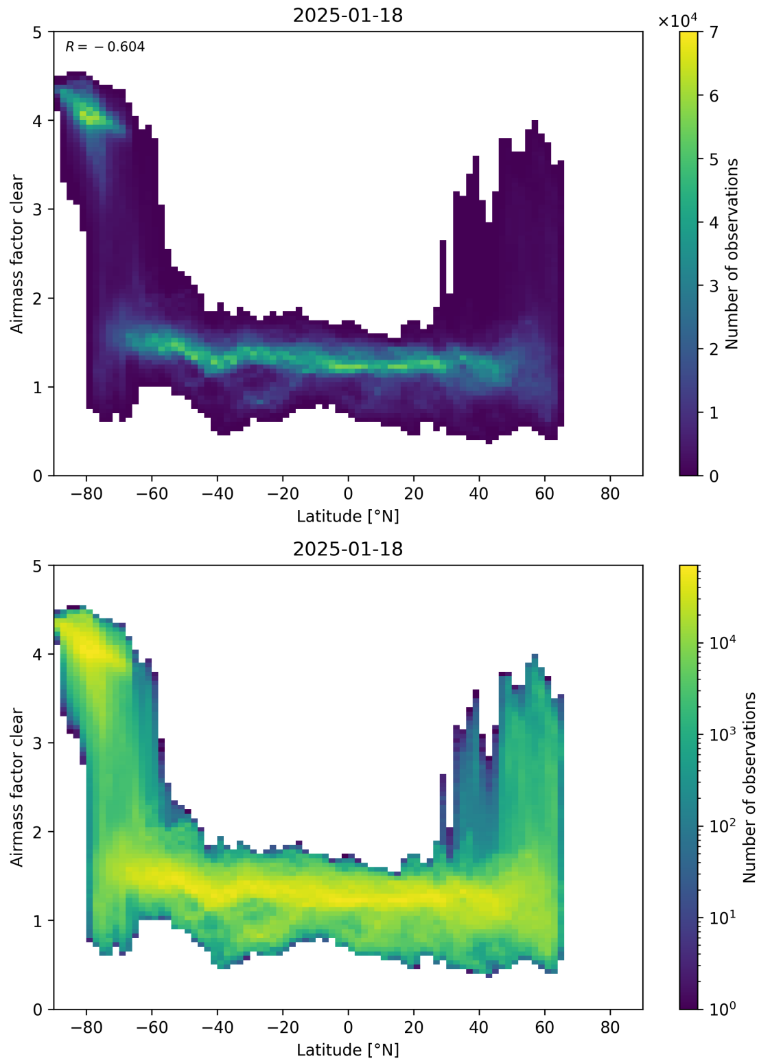
Figure 156: Scatter density plot of “Latitude” against “Airmass factor clear” for 2025-01-17 to 2025-01-19.
