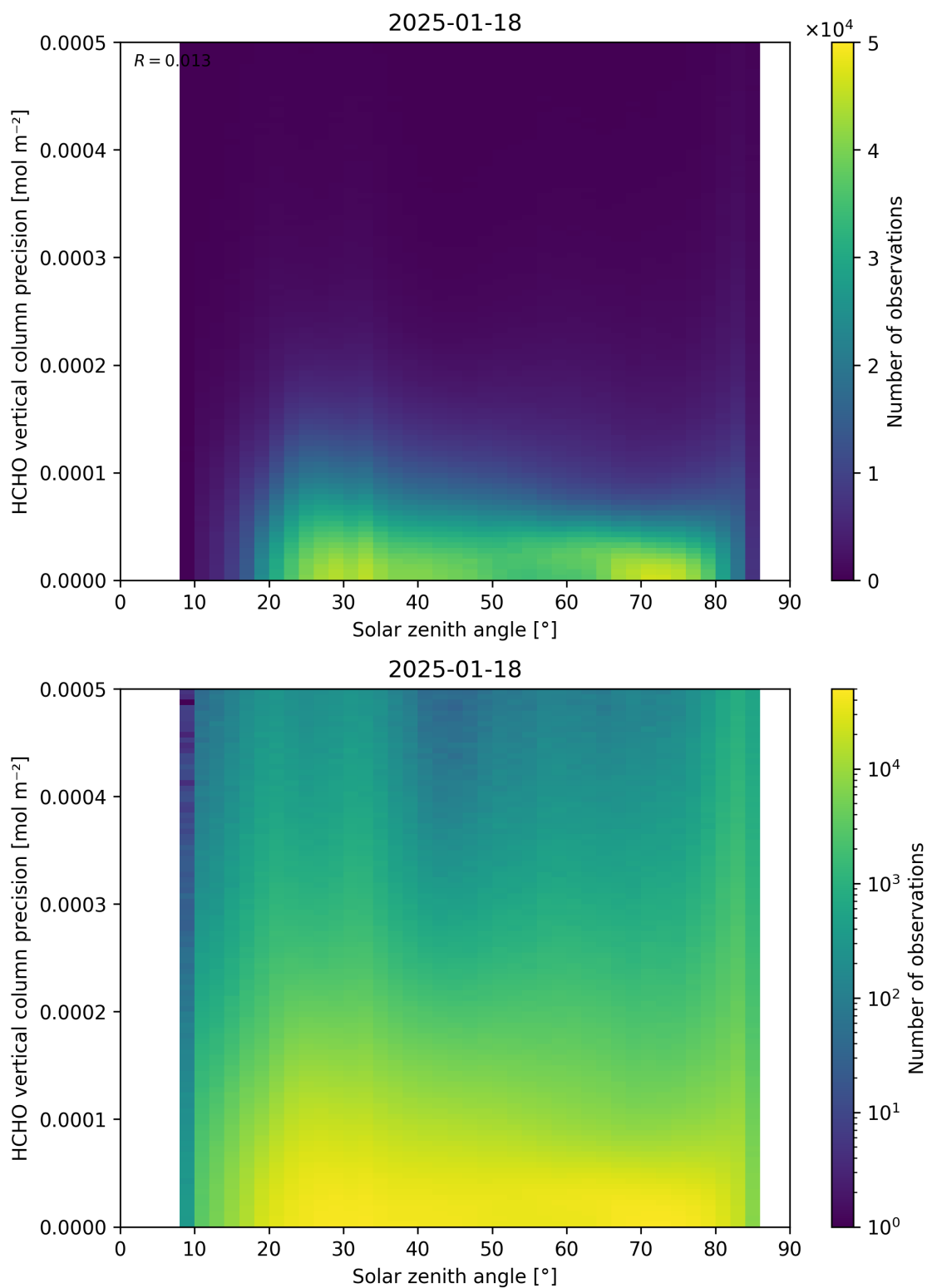
Figure 179: Scatter density plot of “Solar zenith angle” against “HCHO vertical column precision” for 2025-01-17 to 2025-01-19.
