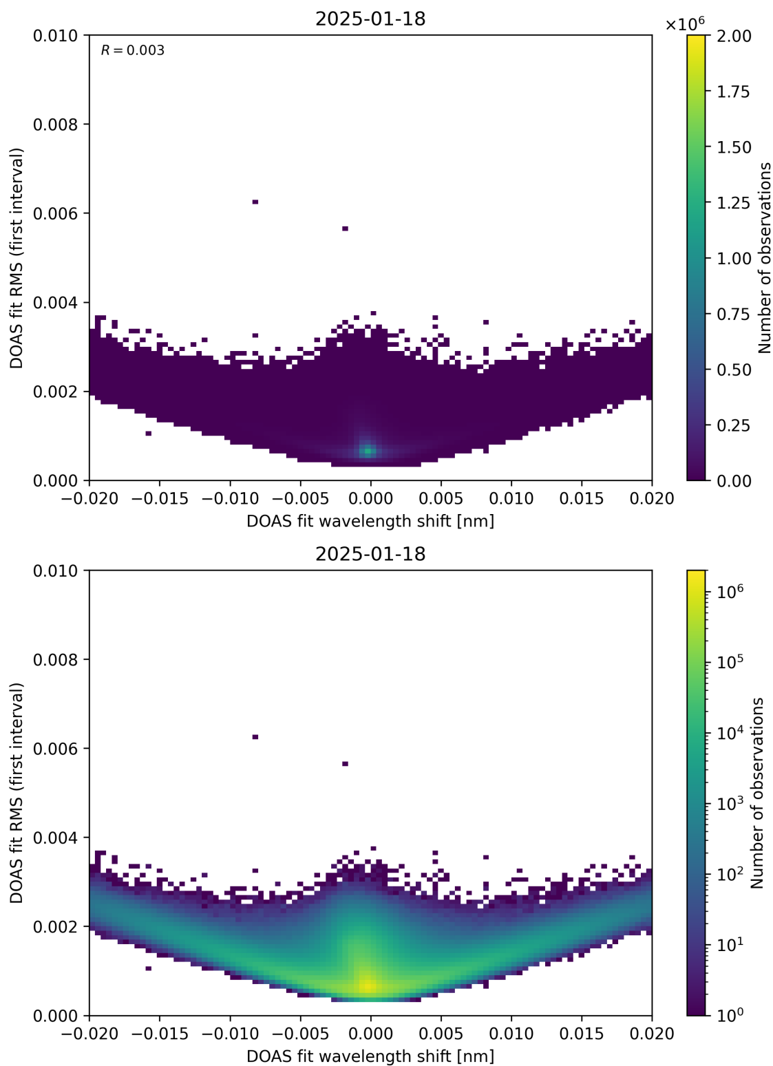
Figure 64: Scatter density plot of “DOAS fit wavelength shift” against “DOAS fit RMS (first interval)” for 2025-01-17 to 2025-01-19.
