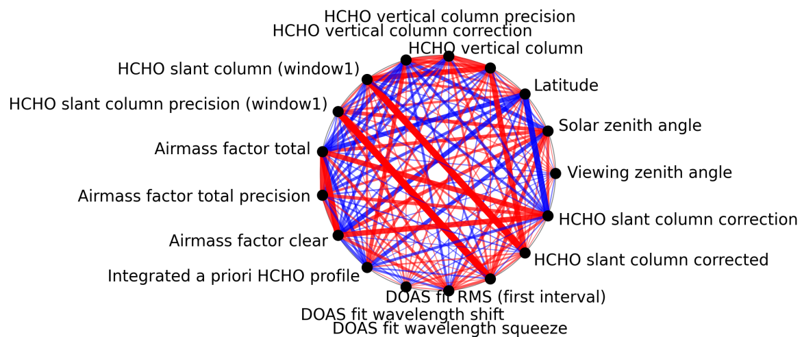
Figure 1: Map of correlation graph for 2025-01-17 to 2025-01-19.
