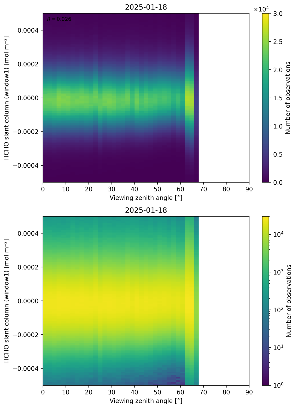
Figure 188: Scatter density plot of “Viewing zenith angle” against “HCHO slant column (window1)” for 2025-01-17 to 2025-01-19.
