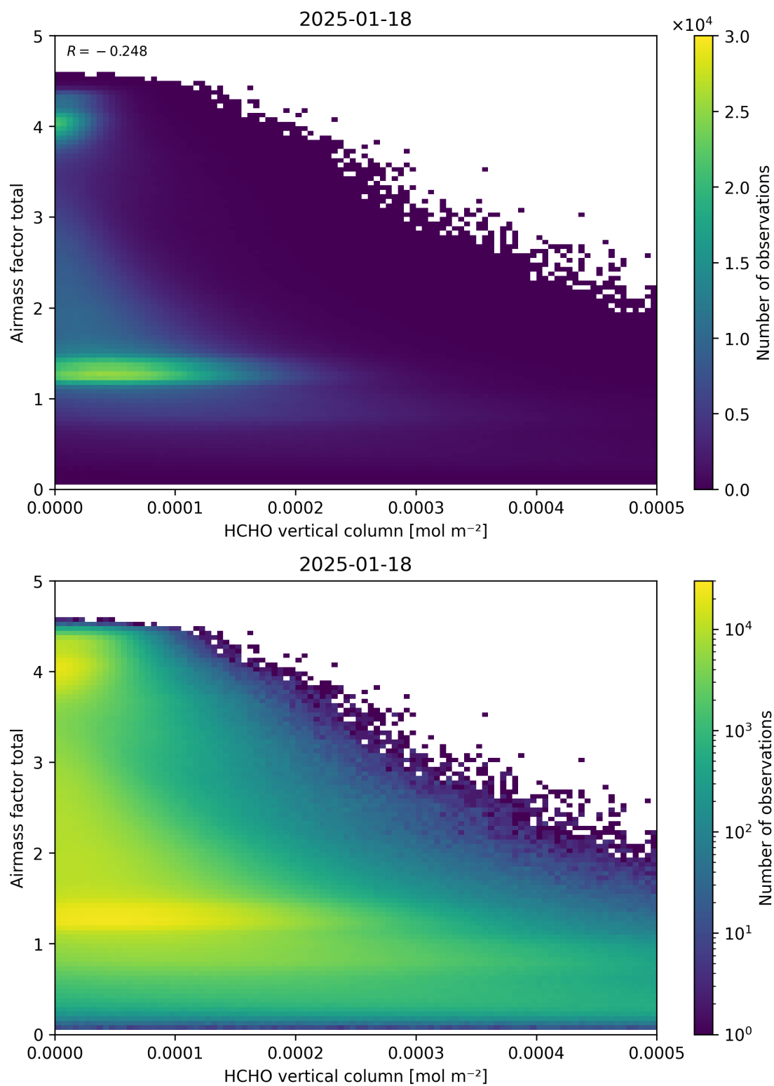
Figure 131: Scatter density plot of “HCHO vertical column” against “Airmass factor total” for 2025-01-17 to 2025-01-19.
