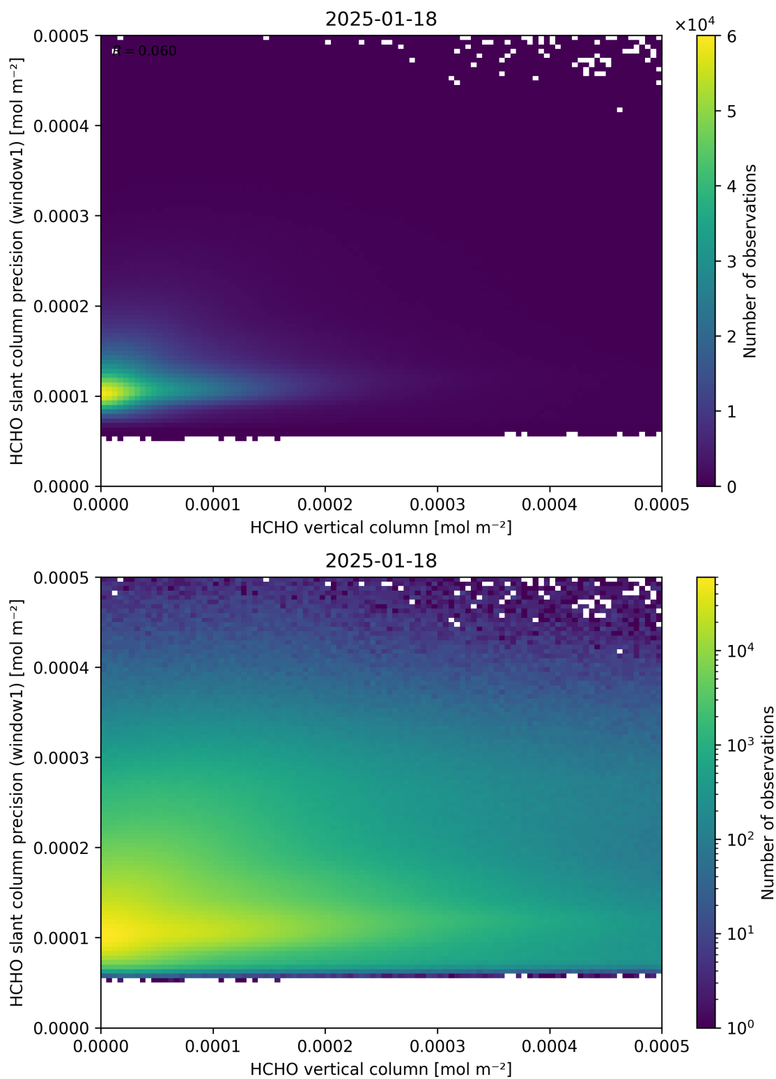
Figure 130: Scatter density plot of “HCHO vertical column” against “HCHO slant column precision (window1)” for 2025-01-17 to 2025-01-19.
