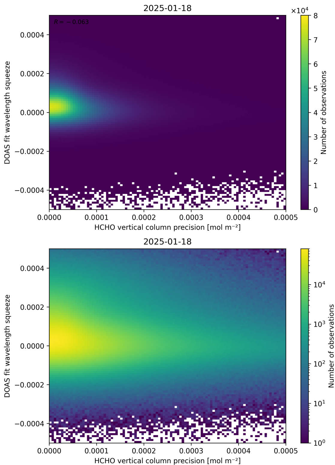
Figure 138: Scatter density plot of “HCHO vertical column precision” against “DOAS fit wavelength squeeze” for 2025-01-17 to 2025-01-19.
