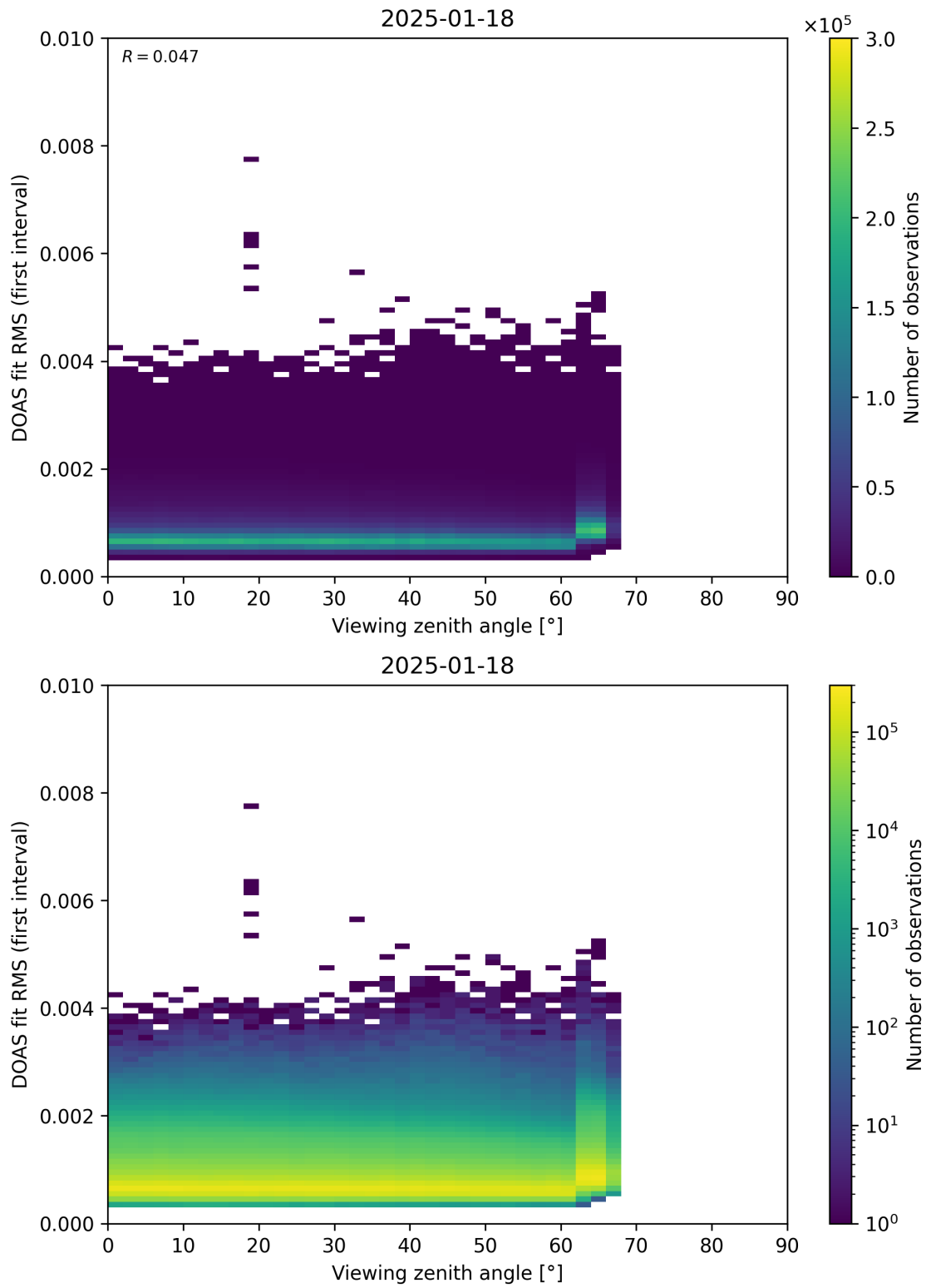
Figure 182: Scatter density plot of “Viewing zenith angle” against “DOAS fit RMS (first interval)” for 2025-01-17 to 2025-01-19.
