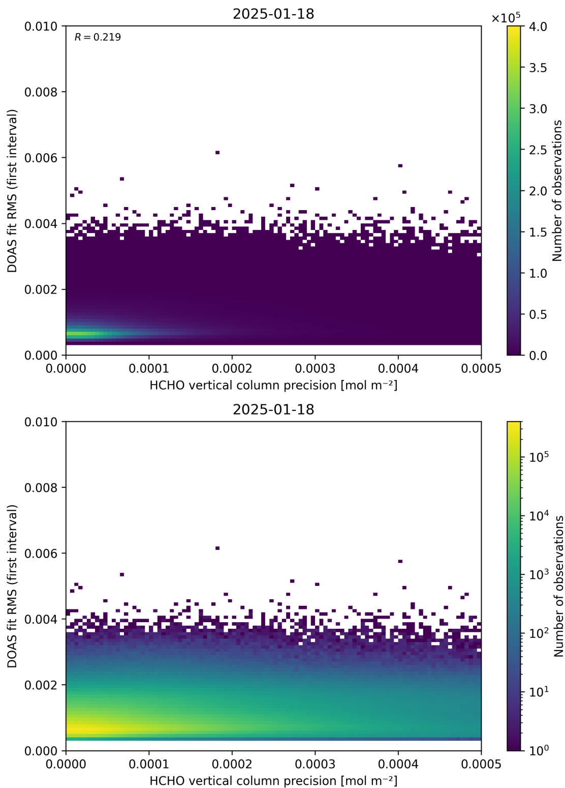
Figure 136: Scatter density plot of “HCHO vertical column precision” against “DOAS fit RMS (first interval)” for 2025-01-17 to 2025-01-19.
