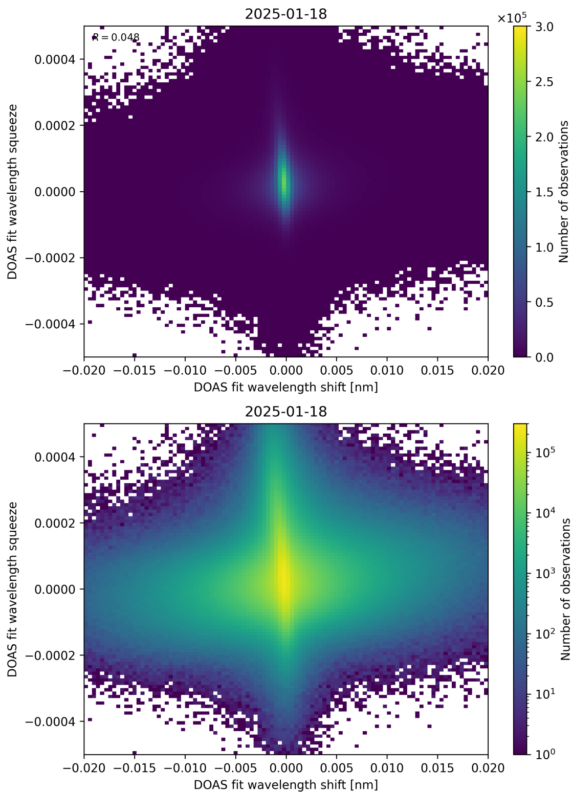
Figure 65: Scatter density plot of “DOAS fit wavelength shift” against “DOAS fit wavelength squeeze” for 2025-01-17 to 2025-01-19.
