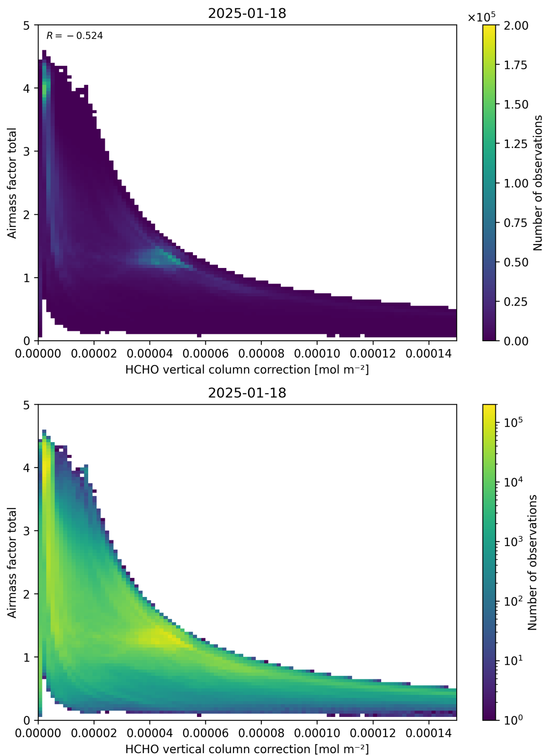
Figure 120: Scatter density plot of “HCHO vertical column correction” against “Airmass factor total” for 2025-01-17 to 2025-01-19.
