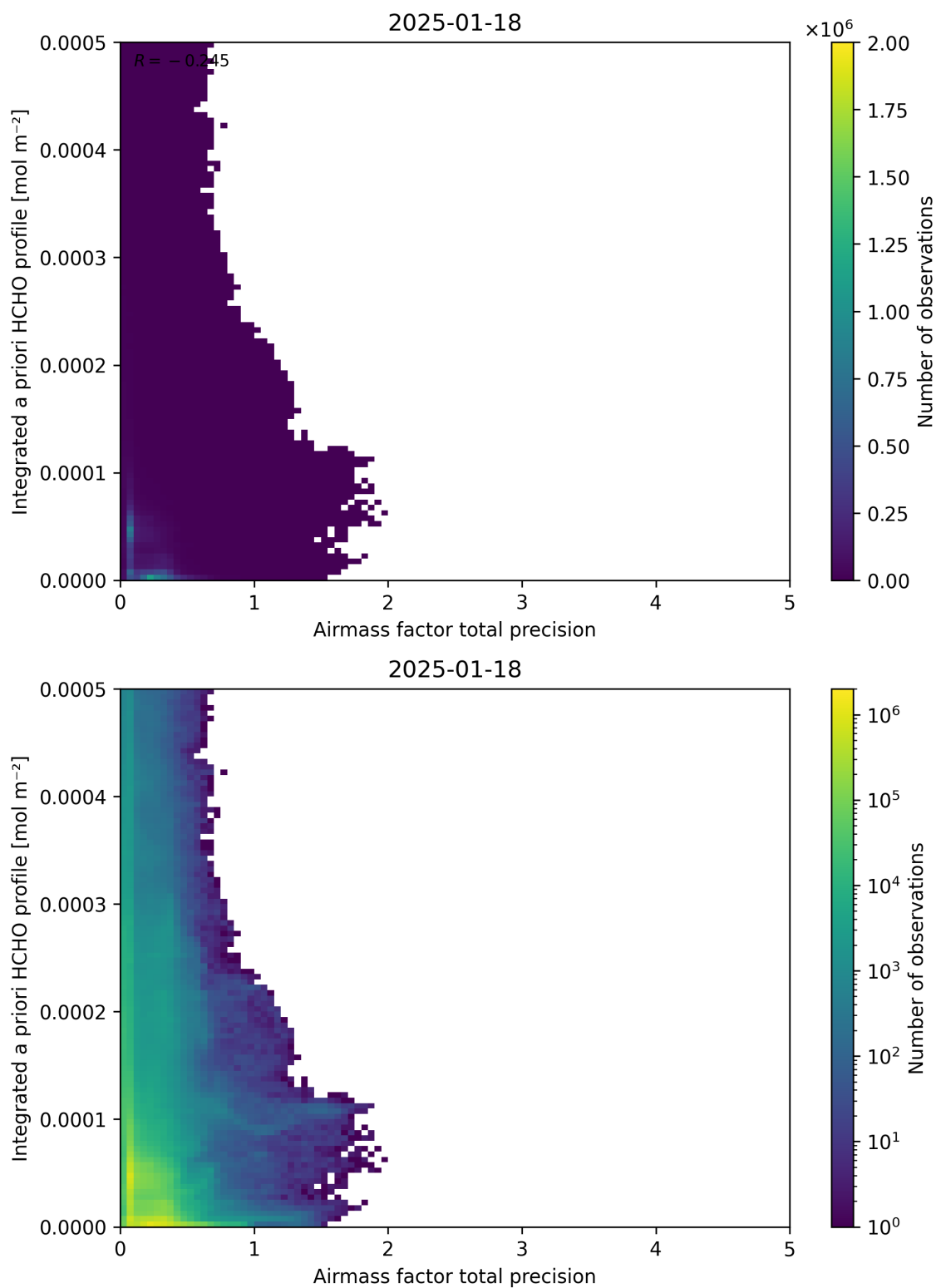
Figure 111: Scatter density plot of “Airmass factor total precision” against “Integrated a priori HCHO profile” for 2025-01-17 to 2025-01-19.
