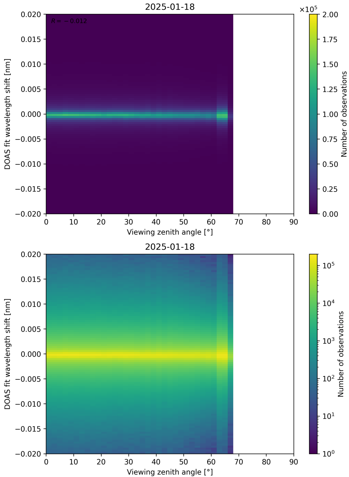
Figure 183: Scatter density plot of “Viewing zenith angle” against “DOAS fit wavelength shift” for 2025-01-17 to 2025-01-19.
