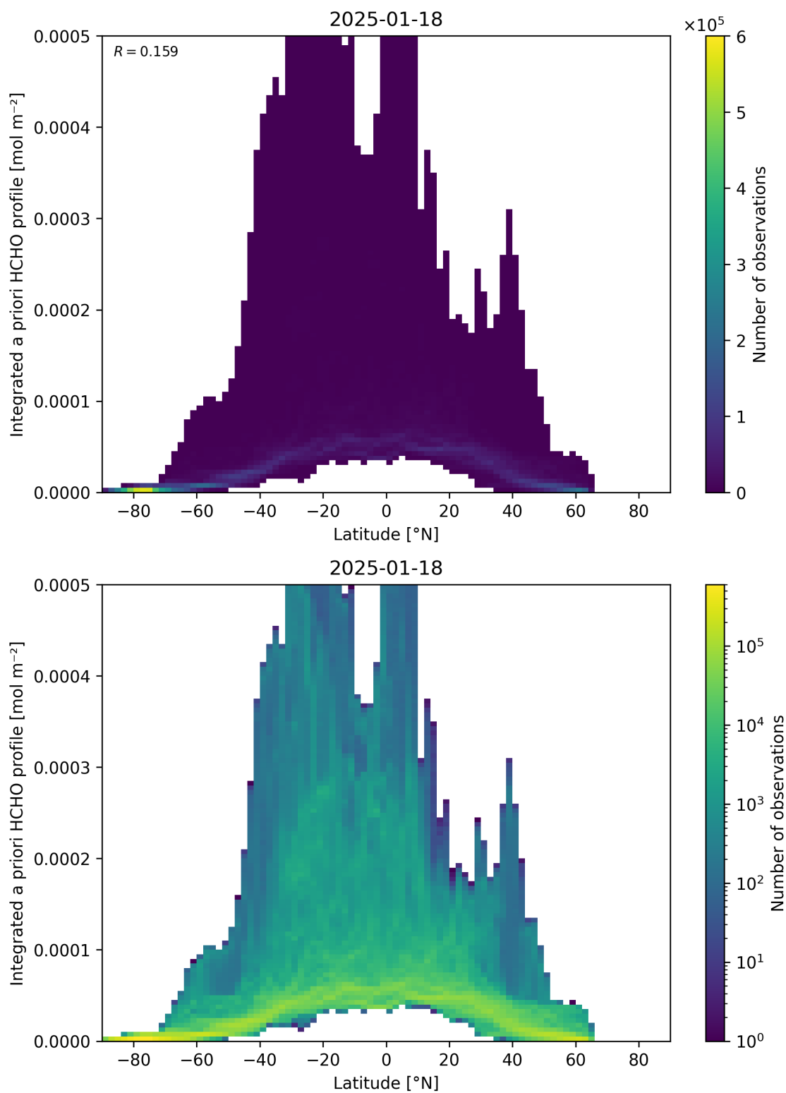
Figure 166: Scatter density plot of “Latitude” against “Integrated a priori HCHO profile” for 2025-01-17 to 2025-01-19.
