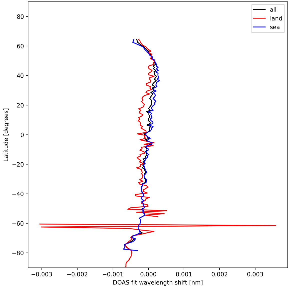
Figure 30: Zonal average of "DOAS fit wavelength shift" for 2025-01-17 to 2025-01-19.
