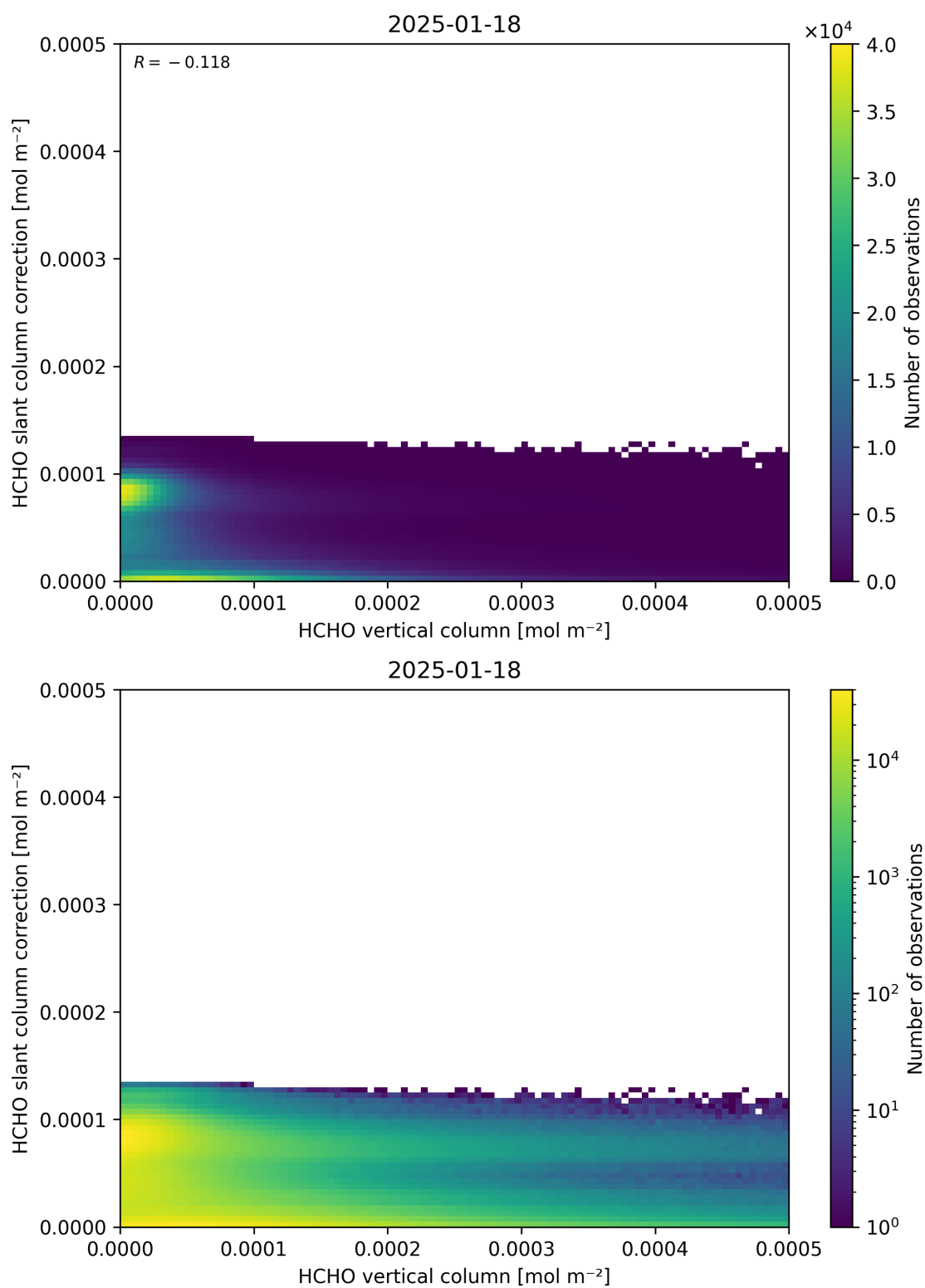
Figure 128: Scatter density plot of “HCHO vertical column” against “HCHO slant column correction” for 2025-01-17 to 2025-01-19.
