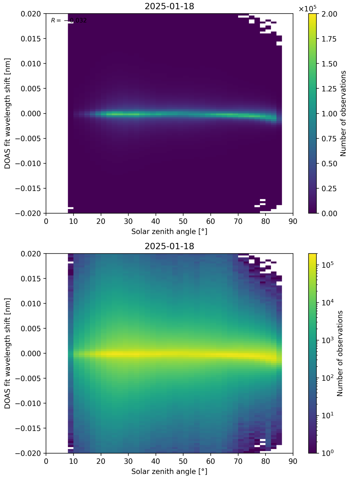
Figure 168: Scatter density plot of “Solar zenith angle” against “DOAS fit wavelength shift” for 2025-01-17 to 2025-01-19.
