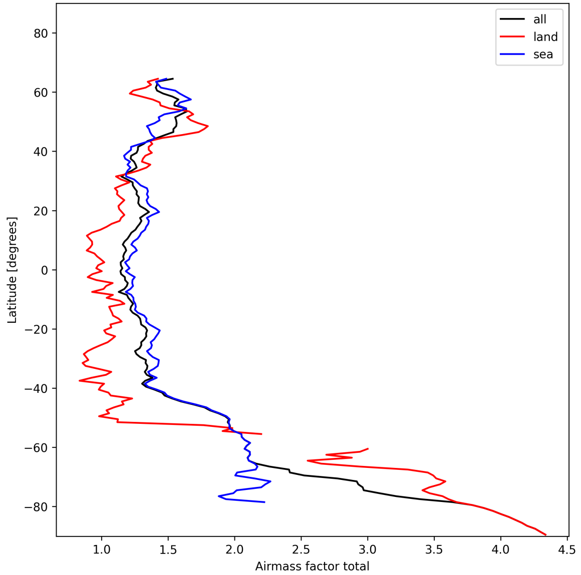
Figure 26: Zonal average of “Airmass factor total” for 2025-01-17 to 2025-01-19.
