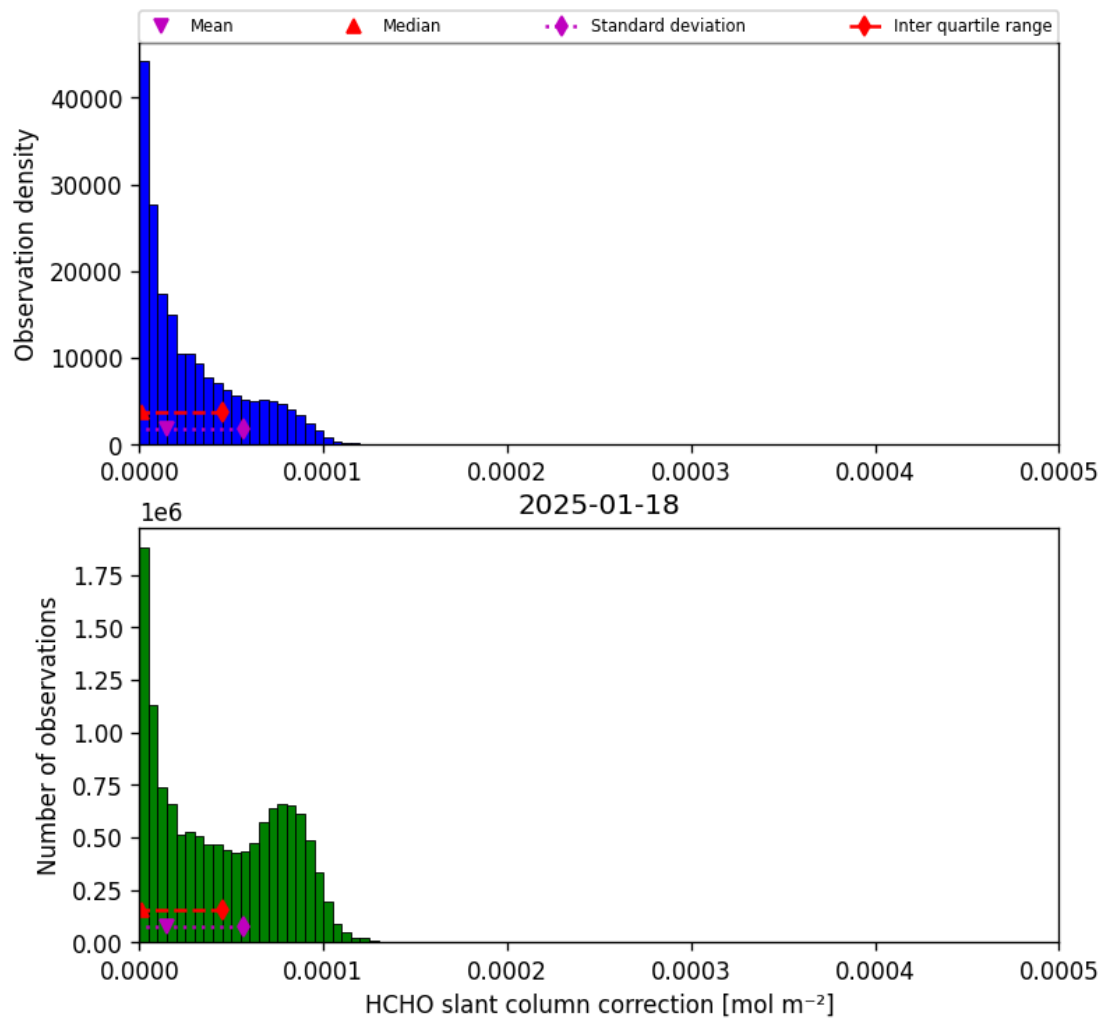
Figure 47: Histogram of “HCHO slant column correction” for 2025-01-17 to 2025-01-19
