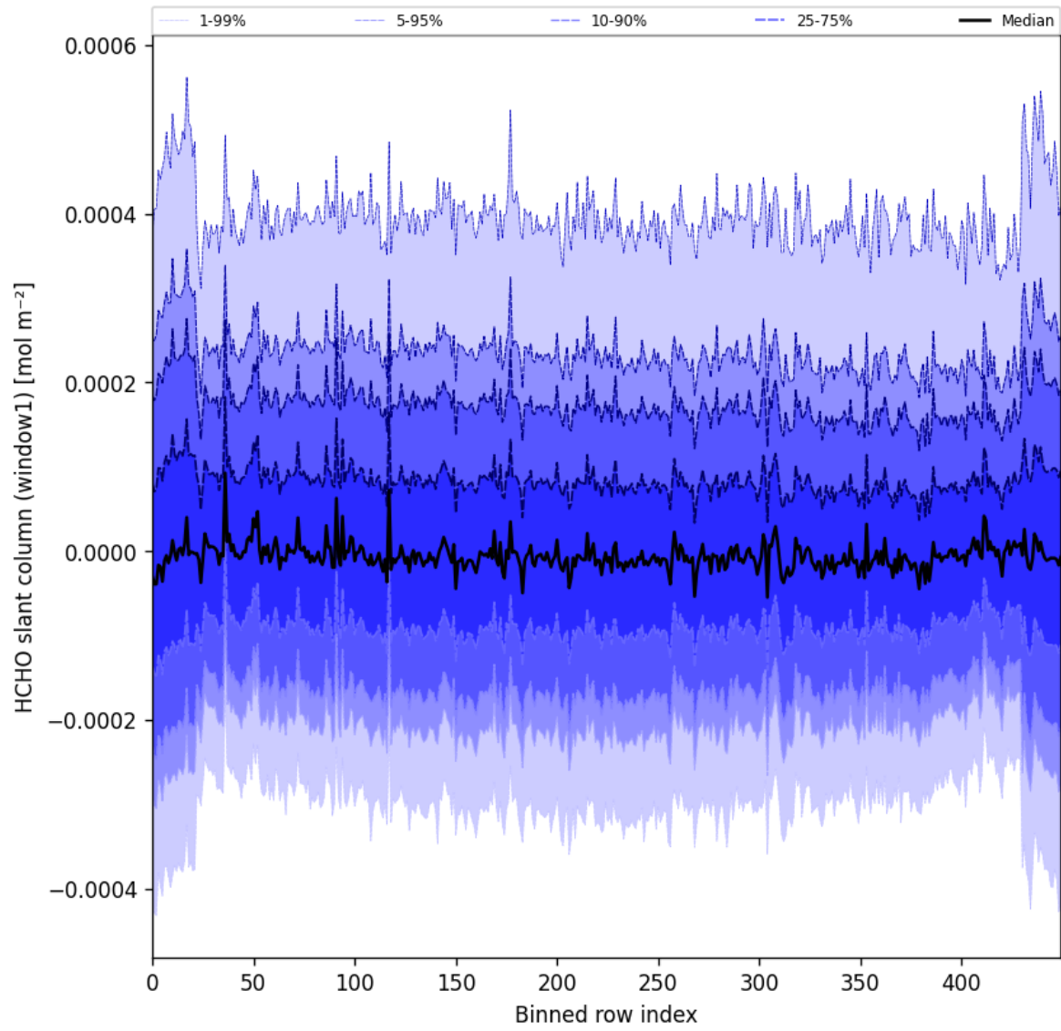
Figure 52: Along track statistics of “HCHO slant column (window1)” for 2025-01-17 to 2025-01-19
