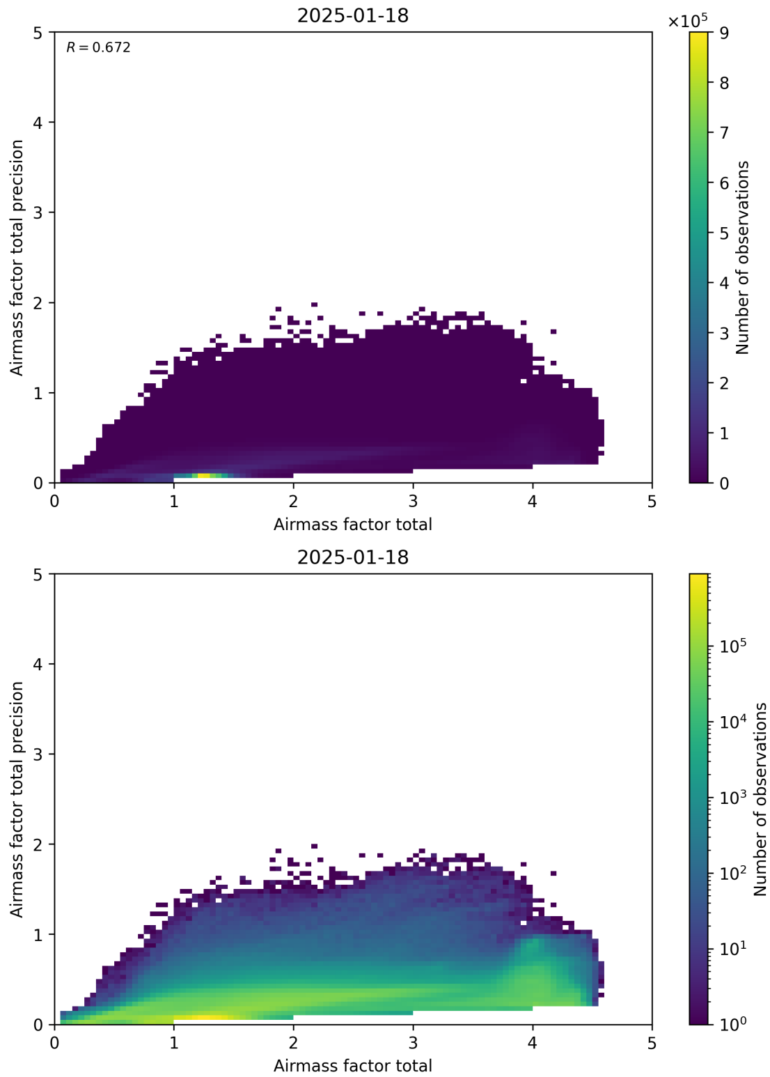
Figure 103: Scatter density plot of “Airmass factor total” against “Airmass factor total precision” for 2025-01-17 to 2025-01-19.
