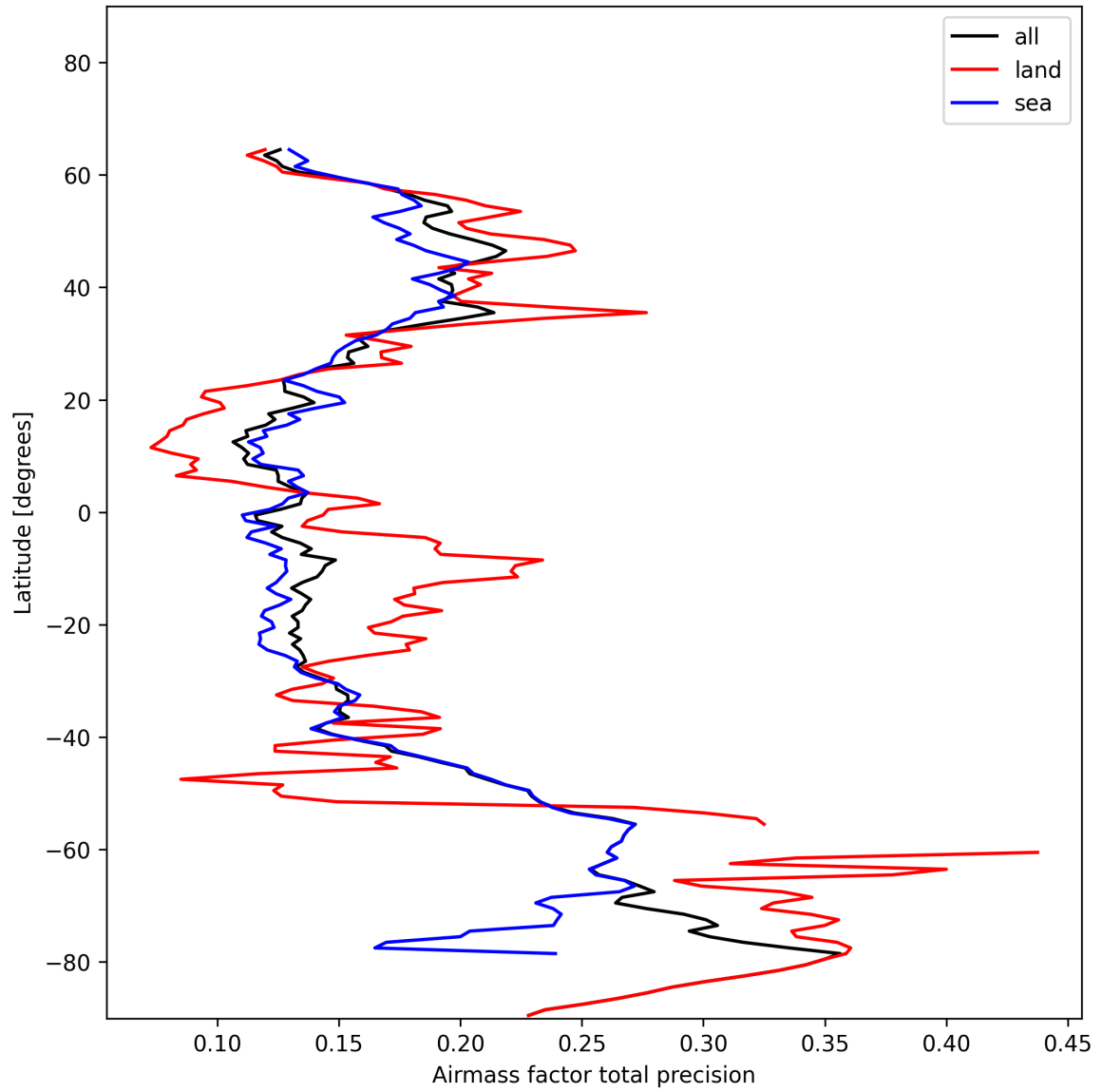
Figure 27: Zonal average of “Airmass factor total precision” for 2025-01-17 to 2025-01-19.
