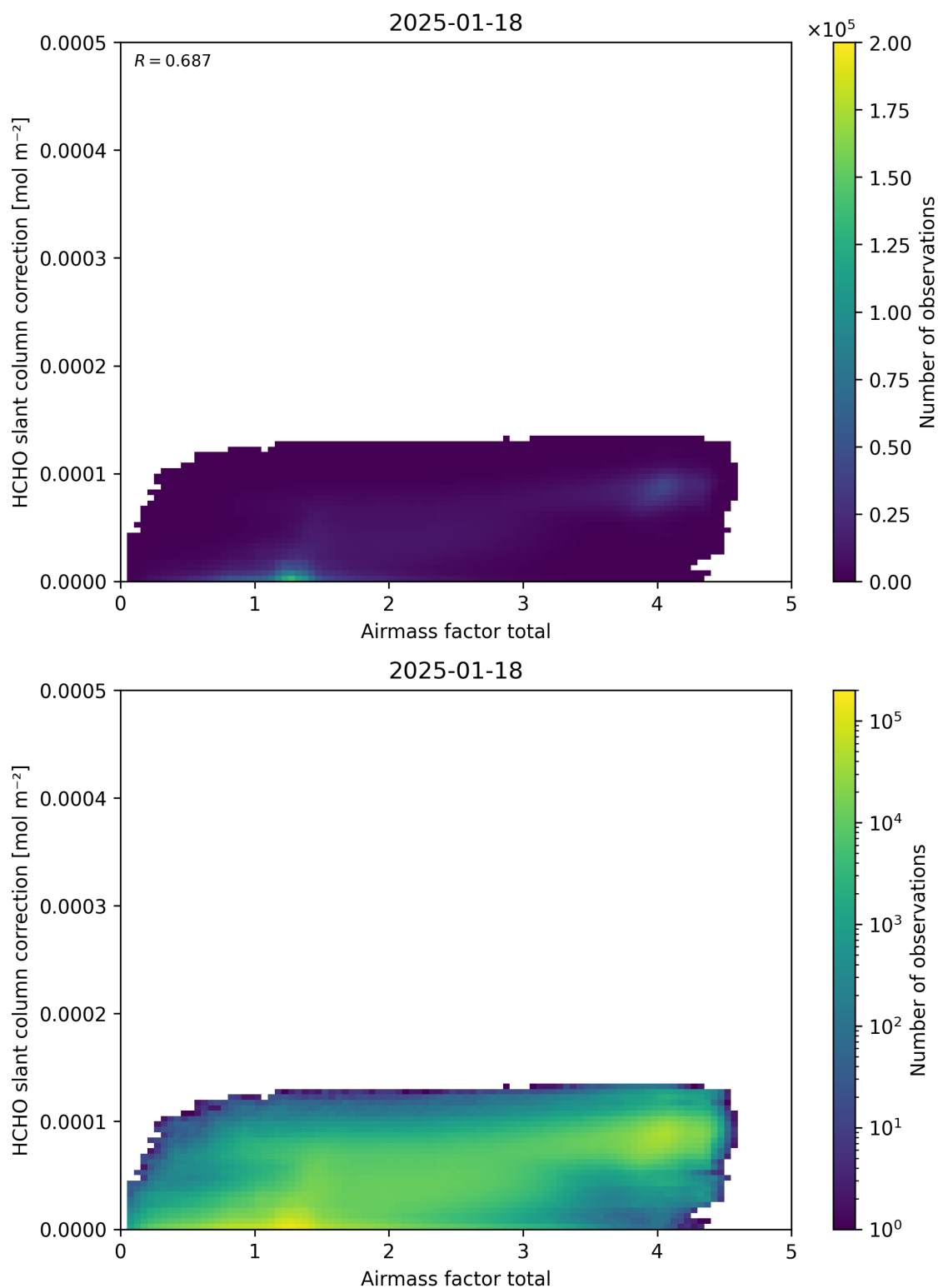
Figure 102: Scatter density plot of “Airmass factor total” against “HCHO slant column correction” for 2025-01-17 to 2025-01-19.
