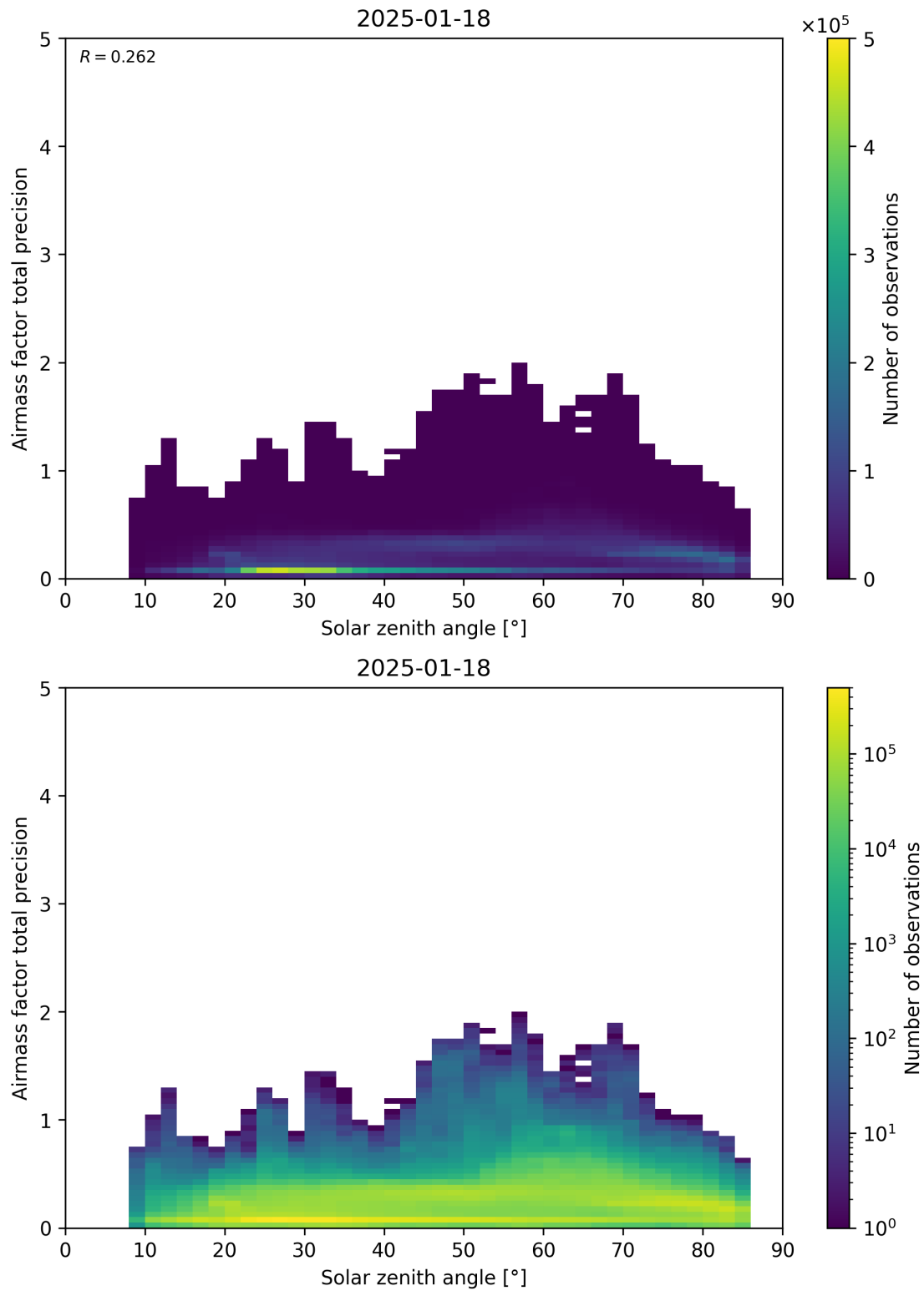
Figure 176: Scatter density plot of “Solar zenith angle” against “Airmass factor total precision” for 2025-01-17 to 2025-01-19.
