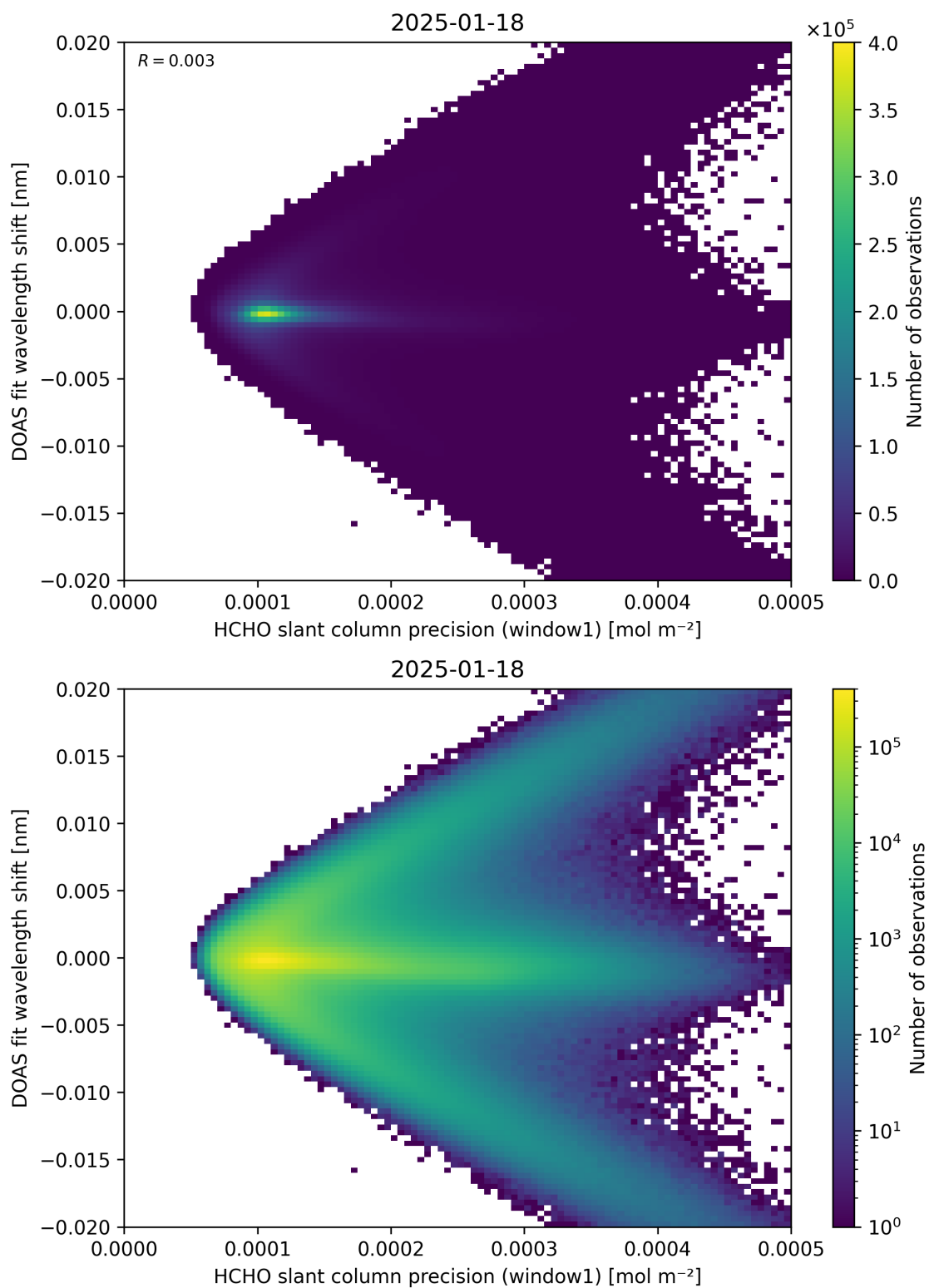
Figure 89: Scatter density plot of “HCHO slant column precision (window1)” against “DOAS fit wavelength shift” for 2025-01-17 to 2025-01-19.
