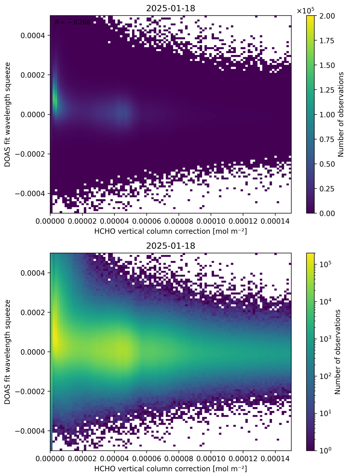
Figure 114: Scatter density plot of “HCHO vertical column correction” against “DOAS fit wavelength squeeze” for 2025-01-17 to 2025-01-19.
