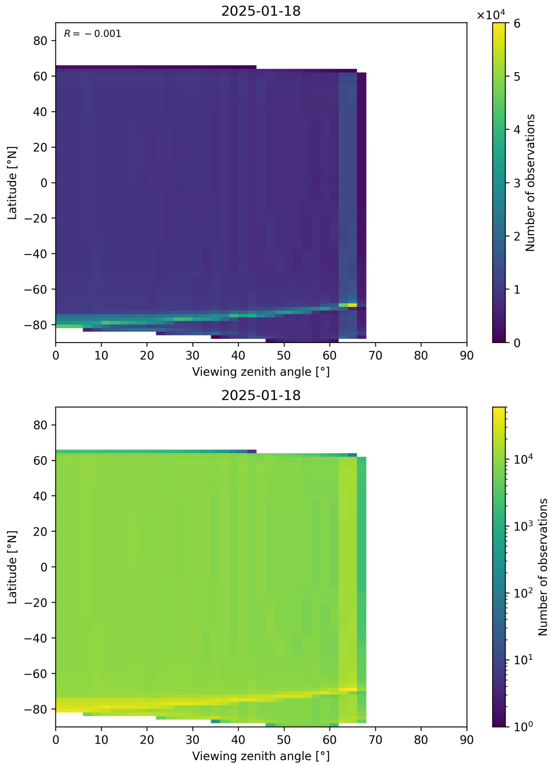
Figure 196: Scatter density plot of “Viewing zenith angle” against “Latitude” for 2025-01-17 to 2025-01-19.
