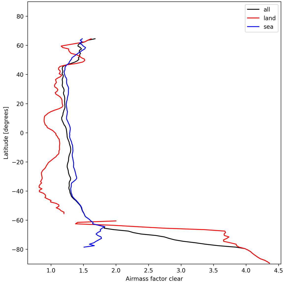
Figure 28: Zonal average of “Airmass factor clear” for 2025-01-17 to 2025-01-19.
