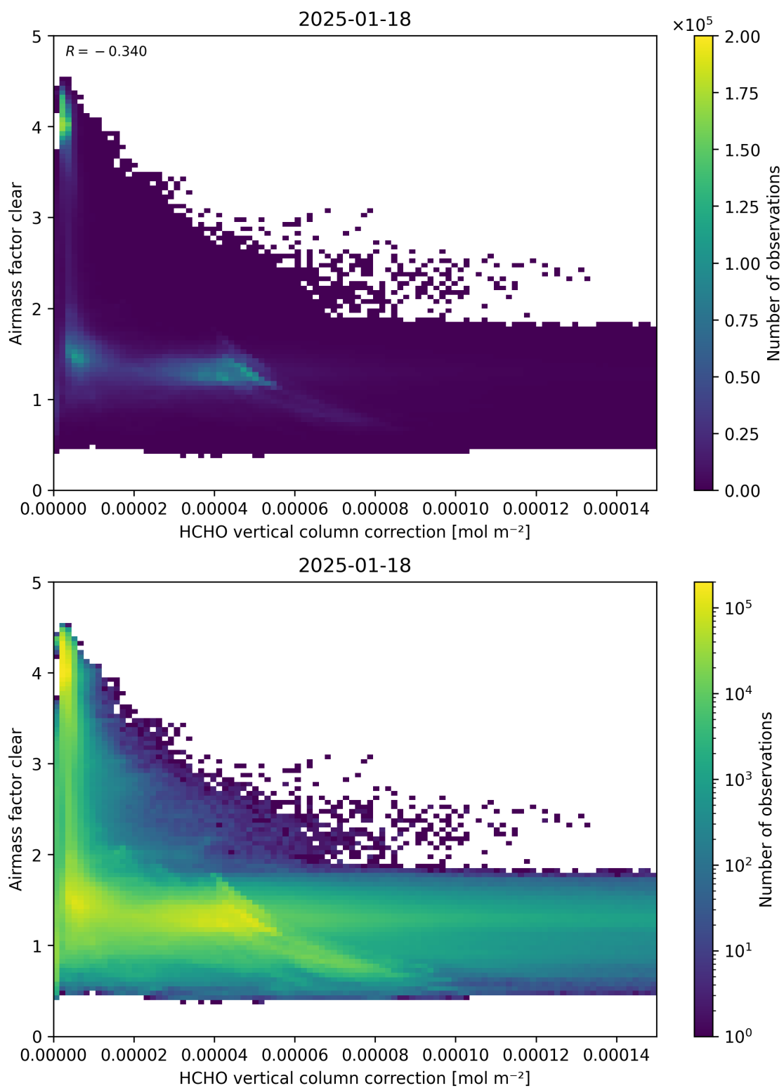
Figure 115: Scatter density plot of “HCHO vertical column correction” against “Airmass factor clear” for 2025-01-17 to 2025-01-19.
