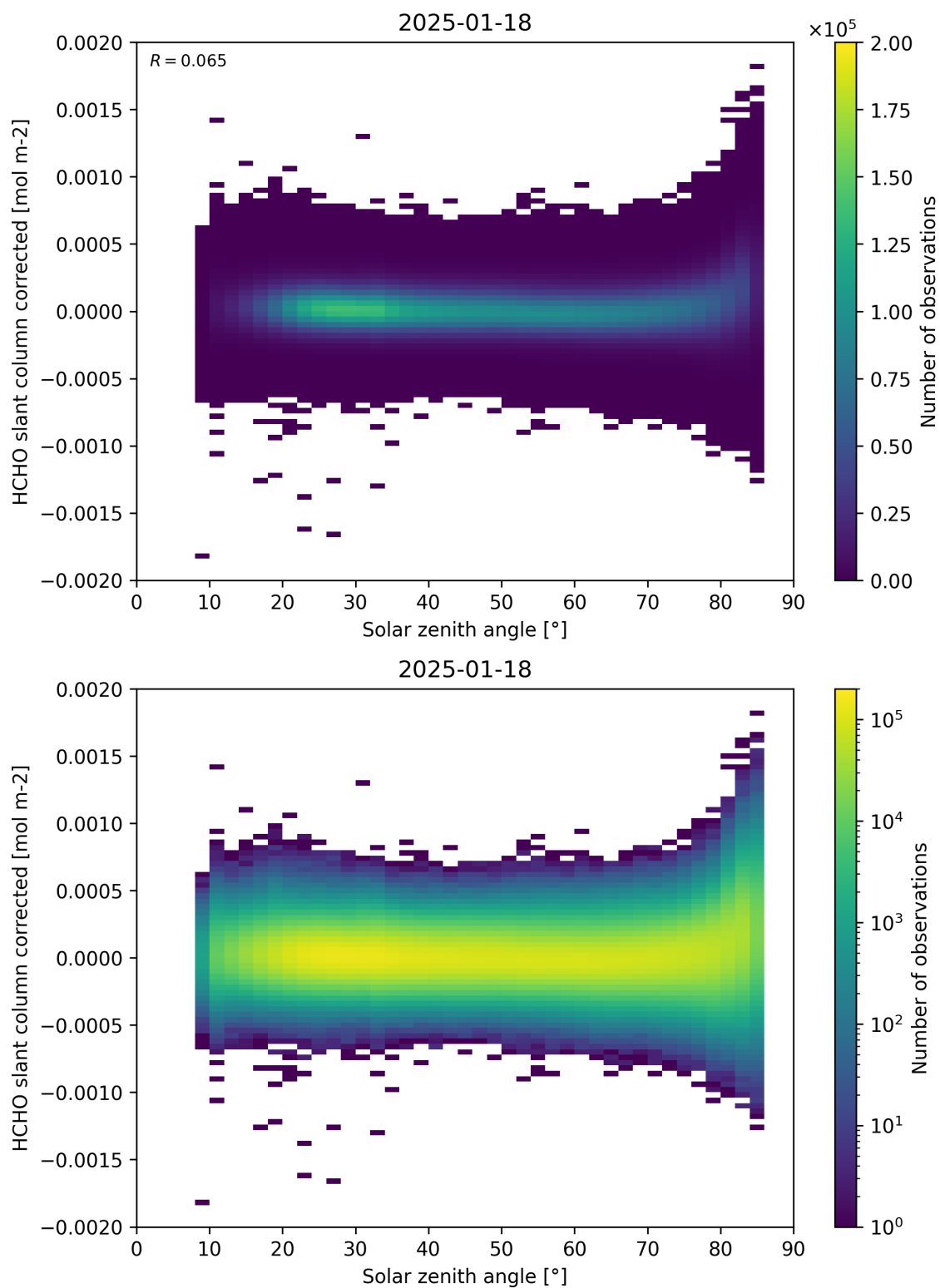
Figure 171: Scatter density plot of “Solar zenith angle” against “HCHO slant column corrected” for 2025-01-17 to 2025-01-19.
