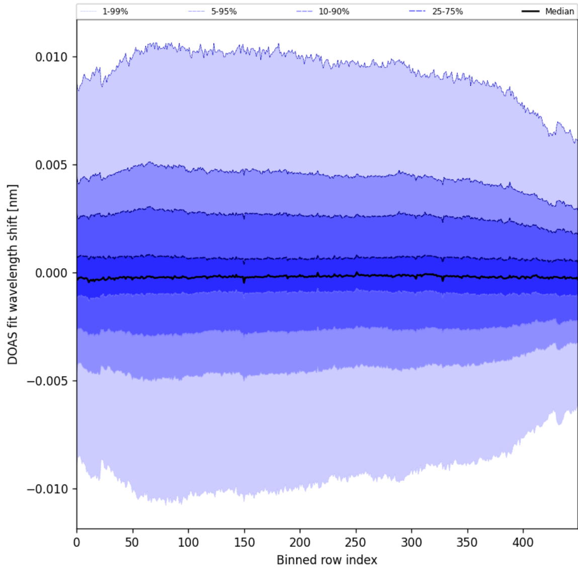
Figure 58: Along track statistics of “DOAS fit wavelength shift” for 2025-01-17 to 2025-01-19
