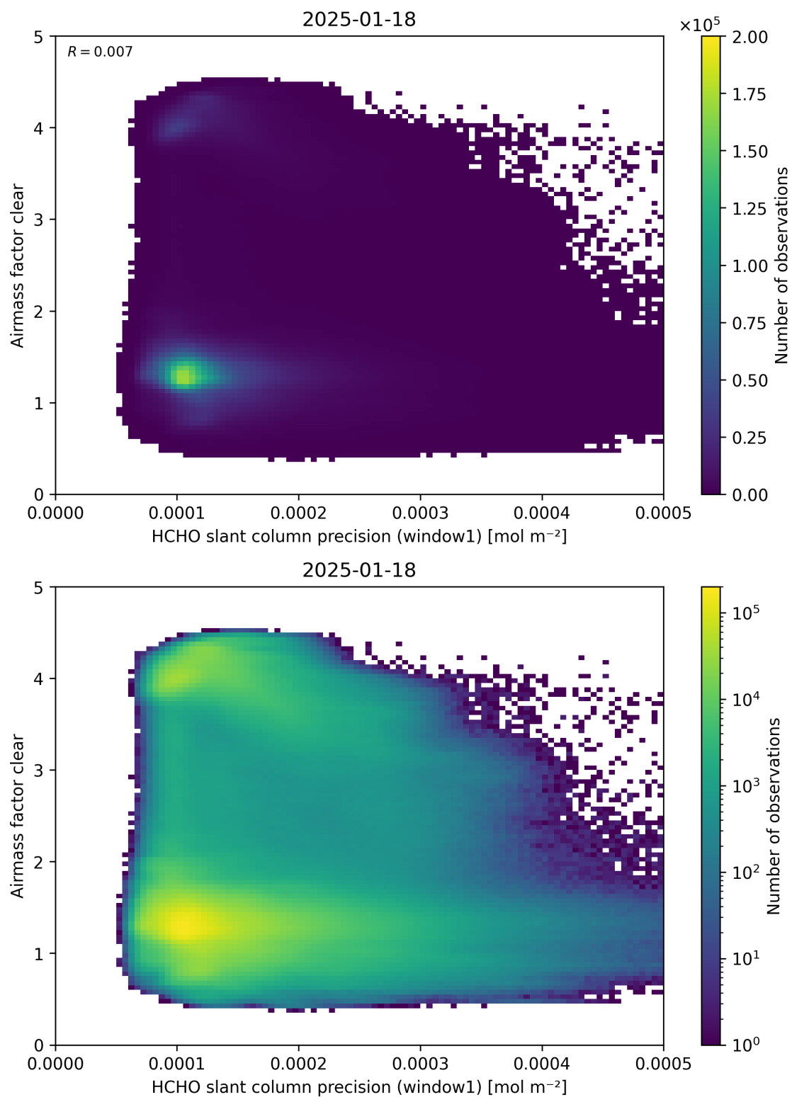
Figure 91: Scatter density plot of “HCHO slant column precision (window1)” against “Airmass factor clear” for 2025-01-17 to 2025-01-19.
