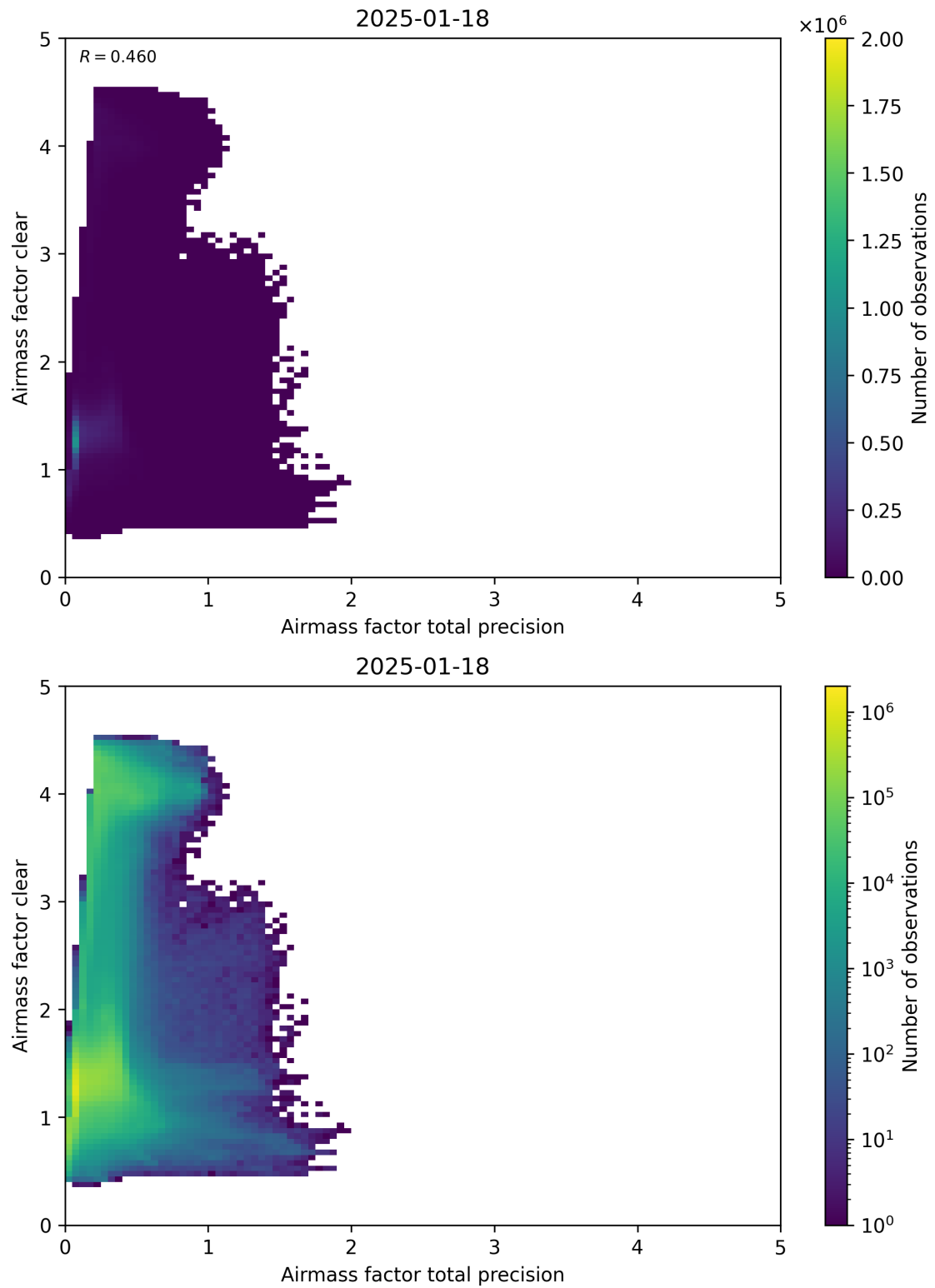
Figure 108: Scatter density plot of “Airmass factor total precision” against “Airmass factor clear” for 2025-01-17 to 2025-01-19.
