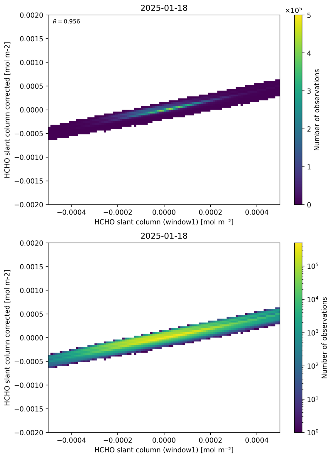
Figure 82: Scatter density plot of “HCHO slant column (window1)” against “HCHO slant column corrected” for 2025-01-17 to 2025-01-19.
