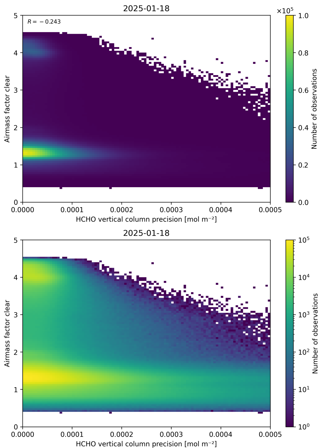
Figure 139: Scatter density plot of “HCHO vertical column precision” against “Airmass factor clear” for 2025-01-17 to 2025-01-19.
