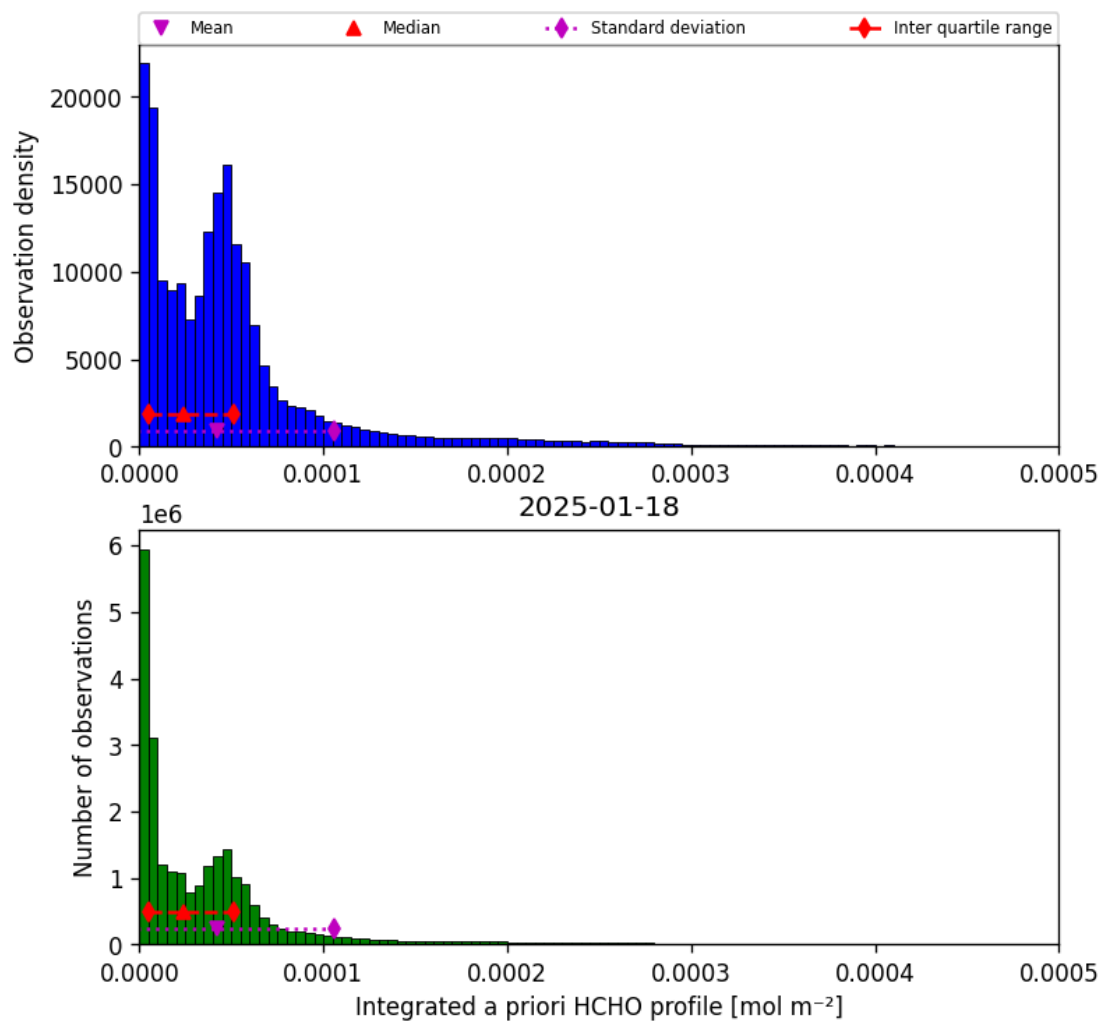
Figure 43: Histogram of “Integrated a priori HCHO profile” for 2025-01-17 to 2025-01-19
