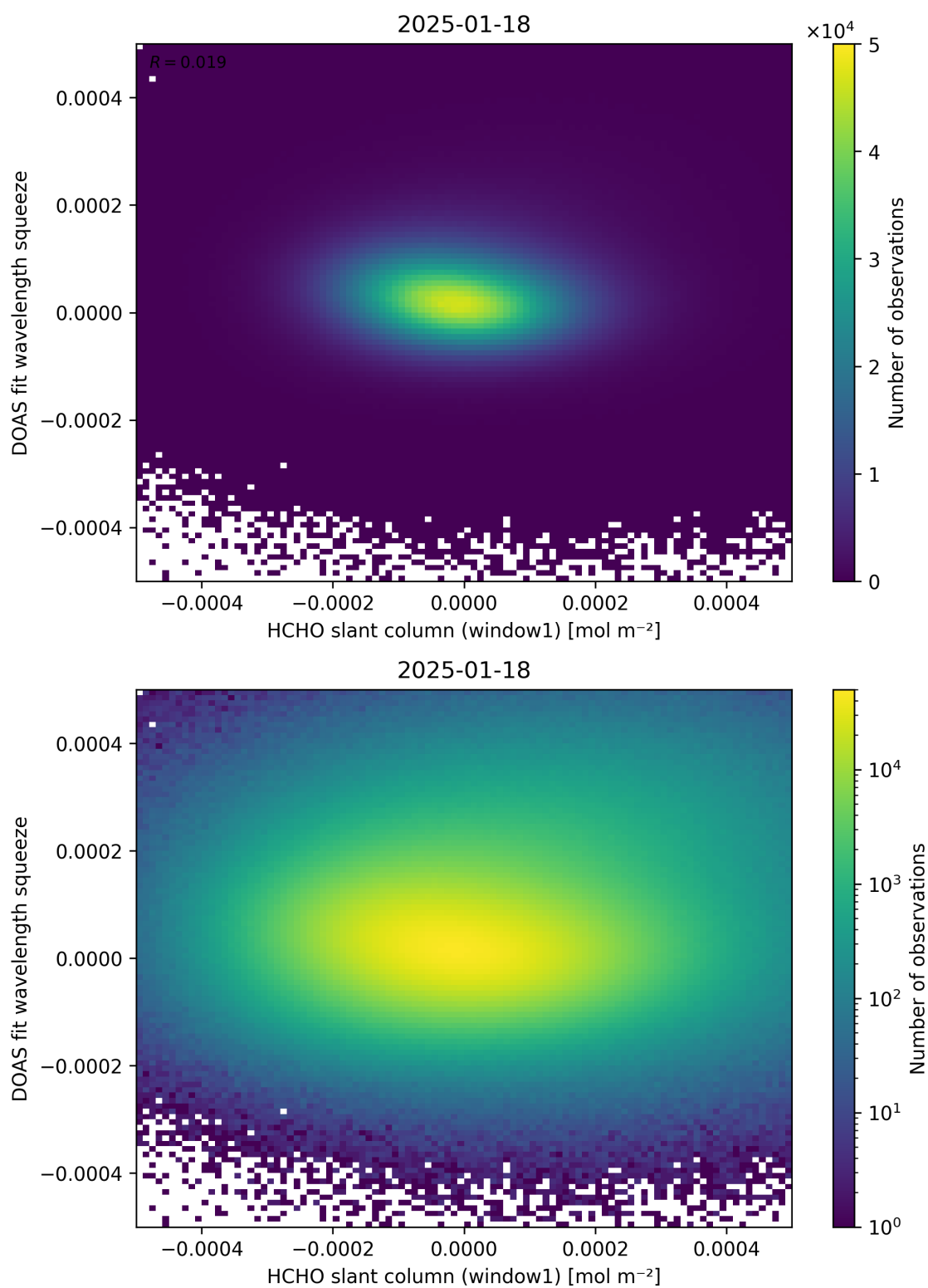
Figure 80: Scatter density plot of “HCHO slant column (window1)” against “DOAS fit wavelength squeeze” for 2025-01-17 to 2025-01-19.
