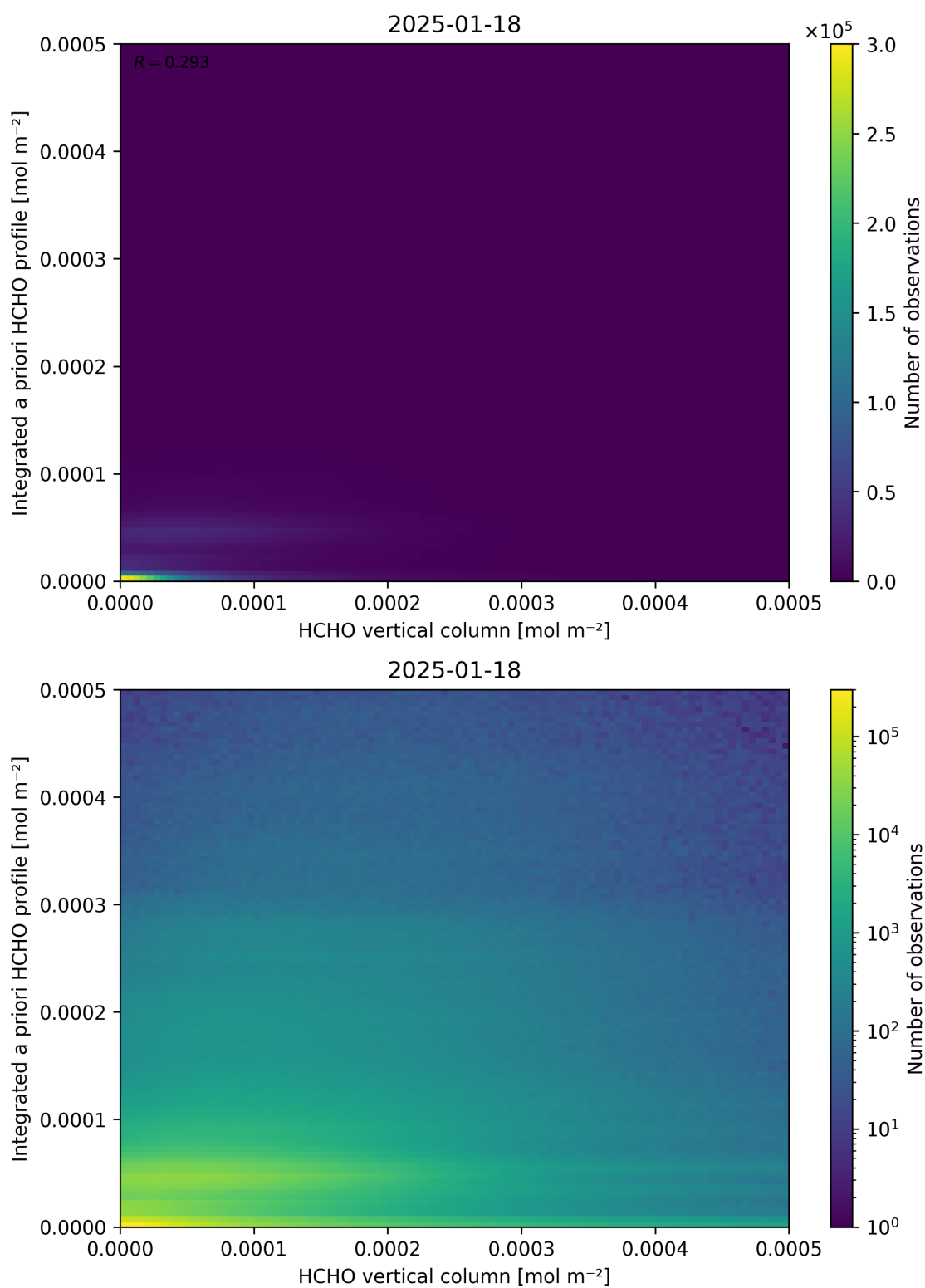
Figure 135: Scatter density plot of “HCHO vertical column” against “Integrated a priori HCHO profile” for 2025-01-17 to 2025-01-19.
