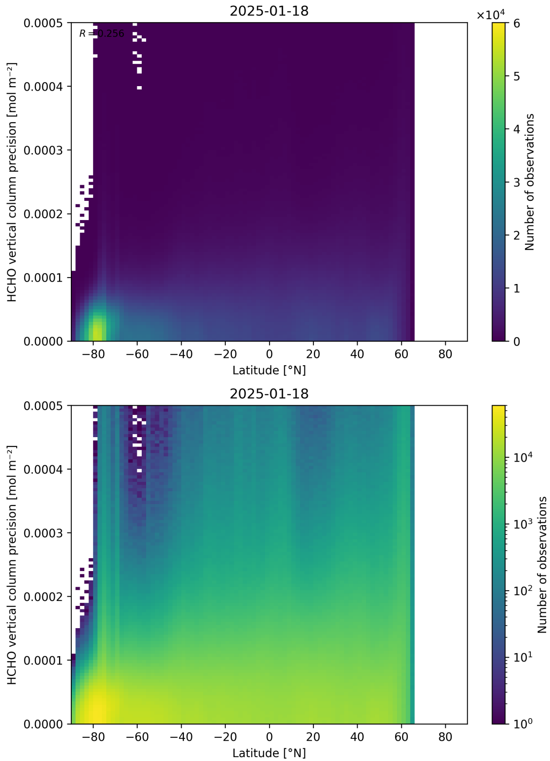
Figure 165: Scatter density plot of “Latitude” against “HCHO vertical column precision” for 2025-01-17 to 2025-01-19.
