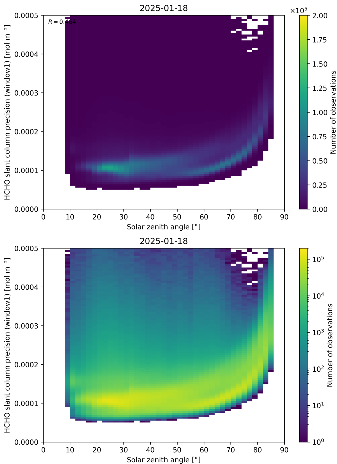
Figure 174: Scatter density plot of “Solar zenith angle” against “HCHO slant column precision (window1)” for 2025-01-17 to 2025-01-19.
