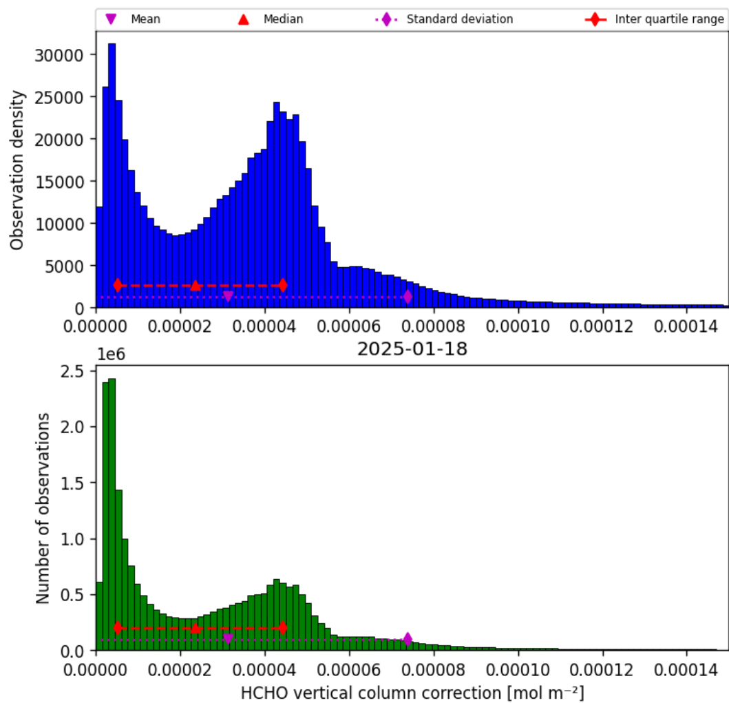
Figure 37: Histogram of “HCHO vertical column correction” for 2025-01-17 to 2025-01-19
