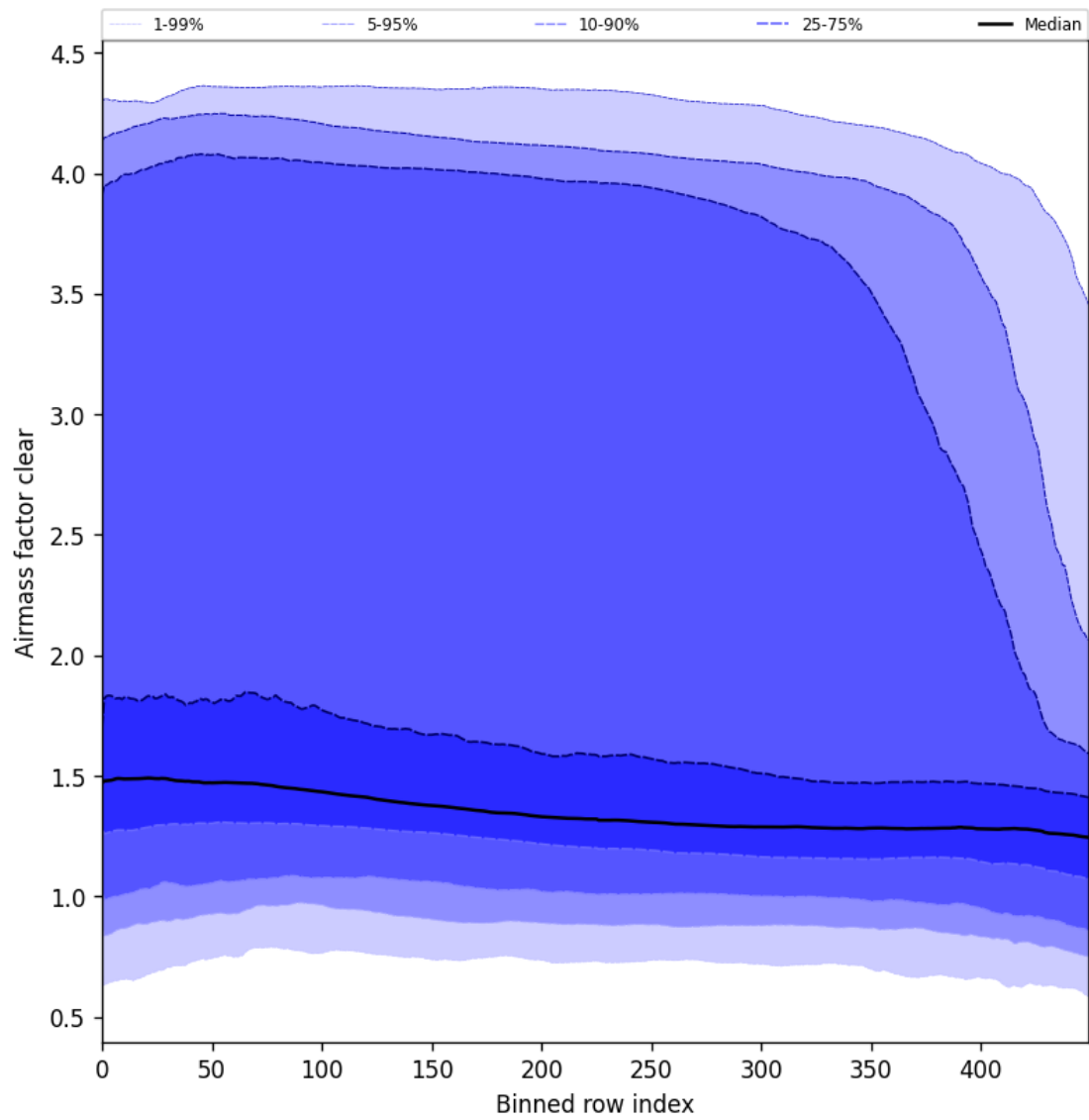
Figure 56: Along track statistics of “Airmass factor clear” for 2025-01-17 to 2025-01-19
