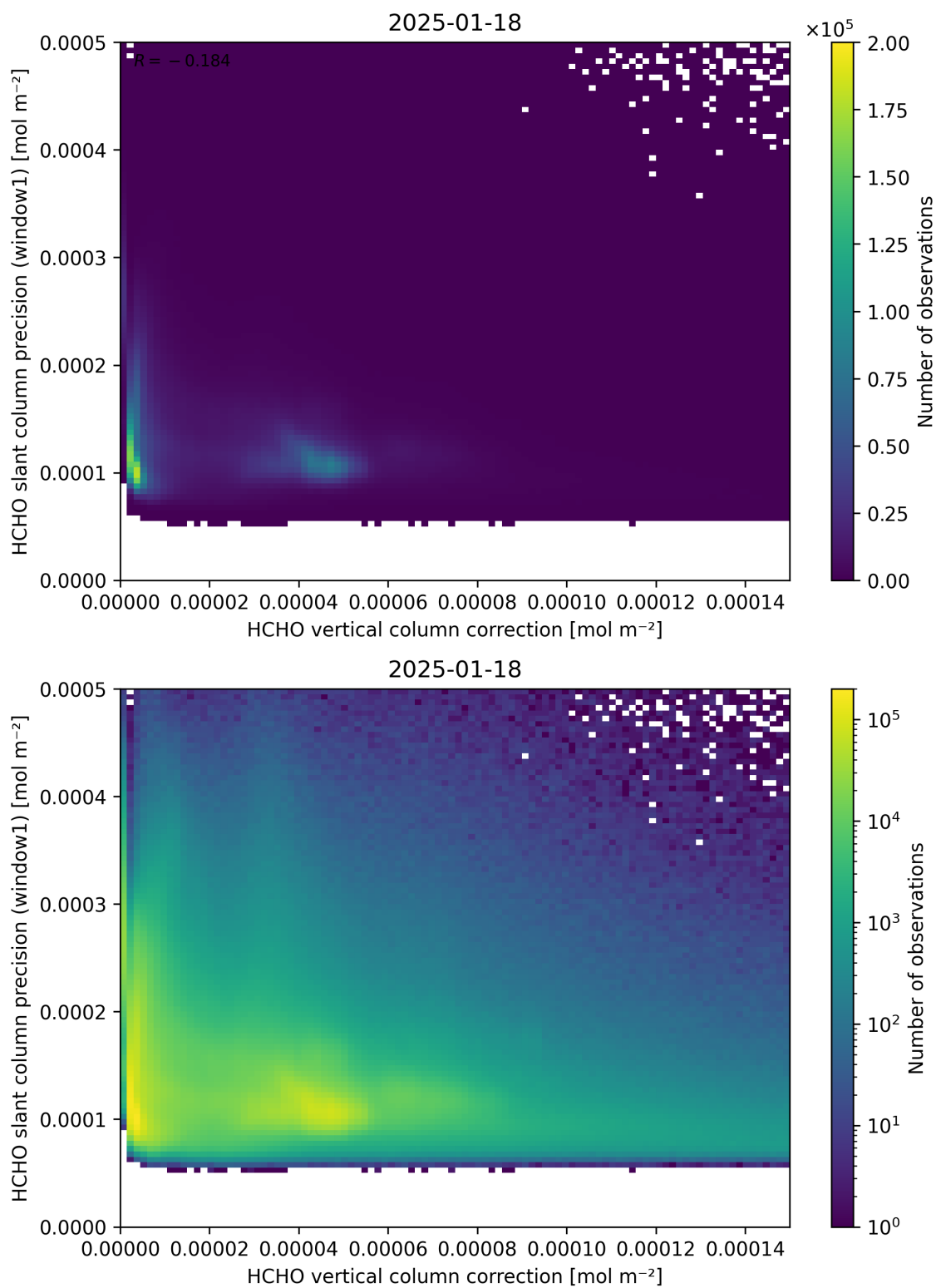
Figure 119: Scatter density plot of “HCHO vertical column correction” against “HCHO slant column precision (window1)” for 2025-01-17 to 2025-01-19.
