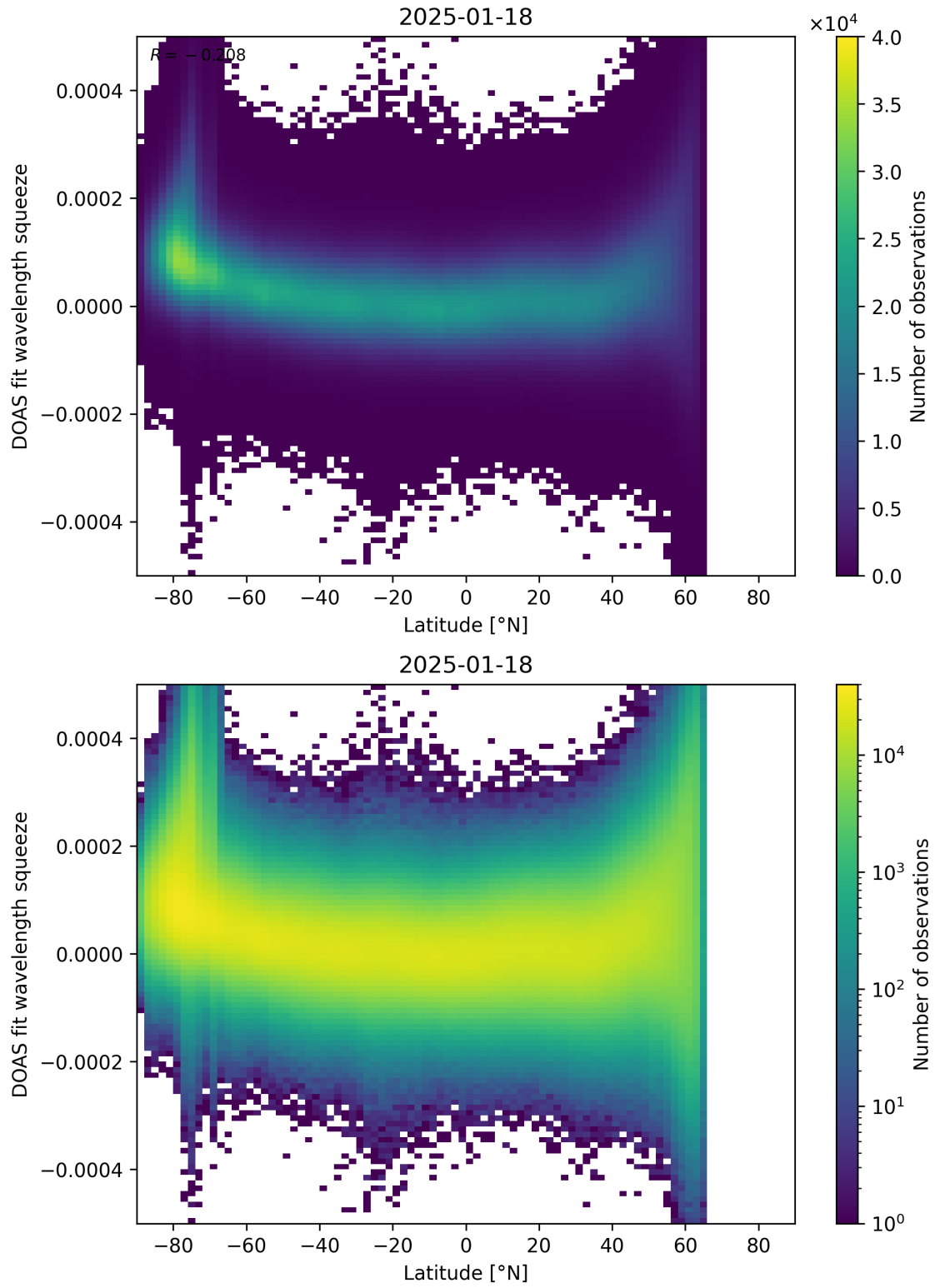
Figure 155: Scatter density plot of “Latitude” against “DOAS fit wavelength squeeze” for 2025-01-17 to 2025-01-19.
