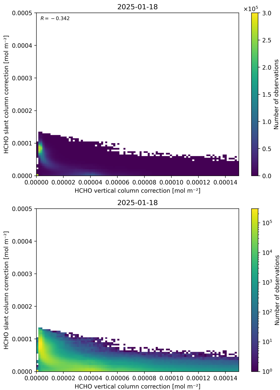
Figure 117: Scatter density plot of “HCHO vertical column correction” against “HCHO slant column correction” for 2025-01-17 to 2025-01-19.
