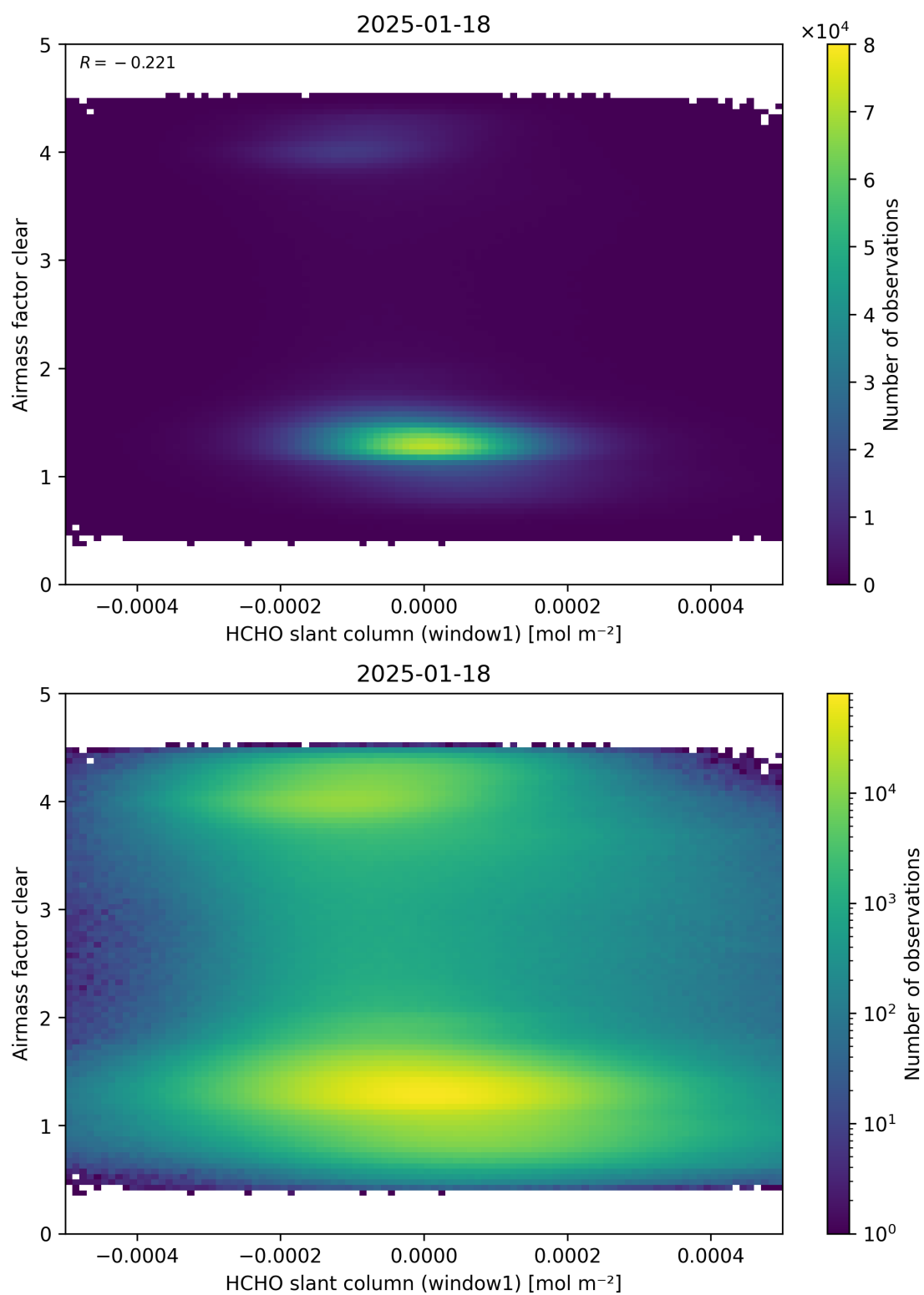
Figure 81: Scatter density plot of “HCHO slant column (window1)” against “Airmass factor clear” for 2025-01-17 to 2025-01-19.
