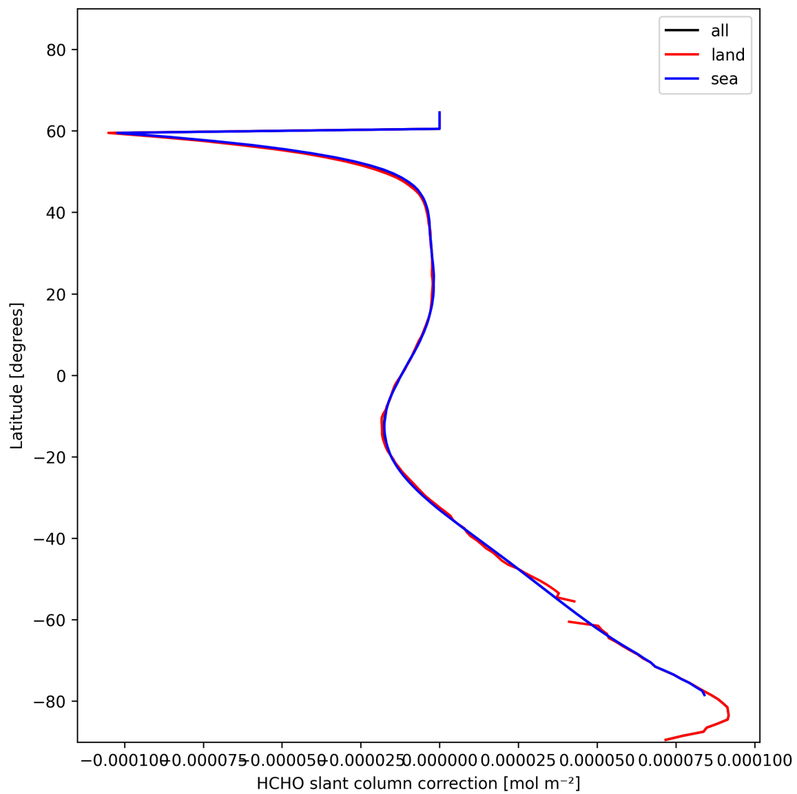
Figure 33: Zonal average of “HCHO slant column correction” for 2025-01-17 to 2025-01-19.
