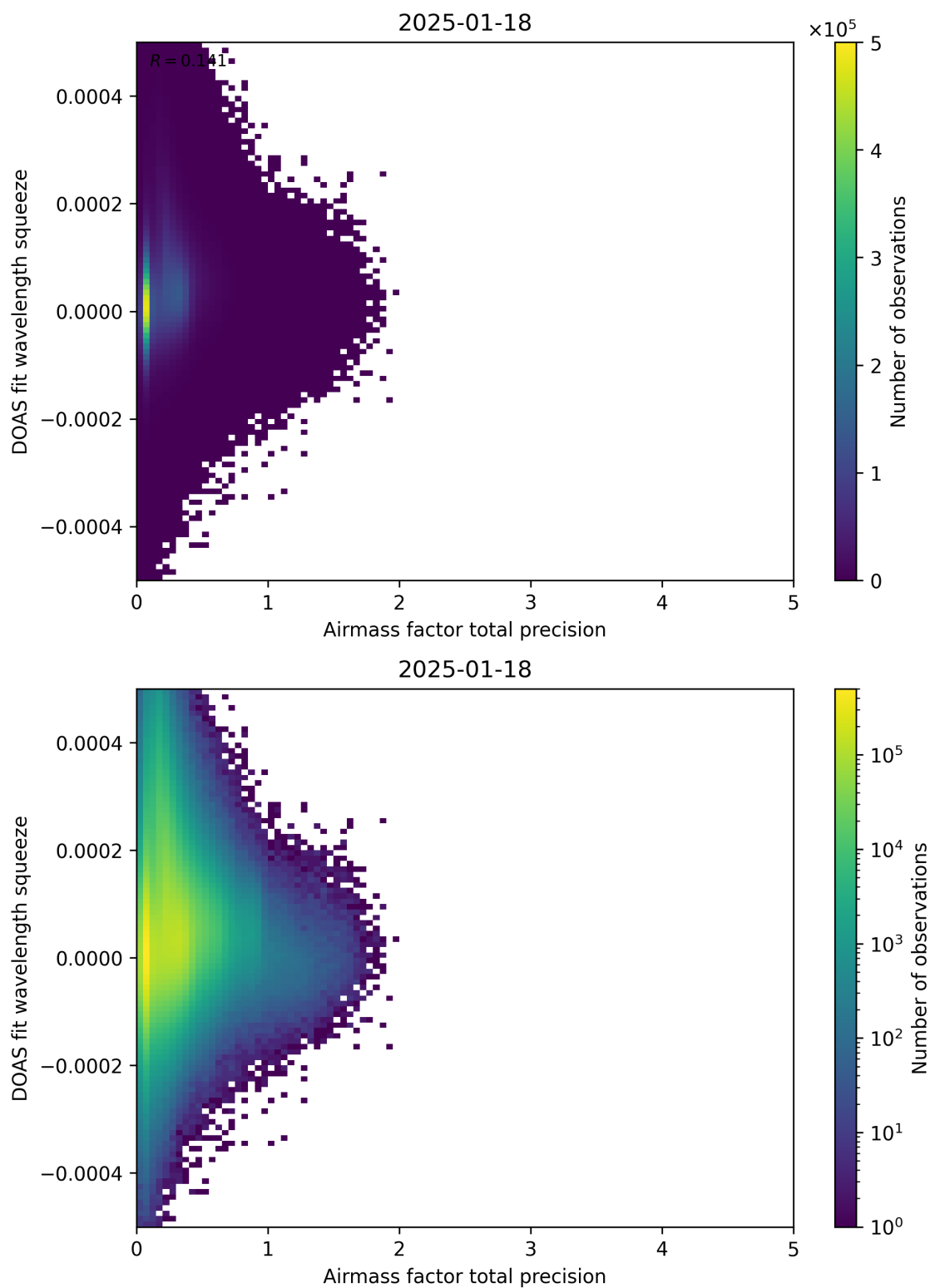
Figure 107: Scatter density plot of “Airmass factor total precision” against “DOAS fit wavelength squeeze” for 2025-01-17 to 2025-01-19.
