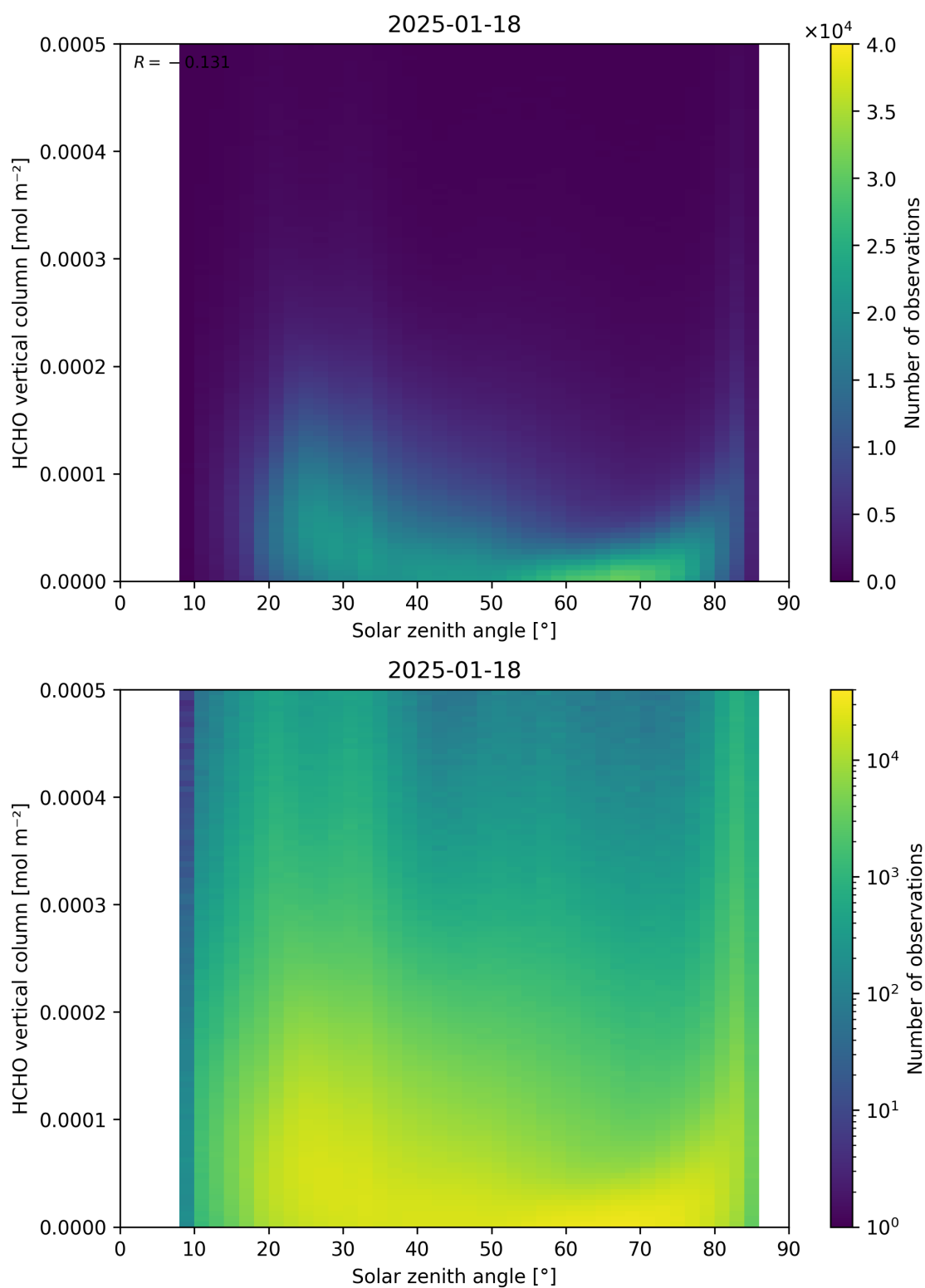
Figure 177: Scatter density plot of “Solar zenith angle” against “HCHO vertical column” for 2025-01-17 to 2025-01-19.
