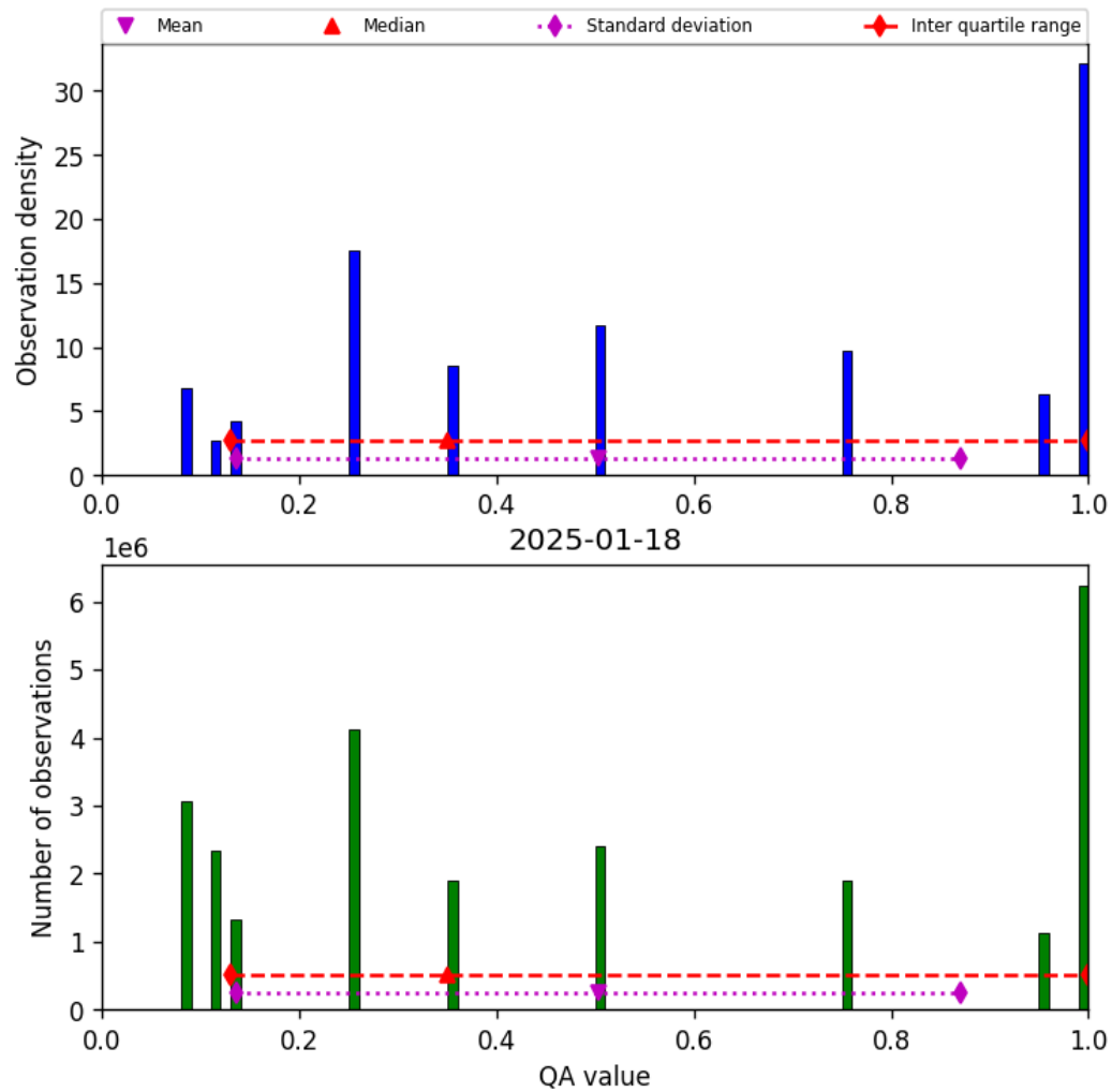
Figure 34: Histogram of “QA value” for 2025-01-17 to 2025-01-19
