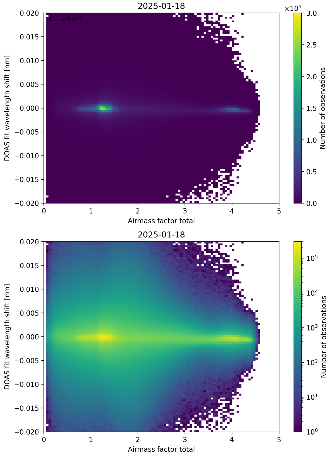
Figure 98: Scatter density plot of “Airmass factor total” against “DOAS fit wavelength shift” for 2025-01-17 to 2025-01-19.
