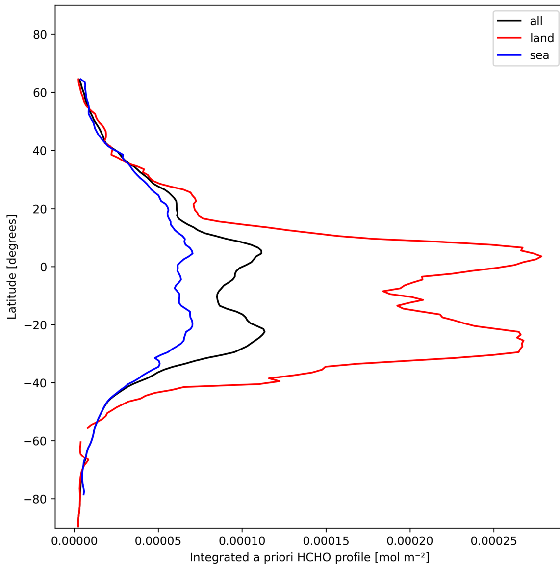
Figure 29: Zonal average of “Integrated a priori HCHO profile” for 2025-01-17 to 2025-01-19.
