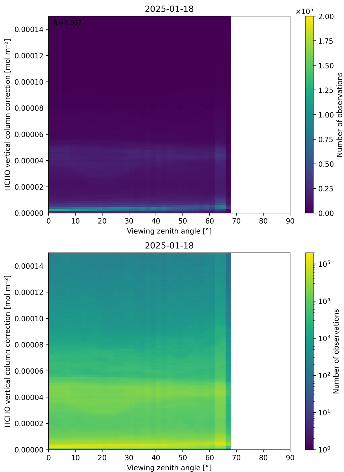
Figure 193: Scatter density plot of “Viewing zenith angle” against “HCHO vertical column correction” for 2025-01-17 to 2025-01-19.
