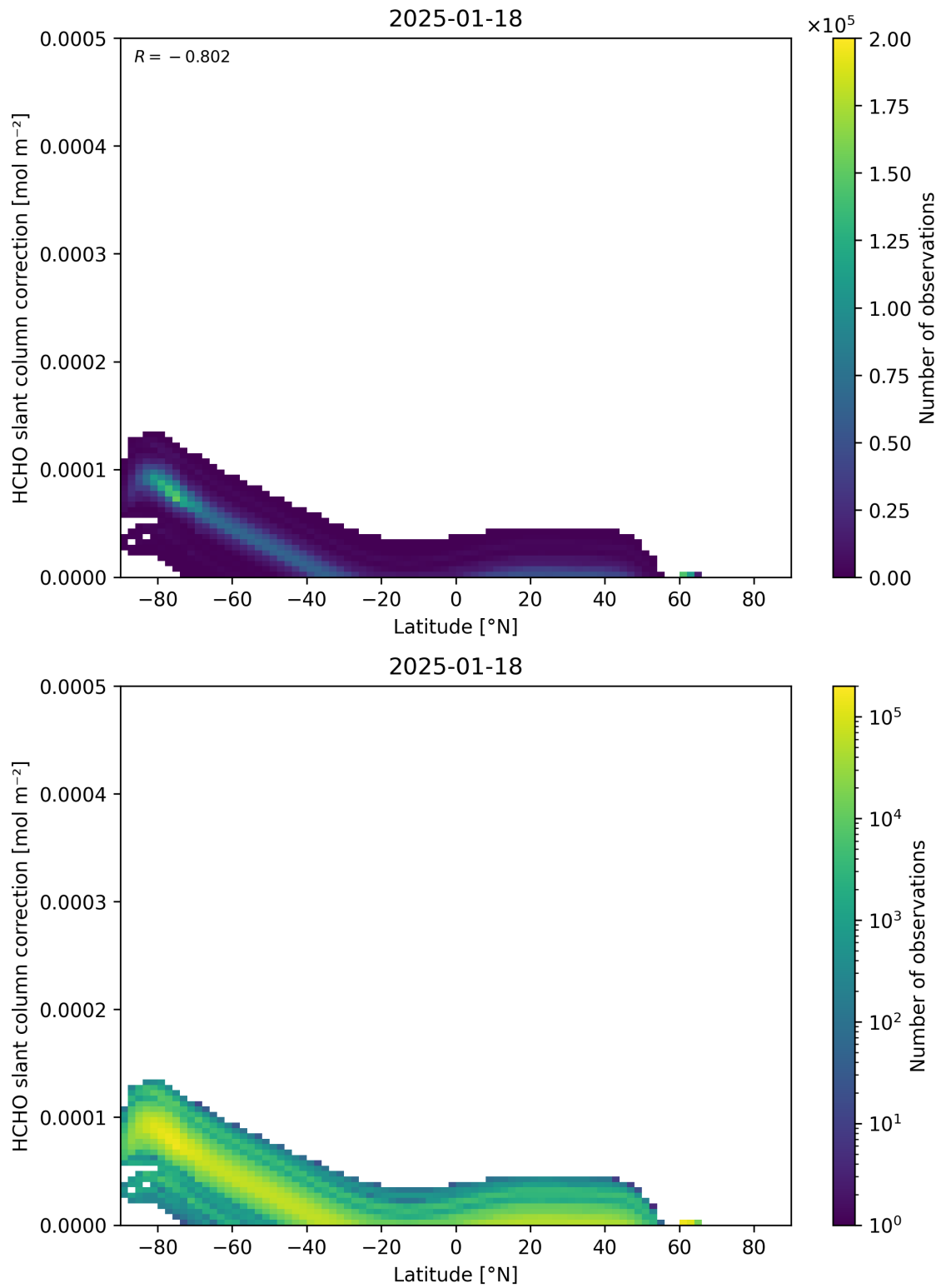
Figure 158: Scatter density plot of “Latitude” against “HCHO slant column correction” for 2025-01-17 to 2025-01-19.
