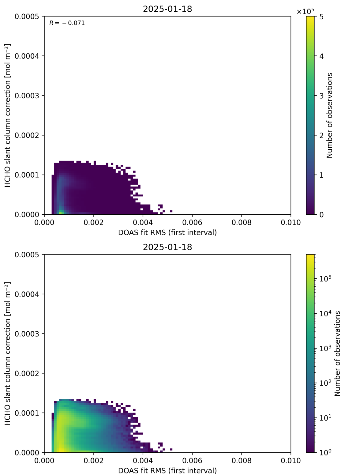
Figure 63: Scatter density plot of “DOAS fit RMS (first interval)” against “HCHO slant column correction” for 2025-01-17 to 2025-01-19.
