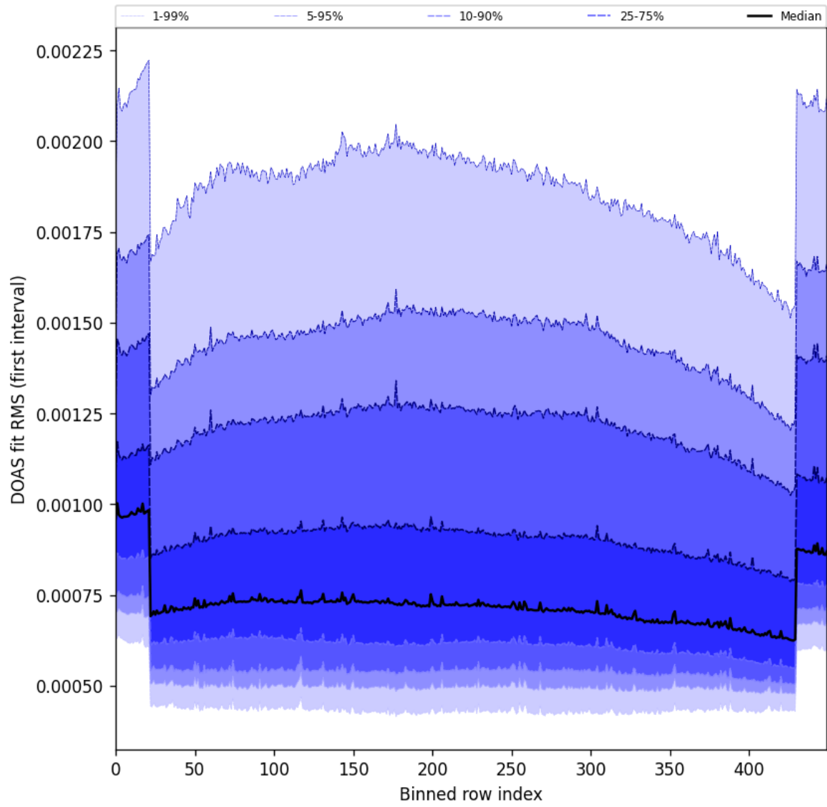
Figure 60: Along track statistics of “DOAS fit RMS (first interval)” for 2025-01-17 to 2025-01-19
