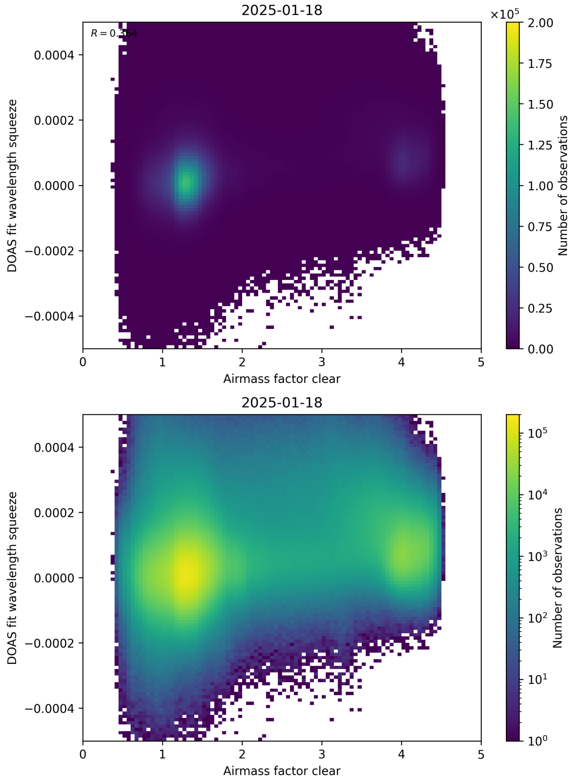
Figure 73: Scatter density plot of “Airmass factor clear” against “DOAS fit wavelength squeeze” for 2025-01-17 to 2025-01-19.
