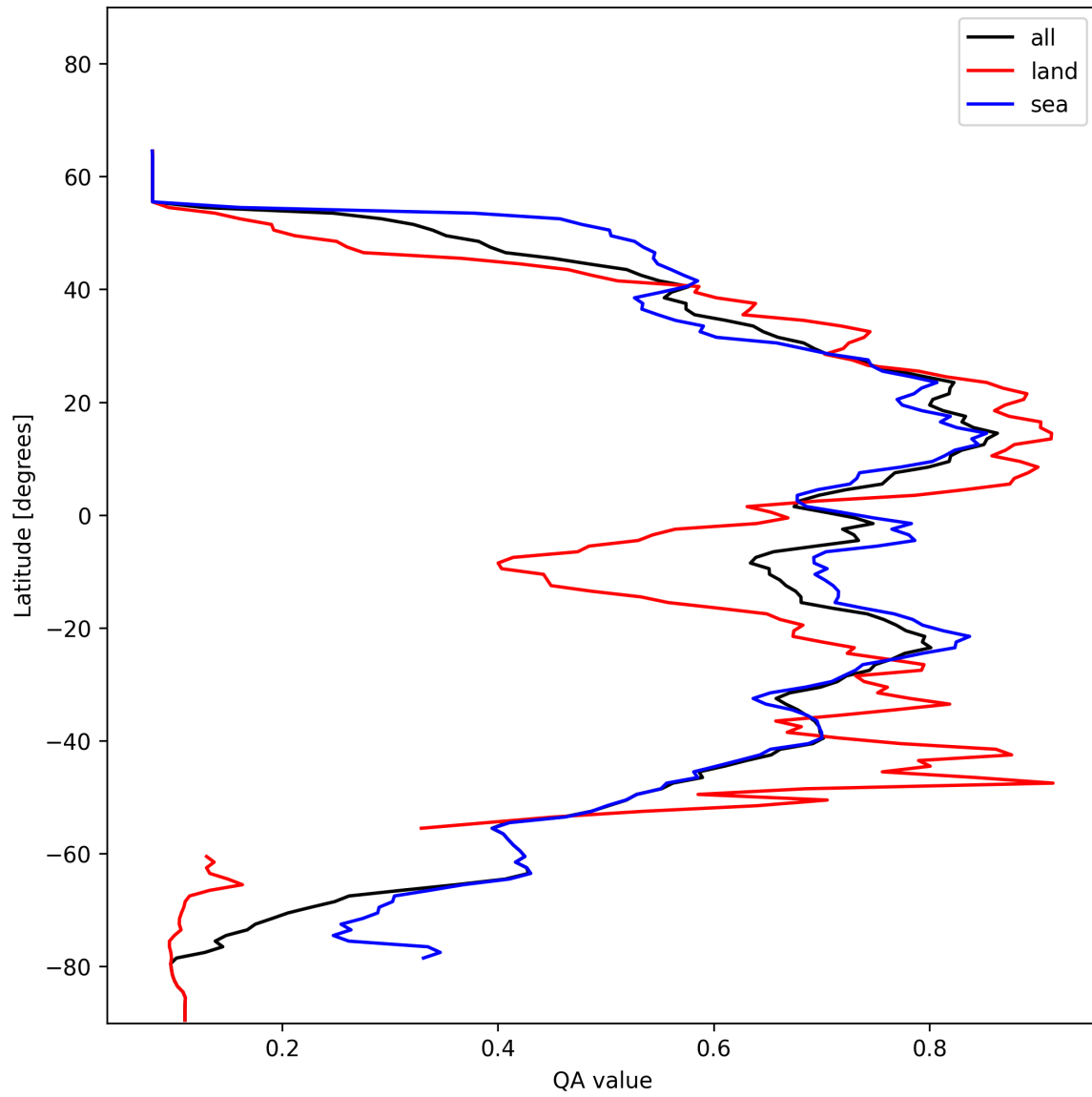
Figure 20: Zonal average of “QA value” for 2025-01-17 to 2025-01-19.
