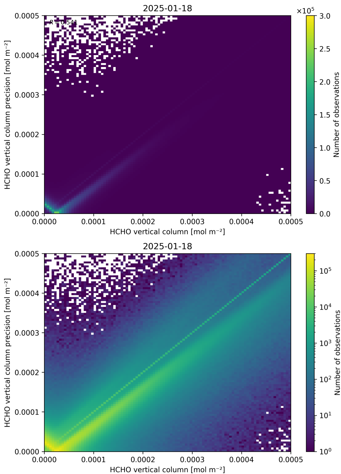
Figure 134: Scatter density plot of “HCHO vertical column” against “HCHO vertical column precision” for 2025-01-17 to 2025-01-19.
