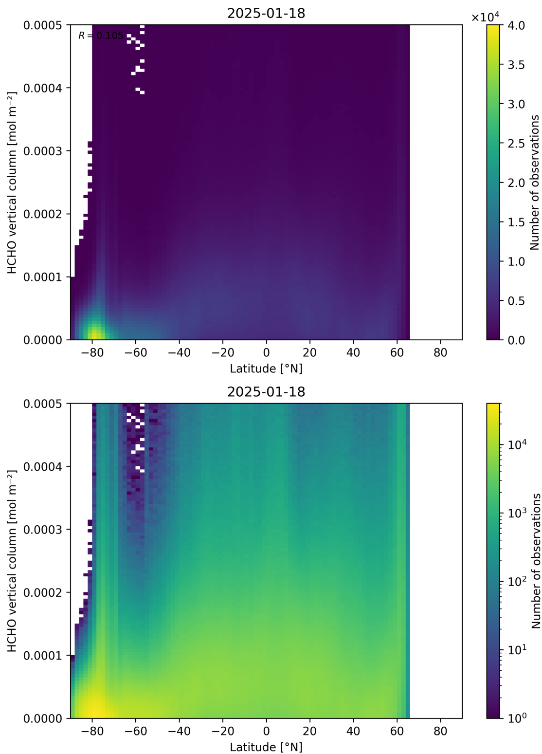
Figure 163: Scatter density plot of “Latitude” against “HCHO vertical column” for 2025-01-17 to 2025-01-19.
