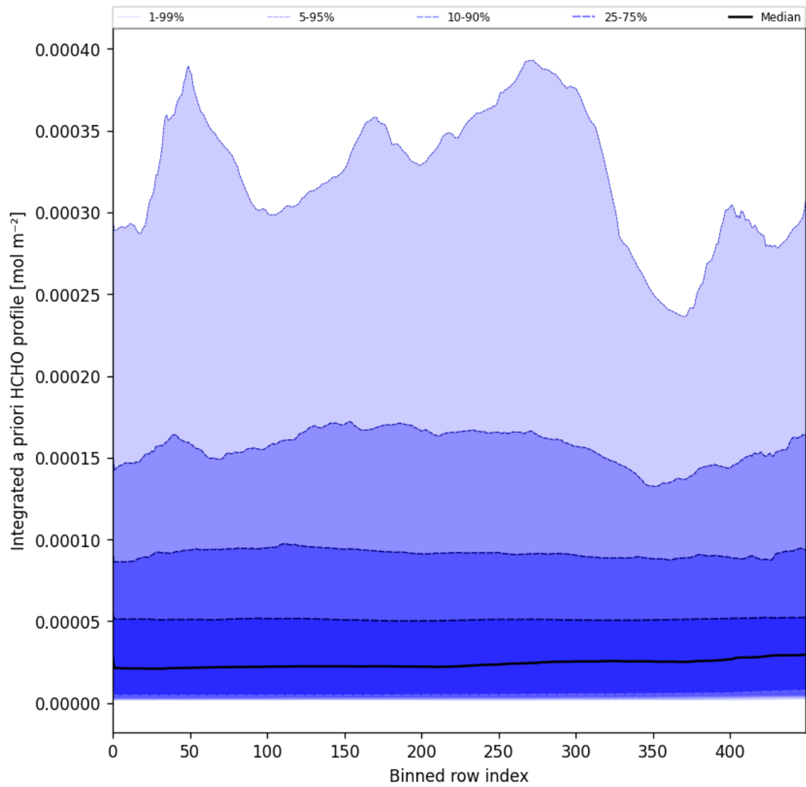
Figure 57: Along track statistics of “Integrated a priori HCHO profile” for 2025-01-17 to 2025-01-19
