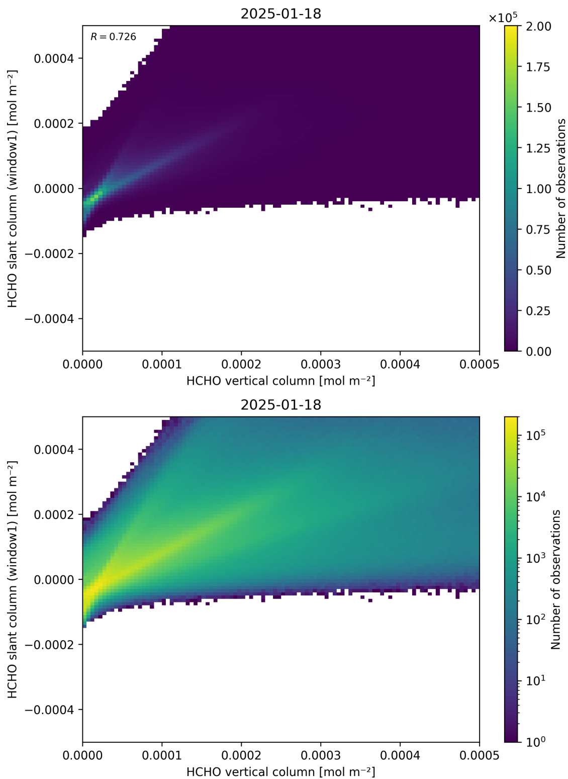
Figure 129: Scatter density plot of “HCHO vertical column” against “HCHO slant column (window1)” for 2025-01-17 to 2025-01-19.
