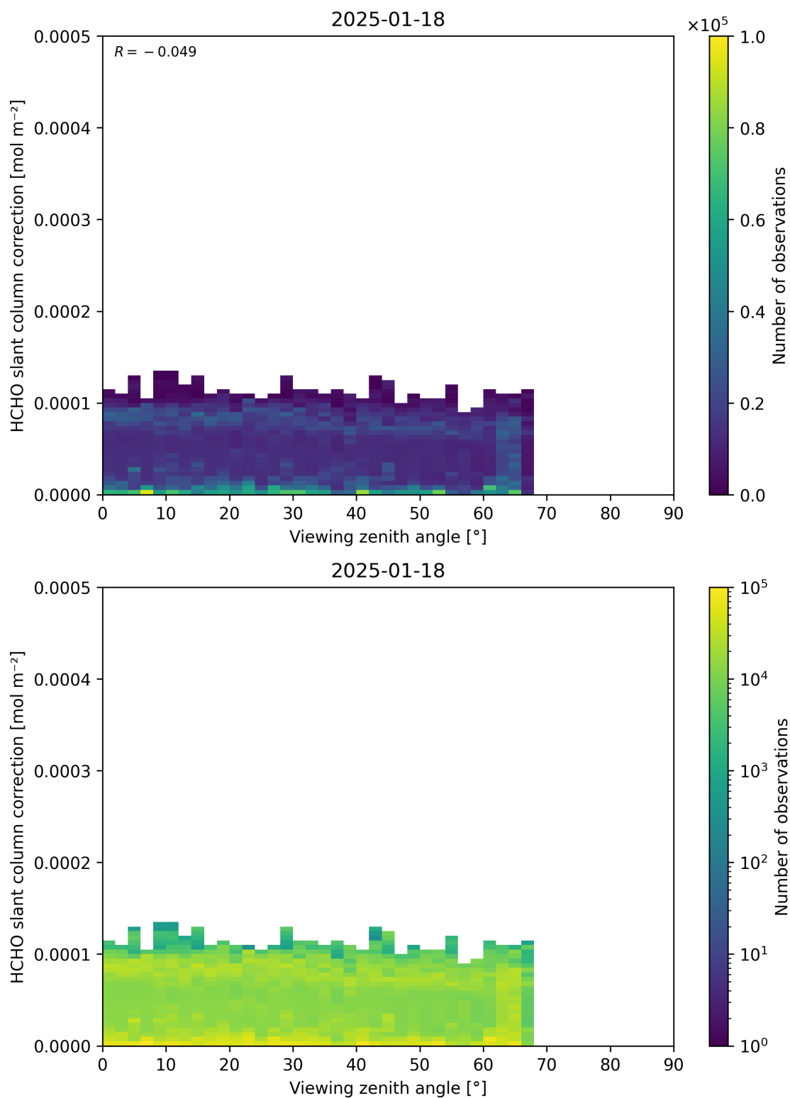
Figure 187: Scatter density plot of “Viewing zenith angle” against “HCHO slant column correction” for 2025-01-17 to 2025-01-19.
