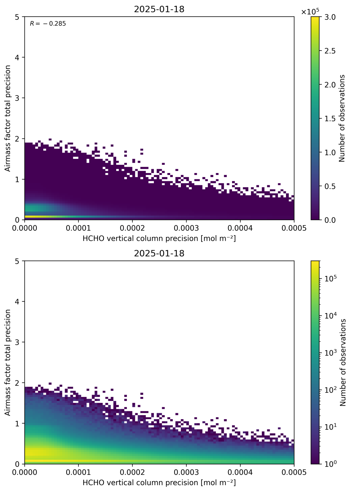
Figure 145: Scatter density plot of “HCHO vertical column precision” against “Airmass factor total precision” for 2025-01-17 to 2025-01-19.
