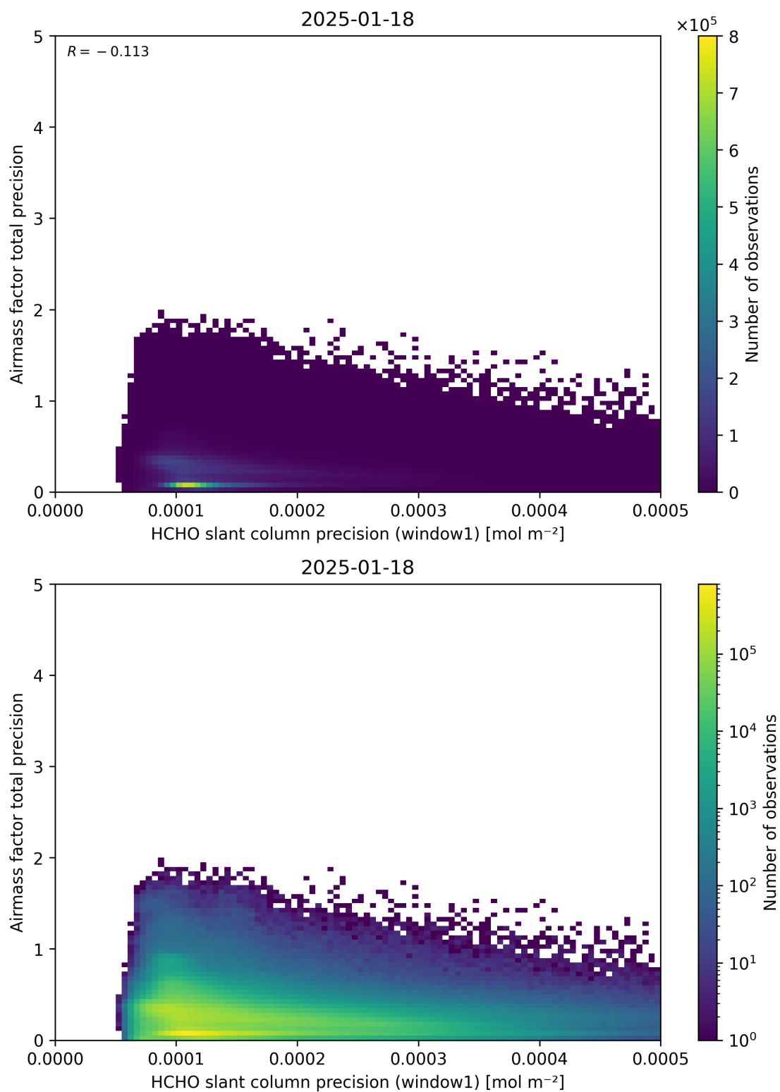
Figure 95: Scatter density plot of “HCHO slant column precision (window1)” against “Airmass factor total precision” for 2025-01-17 to 2025-01-19.
