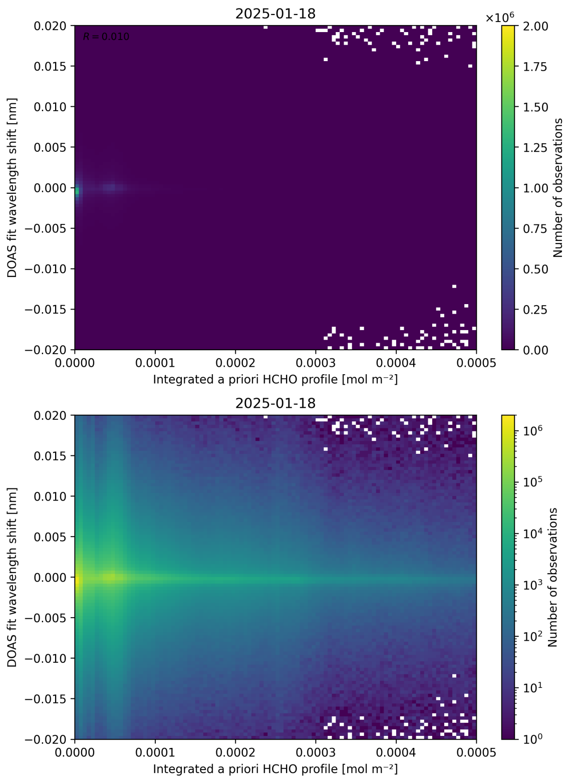
Figure 149: Scatter density plot of “Integrated a priori HCHO profile” against “DOAS fit wavelength shift” for 2025-01-17 to 2025-01-19.
