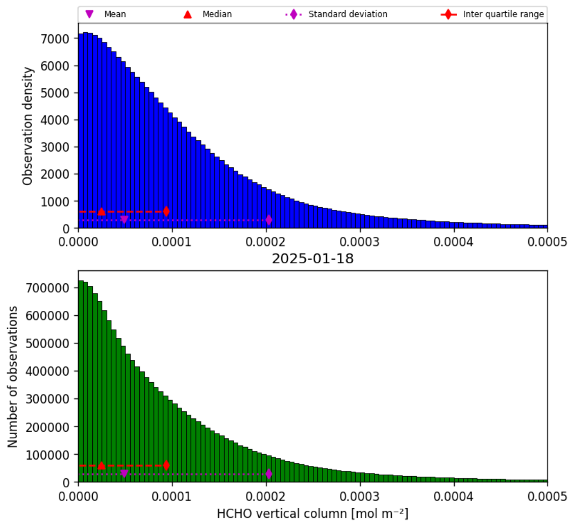
Figure 35: Histogram of “HCHO vertical column” for 2025-01-17 to 2025-01-19
