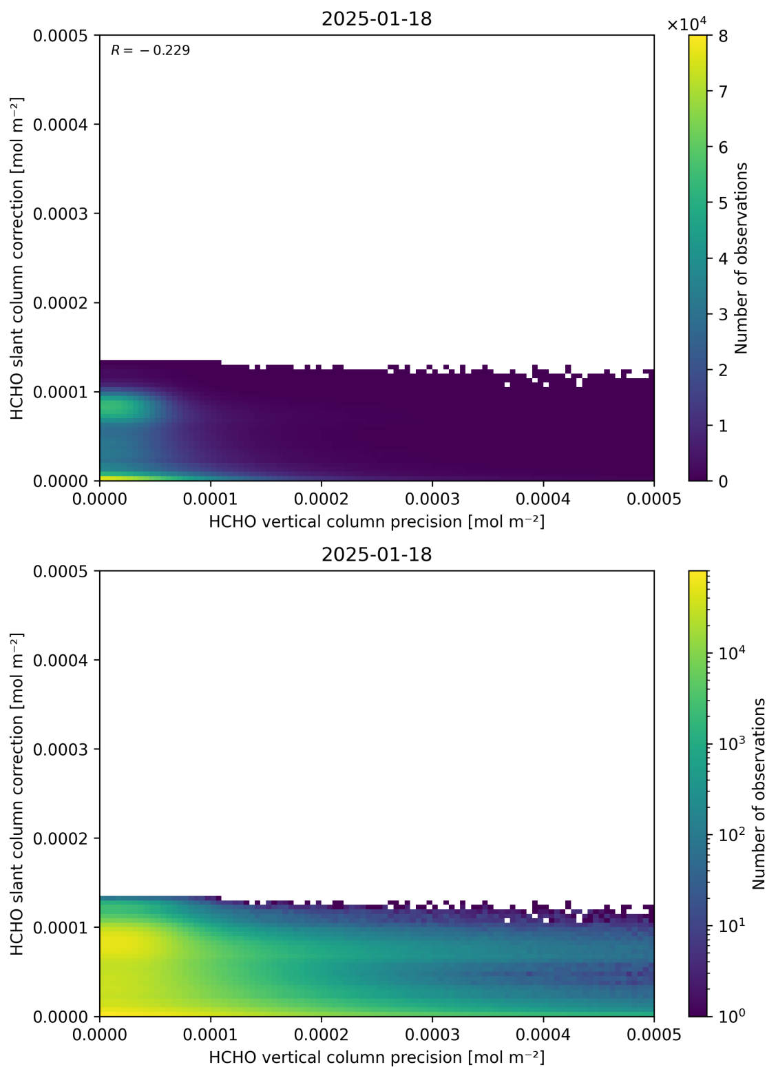
Figure 141: Scatter density plot of “HCHO vertical column precision” against “HCHO slant column correction” for 2025-01-17 to 2025-01-19.
