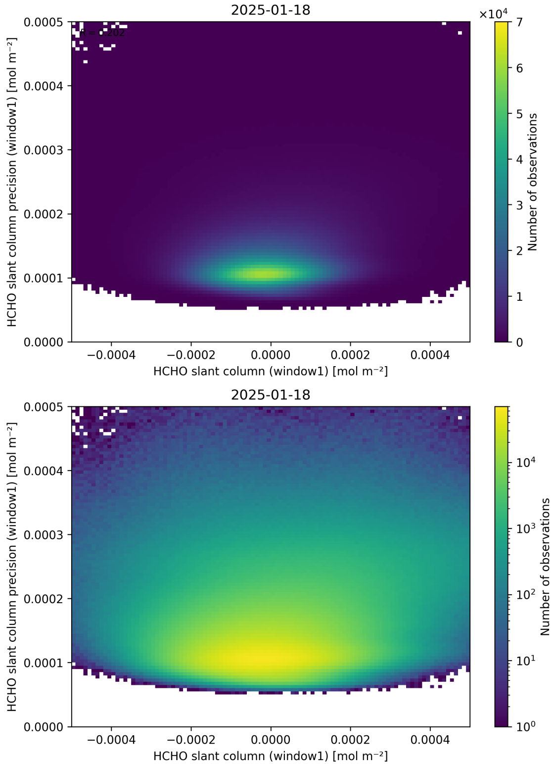
Figure 84: Scatter density plot of “HCHO slant column (window1)” against “HCHO slant column precision (window1)” for 2025-01-17 to 2025-01-19.
