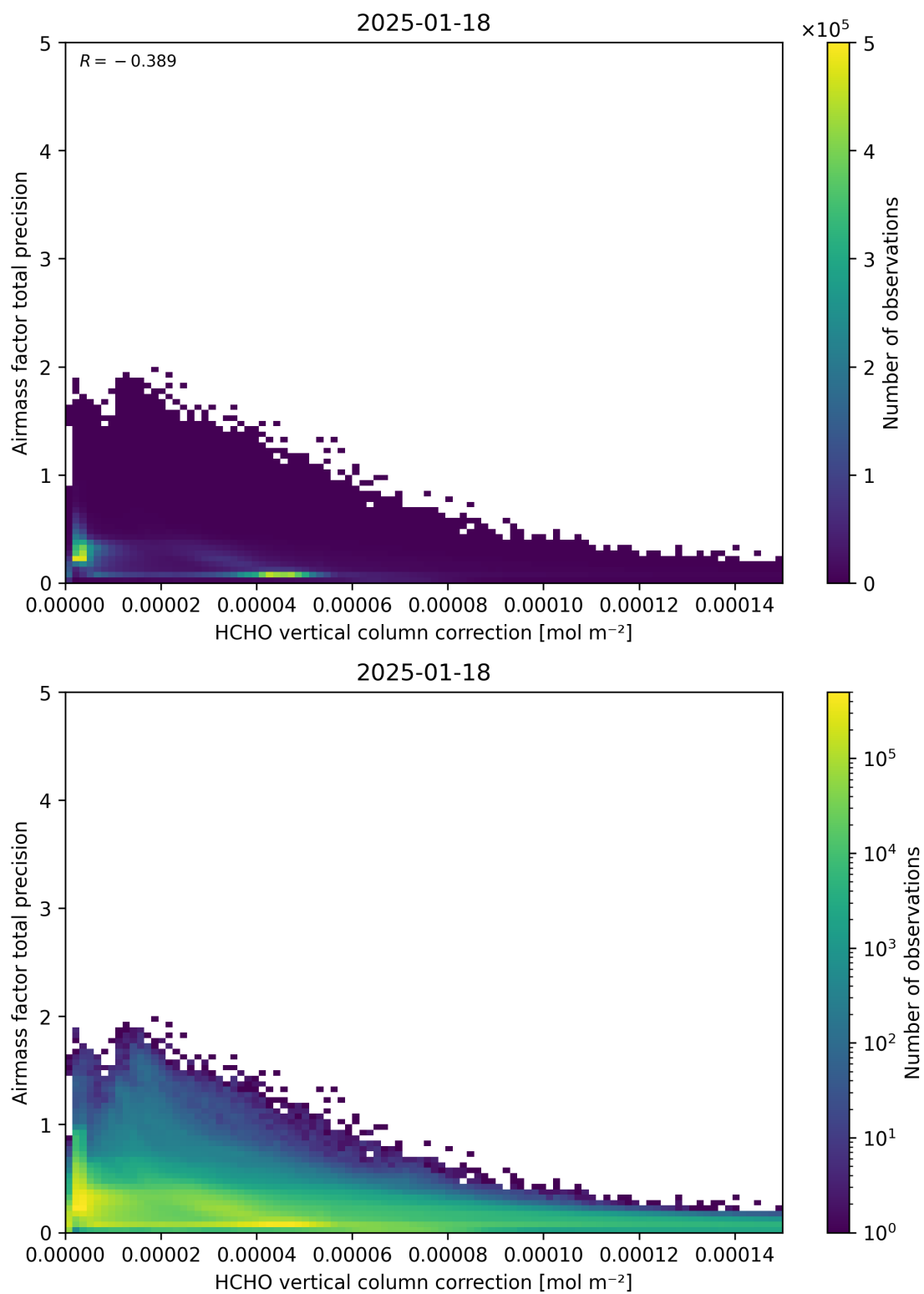
Figure 121: Scatter density plot of “HCHO vertical column correction” against “Airmass factor total precision” for 2025-01-17 to 2025-01-19.
