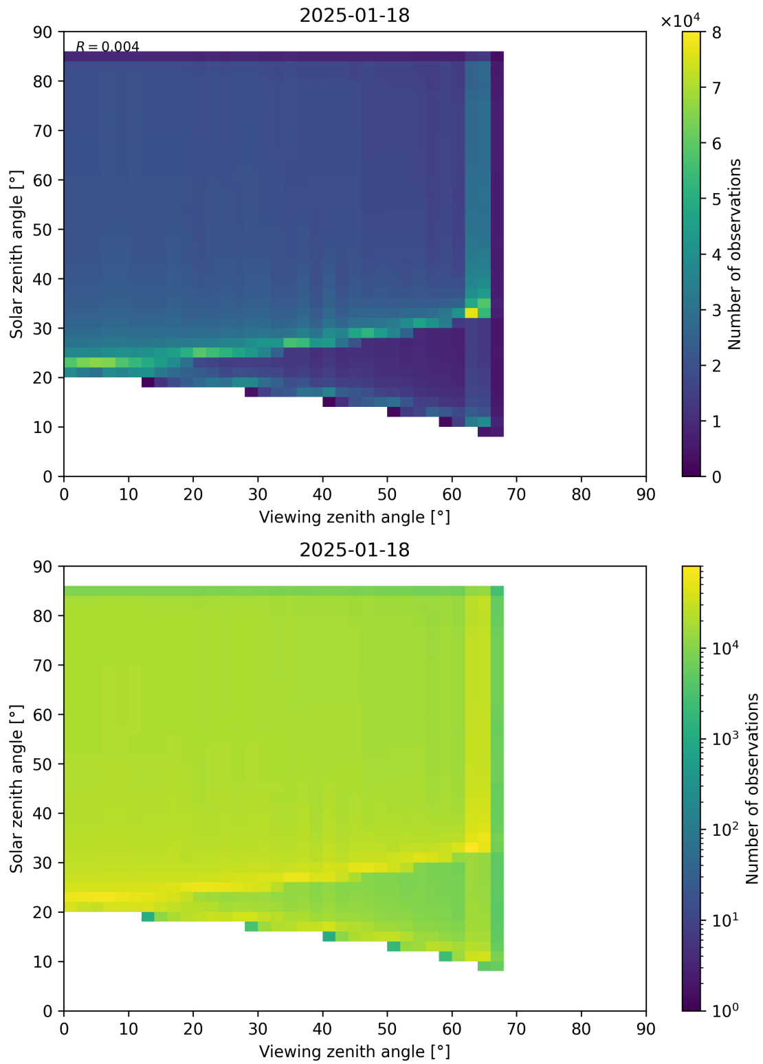
Figure 197: Scatter density plot of “Viewing zenith angle” against “Solar zenith angle” for 2025-01-17 to 2025-01-19.
