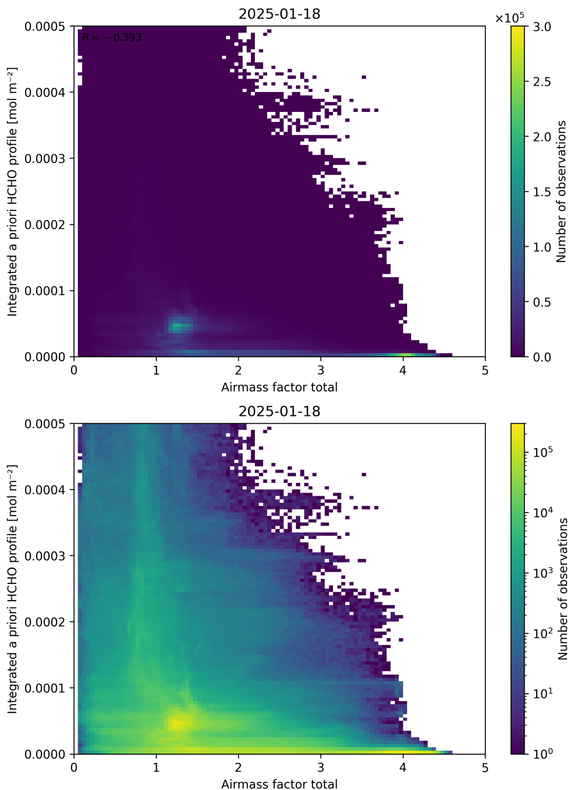
Figure 104: Scatter density plot of “Airmass factor total” against “Integrated a priori HCHO profile” for 2025-01-17 to 2025-01-19.
