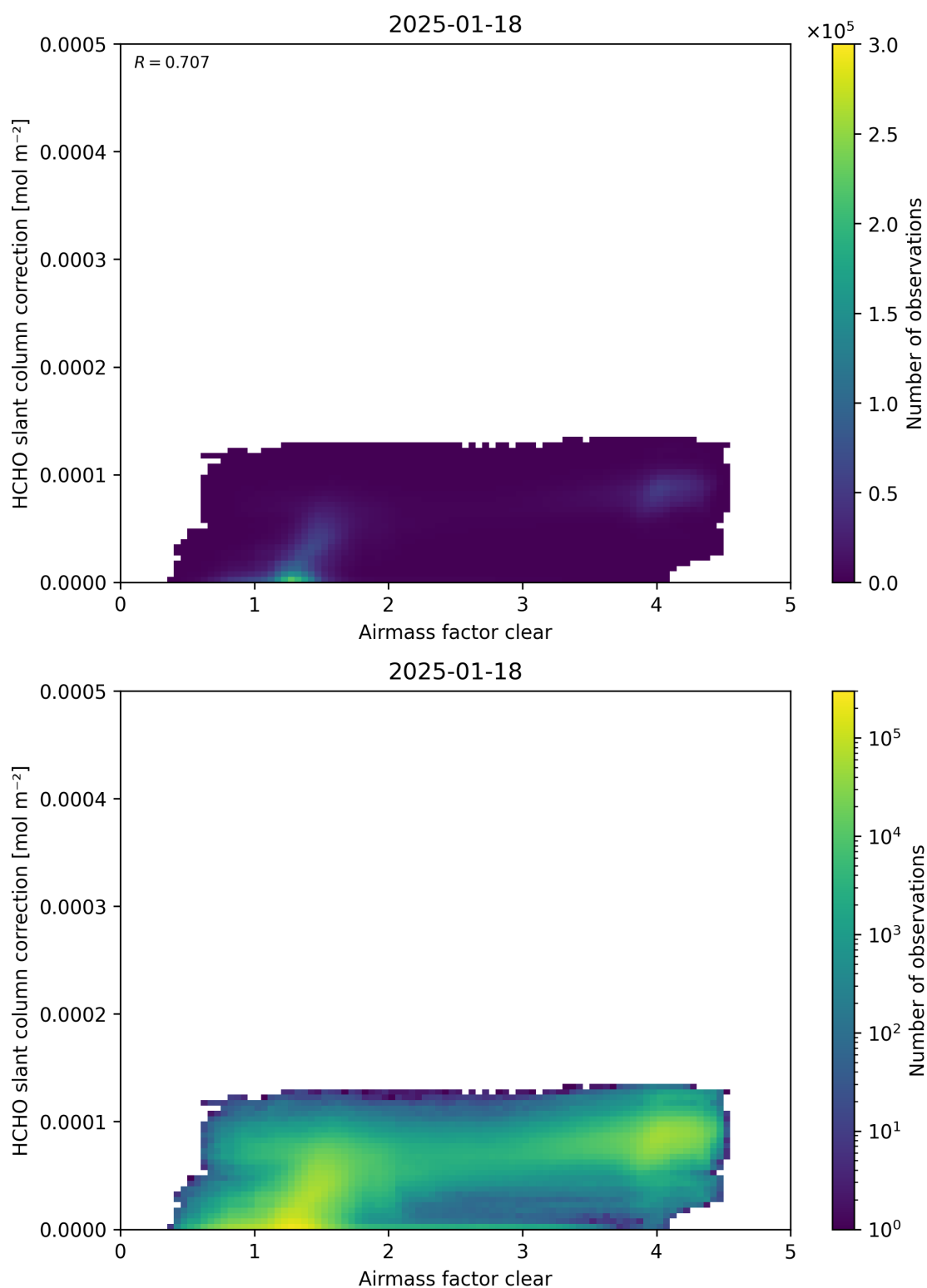
Figure 75: Scatter density plot of “Airmass factor clear” against “HCHO slant column correction” for 2025-01-17 to 2025-01-19.
