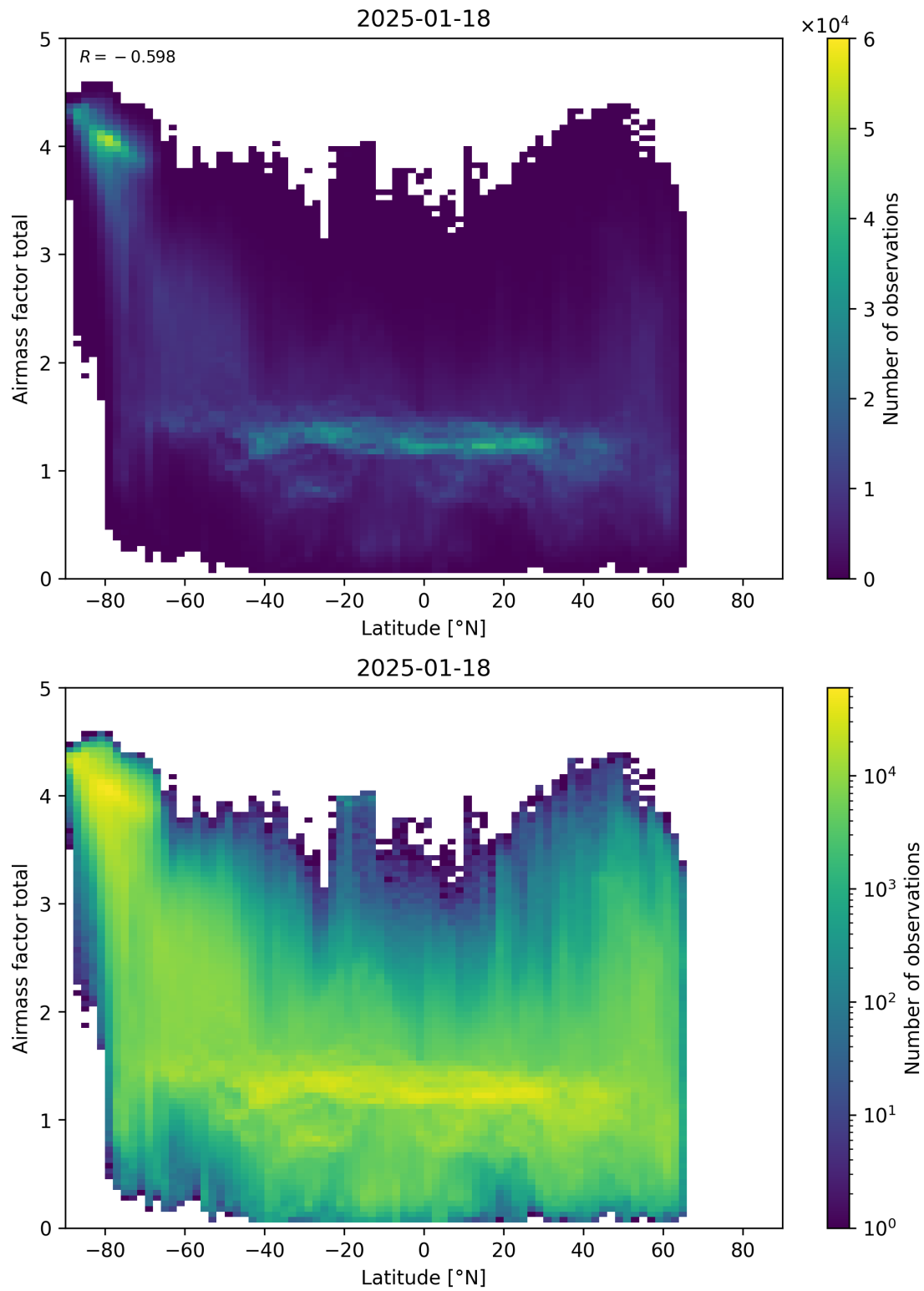
Figure 161: Scatter density plot of “Latitude” against “Airmass factor total” for 2025-01-17 to 2025-01-19.
