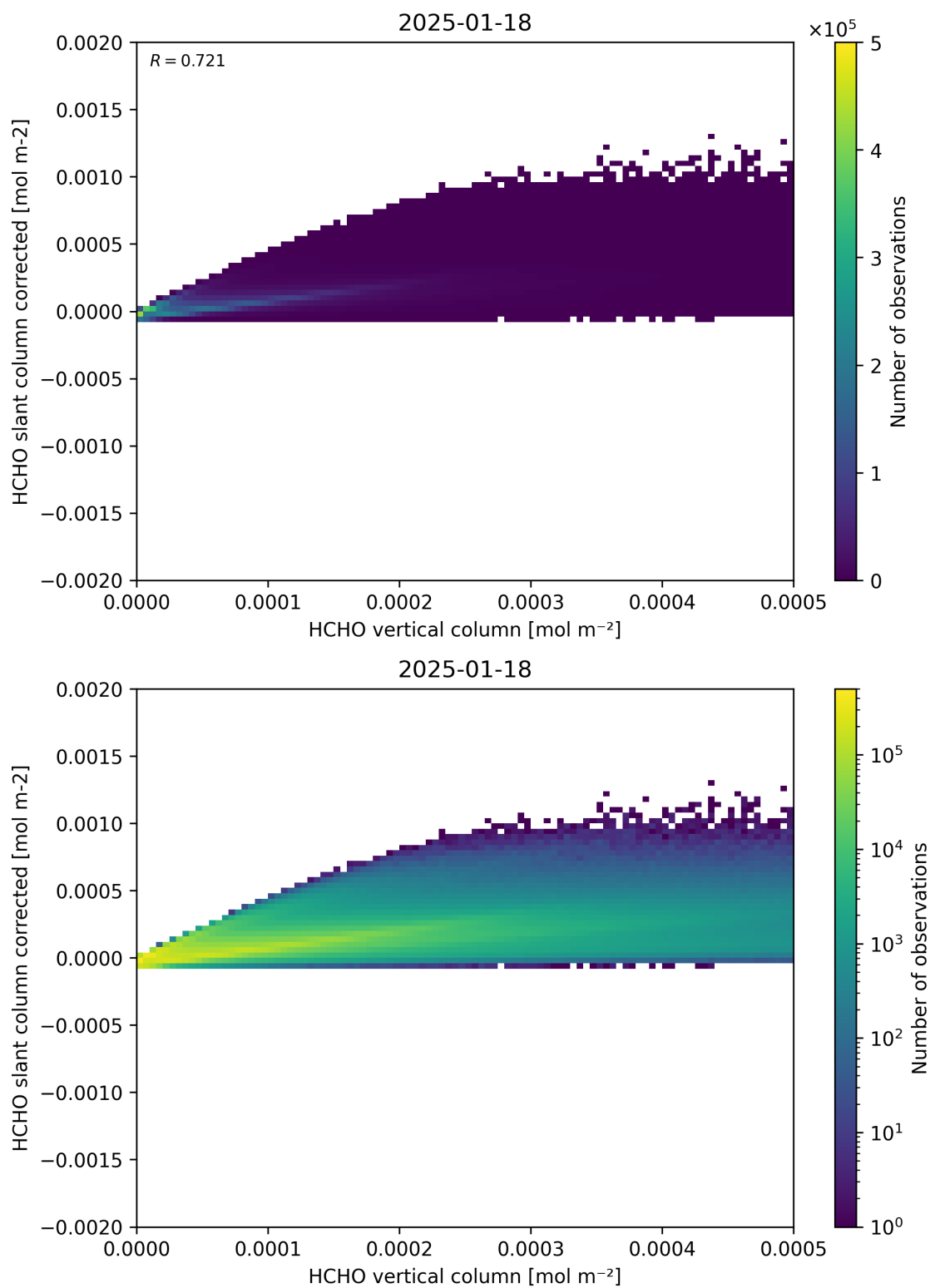
Figure 127: Scatter density plot of “HCHO vertical column” against “HCHO slant column corrected” for 2025-01-17 to 2025-01-19.
