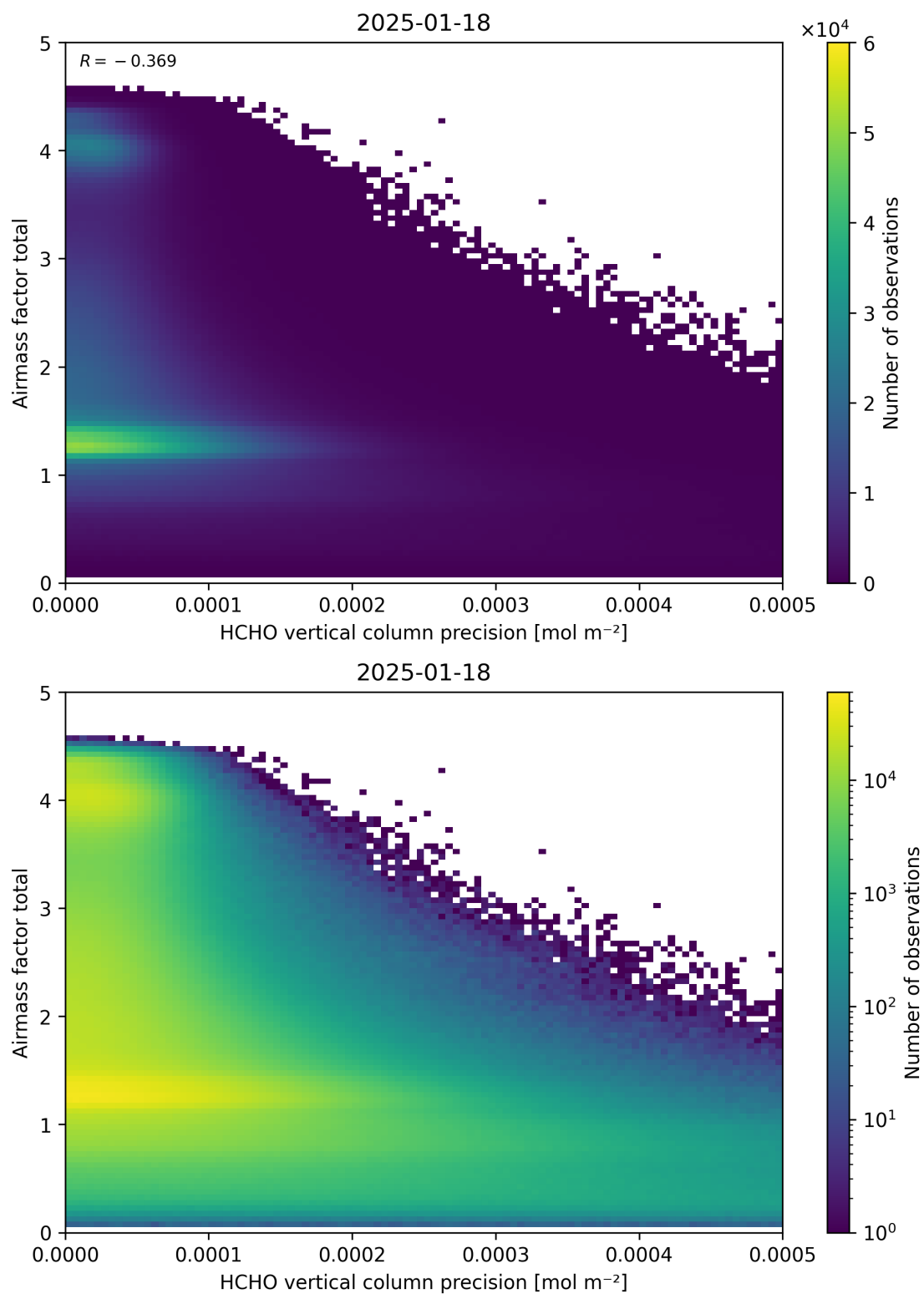
Figure 144: Scatter density plot of “HCHO vertical column precision” against “Airmass factor total” for 2025-01-17 to 2025-01-19.
