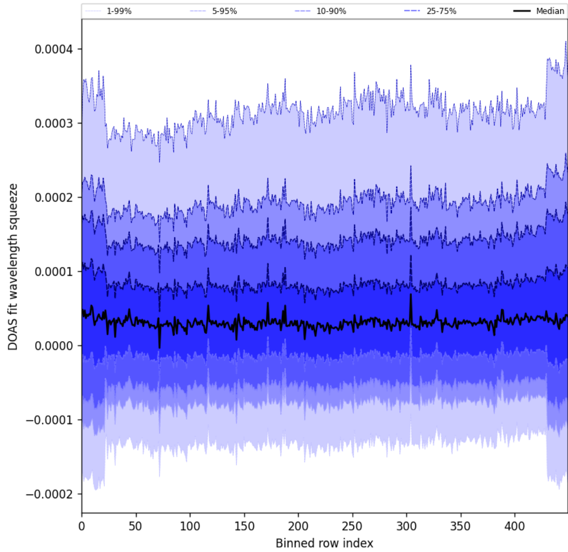
Figure 59: Along track statistics of “DOAS fit wavelength squeeze” for 2025-01-17 to 2025-01-19
