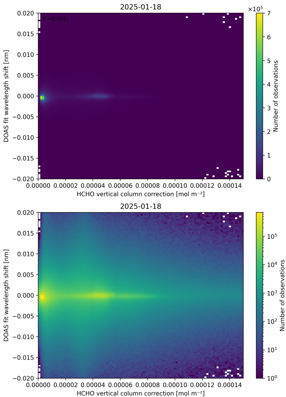
Figure 113: Scatter density plot of “HCHO vertical column correction” against “DOAS fit wavelength shift” for 2025-01-17 to 2025-01-19.
