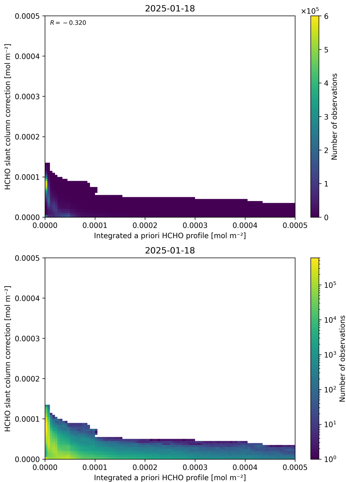
Figure 152: Scatter density plot of “Integrated a priori HCHO profile” against “HCHO slant column correction” for 2025-01-17 to 2025-01-19.
