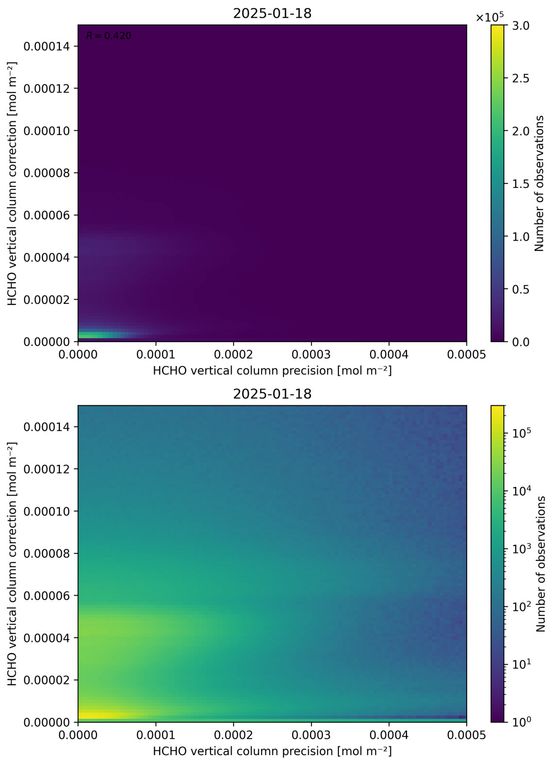
Figure 146: Scatter density plot of “HCHO vertical column precision” against “HCHO vertical column correction” for 2025-01-17 to 2025-01-19.
