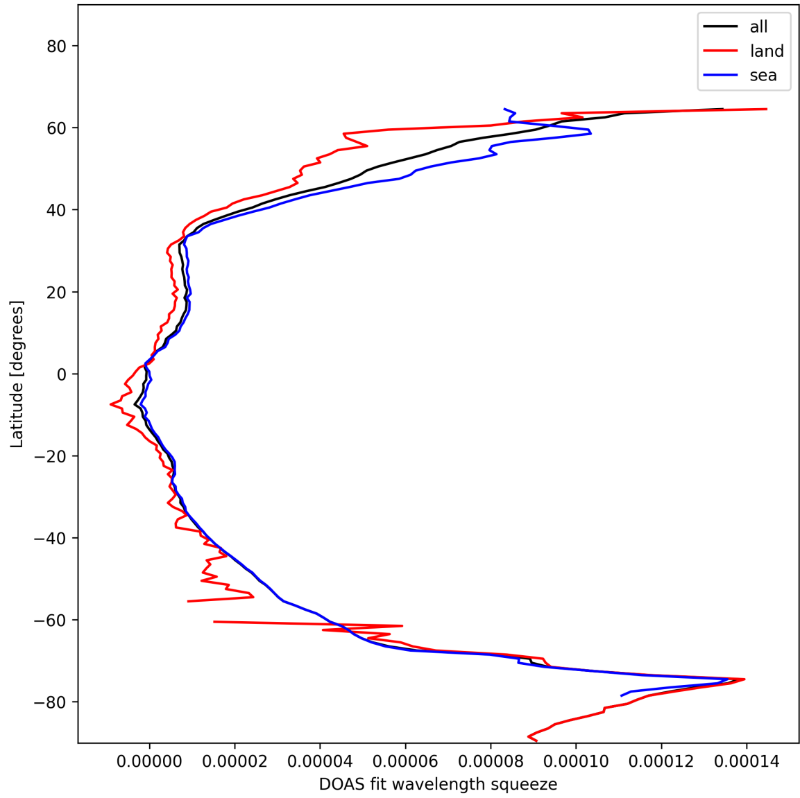
Figure 31: Zonal average of “DOAS fit wavelength squeeze” for 2025-01-17 to 2025-01-19.
