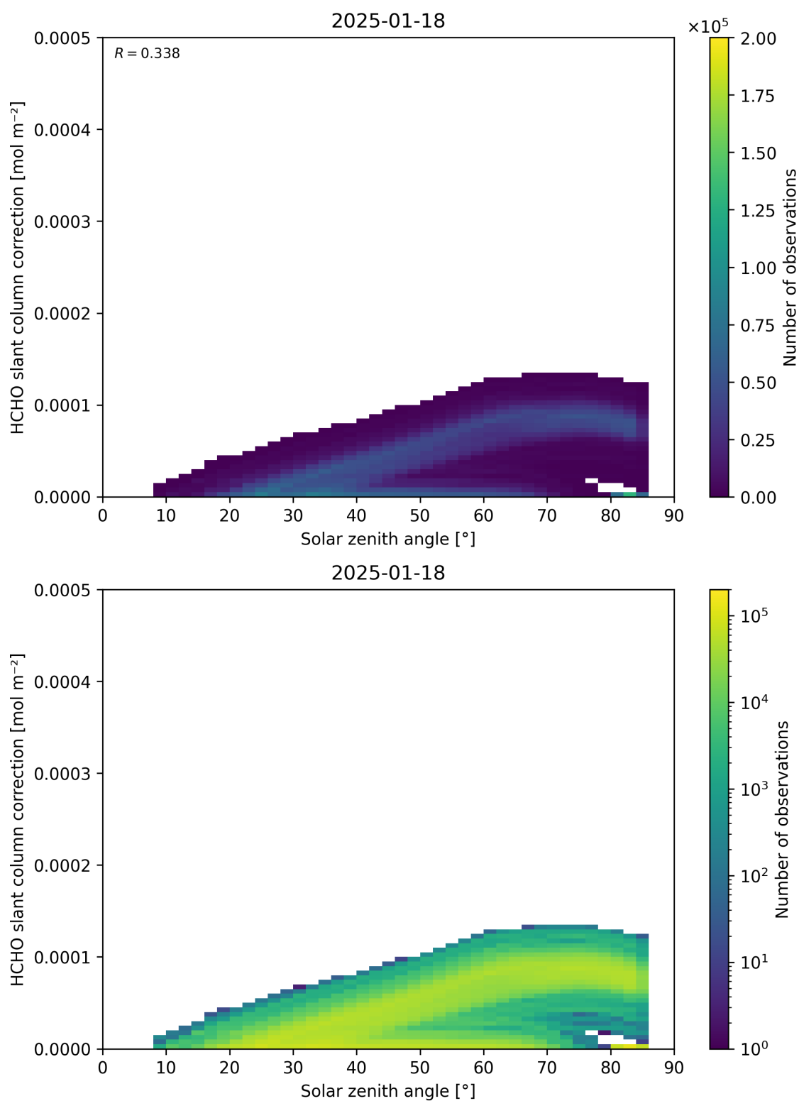
Figure 172: Scatter density plot of “Solar zenith angle” against “HCHO slant column correction” for 2025-01-17 to 2025-01-19.
