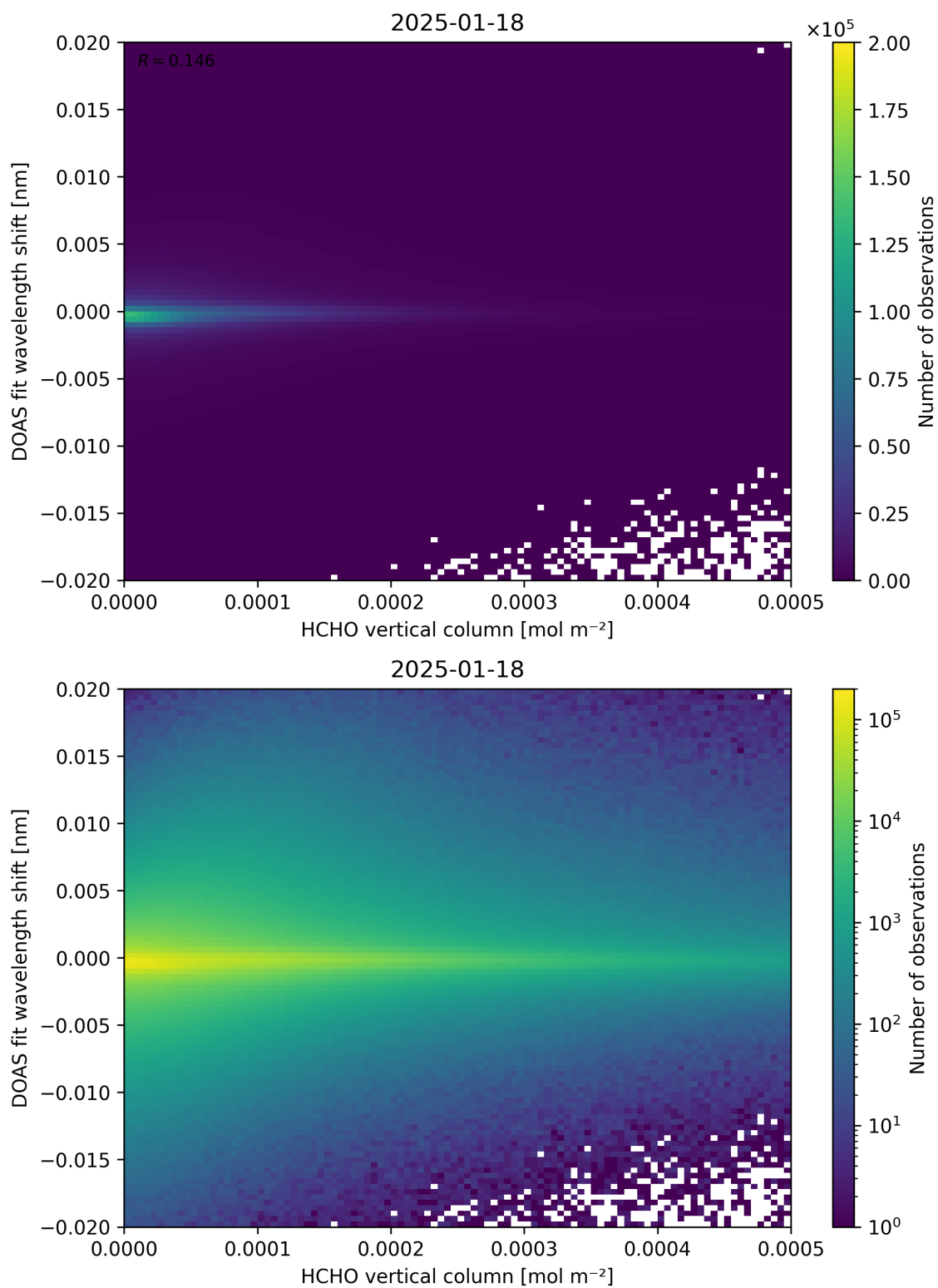
Figure 124: Scatter density plot of “HCHO vertical column” against “DOAS fit wavelength shift” for 2025-01-17 to 2025-01-19.
