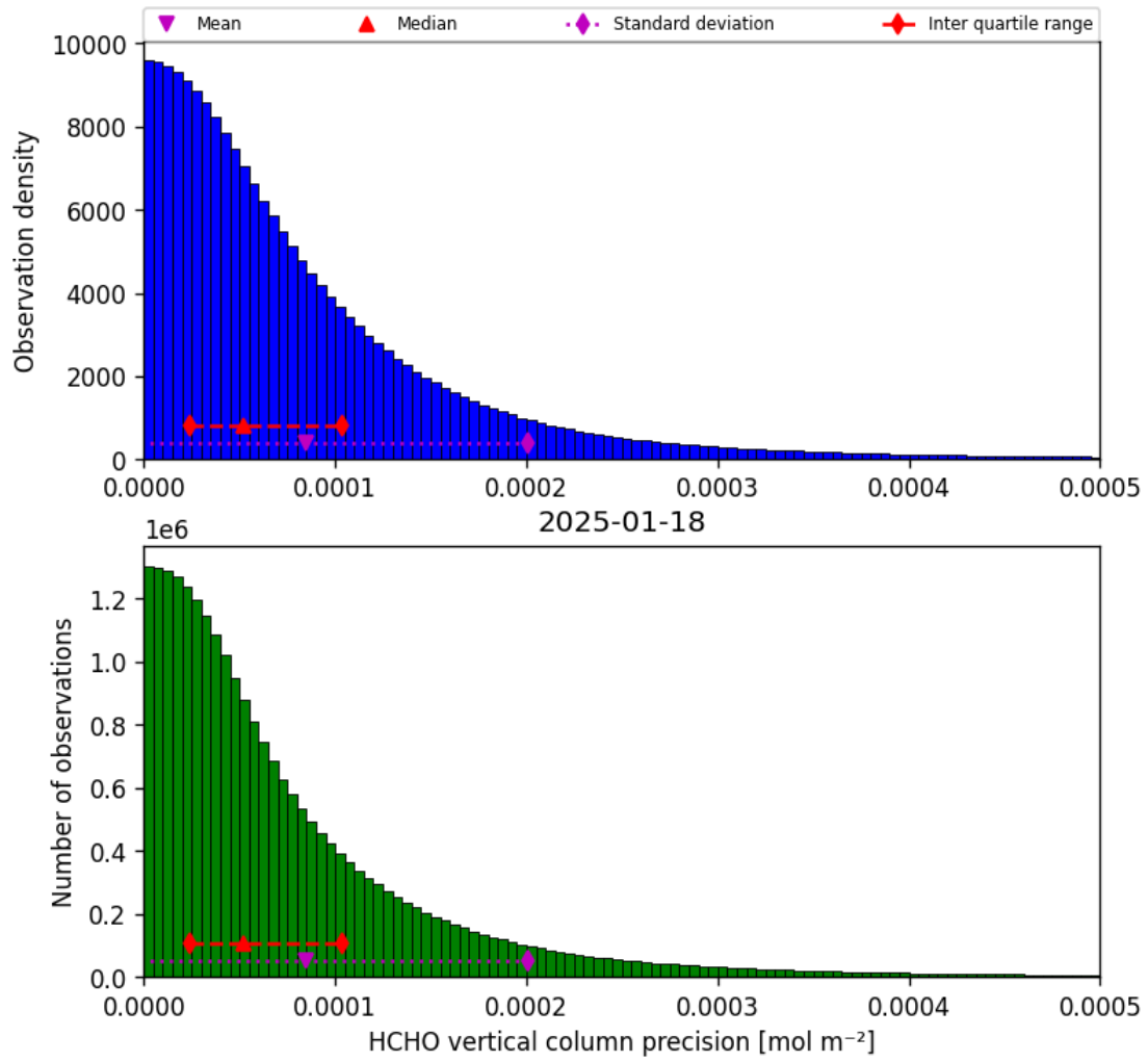
Figure 36: Histogram of “HCHO vertical column precision” for 2025-01-17 to 2025-01-19
