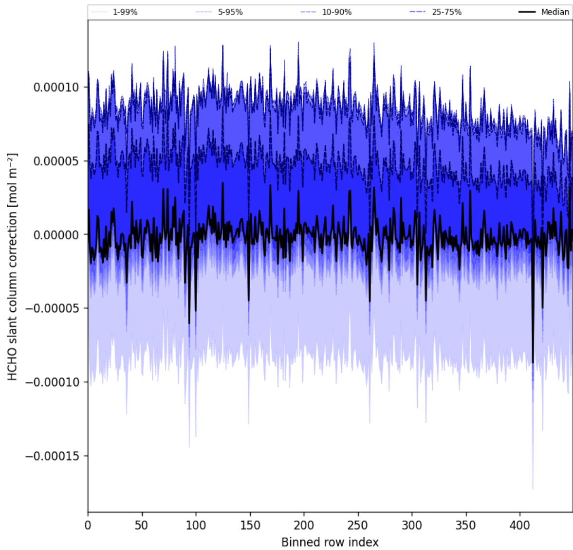
Figure 61: Along track statistics of “HCHO slant column correction” for 2025-01-17 to 2025-01-19
