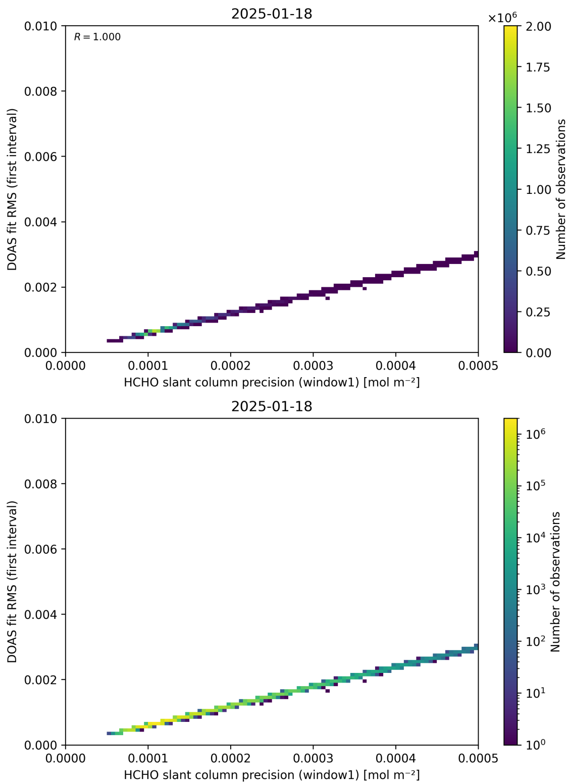
Figure 88: Scatter density plot of “HCHO slant column precision (window1)” against “DOAS fit RMS (first interval)” for 2025-01-17 to 2025-01-19.
