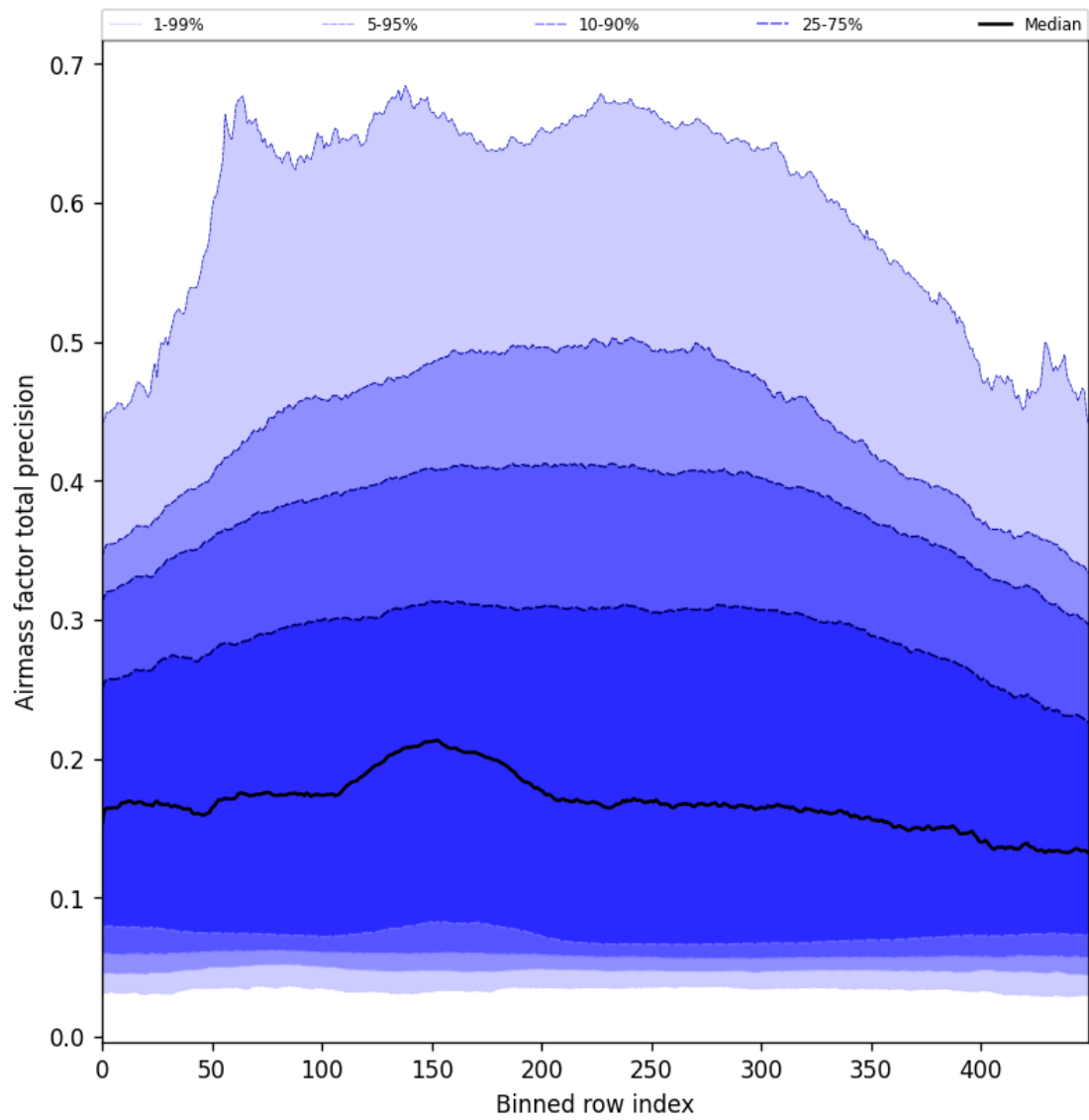
Figure 55: Along track statistics of “Airmass factor total precision” for 2025-01-17 to 2025-01-19
