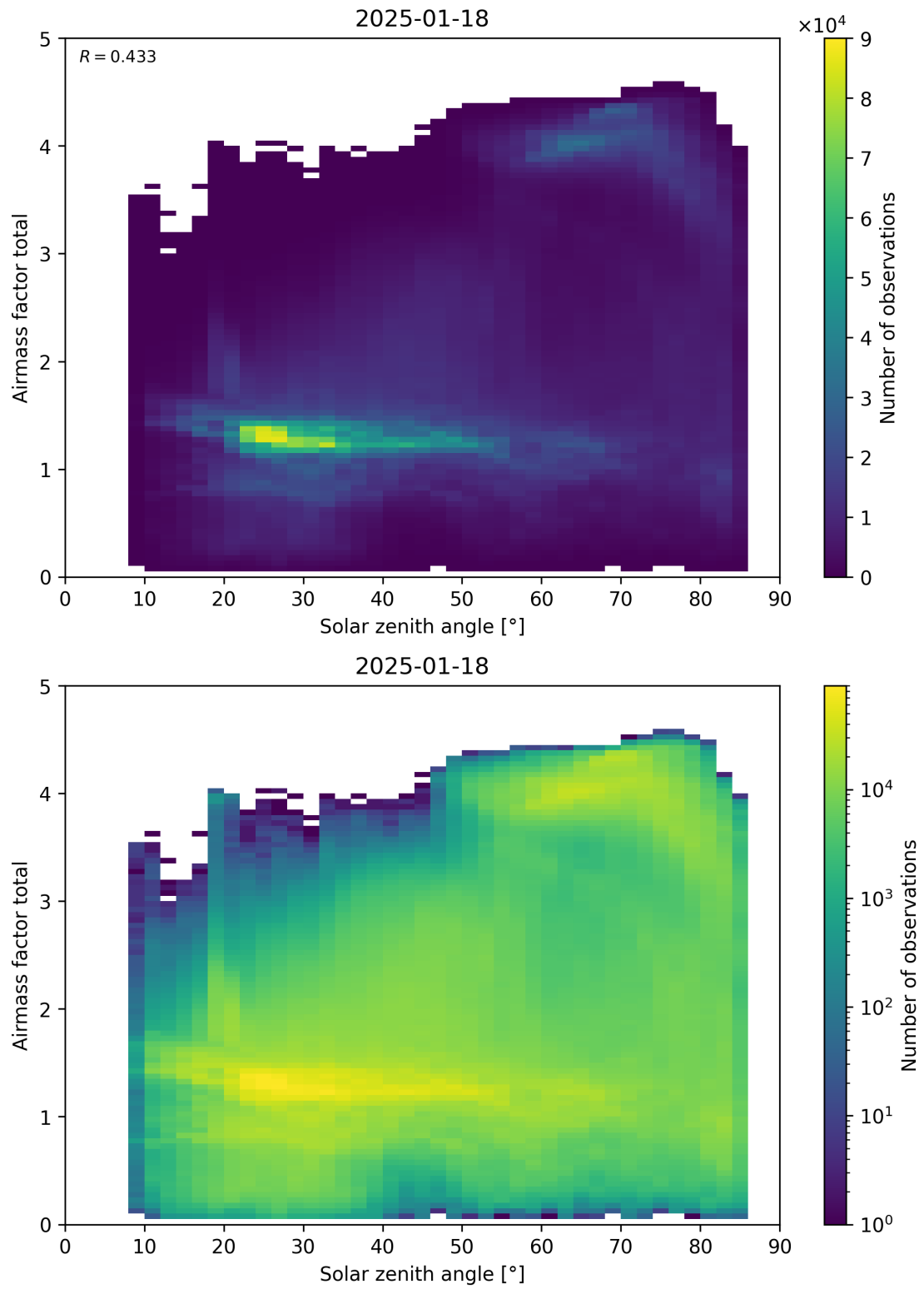
Figure 175: Scatter density plot of “Solar zenith angle” against “Airmass factor total” for 2025-01-17 to 2025-01-19.
