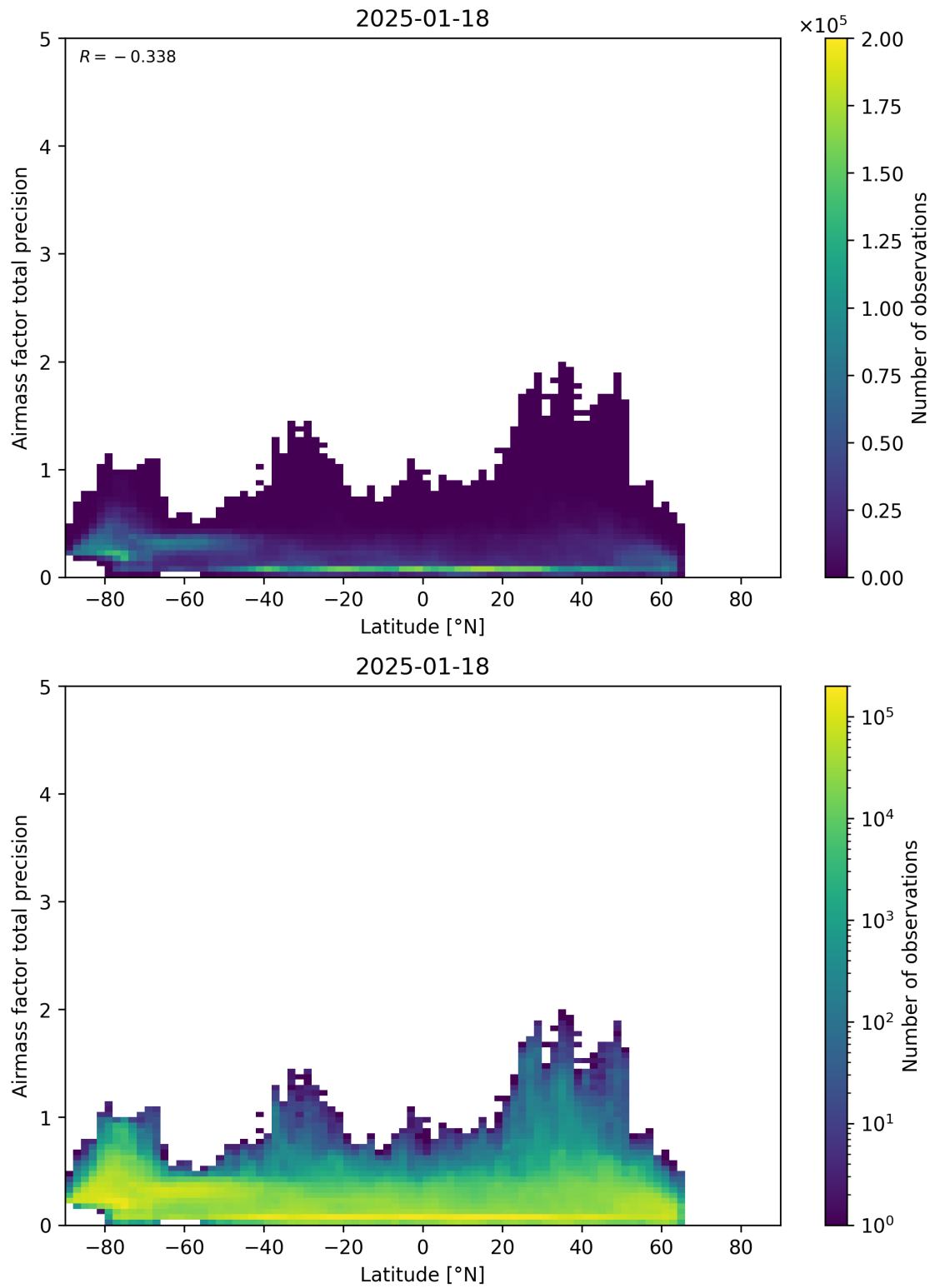
Figure 162: Scatter density plot of “Latitude” against “Airmass factor total precision” for 2025-01-17 to 2025-01-19.
