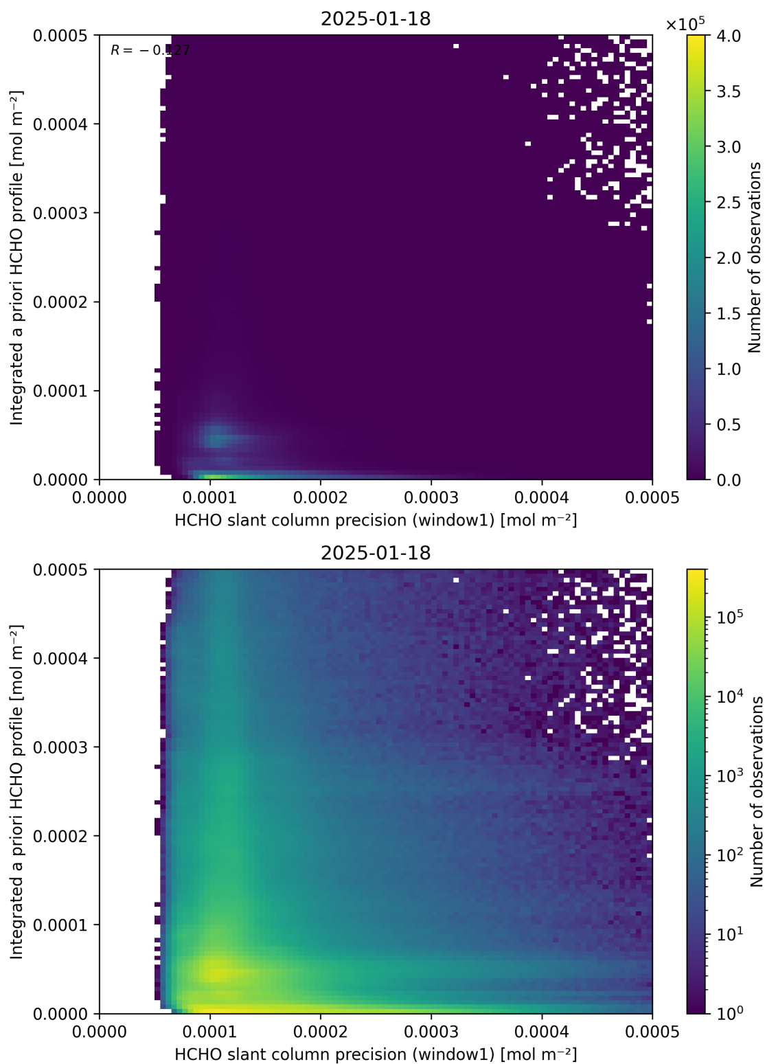
Figure 96: Scatter density plot of “HCHO slant column precision (window1)” against “Integrated a priori HCHO profile” for 2025-01-17 to 2025-01-19.
