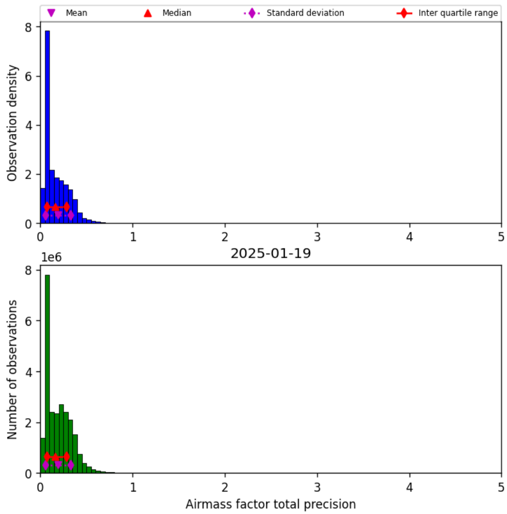
Figure 41: Histogram of “Airmass factor total precision” for 2025-01-18 to 2025-01-20
