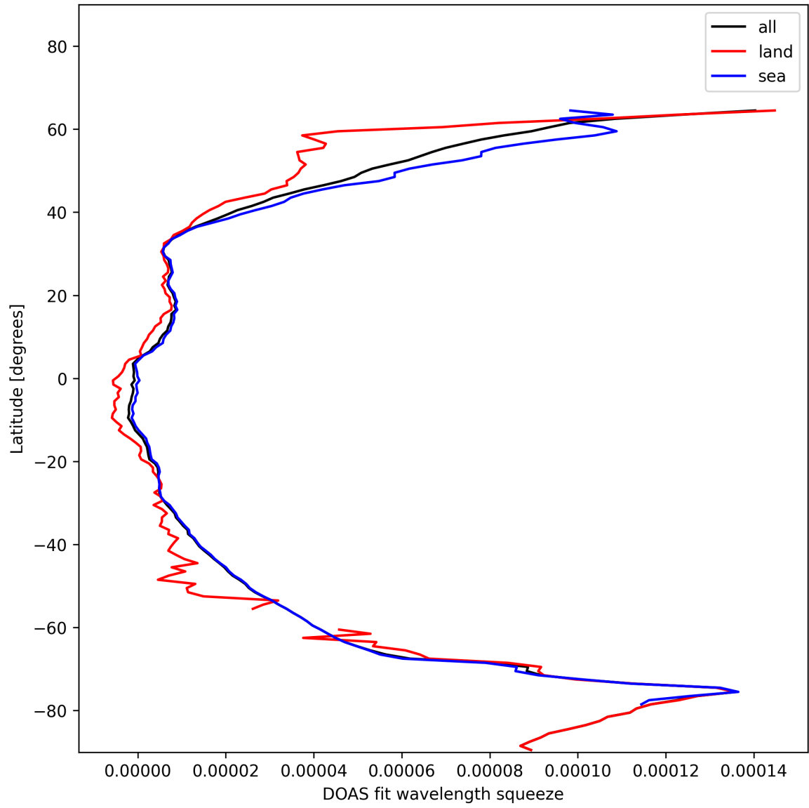
Figure 31: Zonal average of “DOAS fit wavelength squeeze” for 2025-01-18 to 2025-01-20.
