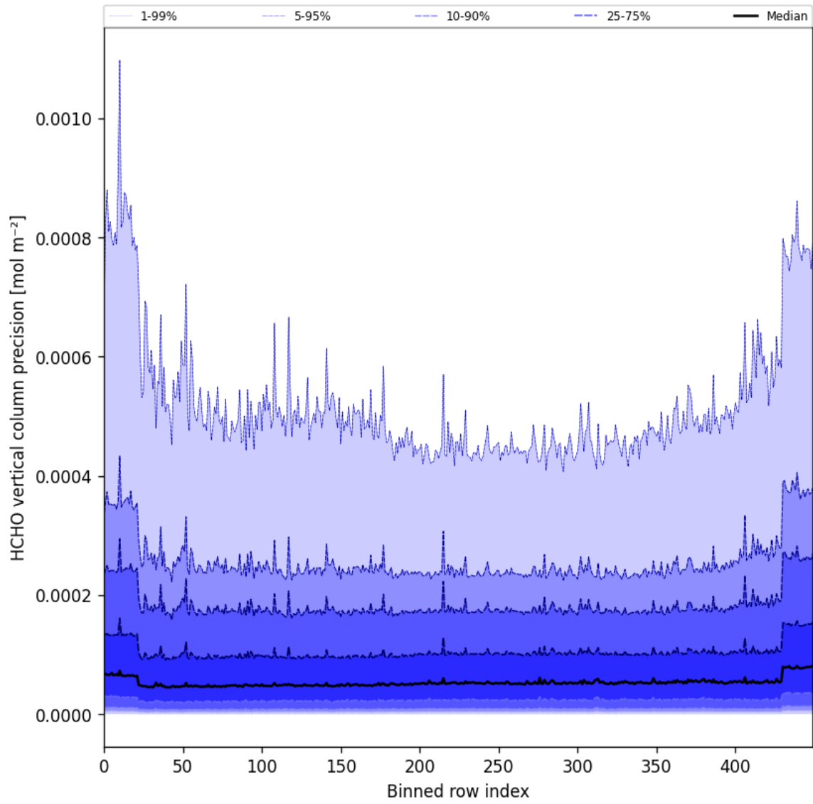
Figure 50: Along track statistics of “HCHO vertical column precision” for 2025-01-18 to 2025-01-20
