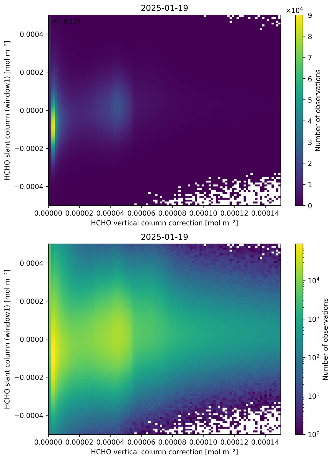
Figure 118: Scatter density plot of “HCHO vertical column correction” against “HCHO slant column (window1)” for 2025-01-18 to 2025-01-20.
