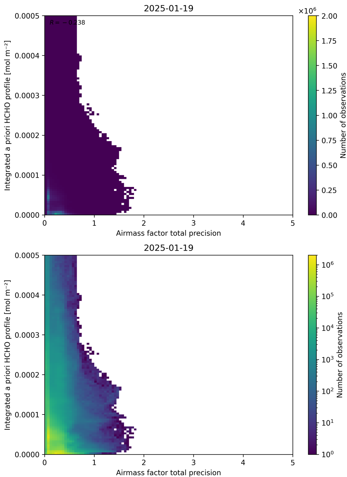
Figure 111: Scatter density plot of “Airmass factor total precision” against “Integrated a priori HCHO profile” for 2025-01-18 to 2025-01-20.
