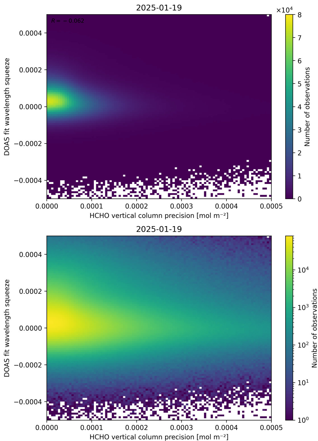
Figure 138: Scatter density plot of “HCHO vertical column precision” against “DOAS fit wavelength squeeze” for 2025-01-18 to 2025-01-20.
