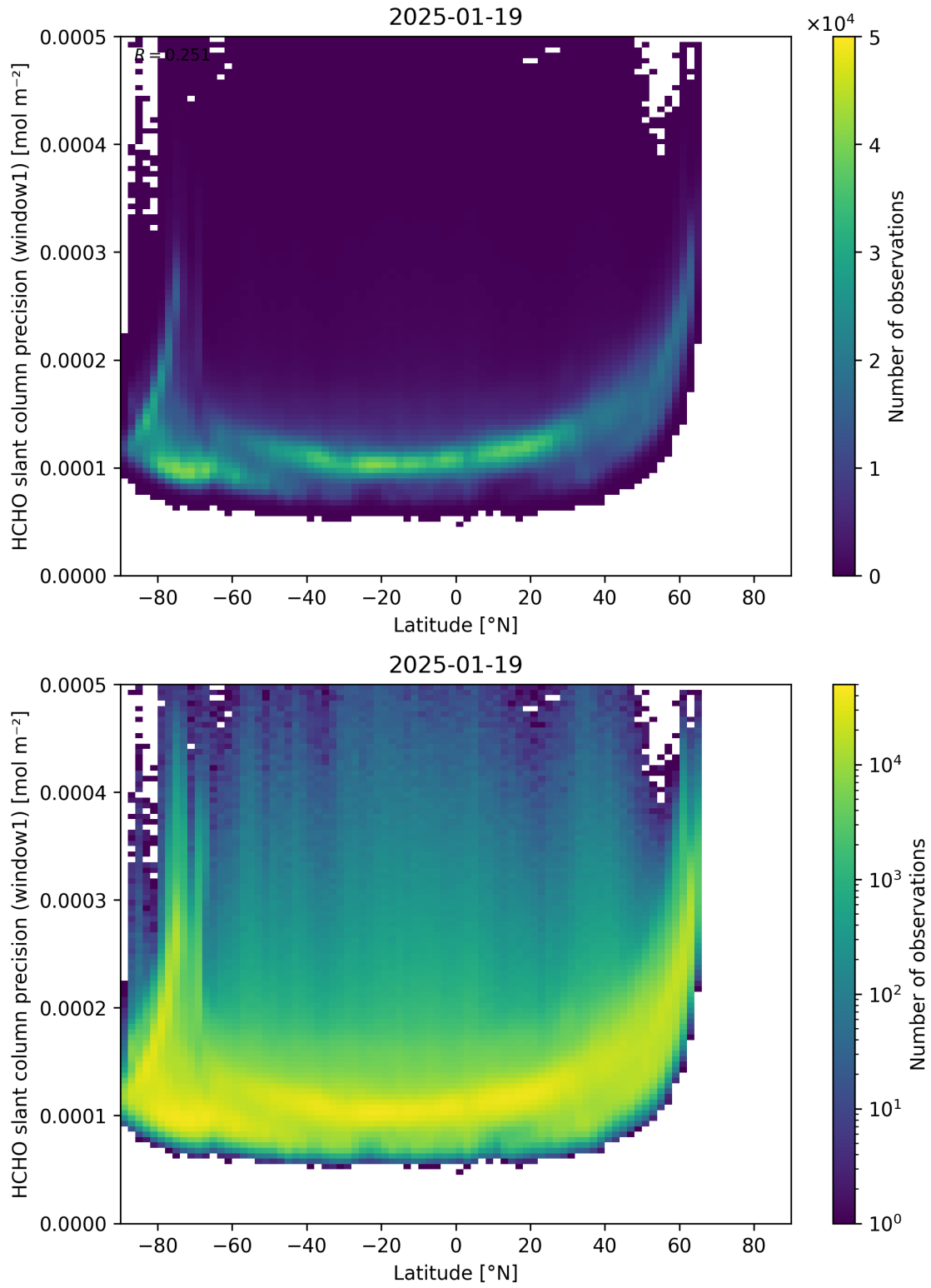
Figure 160: Scatter density plot of “Latitude” against “HCHO slant column precision (window1)” for 2025-01-18 to 2025-01-20.
