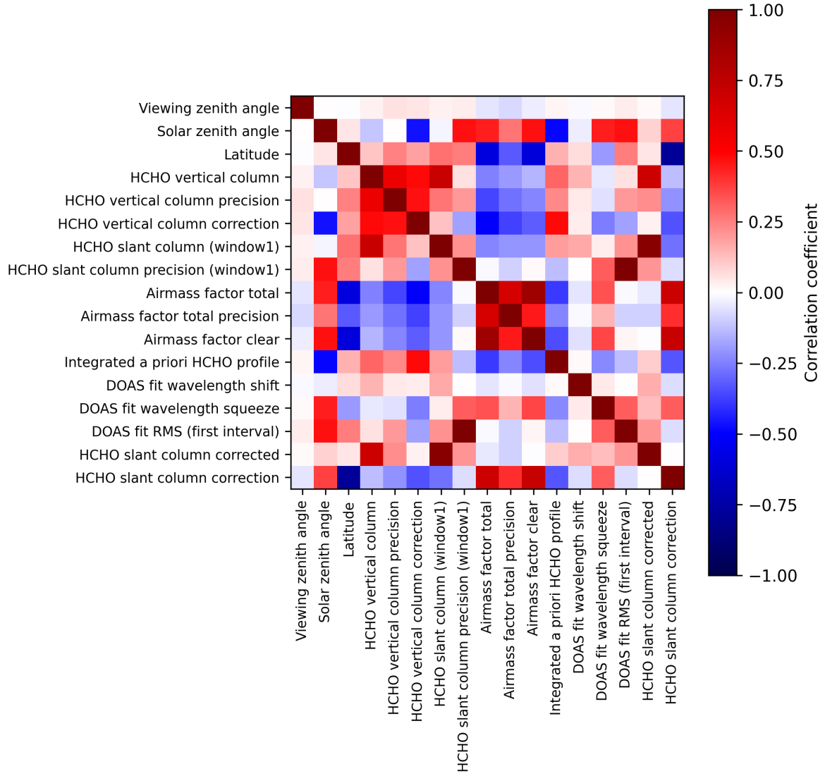
Figure 2: Map of correlation matrix for 2025-01-18 to 2025-01-20.
