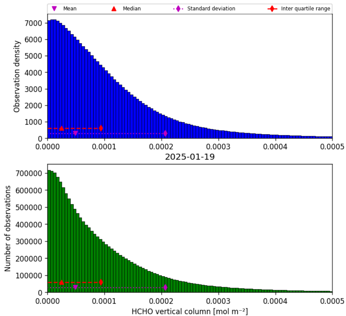
Figure 35: Histogram of “HCHO vertical column” for 2025-01-18 to 2025-01-20
