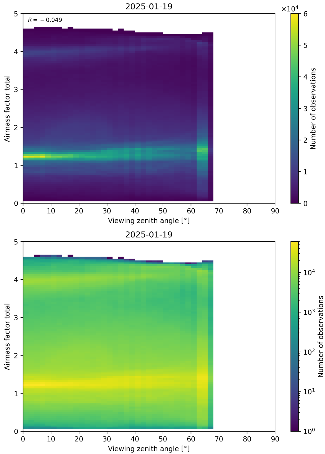
Figure 190: Scatter density plot of “Viewing zenith angle” against “Airmass factor total” for 2025-01-18 to 2025-01-20.
