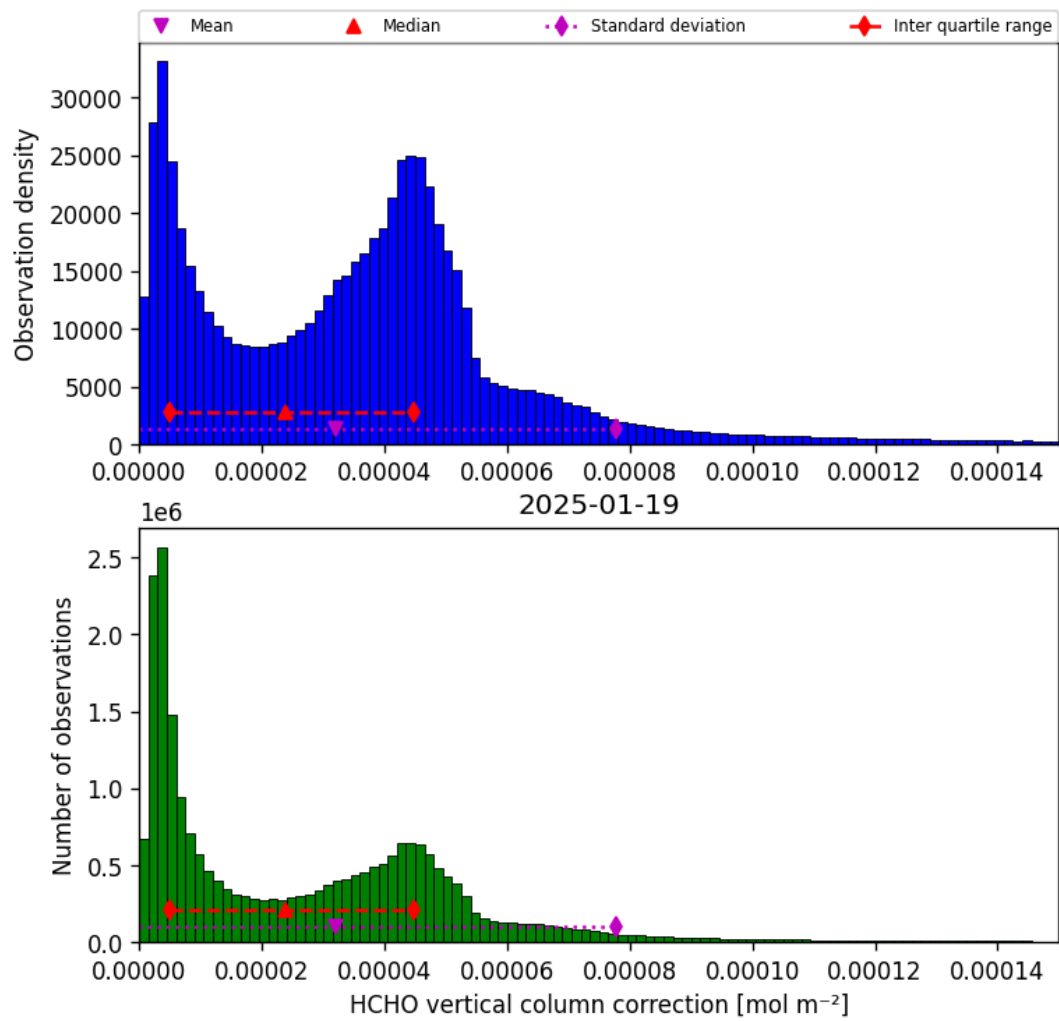
Figure 37: Histogram of “HCHO vertical column correction” for 2025-01-18 to 2025-01-20
