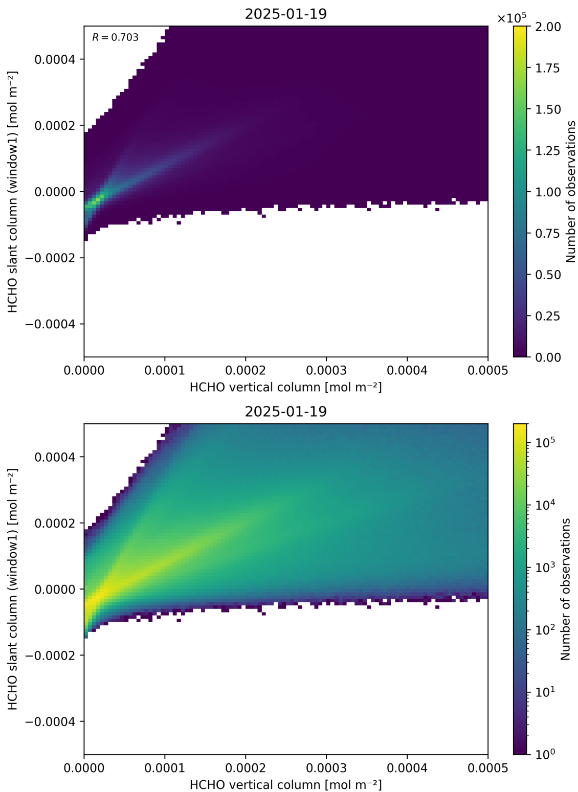
Figure 129: Scatter density plot of “HCHO vertical column” against “HCHO slant column (window1)” for 2025-01-18 to 2025-01-20.
