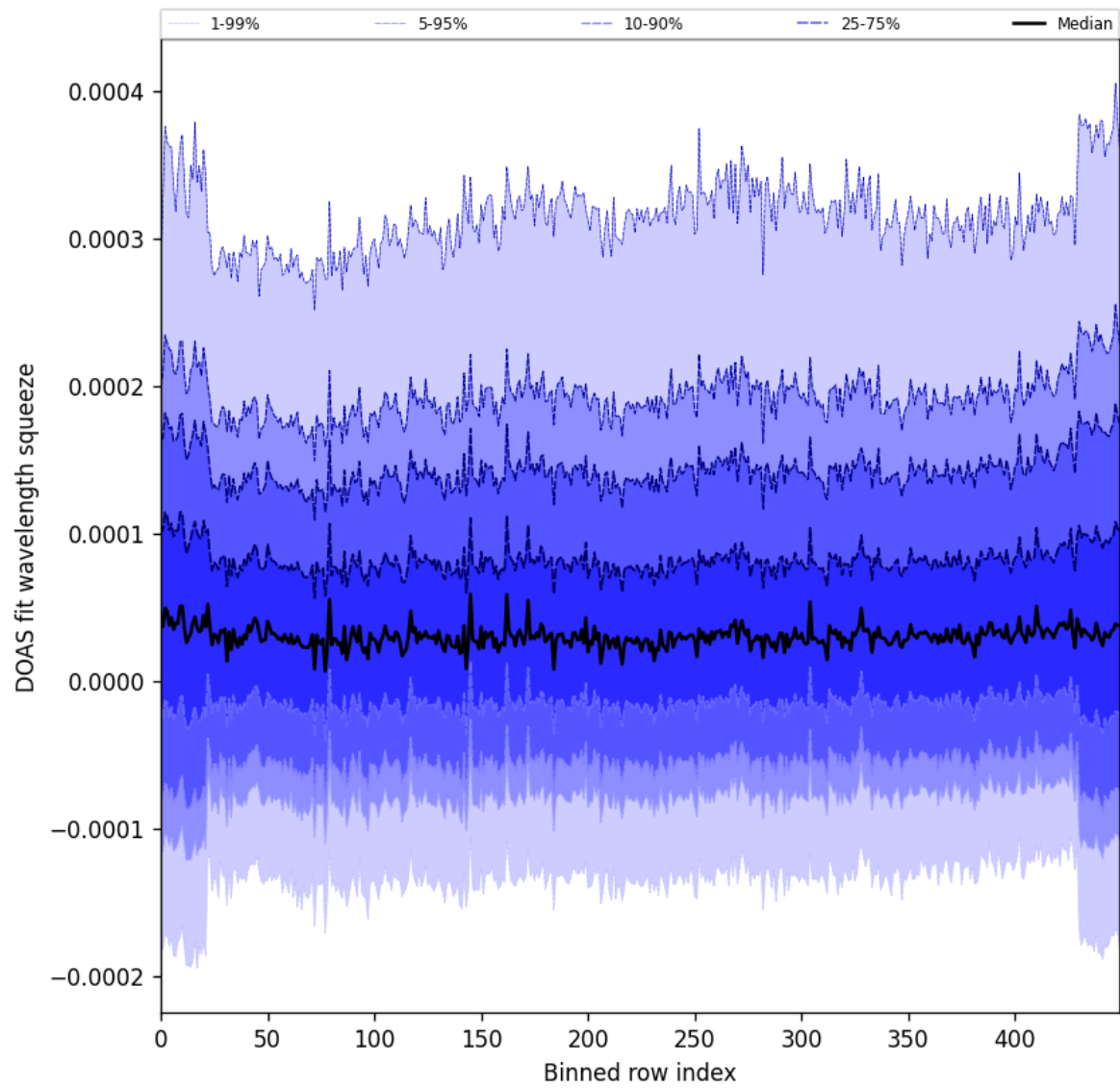
Figure 59: Along track statistics of “DOAS fit wavelength squeeze” for 2025-01-18 to 2025-01-20
