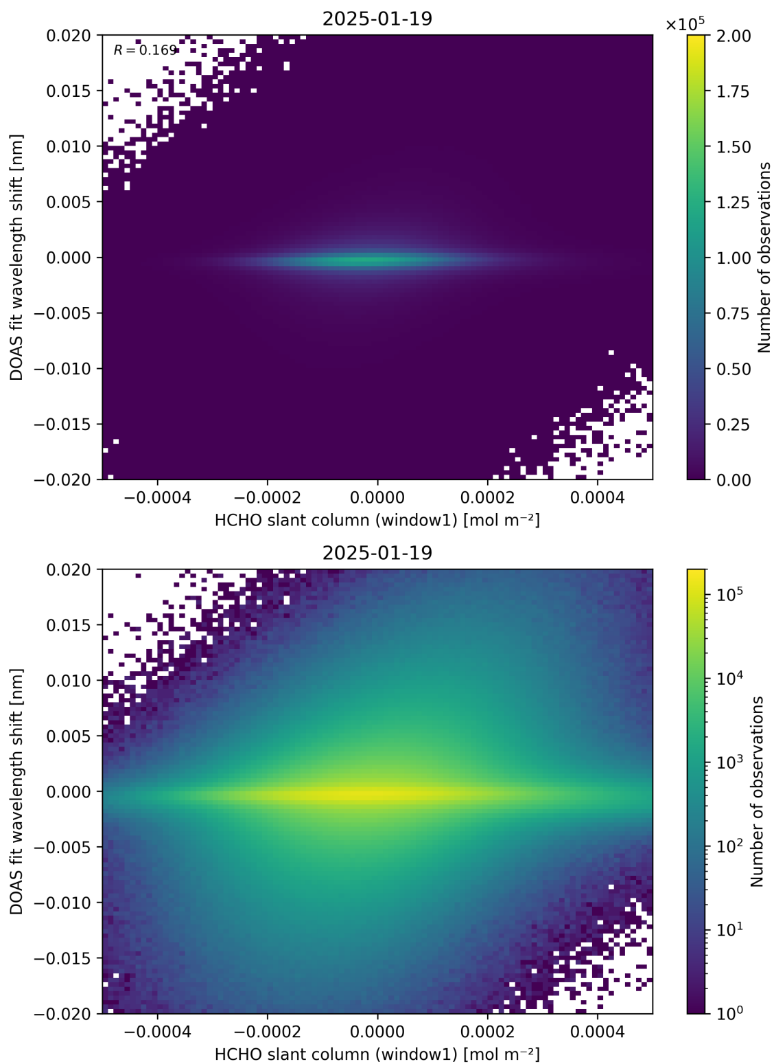
Figure 79: Scatter density plot of “HCHO slant column (window1)” against “DOAS fit wavelength shift” for 2025-01-18 to 2025-01-20.
