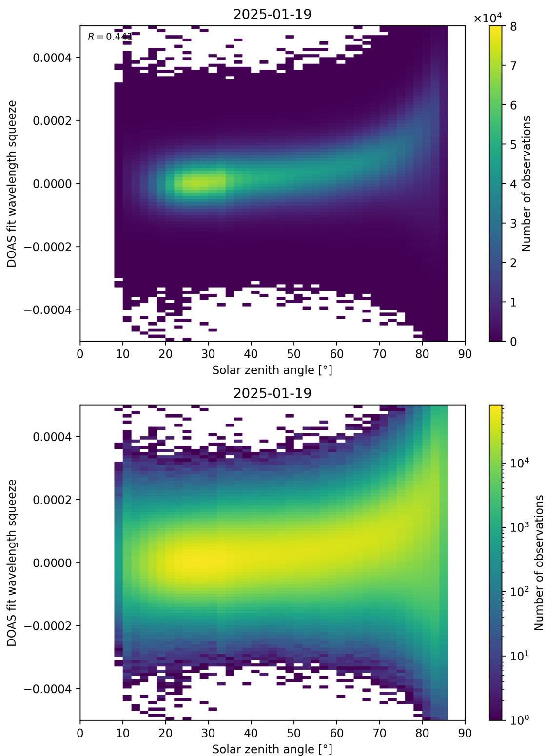
Figure 169: Scatter density plot of “Solar zenith angle” against “DOAS fit wavelength squeeze” for 2025-01-18 to 2025-01-20.
