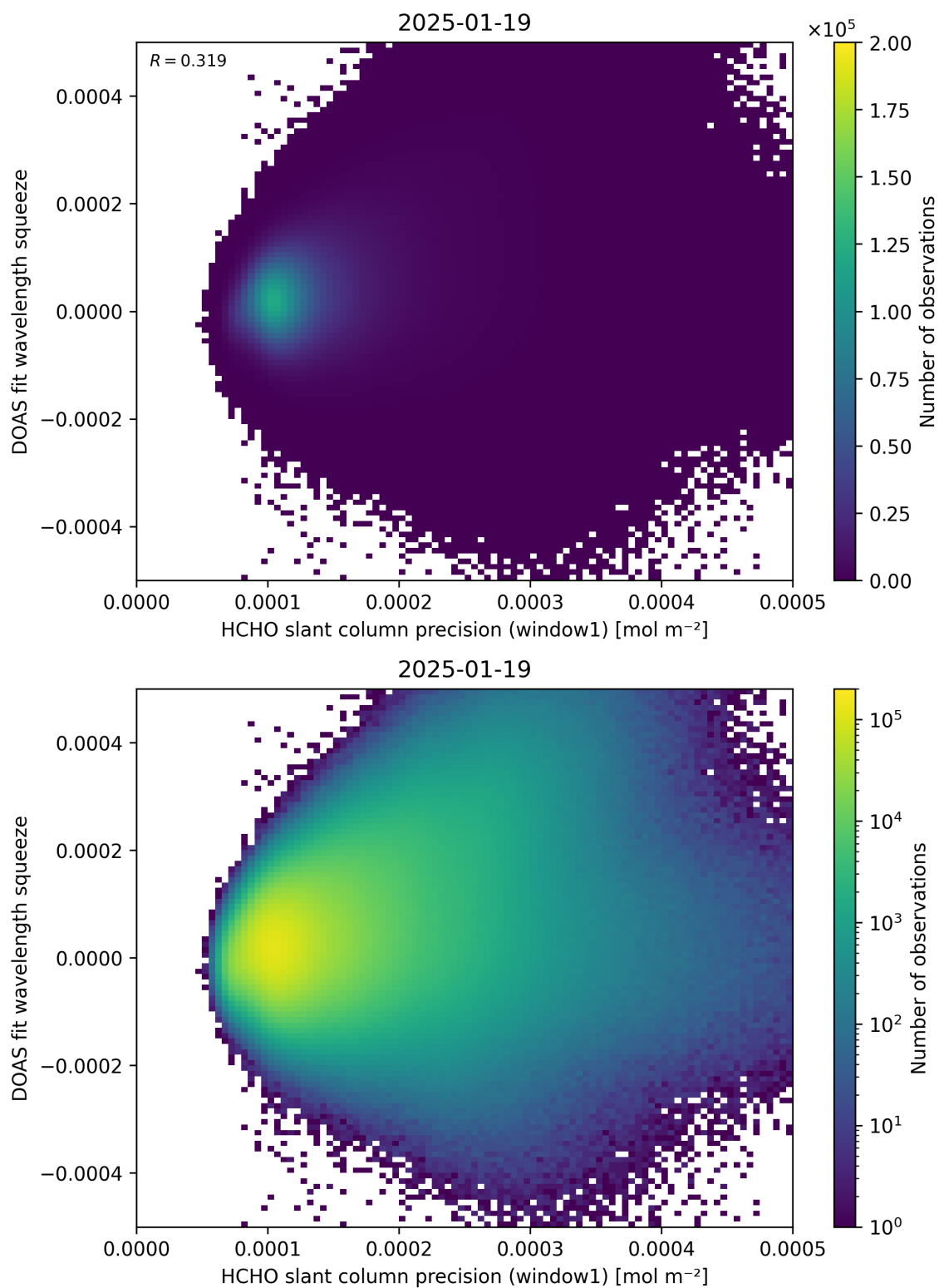
Figure 90: Scatter density plot of “HCHO slant column precision (window1)” against “DOAS fit wavelength squeeze” for 2025-01-18 to 2025-01-20.
