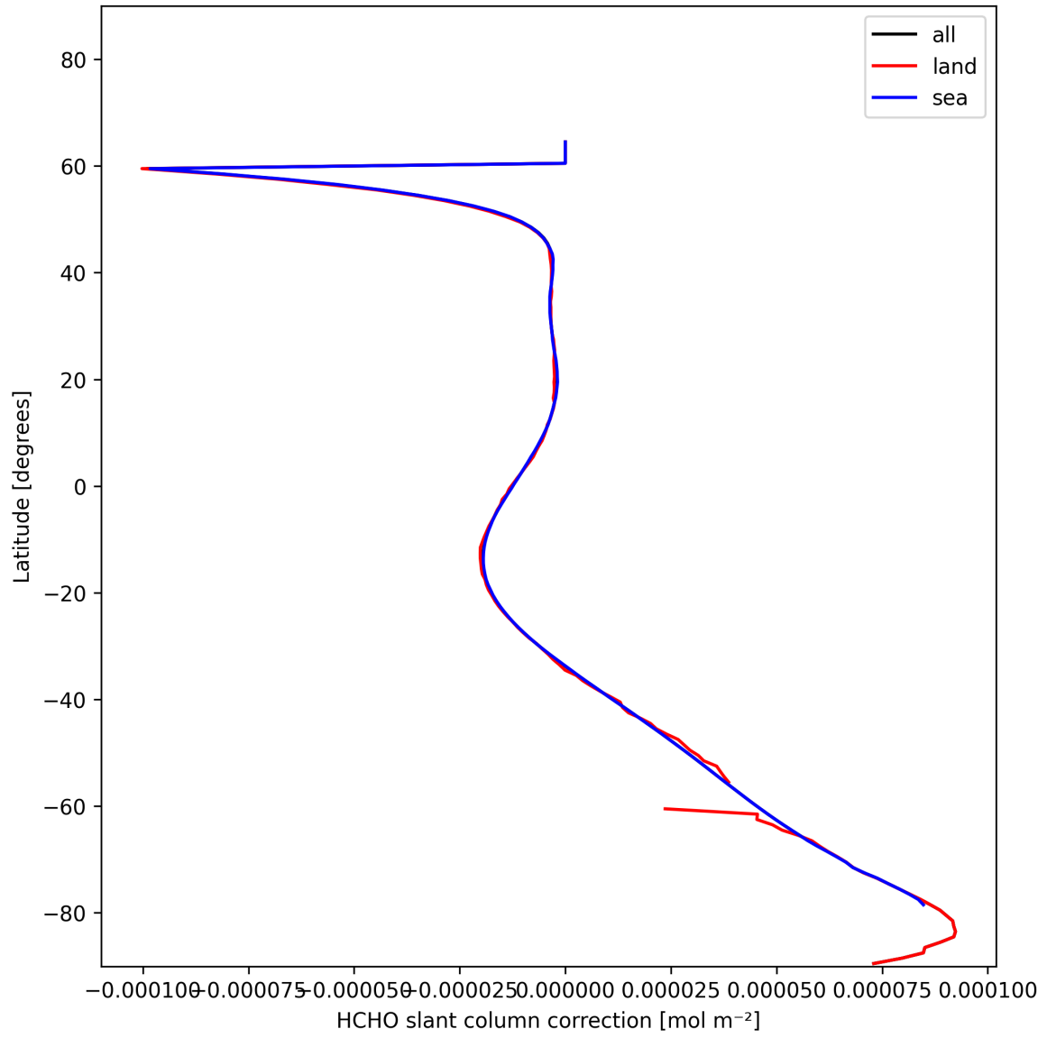
Figure 33: Zonal average of “HCHO slant column correction” for 2025-01-18 to 2025-01-20.
