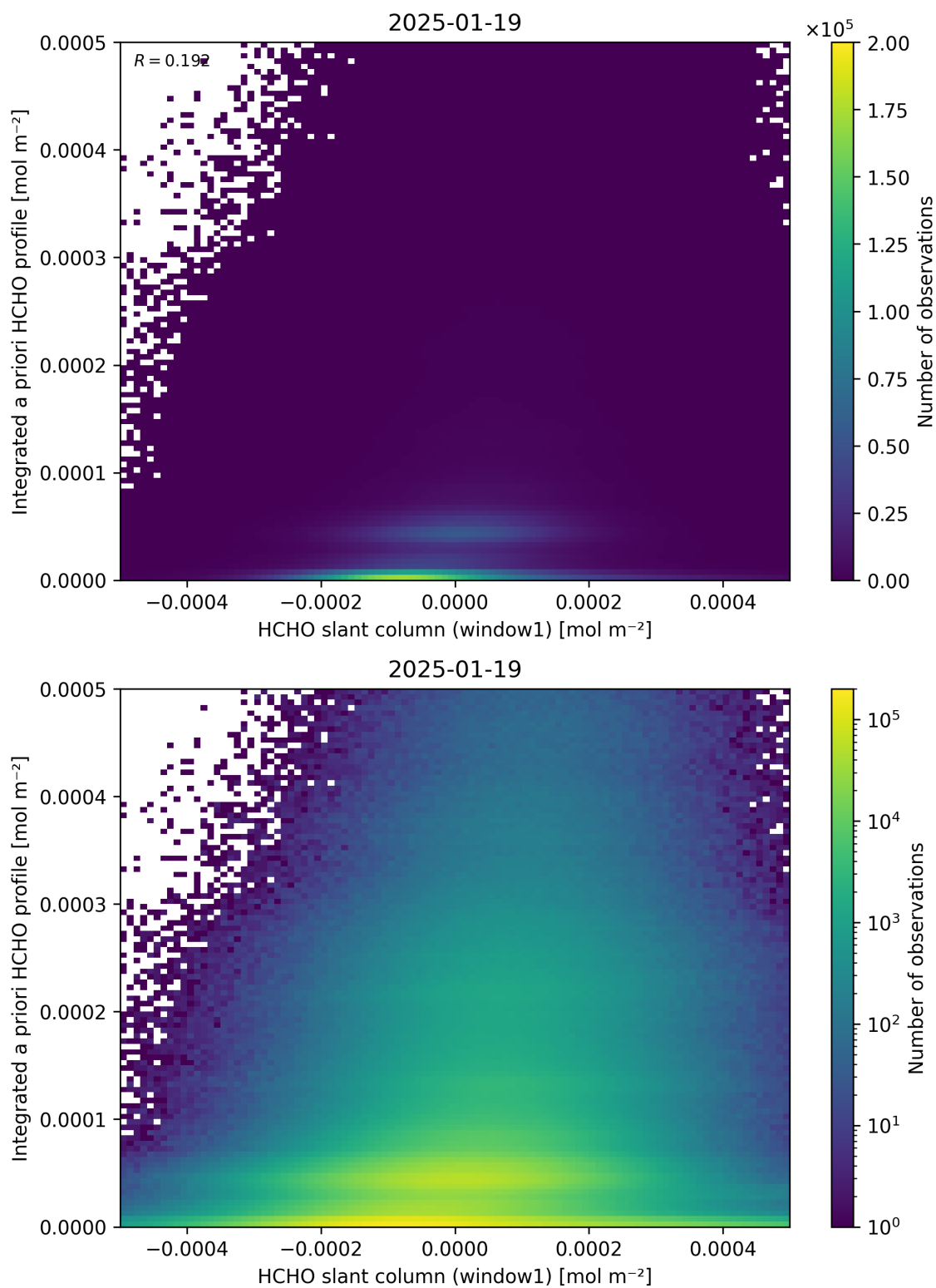
Figure 87: Scatter density plot of “HCHO slant column (window1)” against “Integrated a priori HCHO profile” for 2025-01-18 to 2025-01-20.
