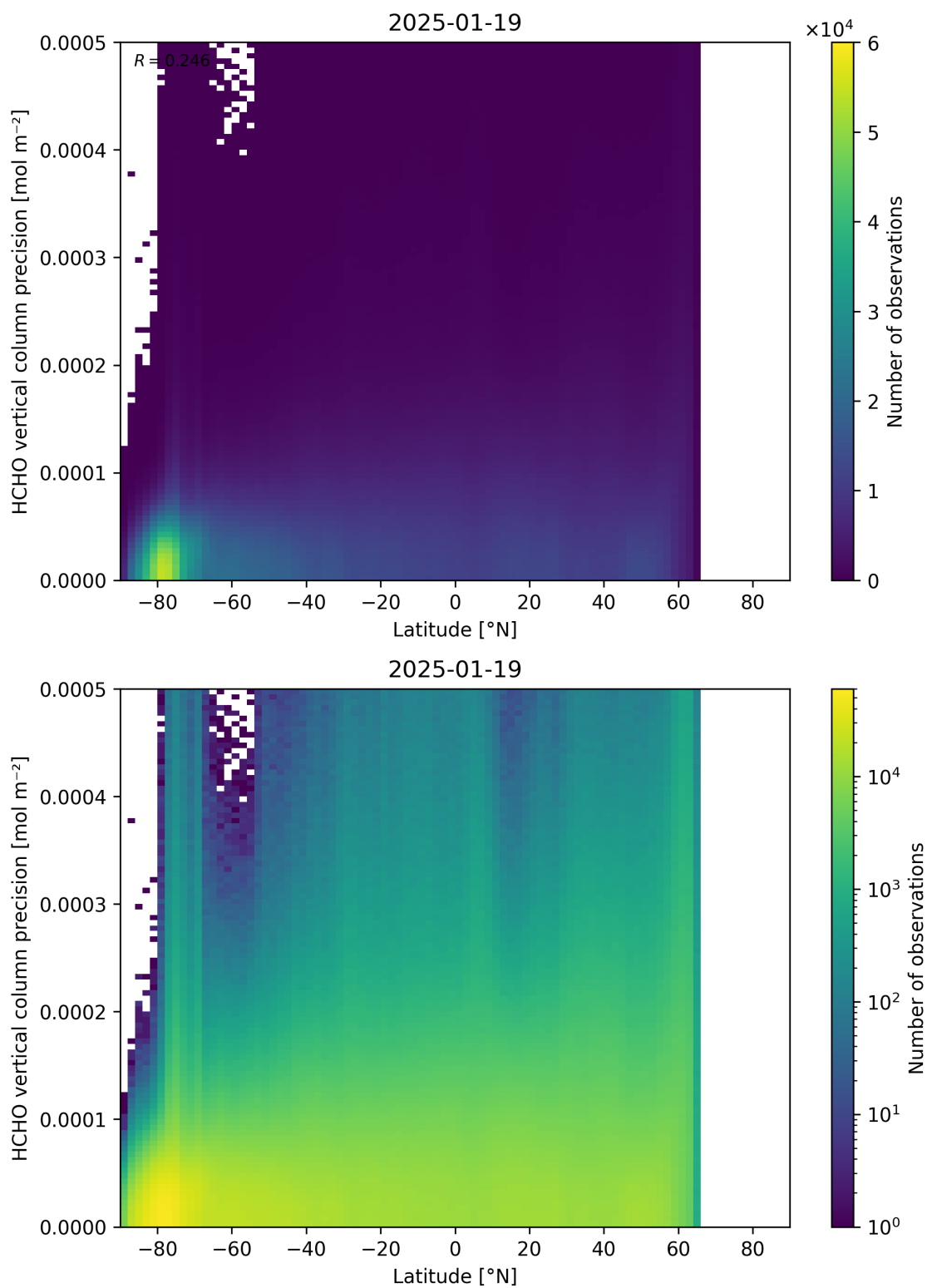
Figure 165: Scatter density plot of “Latitude” against “HCHO vertical column precision” for 2025-01-18 to 2025-01-20.
