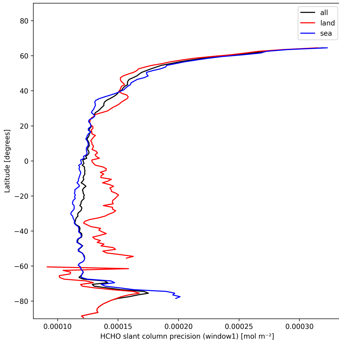
Figure 25: Zonal average of “HCHO slant column precision (window1)” for 2025-01-18 to 2025-01-20.
