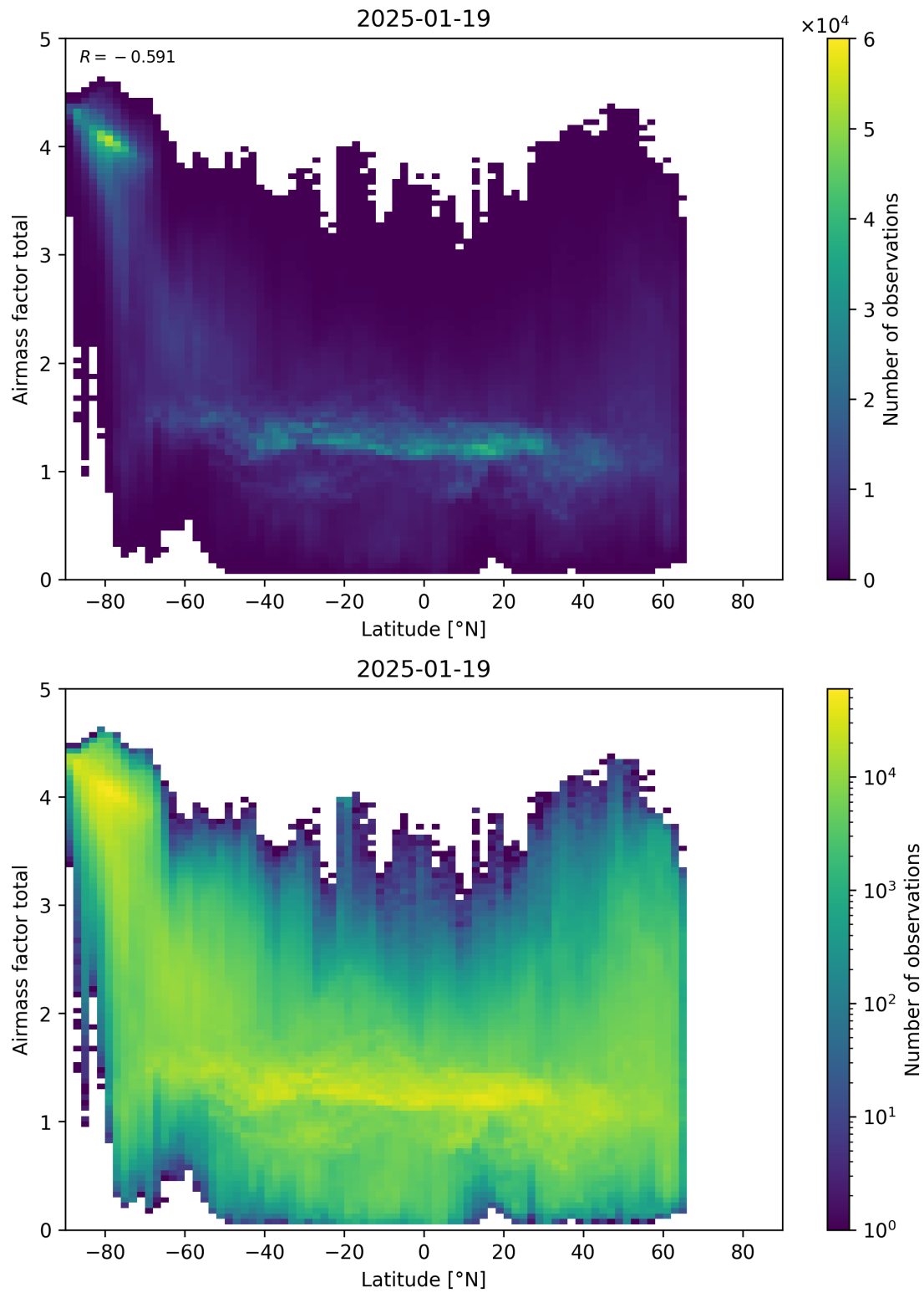
Figure 161: Scatter density plot of “Latitude” against “Airmass factor total” for 2025-01-18 to 2025-01-20.
