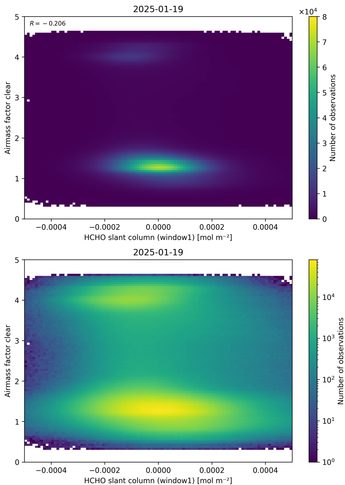
Figure 81: Scatter density plot of “HCHO slant column (window1)” against “Airmass factor clear” for 2025-01-18 to 2025-01-20.
