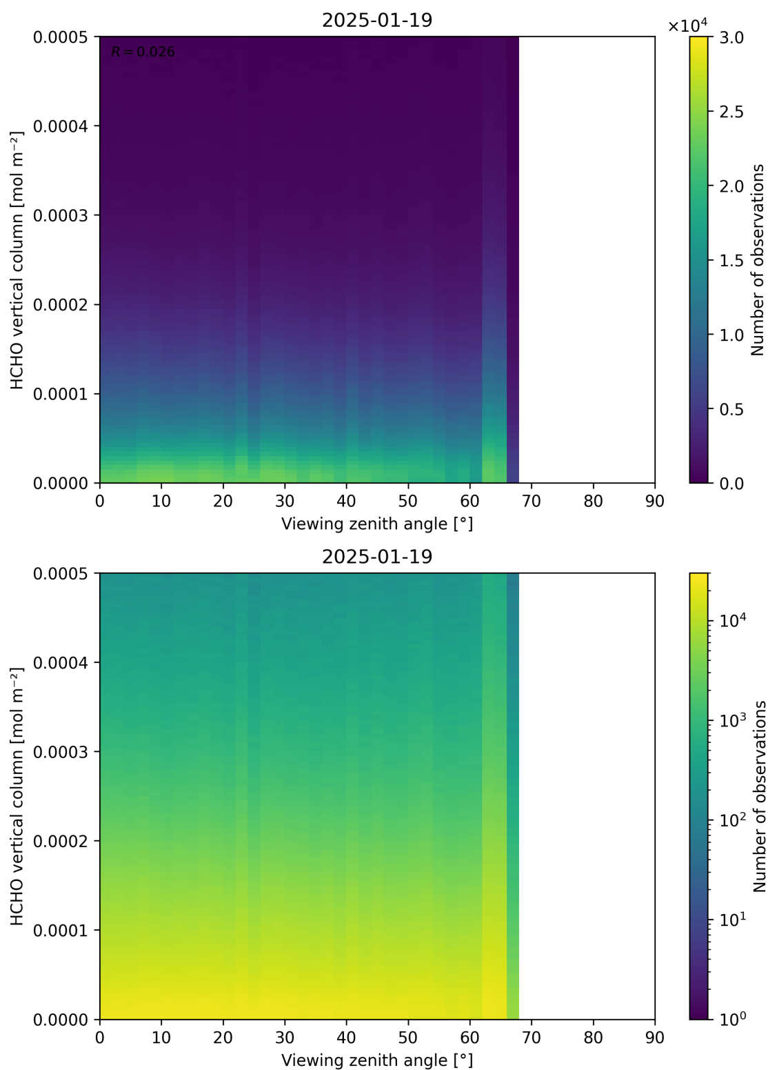
Figure 192: Scatter density plot of “Viewing zenith angle” against “HCHO vertical column” for 2025-01-18 to 2025-01-20.
