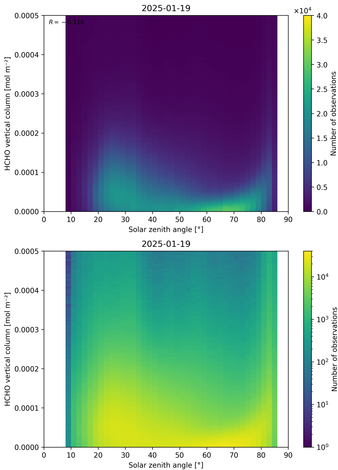
Figure 177: Scatter density plot of “Solar zenith angle” against “HCHO vertical column” for 2025-01-18 to 2025-01-20.
