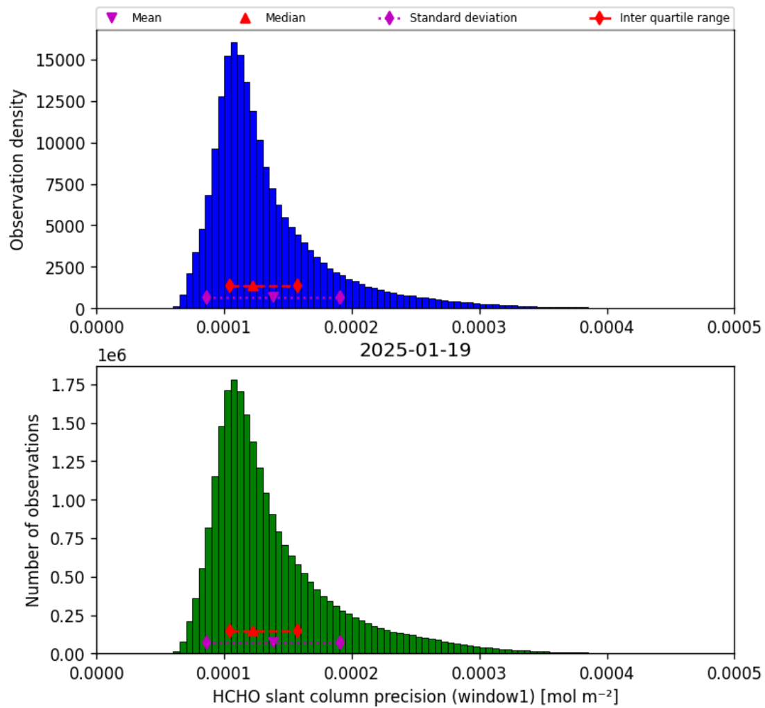
Figure 39: Histogram of “HCHO slant column precision (window1)” for 2025-01-18 to 2025-01-20
