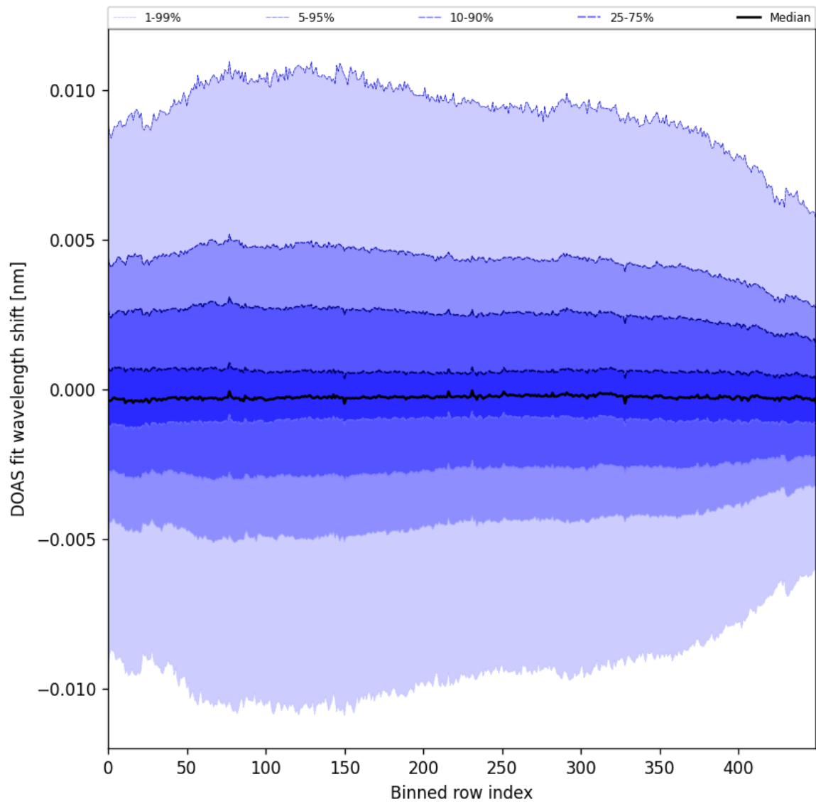
Figure 58: Along track statistics of “DOAS fit wavelength shift” for 2025-01-18 to 2025-01-20
