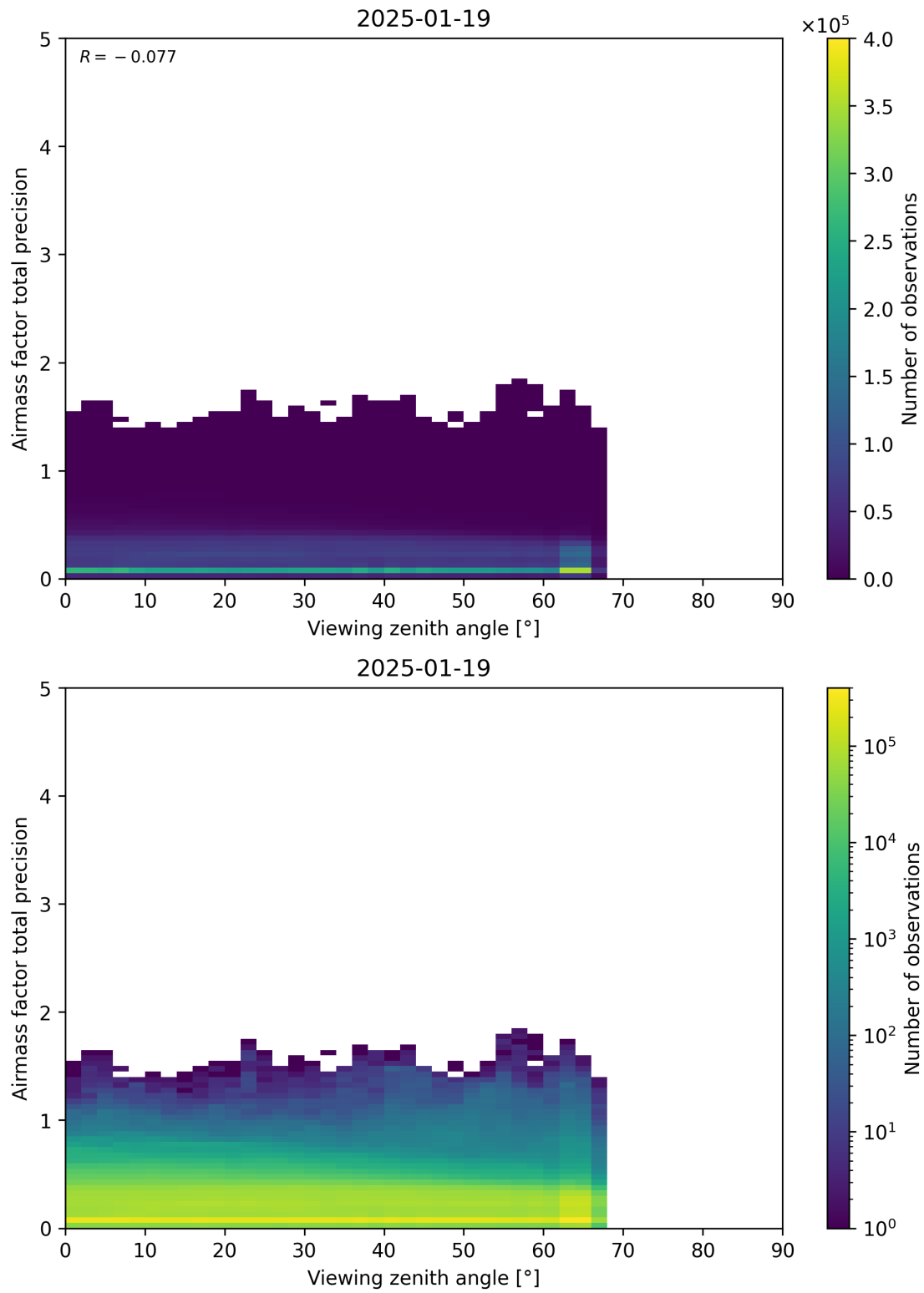
Figure 191: Scatter density plot of “Viewing zenith angle” against “Airmass factor total precision” for 2025-01-18 to 2025-01-20.
