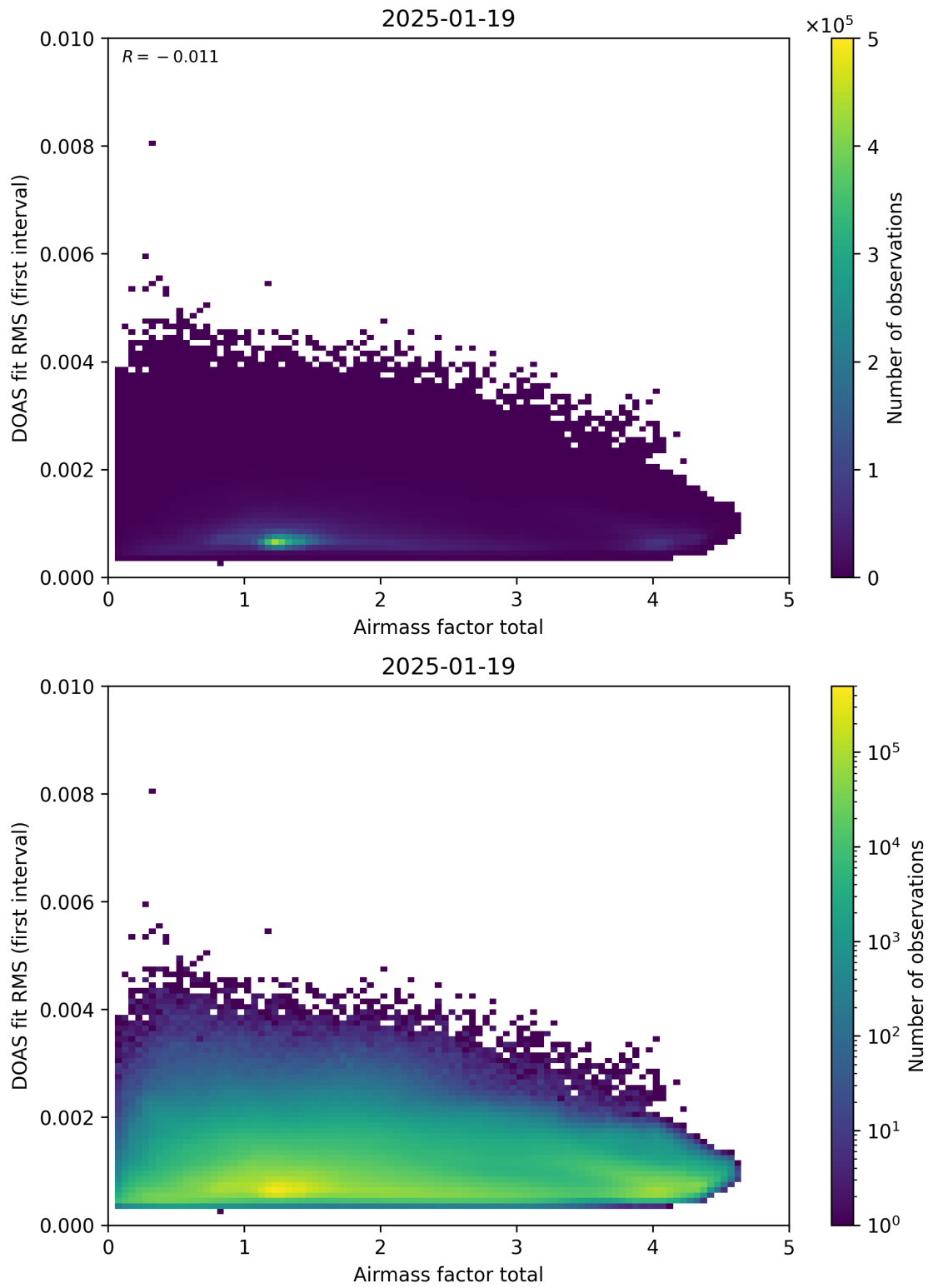
Figure 97: Scatter density plot of “Airmass factor total” against “DOAS fit RMS (first interval)” for 2025-01-18 to 2025-01-20.
