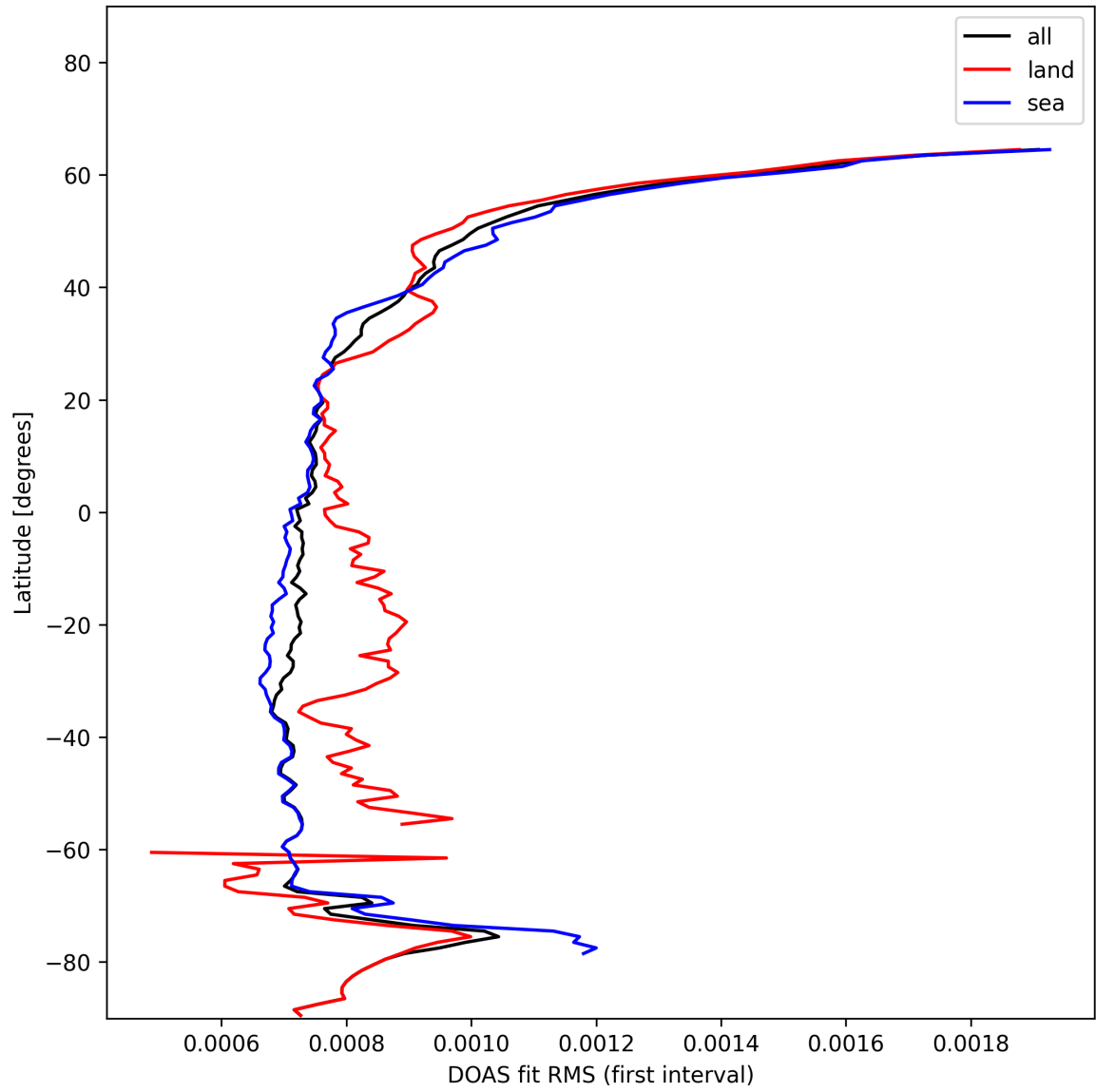
Figure 32: Zonal average of “DOAS fit RMS (first interval)” for 2025-01-18 to 2025-01-20.
