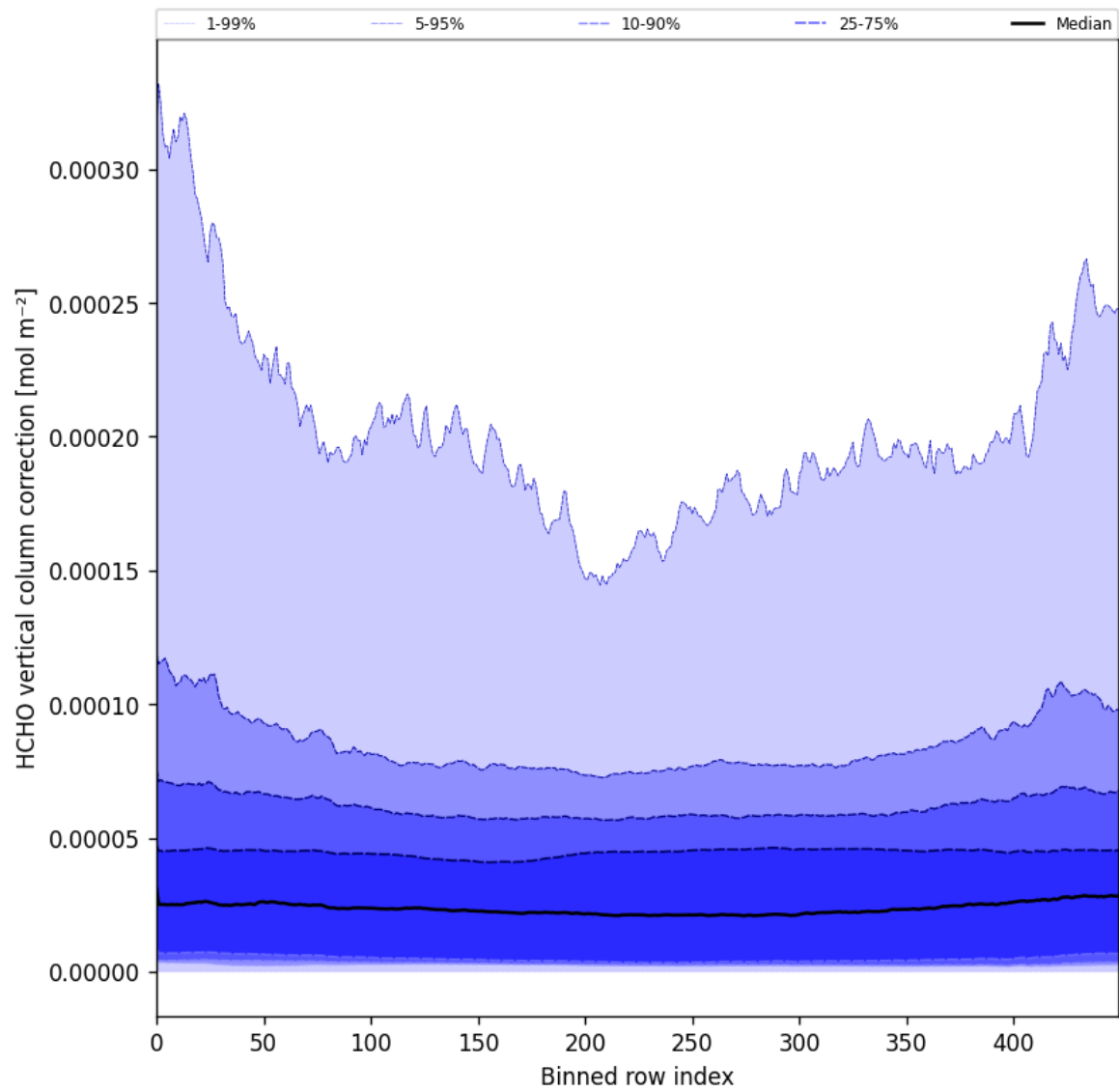
Figure 51: Along track statistics of “HCHO vertical column correction” for 2025-01-18 to 2025-01-20
