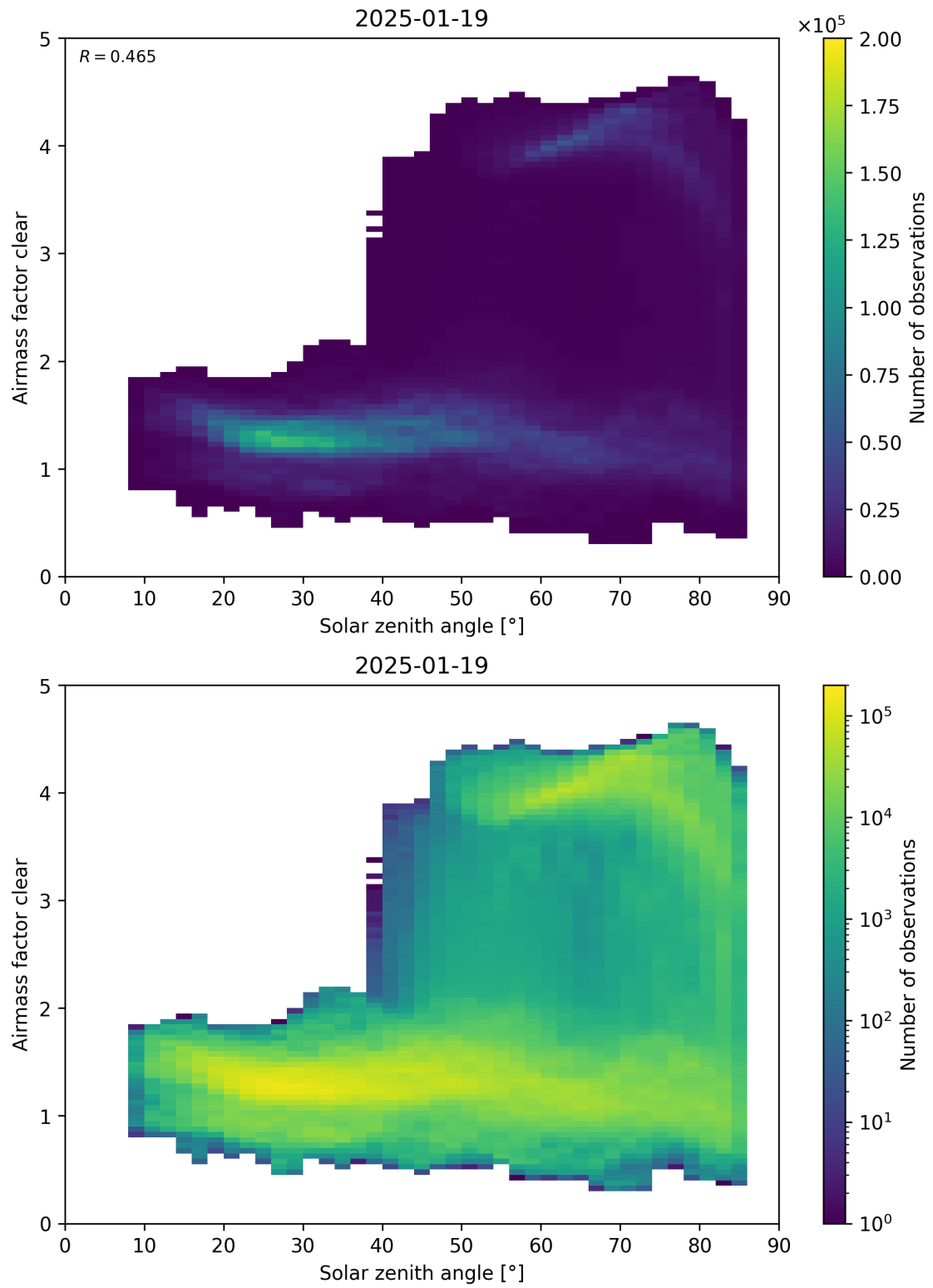
Figure 170: Scatter density plot of “Solar zenith angle” against “Airmass factor clear” for 2025-01-18 to 2025-01-20.
