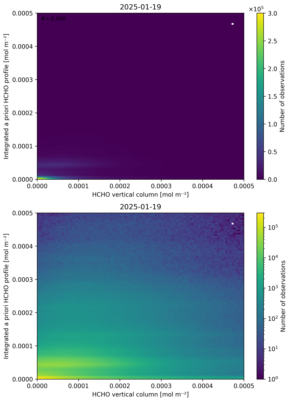
Figure 135: Scatter density plot of “HCHO vertical column” against “Integrated a priori HCHO profile” for 2025-01-18 to 2025-01-20.
