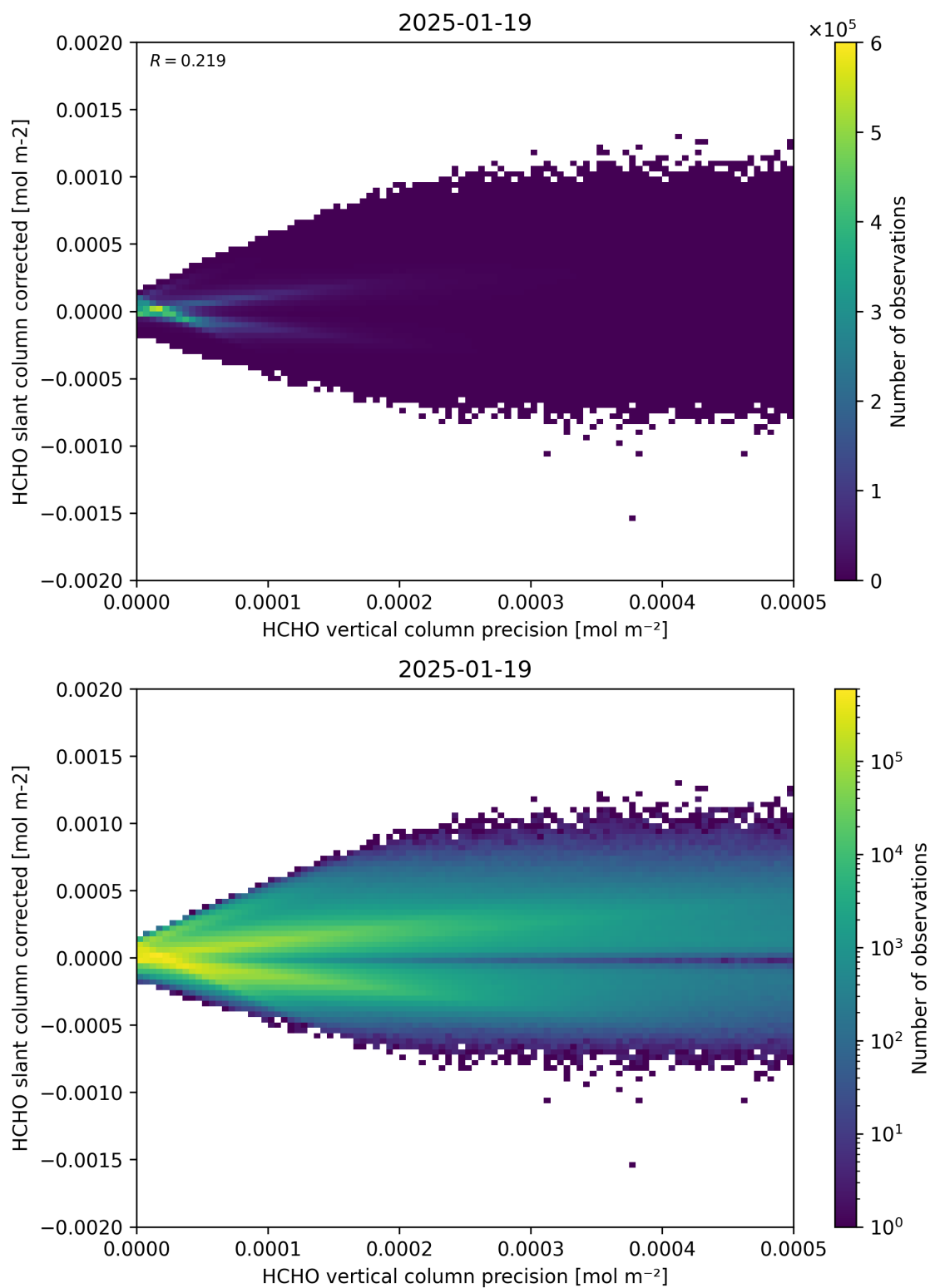
Figure 140: Scatter density plot of “HCHO vertical column precision” against “HCHO slant column corrected” for 2025-01-18 to 2025-01-20.
