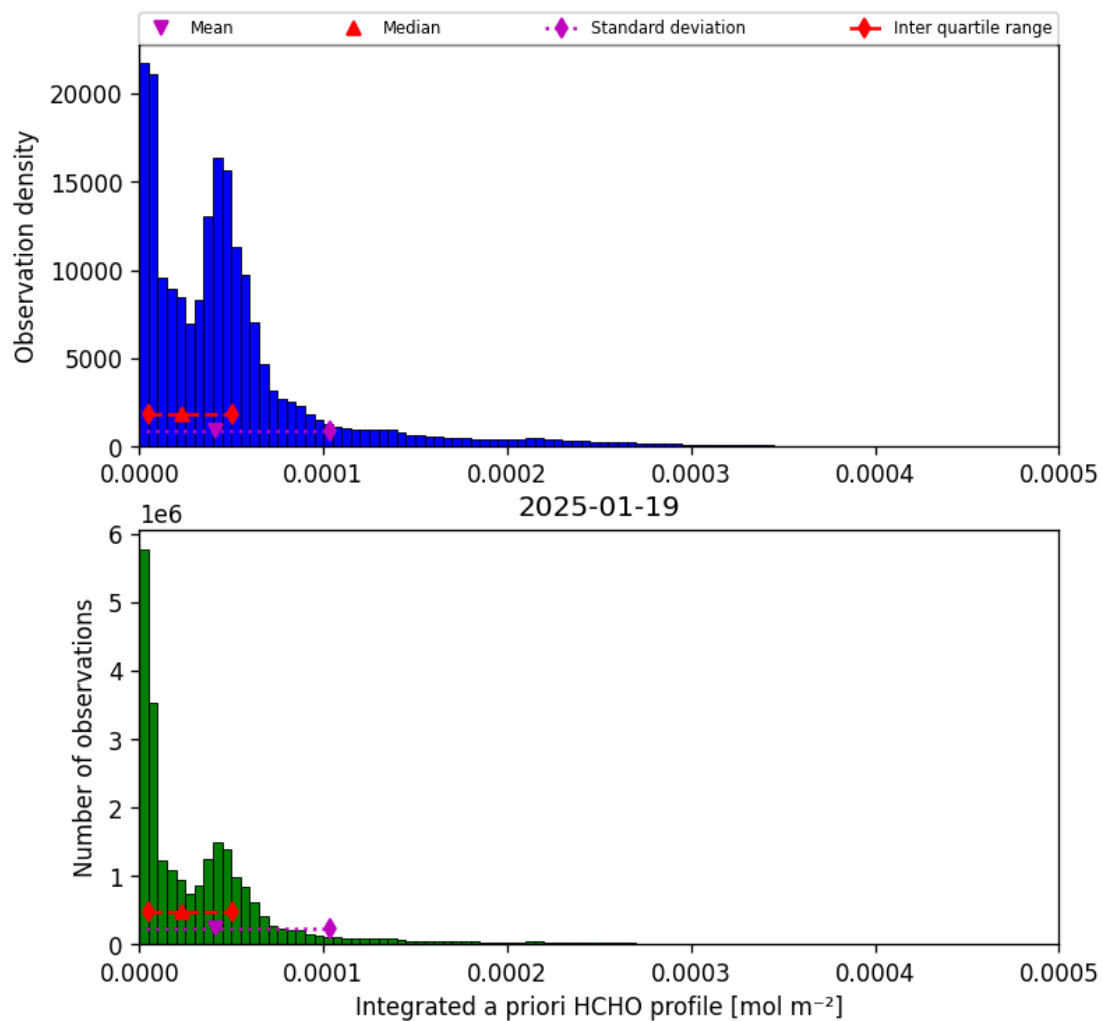
Figure 43: Histogram of “Integrated a priori HCHO profile” for 2025-01-18 to 2025-01-20
