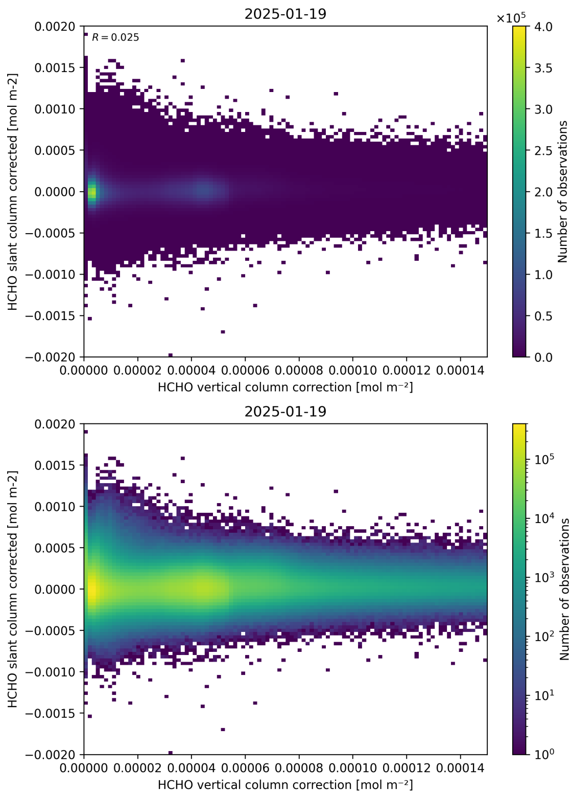
Figure 116: Scatter density plot of “HCHO vertical column correction” against “HCHO slant column corrected” for 2025-01-18 to 2025-01-20.
