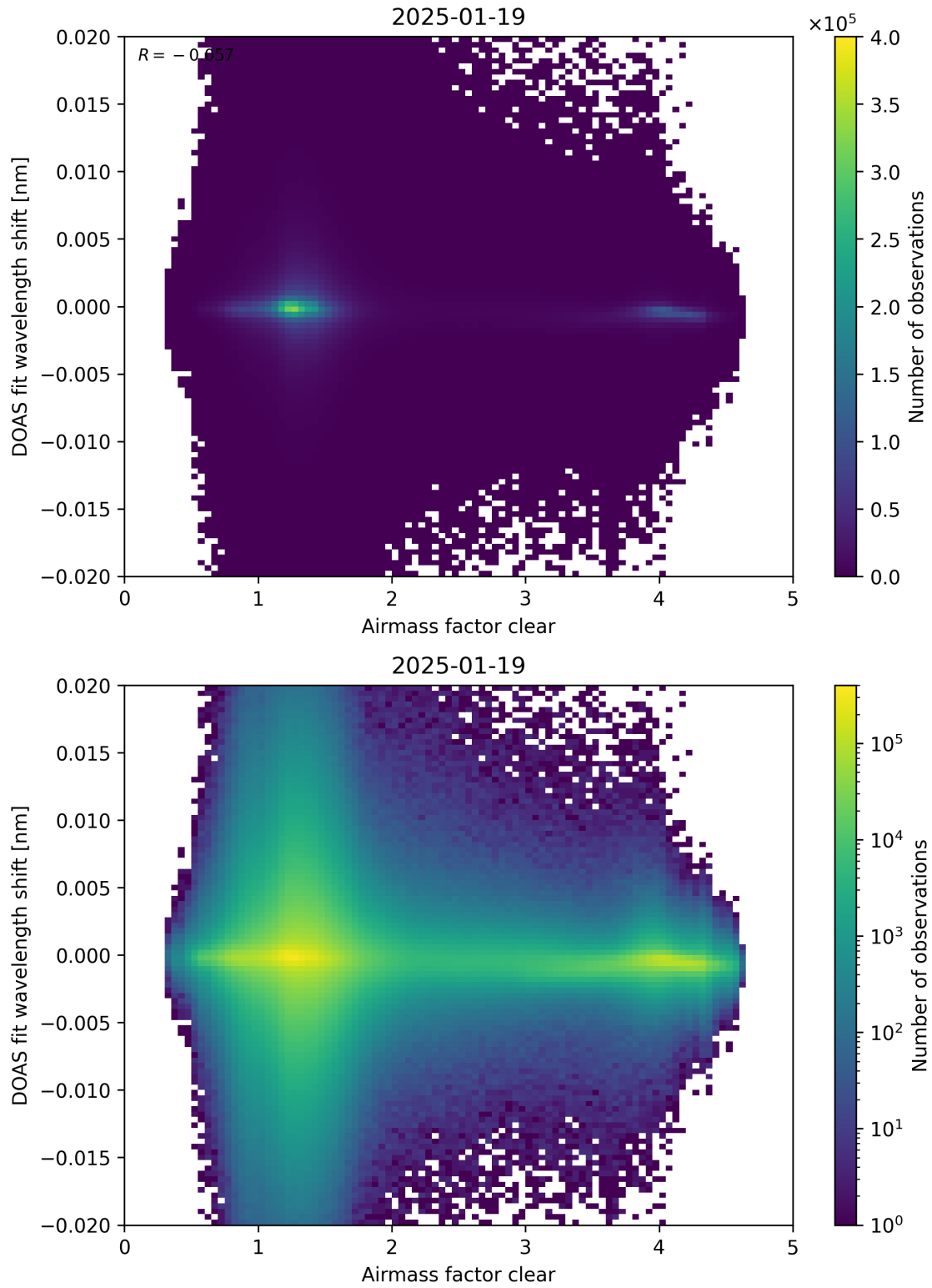
Figure 72: Scatter density plot of “Airmass factor clear” against “DOAS fit wavelength shift” for 2025-01-18 to 2025-01-20.
