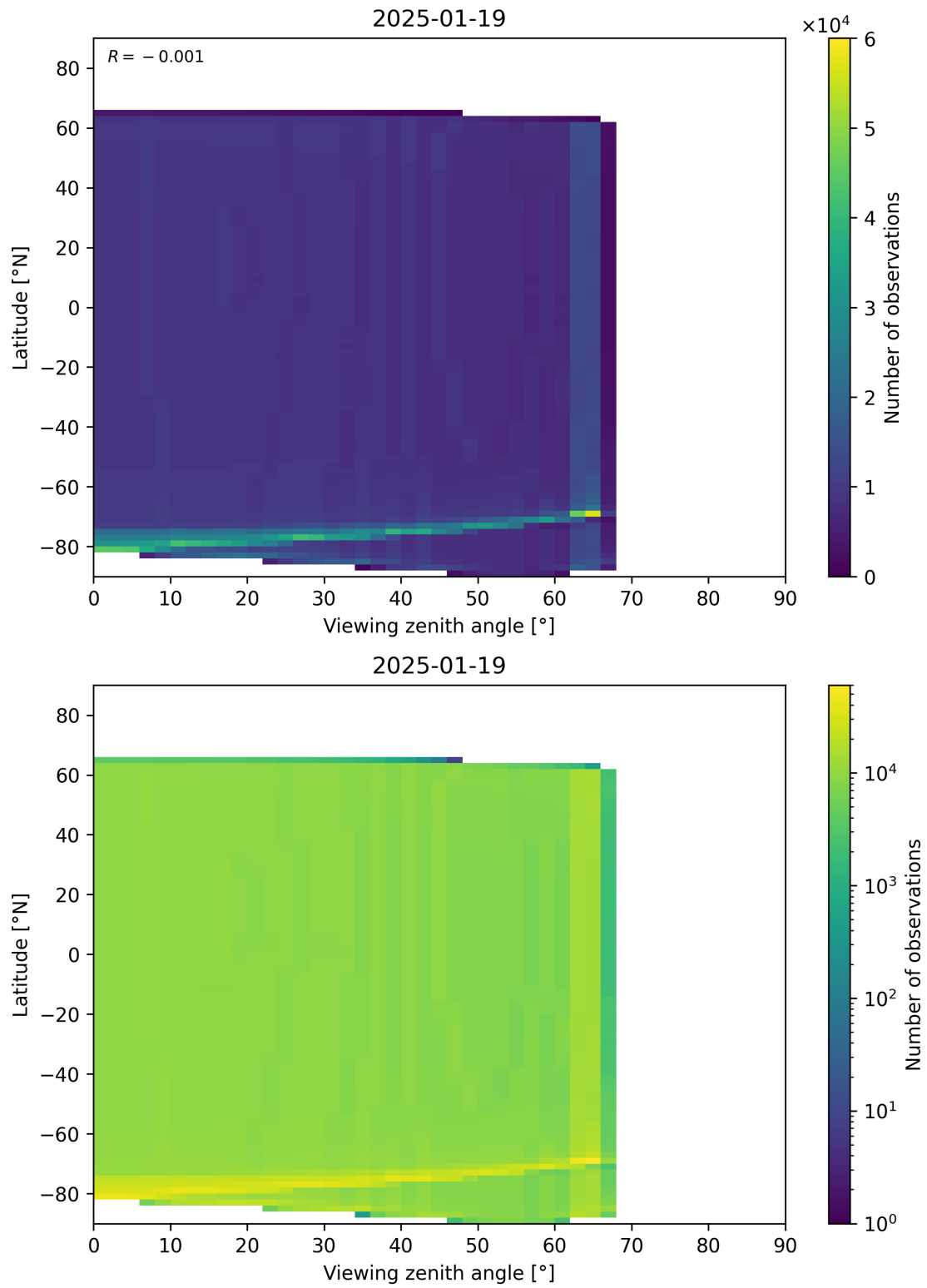
Figure 196: Scatter density plot of “Viewing zenith angle” against “Latitude” for 2025-01-18 to 2025-01-20.
