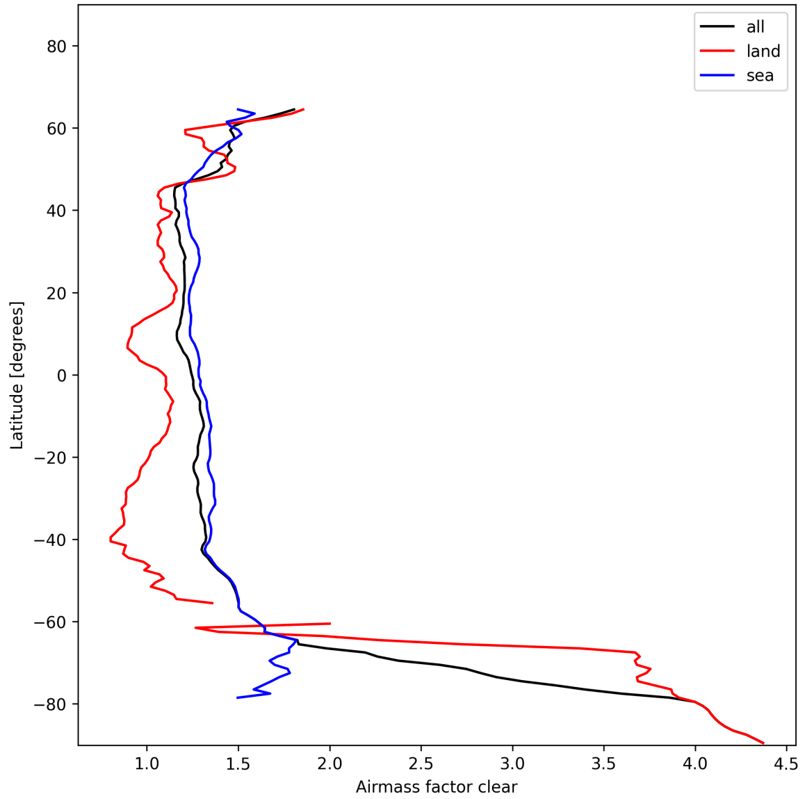
Figure 28: Zonal average of “Airmass factor clear” for 2025-01-18 to 2025-01-20.
