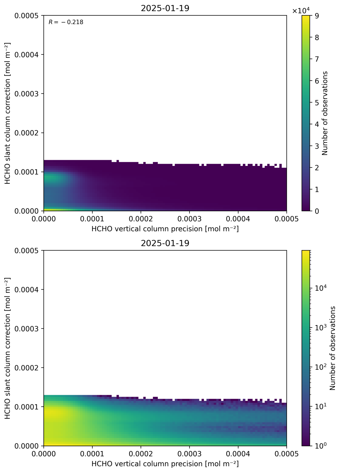
Figure 141: Scatter density plot of “HCHO vertical column precision” against “HCHO slant column correction” for 2025-01-18 to 2025-01-20.
