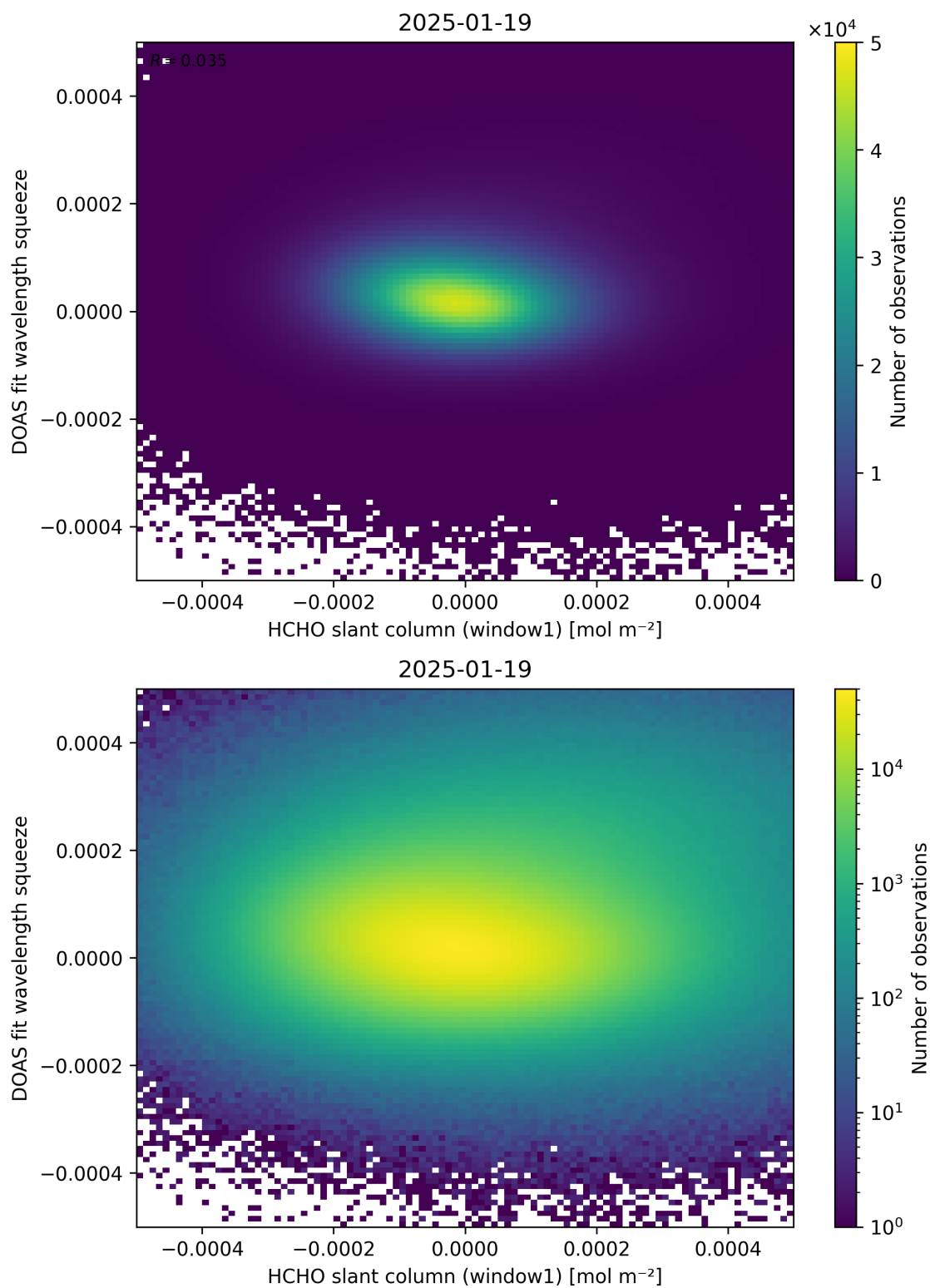
Figure 80: Scatter density plot of “HCHO slant column (window1)” against “DOAS fit wavelength squeeze” for 2025-01-18 to 2025-01-20.
