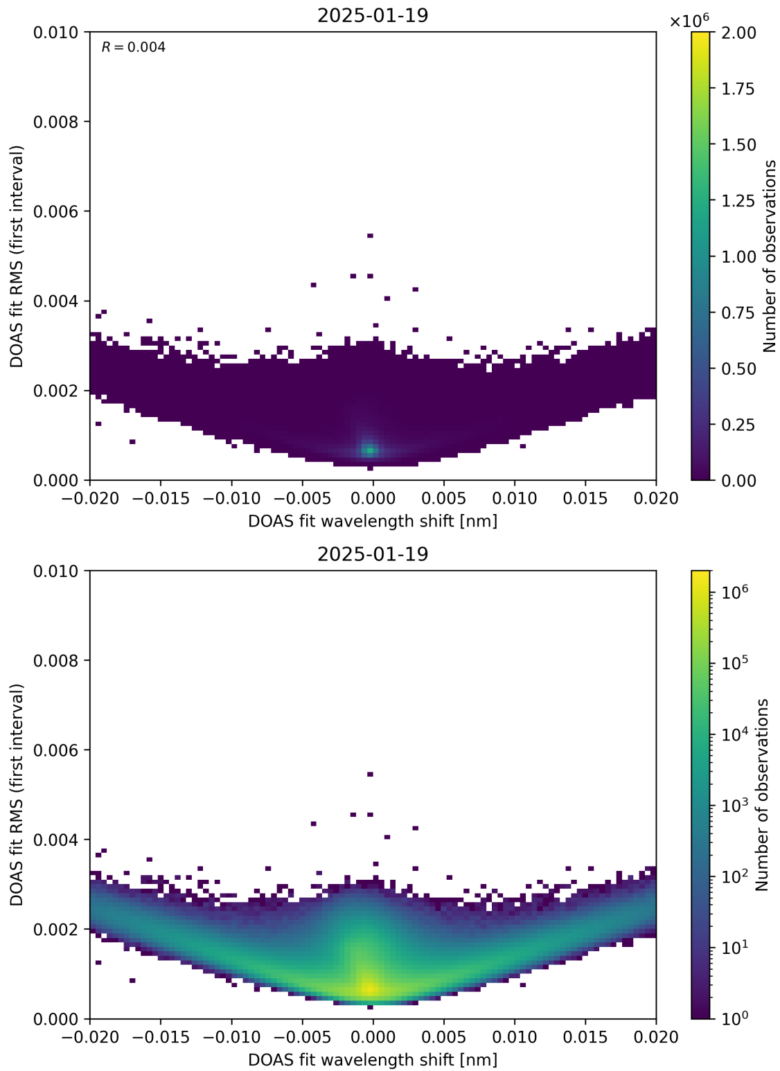
Figure 64: Scatter density plot of “DOAS fit wavelength shift” against “DOAS fit RMS (first interval)” for 2025-01-18 to 2025-01-20.
