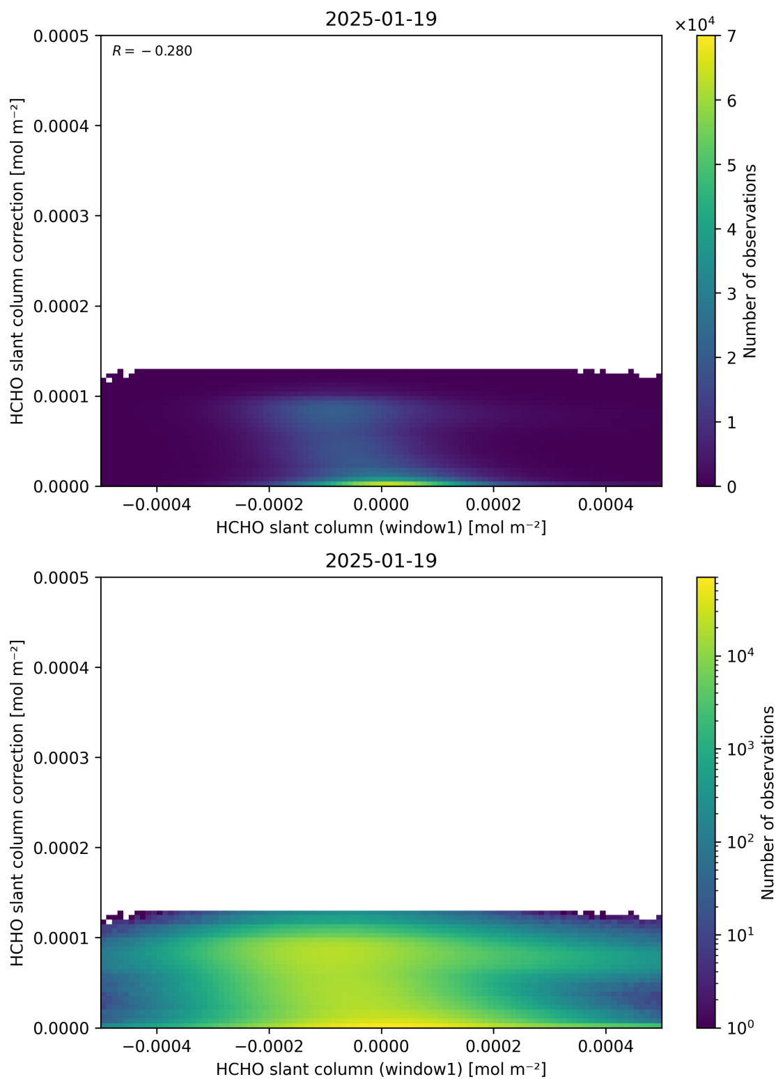
Figure 83: Scatter density plot of “HCHO slant column (window1)” against “HCHO slant column correction” for 2025-01-18 to 2025-01-20.
