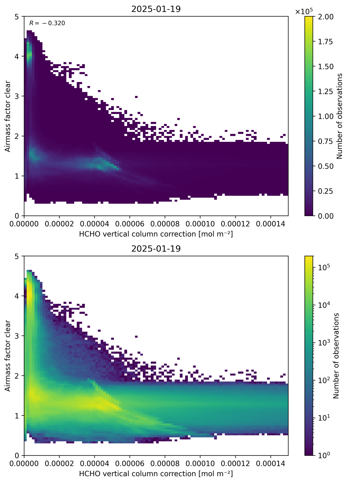
Figure 115: Scatter density plot of “HCHO vertical column correction” against “Airmass factor clear” for 2025-01-18 to 2025-01-20.
