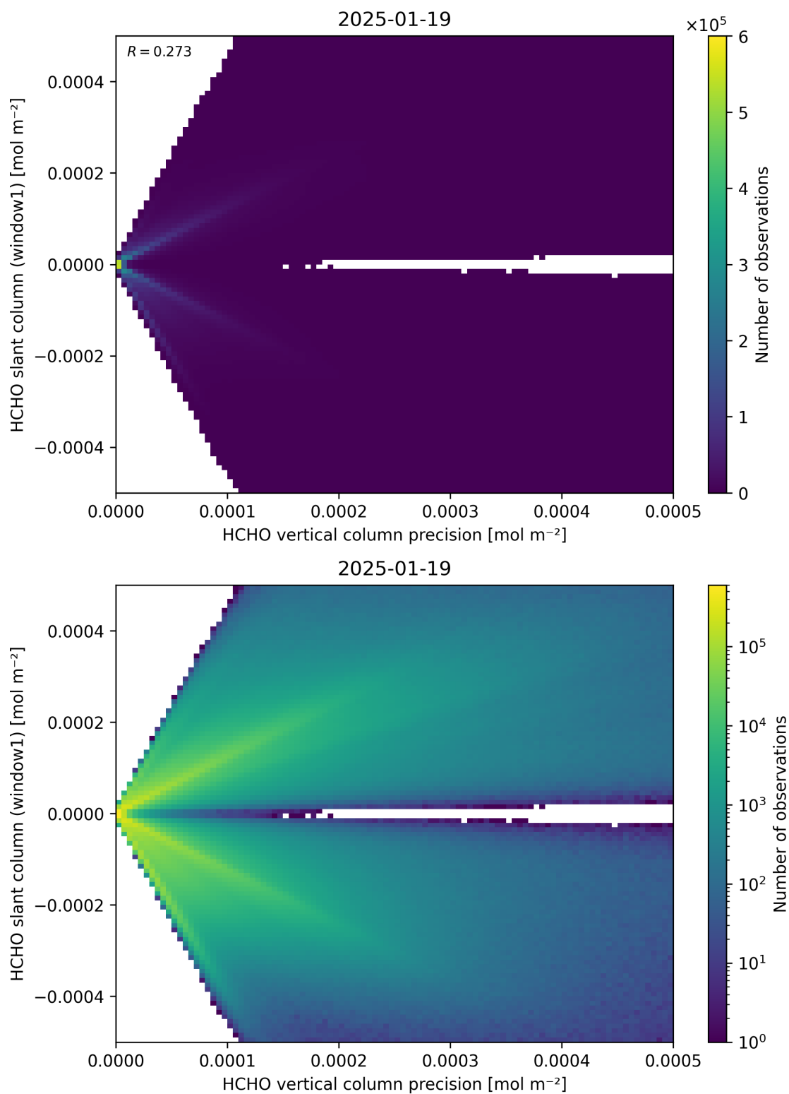
Figure 142: Scatter density plot of “HCHO vertical column precision” against “HCHO slant column (window1)” for 2025-01-18 to 2025-01-20.
