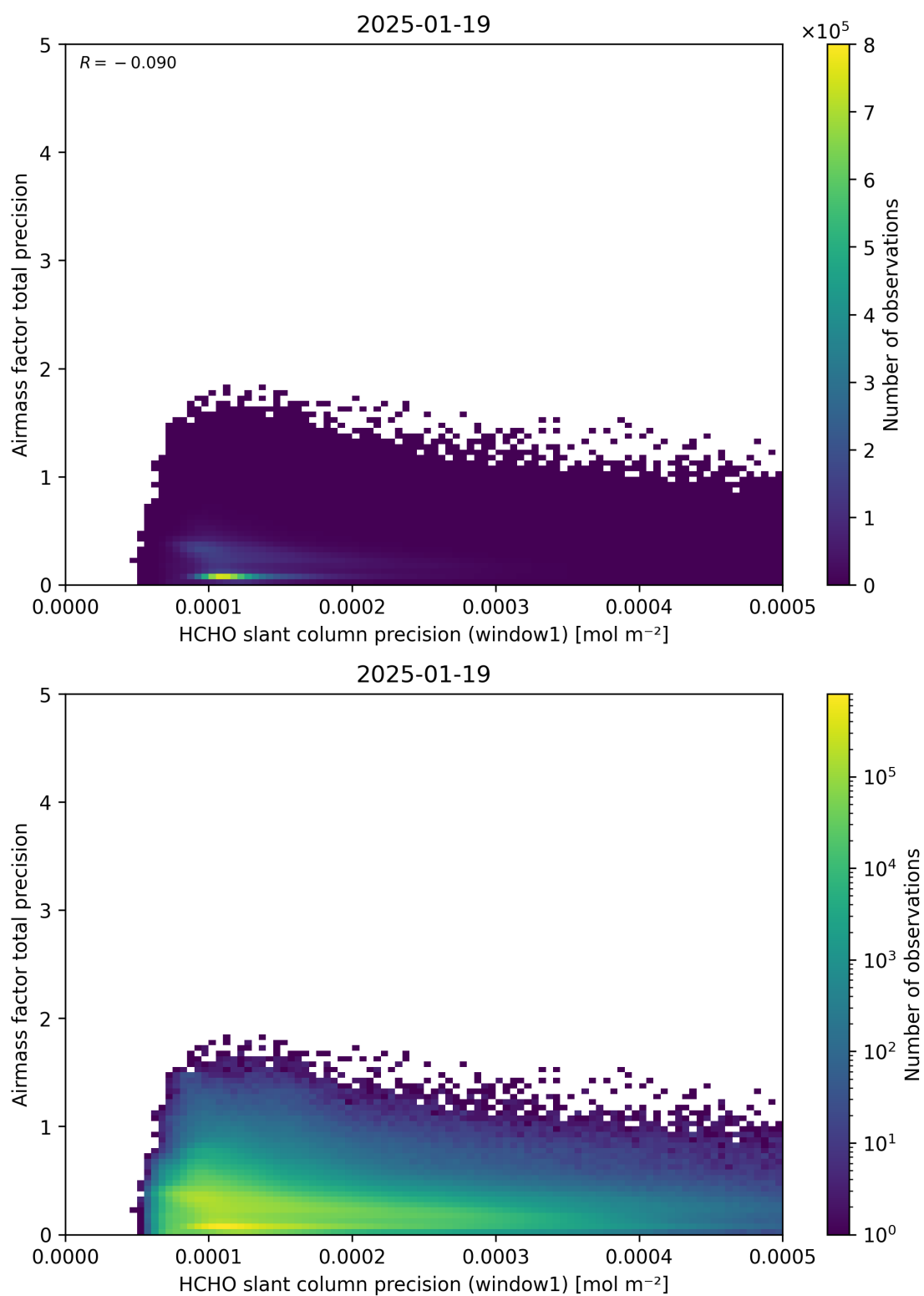
Figure 95: Scatter density plot of “HCHO slant column precision (window1)” against “Airmass factor total precision” for 2025-01-18 to 2025-01-20.
