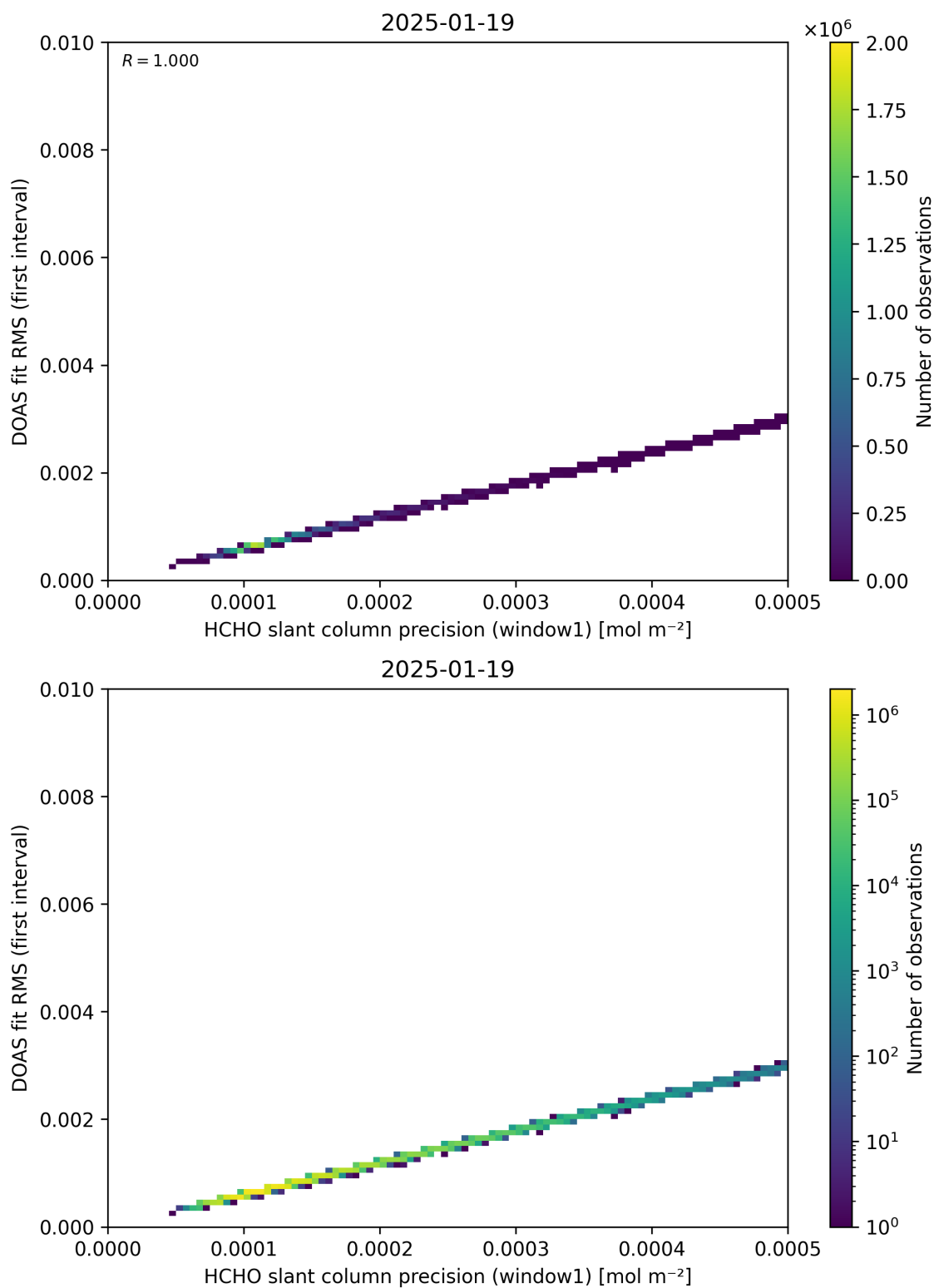
Figure 88: Scatter density plot of “HCHO slant column precision (window1)” against “DOAS fit RMS (first interval)” for 2025-01-18 to 2025-01-20.
