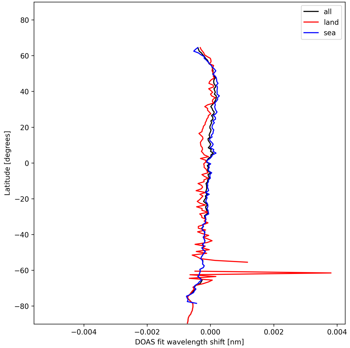
Figure 30: Zonal average of "DOAS fit wavelength shift" for 2025-01-18 to 2025-01-20.
