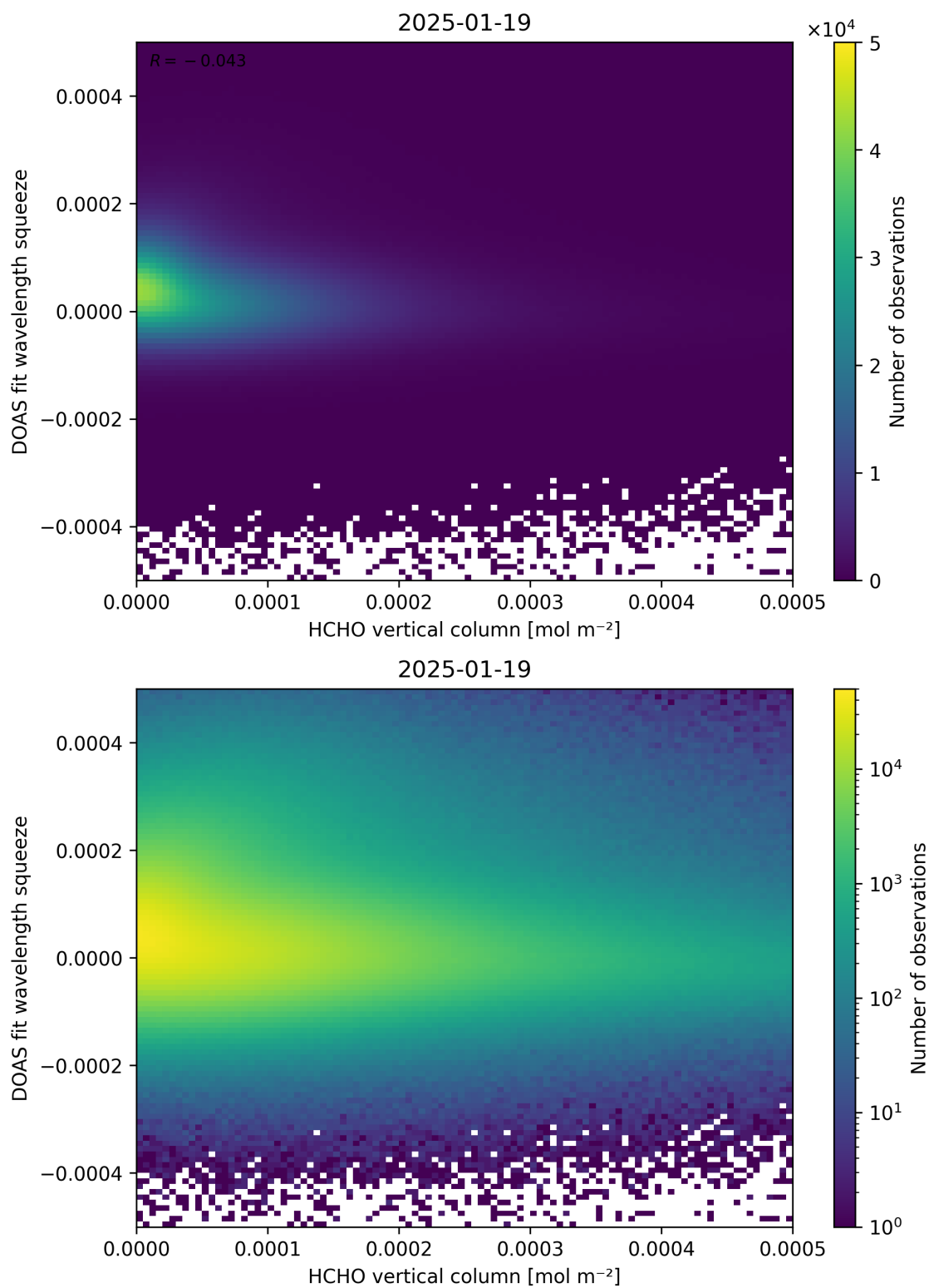
Figure 125: Scatter density plot of “HCHO vertical column” against “DOAS fit wavelength squeeze” for 2025-01-18 to 2025-01-20.
