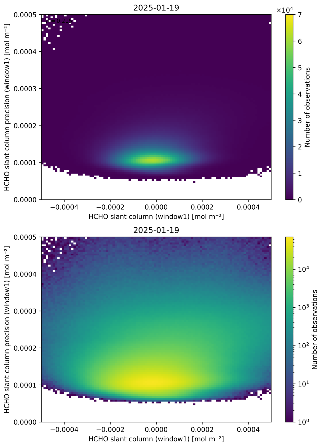
Figure 84: Scatter density plot of “HCHO slant column (window1)” against “HCHO slant column precision (window1)” for 2025-01-18 to 2025-01-20.
