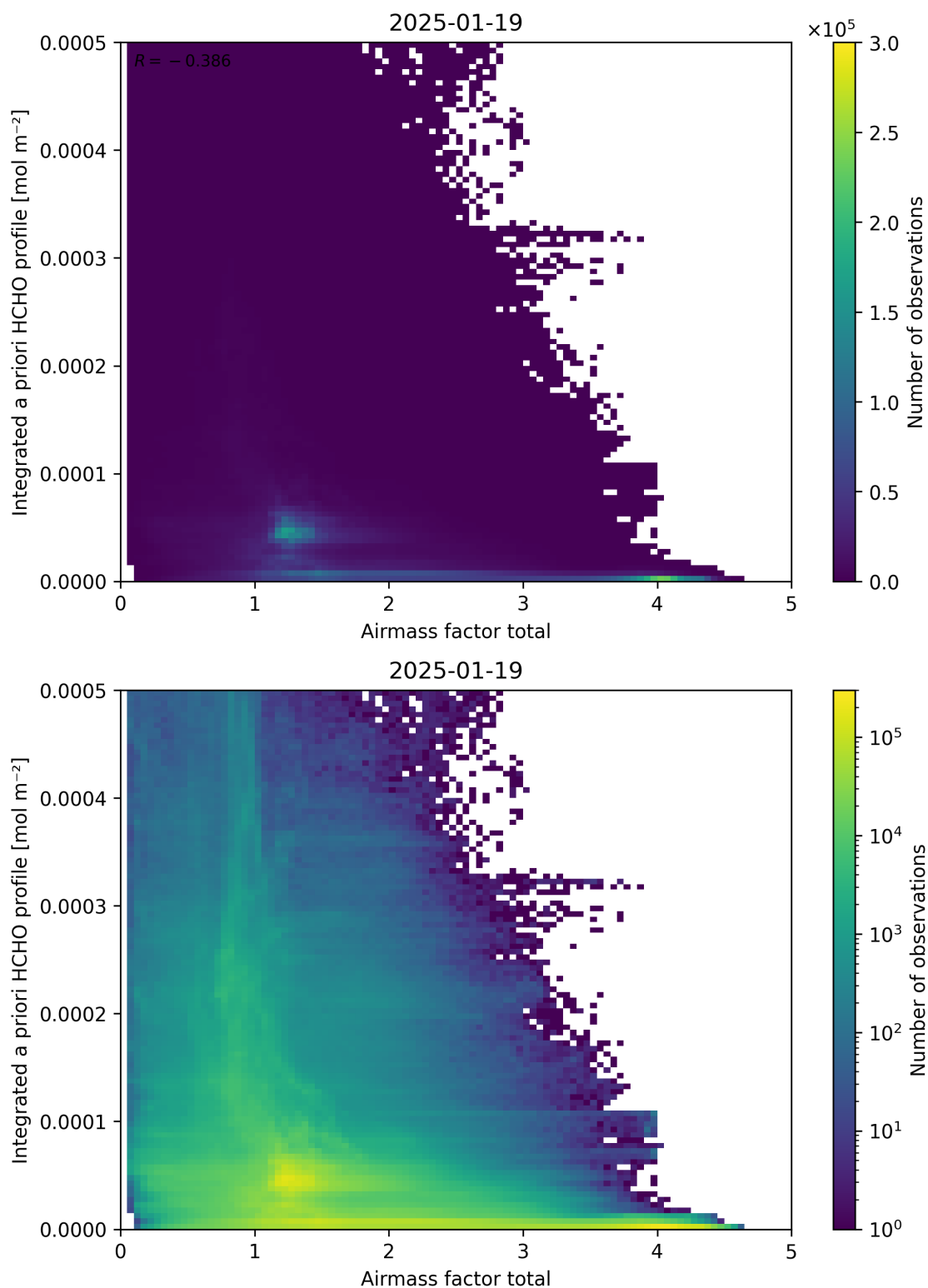
Figure 104: Scatter density plot of “Airmass factor total” against “Integrated a priori HCHO profile” for 2025-01-18 to 2025-01-20.
