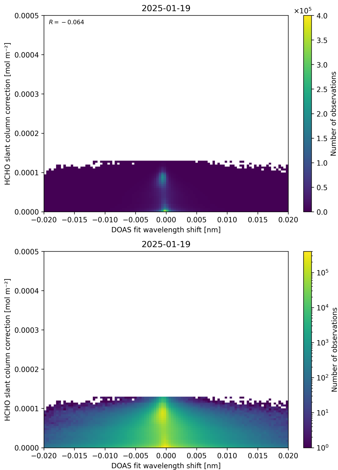
Figure 67: Scatter density plot of “DOAS fit wavelength shift” against “HCHO slant column correction” for 2025-01-18 to 2025-01-20.
