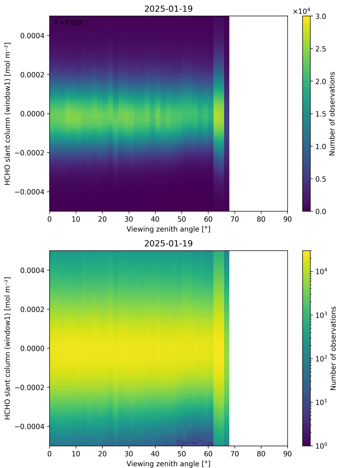
Figure 188: Scatter density plot of “Viewing zenith angle” against “HCHO slant column (window1)” for 2025-01-18 to 2025-01-20.
