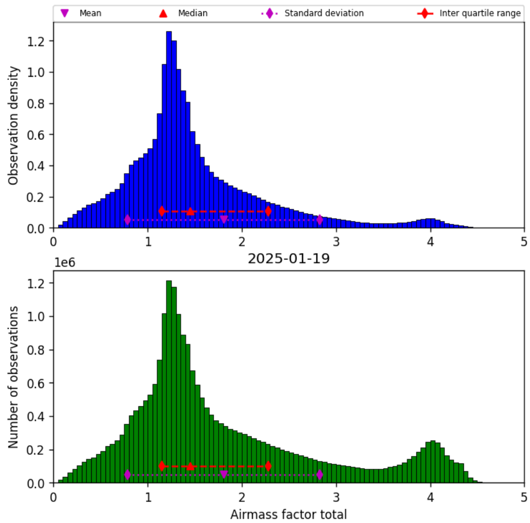
Figure 40: Histogram of “Airmass factor total” for 2025-01-18 to 2025-01-20
