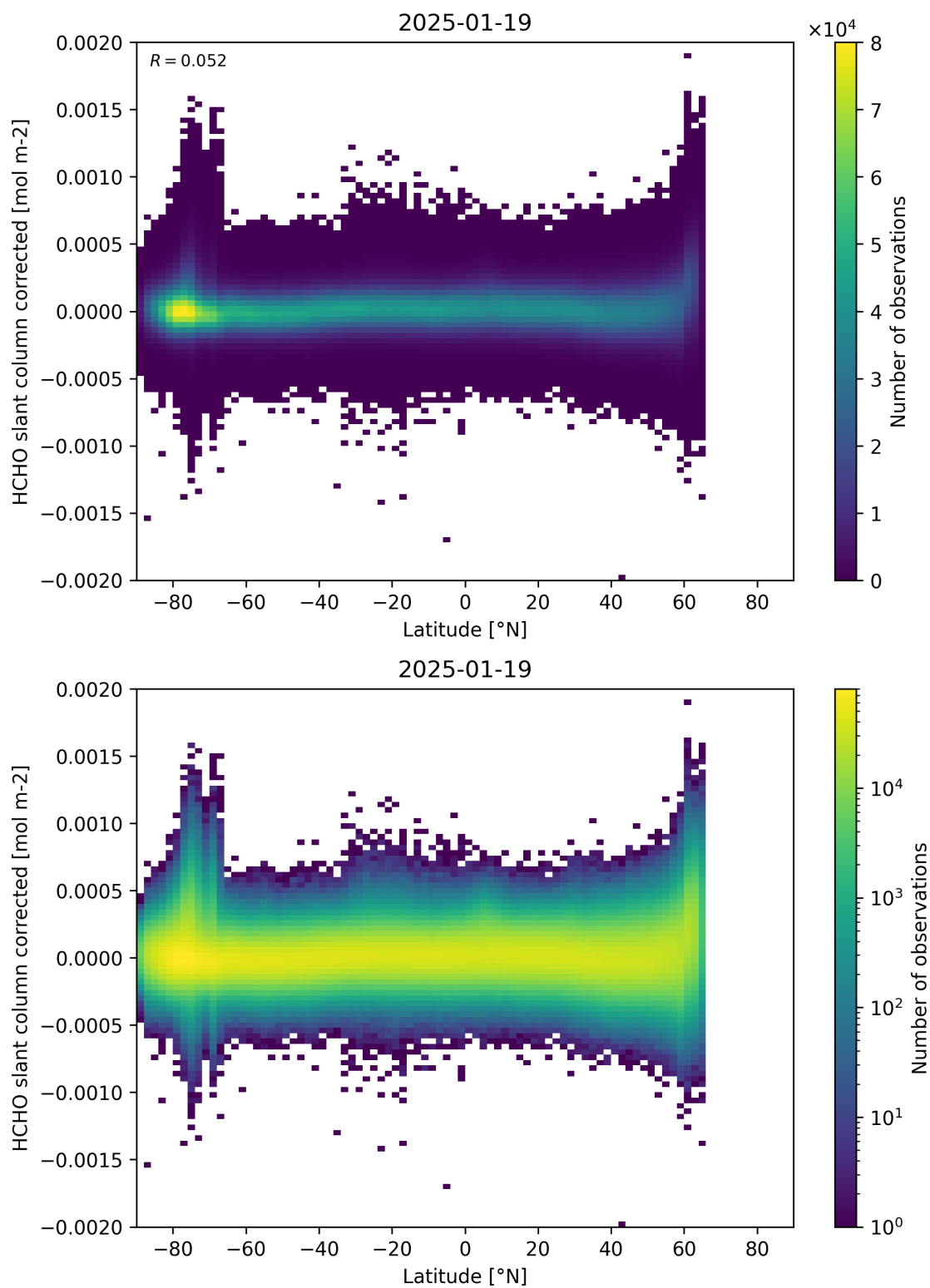
Figure 157: Scatter density plot of “Latitude” against “HCHO slant column corrected” for 2025-01-18 to 2025-01-20.
