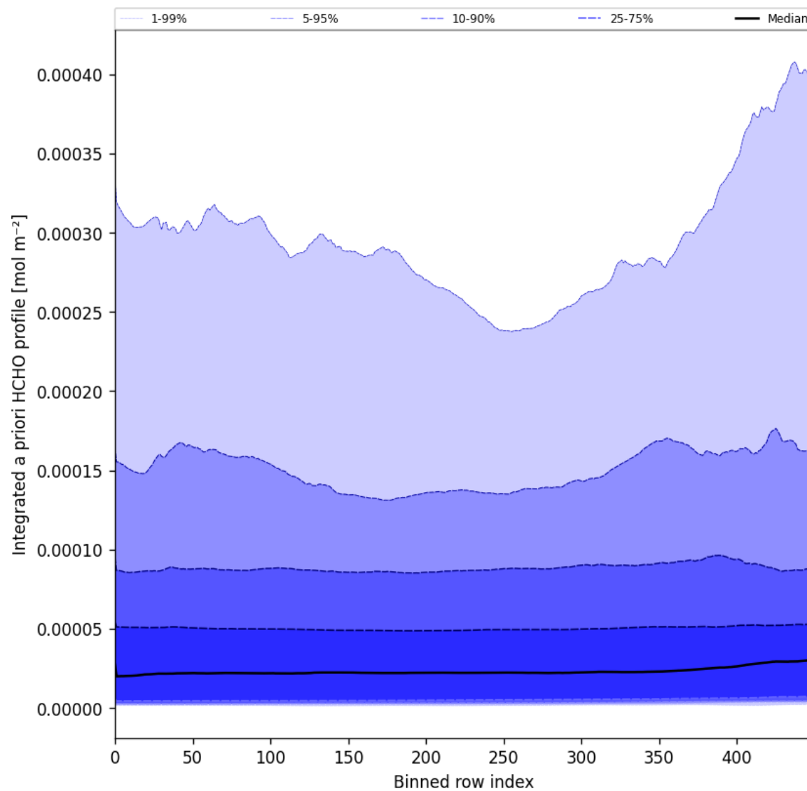
Figure 57: Along track statistics of “Integrated a priori HCHO profile” for 2025-01-18 to 2025-01-20
