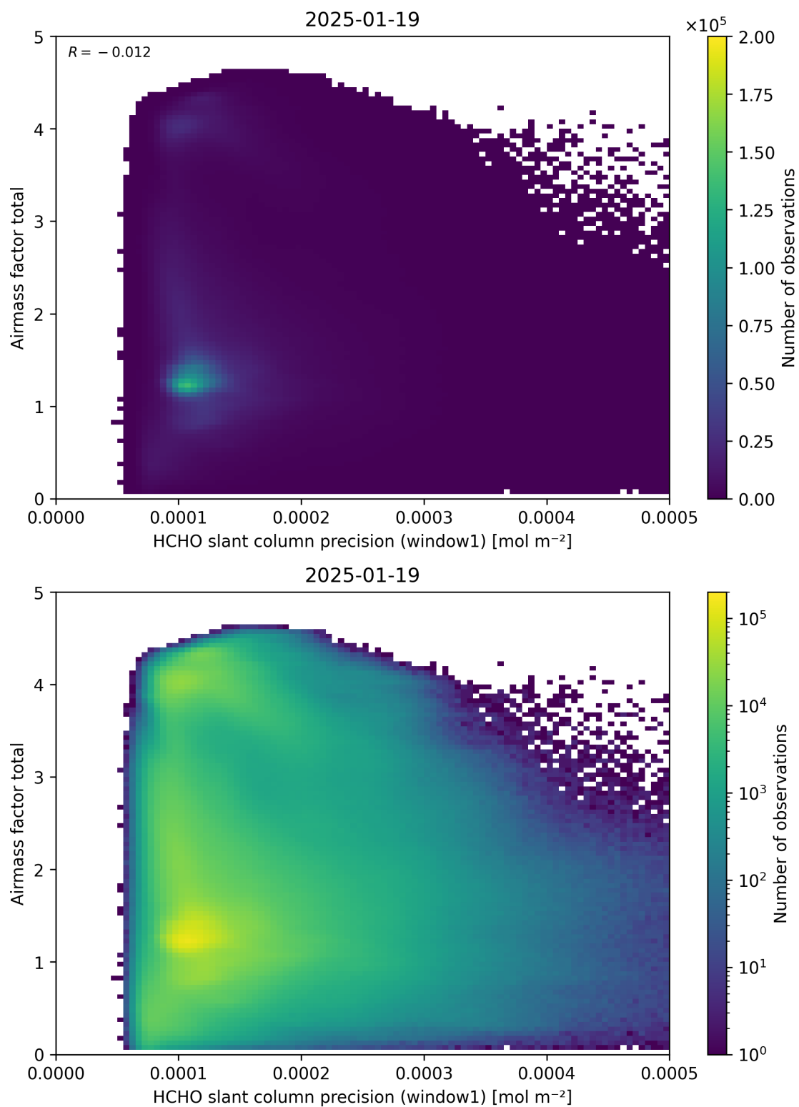
Figure 94: Scatter density plot of “HCHO slant column precision (window1)” against “Airmass factor total” for 2025-01-18 to 2025-01-20.
