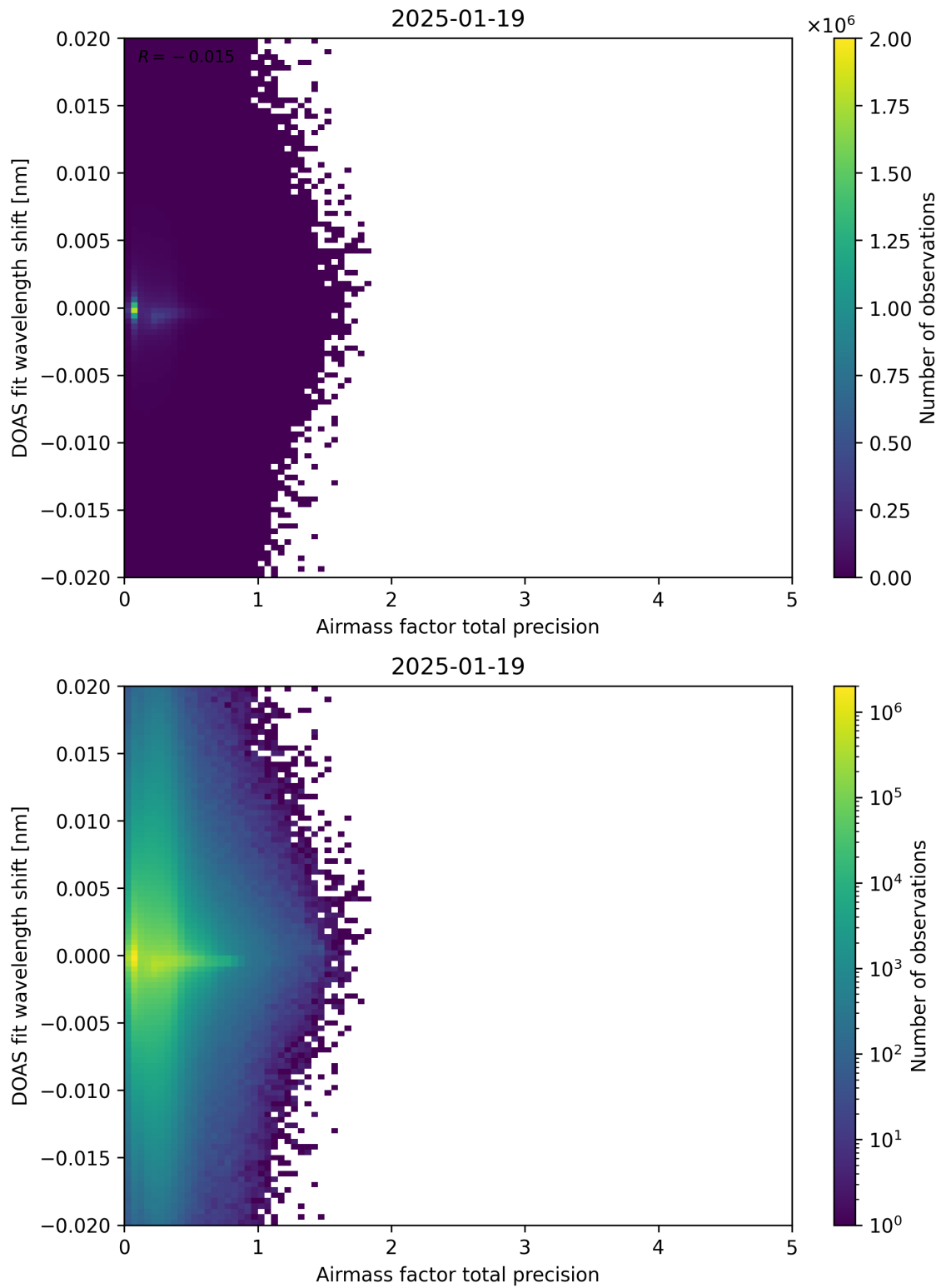
Figure 106: Scatter density plot of “Airmass factor total precision” against “DOAS fit wavelength shift” for 2025-01-18 to 2025-01-20.
