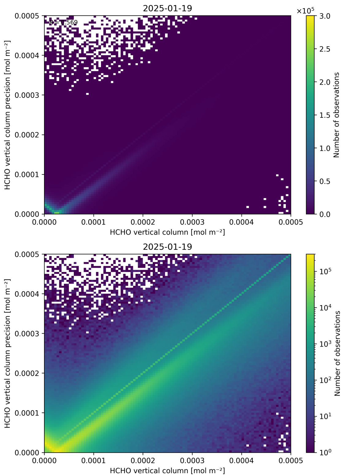
Figure 134: Scatter density plot of “HCHO vertical column” against “HCHO vertical column precision” for 2025-01-18 to 2025-01-20.
