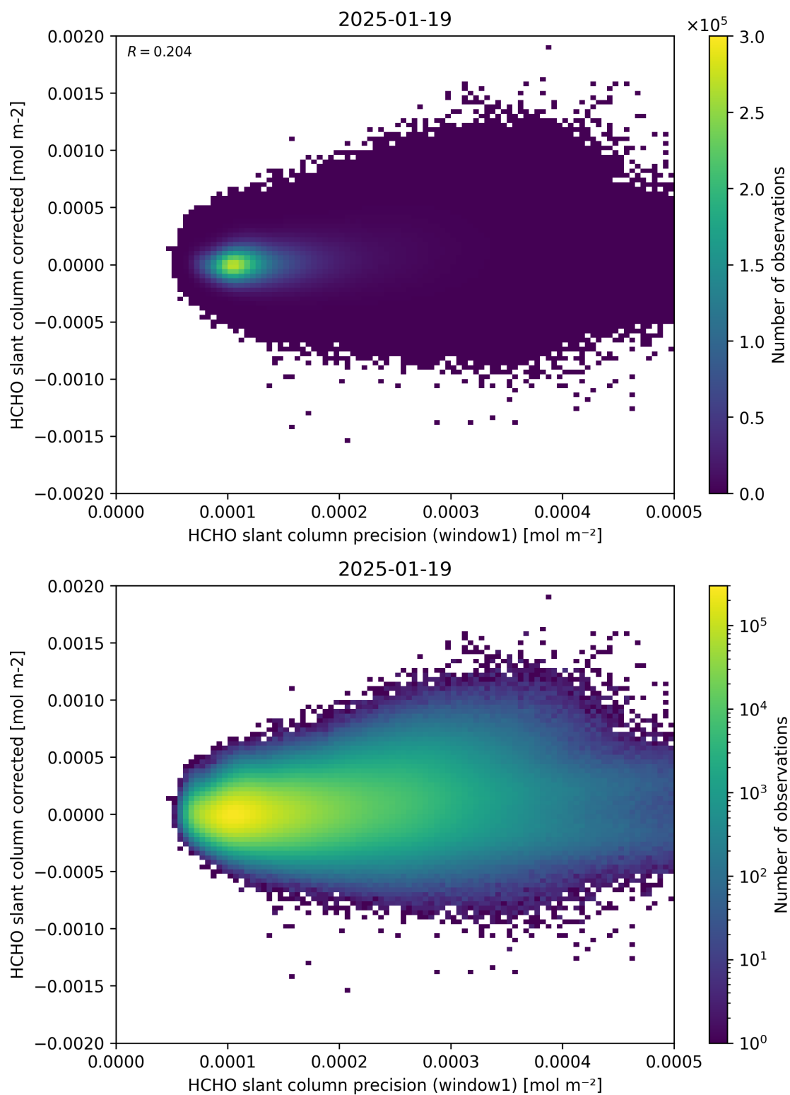
Figure 92: Scatter density plot of “HCHO slant column precision (window1)” against “HCHO slant column corrected” for 2025-01-18 to 2025-01-20.
