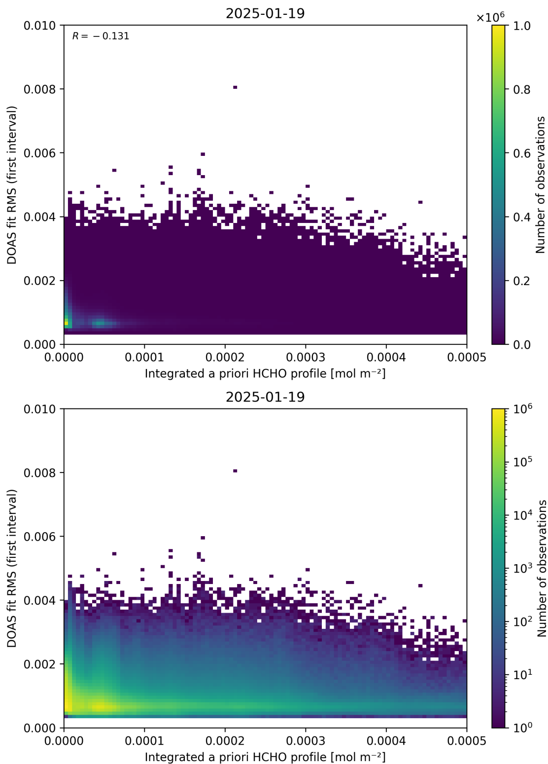
Figure 148: Scatter density plot of “Integrated a priori HCHO profile” against “DOAS fit RMS (first interval)” for 2025-01-18 to 2025-01-20.
