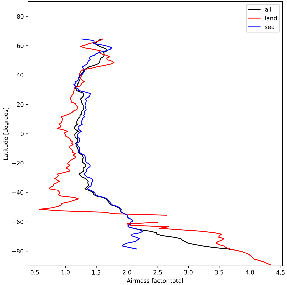
Figure 26: Zonal average of “Airmass factor total” for 2025-01-18 to 2025-01-20.
