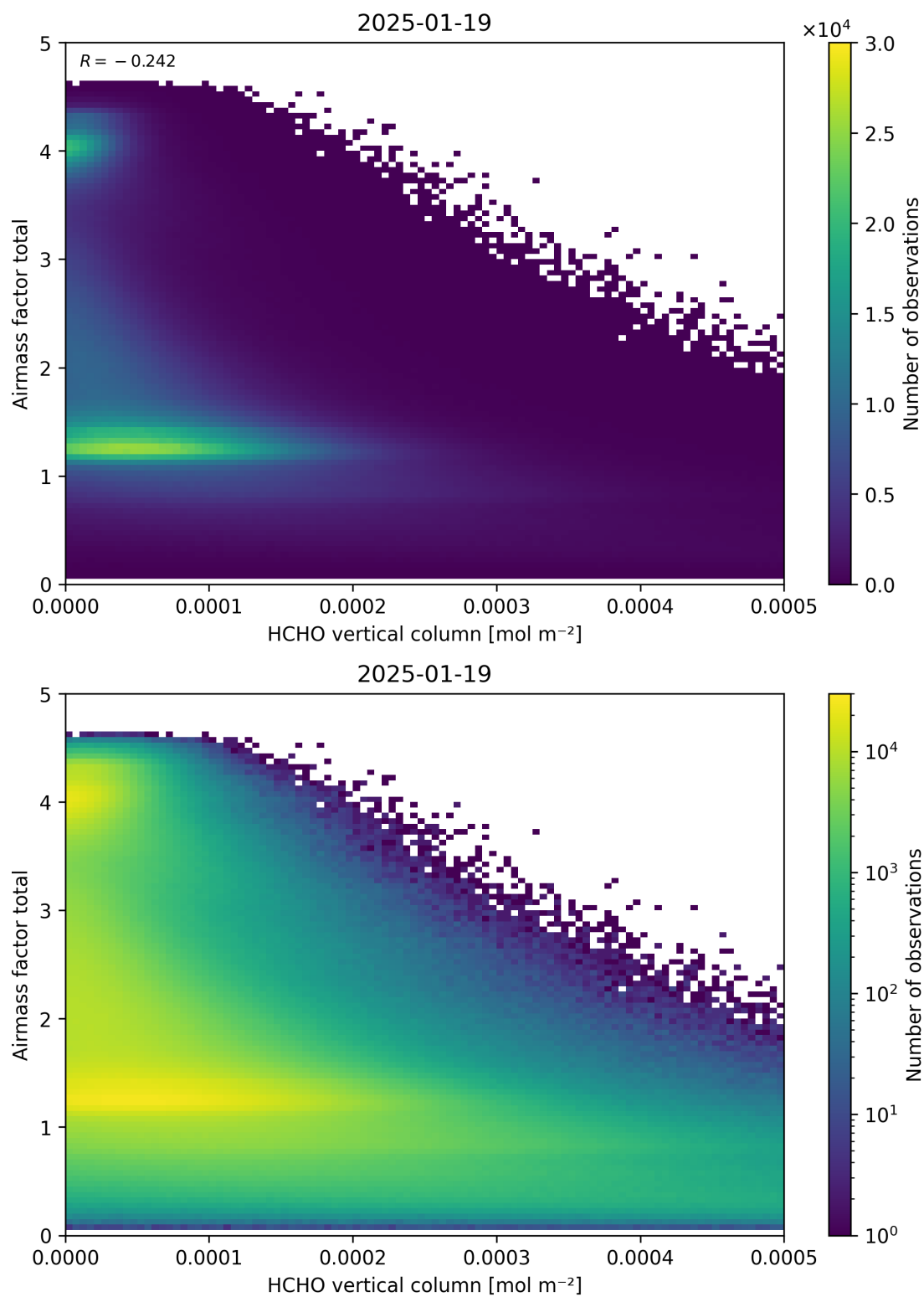
Figure 131: Scatter density plot of “HCHO vertical column” against “Airmass factor total” for 2025-01-18 to 2025-01-20.
