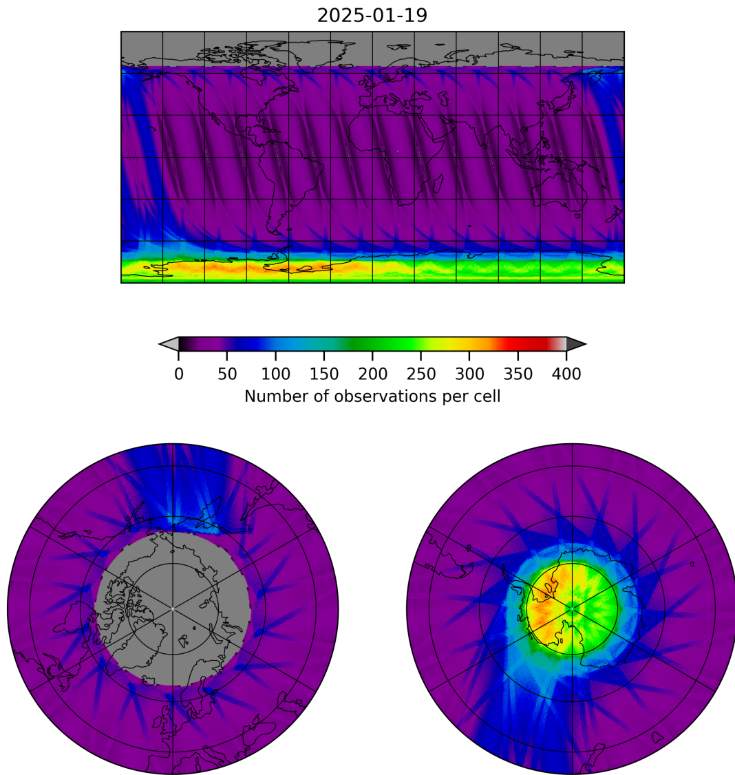
Figure 19: Map of the number of observations for 2025-01-18 to 2025-01-20
