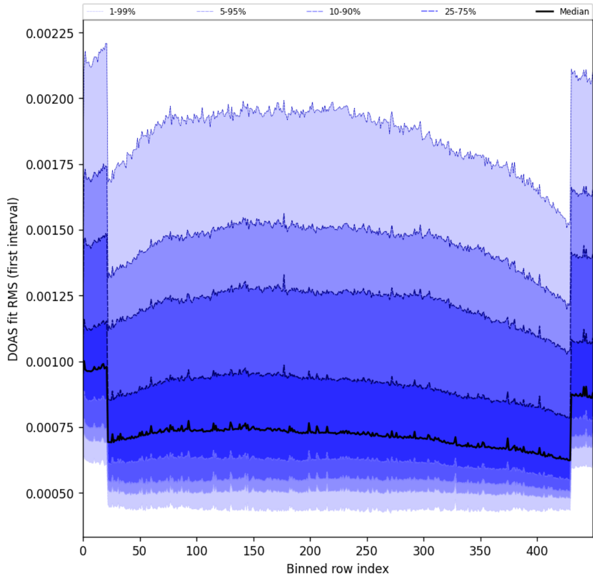
Figure 60: Along track statistics of “DOAS fit RMS (first interval)” for 2025-01-18 to 2025-01-20
