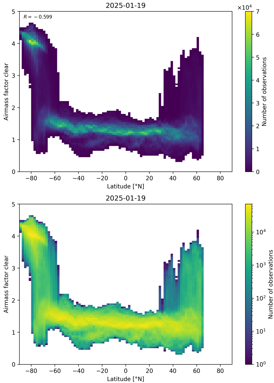
Figure 156: Scatter density plot of “Latitude” against “Airmass factor clear” for 2025-01-18 to 2025-01-20.
