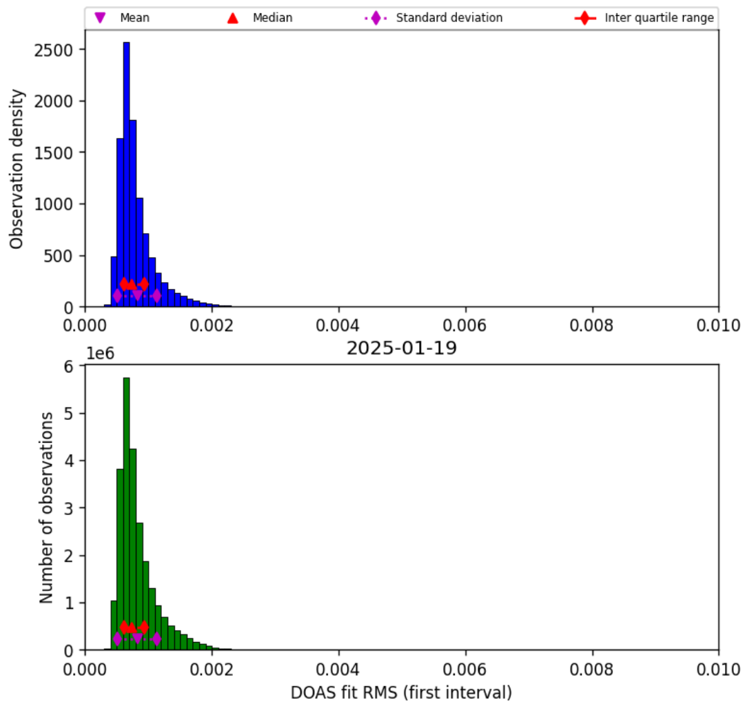
Figure 46: Histogram of “DOAS fit RMS (first interval)” for 2025-01-18 to 2025-01-20
