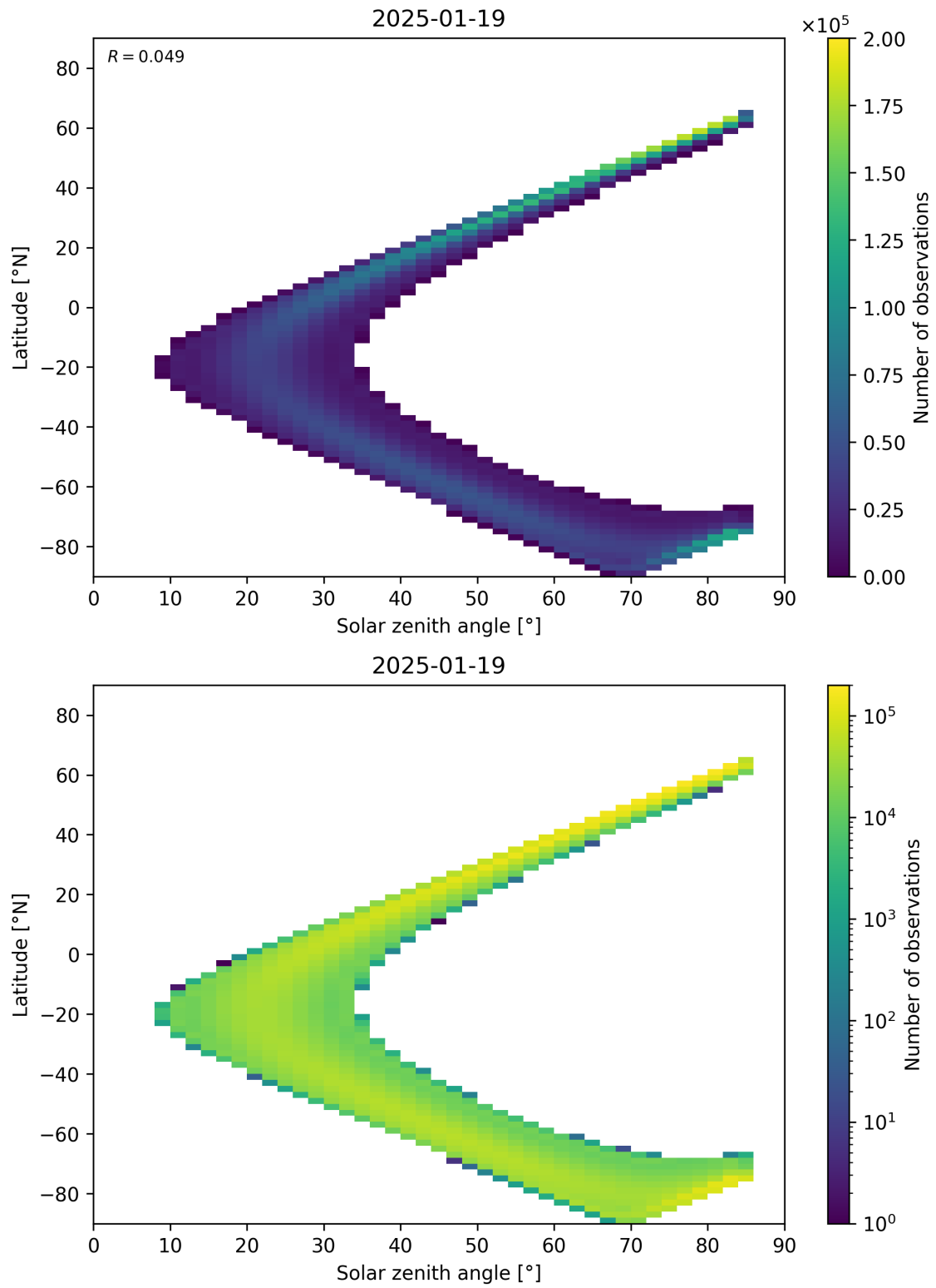
Figure 181: Scatter density plot of “Solar zenith angle” against “Latitude” for 2025-01-18 to 2025-01-20.
