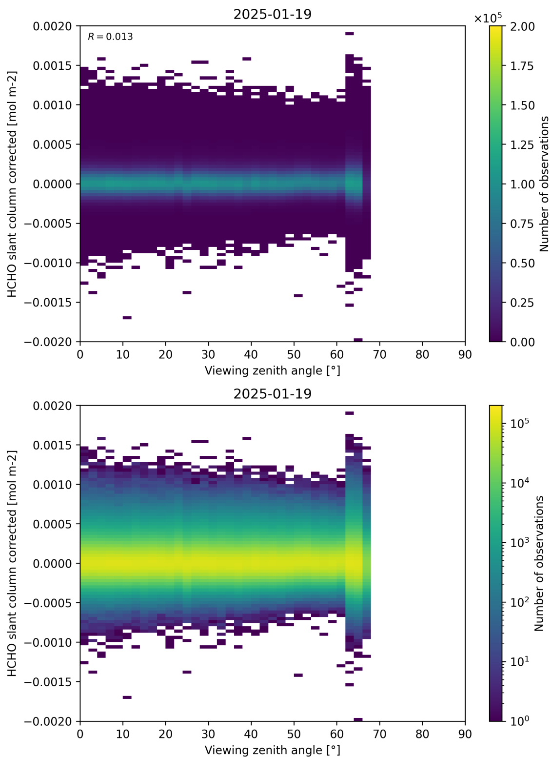
Figure 186: Scatter density plot of “Viewing zenith angle” against “HCHO slant column corrected” for 2025-01-18 to 2025-01-20.
