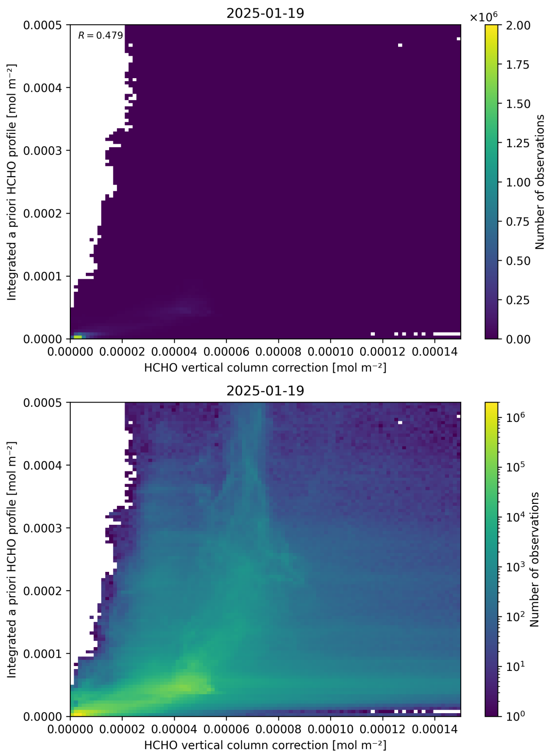
Figure 122: Scatter density plot of “HCHO vertical column correction” against “Integrated a priori HCHO profile” for 2025-01-18 to 2025-01-20.
