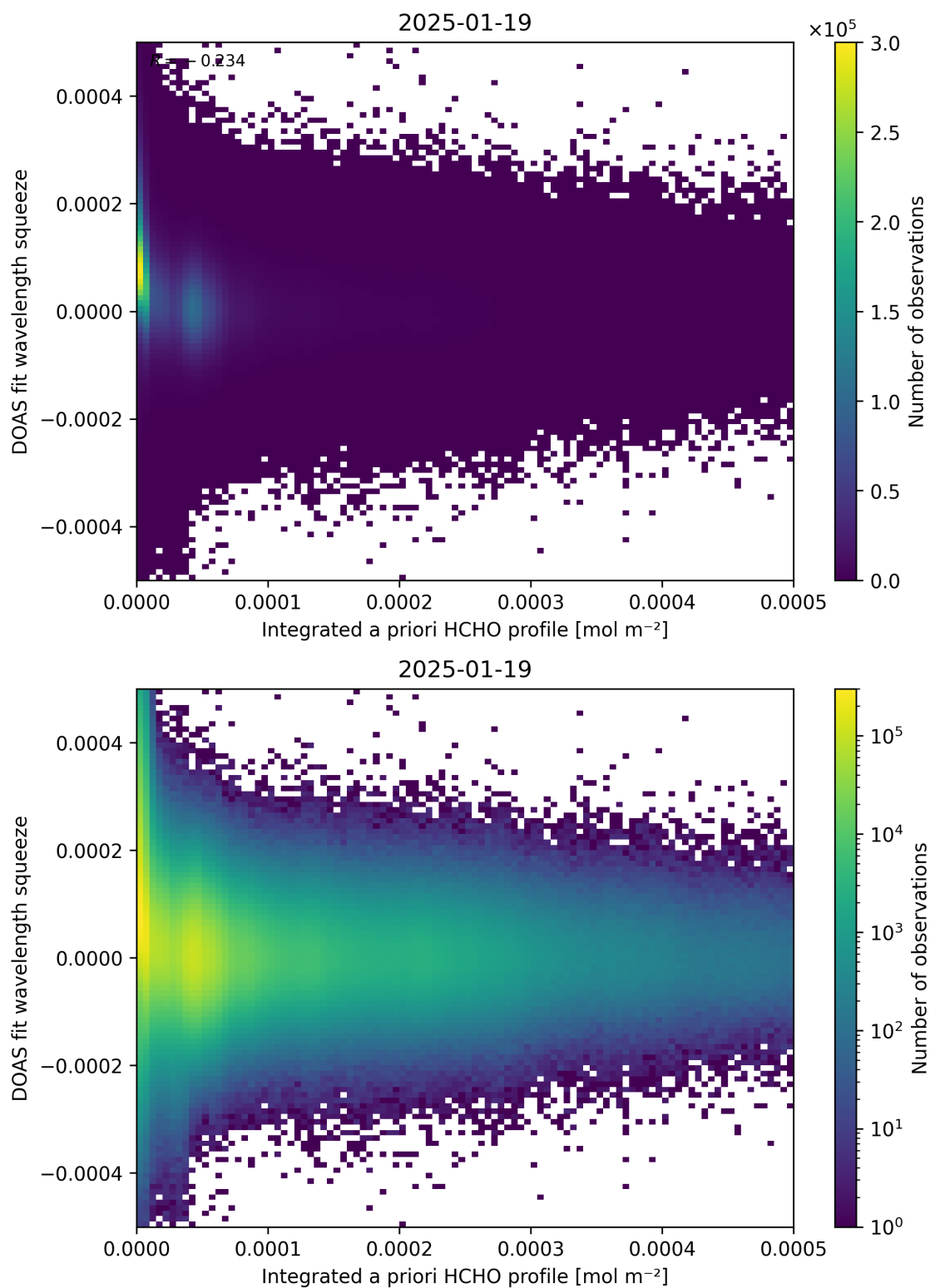
Figure 150: Scatter density plot of “Integrated a priori HCHO profile” against “DOAS fit wavelength squeeze” for 2025-01-18 to 2025-01-20.
