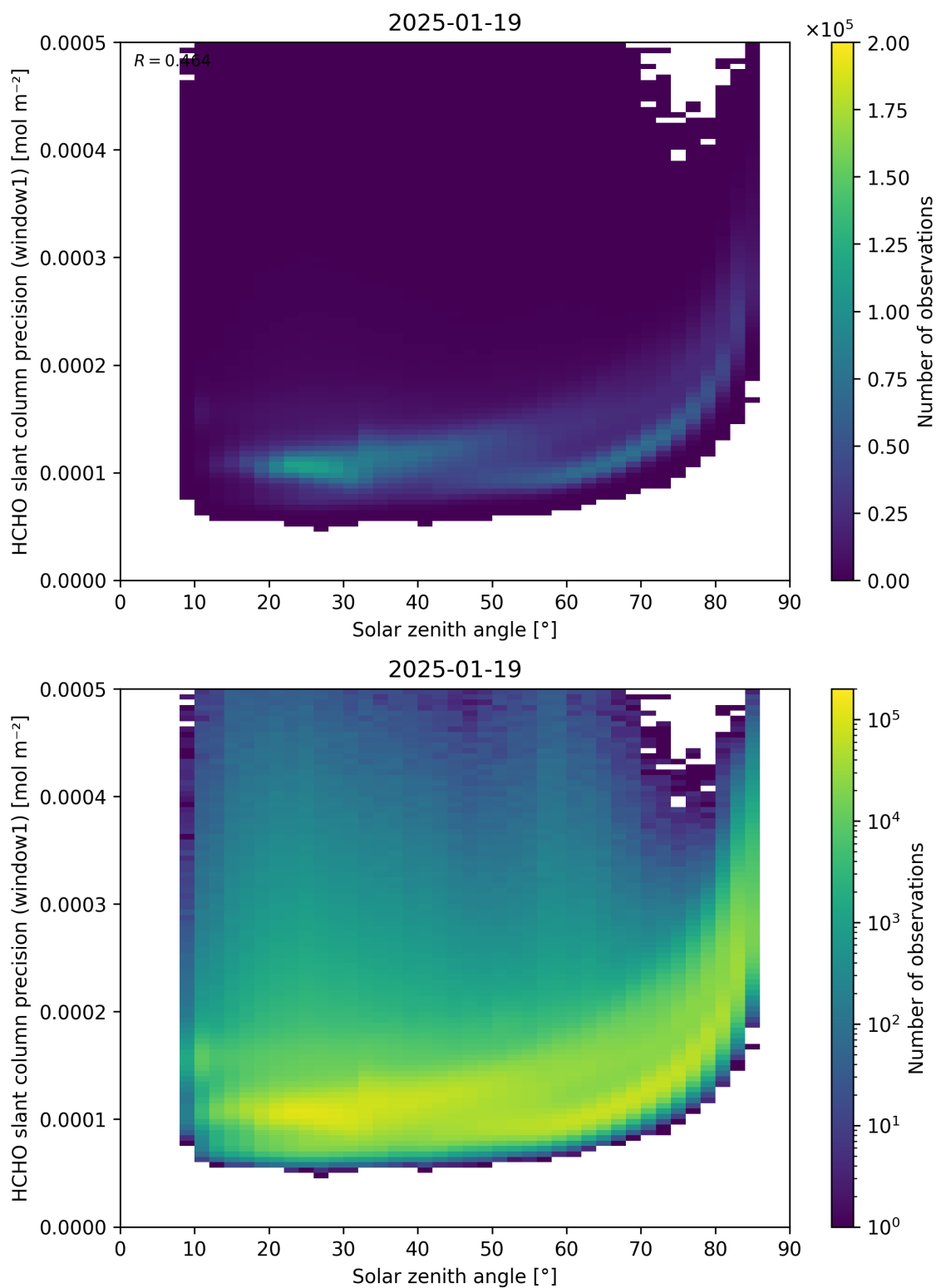
Figure 174: Scatter density plot of “Solar zenith angle” against “HCHO slant column precision (window1)” for 2025-01-18 to 2025-01-20.
