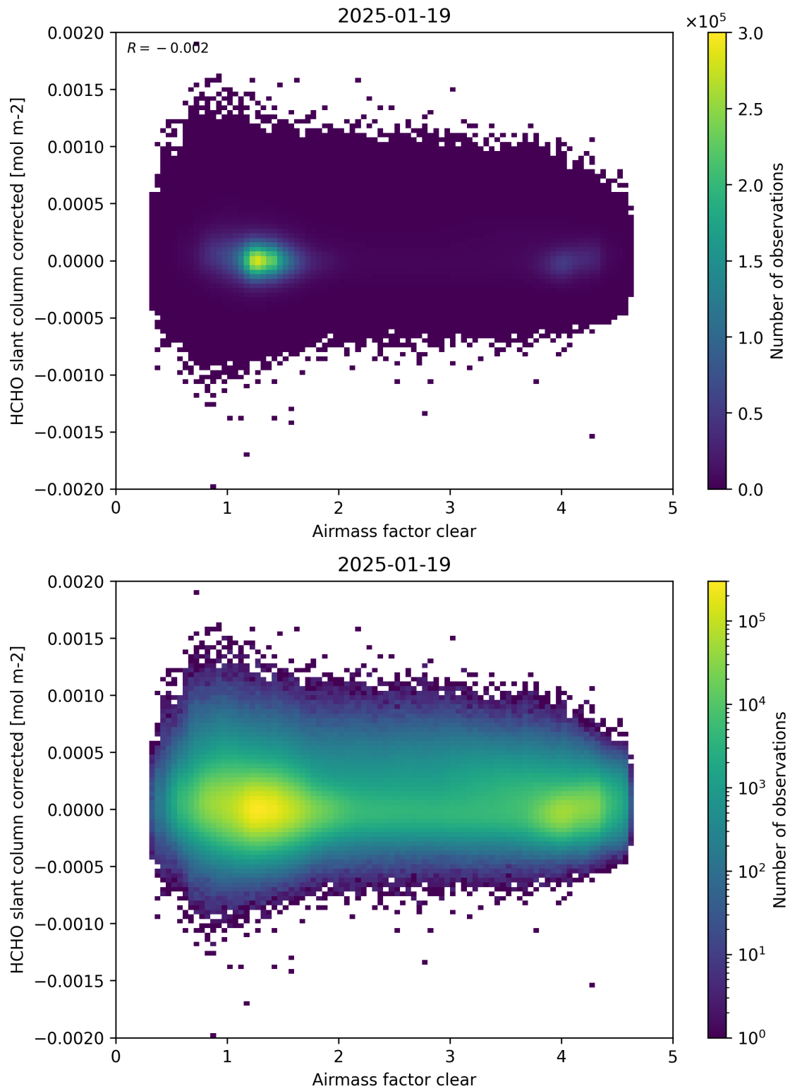
Figure 74: Scatter density plot of “Airmass factor clear” against “HCHO slant column corrected” for 2025-01-18 to 2025-01-20.
