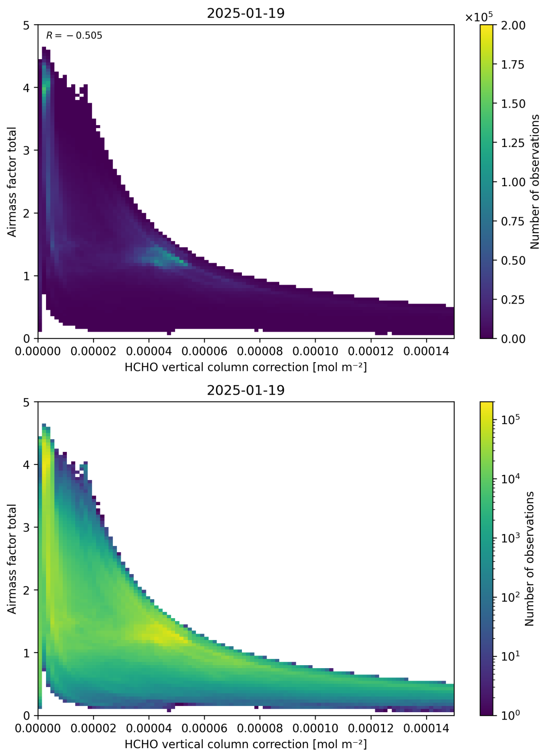
Figure 120: Scatter density plot of “HCHO vertical column correction” against “Airmass factor total” for 2025-01-18 to 2025-01-20.
