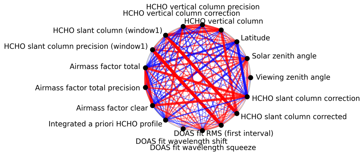
Figure 1: Map of correlation graph for 2025-01-18 to 2025-01-20.
