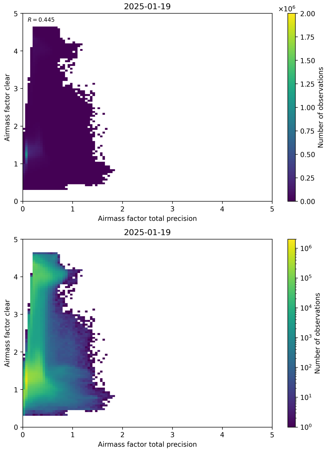
Figure 108: Scatter density plot of “Airmass factor total precision” against “Airmass factor clear” for 2025-01-18 to 2025-01-20.
