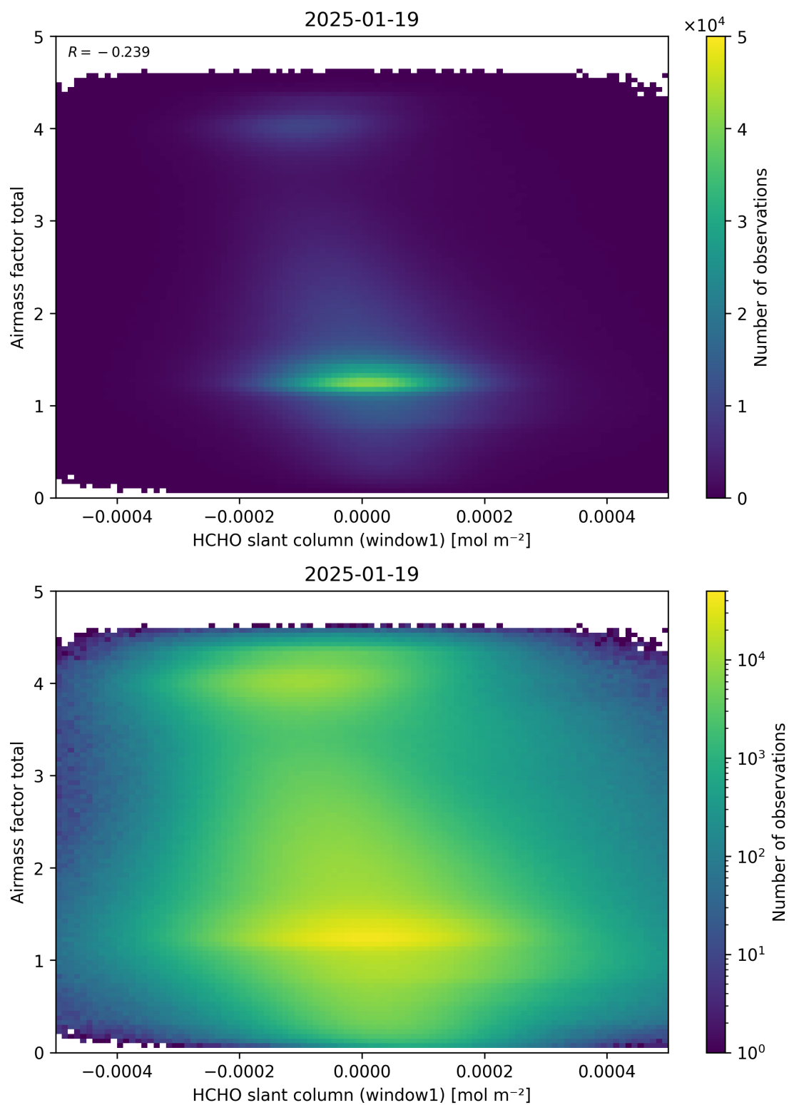
Figure 85: Scatter density plot of “HCHO slant column (window1)” against “Airmass factor total” for 2025-01-18 to 2025-01-20.
