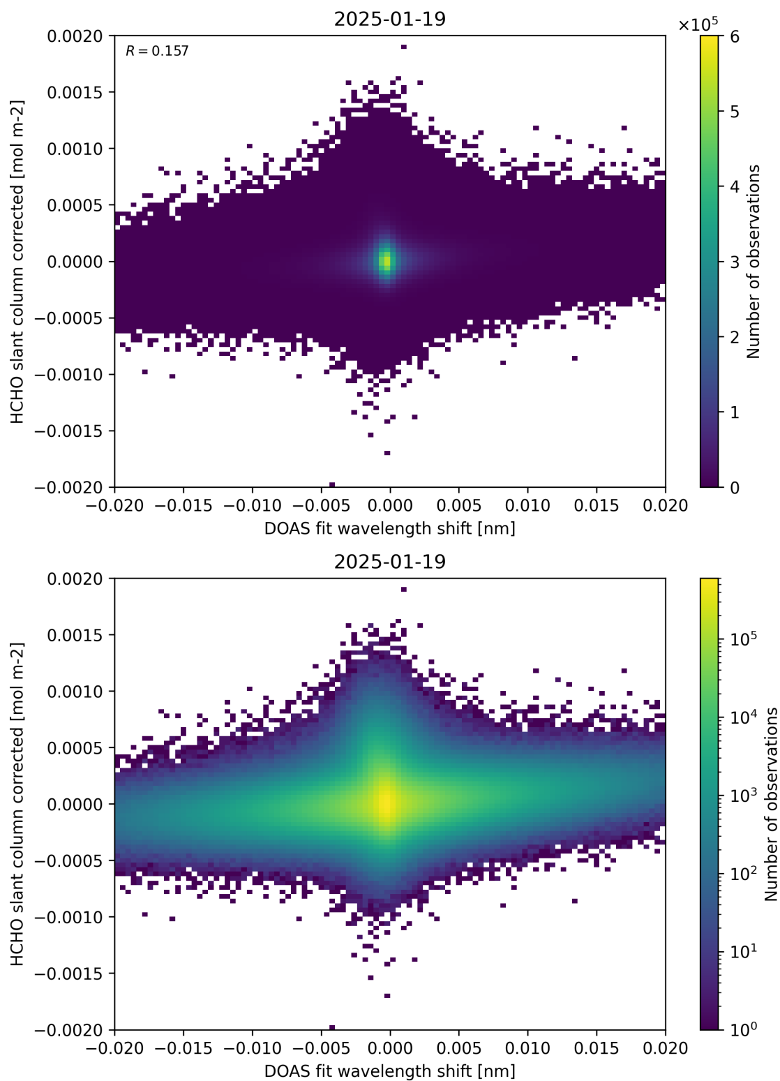
Figure 66: Scatter density plot of “DOAS fit wavelength shift” against “HCHO slant column corrected” for 2025-01-18 to 2025-01-20.
