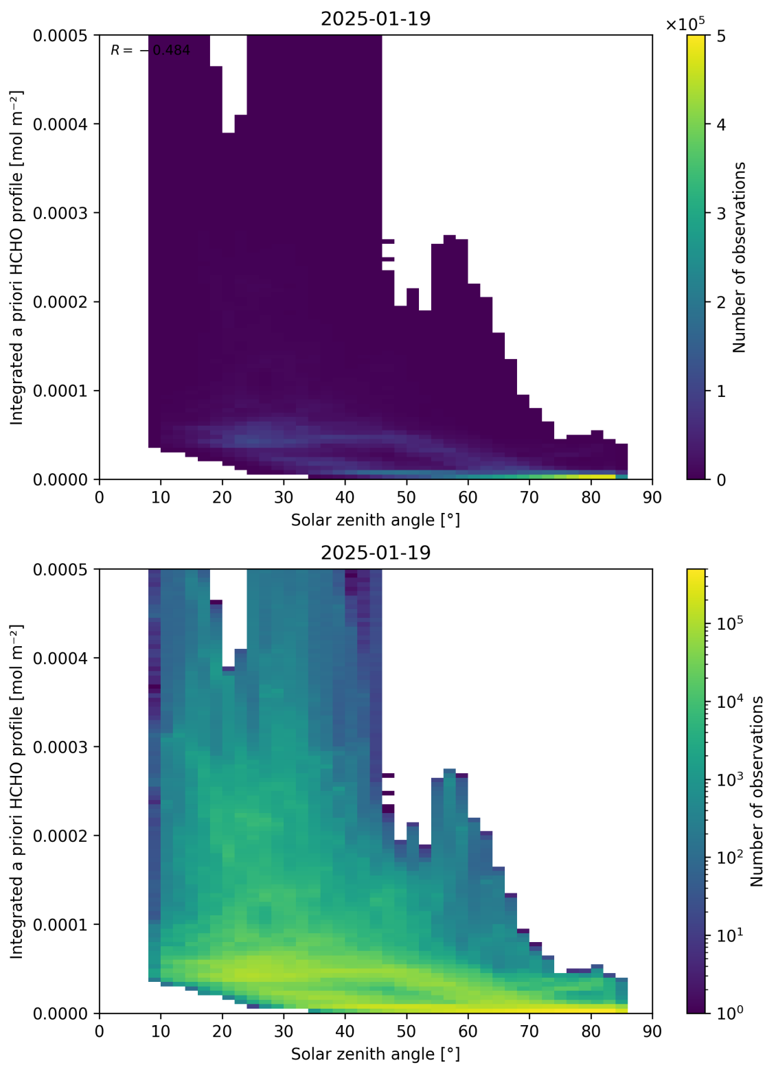
Figure 180: Scatter density plot of “Solar zenith angle” against “Integrated a priori HCHO profile” for 2025-01-18 to 2025-01-20.
