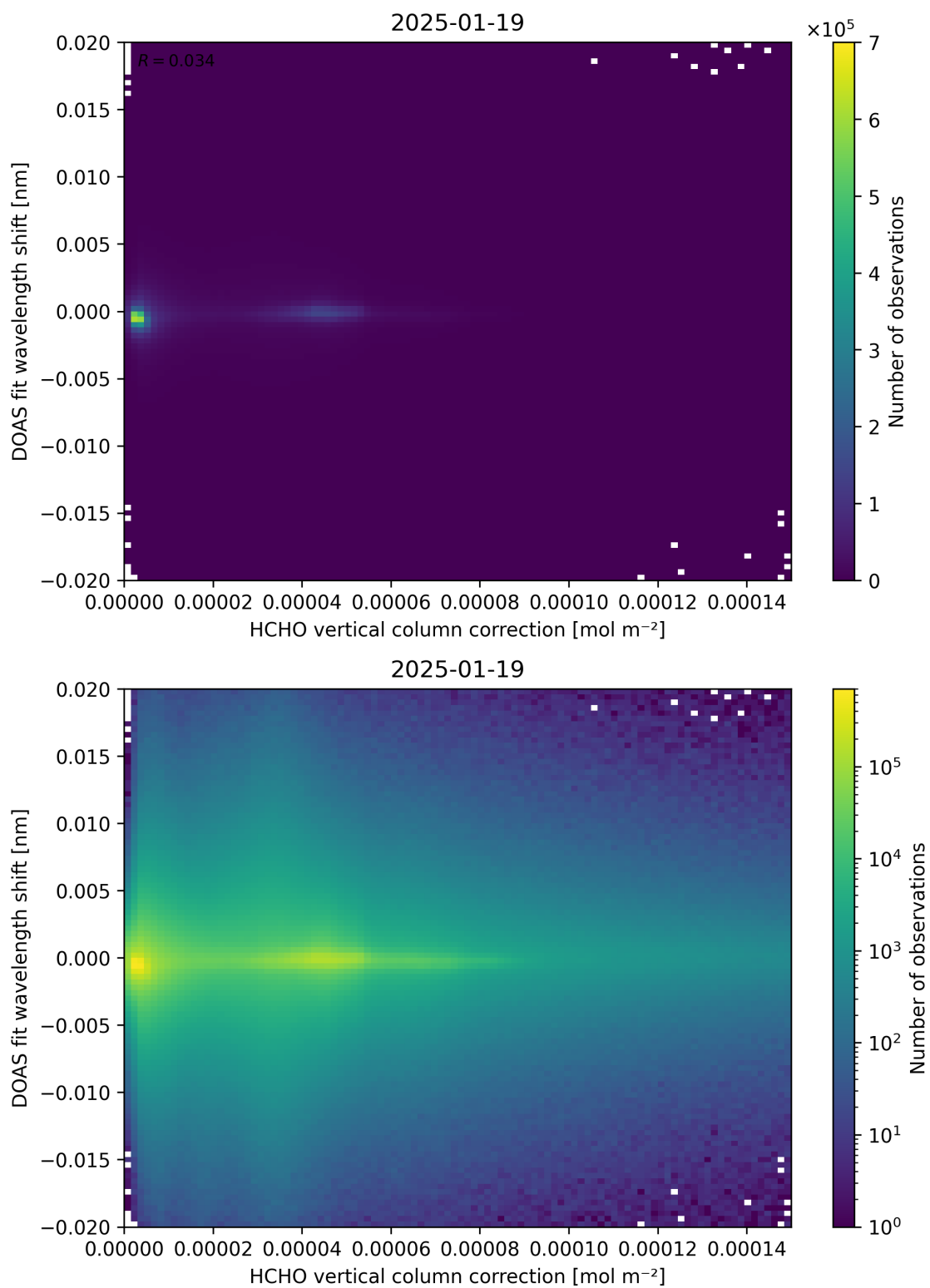
Figure 113: Scatter density plot of “HCHO vertical column correction” against “DOAS fit wavelength shift” for 2025-01-18 to 2025-01-20.
