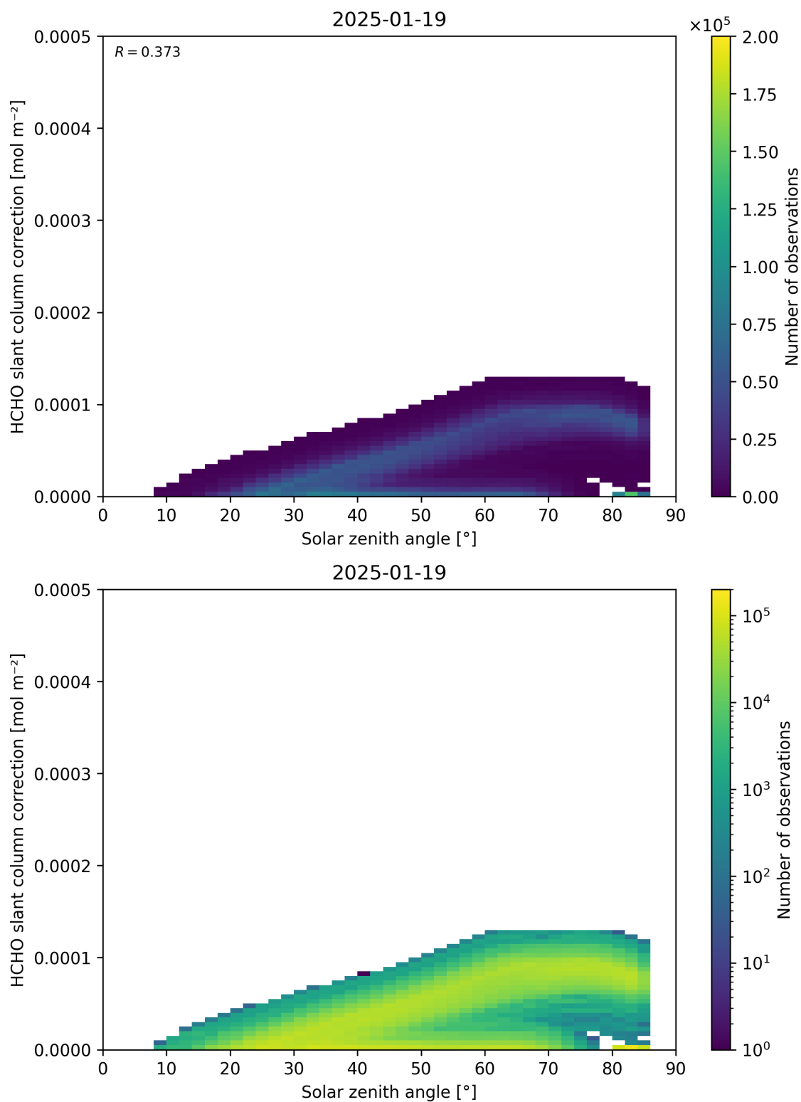
Figure 172: Scatter density plot of “Solar zenith angle” against “HCHO slant column correction” for 2025-01-18 to 2025-01-20.
