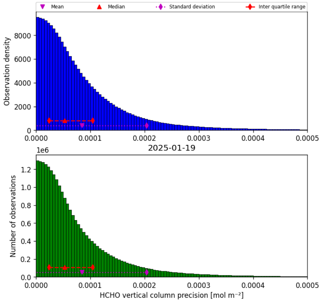
Figure 36: Histogram of “HCHO vertical column precision” for 2025-01-18 to 2025-01-20
