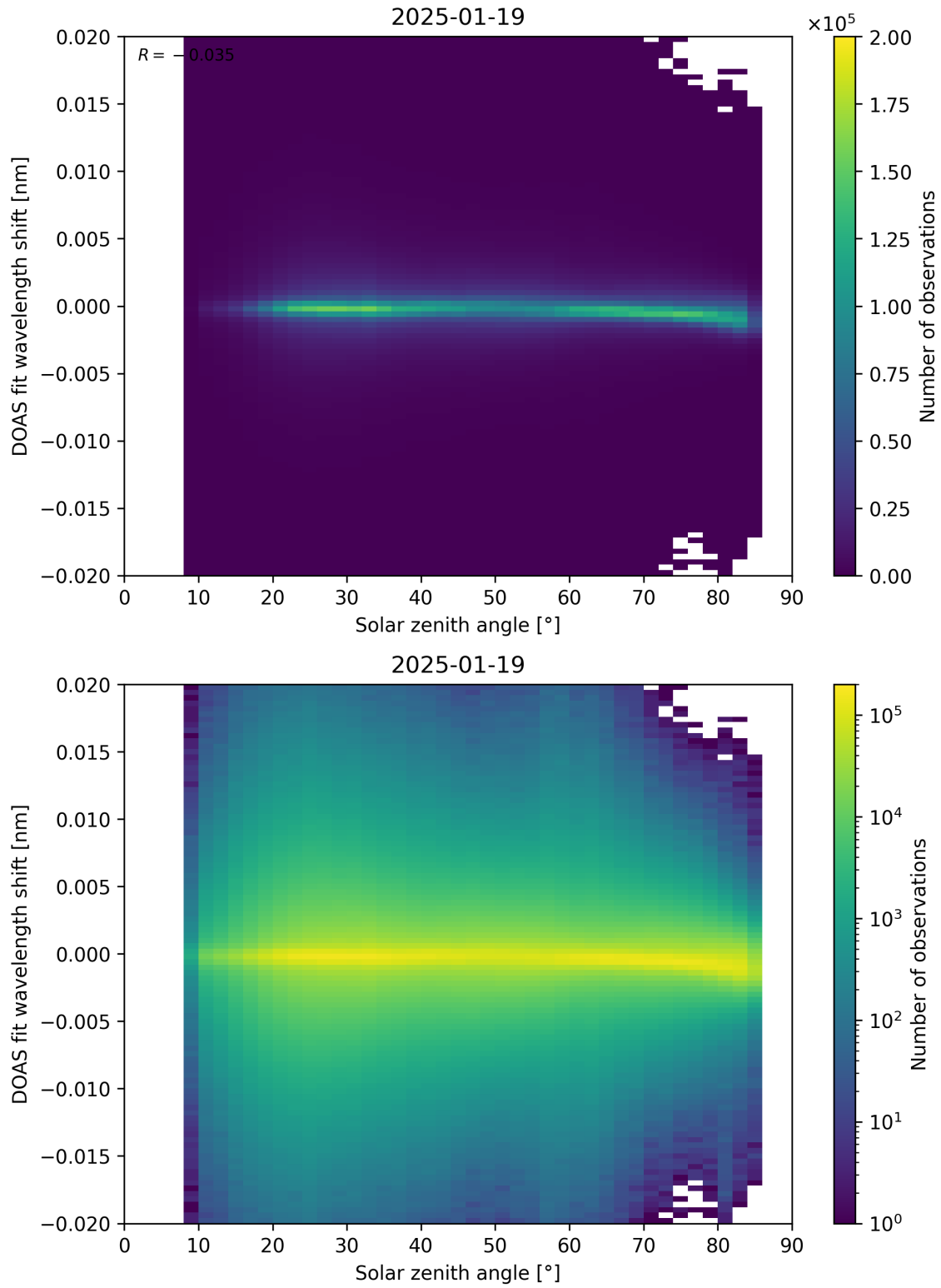
Figure 168: Scatter density plot of “Solar zenith angle” against “DOAS fit wavelength shift” for 2025-01-18 to 2025-01-20.
