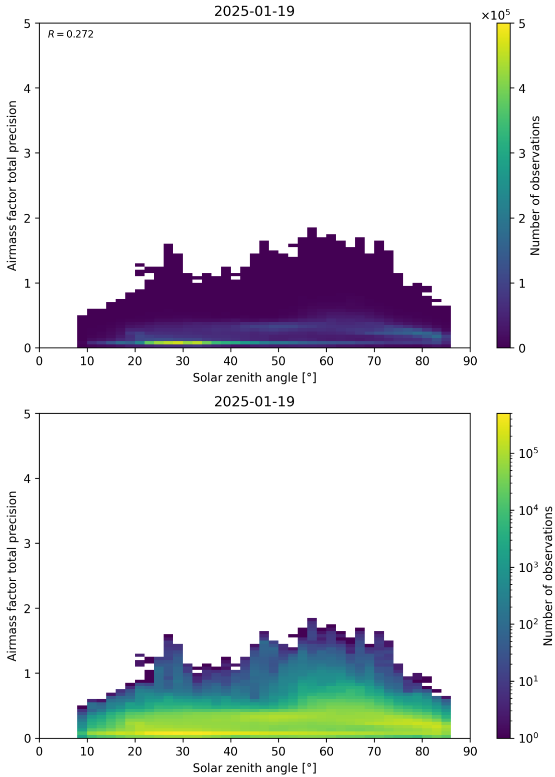
Figure 176: Scatter density plot of “Solar zenith angle” against “Airmass factor total precision” for 2025-01-18 to 2025-01-20.
