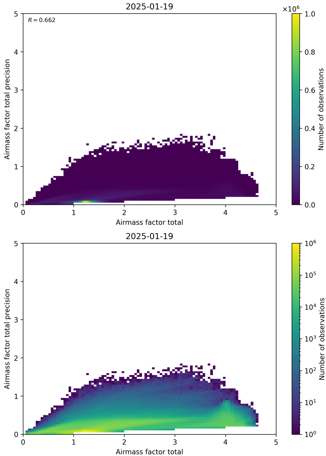
Figure 103: Scatter density plot of “Airmass factor total” against “Airmass factor total precision” for 2025-01-18 to 2025-01-20.
