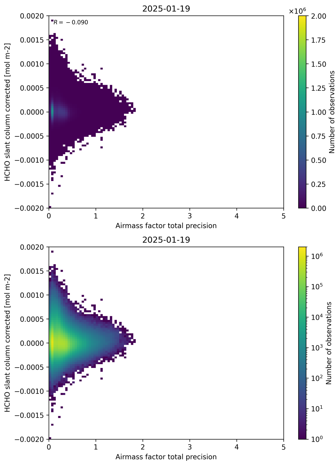
Figure 109: Scatter density plot of “Airmass factor total precision” against “HCHO slant column corrected” for 2025-01-18 to 2025-01-20.
