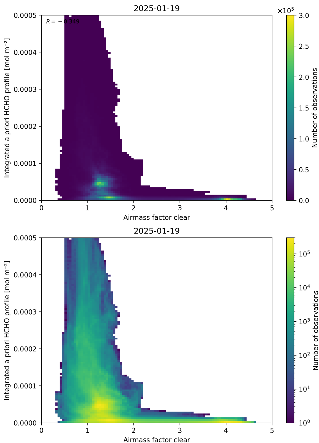
Figure 76: Scatter density plot of “Airmass factor clear” against “Integrated a priori HCHO profile” for 2025-01-18 to 2025-01-20.
