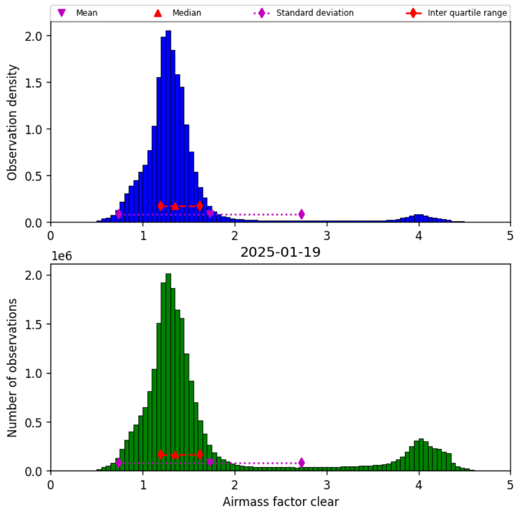
Figure 42: Histogram of “Airmass factor clear” for 2025-01-18 to 2025-01-20
