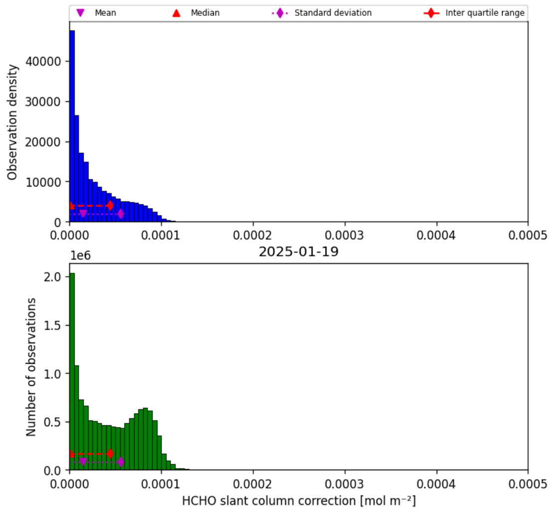
Figure 47: Histogram of “HCHO slant column correction” for 2025-01-18 to 2025-01-20
