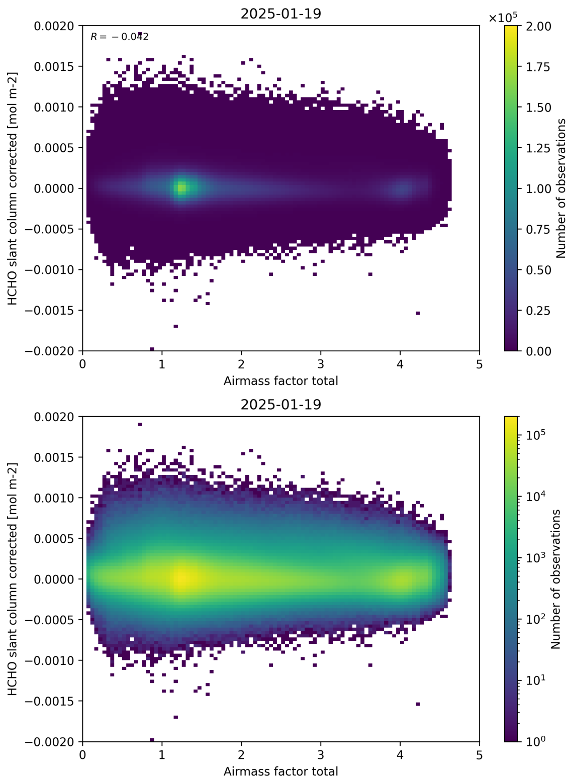
Figure 101: Scatter density plot of “Airmass factor total” against “HCHO slant column corrected” for 2025-01-18 to 2025-01-20.
