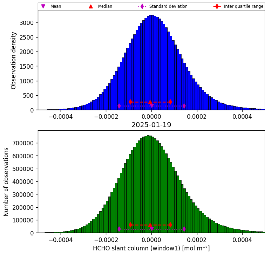
Figure 38: Histogram of “HCHO slant column (window1)” for 2025-01-18 to 2025-01-20
