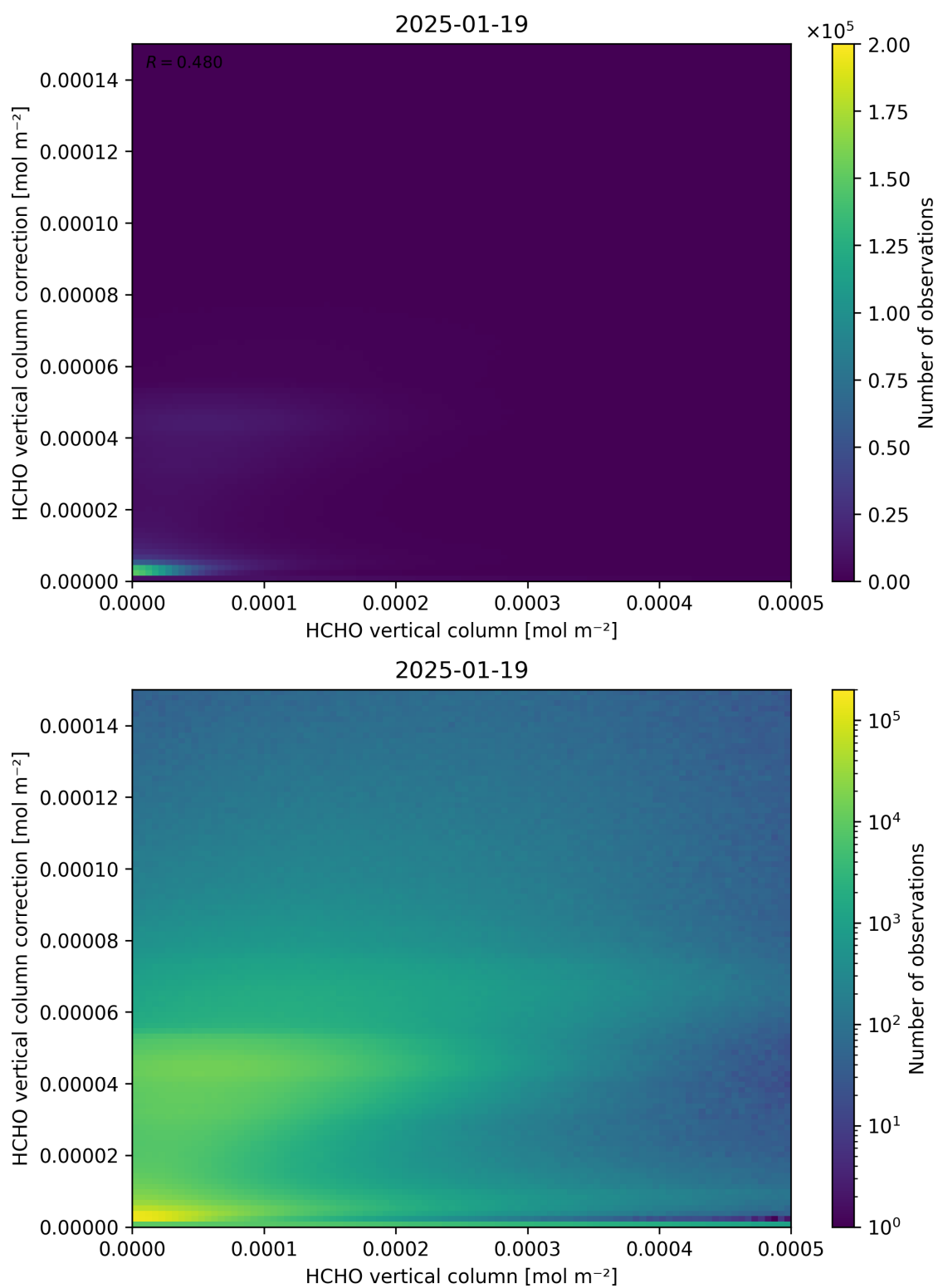
Figure 133: Scatter density plot of “HCHO vertical column” against “HCHO vertical column correction” for 2025-01-18 to 2025-01-20.
