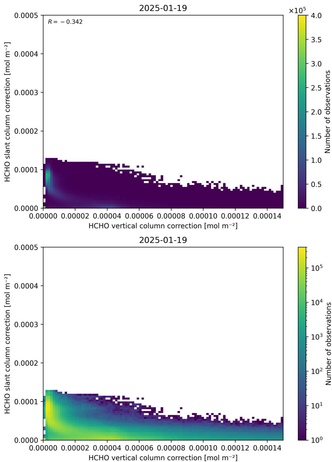
Figure 117: Scatter density plot of “HCHO vertical column correction” against “HCHO slant column correction” for 2025-01-18 to 2025-01-20.
