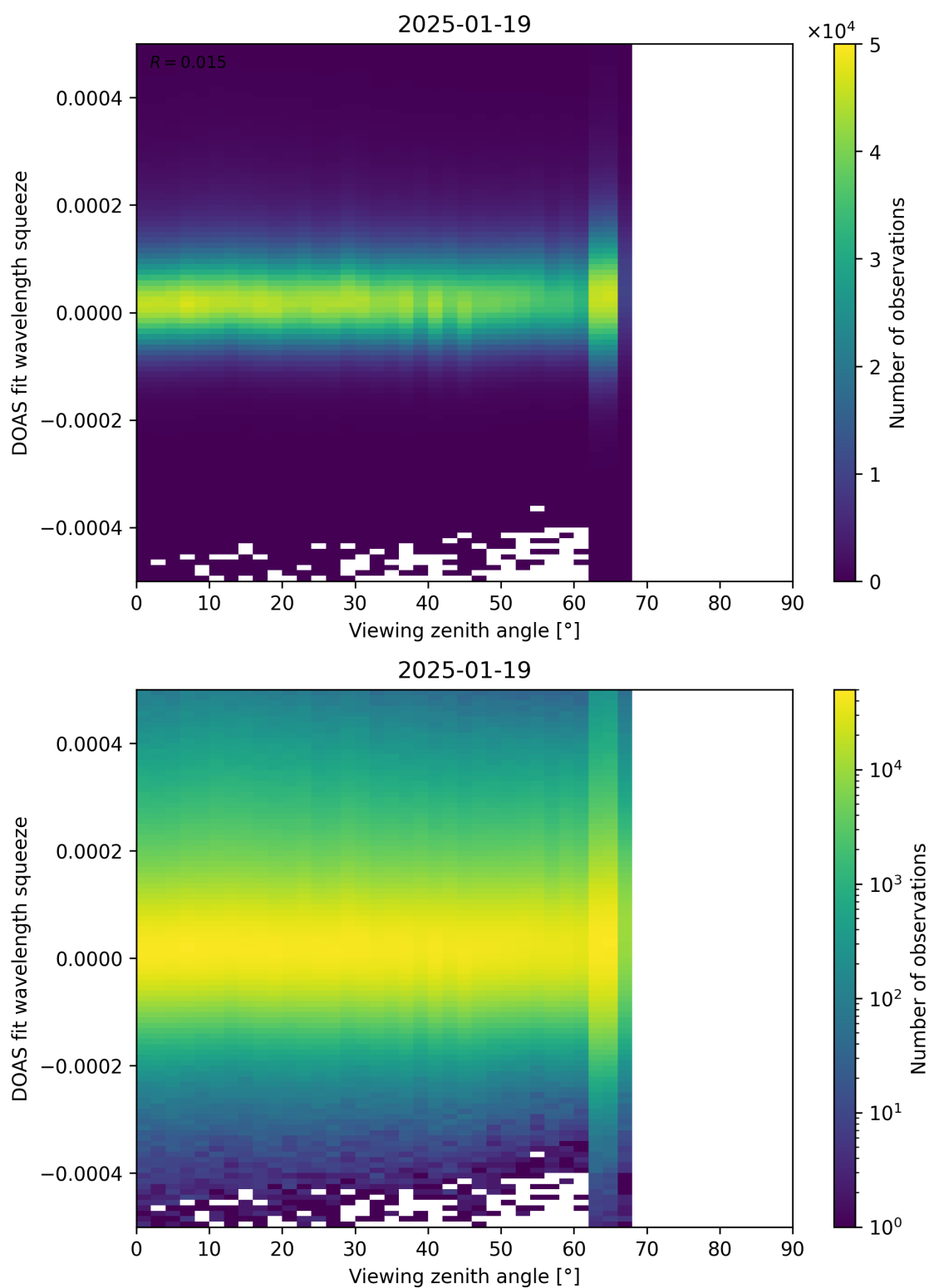
Figure 184: Scatter density plot of “Viewing zenith angle” against “DOAS fit wavelength squeeze” for 2025-01-18 to 2025-01-20.
