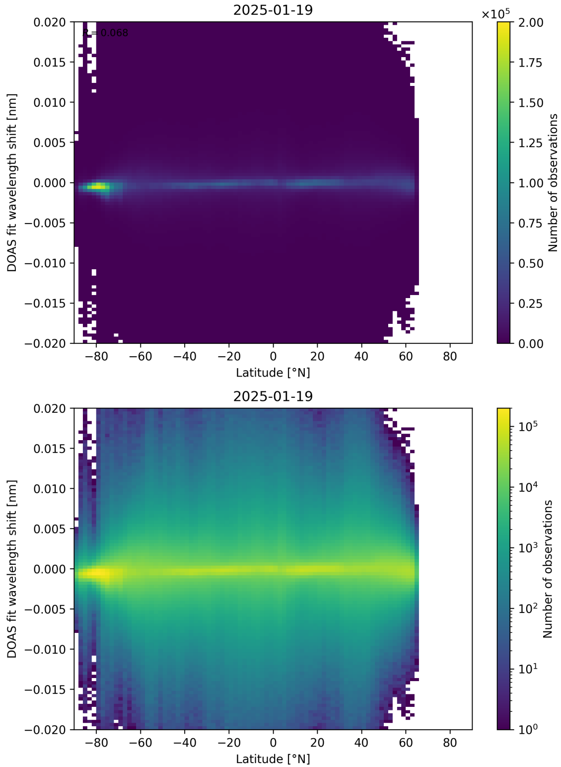
Figure 154: Scatter density plot of “Latitude” against “DOAS fit wavelength shift” for 2025-01-18 to 2025-01-20.
