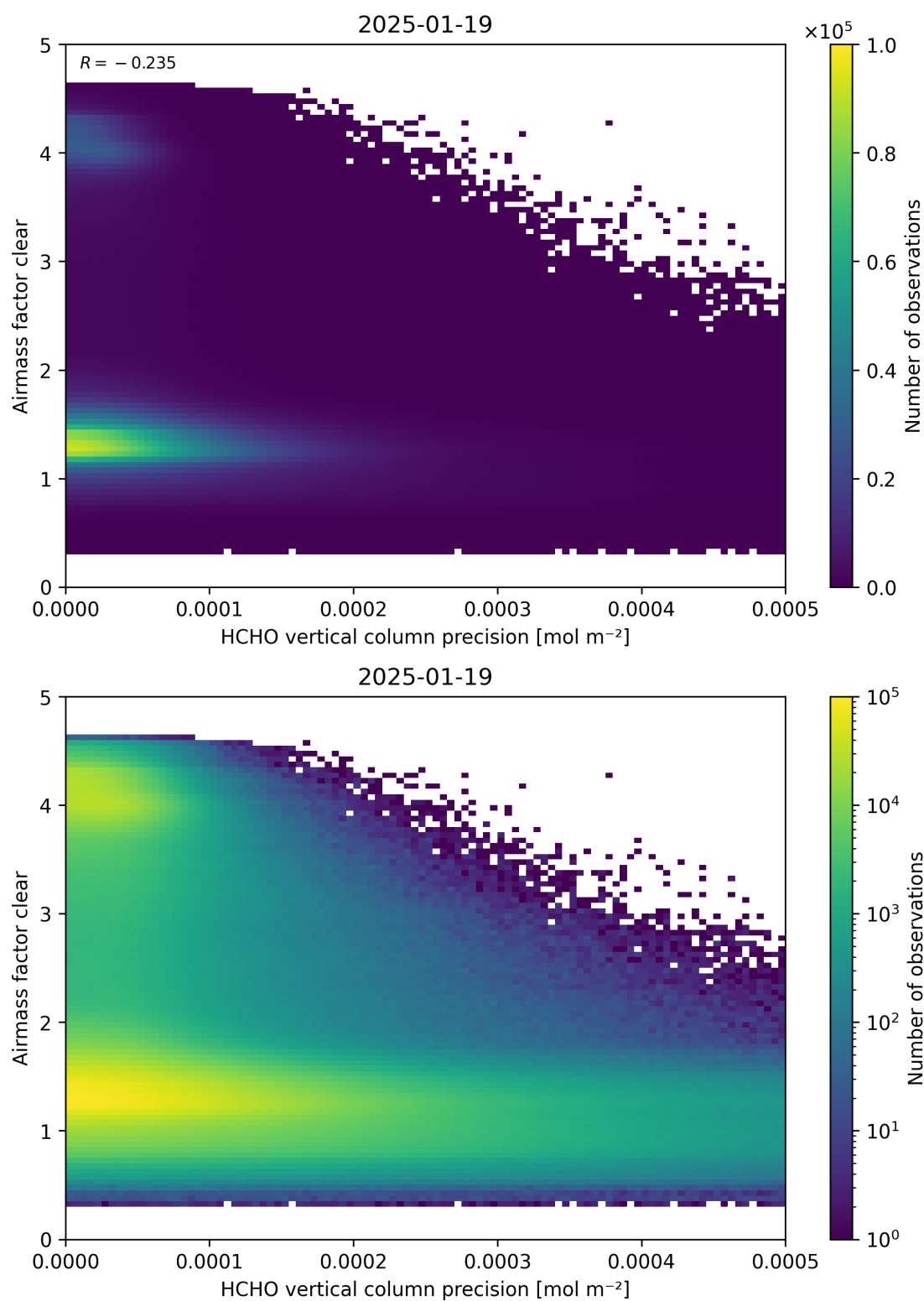
Figure 139: Scatter density plot of “HCHO vertical column precision” against “Airmass factor clear” for 2025-01-18 to 2025-01-20.
