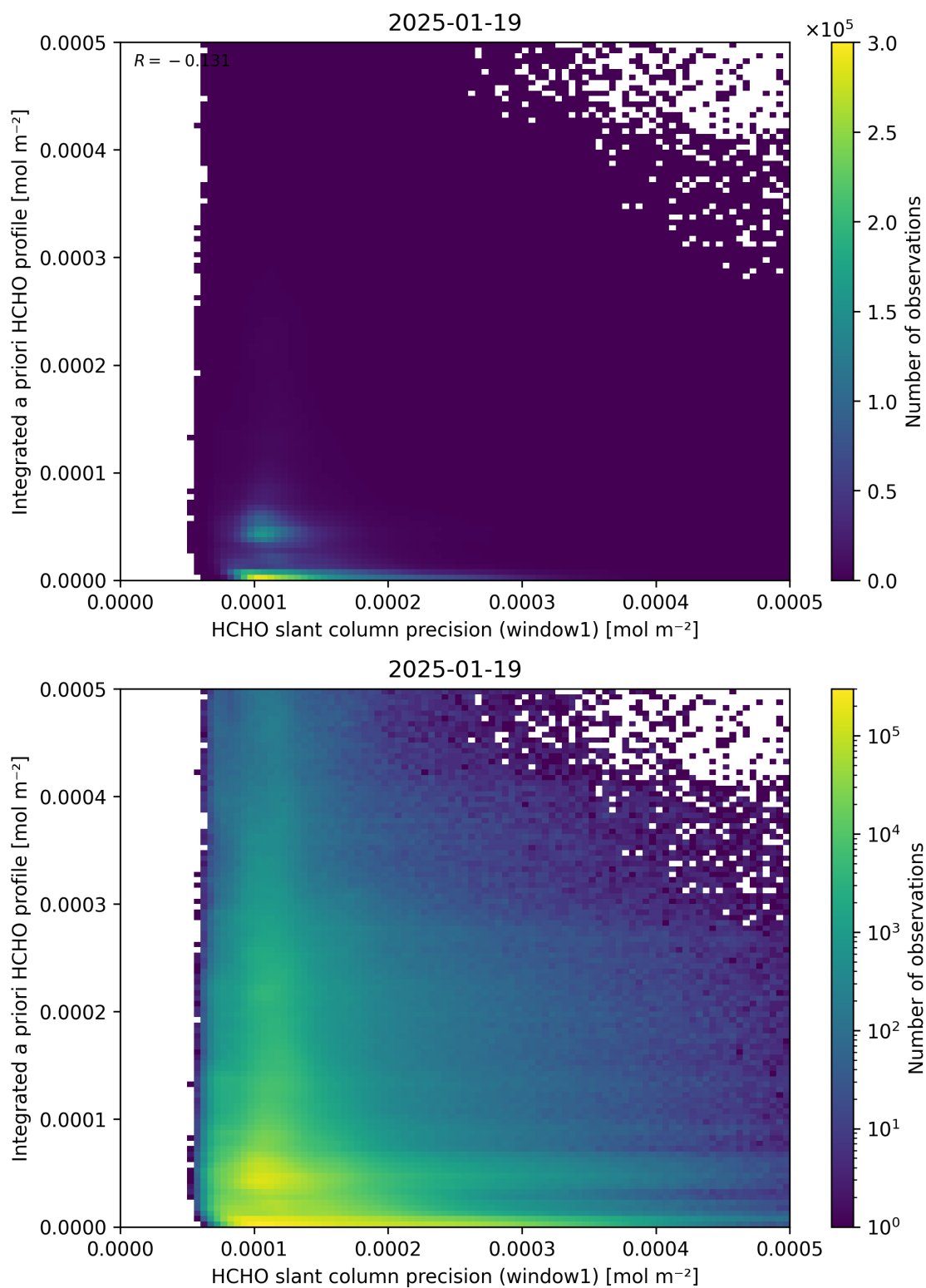
Figure 96: Scatter density plot of “HCHO slant column precision (window1)” against “Integrated a priori HCHO profile” for 2025-01-18 to 2025-01-20.
