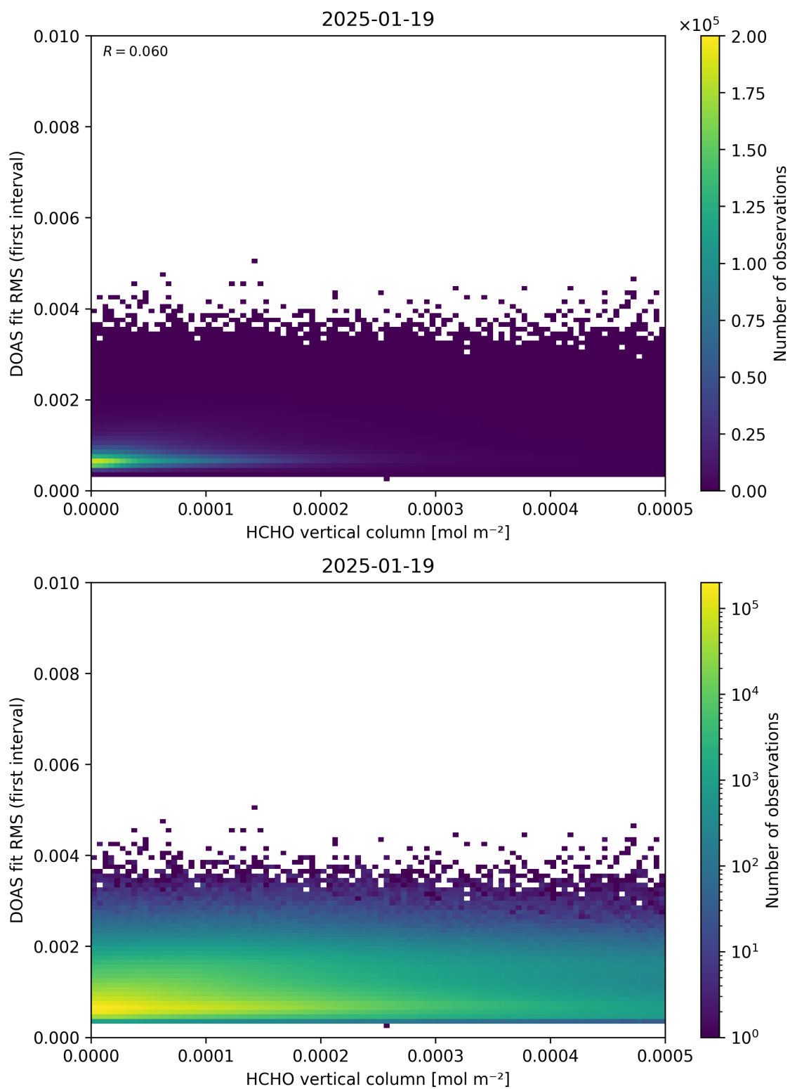
Figure 123: Scatter density plot of “HCHO vertical column” against “DOAS fit RMS (first interval)” for 2025-01-18 to 2025-01-20.
