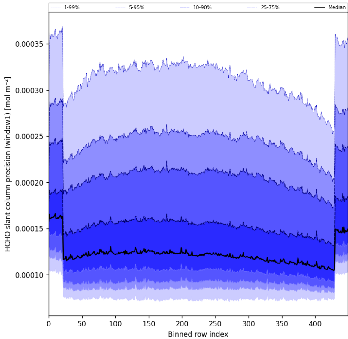
Figure 53: Along track statistics of “HCHO slant column precision (window1)” for 2025-01-18 to 2025-01-20
