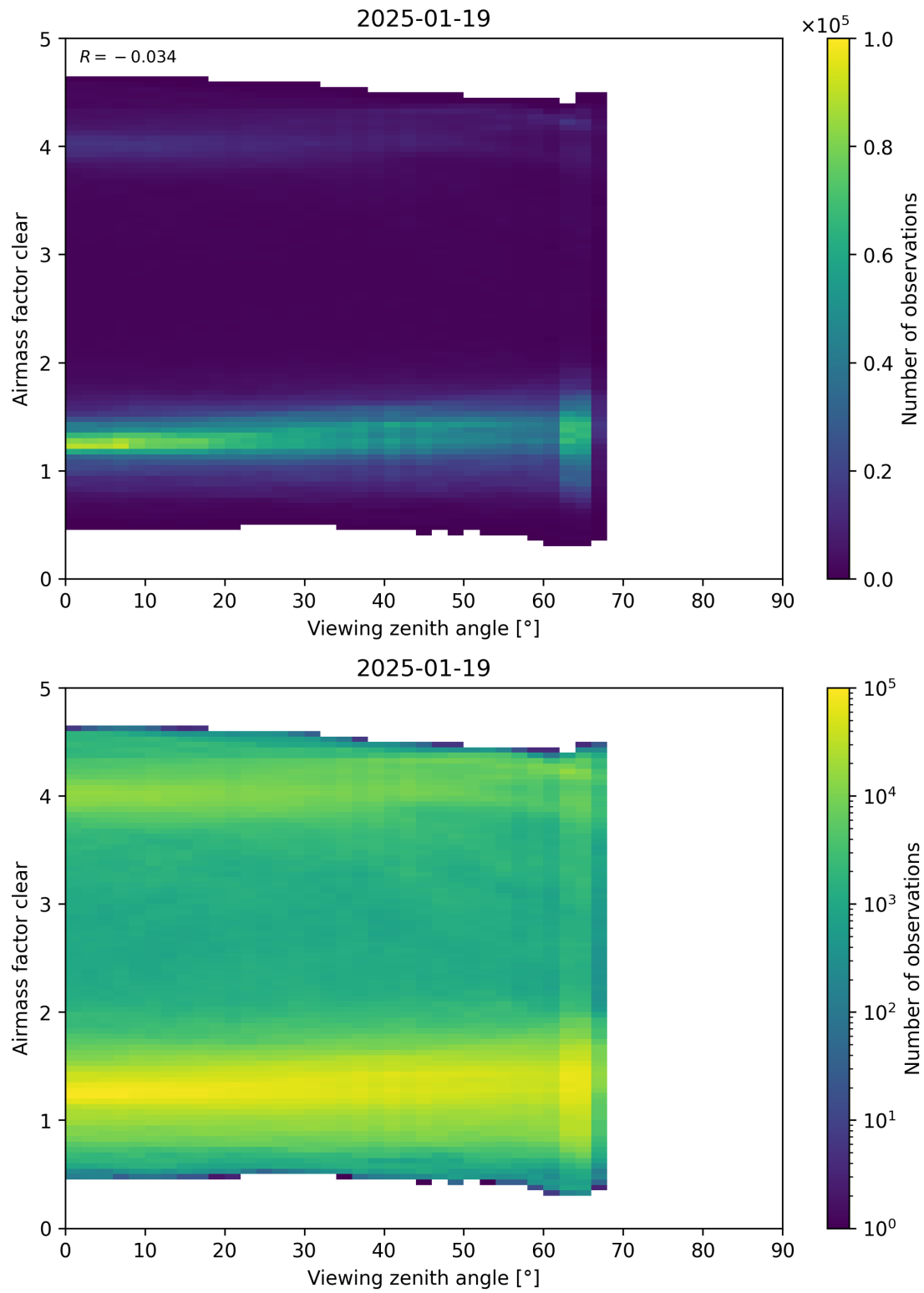
Figure 185: Scatter density plot of “Viewing zenith angle” against “Airmass factor clear” for 2025-01-18 to 2025-01-20.
