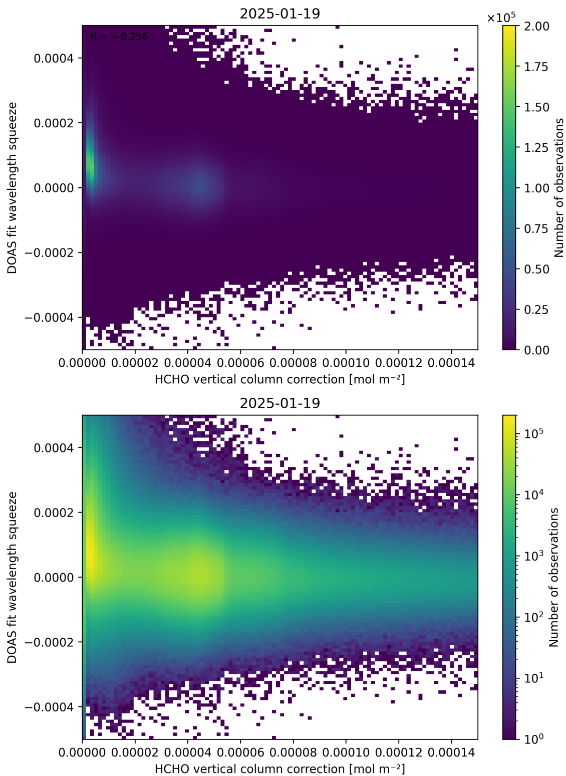
Figure 114: Scatter density plot of “HCHO vertical column correction” against “DOAS fit wavelength squeeze” for 2025-01-18 to 2025-01-20.
