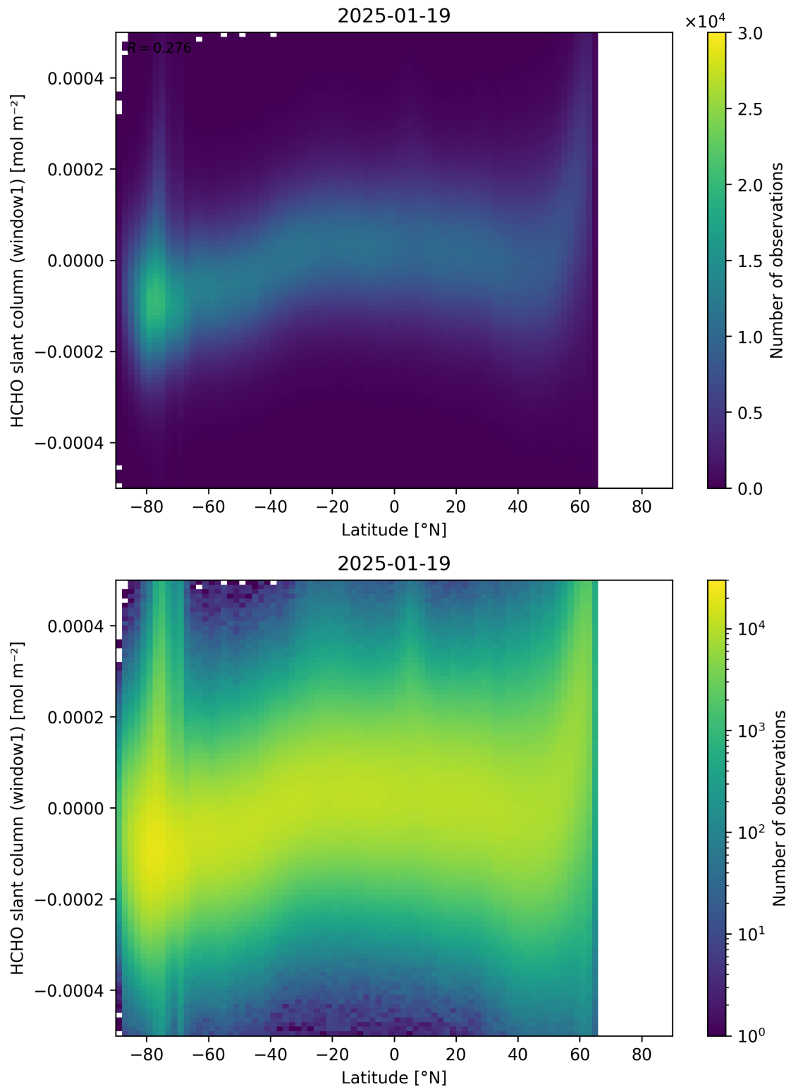
Figure 159: Scatter density plot of “Latitude” against “HCHO slant column (window1)” for 2025-01-18 to 2025-01-20.
