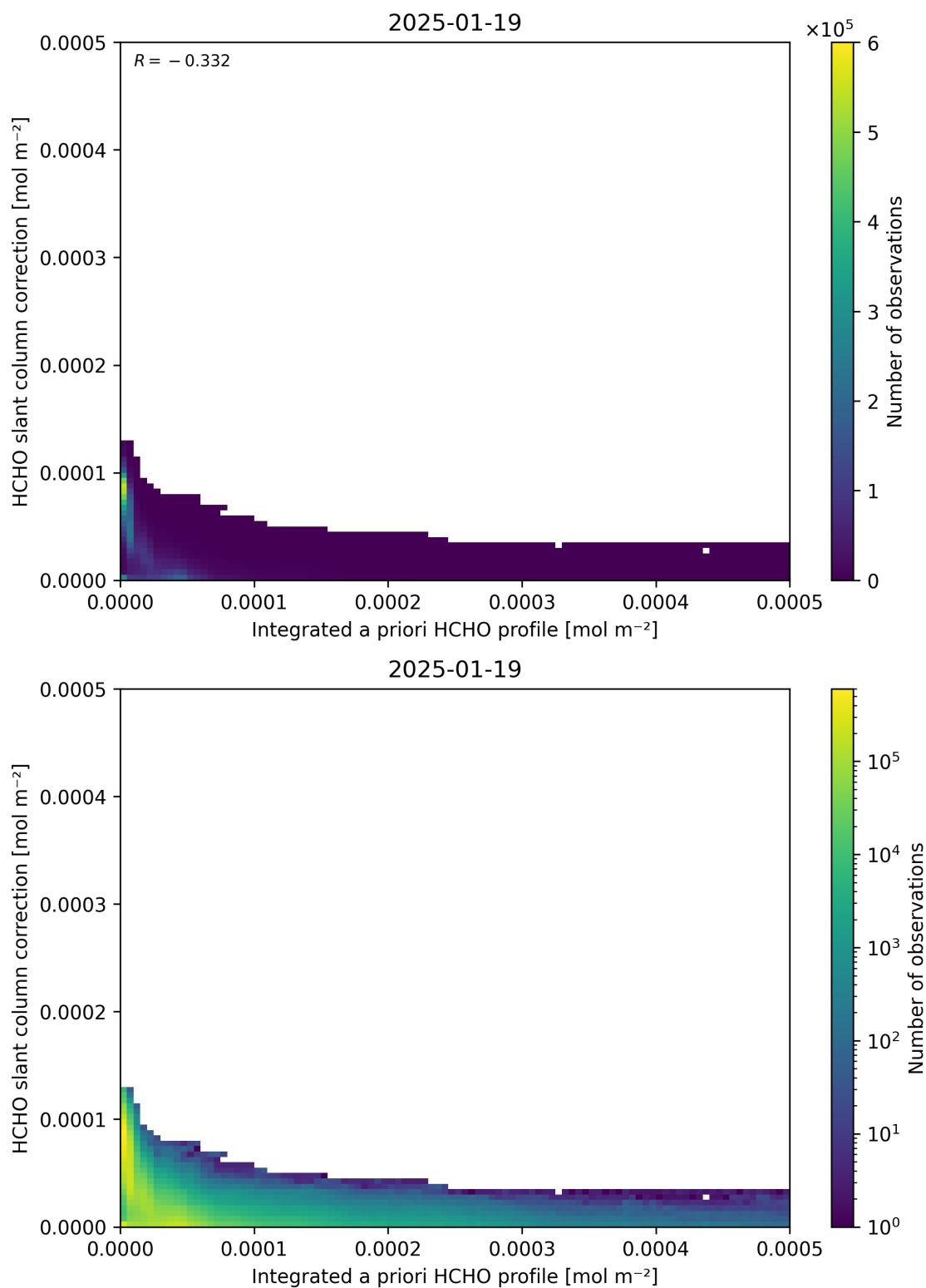
Figure 152: Scatter density plot of “Integrated a priori HCHO profile” against “HCHO slant column correction” for 2025-01-18 to 2025-01-20.
