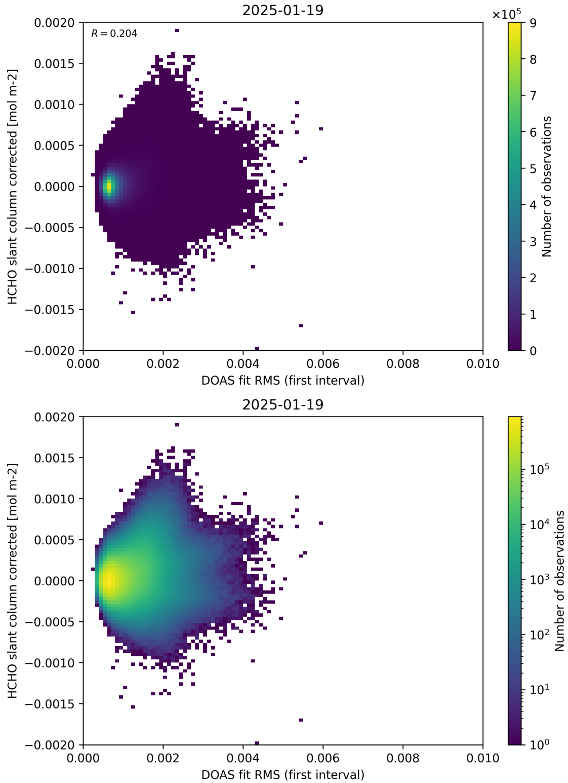
Figure 62: Scatter density plot of “DOAS fit RMS (first interval)” against “HCHO slant column corrected” for 2025-01-18 to 2025-01-20.
