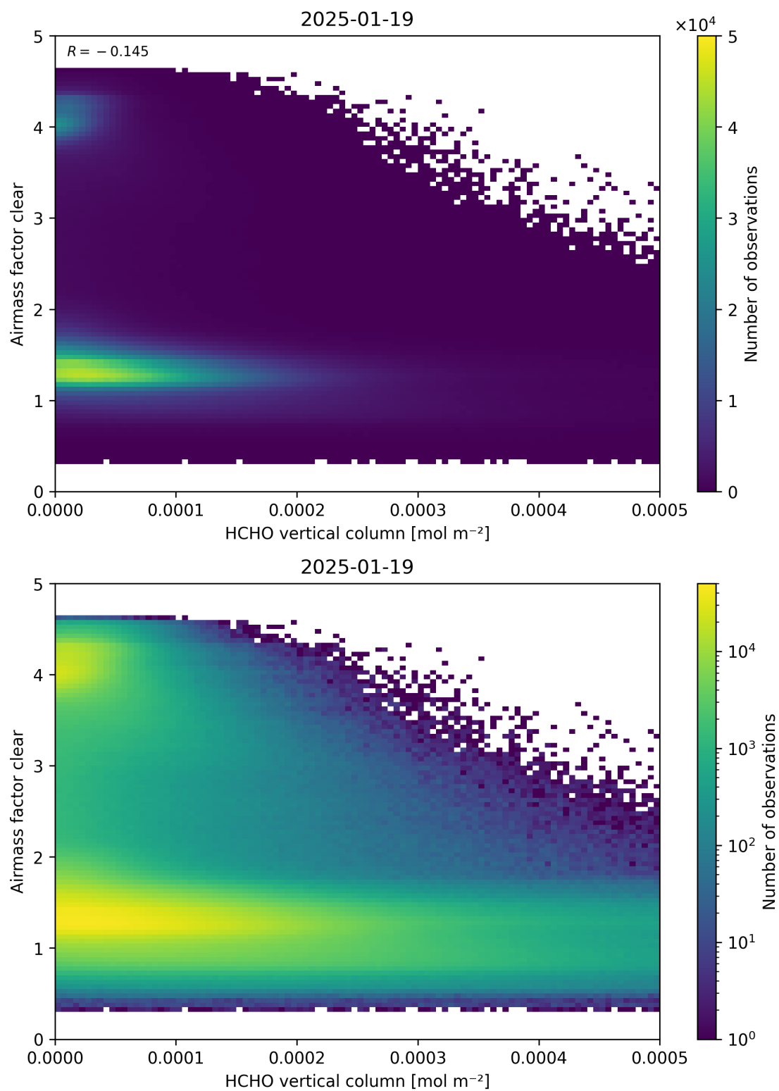
Figure 126: Scatter density plot of “HCHO vertical column” against “Airmass factor clear” for 2025-01-18 to 2025-01-20.
