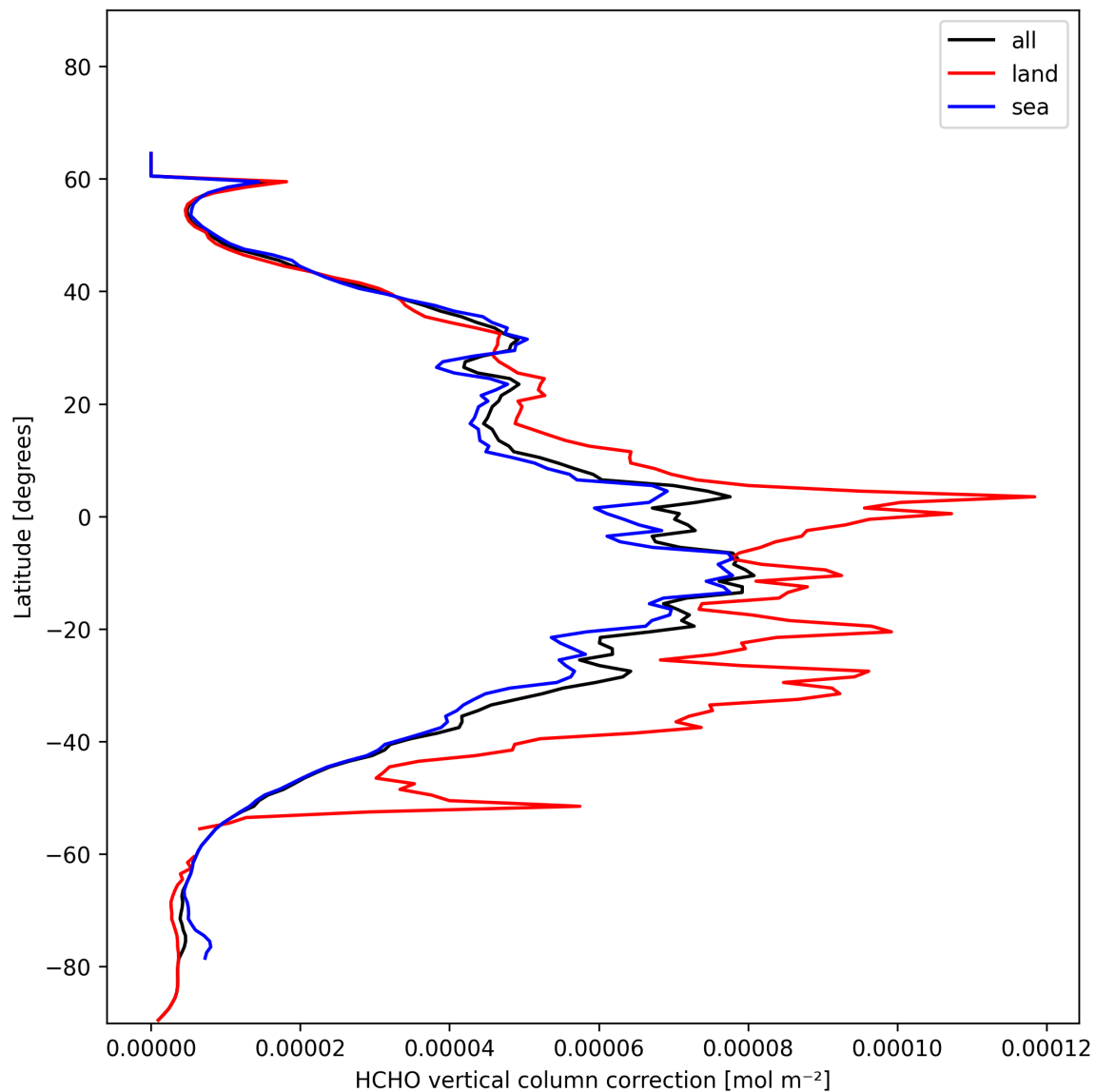
Figure 23: Zonal average of “HCHO vertical column correction” for 2025-01-18 to 2025-01-20.
