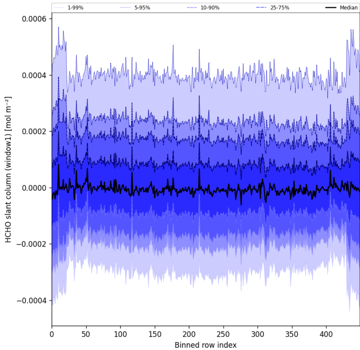
Figure 52: Along track statistics of "HCHO slant column (window1)" for 2025-01-18 to 2025-01-20
