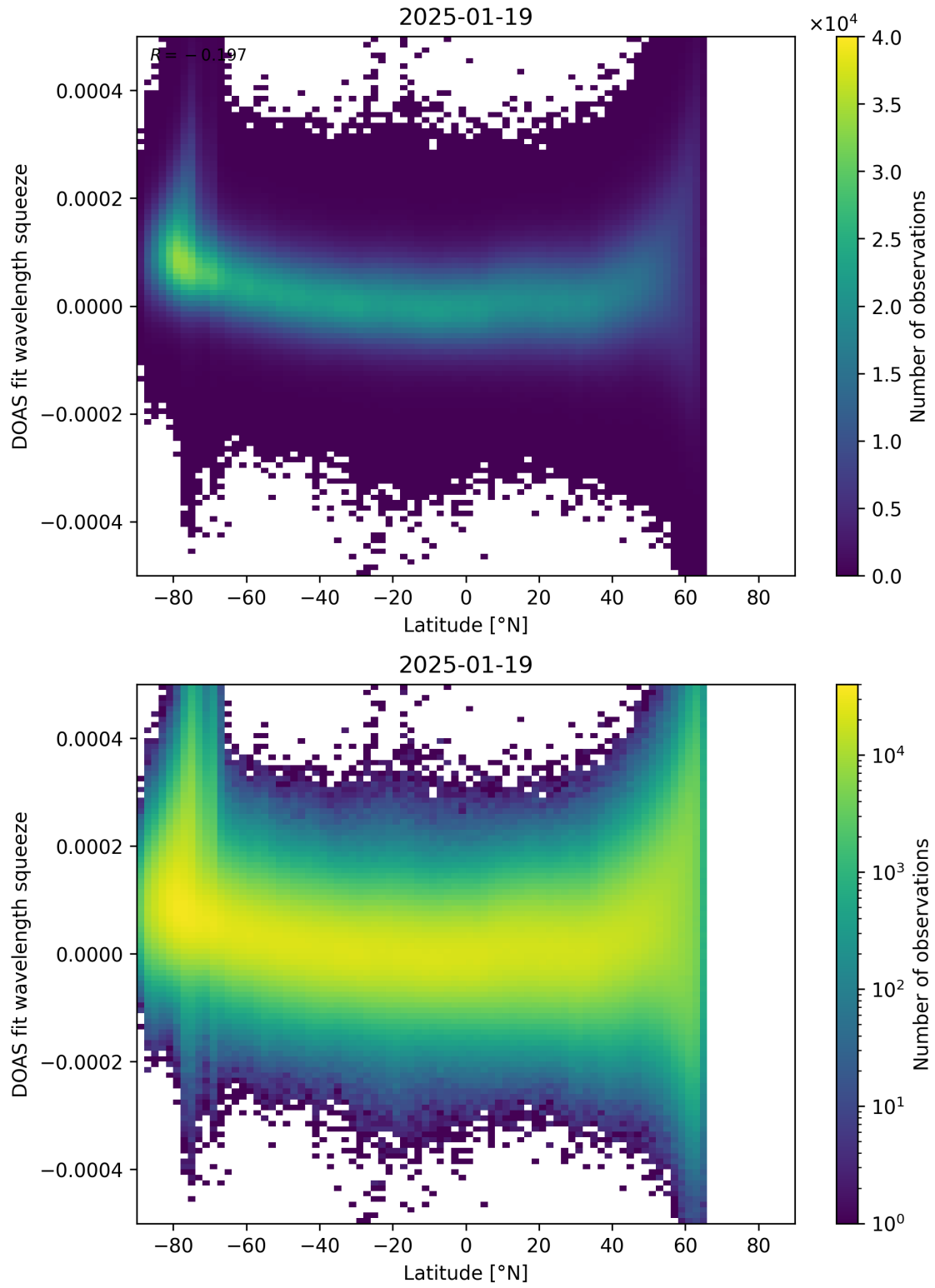
Figure 155: Scatter density plot of “Latitude” against “DOAS fit wavelength squeeze” for 2025-01-18 to 2025-01-20.
