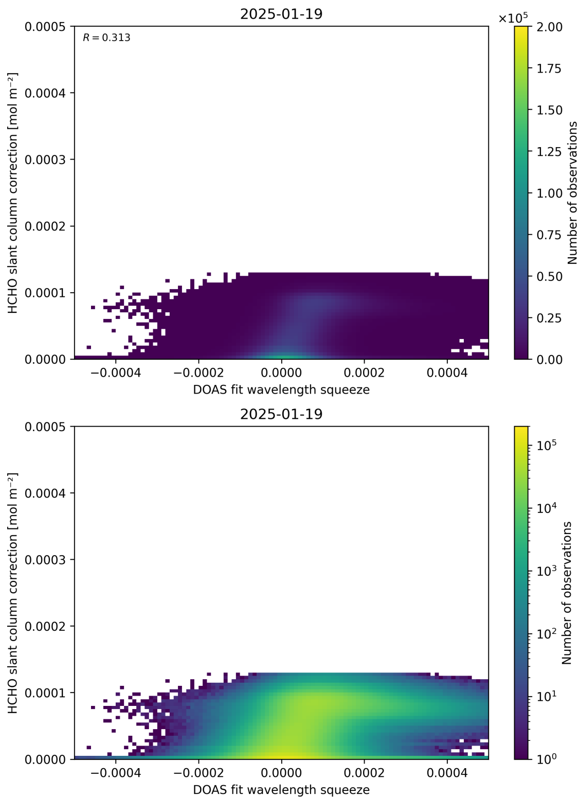
Figure 70: Scatter density plot of “DOAS fit wavelength squeeze” against “HCHO slant column correction” for 2025-01-18 to 2025-01-20.
