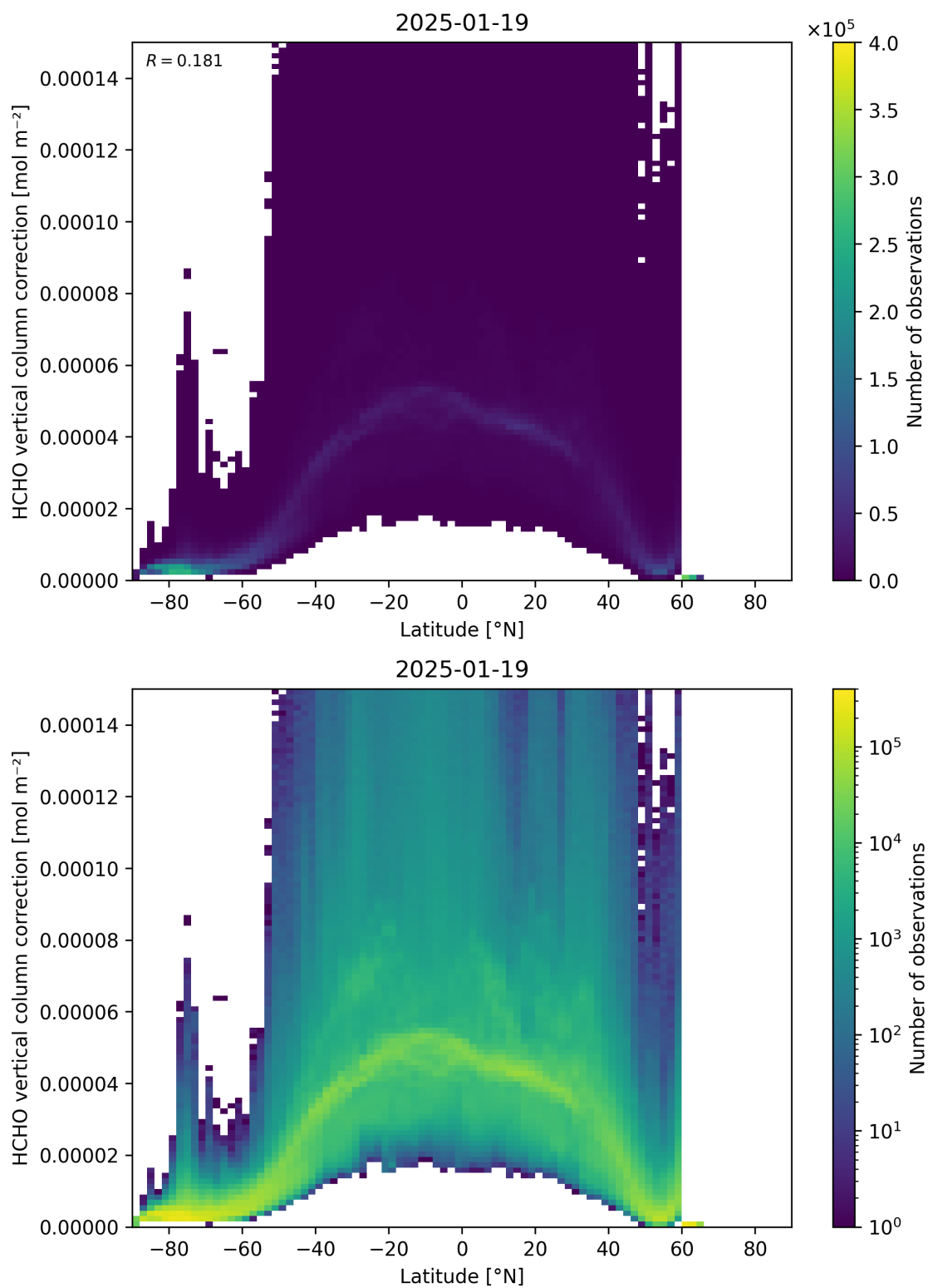
Figure 164: Scatter density plot of “Latitude” against “HCHO vertical column correction” for 2025-01-18 to 2025-01-20.
