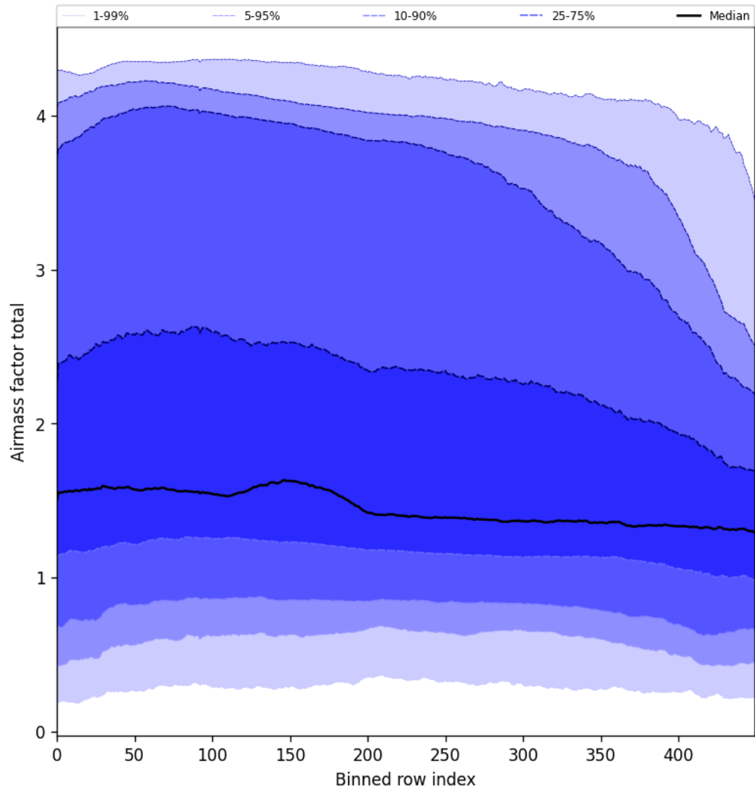
Figure 54: Along track statistics of “Airmass factor total” for 2025-01-18 to 2025-01-20
