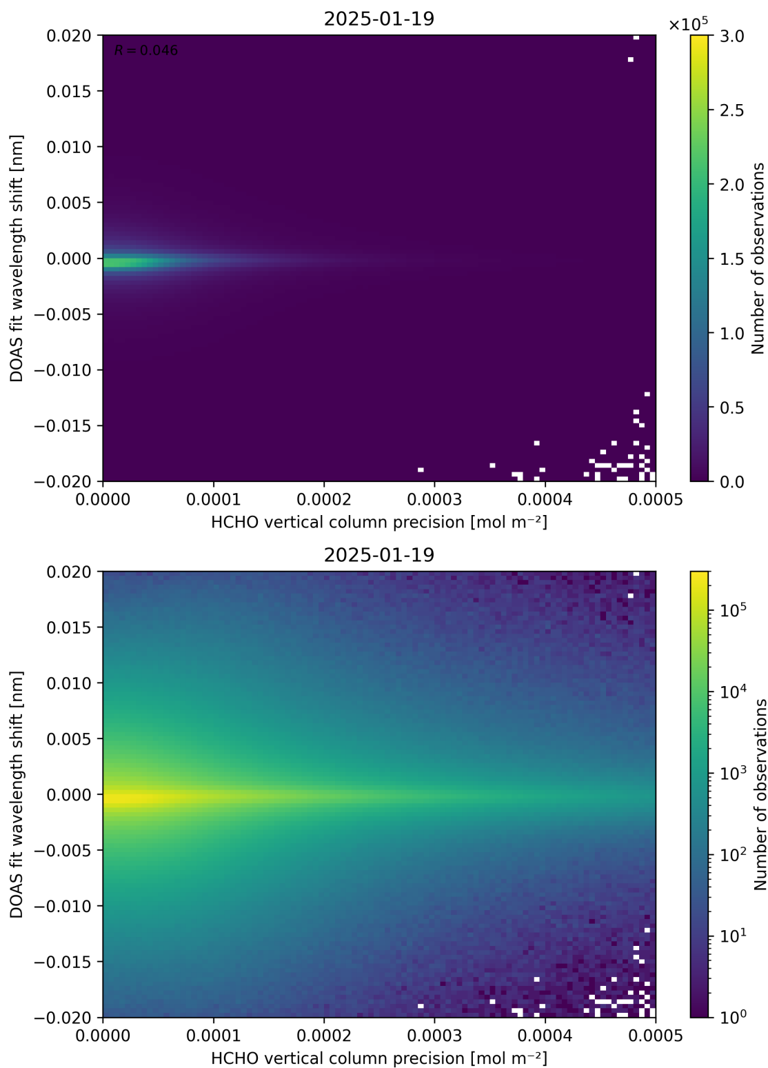
Figure 137: Scatter density plot of “HCHO vertical column precision” against “DOAS fit wavelength shift” for 2025-01-18 to 2025-01-20.
