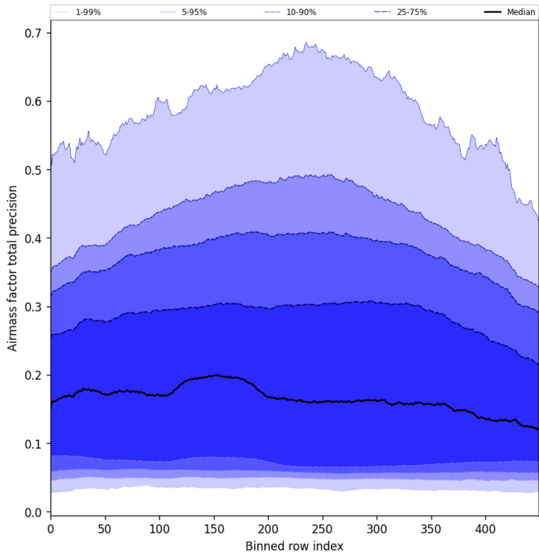
Figure 55: Along track statistics of “Airmass factor total precision” for 2025-01-18 to 2025-01-20
