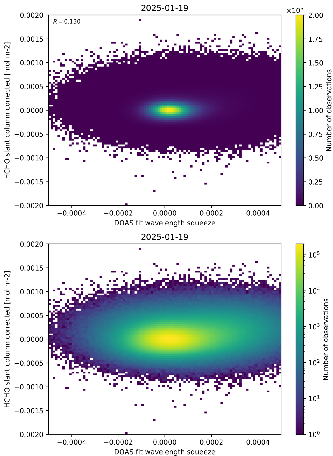
Figure 69: Scatter density plot of “DOAS fit wavelength squeeze” against “HCHO slant column corrected” for 2025-01-18 to 2025-01-20.
