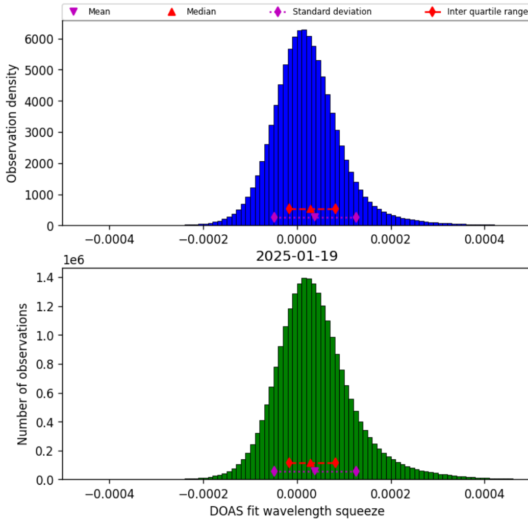
Figure 45: Histogram of “DOAS fit wavelength squeeze” for 2025-01-18 to 2025-01-20
