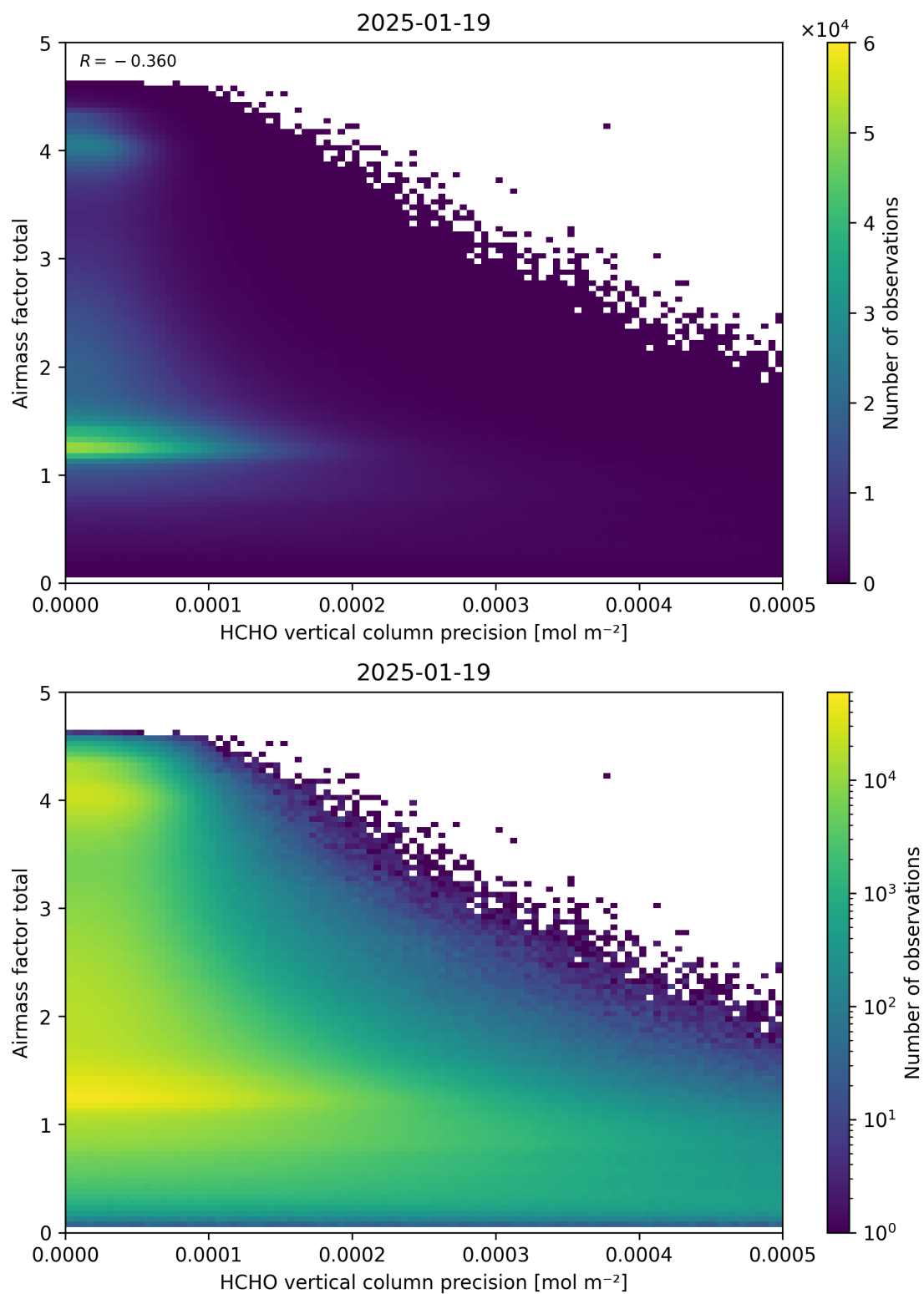
Figure 144: Scatter density plot of “HCHO vertical column precision” against “Airmass factor total” for 2025-01-18 to 2025-01-20.
