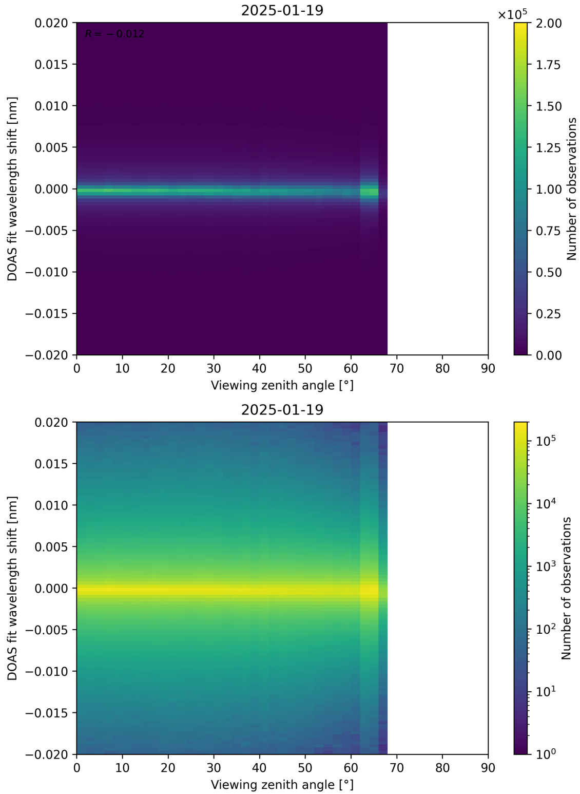
Figure 183: Scatter density plot of “Viewing zenith angle” against “DOAS fit wavelength shift” for 2025-01-18 to 2025-01-20.
