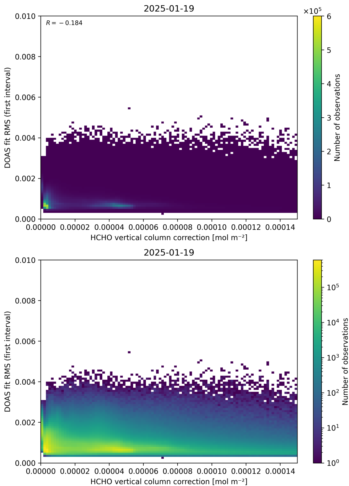
Figure 112: Scatter density plot of “HCHO vertical column correction” against “DOAS fit RMS (first interval)” for 2025-01-18 to 2025-01-20.
