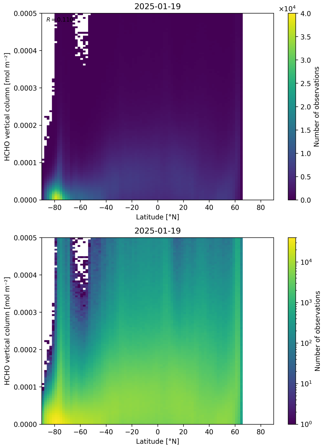
Figure 163: Scatter density plot of “Latitude” against “HCHO vertical column” for 2025-01-18 to 2025-01-20.
