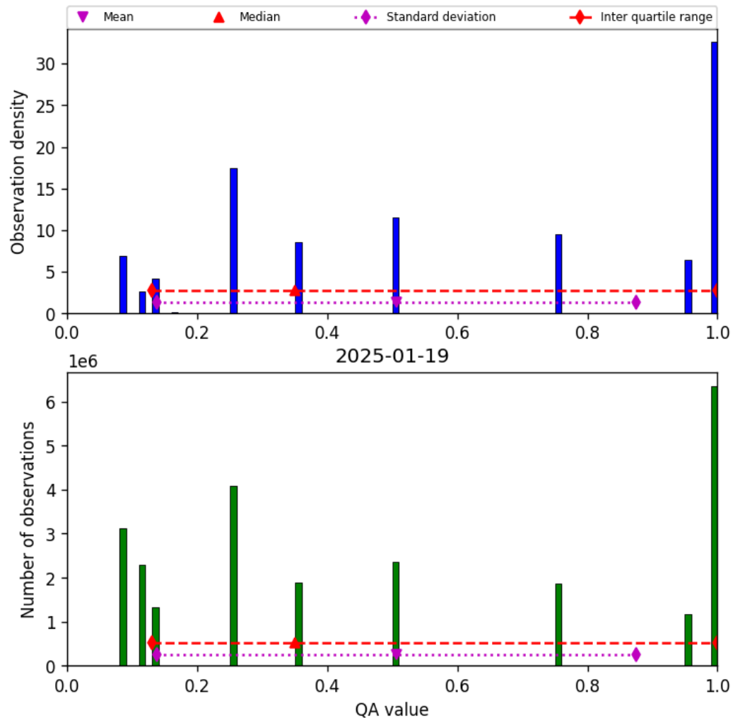
Figure 34: Histogram of “QA value” for 2025-01-18 to 2025-01-20
