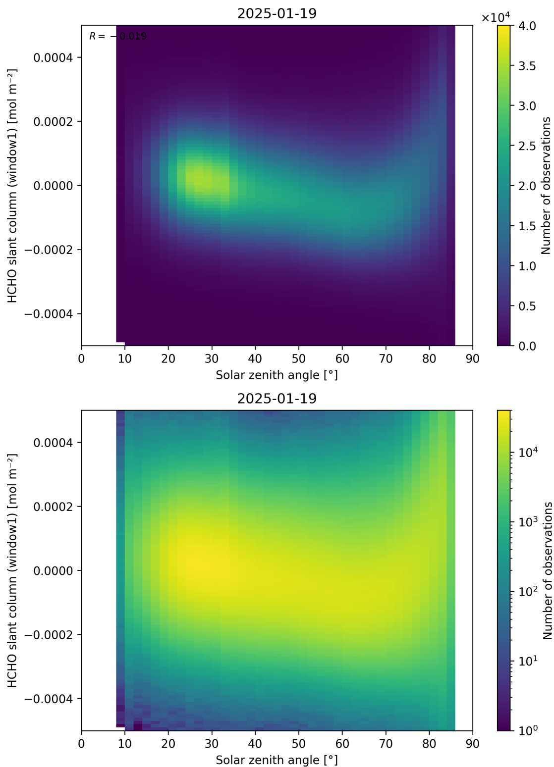
Figure 173: Scatter density plot of “Solar zenith angle” against “HCHO slant column (window1)” for 2025-01-18 to 2025-01-20.
