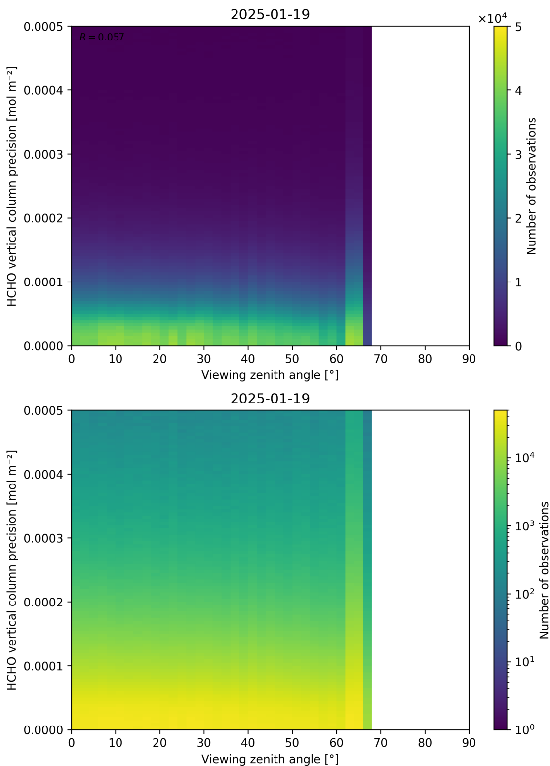
Figure 194: Scatter density plot of “Viewing zenith angle” against “HCHO vertical column precision” for 2025-01-18 to 2025-01-20.
