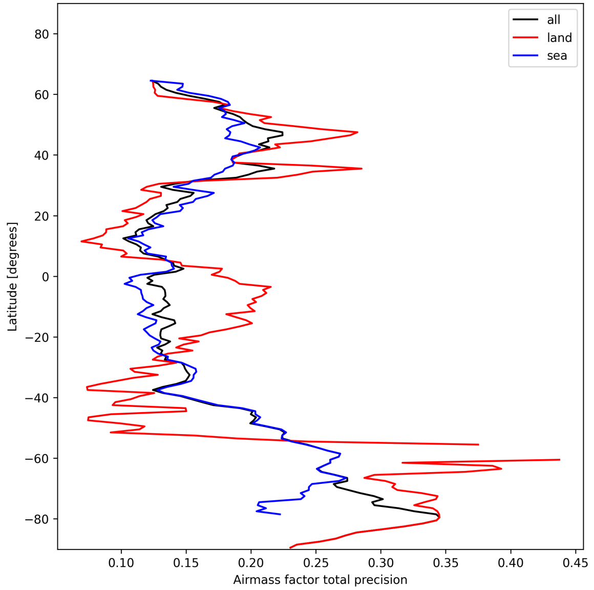
Figure 27: Zonal average of “Airmass factor total precision” for 2025-01-18 to 2025-01-20.
