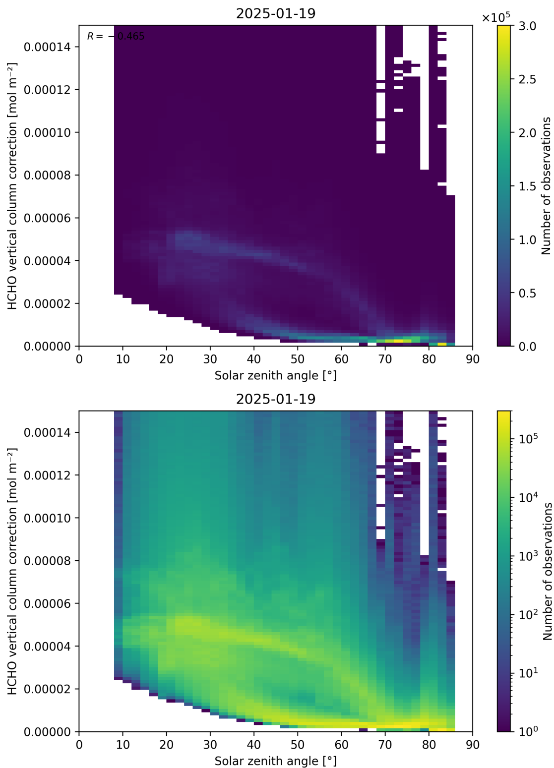
Figure 178: Scatter density plot of “Solar zenith angle” against “HCHO vertical column correction” for 2025-01-18 to 2025-01-20.
