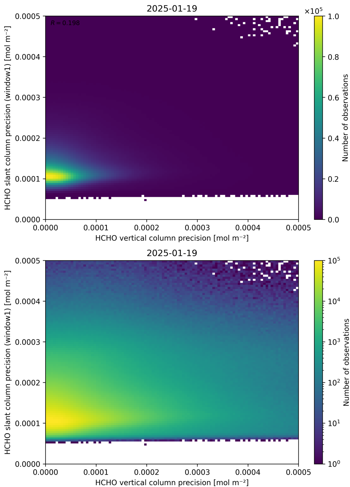
Figure 143: Scatter density plot of “HCHO vertical column precision” against “HCHO slant column precision (window1)” for 2025-01-18 to 2025-01-20.
