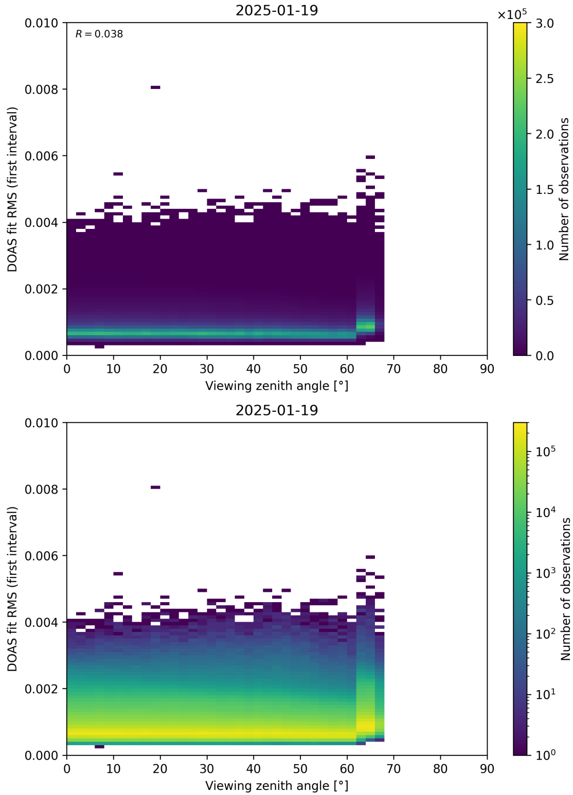
Figure 182: Scatter density plot of “Viewing zenith angle” against “DOAS fit RMS (first interval)” for 2025-01-18 to 2025-01-20.
