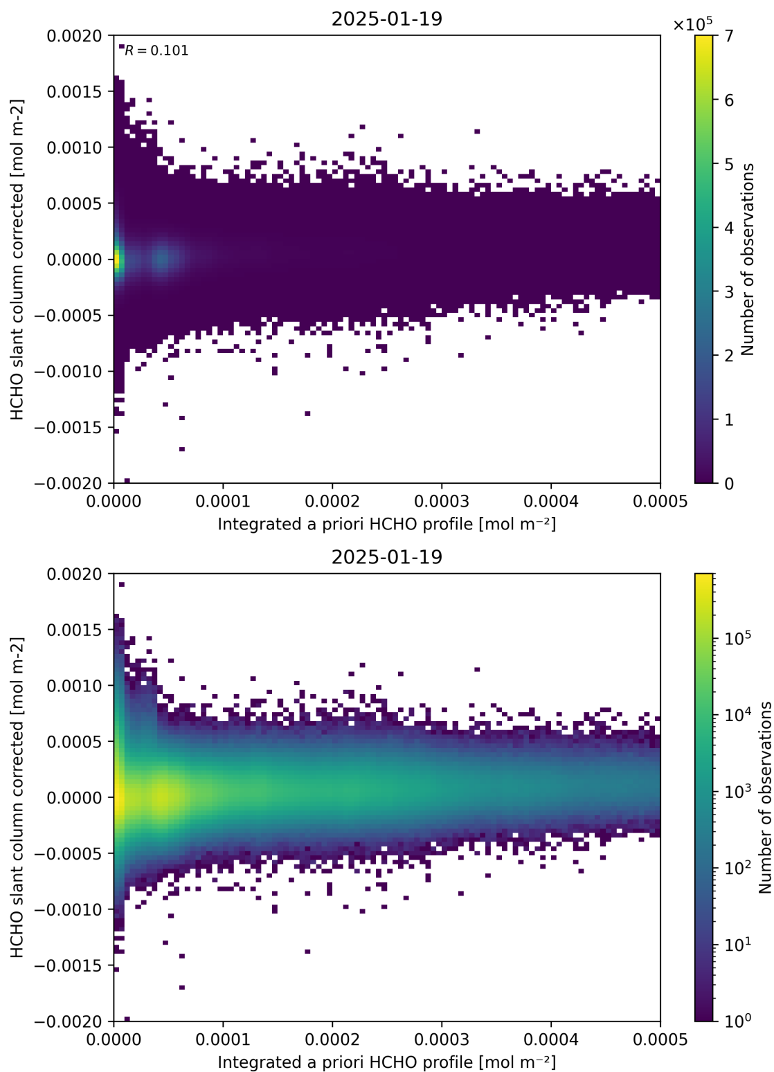
Figure 151: Scatter density plot of “Integrated a priori HCHO profile” against “HCHO slant column corrected” for 2025-01-18 to 2025-01-20.
