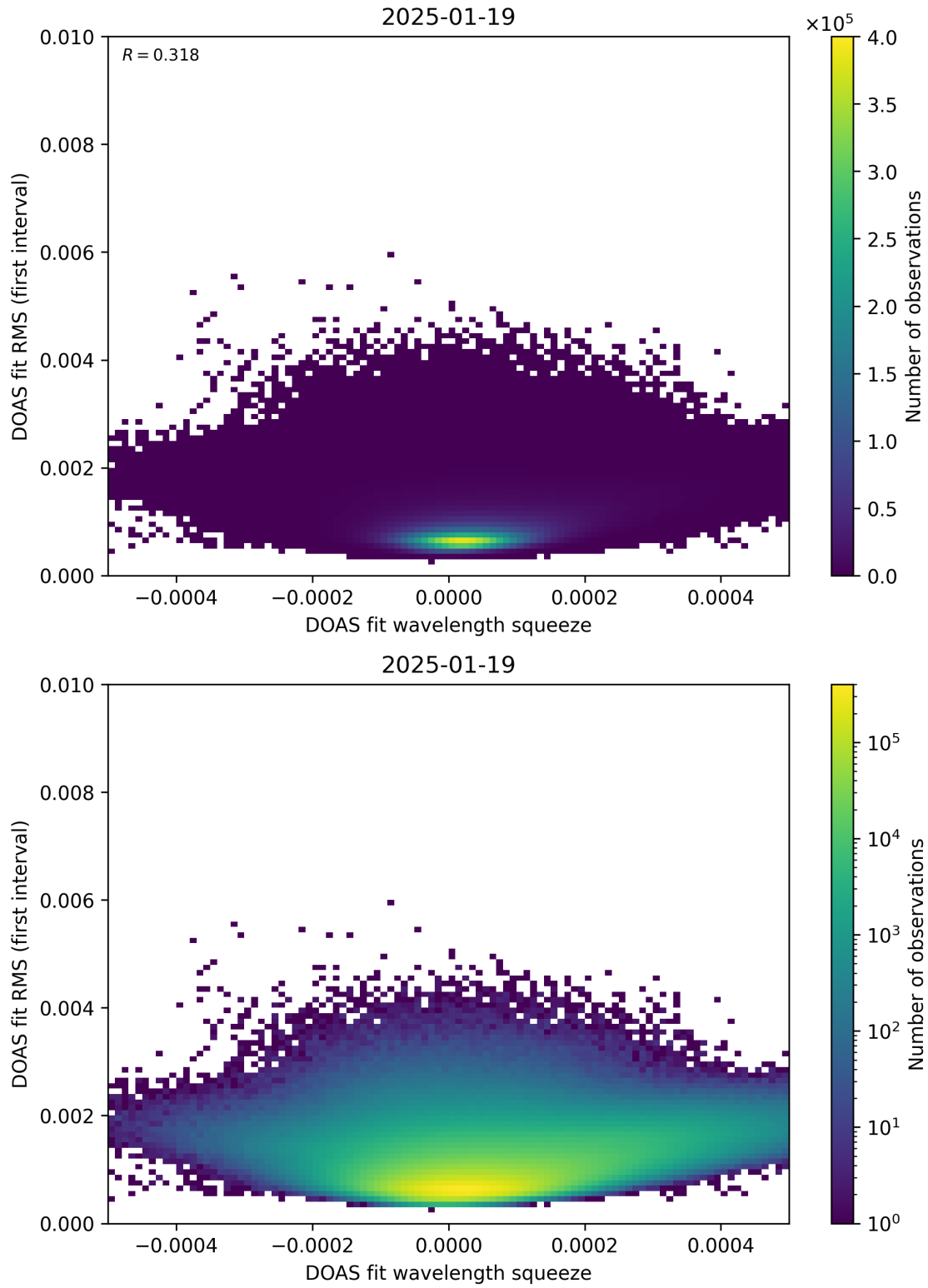
Figure 68: Scatter density plot of “DOAS fit wavelength squeeze” against “DOAS fit RMS (first interval)” for 2025-01-18 to 2025-01-20.
