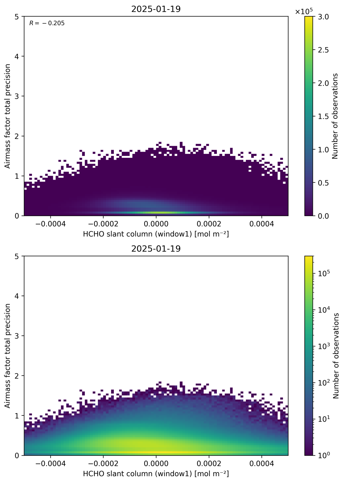
Figure 86: Scatter density plot of “HCHO slant column (window1)” against “Airmass factor total precision” for 2025-01-18 to 2025-01-20.
