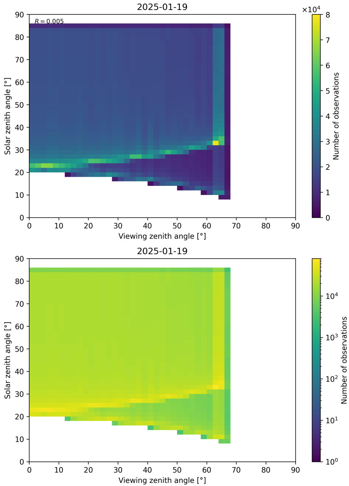
Figure 197: Scatter density plot of “Viewing zenith angle” against “Solar zenith angle” for 2025-01-18 to 2025-01-20.
