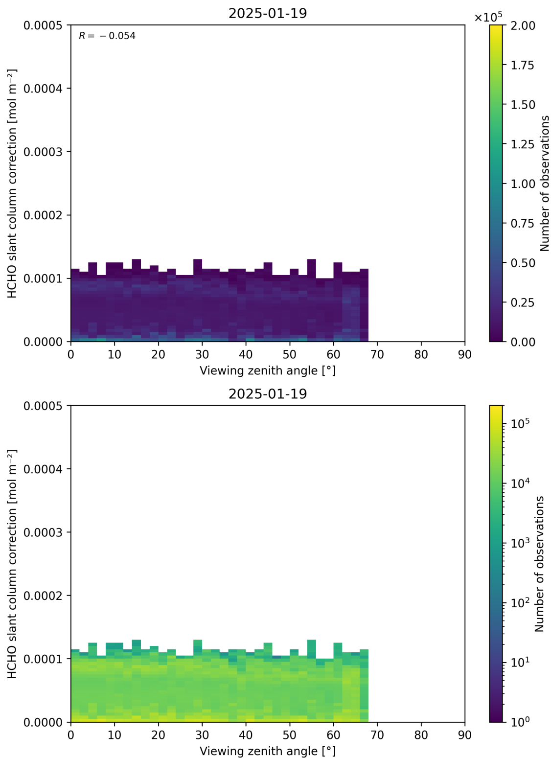
Figure 187: Scatter density plot of “Viewing zenith angle” against “HCHO slant column correction” for 2025-01-18 to 2025-01-20.
