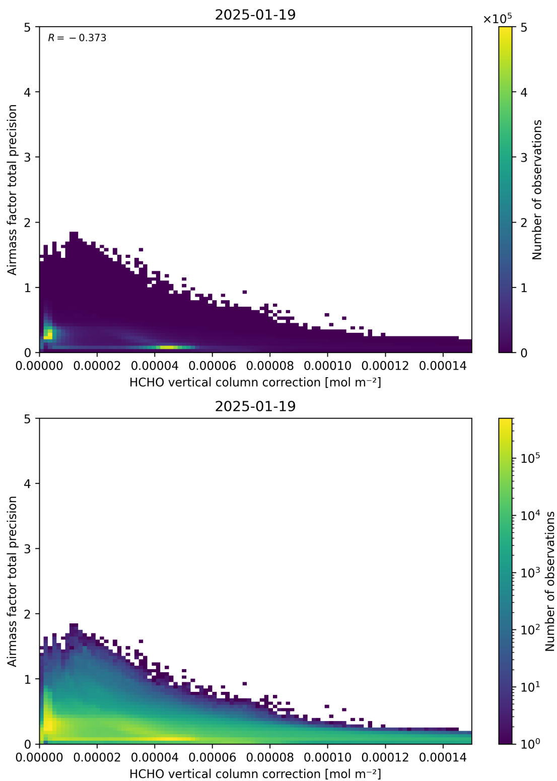
Figure 121: Scatter density plot of “HCHO vertical column correction” against “Airmass factor total precision” for 2025-01-18 to 2025-01-20.
