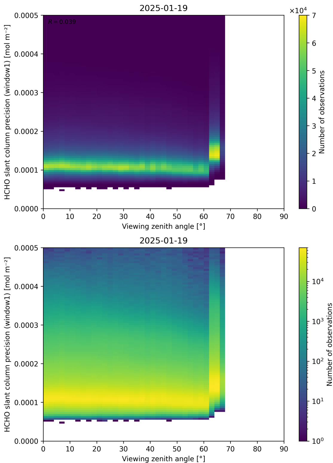
Figure 189: Scatter density plot of “Viewing zenith angle” against “HCHO slant column precision (window1)” for 2025-01-18 to 2025-01-20.
