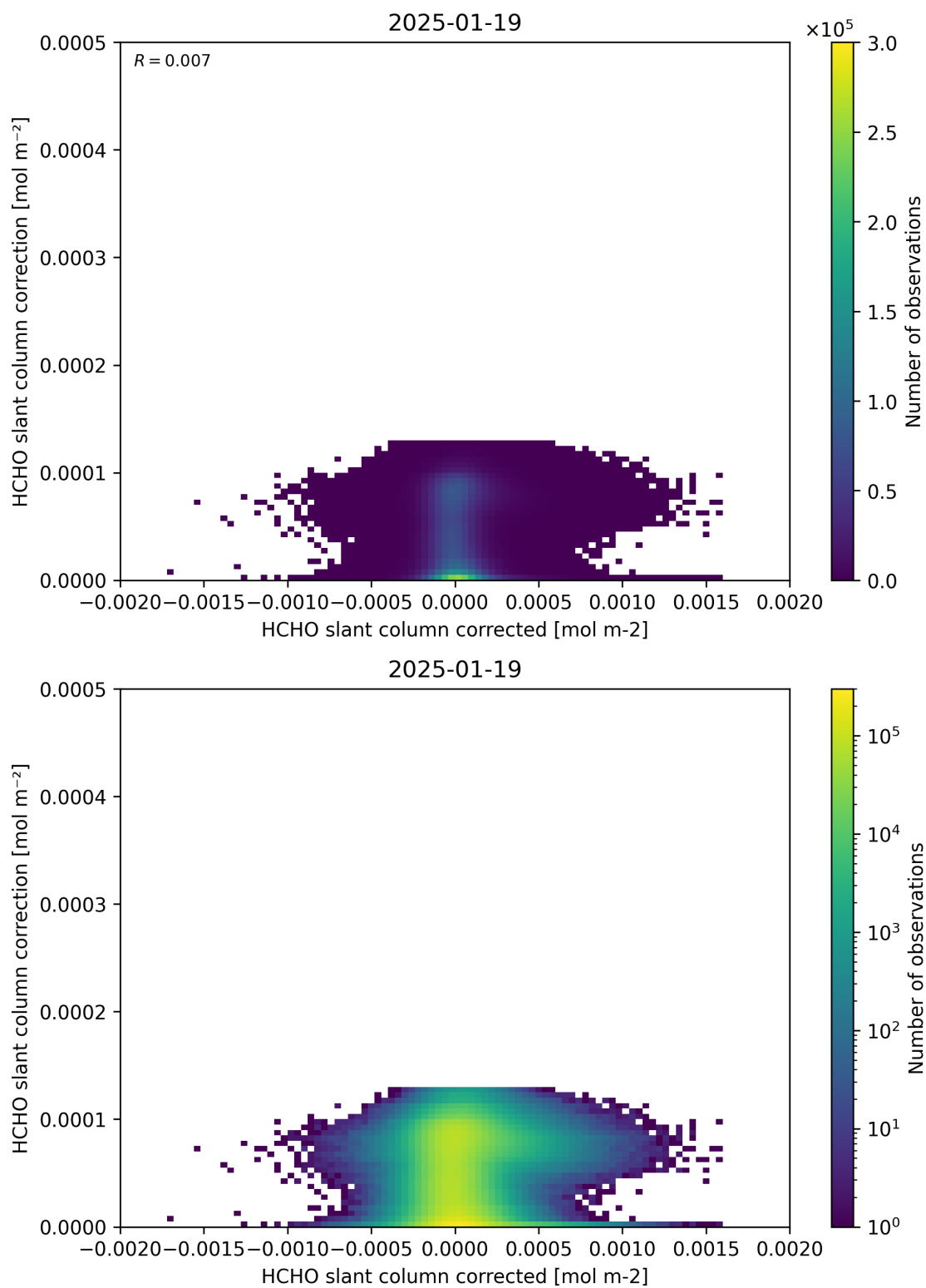
Figure 77: Scatter density plot of “HCHO slant column corrected” against “HCHO slant column correction” for 2025-01-18 to 2025-01-20.
