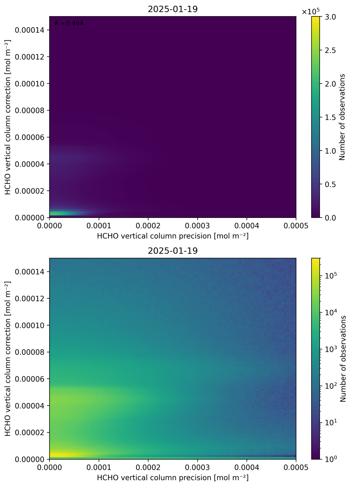
Figure 146: Scatter density plot of “HCHO vertical column precision” against “HCHO vertical column correction” for 2025-01-18 to 2025-01-20.
