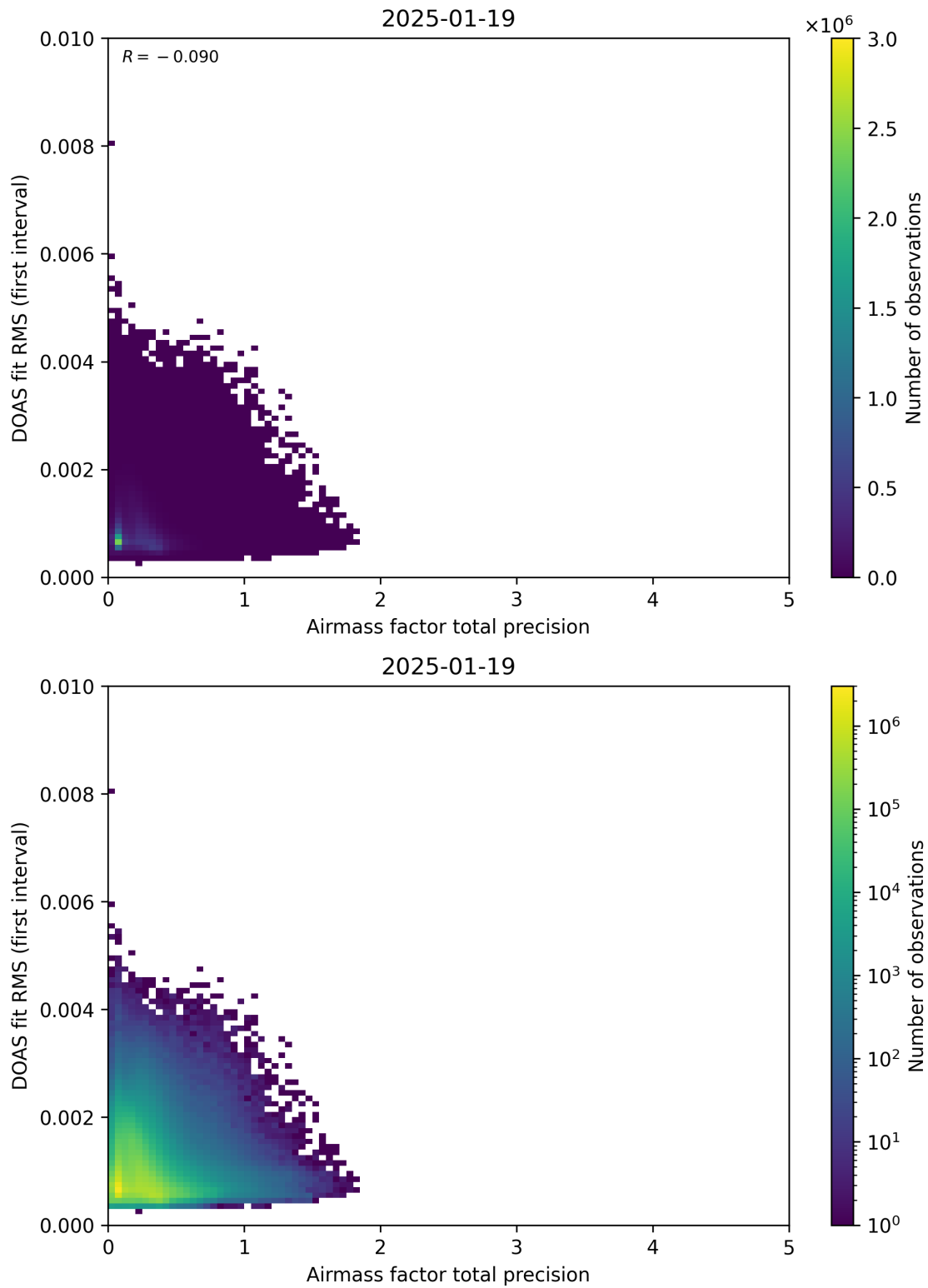
Figure 105: Scatter density plot of “Airmass factor total precision” against “DOAS fit RMS (first interval)” for 2025-01-18 to 2025-01-20.
