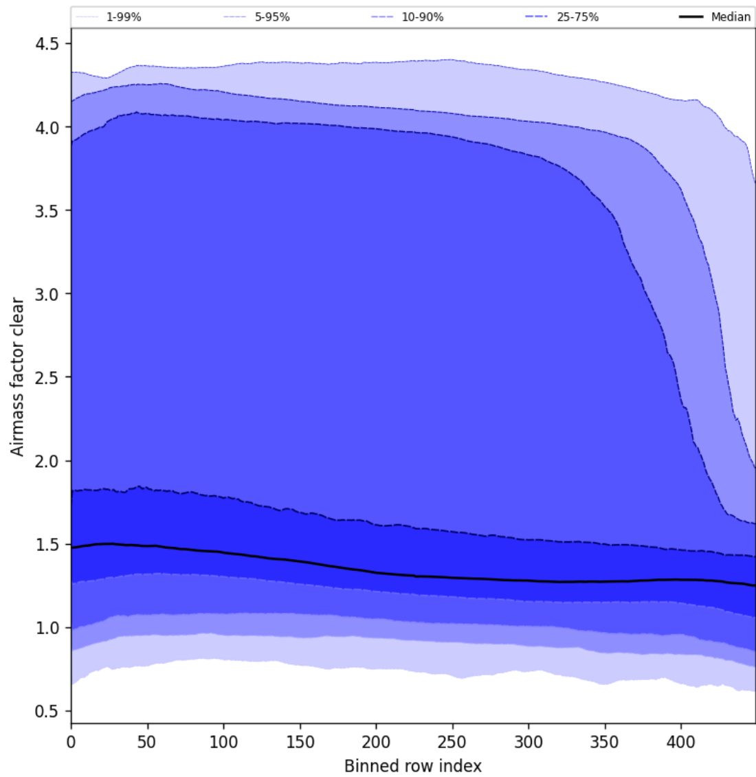
Figure 56: Along track statistics of “Airmass factor clear” for 2025-01-18 to 2025-01-20
