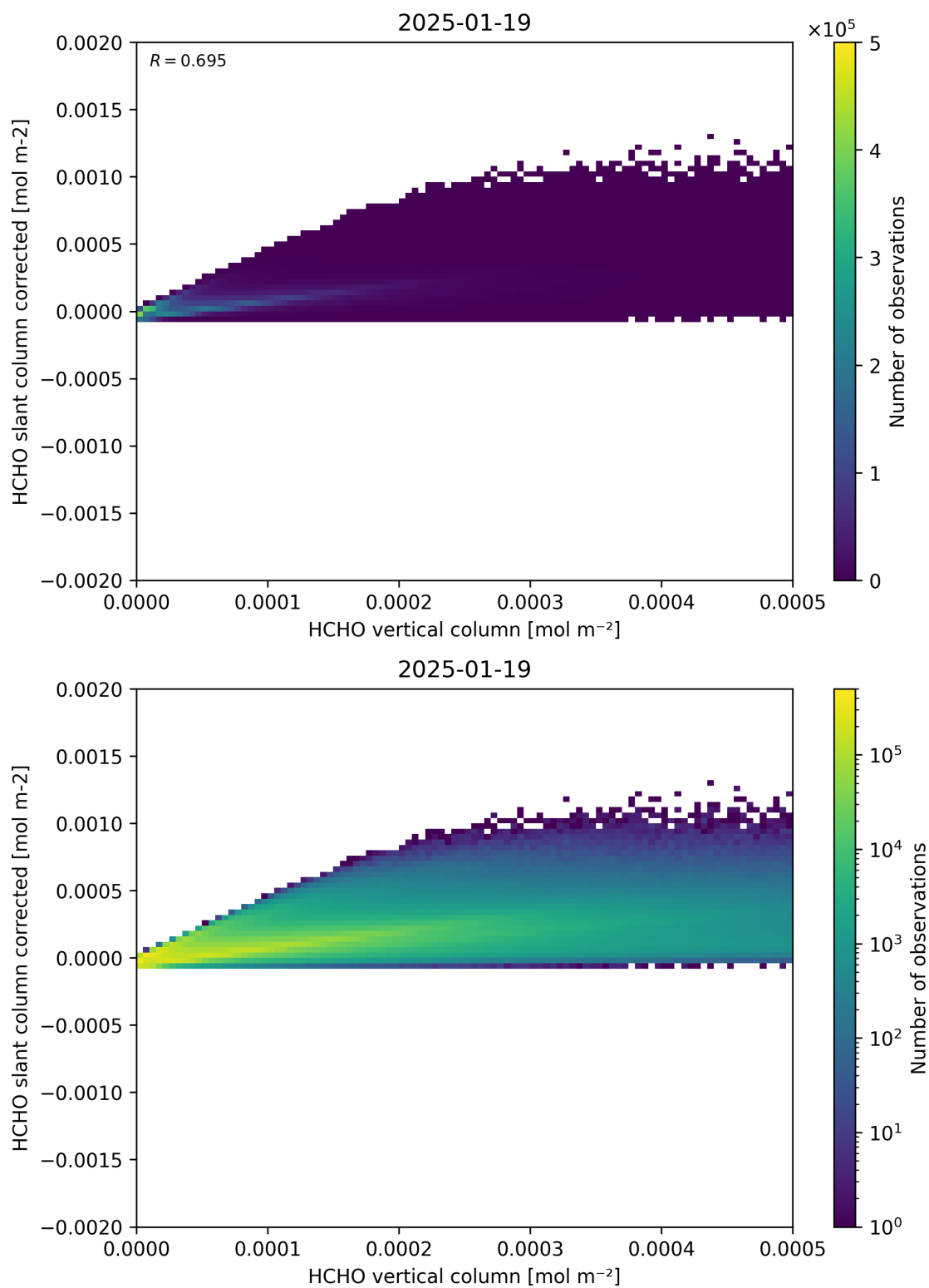
Figure 127: Scatter density plot of “HCHO vertical column” against “HCHO slant column corrected” for 2025-01-18 to 2025-01-20.
