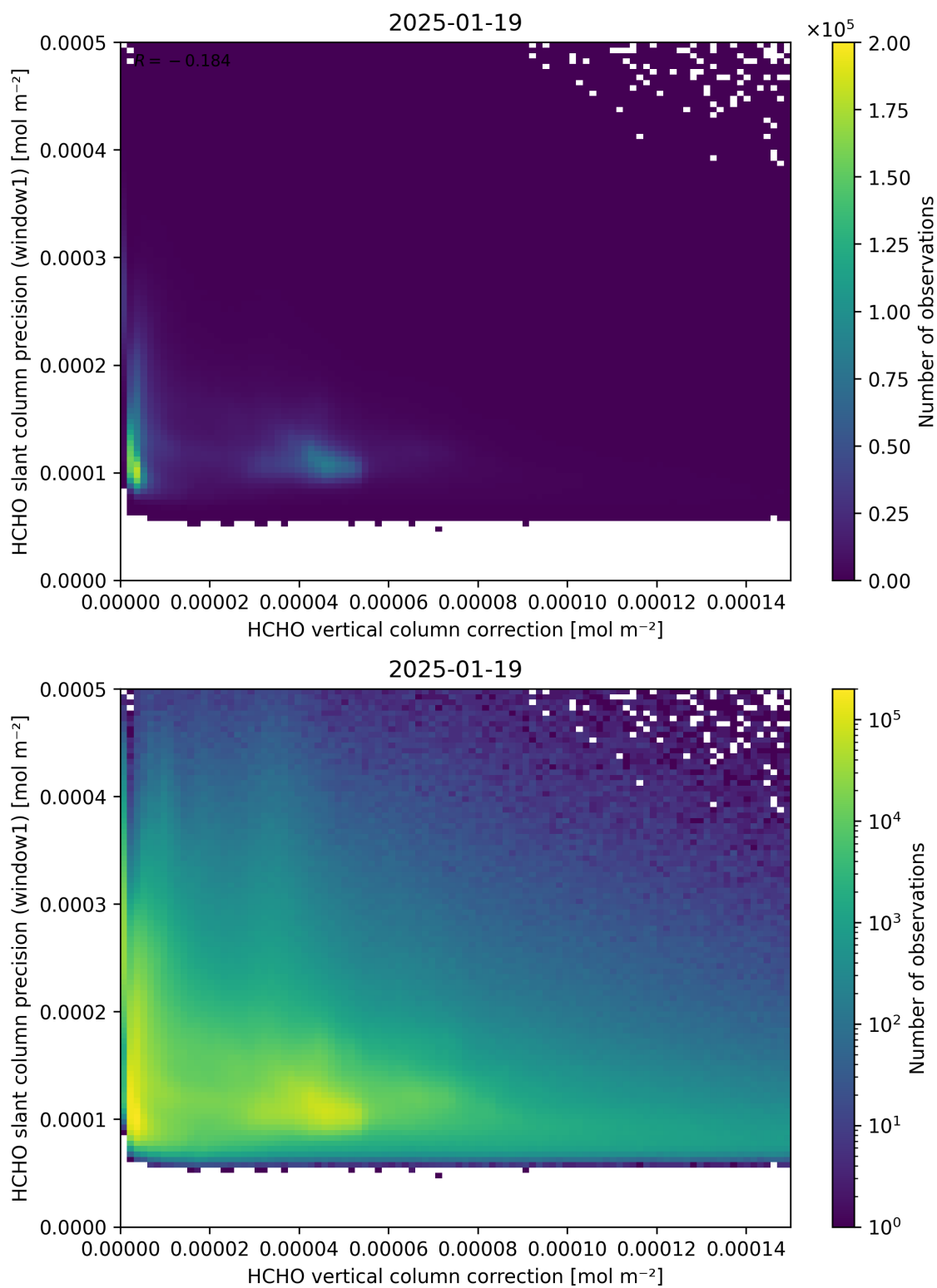
Figure 119: Scatter density plot of “HCHO vertical column correction” against “HCHO slant column precision (window1)” for 2025-01-18 to 2025-01-20.
