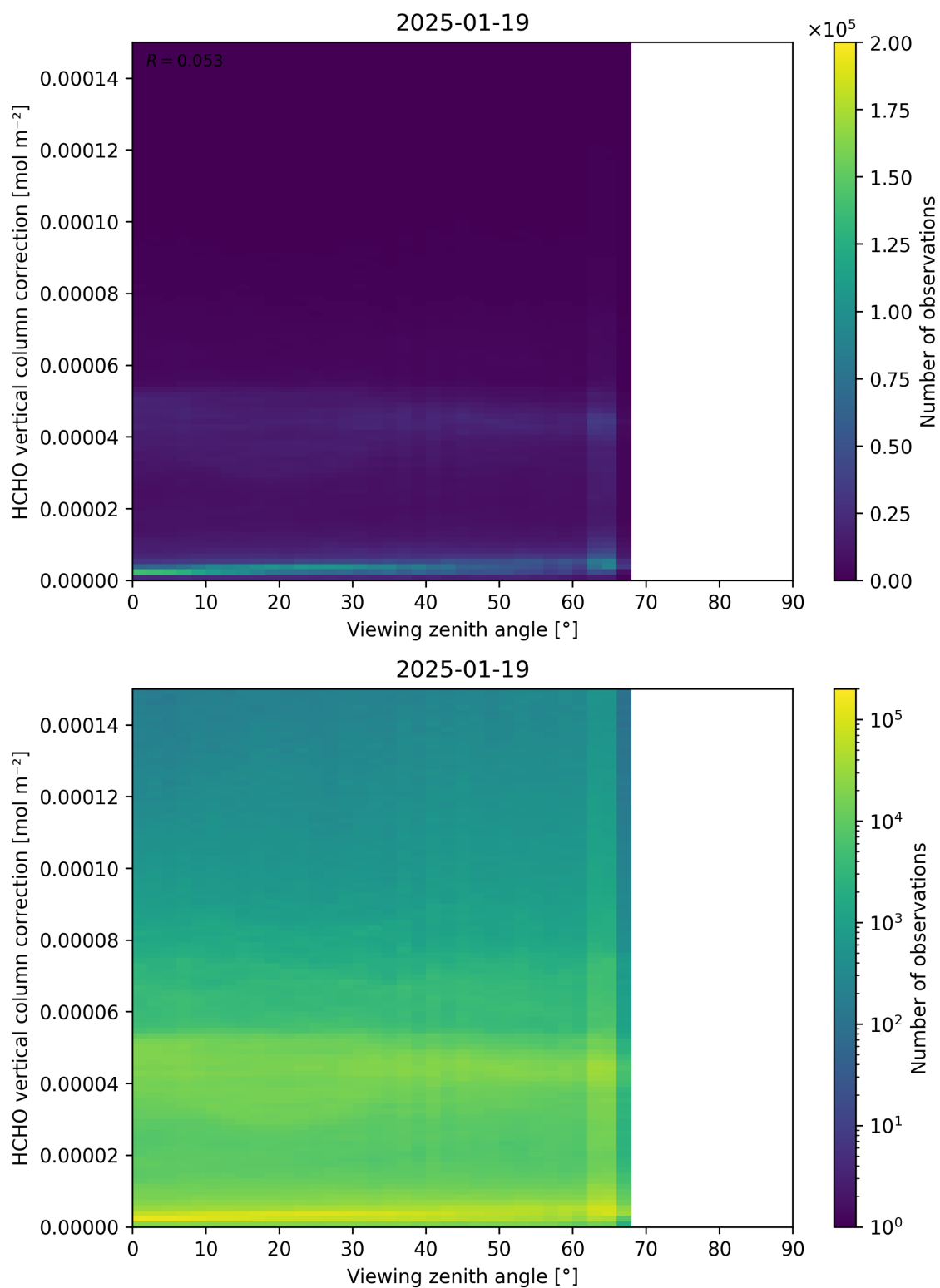
Figure 193: Scatter density plot of “Viewing zenith angle” against “HCHO vertical column correction” for 2025-01-18 to 2025-01-20.
