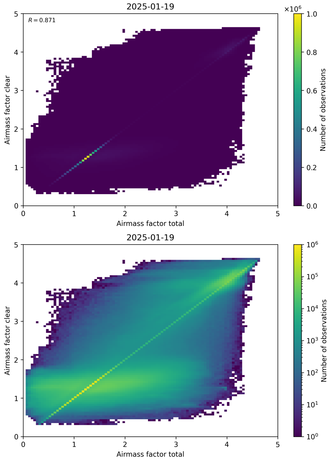
Figure 100: Scatter density plot of “Airmass factor total” against “Airmass factor clear” for 2025-01-18 to 2025-01-20.
