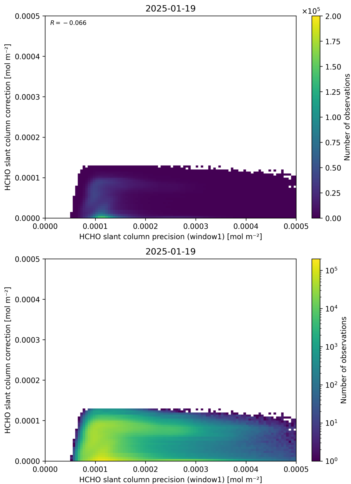
Figure 93: Scatter density plot of “HCHO slant column precision (window1)” against “HCHO slant column correction” for 2025-01-18 to 2025-01-20.
