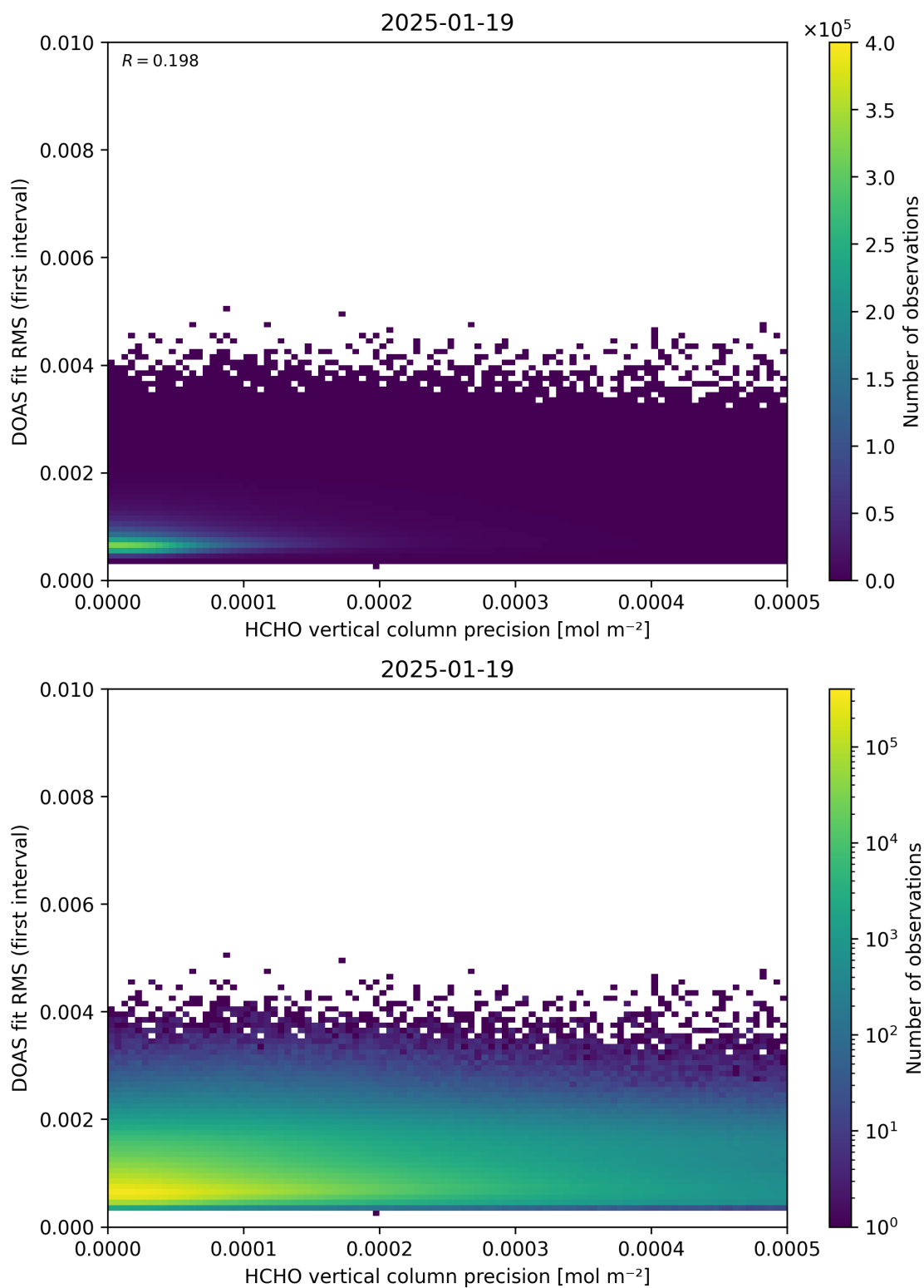
Figure 136: Scatter density plot of “HCHO vertical column precision” against “DOAS fit RMS (first interval)” for 2025-01-18 to 2025-01-20.
