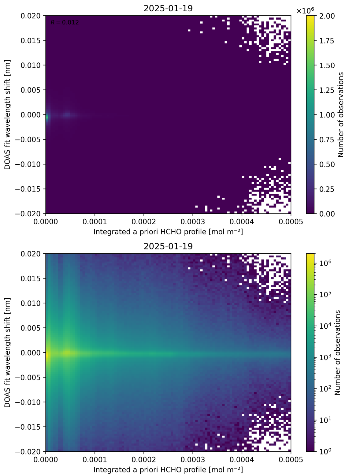
Figure 149: Scatter density plot of “Integrated a priori HCHO profile” against “DOAS fit wavelength shift” for 2025-01-18 to 2025-01-20.
