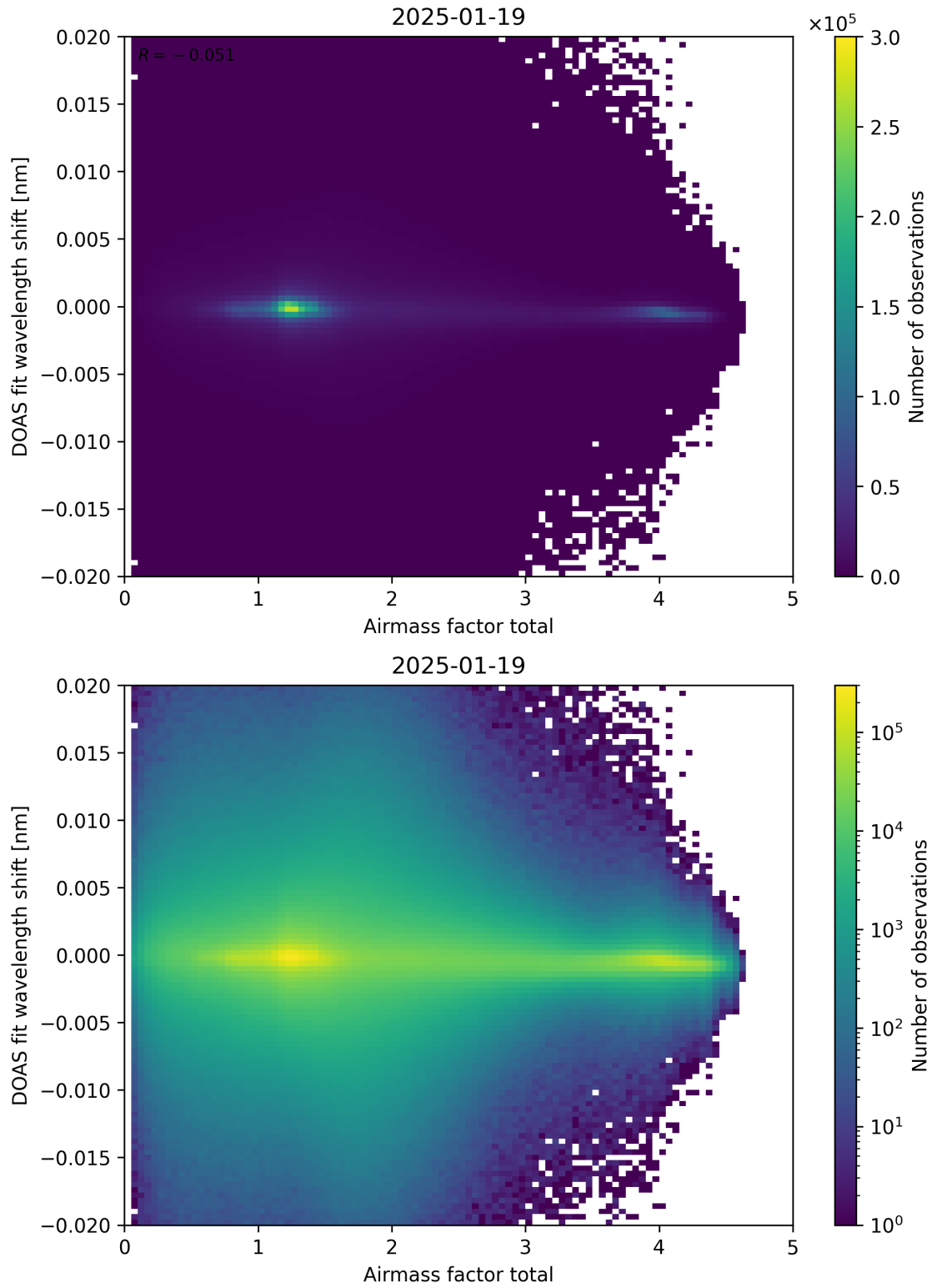
Figure 98: Scatter density plot of “Airmass factor total” against “DOAS fit wavelength shift” for 2025-01-18 to 2025-01-20.
