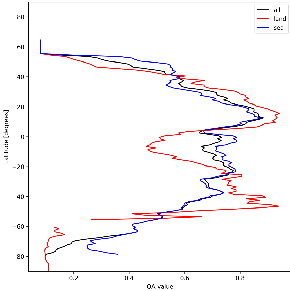
Figure 20: Zonal average of “QA value” for 2025-01-18 to 2025-01-20.
