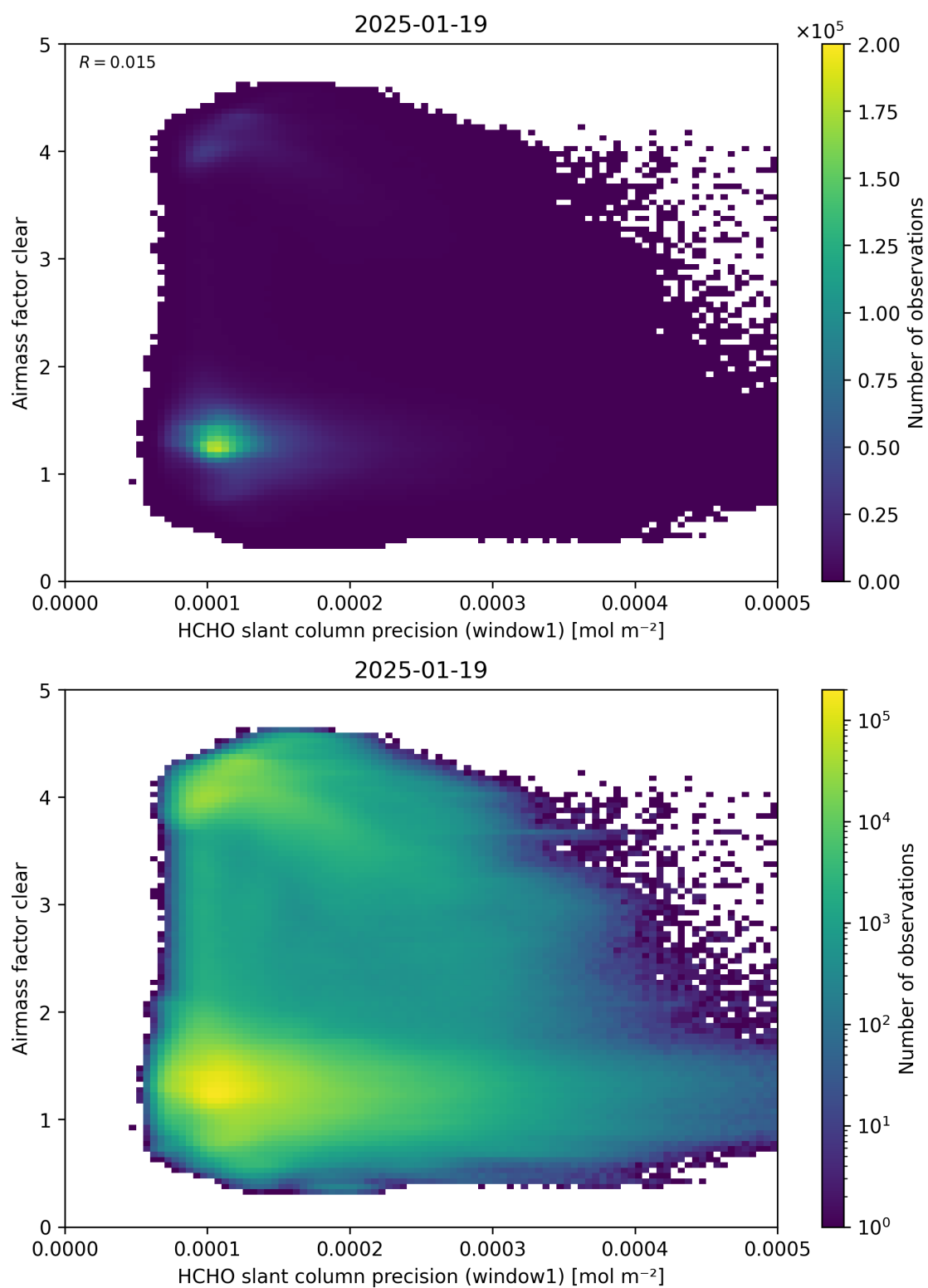
Figure 91: Scatter density plot of “HCHO slant column precision (window1)” against “Airmass factor clear” for 2025-01-18 to 2025-01-20.
