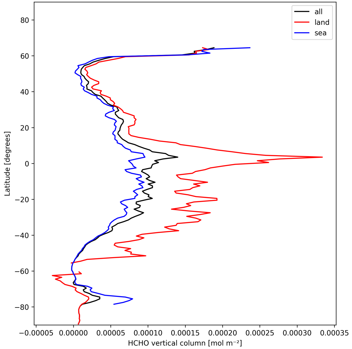
Figure 21: Zonal average of “HCHO vertical column” for 2025-01-18 to 2025-01-20.
