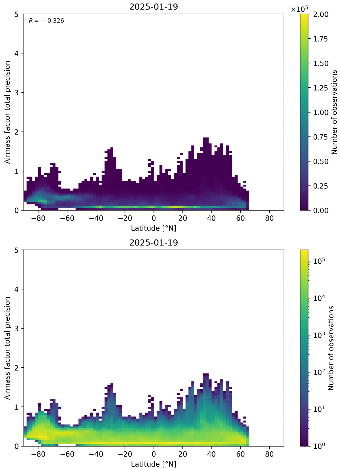
Figure 162: Scatter density plot of “Latitude” against “Airmass factor total precision” for 2025-01-18 to 2025-01-20.
