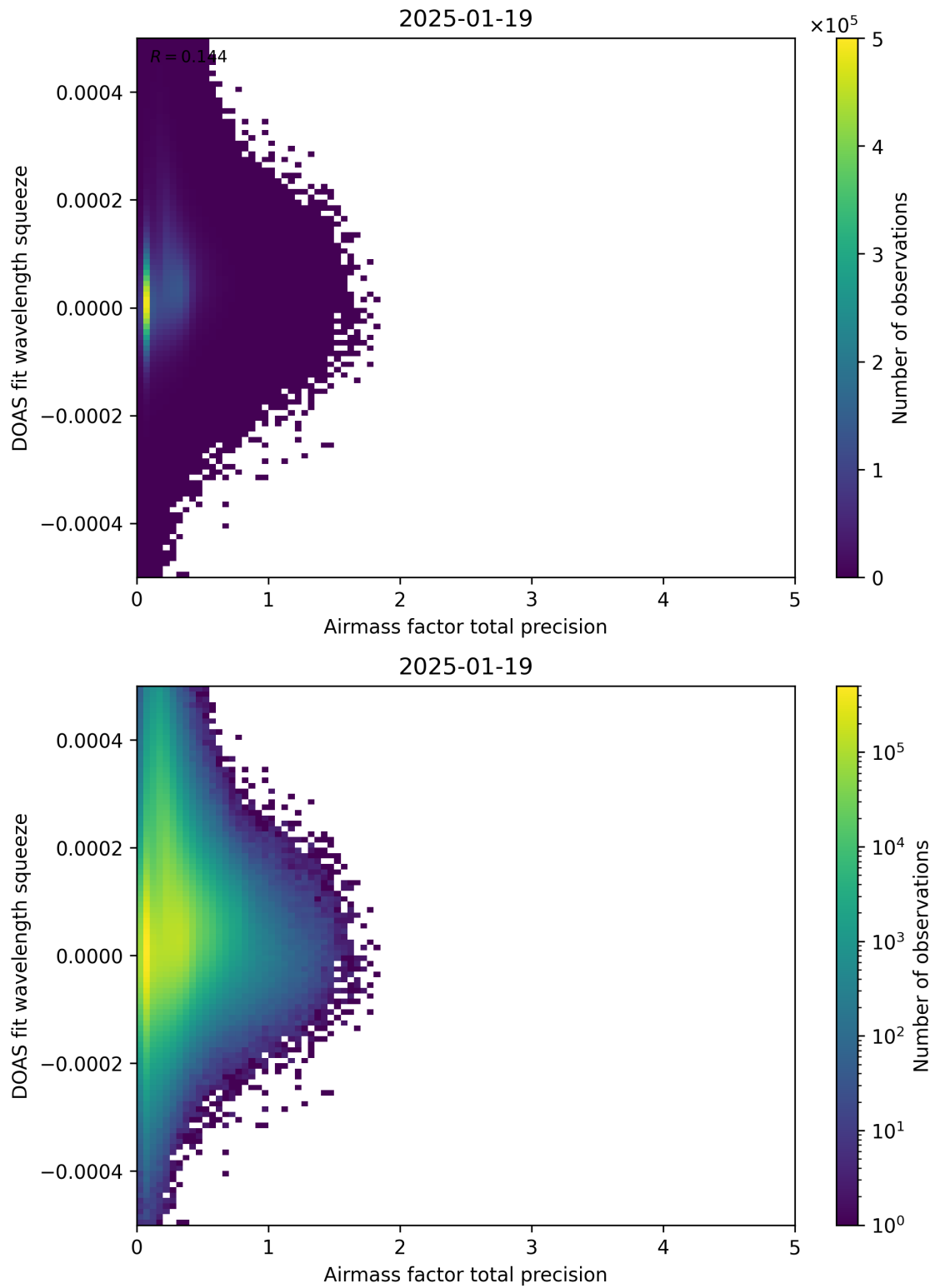
Figure 107: Scatter density plot of “Airmass factor total precision” against “DOAS fit wavelength squeeze” for 2025-01-18 to 2025-01-20.
