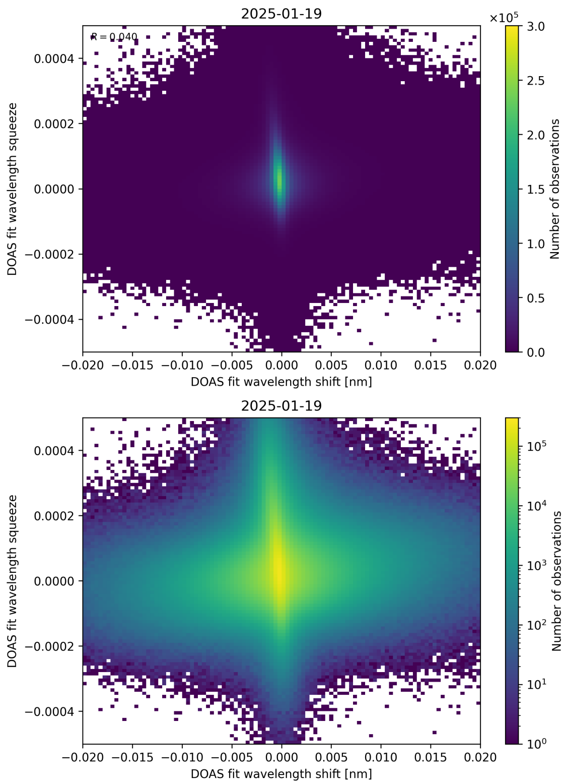
Figure 65: Scatter density plot of “DOAS fit wavelength shift” against “DOAS fit wavelength squeeze” for 2025-01-18 to 2025-01-20.
