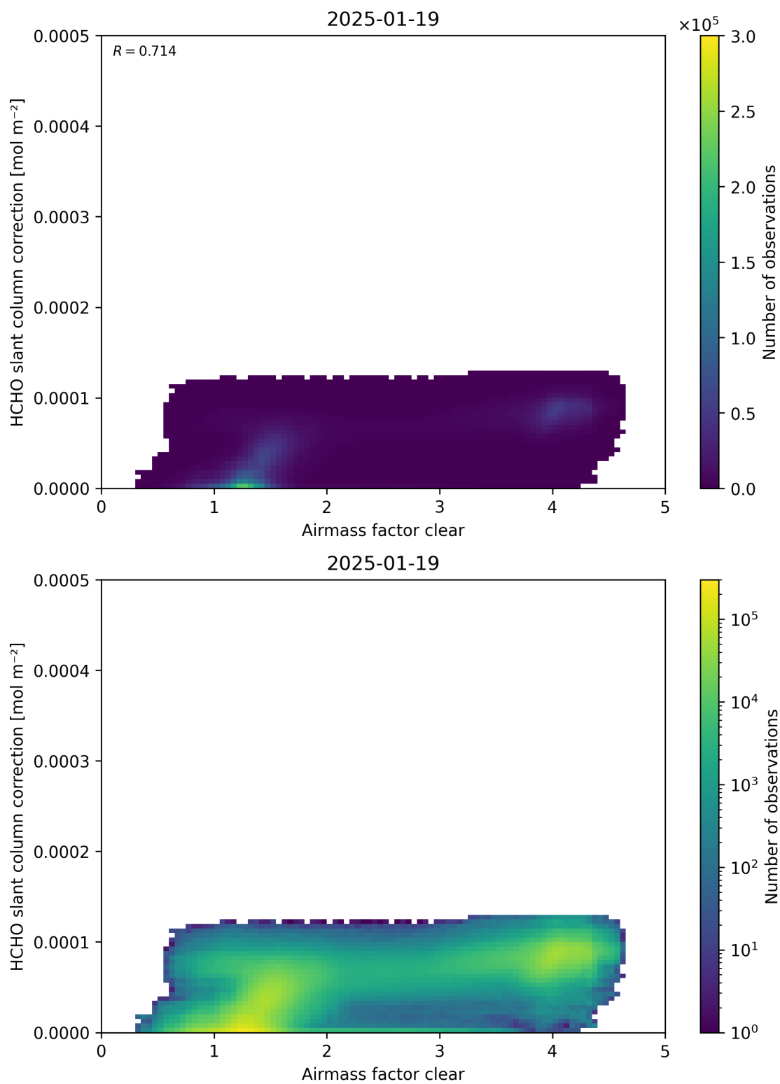
Figure 75: Scatter density plot of “Airmass factor clear” against “HCHO slant column correction” for 2025-01-18 to 2025-01-20.
