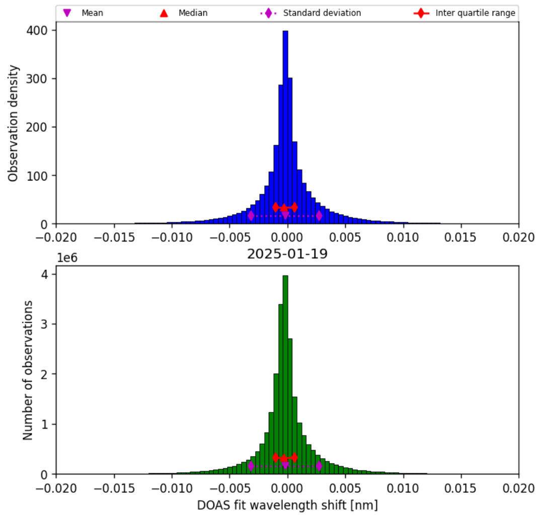
Figure 44: Histogram of “DOAS fit wavelength shift” for 2025-01-18 to 2025-01-20
