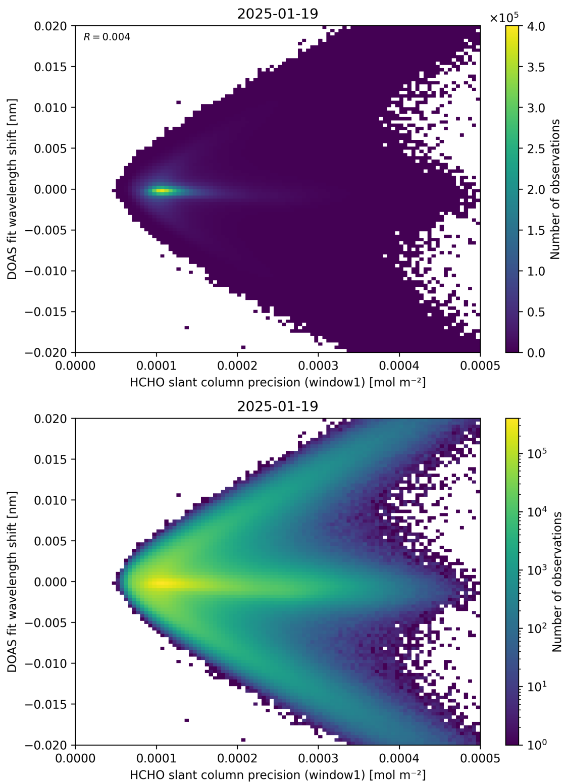
Figure 89: Scatter density plot of “HCHO slant column precision (window1)” against “DOAS fit wavelength shift” for 2025-01-18 to 2025-01-20.
