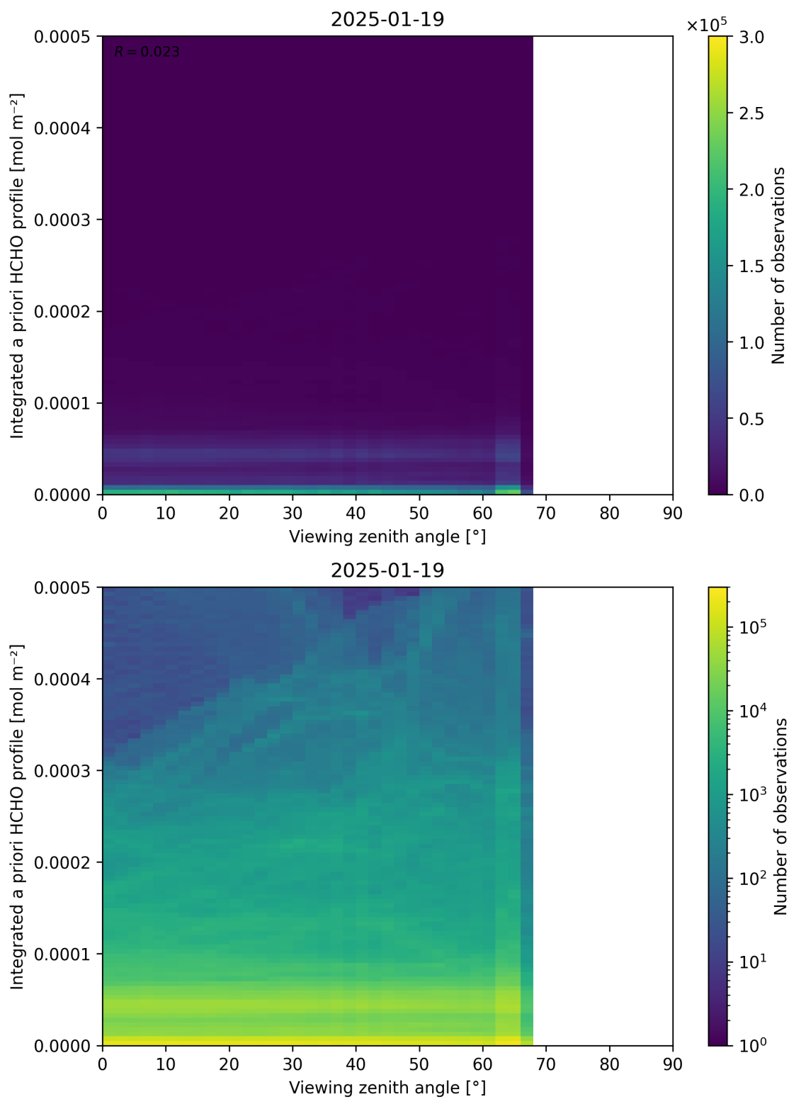
Figure 195: Scatter density plot of “Viewing zenith angle” against “Integrated a priori HCHO profile” for 2025-01-18 to 2025-01-20.
