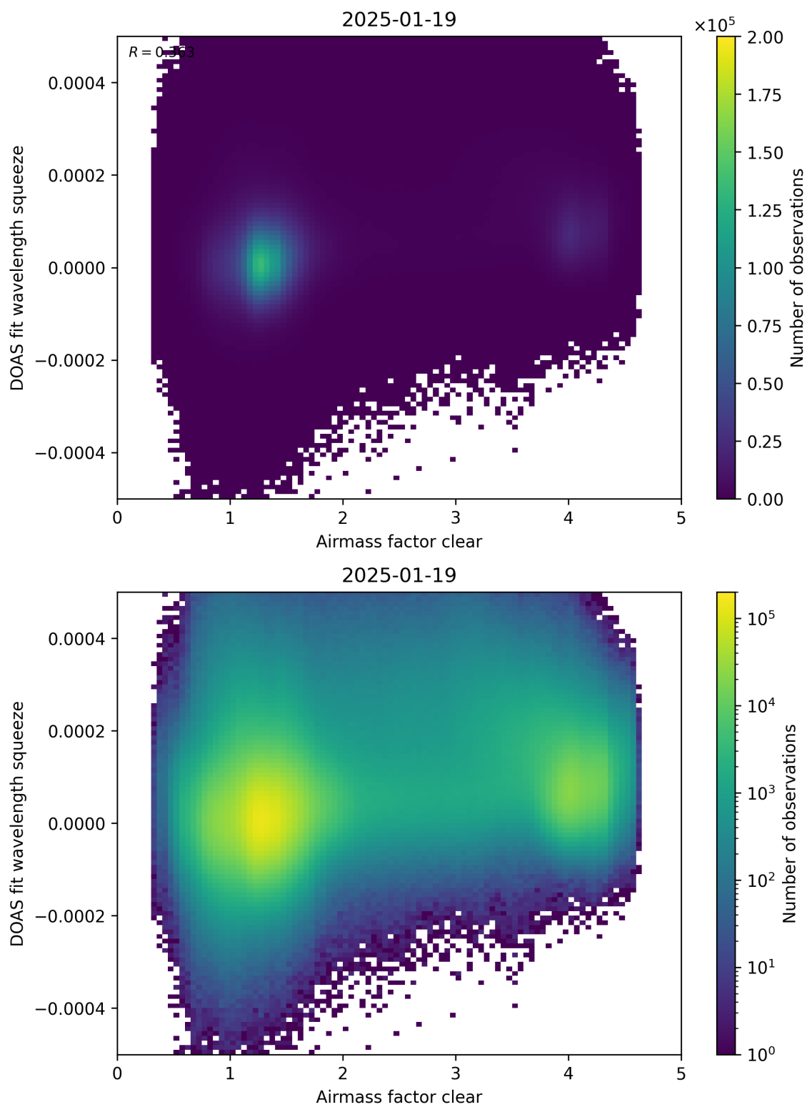
Figure 73: Scatter density plot of “Airmass factor clear” against “DOAS fit wavelength squeeze” for 2025-01-18 to 2025-01-20.
