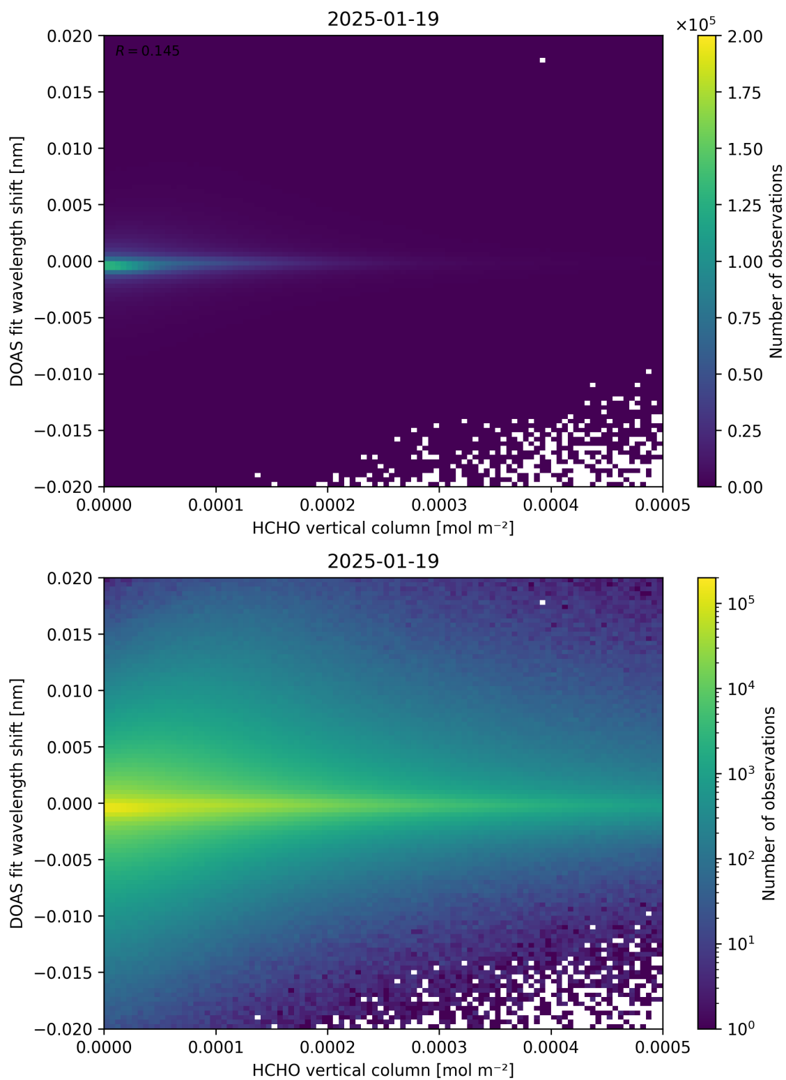
Figure 124: Scatter density plot of “HCHO vertical column” against “DOAS fit wavelength shift” for 2025-01-18 to 2025-01-20.
