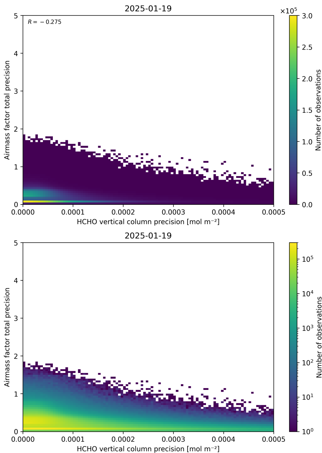
Figure 145: Scatter density plot of “HCHO vertical column precision” against “Airmass factor total precision” for 2025-01-18 to 2025-01-20.
