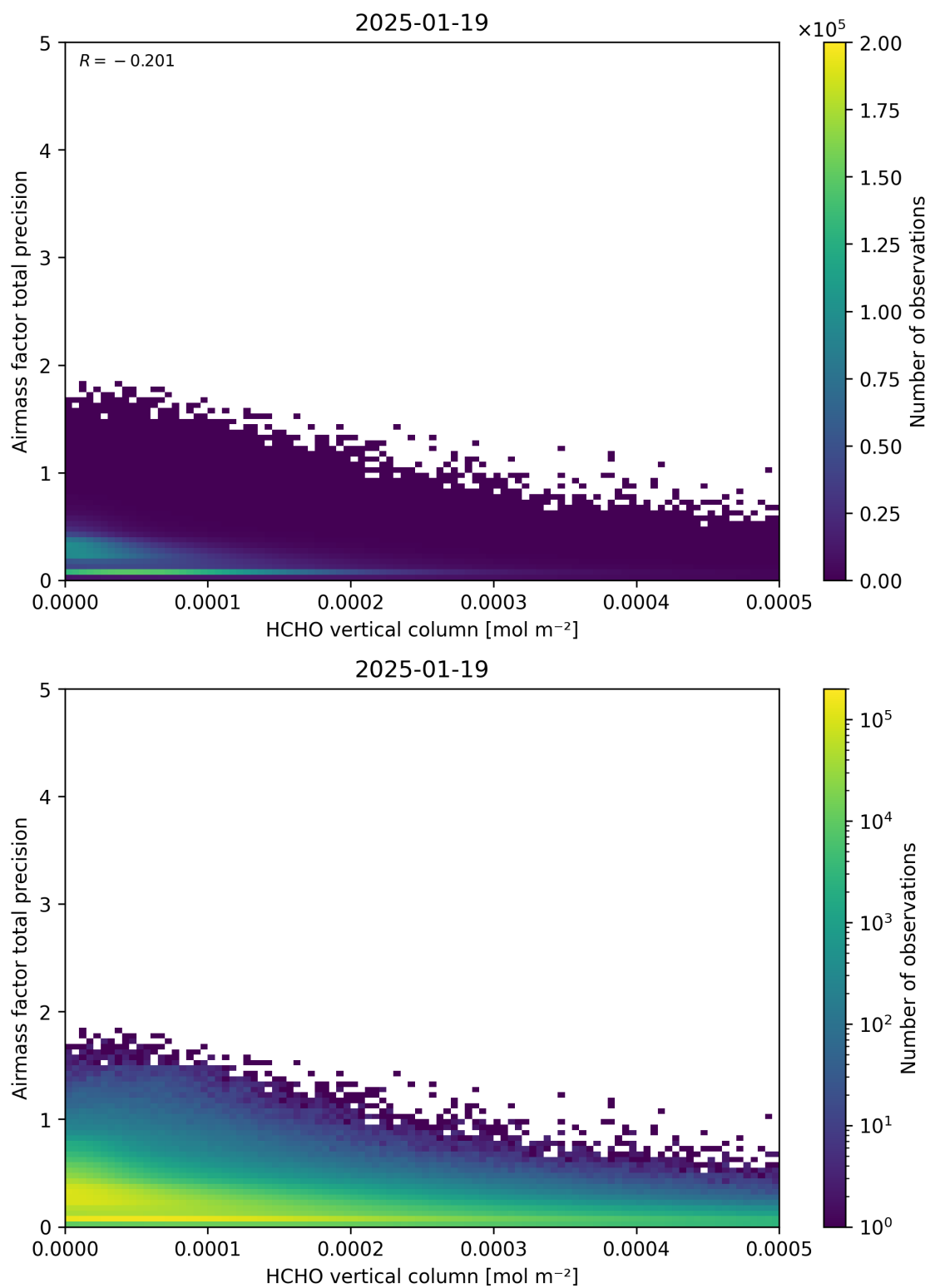
Figure 132: Scatter density plot of “HCHO vertical column” against “Airmass factor total precision” for 2025-01-18 to 2025-01-20.
