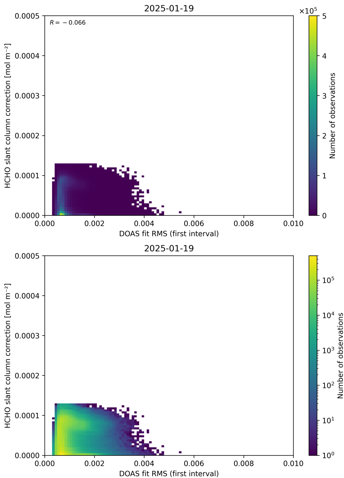
Figure 63: Scatter density plot of “DOAS fit RMS (first interval)” against “HCHO slant column correction” for 2025-01-18 to 2025-01-20.
