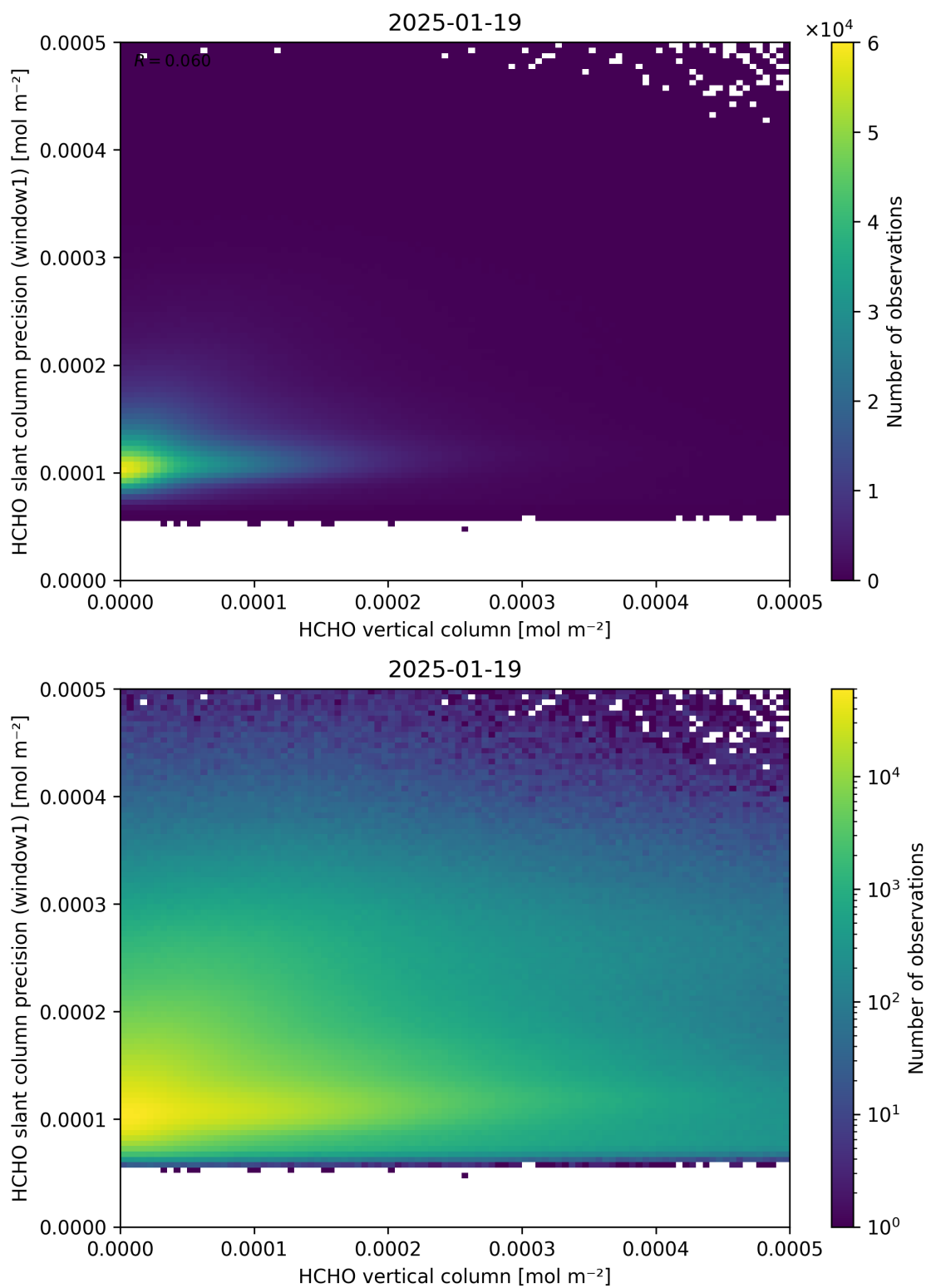
Figure 130: Scatter density plot of “HCHO vertical column” against “HCHO slant column precision (window1)” for 2025-01-18 to 2025-01-20.
