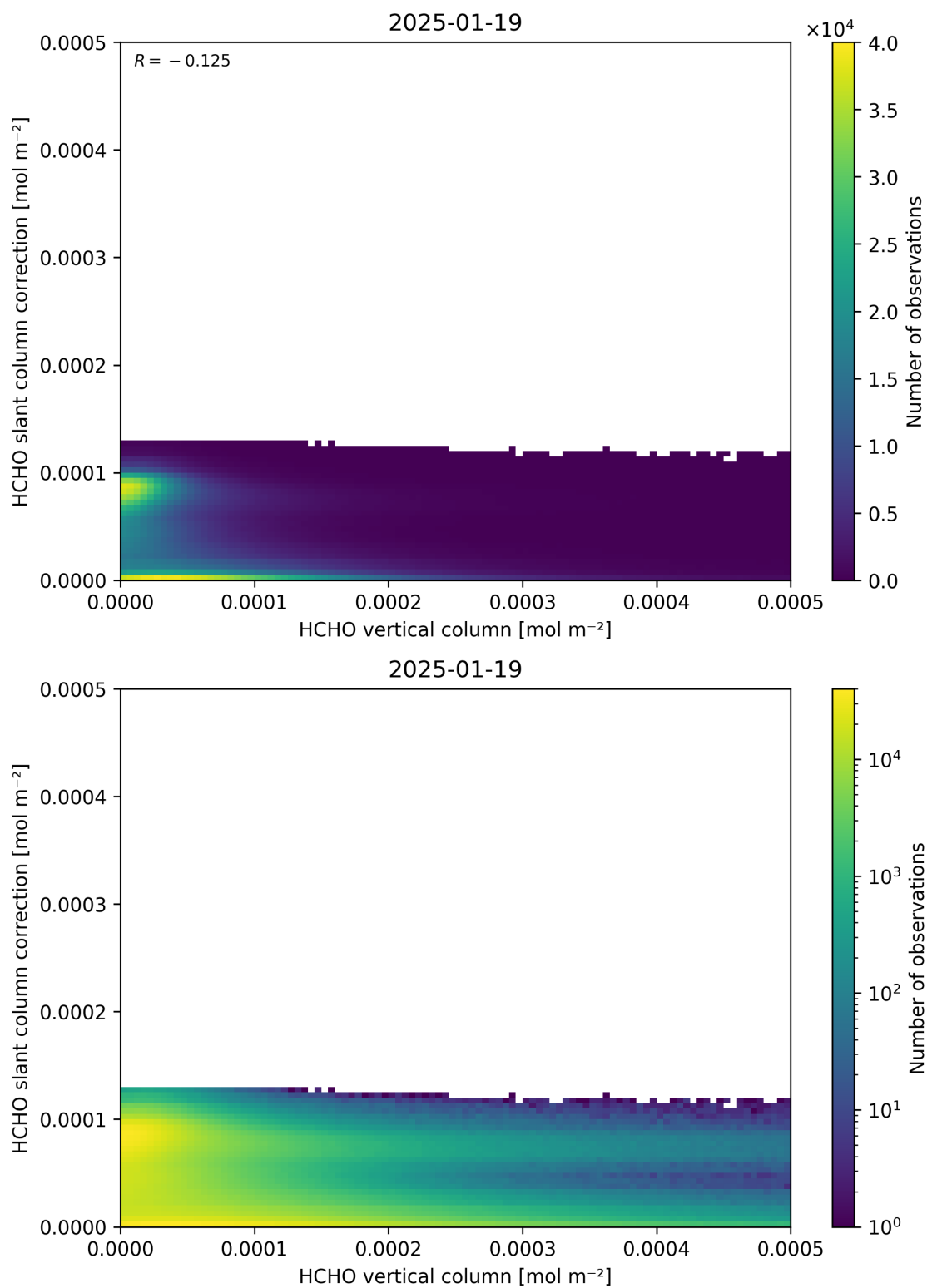
Figure 128: Scatter density plot of “HCHO vertical column” against “HCHO slant column correction” for 2025-01-18 to 2025-01-20.
