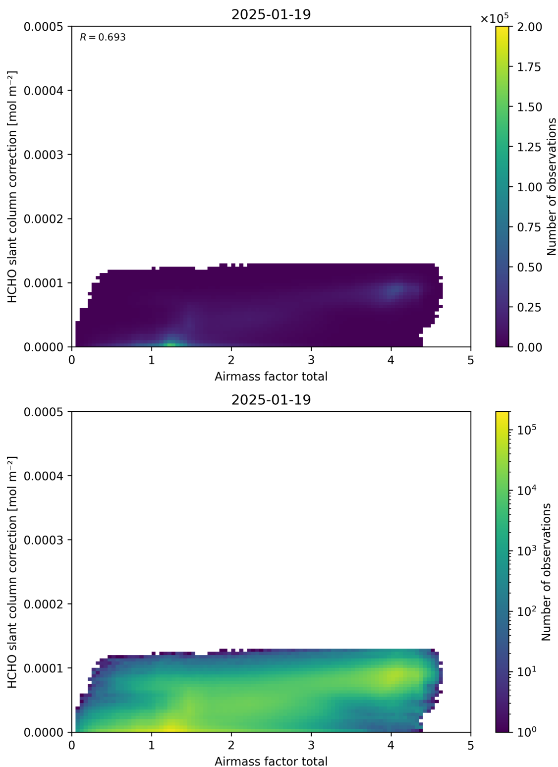
Figure 102: Scatter density plot of “Airmass factor total” against “HCHO slant column correction” for 2025-01-18 to 2025-01-20.
