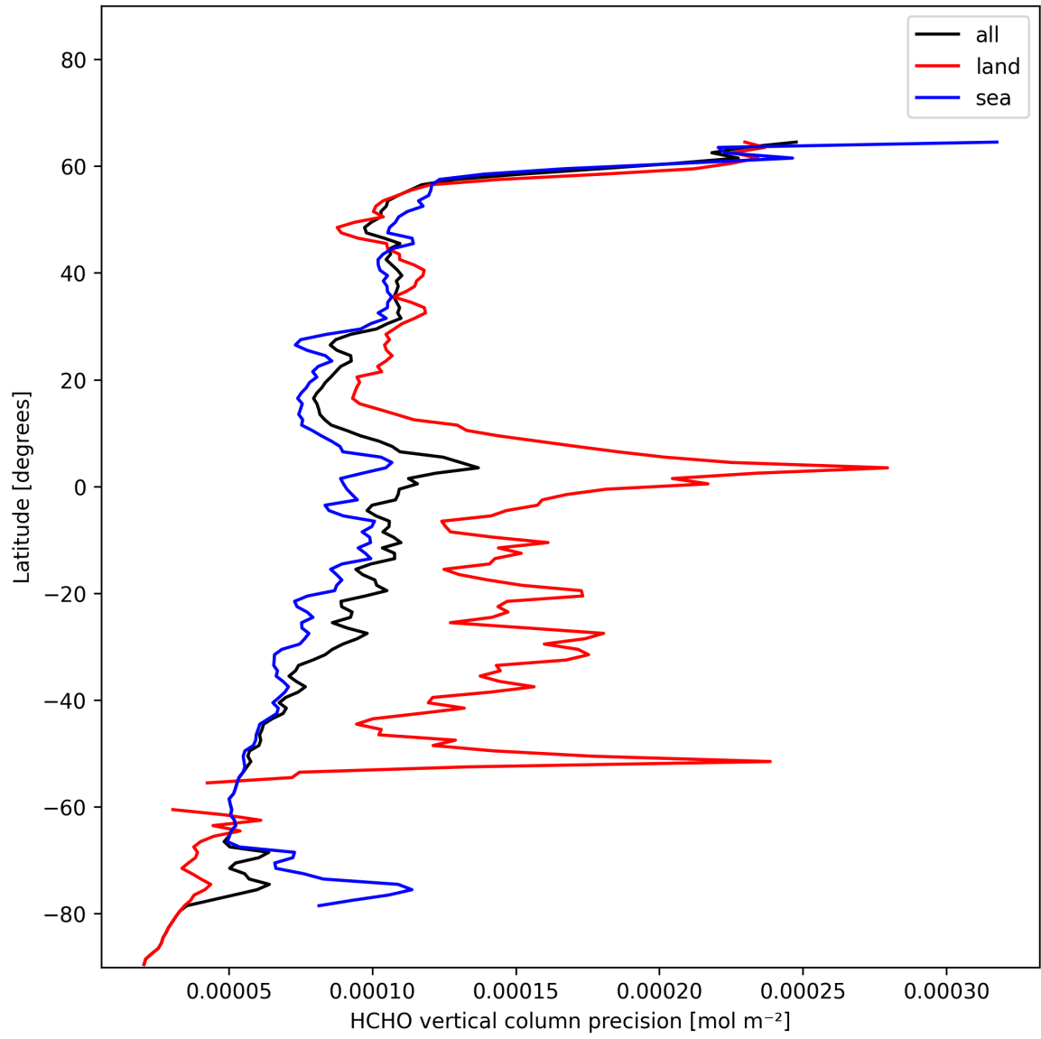
Figure 22: Zonal average of “HCHO vertical column precision” for 2025-01-18 to 2025-01-20.
