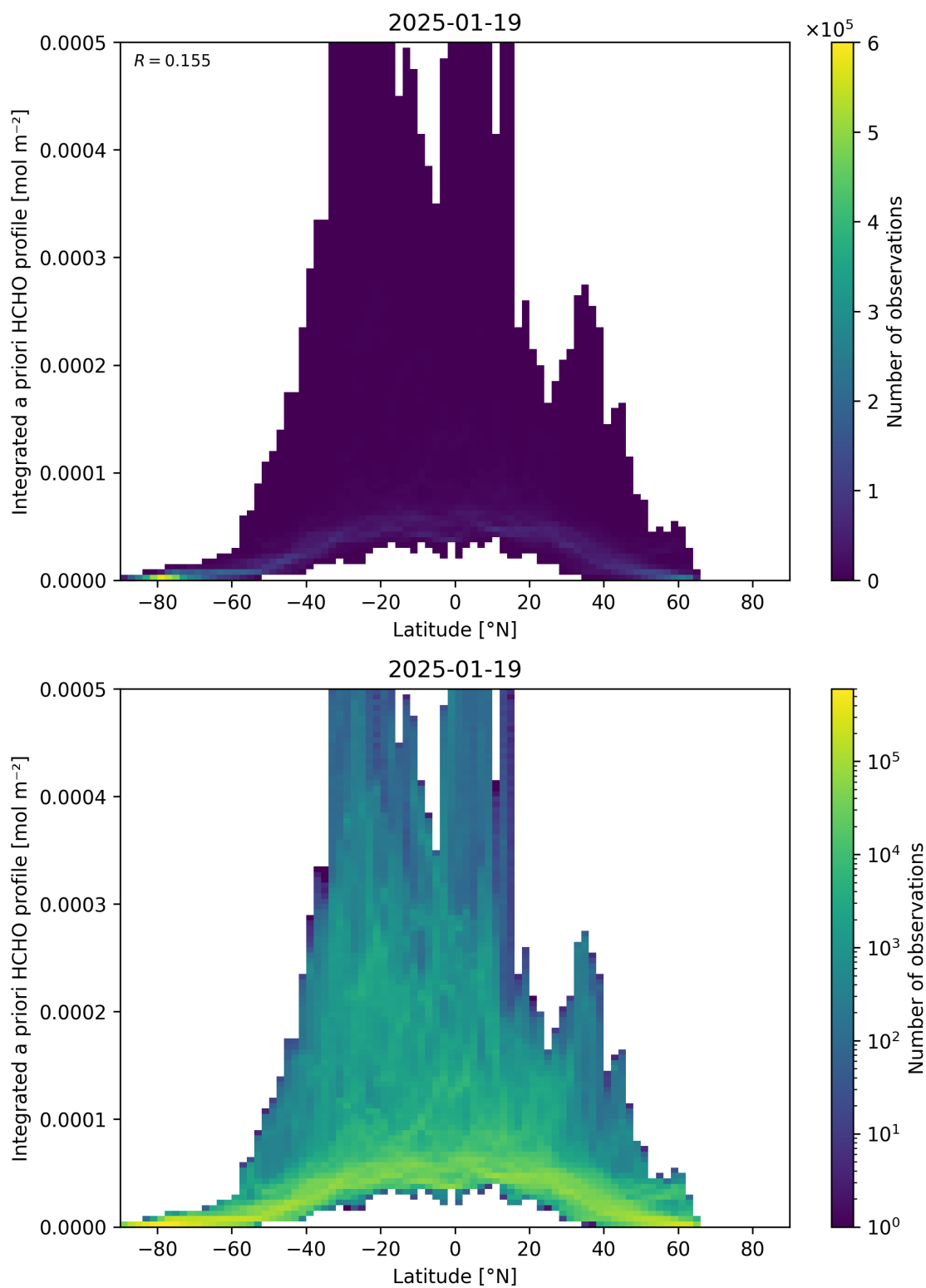
Figure 166: Scatter density plot of “Latitude” against “Integrated a priori HCHO profile” for 2025-01-18 to 2025-01-20.
