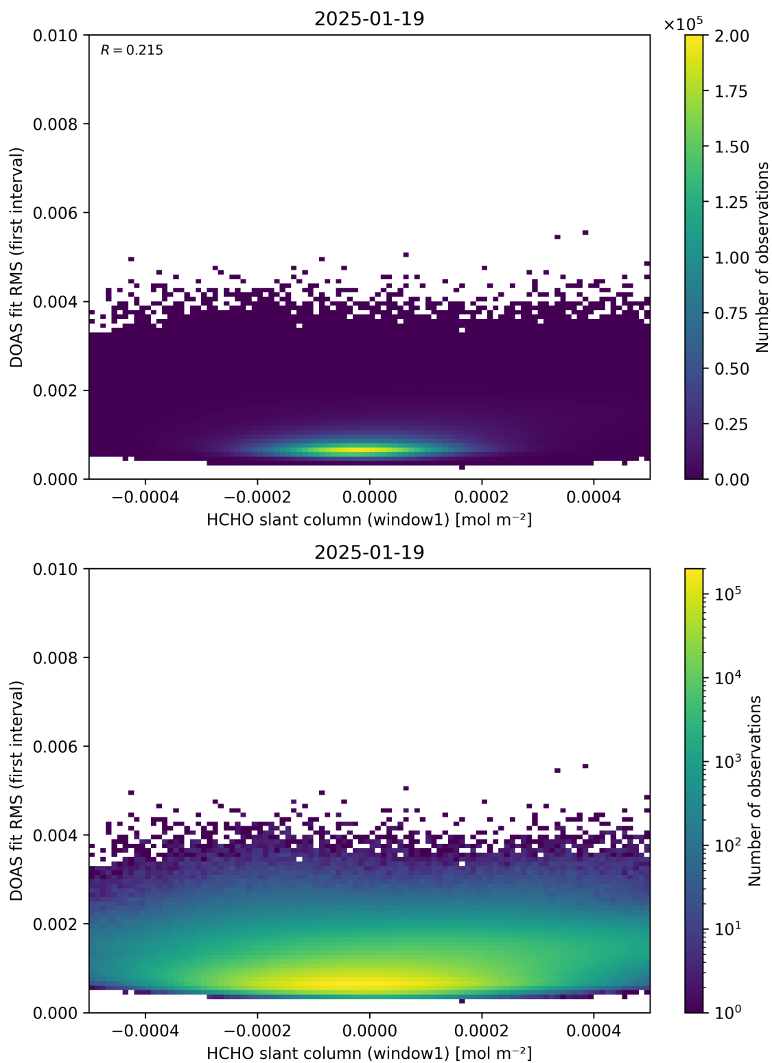
Figure 78: Scatter density plot of “HCHO slant column (window1)” against “DOAS fit RMS (first interval)” for 2025-01-18 to 2025-01-20.
