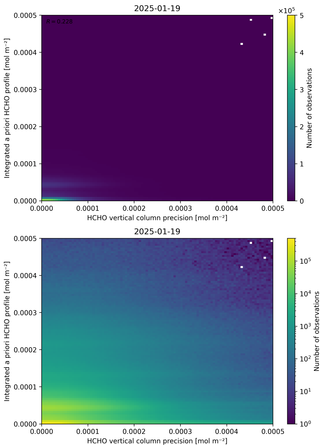
Figure 147: Scatter density plot of “HCHO vertical column precision” against “Integrated a priori HCHO profile” for 2025-01-18 to 2025-01-20.
