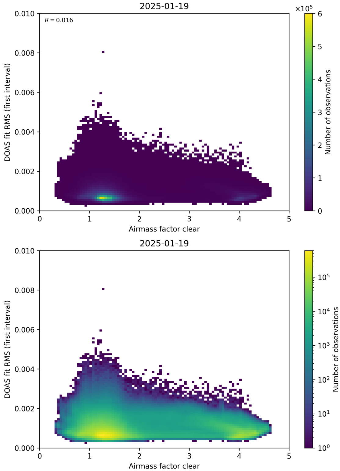
Figure 71: Scatter density plot of “Airmass factor clear” against “DOAS fit RMS (first interval)” for 2025-01-18 to 2025-01-20.
