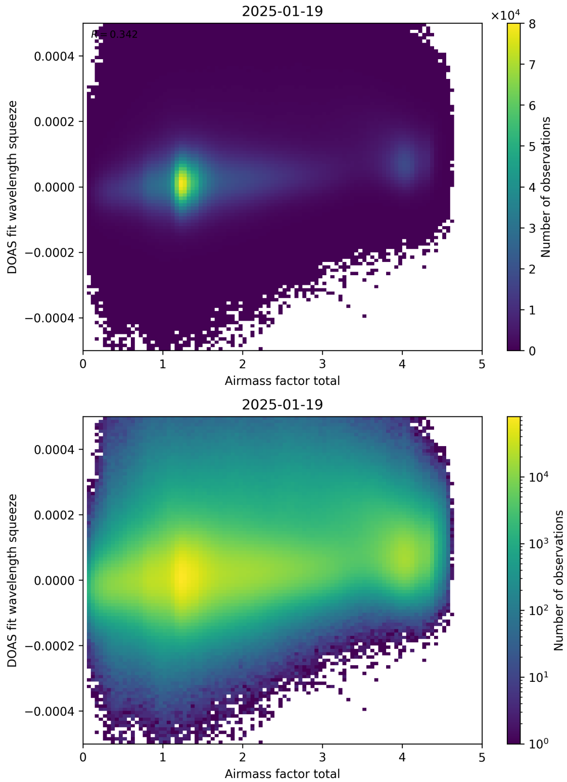
Figure 99: Scatter density plot of “Airmass factor total” against “DOAS fit wavelength squeeze” for 2025-01-18 to 2025-01-20.
