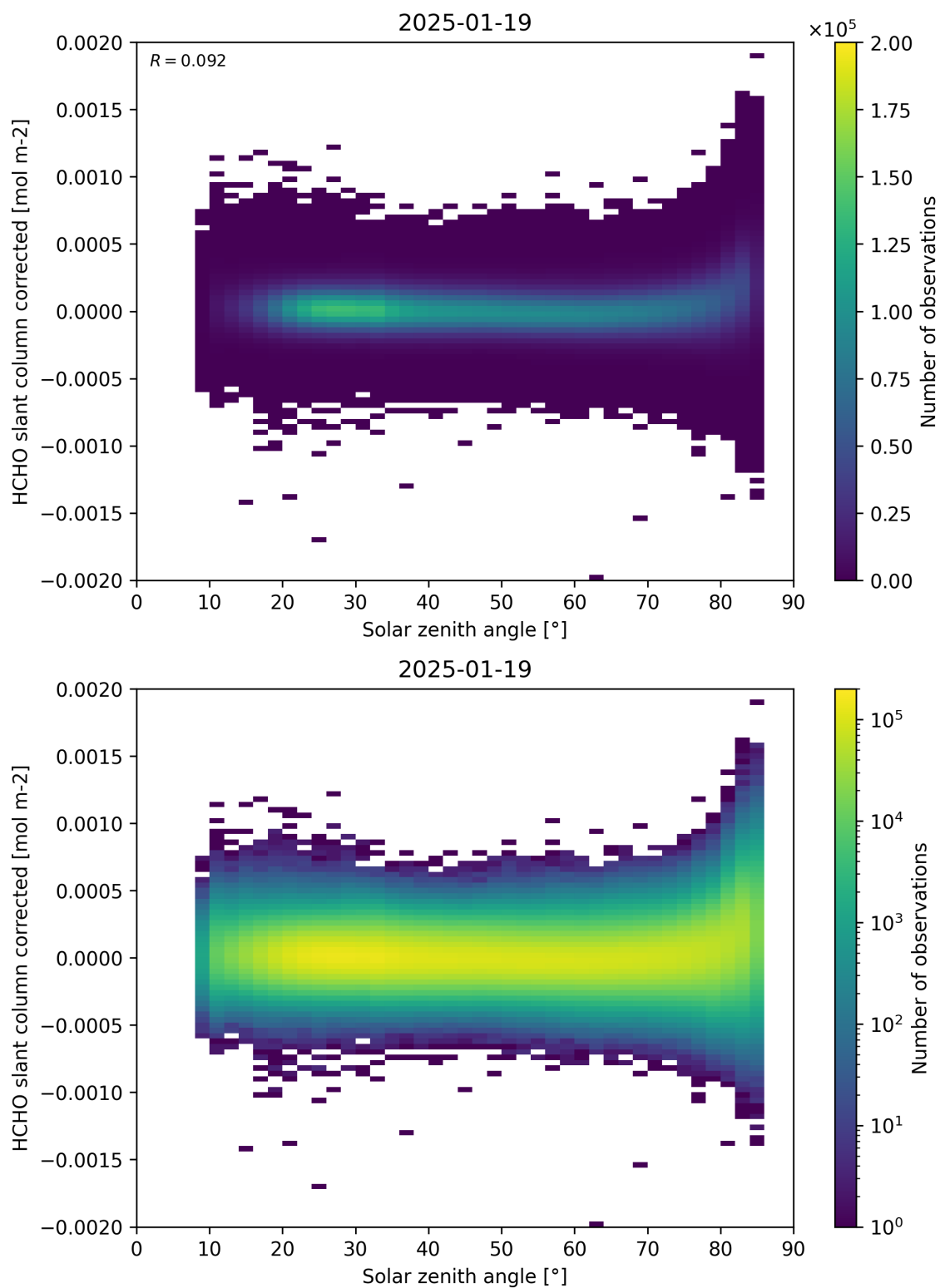
Figure 171: Scatter density plot of “Solar zenith angle” against “HCHO slant column corrected” for 2025-01-18 to 2025-01-20.
