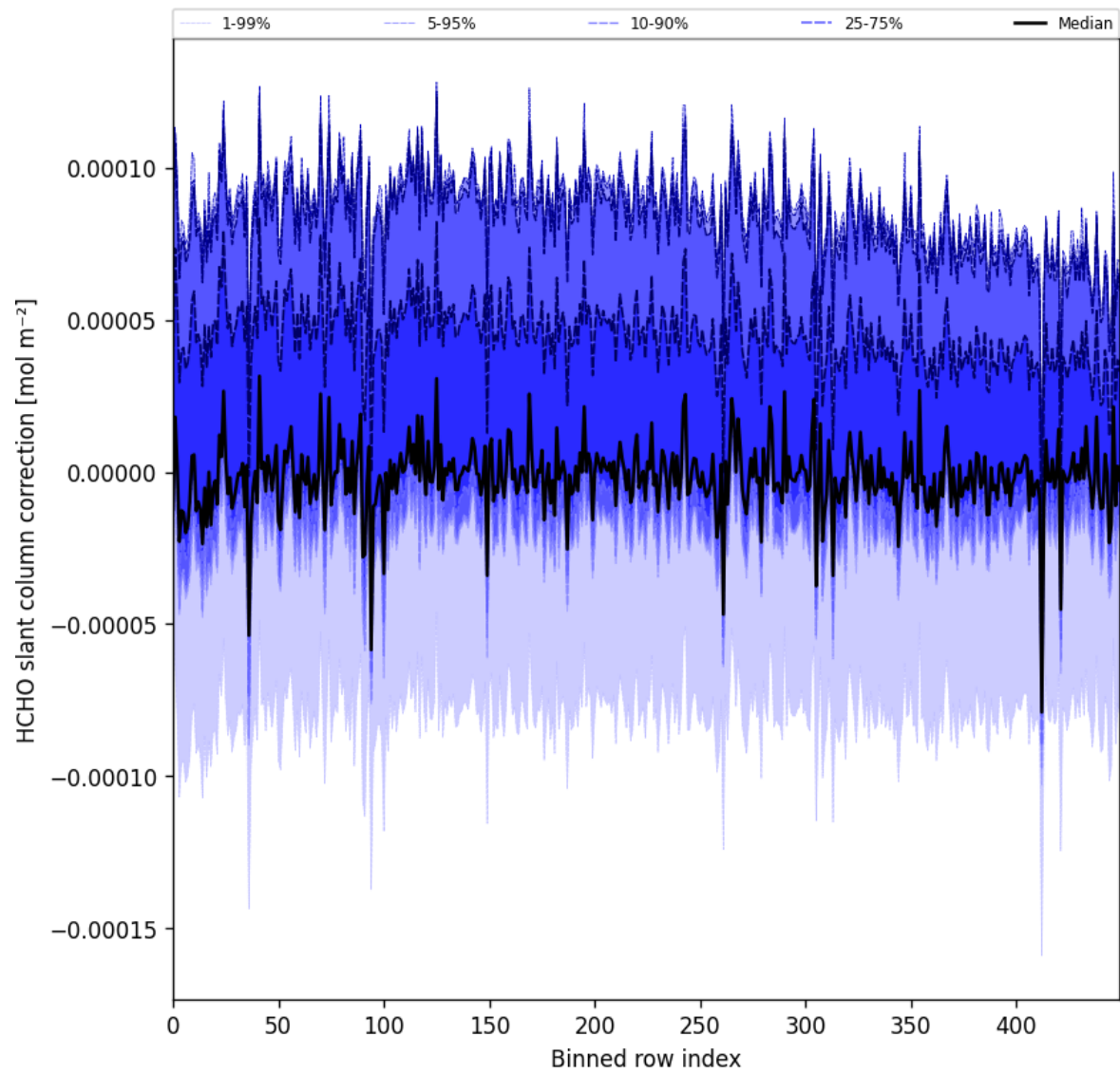
Figure 61: Along track statistics of “HCHO slant column correction” for 2025-01-18 to 2025-01-20
