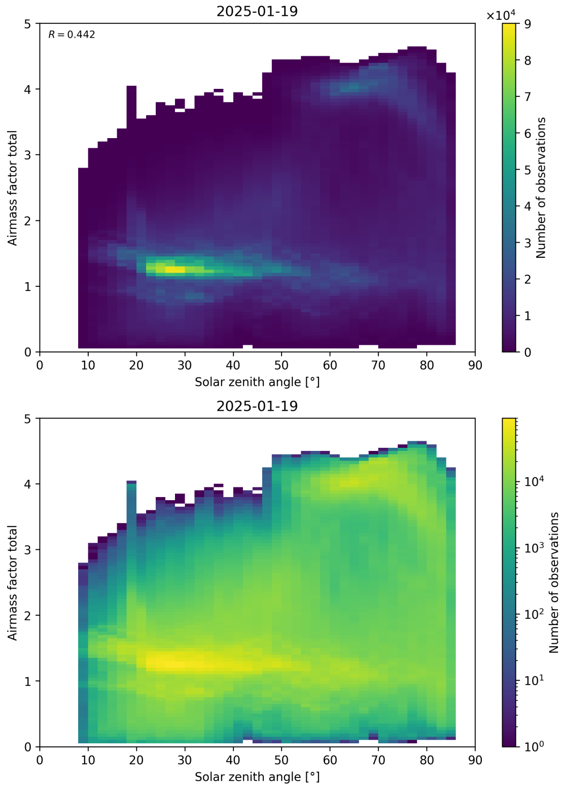
Figure 175: Scatter density plot of “Solar zenith angle” against “Airmass factor total” for 2025-01-18 to 2025-01-20.
