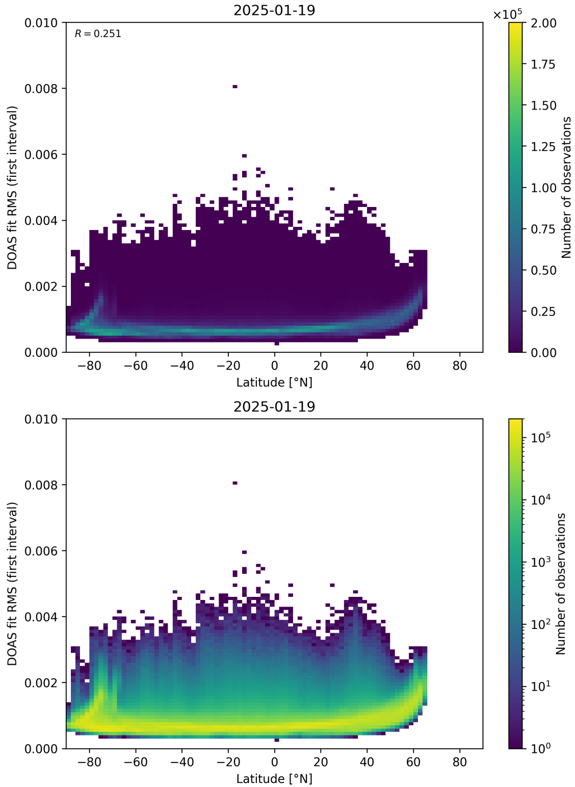
Figure 153: Scatter density plot of “Latitude” against “DOAS fit RMS (first interval)” for 2025-01-18 to 2025-01-20.
