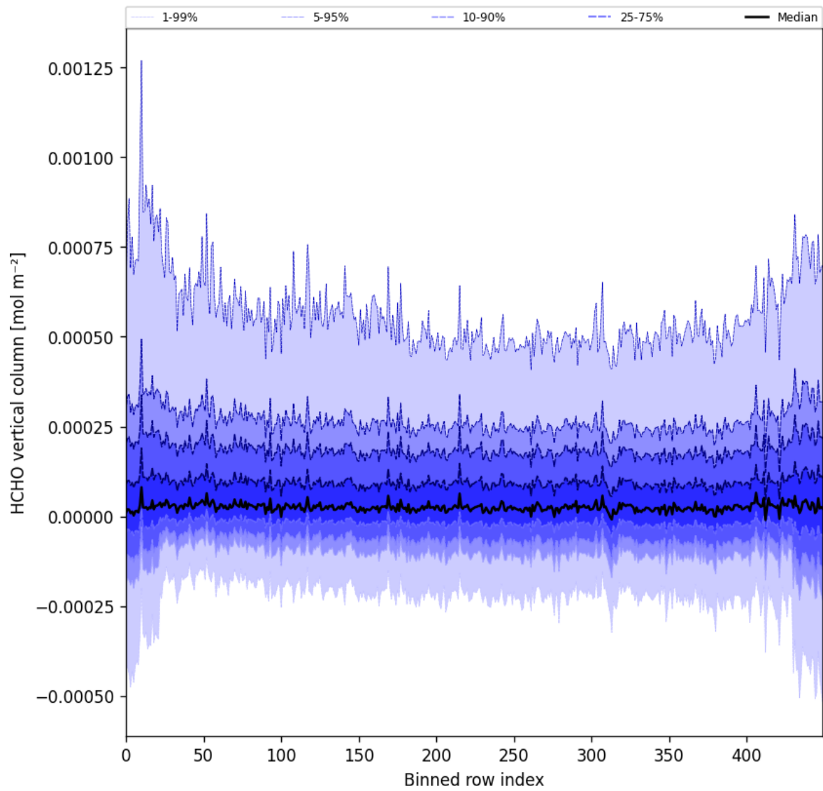
Figure 49: Along track statistics of “HCHO vertical column” for 2025-01-18 to 2025-01-20
