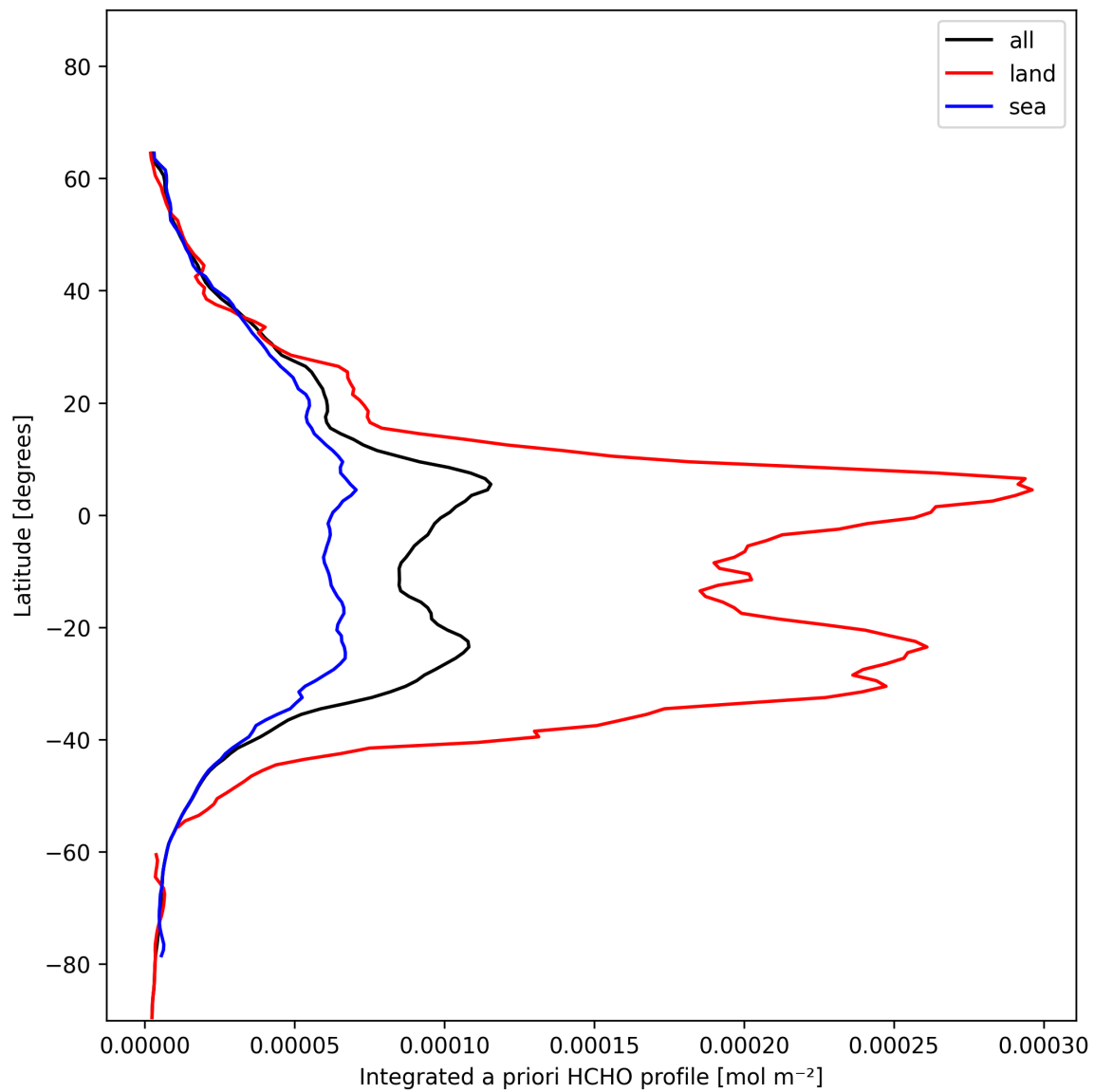
Figure 29: Zonal average of “Integrated a priori HCHO profile” for 2025-01-18 to 2025-01-20.
