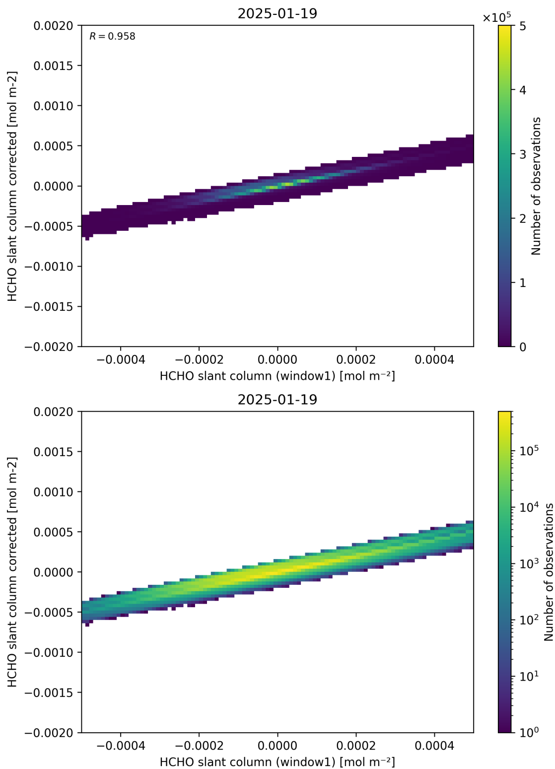
Figure 82: Scatter density plot of “HCHO slant column (window1)” against “HCHO slant column corrected” for 2025-01-18 to 2025-01-20.
