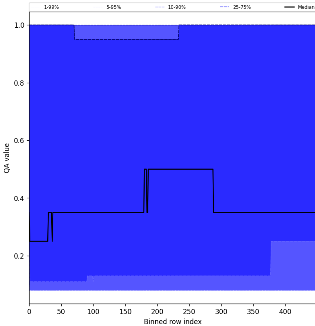
Figure 48: Along track statistics of “QA value” for 2025-01-18 to 2025-01-20
