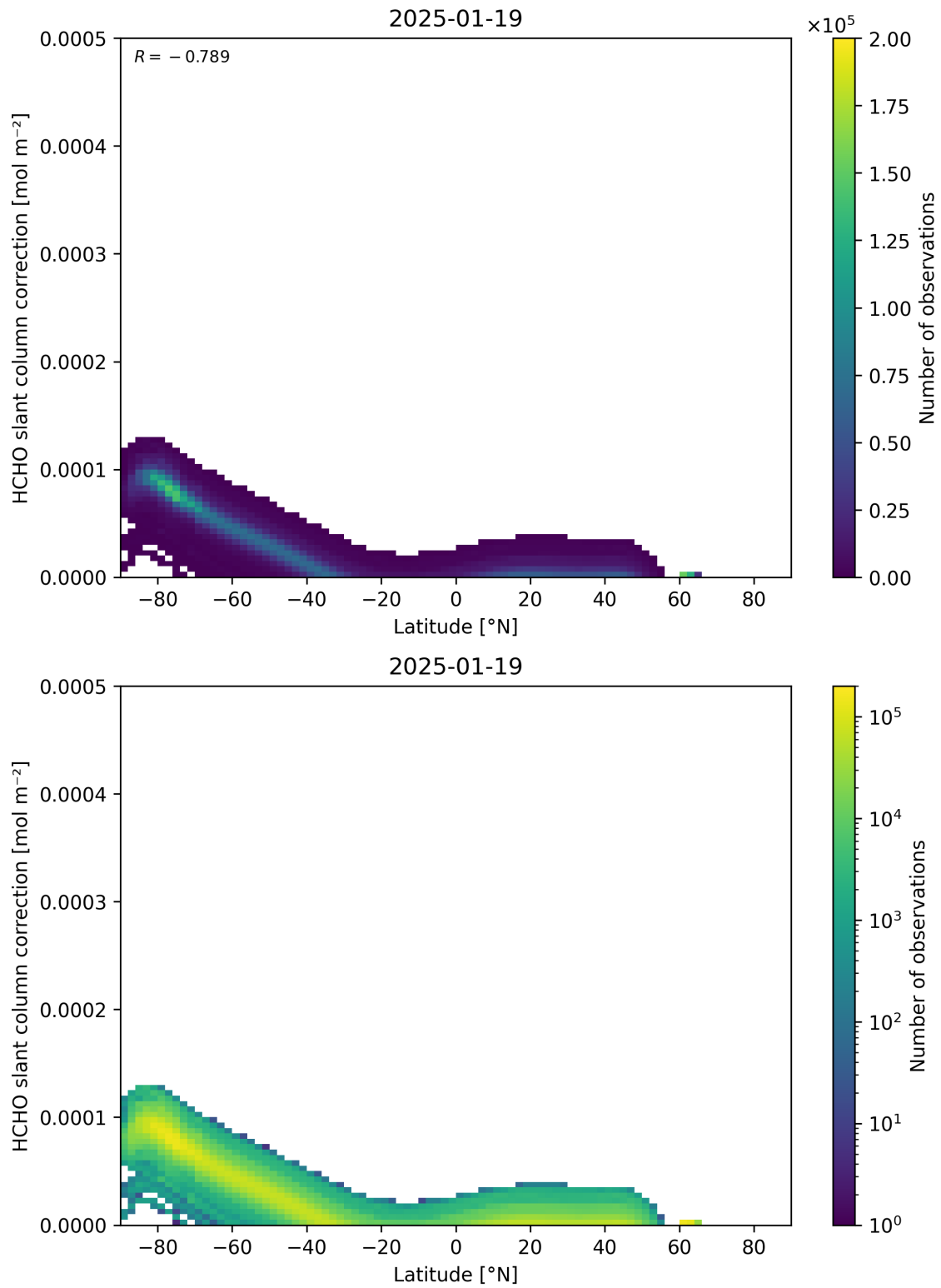
Figure 158: Scatter density plot of “Latitude” against “HCHO slant column correction” for 2025-01-18 to 2025-01-20.
