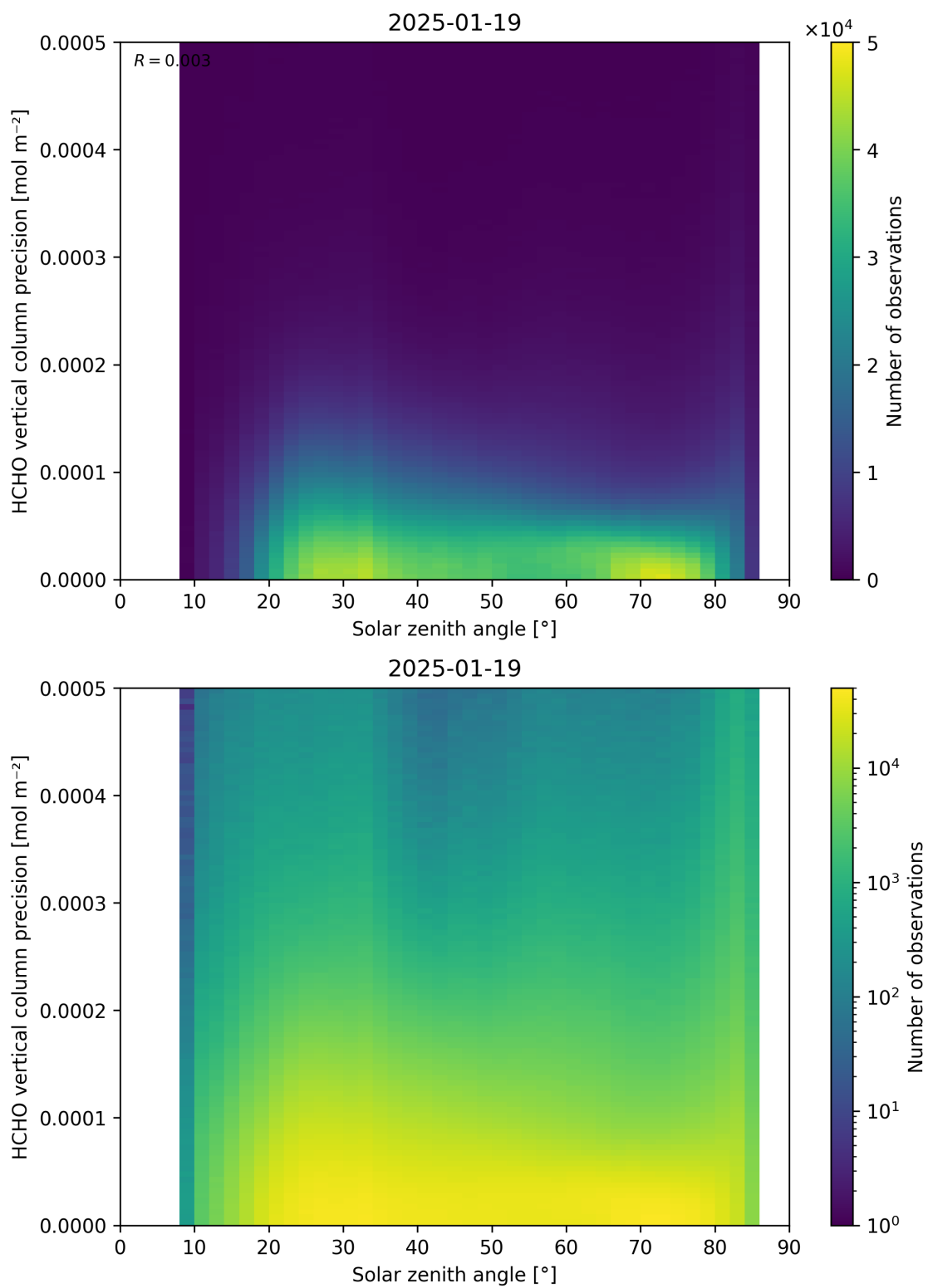
Figure 179: Scatter density plot of “Solar zenith angle” against “HCHO vertical column precision” for 2025-01-18 to 2025-01-20.
