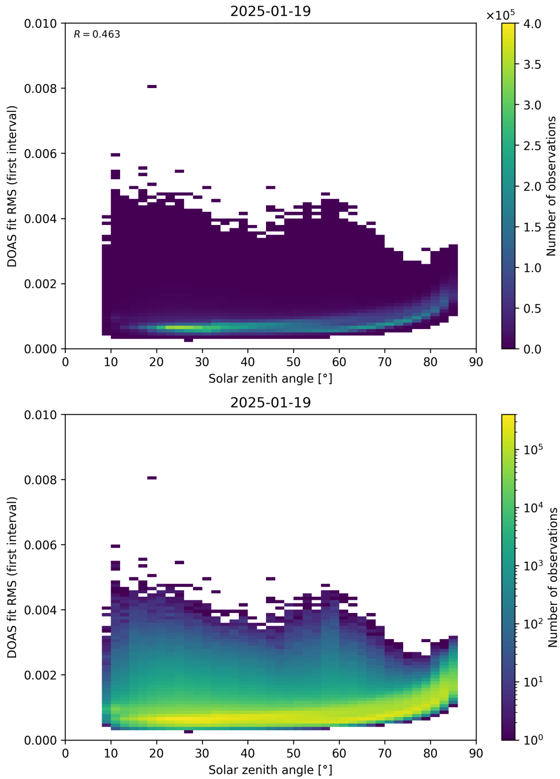
Figure 167: Scatter density plot of “Solar zenith angle” against “DOAS fit RMS (first interval)” for 2025-01-18 to 2025-01-20.
