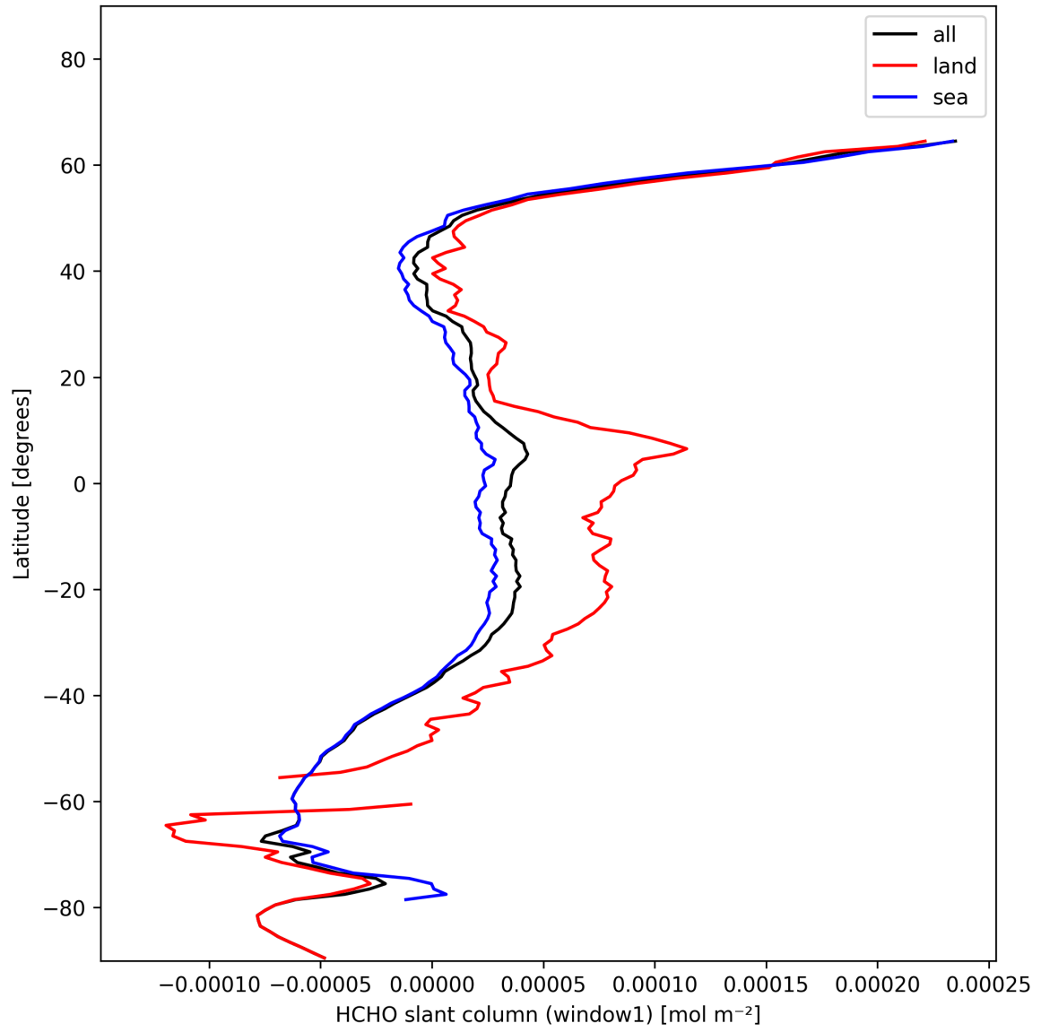
Figure 24: Zonal average of “HCHO slant column (window1)” for 2025-01-18 to 2025-01-20.
