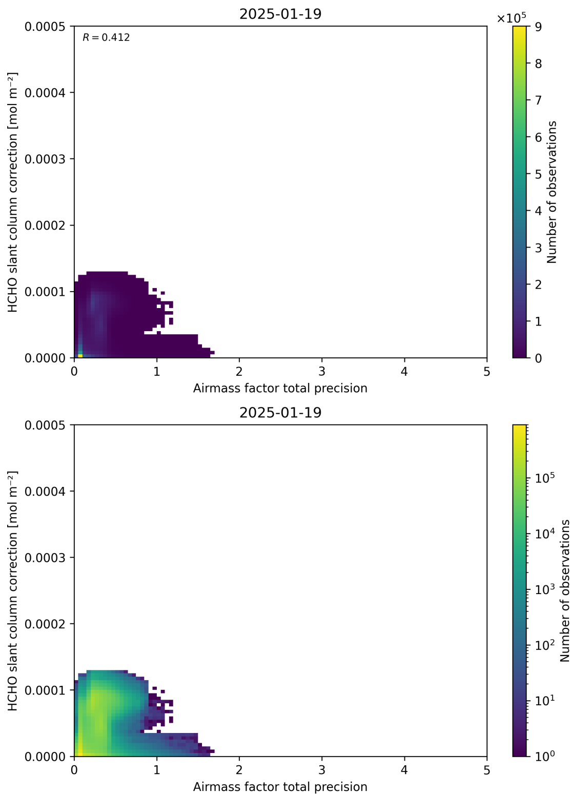
Figure 110: Scatter density plot of “Airmass factor total precision” against “HCHO slant column correction” for 2025-01-18 to 2025-01-20.
