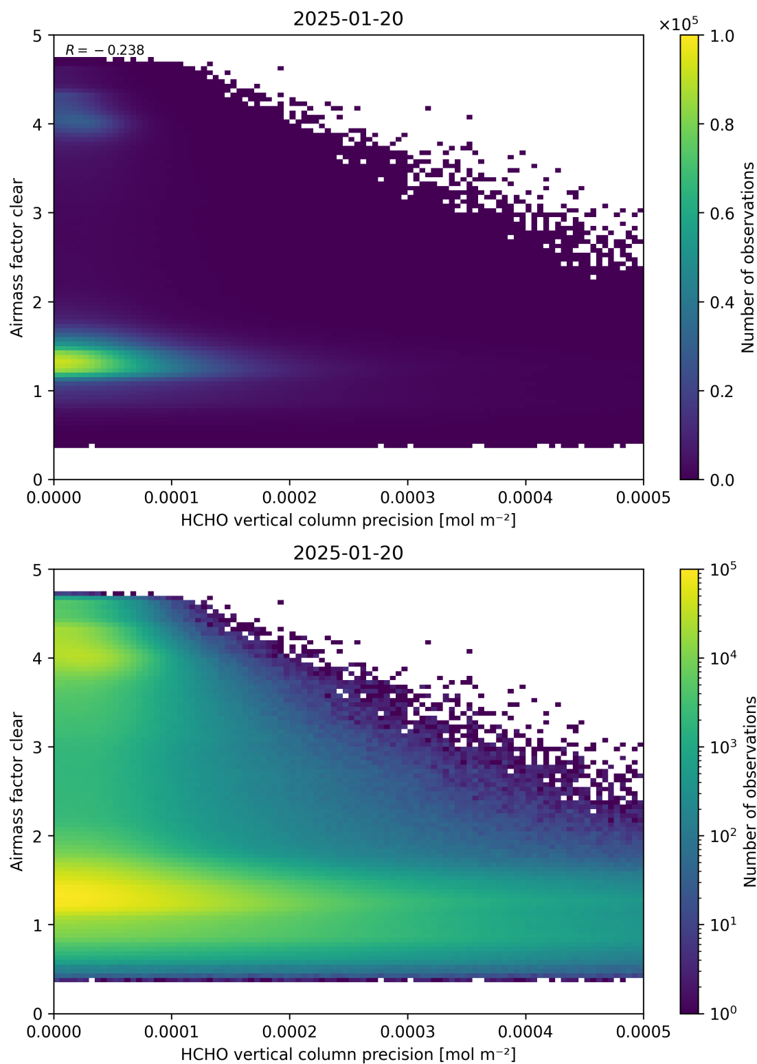
Figure 139: Scatter density plot of “HCHO vertical column precision” against “Airmass factor clear” for 2025-01-19 to 2025-01-21.
