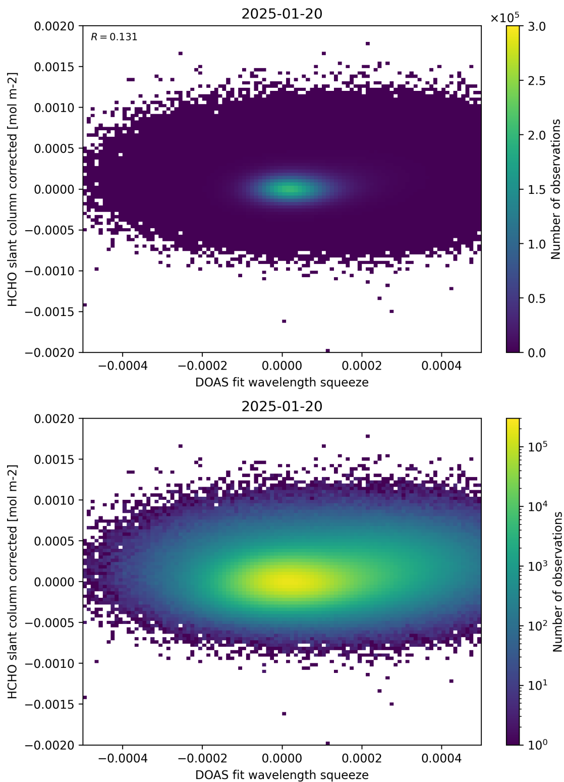
Figure 69: Scatter density plot of “DOAS fit wavelength squeeze” against “HCHO slant column corrected” for 2025-01-19 to 2025-01-21.
