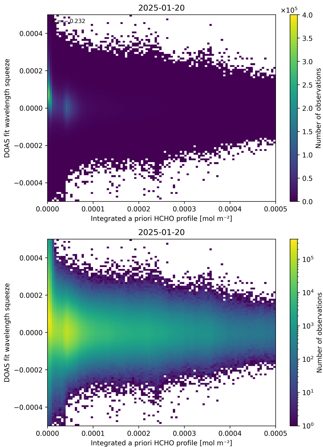
Figure 150: Scatter density plot of “Integrated a priori HCHO profile” against “DOAS fit wavelength squeeze” for 2025-01-19 to 2025-01-21.
