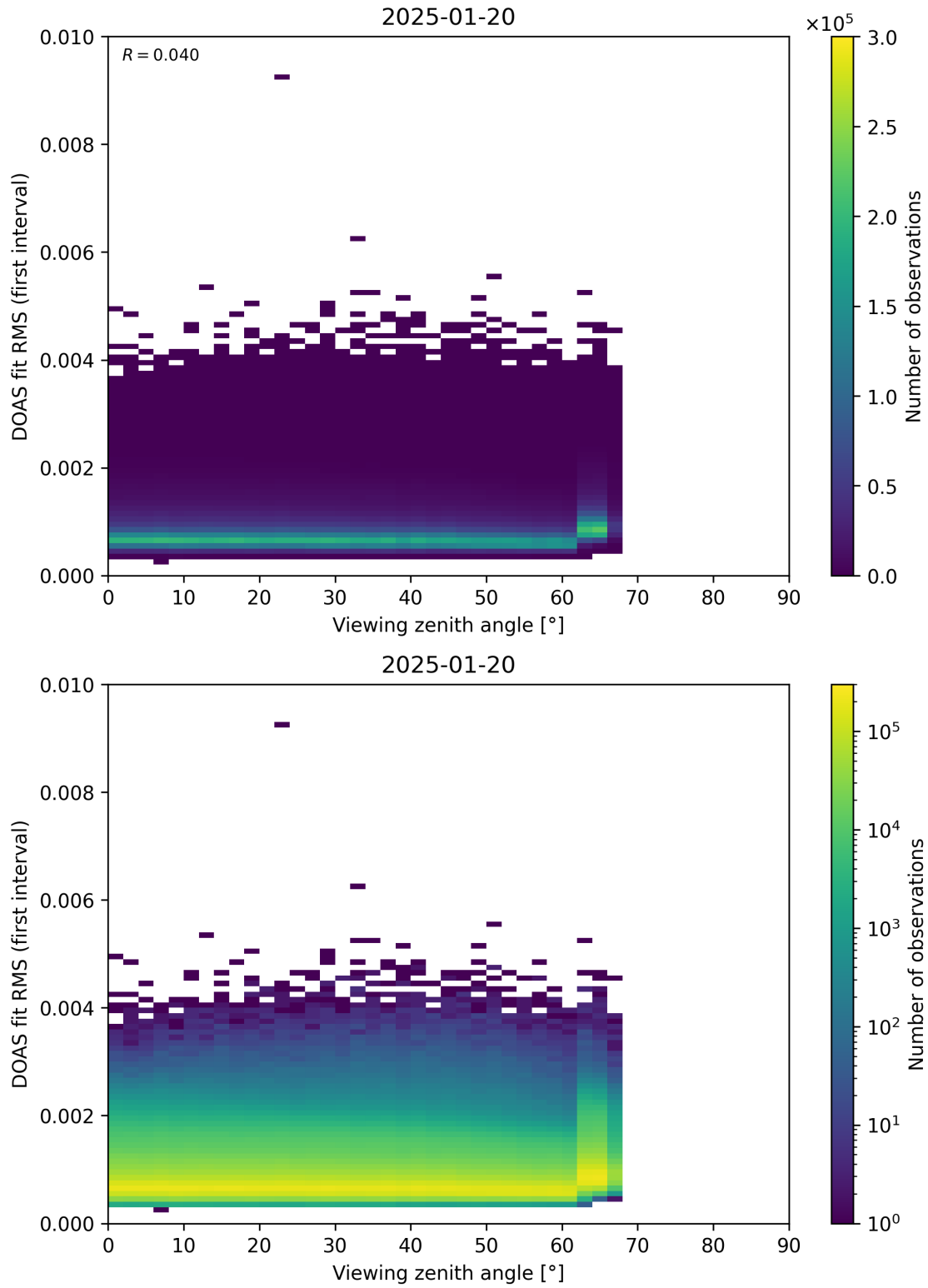
Figure 182: Scatter density plot of “Viewing zenith angle” against “DOAS fit RMS (first interval)” for 2025-01-19 to 2025-01-21.
