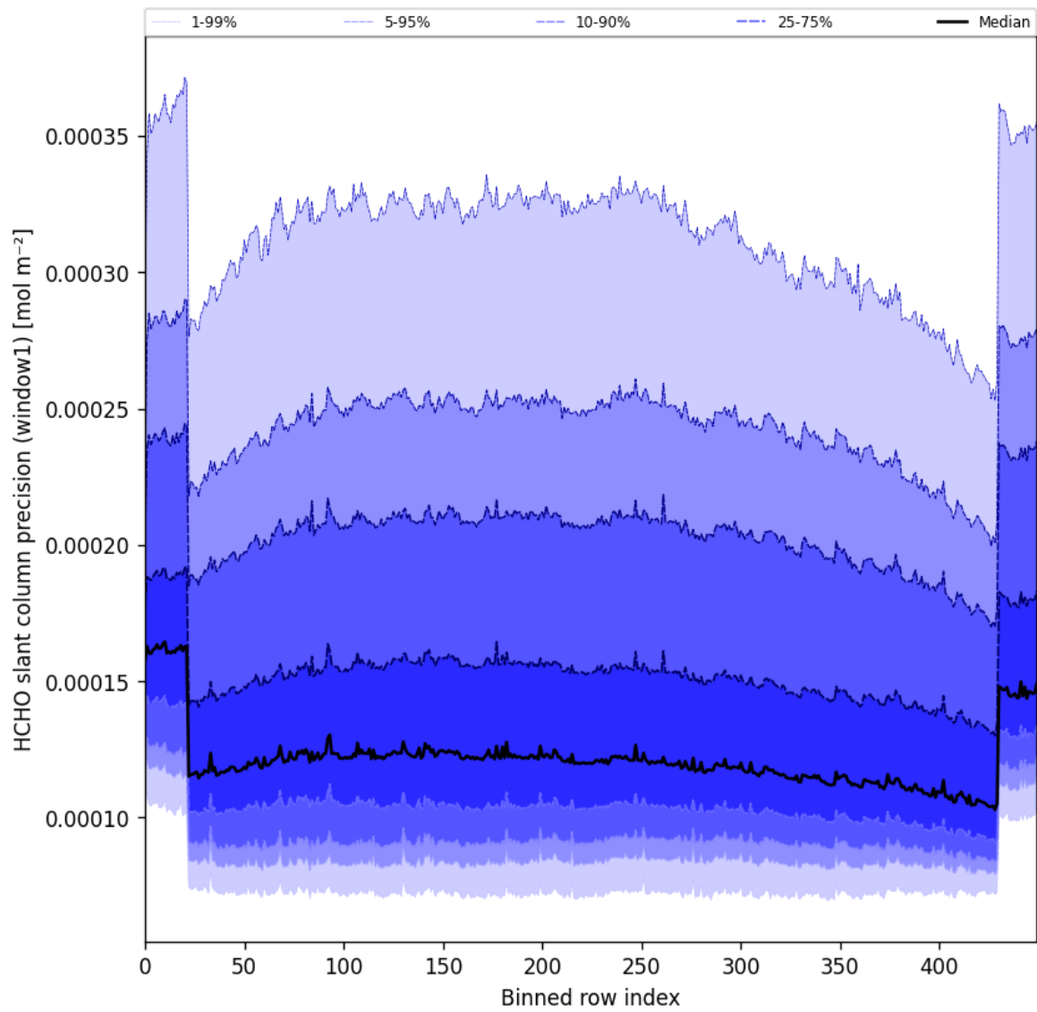
Figure 53: Along track statistics of “HCHO slant column precision (window1)” for 2025-01-19 to 2025-01-21
