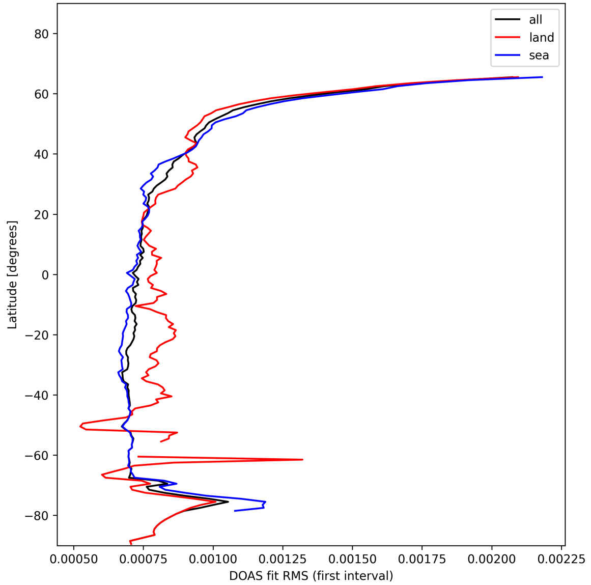
Figure 32: Zonal average of “DOAS fit RMS (first interval)” for 2025-01-19 to 2025-01-21.
