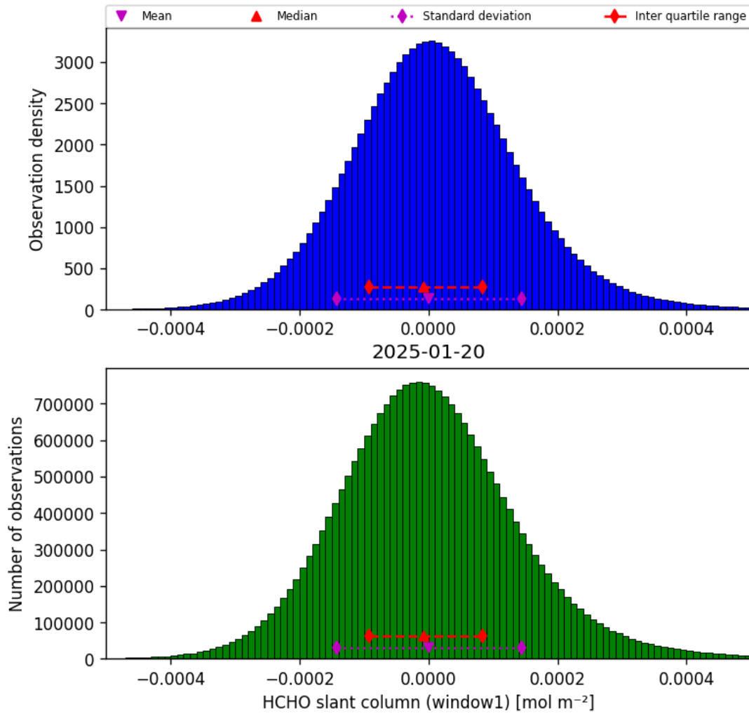
Figure 38: Histogram of “HCHO slant column (window1)” for 2025-01-19 to 2025-01-21
