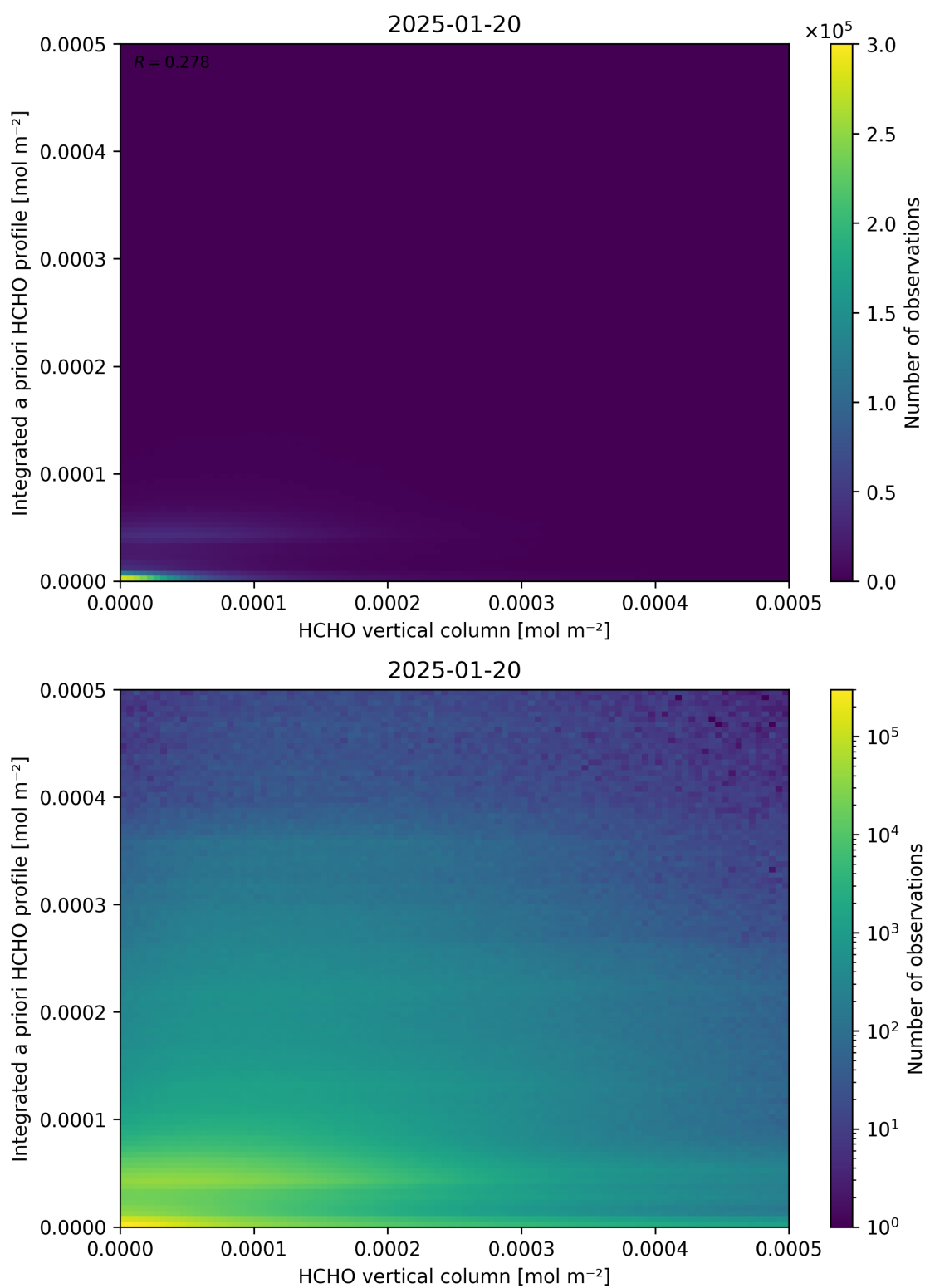
Figure 135: Scatter density plot of “HCHO vertical column” against “Integrated a priori HCHO profile” for 2025-01-19 to 2025-01-21.
