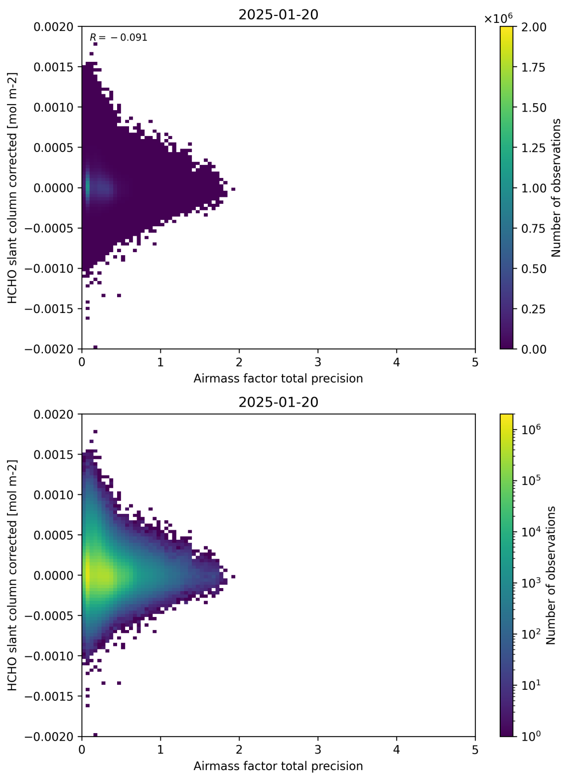
Figure 109: Scatter density plot of “Airmass factor total precision” against “HCHO slant column corrected” for 2025-01-19 to 2025-01-21.
