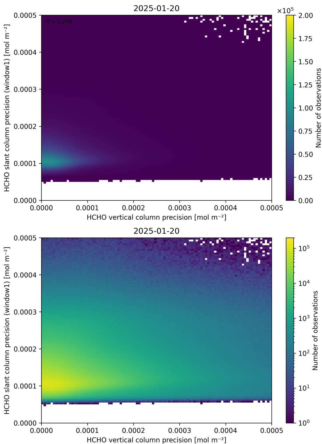
Figure 143: Scatter density plot of “HCHO vertical column precision” against “HCHO slant column precision (window1)” for 2025-01-19 to 2025-01-21.
