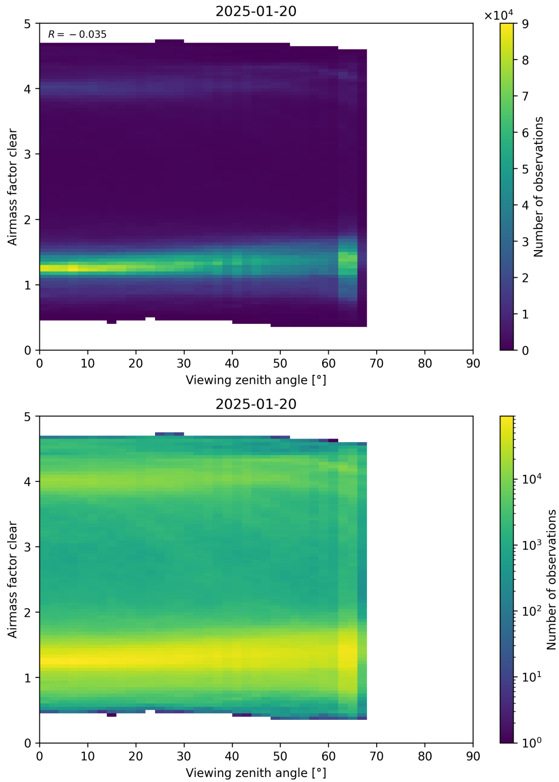
Figure 185: Scatter density plot of “Viewing zenith angle” against “Airmass factor clear” for 2025-01-19 to 2025-01-21.
