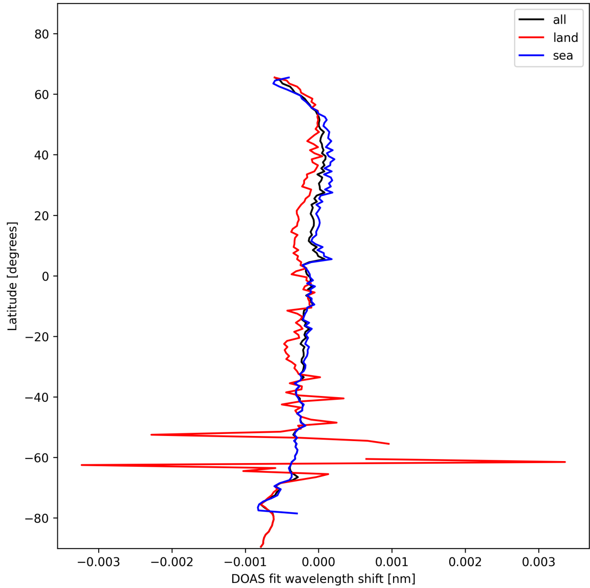
Figure 30: Zonal average of "DOAS fit wavelength shift" for 2025-01-19 to 2025-01-21.
