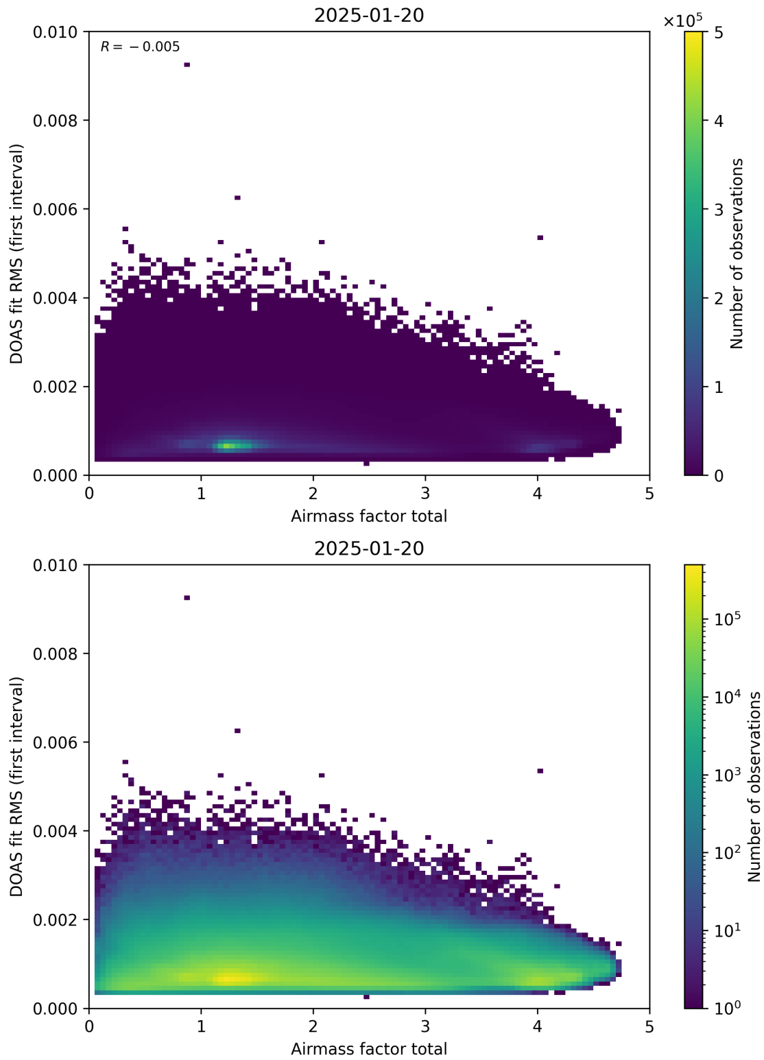
Figure 97: Scatter density plot of “Airmass factor total” against “DOAS fit RMS (first interval)” for 2025-01-19 to 2025-01-21.
