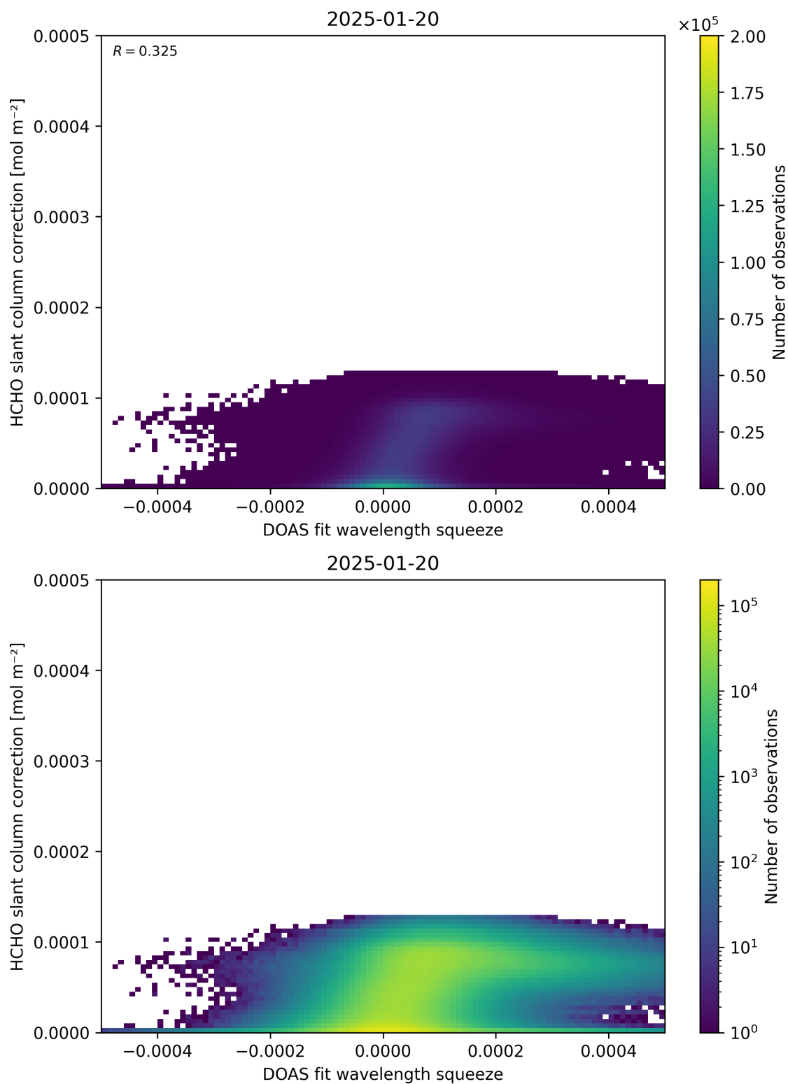
Figure 70: Scatter density plot of “DOAS fit wavelength squeeze” against “HCHO slant column correction” for 2025-01-19 to 2025-01-21.
