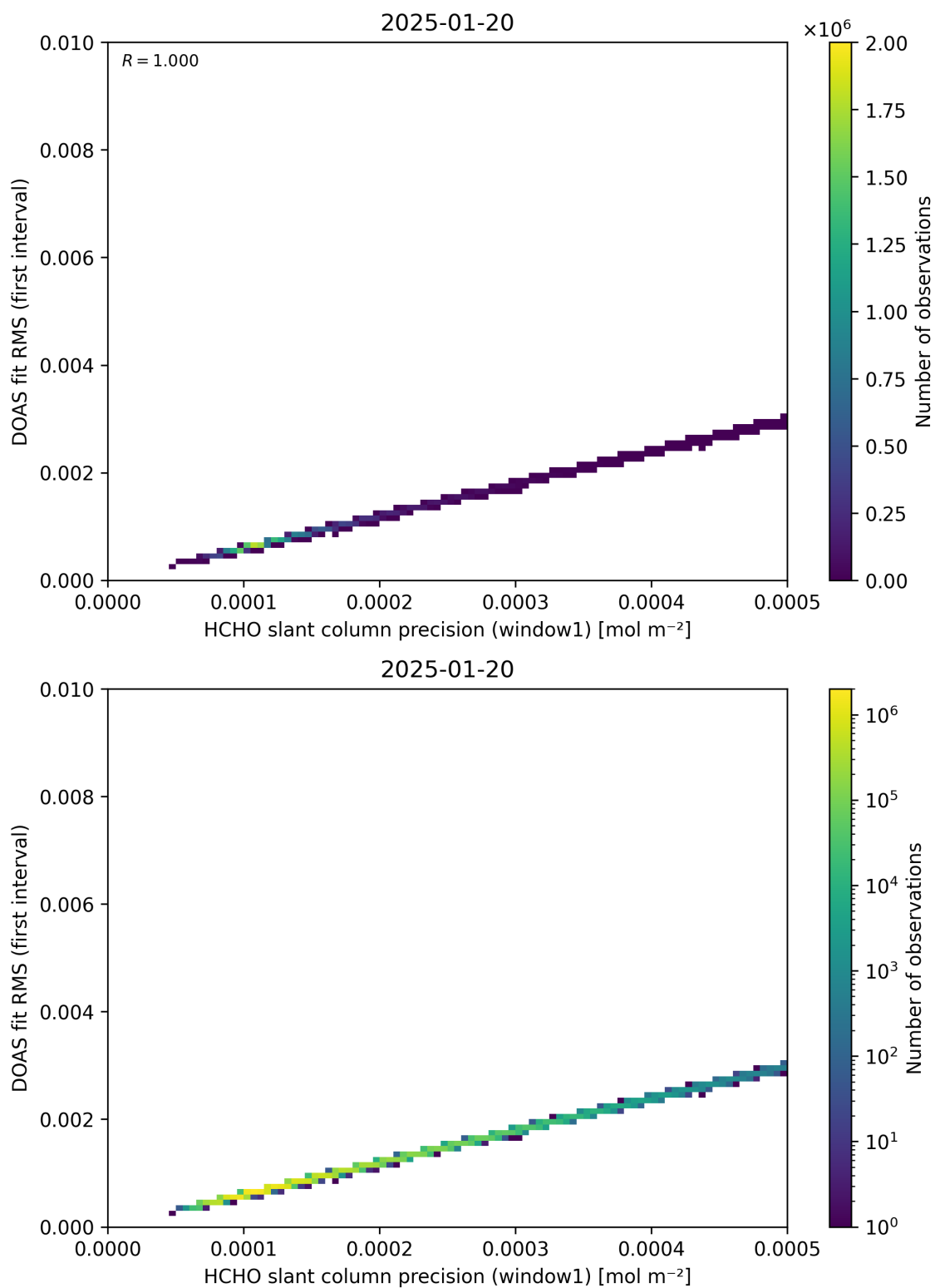
Figure 88: Scatter density plot of “HCHO slant column precision (window1)” against “DOAS fit RMS (first interval)” for 2025-01-19 to 2025-01-21.
