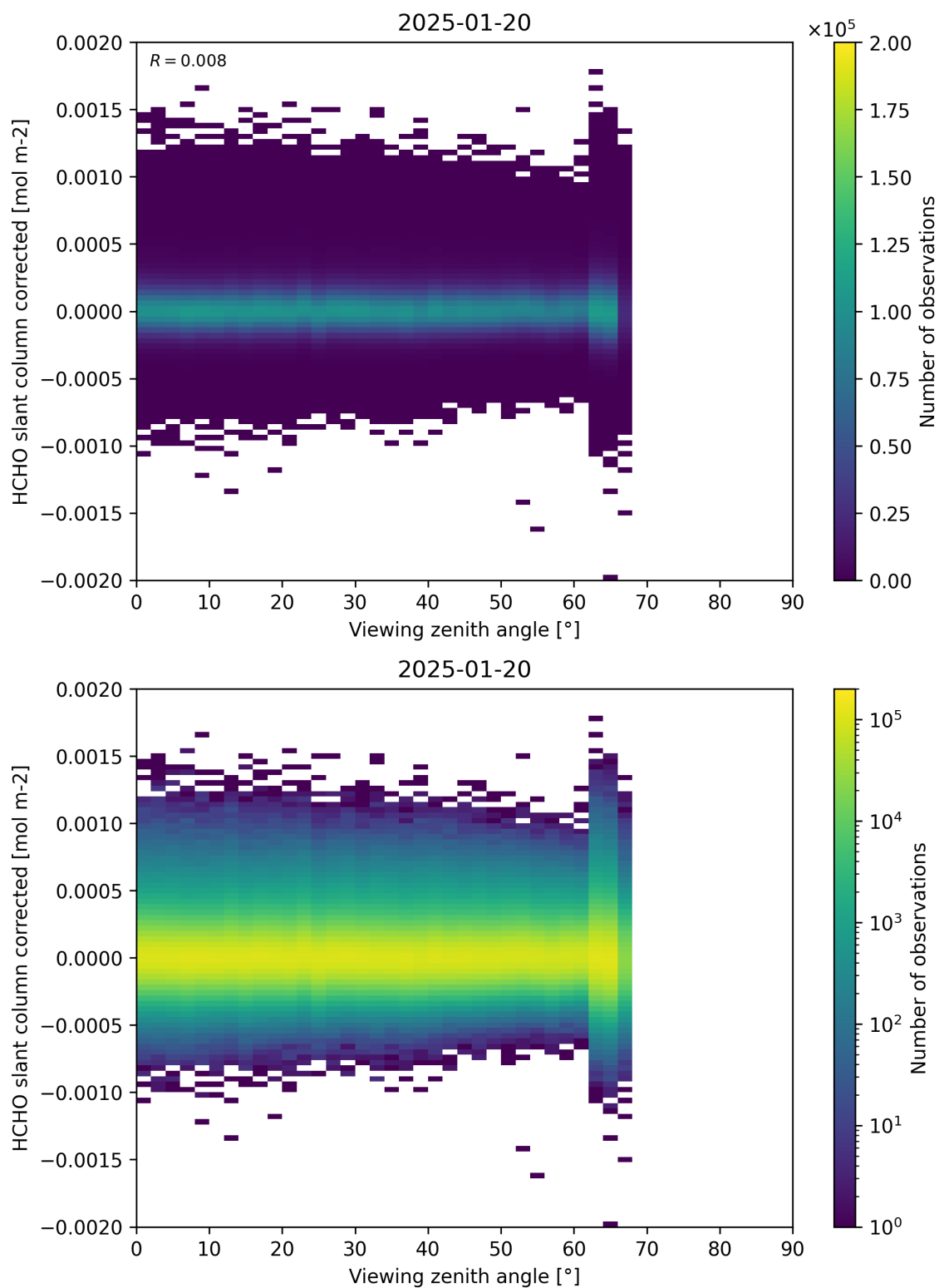
Figure 186: Scatter density plot of “Viewing zenith angle” against “HCHO slant column corrected” for 2025-01-19 to 2025-01-21.
