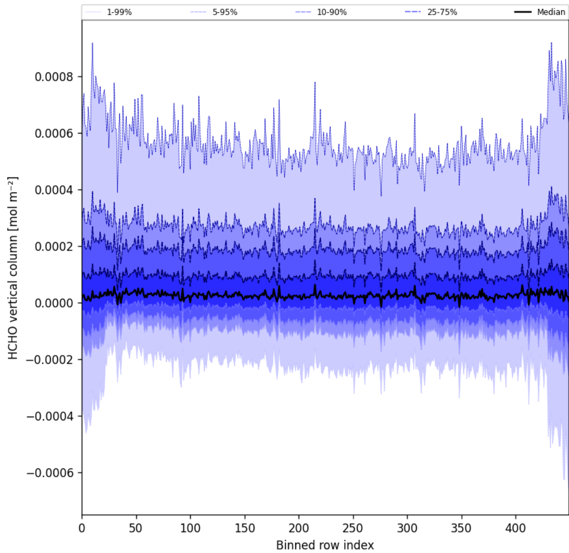
Figure 49: Along track statistics of “HCHO vertical column” for 2025-01-19 to 2025-01-21
