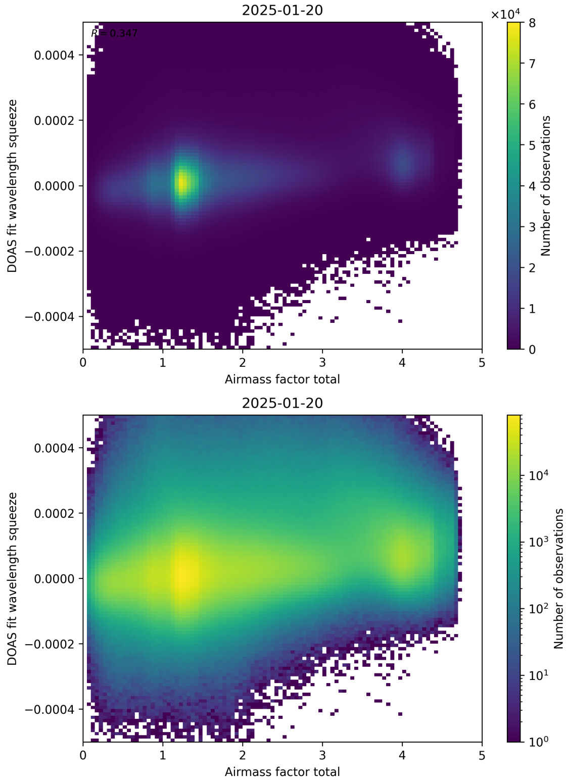
Figure 99: Scatter density plot of “Airmass factor total” against “DOAS fit wavelength squeeze” for 2025-01-19 to 2025-01-21.
