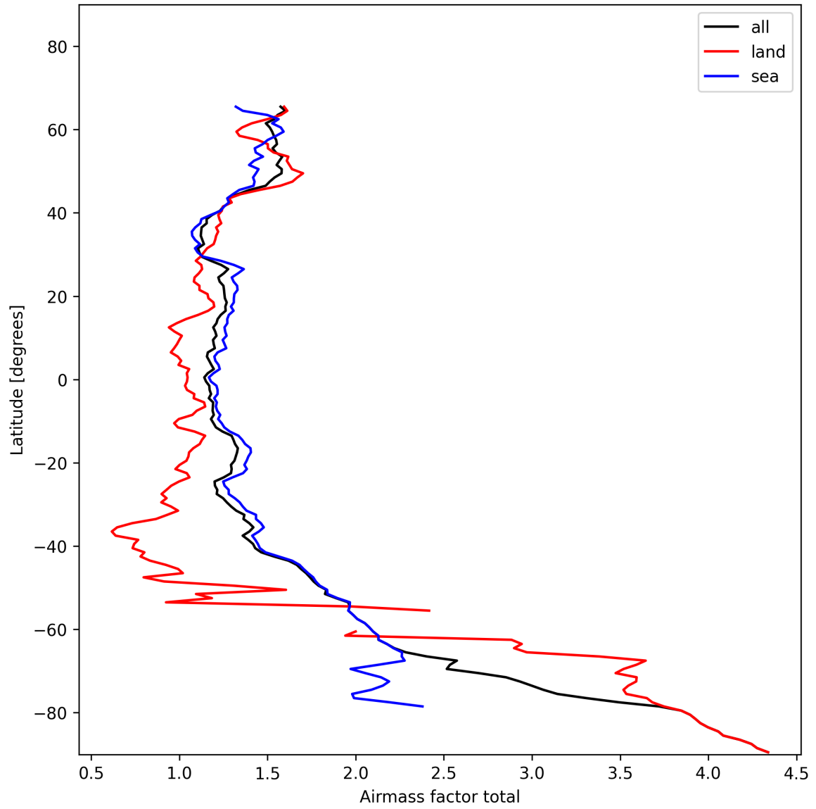
Figure 26: Zonal average of “Airmass factor total” for 2025-01-19 to 2025-01-21.
