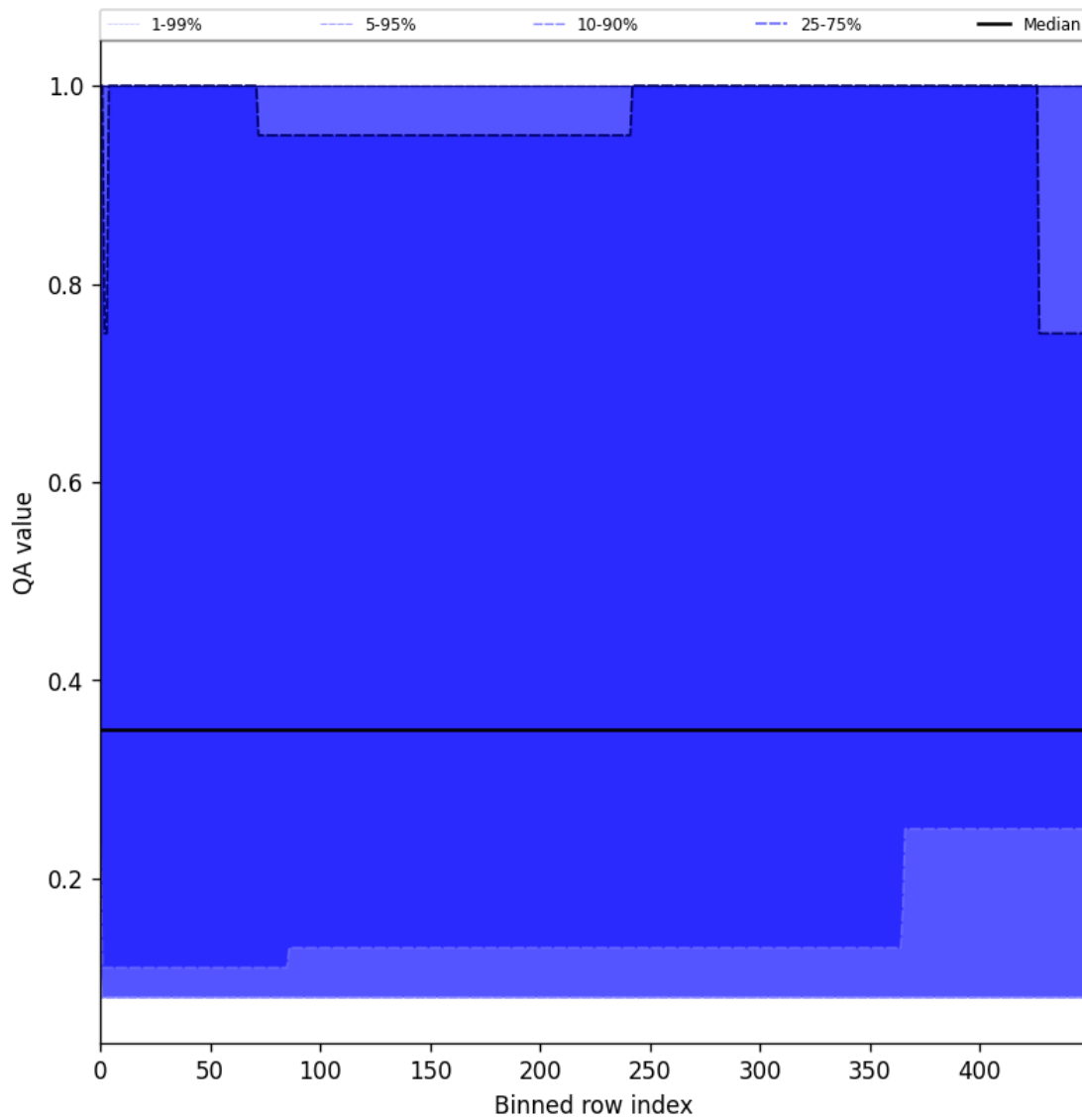
Figure 48: Along track statistics of “QA value” for 2025-01-19 to 2025-01-21
