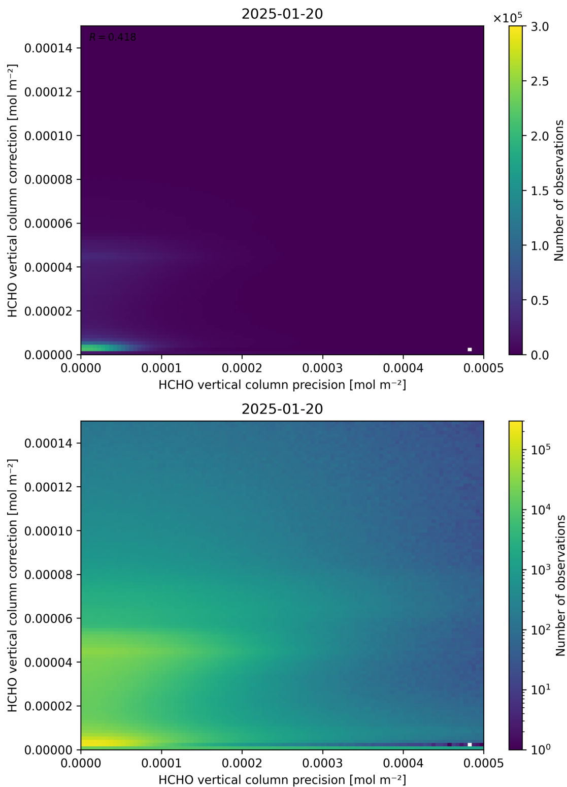
Figure 146: Scatter density plot of “HCHO vertical column precision” against “HCHO vertical column correction” for 2025-01-19 to 2025-01-21.
