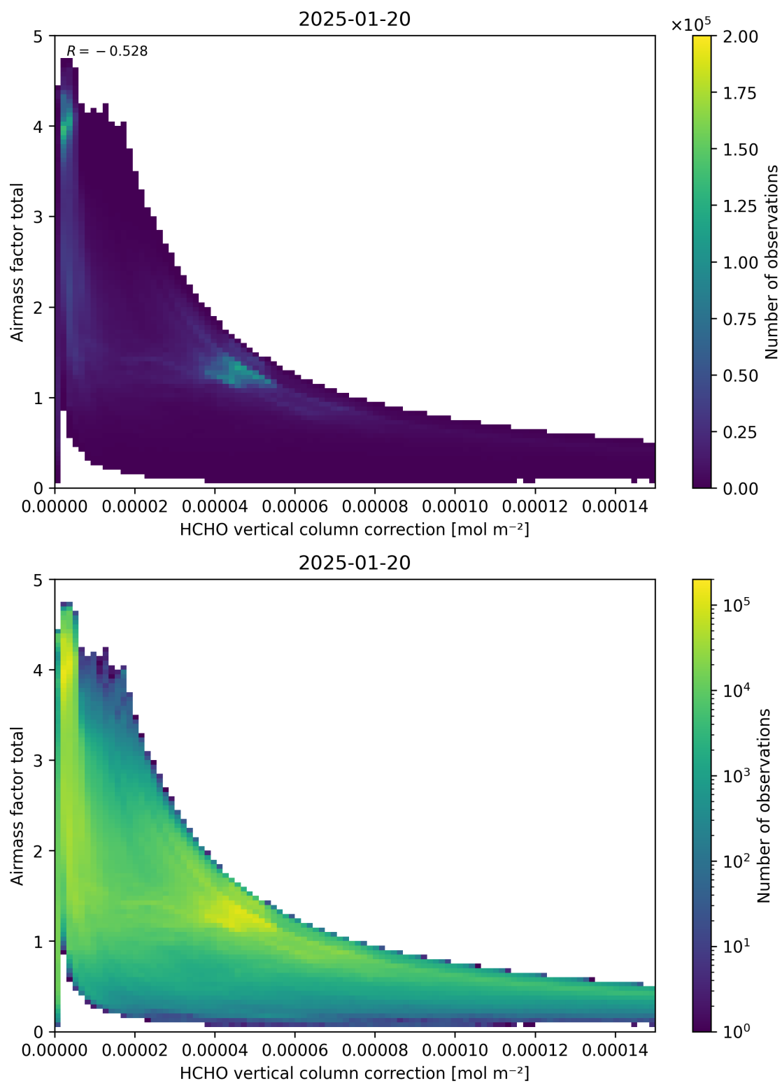
Figure 120: Scatter density plot of “HCHO vertical column correction” against “Airmass factor total” for 2025-01-19 to 2025-01-21.
