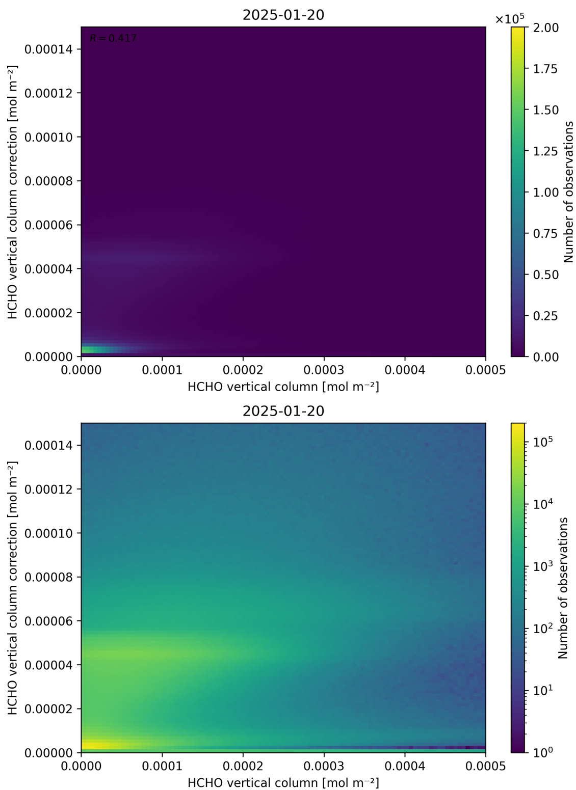
Figure 133: Scatter density plot of “HCHO vertical column” against “HCHO vertical column correction” for 2025-01-19 to 2025-01-21.
