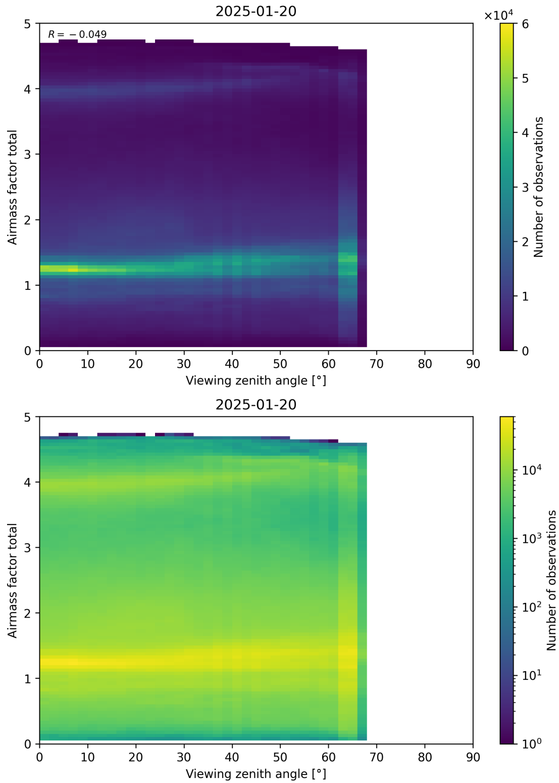
Figure 190: Scatter density plot of “Viewing zenith angle” against “Airmass factor total” for 2025-01-19 to 2025-01-21.
