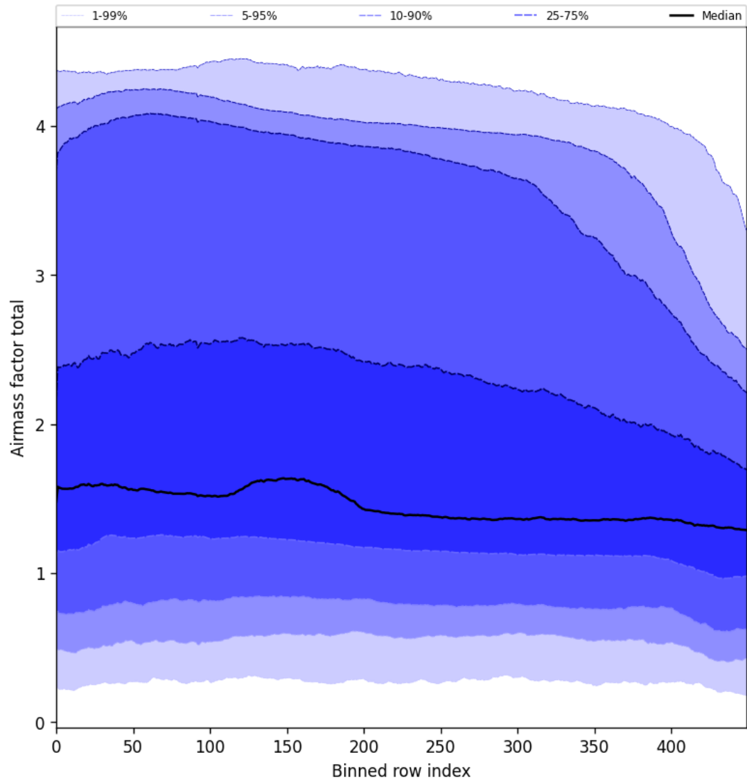
Figure 54: Along track statistics of “Airmass factor total” for 2025-01-19 to 2025-01-21
