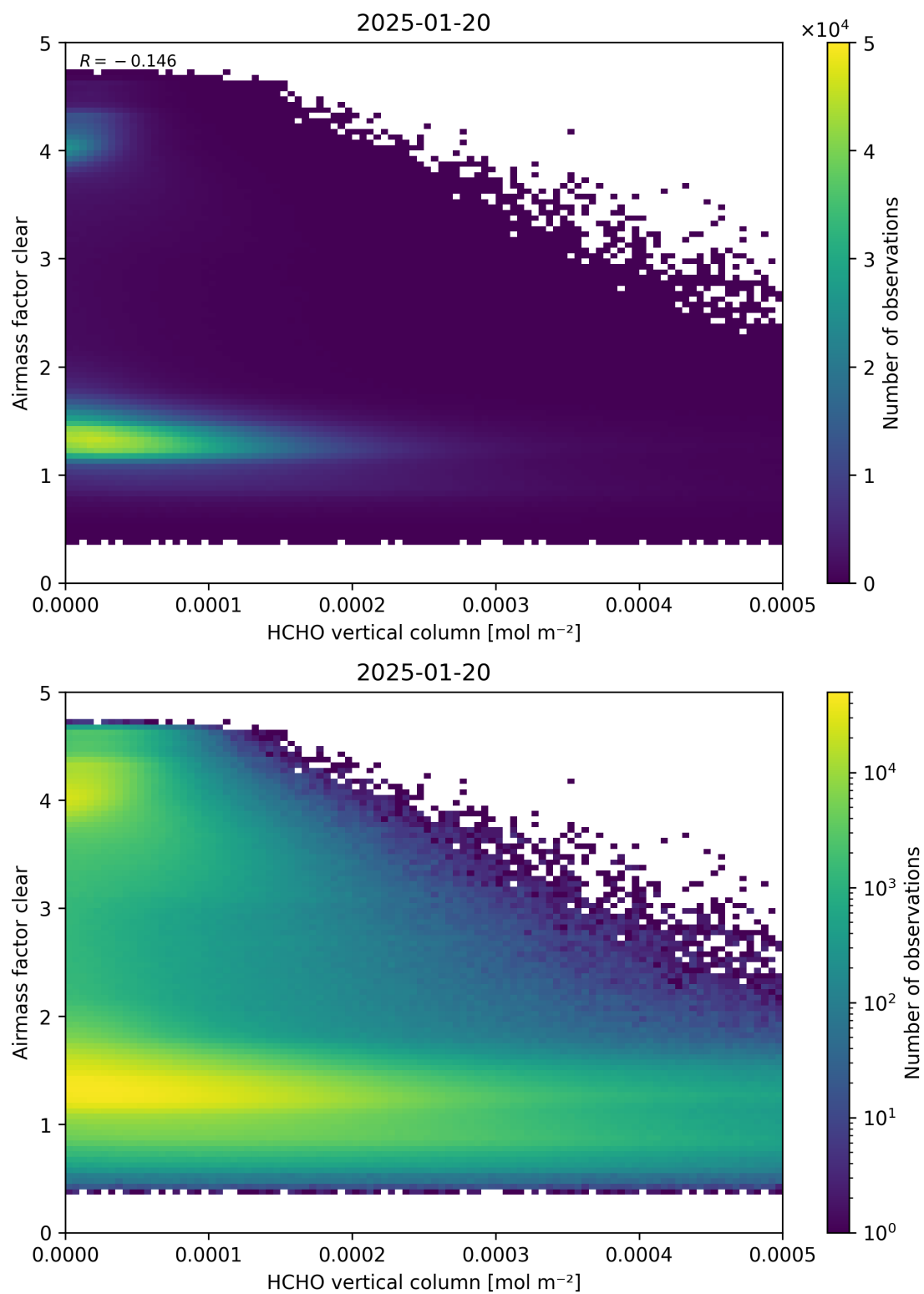
Figure 126: Scatter density plot of “HCHO vertical column” against “Airmass factor clear” for 2025-01-19 to 2025-01-21.
