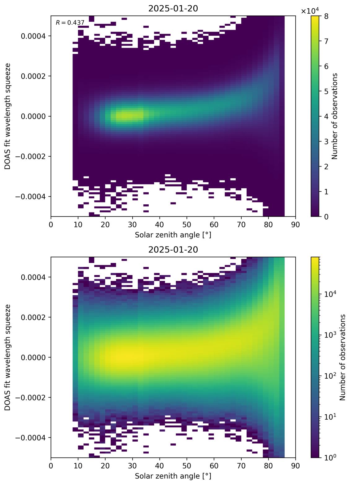
Figure 169: Scatter density plot of “Solar zenith angle” against “DOAS fit wavelength squeeze” for 2025-01-19 to 2025-01-21.
