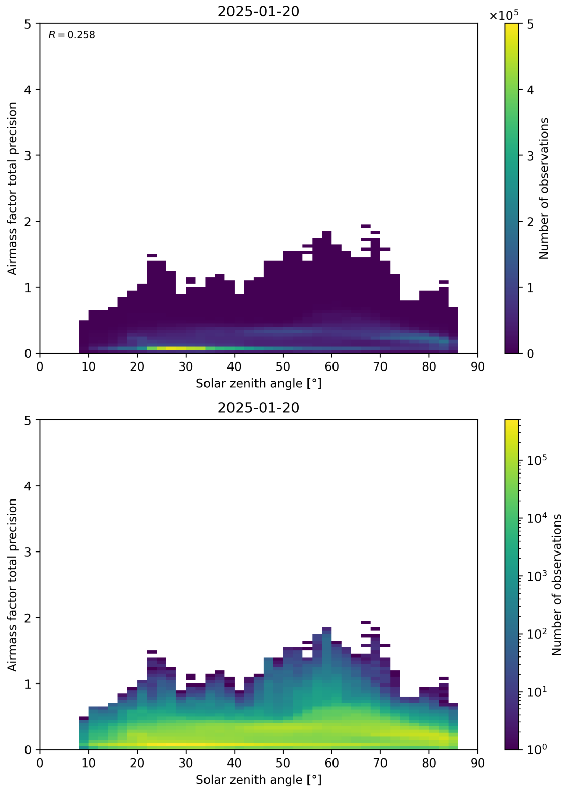
Figure 176: Scatter density plot of “Solar zenith angle” against “Airmass factor total precision” for 2025-01-19 to 2025-01-21.
