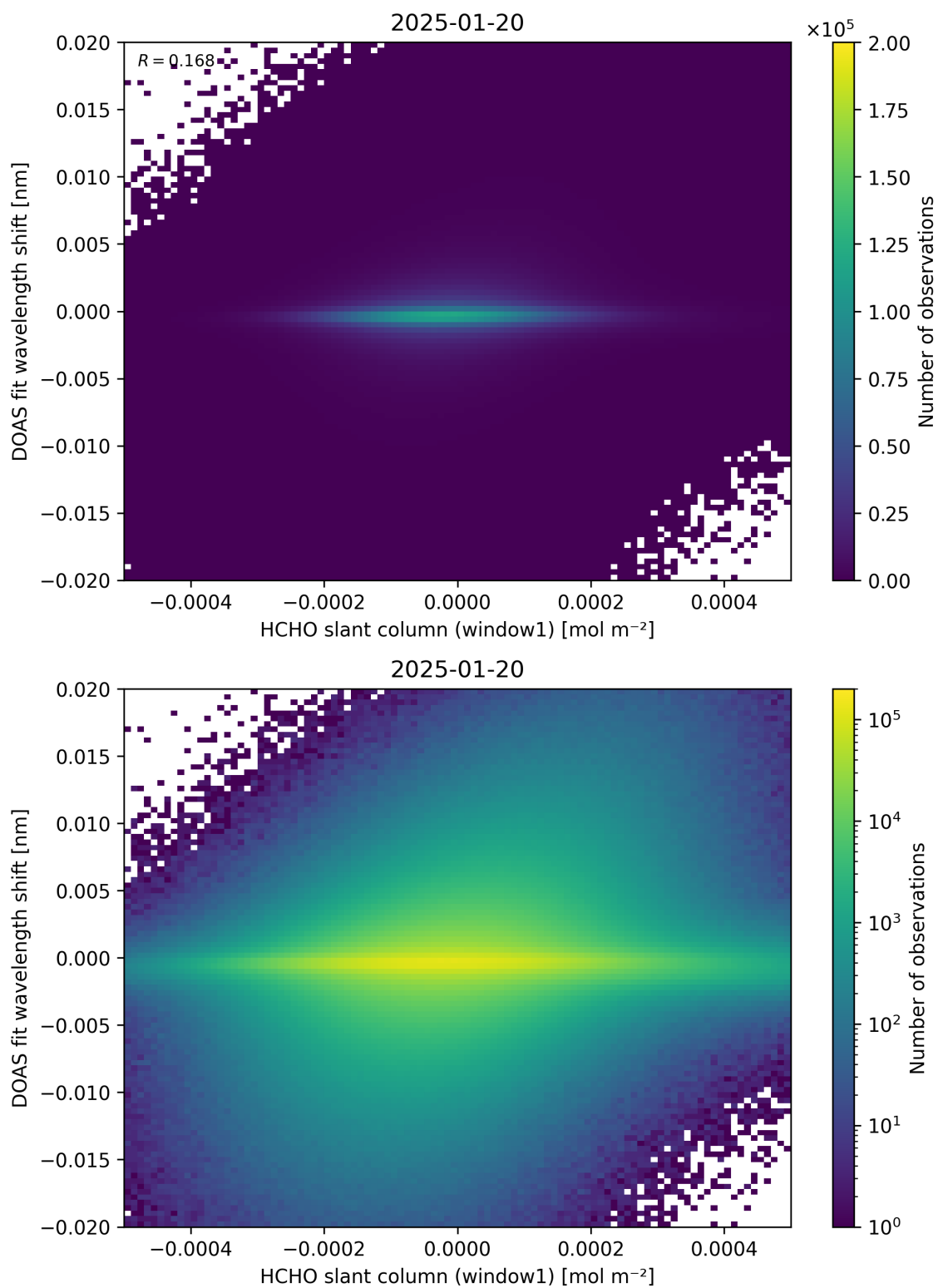
Figure 79: Scatter density plot of “HCHO slant column (window1)” against “DOAS fit wavelength shift” for 2025-01-19 to 2025-01-21.
