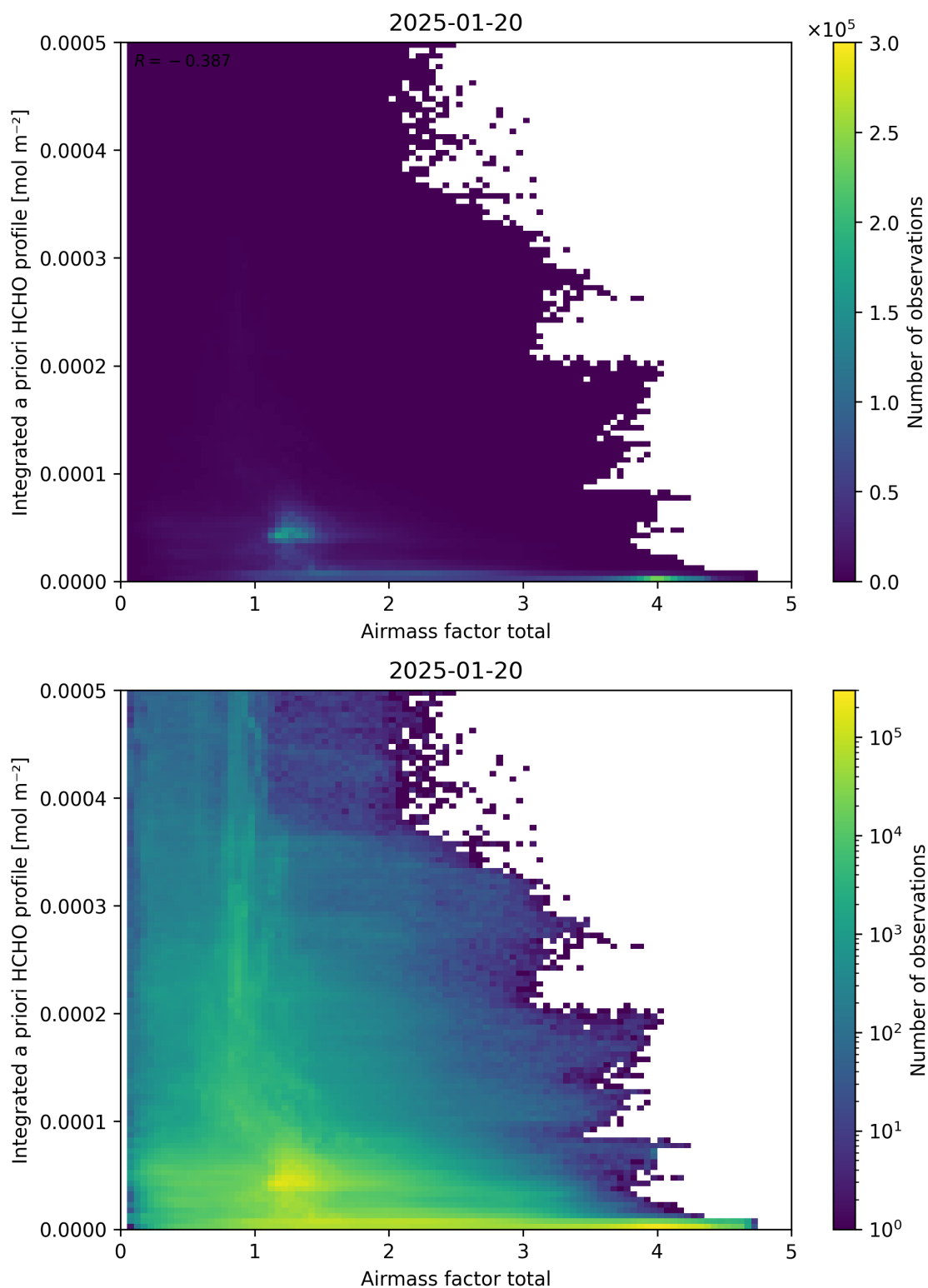
Figure 104: Scatter density plot of “Airmass factor total” against “Integrated a priori HCHO profile” for 2025-01-19 to 2025-01-21.
