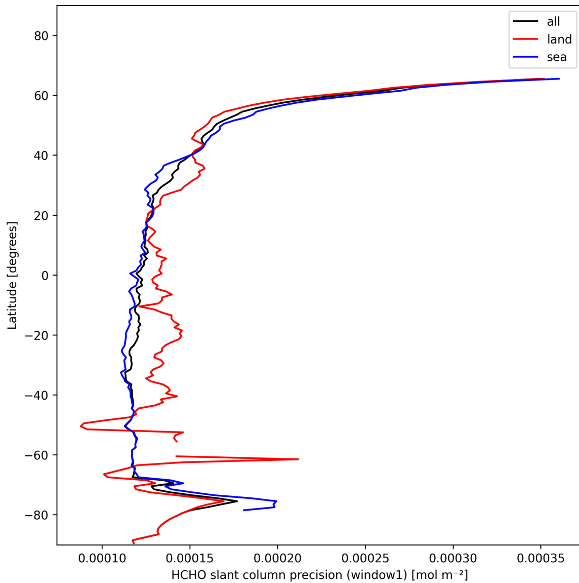
Figure 25: Zonal average of “HCHO slant column precision (window1)” for 2025-01-19 to 2025-01-21.
