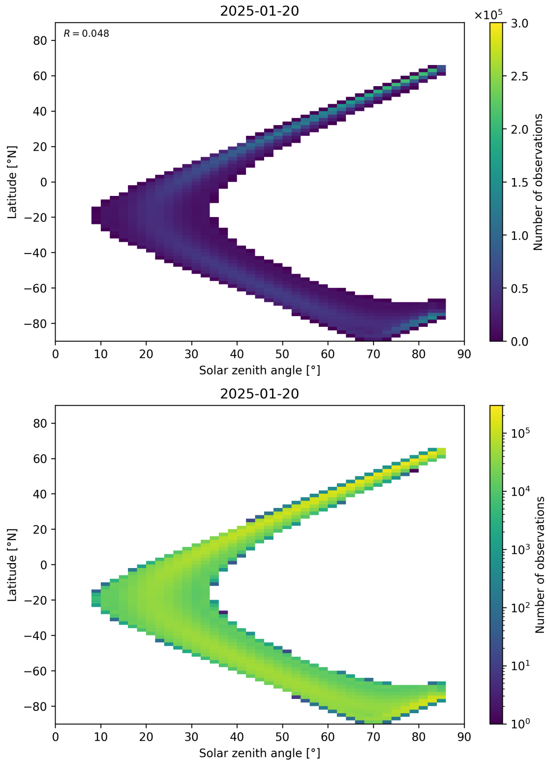
Figure 181: Scatter density plot of “Solar zenith angle” against “Latitude” for 2025-01-19 to 2025-01-21.
