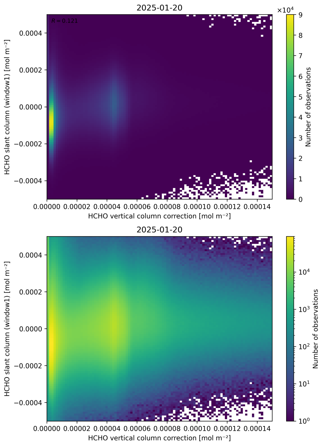
Figure 118: Scatter density plot of “HCHO vertical column correction” against “HCHO slant column (window1)” for 2025-01-19 to 2025-01-21.
