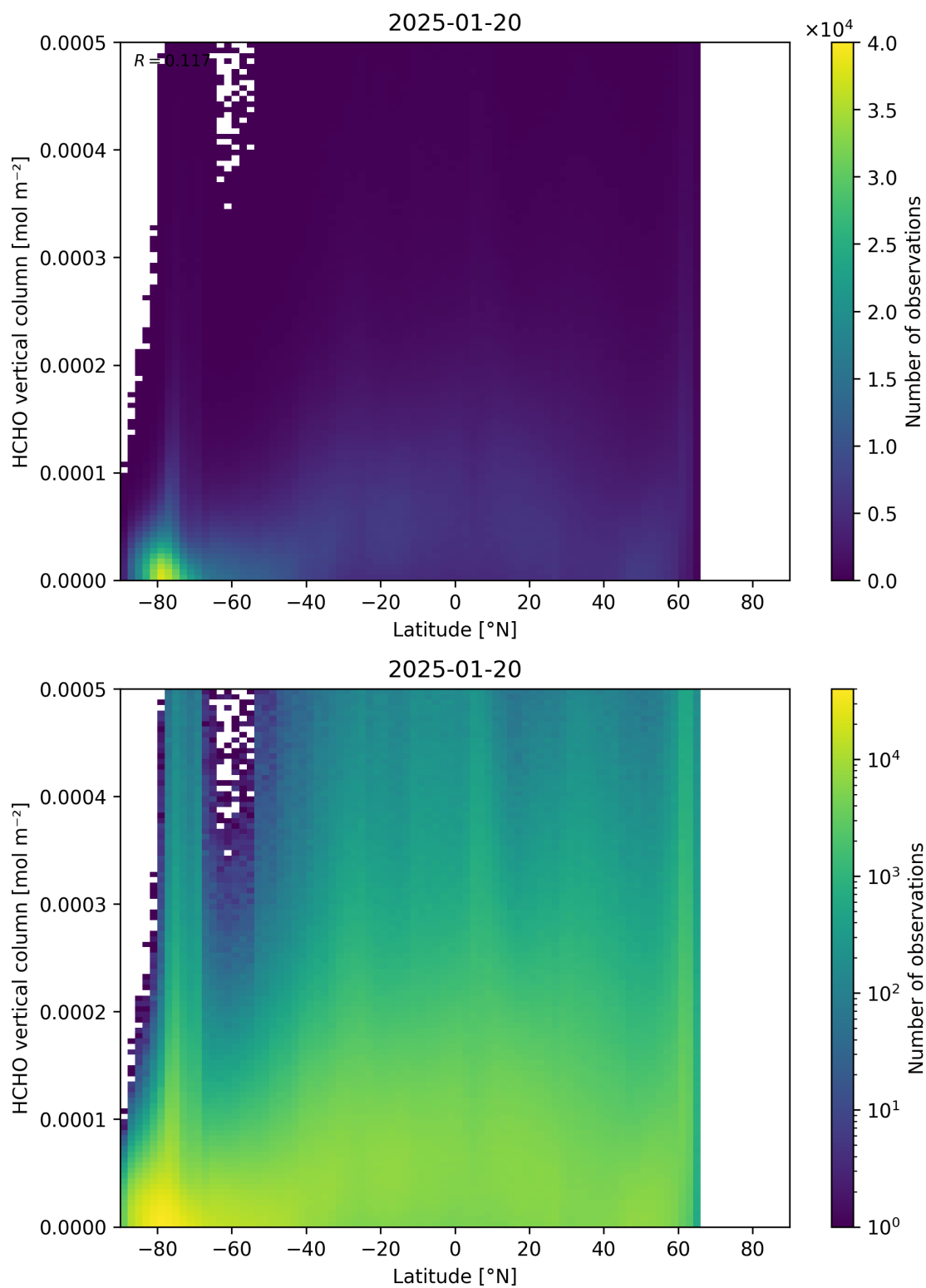
Figure 163: Scatter density plot of “Latitude” against “HCHO vertical column” for 2025-01-19 to 2025-01-21.
