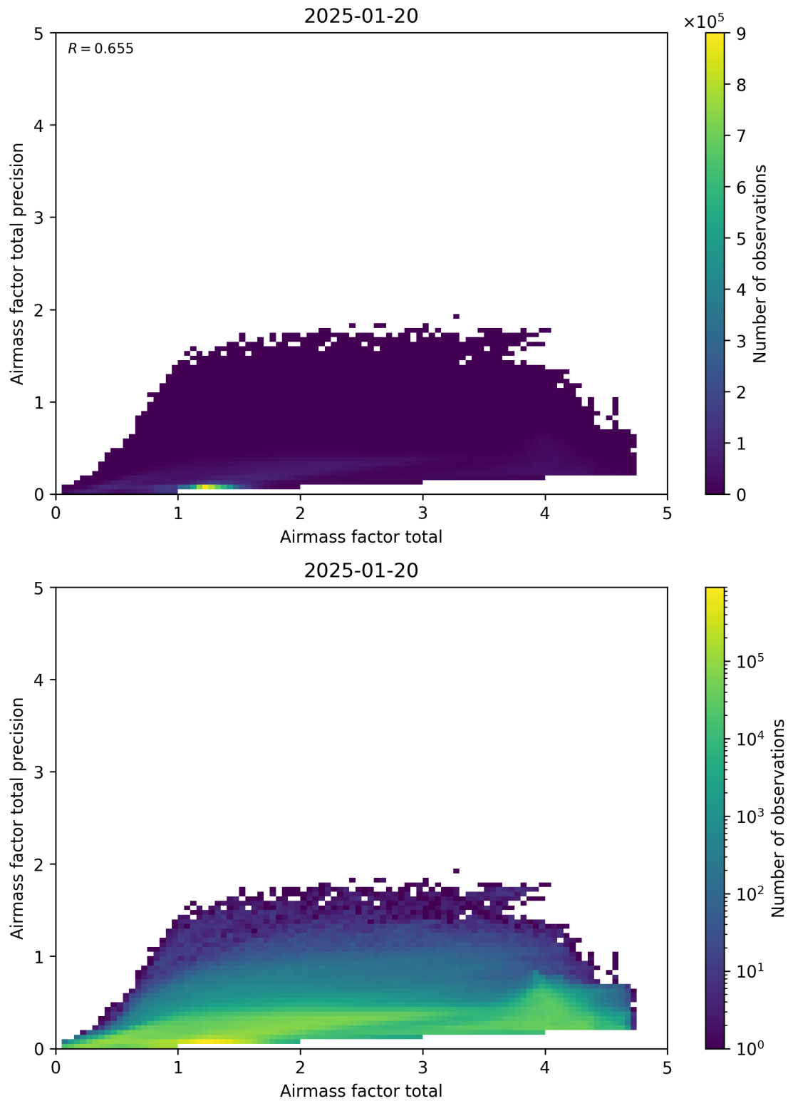
Figure 103: Scatter density plot of “Airmass factor total” against “Airmass factor total precision” for 2025-01-19 to 2025-01-21.
