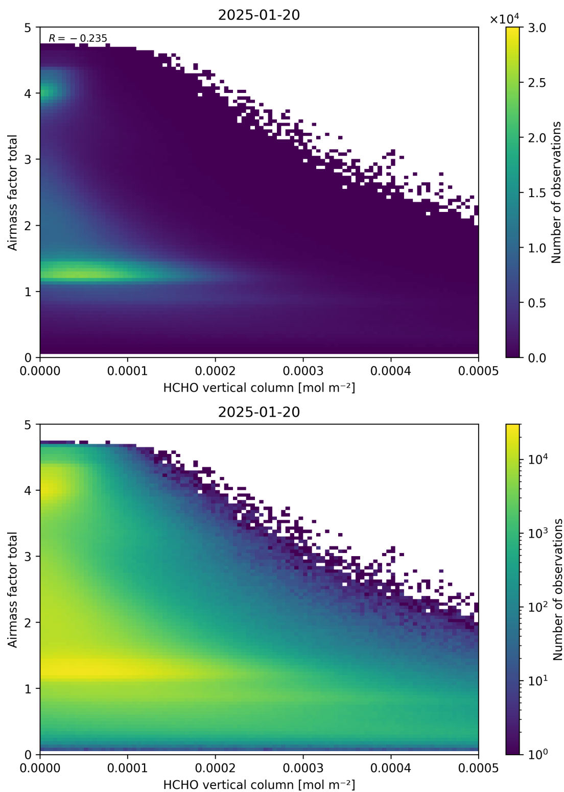
Figure 131: Scatter density plot of “HCHO vertical column” against “Airmass factor total” for 2025-01-19 to 2025-01-21.
