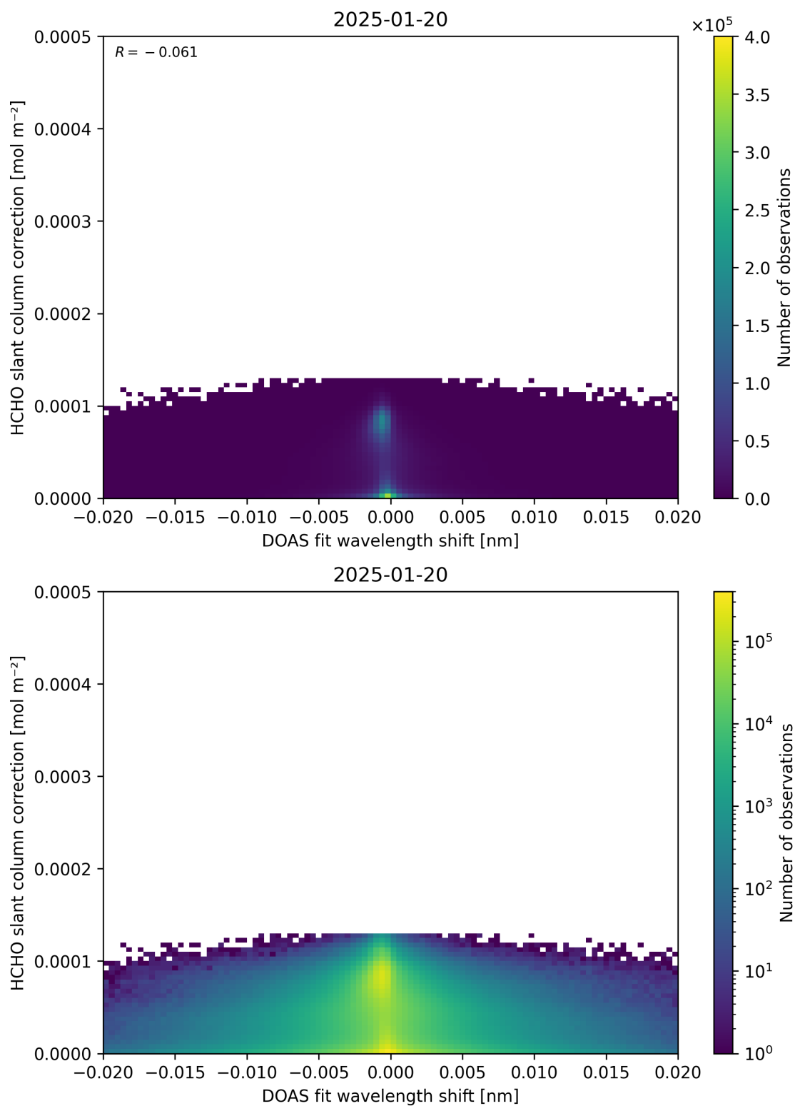
Figure 67: Scatter density plot of “DOAS fit wavelength shift” against “HCHO slant column correction” for 2025-01-19 to 2025-01-21.
