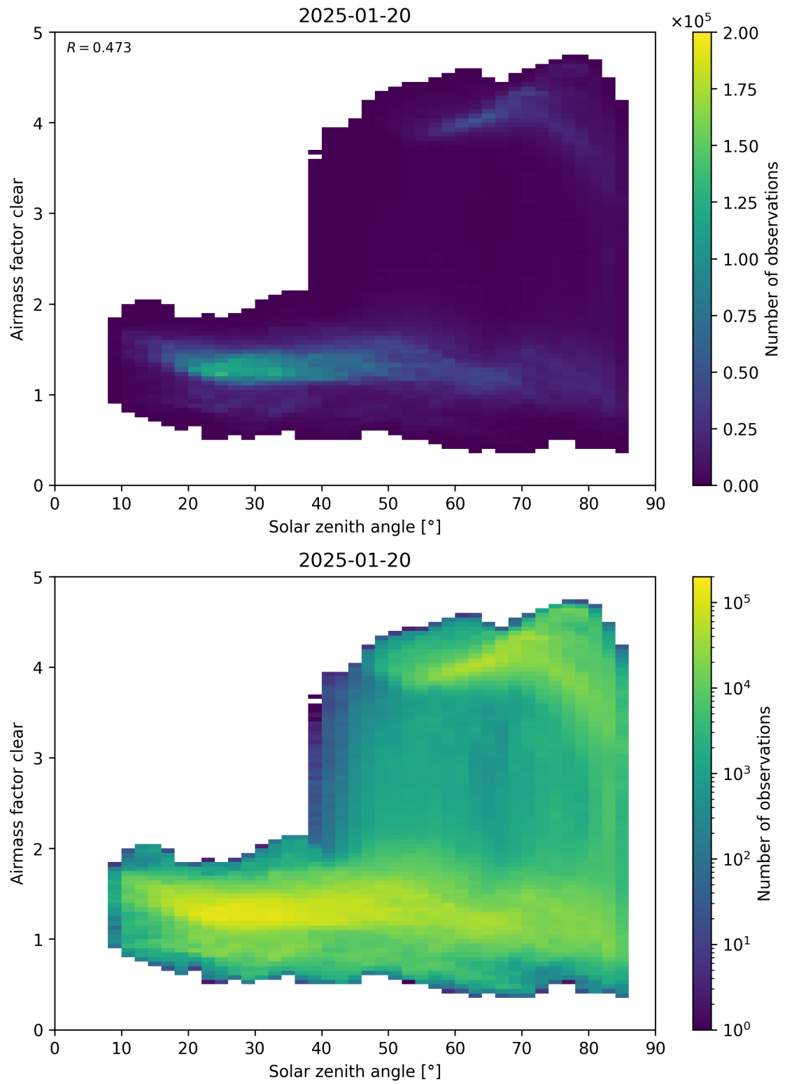
Figure 170: Scatter density plot of “Solar zenith angle” against “Airmass factor clear” for 2025-01-19 to 2025-01-21.
