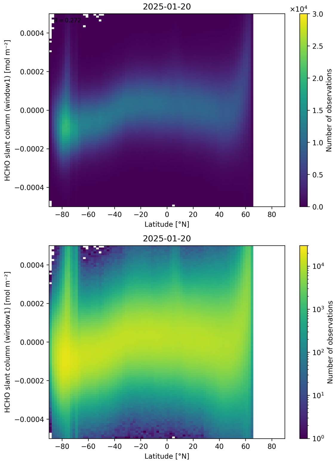
Figure 159: Scatter density plot of “Latitude” against “HCHO slant column (window1)” for 2025-01-19 to 2025-01-21.
