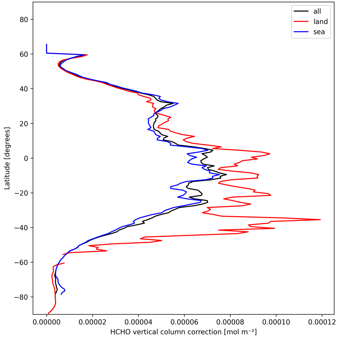
Figure 23: Zonal average of “HCHO vertical column correction” for 2025-01-19 to 2025-01-21.
