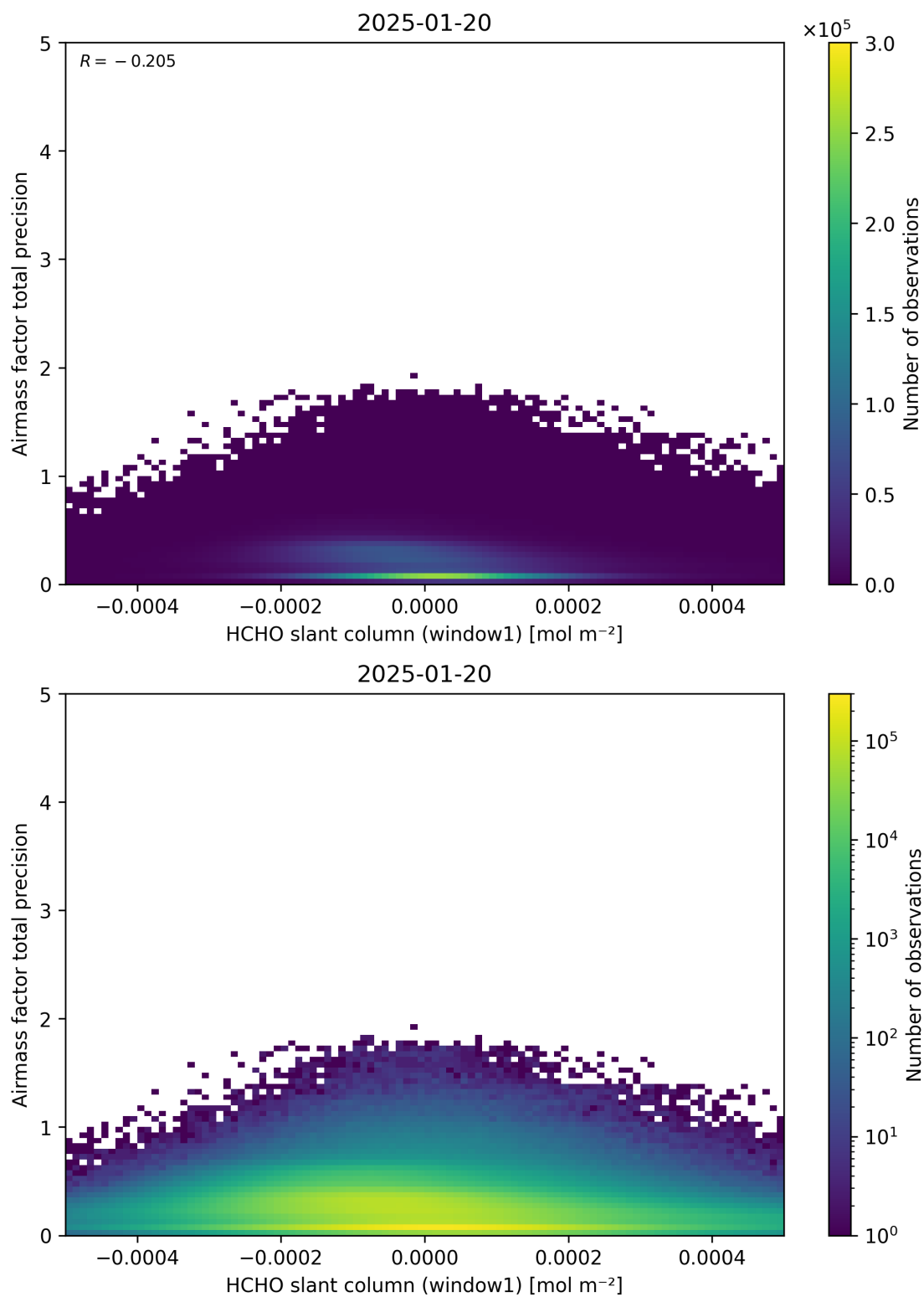
Figure 86: Scatter density plot of “HCHO slant column (window1)” against “Airmass factor total precision” for 2025-01-19 to 2025-01-21.
