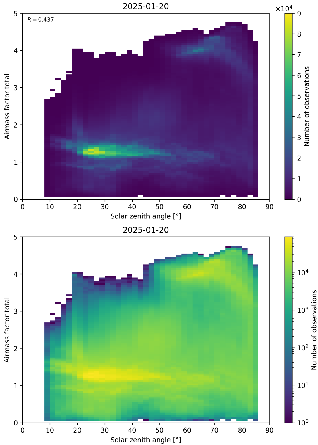
Figure 175: Scatter density plot of “Solar zenith angle” against “Airmass factor total” for 2025-01-19 to 2025-01-21.
