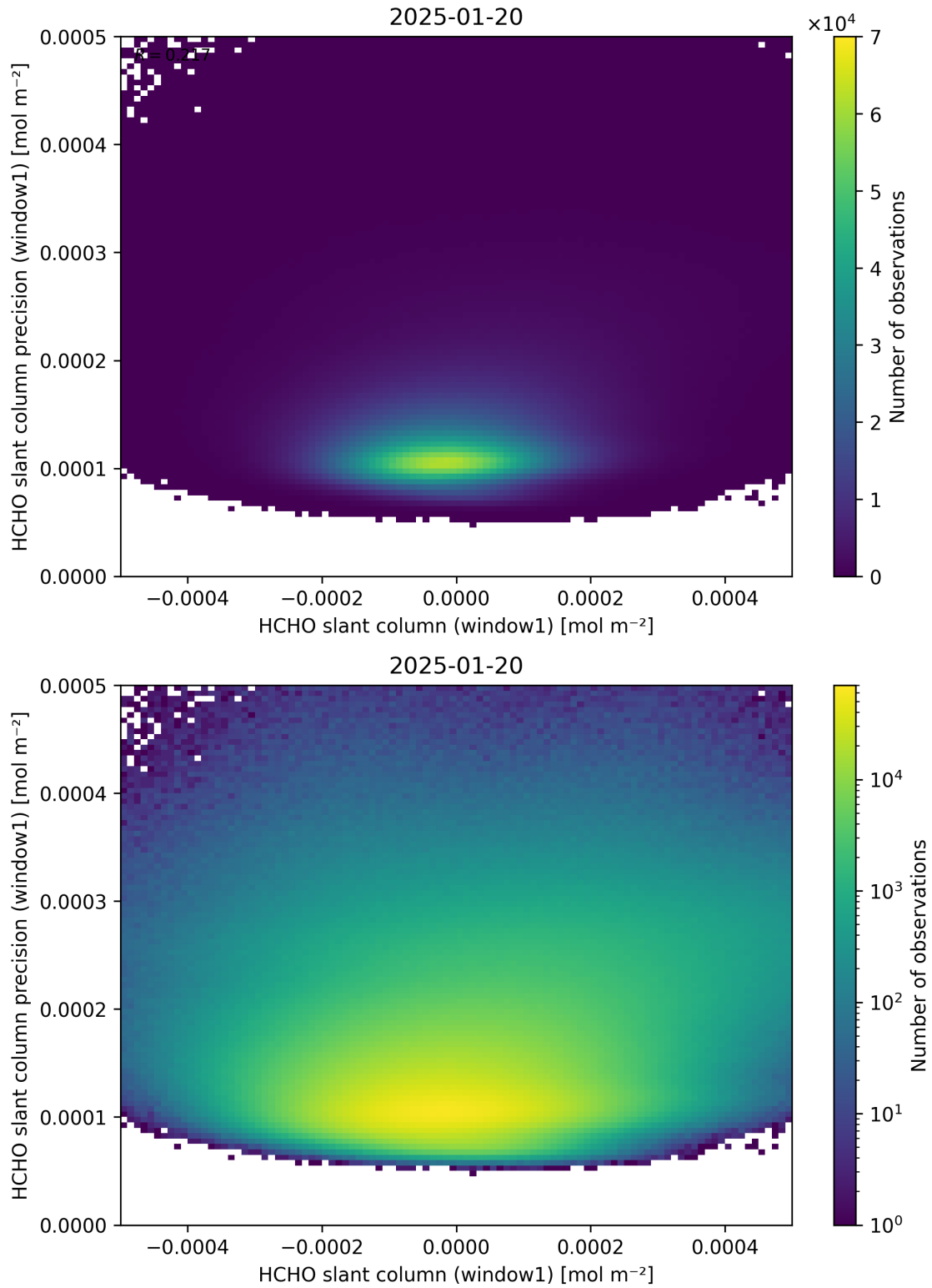
Figure 84: Scatter density plot of “HCHO slant column (window1)” against “HCHO slant column precision (window1)” for 2025-01-19 to 2025-01-21.
