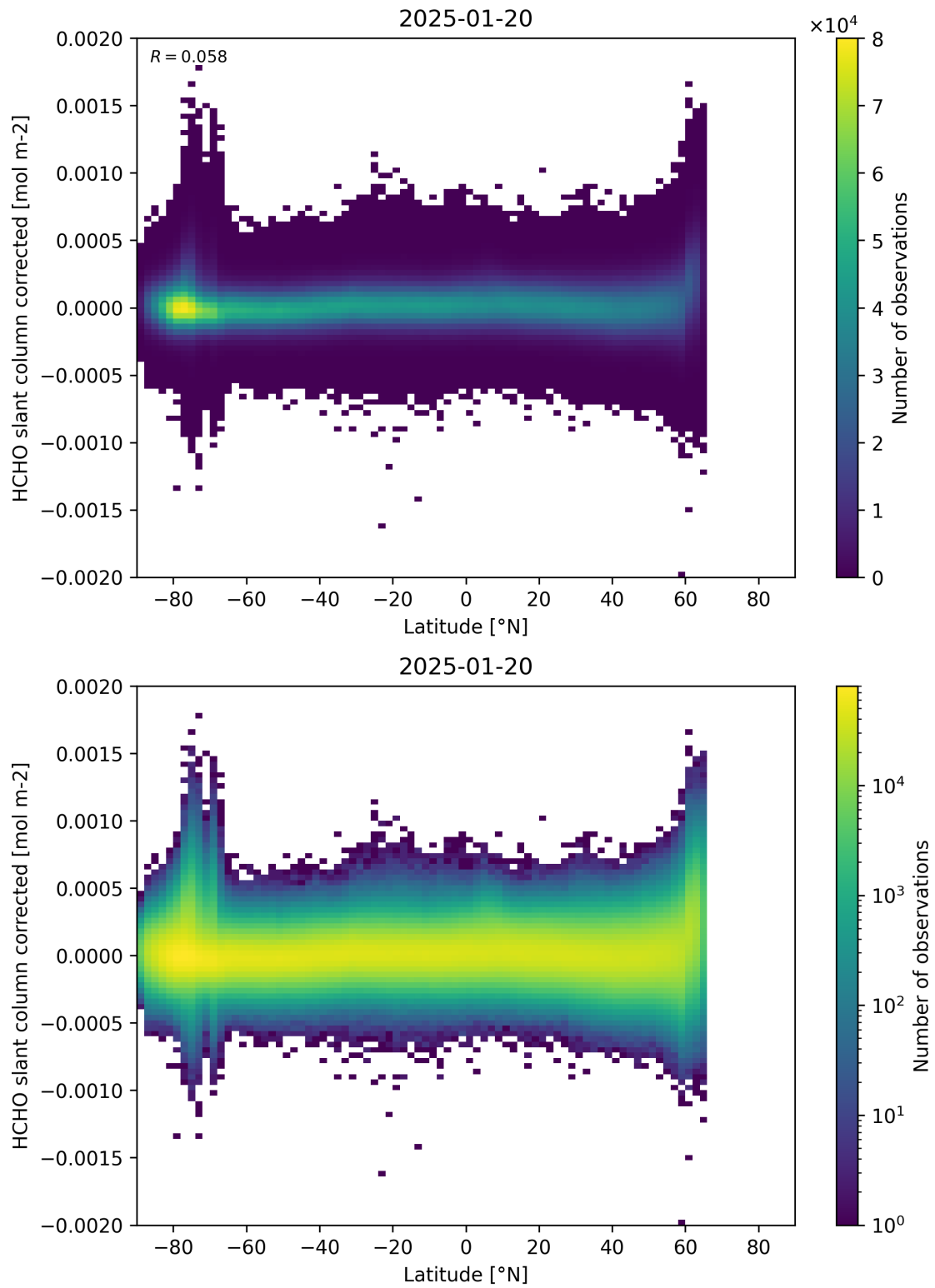
Figure 157: Scatter density plot of “Latitude” against “HCHO slant column corrected” for 2025-01-19 to 2025-01-21.
