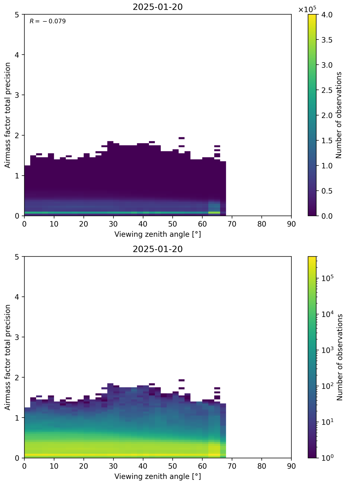
Figure 191: Scatter density plot of “Viewing zenith angle” against “Airmass factor total precision” for 2025-01-19 to 2025-01-21.
