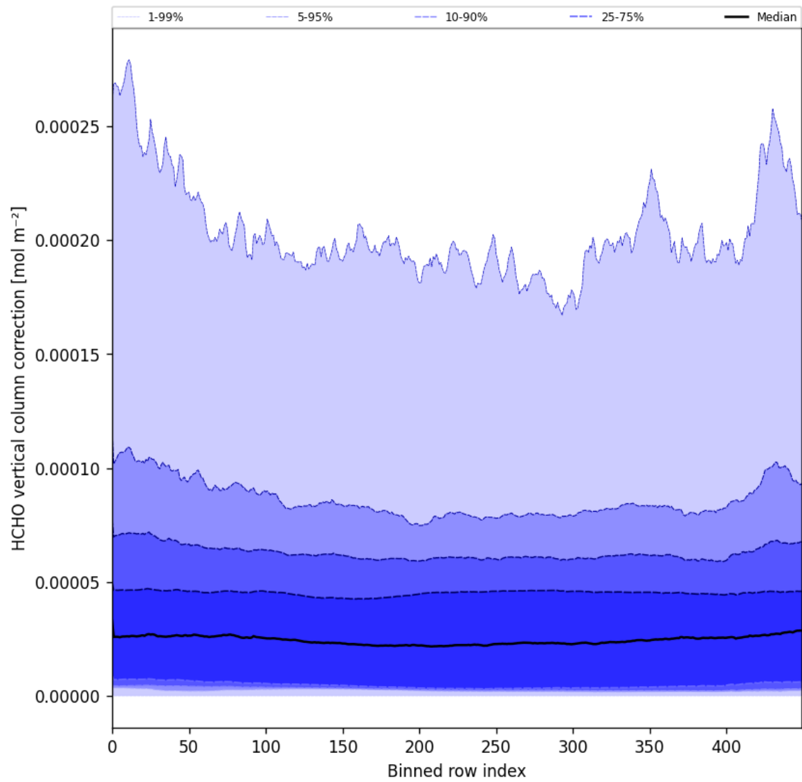
Figure 51: Along track statistics of “HCHO vertical column correction” for 2025-01-19 to 2025-01-21
