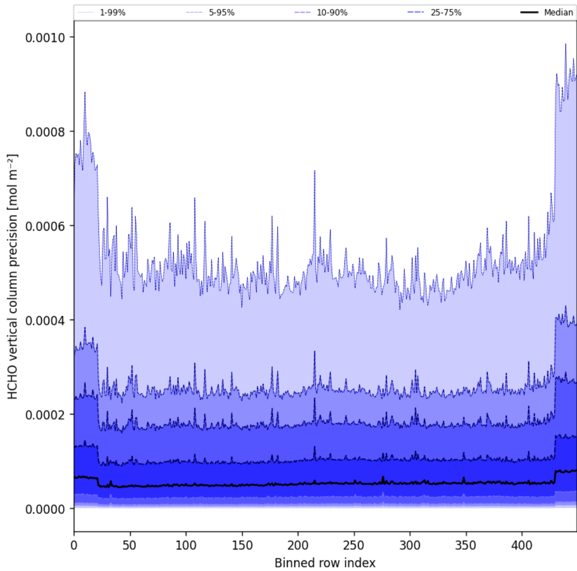
Figure 50: Along track statistics of “HCHO vertical column precision” for 2025-01-19 to 2025-01-21
