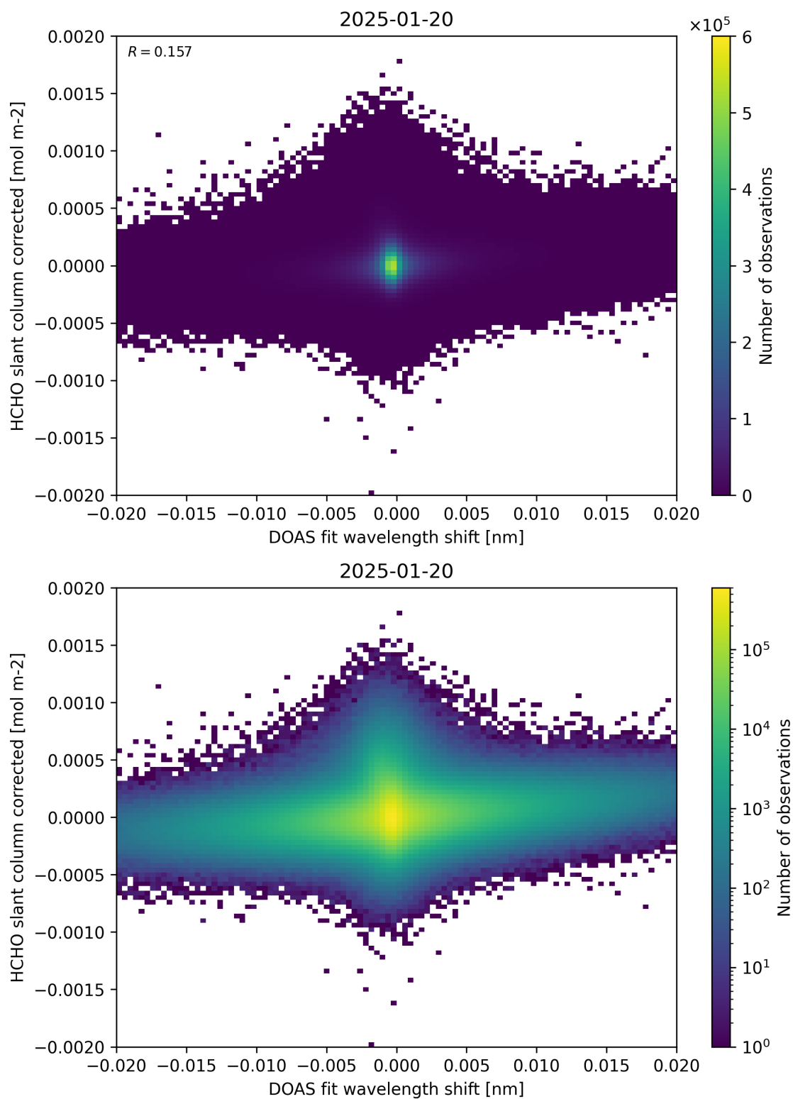
Figure 66: Scatter density plot of “DOAS fit wavelength shift” against “HCHO slant column corrected” for 2025-01-19 to 2025-01-21.
