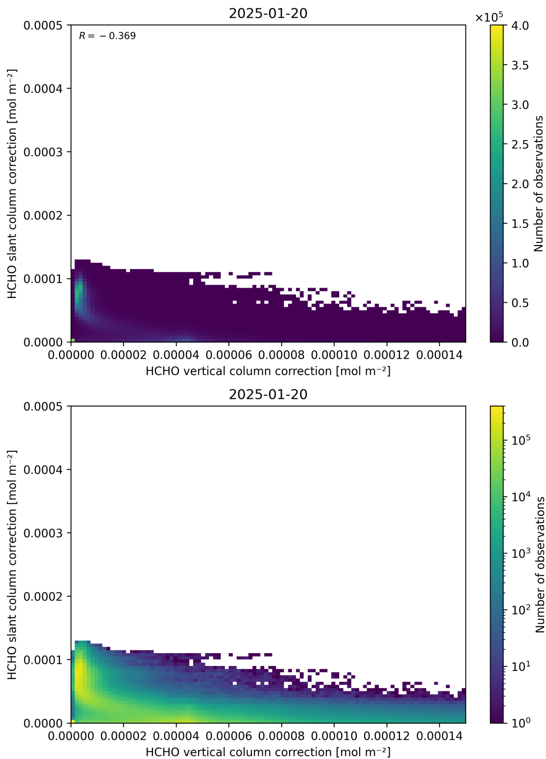
Figure 117: Scatter density plot of “HCHO vertical column correction” against “HCHO slant column correction” for 2025-01-19 to 2025-01-21.
