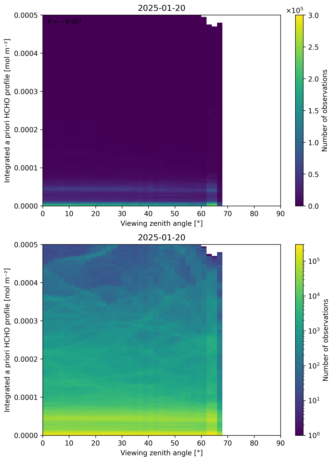
Figure 195: Scatter density plot of “Viewing zenith angle” against “Integrated a priori HCHO profile” for 2025-01-19 to 2025-01-21.
