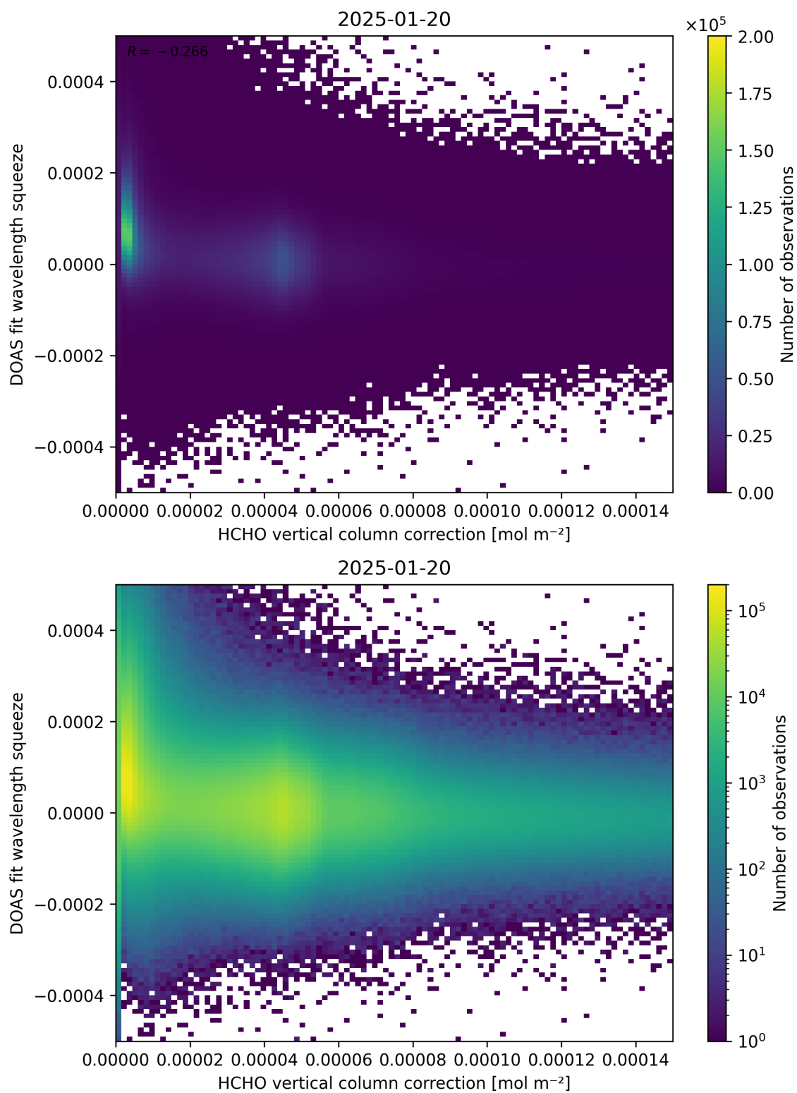
Figure 114: Scatter density plot of “HCHO vertical column correction” against “DOAS fit wavelength squeeze” for 2025-01-19 to 2025-01-21.
