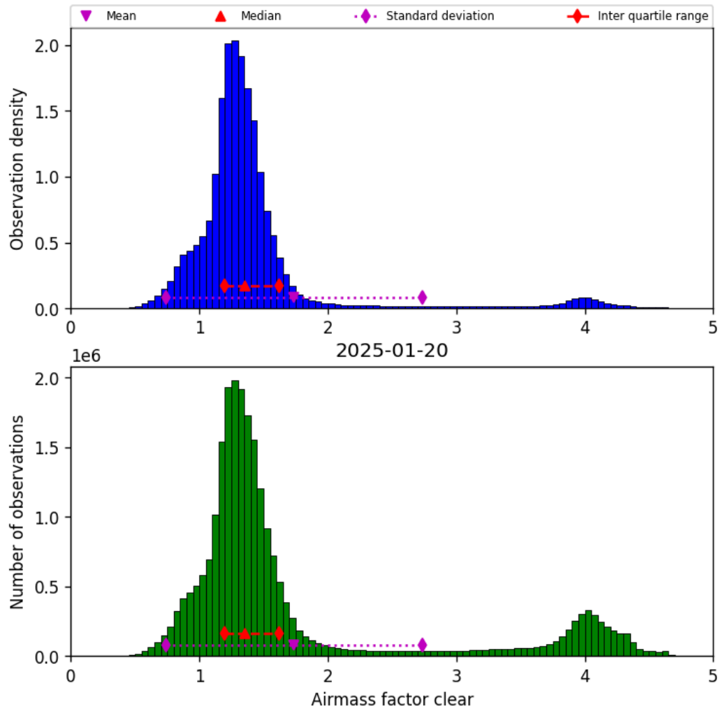
Figure 42: Histogram of “Airmass factor clear” for 2025-01-19 to 2025-01-21
