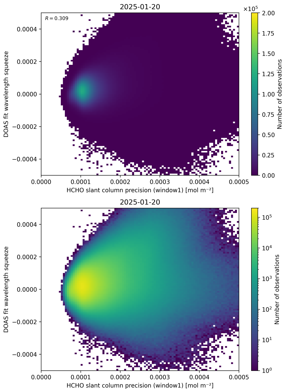
Figure 90: Scatter density plot of “HCHO slant column precision (window1)” against “DOAS fit wavelength squeeze” for 2025-01-19 to 2025-01-21.
