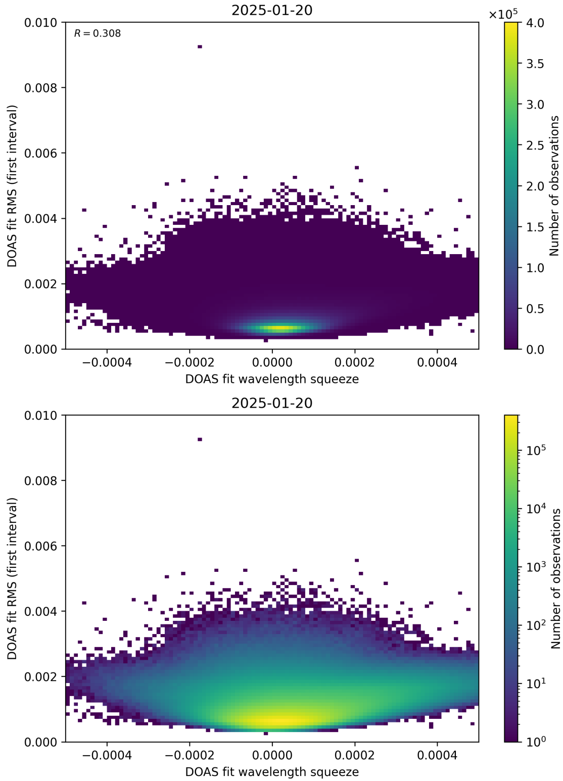
Figure 68: Scatter density plot of “DOAS fit wavelength squeeze” against “DOAS fit RMS (first interval)” for 2025-01-19 to 2025-01-21.
