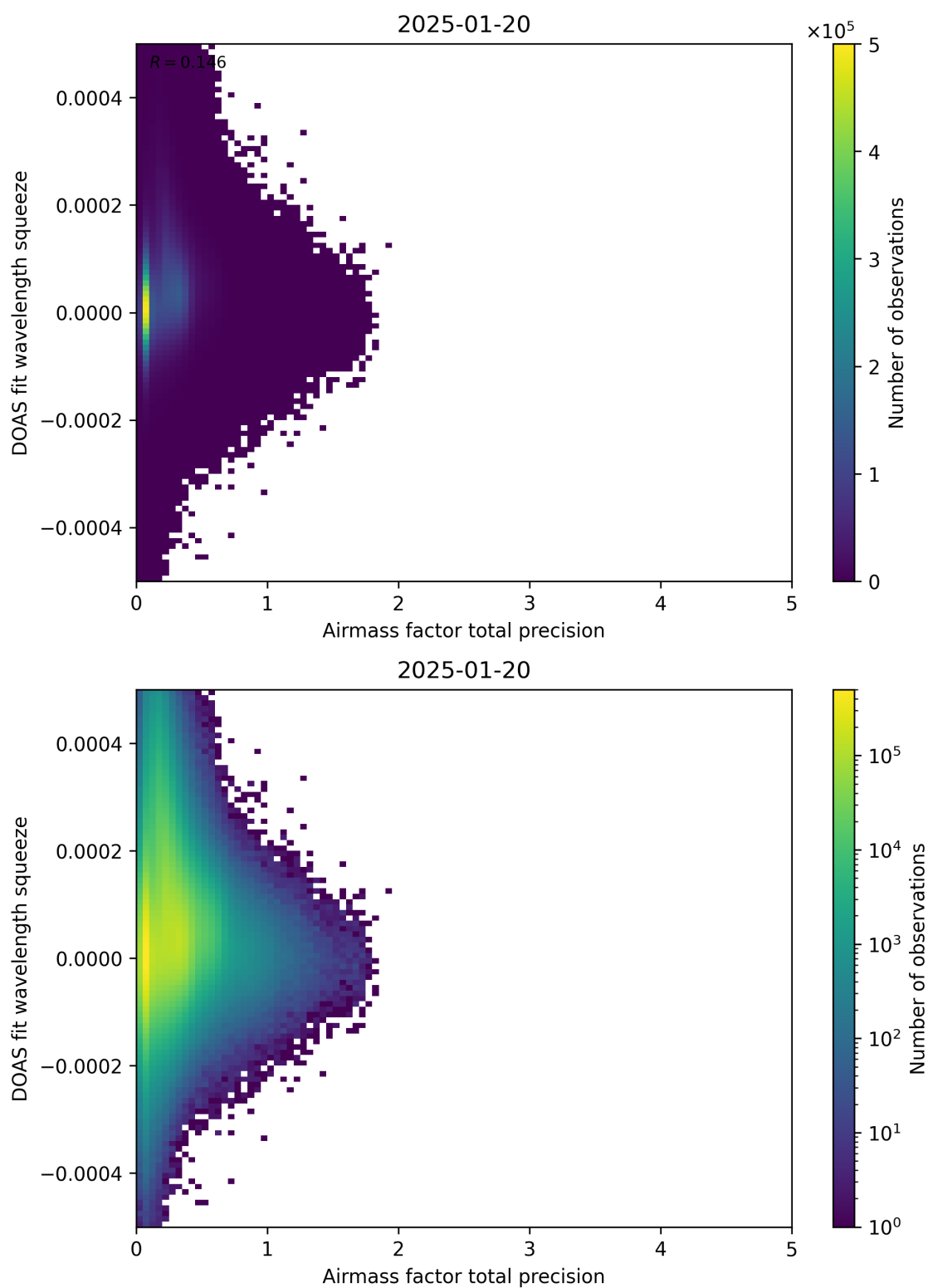
Figure 107: Scatter density plot of “Airmass factor total precision” against “DOAS fit wavelength squeeze” for 2025-01-19 to 2025-01-21.
