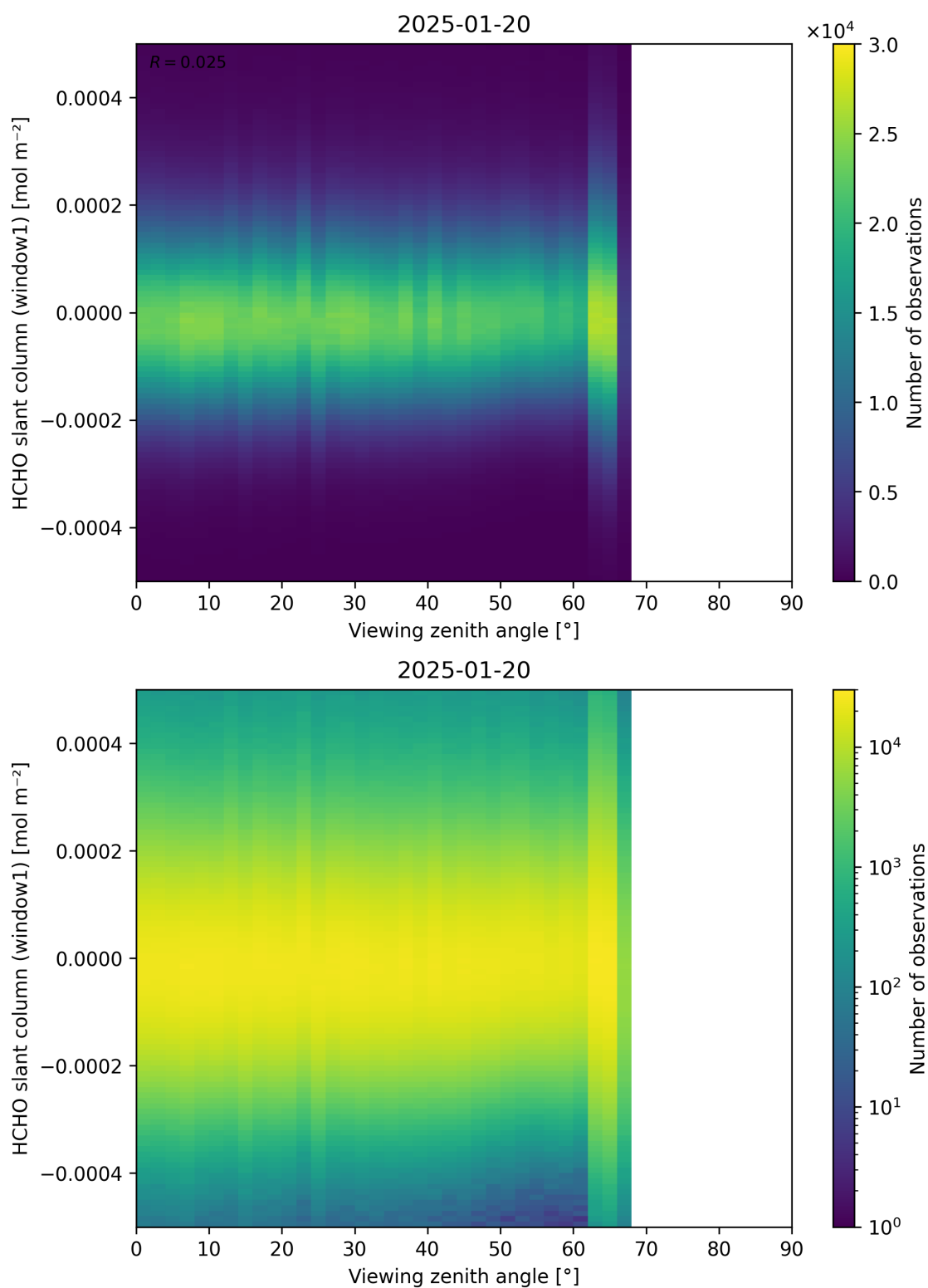
Figure 188: Scatter density plot of “Viewing zenith angle” against “HCHO slant column (window1)” for 2025-01-19 to 2025-01-21.
