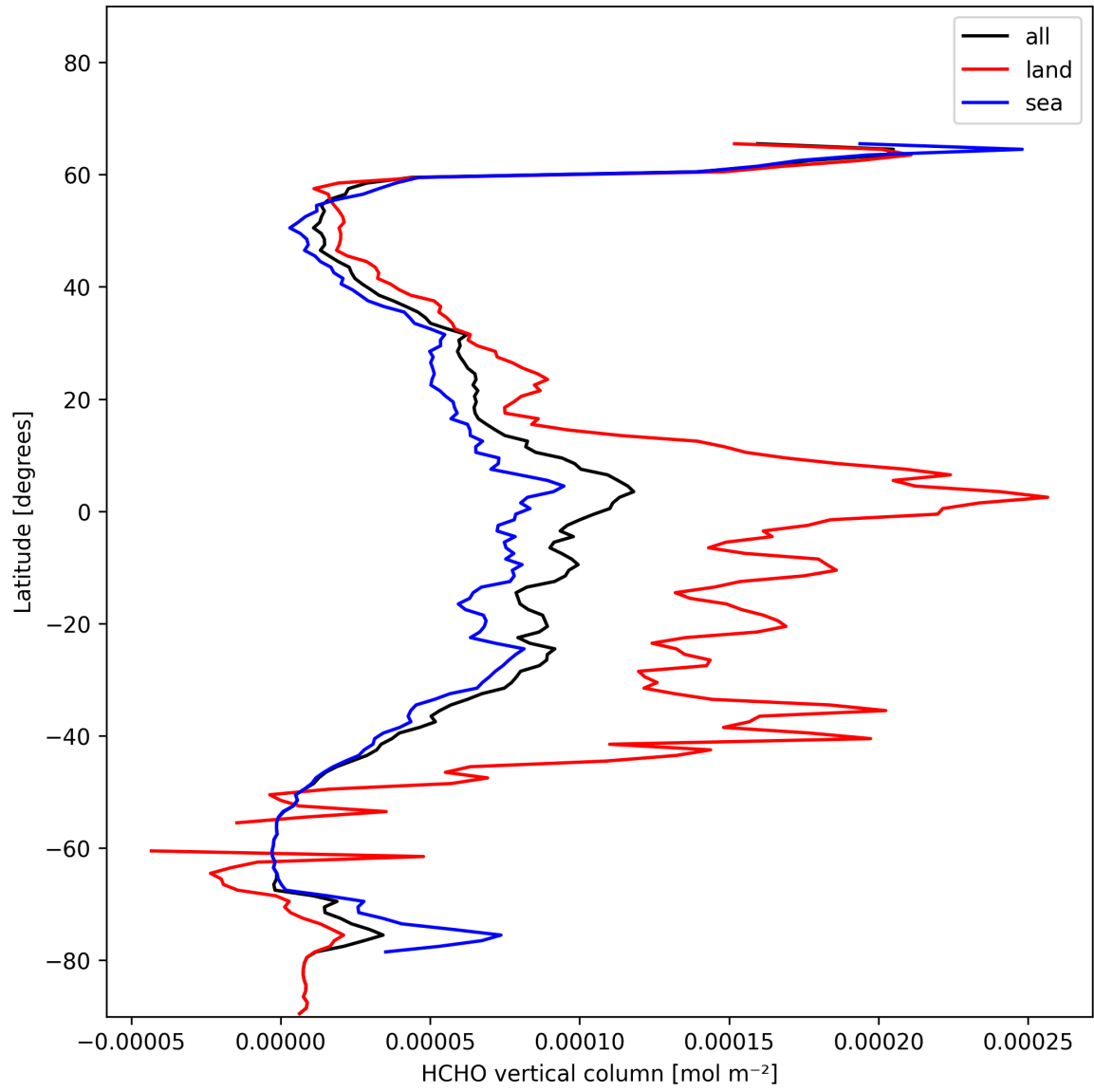
Figure 21: Zonal average of “HCHO vertical column” for 2025-01-19 to 2025-01-21.
