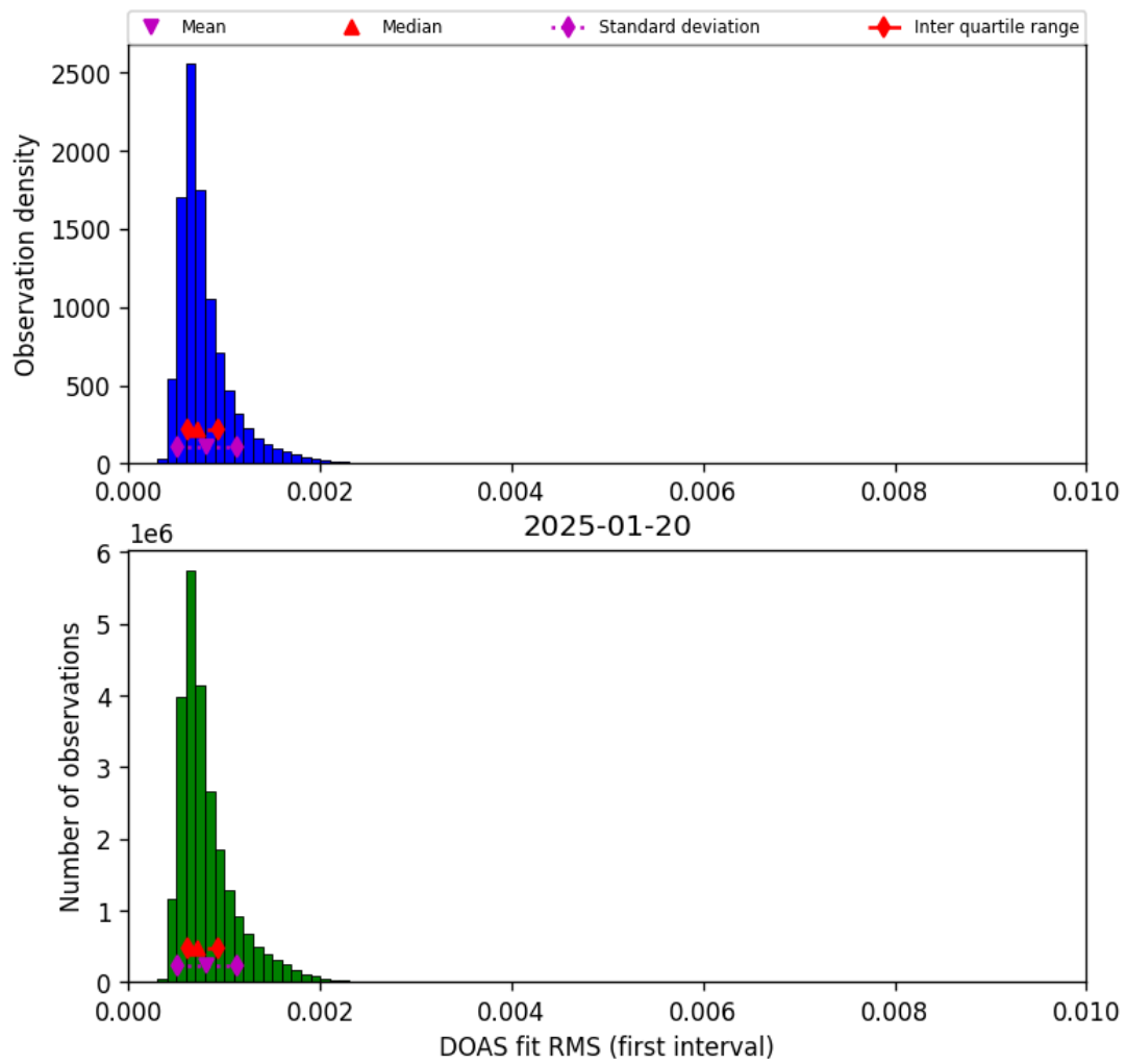
Figure 46: Histogram of “DOAS fit RMS (first interval)” for 2025-01-19 to 2025-01-21
