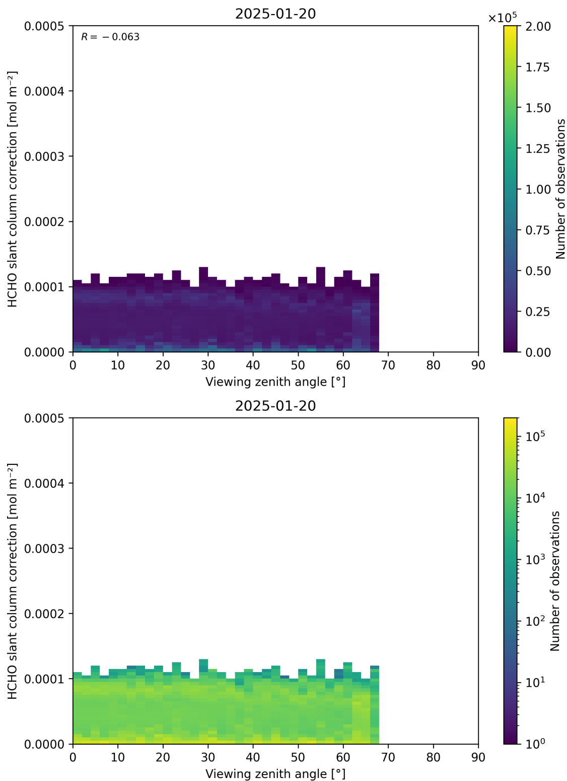
Figure 187: Scatter density plot of “Viewing zenith angle” against “HCHO slant column correction” for 2025-01-19 to 2025-01-21.
