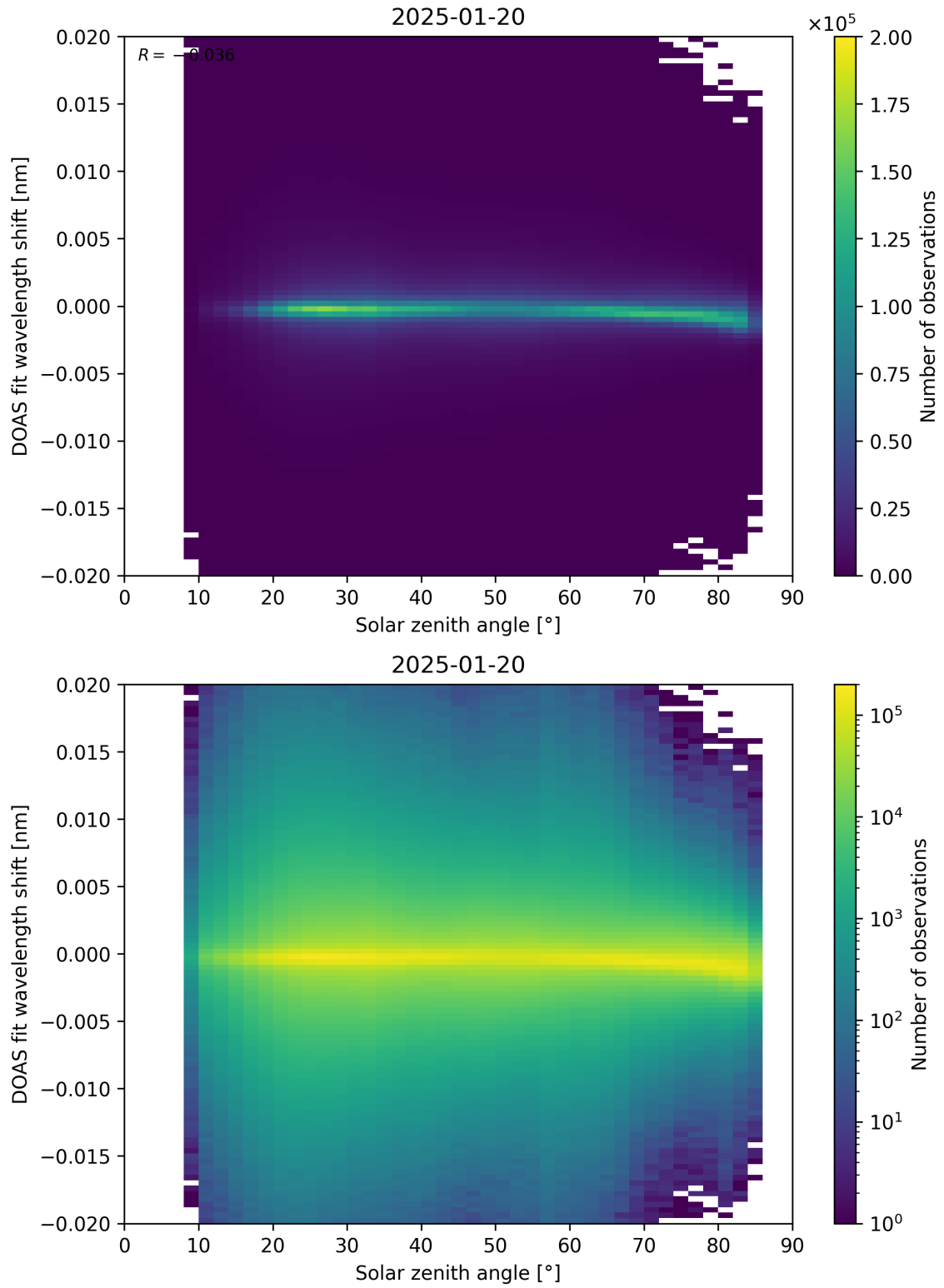
Figure 168: Scatter density plot of “Solar zenith angle” against “DOAS fit wavelength shift” for 2025-01-19 to 2025-01-21.
