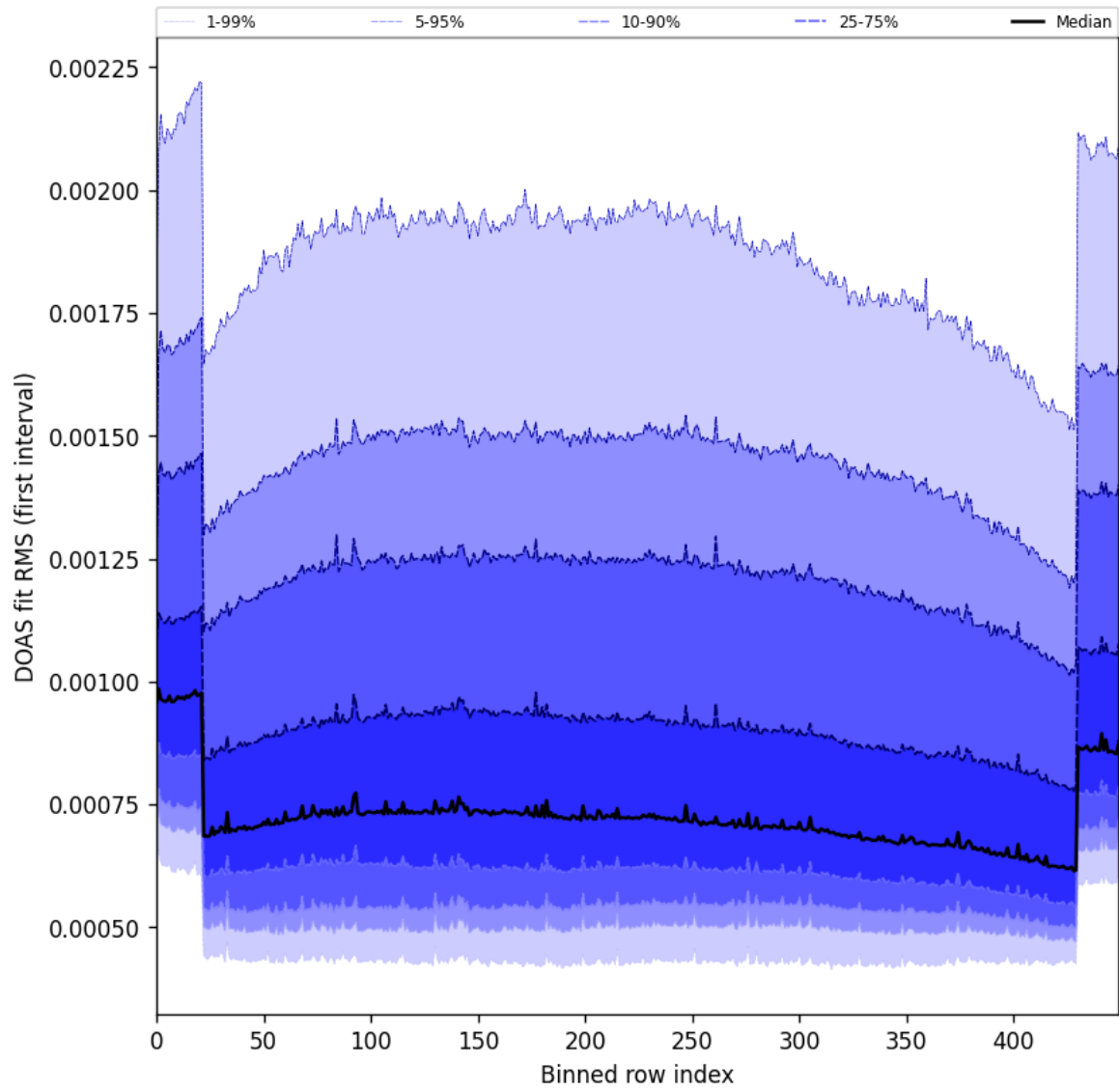
Figure 60: Along track statistics of “DOAS fit RMS (first interval)” for 2025-01-19 to 2025-01-21
