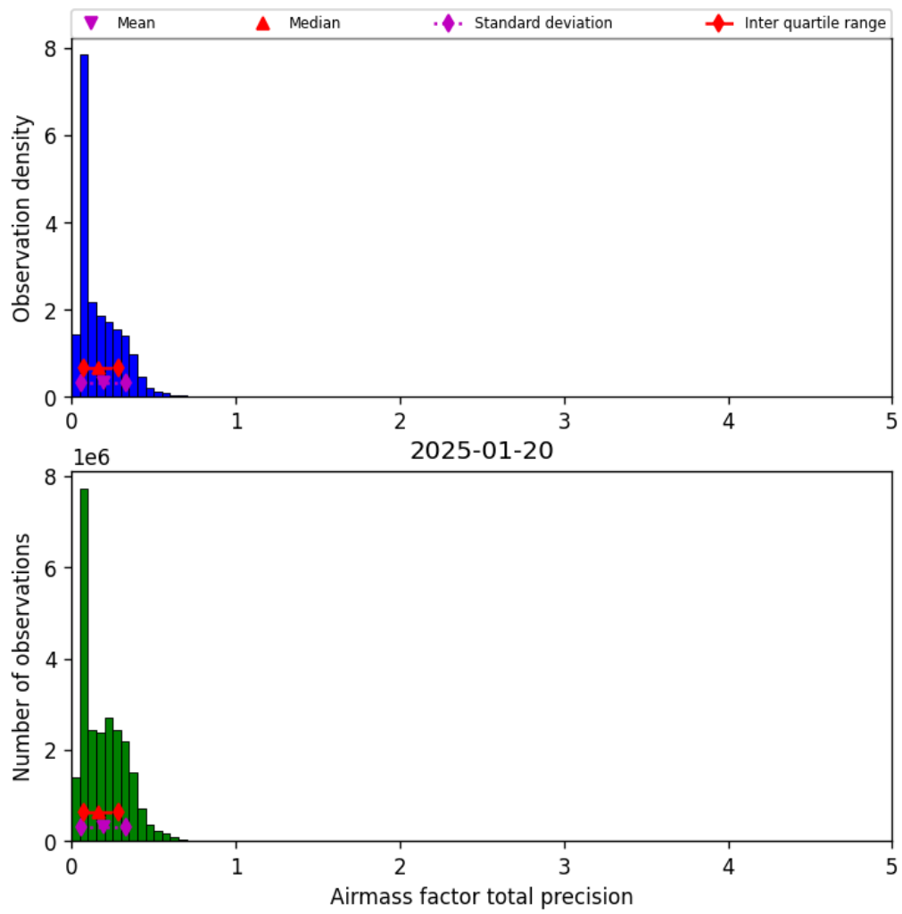
Figure 41: Histogram of “Airmass factor total precision” for 2025-01-19 to 2025-01-21
