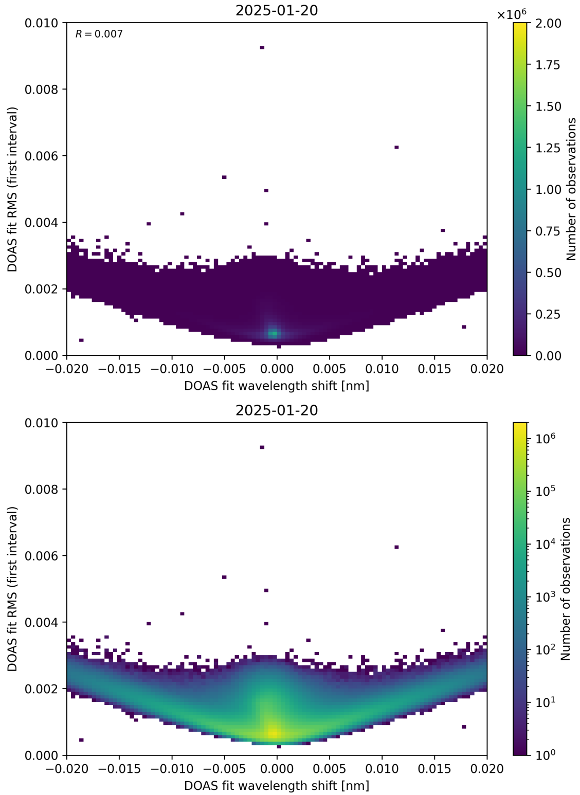
Figure 64: Scatter density plot of “DOAS fit wavelength shift” against “DOAS fit RMS (first interval)” for 2025-01-19 to 2025-01-21.
