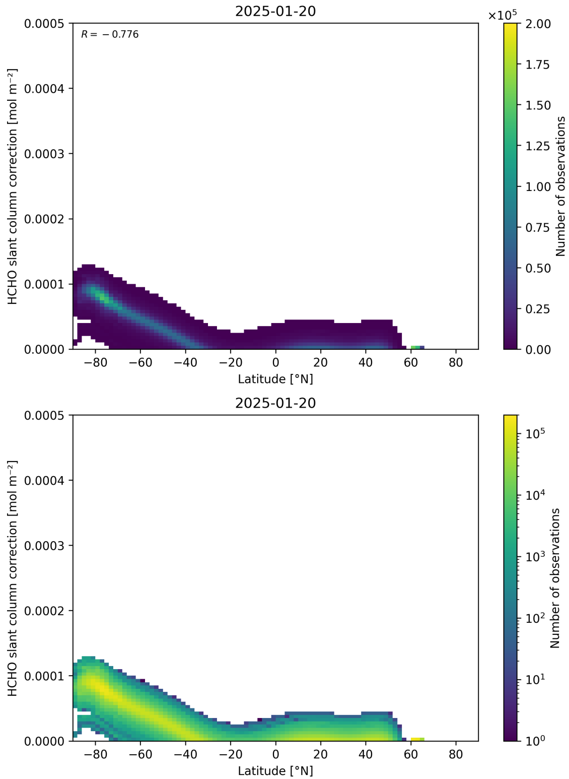
Figure 158: Scatter density plot of “Latitude” against “HCHO slant column correction” for 2025-01-19 to 2025-01-21.
