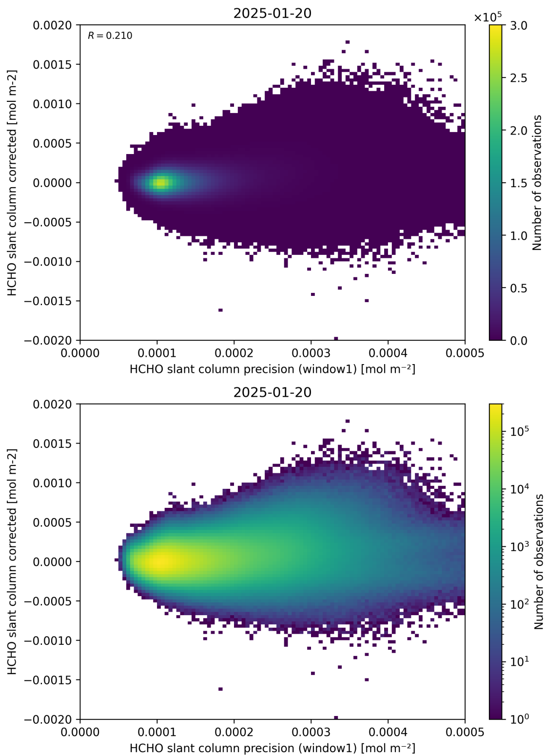
Figure 92: Scatter density plot of “HCHO slant column precision (window1)” against “HCHO slant column corrected” for 2025-01-19 to 2025-01-21.
