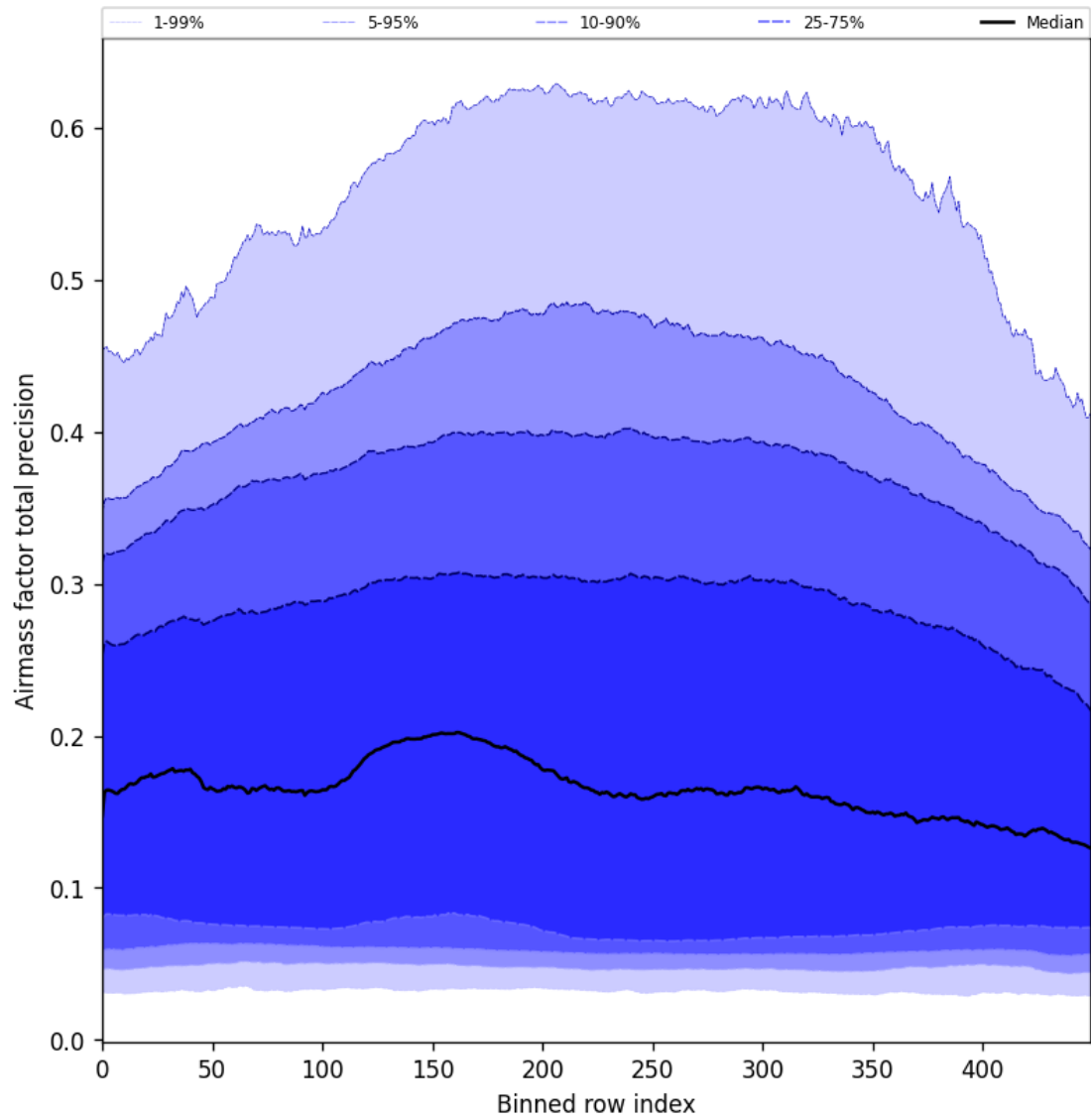
Figure 55: Along track statistics of “Airmass factor total precision” for 2025-01-19 to 2025-01-21
