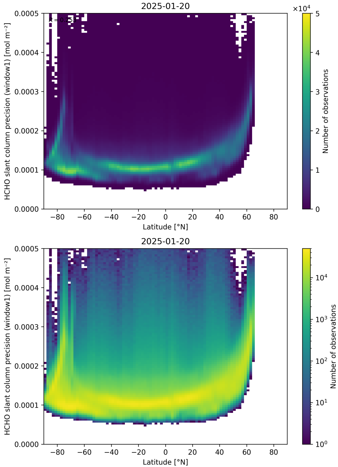
Figure 160: Scatter density plot of “Latitude” against “HCHO slant column precision (window1)” for 2025-01-19 to 2025-01-21.
