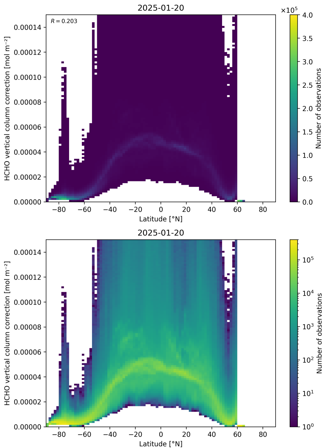
Figure 164: Scatter density plot of “Latitude” against “HCHO vertical column correction” for 2025-01-19 to 2025-01-21.
