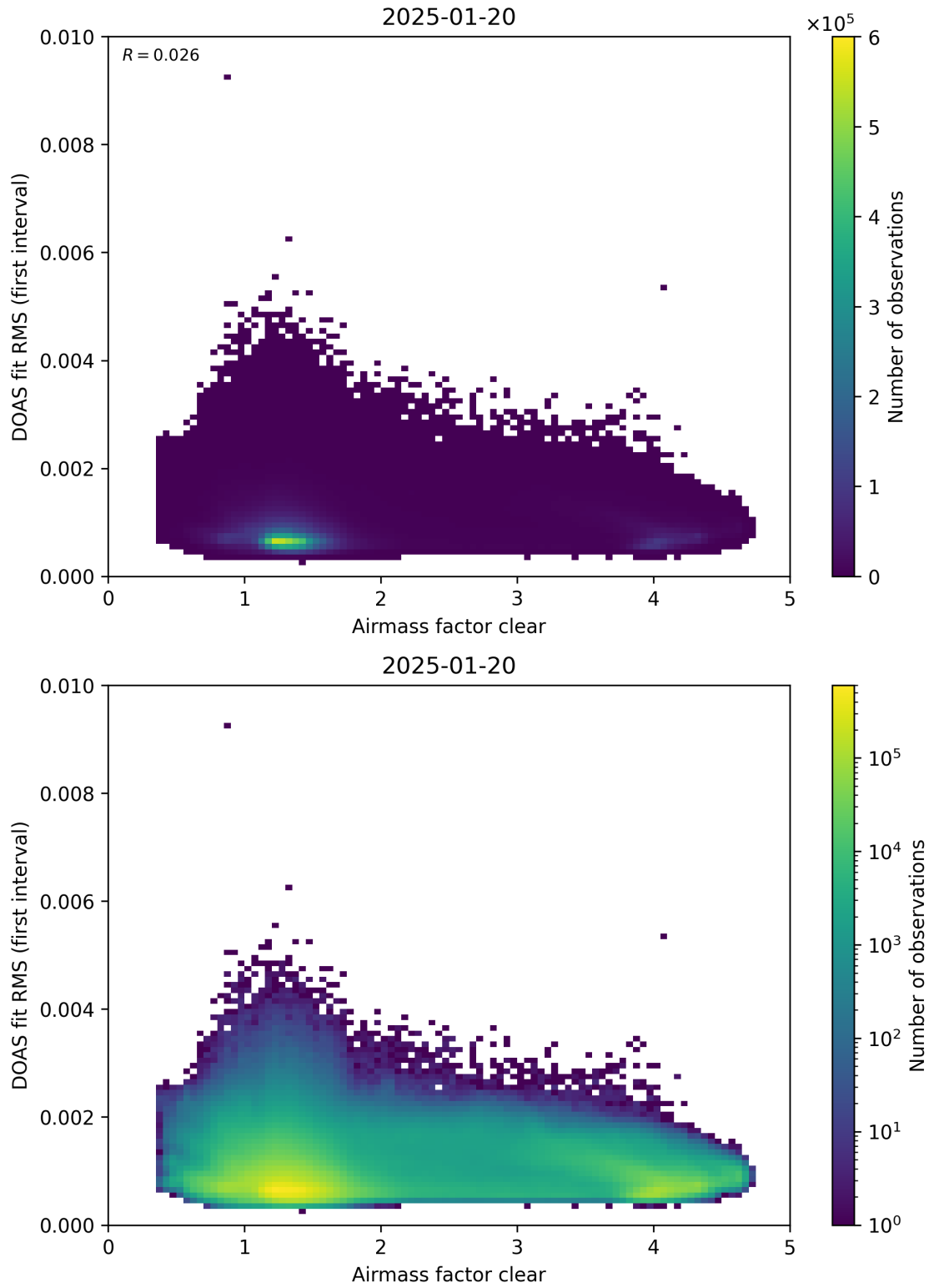
Figure 71: Scatter density plot of “Airmass factor clear” against “DOAS fit RMS (first interval)” for 2025-01-19 to 2025-01-21.
