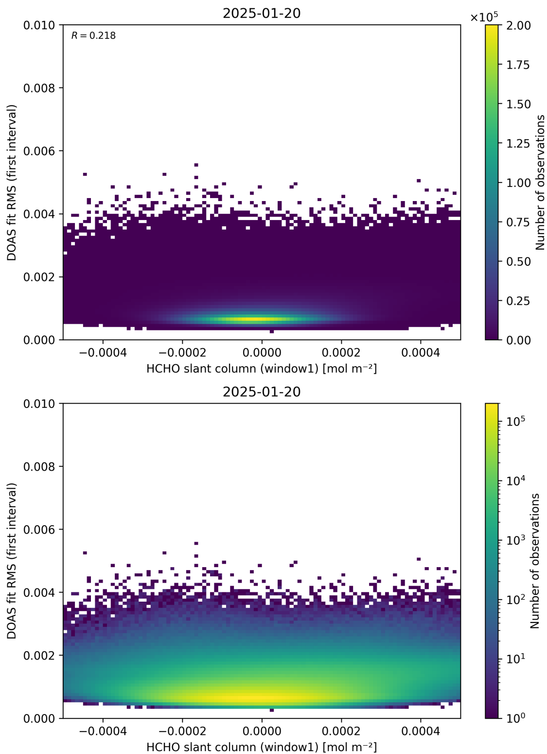
Figure 78: Scatter density plot of “HCHO slant column (window1)” against “DOAS fit RMS (first interval)” for 2025-01-19 to 2025-01-21.
