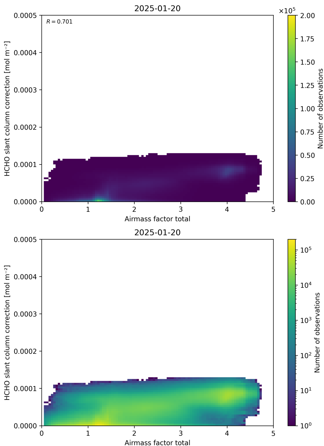
Figure 102: Scatter density plot of “Airmass factor total” against “HCHO slant column correction” for 2025-01-19 to 2025-01-21.
