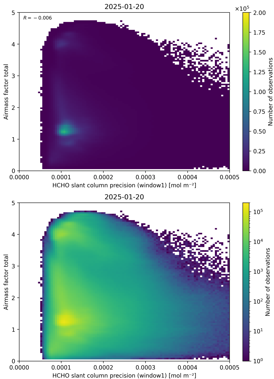
Figure 94: Scatter density plot of “HCHO slant column precision (window1)” against “Airmass factor total” for 2025-01-19 to 2025-01-21.
