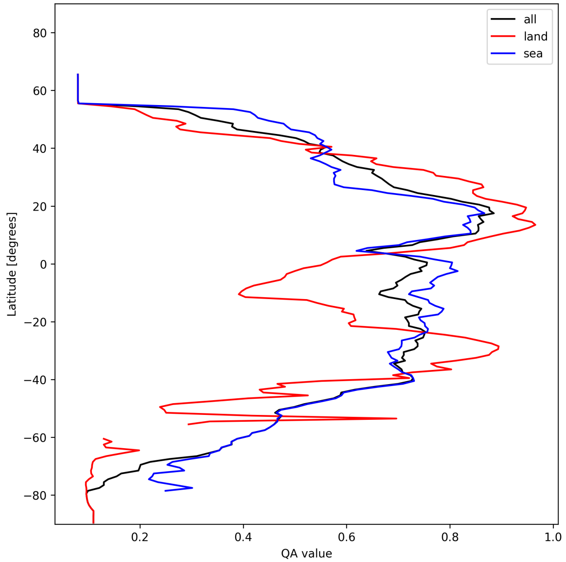
Figure 20: Zonal average of “QA value” for 2025-01-19 to 2025-01-21.
