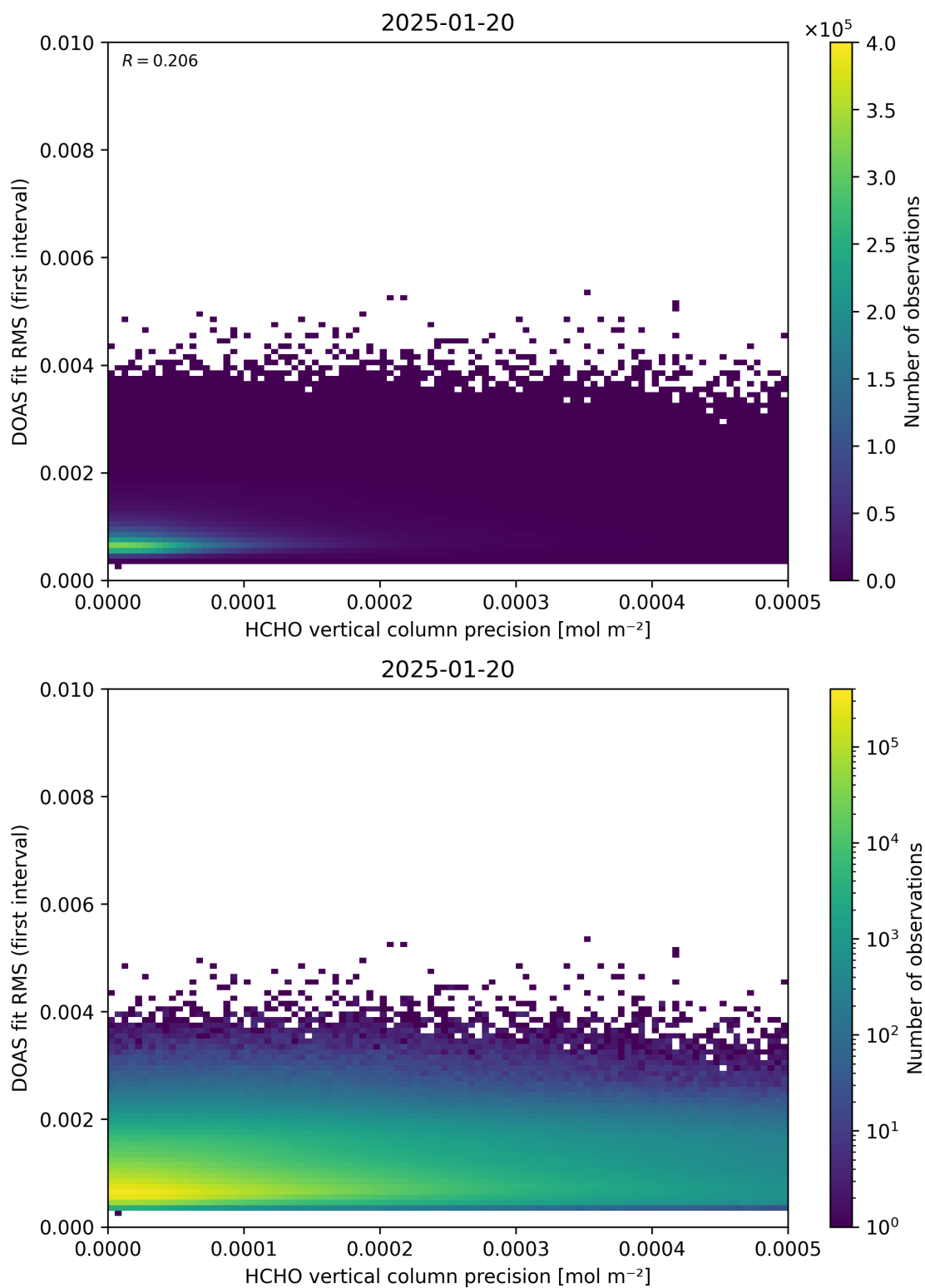
Figure 136: Scatter density plot of “HCHO vertical column precision” against “DOAS fit RMS (first interval)” for 2025-01-19 to 2025-01-21.
