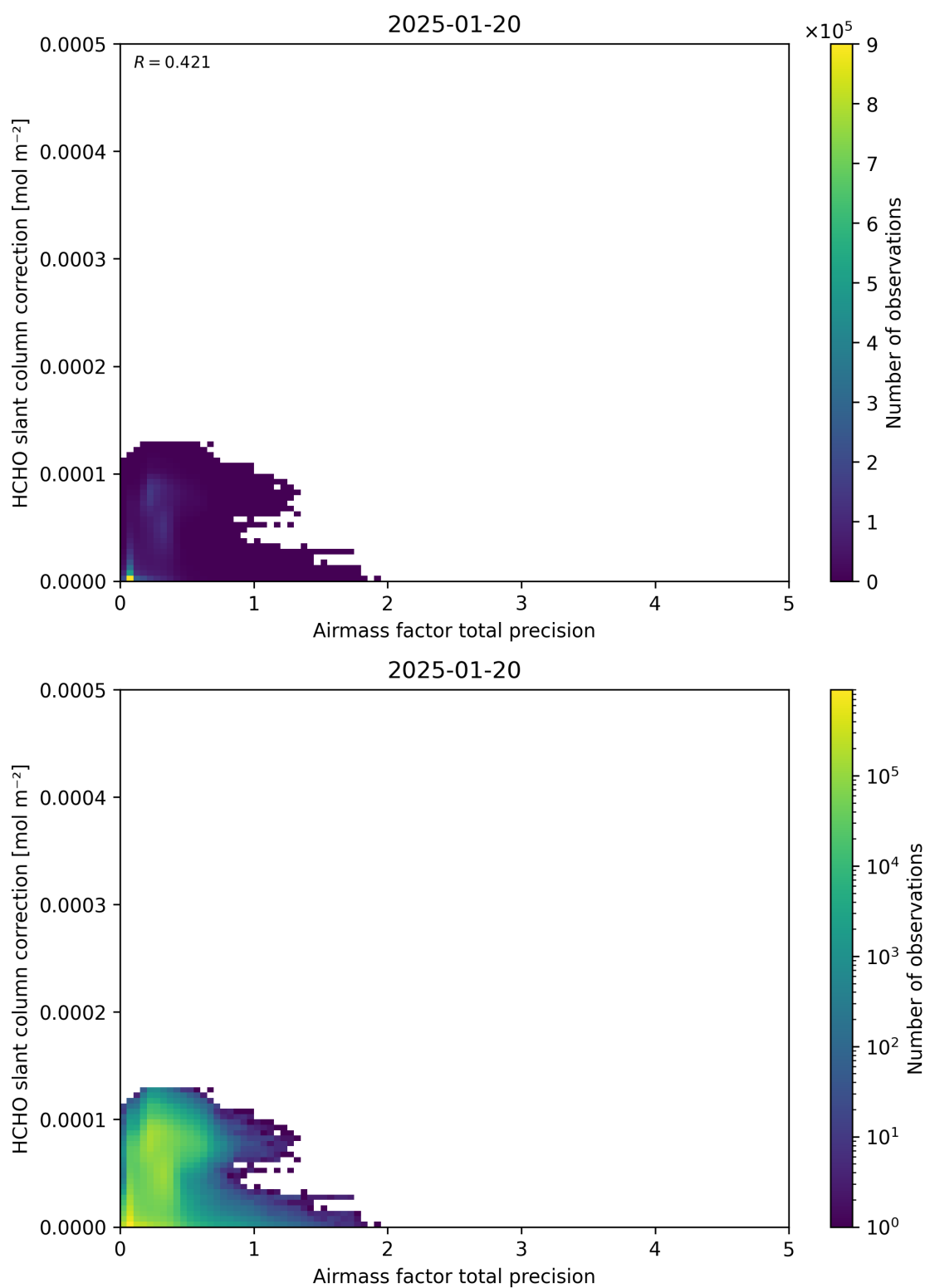
Figure 110: Scatter density plot of “Airmass factor total precision” against “HCHO slant column correction” for 2025-01-19 to 2025-01-21.
