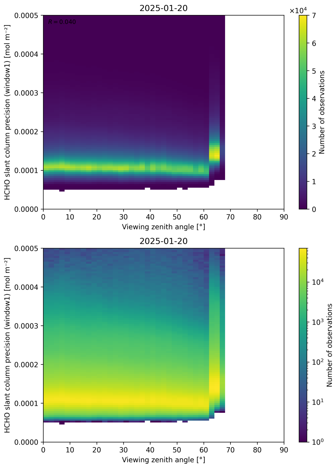
Figure 189: Scatter density plot of “Viewing zenith angle” against “HCHO slant column precision (window1)” for 2025-01-19 to 2025-01-21.
