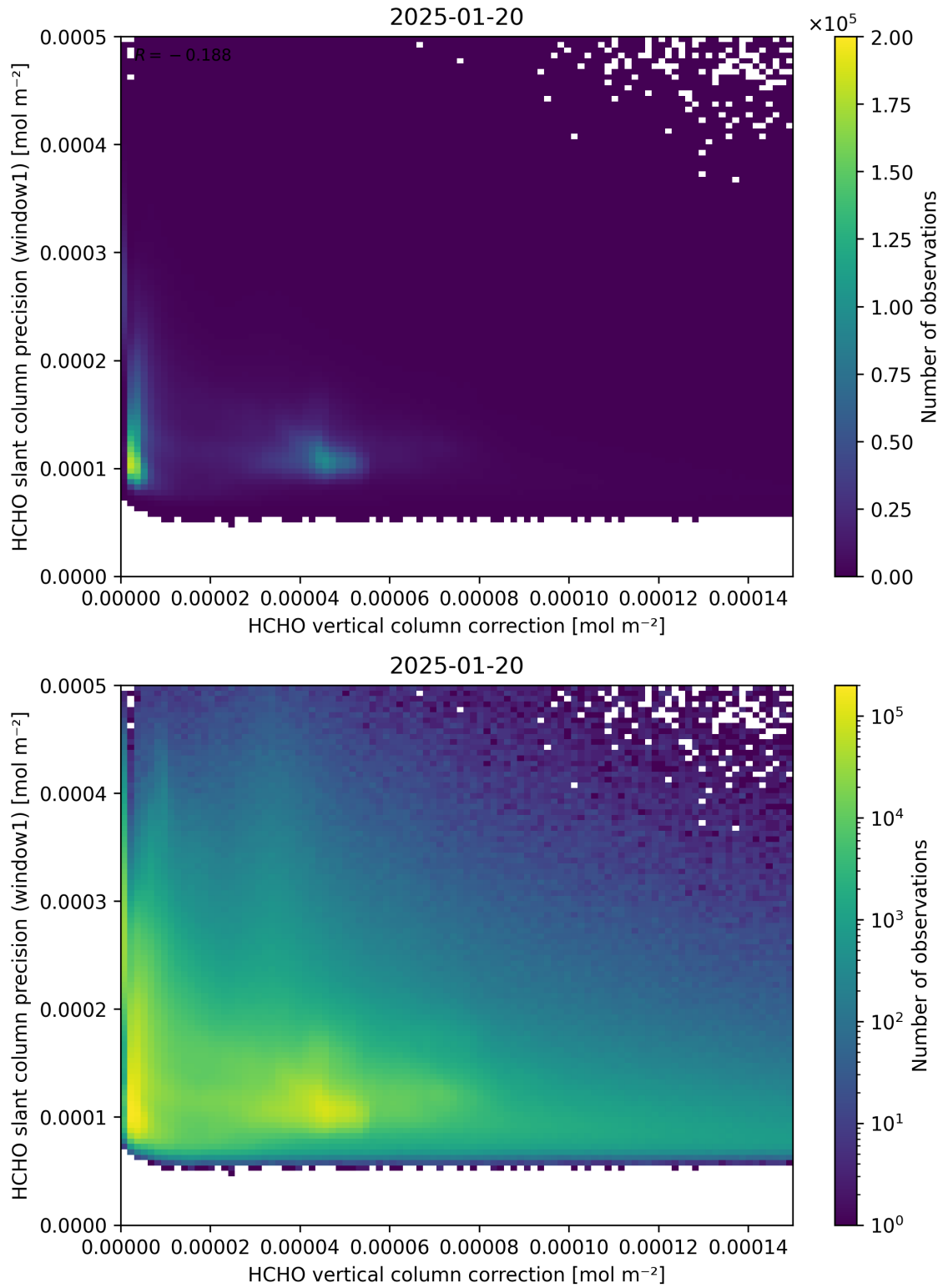
Figure 119: Scatter density plot of “HCHO vertical column correction” against “HCHO slant column precision (window1)” for 2025-01-19 to 2025-01-21.
