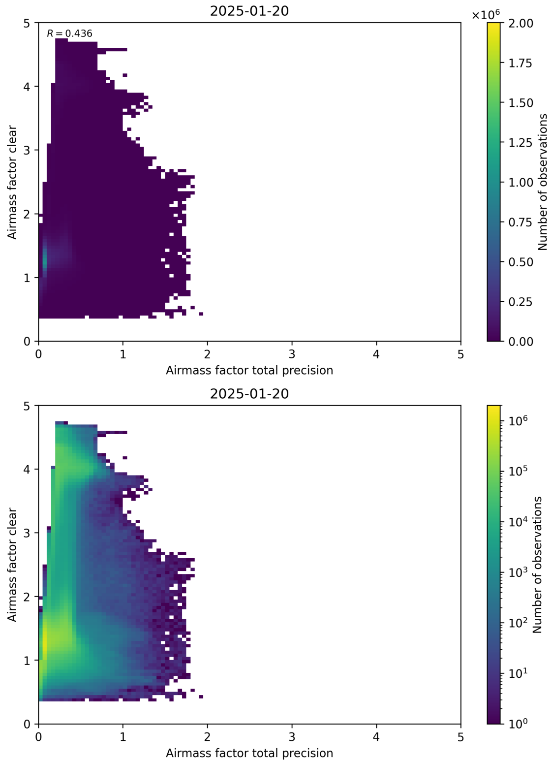
Figure 108: Scatter density plot of “Airmass factor total precision” against “Airmass factor clear” for 2025-01-19 to 2025-01-21.
