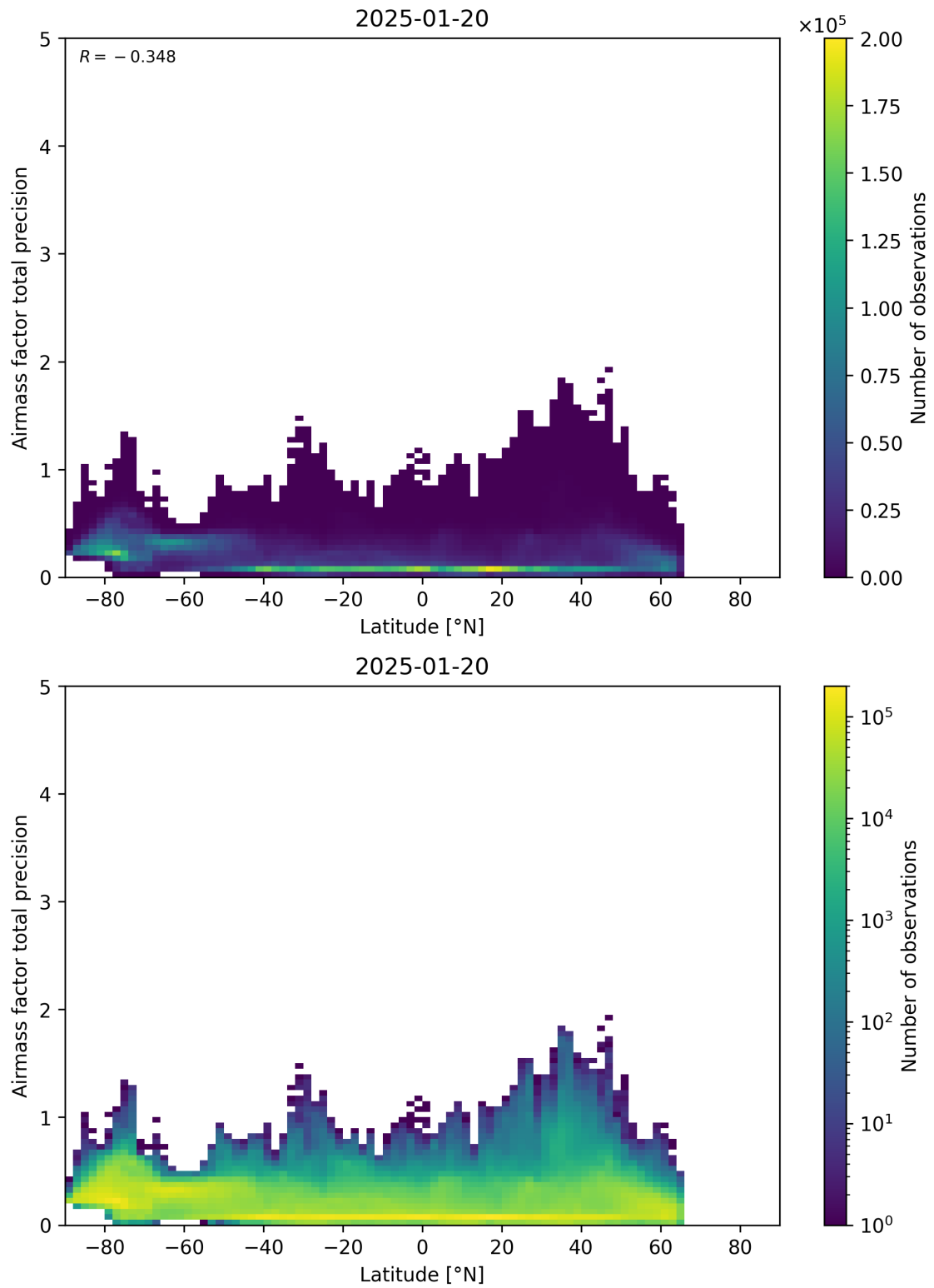
Figure 162: Scatter density plot of “Latitude” against “Airmass factor total precision” for 2025-01-19 to 2025-01-21.
