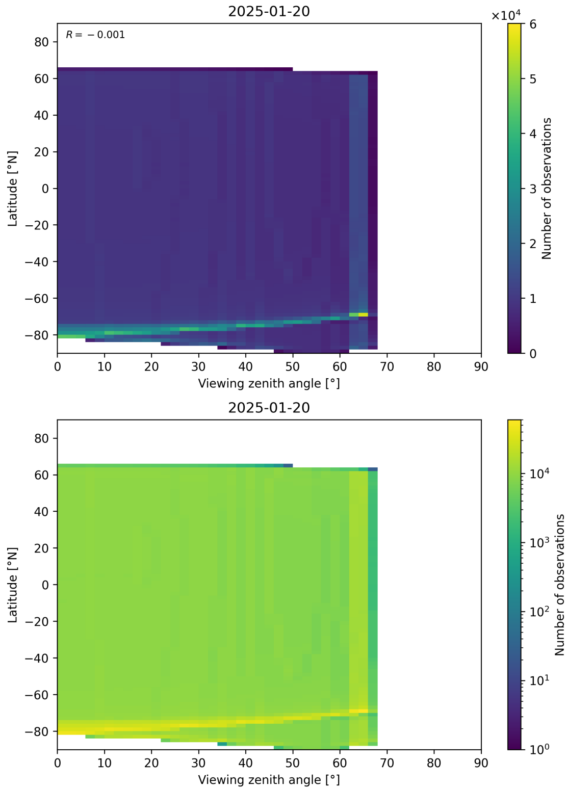
Figure 196: Scatter density plot of “Viewing zenith angle” against “Latitude” for 2025-01-19 to 2025-01-21.
