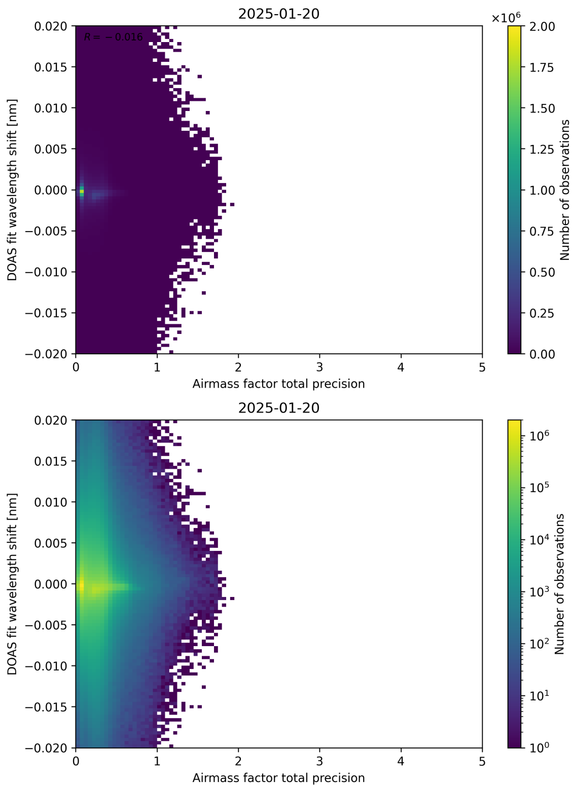
Figure 106: Scatter density plot of “Airmass factor total precision” against “DOAS fit wavelength shift” for 2025-01-19 to 2025-01-21.
