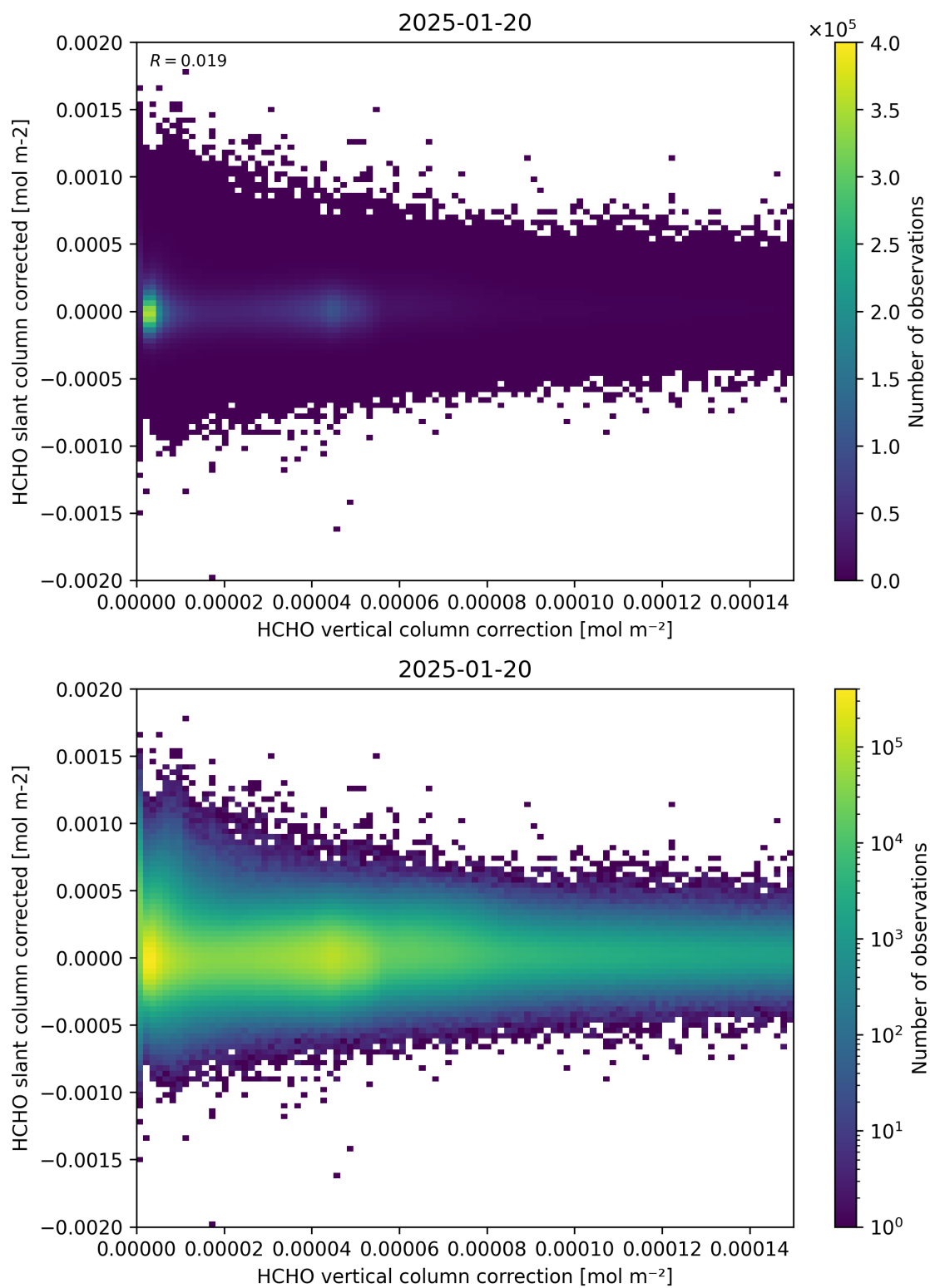
Figure 116: Scatter density plot of “HCHO vertical column correction” against “HCHO slant column corrected” for 2025-01-19 to 2025-01-21.
