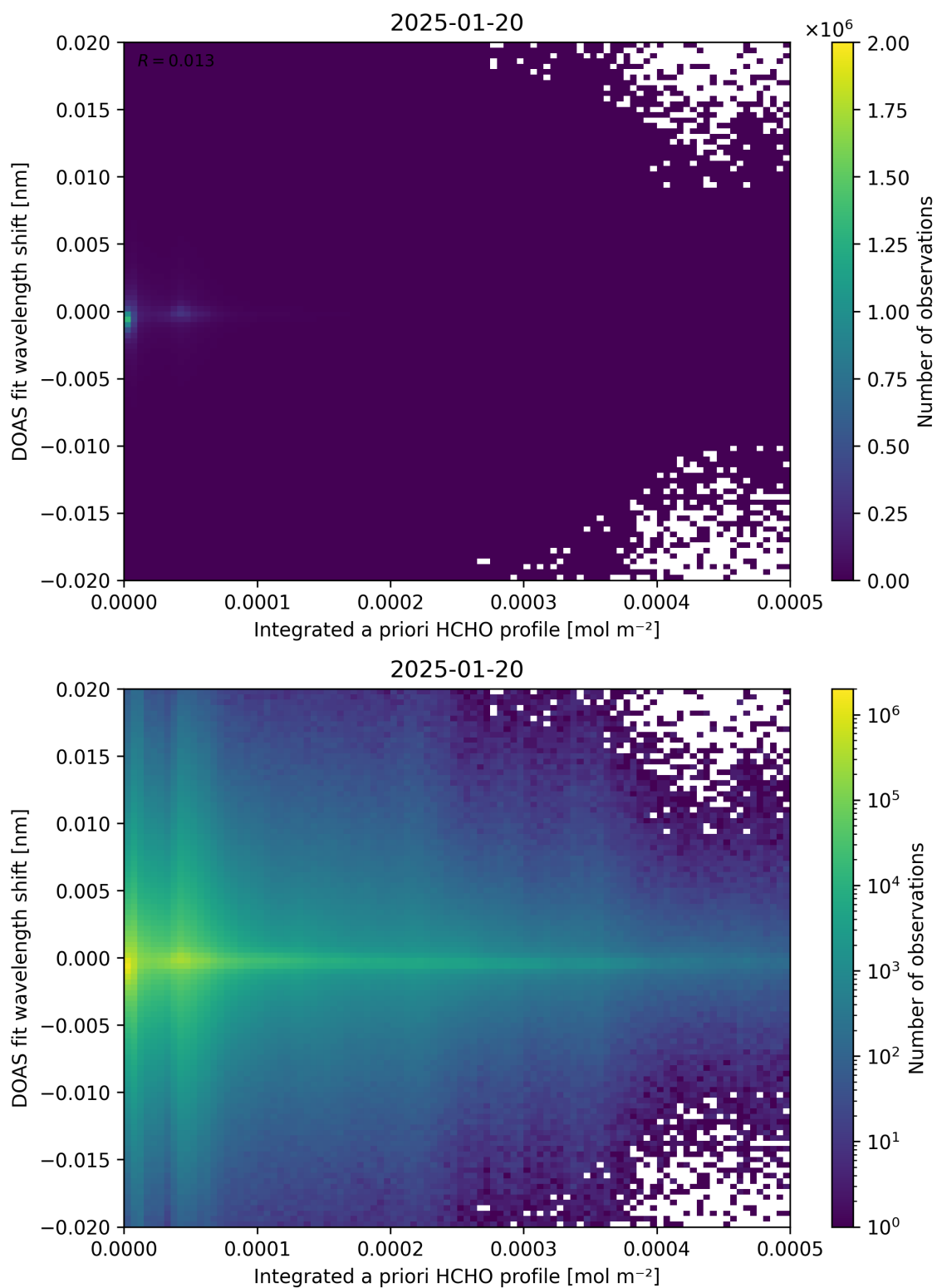
Figure 149: Scatter density plot of “Integrated a priori HCHO profile” against “DOAS fit wavelength shift” for 2025-01-19 to 2025-01-21.
