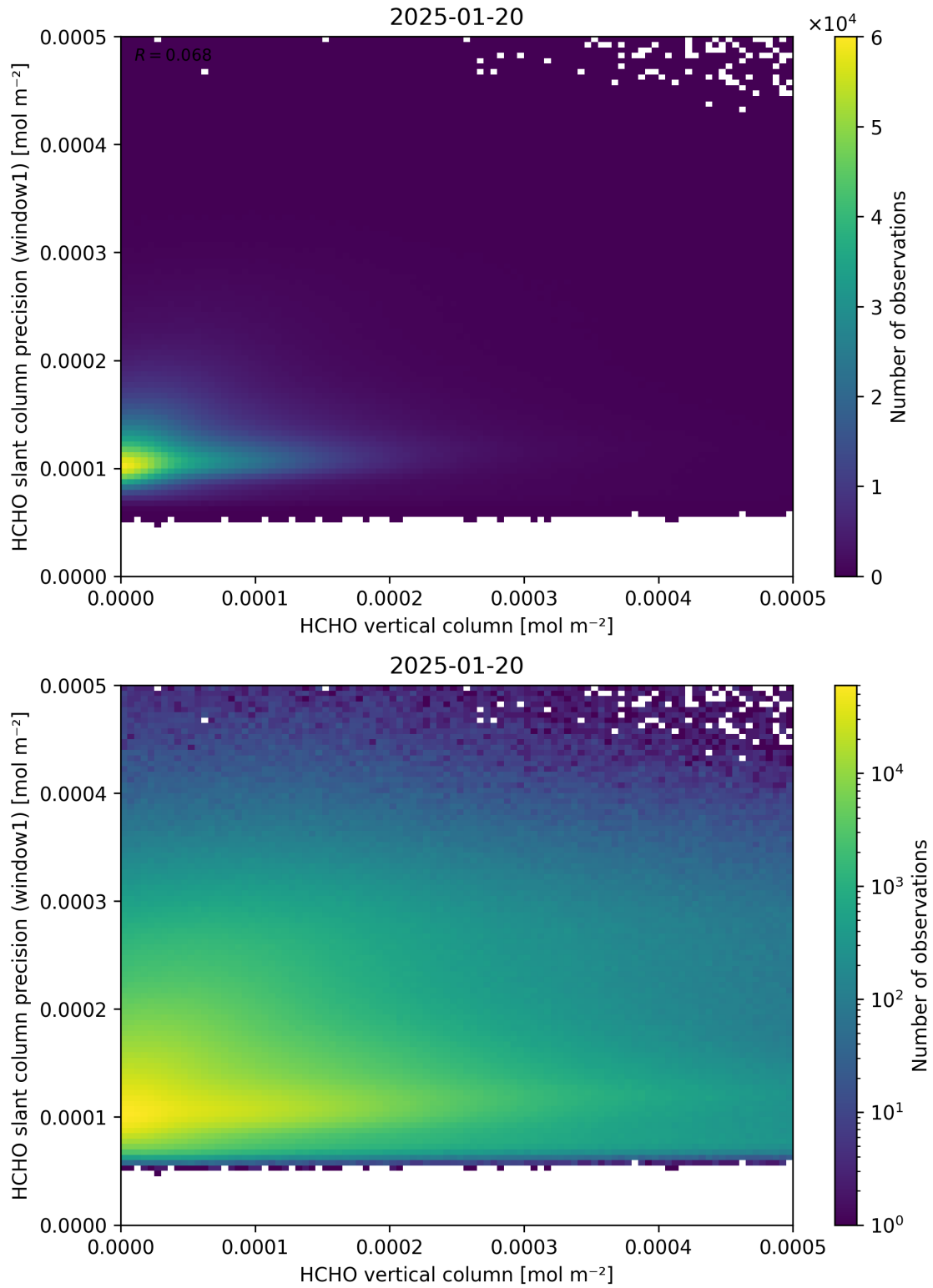
Figure 130: Scatter density plot of “HCHO vertical column” against “HCHO slant column precision (window1)” for 2025-01-19 to 2025-01-21.
