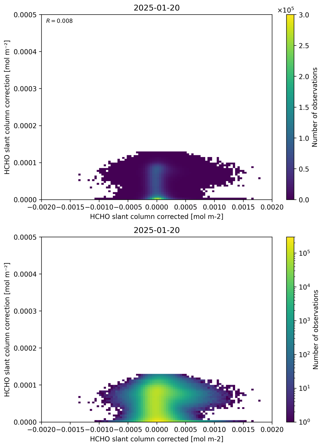
Figure 77: Scatter density plot of “HCHO slant column corrected” against “HCHO slant column correction” for 2025-01-19 to 2025-01-21.
