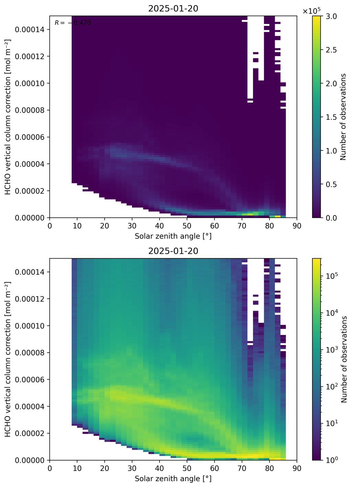
Figure 178: Scatter density plot of “Solar zenith angle” against “HCHO vertical column correction” for 2025-01-19 to 2025-01-21.
