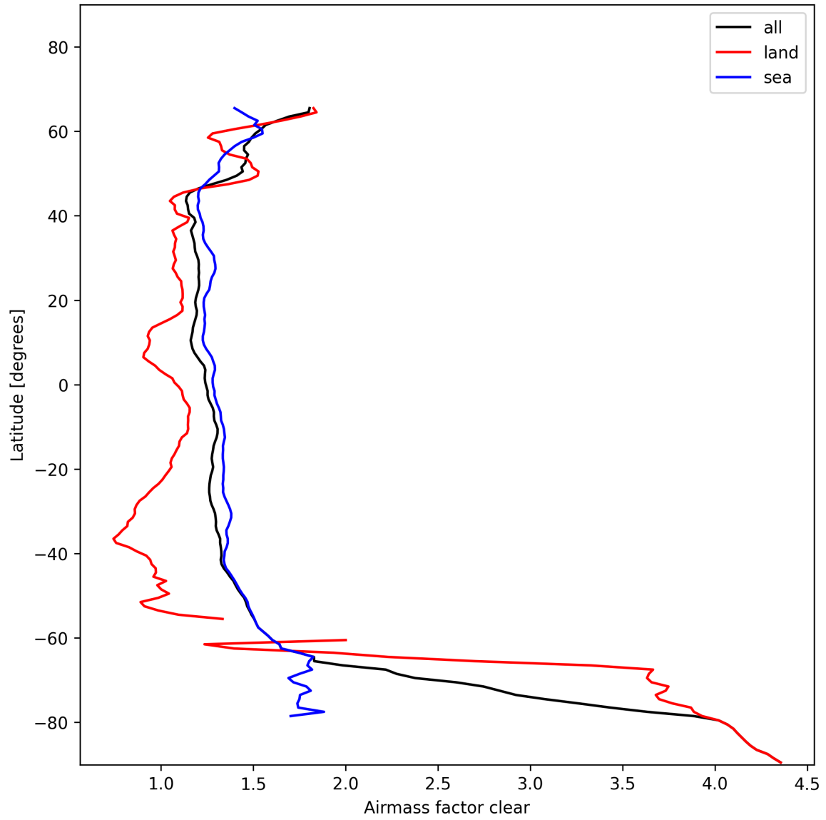
Figure 28: Zonal average of “Airmass factor clear” for 2025-01-19 to 2025-01-21.
