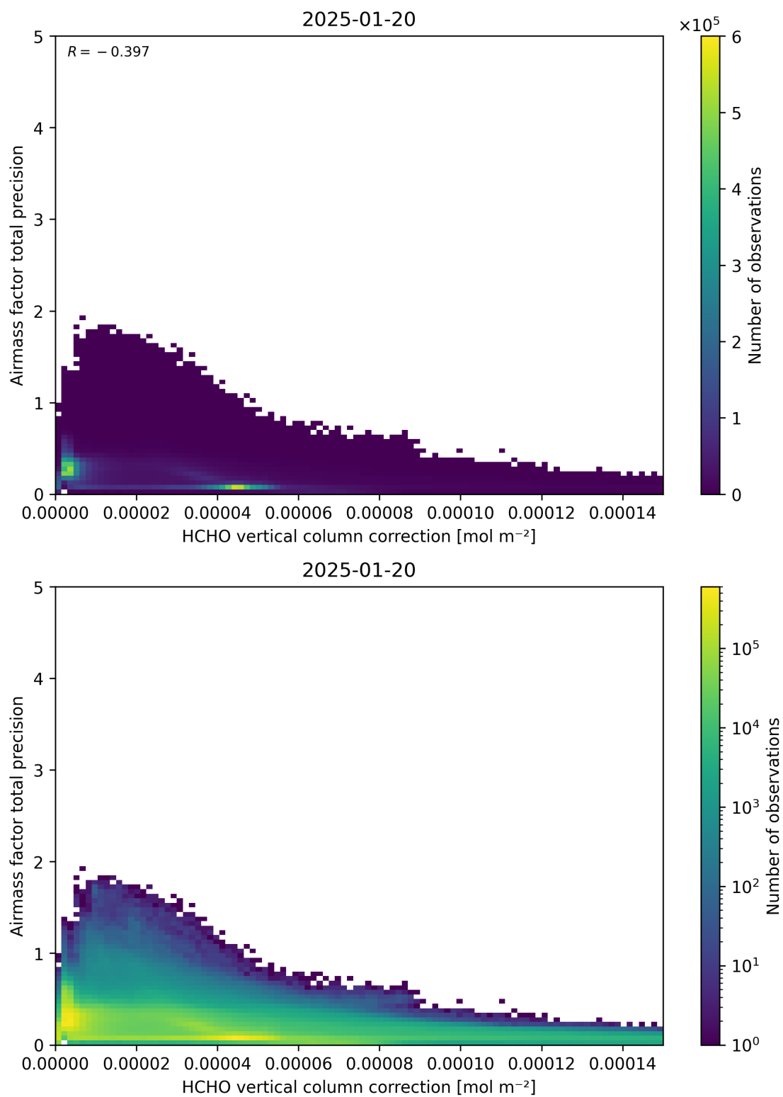
Figure 121: Scatter density plot of “HCHO vertical column correction” against “Airmass factor total precision” for 2025-01-19 to 2025-01-21.
