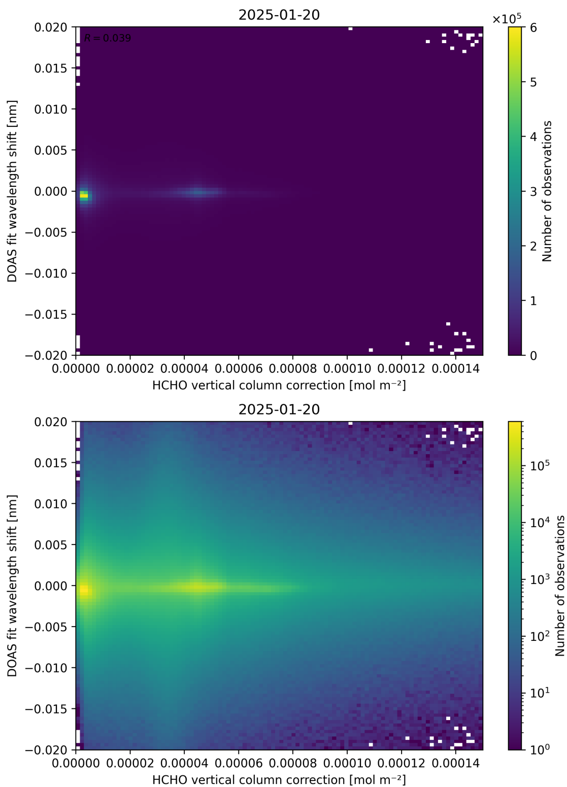
Figure 113: Scatter density plot of “HCHO vertical column correction” against “DOAS fit wavelength shift” for 2025-01-19 to 2025-01-21.
