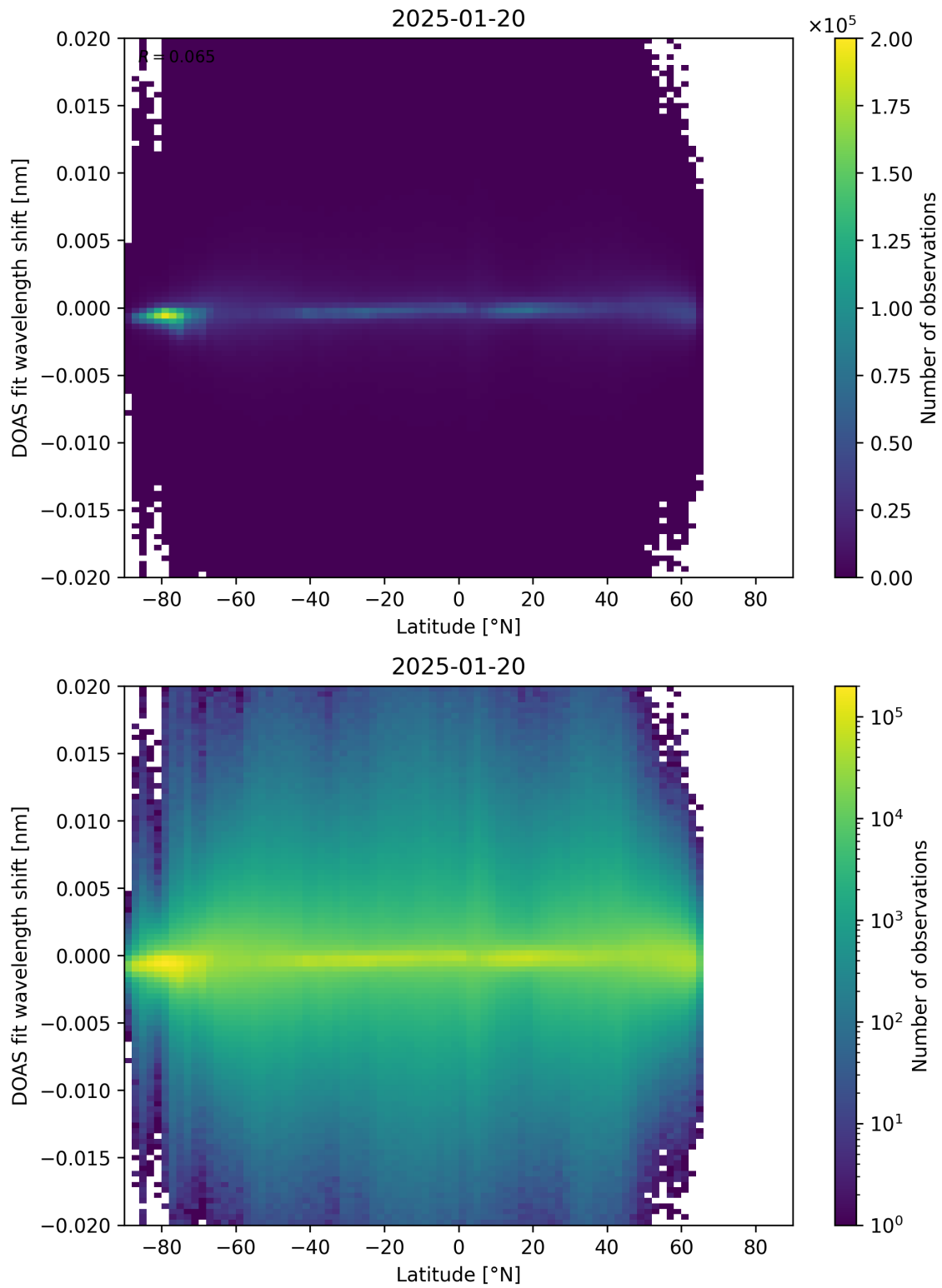
Figure 154: Scatter density plot of “Latitude” against “DOAS fit wavelength shift” for 2025-01-19 to 2025-01-21.
