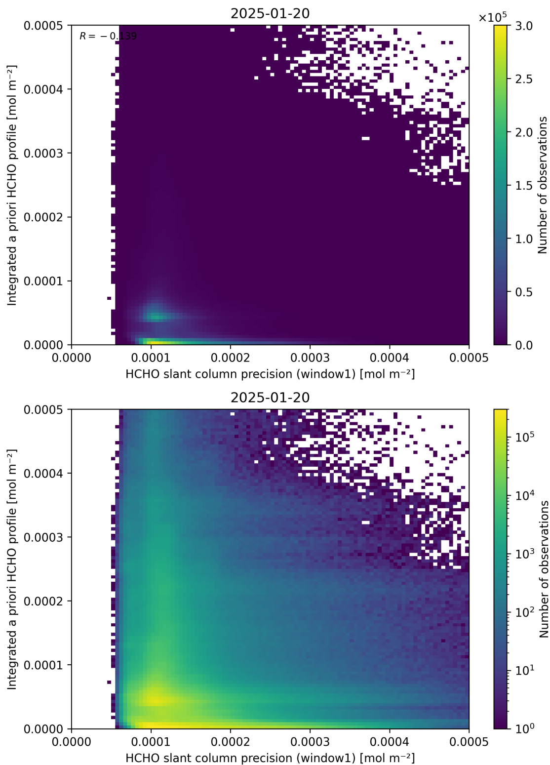
Figure 96: Scatter density plot of “HCHO slant column precision (window1)” against “Integrated a priori HCHO profile” for 2025-01-19 to 2025-01-21.
