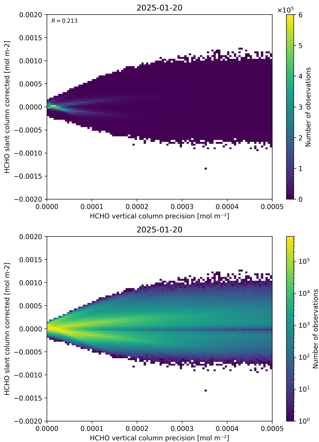
Figure 140: Scatter density plot of “HCHO vertical column precision” against “HCHO slant column corrected” for 2025-01-19 to 2025-01-21.
