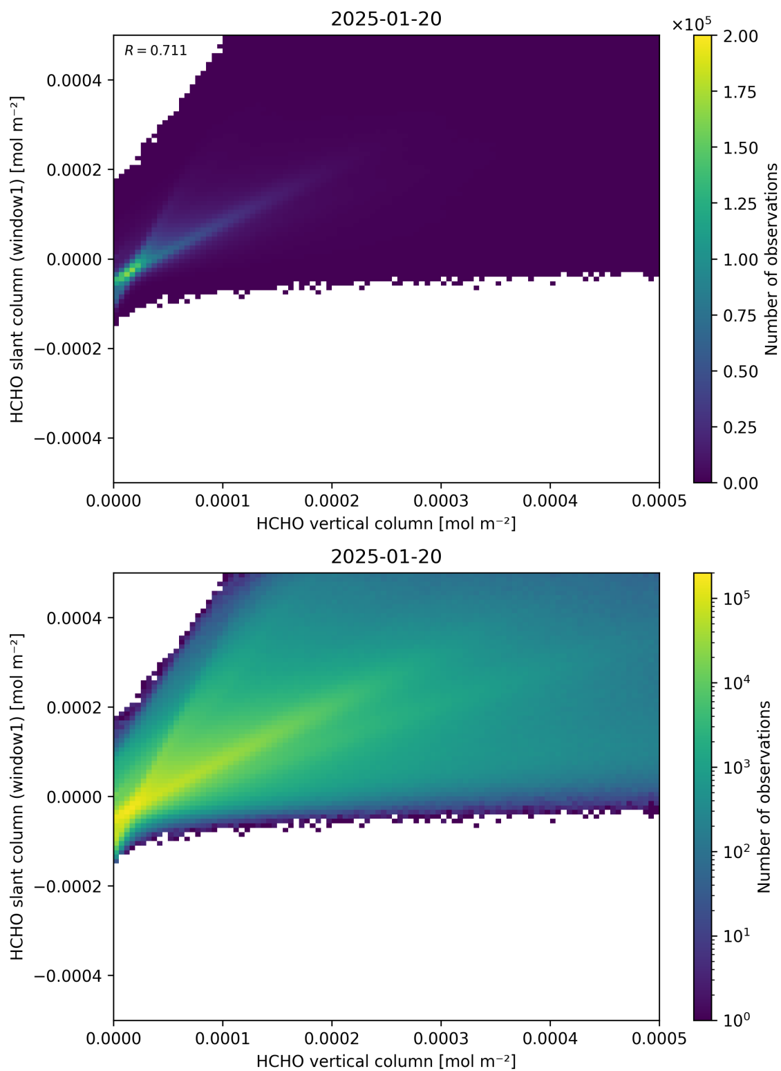
Figure 129: Scatter density plot of “HCHO vertical column” against “HCHO slant column (window1)” for 2025-01-19 to 2025-01-21.
