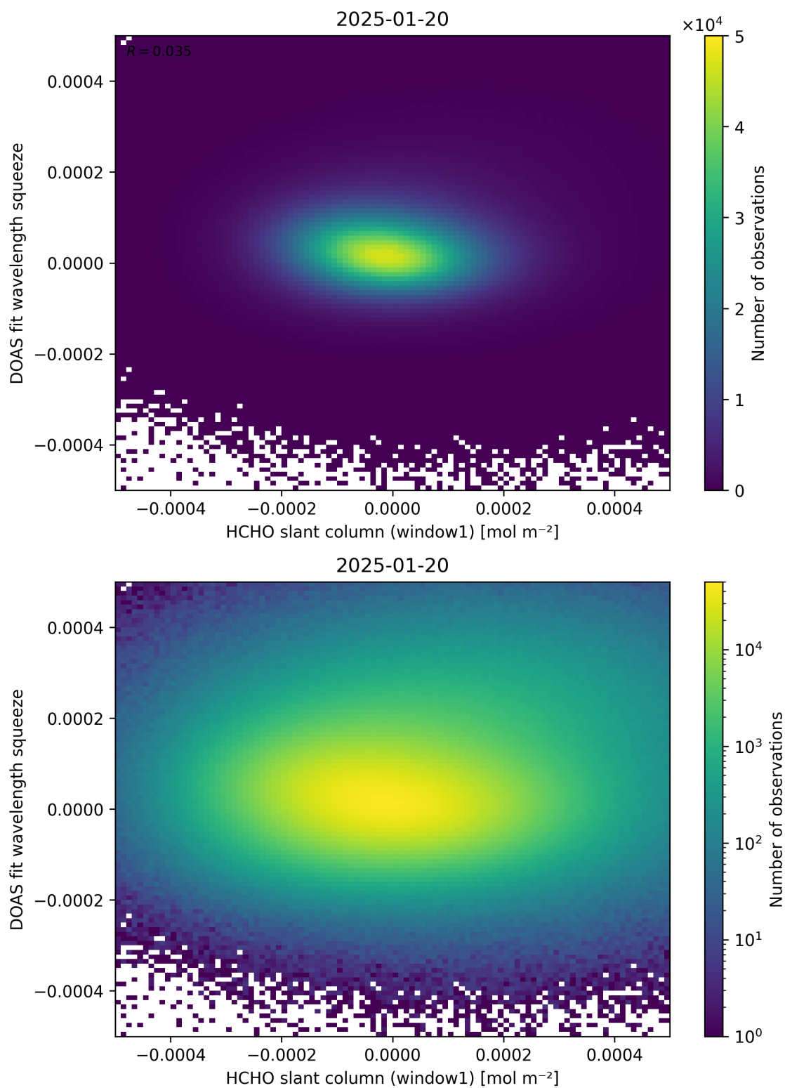
Figure 80: Scatter density plot of “HCHO slant column (window1)” against “DOAS fit wavelength squeeze” for 2025-01-19 to 2025-01-21.
