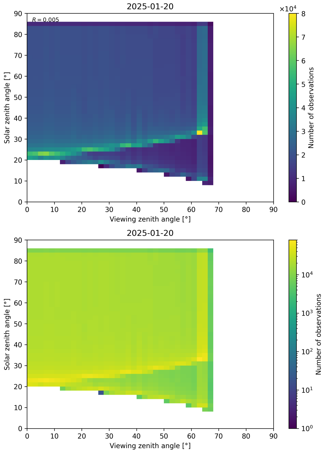
Figure 197: Scatter density plot of “Viewing zenith angle” against “Solar zenith angle” for 2025-01-19 to 2025-01-21.
