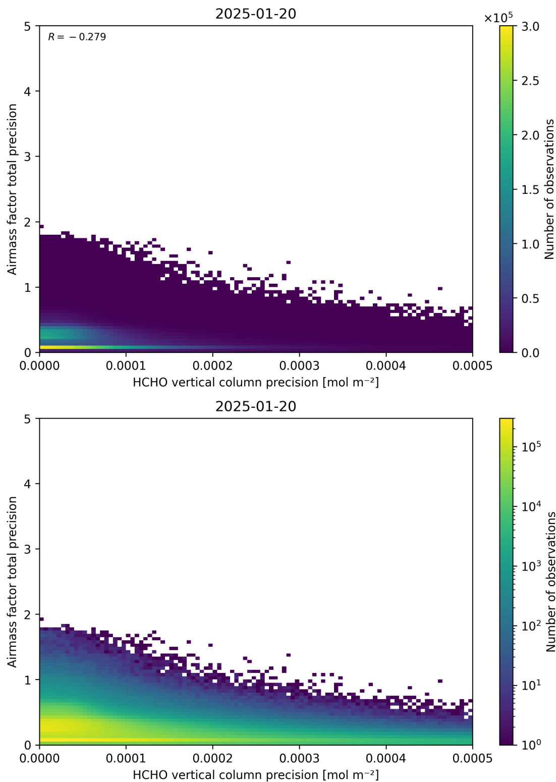
Figure 145: Scatter density plot of “HCHO vertical column precision” against “Airmass factor total precision” for 2025-01-19 to 2025-01-21.
