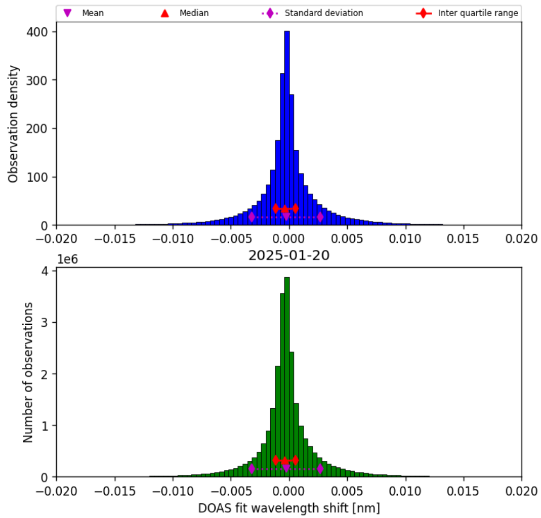
Figure 44: Histogram of “DOAS fit wavelength shift” for 2025-01-19 to 2025-01-21
