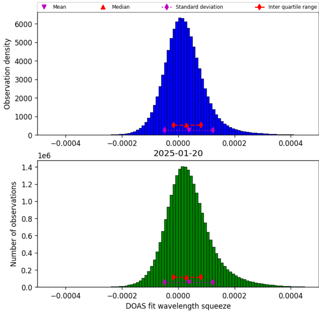
Figure 45: Histogram of “DOAS fit wavelength squeeze” for 2025-01-19 to 2025-01-21
