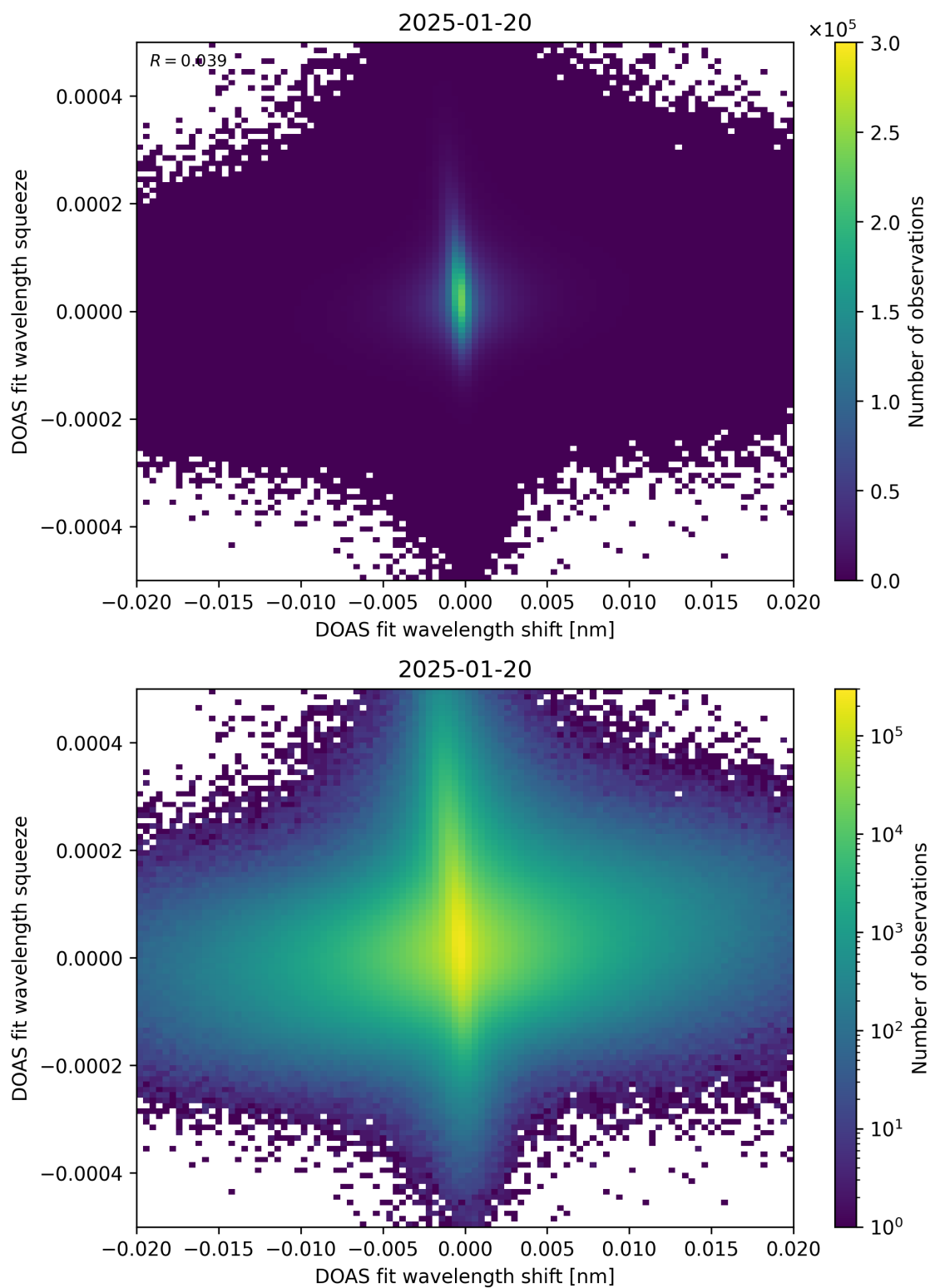
Figure 65: Scatter density plot of “DOAS fit wavelength shift” against “DOAS fit wavelength squeeze” for 2025-01-19 to 2025-01-21.
