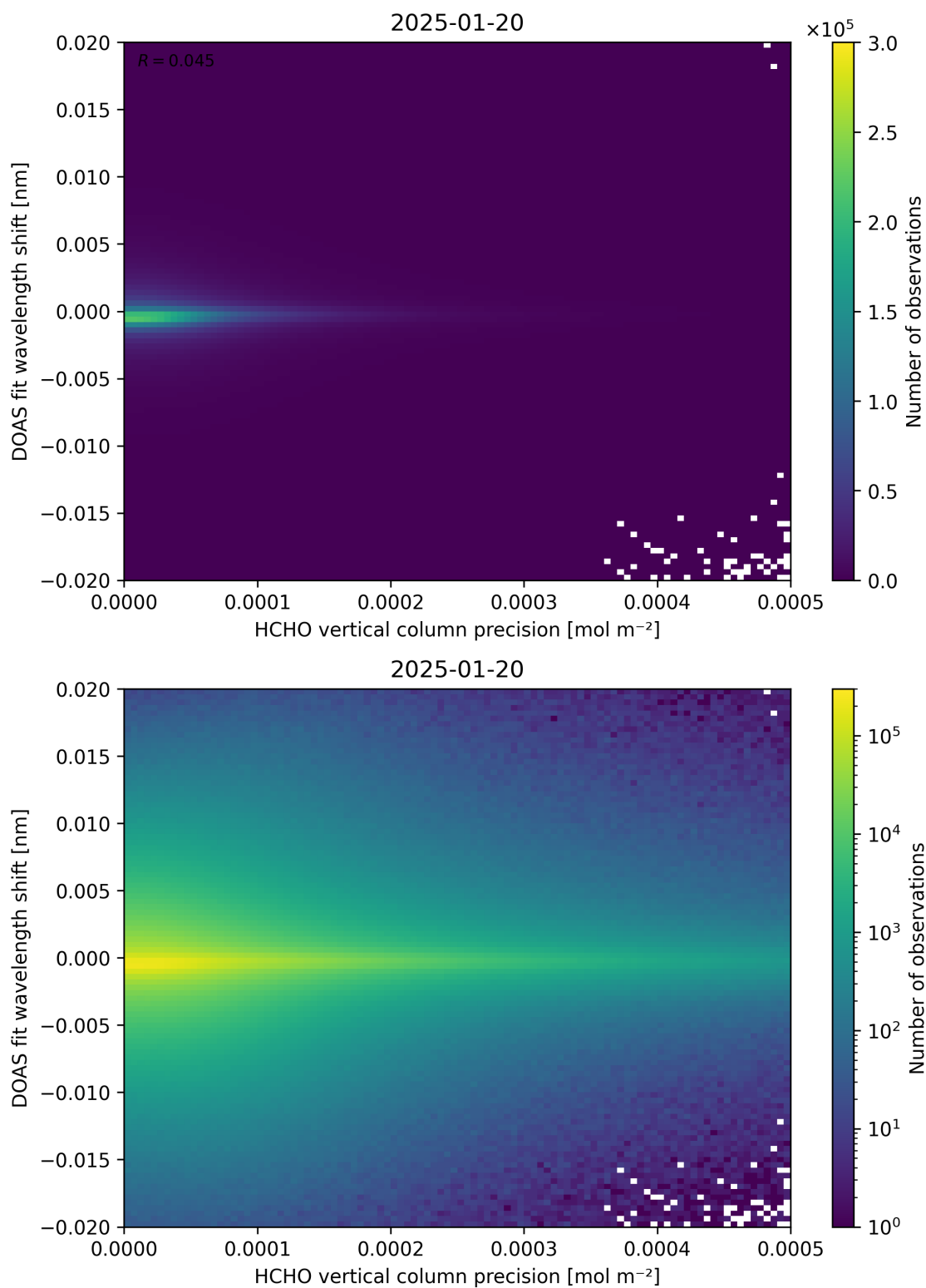
Figure 137: Scatter density plot of “HCHO vertical column precision” against “DOAS fit wavelength shift” for 2025-01-19 to 2025-01-21.
