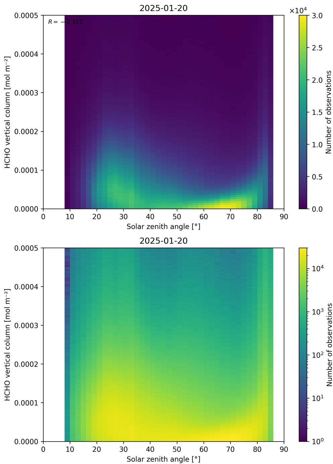
Figure 177: Scatter density plot of “Solar zenith angle” against “HCHO vertical column” for 2025-01-19 to 2025-01-21.
