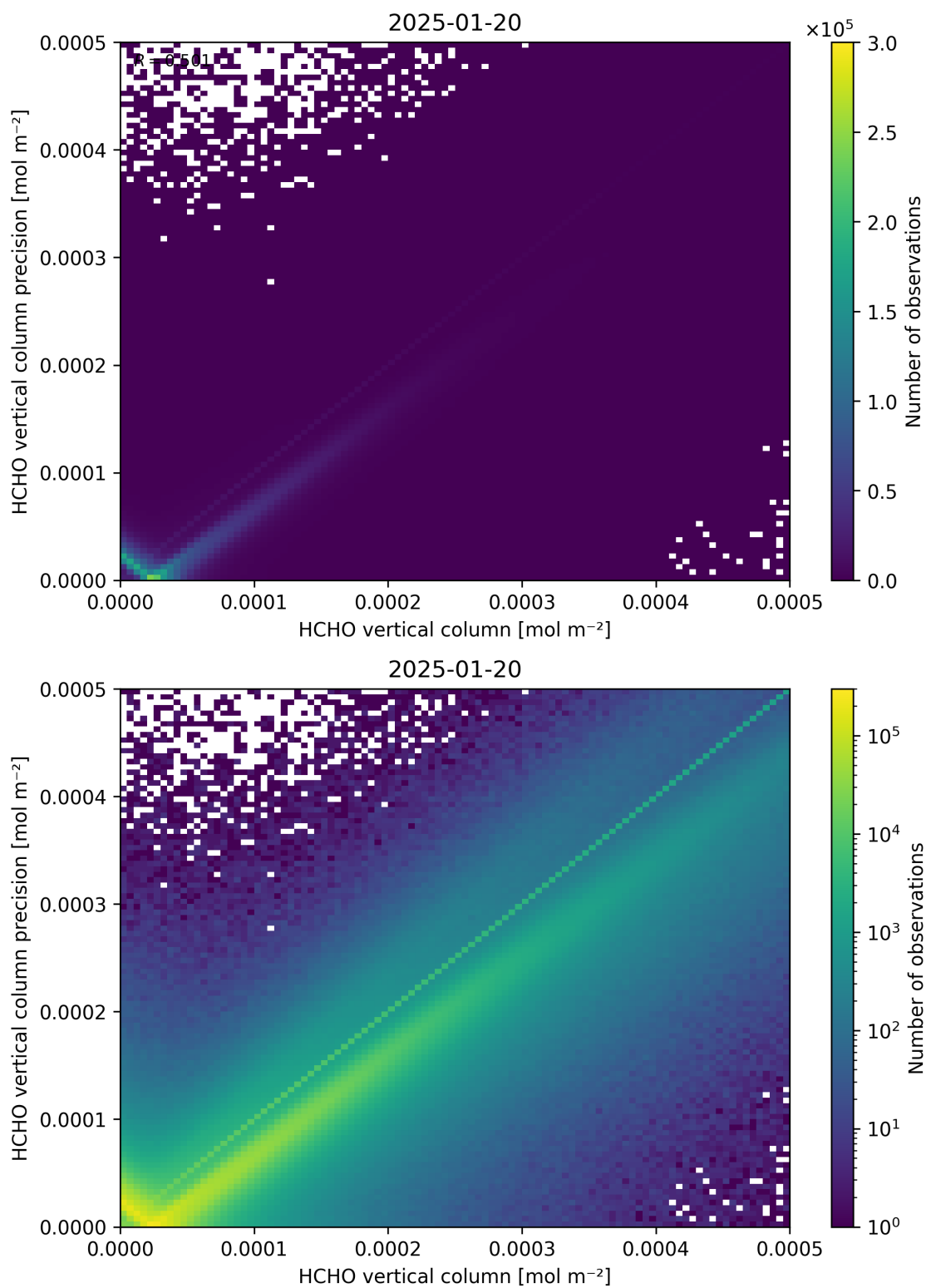
Figure 134: Scatter density plot of “HCHO vertical column” against “HCHO vertical column precision” for 2025-01-19 to 2025-01-21.
