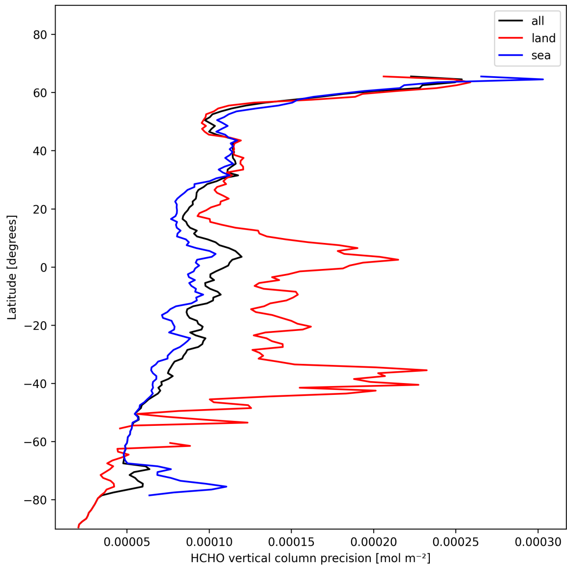
Figure 22: Zonal average of “HCHO vertical column precision” for 2025-01-19 to 2025-01-21.
