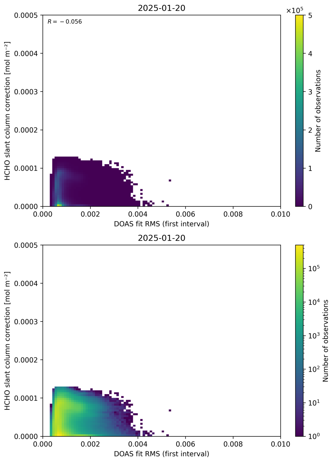
Figure 63: Scatter density plot of “DOAS fit RMS (first interval)” against “HCHO slant column correction” for 2025-01-19 to 2025-01-21.
