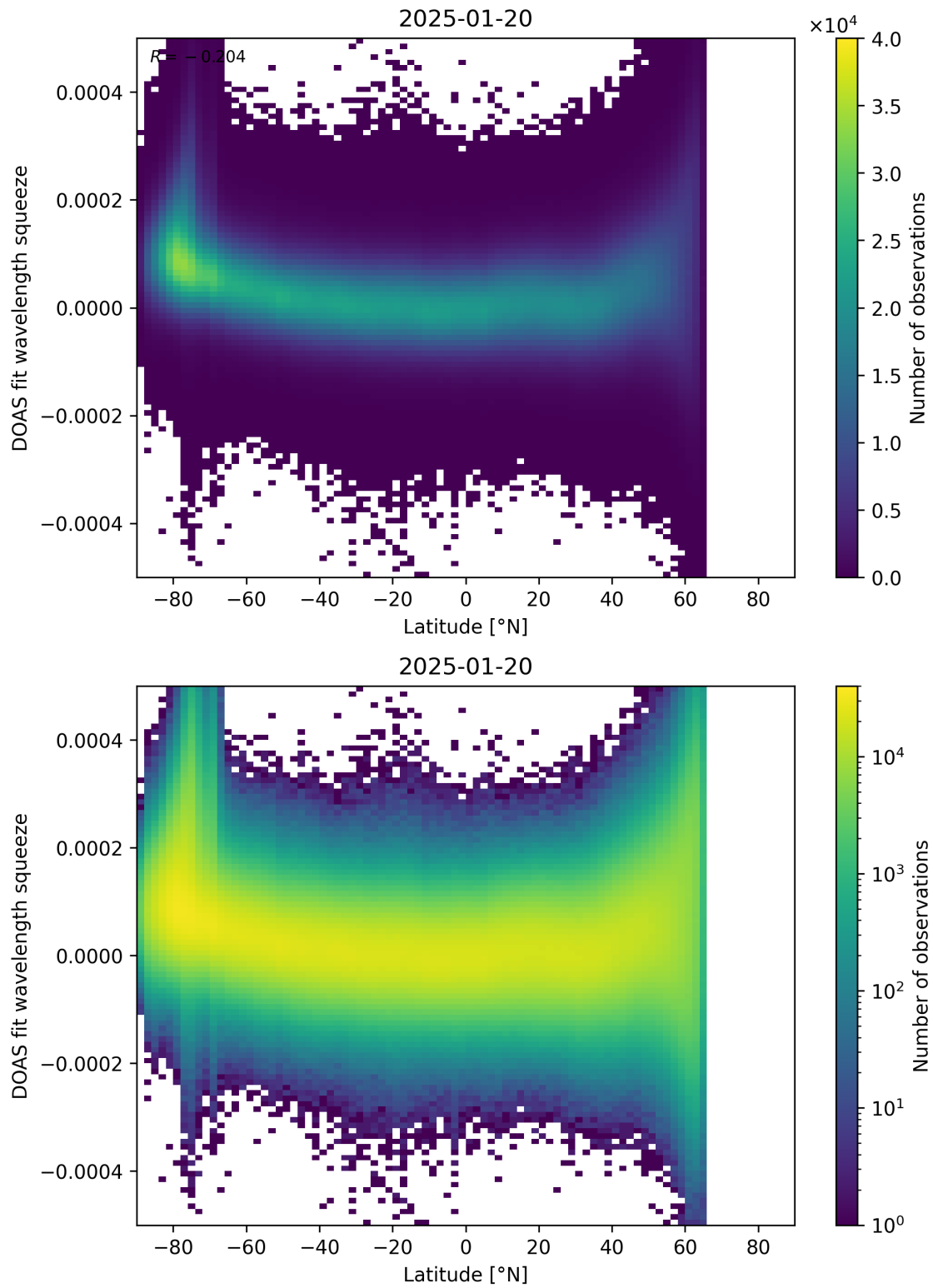
Figure 155: Scatter density plot of “Latitude” against “DOAS fit wavelength squeeze” for 2025-01-19 to 2025-01-21.
