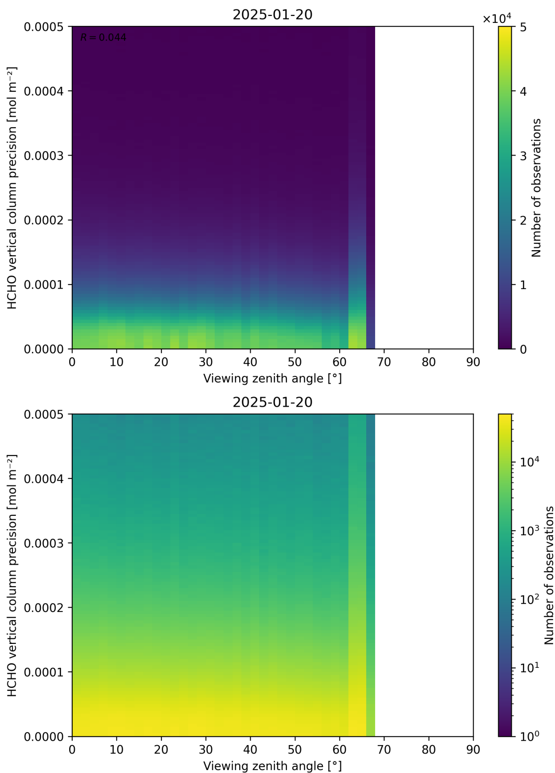
Figure 194: Scatter density plot of “Viewing zenith angle” against “HCHO vertical column precision” for 2025-01-19 to 2025-01-21.
