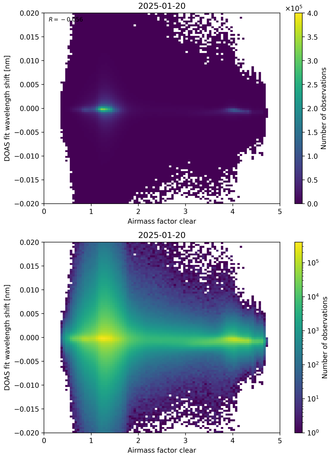
Figure 72: Scatter density plot of “Airmass factor clear” against “DOAS fit wavelength shift” for 2025-01-19 to 2025-01-21.
