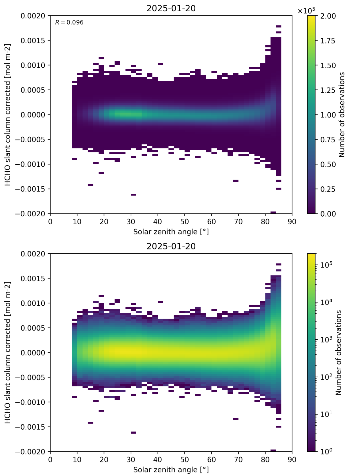
Figure 171: Scatter density plot of “Solar zenith angle” against “HCHO slant column corrected” for 2025-01-19 to 2025-01-21.
