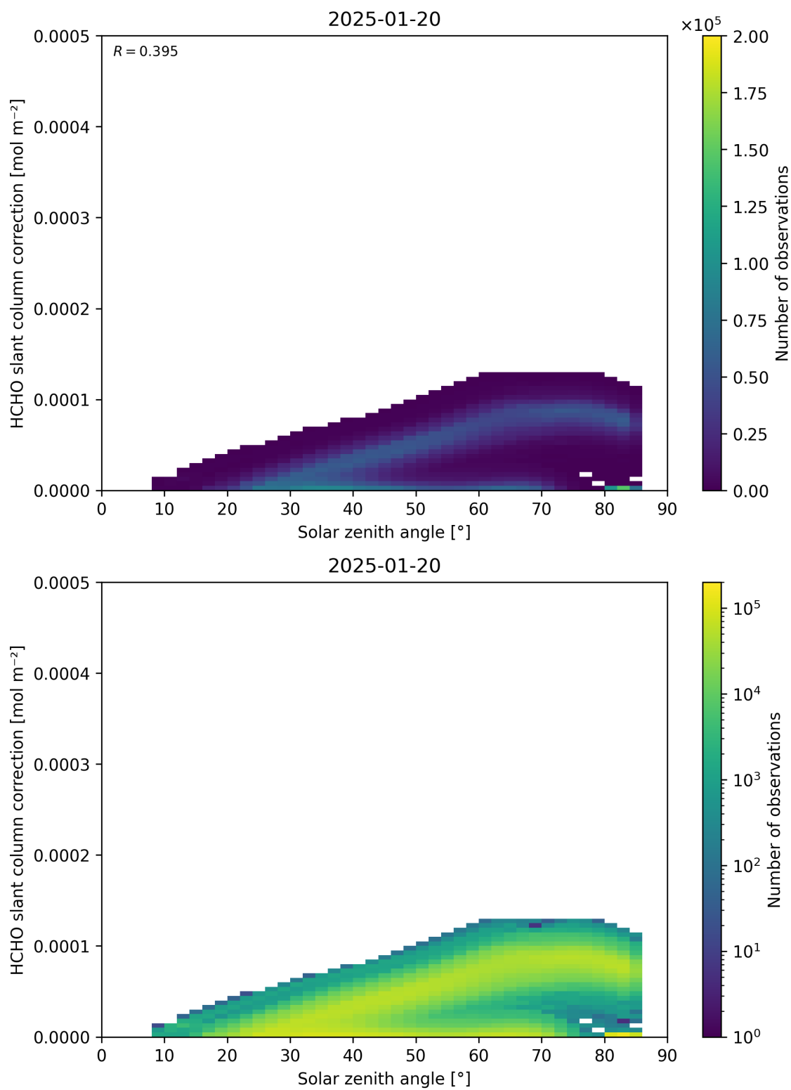
Figure 172: Scatter density plot of “Solar zenith angle” against “HCHO slant column correction” for 2025-01-19 to 2025-01-21.
