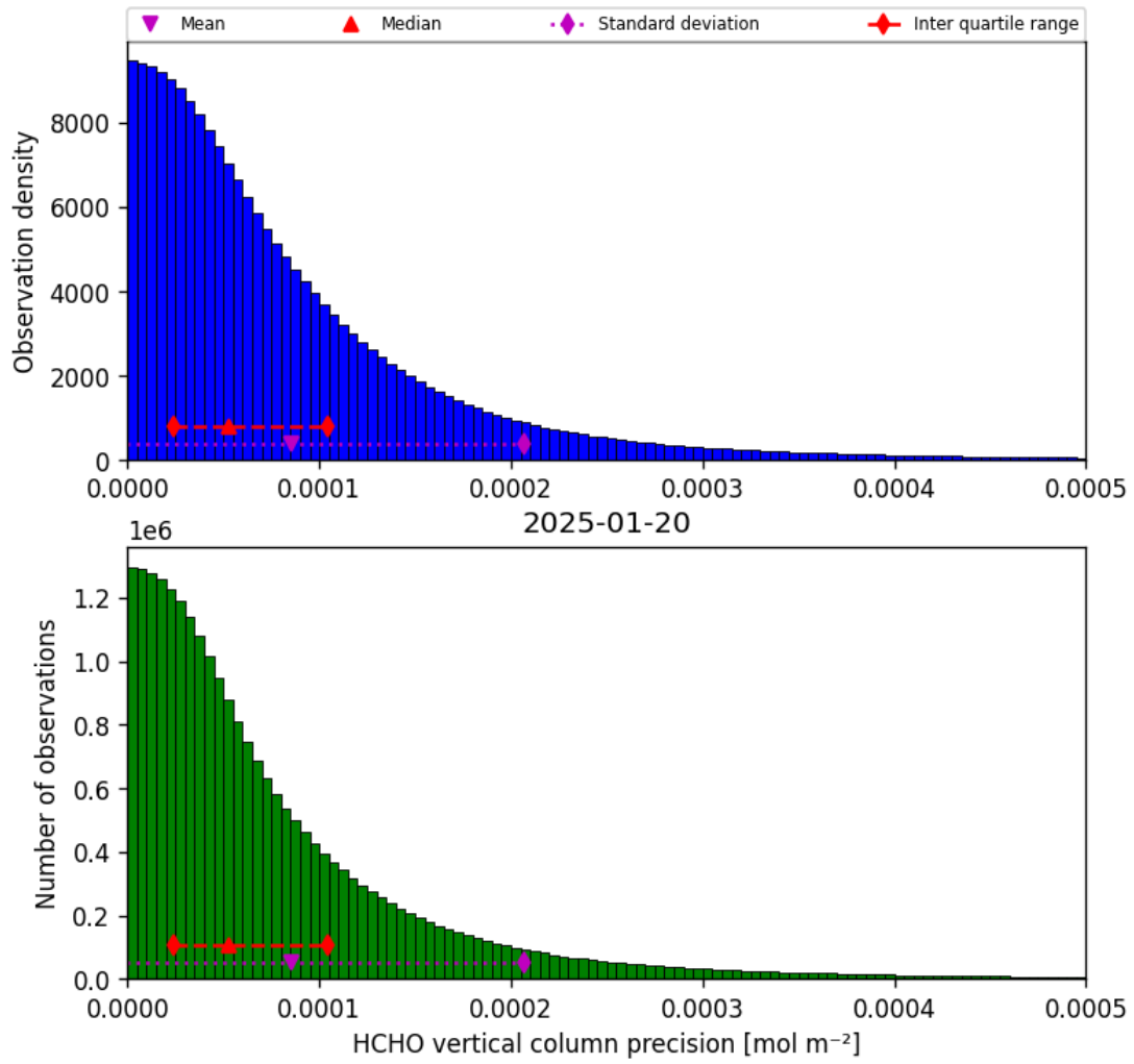
Figure 36: Histogram of “HCHO vertical column precision” for 2025-01-19 to 2025-01-21
