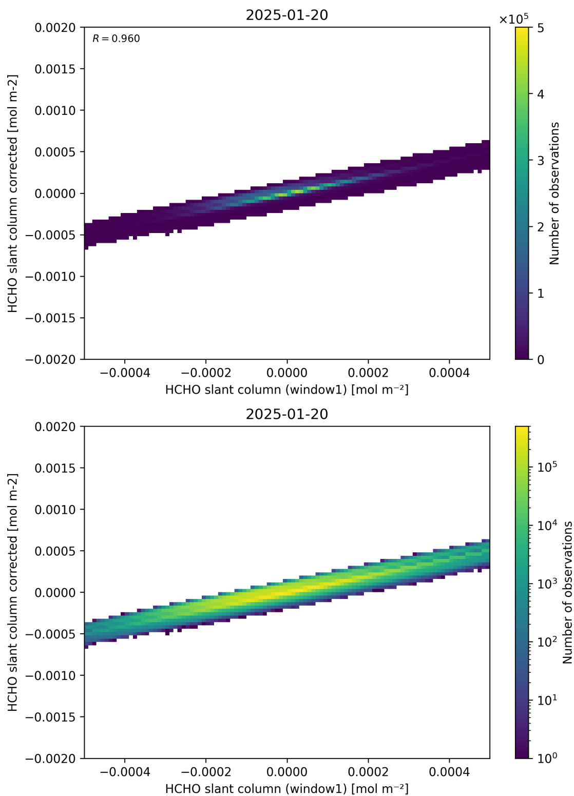
Figure 82: Scatter density plot of “HCHO slant column (window1)” against “HCHO slant column corrected” for 2025-01-19 to 2025-01-21.
