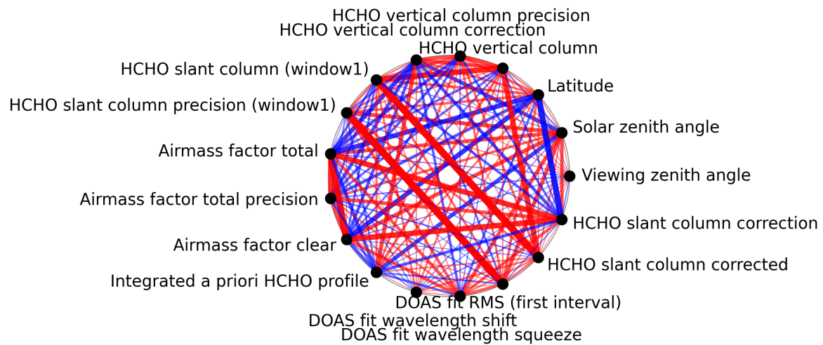
Figure 1: Map of correlation graph for 2025-01-19 to 2025-01-21.
