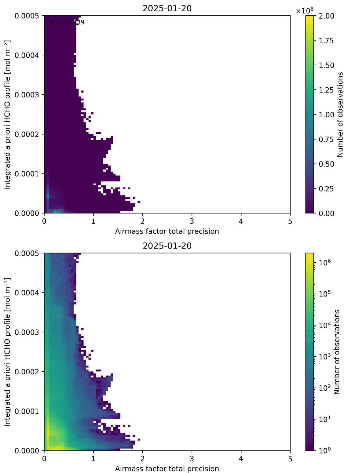
Figure 111: Scatter density plot of “Airmass factor total precision” against “Integrated a priori HCHO profile” for 2025-01-19 to 2025-01-21.
