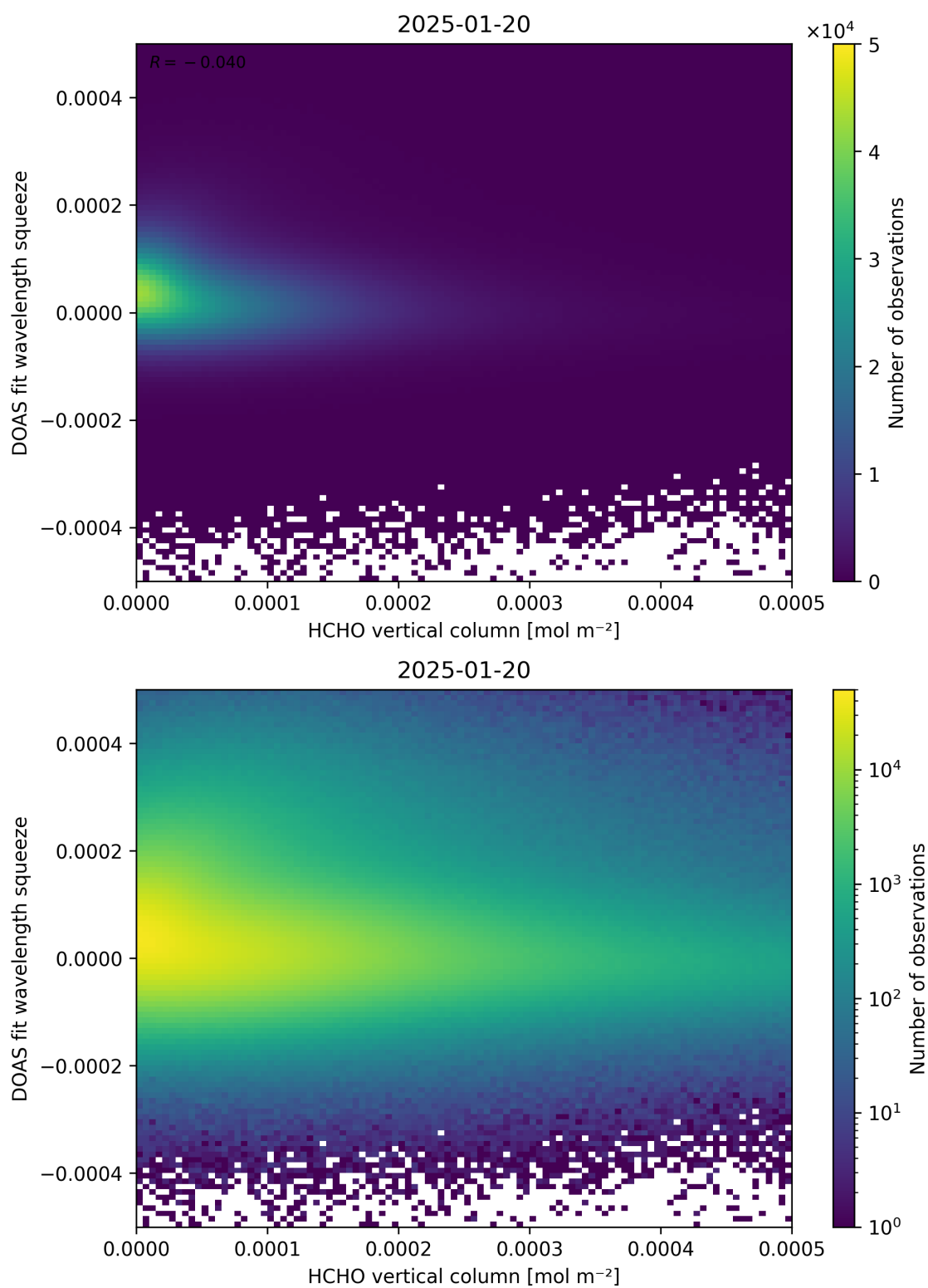
Figure 125: Scatter density plot of “HCHO vertical column” against “DOAS fit wavelength squeeze” for 2025-01-19 to 2025-01-21.
