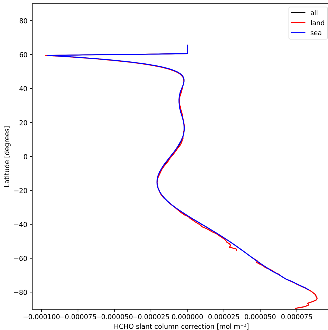
Figure 33: Zonal average of “HCHO slant column correction” for 2025-01-19 to 2025-01-21.
