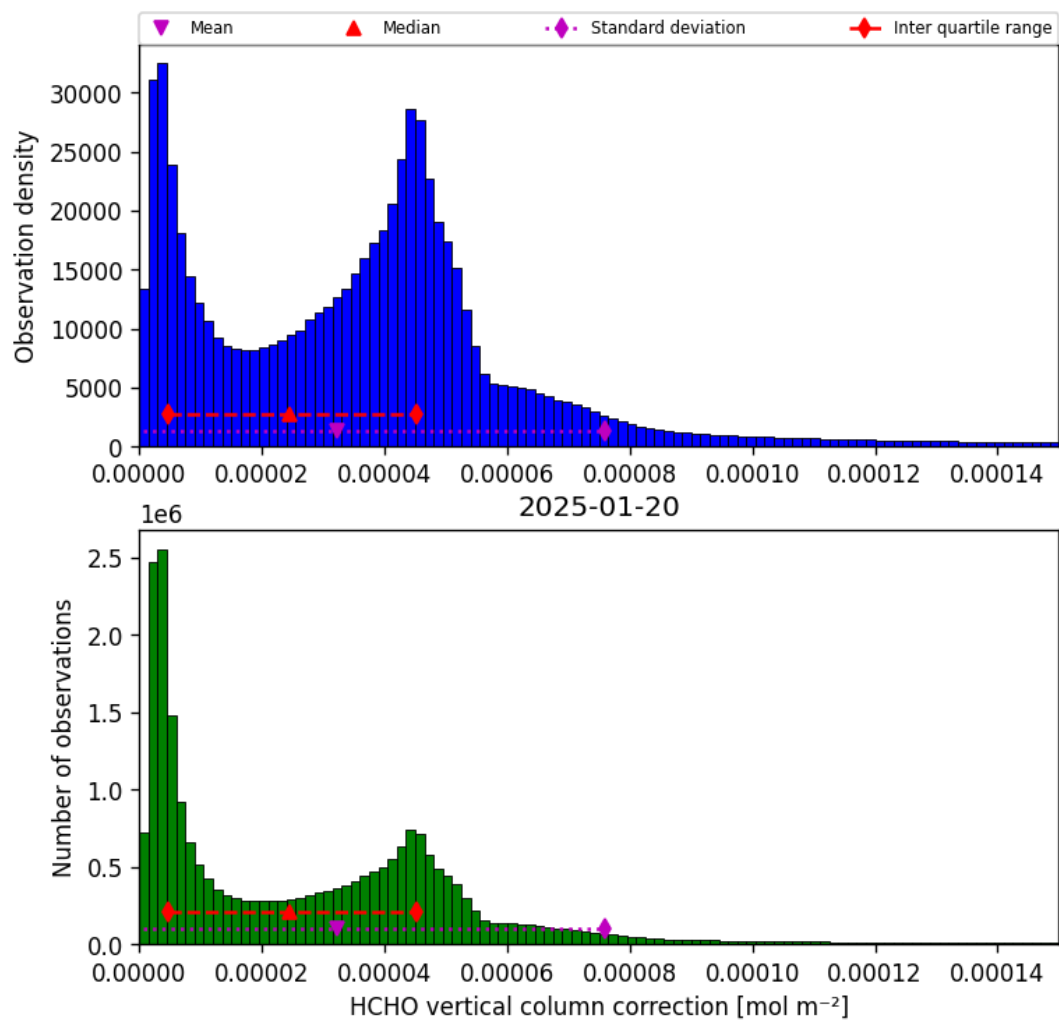
Figure 37: Histogram of “HCHO vertical column correction” for 2025-01-19 to 2025-01-21
