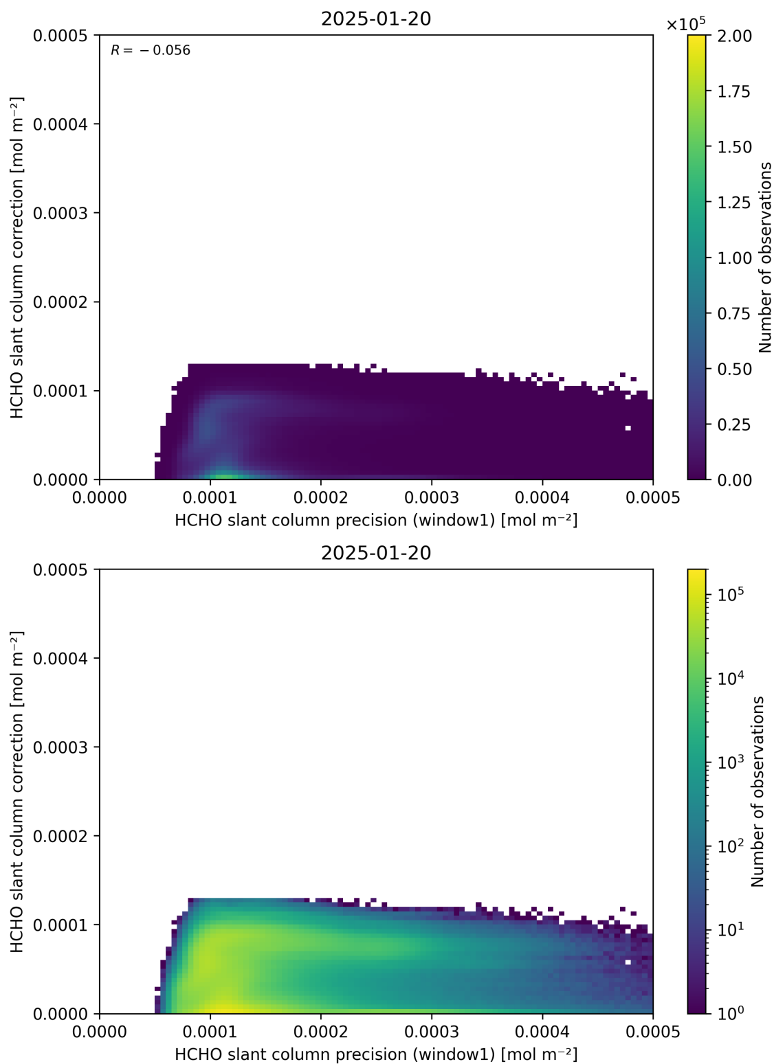
Figure 93: Scatter density plot of “HCHO slant column precision (window1)” against “HCHO slant column correction” for 2025-01-19 to 2025-01-21.
