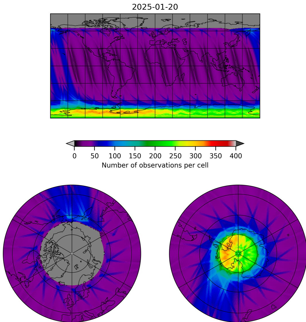
Figure 19: Map of the number of observations for 2025-01-19 to 2025-01-21
