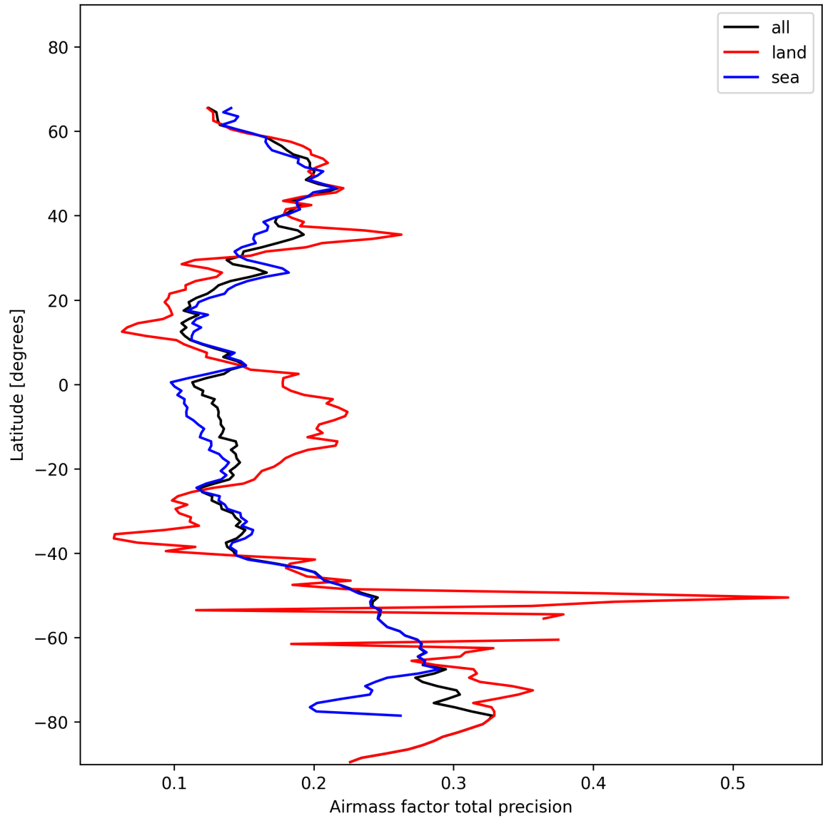
Figure 27: Zonal average of “Airmass factor total precision” for 2025-01-19 to 2025-01-21.
