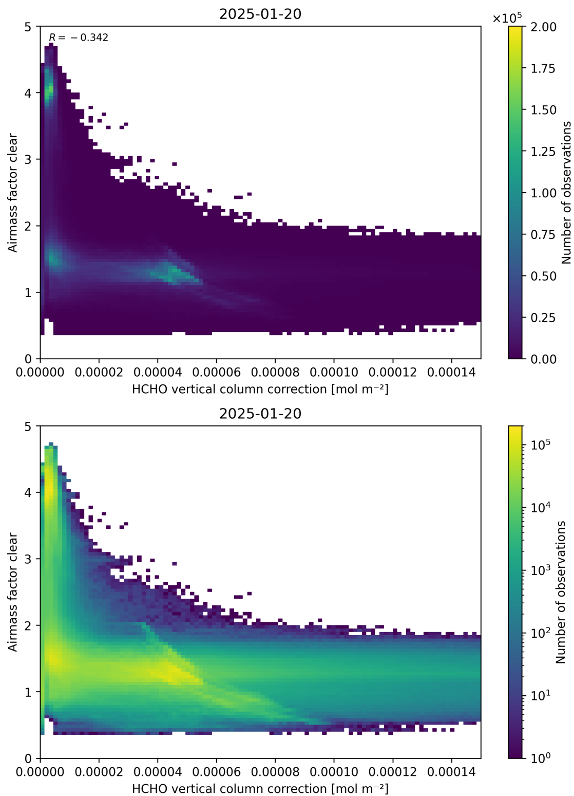
Figure 115: Scatter density plot of “HCHO vertical column correction” against “Airmass factor clear” for 2025-01-19 to 2025-01-21.
