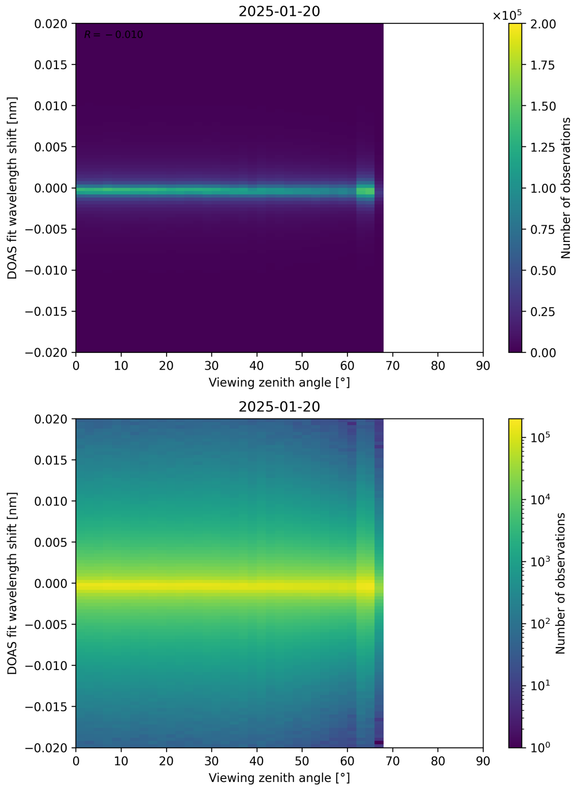
Figure 183: Scatter density plot of “Viewing zenith angle” against “DOAS fit wavelength shift” for 2025-01-19 to 2025-01-21.
