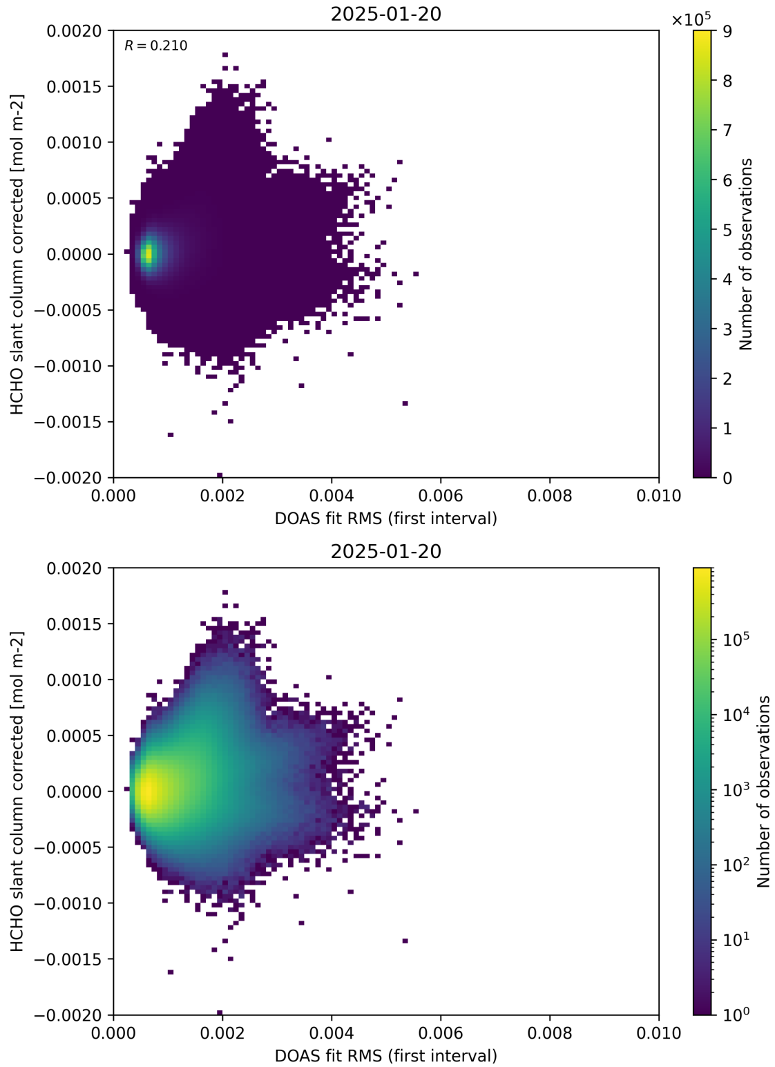
Figure 62: Scatter density plot of “DOAS fit RMS (first interval)” against “HCHO slant column corrected” for 2025-01-19 to 2025-01-21.
