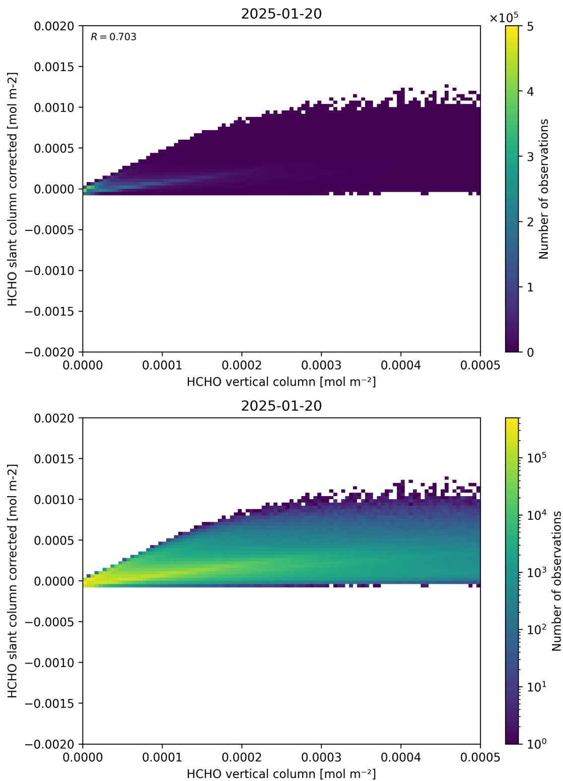
Figure 127: Scatter density plot of “HCHO vertical column” against “HCHO slant column corrected” for 2025-01-19 to 2025-01-21.
