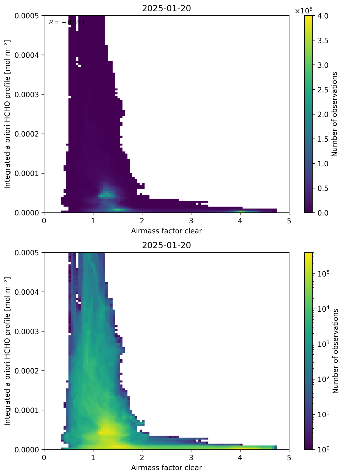
Figure 76: Scatter density plot of “Airmass factor clear” against “Integrated a priori HCHO profile” for 2025-01-19 to 2025-01-21.
