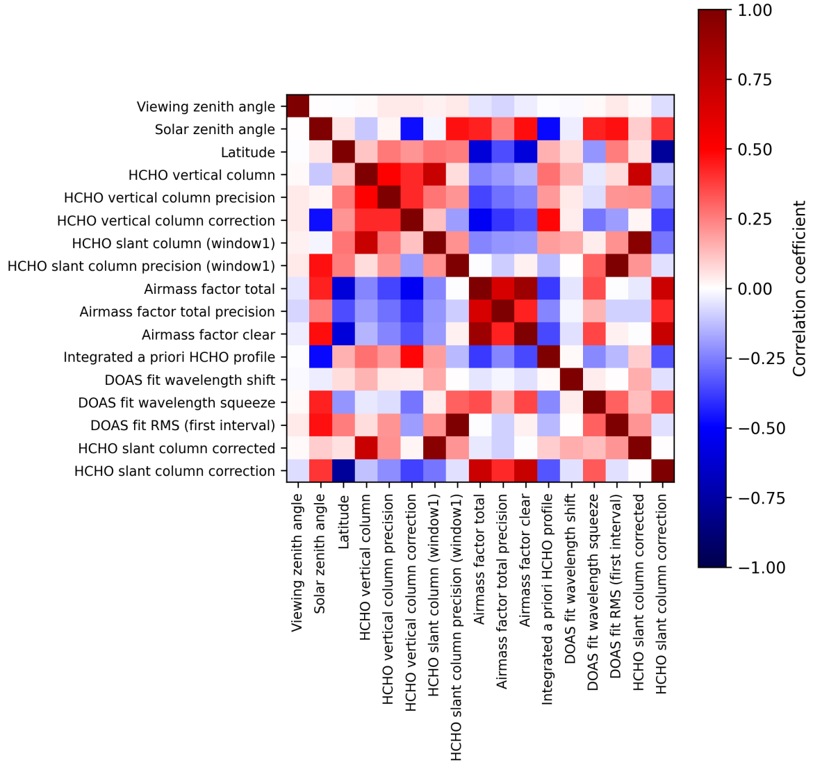
Figure 2: Map of correlation matrix for 2025-01-19 to 2025-01-21.
