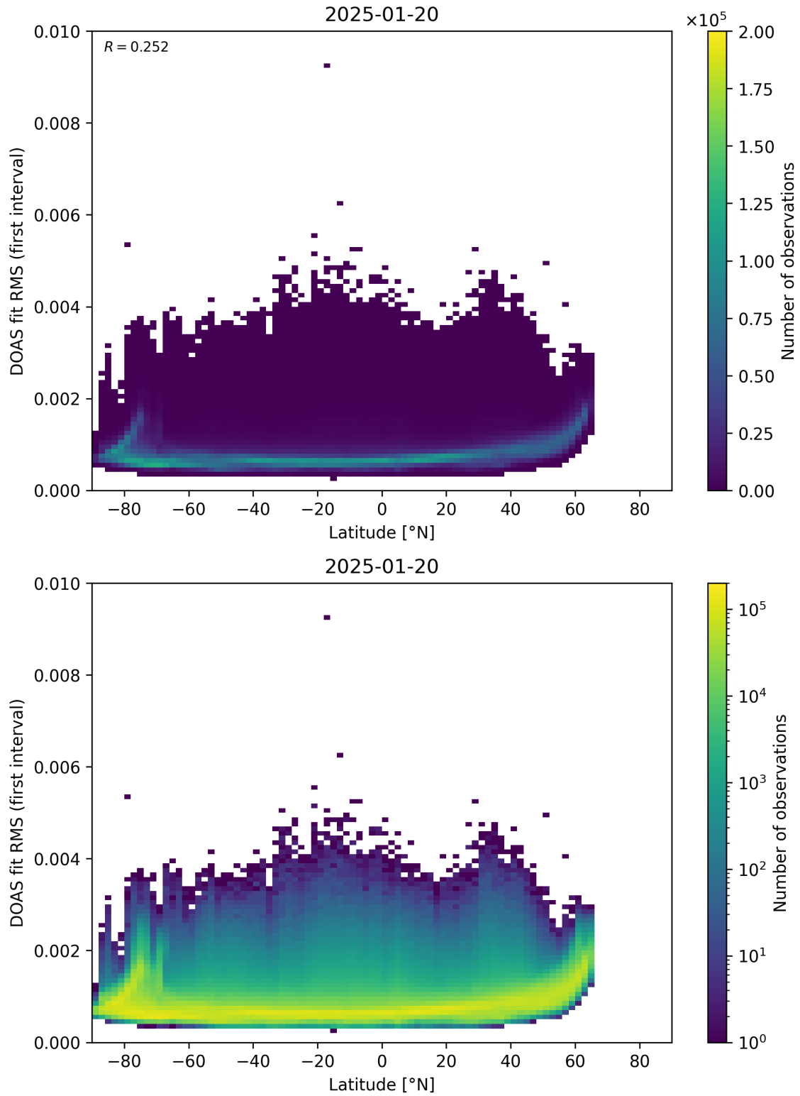
Figure 153: Scatter density plot of “Latitude” against “DOAS fit RMS (first interval)” for 2025-01-19 to 2025-01-21.
