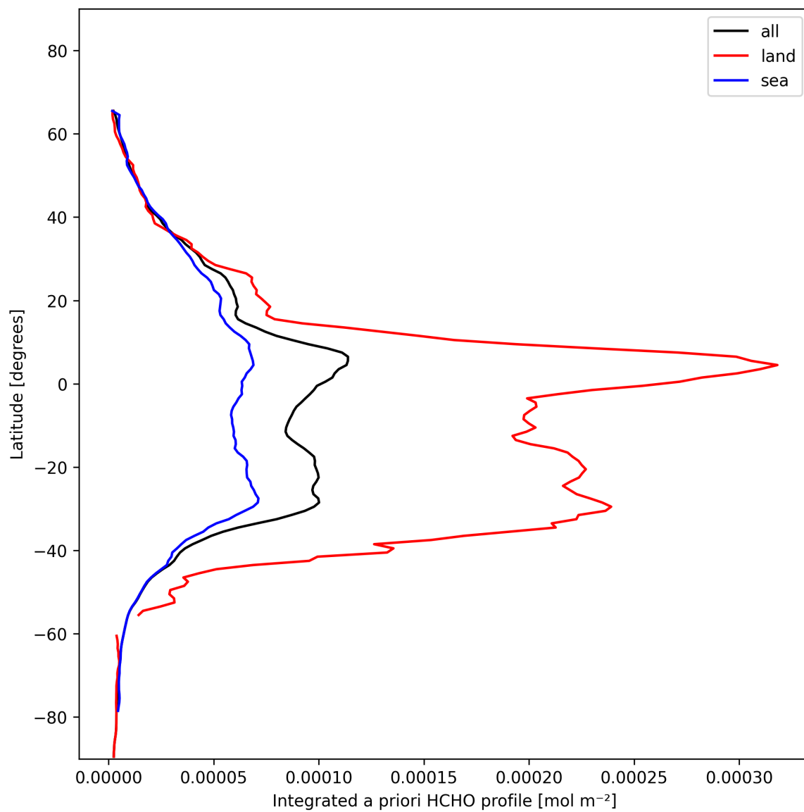
Figure 29: Zonal average of “Integrated a priori HCHO profile” for 2025-01-19 to 2025-01-21.
