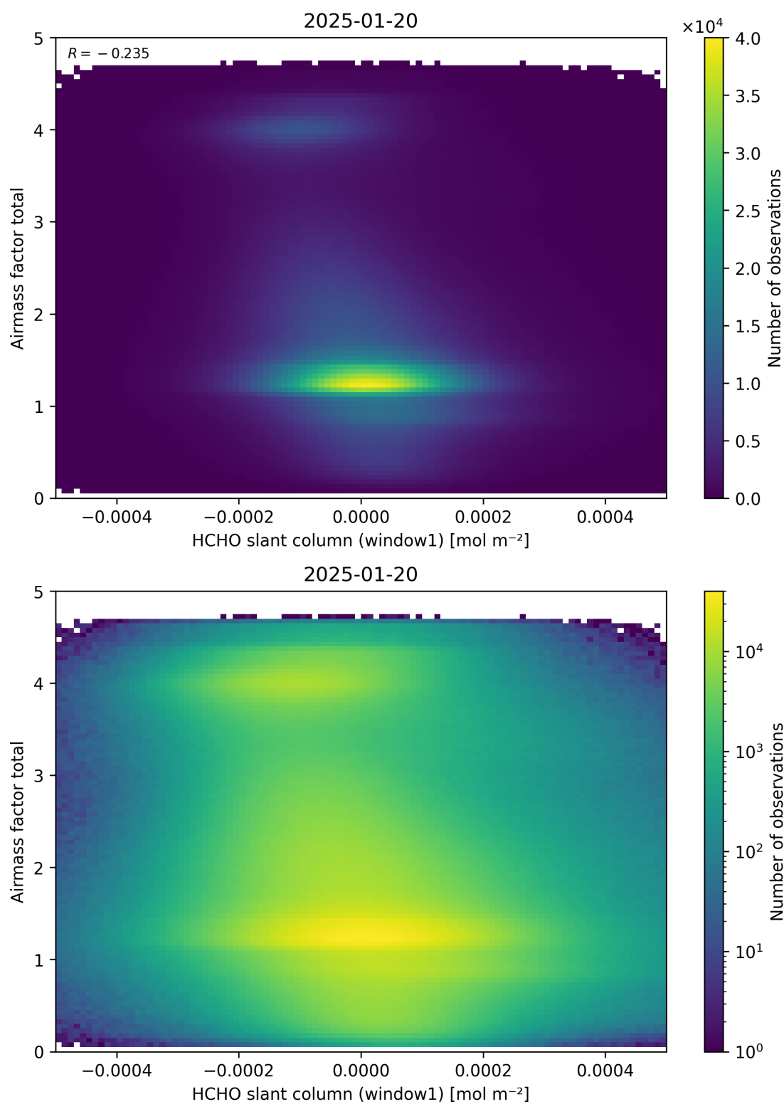
Figure 85: Scatter density plot of “HCHO slant column (window1)” against “Airmass factor total” for 2025-01-19 to 2025-01-21.
