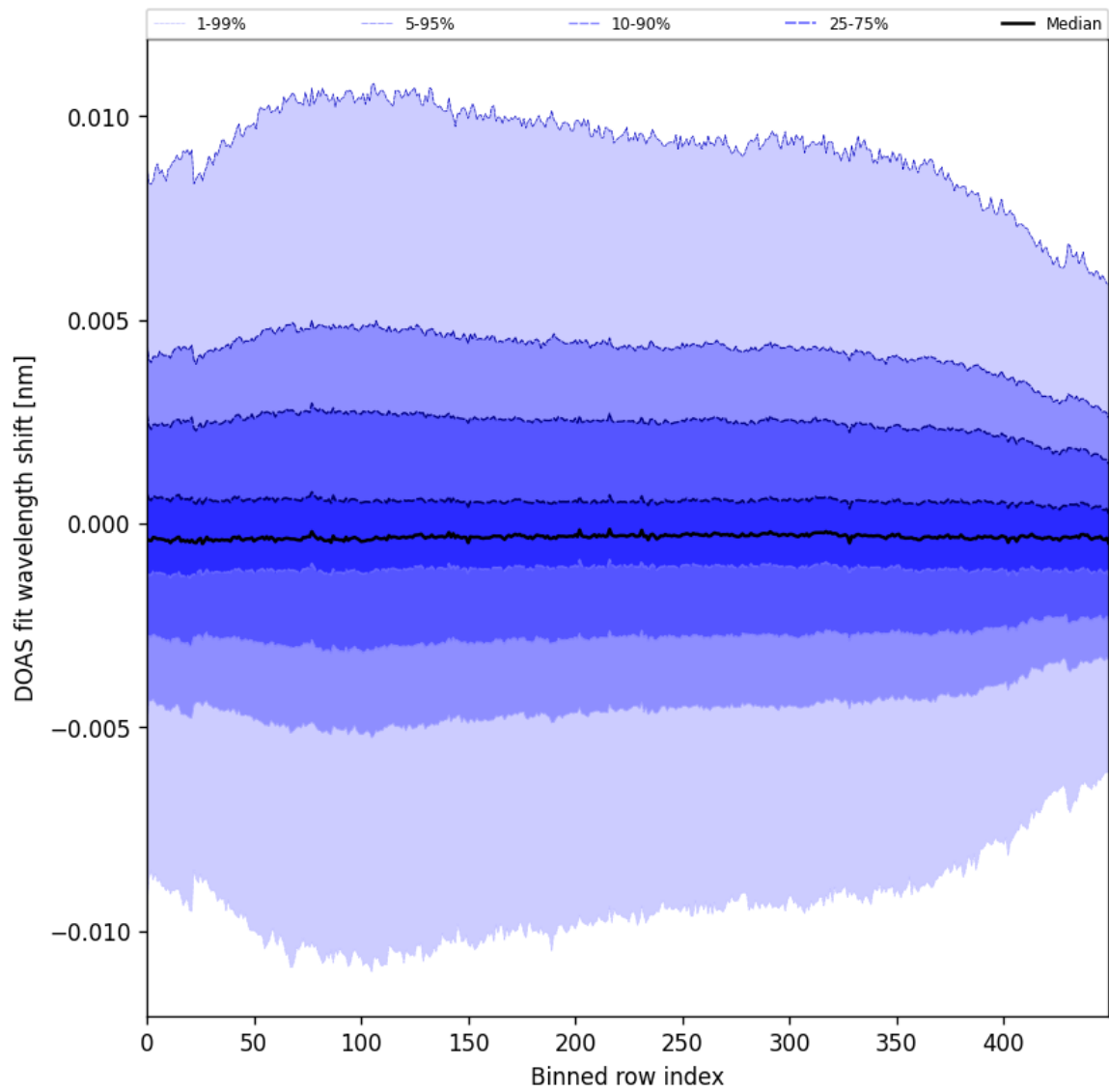
Figure 58: Along track statistics of “DOAS fit wavelength shift” for 2025-01-19 to 2025-01-21
