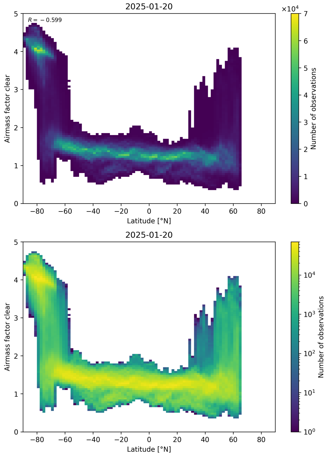
Figure 156: Scatter density plot of “Latitude” against “Airmass factor clear” for 2025-01-19 to 2025-01-21.
