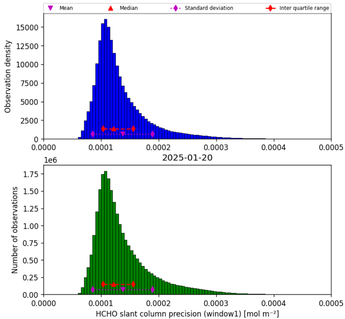
Figure 39: Histogram of “HCHO slant column precision (window1)” for 2025-01-19 to 2025-01-21
