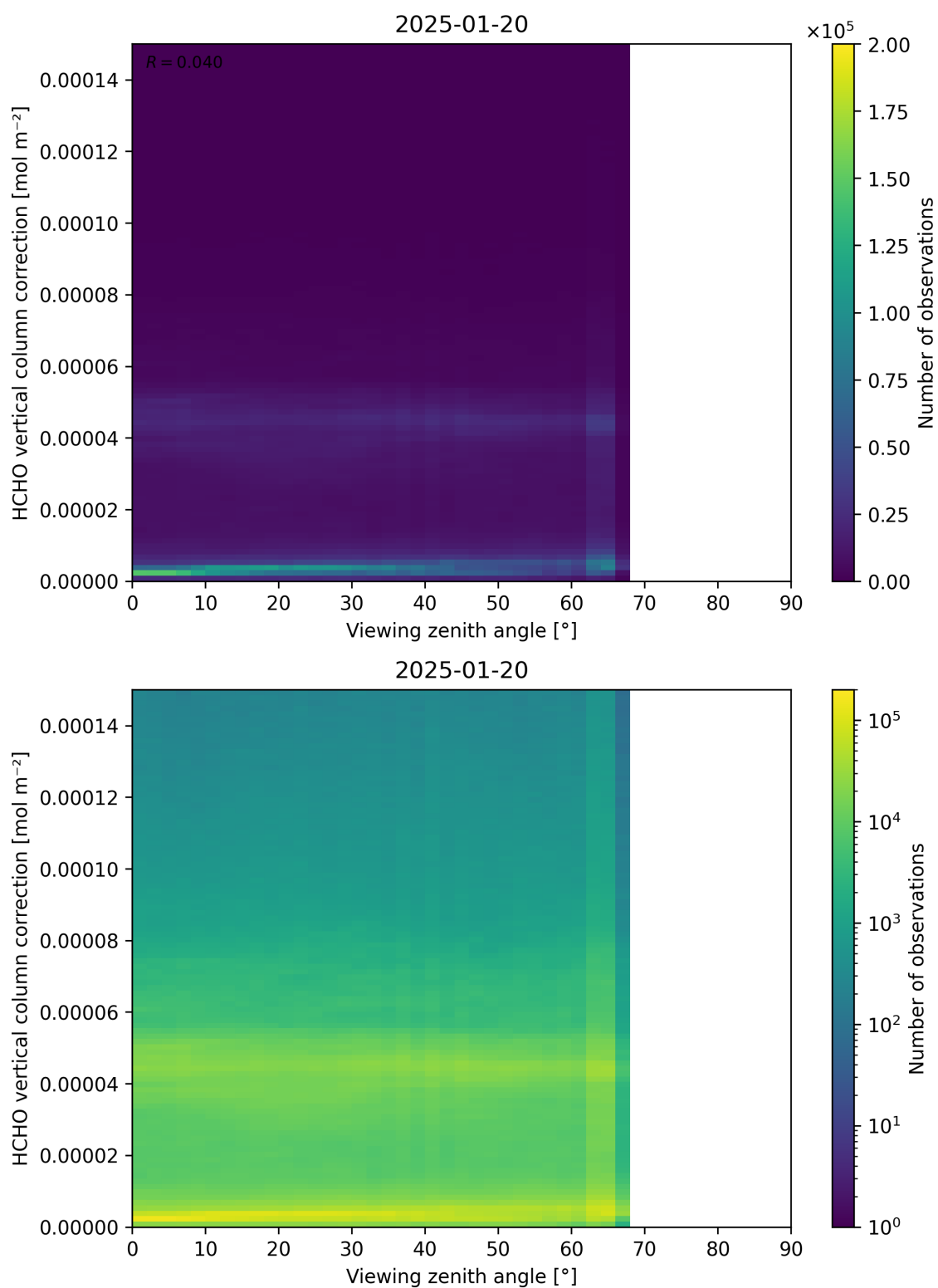
Figure 193: Scatter density plot of “Viewing zenith angle” against “HCHO vertical column correction” for 2025-01-19 to 2025-01-21.
