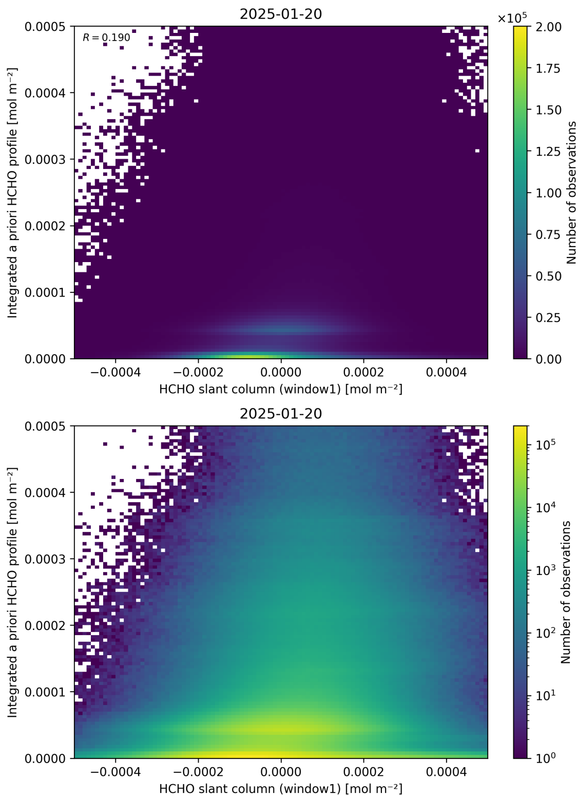
Figure 87: Scatter density plot of “HCHO slant column (window1)” against “Integrated a priori HCHO profile” for 2025-01-19 to 2025-01-21.
