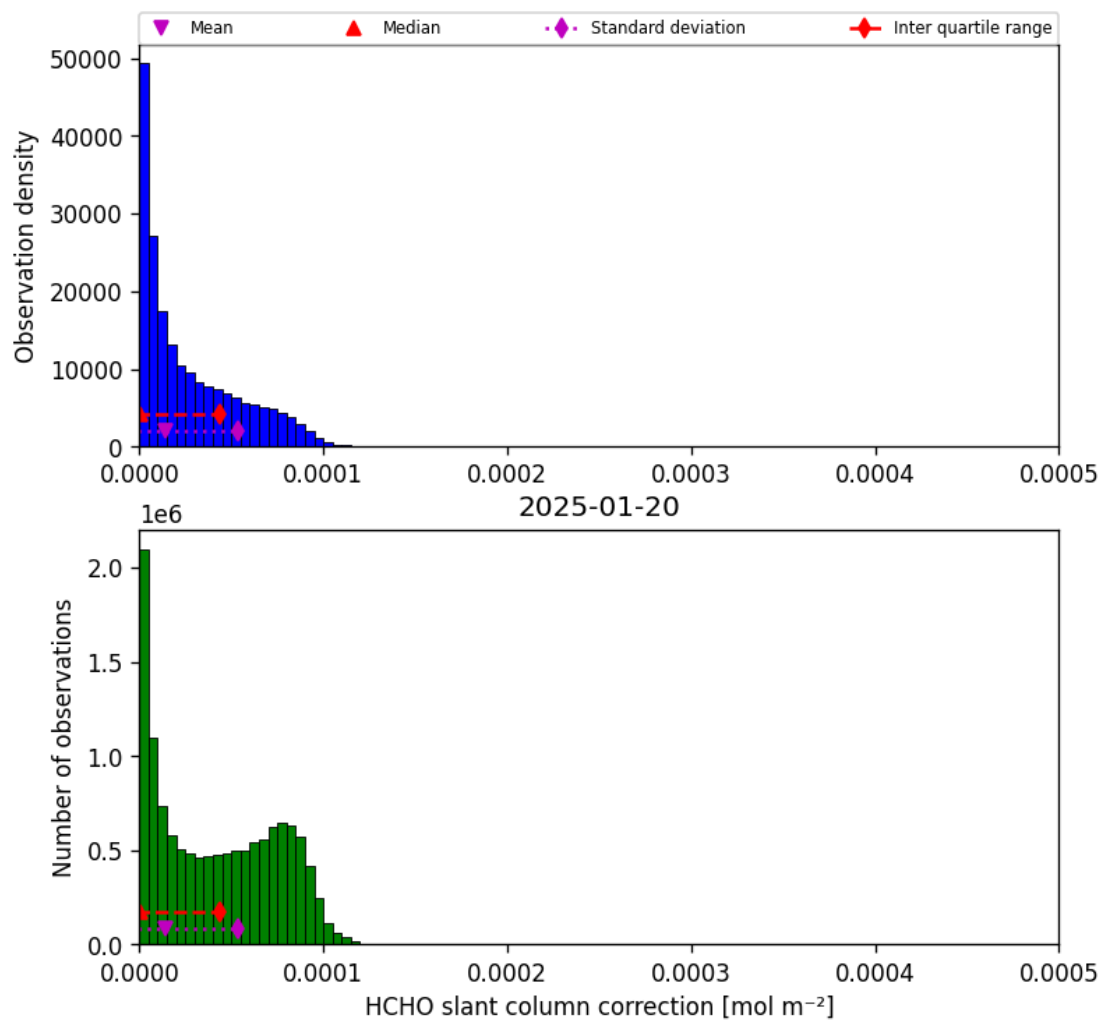
Figure 47: Histogram of “HCHO slant column correction” for 2025-01-19 to 2025-01-21
