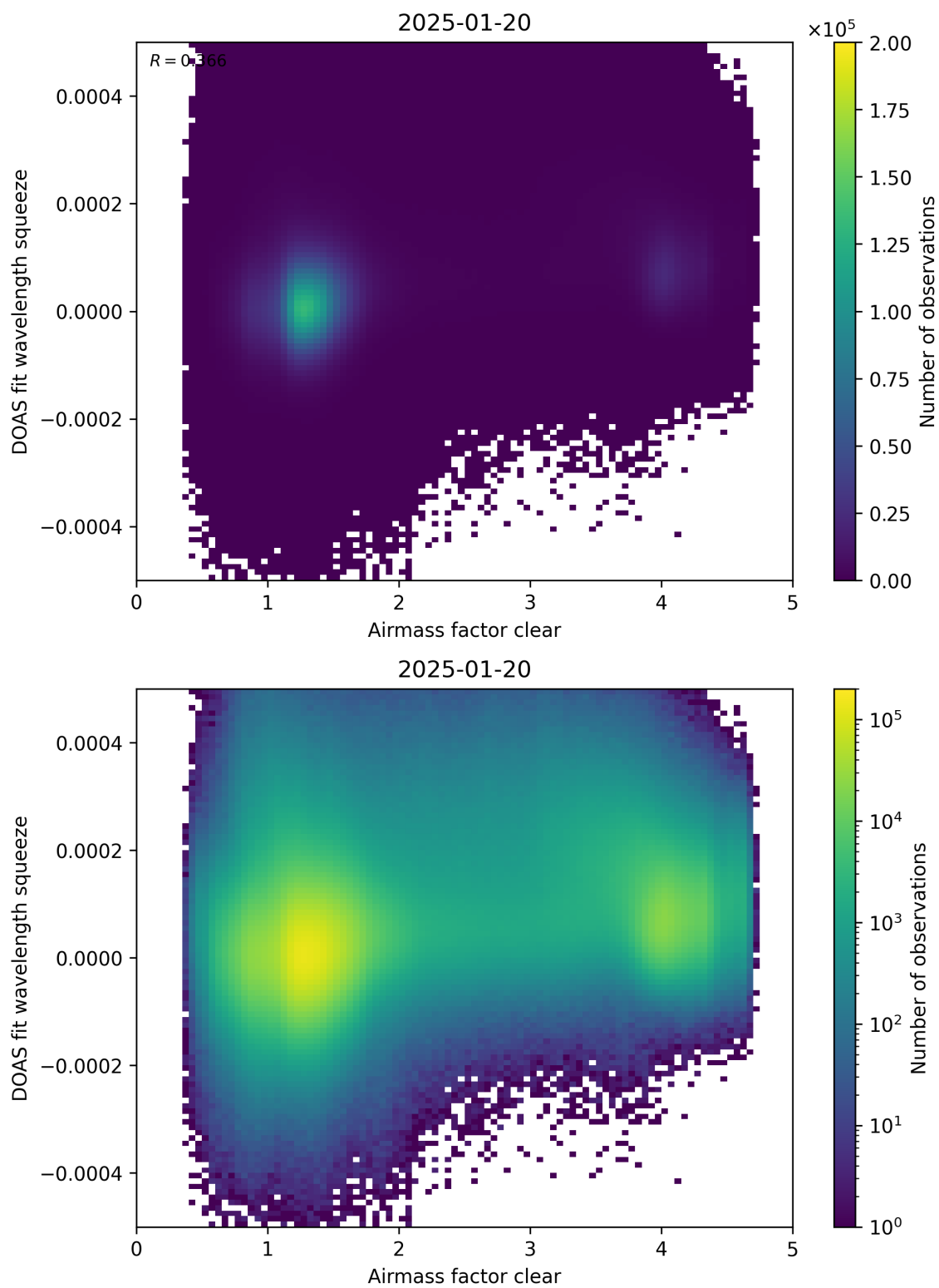
Figure 73: Scatter density plot of “Airmass factor clear” against “DOAS fit wavelength squeeze” for 2025-01-19 to 2025-01-21.
