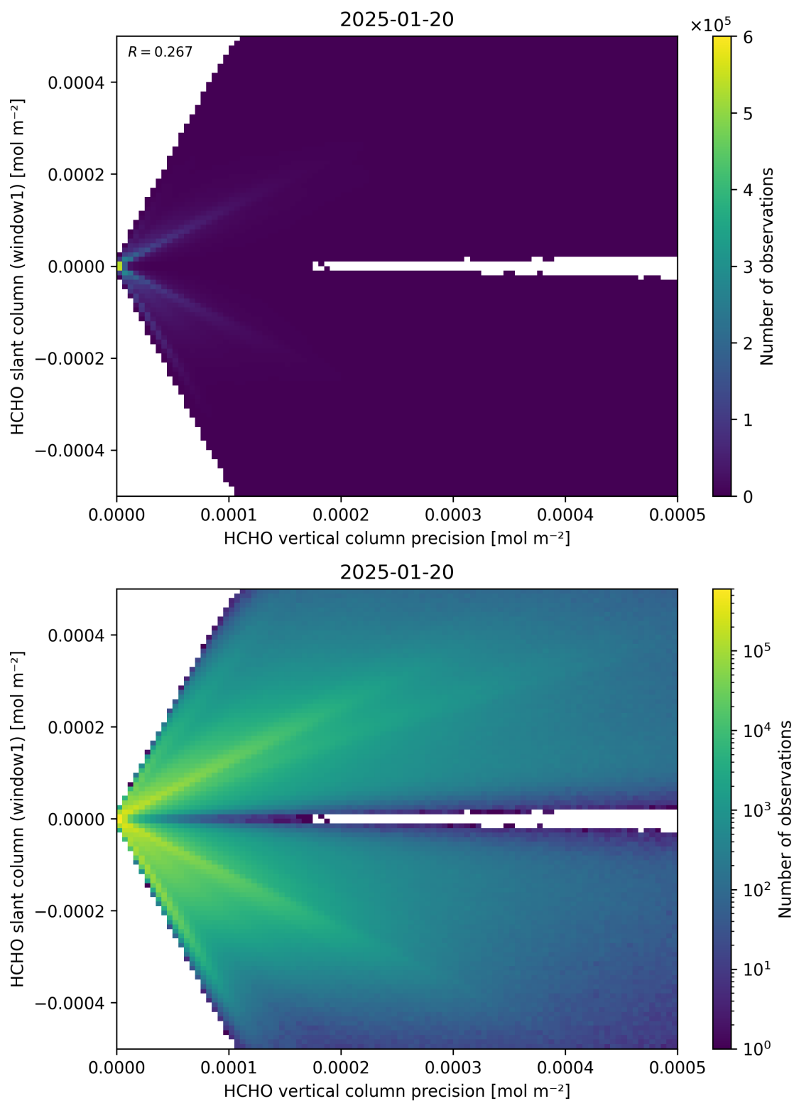
Figure 142: Scatter density plot of “HCHO vertical column precision” against “HCHO slant column (window1)” for 2025-01-19 to 2025-01-21.
