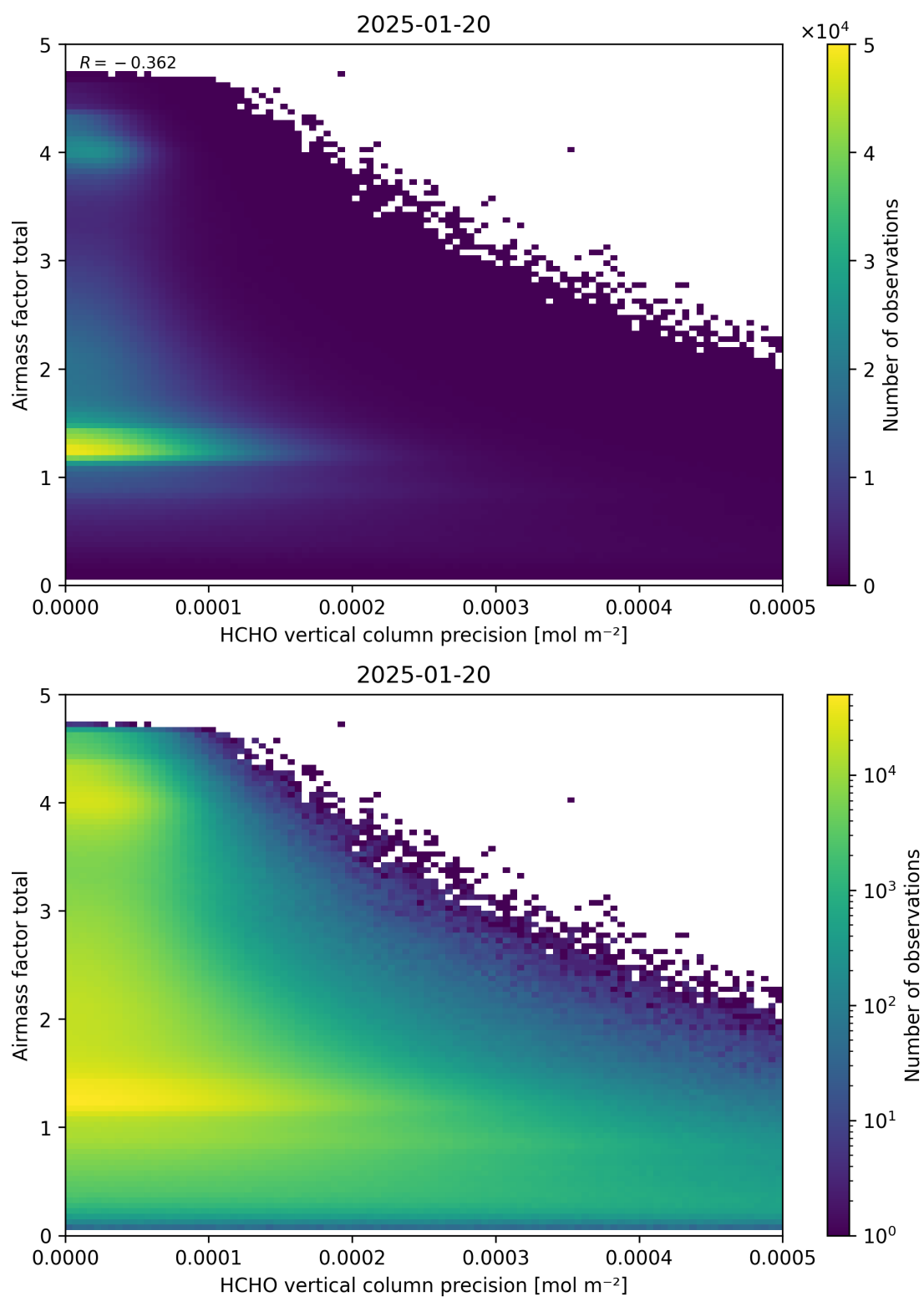
Figure 144: Scatter density plot of “HCHO vertical column precision” against “Airmass factor total” for 2025-01-19 to 2025-01-21.
