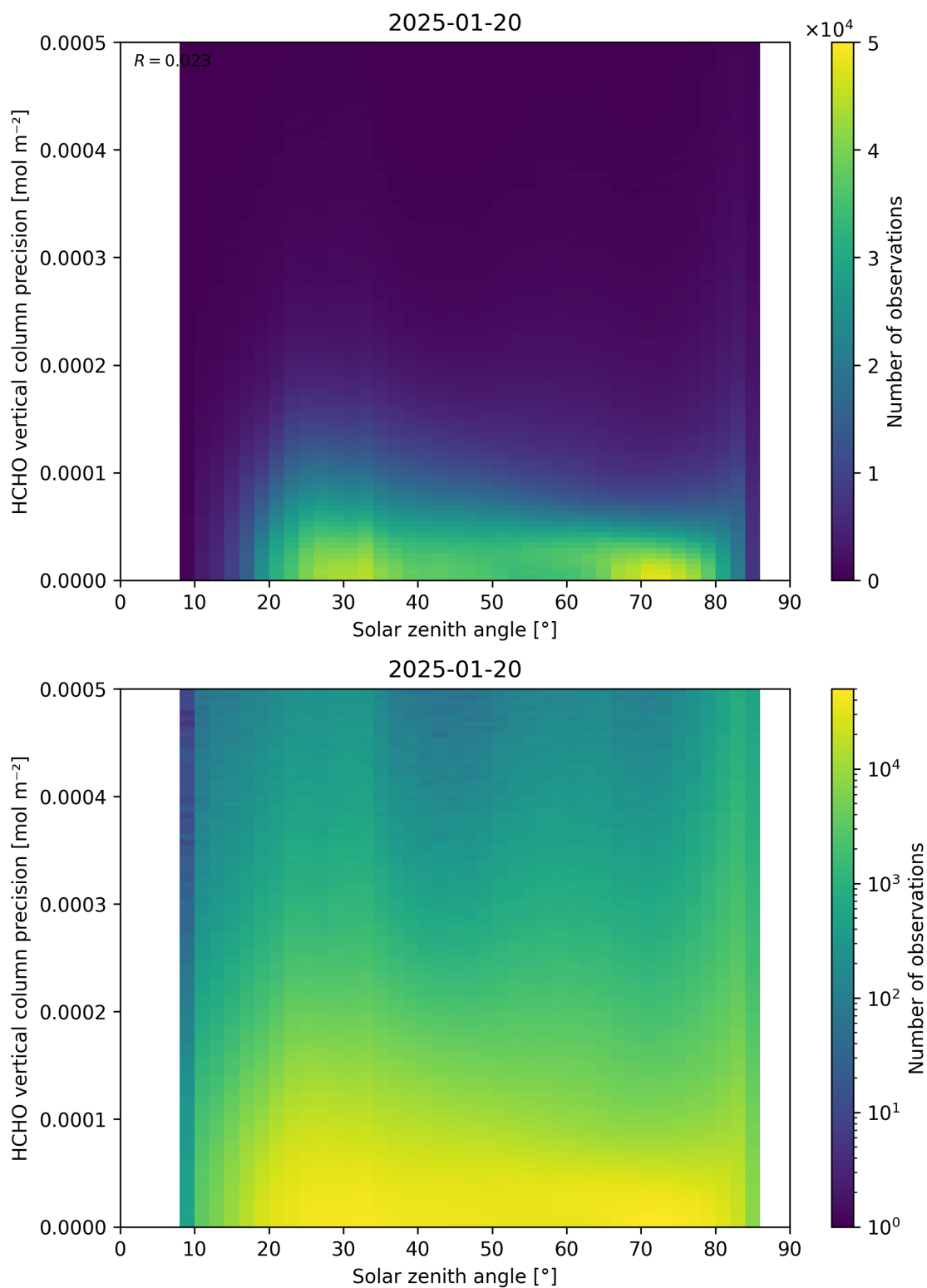
Figure 179: Scatter density plot of “Solar zenith angle” against “HCHO vertical column precision” for 2025-01-19 to 2025-01-21.
