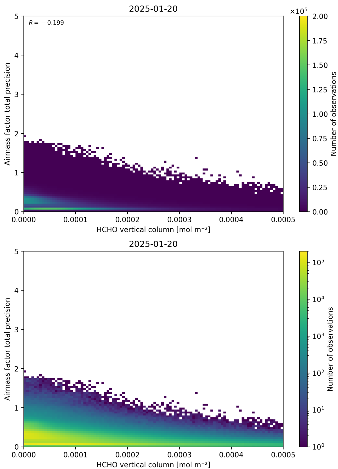
Figure 132: Scatter density plot of “HCHO vertical column” against “Airmass factor total precision” for 2025-01-19 to 2025-01-21.
