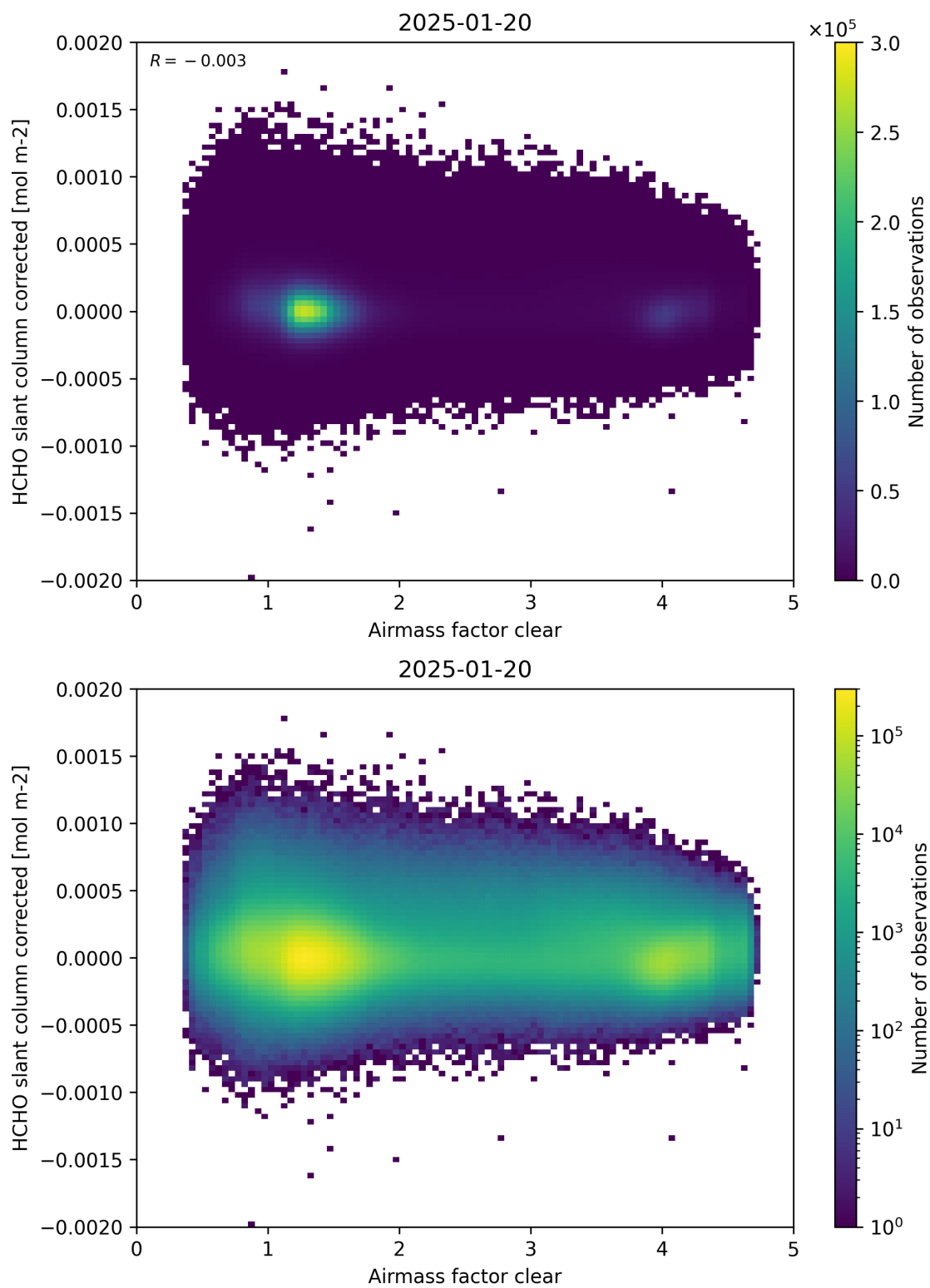
Figure 74: Scatter density plot of “Airmass factor clear” against “HCHO slant column corrected” for 2025-01-19 to 2025-01-21.
