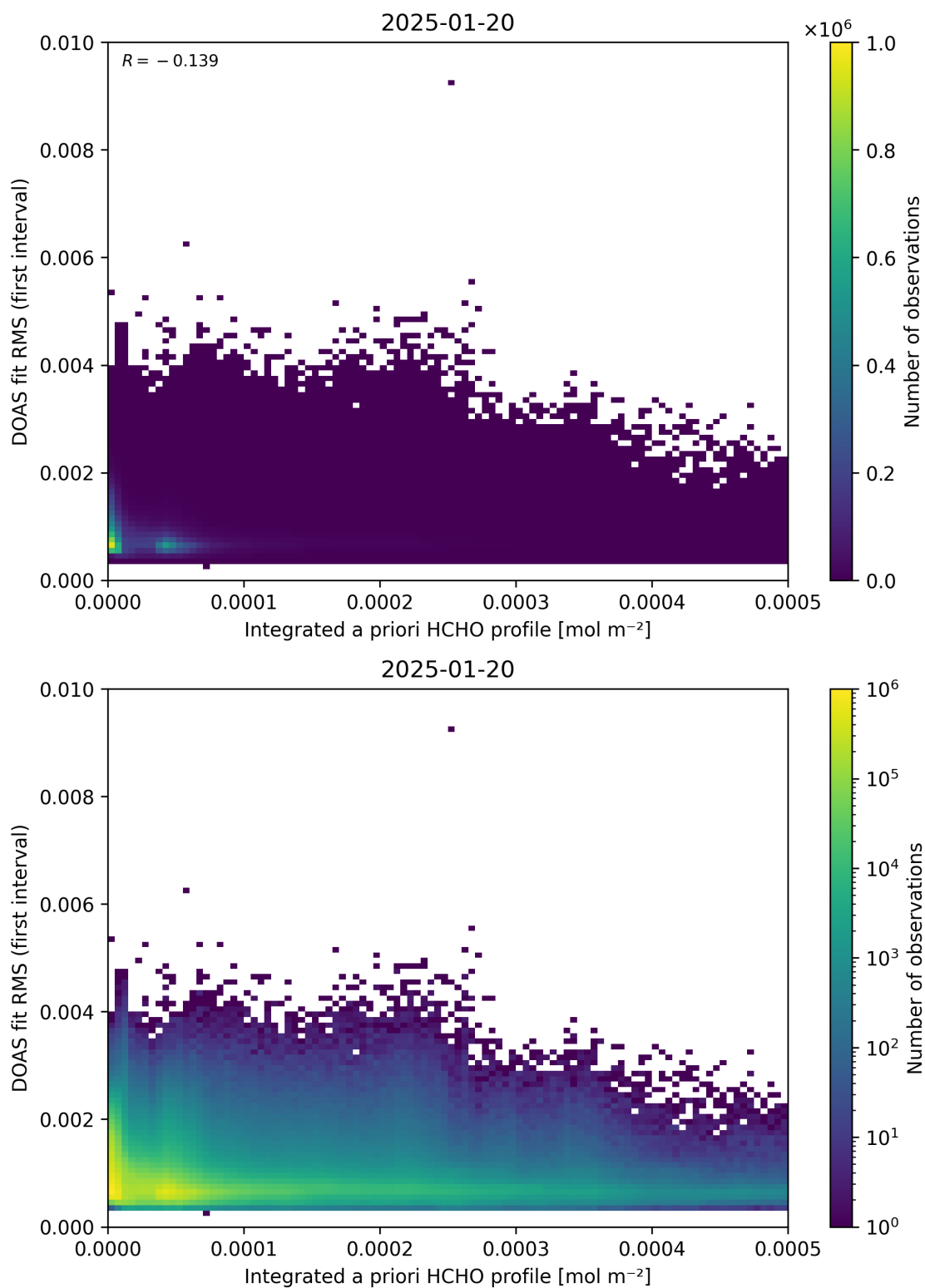
Figure 148: Scatter density plot of “Integrated a priori HCHO profile” against “DOAS fit RMS (first interval)” for 2025-01-19 to 2025-01-21.
