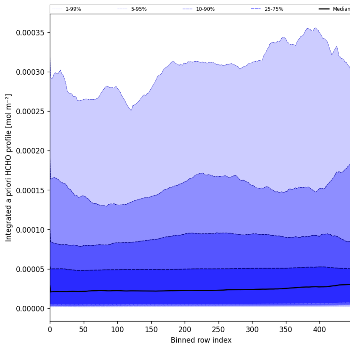
Figure 57: Along track statistics of “Integrated a priori HCHO profile” for 2025-01-19 to 2025-01-21
