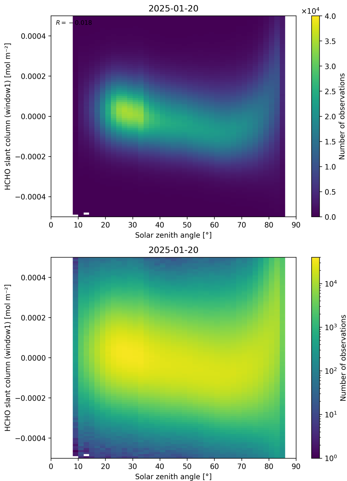
Figure 173: Scatter density plot of “Solar zenith angle” against “HCHO slant column (window1)” for 2025-01-19 to 2025-01-21.
