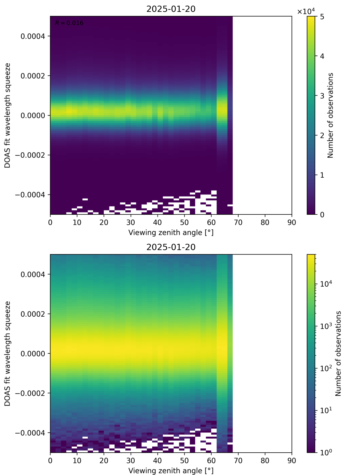
Figure 184: Scatter density plot of “Viewing zenith angle” against “DOAS fit wavelength squeeze” for 2025-01-19 to 2025-01-21.
