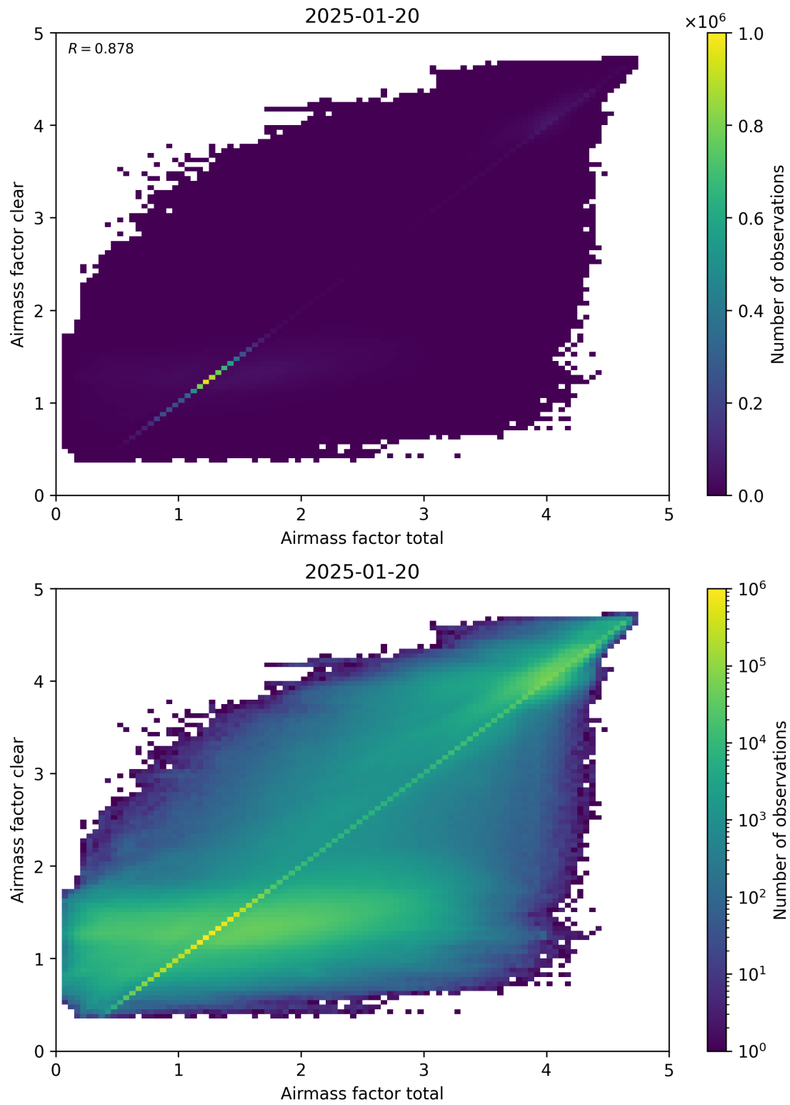
Figure 100: Scatter density plot of “Airmass factor total” against “Airmass factor clear” for 2025-01-19 to 2025-01-21.
