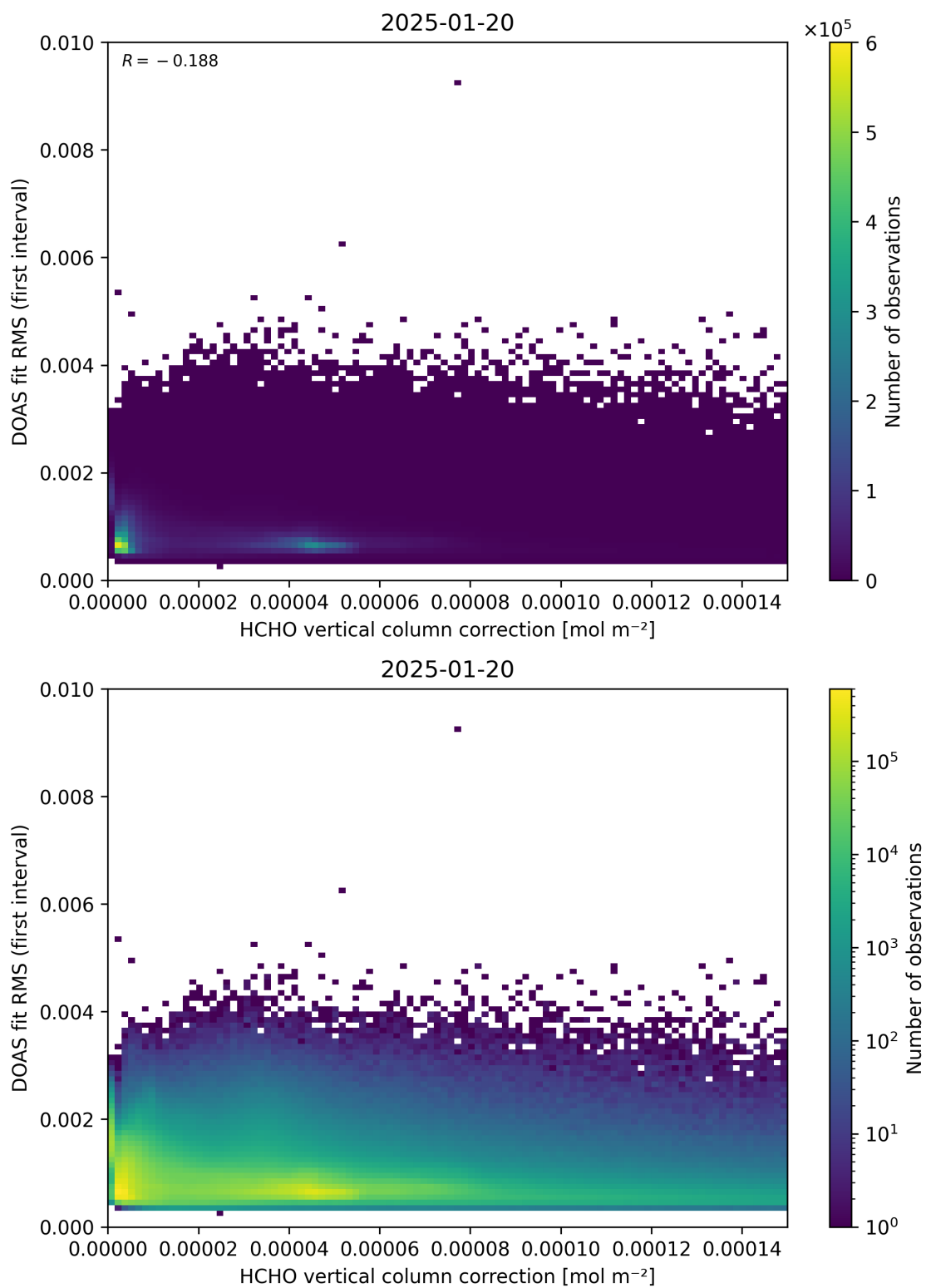
Figure 112: Scatter density plot of “HCHO vertical column correction” against “DOAS fit RMS (first interval)” for 2025-01-19 to 2025-01-21.
