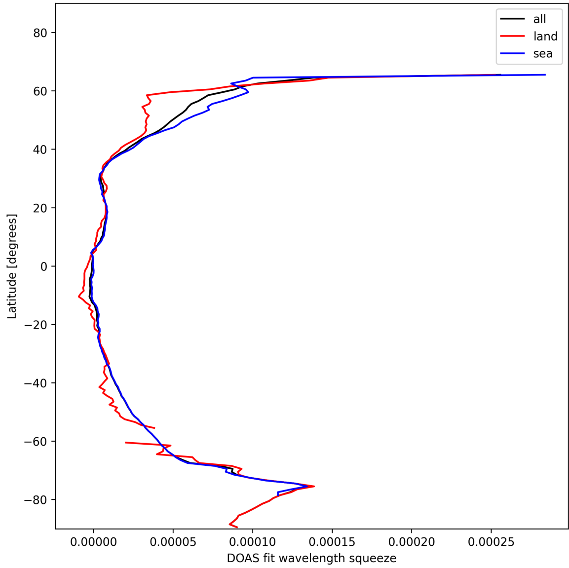
Figure 31: Zonal average of “DOAS fit wavelength squeeze” for 2025-01-19 to 2025-01-21.
