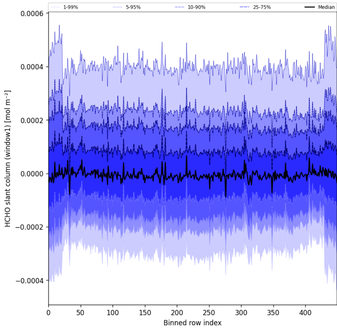
Figure 52: Along track statistics of “HCHO slant column (window1)” for 2025-01-19 to 2025-01-21
