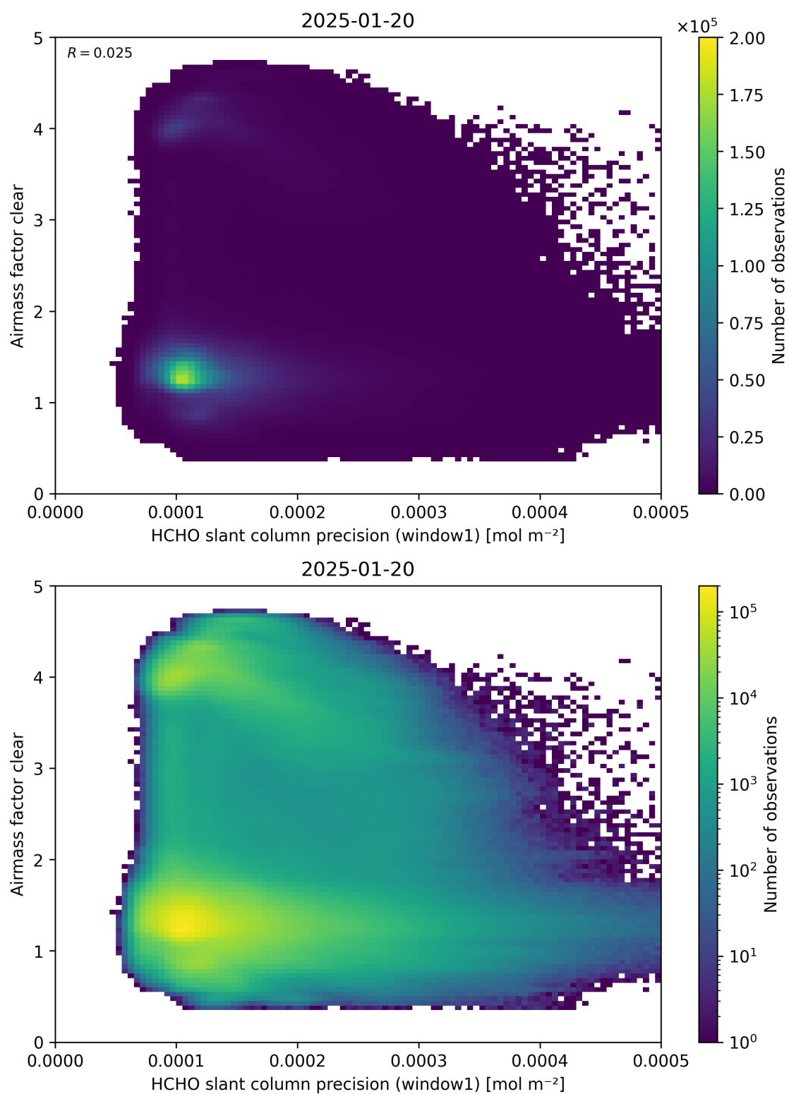
Figure 91: Scatter density plot of “HCHO slant column precision (window1)” against “Airmass factor clear” for 2025-01-19 to 2025-01-21.
