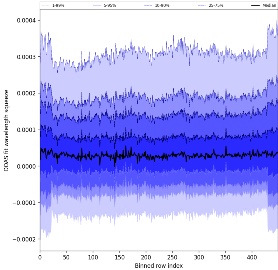
Figure 59: Along track statistics of “DOAS fit wavelength squeeze” for 2025-01-19 to 2025-01-21
