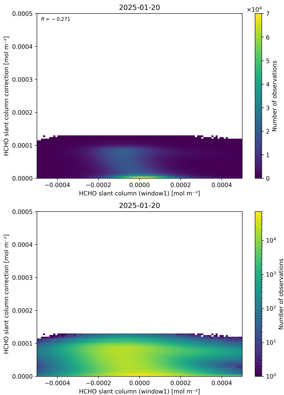
Figure 83: Scatter density plot of “HCHO slant column (window1)” against “HCHO slant column correction” for 2025-01-19 to 2025-01-21.
