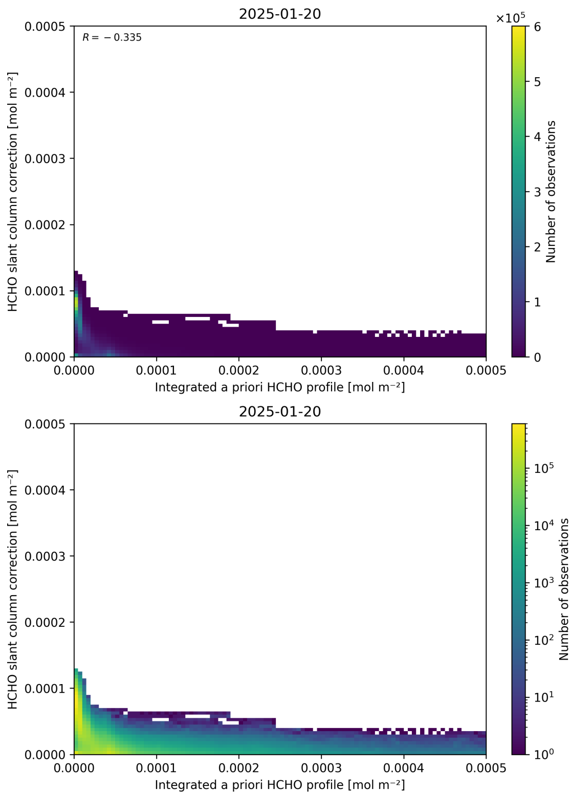
Figure 152: Scatter density plot of “Integrated a priori HCHO profile” against “HCHO slant column correction” for 2025-01-19 to 2025-01-21.
