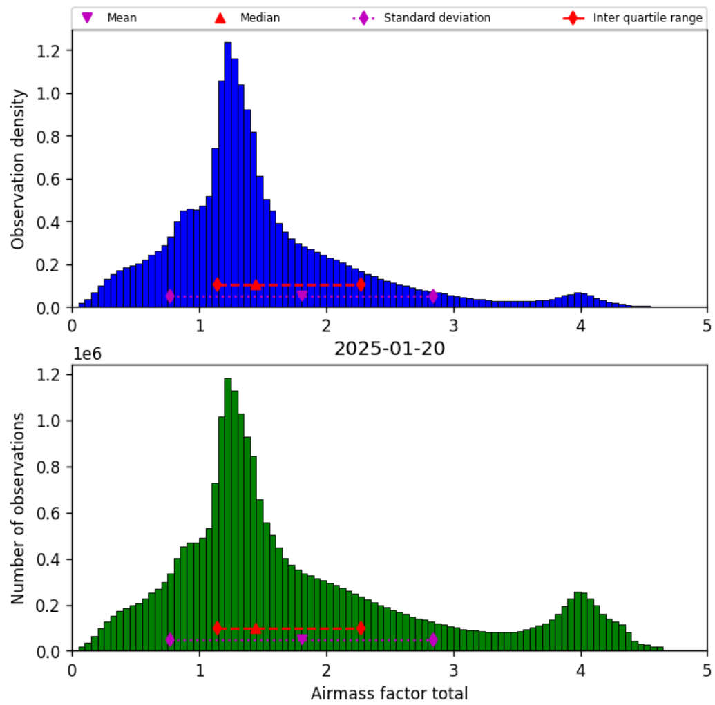
Figure 40: Histogram of “Airmass factor total” for 2025-01-19 to 2025-01-21
