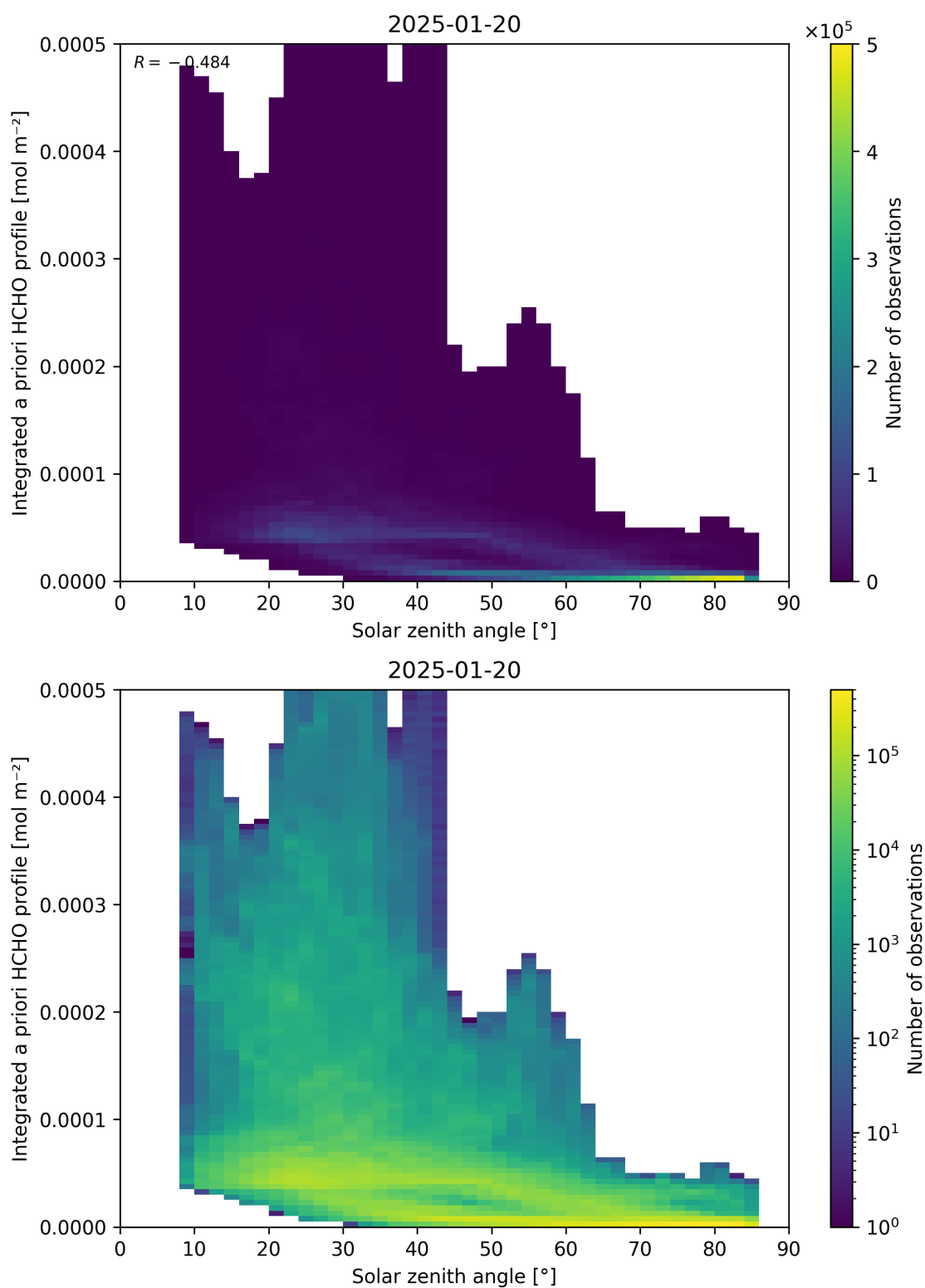
Figure 180: Scatter density plot of “Solar zenith angle” against “Integrated a priori HCHO profile” for 2025-01-19 to 2025-01-21.
