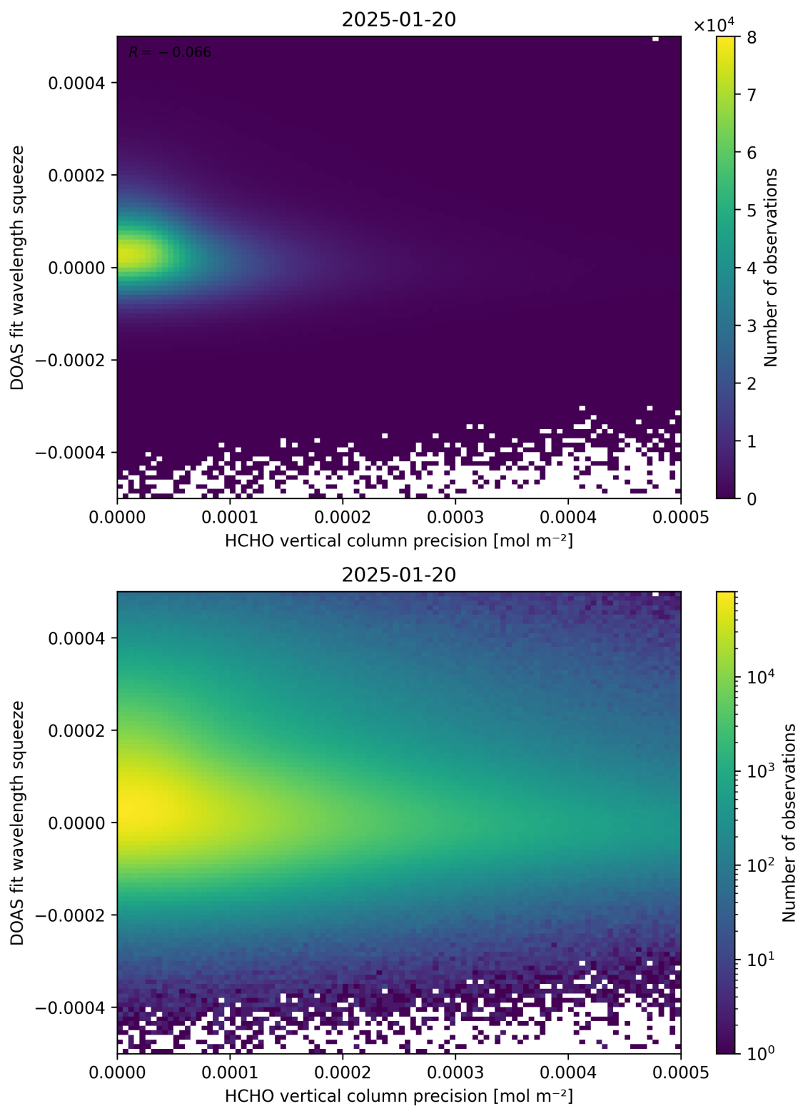
Figure 138: Scatter density plot of “HCHO vertical column precision” against “DOAS fit wavelength squeeze” for 2025-01-19 to 2025-01-21.
