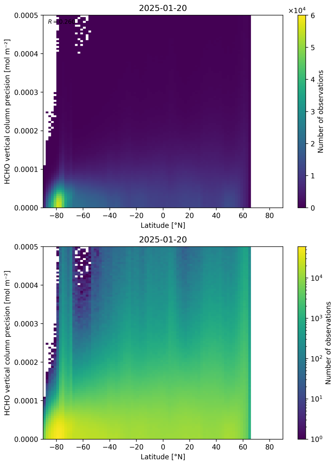
Figure 165: Scatter density plot of “Latitude” against “HCHO vertical column precision” for 2025-01-19 to 2025-01-21.
