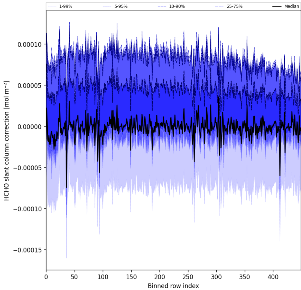
Figure 61: Along track statistics of "HCHO slant column correction" for 2025-01-19 to 2025-01-21
