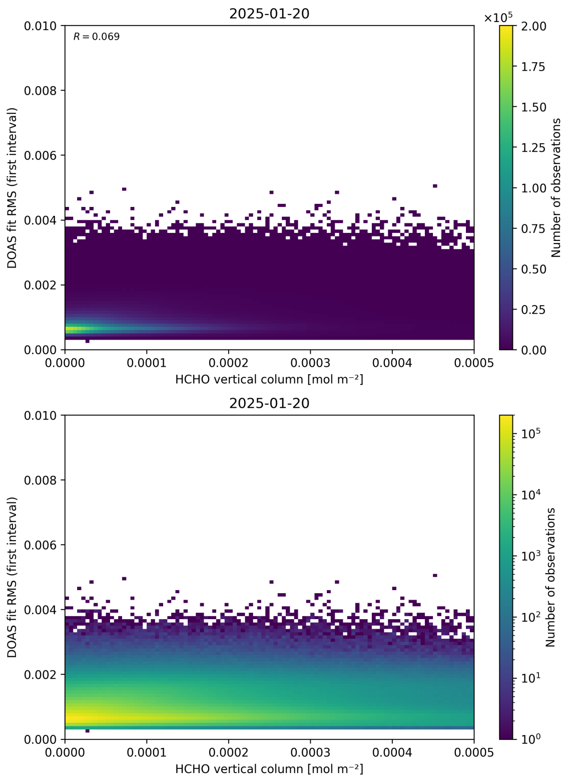
Figure 123: Scatter density plot of “HCHO vertical column” against “DOAS fit RMS (first interval)” for 2025-01-19 to 2025-01-21.
