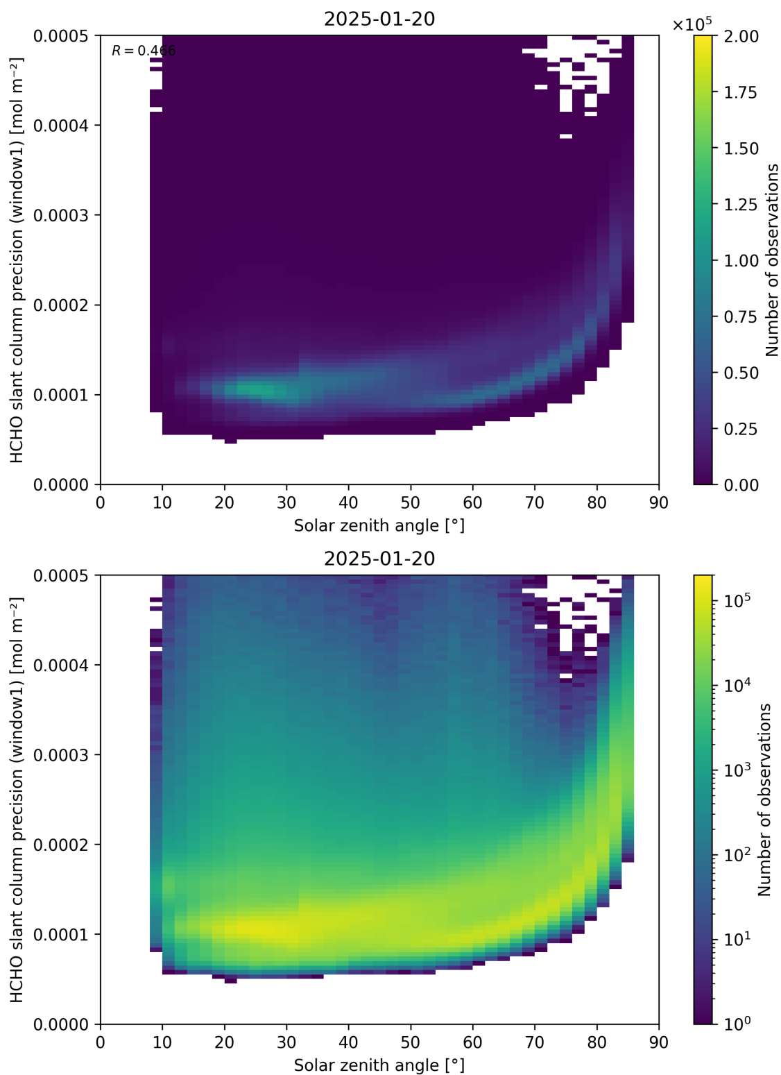
Figure 174: Scatter density plot of “Solar zenith angle” against “HCHO slant column precision (window1)” for 2025-01-19 to 2025-01-21.
