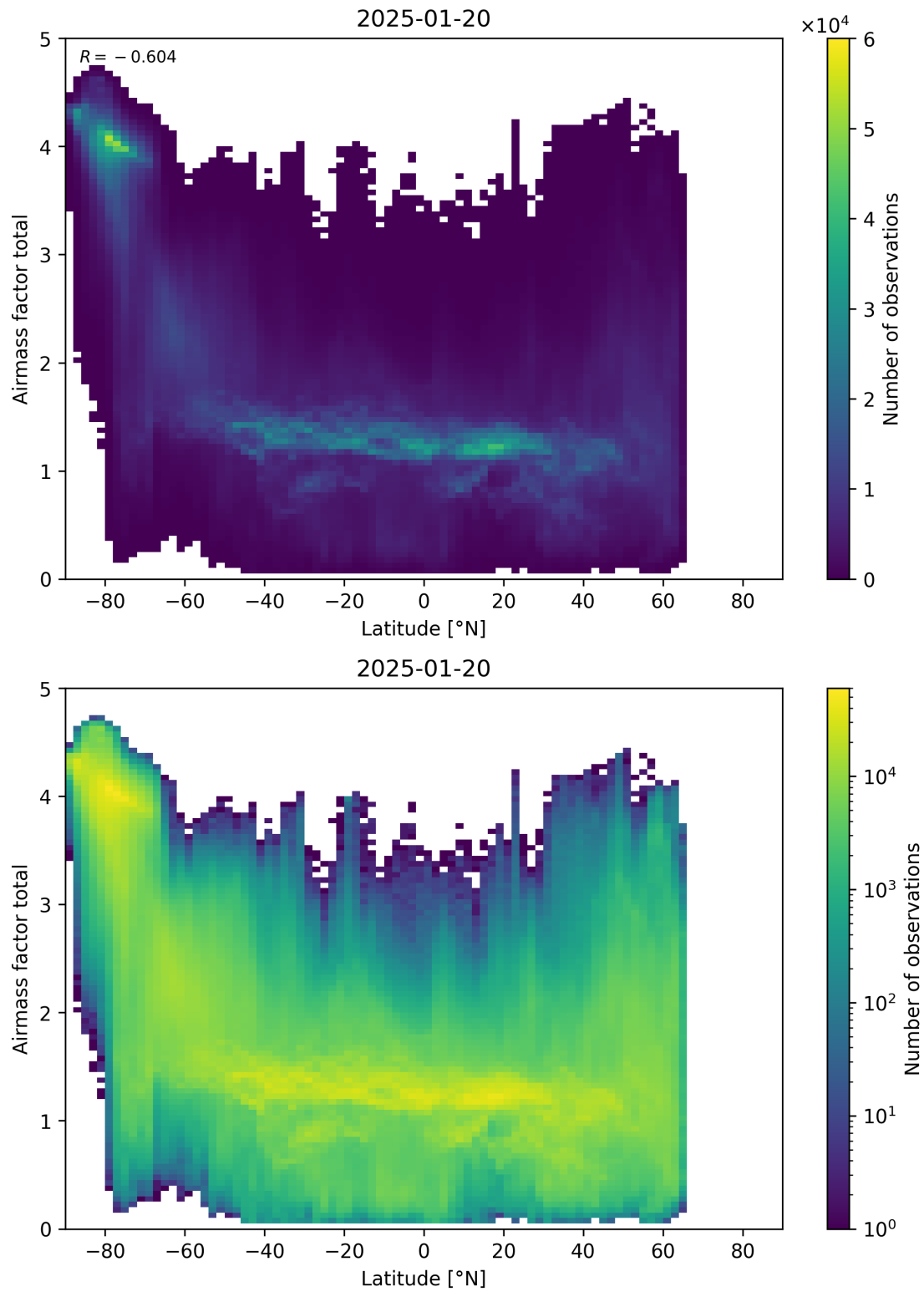
Figure 161: Scatter density plot of “Latitude” against “Airmass factor total” for 2025-01-19 to 2025-01-21.
