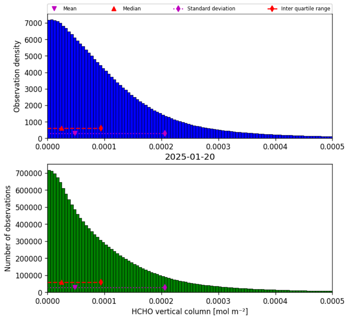
Figure 35: Histogram of “HCHO vertical column” for 2025-01-19 to 2025-01-21
