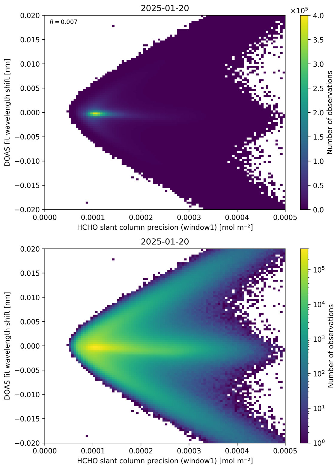
Figure 89: Scatter density plot of “HCHO slant column precision (window1)” against “DOAS fit wavelength shift” for 2025-01-19 to 2025-01-21.
