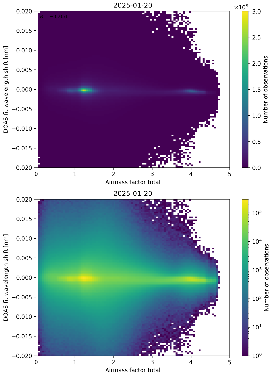
Figure 98: Scatter density plot of “Airmass factor total” against “DOAS fit wavelength shift” for 2025-01-19 to 2025-01-21.
