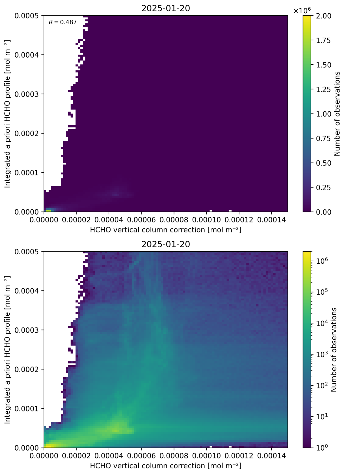
Figure 122: Scatter density plot of “HCHO vertical column correction” against “Integrated a priori HCHO profile” for 2025-01-19 to 2025-01-21.
