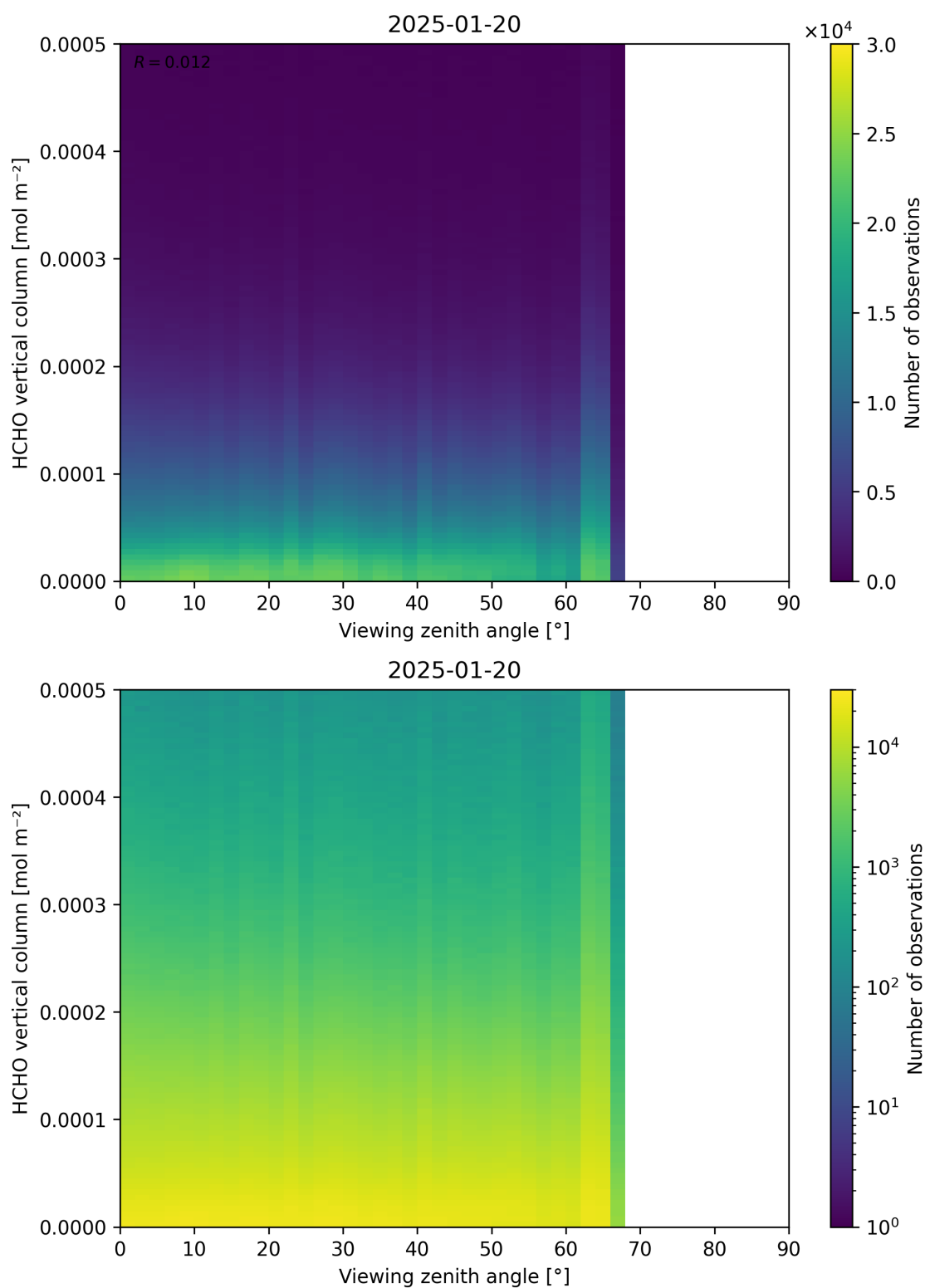
Figure 192: Scatter density plot of “Viewing zenith angle” against “HCHO vertical column” for 2025-01-19 to 2025-01-21.
