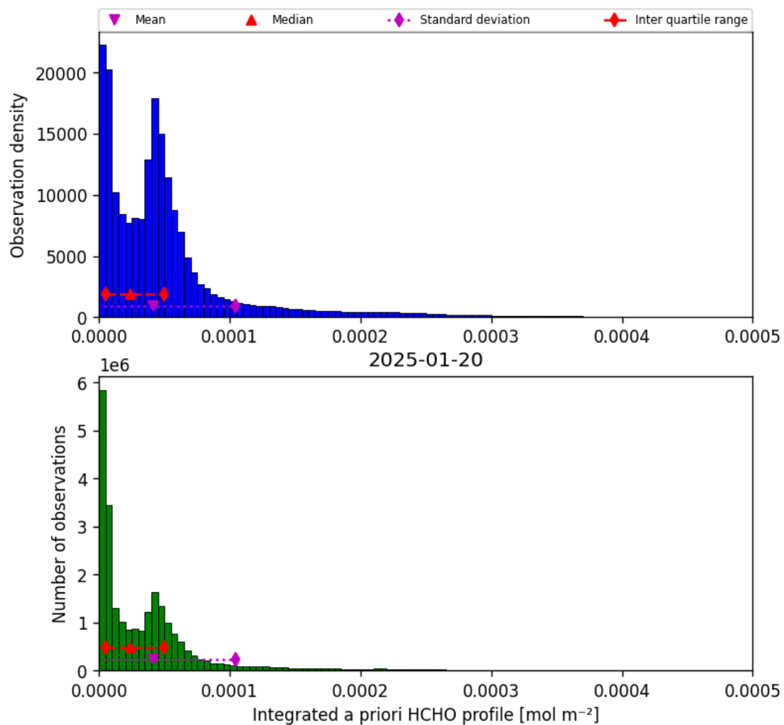
Figure 43: Histogram of “Integrated a priori HCHO profile” for 2025-01-19 to 2025-01-21
