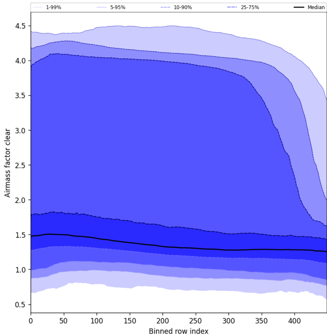
Figure 56: Along track statistics of “Airmass factor clear” for 2025-01-19 to 2025-01-21
