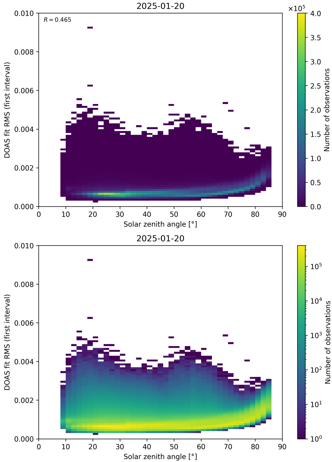
Figure 167: Scatter density plot of “Solar zenith angle” against “DOAS fit RMS (first interval)” for 2025-01-19 to 2025-01-21.
