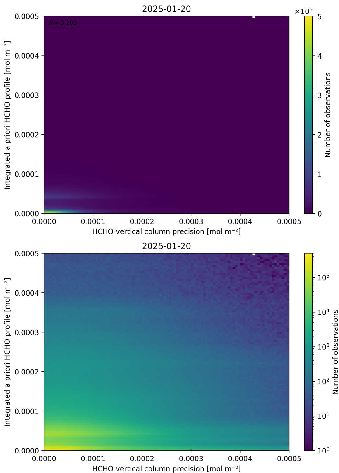
Figure 147: Scatter density plot of “HCHO vertical column precision” against “Integrated a priori HCHO profile” for 2025-01-19 to 2025-01-21.
