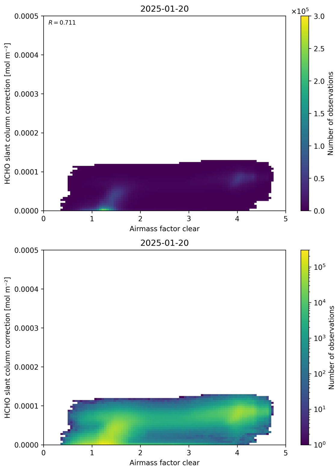
Figure 75: Scatter density plot of “Airmass factor clear” against “HCHO slant column correction” for 2025-01-19 to 2025-01-21.
