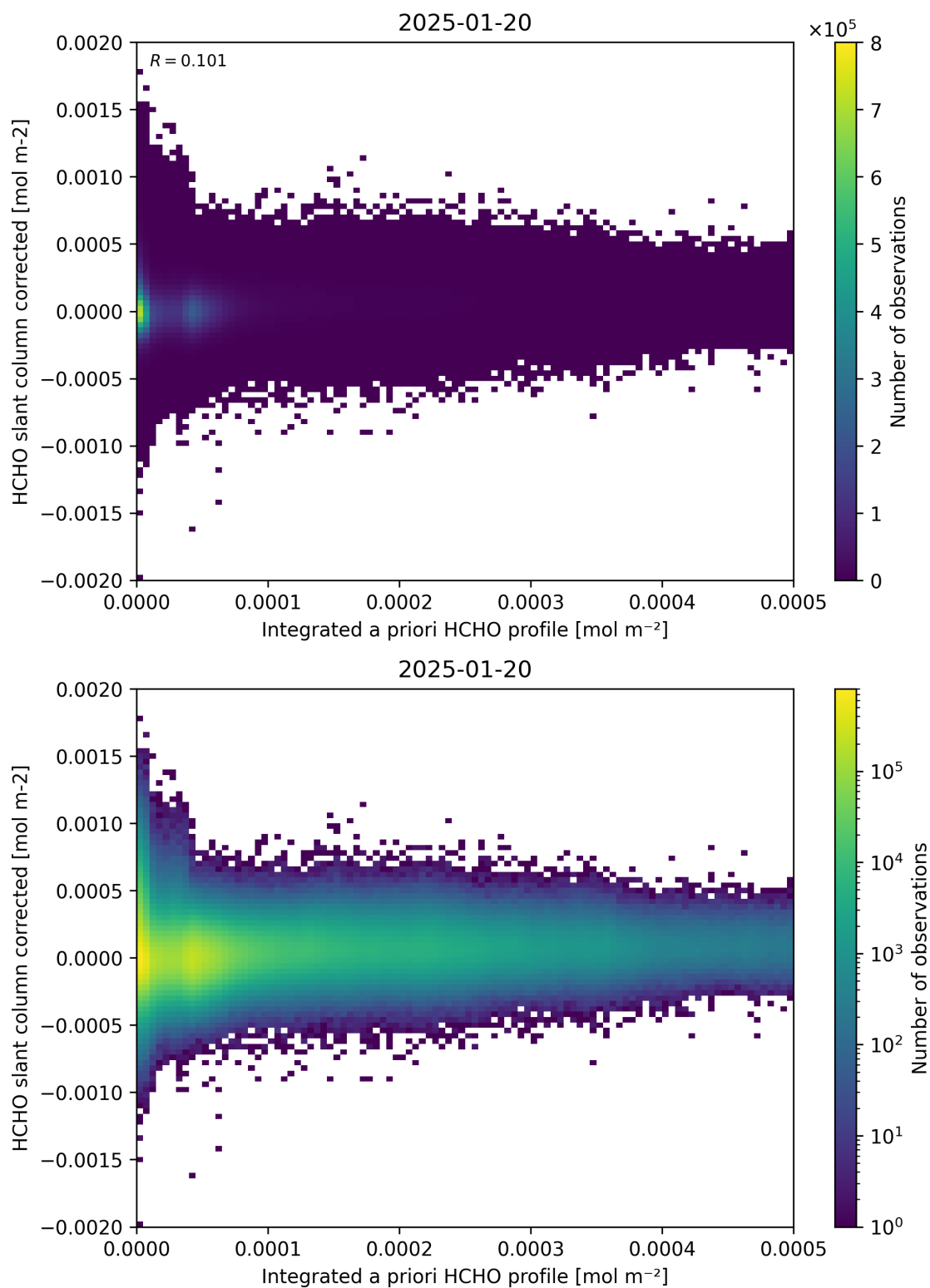
Figure 151: Scatter density plot of “Integrated a priori HCHO profile” against “HCHO slant column corrected” for 2025-01-19 to 2025-01-21.
