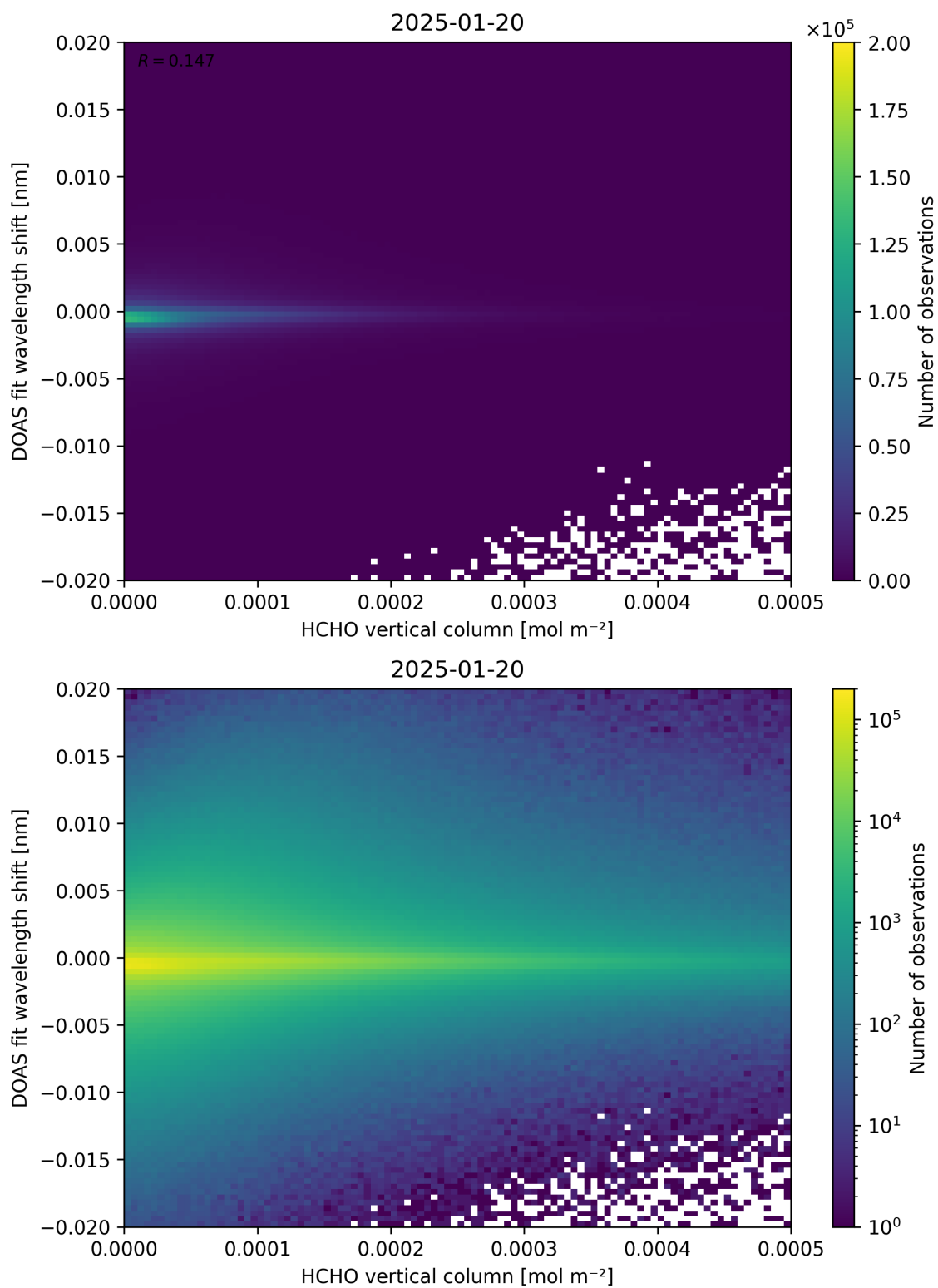
Figure 124: Scatter density plot of “HCHO vertical column” against “DOAS fit wavelength shift” for 2025-01-19 to 2025-01-21.
