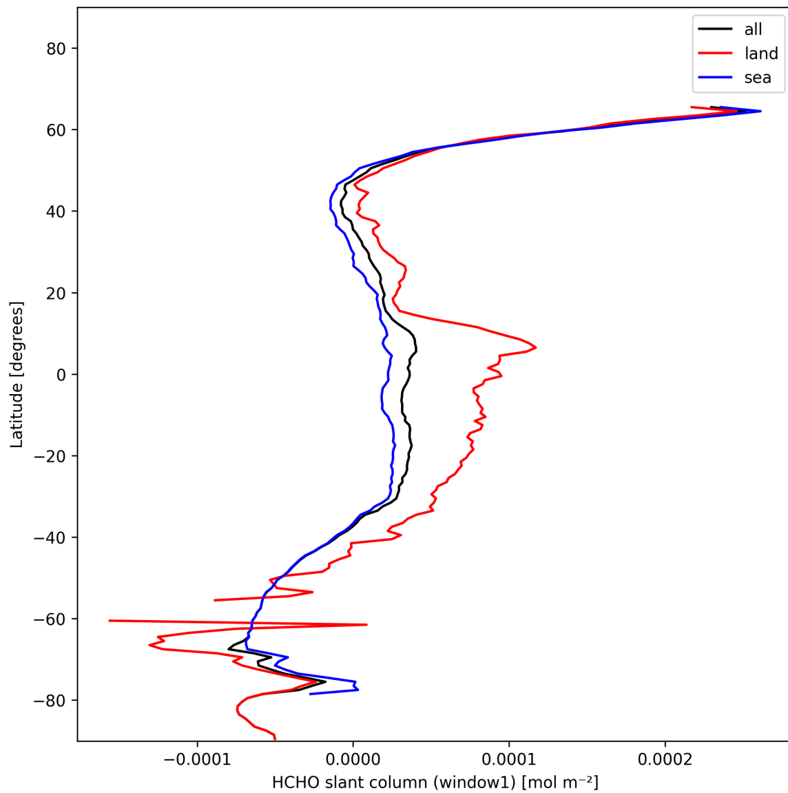
Figure 24: Zonal average of “HCHO slant column (window1)” for 2025-01-19 to 2025-01-21.
