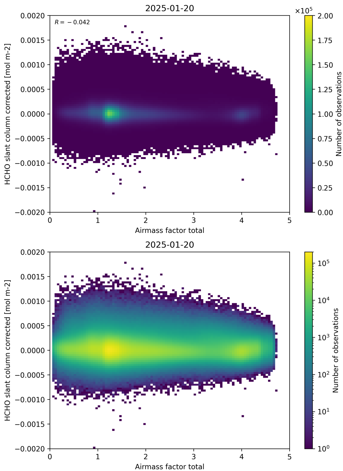
Figure 101: Scatter density plot of “Airmass factor total” against “HCHO slant column corrected” for 2025-01-19 to 2025-01-21.
