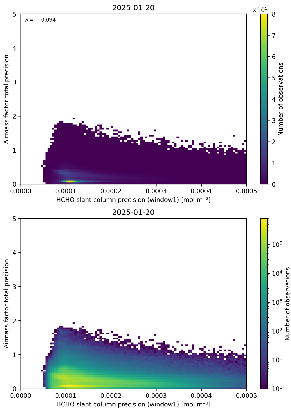
Figure 95: Scatter density plot of “HCHO slant column precision (window1)” against “Airmass factor total precision” for 2025-01-19 to 2025-01-21.
