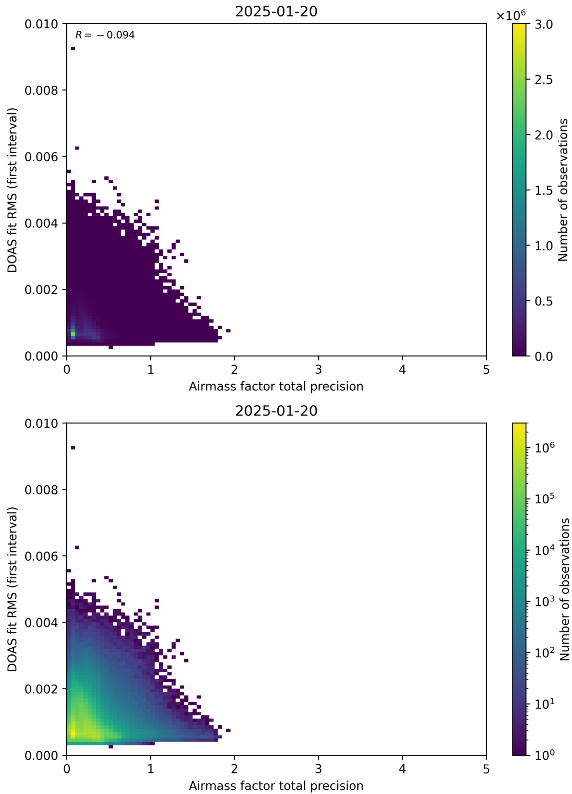
Figure 105: Scatter density plot of “Airmass factor total precision” against “DOAS fit RMS (first interval)” for 2025-01-19 to 2025-01-21.
