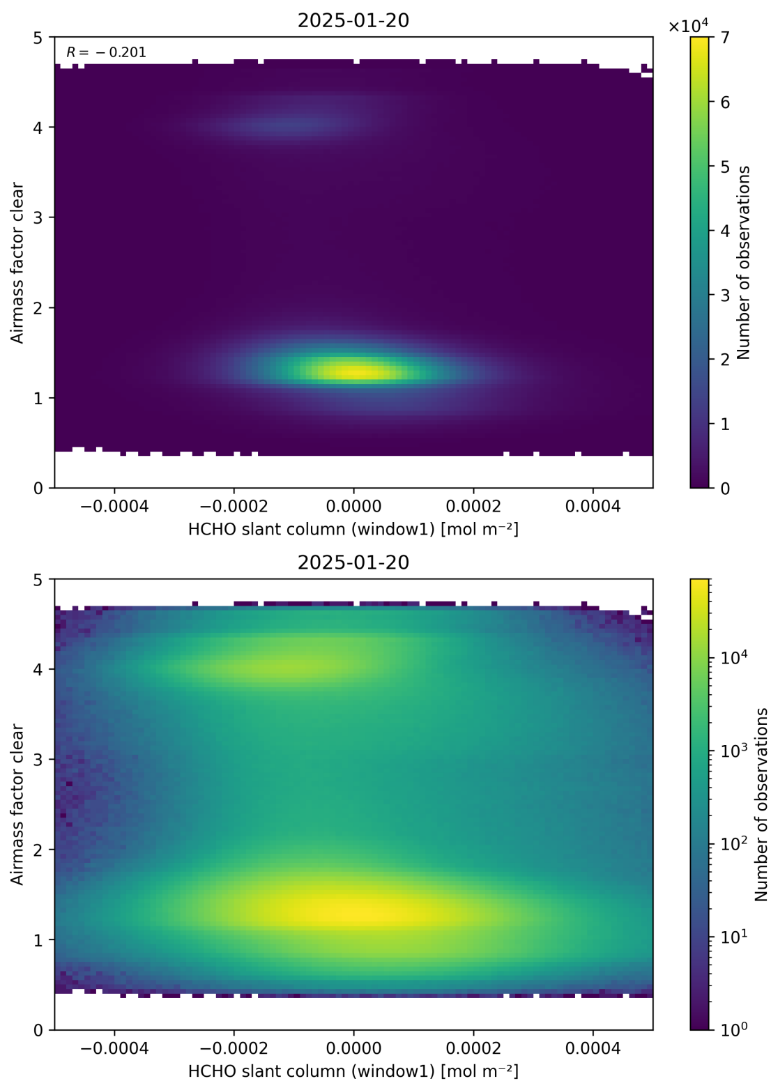
Figure 81: Scatter density plot of “HCHO slant column (window1)” against “Airmass factor clear” for 2025-01-19 to 2025-01-21.
