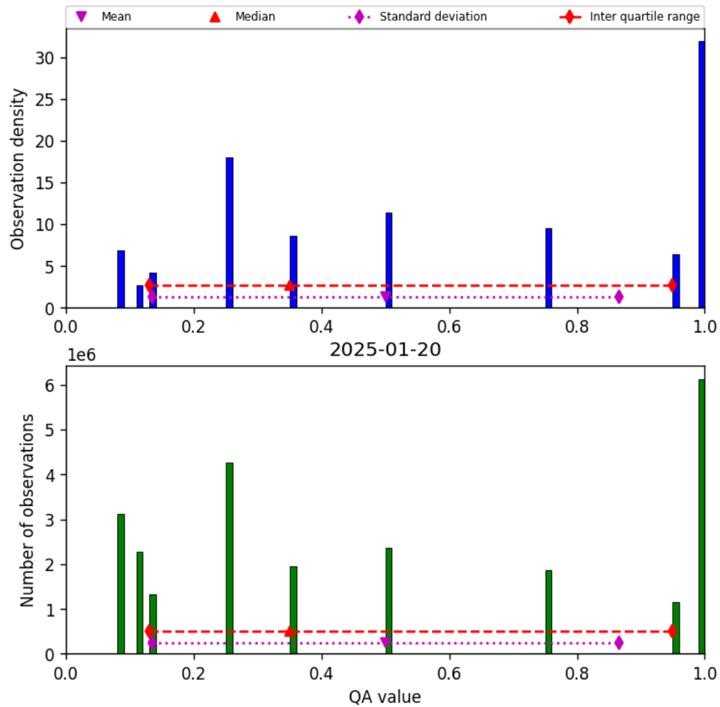
Figure 34: Histogram of “QA value” for 2025-01-19 to 2025-01-21
