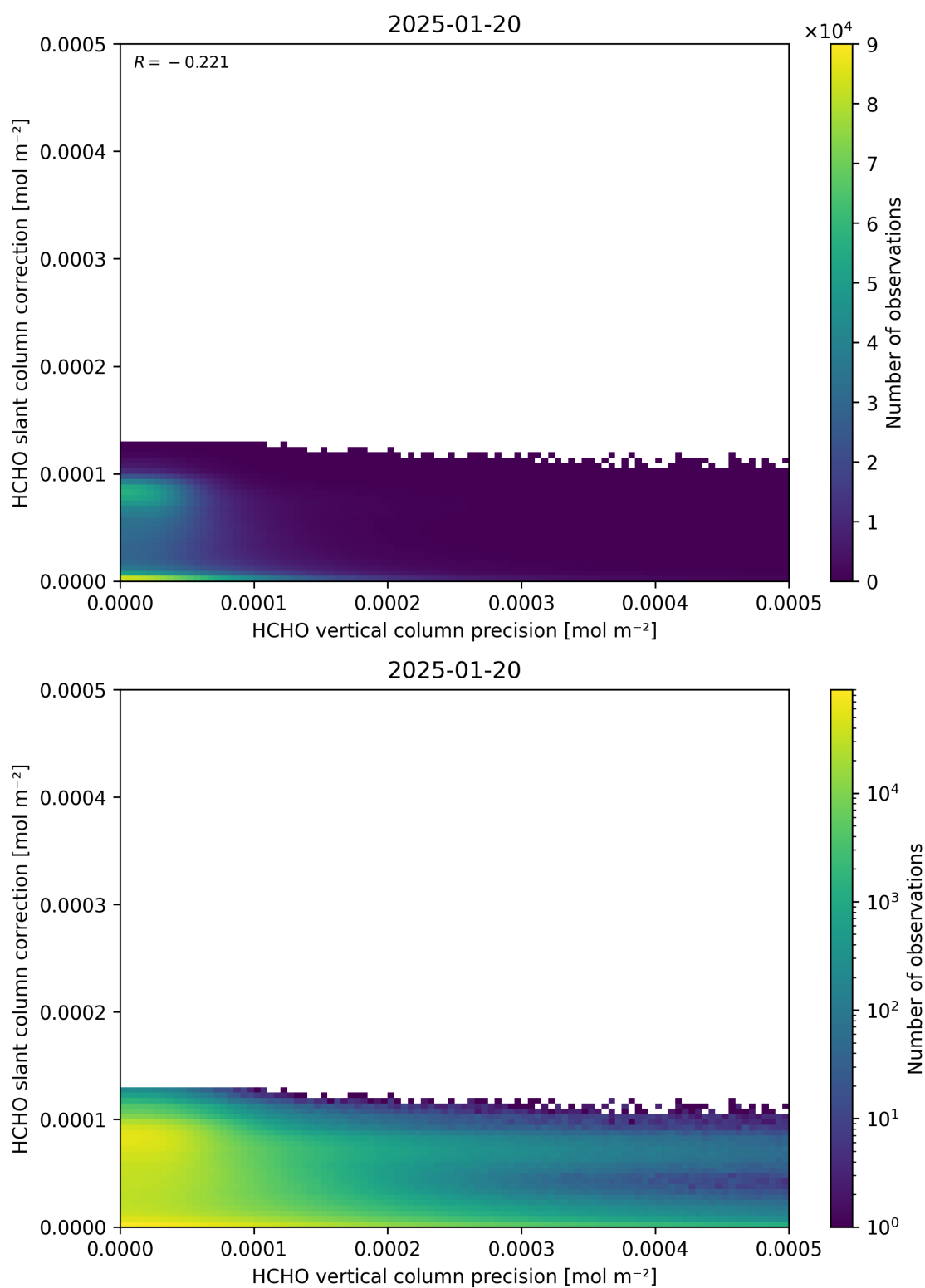
Figure 141: Scatter density plot of “HCHO vertical column precision” against “HCHO slant column correction” for 2025-01-19 to 2025-01-21.
