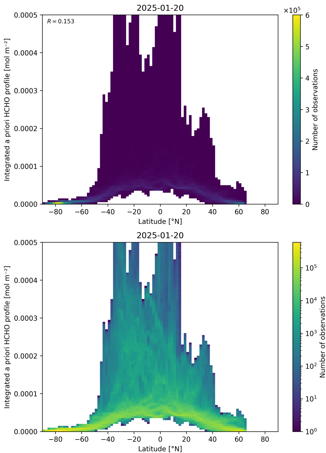
Figure 166: Scatter density plot of “Latitude” against “Integrated a priori HCHO profile” for 2025-01-19 to 2025-01-21.
