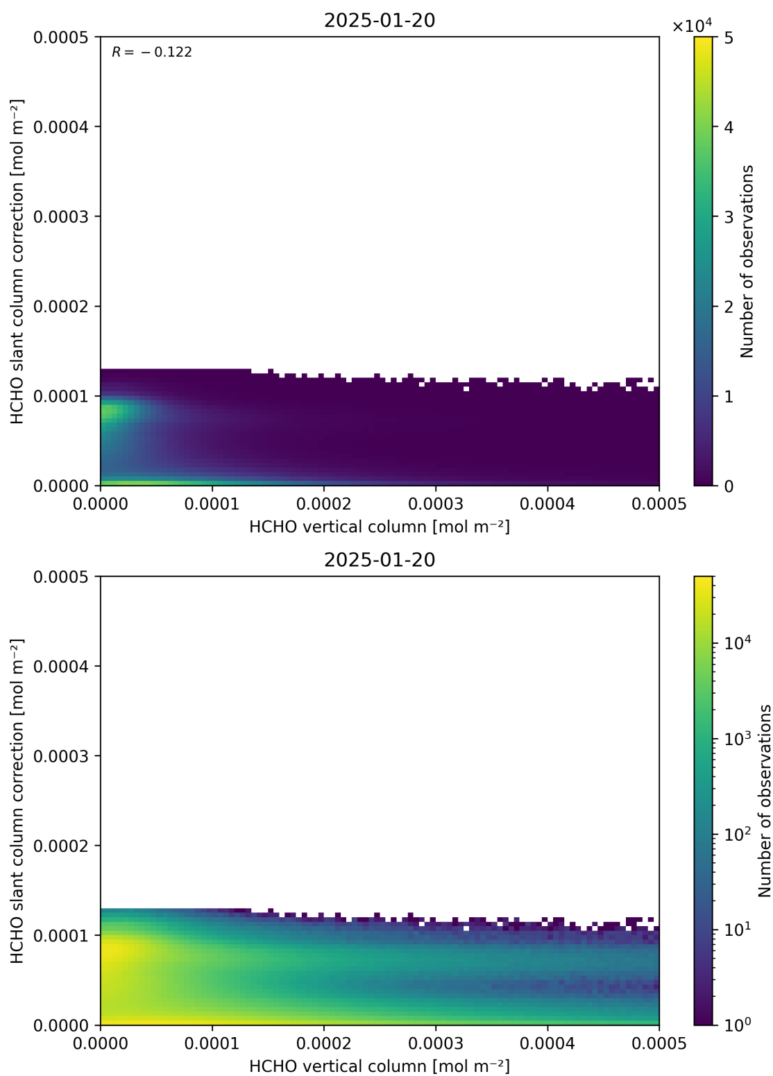
Figure 128: Scatter density plot of “HCHO vertical column” against “HCHO slant column correction” for 2025-01-19 to 2025-01-21.
