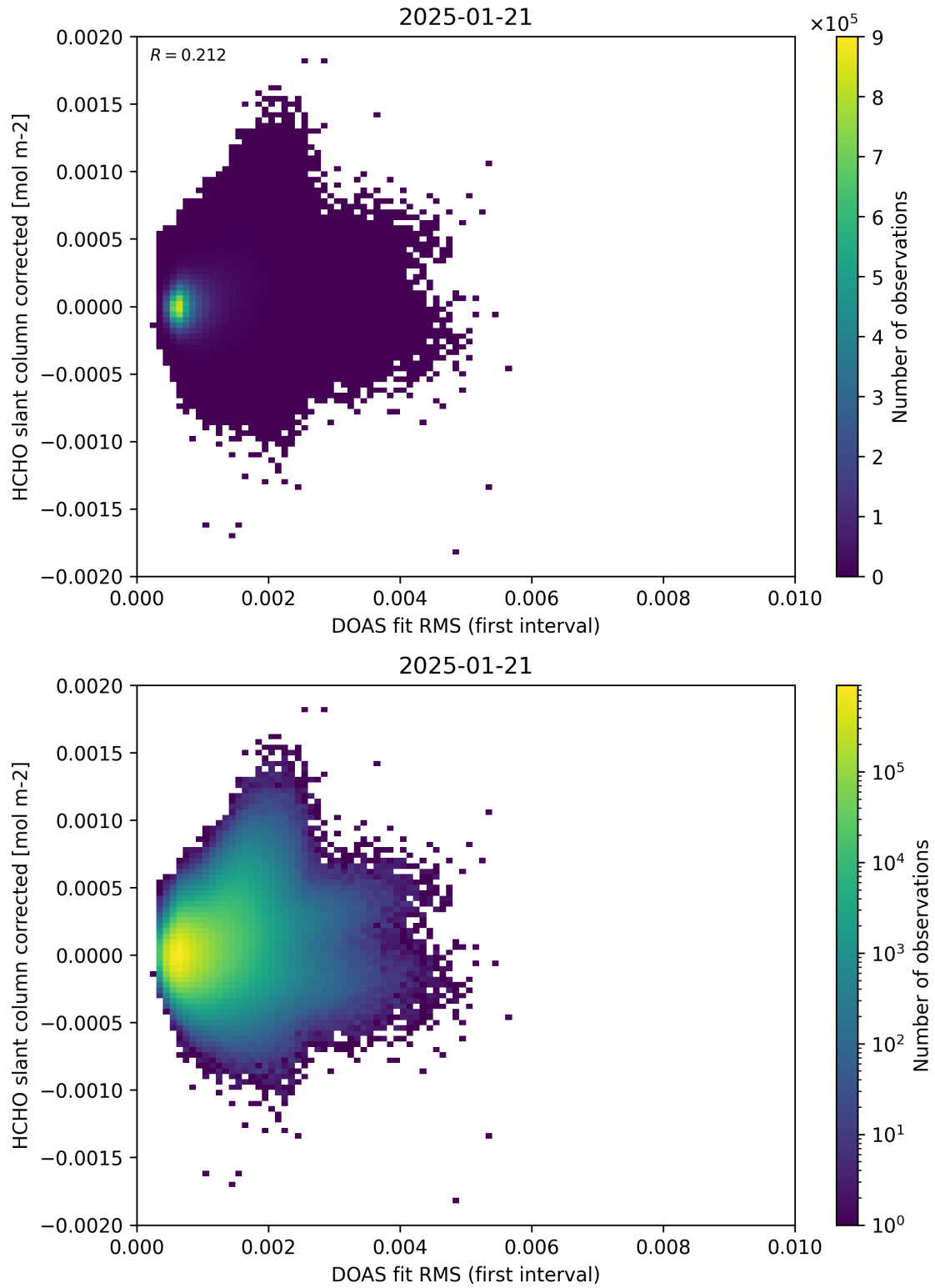
Figure 62: Scatter density plot of “DOAS fit RMS (first interval)” against “HCHO slant column corrected” for 2025-01-20 to 2025-01-22.
