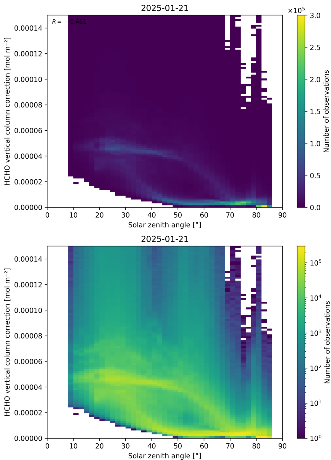
Figure 178: Scatter density plot of “Solar zenith angle” against “HCHO vertical column correction” for 2025-01-20 to 2025-01-22.
