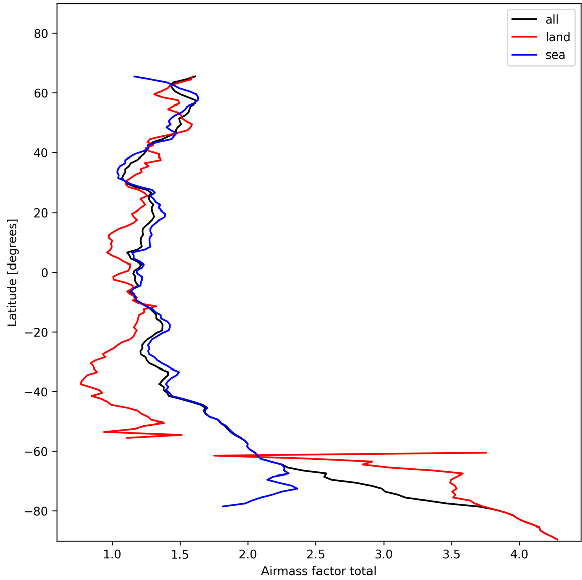
Figure 26: Zonal average of “Airmass factor total” for 2025-01-20 to 2025-01-22.
