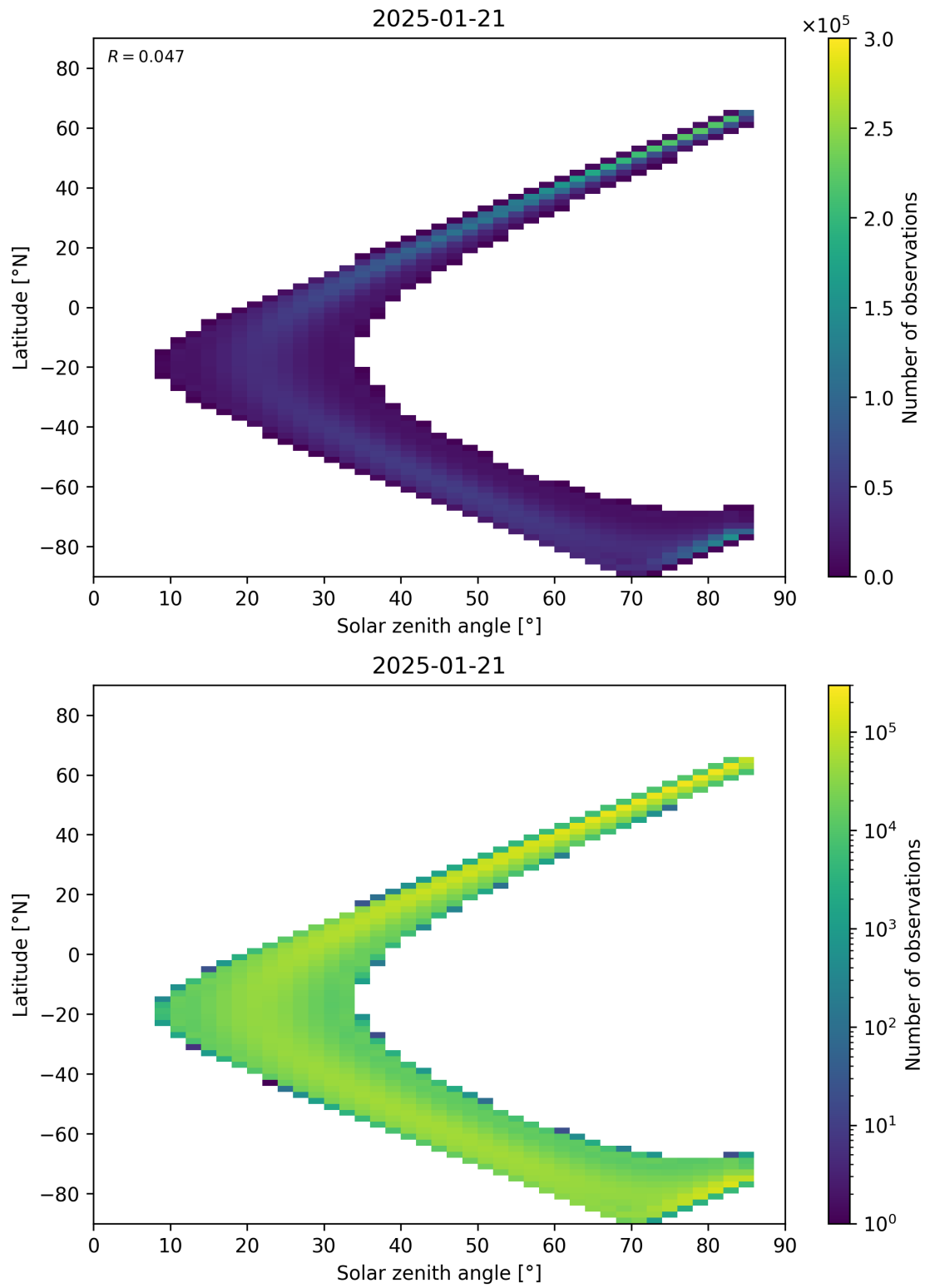
Figure 181: Scatter density plot of “Solar zenith angle” against “Latitude” for 2025-01-20 to 2025-01-22.
