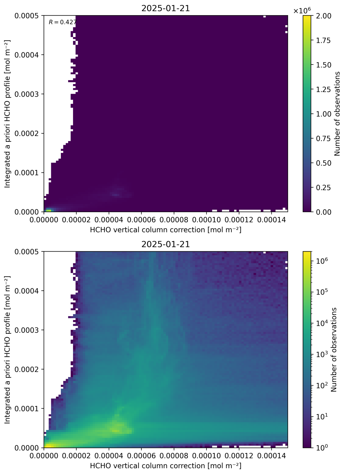
Figure 122: Scatter density plot of “HCHO vertical column correction” against “Integrated a priori HCHO profile” for 2025-01-20 to 2025-01-22.
