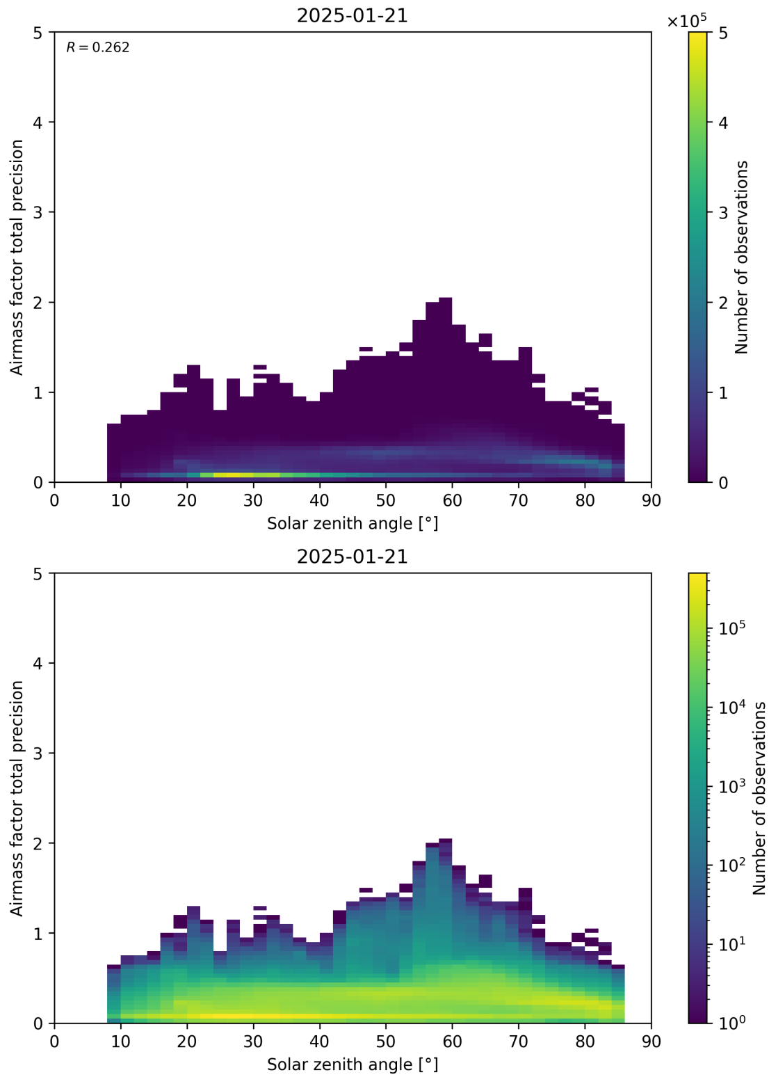
Figure 176: Scatter density plot of “Solar zenith angle” against “Airmass factor total precision” for 2025-01-20 to 2025-01-22.
