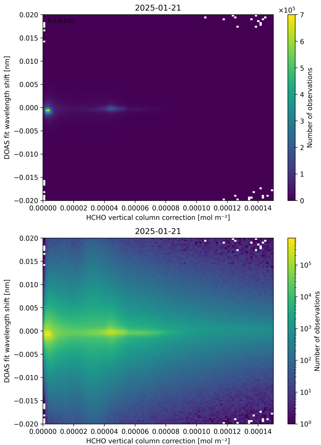
Figure 113: Scatter density plot of “HCHO vertical column correction” against “DOAS fit wavelength shift” for 2025-01-20 to 2025-01-22.
