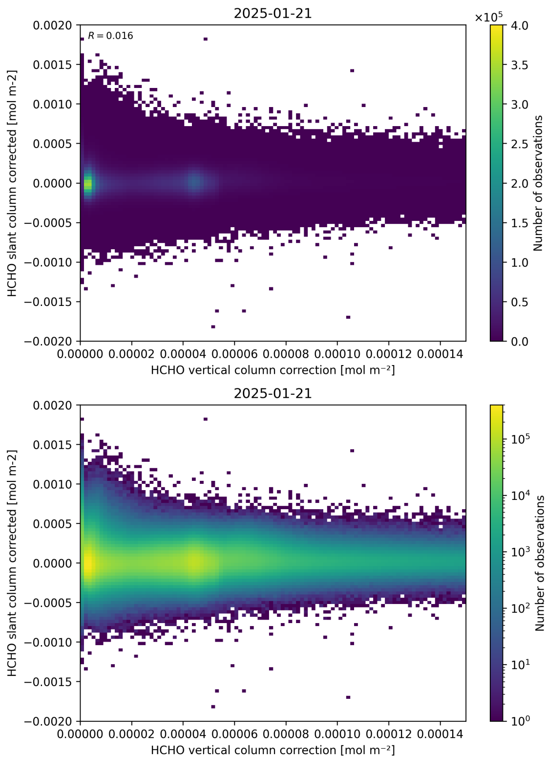
Figure 116: Scatter density plot of “HCHO vertical column correction” against “HCHO slant column corrected” for 2025-01-20 to 2025-01-22.
