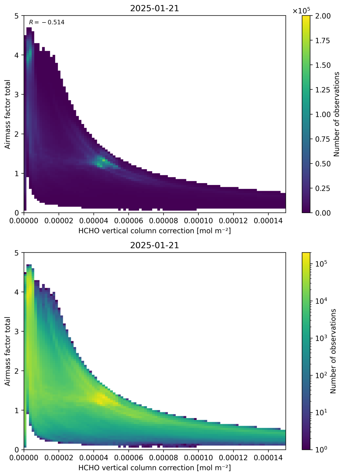
Figure 120: Scatter density plot of “HCHO vertical column correction” against “Airmass factor total” for 2025-01-20 to 2025-01-22.
