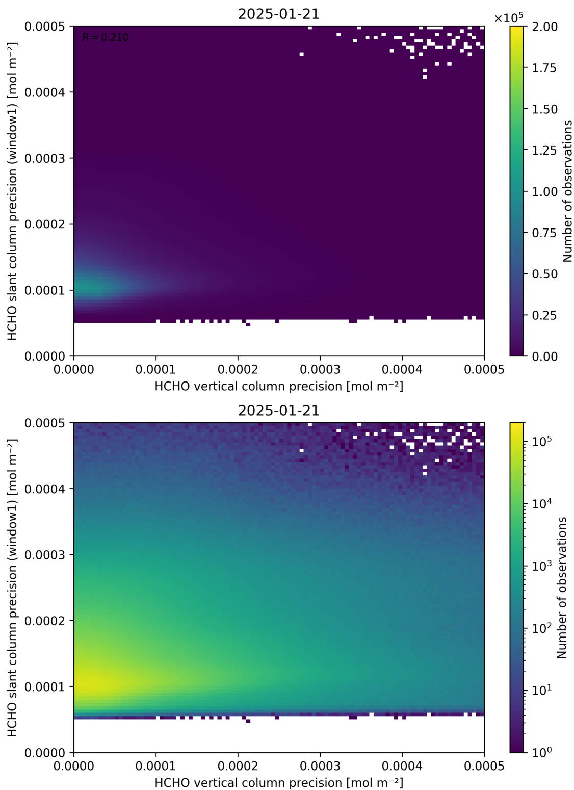
Figure 143: Scatter density plot of “HCHO vertical column precision” against “HCHO slant column precision (window1)” for 2025-01-20 to 2025-01-22.
