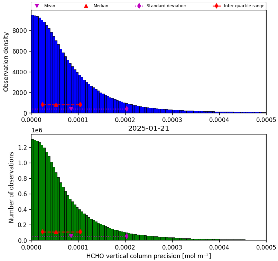
Figure 36: Histogram of “HCHO vertical column precision” for 2025-01-20 to 2025-01-22
