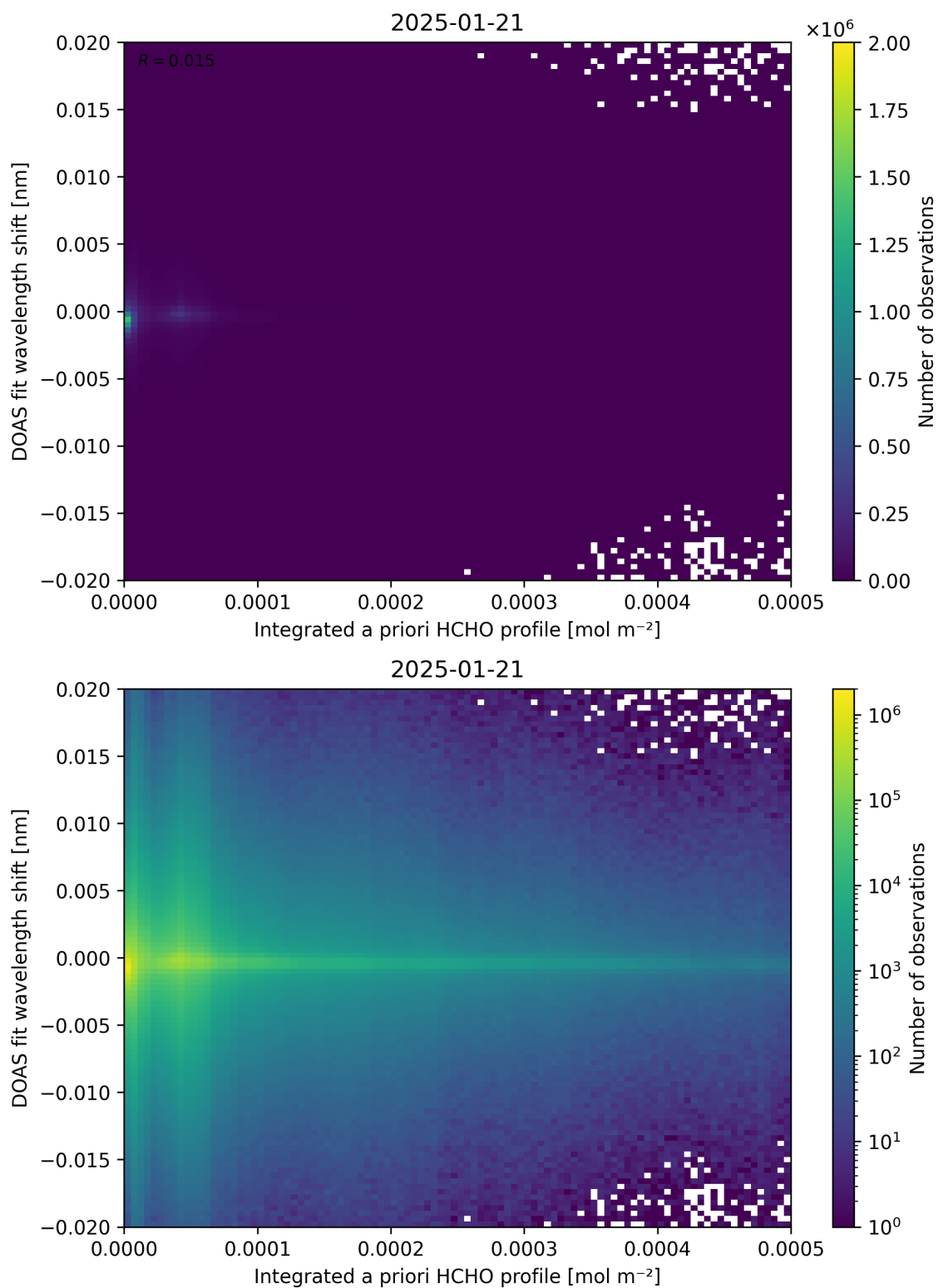
Figure 149: Scatter density plot of “Integrated a priori HCHO profile” against “DOAS fit wavelength shift” for 2025-01-20 to 2025-01-22.
