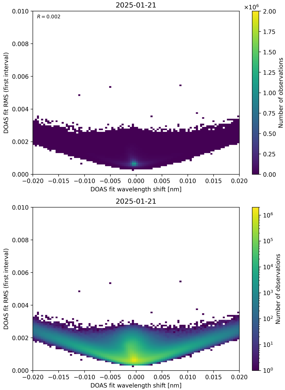
Figure 64: Scatter density plot of “DOAS fit wavelength shift” against “DOAS fit RMS (first interval)” for 2025-01-20 to 2025-01-22.
