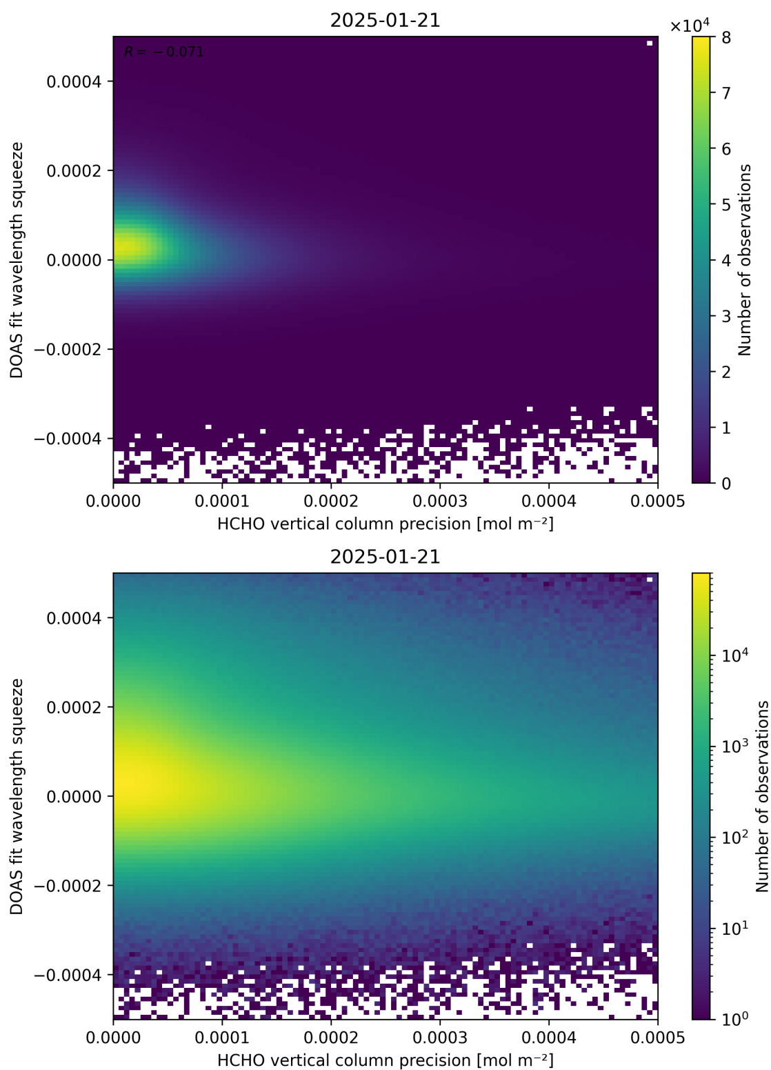
Figure 138: Scatter density plot of “HCHO vertical column precision” against “DOAS fit wavelength squeeze” for 2025-01-20 to 2025-01-22.
