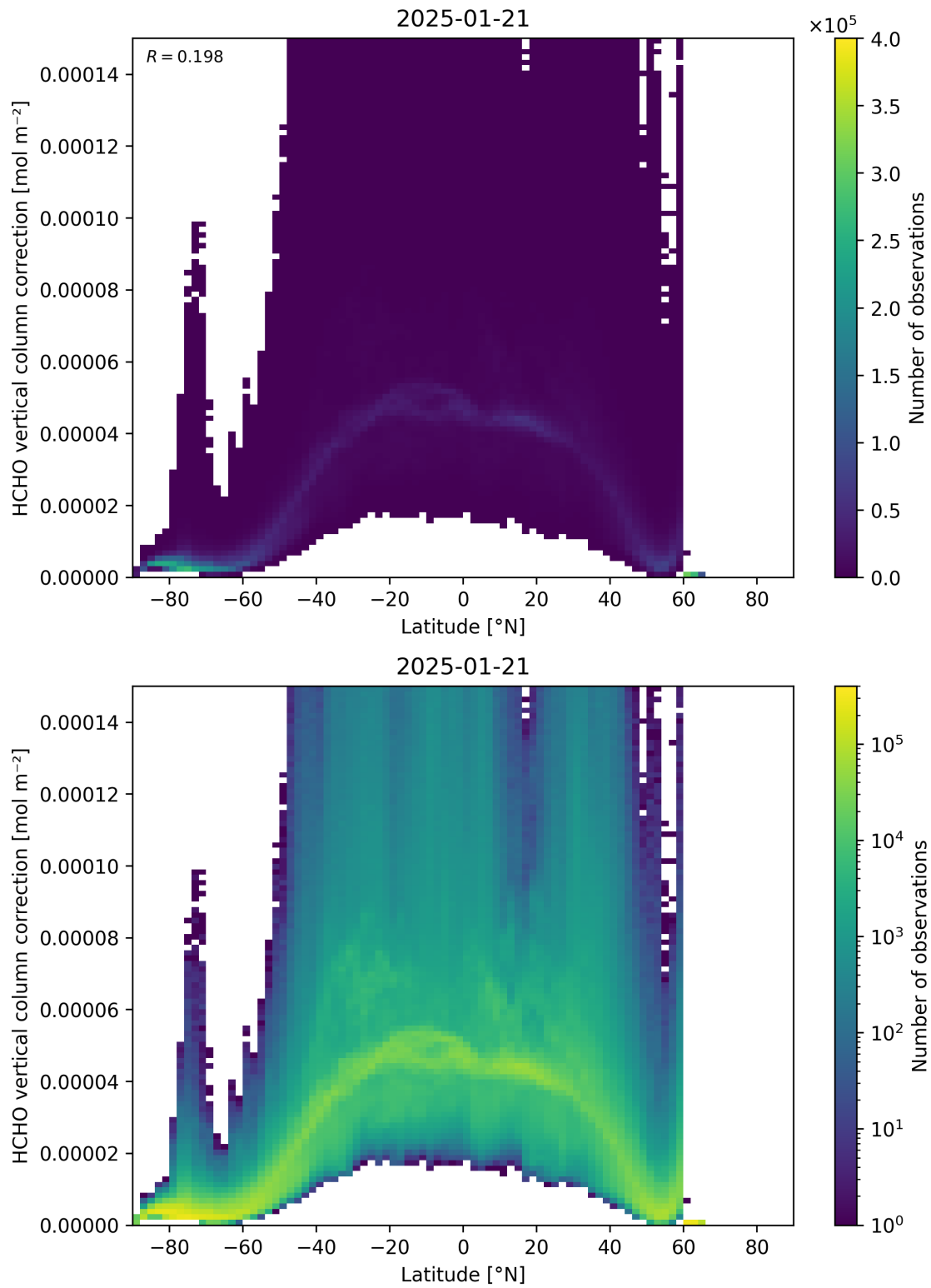
Figure 164: Scatter density plot of “Latitude” against “HCHO vertical column correction” for 2025-01-20 to 2025-01-22.
