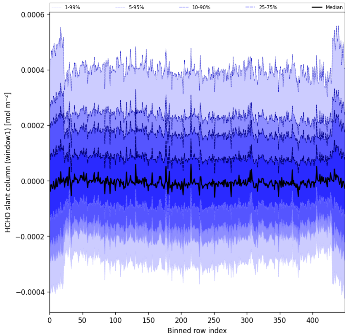
Figure 52: Along track statistics of "HCHO slant column (window1)" for 2025-01-20 to 2025-01-22
