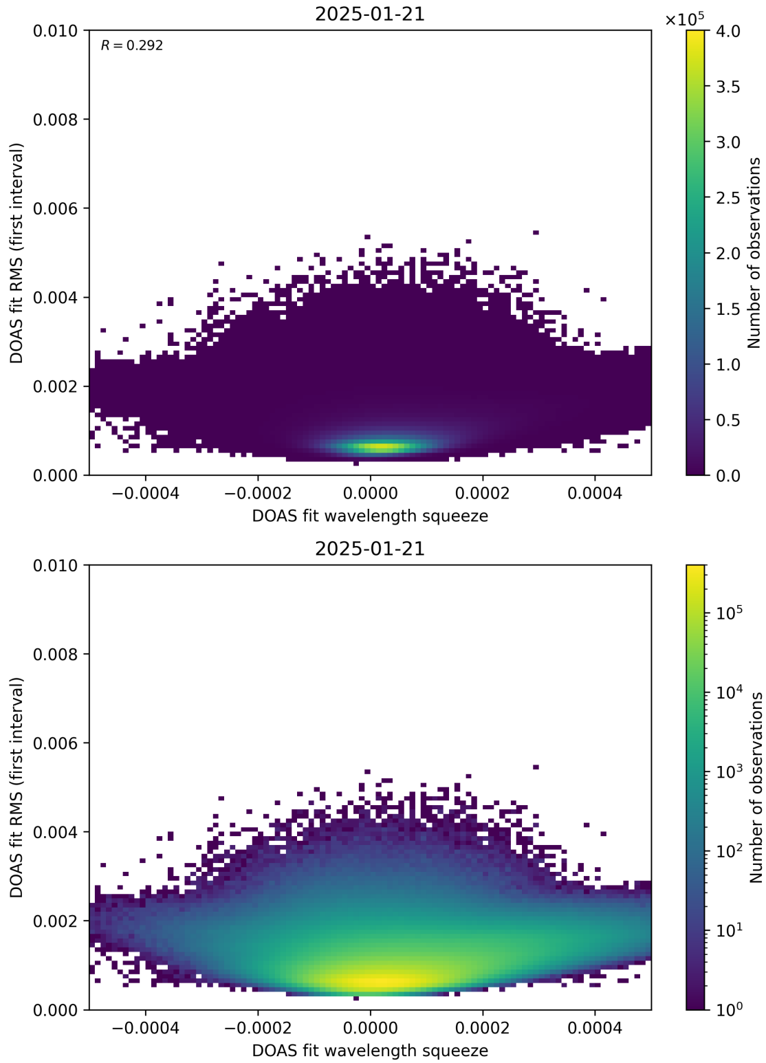
Figure 68: Scatter density plot of “DOAS fit wavelength squeeze” against “DOAS fit RMS (first interval)” for 2025-01-20 to 2025-01-22.
