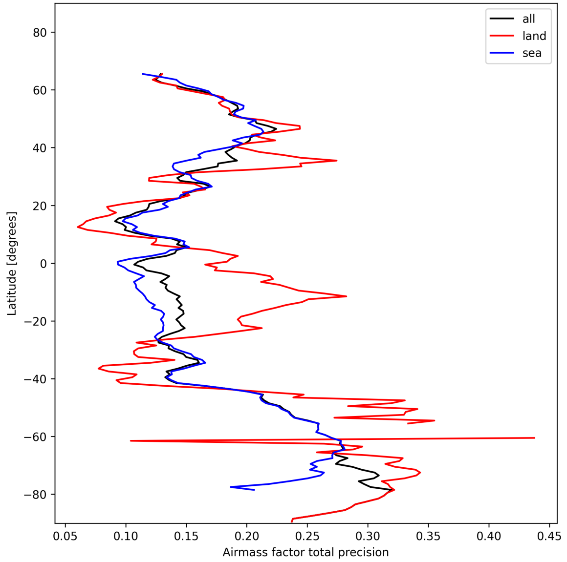
Figure 27: Zonal average of “Airmass factor total precision” for 2025-01-20 to 2025-01-22.
