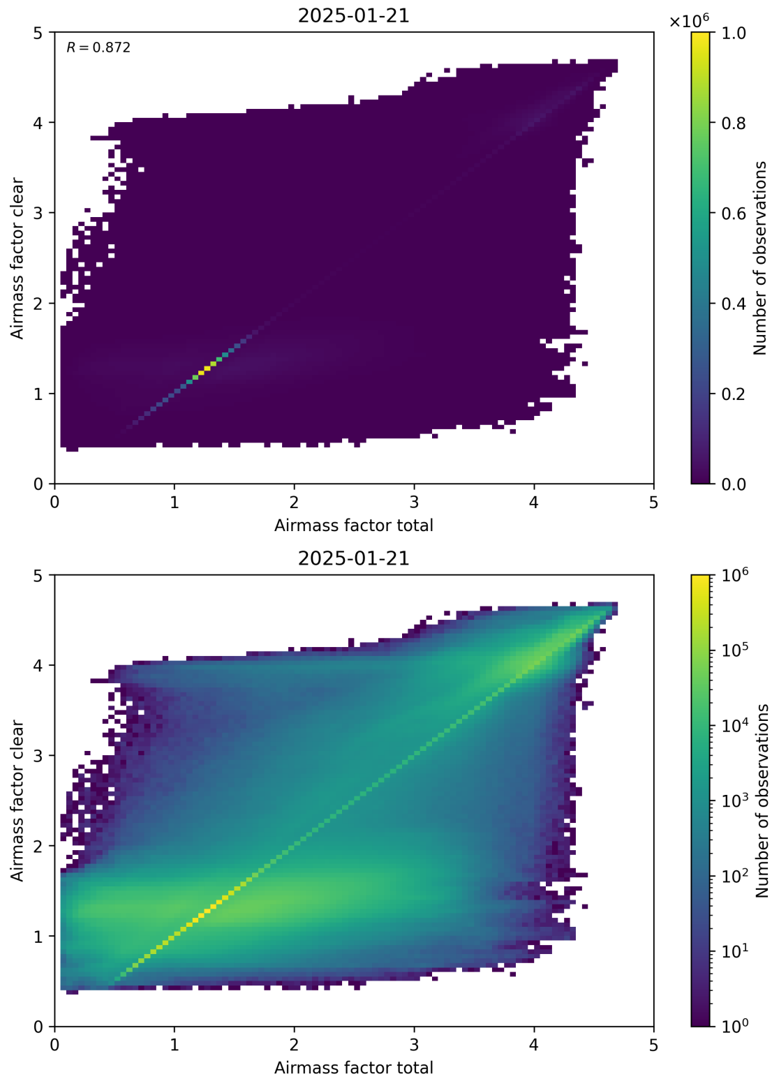
Figure 100: Scatter density plot of “Airmass factor total” against “Airmass factor clear” for 2025-01-20 to 2025-01-22.
