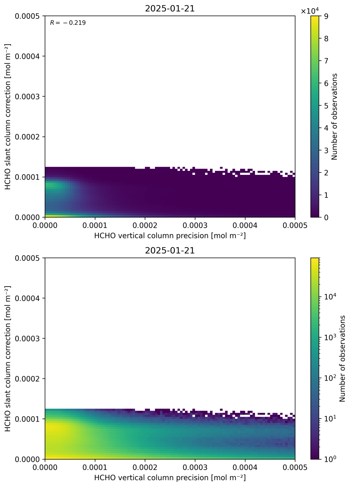
Figure 141: Scatter density plot of “HCHO vertical column precision” against “HCHO slant column correction” for 2025-01-20 to 2025-01-22.
