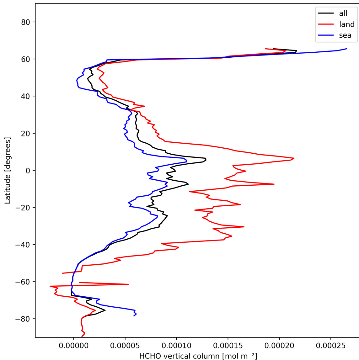
Figure 21: Zonal average of “HCHO vertical column” for 2025-01-20 to 2025-01-22.
