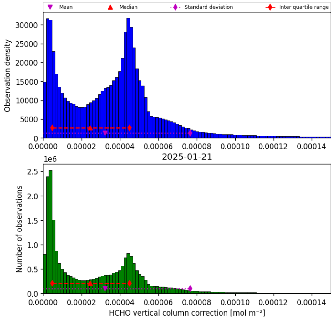
Figure 37: Histogram of “HCHO vertical column correction” for 2025-01-20 to 2025-01-22
