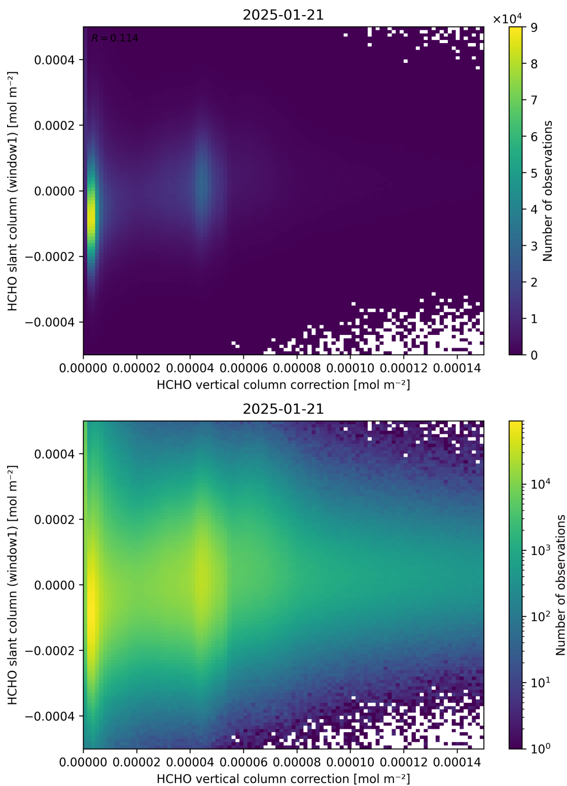
Figure 118: Scatter density plot of “HCHO vertical column correction” against “HCHO slant column (window1)” for 2025-01-20 to 2025-01-22.
