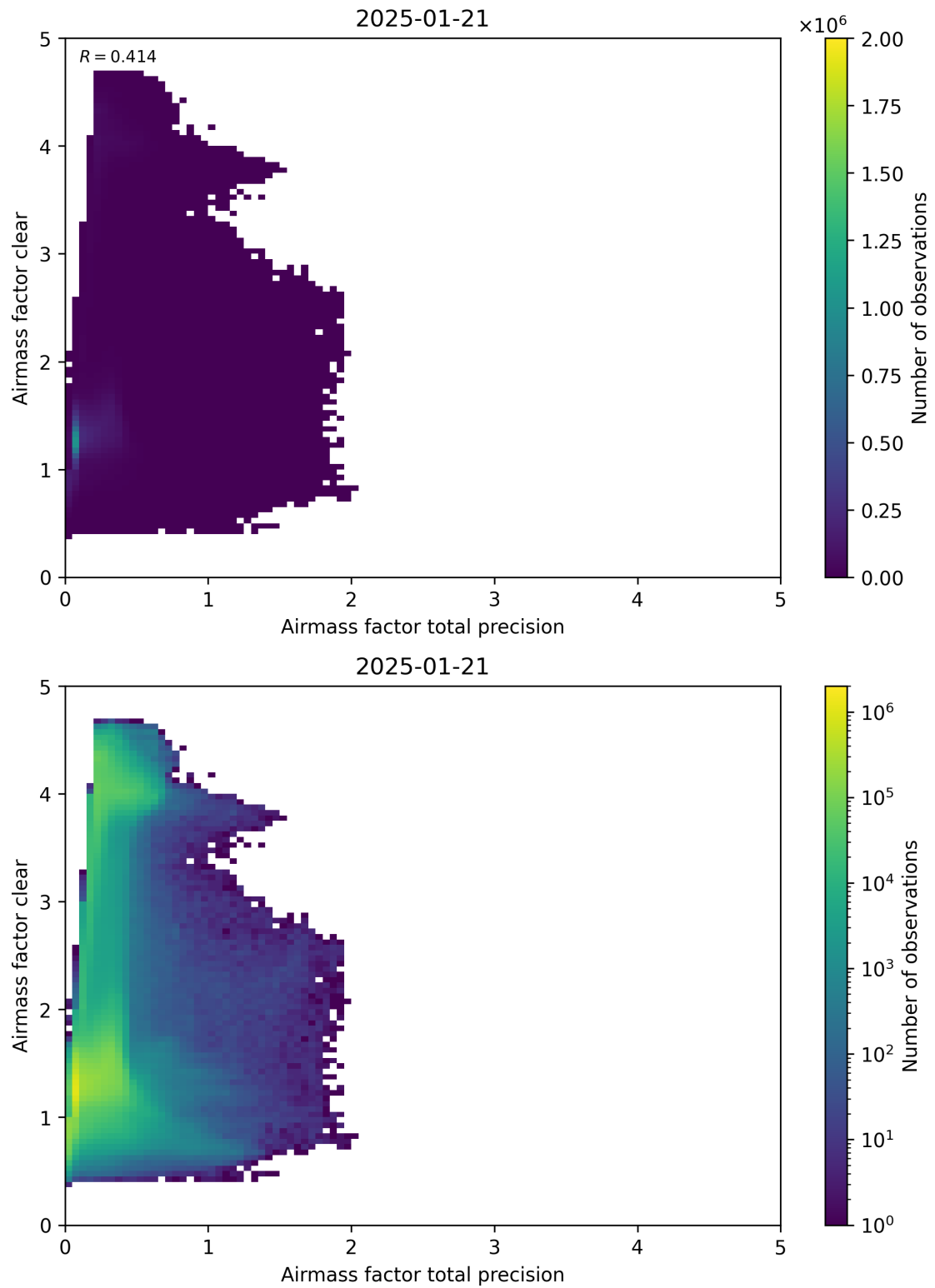
Figure 108: Scatter density plot of “Airmass factor total precision” against “Airmass factor clear” for 2025-01-20 to 2025-01-22.
