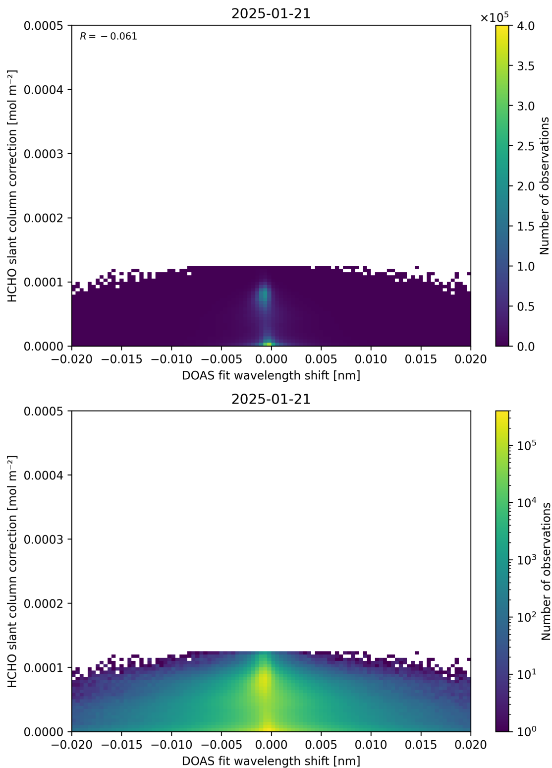
Figure 67: Scatter density plot of “DOAS fit wavelength shift” against “HCHO slant column correction” for 2025-01-20 to 2025-01-22.
