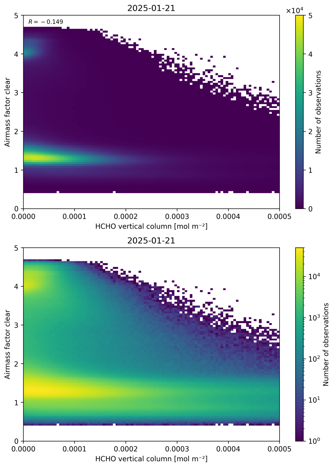
Figure 126: Scatter density plot of “HCHO vertical column” against “Airmass factor clear” for 2025-01-20 to 2025-01-22.
