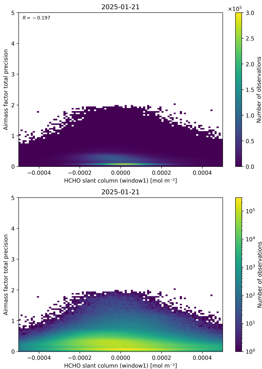
Figure 86: Scatter density plot of “HCHO slant column (window1)” against “Airmass factor total precision” for 2025-01-20 to 2025-01-22.
