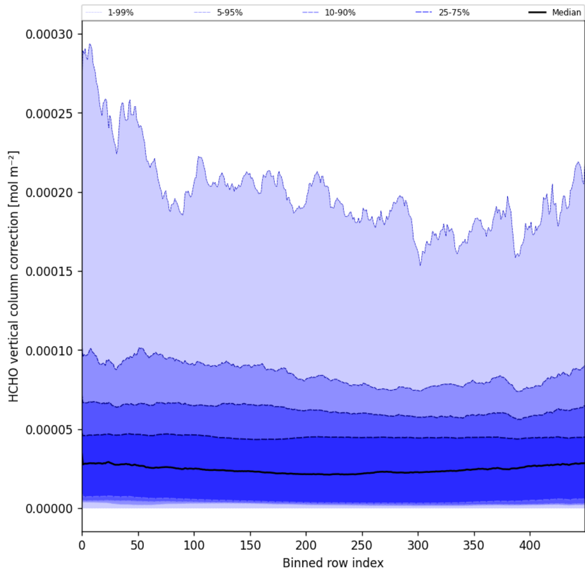
Figure 51: Along track statistics of “HCHO vertical column correction” for 2025-01-20 to 2025-01-22
