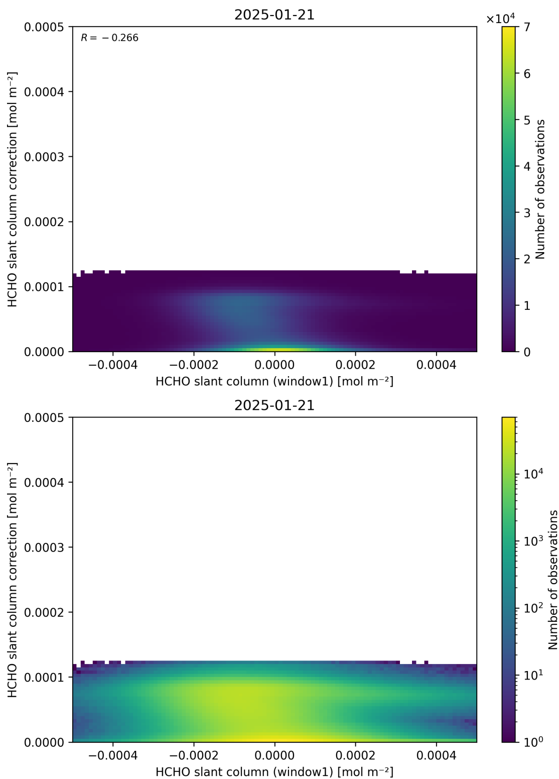
Figure 83: Scatter density plot of “HCHO slant column (window1)” against “HCHO slant column correction” for 2025-01-20 to 2025-01-22.
