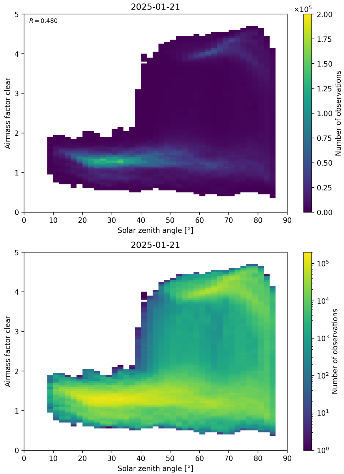
Figure 170: Scatter density plot of “Solar zenith angle” against “Airmass factor clear” for 2025-01-20 to 2025-01-22.
