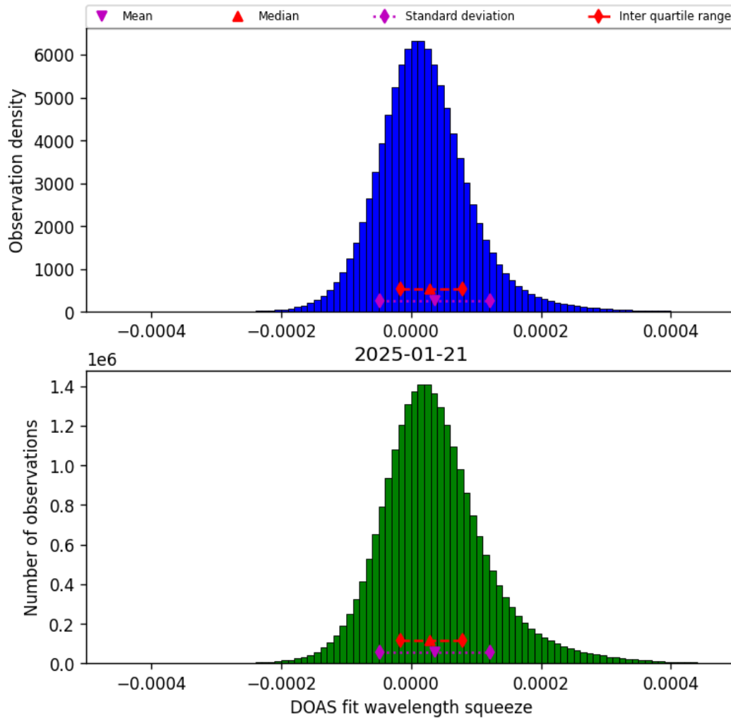
Figure 45: Histogram of “DOAS fit wavelength squeeze” for 2025-01-20 to 2025-01-22
