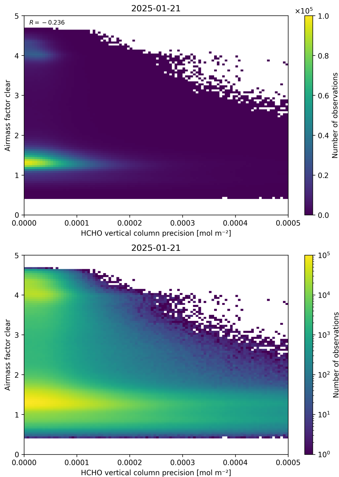
Figure 139: Scatter density plot of “HCHO vertical column precision” against “Airmass factor clear” for 2025-01-20 to 2025-01-22.
