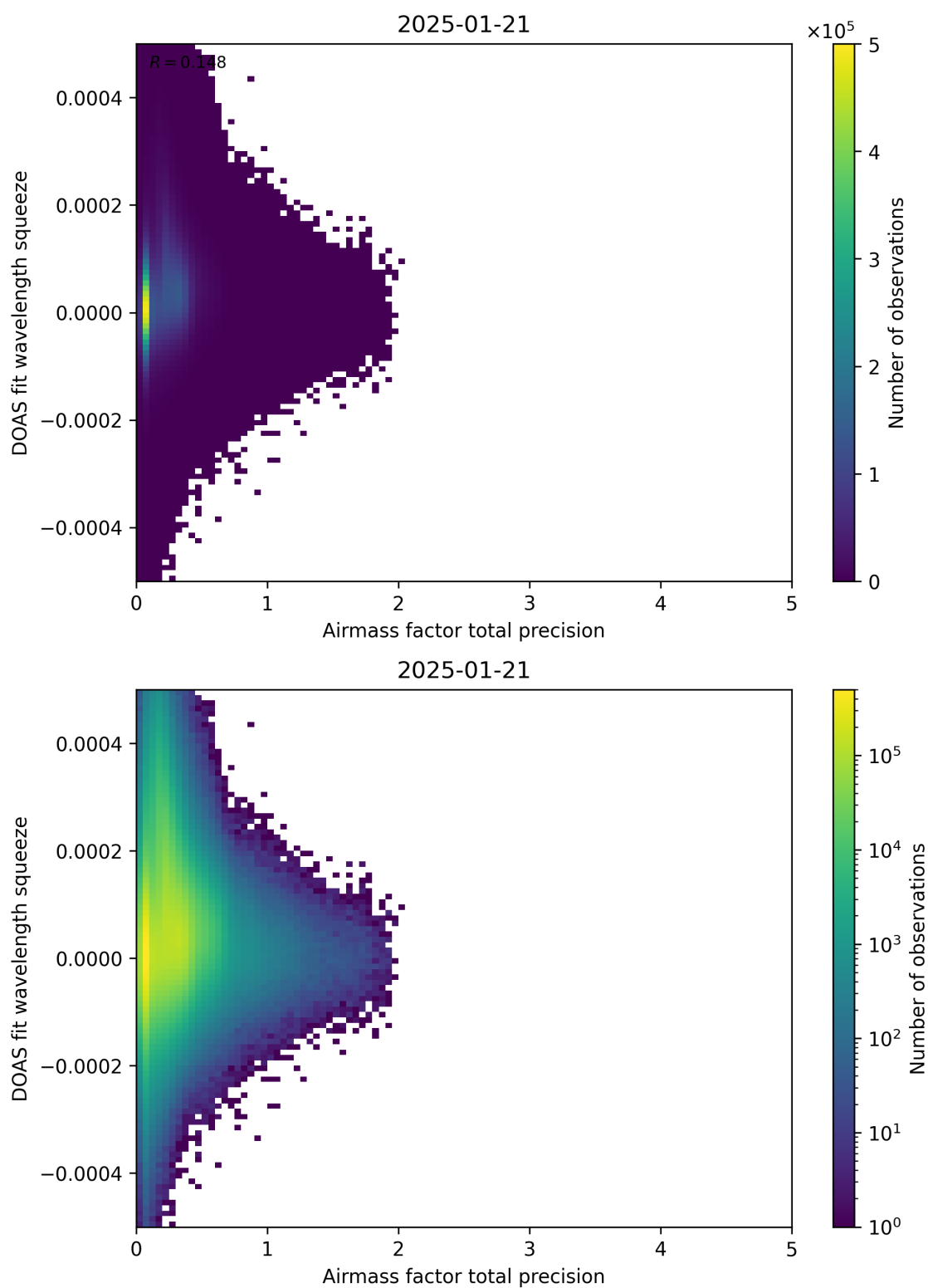
Figure 107: Scatter density plot of “Airmass factor total precision” against “DOAS fit wavelength squeeze” for 2025-01-20 to 2025-01-22.
