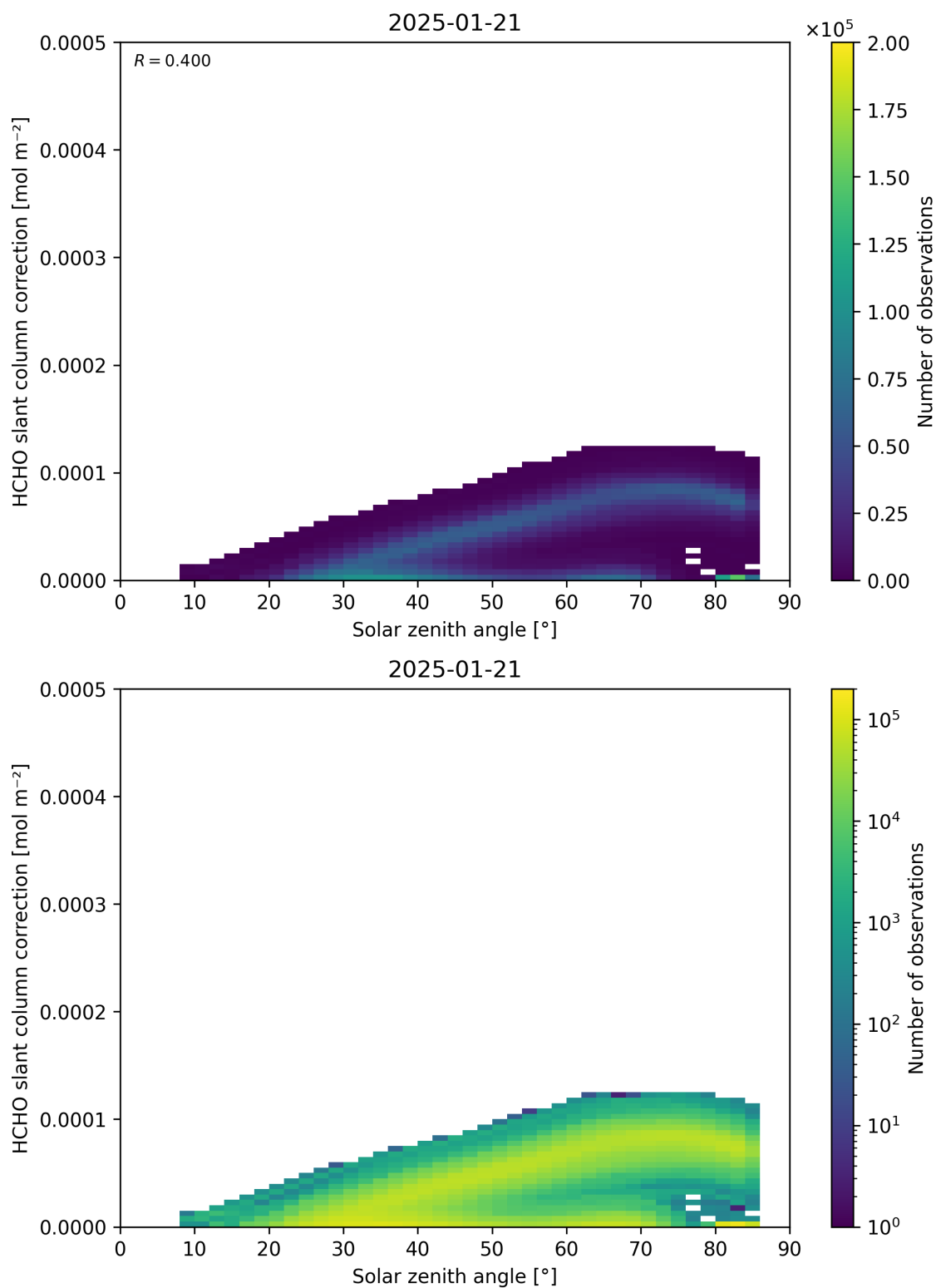
Figure 172: Scatter density plot of “Solar zenith angle” against “HCHO slant column correction” for 2025-01-20 to 2025-01-22.
