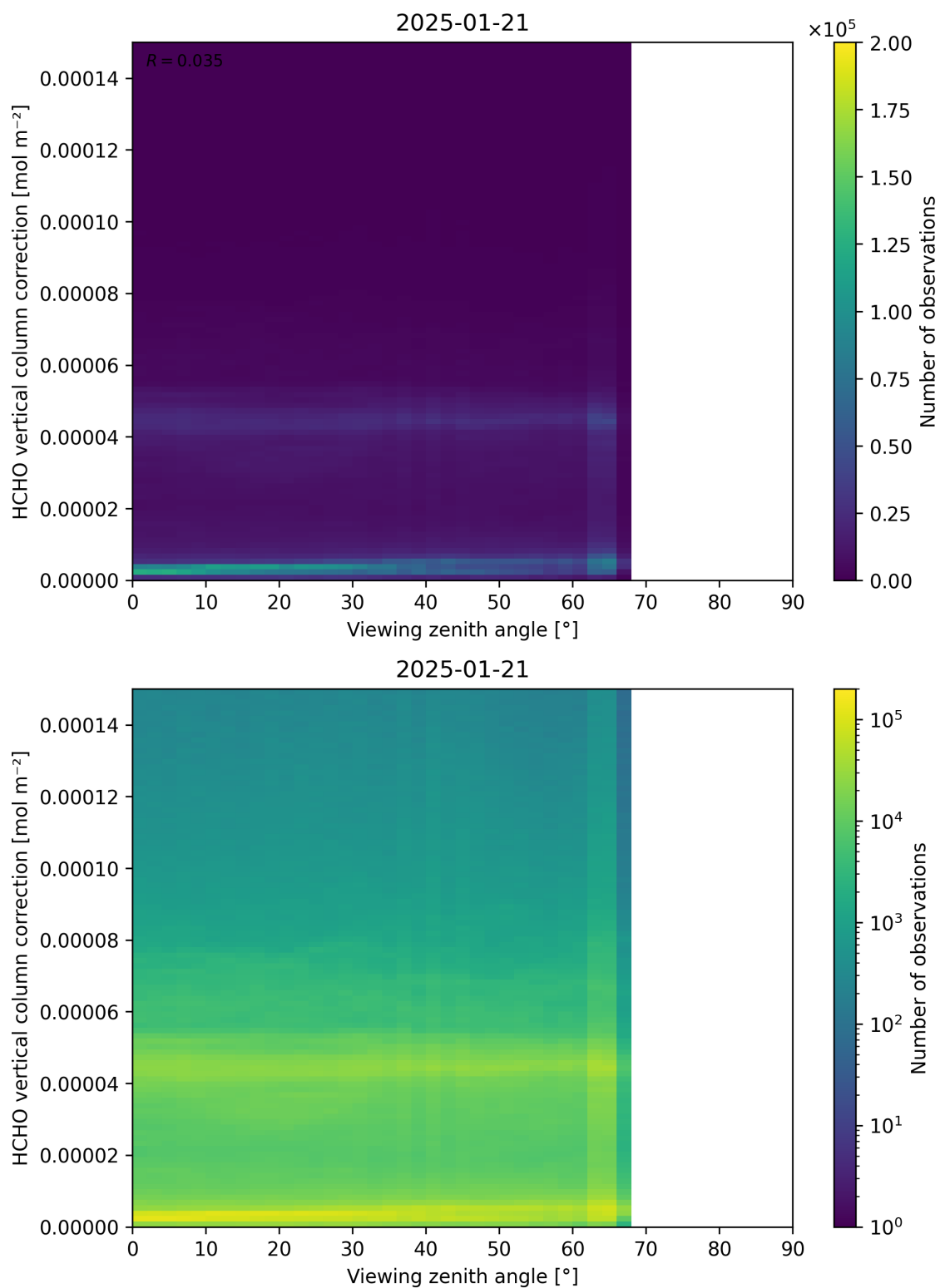
Figure 193: Scatter density plot of “Viewing zenith angle” against “HCHO vertical column correction” for 2025-01-20 to 2025-01-22.
