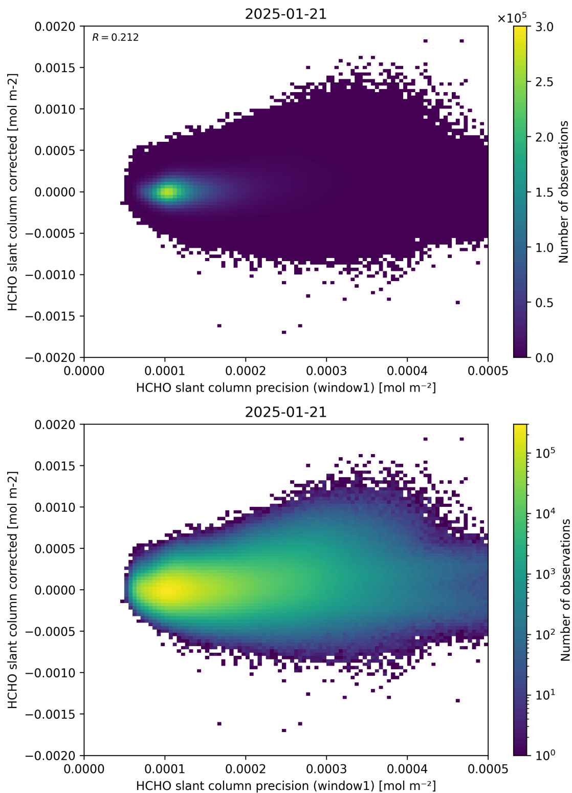
Figure 92: Scatter density plot of “HCHO slant column precision (window1)” against “HCHO slant column corrected” for 2025-01-20 to 2025-01-22.
