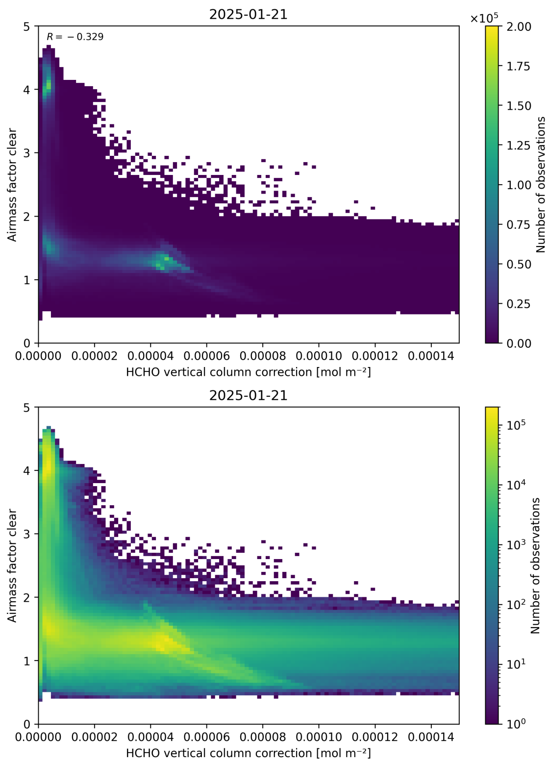
Figure 115: Scatter density plot of “HCHO vertical column correction” against “Airmass factor clear” for 2025-01-20 to 2025-01-22.
