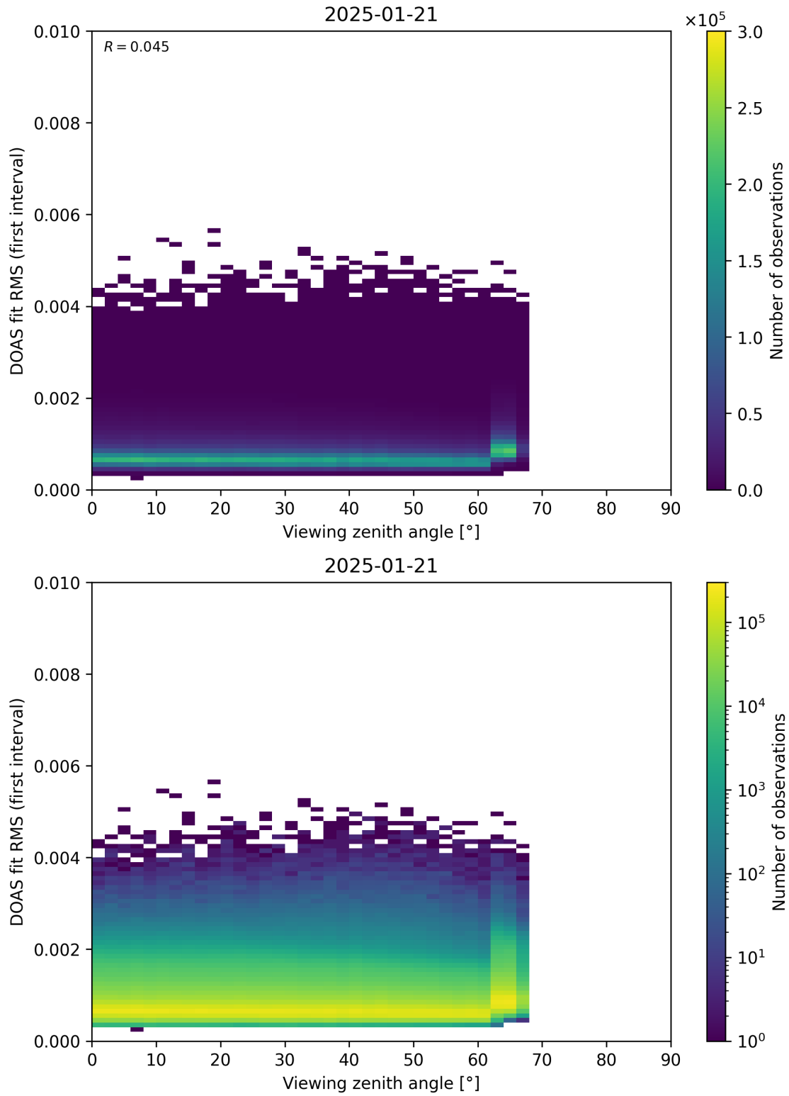
Figure 182: Scatter density plot of “Viewing zenith angle” against “DOAS fit RMS (first interval)” for 2025-01-20 to 2025-01-22.
