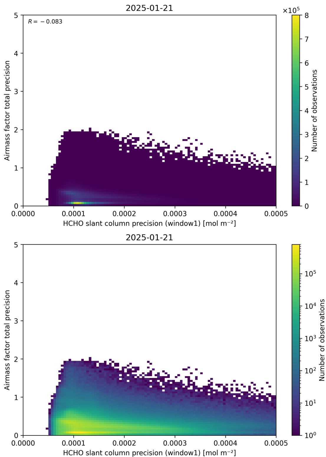
Figure 95: Scatter density plot of “HCHO slant column precision (window1)” against “Airmass factor total precision” for 2025-01-20 to 2025-01-22.
