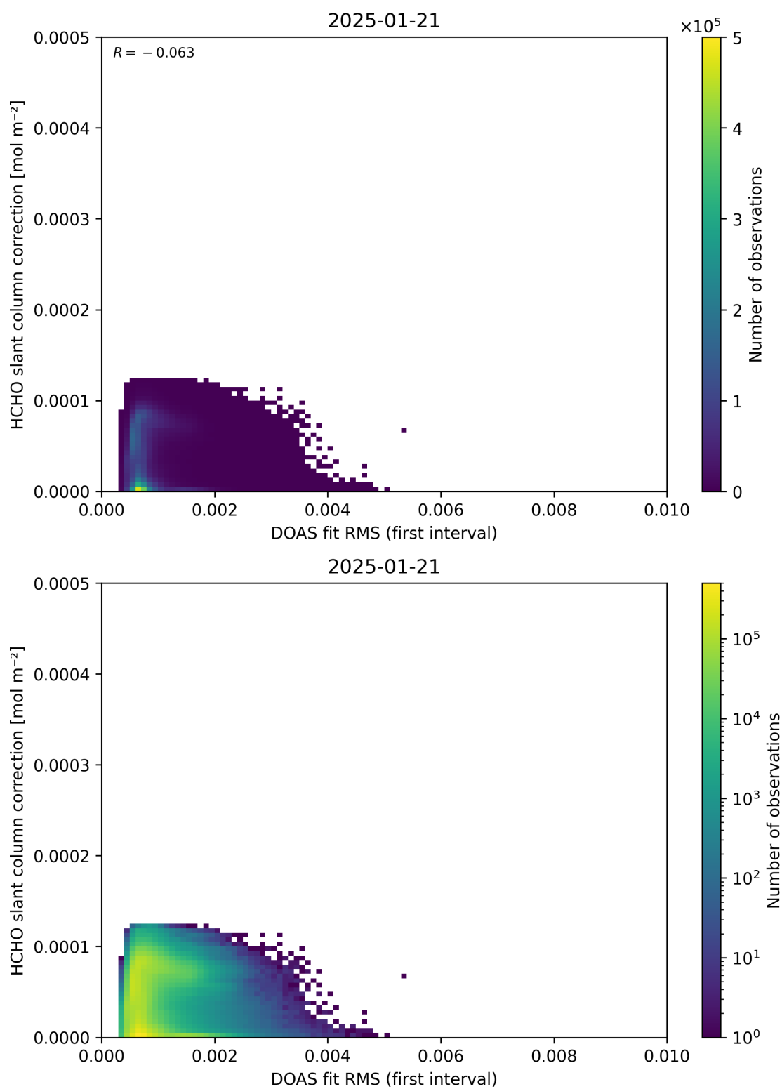
Figure 63: Scatter density plot of “DOAS fit RMS (first interval)” against “HCHO slant column correction” for 2025-01-20 to 2025-01-22.
