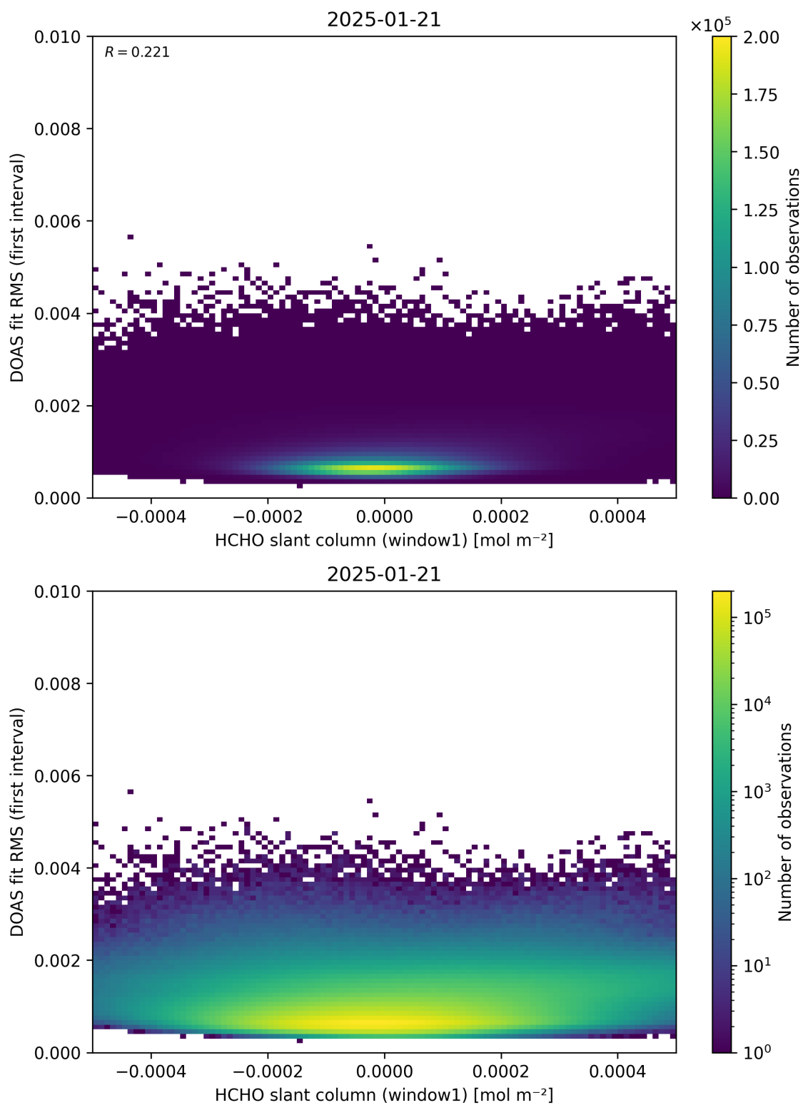
Figure 78: Scatter density plot of “HCHO slant column (window1)” against “DOAS fit RMS (first interval)” for 2025-01-20 to 2025-01-22.
