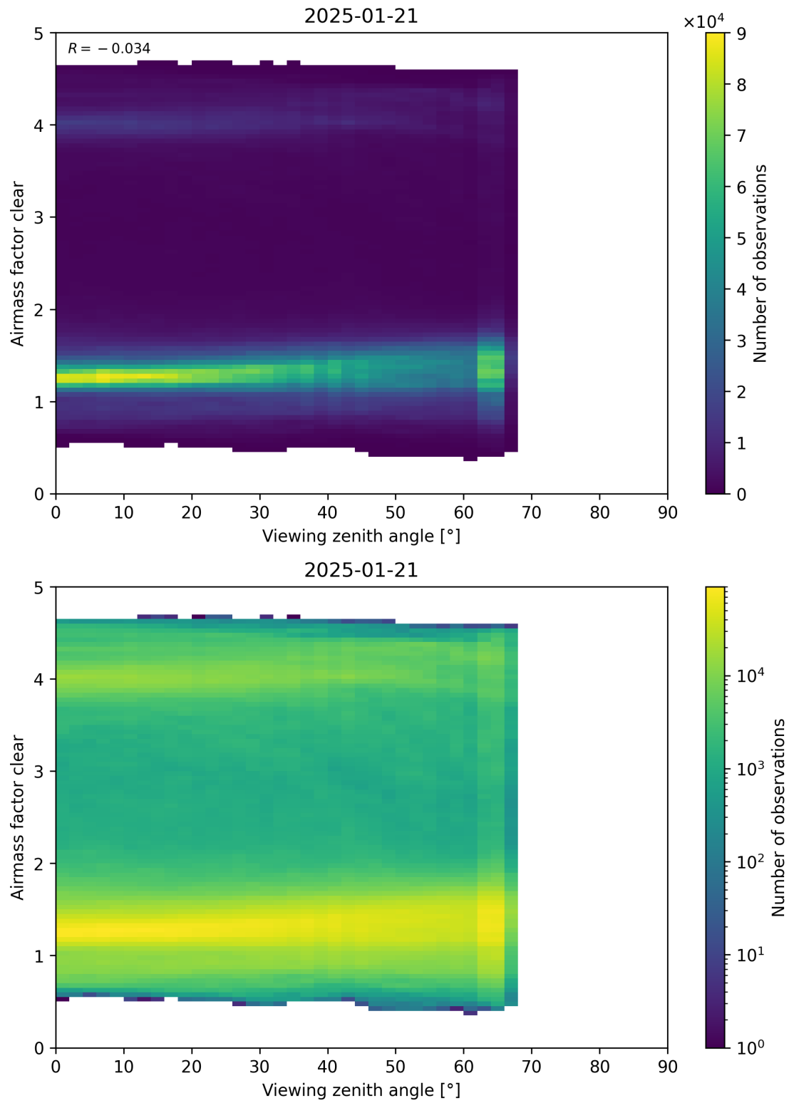
Figure 185: Scatter density plot of “Viewing zenith angle” against “Airmass factor clear” for 2025-01-20 to 2025-01-22.
