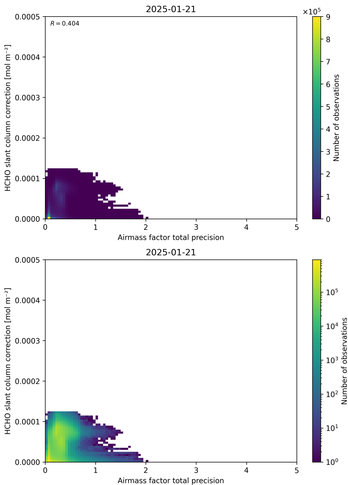
Figure 110: Scatter density plot of “Airmass factor total precision” against “HCHO slant column correction” for 2025-01-20 to 2025-01-22.
