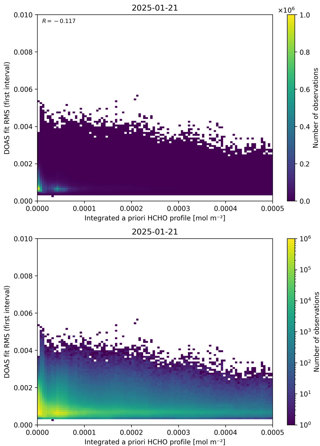
Figure 148: Scatter density plot of “Integrated a priori HCHO profile” against “DOAS fit RMS (first interval)” for 2025-01-20 to 2025-01-22.
