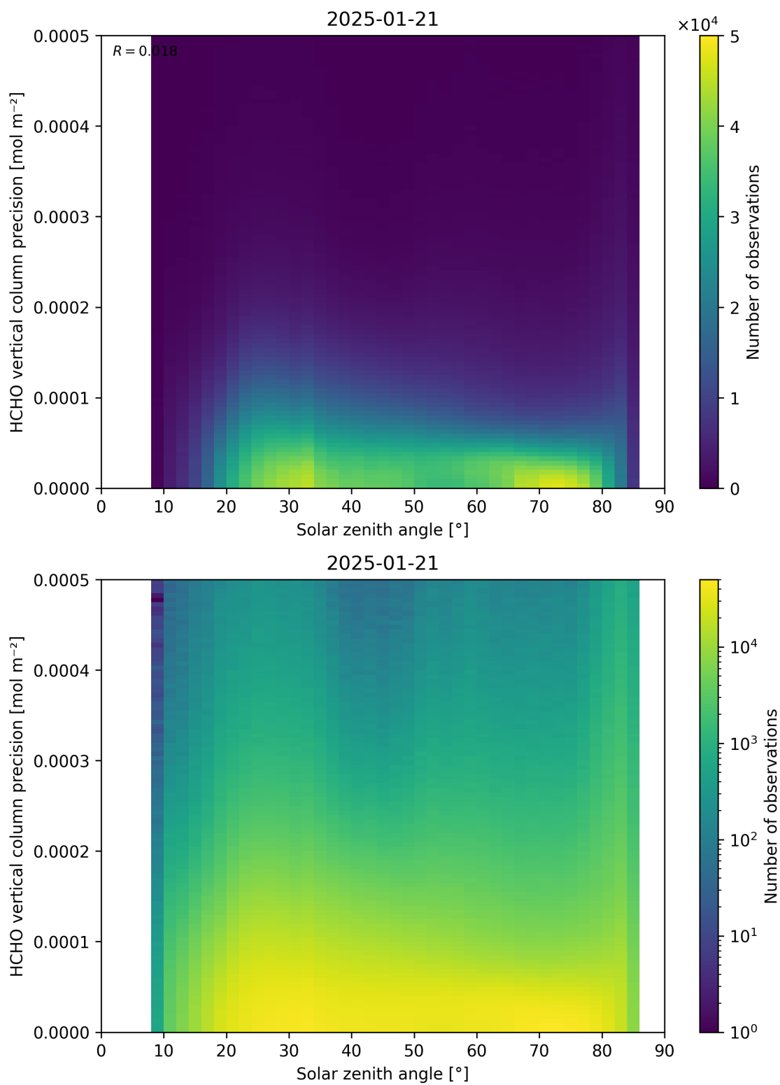
Figure 179: Scatter density plot of “Solar zenith angle” against “HCHO vertical column precision” for 2025-01-20 to 2025-01-22.
