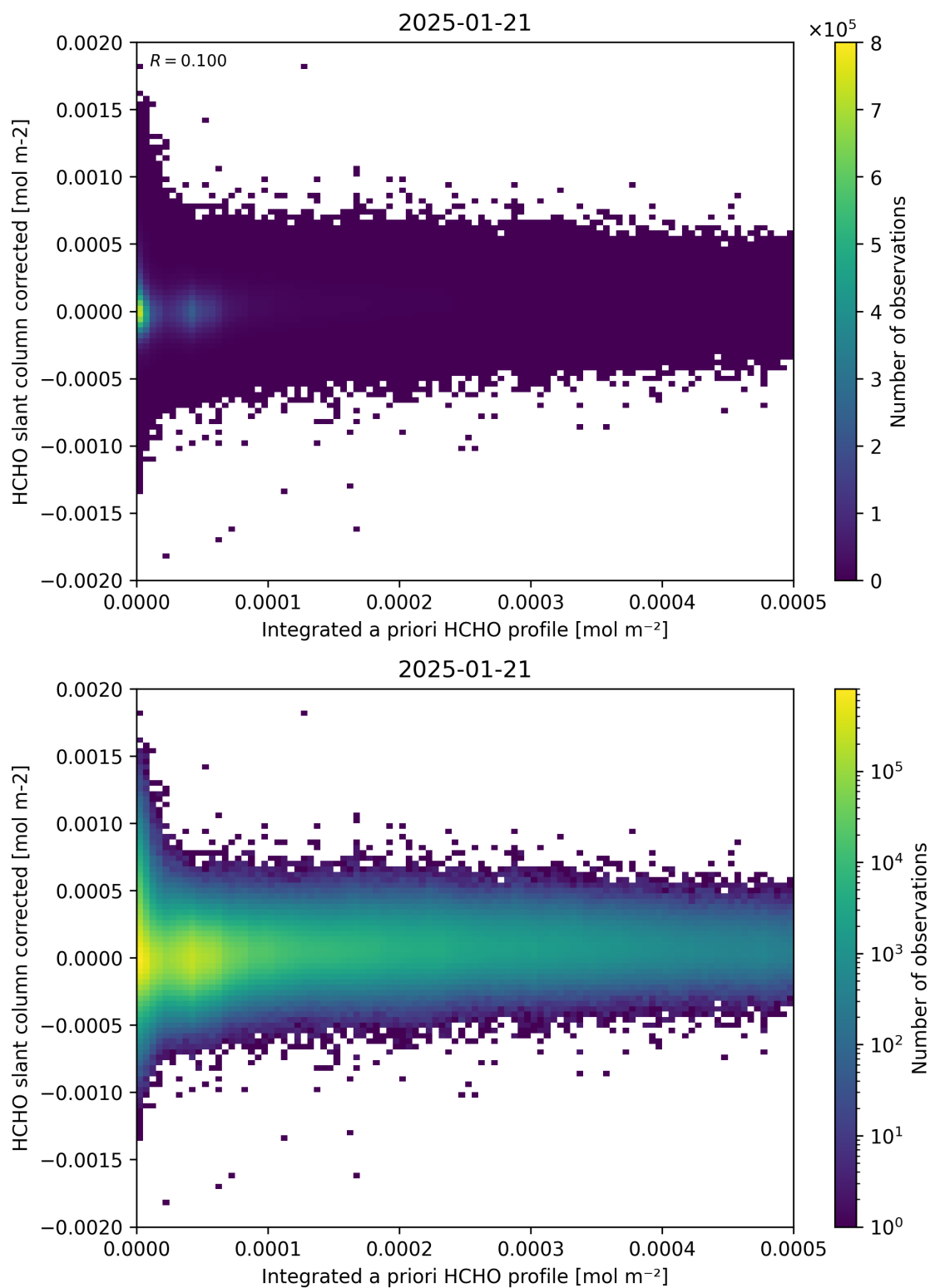
Figure 151: Scatter density plot of “Integrated a priori HCHO profile” against “HCHO slant column corrected” for 2025-01-20 to 2025-01-22.
