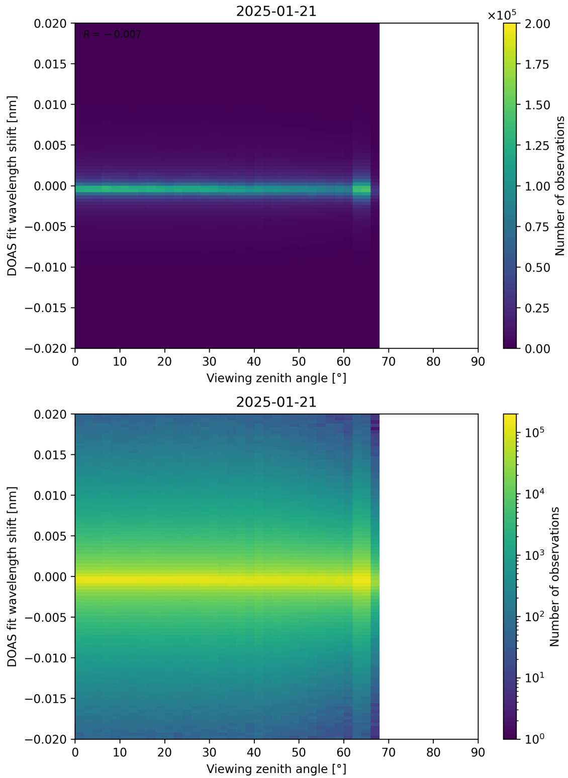
Figure 183: Scatter density plot of “Viewing zenith angle” against “DOAS fit wavelength shift” for 2025-01-20 to 2025-01-22.
