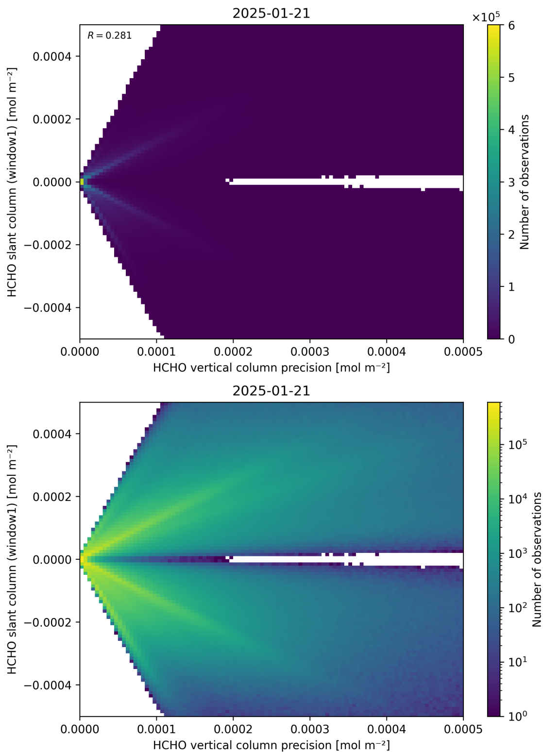
Figure 142: Scatter density plot of “HCHO vertical column precision” against “HCHO slant column (window1)” for 2025-01-20 to 2025-01-22.
