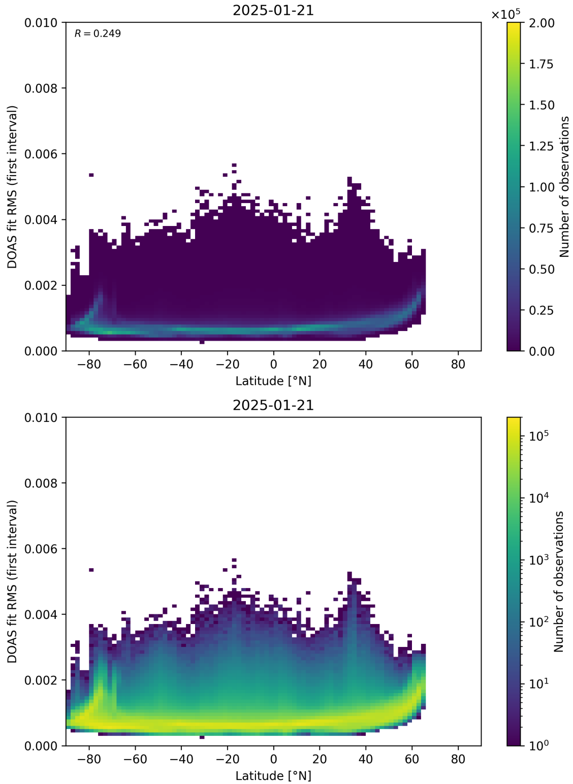
Figure 153: Scatter density plot of “Latitude” against “DOAS fit RMS (first interval)” for 2025-01-20 to 2025-01-22.
