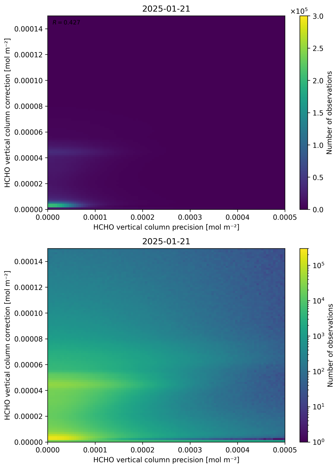
Figure 146: Scatter density plot of “HCHO vertical column precision” against “HCHO vertical column correction” for 2025-01-20 to 2025-01-22.
