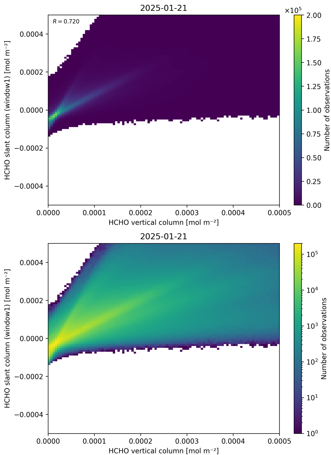
Figure 129: Scatter density plot of “HCHO vertical column” against “HCHO slant column (window1)” for 2025-01-20 to 2025-01-22.
