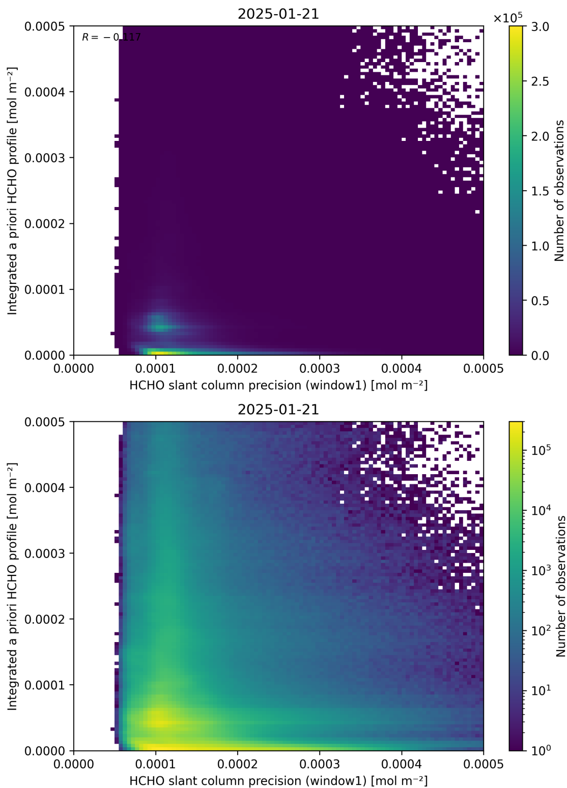
Figure 96: Scatter density plot of “HCHO slant column precision (window1)” against “Integrated a priori HCHO profile” for 2025-01-20 to 2025-01-22.
