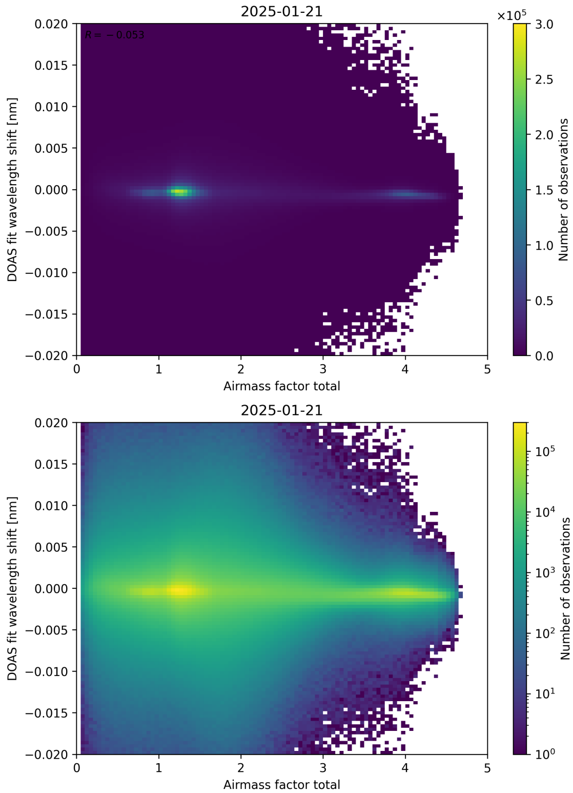
Figure 98: Scatter density plot of “Airmass factor total” against “DOAS fit wavelength shift” for 2025-01-20 to 2025-01-22.
