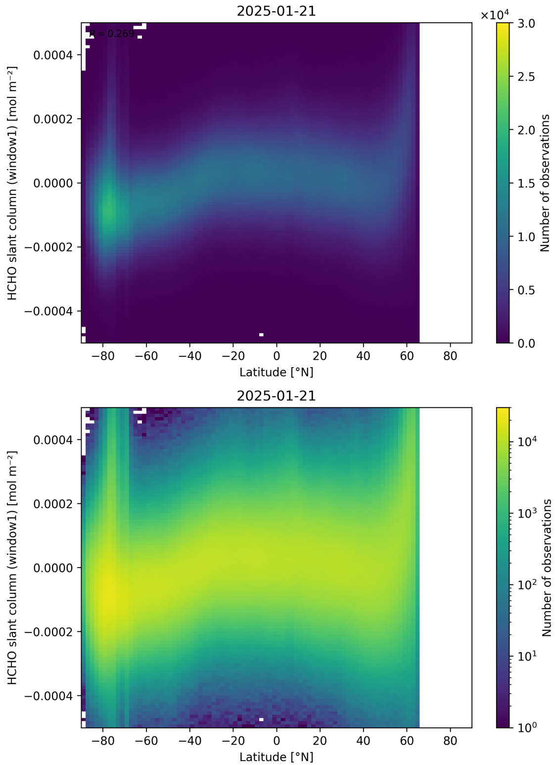
Figure 159: Scatter density plot of “Latitude” against “HCHO slant column (window1)” for 2025-01-20 to 2025-01-22.
