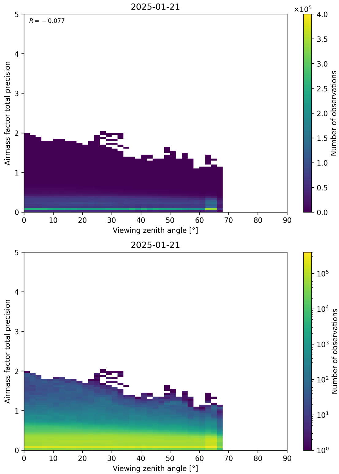
Figure 191: Scatter density plot of “Viewing zenith angle” against “Airmass factor total precision” for 2025-01-20 to 2025-01-22.
