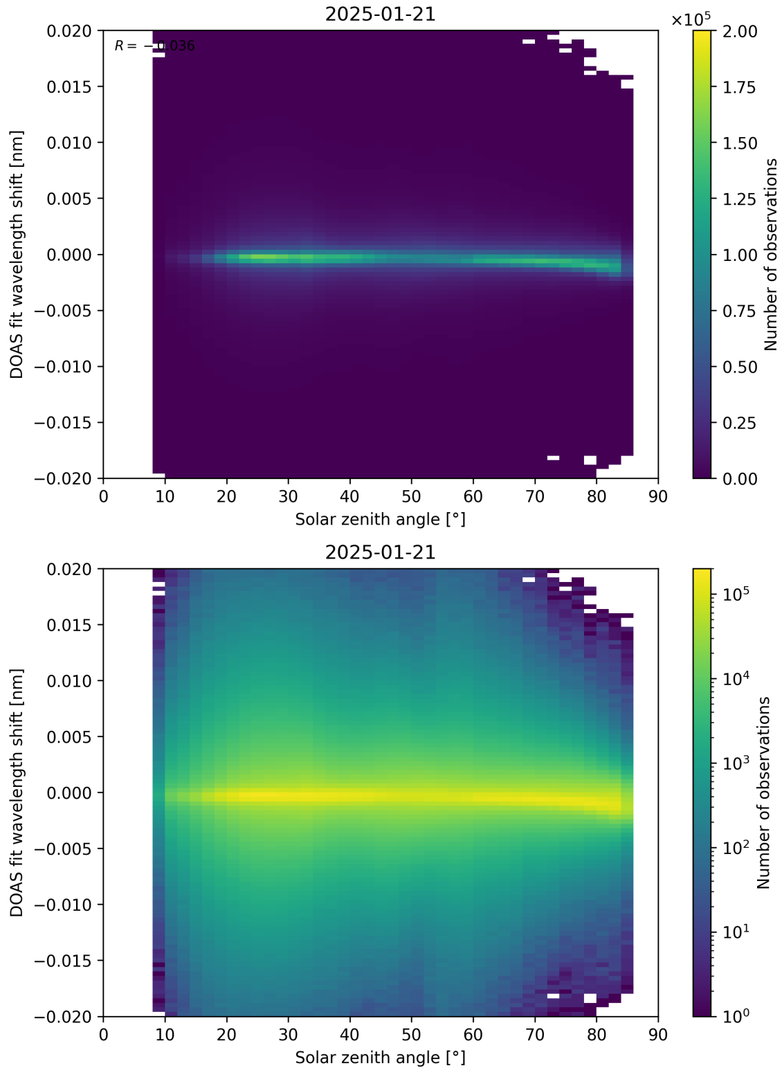
Figure 168: Scatter density plot of “Solar zenith angle” against “DOAS fit wavelength shift” for 2025-01-20 to 2025-01-22.
