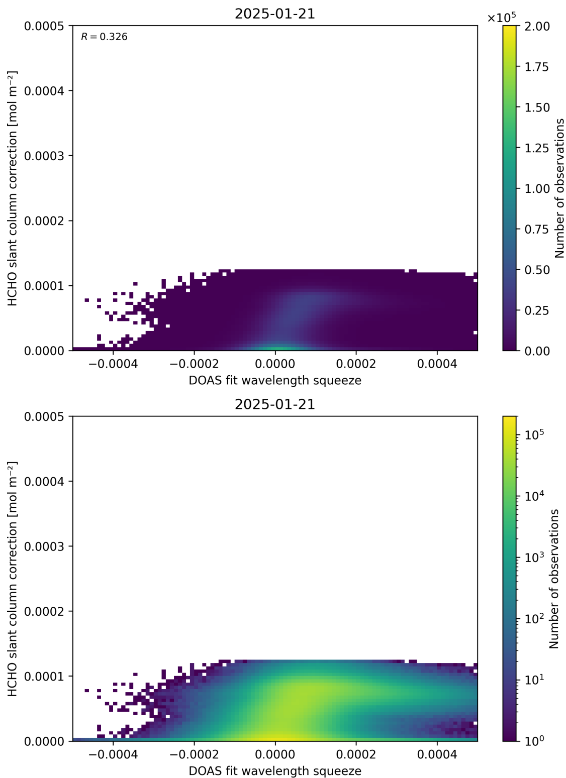
Figure 70: Scatter density plot of “DOAS fit wavelength squeeze” against “HCHO slant column correction” for 2025-01-20 to 2025-01-22.
