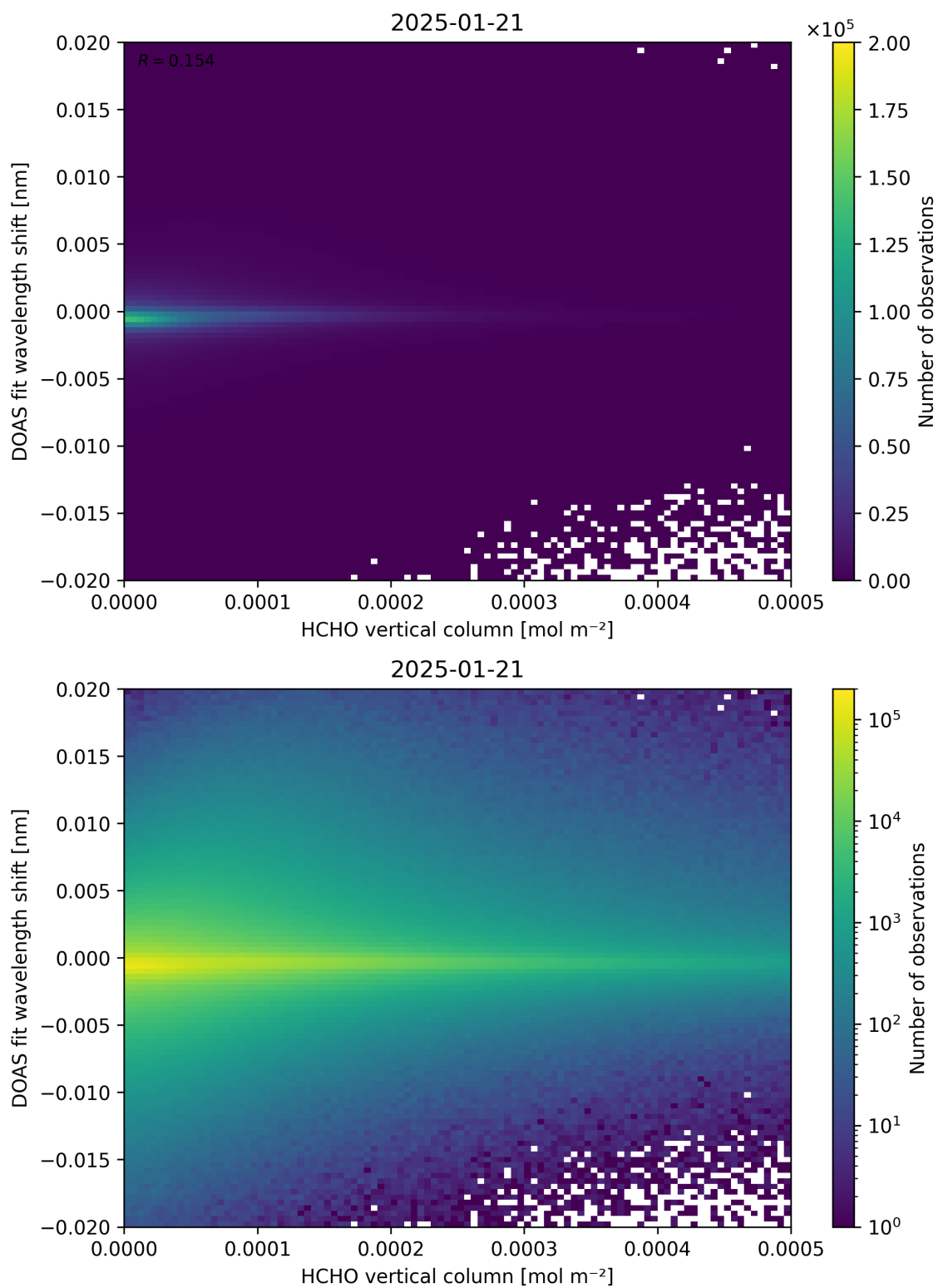
Figure 124: Scatter density plot of “HCHO vertical column” against “DOAS fit wavelength shift” for 2025-01-20 to 2025-01-22.
