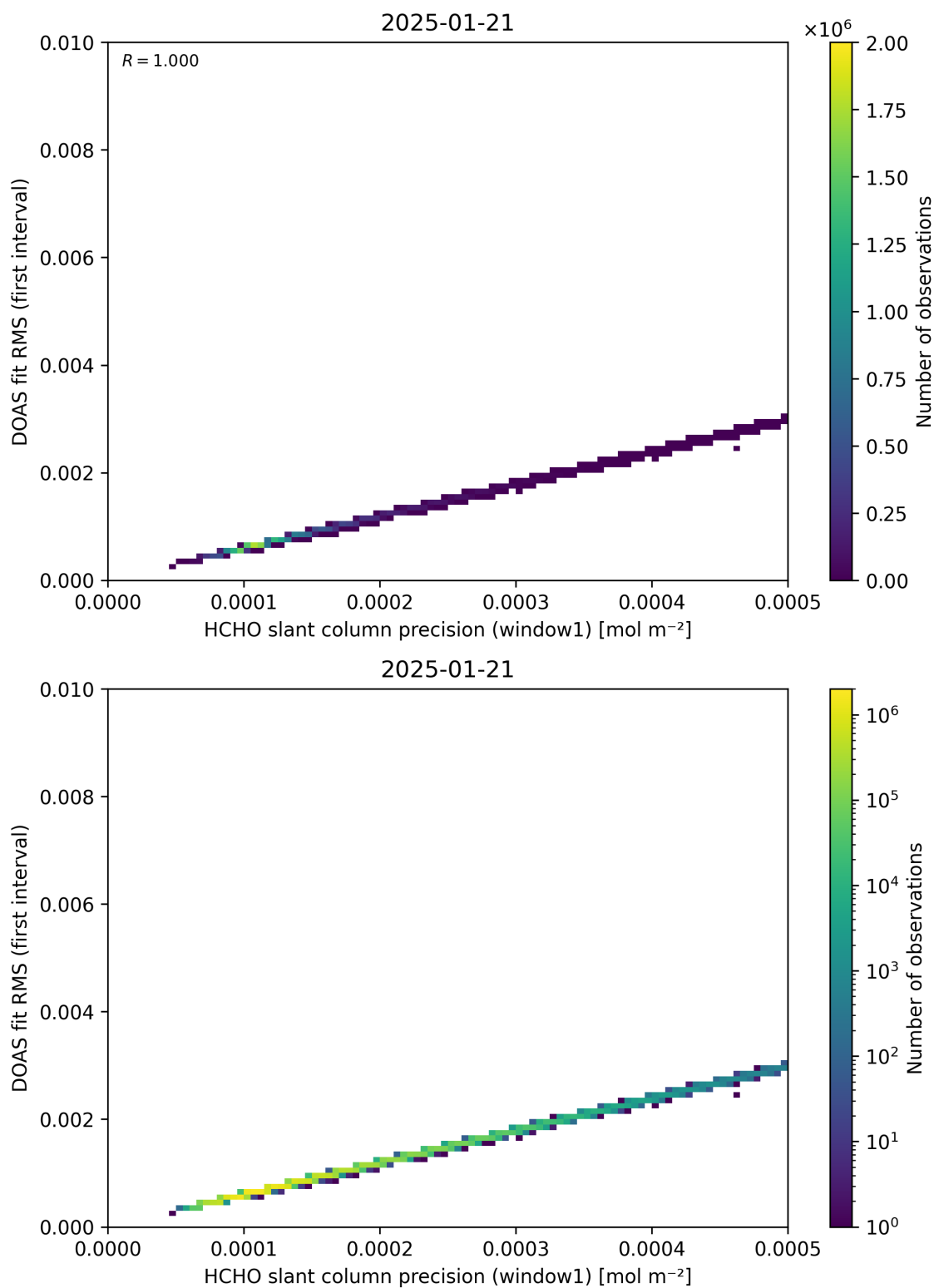
Figure 88: Scatter density plot of “HCHO slant column precision (window1)” against “DOAS fit RMS (first interval)” for 2025-01-20 to 2025-01-22.
