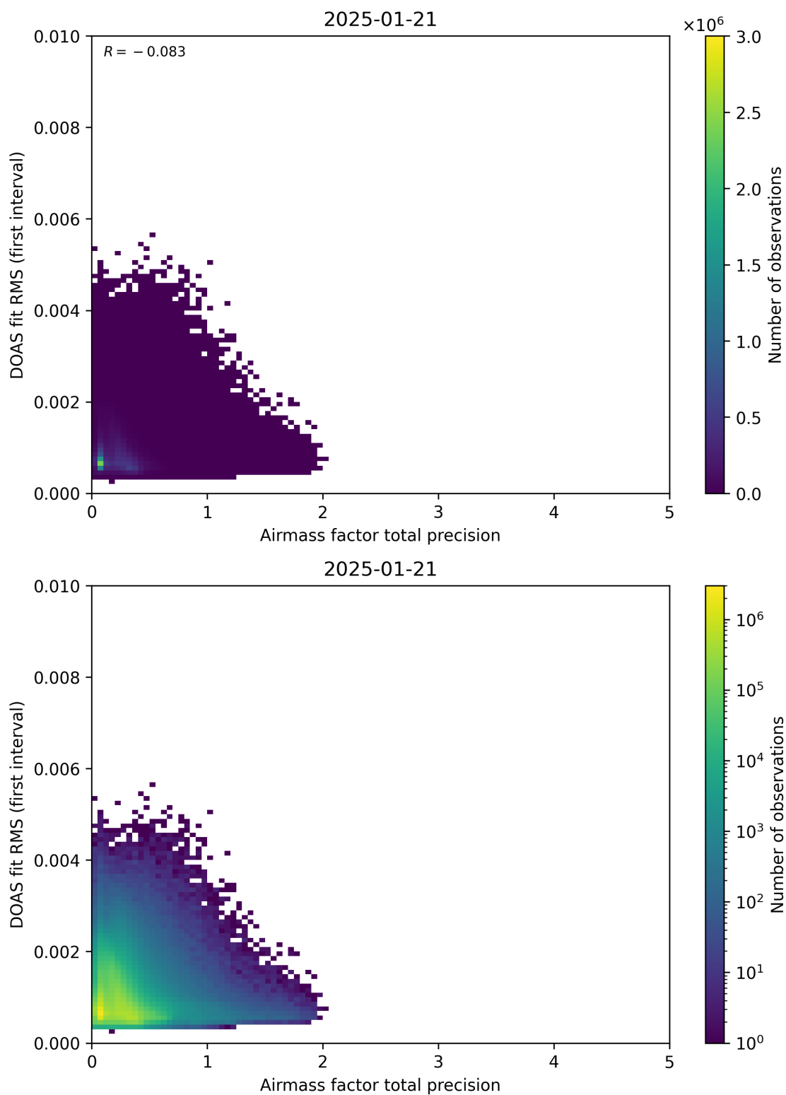
Figure 105: Scatter density plot of “Airmass factor total precision” against “DOAS fit RMS (first interval)” for 2025-01-20 to 2025-01-22.
