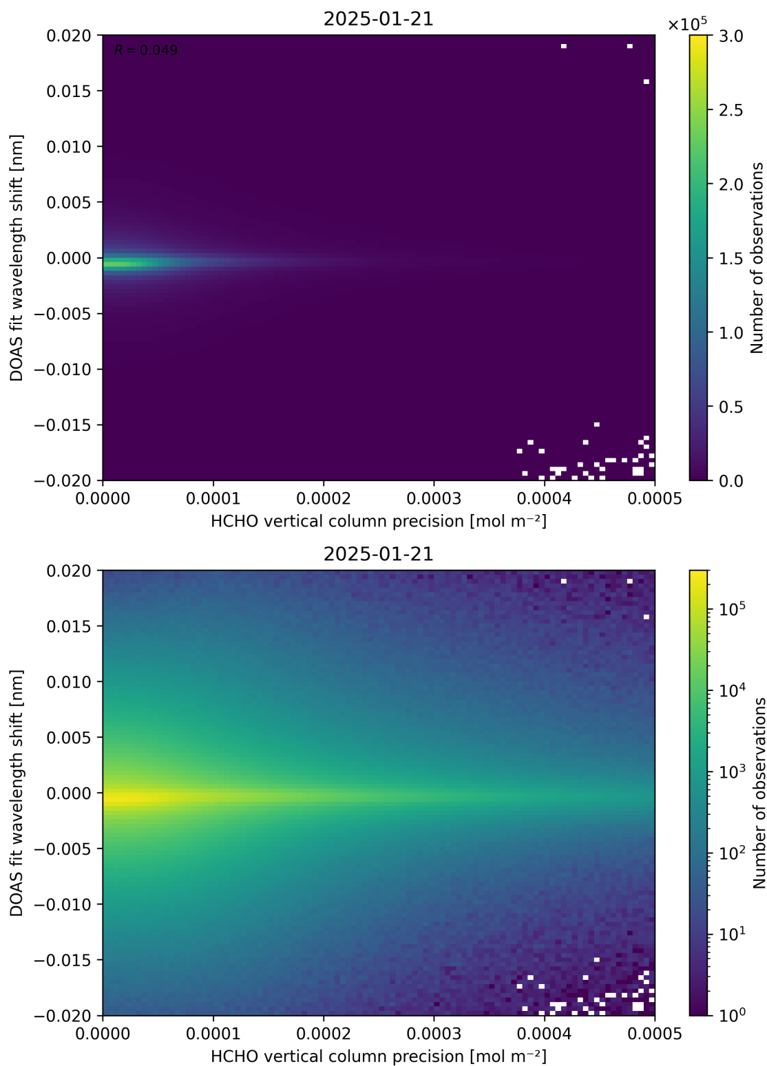
Figure 137: Scatter density plot of “HCHO vertical column precision” against “DOAS fit wavelength shift” for 2025-01-20 to 2025-01-22.
