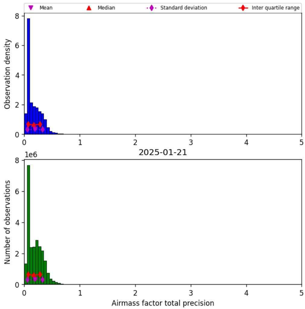
Figure 41: Histogram of “Airmass factor total precision” for 2025-01-20 to 2025-01-22
