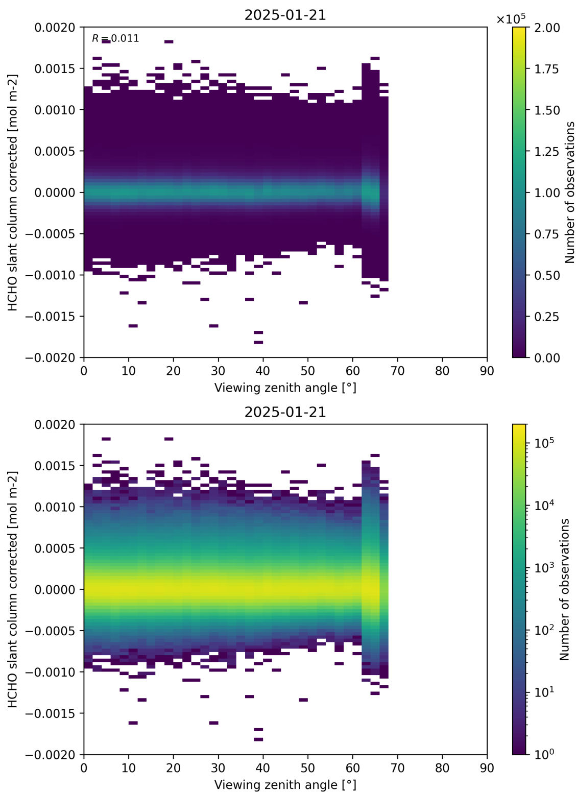
Figure 186: Scatter density plot of “Viewing zenith angle” against “HCHO slant column corrected” for 2025-01-20 to 2025-01-22.
