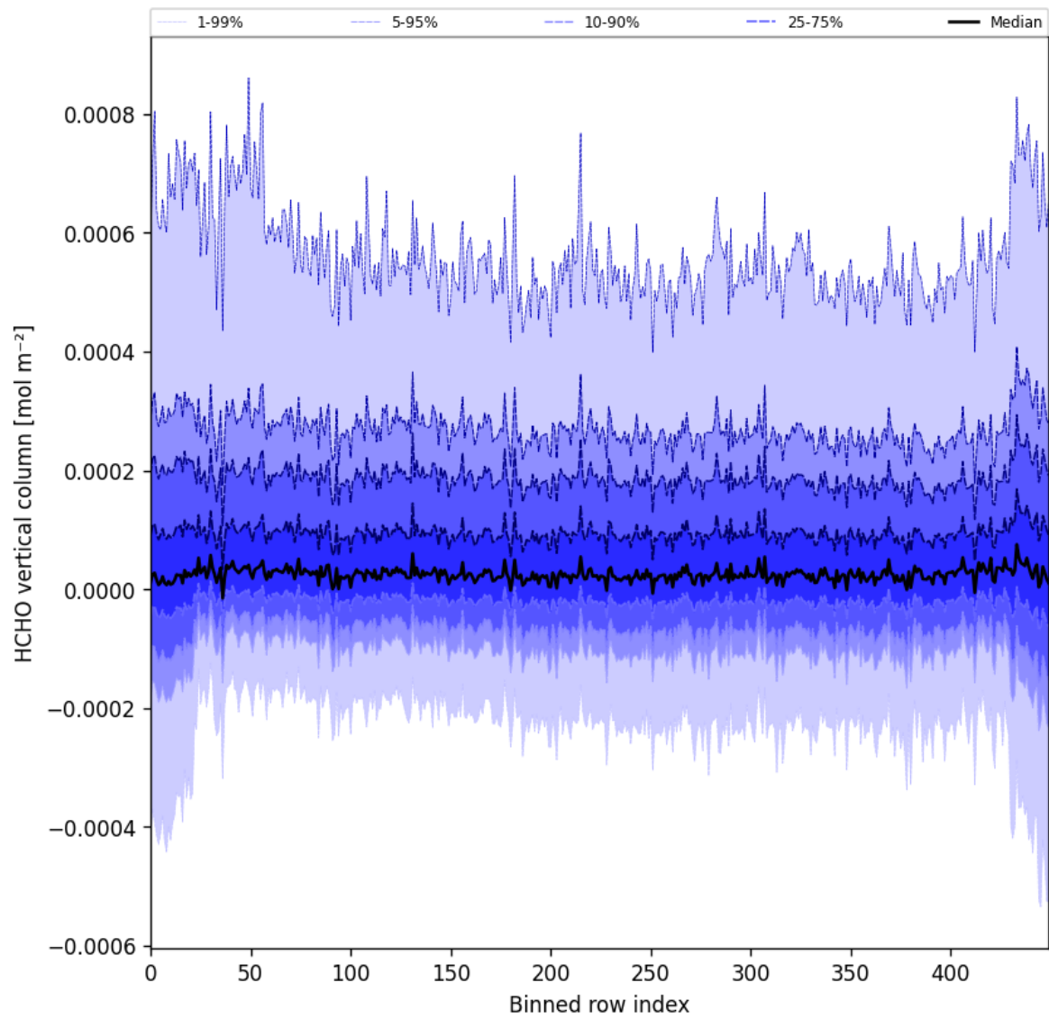
Figure 49: Along track statistics of “HCHO vertical column” for 2025-01-20 to 2025-01-22
