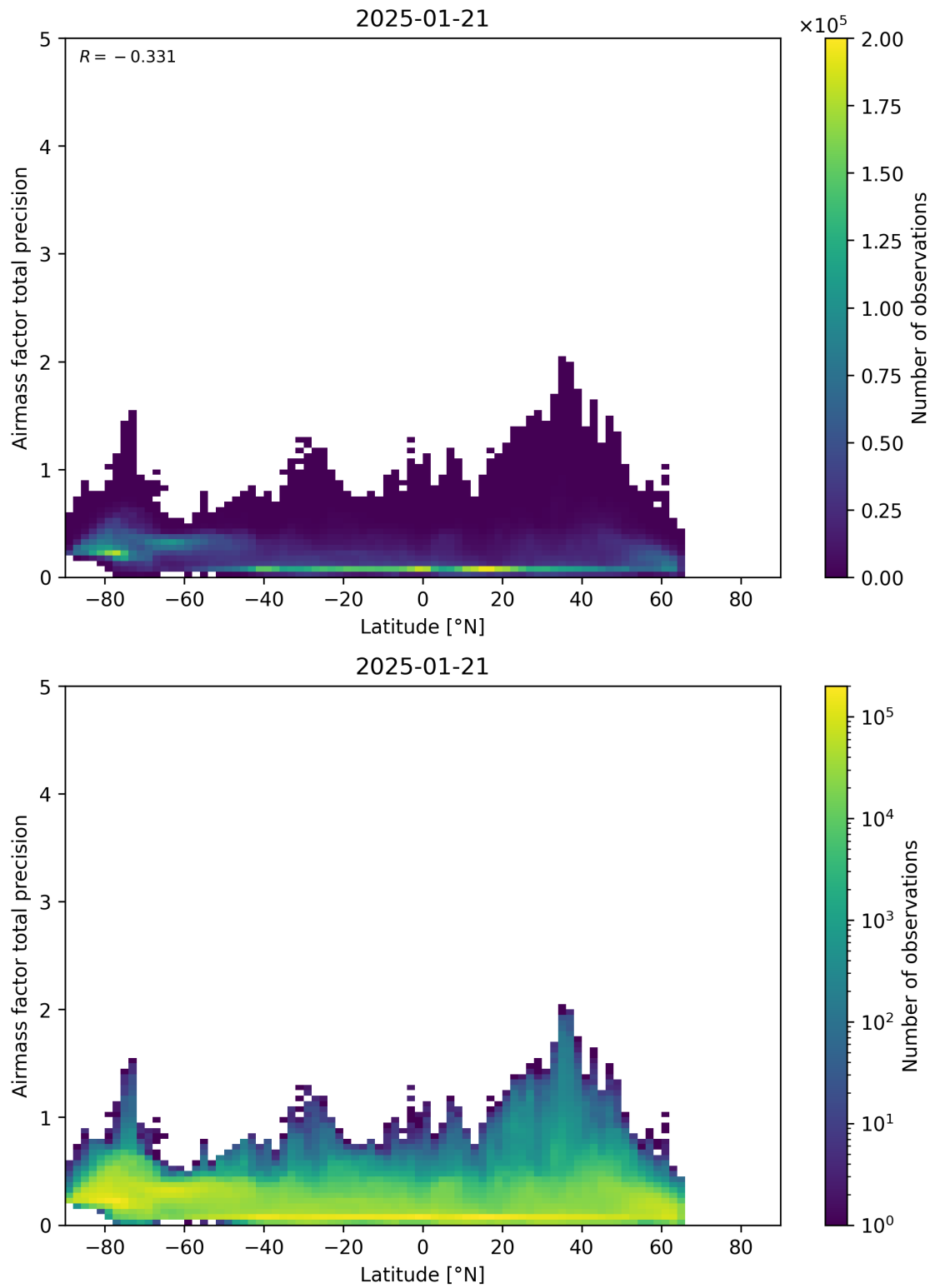
Figure 162: Scatter density plot of “Latitude” against “Airmass factor total precision” for 2025-01-20 to 2025-01-22.
