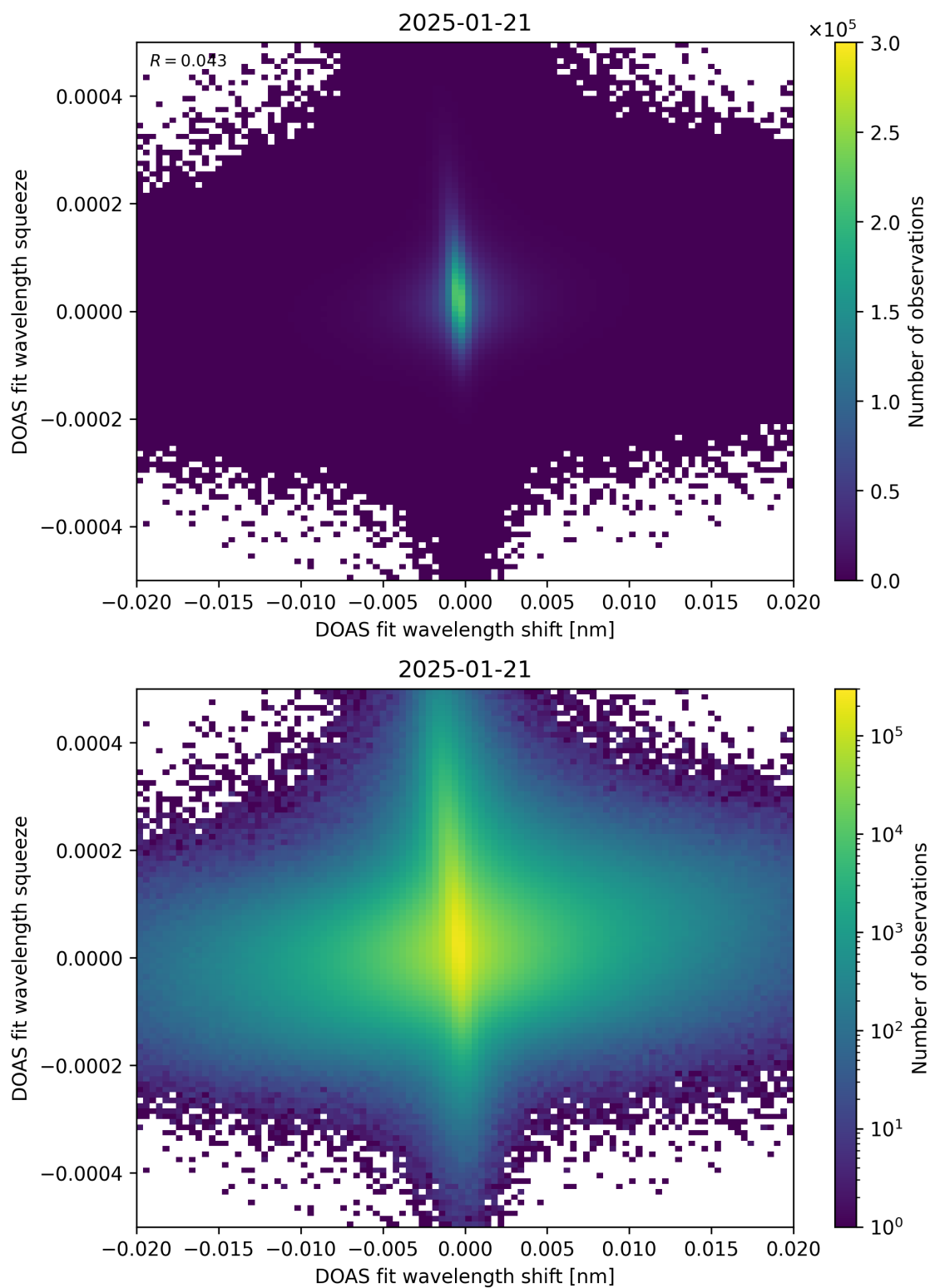
Figure 65: Scatter density plot of “DOAS fit wavelength shift” against “DOAS fit wavelength squeeze” for 2025-01-20 to 2025-01-22.
