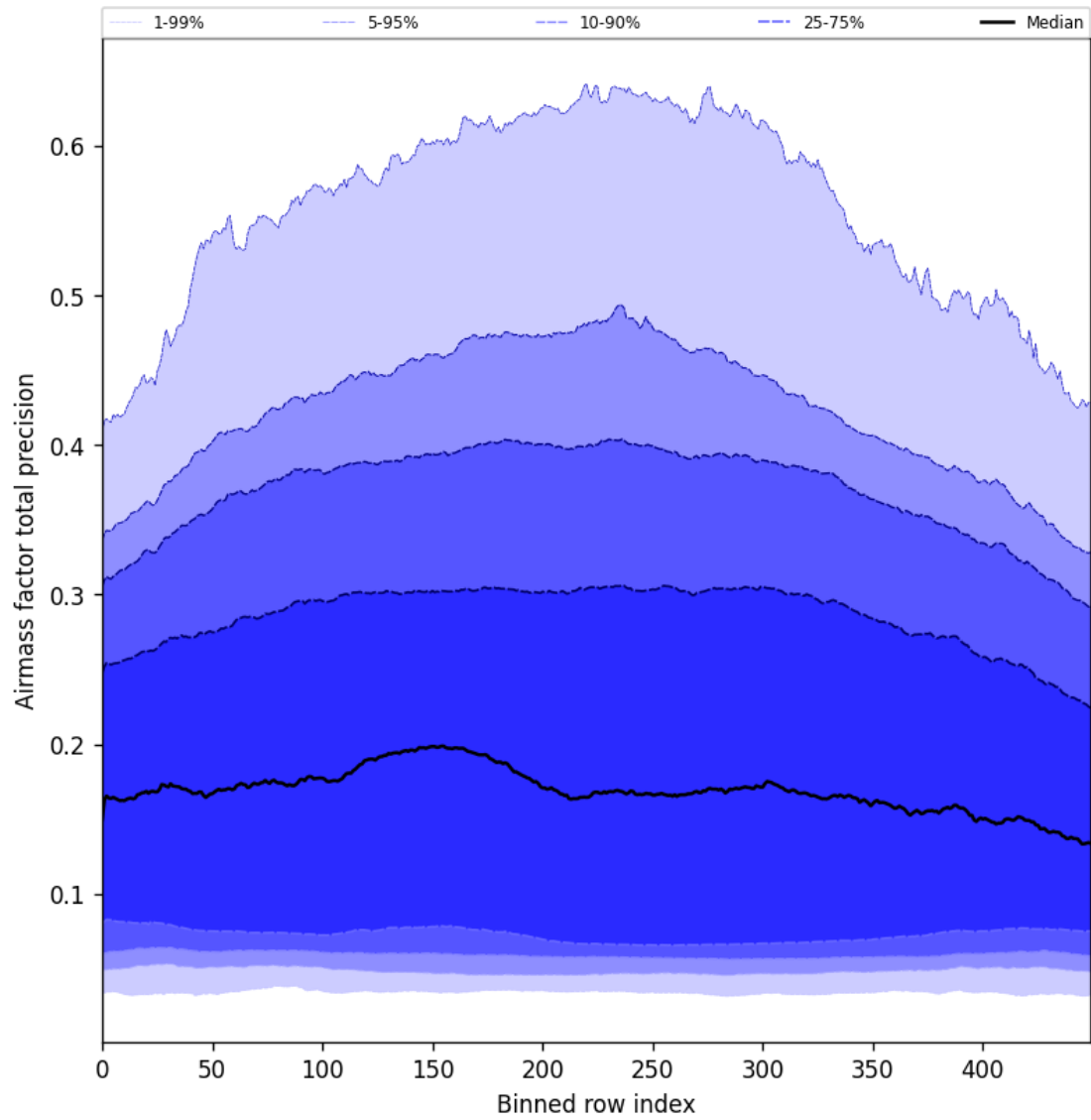
Figure 55: Along track statistics of “Airmass factor total precision” for 2025-01-20 to 2025-01-22
