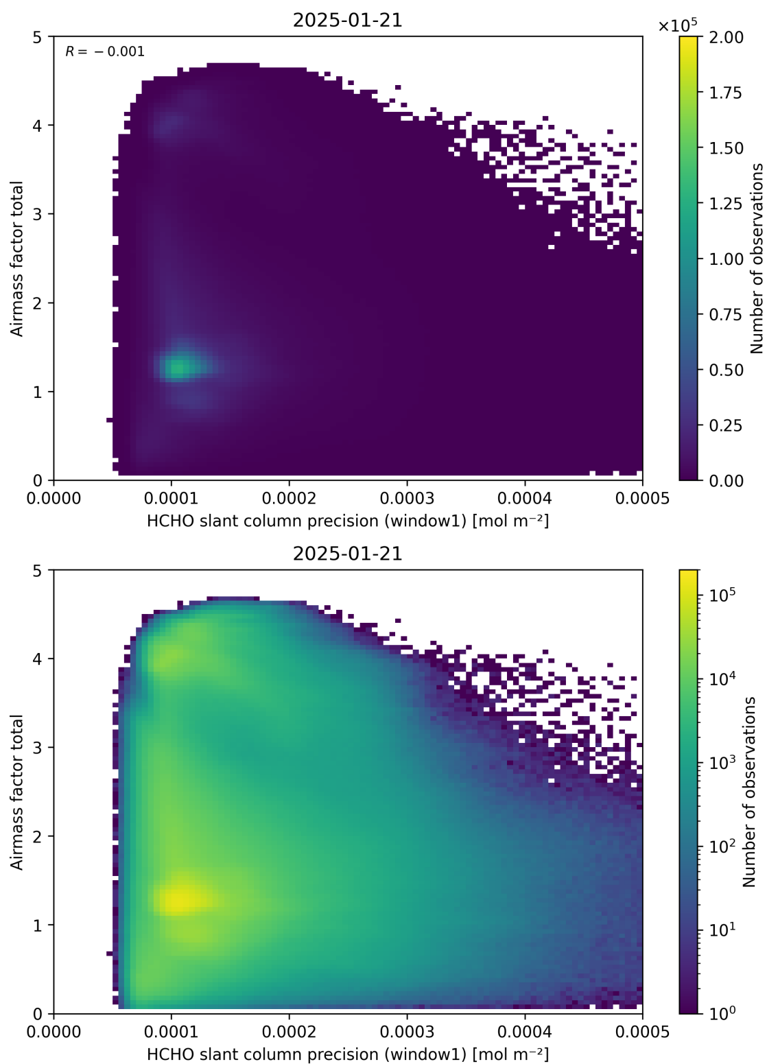
Figure 94: Scatter density plot of “HCHO slant column precision (window1)” against “Airmass factor total” for 2025-01-20 to 2025-01-22.
