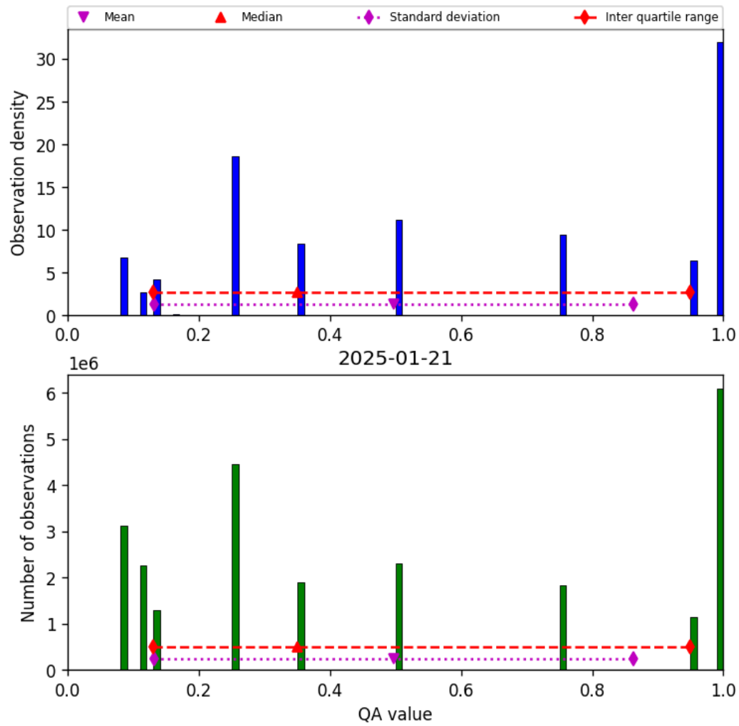
Figure 34: Histogram of “QA value” for 2025-01-20 to 2025-01-22
