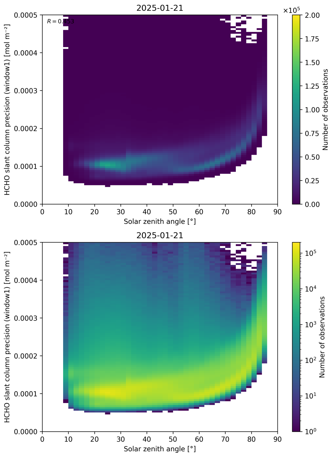
Figure 174: Scatter density plot of “Solar zenith angle” against “HCHO slant column precision (window1)” for 2025-01-20 to 2025-01-22.
