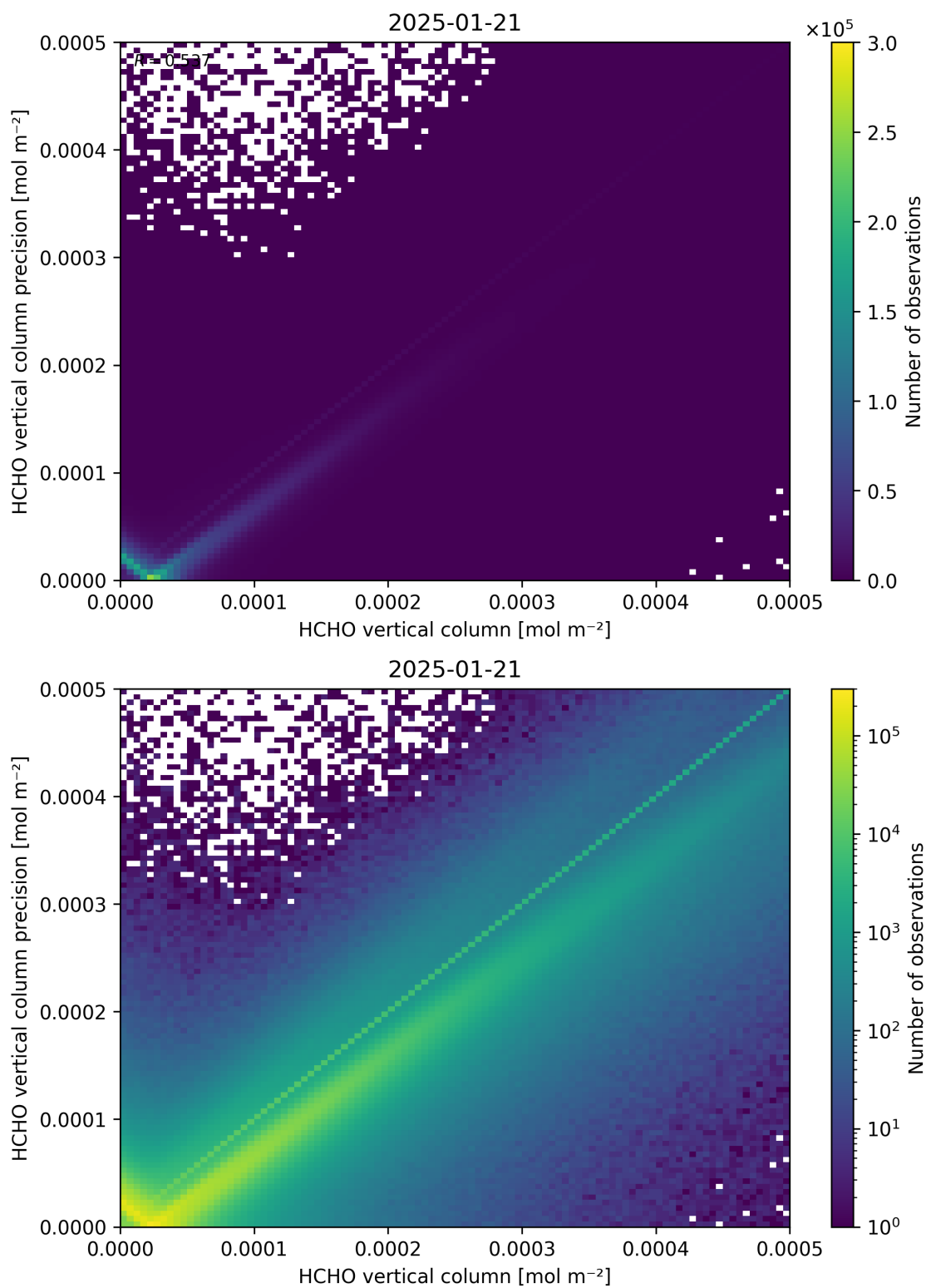
Figure 134: Scatter density plot of “HCHO vertical column” against “HCHO vertical column precision” for 2025-01-20 to 2025-01-22.
