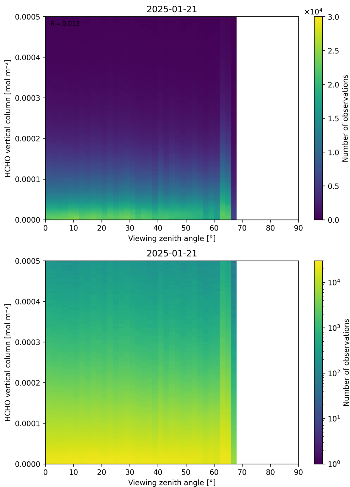
Figure 192: Scatter density plot of “Viewing zenith angle” against “HCHO vertical column” for 2025-01-20 to 2025-01-22.
