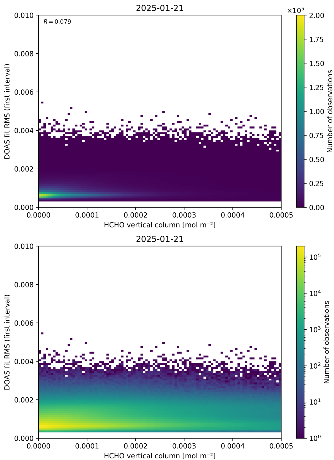
Figure 123: Scatter density plot of “HCHO vertical column” against “DOAS fit RMS (first interval)” for 2025-01-20 to 2025-01-22.
