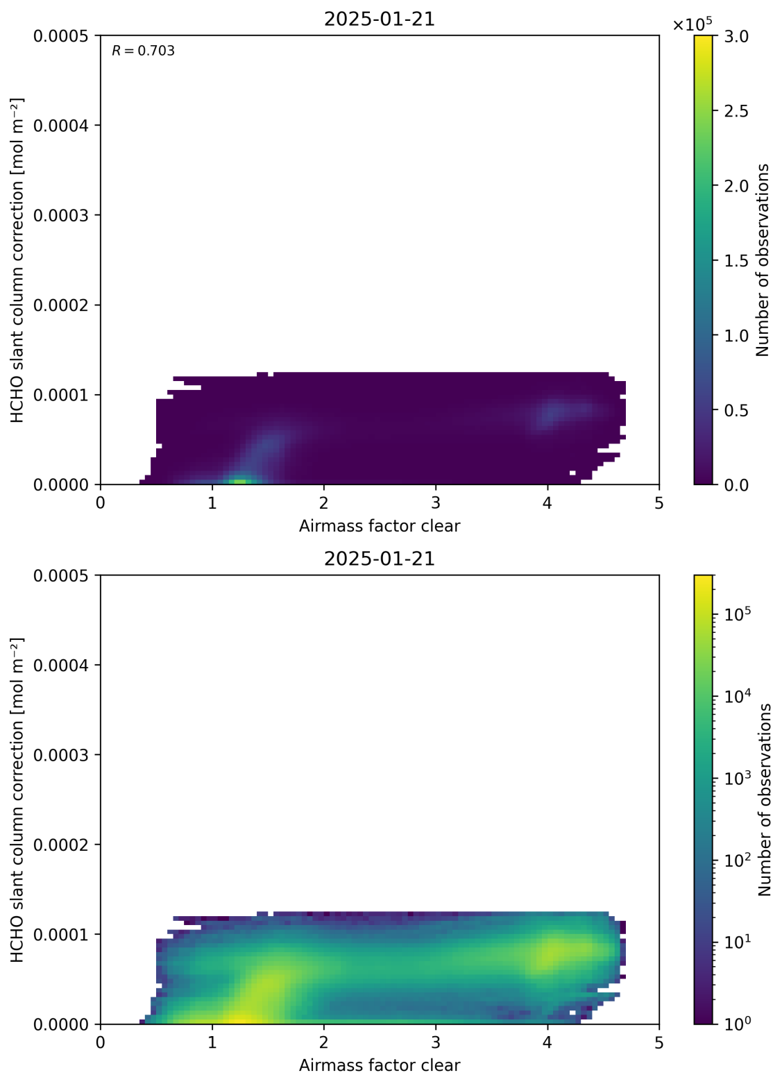
Figure 75: Scatter density plot of “Airmass factor clear” against “HCHO slant column correction” for 2025-01-20 to 2025-01-22.
