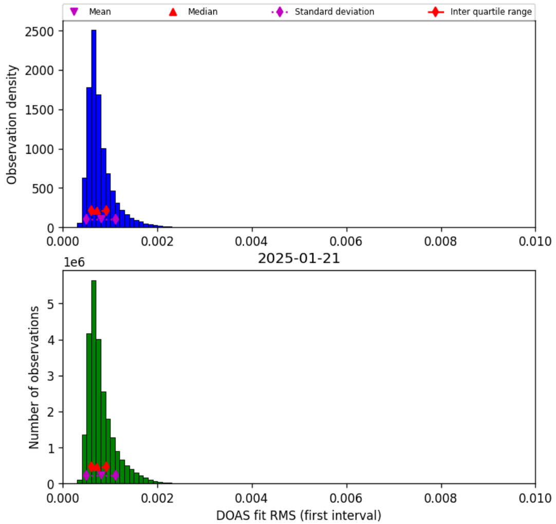
Figure 46: Histogram of “DOAS fit RMS (first interval)” for 2025-01-20 to 2025-01-22
