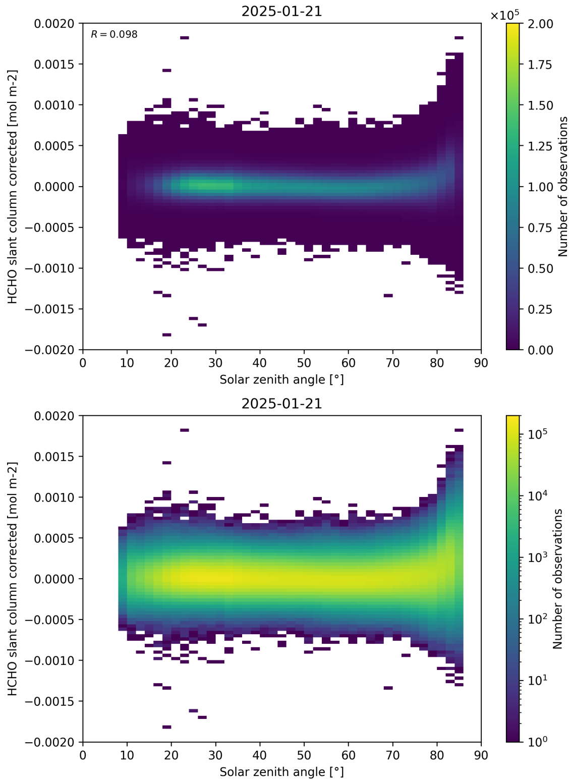
Figure 171: Scatter density plot of “Solar zenith angle” against “HCHO slant column corrected” for 2025-01-20 to 2025-01-22.
