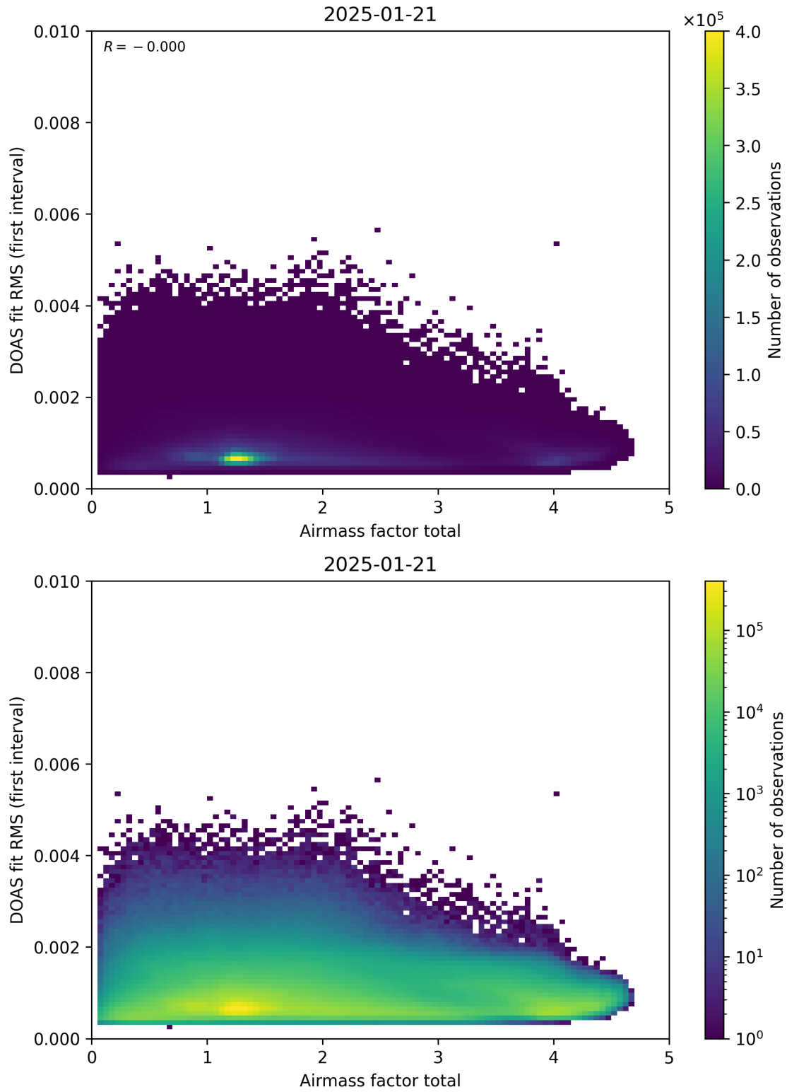
Figure 97: Scatter density plot of “Airmass factor total” against “DOAS fit RMS (first interval)” for 2025-01-20 to 2025-01-22.
