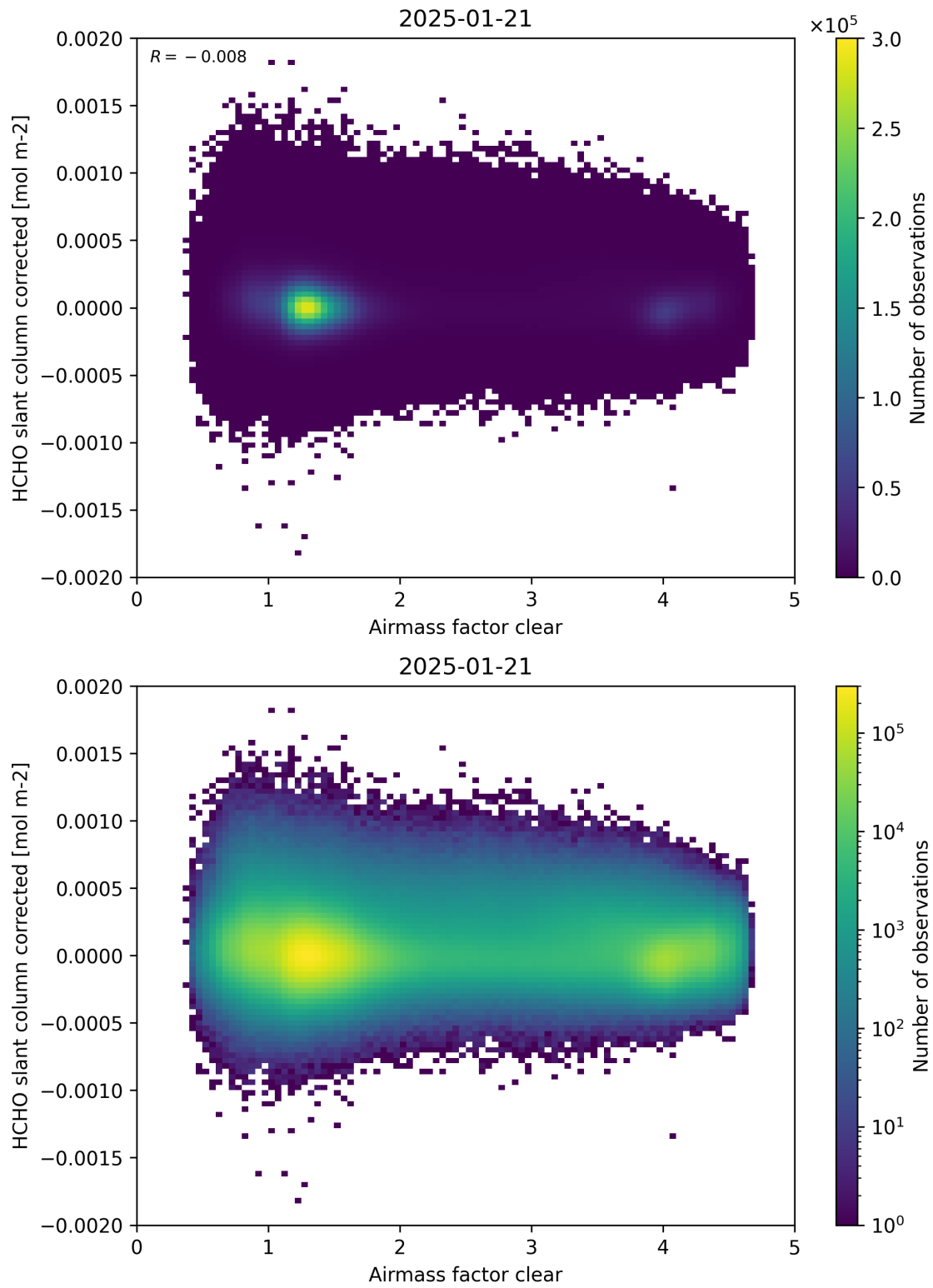
Figure 74: Scatter density plot of “Airmass factor clear” against “HCHO slant column corrected” for 2025-01-20 to 2025-01-22.
