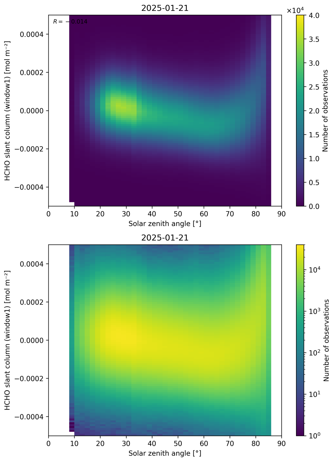
Figure 173: Scatter density plot of “Solar zenith angle” against “HCHO slant column (window1)” for 2025-01-20 to 2025-01-22.
