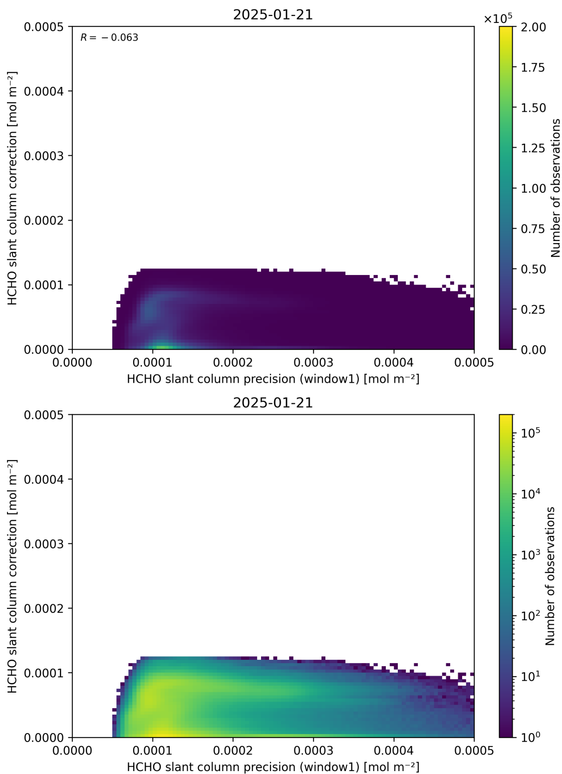
Figure 93: Scatter density plot of “HCHO slant column precision (window1)” against “HCHO slant column correction” for 2025-01-20 to 2025-01-22.
