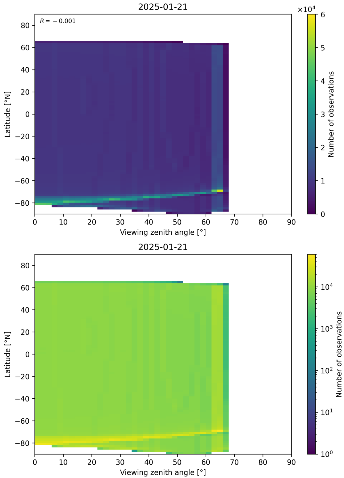
Figure 196: Scatter density plot of “Viewing zenith angle” against “Latitude” for 2025-01-20 to 2025-01-22.
