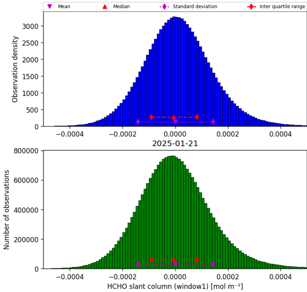
Figure 38: Histogram of “HCHO slant column (window1)” for 2025-01-20 to 2025-01-22
