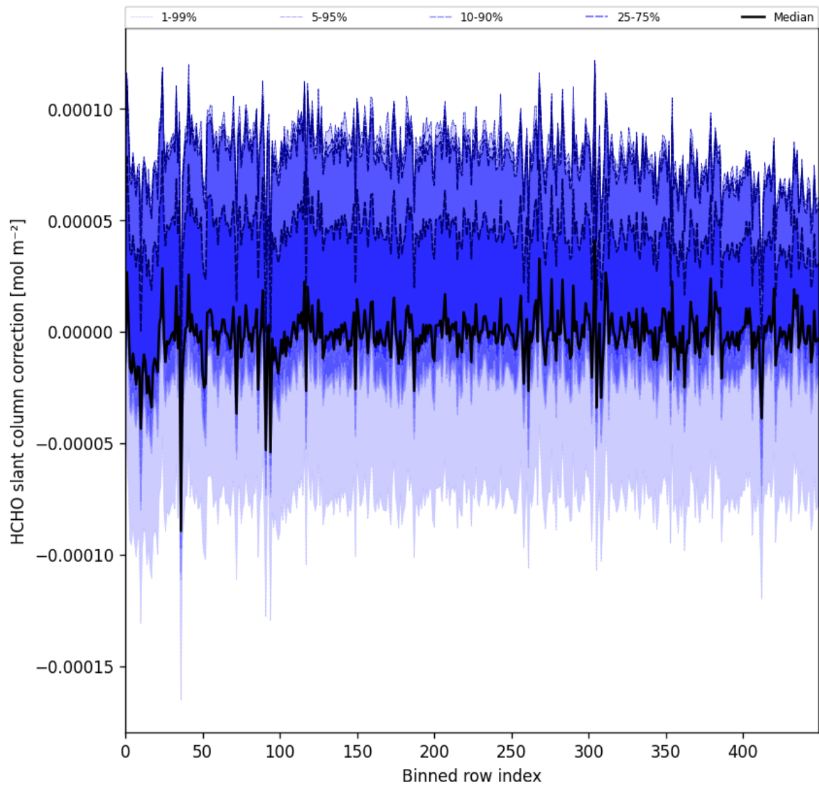
Figure 61: Along track statistics of “HCHO slant column correction” for 2025-01-20 to 2025-01-22
