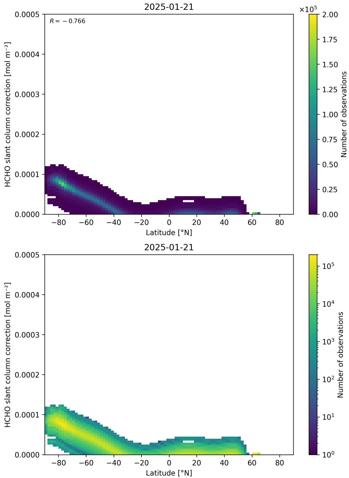
Figure 158: Scatter density plot of “Latitude” against “HCHO slant column correction” for 2025-01-20 to 2025-01-22.
