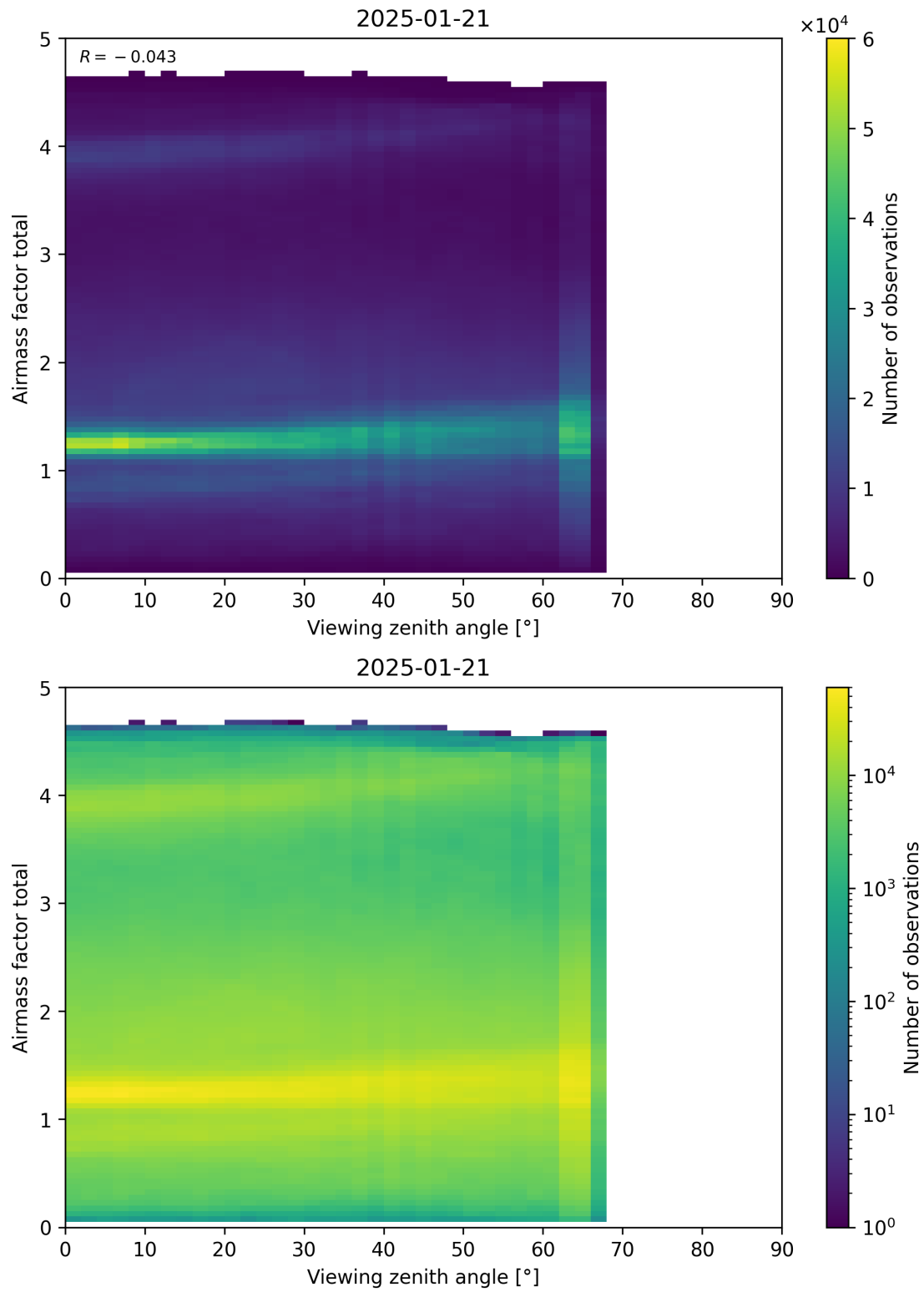
Figure 190: Scatter density plot of “Viewing zenith angle” against “Airmass factor total” for 2025-01-20 to 2025-01-22.
