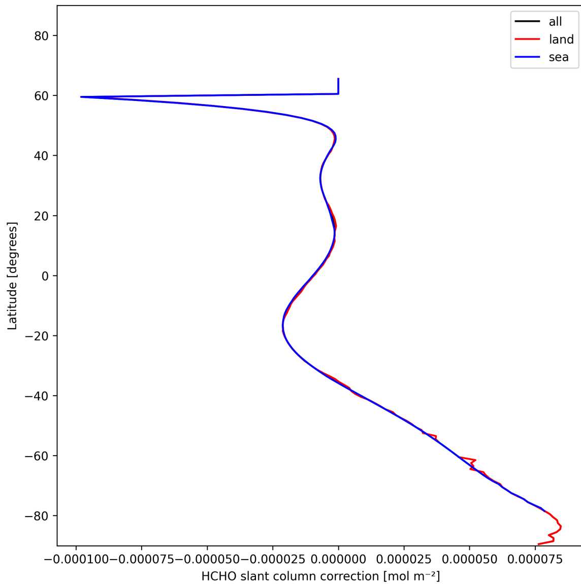
Figure 33: Zonal average of “HCHO slant column correction” for 2025-01-20 to 2025-01-22.
