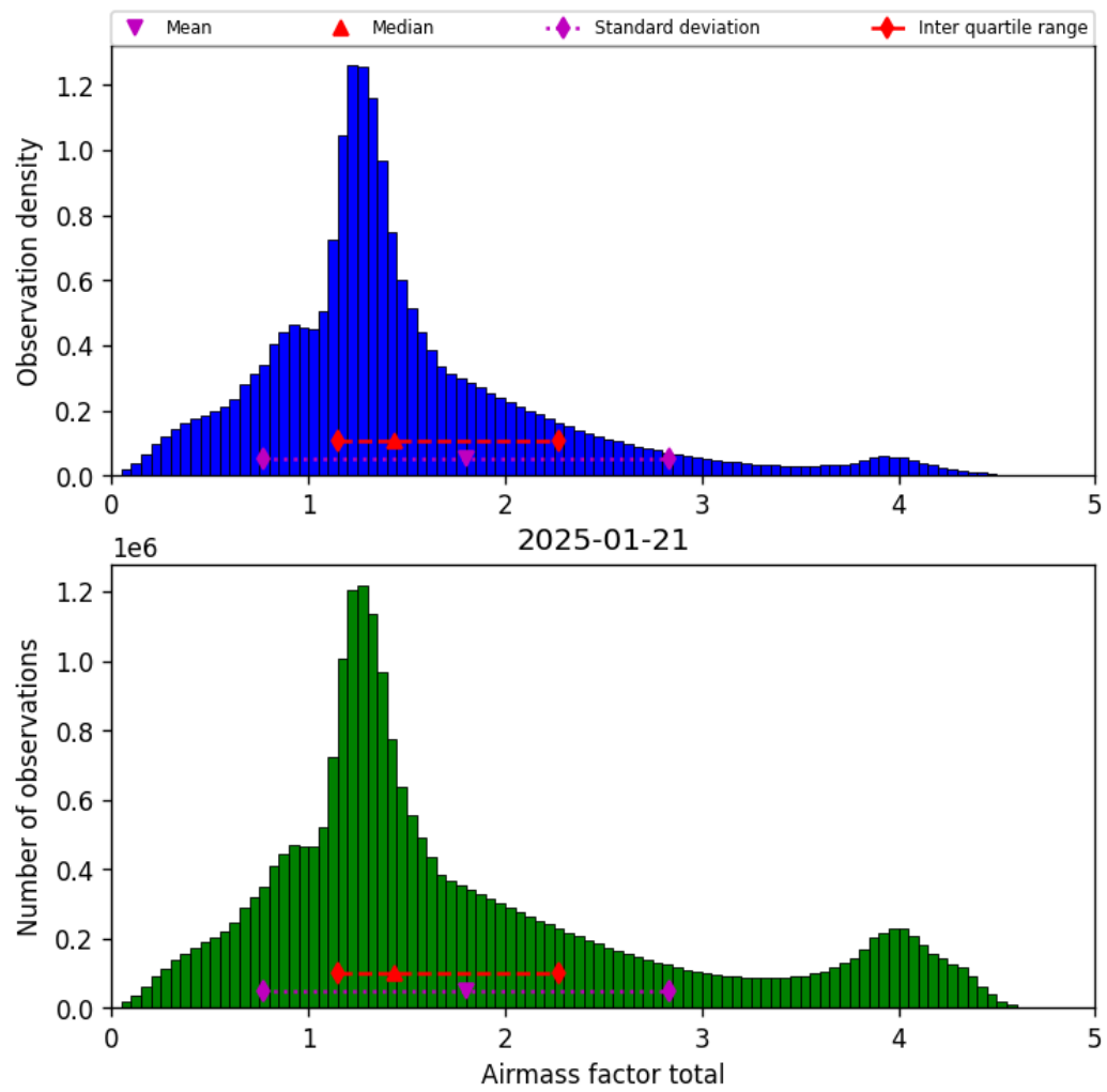
Figure 40: Histogram of “Airmass factor total” for 2025-01-20 to 2025-01-22
