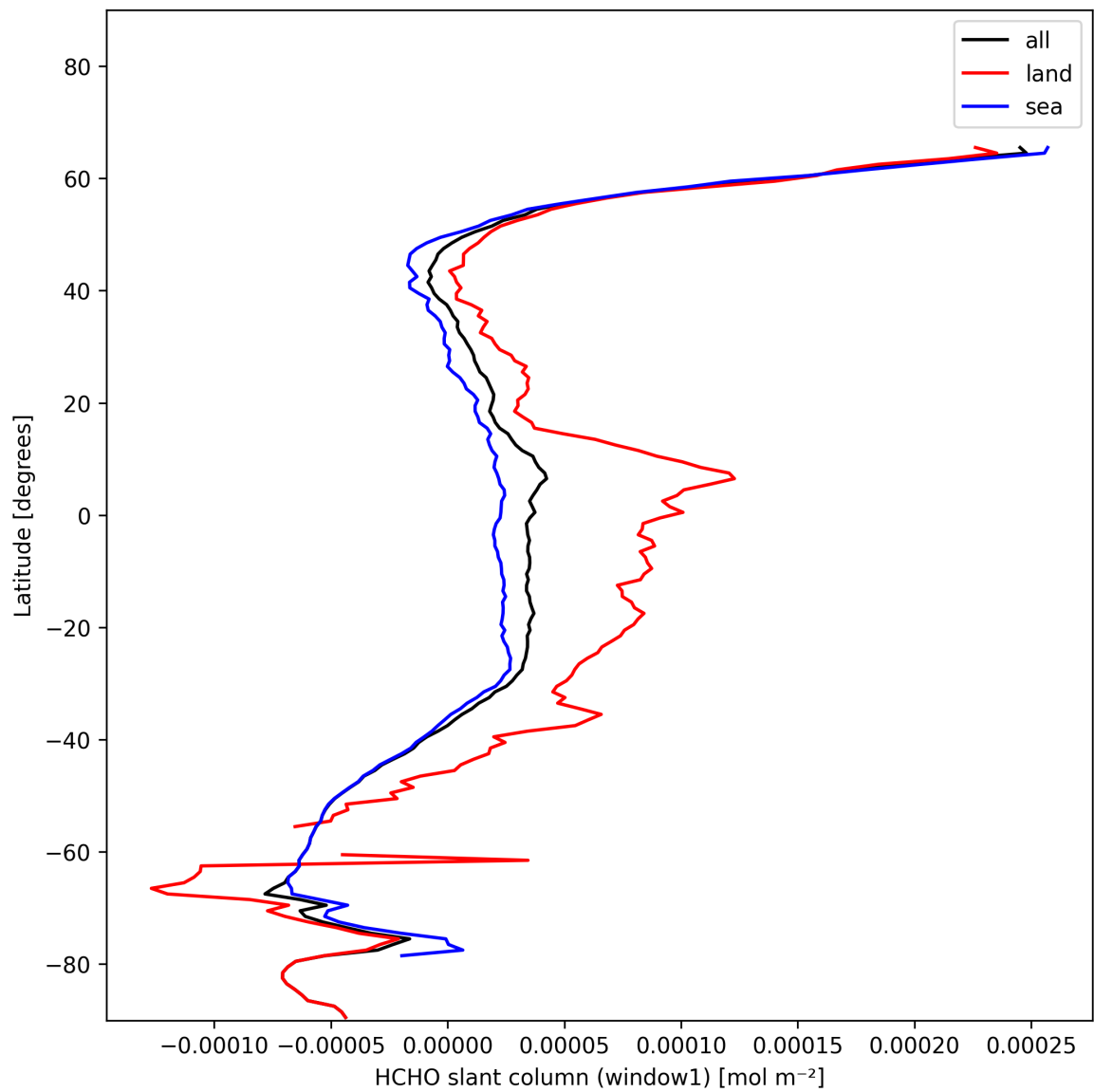
Figure 24: Zonal average of “HCHO slant column (window1)” for 2025-01-20 to 2025-01-22.
