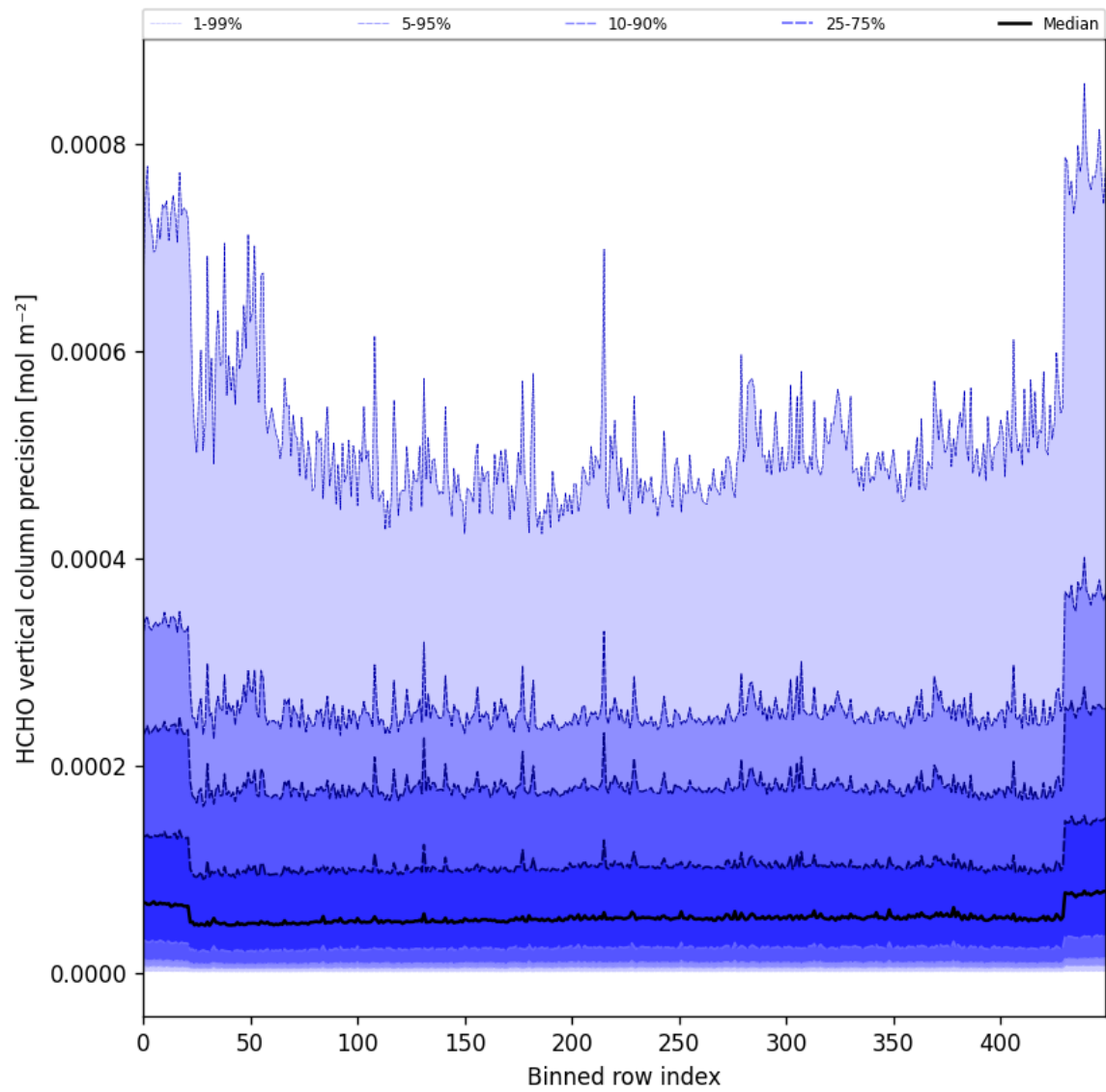
Figure 50: Along track statistics of “HCHO vertical column precision” for 2025-01-20 to 2025-01-22
