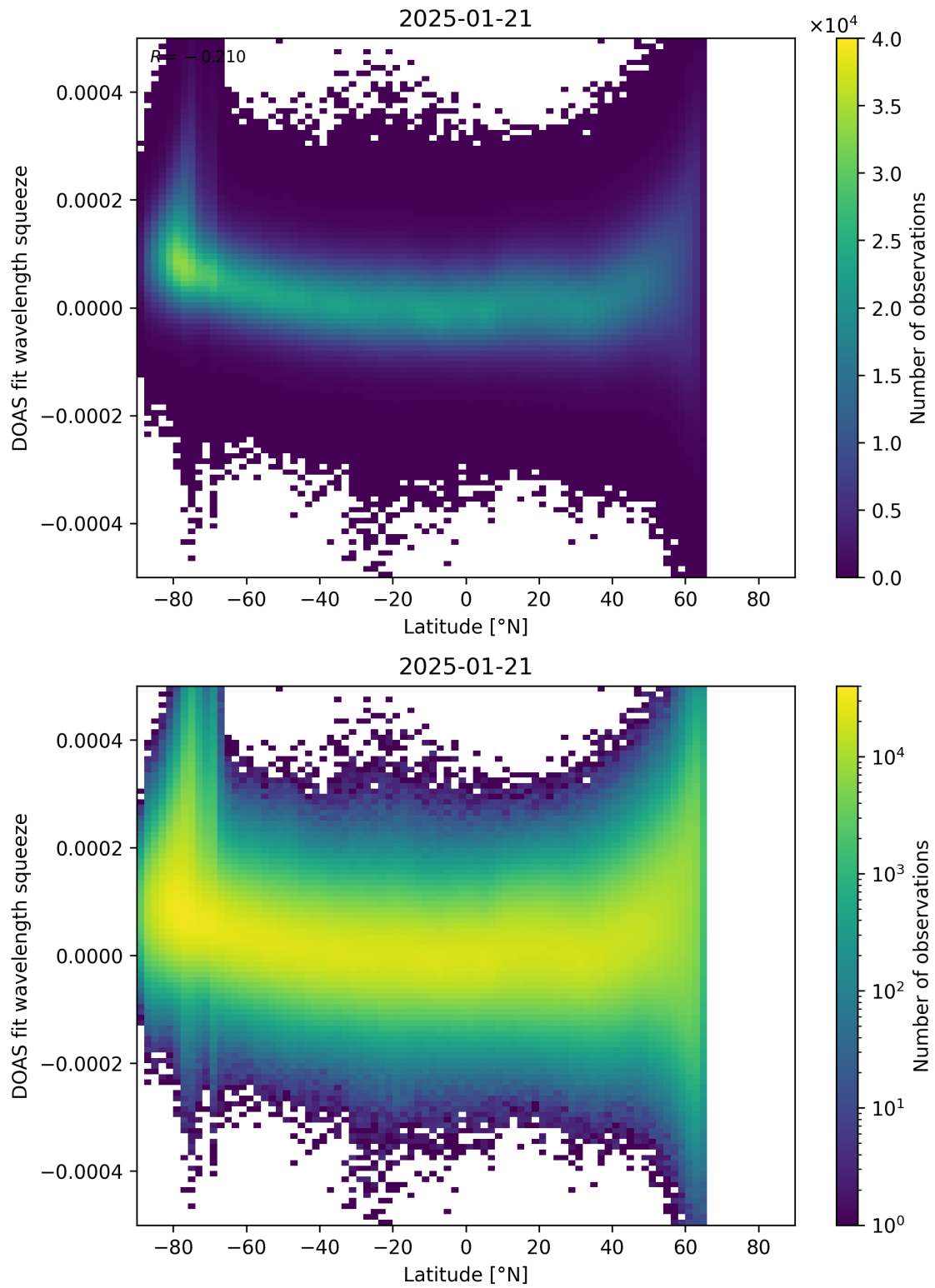
Figure 155: Scatter density plot of “Latitude” against “DOAS fit wavelength squeeze” for 2025-01-20 to 2025-01-22.
