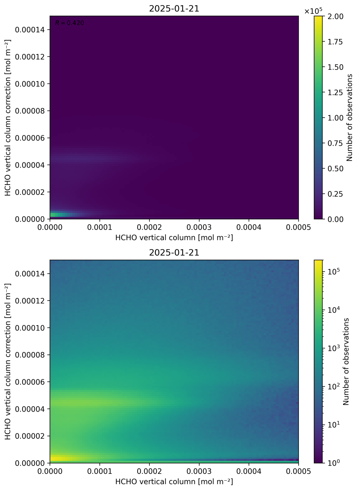
Figure 133: Scatter density plot of “HCHO vertical column” against “HCHO vertical column correction” for 2025-01-20 to 2025-01-22.
