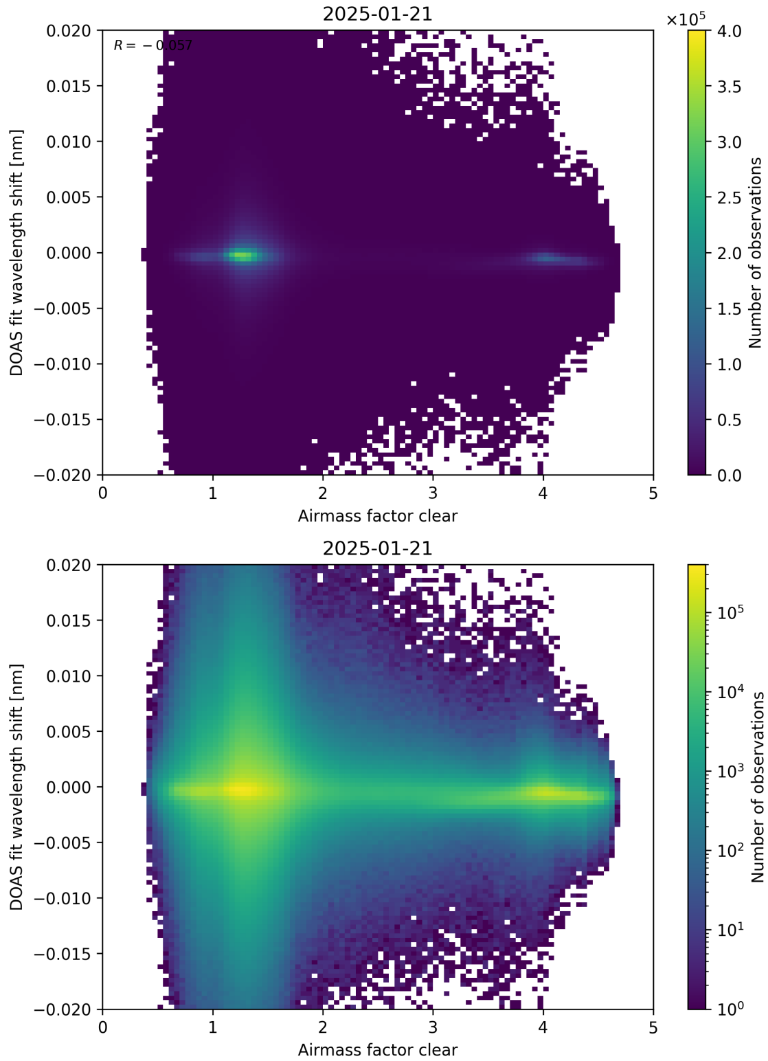
Figure 72: Scatter density plot of “Airmass factor clear” against “DOAS fit wavelength shift” for 2025-01-20 to 2025-01-22.
