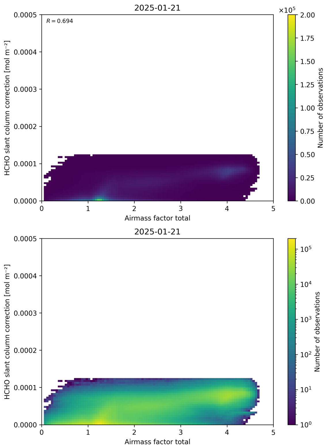
Figure 102: Scatter density plot of “Airmass factor total” against “HCHO slant column correction” for 2025-01-20 to 2025-01-22.
