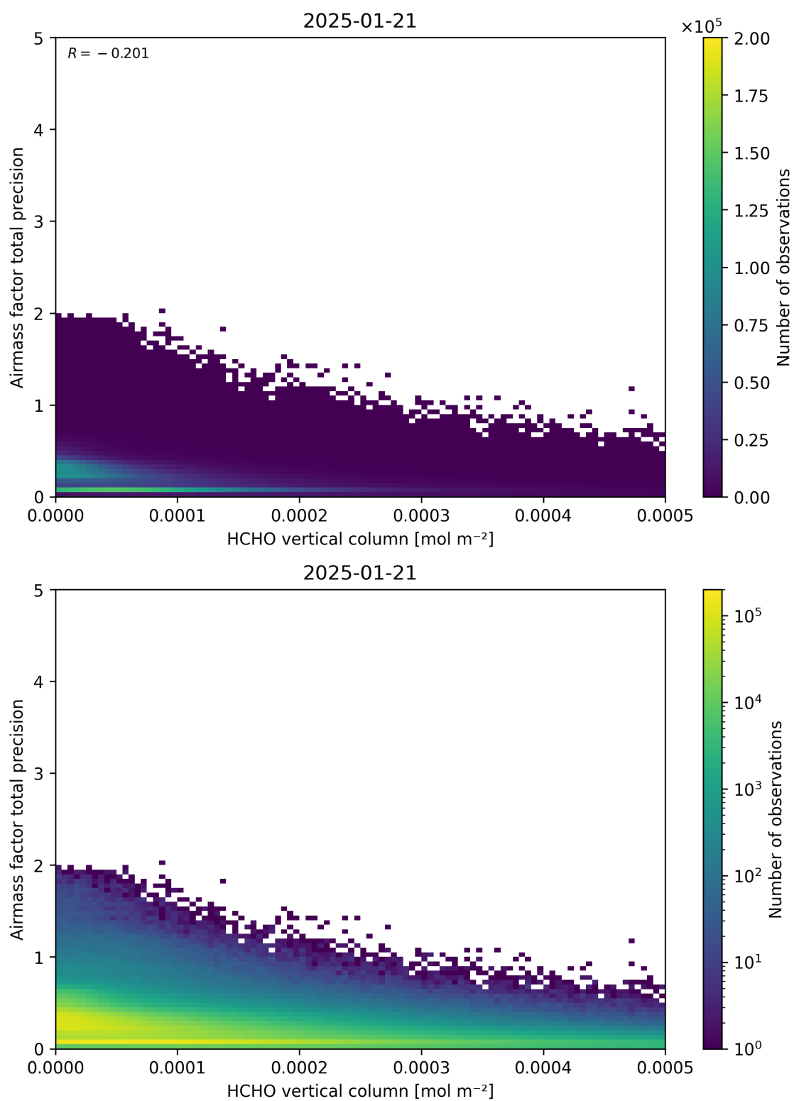
Figure 132: Scatter density plot of “HCHO vertical column” against “Airmass factor total precision” for 2025-01-20 to 2025-01-22.
