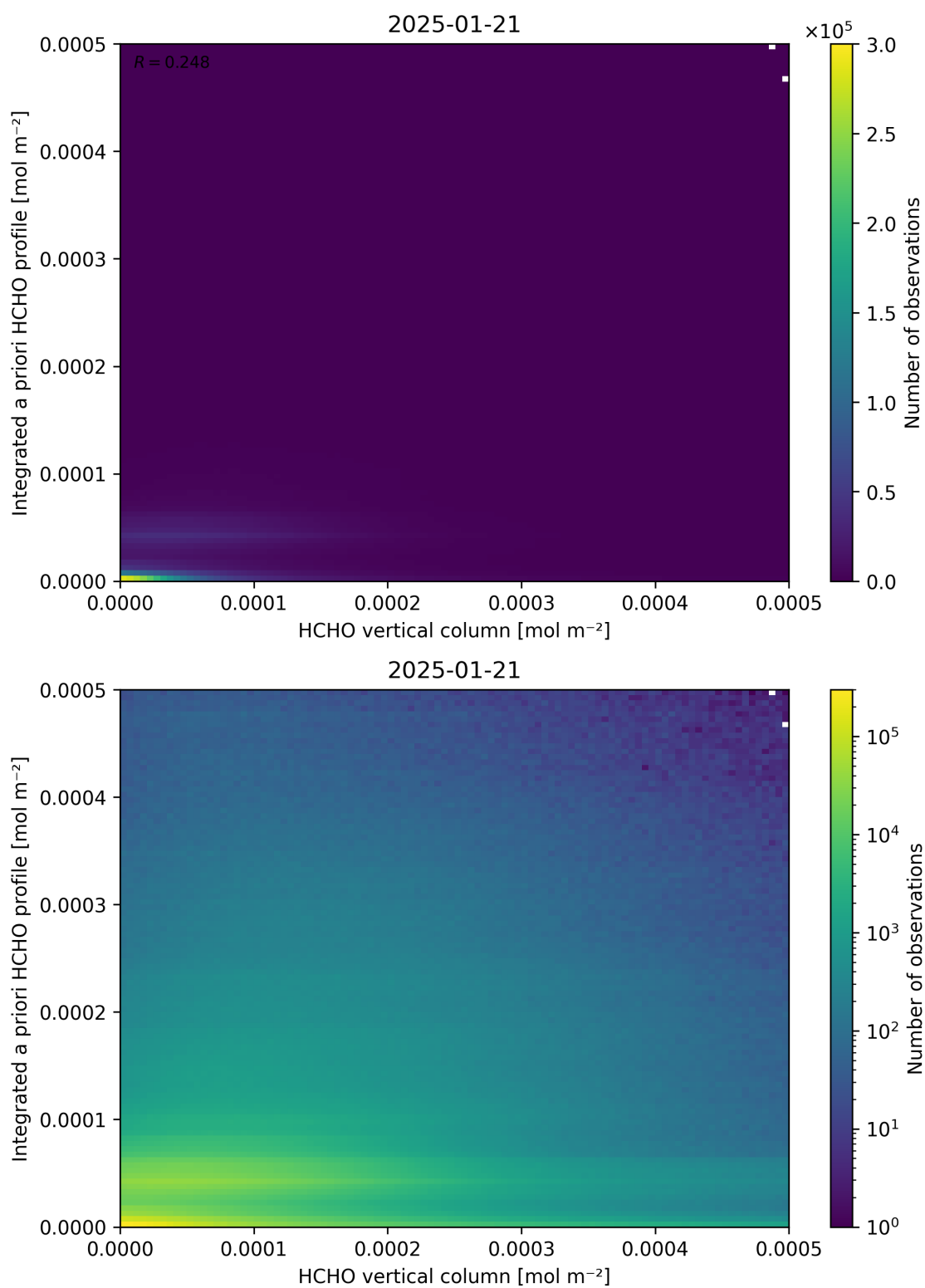
Figure 135: Scatter density plot of “HCHO vertical column” against “Integrated a priori HCHO profile” for 2025-01-20 to 2025-01-22.
