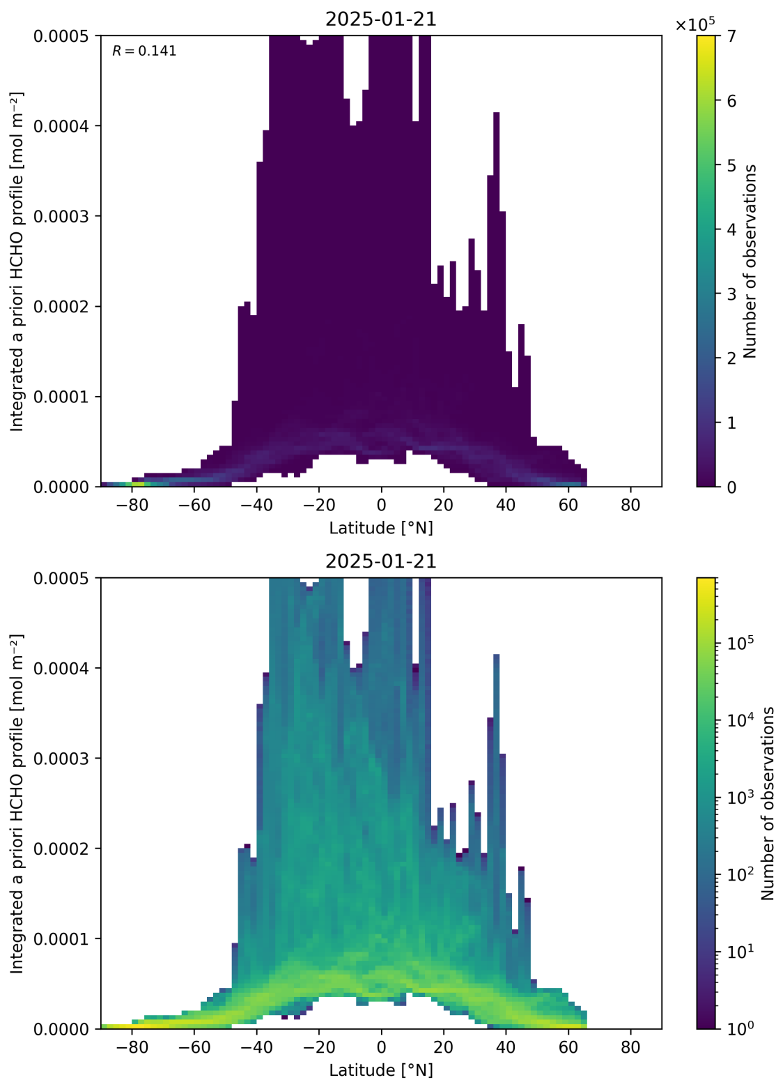
Figure 166: Scatter density plot of “Latitude” against “Integrated a priori HCHO profile” for 2025-01-20 to 2025-01-22.
