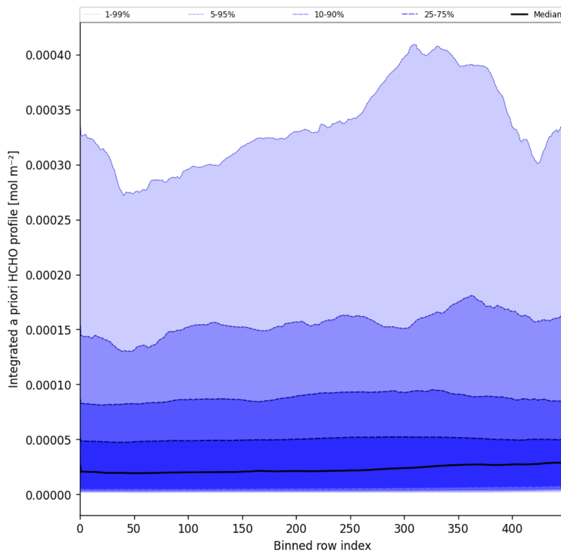
Figure 57: Along track statistics of “Integrated a priori HCHO profile” for 2025-01-20 to 2025-01-22
