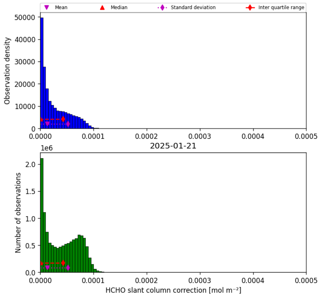
Figure 47: Histogram of “HCHO slant column correction” for 2025-01-20 to 2025-01-22
