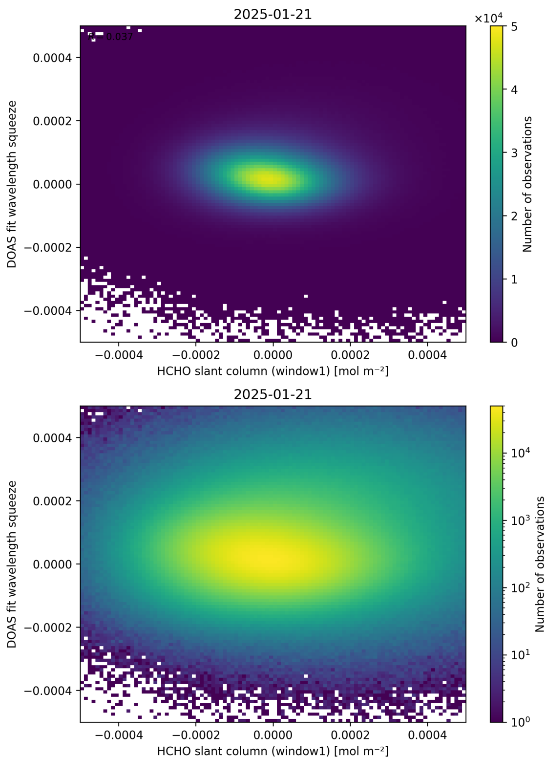
Figure 80: Scatter density plot of “HCHO slant column (window1)” against “DOAS fit wavelength squeeze” for 2025-01-20 to 2025-01-22.
