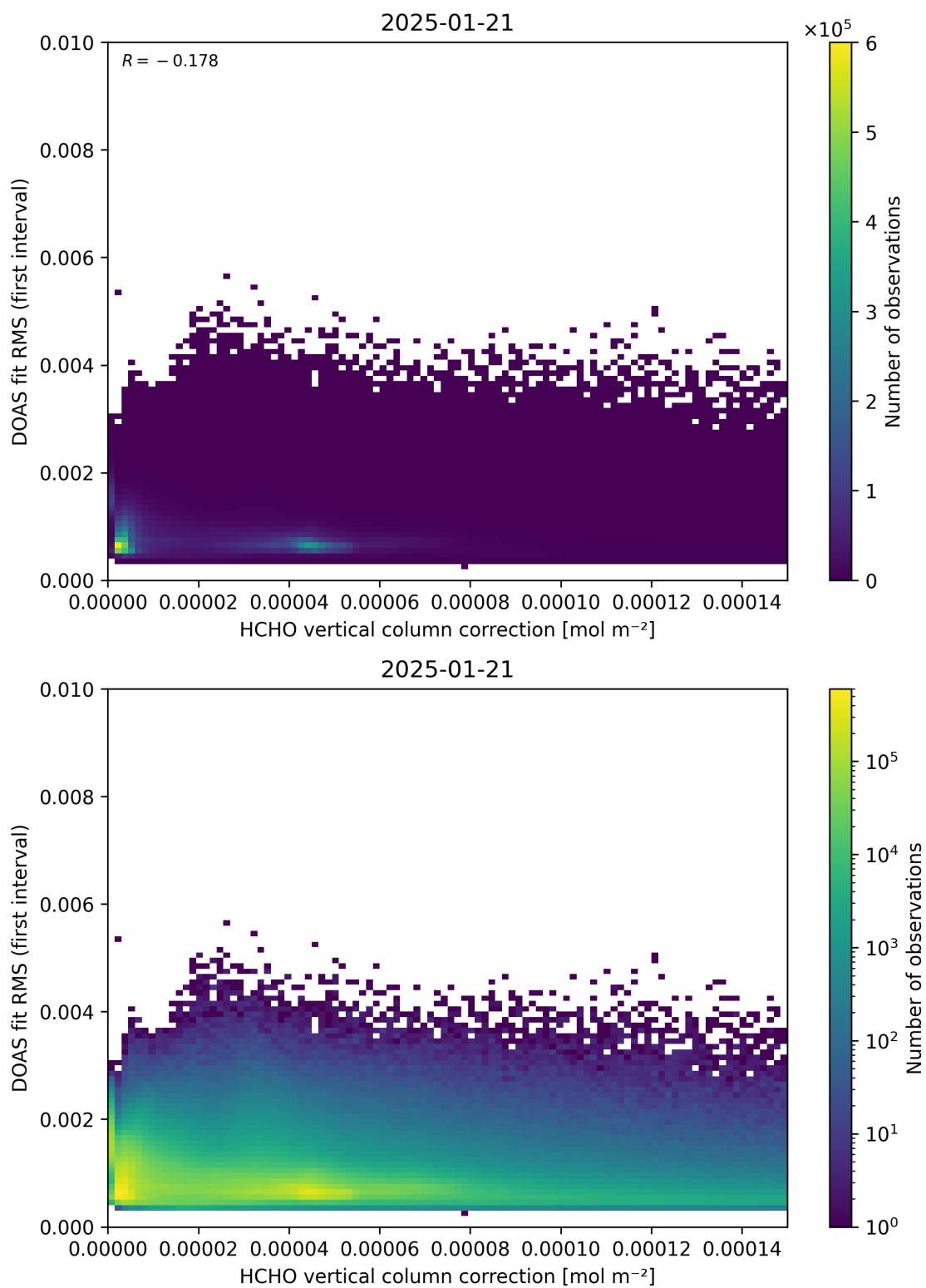
Figure 112: Scatter density plot of “HCHO vertical column correction” against “DOAS fit RMS (first interval)” for 2025-01-20 to 2025-01-22.
