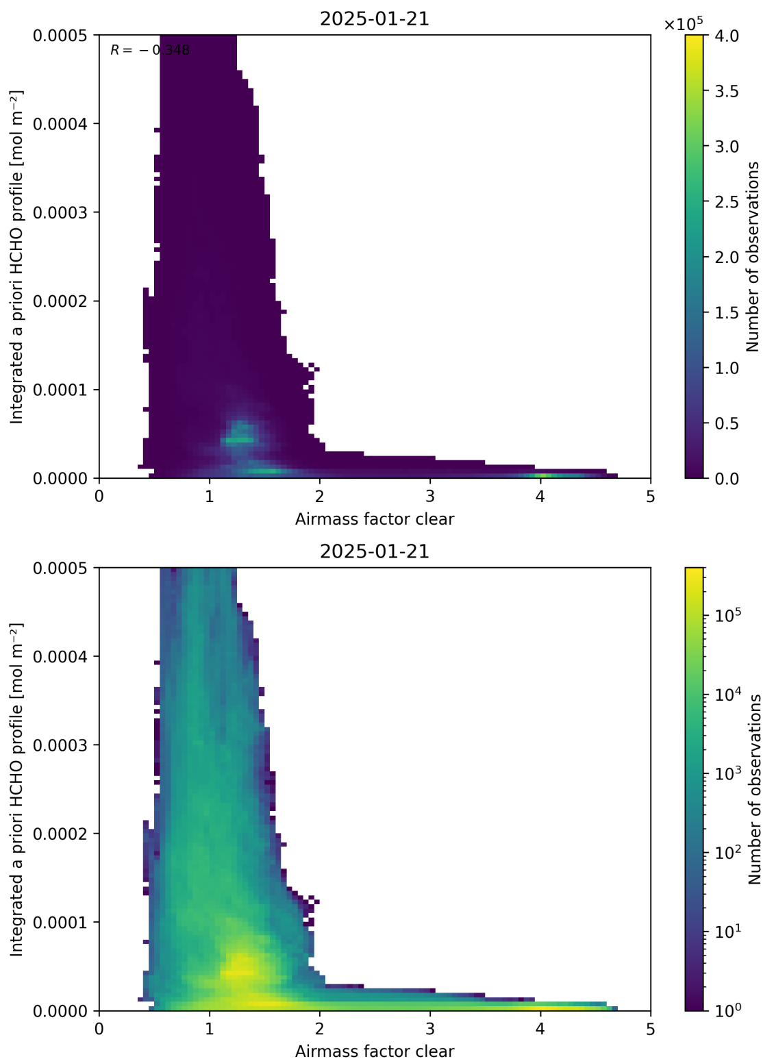
Figure 76: Scatter density plot of “Airmass factor clear” against “Integrated a priori HCHO profile” for 2025-01-20 to 2025-01-22.
