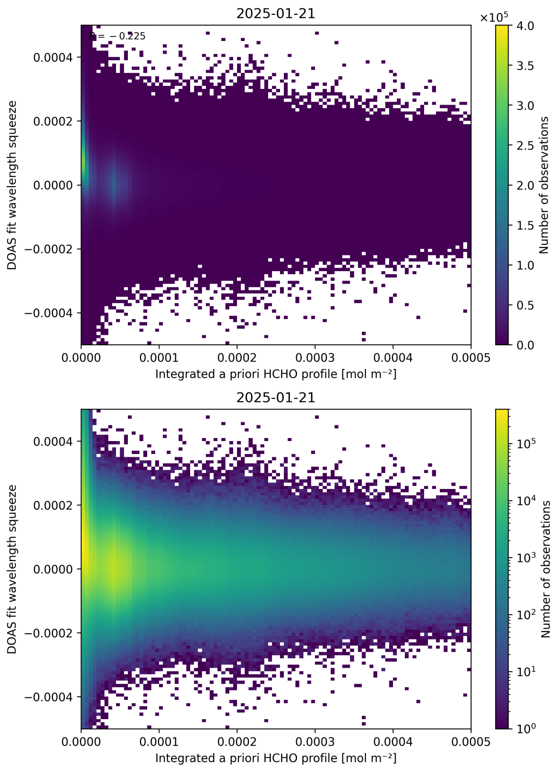
Figure 150: Scatter density plot of “Integrated a priori HCHO profile” against “DOAS fit wavelength squeeze” for 2025-01-20 to 2025-01-22.
