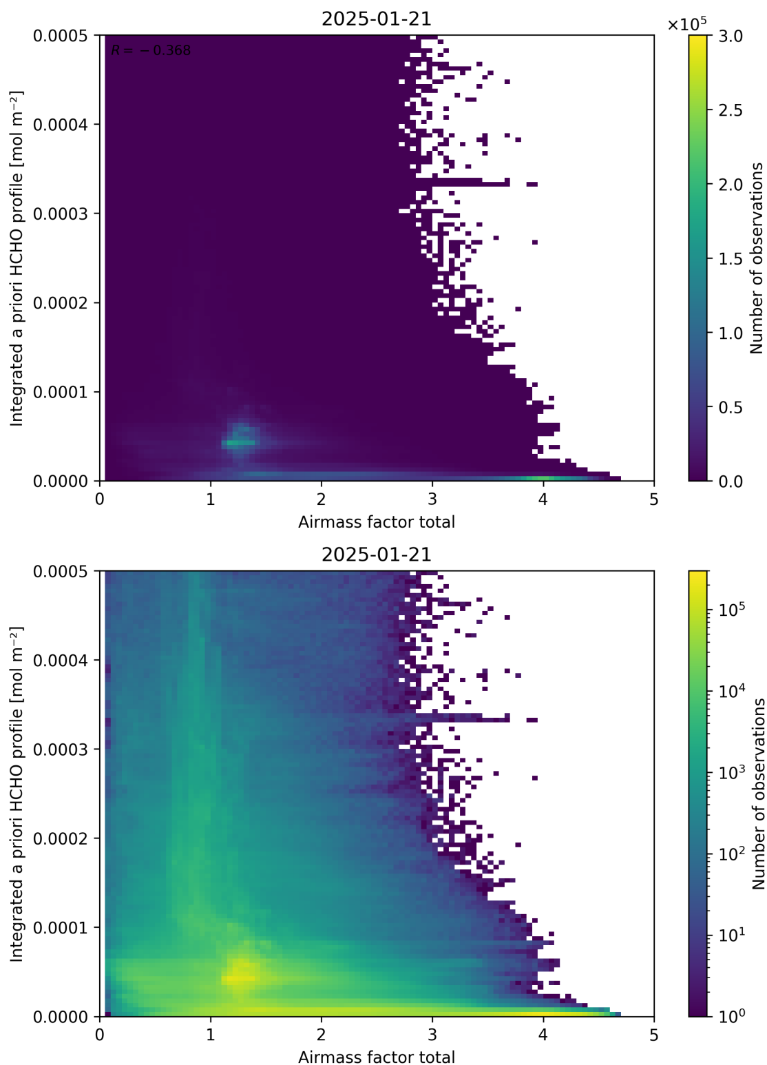
Figure 104: Scatter density plot of “Airmass factor total” against “Integrated a priori HCHO profile” for 2025-01-20 to 2025-01-22.
