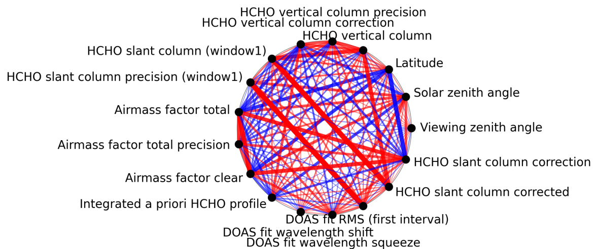
Figure 1: Map of correlation graph for 2025-01-20 to 2025-01-22.
