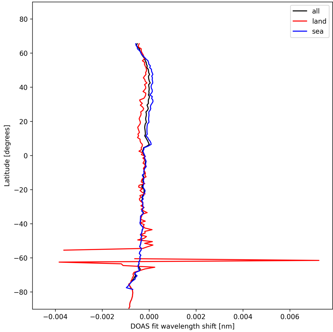
Figure 30: Zonal average of “DOAS fit wavelength shift” for 2025-01-20 to 2025-01-22.
