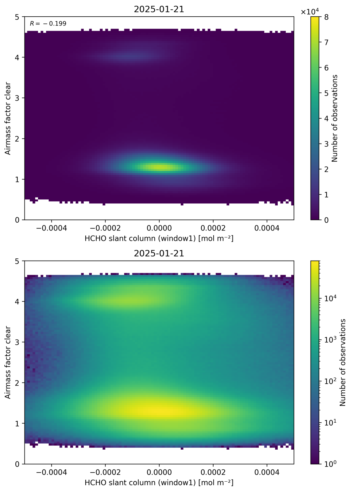
Figure 81: Scatter density plot of “HCHO slant column (window1)” against “Airmass factor clear” for 2025-01-20 to 2025-01-22.
