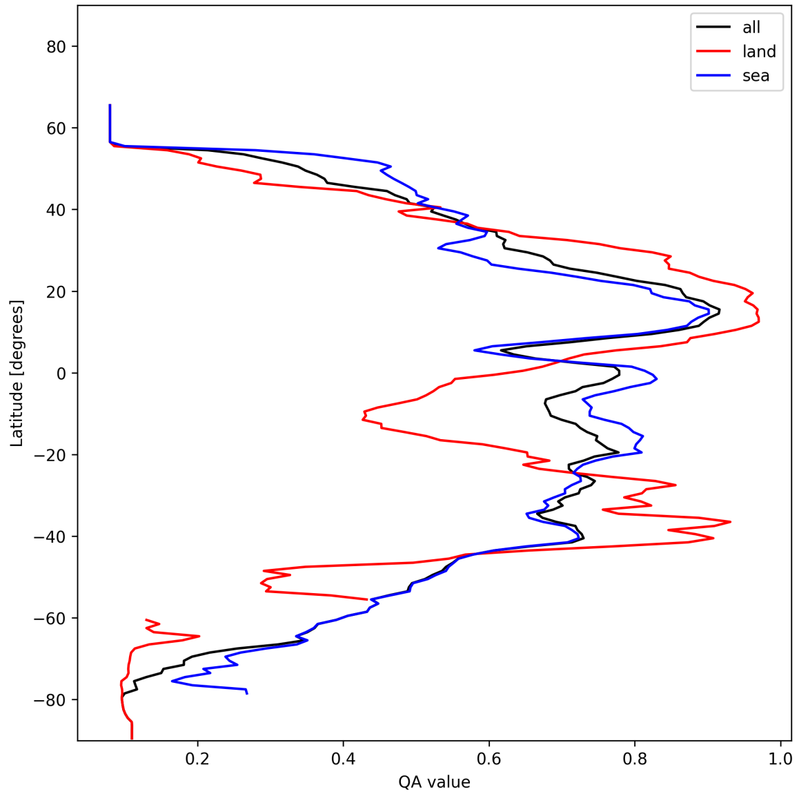
Figure 20: Zonal average of “QA value” for 2025-01-20 to 2025-01-22.
