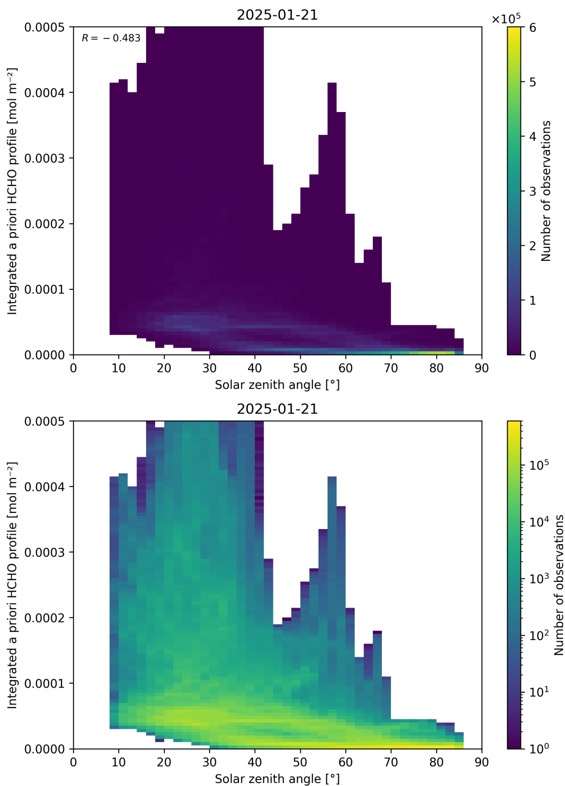
Figure 180: Scatter density plot of “Solar zenith angle” against “Integrated a priori HCHO profile” for 2025-01-20 to 2025-01-22.
