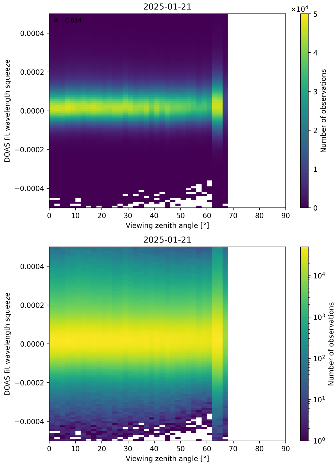
Figure 184: Scatter density plot of “Viewing zenith angle” against “DOAS fit wavelength squeeze” for 2025-01-20 to 2025-01-22.
