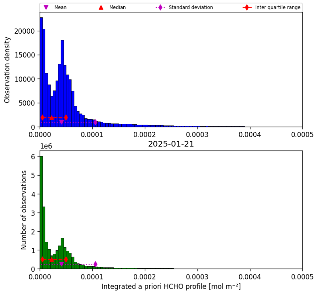
Figure 43: Histogram of “Integrated a priori HCHO profile” for 2025-01-20 to 2025-01-22
