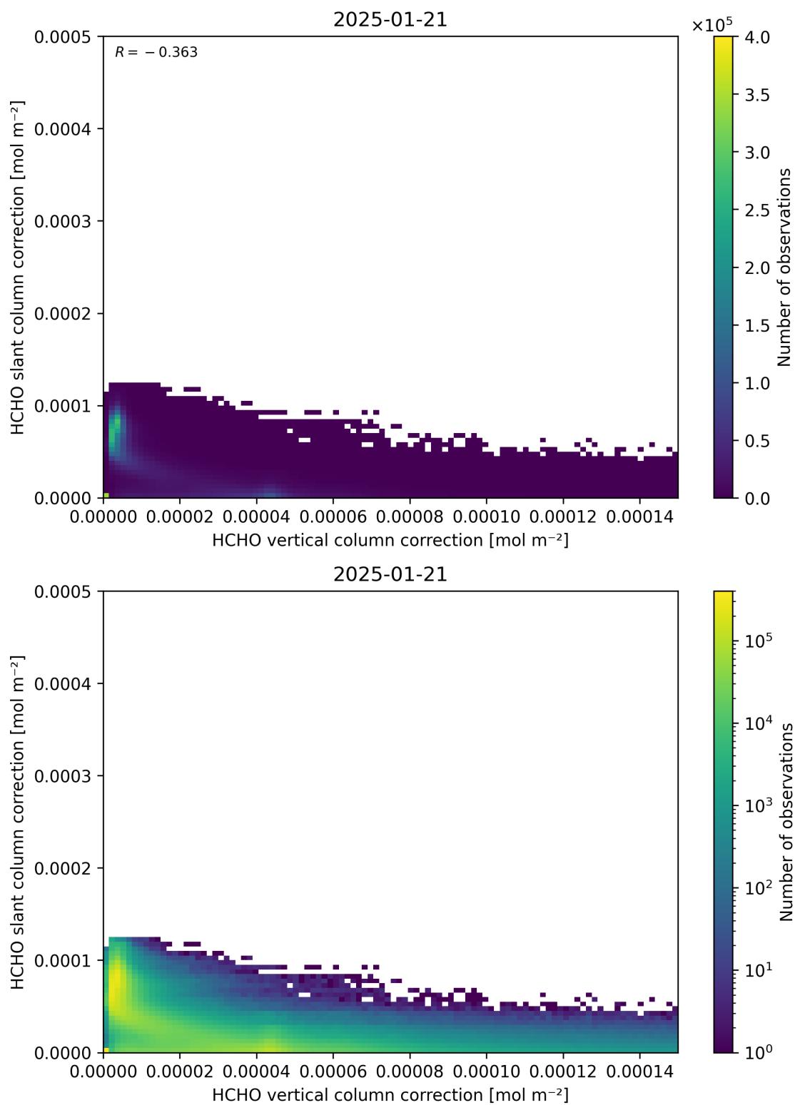
Figure 117: Scatter density plot of “HCHO vertical column correction” against “HCHO slant column correction” for 2025-01-20 to 2025-01-22.
