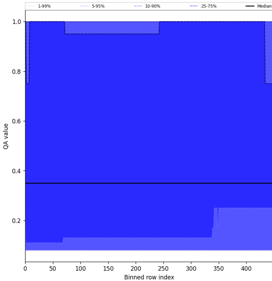
Figure 48: Along track statistics of “QA value” for 2025-01-20 to 2025-01-22
