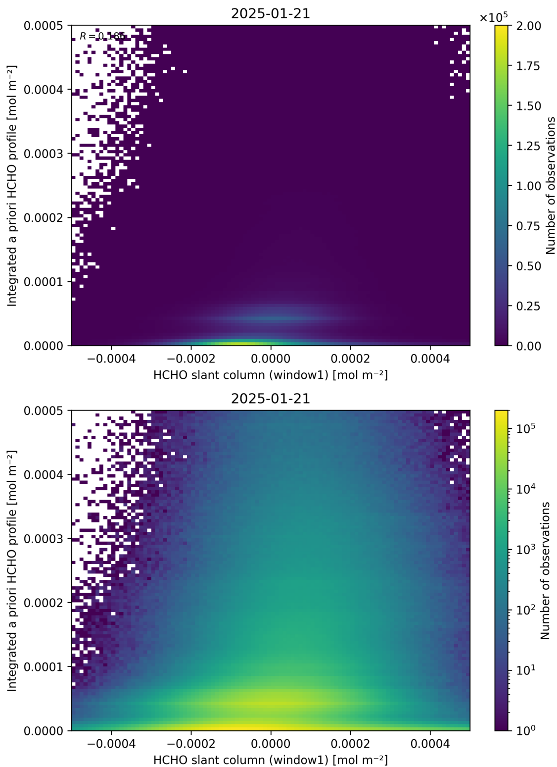
Figure 87: Scatter density plot of “HCHO slant column (window1)” against “Integrated a priori HCHO profile” for 2025-01-20 to 2025-01-22.
