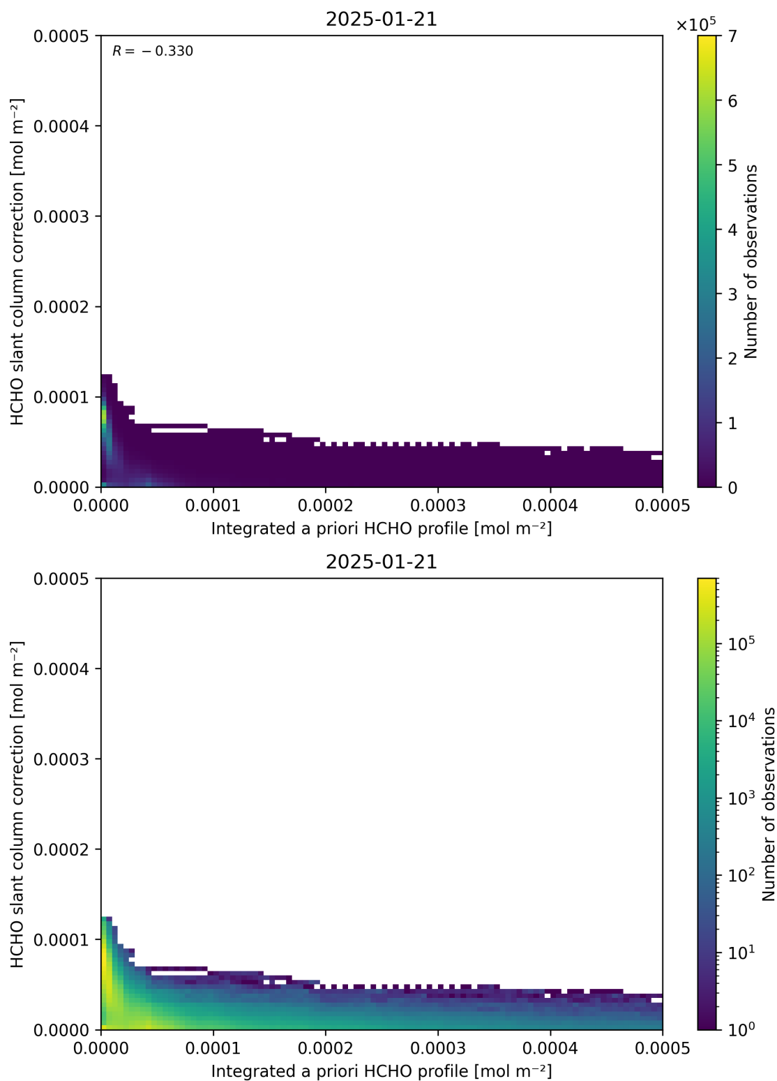
Figure 152: Scatter density plot of “Integrated a priori HCHO profile” against “HCHO slant column correction” for 2025-01-20 to 2025-01-22.
