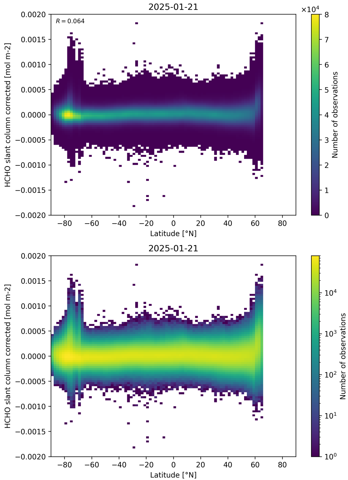
Figure 157: Scatter density plot of “Latitude” against “HCHO slant column corrected” for 2025-01-20 to 2025-01-22.
