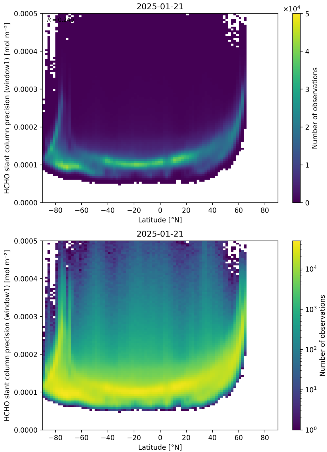
Figure 160: Scatter density plot of “Latitude” against “HCHO slant column precision (window1)” for 2025-01-20 to 2025-01-22.
