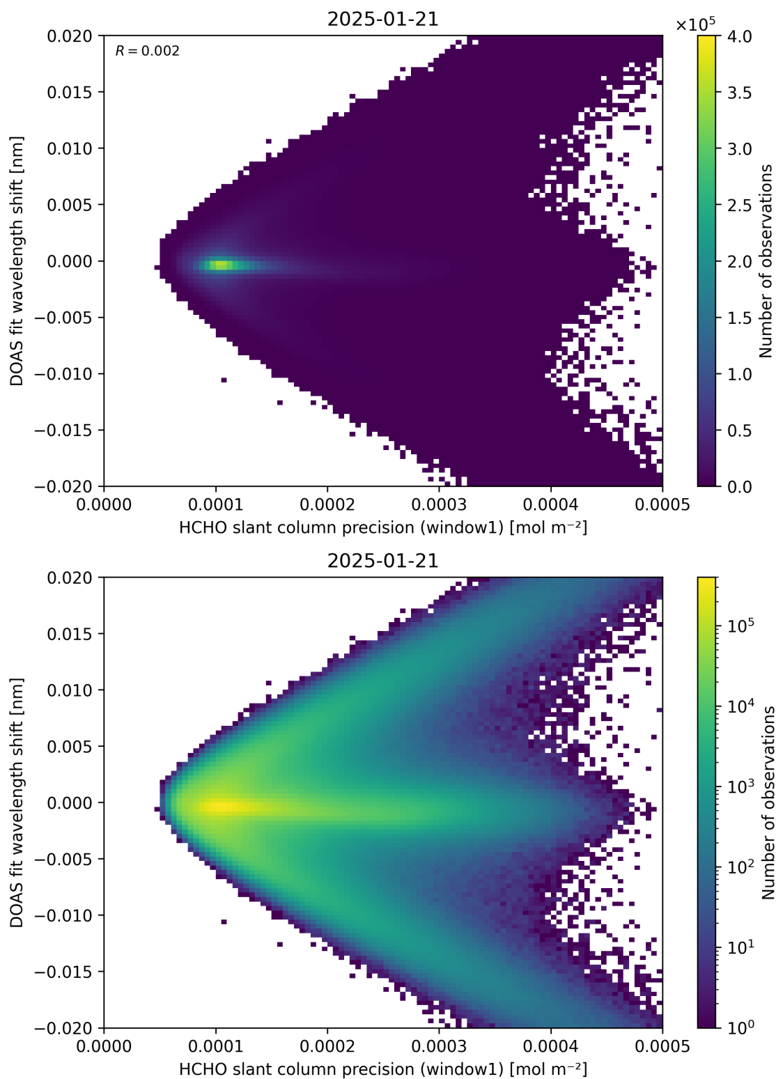
Figure 89: Scatter density plot of “HCHO slant column precision (window1)” against “DOAS fit wavelength shift” for 2025-01-20 to 2025-01-22.
