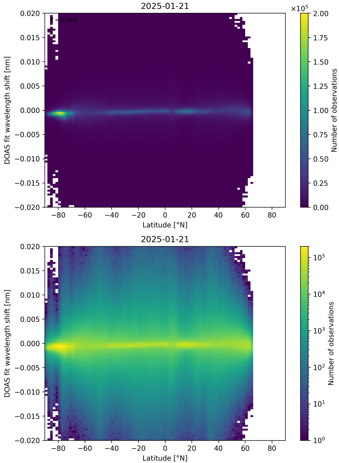
Figure 154: Scatter density plot of “Latitude” against “DOAS fit wavelength shift” for 2025-01-20 to 2025-01-22.
