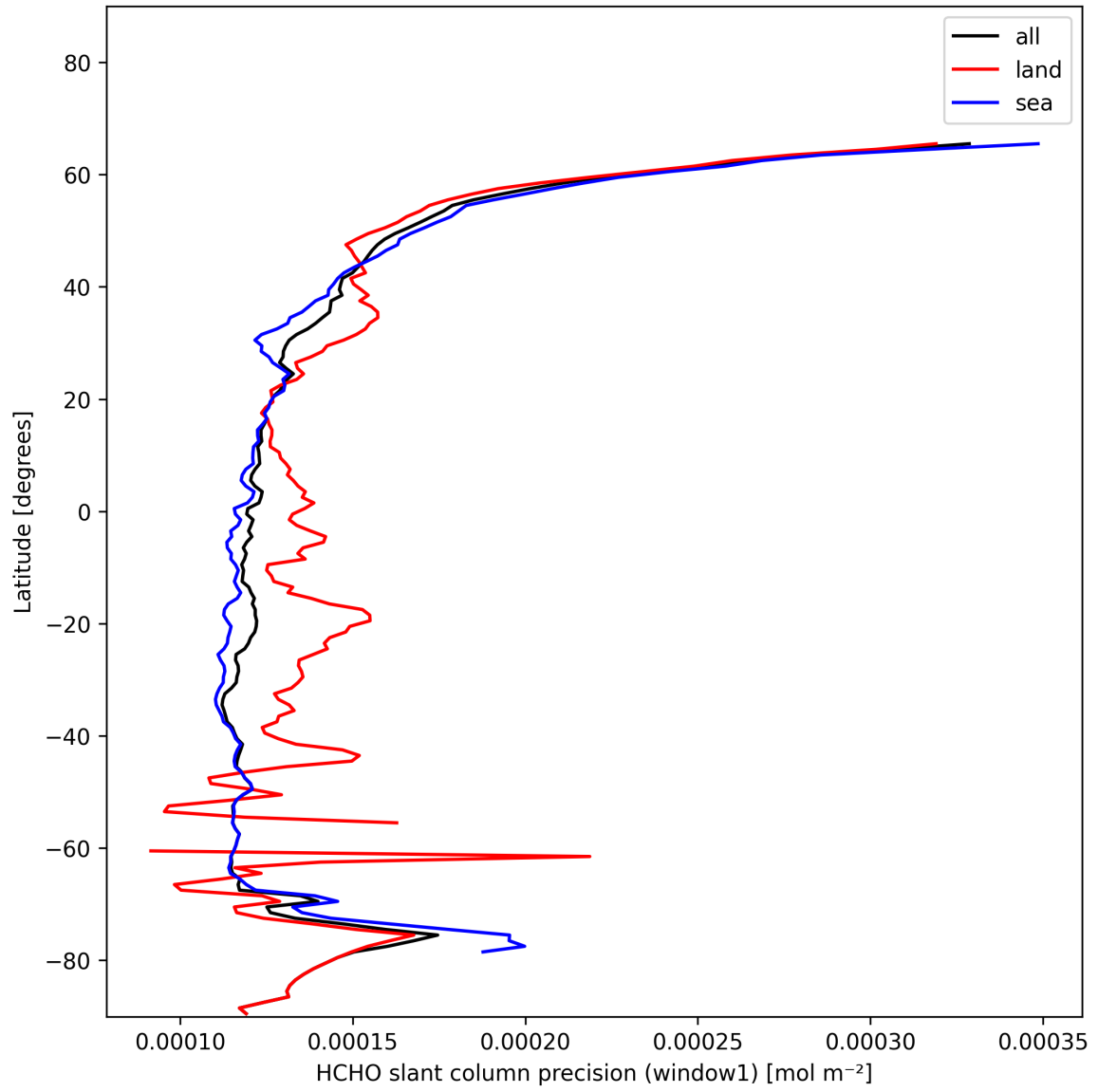
Figure 25: Zonal average of “HCHO slant column precision (window1)” for 2025-01-20 to 2025-01-22.
