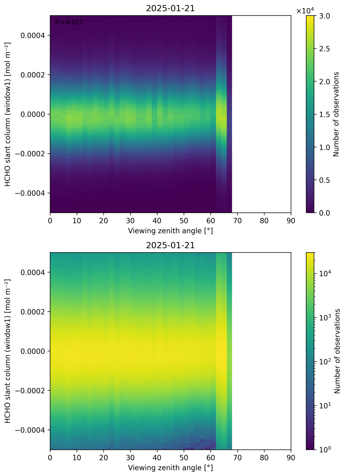
Figure 188: Scatter density plot of “Viewing zenith angle” against “HCHO slant column (window1)” for 2025-01-20 to 2025-01-22.
