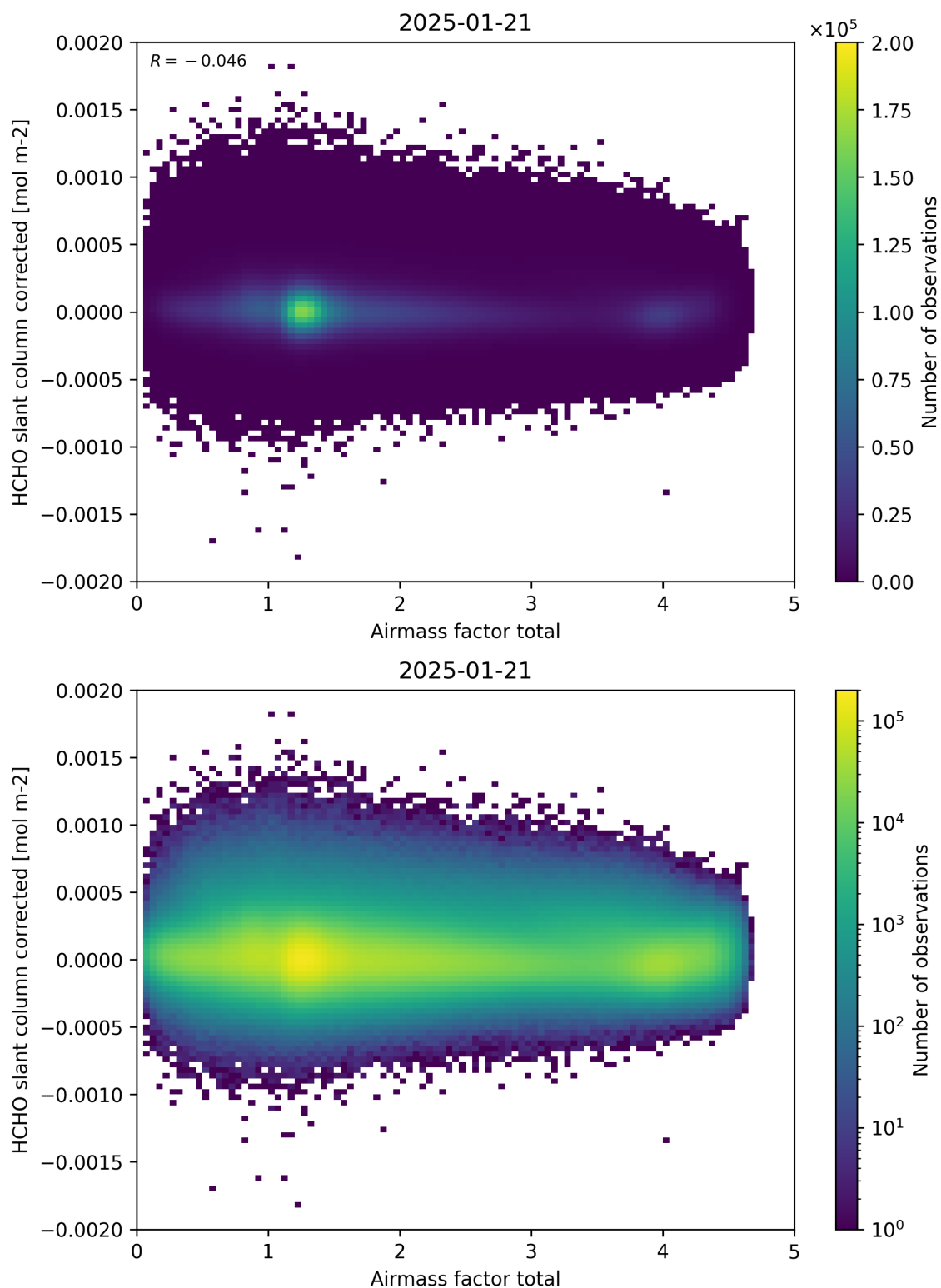
Figure 101: Scatter density plot of “Airmass factor total” against “HCHO slant column corrected” for 2025-01-20 to 2025-01-22.
