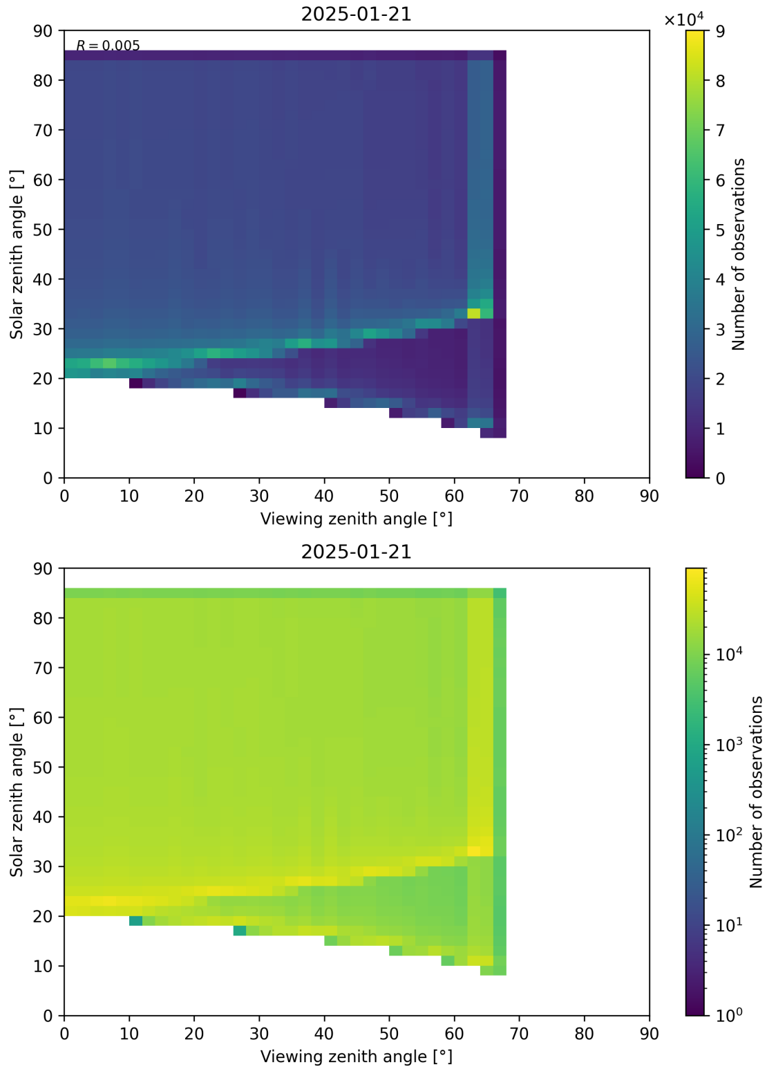
Figure 197: Scatter density plot of “Viewing zenith angle” against “Solar zenith angle” for 2025-01-20 to 2025-01-22.
