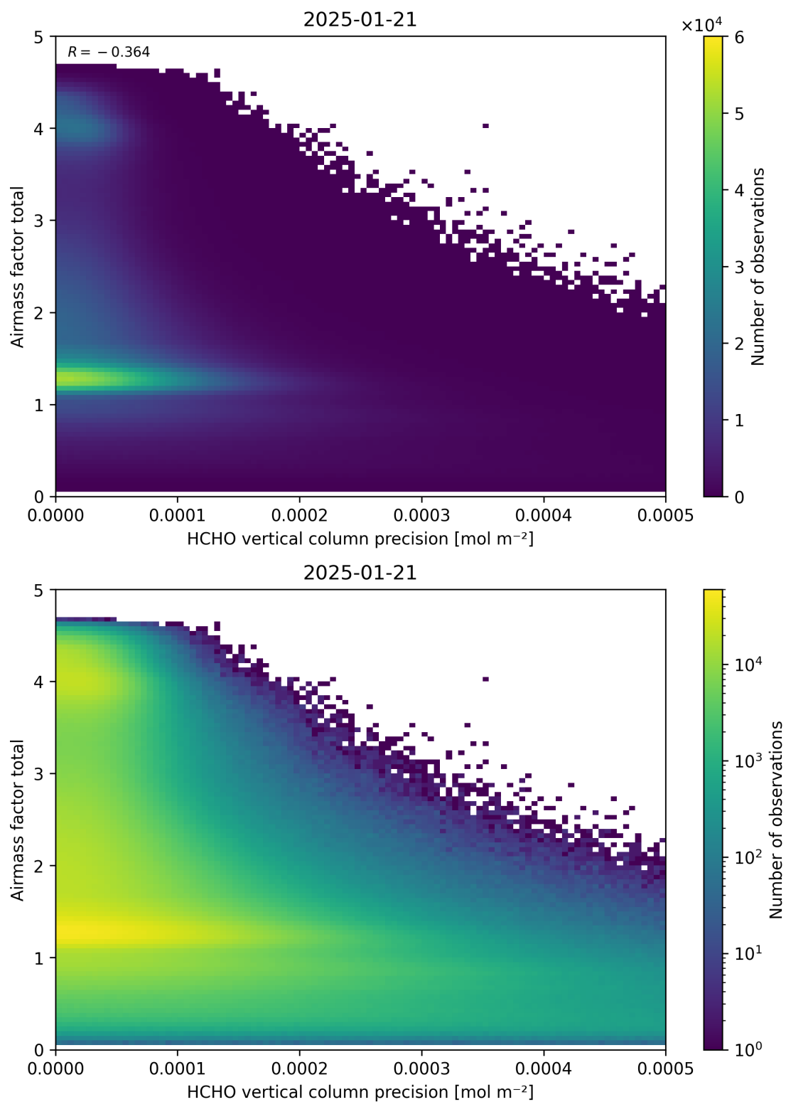
Figure 144: Scatter density plot of “HCHO vertical column precision” against “Airmass factor total” for 2025-01-20 to 2025-01-22.
