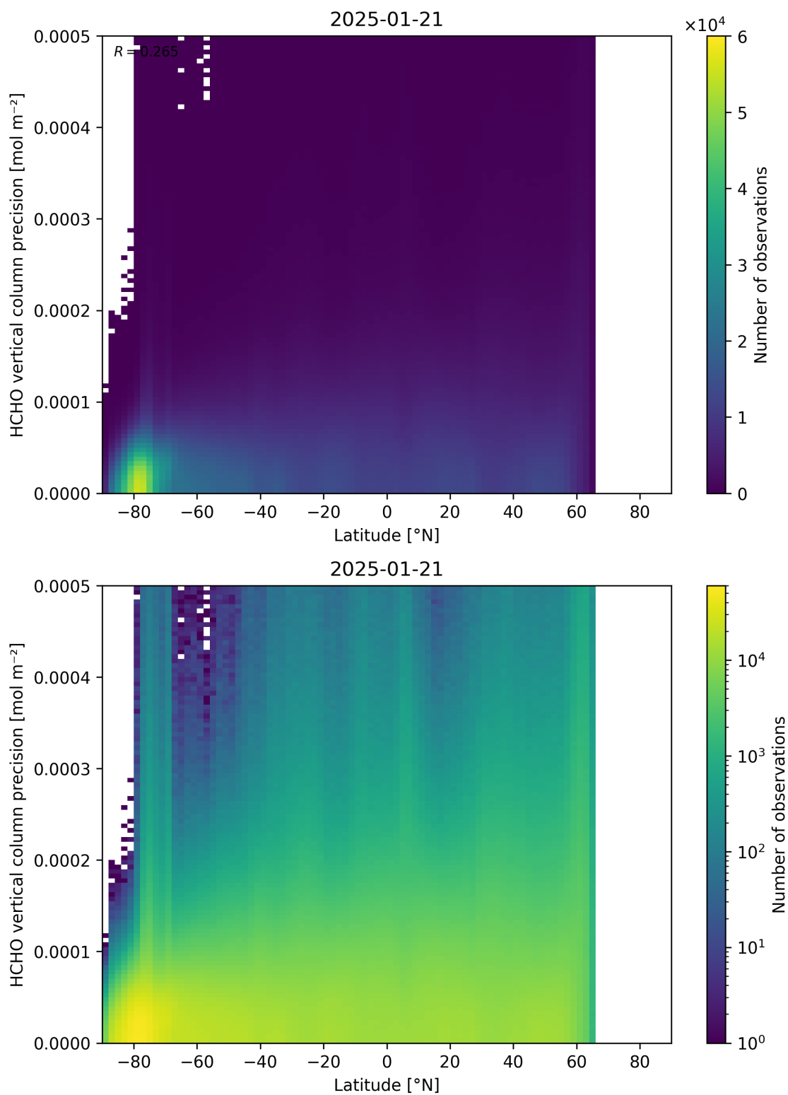
Figure 165: Scatter density plot of “Latitude” against “HCHO vertical column precision” for 2025-01-20 to 2025-01-22.
