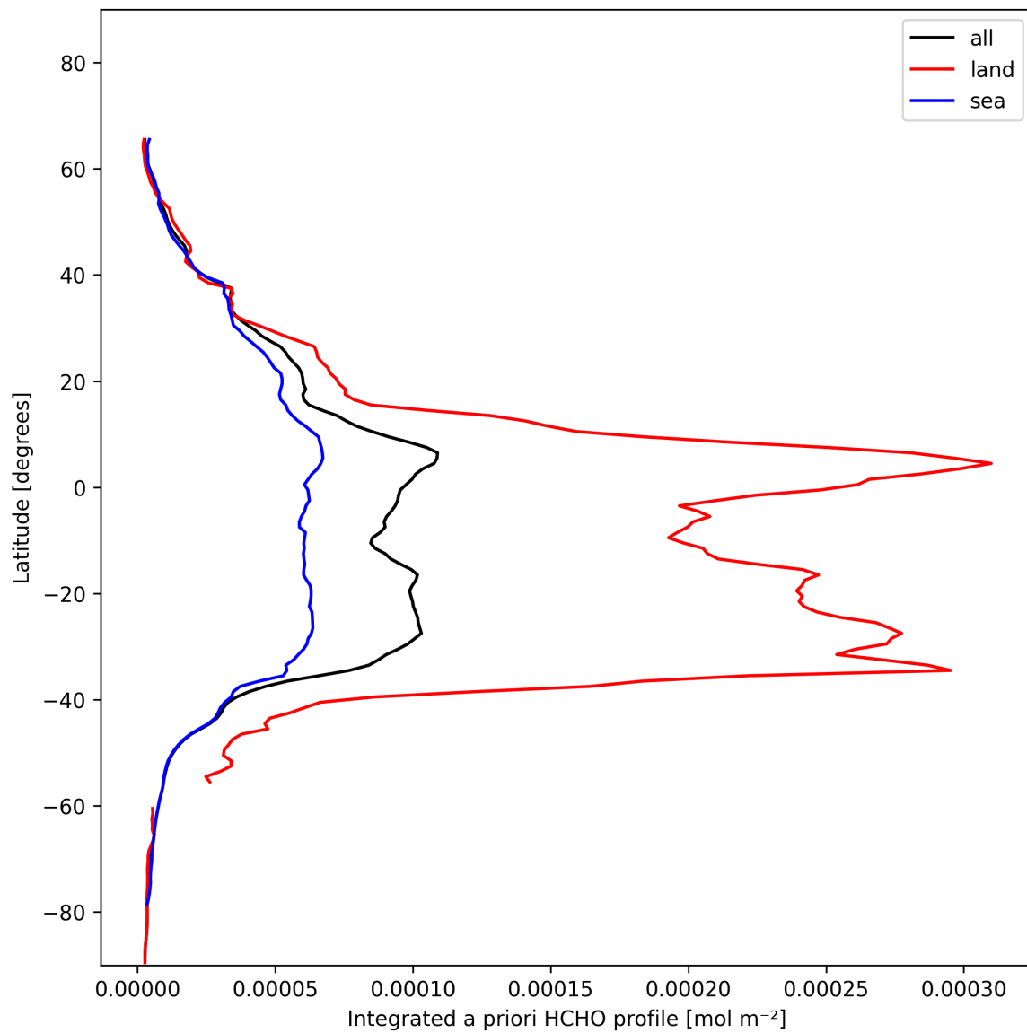
Figure 29: Zonal average of “Integrated a priori HCHO profile” for 2025-01-20 to 2025-01-22.
