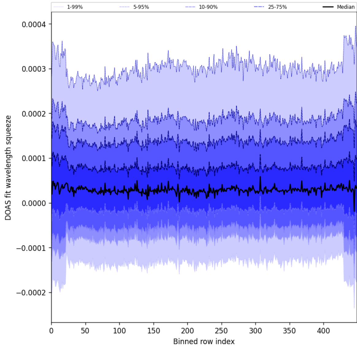
Figure 59: Along track statistics of “DOAS fit wavelength squeeze” for 2025-01-20 to 2025-01-22
