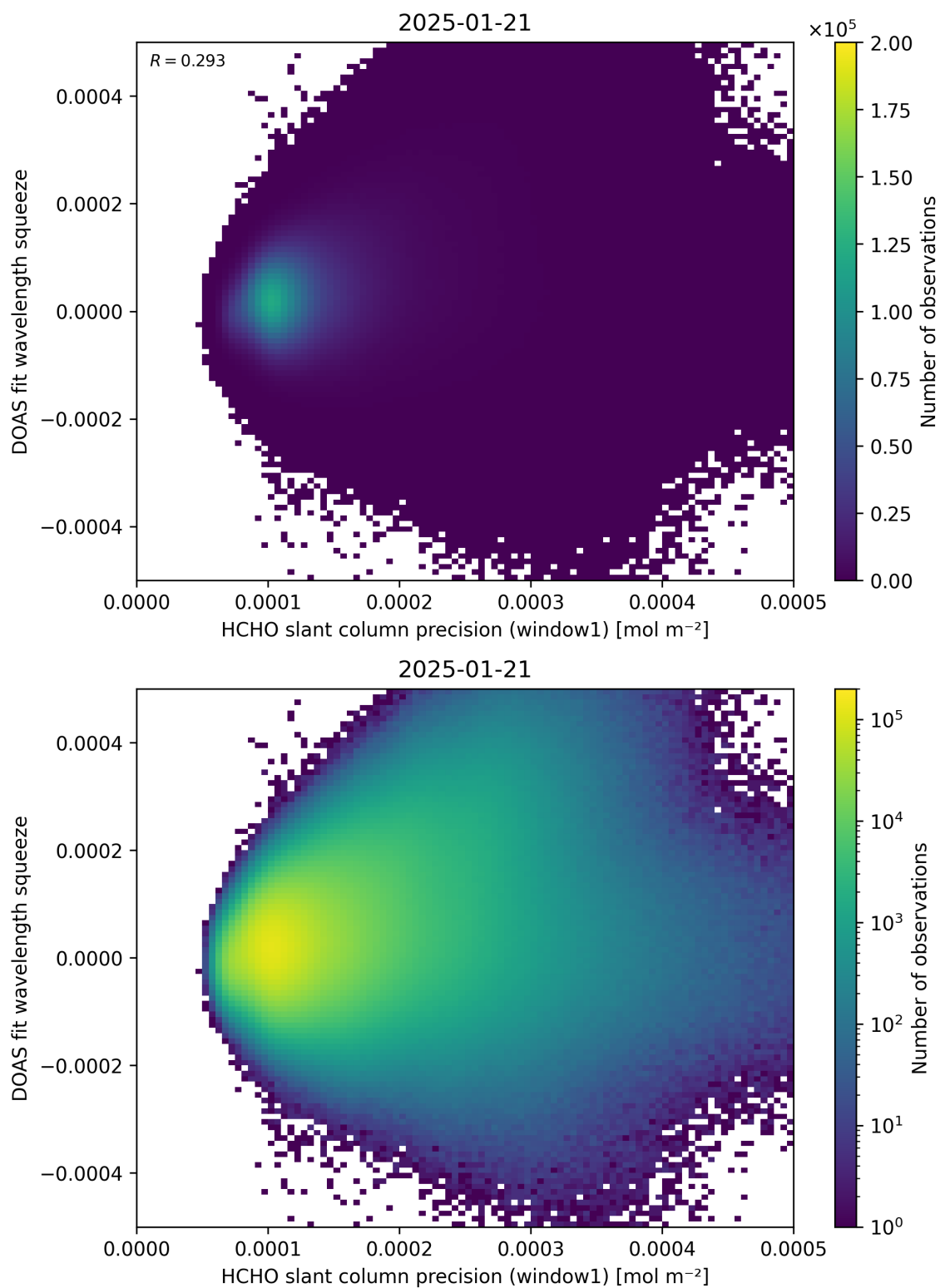
Figure 90: Scatter density plot of “HCHO slant column precision (window1)” against “DOAS fit wavelength squeeze” for 2025-01-20 to 2025-01-22.
