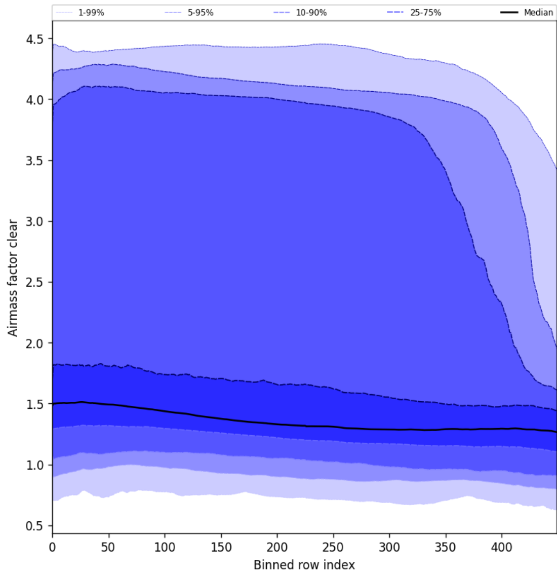
Figure 56: Along track statistics of “Airmass factor clear” for 2025-01-20 to 2025-01-22
