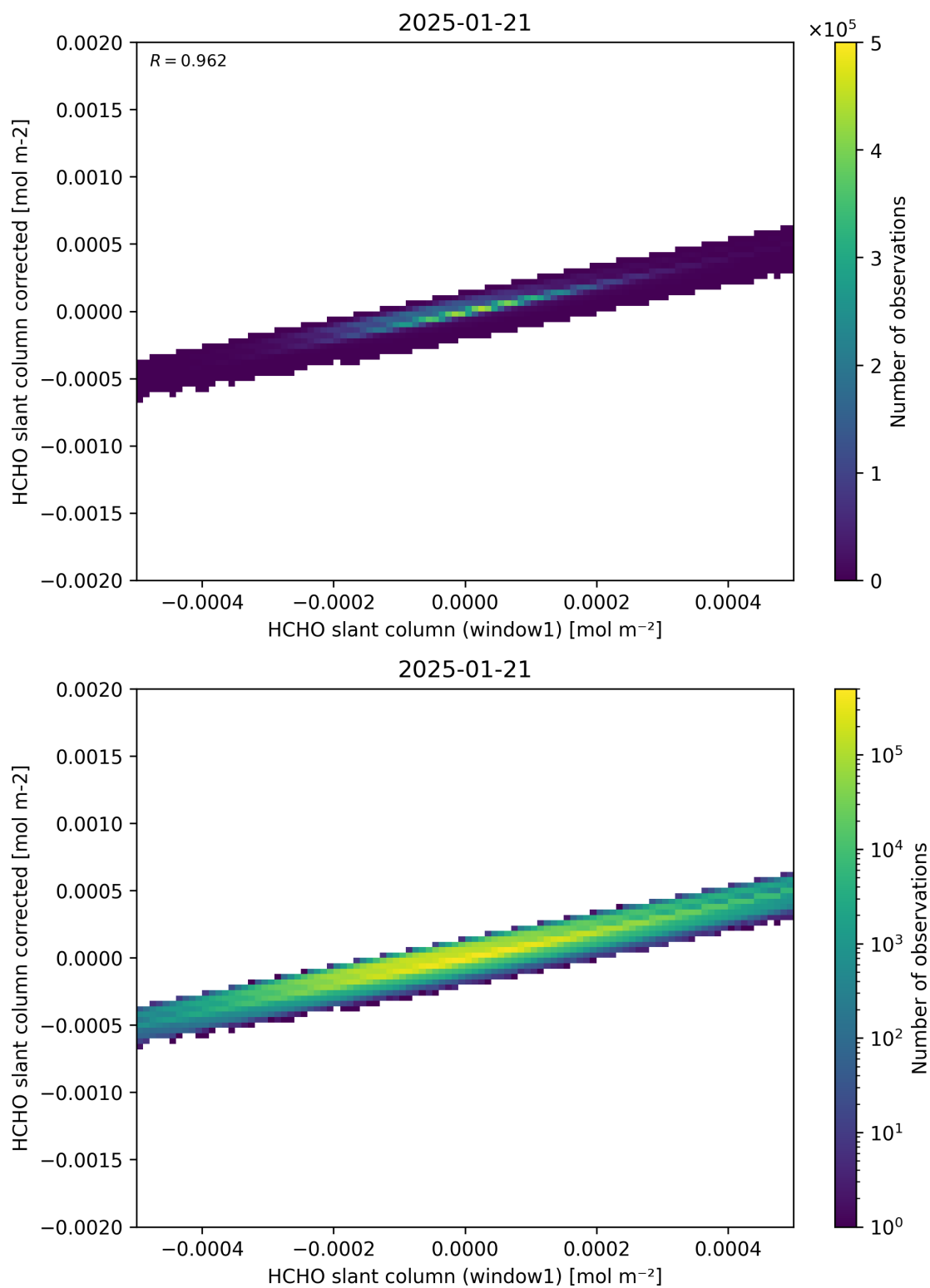
Figure 82: Scatter density plot of “HCHO slant column (window1)” against “HCHO slant column corrected” for 2025-01-20 to 2025-01-22.
