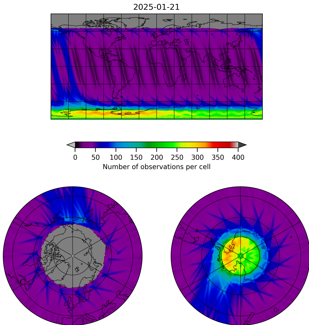
Figure 19: Map of the number of observations for 2025-01-20 to 2025-01-22
