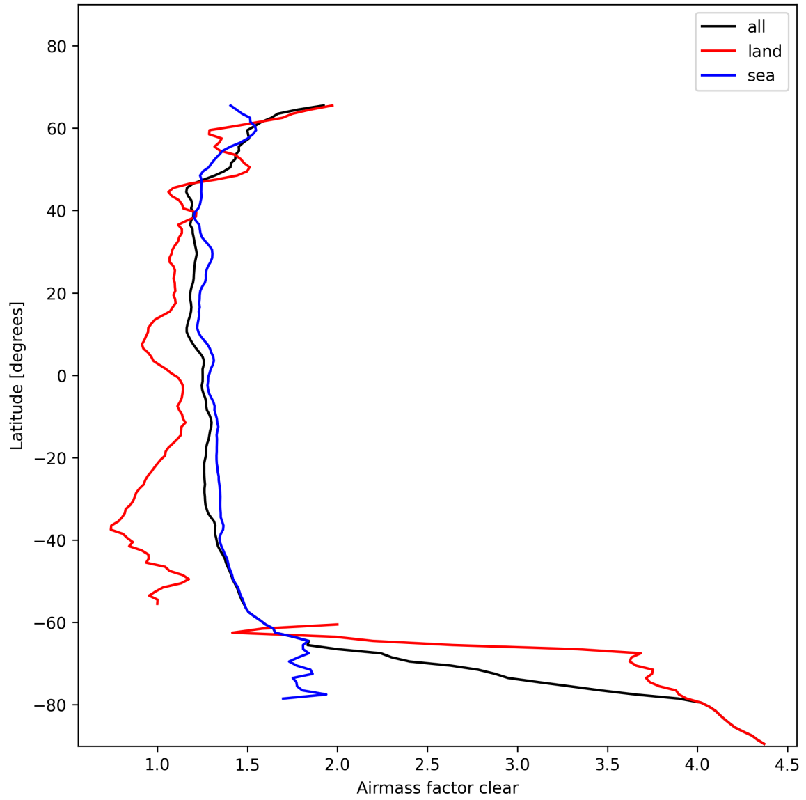
Figure 28: Zonal average of “Airmass factor clear” for 2025-01-20 to 2025-01-22.
