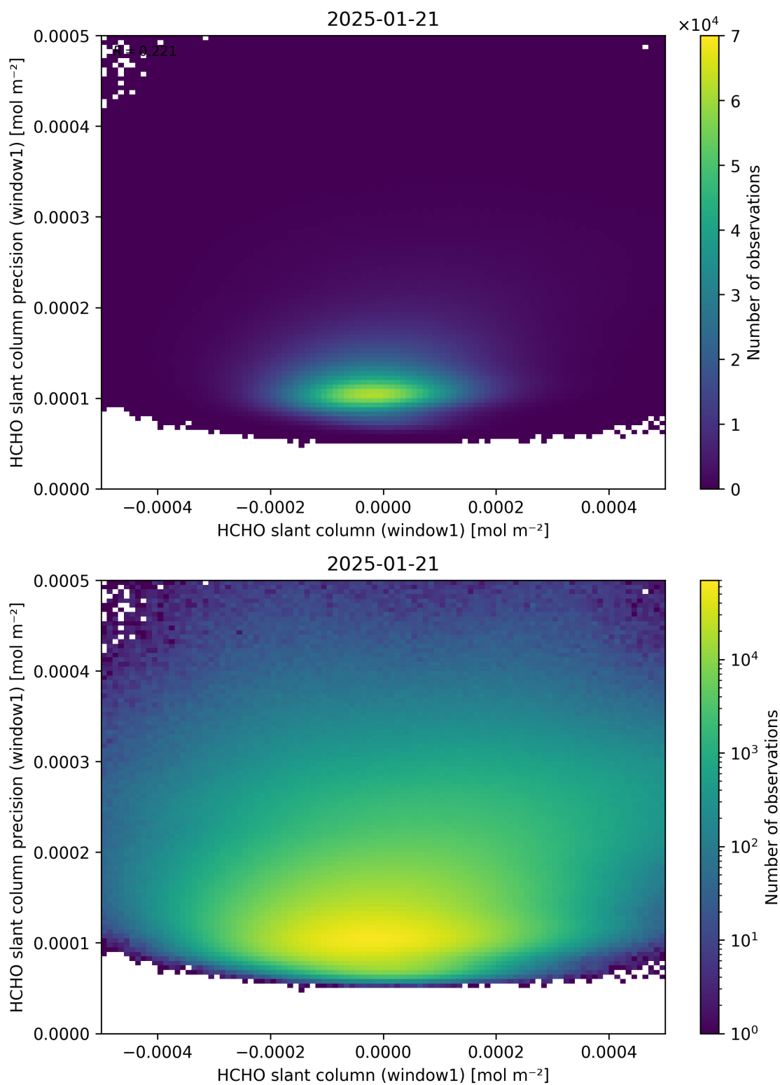
Figure 84: Scatter density plot of “HCHO slant column (window1)” against “HCHO slant column precision (window1)” for 2025-01-20 to 2025-01-22.
