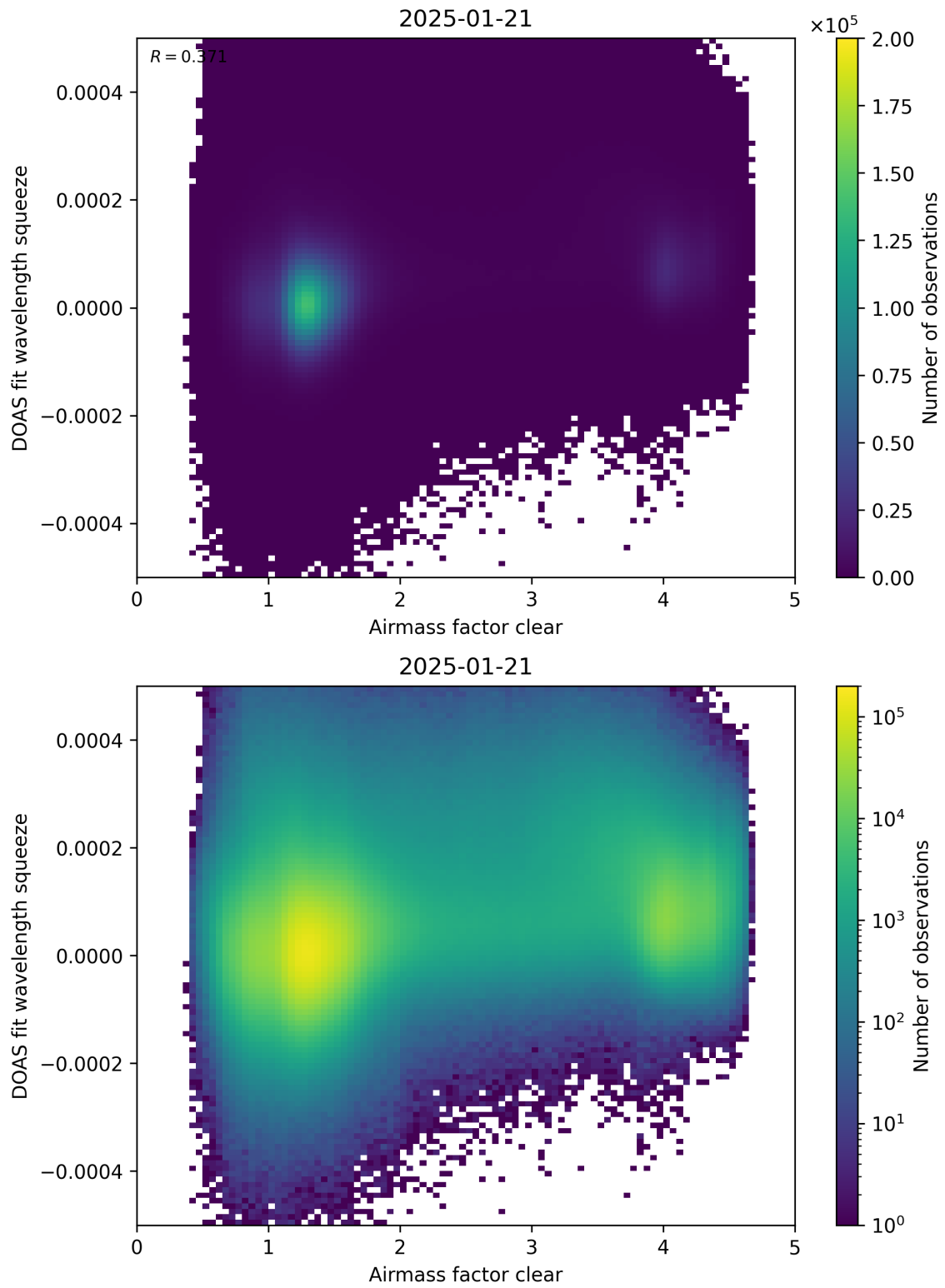
Figure 73: Scatter density plot of “Airmass factor clear” against “DOAS fit wavelength squeeze” for 2025-01-20 to 2025-01-22.
