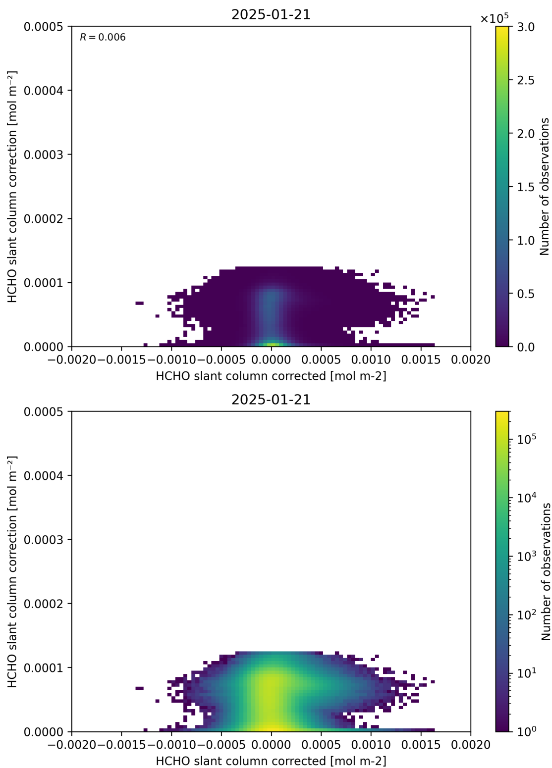
Figure 77: Scatter density plot of “HCHO slant column corrected” against “HCHO slant column correction” for 2025-01-20 to 2025-01-22.
