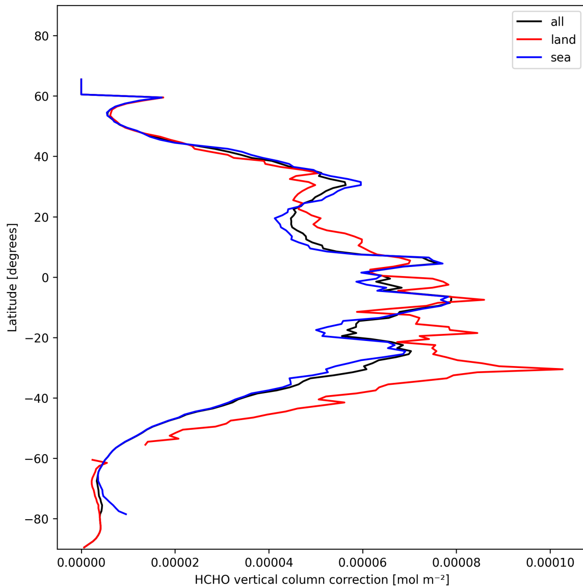
Figure 23: Zonal average of “HCHO vertical column correction” for 2025-01-20 to 2025-01-22.
