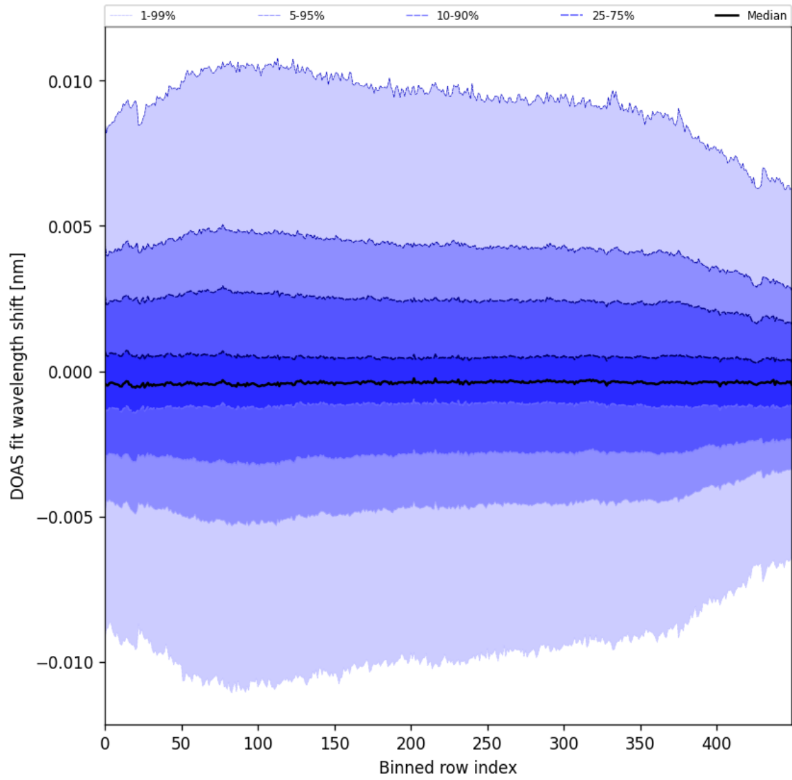
Figure 58: Along track statistics of “DOAS fit wavelength shift” for 2025-01-20 to 2025-01-22
