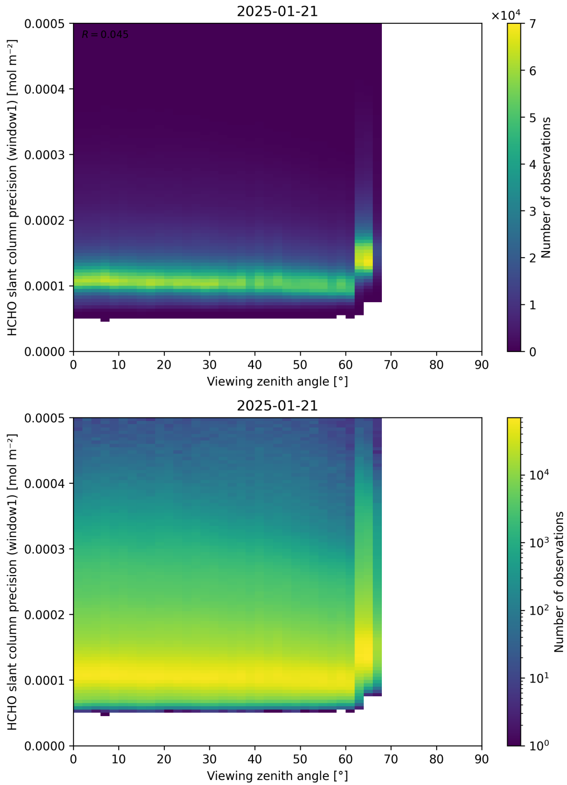
Figure 189: Scatter density plot of “Viewing zenith angle” against “HCHO slant column precision (window1)” for 2025-01-20 to 2025-01-22.
