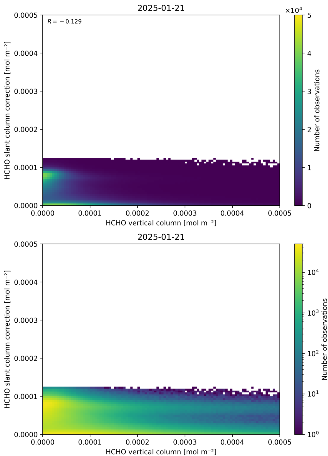
Figure 128: Scatter density plot of “HCHO vertical column” against “HCHO slant column correction” for 2025-01-20 to 2025-01-22.
