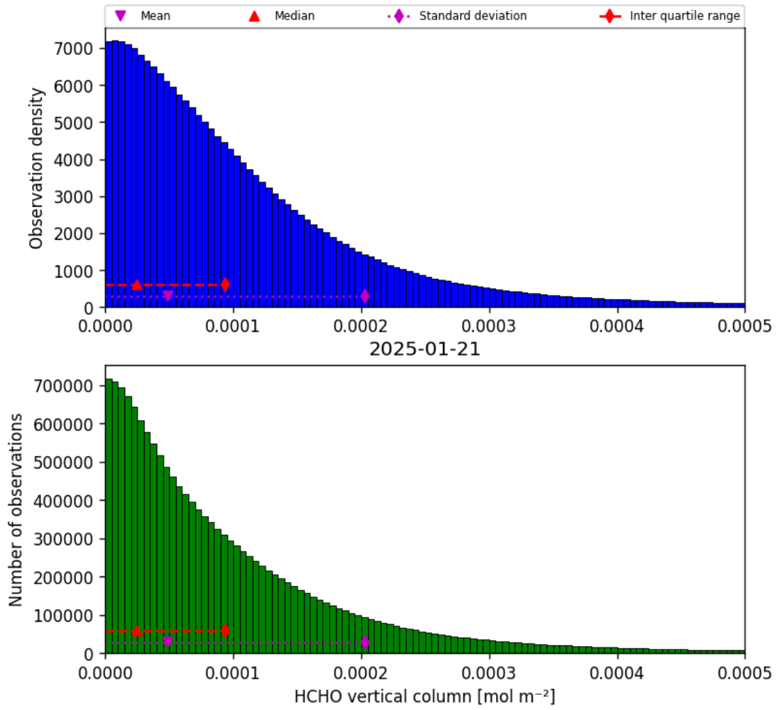
Figure 35: Histogram of “HCHO vertical column” for 2025-01-20 to 2025-01-22
