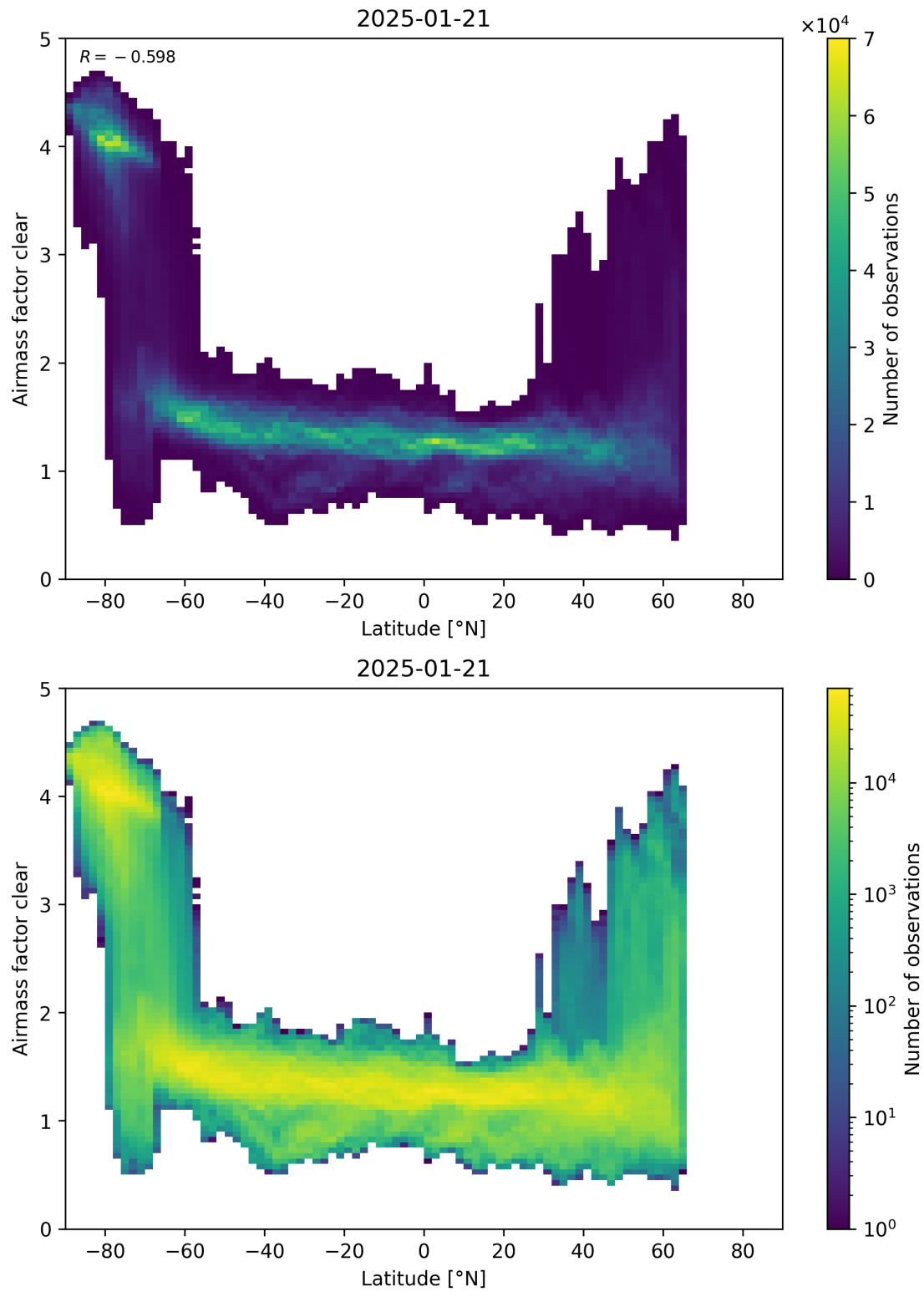
Figure 156: Scatter density plot of “Latitude” against “Airmass factor clear” for 2025-01-20 to 2025-01-22.
