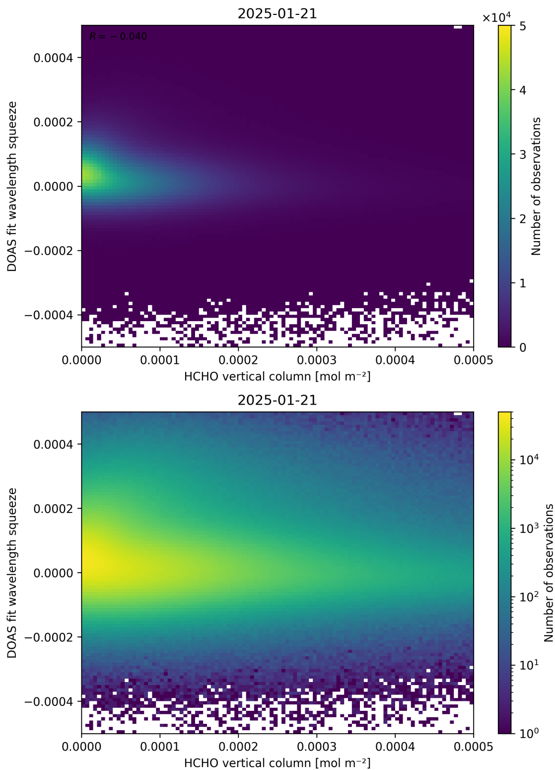
Figure 125: Scatter density plot of “HCHO vertical column” against “DOAS fit wavelength squeeze” for 2025-01-20 to 2025-01-22.
