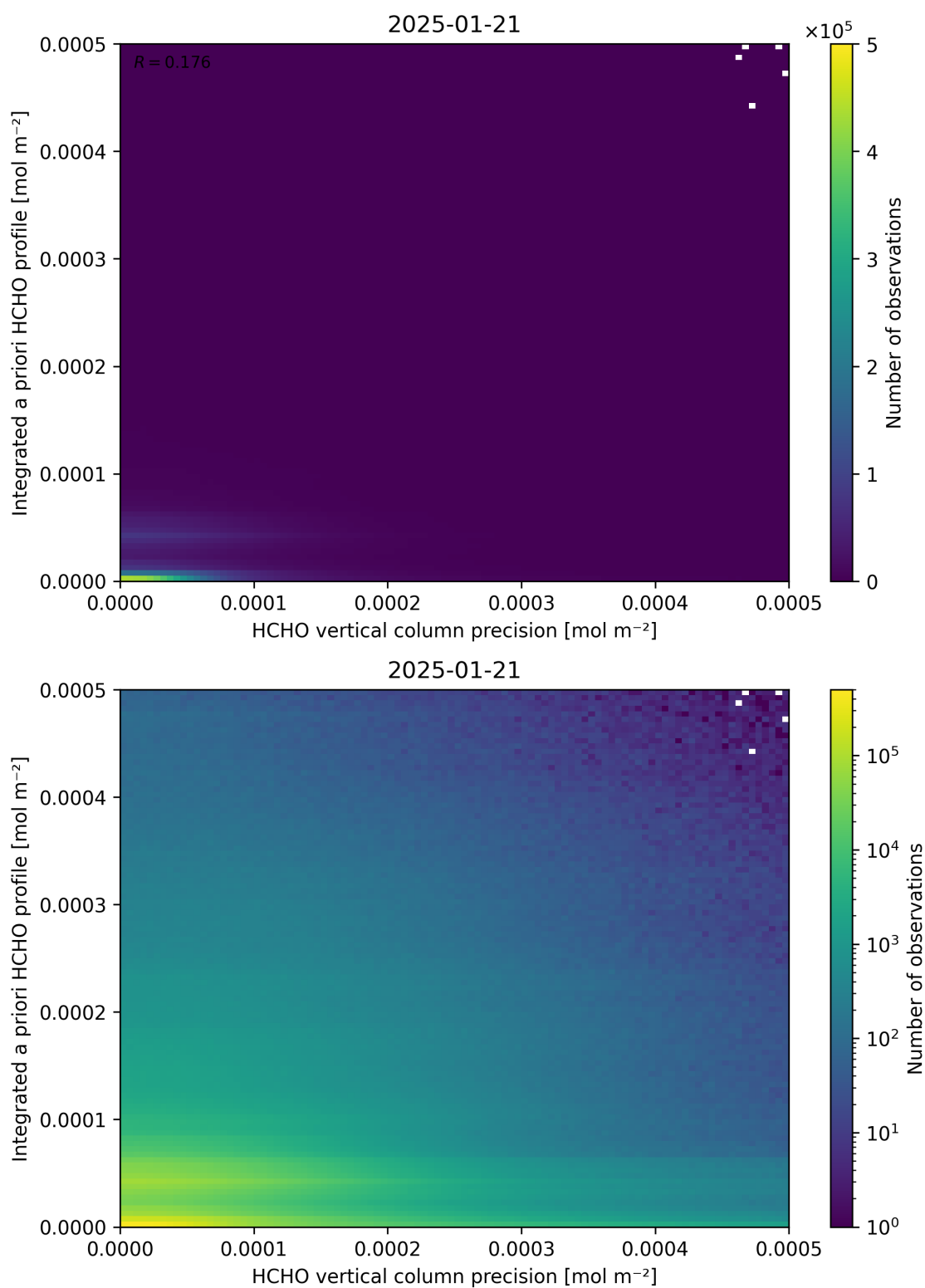
Figure 147: Scatter density plot of “HCHO vertical column precision” against “Integrated a priori HCHO profile” for 2025-01-20 to 2025-01-22.
