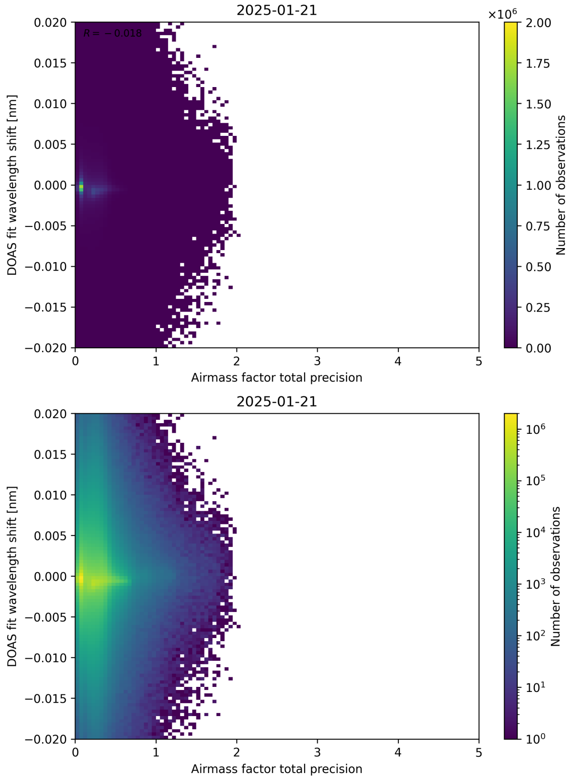
Figure 106: Scatter density plot of “Airmass factor total precision” against “DOAS fit wavelength shift” for 2025-01-20 to 2025-01-22.
