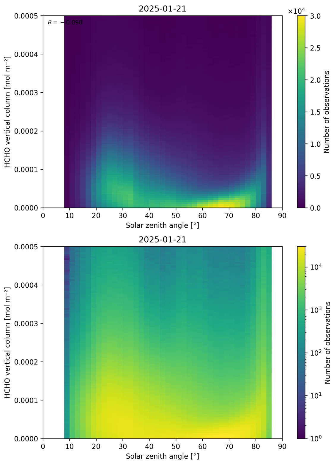
Figure 177: Scatter density plot of “Solar zenith angle” against “HCHO vertical column” for 2025-01-20 to 2025-01-22.
