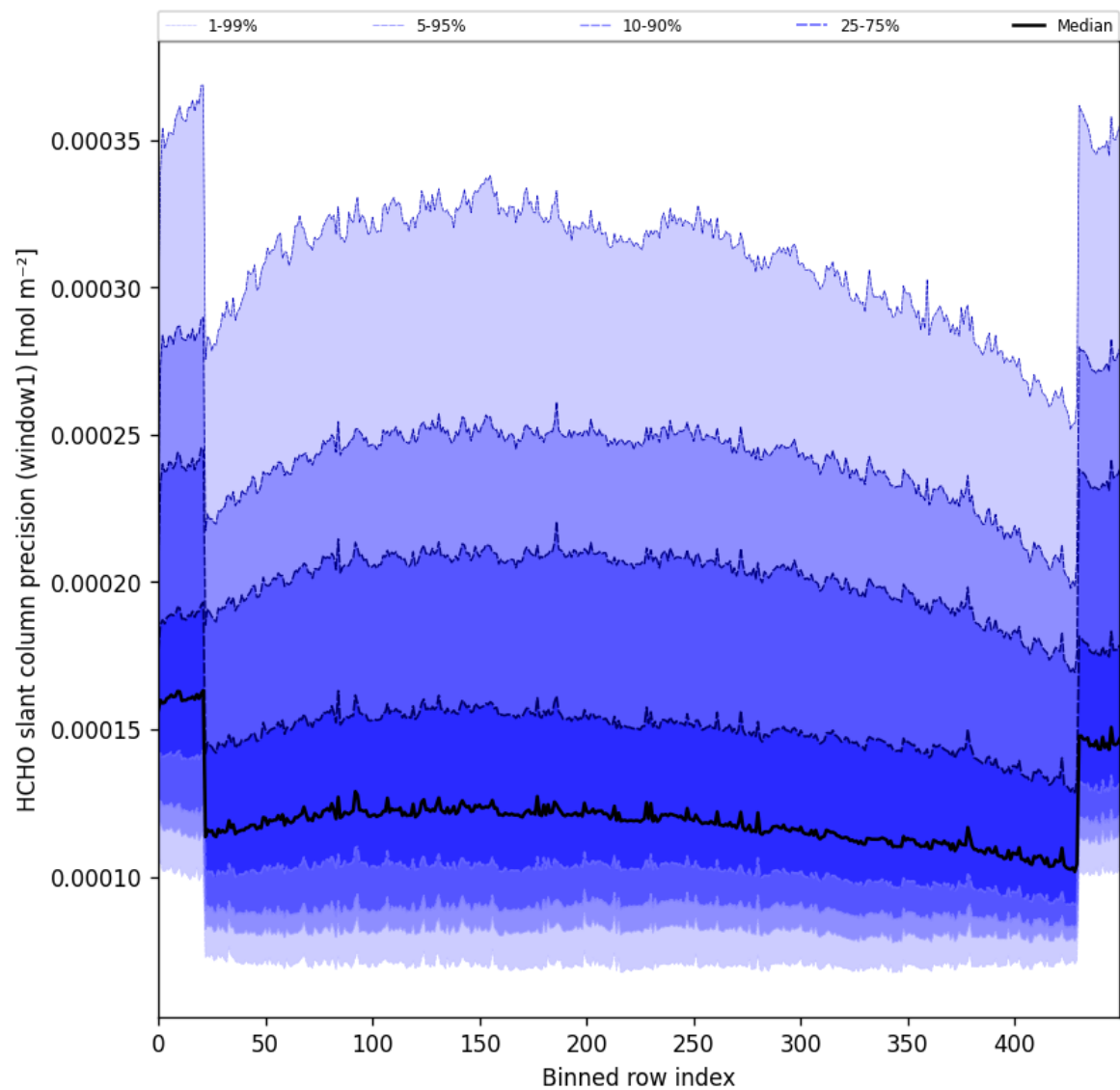
Figure 53: Along track statistics of “HCHO slant column precision (window1)” for 2025-01-20 to 2025-01-22
