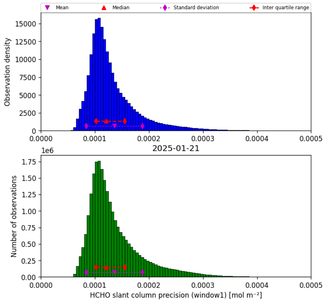
Figure 39: Histogram of “HCHO slant column precision (window1)” for 2025-01-20 to 2025-01-22
