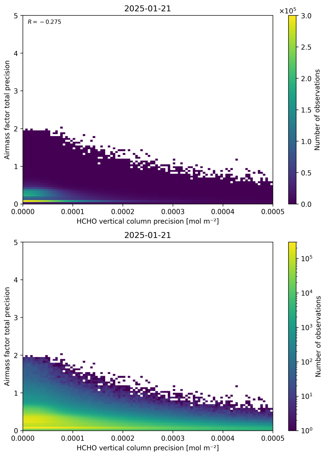
Figure 145: Scatter density plot of “HCHO vertical column precision” against “Airmass factor total precision” for 2025-01-20 to 2025-01-22.
