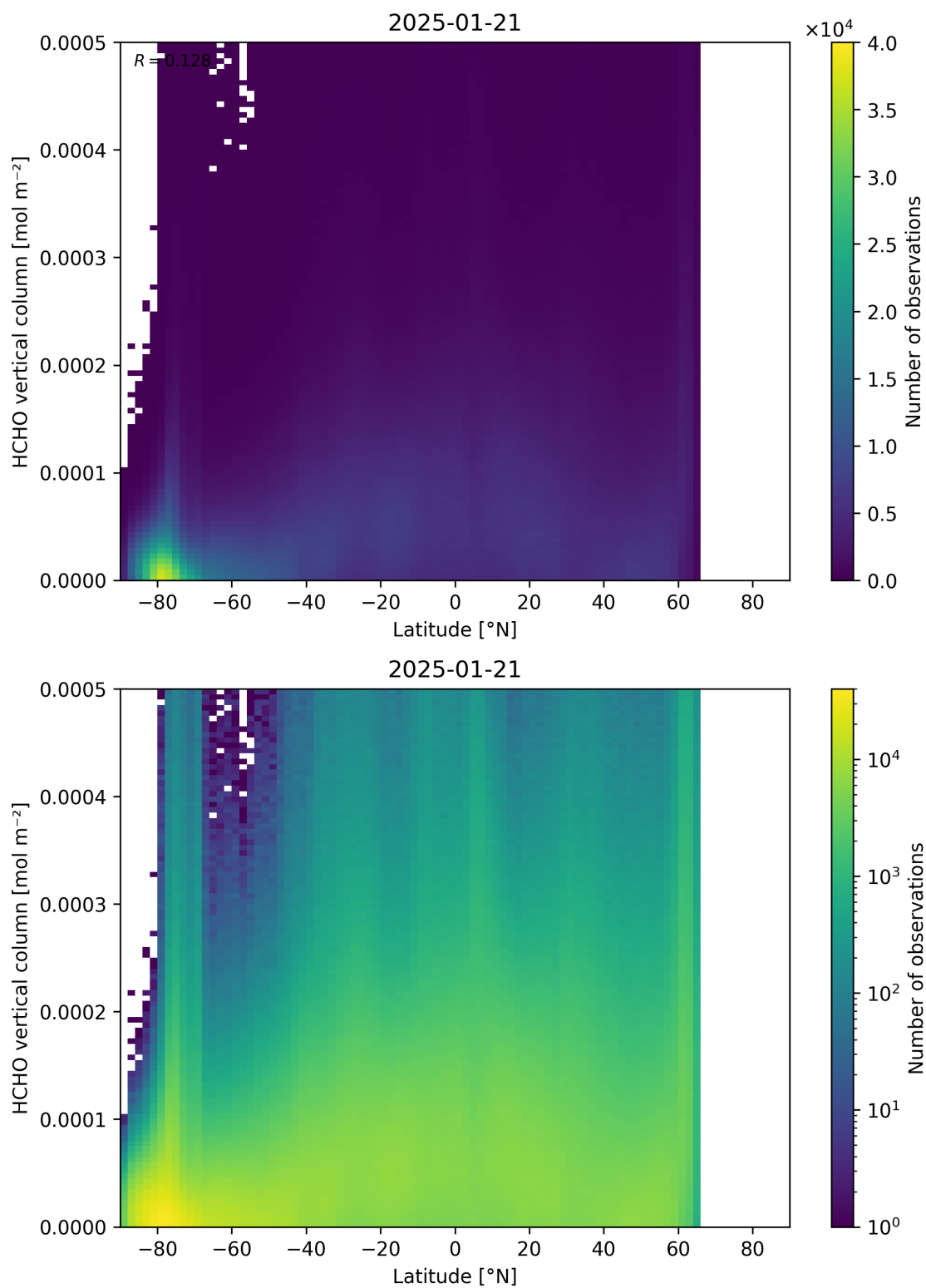
Figure 163: Scatter density plot of “Latitude” against “HCHO vertical column” for 2025-01-20 to 2025-01-22.
