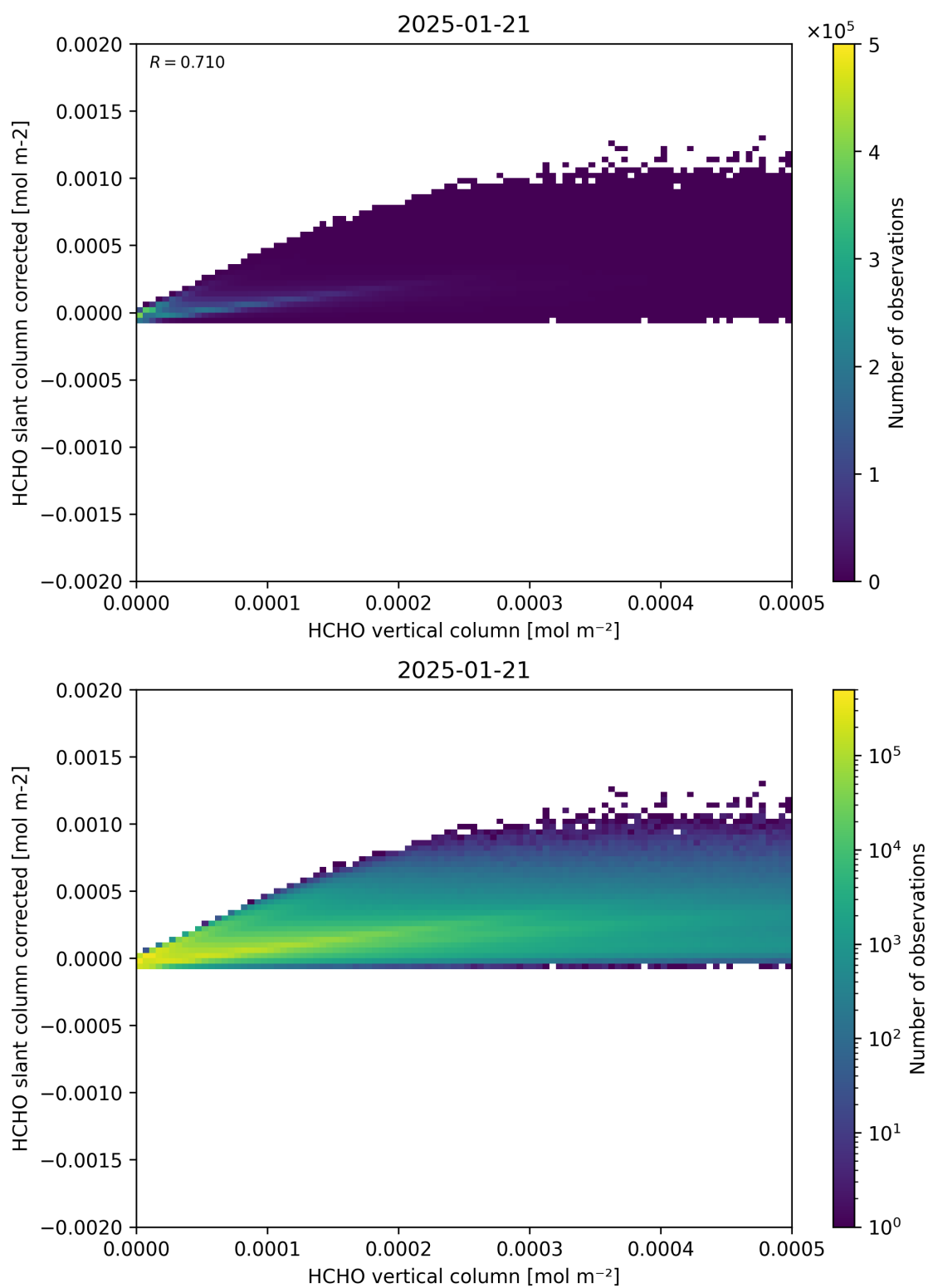
Figure 127: Scatter density plot of “HCHO vertical column” against “HCHO slant column corrected” for 2025-01-20 to 2025-01-22.
