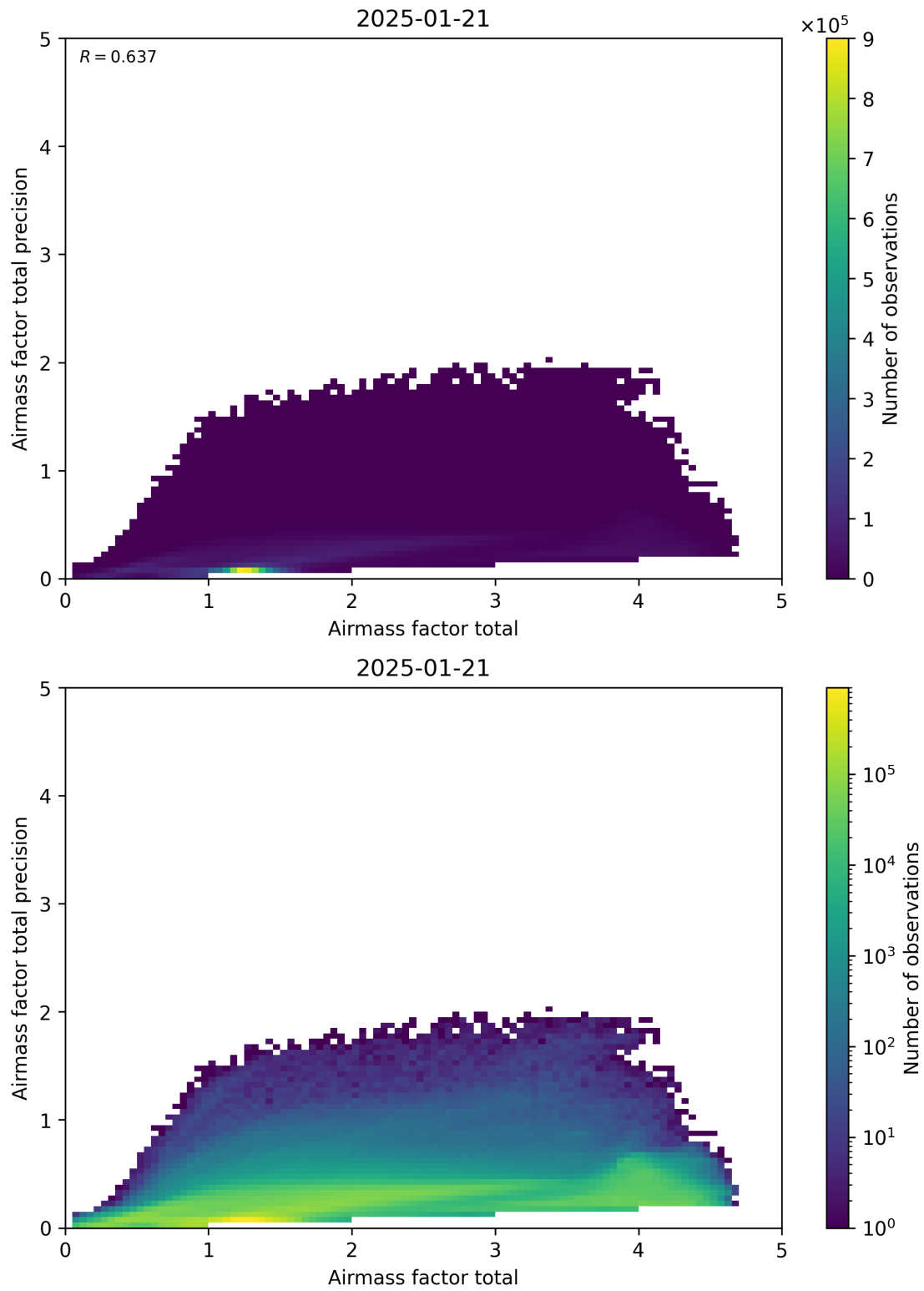
Figure 103: Scatter density plot of “Airmass factor total” against “Airmass factor total precision” for 2025-01-20 to 2025-01-22.
