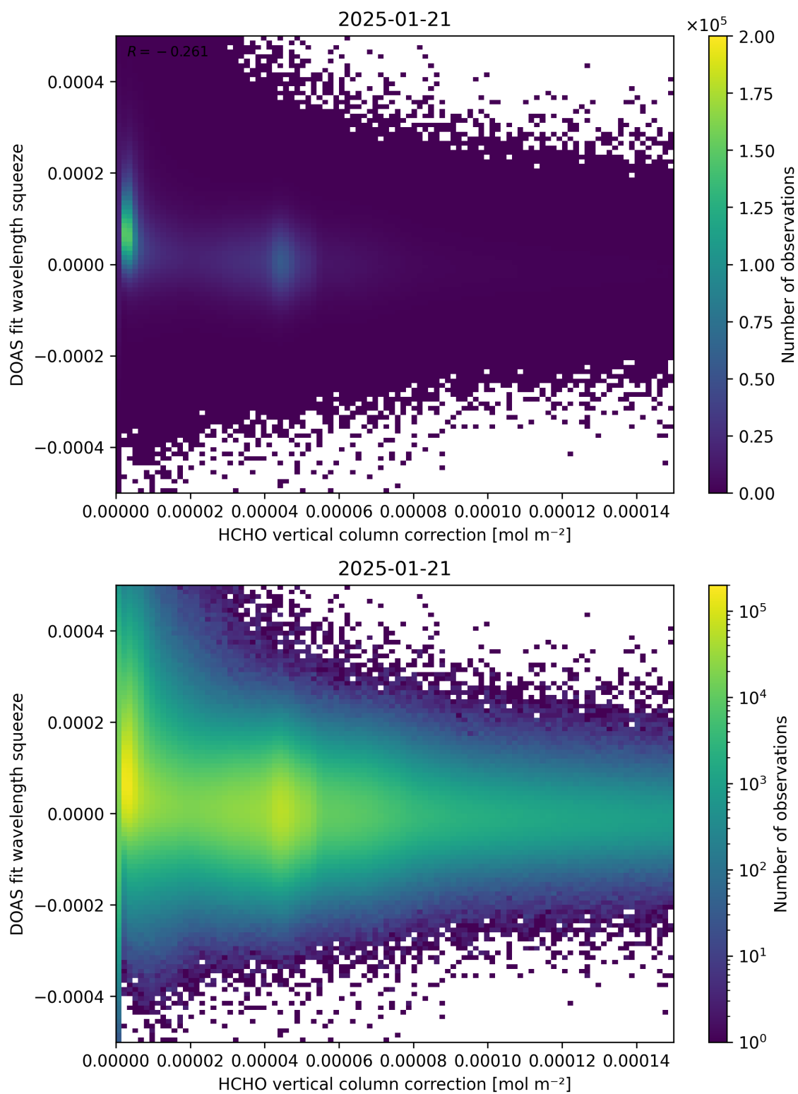
Figure 114: Scatter density plot of “HCHO vertical column correction” against “DOAS fit wavelength squeeze” for 2025-01-20 to 2025-01-22.
