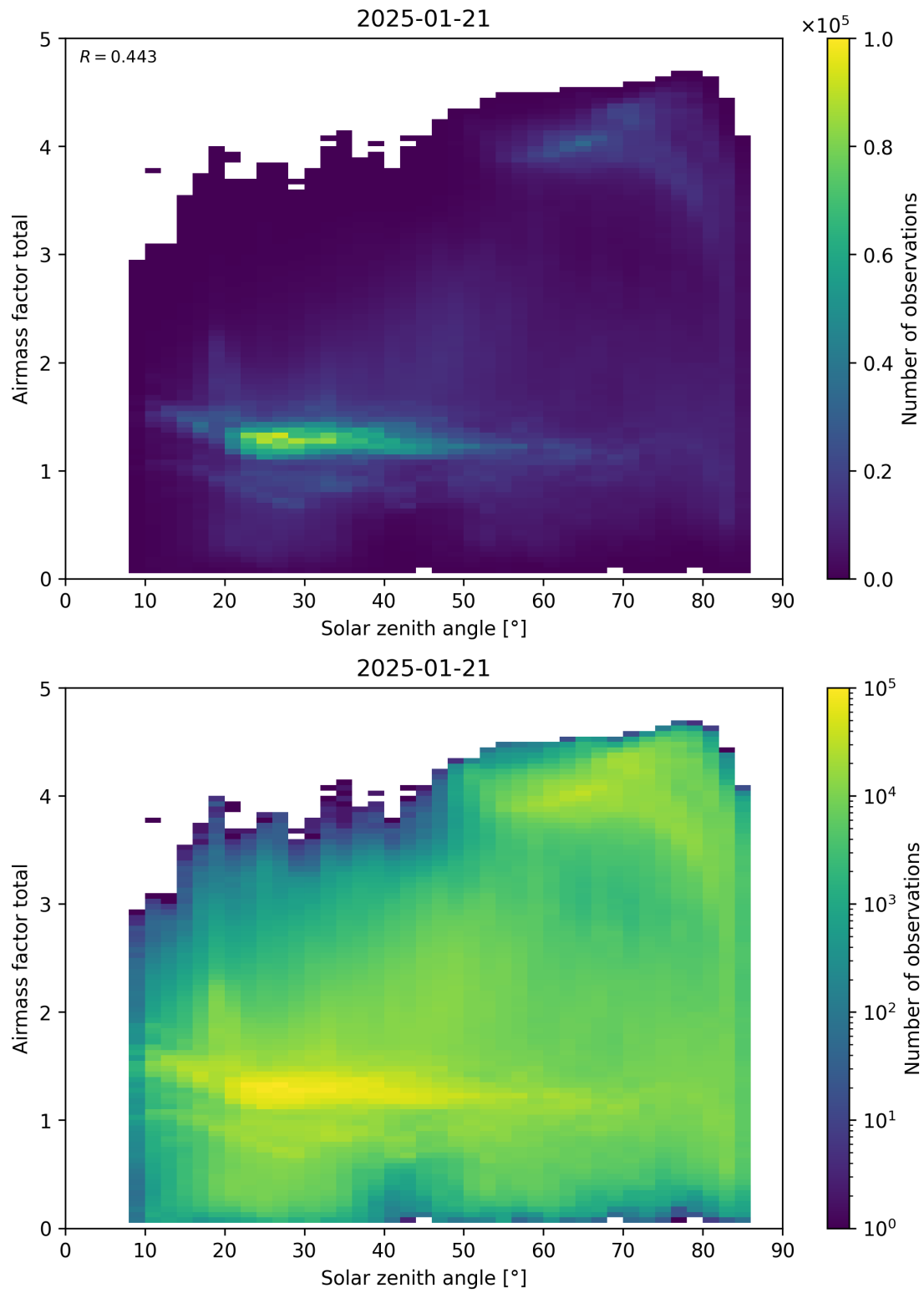
Figure 175: Scatter density plot of “Solar zenith angle” against “Airmass factor total” for 2025-01-20 to 2025-01-22.
