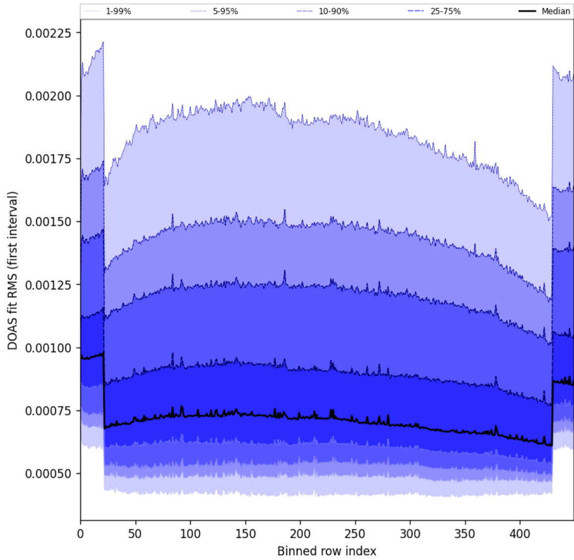
Figure 60: Along track statistics of “DOAS fit RMS (first interval)” for 2025-01-20 to 2025-01-22
