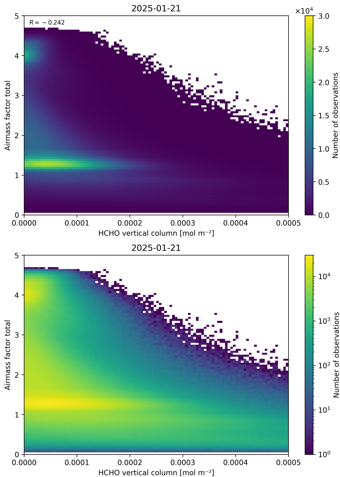
Figure 131: Scatter density plot of “HCHO vertical column” against “Airmass factor total” for 2025-01-20 to 2025-01-22.
