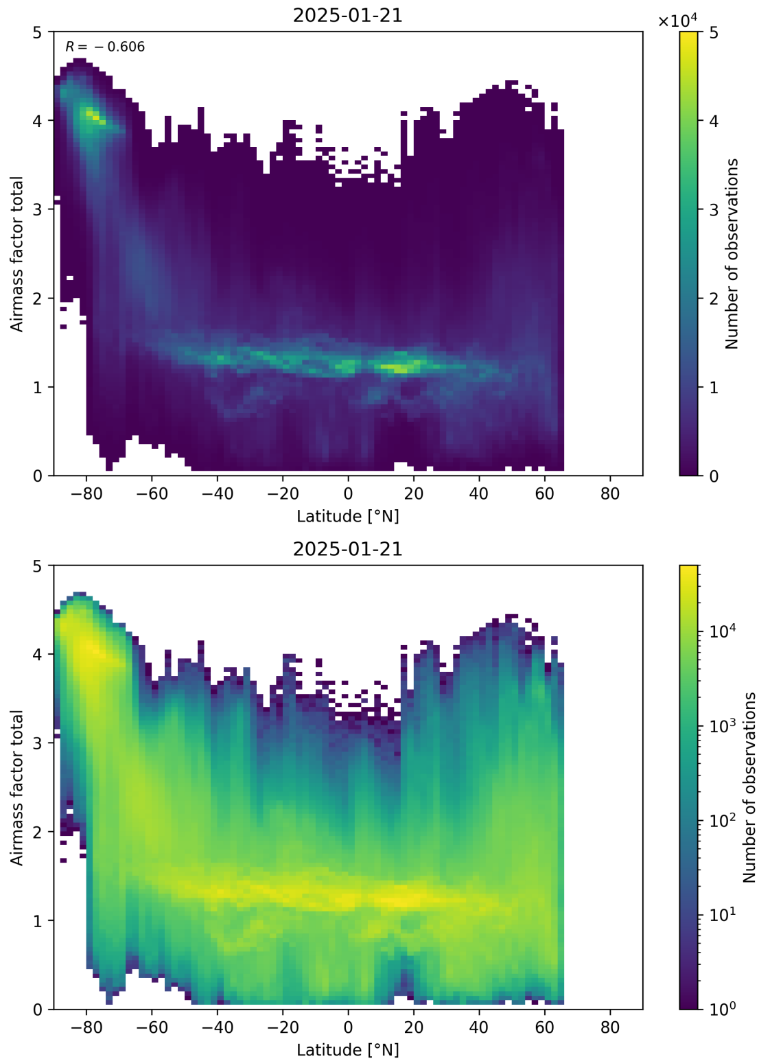
Figure 161: Scatter density plot of “Latitude” against “Airmass factor total” for 2025-01-20 to 2025-01-22.
