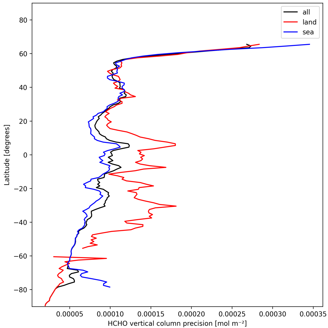
Figure 22: Zonal average of “HCHO vertical column precision” for 2025-01-20 to 2025-01-22.
