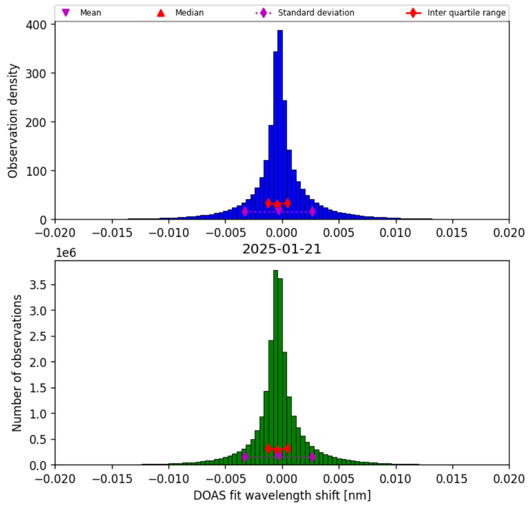
Figure 44: Histogram of “DOAS fit wavelength shift” for 2025-01-20 to 2025-01-22
