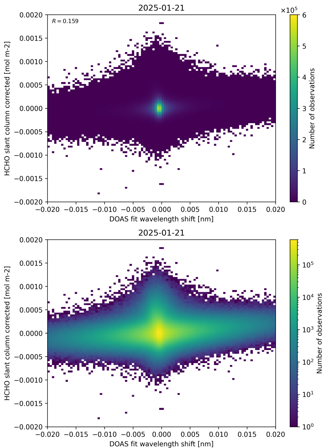
Figure 66: Scatter density plot of “DOAS fit wavelength shift” against “HCHO slant column corrected” for 2025-01-20 to 2025-01-22.
