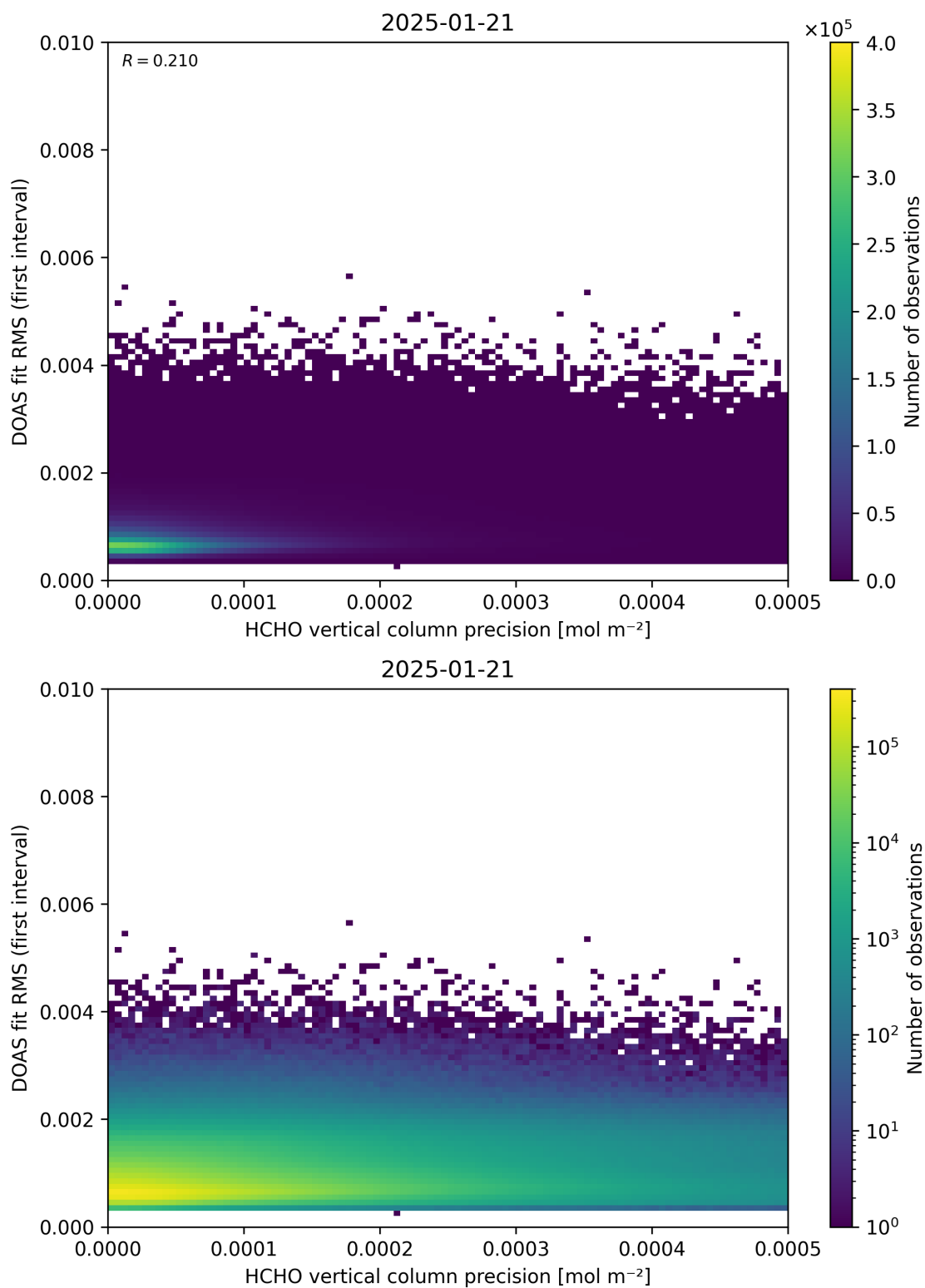
Figure 136: Scatter density plot of “HCHO vertical column precision” against “DOAS fit RMS (first interval)” for 2025-01-20 to 2025-01-22.
