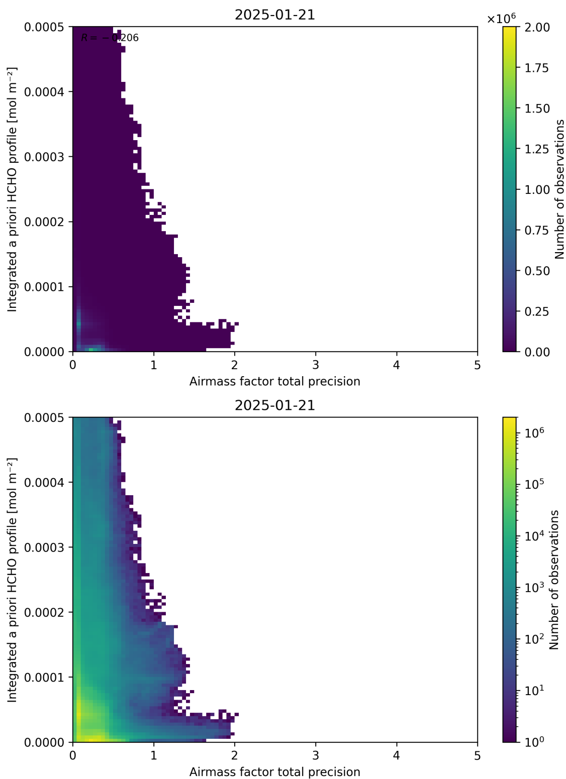
Figure 111: Scatter density plot of “Airmass factor total precision” against “Integrated a priori HCHO profile” for 2025-01-20 to 2025-01-22.
