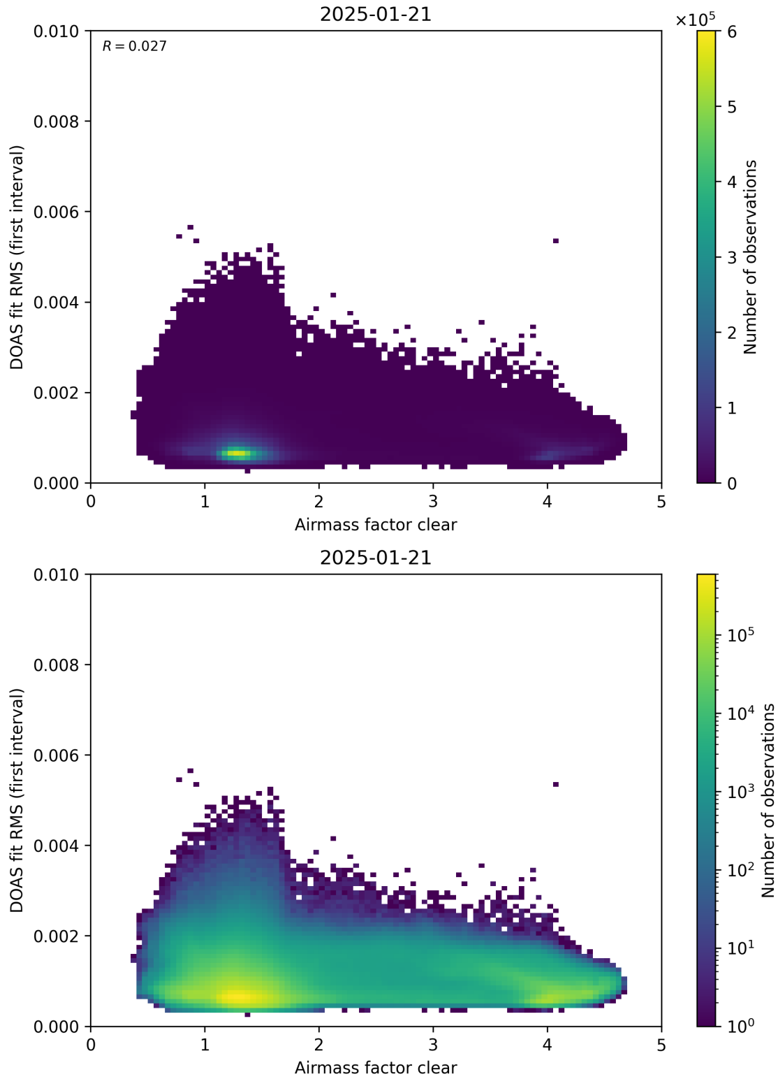
Figure 71: Scatter density plot of “Airmass factor clear” against “DOAS fit RMS (first interval)” for 2025-01-20 to 2025-01-22.
