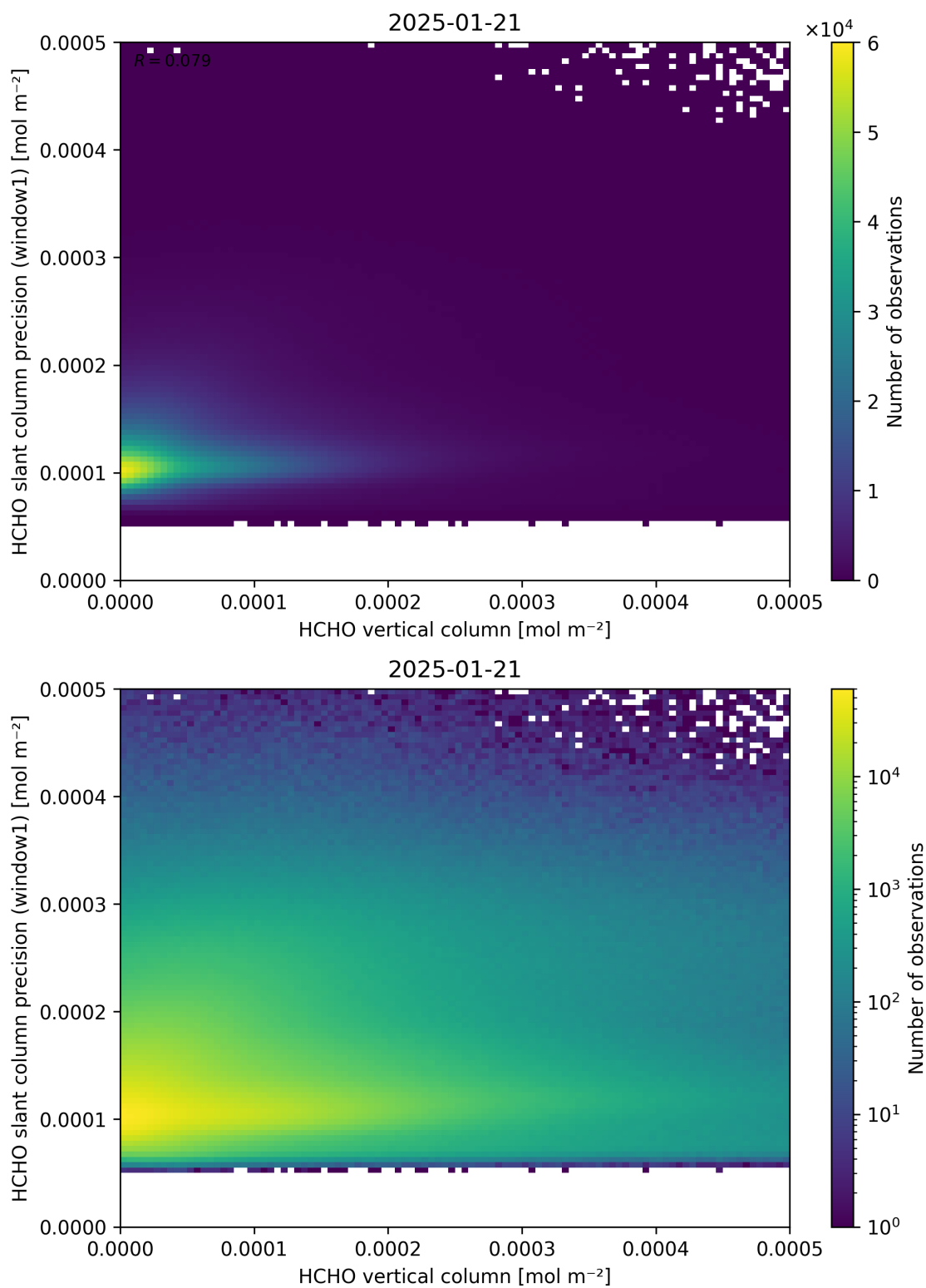
Figure 130: Scatter density plot of “HCHO vertical column” against “HCHO slant column precision (window1)” for 2025-01-20 to 2025-01-22.
