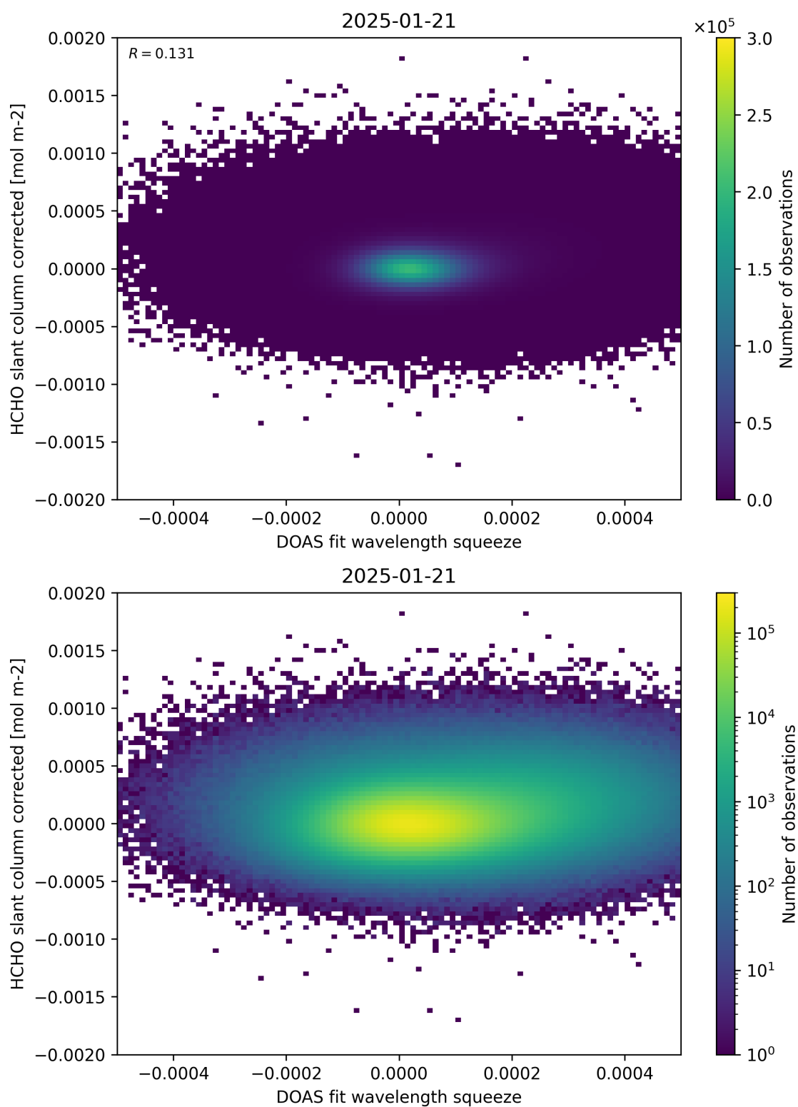
Figure 69: Scatter density plot of “DOAS fit wavelength squeeze” against “HCHO slant column corrected” for 2025-01-20 to 2025-01-22.
