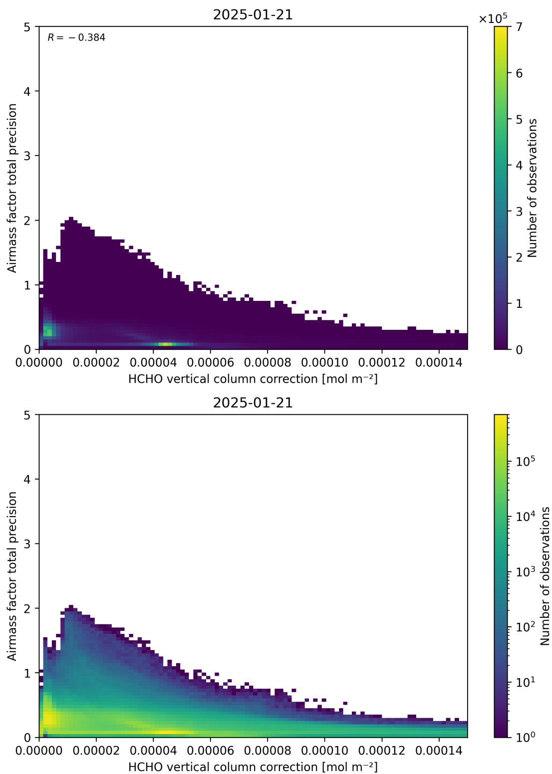
Figure 121: Scatter density plot of “HCHO vertical column correction” against “Airmass factor total precision” for 2025-01-20 to 2025-01-22.
