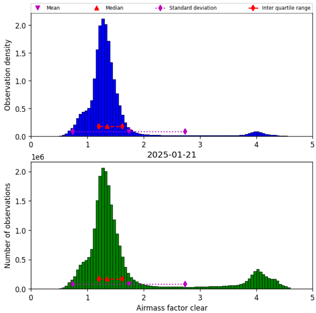
Figure 42: Histogram of “Airmass factor clear” for 2025-01-20 to 2025-01-22
