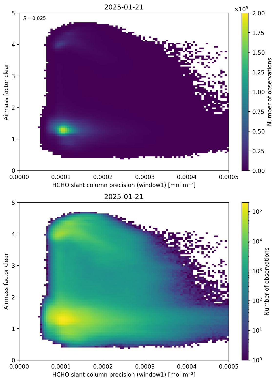
Figure 91: Scatter density plot of “HCHO slant column precision (window1)” against “Airmass factor clear” for 2025-01-20 to 2025-01-22.
