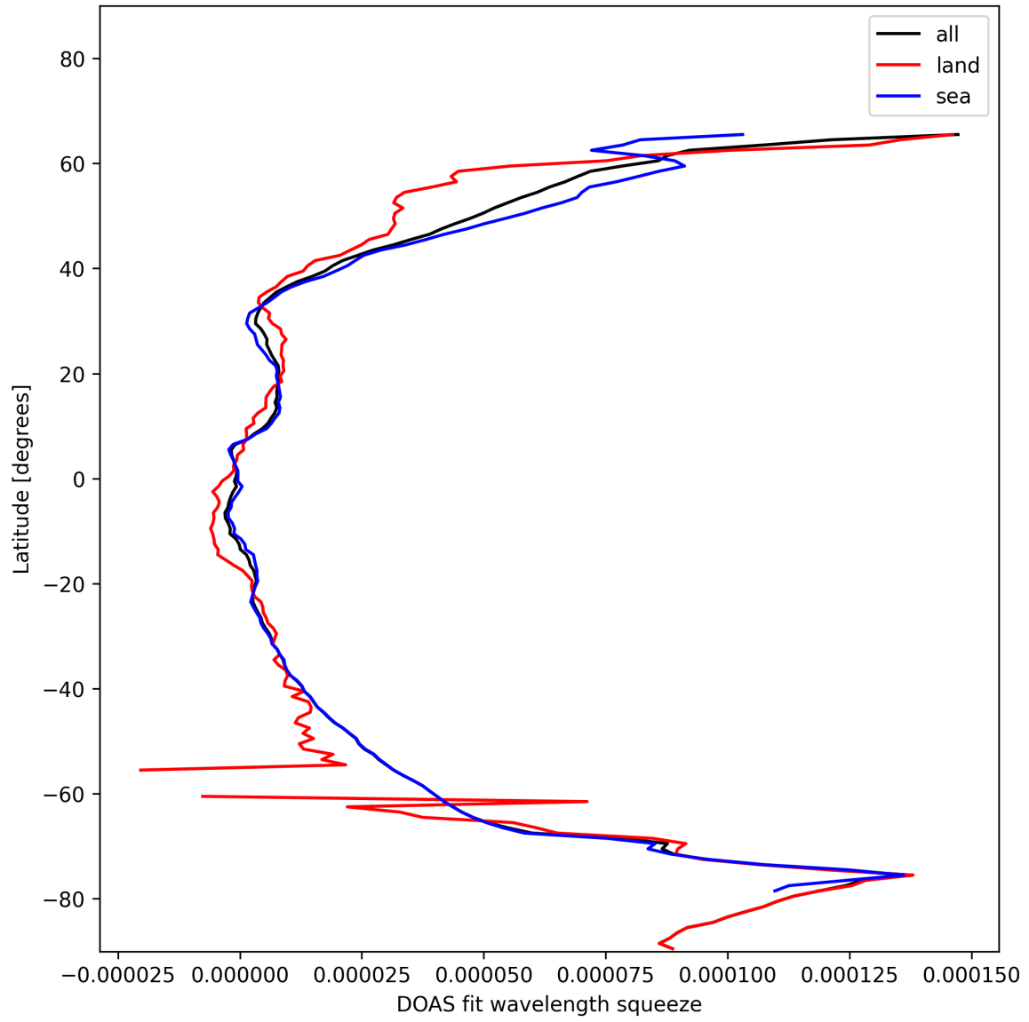
Figure 31: Zonal average of “DOAS fit wavelength squeeze” for 2025-01-20 to 2025-01-22.
