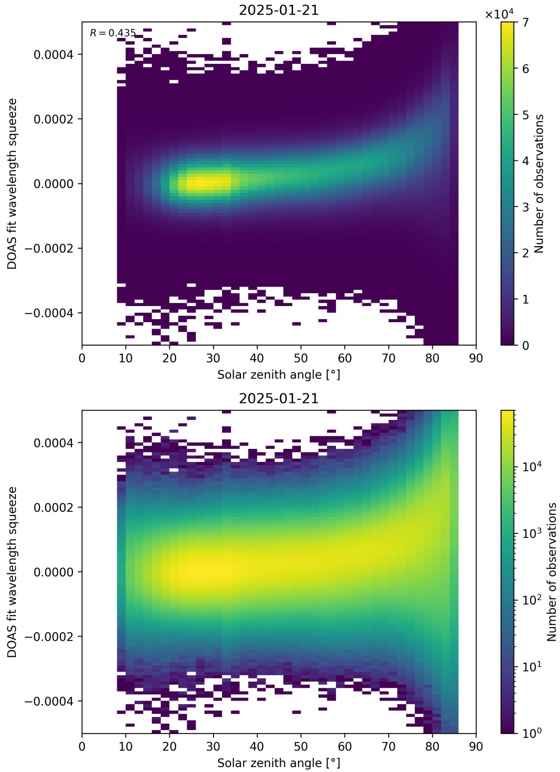
Figure 169: Scatter density plot of “Solar zenith angle” against “DOAS fit wavelength squeeze” for 2025-01-20 to 2025-01-22.
