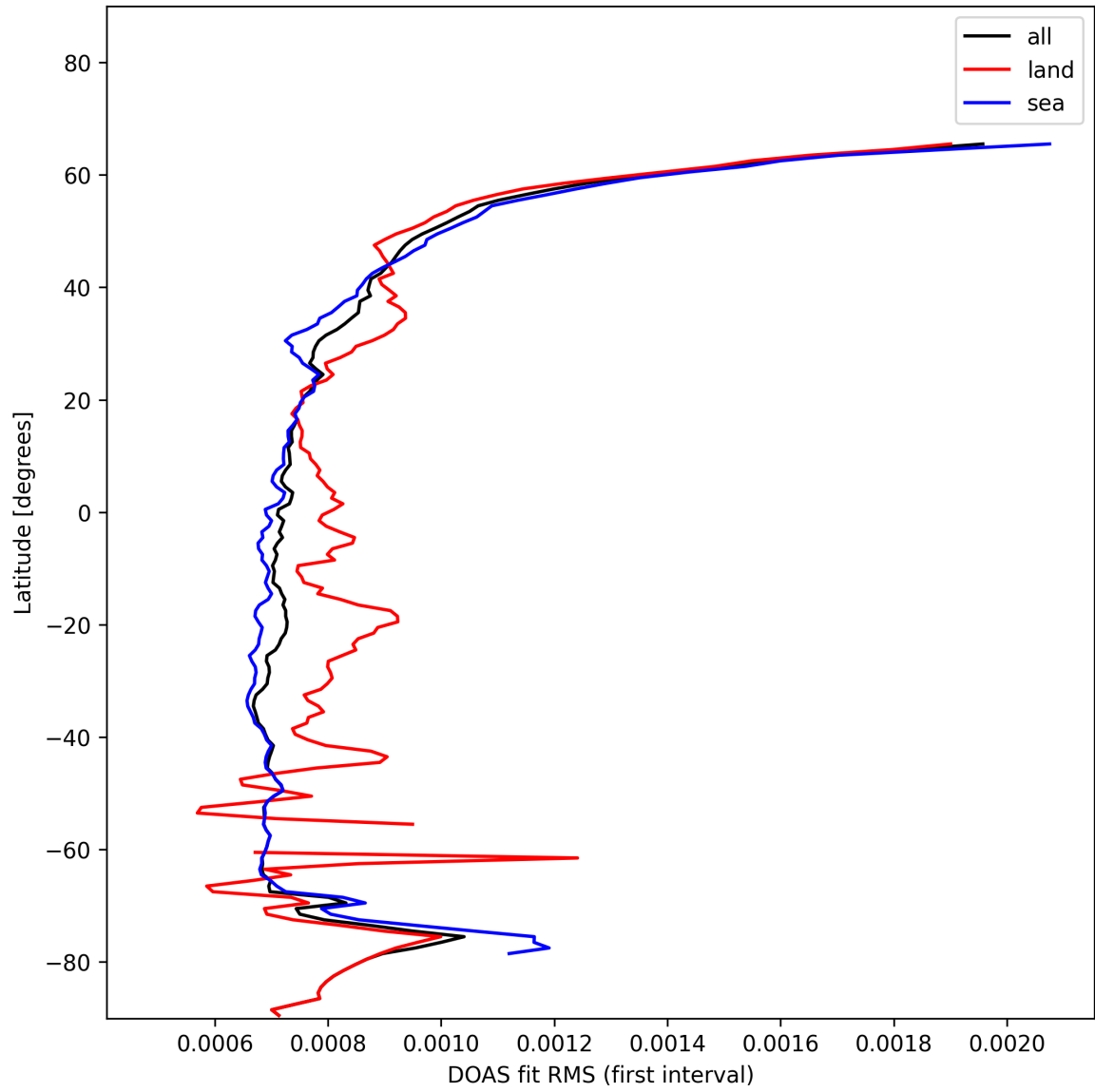
Figure 32: Zonal average of “DOAS fit RMS (first interval)” for 2025-01-20 to 2025-01-22.
