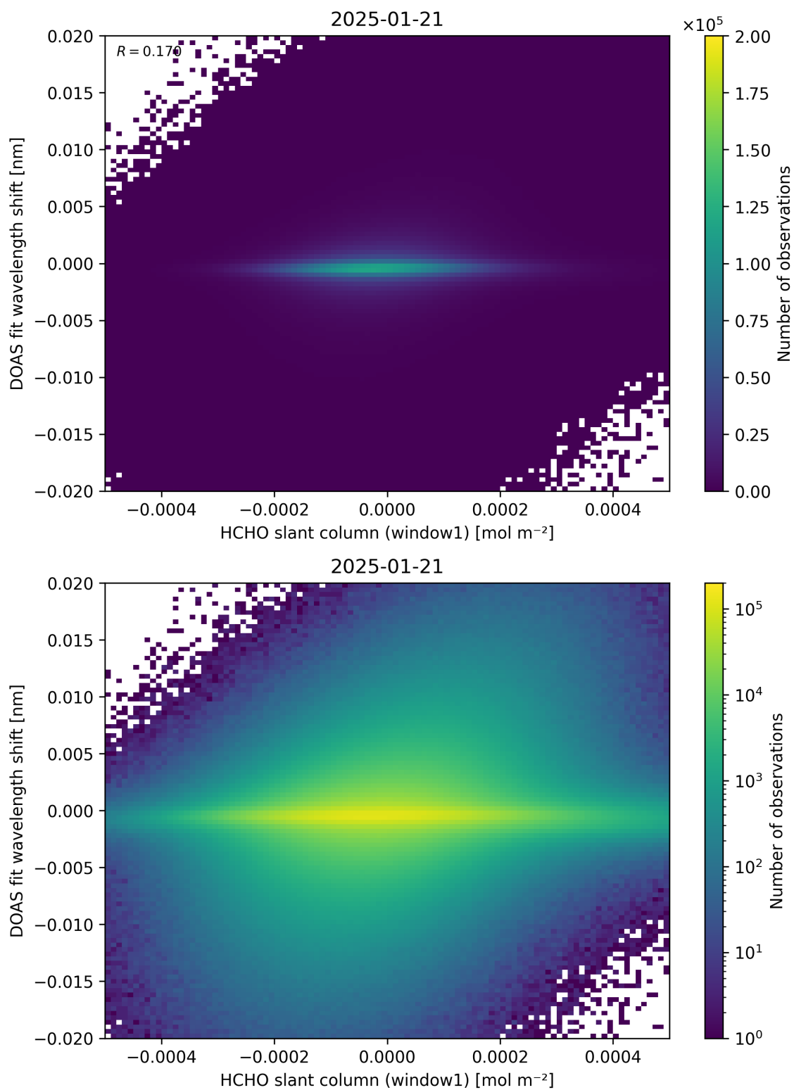
Figure 79: Scatter density plot of “HCHO slant column (window1)” against “DOAS fit wavelength shift” for 2025-01-20 to 2025-01-22.
