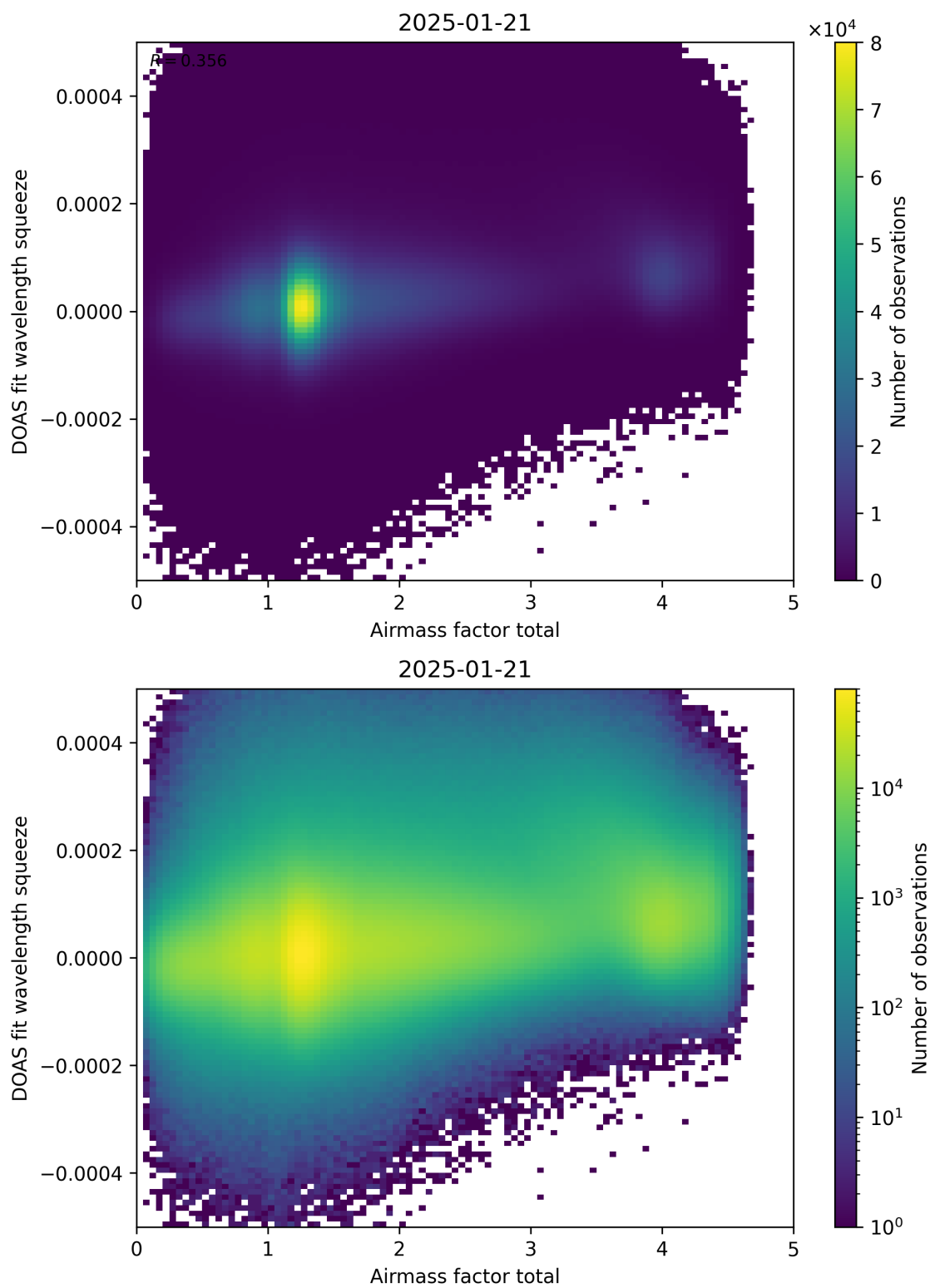
Figure 99: Scatter density plot of “Airmass factor total” against “DOAS fit wavelength squeeze” for 2025-01-20 to 2025-01-22.
