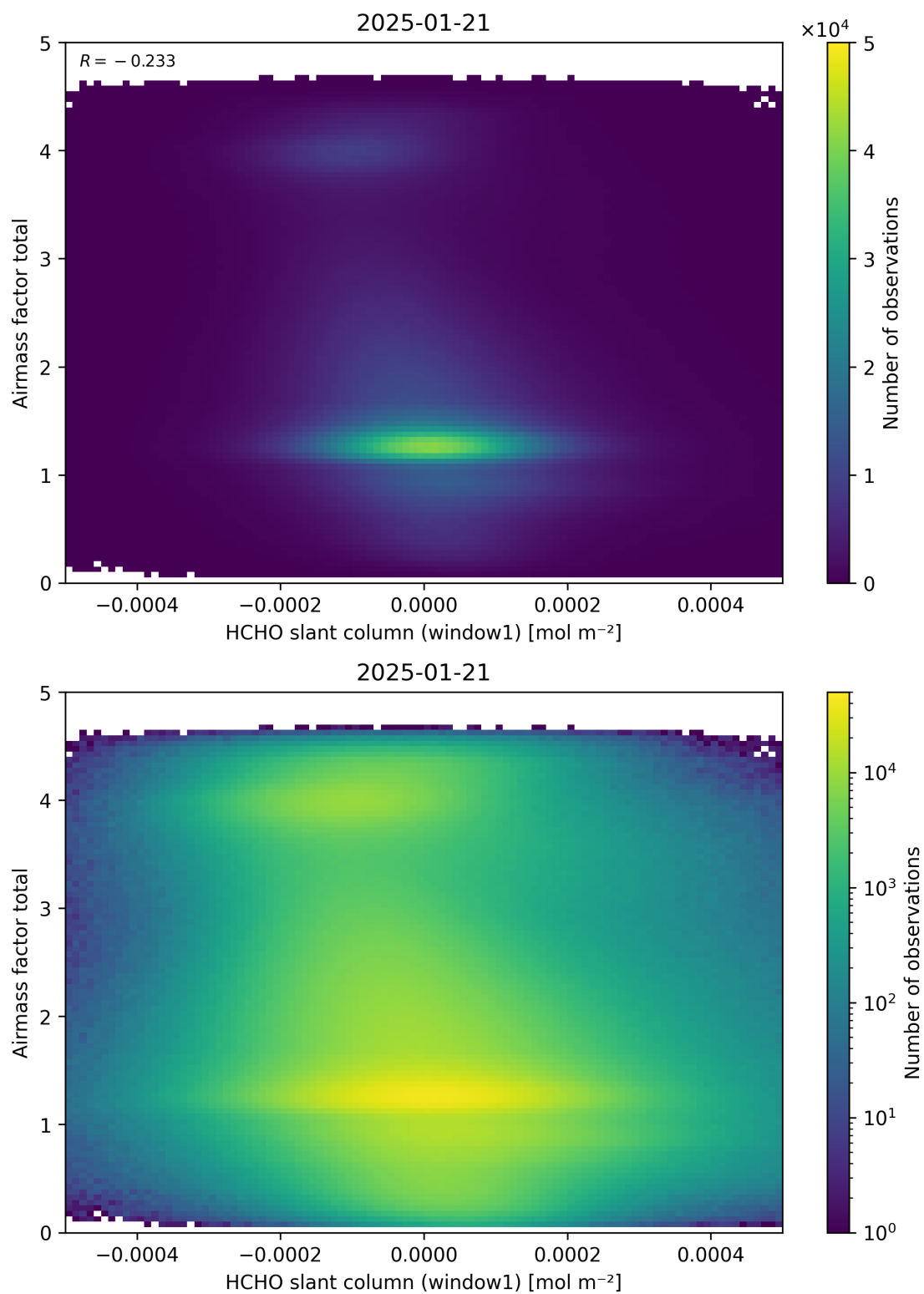
Figure 85: Scatter density plot of “HCHO slant column (window1)” against “Airmass factor total” for 2025-01-20 to 2025-01-22.
