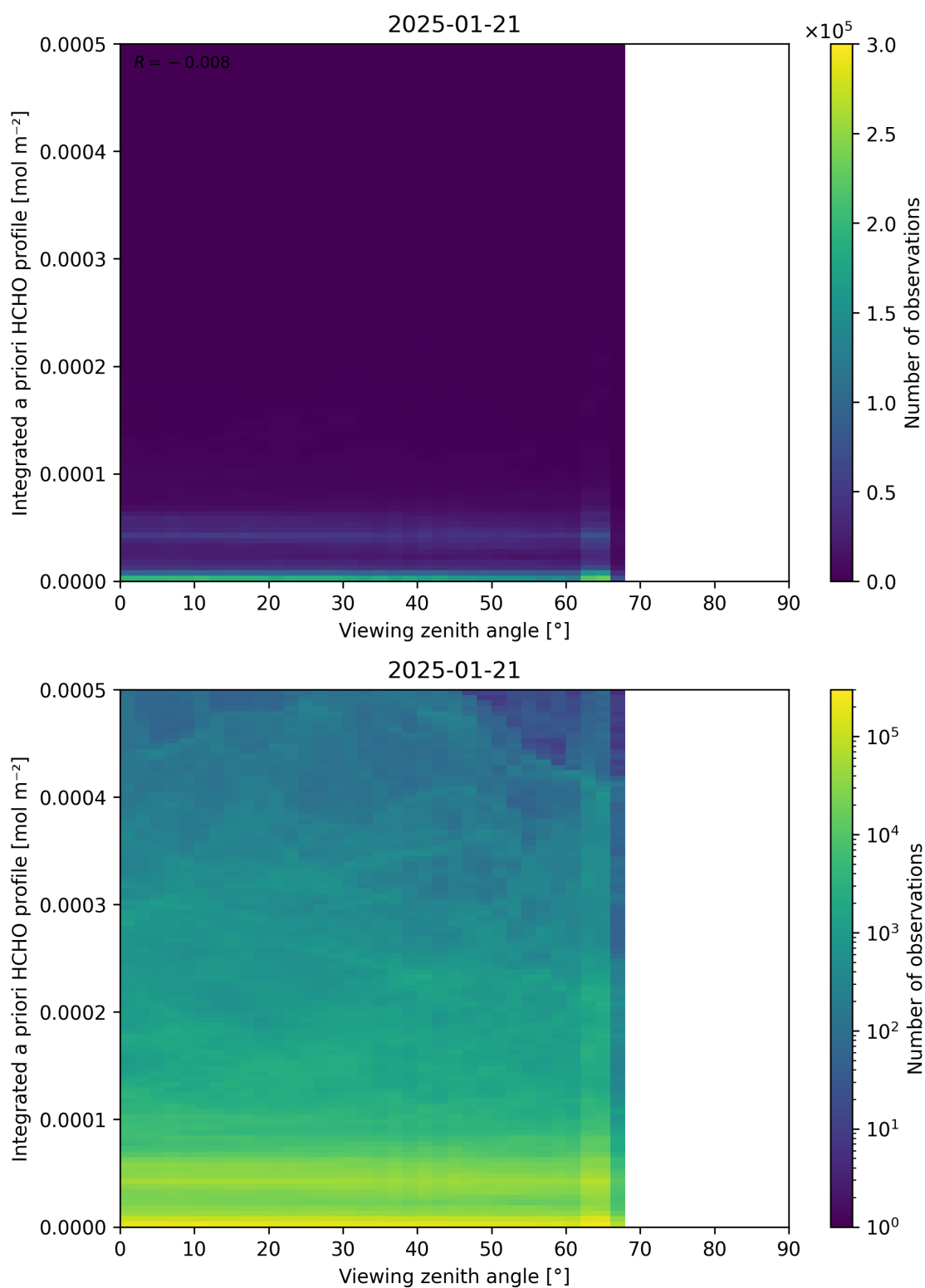
Figure 195: Scatter density plot of “Viewing zenith angle” against “Integrated a priori HCHO profile” for 2025-01-20 to 2025-01-22.
