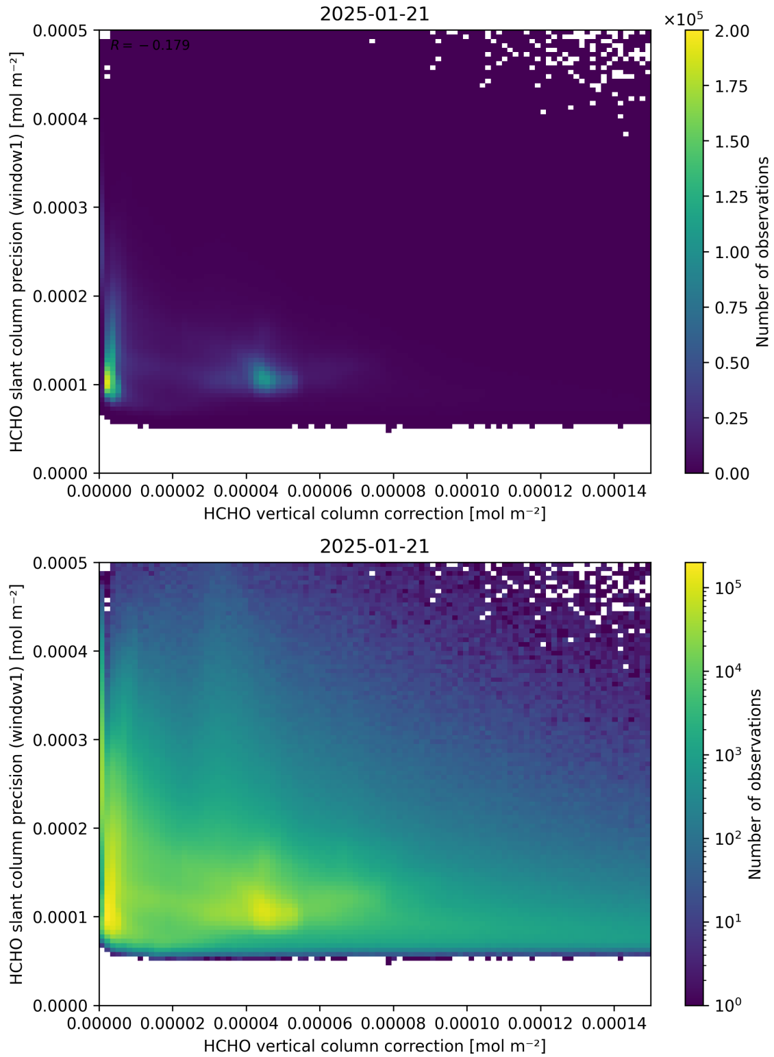
Figure 119: Scatter density plot of “HCHO vertical column correction” against “HCHO slant column precision (window1)” for 2025-01-20 to 2025-01-22.
