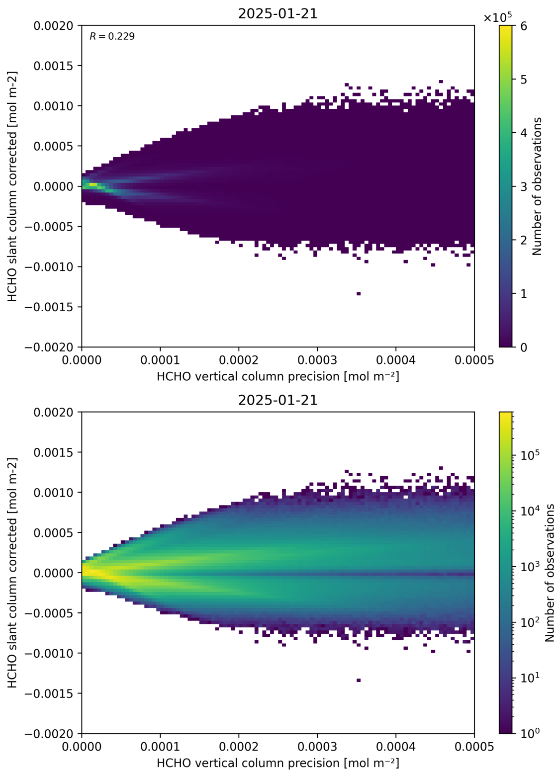
Figure 140: Scatter density plot of “HCHO vertical column precision” against “HCHO slant column corrected” for 2025-01-20 to 2025-01-22.
