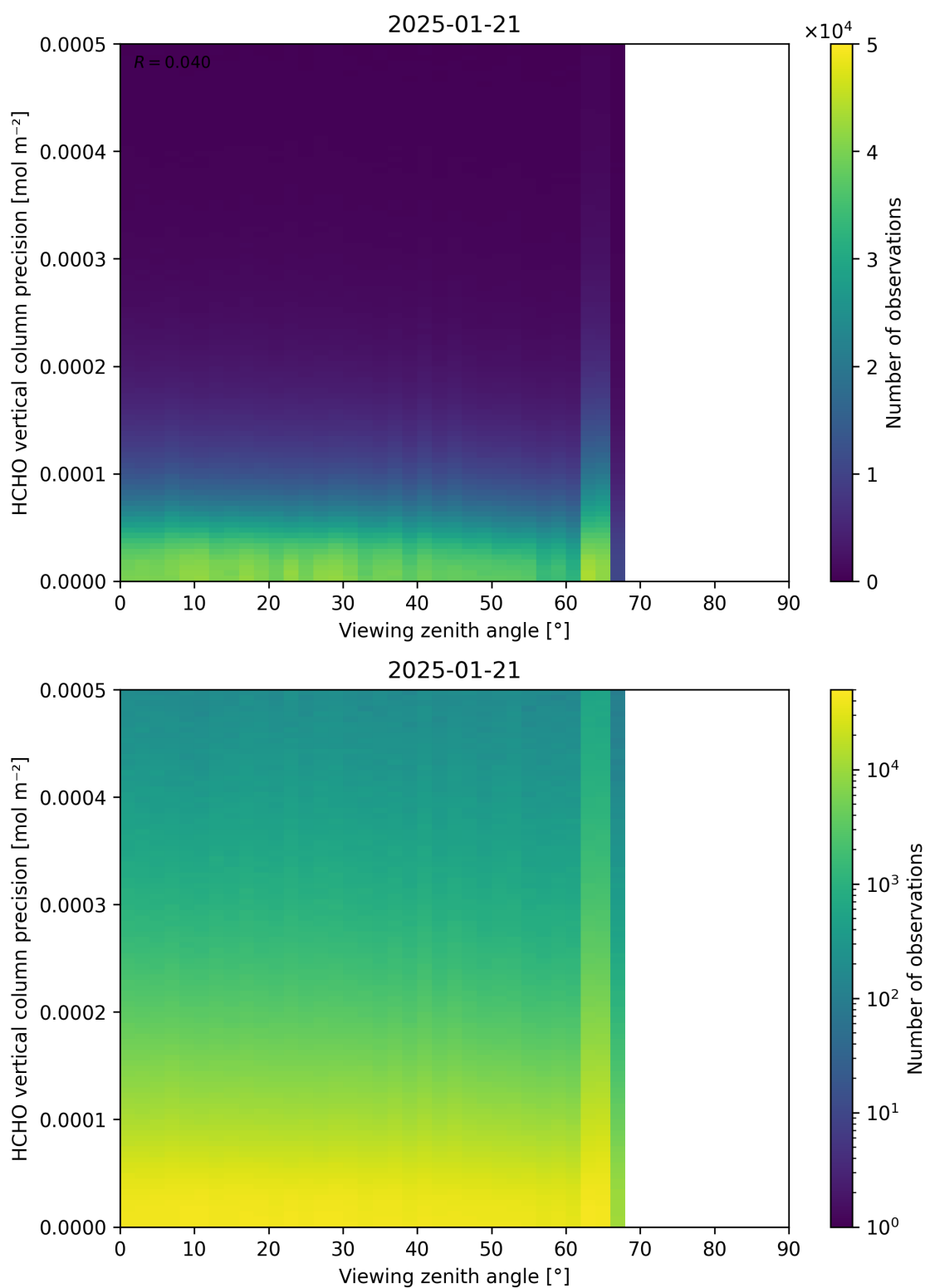
Figure 194: Scatter density plot of “Viewing zenith angle” against “HCHO vertical column precision” for 2025-01-20 to 2025-01-22.
