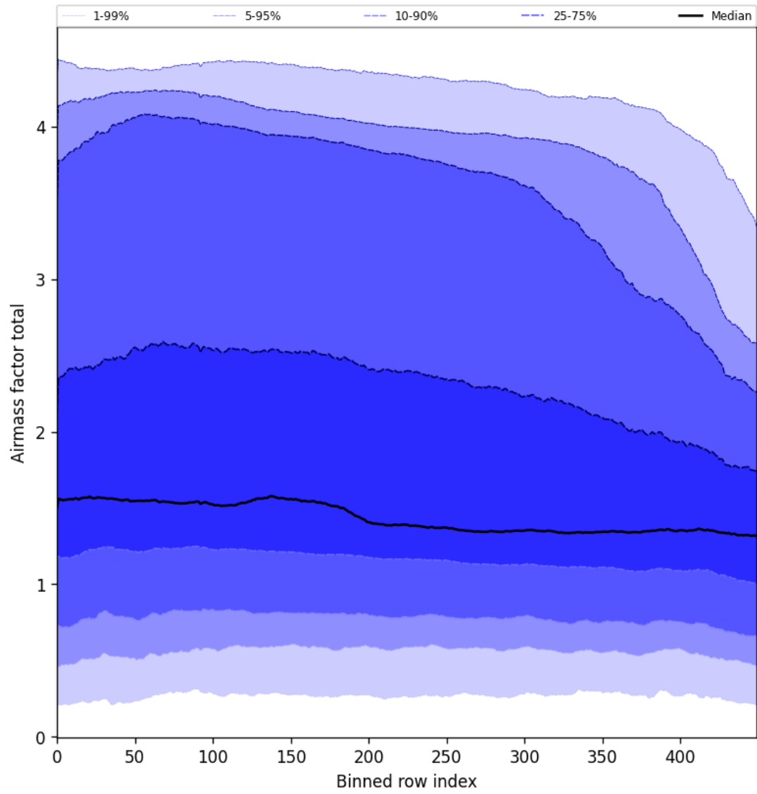
Figure 54: Along track statistics of “Airmass factor total” for 2025-01-20 to 2025-01-22
