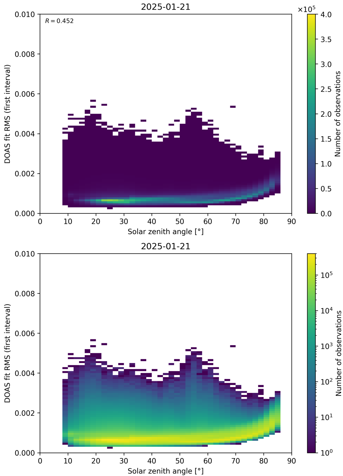
Figure 167: Scatter density plot of “Solar zenith angle” against “DOAS fit RMS (first interval)” for 2025-01-20 to 2025-01-22.
