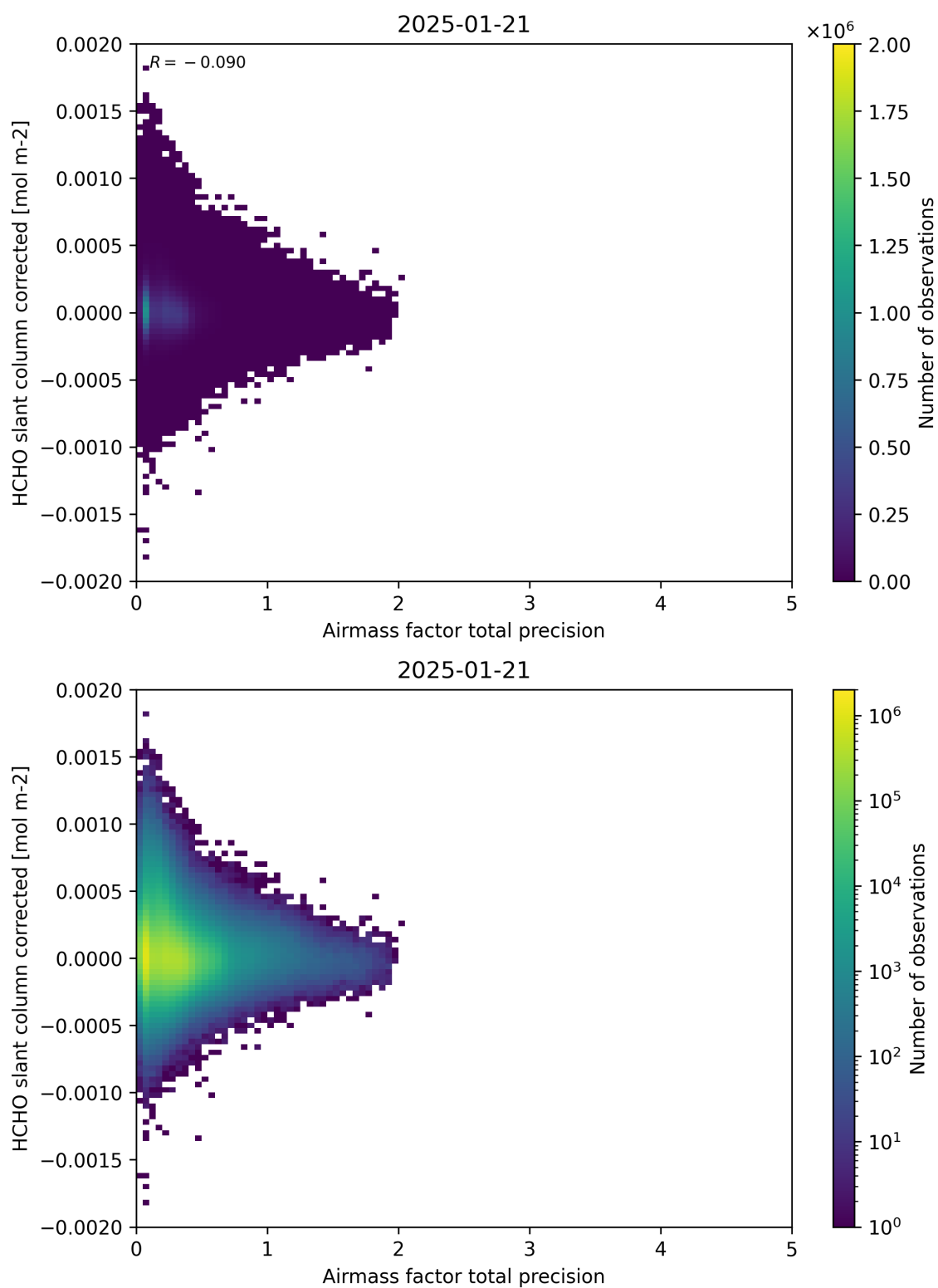
Figure 109: Scatter density plot of “Airmass factor total precision” against “HCHO slant column corrected” for 2025-01-20 to 2025-01-22.
