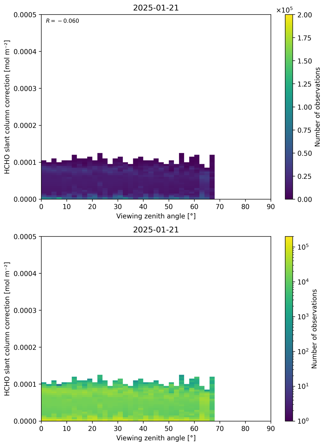
Figure 187: Scatter density plot of “Viewing zenith angle” against “HCHO slant column correction” for 2025-01-20 to 2025-01-22.
