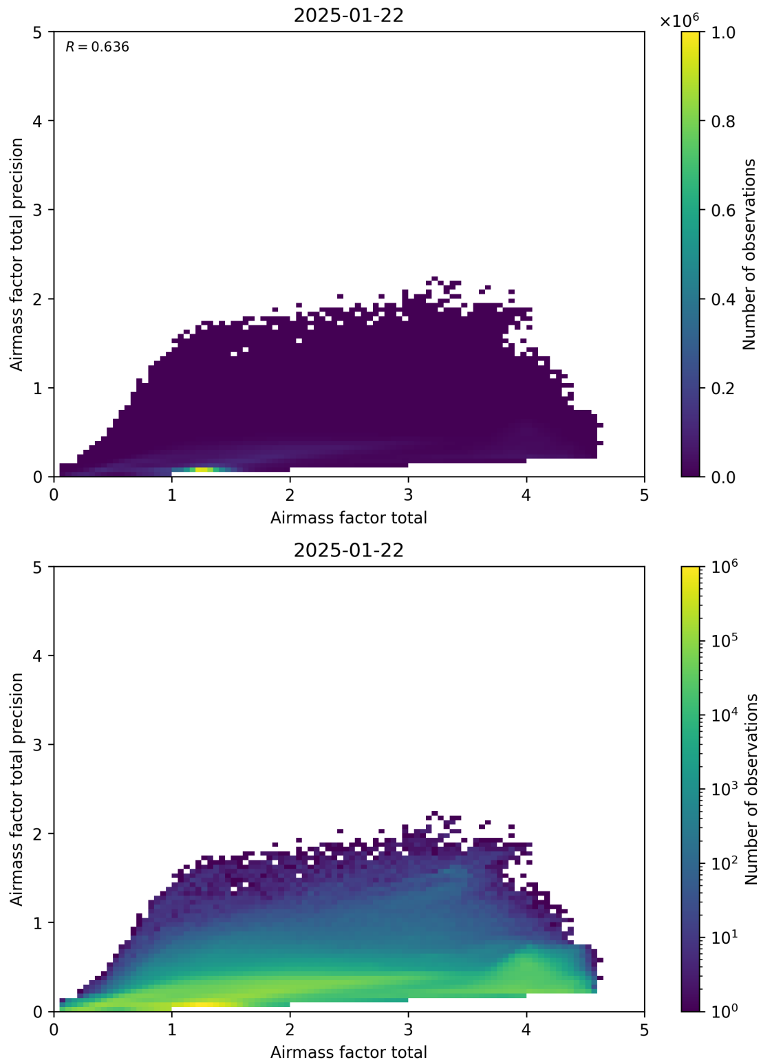
Figure 103: Scatter density plot of “Airmass factor total” against “Airmass factor total precision” for 2025-01-21 to 2025-01-23.
