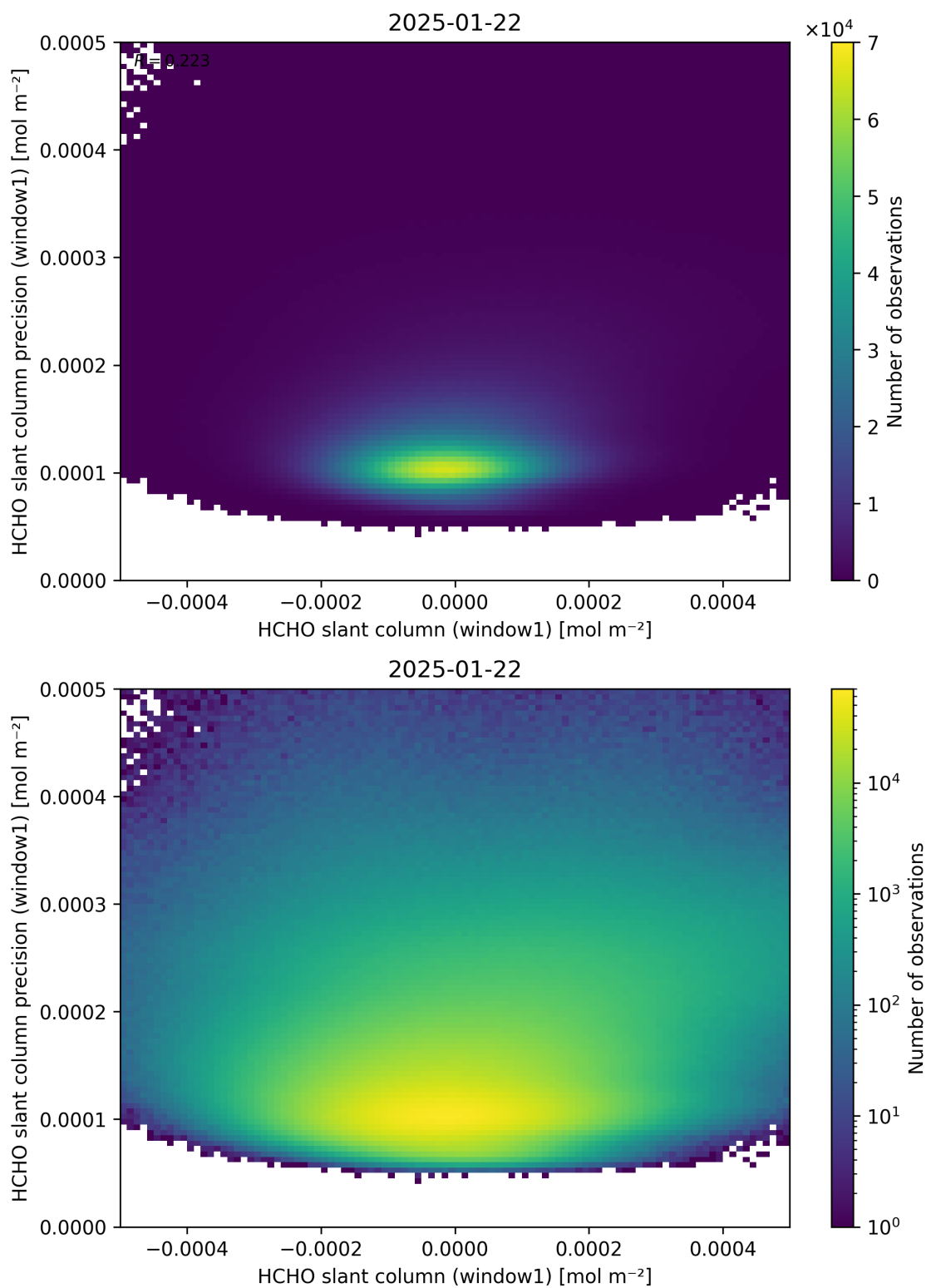
Figure 84: Scatter density plot of “HCHO slant column (window1)” against “HCHO slant column precision (window1)” for 2025-01-21 to 2025-01-23.
