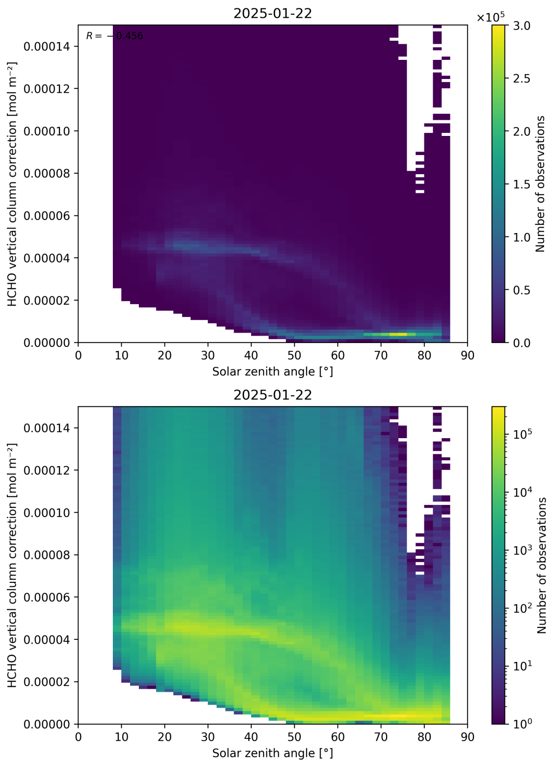
Figure 178: Scatter density plot of “Solar zenith angle” against “HCHO vertical column correction” for 2025-01-21 to 2025-01-23.
