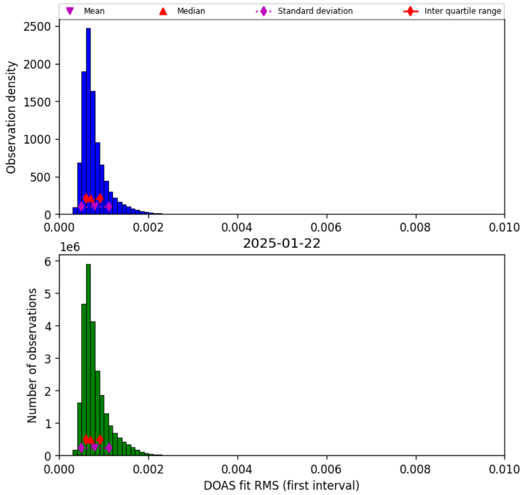
Figure 46: Histogram of “DOAS fit RMS (first interval)” for 2025-01-21 to 2025-01-23
