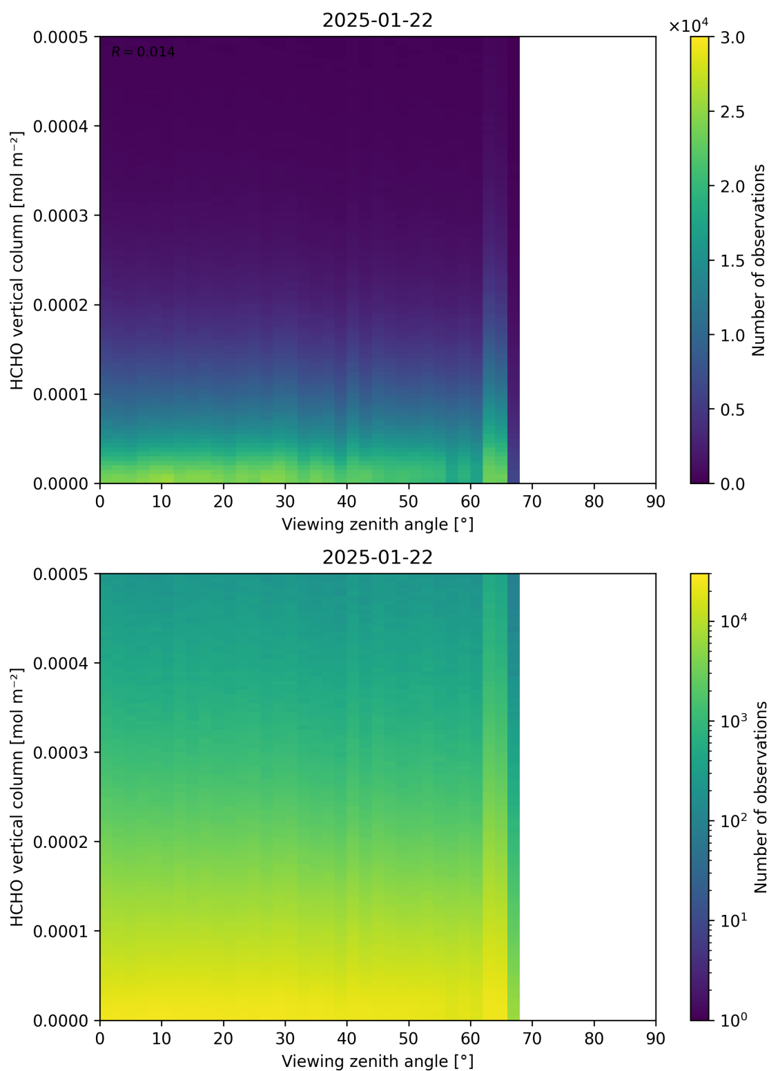
Figure 192: Scatter density plot of “Viewing zenith angle” against “HCHO vertical column” for 2025-01-21 to 2025-01-23.
