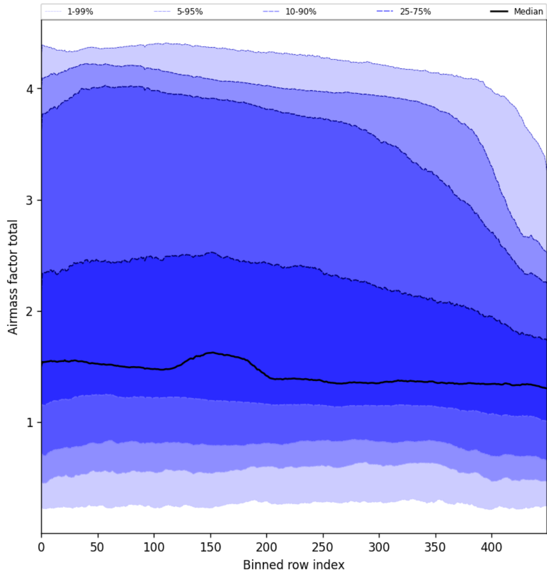
Figure 54: Along track statistics of “Airmass factor total” for 2025-01-21 to 2025-01-23
