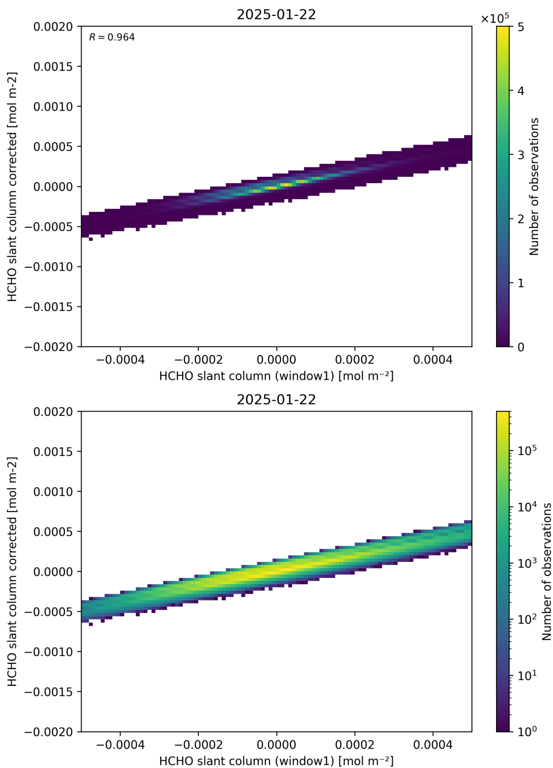
Figure 82: Scatter density plot of “HCHO slant column (window1)” against “HCHO slant column corrected” for 2025-01-21 to 2025-01-23.
