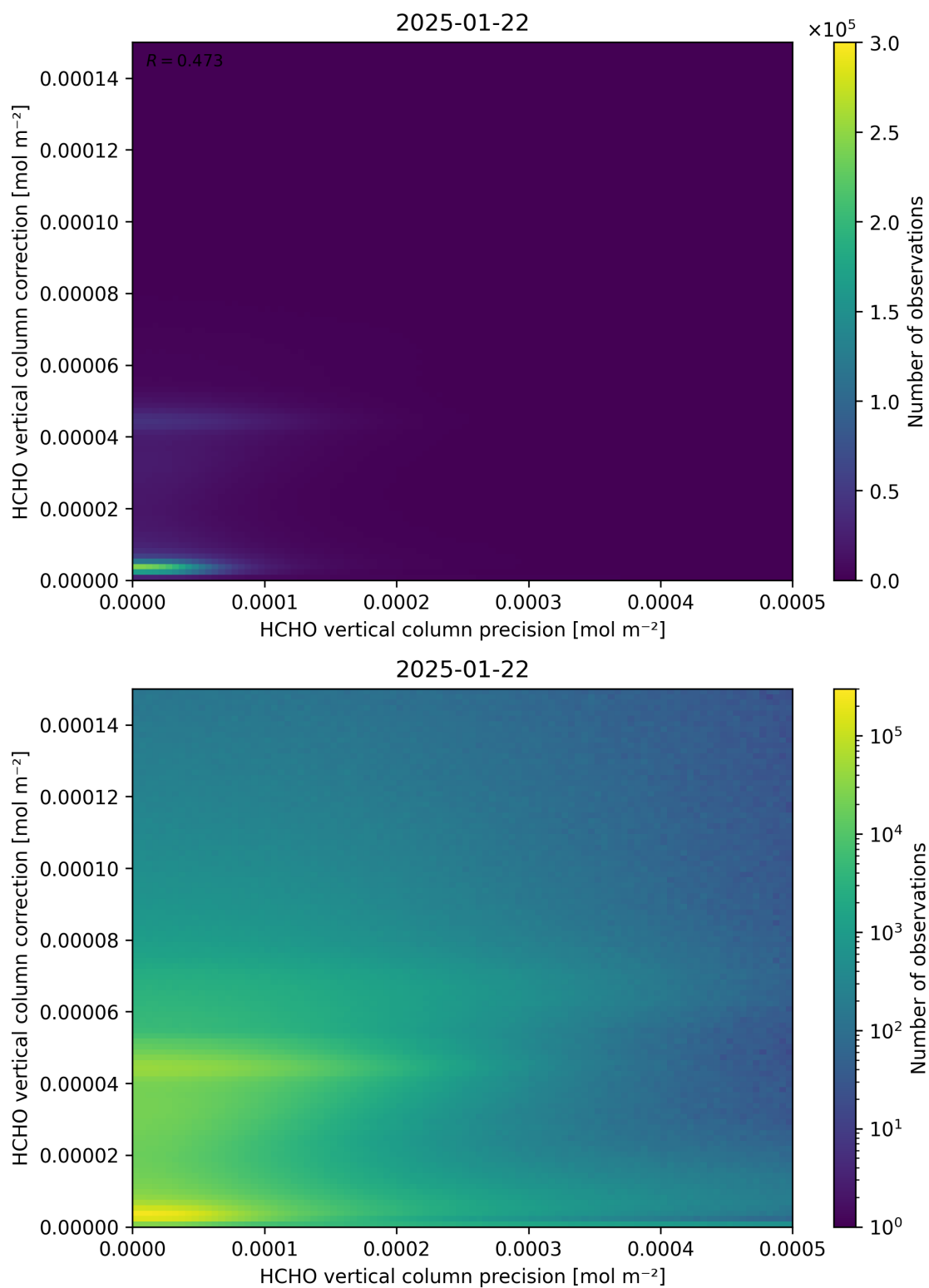
Figure 146: Scatter density plot of “HCHO vertical column precision” against “HCHO vertical column correction” for 2025-01-21 to 2025-01-23.
