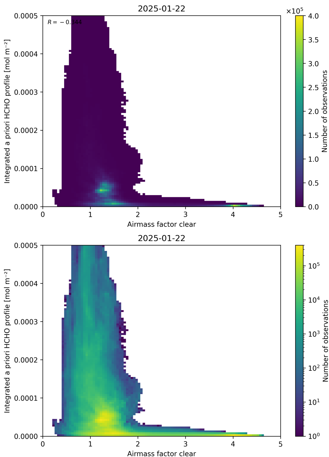
Figure 76: Scatter density plot of “Airmass factor clear” against “Integrated a priori HCHO profile” for 2025-01-21 to 2025-01-23.
