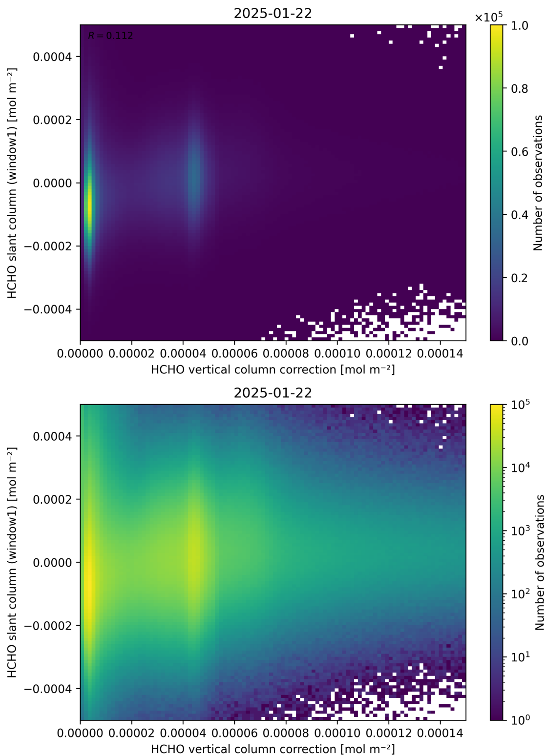
Figure 118: Scatter density plot of “HCHO vertical column correction” against “HCHO slant column (window1)” for 2025-01-21 to 2025-01-23.
