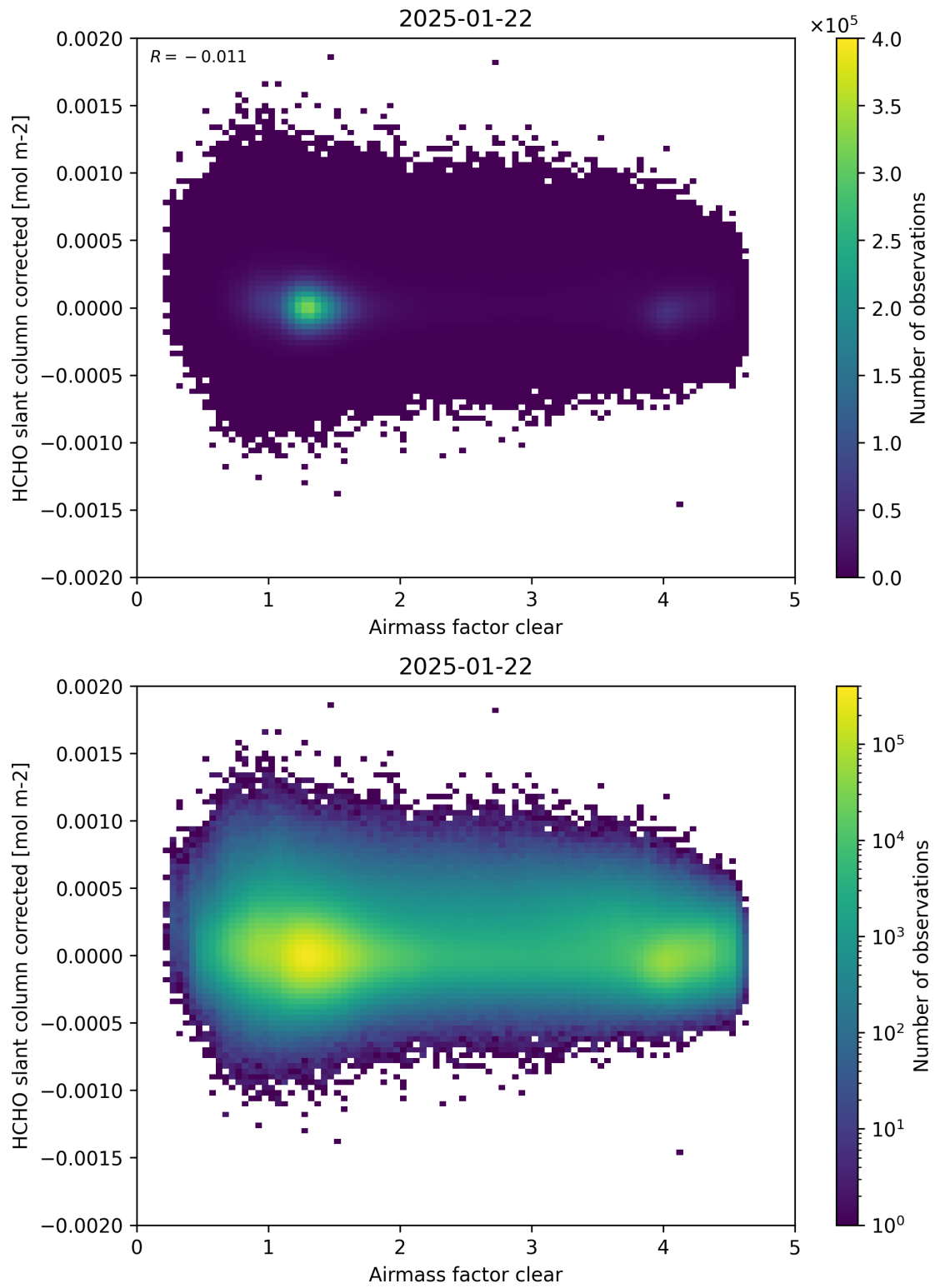
Figure 74: Scatter density plot of “Airmass factor clear” against “HCHO slant column corrected” for 2025-01-21 to 2025-01-23.
