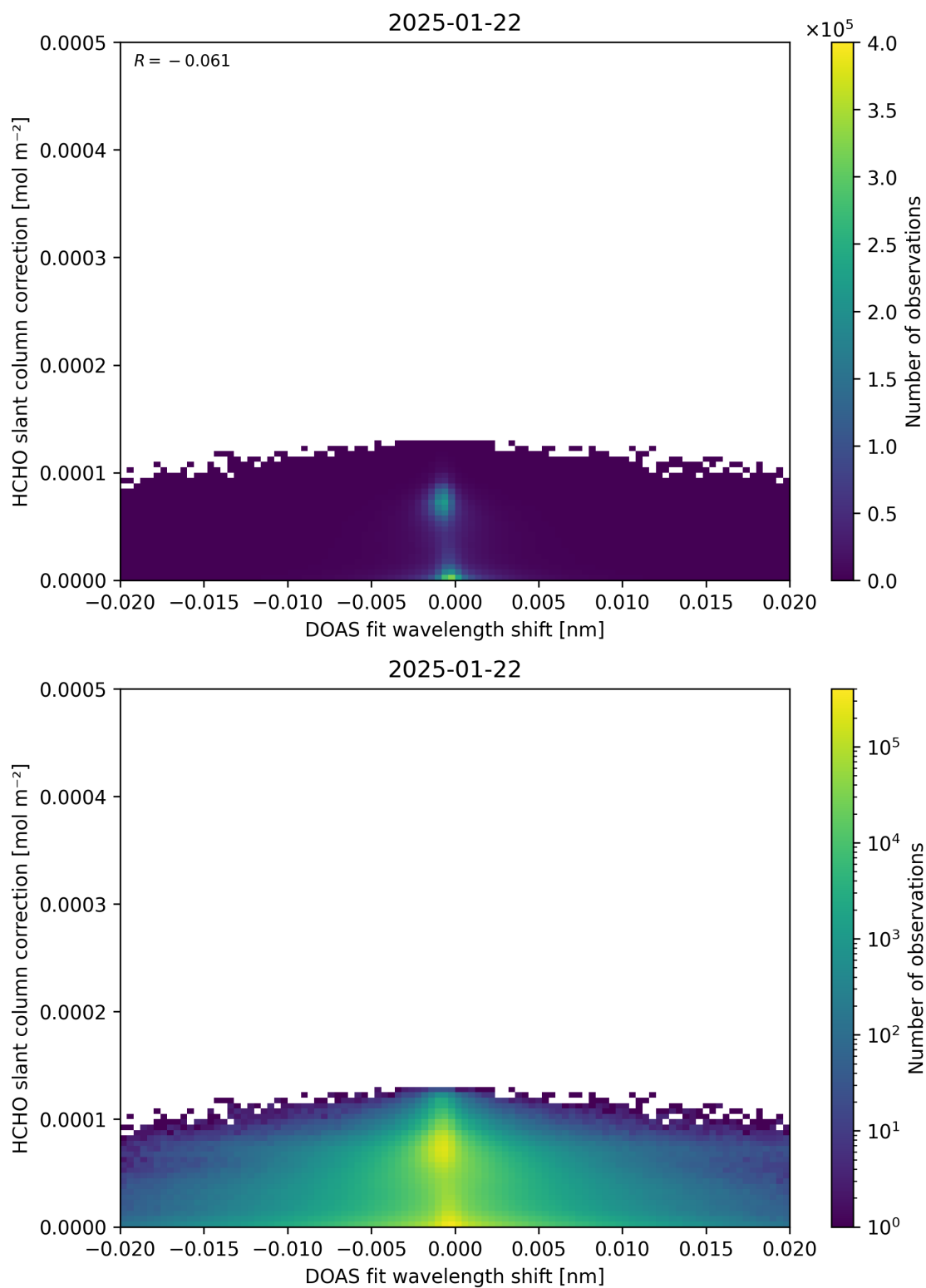
Figure 67: Scatter density plot of “DOAS fit wavelength shift” against “HCHO slant column correction” for 2025-01-21 to 2025-01-23.
