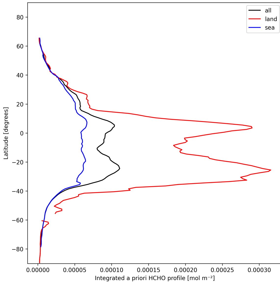
Figure 29: Zonal average of “Integrated a priori HCHO profile” for 2025-01-21 to 2025-01-23.
