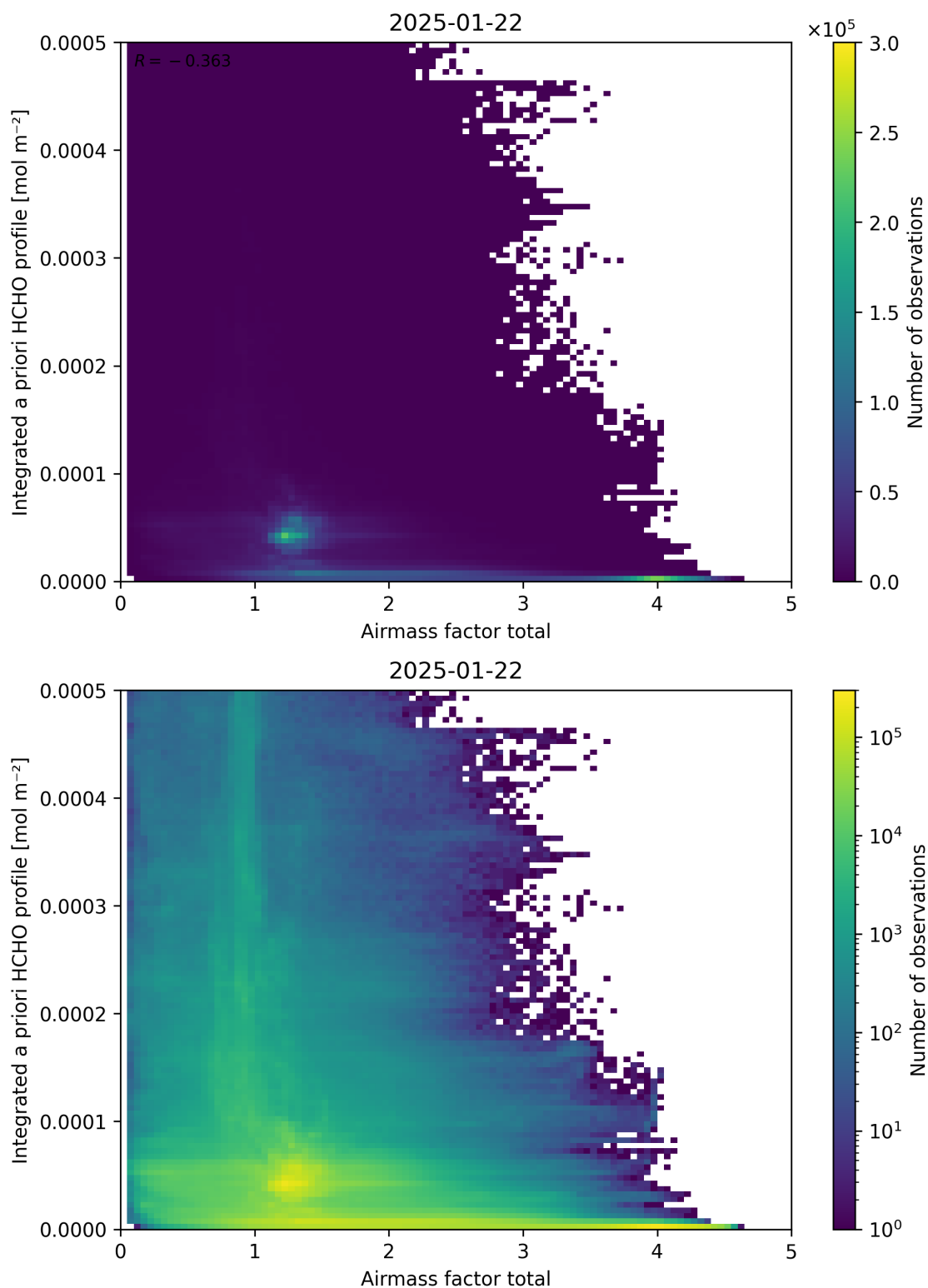
Figure 104: Scatter density plot of “Airmass factor total” against “Integrated a priori HCHO profile” for 2025-01-21 to 2025-01-23.
