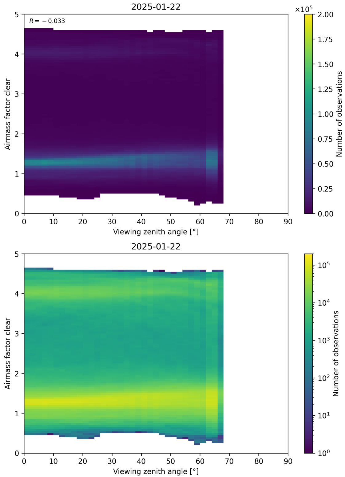
Figure 185: Scatter density plot of “Viewing zenith angle” against “Airmass factor clear” for 2025-01-21 to 2025-01-23.
