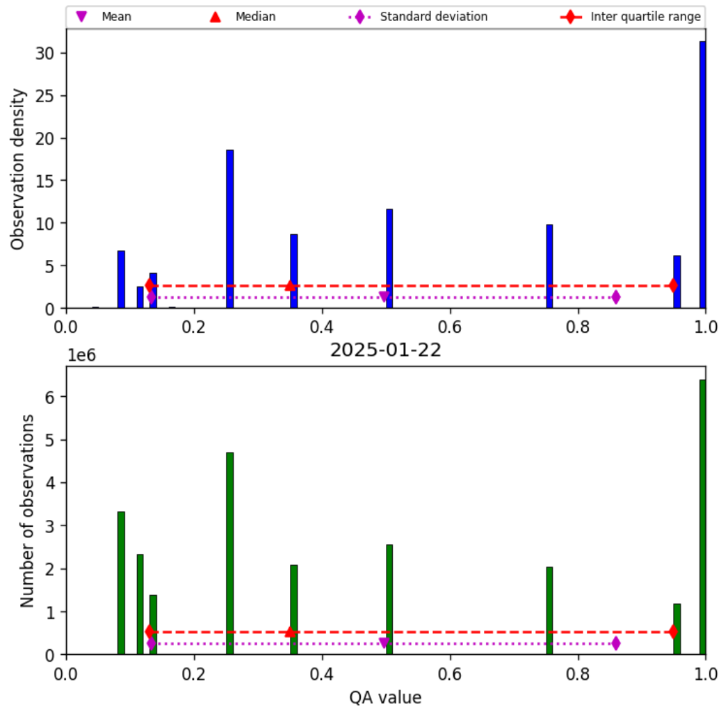
Figure 34: Histogram of “QA value” for 2025-01-21 to 2025-01-23
