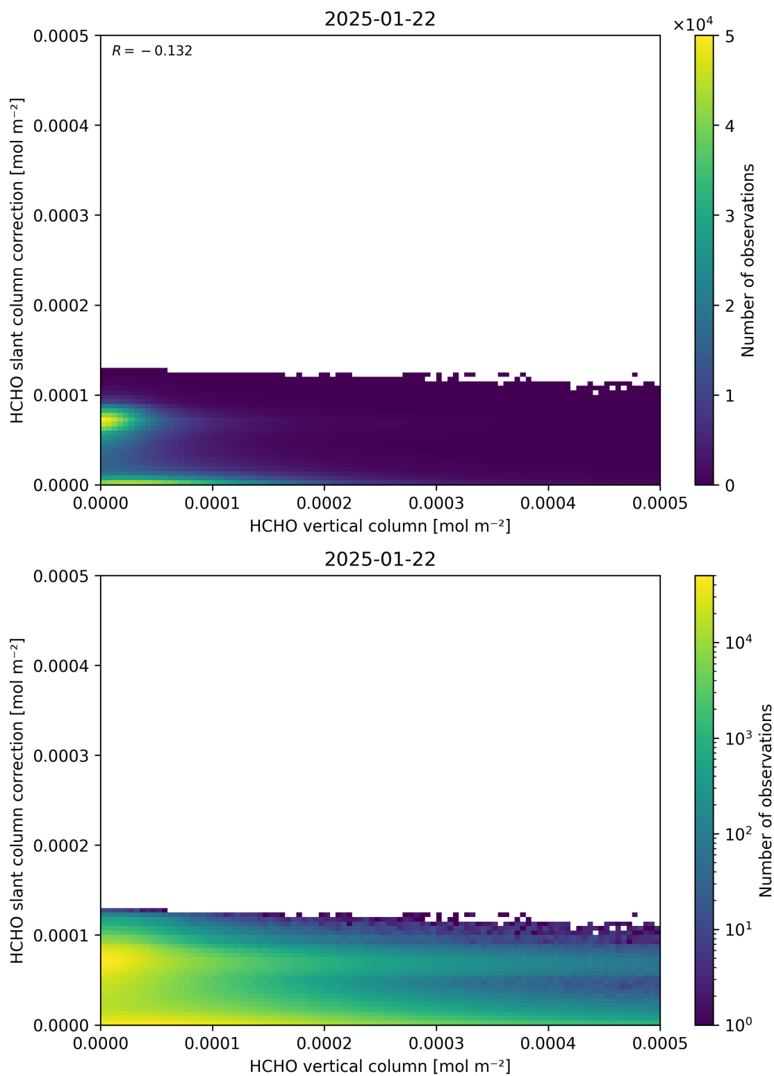
Figure 128: Scatter density plot of “HCHO vertical column” against “HCHO slant column correction” for 2025-01-21 to 2025-01-23.
