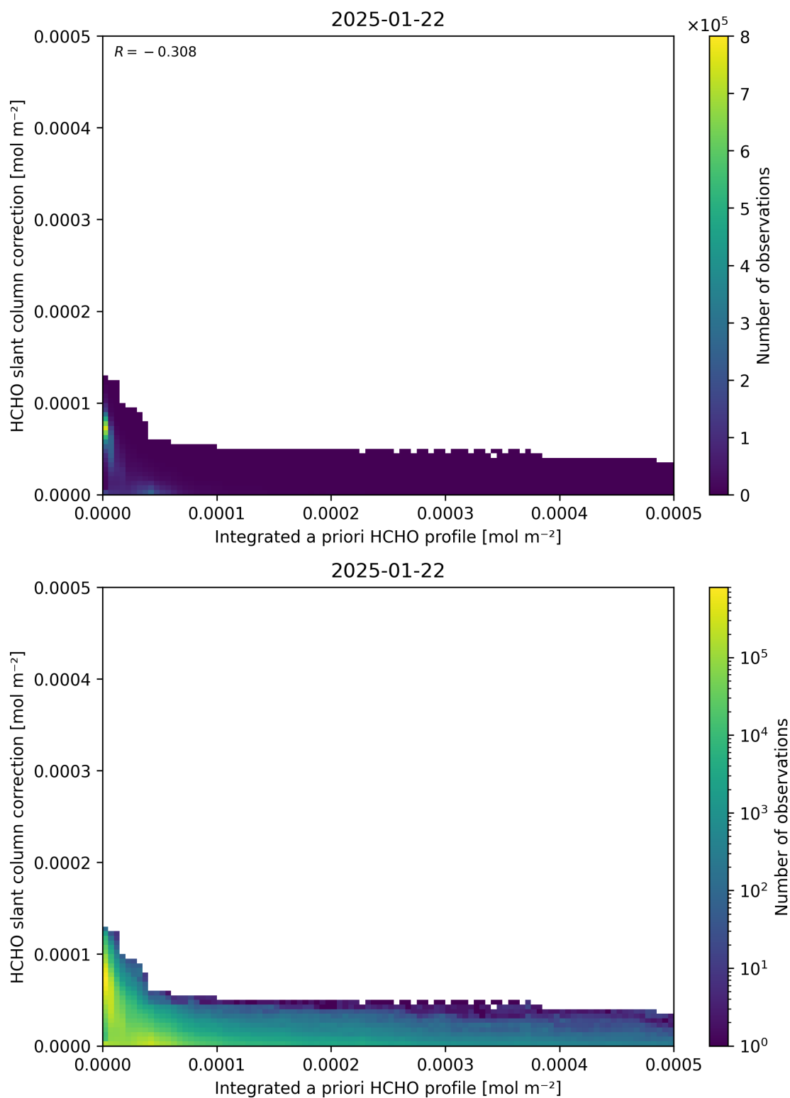
Figure 152: Scatter density plot of “Integrated a priori HCHO profile” against “HCHO slant column correction” for 2025-01-21 to 2025-01-23.
