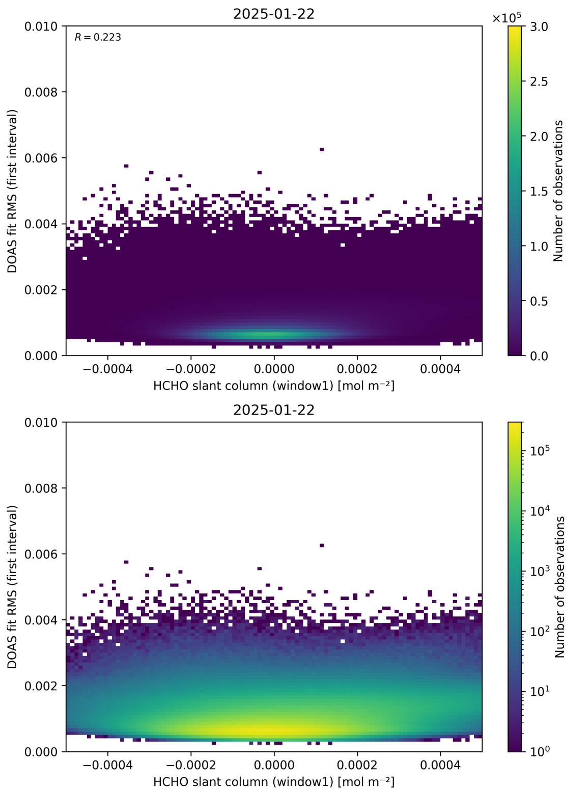
Figure 78: Scatter density plot of “HCHO slant column (window1)” against “DOAS fit RMS (first interval)” for 2025-01-21 to 2025-01-23.
