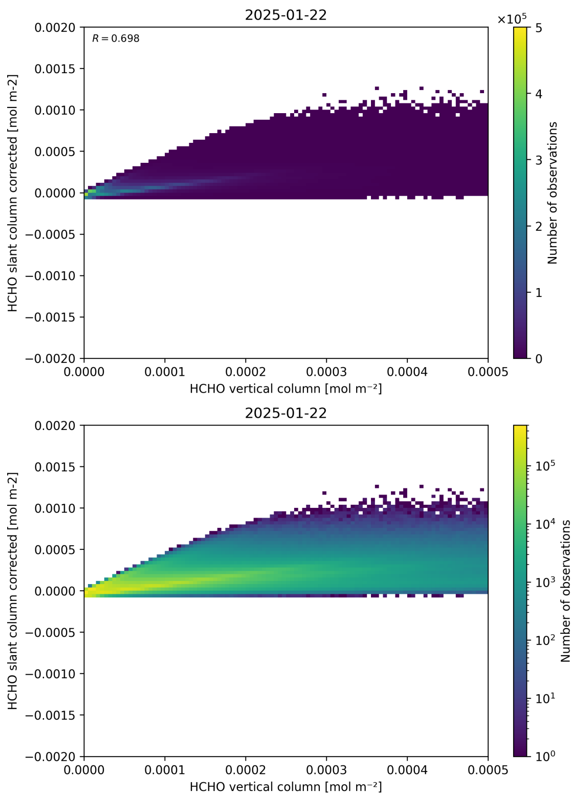
Figure 127: Scatter density plot of “HCHO vertical column” against “HCHO slant column corrected” for 2025-01-21 to 2025-01-23.
