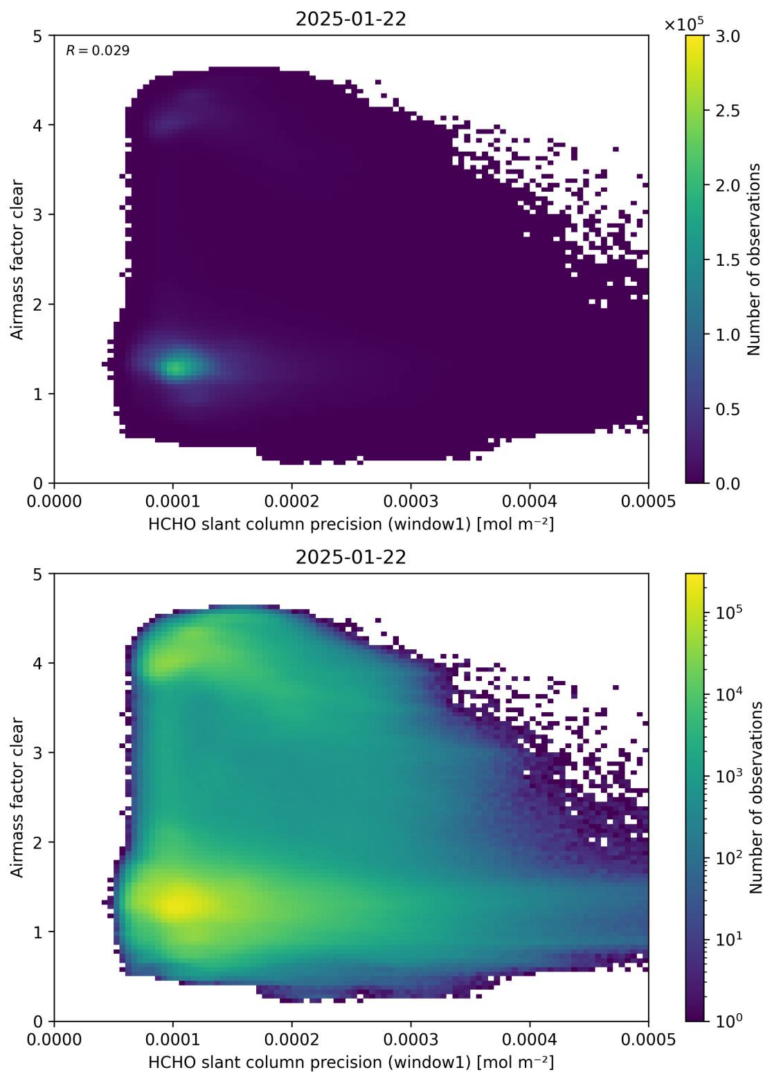
Figure 91: Scatter density plot of “HCHO slant column precision (window1)” against “Airmass factor clear” for 2025-01-21 to 2025-01-23.
