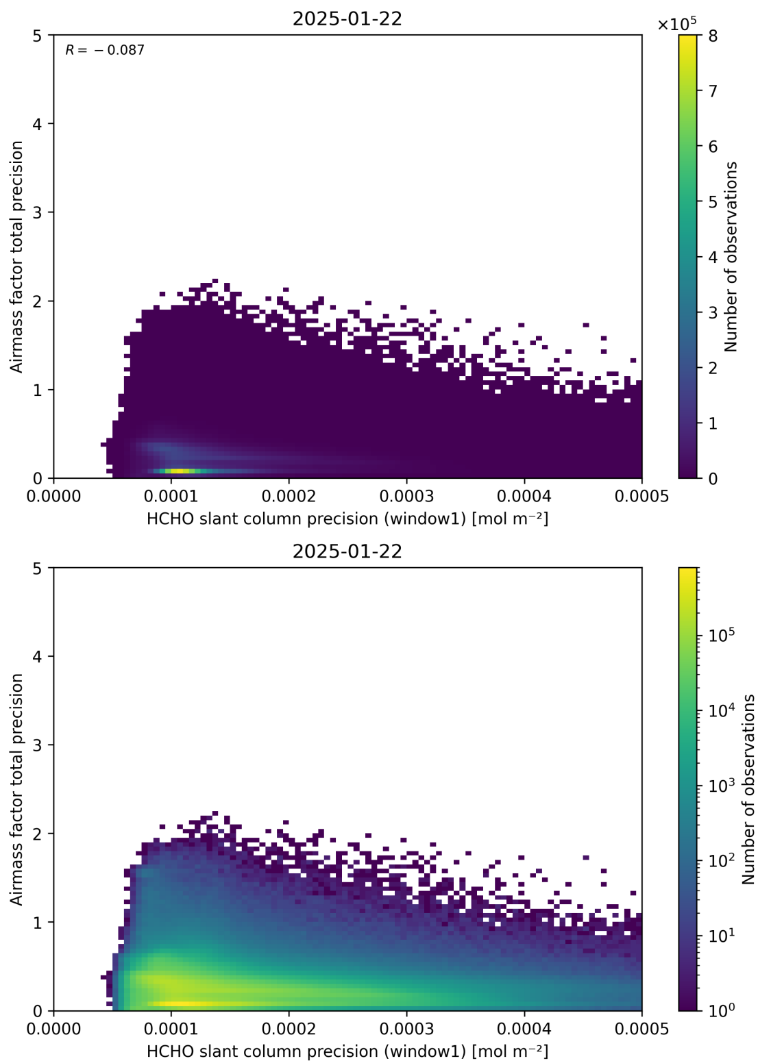
Figure 95: Scatter density plot of “HCHO slant column precision (window1)” against “Airmass factor total precision” for 2025-01-21 to 2025-01-23.
