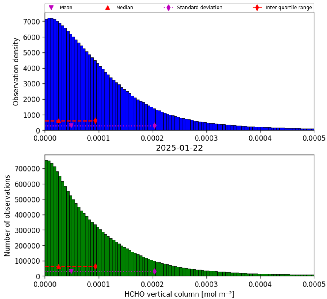
Figure 35: Histogram of “HCHO vertical column” for 2025-01-21 to 2025-01-23
