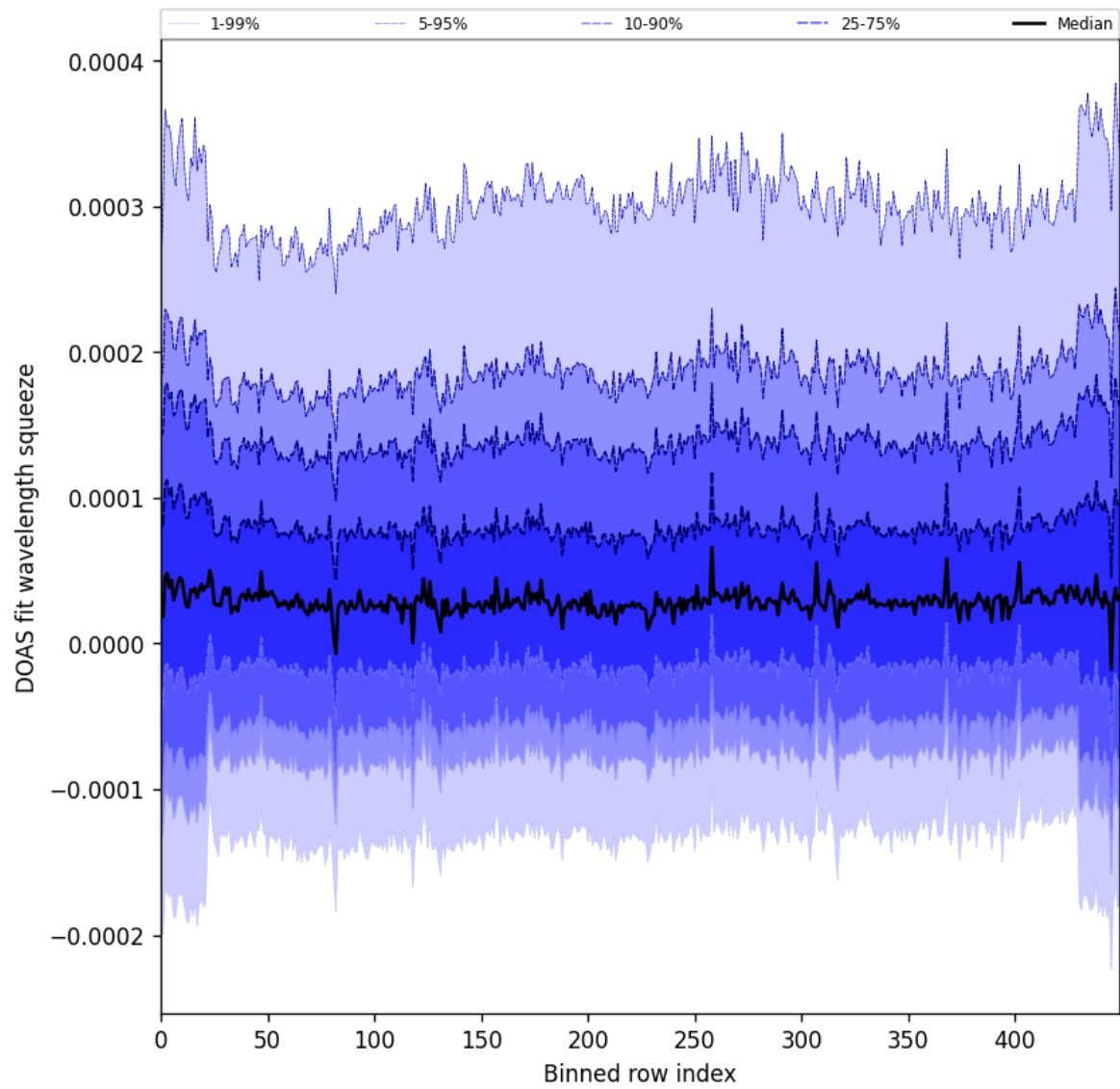
Figure 59: Along track statistics of “DOAS fit wavelength squeeze” for 2025-01-21 to 2025-01-23
