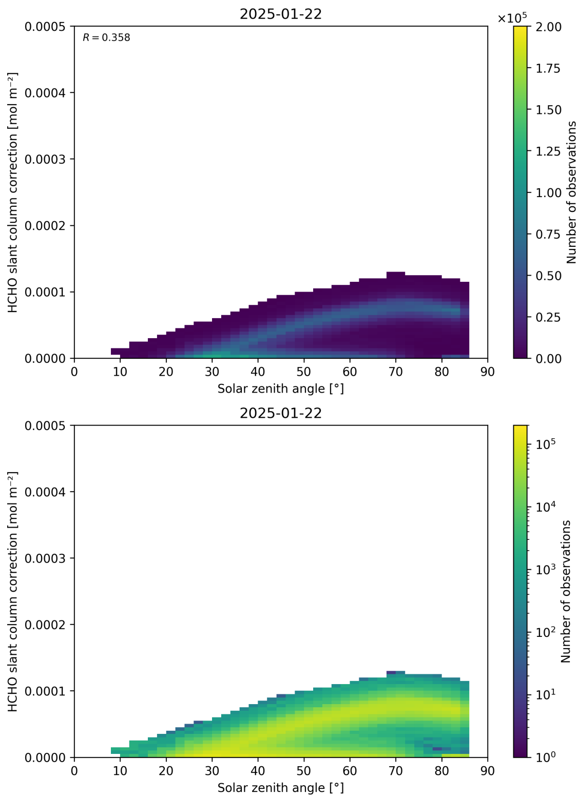
Figure 172: Scatter density plot of “Solar zenith angle” against “HCHO slant column correction” for 2025-01-21 to 2025-01-23.
