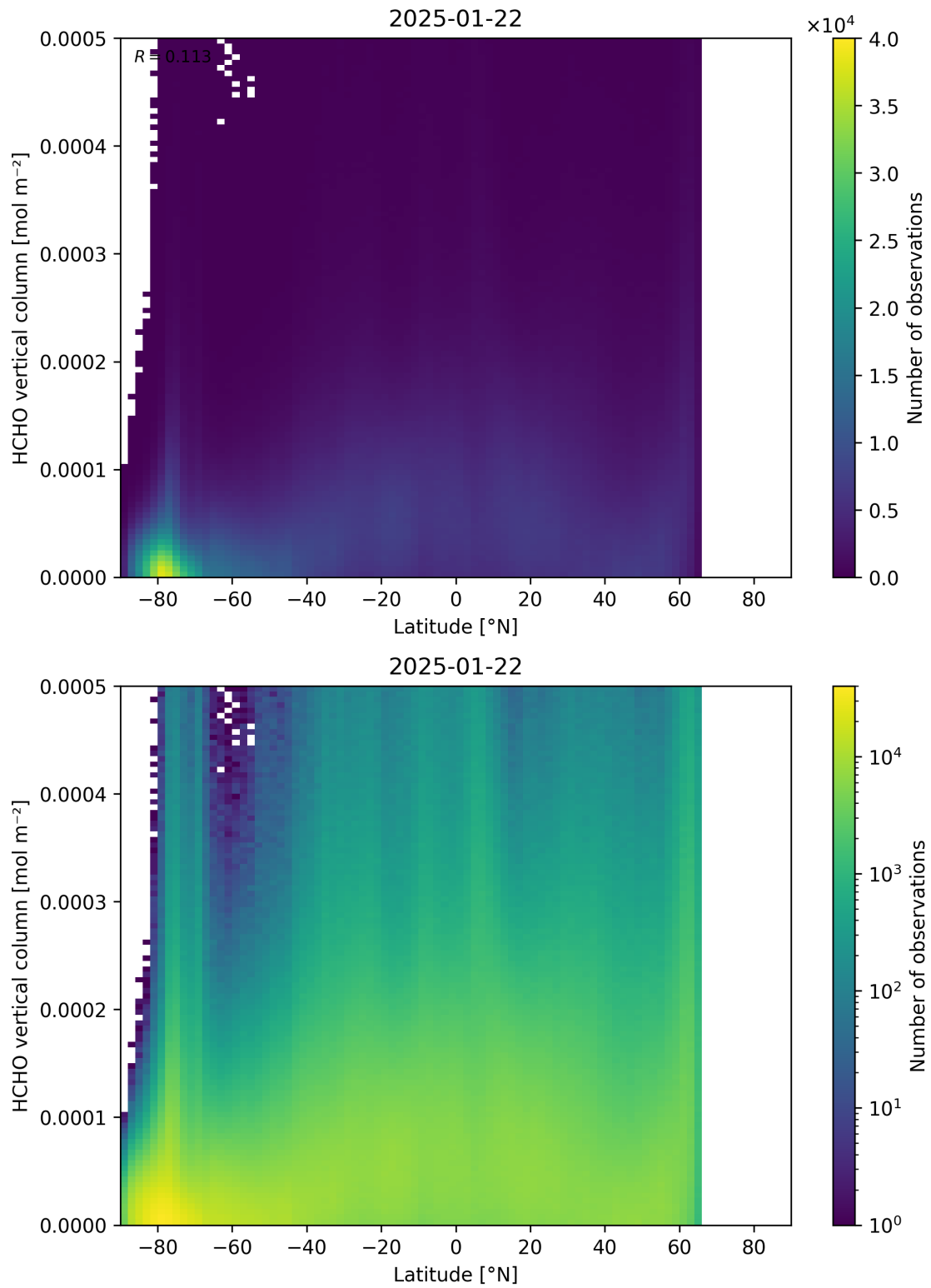
Figure 163: Scatter density plot of “Latitude” against “HCHO vertical column” for 2025-01-21 to 2025-01-23.
