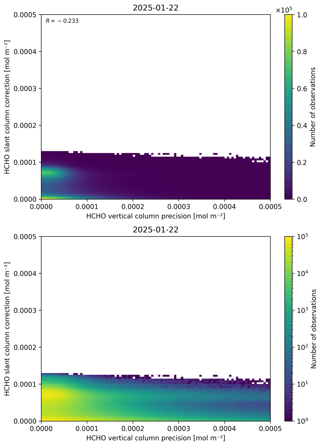
Figure 141: Scatter density plot of “HCHO vertical column precision” against “HCHO slant column correction” for 2025-01-21 to 2025-01-23.
