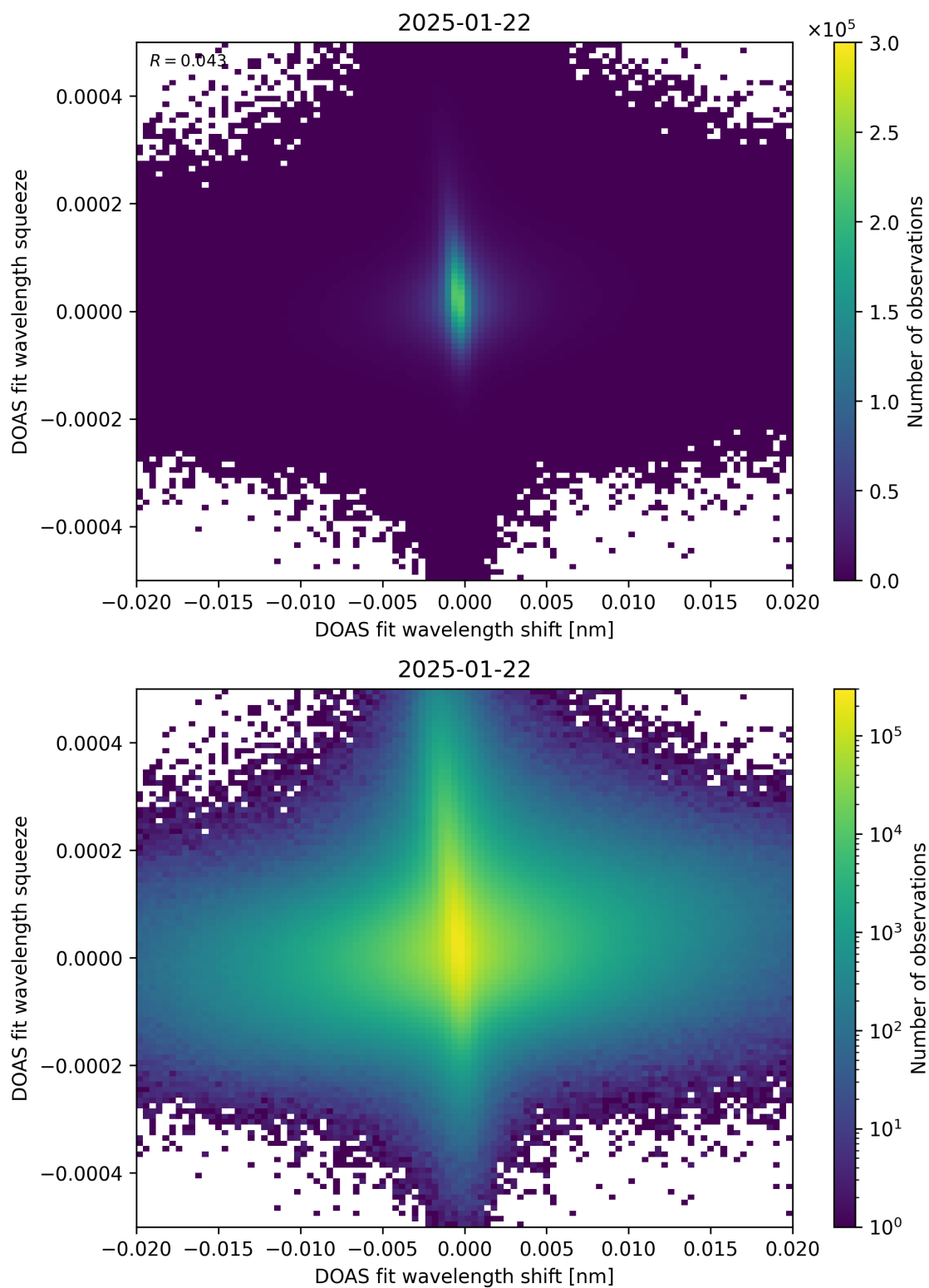
Figure 65: Scatter density plot of “DOAS fit wavelength shift” against “DOAS fit wavelength squeeze” for 2025-01-21 to 2025-01-23.
