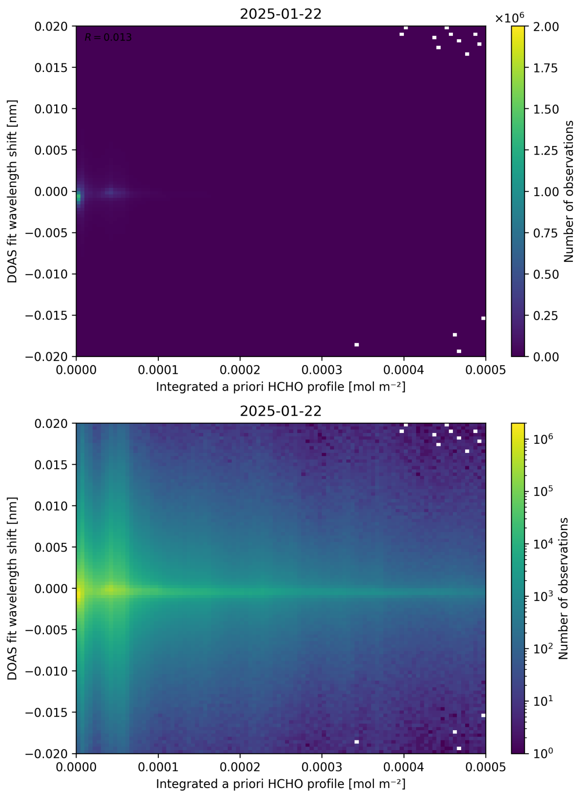
Figure 149: Scatter density plot of “Integrated a priori HCHO profile” against “DOAS fit wavelength shift” for 2025-01-21 to 2025-01-23.
