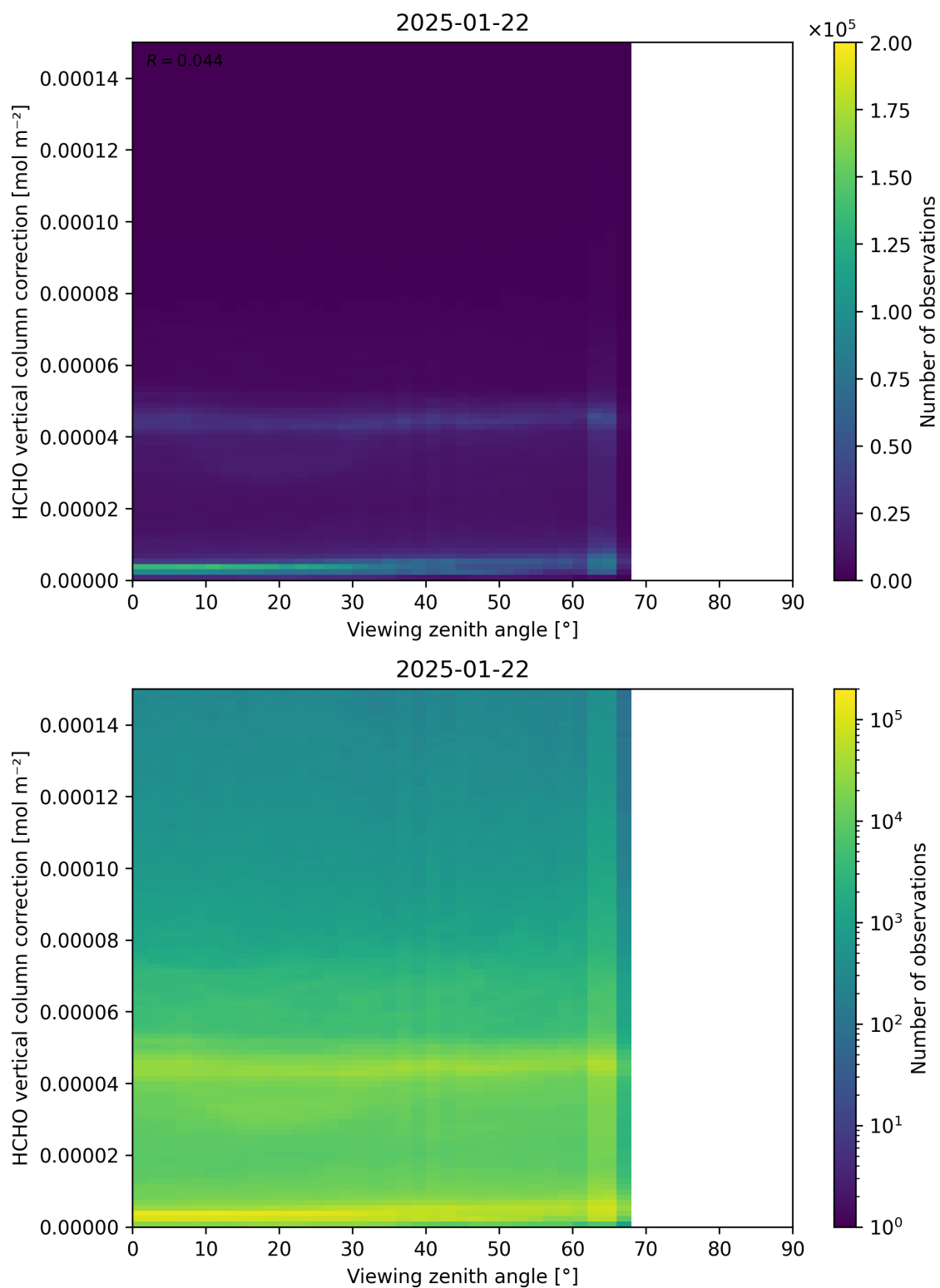
Figure 193: Scatter density plot of “Viewing zenith angle” against “HCHO vertical column correction” for 2025-01-21 to 2025-01-23.
