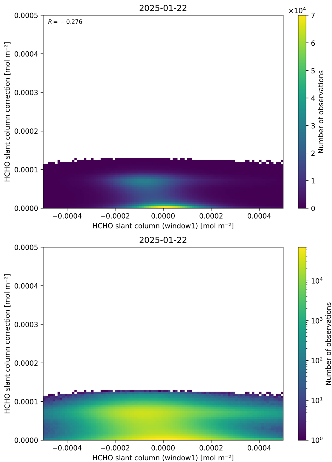
Figure 83: Scatter density plot of “HCHO slant column (window1)” against “HCHO slant column correction” for 2025-01-21 to 2025-01-23.
