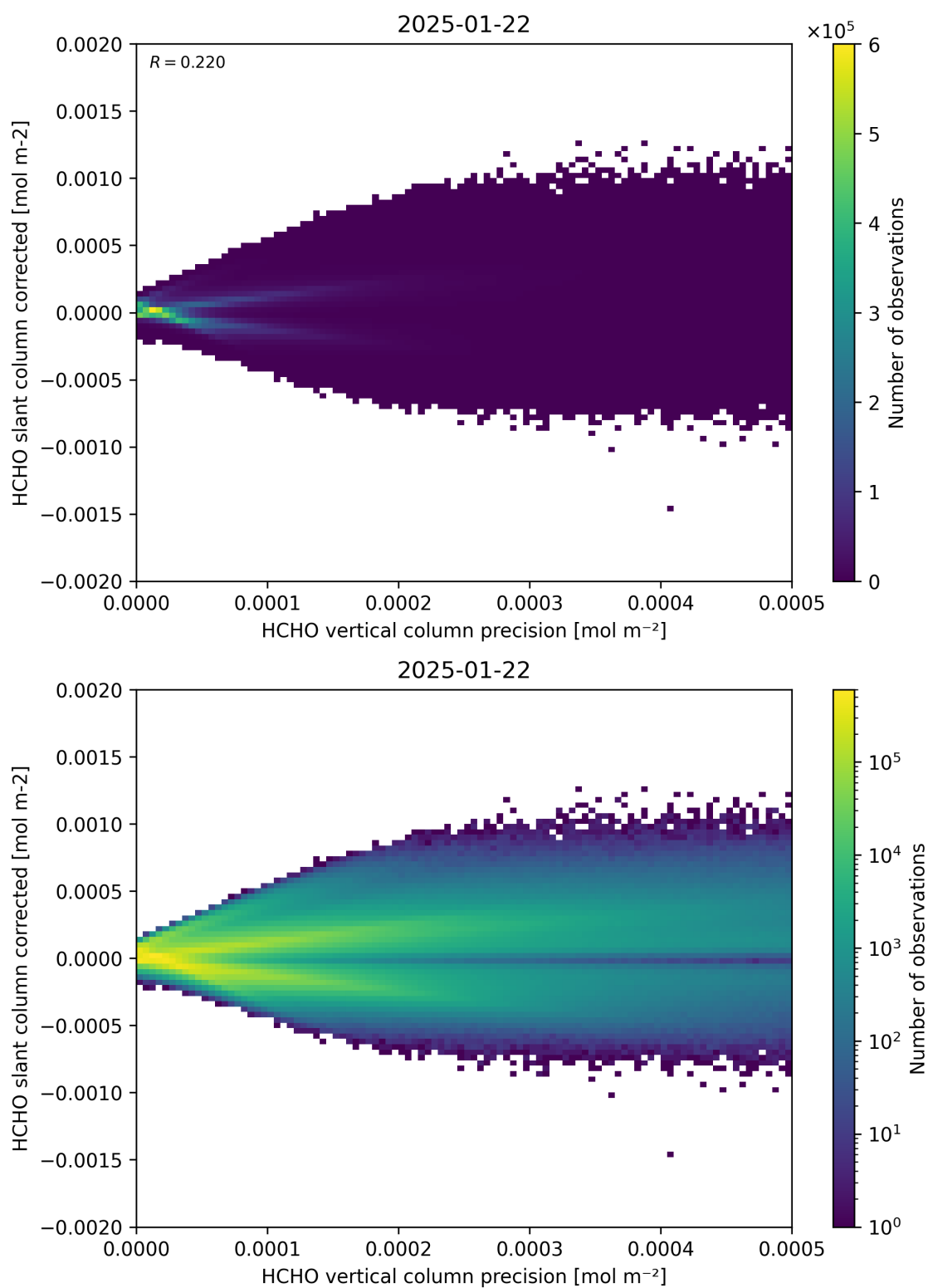
Figure 140: Scatter density plot of “HCHO vertical column precision” against “HCHO slant column corrected” for 2025-01-21 to 2025-01-23.
