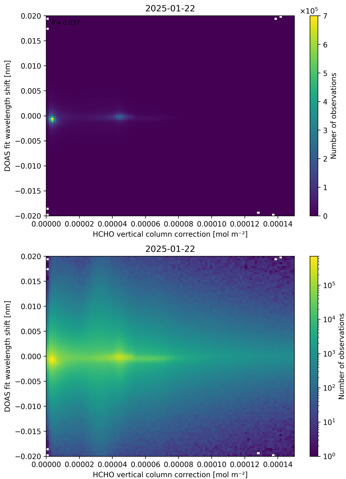
Figure 113: Scatter density plot of “HCHO vertical column correction” against “DOAS fit wavelength shift” for 2025-01-21 to 2025-01-23.
