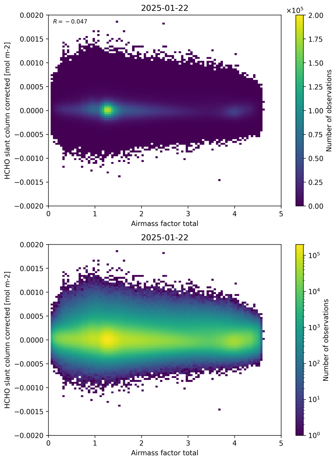
Figure 101: Scatter density plot of “Airmass factor total” against “HCHO slant column corrected” for 2025-01-21 to 2025-01-23.
