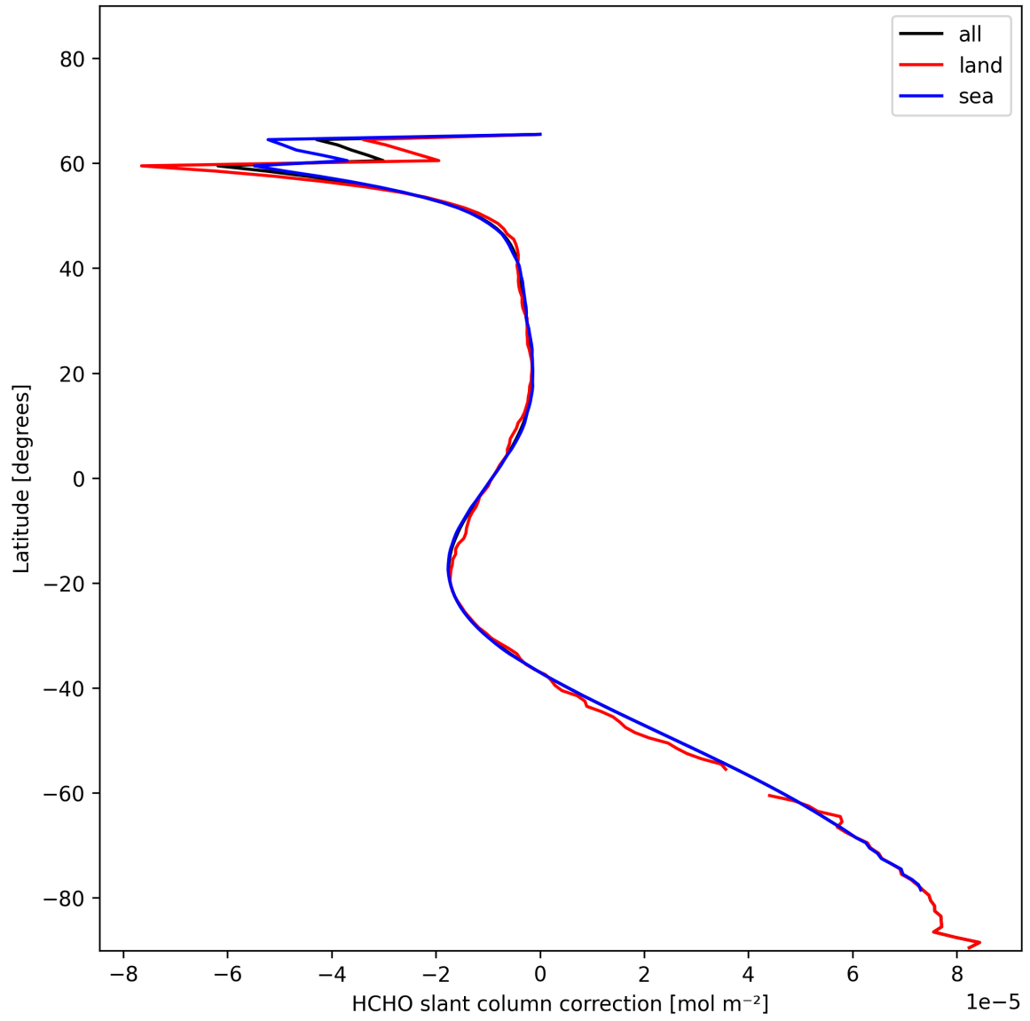
Figure 33: Zonal average of “HCHO slant column correction” for 2025-01-21 to 2025-01-23.
