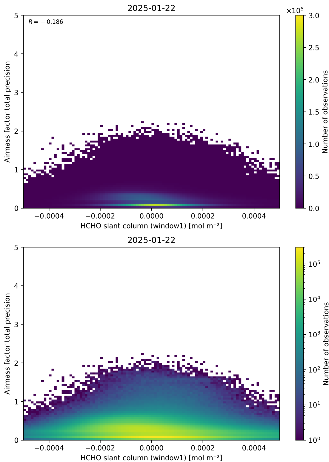
Figure 86: Scatter density plot of “HCHO slant column (window1)” against “Airmass factor total precision” for 2025-01-21 to 2025-01-23.
