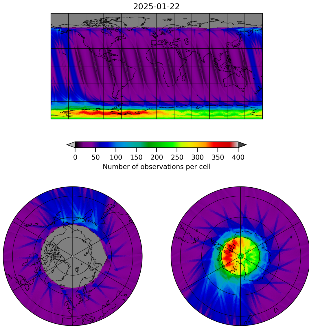
Figure 19: Map of the number of observations for 2025-01-21 to 2025-01-23
