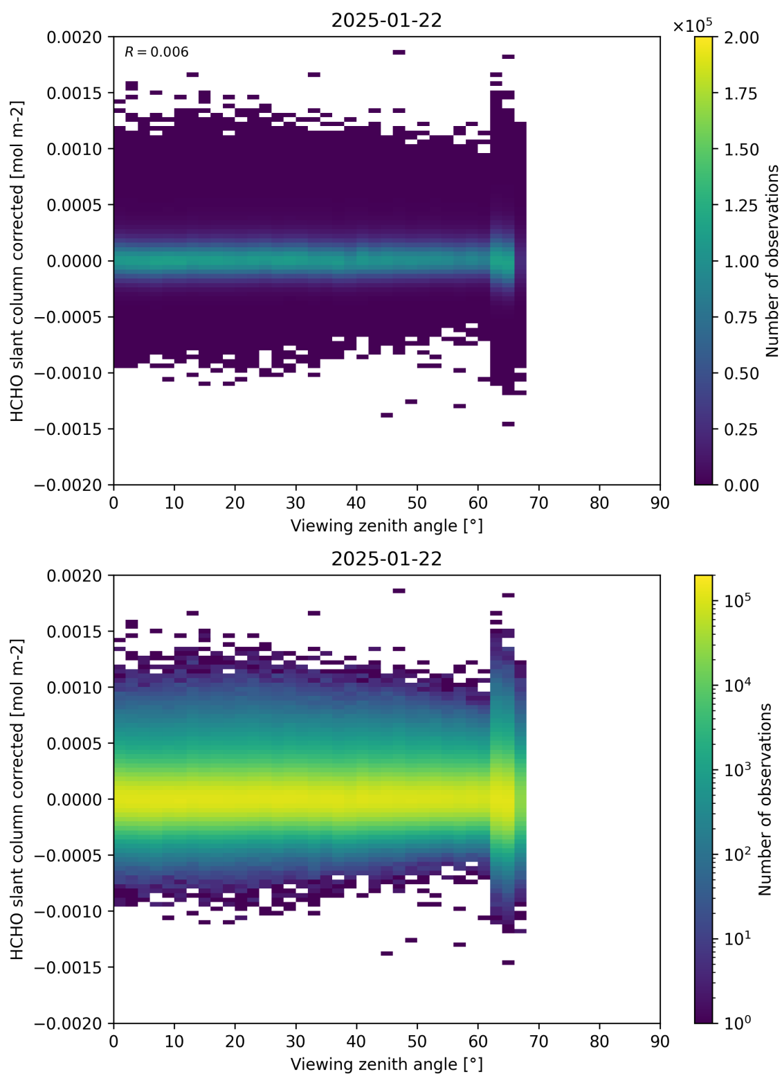
Figure 186: Scatter density plot of “Viewing zenith angle” against “HCHO slant column corrected” for 2025-01-21 to 2025-01-23.
