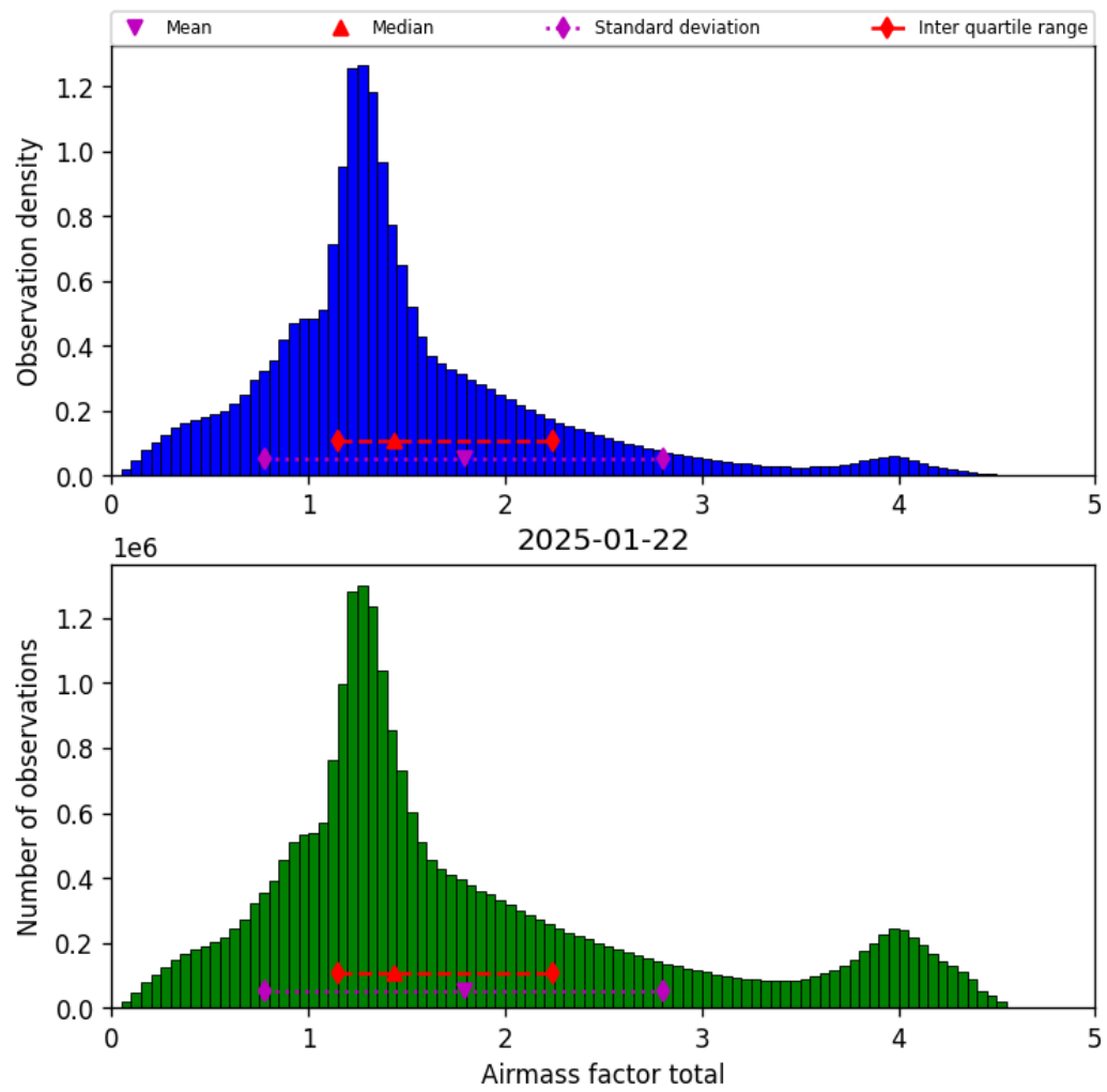
Figure 40: Histogram of “Airmass factor total” for 2025-01-21 to 2025-01-23
