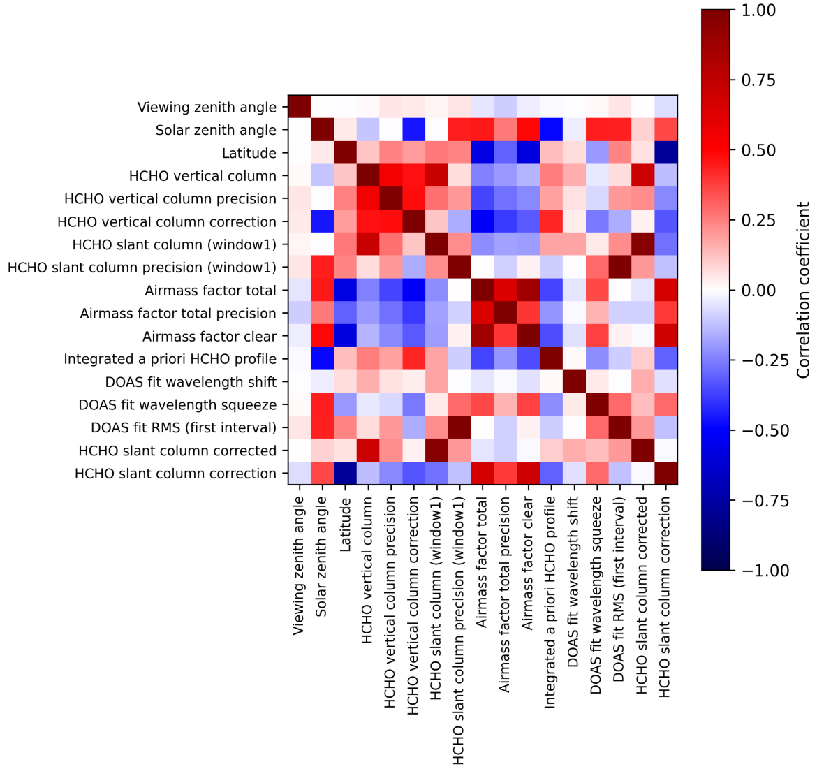
Figure 2: Map of correlation matrix for 2025-01-21 to 2025-01-23.
