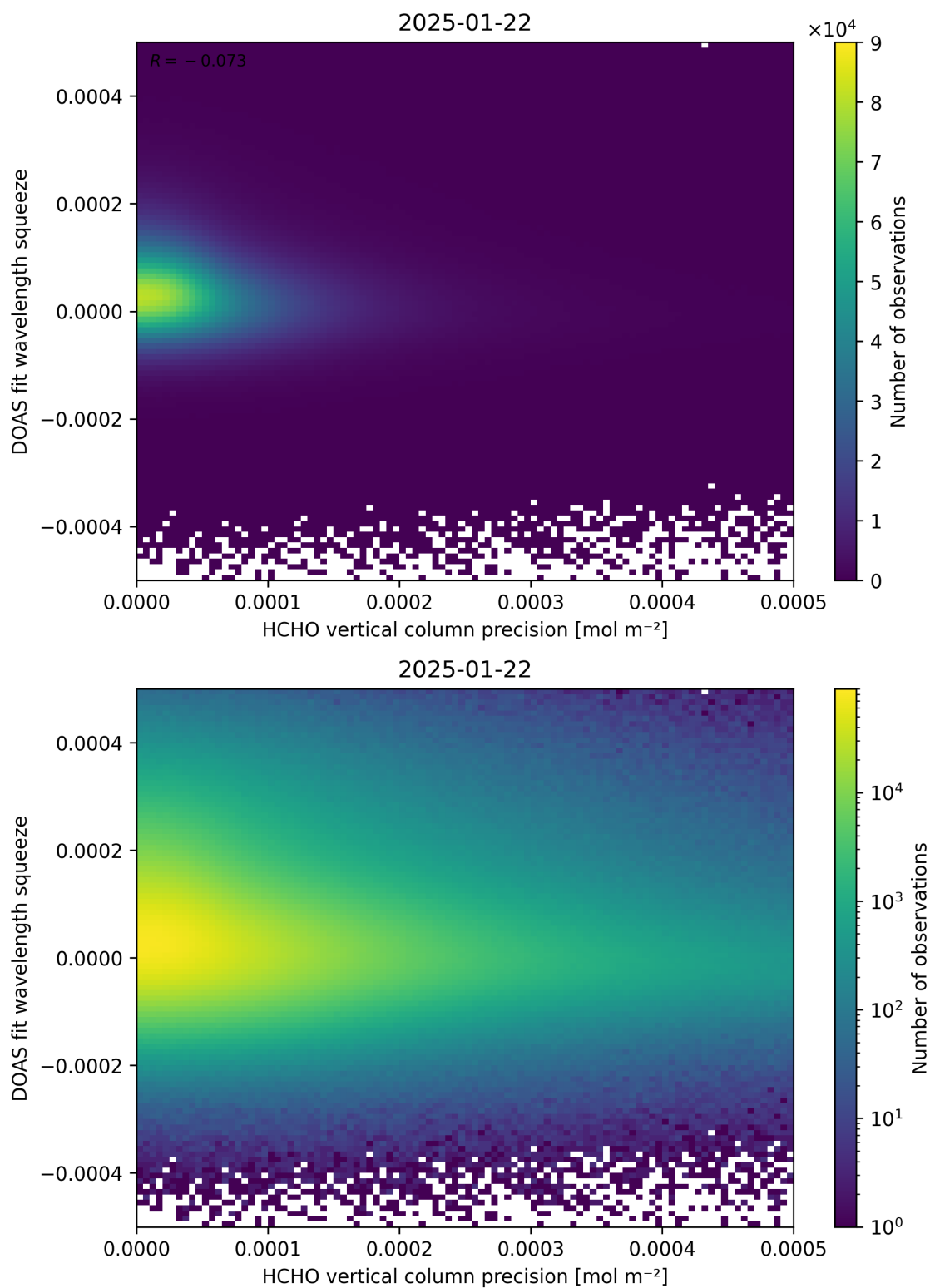
Figure 138: Scatter density plot of “HCHO vertical column precision” against “DOAS fit wavelength squeeze” for 2025-01-21 to 2025-01-23.
