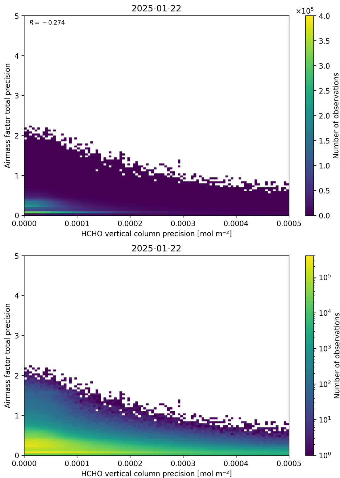
Figure 145: Scatter density plot of “HCHO vertical column precision” against “Airmass factor total precision” for 2025-01-21 to 2025-01-23.
