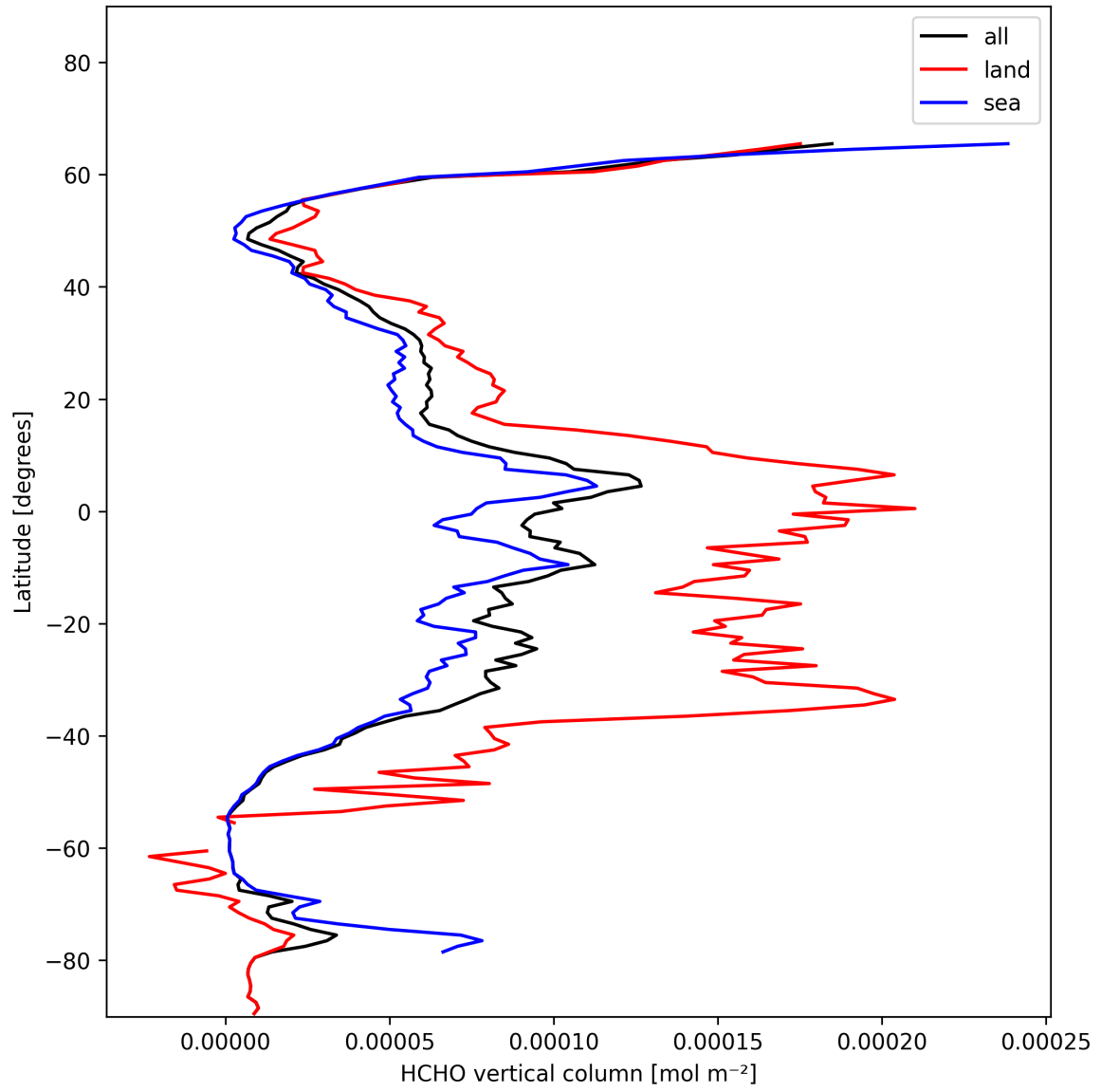
Figure 21: Zonal average of “HCHO vertical column” for 2025-01-21 to 2025-01-23.
