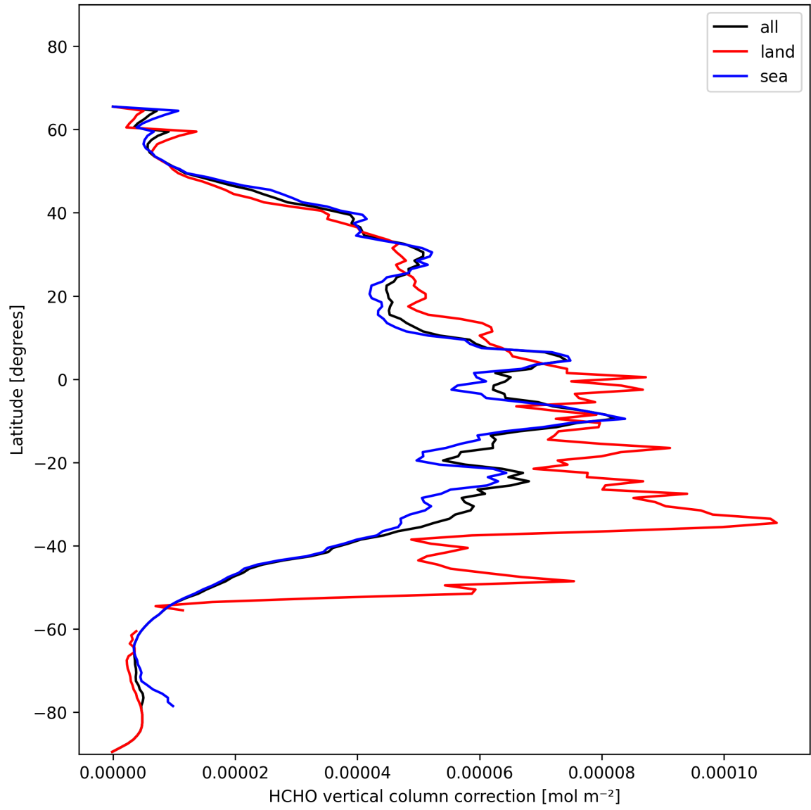
Figure 23: Zonal average of “HCHO vertical column correction” for 2025-01-21 to 2025-01-23.
