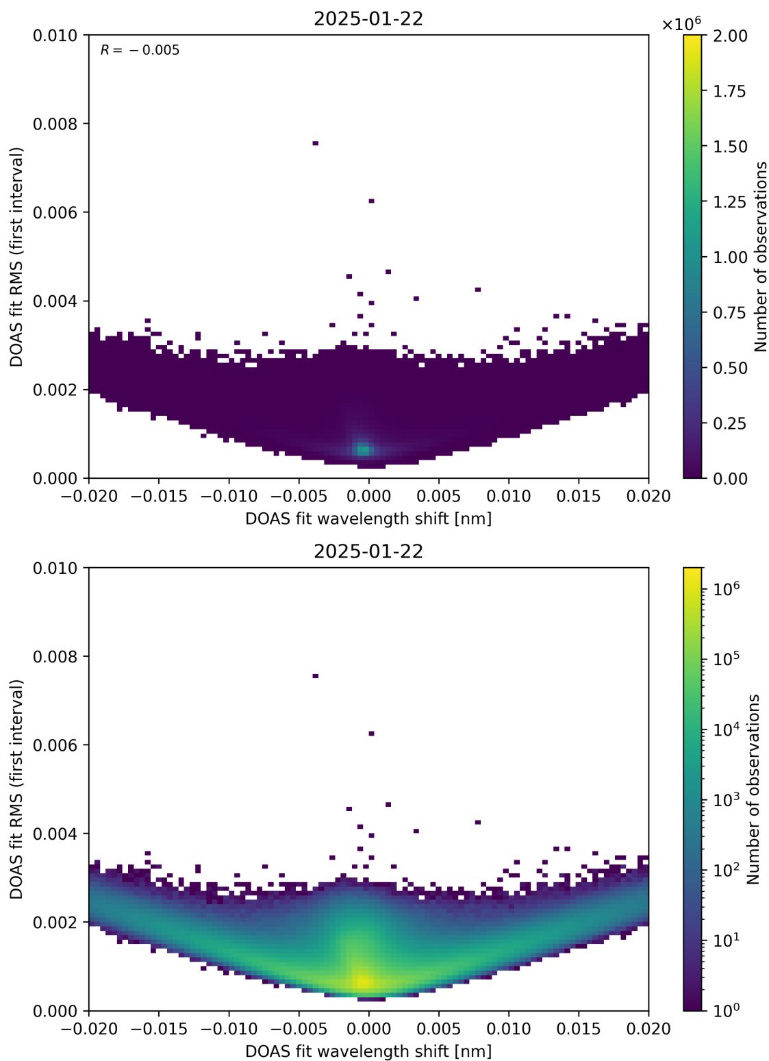
Figure 64: Scatter density plot of “DOAS fit wavelength shift” against “DOAS fit RMS (first interval)” for 2025-01-21 to 2025-01-23.
