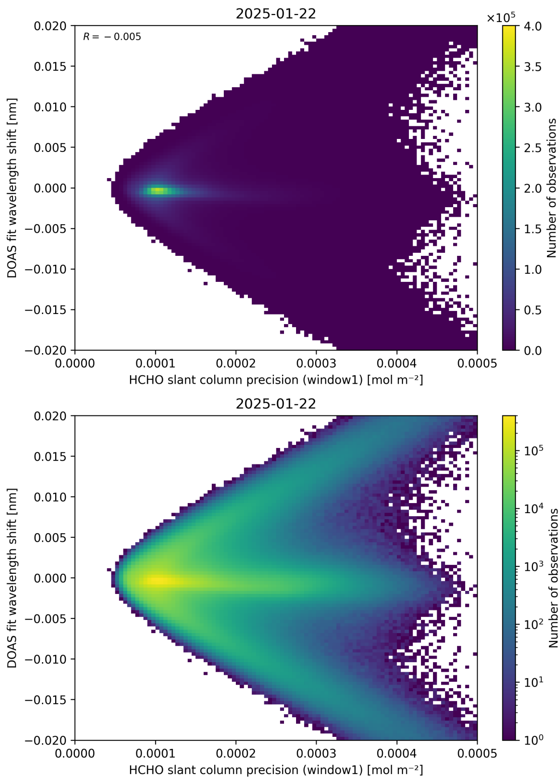
Figure 89: Scatter density plot of “HCHO slant column precision (window1)” against “DOAS fit wavelength shift” for 2025-01-21 to 2025-01-23.
