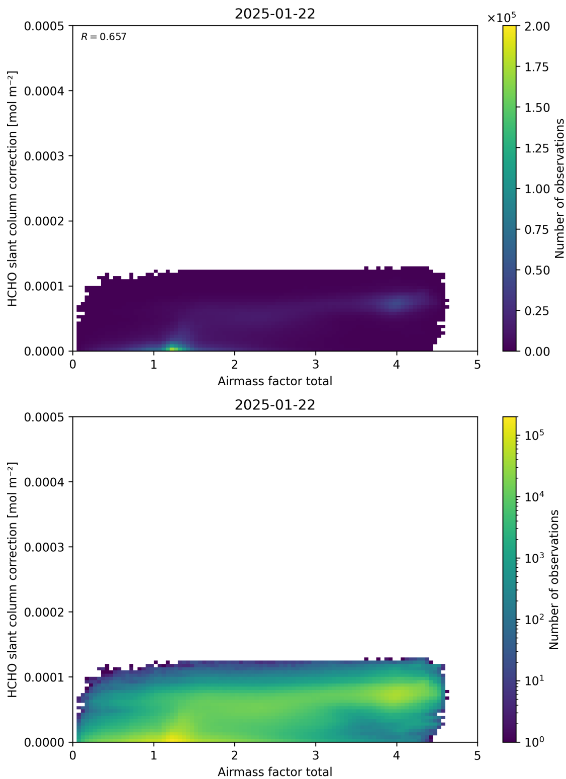
Figure 102: Scatter density plot of “Airmass factor total” against “HCHO slant column correction” for 2025-01-21 to 2025-01-23.
