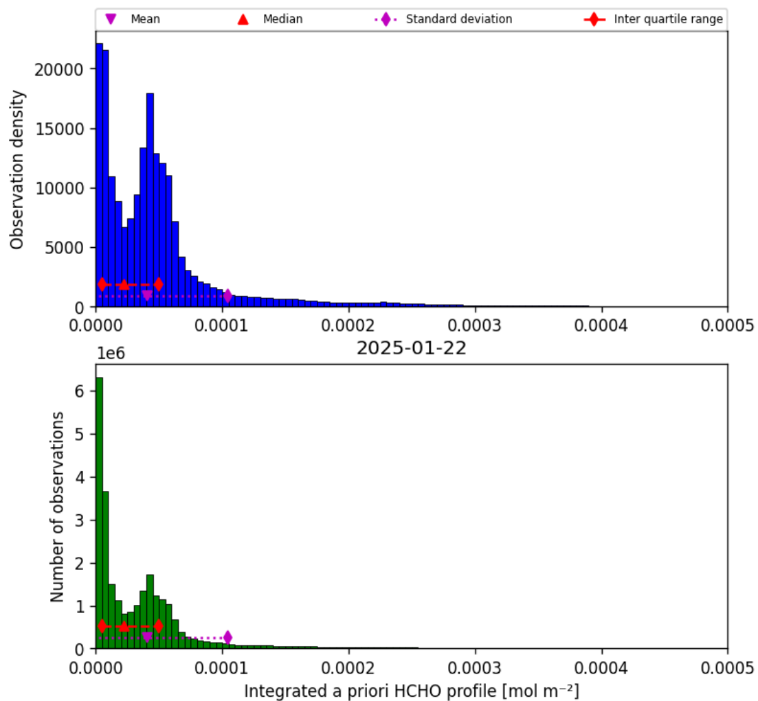
Figure 43: Histogram of “Integrated a priori HCHO profile” for 2025-01-21 to 2025-01-23
