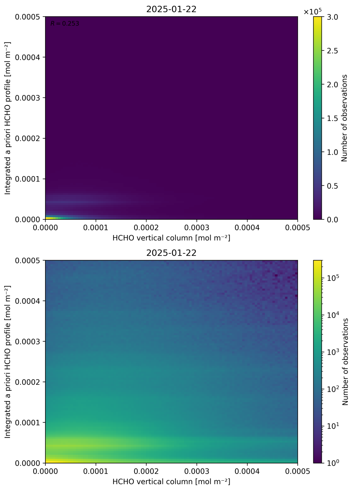
Figure 135: Scatter density plot of “HCHO vertical column” against “Integrated a priori HCHO profile” for 2025-01-21 to 2025-01-23.
