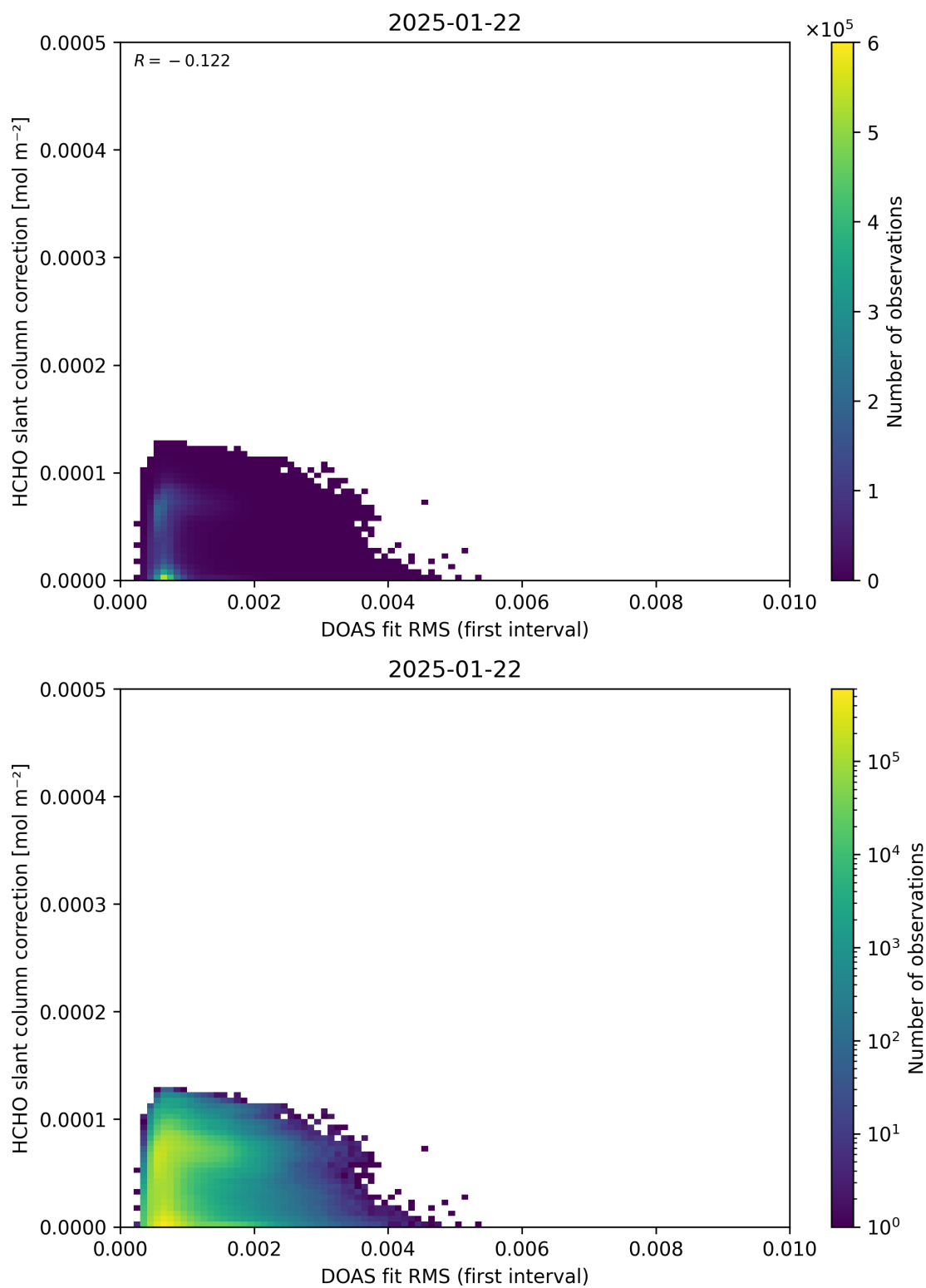
Figure 63: Scatter density plot of “DOAS fit RMS (first interval)” against “HCHO slant column correction” for 2025-01-21 to 2025-01-23.
