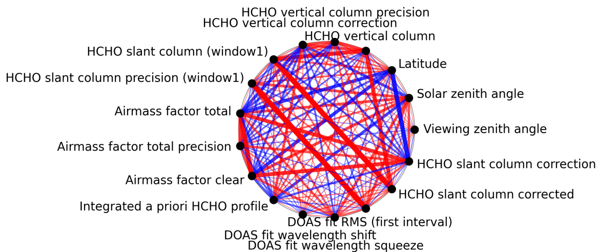
Figure 1: Map of correlation graph for 2025-01-21 to 2025-01-23.
