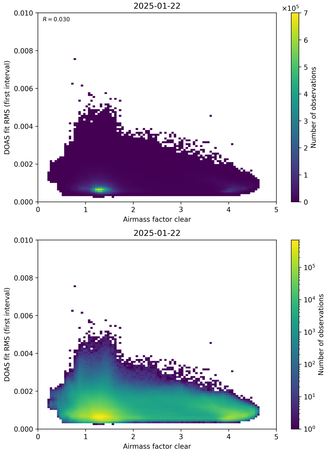
Figure 71: Scatter density plot of “Airmass factor clear” against “DOAS fit RMS (first interval)” for 2025-01-21 to 2025-01-23.
