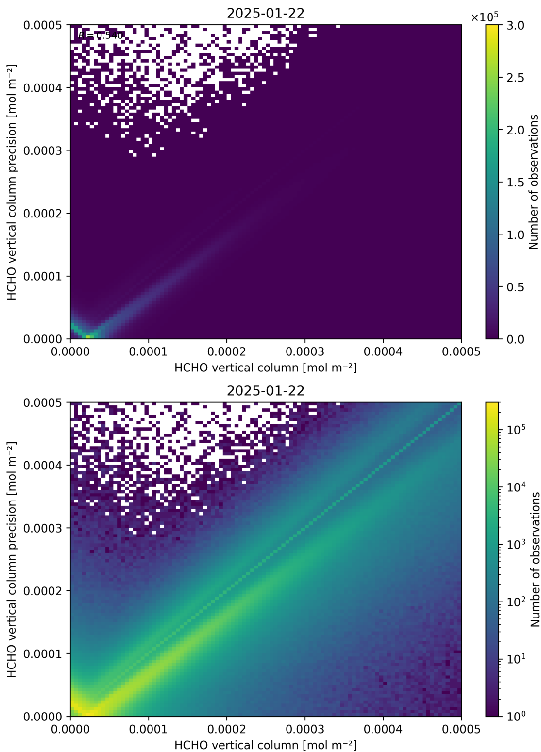
Figure 134: Scatter density plot of “HCHO vertical column” against “HCHO vertical column precision” for 2025-01-21 to 2025-01-23.
