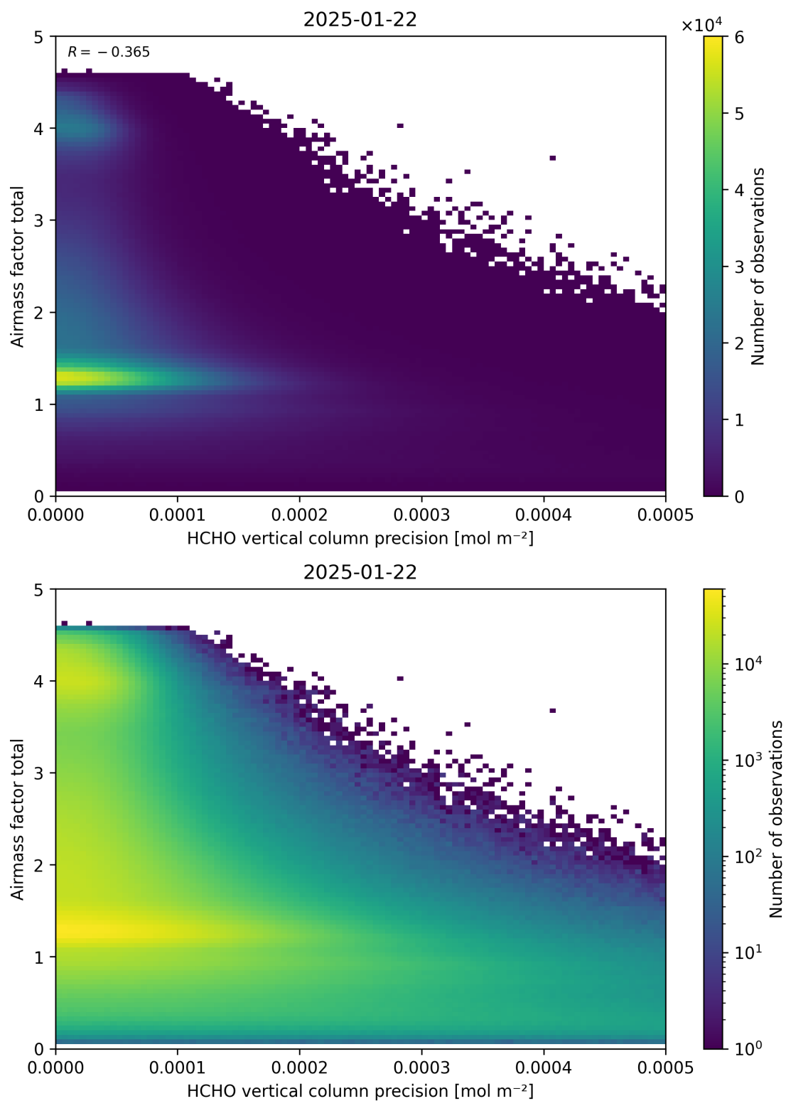
Figure 144: Scatter density plot of “HCHO vertical column precision” against “Airmass factor total” for 2025-01-21 to 2025-01-23.
