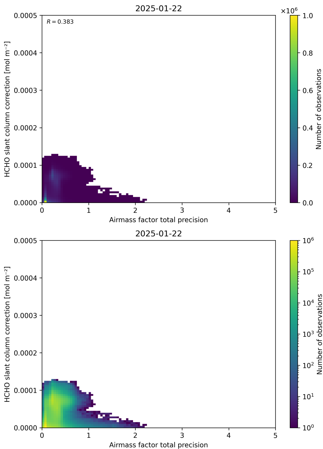
Figure 110: Scatter density plot of “Airmass factor total precision” against “HCHO slant column correction” for 2025-01-21 to 2025-01-23.
