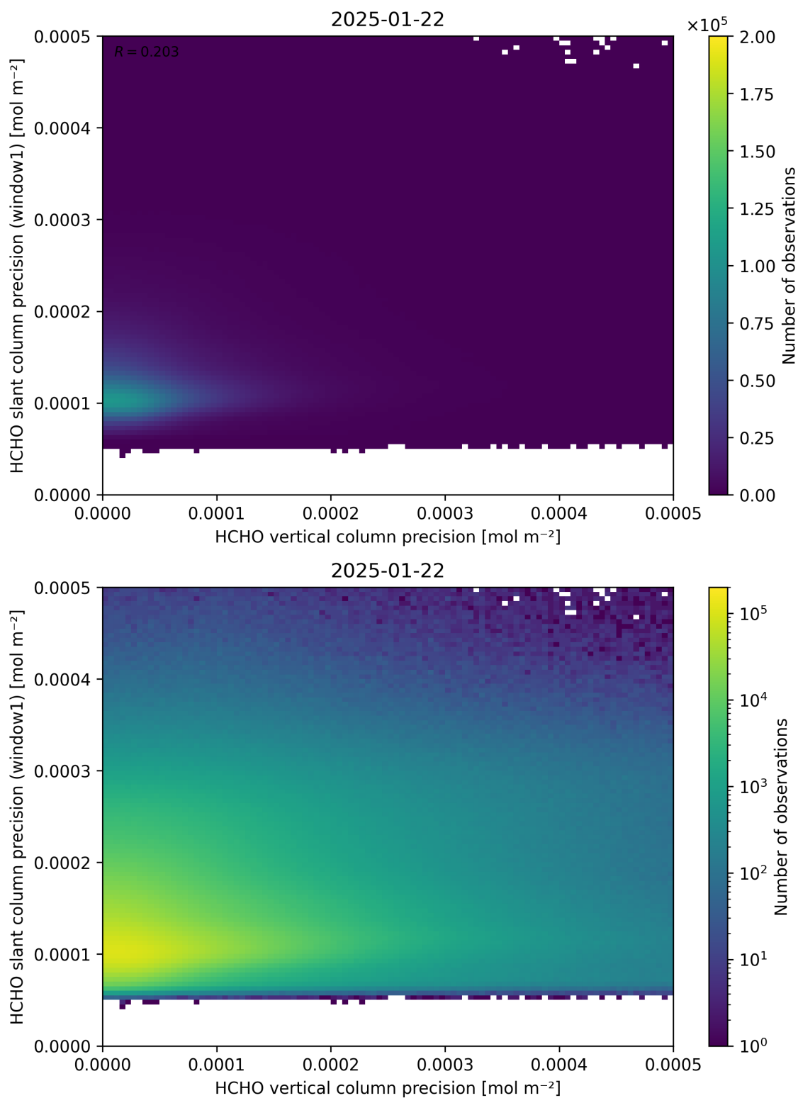
Figure 143: Scatter density plot of “HCHO vertical column precision” against “HCHO slant column precision (window1)” for 2025-01-21 to 2025-01-23.
