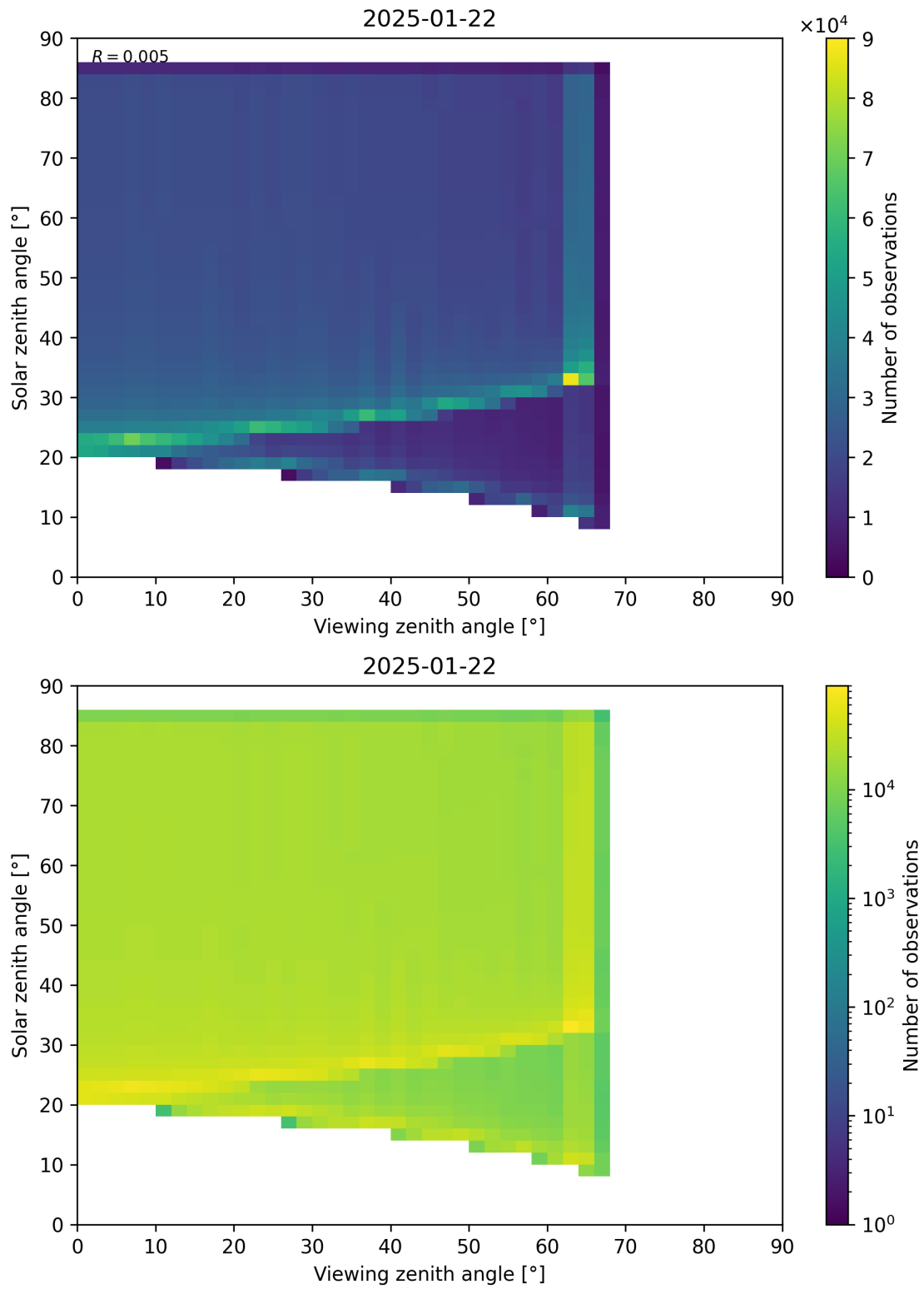
Figure 197: Scatter density plot of “Viewing zenith angle” against “Solar zenith angle” for 2025-01-21 to 2025-01-23.
