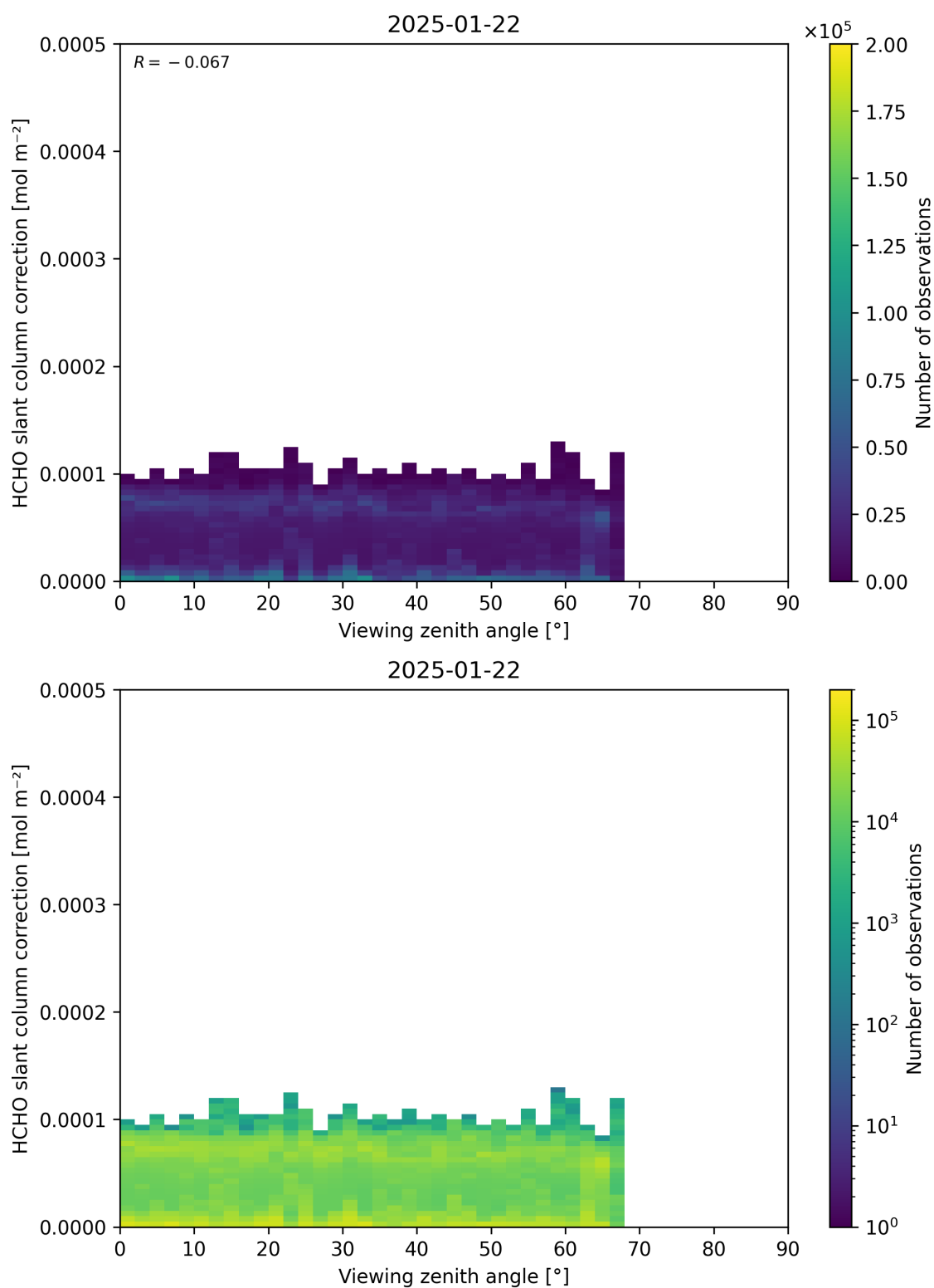
Figure 187: Scatter density plot of “Viewing zenith angle” against “HCHO slant column correction” for 2025-01-21 to 2025-01-23.
