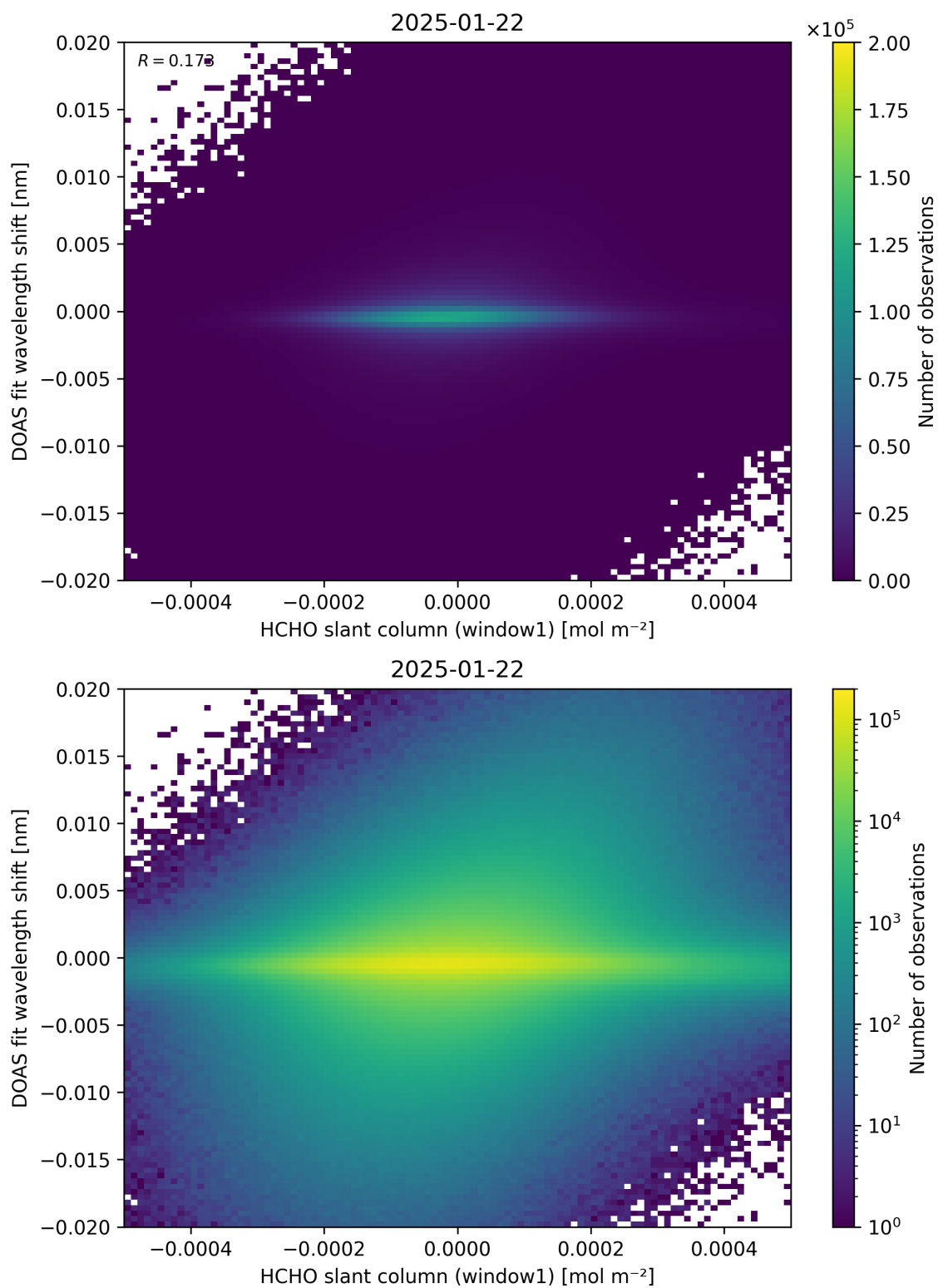
Figure 79: Scatter density plot of “HCHO slant column (window1)” against “DOAS fit wavelength shift” for 2025-01-21 to 2025-01-23.
