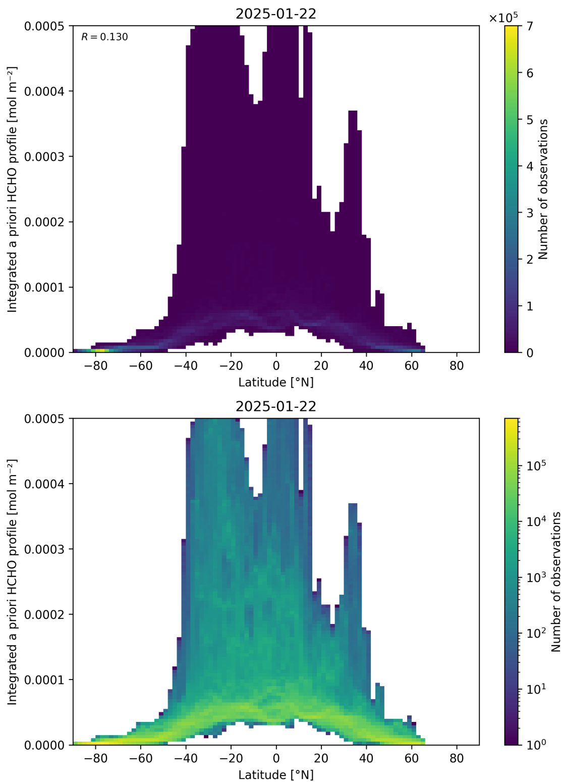
Figure 166: Scatter density plot of “Latitude” against “Integrated a priori HCHO profile” for 2025-01-21 to 2025-01-23.
