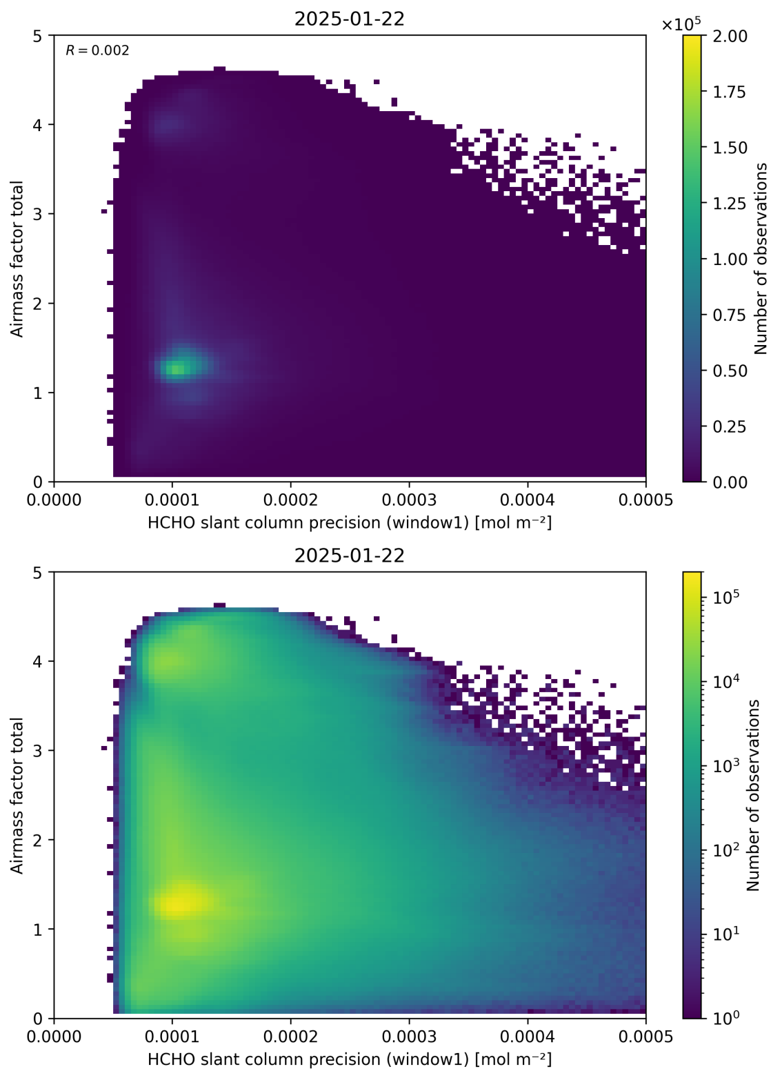
Figure 94: Scatter density plot of “HCHO slant column precision (window1)” against “Airmass factor total” for 2025-01-21 to 2025-01-23.
