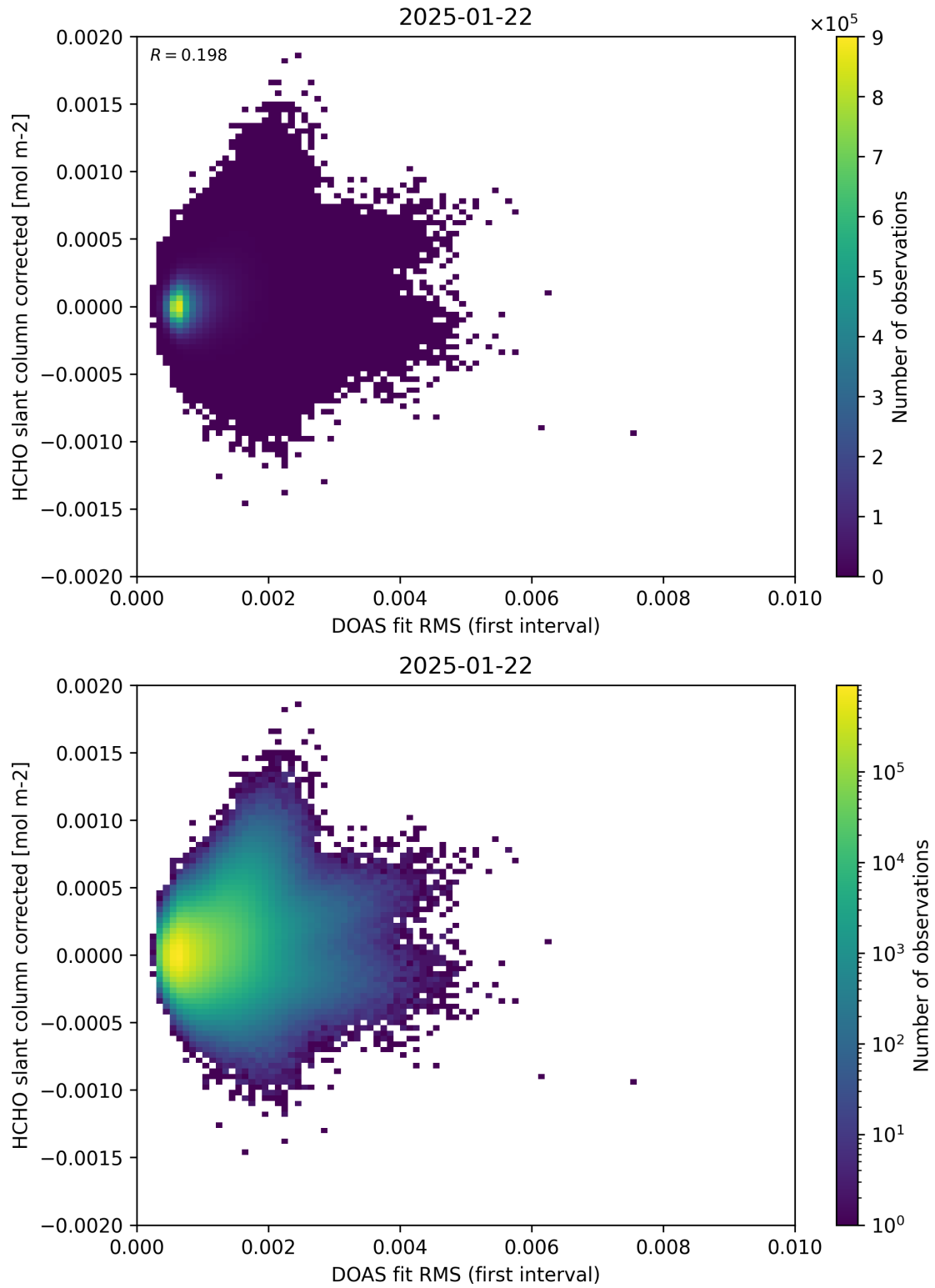
Figure 62: Scatter density plot of “DOAS fit RMS (first interval)” against “HCHO slant column corrected” for 2025-01-21 to 2025-01-23.
