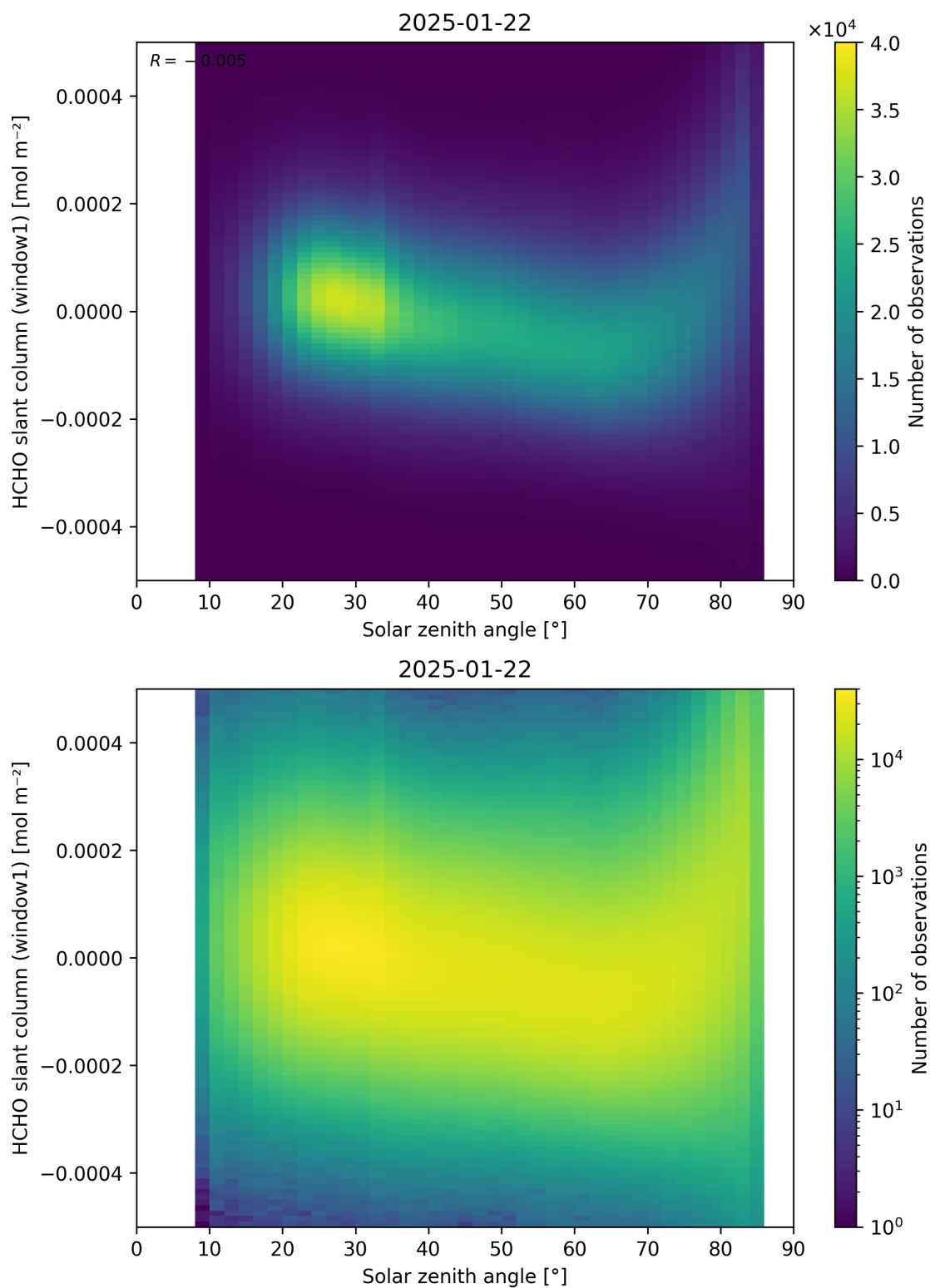
Figure 173: Scatter density plot of “Solar zenith angle” against “HCHO slant column (window1)” for 2025-01-21 to 2025-01-23.
