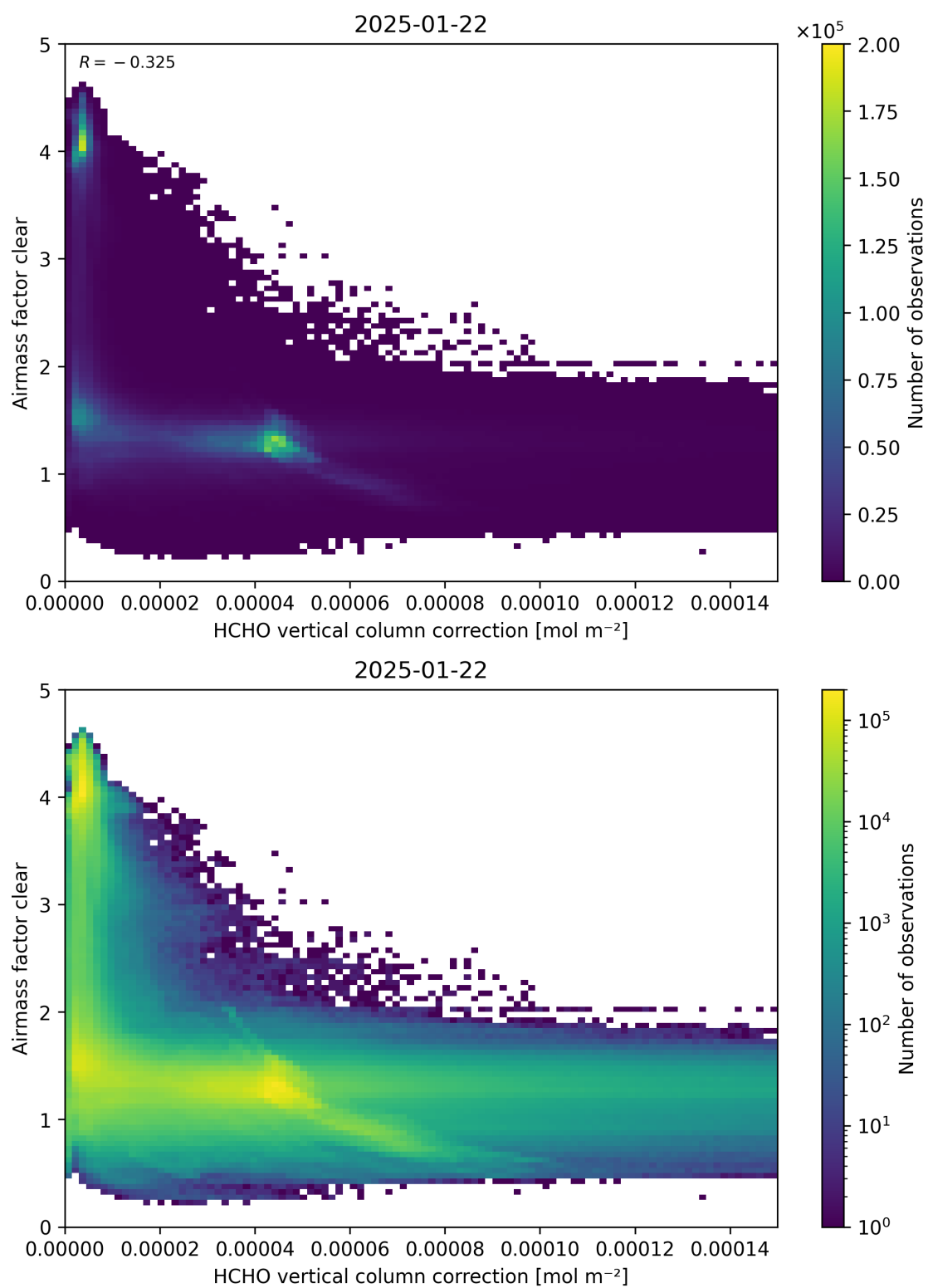
Figure 115: Scatter density plot of “HCHO vertical column correction” against “Airmass factor clear” for 2025-01-21 to 2025-01-23.
