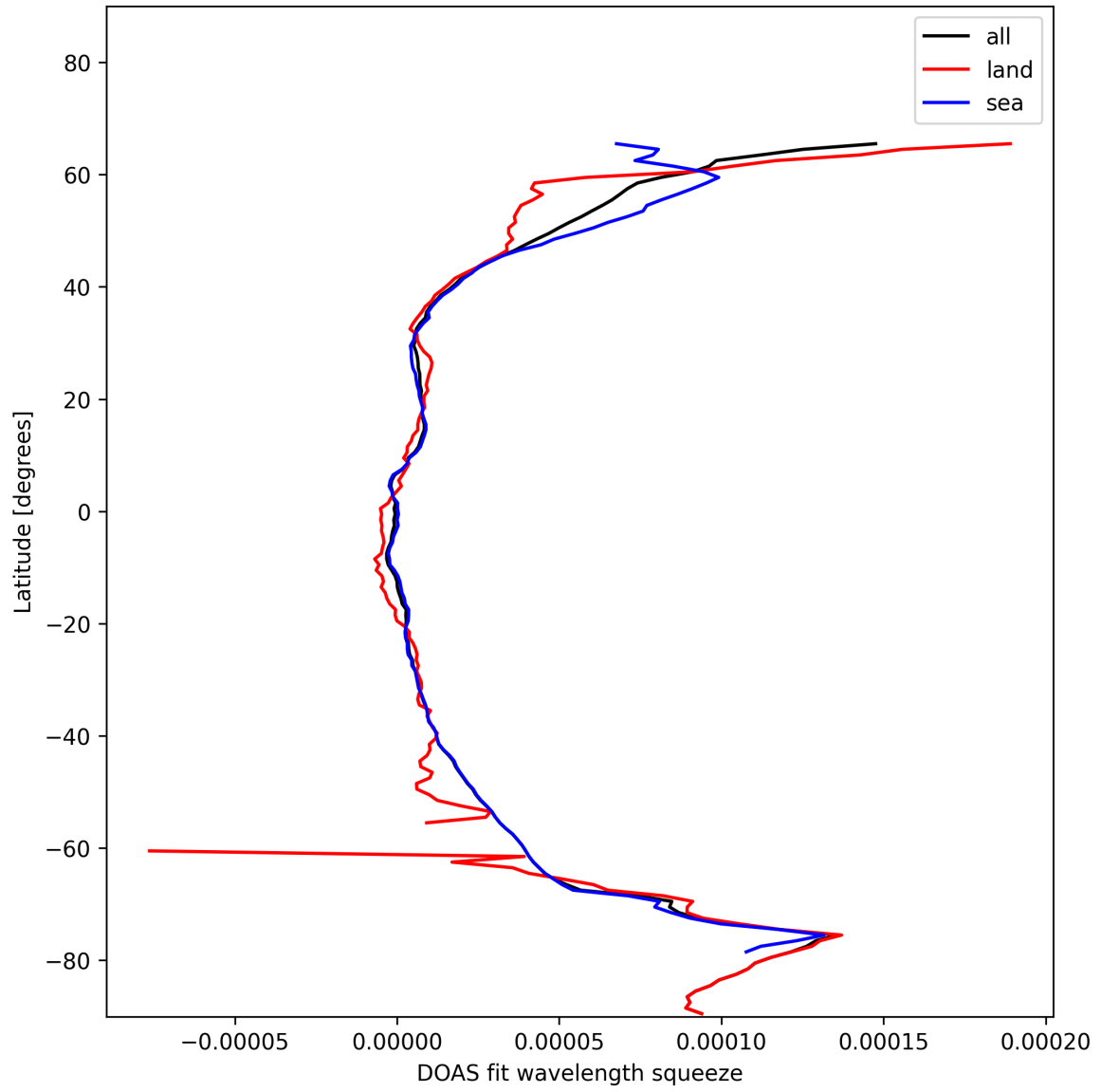
Figure 31: Zonal average of “DOAS fit wavelength squeeze” for 2025-01-21 to 2025-01-23.
