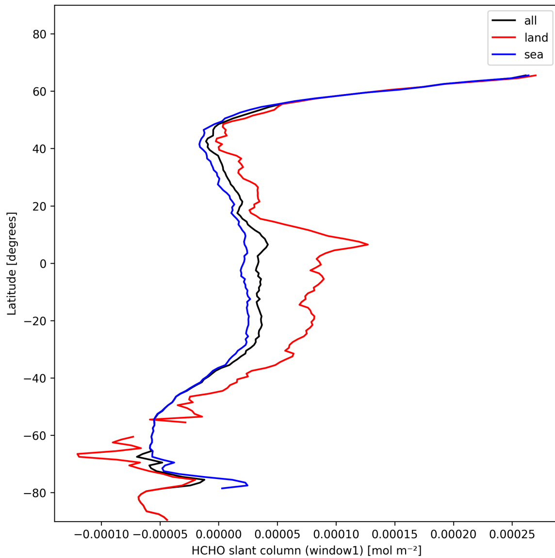
Figure 24: Zonal average of “HCHO slant column (window1)” for 2025-01-21 to 2025-01-23.
