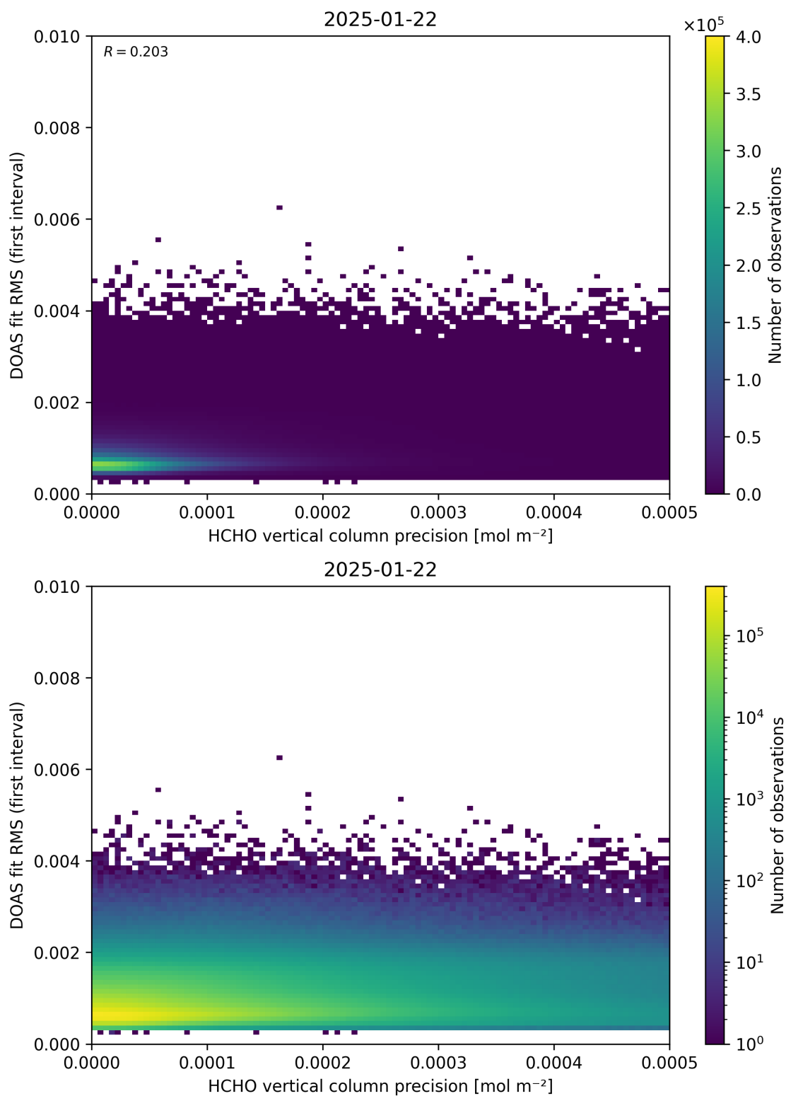
Figure 136: Scatter density plot of “HCHO vertical column precision” against “DOAS fit RMS (first interval)” for 2025-01-21 to 2025-01-23.
