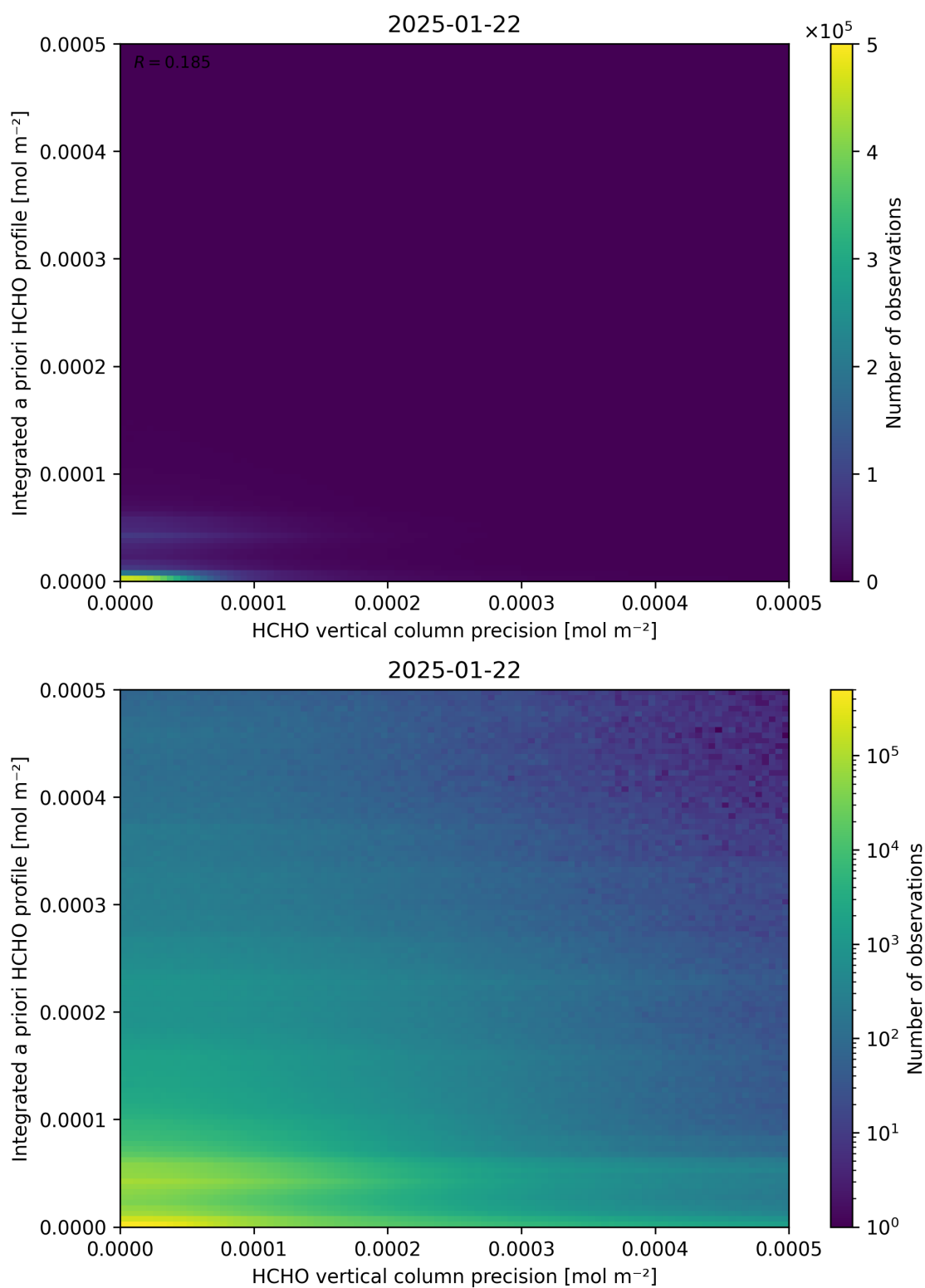
Figure 147: Scatter density plot of “HCHO vertical column precision” against “Integrated a priori HCHO profile” for 2025-01-21 to 2025-01-23.
