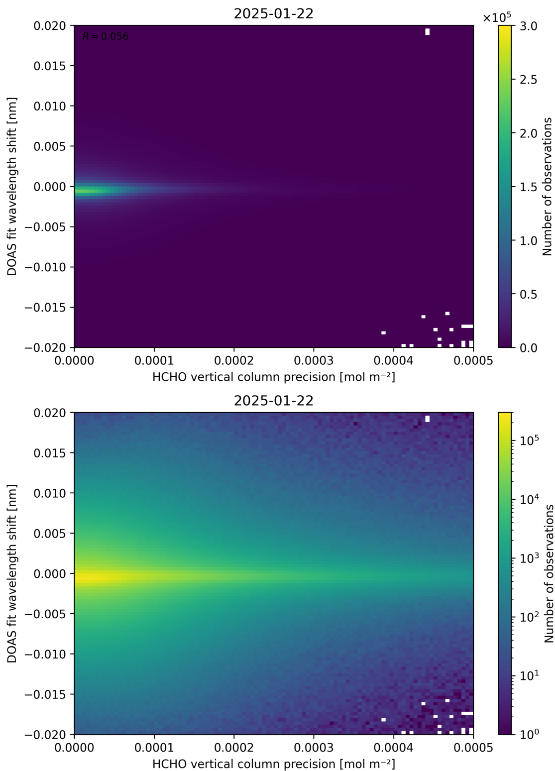
Figure 137: Scatter density plot of “HCHO vertical column precision” against “DOAS fit wavelength shift” for 2025-01-21 to 2025-01-23.
