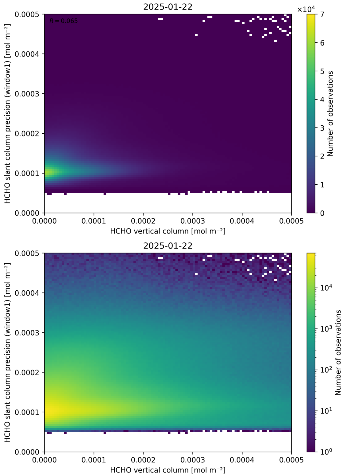
Figure 130: Scatter density plot of “HCHO vertical column” against “HCHO slant column precision (window1)” for 2025-01-21 to 2025-01-23.
