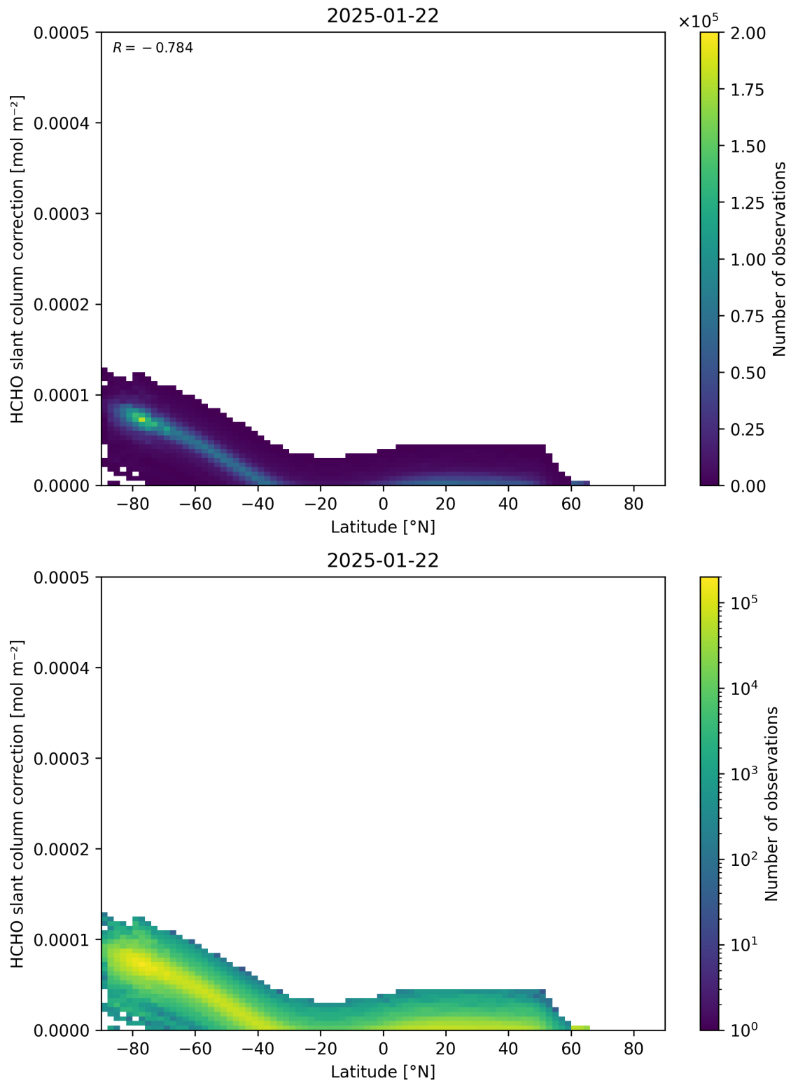
Figure 158: Scatter density plot of “Latitude” against “HCHO slant column correction” for 2025-01-21 to 2025-01-23.
