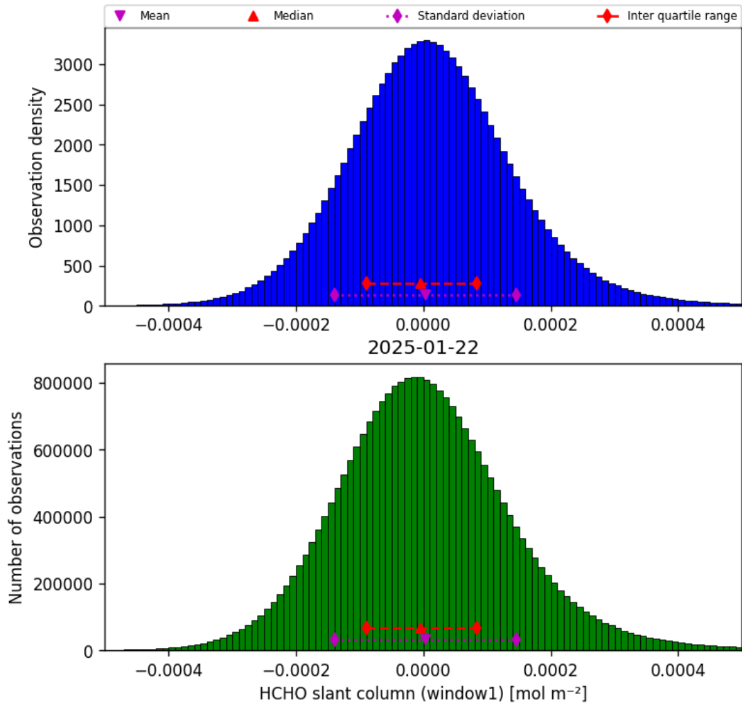
Figure 38: Histogram of “HCHO slant column (window1)” for 2025-01-21 to 2025-01-23
