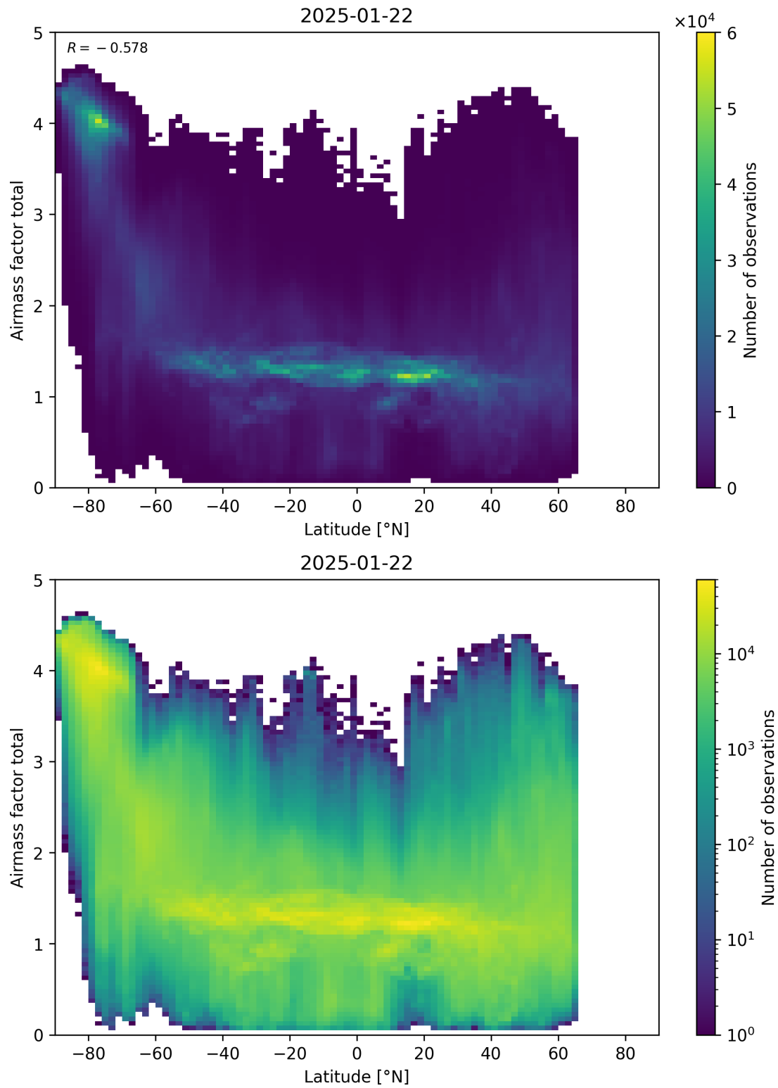
Figure 161: Scatter density plot of “Latitude” against “Airmass factor total” for 2025-01-21 to 2025-01-23.
