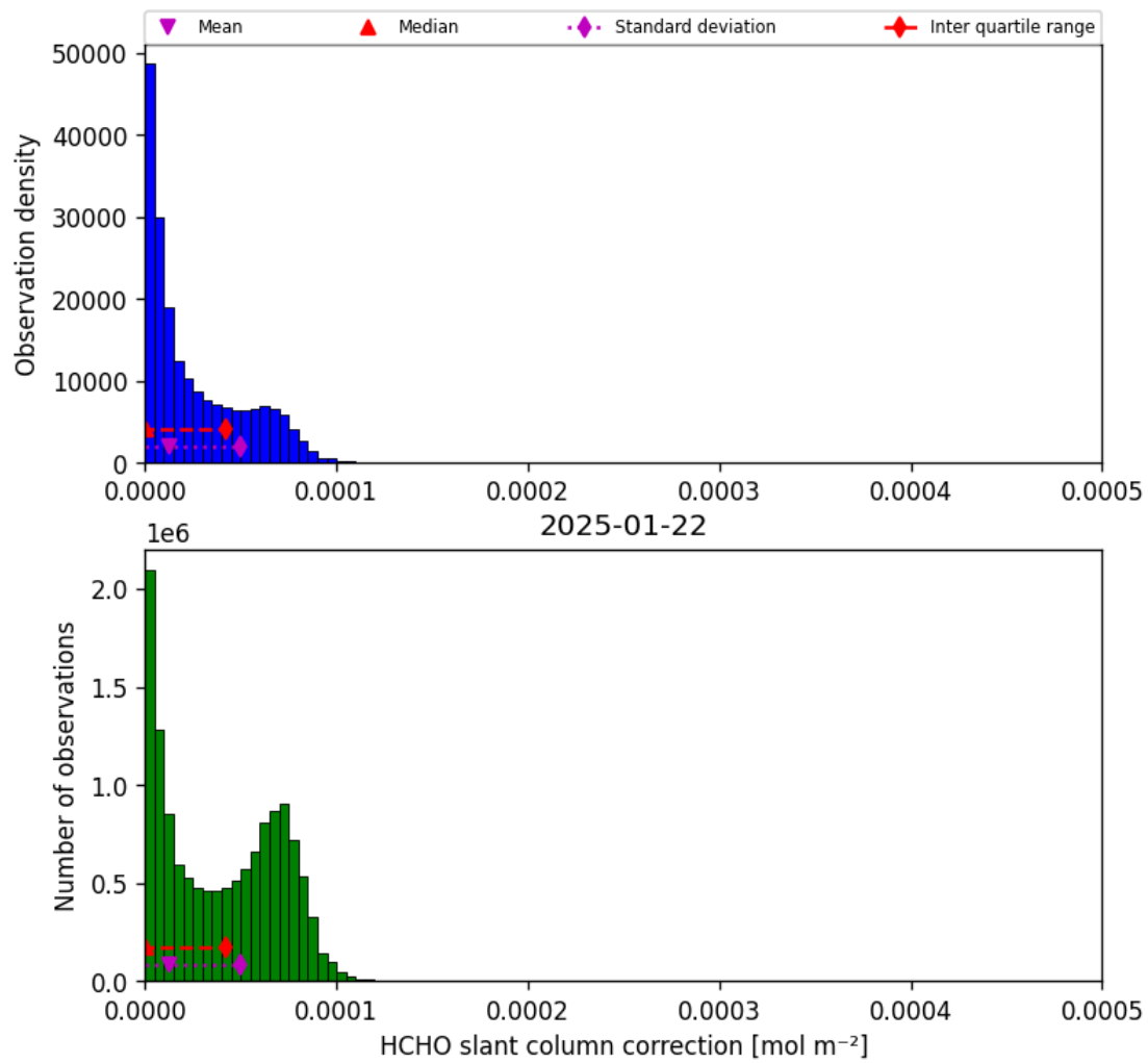
Figure 47: Histogram of “HCHO slant column correction” for 2025-01-21 to 2025-01-23
