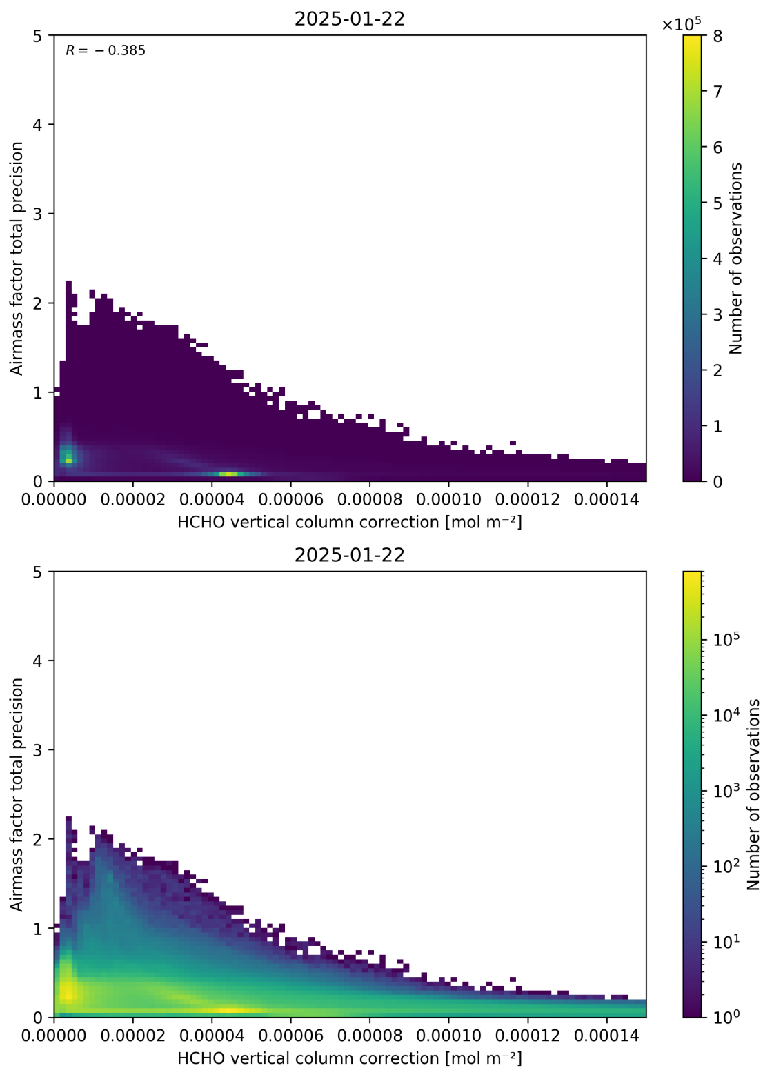
Figure 121: Scatter density plot of “HCHO vertical column correction” against “Airmass factor total precision” for 2025-01-21 to 2025-01-23.
