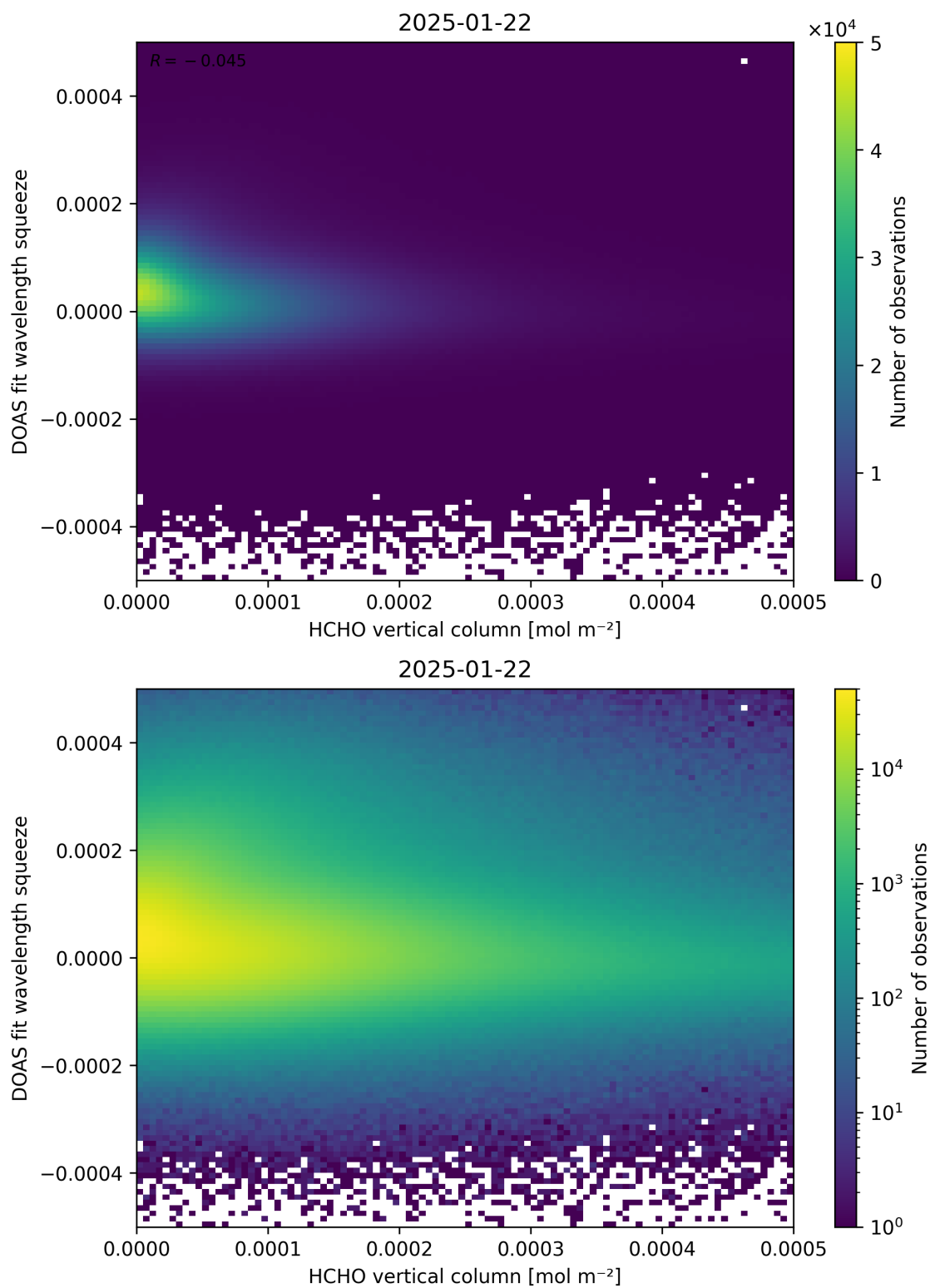
Figure 125: Scatter density plot of “HCHO vertical column” against “DOAS fit wavelength squeeze” for 2025-01-21 to 2025-01-23.
