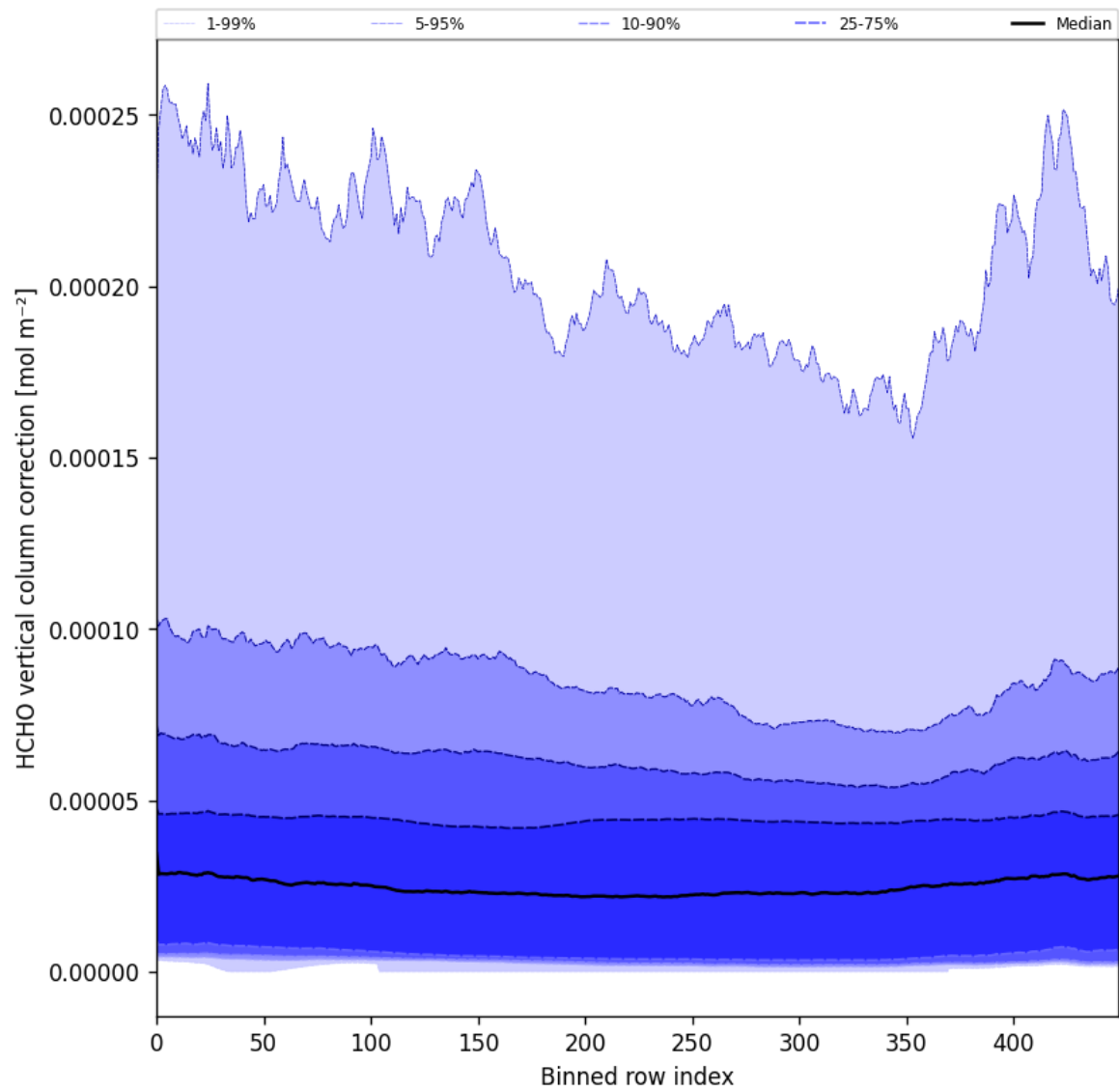
Figure 51: Along track statistics of “HCHO vertical column correction” for 2025-01-21 to 2025-01-23
