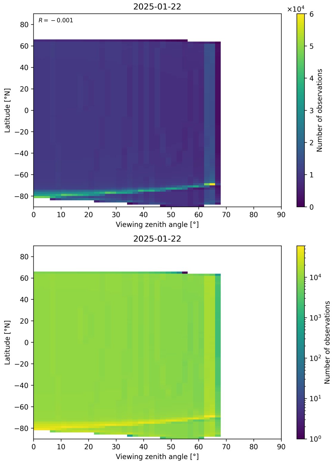
Figure 196: Scatter density plot of “Viewing zenith angle” against “Latitude” for 2025-01-21 to 2025-01-23.
