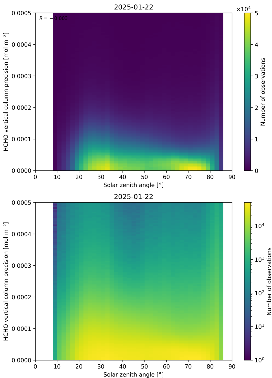
Figure 179: Scatter density plot of “Solar zenith angle” against “HCHO vertical column precision” for 2025-01-21 to 2025-01-23.
