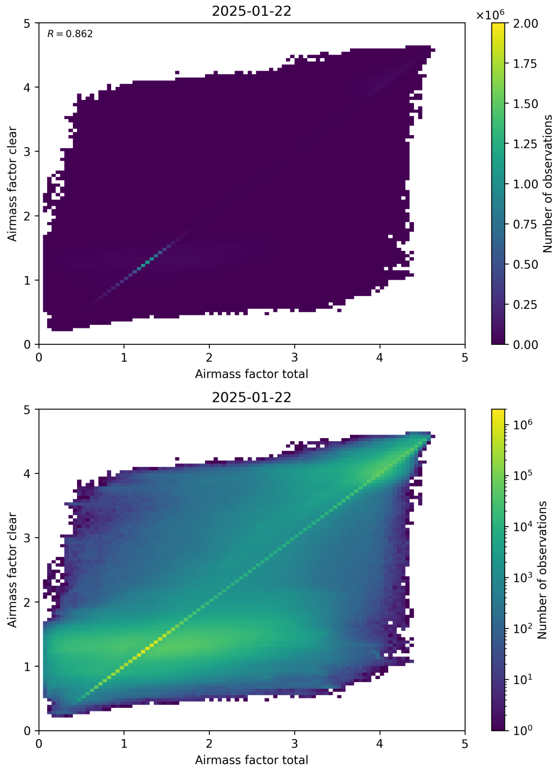
Figure 100: Scatter density plot of “Airmass factor total” against “Airmass factor clear” for 2025-01-21 to 2025-01-23.
