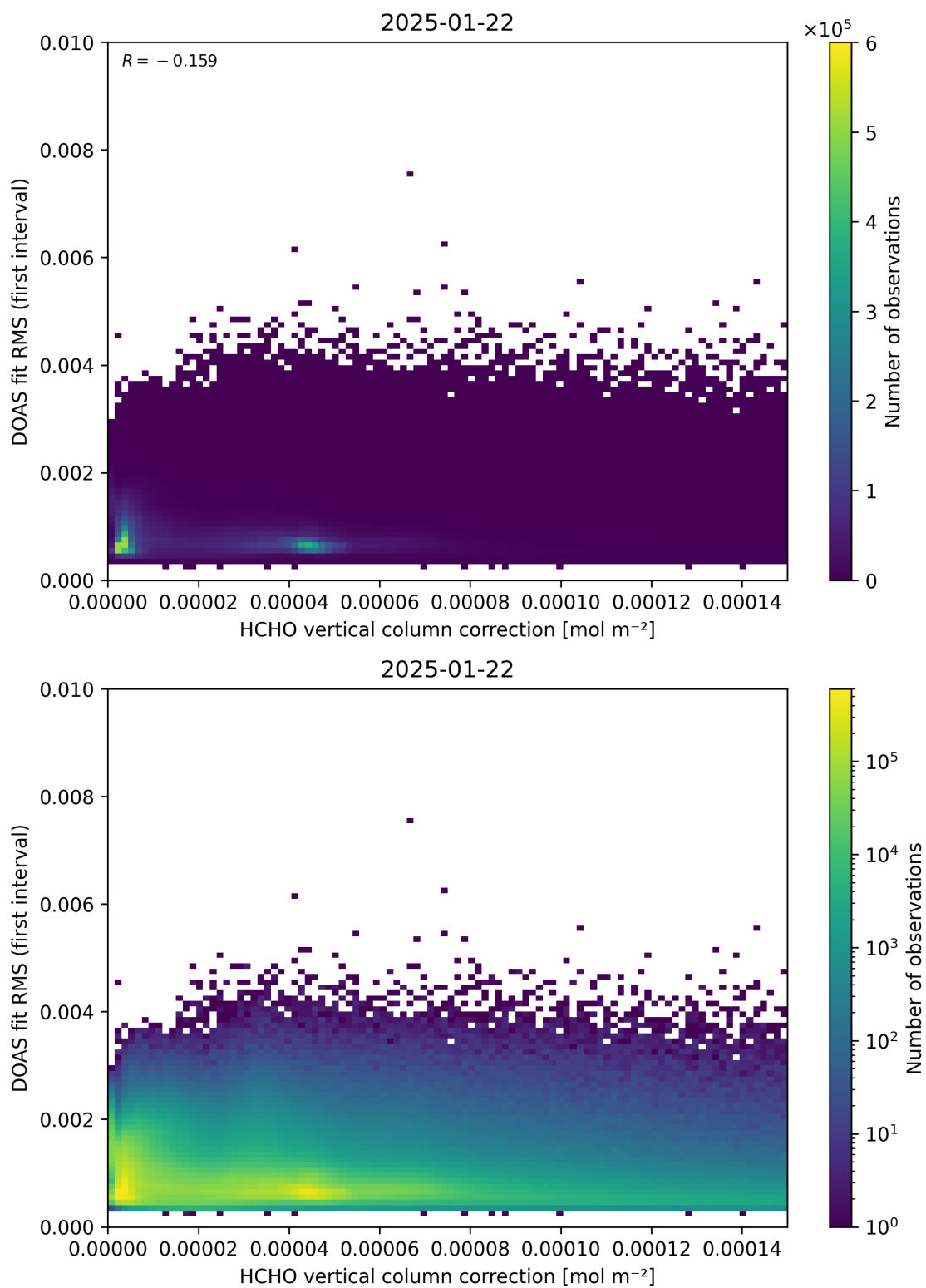
Figure 112: Scatter density plot of “HCHO vertical column correction” against “DOAS fit RMS (first interval)” for 2025-01-21 to 2025-01-23.
