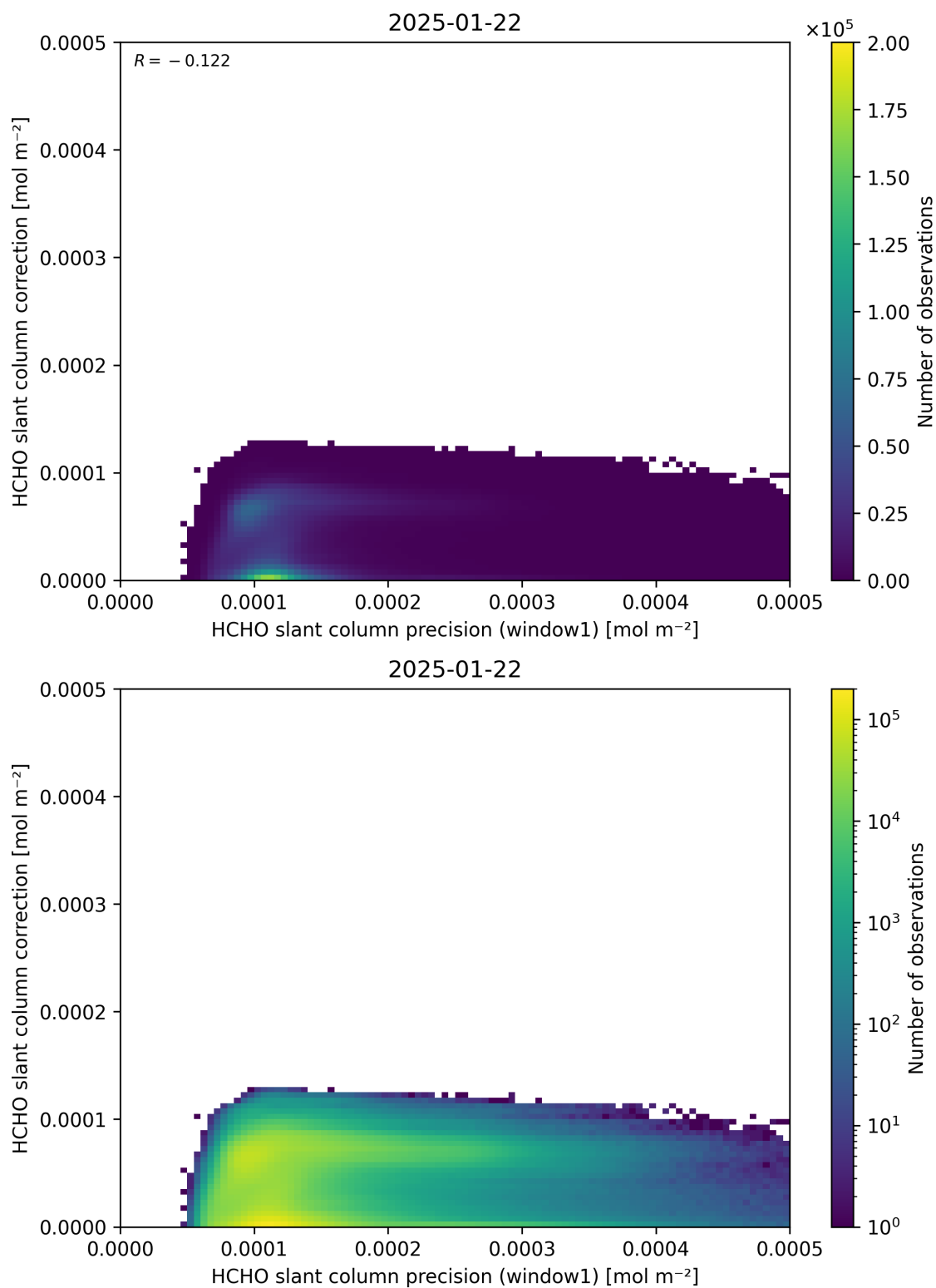
Figure 93: Scatter density plot of “HCHO slant column precision (window1)” against “HCHO slant column correction” for 2025-01-21 to 2025-01-23.
