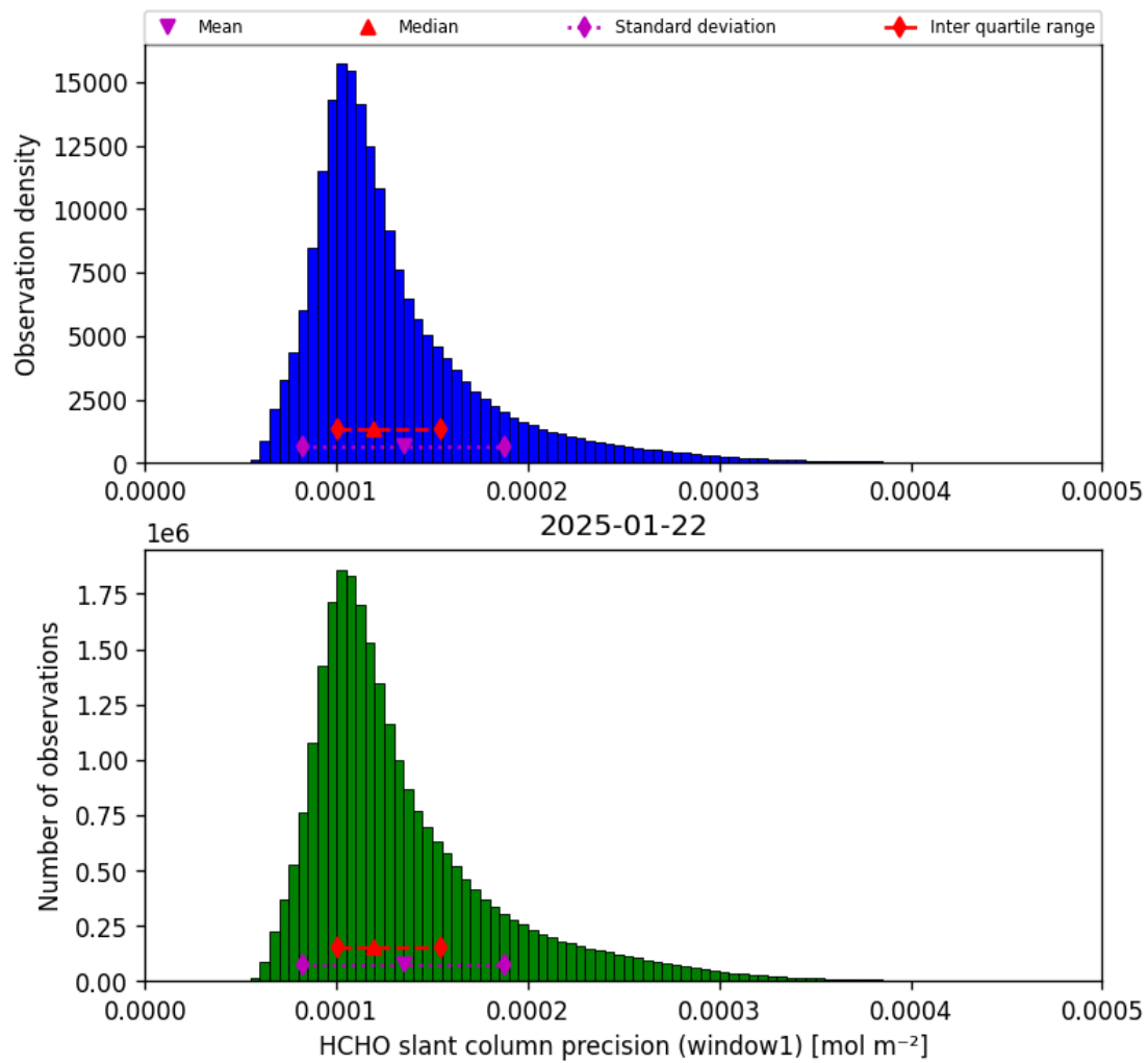
Figure 39: Histogram of “HCHO slant column precision (window1)” for 2025-01-21 to 2025-01-23
