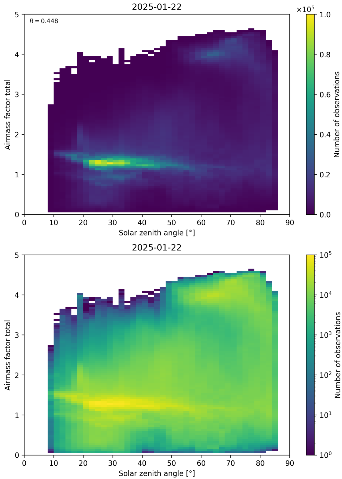
Figure 175: Scatter density plot of “Solar zenith angle” against “Airmass factor total” for 2025-01-21 to 2025-01-23.
