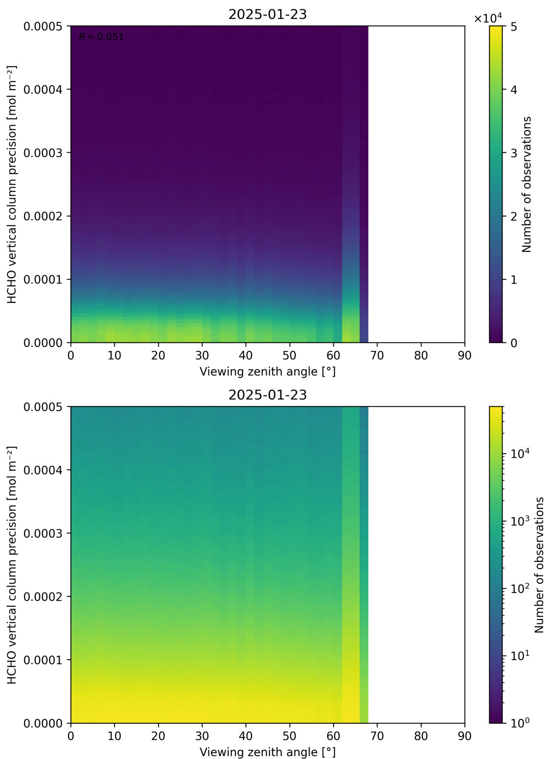
Figure 194: Scatter density plot of “Viewing zenith angle” against “HCHO vertical column precision” for 2025-01-23 to 2025-01-24.
