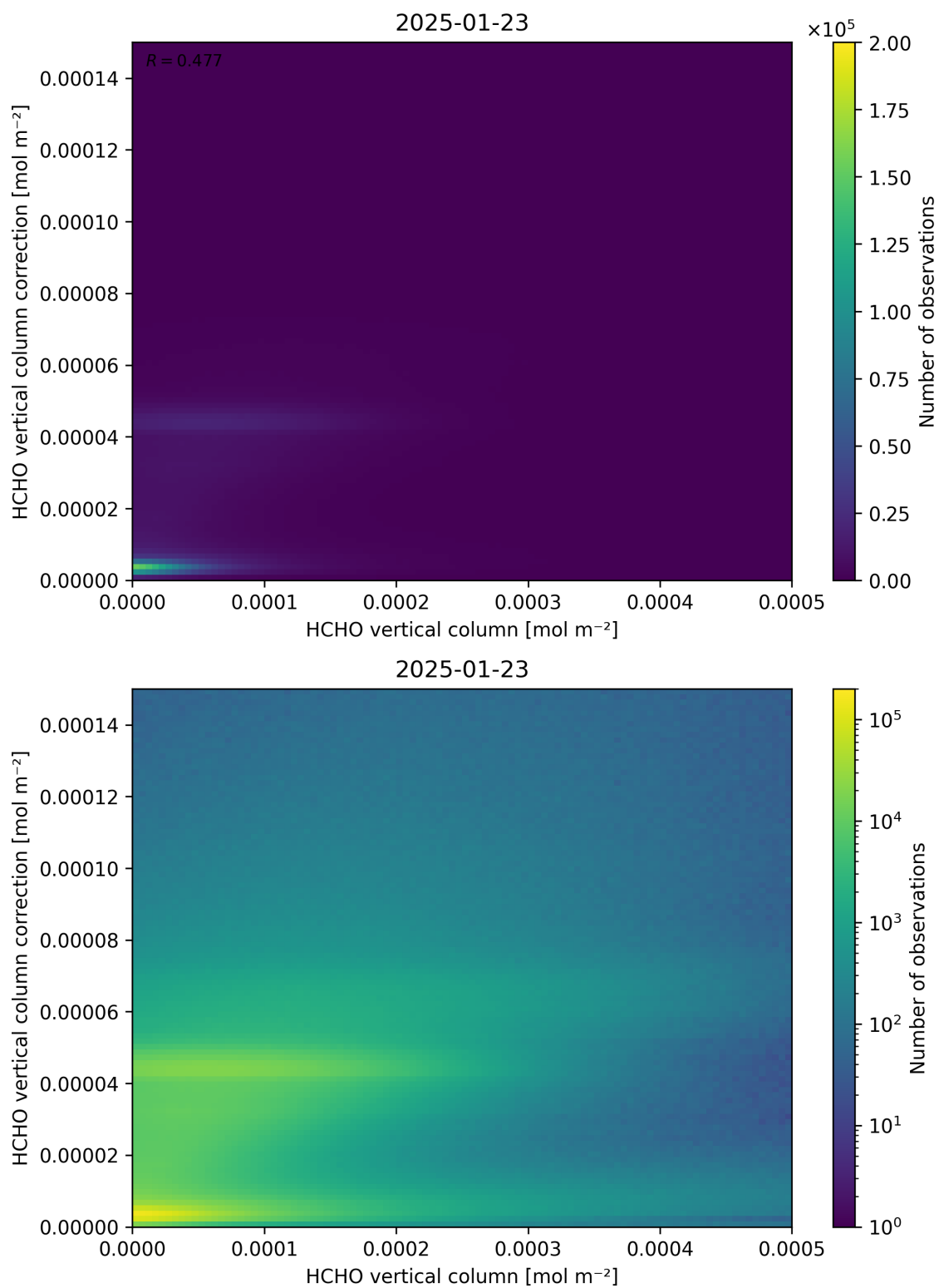
Figure 133: Scatter density plot of “HCHO vertical column” against “HCHO vertical column correction” for 2025-01-23 to 2025-01-24.
