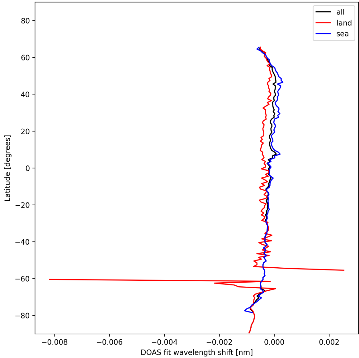
Figure 30: Zonal average of “DOAS fit wavelength shift” for 2025-01-23 to 2025-01-24.
