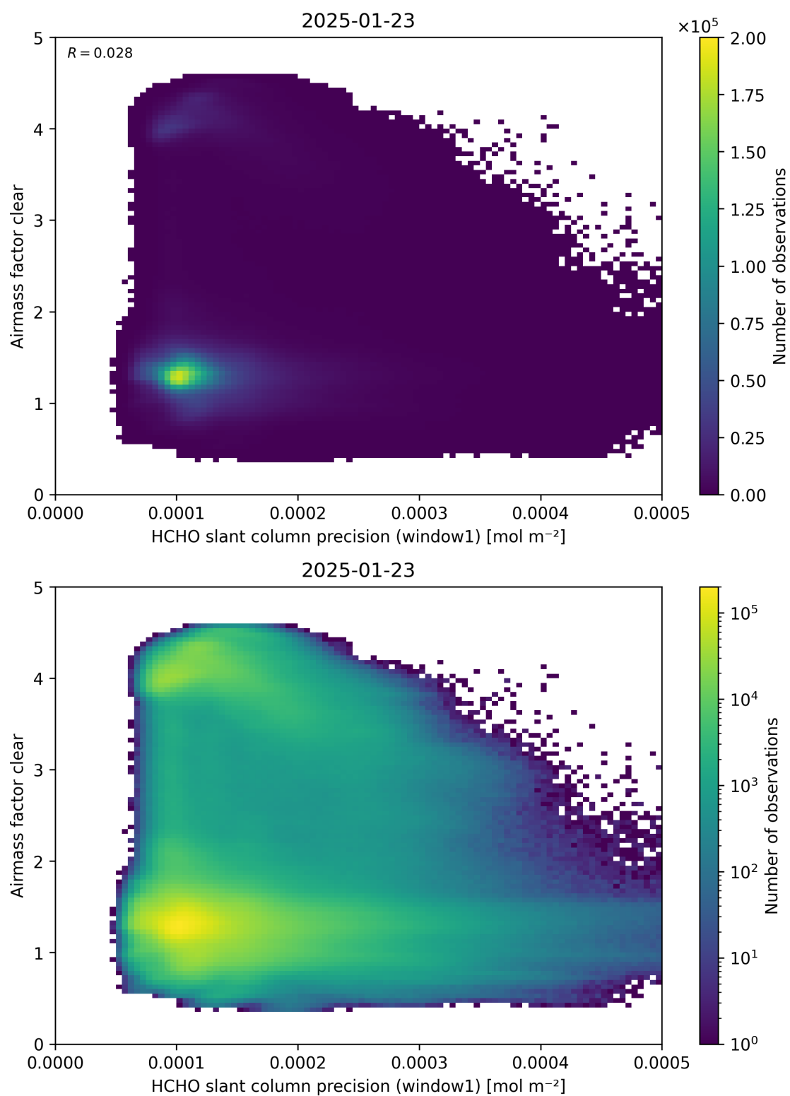
Figure 91: Scatter density plot of “HCHO slant column precision (window1)” against “Airmass factor clear” for 2025-01-23 to 2025-01-24.
