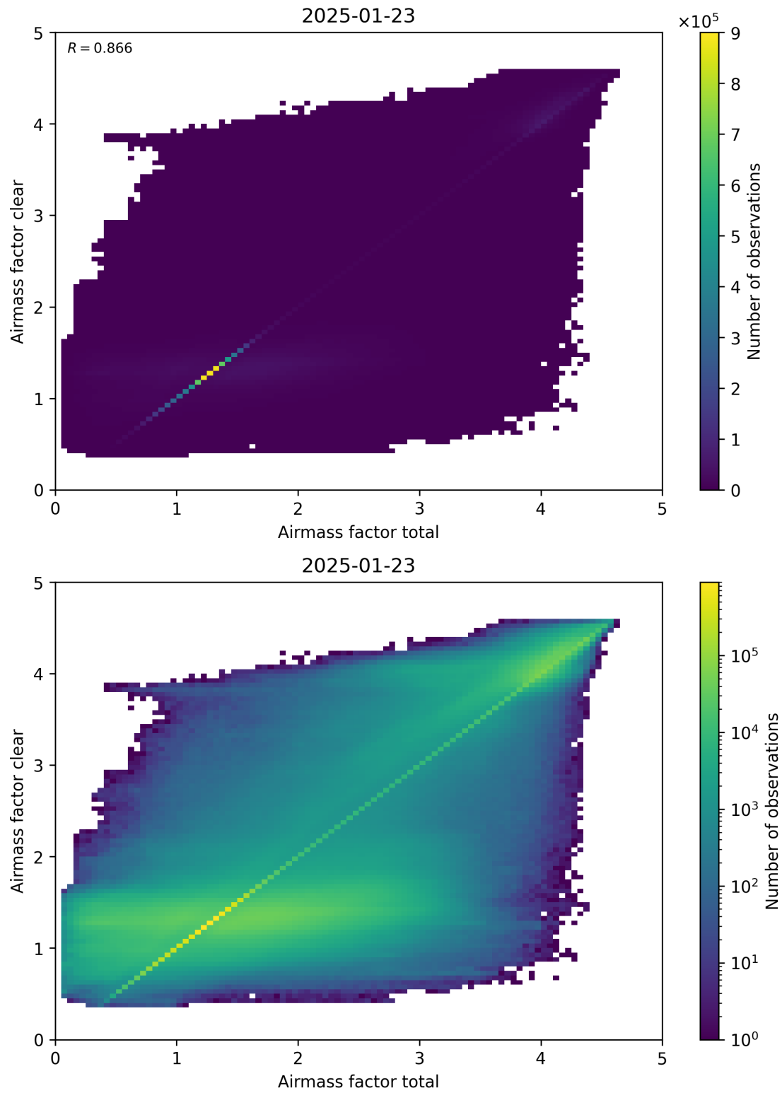
Figure 100: Scatter density plot of “Airmass factor total” against “Airmass factor clear” for 2025-01-23 to 2025-01-24.
