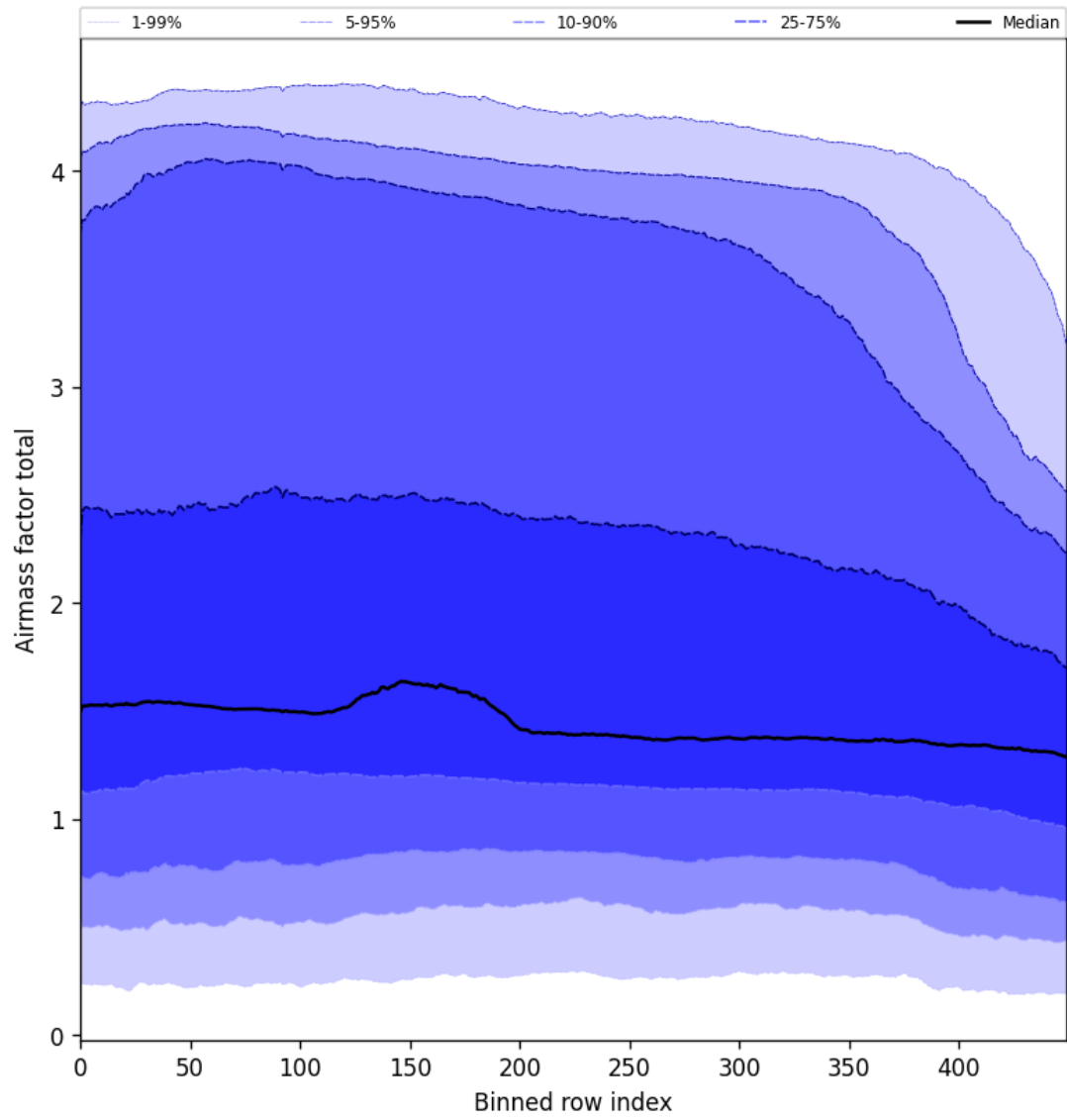
Figure 54: Along track statistics of “Airmass factor total” for 2025-01-23 to 2025-01-24
