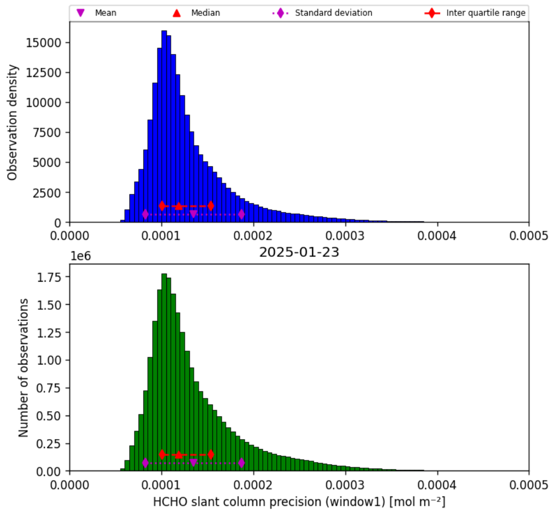
Figure 39: Histogram of “HCHO slant column precision (window1)” for 2025-01-23 to 2025-01-24
