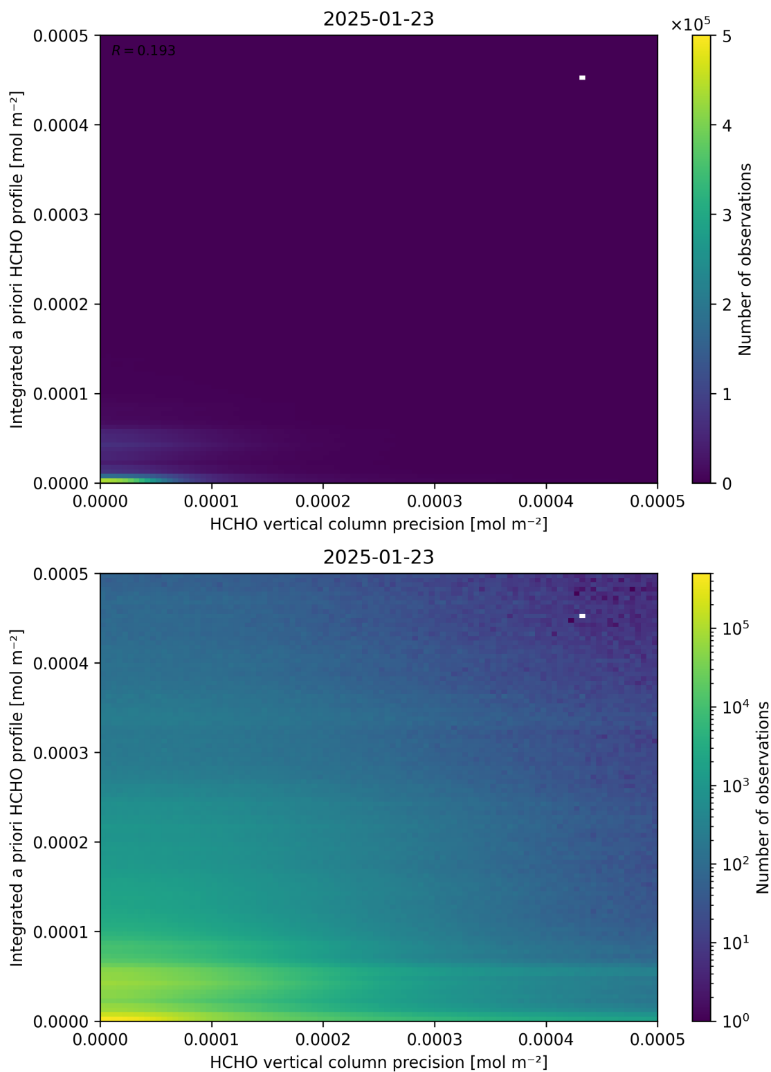
Figure 147: Scatter density plot of “HCHO vertical column precision” against “Integrated a priori HCHO profile” for 2025-01-23 to 2025-01-24.
