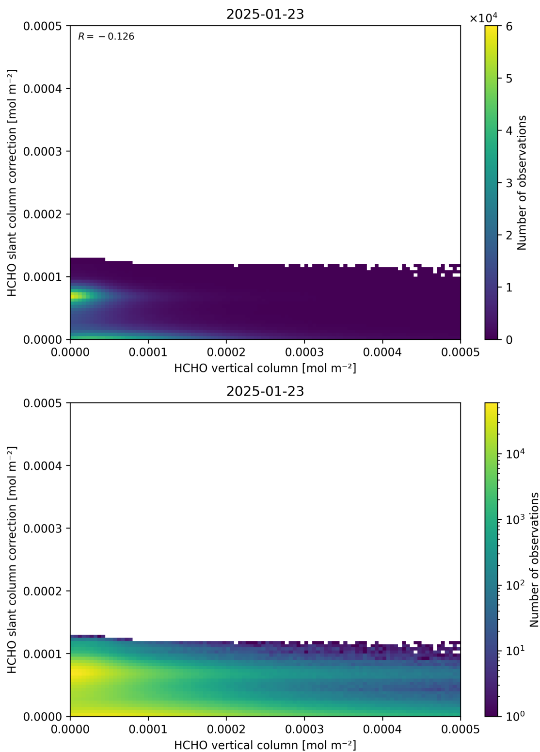
Figure 128: Scatter density plot of “HCHO vertical column” against “HCHO slant column correction” for 2025-01-23 to 2025-01-24.
