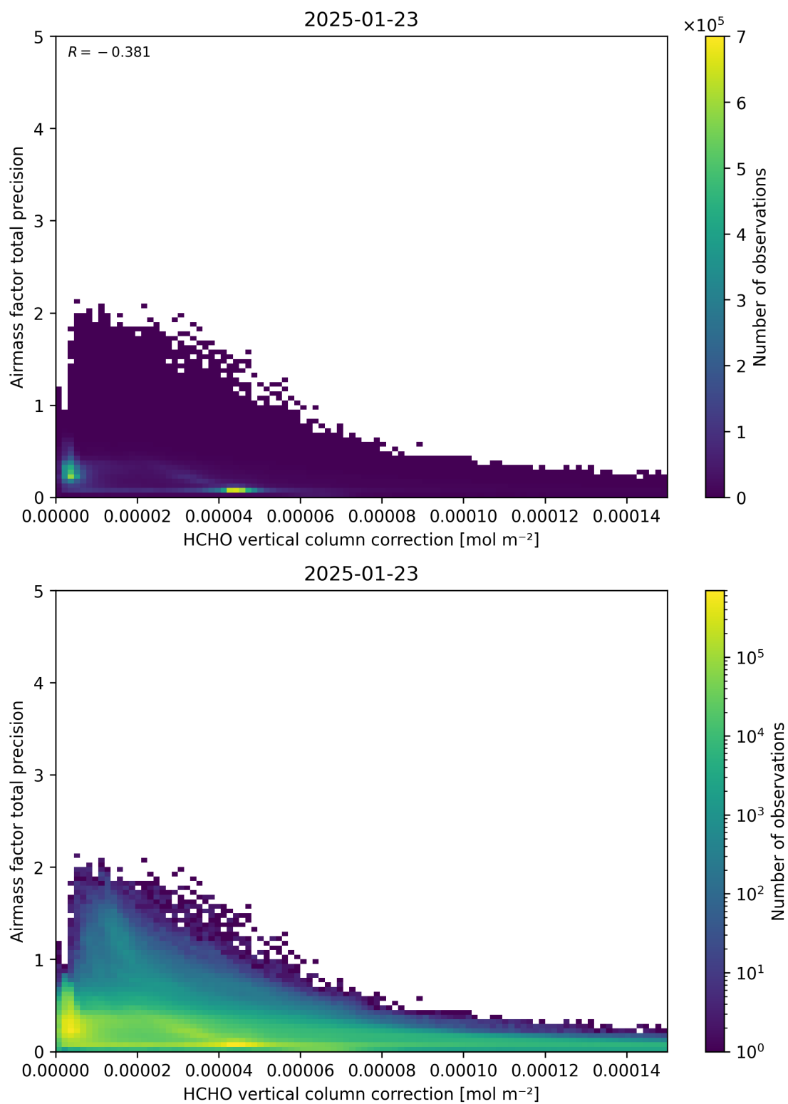
Figure 121: Scatter density plot of “HCHO vertical column correction” against “Airmass factor total precision” for 2025-01-23 to 2025-01-24.
