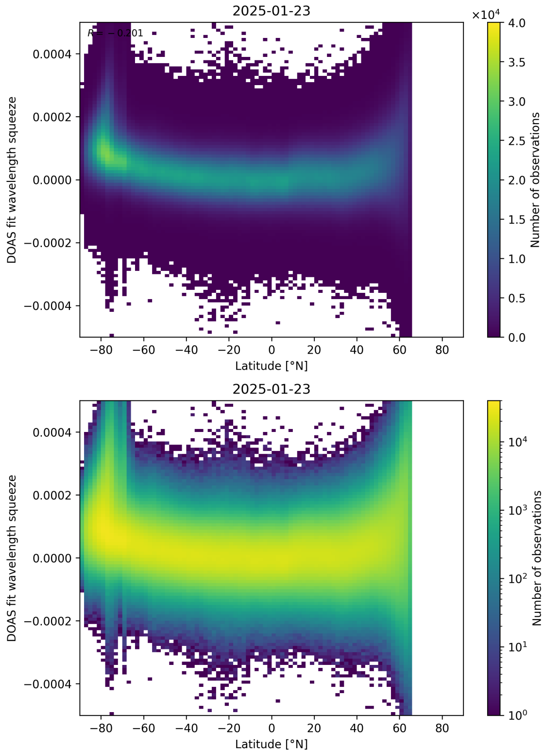
Figure 155: Scatter density plot of “Latitude” against “DOAS fit wavelength squeeze” for 2025-01-23 to 2025-01-24.
