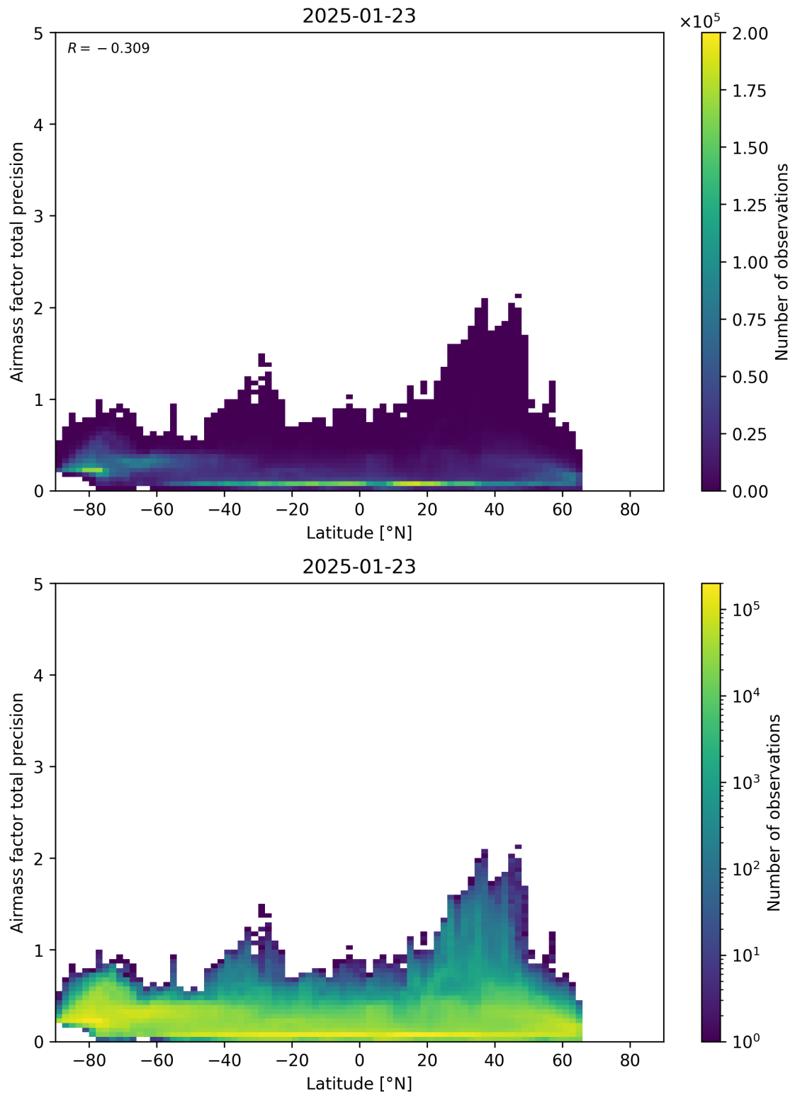
Figure 162: Scatter density plot of “Latitude” against “Airmass factor total precision” for 2025-01-23 to 2025-01-24.
