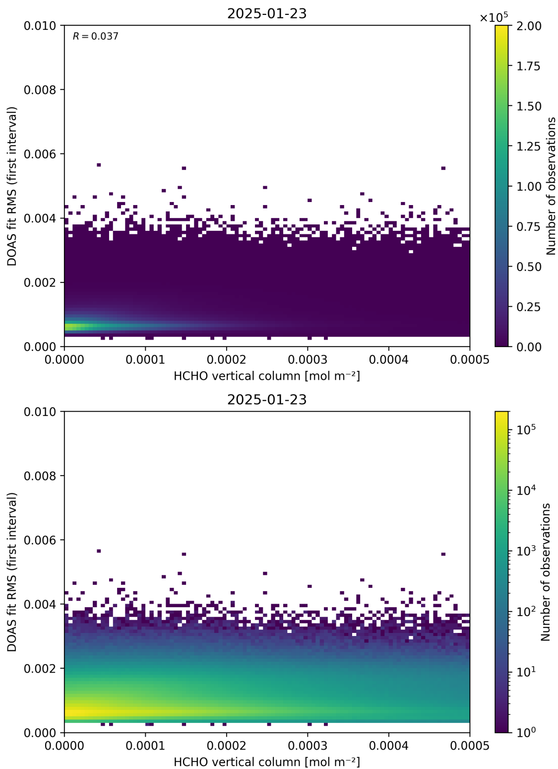
Figure 123: Scatter density plot of “HCHO vertical column” against “DOAS fit RMS (first interval)” for 2025-01-23 to 2025-01-24.
