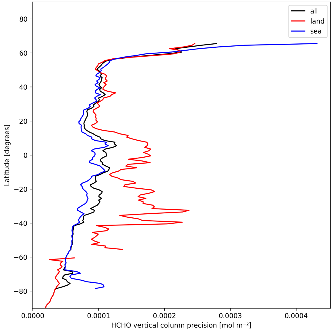
Figure 22: Zonal average of “HCHO vertical column precision” for 2025-01-23 to 2025-01-24.
