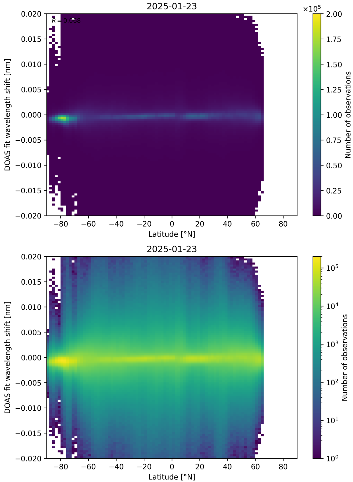
Figure 154: Scatter density plot of “Latitude” against “DOAS fit wavelength shift” for 2025-01-23 to 2025-01-24.
