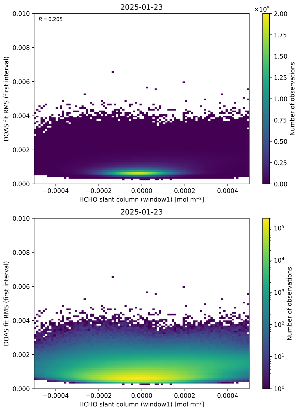
Figure 78: Scatter density plot of “HCHO slant column (window1)” against “DOAS fit RMS (first interval)” for 2025-01-23 to 2025-01-24.
