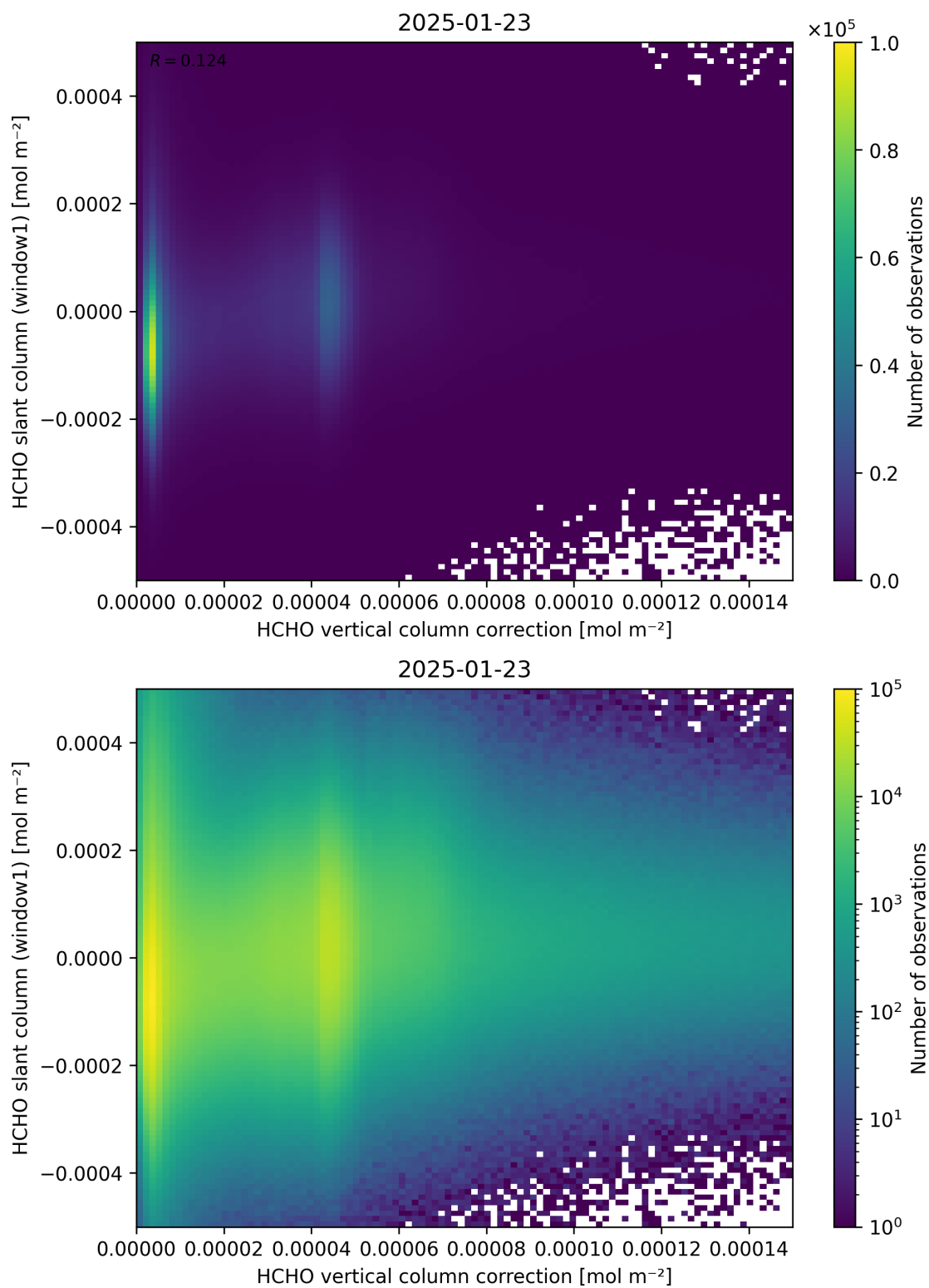
Figure 118: Scatter density plot of “HCHO vertical column correction” against “HCHO slant column (window1)” for 2025-01-23 to 2025-01-24.
