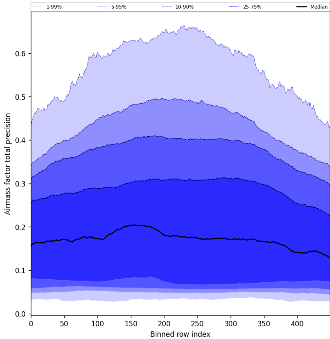
Figure 55: Along track statistics of “Airmass factor total precision” for 2025-01-23 to 2025-01-24
