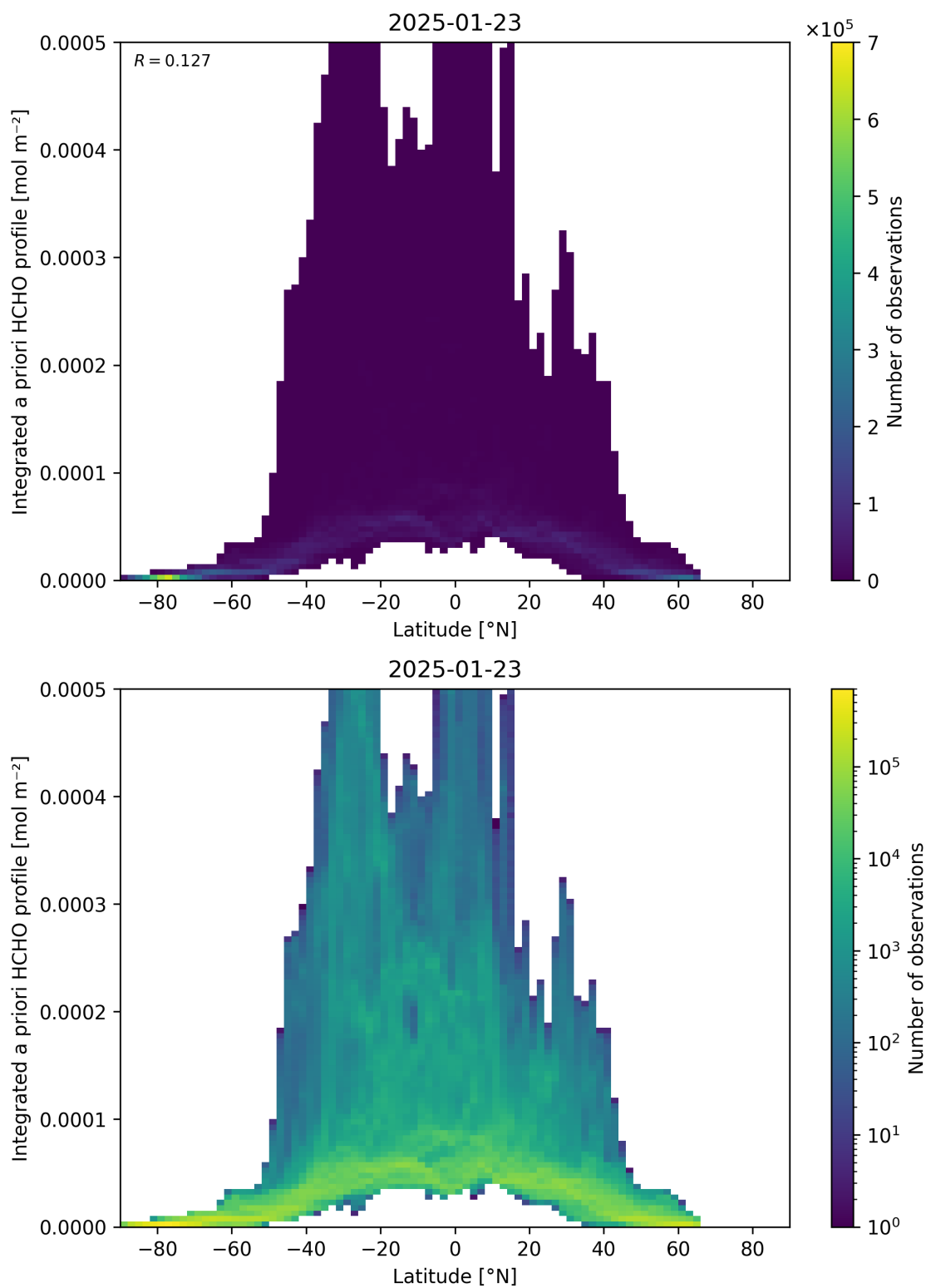
Figure 166: Scatter density plot of “Latitude” against “Integrated a priori HCHO profile” for 2025-01-23 to 2025-01-24.
