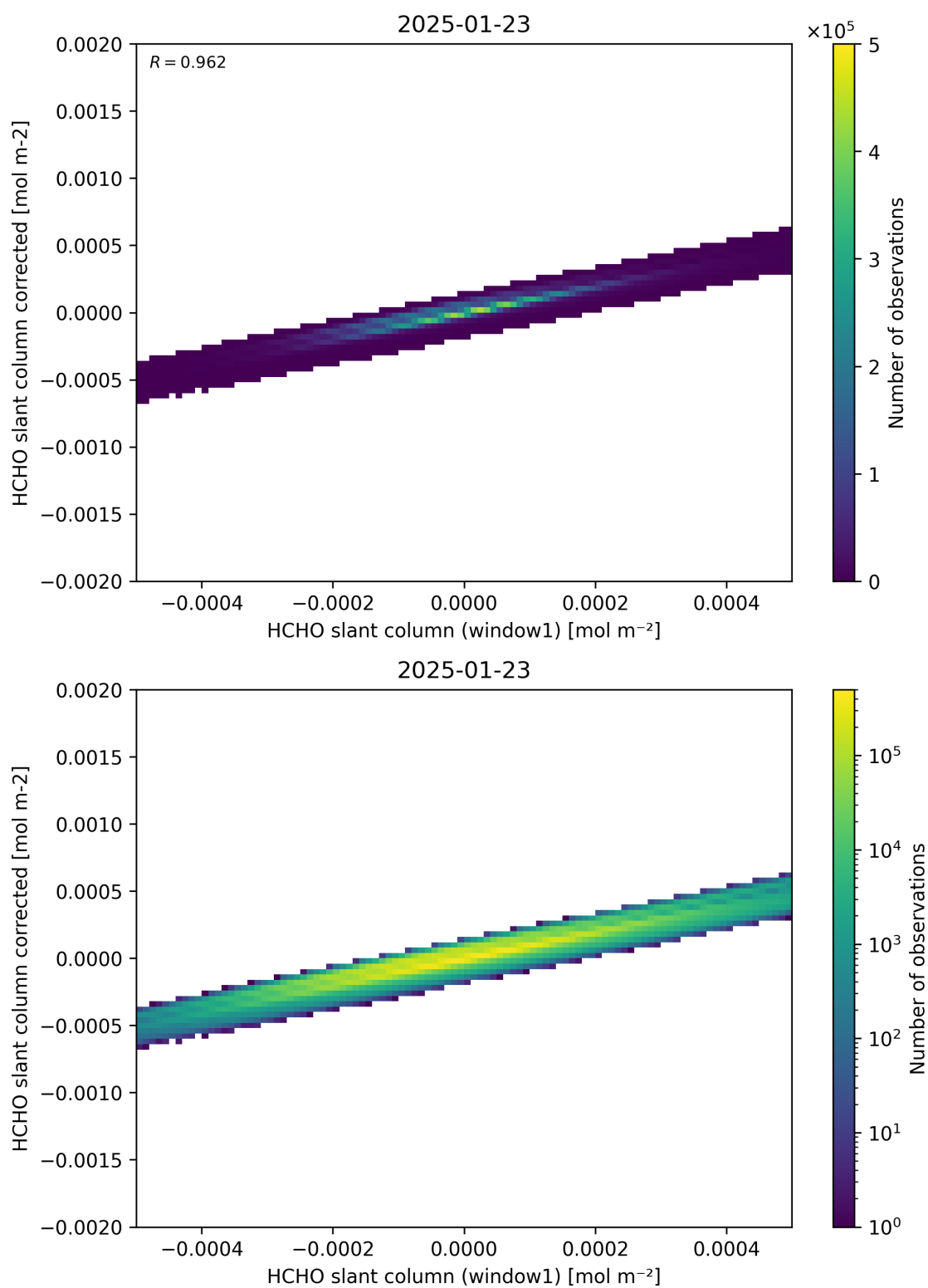
Figure 82: Scatter density plot of “HCHO slant column (window1)” against “HCHO slant column corrected” for 2025-01-23 to 2025-01-24.
