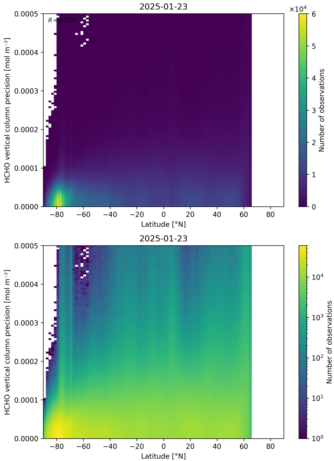
Figure 165: Scatter density plot of “Latitude” against “HCHO vertical column precision” for 2025-01-23 to 2025-01-24.
