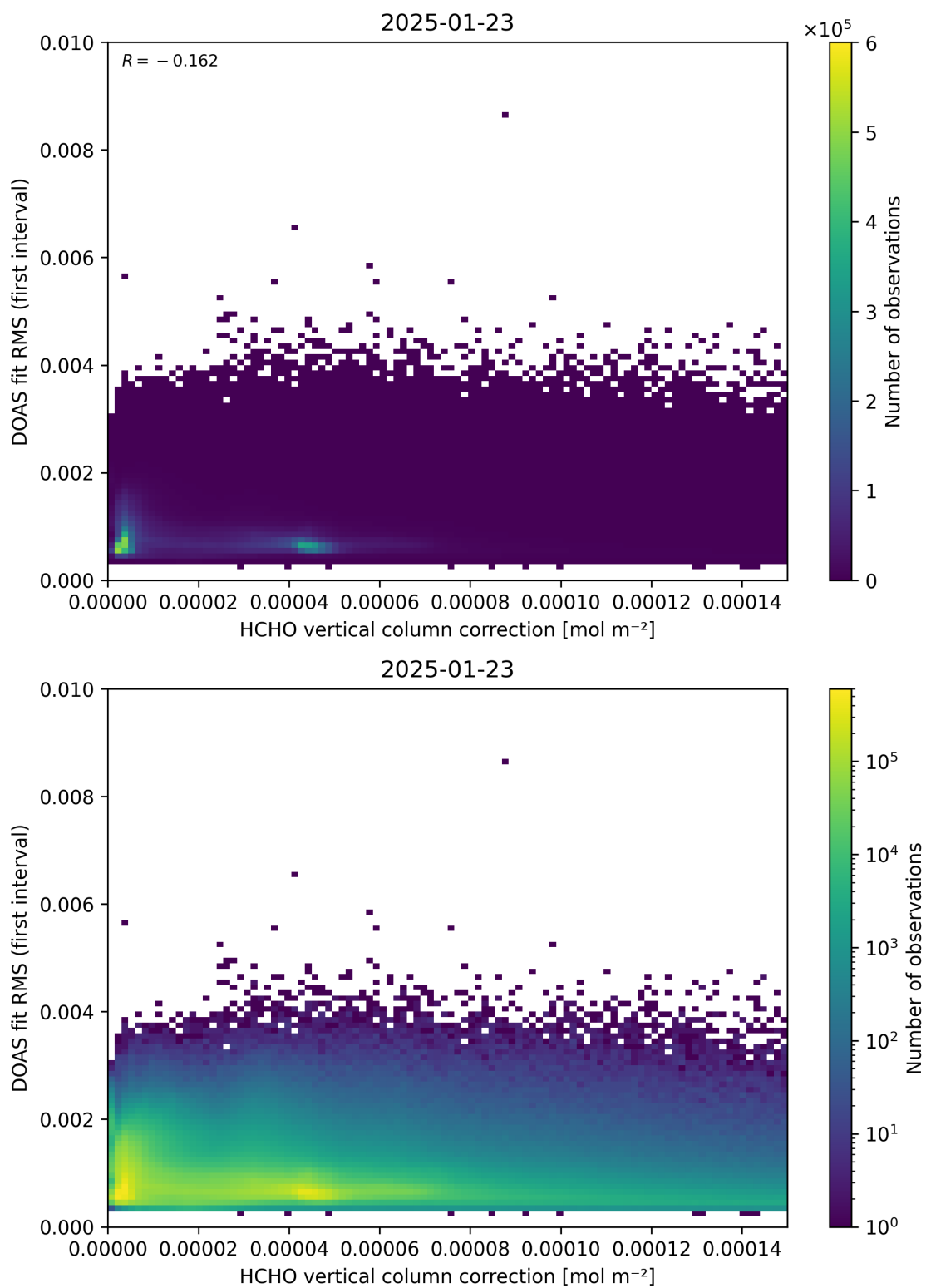
Figure 112: Scatter density plot of “HCHO vertical column correction” against “DOAS fit RMS (first interval)” for 2025-01-23 to 2025-01-24.
