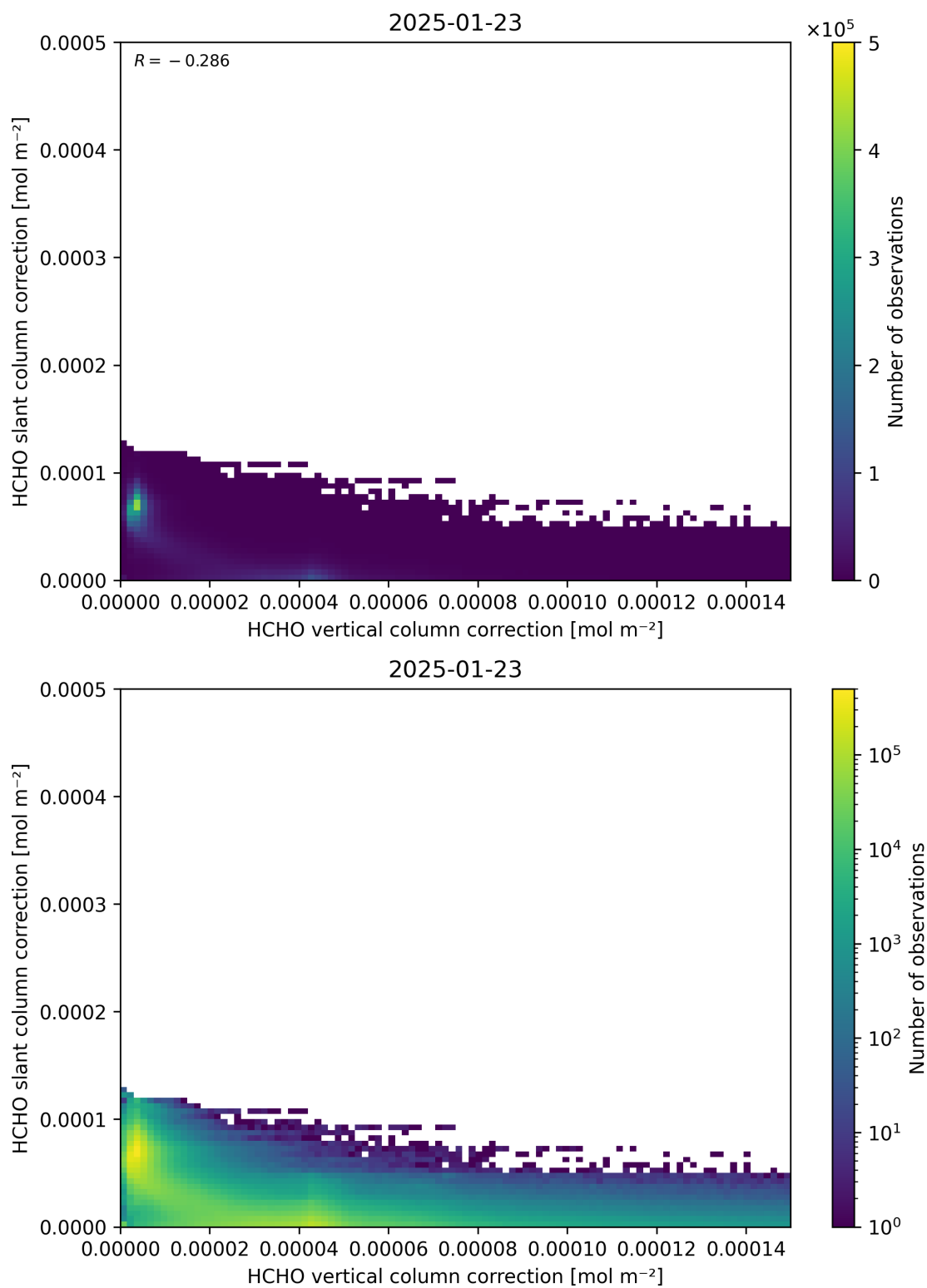
Figure 117: Scatter density plot of “HCHO vertical column correction” against “HCHO slant column correction” for 2025-01-23 to 2025-01-24.
