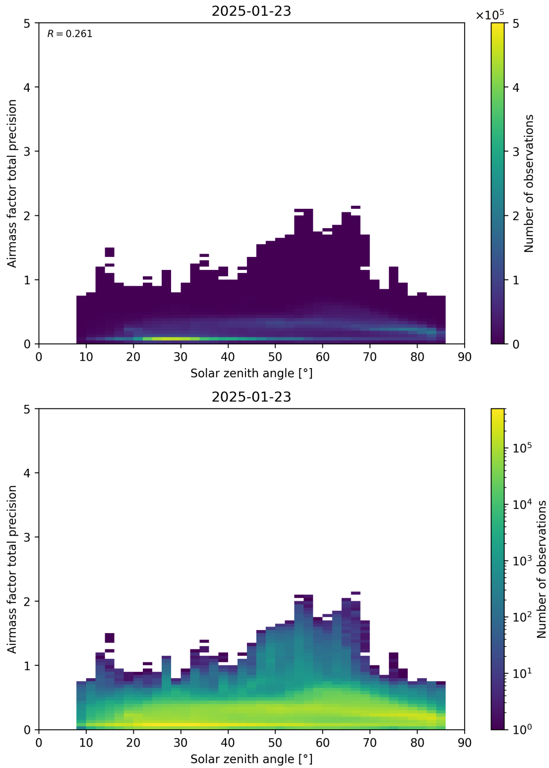
Figure 176: Scatter density plot of “Solar zenith angle” against “Airmass factor total precision” for 2025-01-23 to 2025-01-24.
