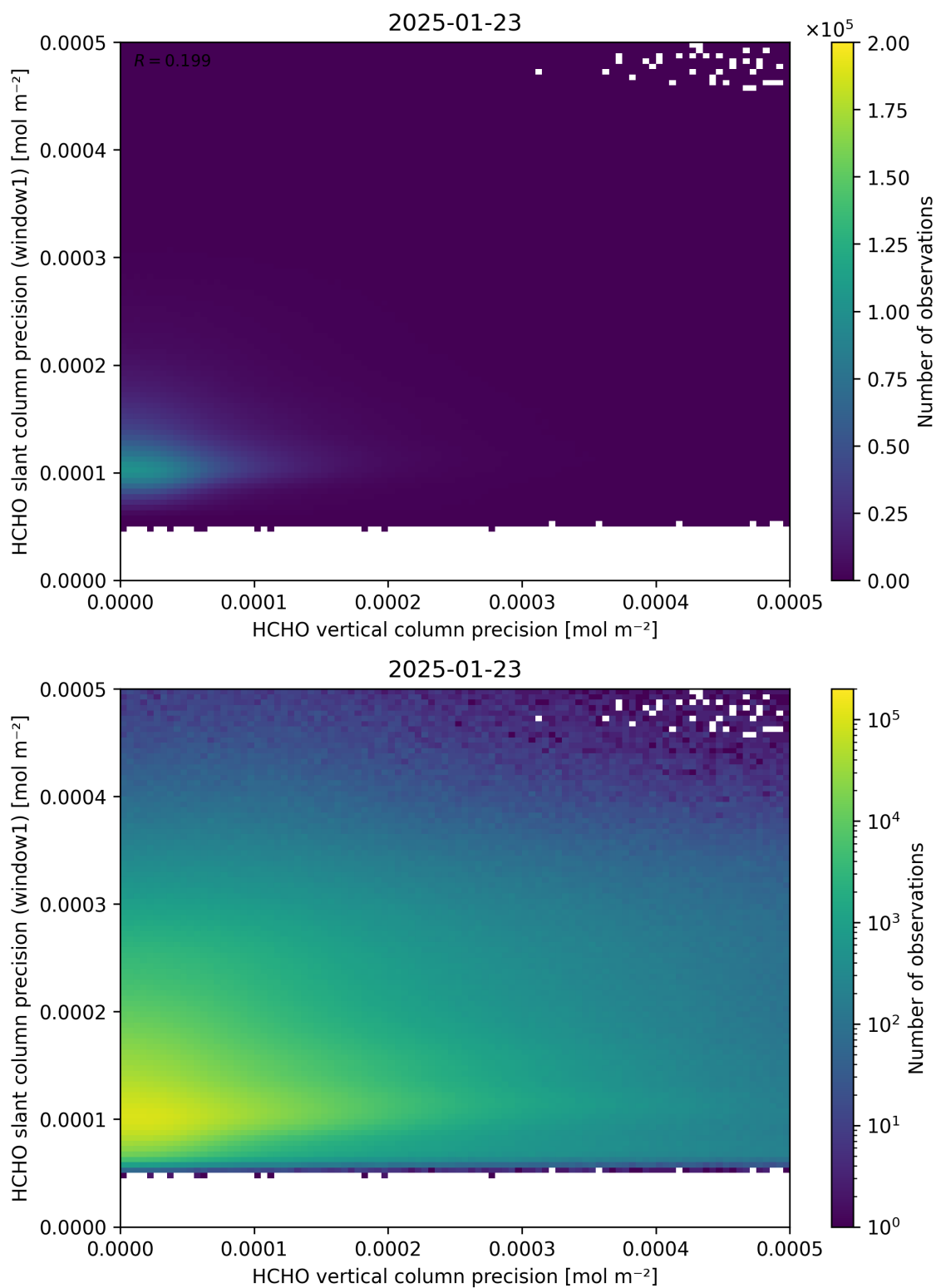
Figure 143: Scatter density plot of “HCHO vertical column precision” against “HCHO slant column precision (window1)” for 2025-01-23 to 2025-01-24.
