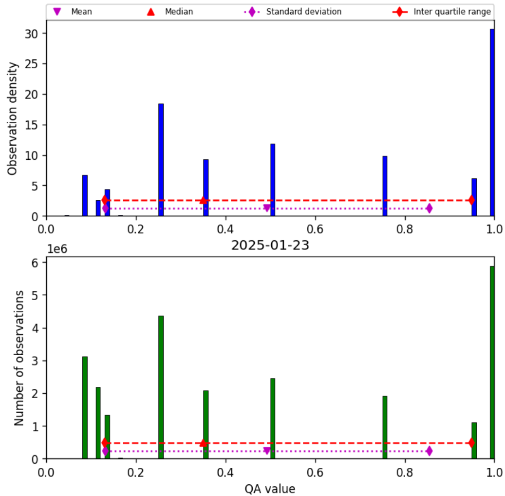
Figure 34: Histogram of “QA value” for 2025-01-23 to 2025-01-24
