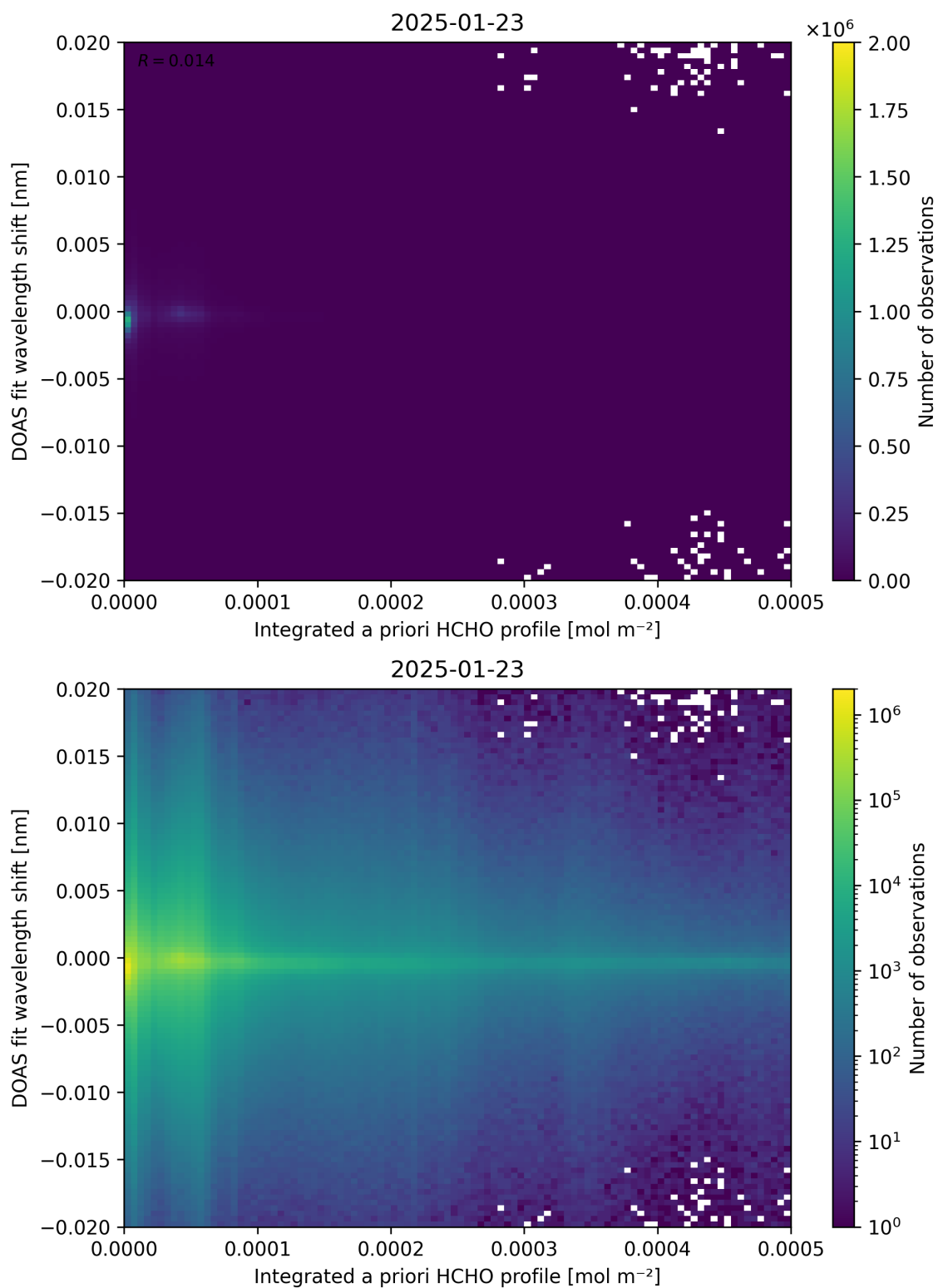
Figure 149: Scatter density plot of “Integrated a priori HCHO profile” against “DOAS fit wavelength shift” for 2025-01-23 to 2025-01-24.
