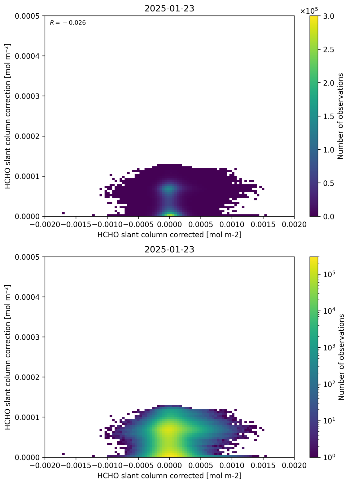
Figure 77: Scatter density plot of “HCHO slant column corrected” against “HCHO slant column correction” for 2025-01-23 to 2025-01-24.
