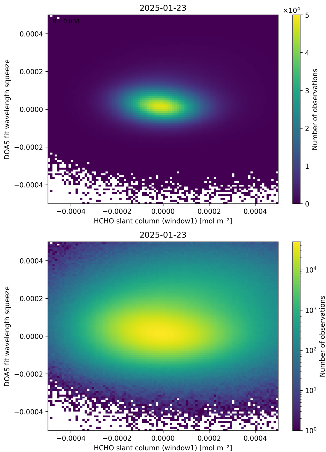
Figure 80: Scatter density plot of “HCHO slant column (window1)” against “DOAS fit wavelength squeeze” for 2025-01-23 to 2025-01-24.
