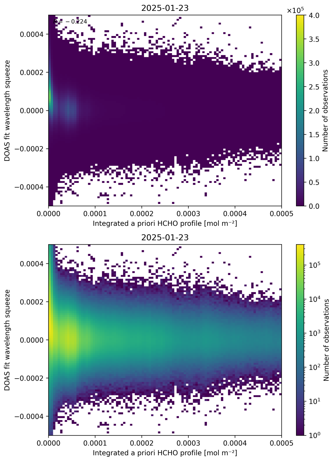
Figure 150: Scatter density plot of “Integrated a priori HCHO profile” against “DOAS fit wavelength squeeze” for 2025-01-23 to 2025-01-24.
