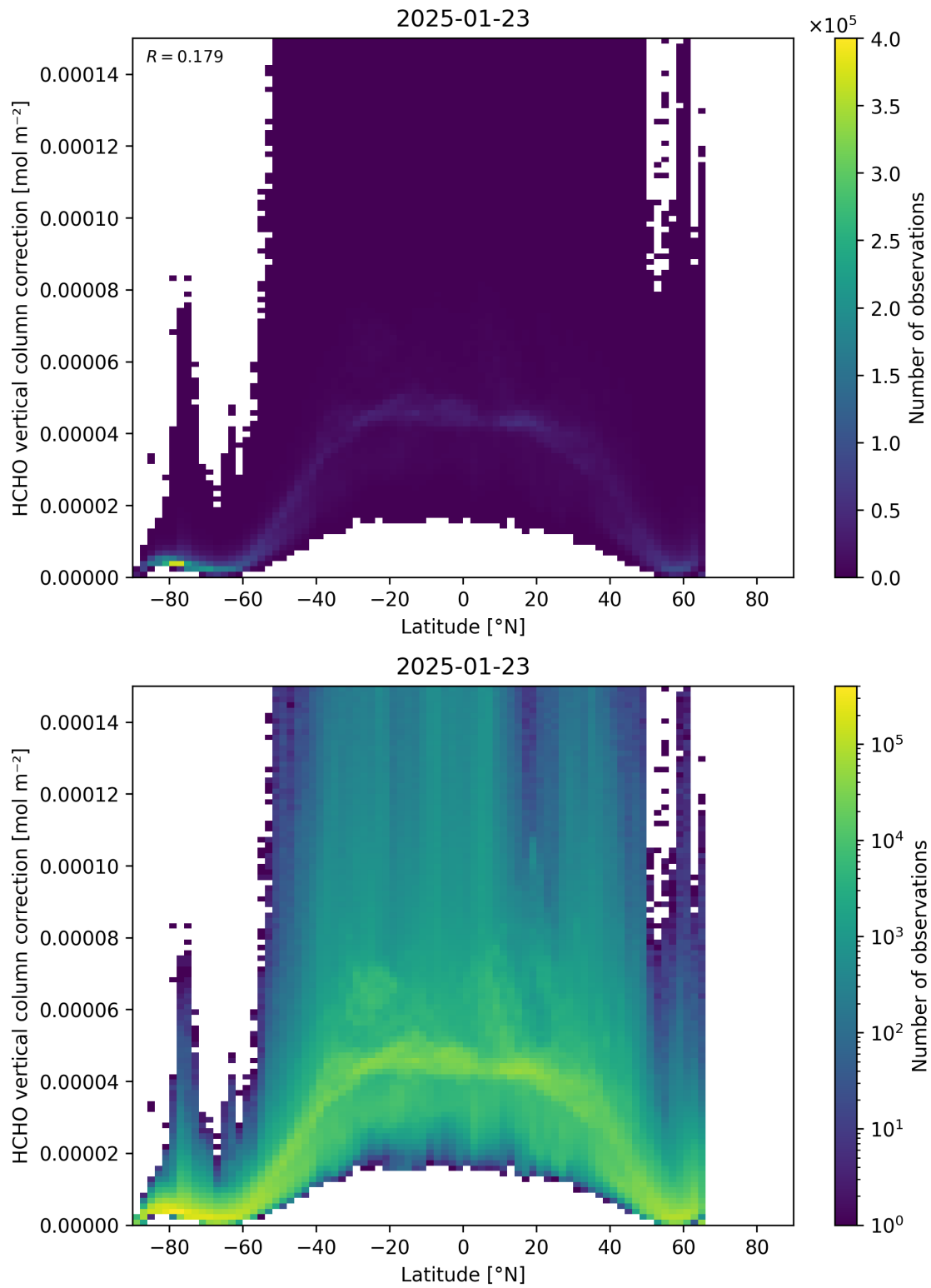
Figure 164: Scatter density plot of “Latitude” against “HCHO vertical column correction” for 2025-01-23 to 2025-01-24.
