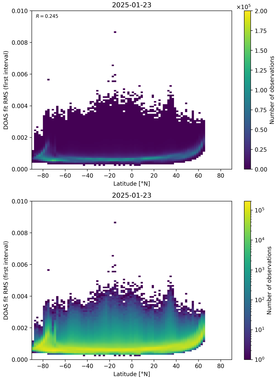
Figure 153: Scatter density plot of “Latitude” against “DOAS fit RMS (first interval)” for 2025-01-23 to 2025-01-24.
