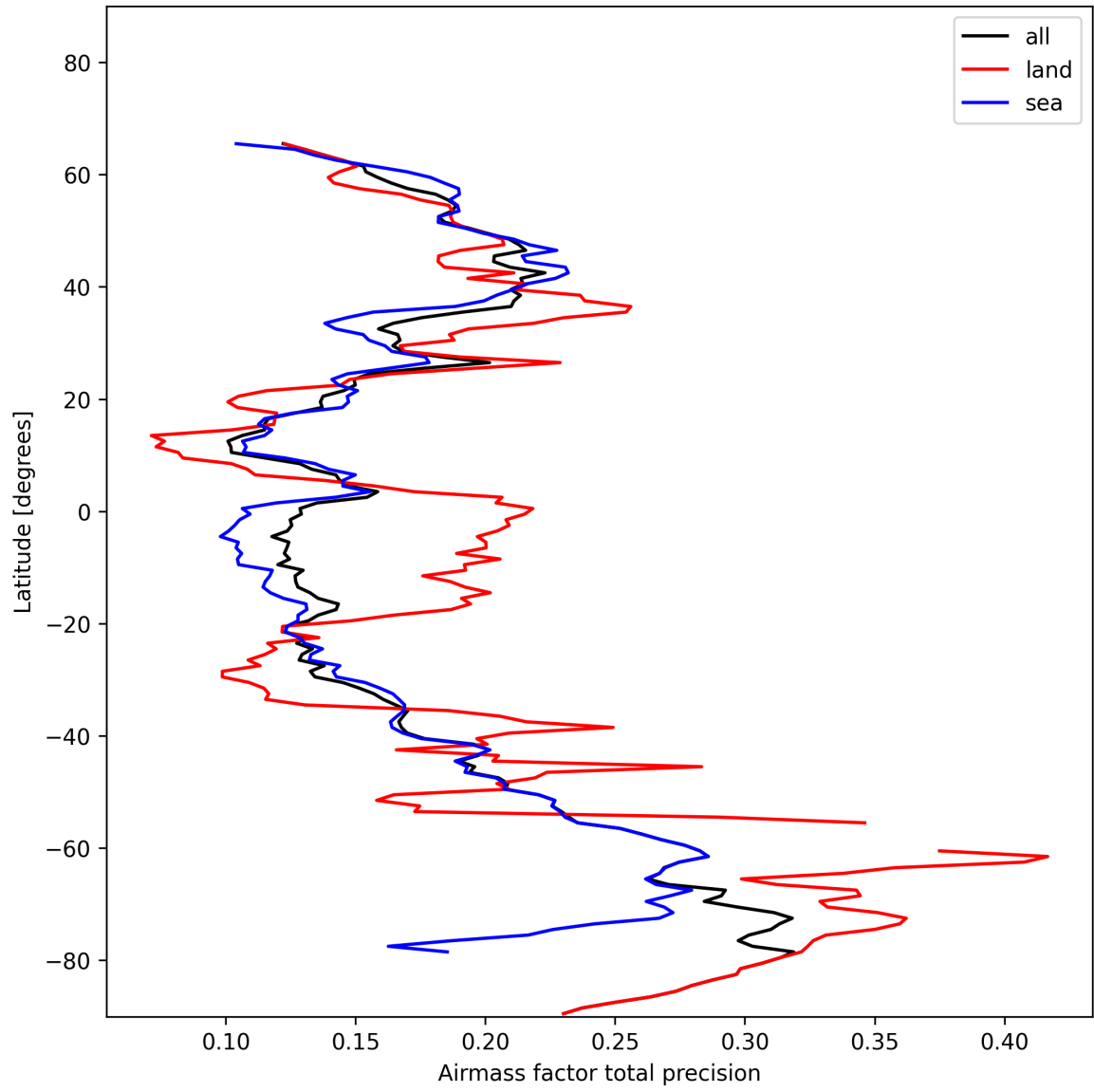
Figure 27: Zonal average of “Airmass factor total precision” for 2025-01-23 to 2025-01-24.
