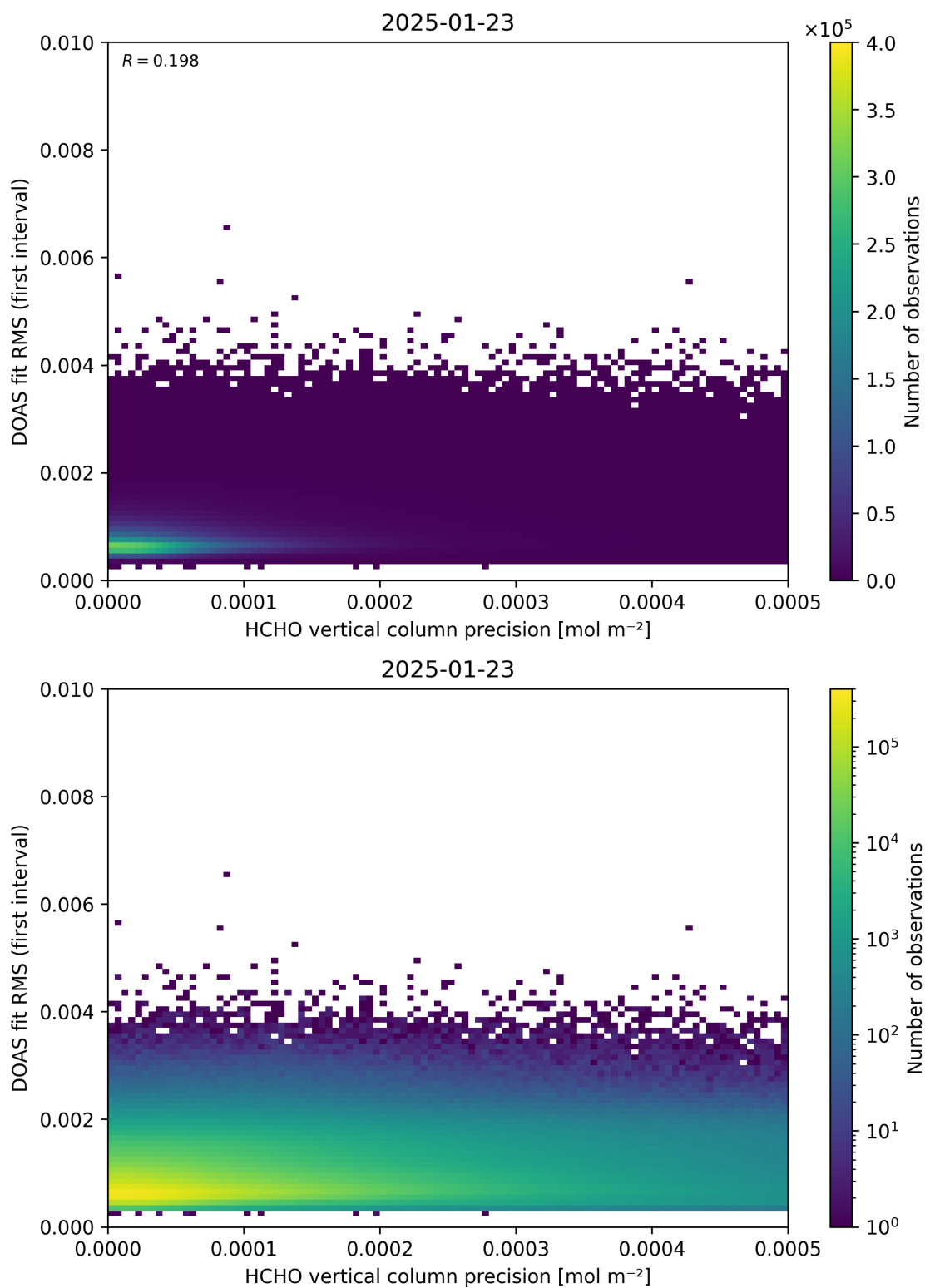
Figure 136: Scatter density plot of “HCHO vertical column precision” against “DOAS fit RMS (first interval)” for 2025-01-23 to 2025-01-24.
