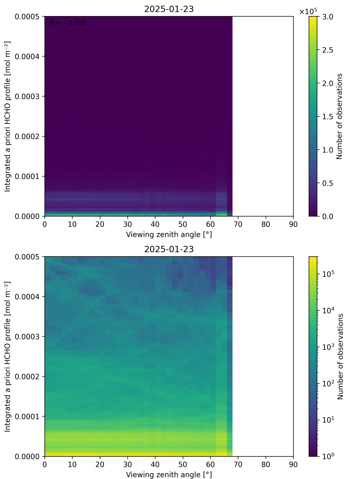
Figure 195: Scatter density plot of “Viewing zenith angle” against “Integrated a priori HCHO profile” for 2025-01-23 to 2025-01-24.
