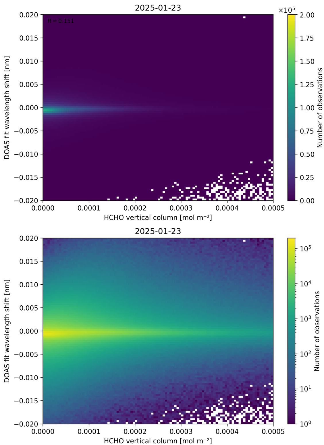
Figure 124: Scatter density plot of “HCHO vertical column” against “DOAS fit wavelength shift” for 2025-01-23 to 2025-01-24.
