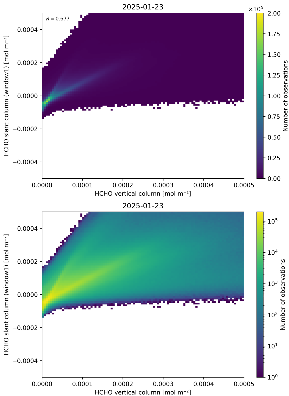
Figure 129: Scatter density plot of “HCHO vertical column” against “HCHO slant column (window1)” for 2025-01-23 to 2025-01-24.
