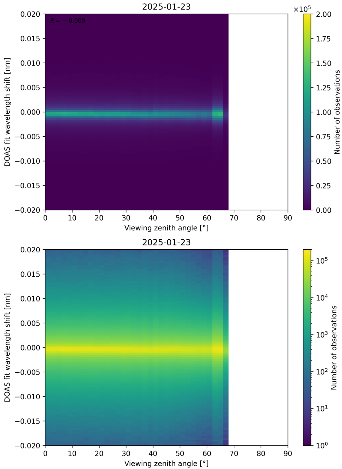
Figure 183: Scatter density plot of “Viewing zenith angle” against “DOAS fit wavelength shift” for 2025-01-23 to 2025-01-24.
