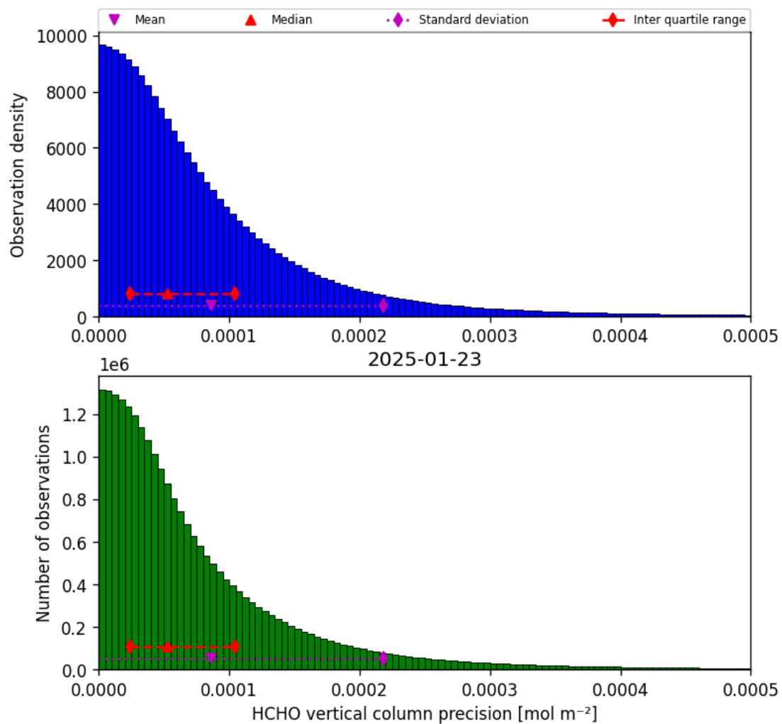
Figure 36: Histogram of “HCHO vertical column precision” for 2025-01-23 to 2025-01-24
