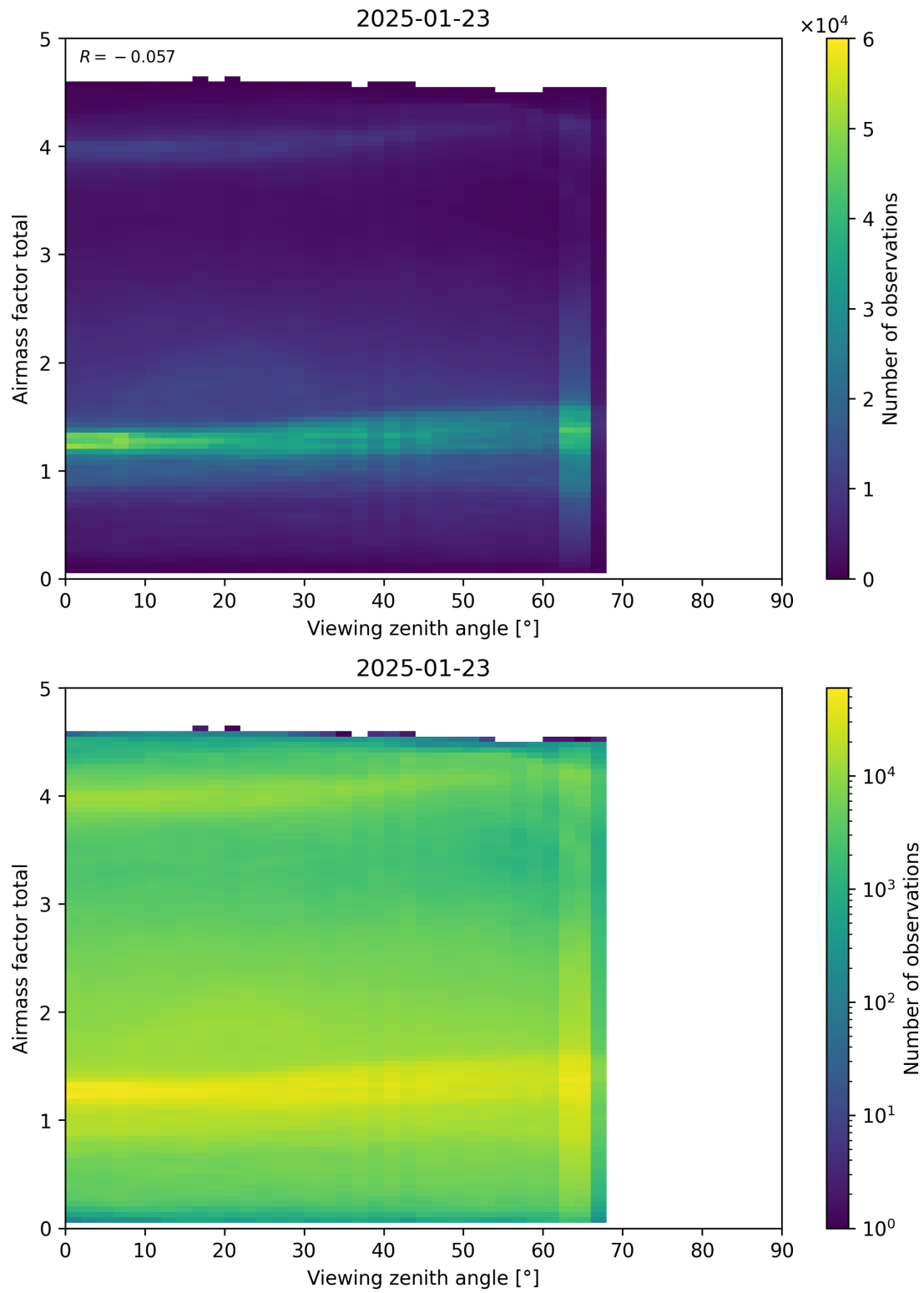
Figure 190: Scatter density plot of “Viewing zenith angle” against “Airmass factor total” for 2025-01-23 to 2025-01-24.
