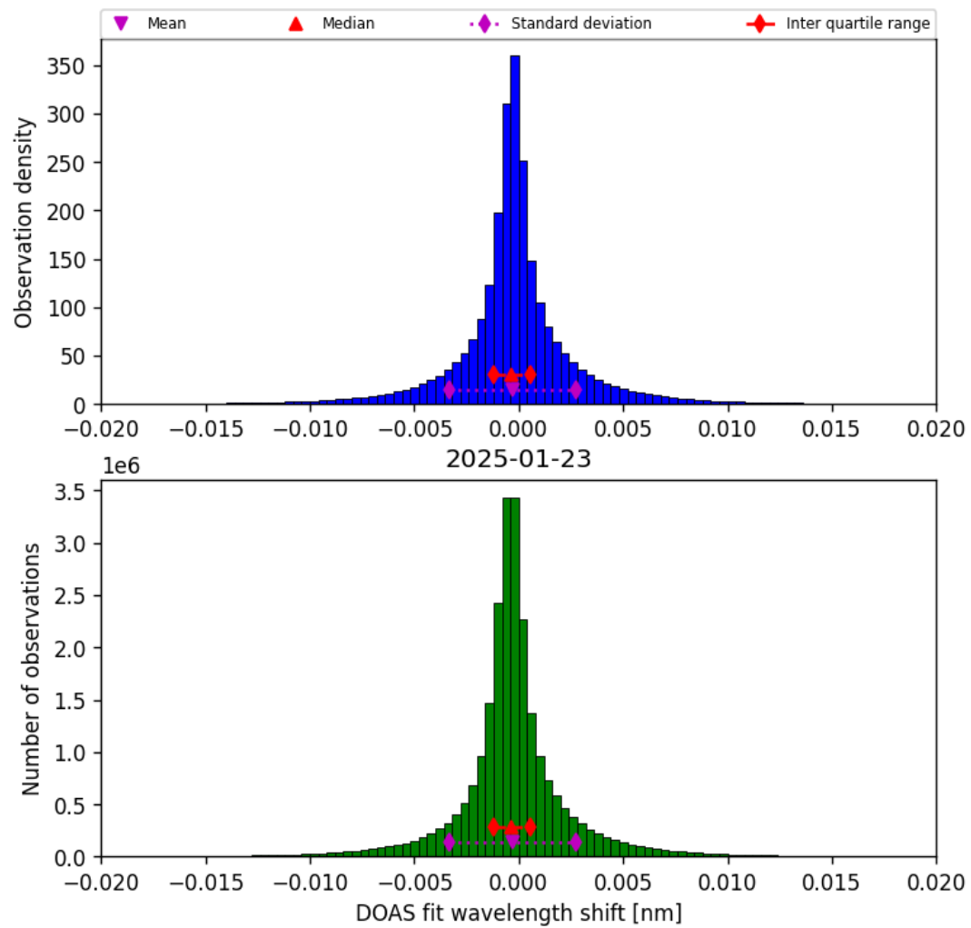
Figure 44: Histogram of “DOAS fit wavelength shift” for 2025-01-23 to 2025-01-24
