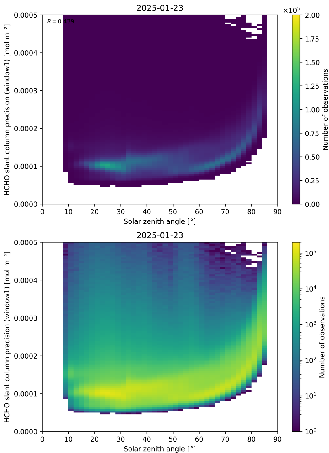
Figure 174: Scatter density plot of “Solar zenith angle” against “HCHO slant column precision (window1)” for 2025-01-23 to 2025-01-24.
