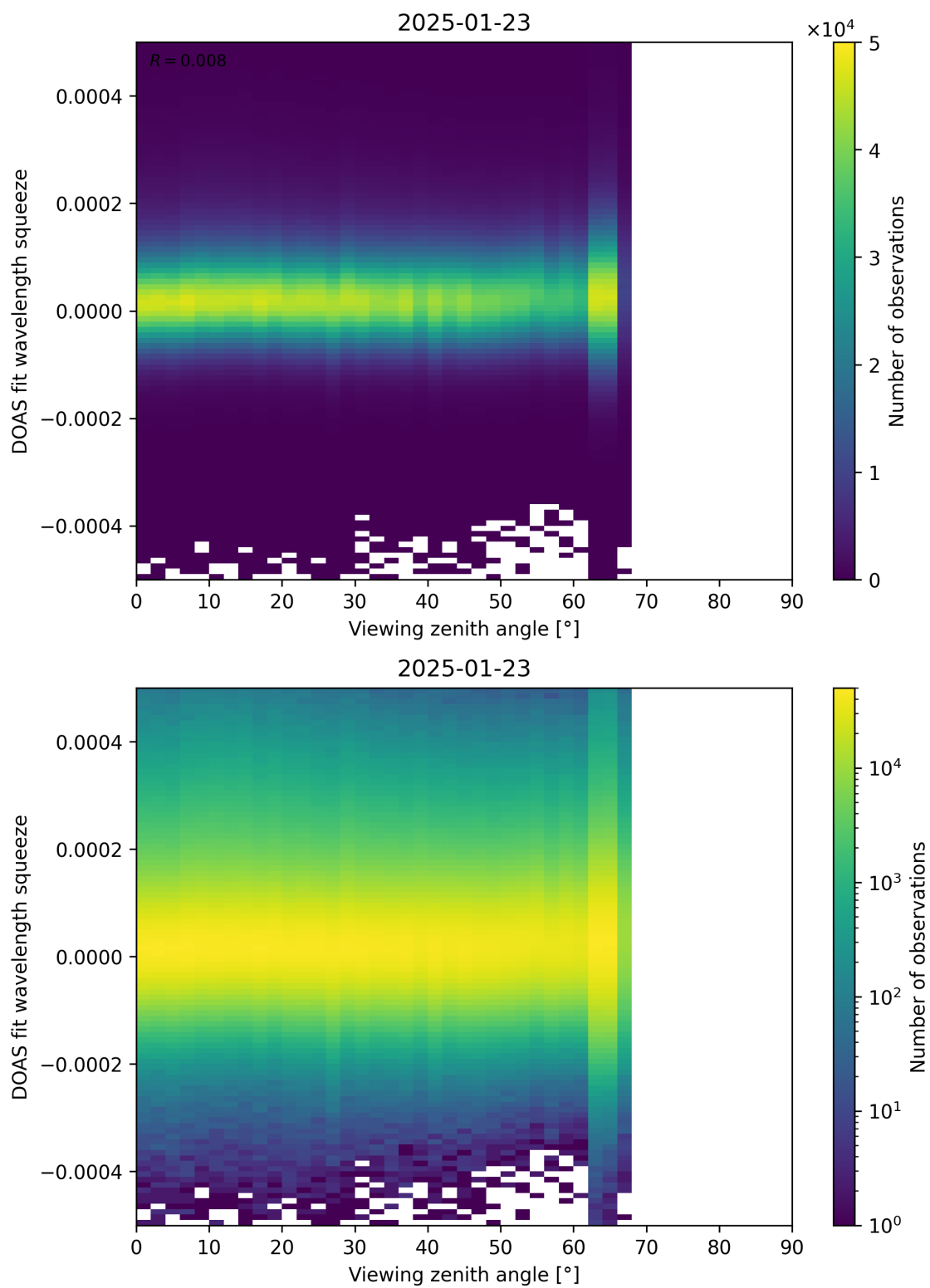
Figure 184: Scatter density plot of “Viewing zenith angle” against “DOAS fit wavelength squeeze” for 2025-01-23 to 2025-01-24.
