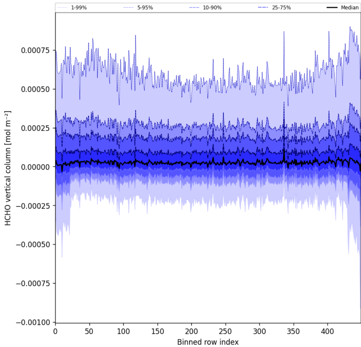
Figure 49: Along track statistics of “HCHO vertical column” for 2025-01-23 to 2025-01-24
