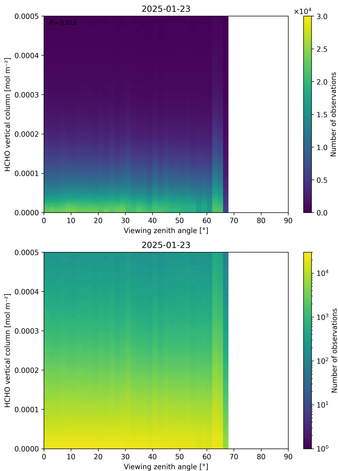
Figure 192: Scatter density plot of “Viewing zenith angle” against “HCHO vertical column” for 2025-01-23 to 2025-01-24.
