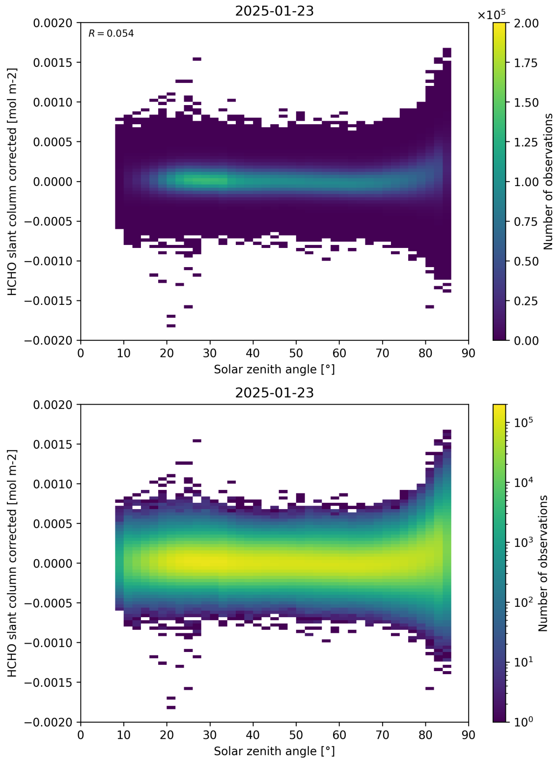
Figure 171: Scatter density plot of “Solar zenith angle” against “HCHO slant column corrected” for 2025-01-23 to 2025-01-24.
