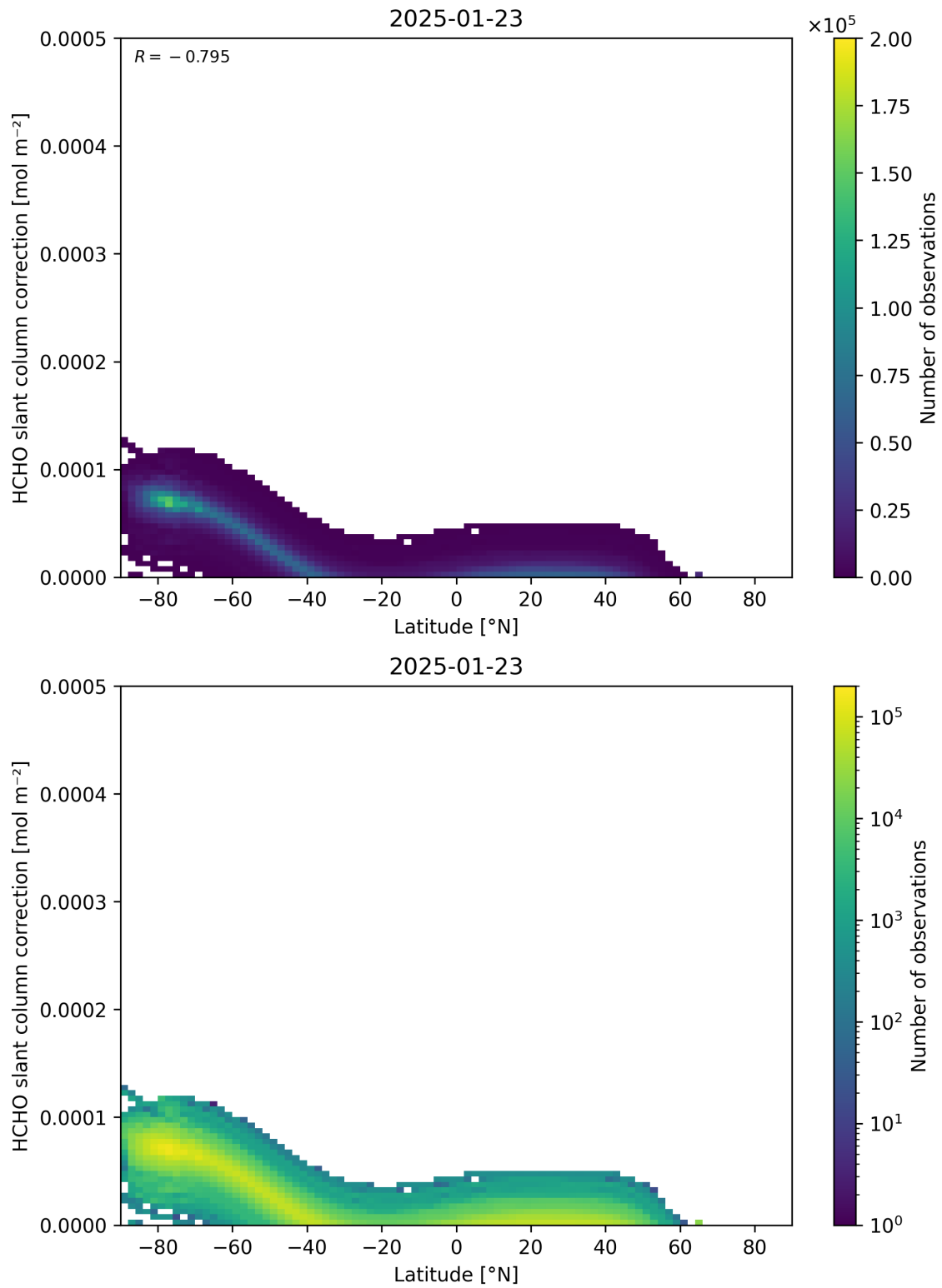
Figure 158: Scatter density plot of “Latitude” against “HCHO slant column correction” for 2025-01-23 to 2025-01-24.
