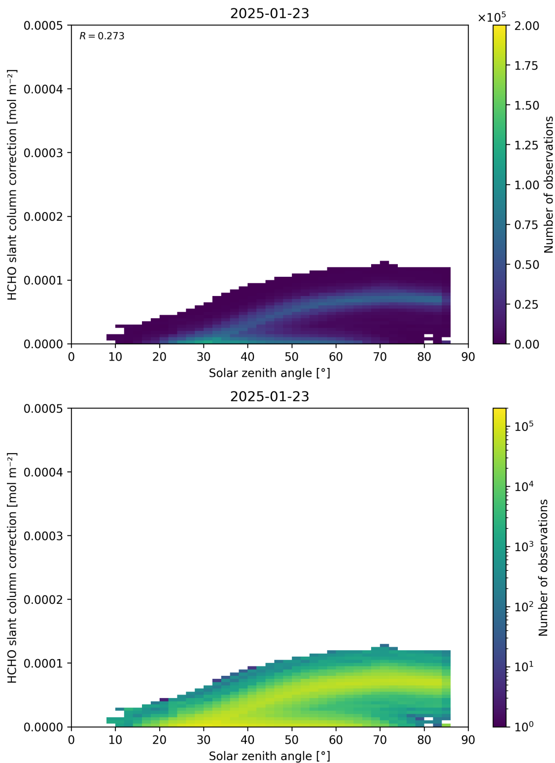
Figure 172: Scatter density plot of “Solar zenith angle” against “HCHO slant column correction” for 2025-01-23 to 2025-01-24.
