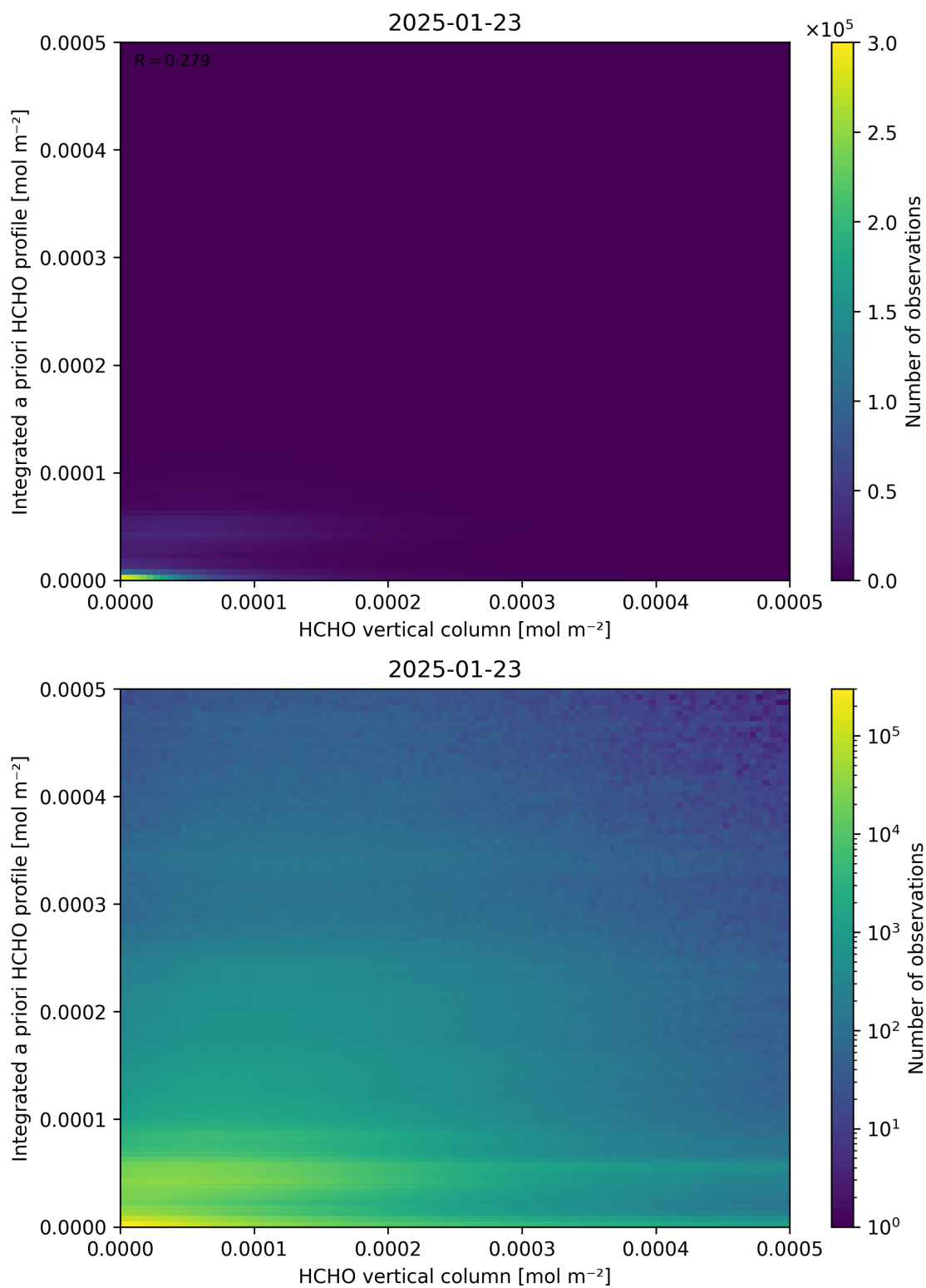
Figure 135: Scatter density plot of “HCHO vertical column” against “Integrated a priori HCHO profile” for 2025-01-23 to 2025-01-24.
