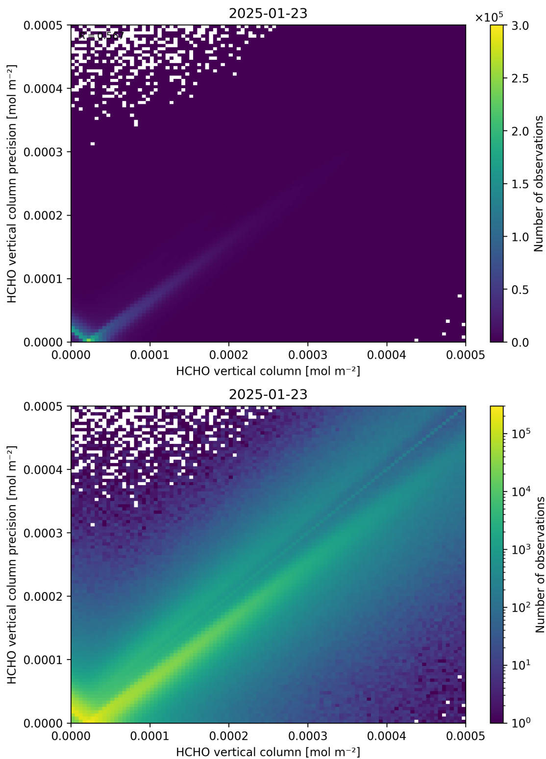
Figure 134: Scatter density plot of “HCHO vertical column” against “HCHO vertical column precision” for 2025-01-23 to 2025-01-24.
