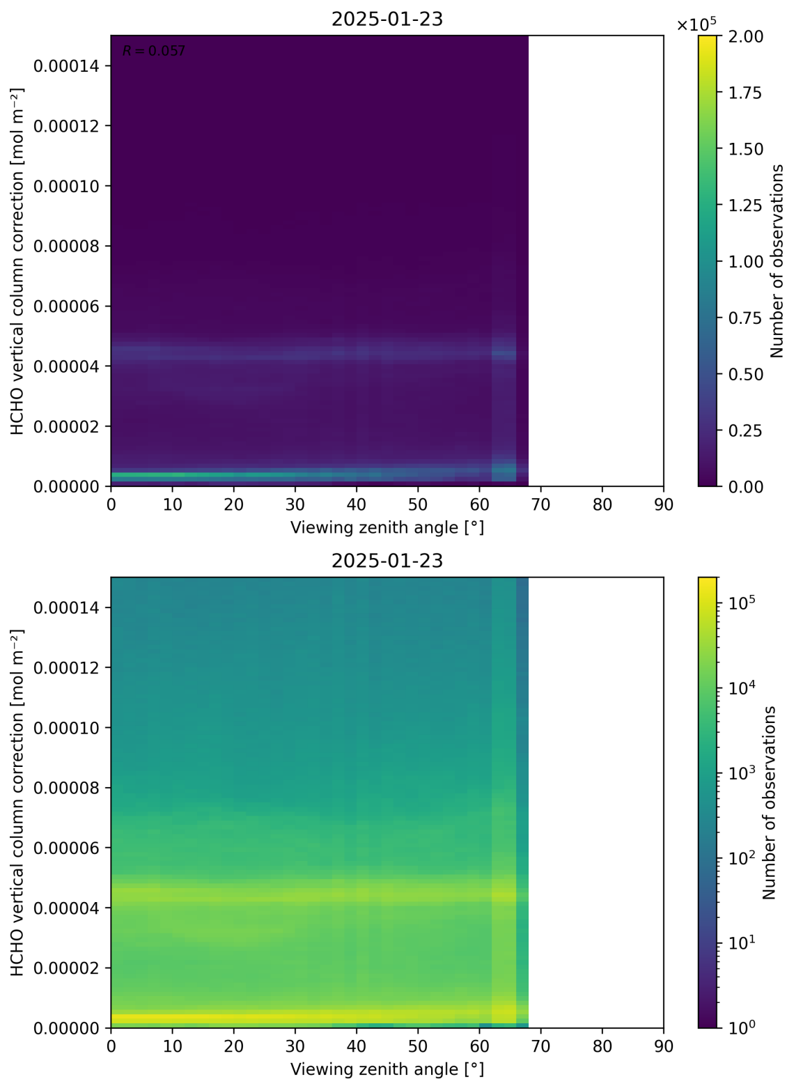
Figure 193: Scatter density plot of “Viewing zenith angle” against “HCHO vertical column correction” for 2025-01-23 to 2025-01-24.
