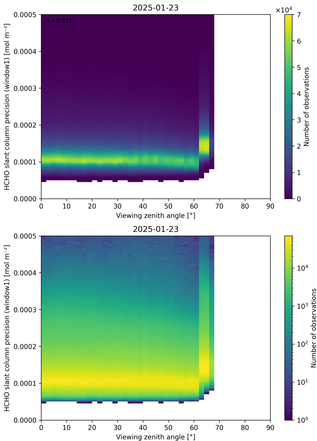
Figure 189: Scatter density plot of “Viewing zenith angle” against “HCHO slant column precision (window1)” for 2025-01-23 to 2025-01-24.
