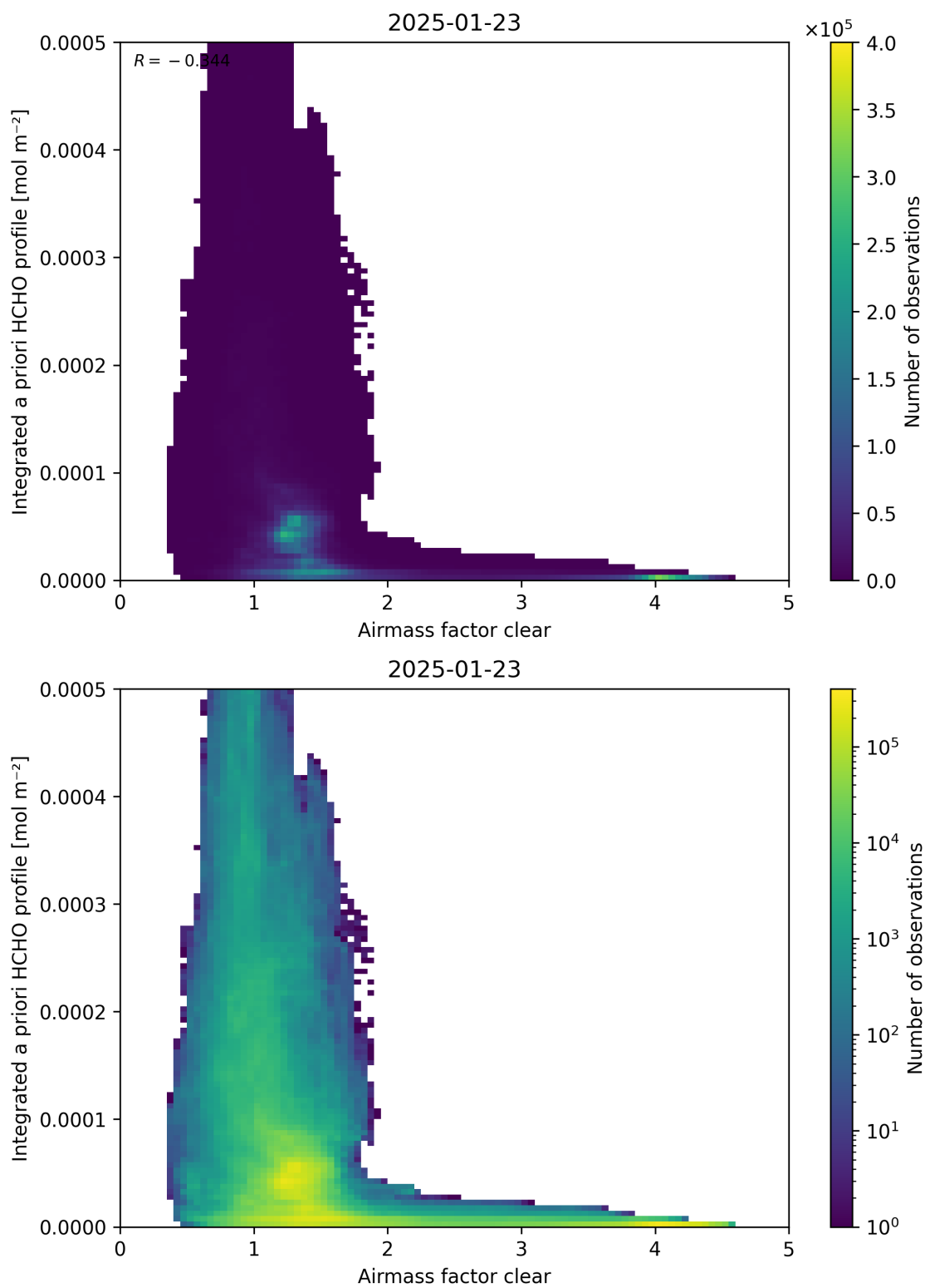
Figure 76: Scatter density plot of “Airmass factor clear” against “Integrated a priori HCHO profile” for 2025-01-23 to 2025-01-24.
