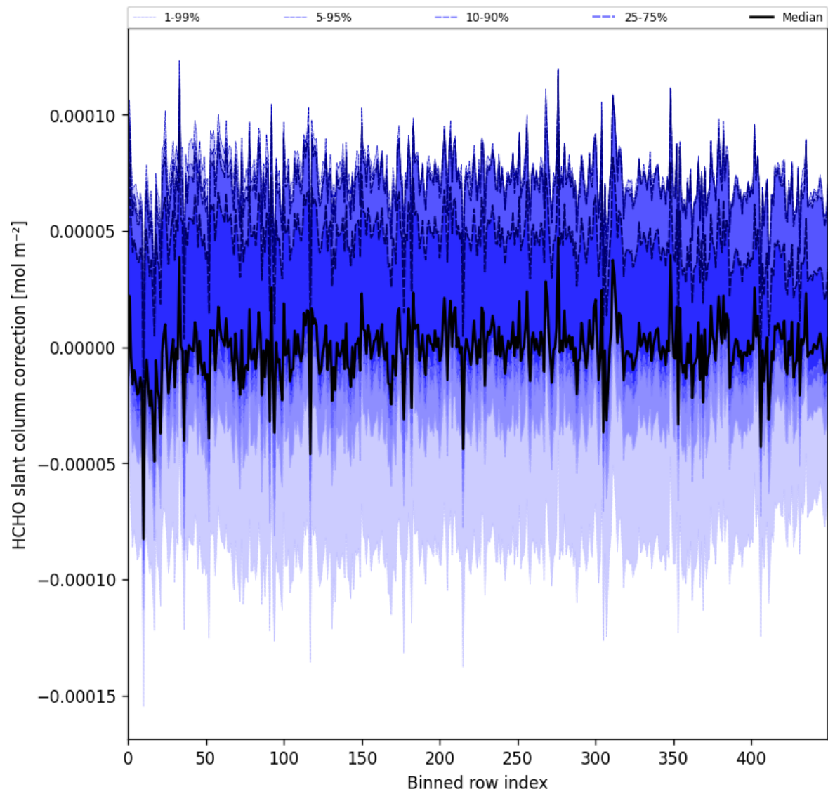
Figure 61: Along track statistics of “HCHO slant column correction” for 2025-01-23 to 2025-01-24
