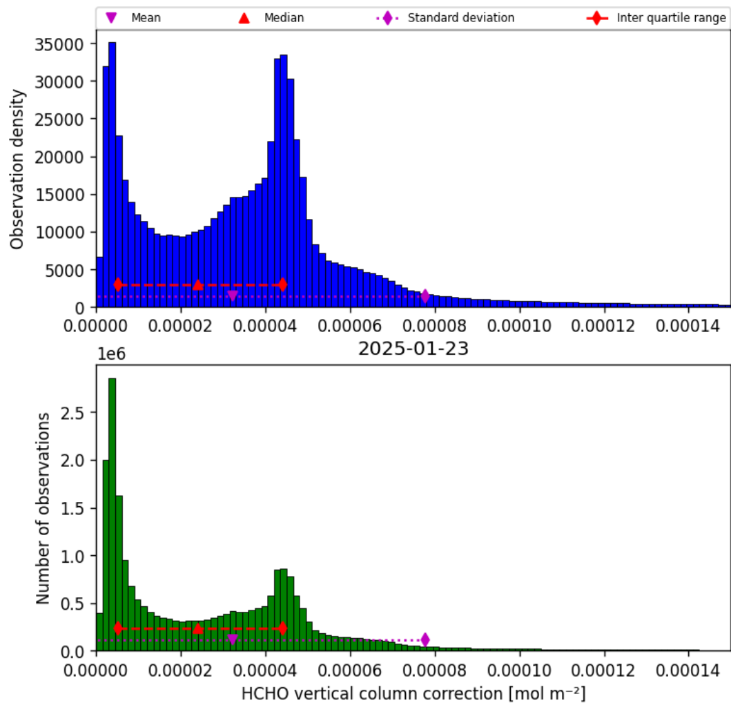
Figure 37: Histogram of “HCHO vertical column correction” for 2025-01-23 to 2025-01-24
