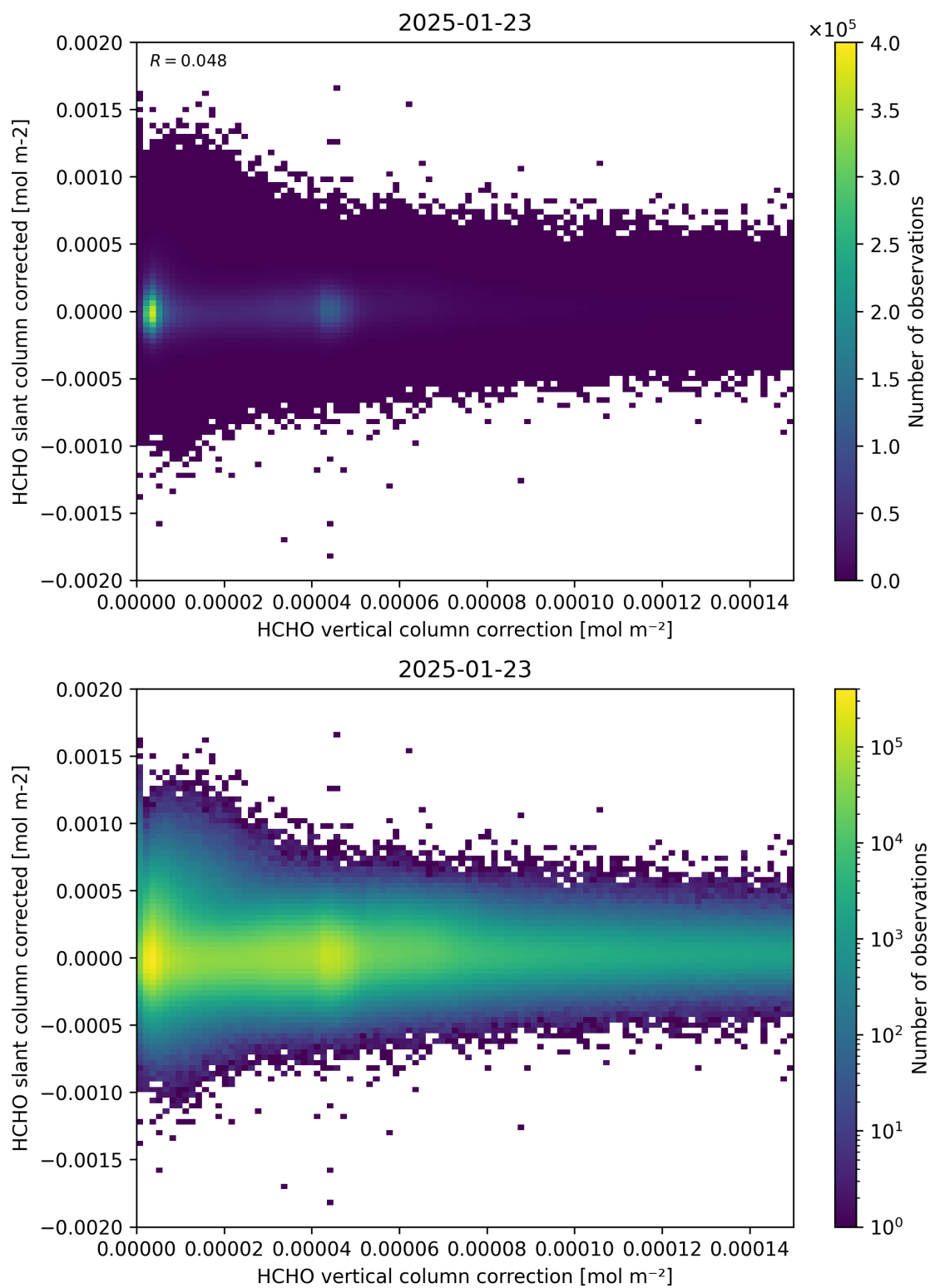
Figure 116: Scatter density plot of “HCHO vertical column correction” against “HCHO slant column corrected” for 2025-01-23 to 2025-01-24.
