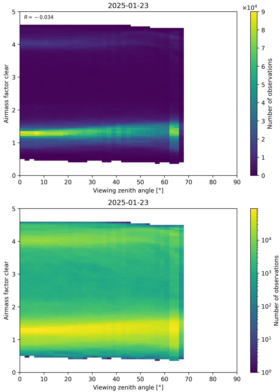
Figure 185: Scatter density plot of “Viewing zenith angle” against “Airmass factor clear” for 2025-01-23 to 2025-01-24.
