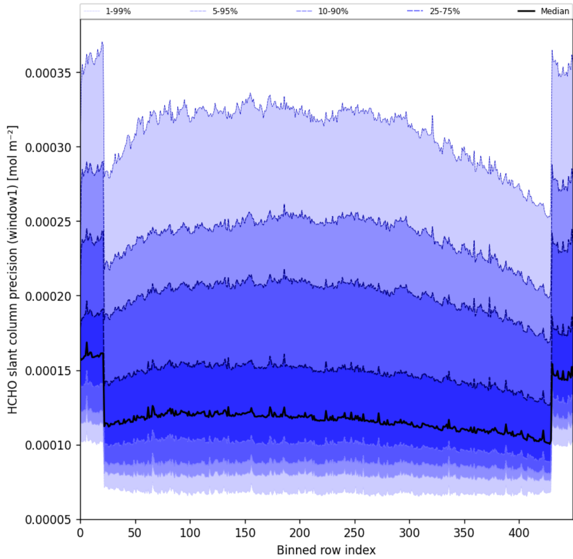
Figure 53: Along track statistics of “HCHO slant column precision (window1)” for 2025-01-23 to 2025-01-24
