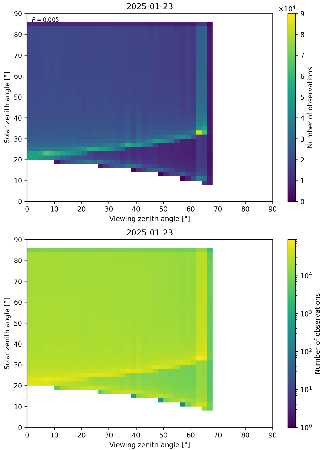
Figure 197: Scatter density plot of “Viewing zenith angle” against “Solar zenith angle” for 2025-01-23 to 2025-01-24.
