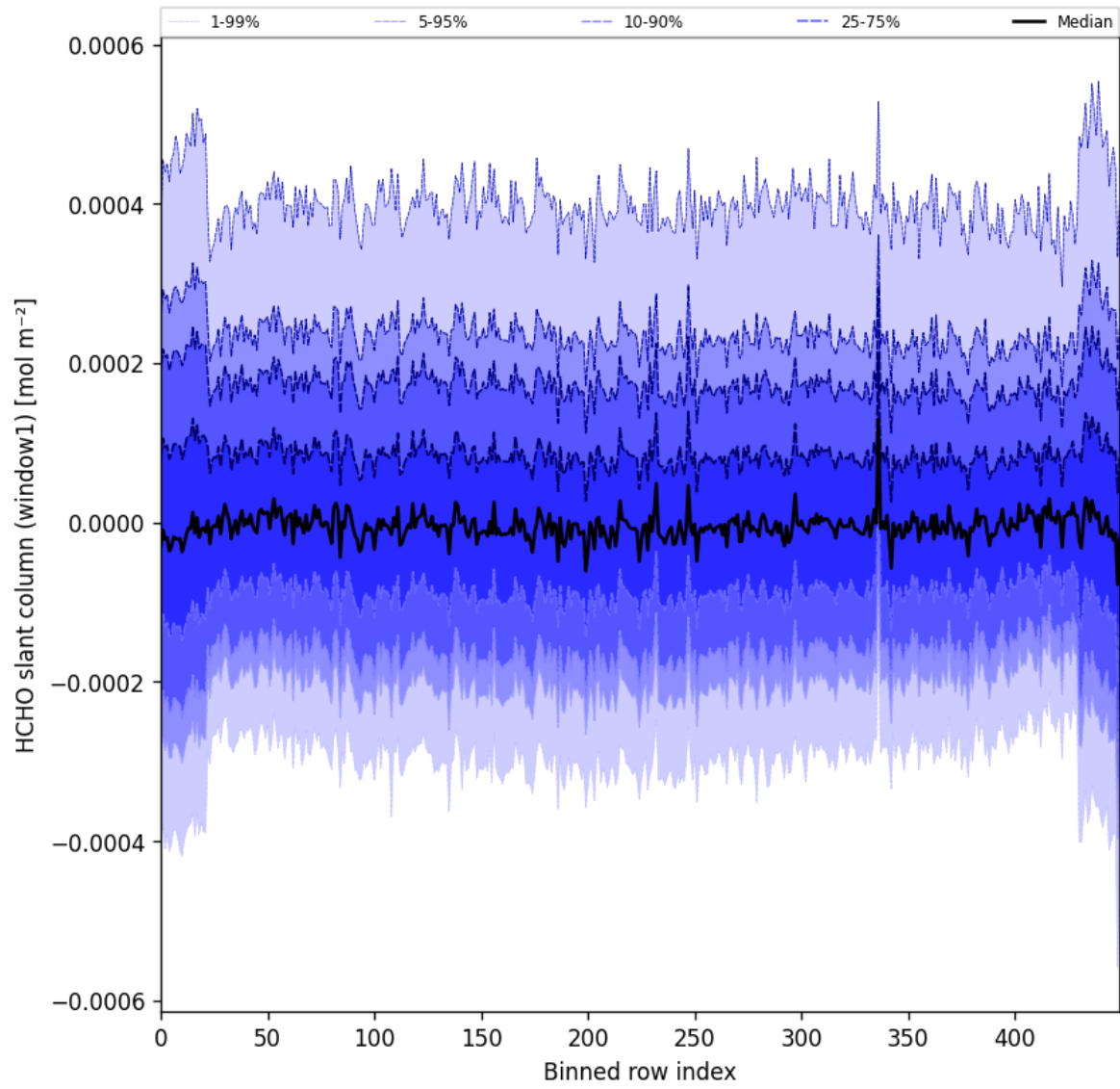
Figure 52: Along track statistics of “HCHO slant column (window1)” for 2025-01-23 to 2025-01-24
