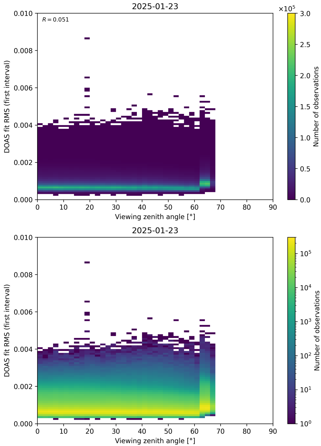
Figure 182: Scatter density plot of “Viewing zenith angle” against “DOAS fit RMS (first interval)” for 2025-01-23 to 2025-01-24.
