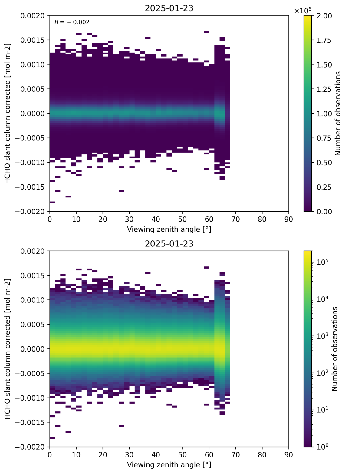
Figure 186: Scatter density plot of “Viewing zenith angle” against “HCHO slant column corrected” for 2025-01-23 to 2025-01-24.
