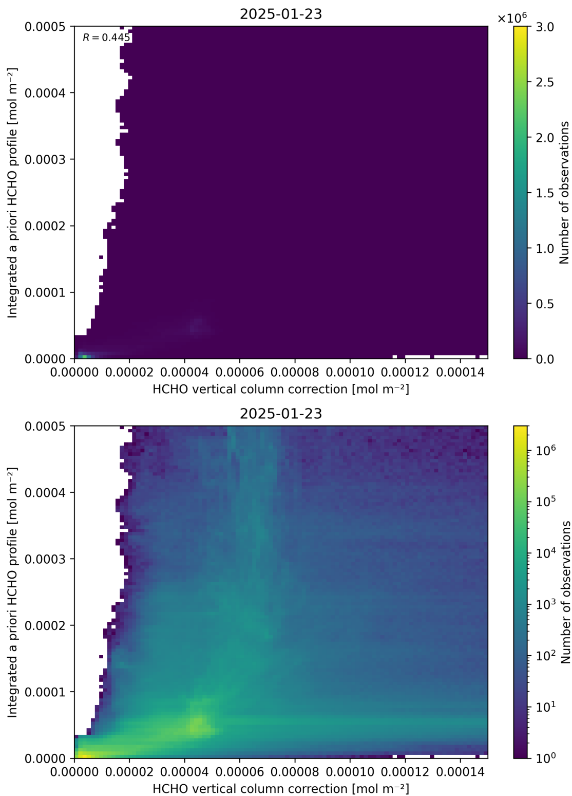
Figure 122: Scatter density plot of “HCHO vertical column correction” against “Integrated a priori HCHO profile” for 2025-01-23 to 2025-01-24.
