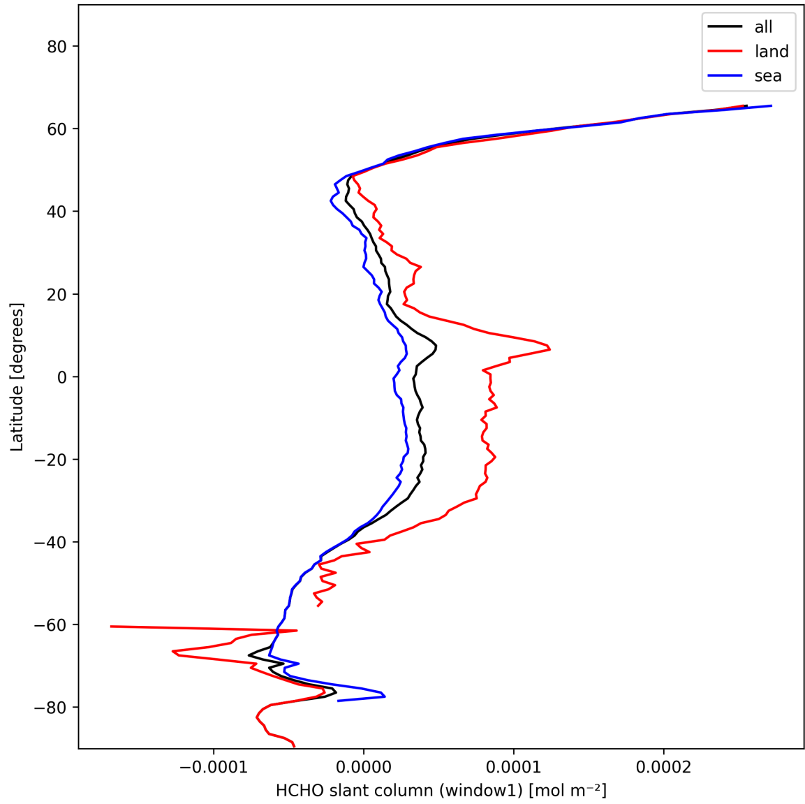
Figure 24: Zonal average of “HCHO slant column (window1)” for 2025-01-23 to 2025-01-24.
