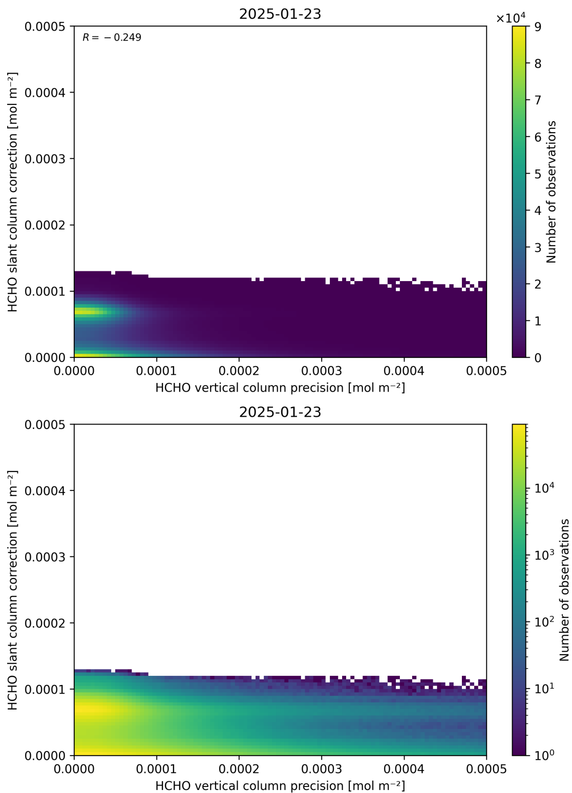
Figure 141: Scatter density plot of “HCHO vertical column precision” against “HCHO slant column correction” for 2025-01-23 to 2025-01-24.
