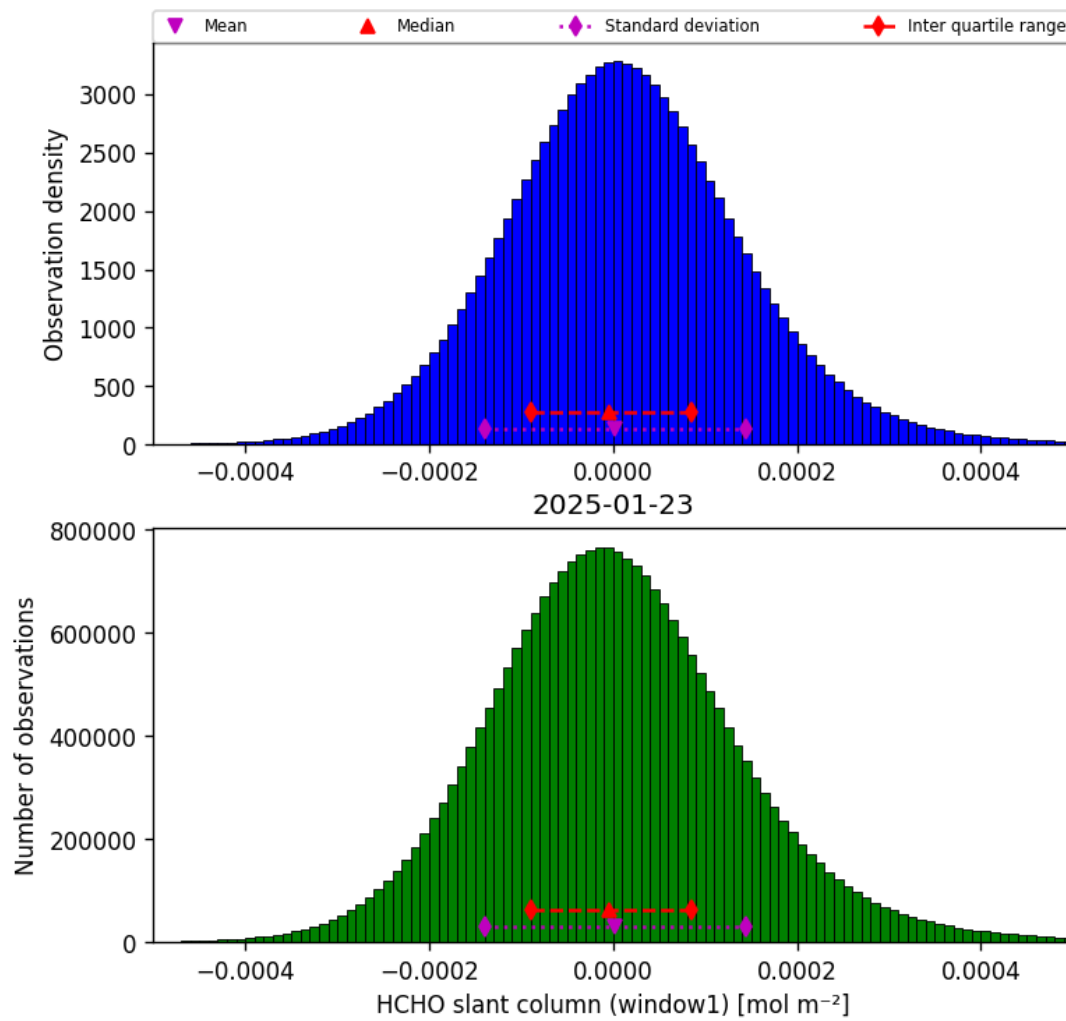
Figure 38: Histogram of “HCHO slant column (window1)” for 2025-01-23 to 2025-01-24
