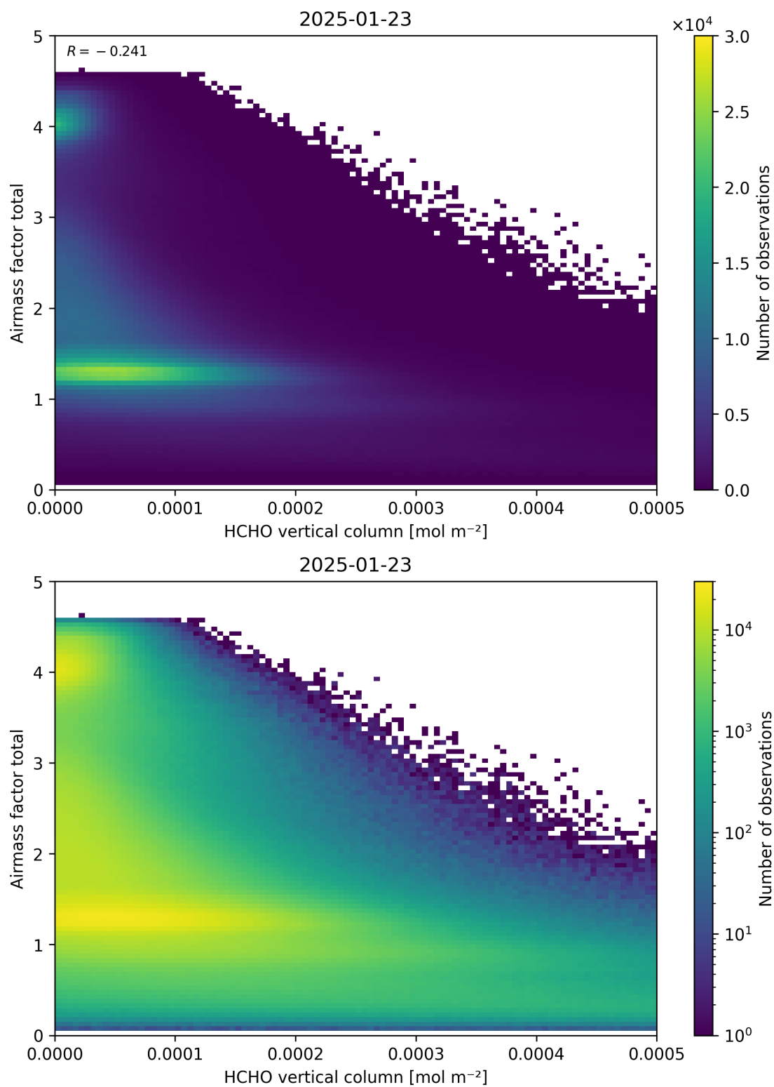
Figure 131: Scatter density plot of “HCHO vertical column” against “Airmass factor total” for 2025-01-23 to 2025-01-24.
