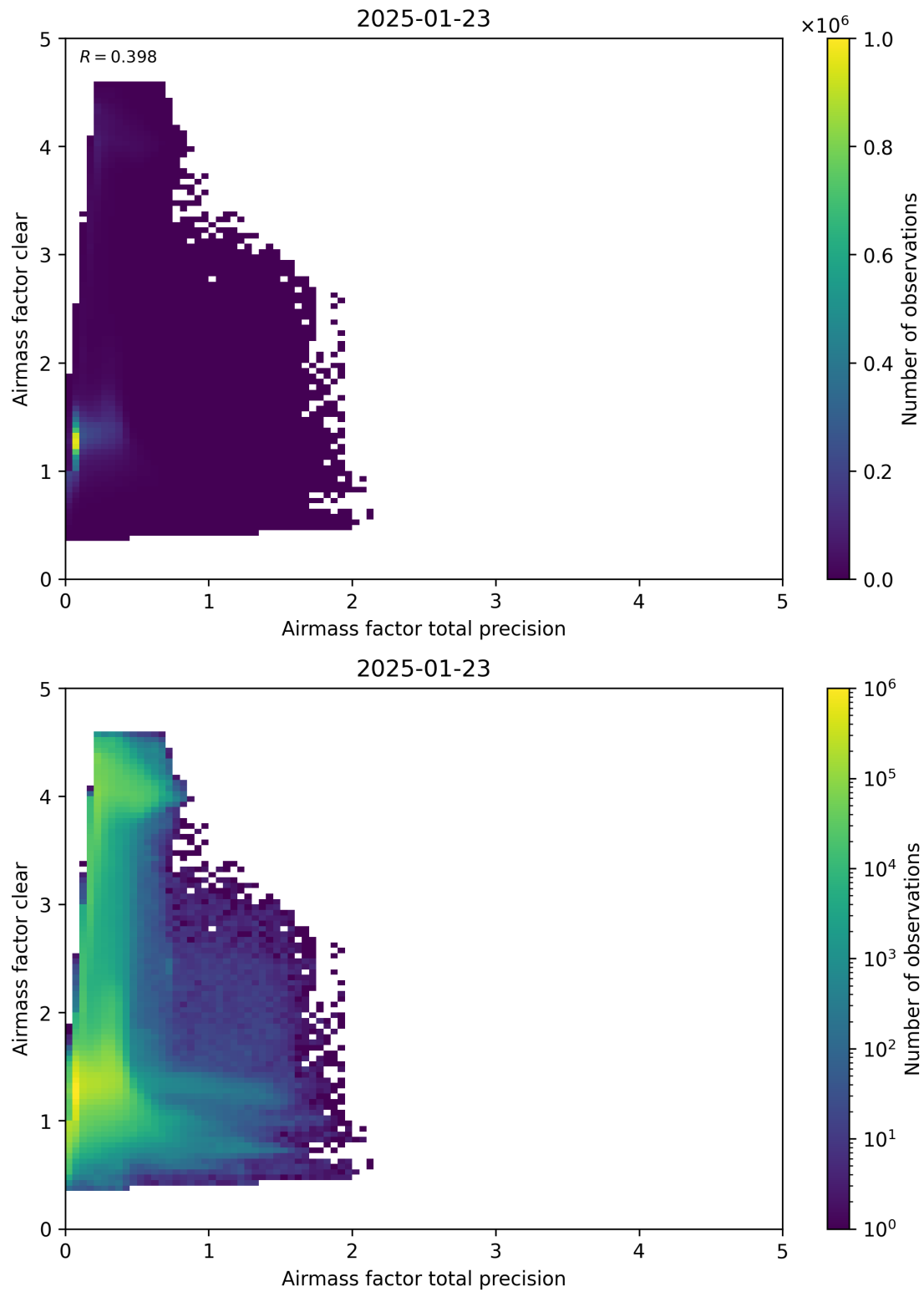
Figure 108: Scatter density plot of “Airmass factor total precision” against “Airmass factor clear” for 2025-01-23 to 2025-01-24.
