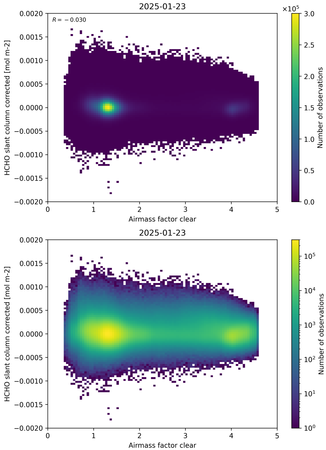
Figure 74: Scatter density plot of “Airmass factor clear” against “HCHO slant column corrected” for 2025-01-23 to 2025-01-24.
