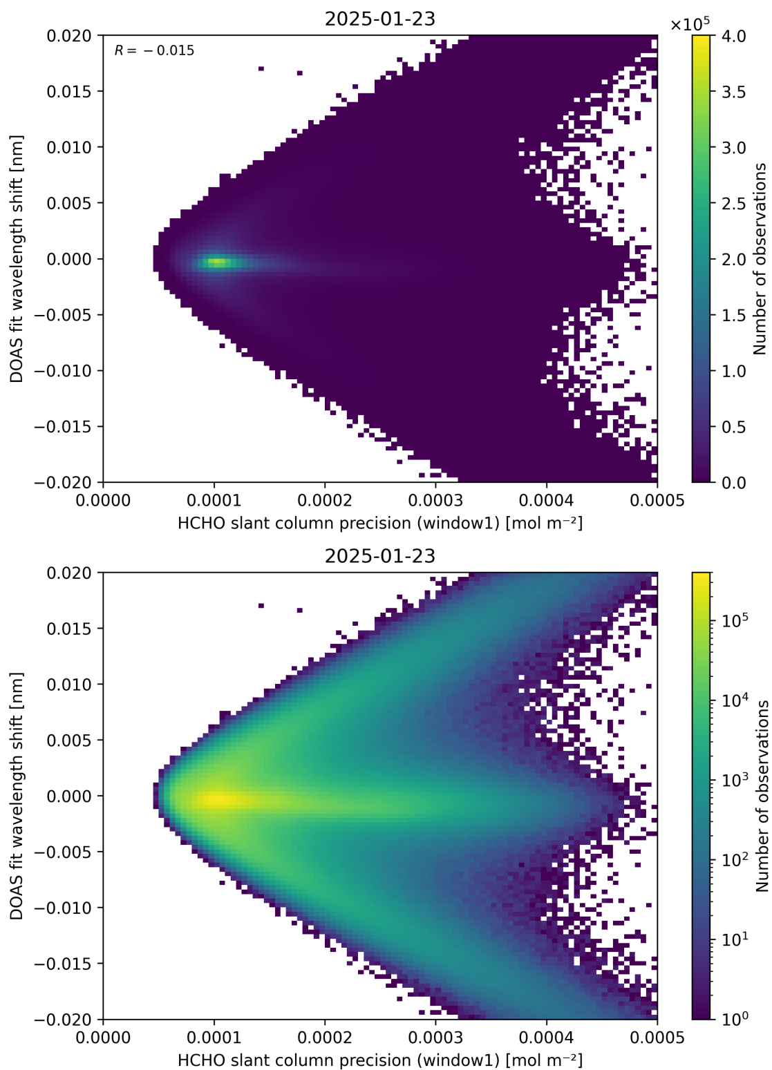
Figure 89: Scatter density plot of “HCHO slant column precision (window1)” against “DOAS fit wavelength shift” for 2025-01-23 to 2025-01-24.
