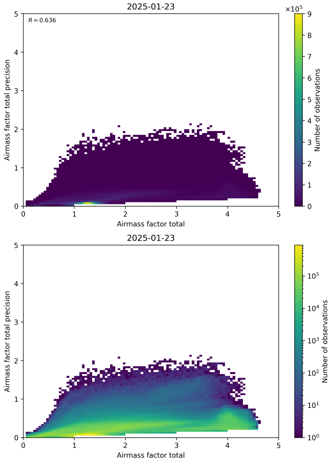
Figure 103: Scatter density plot of “Airmass factor total” against “Airmass factor total precision” for 2025-01-23 to 2025-01-24.
