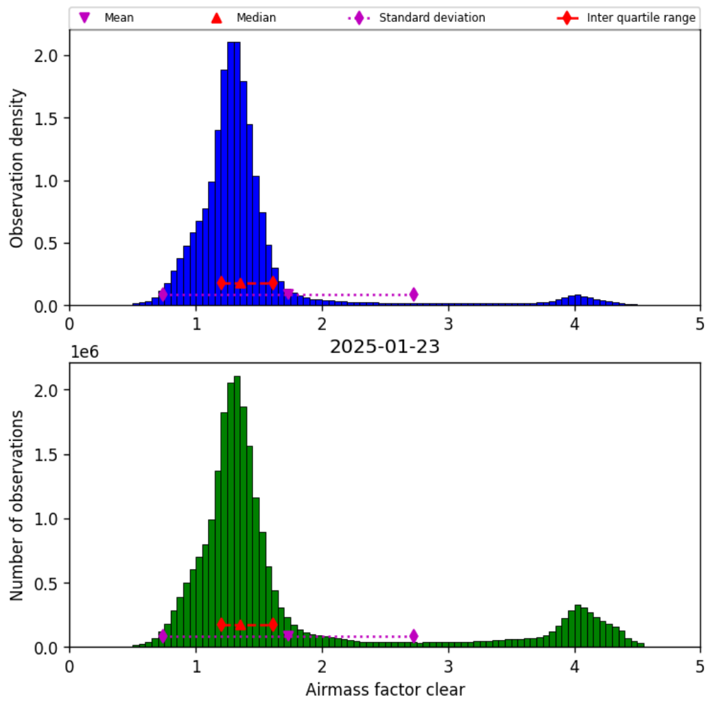
Figure 42: Histogram of “Airmass factor clear” for 2025-01-23 to 2025-01-24
