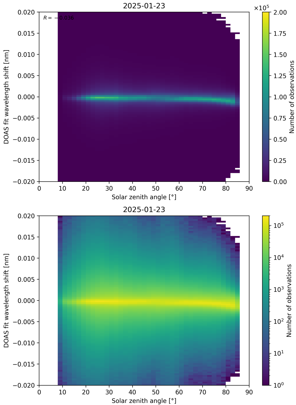
Figure 168: Scatter density plot of “Solar zenith angle” against “DOAS fit wavelength shift” for 2025-01-23 to 2025-01-24.
