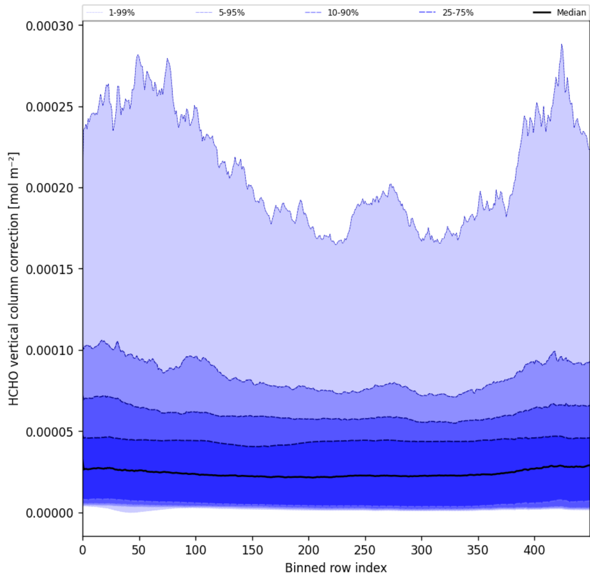
Figure 51: Along track statistics of "HCHO vertical column correction" for 2025-01-23 to 2025-01-24
