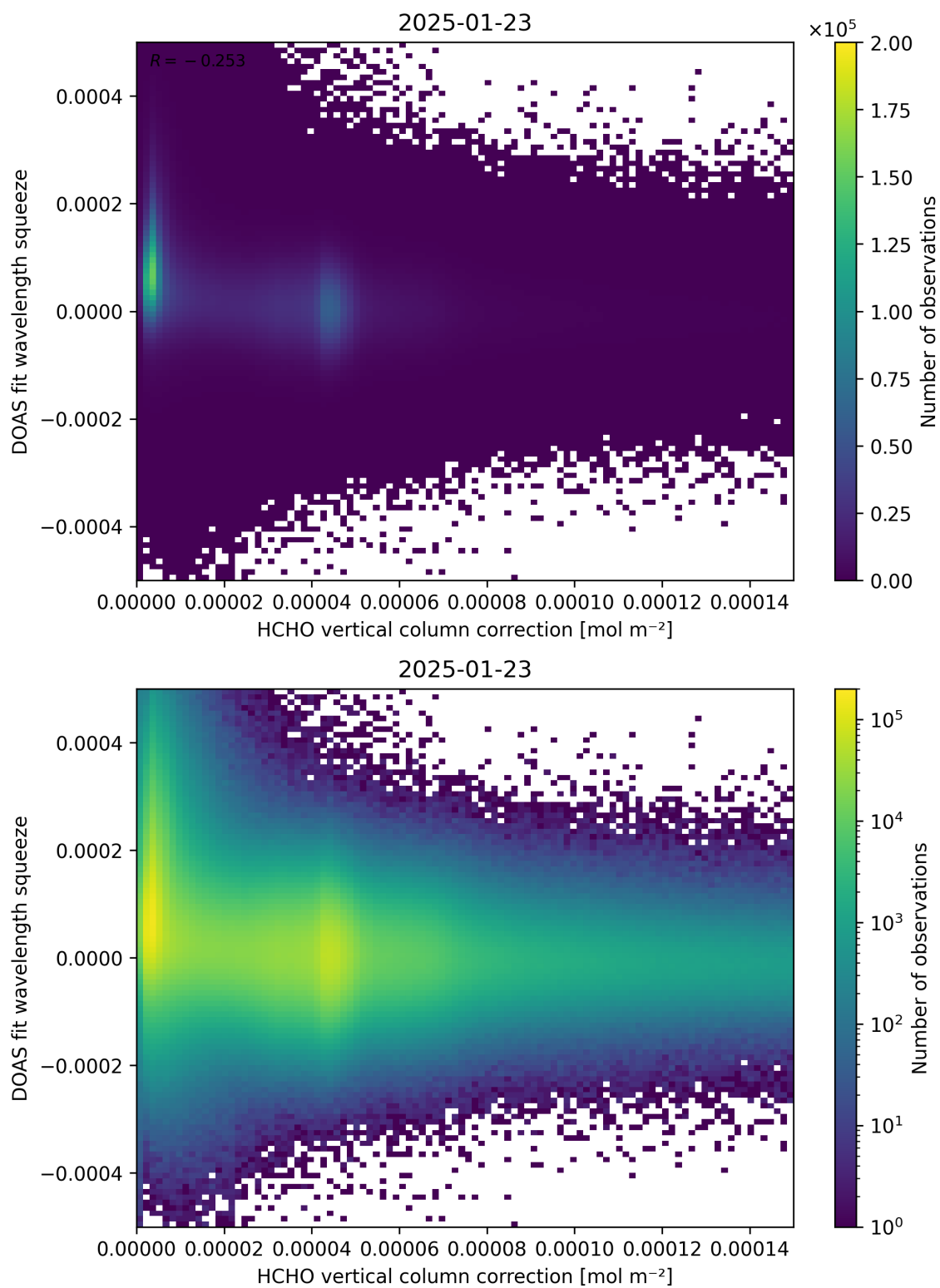
Figure 114: Scatter density plot of “HCHO vertical column correction” against “DOAS fit wavelength squeeze” for 2025-01-23 to 2025-01-24.
