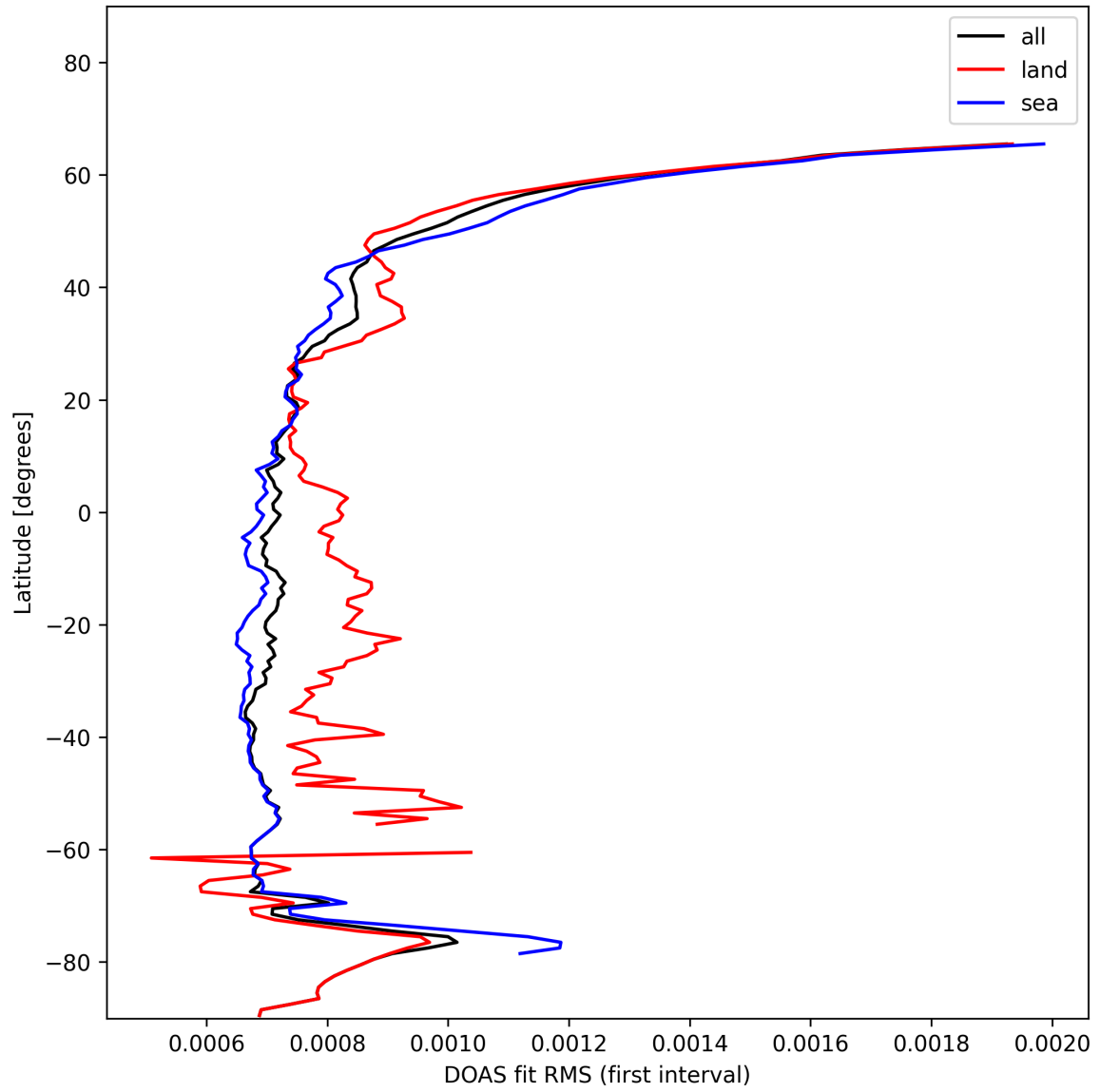
Figure 32: Zonal average of “DOAS fit RMS (first interval)” for 2025-01-23 to 2025-01-24.
