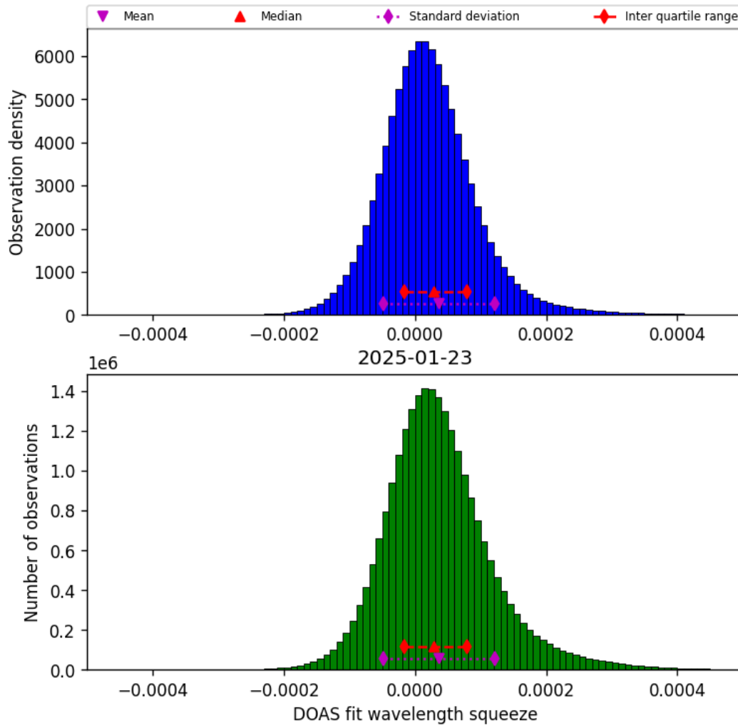
Figure 45: Histogram of “DOAS fit wavelength squeeze” for 2025-01-23 to 2025-01-24
