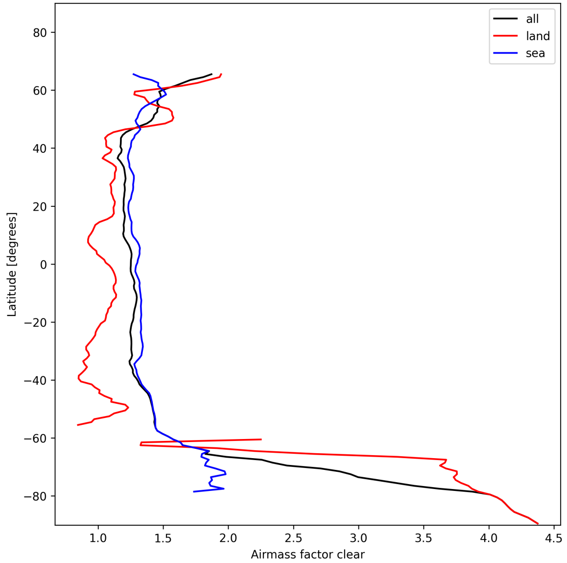
Figure 28: Zonal average of “Airmass factor clear” for 2025-01-23 to 2025-01-24.
