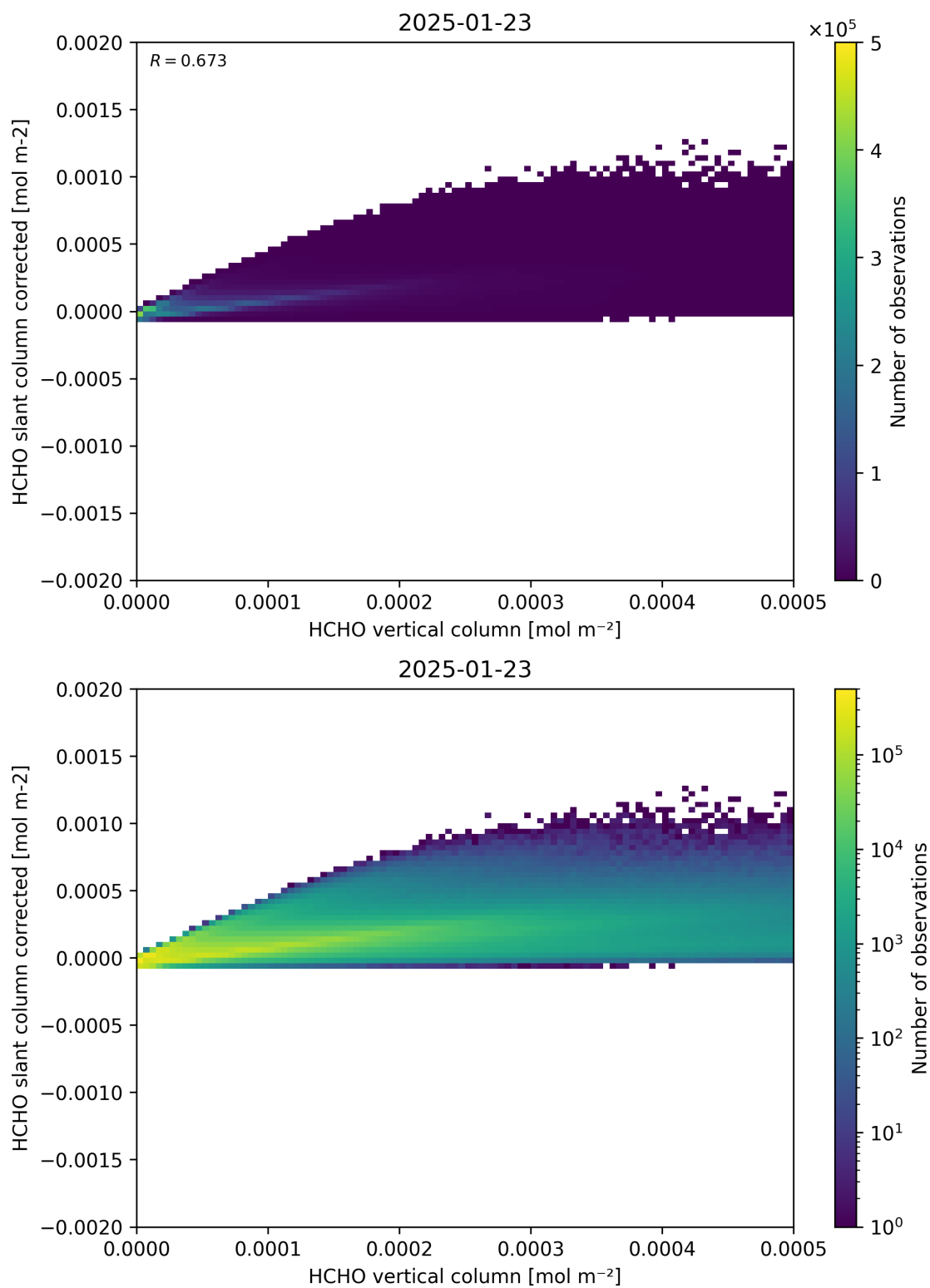
Figure 127: Scatter density plot of “HCHO vertical column” against “HCHO slant column corrected” for 2025-01-23 to 2025-01-24.
