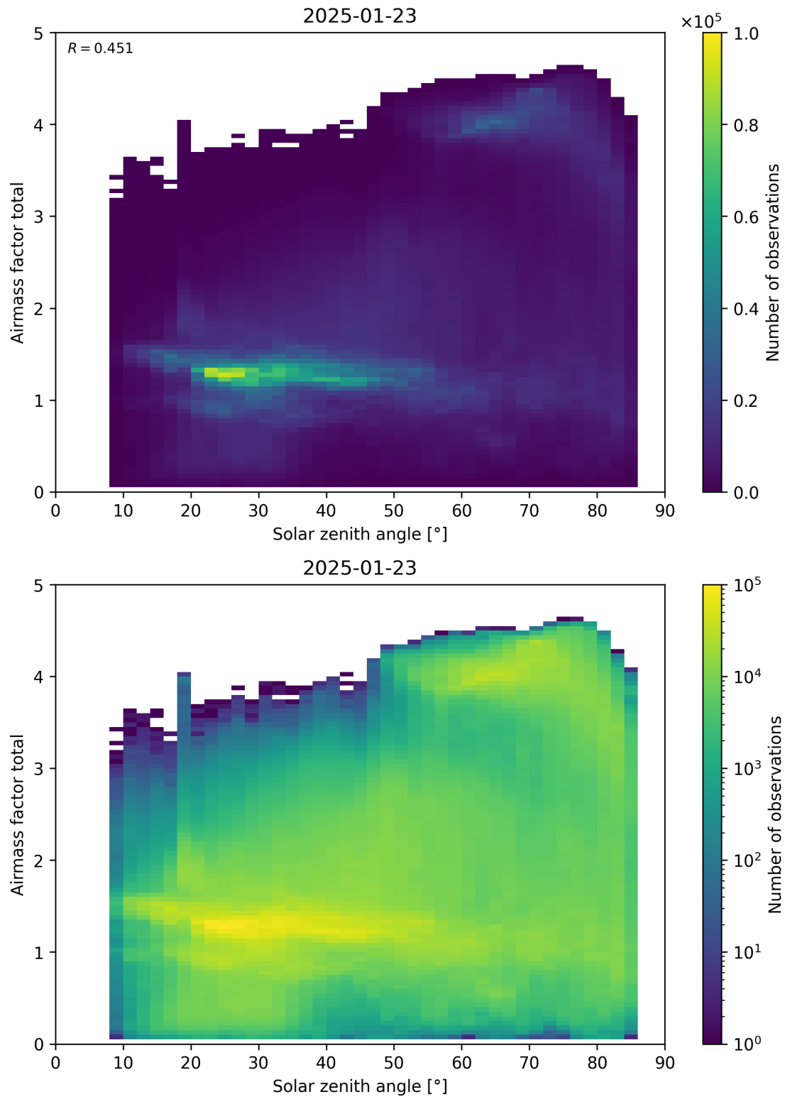
Figure 175: Scatter density plot of “Solar zenith angle” against “Airmass factor total” for 2025-01-23 to 2025-01-24.
