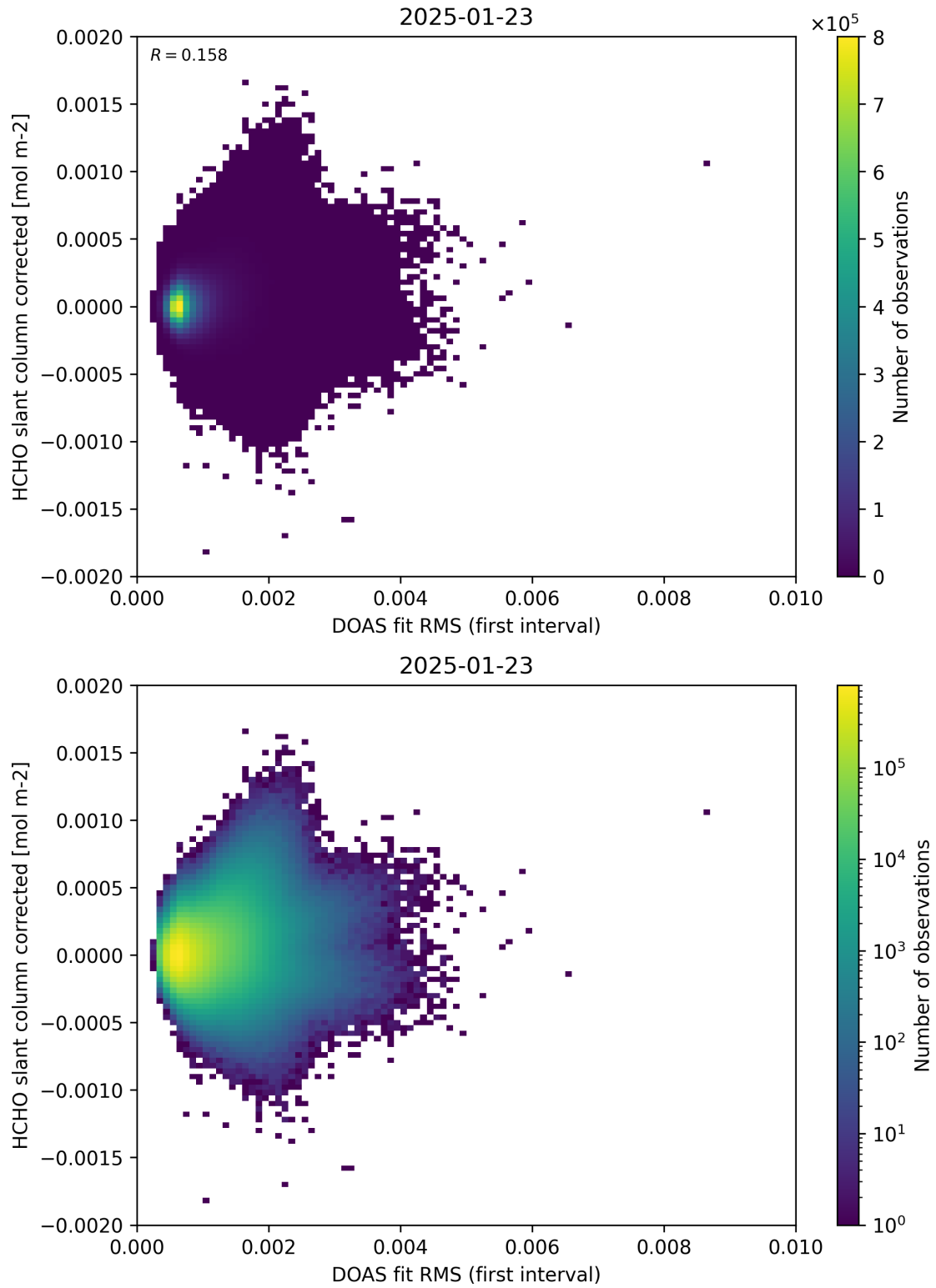
Figure 62: Scatter density plot of “DOAS fit RMS (first interval)” against “HCHO slant column corrected” for 2025-01-23 to 2025-01-24.
