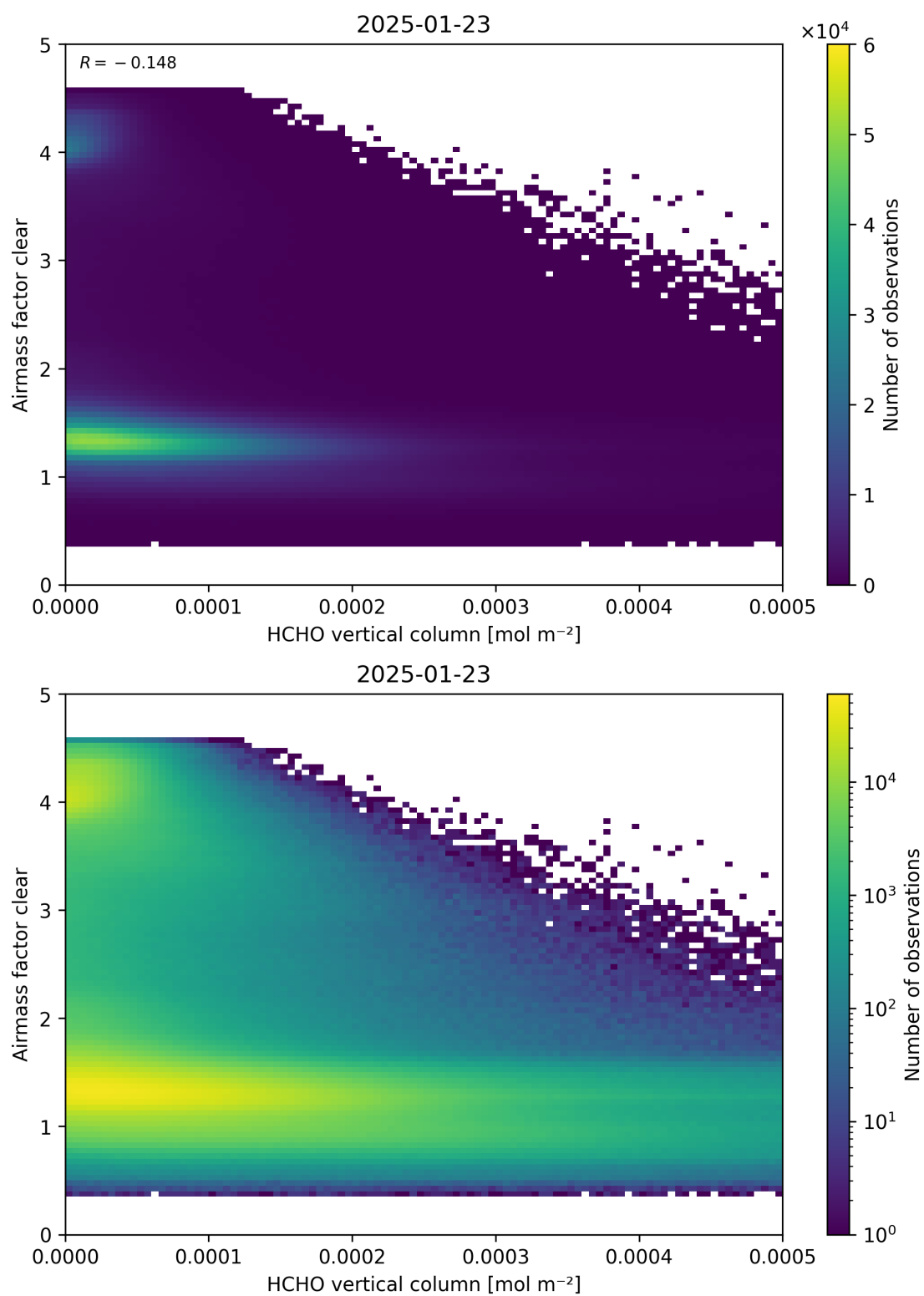
Figure 126: Scatter density plot of “HCHO vertical column” against “Airmass factor clear” for 2025-01-23 to 2025-01-24.
