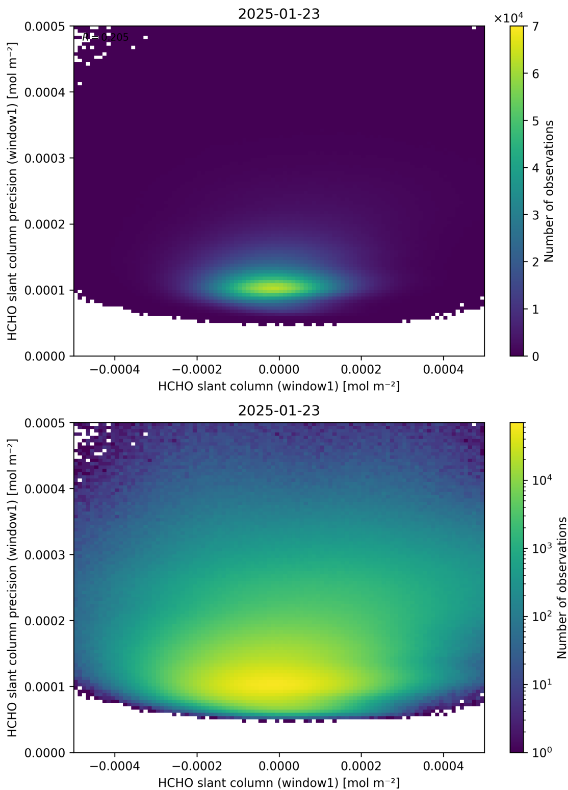
Figure 84: Scatter density plot of “HCHO slant column (window1)” against “HCHO slant column precision (window1)” for 2025-01-23 to 2025-01-24.
