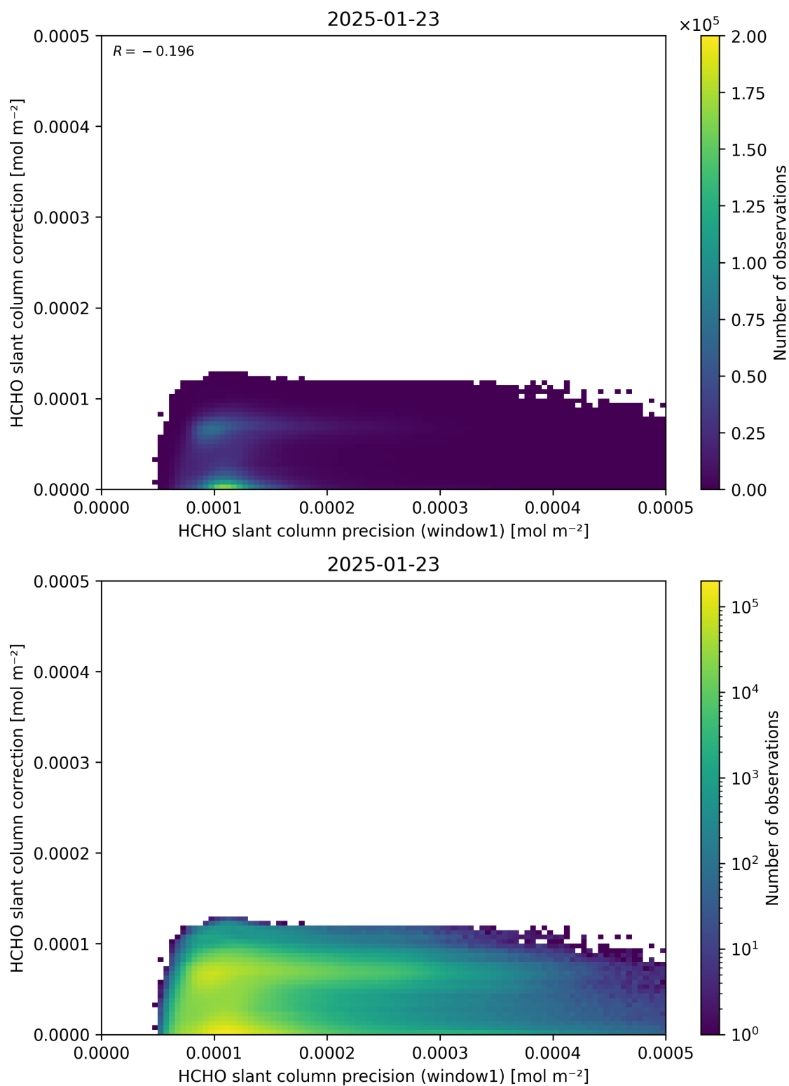
Figure 93: Scatter density plot of “HCHO slant column precision (window1)” against “HCHO slant column correction” for 2025-01-23 to 2025-01-24.
