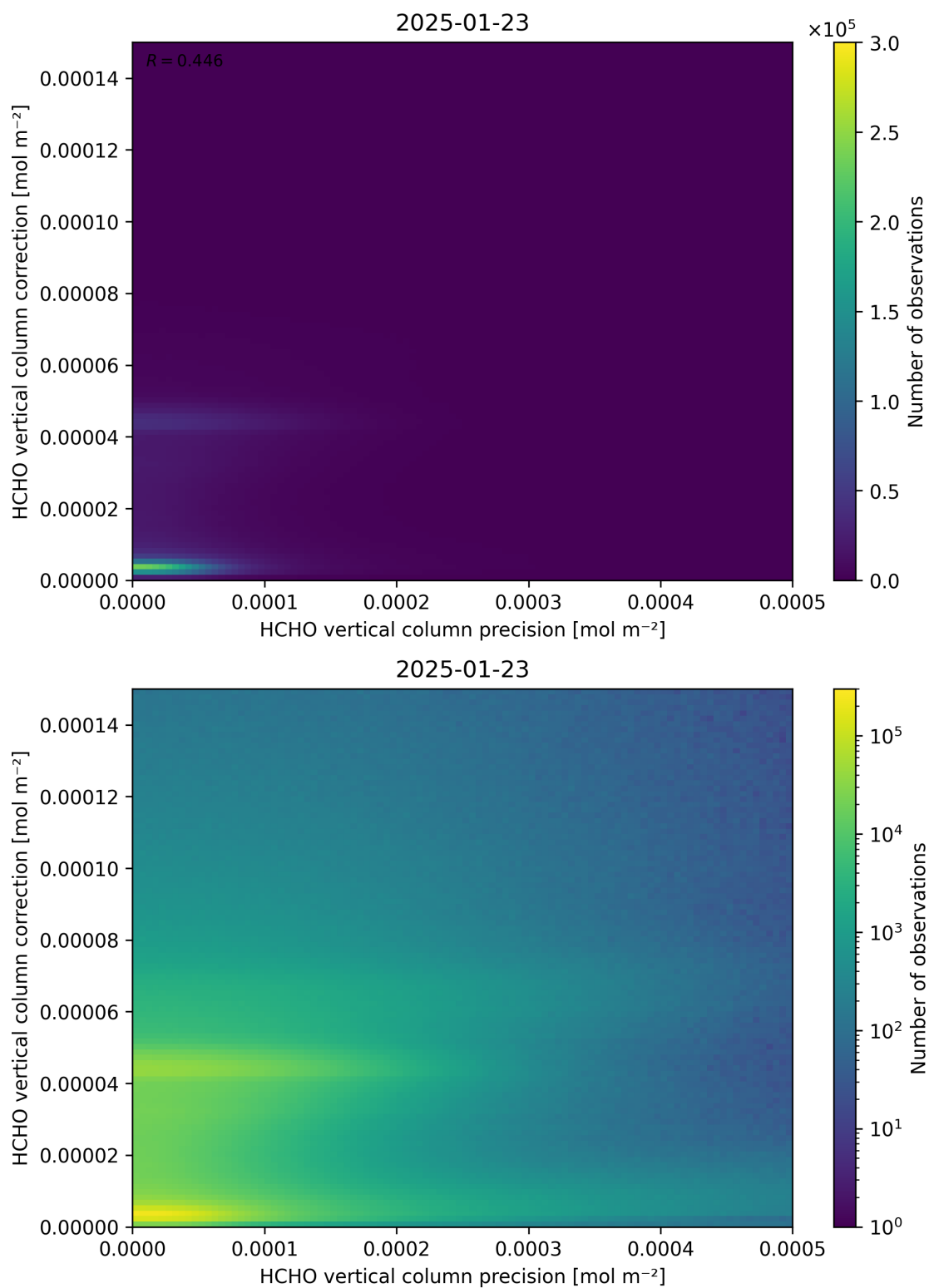
Figure 146: Scatter density plot of “HCHO vertical column precision” against “HCHO vertical column correction” for 2025-01-23 to 2025-01-24.
