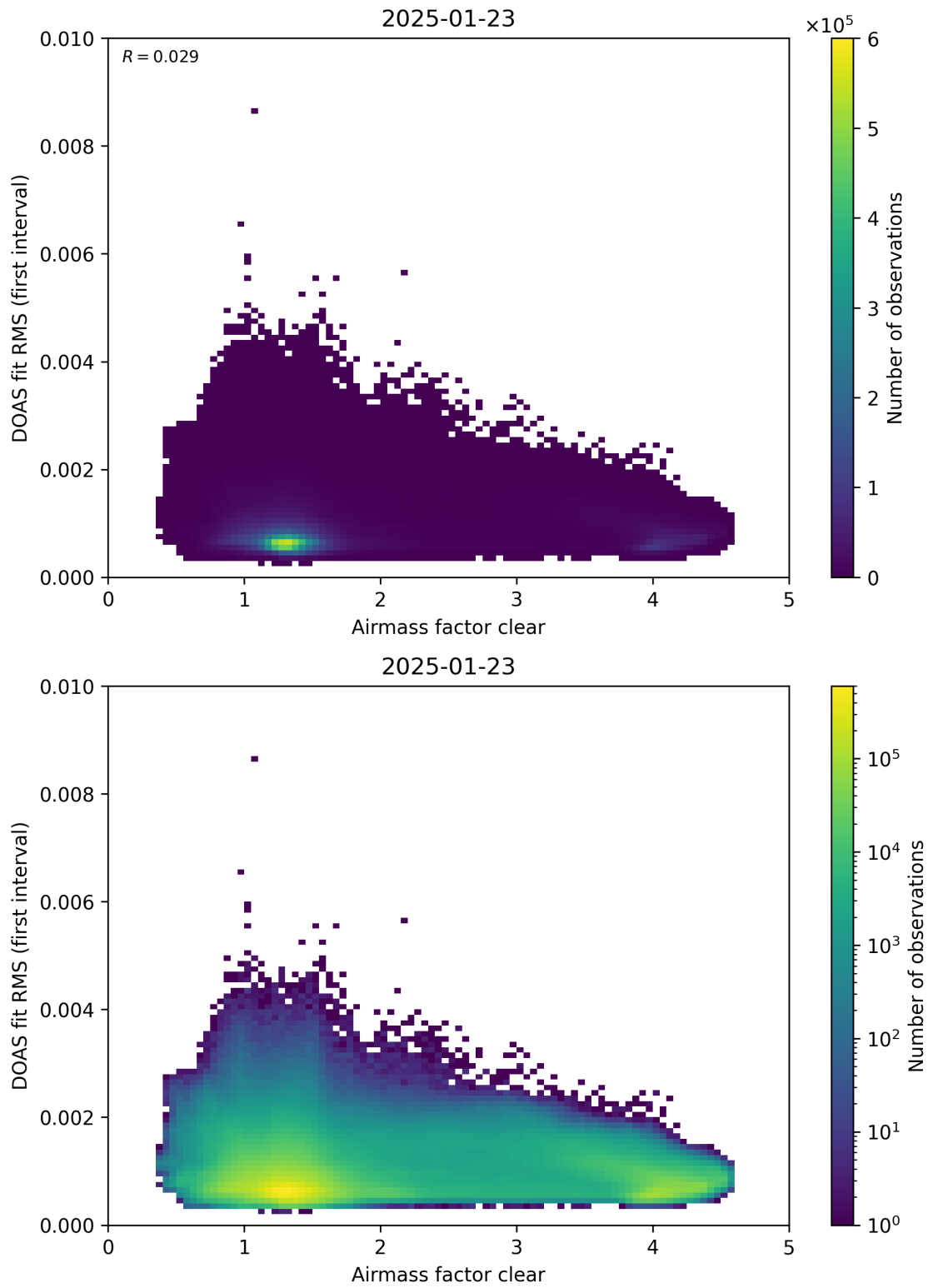
Figure 71: Scatter density plot of “Airmass factor clear” against “DOAS fit RMS (first interval)” for 2025-01-23 to 2025-01-24.
