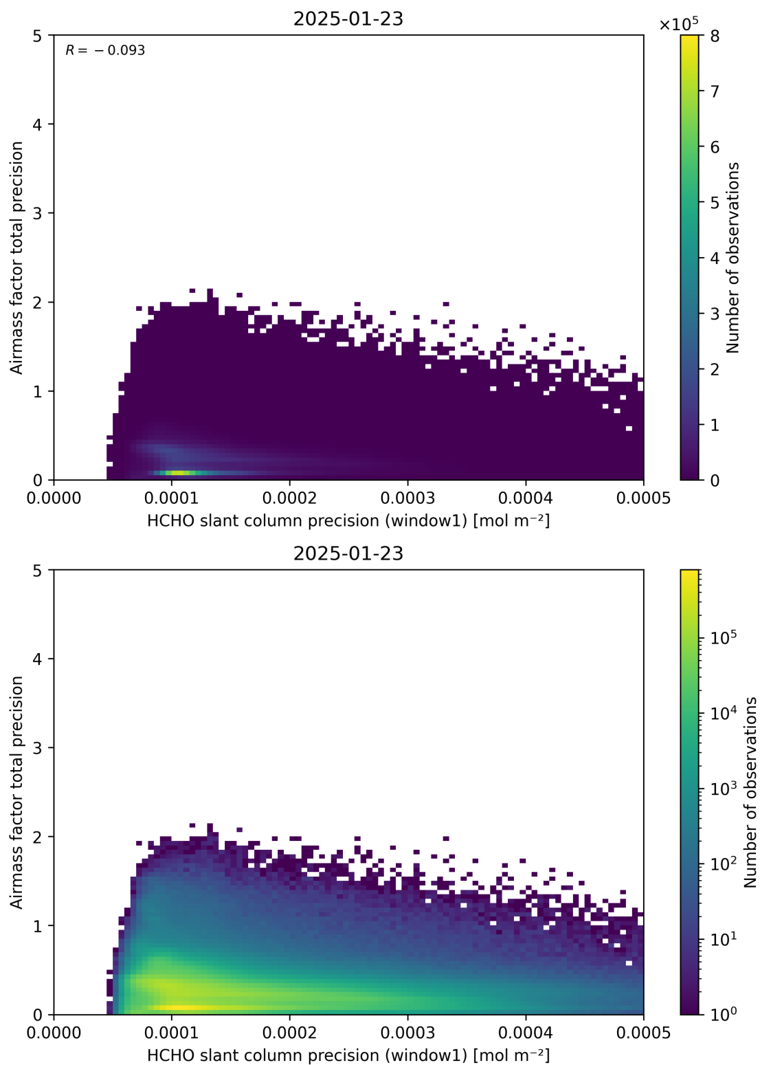
Figure 95: Scatter density plot of “HCHO slant column precision (window1)” against “Airmass factor total precision” for 2025-01-23 to 2025-01-24.
