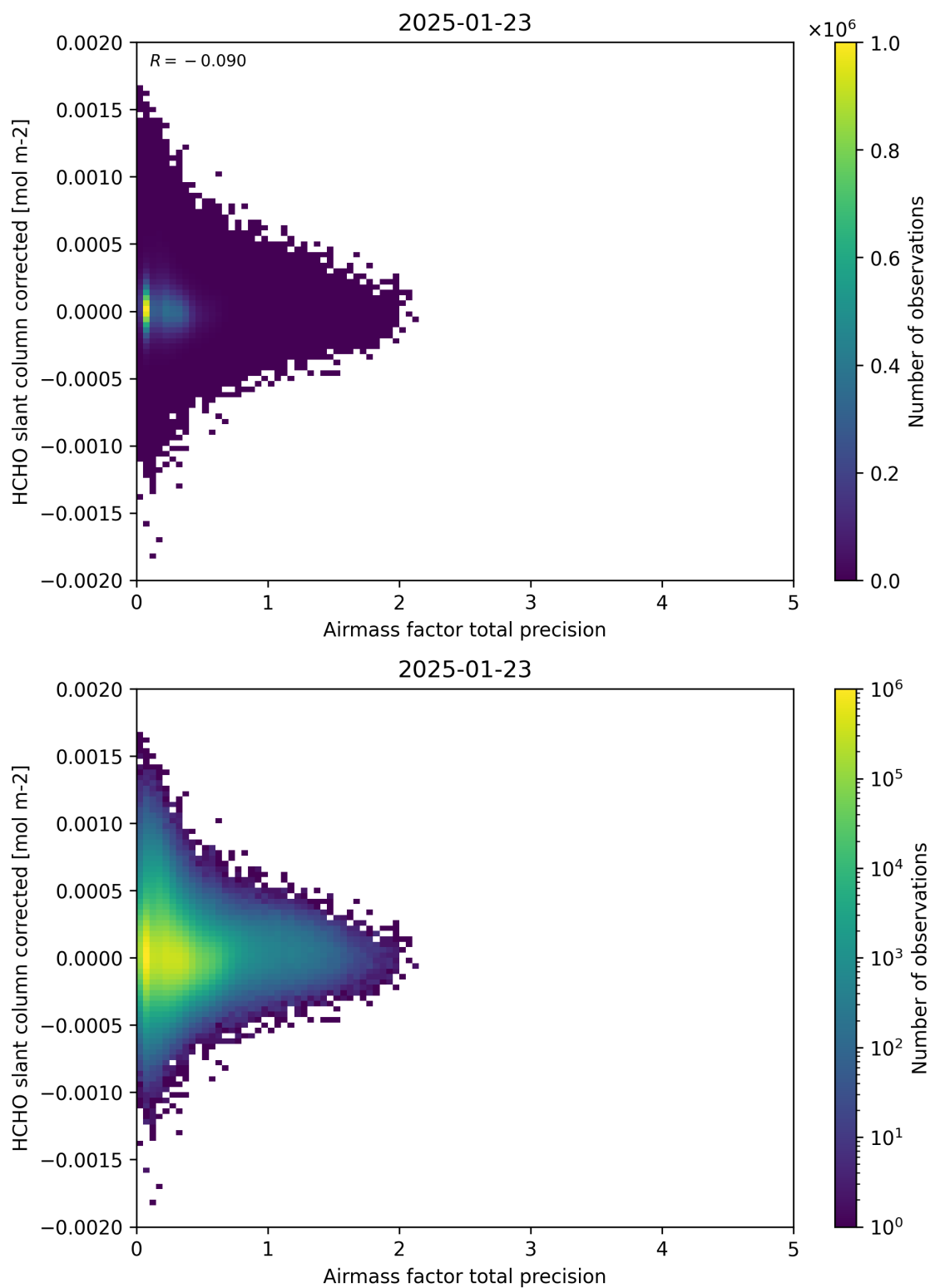
Figure 109: Scatter density plot of “Airmass factor total precision” against “HCHO slant column corrected” for 2025-01-23 to 2025-01-24.
