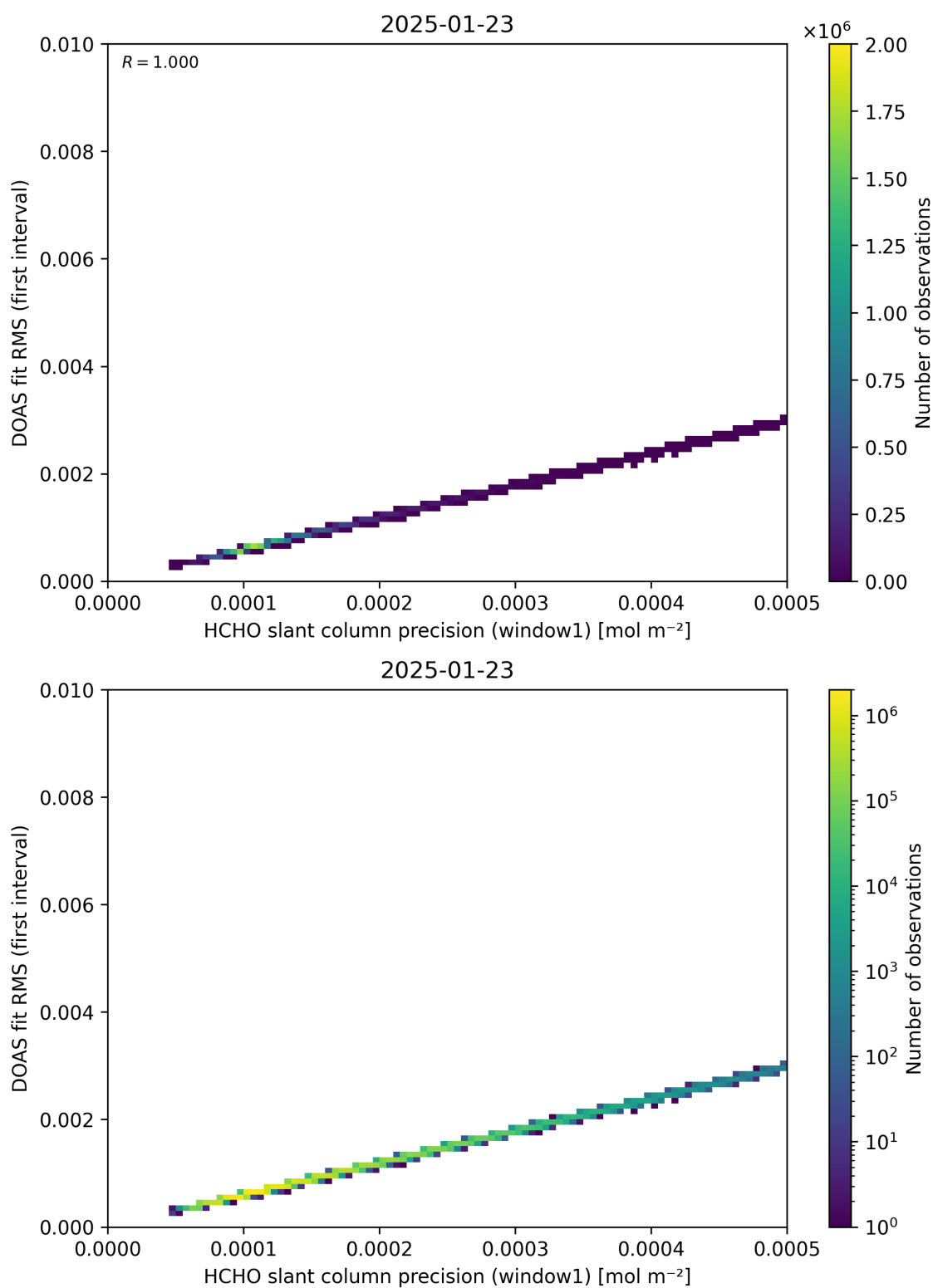
Figure 88: Scatter density plot of “HCHO slant column precision (window1)” against “DOAS fit RMS (first interval)” for 2025-01-23 to 2025-01-24.
