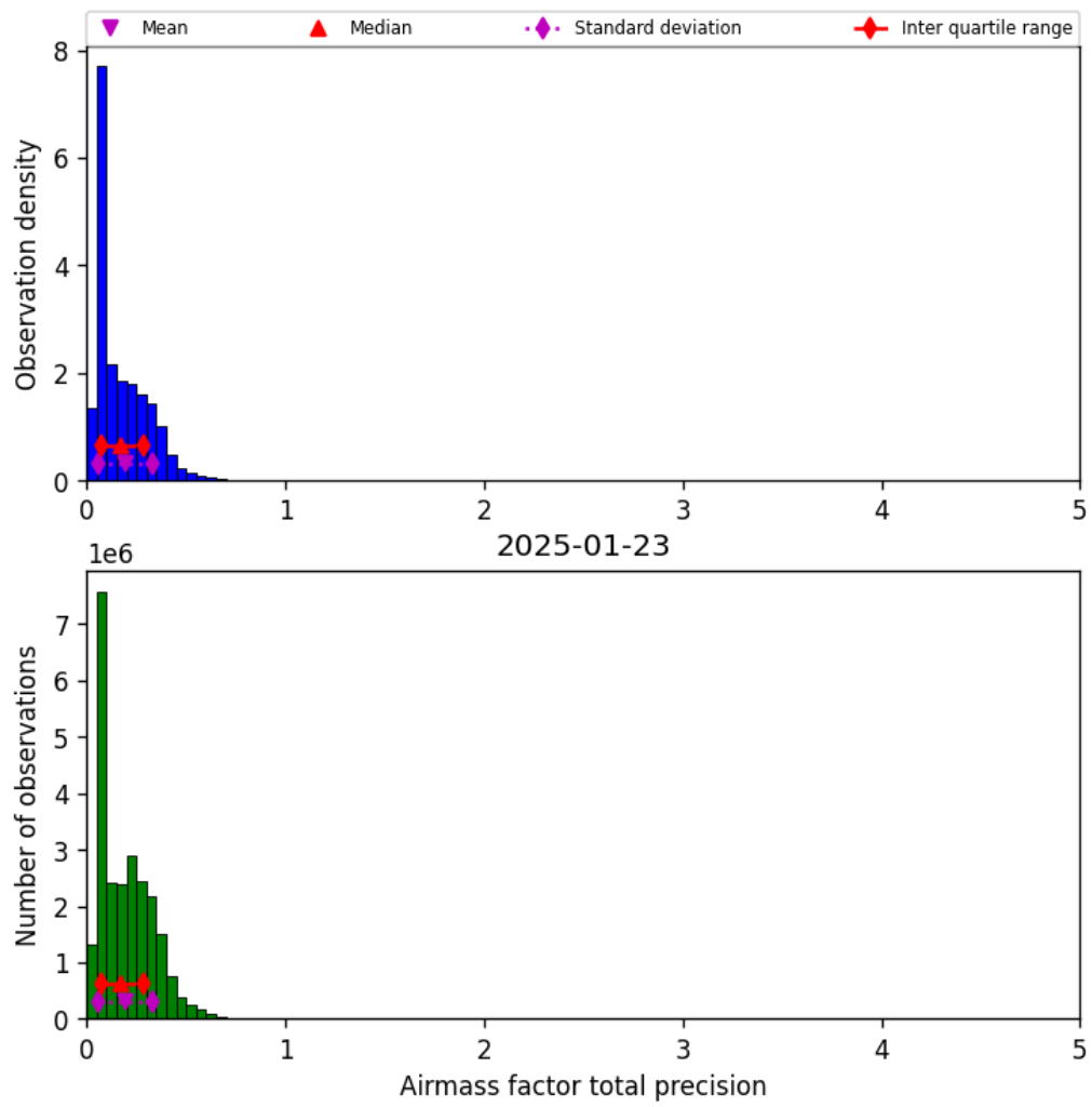
Figure 41: Histogram of “Airmass factor total precision” for 2025-01-23 to 2025-01-24
