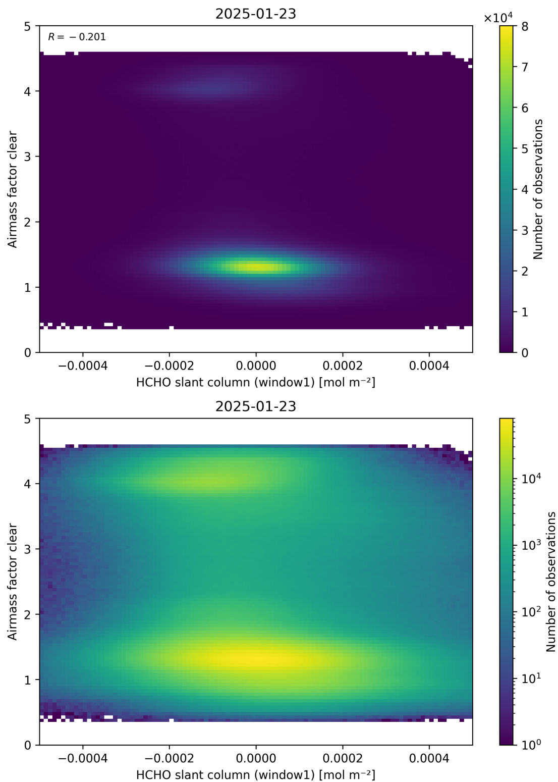
Figure 81: Scatter density plot of “HCHO slant column (window1)” against “Airmass factor clear” for 2025-01-23 to 2025-01-24.
