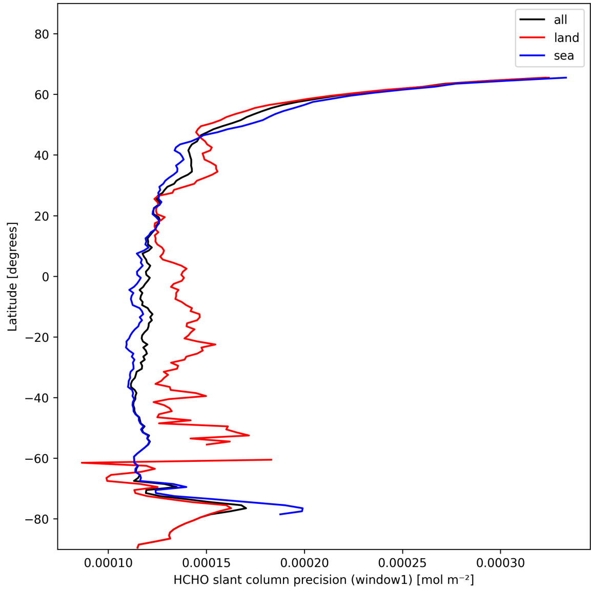
Figure 25: Zonal average of “HCHO slant column precision (window1)” for 2025-01-23 to 2025-01-24.
