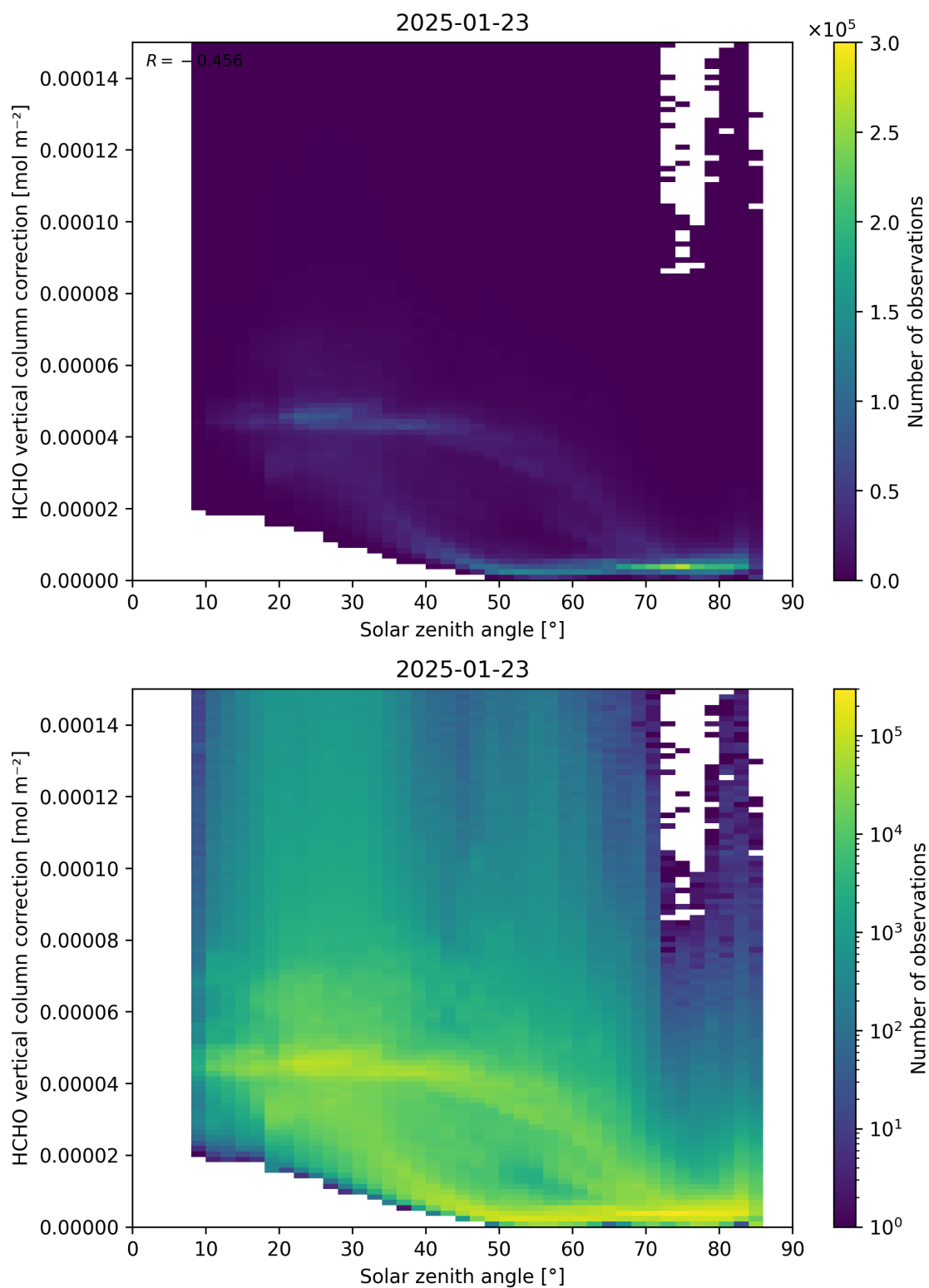
Figure 178: Scatter density plot of “Solar zenith angle” against “HCHO vertical column correction” for 2025-01-23 to 2025-01-24.
