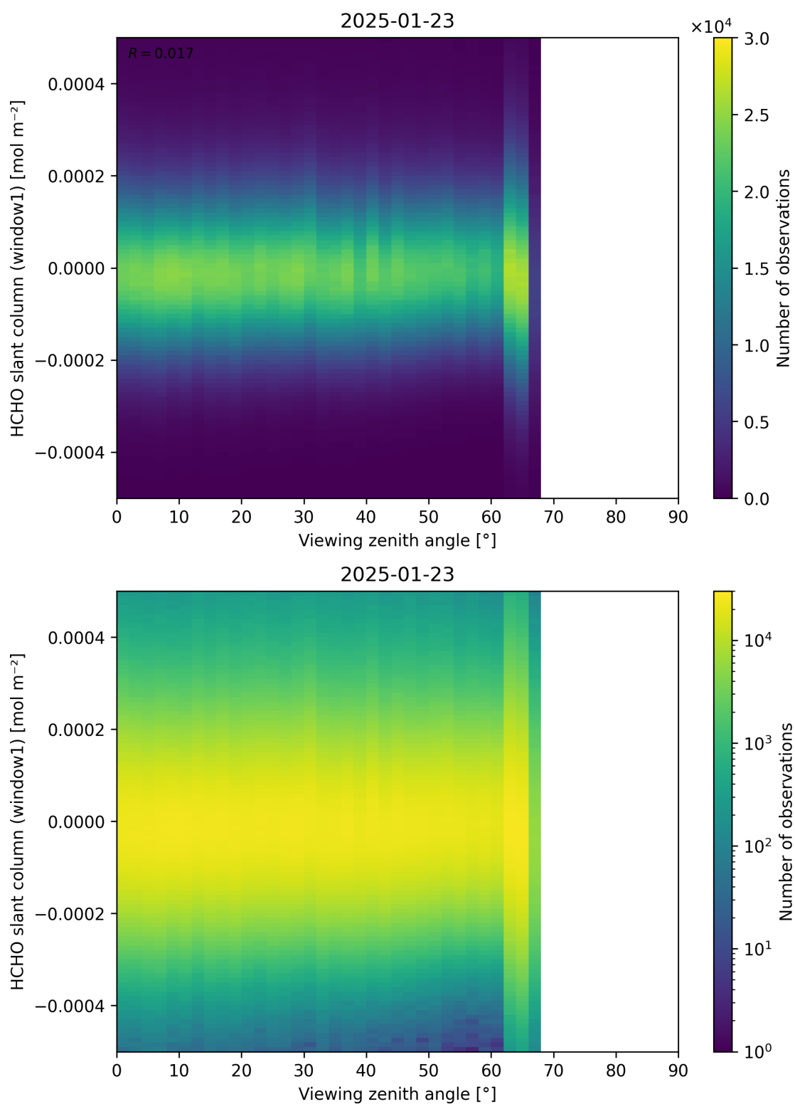
Figure 188: Scatter density plot of “Viewing zenith angle” against “HCHO slant column (window1)” for 2025-01-23 to 2025-01-24.
