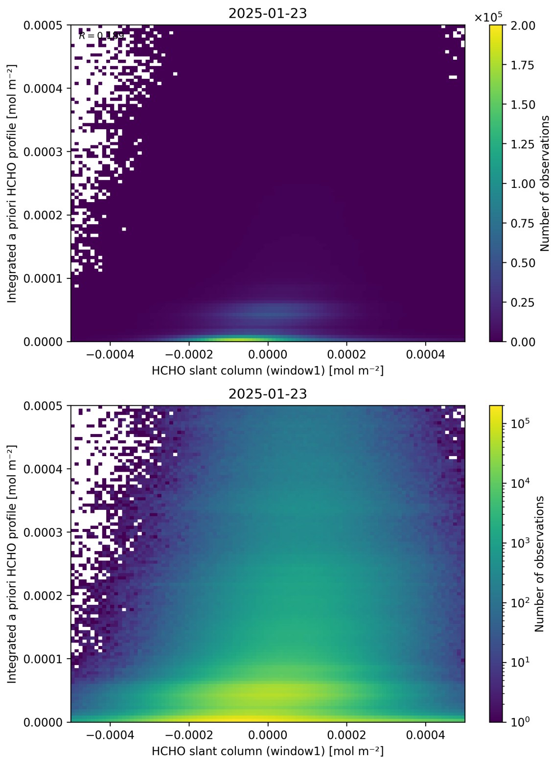
Figure 87: Scatter density plot of “HCHO slant column (window1)” against “Integrated a priori HCHO profile” for 2025-01-23 to 2025-01-24.
