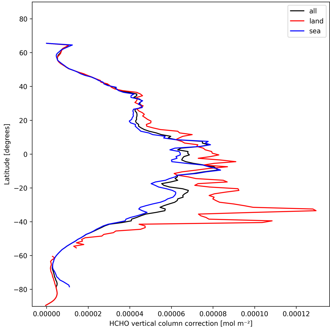
Figure 23: Zonal average of “HCHO vertical column correction” for 2025-01-23 to 2025-01-24.
