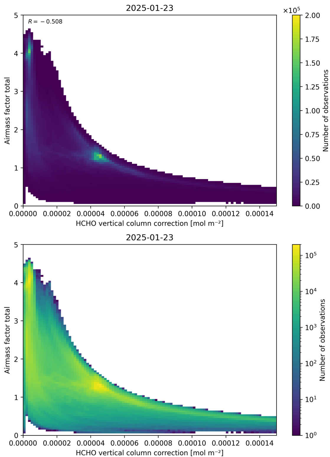
Figure 120: Scatter density plot of “HCHO vertical column correction” against “Airmass factor total” for 2025-01-23 to 2025-01-24.
