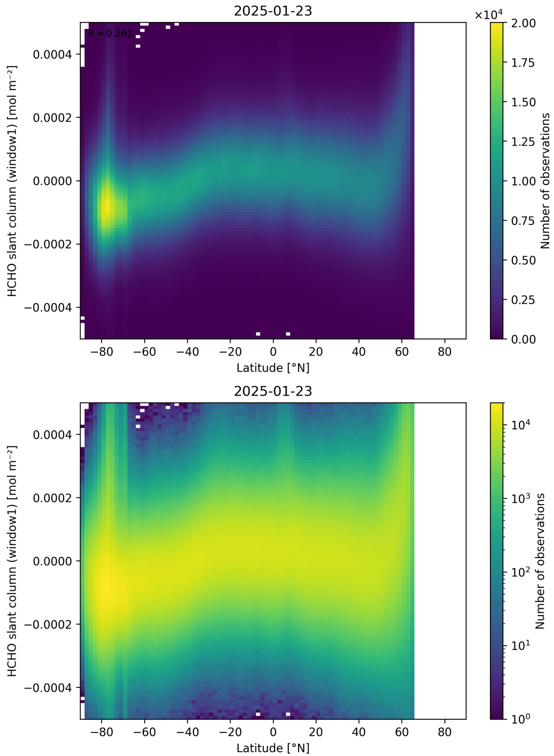
Figure 159: Scatter density plot of “Latitude” against “HCHO slant column (window1)” for 2025-01-23 to 2025-01-24.
