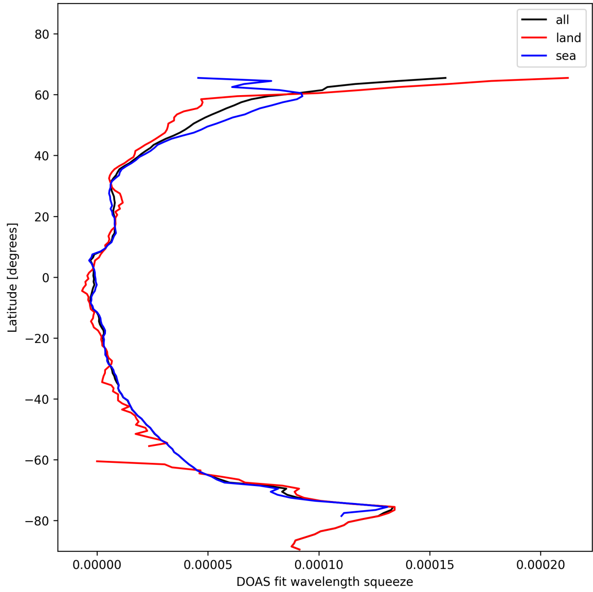
Figure 31: Zonal average of “DOAS fit wavelength squeeze” for 2025-01-23 to 2025-01-24.
