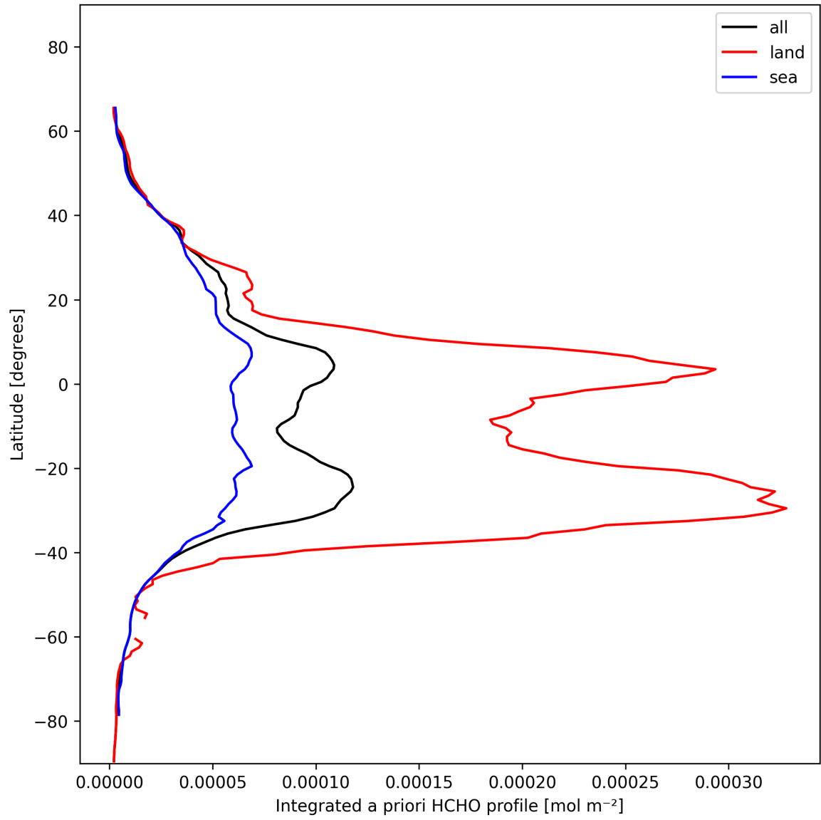
Figure 29: Zonal average of “Integrated a priori HCHO profile” for 2025-01-23 to 2025-01-24.
