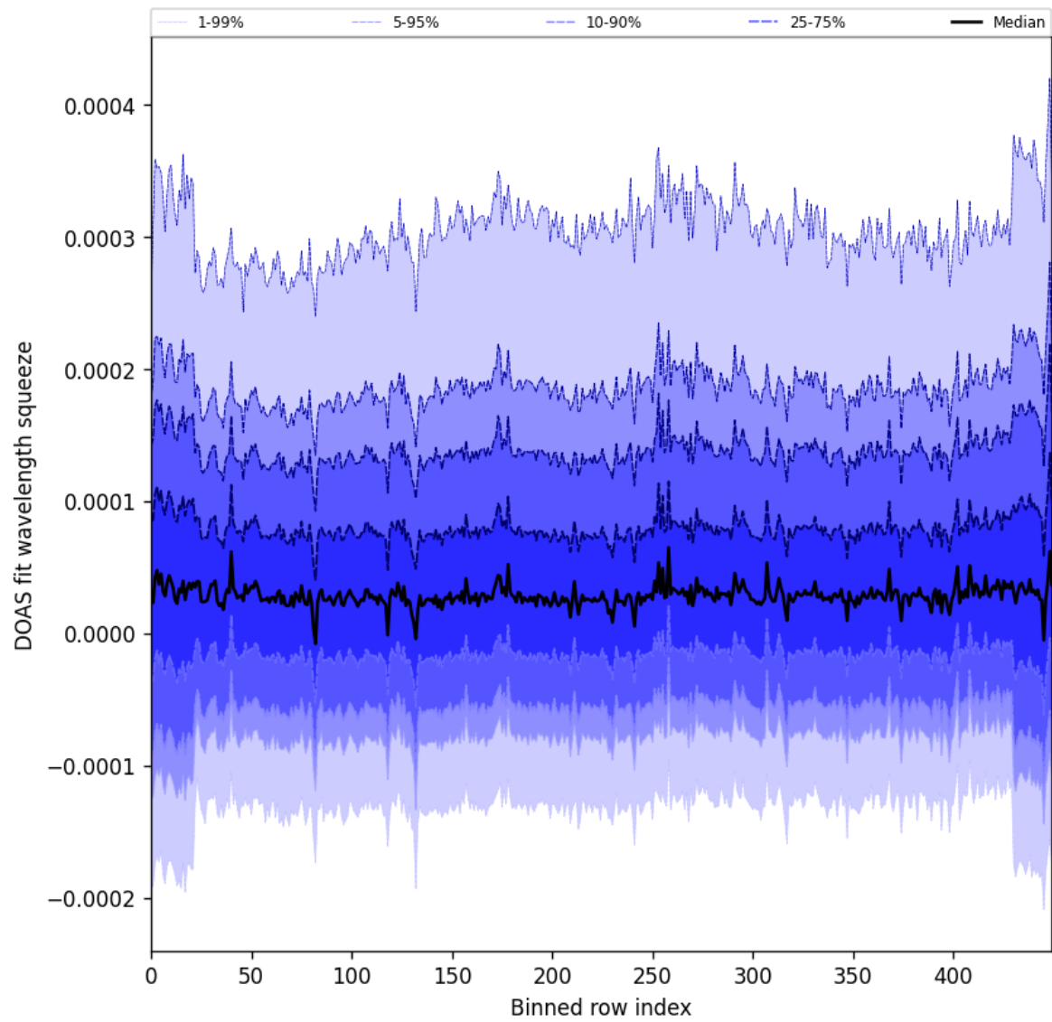
Figure 59: Along track statistics of “DOAS fit wavelength squeeze” for 2025-01-23 to 2025-01-24
