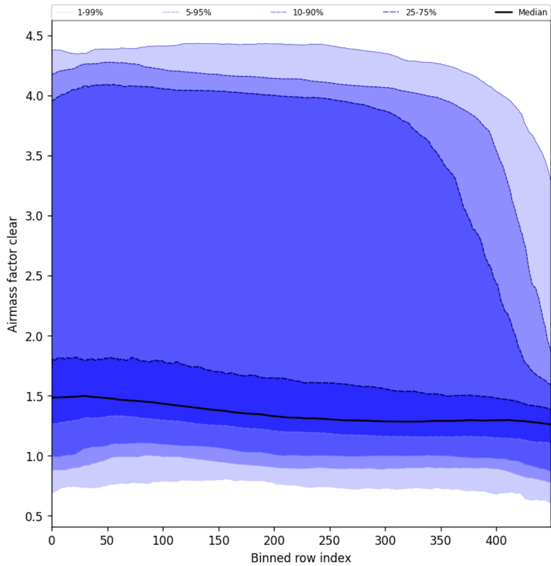
Figure 56: Along track statistics of “Airmass factor clear” for 2025-01-23 to 2025-01-24
