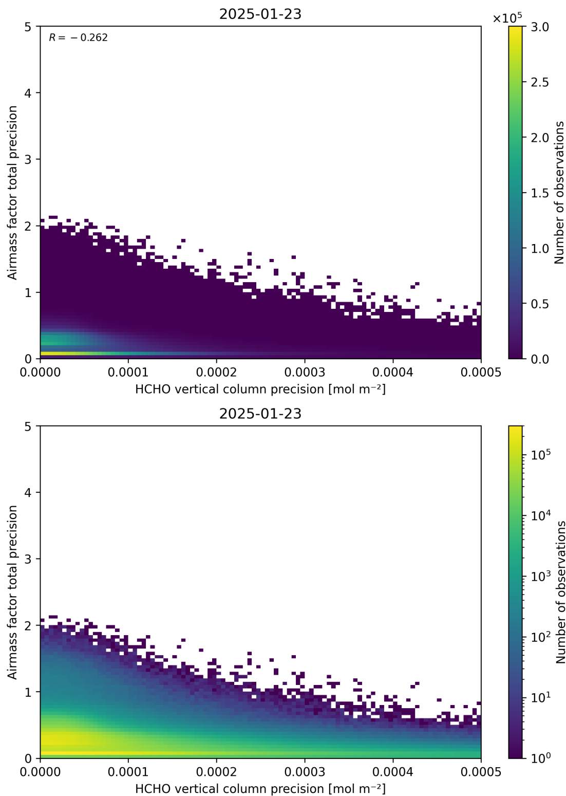
Figure 145: Scatter density plot of “HCHO vertical column precision” against “Airmass factor total precision” for 2025-01-23 to 2025-01-24.
