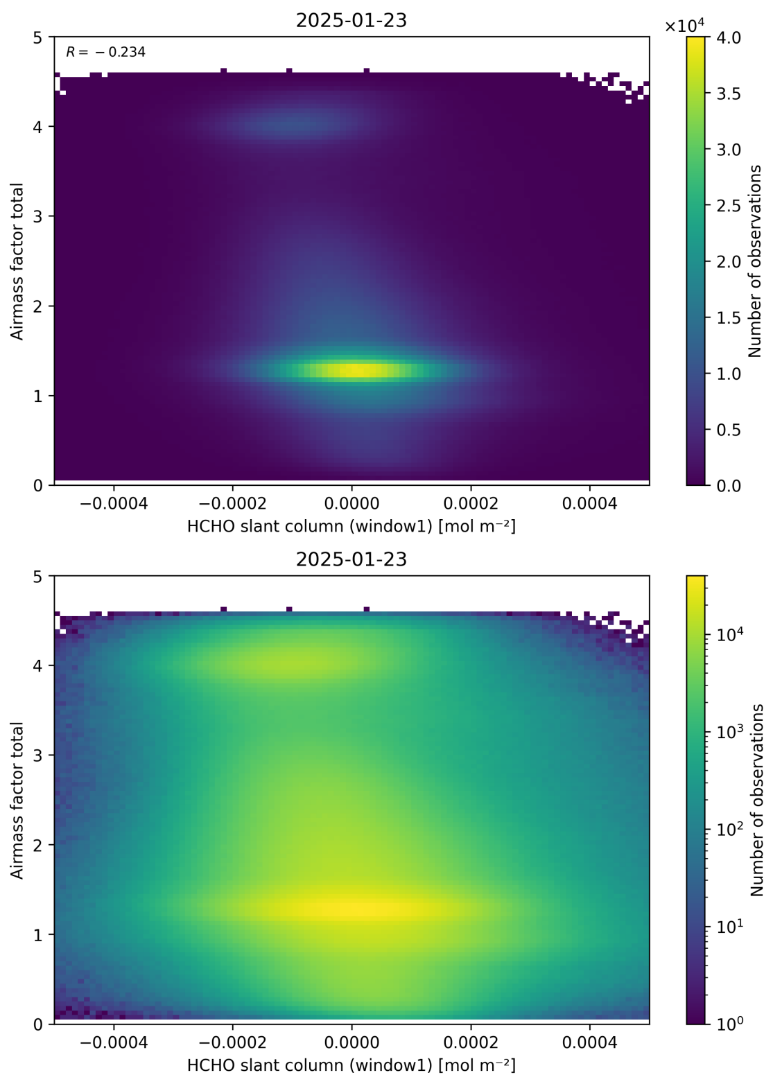
Figure 85: Scatter density plot of “HCHO slant column (window1)” against “Airmass factor total” for 2025-01-23 to 2025-01-24.
