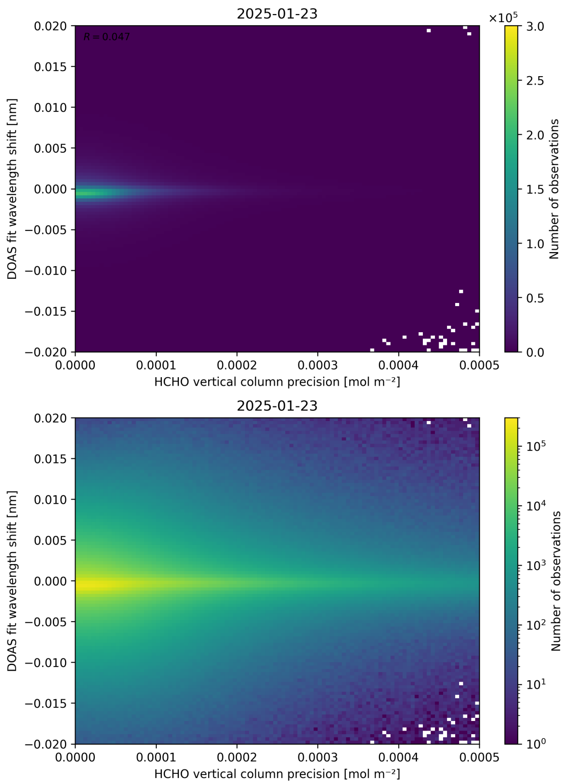
Figure 137: Scatter density plot of “HCHO vertical column precision” against “DOAS fit wavelength shift” for 2025-01-23 to 2025-01-24.
