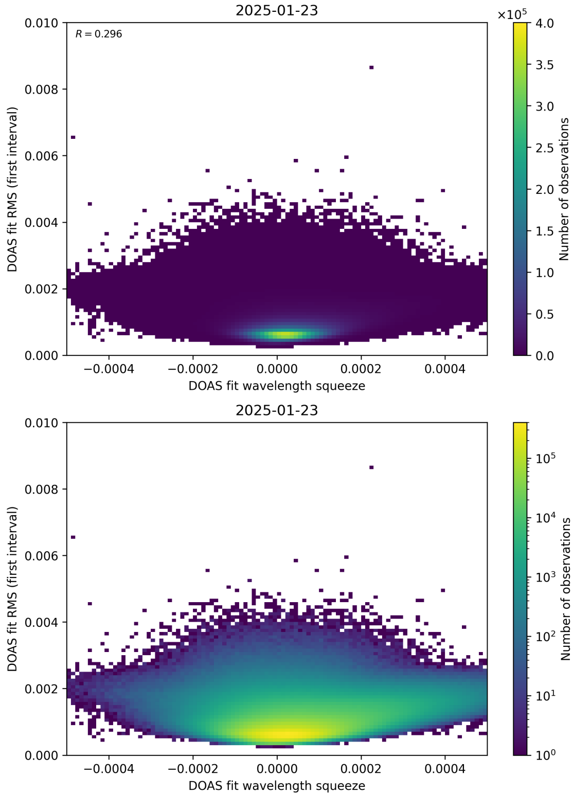
Figure 68: Scatter density plot of “DOAS fit wavelength squeeze” against “DOAS fit RMS (first interval)” for 2025-01-23 to 2025-01-24.
