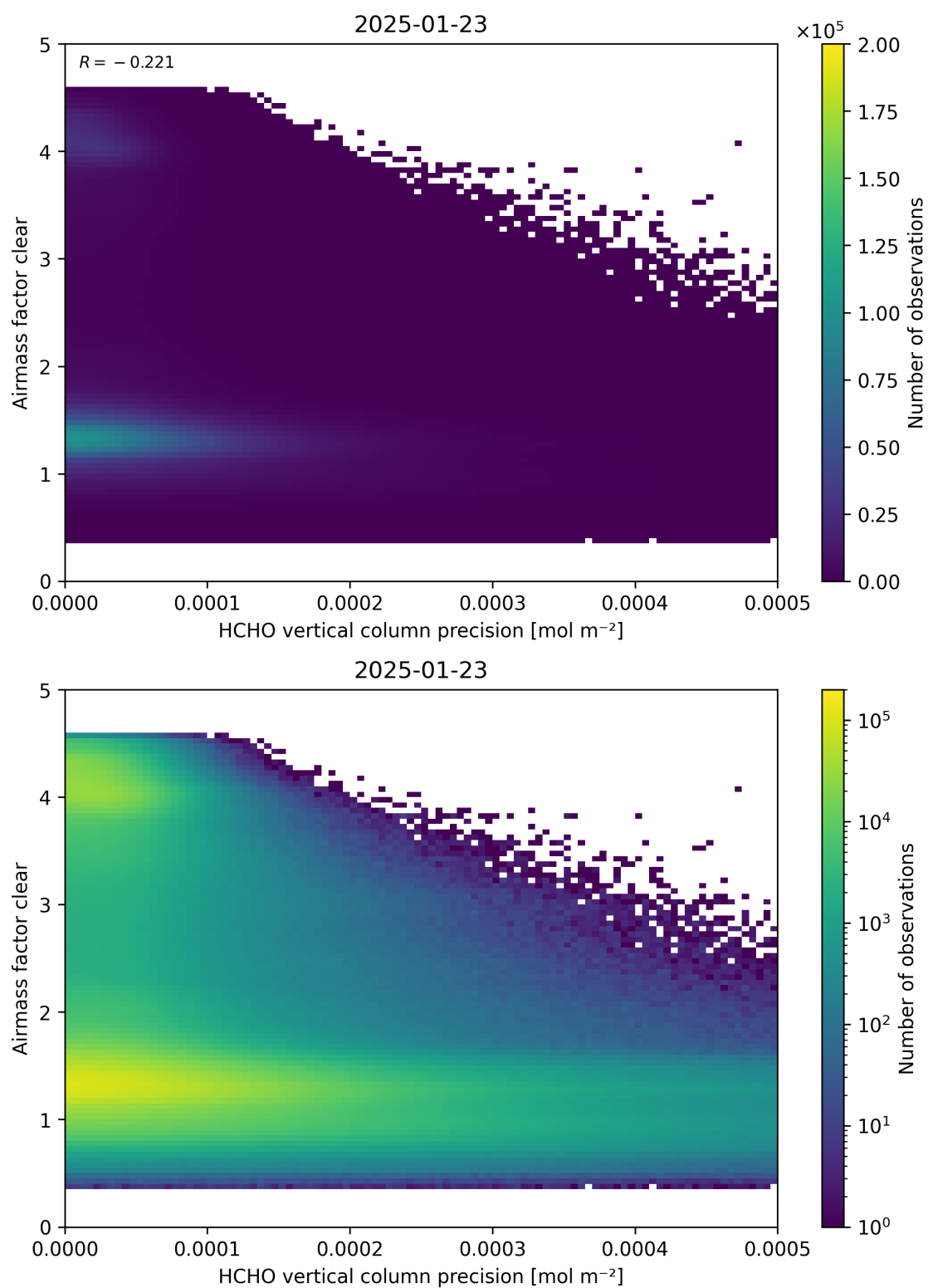
Figure 139: Scatter density plot of “HCHO vertical column precision” against “Airmass factor clear” for 2025-01-23 to 2025-01-24.
