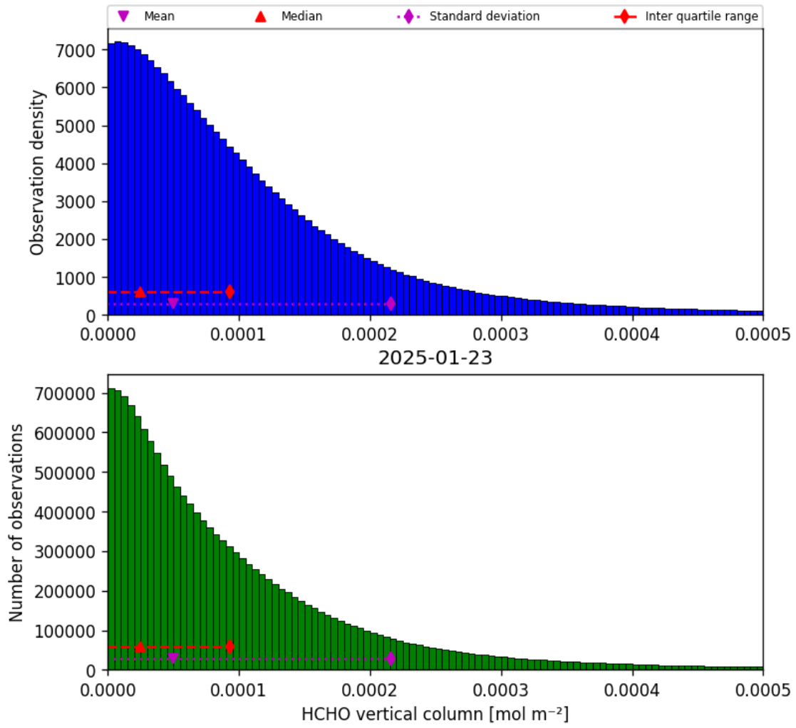
Figure 35: Histogram of “HCHO vertical column” for 2025-01-23 to 2025-01-24
