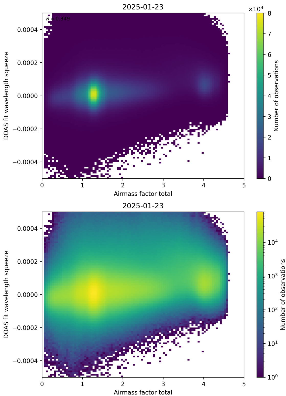
Figure 99: Scatter density plot of “Airmass factor total” against “DOAS fit wavelength squeeze” for 2025-01-23 to 2025-01-24.
