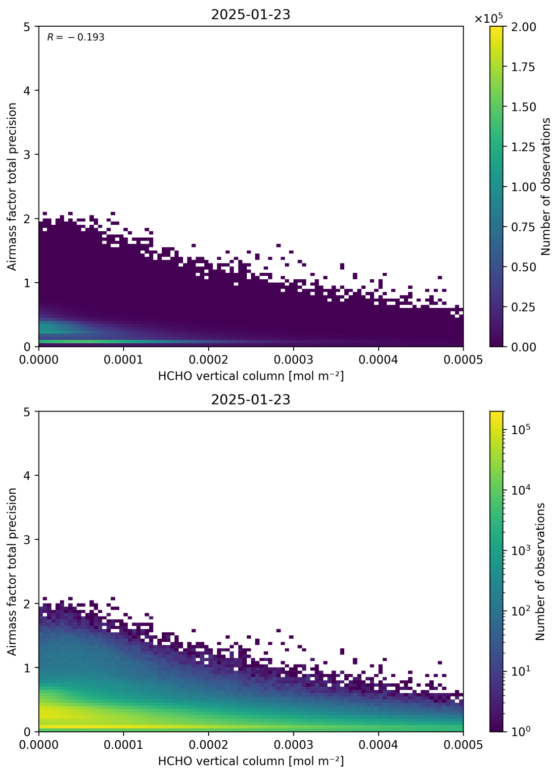
Figure 132: Scatter density plot of “HCHO vertical column” against “Airmass factor total precision” for 2025-01-23 to 2025-01-24.
