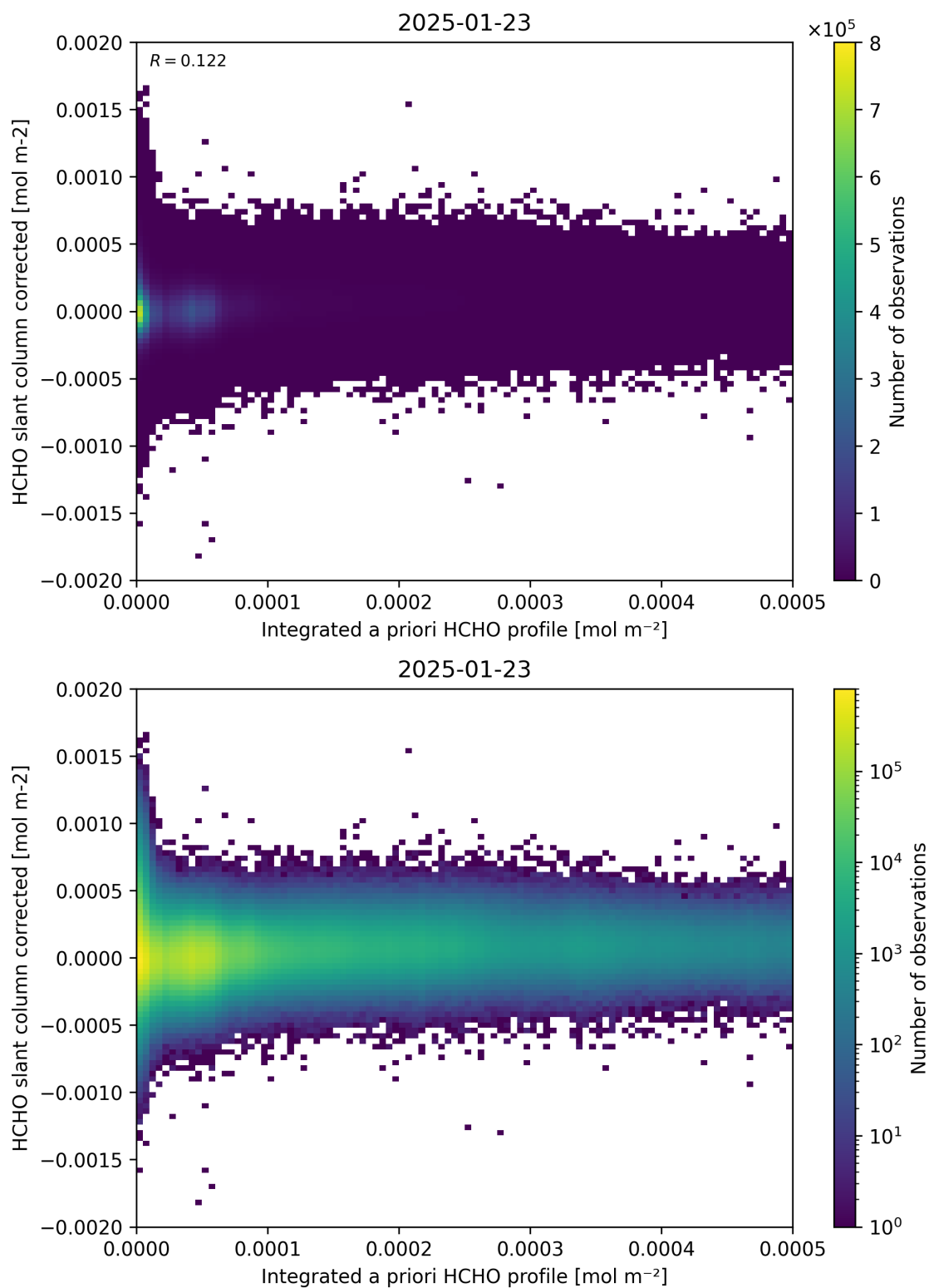
Figure 151: Scatter density plot of “Integrated a priori HCHO profile” against “HCHO slant column corrected” for 2025-01-23 to 2025-01-24.
