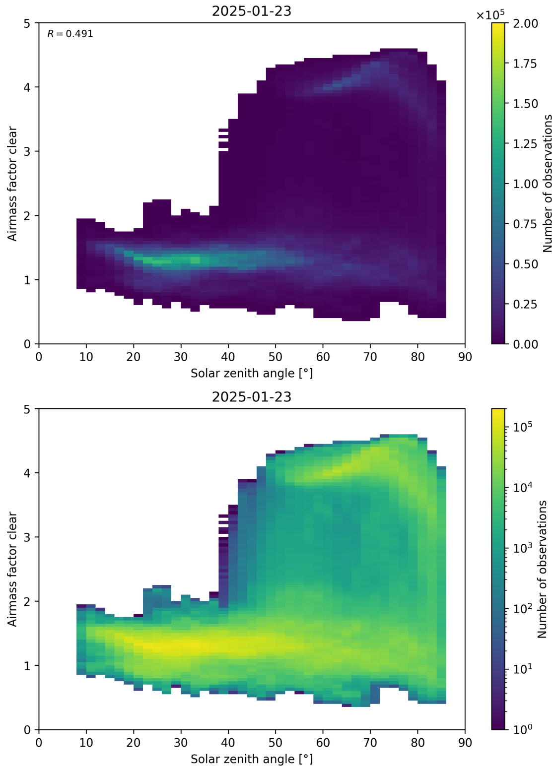
Figure 170: Scatter density plot of “Solar zenith angle” against “Airmass factor clear” for 2025-01-23 to 2025-01-24.
