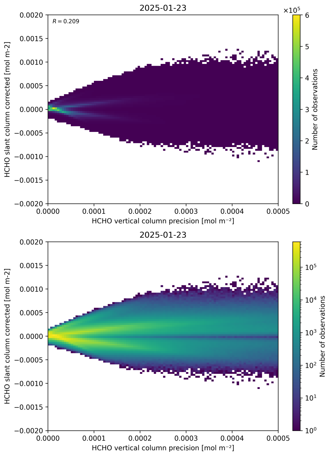
Figure 140: Scatter density plot of “HCHO vertical column precision” against “HCHO slant column corrected” for 2025-01-23 to 2025-01-24.
