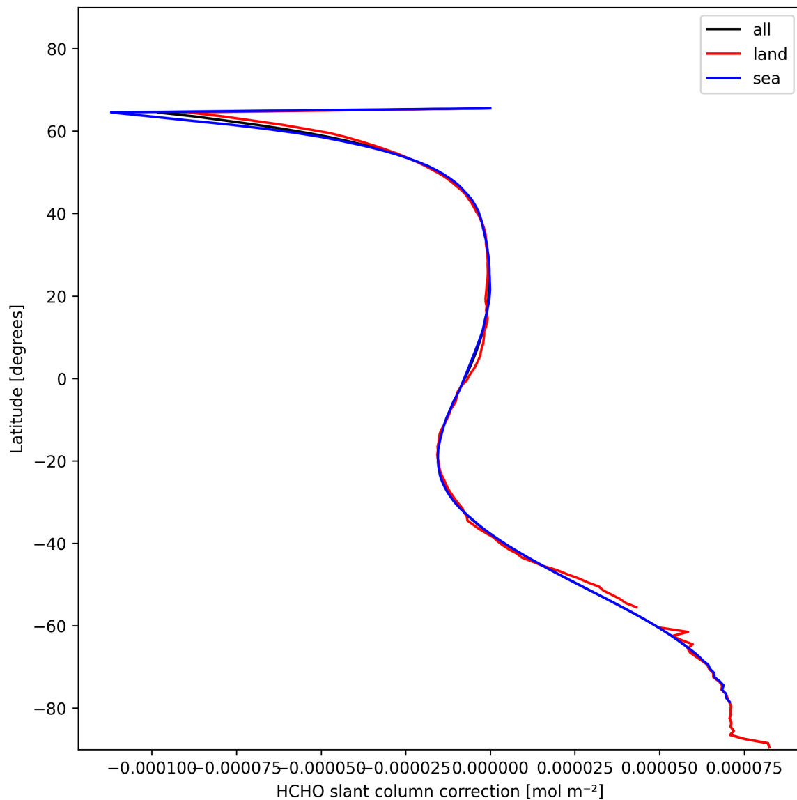
Figure 33: Zonal average of “HCHO slant column correction” for 2025-01-23 to 2025-01-24.
