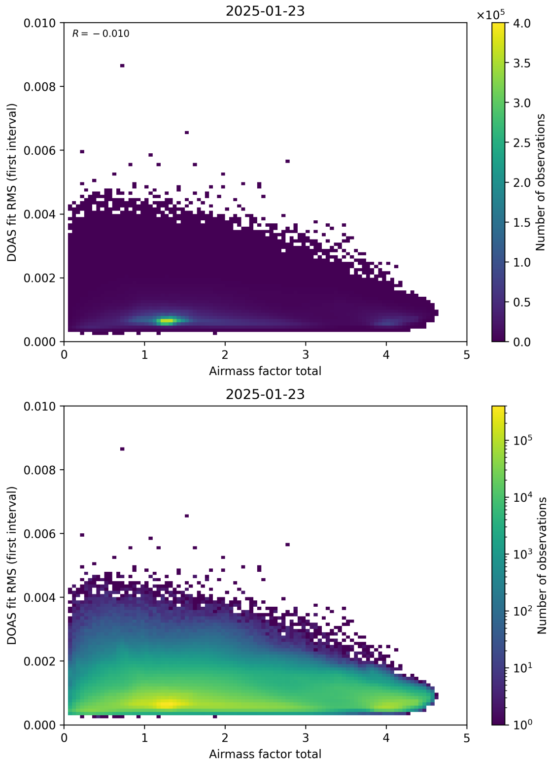
Figure 97: Scatter density plot of “Airmass factor total” against “DOAS fit RMS (first interval)” for 2025-01-23 to 2025-01-24.
