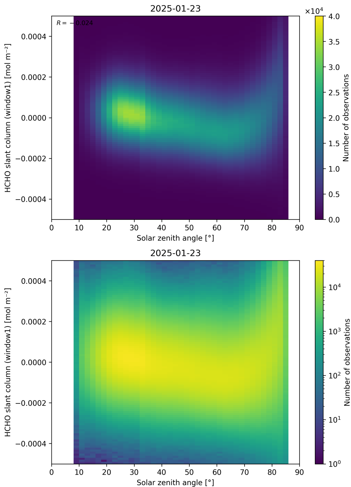
Figure 173: Scatter density plot of “Solar zenith angle” against “HCHO slant column (window1)” for 2025-01-23 to 2025-01-24.
