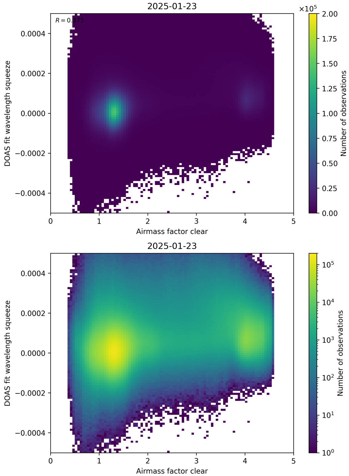
Figure 73: Scatter density plot of “Airmass factor clear” against “DOAS fit wavelength squeeze” for 2025-01-23 to 2025-01-24.
