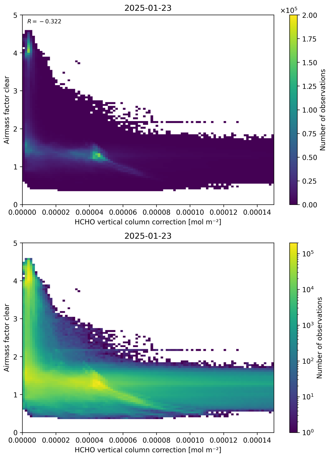
Figure 115: Scatter density plot of “HCHO vertical column correction” against “Airmass factor clear” for 2025-01-23 to 2025-01-24.
