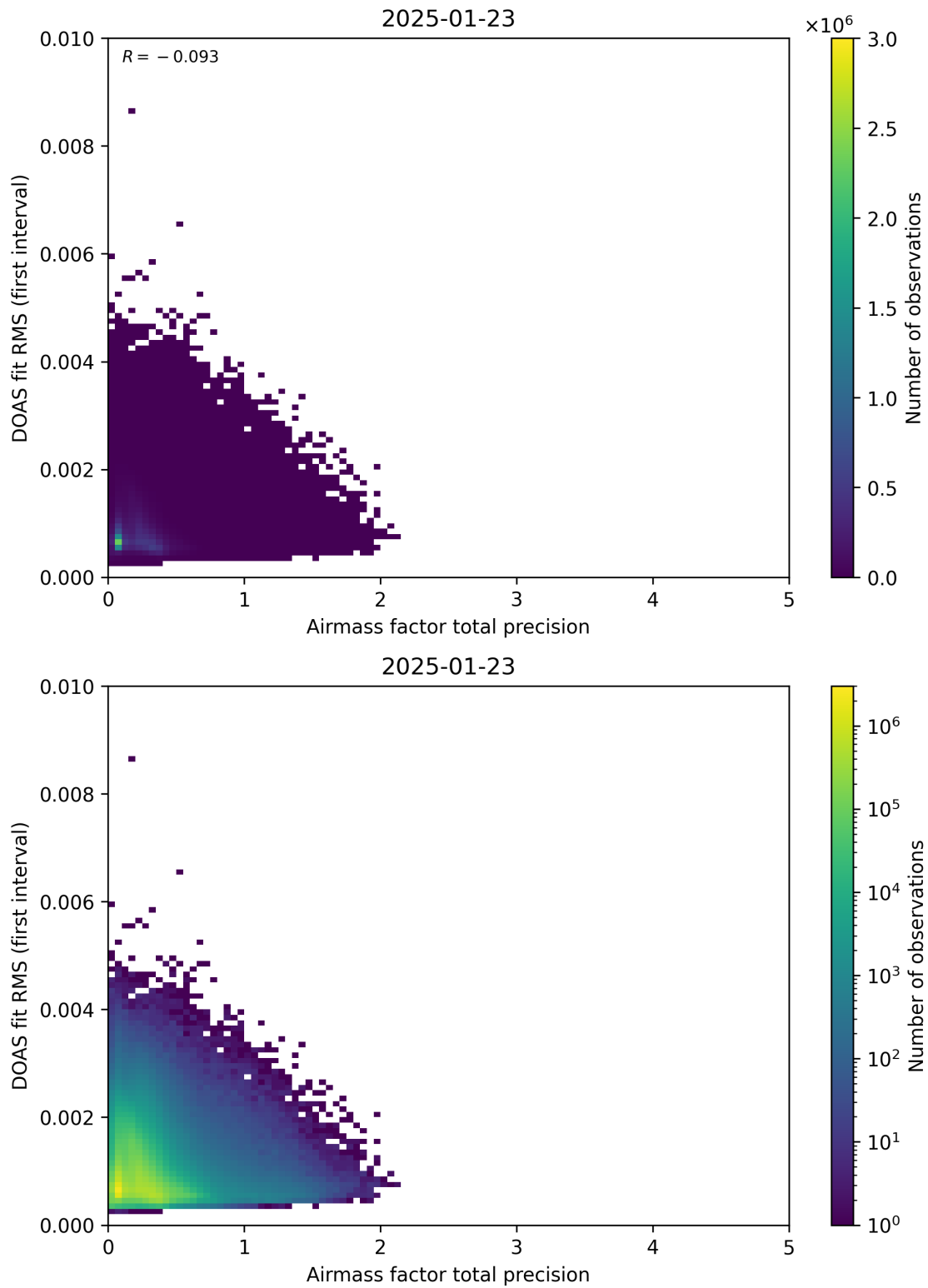
Figure 105: Scatter density plot of “Airmass factor total precision” against “DOAS fit RMS (first interval)” for 2025-01-23 to 2025-01-24.
