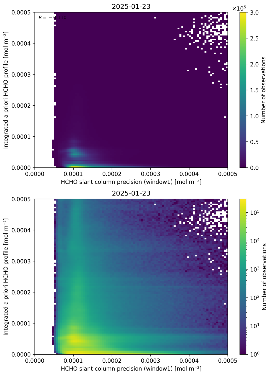
Figure 96: Scatter density plot of “HCHO slant column precision (window1)” against “Integrated a priori HCHO profile” for 2025-01-23 to 2025-01-24.
