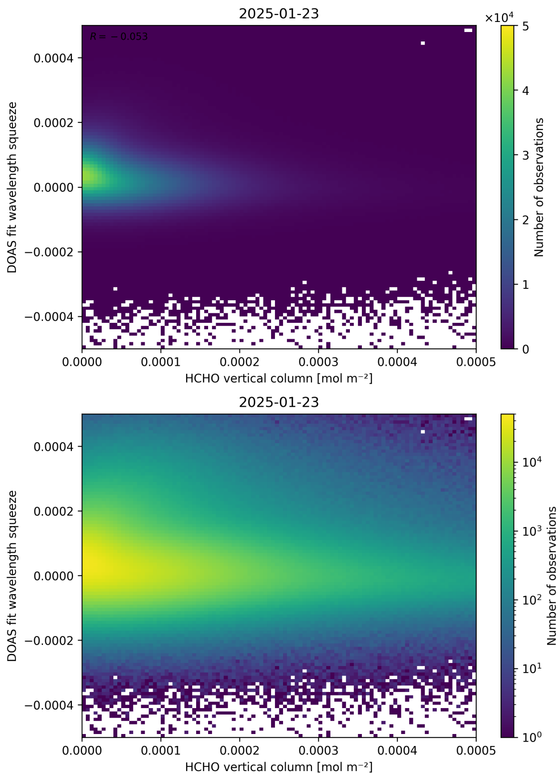
Figure 125: Scatter density plot of “HCHO vertical column” against “DOAS fit wavelength squeeze” for 2025-01-23 to 2025-01-24.
