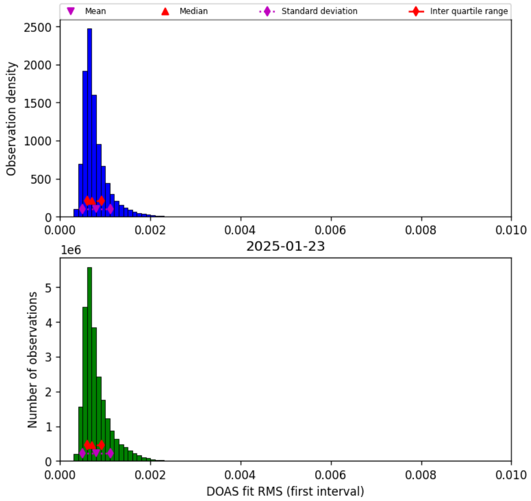
Figure 46: Histogram of “DOAS fit RMS (first interval)” for 2025-01-23 to 2025-01-24
