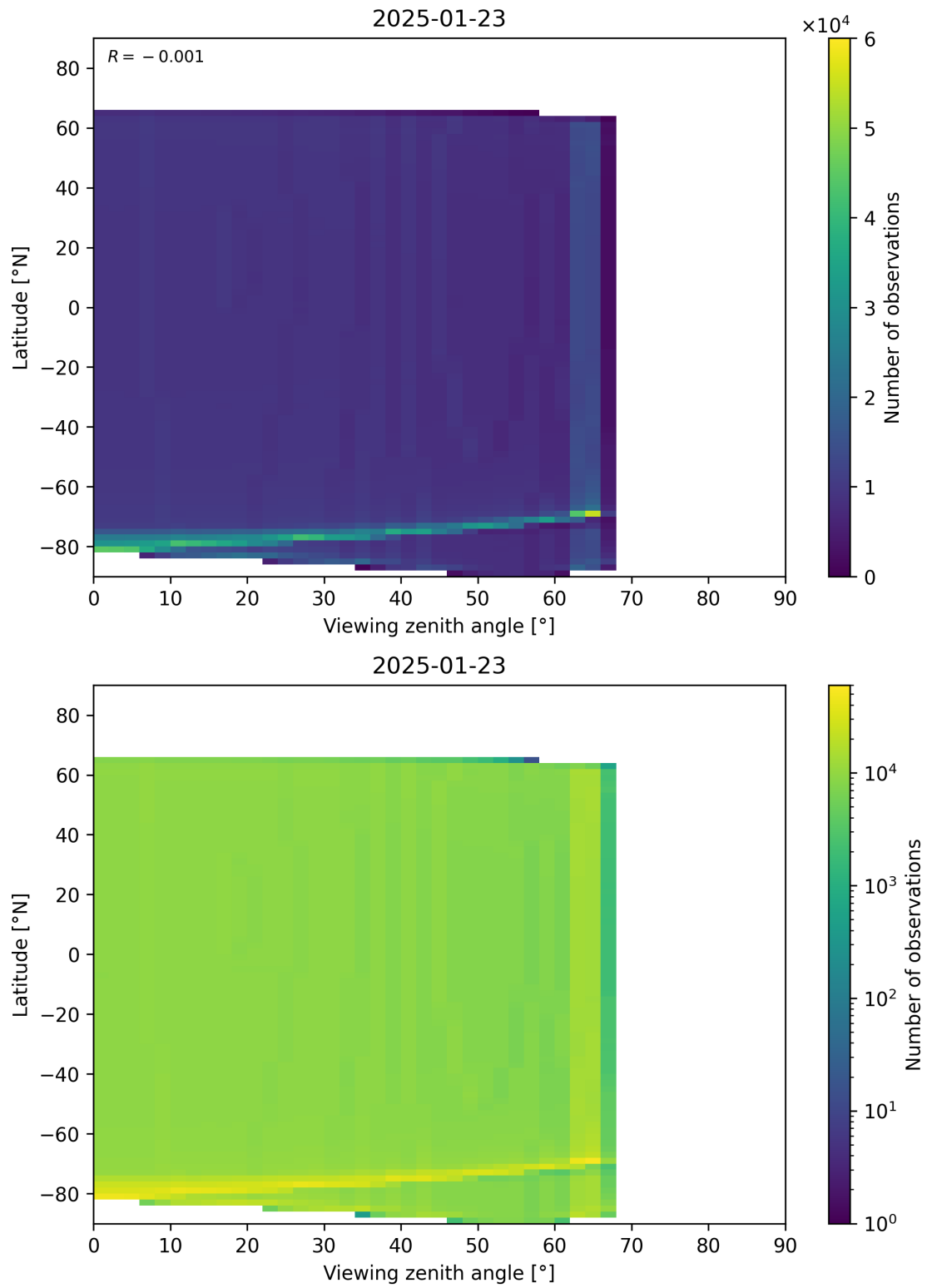
Figure 196: Scatter density plot of “Viewing zenith angle” against “Latitude” for 2025-01-23 to 2025-01-24.
