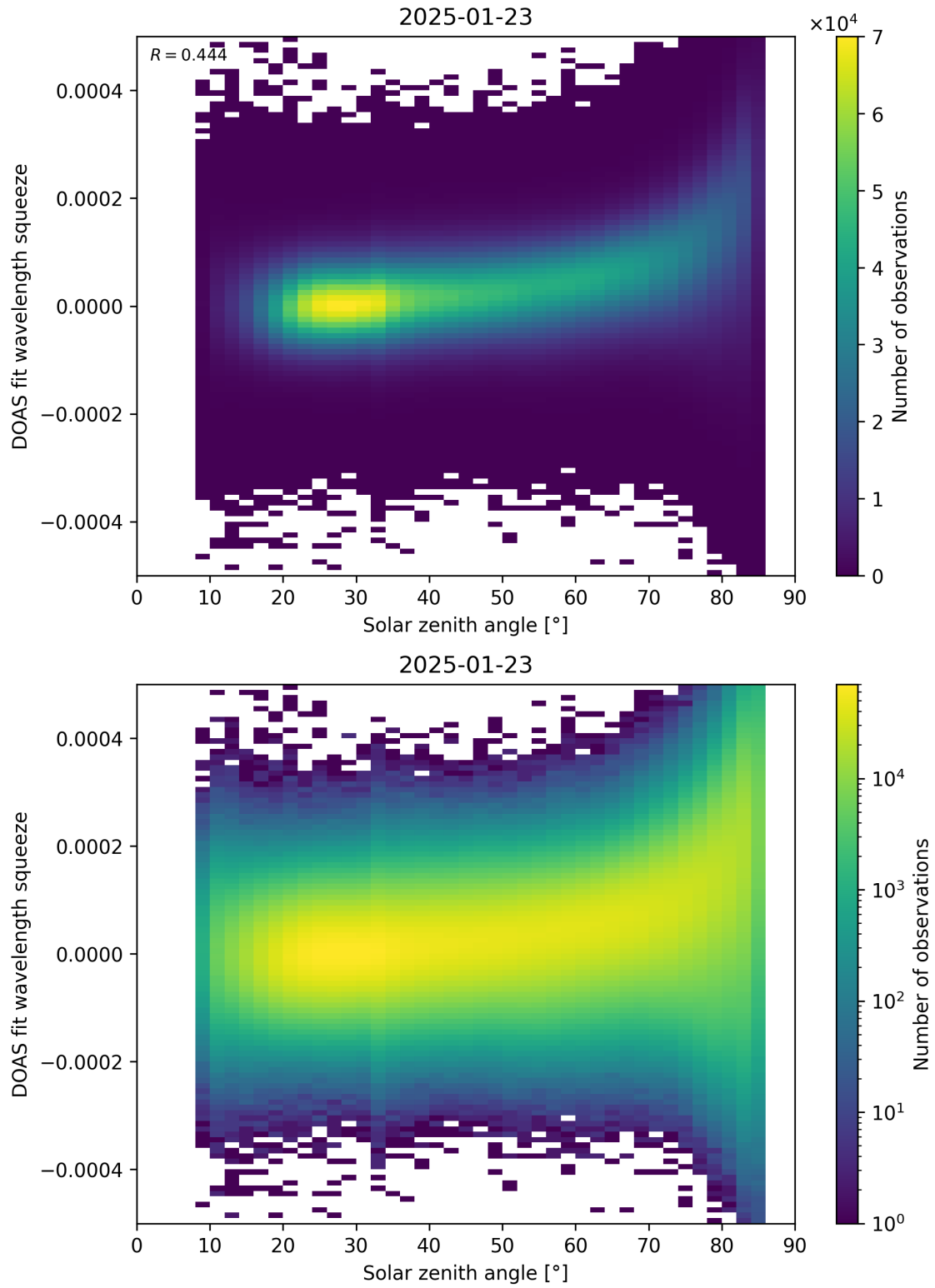
Figure 169: Scatter density plot of “Solar zenith angle” against “DOAS fit wavelength squeeze” for 2025-01-23 to 2025-01-24.
