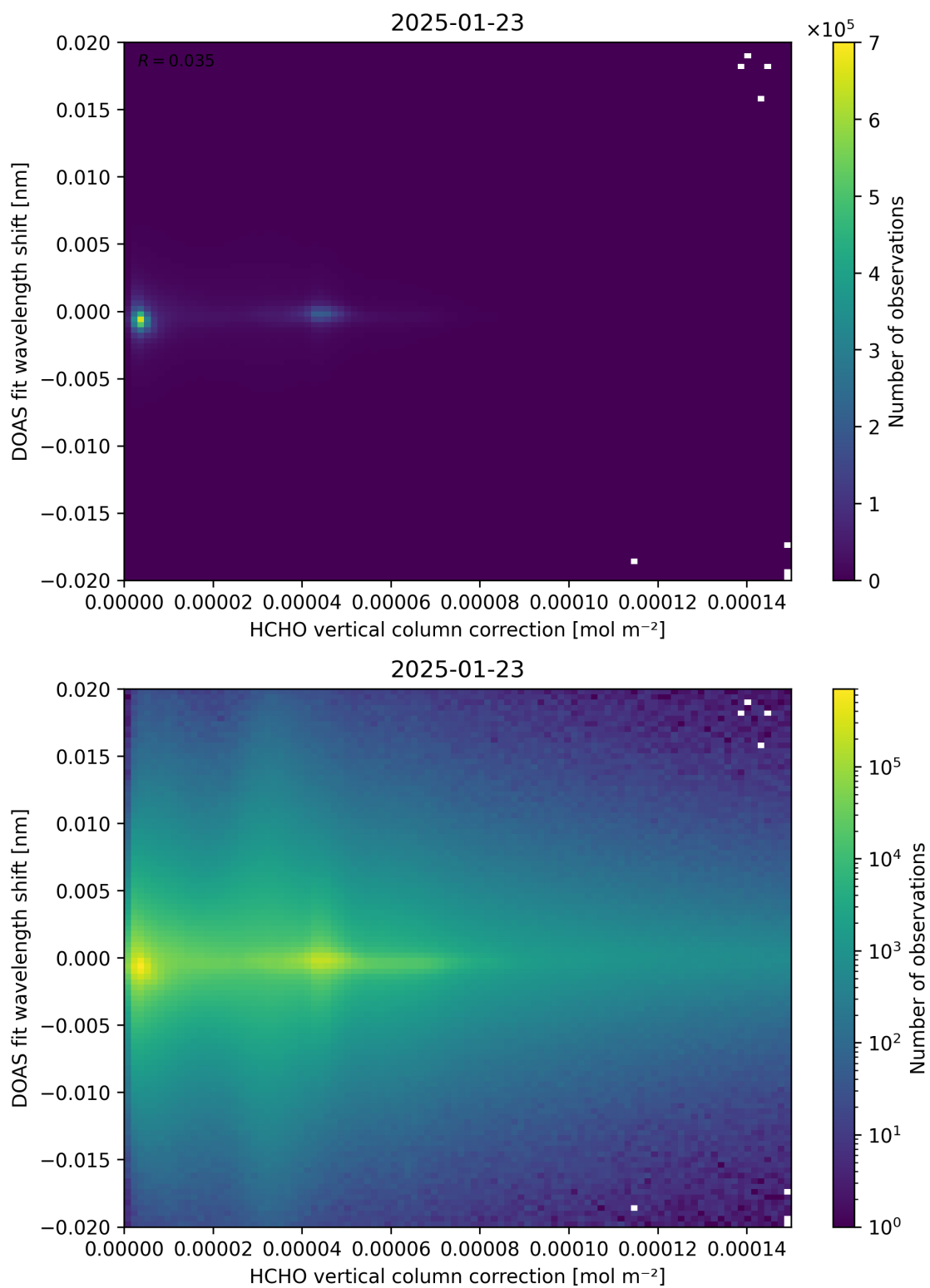
Figure 113: Scatter density plot of “HCHO vertical column correction” against “DOAS fit wavelength shift” for 2025-01-23 to 2025-01-24.
