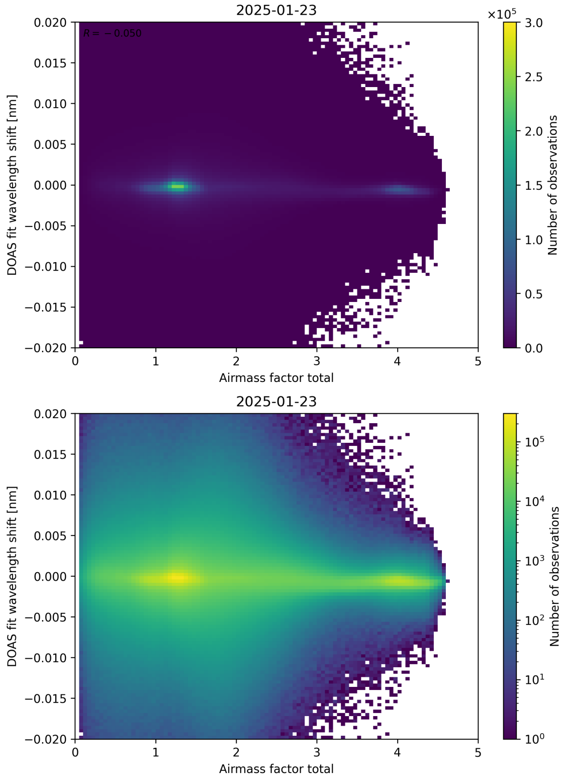
Figure 98: Scatter density plot of “Airmass factor total” against “DOAS fit wavelength shift” for 2025-01-23 to 2025-01-24.
