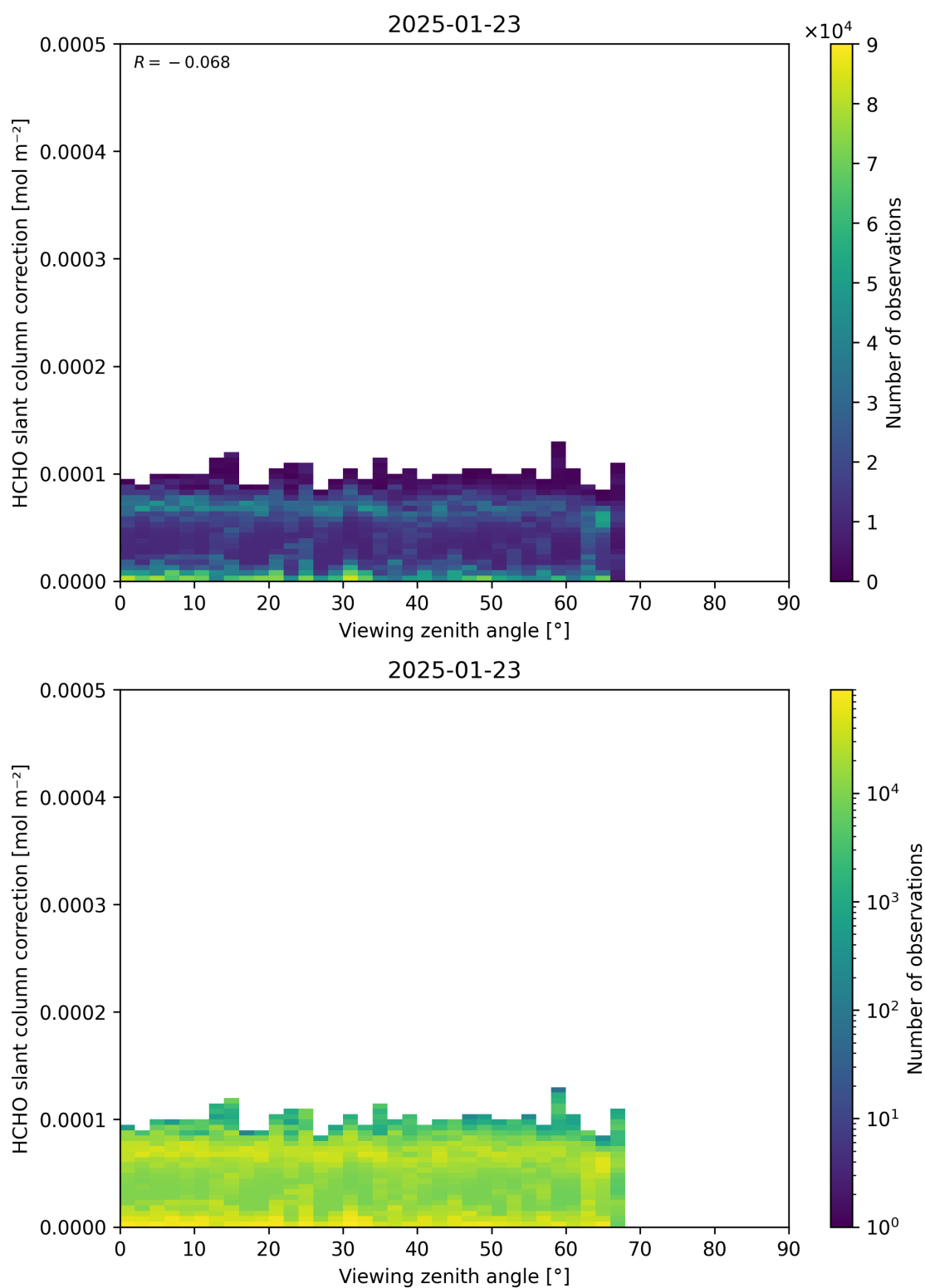
Figure 187: Scatter density plot of “Viewing zenith angle” against “HCHO slant column correction” for 2025-01-23 to 2025-01-24.
