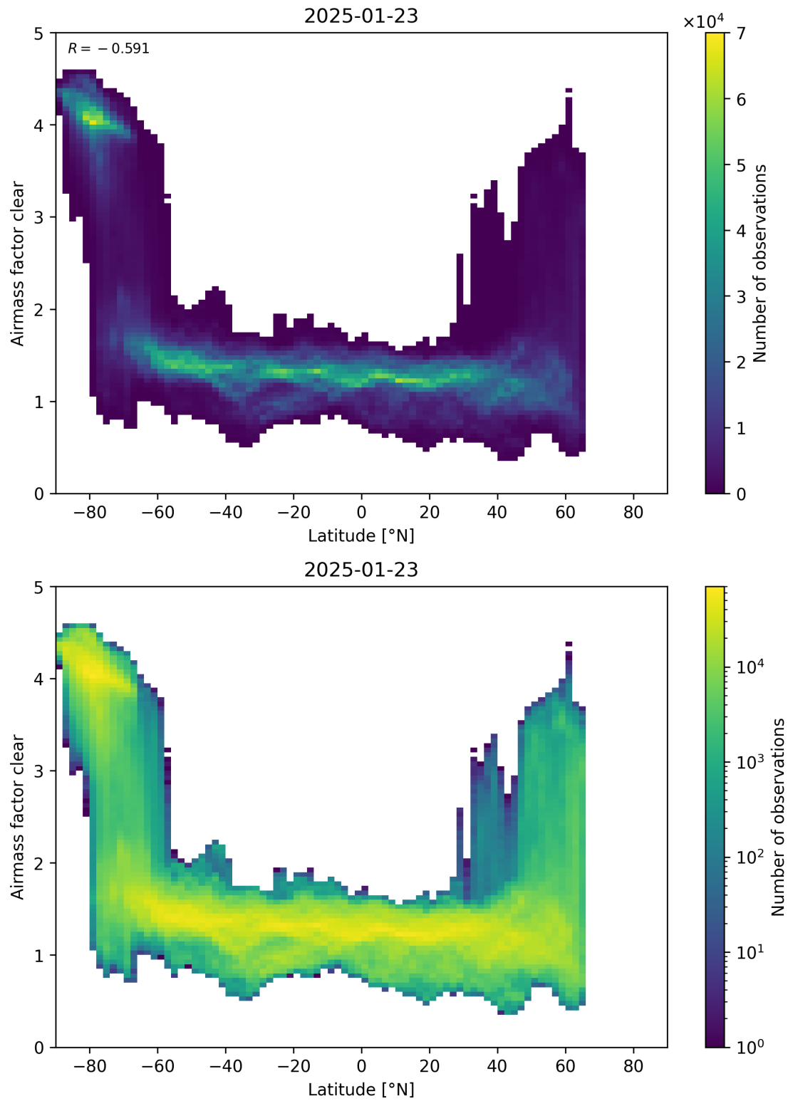
Figure 156: Scatter density plot of “Latitude” against “Airmass factor clear” for 2025-01-23 to 2025-01-24.
