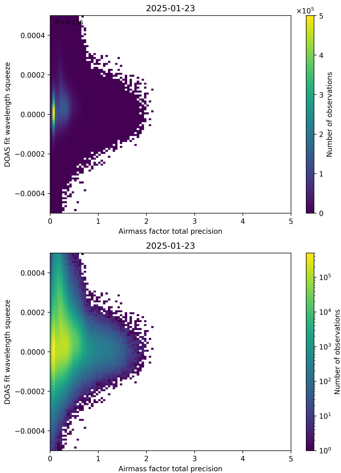
Figure 107: Scatter density plot of “Airmass factor total precision” against “DOAS fit wavelength squeeze” for 2025-01-23 to 2025-01-24.
