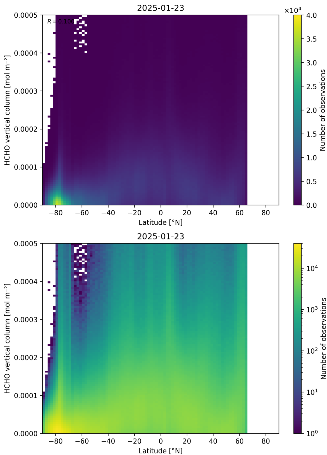
Figure 163: Scatter density plot of “Latitude” against “HCHO vertical column” for 2025-01-23 to 2025-01-24.
