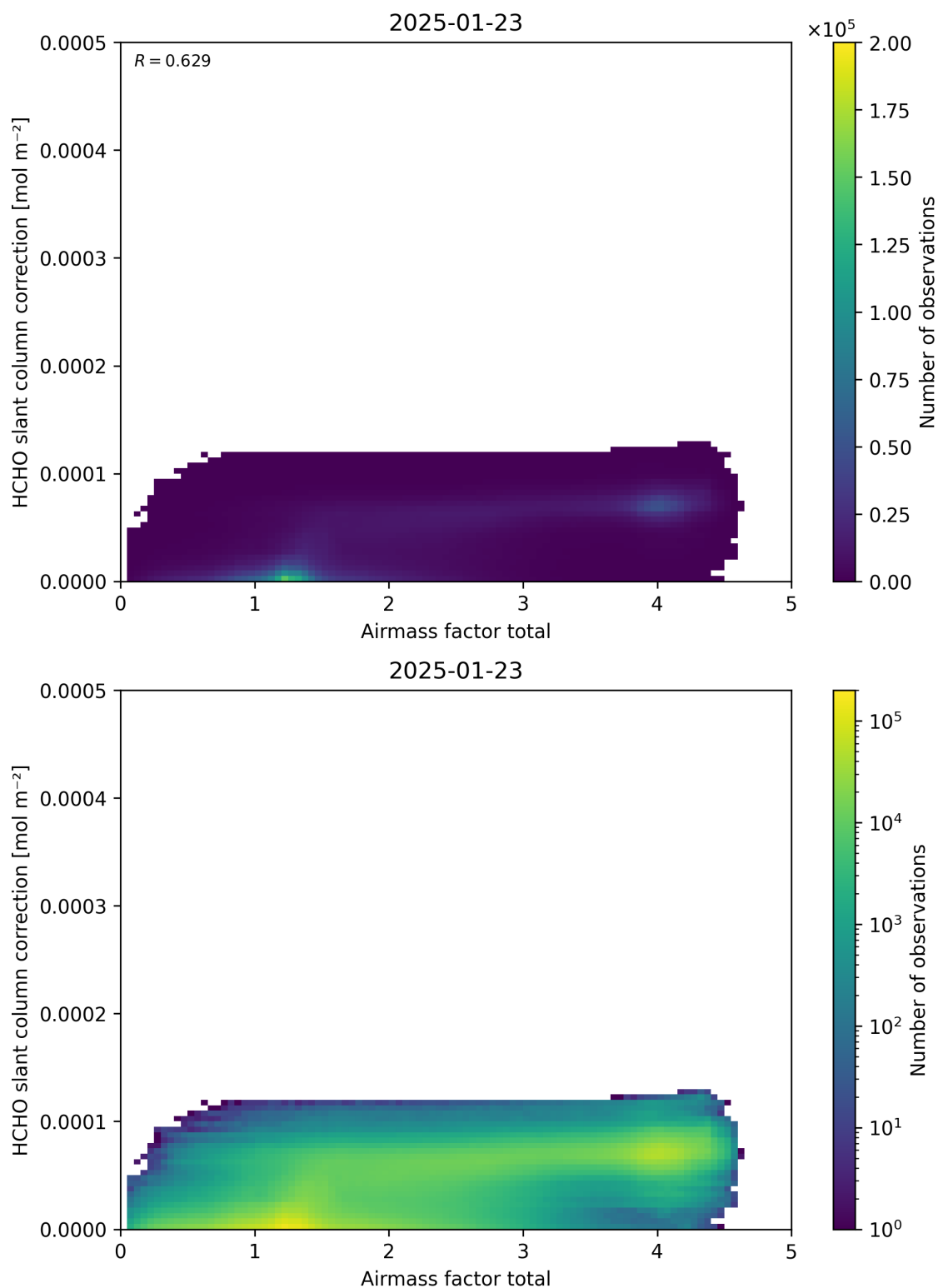
Figure 102: Scatter density plot of “Airmass factor total” against “HCHO slant column correction” for 2025-01-23 to 2025-01-24.
