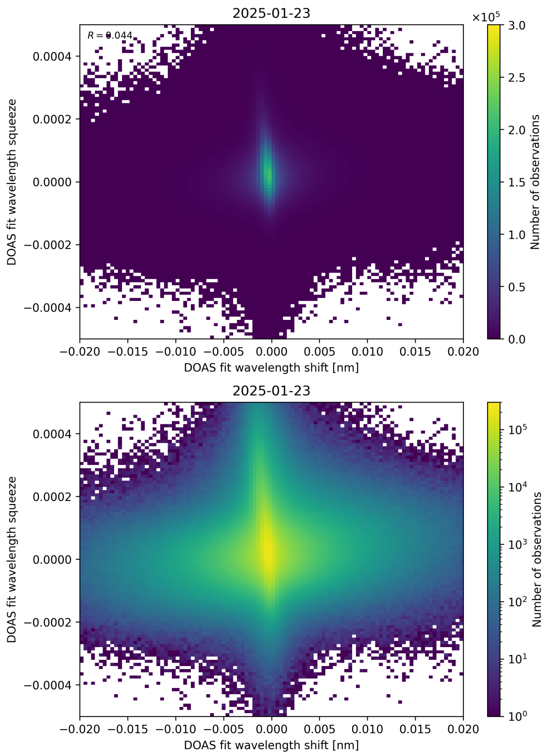
Figure 65: Scatter density plot of “DOAS fit wavelength shift” against “DOAS fit wavelength squeeze” for 2025-01-23 to 2025-01-24.
