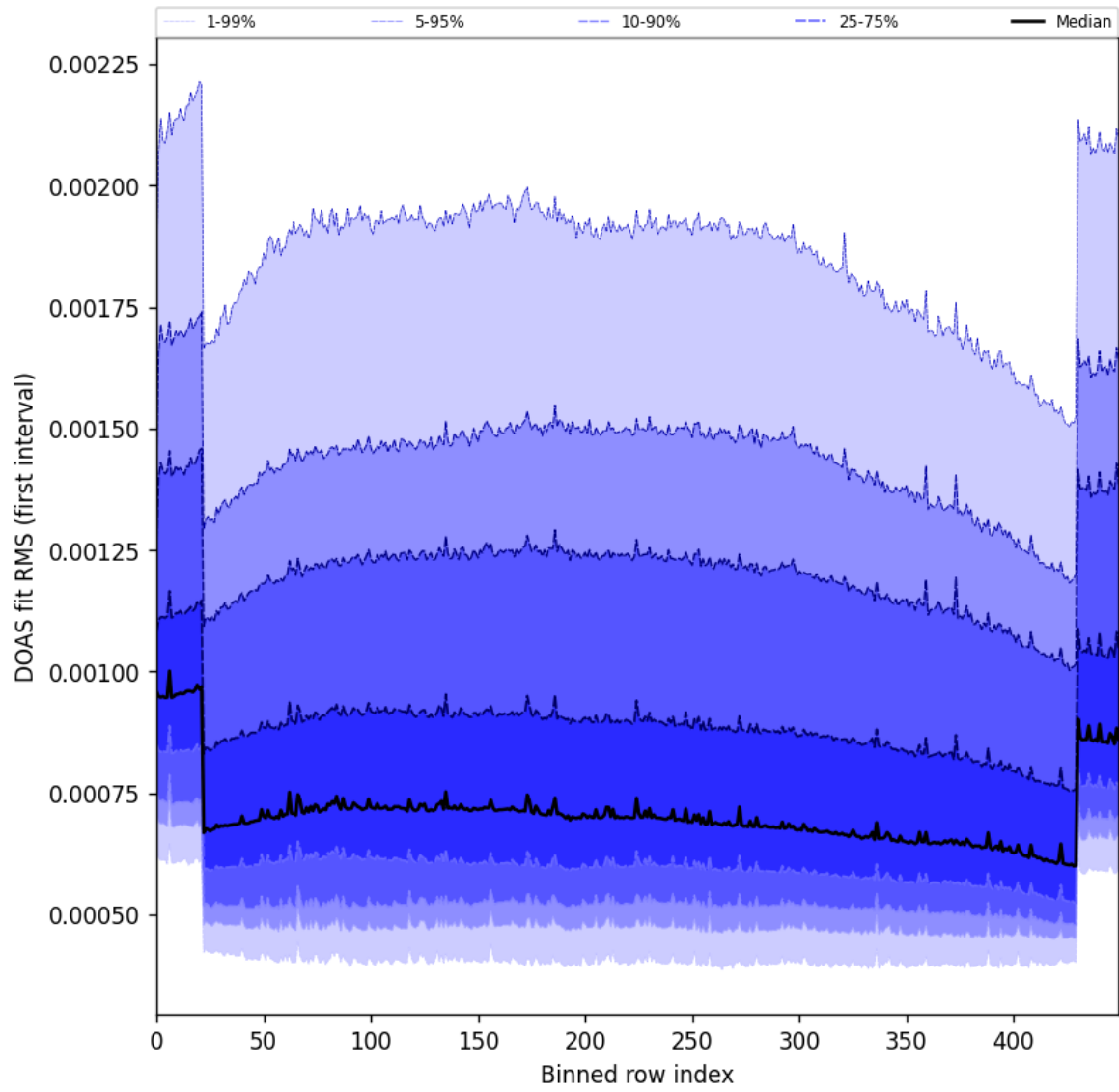
Figure 60: Along track statistics of “DOAS fit RMS (first interval)” for 2025-01-23 to 2025-01-24
