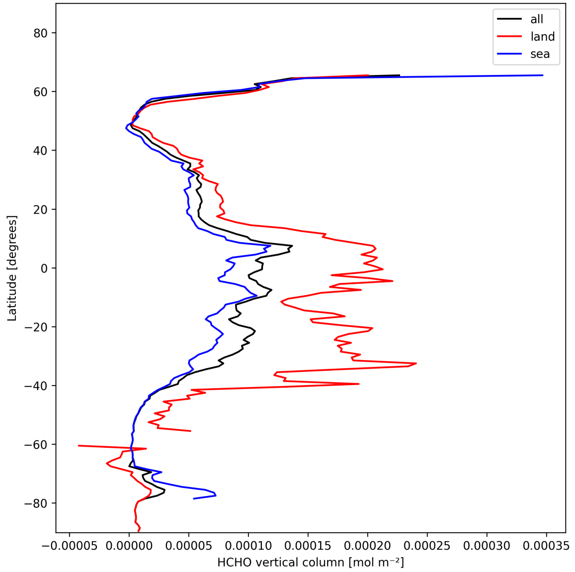
Figure 21: Zonal average of “HCHO vertical column” for 2025-01-23 to 2025-01-24.
