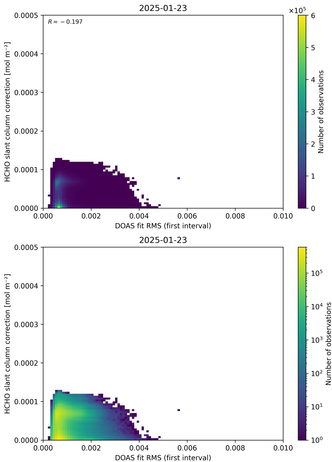
Figure 63: Scatter density plot of “DOAS fit RMS (first interval)” against “HCHO slant column correction” for 2025-01-23 to 2025-01-24.
