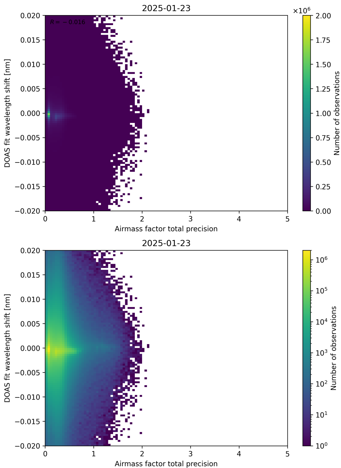
Figure 106: Scatter density plot of “Airmass factor total precision” against “DOAS fit wavelength shift” for 2025-01-23 to 2025-01-24.
