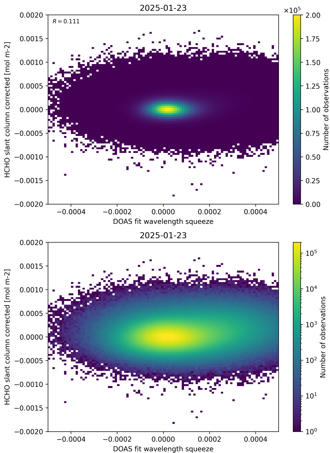
Figure 69: Scatter density plot of “DOAS fit wavelength squeeze” against “HCHO slant column corrected” for 2025-01-23 to 2025-01-24.
