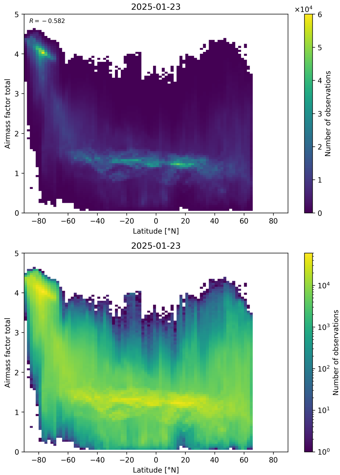
Figure 161: Scatter density plot of “Latitude” against “Airmass factor total” for 2025-01-23 to 2025-01-24.
