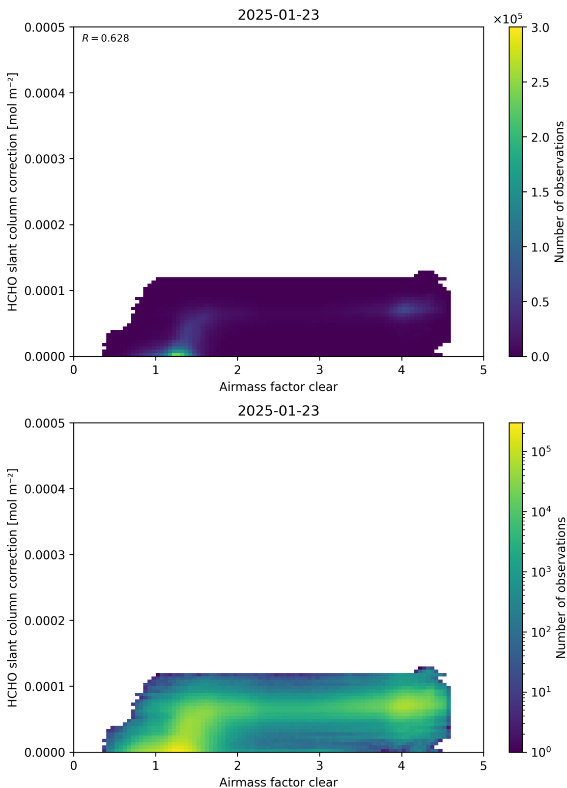
Figure 75: Scatter density plot of “Airmass factor clear” against “HCHO slant column correction” for 2025-01-23 to 2025-01-24.
