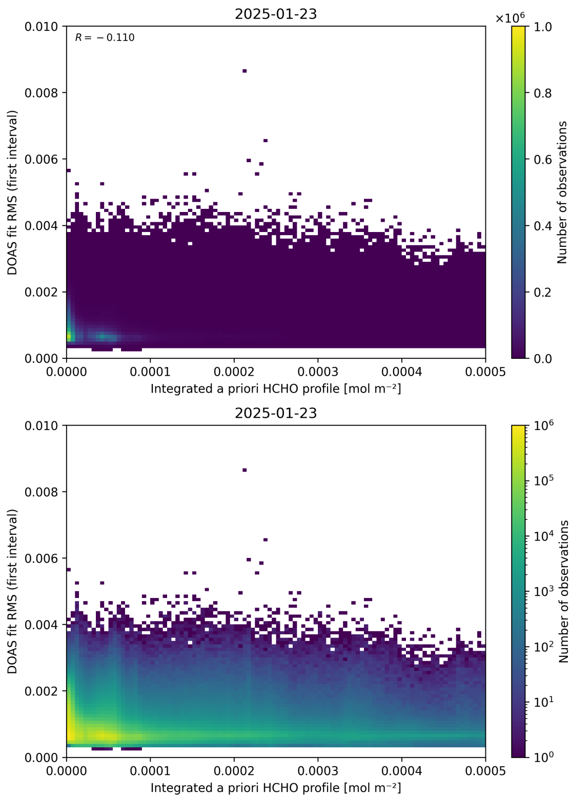
Figure 148: Scatter density plot of “Integrated a priori HCHO profile” against “DOAS fit RMS (first interval)” for 2025-01-23 to 2025-01-24.
