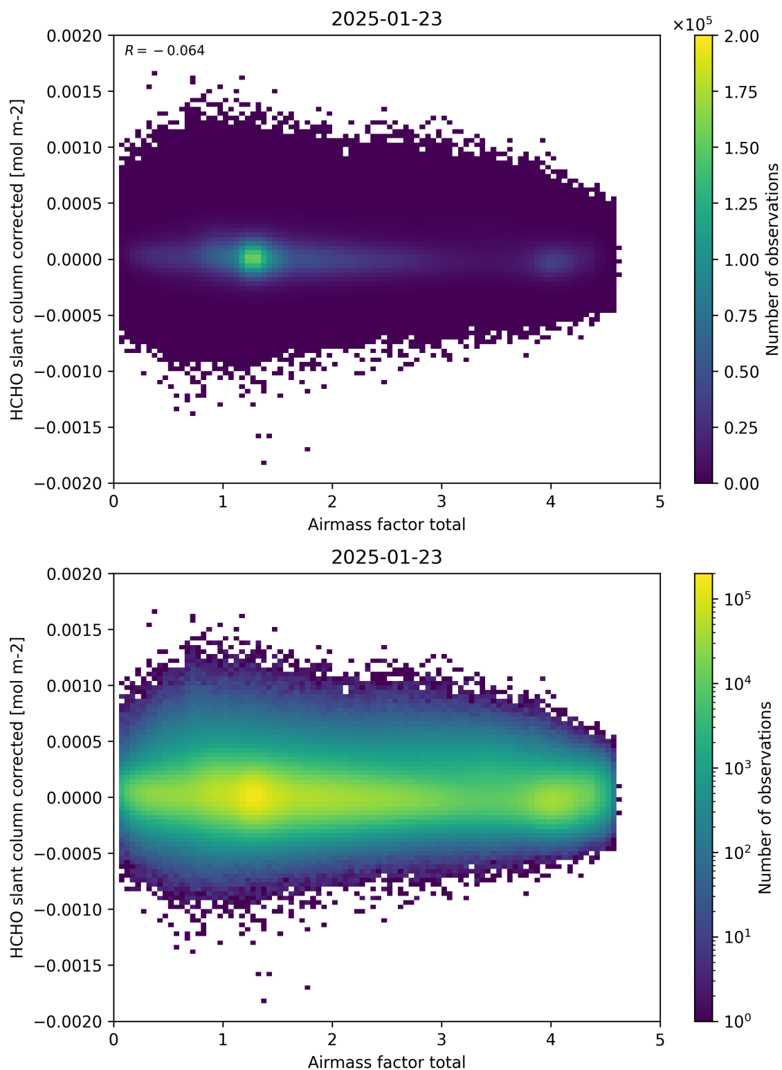
Figure 101: Scatter density plot of “Airmass factor total” against “HCHO slant column corrected” for 2025-01-23 to 2025-01-24.
