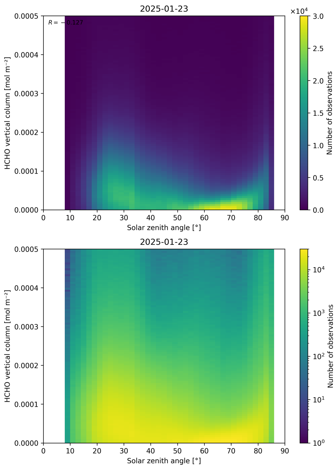
Figure 177: Scatter density plot of “Solar zenith angle” against “HCHO vertical column” for 2025-01-23 to 2025-01-24.
