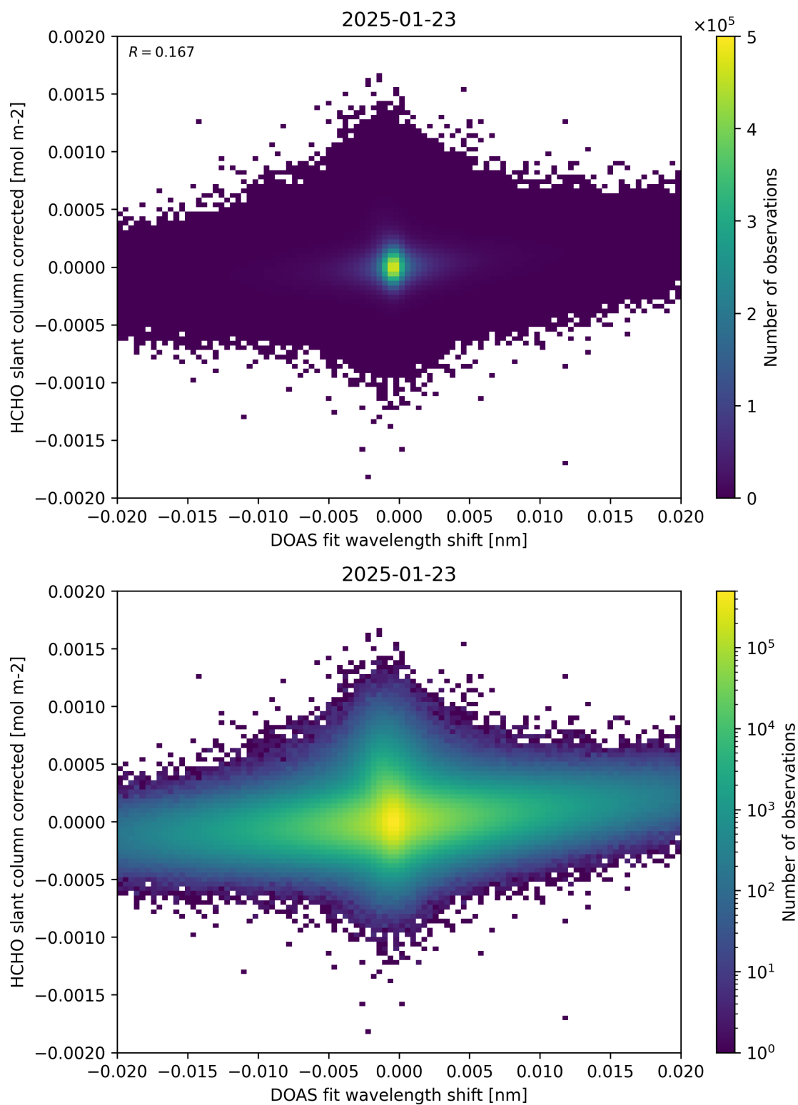
Figure 66: Scatter density plot of “DOAS fit wavelength shift” against “HCHO slant column corrected” for 2025-01-23 to 2025-01-24.
