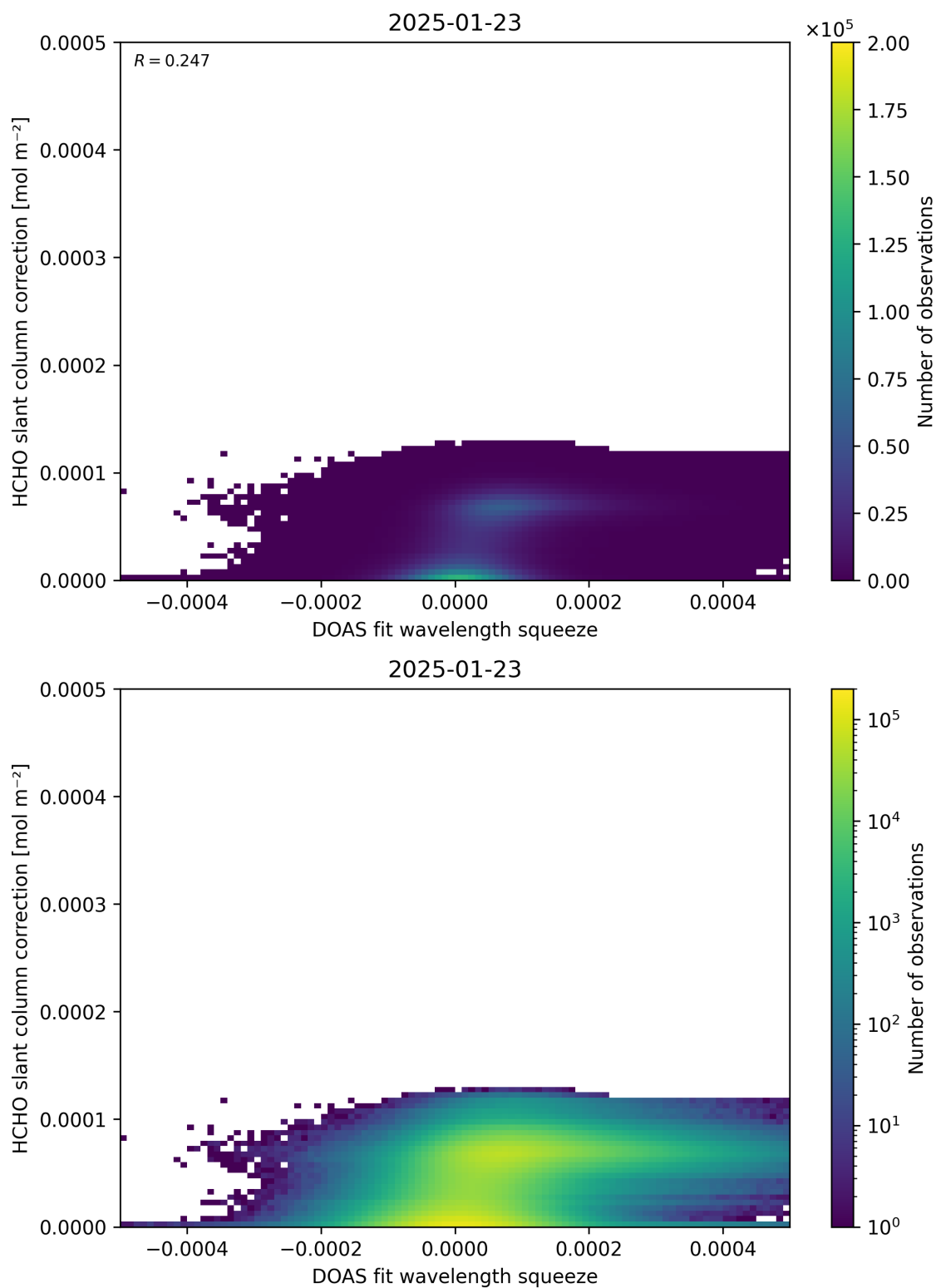
Figure 70: Scatter density plot of “DOAS fit wavelength squeeze” against “HCHO slant column correction” for 2025-01-23 to 2025-01-24.
