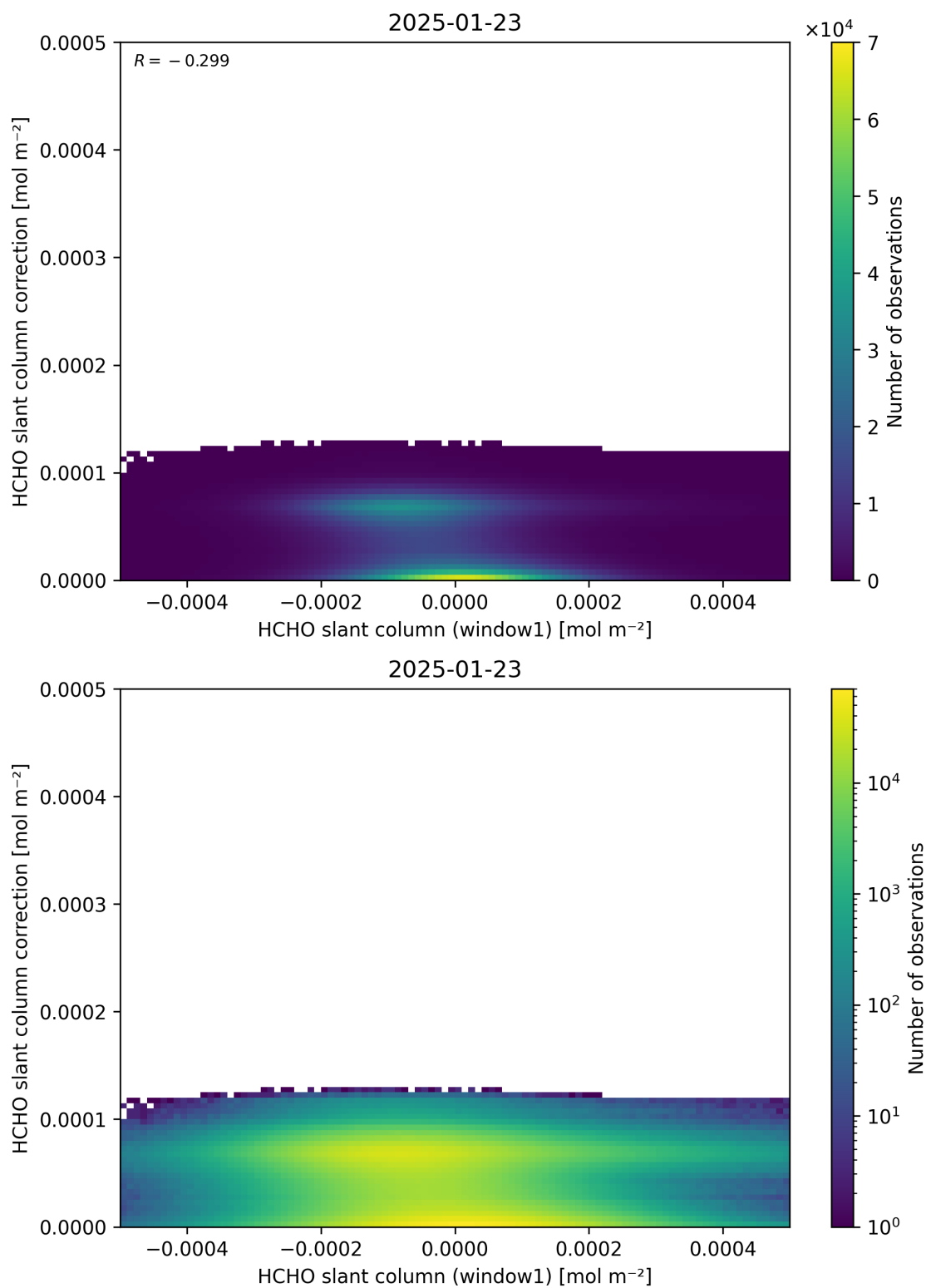
Figure 83: Scatter density plot of “HCHO slant column (window1)” against “HCHO slant column correction” for 2025-01-23 to 2025-01-24.
