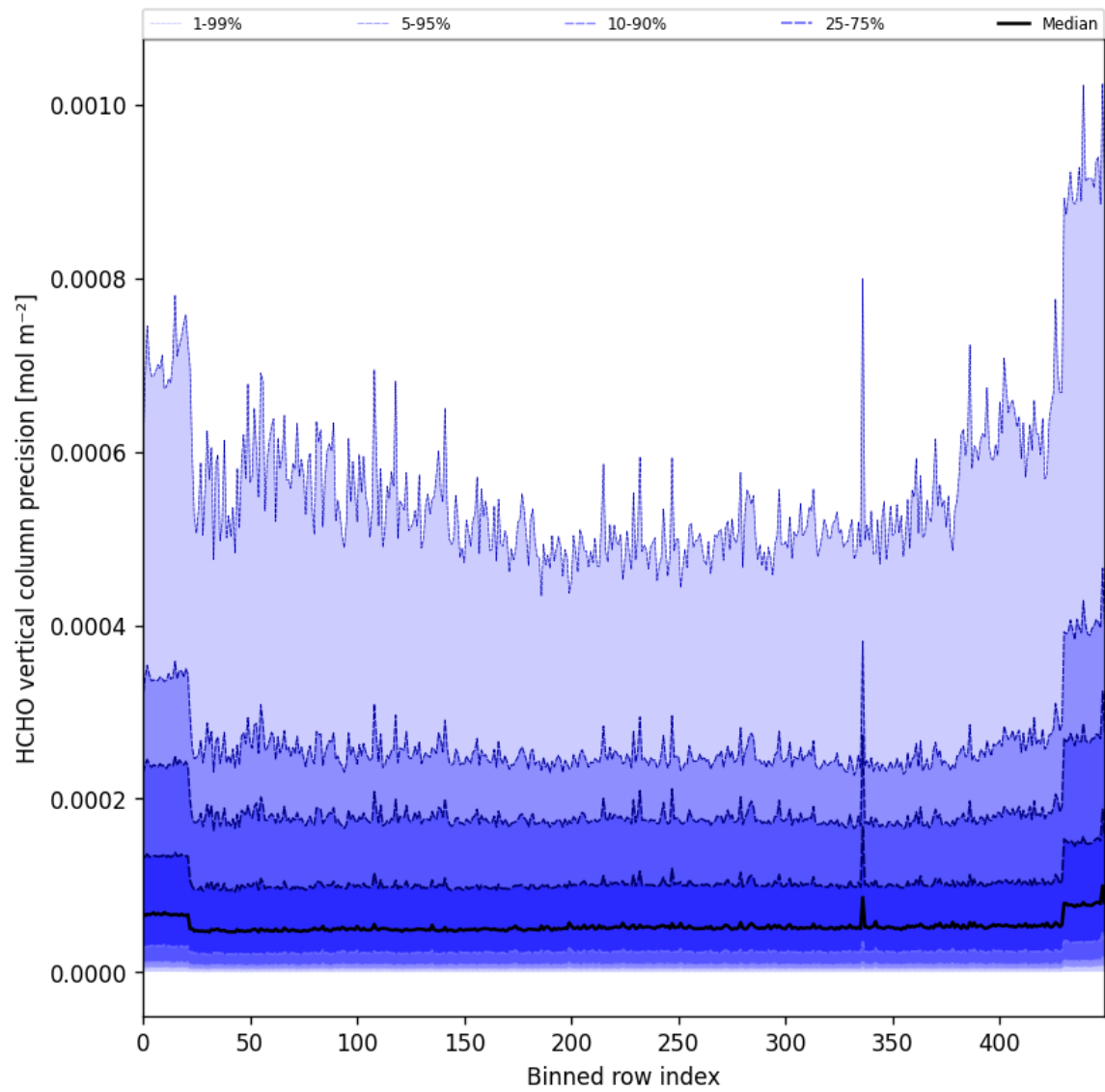
Figure 50: Along track statistics of “HCHO vertical column precision” for 2025-01-23 to 2025-01-24
