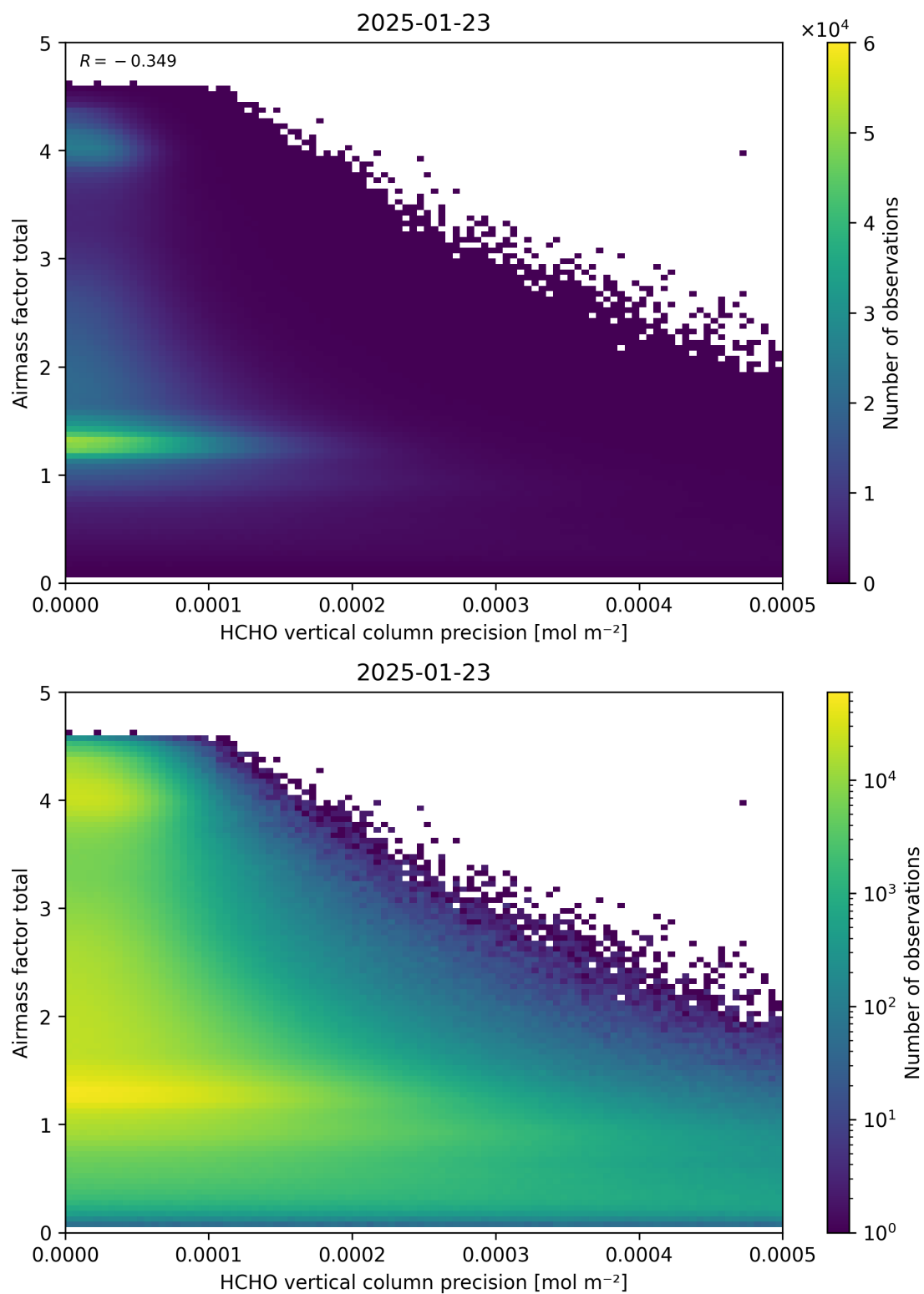
Figure 144: Scatter density plot of “HCHO vertical column precision” against “Airmass factor total” for 2025-01-23 to 2025-01-24.
