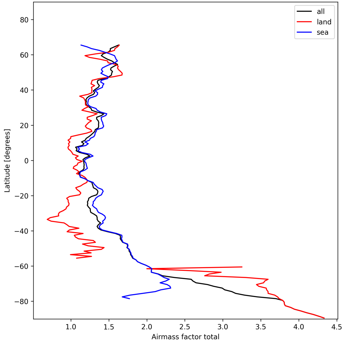
Figure 26: Zonal average of “Airmass factor total” for 2025-01-23 to 2025-01-24.
