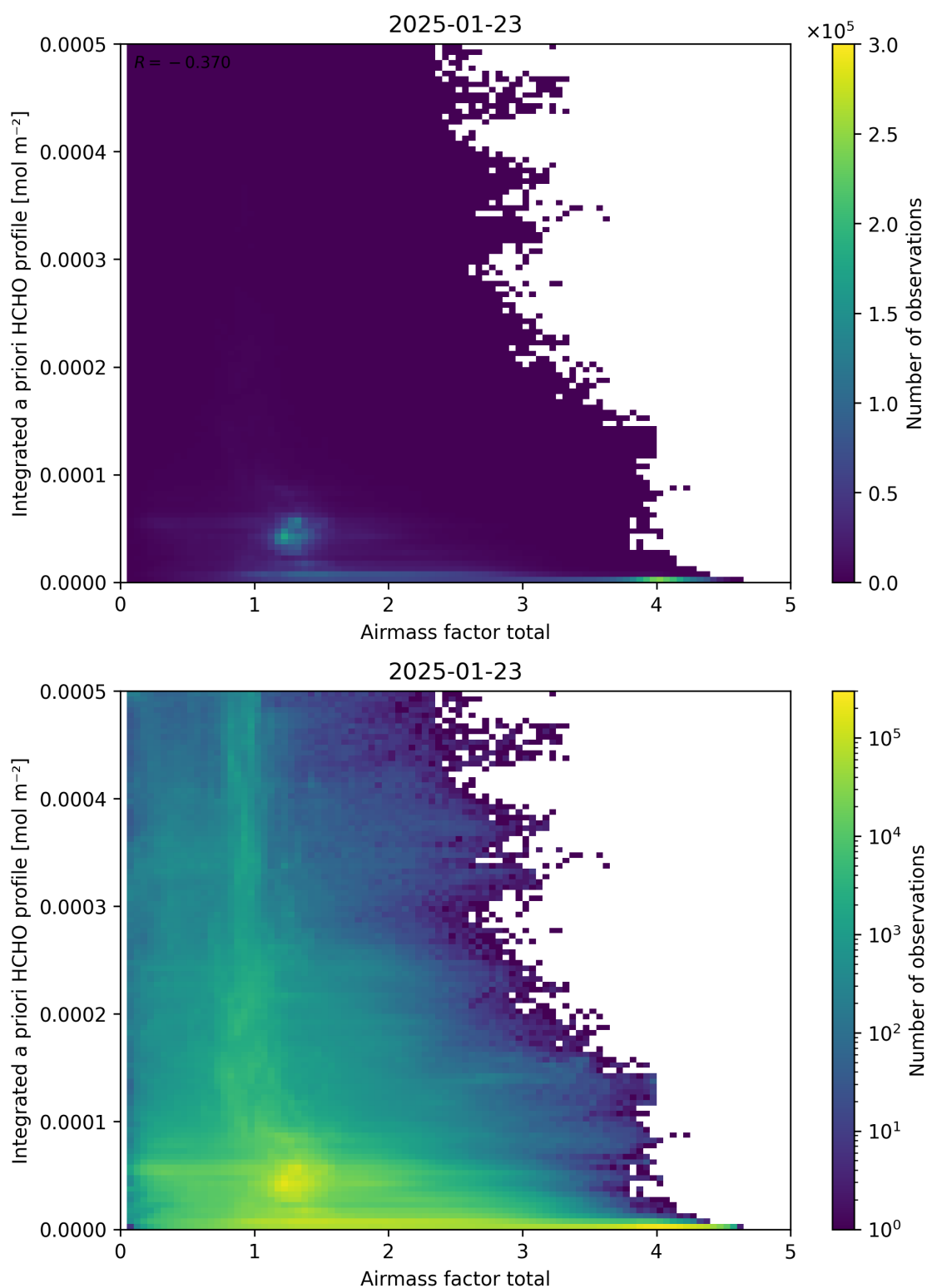
Figure 104: Scatter density plot of “Airmass factor total” against “Integrated a priori HCHO profile” for 2025-01-23 to 2025-01-24.
