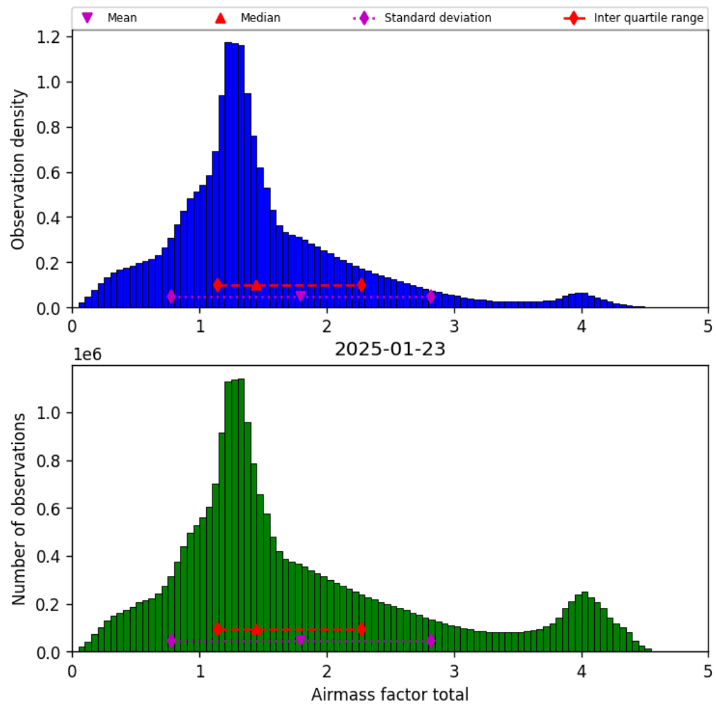
Figure 40: Histogram of “Airmass factor total” for 2025-01-23 to 2025-01-24
