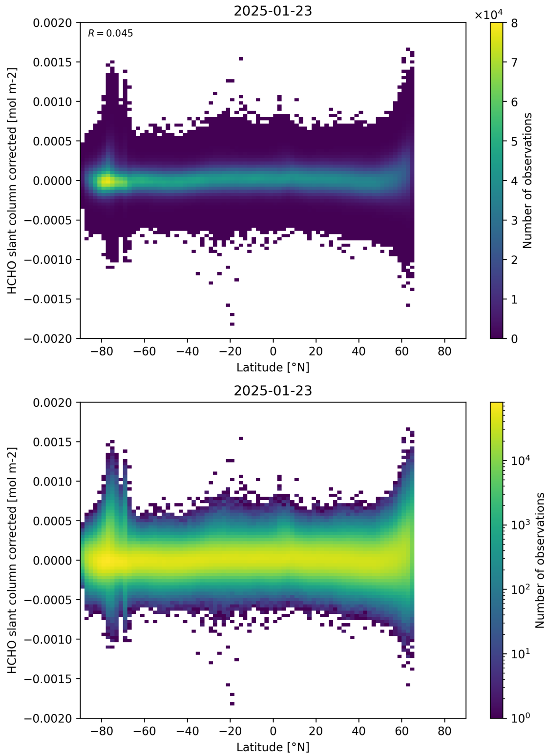
Figure 157: Scatter density plot of “Latitude” against “HCHO slant column corrected” for 2025-01-23 to 2025-01-24.
