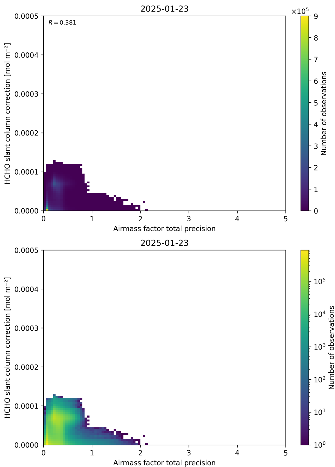
Figure 110: Scatter density plot of “Airmass factor total precision” against “HCHO slant column correction” for 2025-01-23 to 2025-01-24.
