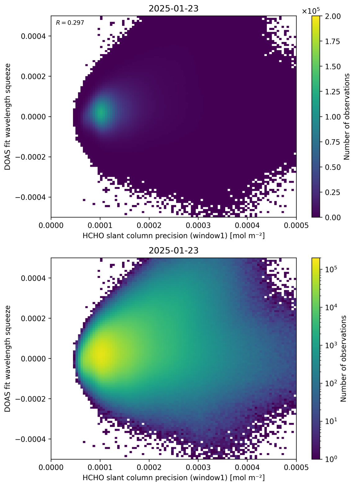
Figure 90: Scatter density plot of “HCHO slant column precision (window1)” against “DOAS fit wavelength squeeze” for 2025-01-23 to 2025-01-24.
