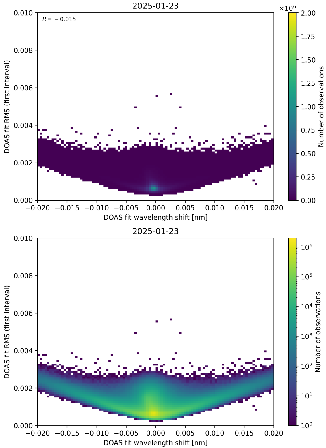
Figure 64: Scatter density plot of “DOAS fit wavelength shift” against “DOAS fit RMS (first interval)” for 2025-01-23 to 2025-01-24.
