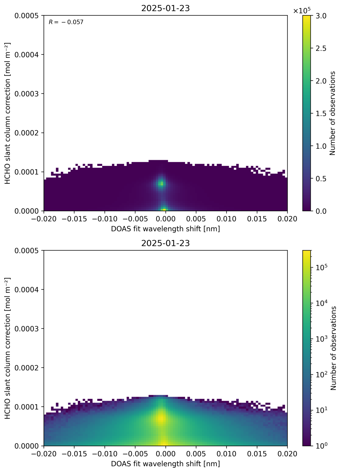
Figure 67: Scatter density plot of “DOAS fit wavelength shift” against “HCHO slant column correction” for 2025-01-23 to 2025-01-24.
