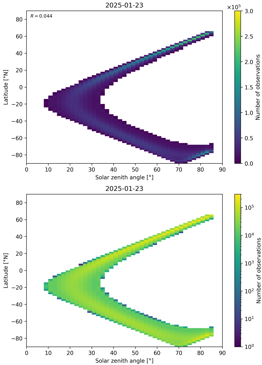
Figure 181: Scatter density plot of “Solar zenith angle” against “Latitude” for 2025-01-23 to 2025-01-24.
