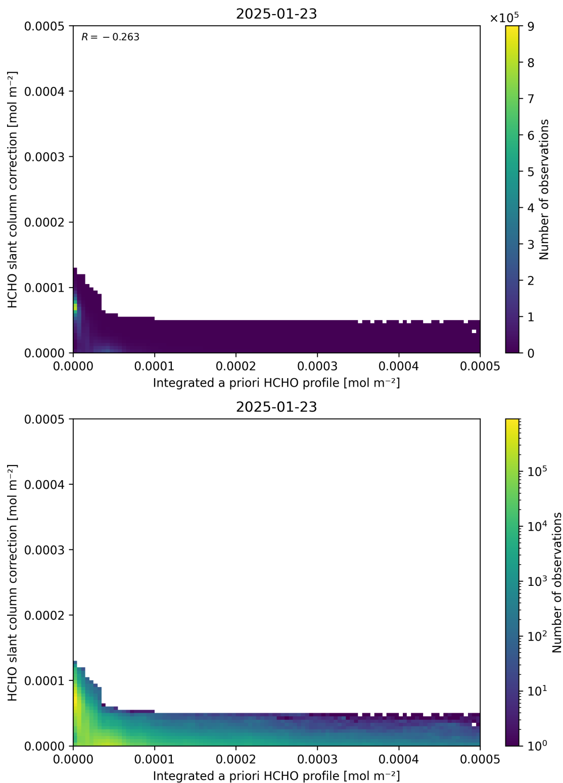
Figure 152: Scatter density plot of “Integrated a priori HCHO profile” against “HCHO slant column correction” for 2025-01-23 to 2025-01-24.
