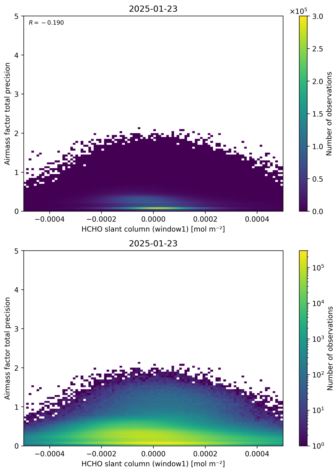
Figure 86: Scatter density plot of “HCHO slant column (window1)” against “Airmass factor total precision” for 2025-01-23 to 2025-01-24.
