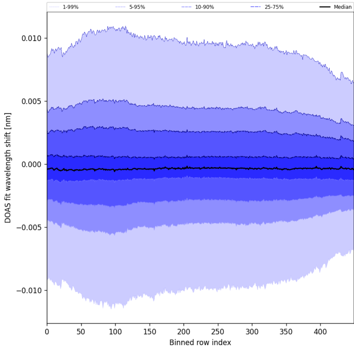
Figure 58: Along track statistics of “DOAS fit wavelength shift” for 2025-01-23 to 2025-01-24
