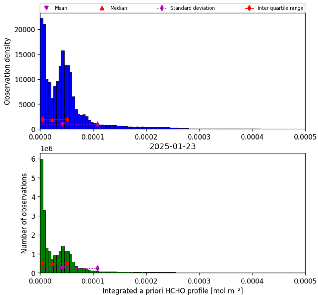
Figure 43: Histogram of “Integrated a priori HCHO profile” for 2025-01-23 to 2025-01-24
