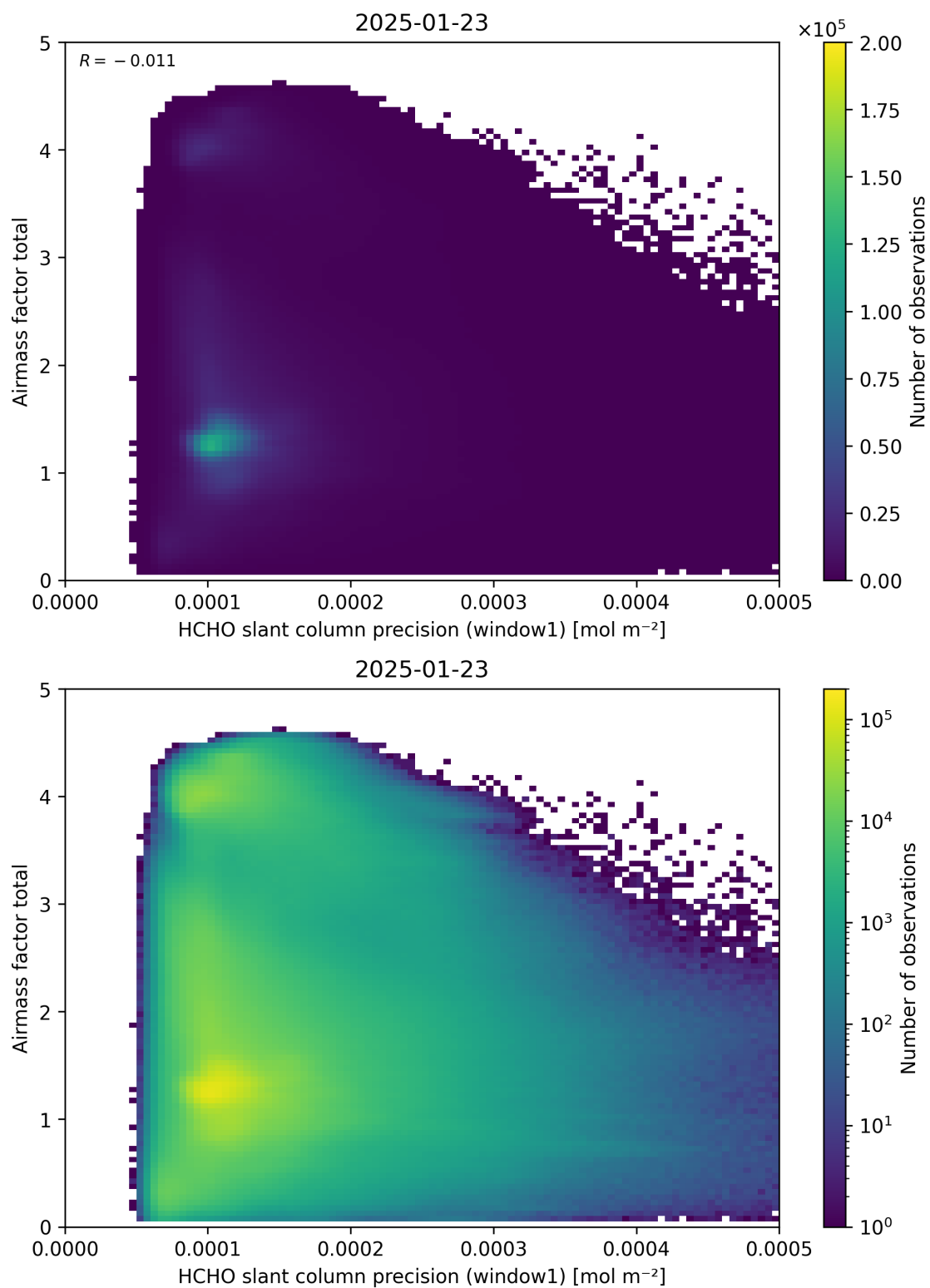
Figure 94: Scatter density plot of “HCHO slant column precision (window1)” against “Airmass factor total” for 2025-01-23 to 2025-01-24.
