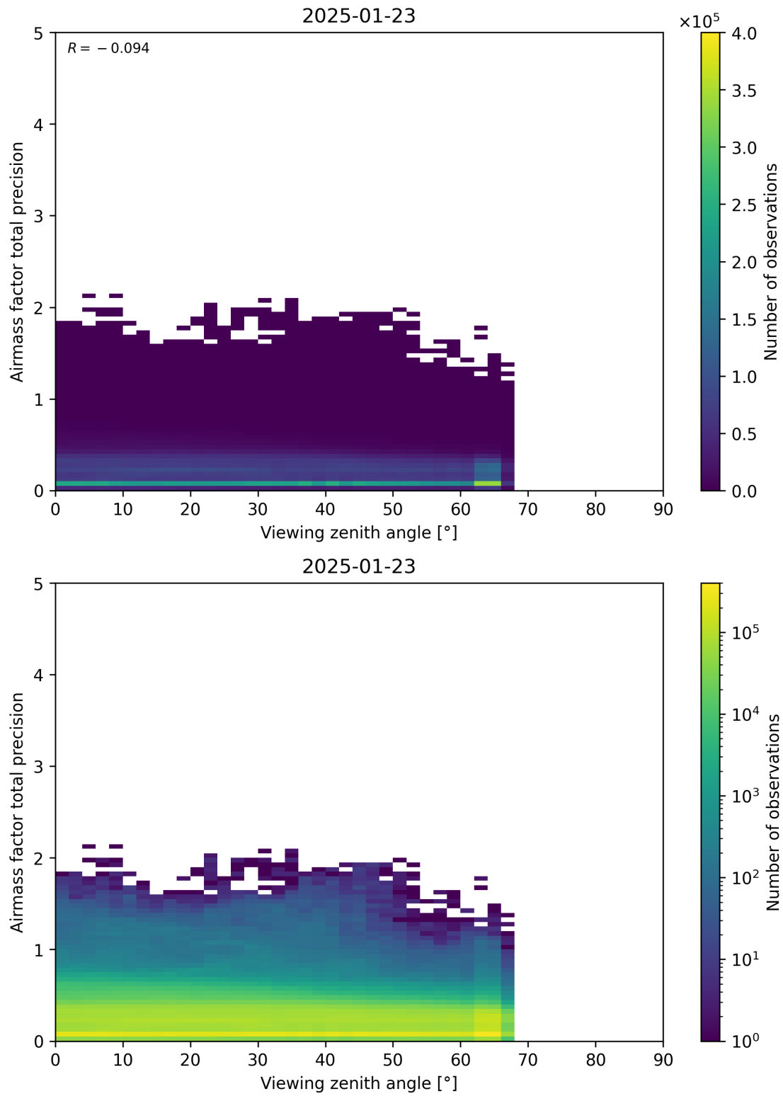
Figure 191: Scatter density plot of “Viewing zenith angle” against “Airmass factor total precision” for 2025-01-23 to 2025-01-24.
