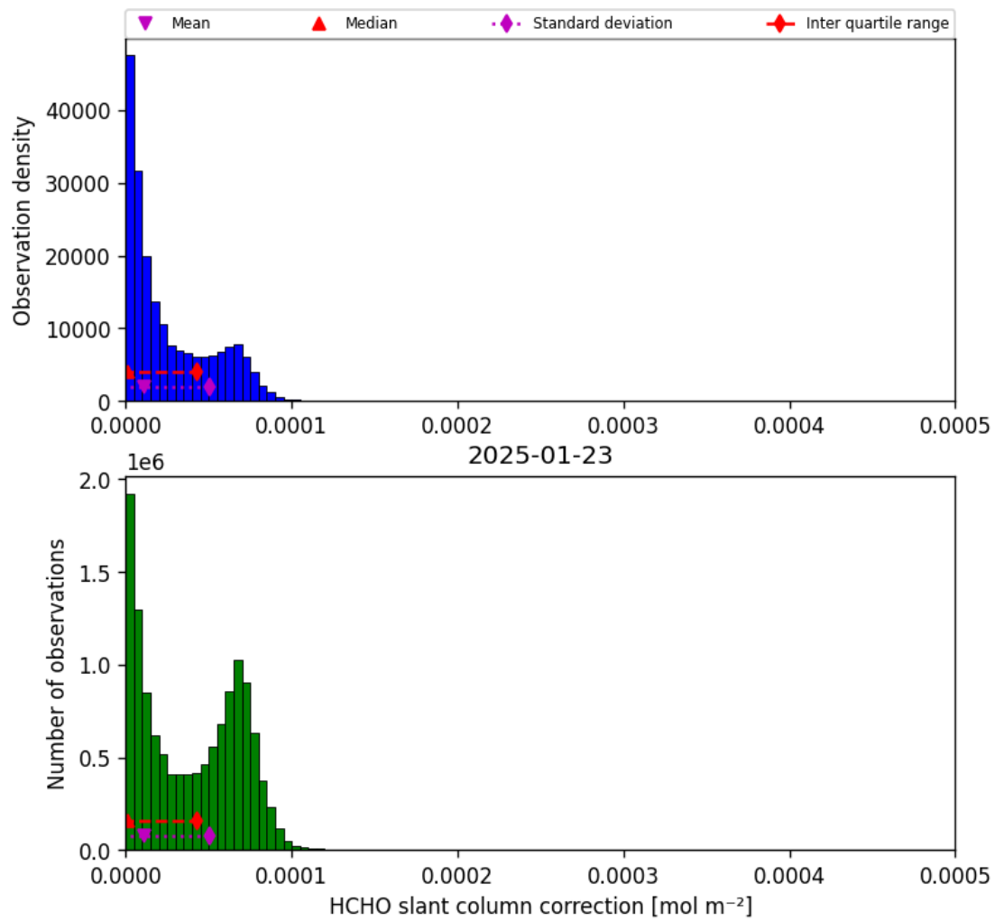
Figure 47: Histogram of “HCHO slant column correction” for 2025-01-23 to 2025-01-24
