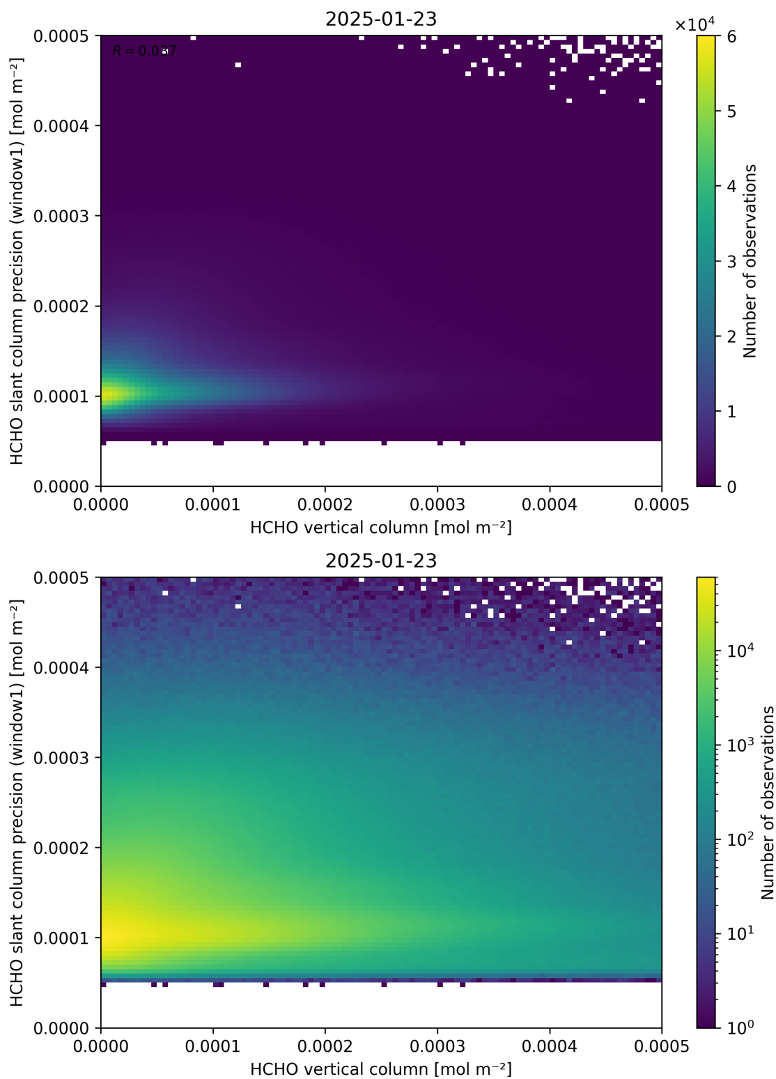
Figure 130: Scatter density plot of “HCHO vertical column” against “HCHO slant column precision (window1)” for 2025-01-23 to 2025-01-24.
