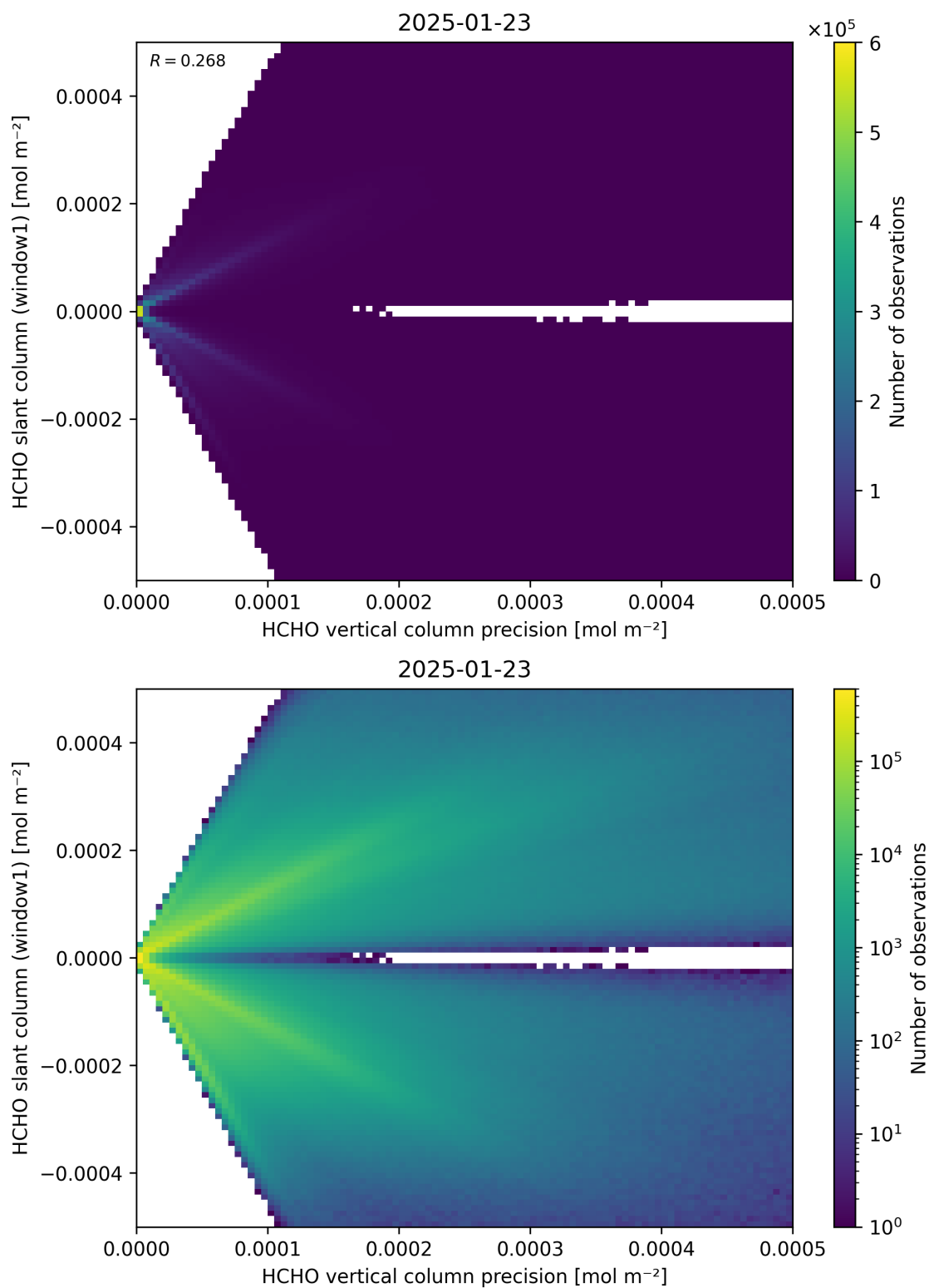
Figure 142: Scatter density plot of “HCHO vertical column precision” against “HCHO slant column (window1)” for 2025-01-23 to 2025-01-24.
