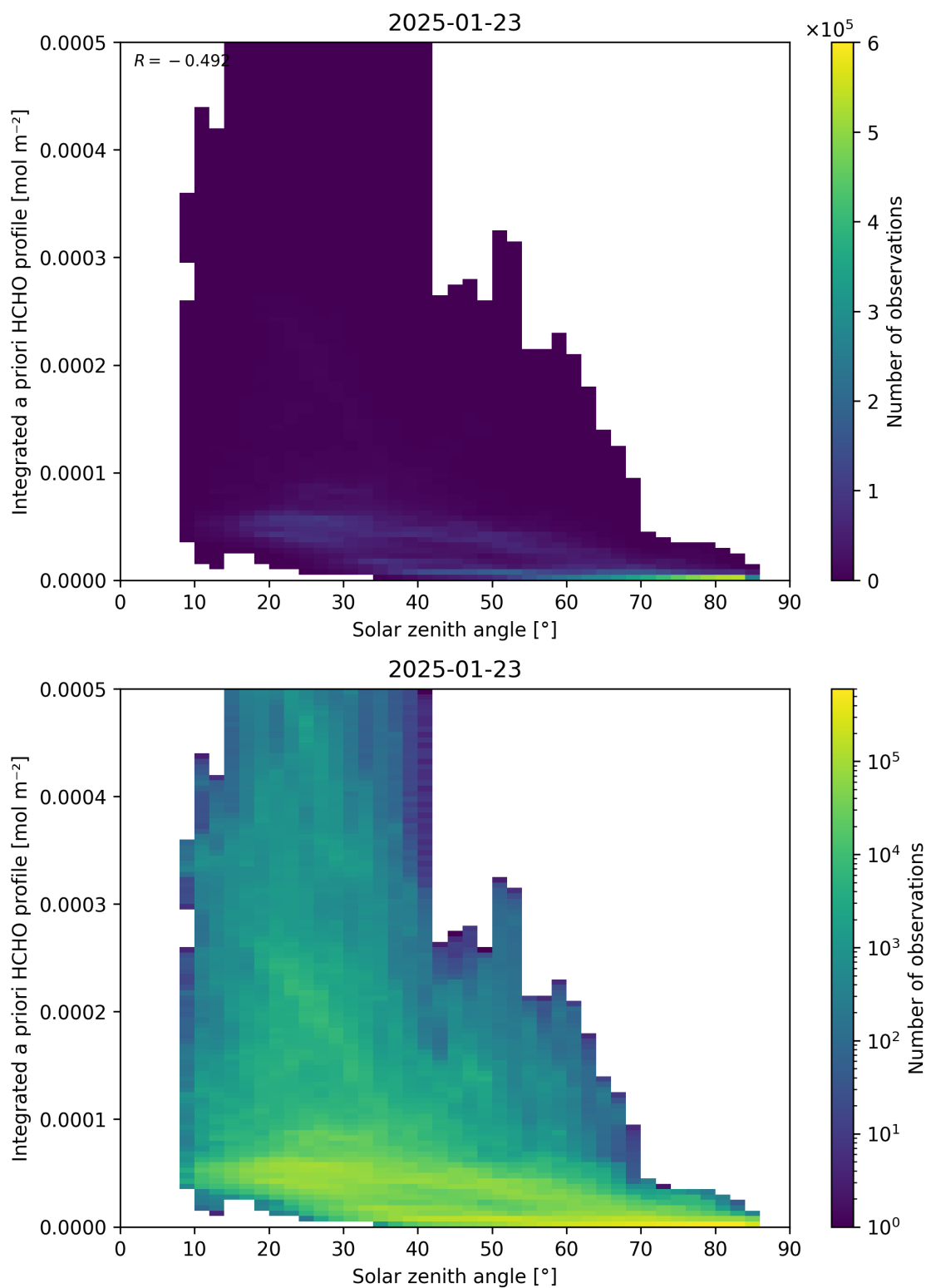
Figure 180: Scatter density plot of “Solar zenith angle” against “Integrated a priori HCHO profile” for 2025-01-23 to 2025-01-24.
