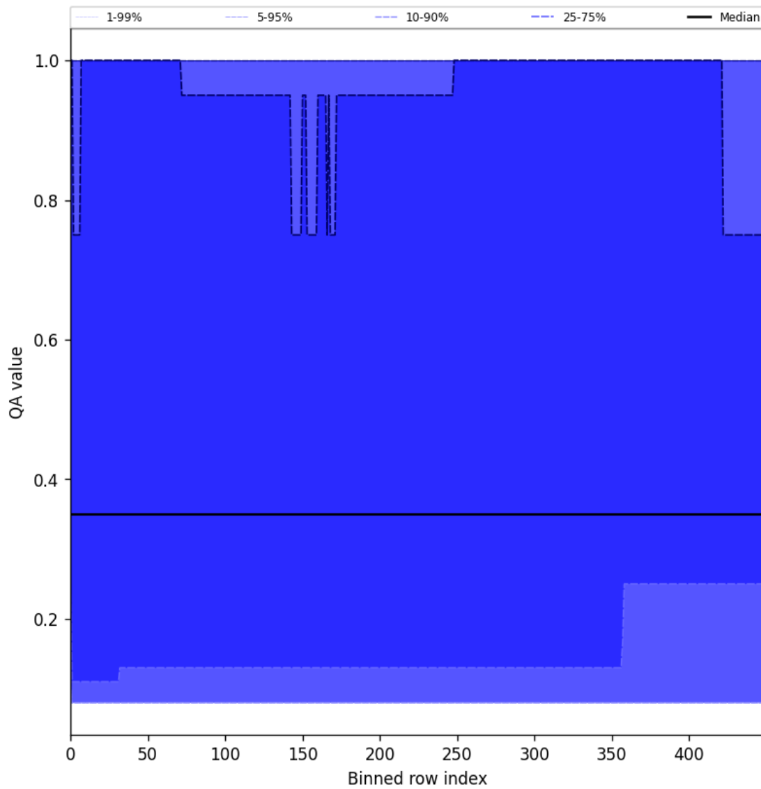
Figure 48: Along track statistics of “QA value” for 2025-01-23 to 2025-01-24
