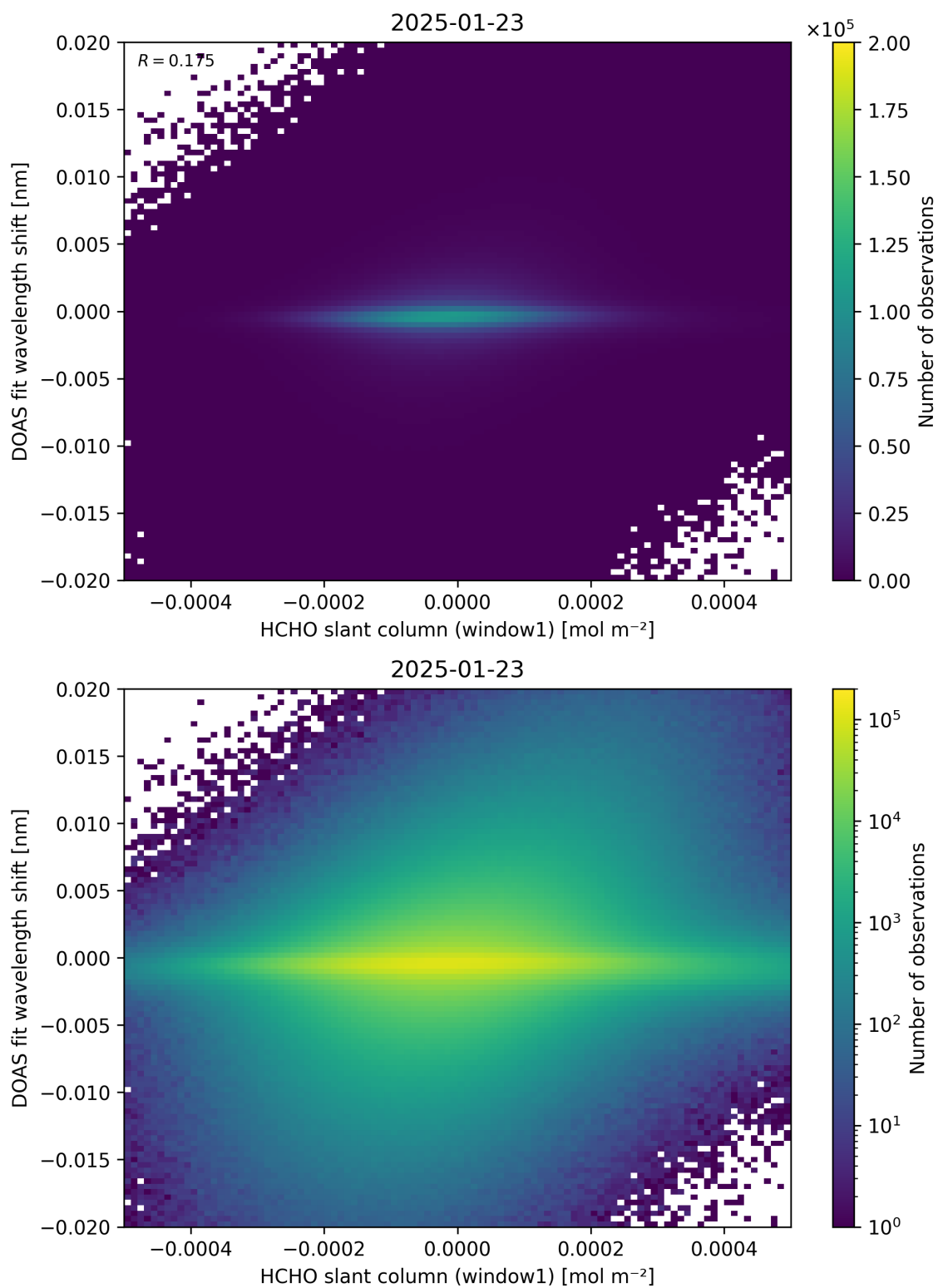
Figure 79: Scatter density plot of “HCHO slant column (window1)” against “DOAS fit wavelength shift” for 2025-01-23 to 2025-01-24.
