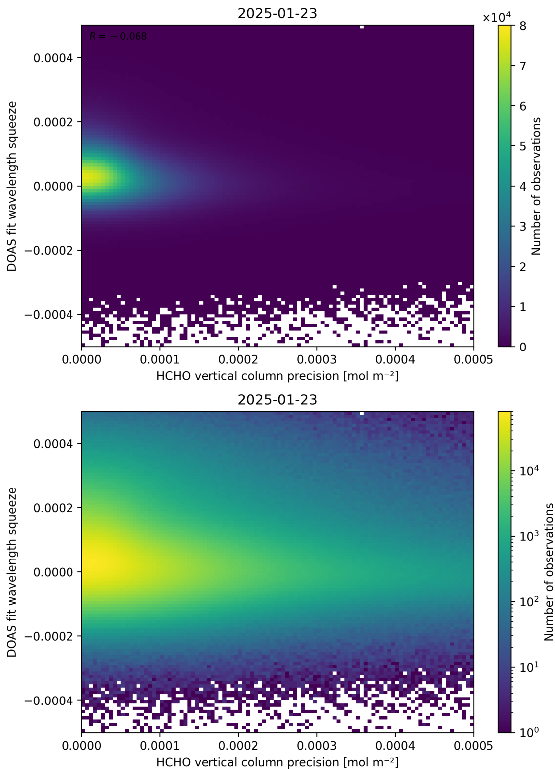
Figure 138: Scatter density plot of “HCHO vertical column precision” against “DOAS fit wavelength squeeze” for 2025-01-23 to 2025-01-24.
