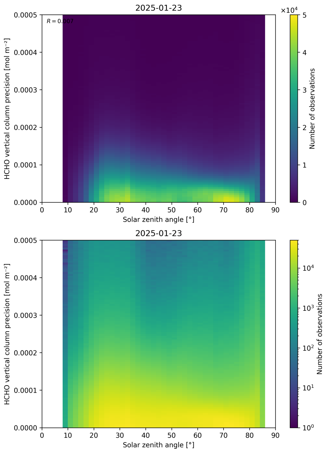
Figure 179: Scatter density plot of “Solar zenith angle” against “HCHO vertical column precision” for 2025-01-23 to 2025-01-24.
