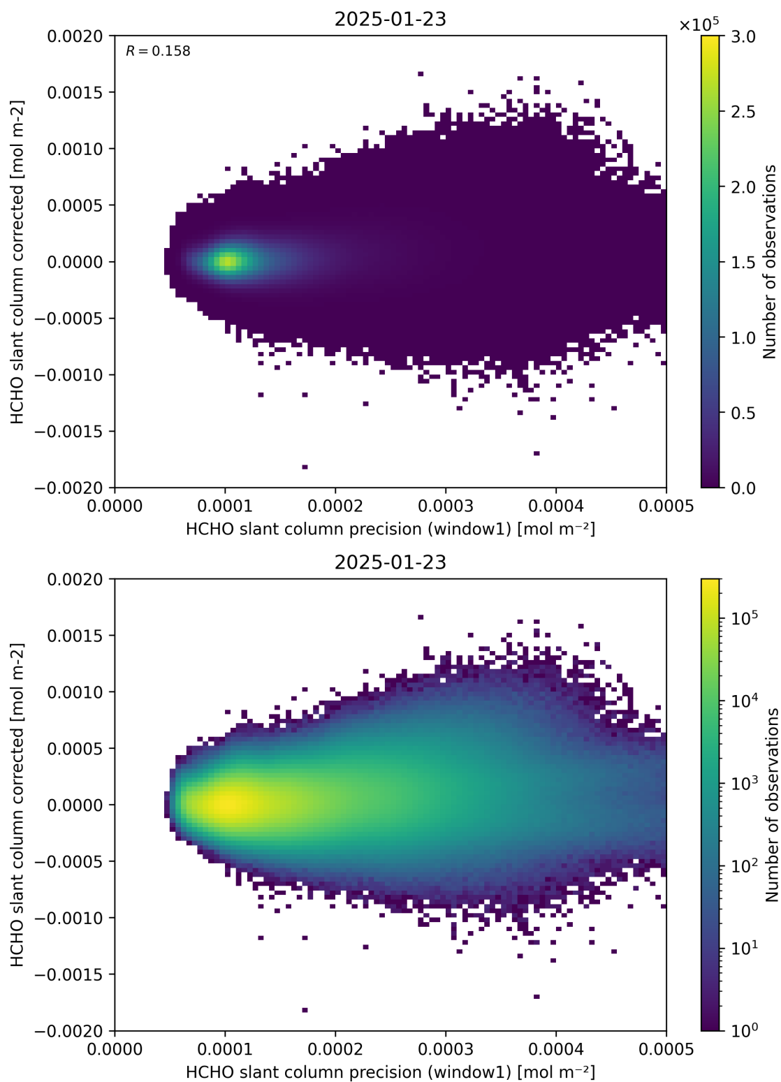
Figure 92: Scatter density plot of “HCHO slant column precision (window1)” against “HCHO slant column corrected” for 2025-01-23 to 2025-01-24.
