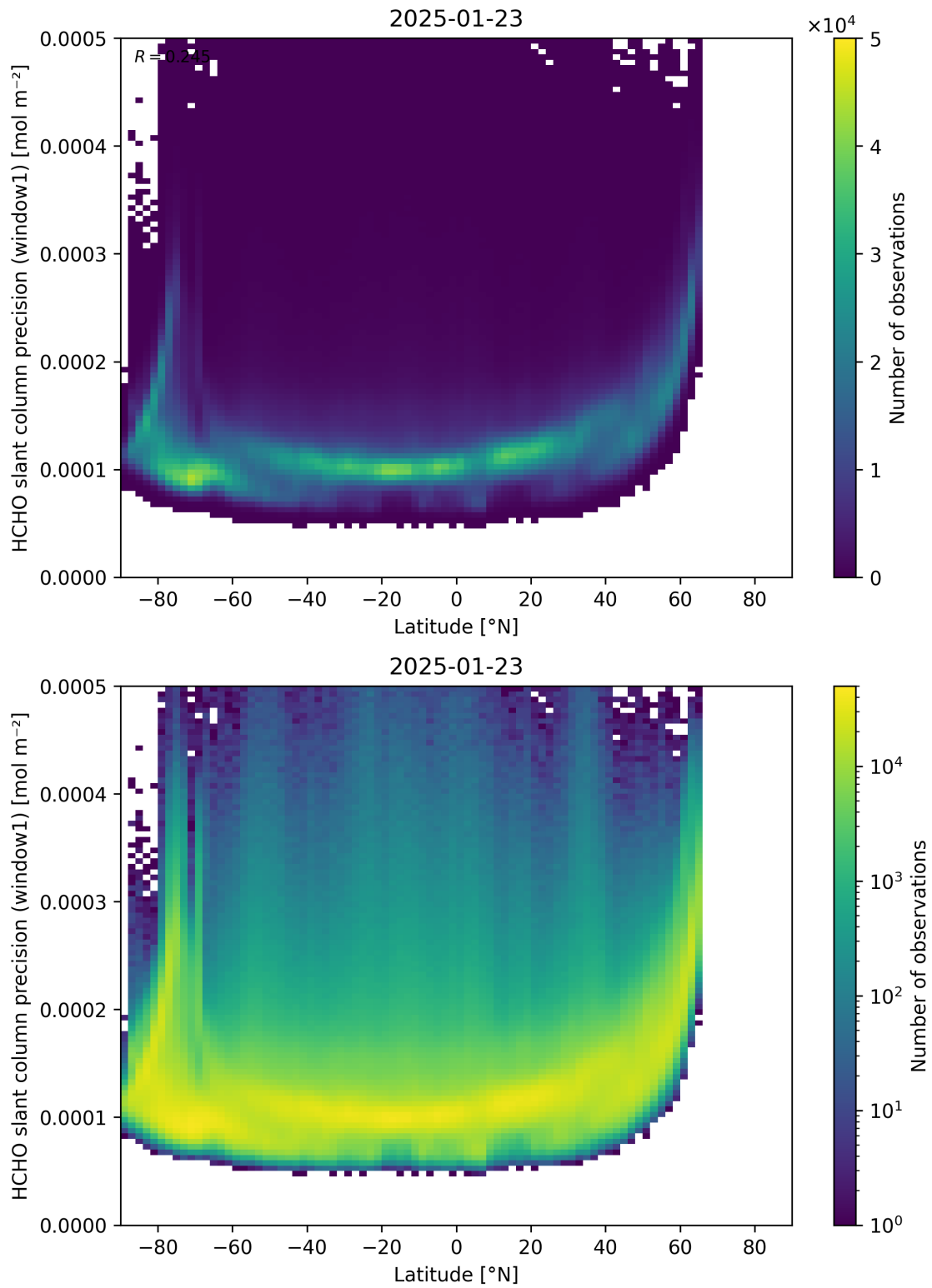
Figure 160: Scatter density plot of “Latitude” against “HCHO slant column precision (window1)” for 2025-01-23 to 2025-01-24.
