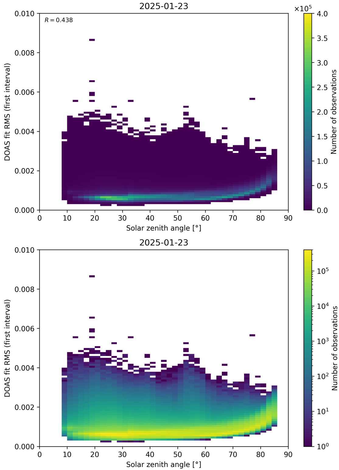
Figure 167: Scatter density plot of “Solar zenith angle” against “DOAS fit RMS (first interval)” for 2025-01-23 to 2025-01-24.
