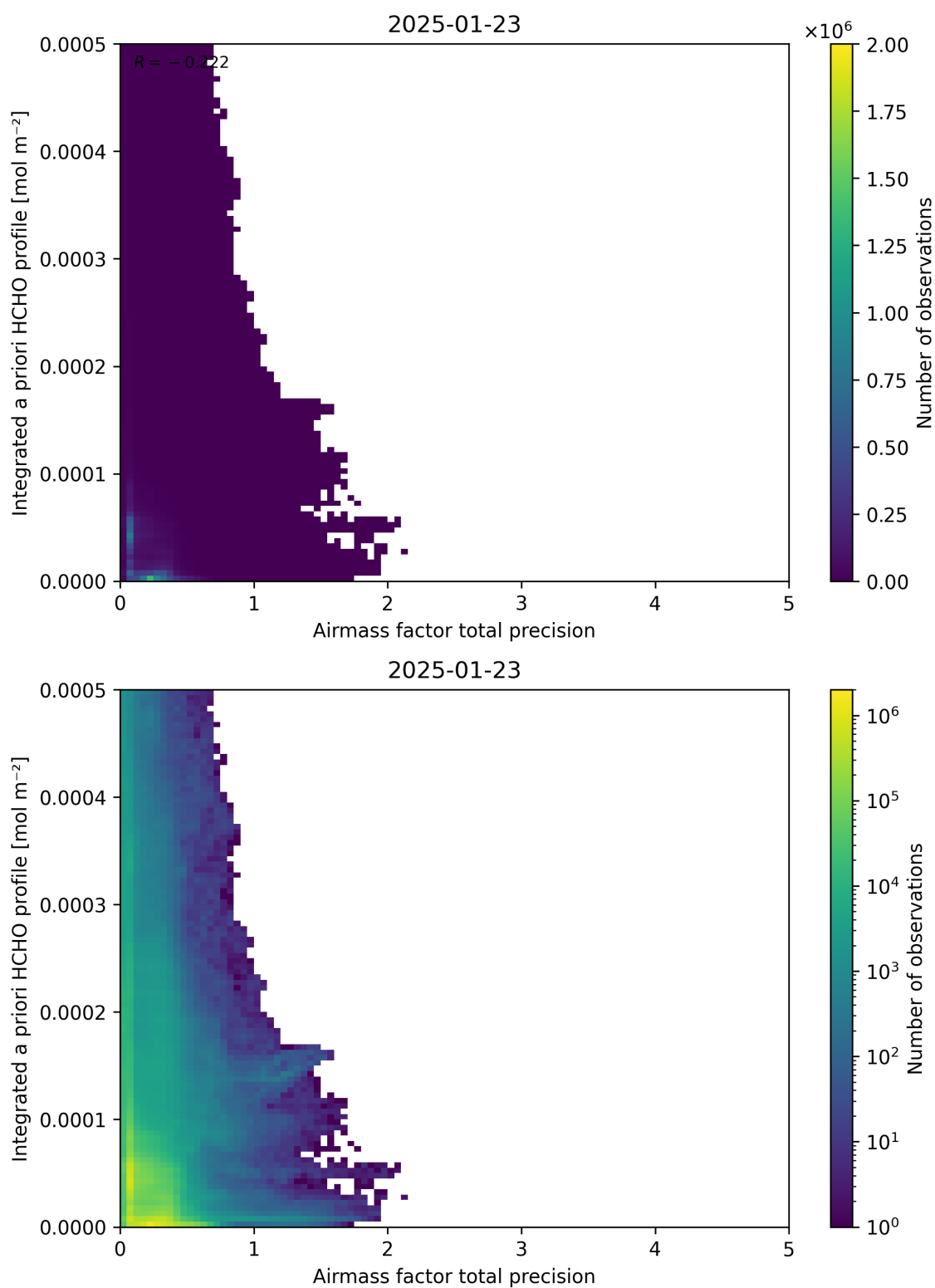
Figure 111: Scatter density plot of “Airmass factor total precision” against “Integrated a priori HCHO profile” for 2025-01-23 to 2025-01-24.
