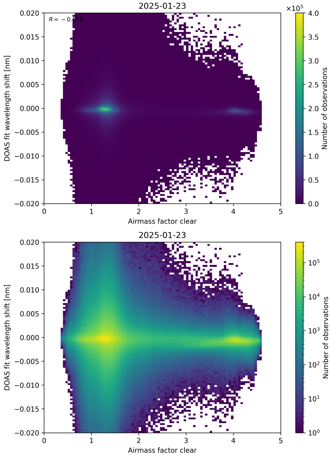
Figure 72: Scatter density plot of “Airmass factor clear” against “DOAS fit wavelength shift” for 2025-01-23 to 2025-01-24.
