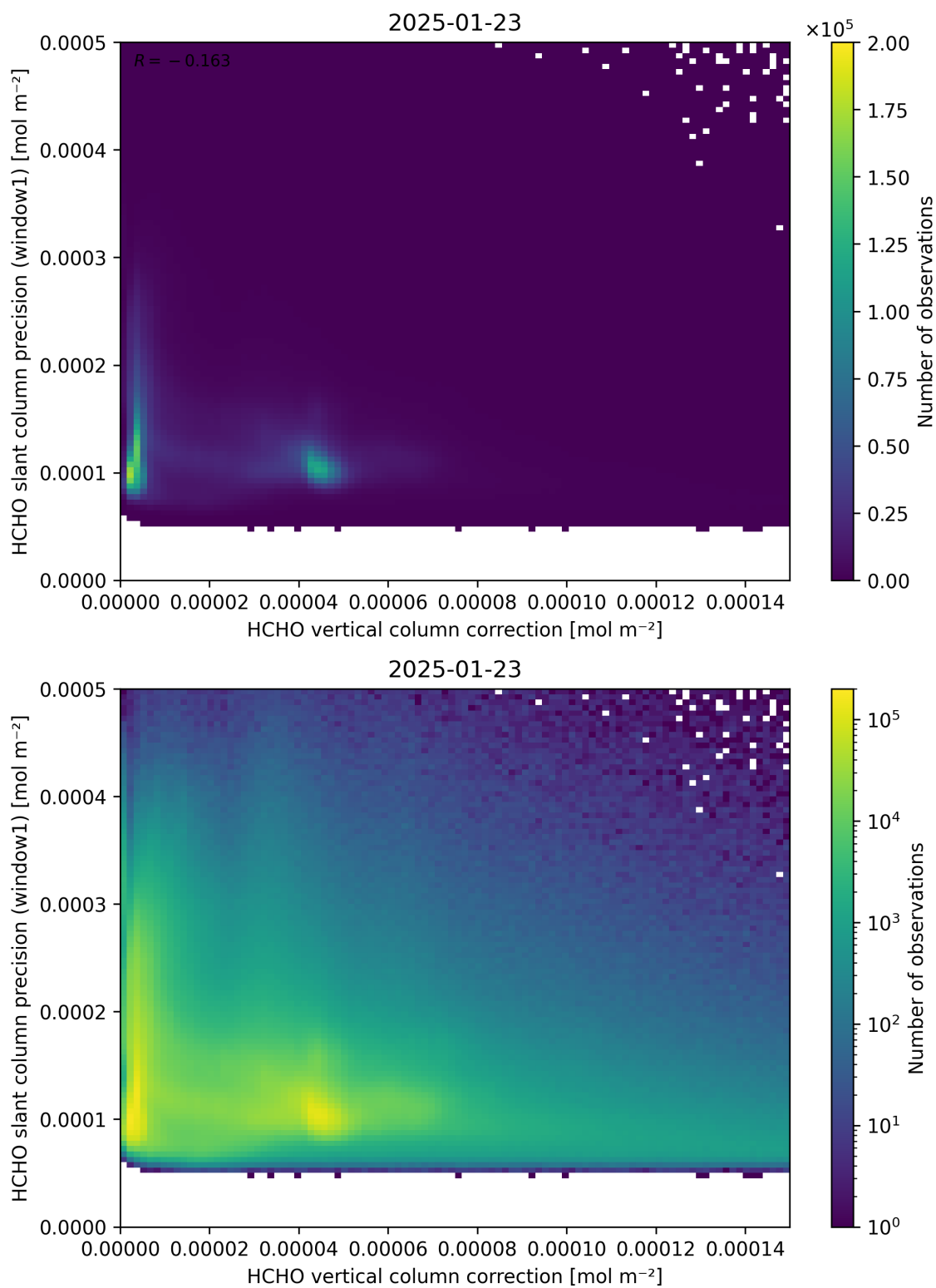
Figure 119: Scatter density plot of “HCHO vertical column correction” against “HCHO slant column precision (window1)” for 2025-01-23 to 2025-01-24.
