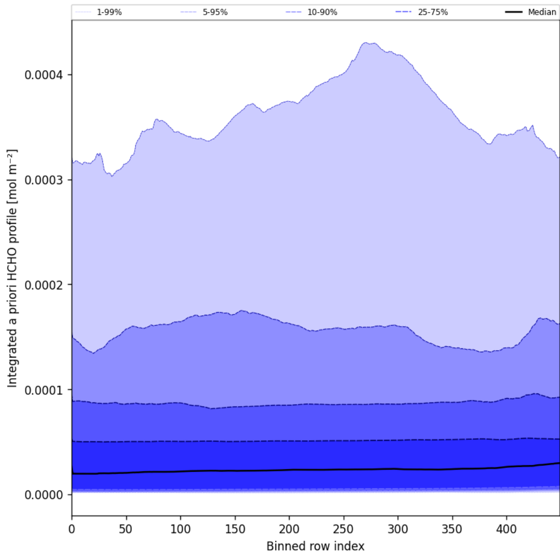
Figure 57: Along track statistics of “Integrated a priori HCHO profile” for 2025-01-23 to 2025-01-24
