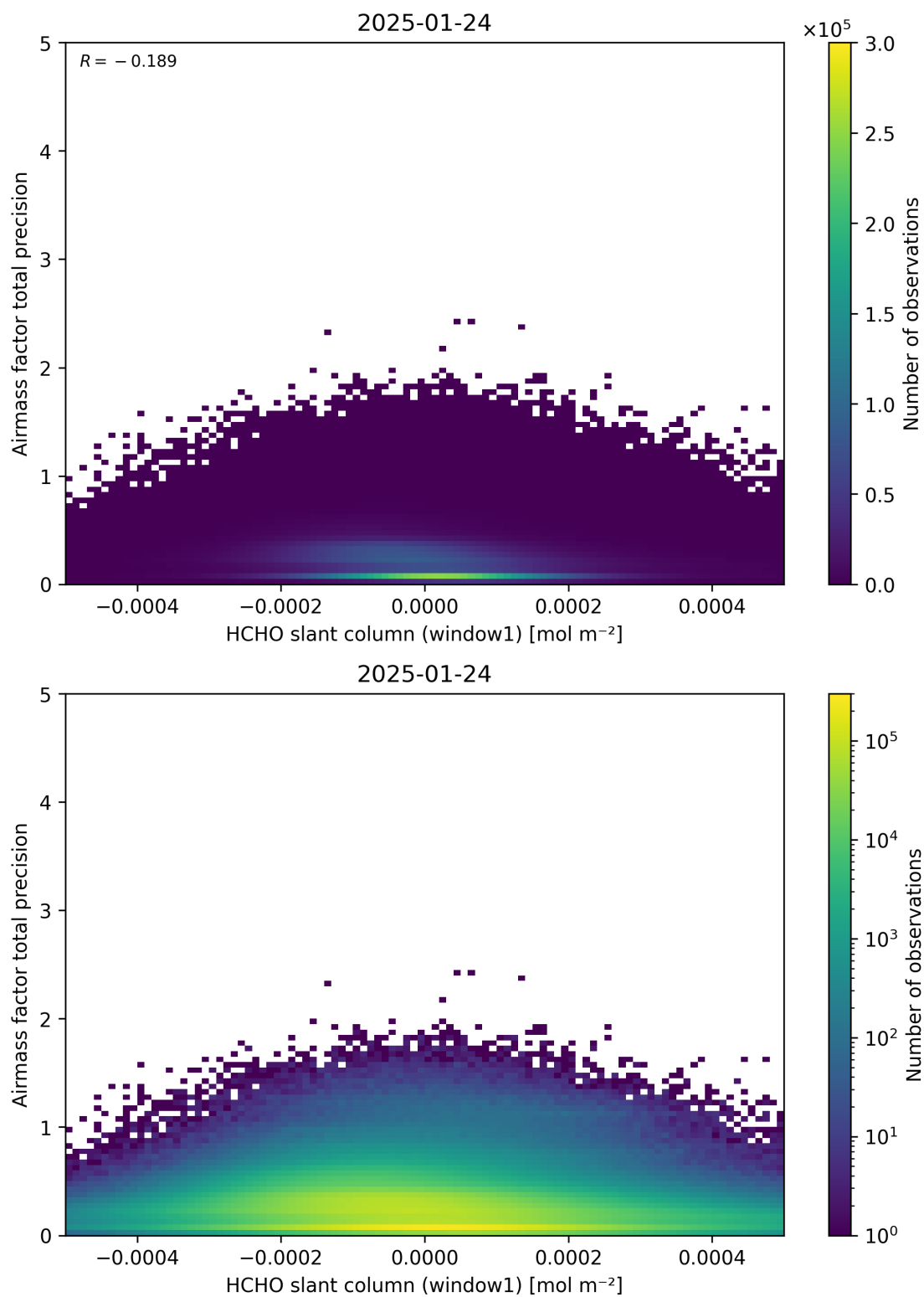
Figure 86: Scatter density plot of “HCHO slant column (window1)” against “Airmass factor total precision” for 2025-01-23 to 2025-01-25.
