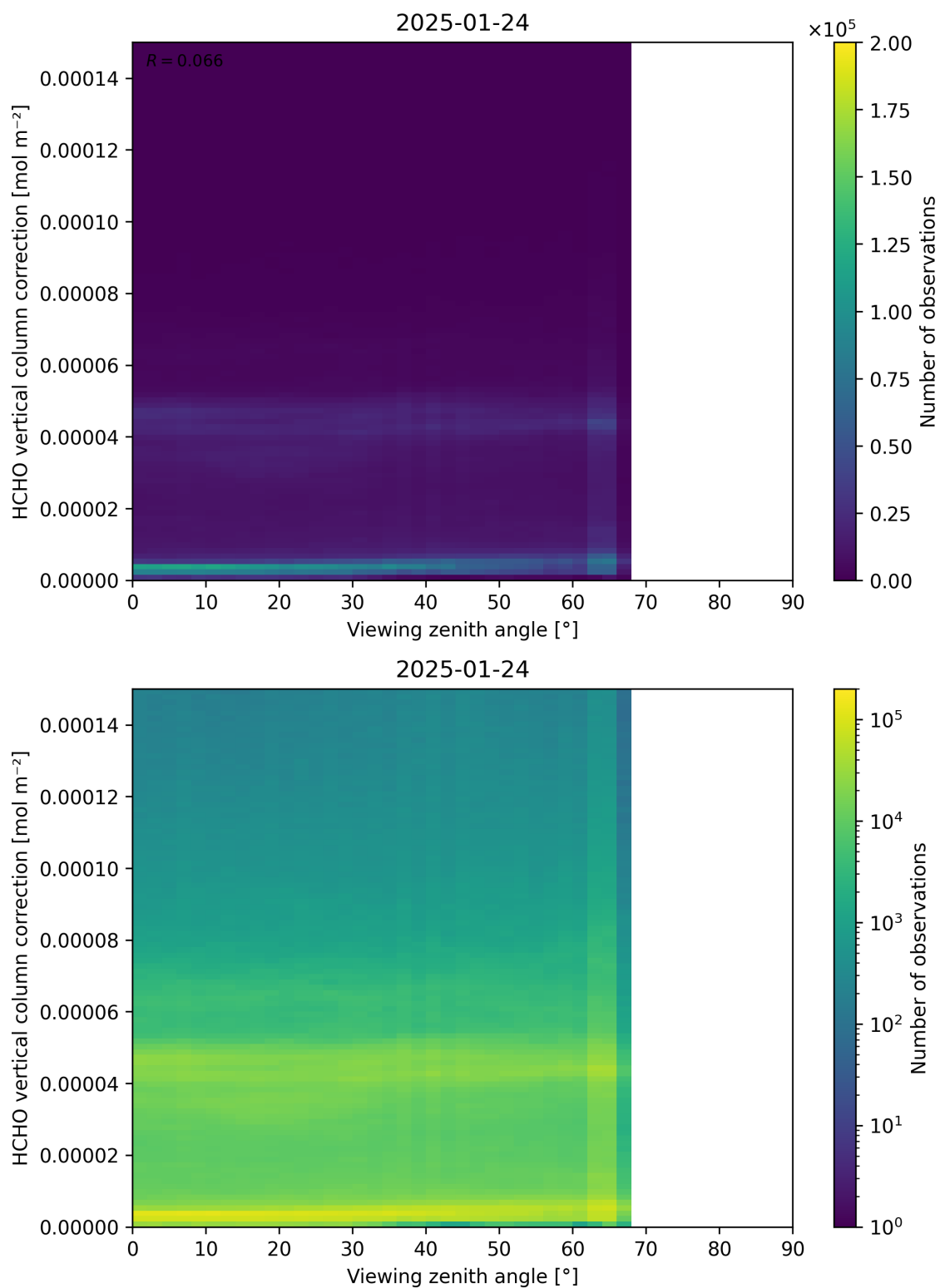
Figure 193: Scatter density plot of “Viewing zenith angle” against “HCHO vertical column correction” for 2025-01-23 to 2025-01-25.
