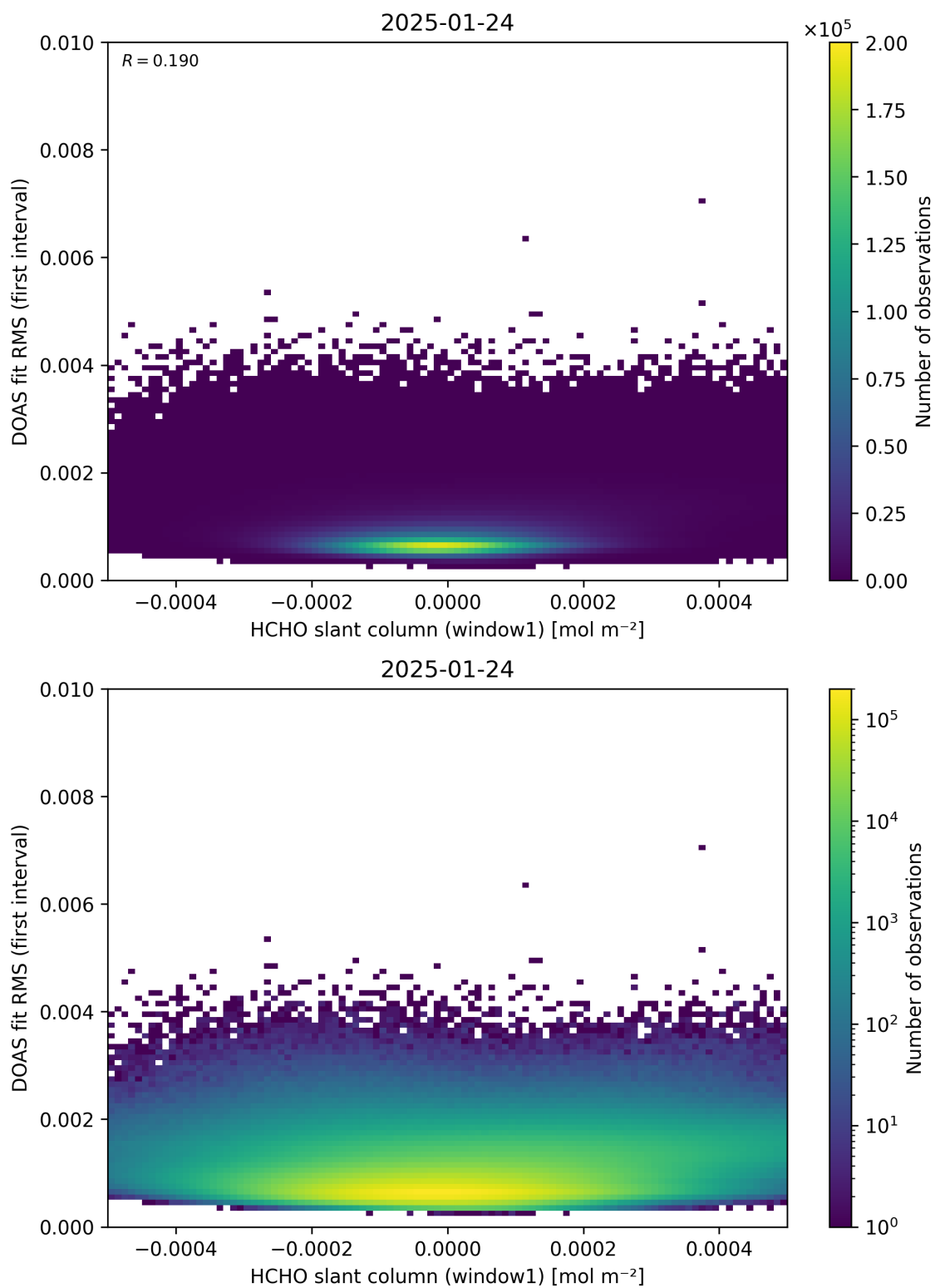
Figure 78: Scatter density plot of “HCHO slant column (window1)” against “DOAS fit RMS (first interval)” for 2025-01-23 to 2025-01-25.
