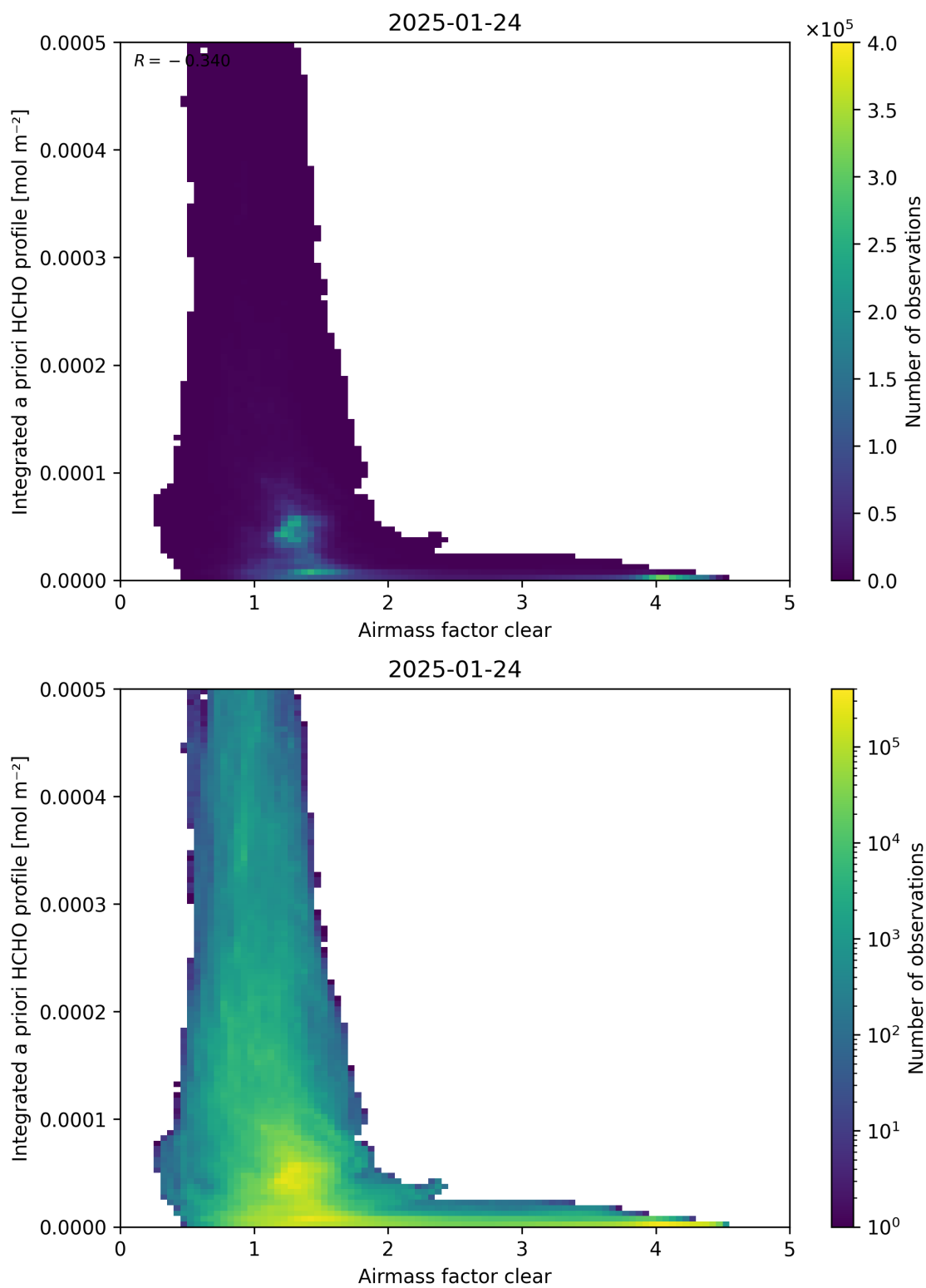
Figure 76: Scatter density plot of “Airmass factor clear” against “Integrated a priori HCHO profile” for 2025-01-23 to 2025-01-25.
