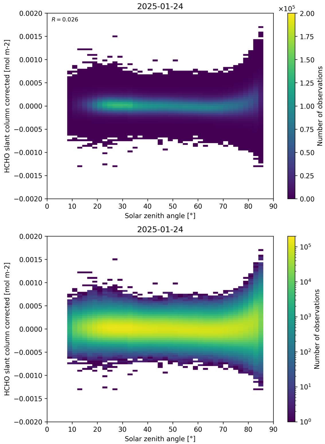
Figure 171: Scatter density plot of “Solar zenith angle” against “HCHO slant column corrected” for 2025-01-23 to 2025-01-25.
