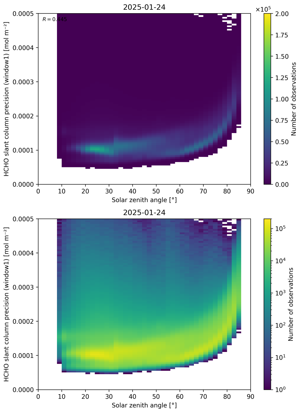
Figure 174: Scatter density plot of “Solar zenith angle” against “HCHO slant column precision (window1)” for 2025-01-23 to 2025-01-25.
