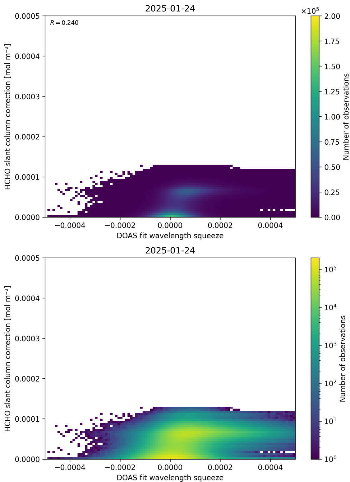
Figure 70: Scatter density plot of “DOAS fit wavelength squeeze” against “HCHO slant column correction” for 2025-01-23 to 2025-01-25.
