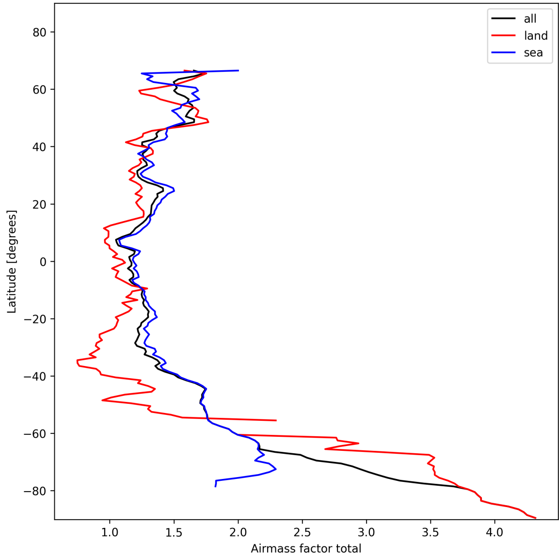
Figure 26: Zonal average of “Airmass factor total” for 2025-01-23 to 2025-01-25.
