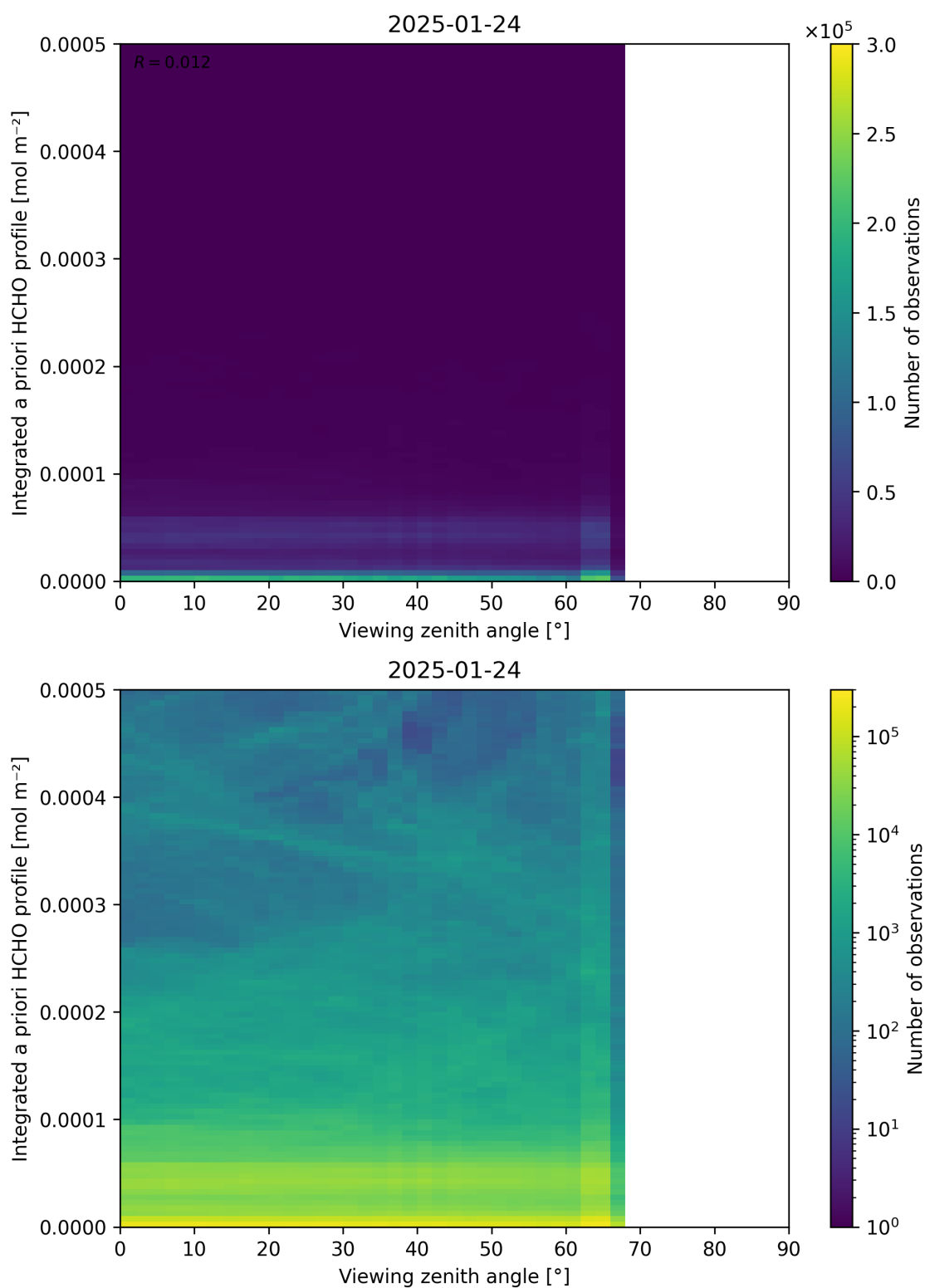
Figure 195: Scatter density plot of “Viewing zenith angle” against “Integrated a priori HCHO profile” for 2025-01-23 to 2025-01-25.
