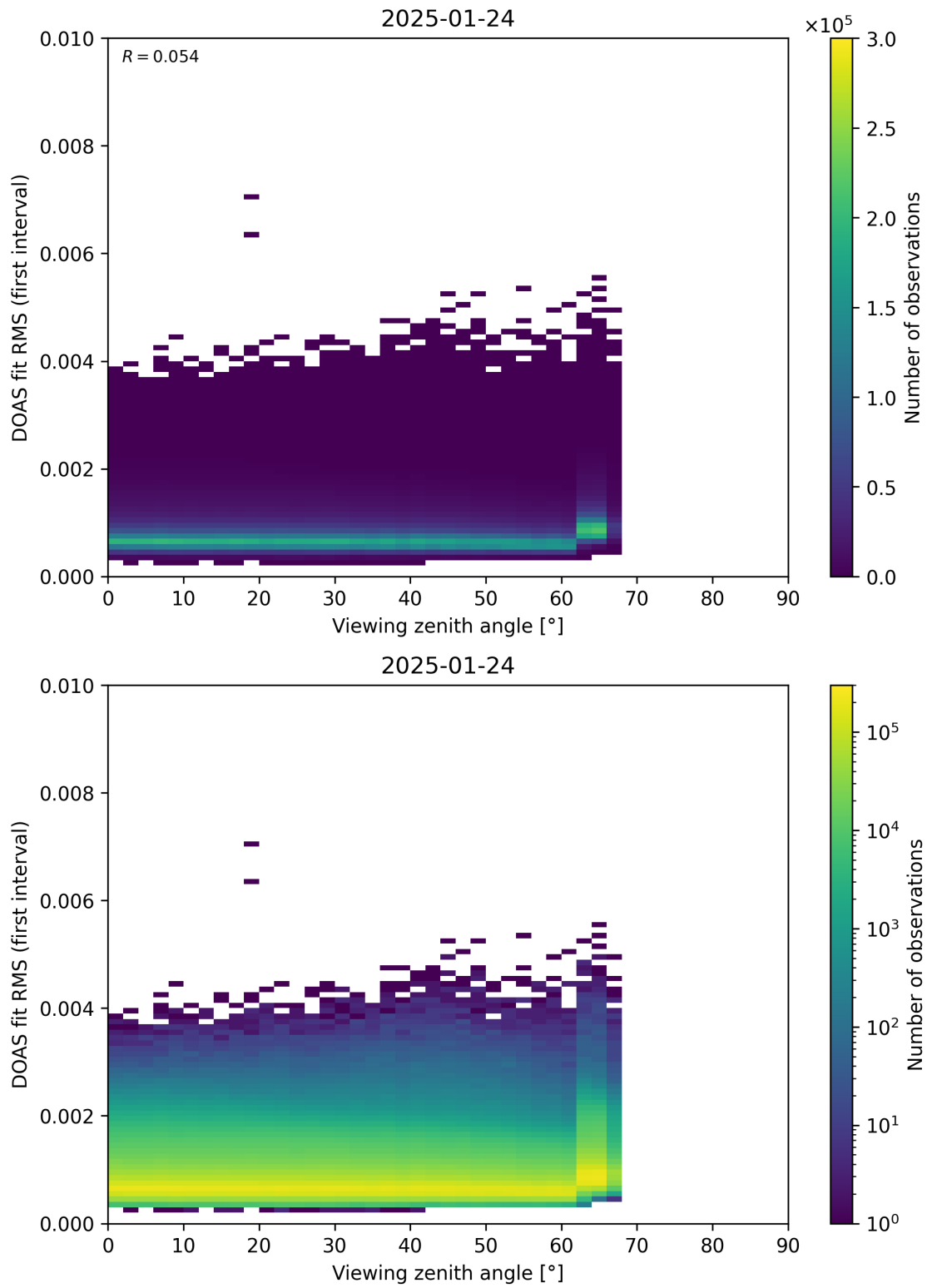
Figure 182: Scatter density plot of “Viewing zenith angle” against “DOAS fit RMS (first interval)” for 2025-01-23 to 2025-01-25.
