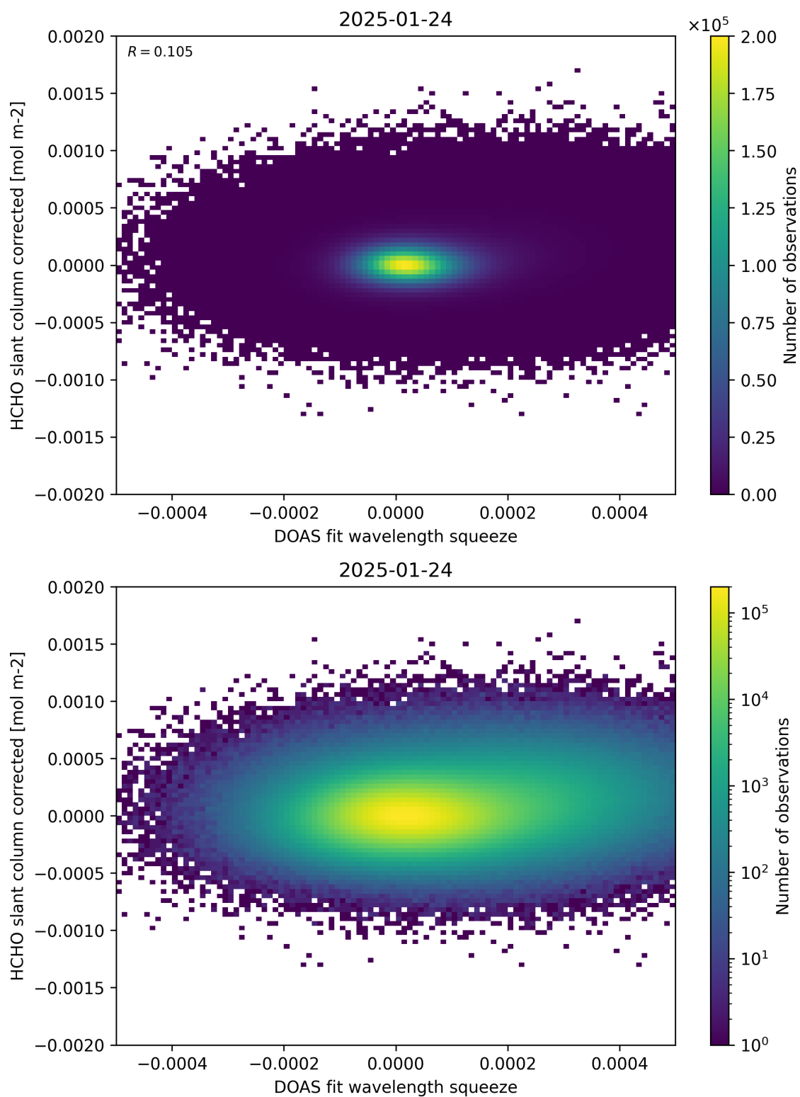
Figure 69: Scatter density plot of “DOAS fit wavelength squeeze” against “HCHO slant column corrected” for 2025-01-23 to 2025-01-25.
