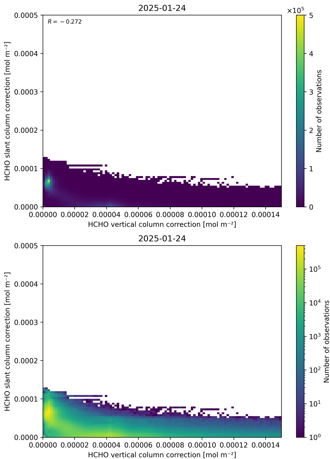
Figure 117: Scatter density plot of “HCHO vertical column correction” against “HCHO slant column correction” for 2025-01-23 to 2025-01-25.
