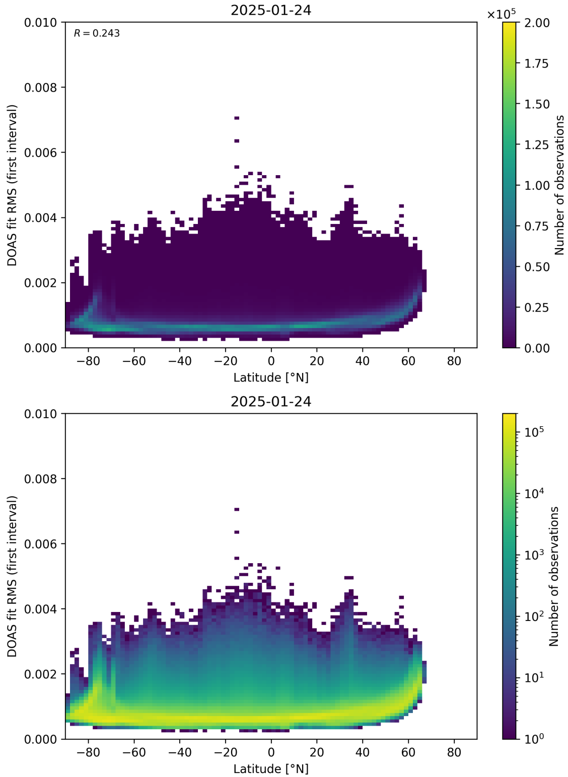
Figure 153: Scatter density plot of “Latitude” against “DOAS fit RMS (first interval)” for 2025-01-23 to 2025-01-25.
