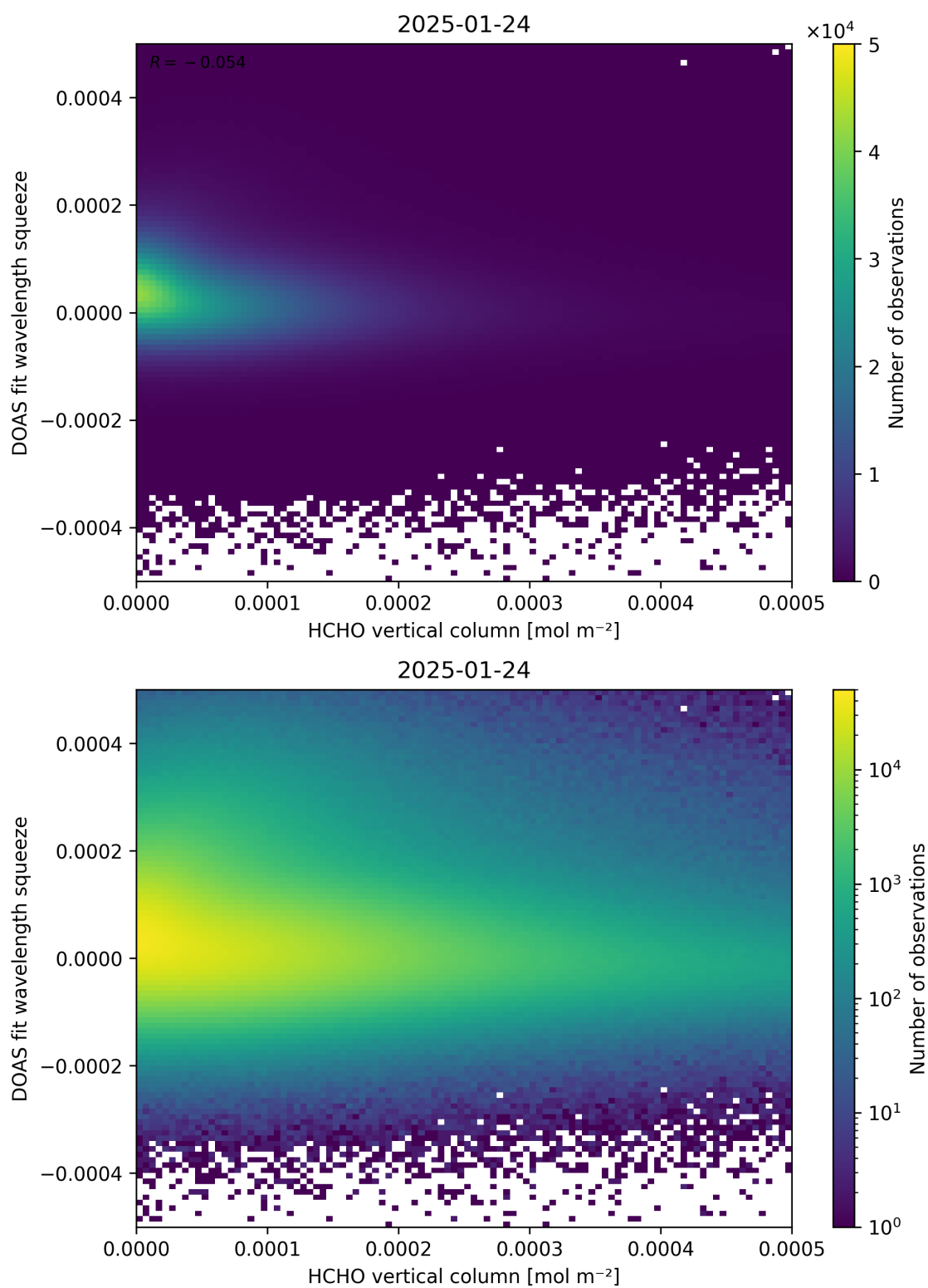
Figure 125: Scatter density plot of “HCHO vertical column” against “DOAS fit wavelength squeeze” for 2025-01-23 to 2025-01-25.
