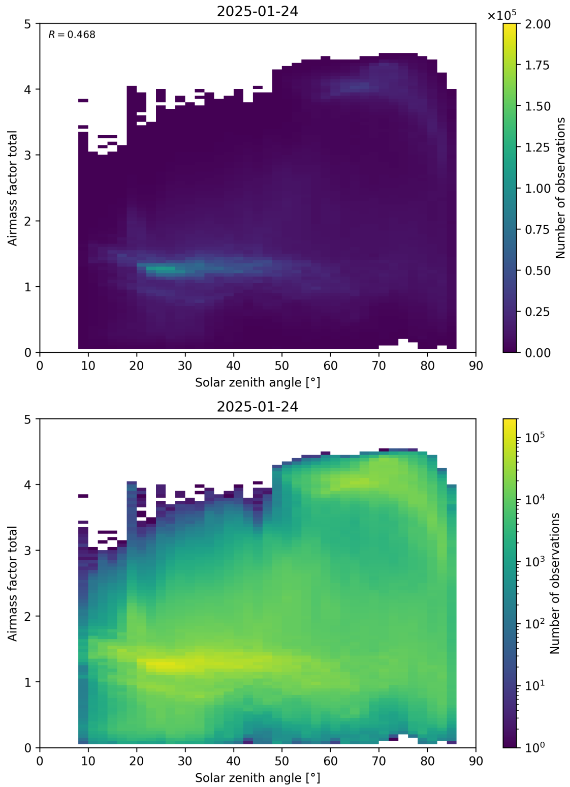
Figure 175: Scatter density plot of “Solar zenith angle” against “Airmass factor total” for 2025-01-23 to 2025-01-25.
