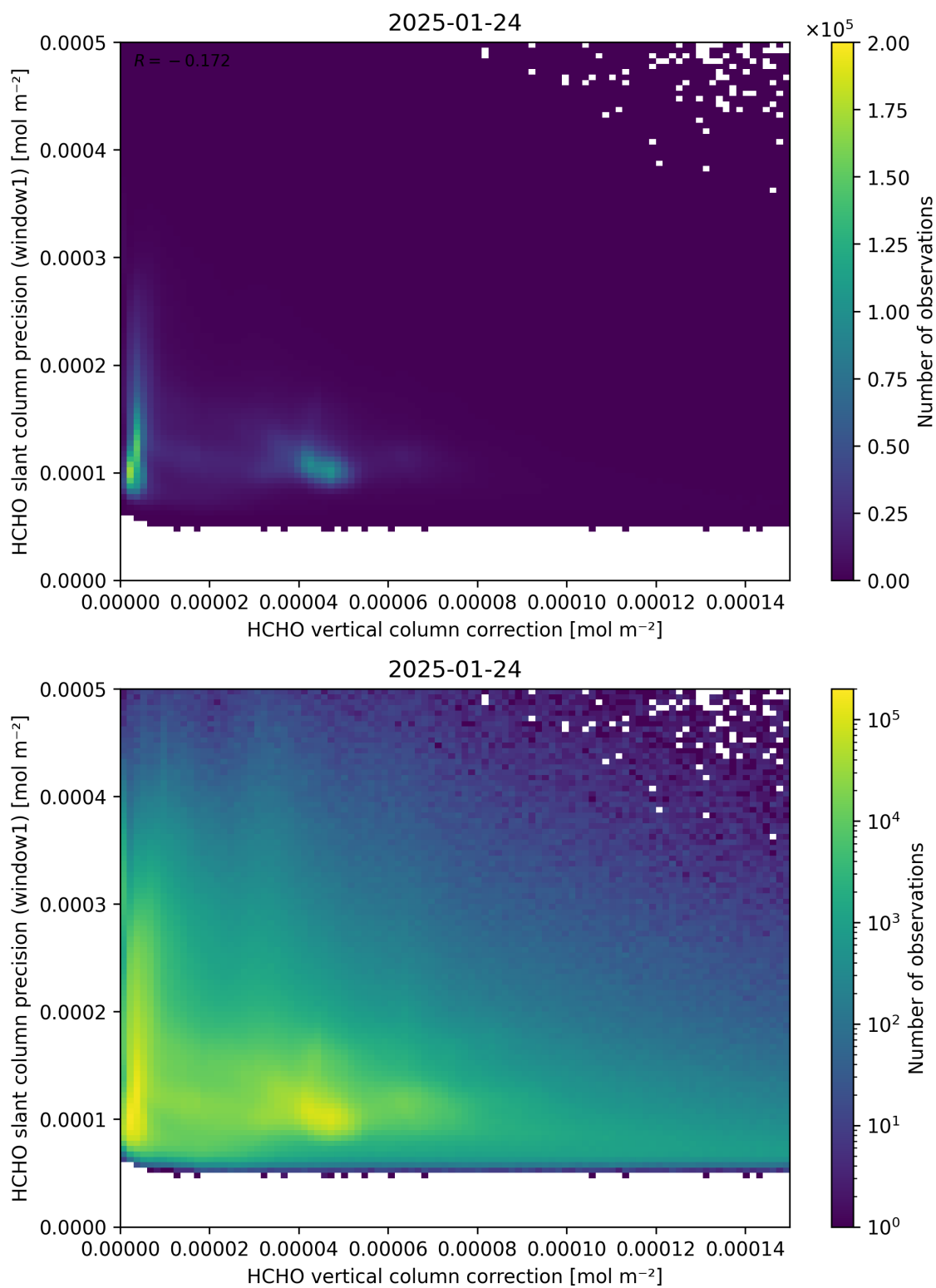
Figure 119: Scatter density plot of “HCHO vertical column correction” against “HCHO slant column precision (window1)” for 2025-01-23 to 2025-01-25.
