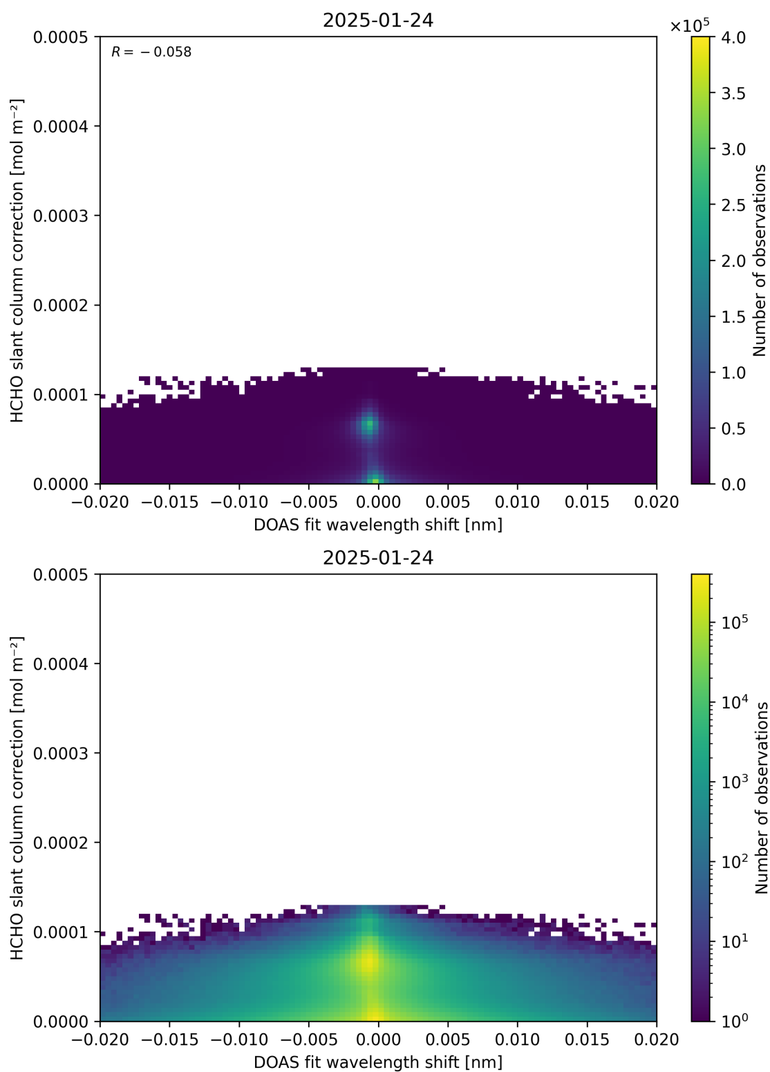
Figure 67: Scatter density plot of “DOAS fit wavelength shift” against “HCHO slant column correction” for 2025-01-23 to 2025-01-25.
