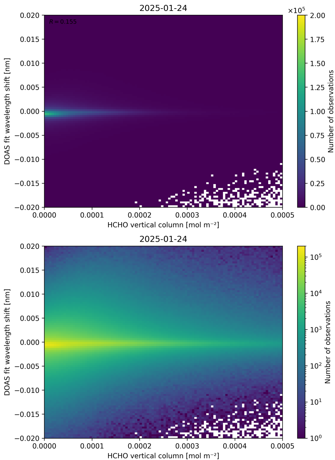
Figure 124: Scatter density plot of “HCHO vertical column” against “DOAS fit wavelength shift” for 2025-01-23 to 2025-01-25.
