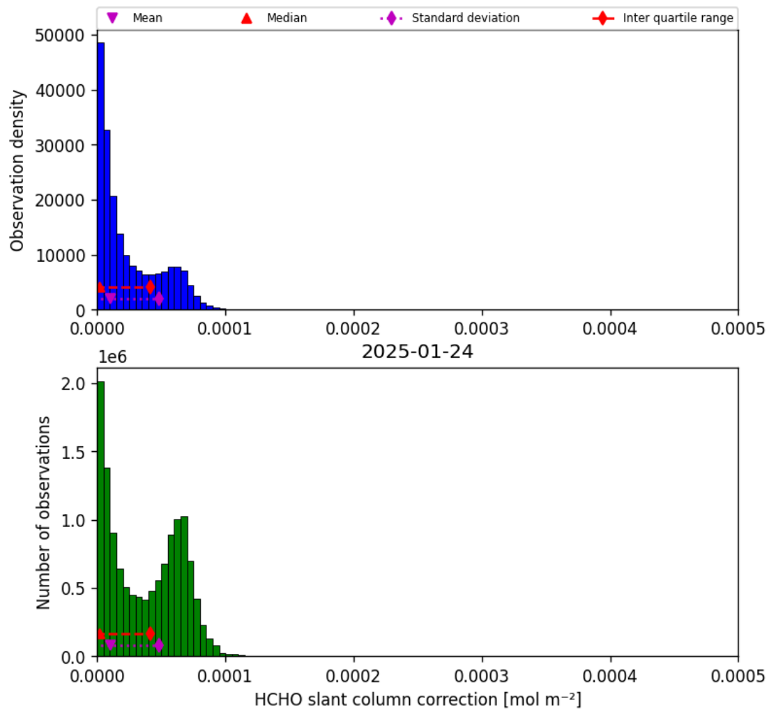
Figure 47: Histogram of “HCHO slant column correction” for 2025-01-23 to 2025-01-25
