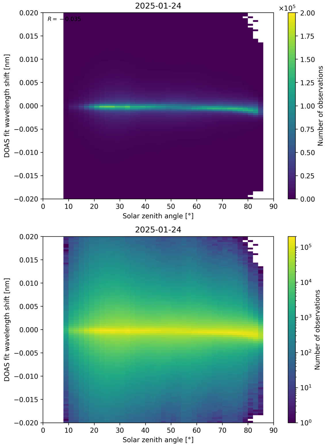
Figure 168: Scatter density plot of “Solar zenith angle” against “DOAS fit wavelength shift” for 2025-01-23 to 2025-01-25.
