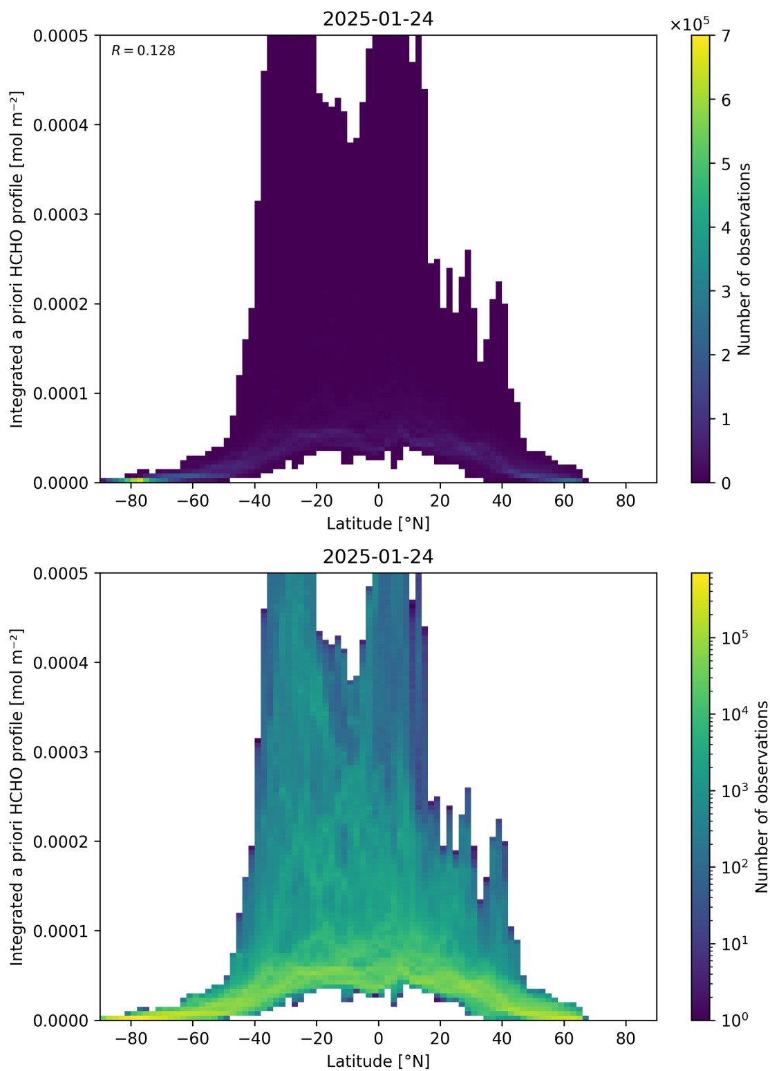
Figure 166: Scatter density plot of “Latitude” against “Integrated a priori HCHO profile” for 2025-01-23 to 2025-01-25.
