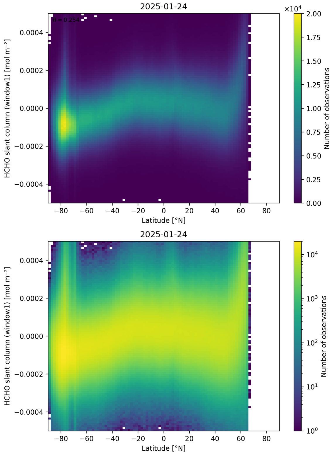
Figure 159: Scatter density plot of “Latitude” against “HCHO slant column (window1)” for 2025-01-23 to 2025-01-25.
