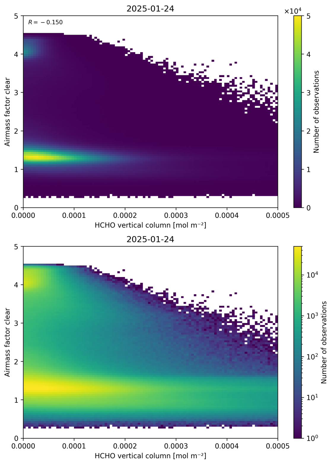
Figure 126: Scatter density plot of “HCHO vertical column” against “Airmass factor clear” for 2025-01-23 to 2025-01-25.
