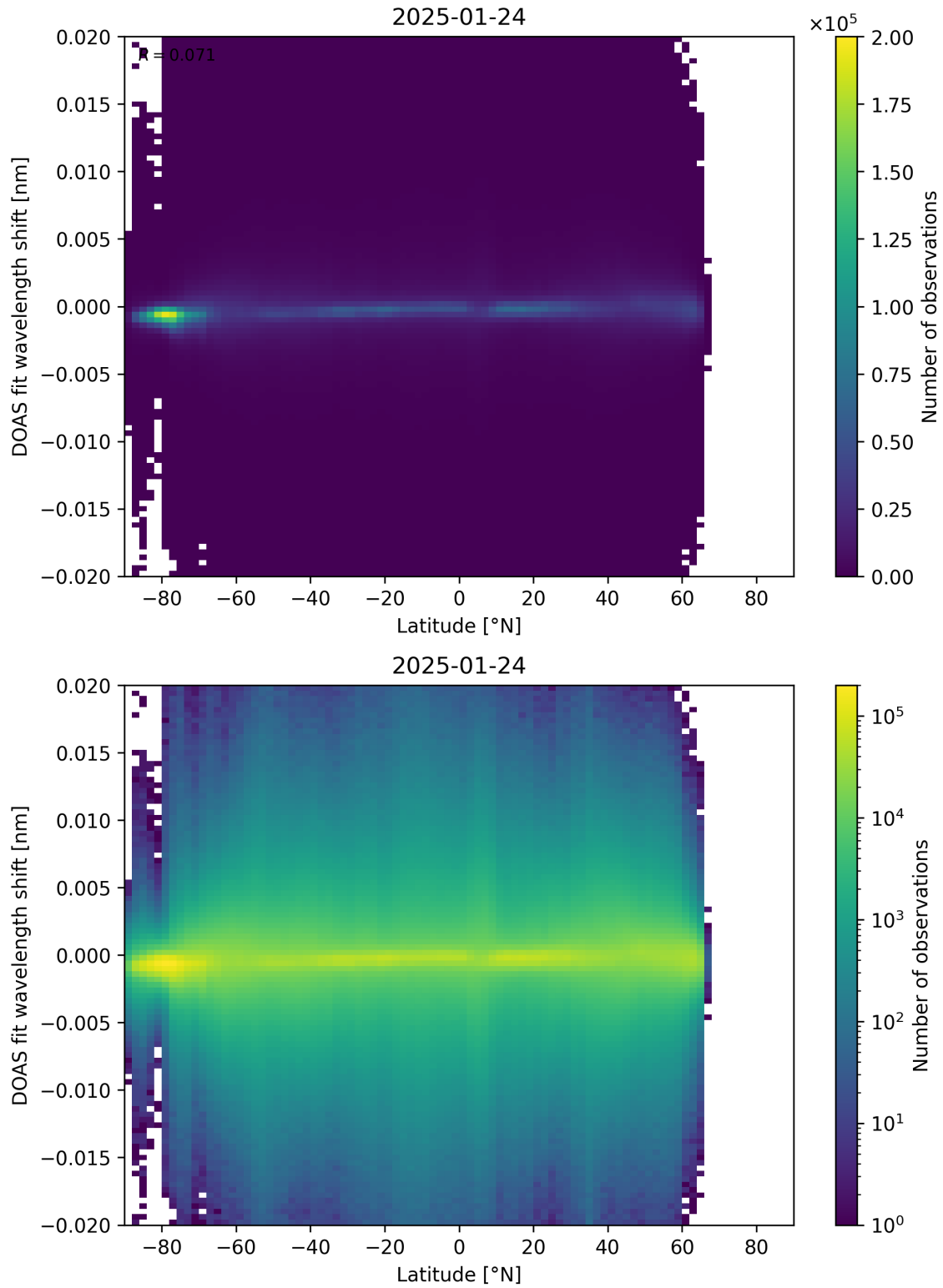
Figure 154: Scatter density plot of “Latitude” against “DOAS fit wavelength shift” for 2025-01-23 to 2025-01-25.
