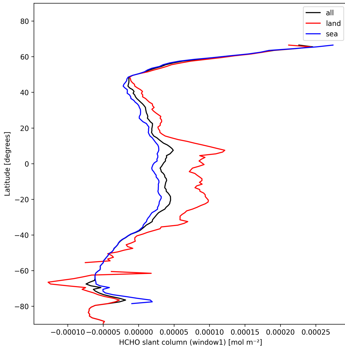
Figure 24: Zonal average of “HCHO slant column (window1)” for 2025-01-23 to 2025-01-25.
