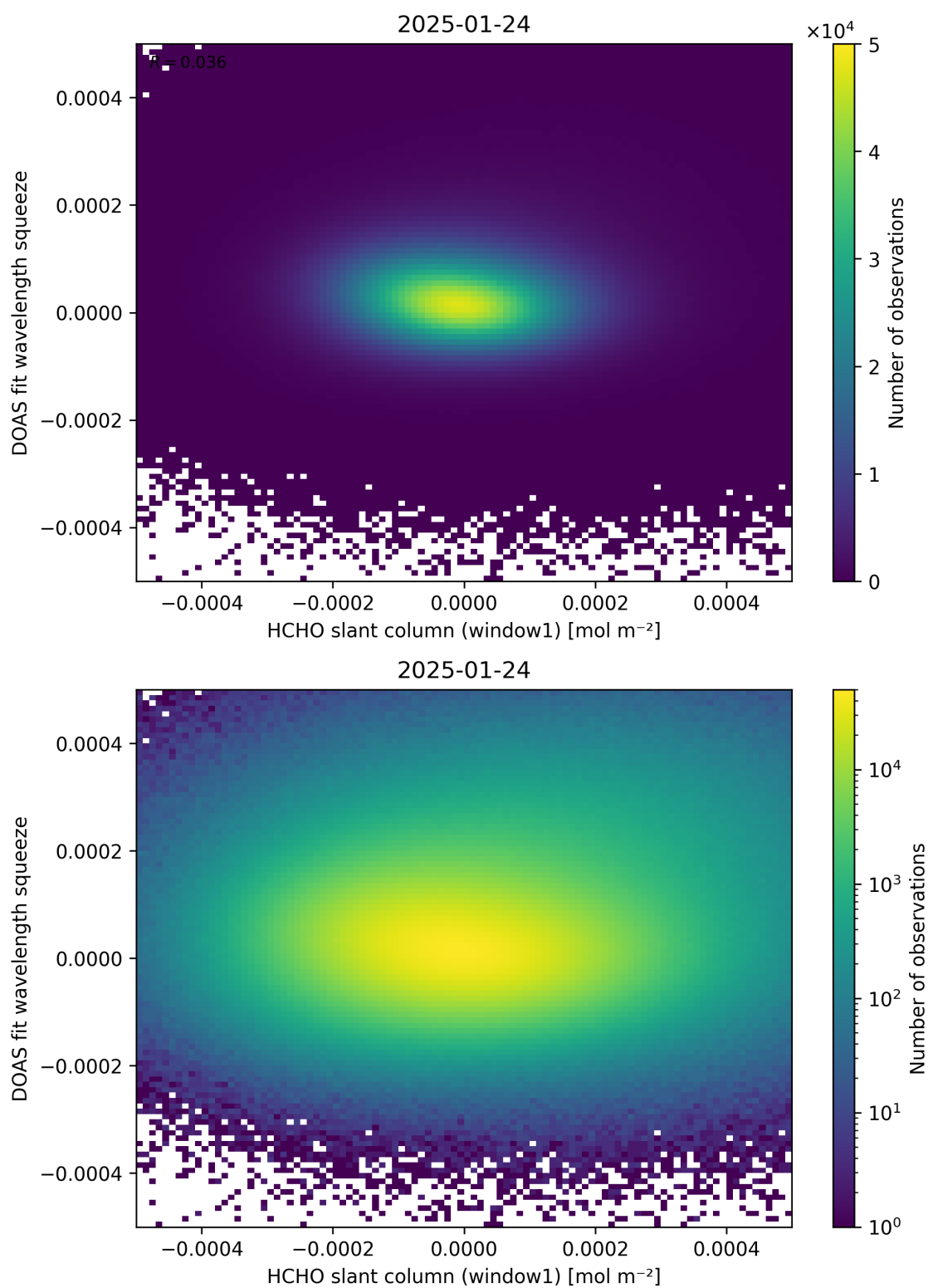
Figure 80: Scatter density plot of “HCHO slant column (window1)” against “DOAS fit wavelength squeeze” for 2025-01-23 to 2025-01-25.
