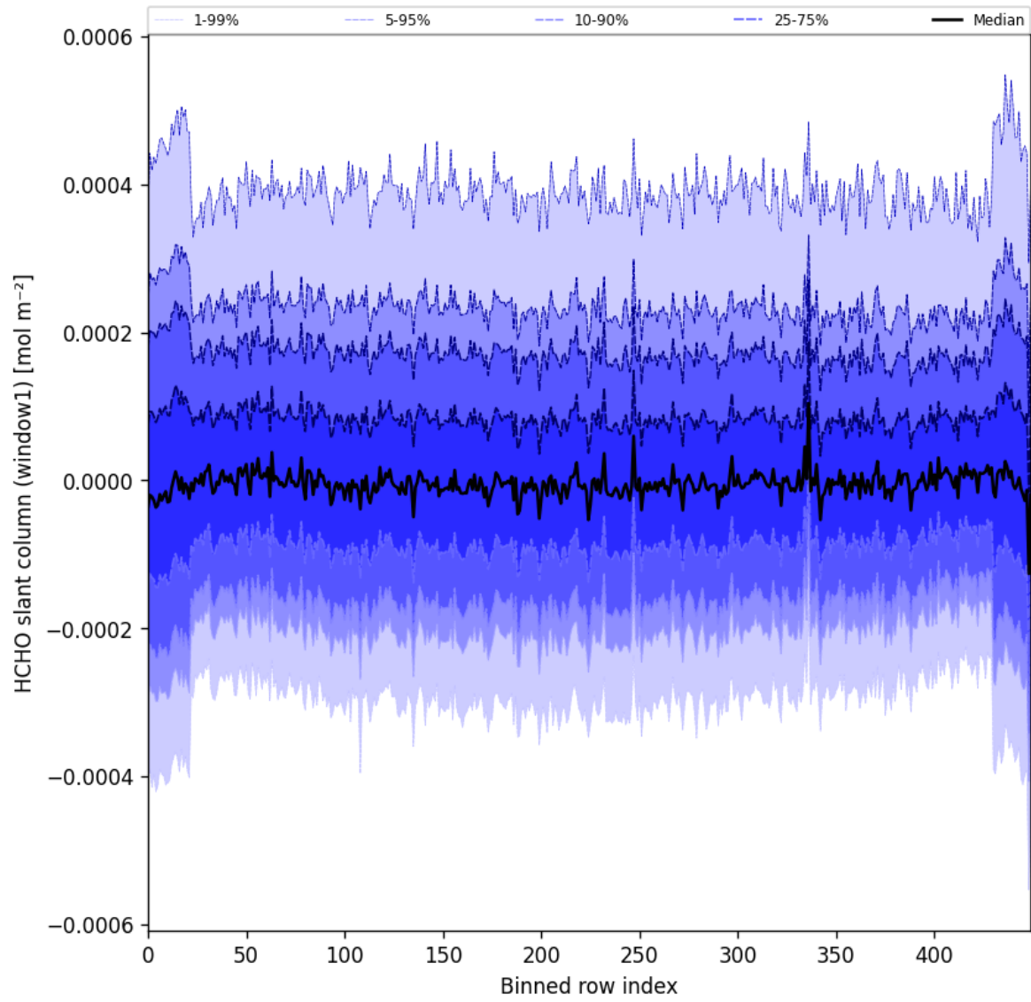
Figure 52: Along track statistics of “HCHO slant column (window1)” for 2025-01-23 to 2025-01-25
