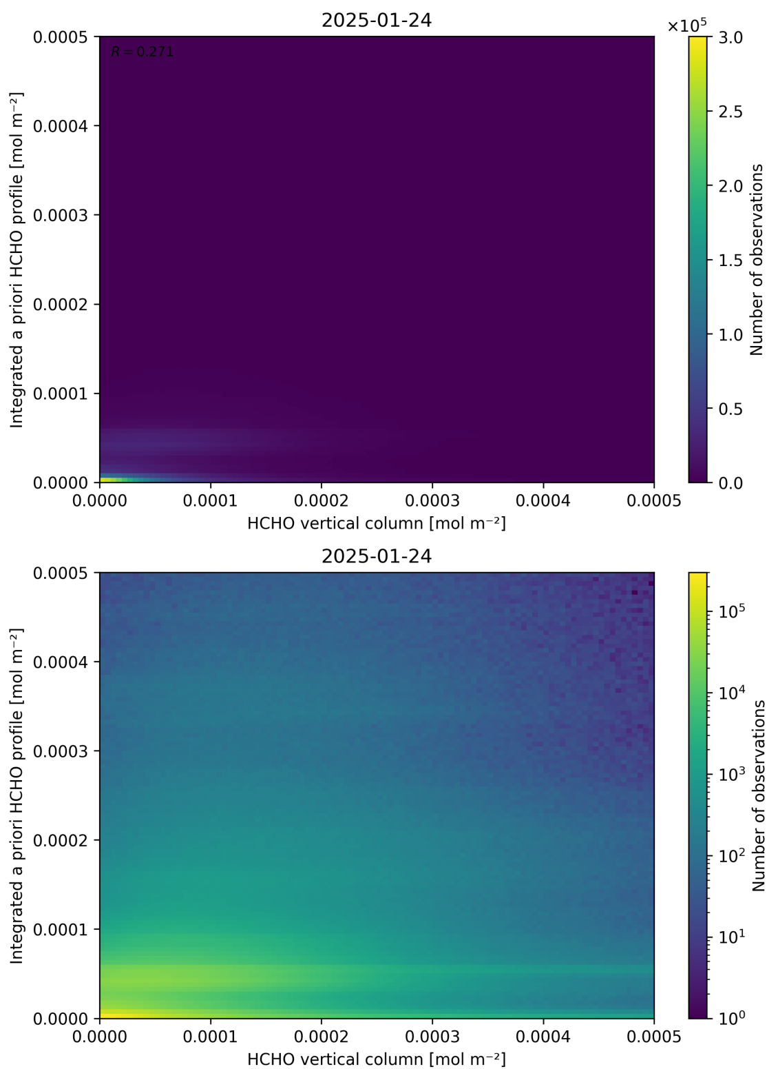
Figure 135: Scatter density plot of “HCHO vertical column” against “Integrated a priori HCHO profile” for 2025-01-23 to 2025-01-25.
