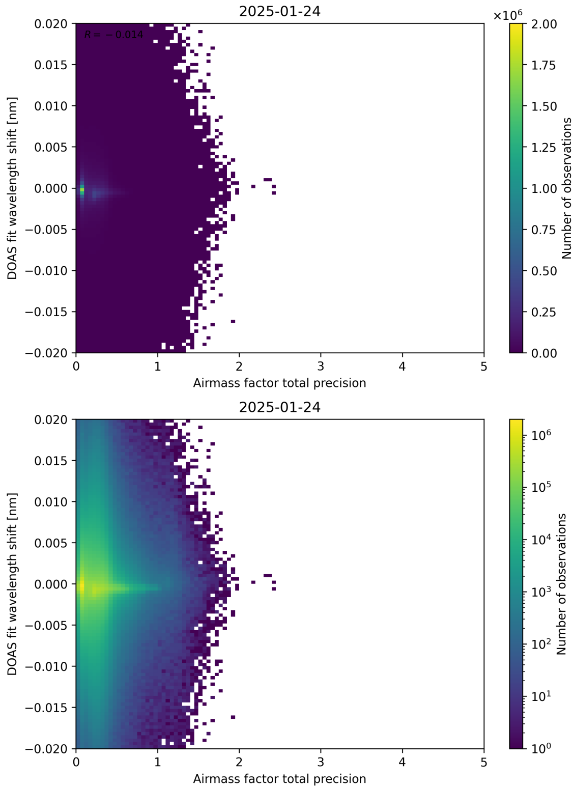
Figure 106: Scatter density plot of “Airmass factor total precision” against “DOAS fit wavelength shift” for 2025-01-23 to 2025-01-25.
