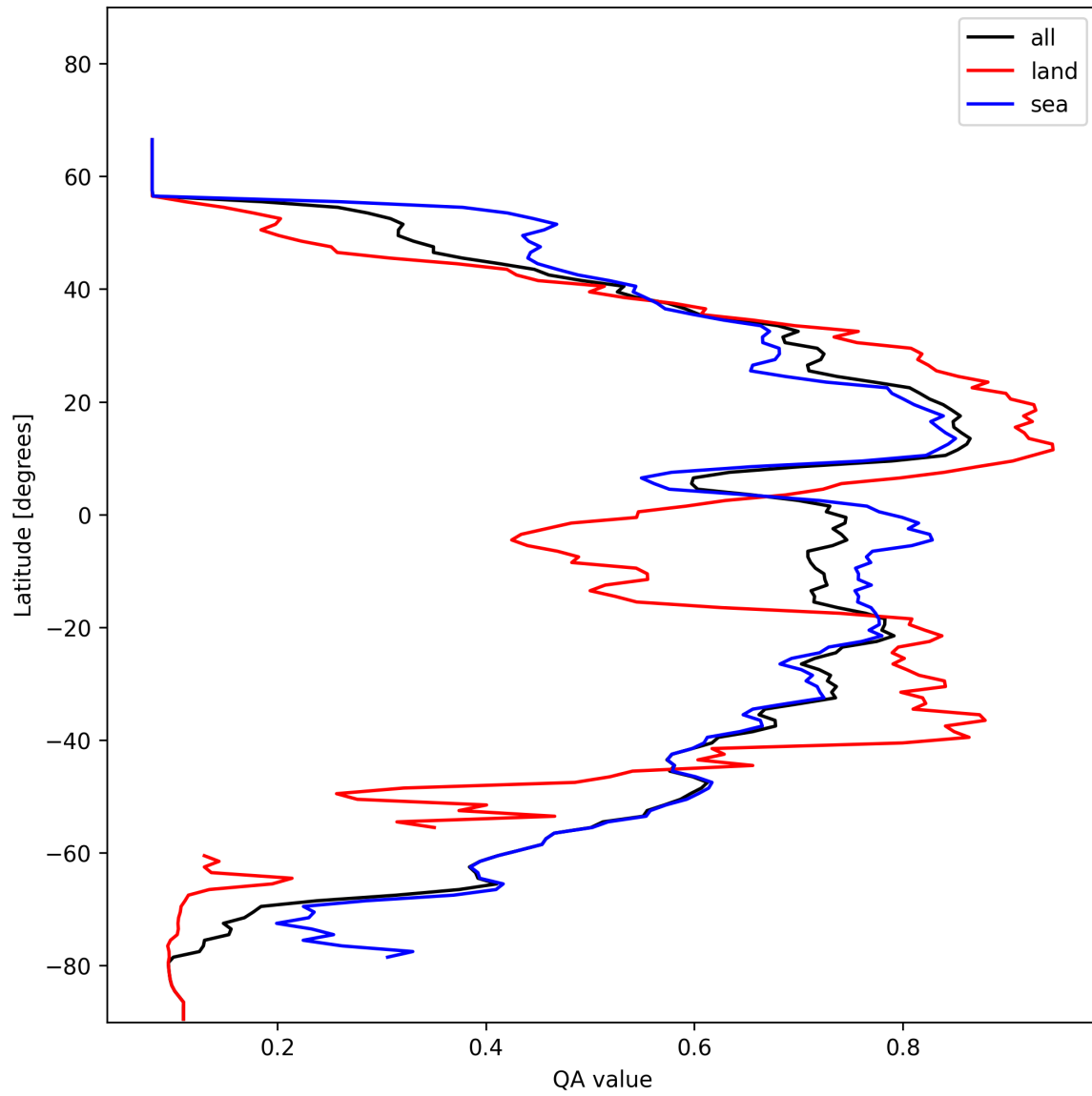
Figure 20: Zonal average of “QA value” for 2025-01-23 to 2025-01-25.
