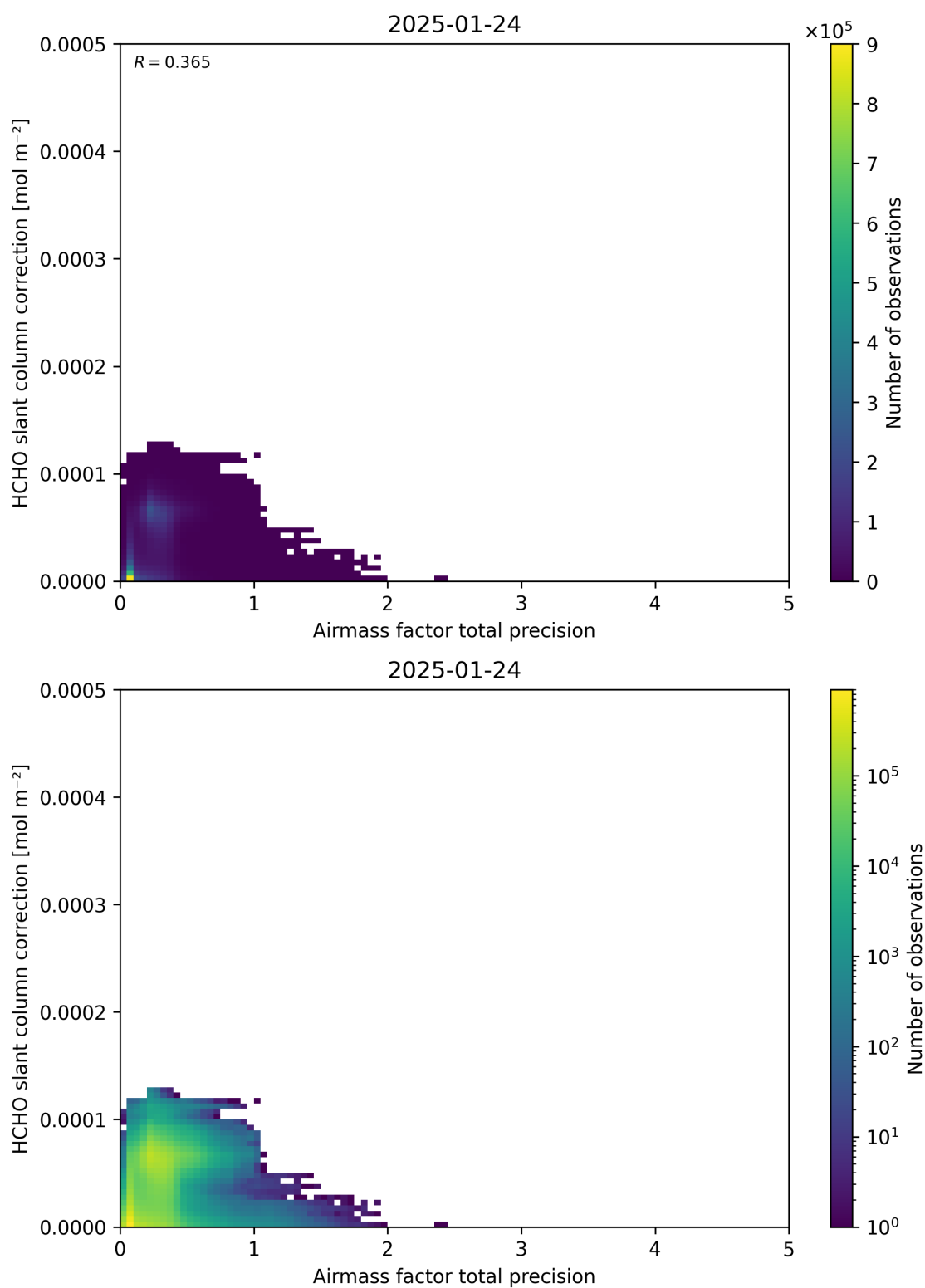
Figure 110: Scatter density plot of “Airmass factor total precision” against “HCHO slant column correction” for 2025-01-23 to 2025-01-25.
