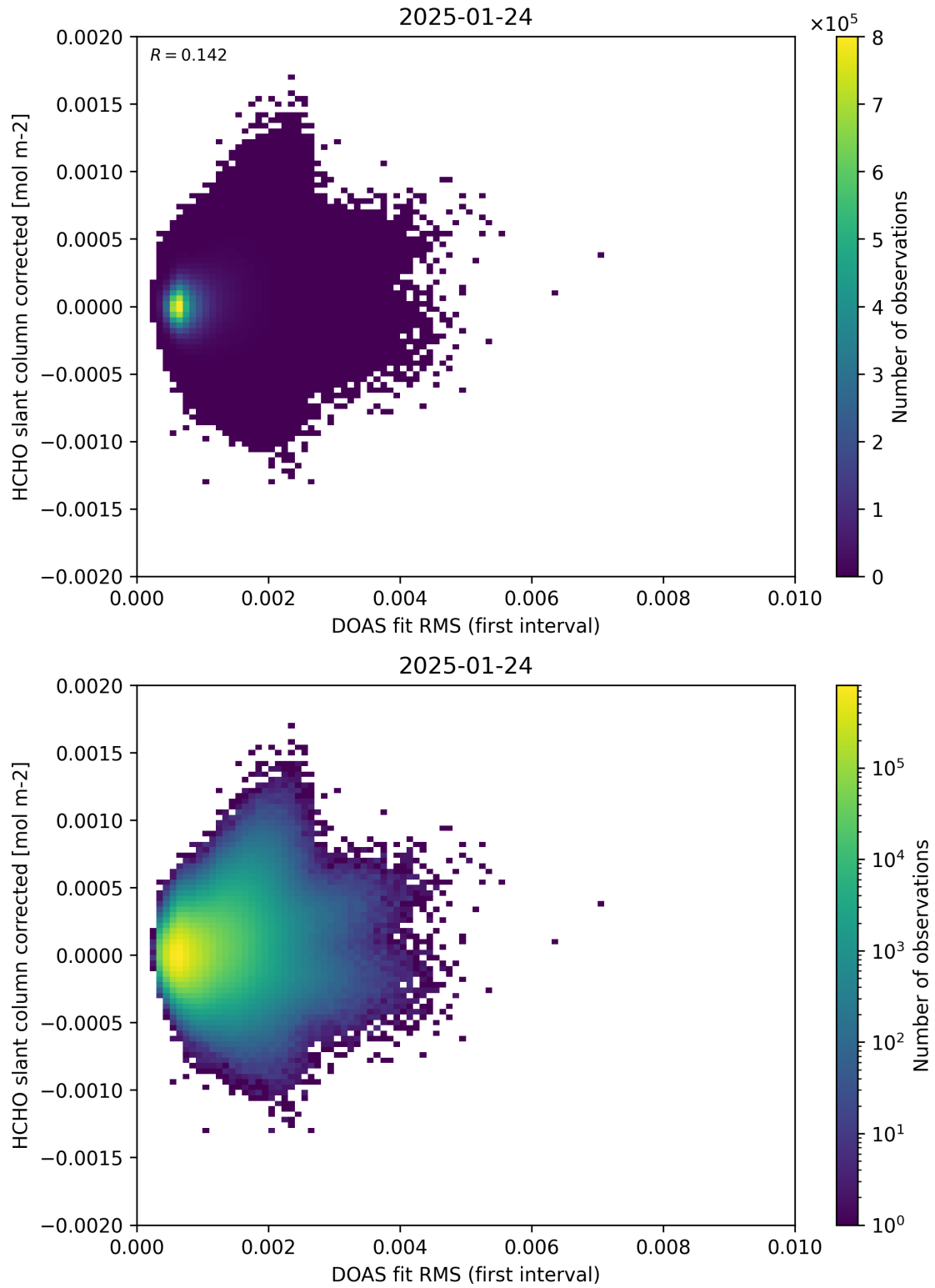
Figure 62: Scatter density plot of “DOAS fit RMS (first interval)” against “HCHO slant column corrected” for 2025-01-23 to 2025-01-25.
