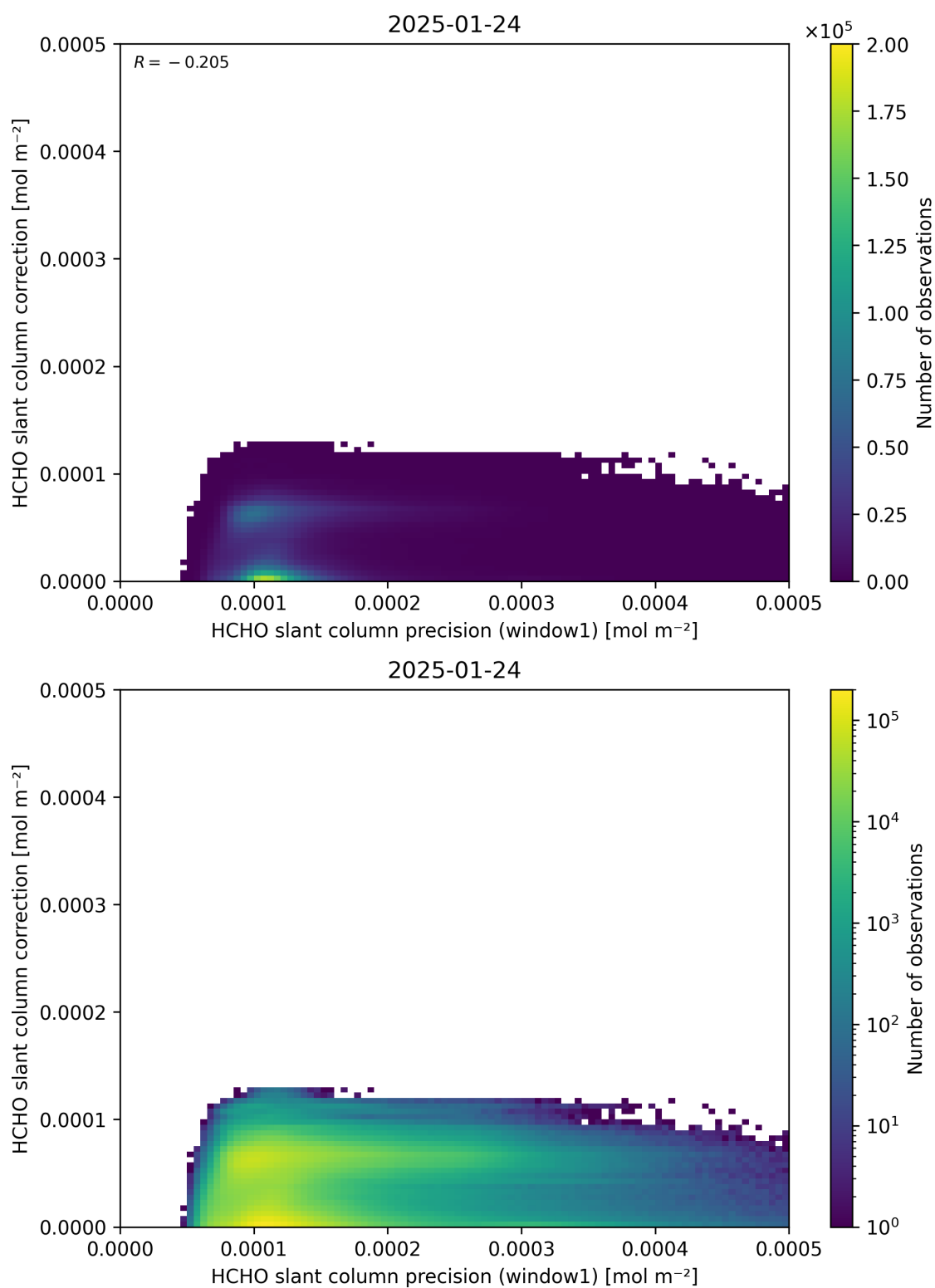
Figure 93: Scatter density plot of “HCHO slant column precision (window1)” against “HCHO slant column correction” for 2025-01-23 to 2025-01-25.
