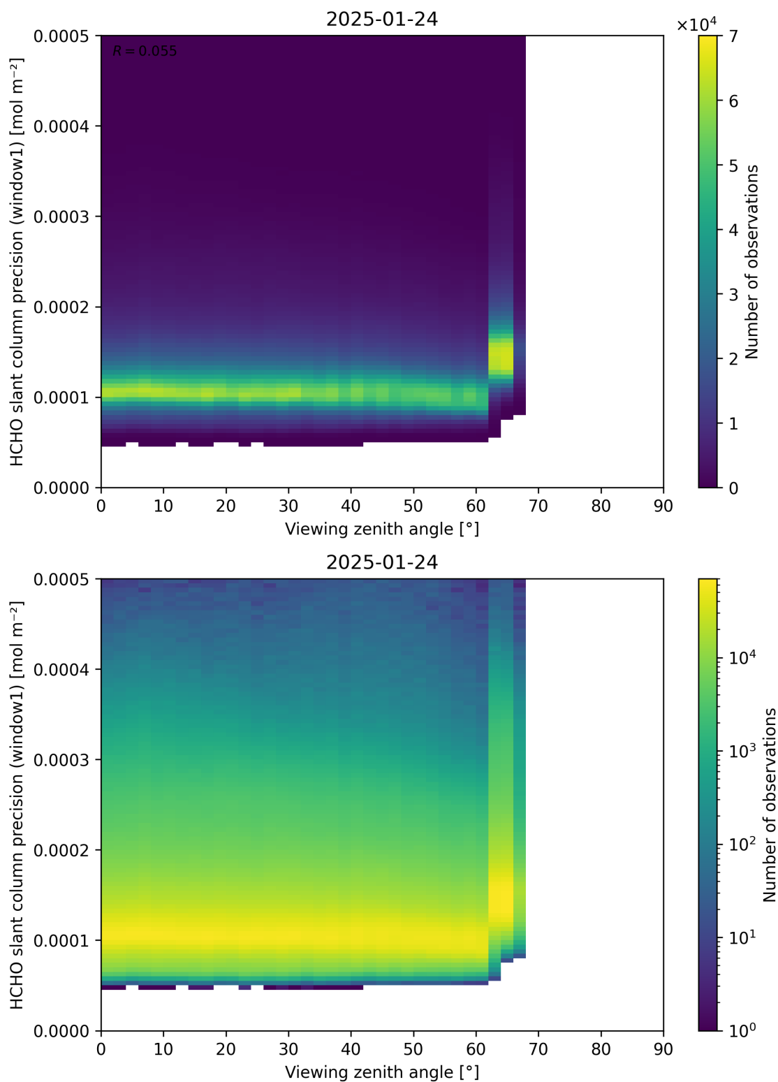
Figure 189: Scatter density plot of “Viewing zenith angle” against “HCHO slant column precision (window1)” for 2025-01-23 to 2025-01-25.
