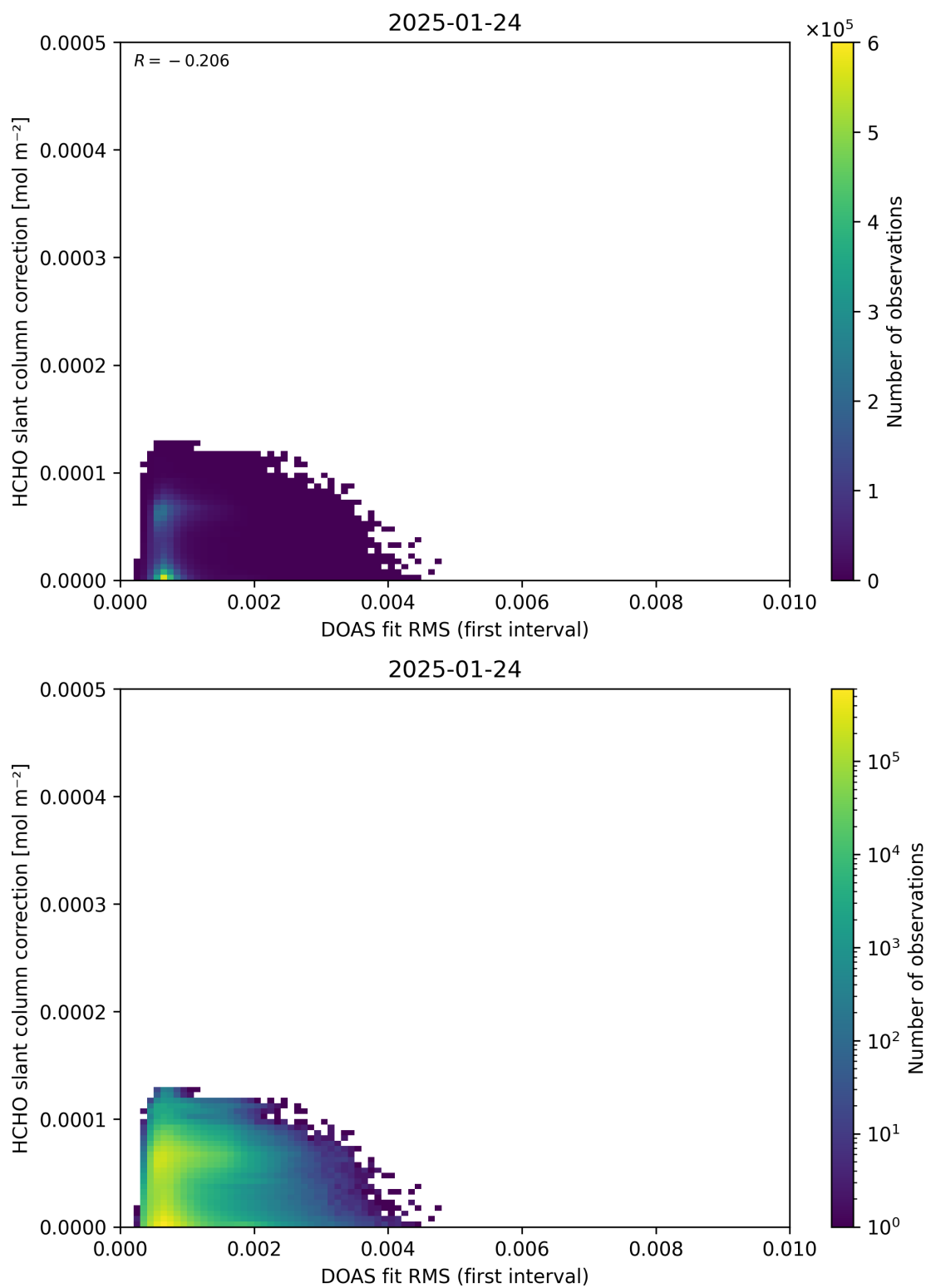
Figure 63: Scatter density plot of “DOAS fit RMS (first interval)” against “HCHO slant column correction” for 2025-01-23 to 2025-01-25.
