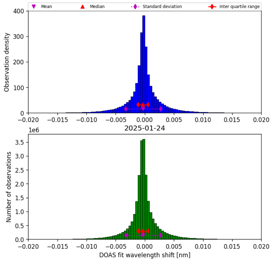
Figure 44: Histogram of “DOAS fit wavelength shift” for 2025-01-23 to 2025-01-25
