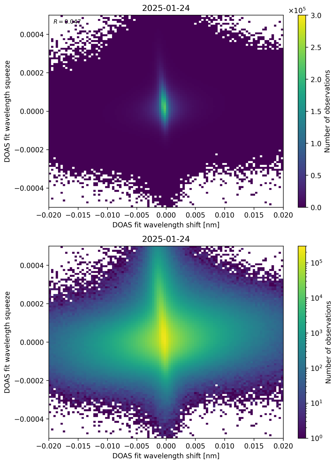
Figure 65: Scatter density plot of “DOAS fit wavelength shift” against “DOAS fit wavelength squeeze” for 2025-01-23 to 2025-01-25.
