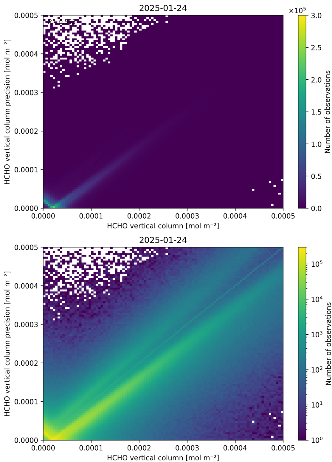
Figure 134: Scatter density plot of “HCHO vertical column” against “HCHO vertical column precision” for 2025-01-23 to 2025-01-25.
