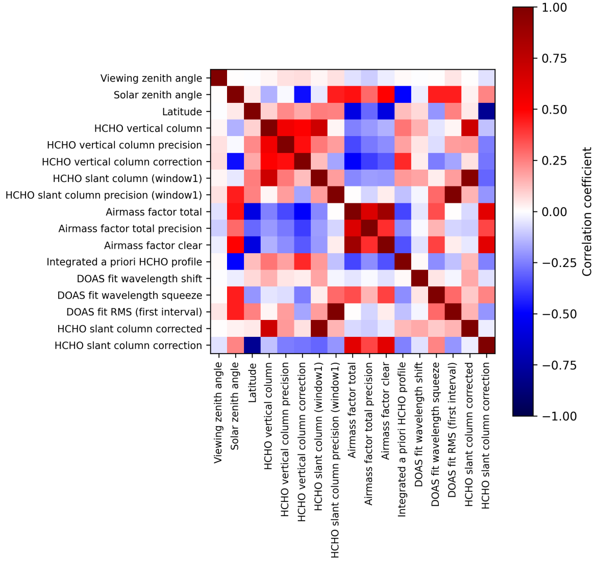
Figure 2: Map of correlation matrix for 2025-01-23 to 2025-01-25.
