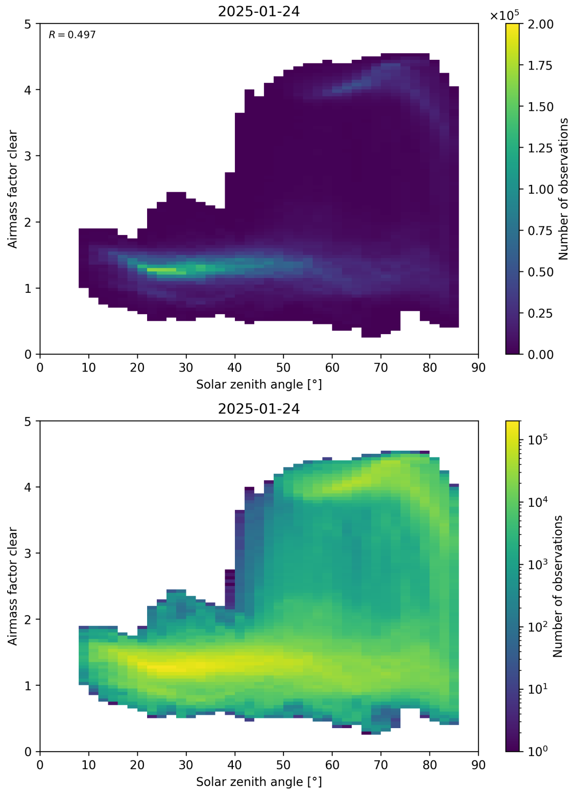
Figure 170: Scatter density plot of “Solar zenith angle” against “Airmass factor clear” for 2025-01-23 to 2025-01-25.
