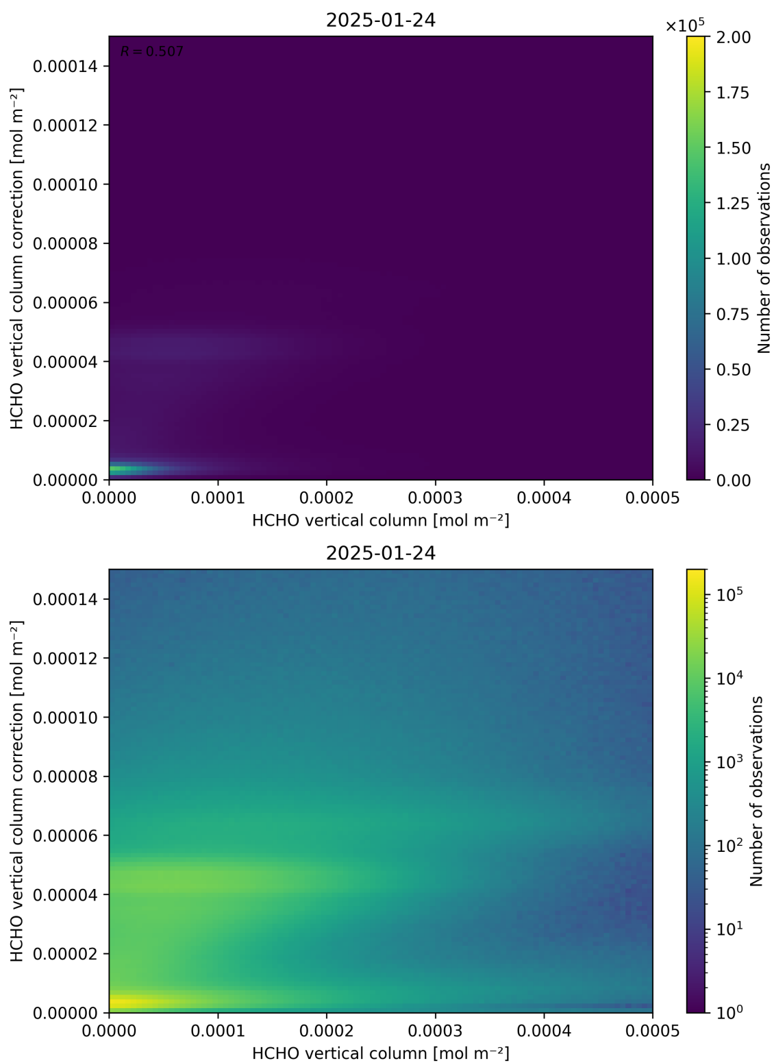
Figure 133: Scatter density plot of “HCHO vertical column” against “HCHO vertical column correction” for 2025-01-23 to 2025-01-25.
