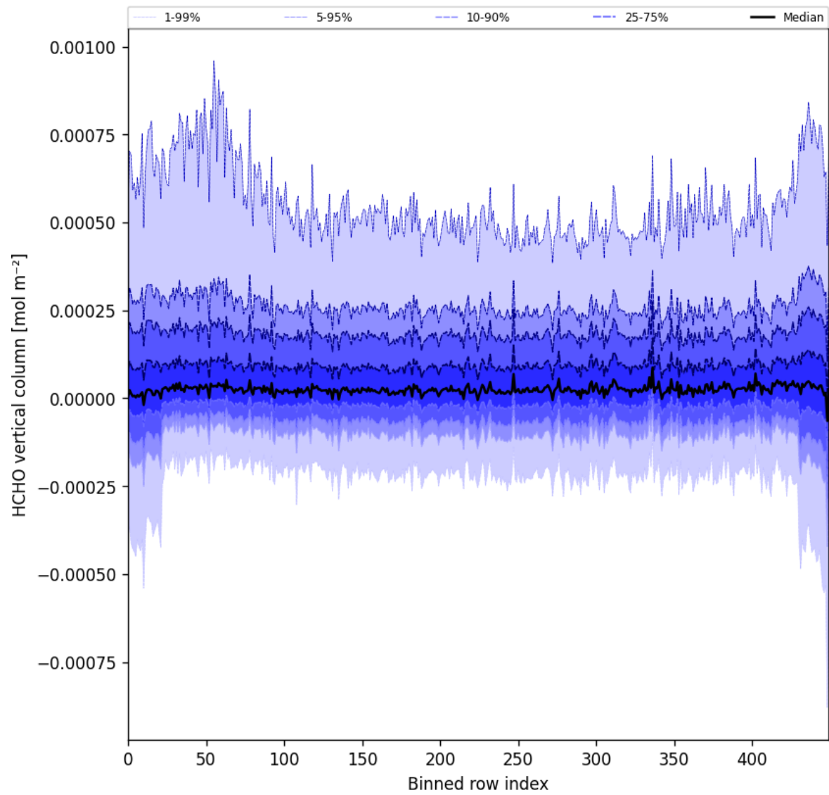
Figure 49: Along track statistics of “HCHO vertical column” for 2025-01-23 to 2025-01-25
