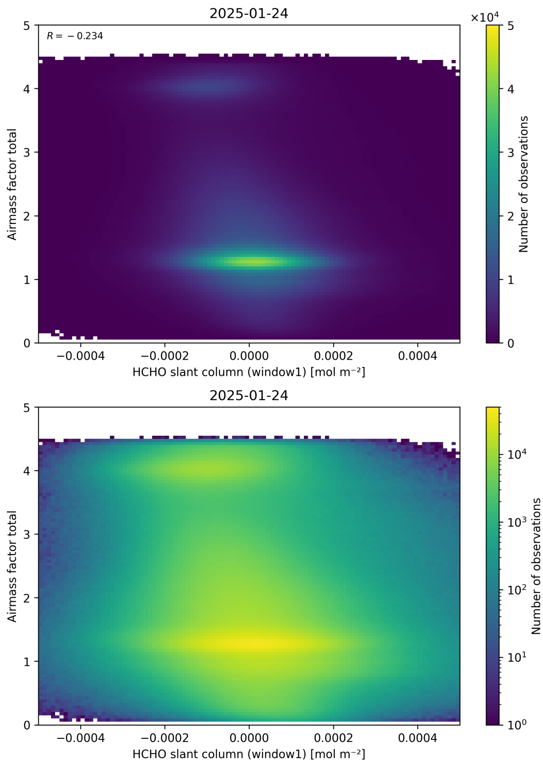
Figure 85: Scatter density plot of “HCHO slant column (window1)” against “Airmass factor total” for 2025-01-23 to 2025-01-25.
