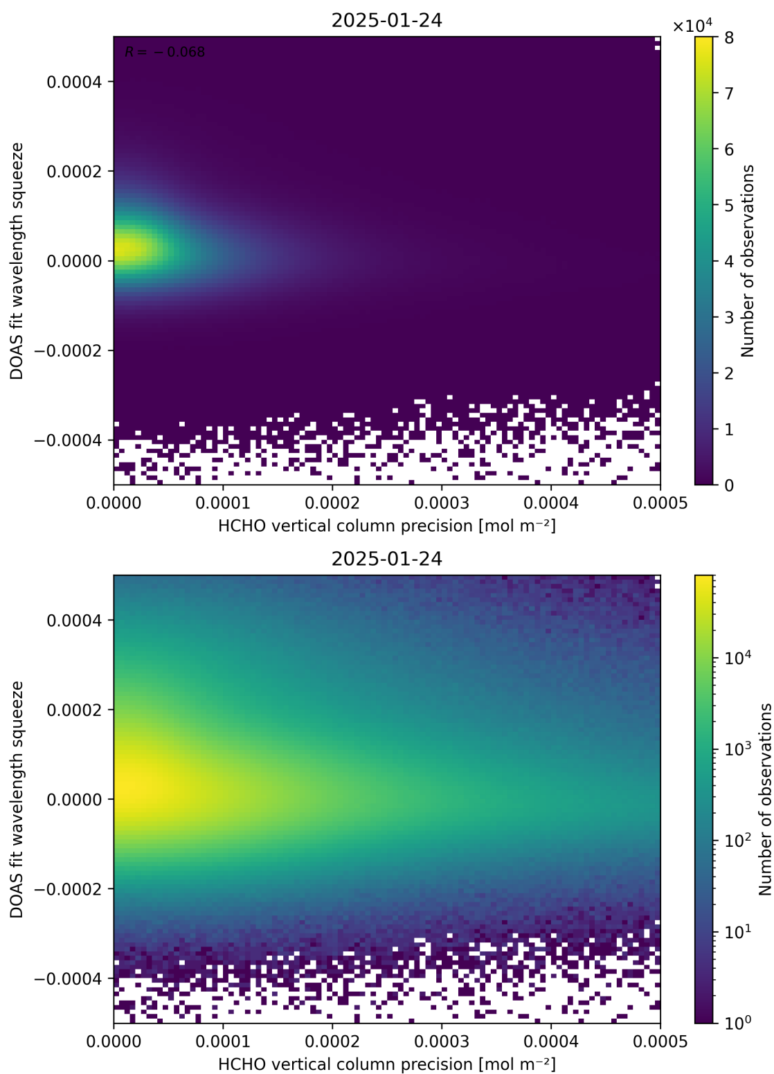
Figure 138: Scatter density plot of “HCHO vertical column precision” against “DOAS fit wavelength squeeze” for 2025-01-23 to 2025-01-25.
