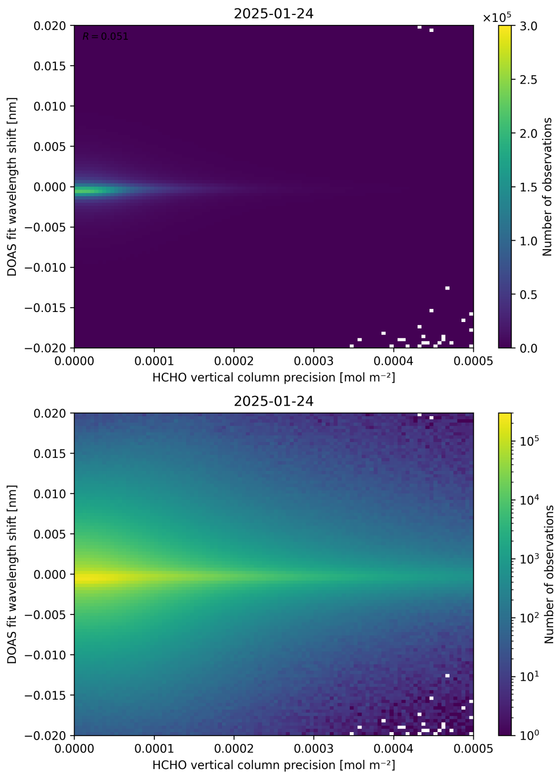
Figure 137: Scatter density plot of “HCHO vertical column precision” against “DOAS fit wavelength shift” for 2025-01-23 to 2025-01-25.
