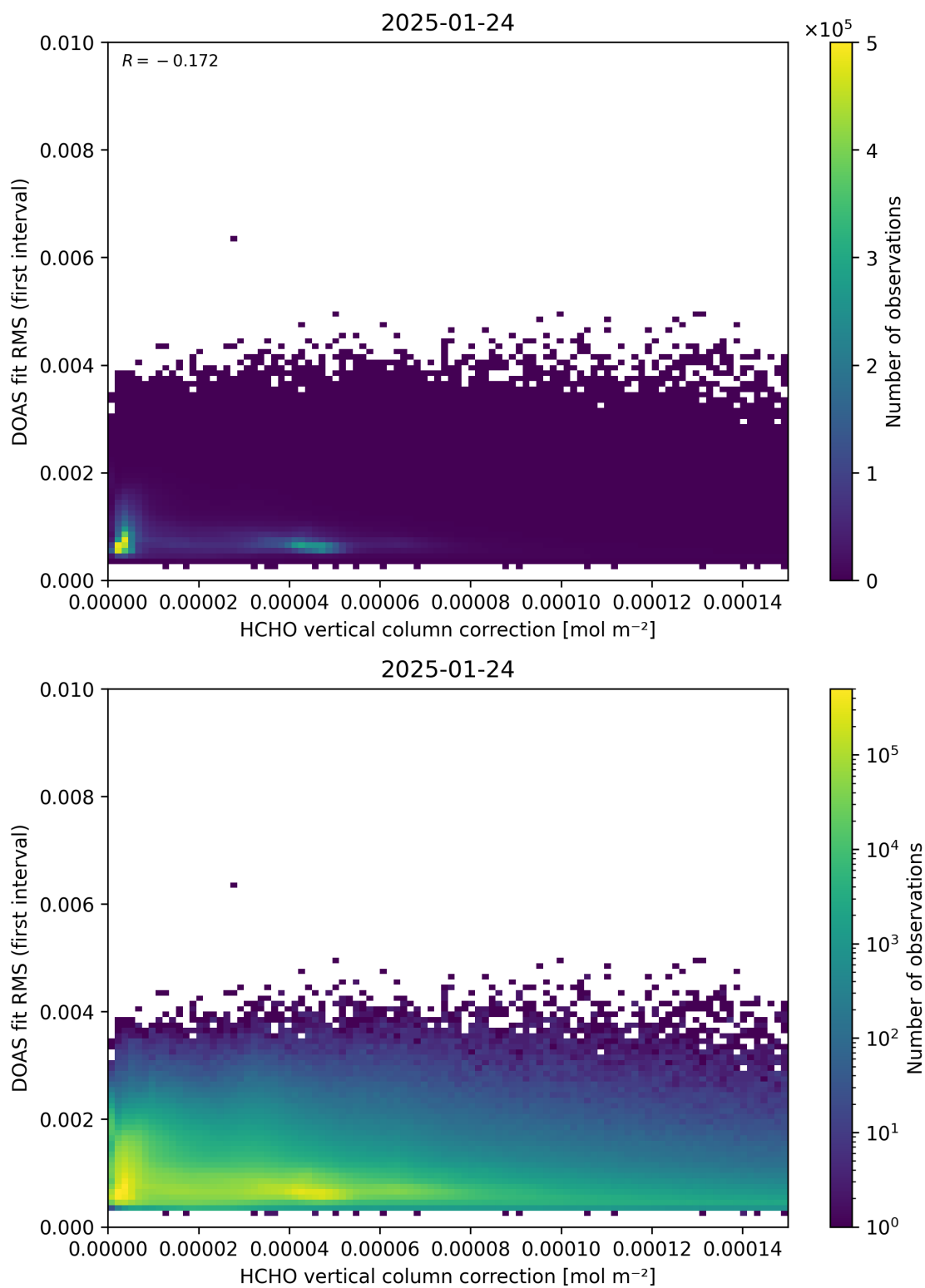
Figure 112: Scatter density plot of “HCHO vertical column correction” against “DOAS fit RMS (first interval)” for 2025-01-23 to 2025-01-25.
