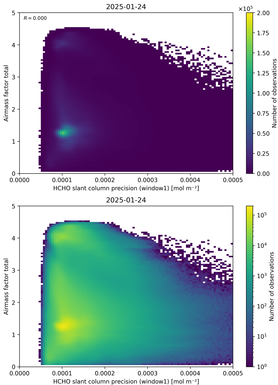
Figure 94: Scatter density plot of “HCHO slant column precision (window1)” against “Airmass factor total” for 2025-01-23 to 2025-01-25.
