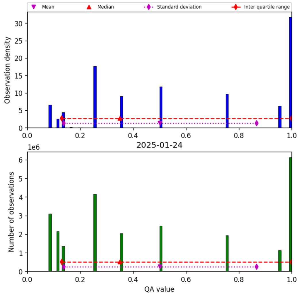
Figure 34: Histogram of “QA value” for 2025-01-23 to 2025-01-25
