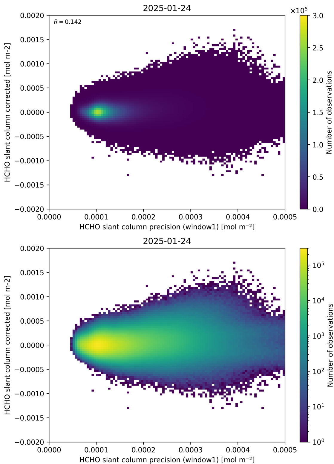
Figure 92: Scatter density plot of “HCHO slant column precision (window1)” against “HCHO slant column corrected” for 2025-01-23 to 2025-01-25.
