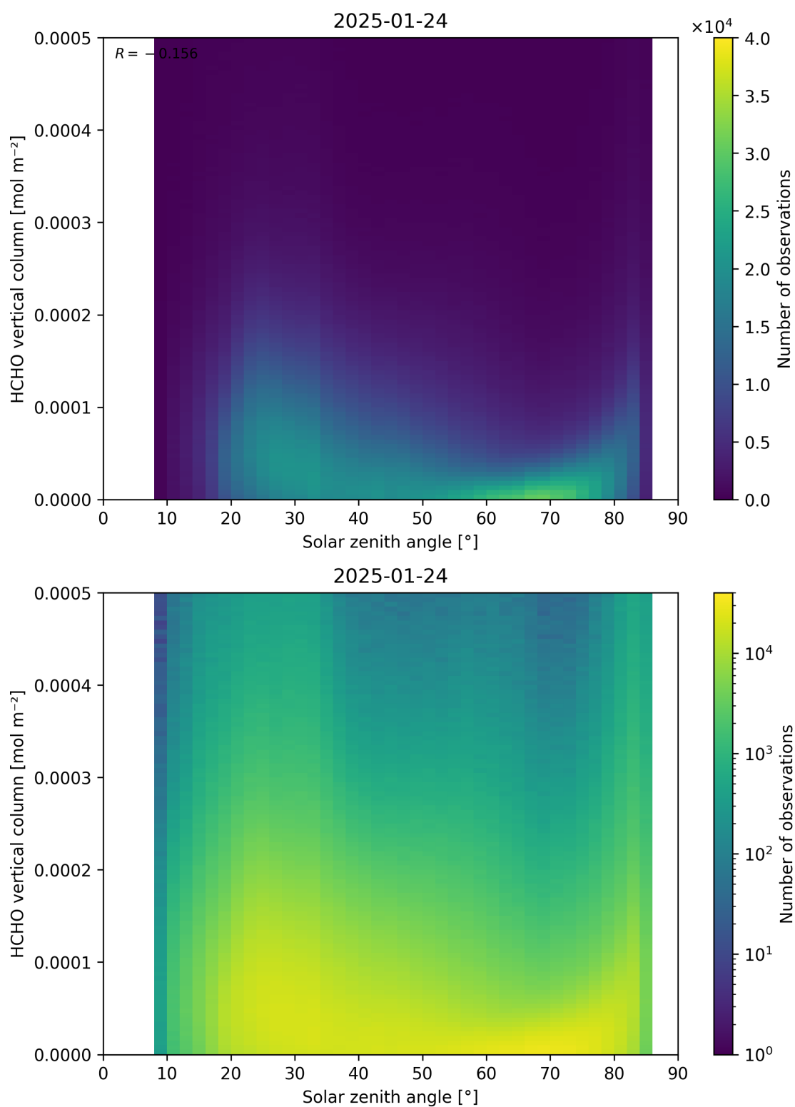
Figure 177: Scatter density plot of “Solar zenith angle” against “HCHO vertical column” for 2025-01-23 to 2025-01-25.
