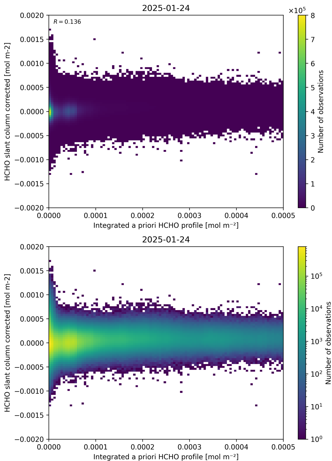
Figure 151: Scatter density plot of “Integrated a priori HCHO profile” against “HCHO slant column corrected” for 2025-01-23 to 2025-01-25.
