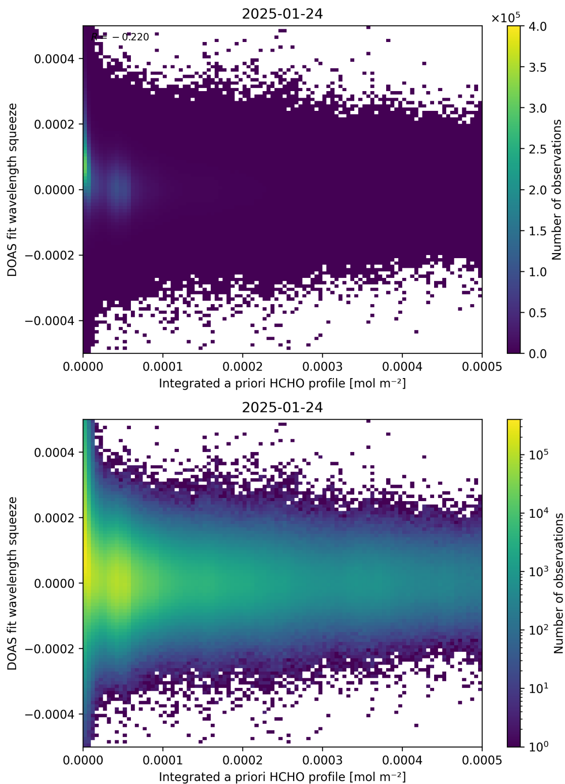
Figure 150: Scatter density plot of “Integrated a priori HCHO profile” against “DOAS fit wavelength squeeze” for 2025-01-23 to 2025-01-25.
