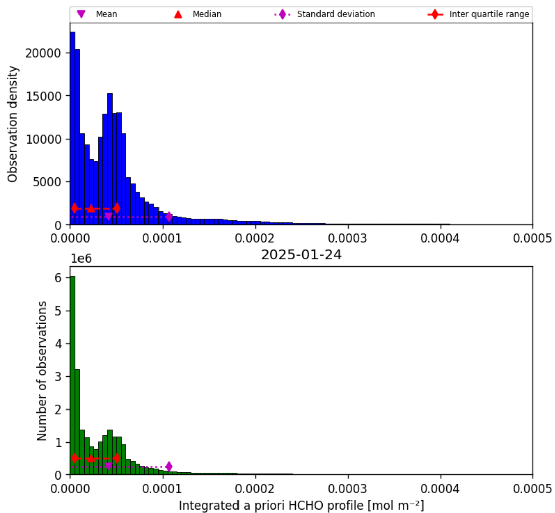
Figure 43: Histogram of “Integrated a priori HCHO profile” for 2025-01-23 to 2025-01-25
