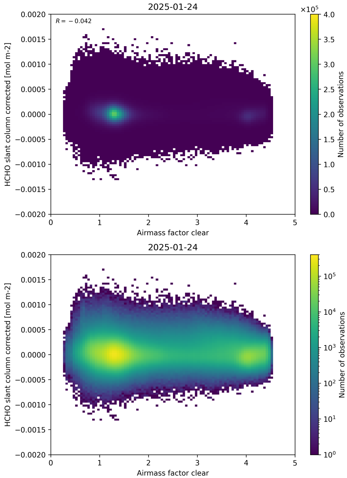
Figure 74: Scatter density plot of “Airmass factor clear” against “HCHO slant column corrected” for 2025-01-23 to 2025-01-25.
