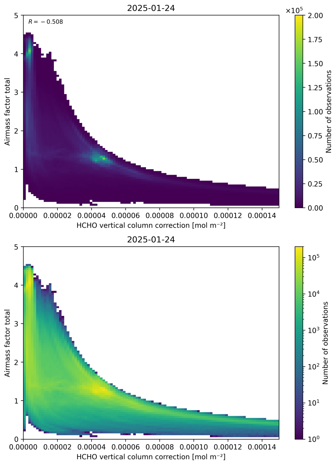
Figure 120: Scatter density plot of “HCHO vertical column correction” against “Airmass factor total” for 2025-01-23 to 2025-01-25.
