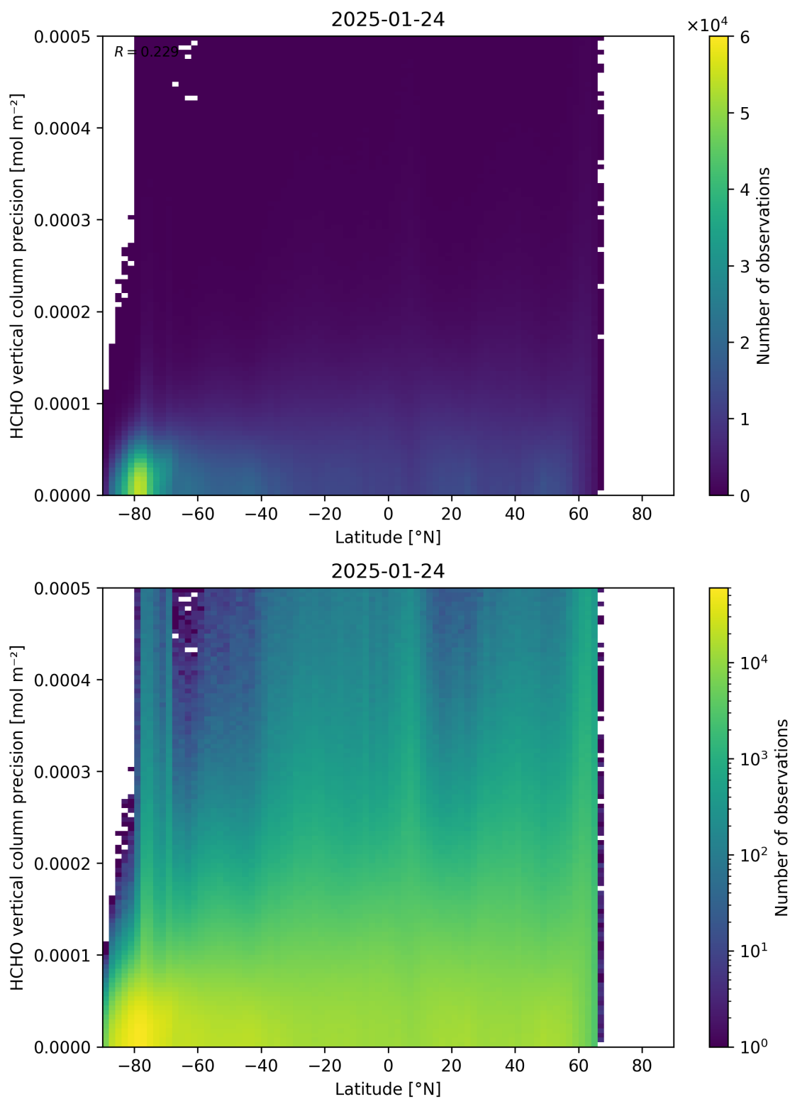
Figure 165: Scatter density plot of “Latitude” against “HCHO vertical column precision” for 2025-01-23 to 2025-01-25.
