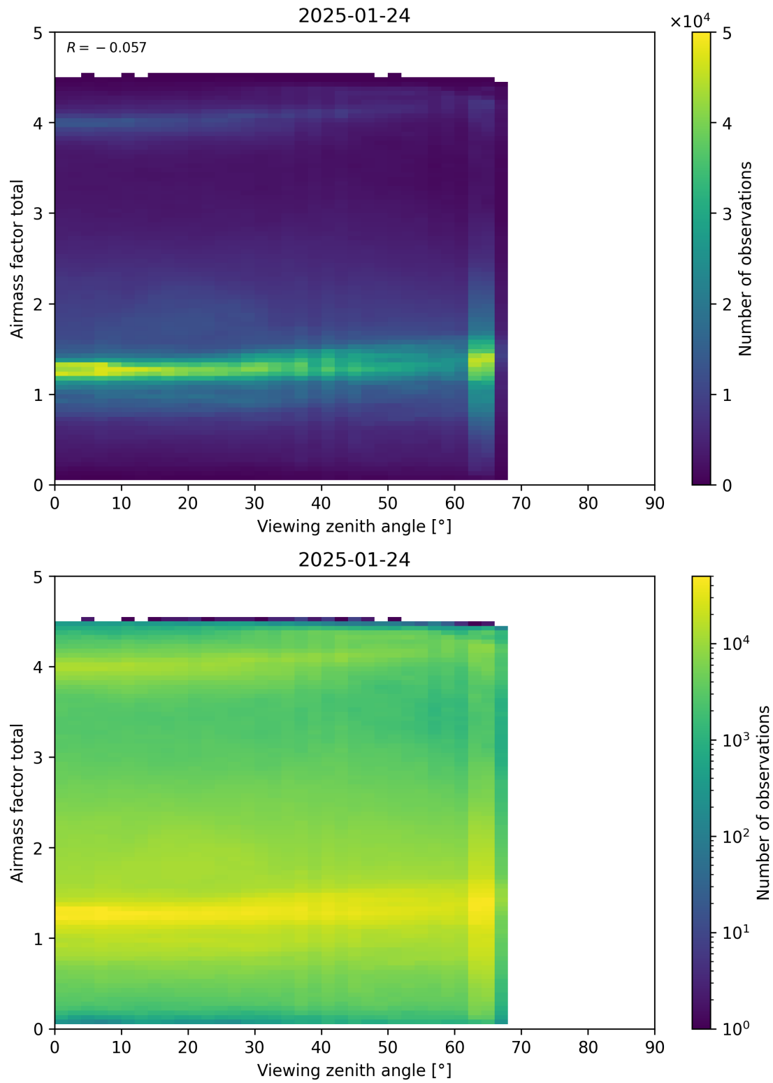
Figure 190: Scatter density plot of “Viewing zenith angle” against “Airmass factor total” for 2025-01-23 to 2025-01-25.
