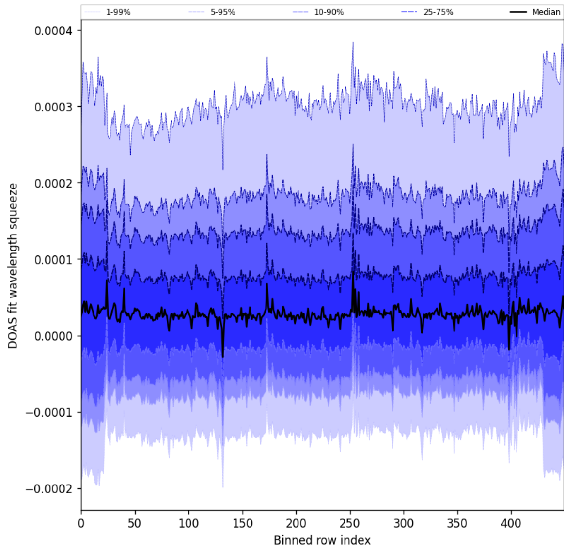
Figure 59: Along track statistics of “DOAS fit wavelength squeeze” for 2025-01-23 to 2025-01-25
