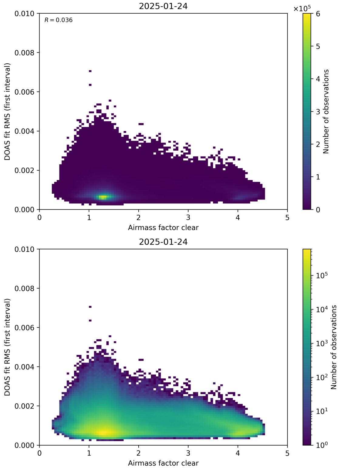
Figure 71: Scatter density plot of “Airmass factor clear” against “DOAS fit RMS (first interval)” for 2025-01-23 to 2025-01-25.
