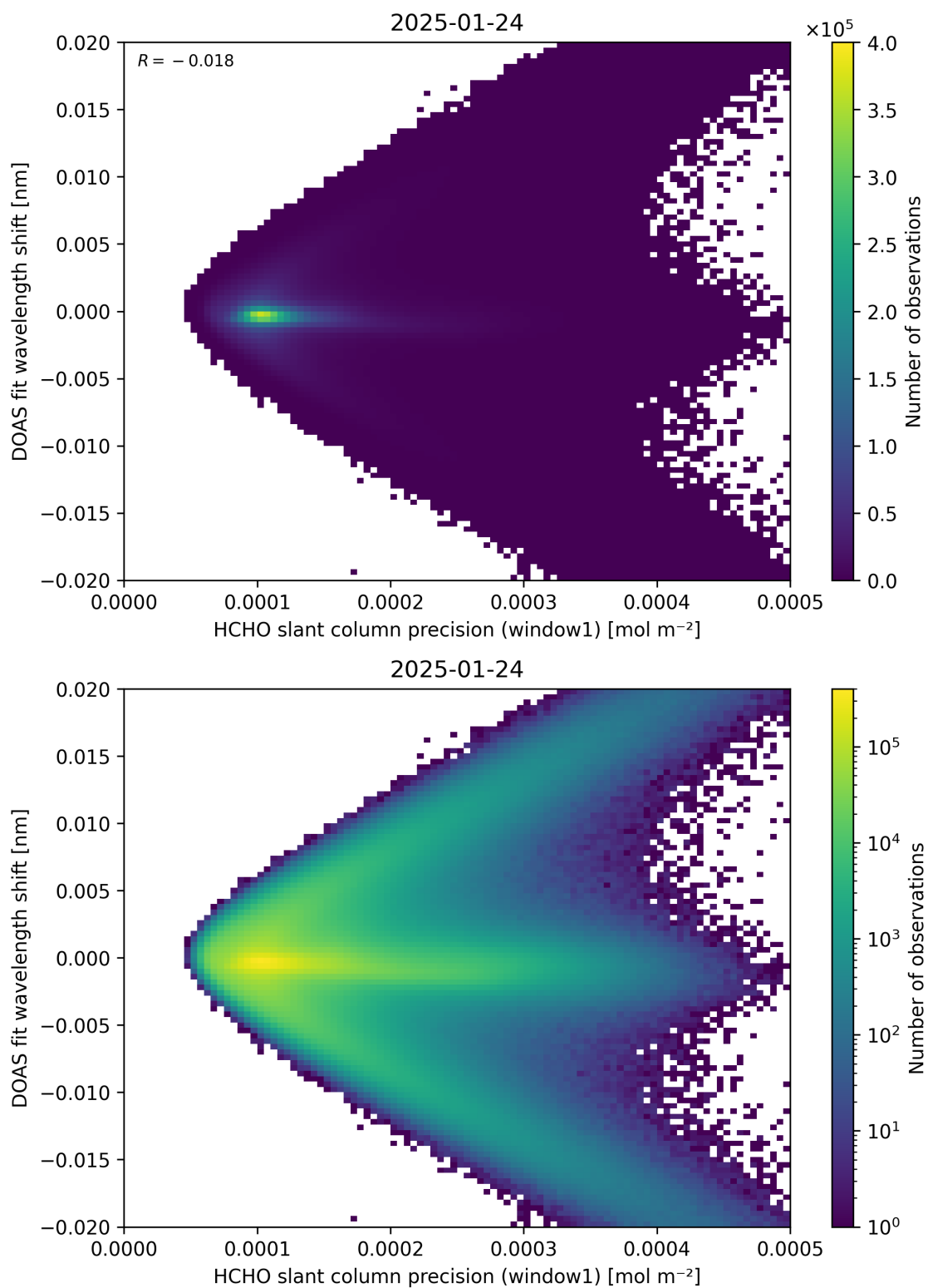
Figure 89: Scatter density plot of “HCHO slant column precision (window1)” against “DOAS fit wavelength shift” for 2025-01-23 to 2025-01-25.
