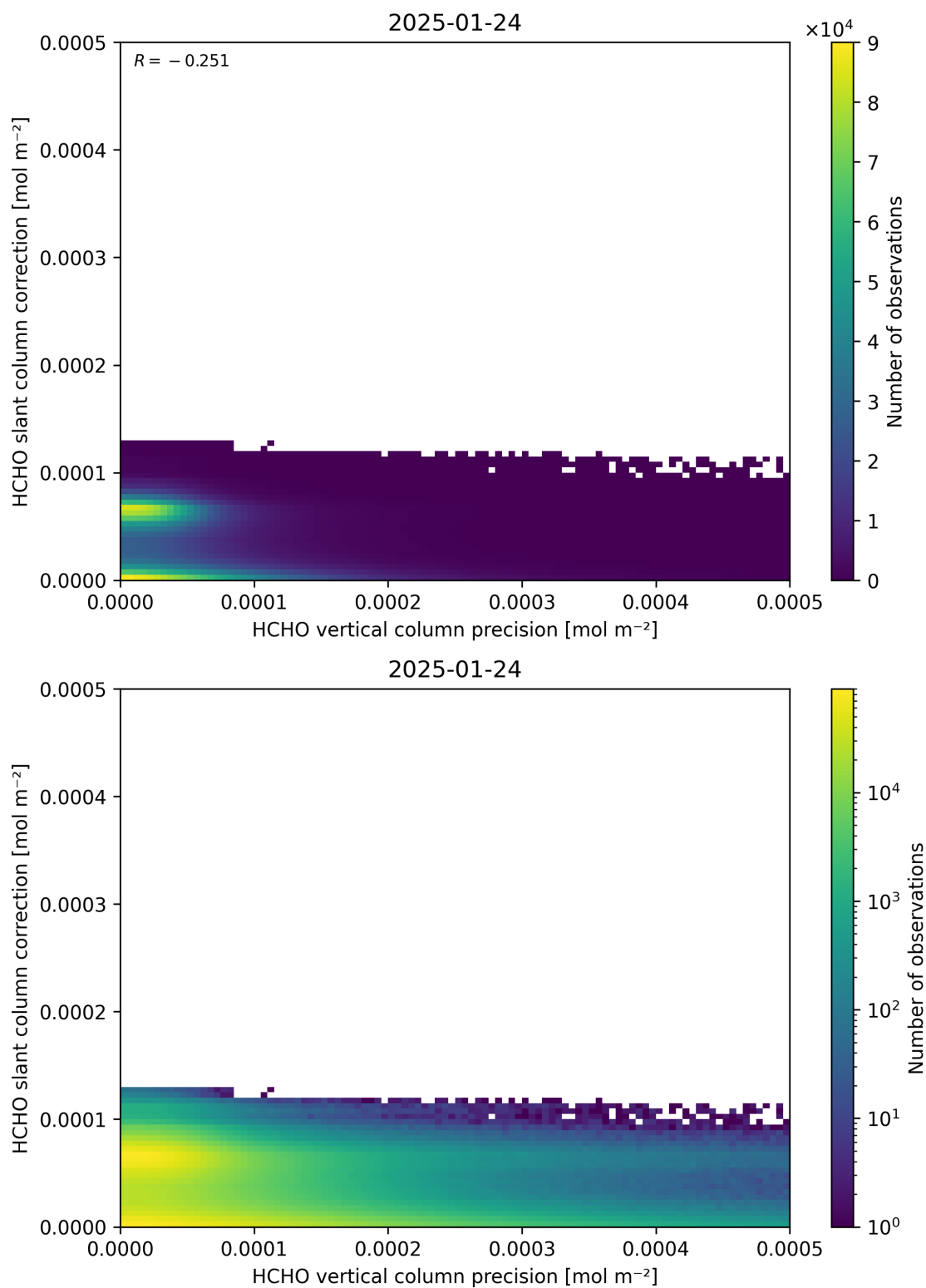
Figure 141: Scatter density plot of “HCHO vertical column precision” against “HCHO slant column correction” for 2025-01-23 to 2025-01-25.
