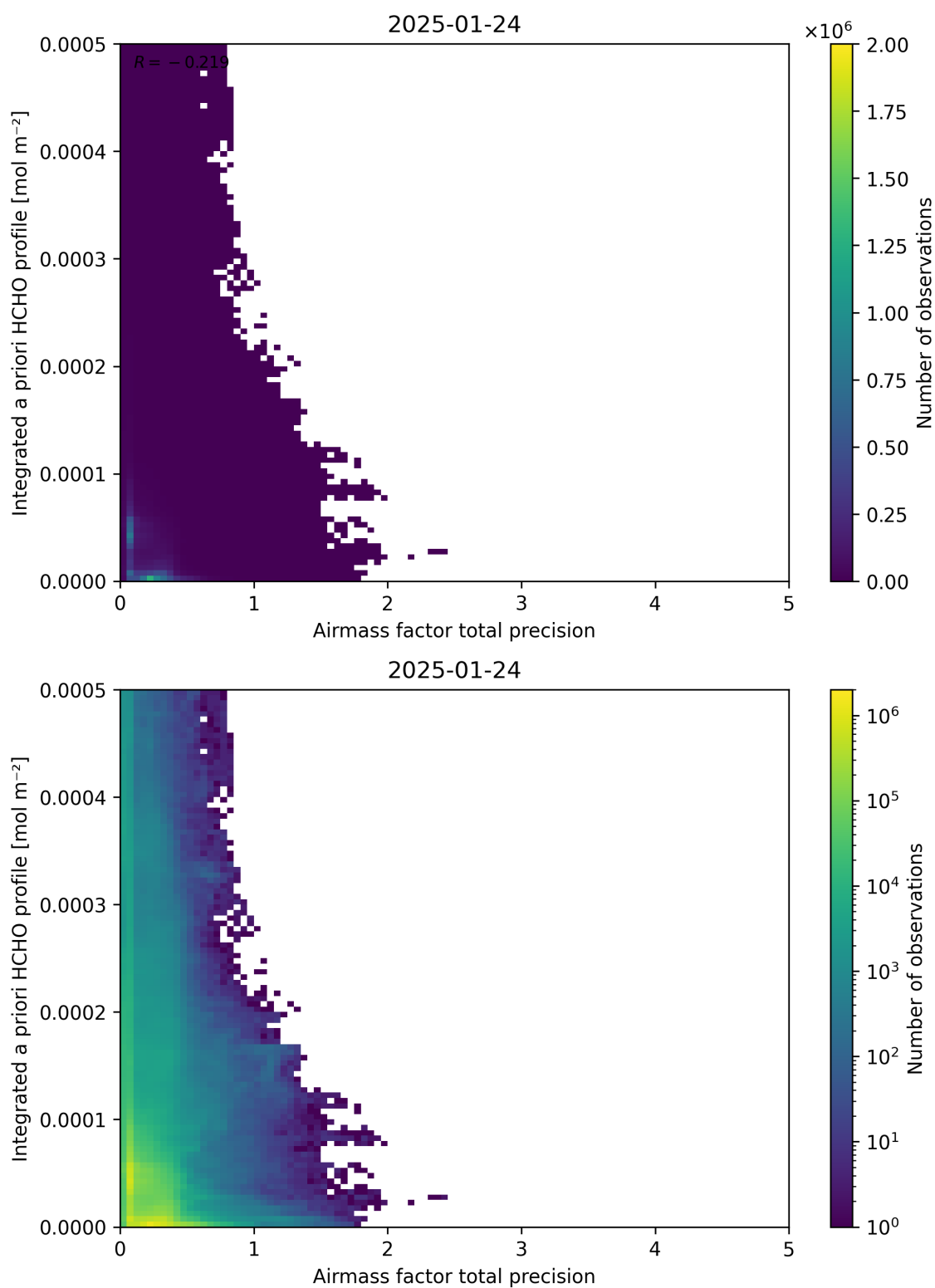
Figure 111: Scatter density plot of “Airmass factor total precision” against “Integrated a priori HCHO profile” for 2025-01-23 to 2025-01-25.
