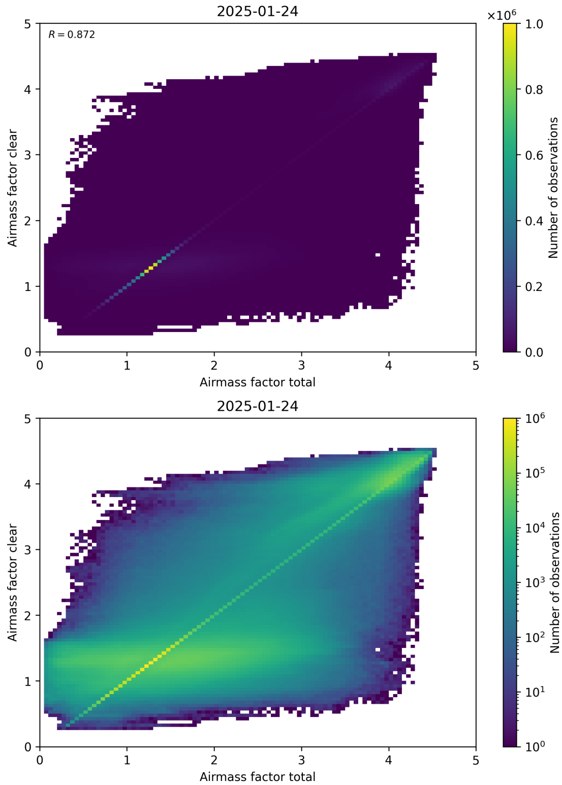
Figure 100: Scatter density plot of “Airmass factor total” against “Airmass factor clear” for 2025-01-23 to 2025-01-25.
