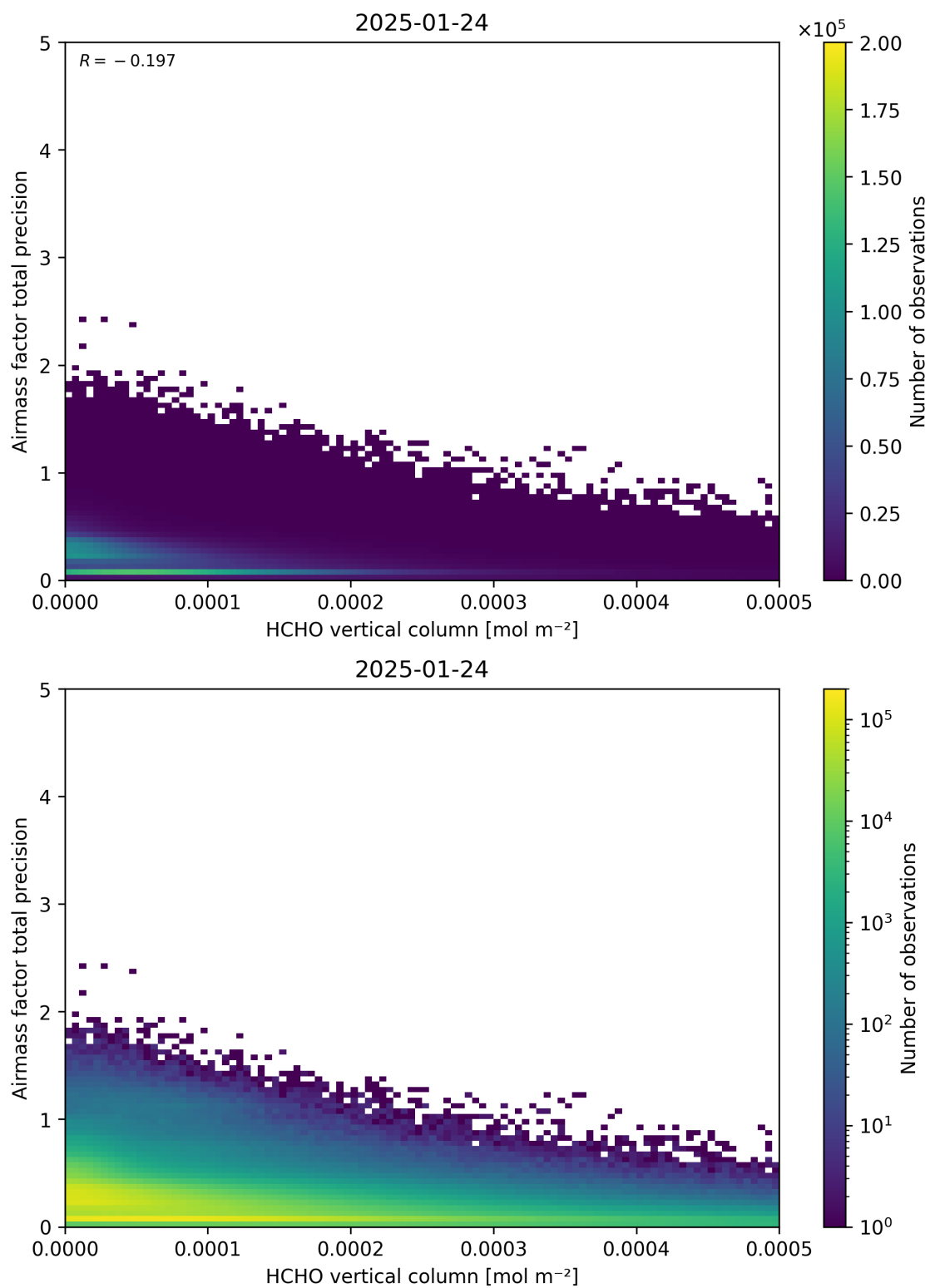
Figure 132: Scatter density plot of “HCHO vertical column” against “Airmass factor total precision” for 2025-01-23 to 2025-01-25.
