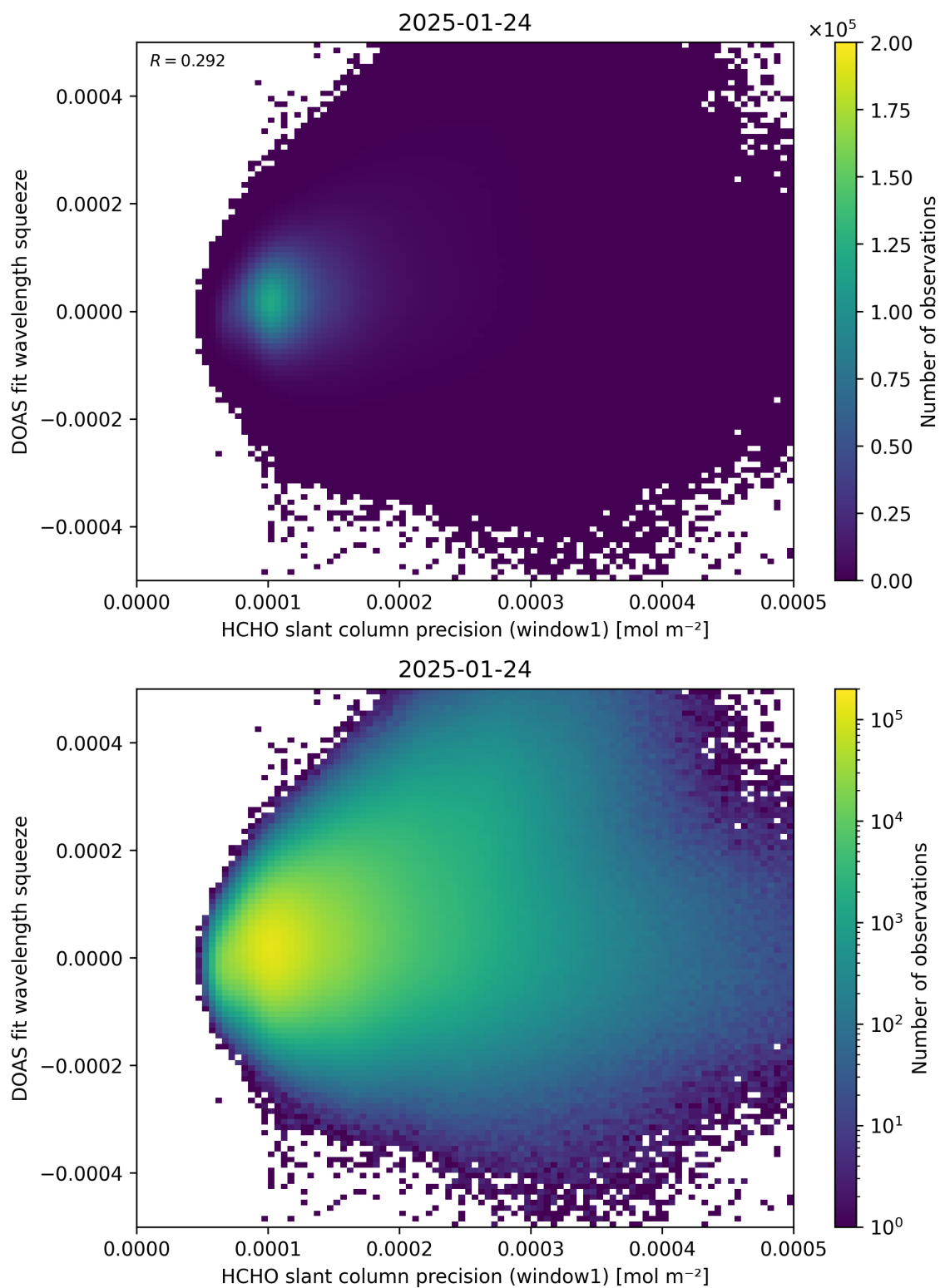
Figure 90: Scatter density plot of “HCHO slant column precision (window1)” against “DOAS fit wavelength squeeze” for 2025-01-23 to 2025-01-25.
