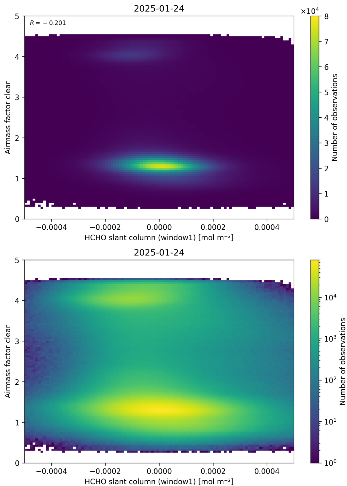
Figure 81: Scatter density plot of “HCHO slant column (window1)” against “Airmass factor clear” for 2025-01-23 to 2025-01-25.
