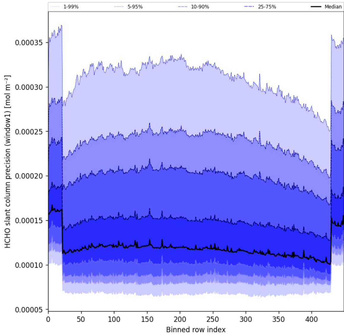
Figure 53: Along track statistics of “HCHO slant column precision (window1)” for 2025-01-23 to 2025-01-25
