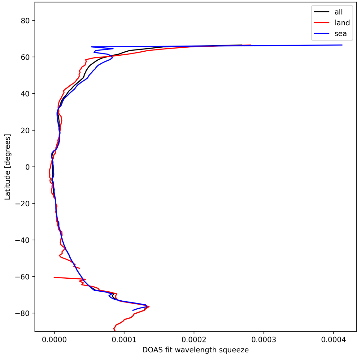
Figure 31: Zonal average of “DOAS fit wavelength squeeze” for 2025-01-23 to 2025-01-25.
