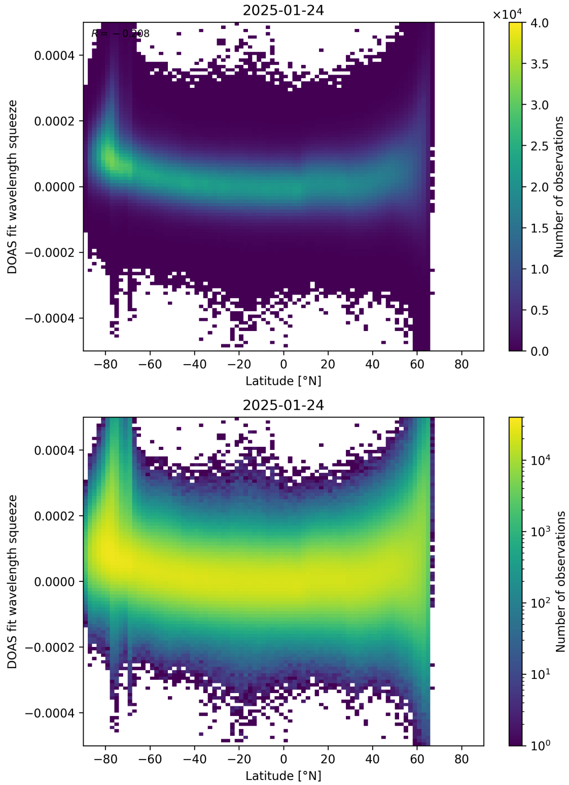
Figure 155: Scatter density plot of “Latitude” against “DOAS fit wavelength squeeze” for 2025-01-23 to 2025-01-25.
