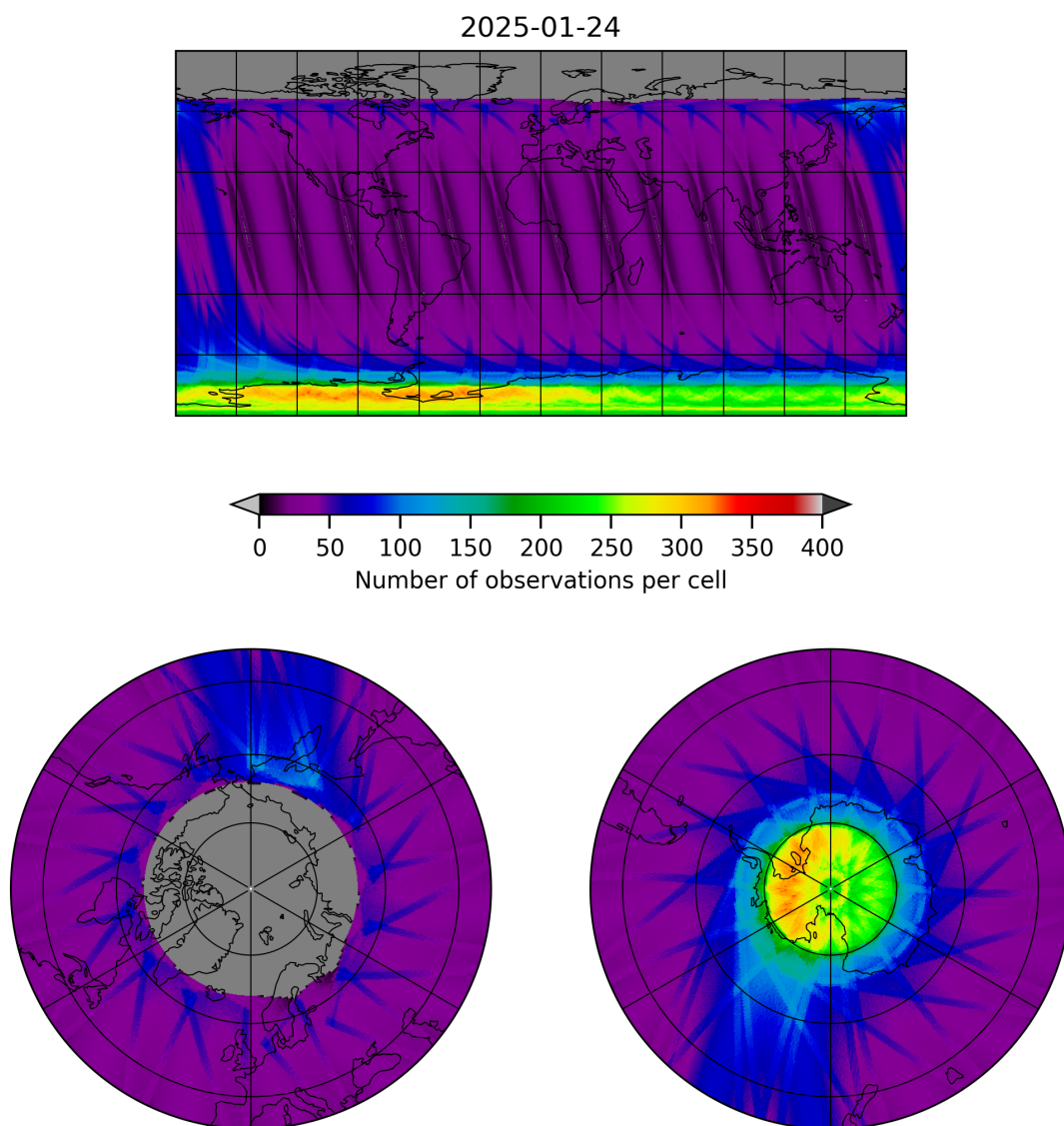
Figure 19: Map of the number of observations for 2025-01-23 to 2025-01-25
