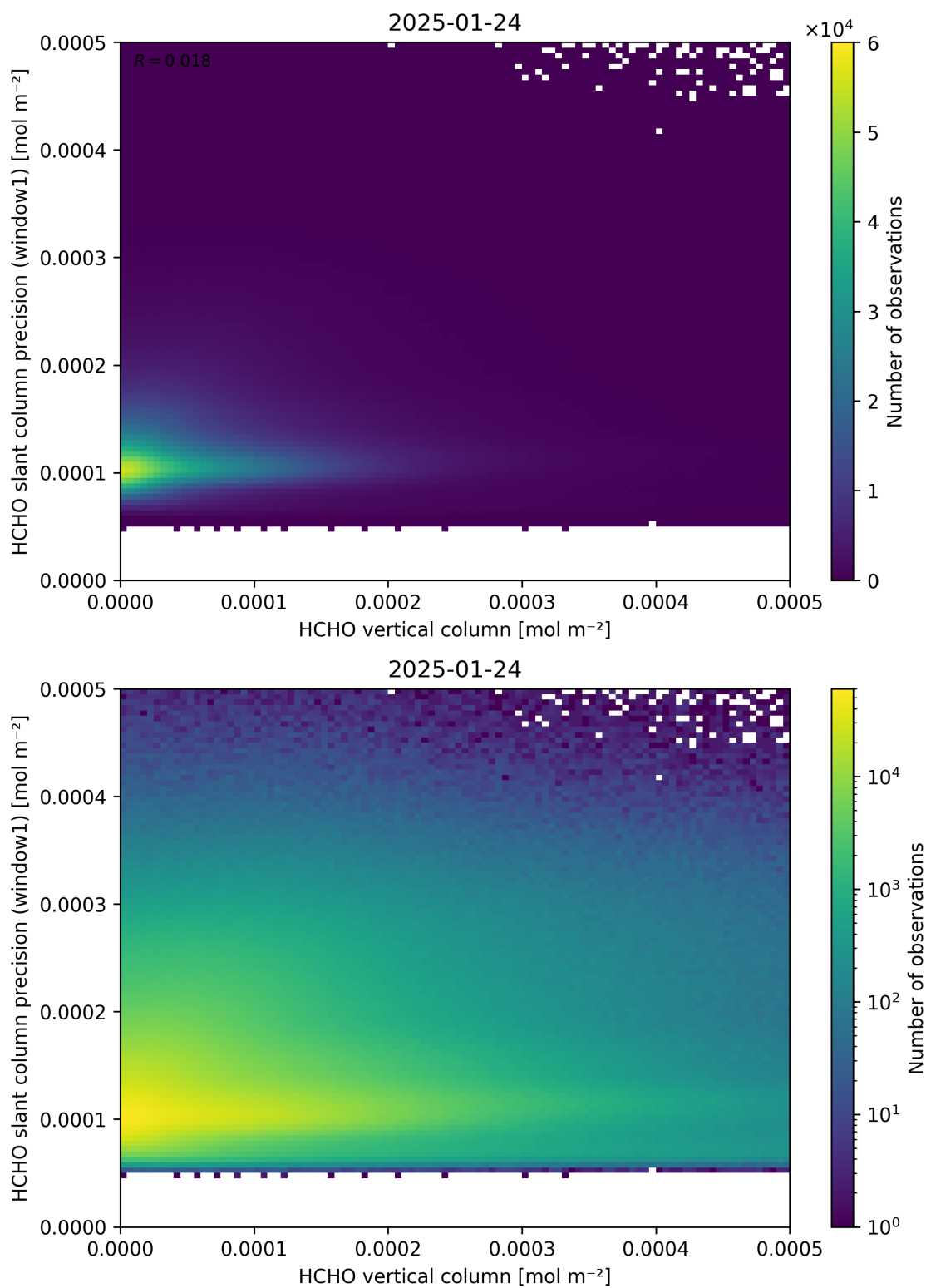
Figure 130: Scatter density plot of “HCHO vertical column” against “HCHO slant column precision (window1)” for 2025-01-23 to 2025-01-25.
