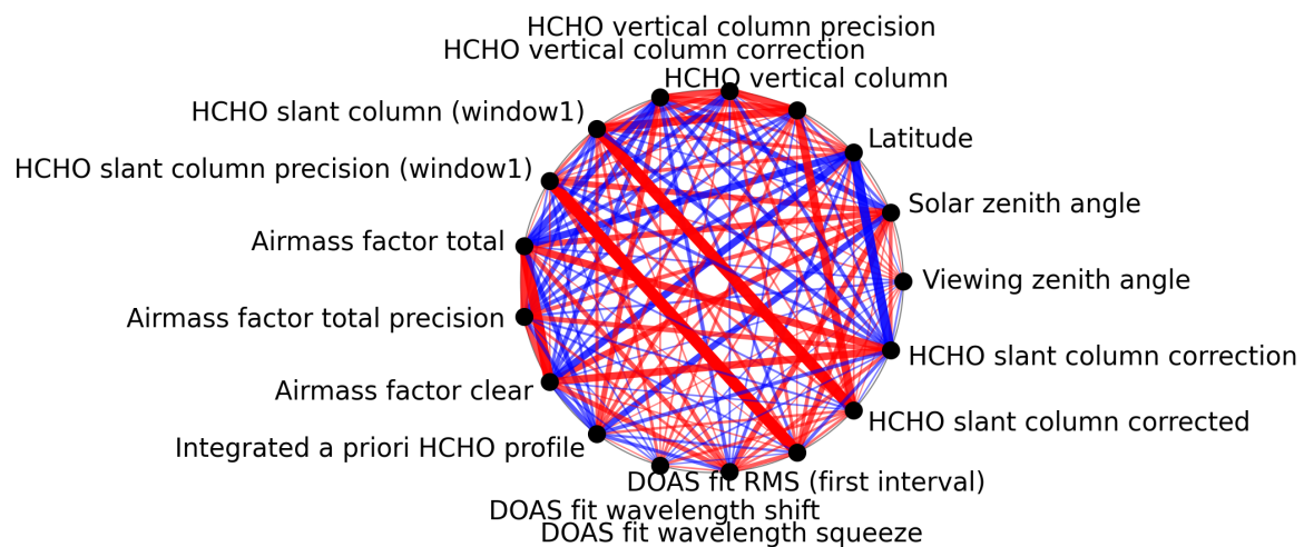
Figure 1: Map of correlation graph for 2025-01-23 to 2025-01-25.
