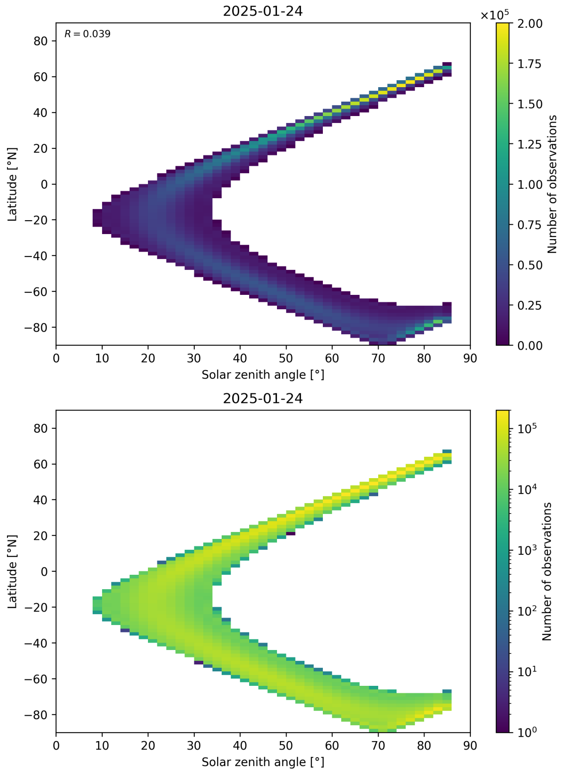
Figure 181: Scatter density plot of “Solar zenith angle” against “Latitude” for 2025-01-23 to 2025-01-25.
