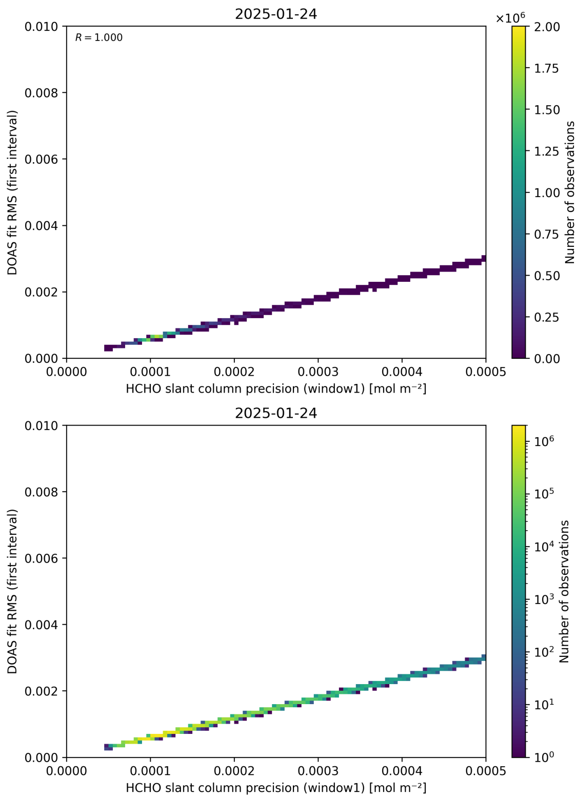
Figure 88: Scatter density plot of “HCHO slant column precision (window1)” against “DOAS fit RMS (first interval)” for 2025-01-23 to 2025-01-25.
