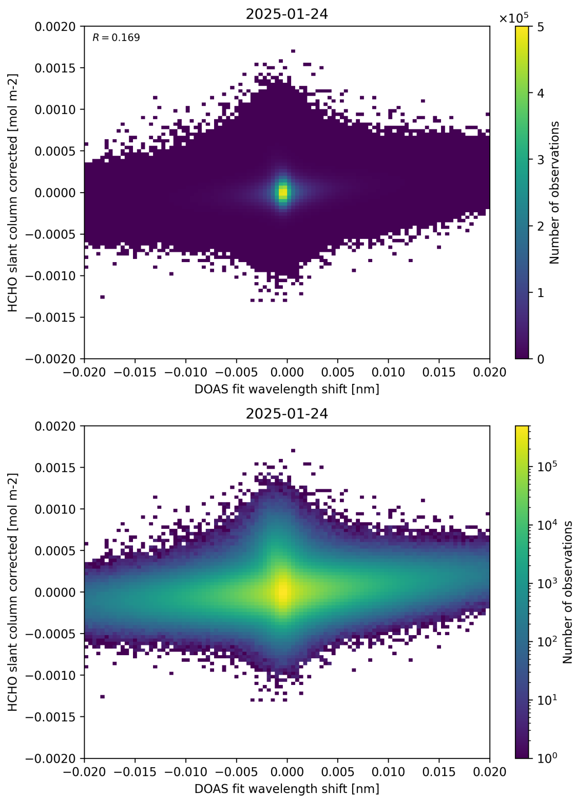
Figure 66: Scatter density plot of “DOAS fit wavelength shift” against “HCHO slant column corrected” for 2025-01-23 to 2025-01-25.
