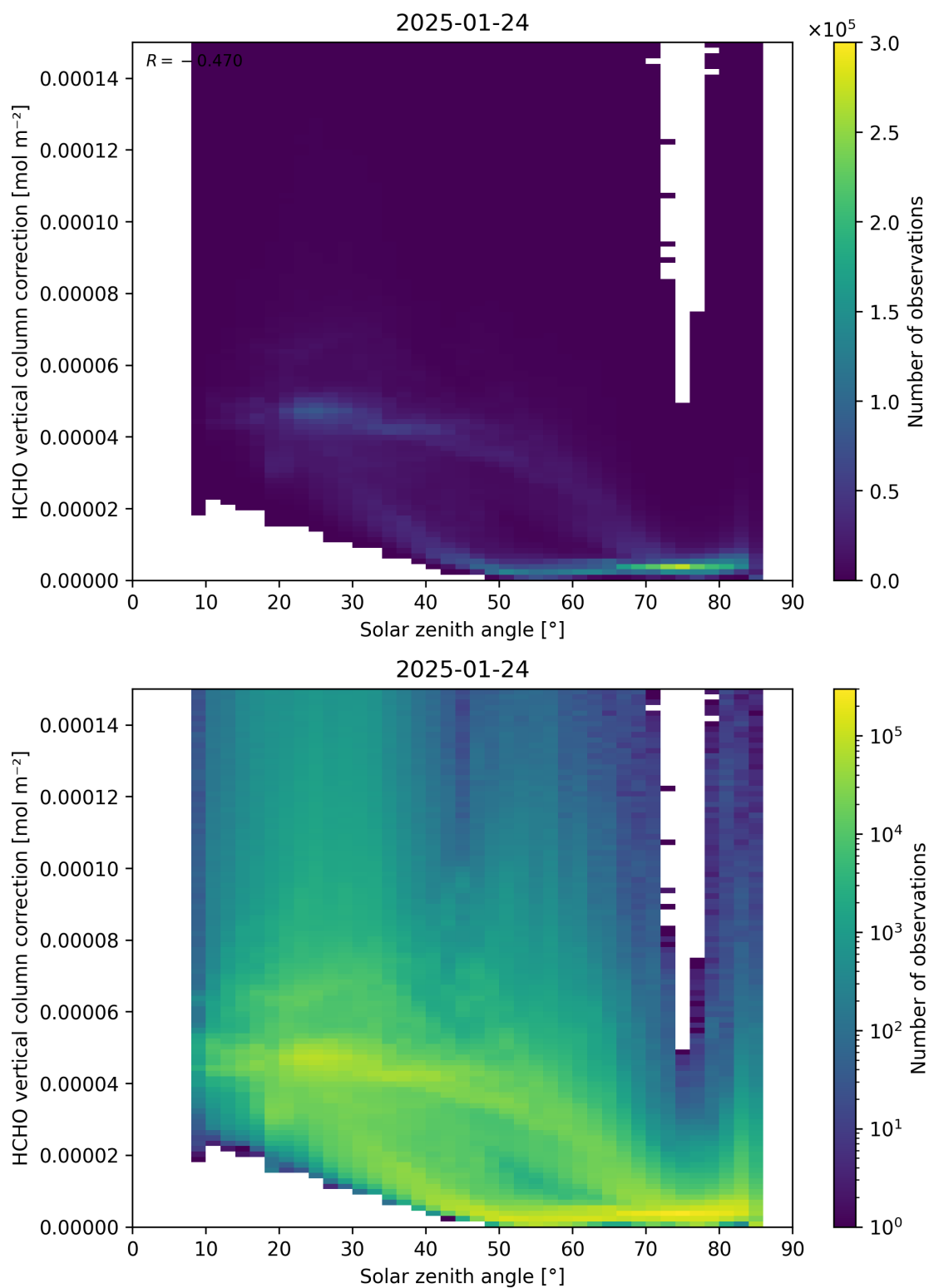
Figure 178: Scatter density plot of “Solar zenith angle” against “HCHO vertical column correction” for 2025-01-23 to 2025-01-25.
