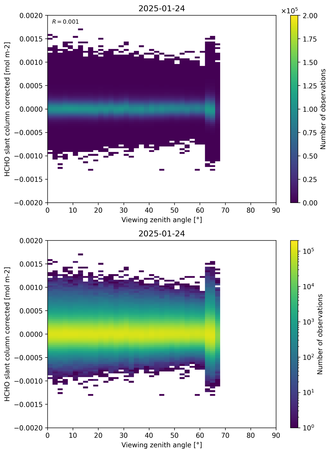
Figure 186: Scatter density plot of “Viewing zenith angle” against “HCHO slant column corrected” for 2025-01-23 to 2025-01-25.
