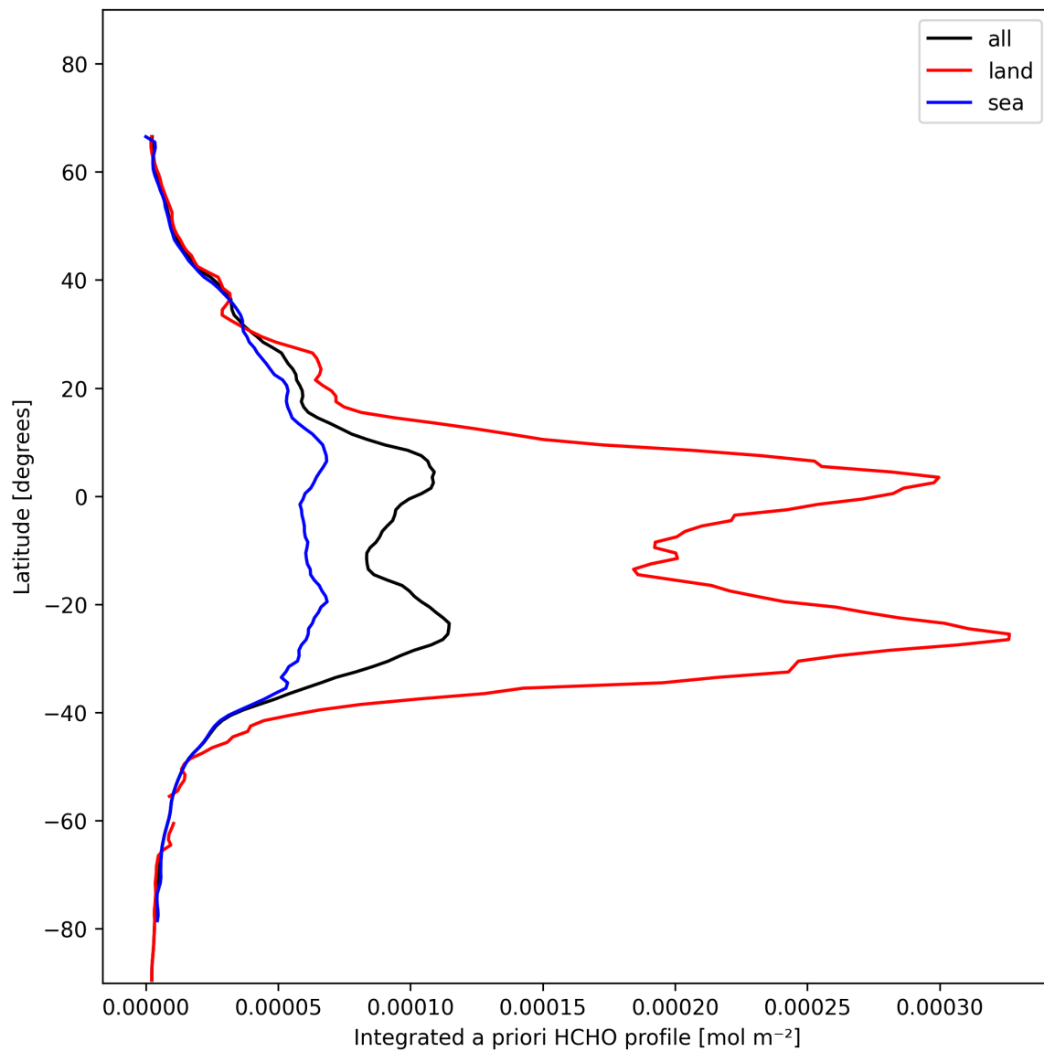
Figure 29: Zonal average of “Integrated a priori HCHO profile” for 2025-01-23 to 2025-01-25.
