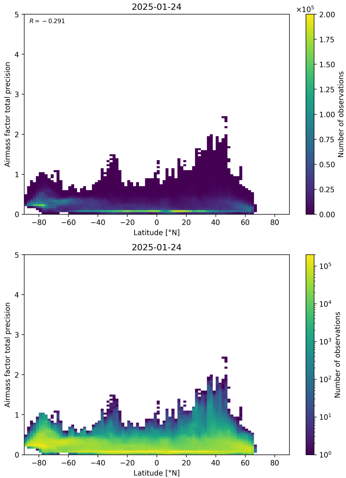
Figure 162: Scatter density plot of “Latitude” against “Airmass factor total precision” for 2025-01-23 to 2025-01-25.
