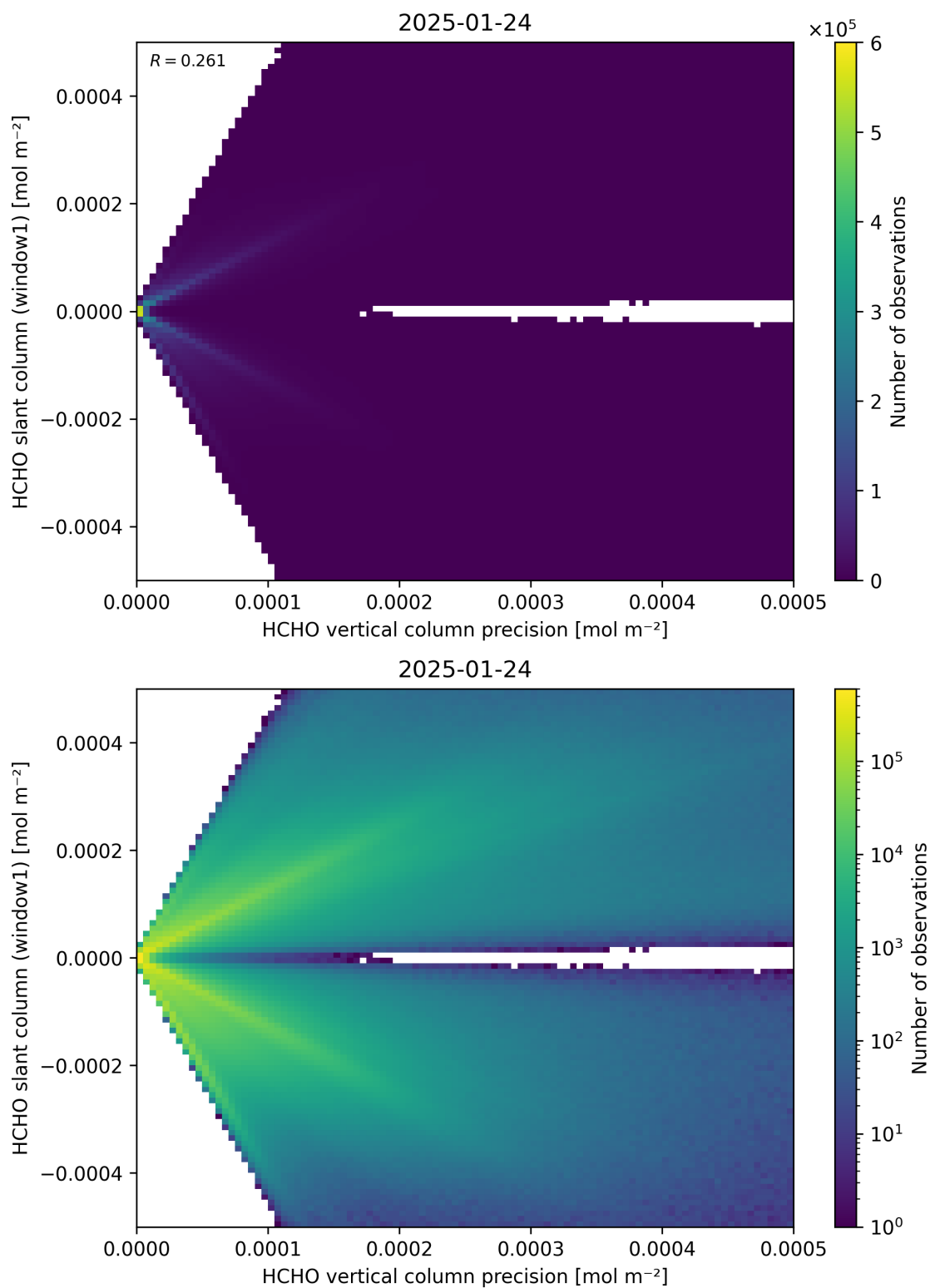
Figure 142: Scatter density plot of “HCHO vertical column precision” against “HCHO slant column (window1)” for 2025-01-23 to 2025-01-25.
