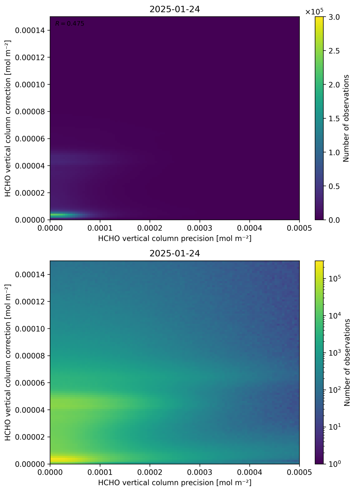
Figure 146: Scatter density plot of “HCHO vertical column precision” against “HCHO vertical column correction” for 2025-01-23 to 2025-01-25.
