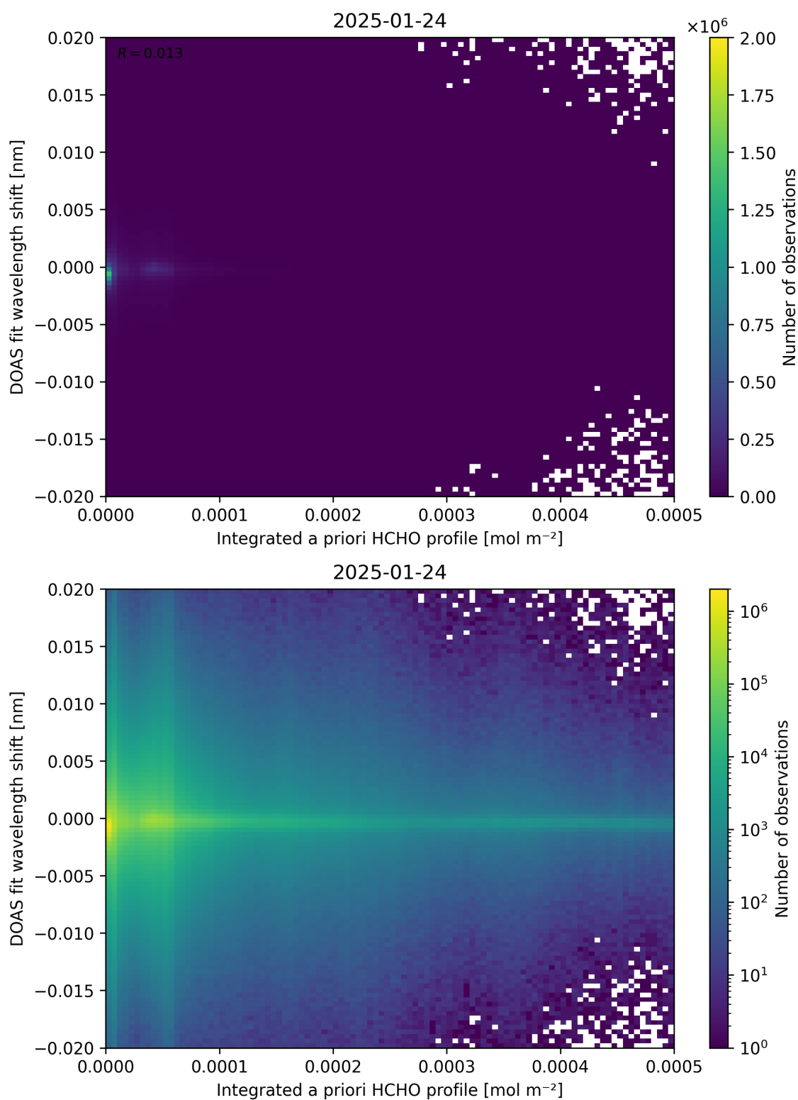
Figure 149: Scatter density plot of “Integrated a priori HCHO profile” against “DOAS fit wavelength shift” for 2025-01-23 to 2025-01-25.
