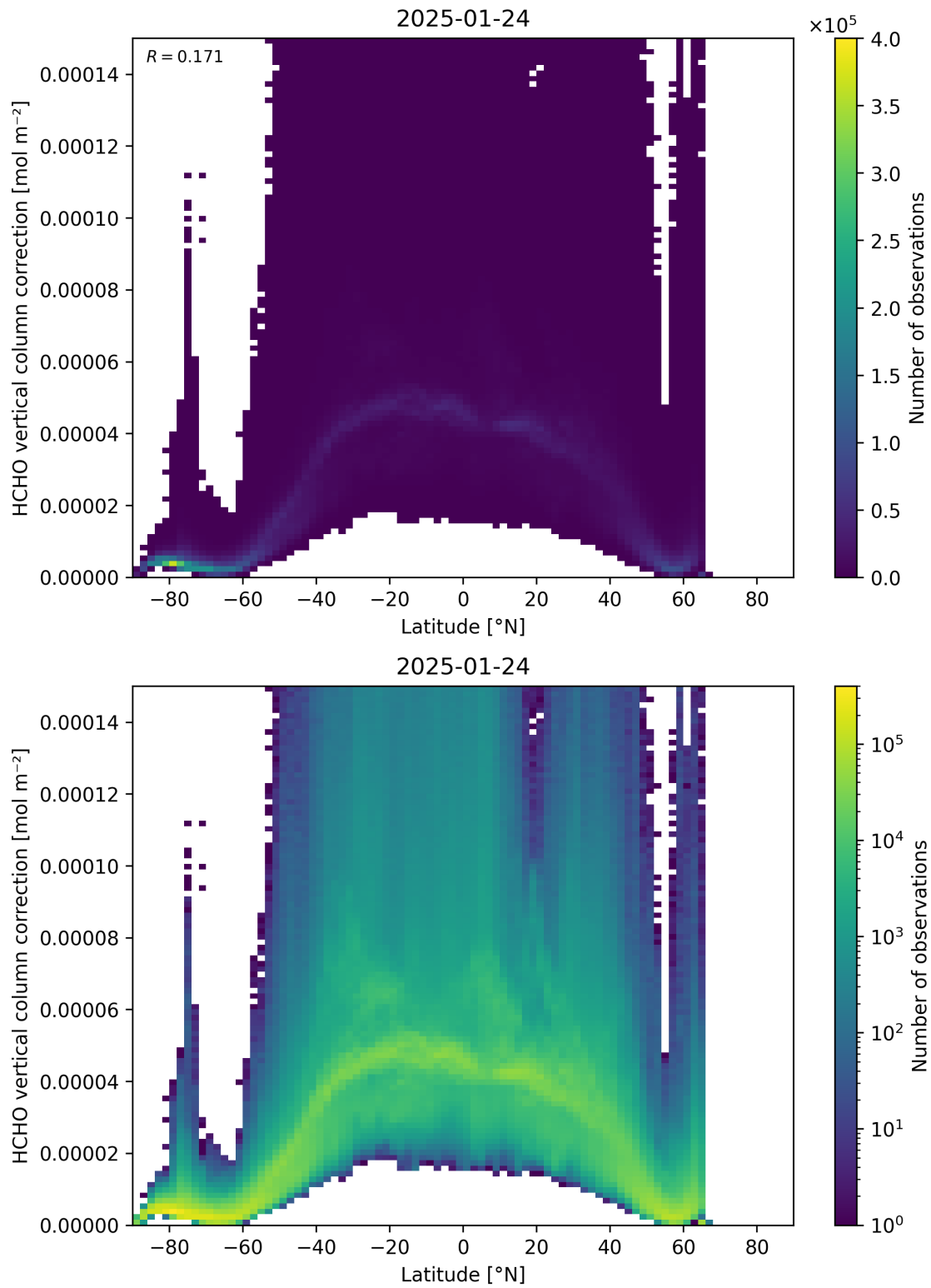
Figure 164: Scatter density plot of “Latitude” against “HCHO vertical column correction” for 2025-01-23 to 2025-01-25.
