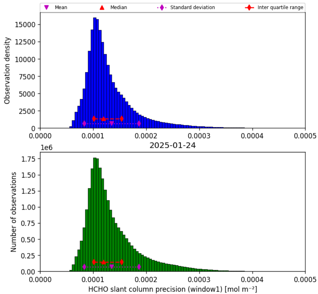
Figure 39: Histogram of “HCHO slant column precision (window1)” for 2025-01-23 to 2025-01-25
