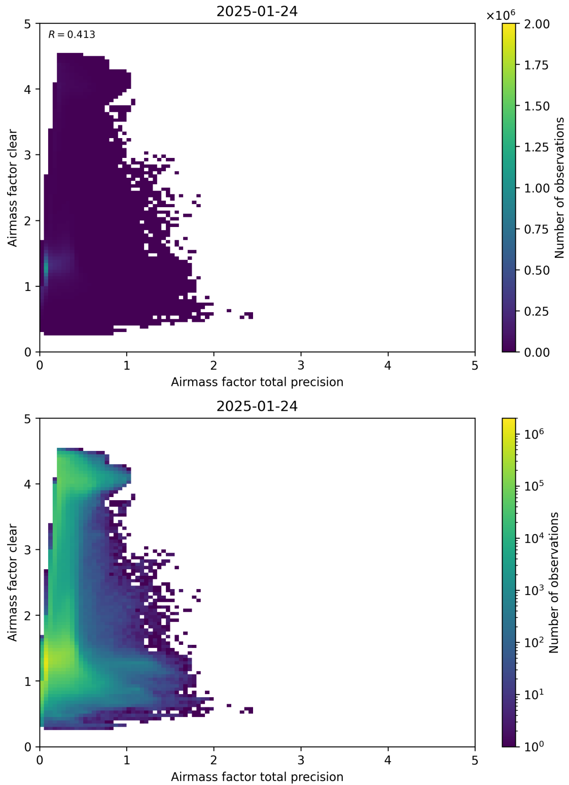
Figure 108: Scatter density plot of “Airmass factor total precision” against “Airmass factor clear” for 2025-01-23 to 2025-01-25.
