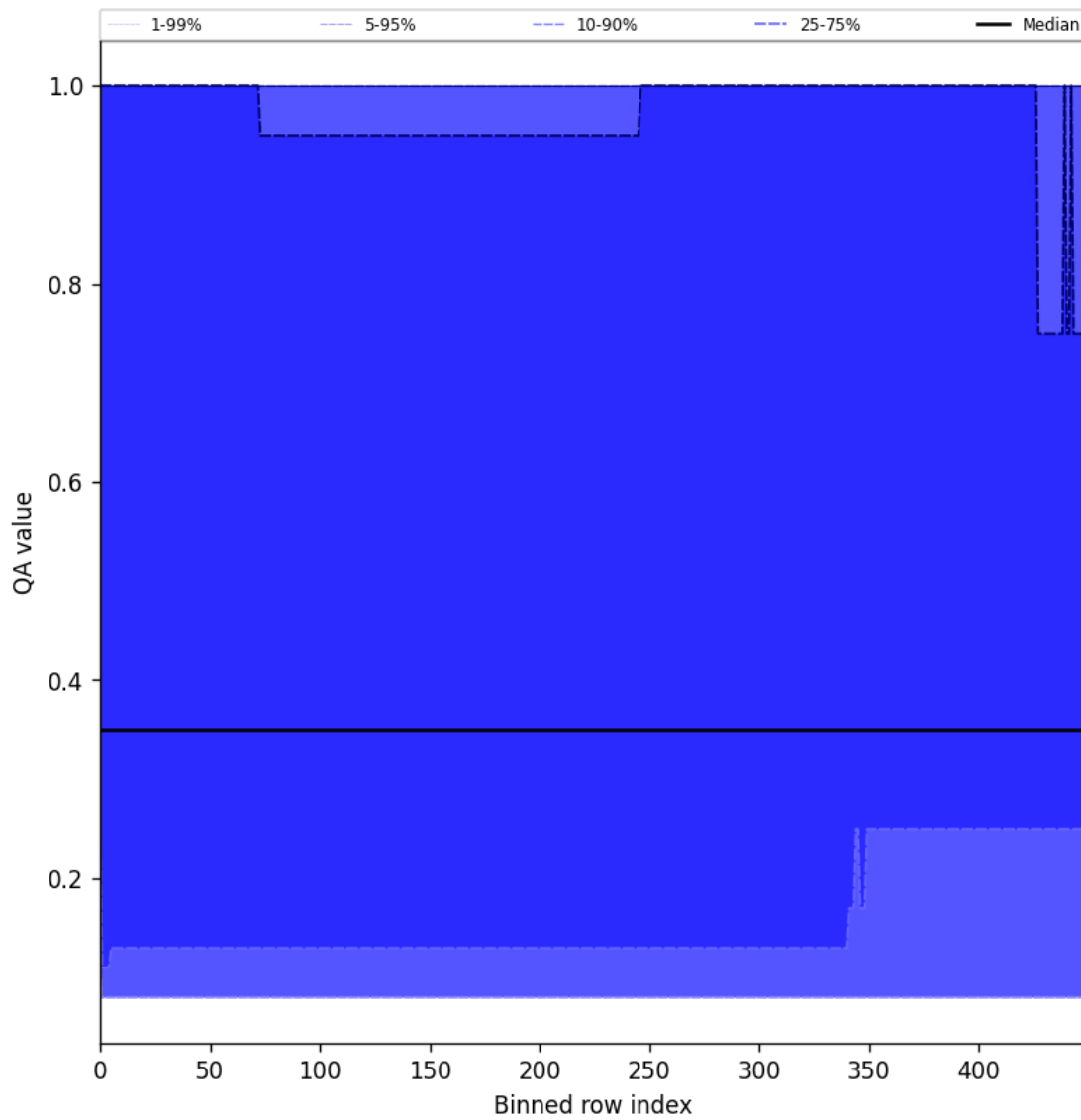
Figure 48: Along track statistics of “QA value” for 2025-01-23 to 2025-01-25
