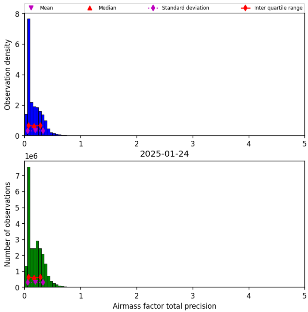
Figure 41: Histogram of “Airmass factor total precision” for 2025-01-23 to 2025-01-25
