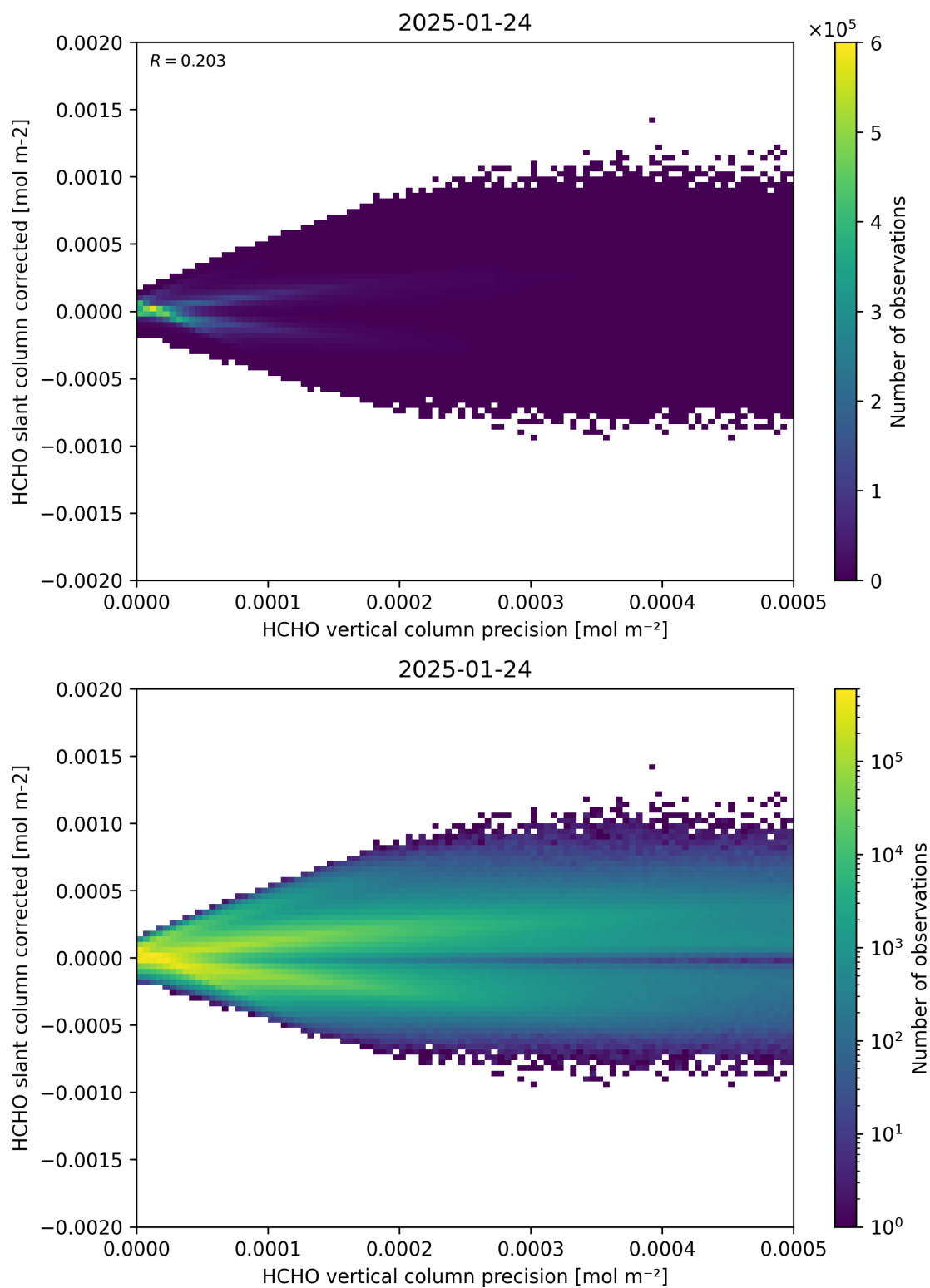
Figure 140: Scatter density plot of “HCHO vertical column precision” against “HCHO slant column corrected” for 2025-01-23 to 2025-01-25.
