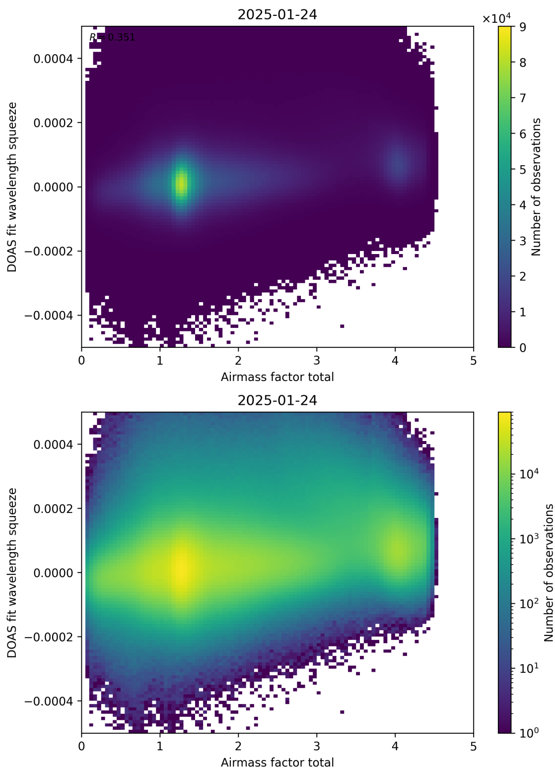
Figure 99: Scatter density plot of “Airmass factor total” against “DOAS fit wavelength squeeze” for 2025-01-23 to 2025-01-25.
