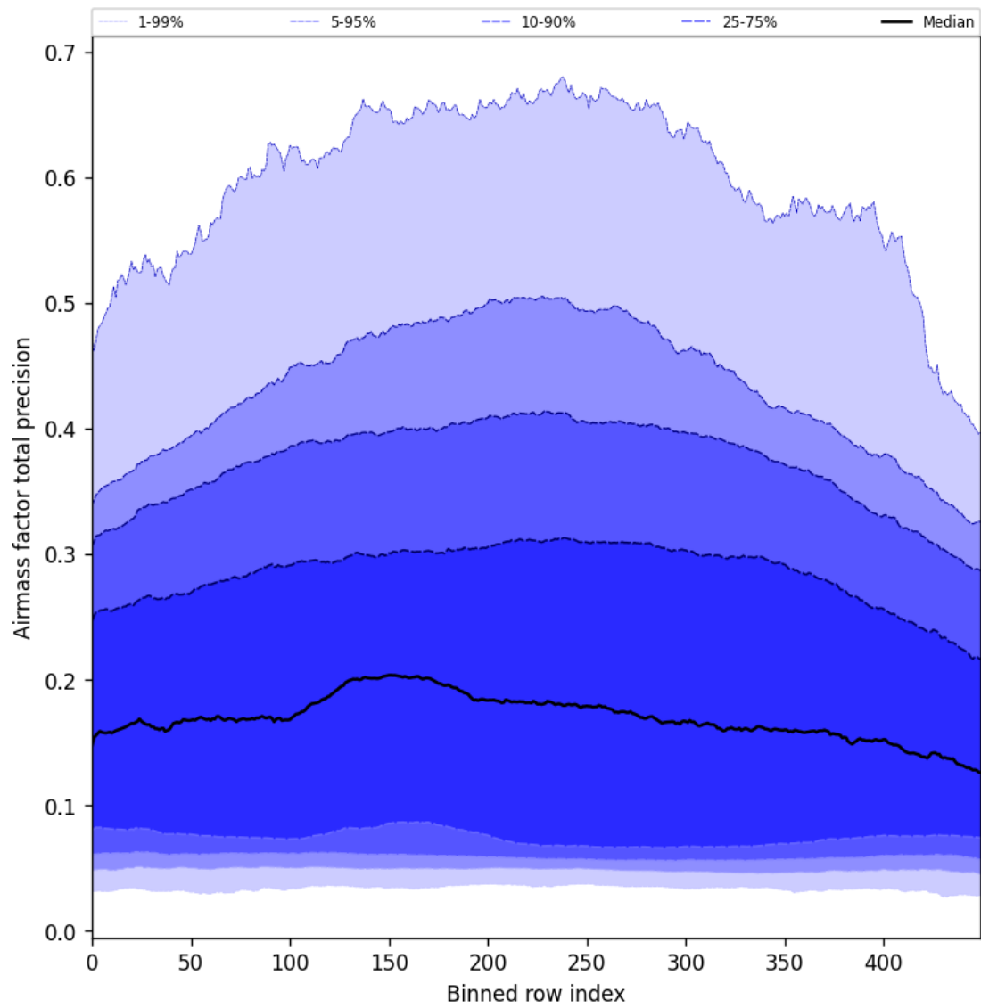
Figure 55: Along track statistics of “Airmass factor total precision” for 2025-01-23 to 2025-01-25
