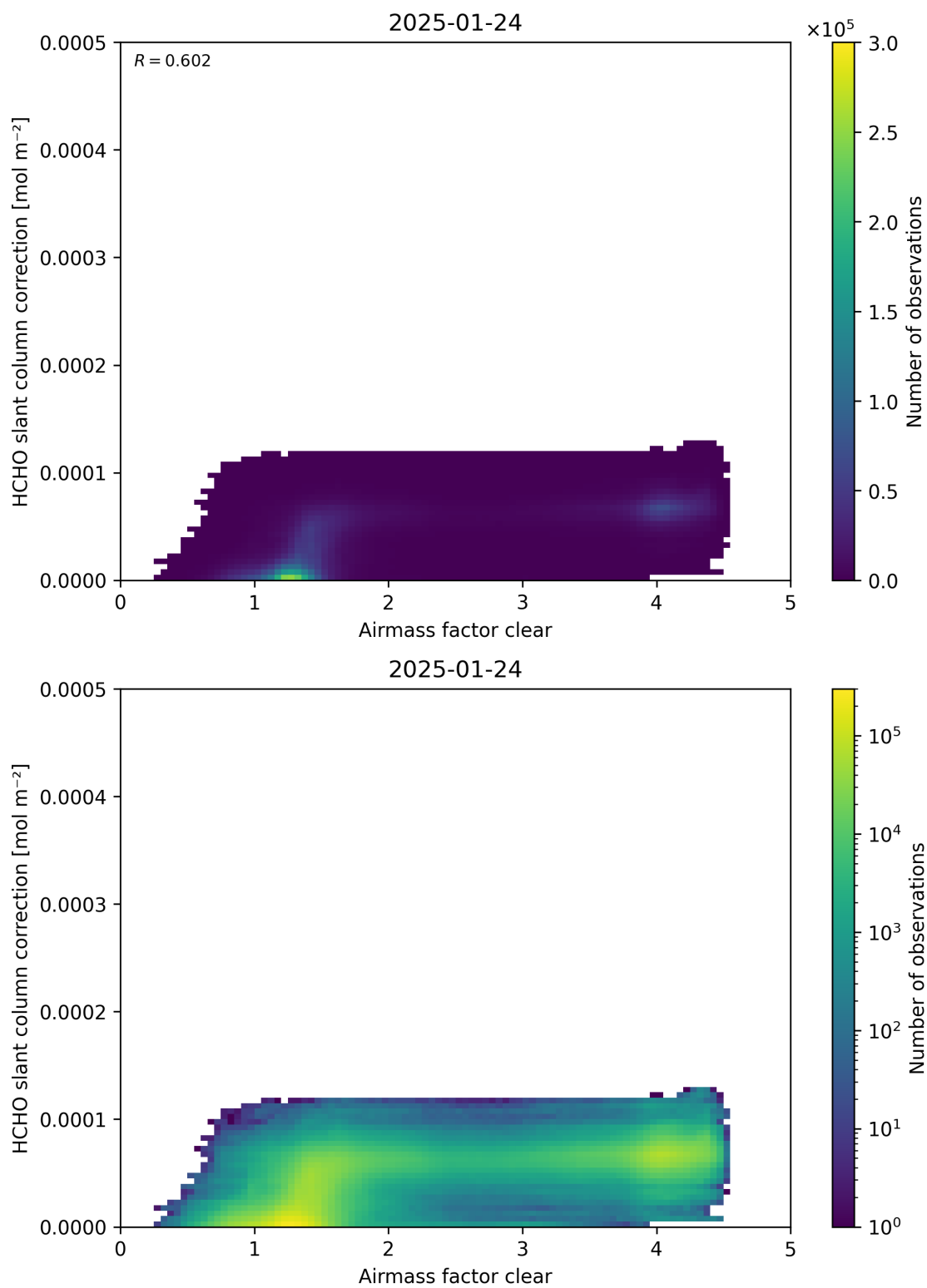
Figure 75: Scatter density plot of “Airmass factor clear” against “HCHO slant column correction” for 2025-01-23 to 2025-01-25.
