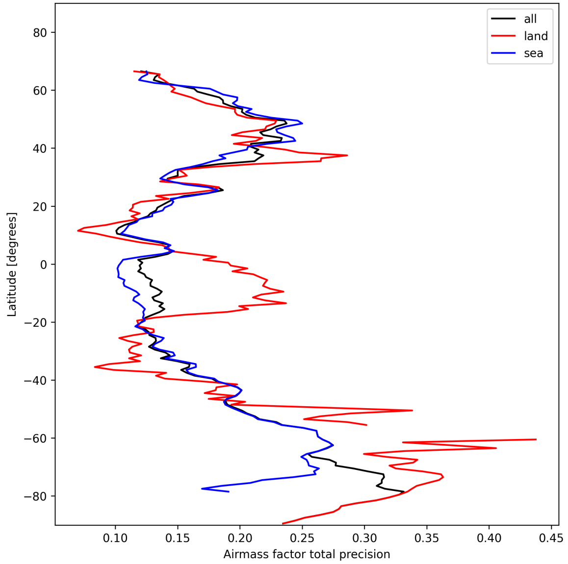
Figure 27: Zonal average of “Airmass factor total precision” for 2025-01-23 to 2025-01-25.
