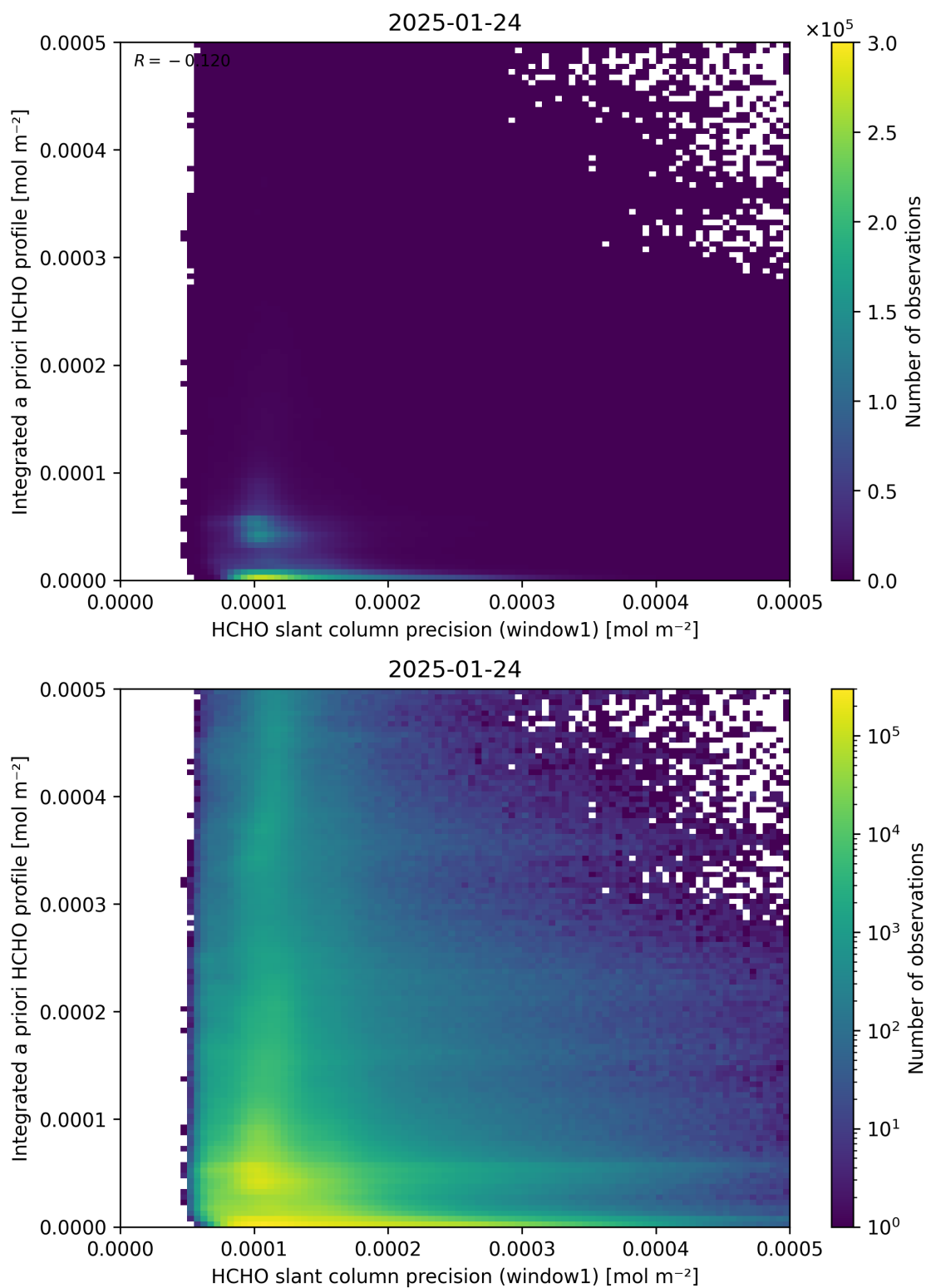
Figure 96: Scatter density plot of “HCHO slant column precision (window1)” against “Integrated a priori HCHO profile” for 2025-01-23 to 2025-01-25.
