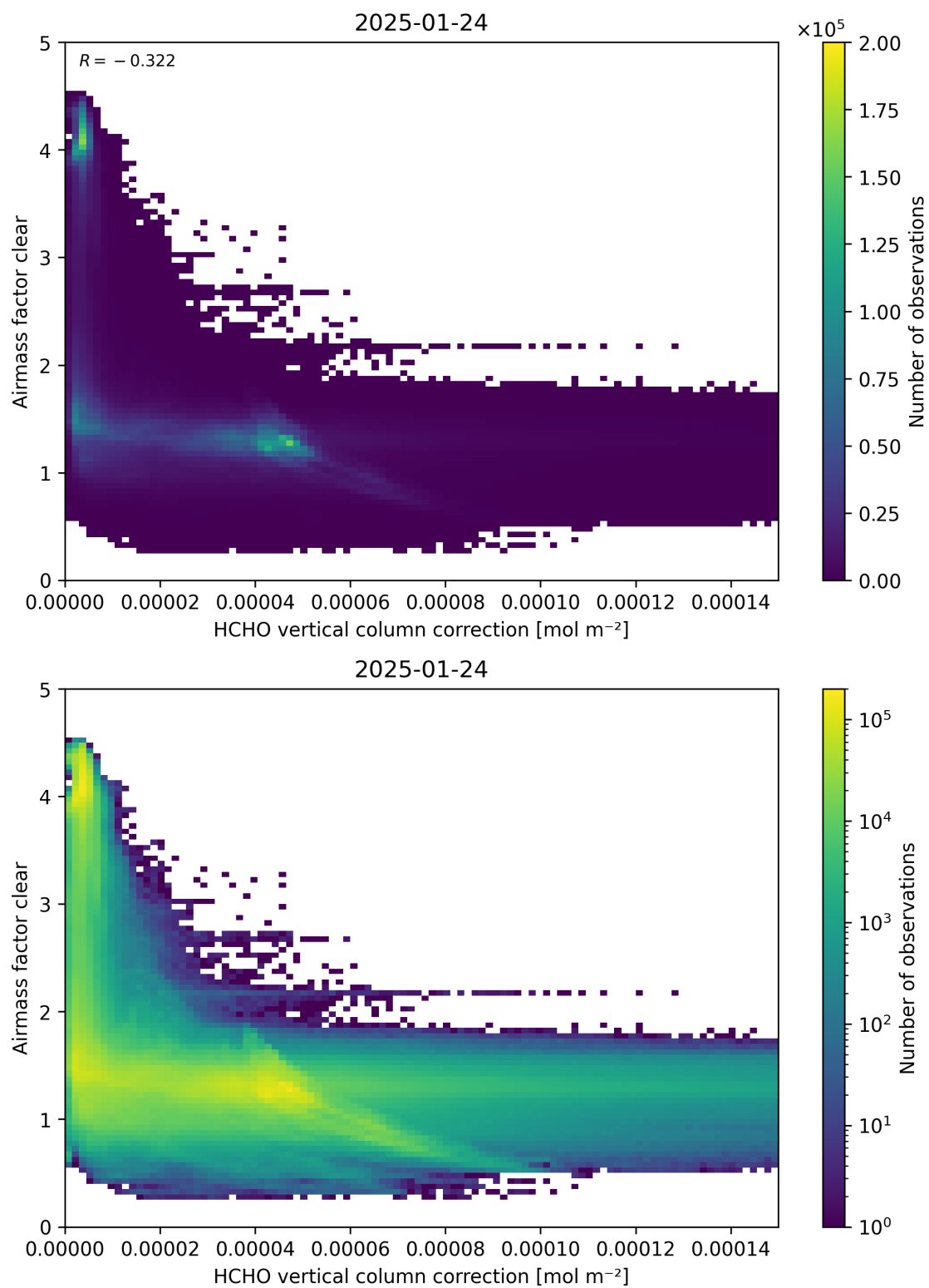
Figure 115: Scatter density plot of “HCHO vertical column correction” against “Airmass factor clear” for 2025-01-23 to 2025-01-25.
