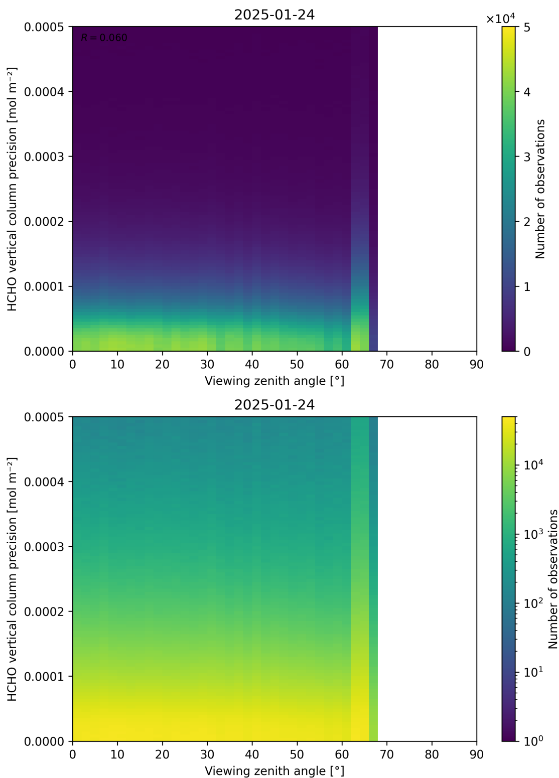
Figure 194: Scatter density plot of “Viewing zenith angle” against “HCHO vertical column precision” for 2025-01-23 to 2025-01-25.
