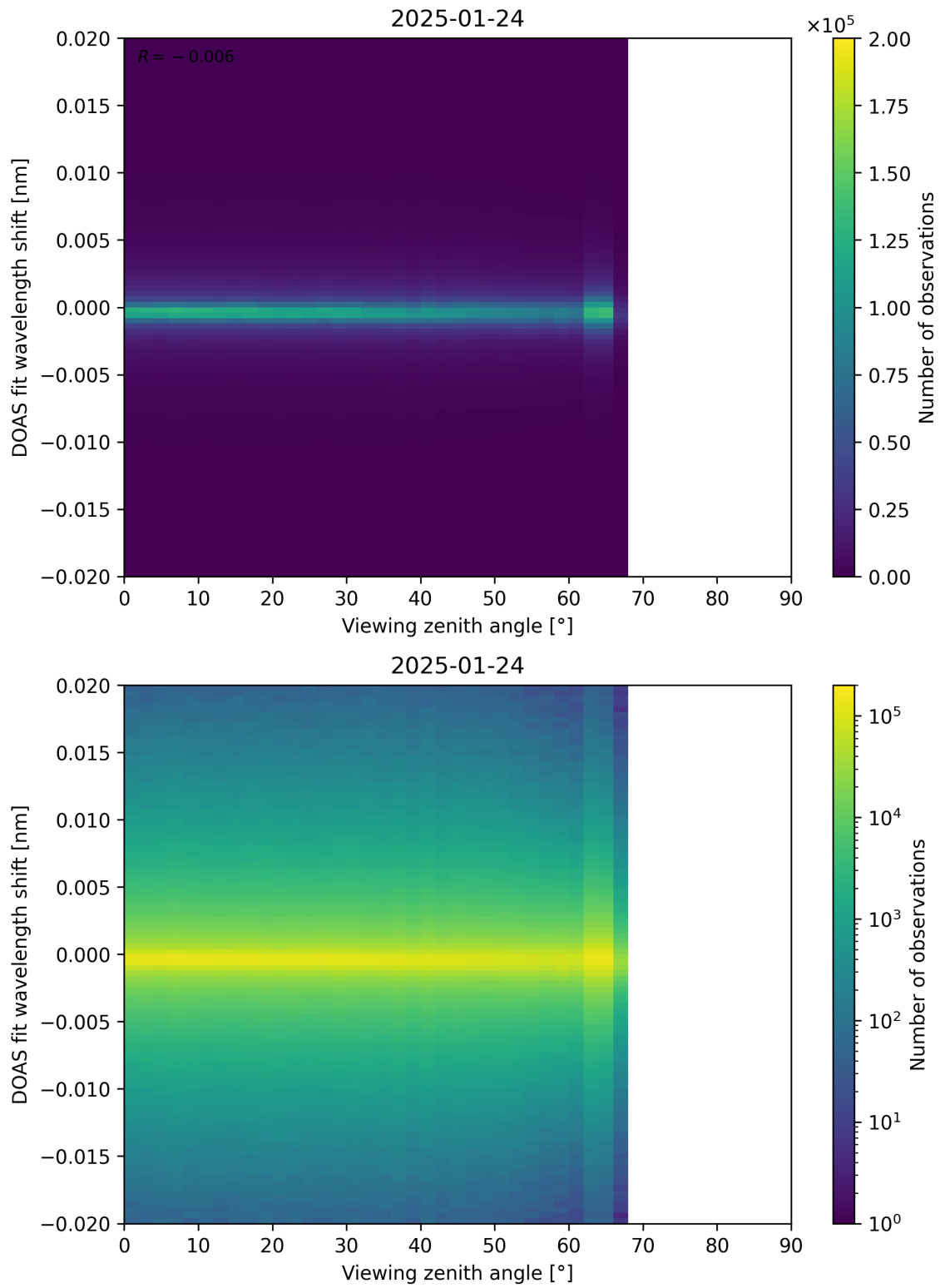
Figure 183: Scatter density plot of “Viewing zenith angle” against “DOAS fit wavelength shift” for 2025-01-23 to 2025-01-25.
