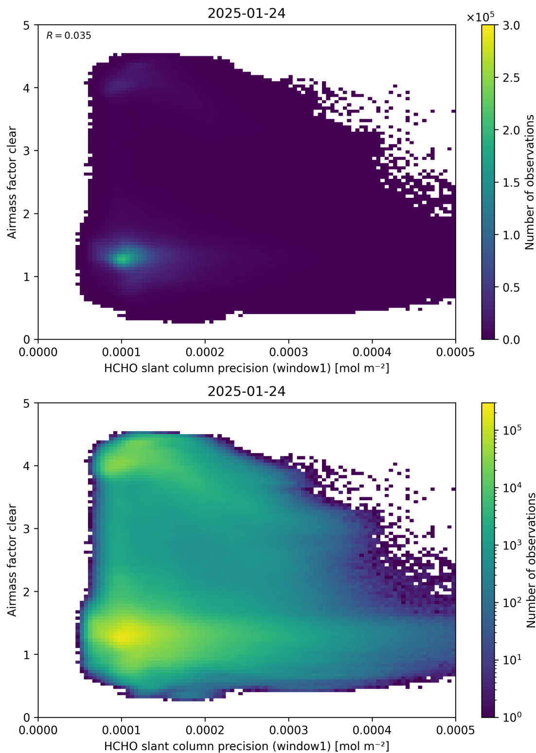
Figure 91: Scatter density plot of “HCHO slant column precision (window1)” against “Airmass factor clear” for 2025-01-23 to 2025-01-25.
