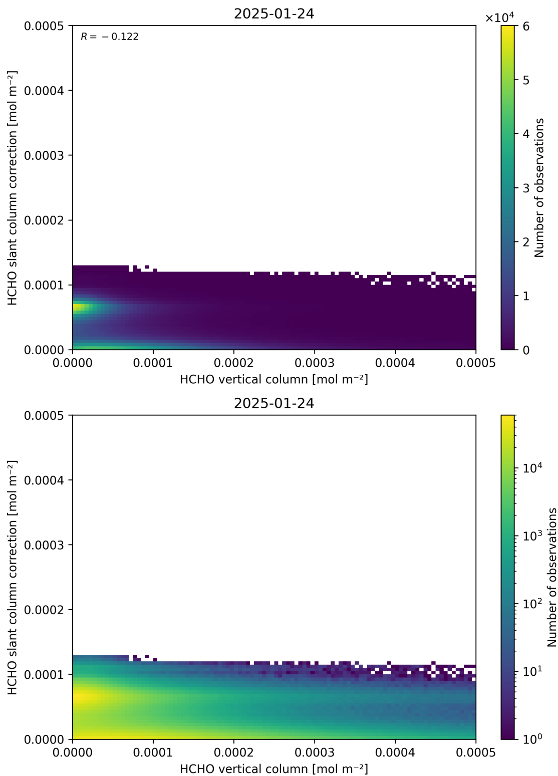
Figure 128: Scatter density plot of “HCHO vertical column” against “HCHO slant column correction” for 2025-01-23 to 2025-01-25.
