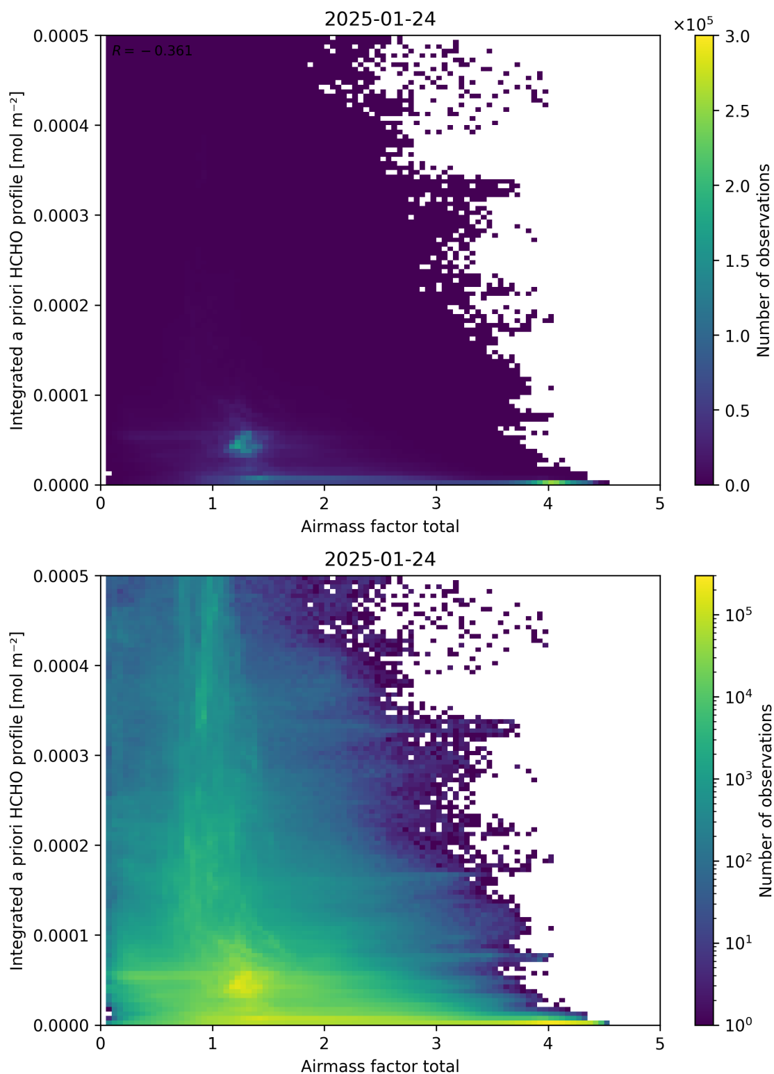
Figure 104: Scatter density plot of “Airmass factor total” against “Integrated a priori HCHO profile” for 2025-01-23 to 2025-01-25.
