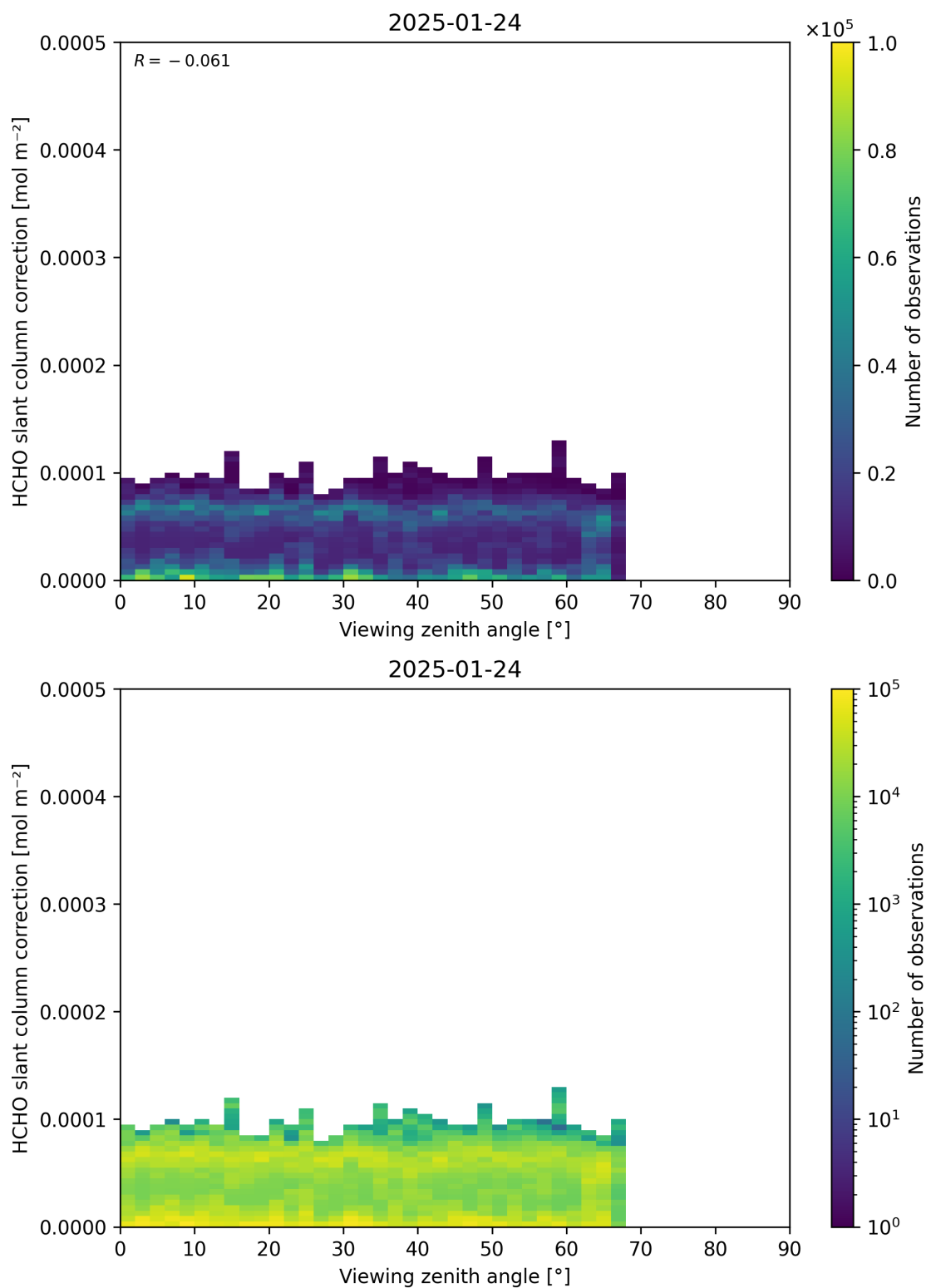
Figure 187: Scatter density plot of “Viewing zenith angle” against “HCHO slant column correction” for 2025-01-23 to 2025-01-25.
