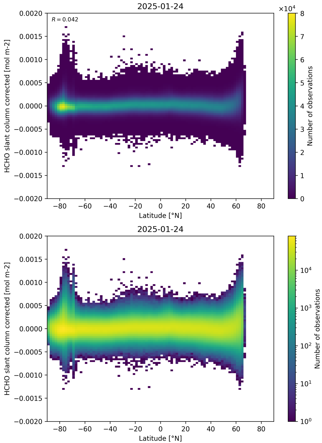
Figure 157: Scatter density plot of “Latitude” against “HCHO slant column corrected” for 2025-01-23 to 2025-01-25.
