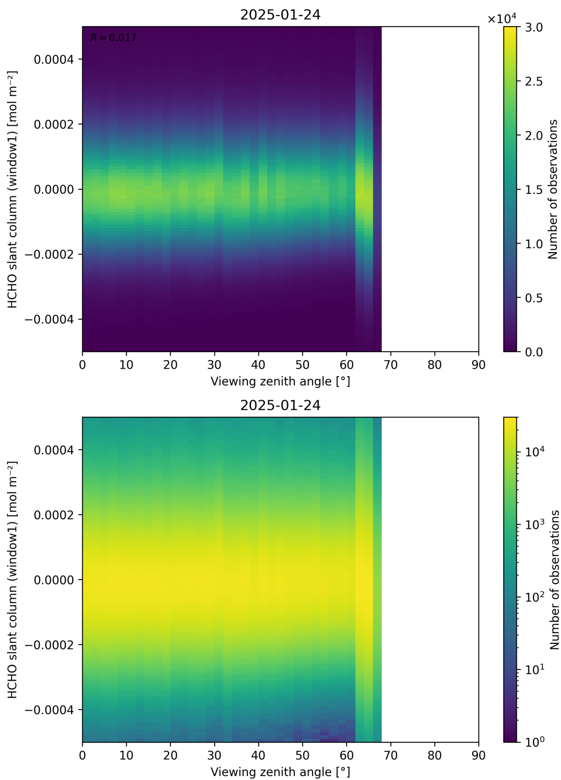
Figure 188: Scatter density plot of “Viewing zenith angle” against “HCHO slant column (window1)” for 2025-01-23 to 2025-01-25.
