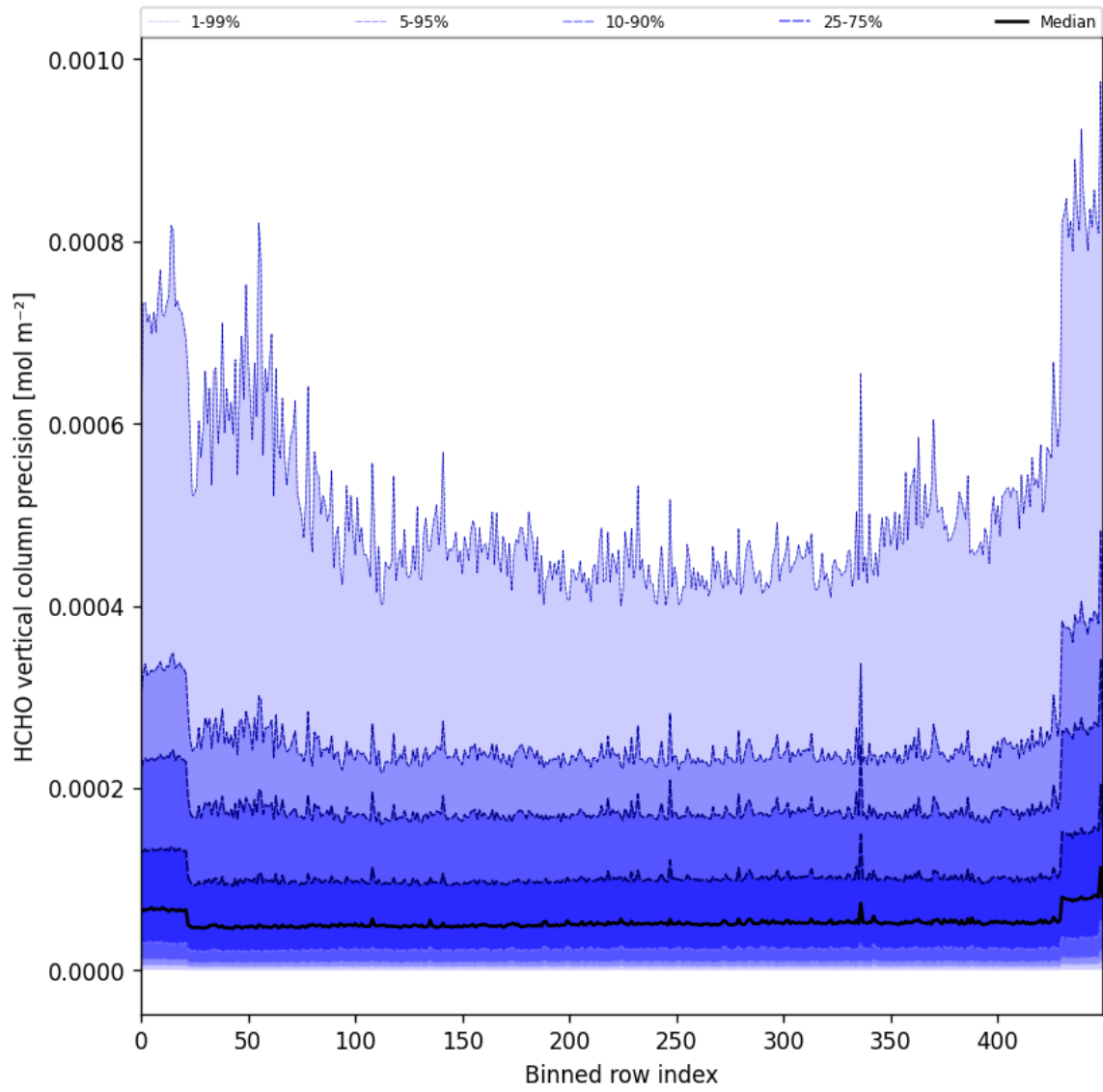
Figure 50: Along track statistics of “HCHO vertical column precision” for 2025-01-23 to 2025-01-25
