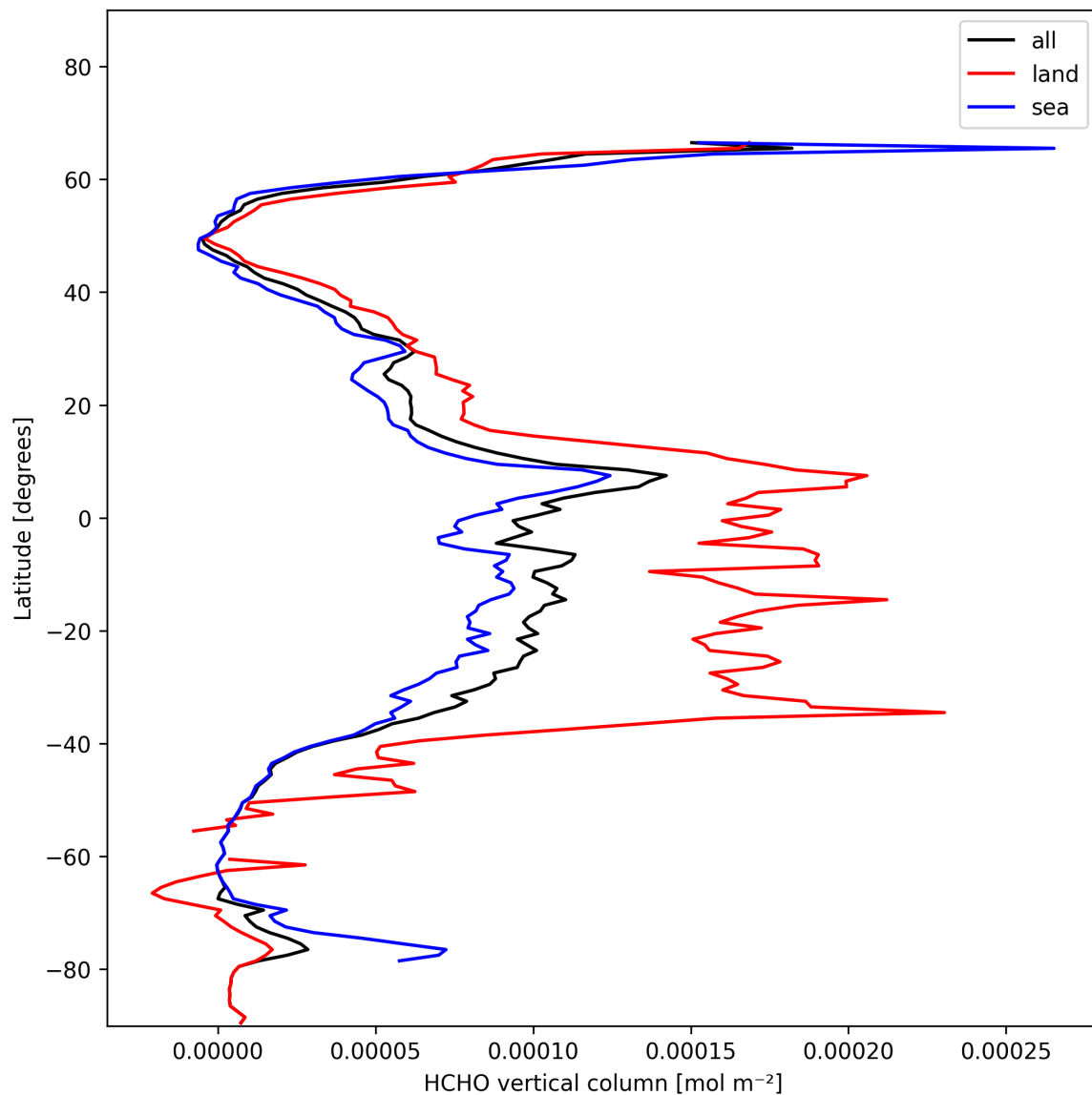
Figure 21: Zonal average of “HCHO vertical column” for 2025-01-23 to 2025-01-25.
