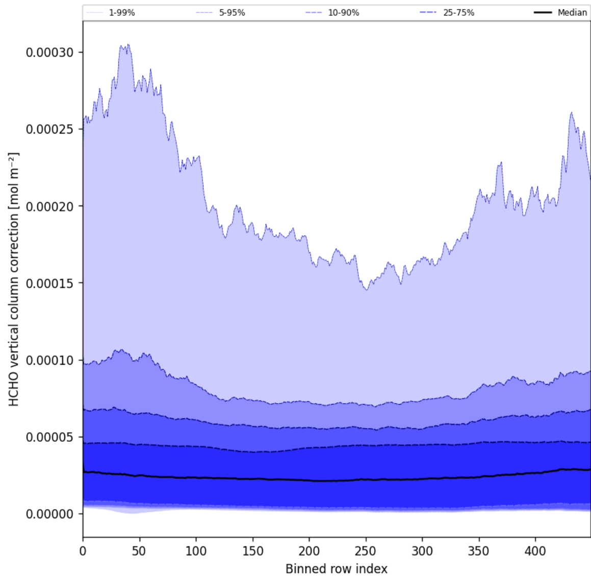
Figure 51: Along track statistics of “HCHO vertical column correction” for 2025-01-23 to 2025-01-25
