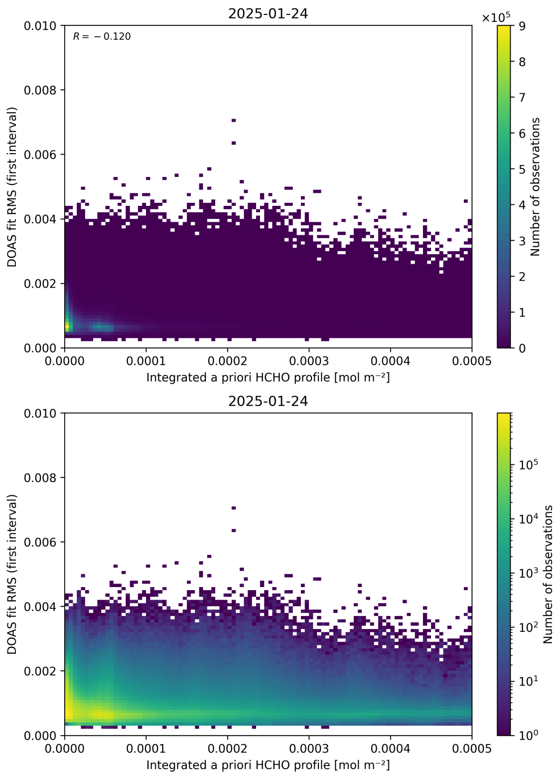
Figure 148: Scatter density plot of “Integrated a priori HCHO profile” against “DOAS fit RMS (first interval)” for 2025-01-23 to 2025-01-25.
