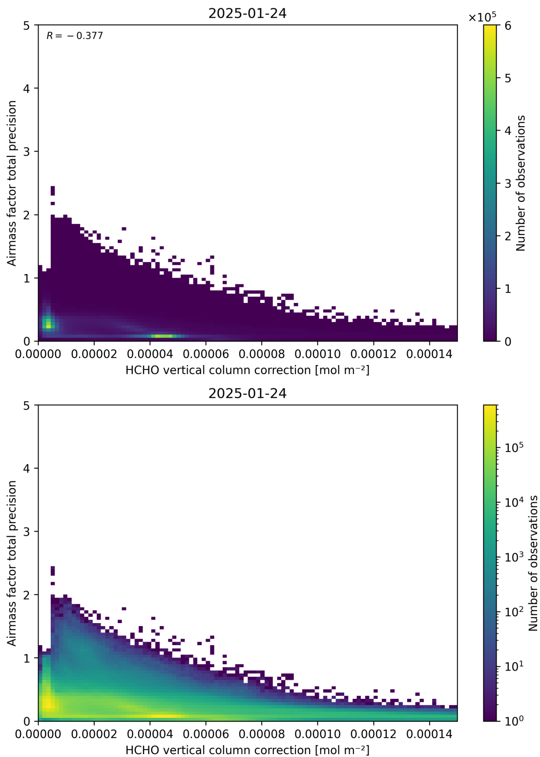
Figure 121: Scatter density plot of “HCHO vertical column correction” against “Airmass factor total precision” for 2025-01-23 to 2025-01-25.
