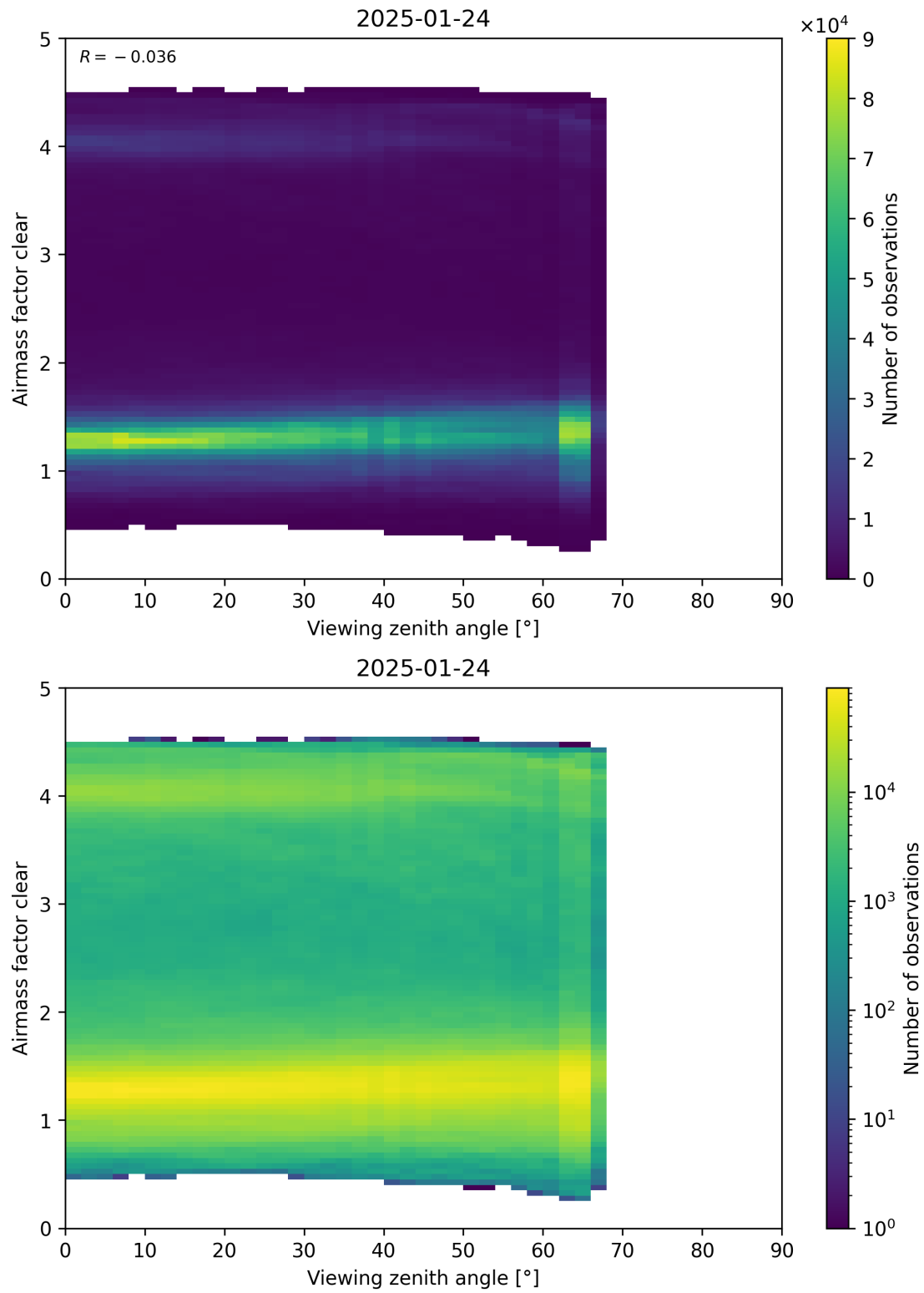
Figure 185: Scatter density plot of “Viewing zenith angle” against “Airmass factor clear” for 2025-01-23 to 2025-01-25.
