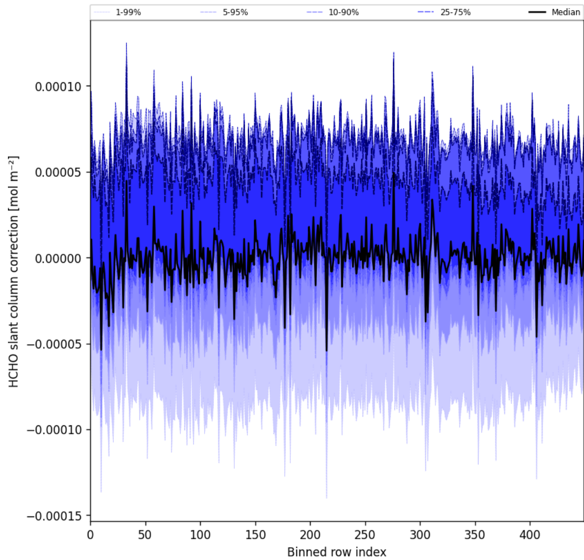
Figure 61: Along track statistics of “HCHO slant column correction” for 2025-01-23 to 2025-01-25
