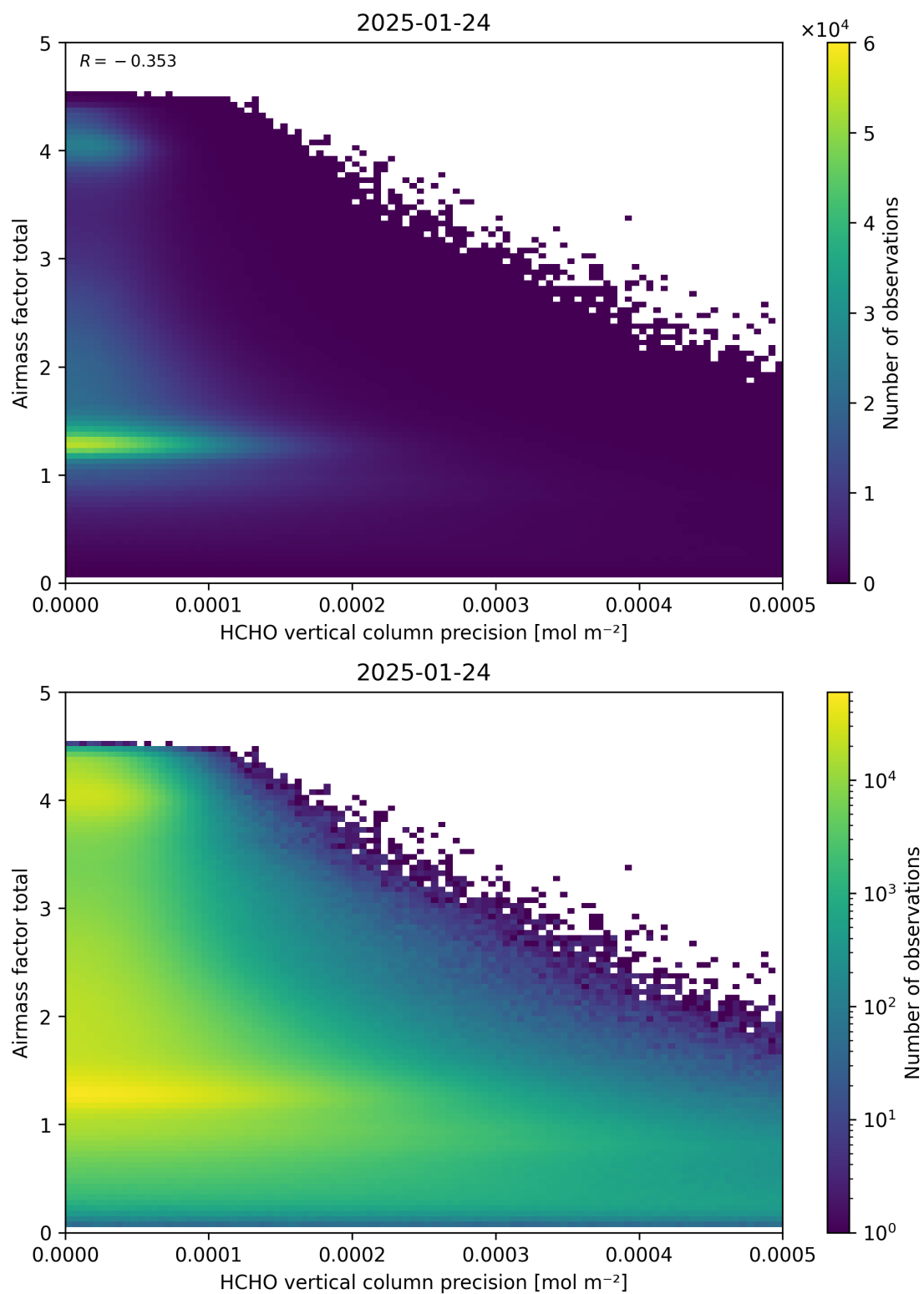
Figure 144: Scatter density plot of “HCHO vertical column precision” against “Airmass factor total” for 2025-01-23 to 2025-01-25.
