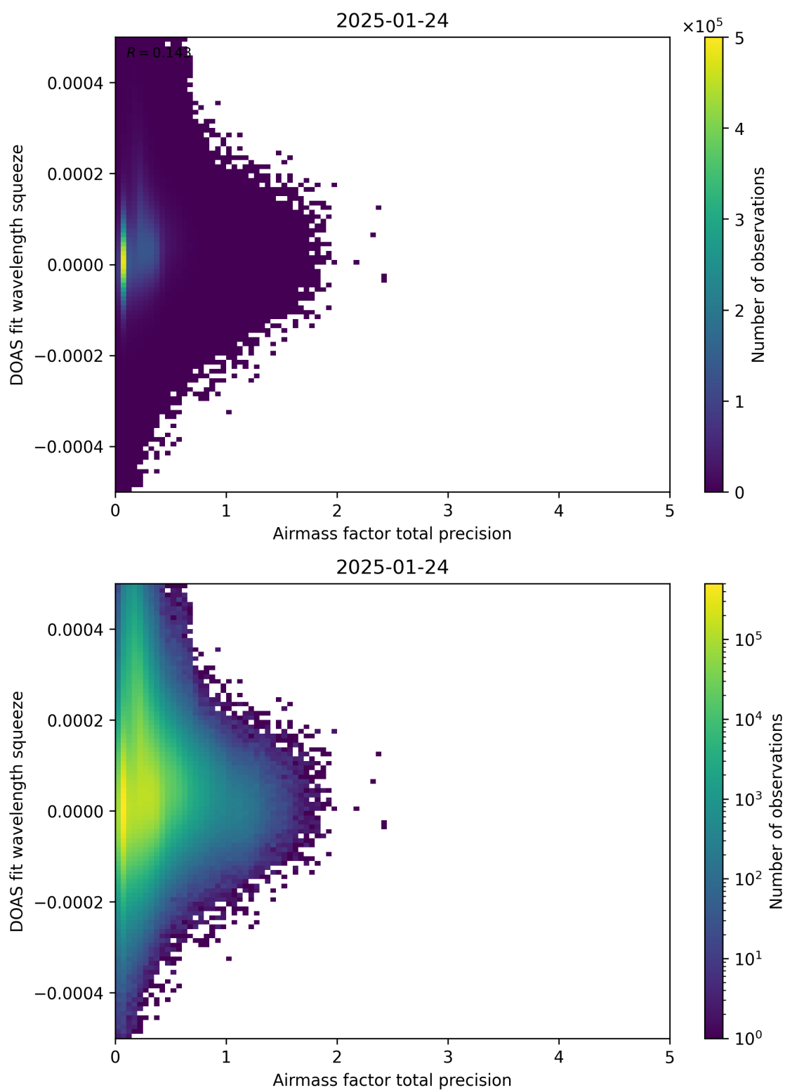
Figure 107: Scatter density plot of “Airmass factor total precision” against “DOAS fit wavelength squeeze” for 2025-01-23 to 2025-01-25.
