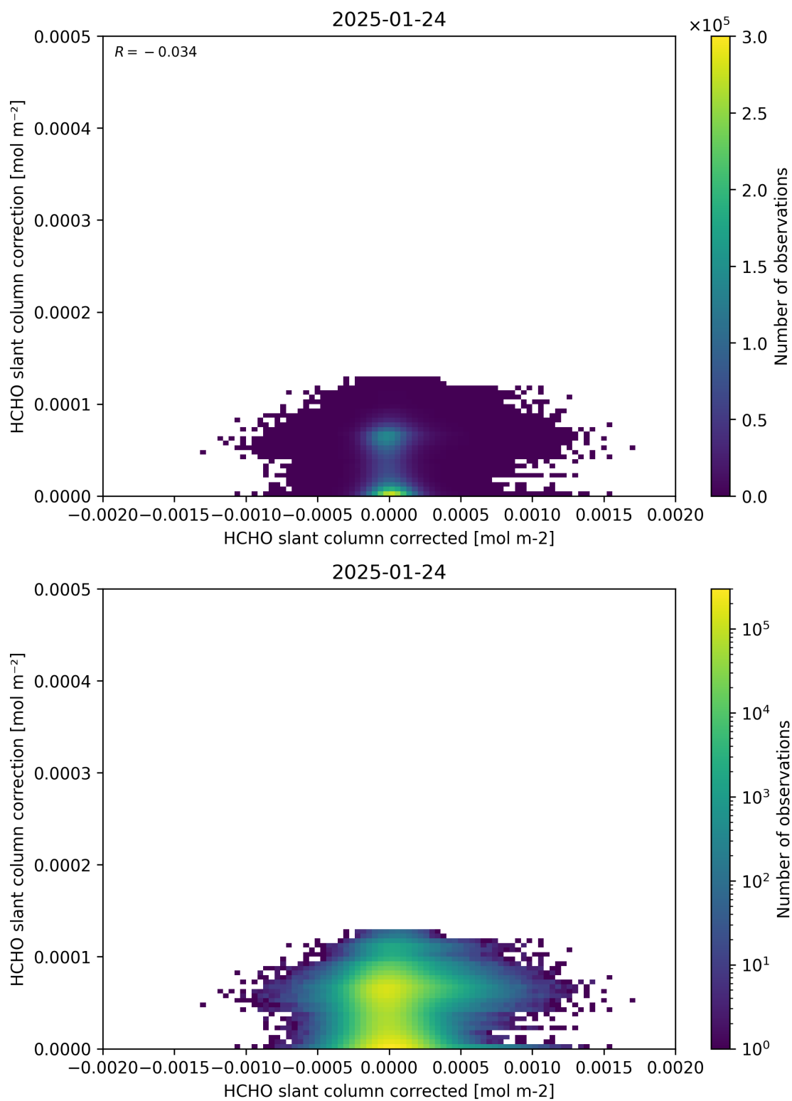
Figure 77: Scatter density plot of “HCHO slant column corrected” against “HCHO slant column correction” for 2025-01-23 to 2025-01-25.
