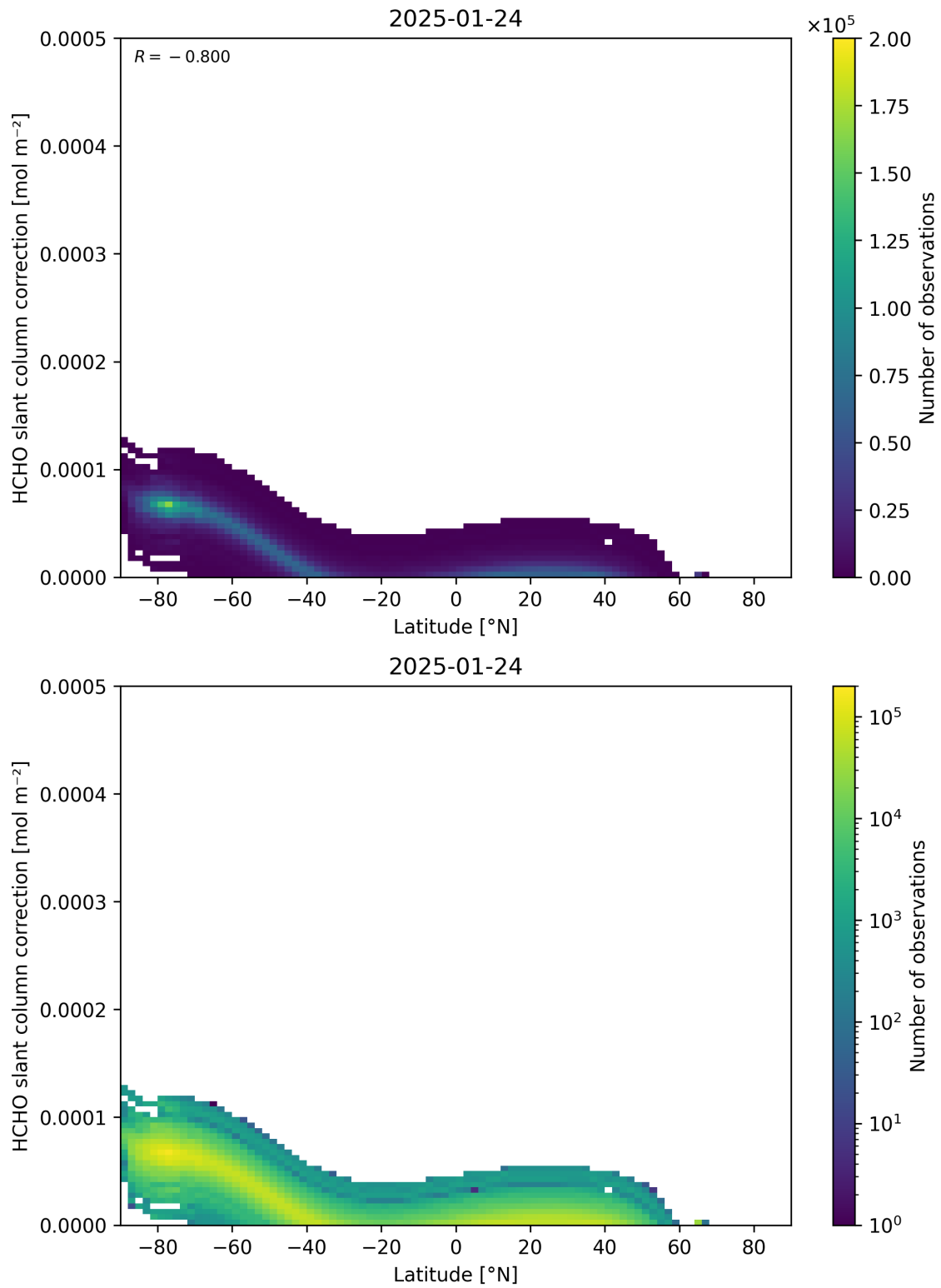
Figure 158: Scatter density plot of “Latitude” against “HCHO slant column correction” for 2025-01-23 to 2025-01-25.
