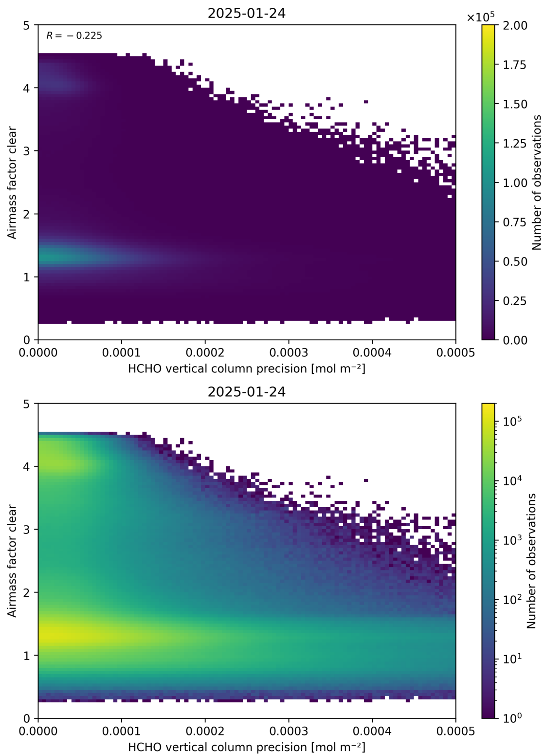
Figure 139: Scatter density plot of “HCHO vertical column precision” against “Airmass factor clear” for 2025-01-23 to 2025-01-25.
