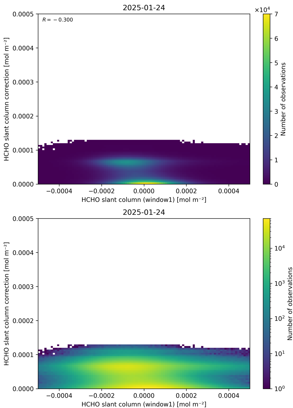
Figure 83: Scatter density plot of “HCHO slant column (window1)” against “HCHO slant column correction” for 2025-01-23 to 2025-01-25.
