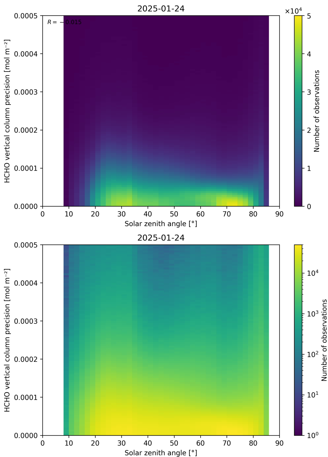
Figure 179: Scatter density plot of “Solar zenith angle” against “HCHO vertical column precision” for 2025-01-23 to 2025-01-25.
