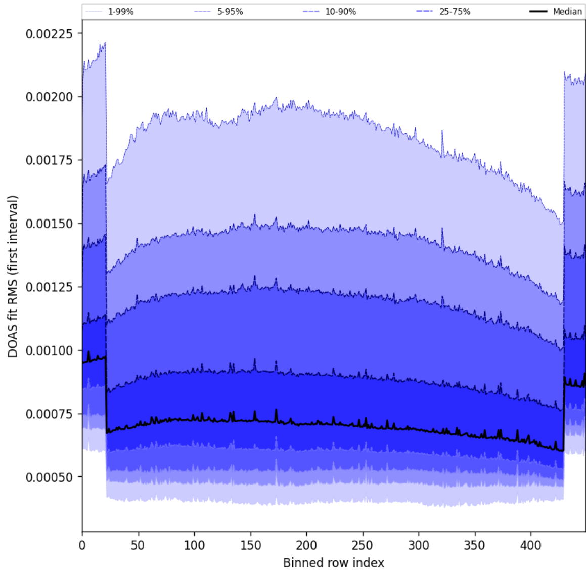
Figure 60: Along track statistics of “DOAS fit RMS (first interval)” for 2025-01-23 to 2025-01-25
