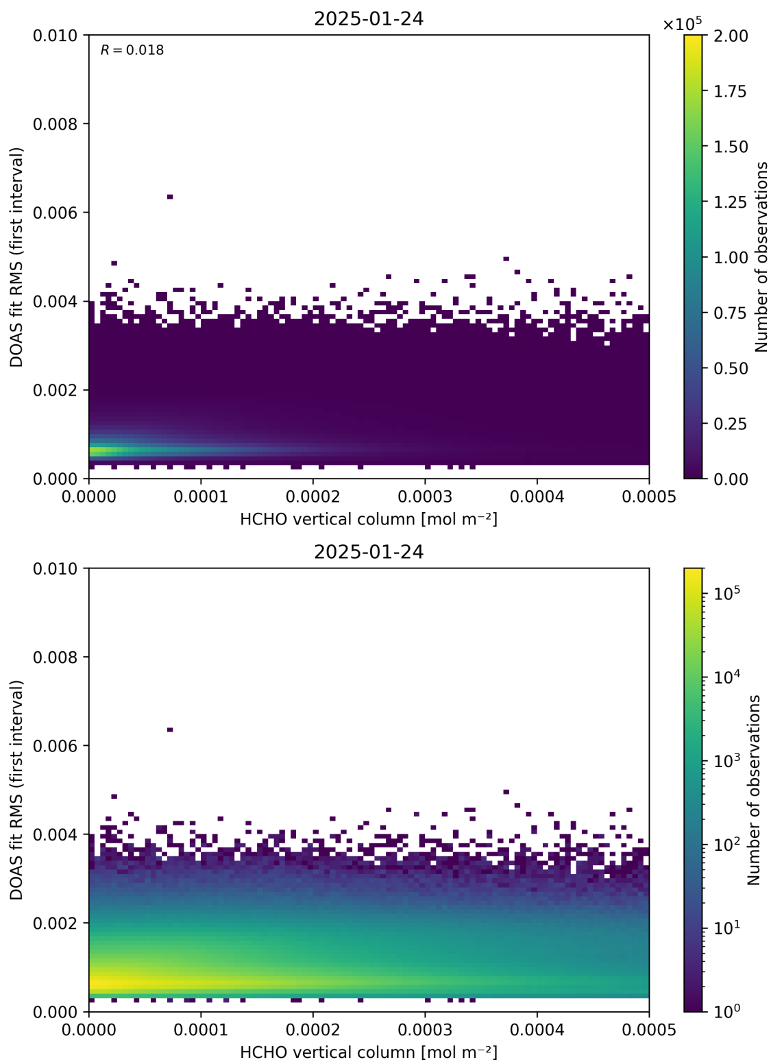
Figure 123: Scatter density plot of “HCHO vertical column” against “DOAS fit RMS (first interval)” for 2025-01-23 to 2025-01-25.
