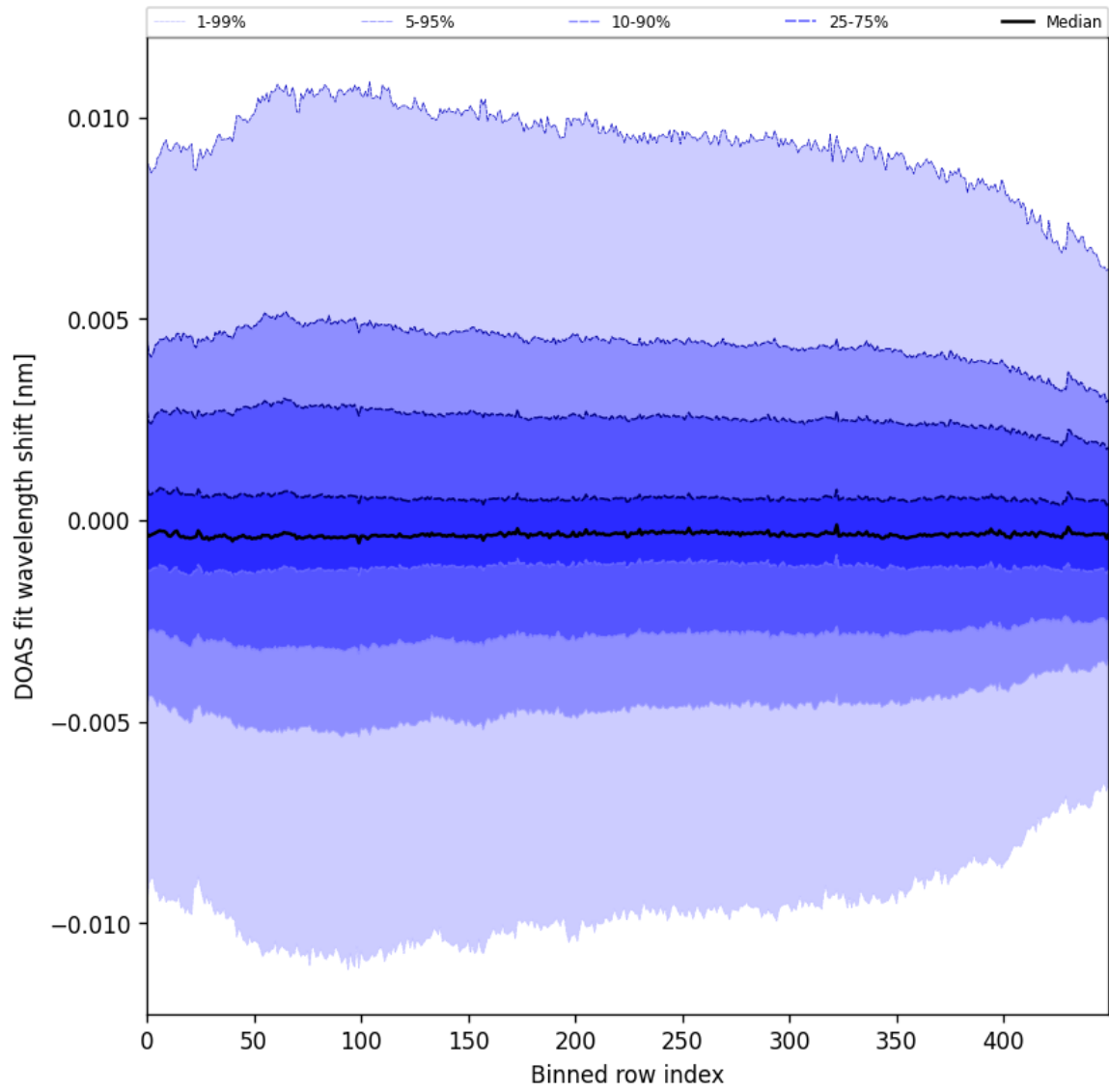
Figure 58: Along track statistics of “DOAS fit wavelength shift” for 2025-01-23 to 2025-01-25
