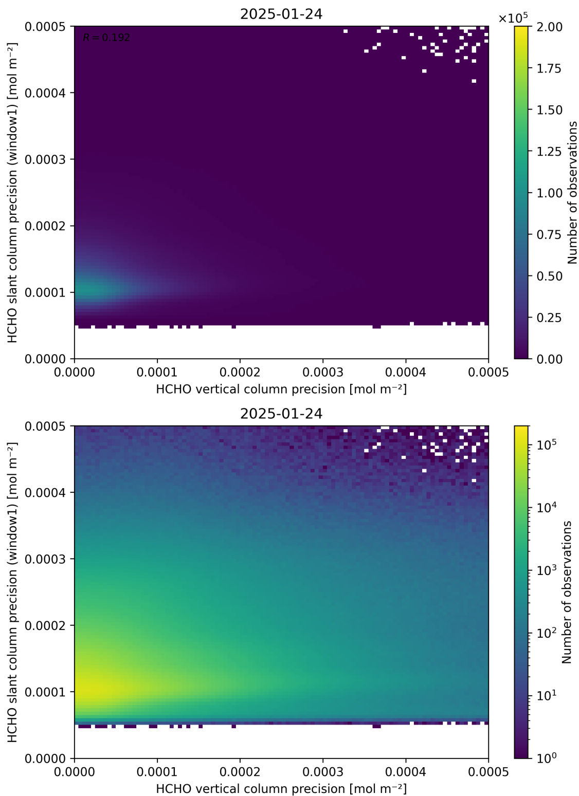
Figure 143: Scatter density plot of “HCHO vertical column precision” against “HCHO slant column precision (window1)” for 2025-01-23 to 2025-01-25.
