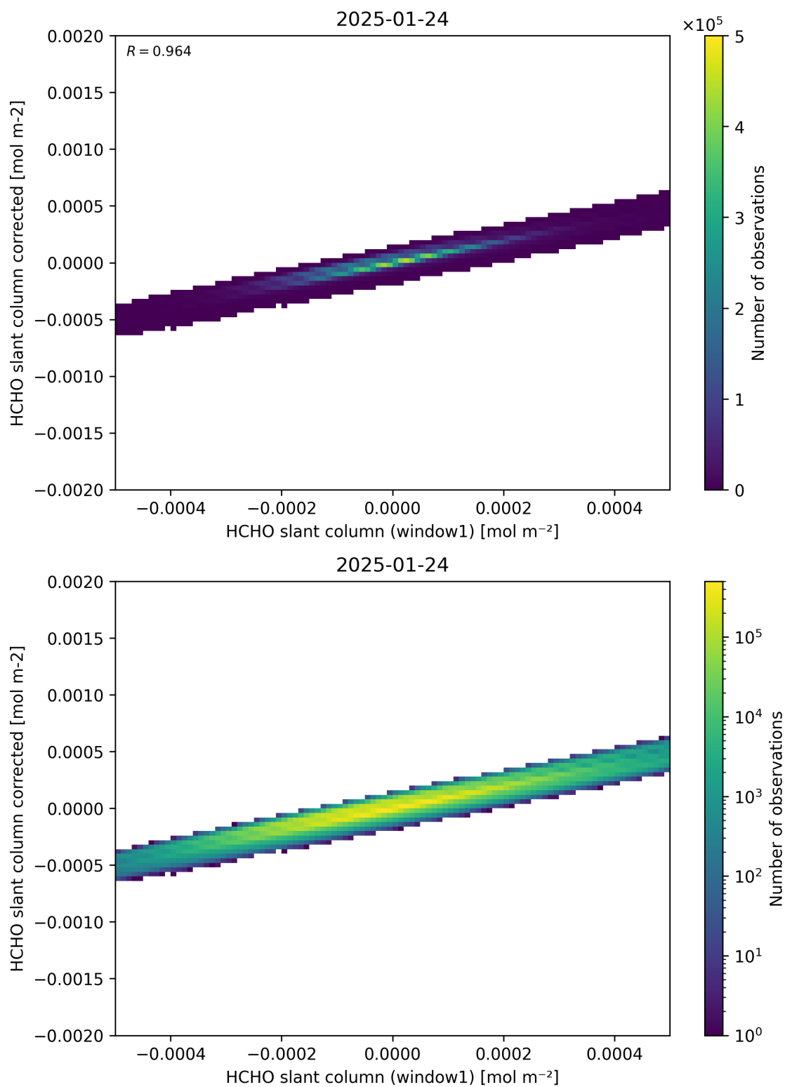
Figure 82: Scatter density plot of “HCHO slant column (window1)” against “HCHO slant column corrected” for 2025-01-23 to 2025-01-25.
