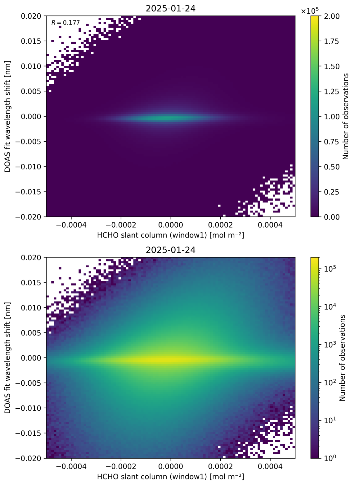
Figure 79: Scatter density plot of “HCHO slant column (window1)” against “DOAS fit wavelength shift” for 2025-01-23 to 2025-01-25.
