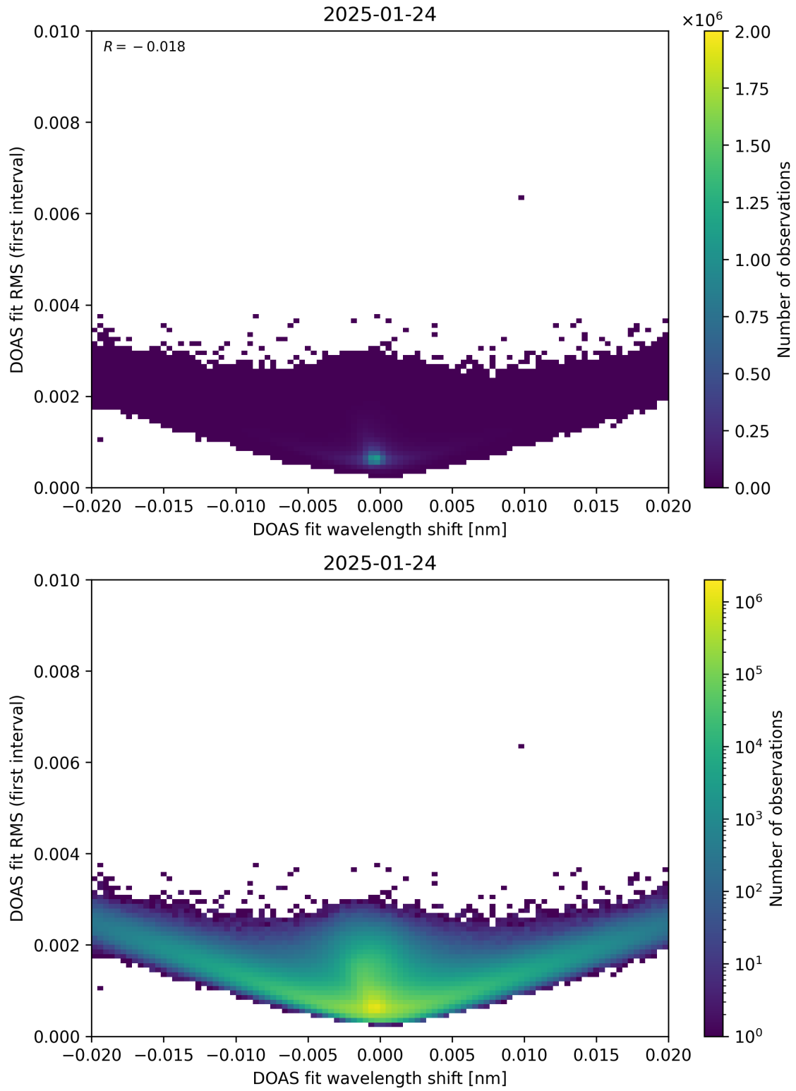
Figure 64: Scatter density plot of “DOAS fit wavelength shift” against “DOAS fit RMS (first interval)” for 2025-01-23 to 2025-01-25.
