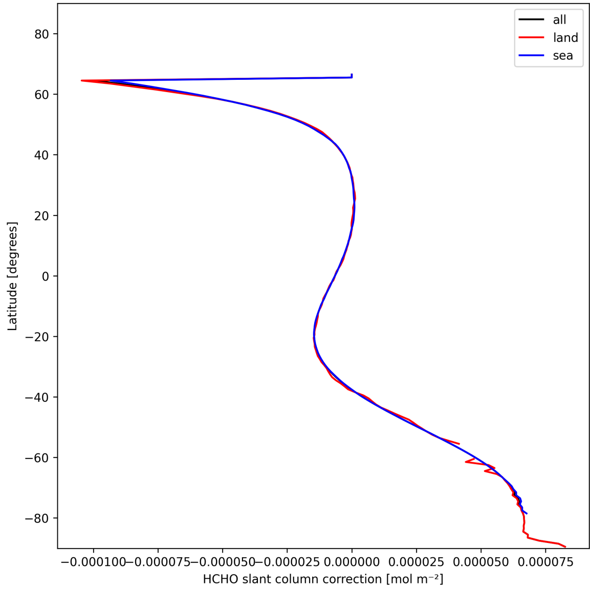
Figure 33: Zonal average of “HCHO slant column correction” for 2025-01-23 to 2025-01-25.
