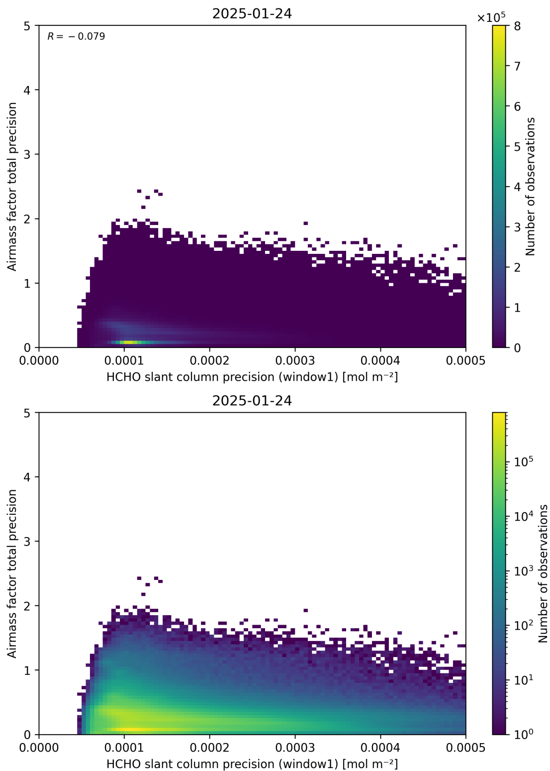
Figure 95: Scatter density plot of “HCHO slant column precision (window1)” against “Airmass factor total precision” for 2025-01-23 to 2025-01-25.
