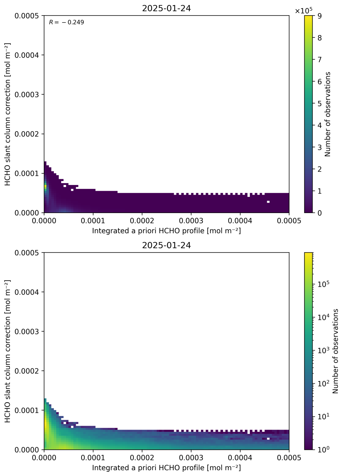
Figure 152: Scatter density plot of “Integrated a priori HCHO profile” against “HCHO slant column correction” for 2025-01-23 to 2025-01-25.
