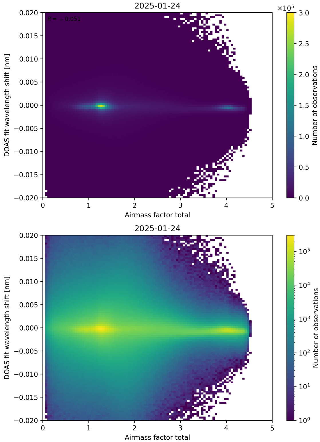
Figure 98: Scatter density plot of “Airmass factor total” against “DOAS fit wavelength shift” for 2025-01-23 to 2025-01-25.
