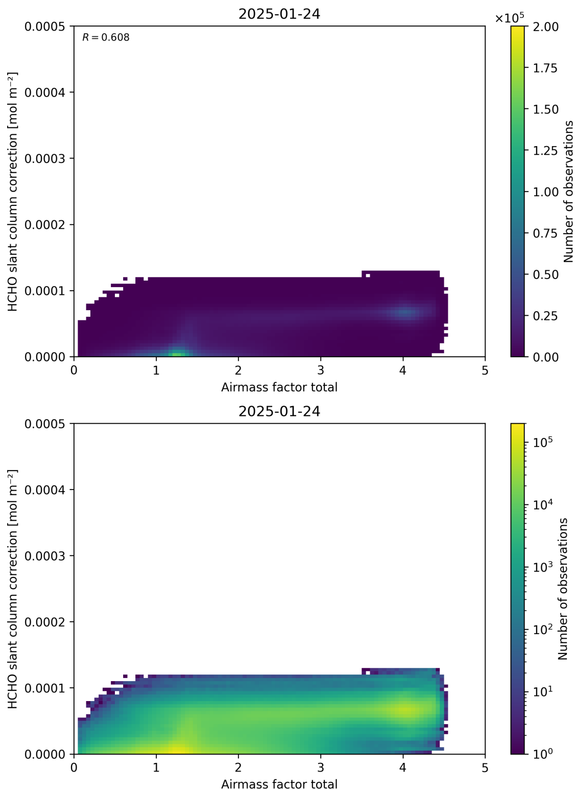
Figure 102: Scatter density plot of “Airmass factor total” against “HCHO slant column correction” for 2025-01-23 to 2025-01-25.
