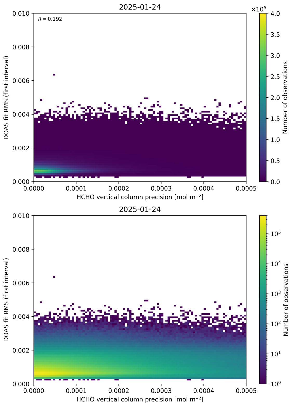
Figure 136: Scatter density plot of “HCHO vertical column precision” against “DOAS fit RMS (first interval)” for 2025-01-23 to 2025-01-25.
