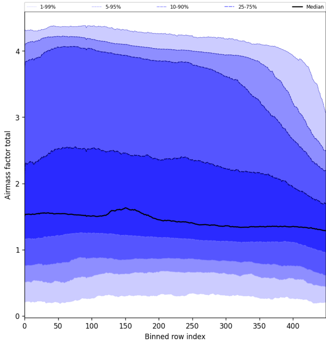
Figure 54: Along track statistics of “Airmass factor total” for 2025-01-23 to 2025-01-25
