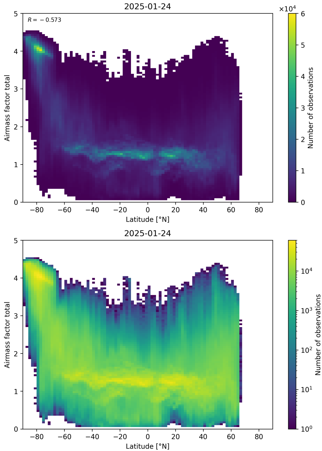
Figure 161: Scatter density plot of “Latitude” against “Airmass factor total” for 2025-01-23 to 2025-01-25.
