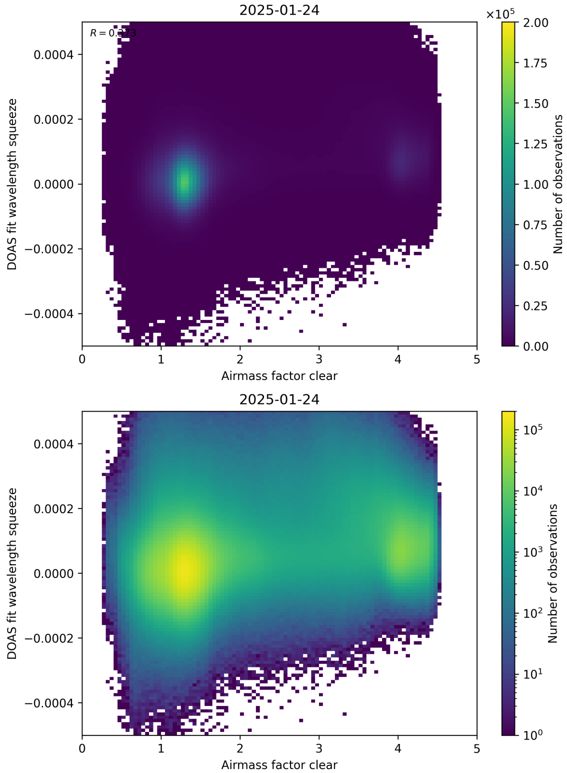
Figure 73: Scatter density plot of “Airmass factor clear” against “DOAS fit wavelength squeeze” for 2025-01-23 to 2025-01-25.
