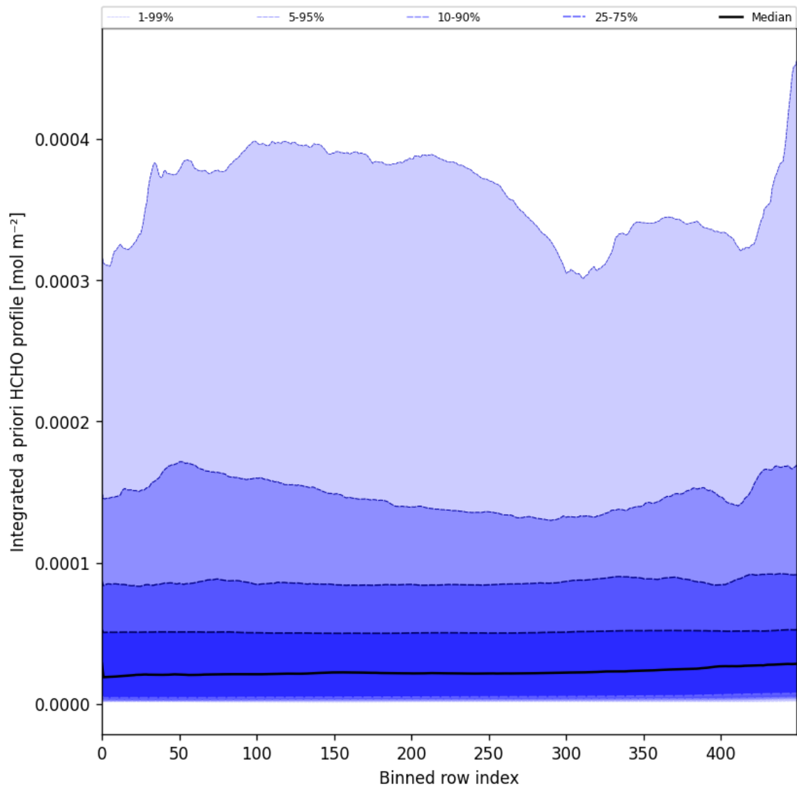
Figure 57: Along track statistics of “Integrated a priori HCHO profile” for 2025-01-23 to 2025-01-25
