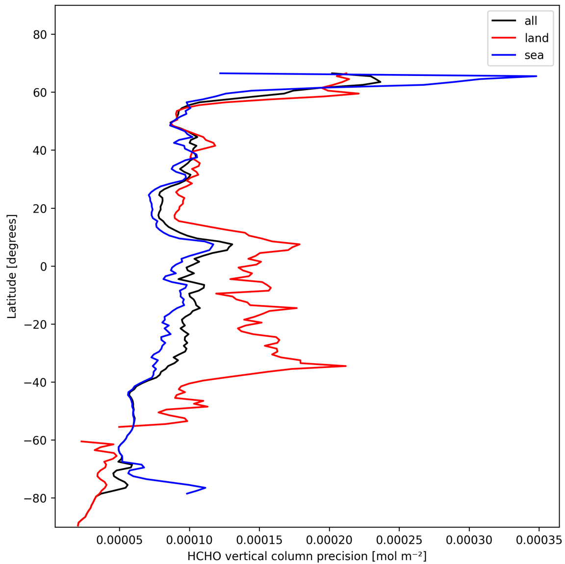
Figure 22: Zonal average of “HCHO vertical column precision” for 2025-01-23 to 2025-01-25.
