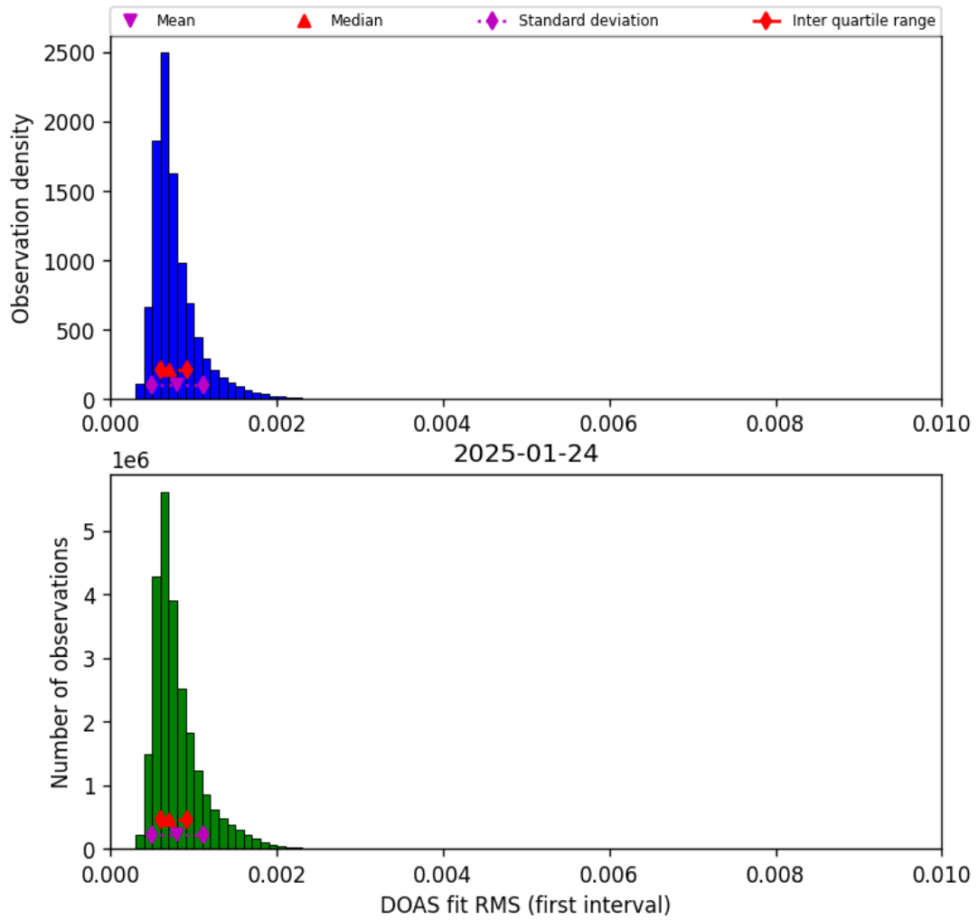
Figure 46: Histogram of “DOAS fit RMS (first interval)” for 2025-01-23 to 2025-01-25
