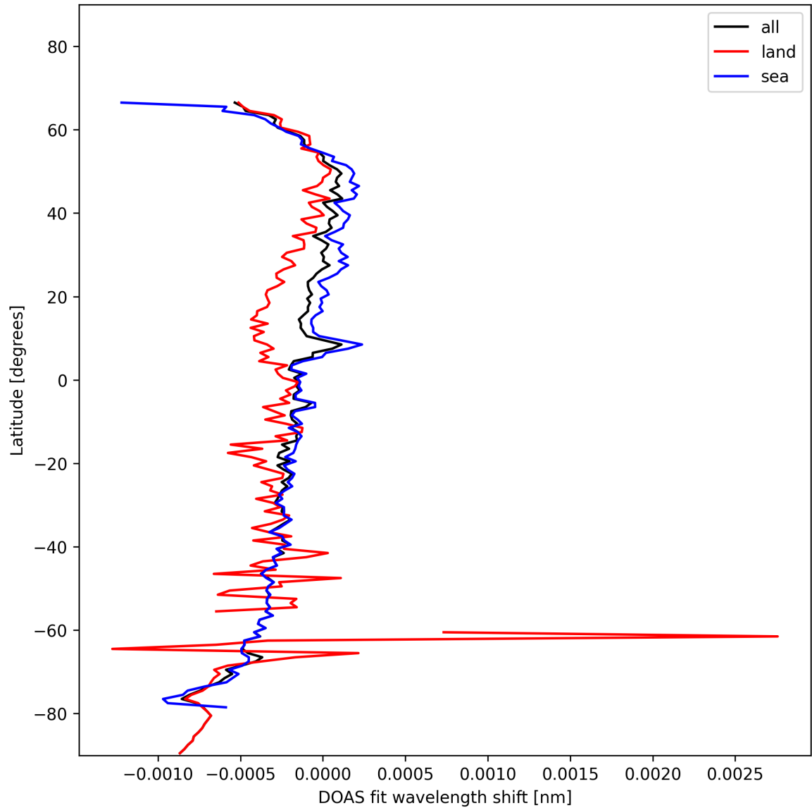
Figure 30: Zonal average of “DOAS fit wavelength shift” for 2025-01-23 to 2025-01-25.
