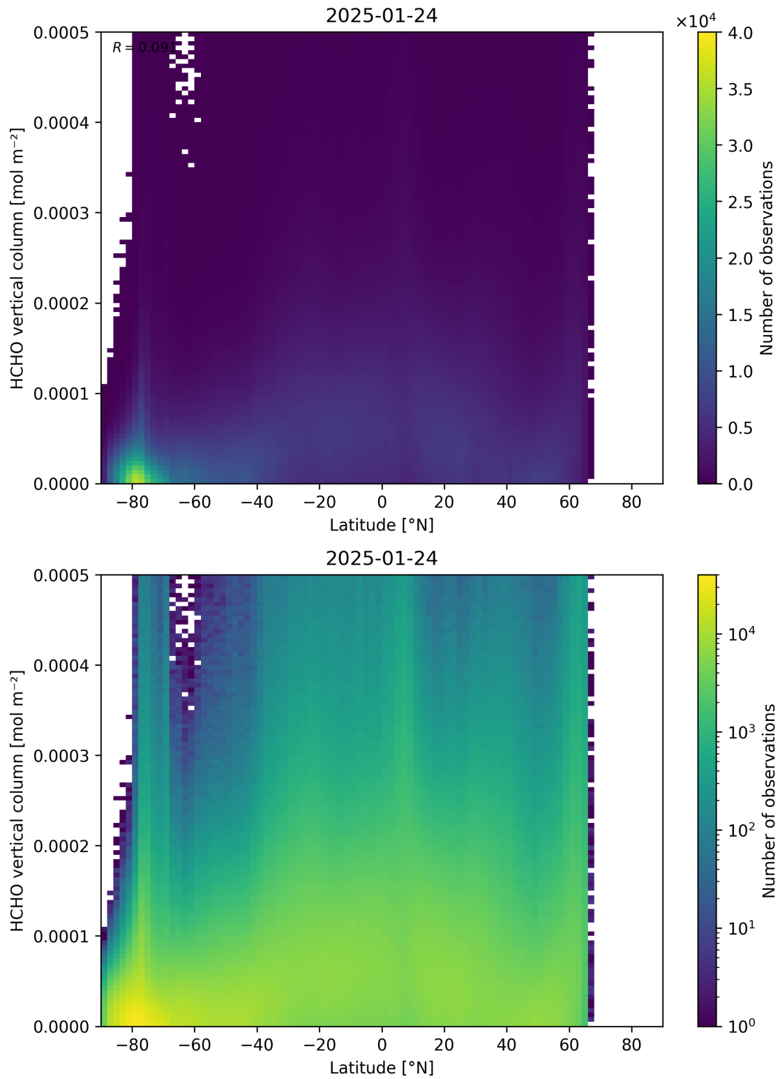
Figure 163: Scatter density plot of “Latitude” against “HCHO vertical column” for 2025-01-23 to 2025-01-25.
