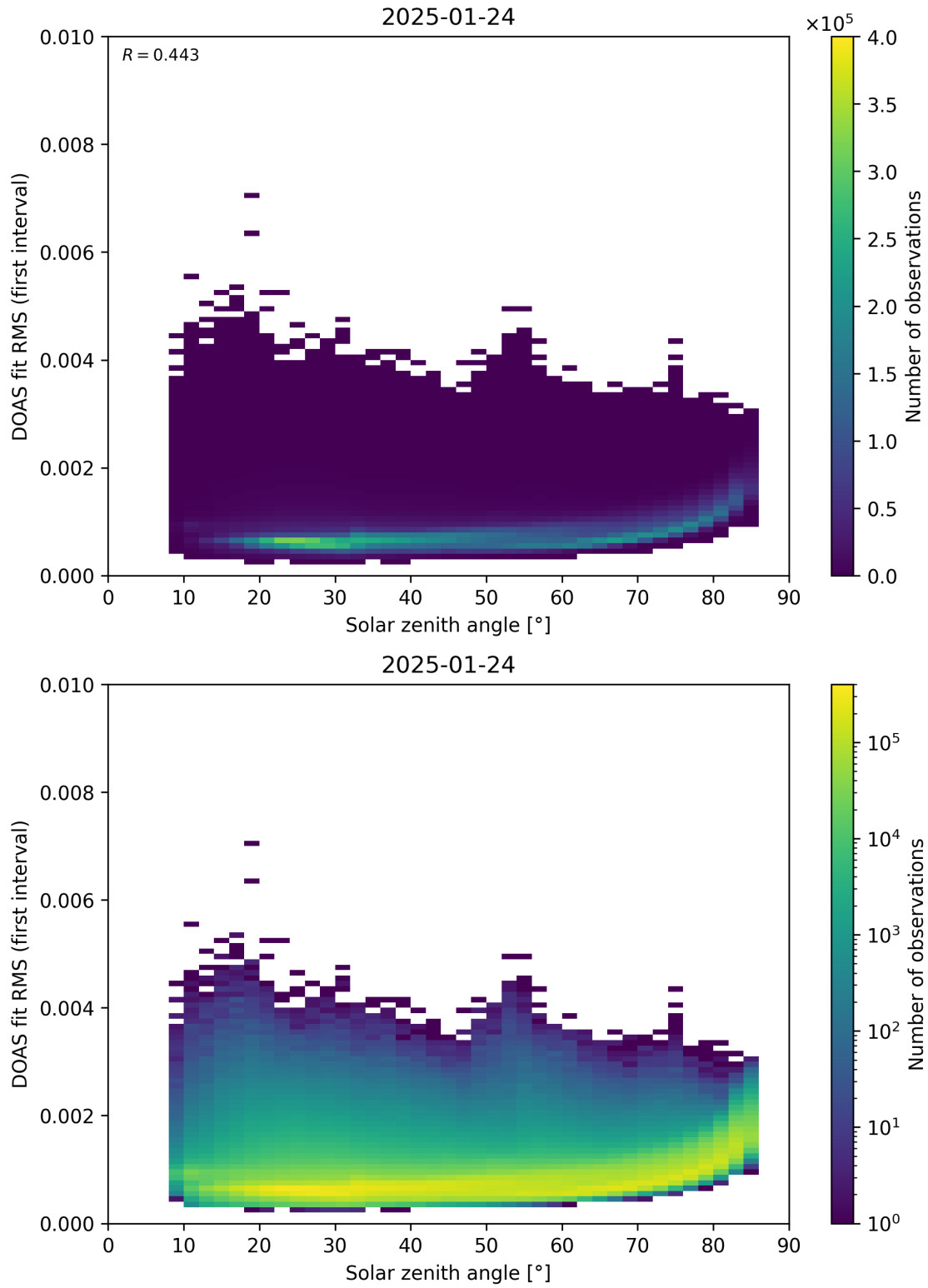
Figure 167: Scatter density plot of “Solar zenith angle” against “DOAS fit RMS (first interval)” for 2025-01-23 to 2025-01-25.
