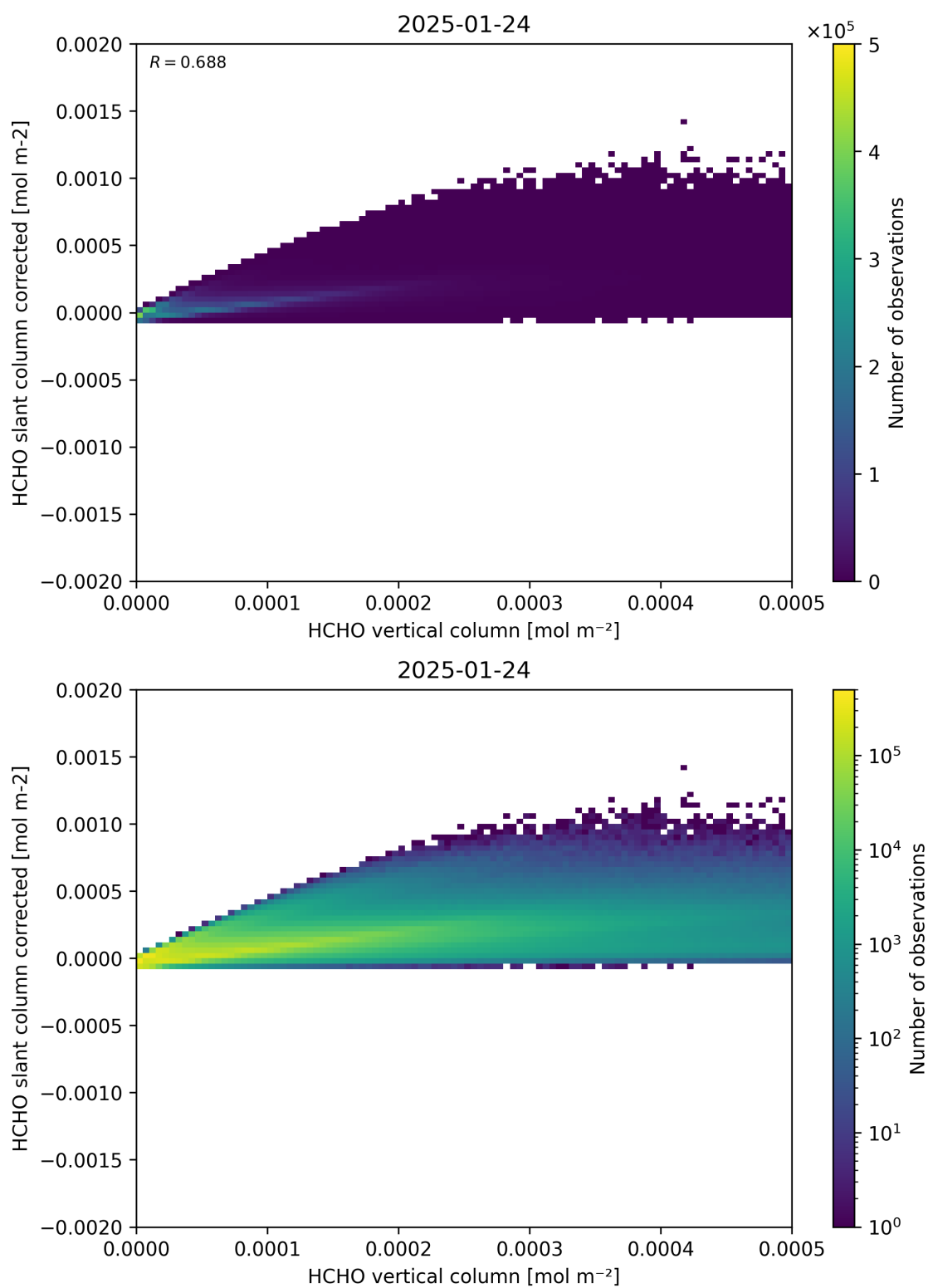
Figure 127: Scatter density plot of “HCHO vertical column” against “HCHO slant column corrected” for 2025-01-23 to 2025-01-25.
