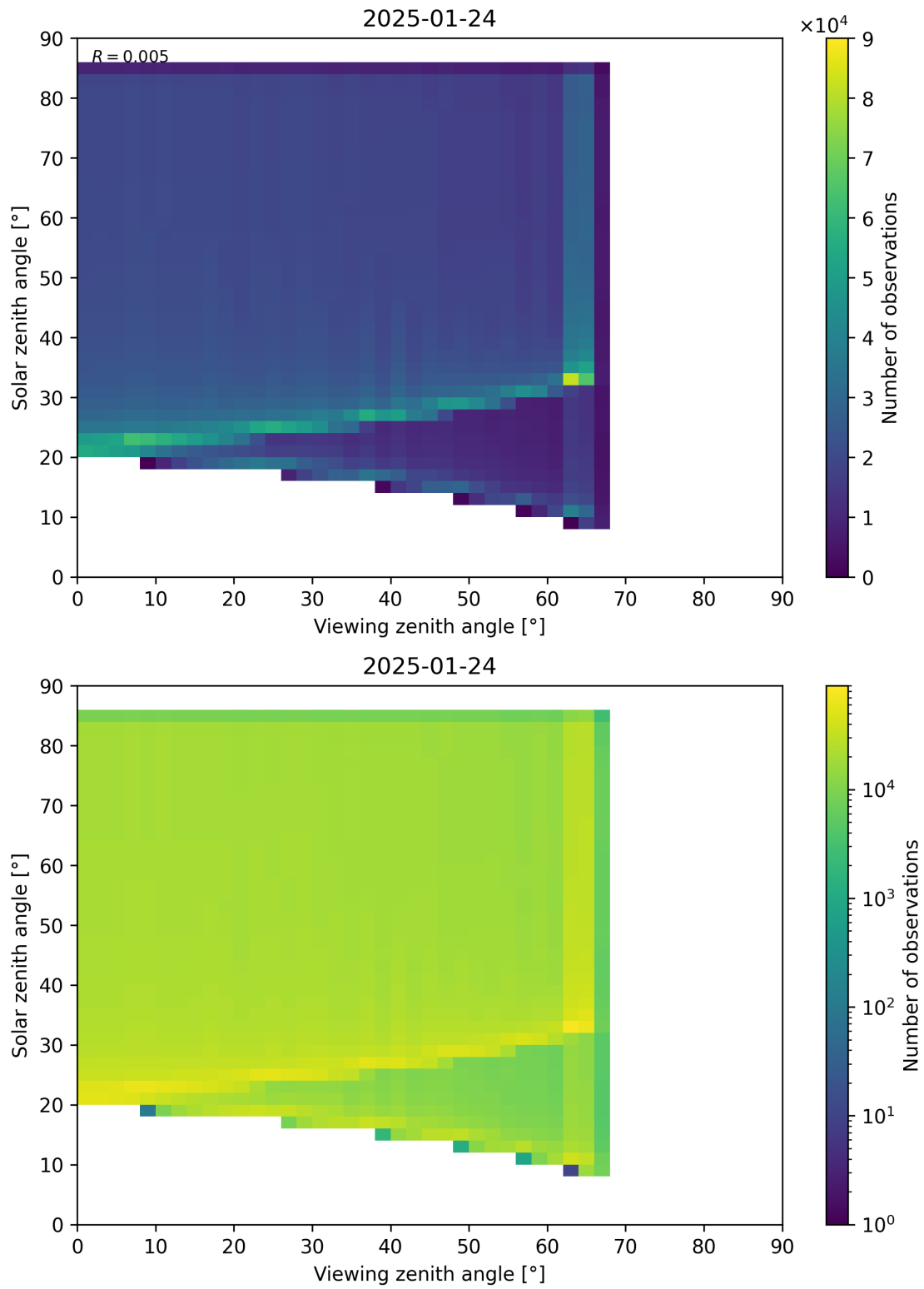
Figure 197: Scatter density plot of “Viewing zenith angle” against “Solar zenith angle” for 2025-01-23 to 2025-01-25.
