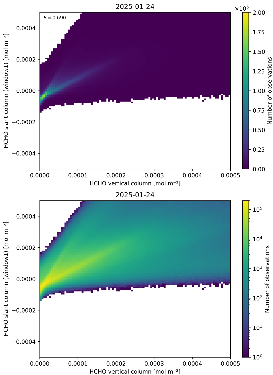
Figure 129: Scatter density plot of “HCHO vertical column” against “HCHO slant column (window1)” for 2025-01-23 to 2025-01-25.
