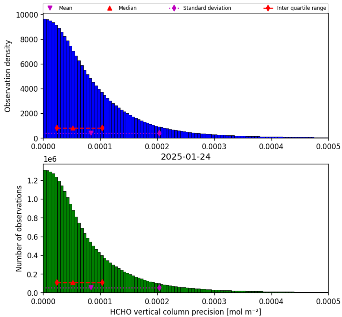
Figure 36: Histogram of “HCHO vertical column precision” for 2025-01-23 to 2025-01-25
