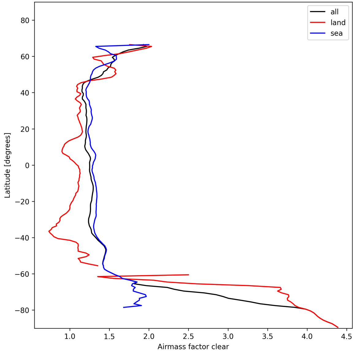
Figure 28: Zonal average of “Airmass factor clear” for 2025-01-23 to 2025-01-25.
