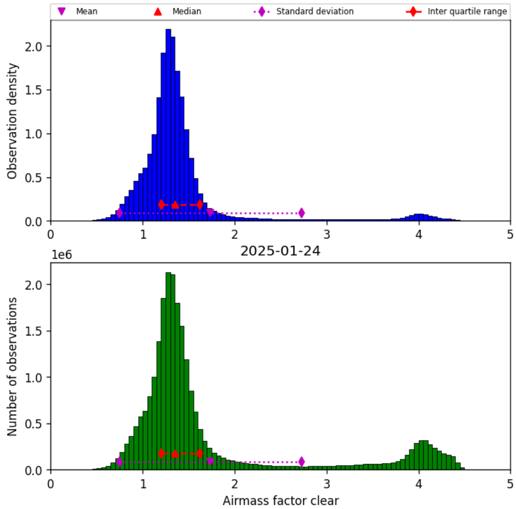
Figure 42: Histogram of “Airmass factor clear” for 2025-01-23 to 2025-01-25
