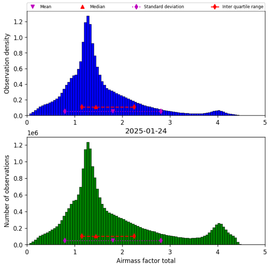
Figure 40: Histogram of “Airmass factor total” for 2025-01-23 to 2025-01-25
