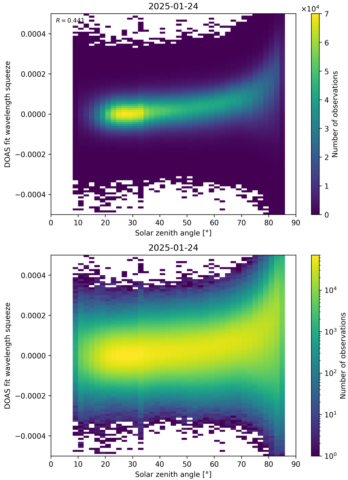
Figure 169: Scatter density plot of “Solar zenith angle” against “DOAS fit wavelength squeeze” for 2025-01-23 to 2025-01-25.
