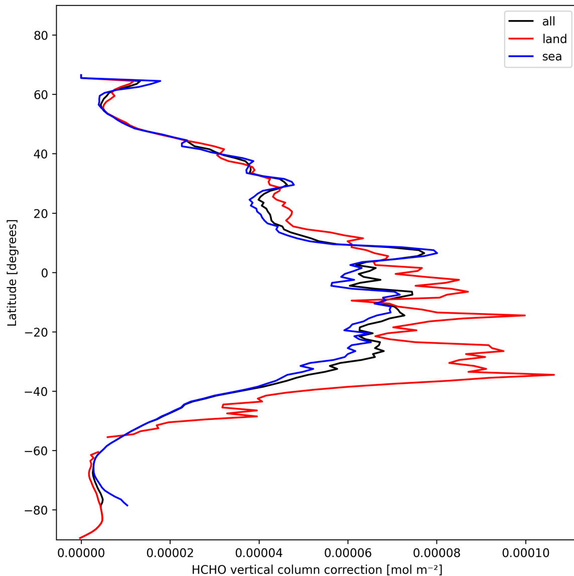
Figure 23: Zonal average of “HCHO vertical column correction” for 2025-01-23 to 2025-01-25.
