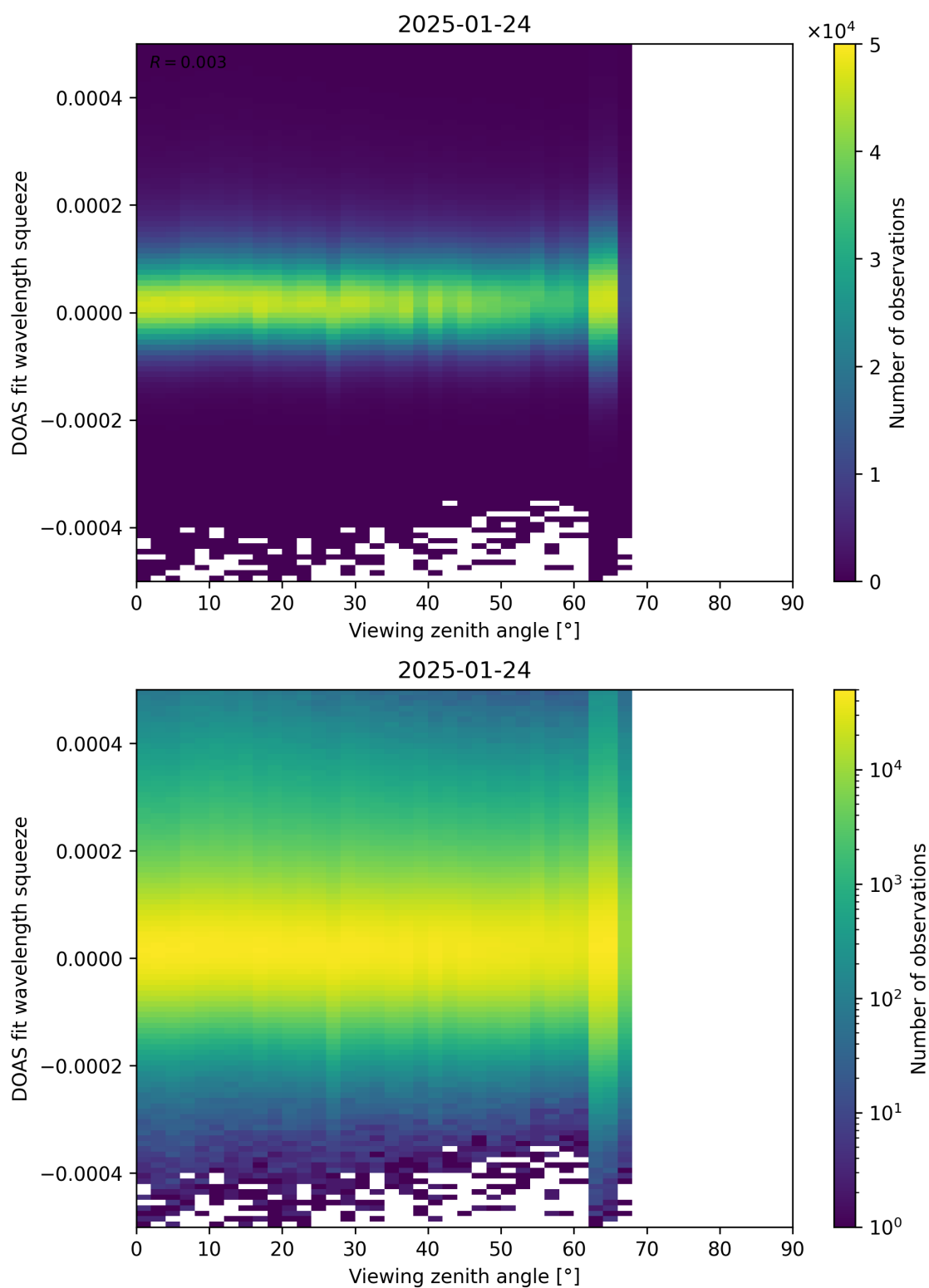
Figure 184: Scatter density plot of “Viewing zenith angle” against “DOAS fit wavelength squeeze” for 2025-01-23 to 2025-01-25.
