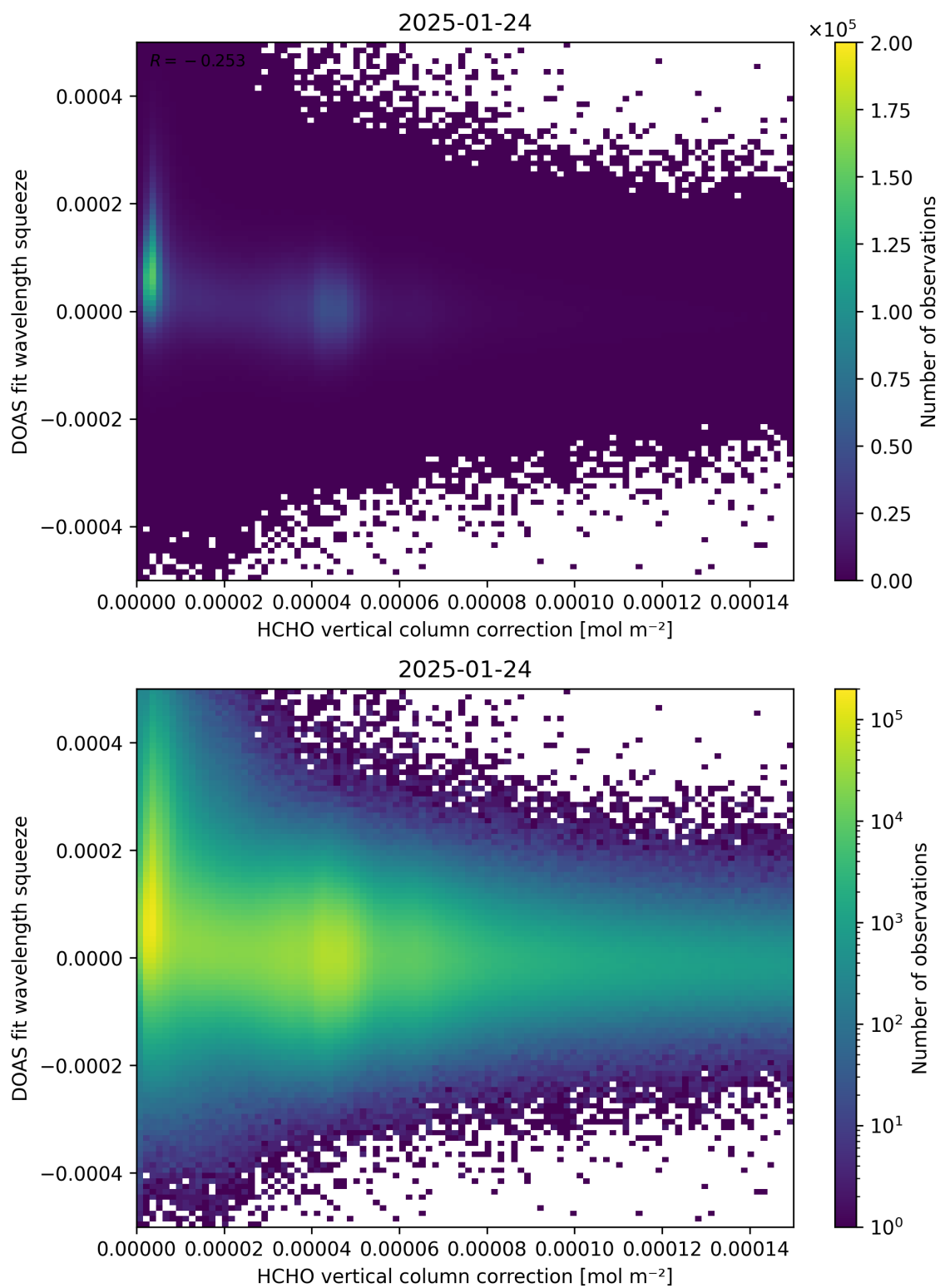
Figure 114: Scatter density plot of “HCHO vertical column correction” against “DOAS fit wavelength squeeze” for 2025-01-23 to 2025-01-25.
