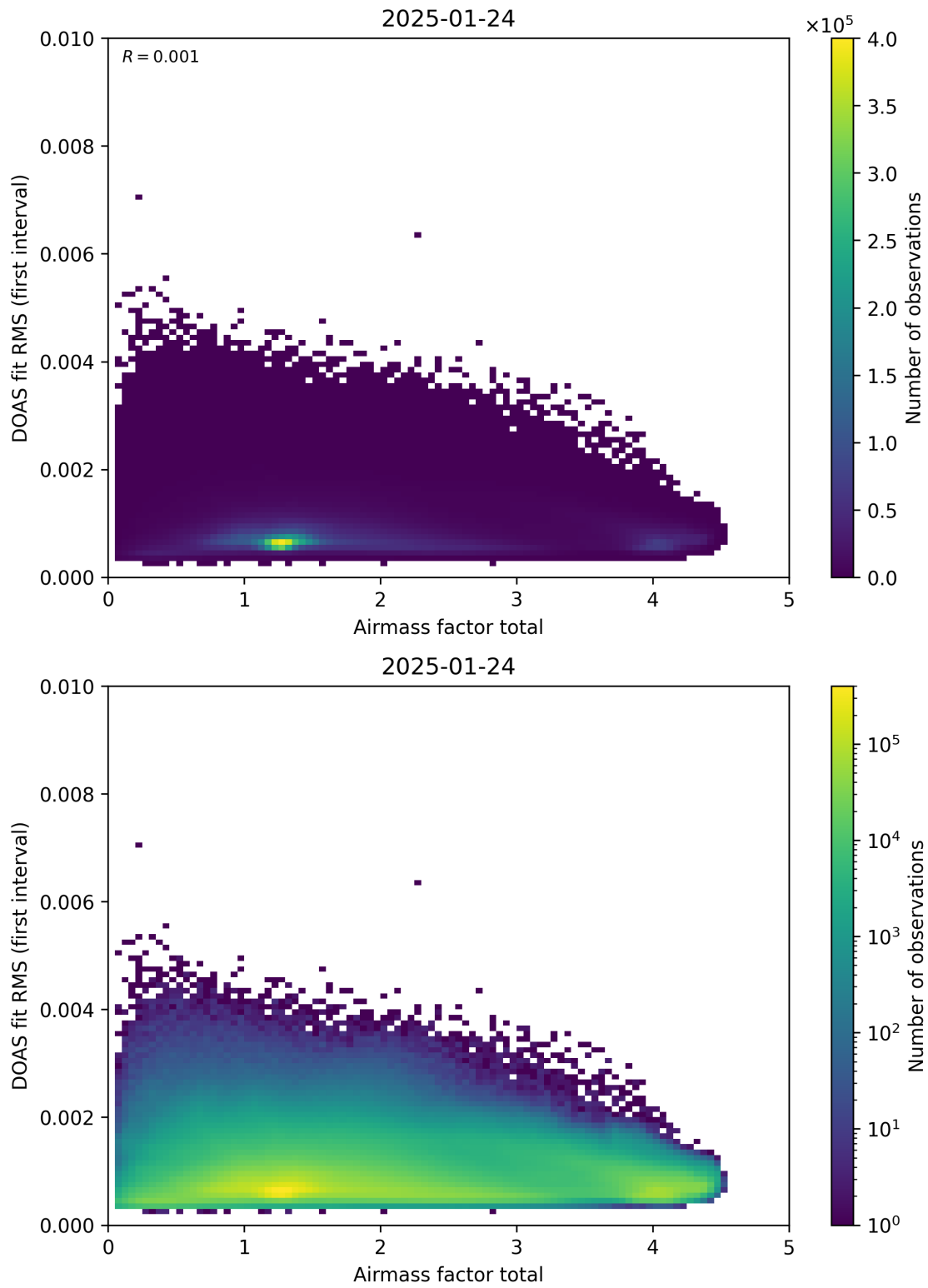
Figure 97: Scatter density plot of “Airmass factor total” against “DOAS fit RMS (first interval)” for 2025-01-23 to 2025-01-25.
