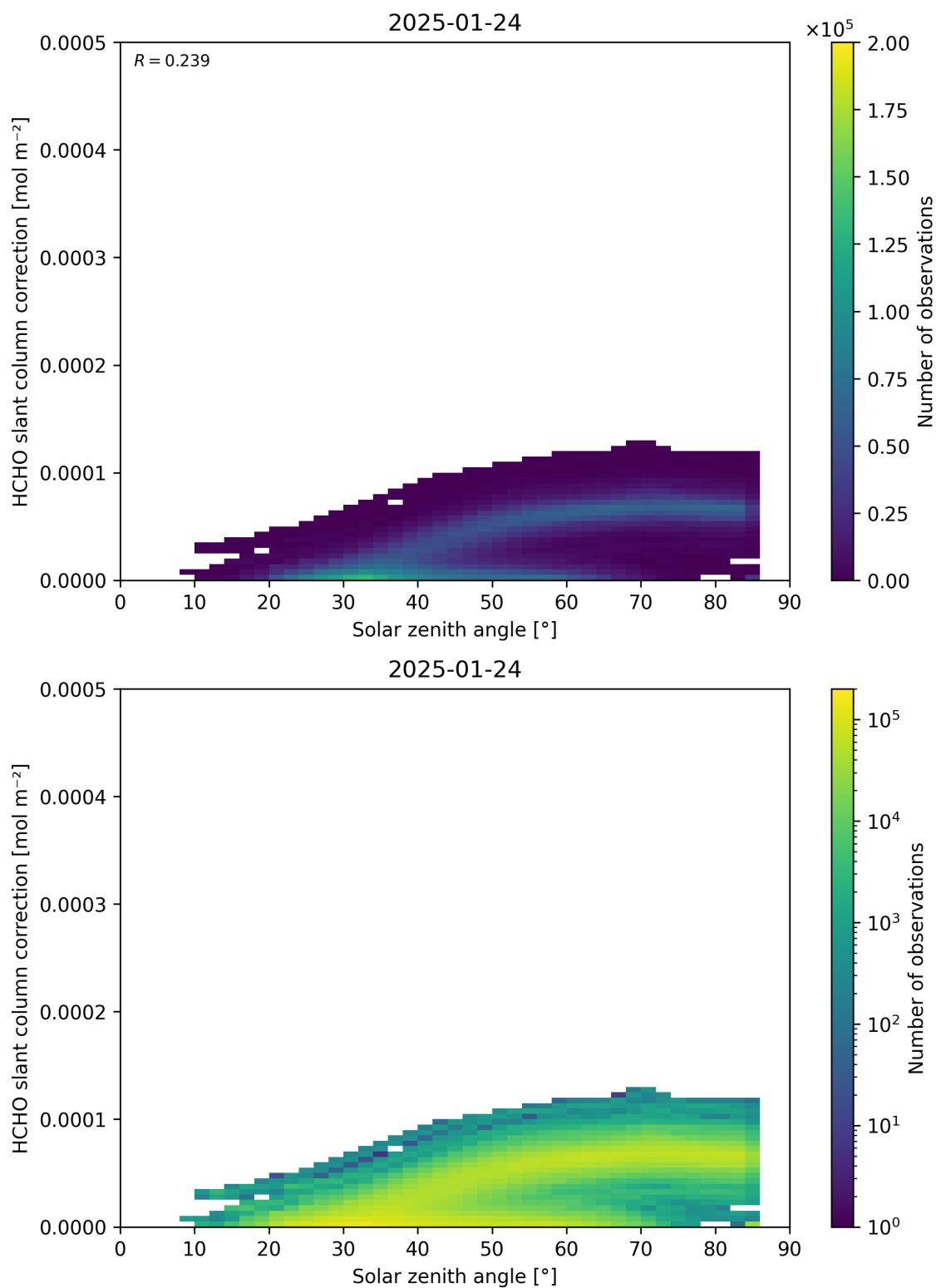
Figure 172: Scatter density plot of “Solar zenith angle” against “HCHO slant column correction” for 2025-01-23 to 2025-01-25.
