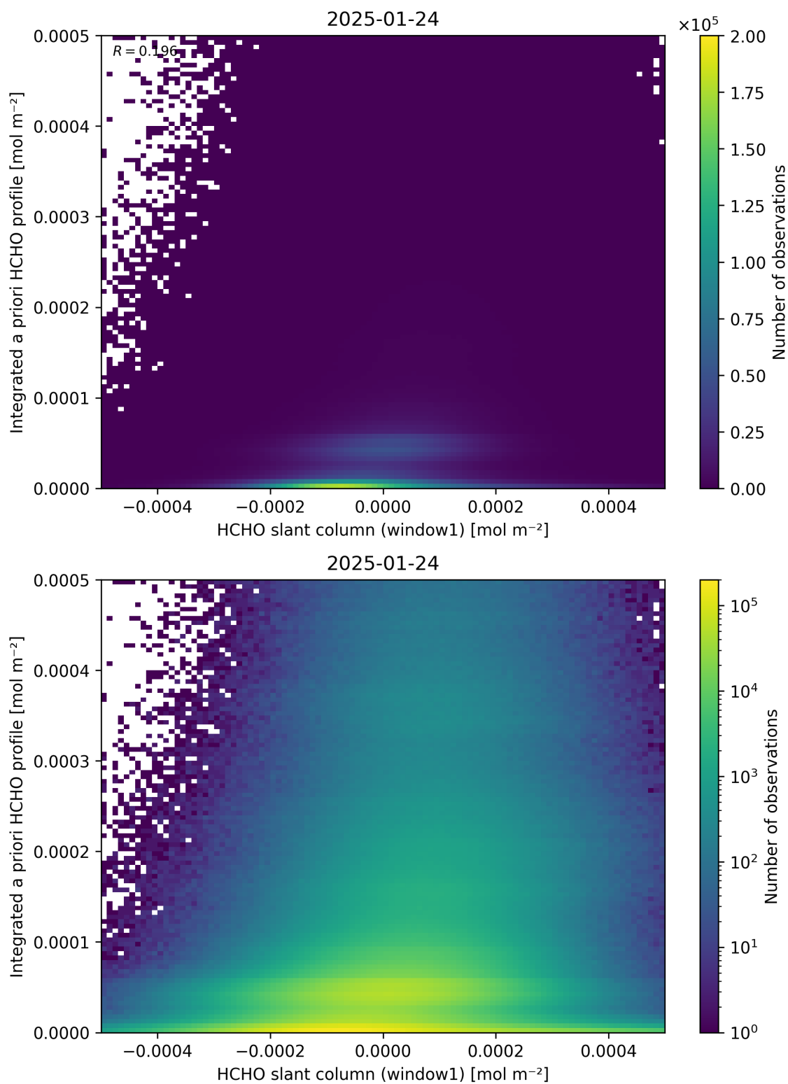
Figure 87: Scatter density plot of “HCHO slant column (window1)” against “Integrated a priori HCHO profile” for 2025-01-23 to 2025-01-25.
