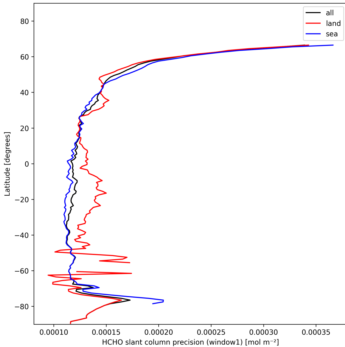
Figure 25: Zonal average of “HCHO slant column precision (window1)” for 2025-01-23 to 2025-01-25.
