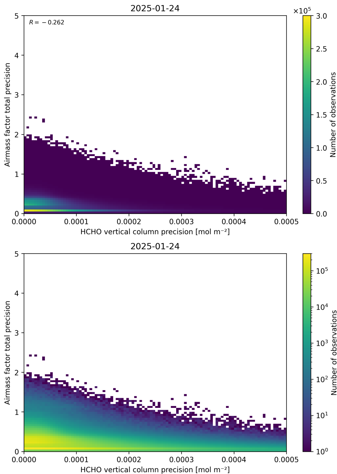
Figure 145: Scatter density plot of “HCHO vertical column precision” against “Airmass factor total precision” for 2025-01-23 to 2025-01-25.
