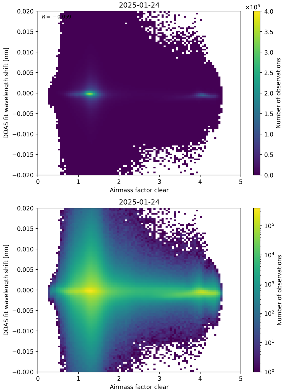
Figure 72: Scatter density plot of “Airmass factor clear” against “DOAS fit wavelength shift” for 2025-01-23 to 2025-01-25.
