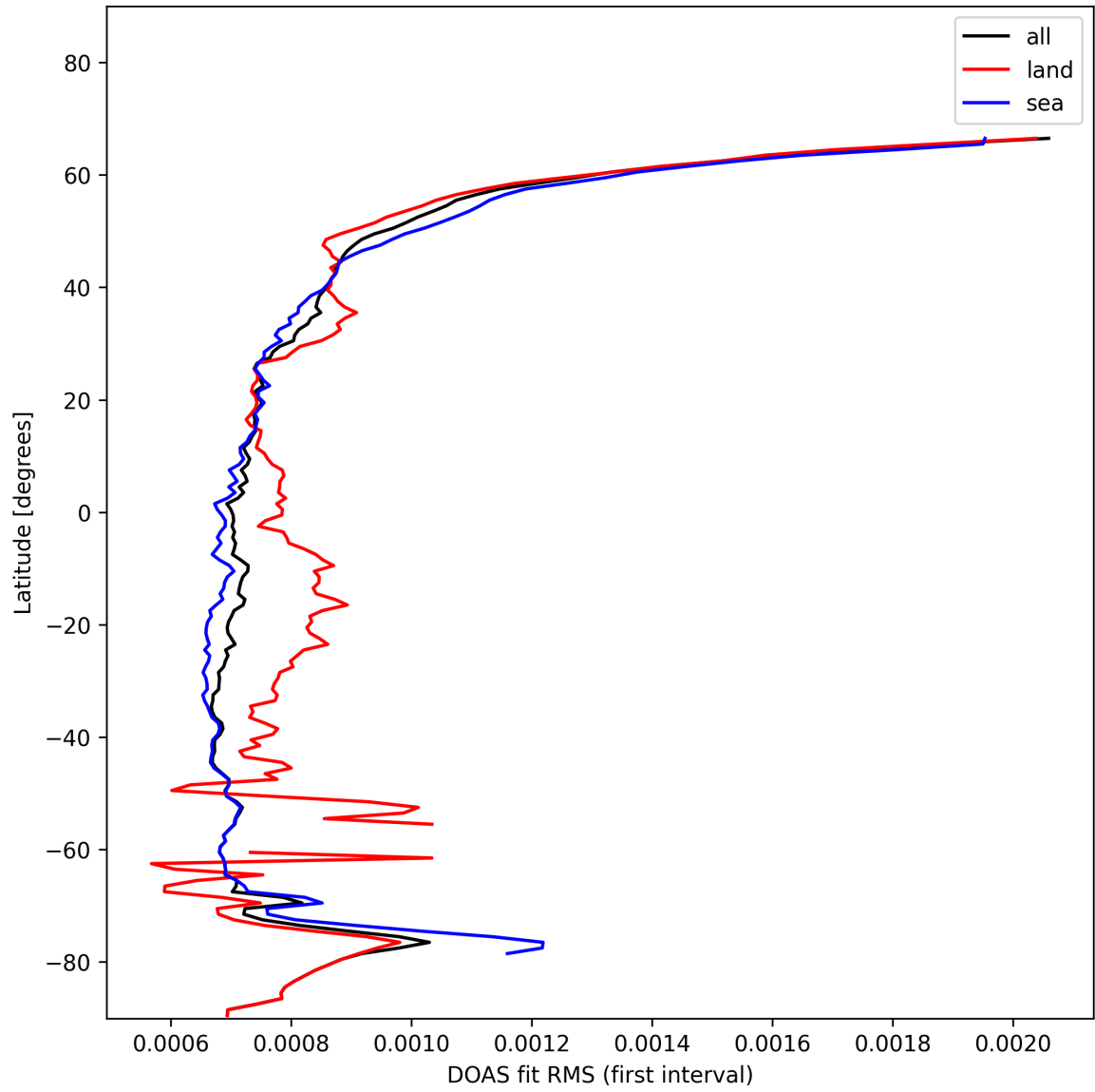
Figure 32: Zonal average of “DOAS fit RMS (first interval)” for 2025-01-23 to 2025-01-25.
