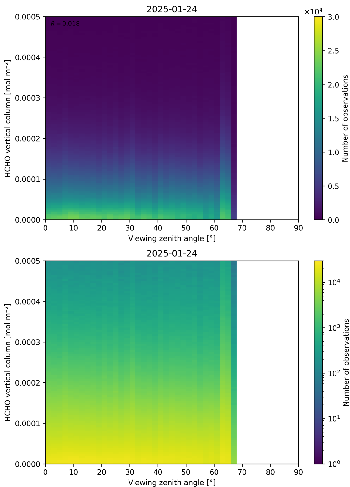
Figure 192: Scatter density plot of “Viewing zenith angle” against “HCHO vertical column” for 2025-01-23 to 2025-01-25.
