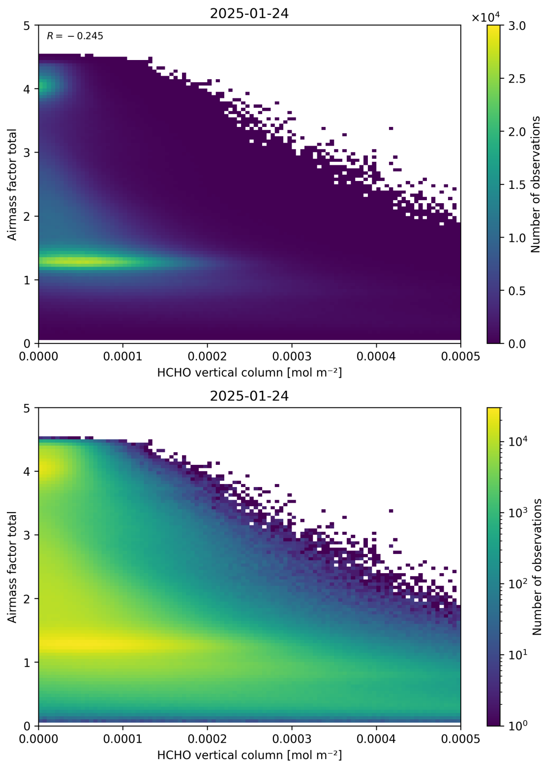
Figure 131: Scatter density plot of “HCHO vertical column” against “Airmass factor total” for 2025-01-23 to 2025-01-25.
