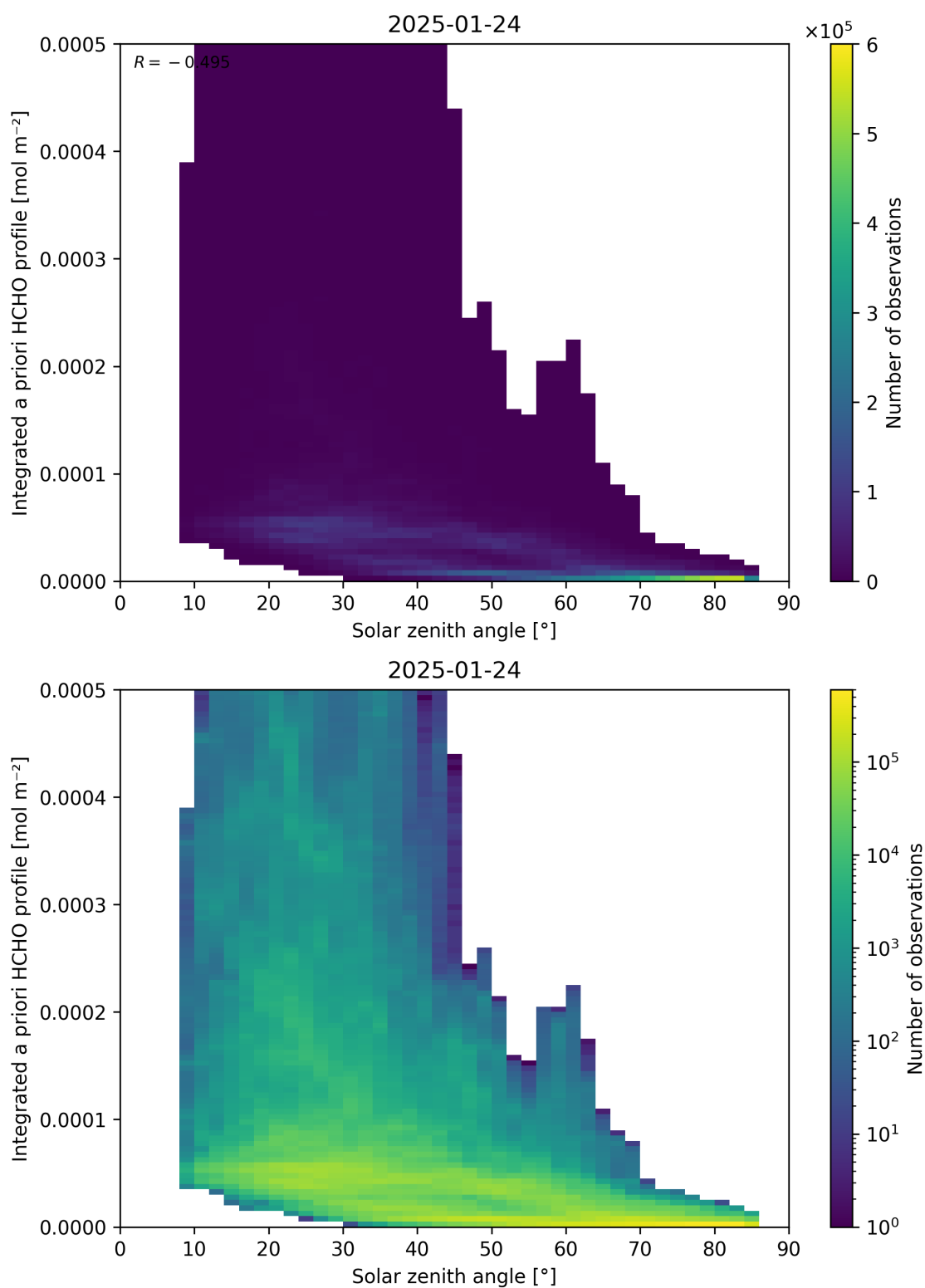
Figure 180: Scatter density plot of “Solar zenith angle” against “Integrated a priori HCHO profile” for 2025-01-23 to 2025-01-25.
