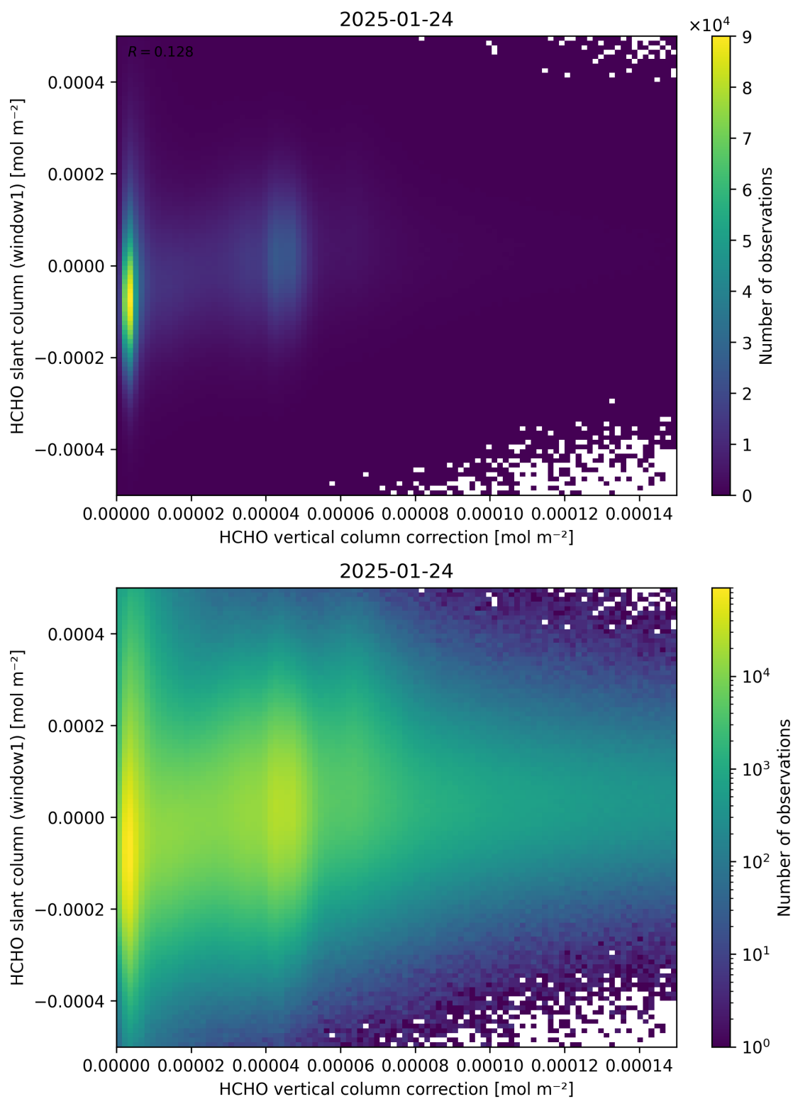
Figure 118: Scatter density plot of “HCHO vertical column correction” against “HCHO slant column (window1)” for 2025-01-23 to 2025-01-25.
