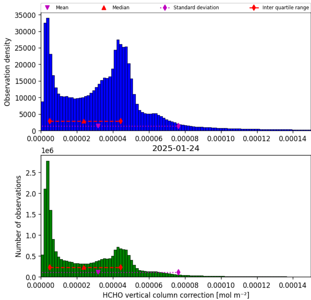
Figure 37: Histogram of “HCHO vertical column correction” for 2025-01-23 to 2025-01-25
