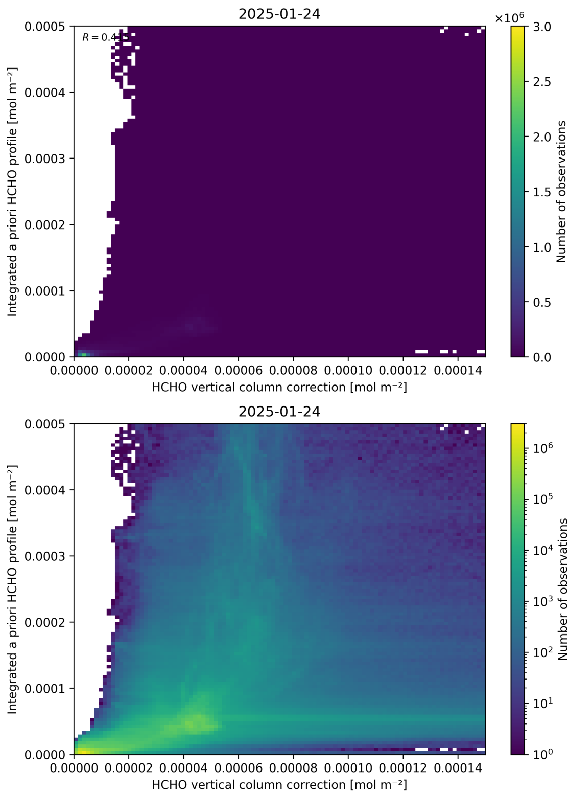
Figure 122: Scatter density plot of “HCHO vertical column correction” against “Integrated a priori HCHO profile” for 2025-01-23 to 2025-01-25.
