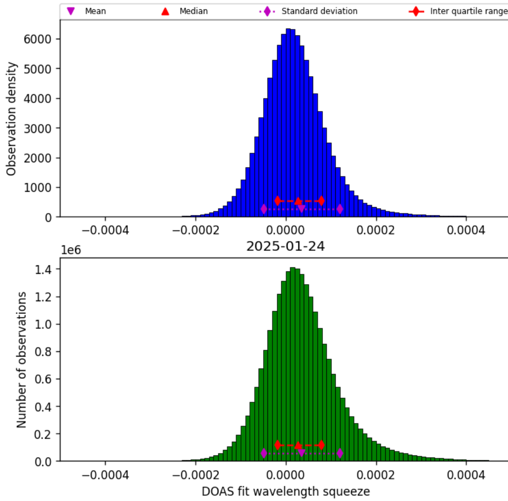
Figure 45: Histogram of “DOAS fit wavelength squeeze” for 2025-01-23 to 2025-01-25
