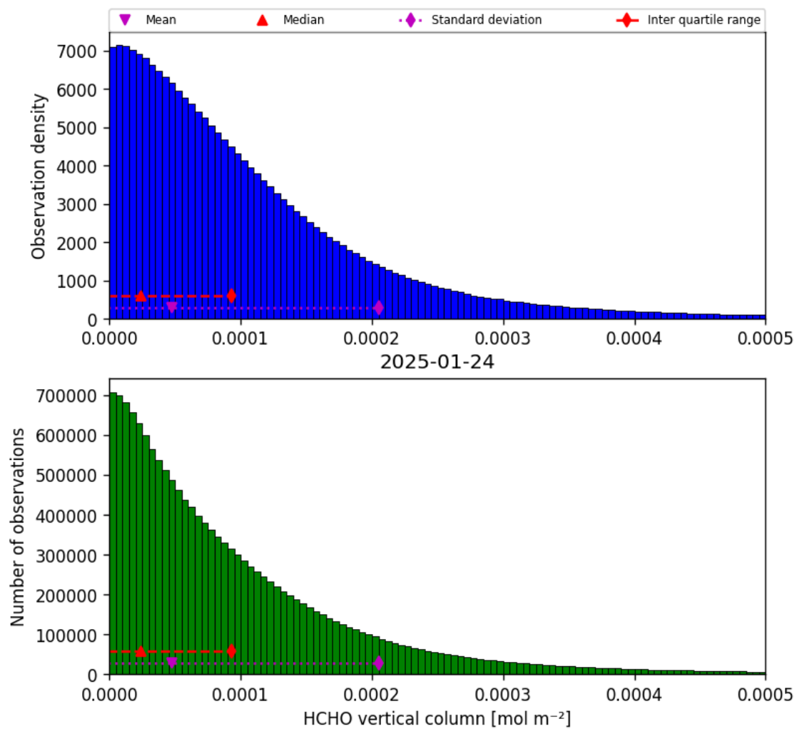
Figure 35: Histogram of “HCHO vertical column” for 2025-01-23 to 2025-01-25
