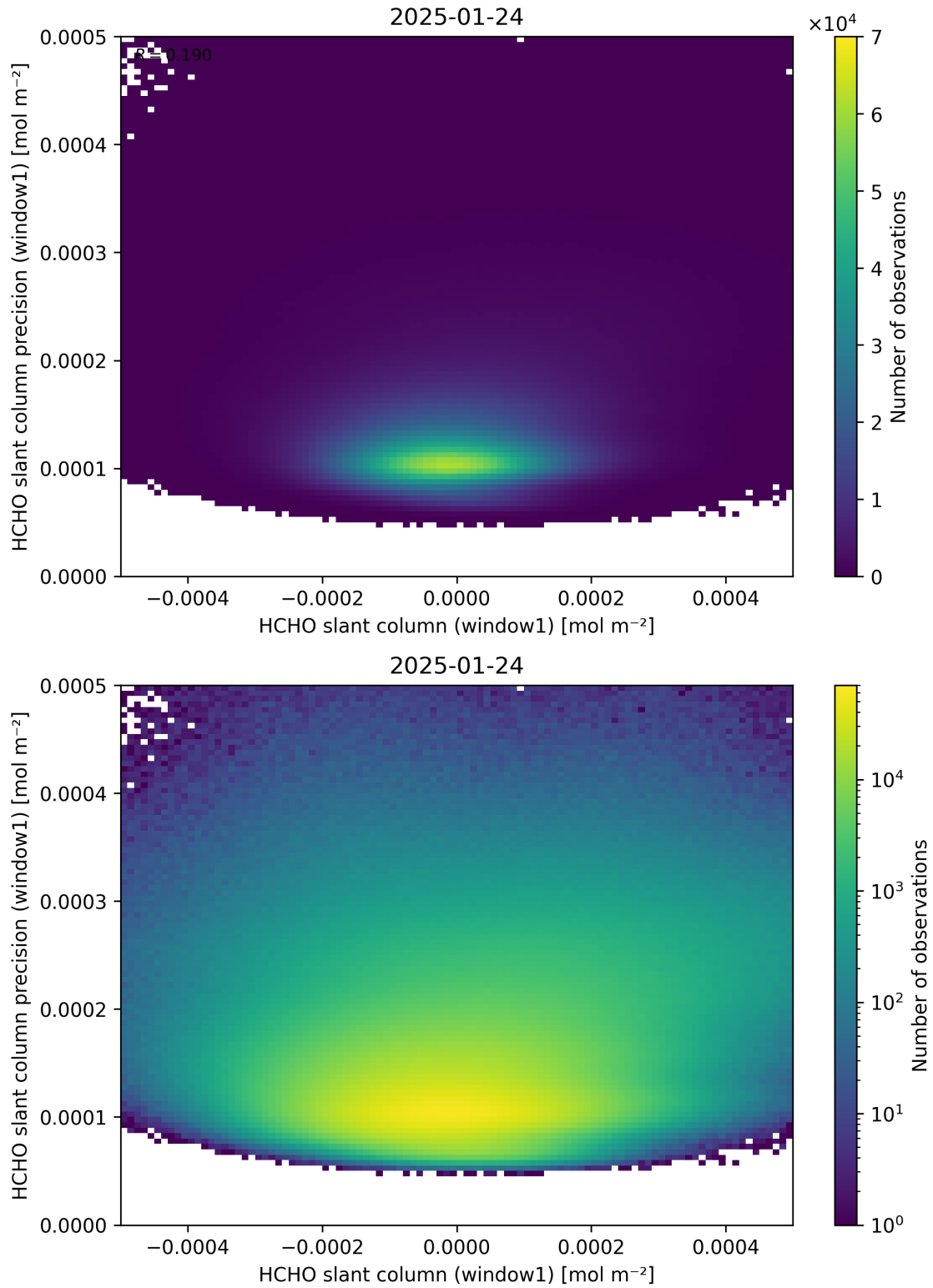
Figure 84: Scatter density plot of “HCHO slant column (window1)” against “HCHO slant column precision (window1)” for 2025-01-23 to 2025-01-25.
