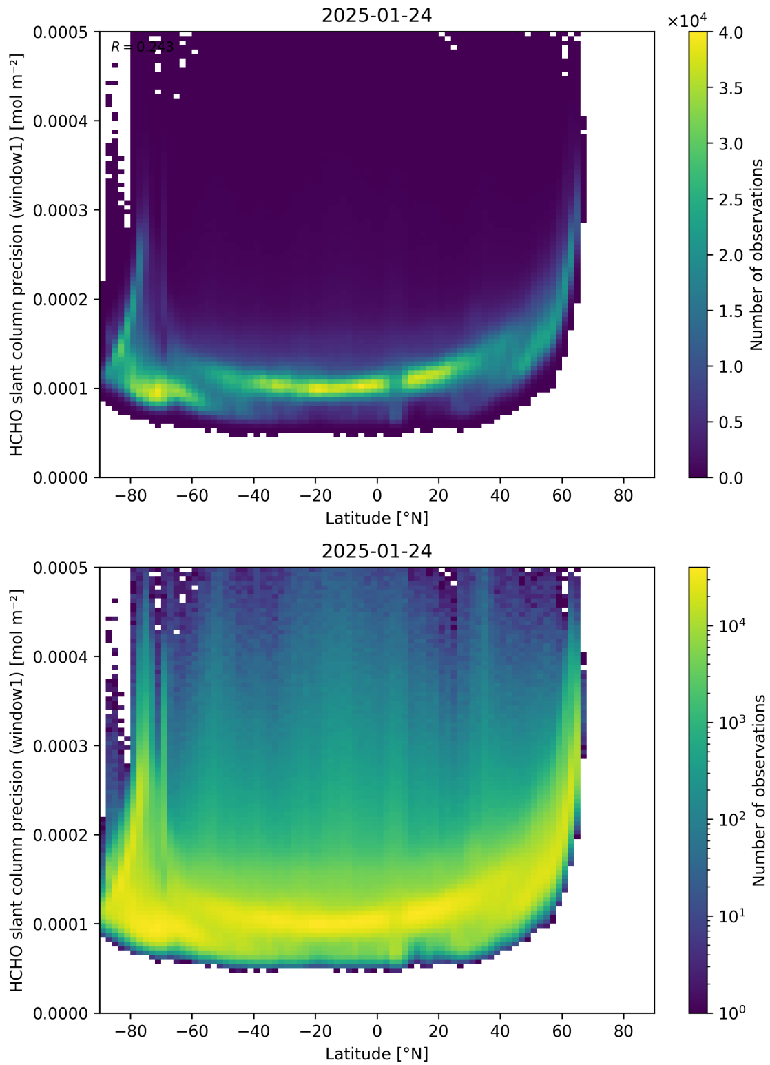
Figure 160: Scatter density plot of “Latitude” against “HCHO slant column precision (window1)” for 2025-01-23 to 2025-01-25.
