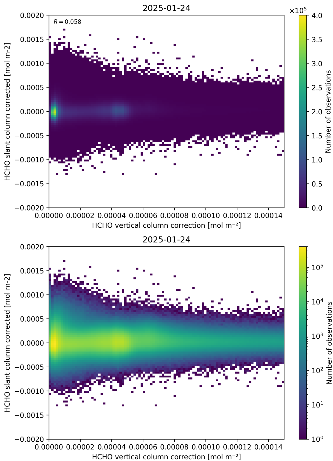
Figure 116: Scatter density plot of “HCHO vertical column correction” against “HCHO slant column corrected” for 2025-01-23 to 2025-01-25.
