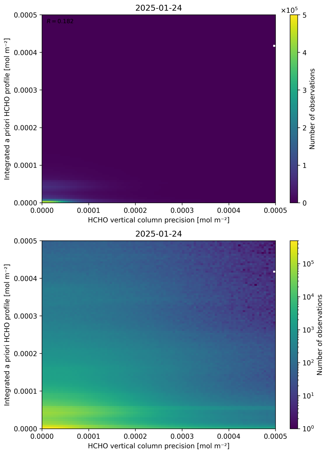
Figure 147: Scatter density plot of “HCHO vertical column precision” against “Integrated a priori HCHO profile” for 2025-01-23 to 2025-01-25.
