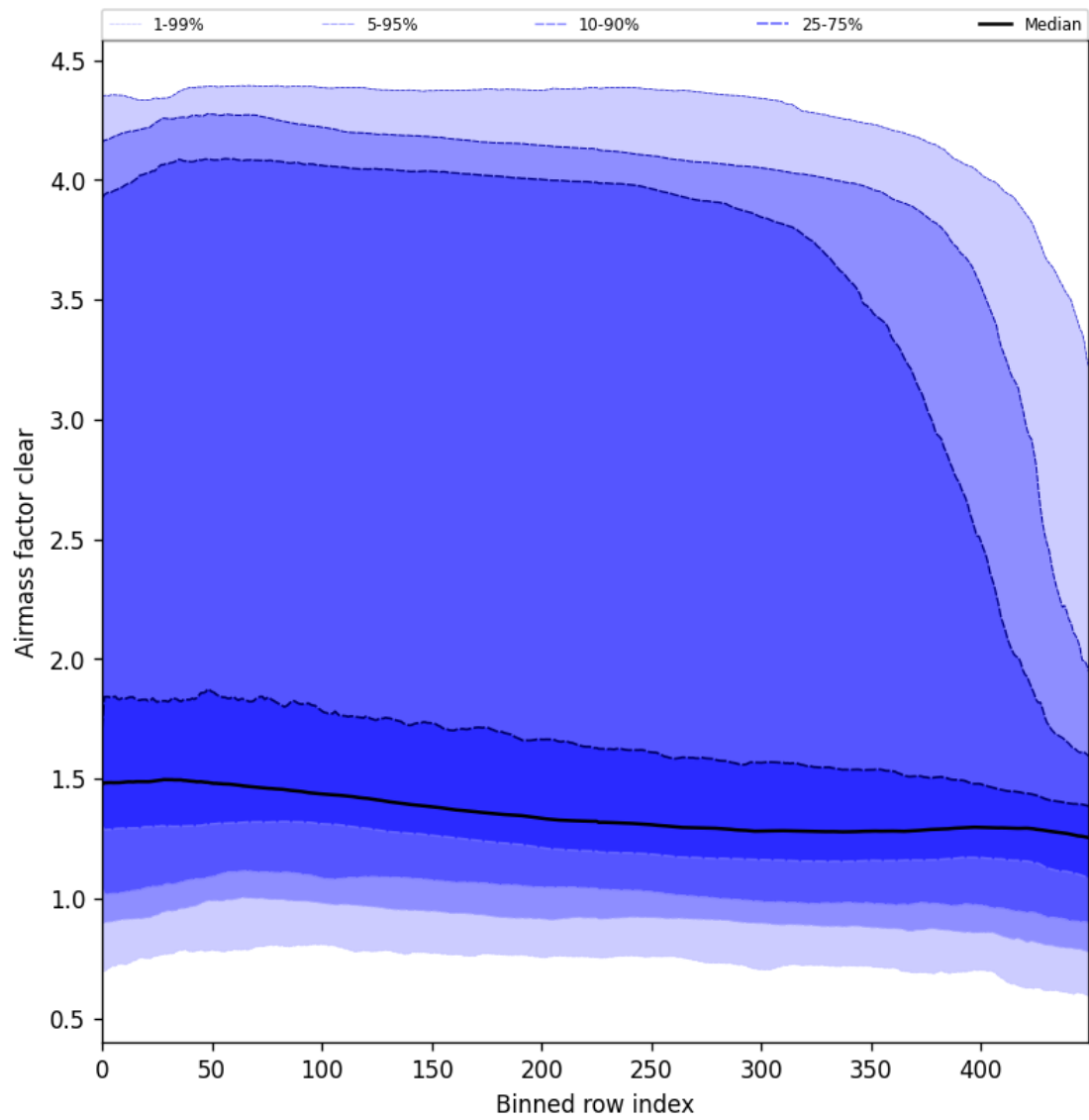
Figure 56: Along track statistics of “Airmass factor clear” for 2025-01-23 to 2025-01-25
