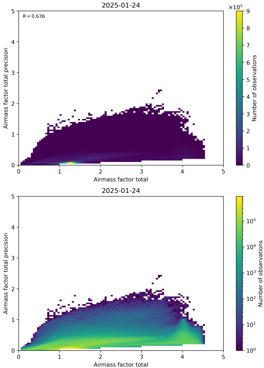
Figure 103: Scatter density plot of “Airmass factor total” against “Airmass factor total precision” for 2025-01-23 to 2025-01-25.
