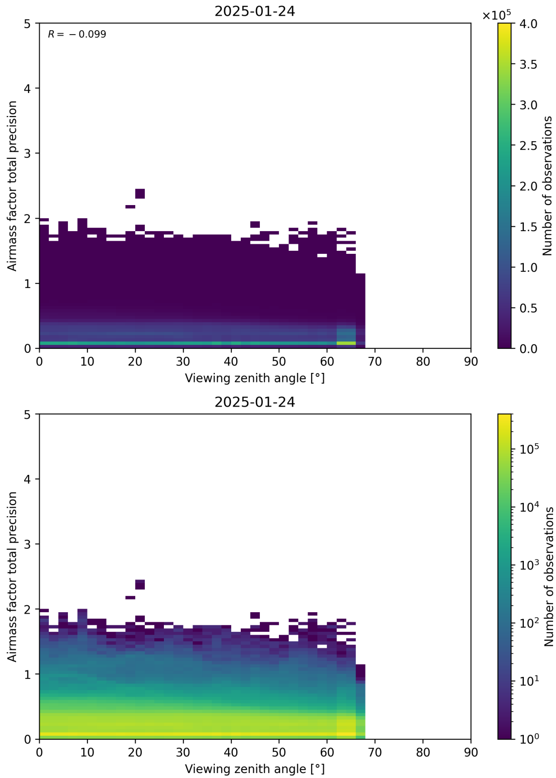
Figure 191: Scatter density plot of “Viewing zenith angle” against “Airmass factor total precision” for 2025-01-23 to 2025-01-25.
