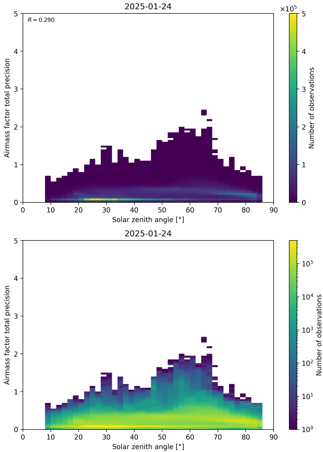
Figure 176: Scatter density plot of “Solar zenith angle” against “Airmass factor total precision” for 2025-01-23 to 2025-01-25.
