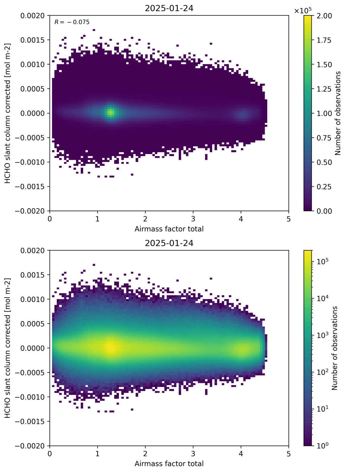
Figure 101: Scatter density plot of “Airmass factor total” against “HCHO slant column corrected” for 2025-01-23 to 2025-01-25.
