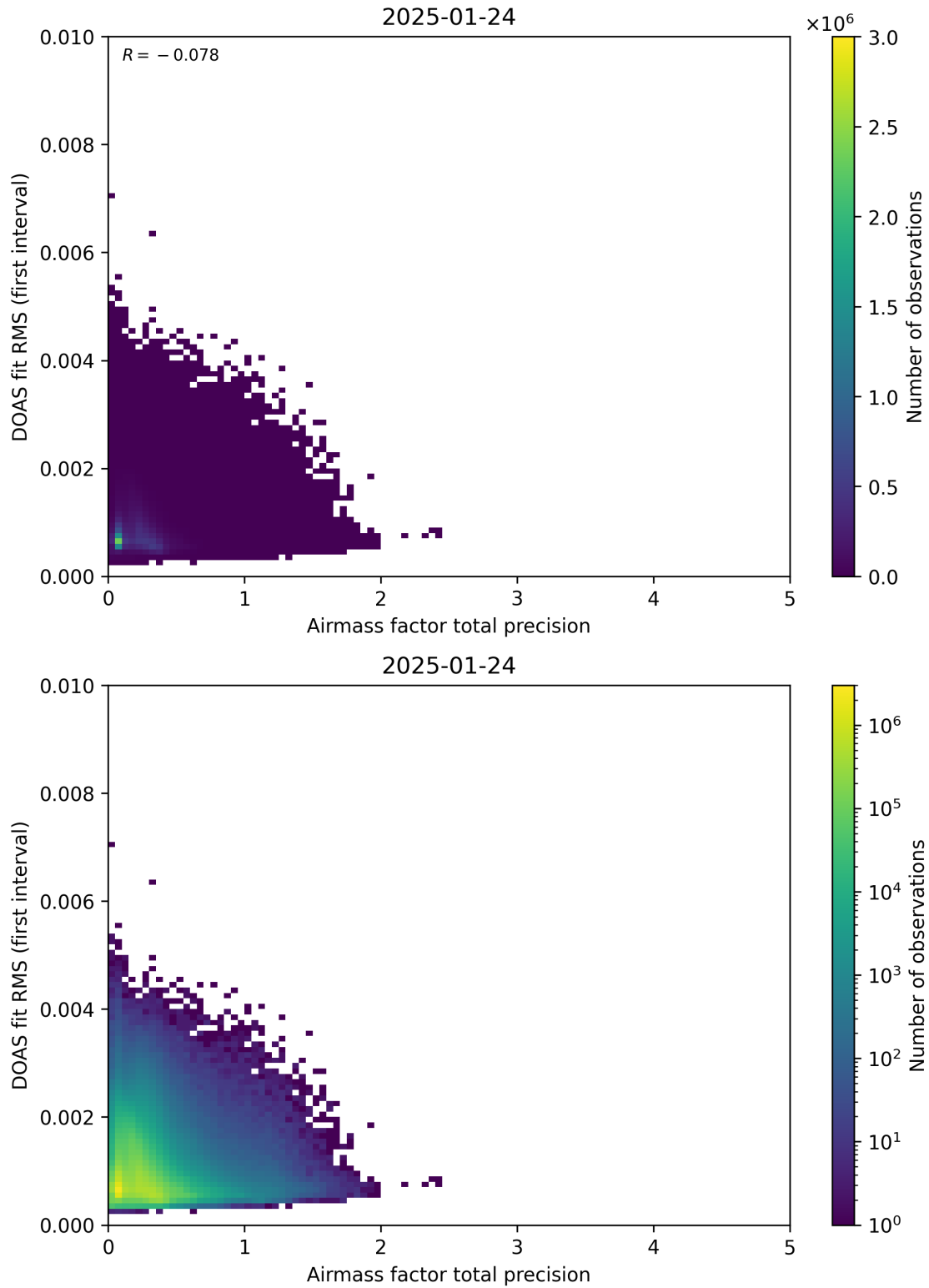
Figure 105: Scatter density plot of “Airmass factor total precision” against “DOAS fit RMS (first interval)” for 2025-01-23 to 2025-01-25.
