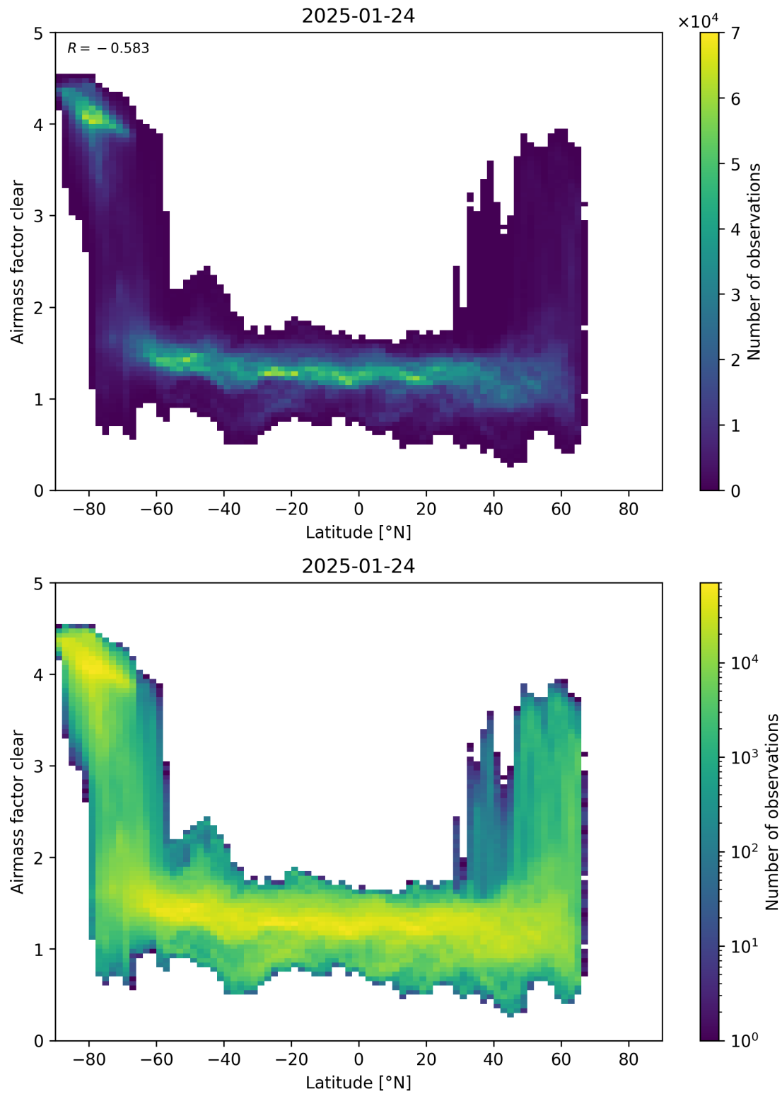
Figure 156: Scatter density plot of “Latitude” against “Airmass factor clear” for 2025-01-23 to 2025-01-25.
