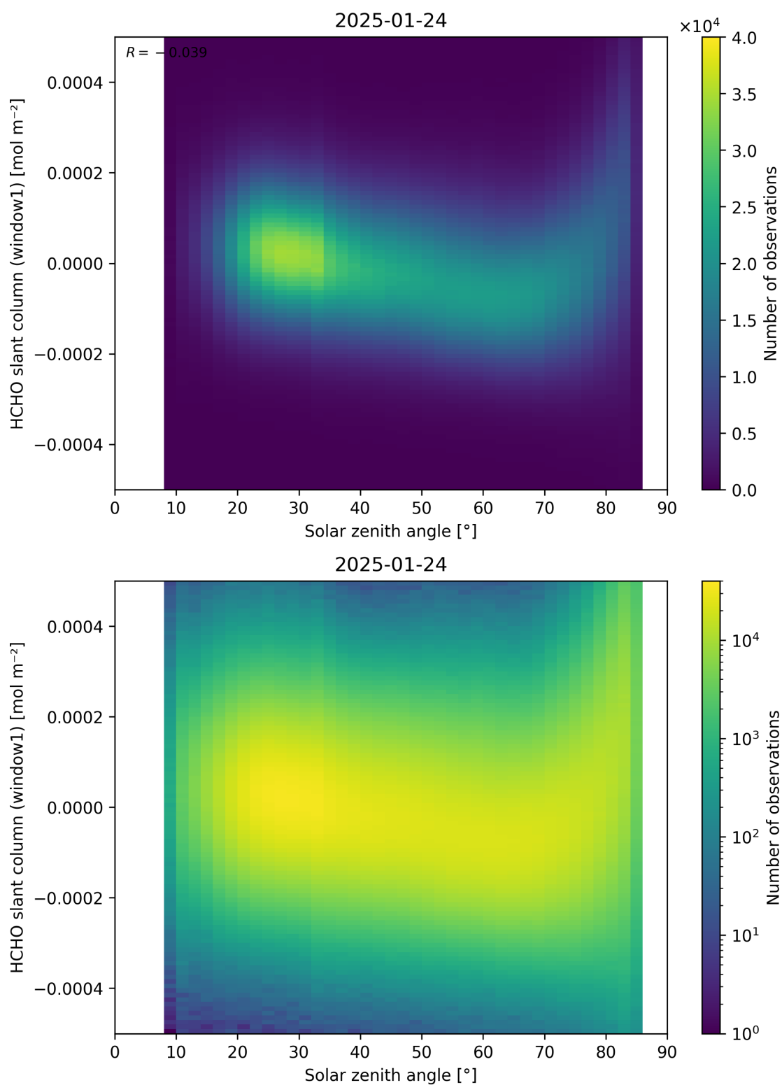
Figure 173: Scatter density plot of “Solar zenith angle” against “HCHO slant column (window1)” for 2025-01-23 to 2025-01-25.
