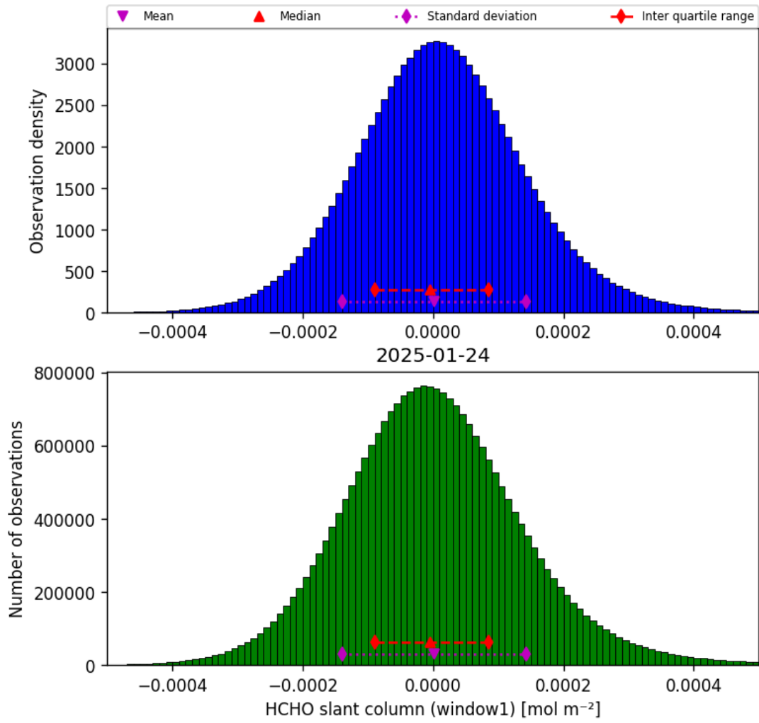
Figure 38: Histogram of “HCHO slant column (window1)” for 2025-01-23 to 2025-01-25
