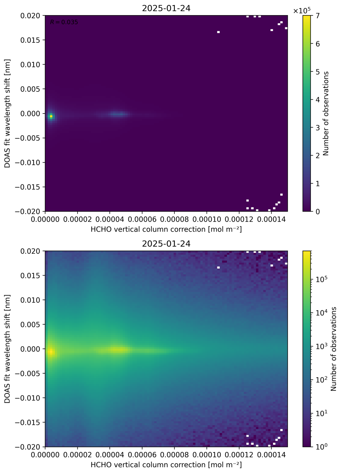
Figure 113: Scatter density plot of “HCHO vertical column correction” against “DOAS fit wavelength shift” for 2025-01-23 to 2025-01-25.
