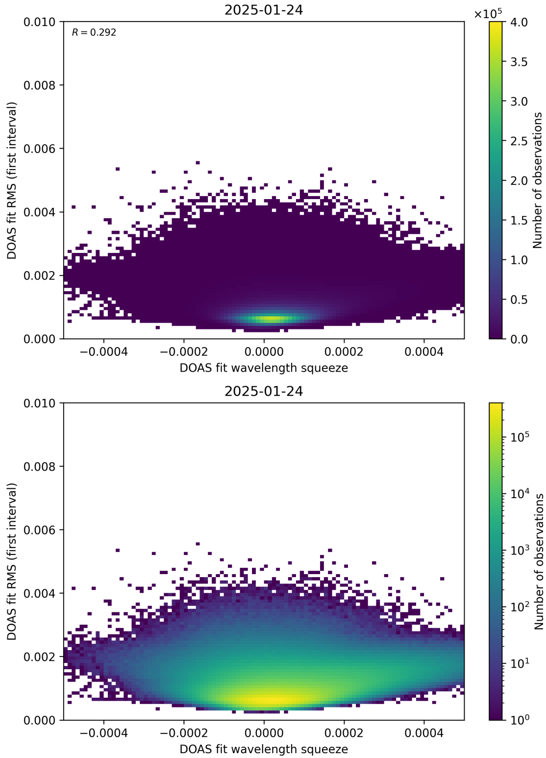
Figure 68: Scatter density plot of “DOAS fit wavelength squeeze” against “DOAS fit RMS (first interval)” for 2025-01-23 to 2025-01-25.
