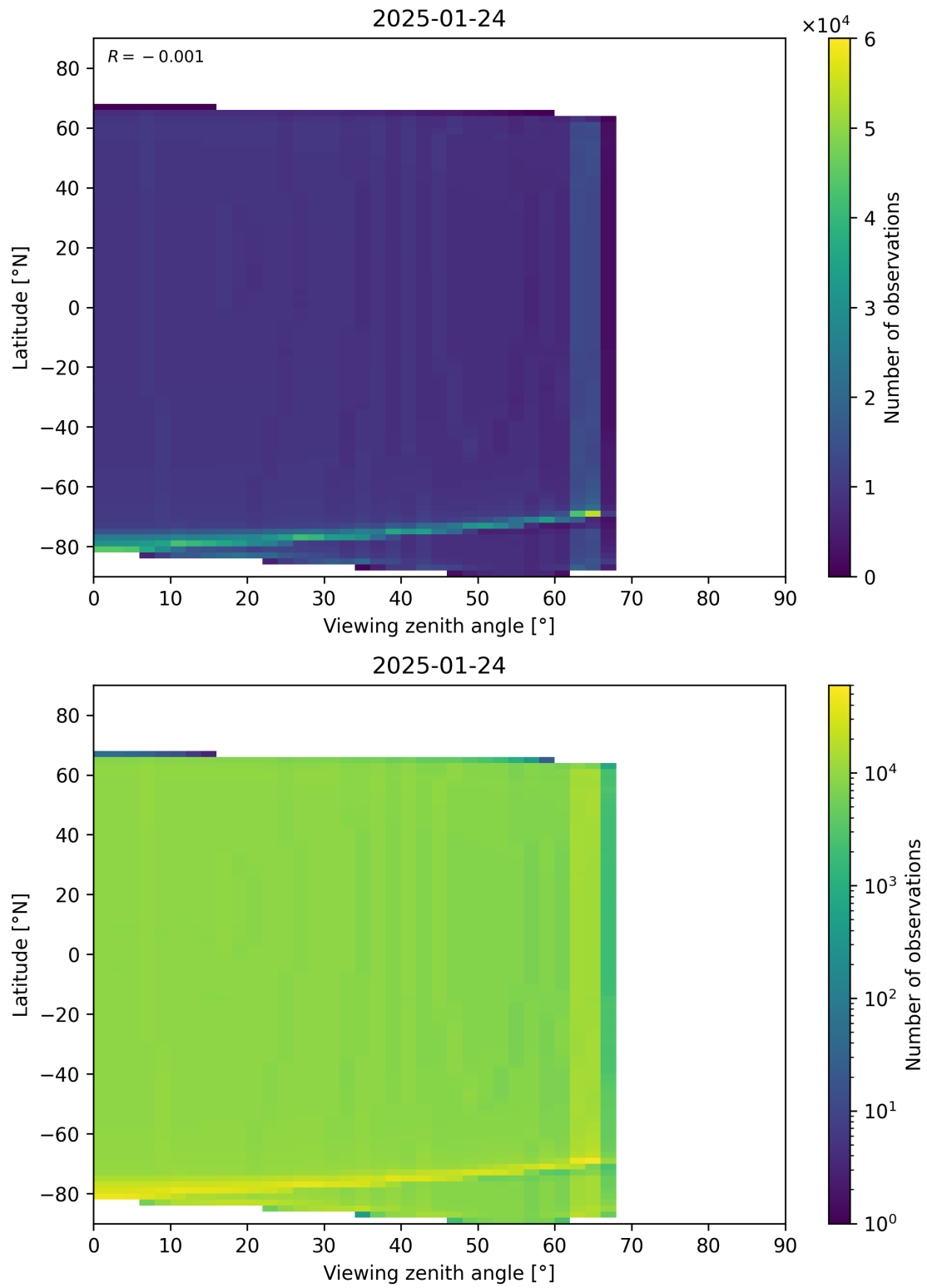
Figure 196: Scatter density plot of “Viewing zenith angle” against “Latitude” for 2025-01-23 to 2025-01-25.
