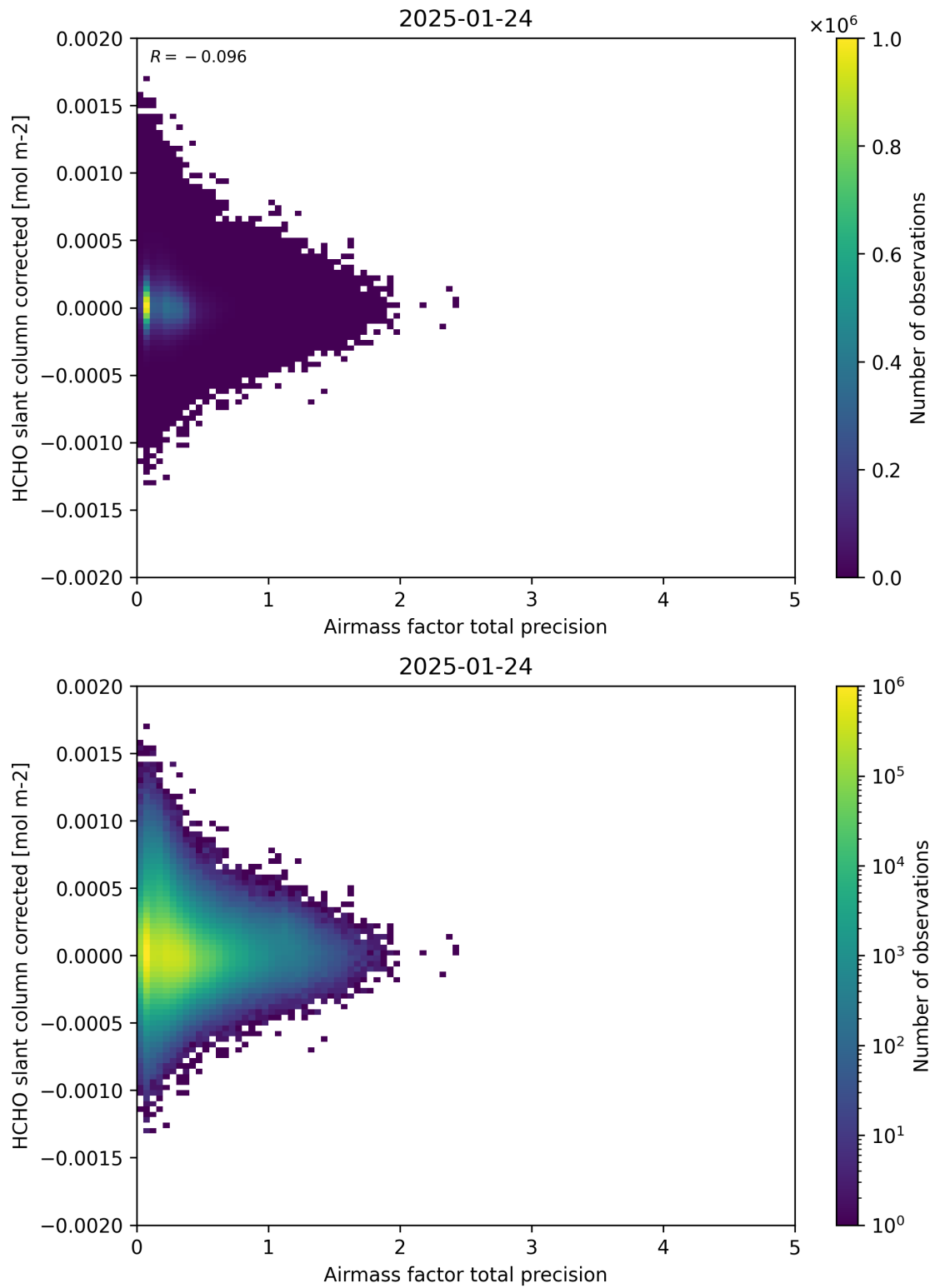
Figure 109: Scatter density plot of “Airmass factor total precision” against “HCHO slant column corrected” for 2025-01-23 to 2025-01-25.
