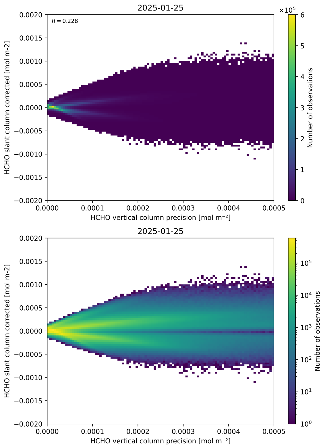
Figure 140: Scatter density plot of “HCHO vertical column precision” against “HCHO slant column corrected” for 2025-01-24 to 2025-01-26.
