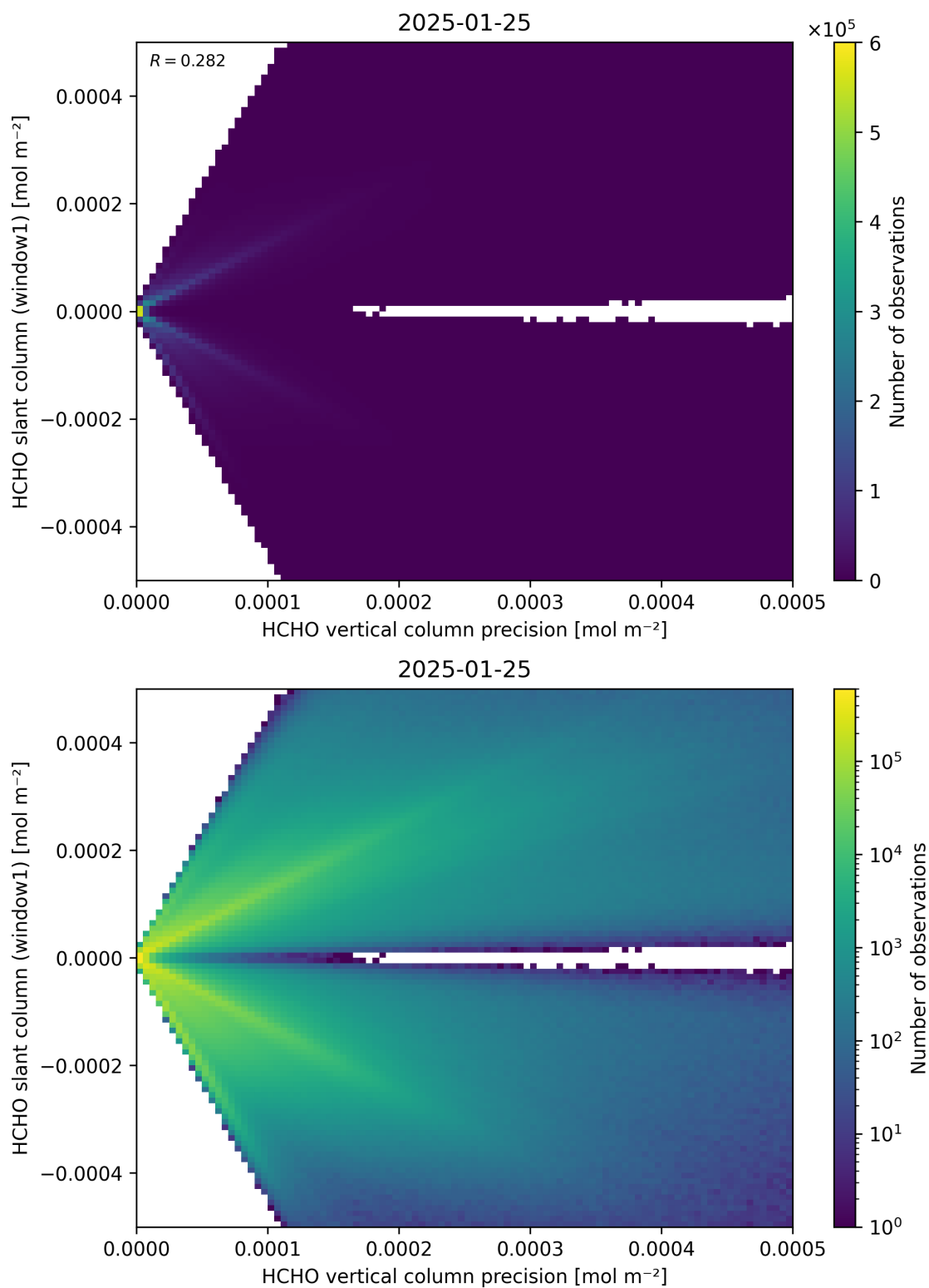
Figure 142: Scatter density plot of “HCHO vertical column precision” against “HCHO slant column (window1)” for 2025-01-24 to 2025-01-26.
