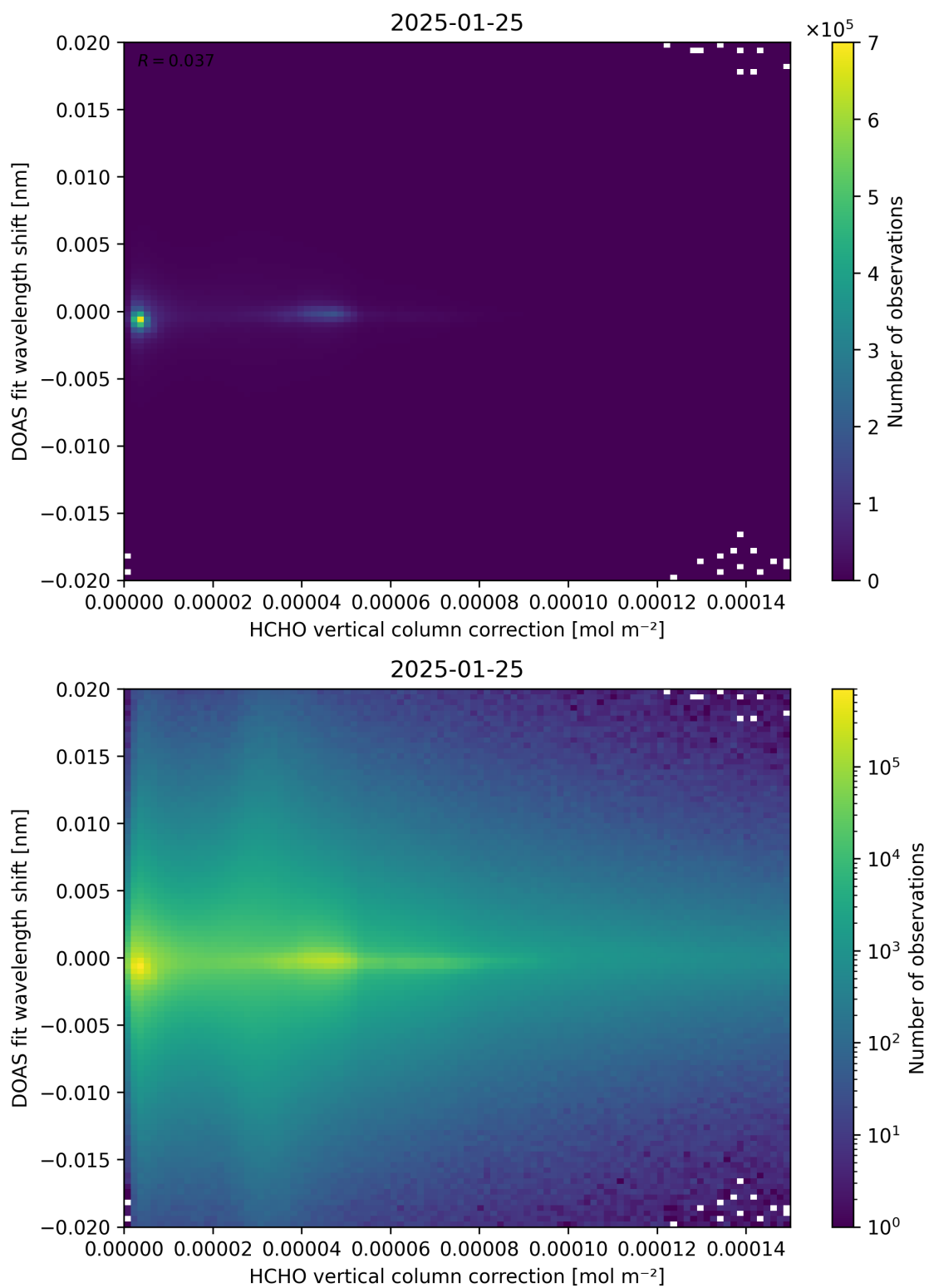
Figure 113: Scatter density plot of “HCHO vertical column correction” against “DOAS fit wavelength shift” for 2025-01-24 to 2025-01-26.
