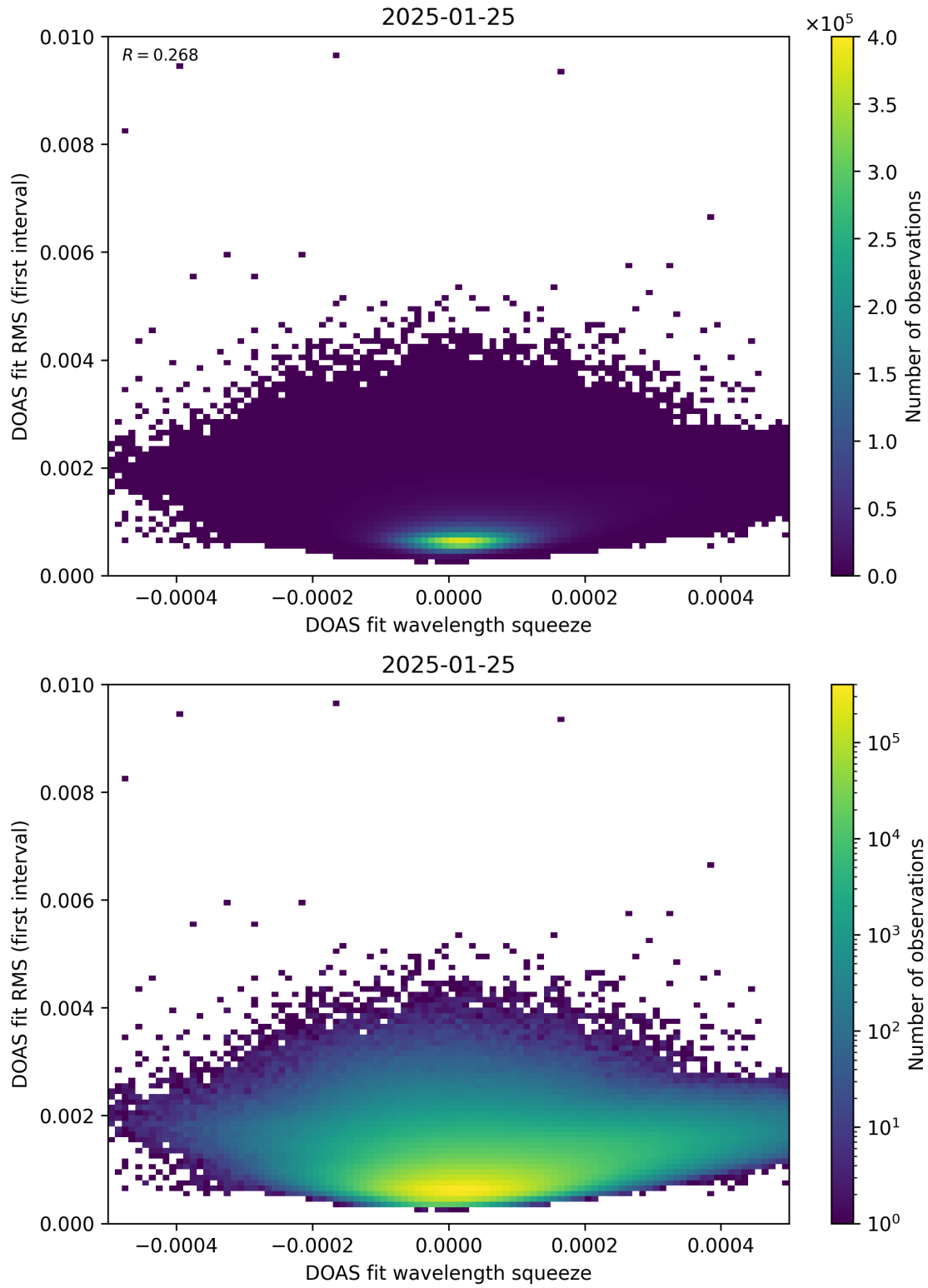
Figure 68: Scatter density plot of “DOAS fit wavelength squeeze” against “DOAS fit RMS (first interval)” for 2025-01-24 to 2025-01-26.
