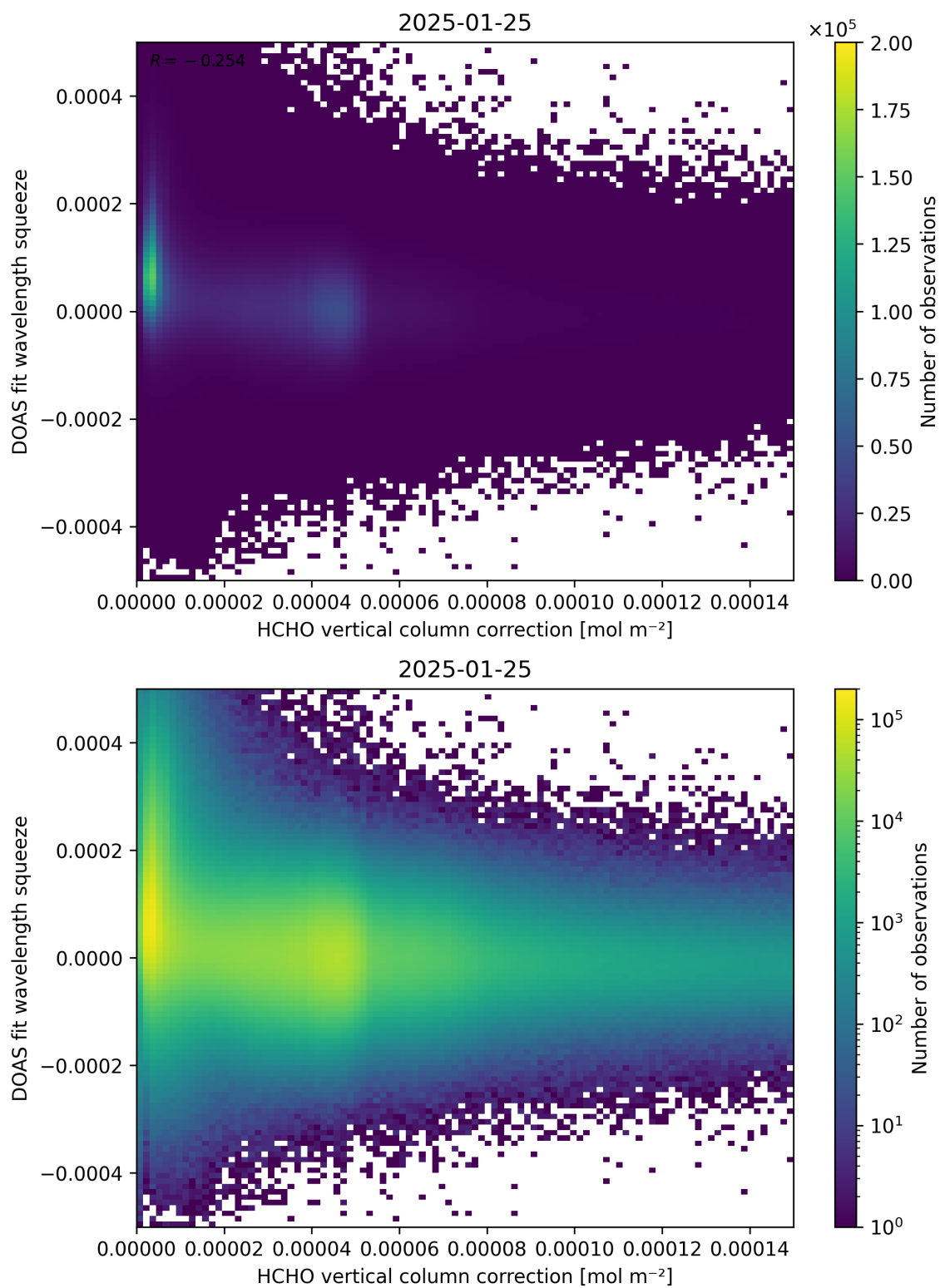
Figure 114: Scatter density plot of “HCHO vertical column correction” against “DOAS fit wavelength squeeze” for 2025-01-24 to 2025-01-26.
