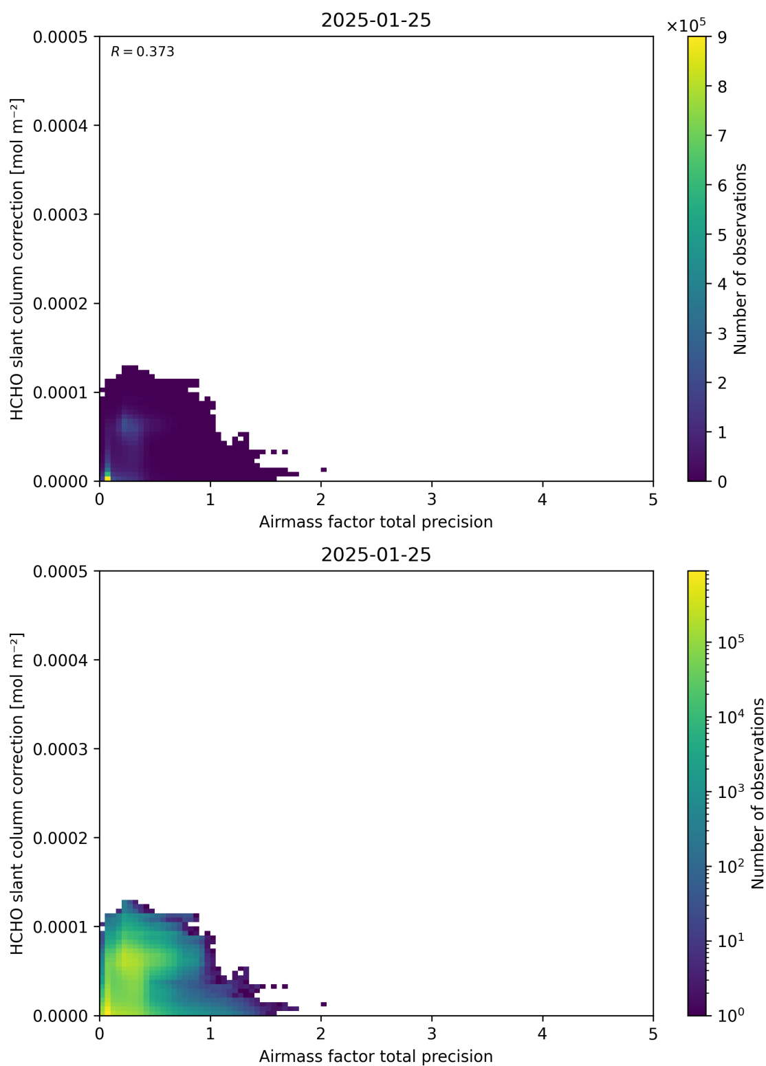
Figure 110: Scatter density plot of “Airmass factor total precision” against “HCHO slant column correction” for 2025-01-24 to 2025-01-26.
