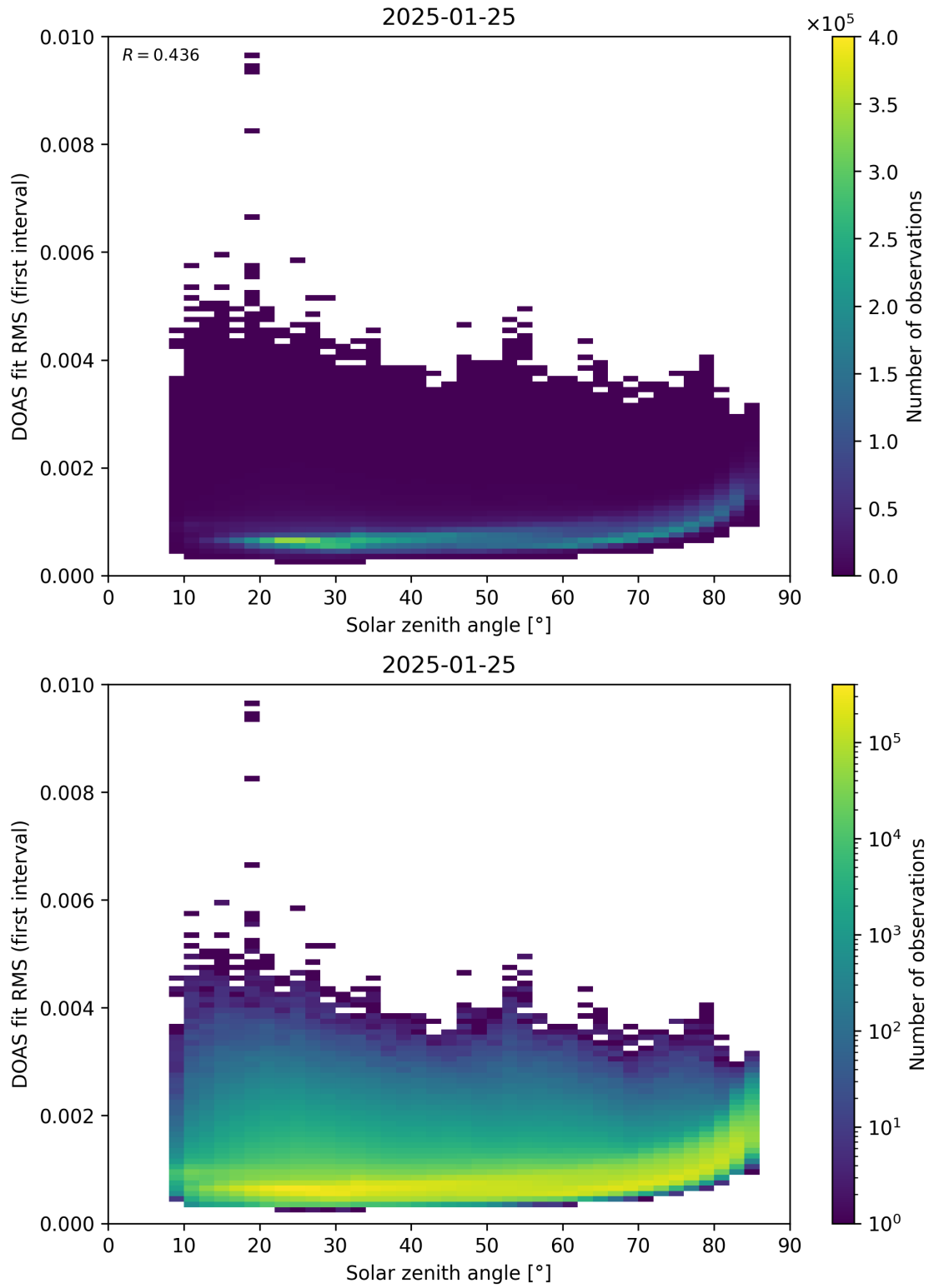
Figure 167: Scatter density plot of “Solar zenith angle” against “DOAS fit RMS (first interval)” for 2025-01-24 to 2025-01-26.
