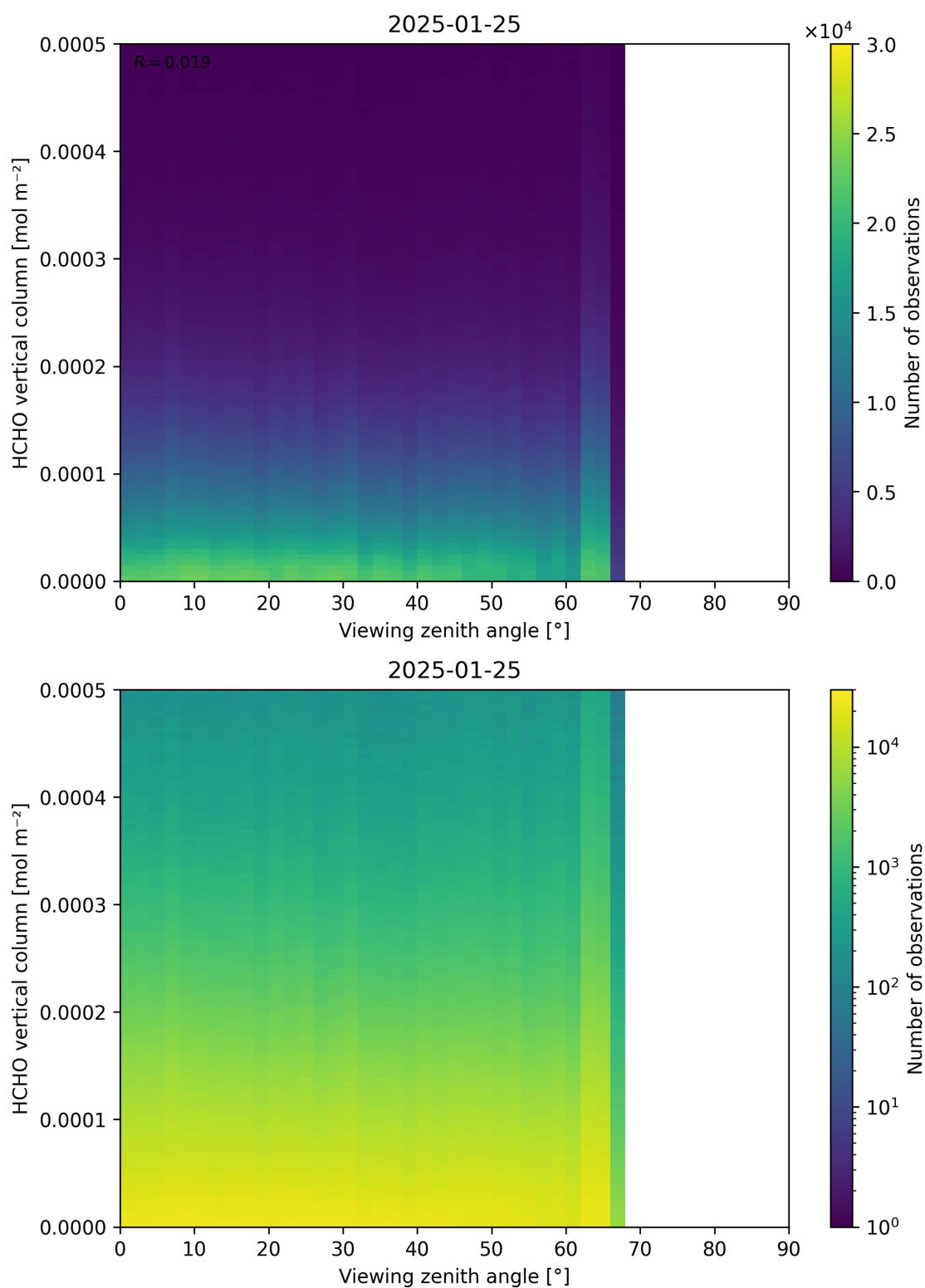
Figure 192: Scatter density plot of “Viewing zenith angle” against “HCHO vertical column” for 2025-01-24 to 2025-01-26.
