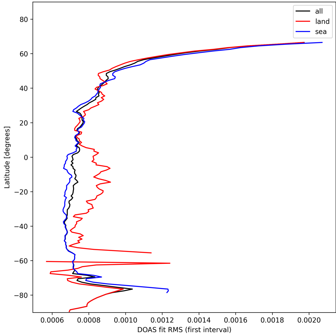
Figure 32: Zonal average of "DOAS fit RMS (first interval)" for 2025-01-24 to 2025-01-26.
