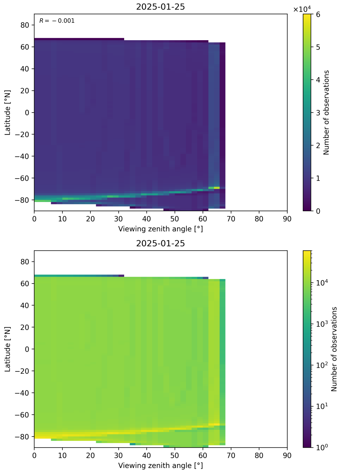
Figure 196: Scatter density plot of “Viewing zenith angle” against “Latitude” for 2025-01-24 to 2025-01-26.
