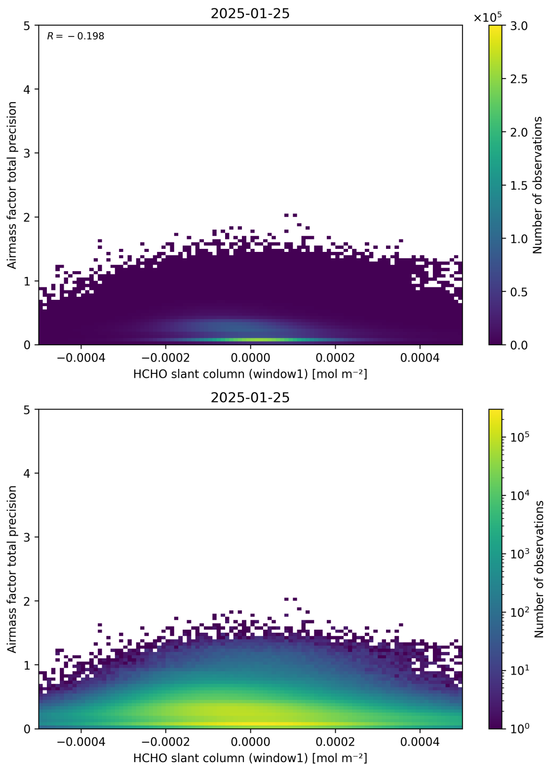
Figure 86: Scatter density plot of “HCHO slant column (window1)” against “Airmass factor total precision” for 2025-01-24 to 2025-01-26.
