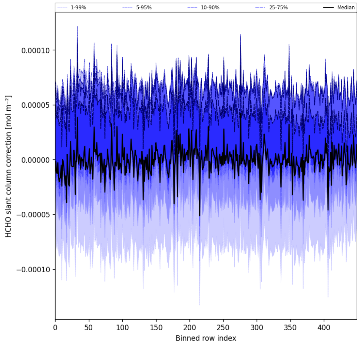
Figure 61: Along track statistics of “HCHO slant column correction” for 2025-01-24 to 2025-01-26
