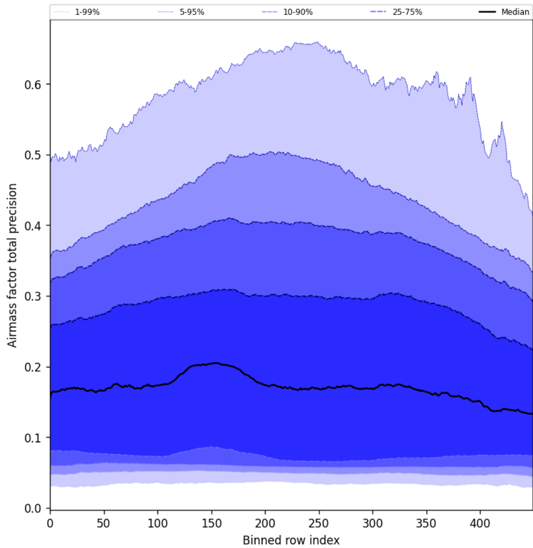
Figure 55: Along track statistics of “Airmass factor total precision” for 2025-01-24 to 2025-01-26
