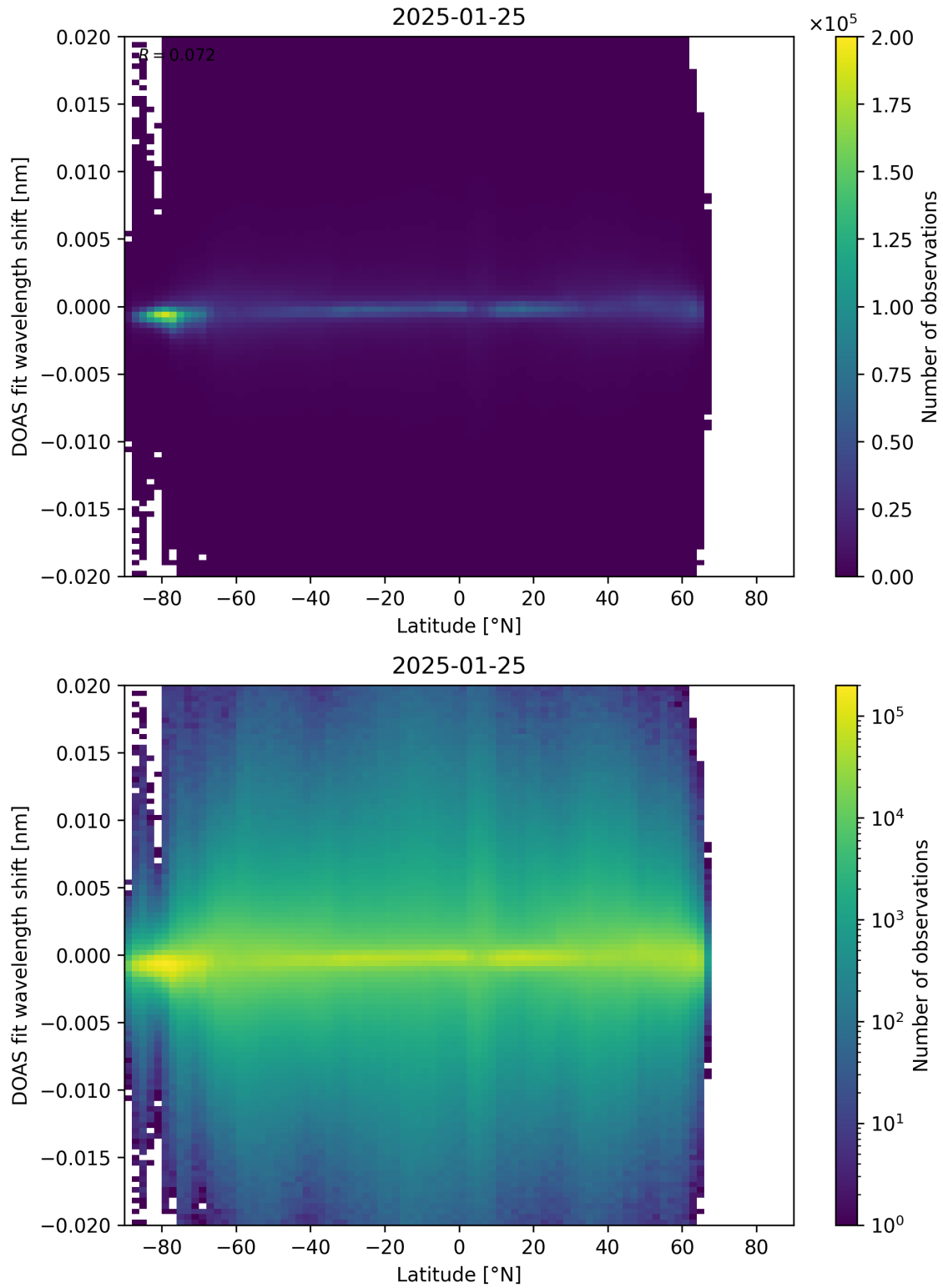
Figure 154: Scatter density plot of “Latitude” against “DOAS fit wavelength shift” for 2025-01-24 to 2025-01-26.
