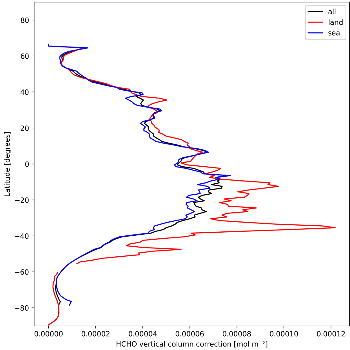
Figure 23: Zonal average of “HCHO vertical column correction” for 2025-01-24 to 2025-01-26.
