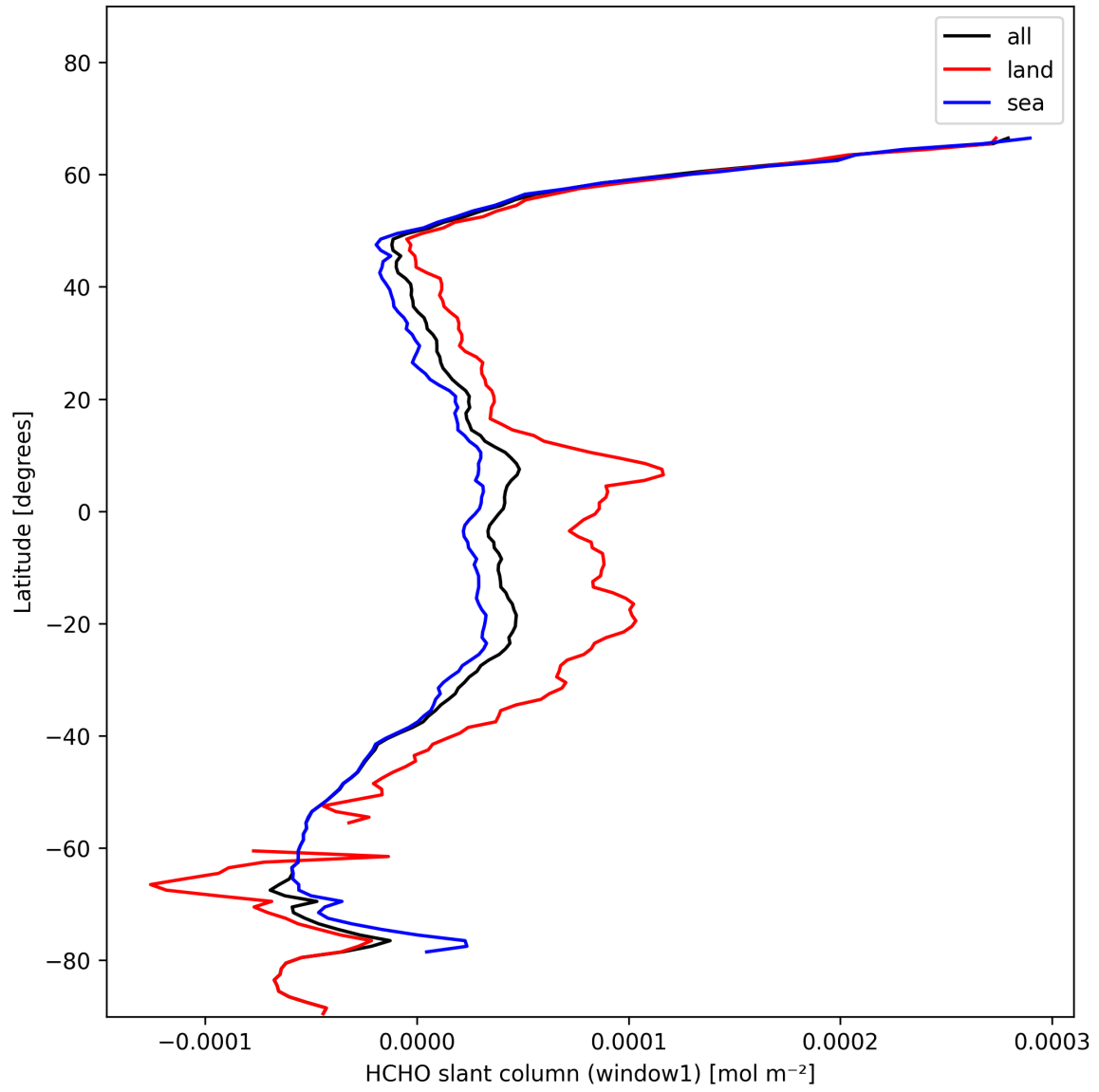
Figure 24: Zonal average of “HCHO slant column (window1)” for 2025-01-24 to 2025-01-26.
