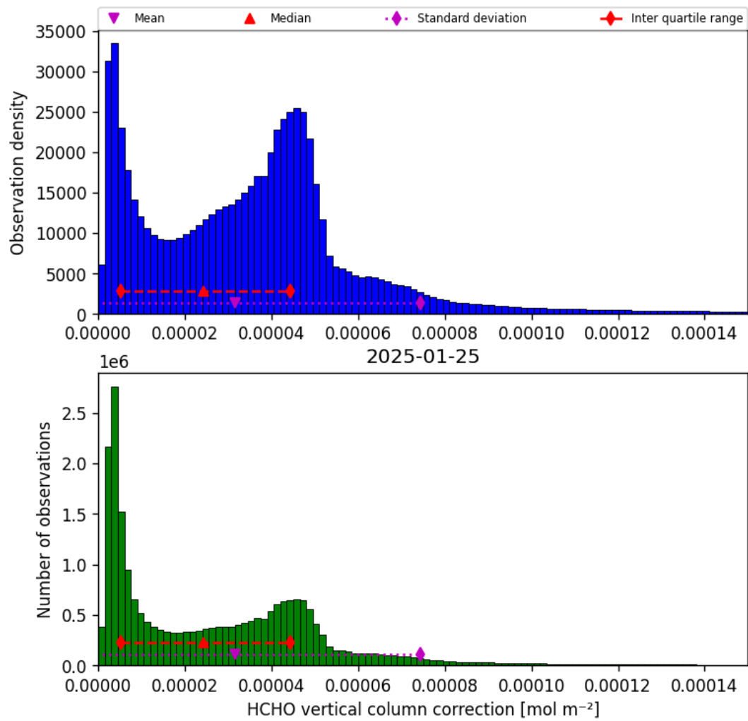
Figure 37: Histogram of “HCHO vertical column correction” for 2025-01-24 to 2025-01-26
