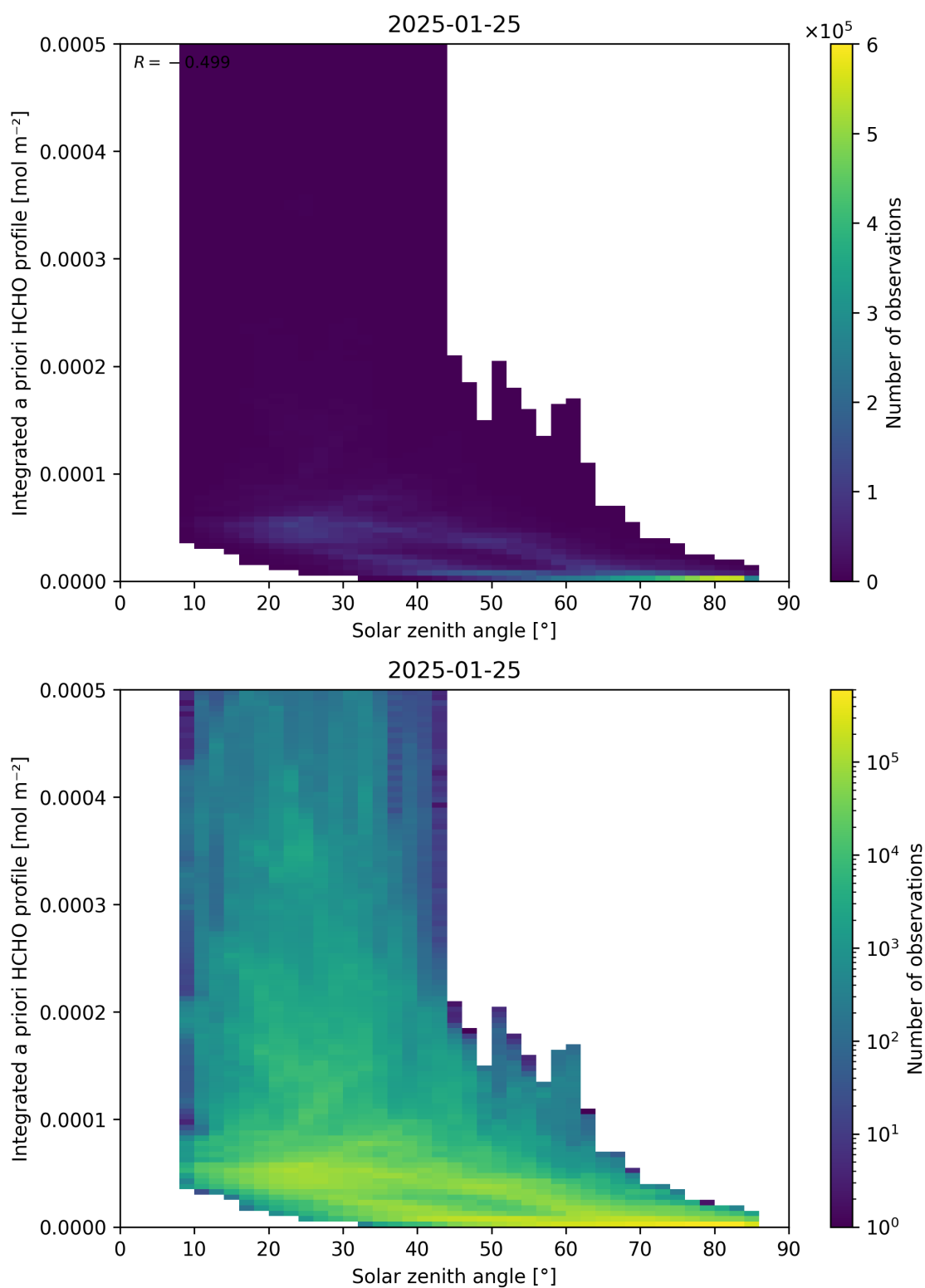
Figure 180: Scatter density plot of “Solar zenith angle” against “Integrated a priori HCHO profile” for 2025-01-24 to 2025-01-26.
