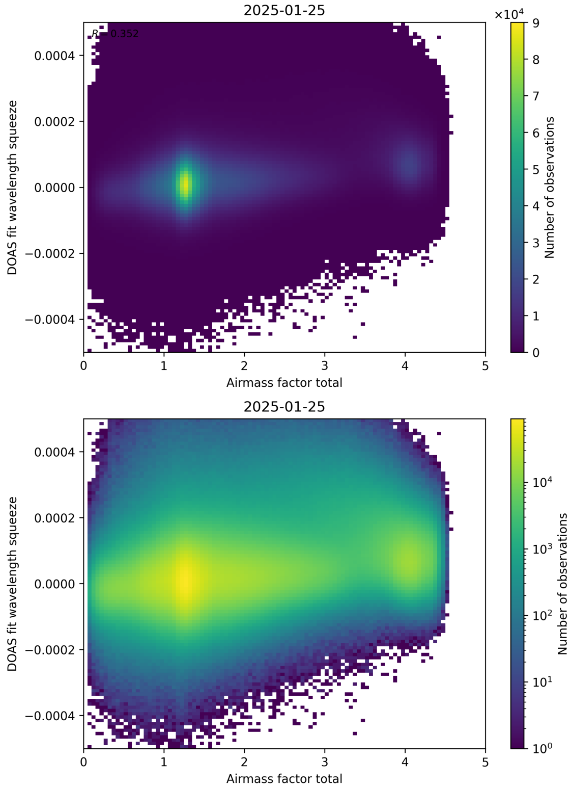
Figure 99: Scatter density plot of “Airmass factor total” against “DOAS fit wavelength squeeze” for 2025-01-24 to 2025-01-26.
