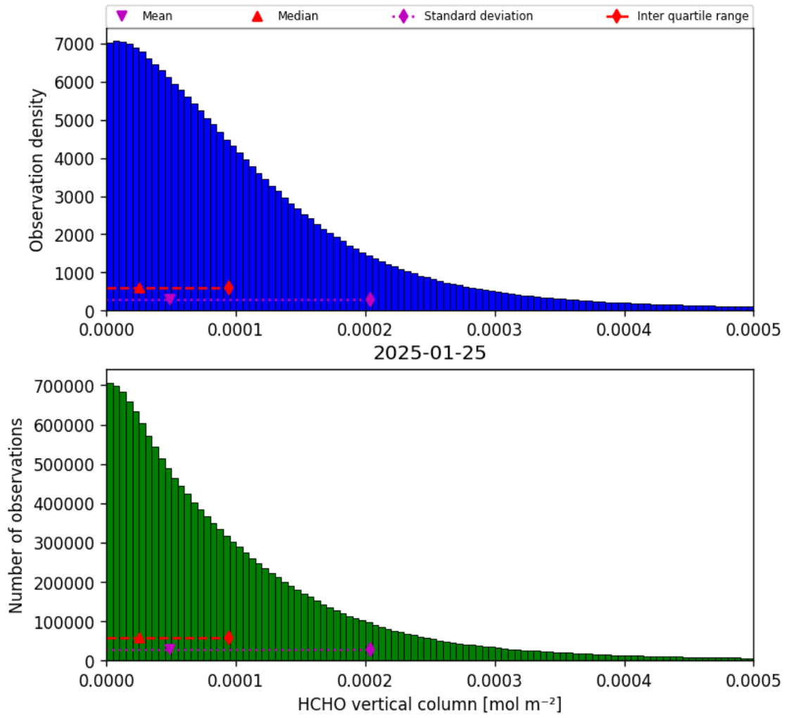
Figure 35: Histogram of “HCHO vertical column” for 2025-01-24 to 2025-01-26
