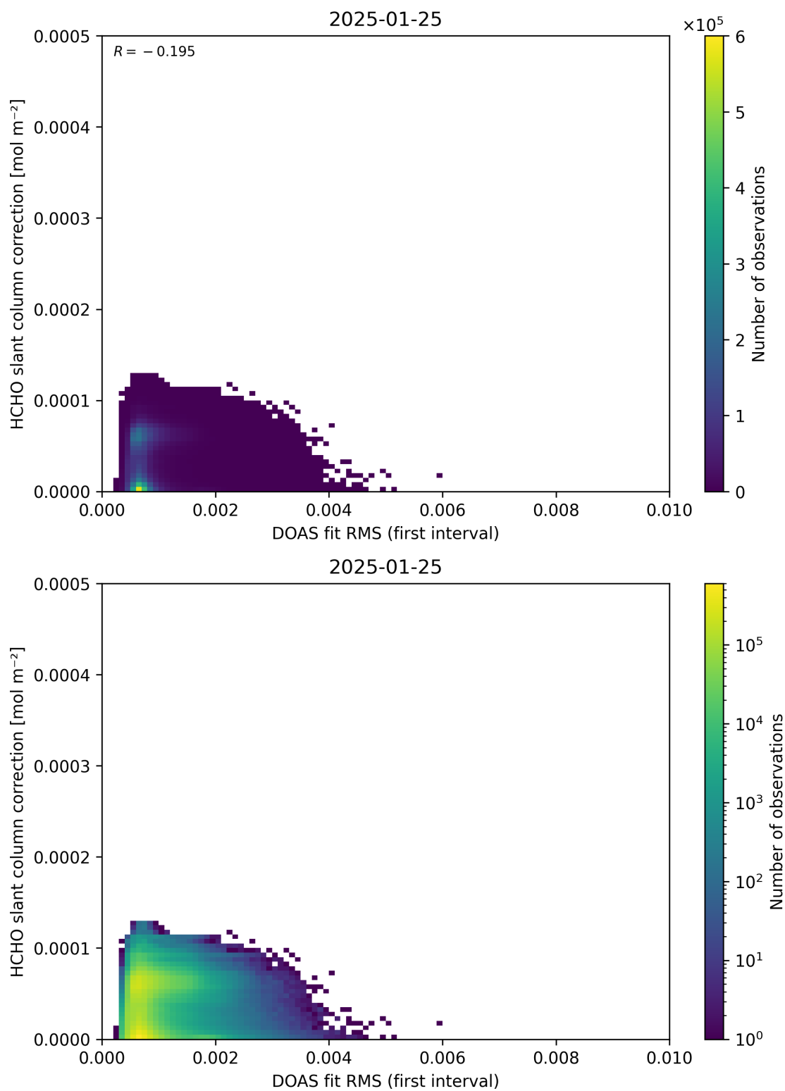
Figure 63: Scatter density plot of “DOAS fit RMS (first interval)” against “HCHO slant column correction” for 2025-01-24 to 2025-01-26.
