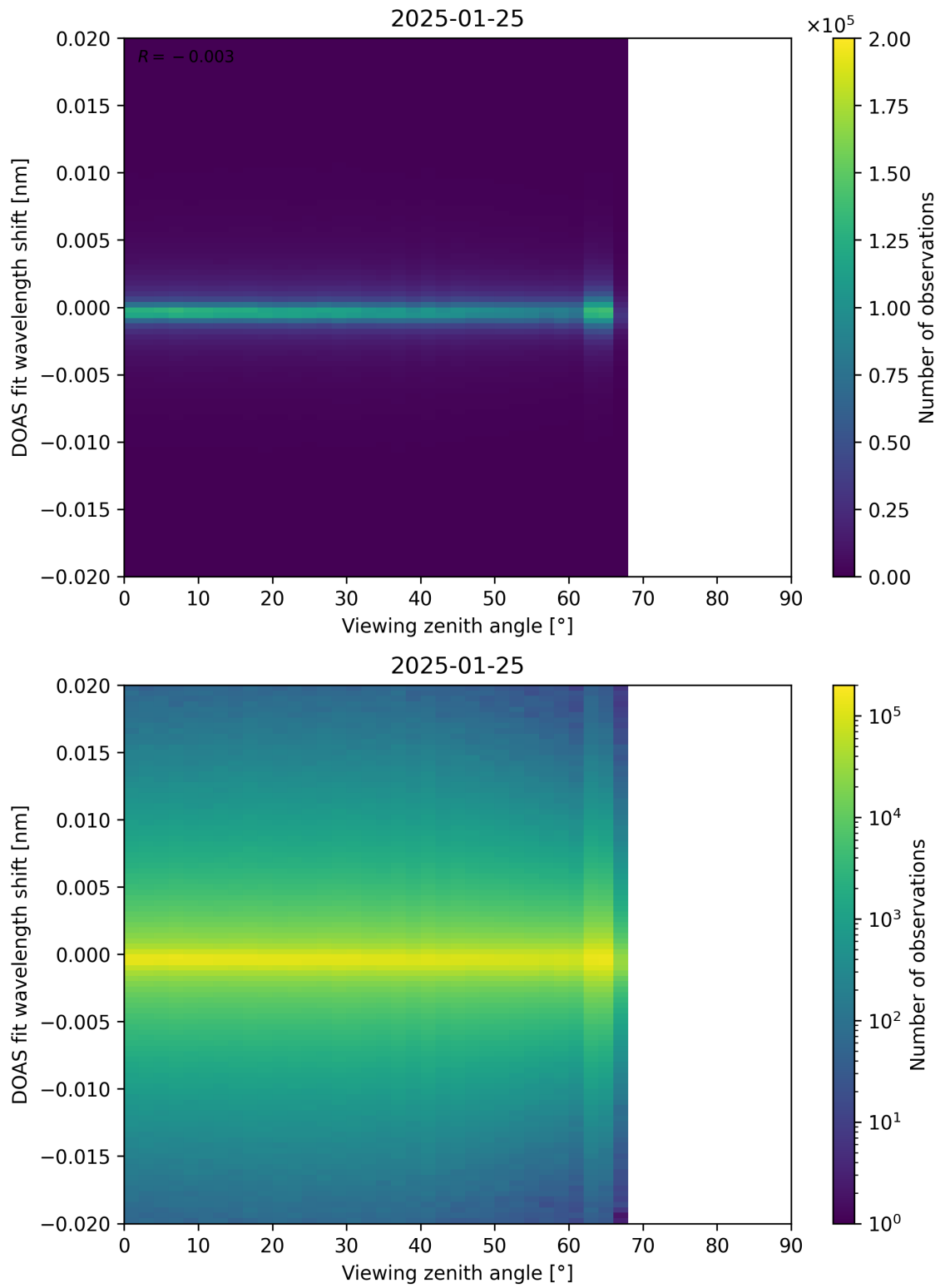
Figure 183: Scatter density plot of “Viewing zenith angle” against “DOAS fit wavelength shift” for 2025-01-24 to 2025-01-26.
