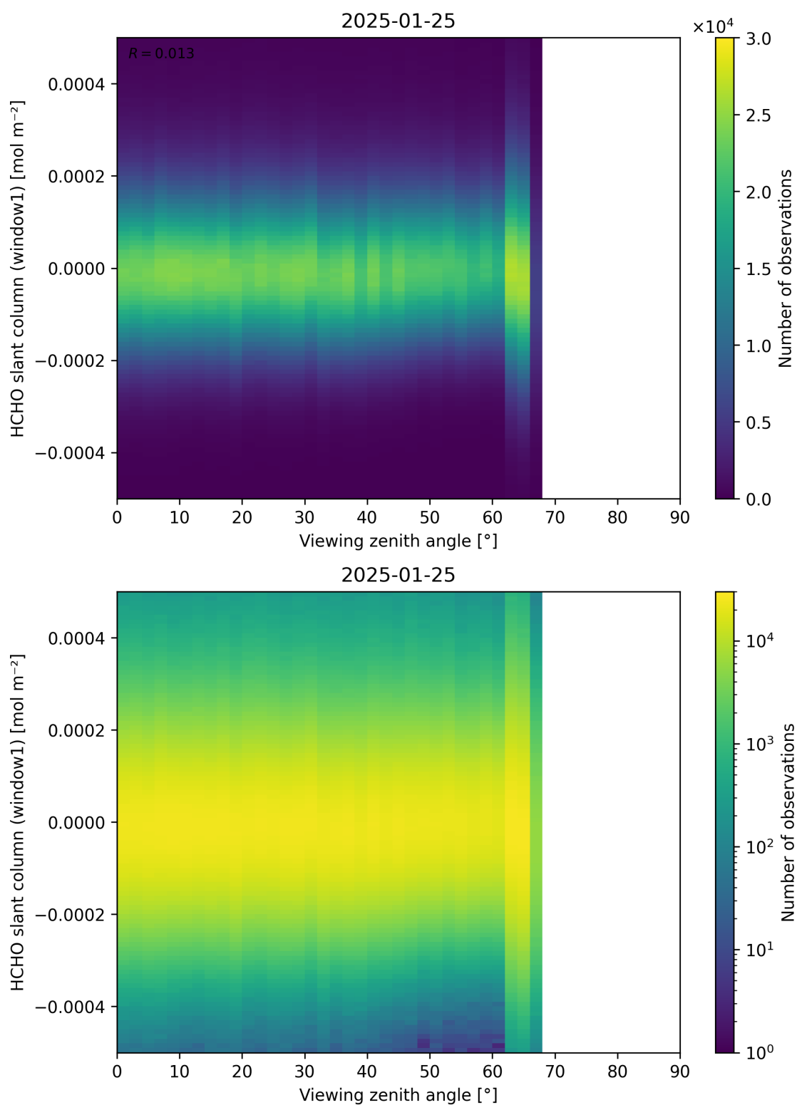
Figure 188: Scatter density plot of “Viewing zenith angle” against “HCHO slant column (window1)” for 2025-01-24 to 2025-01-26.
