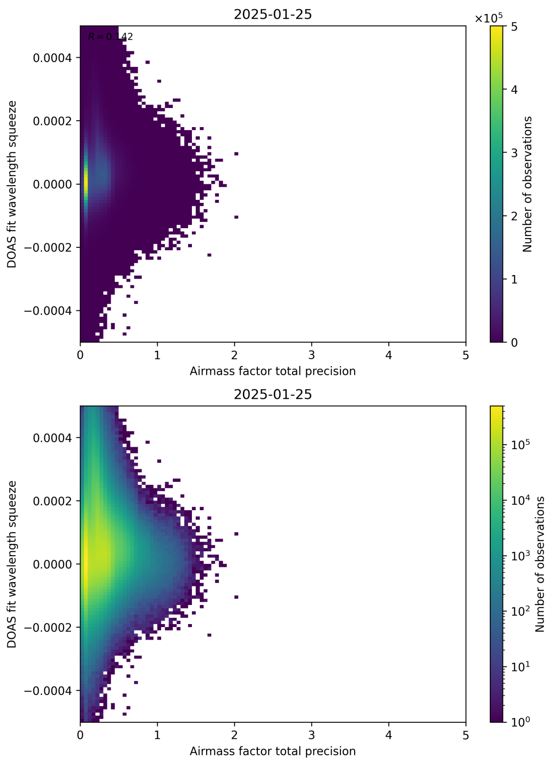
Figure 107: Scatter density plot of “Airmass factor total precision” against “DOAS fit wavelength squeeze” for 2025-01-24 to 2025-01-26.
