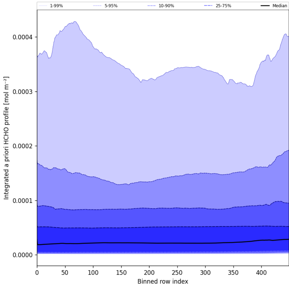
Figure 57: Along track statistics of "Integrated a priori HCHO profile" for 2025-01-24 to 2025-01-26
