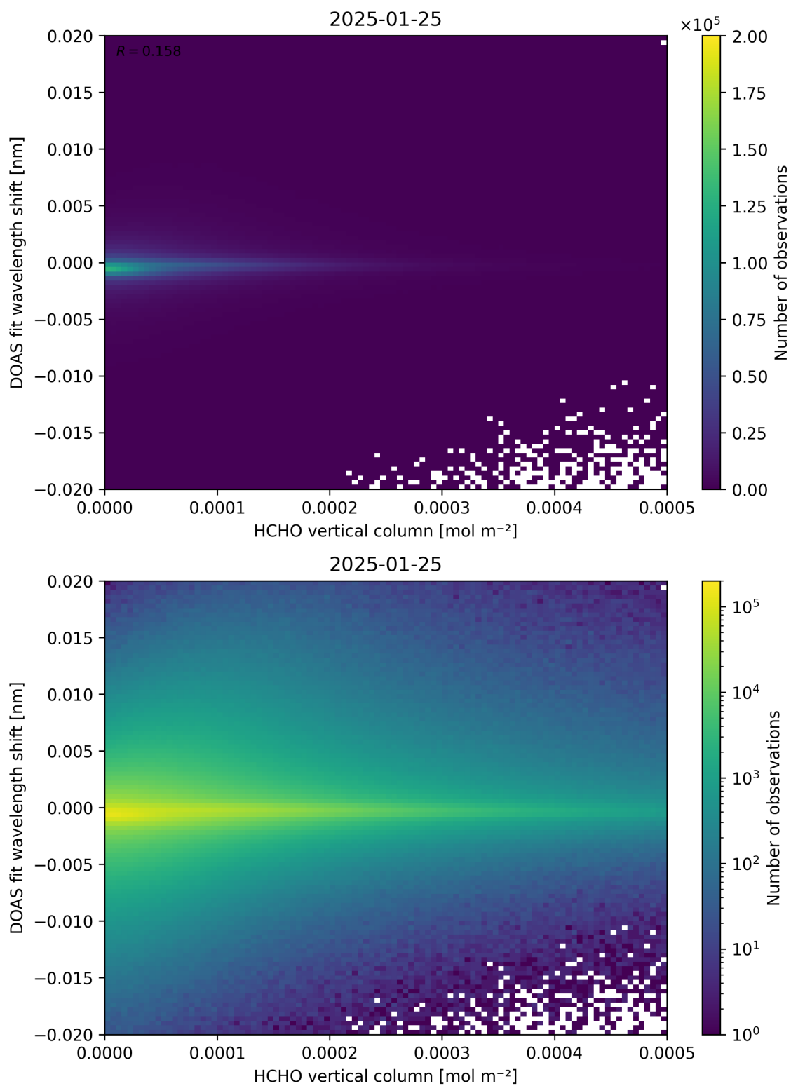
Figure 124: Scatter density plot of “HCHO vertical column” against “DOAS fit wavelength shift” for 2025-01-24 to 2025-01-26.
