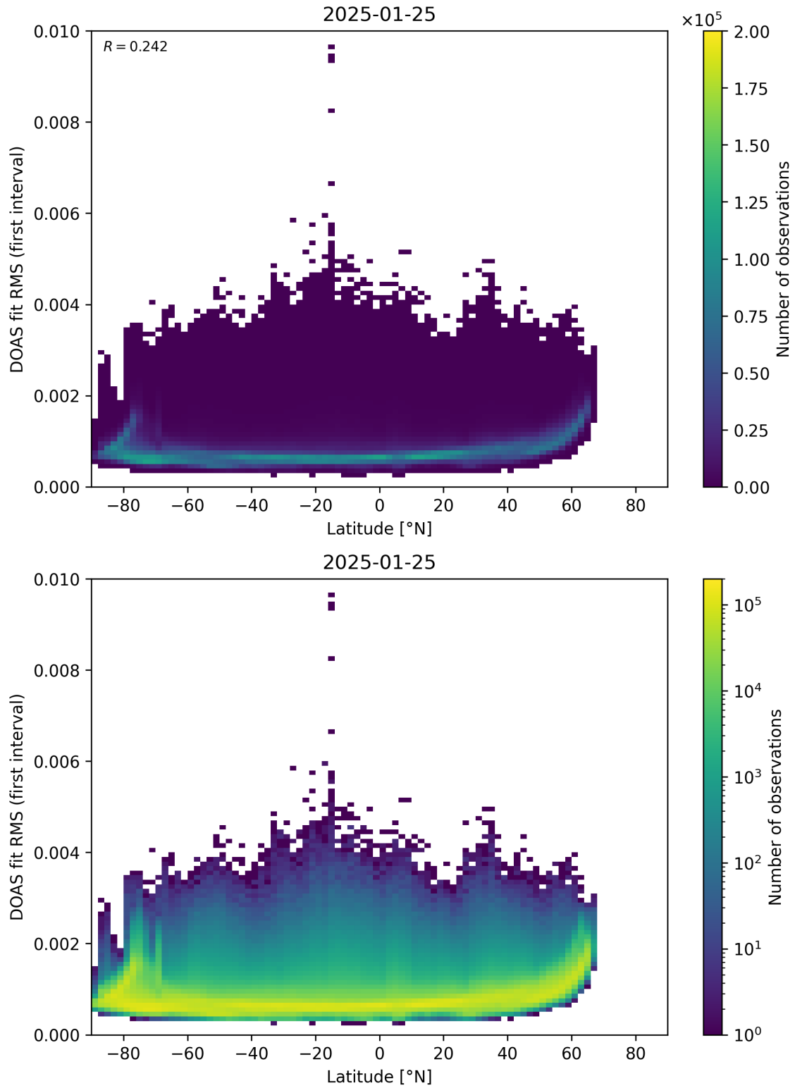
Figure 153: Scatter density plot of “Latitude” against “DOAS fit RMS (first interval)” for 2025-01-24 to 2025-01-26.
