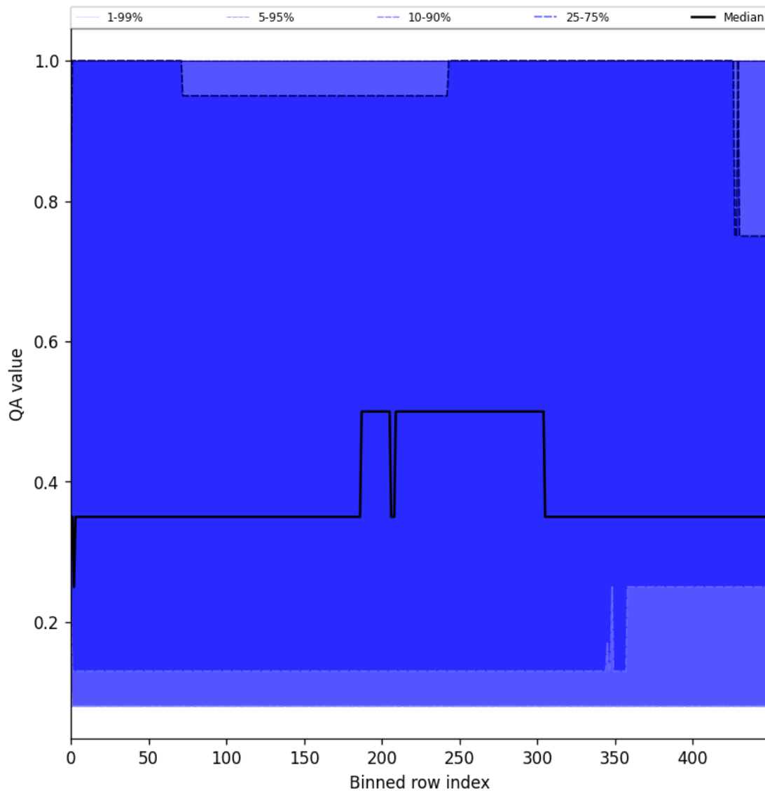
Figure 48: Along track statistics of “QA value” for 2025-01-24 to 2025-01-26
