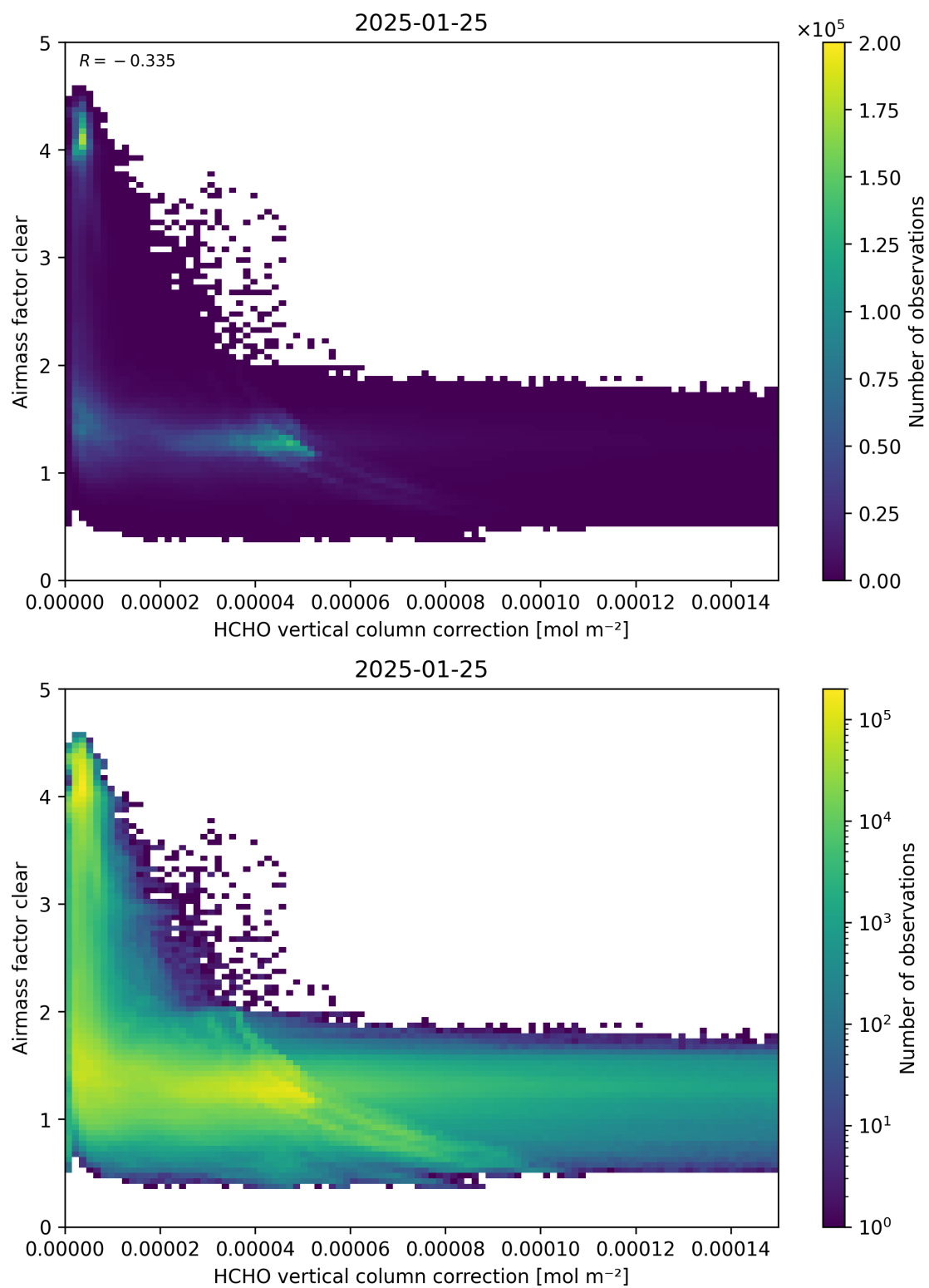
Figure 115: Scatter density plot of “HCHO vertical column correction” against “Airmass factor clear” for 2025-01-24 to 2025-01-26.
