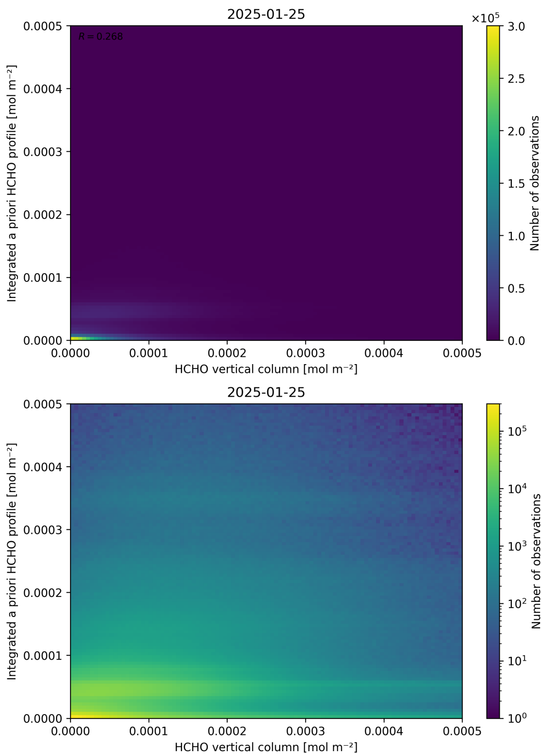
Figure 135: Scatter density plot of “HCHO vertical column” against “Integrated a priori HCHO profile” for 2025-01-24 to 2025-01-26.
