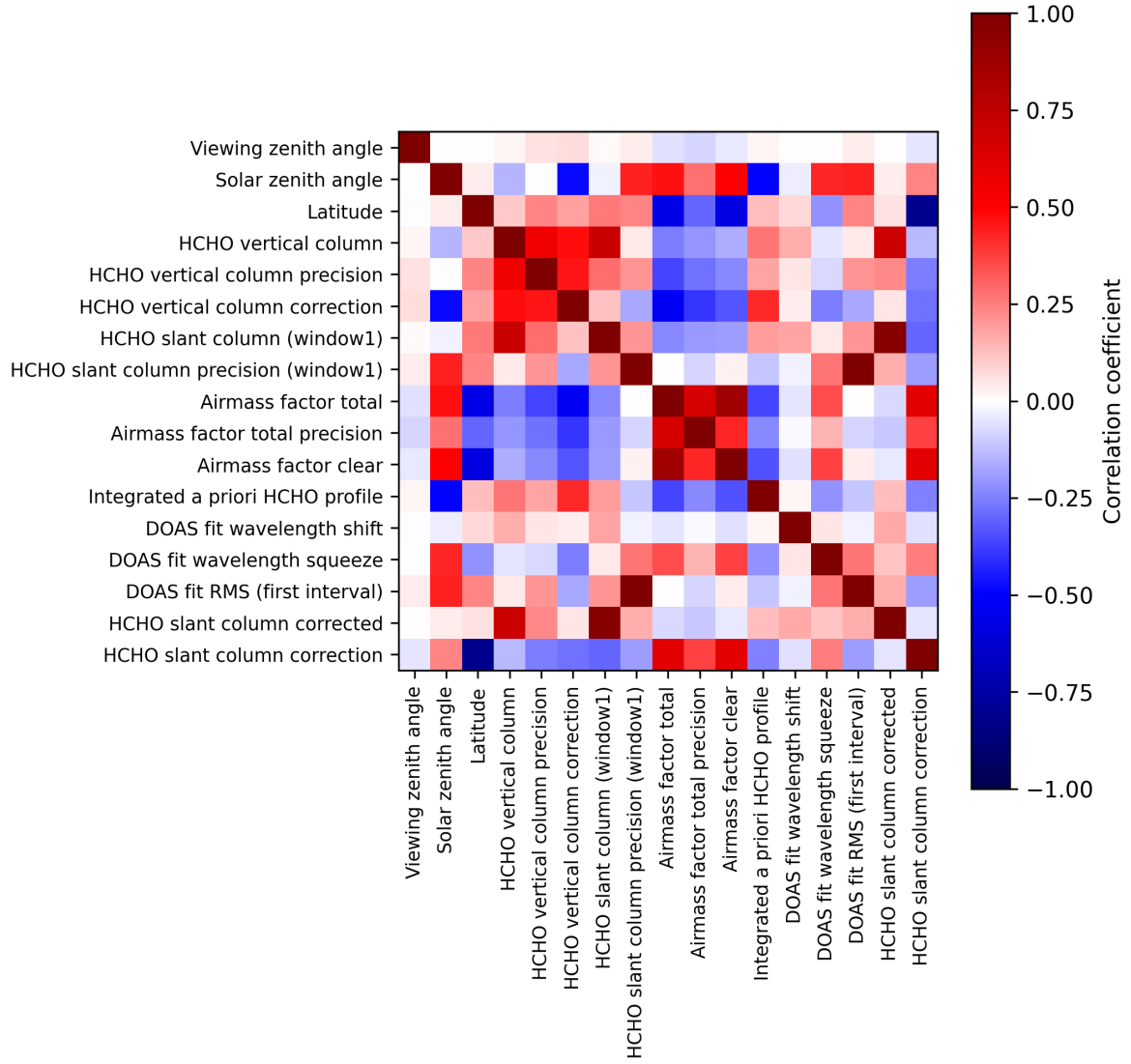
Figure 2: Map of correlation matrix for 2025-01-24 to 2025-01-26.
