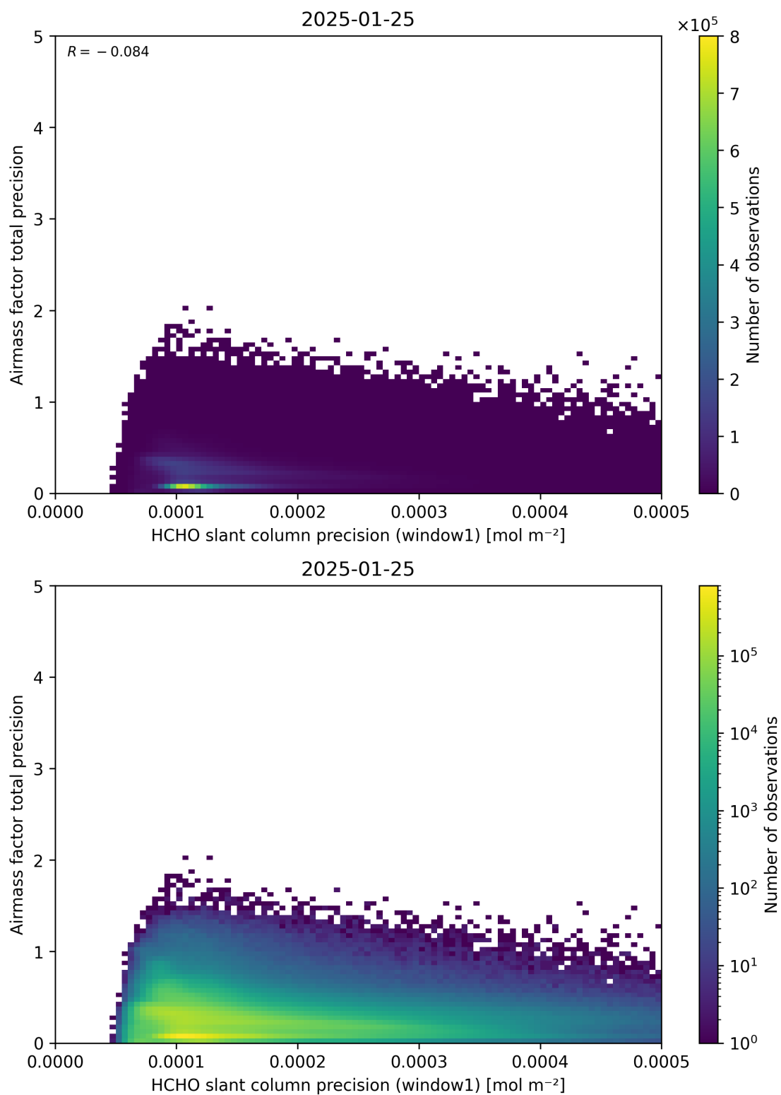
Figure 95: Scatter density plot of “HCHO slant column precision (window1)” against “Airmass factor total precision” for 2025-01-24 to 2025-01-26.
