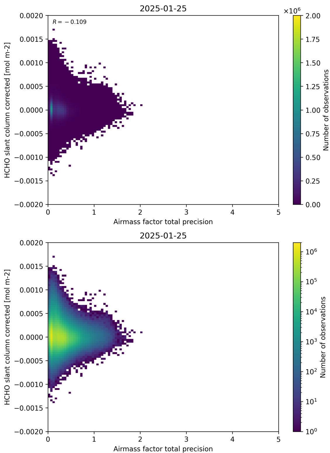
Figure 109: Scatter density plot of “Airmass factor total precision” against “HCHO slant column corrected” for 2025-01-24 to 2025-01-26.
