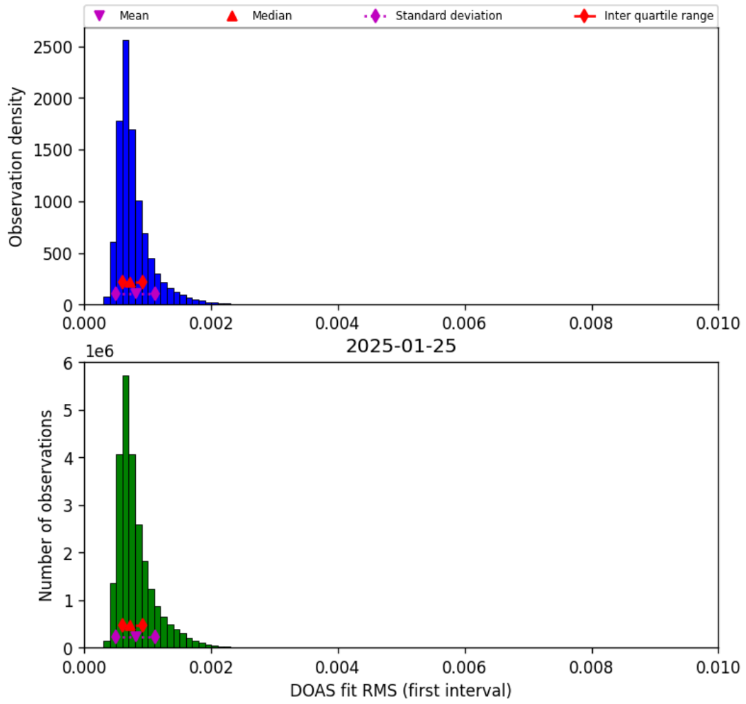
Figure 46: Histogram of “DOAS fit RMS (first interval)” for 2025-01-24 to 2025-01-26
