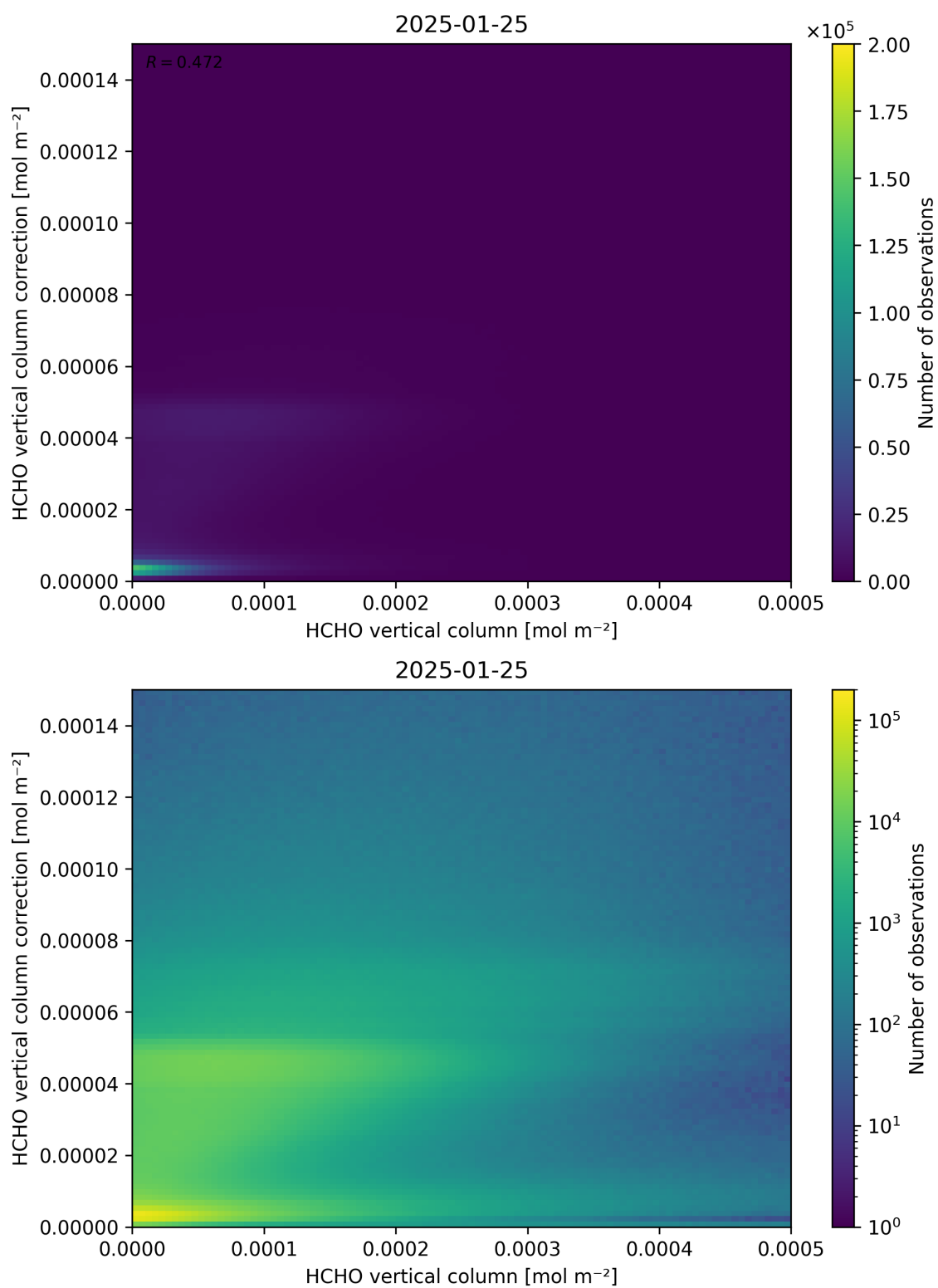
Figure 133: Scatter density plot of “HCHO vertical column” against “HCHO vertical column correction” for 2025-01-24 to 2025-01-26.
