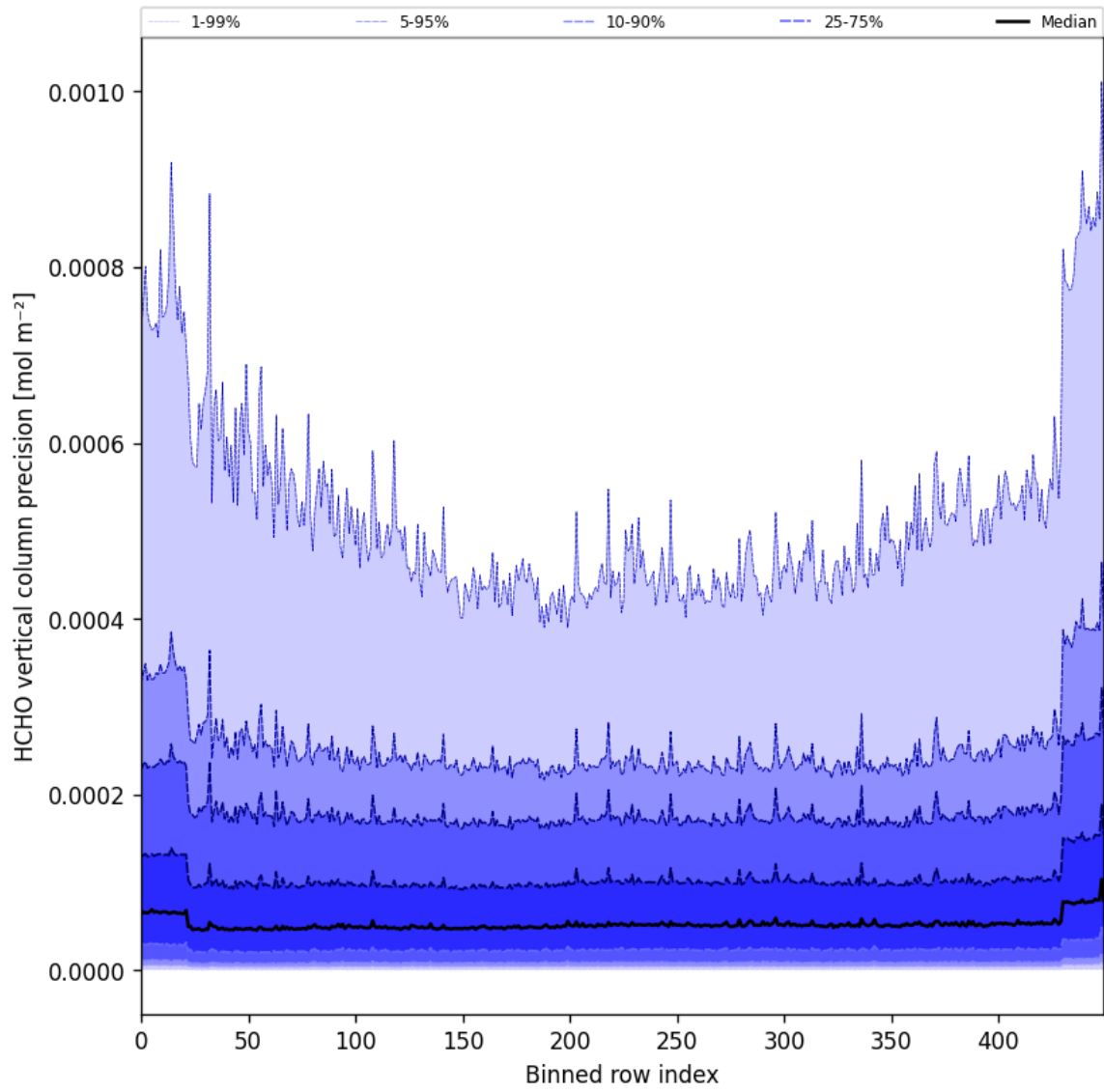
Figure 50: Along track statistics of “HCHO vertical column precision” for 2025-01-24 to 2025-01-26
