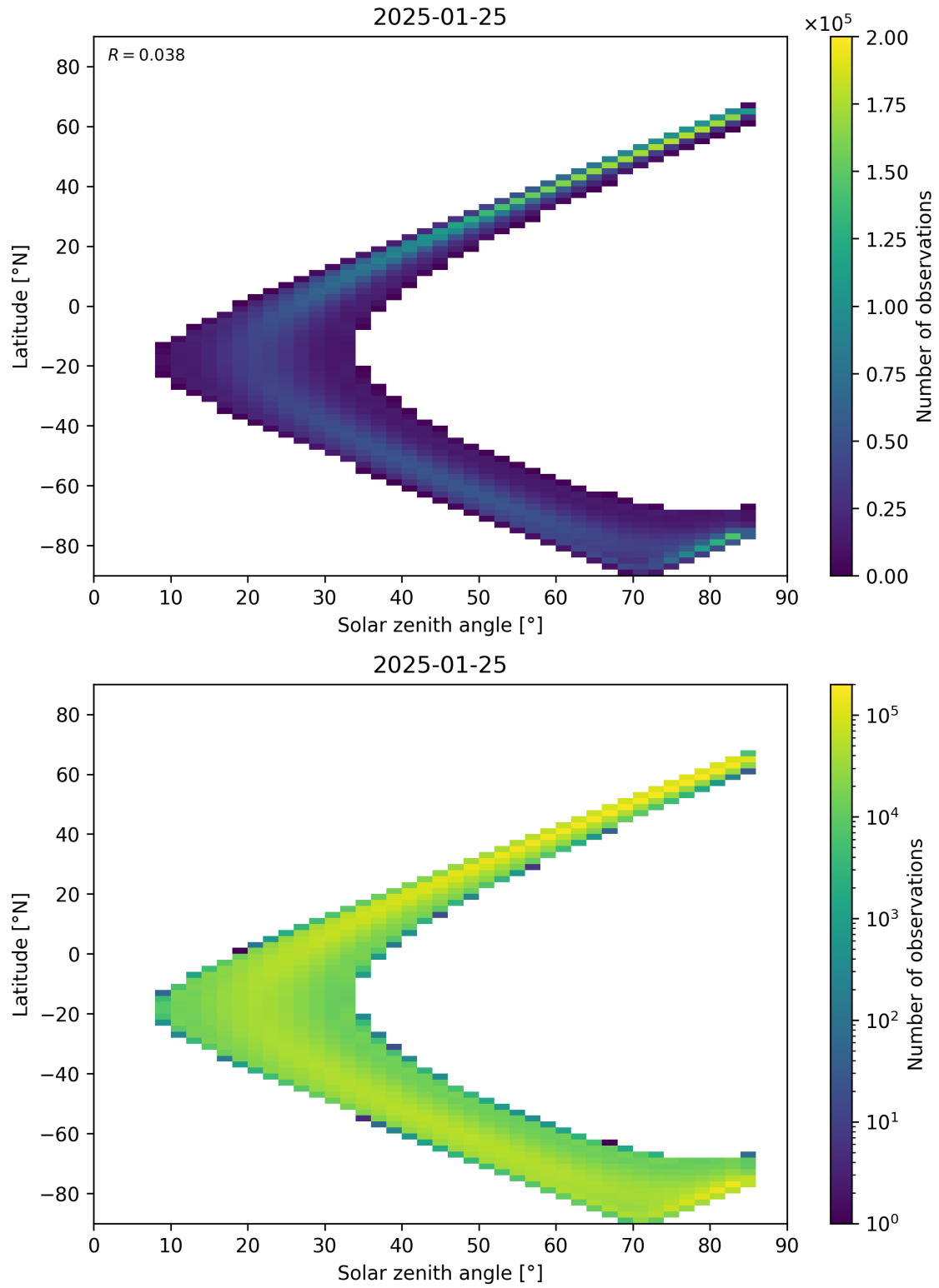
Figure 181: Scatter density plot of “Solar zenith angle” against “Latitude” for 2025-01-24 to 2025-01-26.
