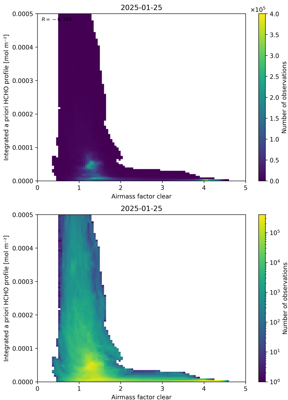
Figure 76: Scatter density plot of “Airmass factor clear” against “Integrated a priori HCHO profile” for 2025-01-24 to 2025-01-26.
