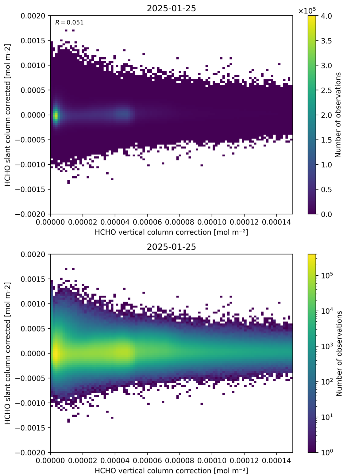
Figure 116: Scatter density plot of “HCHO vertical column correction” against “HCHO slant column corrected” for 2025-01-24 to 2025-01-26.
