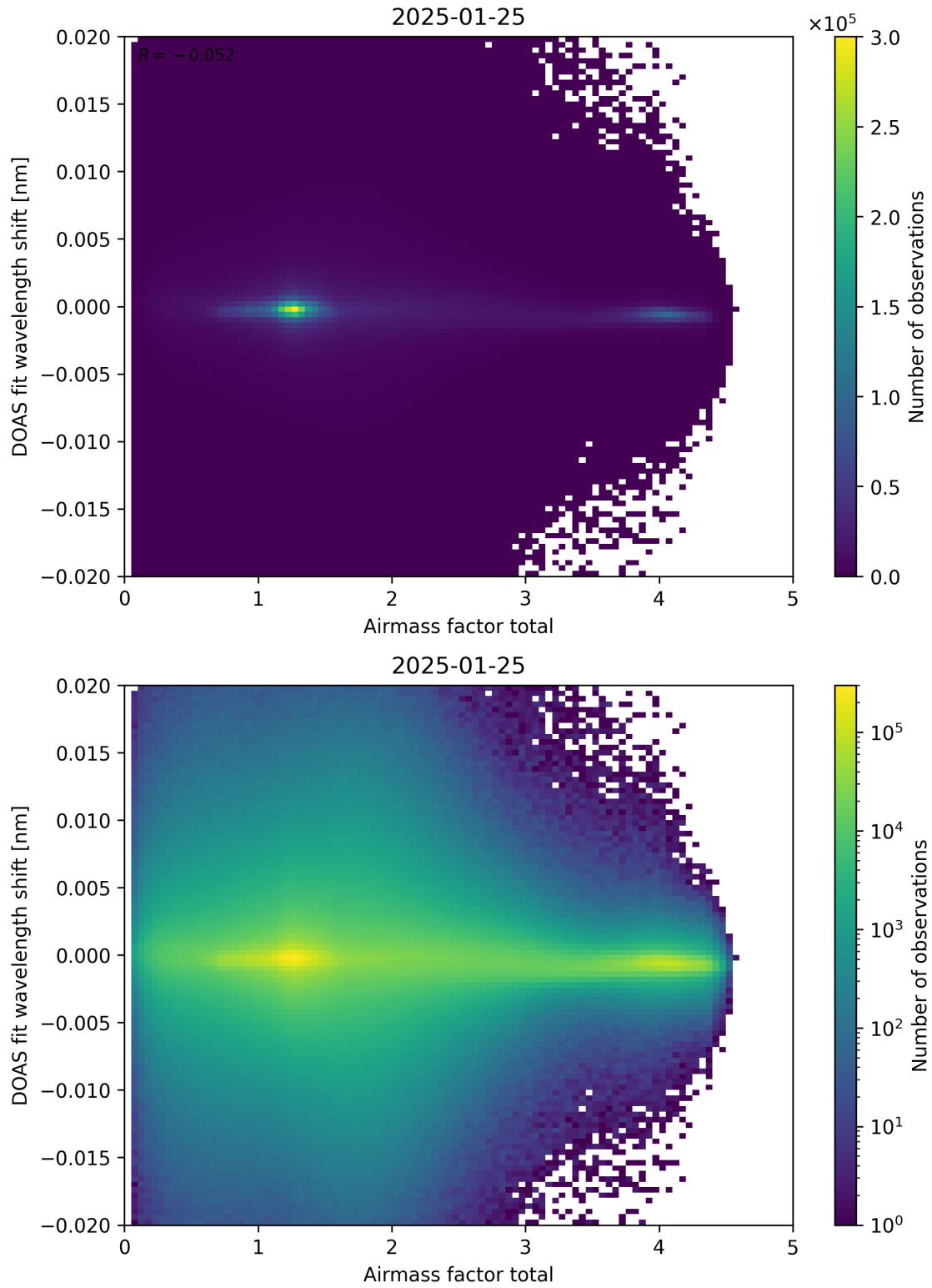
Figure 98: Scatter density plot of “Airmass factor total” against “DOAS fit wavelength shift” for 2025-01-24 to 2025-01-26.
