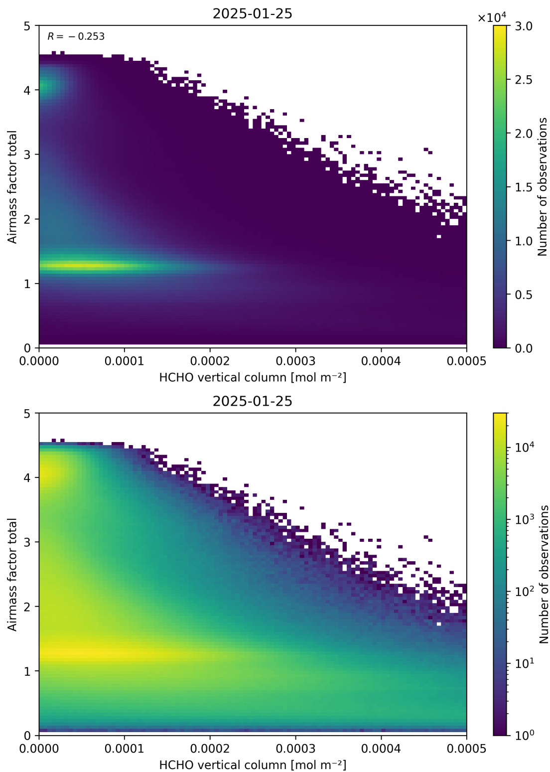
Figure 131: Scatter density plot of “HCHO vertical column” against “Airmass factor total” for 2025-01-24 to 2025-01-26.
