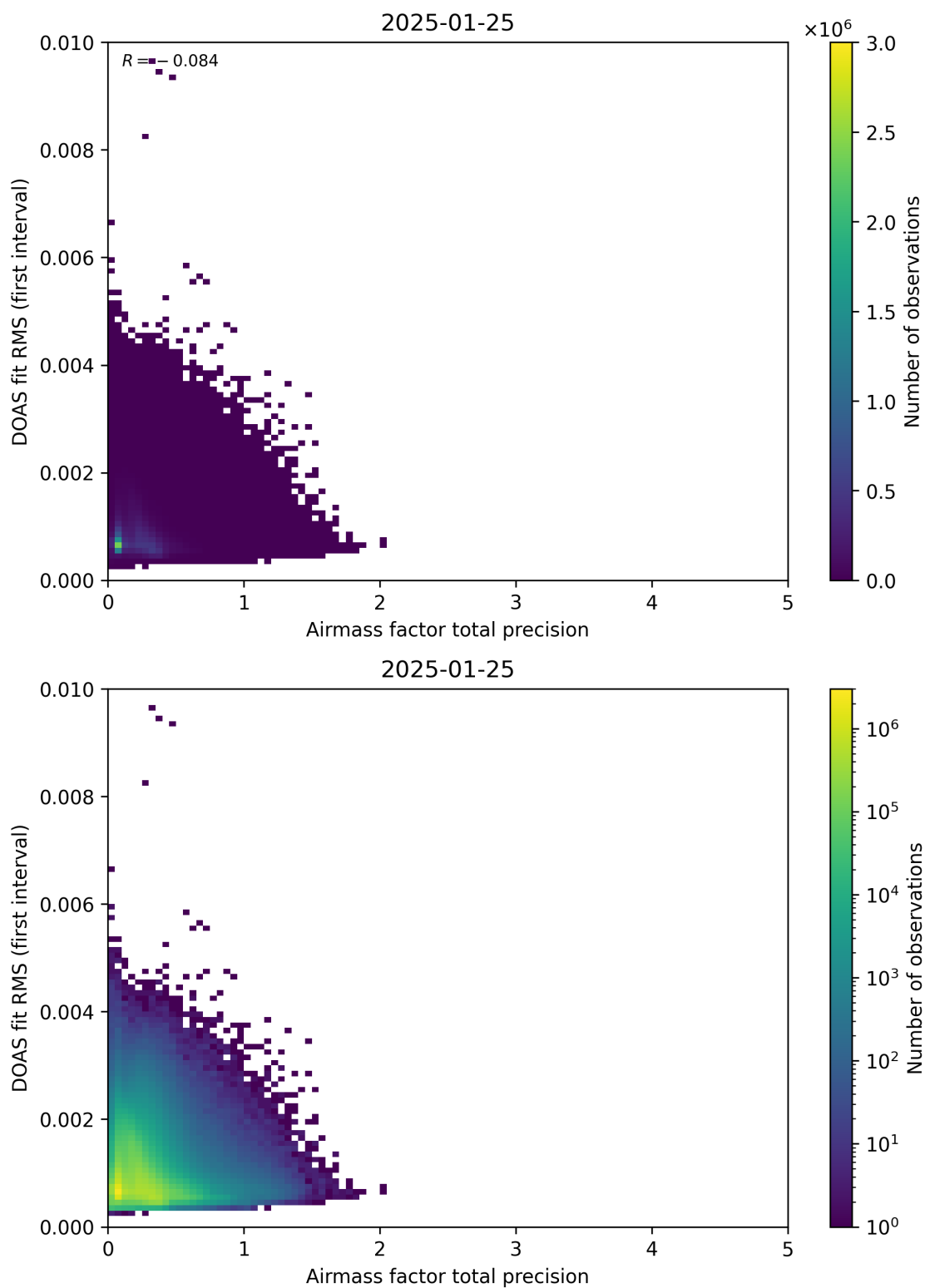
Figure 105: Scatter density plot of “Airmass factor total precision” against “DOAS fit RMS (first interval)” for 2025-01-24 to 2025-01-26.
