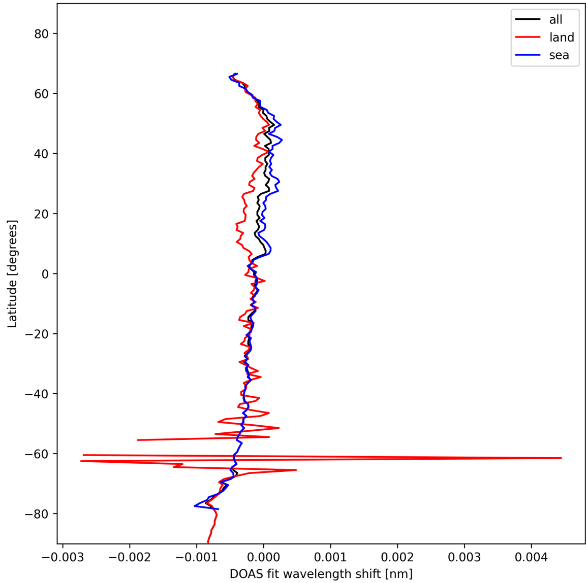
Figure 30: Zonal average of “DOAS fit wavelength shift” for 2025-01-24 to 2025-01-26.
