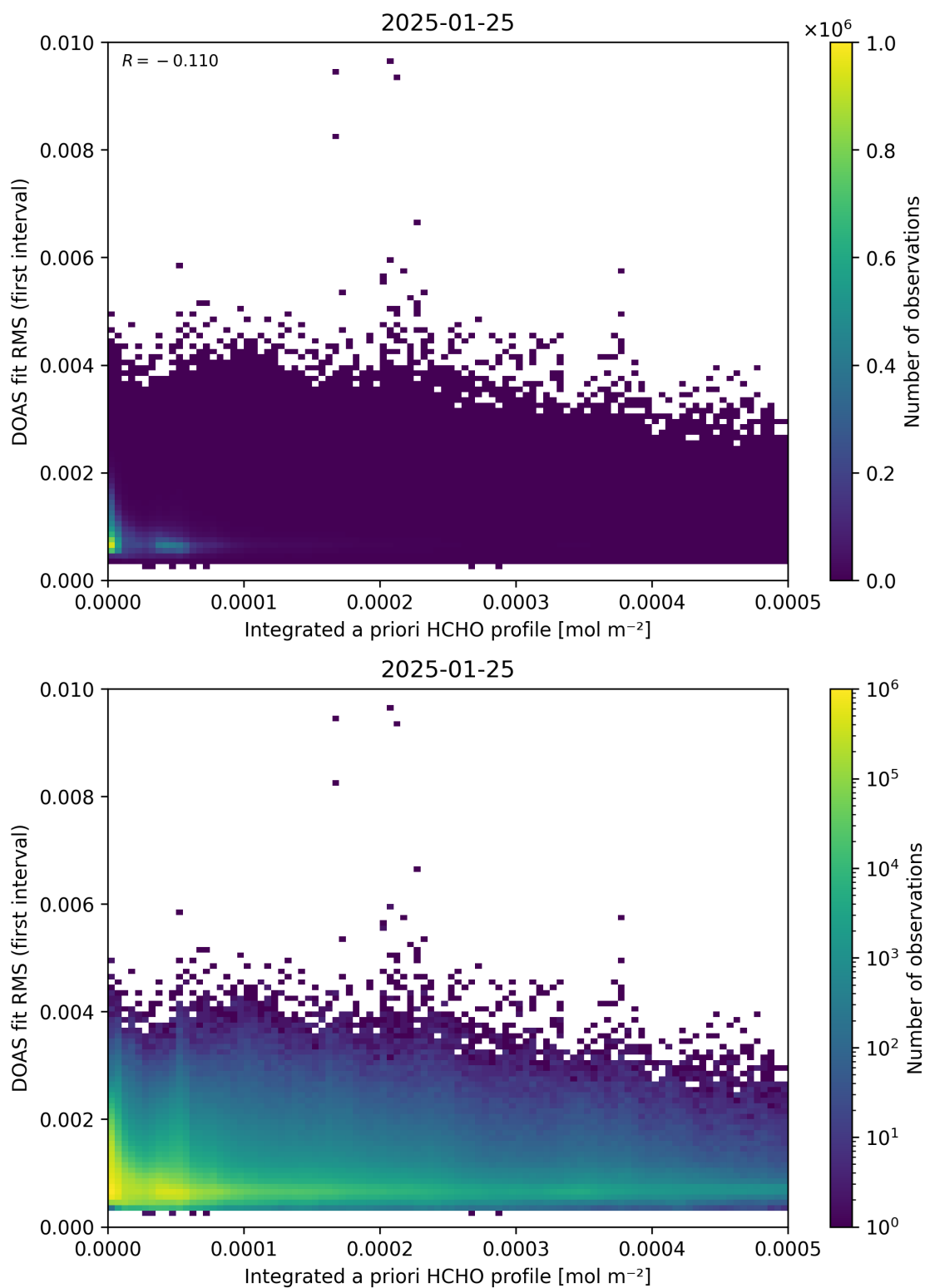
Figure 148: Scatter density plot of “Integrated a priori HCHO profile” against “DOAS fit RMS (first interval)” for 2025-01-24 to 2025-01-26.
