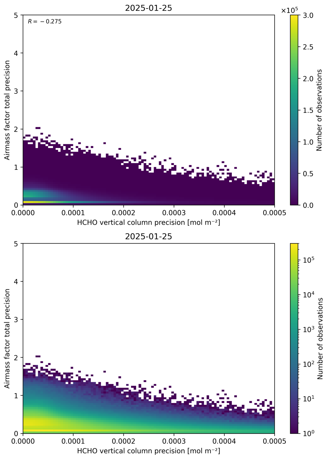
Figure 145: Scatter density plot of “HCHO vertical column precision” against “Airmass factor total precision” for 2025-01-24 to 2025-01-26.
