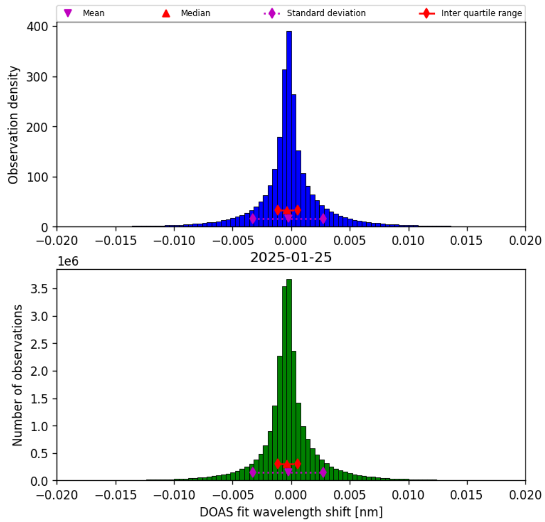
Figure 44: Histogram of “DOAS fit wavelength shift” for 2025-01-24 to 2025-01-26
