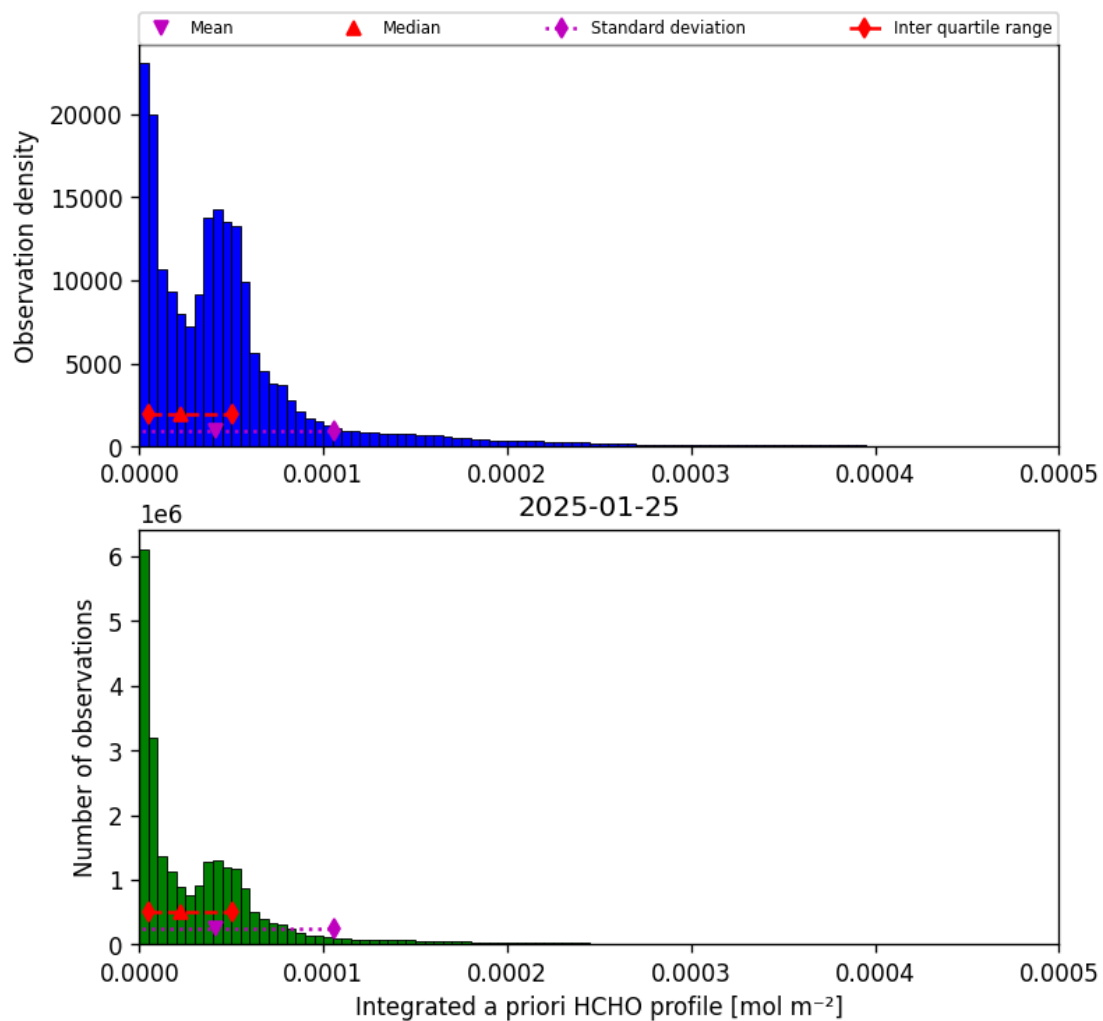
Figure 43: Histogram of “Integrated a priori HCHO profile” for 2025-01-24 to 2025-01-26
