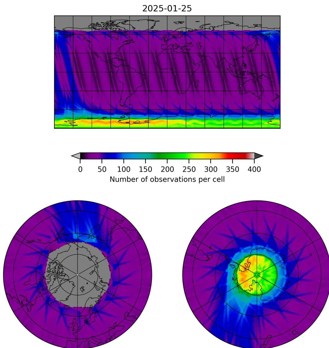
Figure 19: Map of the number of observations for 2025-01-24 to 2025-01-26
