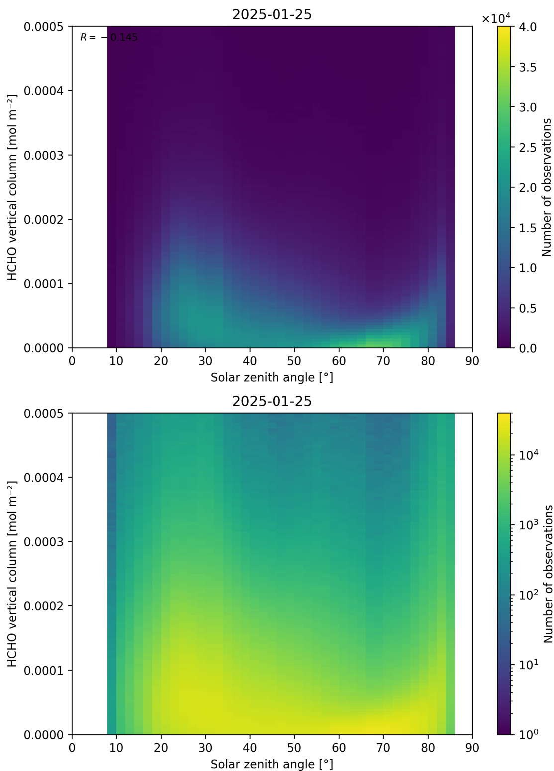
Figure 177: Scatter density plot of “Solar zenith angle” against “HCHO vertical column” for 2025-01-24 to 2025-01-26.
