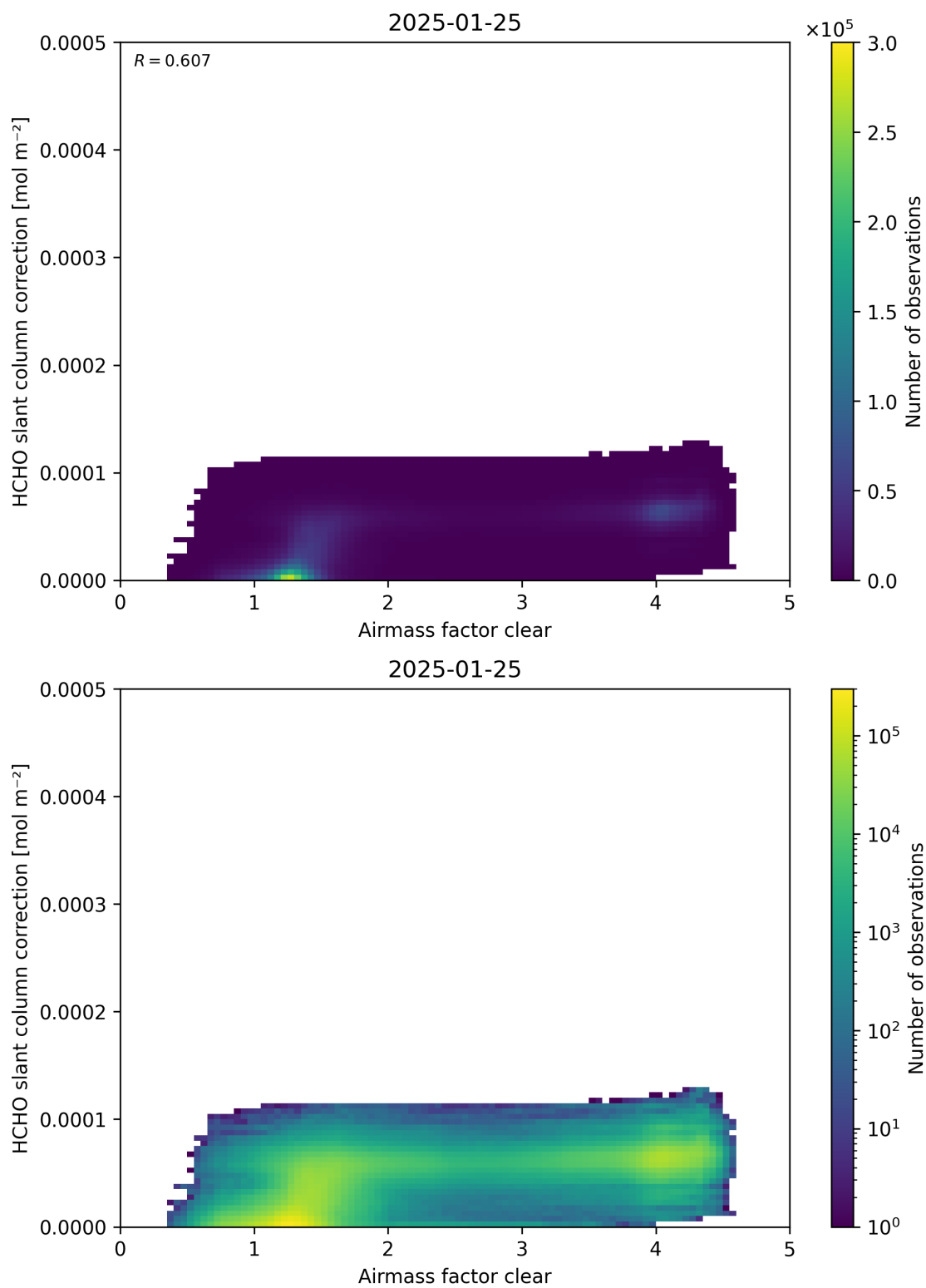
Figure 75: Scatter density plot of “Airmass factor clear” against “HCHO slant column correction” for 2025-01-24 to 2025-01-26.
