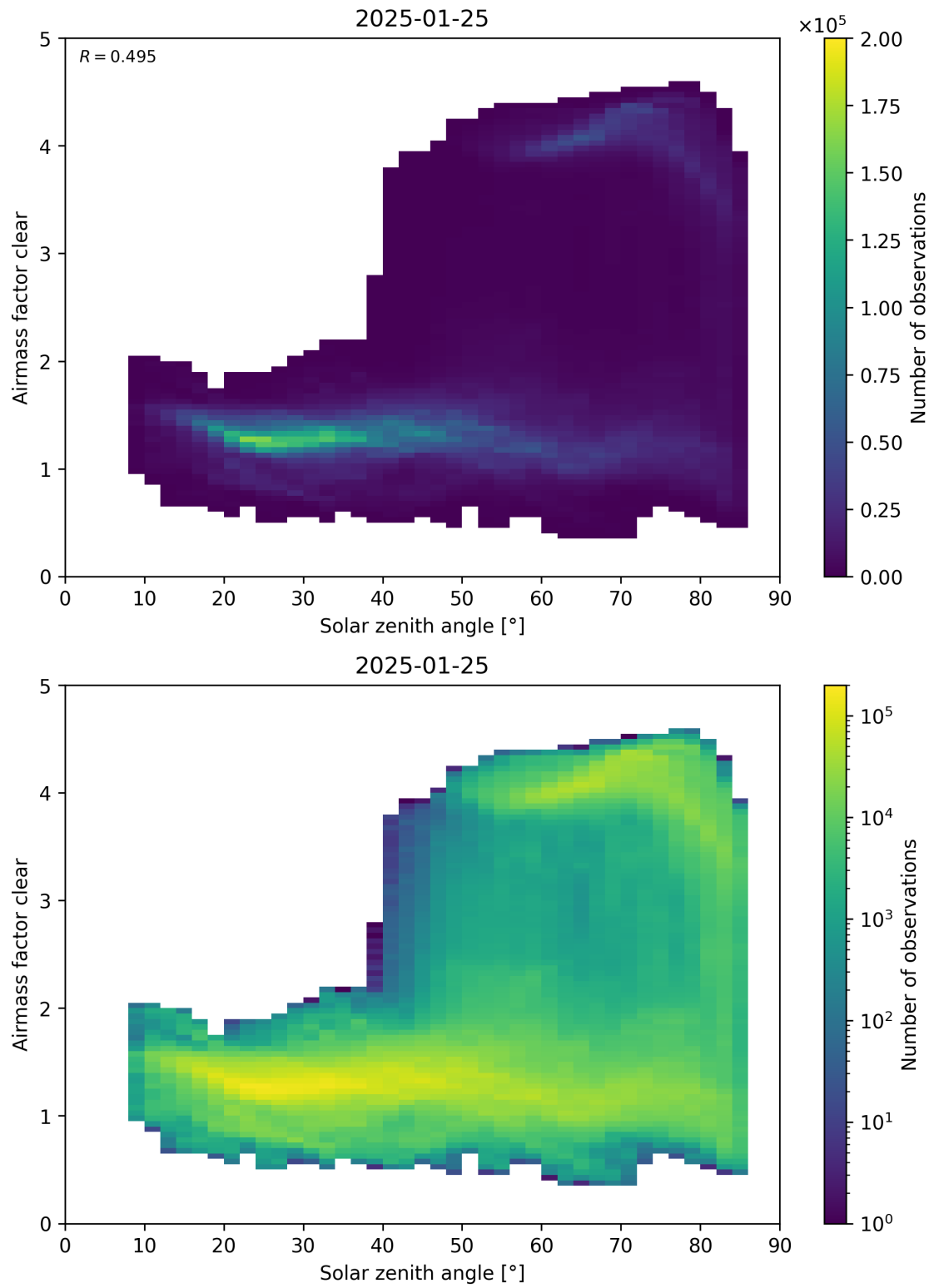
Figure 170: Scatter density plot of “Solar zenith angle” against “Airmass factor clear” for 2025-01-24 to 2025-01-26.
