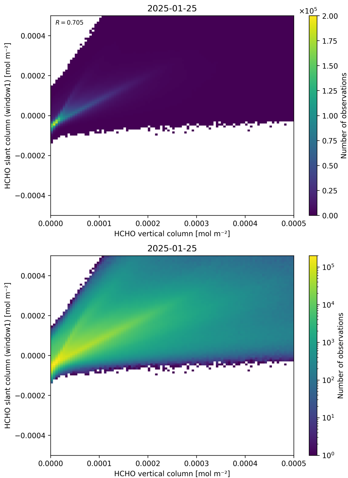
Figure 129: Scatter density plot of “HCHO vertical column” against “HCHO slant column (window1)” for 2025-01-24 to 2025-01-26.
