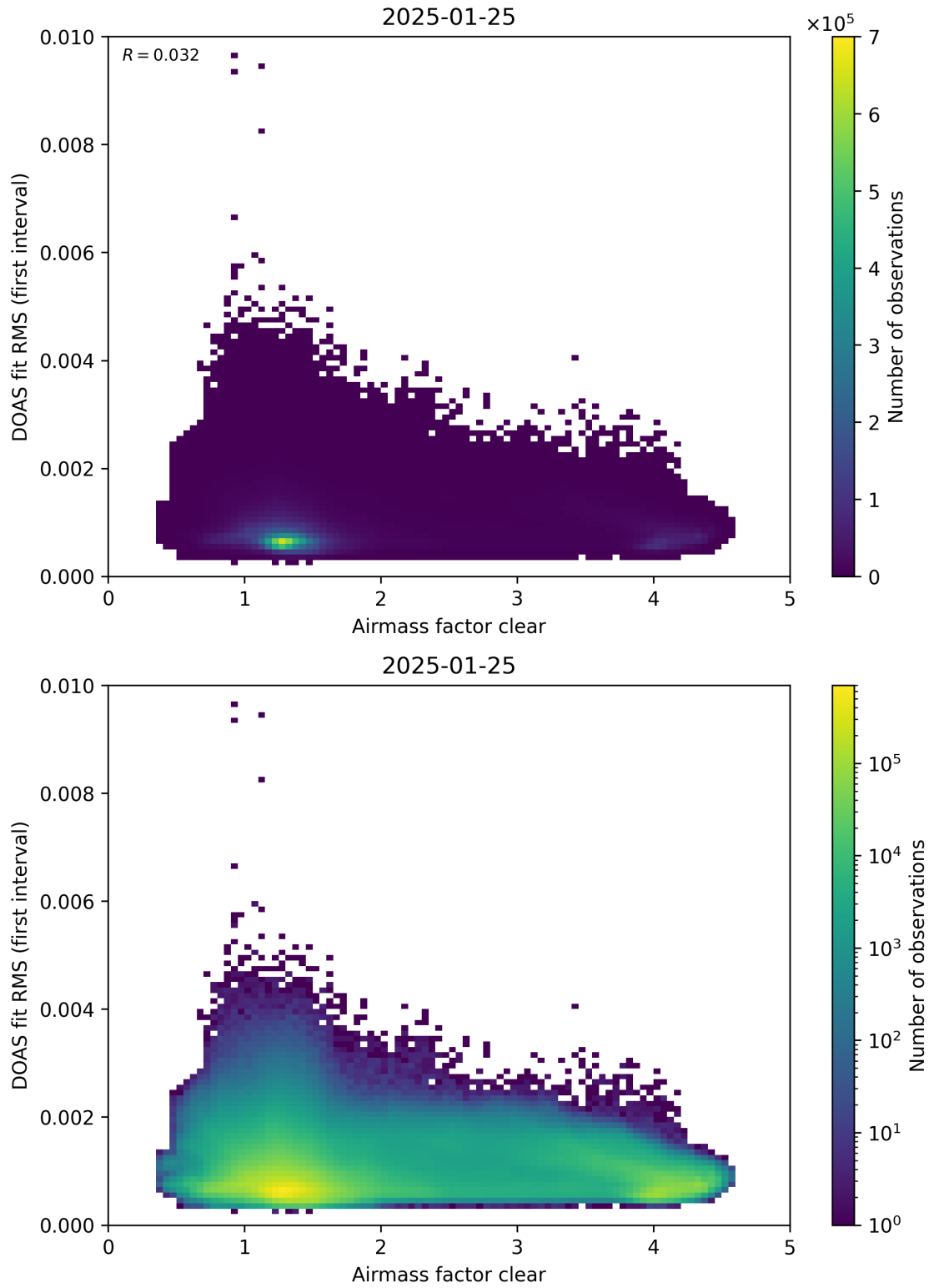
Figure 71: Scatter density plot of “Airmass factor clear” against “DOAS fit RMS (first interval)” for 2025-01-24 to 2025-01-26.
