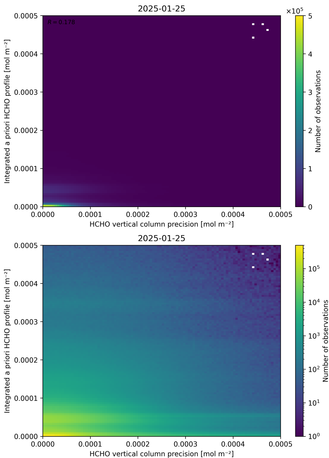
Figure 147: Scatter density plot of “HCHO vertical column precision” against “Integrated a priori HCHO profile” for 2025-01-24 to 2025-01-26.
