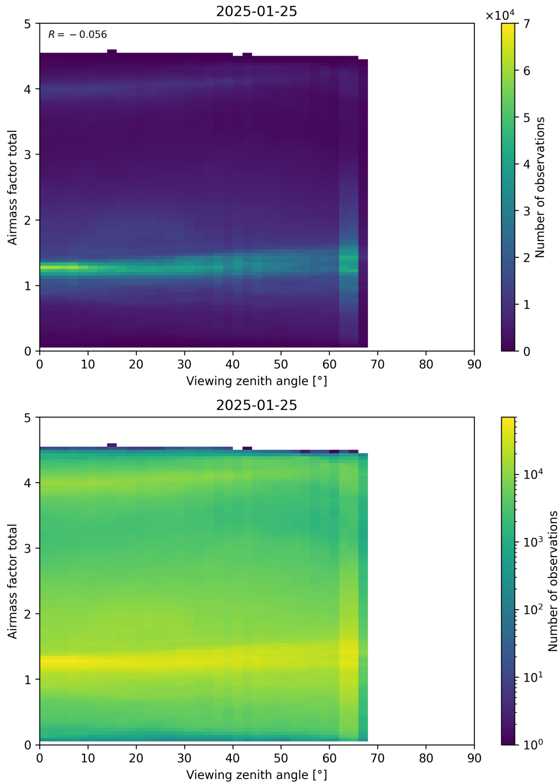
Figure 190: Scatter density plot of “Viewing zenith angle” against “Airmass factor total” for 2025-01-24 to 2025-01-26.
