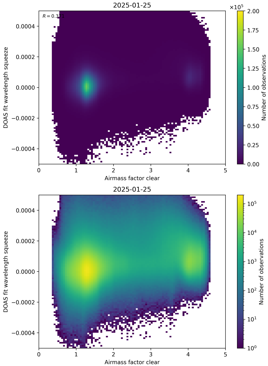
Figure 73: Scatter density plot of “Airmass factor clear” against “DOAS fit wavelength squeeze” for 2025-01-24 to 2025-01-26.
