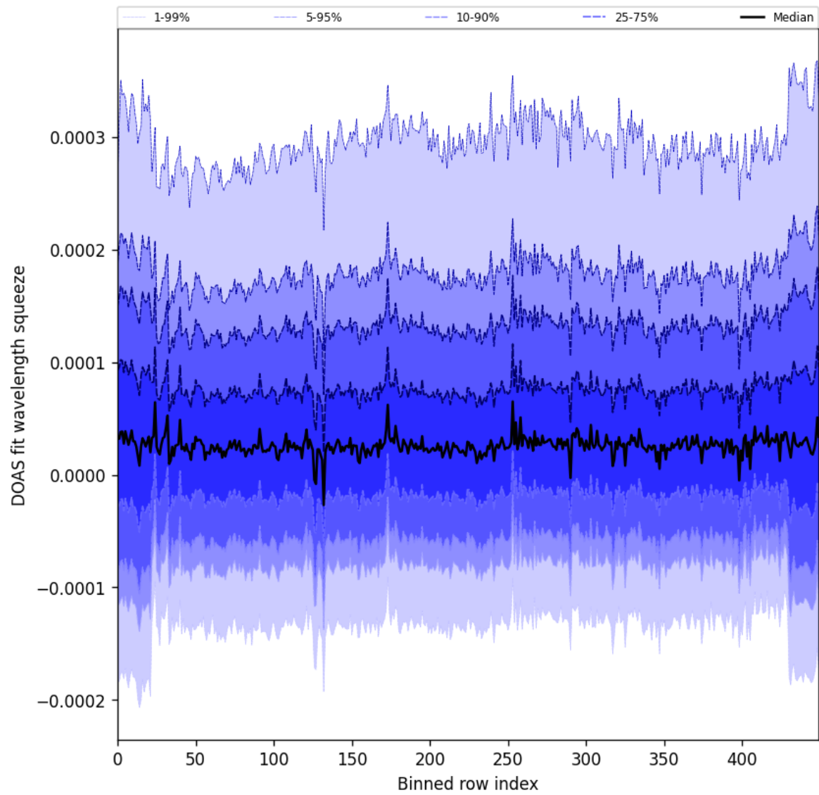
Figure 59: Along track statistics of “DOAS fit wavelength squeeze” for 2025-01-24 to 2025-01-26
