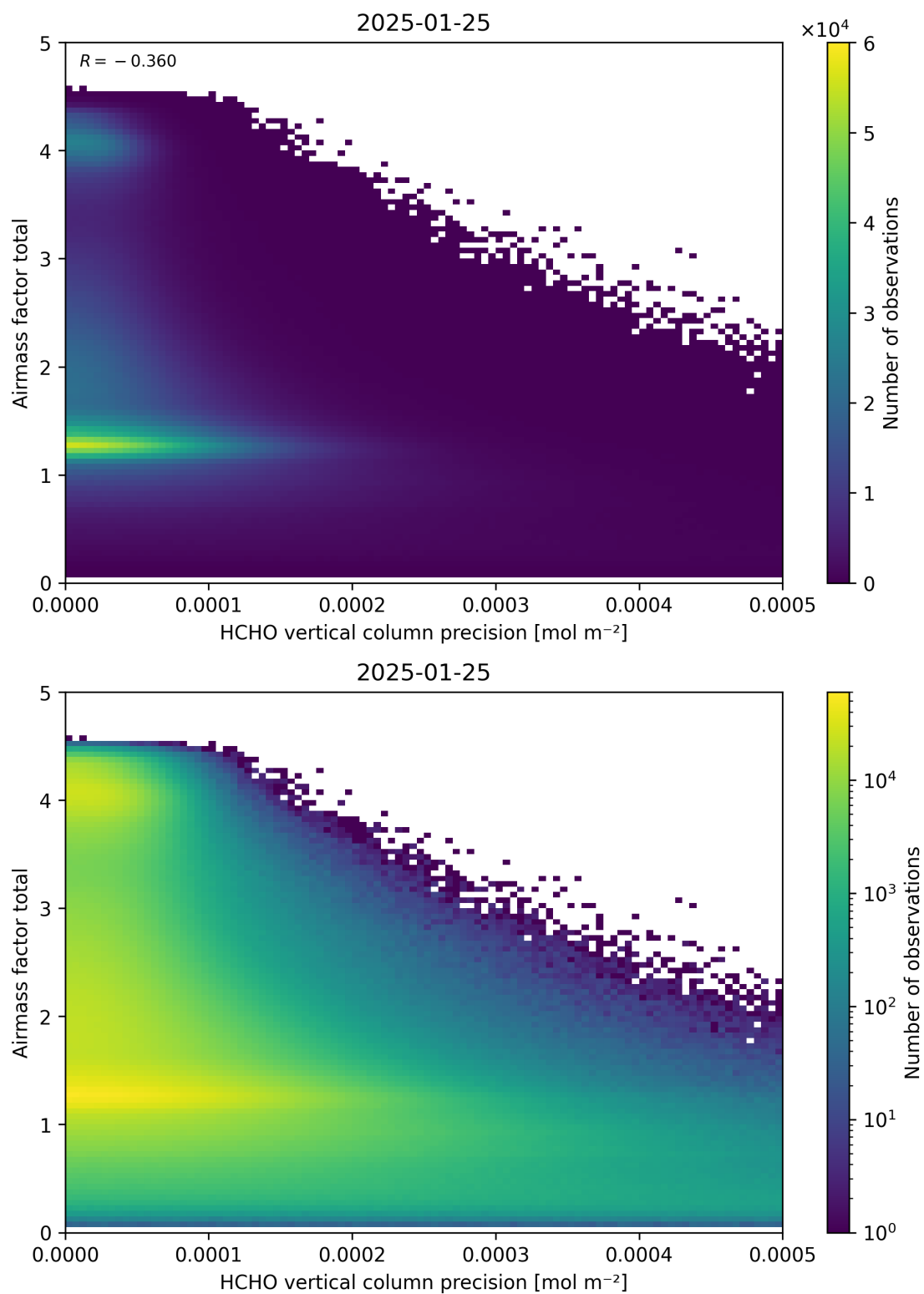
Figure 144: Scatter density plot of “HCHO vertical column precision” against “Airmass factor total” for 2025-01-24 to 2025-01-26.
