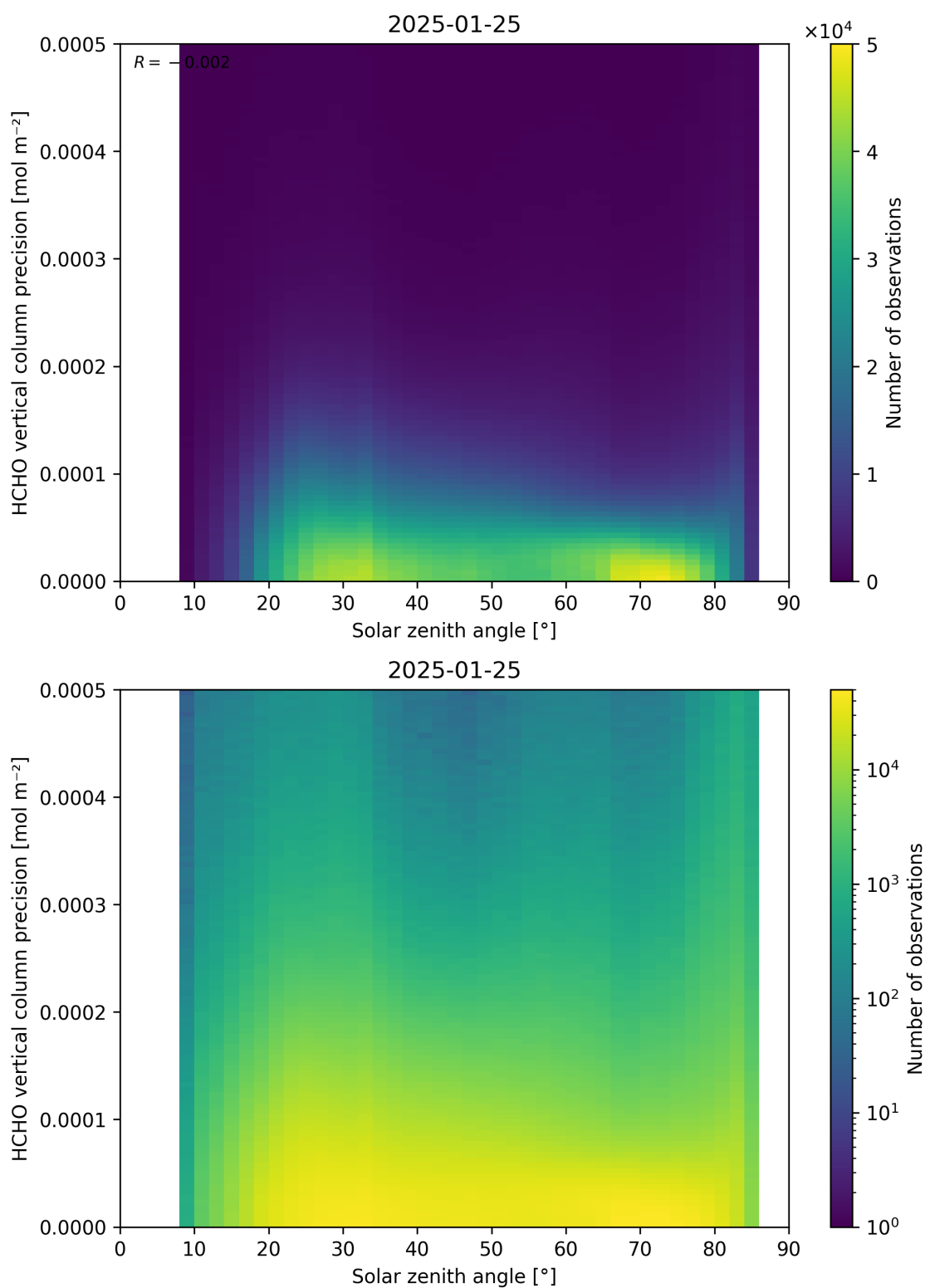
Figure 179: Scatter density plot of “Solar zenith angle” against “HCHO vertical column precision” for 2025-01-24 to 2025-01-26.
