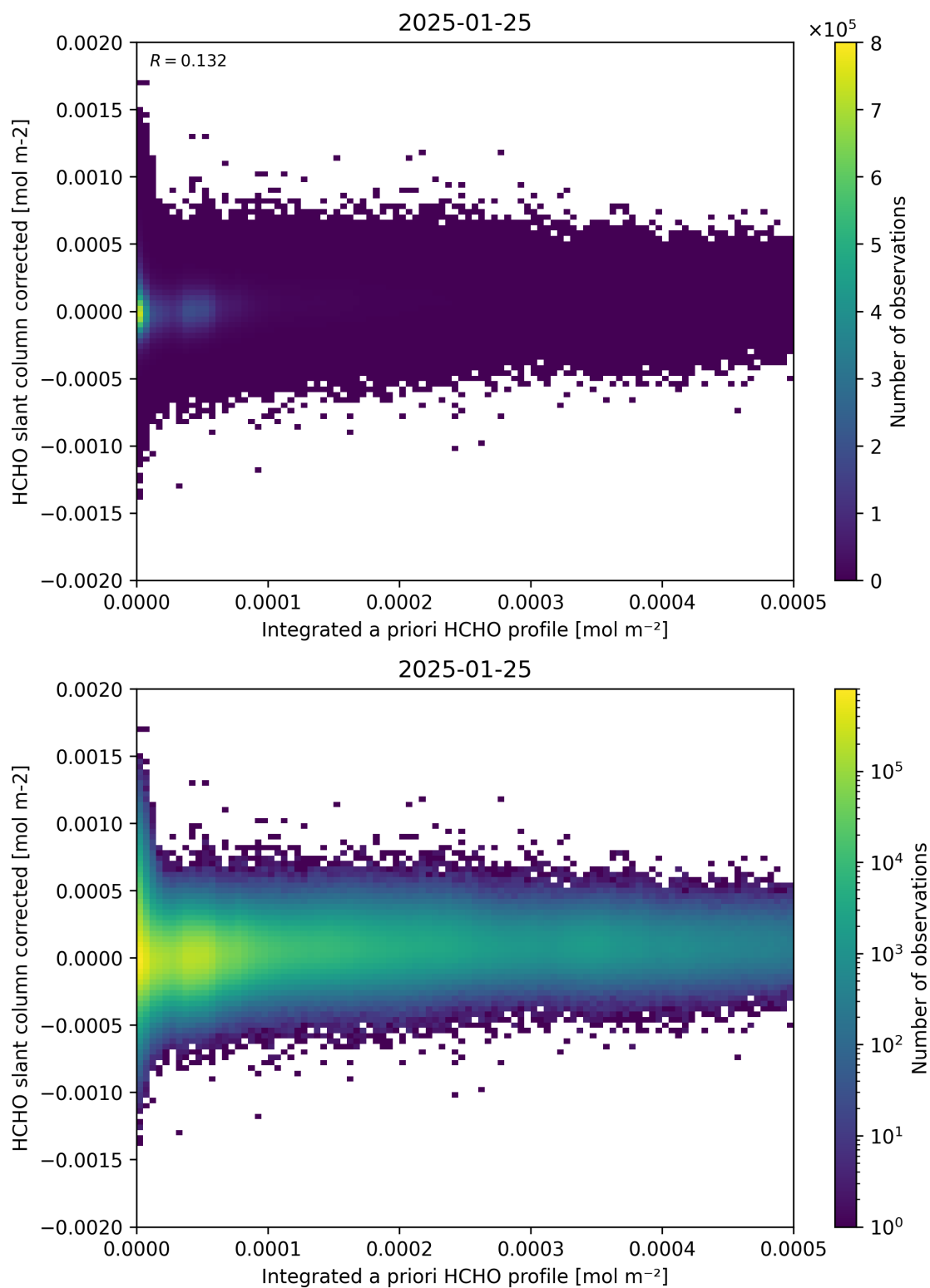
Figure 151: Scatter density plot of “Integrated a priori HCHO profile” against “HCHO slant column corrected” for 2025-01-24 to 2025-01-26.
