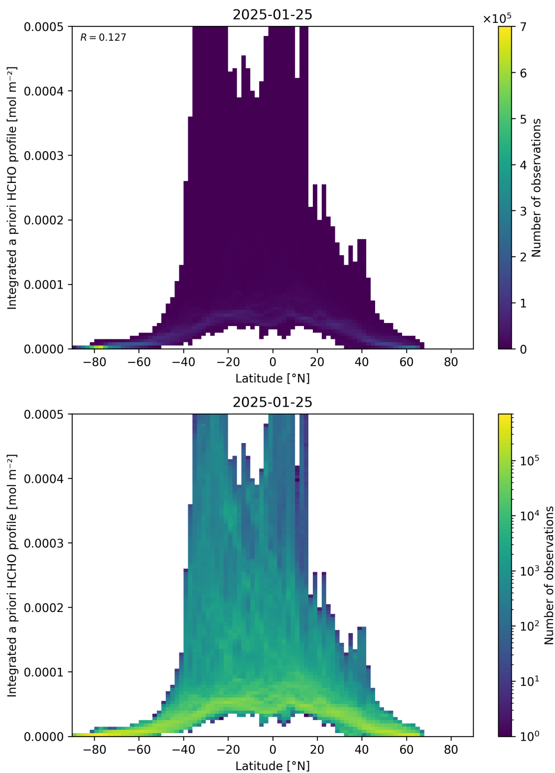
Figure 166: Scatter density plot of “Latitude” against “Integrated a priori HCHO profile” for 2025-01-24 to 2025-01-26.
