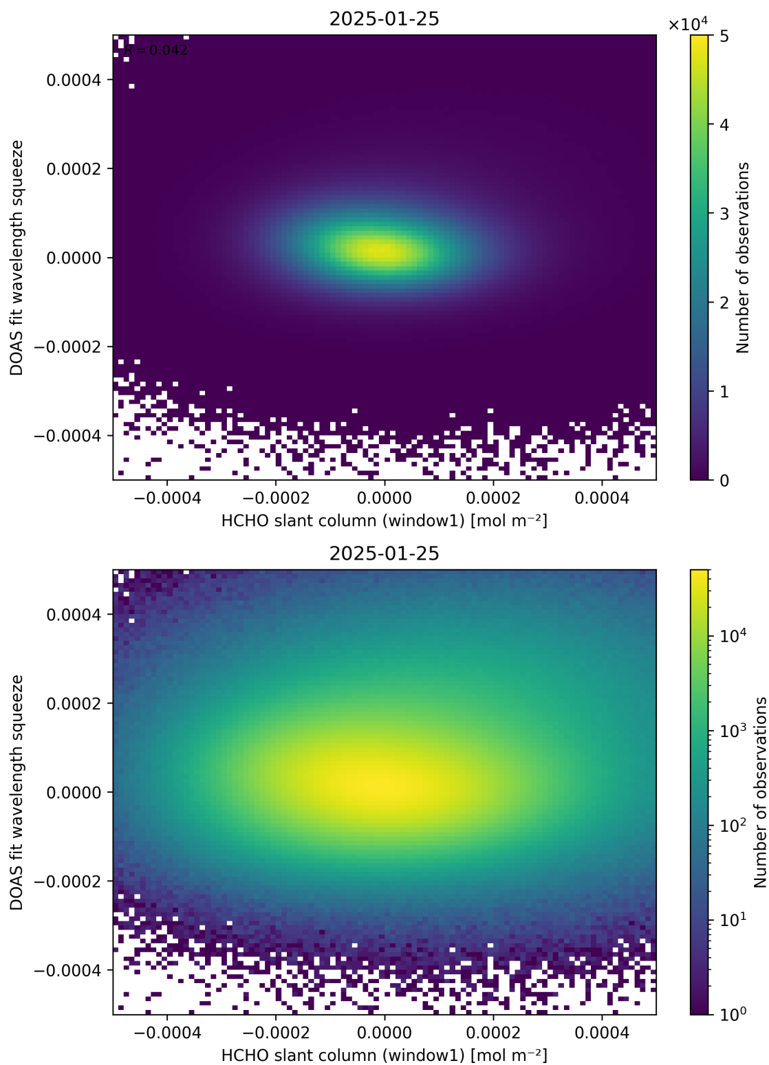
Figure 80: Scatter density plot of “HCHO slant column (window1)” against “DOAS fit wavelength squeeze” for 2025-01-24 to 2025-01-26.
