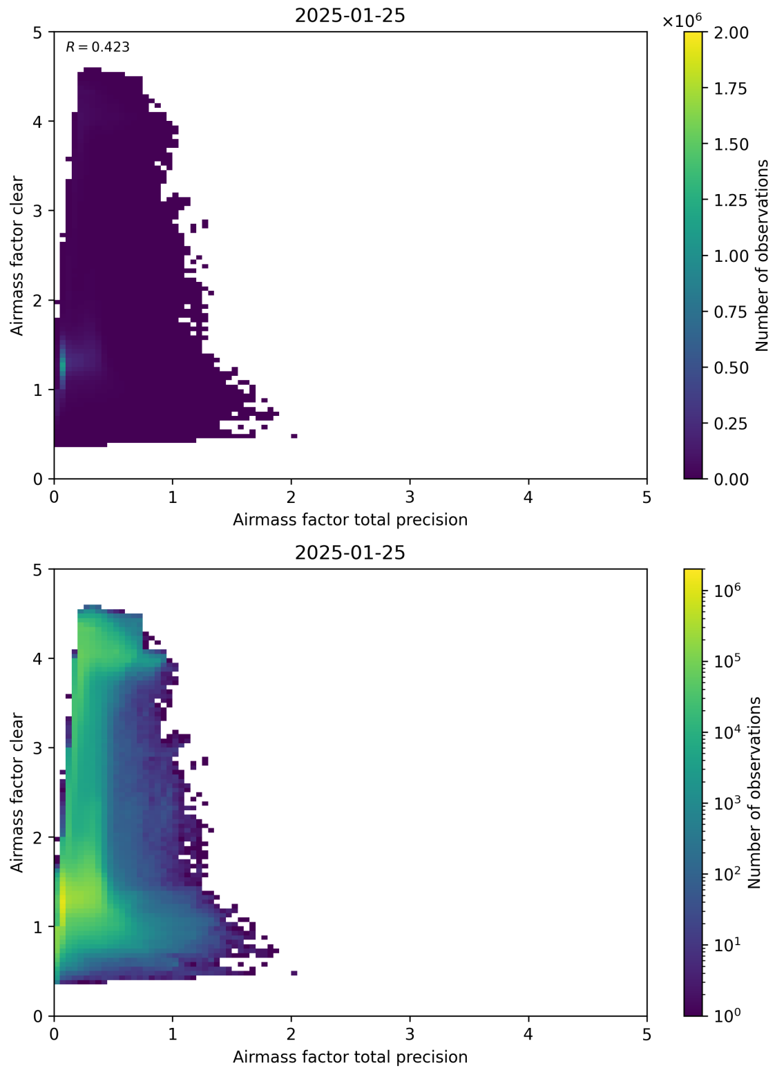
Figure 108: Scatter density plot of “Airmass factor total precision” against “Airmass factor clear” for 2025-01-24 to 2025-01-26.
