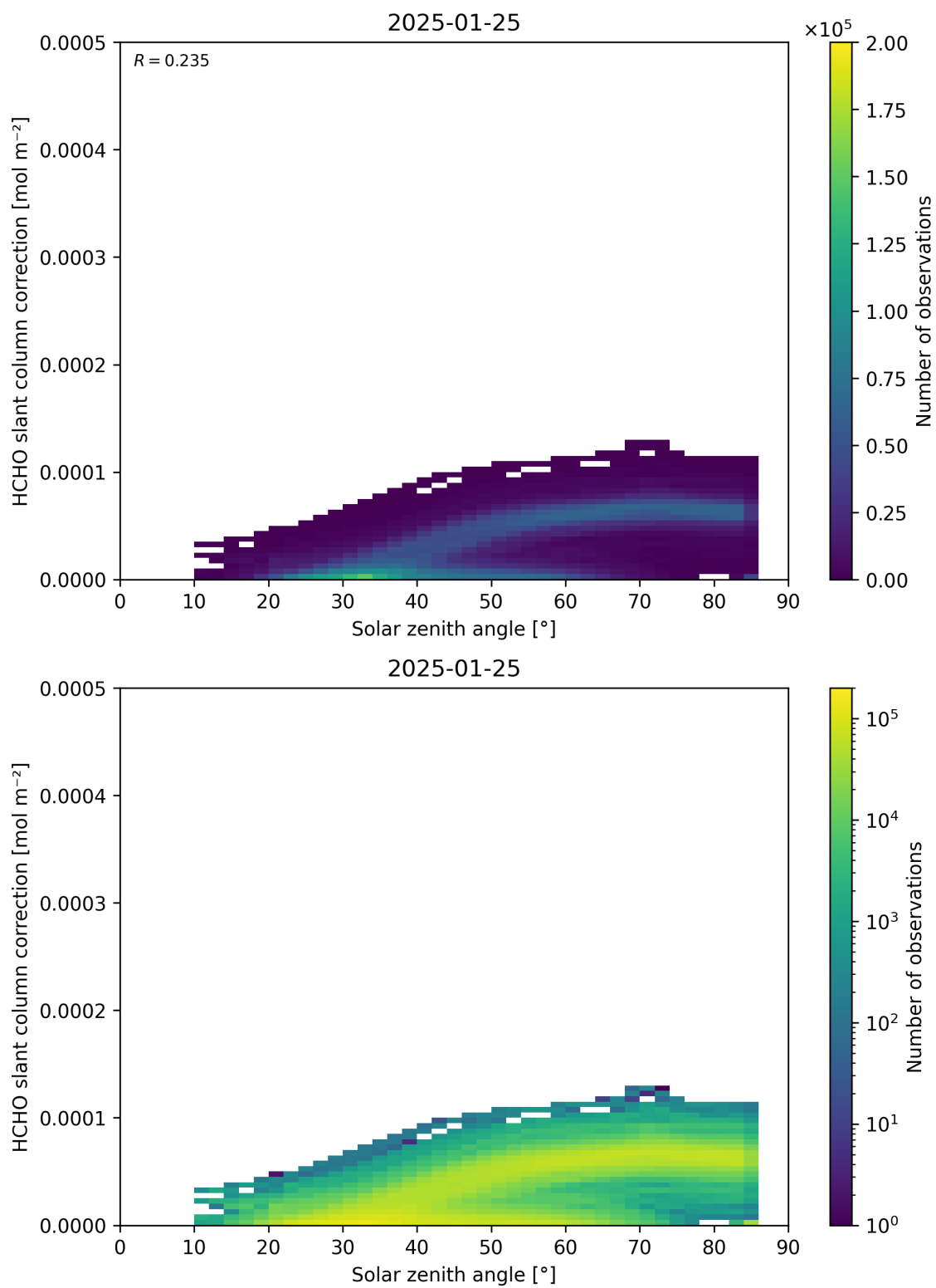
Figure 172: Scatter density plot of “Solar zenith angle” against “HCHO slant column correction” for 2025-01-24 to 2025-01-26.
