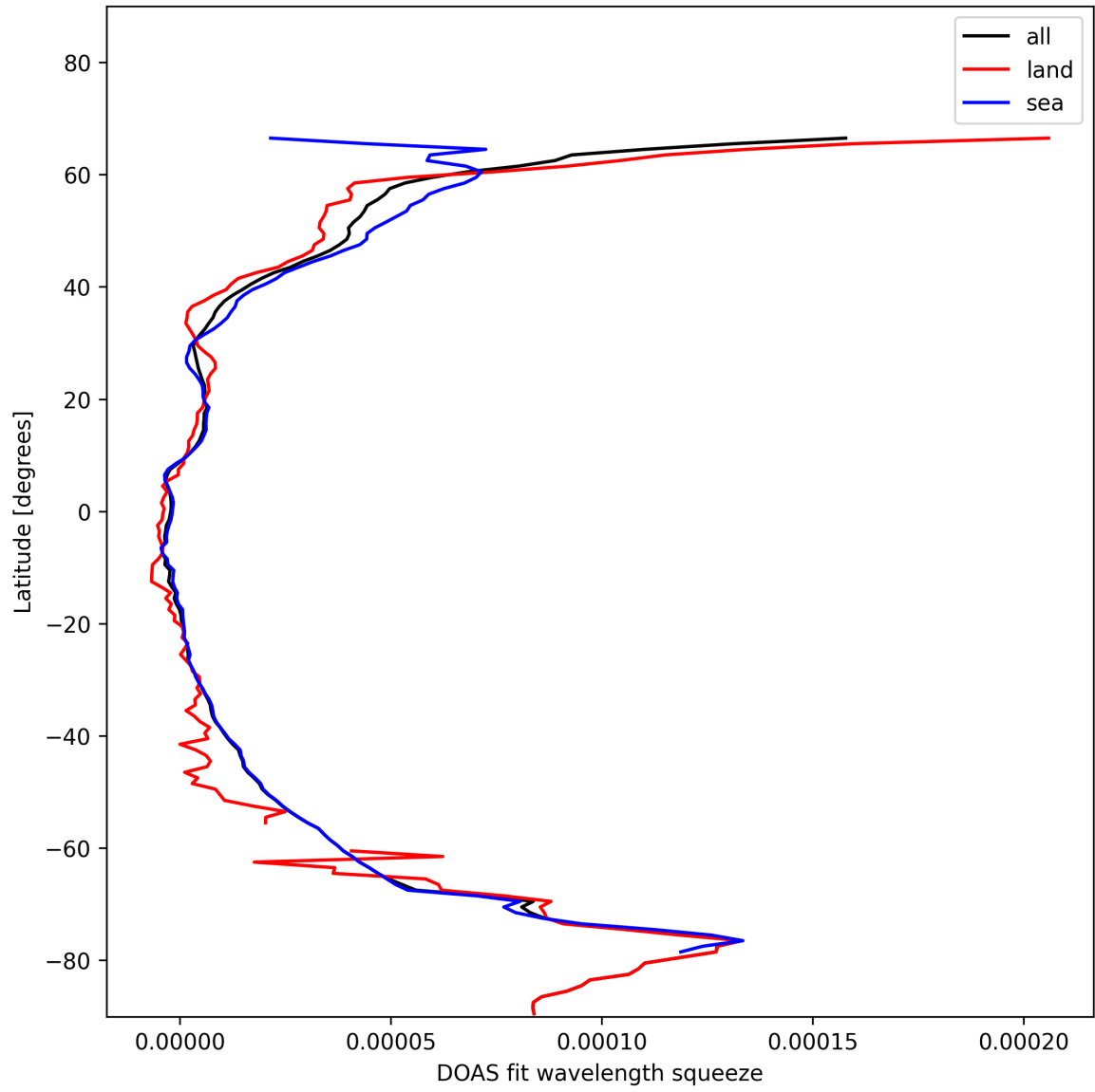
Figure 31: Zonal average of “DOAS fit wavelength squeeze” for 2025-01-24 to 2025-01-26.
