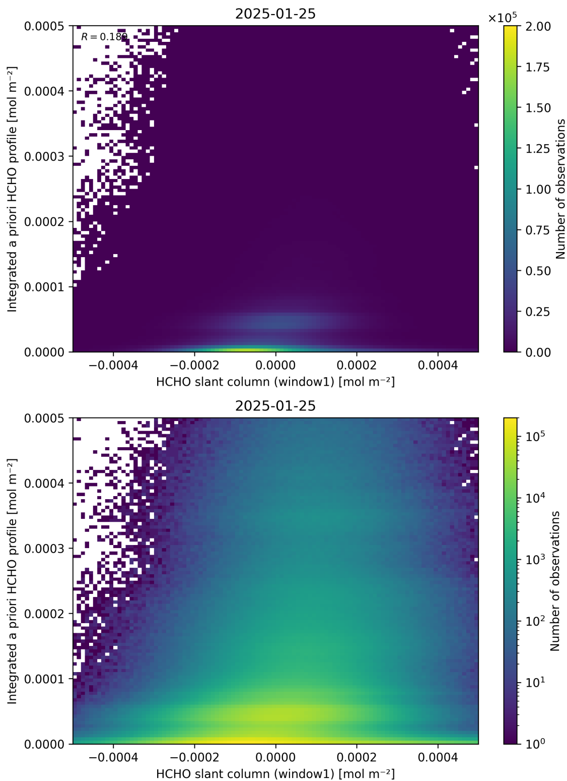
Figure 87: Scatter density plot of “HCHO slant column (window1)” against “Integrated a priori HCHO profile” for 2025-01-24 to 2025-01-26.
