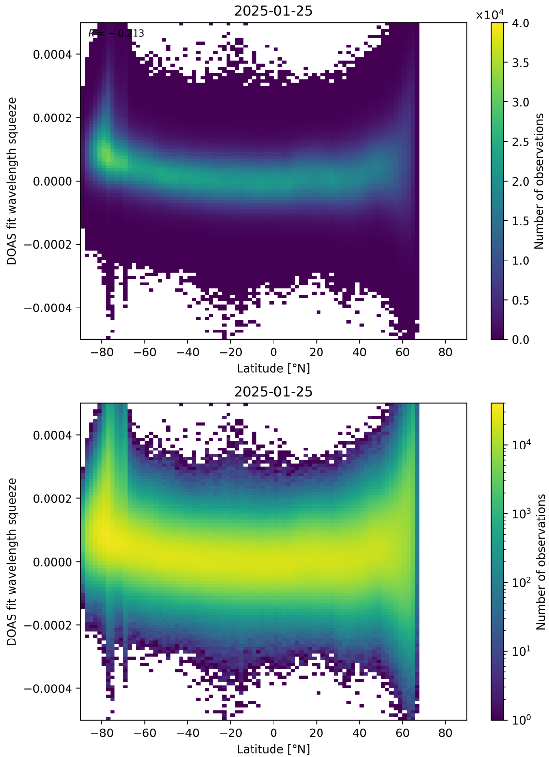
Figure 155: Scatter density plot of “Latitude” against “DOAS fit wavelength squeeze” for 2025-01-24 to 2025-01-26.
