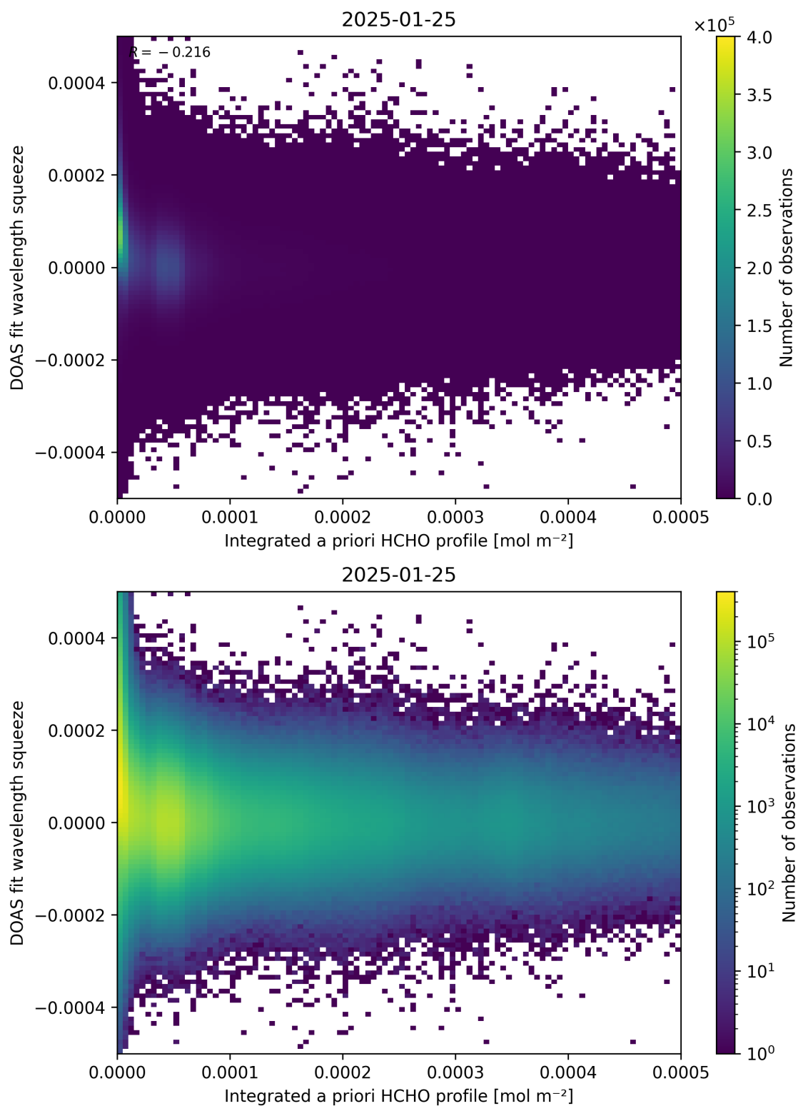
Figure 150: Scatter density plot of “Integrated a priori HCHO profile” against “DOAS fit wavelength squeeze” for 2025-01-24 to 2025-01-26.
