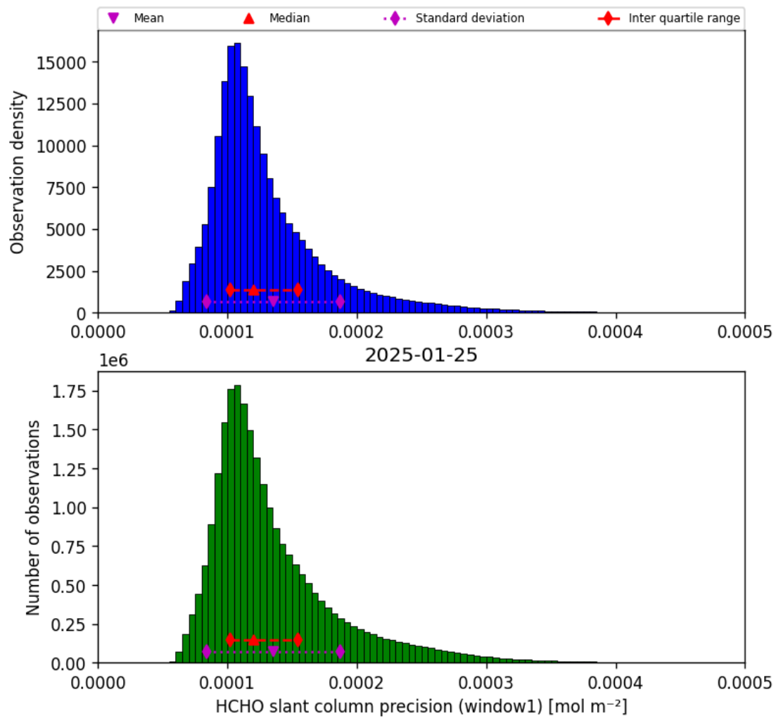
Figure 39: Histogram of “HCHO slant column precision (window1)” for 2025-01-24 to 2025-01-26
