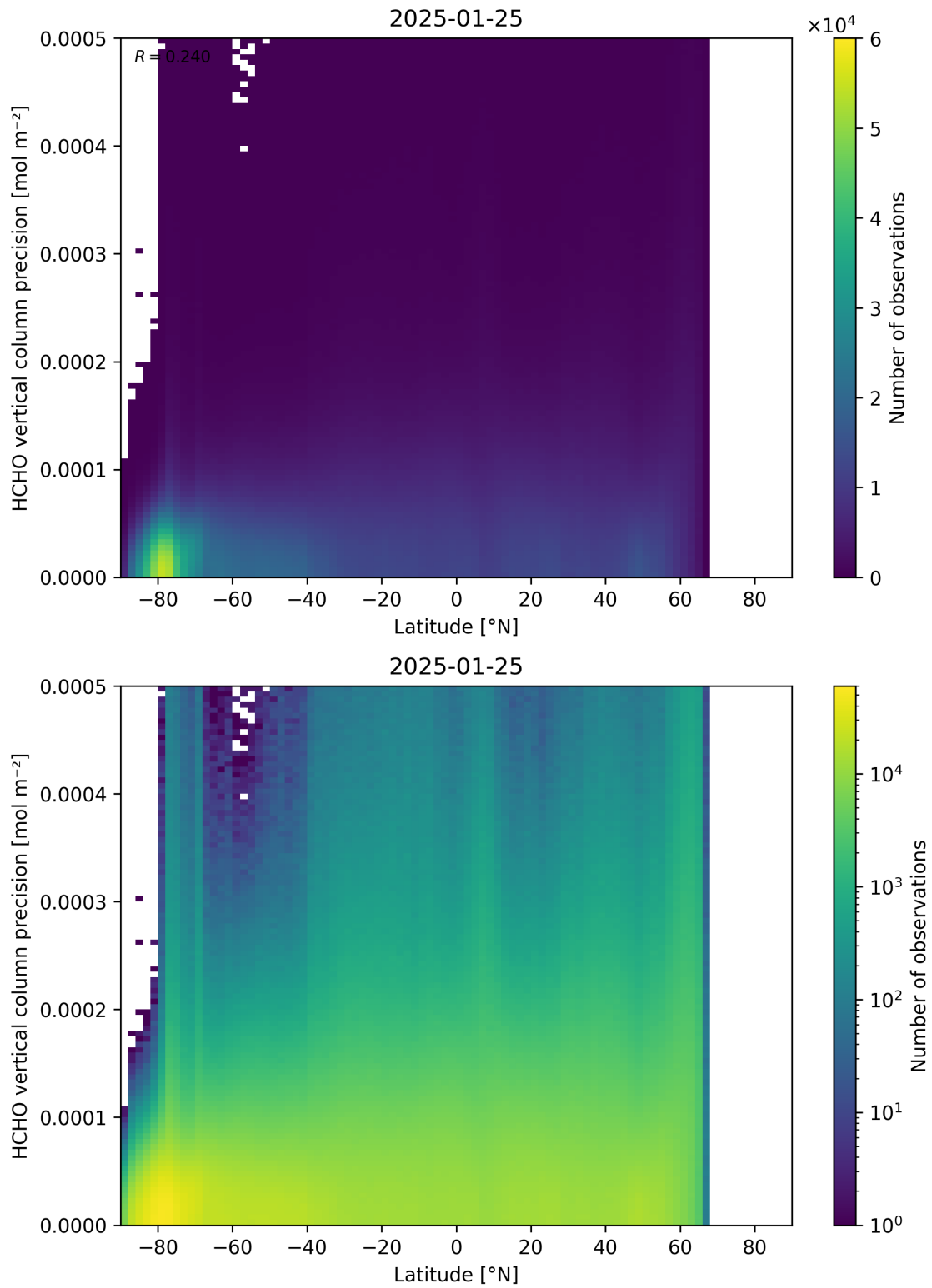
Figure 165: Scatter density plot of “Latitude” against “HCHO vertical column precision” for 2025-01-24 to 2025-01-26.
