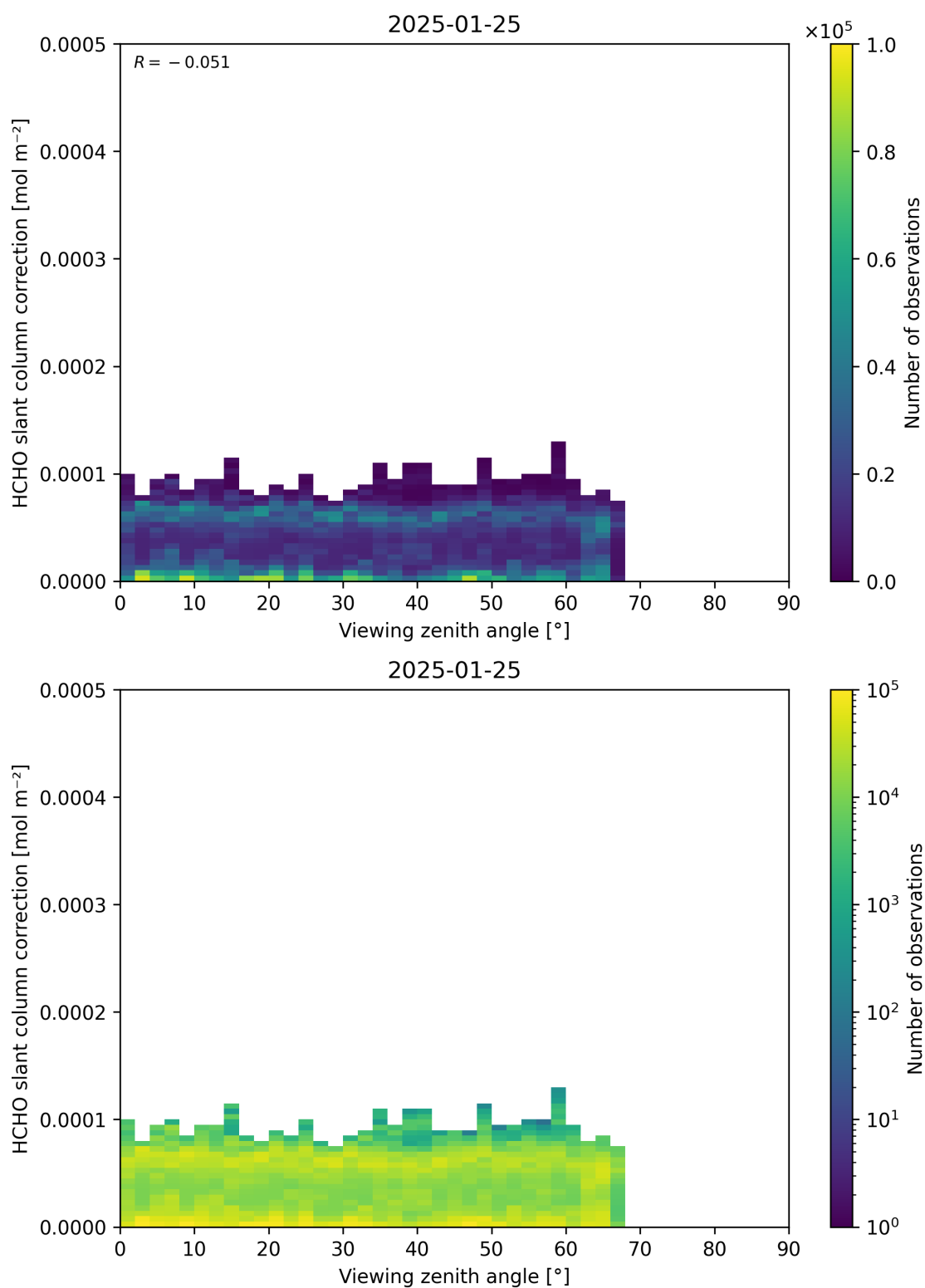
Figure 187: Scatter density plot of “Viewing zenith angle” against “HCHO slant column correction” for 2025-01-24 to 2025-01-26.
