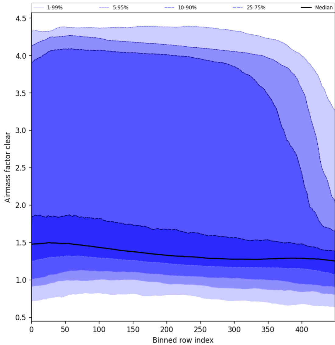
Figure 56: Along track statistics of “Airmass factor clear” for 2025-01-24 to 2025-01-26
