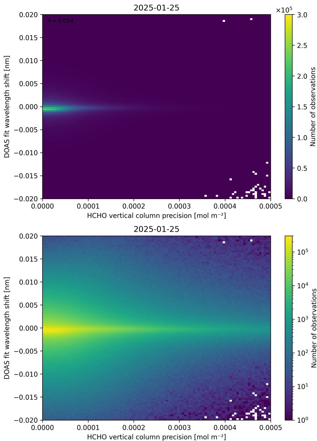
Figure 137: Scatter density plot of “HCHO vertical column precision” against “DOAS fit wavelength shift” for 2025-01-24 to 2025-01-26.
