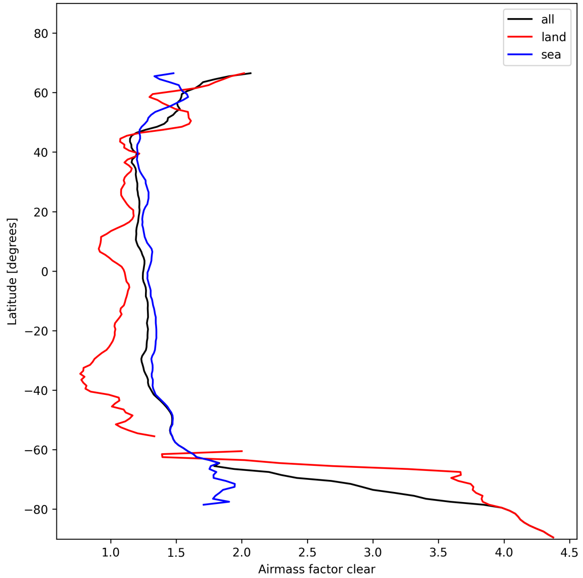
Figure 28: Zonal average of “Airmass factor clear” for 2025-01-24 to 2025-01-26.
