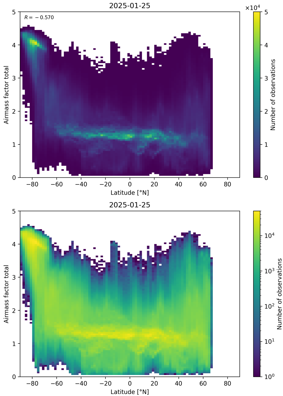
Figure 161: Scatter density plot of “Latitude” against “Airmass factor total” for 2025-01-24 to 2025-01-26.
