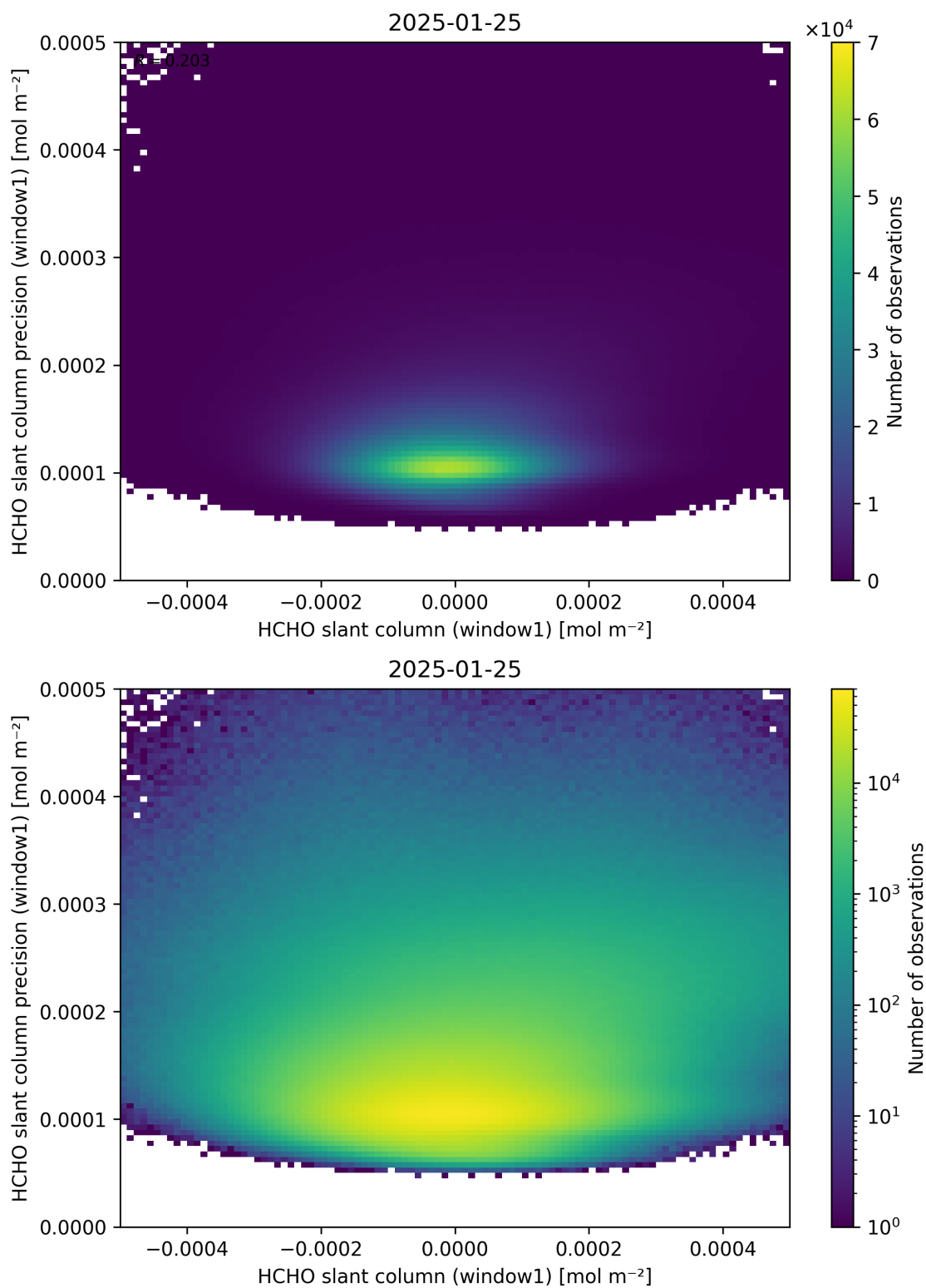
Figure 84: Scatter density plot of “HCHO slant column (window1)” against “HCHO slant column precision (window1)” for 2025-01-24 to 2025-01-26.
