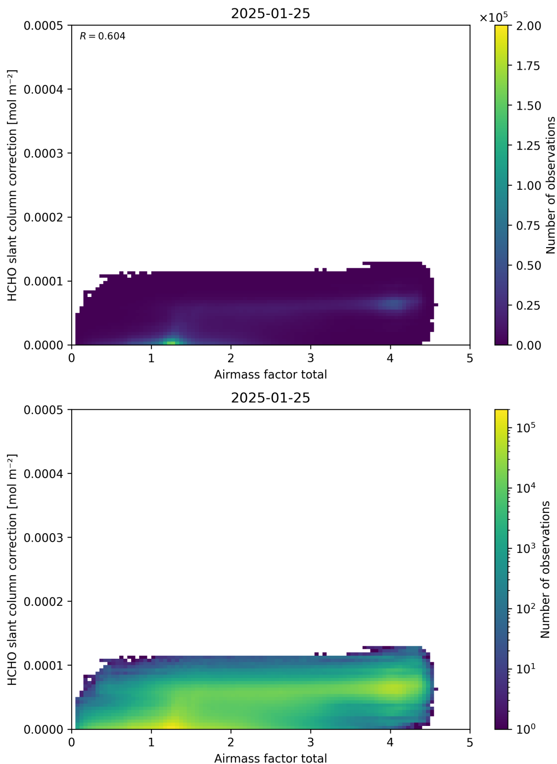
Figure 102: Scatter density plot of “Airmass factor total” against “HCHO slant column correction” for 2025-01-24 to 2025-01-26.
