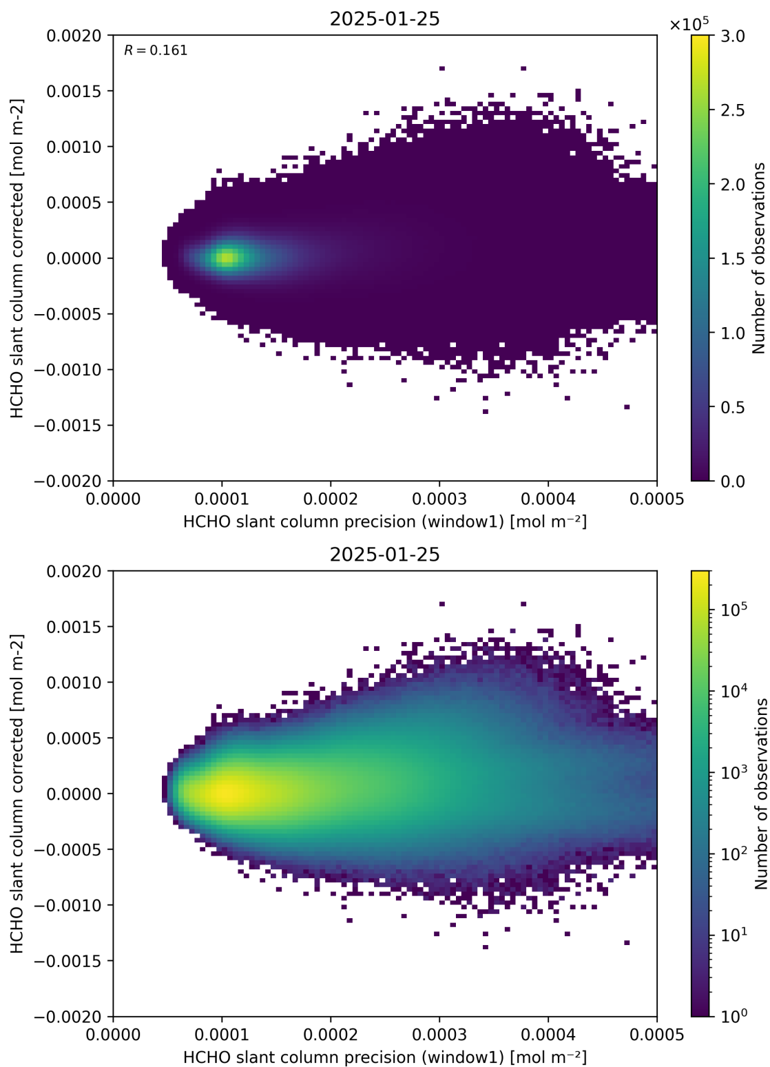
Figure 92: Scatter density plot of “HCHO slant column precision (window1)” against “HCHO slant column corrected” for 2025-01-24 to 2025-01-26.
