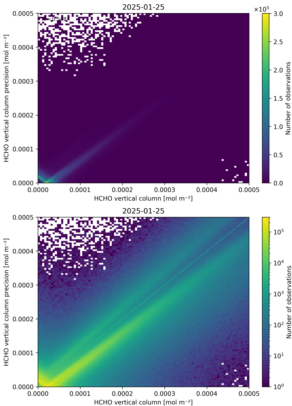
Figure 134: Scatter density plot of “HCHO vertical column” against “HCHO vertical column precision” for 2025-01-24 to 2025-01-26.
