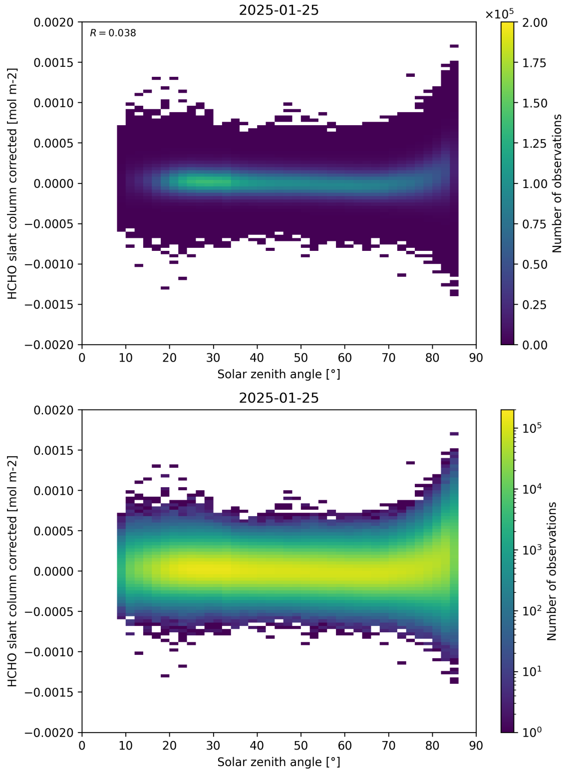
Figure 171: Scatter density plot of “Solar zenith angle” against “HCHO slant column corrected” for 2025-01-24 to 2025-01-26.
