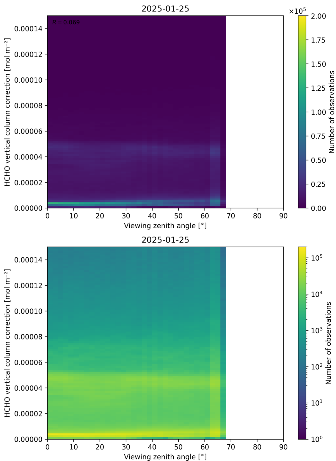
Figure 193: Scatter density plot of “Viewing zenith angle” against “HCHO vertical column correction” for 2025-01-24 to 2025-01-26.
