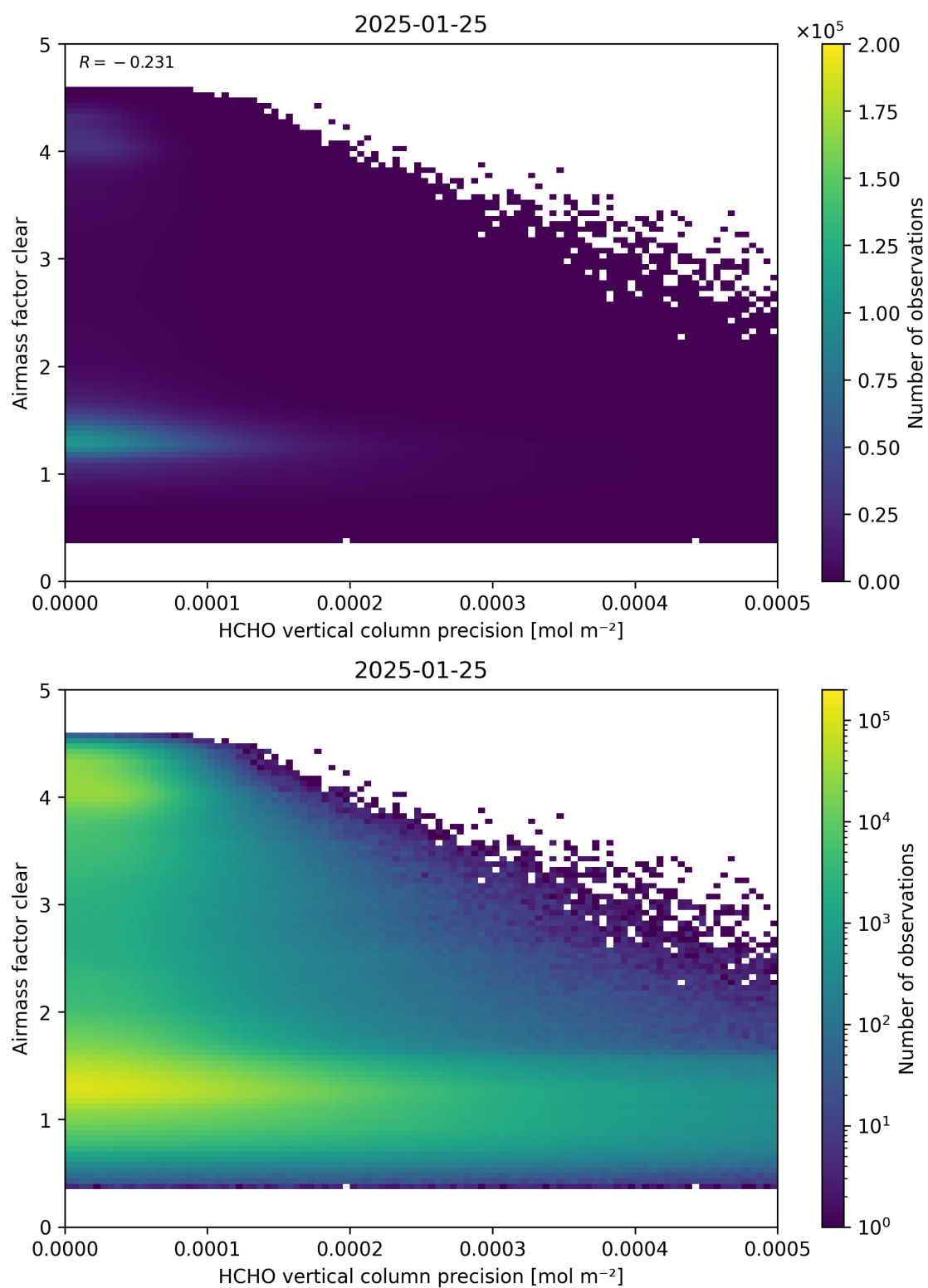
Figure 139: Scatter density plot of “HCHO vertical column precision” against “Airmass factor clear” for 2025-01-24 to 2025-01-26.
