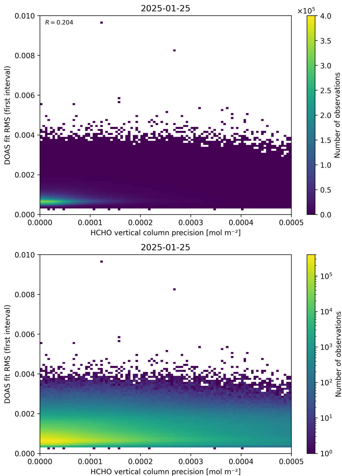
Figure 136: Scatter density plot of “HCHO vertical column precision” against “DOAS fit RMS (first interval)” for 2025-01-24 to 2025-01-26.
