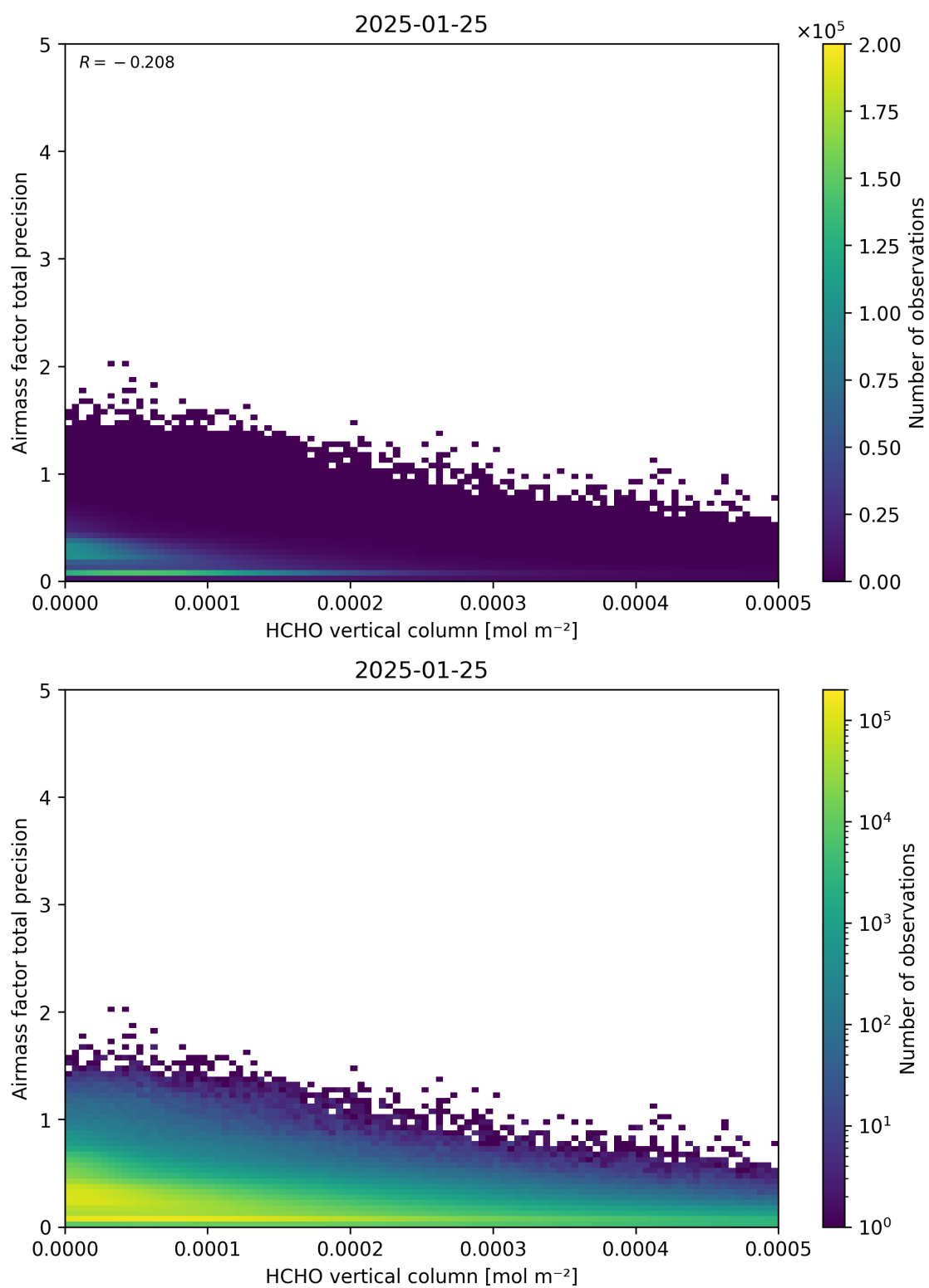
Figure 132: Scatter density plot of “HCHO vertical column” against “Airmass factor total precision” for 2025-01-24 to 2025-01-26.
