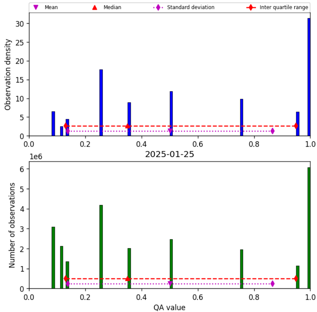
Figure 34: Histogram of “QA value” for 2025-01-24 to 2025-01-26
