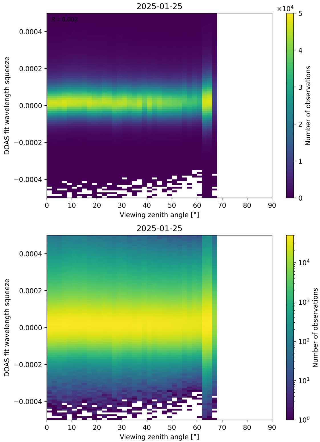
Figure 184: Scatter density plot of “Viewing zenith angle” against “DOAS fit wavelength squeeze” for 2025-01-24 to 2025-01-26.
