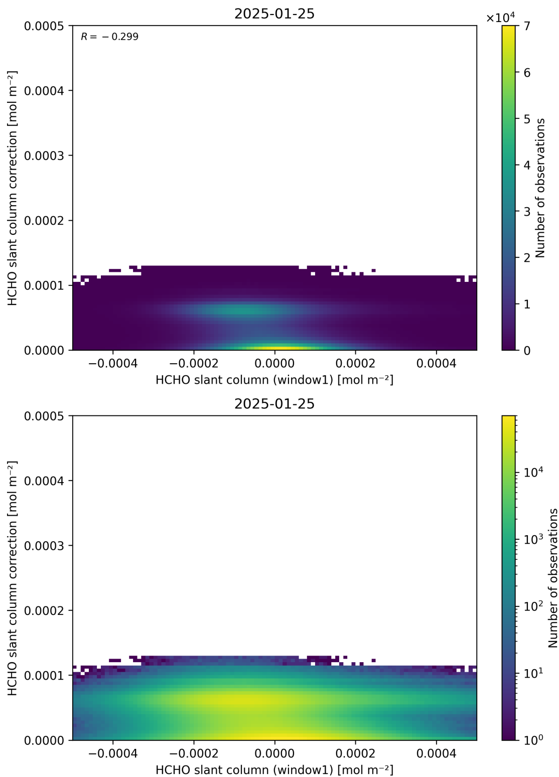
Figure 83: Scatter density plot of “HCHO slant column (window1)” against “HCHO slant column correction” for 2025-01-24 to 2025-01-26.
