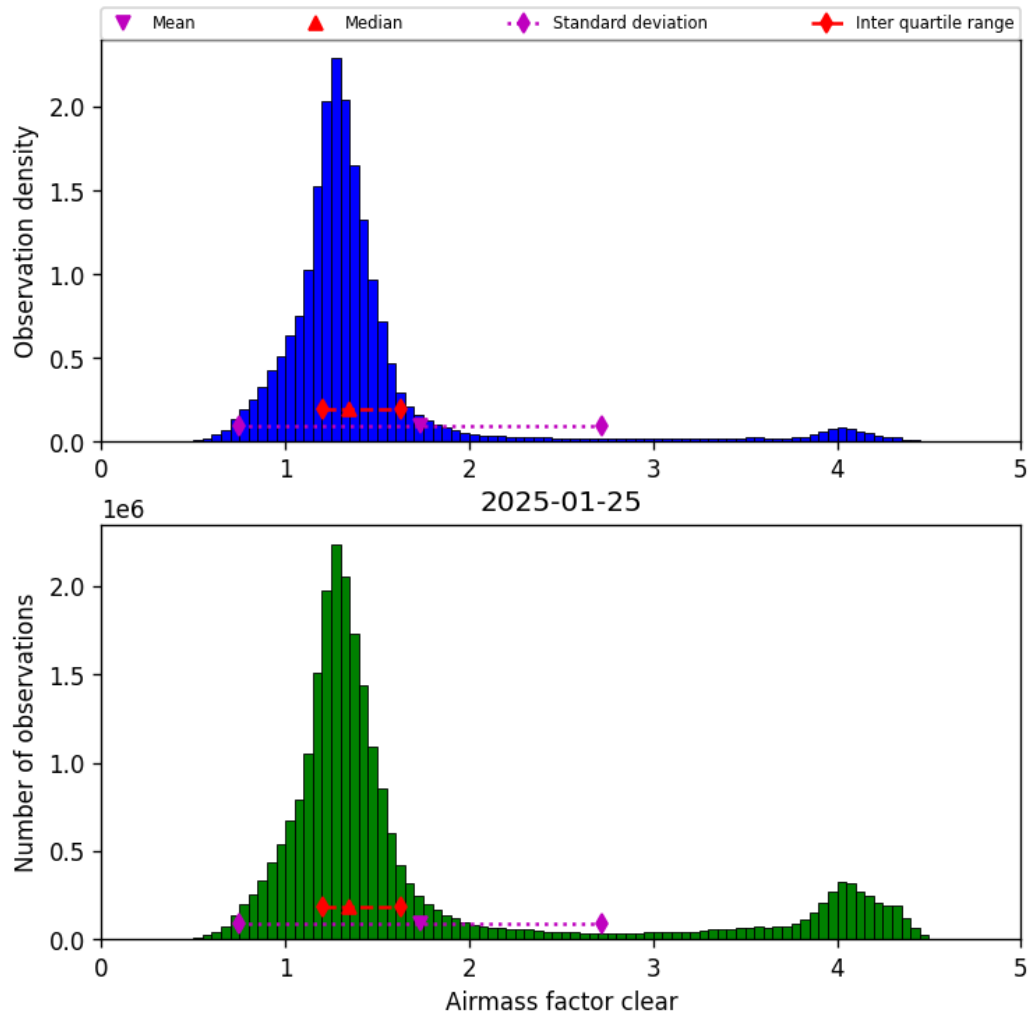
Figure 42: Histogram of “Airmass factor clear” for 2025-01-24 to 2025-01-26
