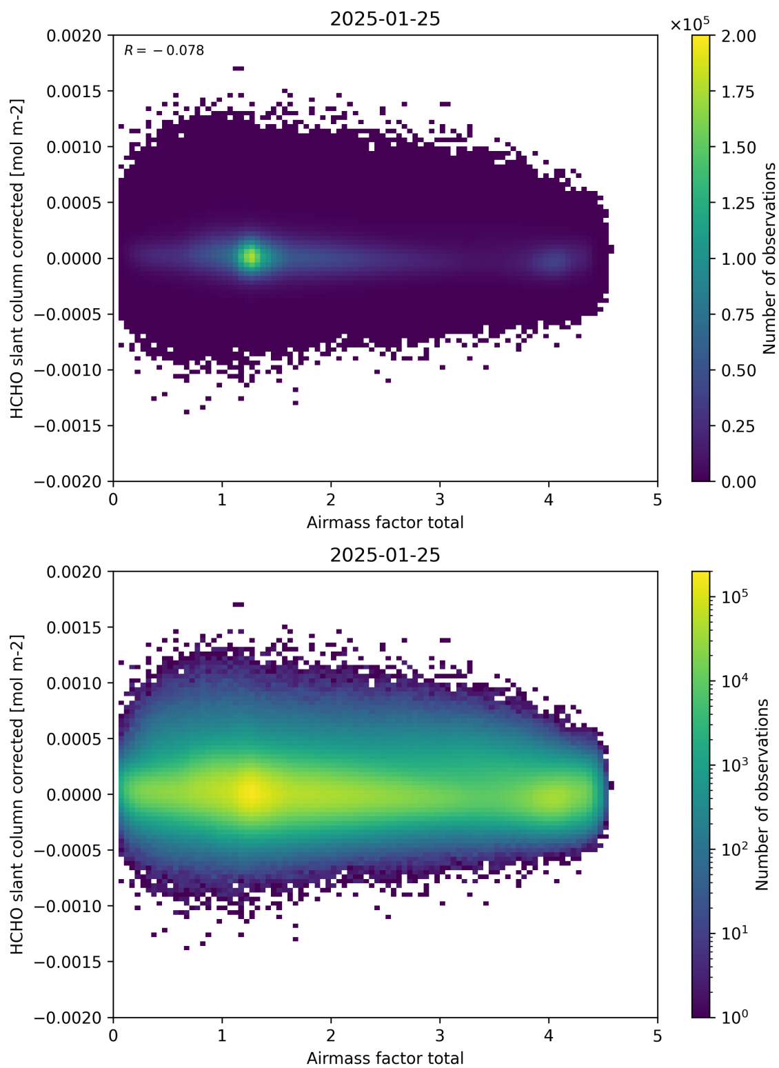
Figure 101: Scatter density plot of “Airmass factor total” against “HCHO slant column corrected” for 2025-01-24 to 2025-01-26.
