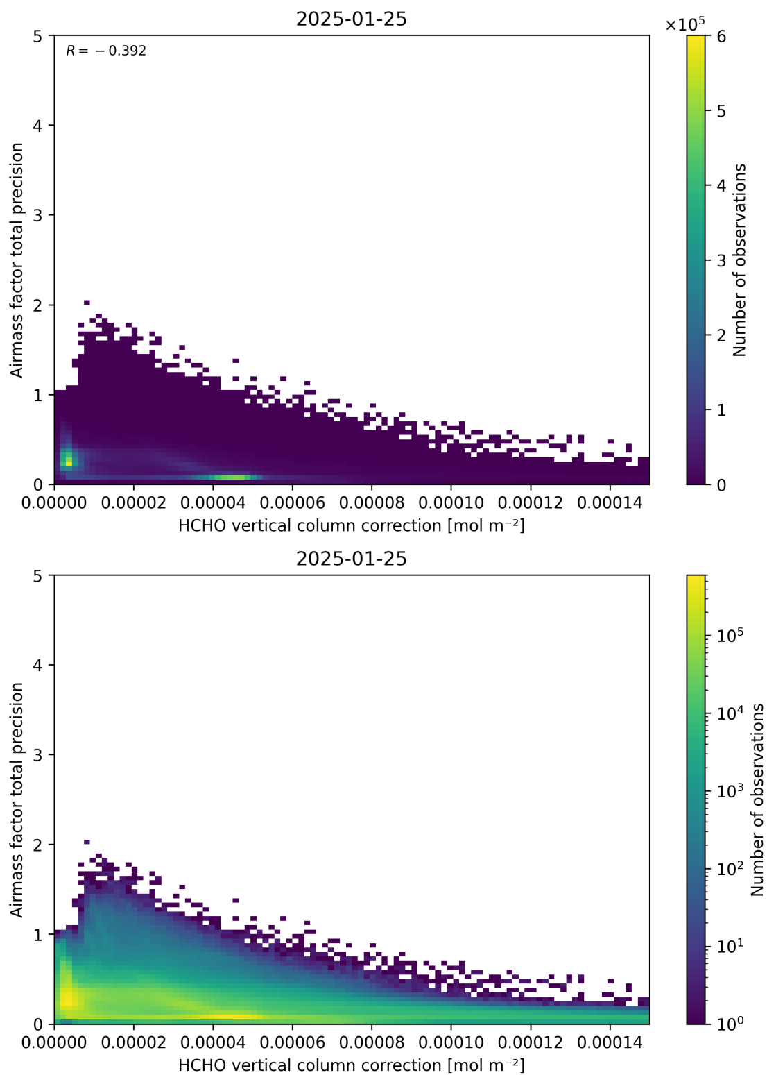
Figure 121: Scatter density plot of “HCHO vertical column correction” against “Airmass factor total precision” for 2025-01-24 to 2025-01-26.
