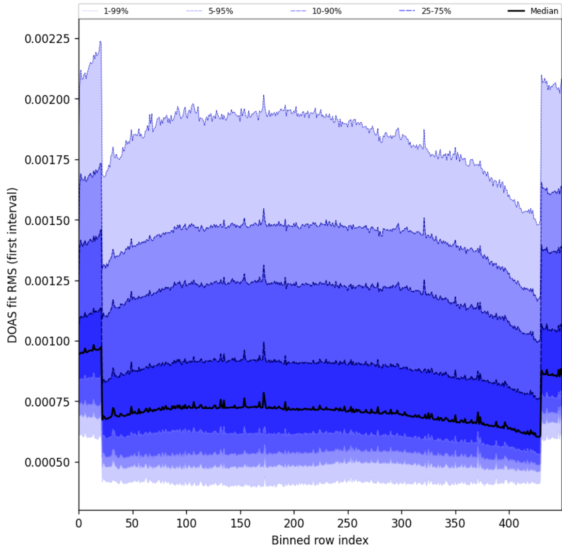
Figure 60: Along track statistics of “DOAS fit RMS (first interval)” for 2025-01-24 to 2025-01-26
