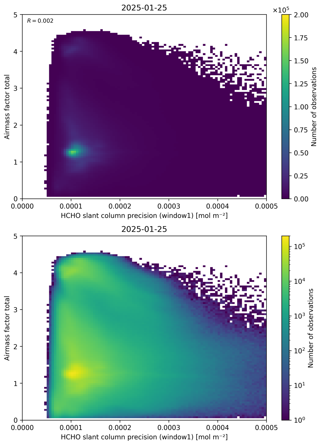
Figure 94: Scatter density plot of “HCHO slant column precision (window1)” against “Airmass factor total” for 2025-01-24 to 2025-01-26.
