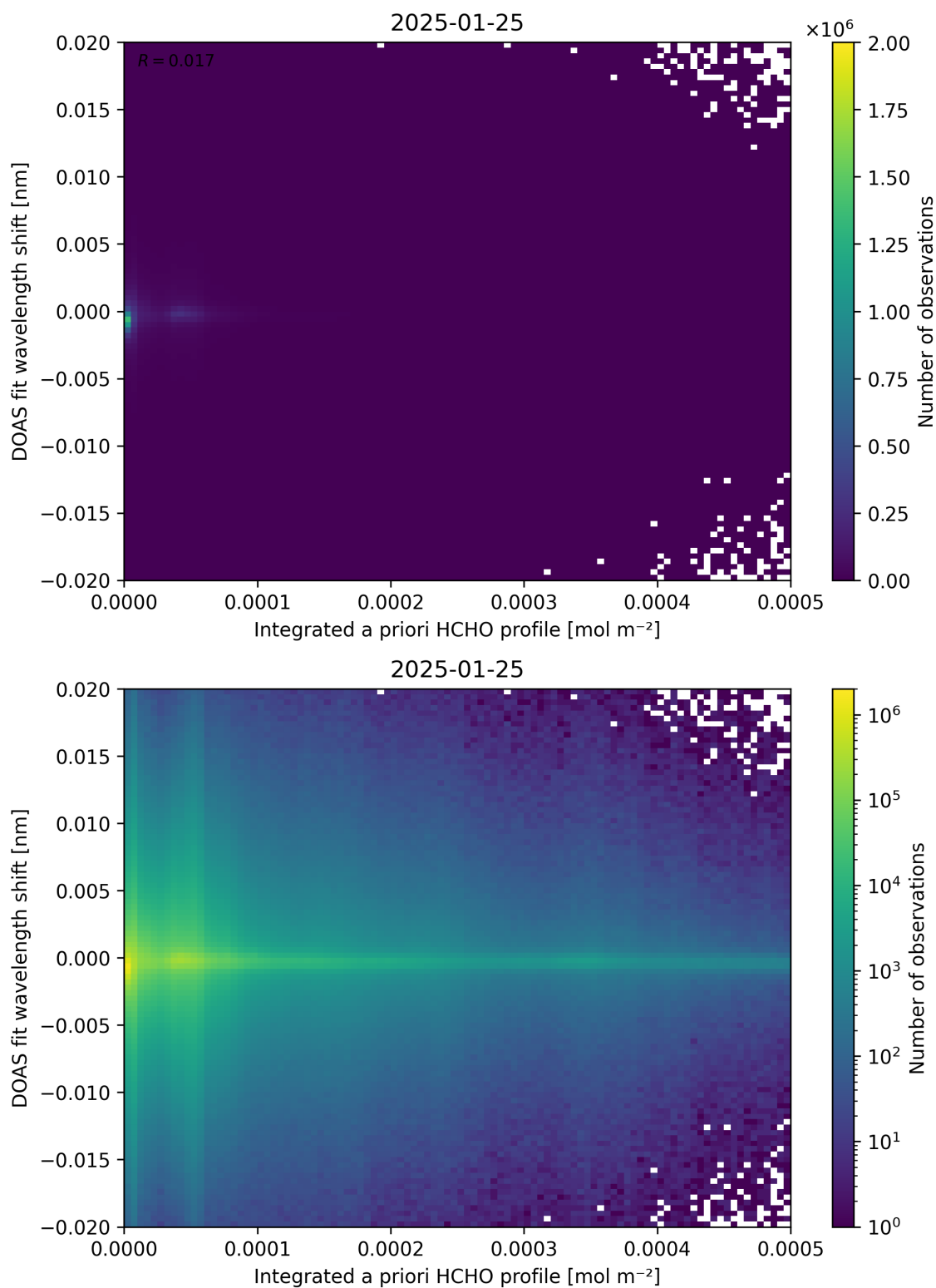
Figure 149: Scatter density plot of “Integrated a priori HCHO profile” against “DOAS fit wavelength shift” for 2025-01-24 to 2025-01-26.
