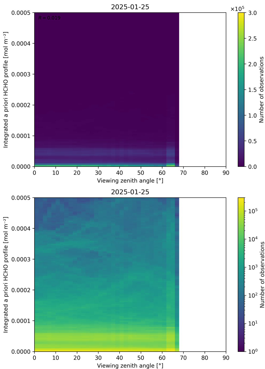
Figure 195: Scatter density plot of “Viewing zenith angle” against “Integrated a priori HCHO profile” for 2025-01-24 to 2025-01-26.
