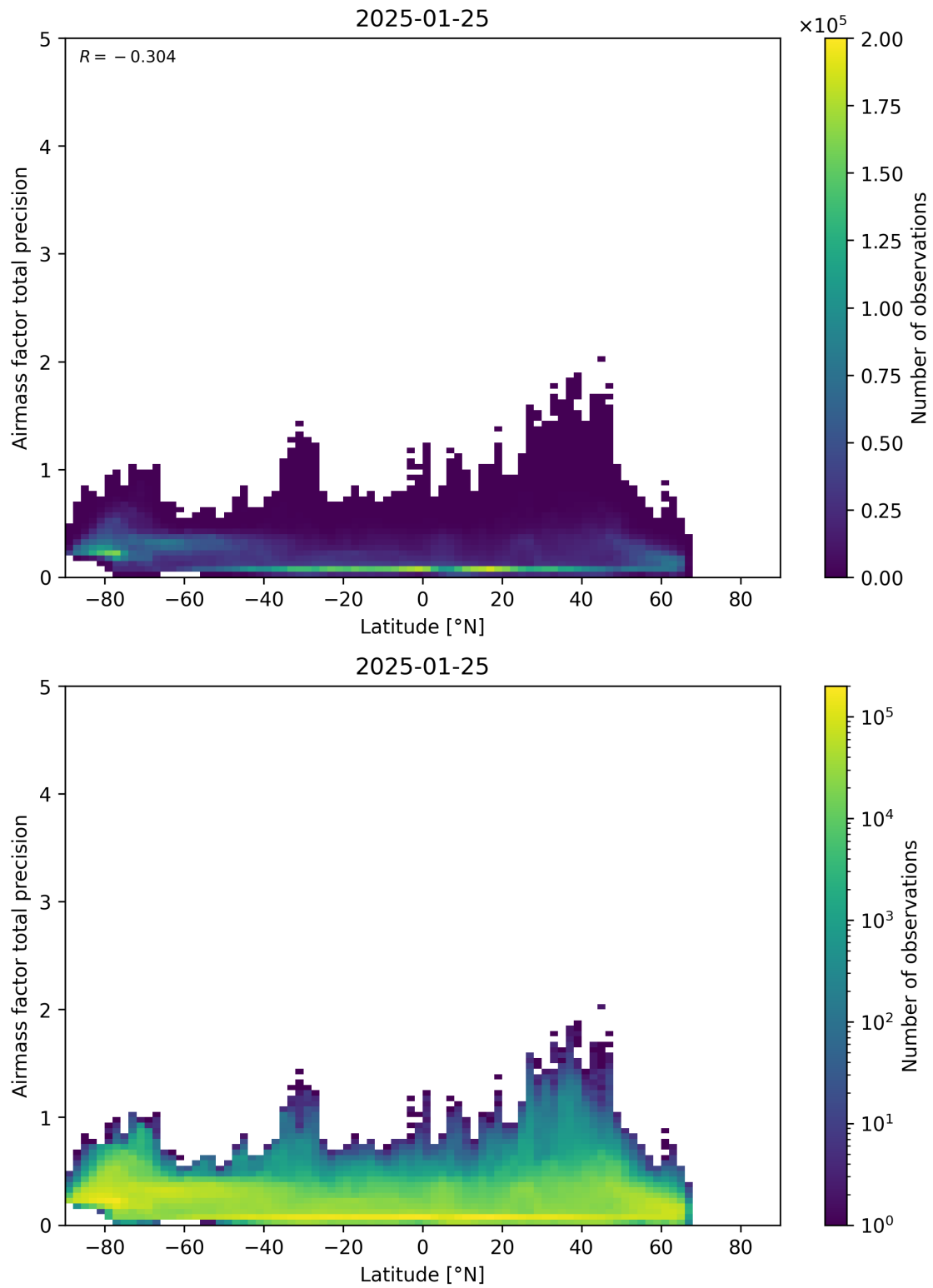
Figure 162: Scatter density plot of “Latitude” against “Airmass factor total precision” for 2025-01-24 to 2025-01-26.
