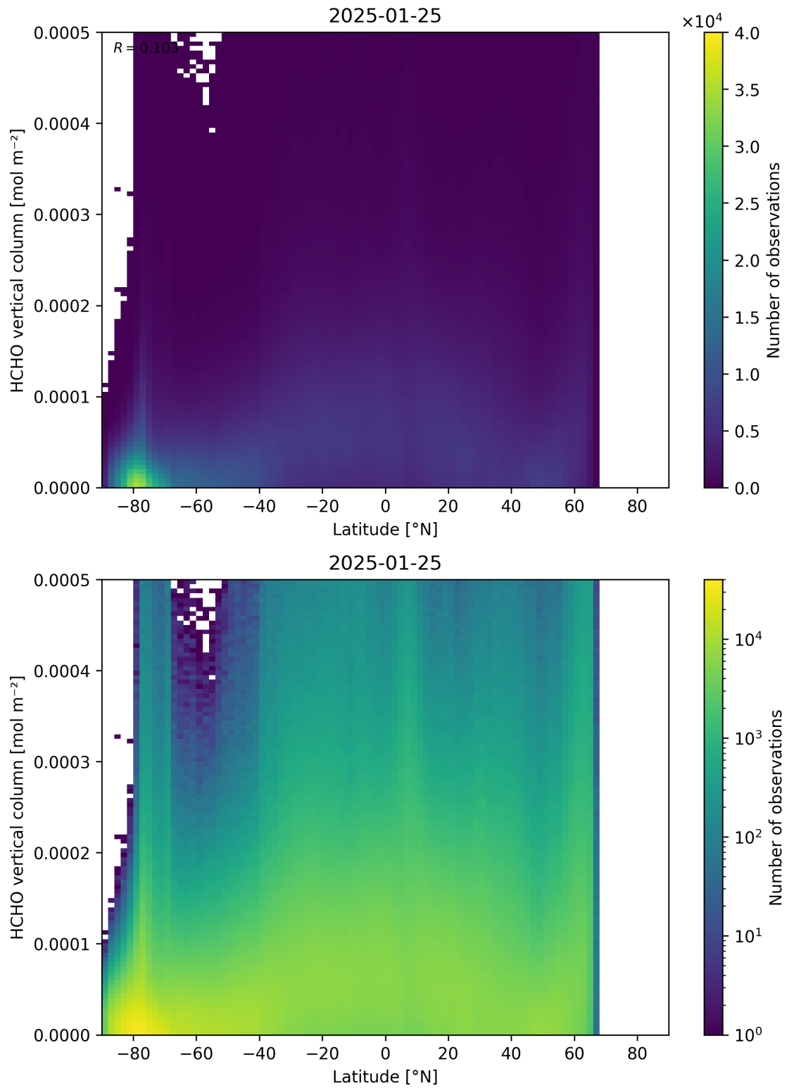
Figure 163: Scatter density plot of “Latitude” against “HCHO vertical column” for 2025-01-24 to 2025-01-26.
