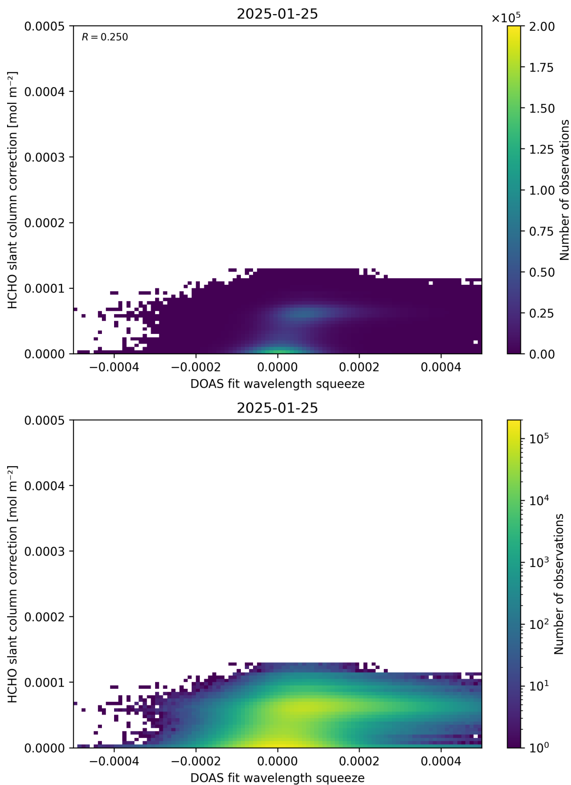
Figure 70: Scatter density plot of “DOAS fit wavelength squeeze” against “HCHO slant column correction” for 2025-01-24 to 2025-01-26.
