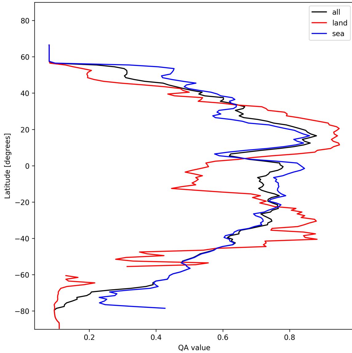
Figure 20: Zonal average of “QA value” for 2025-01-24 to 2025-01-26.
