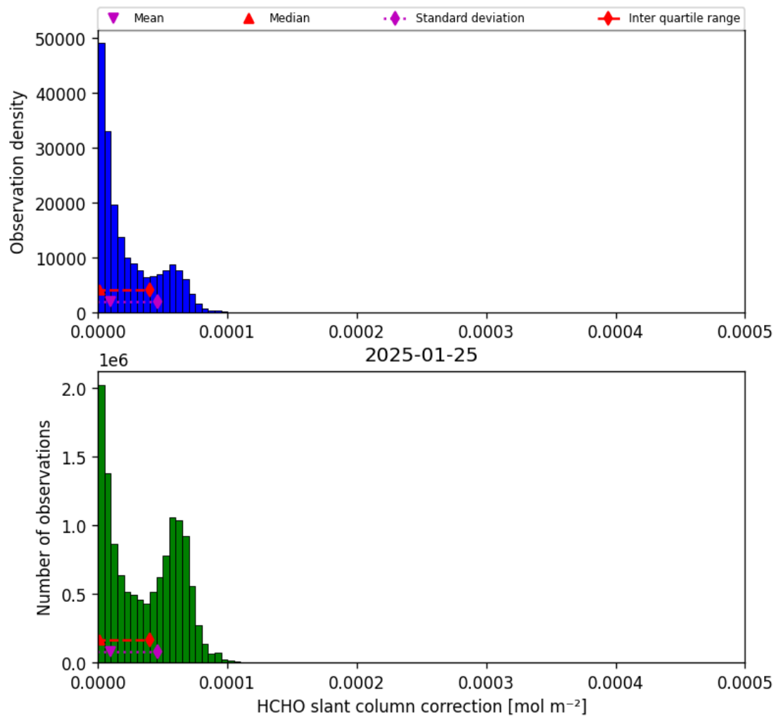
Figure 47: Histogram of “HCHO slant column correction” for 2025-01-24 to 2025-01-26
