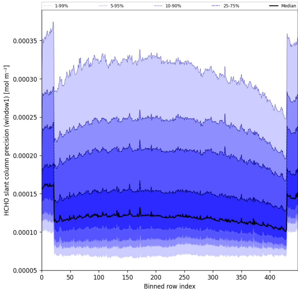
Figure 53: Along track statistics of “HCHO slant column precision (window1)” for 2025-01-24 to 2025-01-26
