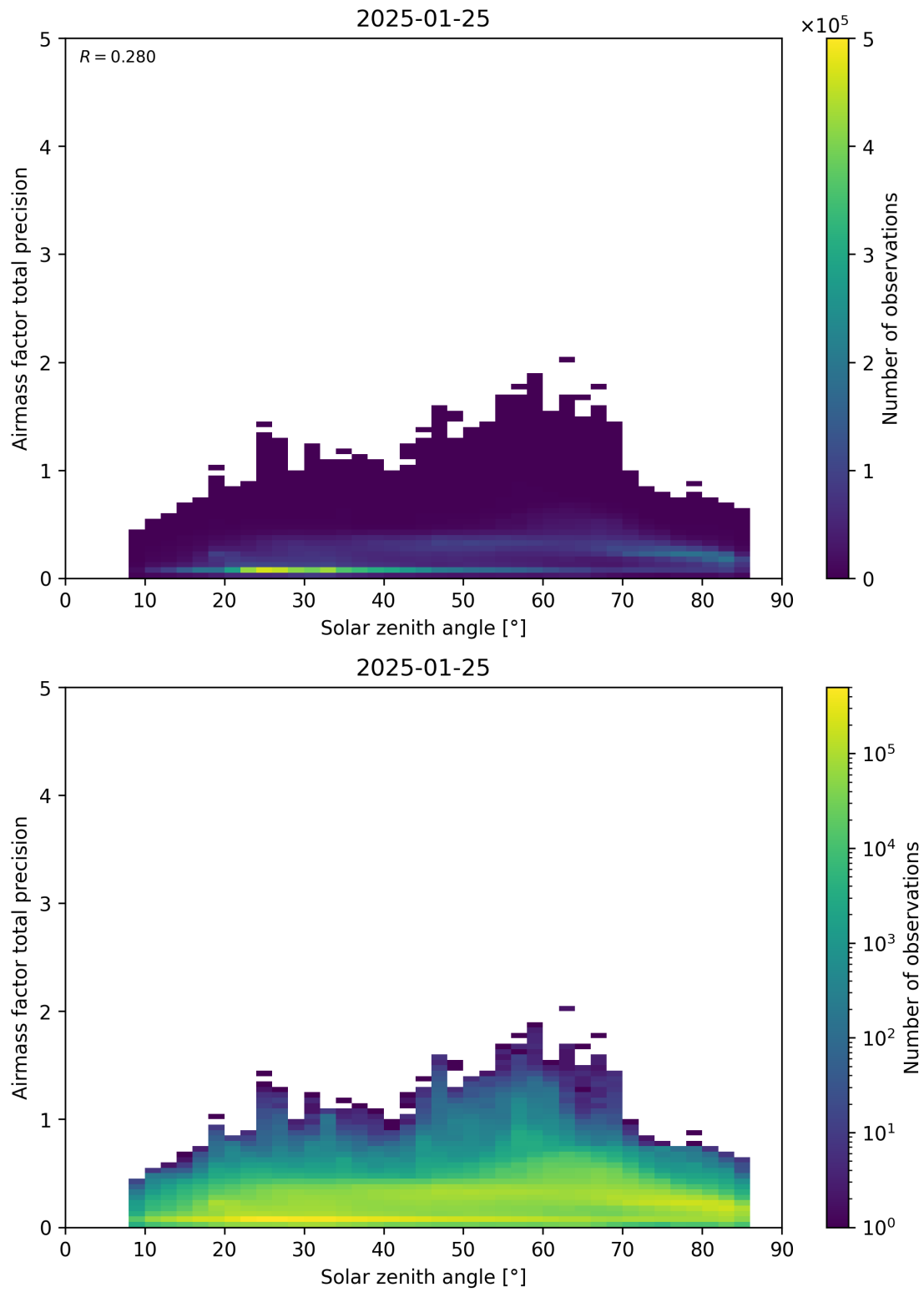
Figure 176: Scatter density plot of “Solar zenith angle” against “Airmass factor total precision” for 2025-01-24 to 2025-01-26.
