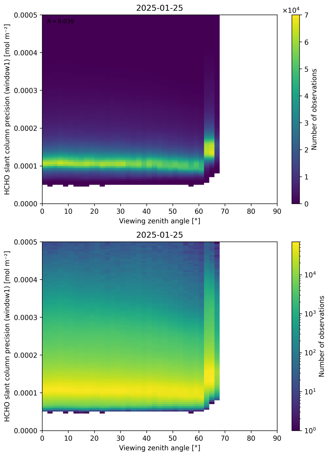
Figure 189: Scatter density plot of “Viewing zenith angle” against “HCHO slant column precision (window1)” for 2025-01-24 to 2025-01-26.
