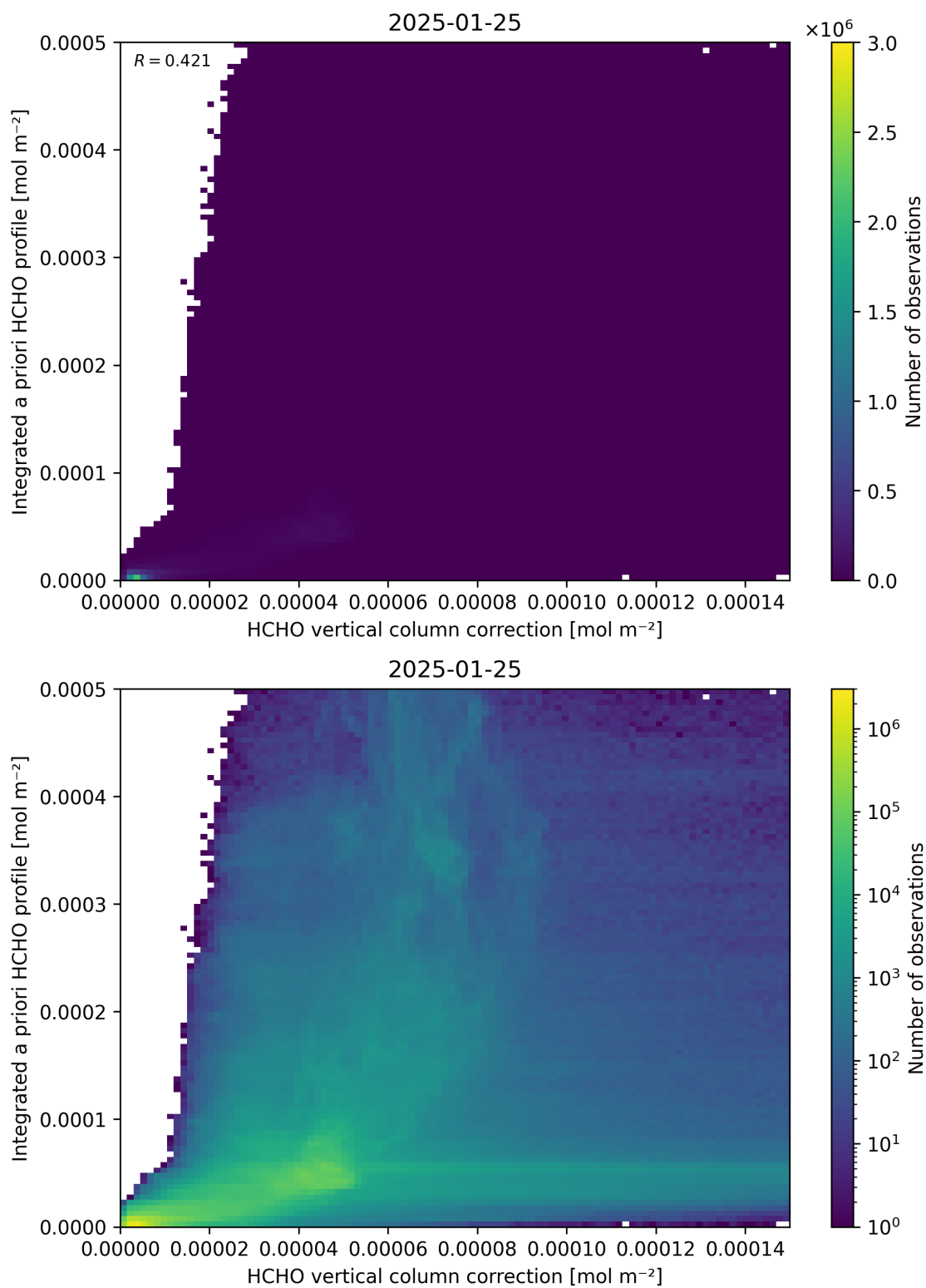
Figure 122: Scatter density plot of “HCHO vertical column correction” against “Integrated a priori HCHO profile” for 2025-01-24 to 2025-01-26.
