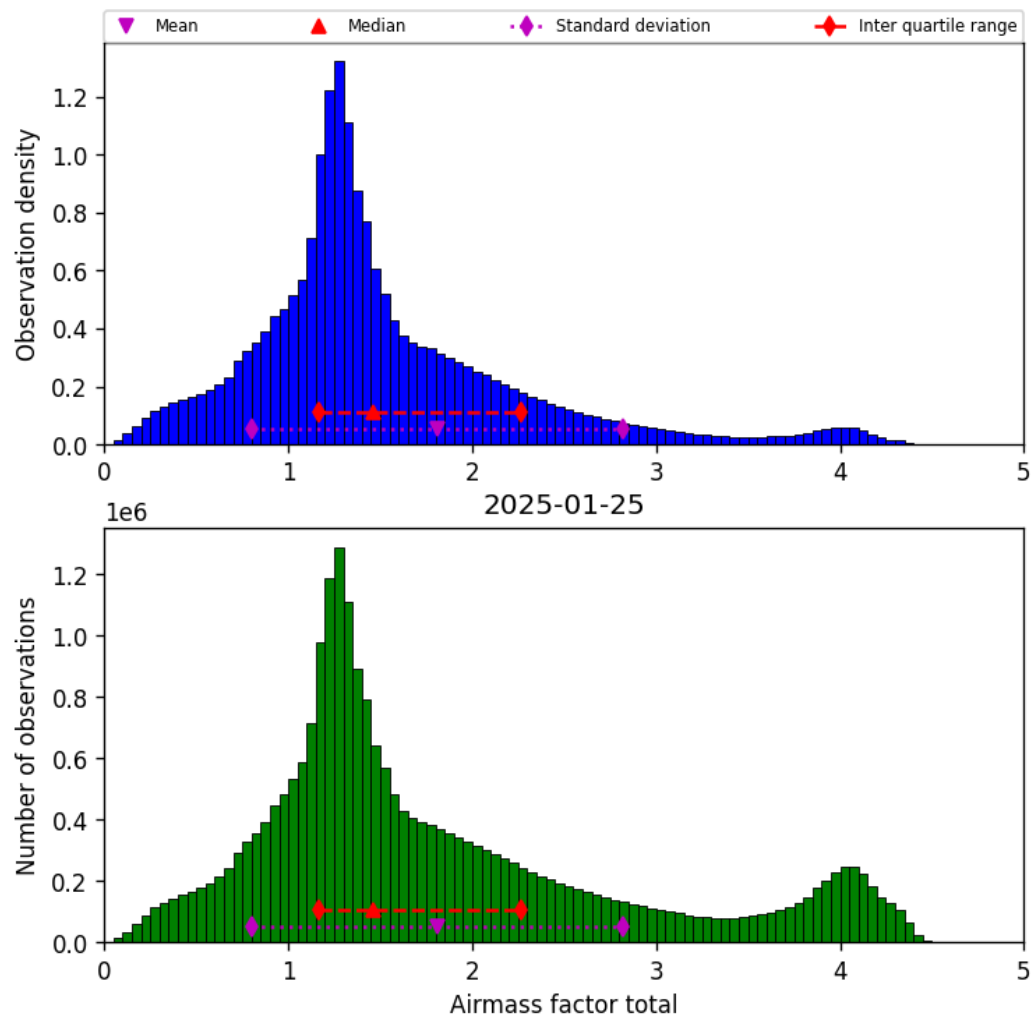
Figure 40: Histogram of “Airmass factor total” for 2025-01-24 to 2025-01-26
