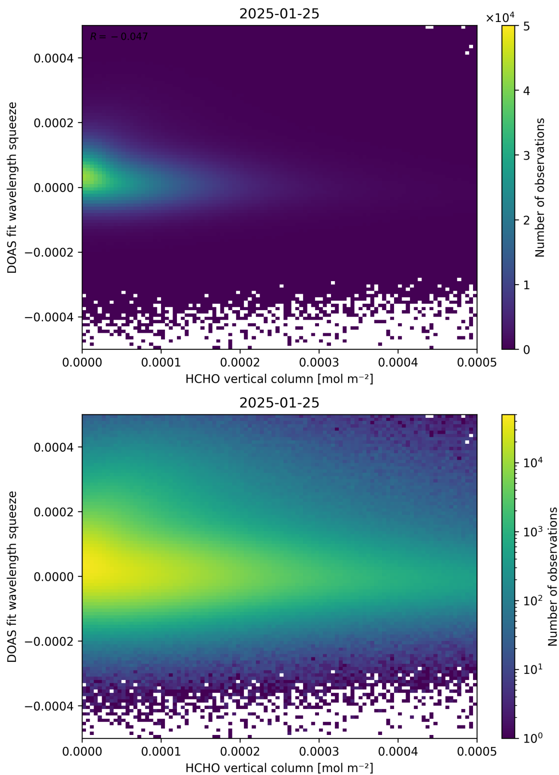
Figure 125: Scatter density plot of “HCHO vertical column” against “DOAS fit wavelength squeeze” for 2025-01-24 to 2025-01-26.
