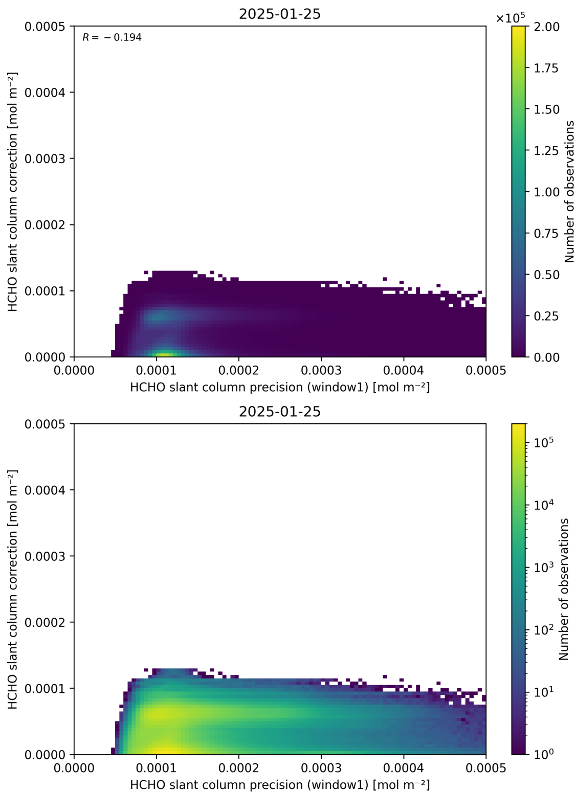
Figure 93: Scatter density plot of “HCHO slant column precision (window1)” against “HCHO slant column correction” for 2025-01-24 to 2025-01-26.
