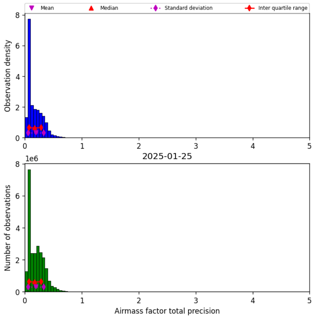
Figure 41: Histogram of “Airmass factor total precision” for 2025-01-24 to 2025-01-26
