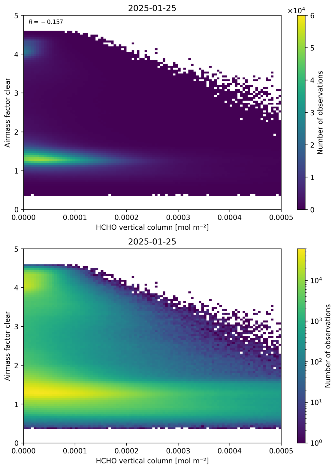
Figure 126: Scatter density plot of “HCHO vertical column” against “Airmass factor clear” for 2025-01-24 to 2025-01-26.
