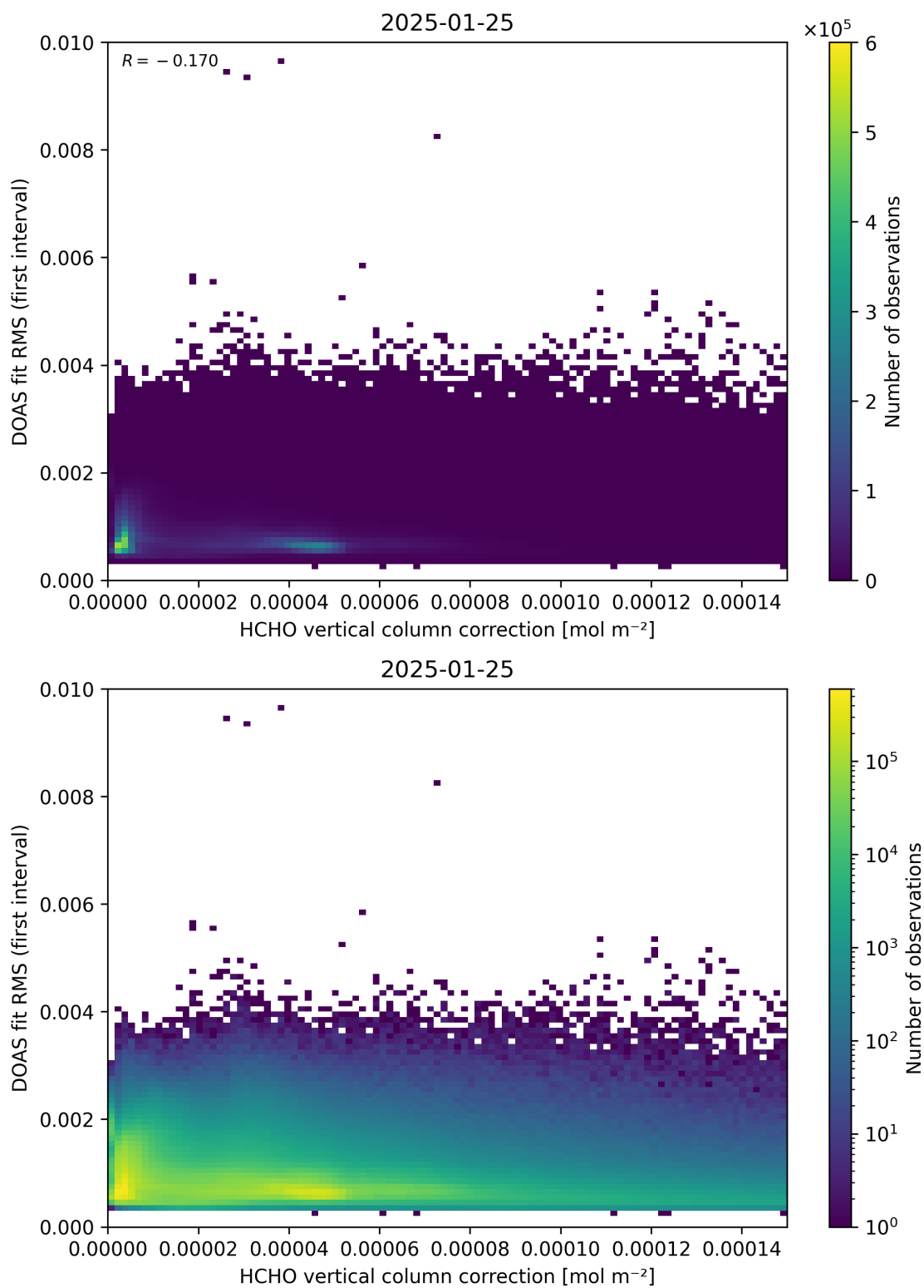
Figure 112: Scatter density plot of “HCHO vertical column correction” against “DOAS fit RMS (first interval)” for 2025-01-24 to 2025-01-26.
