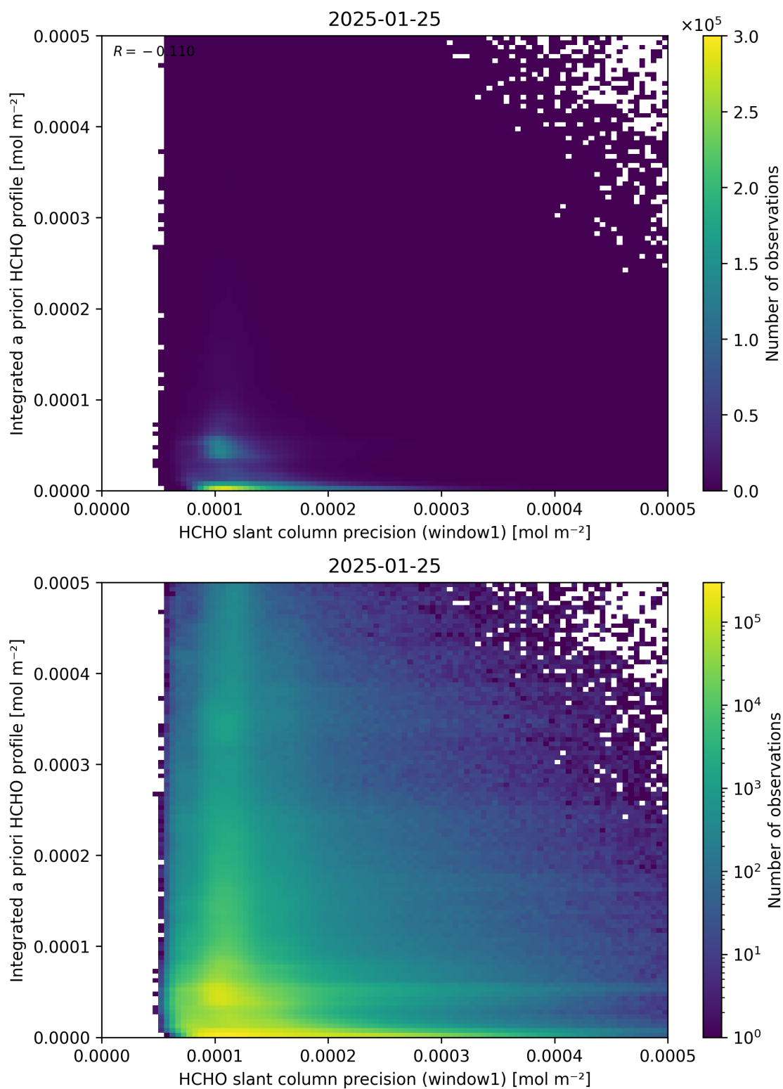
Figure 96: Scatter density plot of “HCHO slant column precision (window1)” against “Integrated a priori HCHO profile” for 2025-01-24 to 2025-01-26.
