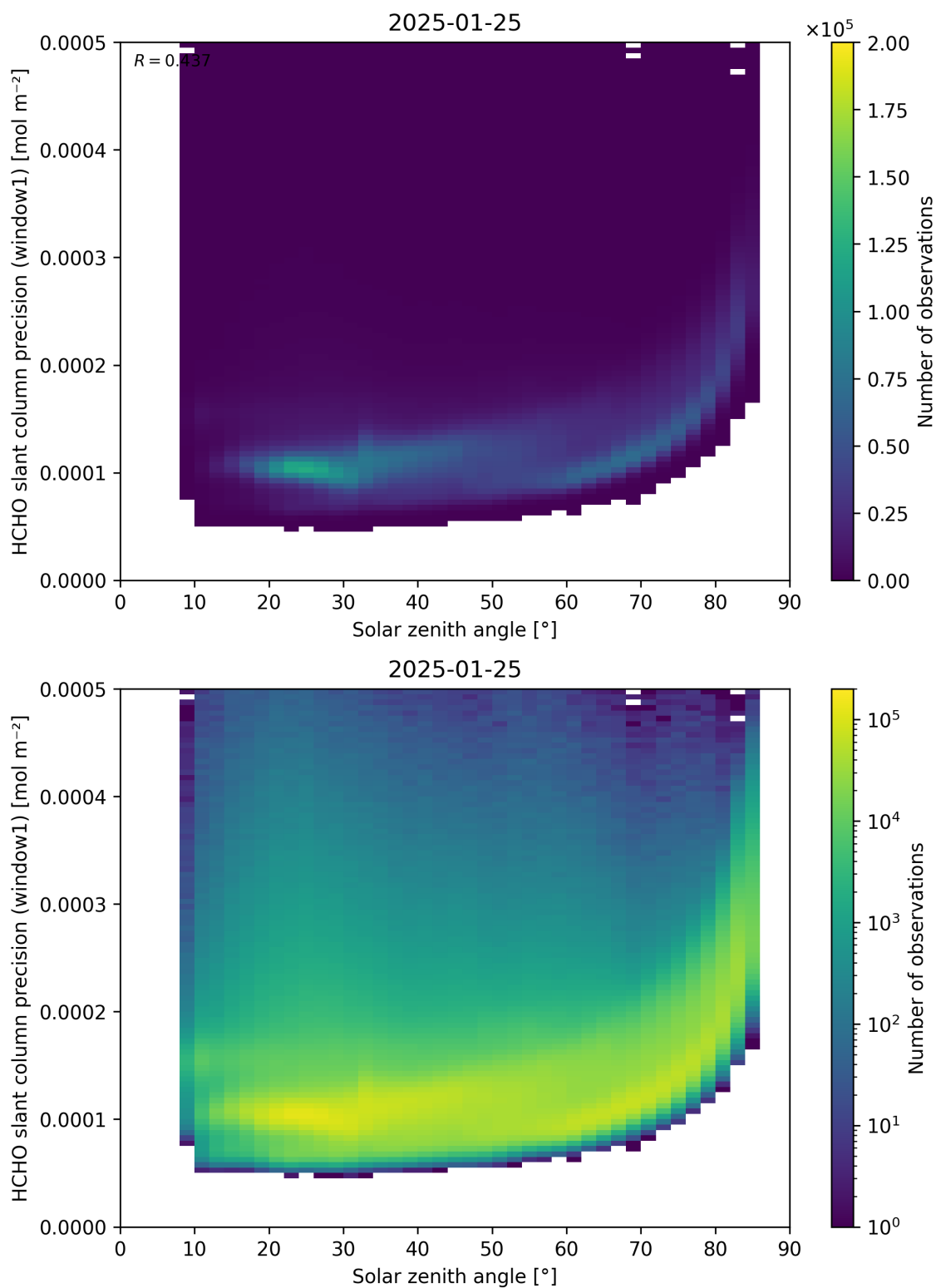
Figure 174: Scatter density plot of “Solar zenith angle” against “HCHO slant column precision (window1)” for 2025-01-24 to 2025-01-26.
