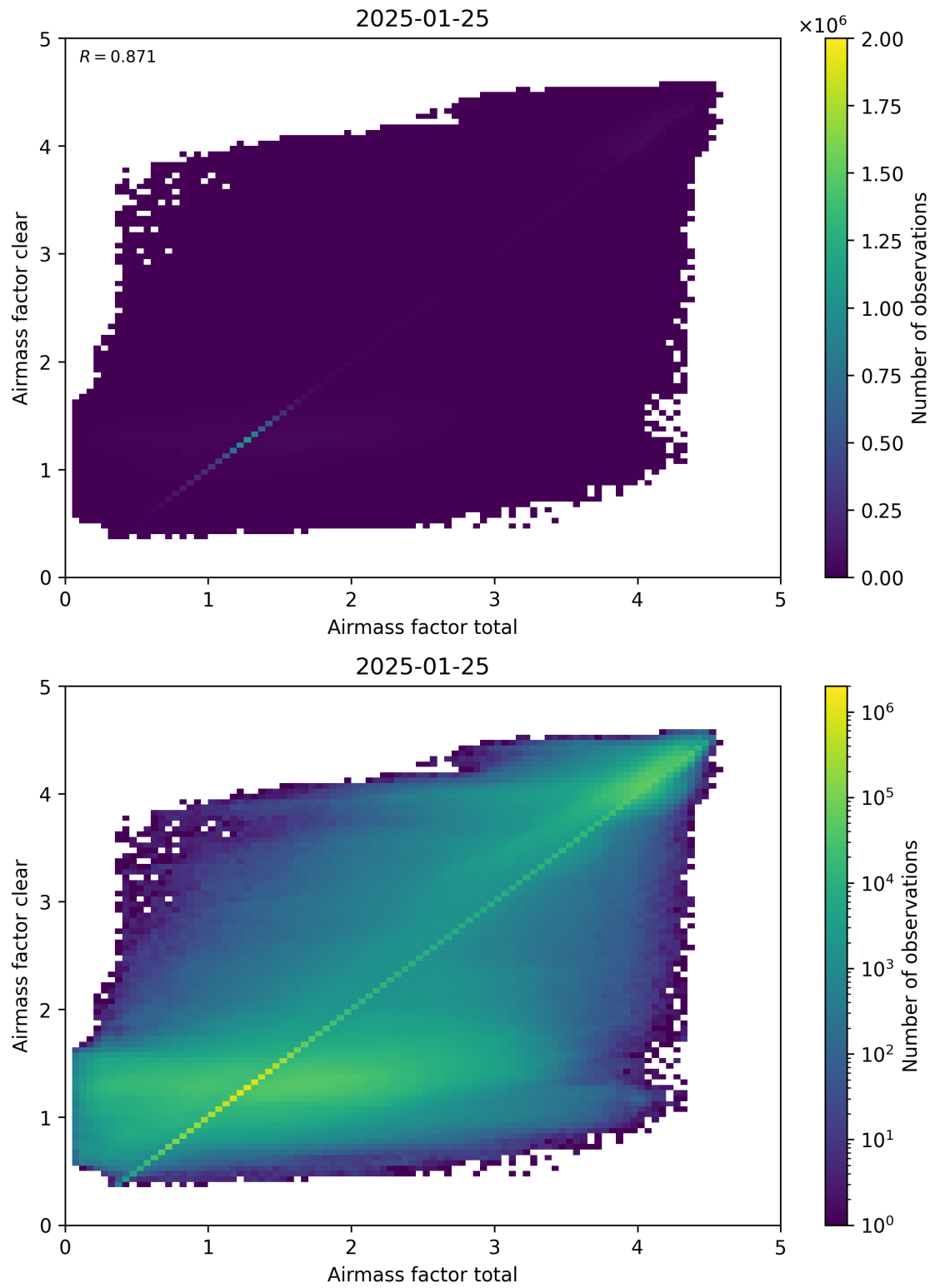
Figure 100: Scatter density plot of “Airmass factor total” against “Airmass factor clear” for 2025-01-24 to 2025-01-26.
