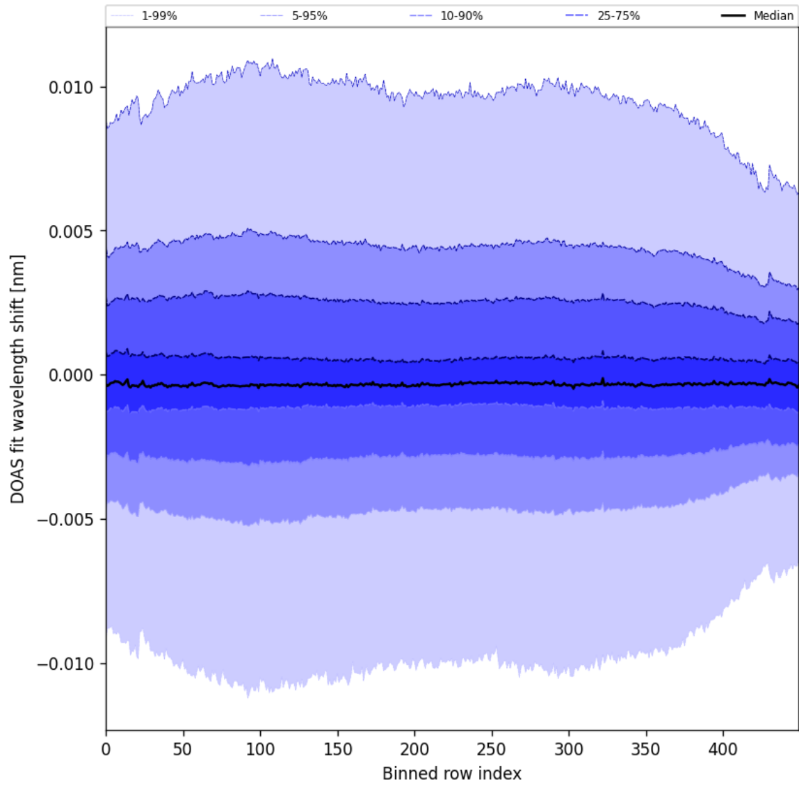
Figure 58: Along track statistics of “DOAS fit wavelength shift” for 2025-01-24 to 2025-01-26
