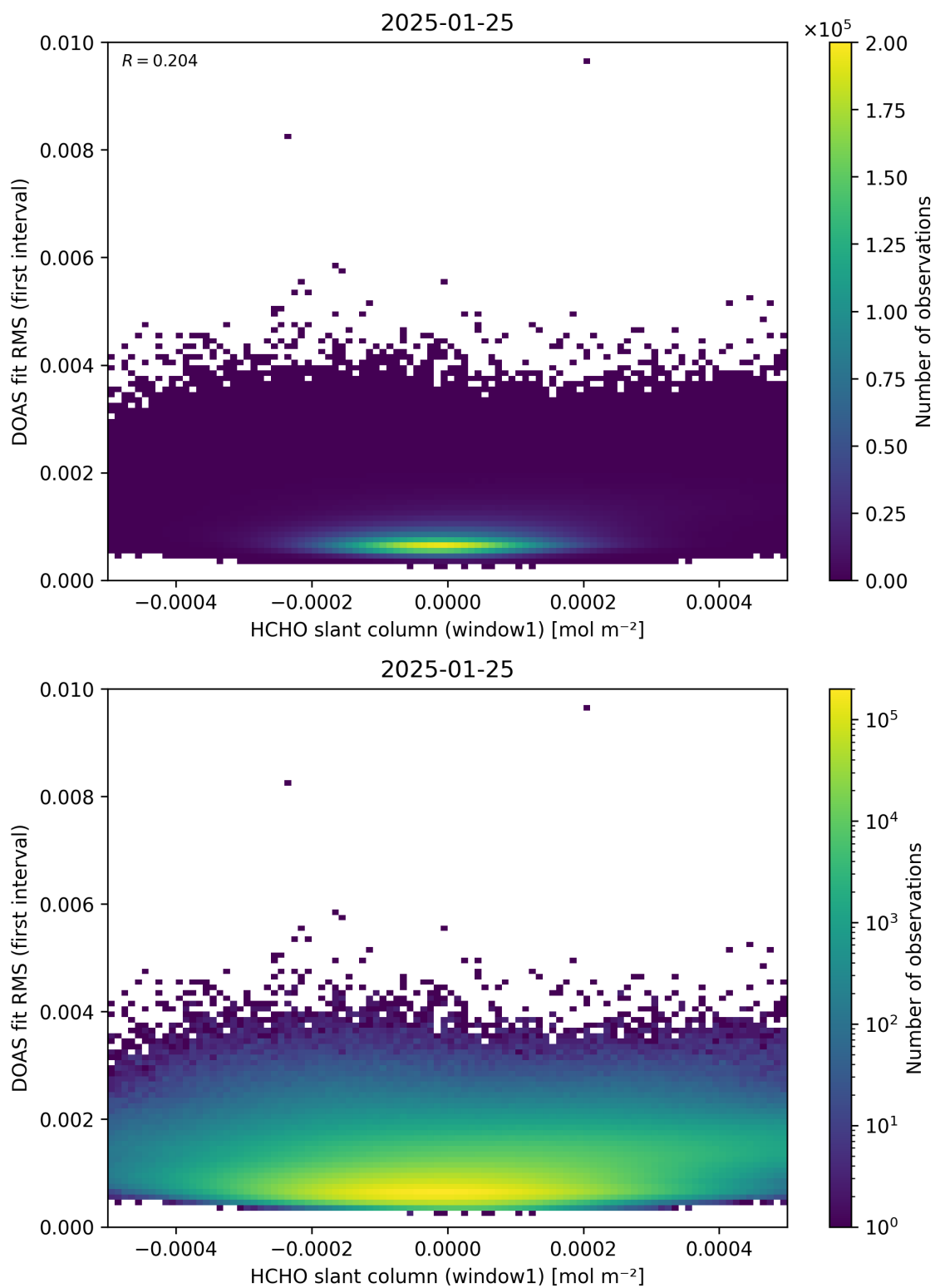
Figure 78: Scatter density plot of “HCHO slant column (window1)” against “DOAS fit RMS (first interval)” for 2025-01-24 to 2025-01-26.
