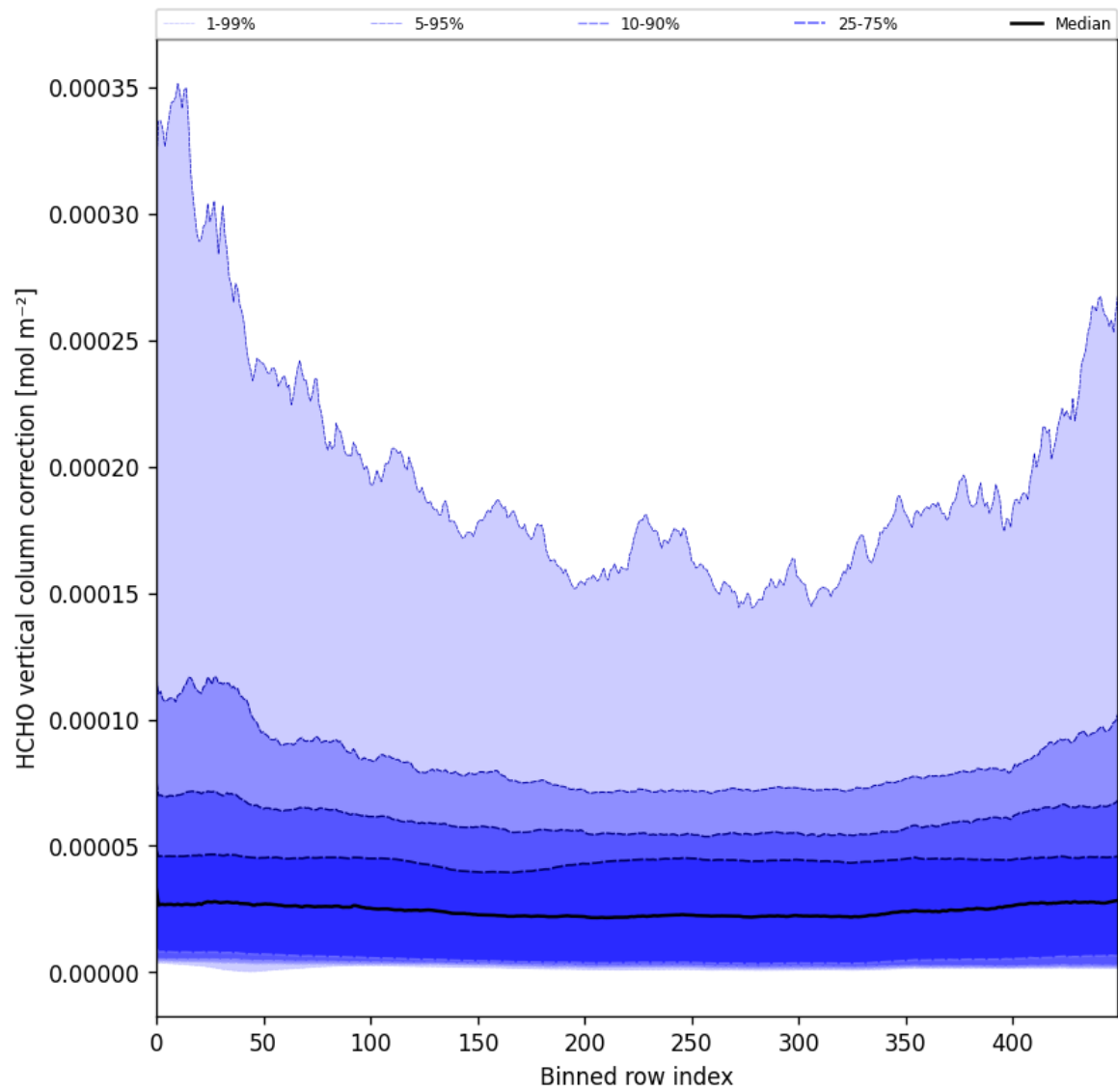
Figure 51: Along track statistics of “HCHO vertical column correction” for 2025-01-24 to 2025-01-26
