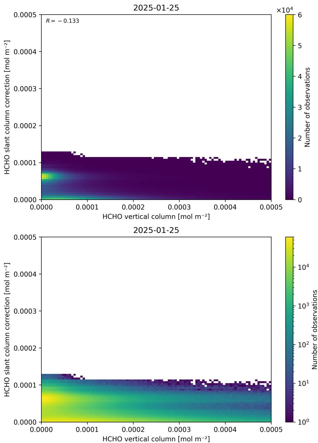
Figure 128: Scatter density plot of “HCHO vertical column” against “HCHO slant column correction” for 2025-01-24 to 2025-01-26.
