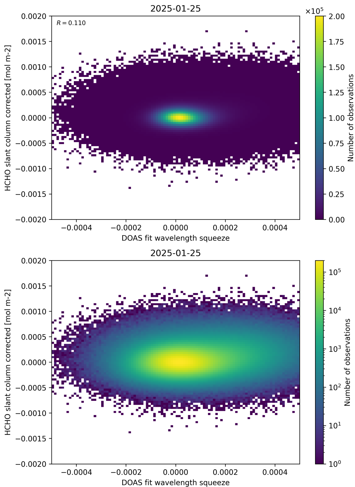
Figure 69: Scatter density plot of “DOAS fit wavelength squeeze” against “HCHO slant column corrected” for 2025-01-24 to 2025-01-26.
