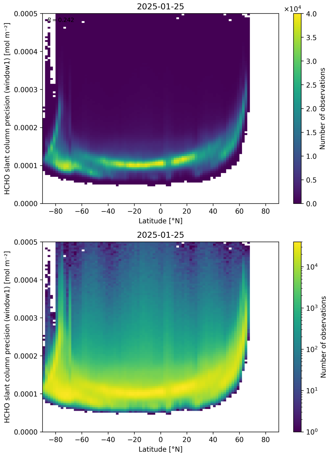
Figure 160: Scatter density plot of “Latitude” against “HCHO slant column precision (window1)” for 2025-01-24 to 2025-01-26.
