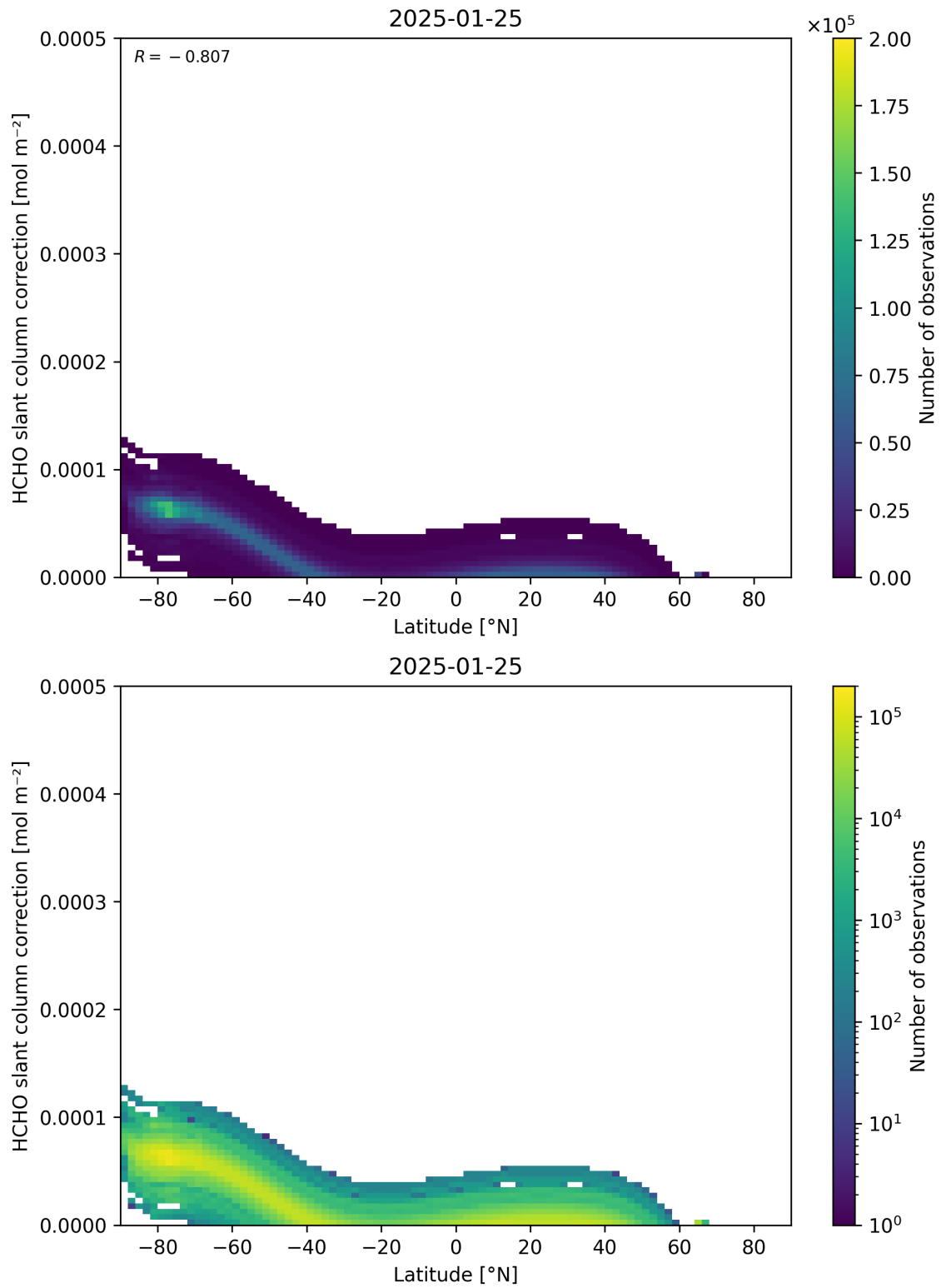
Figure 158: Scatter density plot of “Latitude” against “HCHO slant column correction” for 2025-01-24 to 2025-01-26.
