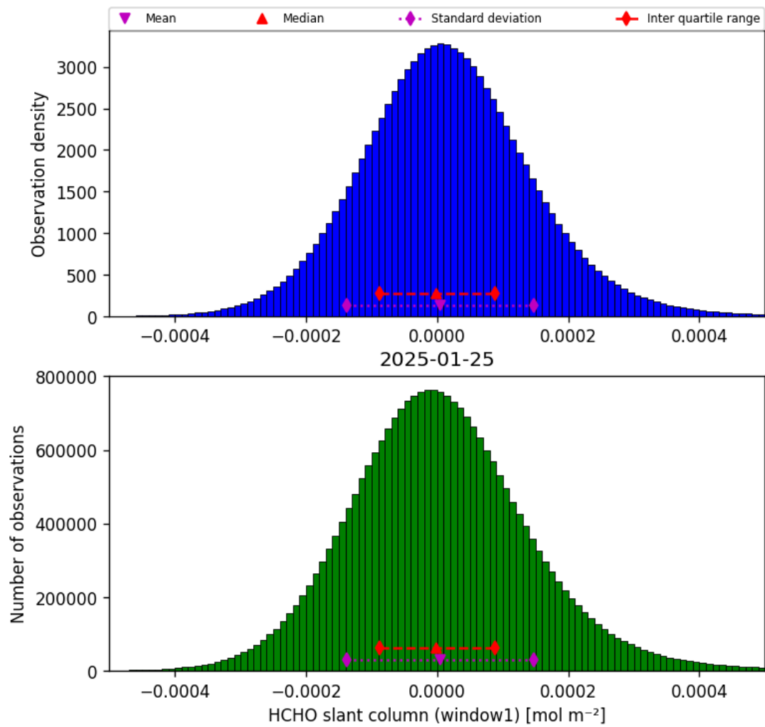
Figure 38: Histogram of “HCHO slant column (window1)” for 2025-01-24 to 2025-01-26
