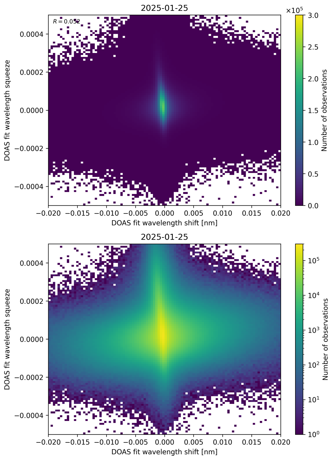
Figure 65: Scatter density plot of “DOAS fit wavelength shift” against “DOAS fit wavelength squeeze” for 2025-01-24 to 2025-01-26.
