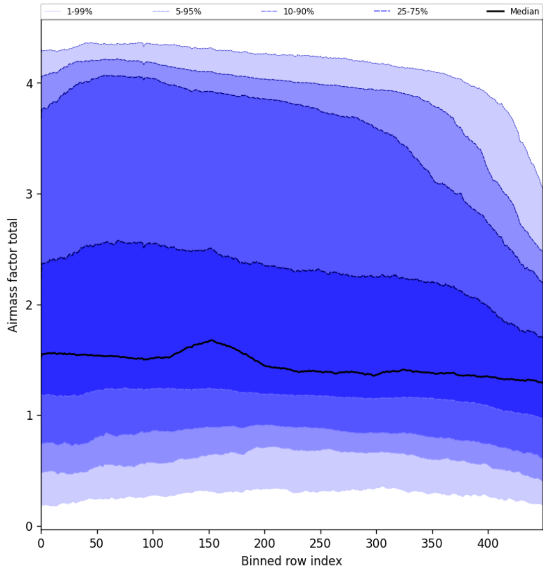
Figure 54: Along track statistics of “Airmass factor total” for 2025-01-24 to 2025-01-26
