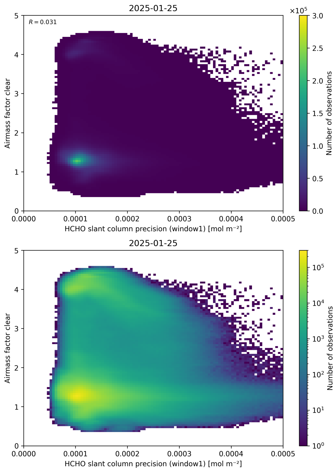
Figure 91: Scatter density plot of “HCHO slant column precision (window1)” against “Airmass factor clear” for 2025-01-24 to 2025-01-26.
