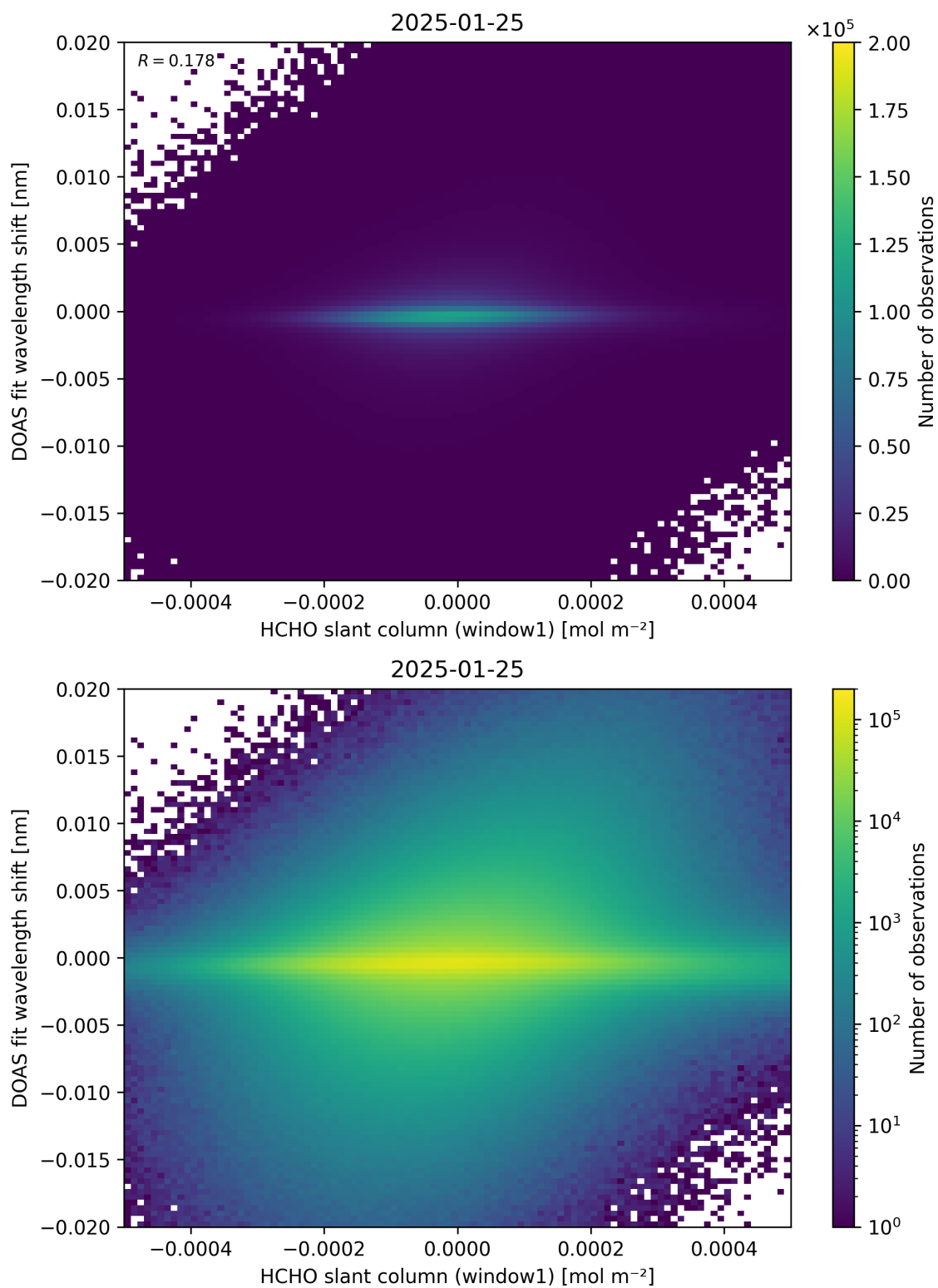
Figure 79: Scatter density plot of “HCHO slant column (window1)” against “DOAS fit wavelength shift” for 2025-01-24 to 2025-01-26.
