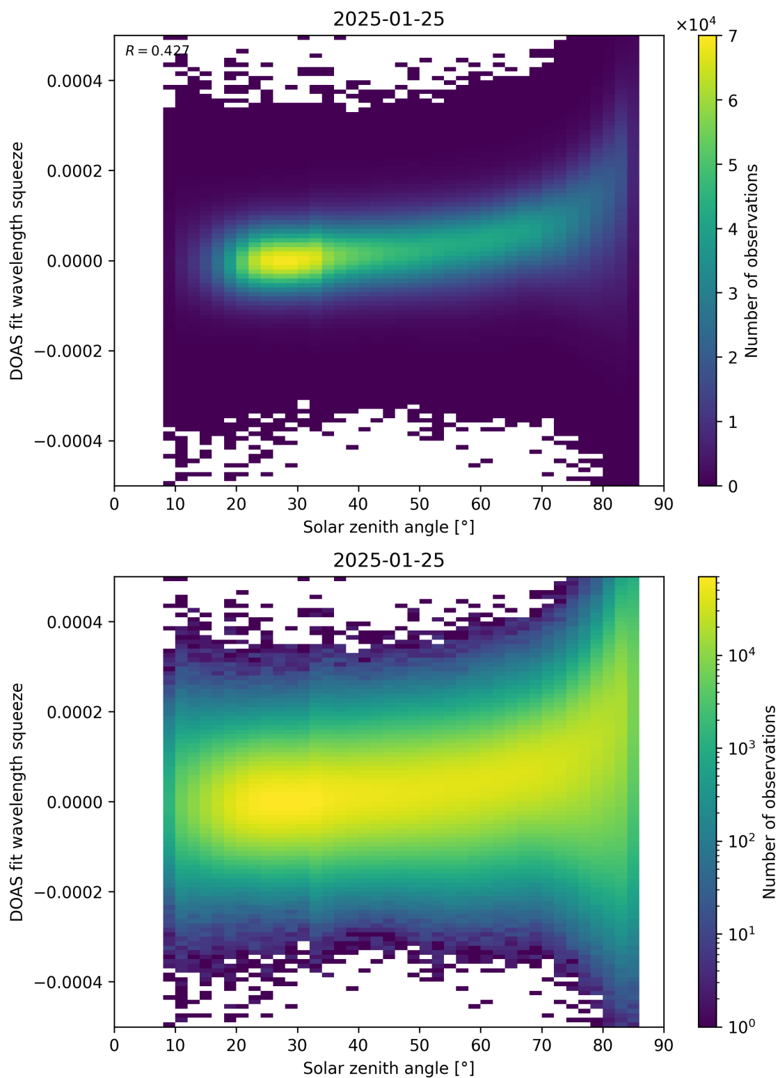
Figure 169: Scatter density plot of “Solar zenith angle” against “DOAS fit wavelength squeeze” for 2025-01-24 to 2025-01-26.
