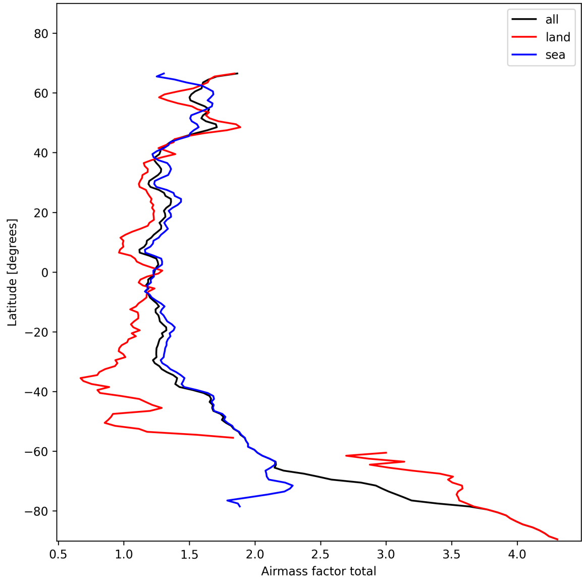
Figure 26: Zonal average of “Airmass factor total” for 2025-01-24 to 2025-01-26.
