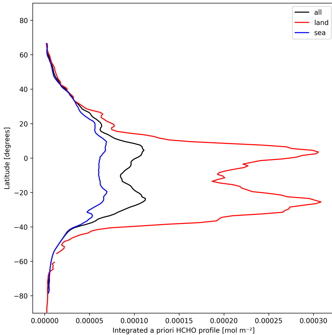
Figure 29: Zonal average of “Integrated a priori HCHO profile” for 2025-01-24 to 2025-01-26.
