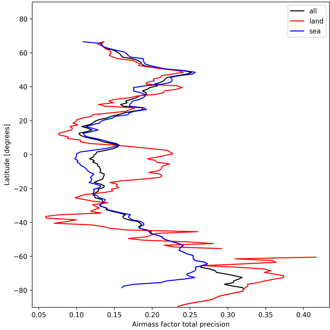
Figure 27: Zonal average of “Airmass factor total precision” for 2025-01-24 to 2025-01-26.
