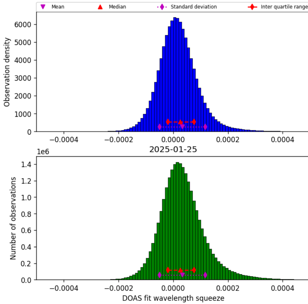
Figure 45: Histogram of “DOAS fit wavelength squeeze” for 2025-01-24 to 2025-01-26
