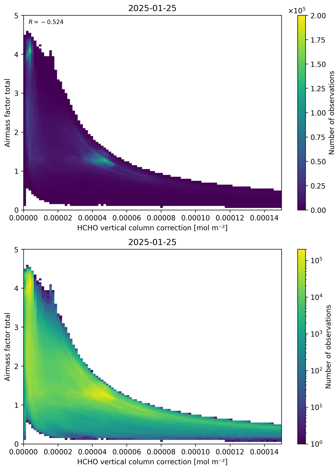
Figure 120: Scatter density plot of “HCHO vertical column correction” against “Airmass factor total” for 2025-01-24 to 2025-01-26.
