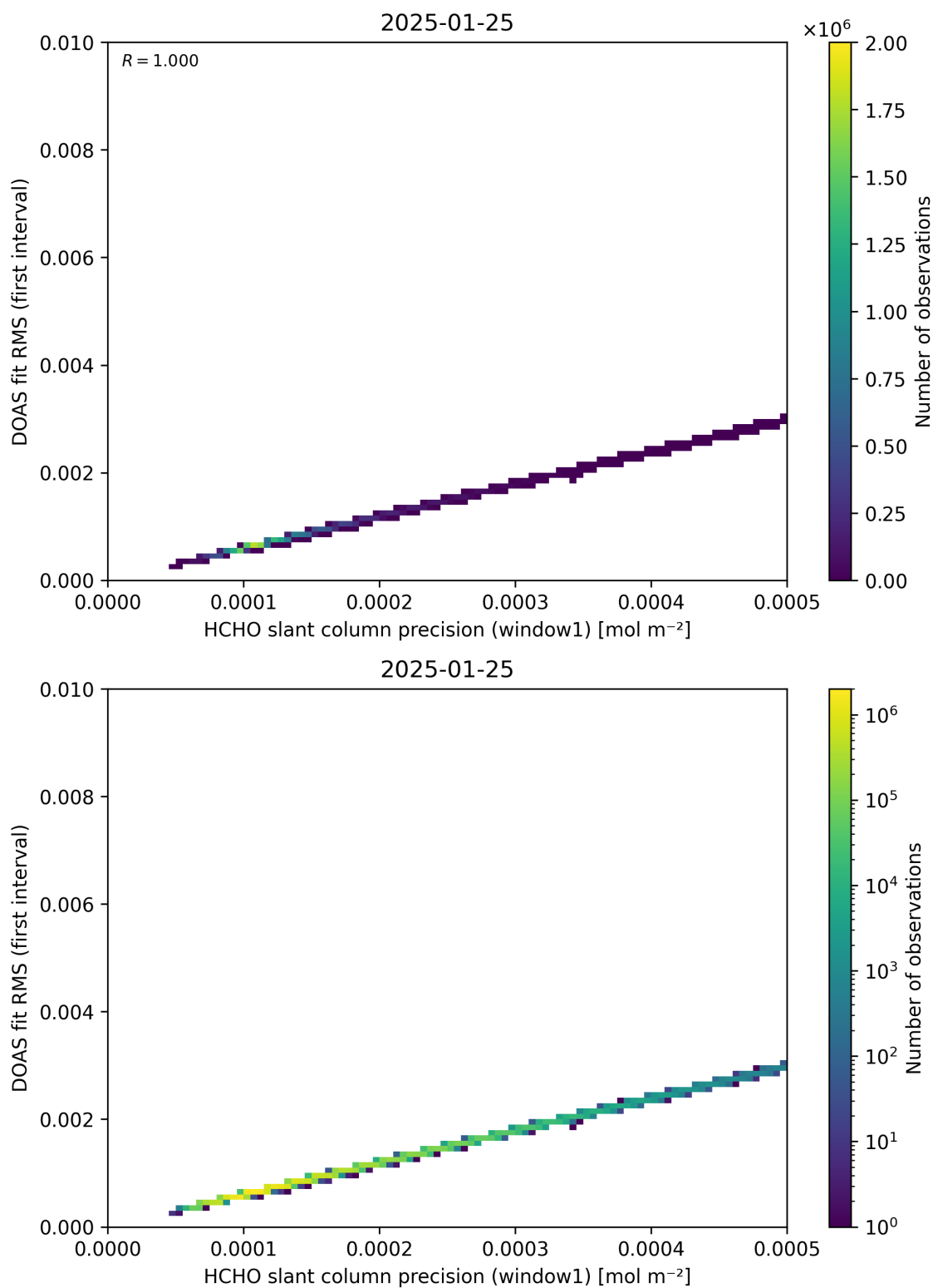
Figure 88: Scatter density plot of “HCHO slant column precision (window1)” against “DOAS fit RMS (first interval)” for 2025-01-24 to 2025-01-26.
