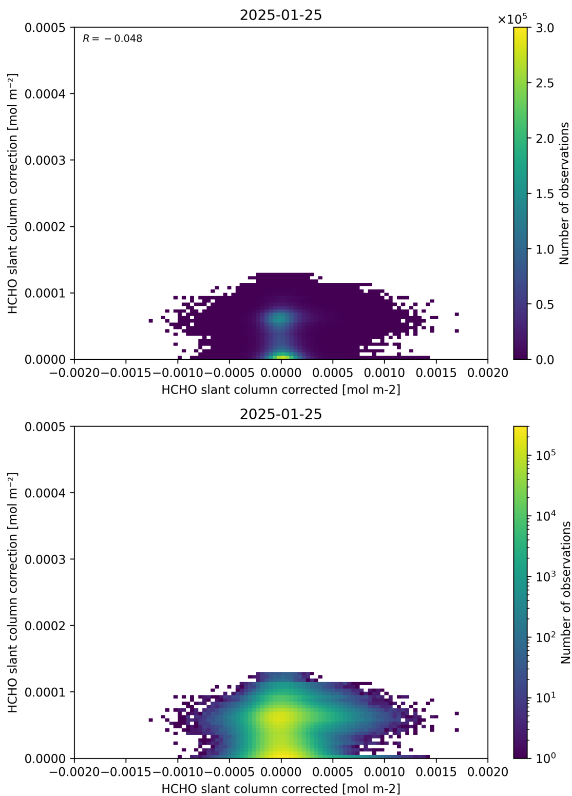
Figure 77: Scatter density plot of “HCHO slant column corrected” against “HCHO slant column correction” for 2025-01-24 to 2025-01-26.
