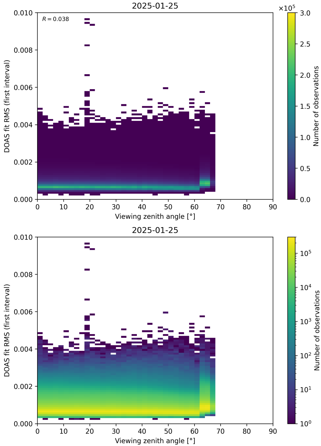
Figure 182: Scatter density plot of “Viewing zenith angle” against “DOAS fit RMS (first interval)” for 2025-01-24 to 2025-01-26.
