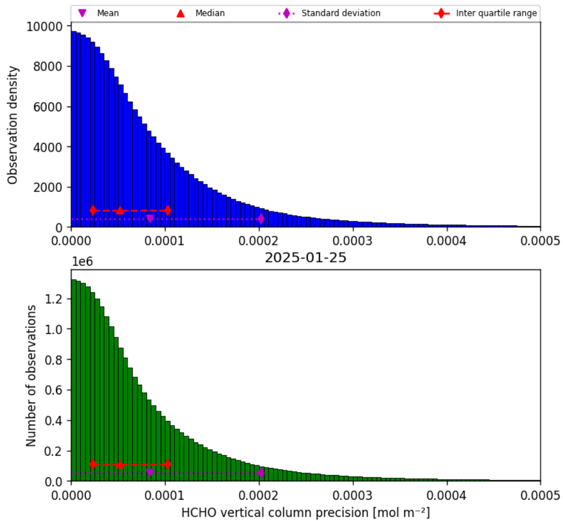
Figure 36: Histogram of “HCHO vertical column precision” for 2025-01-24 to 2025-01-26
