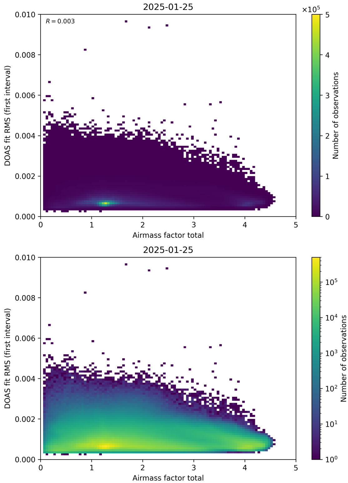
Figure 97: Scatter density plot of “Airmass factor total” against “DOAS fit RMS (first interval)” for 2025-01-24 to 2025-01-26.
