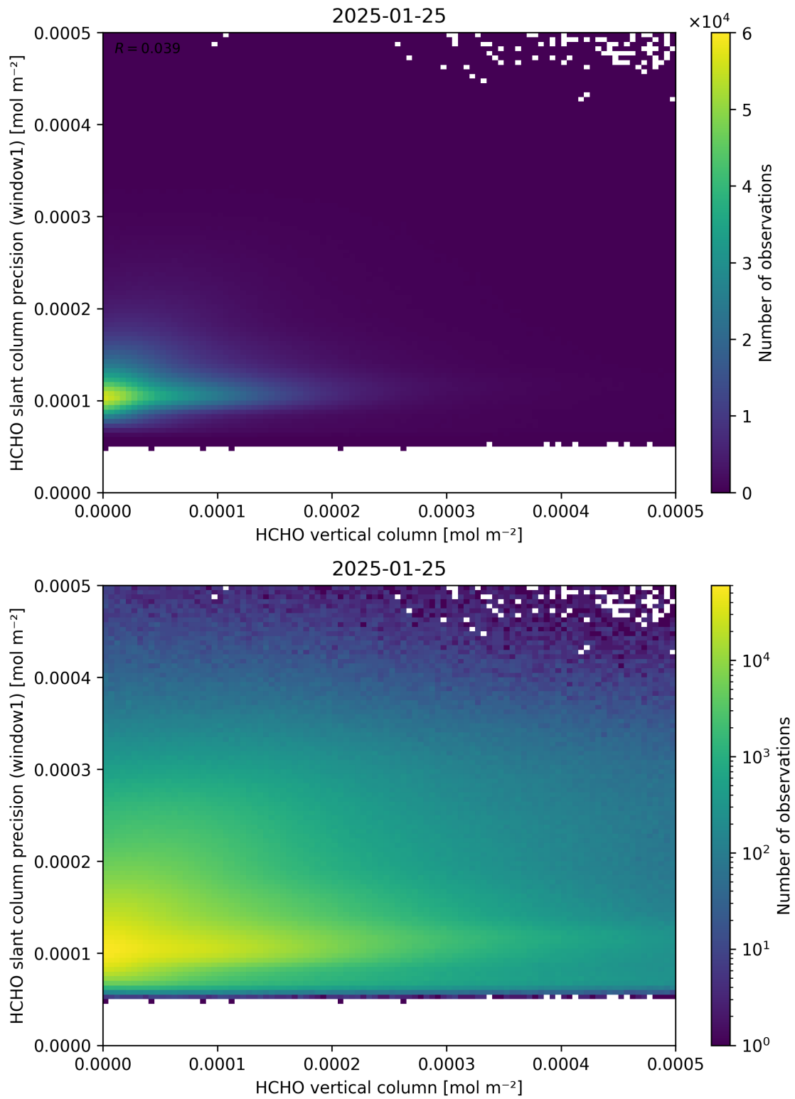
Figure 130: Scatter density plot of “HCHO vertical column” against “HCHO slant column precision (window1)” for 2025-01-24 to 2025-01-26.
