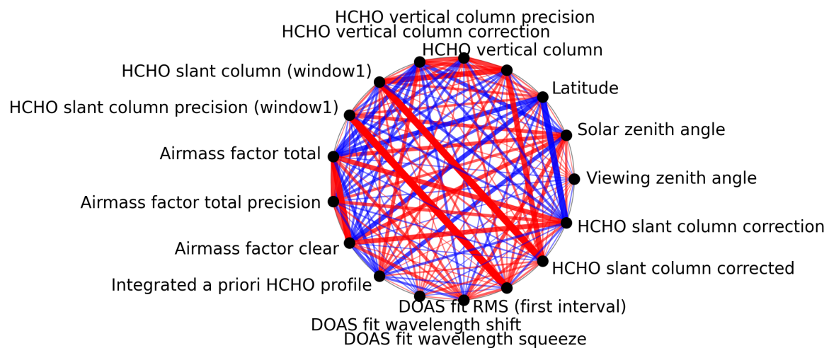
Figure 1: Map of correlation graph for 2025-01-24 to 2025-01-26.
