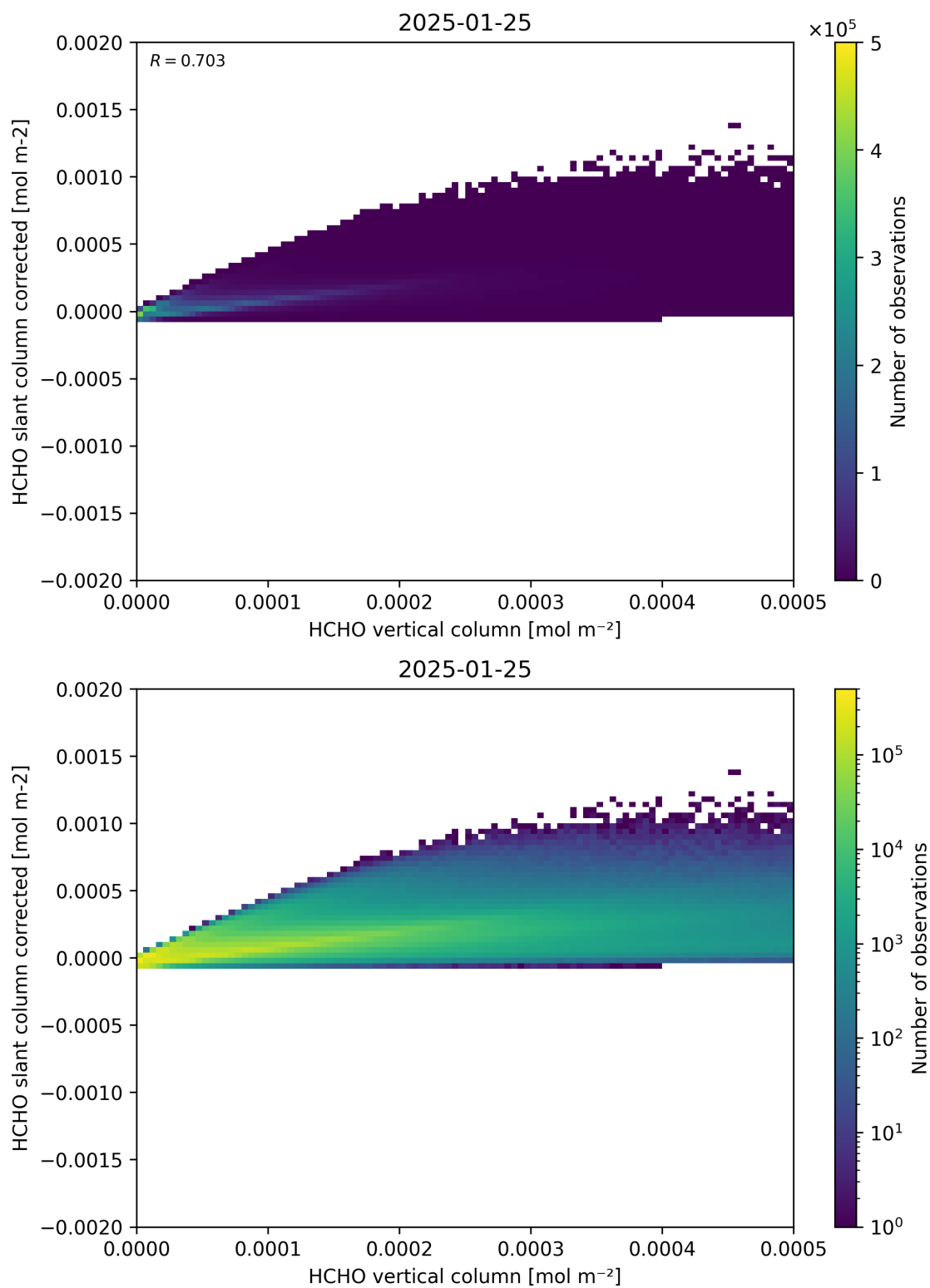
Figure 127: Scatter density plot of “HCHO vertical column” against “HCHO slant column corrected” for 2025-01-24 to 2025-01-26.
