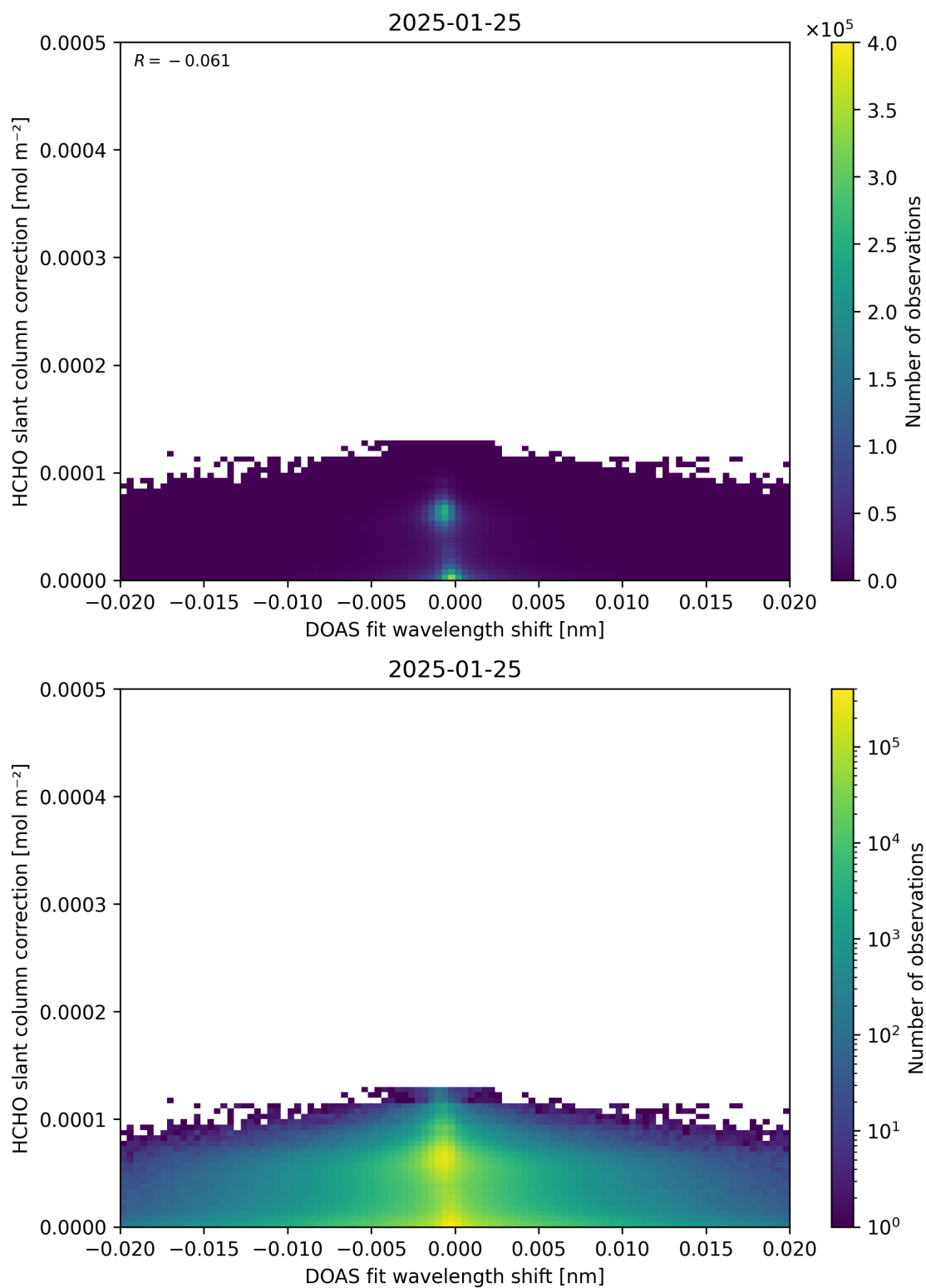
Figure 67: Scatter density plot of “DOAS fit wavelength shift” against “HCHO slant column correction” for 2025-01-24 to 2025-01-26.
