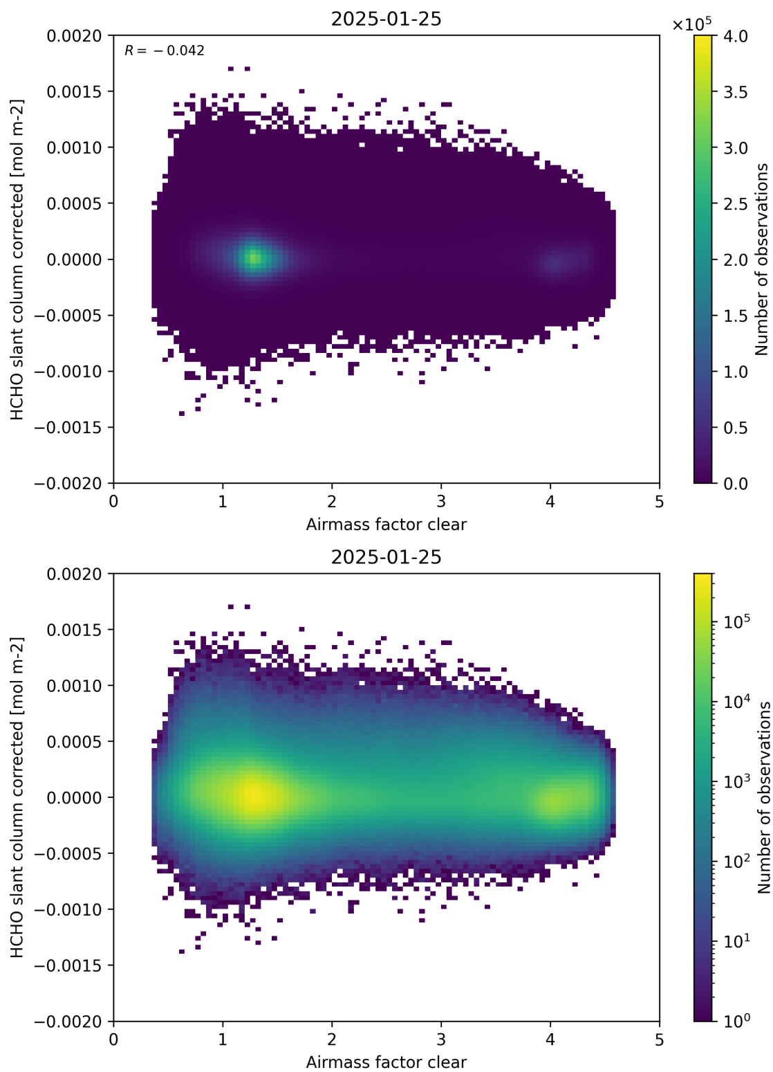
Figure 74: Scatter density plot of “Airmass factor clear” against “HCHO slant column corrected” for 2025-01-24 to 2025-01-26.
