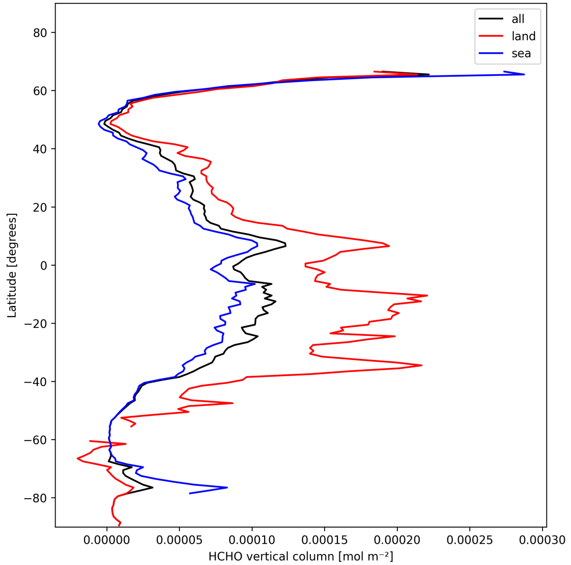
Figure 21: Zonal average of “HCHO vertical column” for 2025-01-24 to 2025-01-26.
