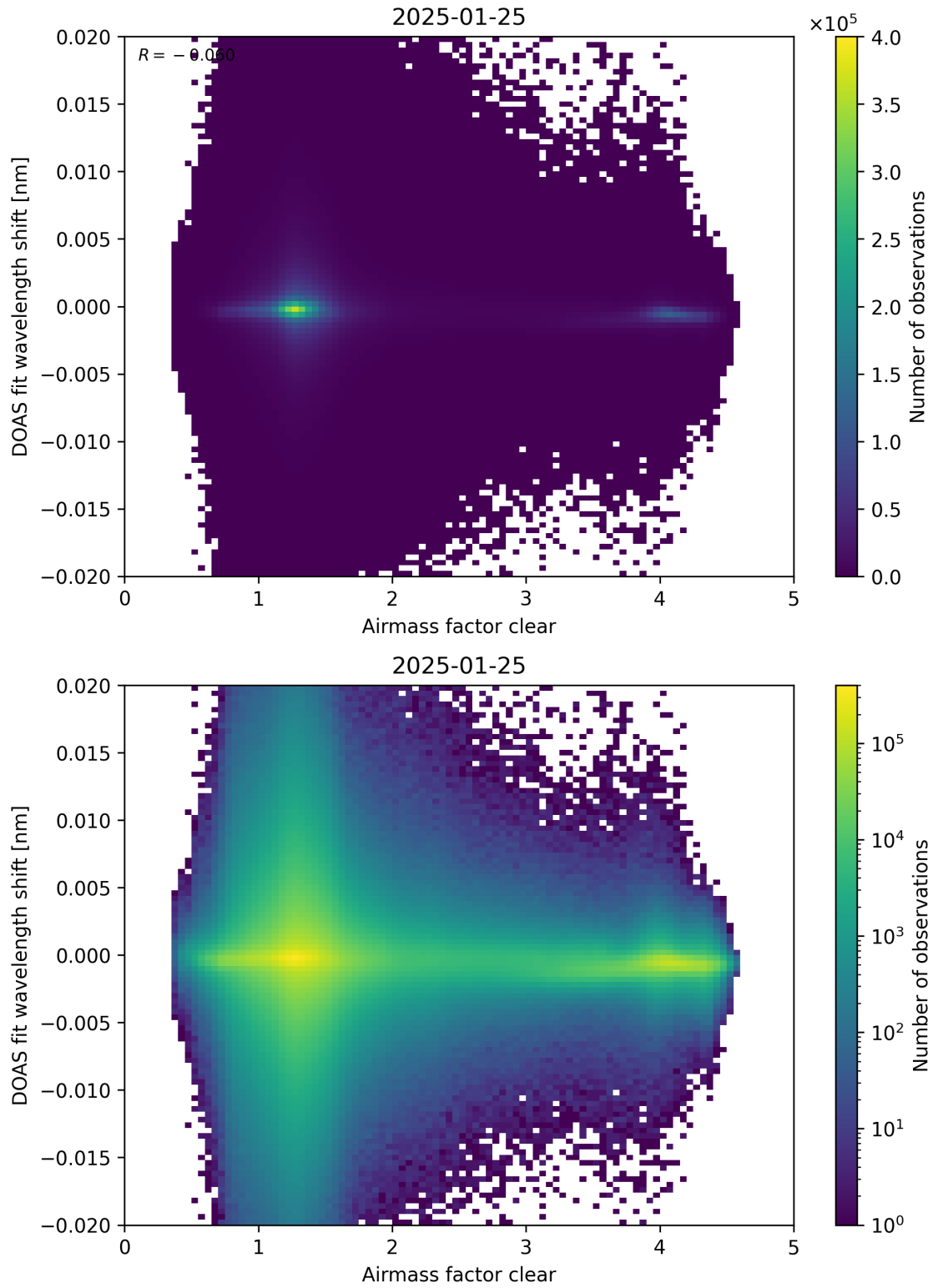
Figure 72: Scatter density plot of “Airmass factor clear” against “DOAS fit wavelength shift” for 2025-01-24 to 2025-01-26.
