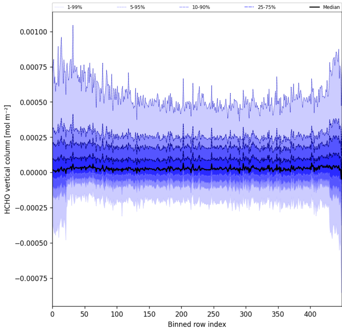
Figure 49: Along track statistics of “HCHO vertical column” for 2025-01-24 to 2025-01-26
