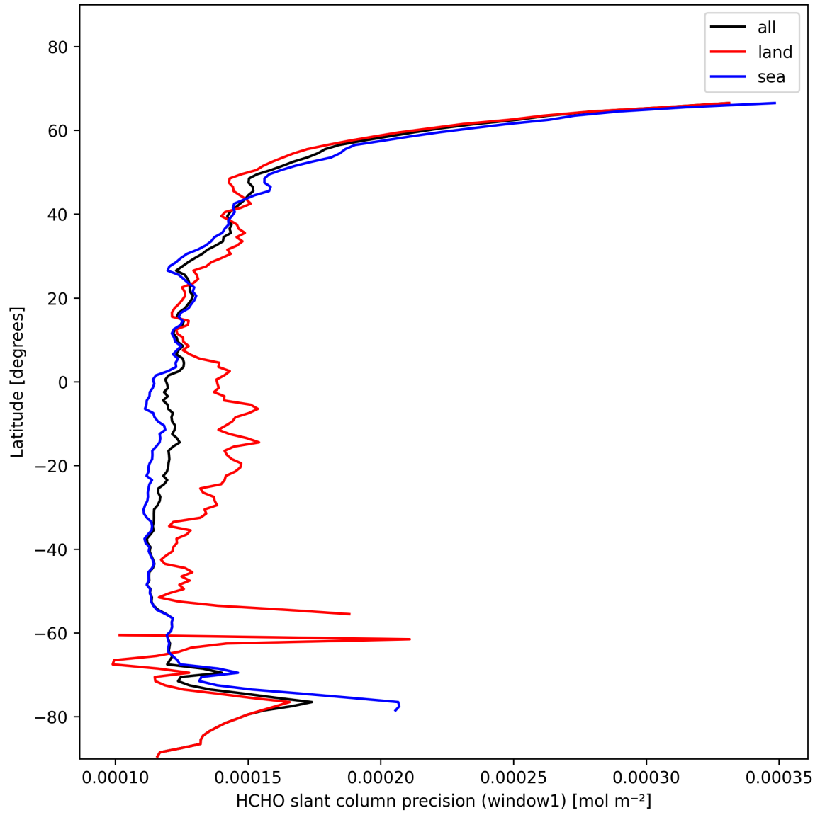
Figure 25: Zonal average of “HCHO slant column precision (window1)” for 2025-01-24 to 2025-01-26.
