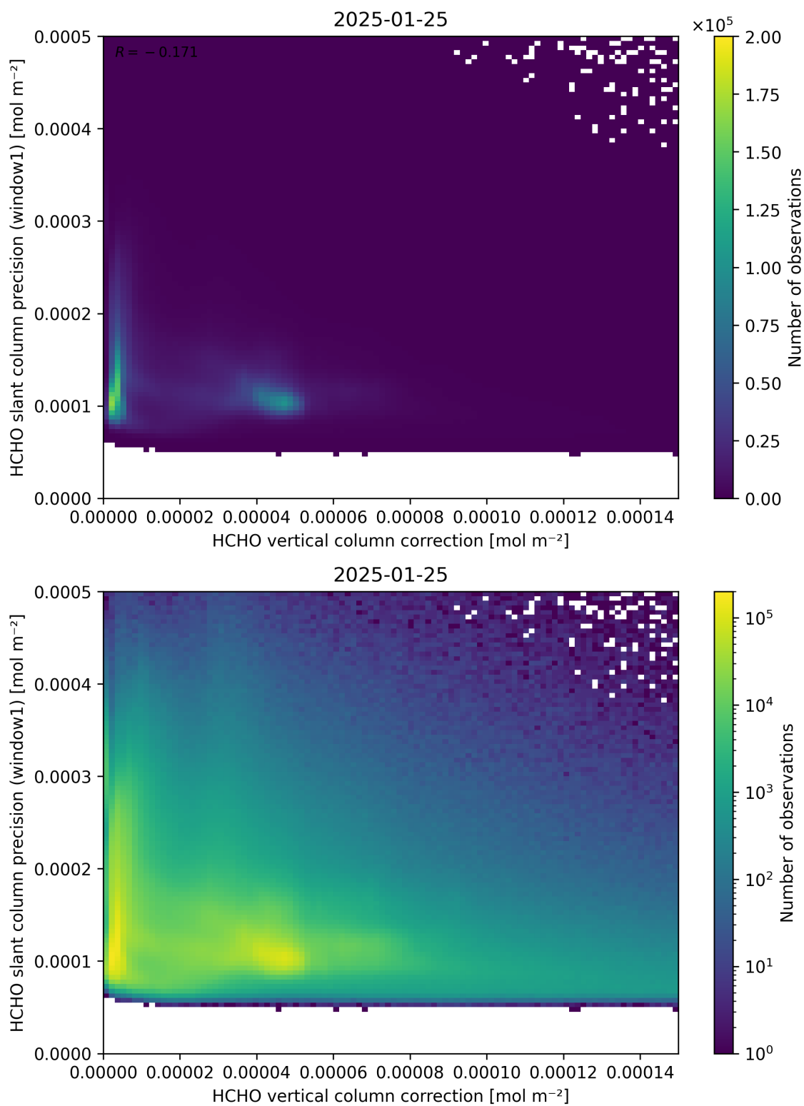
Figure 119: Scatter density plot of “HCHO vertical column correction” against “HCHO slant column precision (window1)” for 2025-01-24 to 2025-01-26.
