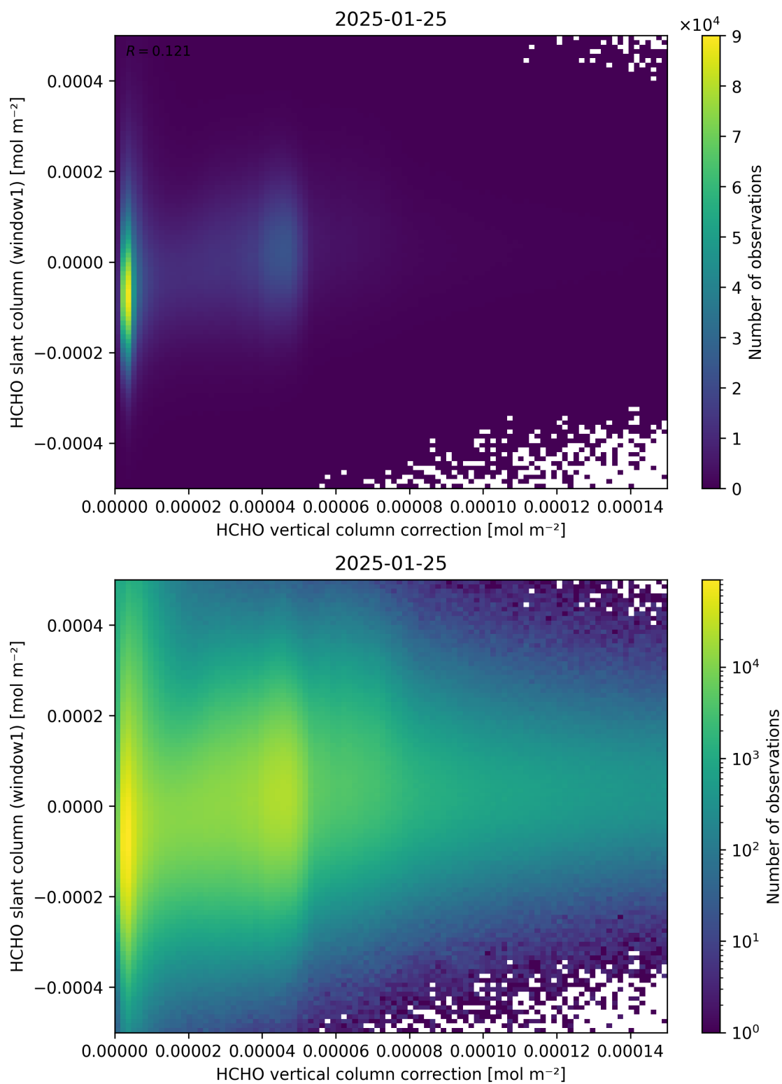
Figure 118: Scatter density plot of “HCHO vertical column correction” against “HCHO slant column (window1)” for 2025-01-24 to 2025-01-26.
