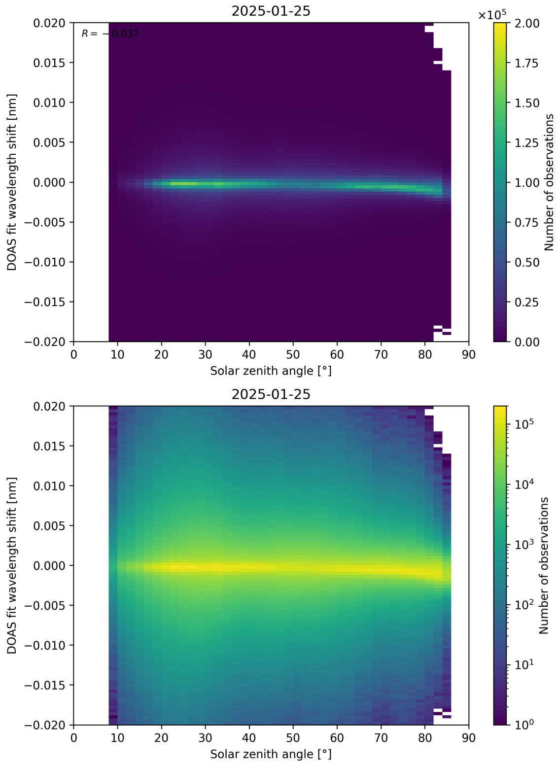
Figure 168: Scatter density plot of “Solar zenith angle” against “DOAS fit wavelength shift” for 2025-01-24 to 2025-01-26.
