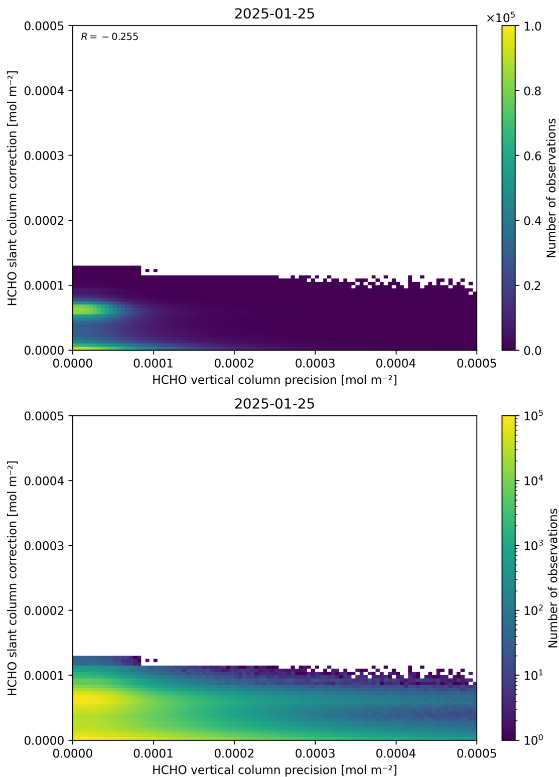
Figure 141: Scatter density plot of “HCHO vertical column precision” against “HCHO slant column correction” for 2025-01-24 to 2025-01-26.
