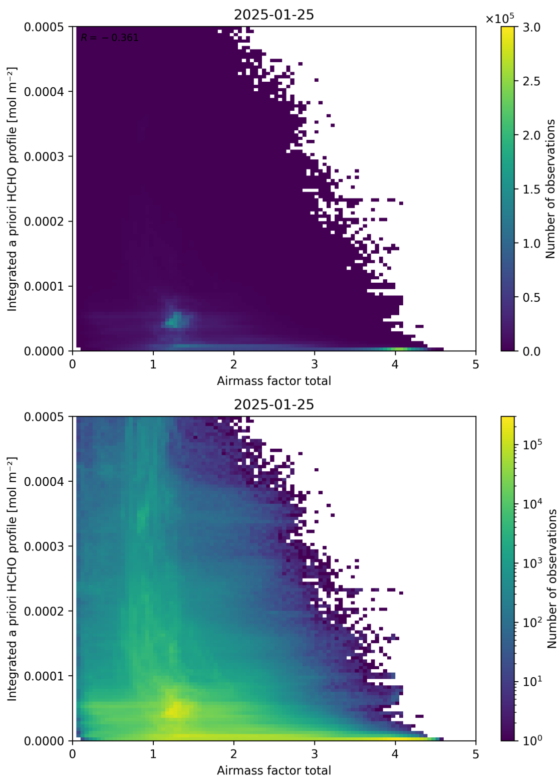
Figure 104: Scatter density plot of “Airmass factor total” against “Integrated a priori HCHO profile” for 2025-01-24 to 2025-01-26.
