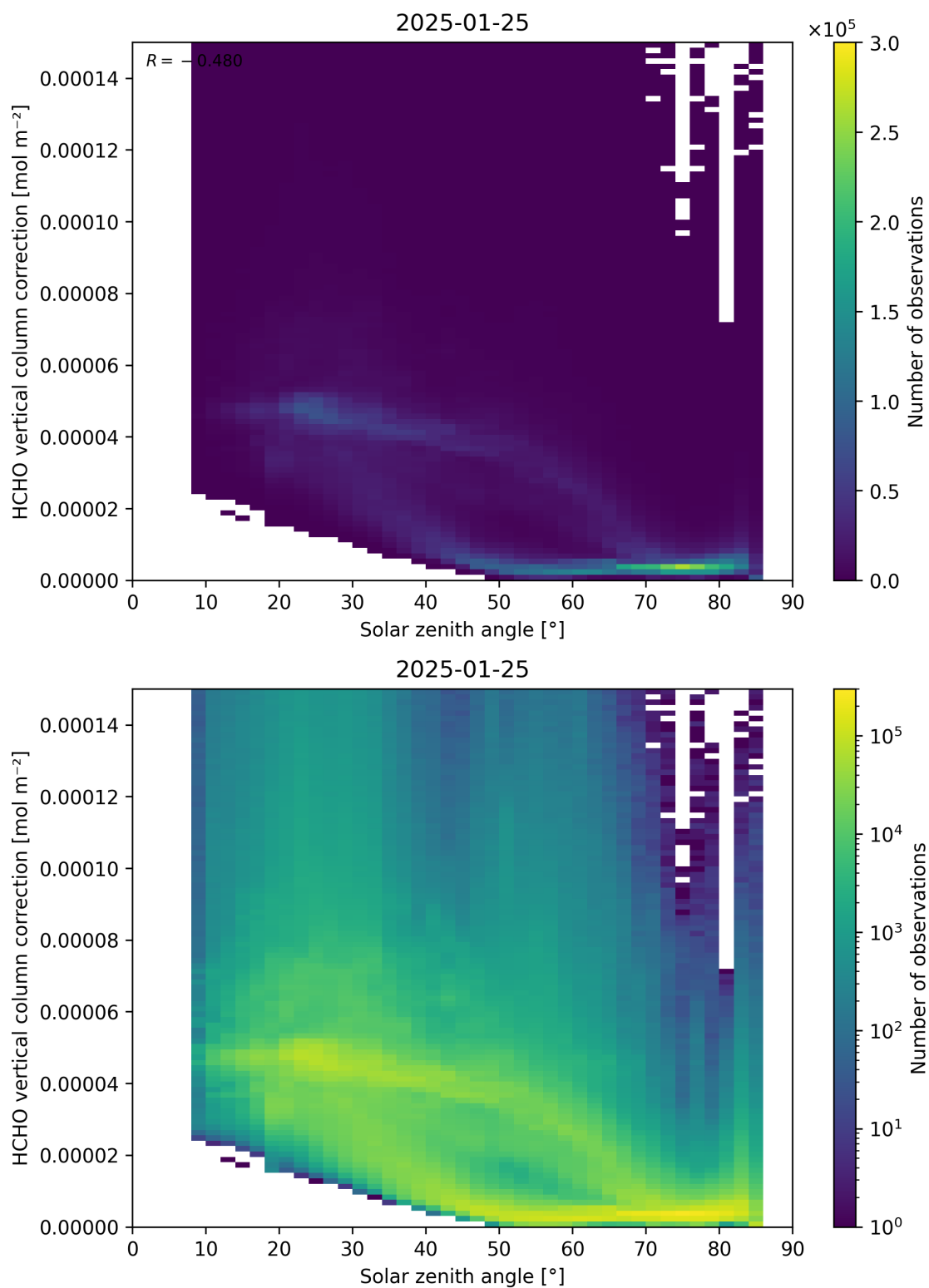
Figure 178: Scatter density plot of “Solar zenith angle” against “HCHO vertical column correction” for 2025-01-24 to 2025-01-26.
