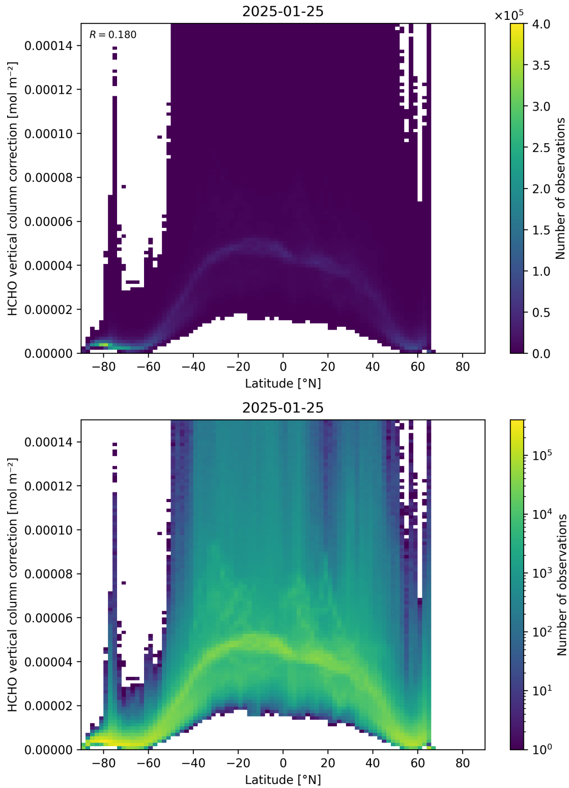
Figure 164: Scatter density plot of “Latitude” against “HCHO vertical column correction” for 2025-01-24 to 2025-01-26.
