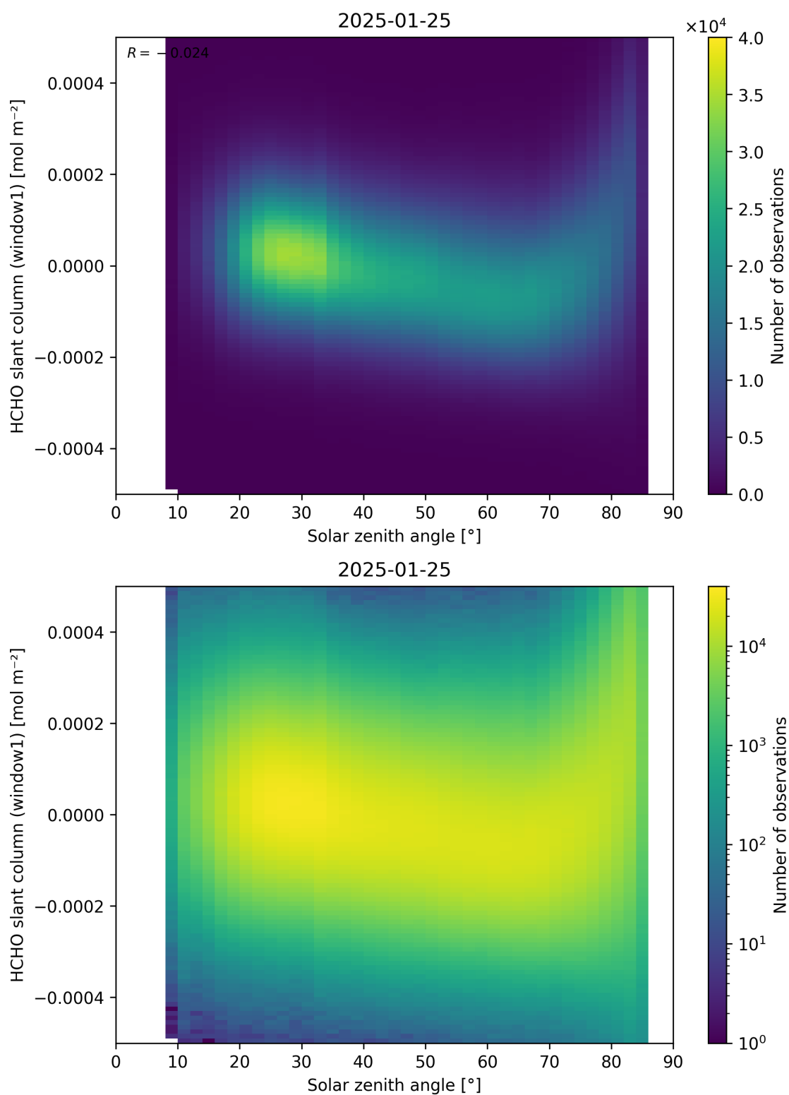
Figure 173: Scatter density plot of “Solar zenith angle” against “HCHO slant column (window1)” for 2025-01-24 to 2025-01-26.
