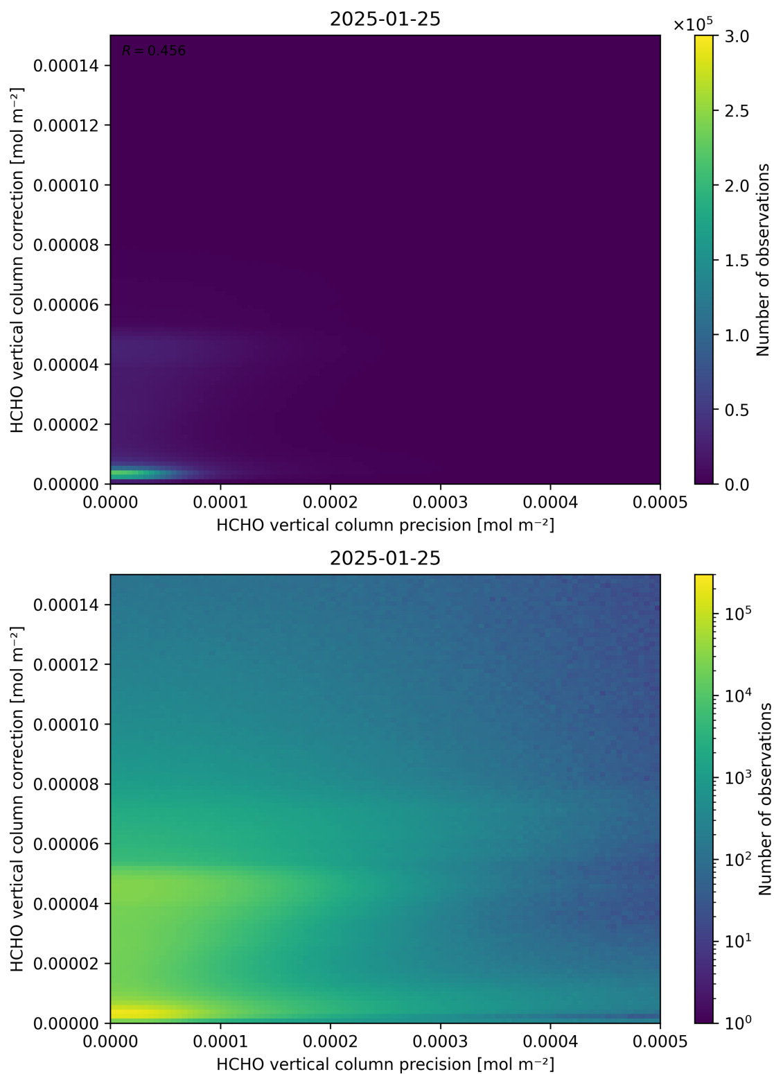
Figure 146: Scatter density plot of “HCHO vertical column precision” against “HCHO vertical column correction” for 2025-01-24 to 2025-01-26.
