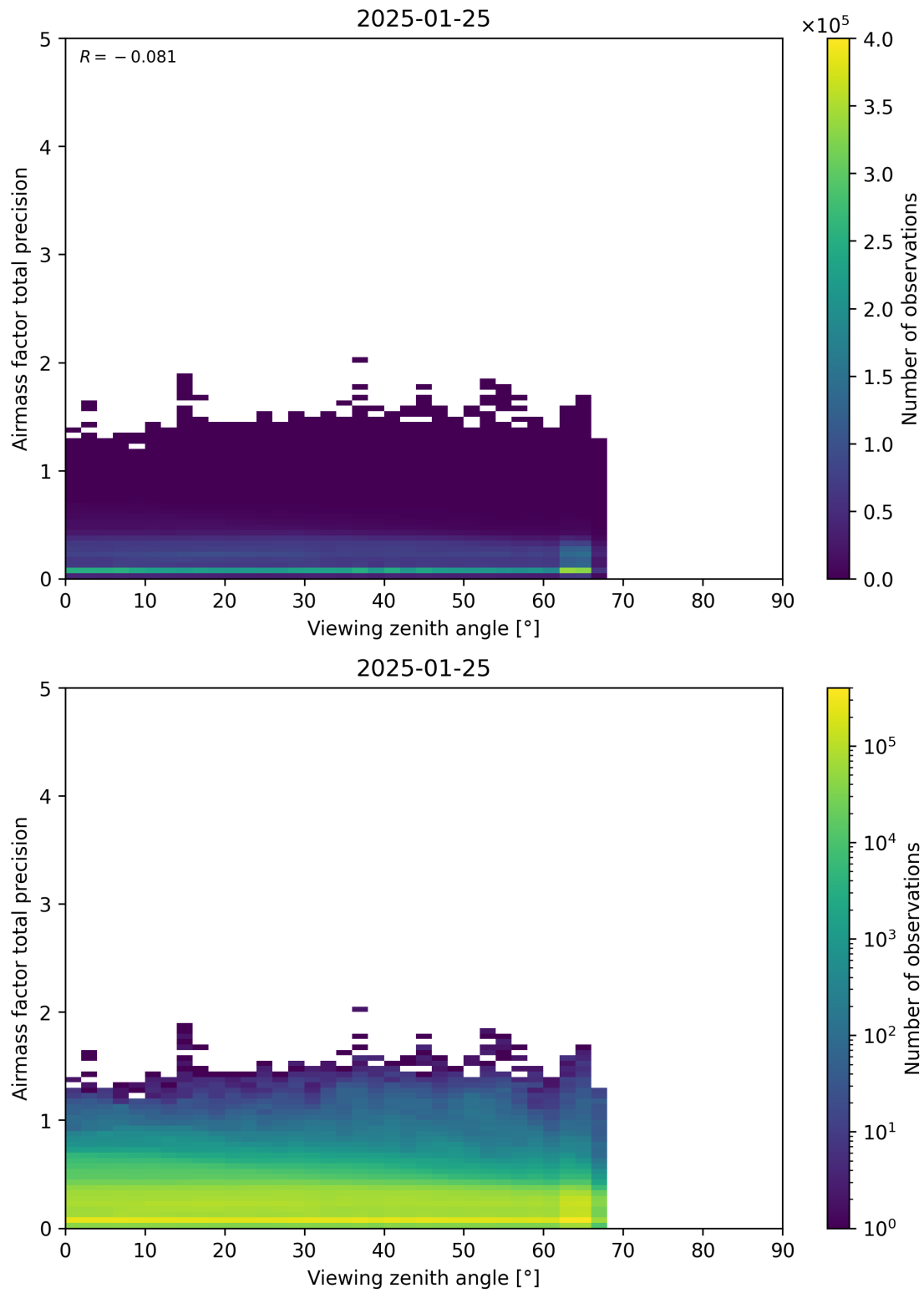
Figure 191: Scatter density plot of “Viewing zenith angle” against “Airmass factor total precision” for 2025-01-24 to 2025-01-26.
