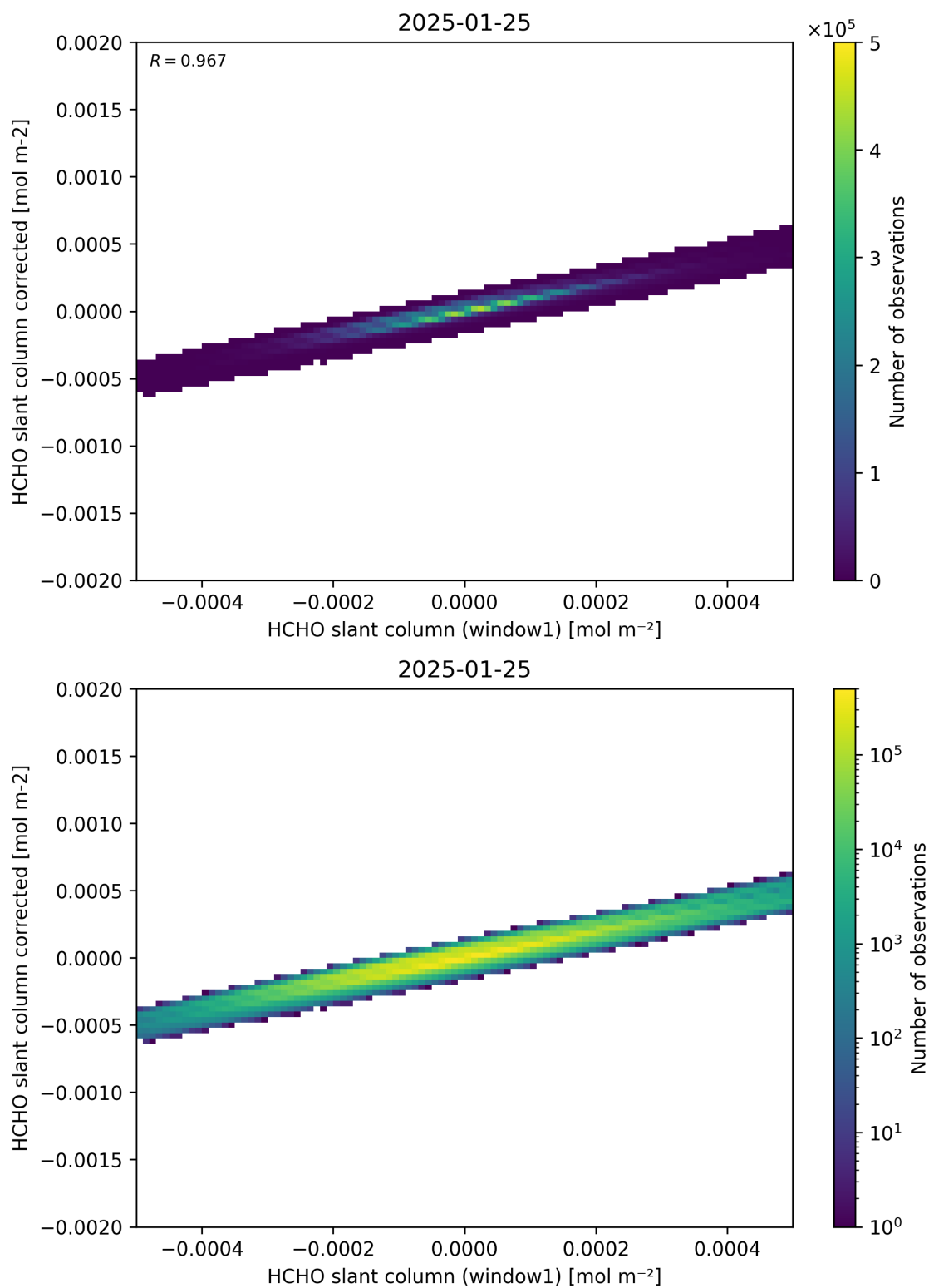
Figure 82: Scatter density plot of “HCHO slant column (window1)” against “HCHO slant column corrected” for 2025-01-24 to 2025-01-26.
