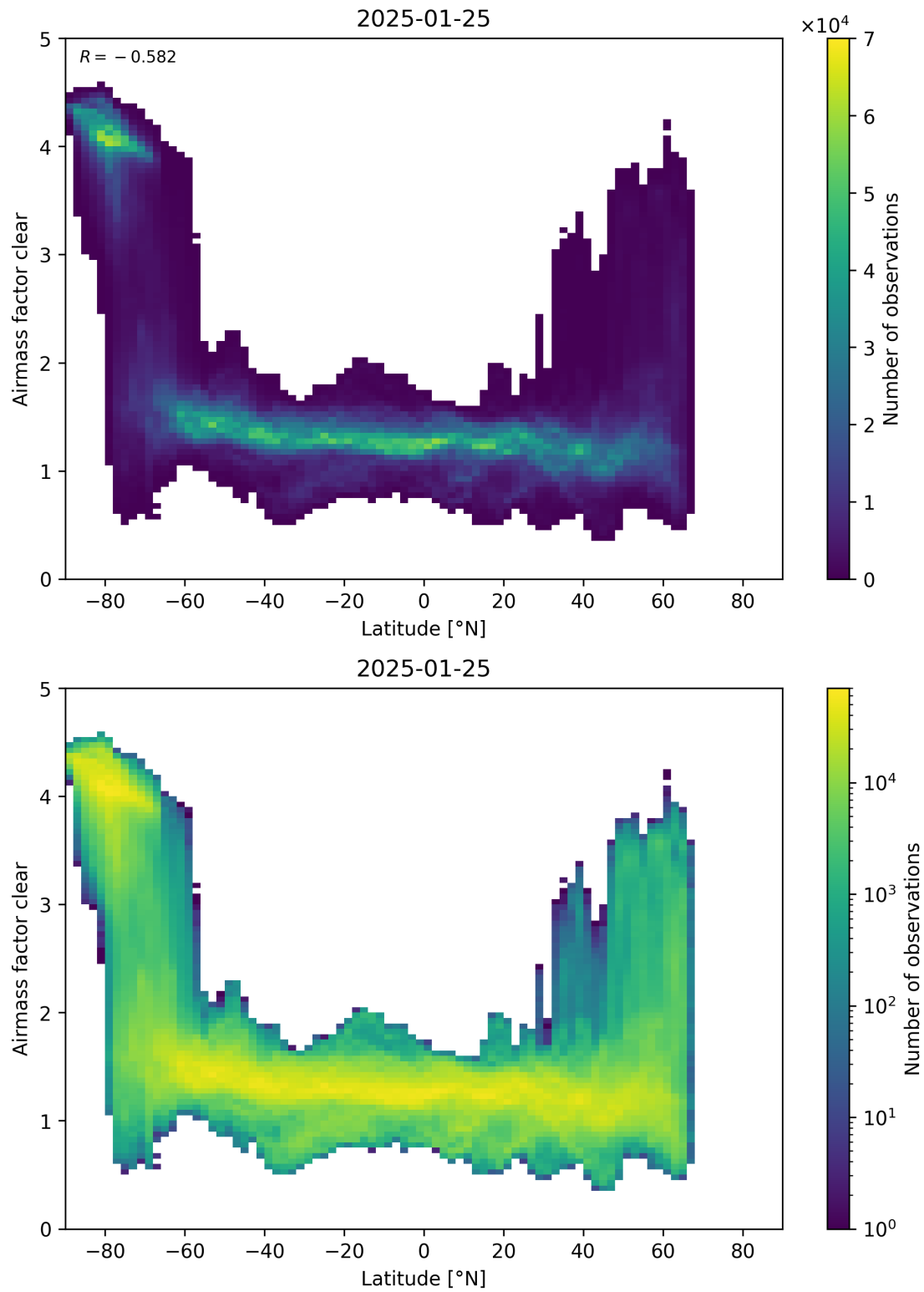
Figure 156: Scatter density plot of “Latitude” against “Airmass factor clear” for 2025-01-24 to 2025-01-26.
