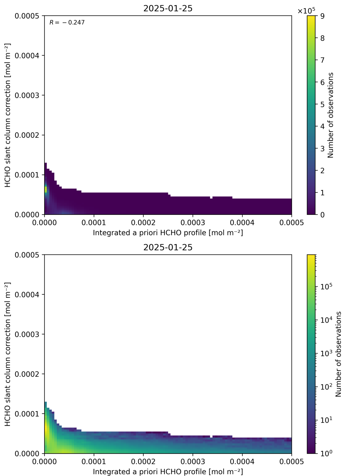
Figure 152: Scatter density plot of “Integrated a priori HCHO profile” against “HCHO slant column correction” for 2025-01-24 to 2025-01-26.
