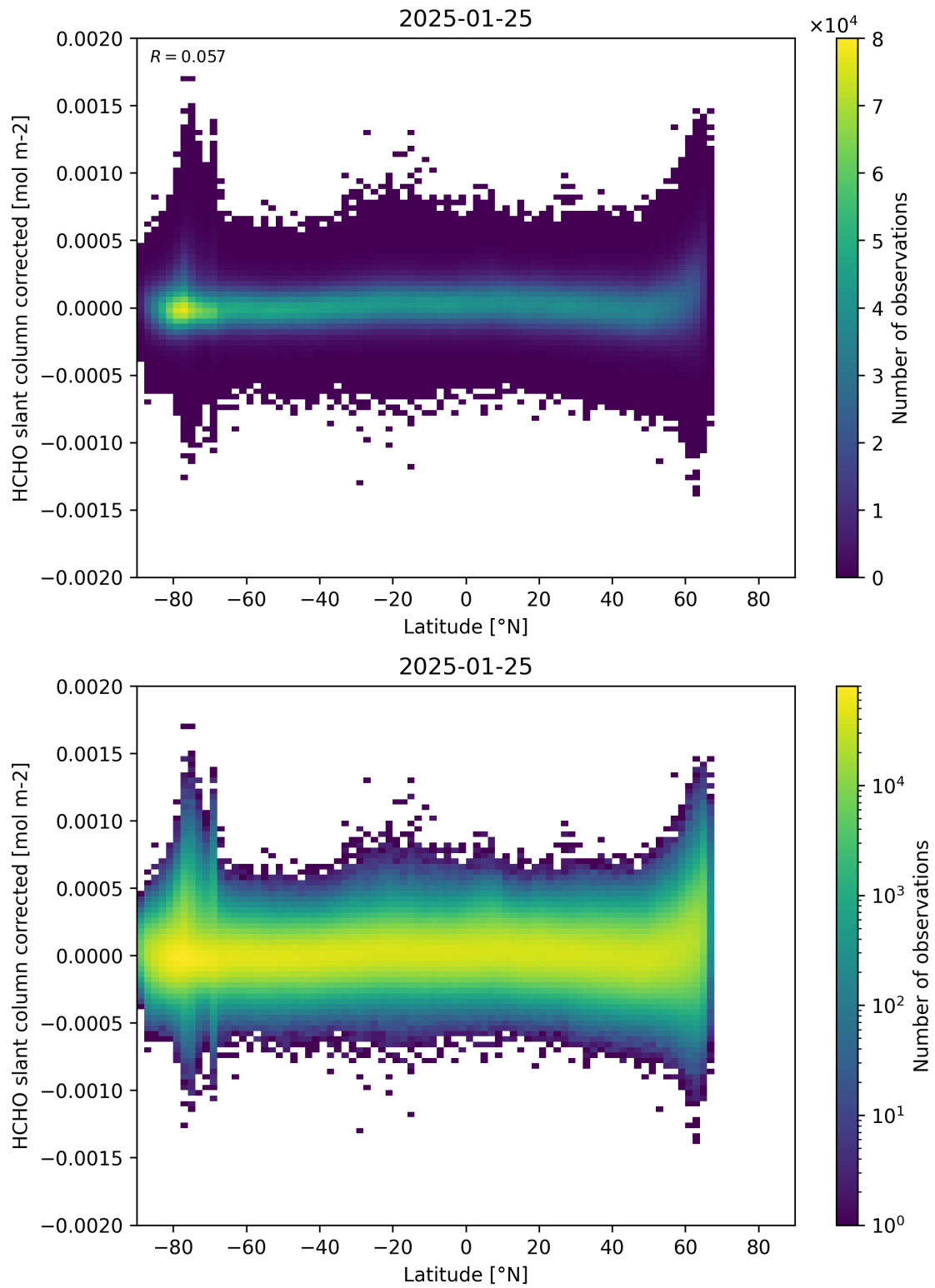
Figure 157: Scatter density plot of “Latitude” against “HCHO slant column corrected” for 2025-01-24 to 2025-01-26.
