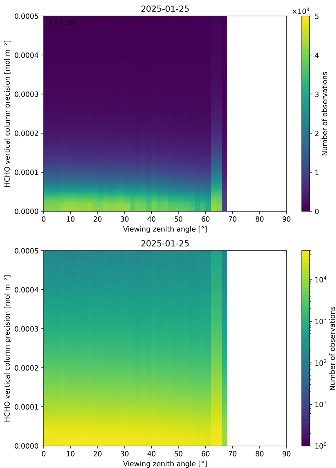
Figure 194: Scatter density plot of “Viewing zenith angle” against “HCHO vertical column precision” for 2025-01-24 to 2025-01-26.
