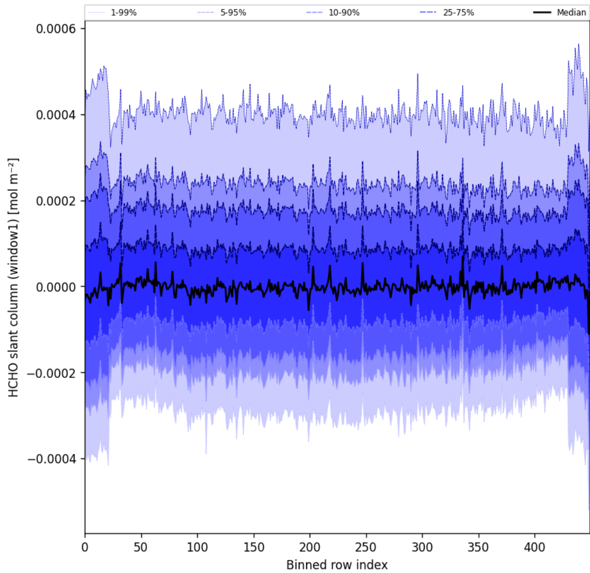
Figure 52: Along track statistics of “HCHO slant column (window1)” for 2025-01-24 to 2025-01-26
