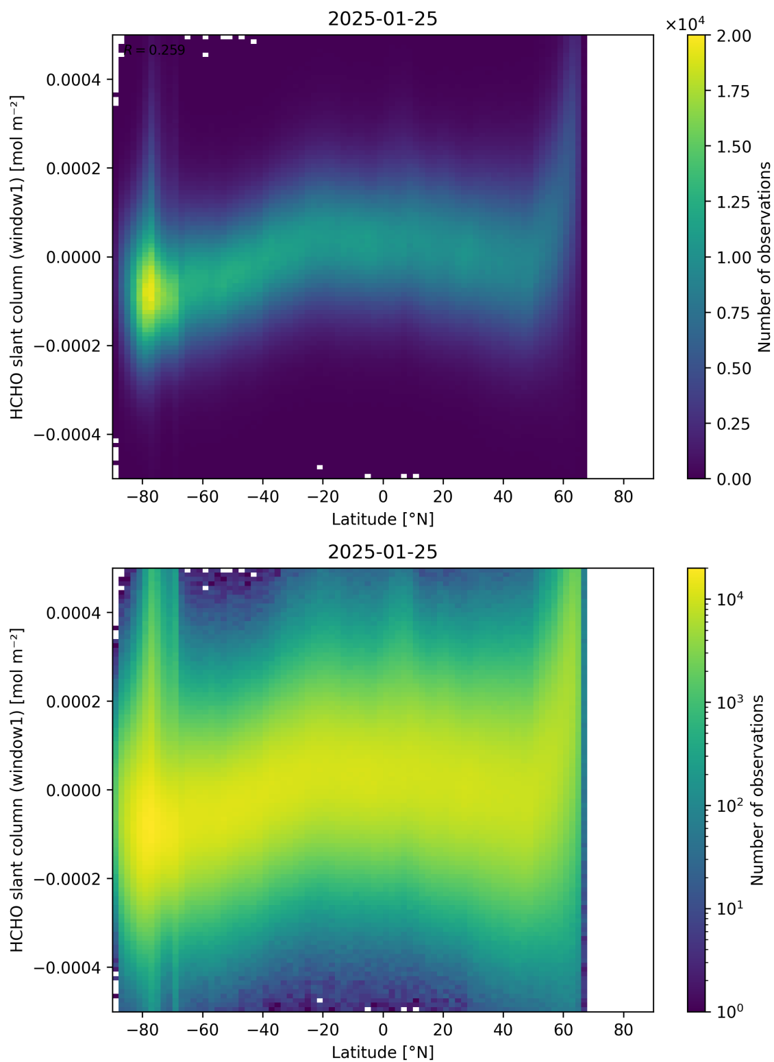
Figure 159: Scatter density plot of “Latitude” against “HCHO slant column (window1)” for 2025-01-24 to 2025-01-26.
