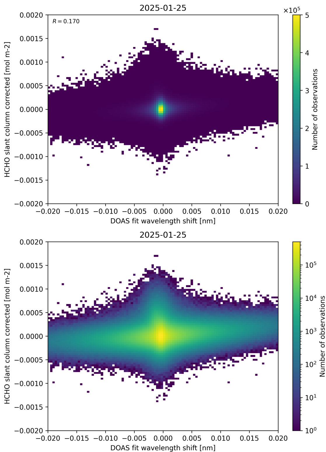
Figure 66: Scatter density plot of “DOAS fit wavelength shift” against “HCHO slant column corrected” for 2025-01-24 to 2025-01-26.
