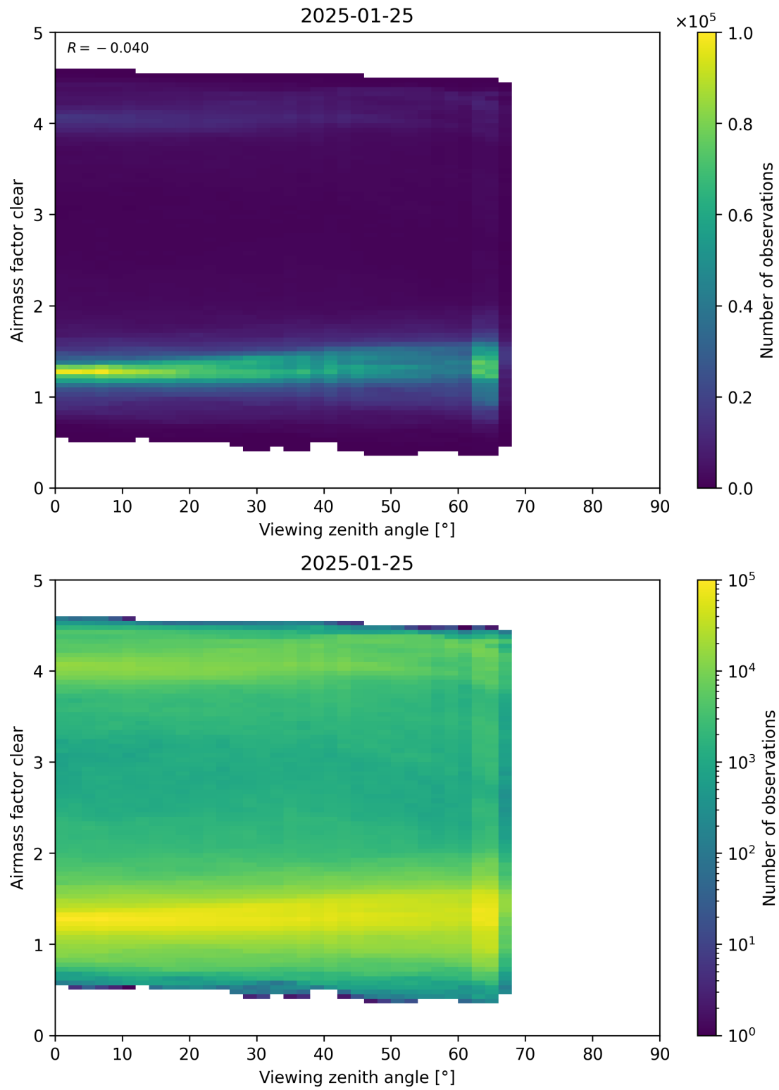
Figure 185: Scatter density plot of “Viewing zenith angle” against “Airmass factor clear” for 2025-01-24 to 2025-01-26.
