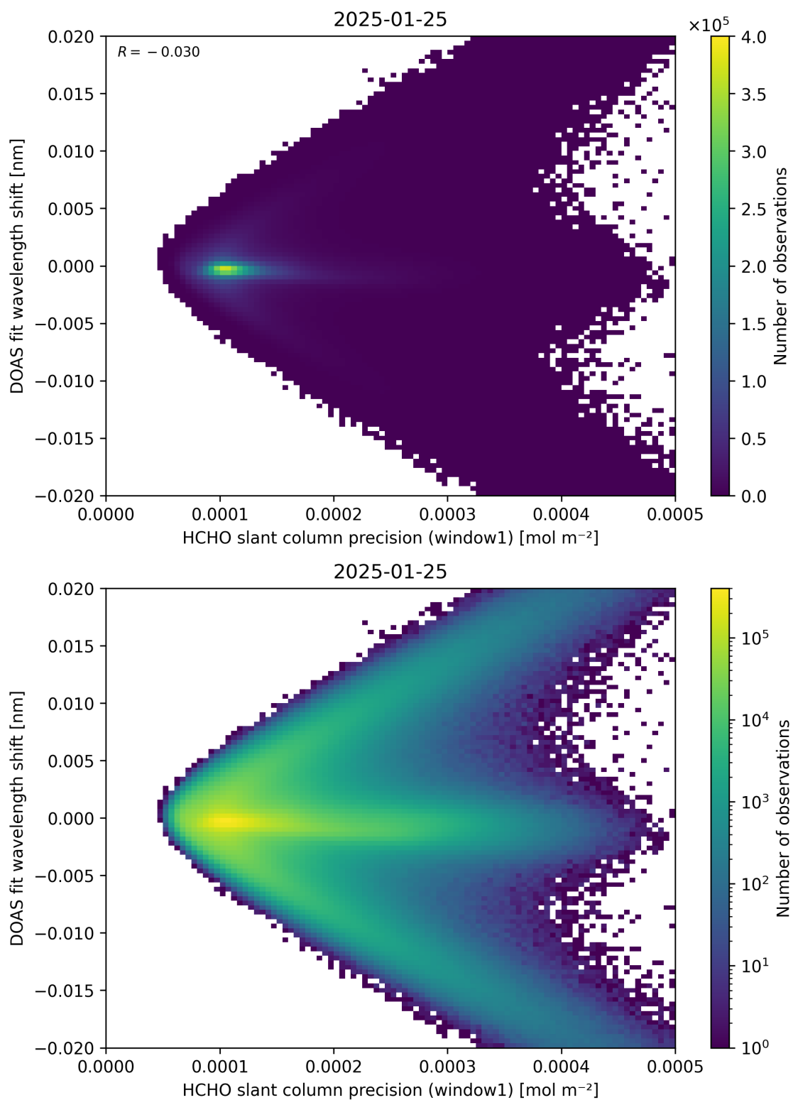
Figure 89: Scatter density plot of “HCHO slant column precision (window1)” against “DOAS fit wavelength shift” for 2025-01-24 to 2025-01-26.
