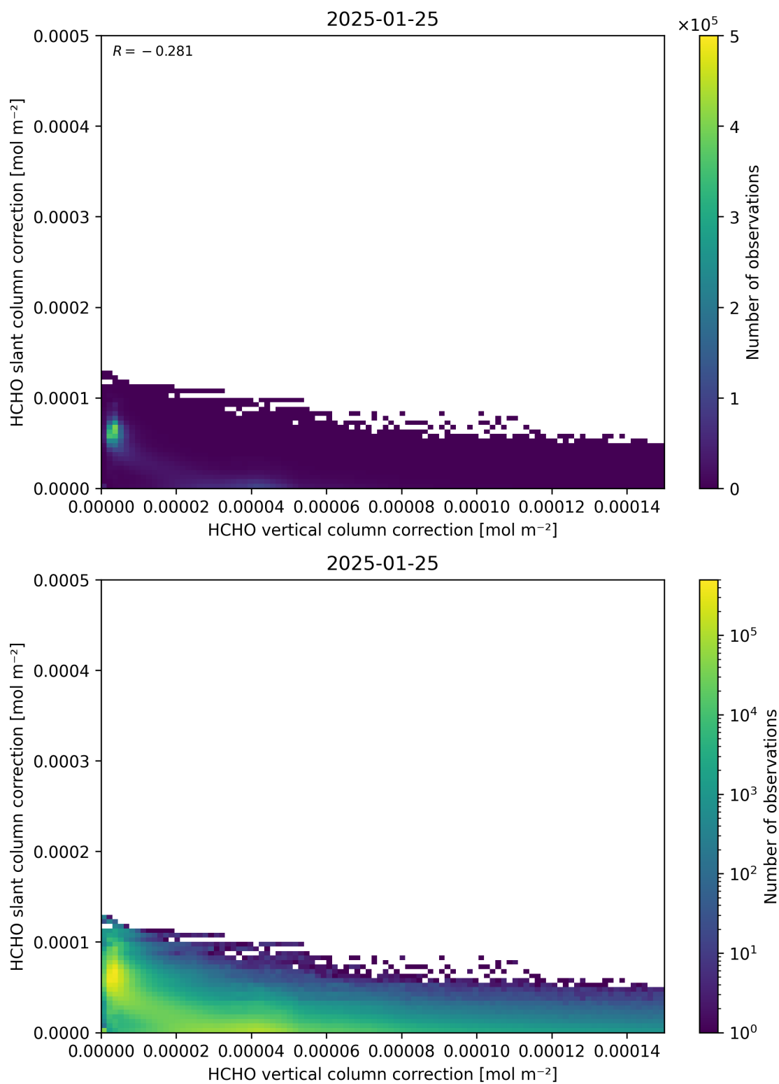
Figure 117: Scatter density plot of “HCHO vertical column correction” against “HCHO slant column correction” for 2025-01-24 to 2025-01-26.
