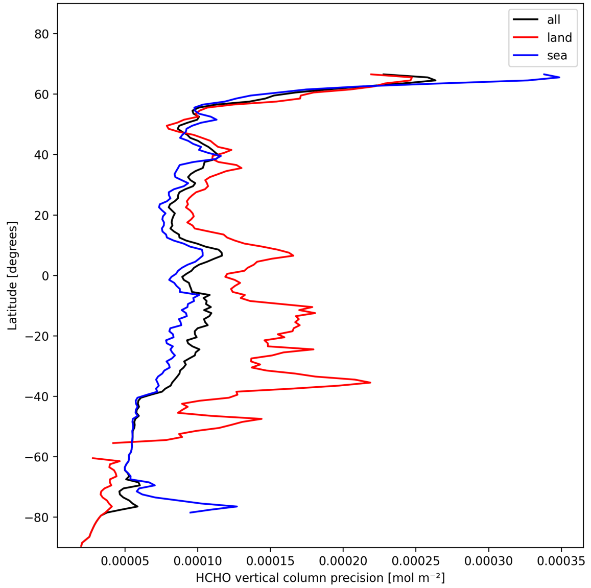
Figure 22: Zonal average of “HCHO vertical column precision” for 2025-01-24 to 2025-01-26.
