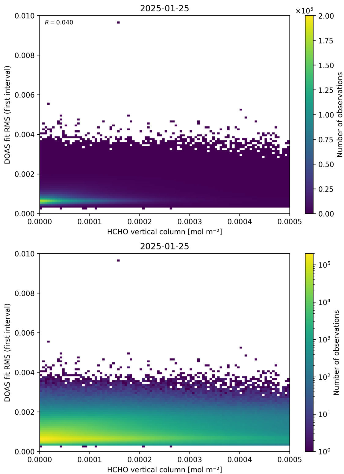
Figure 123: Scatter density plot of “HCHO vertical column” against “DOAS fit RMS (first interval)” for 2025-01-24 to 2025-01-26.
