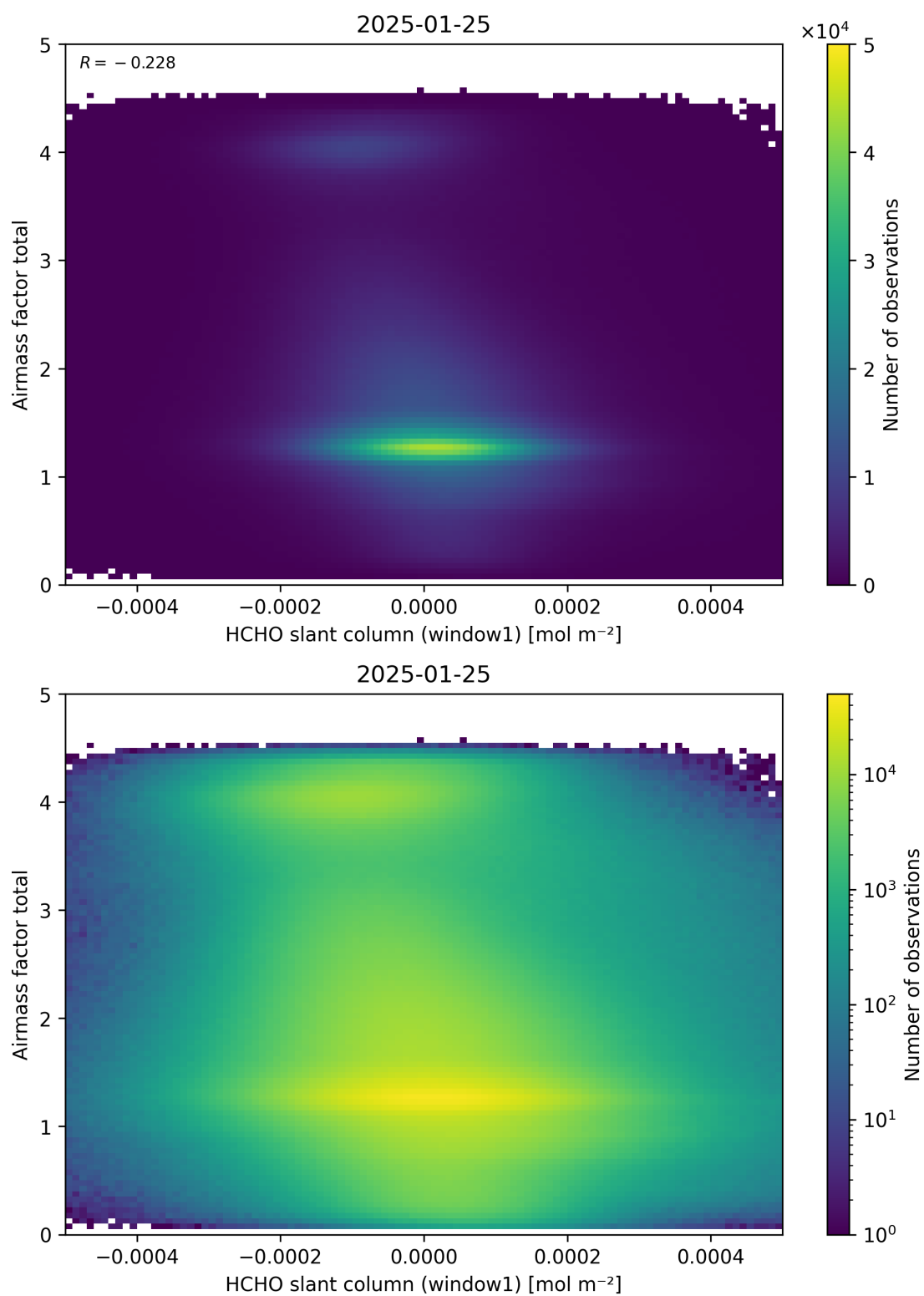
Figure 85: Scatter density plot of “HCHO slant column (window1)” against “Airmass factor total” for 2025-01-24 to 2025-01-26.
