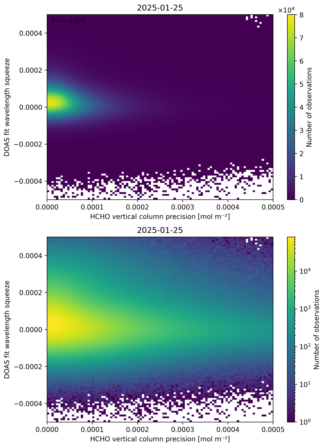
Figure 138: Scatter density plot of “HCHO vertical column precision” against “DOAS fit wavelength squeeze” for 2025-01-24 to 2025-01-26.
