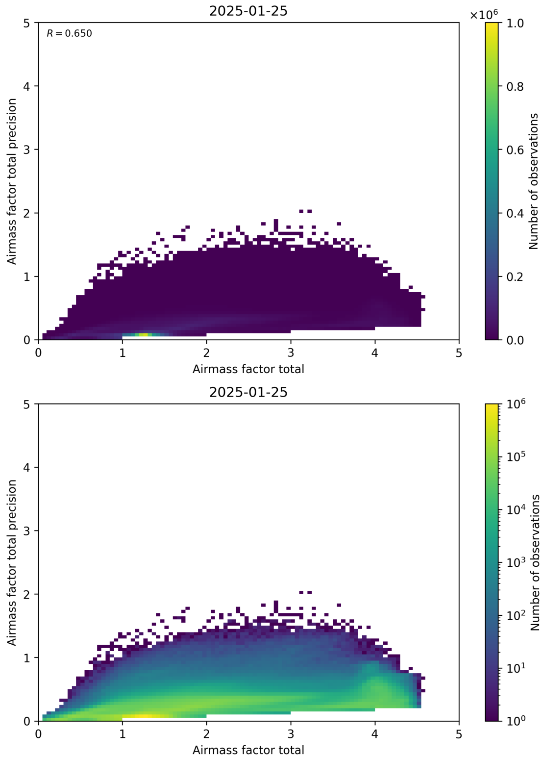
Figure 103: Scatter density plot of “Airmass factor total” against “Airmass factor total precision” for 2025-01-24 to 2025-01-26.
