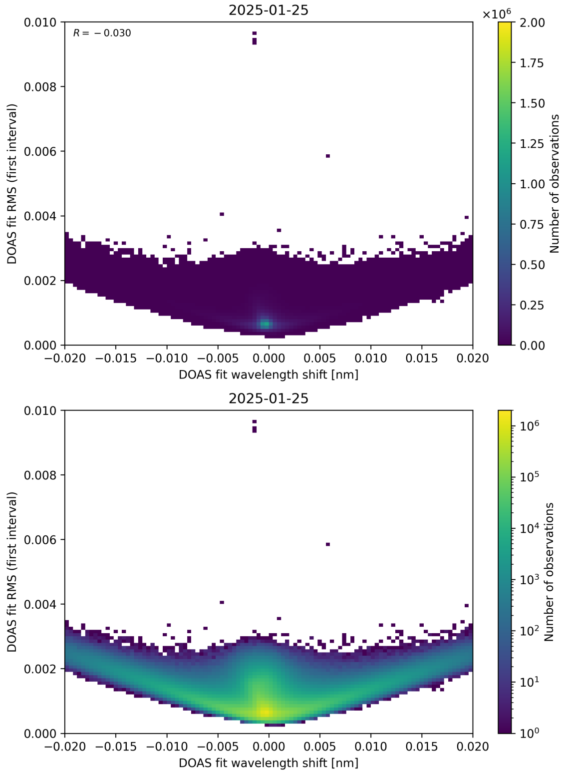
Figure 64: Scatter density plot of “DOAS fit wavelength shift” against “DOAS fit RMS (first interval)” for 2025-01-24 to 2025-01-26.
