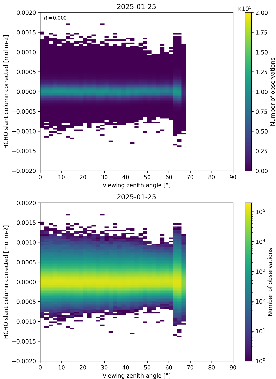
Figure 186: Scatter density plot of “Viewing zenith angle” against “HCHO slant column corrected” for 2025-01-24 to 2025-01-26.
