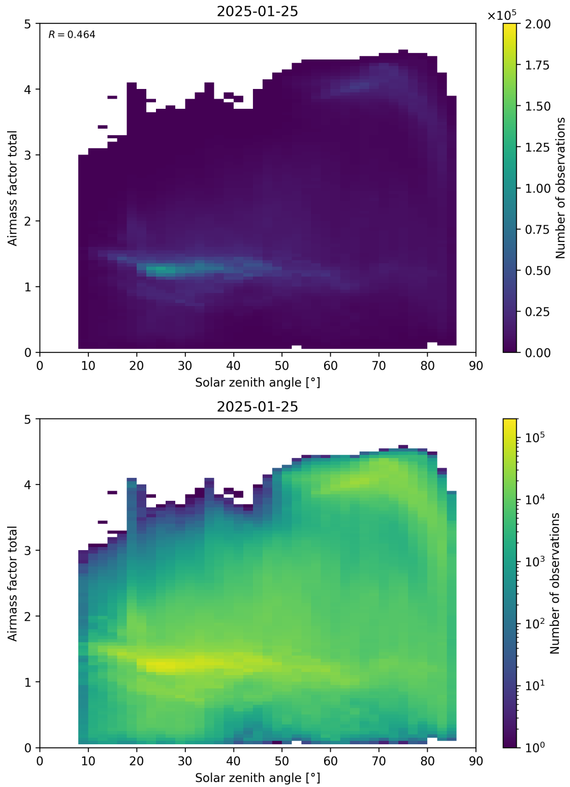
Figure 175: Scatter density plot of “Solar zenith angle” against “Airmass factor total” for 2025-01-24 to 2025-01-26.
