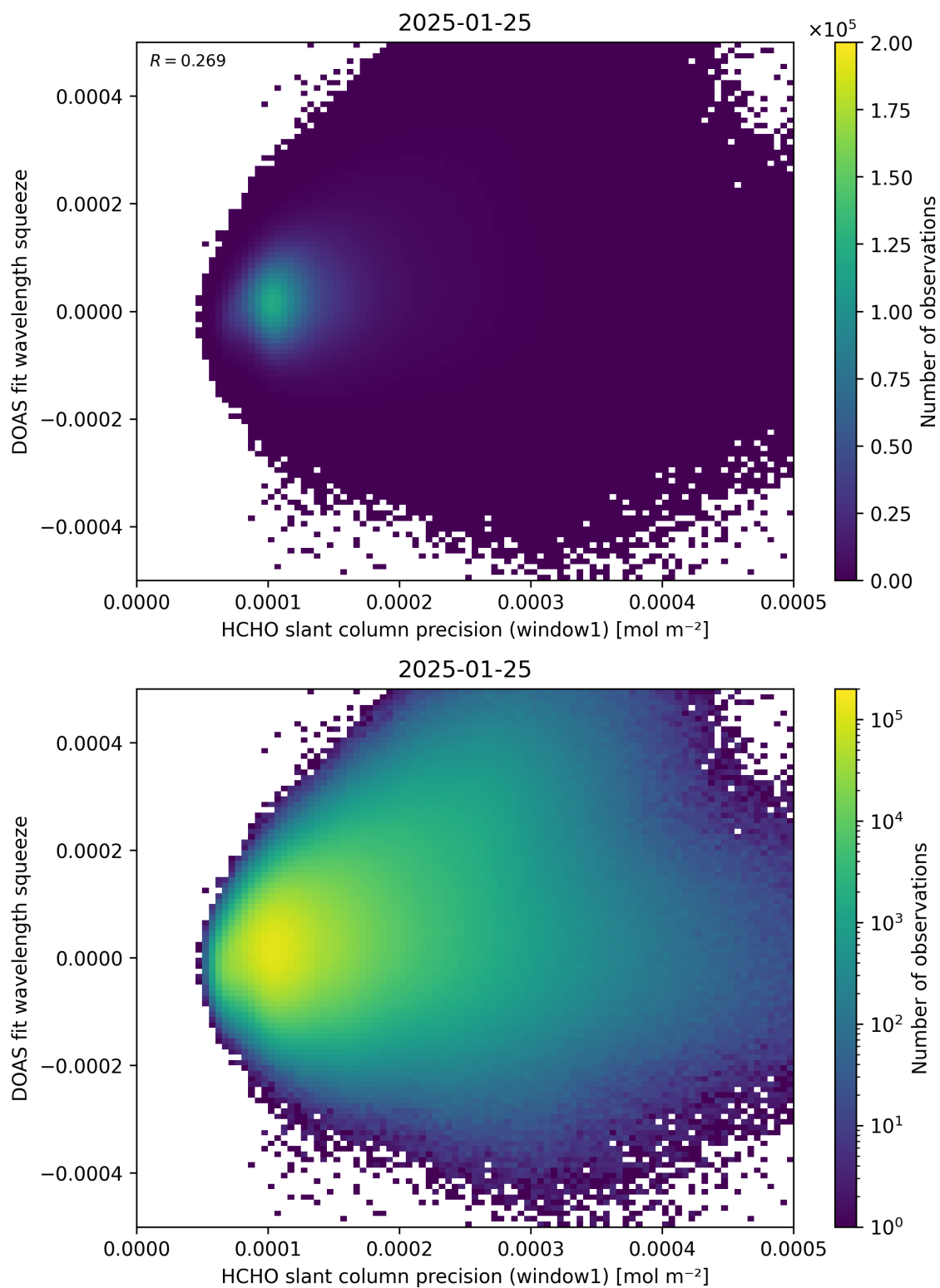
Figure 90: Scatter density plot of “HCHO slant column precision (window1)” against “DOAS fit wavelength squeeze” for 2025-01-24 to 2025-01-26.
