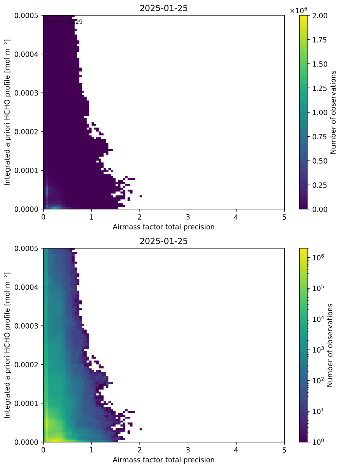
Figure 111: Scatter density plot of “Airmass factor total precision” against “Integrated a priori HCHO profile” for 2025-01-24 to 2025-01-26.
