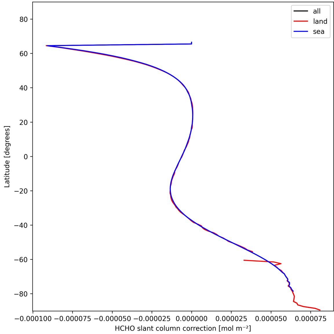
Figure 33: Zonal average of “HCHO slant column correction” for 2025-01-24 to 2025-01-26.
