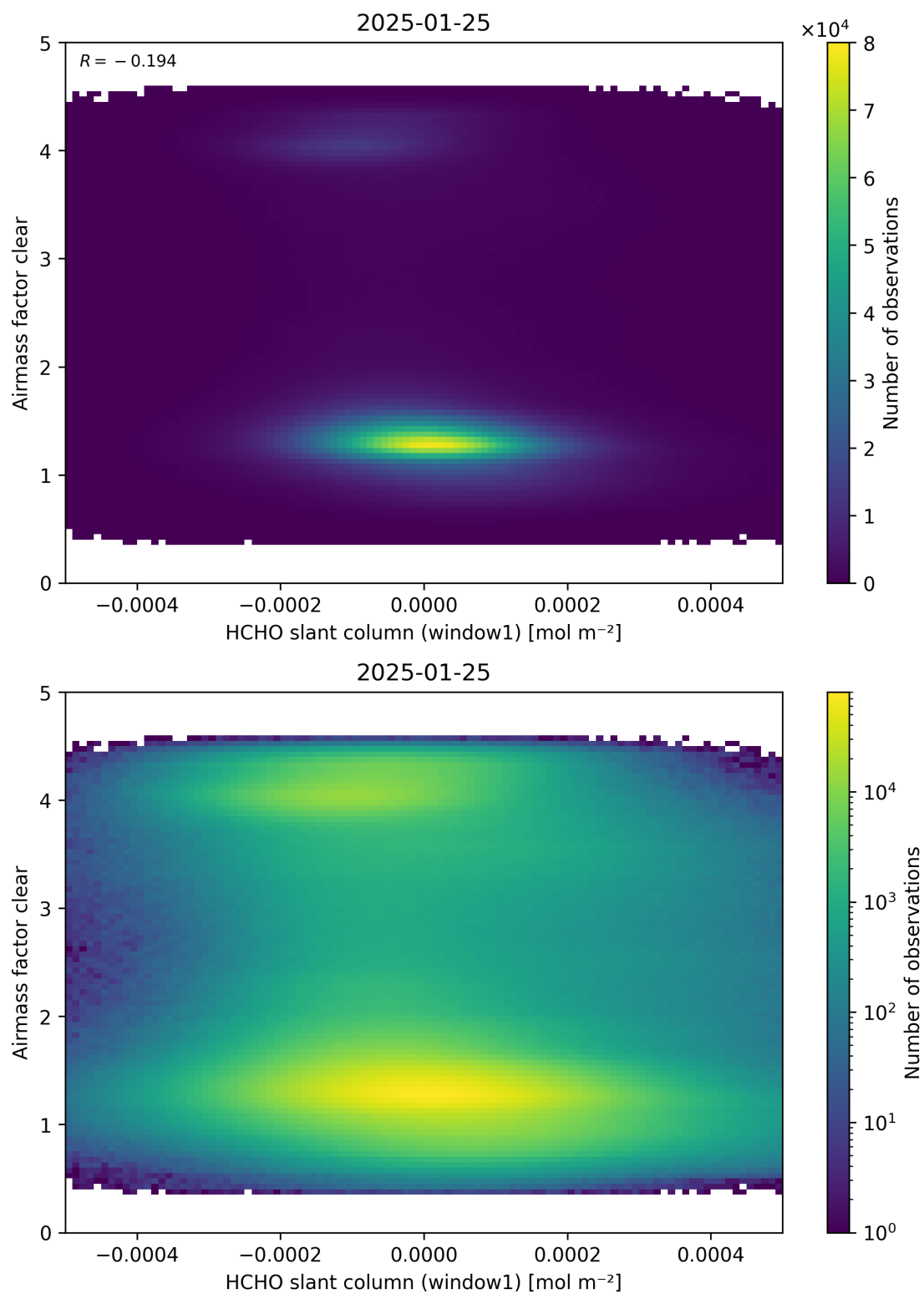
Figure 81: Scatter density plot of “HCHO slant column (window1)” against “Airmass factor clear” for 2025-01-24 to 2025-01-26.
