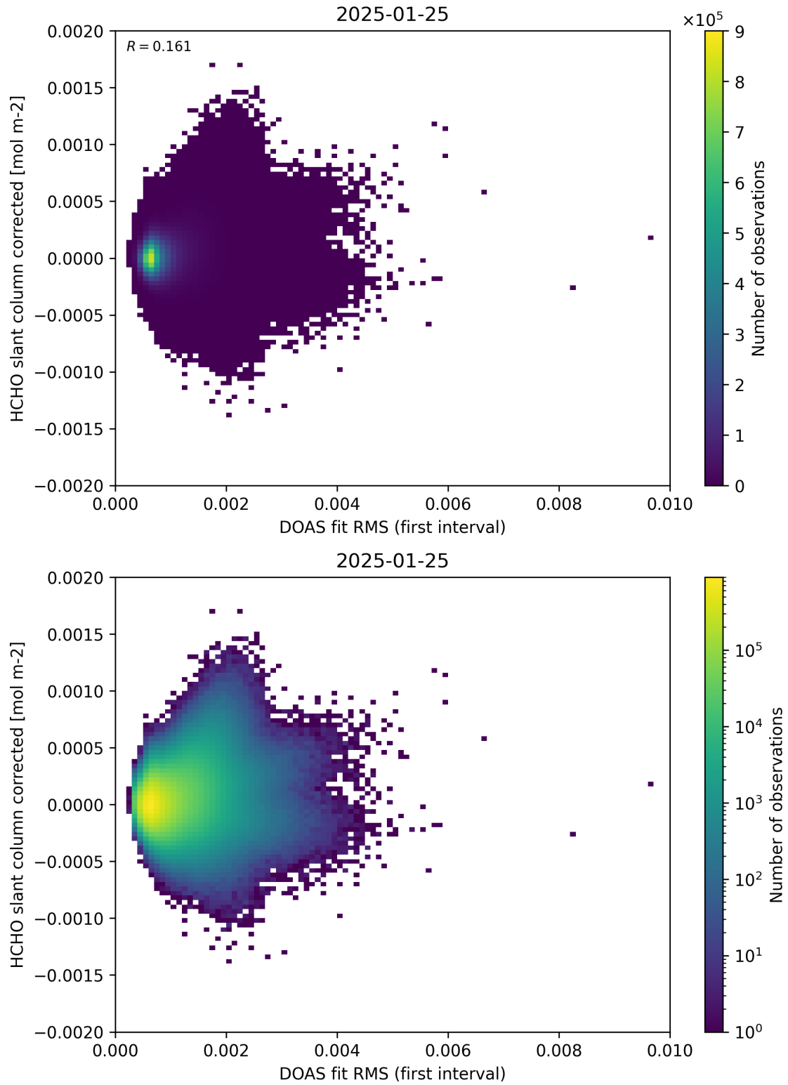
Figure 62: Scatter density plot of “DOAS fit RMS (first interval)” against “HCHO slant column corrected” for 2025-01-24 to 2025-01-26.
