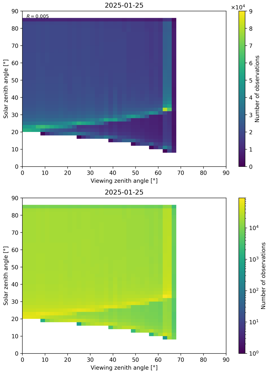
Figure 197: Scatter density plot of “Viewing zenith angle” against “Solar zenith angle” for 2025-01-24 to 2025-01-26.
