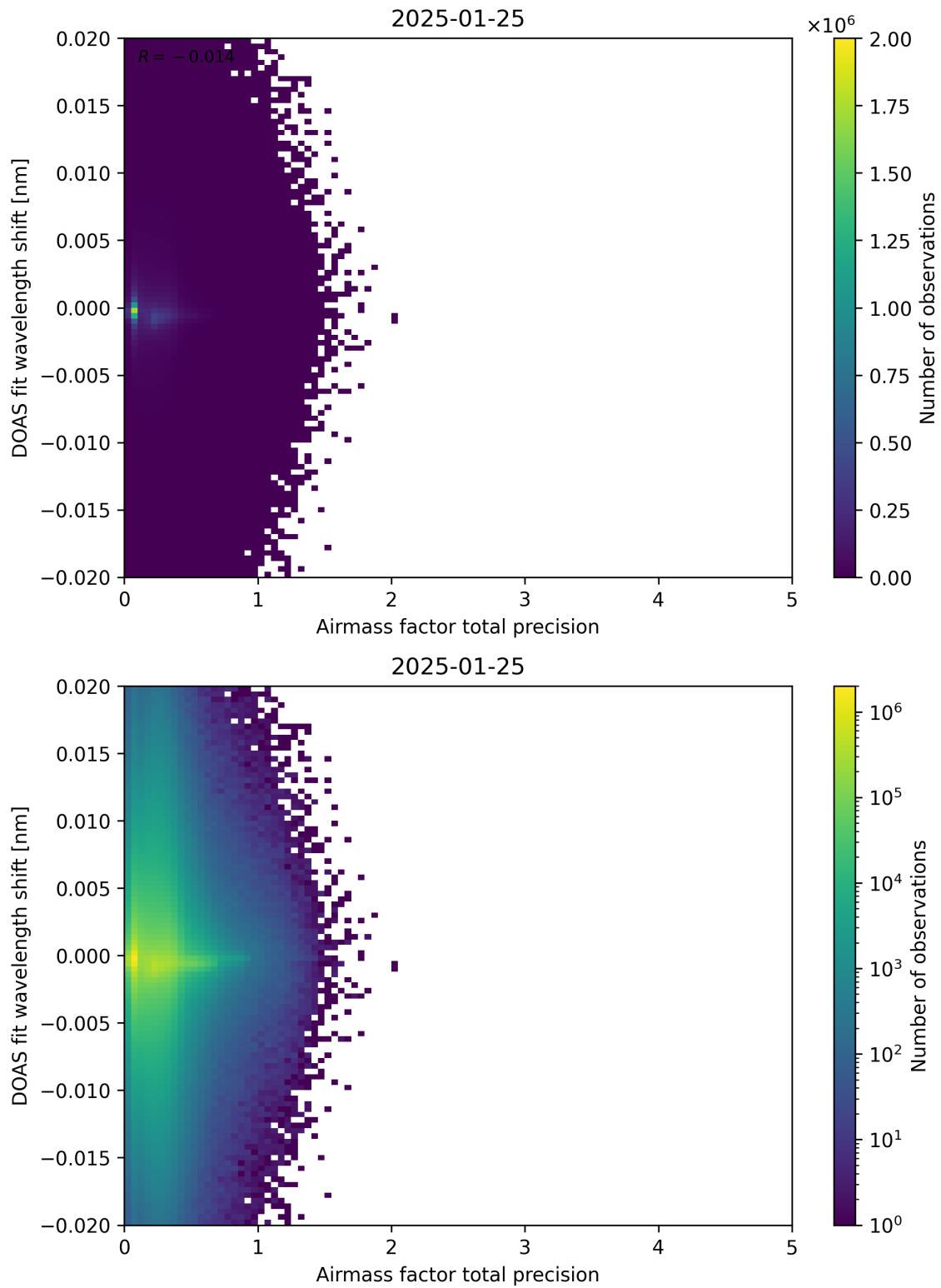
Figure 106: Scatter density plot of “Airmass factor total precision” against “DOAS fit wavelength shift” for 2025-01-24 to 2025-01-26.
