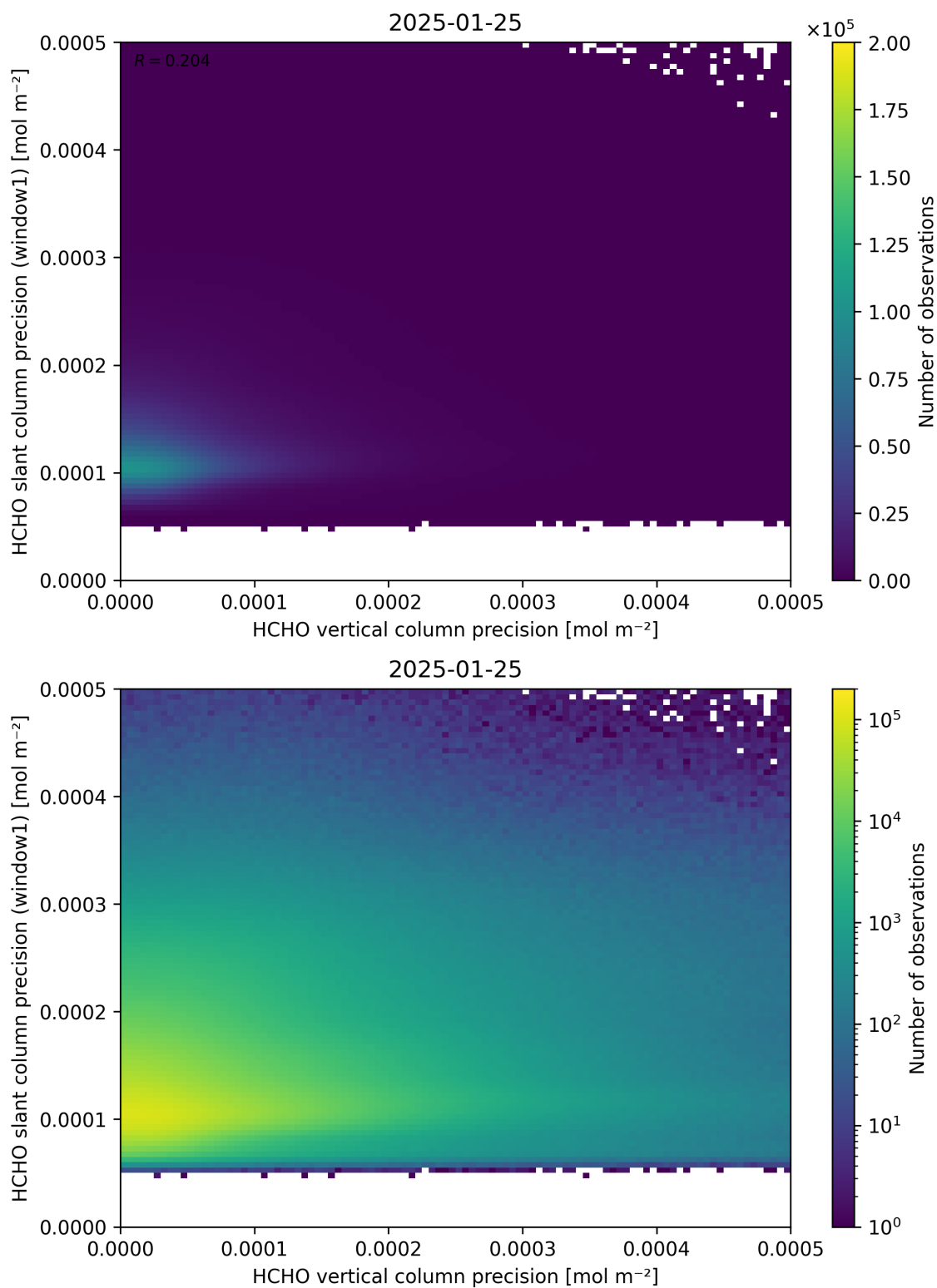
Figure 143: Scatter density plot of “HCHO vertical column precision” against “HCHO slant column precision (window1)” for 2025-01-24 to 2025-01-26.
