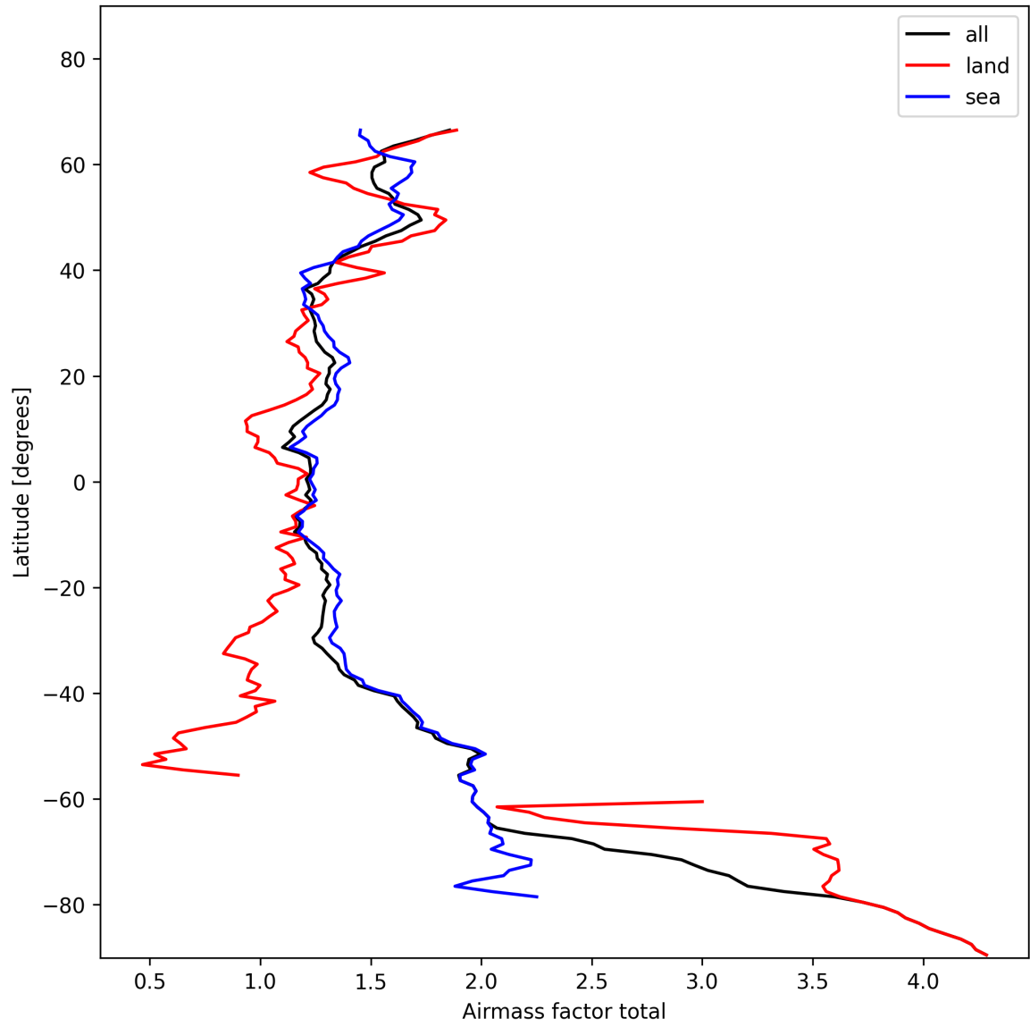
Figure 26: Zonal average of “Airmass factor total” for 2025-01-25 to 2025-01-27.
