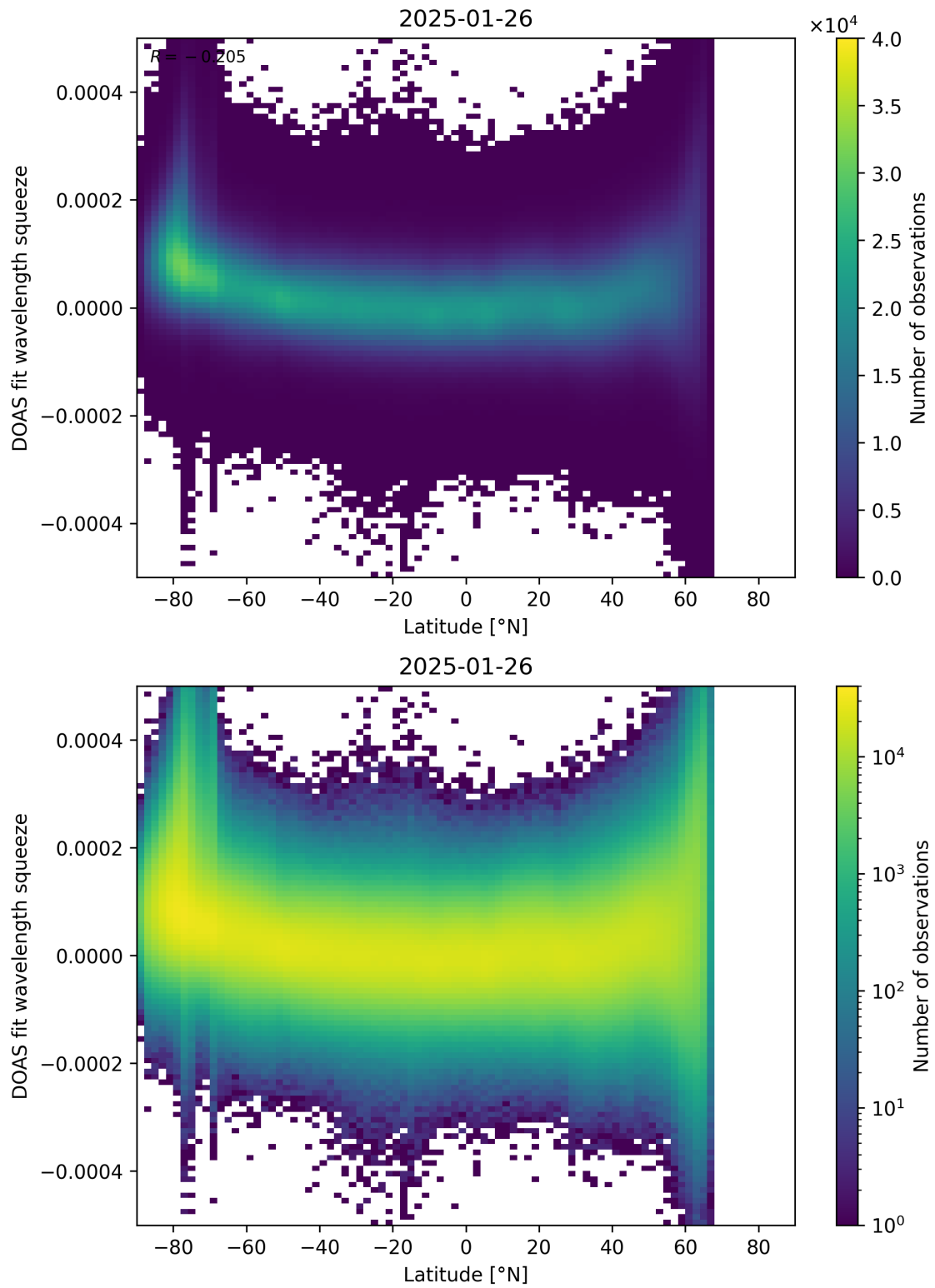
Figure 155: Scatter density plot of “Latitude” against “DOAS fit wavelength squeeze” for 2025-01-25 to 2025-01-27.
