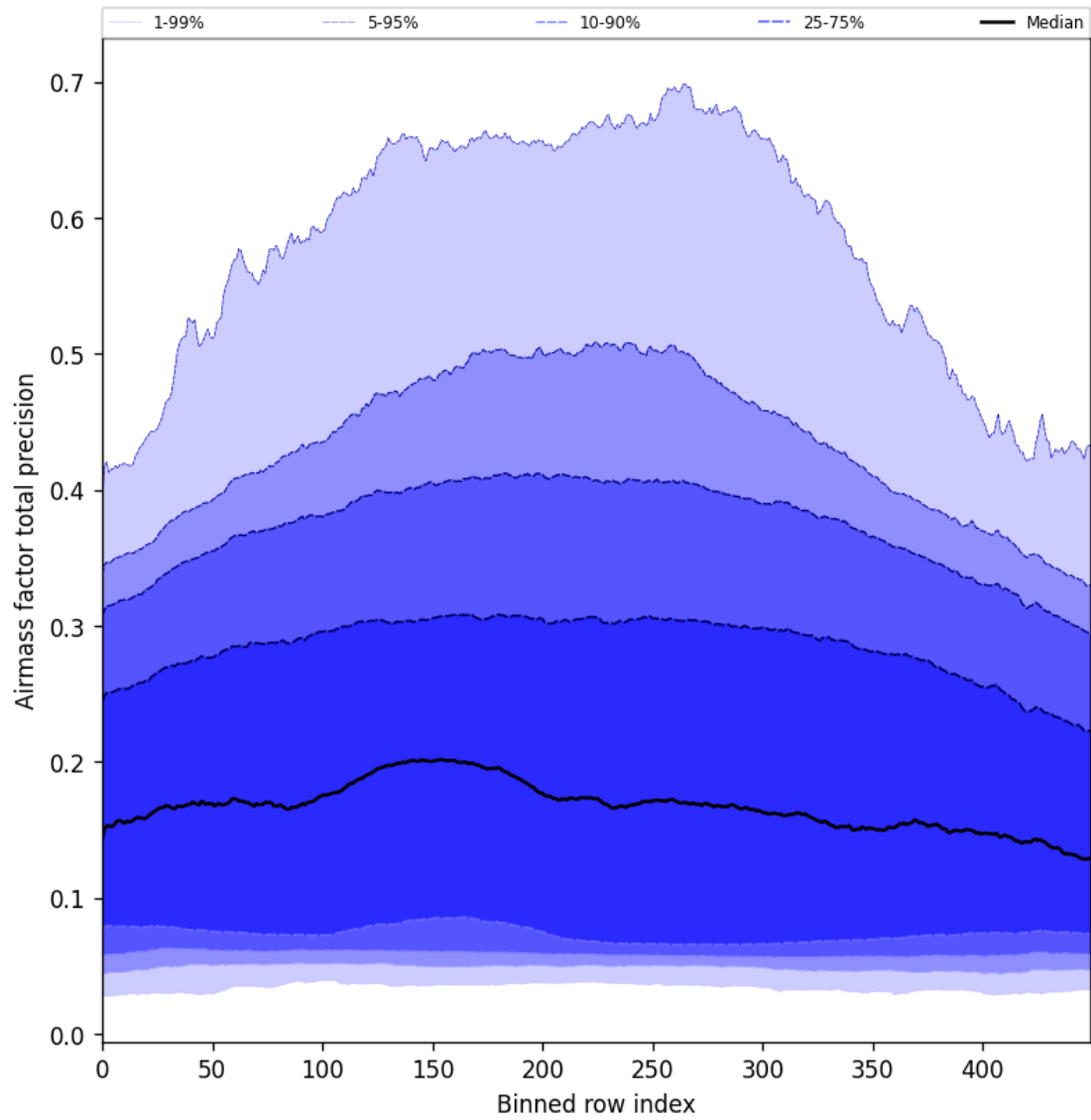
Figure 55: Along track statistics of “Airmass factor total precision” for 2025-01-25 to 2025-01-27
