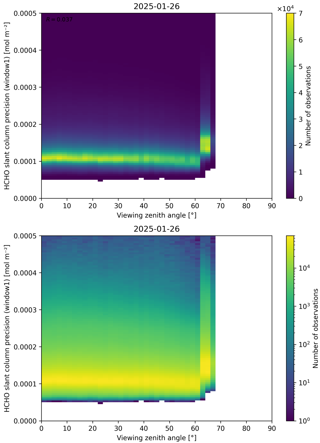
Figure 189: Scatter density plot of “Viewing zenith angle” against “HCHO slant column precision (window1)” for 2025-01-25 to 2025-01-27.
