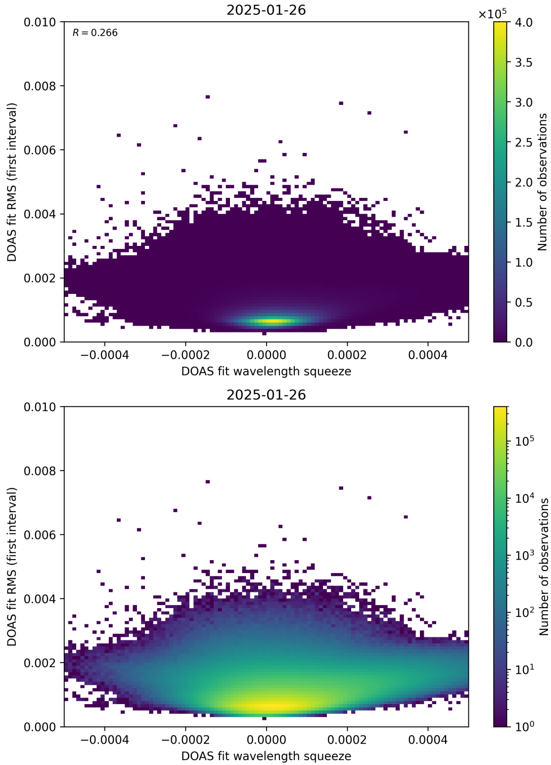
Figure 68: Scatter density plot of “DOAS fit wavelength squeeze” against “DOAS fit RMS (first interval)” for 2025-01-25 to 2025-01-27.
