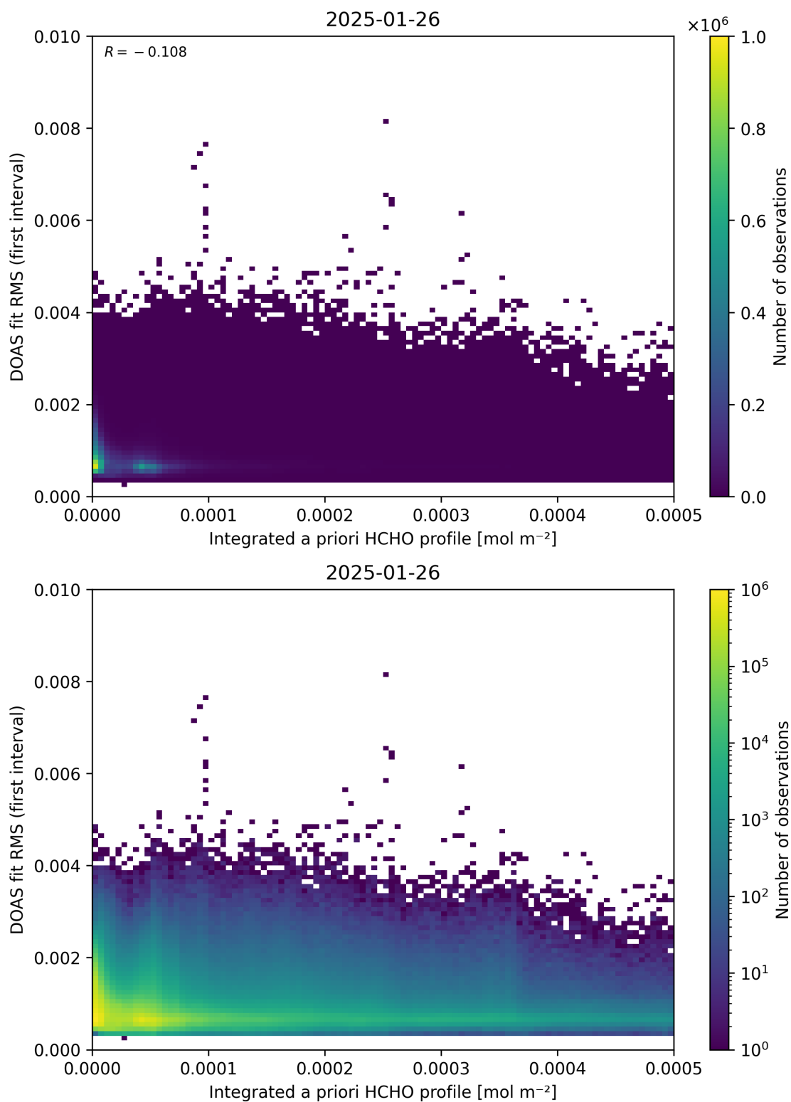
Figure 148: Scatter density plot of “Integrated a priori HCHO profile” against “DOAS fit RMS (first interval)” for 2025-01-25 to 2025-01-27.
