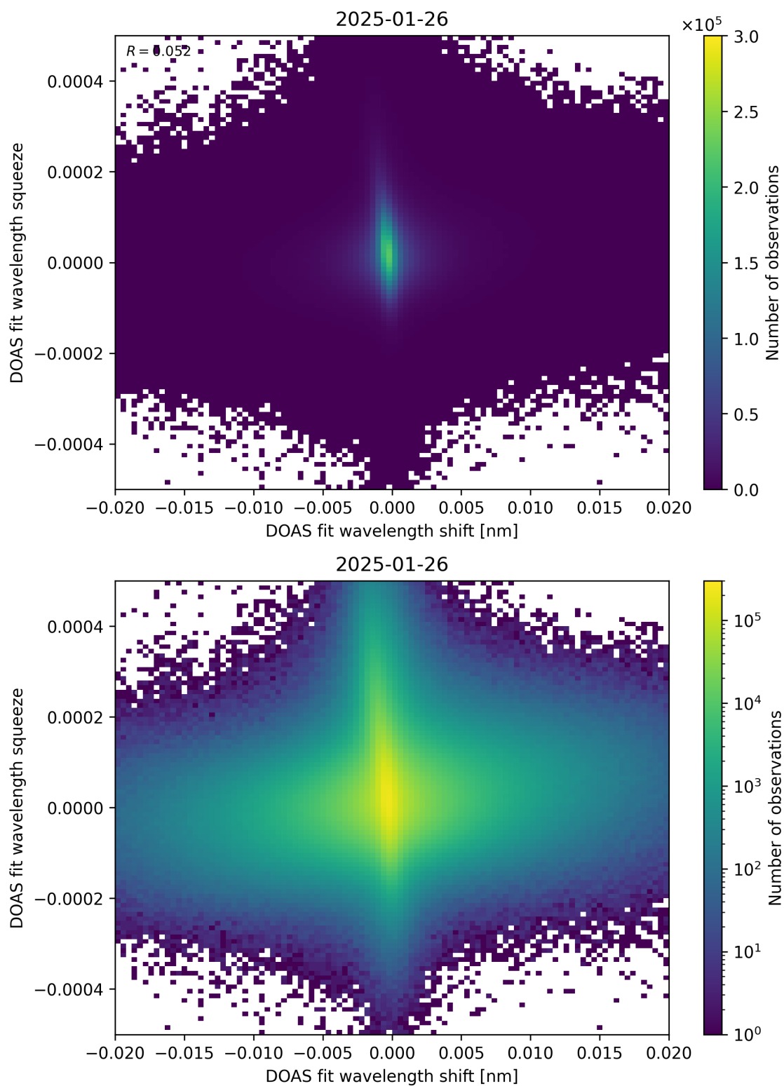
Figure 65: Scatter density plot of “DOAS fit wavelength shift” against “DOAS fit wavelength squeeze” for 2025-01-25 to 2025-01-27.
