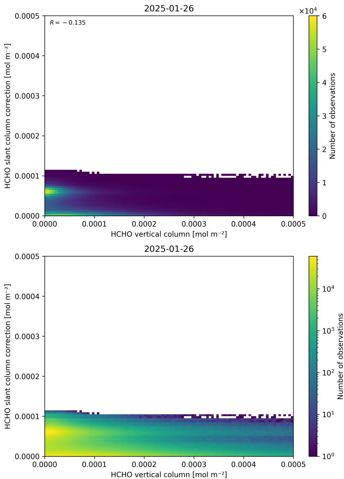
Figure 128: Scatter density plot of “HCHO vertical column” against “HCHO slant column correction” for 2025-01-25 to 2025-01-27.
