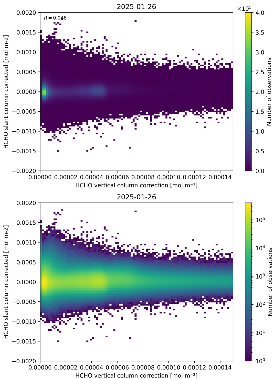
Figure 116: Scatter density plot of “HCHO vertical column correction” against “HCHO slant column corrected” for 2025-01-25 to 2025-01-27.
