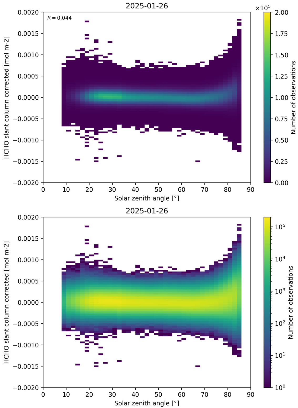
Figure 171: Scatter density plot of “Solar zenith angle” against “HCHO slant column corrected” for 2025-01-25 to 2025-01-27.
