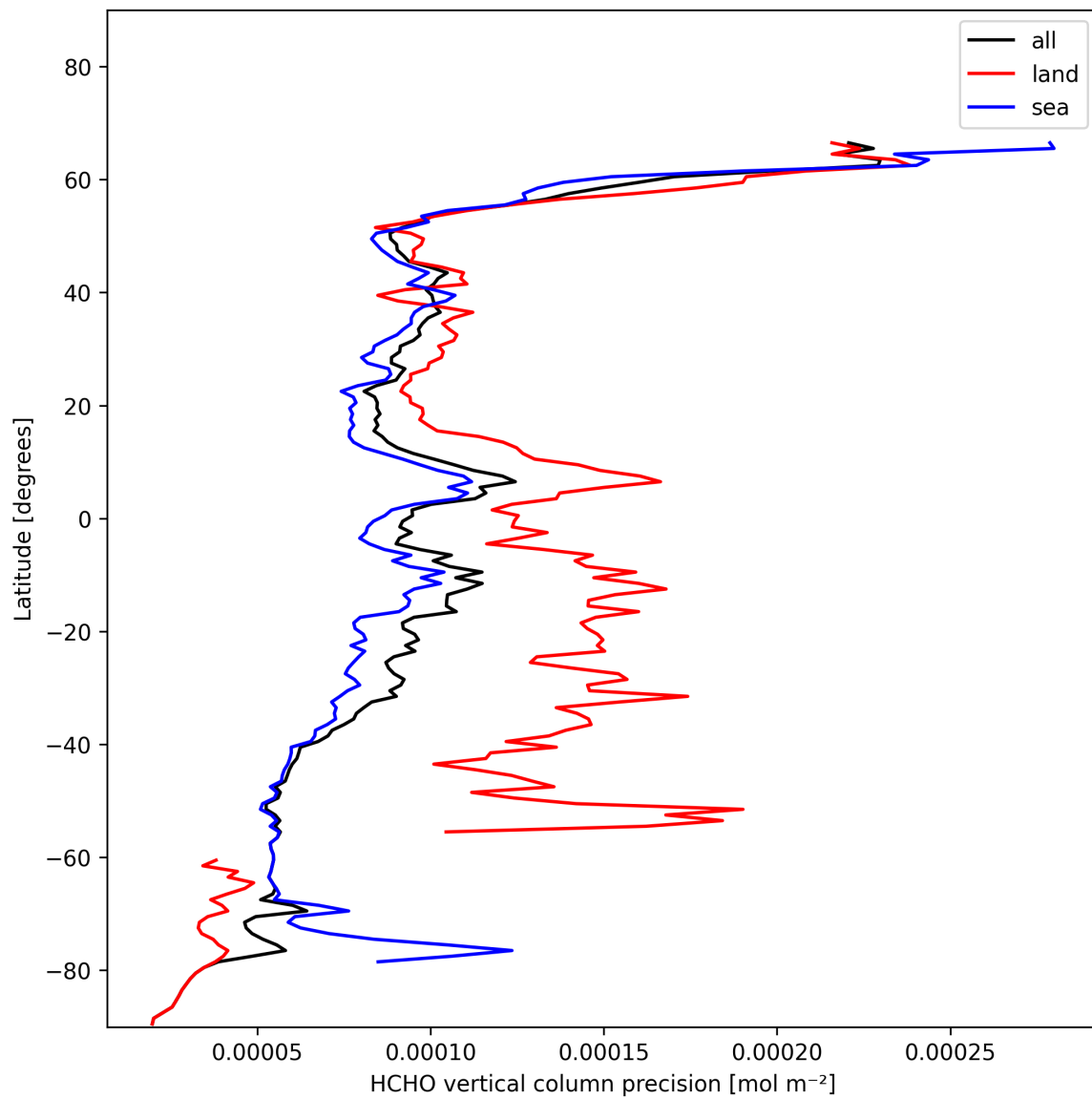
Figure 22: Zonal average of “HCHO vertical column precision” for 2025-01-25 to 2025-01-27.
