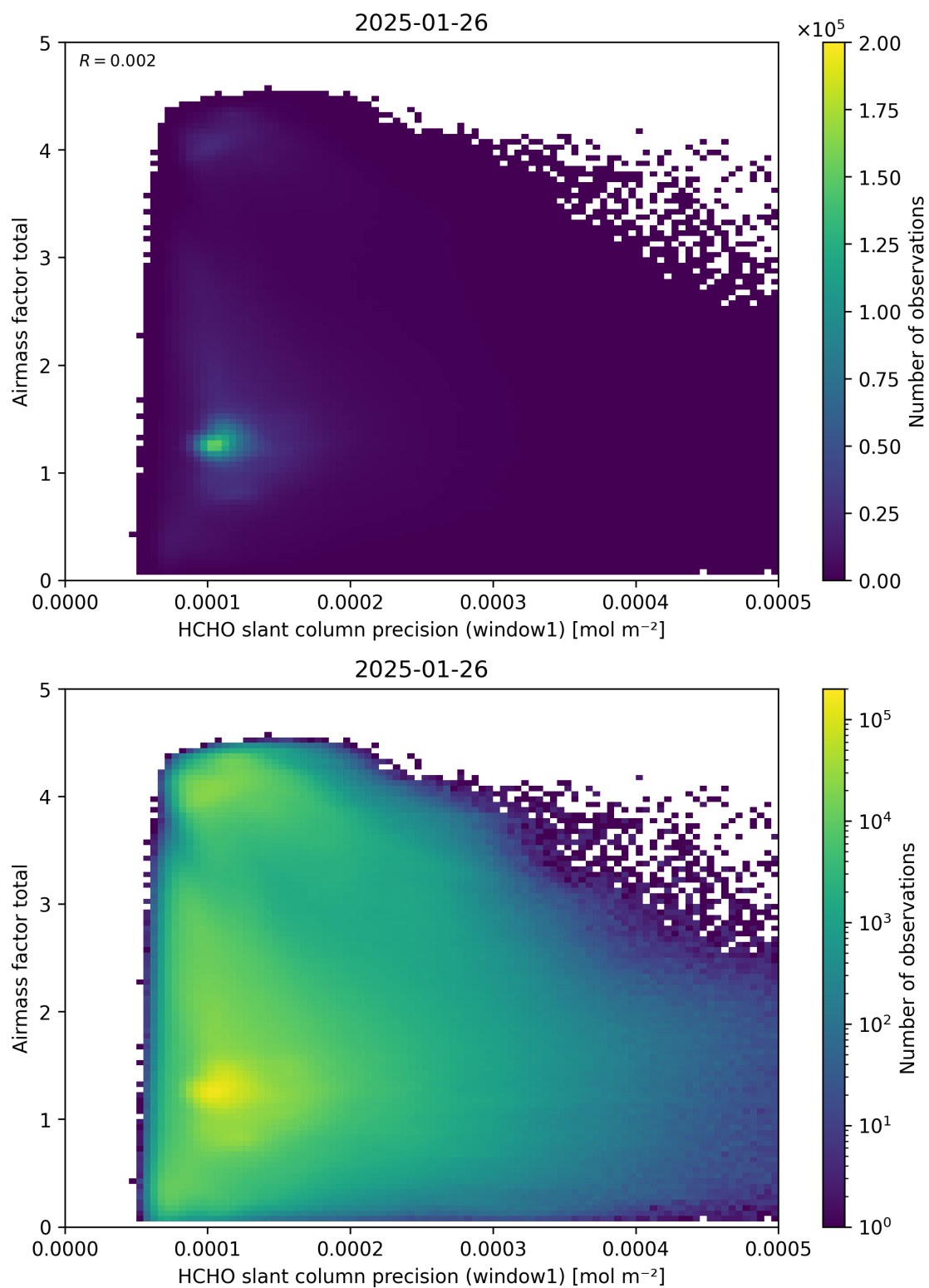
Figure 94: Scatter density plot of “HCHO slant column precision (window1)” against “Airmass factor total” for 2025-01-25 to 2025-01-27.
