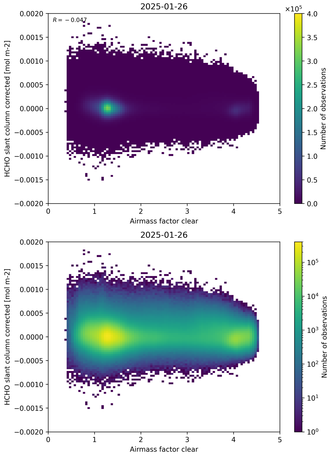
Figure 74: Scatter density plot of “Airmass factor clear” against “HCHO slant column corrected” for 2025-01-25 to 2025-01-27.
