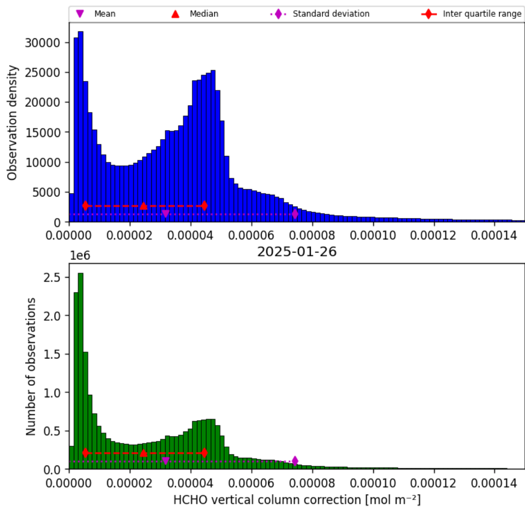
Figure 37: Histogram of “HCHO vertical column correction” for 2025-01-25 to 2025-01-27
