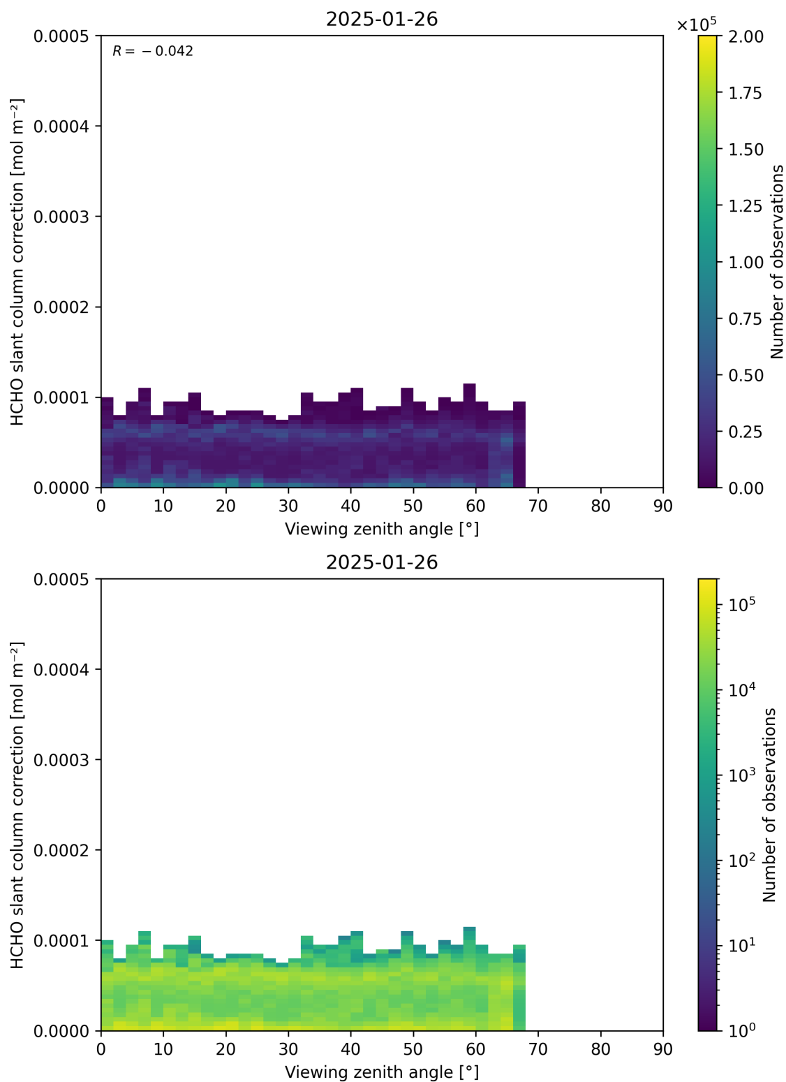
Figure 187: Scatter density plot of “Viewing zenith angle” against “HCHO slant column correction” for 2025-01-25 to 2025-01-27.
