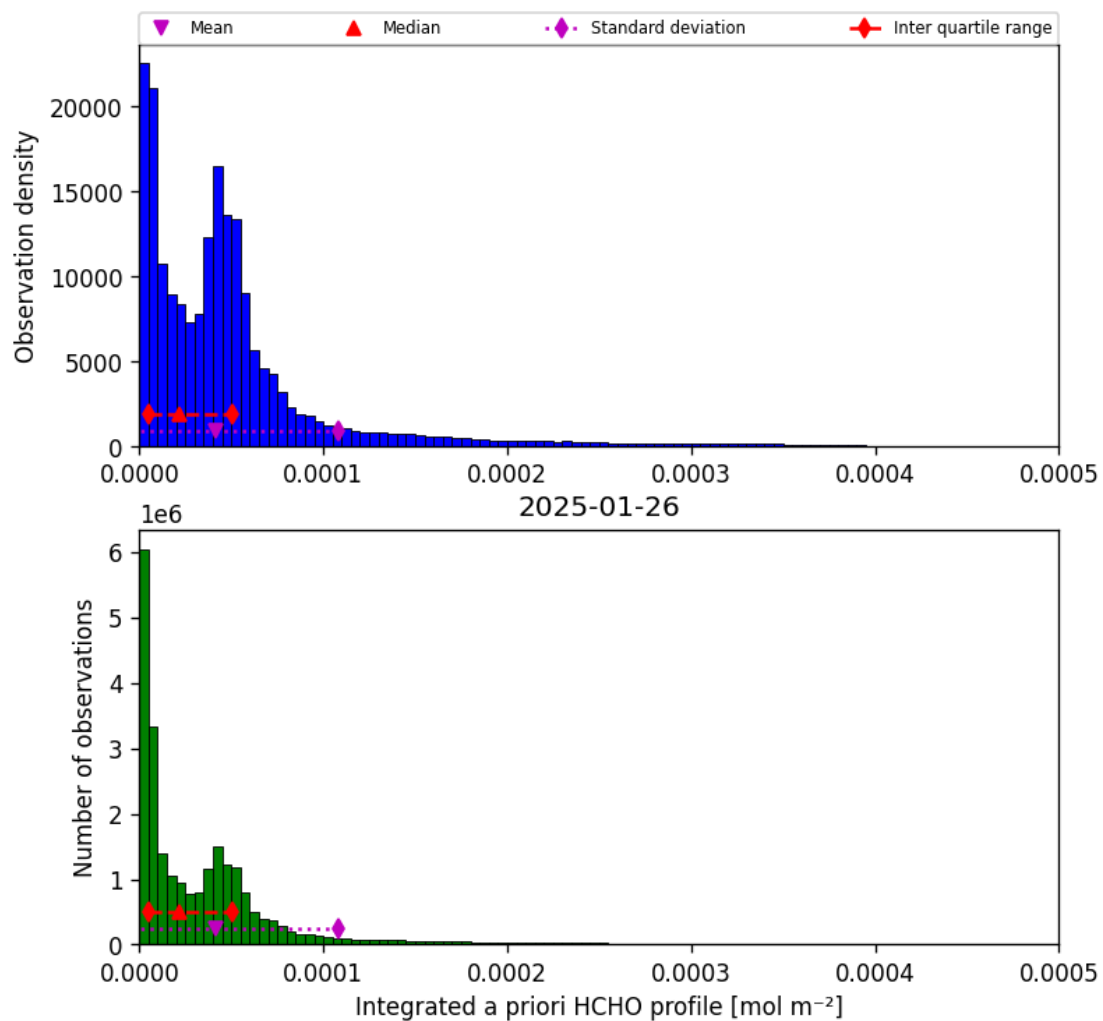
Figure 43: Histogram of “Integrated a priori HCHO profile” for 2025-01-25 to 2025-01-27
