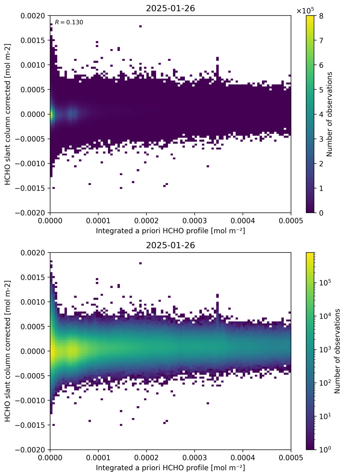
Figure 151: Scatter density plot of “Integrated a priori HCHO profile” against “HCHO slant column corrected” for 2025-01-25 to 2025-01-27.
