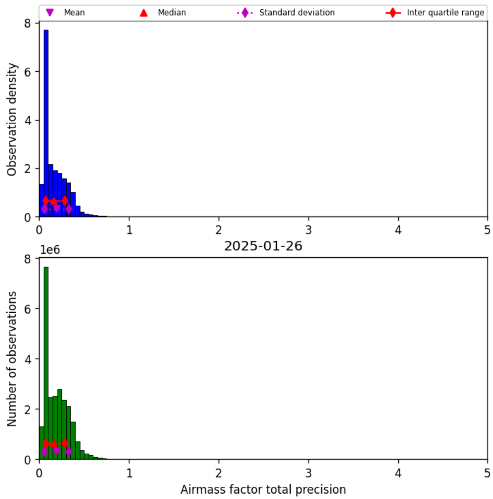
Figure 41: Histogram of “Airmass factor total precision” for 2025-01-25 to 2025-01-27
