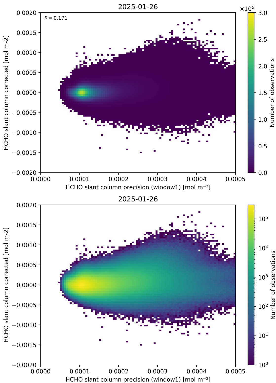
Figure 92: Scatter density plot of “HCHO slant column precision (window1)” against “HCHO slant column corrected” for 2025-01-25 to 2025-01-27.
