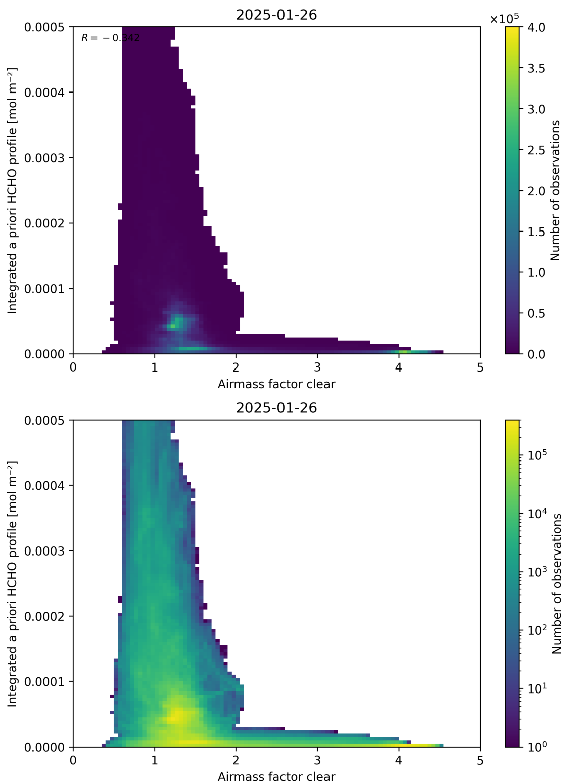
Figure 76: Scatter density plot of “Airmass factor clear” against “Integrated a priori HCHO profile” for 2025-01-25 to 2025-01-27.
