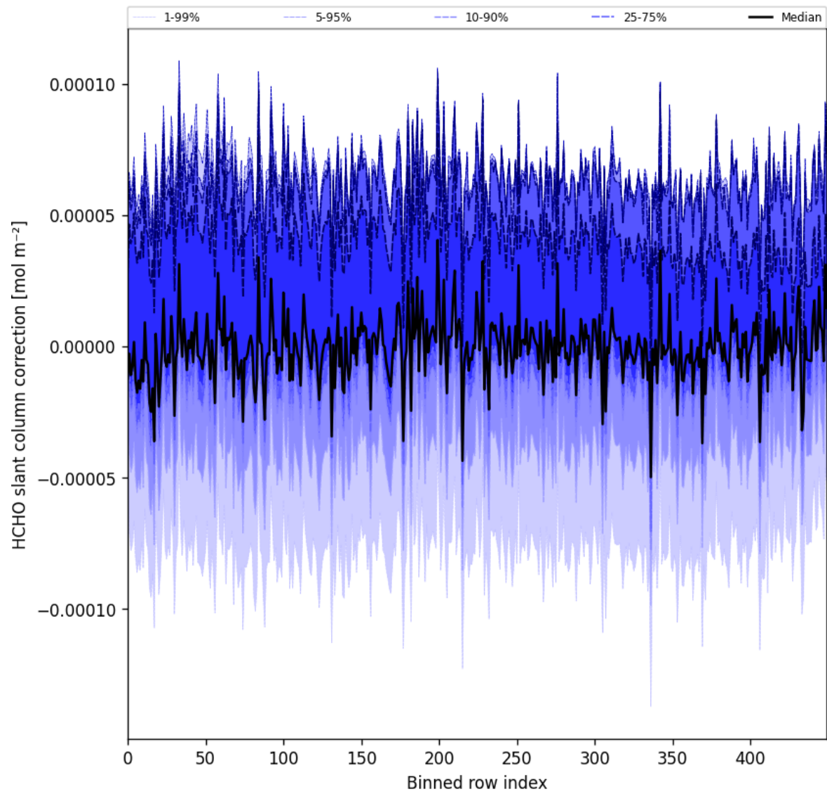
Figure 61: Along track statistics of “HCHO slant column correction” for 2025-01-25 to 2025-01-27
