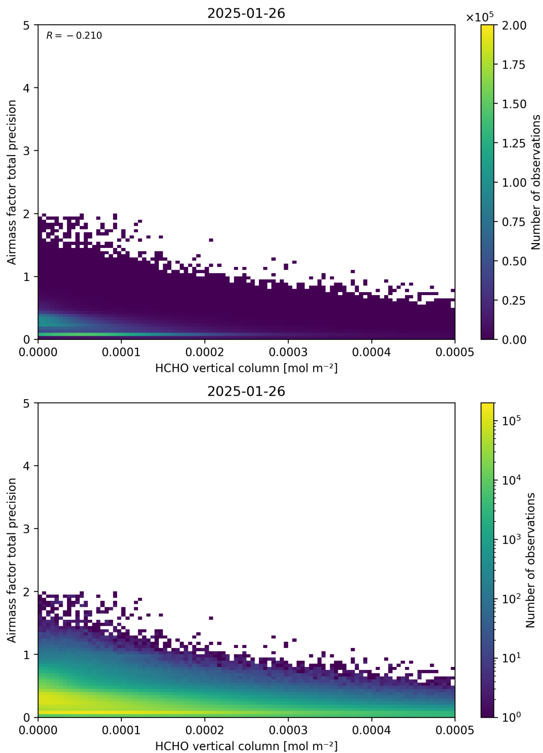
Figure 132: Scatter density plot of “HCHO vertical column” against “Airmass factor total precision” for 2025-01-25 to 2025-01-27.
