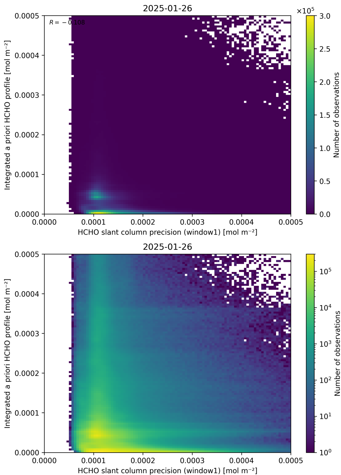
Figure 96: Scatter density plot of “HCHO slant column precision (window1)” against “Integrated a priori HCHO profile” for 2025-01-25 to 2025-01-27.
