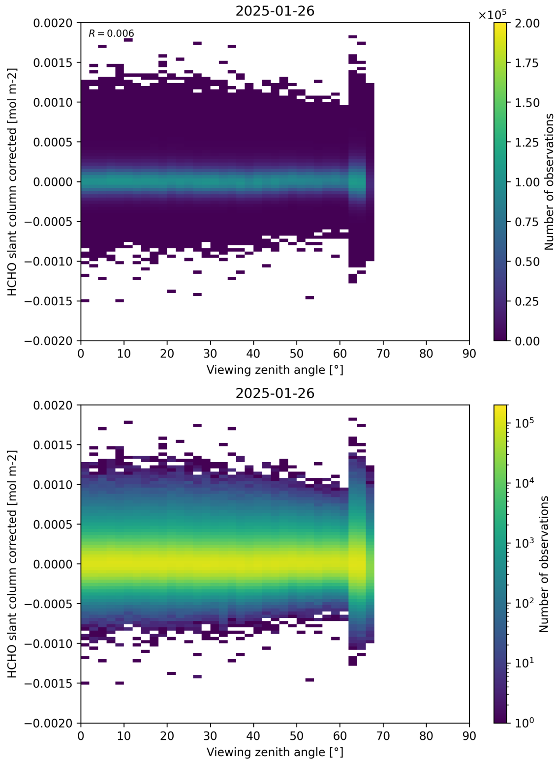
Figure 186: Scatter density plot of “Viewing zenith angle” against “HCHO slant column corrected” for 2025-01-25 to 2025-01-27.
