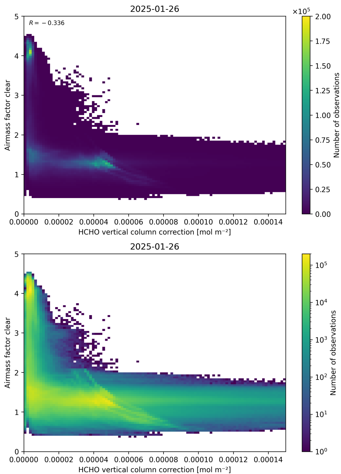
Figure 115: Scatter density plot of “HCHO vertical column correction” against “Airmass factor clear” for 2025-01-25 to 2025-01-27.
