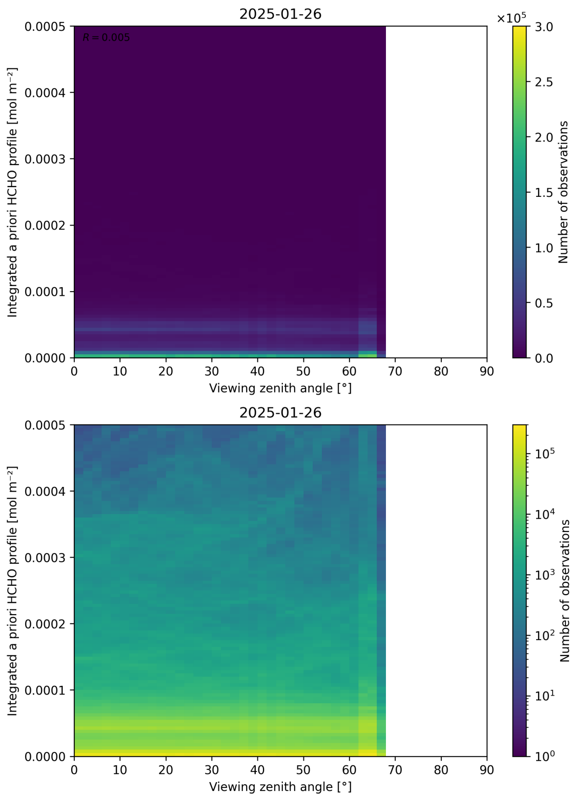
Figure 195: Scatter density plot of “Viewing zenith angle” against “Integrated a priori HCHO profile” for 2025-01-25 to 2025-01-27.
