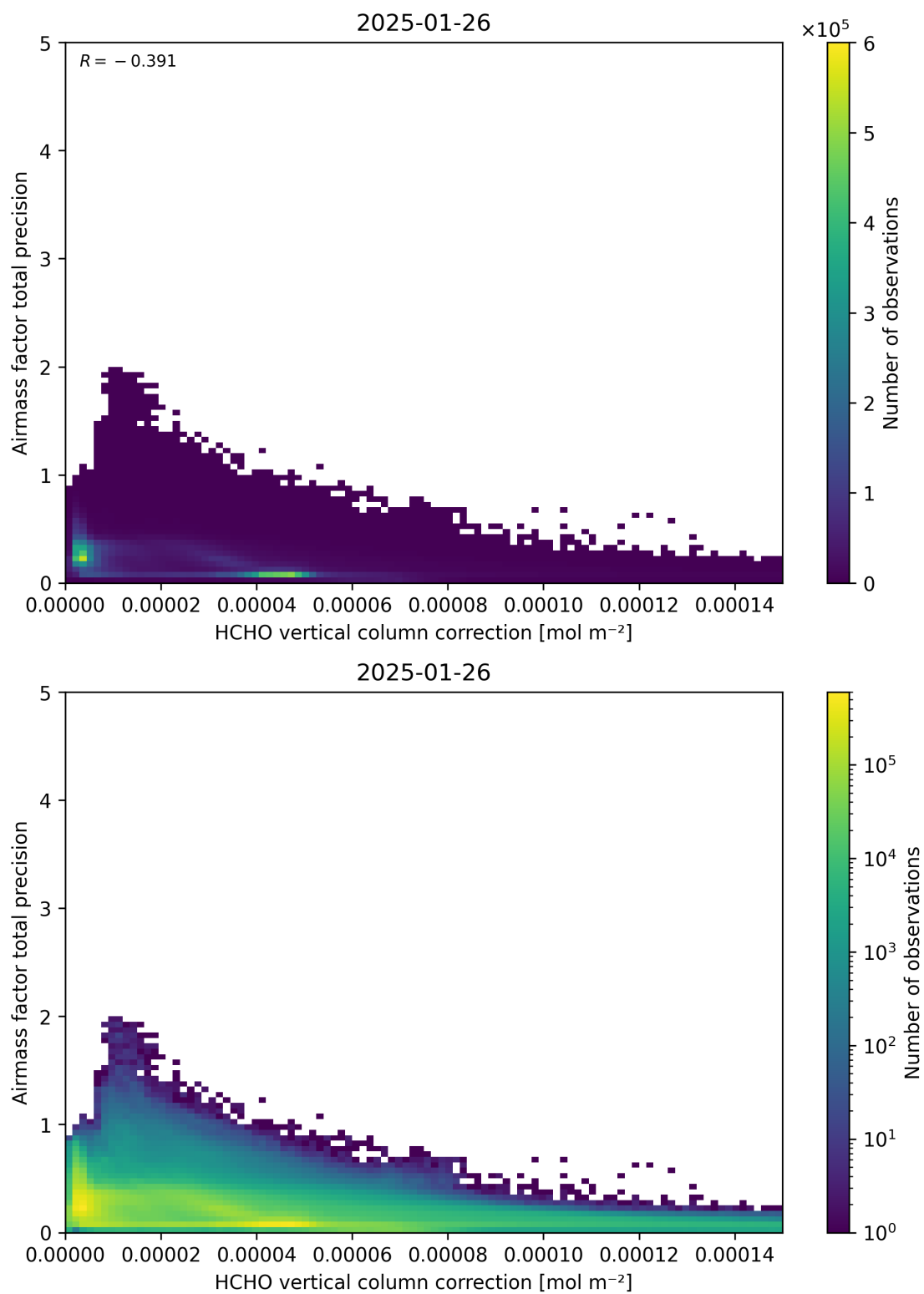
Figure 121: Scatter density plot of “HCHO vertical column correction” against “Airmass factor total precision” for 2025-01-25 to 2025-01-27.
