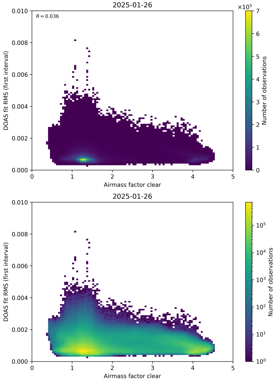
Figure 71: Scatter density plot of “Airmass factor clear” against “DOAS fit RMS (first interval)” for 2025-01-25 to 2025-01-27.
