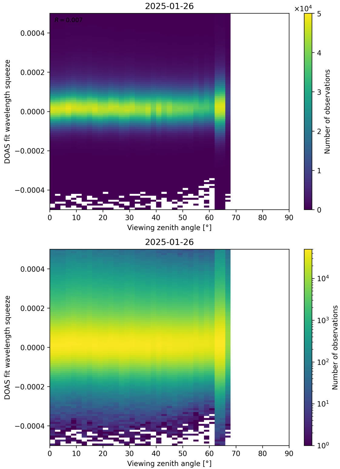
Figure 184: Scatter density plot of “Viewing zenith angle” against “DOAS fit wavelength squeeze” for 2025-01-25 to 2025-01-27.
