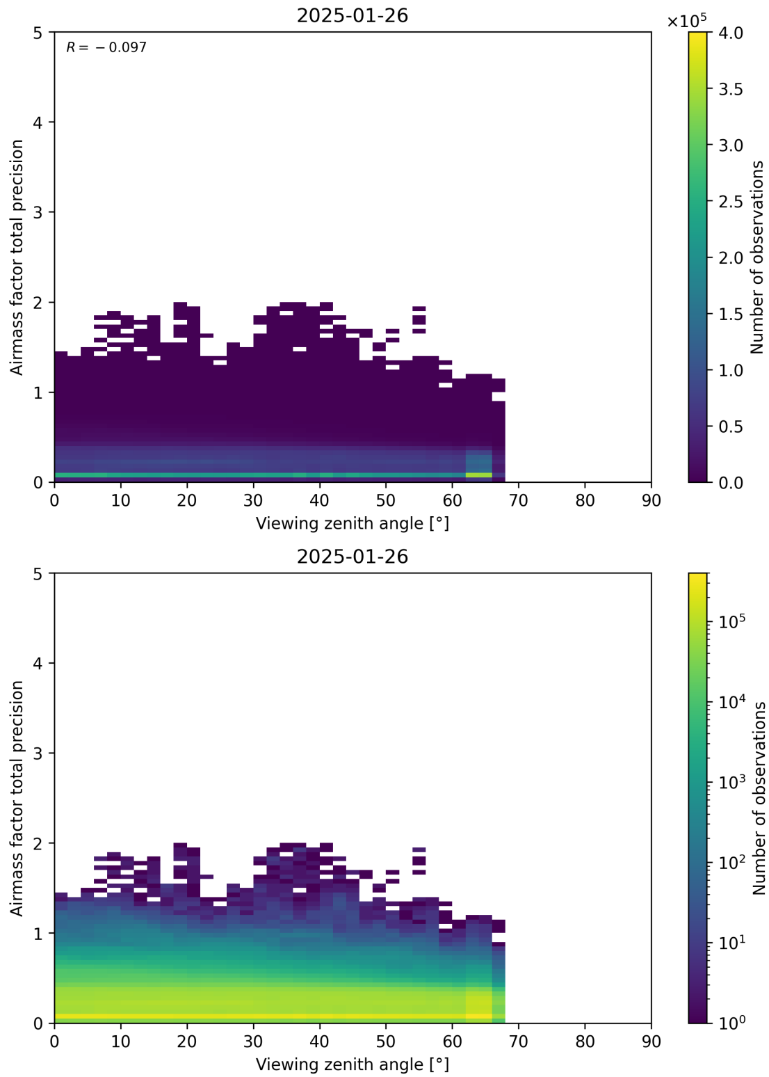
Figure 191: Scatter density plot of “Viewing zenith angle” against “Airmass factor total precision” for 2025-01-25 to 2025-01-27.
