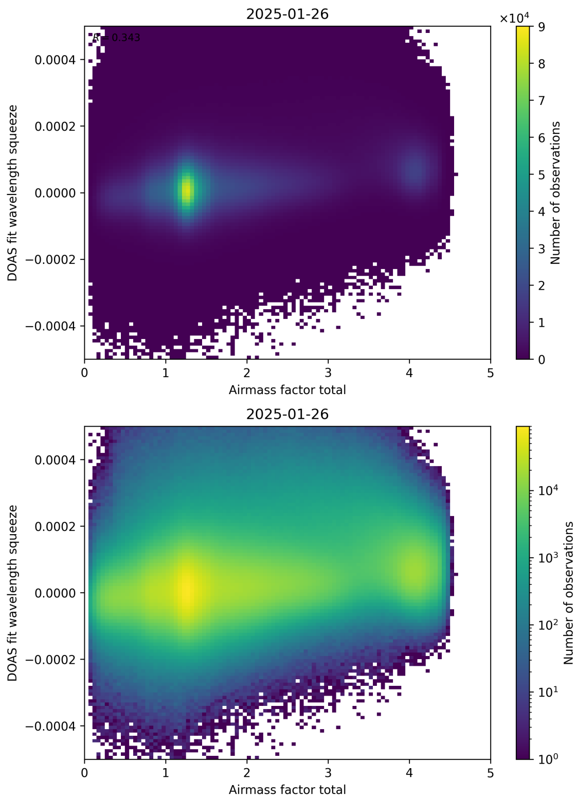
Figure 99: Scatter density plot of “Airmass factor total” against “DOAS fit wavelength squeeze” for 2025-01-25 to 2025-01-27.
