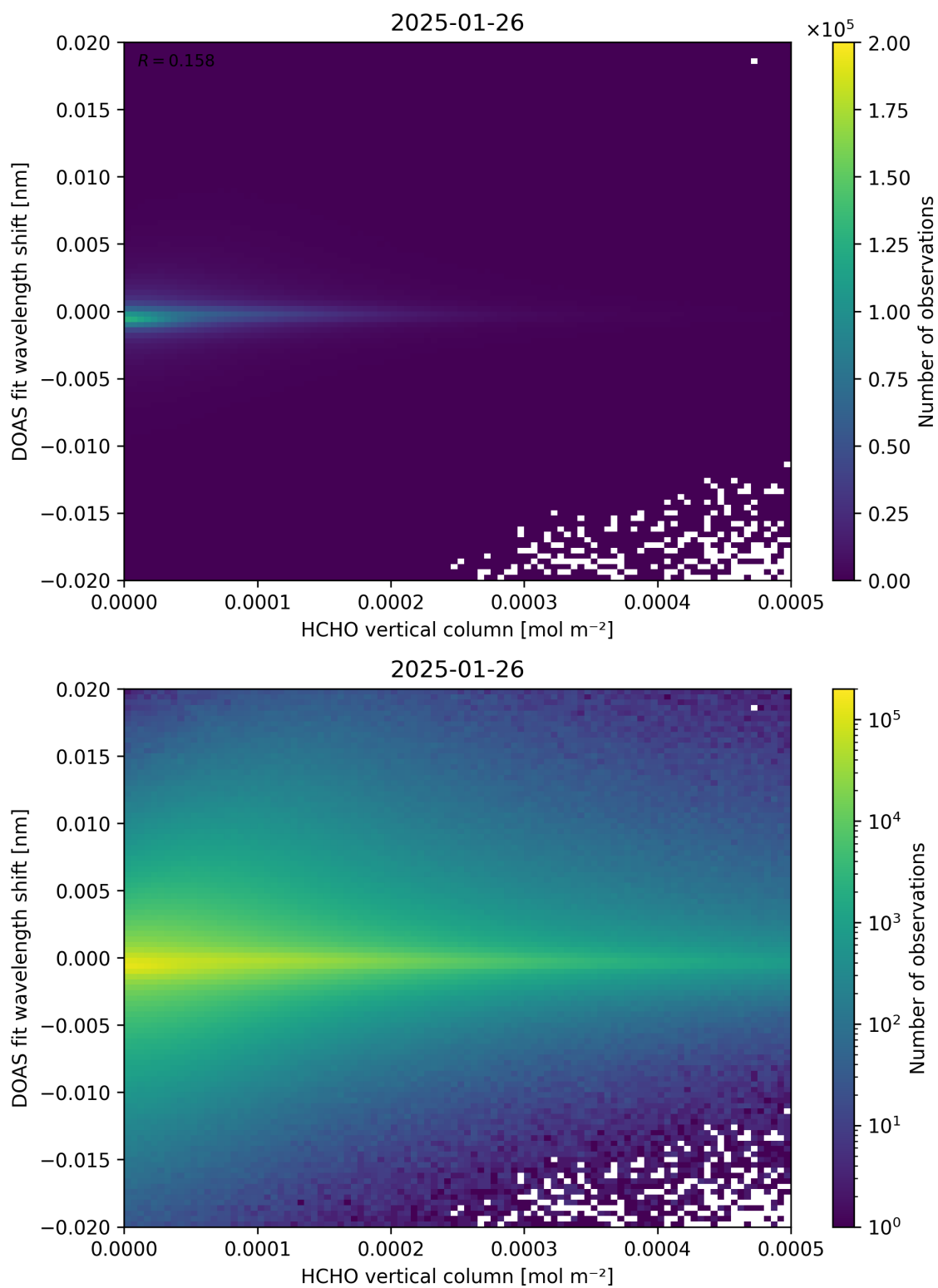
Figure 124: Scatter density plot of “HCHO vertical column” against “DOAS fit wavelength shift” for 2025-01-25 to 2025-01-27.
