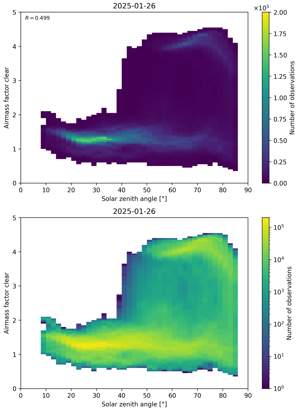
Figure 170: Scatter density plot of “Solar zenith angle” against “Airmass factor clear” for 2025-01-25 to 2025-01-27.
