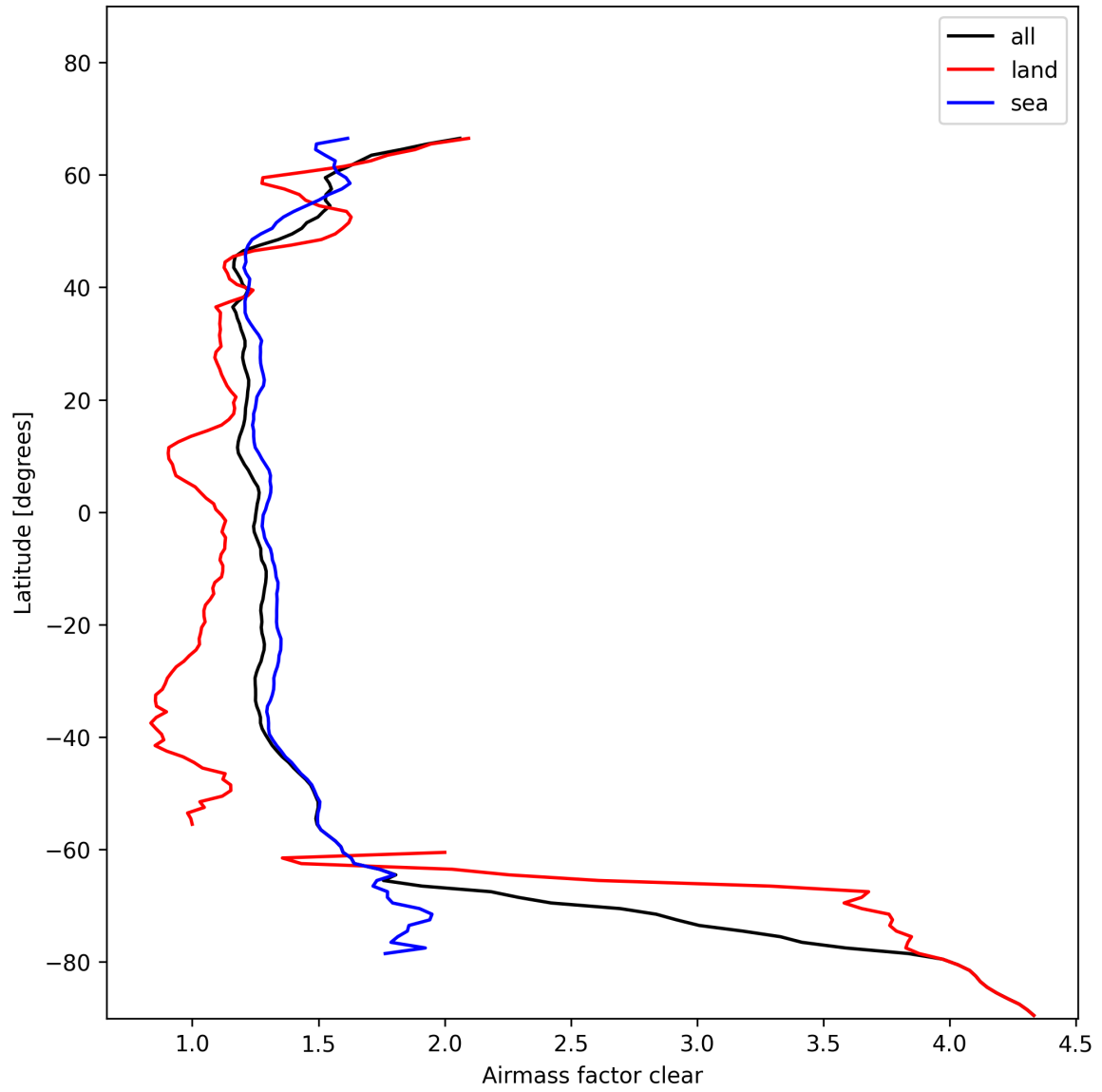
Figure 28: Zonal average of “Airmass factor clear” for 2025-01-25 to 2025-01-27.
