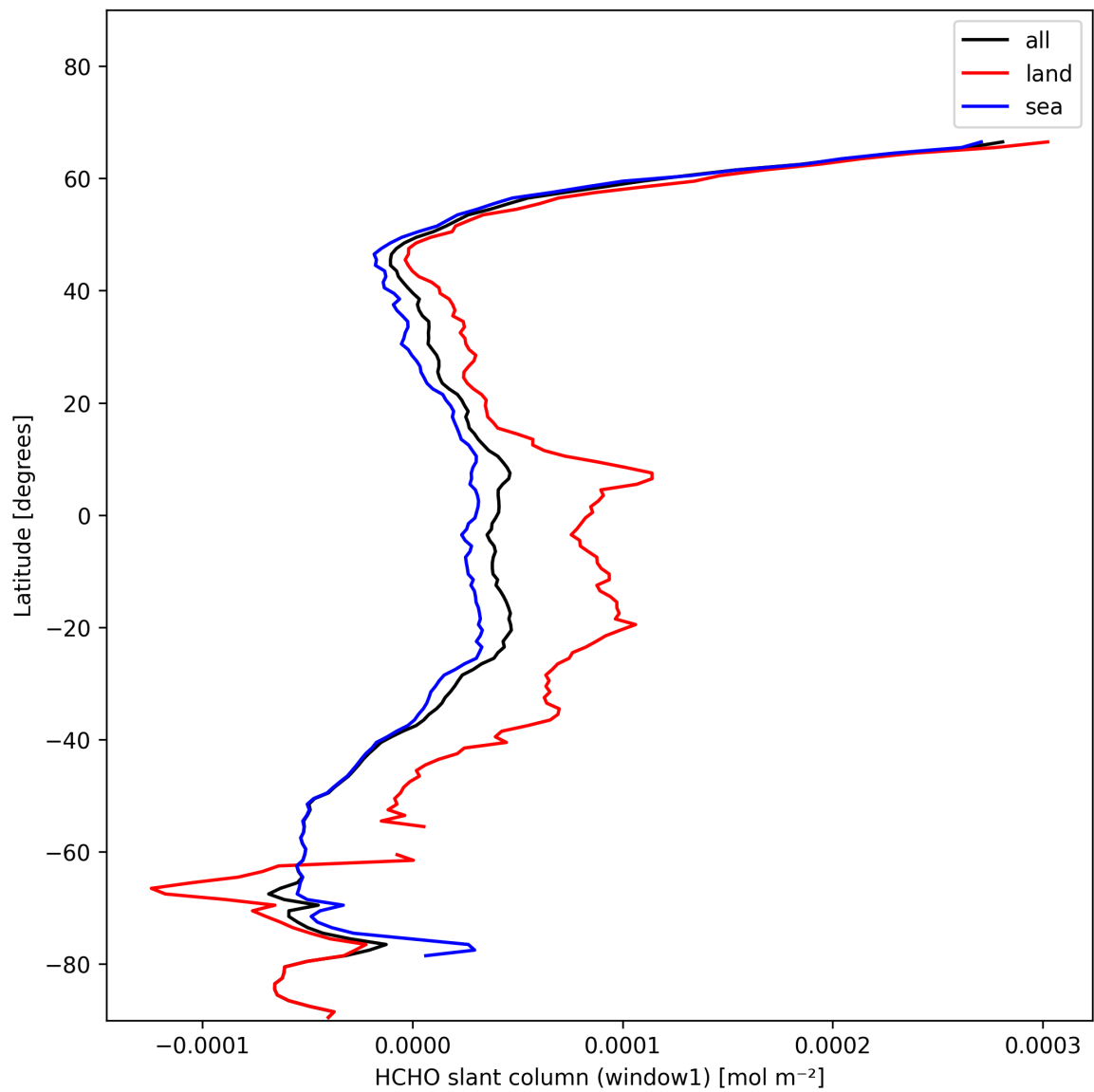
Figure 24: Zonal average of “HCHO slant column (window1)” for 2025-01-25 to 2025-01-27.
