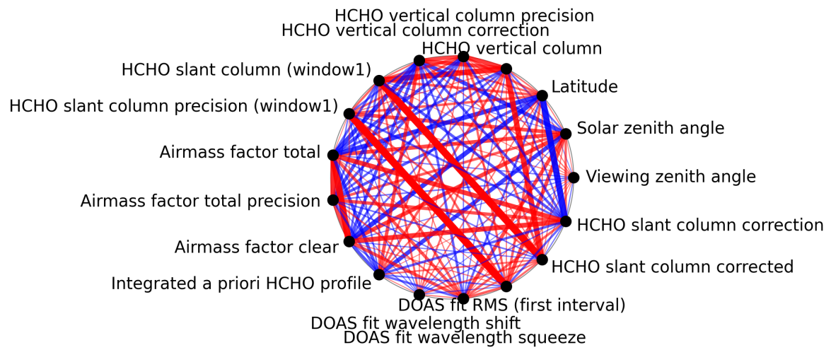
Figure 1: Map of correlation graph for 2025-01-25 to 2025-01-27.
