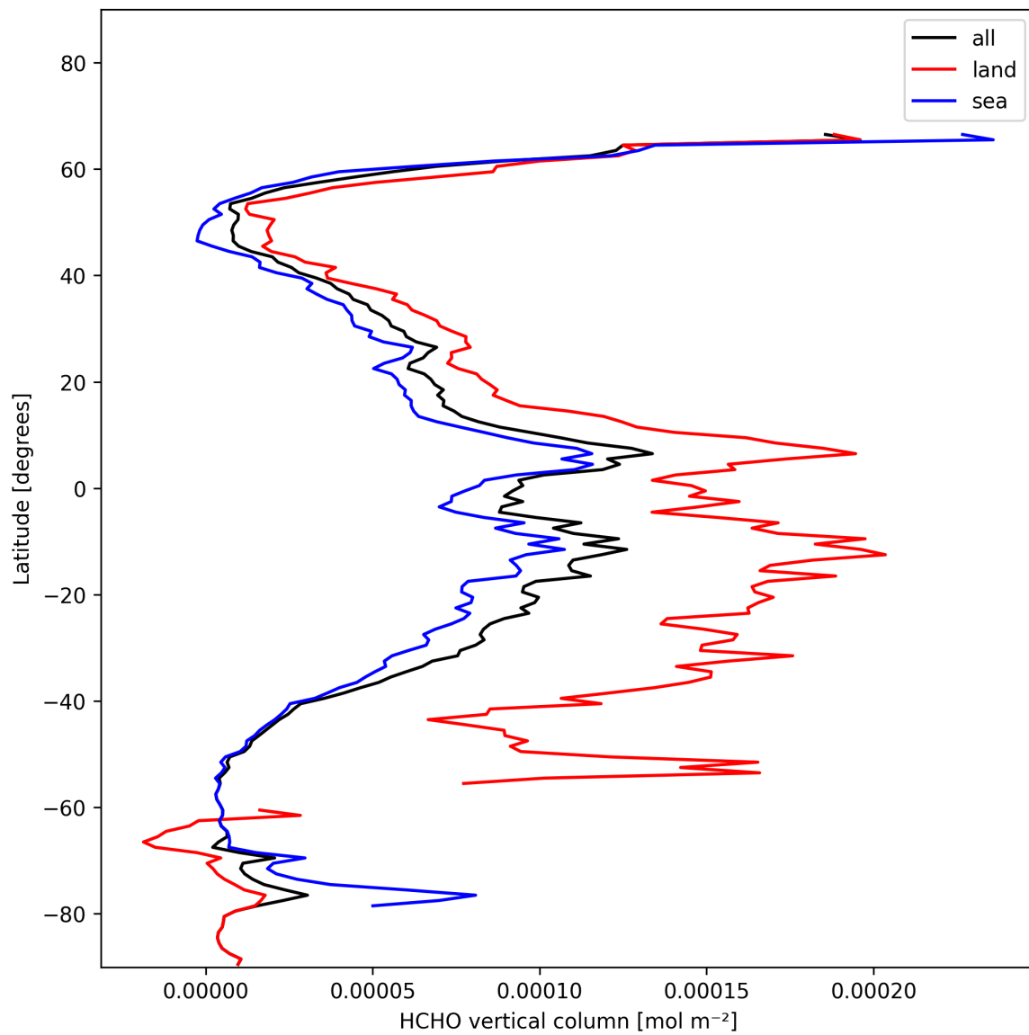
Figure 21: Zonal average of “HCHO vertical column” for 2025-01-25 to 2025-01-27.
