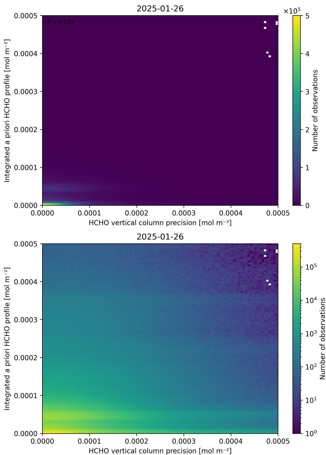
Figure 147: Scatter density plot of “HCHO vertical column precision” against “Integrated a priori HCHO profile” for 2025-01-25 to 2025-01-27.
