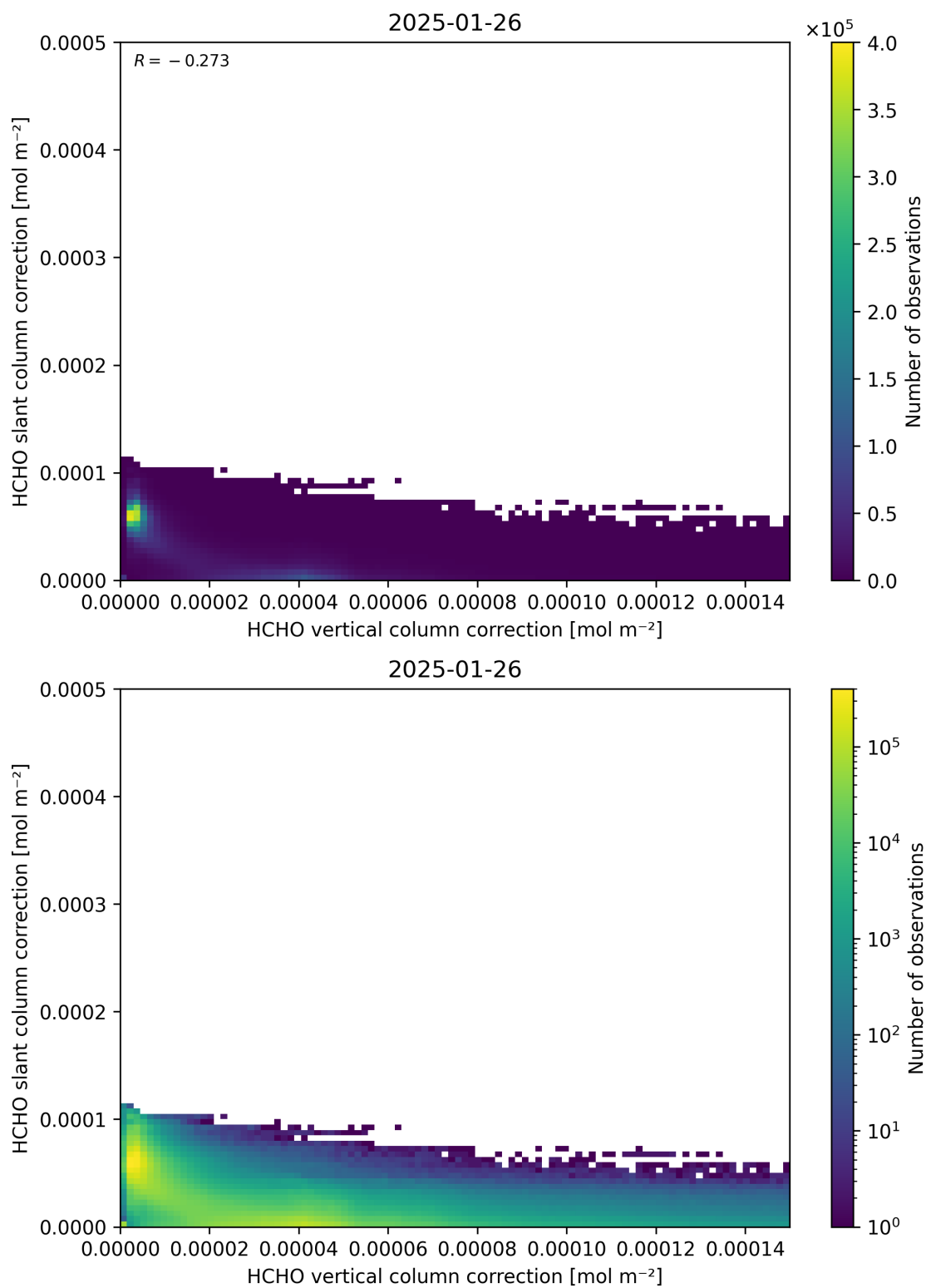
Figure 117: Scatter density plot of “HCHO vertical column correction” against “HCHO slant column correction” for 2025-01-25 to 2025-01-27.
