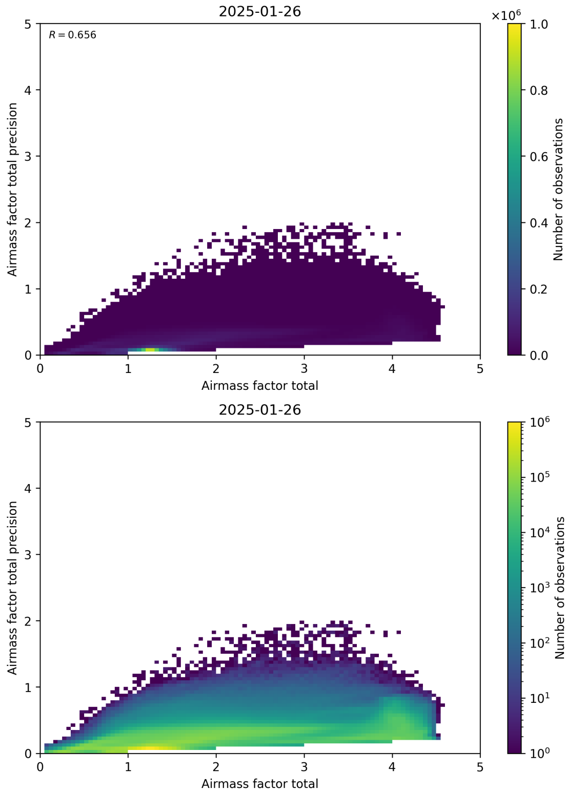
Figure 103: Scatter density plot of “Airmass factor total” against “Airmass factor total precision” for 2025-01-25 to 2025-01-27.
