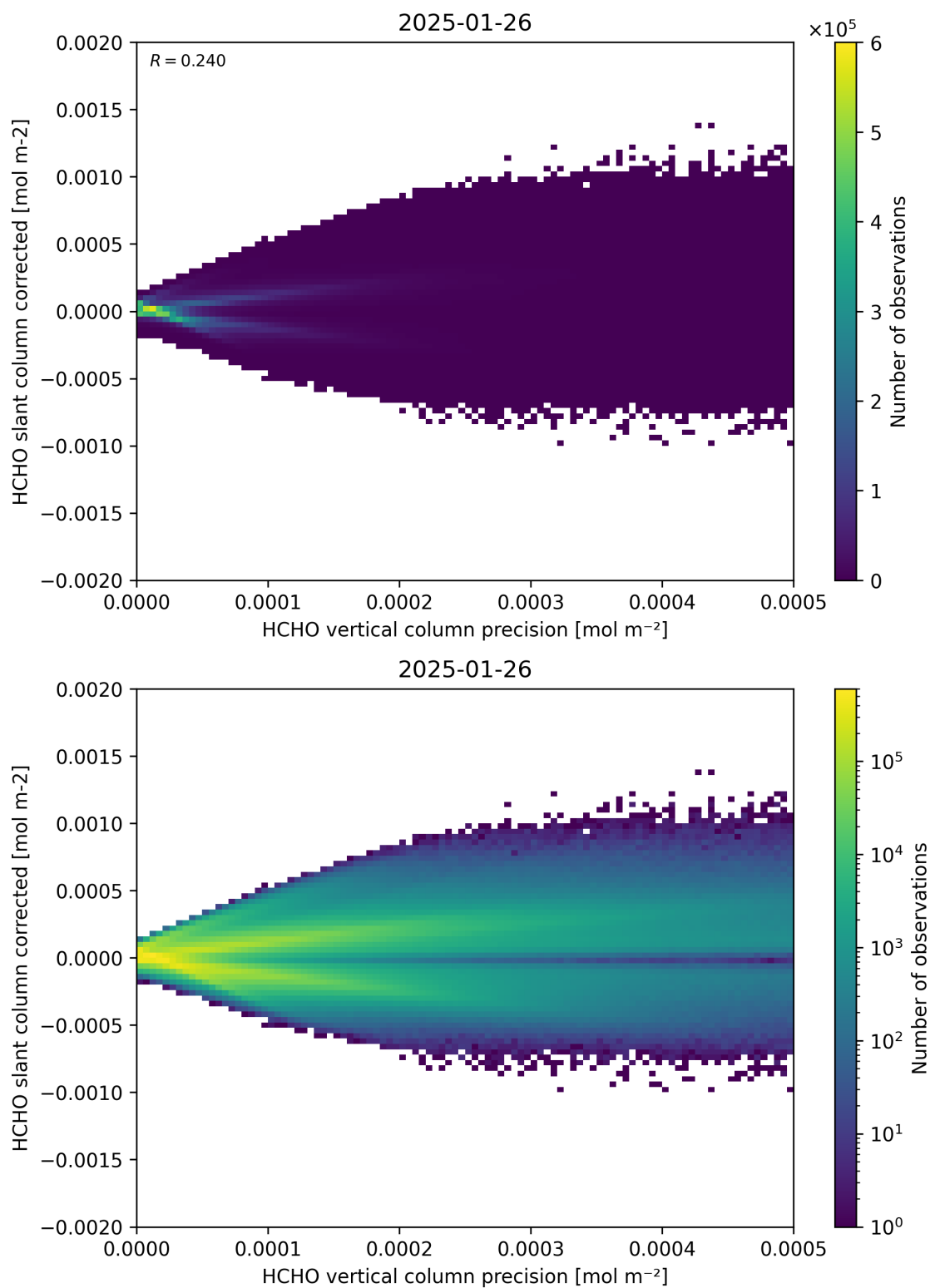
Figure 140: Scatter density plot of “HCHO vertical column precision” against “HCHO slant column corrected” for 2025-01-25 to 2025-01-27.
