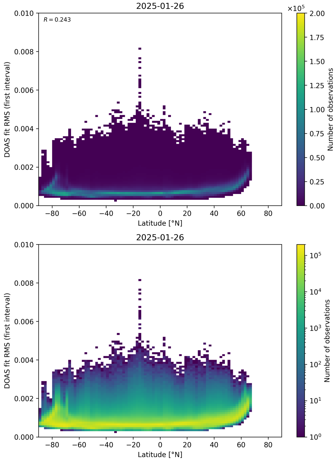
Figure 153: Scatter density plot of “Latitude” against “DOAS fit RMS (first interval)” for 2025-01-25 to 2025-01-27.
