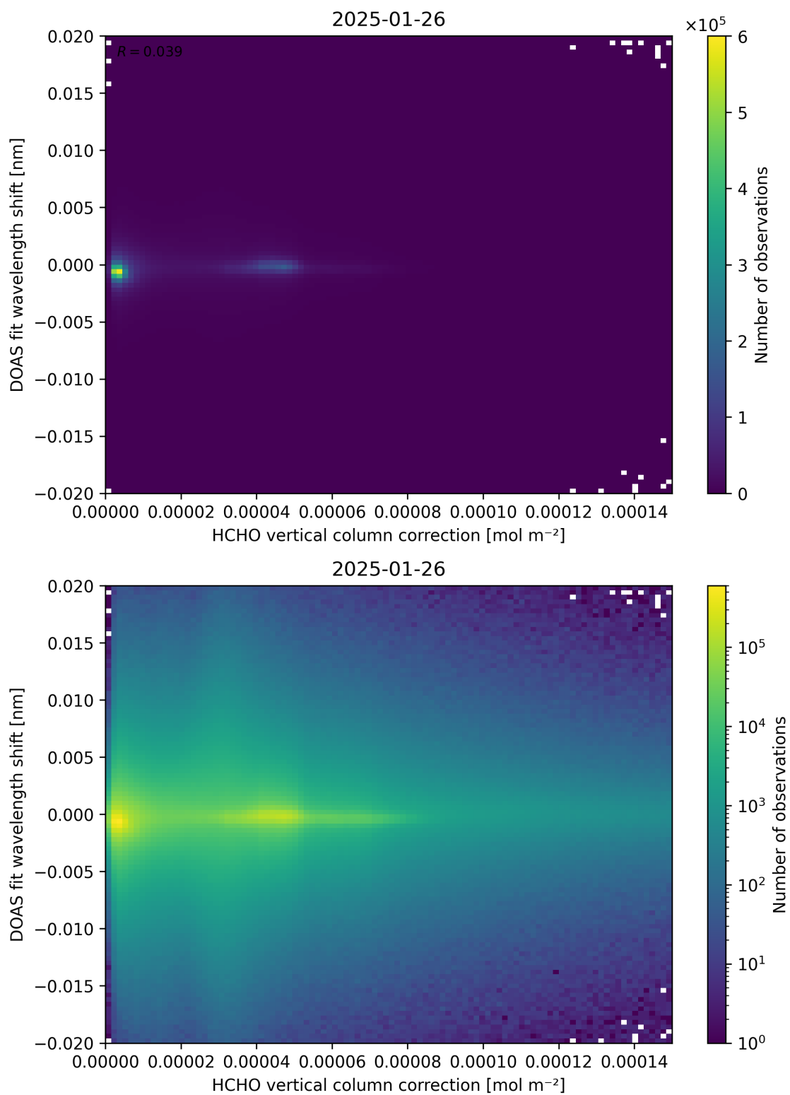
Figure 113: Scatter density plot of “HCHO vertical column correction” against “DOAS fit wavelength shift” for 2025-01-25 to 2025-01-27.
