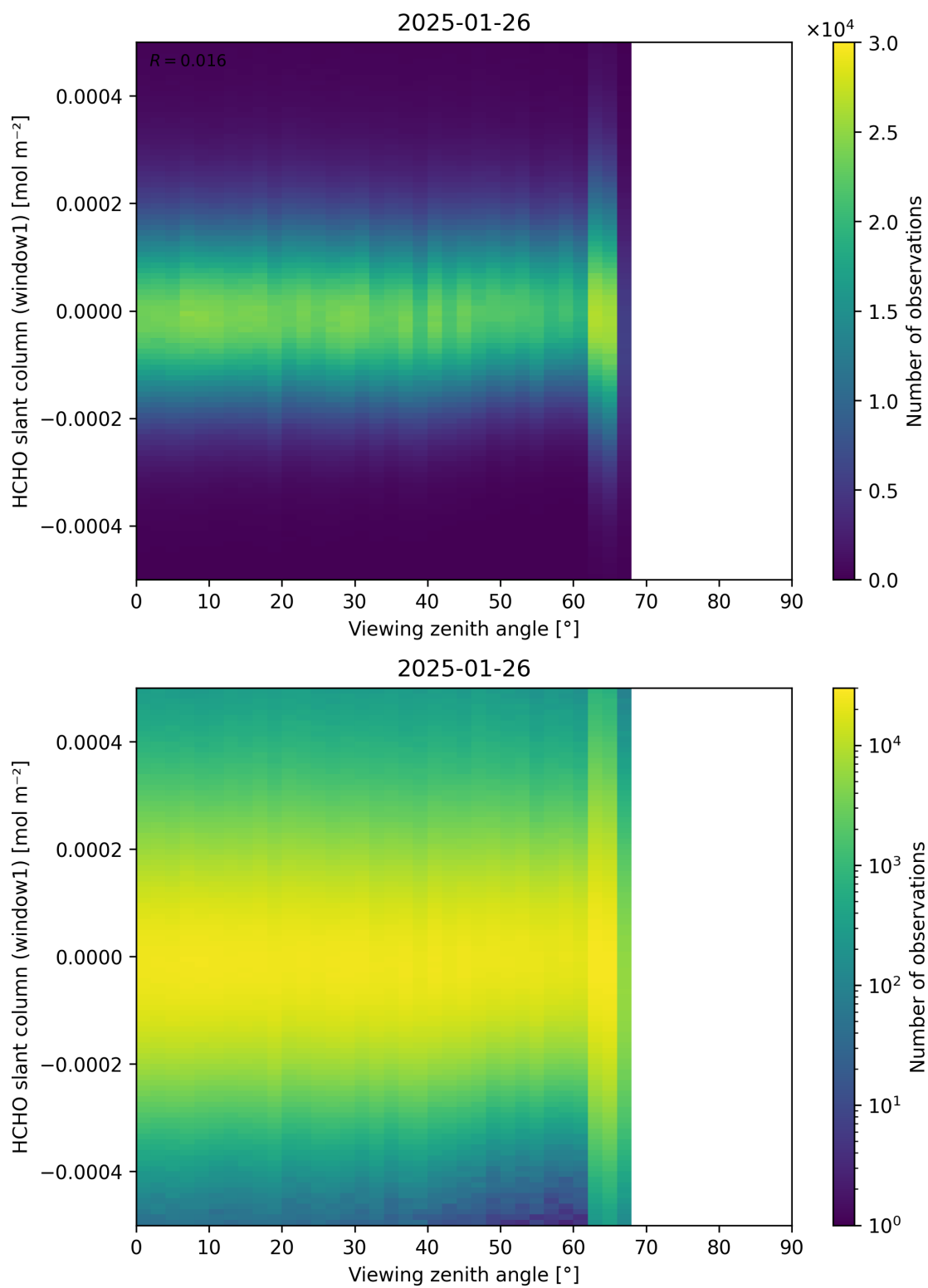
Figure 188: Scatter density plot of “Viewing zenith angle” against “HCHO slant column (window1)” for 2025-01-25 to 2025-01-27.
