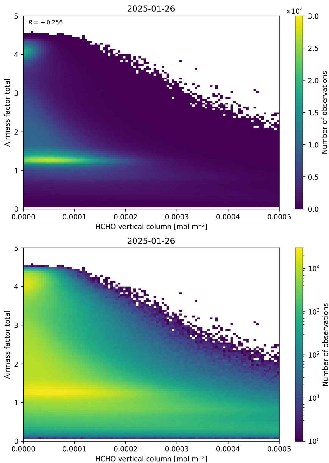
Figure 131: Scatter density plot of “HCHO vertical column” against “Airmass factor total” for 2025-01-25 to 2025-01-27.
