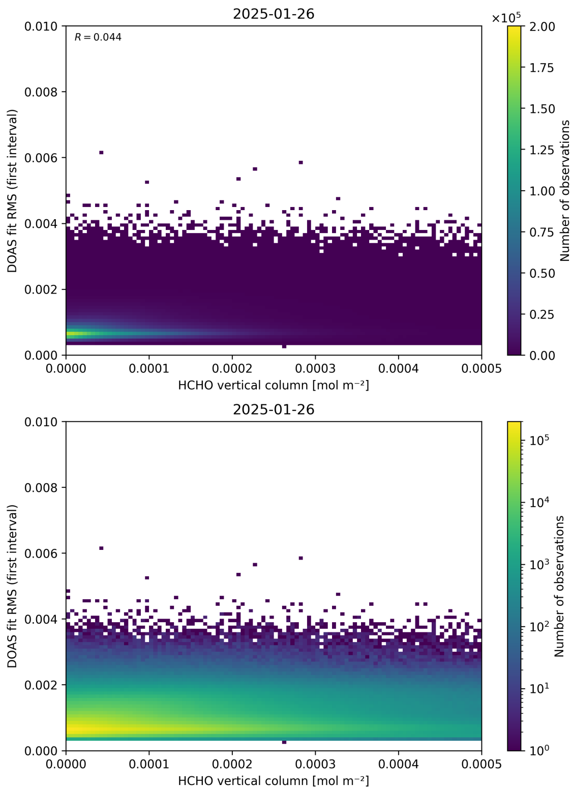
Figure 123: Scatter density plot of “HCHO vertical column” against “DOAS fit RMS (first interval)” for 2025-01-25 to 2025-01-27.
