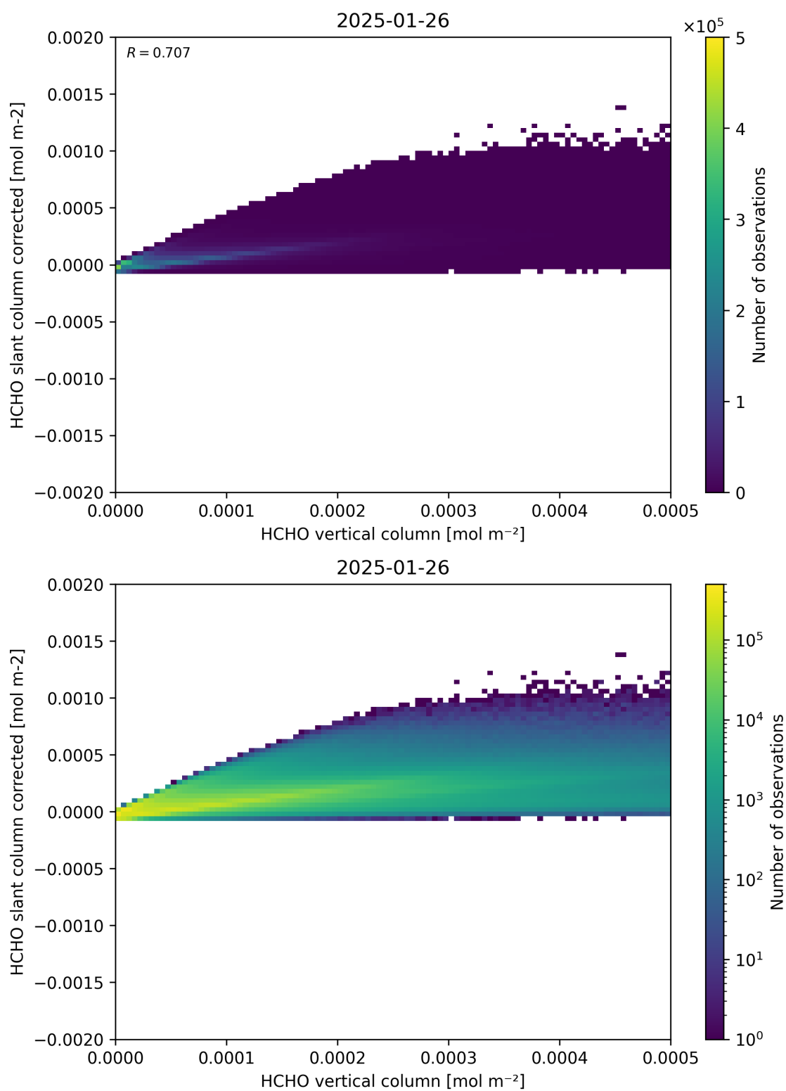
Figure 127: Scatter density plot of “HCHO vertical column” against “HCHO slant column corrected” for 2025-01-25 to 2025-01-27.
