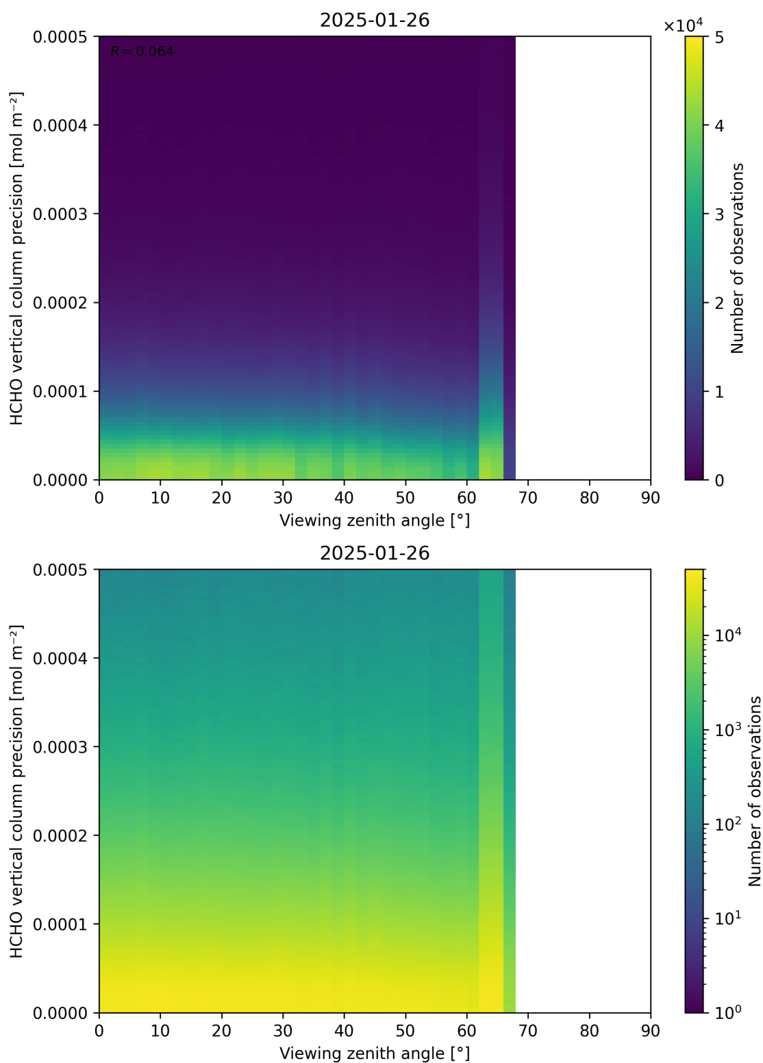
Figure 194: Scatter density plot of “Viewing zenith angle” against “HCHO vertical column precision” for 2025-01-25 to 2025-01-27.
