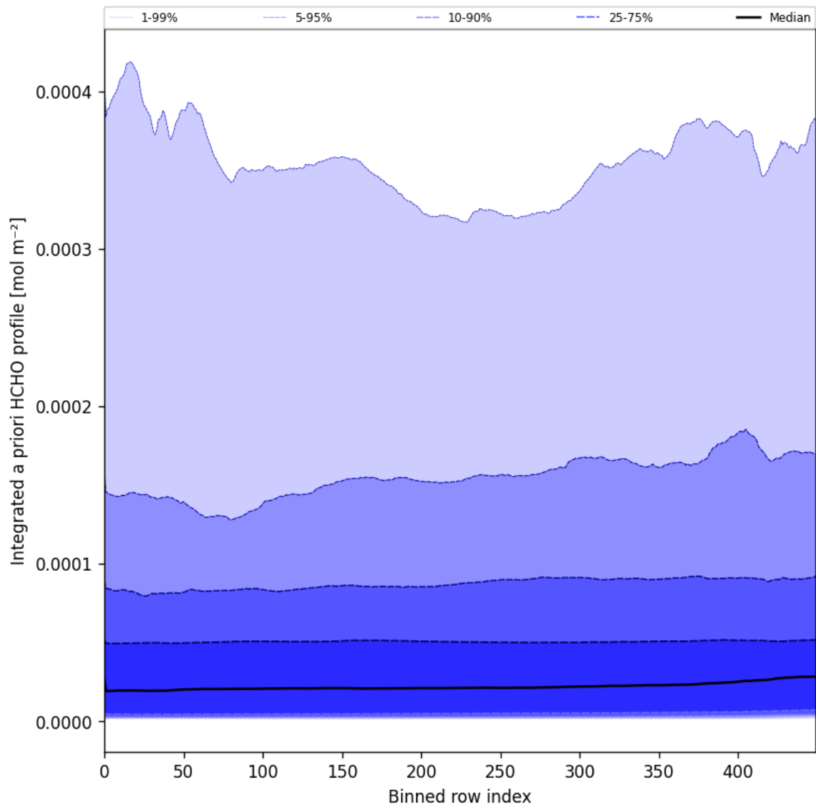
Figure 57: Along track statistics of “Integrated a priori HCHO profile” for 2025-01-25 to 2025-01-27
