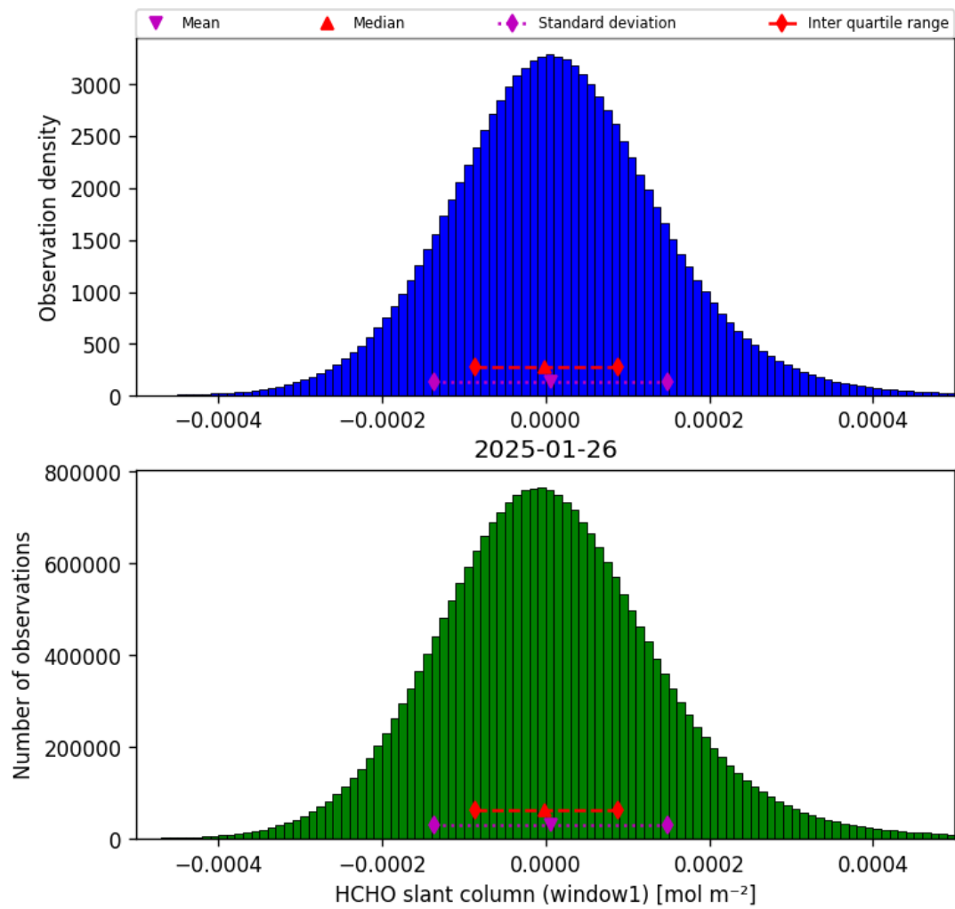
Figure 38: Histogram of “HCHO slant column (window1)” for 2025-01-25 to 2025-01-27
