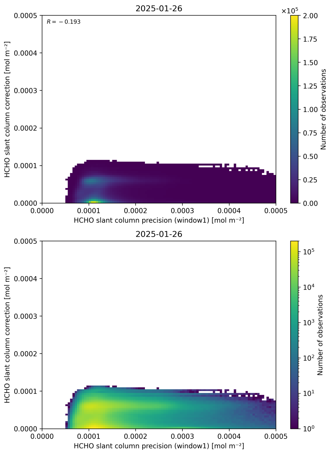
Figure 93: Scatter density plot of “HCHO slant column precision (window1)” against “HCHO slant column correction” for 2025-01-25 to 2025-01-27.
