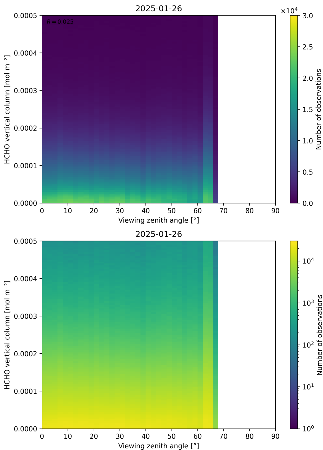
Figure 192: Scatter density plot of “Viewing zenith angle” against “HCHO vertical column” for 2025-01-25 to 2025-01-27.
