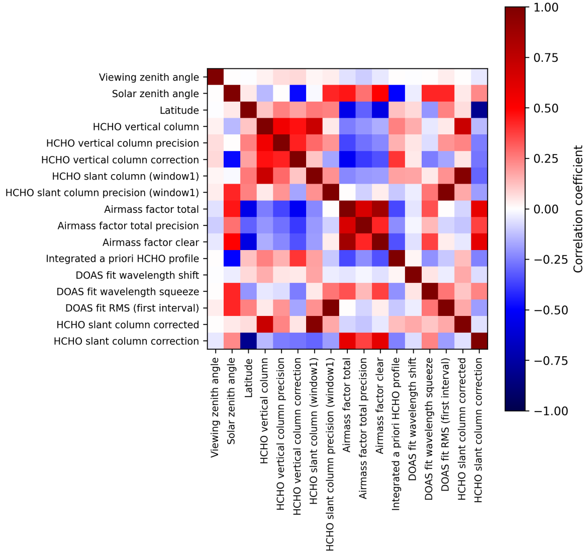
Figure 2: Map of correlation matrix for 2025-01-25 to 2025-01-27.
