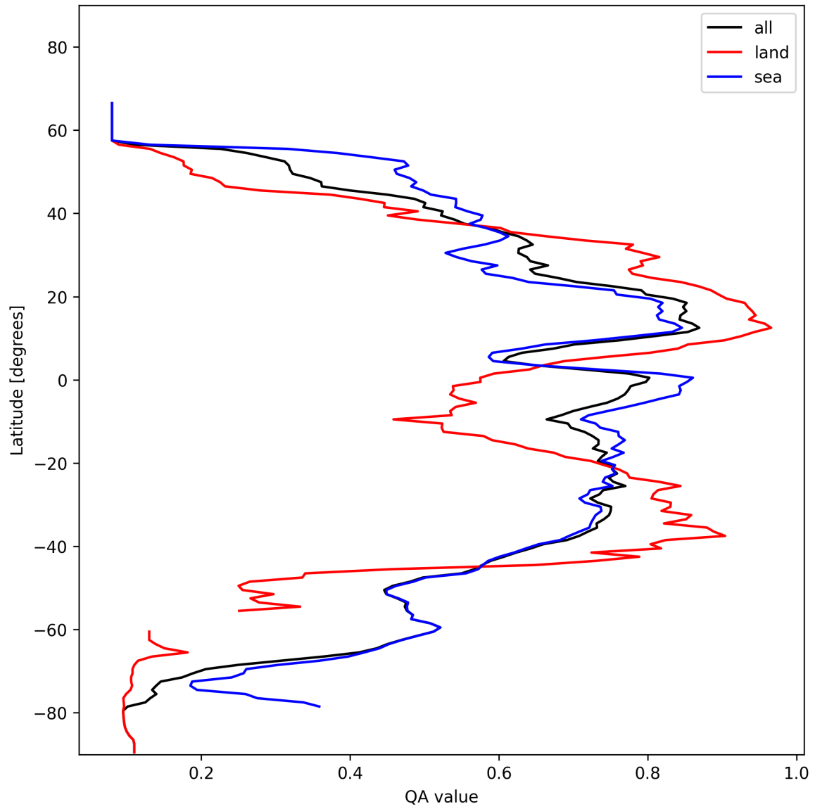
Figure 20: Zonal average of “QA value” for 2025-01-25 to 2025-01-27.
