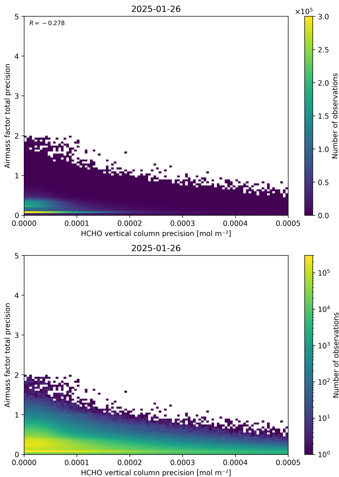
Figure 145: Scatter density plot of “HCHO vertical column precision” against “Airmass factor total precision” for 2025-01-25 to 2025-01-27.
