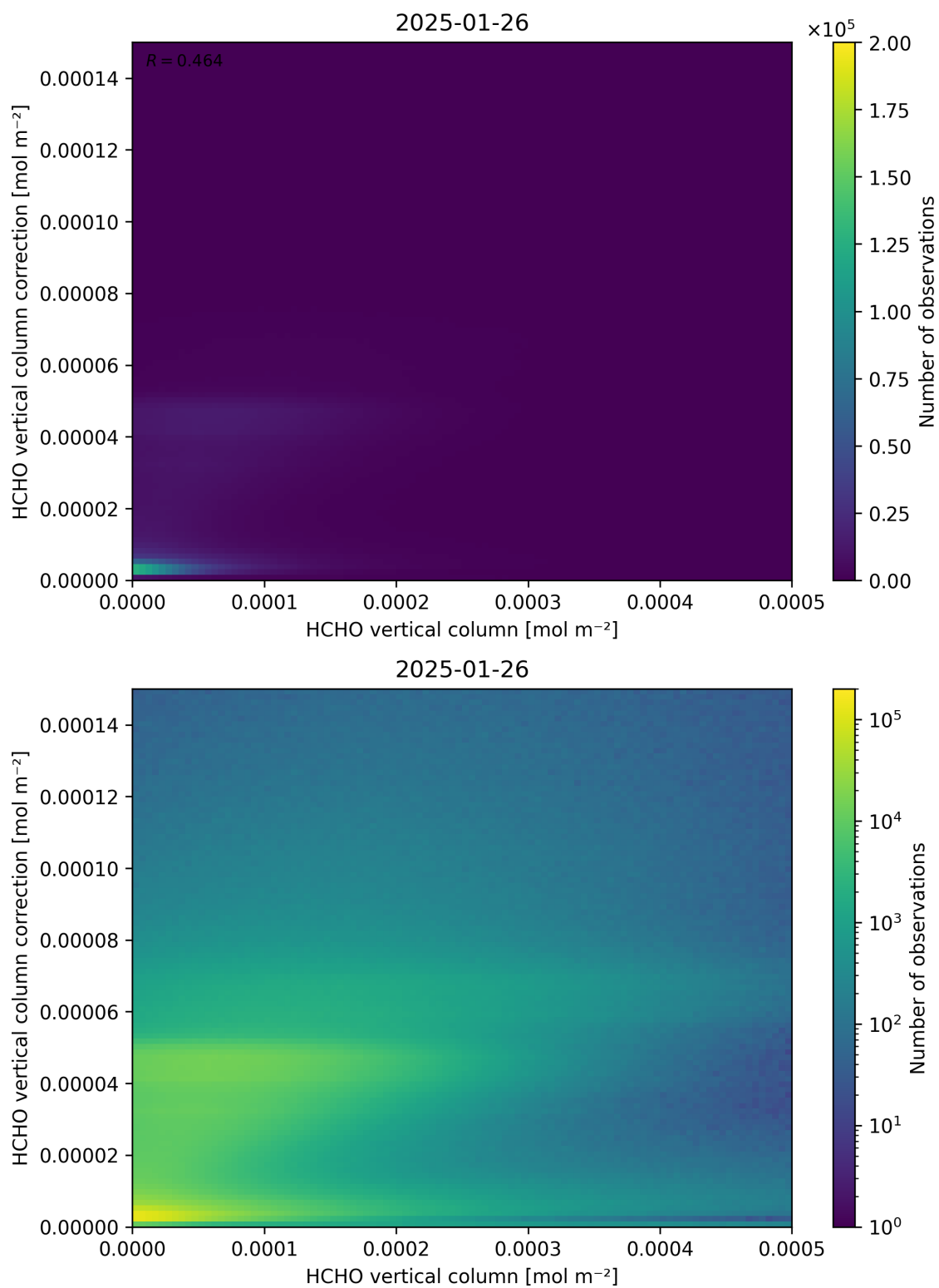
Figure 133: Scatter density plot of “HCHO vertical column” against “HCHO vertical column correction” for 2025-01-25 to 2025-01-27.
