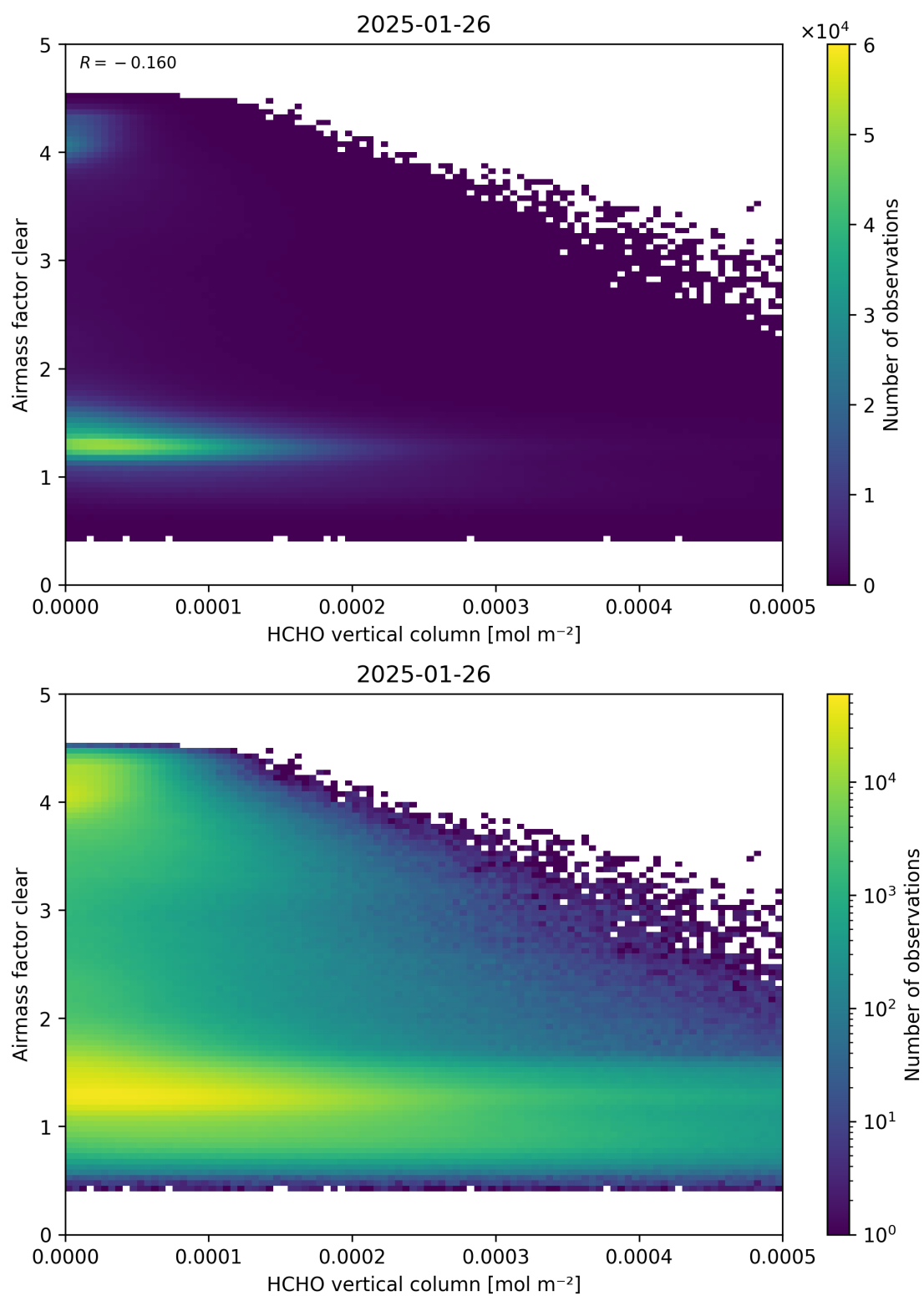
Figure 126: Scatter density plot of “HCHO vertical column” against “Airmass factor clear” for 2025-01-25 to 2025-01-27.
