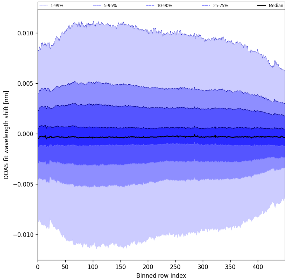
Figure 58: Along track statistics of “DOAS fit wavelength shift” for 2025-01-25 to 2025-01-27
