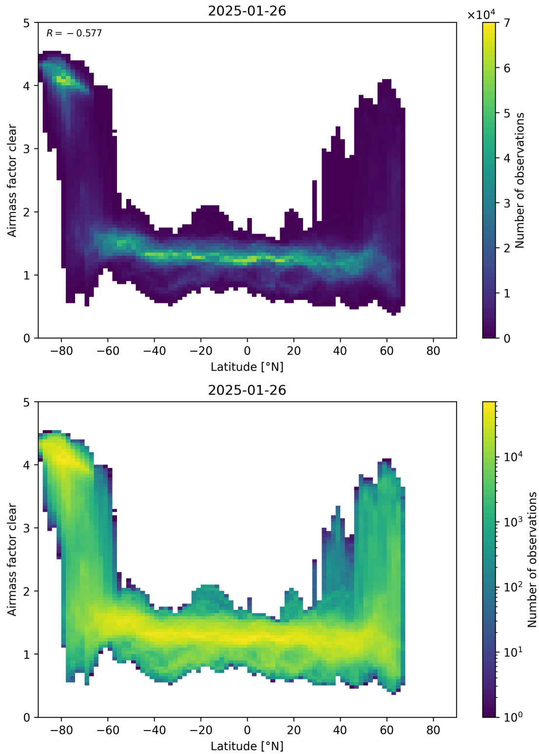
Figure 156: Scatter density plot of “Latitude” against “Airmass factor clear” for 2025-01-25 to 2025-01-27.
