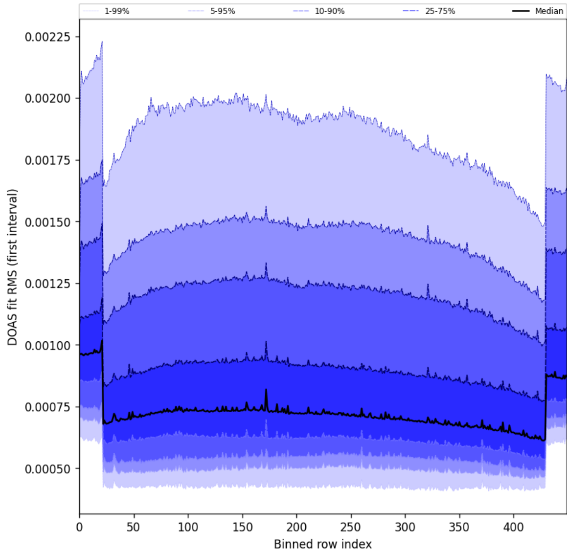
Figure 60: Along track statistics of “DOAS fit RMS (first interval)” for 2025-01-25 to 2025-01-27
