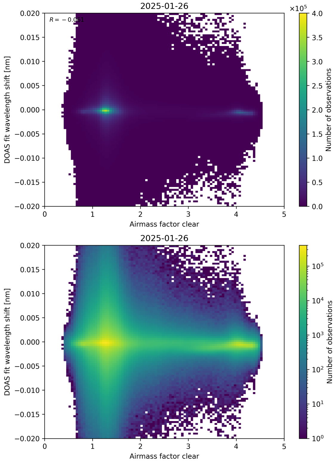
Figure 72: Scatter density plot of “Airmass factor clear” against “DOAS fit wavelength shift” for 2025-01-25 to 2025-01-27.
