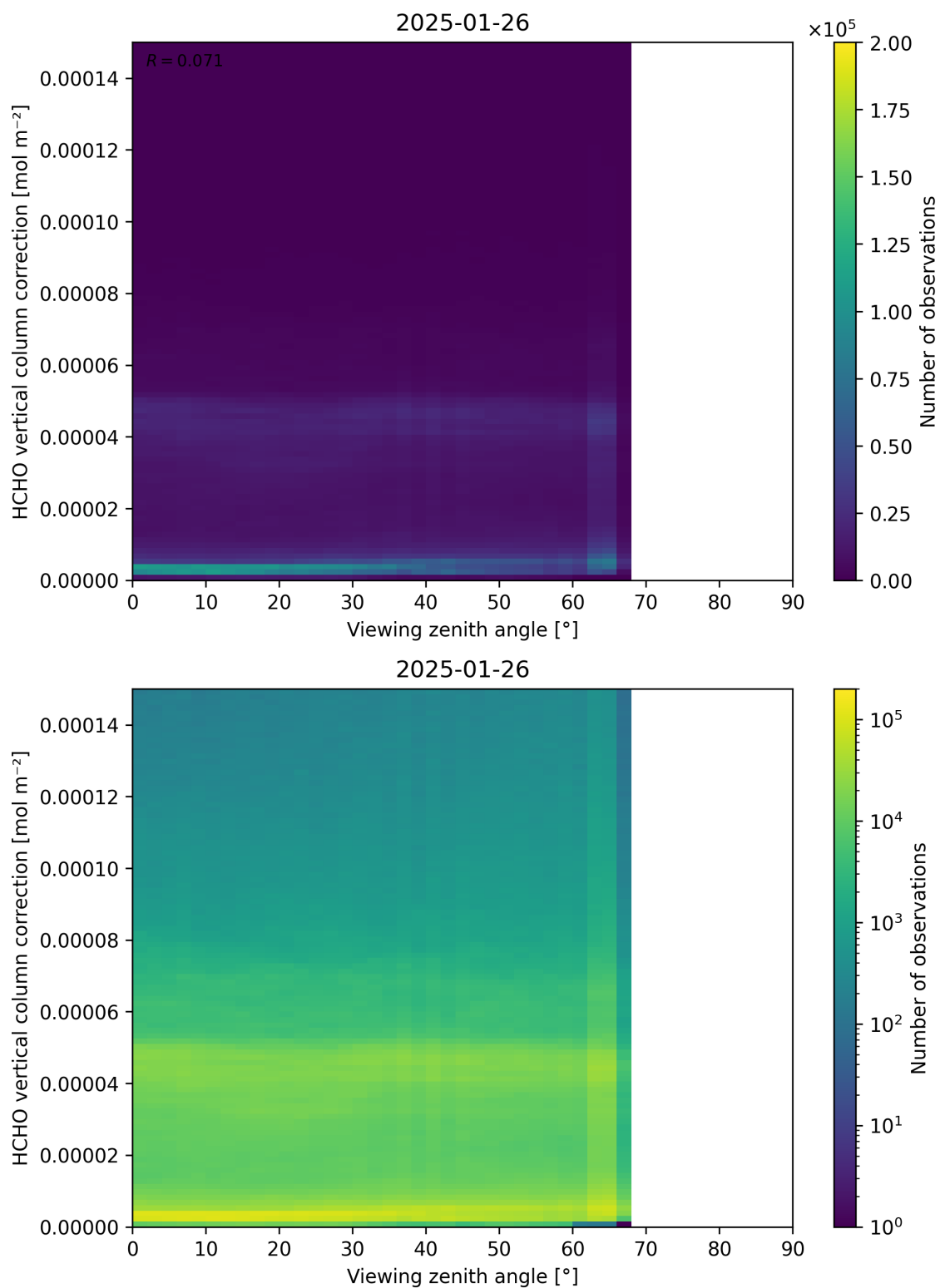
Figure 193: Scatter density plot of “Viewing zenith angle” against “HCHO vertical column correction” for 2025-01-25 to 2025-01-27.
