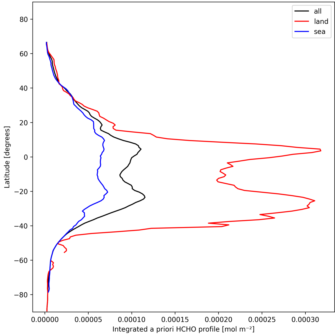
Figure 29: Zonal average of “Integrated a priori HCHO profile” for 2025-01-25 to 2025-01-27.
