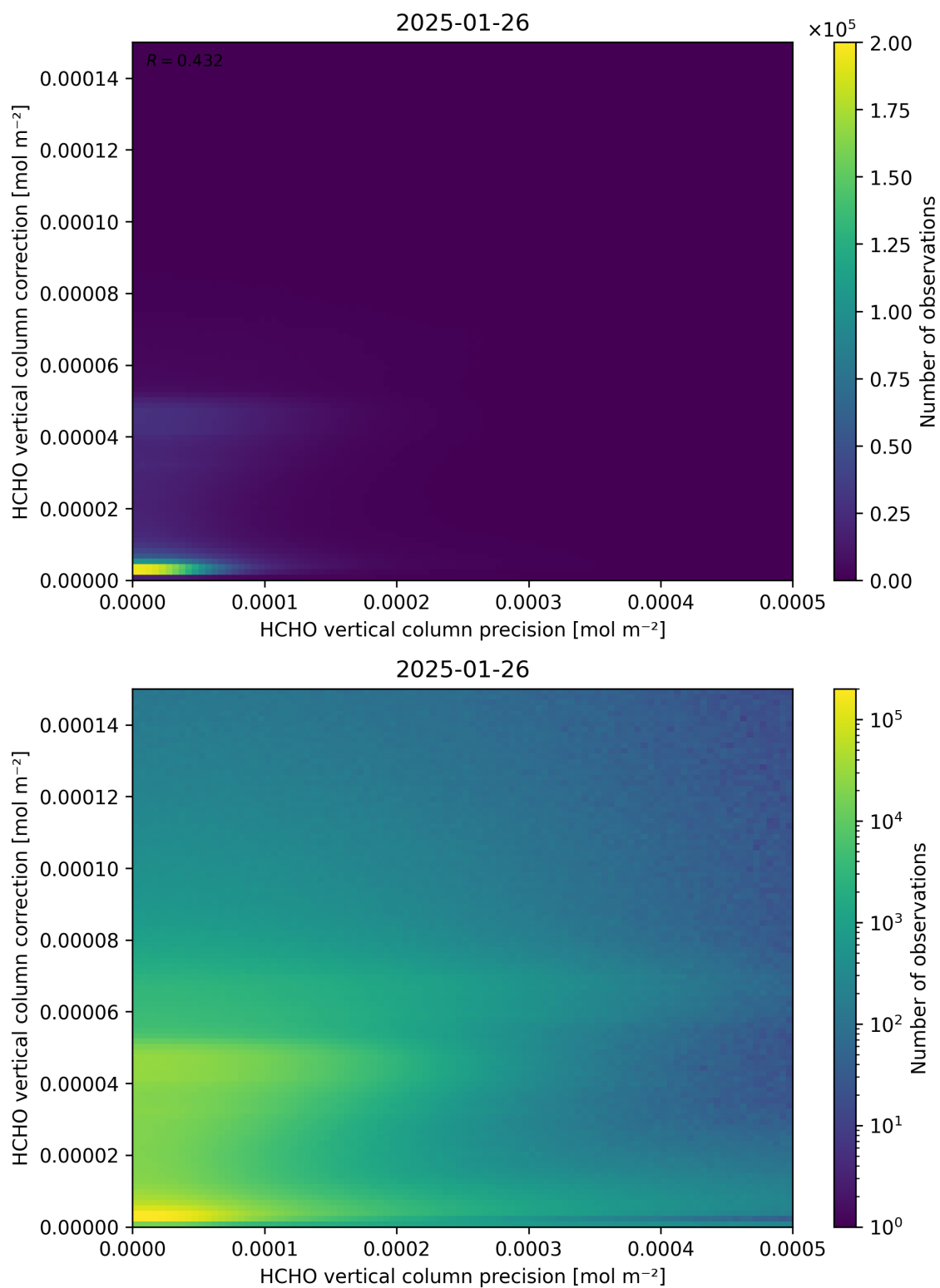
Figure 146: Scatter density plot of “HCHO vertical column precision” against “HCHO vertical column correction” for 2025-01-25 to 2025-01-27.
