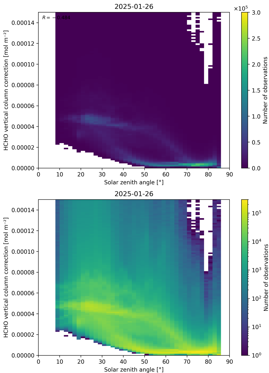
Figure 178: Scatter density plot of “Solar zenith angle” against “HCHO vertical column correction” for 2025-01-25 to 2025-01-27.
