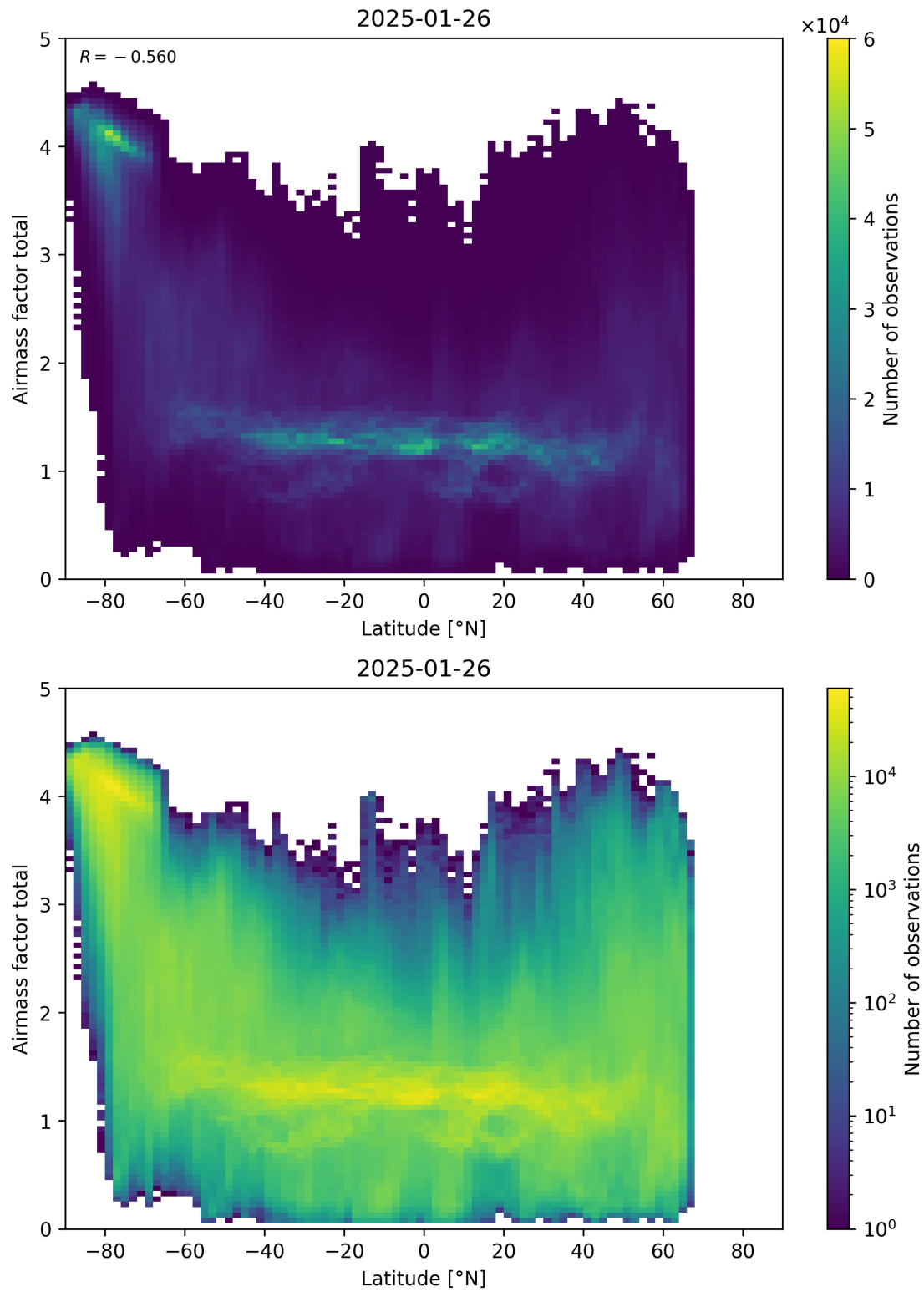
Figure 161: Scatter density plot of “Latitude” against “Airmass factor total” for 2025-01-25 to 2025-01-27.
