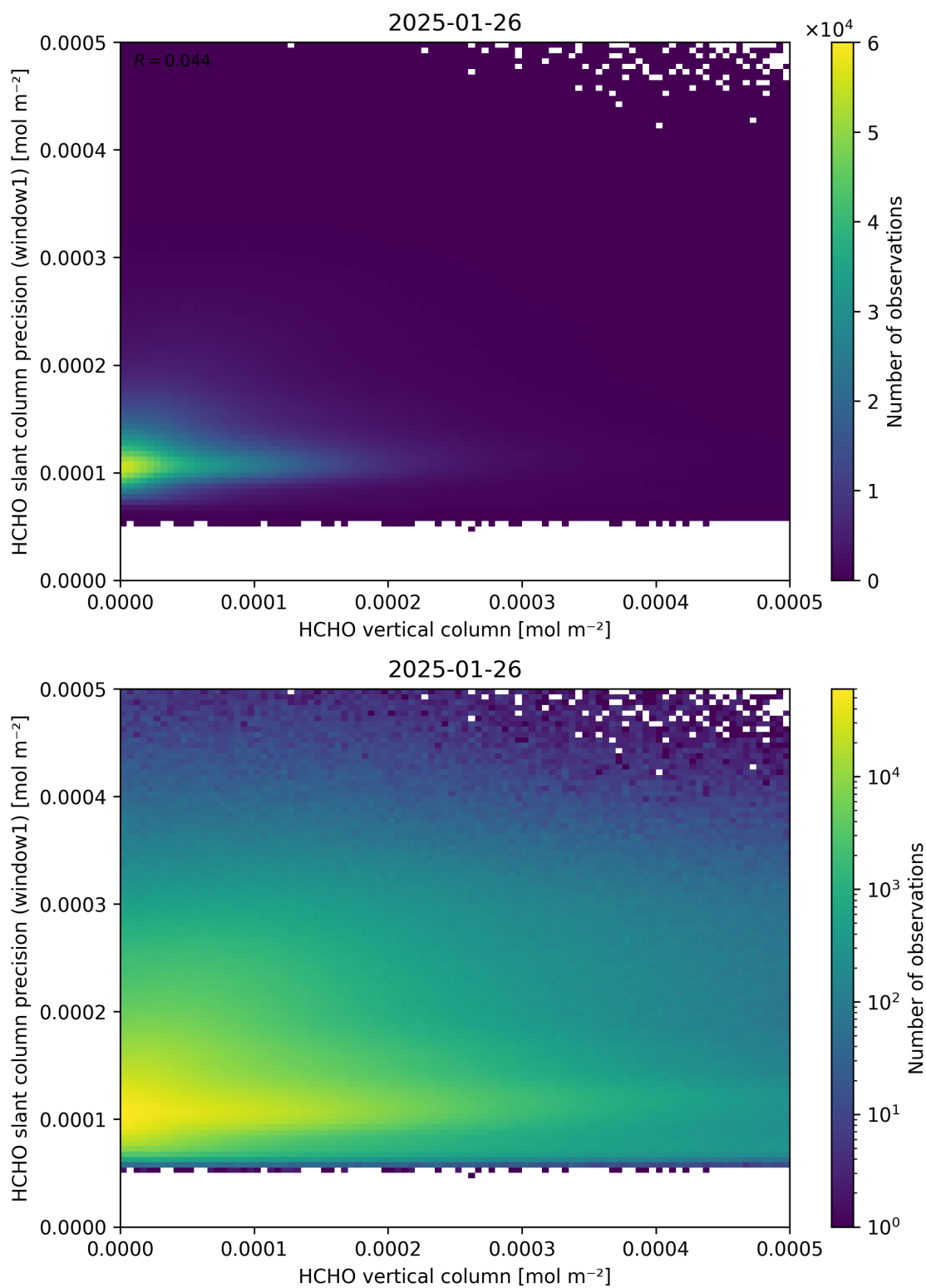
Figure 130: Scatter density plot of “HCHO vertical column” against “HCHO slant column precision (window1)” for 2025-01-25 to 2025-01-27.
