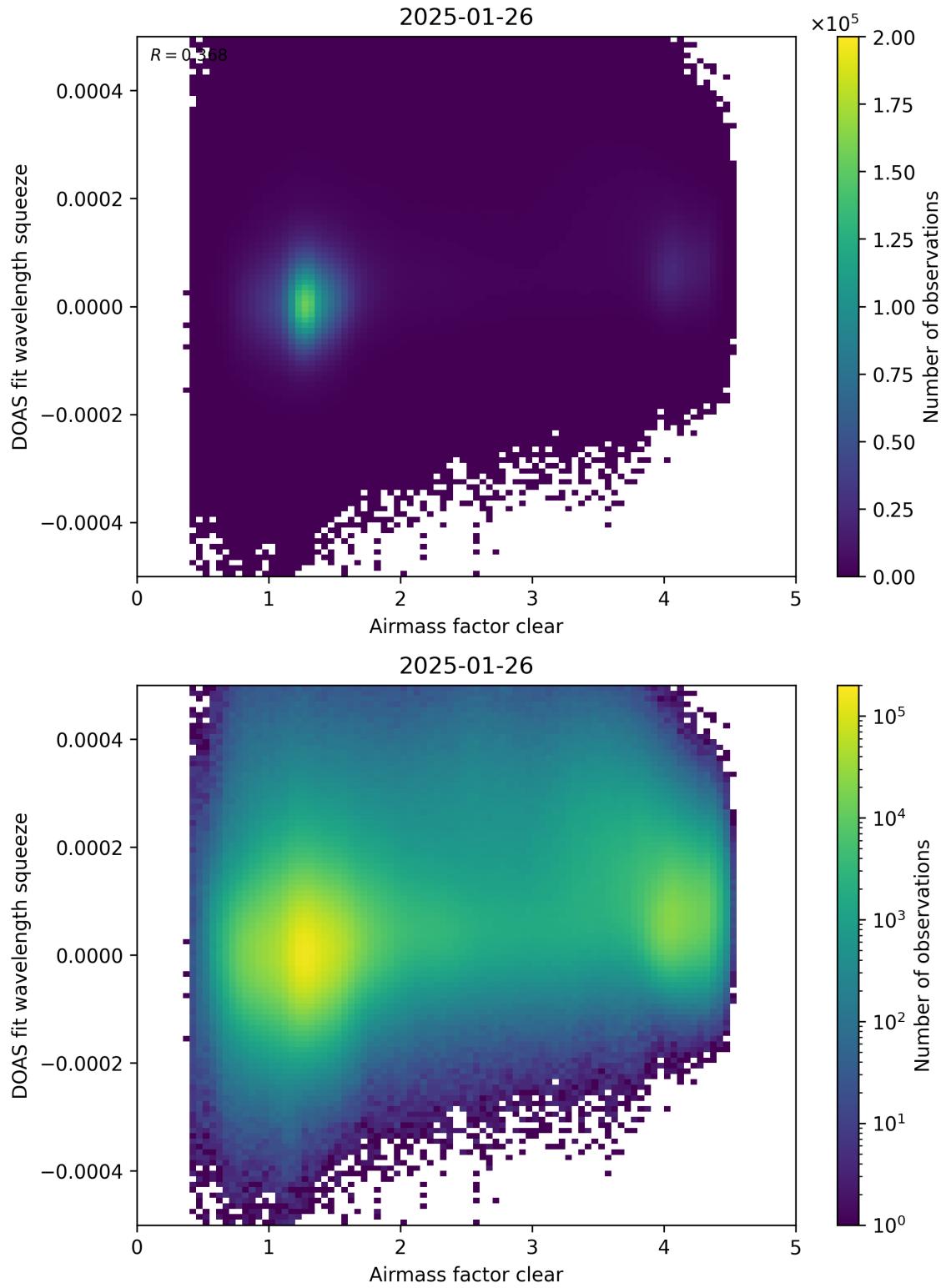
Figure 73: Scatter density plot of “Airmass factor clear” against “DOAS fit wavelength squeeze” for 2025-01-25 to 2025-01-27.
