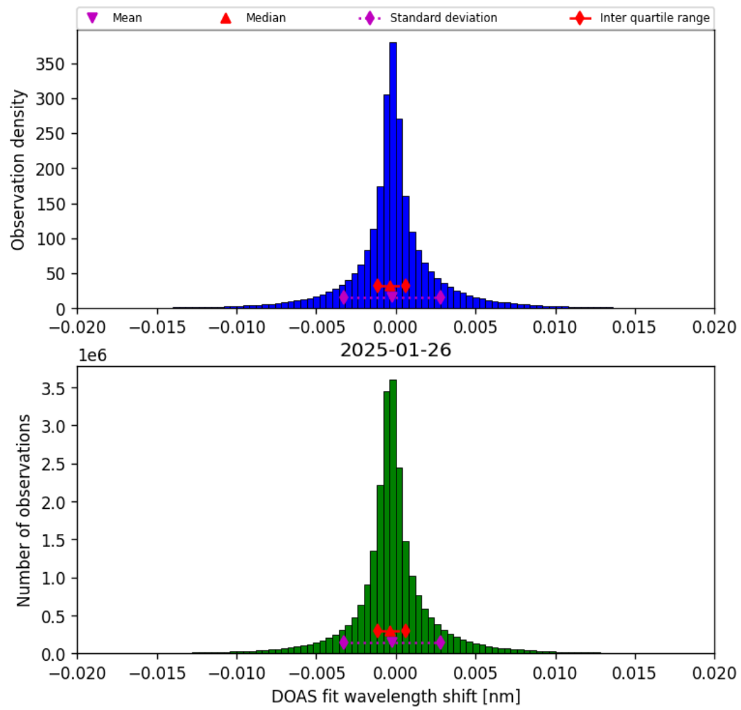
Figure 44: Histogram of “DOAS fit wavelength shift” for 2025-01-25 to 2025-01-27
