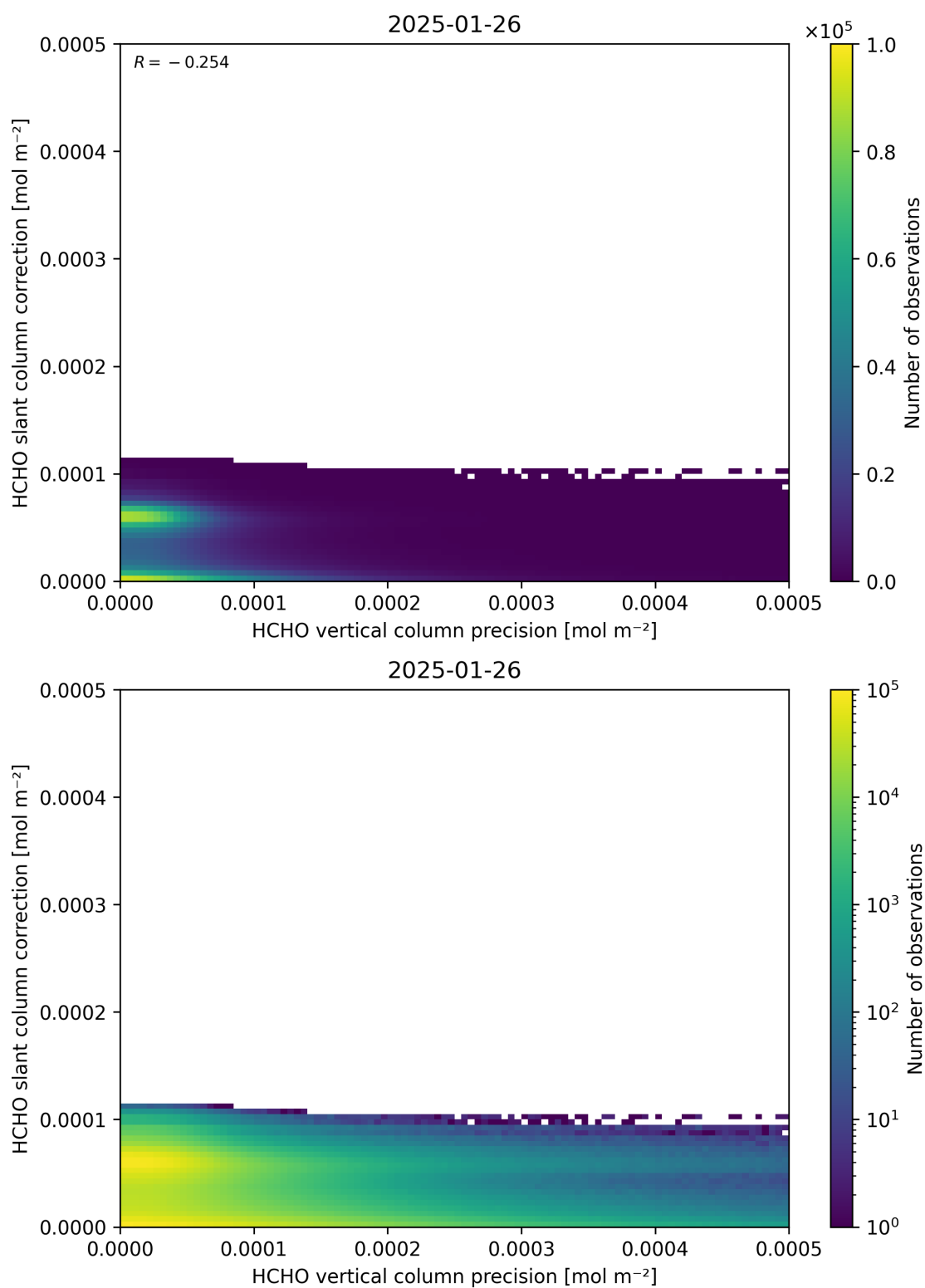
Figure 141: Scatter density plot of “HCHO vertical column precision” against “HCHO slant column correction” for 2025-01-25 to 2025-01-27.
