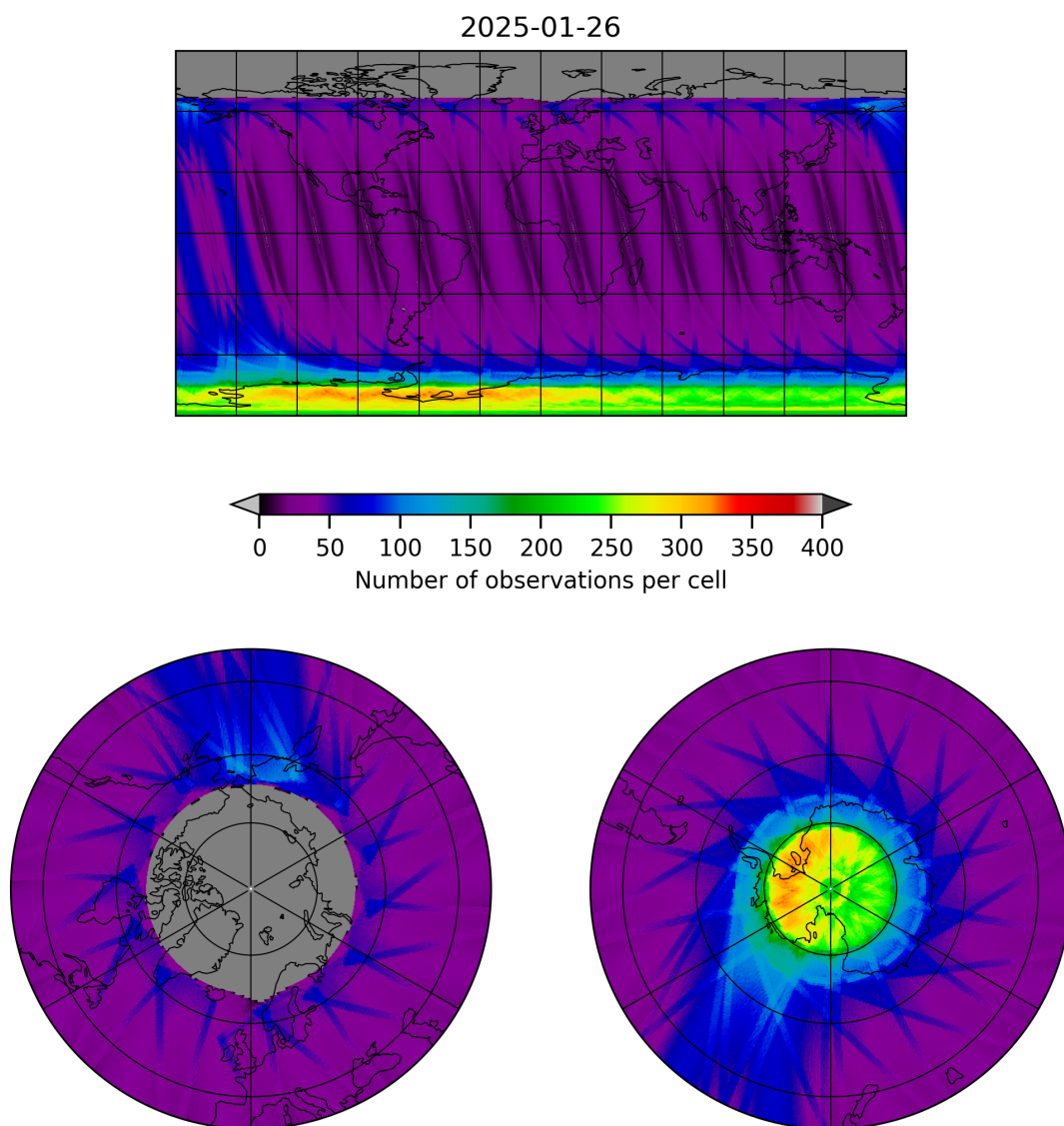
Figure 19: Map of the number of observations for 2025-01-25 to 2025-01-27
