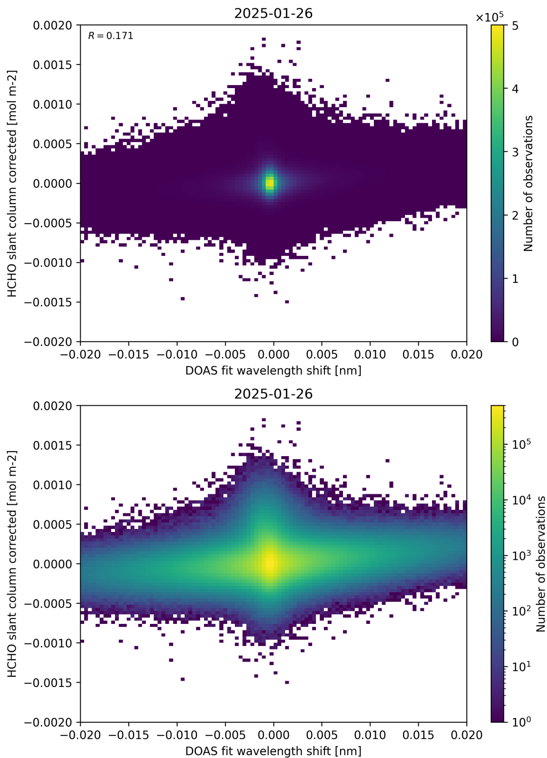
Figure 66: Scatter density plot of “DOAS fit wavelength shift” against “HCHO slant column corrected” for 2025-01-25 to 2025-01-27.
