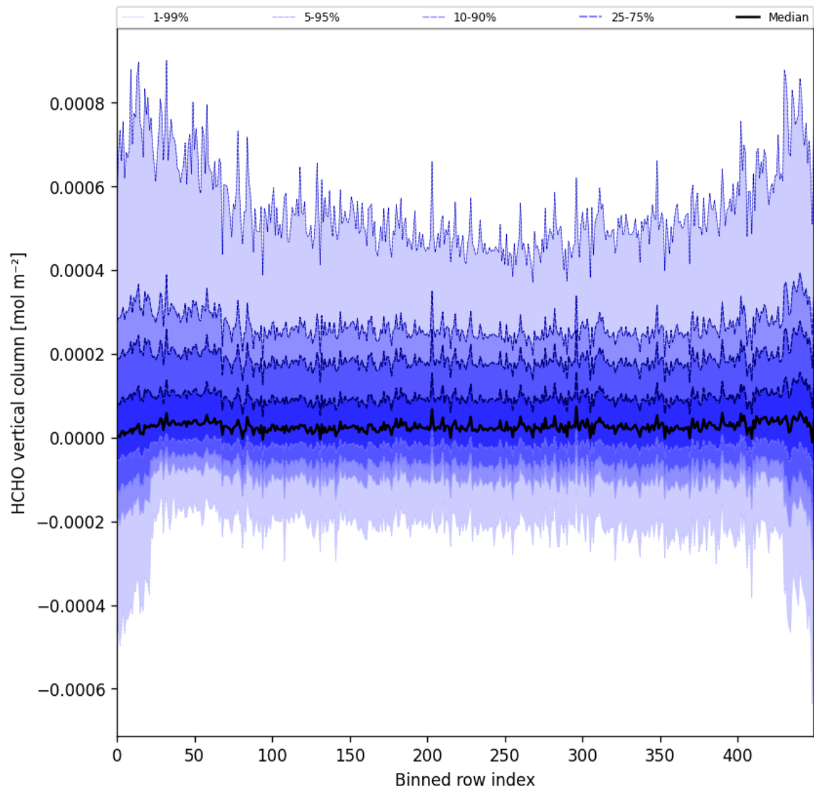
Figure 49: Along track statistics of “HCHO vertical column” for 2025-01-25 to 2025-01-27
