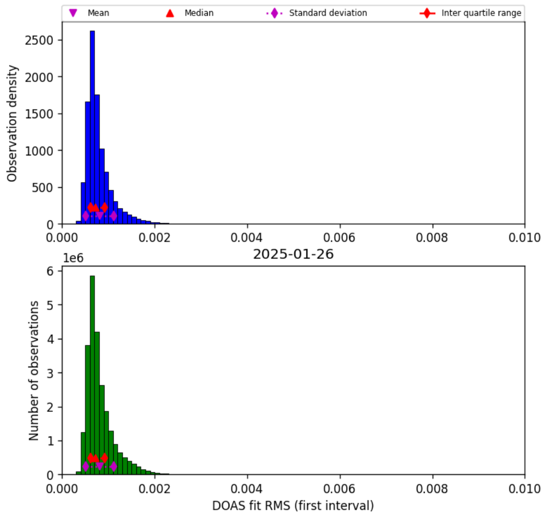
Figure 46: Histogram of “DOAS fit RMS (first interval)” for 2025-01-25 to 2025-01-27
