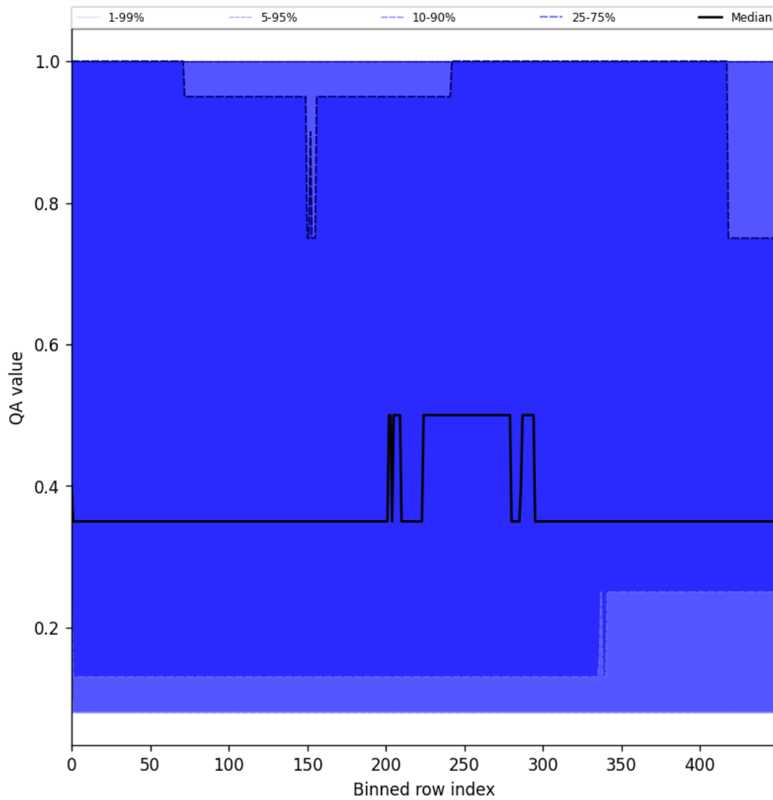
Figure 48: Along track statistics of “QA value” for 2025-01-25 to 2025-01-27
