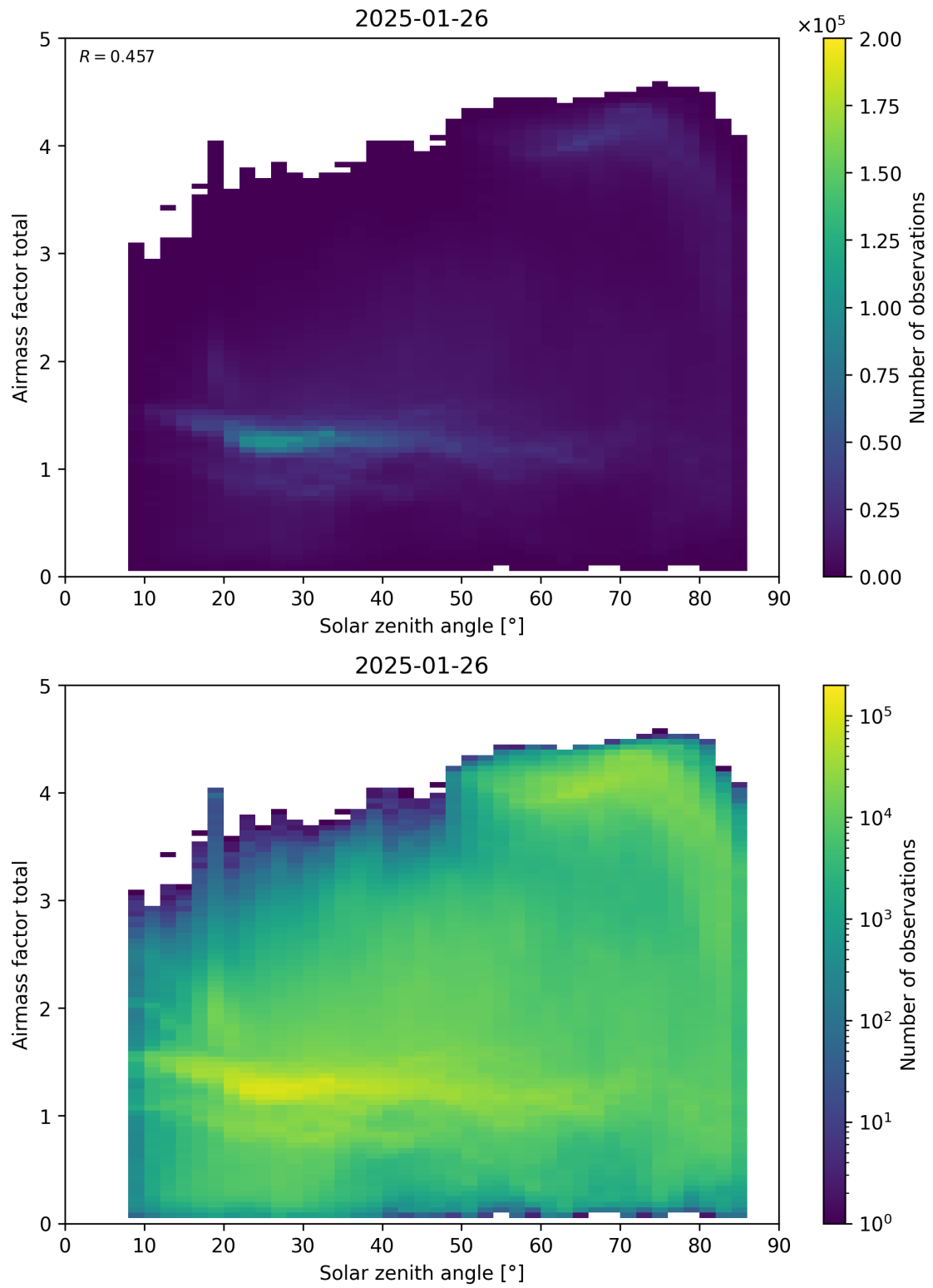
Figure 175: Scatter density plot of “Solar zenith angle” against “Airmass factor total” for 2025-01-25 to 2025-01-27.
