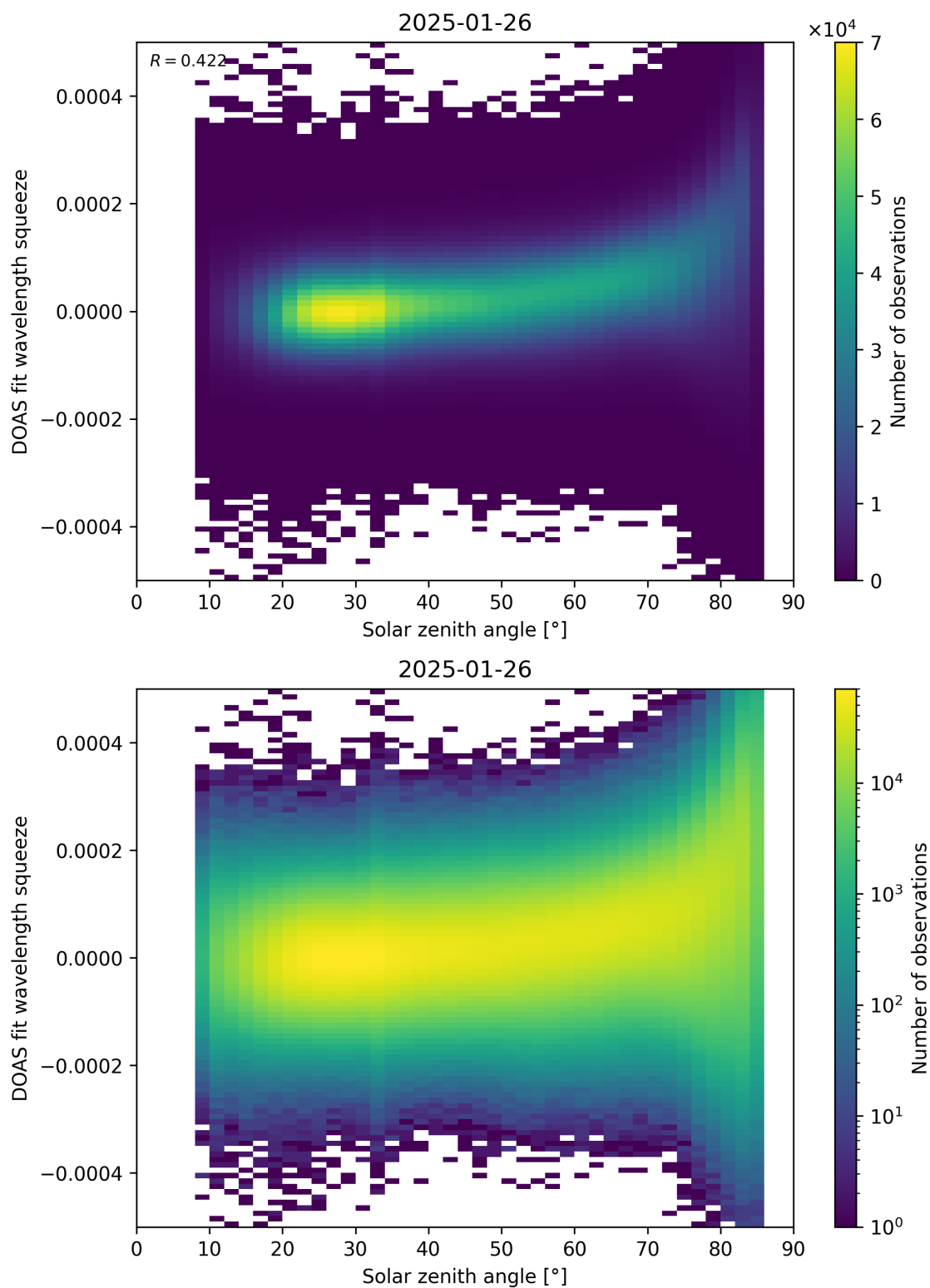
Figure 169: Scatter density plot of “Solar zenith angle” against “DOAS fit wavelength squeeze” for 2025-01-25 to 2025-01-27.
