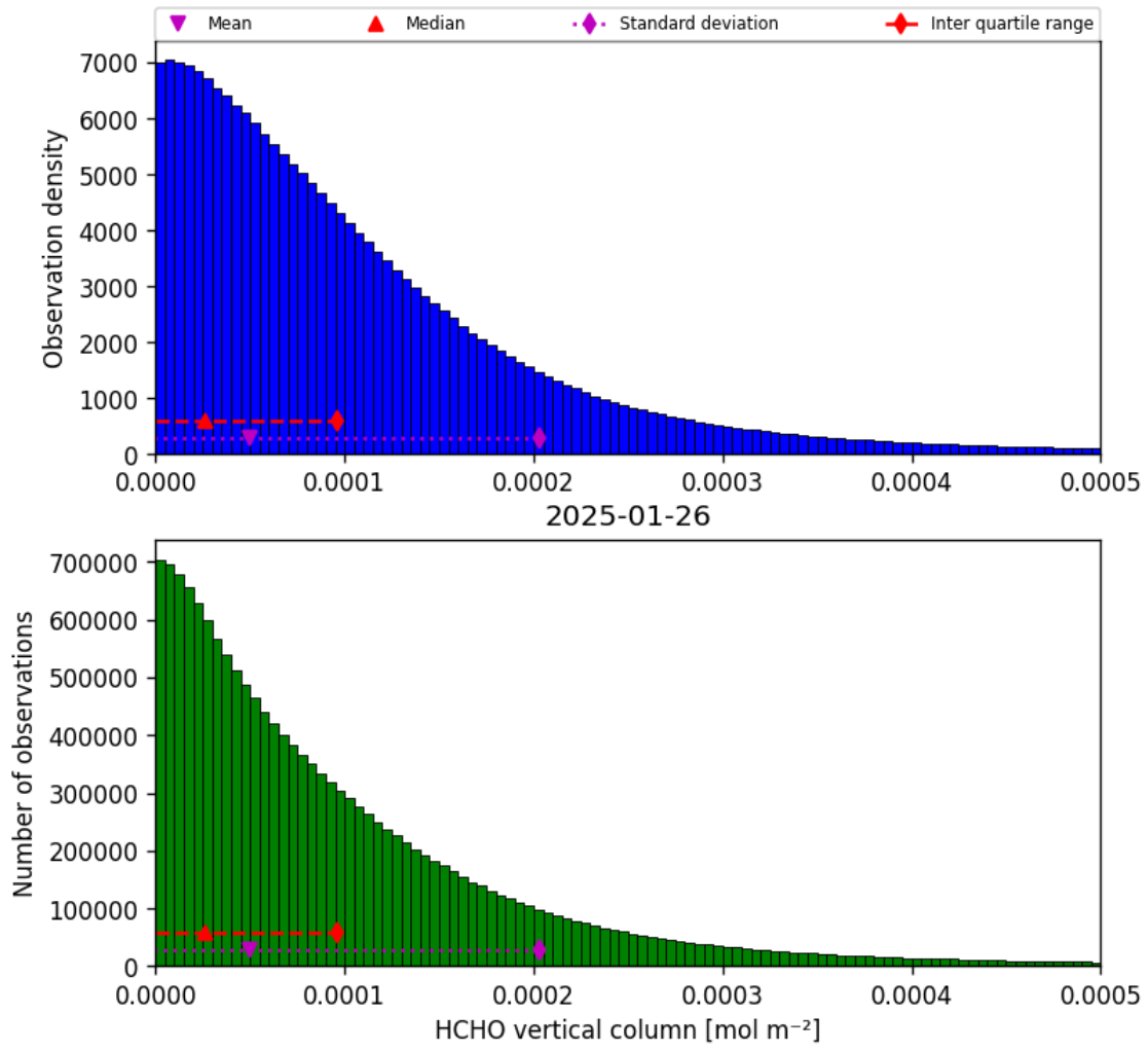
Figure 35: Histogram of “HCHO vertical column” for 2025-01-25 to 2025-01-27
