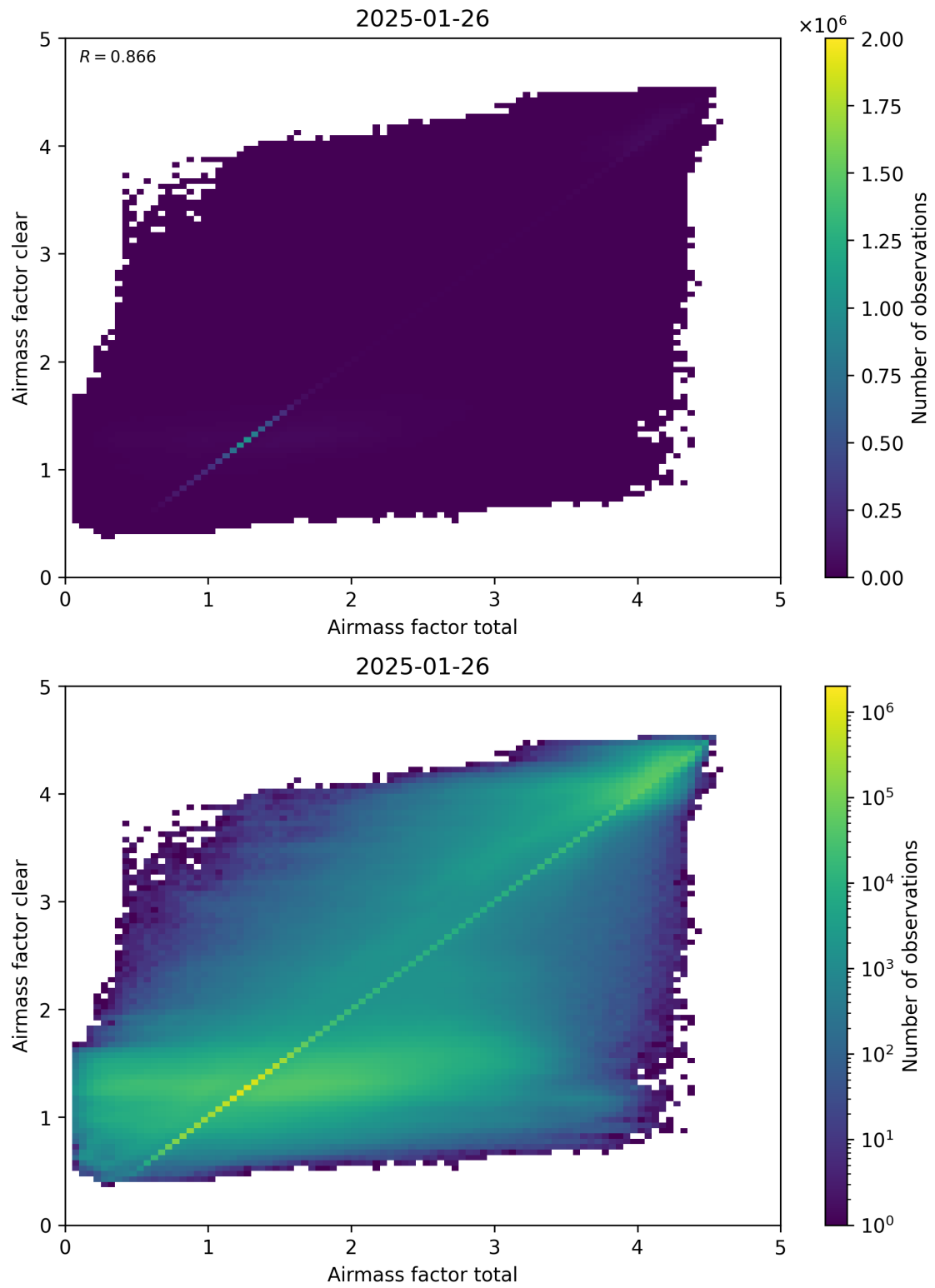
Figure 100: Scatter density plot of “Airmass factor total” against “Airmass factor clear” for 2025-01-25 to 2025-01-27.
