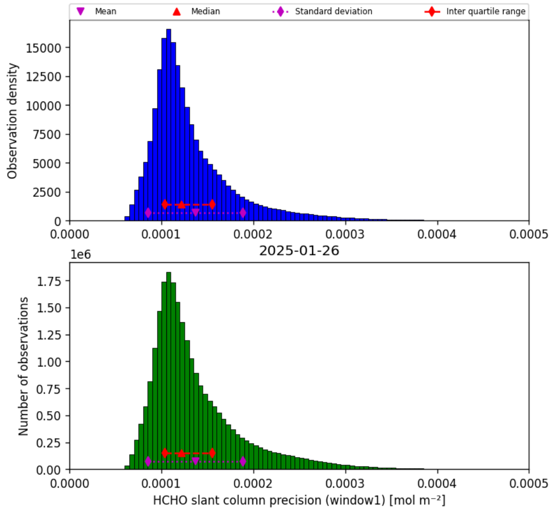
Figure 39: Histogram of “HCHO slant column precision (window1)” for 2025-01-25 to 2025-01-27
