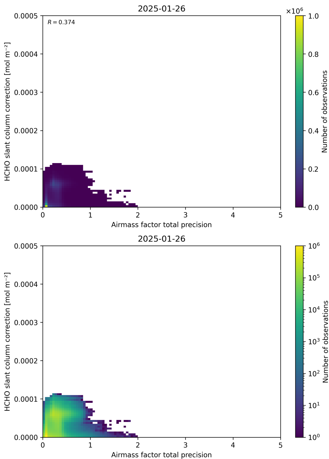
Figure 110: Scatter density plot of “Airmass factor total precision” against “HCHO slant column correction” for 2025-01-25 to 2025-01-27.
