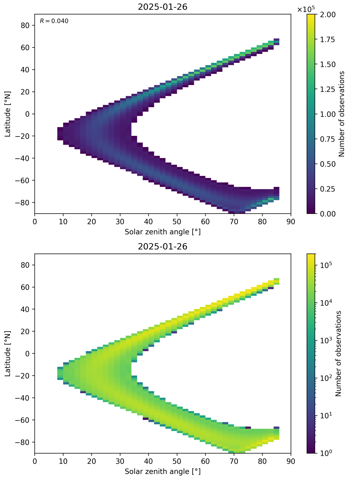
Figure 181: Scatter density plot of “Solar zenith angle” against “Latitude” for 2025-01-25 to 2025-01-27.
