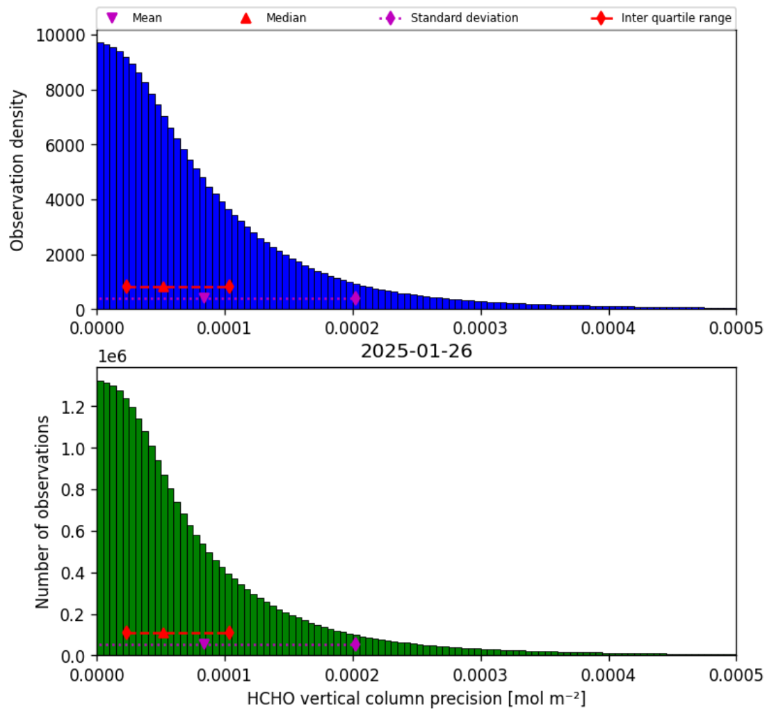
Figure 36: Histogram of “HCHO vertical column precision” for 2025-01-25 to 2025-01-27
