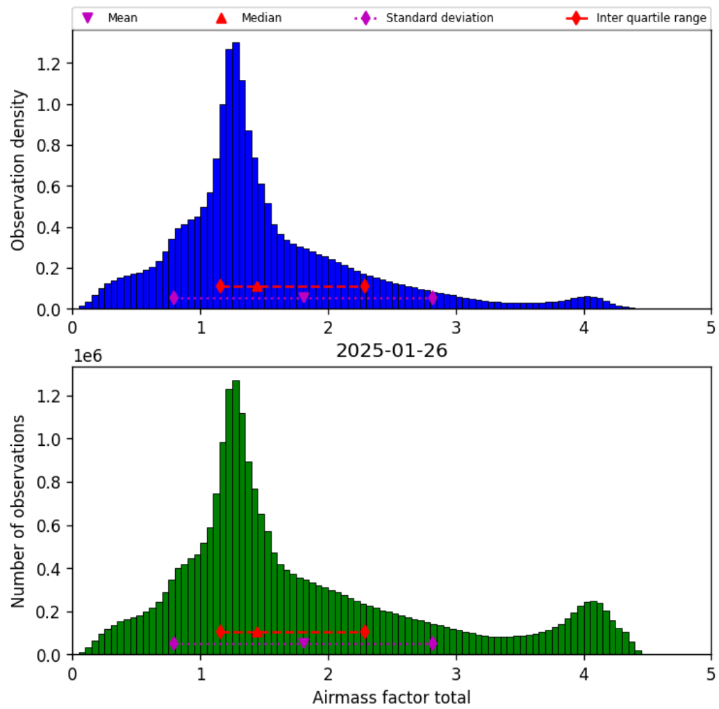
Figure 40: Histogram of “Airmass factor total” for 2025-01-25 to 2025-01-27
