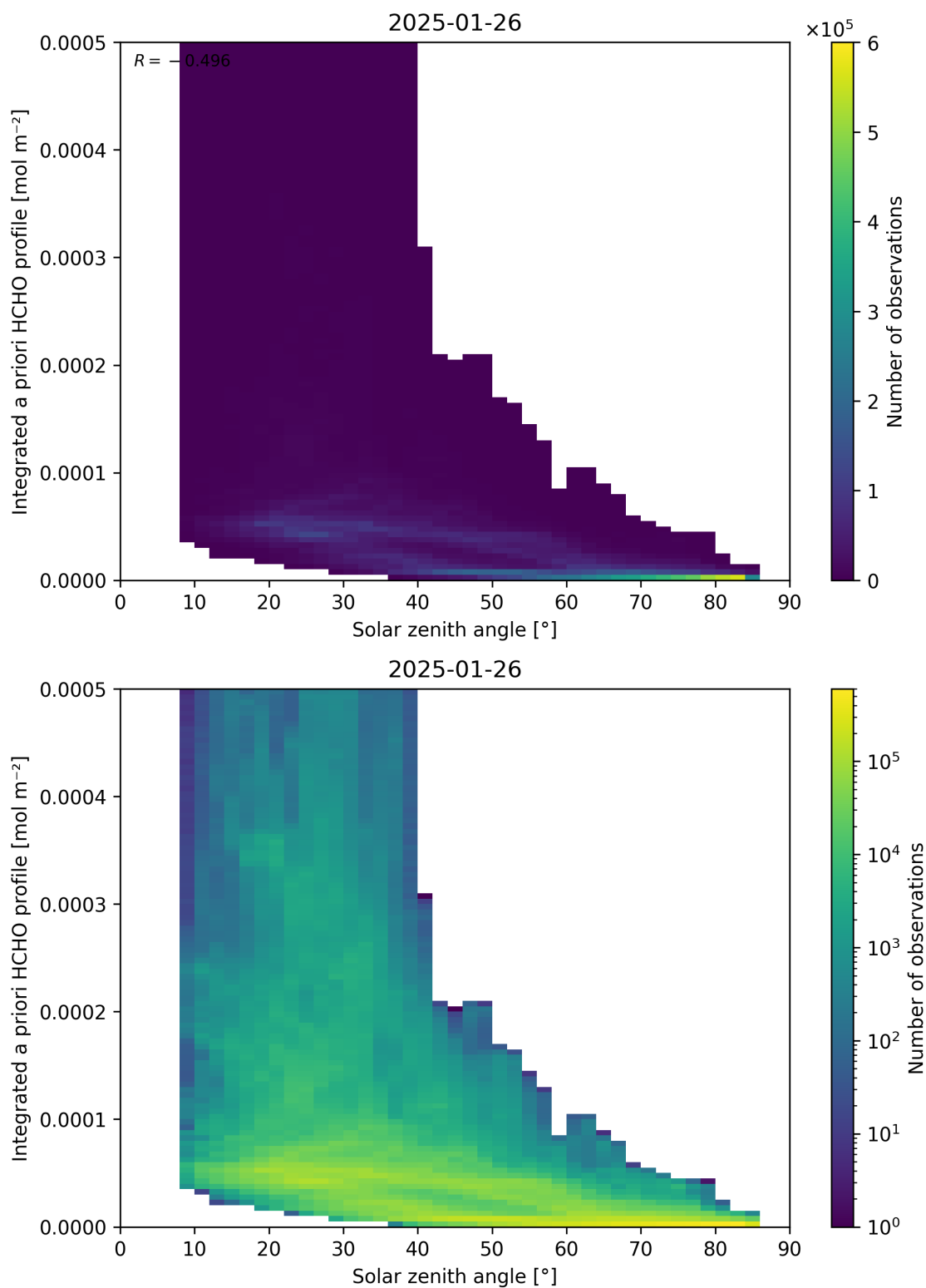
Figure 180: Scatter density plot of “Solar zenith angle” against “Integrated a priori HCHO profile” for 2025-01-25 to 2025-01-27.
