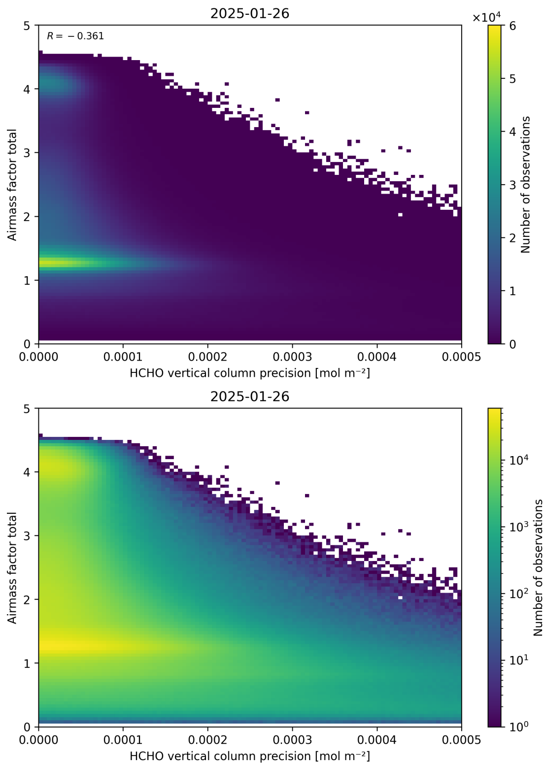
Figure 144: Scatter density plot of “HCHO vertical column precision” against “Airmass factor total” for 2025-01-25 to 2025-01-27.
