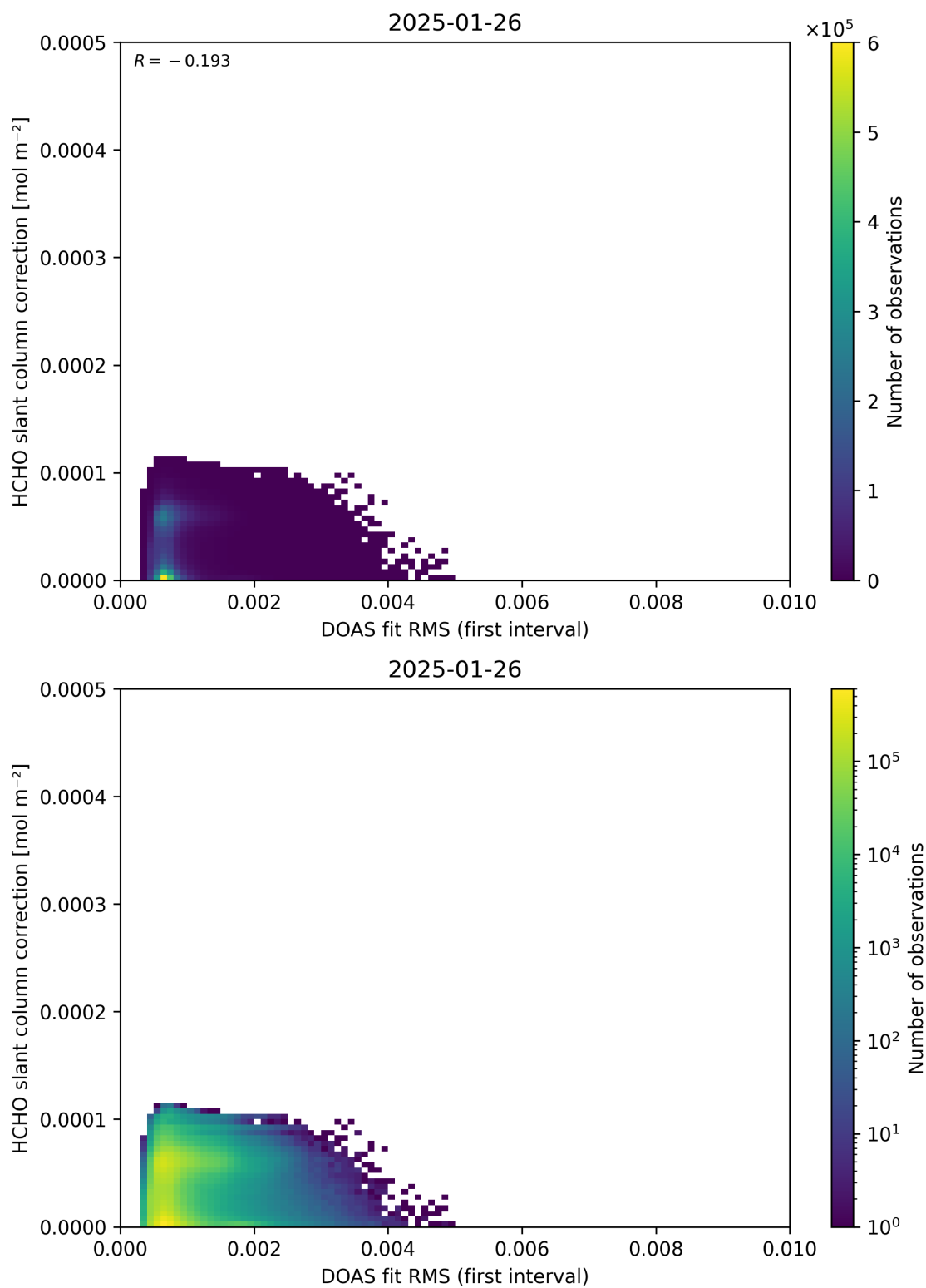
Figure 63: Scatter density plot of “DOAS fit RMS (first interval)” against “HCHO slant column correction” for 2025-01-25 to 2025-01-27.
