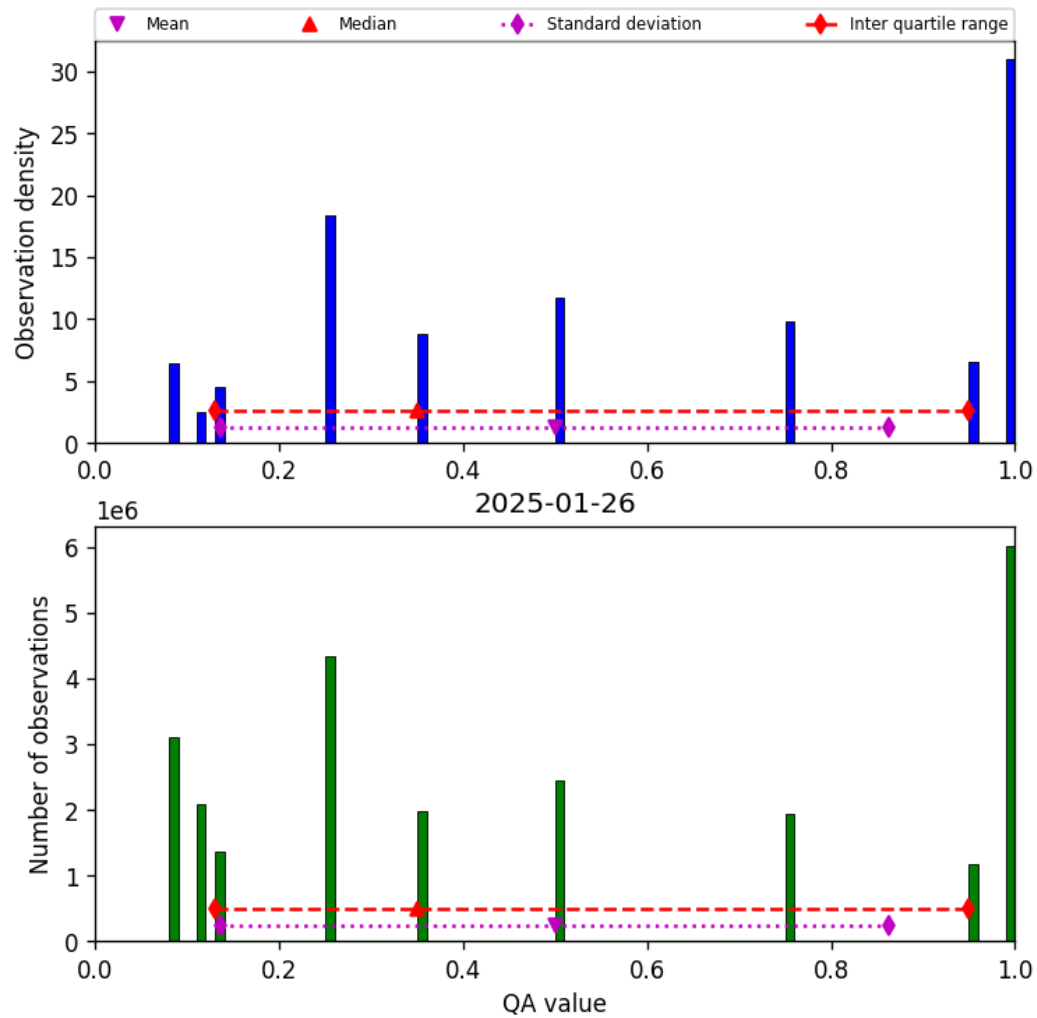
Figure 34: Histogram of “QA value” for 2025-01-25 to 2025-01-27
