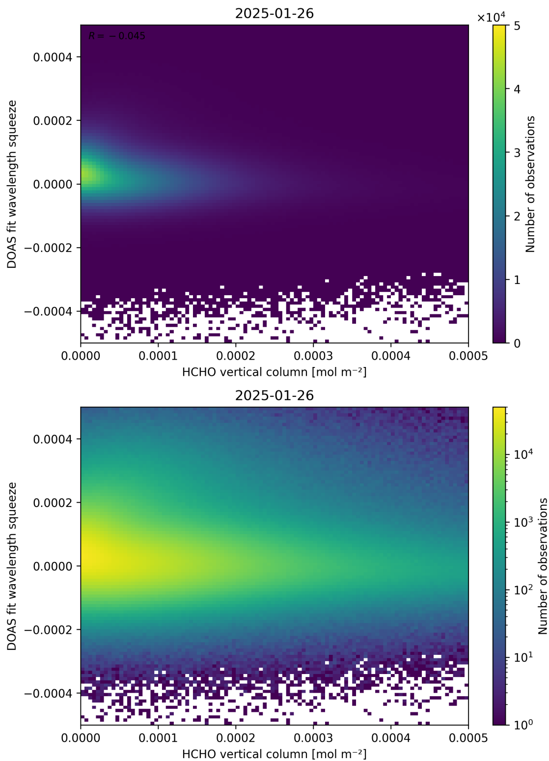
Figure 125: Scatter density plot of “HCHO vertical column” against “DOAS fit wavelength squeeze” for 2025-01-25 to 2025-01-27.
