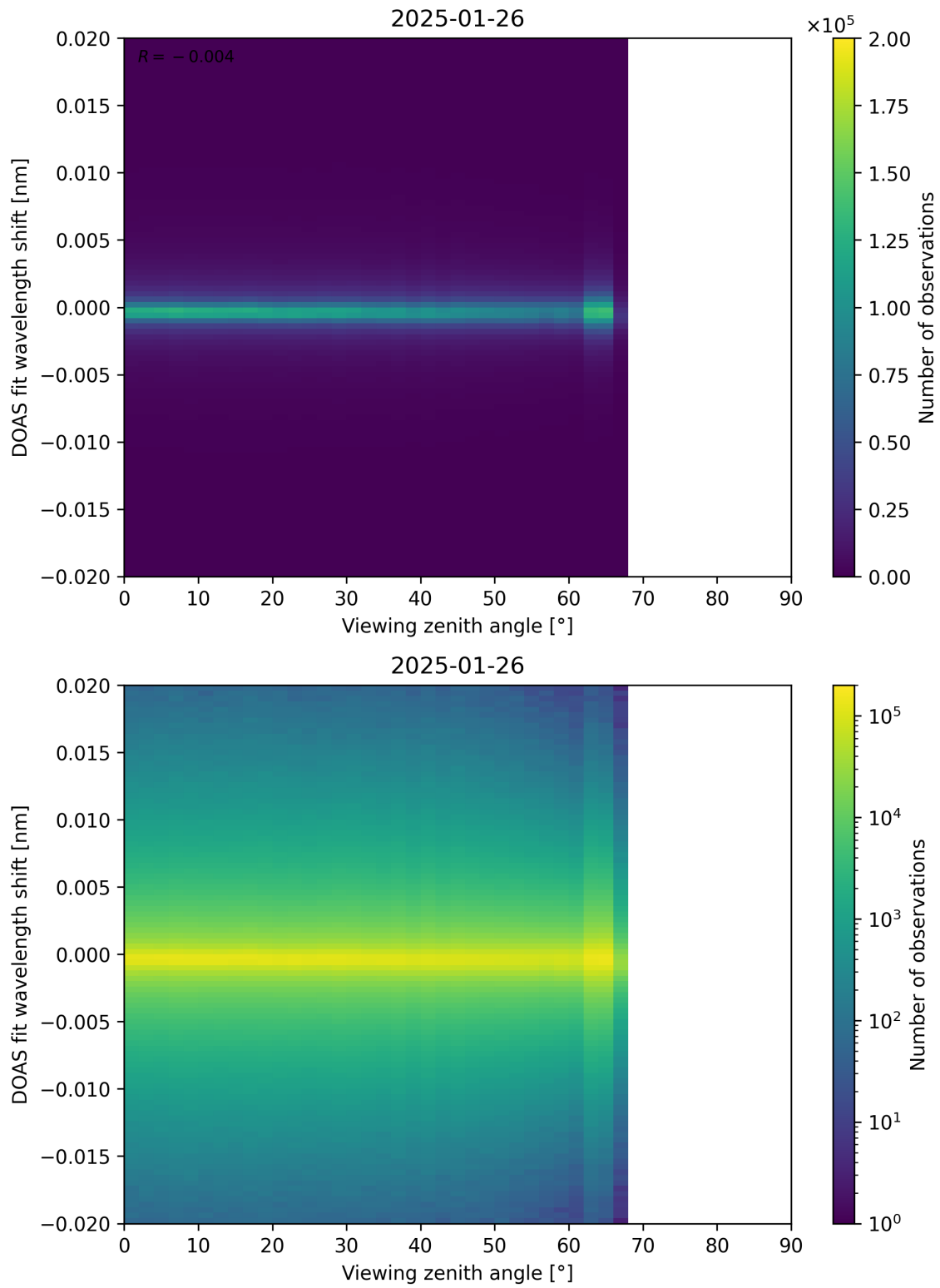
Figure 183: Scatter density plot of “Viewing zenith angle” against “DOAS fit wavelength shift” for 2025-01-25 to 2025-01-27.
