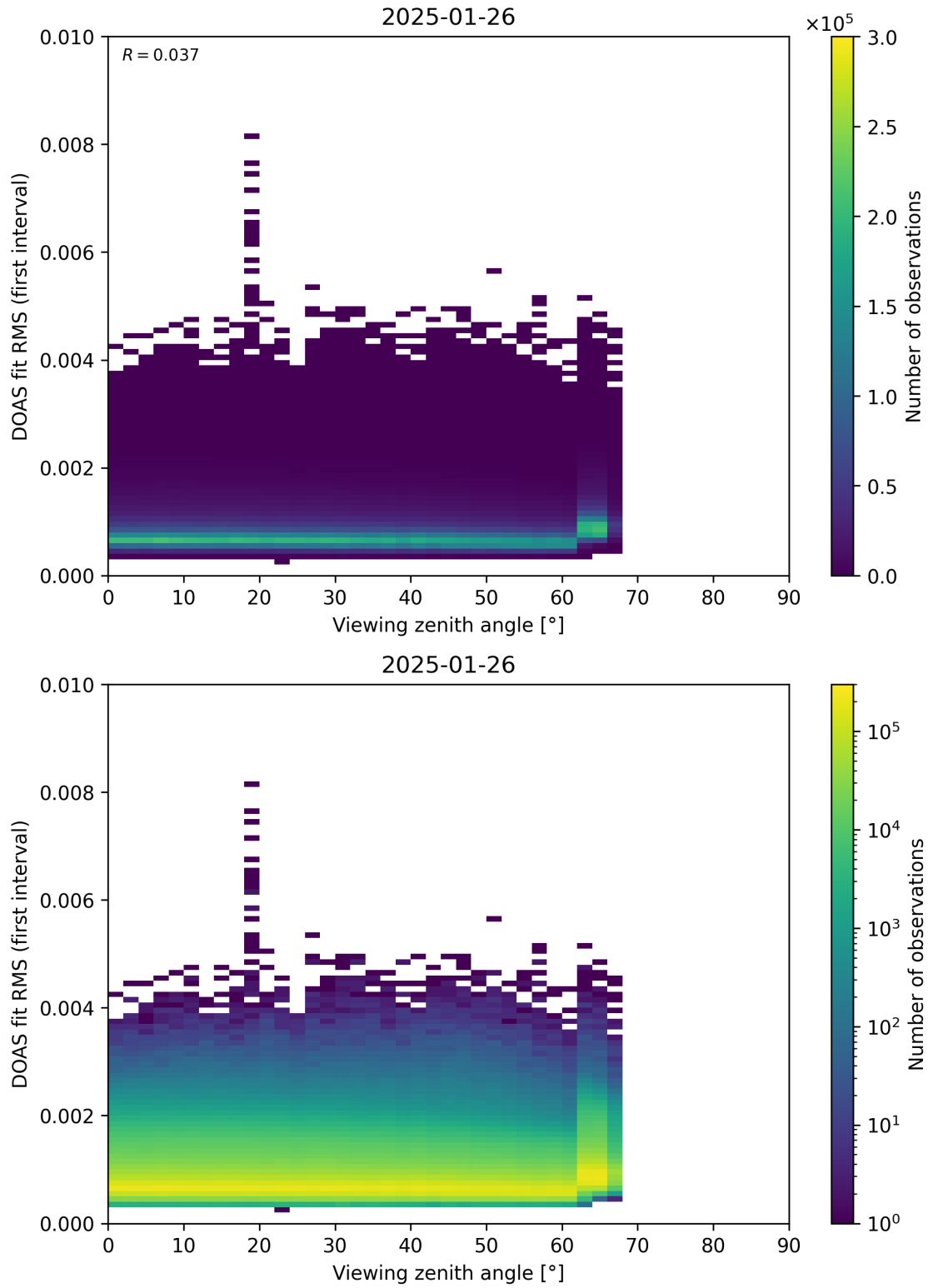
Figure 182: Scatter density plot of “Viewing zenith angle” against “DOAS fit RMS (first interval)” for 2025-01-25 to 2025-01-27.
