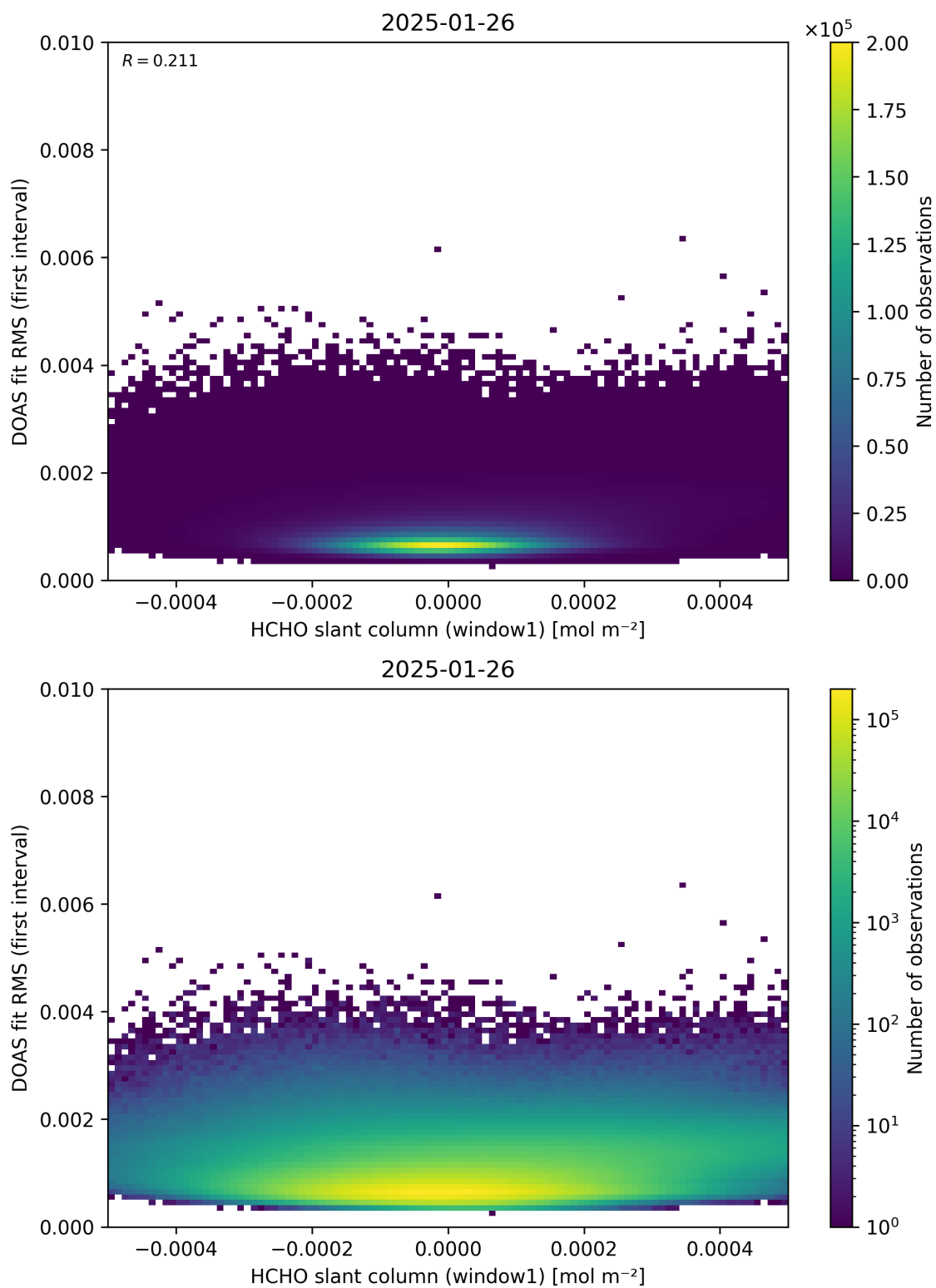
Figure 78: Scatter density plot of “HCHO slant column (window1)” against “DOAS fit RMS (first interval)” for 2025-01-25 to 2025-01-27.
