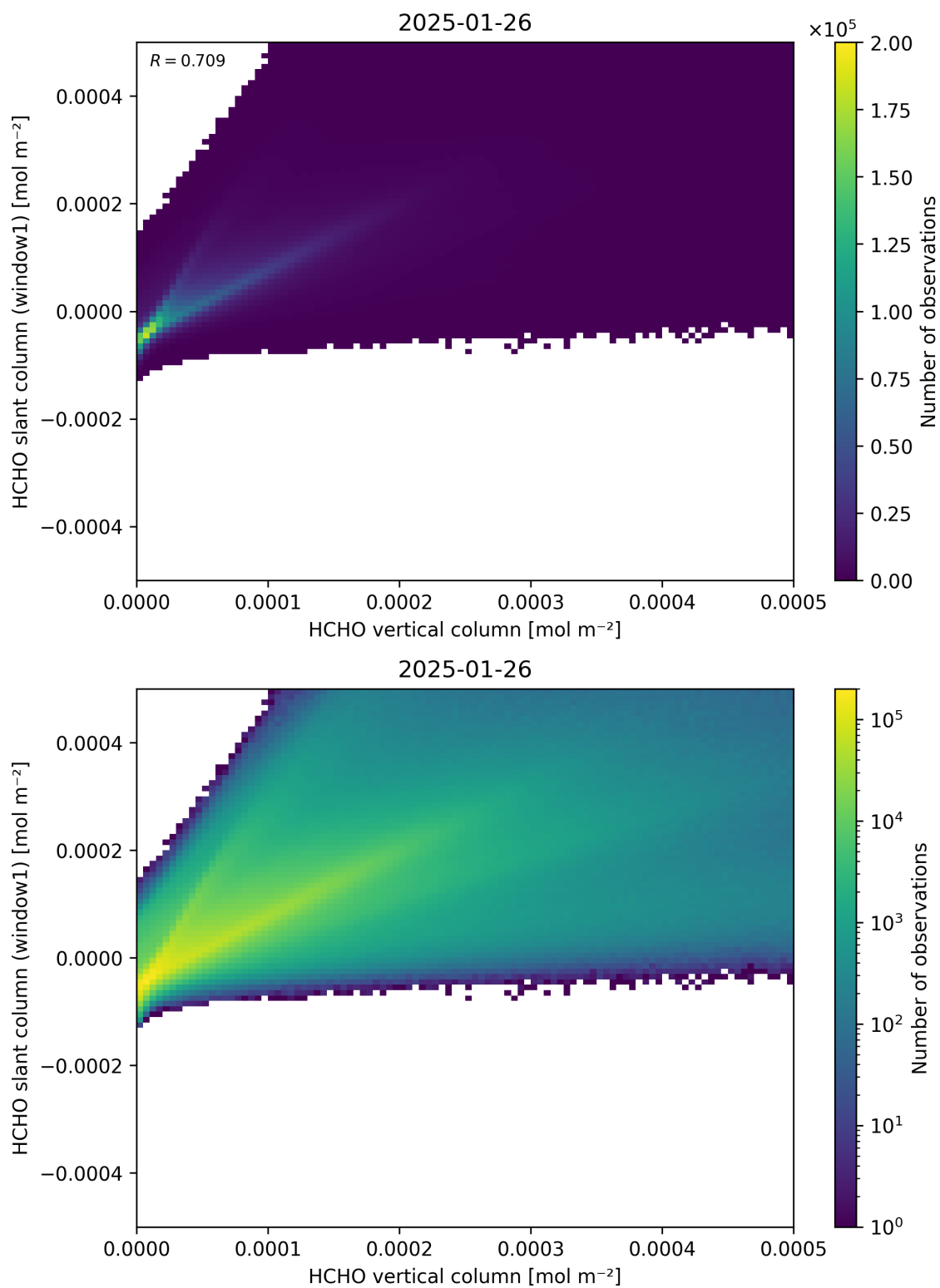
Figure 129: Scatter density plot of “HCHO vertical column” against “HCHO slant column (window1)” for 2025-01-25 to 2025-01-27.
