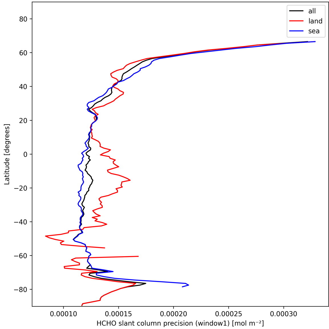
Figure 25: Zonal average of “HCHO slant column precision (window1)” for 2025-01-25 to 2025-01-27.
