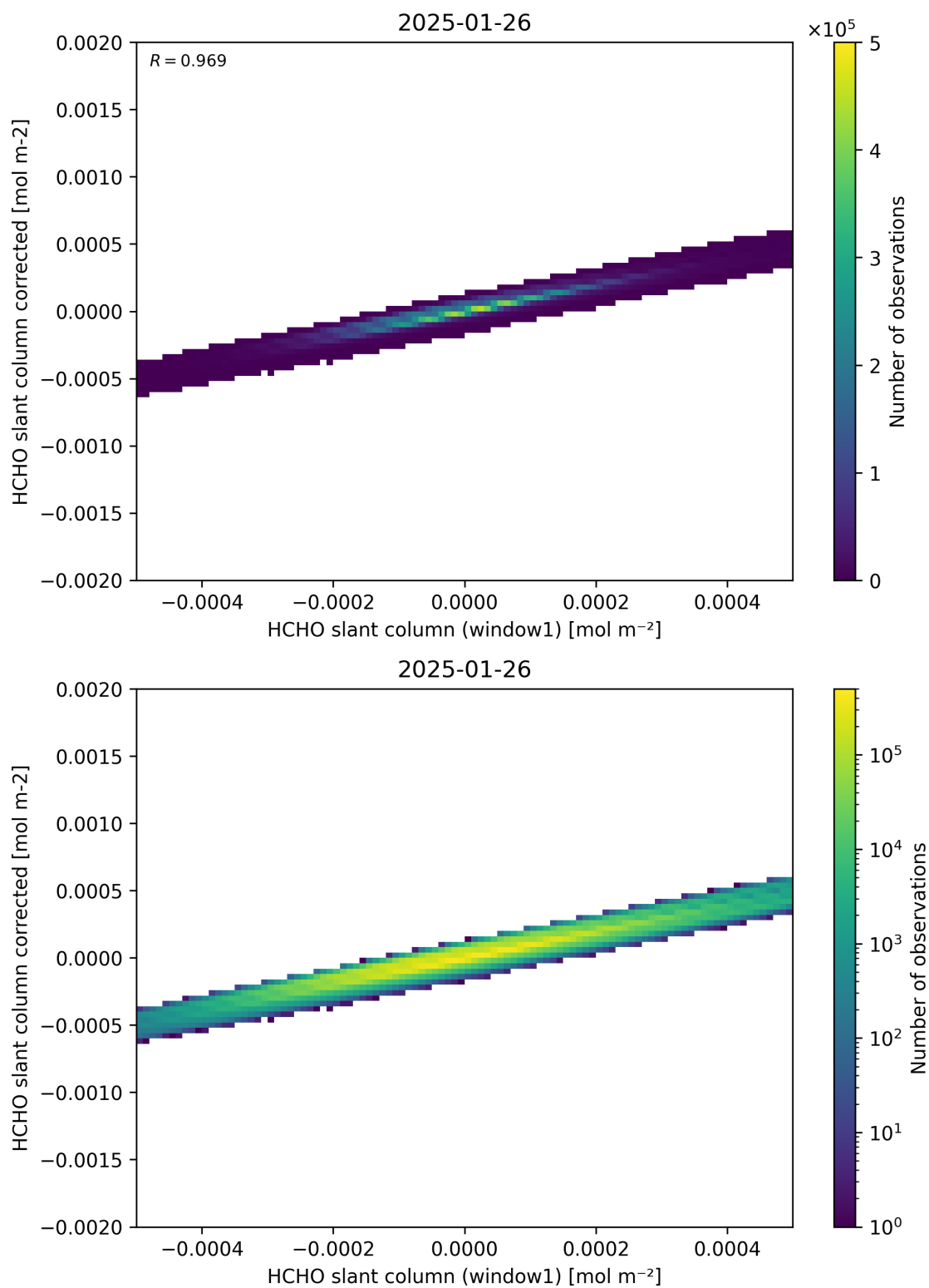
Figure 82: Scatter density plot of “HCHO slant column (window1)” against “HCHO slant column corrected” for 2025-01-25 to 2025-01-27.
