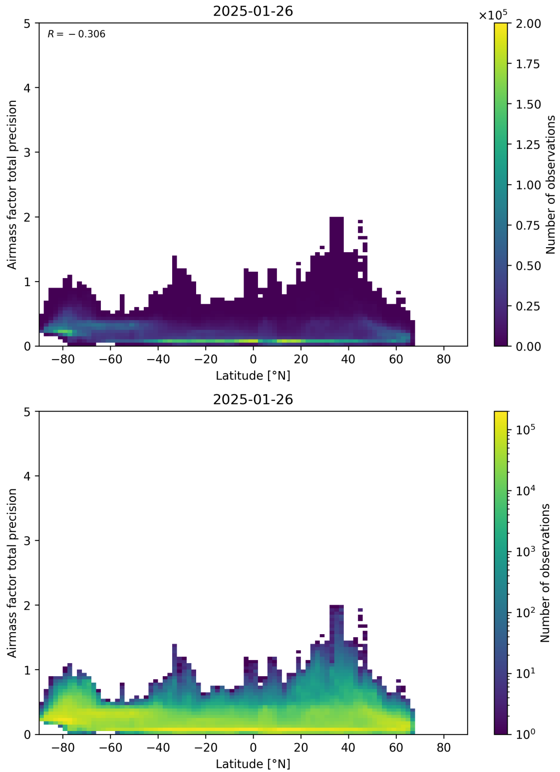
Figure 162: Scatter density plot of “Latitude” against “Airmass factor total precision” for 2025-01-25 to 2025-01-27.
