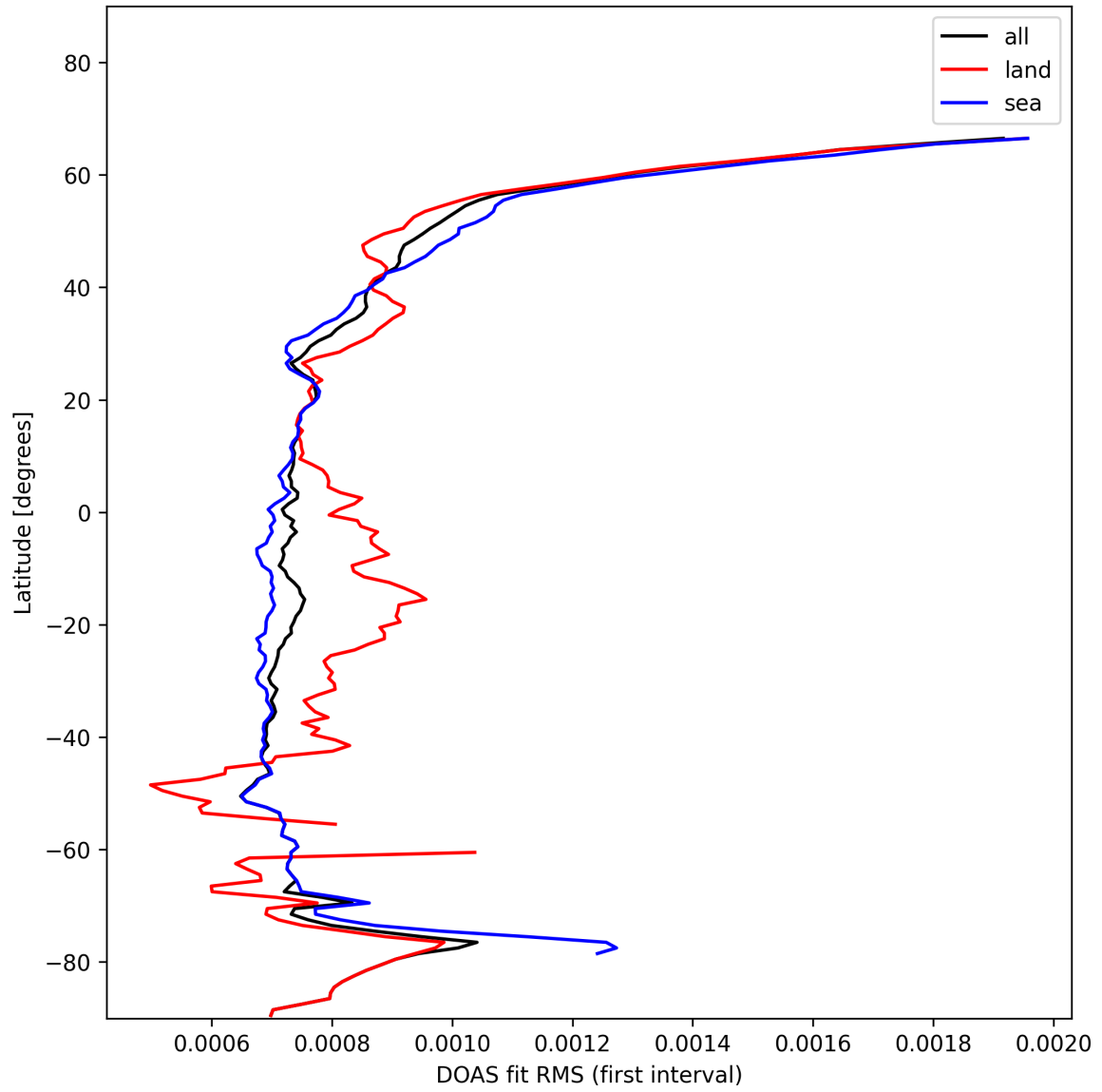
Figure 32: Zonal average of “DOAS fit RMS (first interval)” for 2025-01-25 to 2025-01-27.
