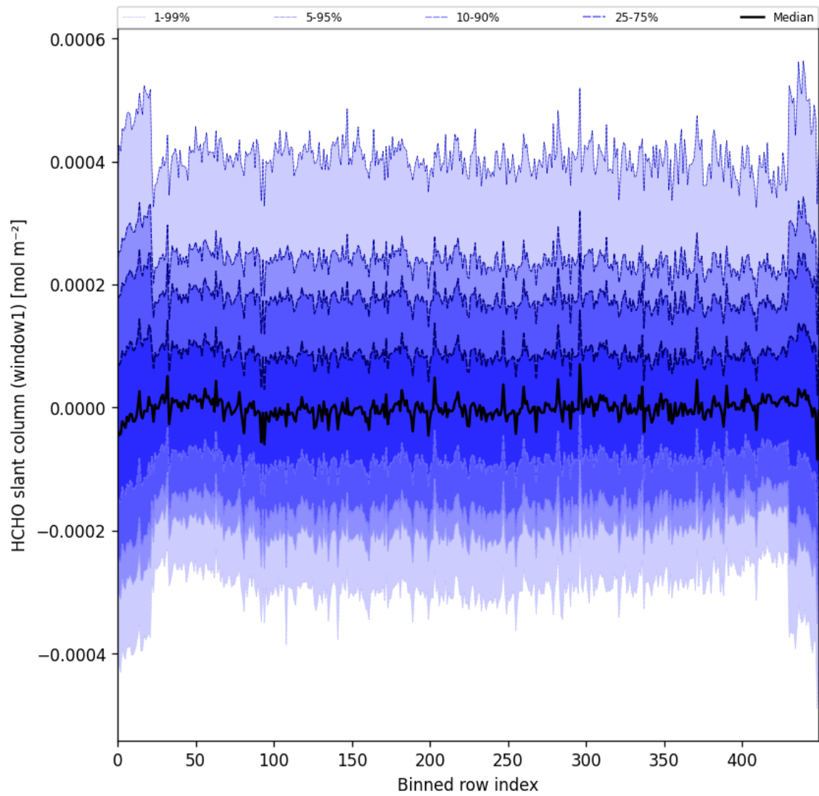
Figure 52: Along track statistics of "HCHO slant column (window1)" for 2025-01-25 to 2025-01-27
