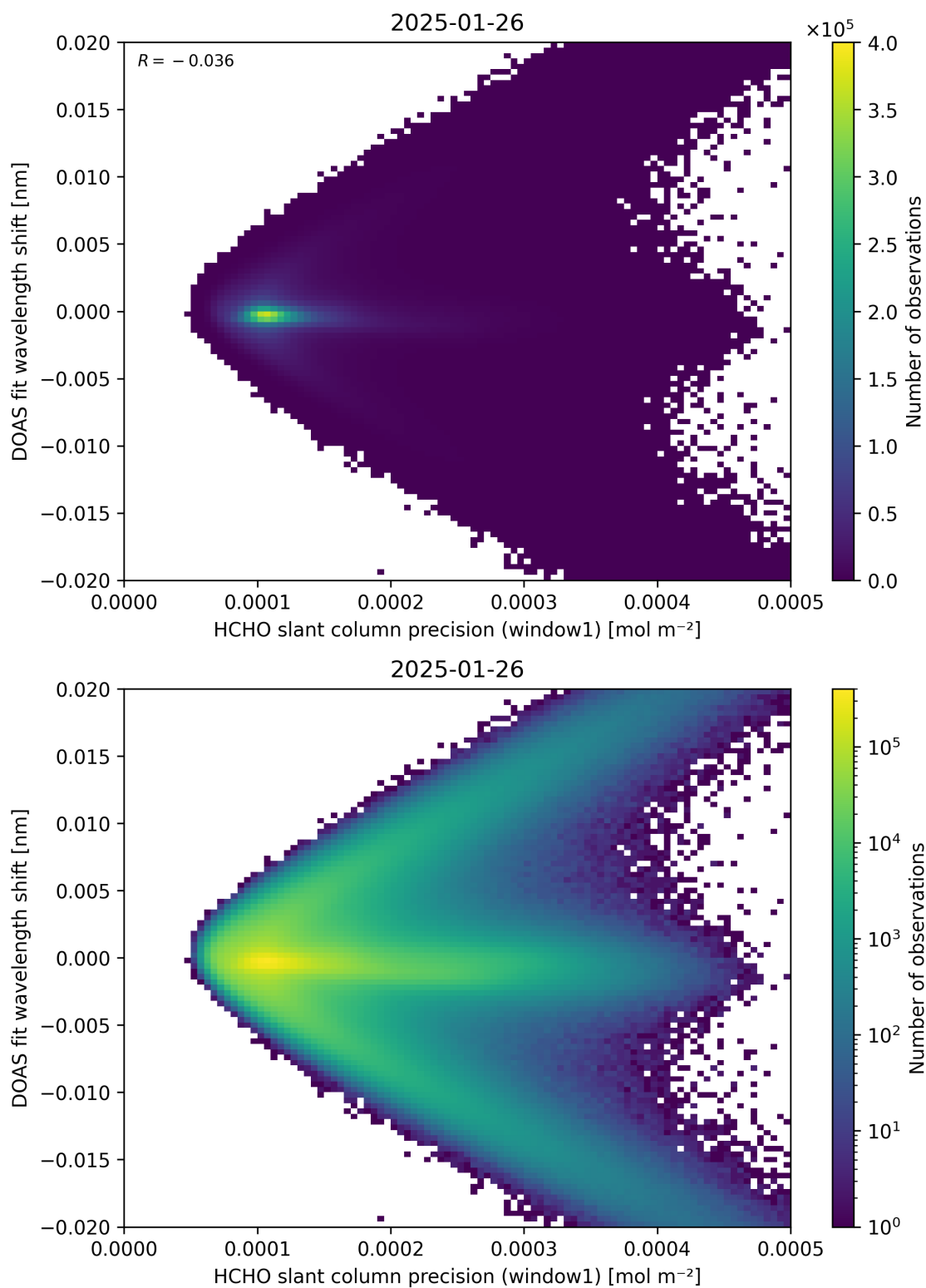
Figure 89: Scatter density plot of “HCHO slant column precision (window1)” against “DOAS fit wavelength shift” for 2025-01-25 to 2025-01-27.
