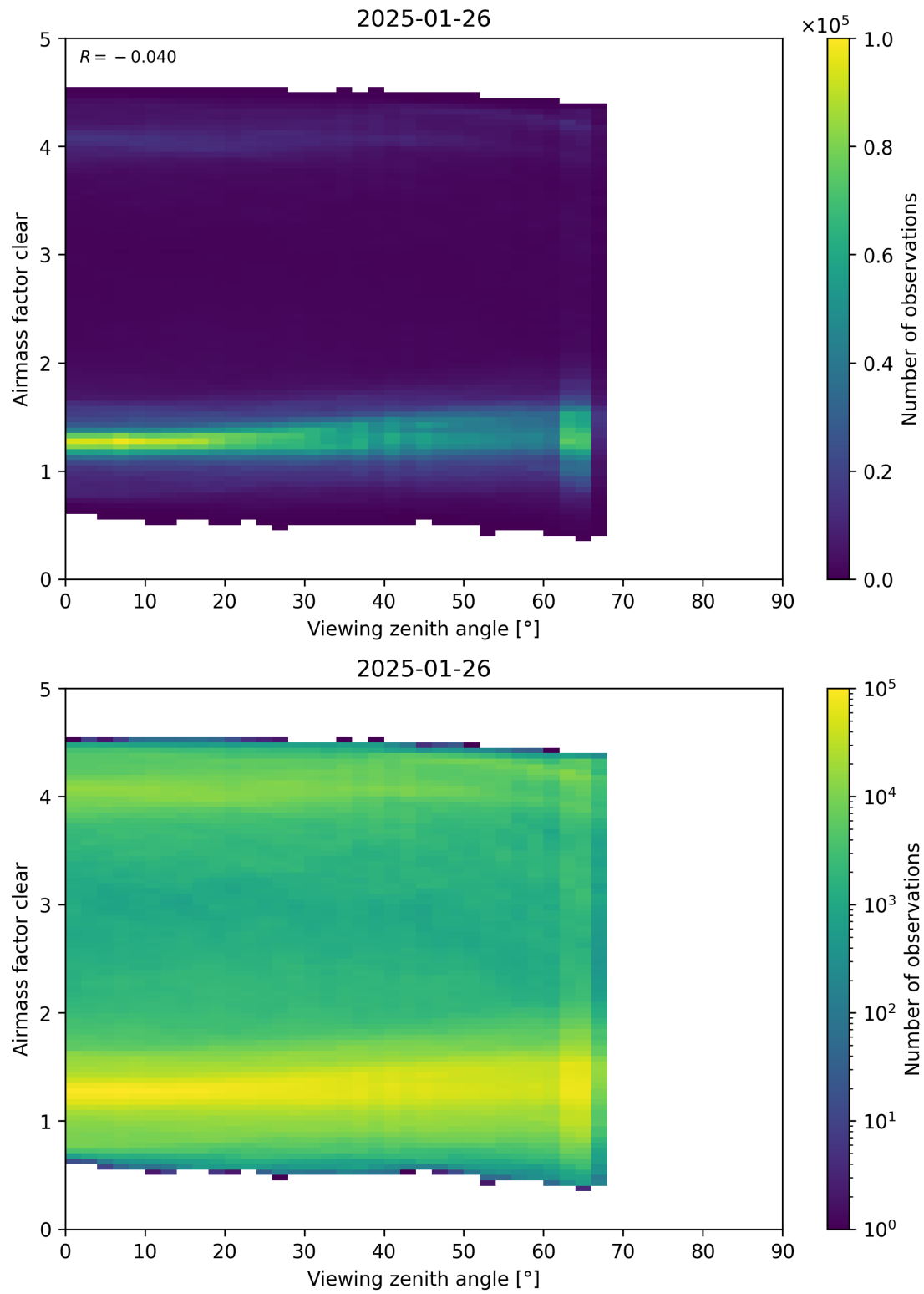
Figure 185: Scatter density plot of “Viewing zenith angle” against “Airmass factor clear” for 2025-01-25 to 2025-01-27.
