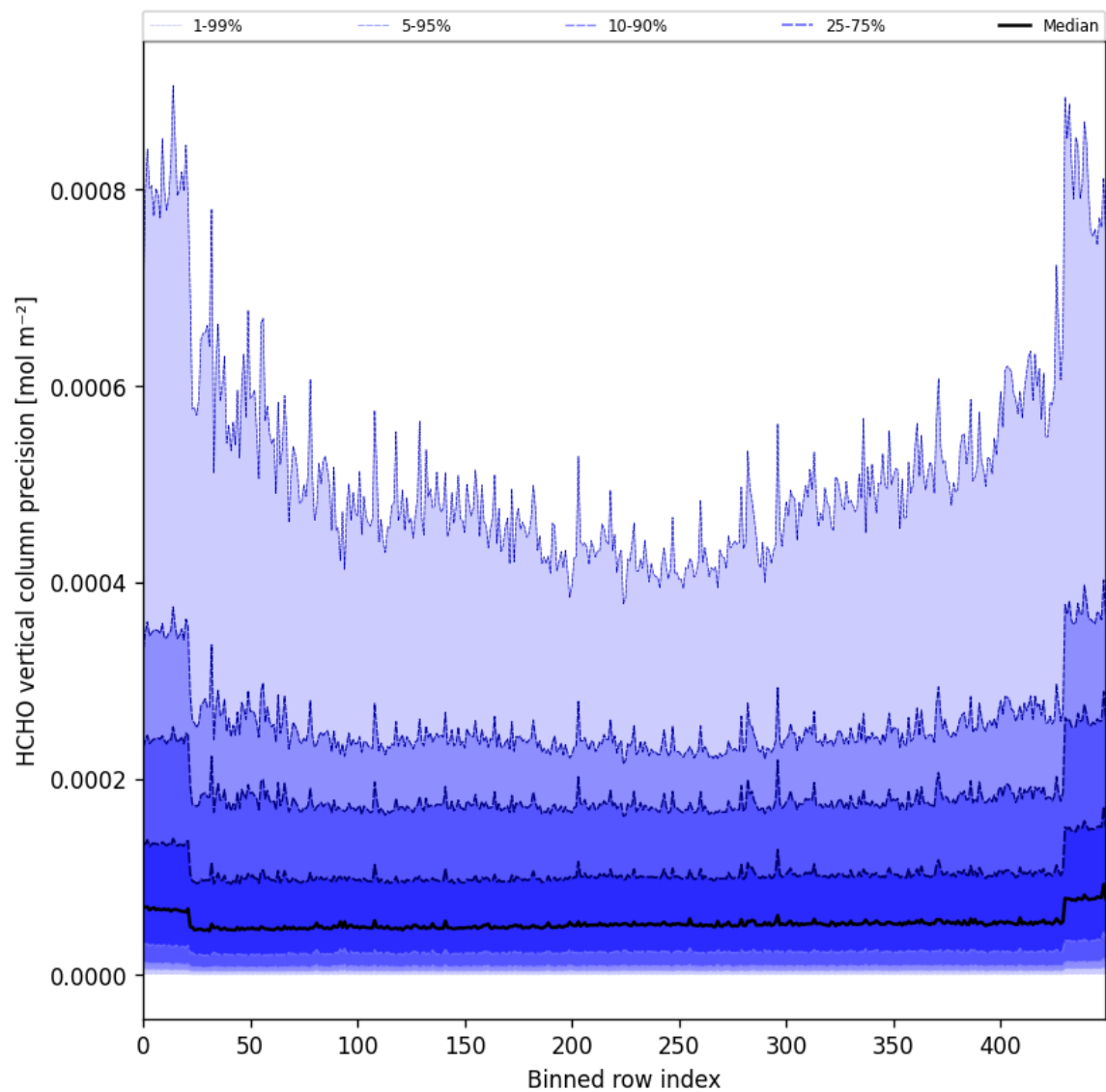
Figure 50: Along track statistics of “HCHO vertical column precision” for 2025-01-25 to 2025-01-27
