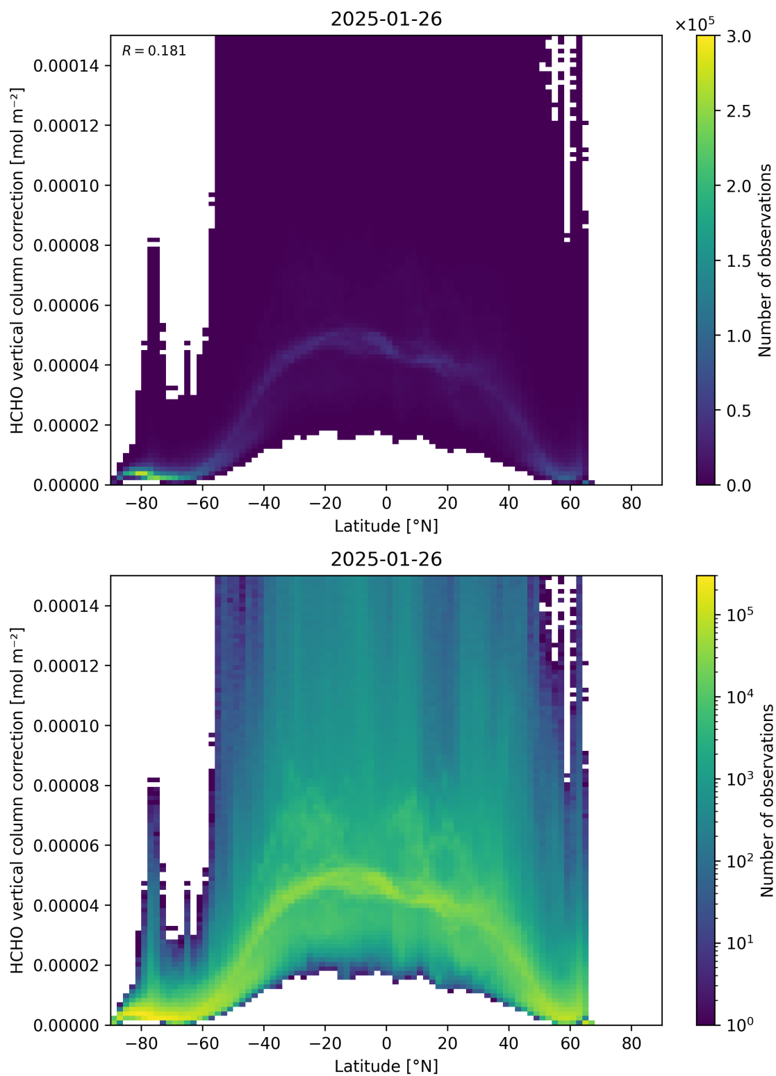
Figure 164: Scatter density plot of “Latitude” against “HCHO vertical column correction” for 2025-01-25 to 2025-01-27.
