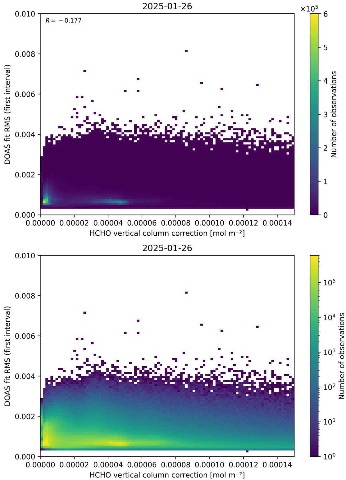
Figure 112: Scatter density plot of “HCHO vertical column correction” against “DOAS fit RMS (first interval)” for 2025-01-25 to 2025-01-27.
