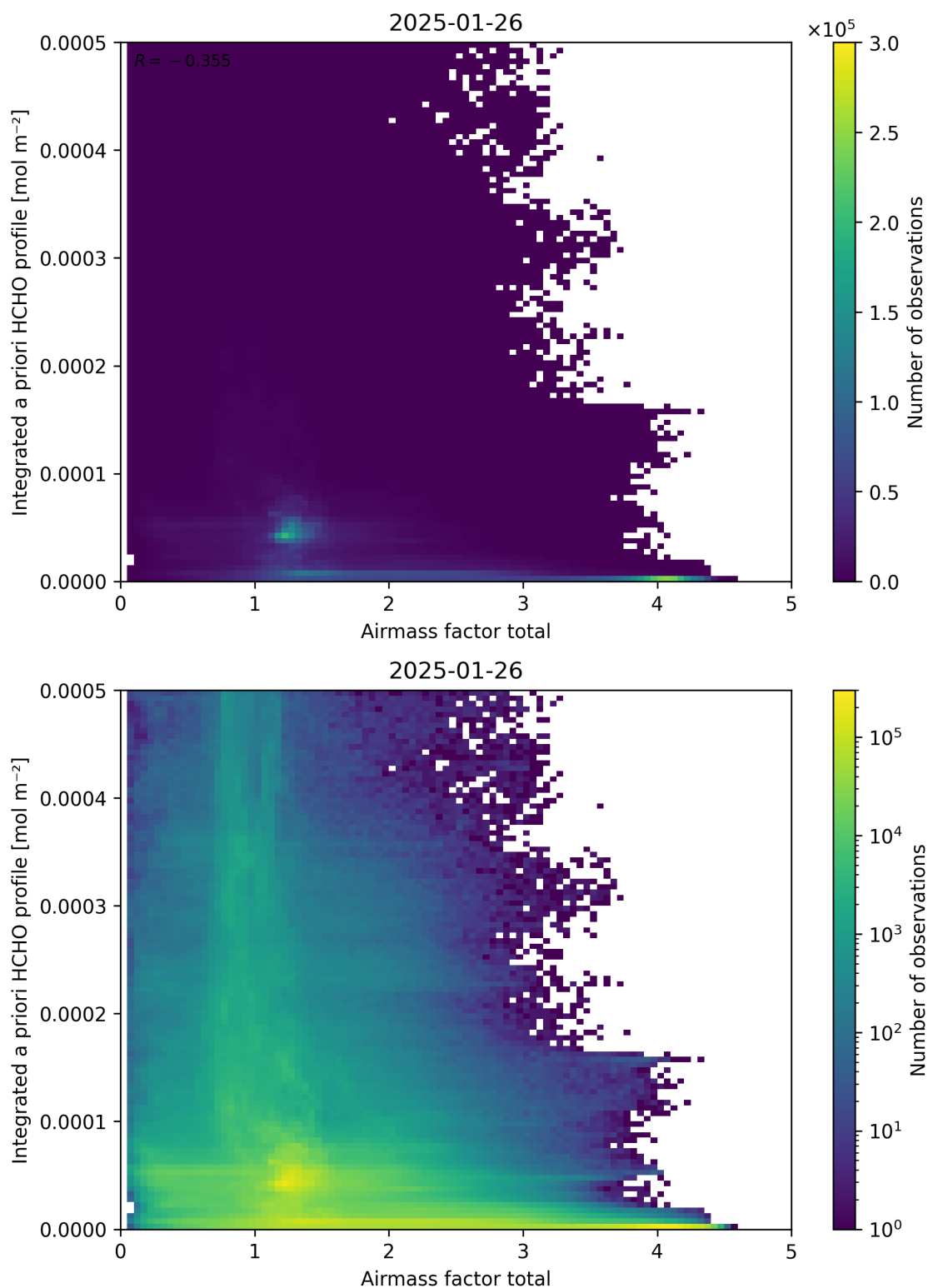
Figure 104: Scatter density plot of “Airmass factor total” against “Integrated a priori HCHO profile” for 2025-01-25 to 2025-01-27.
