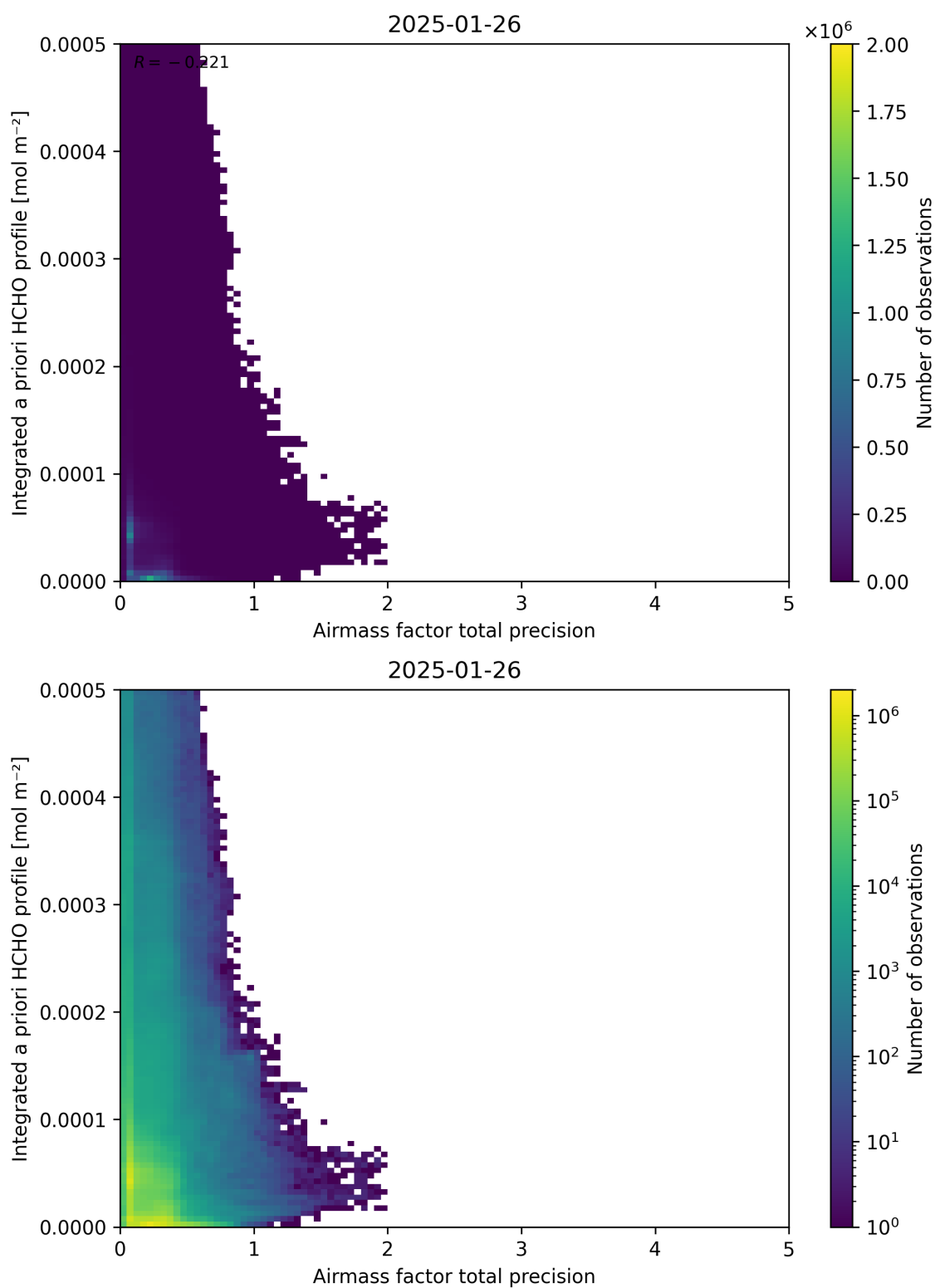
Figure 111: Scatter density plot of “Airmass factor total precision” against “Integrated a priori HCHO profile” for 2025-01-25 to 2025-01-27.
