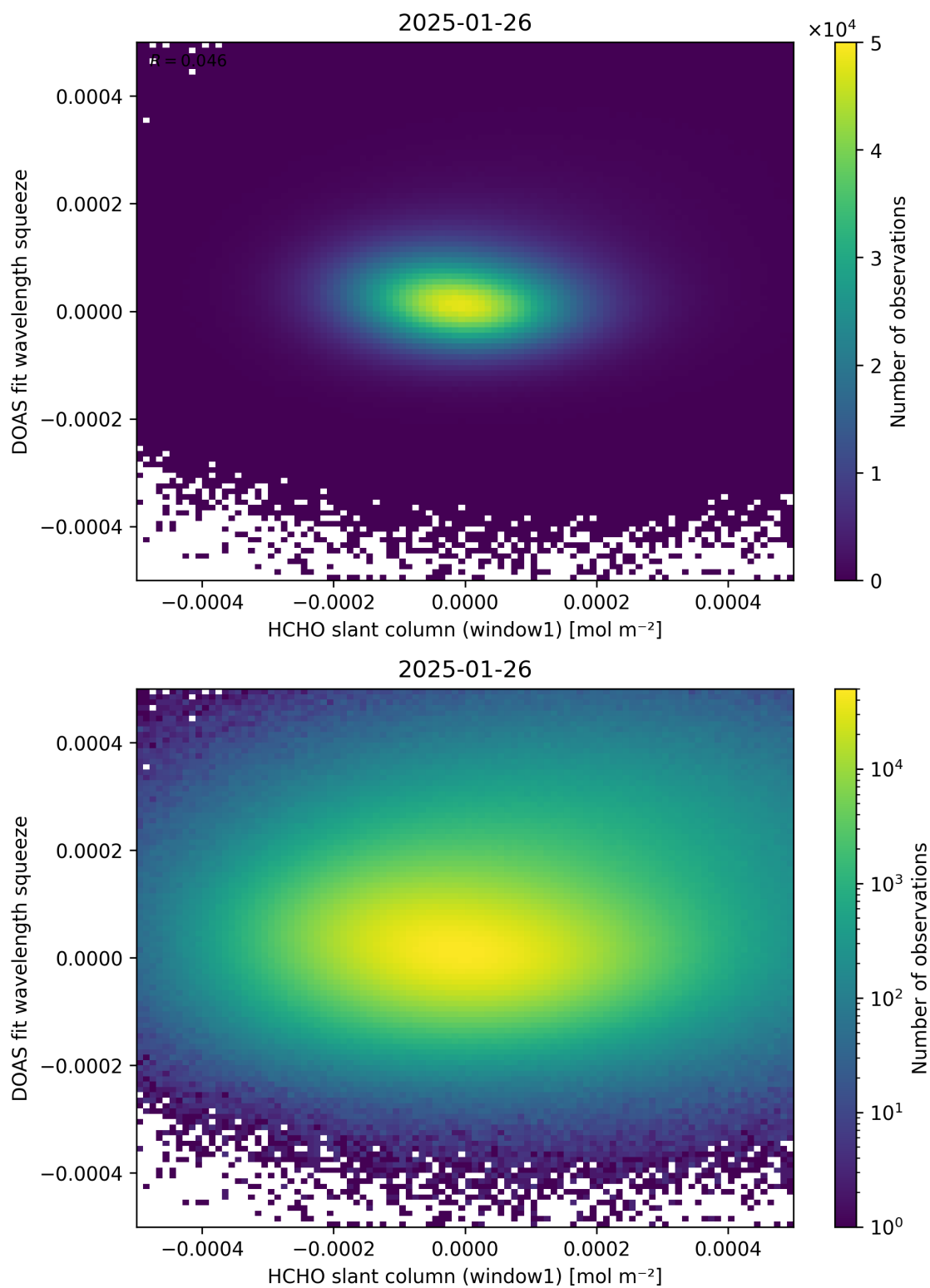
Figure 80: Scatter density plot of “HCHO slant column (window1)” against “DOAS fit wavelength squeeze” for 2025-01-25 to 2025-01-27.
