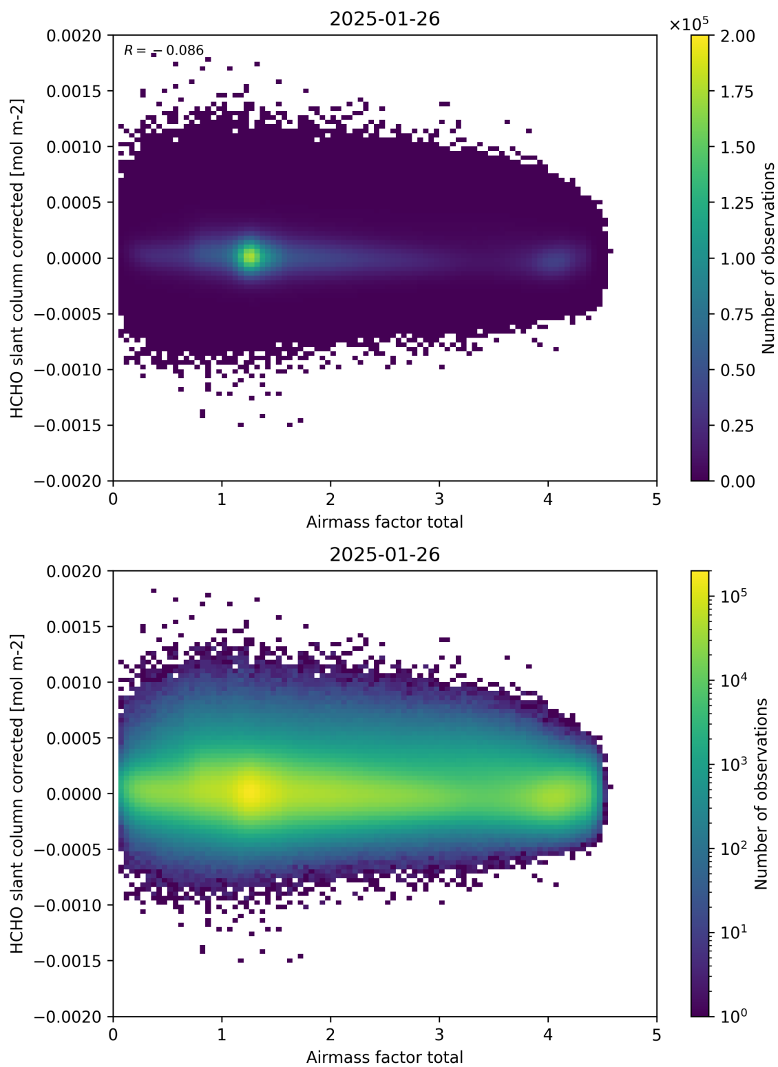
Figure 101: Scatter density plot of “Airmass factor total” against “HCHO slant column corrected” for 2025-01-25 to 2025-01-27.
