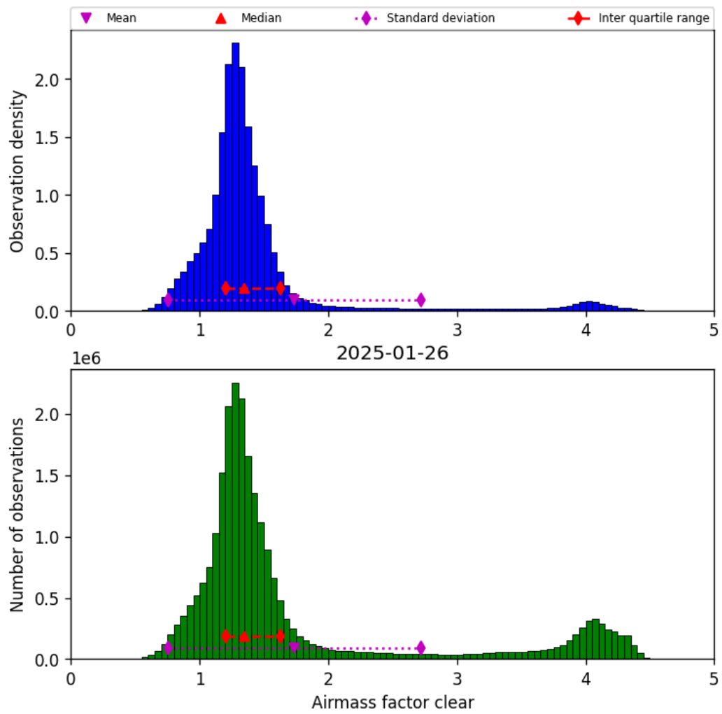
Figure 42: Histogram of “Airmass factor clear” for 2025-01-25 to 2025-01-27
