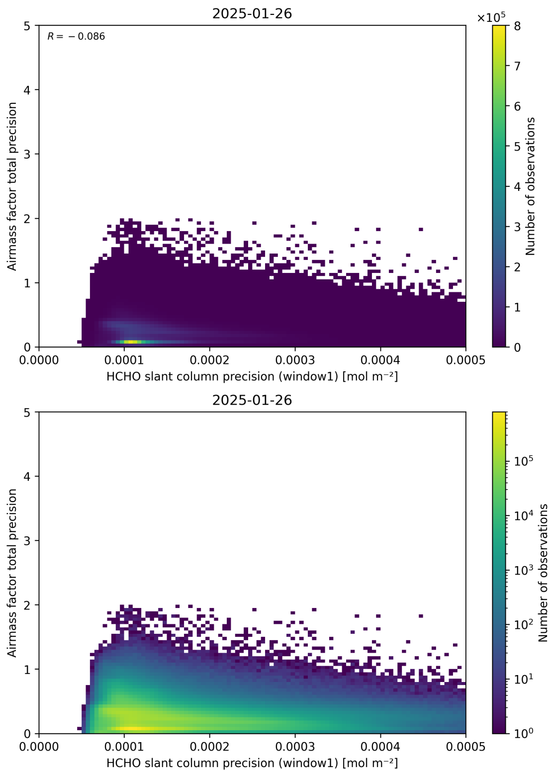
Figure 95: Scatter density plot of “HCHO slant column precision (window1)” against “Airmass factor total precision” for 2025-01-25 to 2025-01-27.
