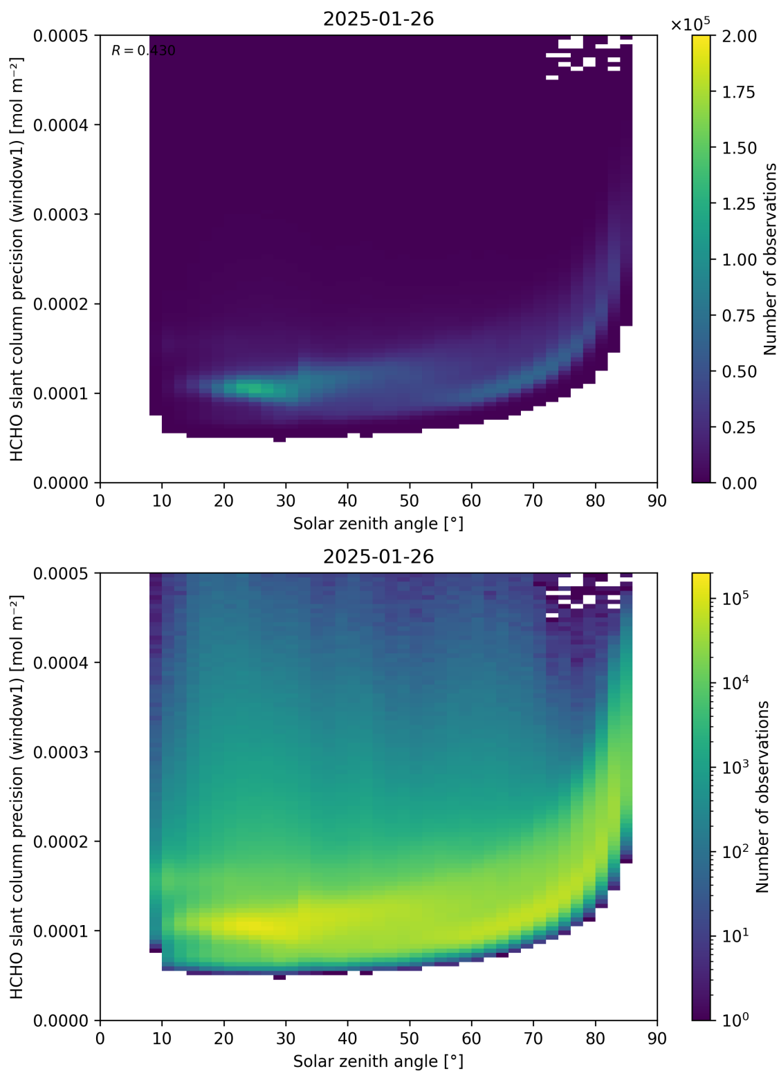
Figure 174: Scatter density plot of “Solar zenith angle” against “HCHO slant column precision (window1)” for 2025-01-25 to 2025-01-27.
