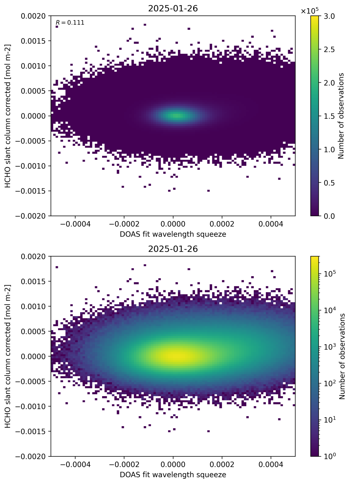
Figure 69: Scatter density plot of “DOAS fit wavelength squeeze” against “HCHO slant column corrected” for 2025-01-25 to 2025-01-27.
