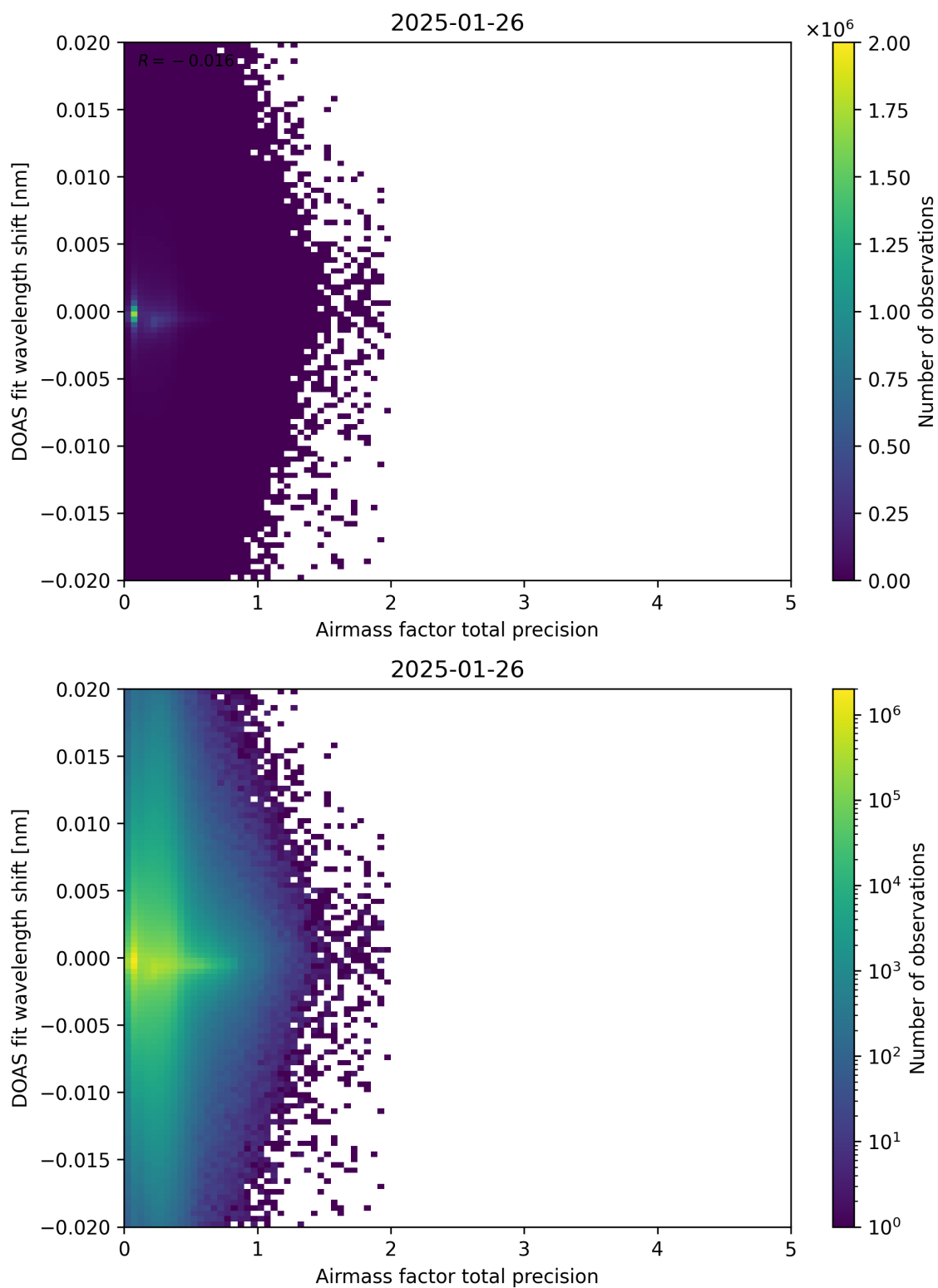
Figure 106: Scatter density plot of “Airmass factor total precision” against “DOAS fit wavelength shift” for 2025-01-25 to 2025-01-27.
