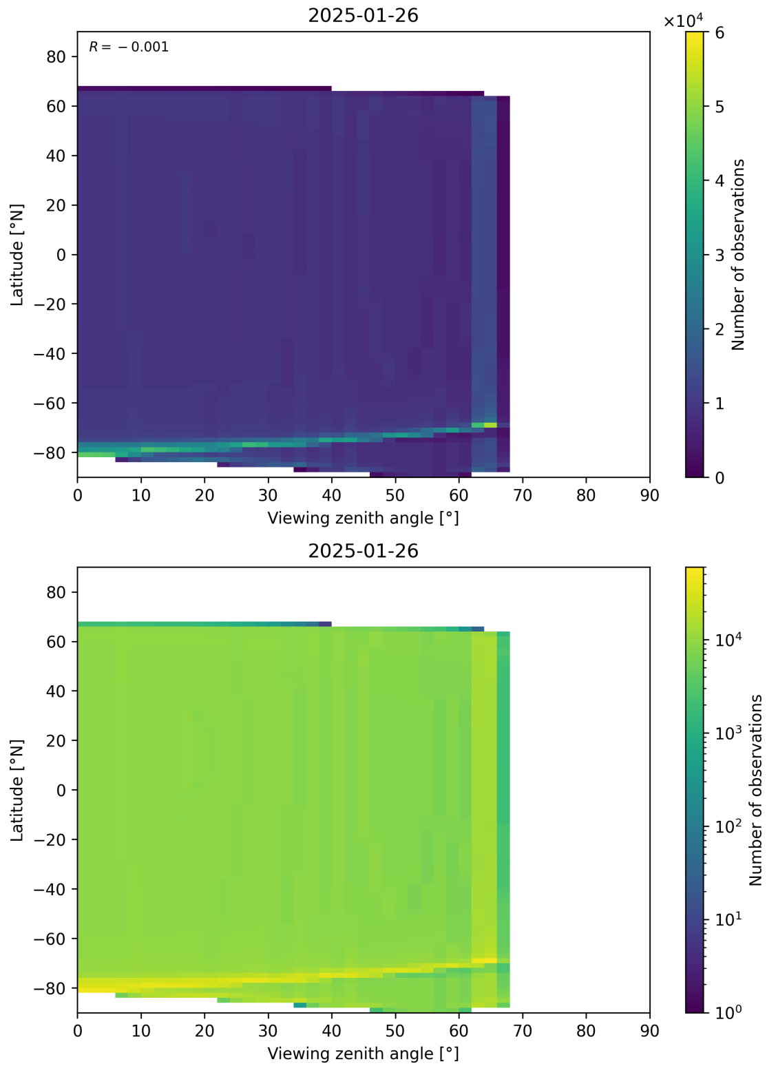
Figure 196: Scatter density plot of “Viewing zenith angle” against “Latitude” for 2025-01-25 to 2025-01-27.
