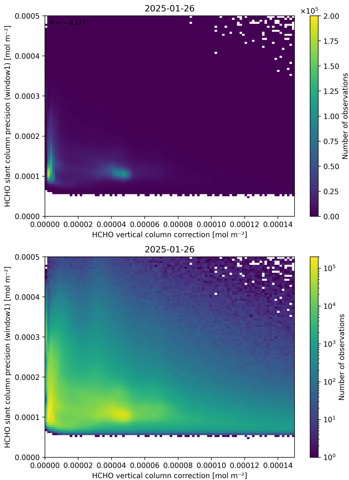
Figure 119: Scatter density plot of “HCHO vertical column correction” against “HCHO slant column precision (window1)” for 2025-01-25 to 2025-01-27.
