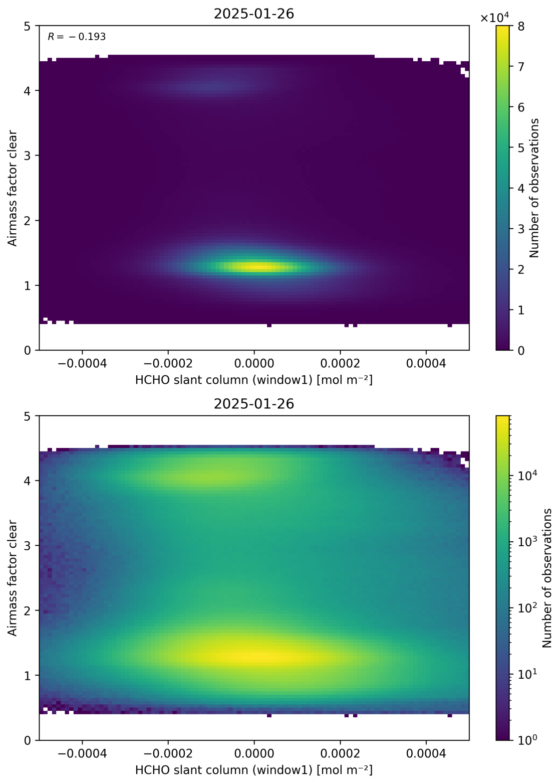
Figure 81: Scatter density plot of “HCHO slant column (window1)” against “Airmass factor clear” for 2025-01-25 to 2025-01-27.
