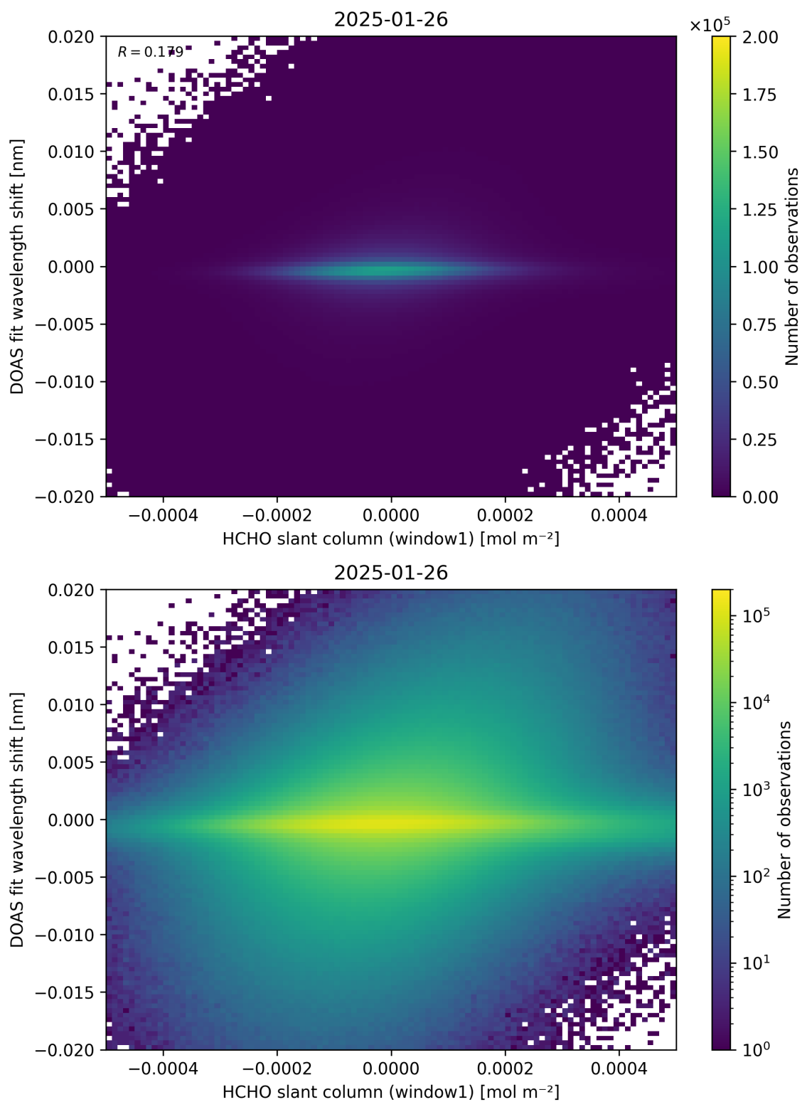
Figure 79: Scatter density plot of “HCHO slant column (window1)” against “DOAS fit wavelength shift” for 2025-01-25 to 2025-01-27.
