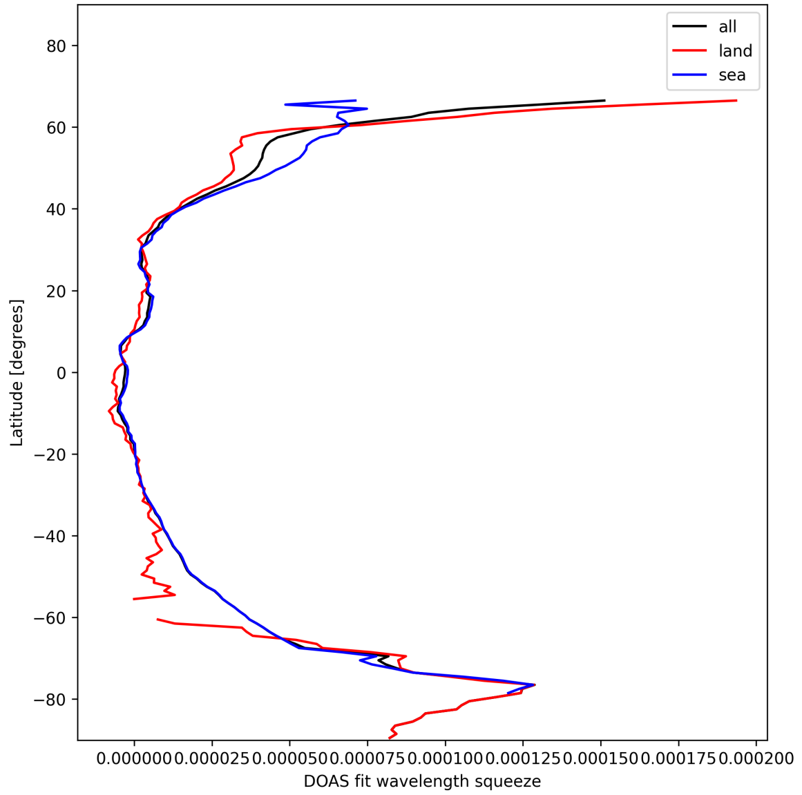
Figure 31: Zonal average of “DOAS fit wavelength squeeze” for 2025-01-25 to 2025-01-27.
