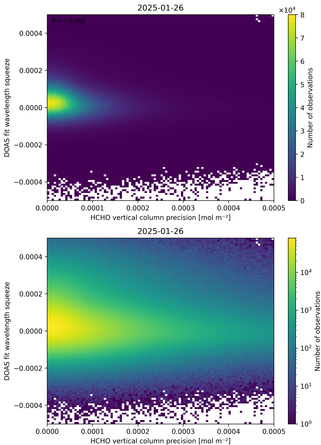
Figure 138: Scatter density plot of “HCHO vertical column precision” against “DOAS fit wavelength squeeze” for 2025-01-25 to 2025-01-27.
