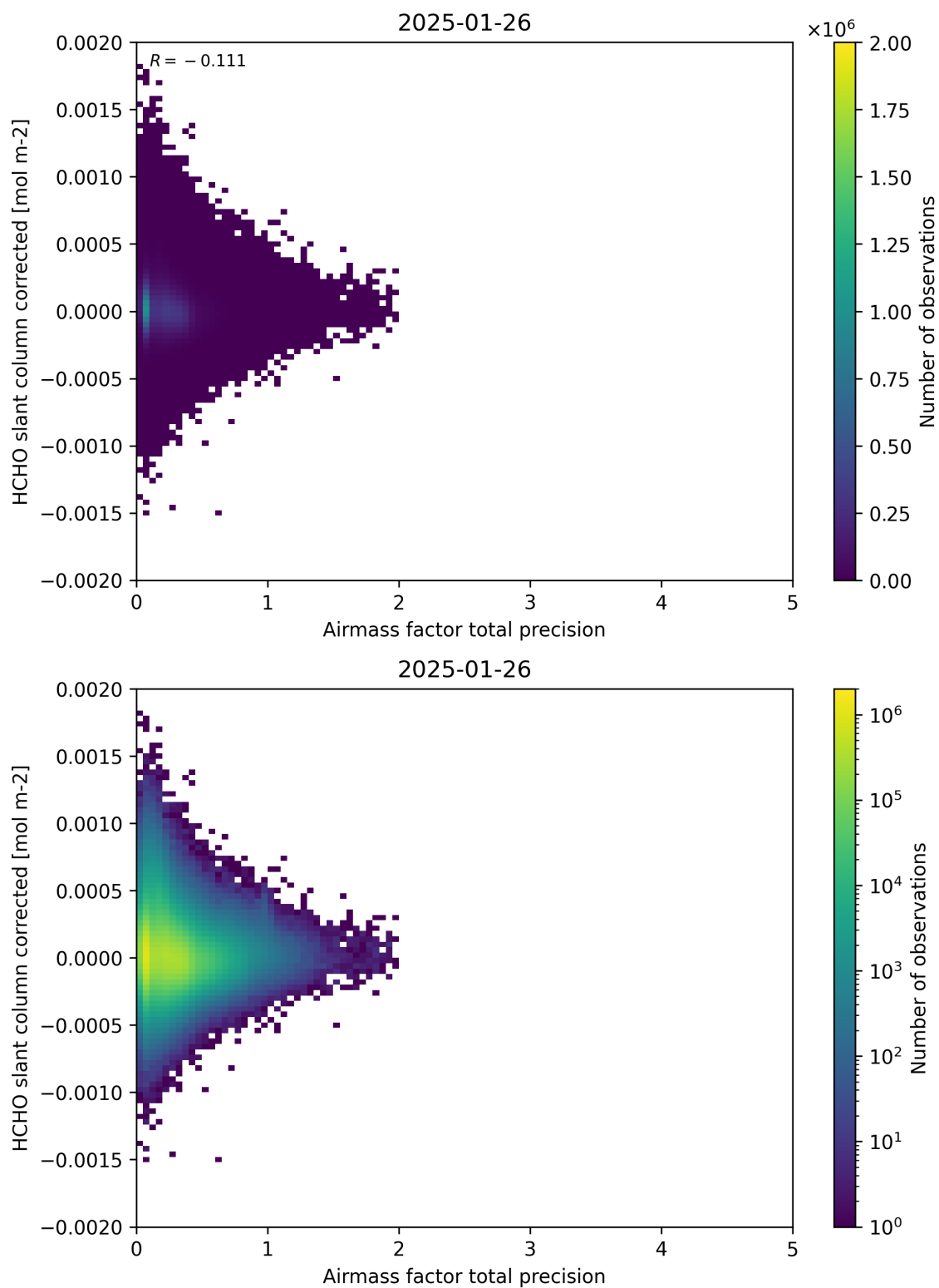
Figure 109: Scatter density plot of “Airmass factor total precision” against “HCHO slant column corrected” for 2025-01-25 to 2025-01-27.
