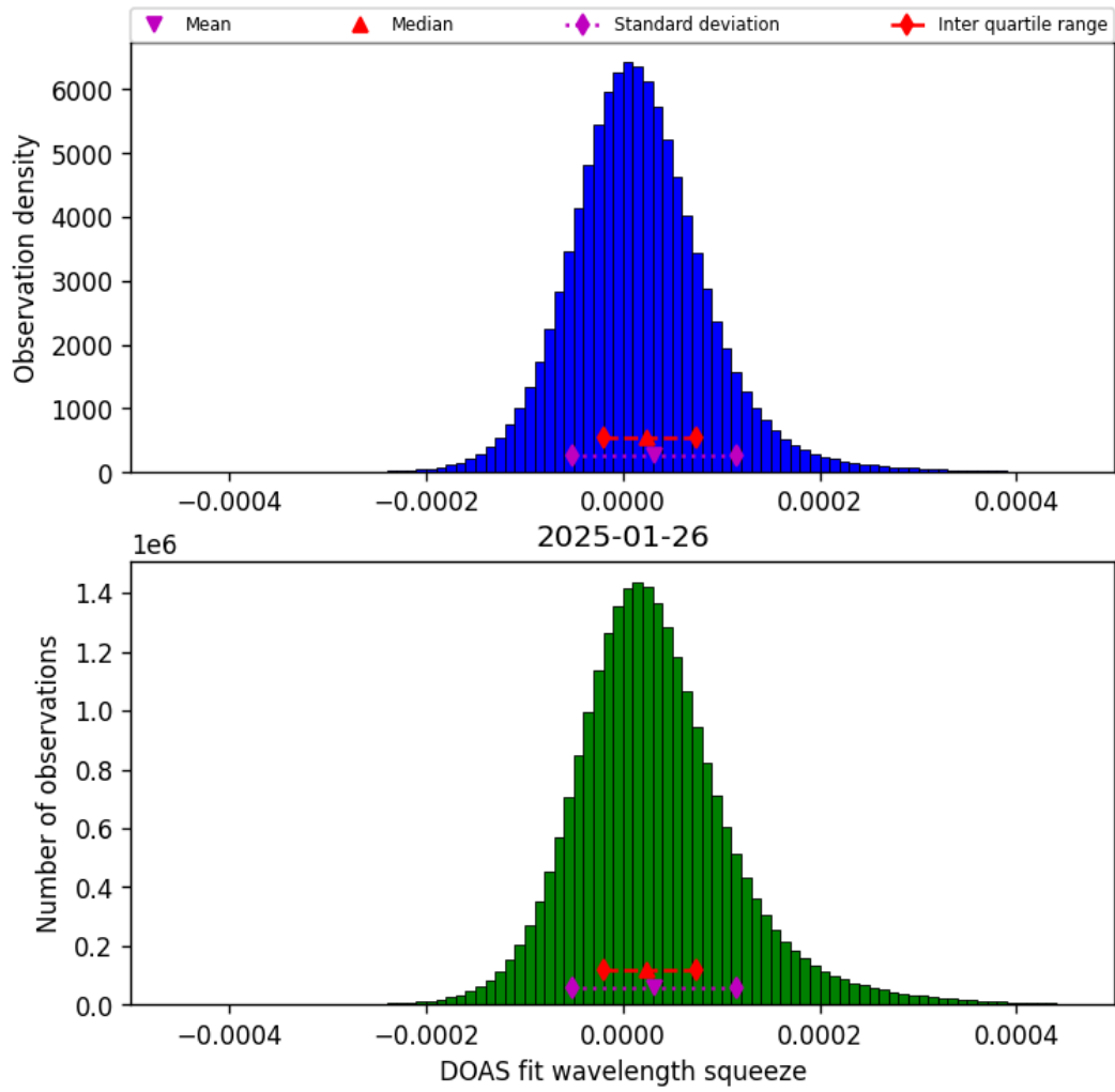
Figure 45: Histogram of “DOAS fit wavelength squeeze” for 2025-01-25 to 2025-01-27
