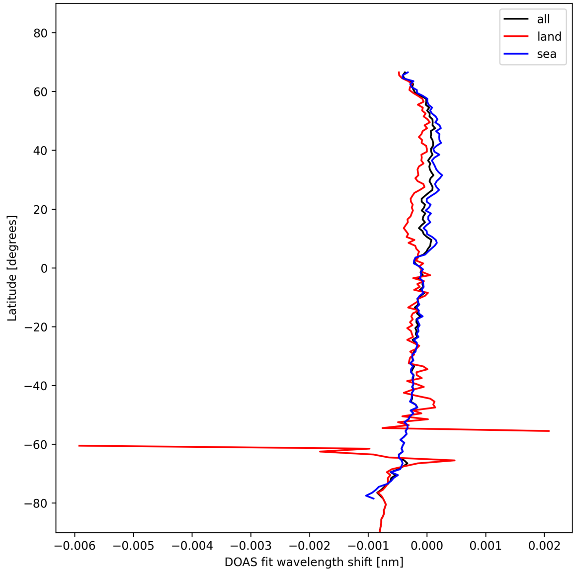
Figure 30: Zonal average of “DOAS fit wavelength shift” for 2025-01-25 to 2025-01-27.
