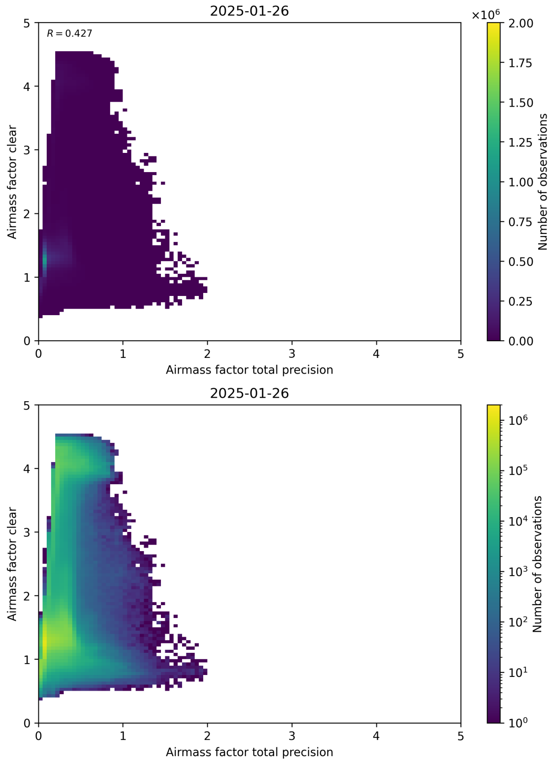
Figure 108: Scatter density plot of “Airmass factor total precision” against “Airmass factor clear” for 2025-01-25 to 2025-01-27.
