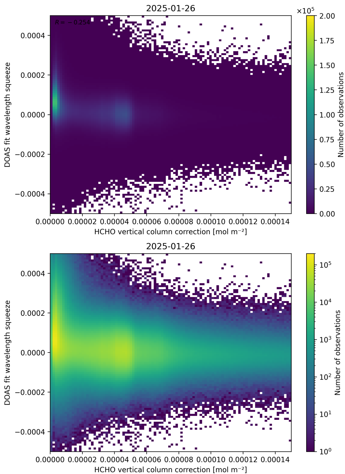
Figure 114: Scatter density plot of “HCHO vertical column correction” against “DOAS fit wavelength squeeze” for 2025-01-25 to 2025-01-27.
