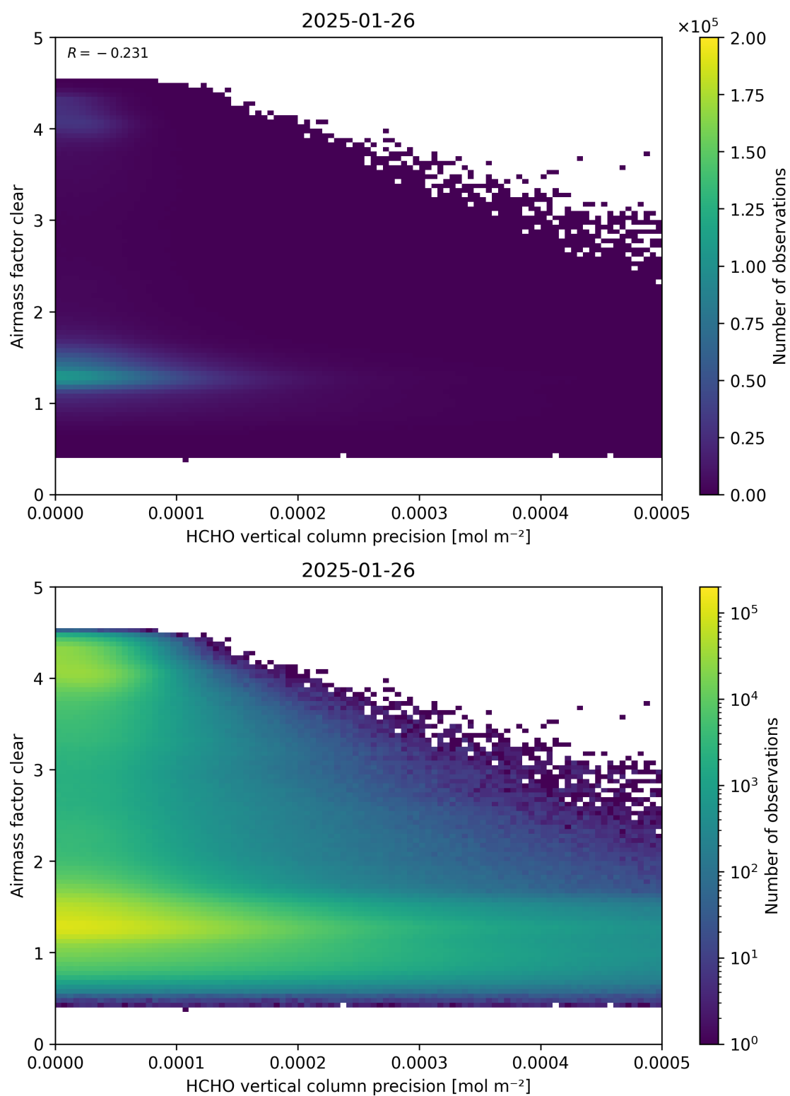
Figure 139: Scatter density plot of “HCHO vertical column precision” against “Airmass factor clear” for 2025-01-25 to 2025-01-27.
