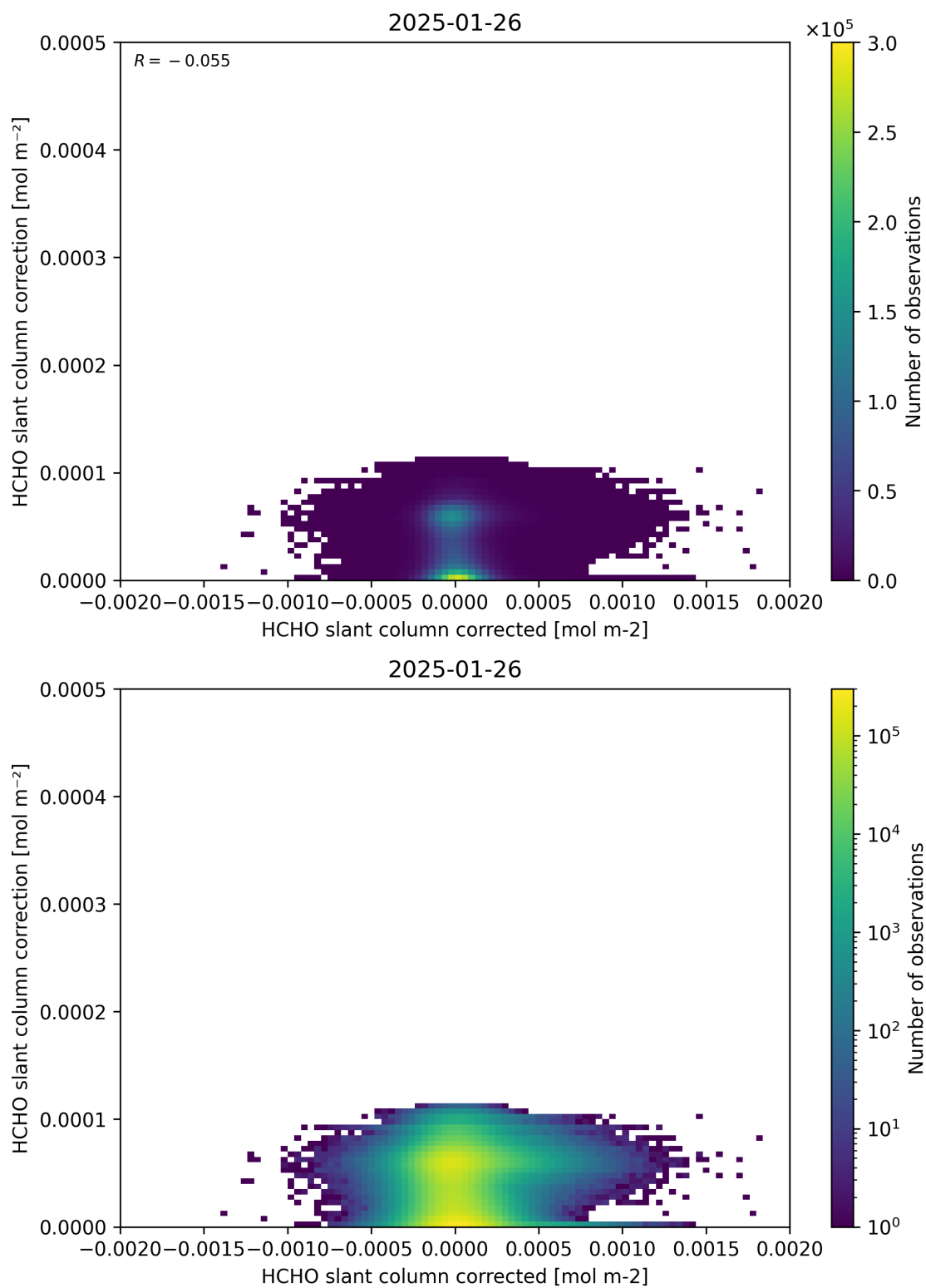
Figure 77: Scatter density plot of “HCHO slant column corrected” against “HCHO slant column correction” for 2025-01-25 to 2025-01-27.
