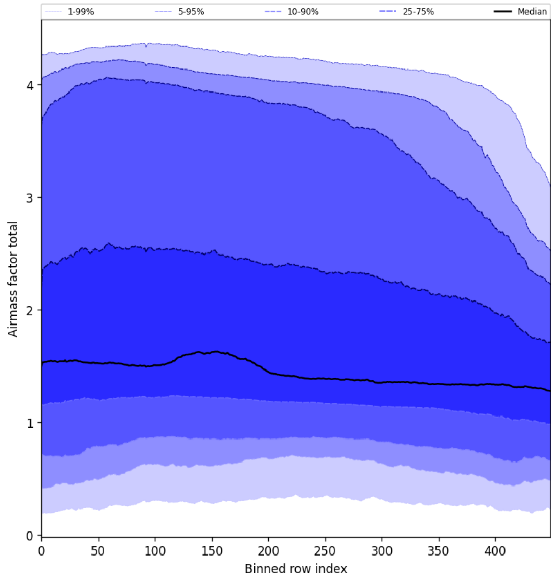
Figure 54: Along track statistics of “Airmass factor total” for 2025-01-25 to 2025-01-27
