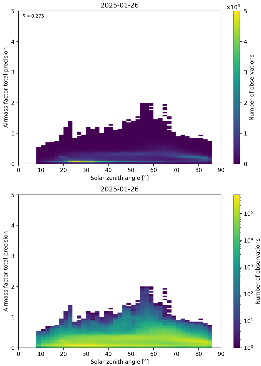
Figure 176: Scatter density plot of “Solar zenith angle” against “Airmass factor total precision” for 2025-01-25 to 2025-01-27.
