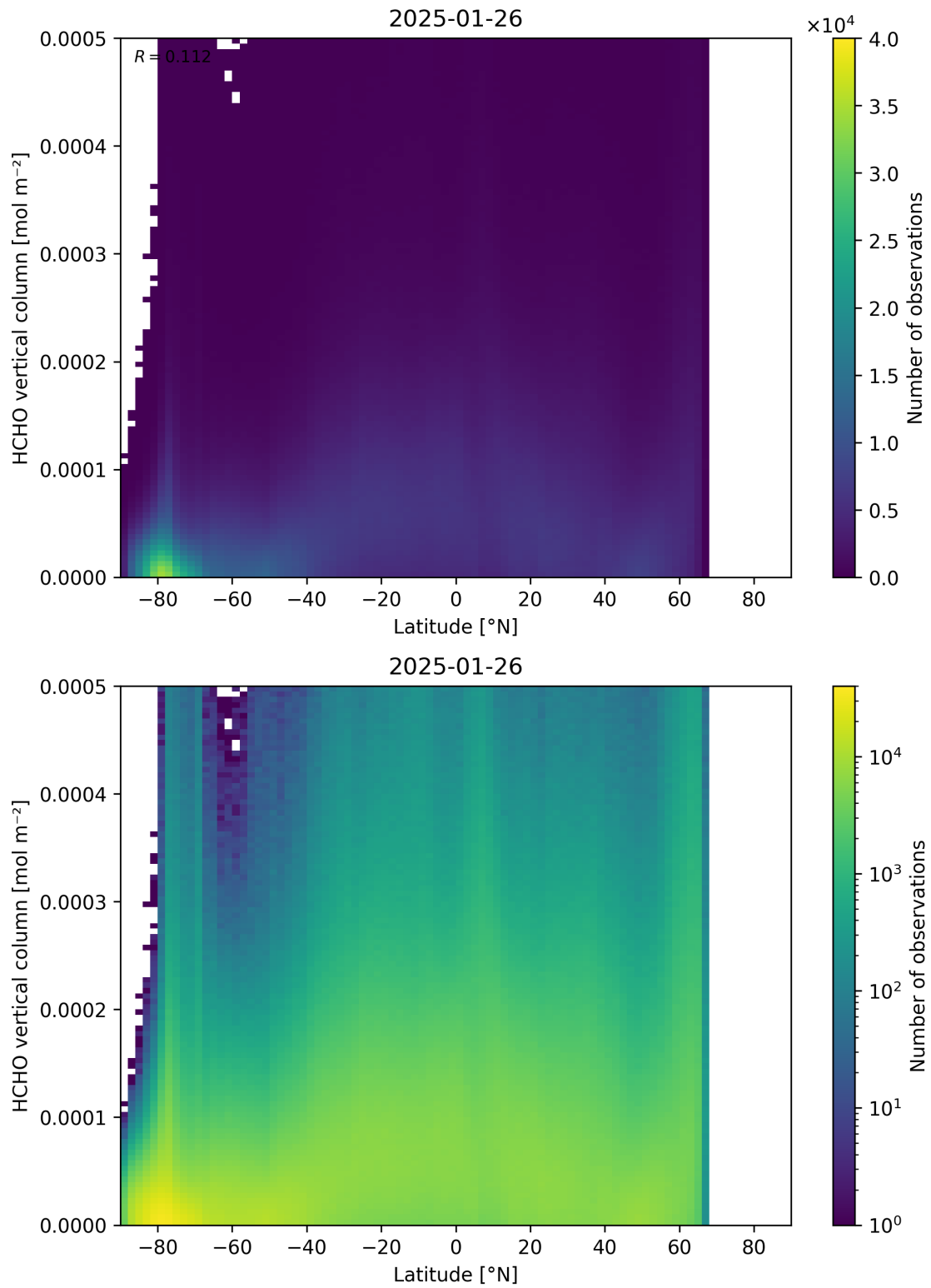
Figure 163: Scatter density plot of “Latitude” against “HCHO vertical column” for 2025-01-25 to 2025-01-27.
