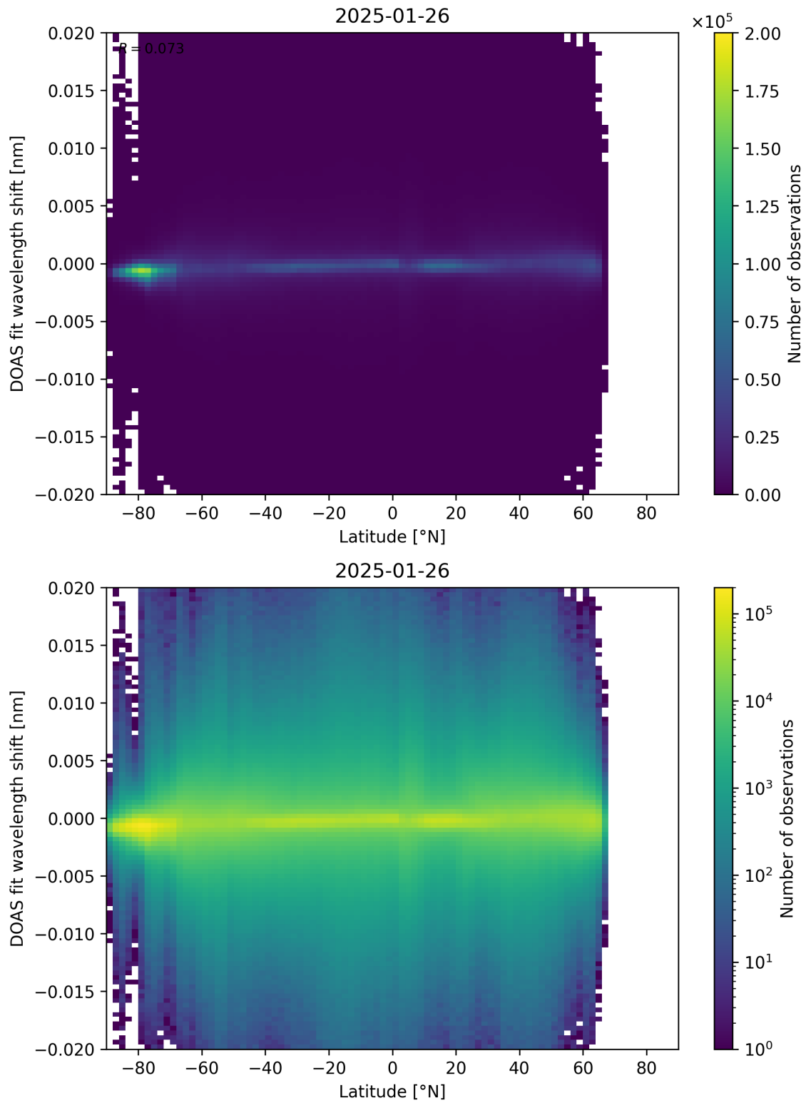
Figure 154: Scatter density plot of “Latitude” against “DOAS fit wavelength shift” for 2025-01-25 to 2025-01-27.
