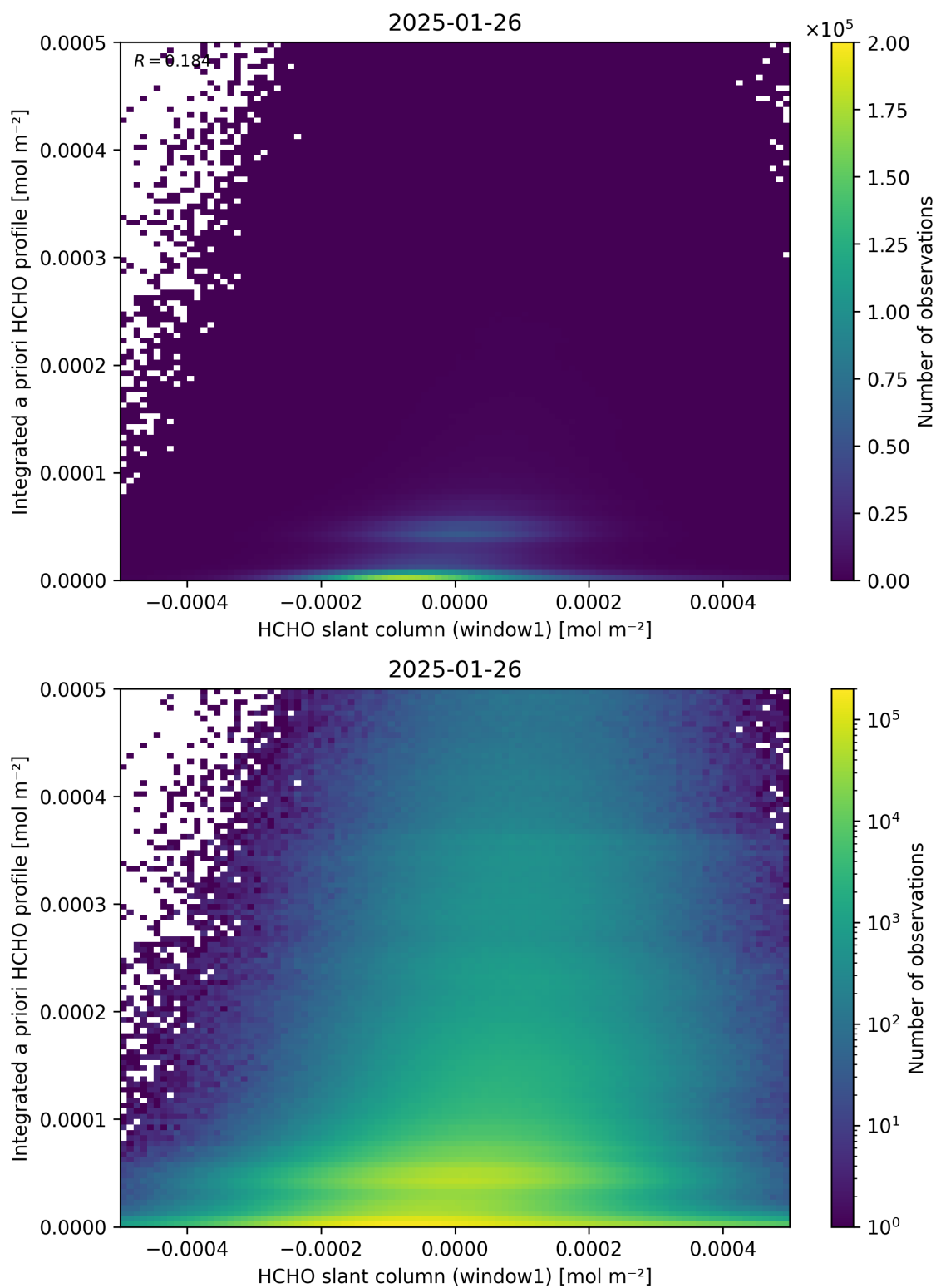
Figure 87: Scatter density plot of “HCHO slant column (window1)” against “Integrated a priori HCHO profile” for 2025-01-25 to 2025-01-27.
