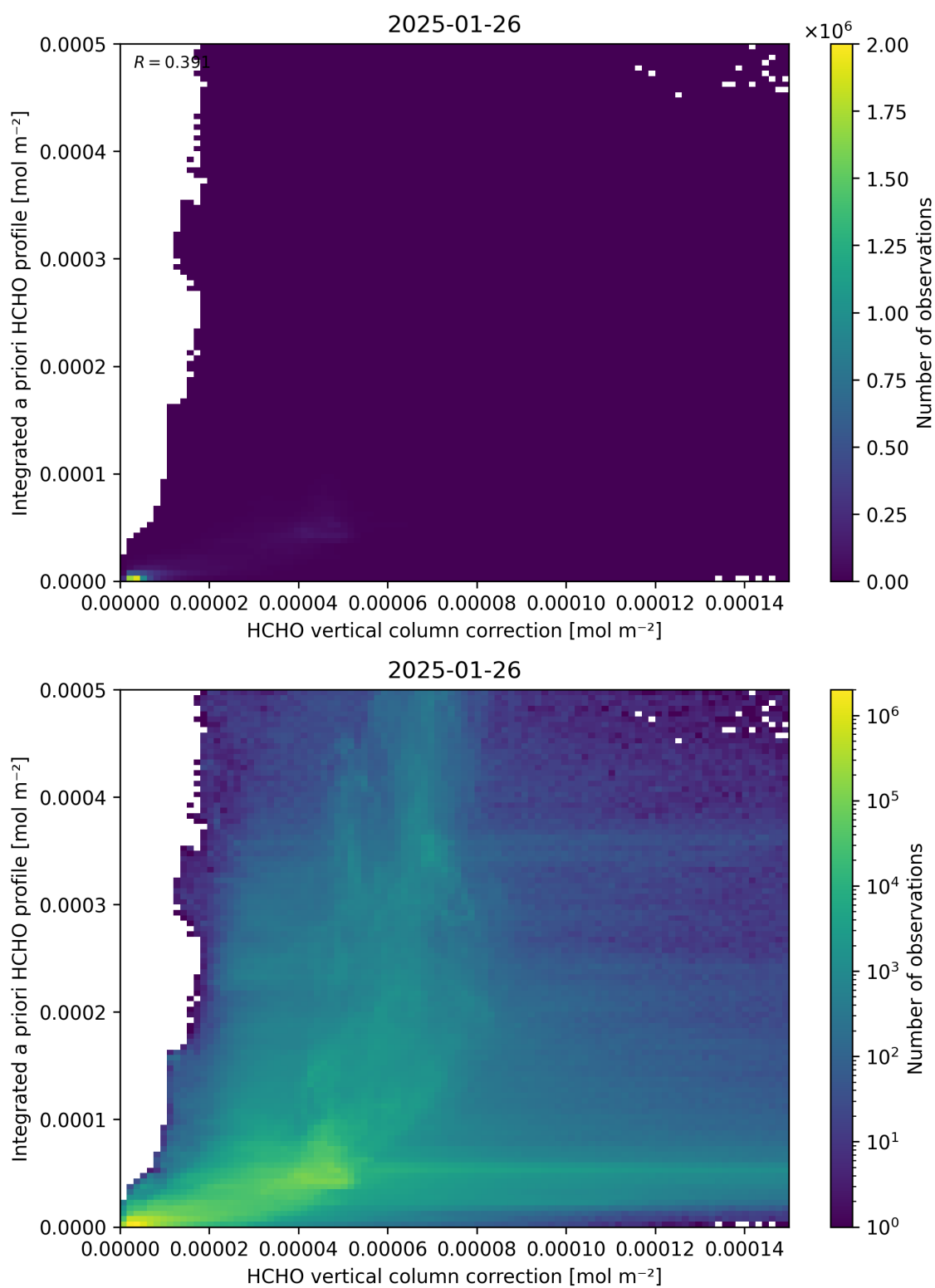
Figure 122: Scatter density plot of “HCHO vertical column correction” against “Integrated a priori HCHO profile” for 2025-01-25 to 2025-01-27.
