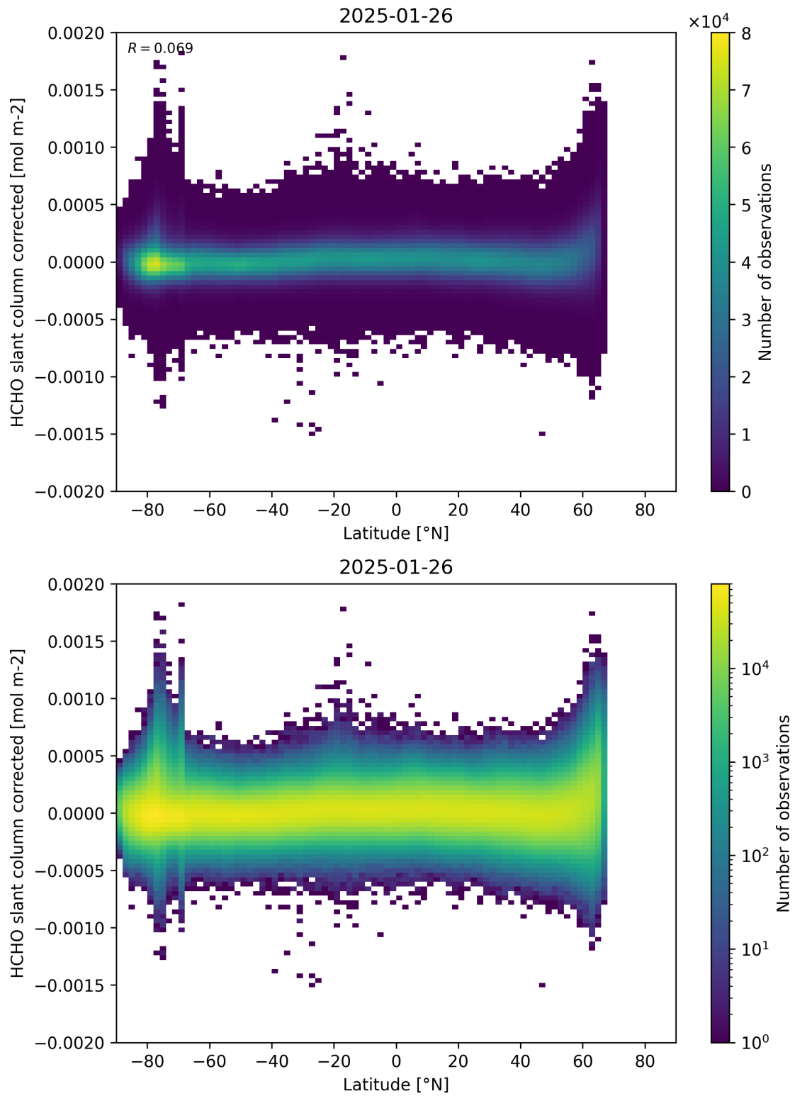
Figure 157: Scatter density plot of “Latitude” against “HCHO slant column corrected” for 2025-01-25 to 2025-01-27.
