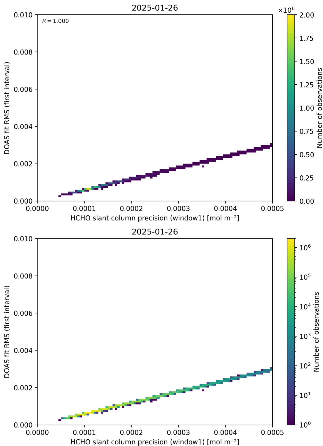
Figure 88: Scatter density plot of “HCHO slant column precision (window1)” against “DOAS fit RMS (first interval)” for 2025-01-25 to 2025-01-27.
