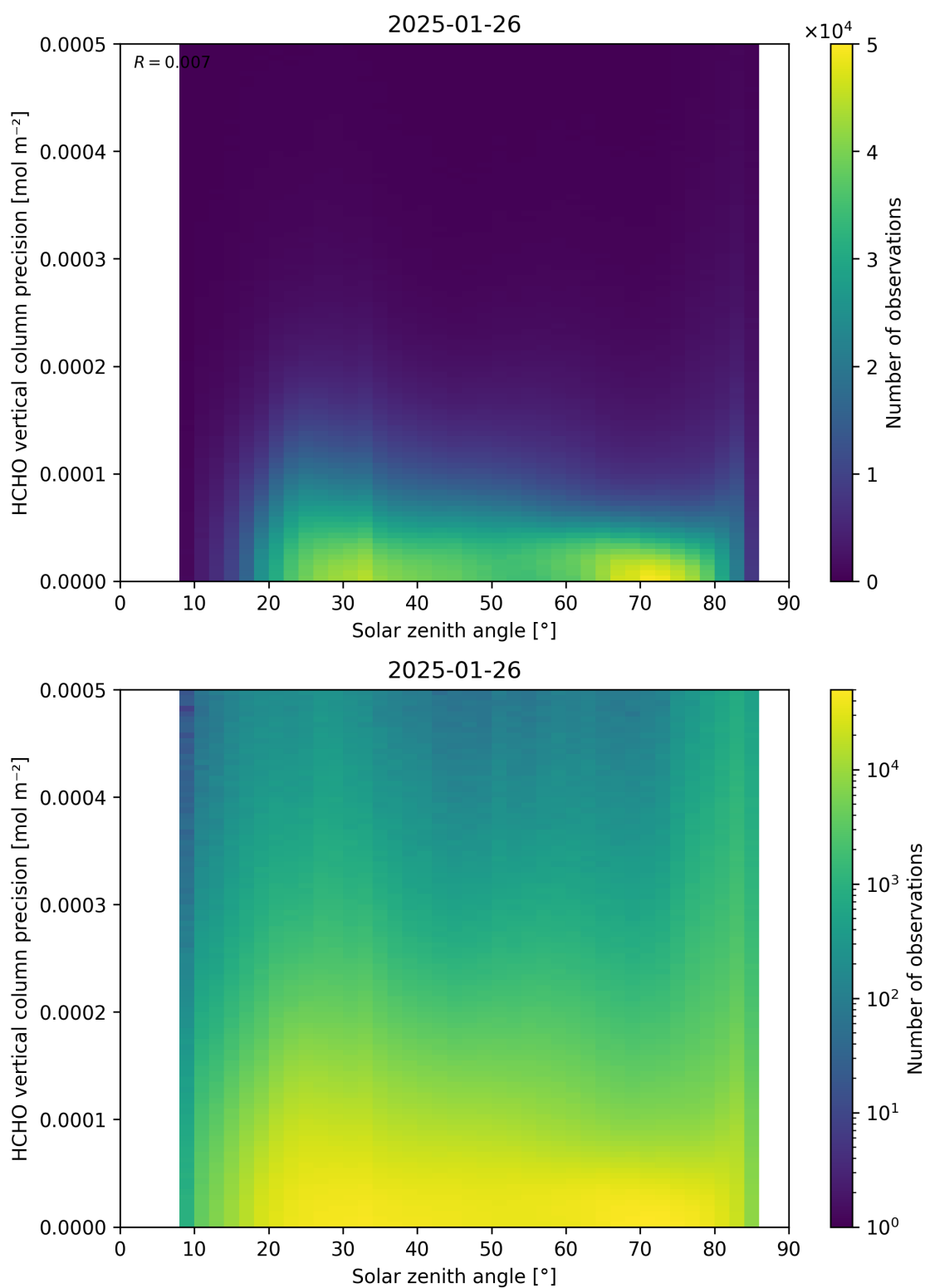
Figure 179: Scatter density plot of “Solar zenith angle” against “HCHO vertical column precision” for 2025-01-25 to 2025-01-27.
