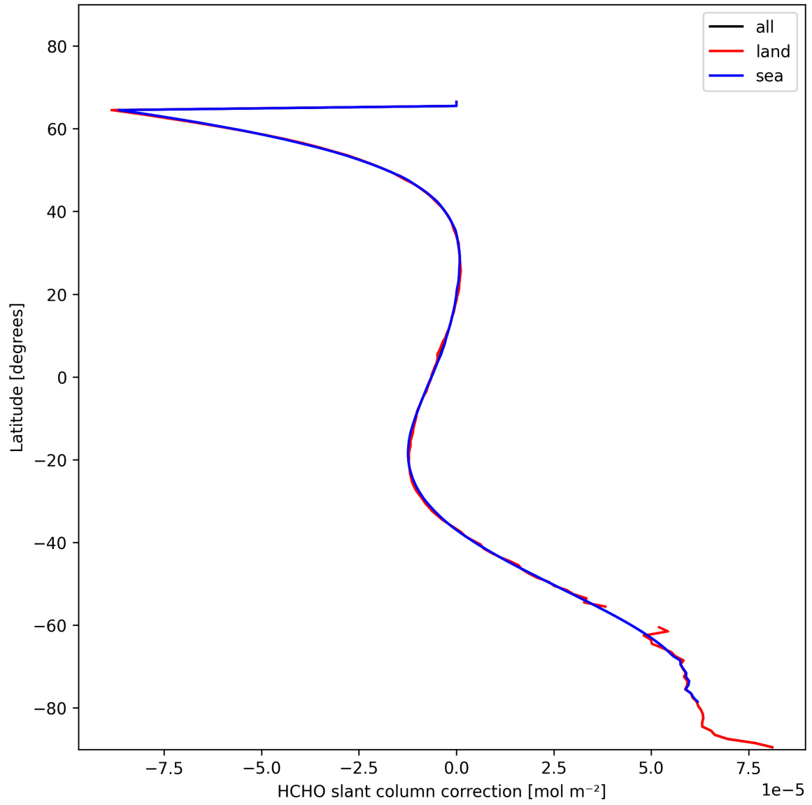
Figure 33: Zonal average of "HCHO slant column correction" for 2025-01-25 to 2025-01-27.
