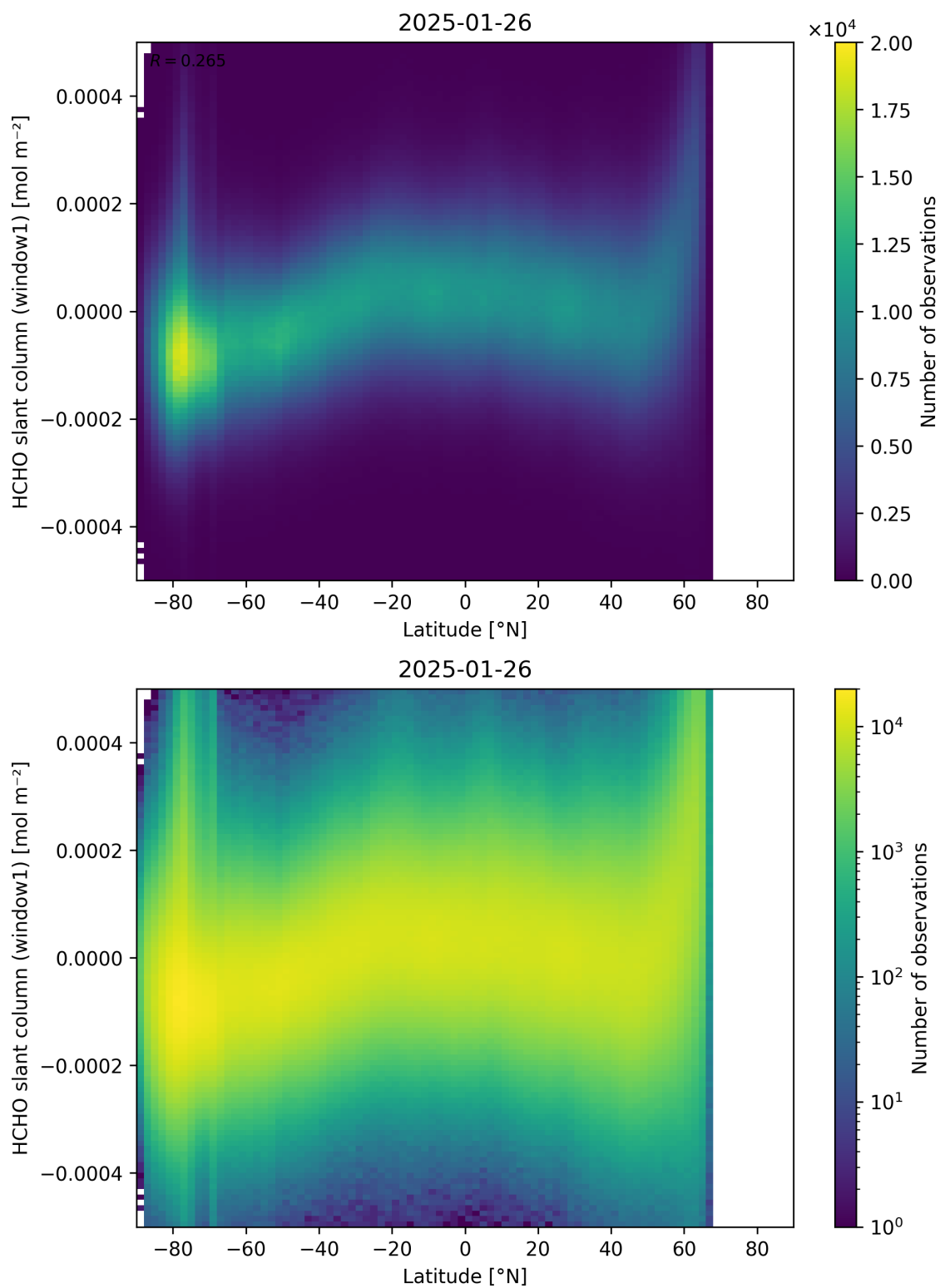
Figure 159: Scatter density plot of “Latitude” against “HCHO slant column (window1)” for 2025-01-25 to 2025-01-27.
