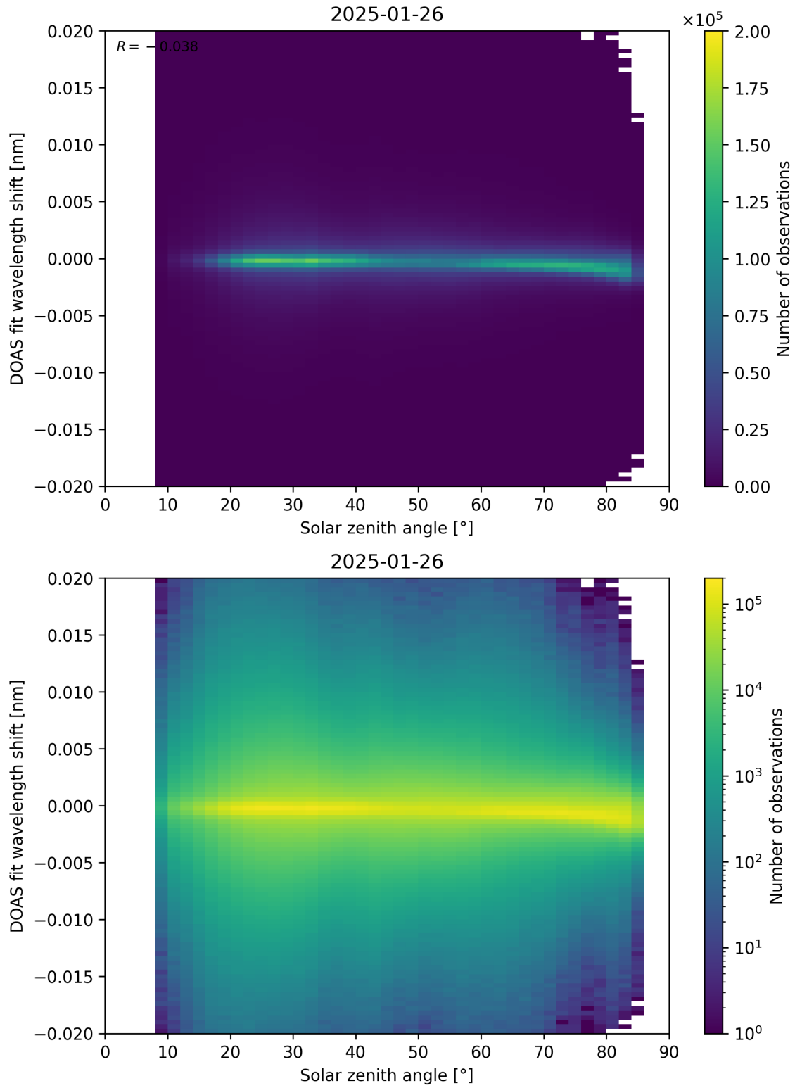
Figure 168: Scatter density plot of “Solar zenith angle” against “DOAS fit wavelength shift” for 2025-01-25 to 2025-01-27.
