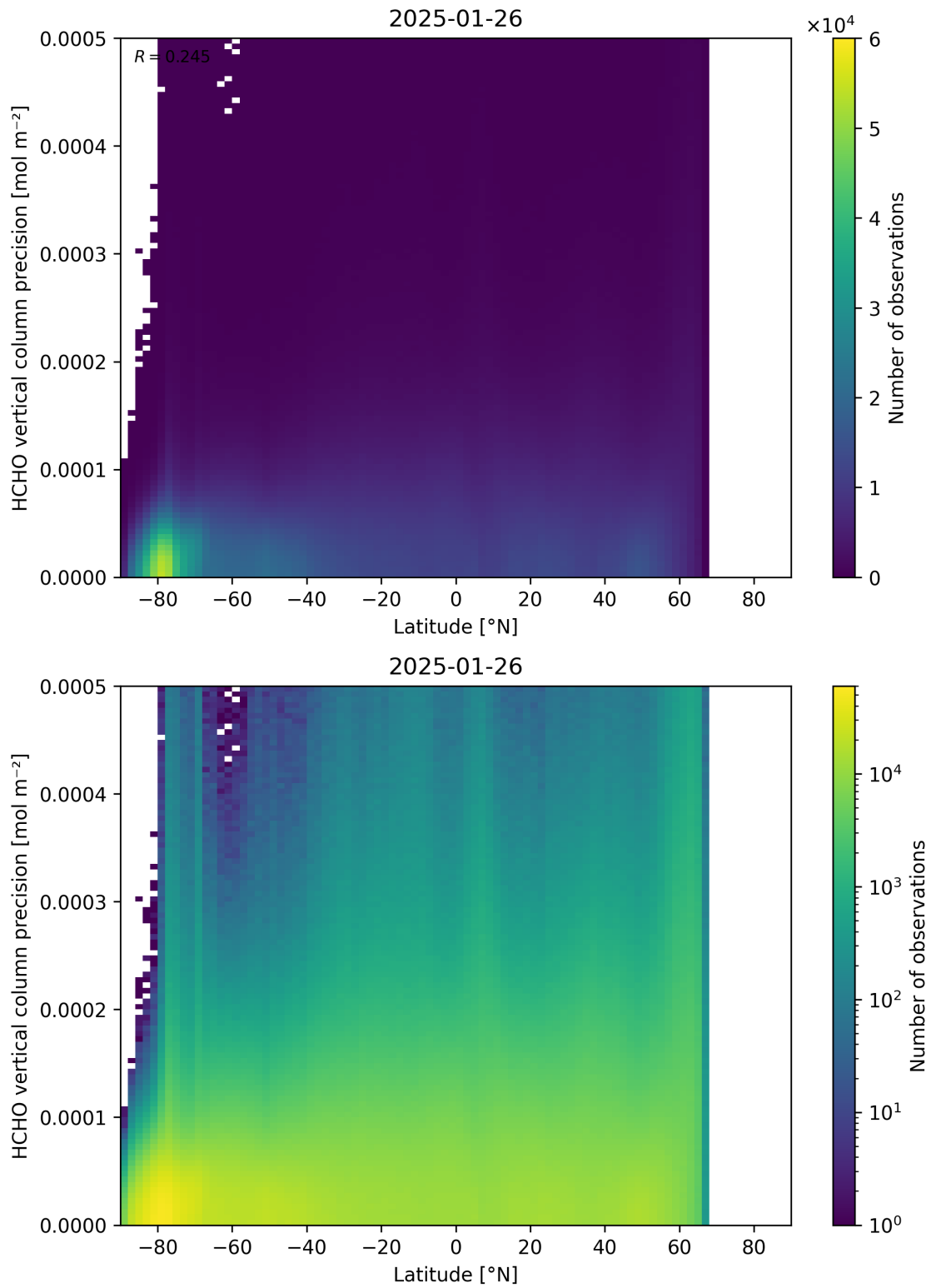
Figure 165: Scatter density plot of “Latitude” against “HCHO vertical column precision” for 2025-01-25 to 2025-01-27.
