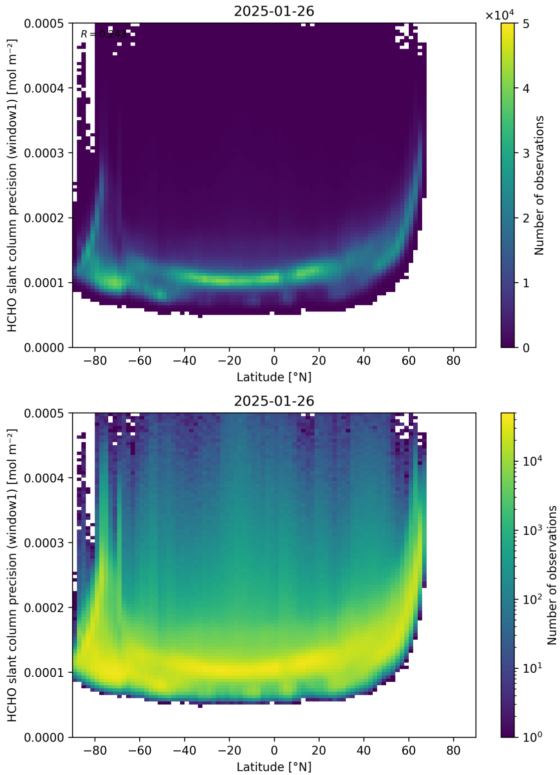
Figure 160: Scatter density plot of “Latitude” against “HCHO slant column precision (window1)” for 2025-01-25 to 2025-01-27.
