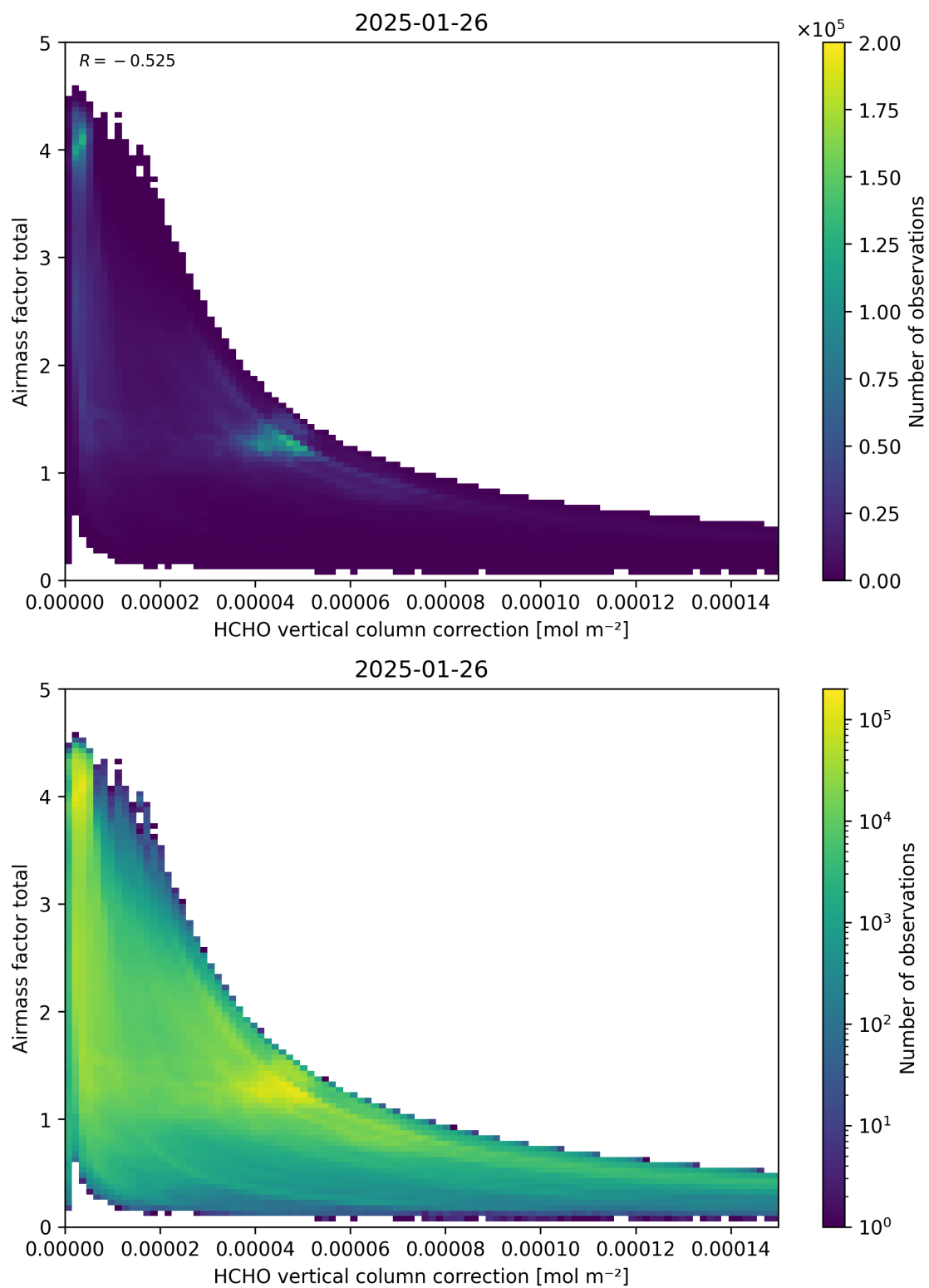
Figure 120: Scatter density plot of “HCHO vertical column correction” against “Airmass factor total” for 2025-01-25 to 2025-01-27.
