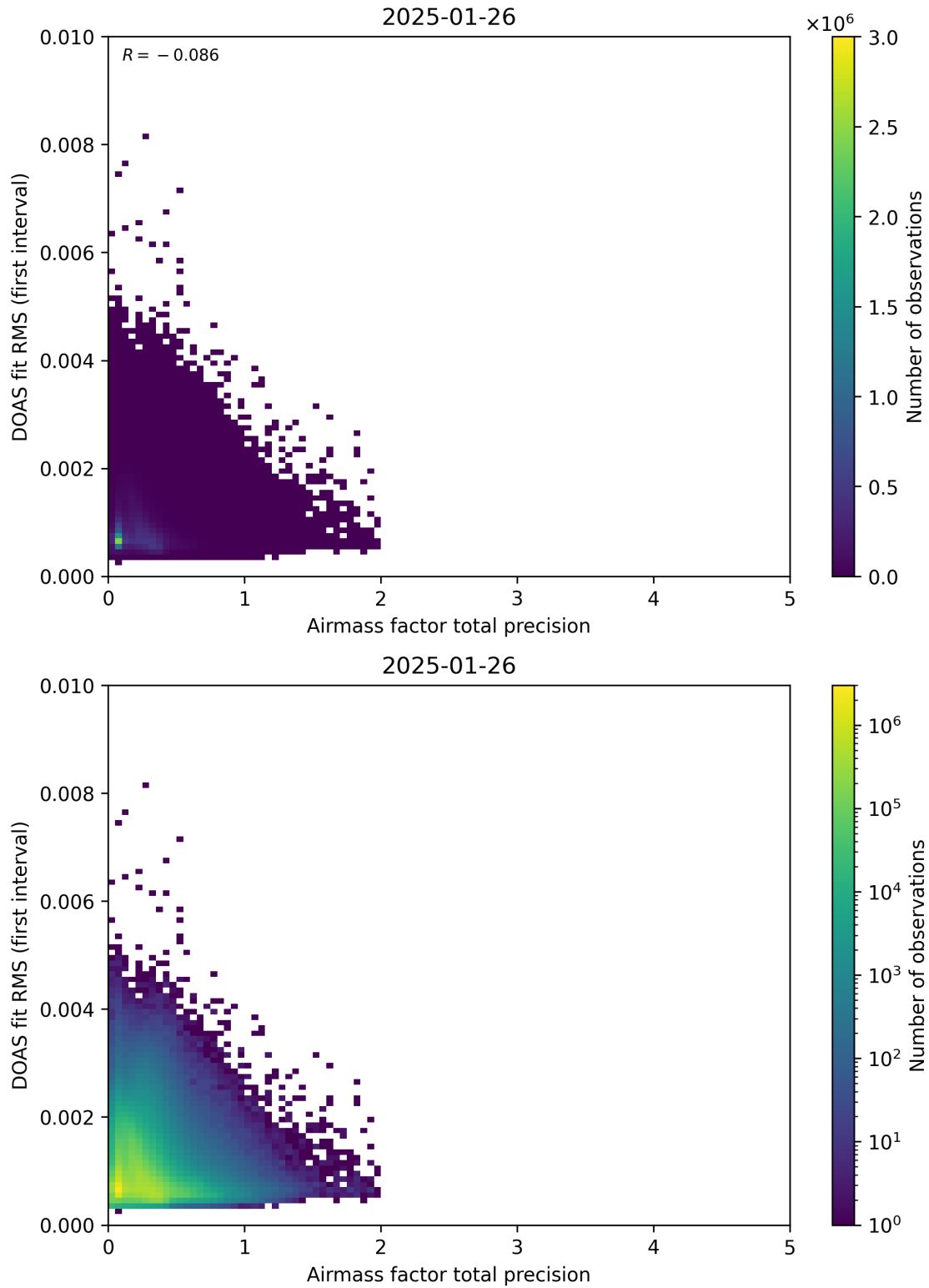
Figure 105: Scatter density plot of “Airmass factor total precision” against “DOAS fit RMS (first interval)” for 2025-01-25 to 2025-01-27.
