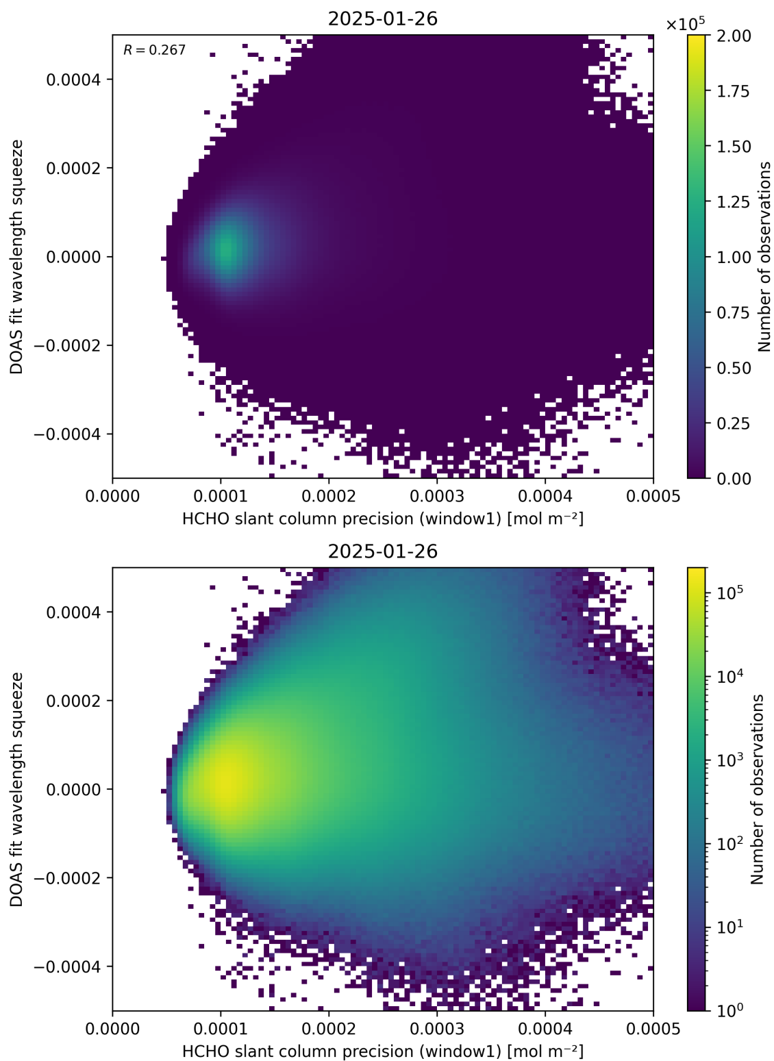
Figure 90: Scatter density plot of “HCHO slant column precision (window1)” against “DOAS fit wavelength squeeze” for 2025-01-25 to 2025-01-27.
