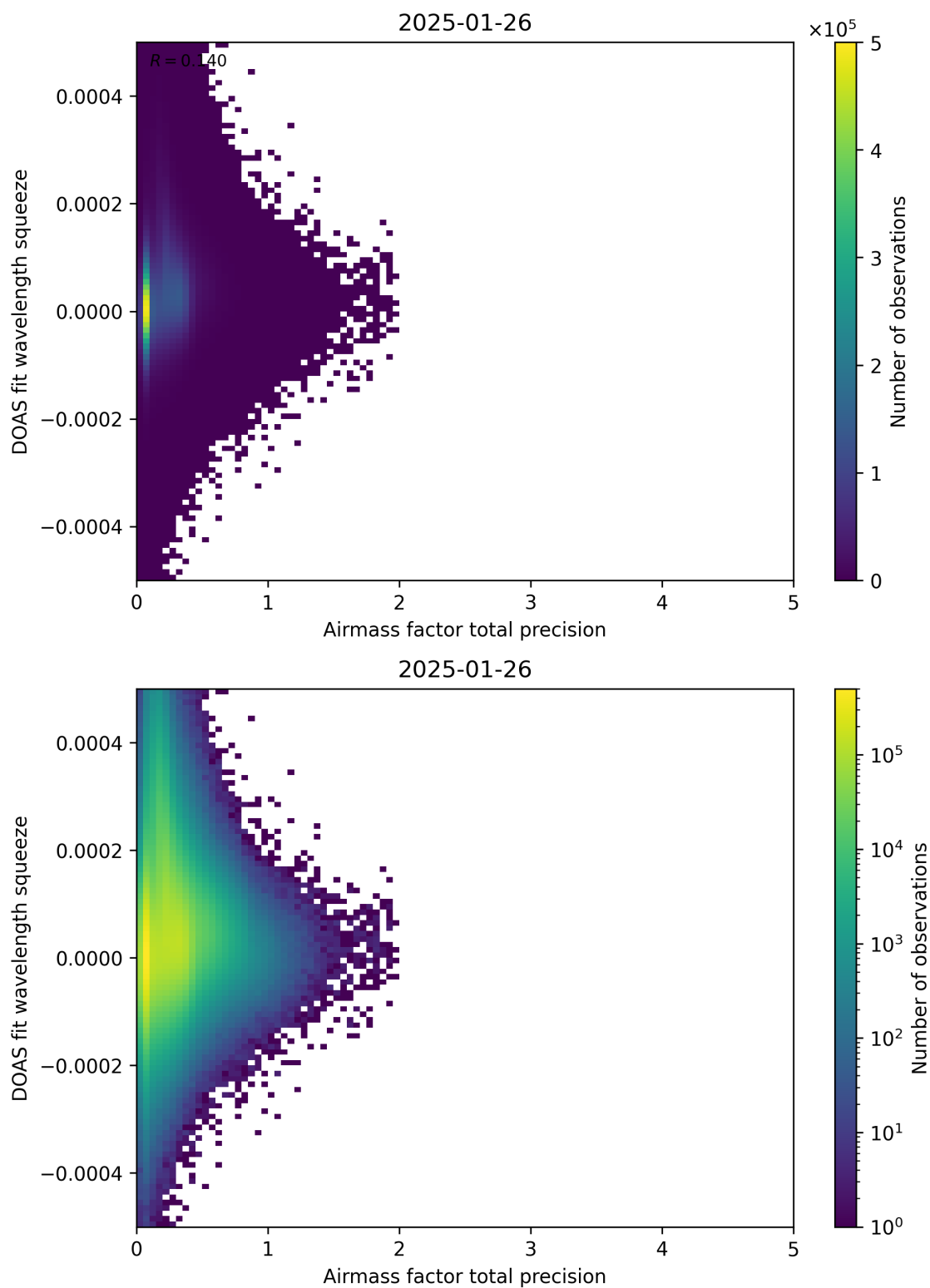
Figure 107: Scatter density plot of “Airmass factor total precision” against “DOAS fit wavelength squeeze” for 2025-01-25 to 2025-01-27.
