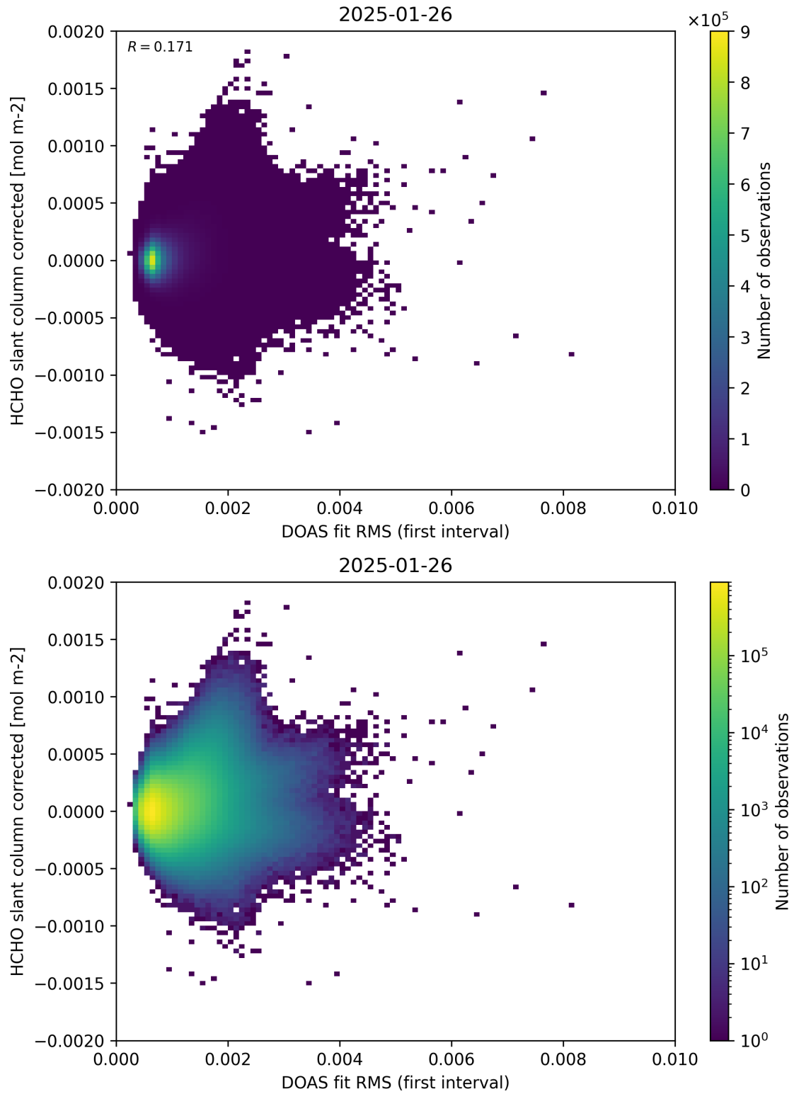
Figure 62: Scatter density plot of “DOAS fit RMS (first interval)” against “HCHO slant column corrected” for 2025-01-25 to 2025-01-27.
