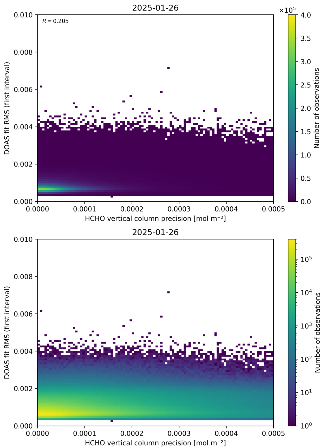
Figure 136: Scatter density plot of “HCHO vertical column precision” against “DOAS fit RMS (first interval)” for 2025-01-25 to 2025-01-27.
