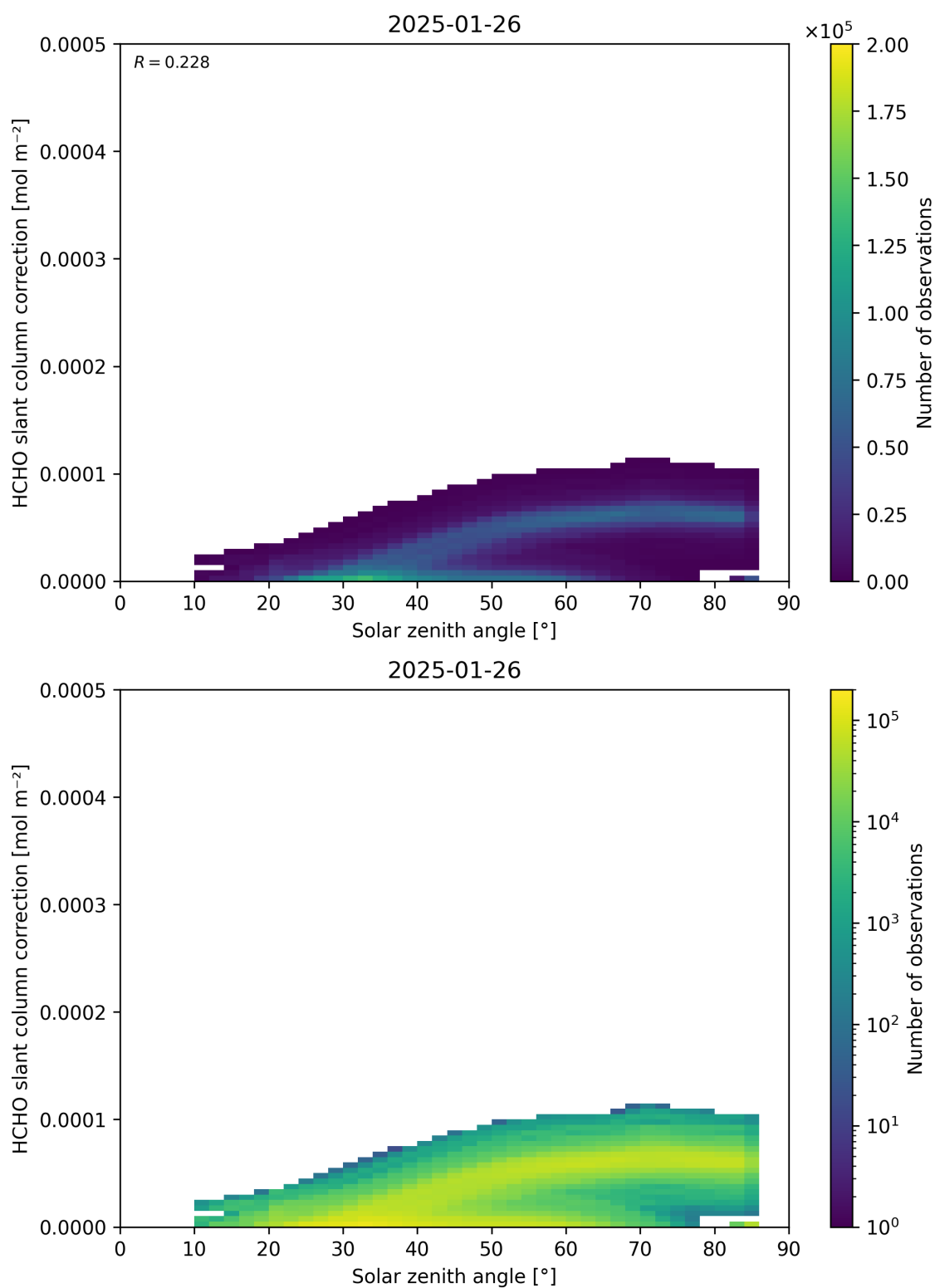
Figure 172: Scatter density plot of “Solar zenith angle” against “HCHO slant column correction” for 2025-01-25 to 2025-01-27.
