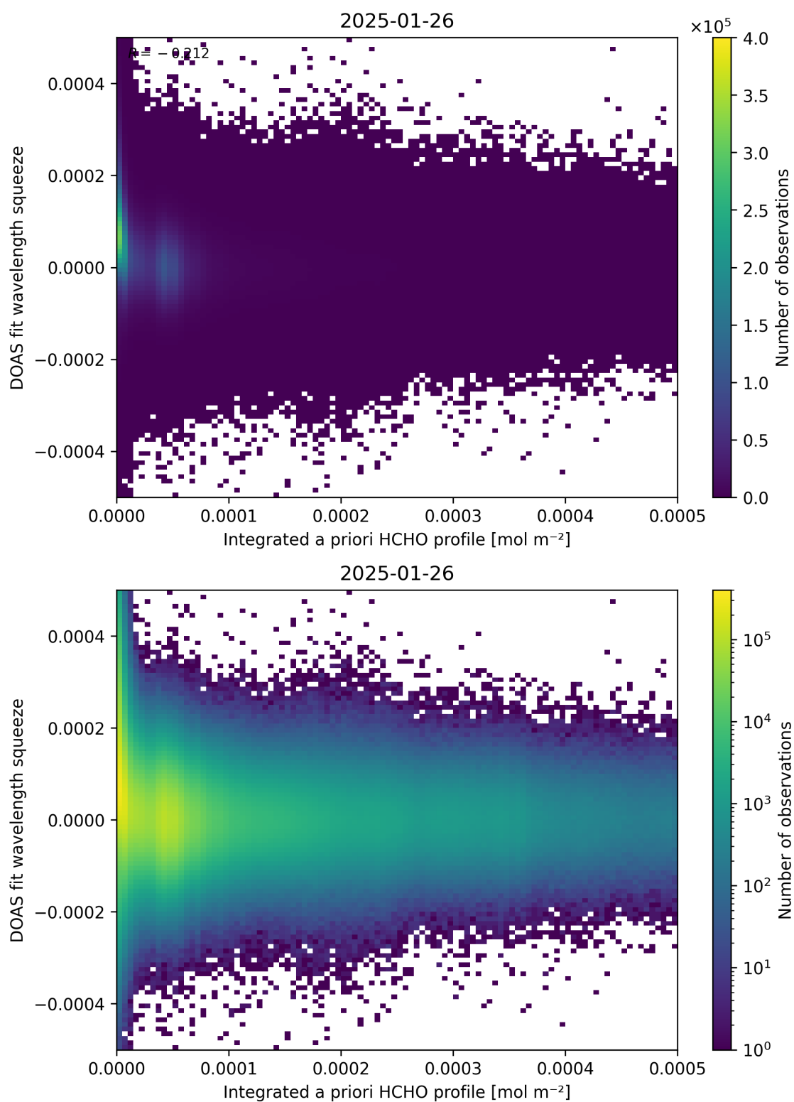
Figure 150: Scatter density plot of “Integrated a priori HCHO profile” against “DOAS fit wavelength squeeze” for 2025-01-25 to 2025-01-27.
