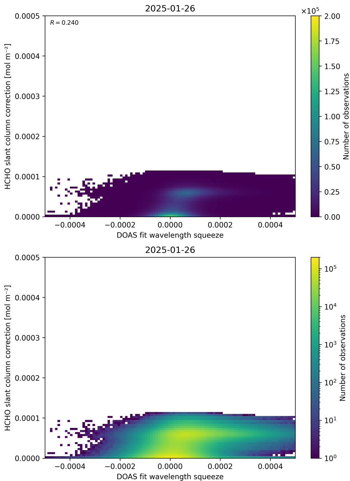
Figure 70: Scatter density plot of “DOAS fit wavelength squeeze” against “HCHO slant column correction” for 2025-01-25 to 2025-01-27.
