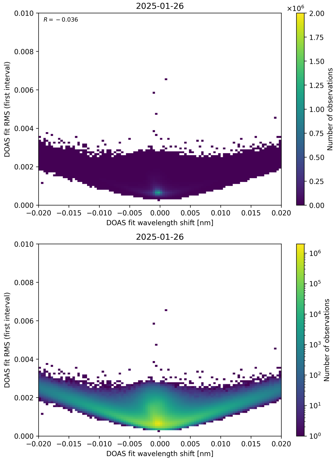
Figure 64: Scatter density plot of “DOAS fit wavelength shift” against “DOAS fit RMS (first interval)” for 2025-01-25 to 2025-01-27.
