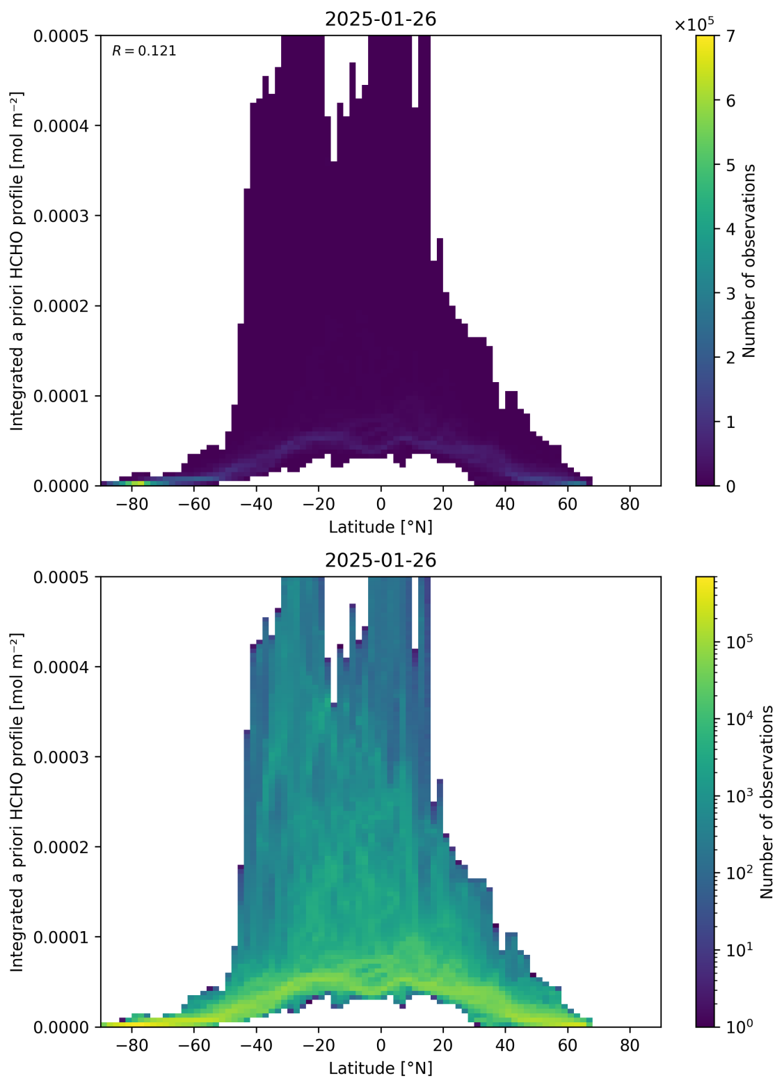
Figure 166: Scatter density plot of “Latitude” against “Integrated a priori HCHO profile” for 2025-01-25 to 2025-01-27.
