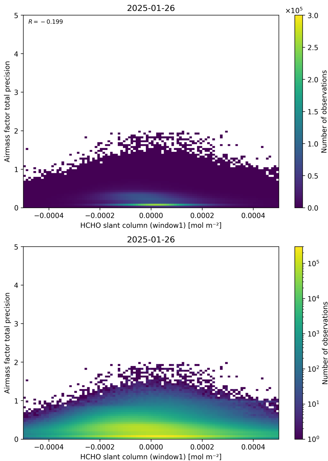
Figure 86: Scatter density plot of “HCHO slant column (window1)” against “Airmass factor total precision” for 2025-01-25 to 2025-01-27.
