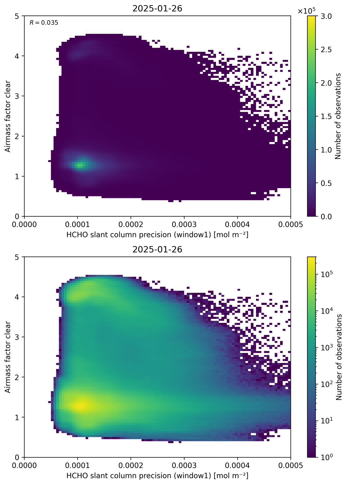
Figure 91: Scatter density plot of “HCHO slant column precision (window1)” against “Airmass factor clear” for 2025-01-25 to 2025-01-27.
