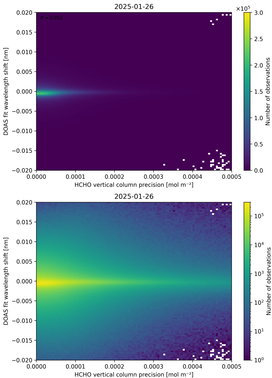
Figure 137: Scatter density plot of “HCHO vertical column precision” against “DOAS fit wavelength shift” for 2025-01-25 to 2025-01-27.
