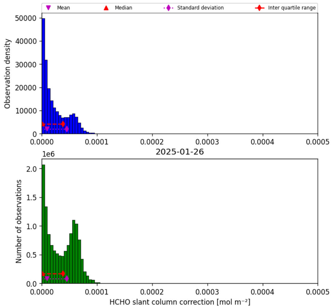
Figure 47: Histogram of "HCHO slant column correction" for 2025-01-25 to 2025-01-27
