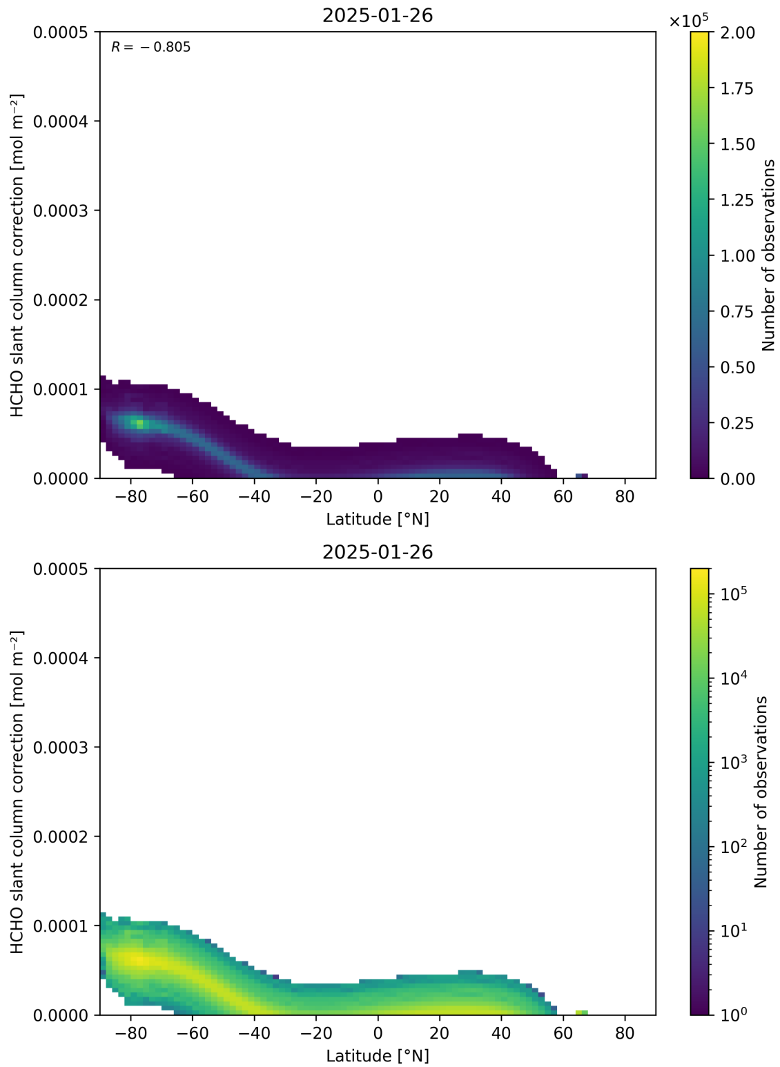
Figure 158: Scatter density plot of “Latitude” against “HCHO slant column correction” for 2025-01-25 to 2025-01-27.
