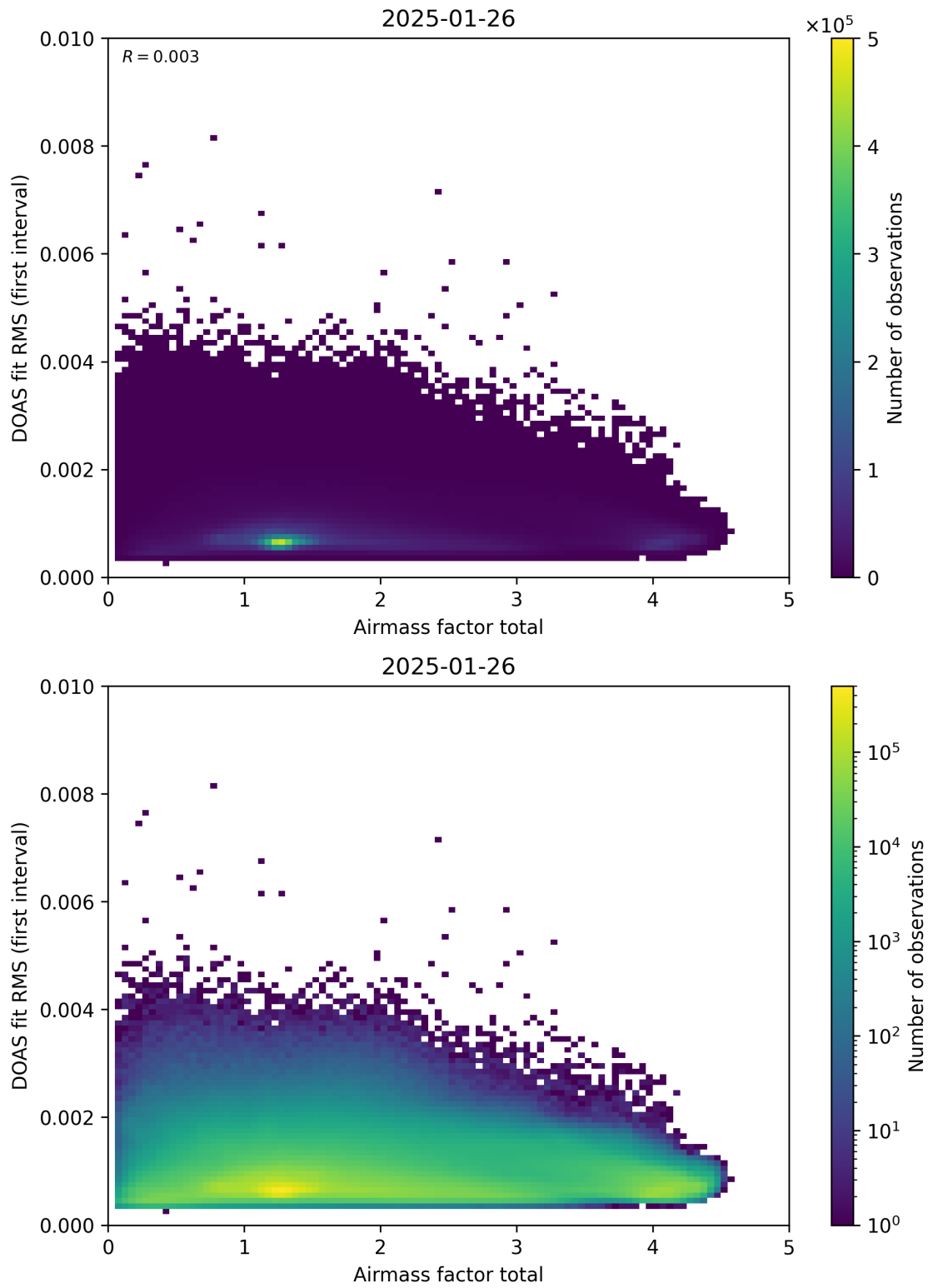
Figure 97: Scatter density plot of “Airmass factor total” against “DOAS fit RMS (first interval)” for 2025-01-25 to 2025-01-27.
