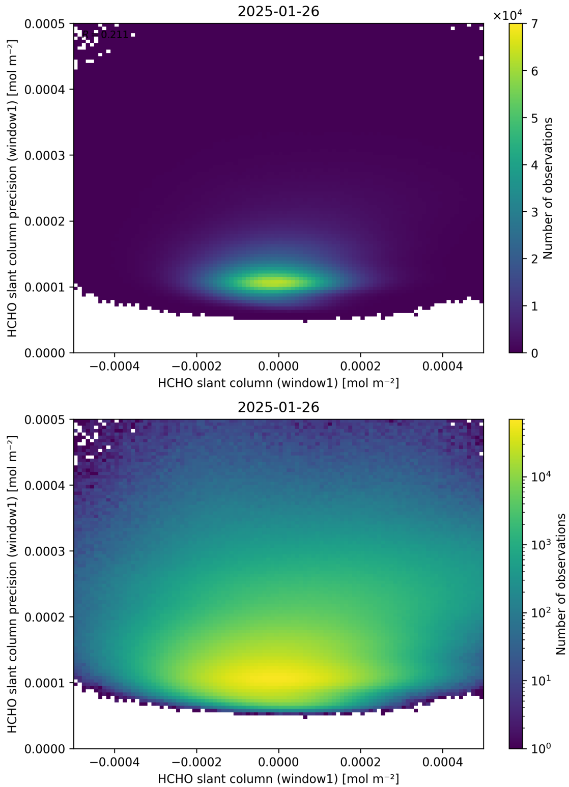
Figure 84: Scatter density plot of “HCHO slant column (window1)” against “HCHO slant column precision (window1)” for 2025-01-25 to 2025-01-27.
