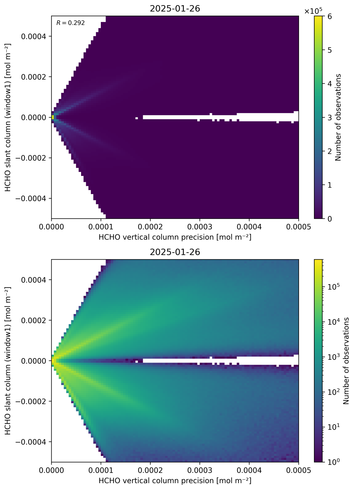
Figure 142: Scatter density plot of “HCHO vertical column precision” against “HCHO slant column (window1)” for 2025-01-25 to 2025-01-27.
