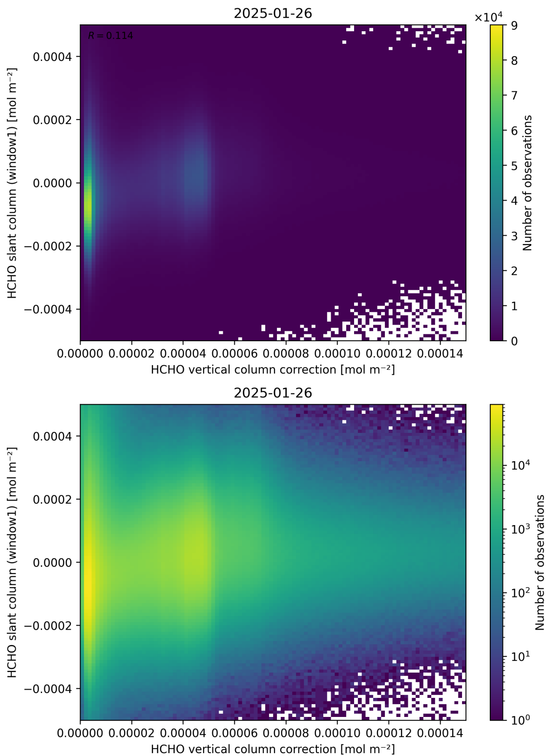
Figure 118: Scatter density plot of “HCHO vertical column correction” against “HCHO slant column (window1)” for 2025-01-25 to 2025-01-27.
