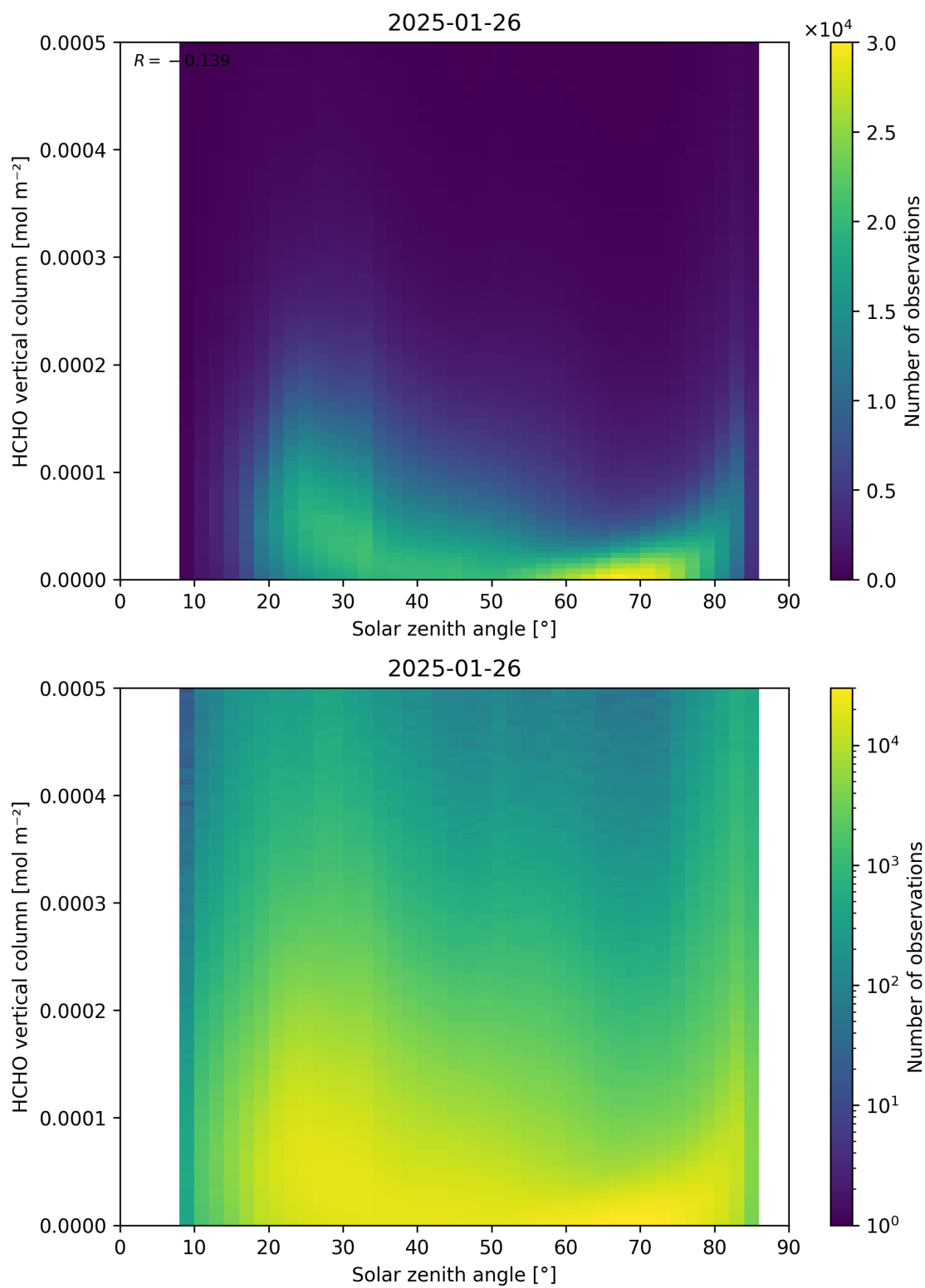
Figure 177: Scatter density plot of “Solar zenith angle” against “HCHO vertical column” for 2025-01-25 to 2025-01-27.
