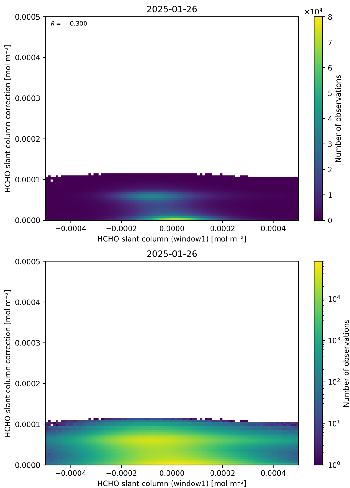
Figure 83: Scatter density plot of “HCHO slant column (window1)” against “HCHO slant column correction” for 2025-01-25 to 2025-01-27.
