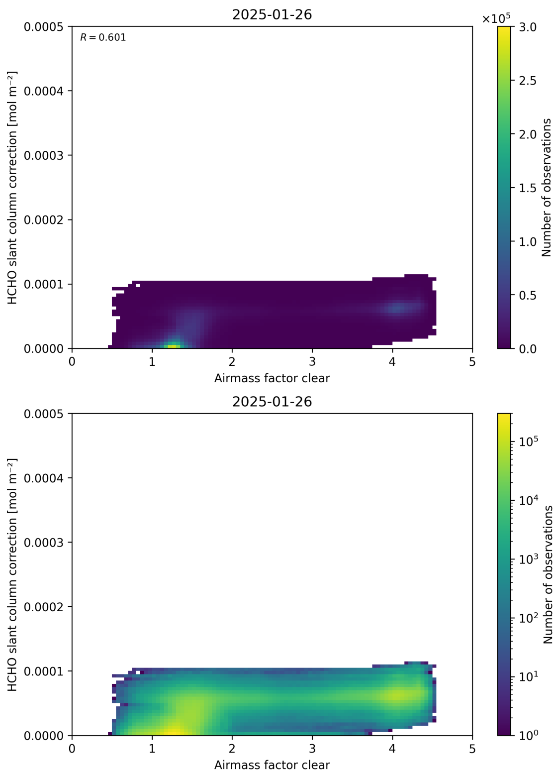
Figure 75: Scatter density plot of “Airmass factor clear” against “HCHO slant column correction” for 2025-01-25 to 2025-01-27.
