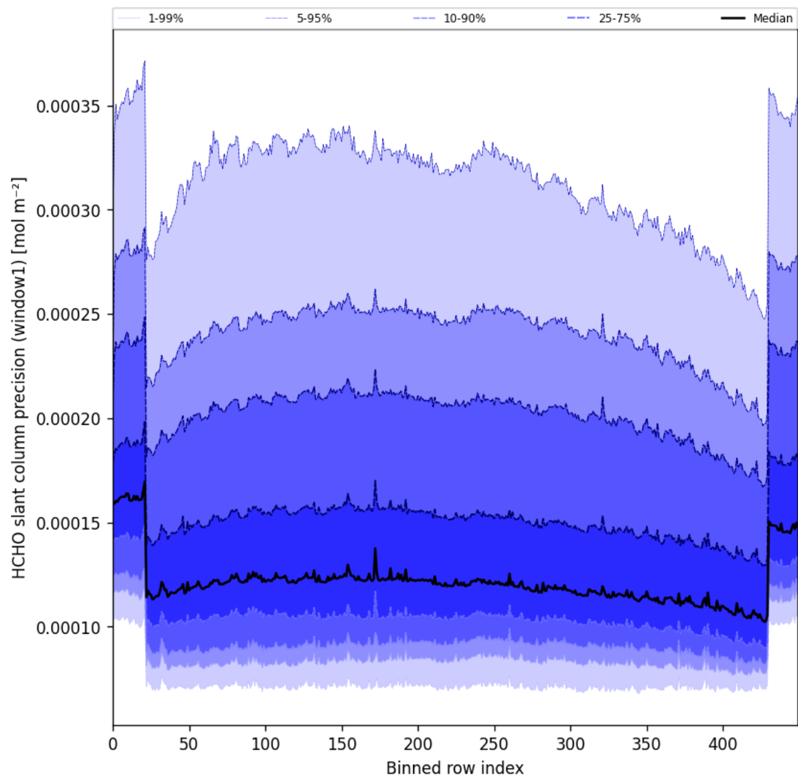
Figure 53: Along track statistics of “HCHO slant column precision (window1)” for 2025-01-25 to 2025-01-27
