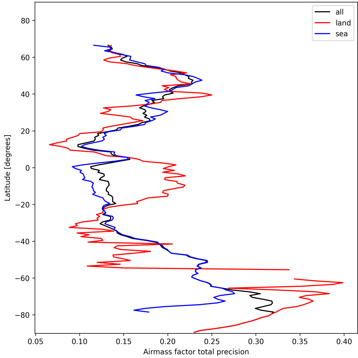
Figure 27: Zonal average of “Airmass factor total precision” for 2025-01-25 to 2025-01-27.
