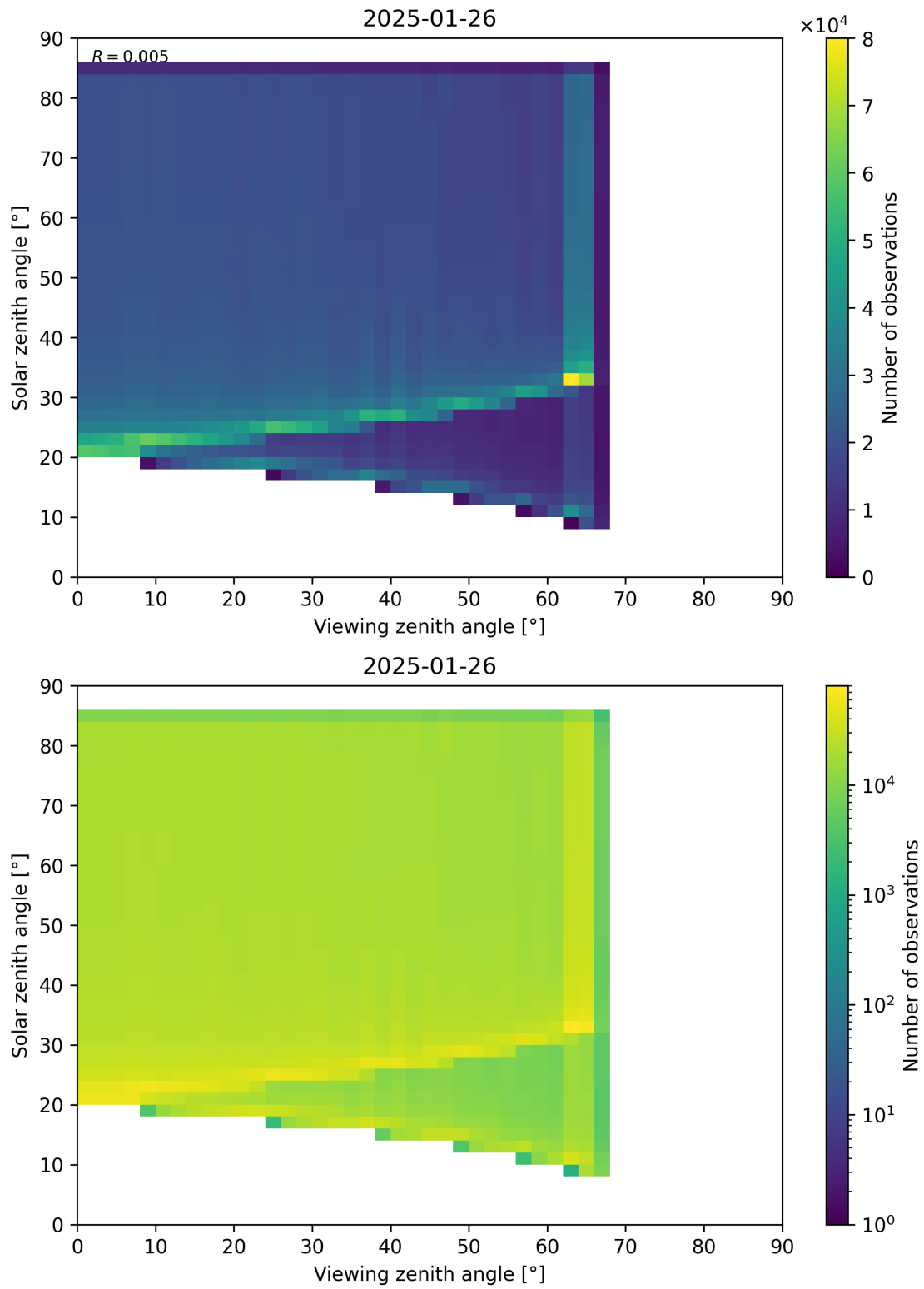
Figure 197: Scatter density plot of “Viewing zenith angle” against “Solar zenith angle” for 2025-01-25 to 2025-01-27.
