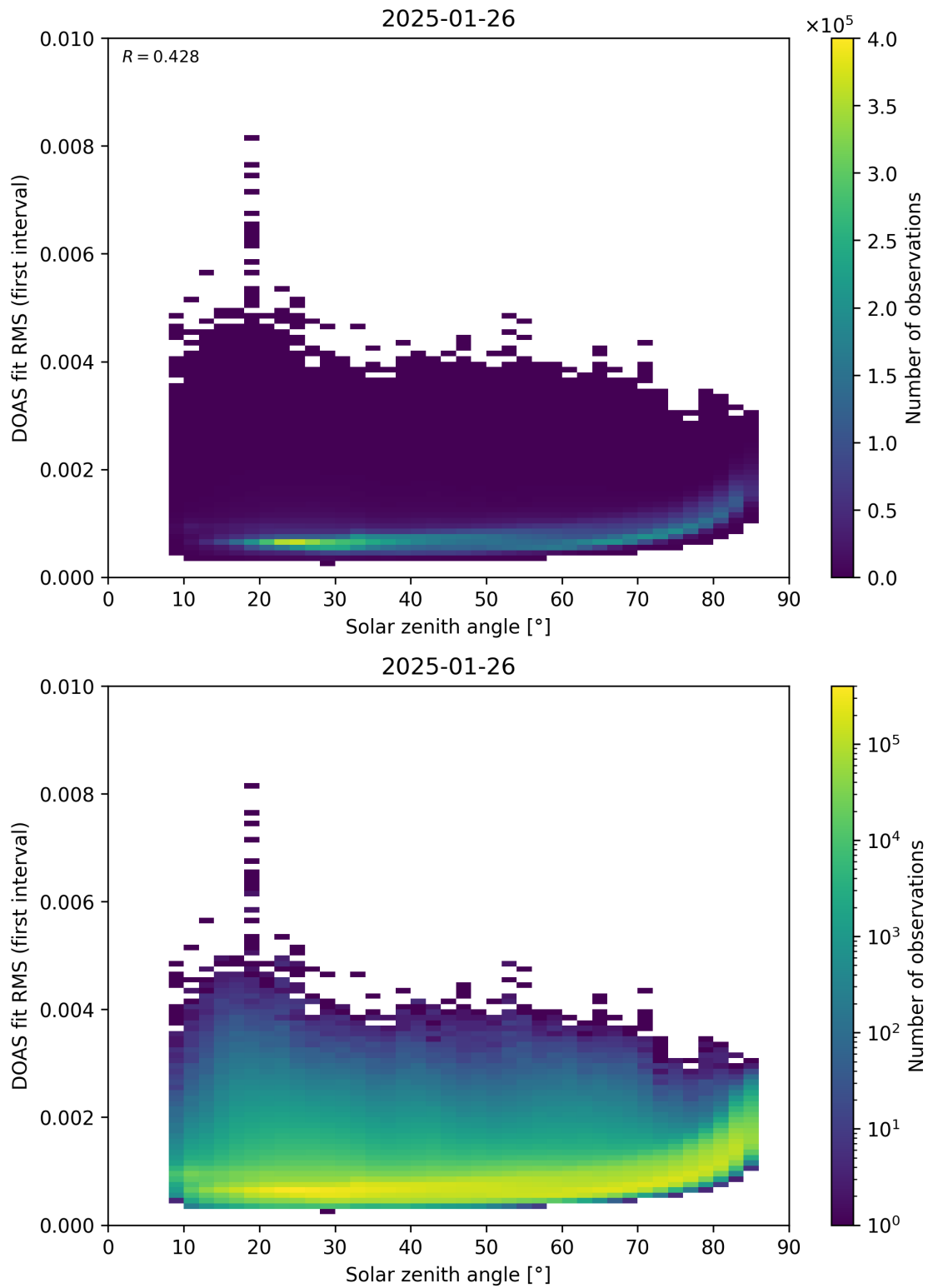
Figure 167: Scatter density plot of “Solar zenith angle” against “DOAS fit RMS (first interval)” for 2025-01-25 to 2025-01-27.
