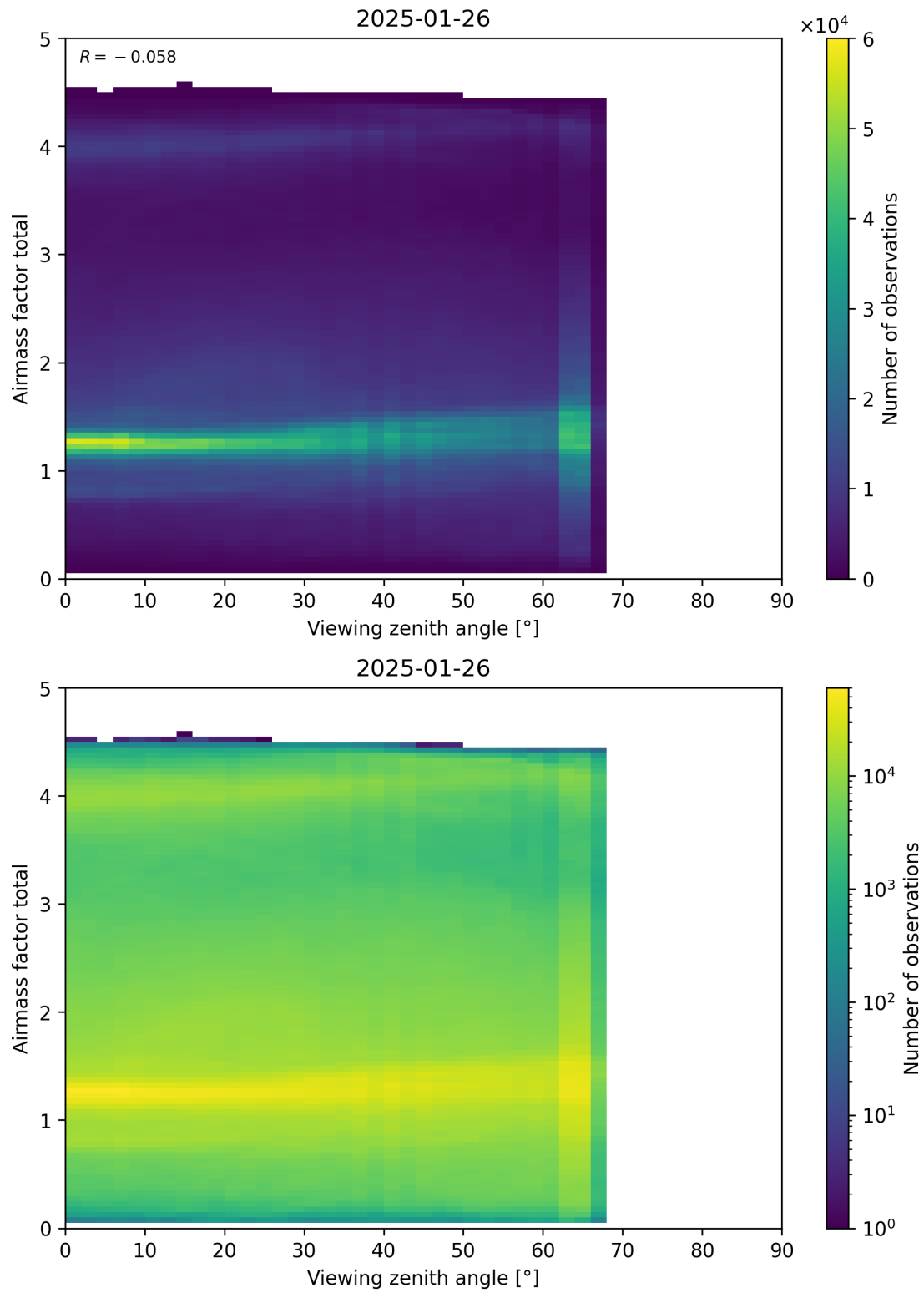
Figure 190: Scatter density plot of “Viewing zenith angle” against “Airmass factor total” for 2025-01-25 to 2025-01-27.
