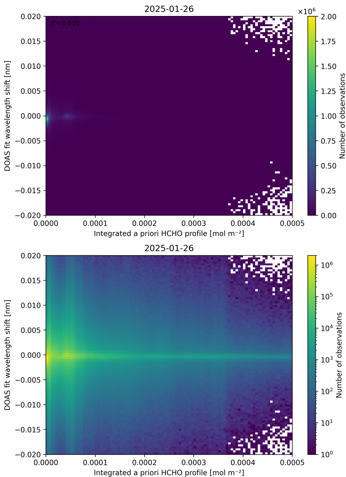
Figure 149: Scatter density plot of “Integrated a priori HCHO profile” against “DOAS fit wavelength shift” for 2025-01-25 to 2025-01-27.
