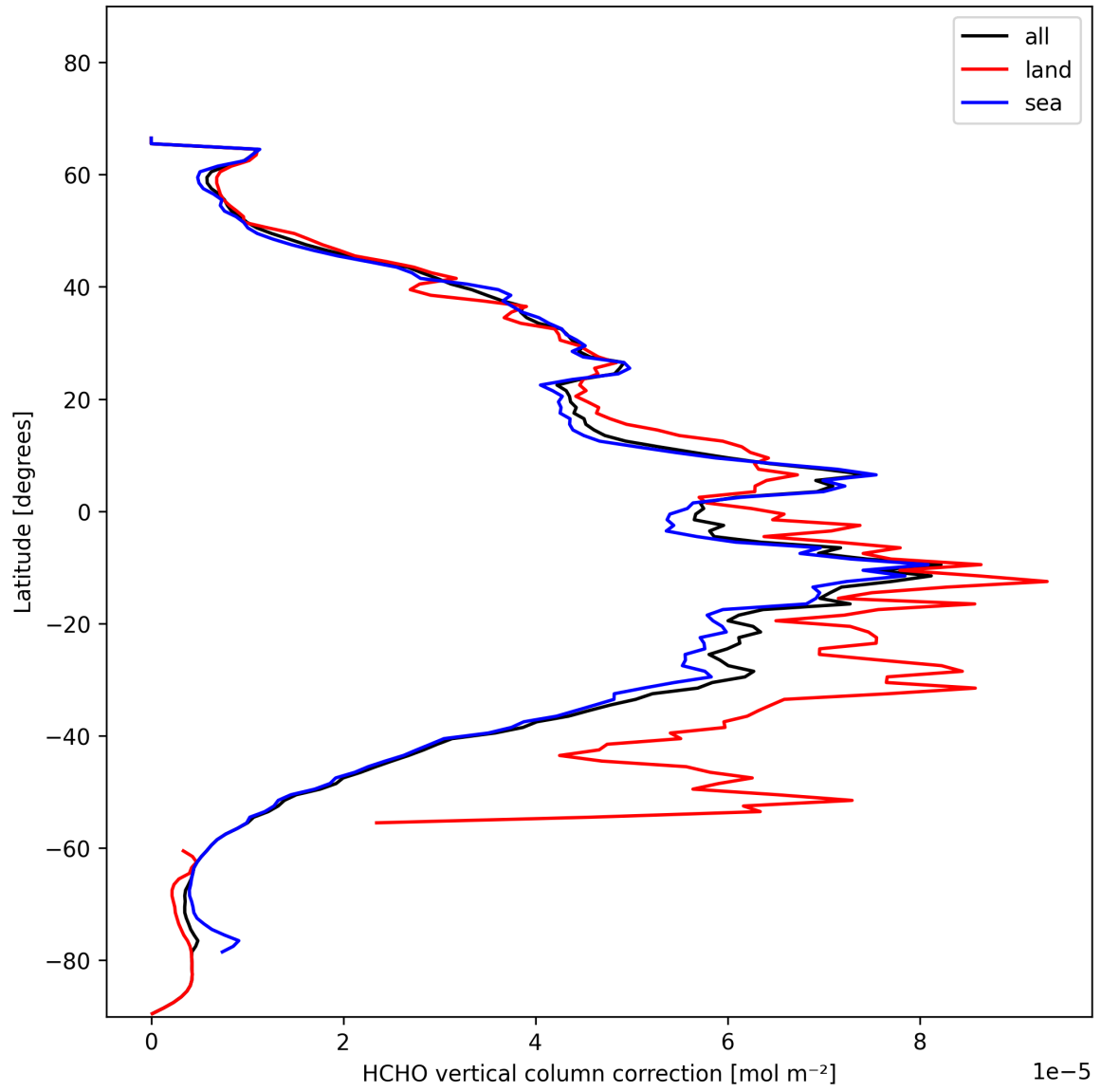
Figure 23: Zonal average of “HCHO vertical column correction” for 2025-01-25 to 2025-01-27.
