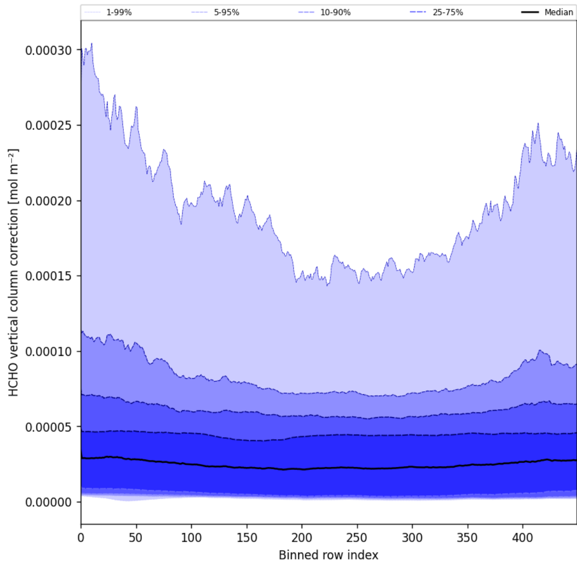
Figure 51: Along track statistics of “HCHO vertical column correction” for 2025-01-25 to 2025-01-27
