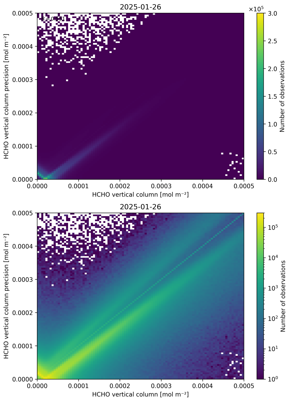
Figure 134: Scatter density plot of “HCHO vertical column” against “HCHO vertical column precision” for 2025-01-25 to 2025-01-27.
