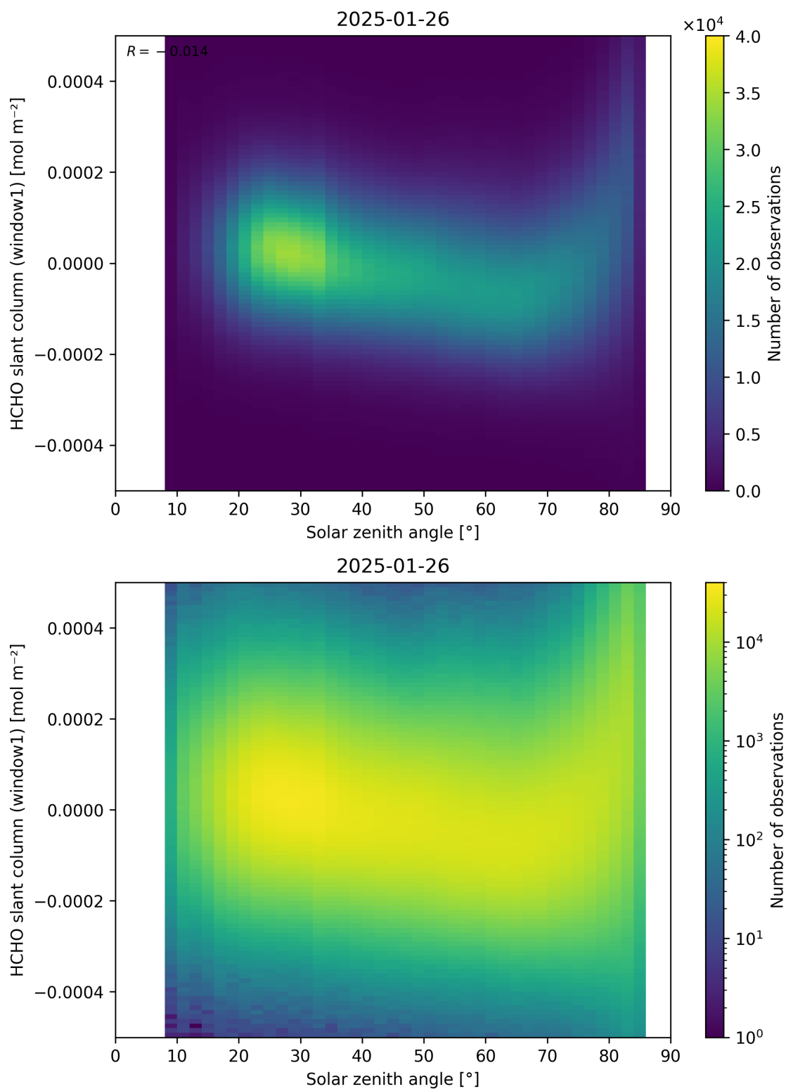
Figure 173: Scatter density plot of “Solar zenith angle” against “HCHO slant column (window1)” for 2025-01-25 to 2025-01-27.
