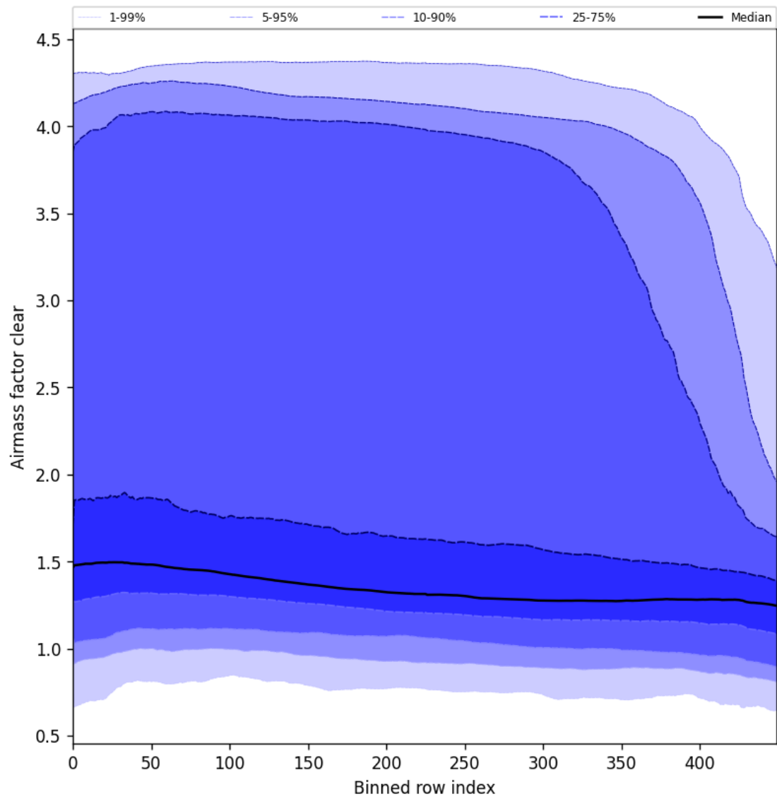
Figure 56: Along track statistics of “Airmass factor clear” for 2025-01-25 to 2025-01-27
