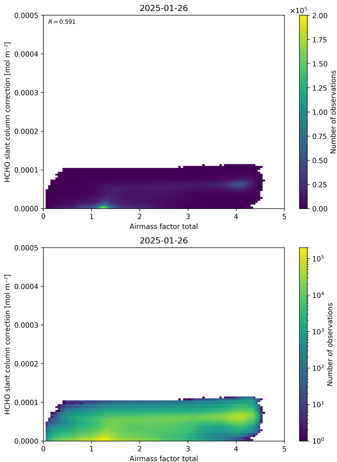
Figure 102: Scatter density plot of “Airmass factor total” against “HCHO slant column correction” for 2025-01-25 to 2025-01-27.
