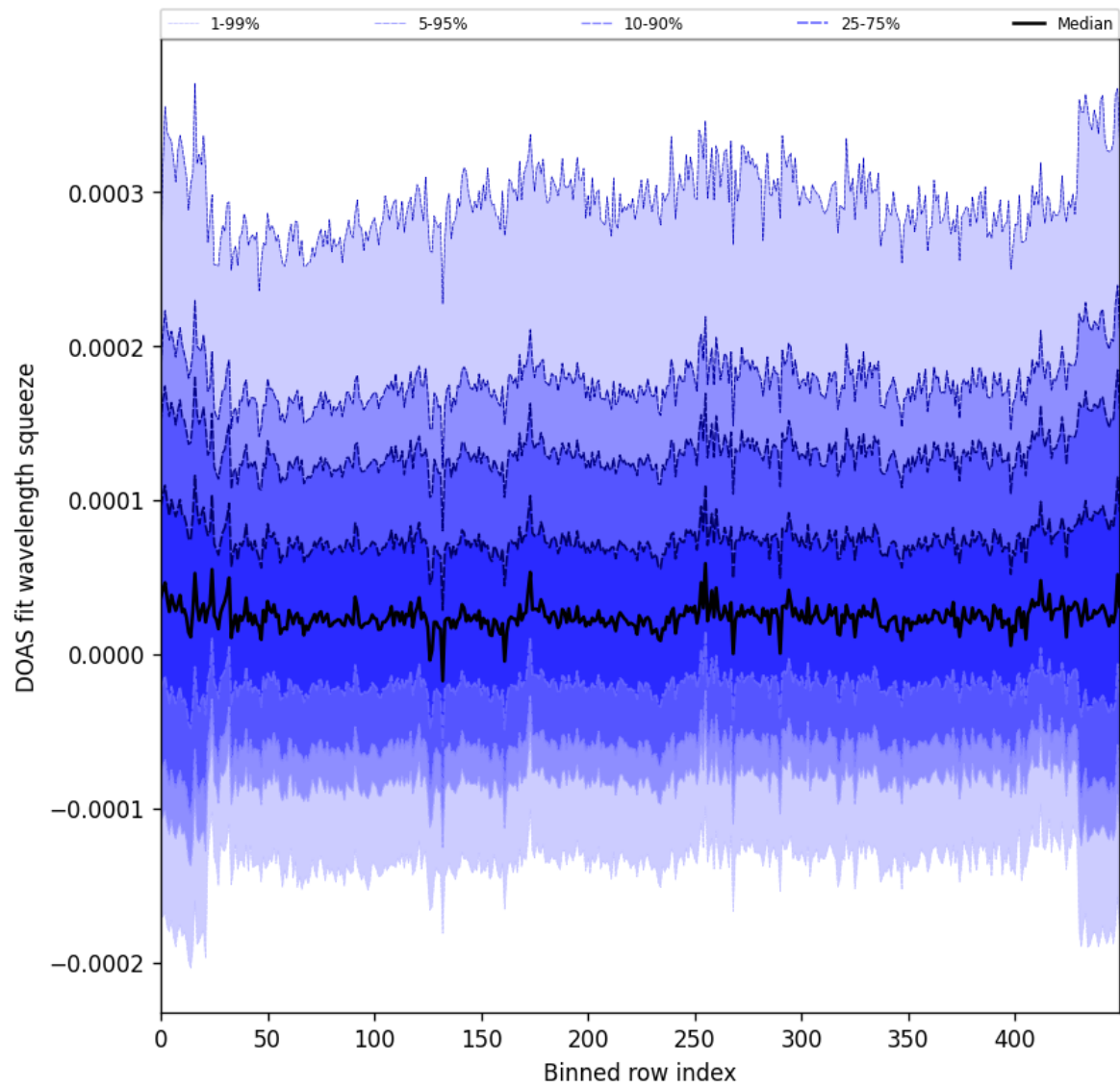
Figure 59: Along track statistics of “DOAS fit wavelength squeeze” for 2025-01-25 to 2025-01-27
