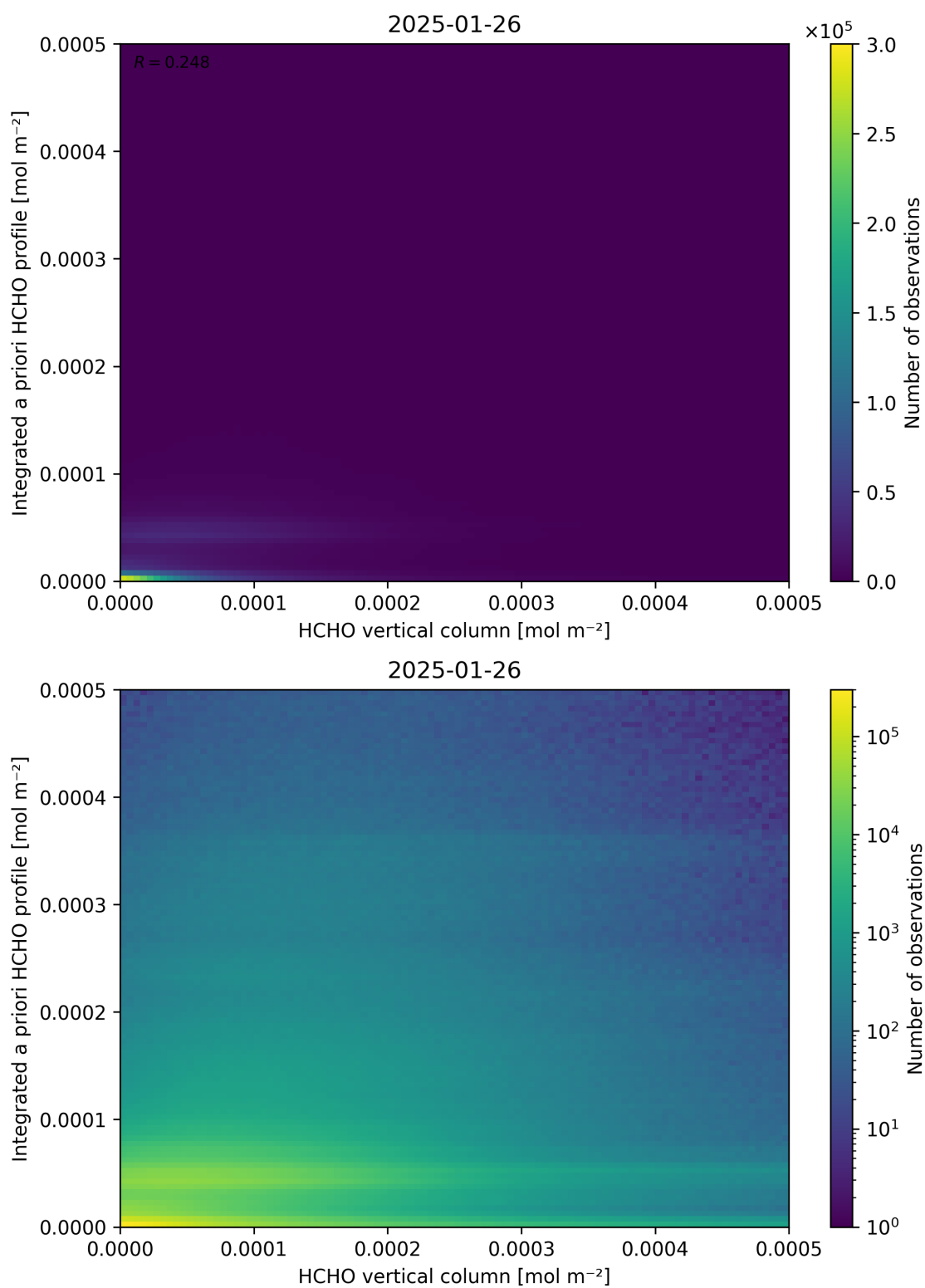
Figure 135: Scatter density plot of “HCHO vertical column” against “Integrated a priori HCHO profile” for 2025-01-25 to 2025-01-27.
