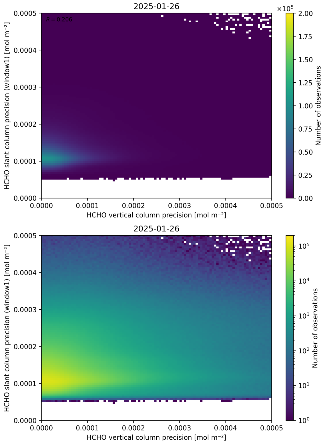
Figure 143: Scatter density plot of “HCHO vertical column precision” against “HCHO slant column precision (window1)” for 2025-01-25 to 2025-01-27.
