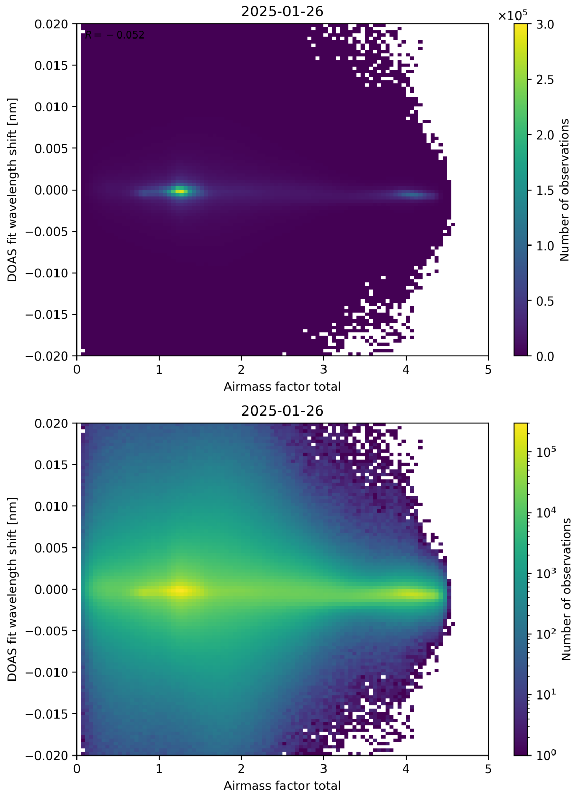
Figure 98: Scatter density plot of “Airmass factor total” against “DOAS fit wavelength shift” for 2025-01-25 to 2025-01-27.
