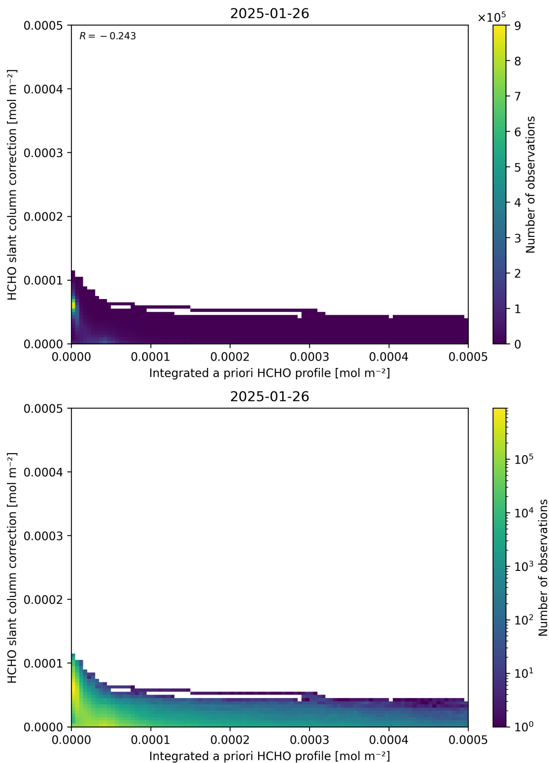
Figure 152: Scatter density plot of “Integrated a priori HCHO profile” against “HCHO slant column correction” for 2025-01-25 to 2025-01-27.
