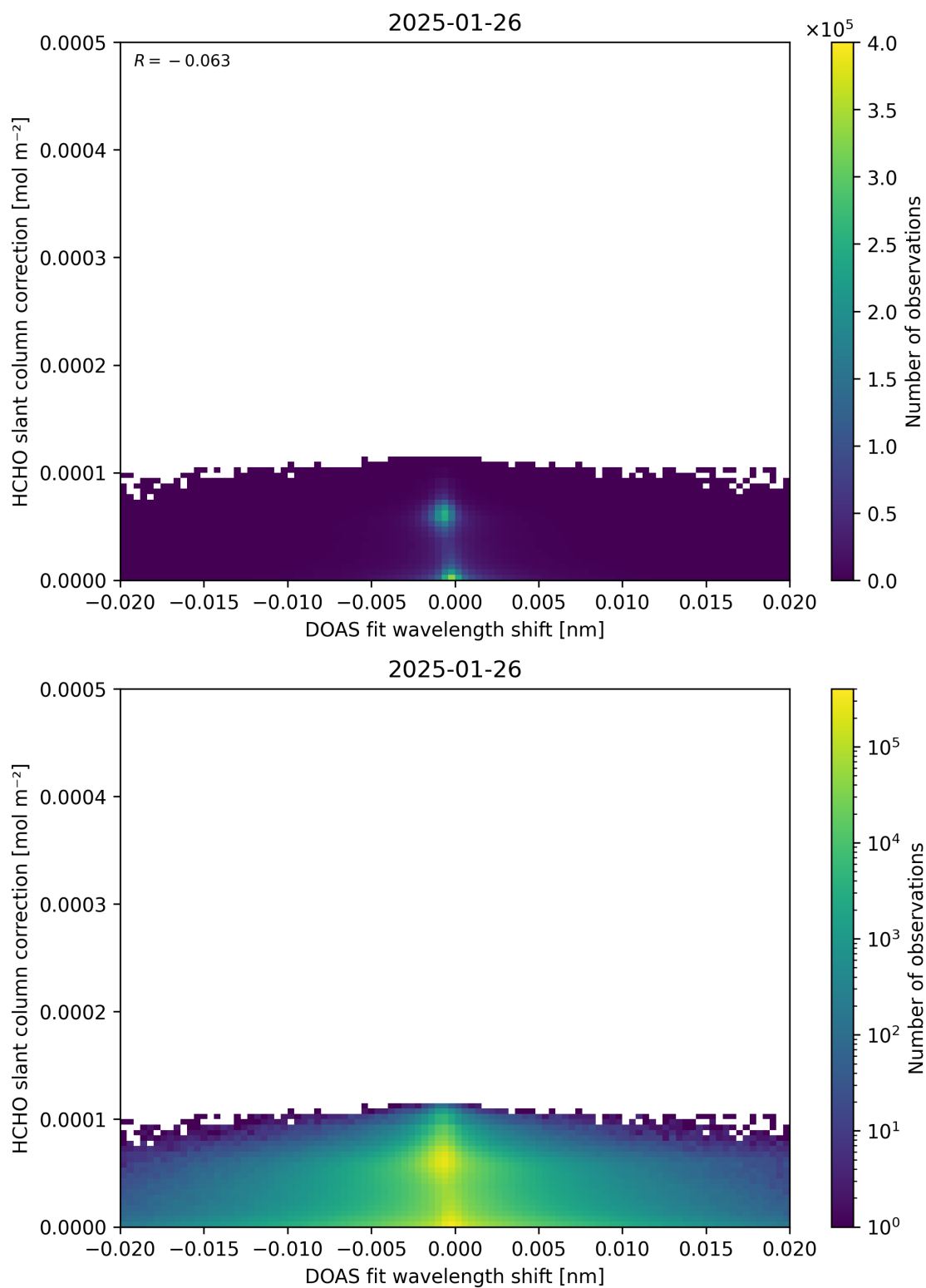
Figure 67: Scatter density plot of “DOAS fit wavelength shift” against “HCHO slant column correction” for 2025-01-25 to 2025-01-27.
