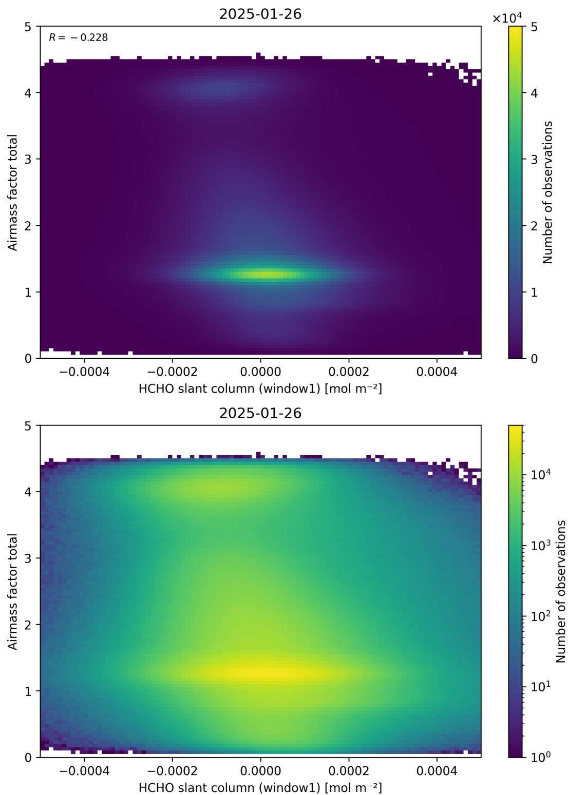
Figure 85: Scatter density plot of “HCHO slant column (window1)” against “Airmass factor total” for 2025-01-25 to 2025-01-27.
