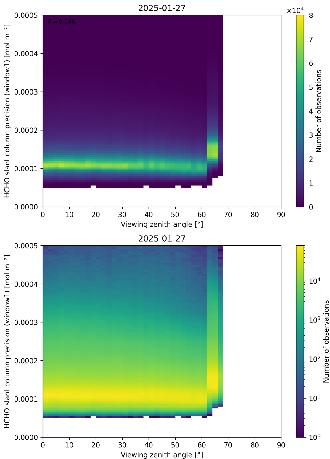
Figure 189: Scatter density plot of “Viewing zenith angle” against “HCHO slant column precision (window1)” for 2025-01-26 to 2025-01-28.
