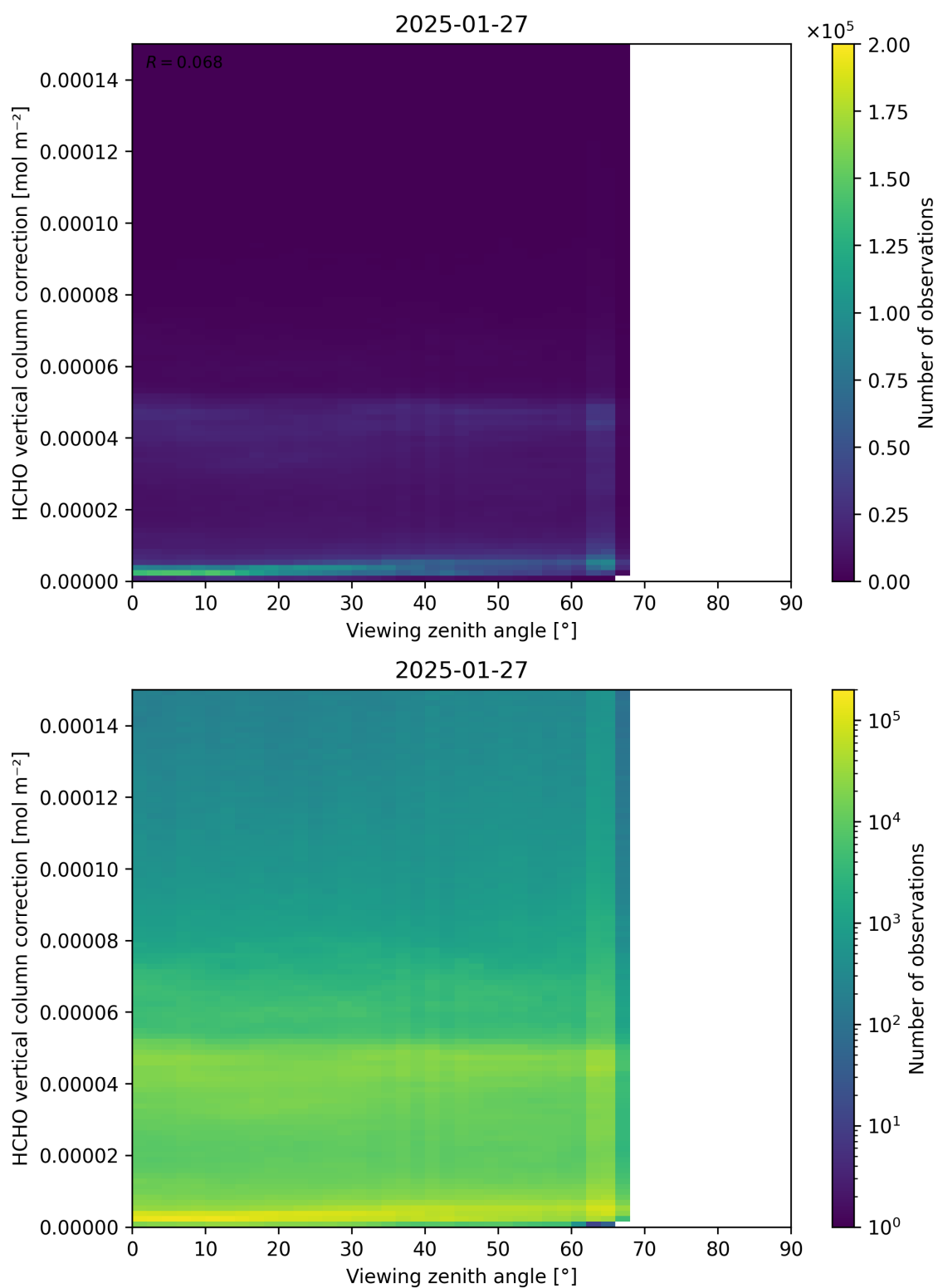
Figure 193: Scatter density plot of “Viewing zenith angle” against “HCHO vertical column correction” for 2025-01-26 to 2025-01-28.
