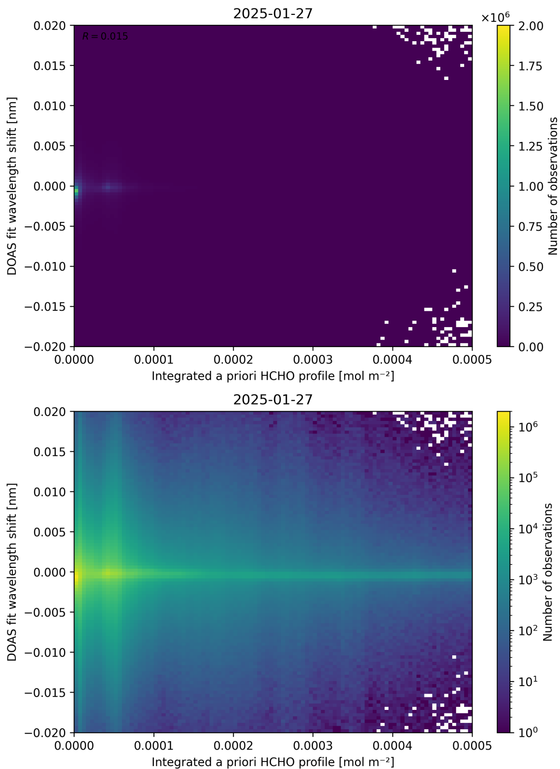
Figure 149: Scatter density plot of “Integrated a priori HCHO profile” against “DOAS fit wavelength shift” for 2025-01-26 to 2025-01-28.
