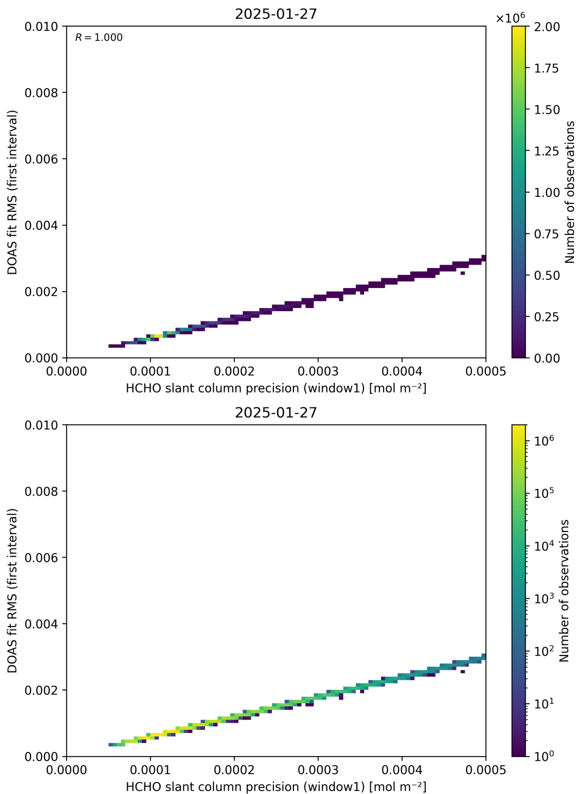
Figure 88: Scatter density plot of “HCHO slant column precision (window1)” against “DOAS fit RMS (first interval)” for 2025-01-26 to 2025-01-28.
