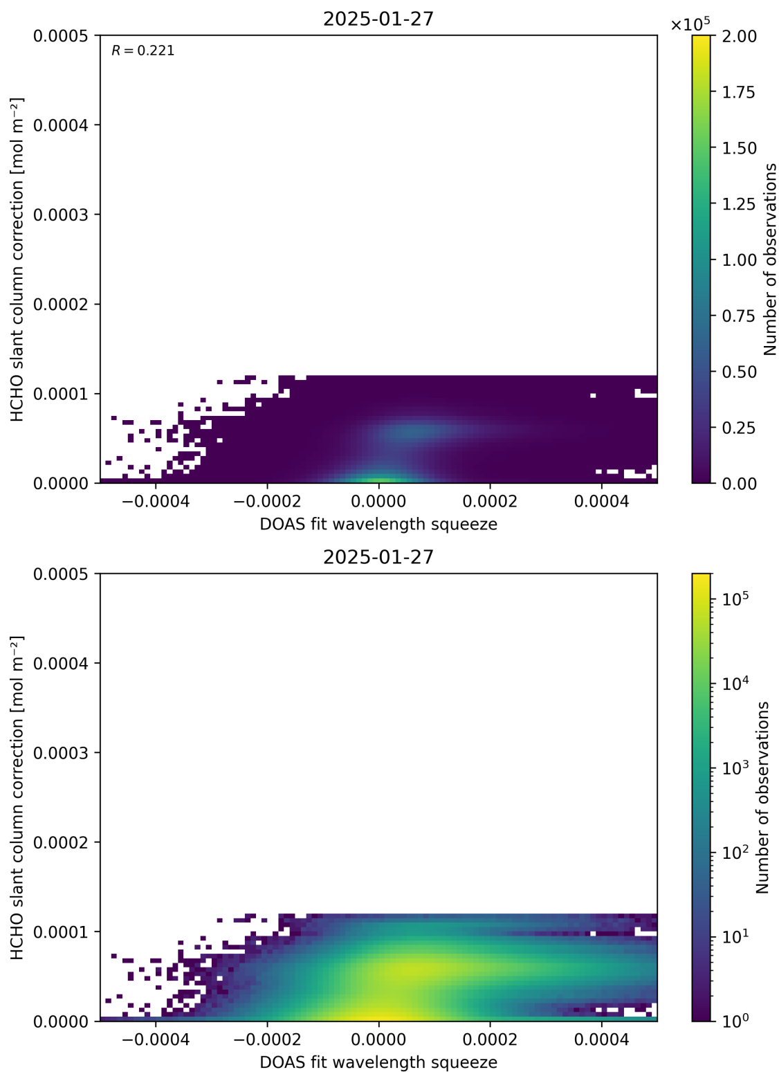
Figure 70: Scatter density plot of “DOAS fit wavelength squeeze” against “HCHO slant column correction” for 2025-01-26 to 2025-01-28.
