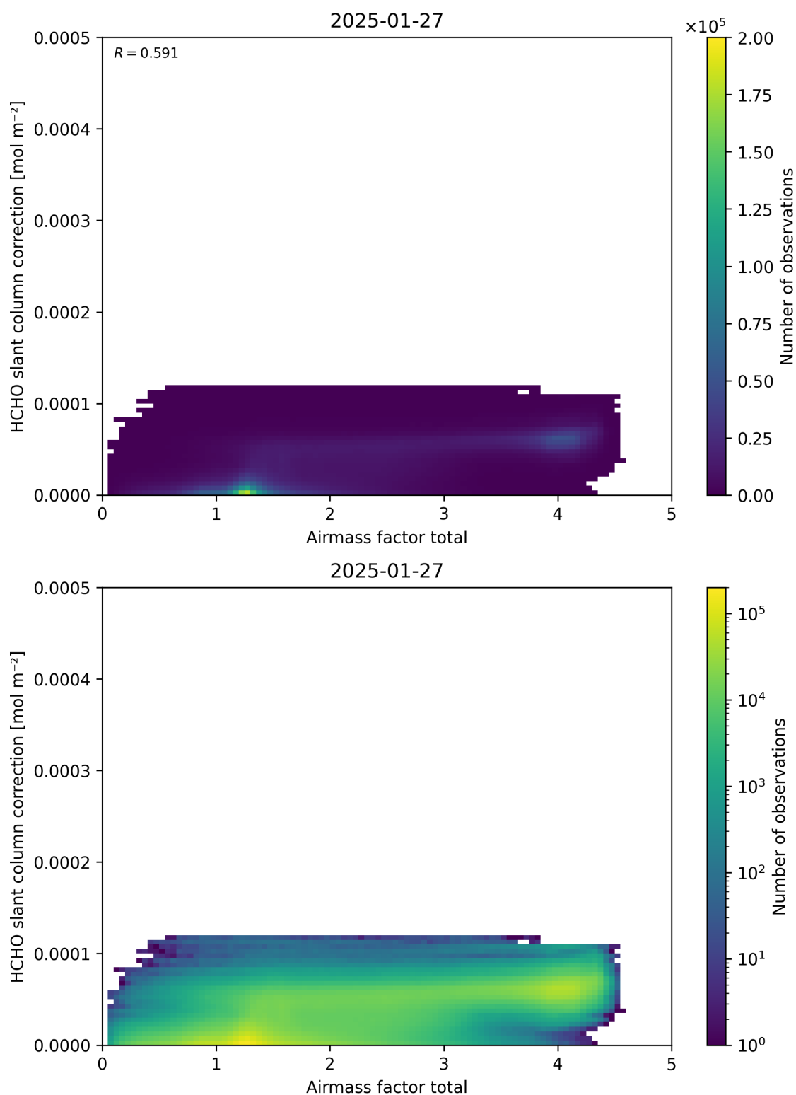
Figure 102: Scatter density plot of “Airmass factor total” against “HCHO slant column correction” for 2025-01-26 to 2025-01-28.
