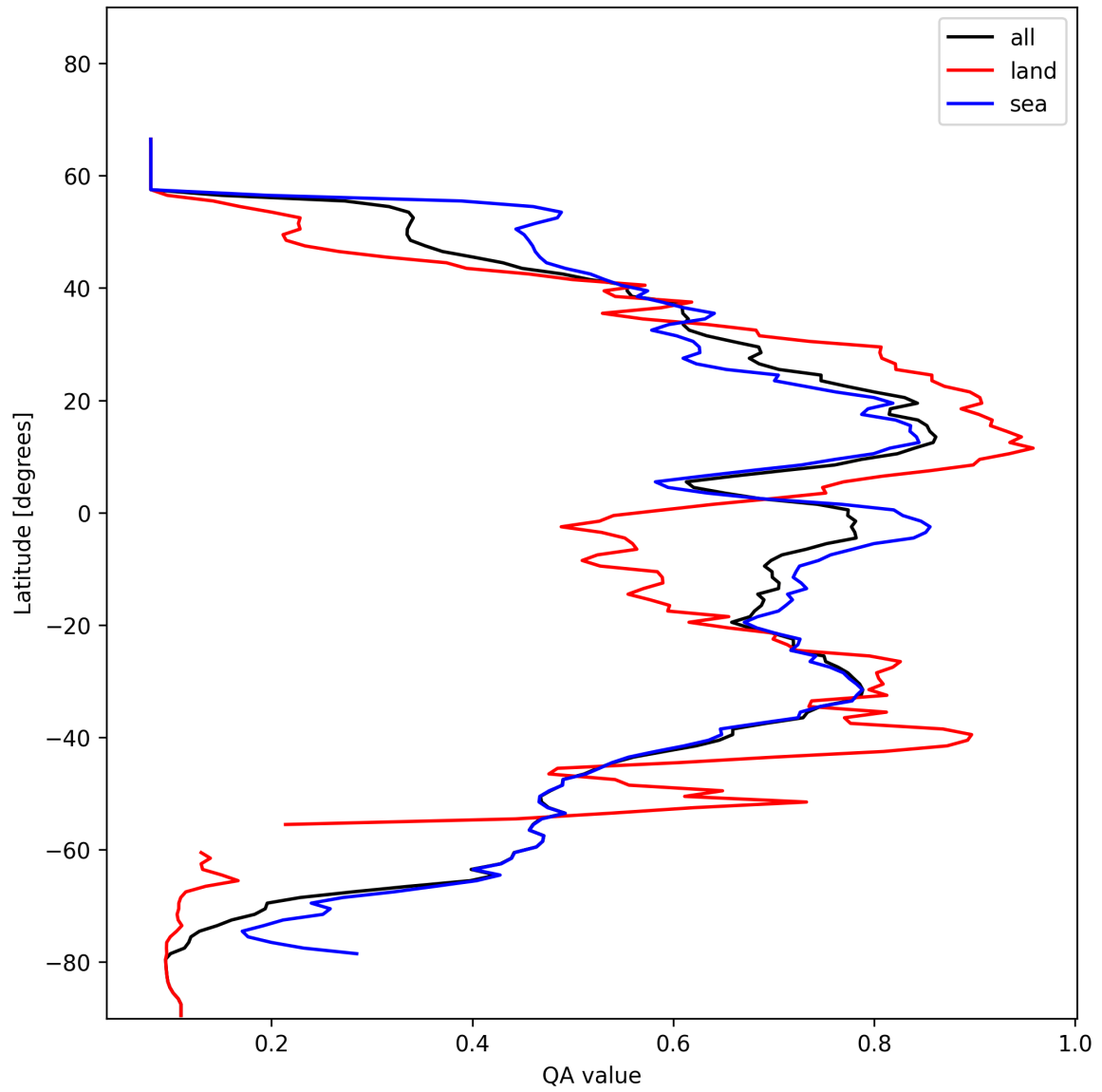
Figure 20: Zonal average of “QA value” for 2025-01-26 to 2025-01-28.
