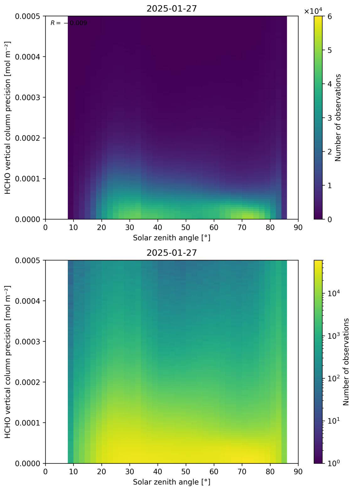
Figure 179: Scatter density plot of “Solar zenith angle” against “HCHO vertical column precision” for 2025-01-26 to 2025-01-28.
