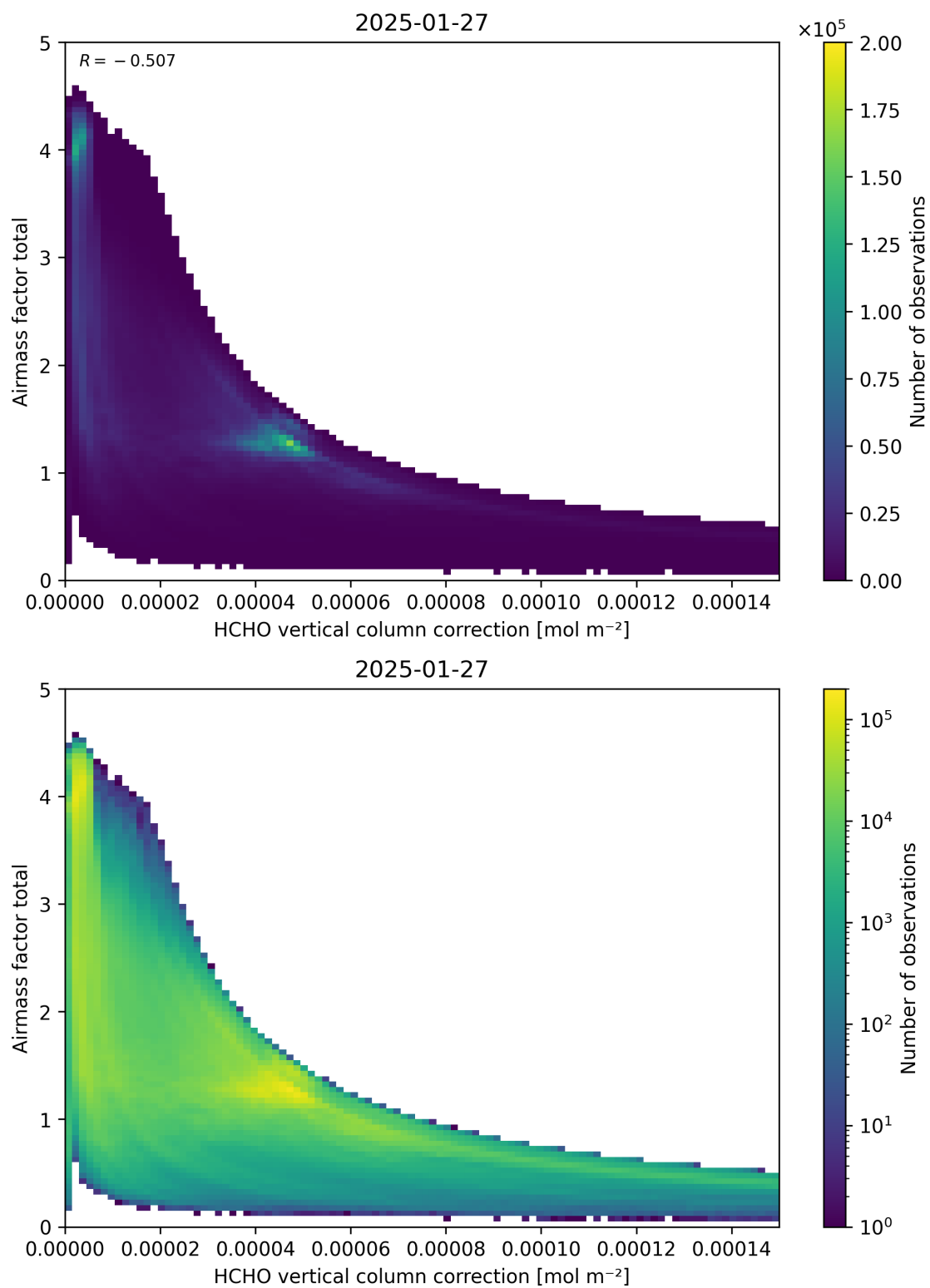
Figure 120: Scatter density plot of “HCHO vertical column correction” against “Airmass factor total” for 2025-01-26 to 2025-01-28.
