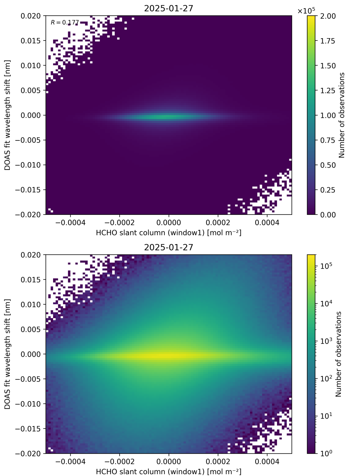
Figure 79: Scatter density plot of “HCHO slant column (window1)” against “DOAS fit wavelength shift” for 2025-01-26 to 2025-01-28.
