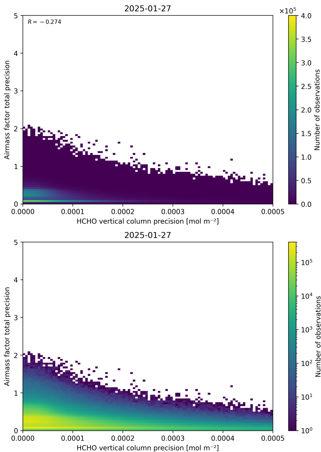
Figure 145: Scatter density plot of “HCHO vertical column precision” against “Airmass factor total precision” for 2025-01-26 to 2025-01-28.
