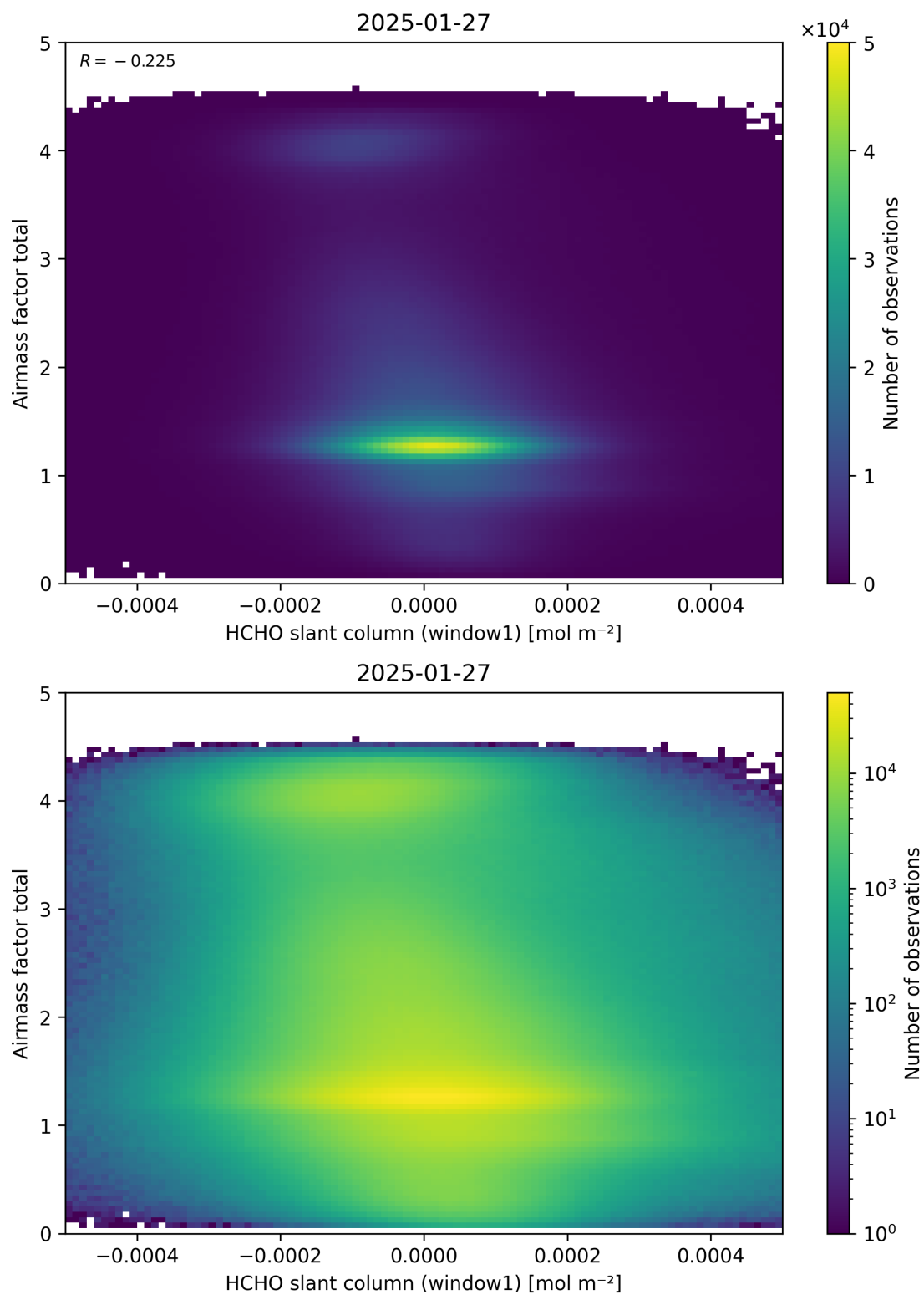
Figure 85: Scatter density plot of “HCHO slant column (window1)” against “Airmass factor total” for 2025-01-26 to 2025-01-28.
