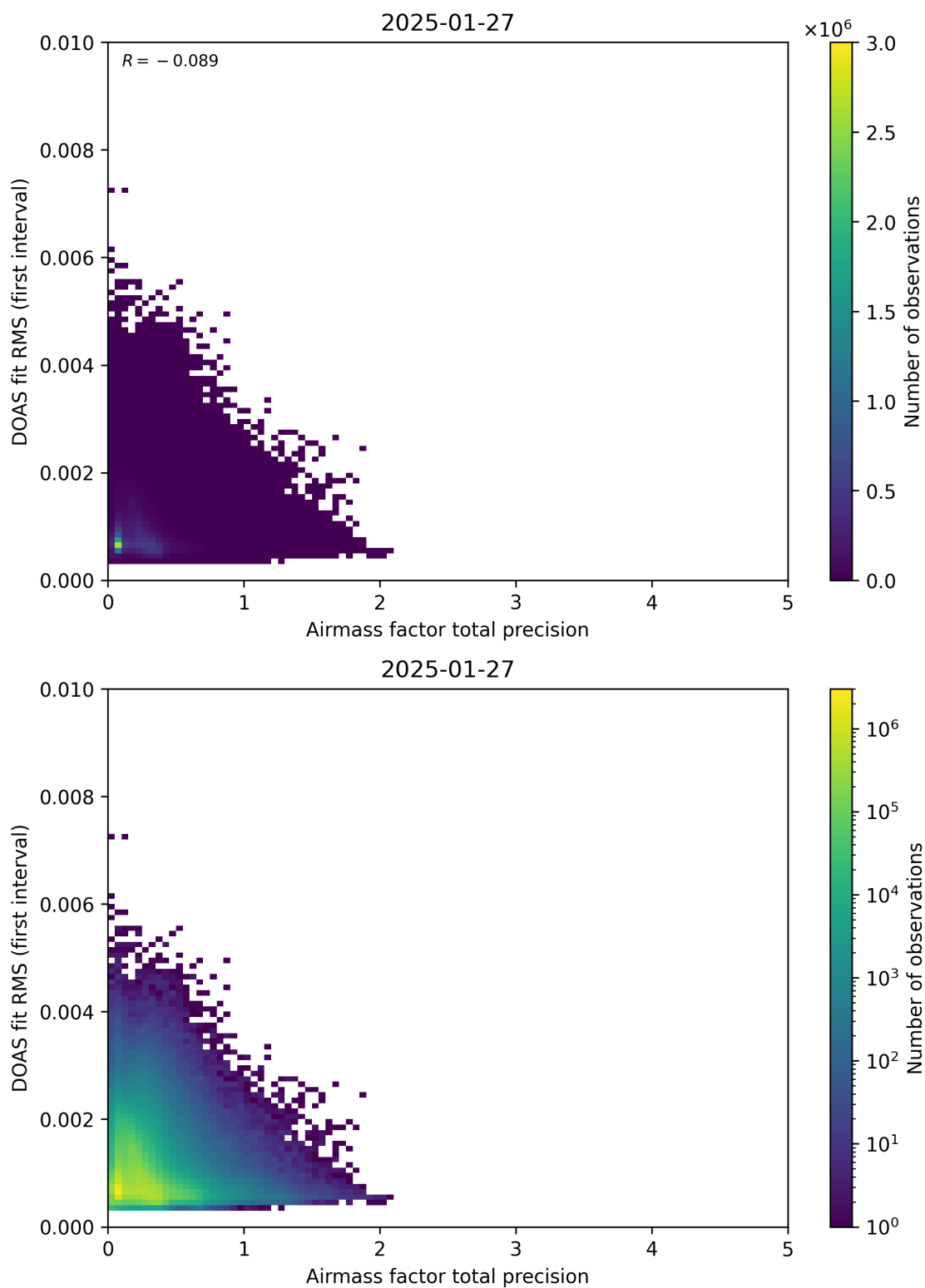
Figure 105: Scatter density plot of “Airmass factor total precision” against “DOAS fit RMS (first interval)” for 2025-01-26 to 2025-01-28.
