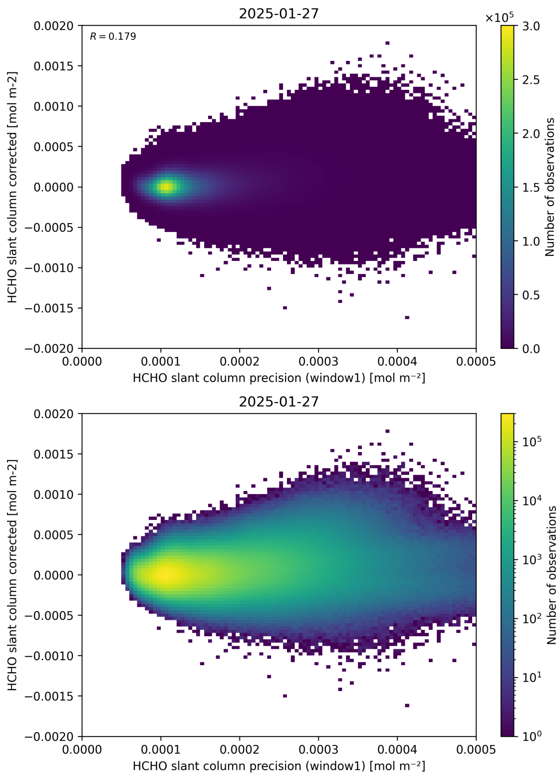
Figure 92: Scatter density plot of “HCHO slant column precision (window1)” against “HCHO slant column corrected” for 2025-01-26 to 2025-01-28.
