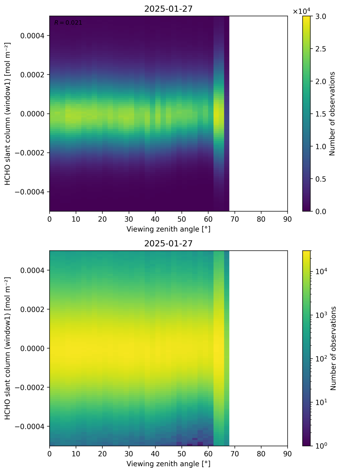
Figure 188: Scatter density plot of “Viewing zenith angle” against “HCHO slant column (window1)” for 2025-01-26 to 2025-01-28.
