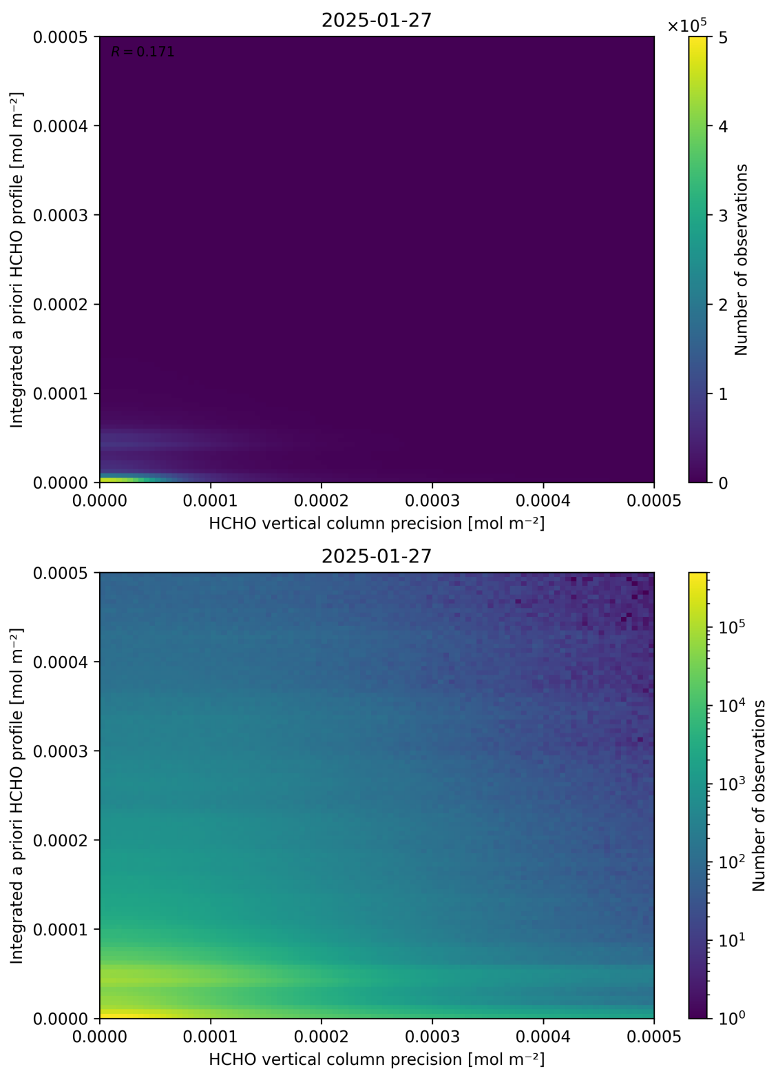
Figure 147: Scatter density plot of “HCHO vertical column precision” against “Integrated a priori HCHO profile” for 2025-01-26 to 2025-01-28.
