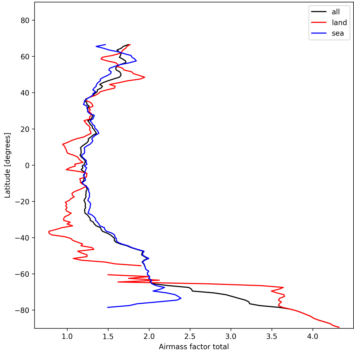
Figure 26: Zonal average of “Airmass factor total” for 2025-01-26 to 2025-01-28.
