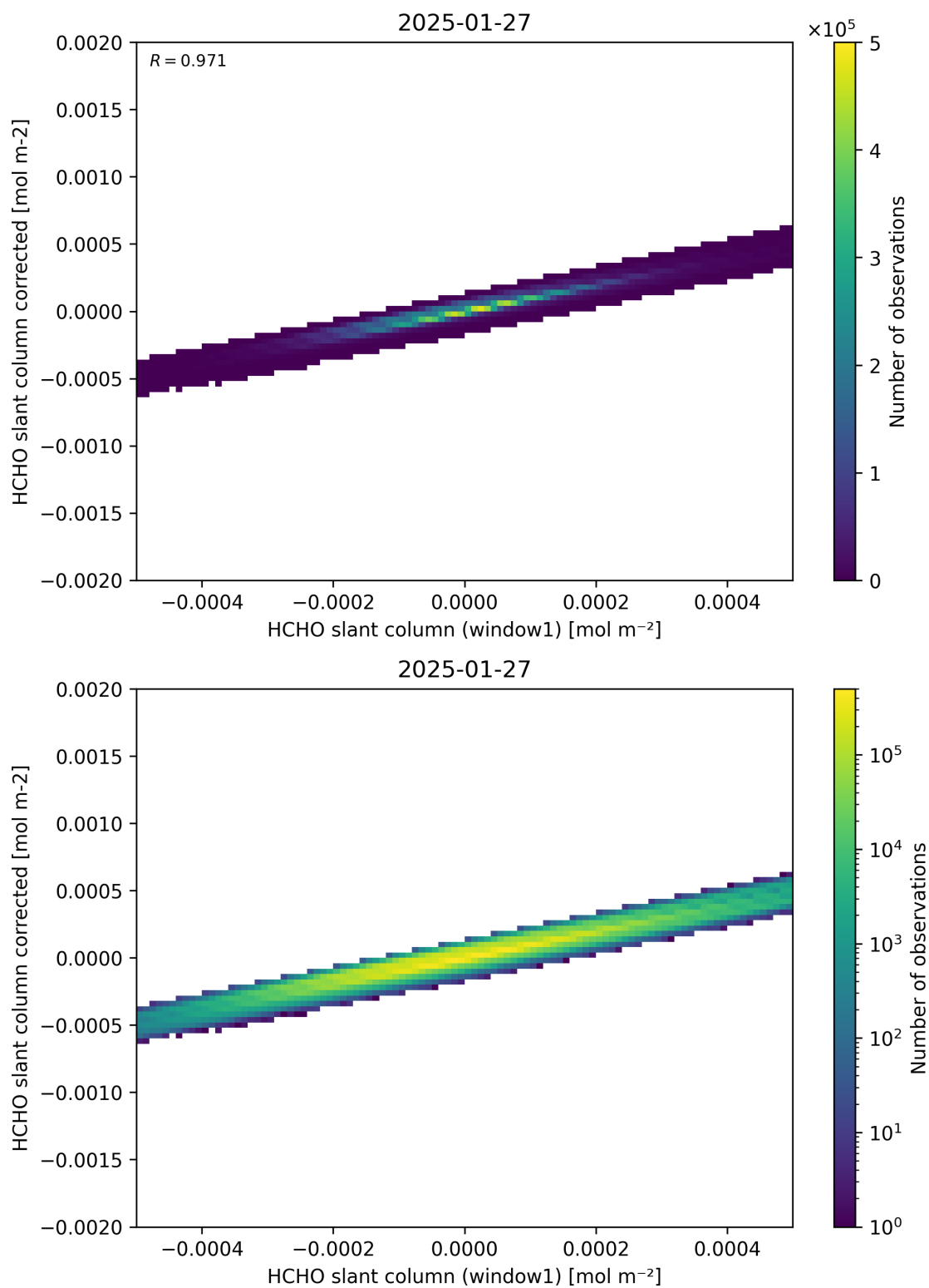
Figure 82: Scatter density plot of “HCHO slant column (window1)” against “HCHO slant column corrected” for 2025-01-26 to 2025-01-28.
