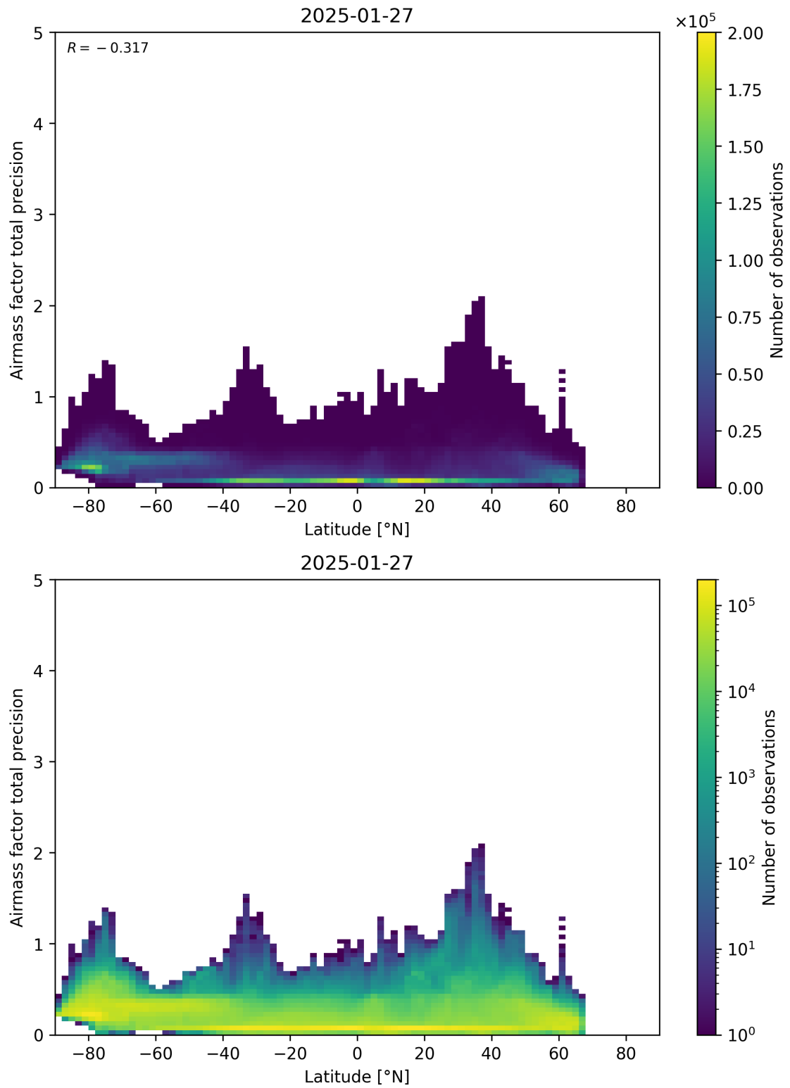
Figure 162: Scatter density plot of “Latitude” against “Airmass factor total precision” for 2025-01-26 to 2025-01-28.
