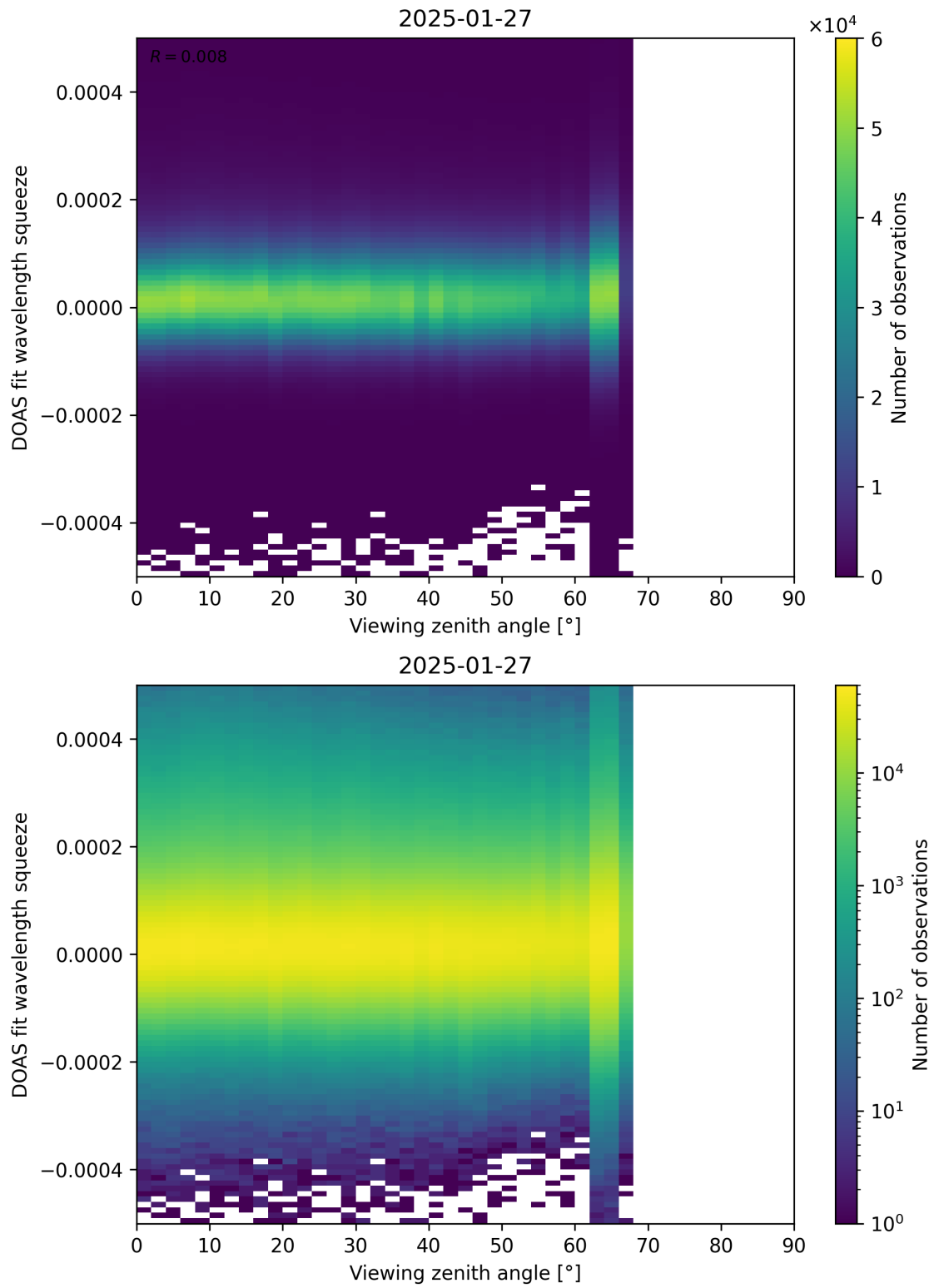
Figure 184: Scatter density plot of “Viewing zenith angle” against “DOAS fit wavelength squeeze” for 2025-01-26 to 2025-01-28.
