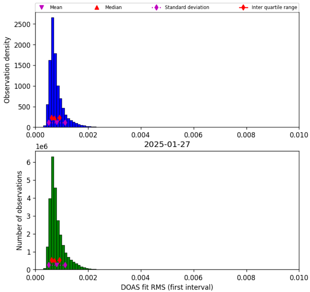
Figure 46: Histogram of “DOAS fit RMS (first interval)” for 2025-01-26 to 2025-01-28
