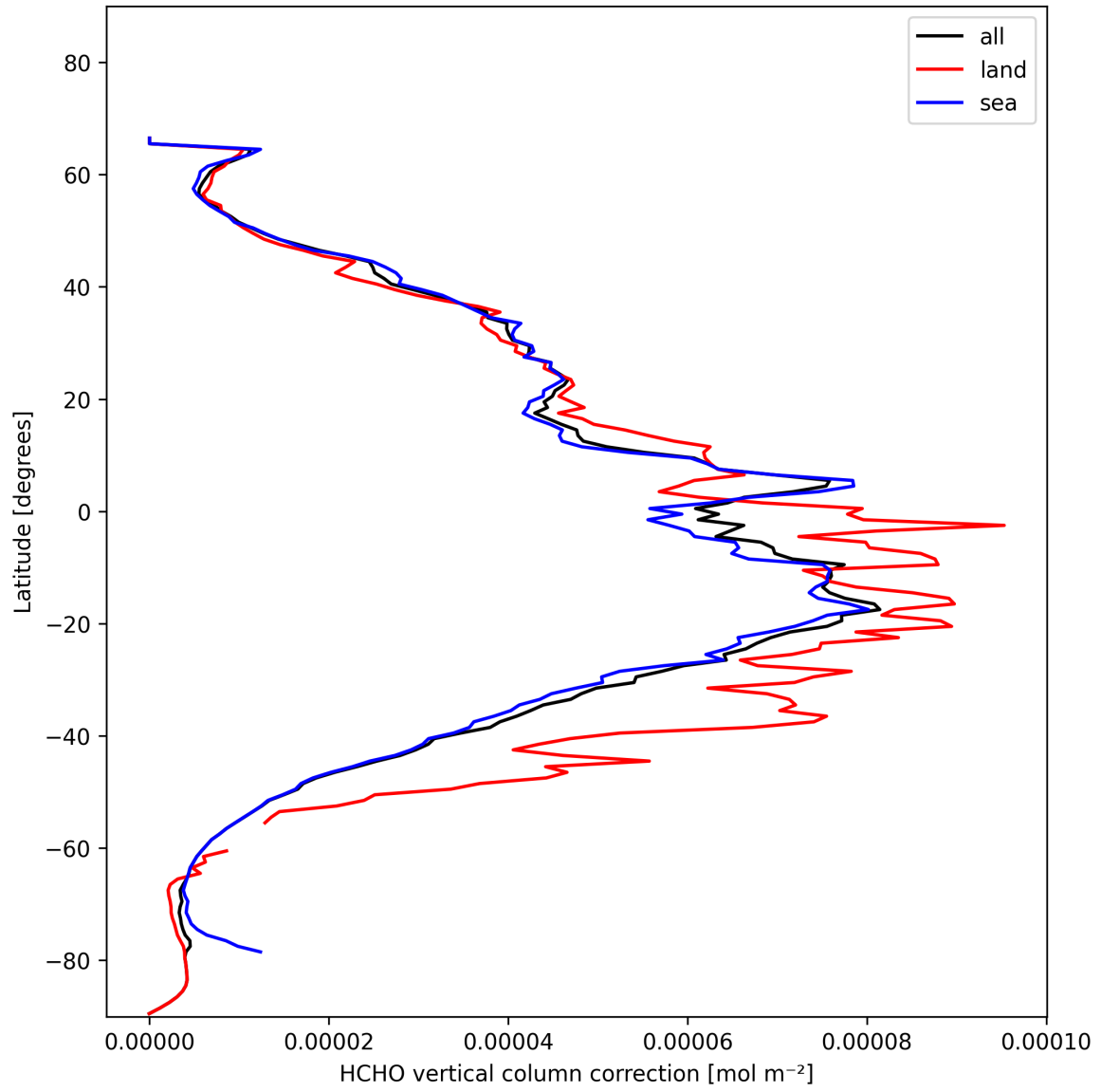
Figure 23: Zonal average of “HCHO vertical column correction” for 2025-01-26 to 2025-01-28.
