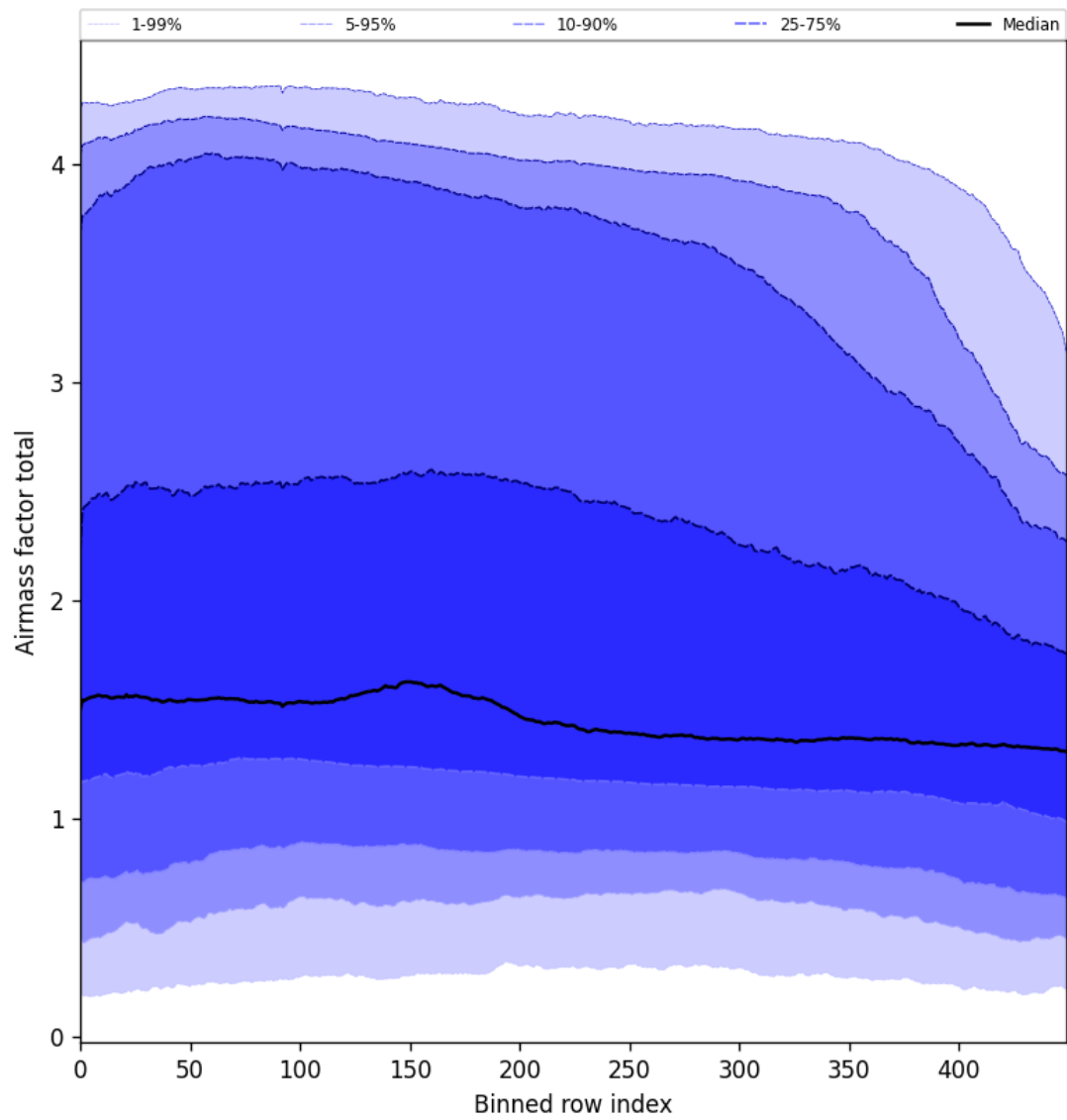
Figure 54: Along track statistics of “Airmass factor total” for 2025-01-26 to 2025-01-28
