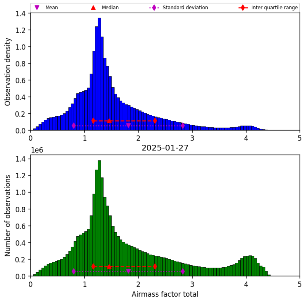
Figure 40: Histogram of “Airmass factor total” for 2025-01-26 to 2025-01-28
