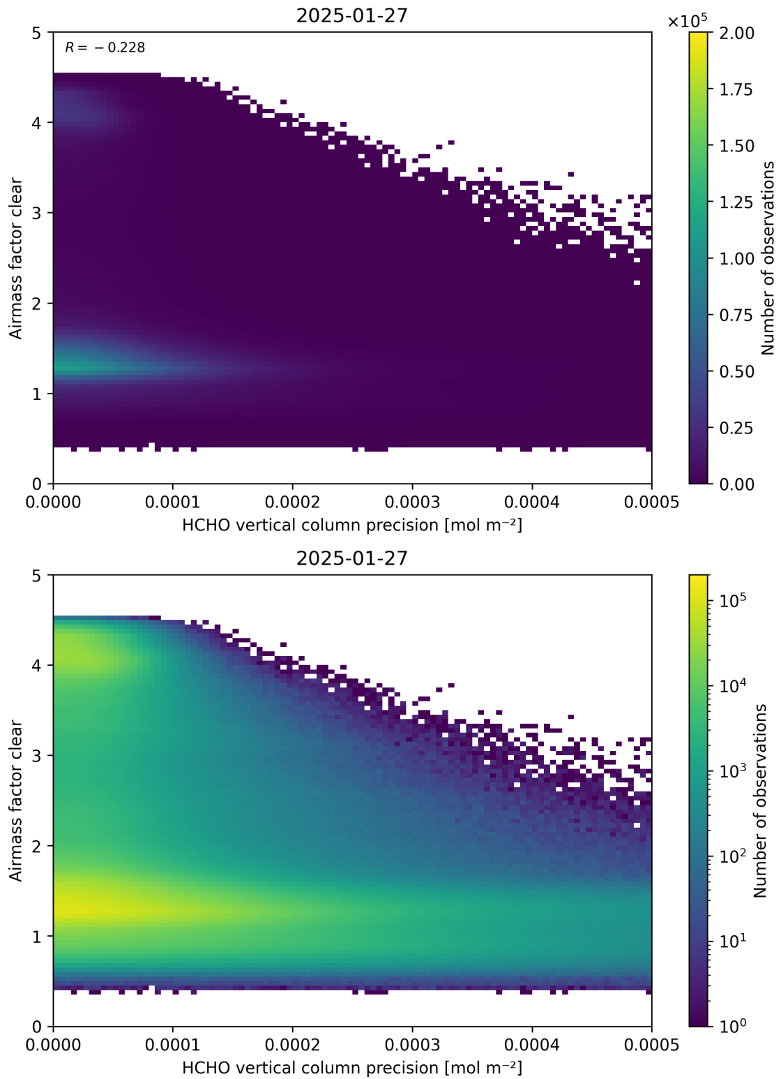
Figure 139: Scatter density plot of “HCHO vertical column precision” against “Airmass factor clear” for 2025-01-26 to 2025-01-28.
