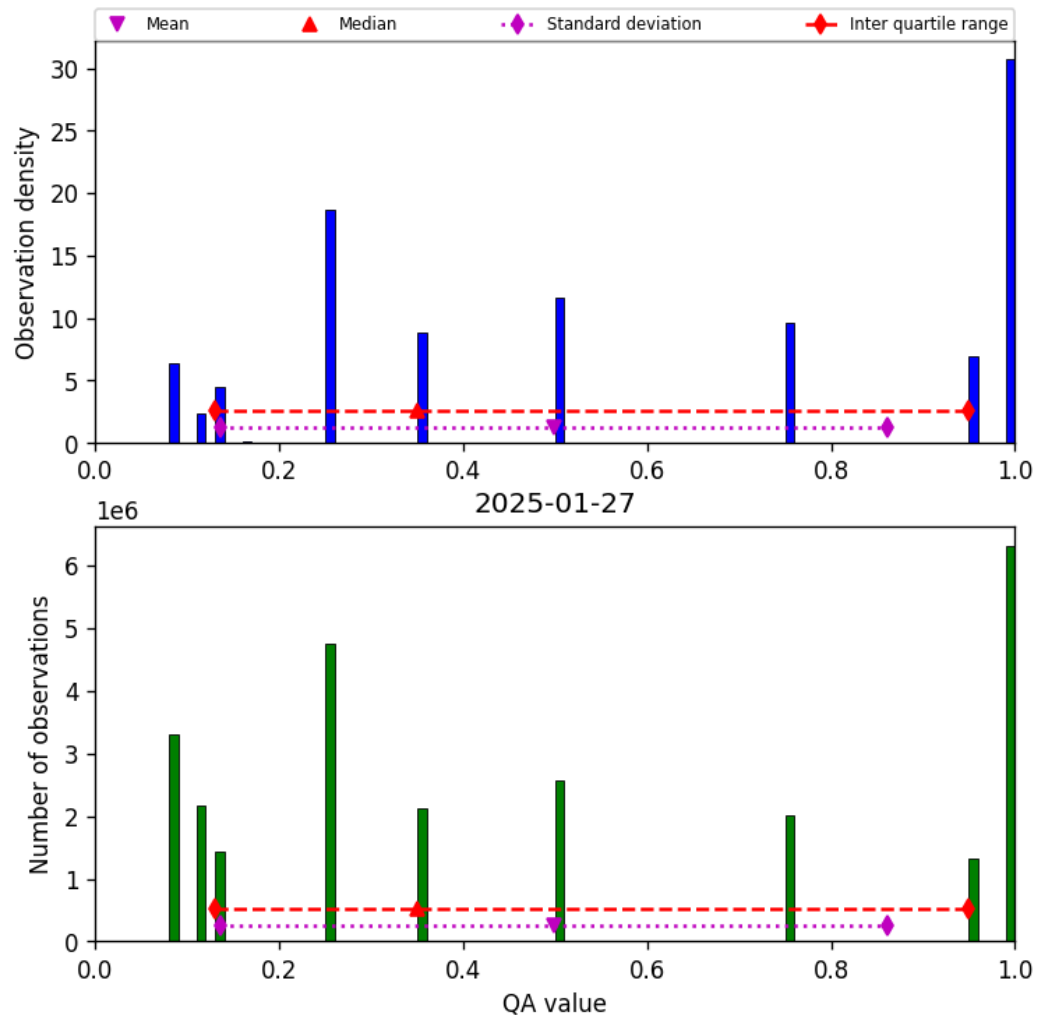
Figure 34: Histogram of “QA value” for 2025-01-26 to 2025-01-28
