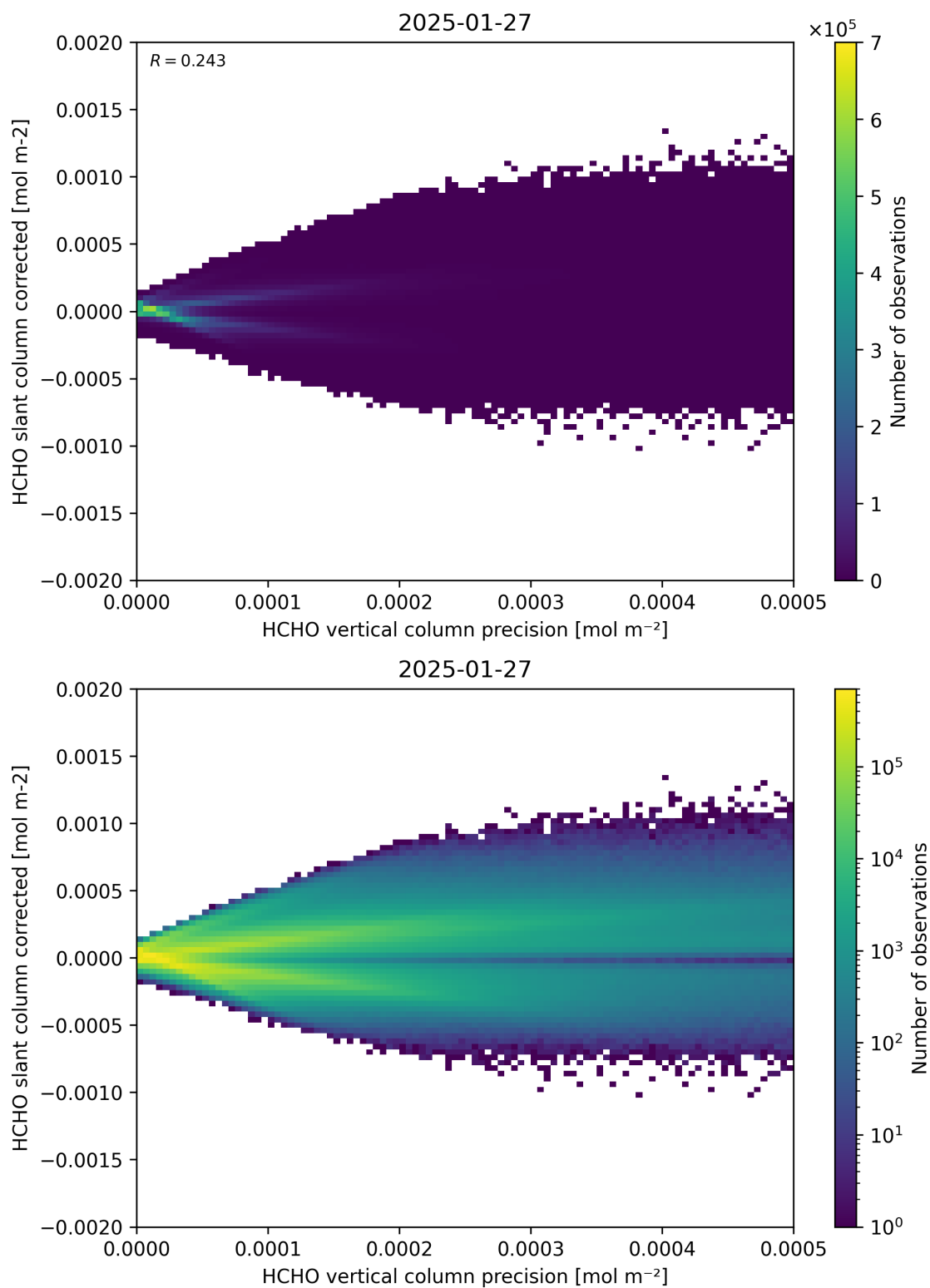
Figure 140: Scatter density plot of “HCHO vertical column precision” against “HCHO slant column corrected” for 2025-01-26 to 2025-01-28.
