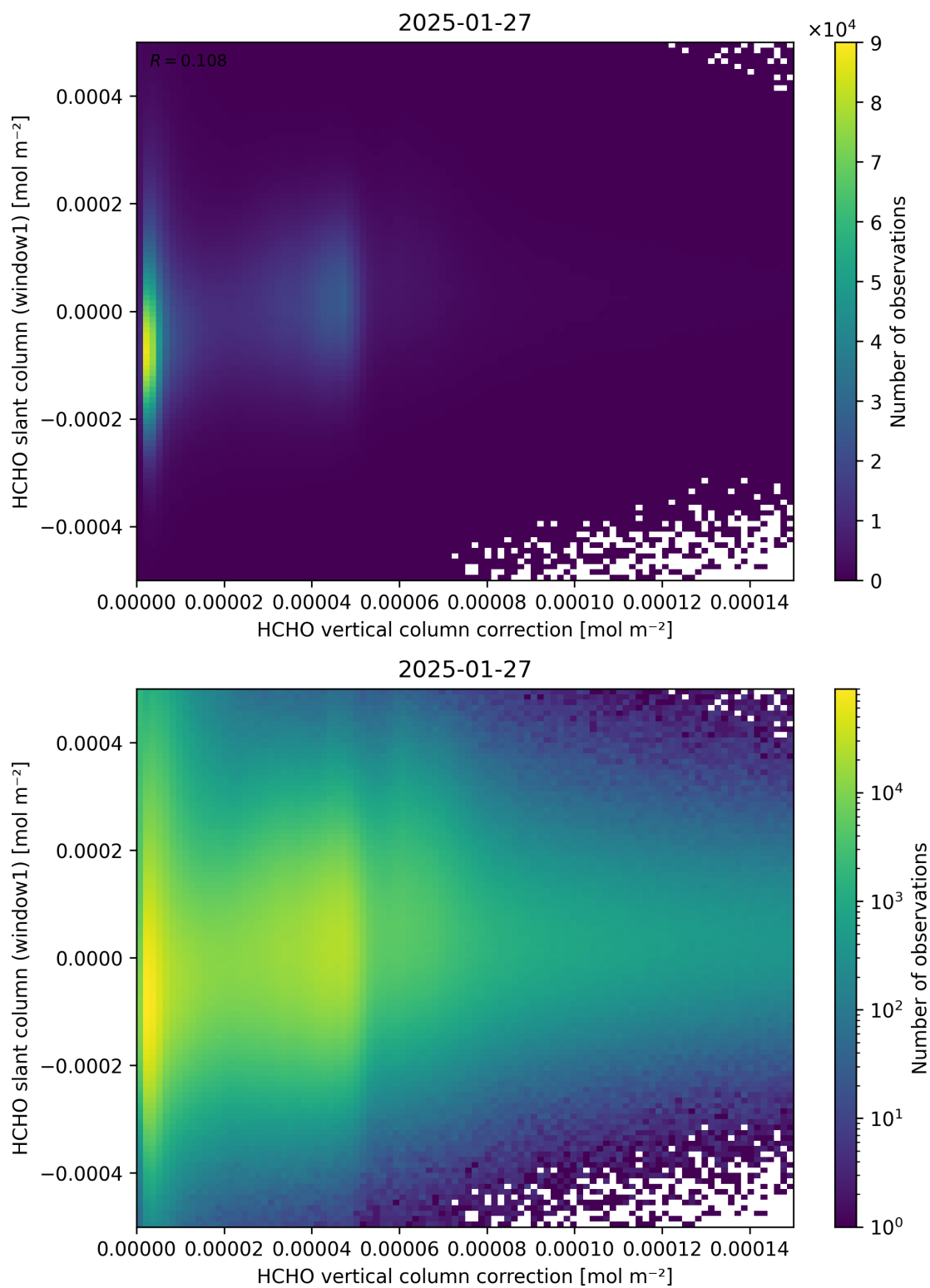
Figure 118: Scatter density plot of “HCHO vertical column correction” against “HCHO slant column (window1)” for 2025-01-26 to 2025-01-28.
