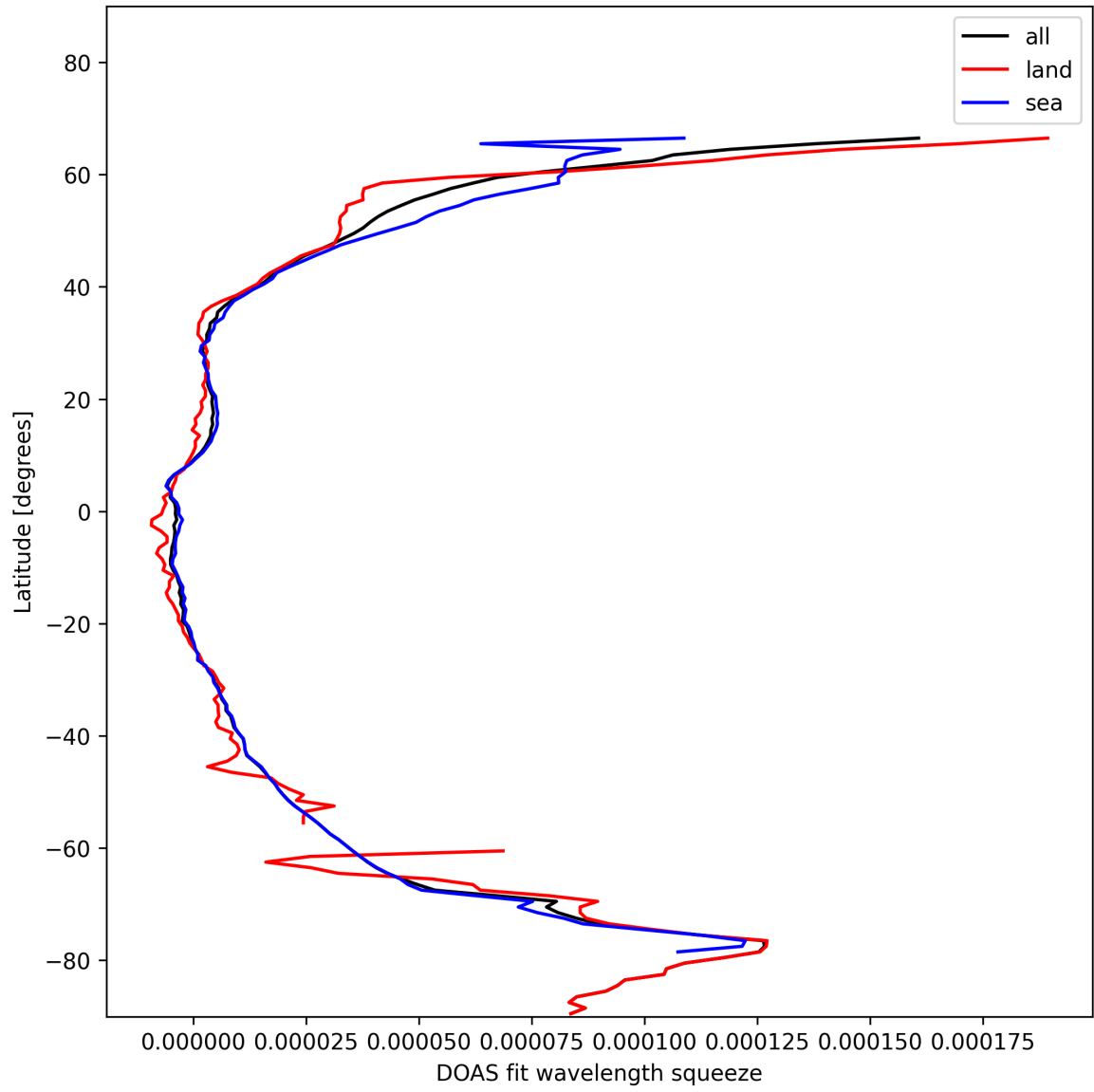
Figure 31: Zonal average of “DOAS fit wavelength squeeze” for 2025-01-26 to 2025-01-28.
