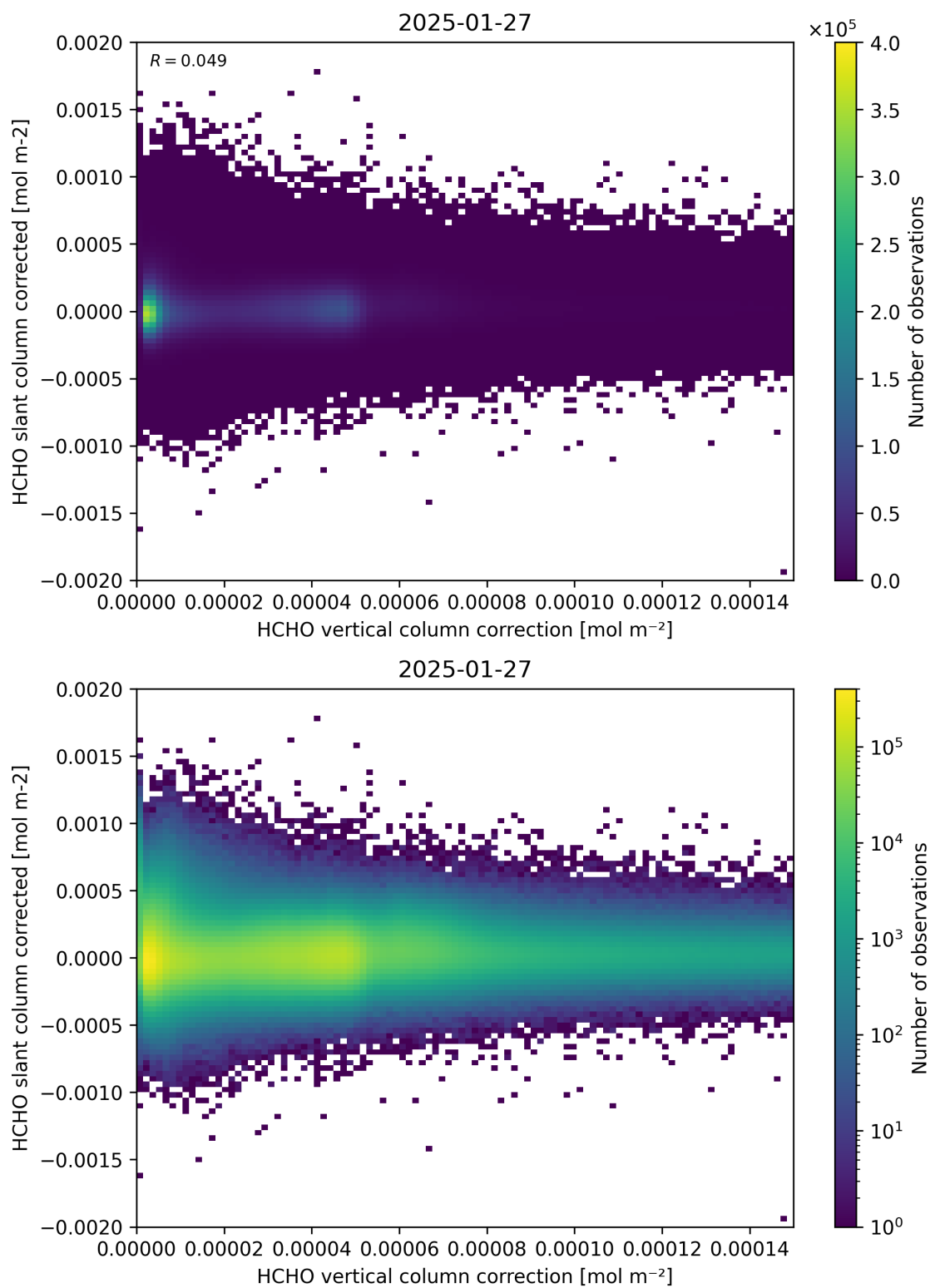
Figure 116: Scatter density plot of “HCHO vertical column correction” against “HCHO slant column corrected” for 2025-01-26 to 2025-01-28.
