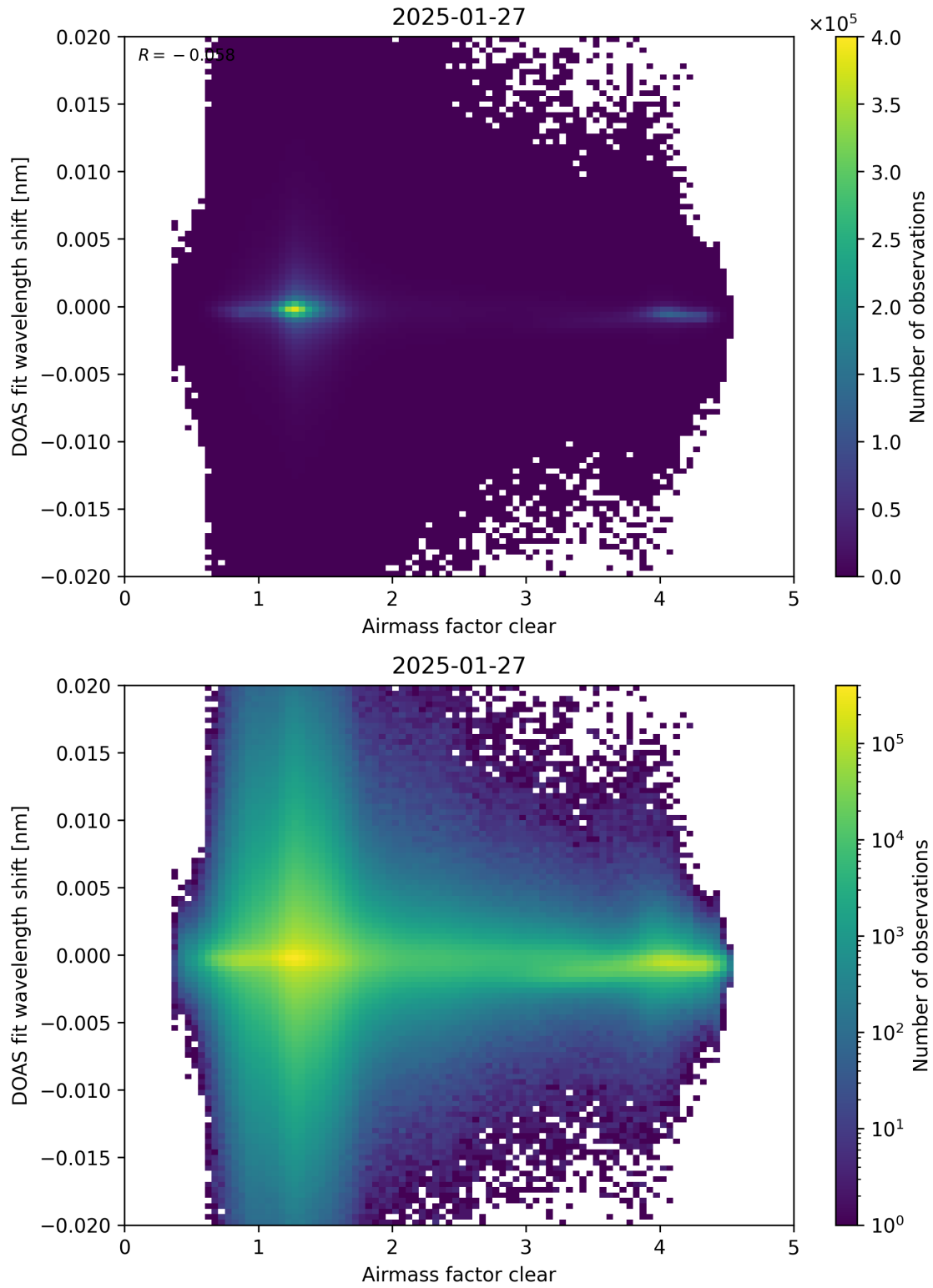
Figure 72: Scatter density plot of “Airmass factor clear” against “DOAS fit wavelength shift” for 2025-01-26 to 2025-01-28.
