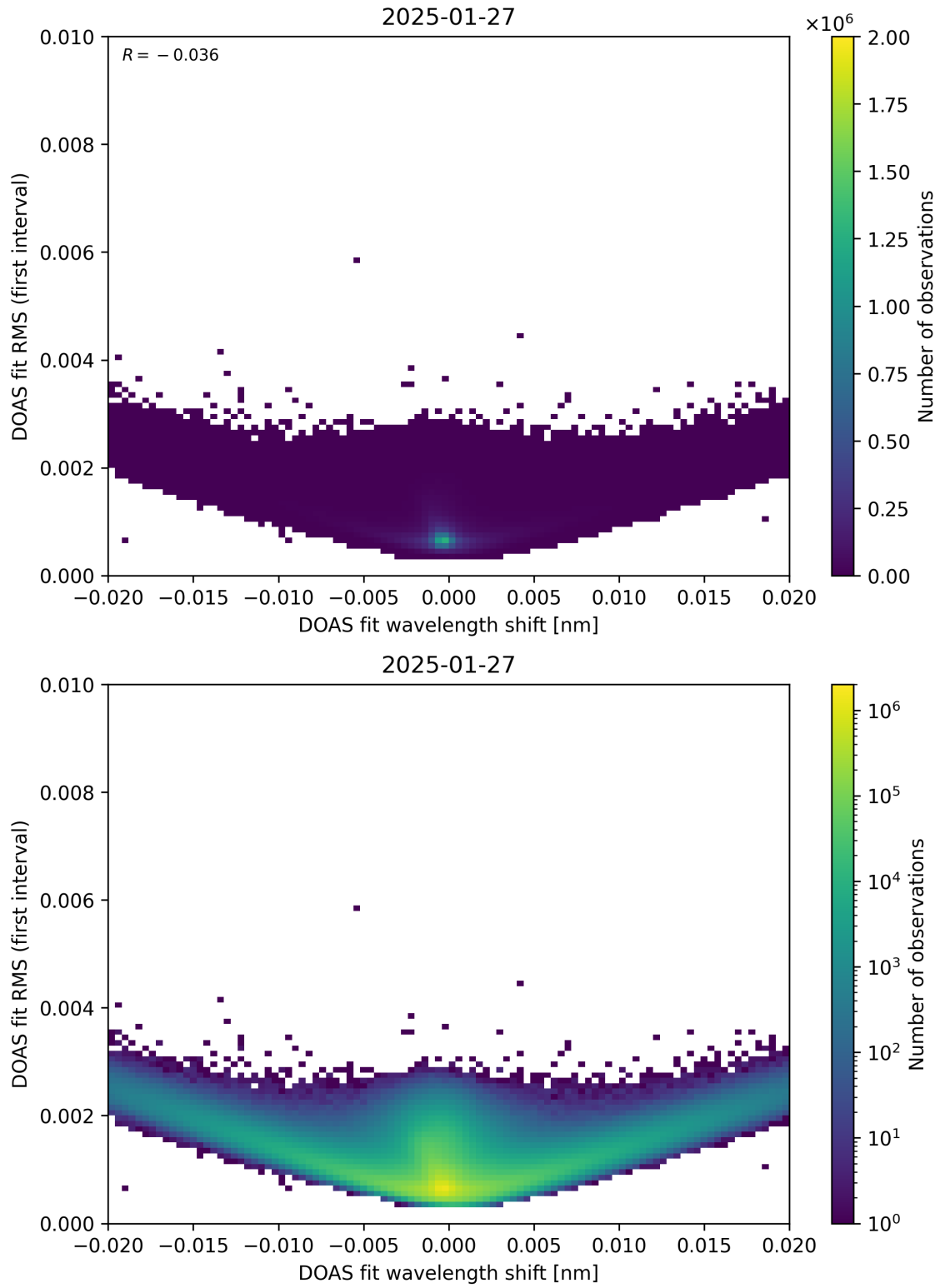
Figure 64: Scatter density plot of “DOAS fit wavelength shift” against “DOAS fit RMS (first interval)” for 2025-01-26 to 2025-01-28.
