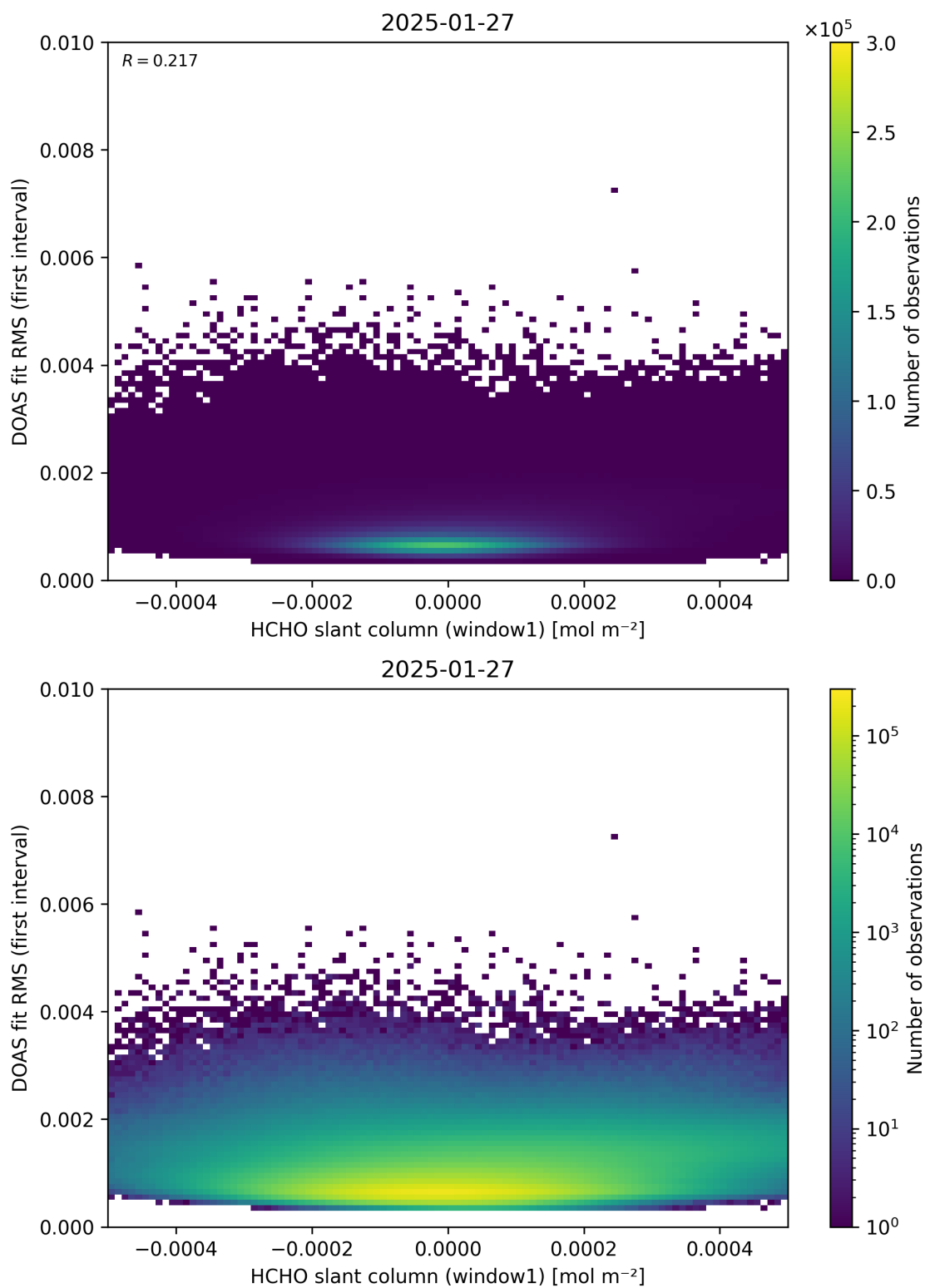
Figure 78: Scatter density plot of “HCHO slant column (window1)” against “DOAS fit RMS (first interval)” for 2025-01-26 to 2025-01-28.
