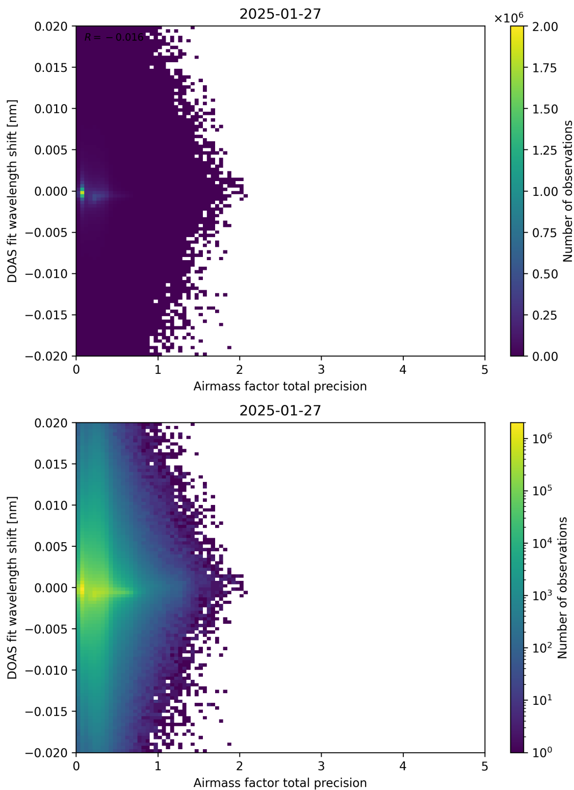
Figure 106: Scatter density plot of “Airmass factor total precision” against “DOAS fit wavelength shift” for 2025-01-26 to 2025-01-28.
