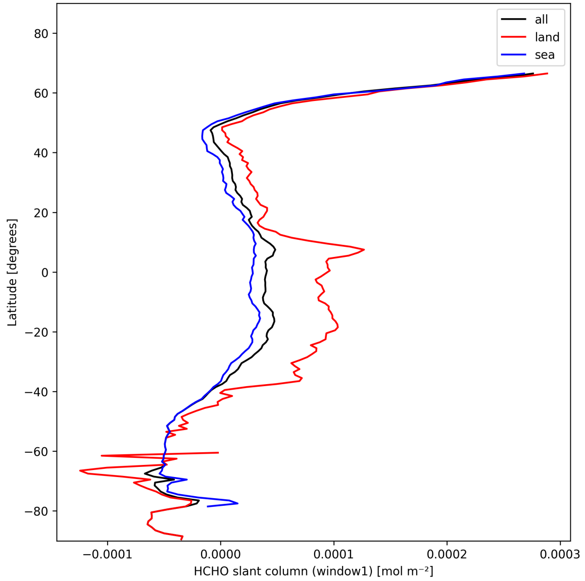
Figure 24: Zonal average of “HCHO slant column (window1)” for 2025-01-26 to 2025-01-28.
