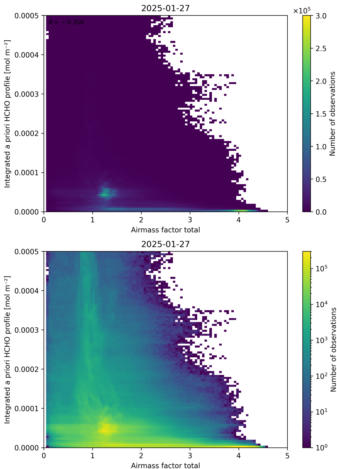
Figure 104: Scatter density plot of “Airmass factor total” against “Integrated a priori HCHO profile” for 2025-01-26 to 2025-01-28.
