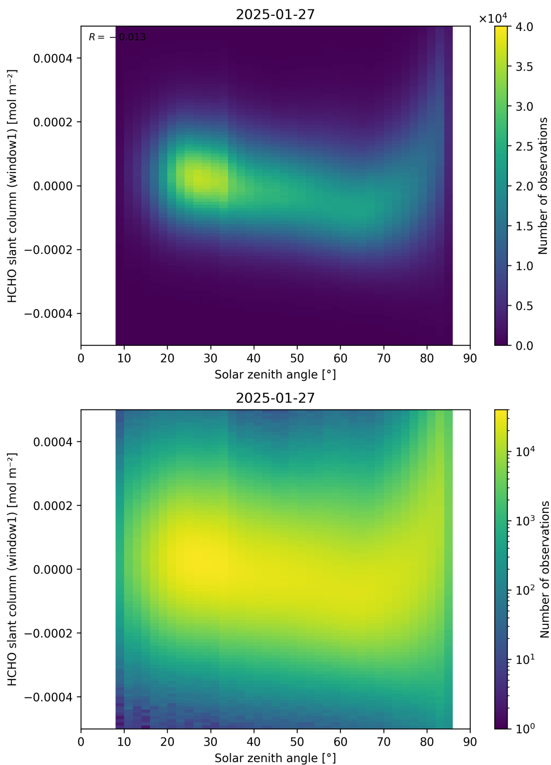
Figure 173: Scatter density plot of “Solar zenith angle” against “HCHO slant column (window1)” for 2025-01-26 to 2025-01-28.
