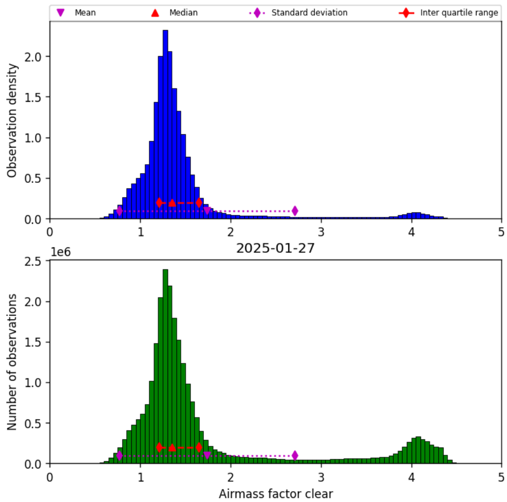
Figure 42: Histogram of “Airmass factor clear” for 2025-01-26 to 2025-01-28
