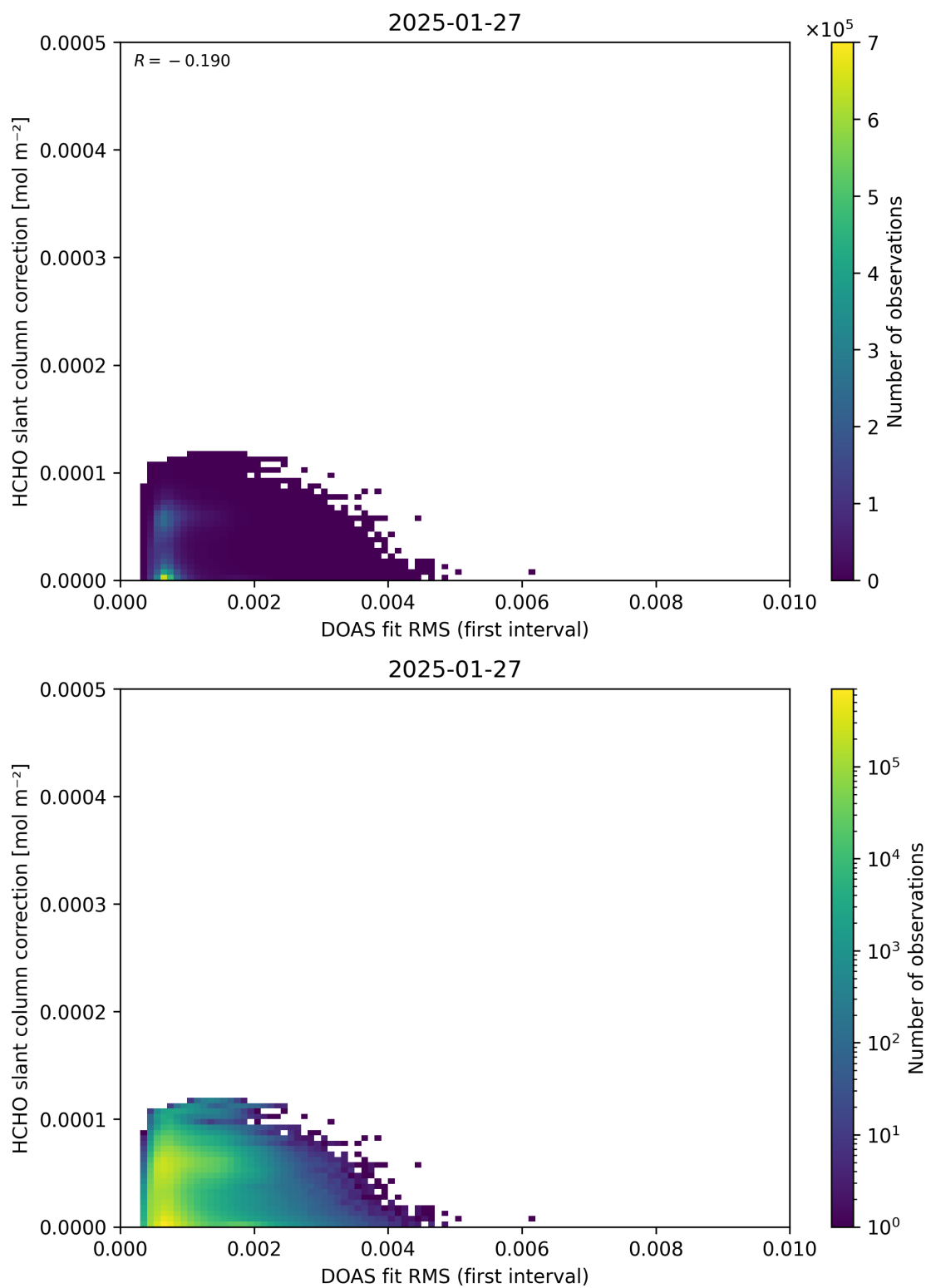
Figure 63: Scatter density plot of “DOAS fit RMS (first interval)” against “HCHO slant column correction” for 2025-01-26 to 2025-01-28.
