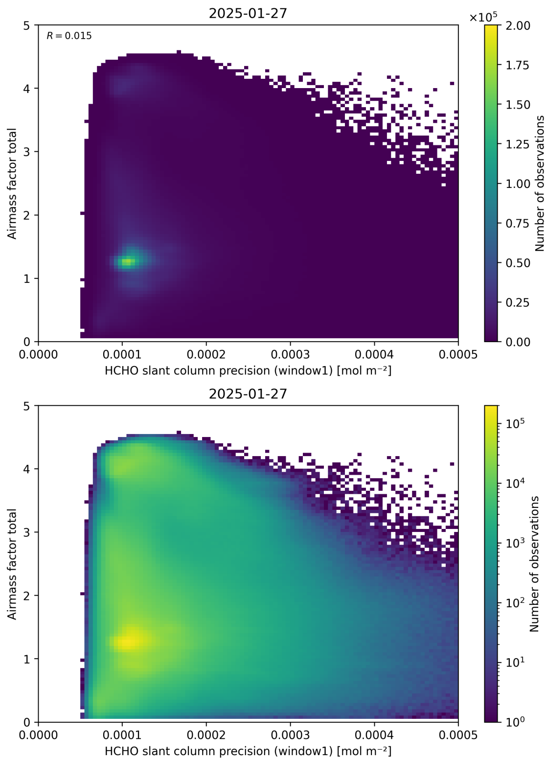
Figure 94: Scatter density plot of “HCHO slant column precision (window1)” against “Airmass factor total” for 2025-01-26 to 2025-01-28.
