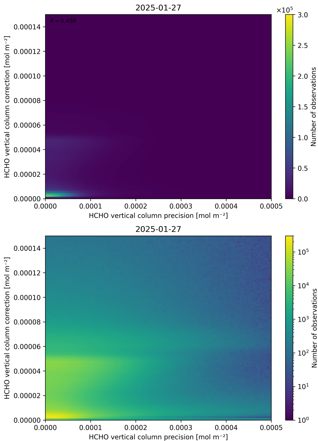
Figure 146: Scatter density plot of “HCHO vertical column precision” against “HCHO vertical column correction” for 2025-01-26 to 2025-01-28.
