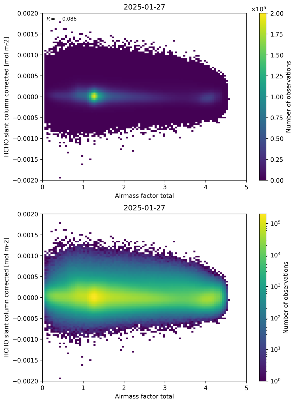
Figure 101: Scatter density plot of “Airmass factor total” against “HCHO slant column corrected” for 2025-01-26 to 2025-01-28.
