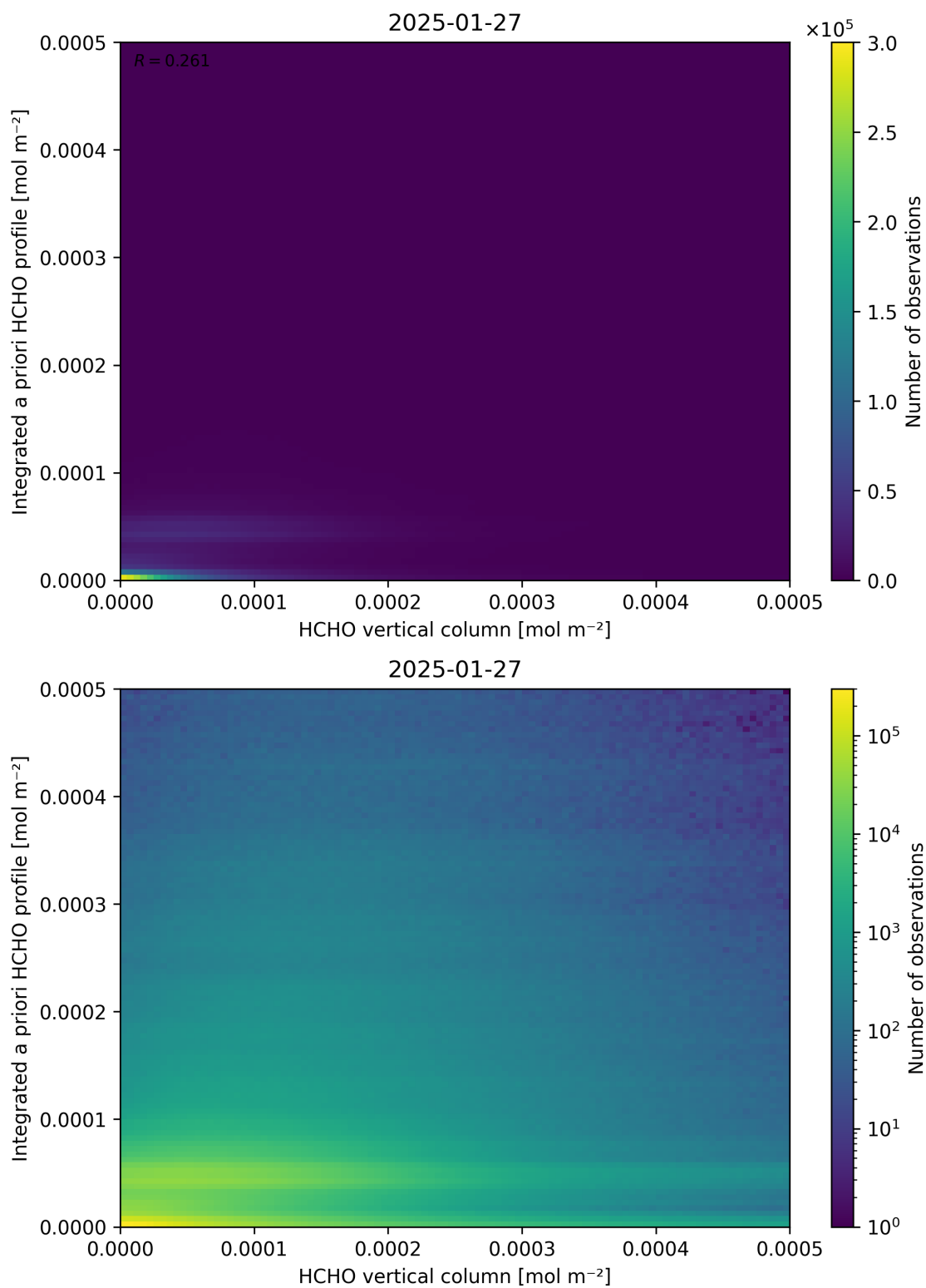
Figure 135: Scatter density plot of “HCHO vertical column” against “Integrated a priori HCHO profile” for 2025-01-26 to 2025-01-28.
