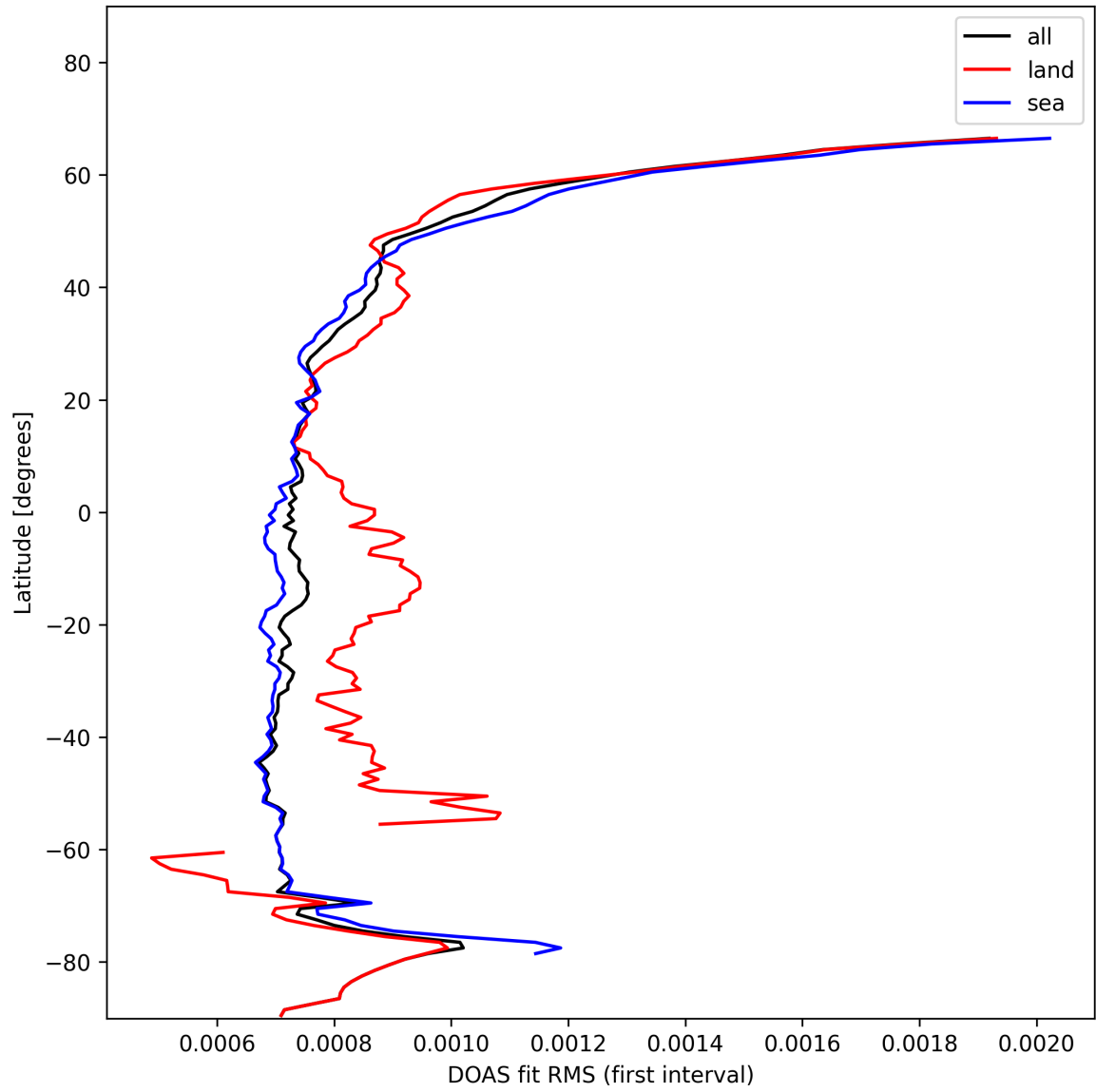
Figure 32: Zonal average of “DOAS fit RMS (first interval)” for 2025-01-26 to 2025-01-28.
