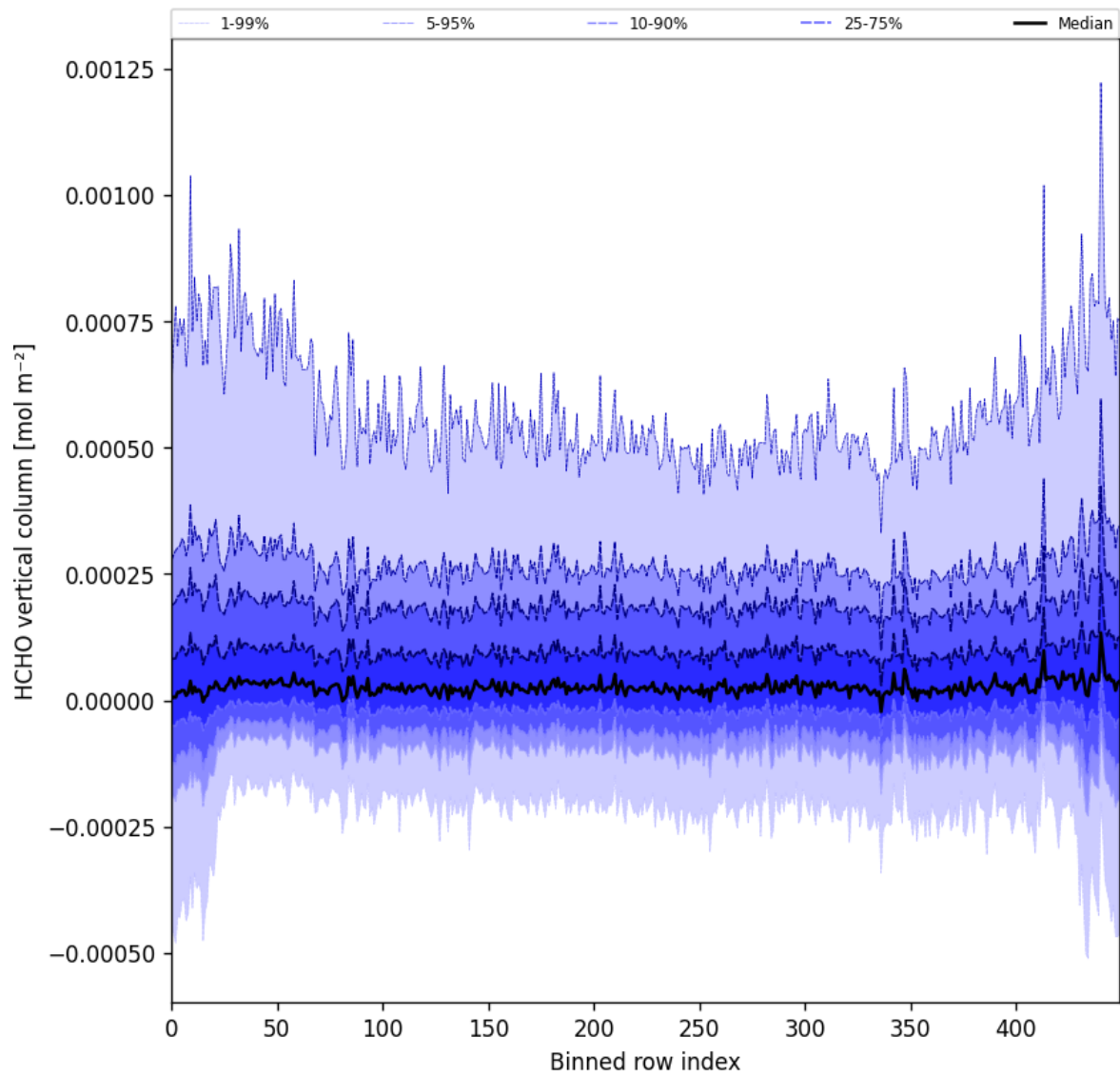
Figure 49: Along track statistics of “HCHO vertical column” for 2025-01-26 to 2025-01-28
