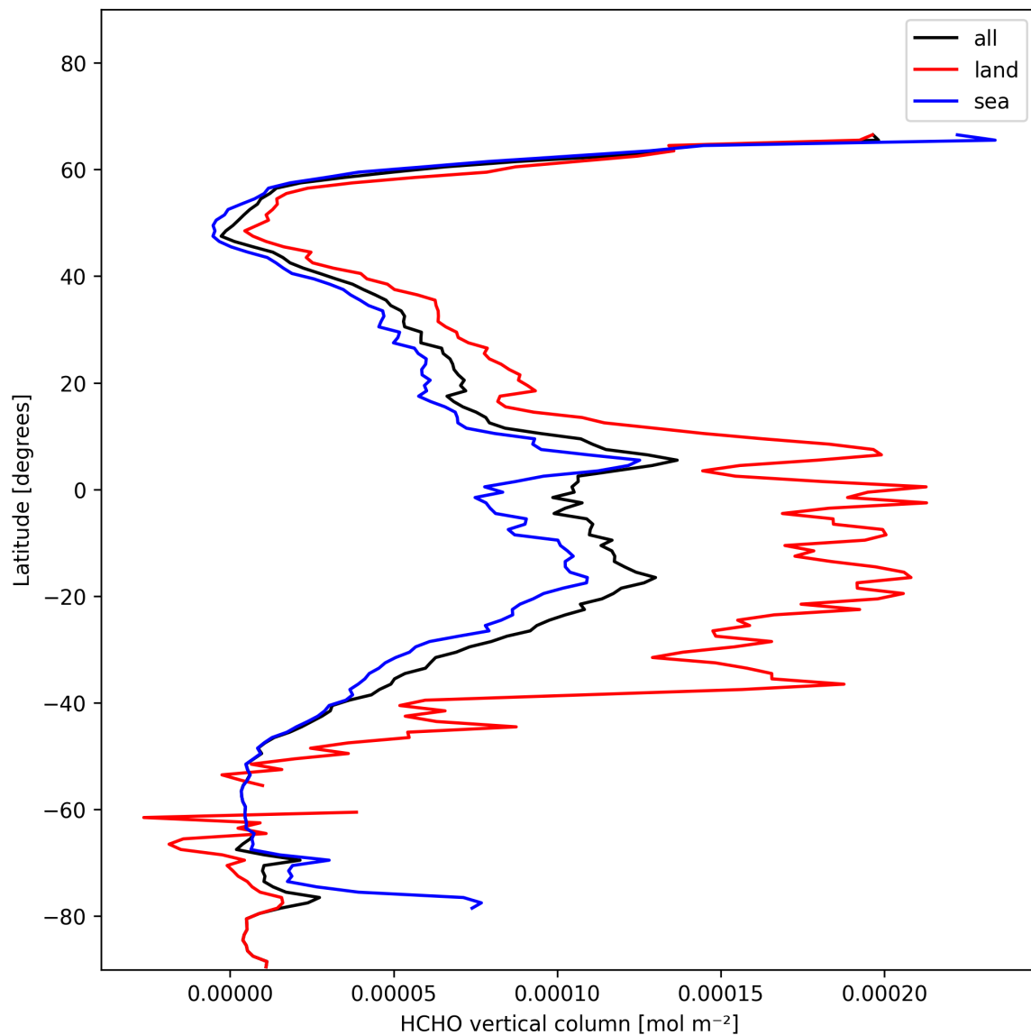
Figure 21: Zonal average of “HCHO vertical column” for 2025-01-26 to 2025-01-28.
