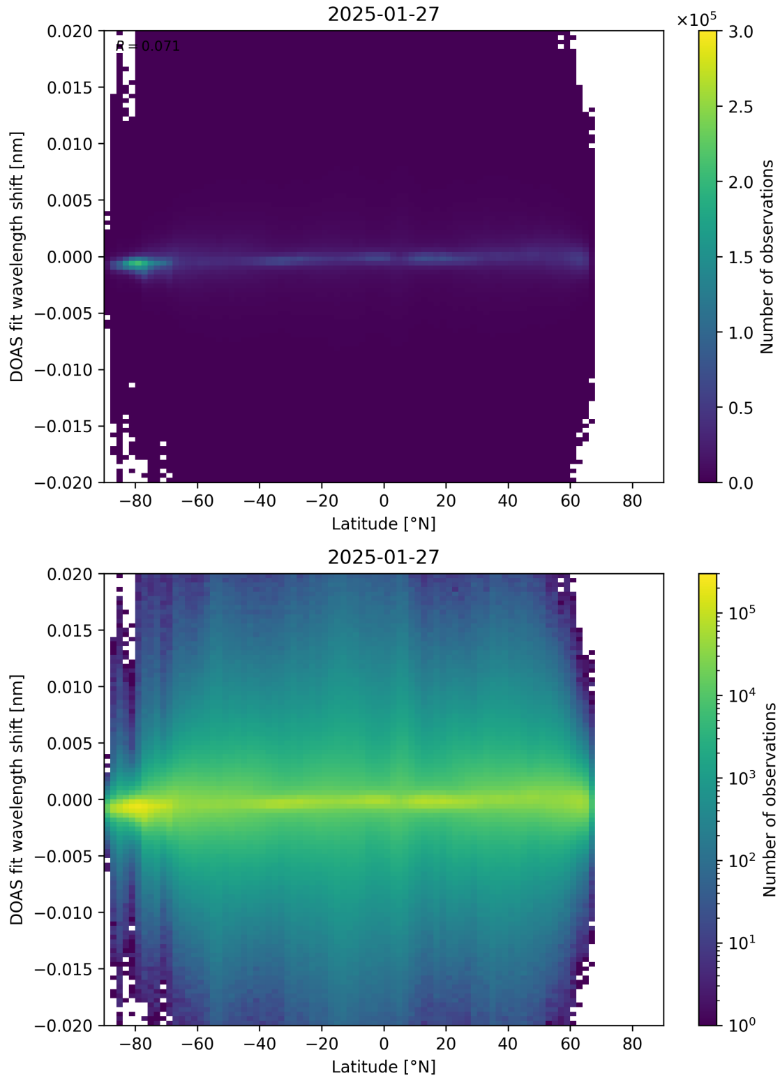
Figure 154: Scatter density plot of “Latitude” against “DOAS fit wavelength shift” for 2025-01-26 to 2025-01-28.
