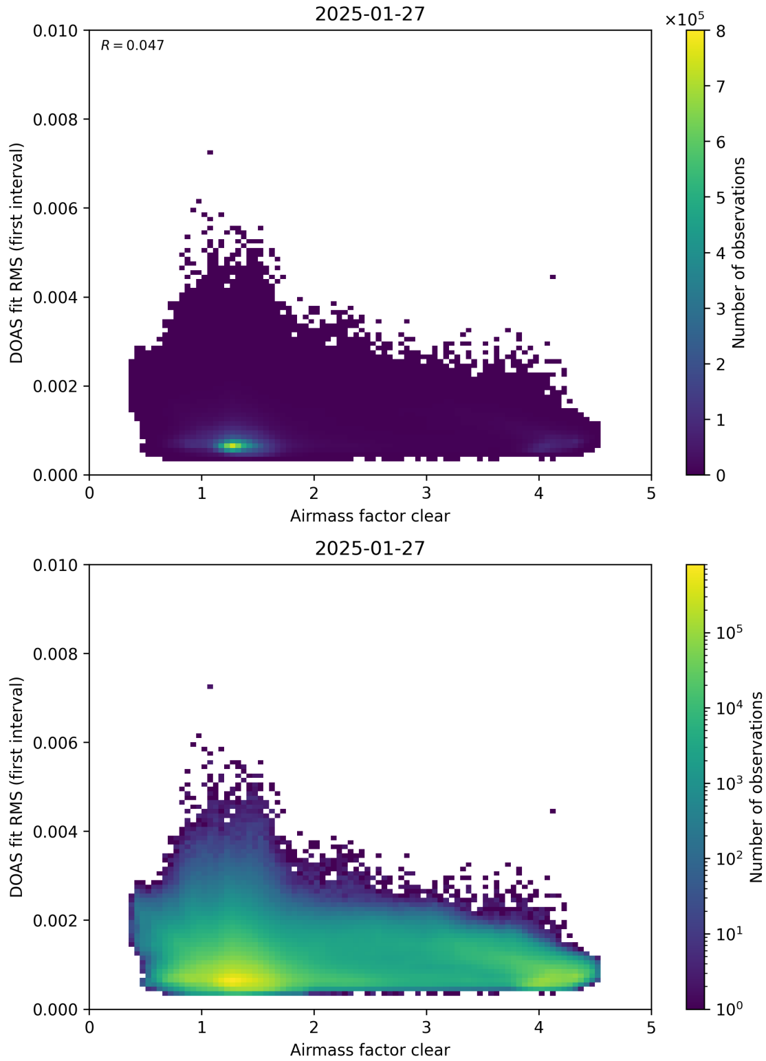
Figure 71: Scatter density plot of “Airmass factor clear” against “DOAS fit RMS (first interval)” for 2025-01-26 to 2025-01-28.
