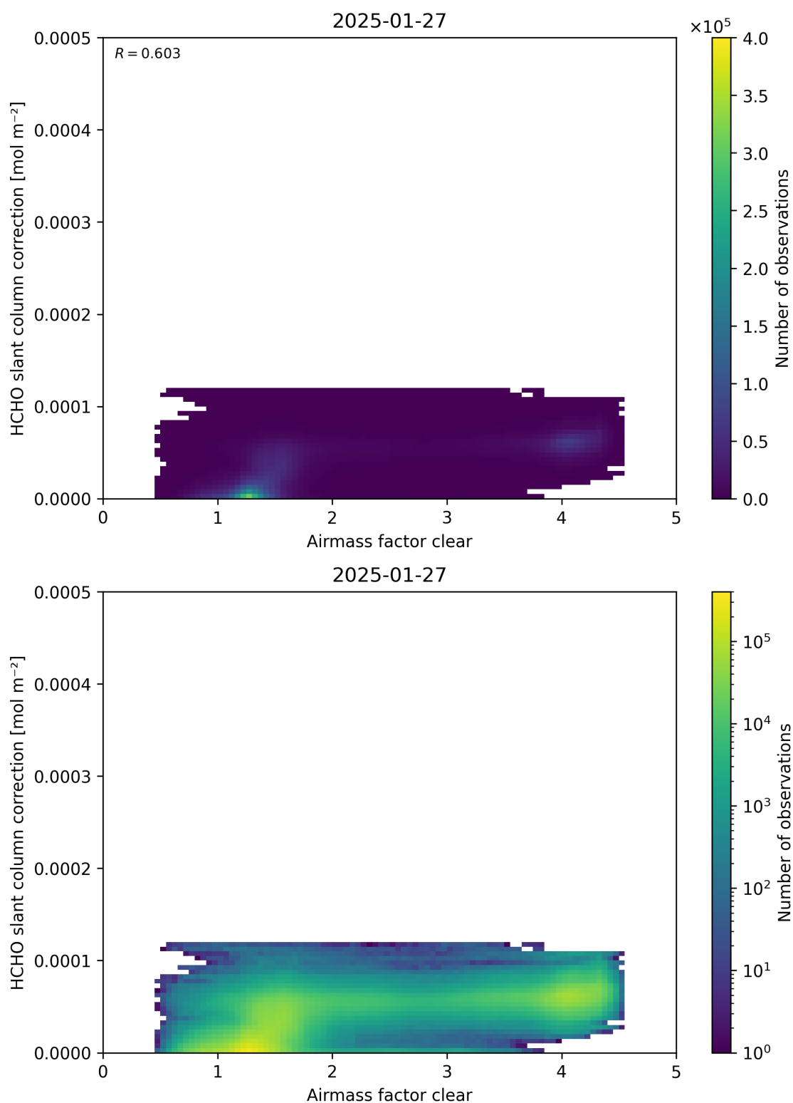
Figure 75: Scatter density plot of “Airmass factor clear” against “HCHO slant column correction” for 2025-01-26 to 2025-01-28.
