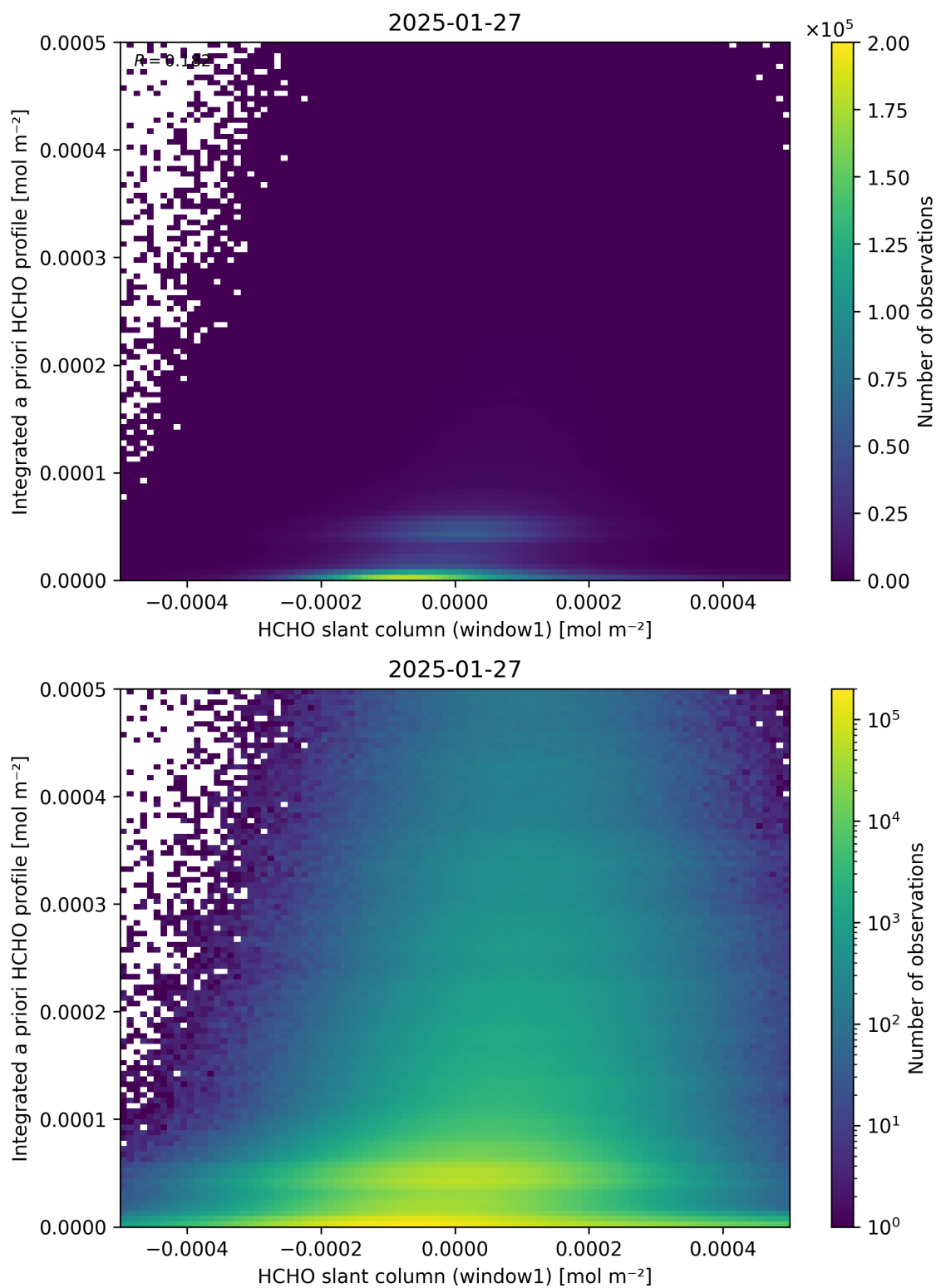
Figure 87: Scatter density plot of “HCHO slant column (window1)” against “Integrated a priori HCHO profile” for 2025-01-26 to 2025-01-28.
