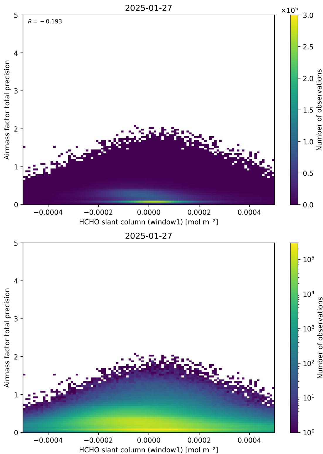
Figure 86: Scatter density plot of “HCHO slant column (window1)” against “Airmass factor total precision” for 2025-01-26 to 2025-01-28.
