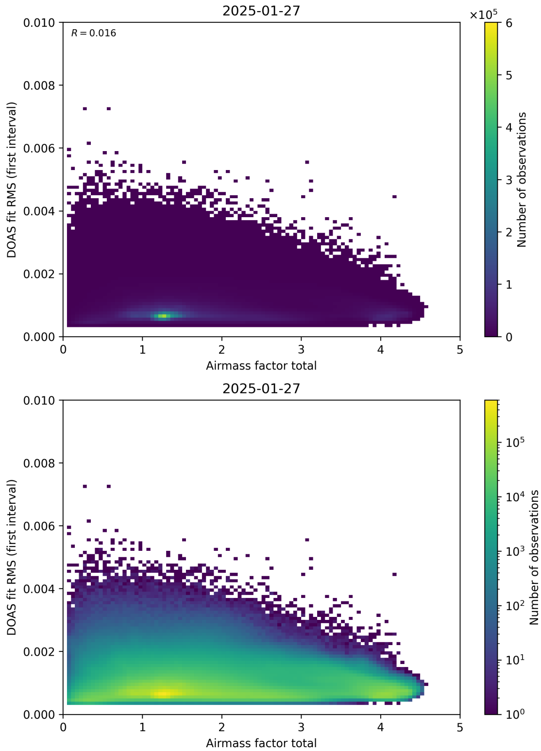
Figure 97: Scatter density plot of “Airmass factor total” against “DOAS fit RMS (first interval)” for 2025-01-26 to 2025-01-28.
