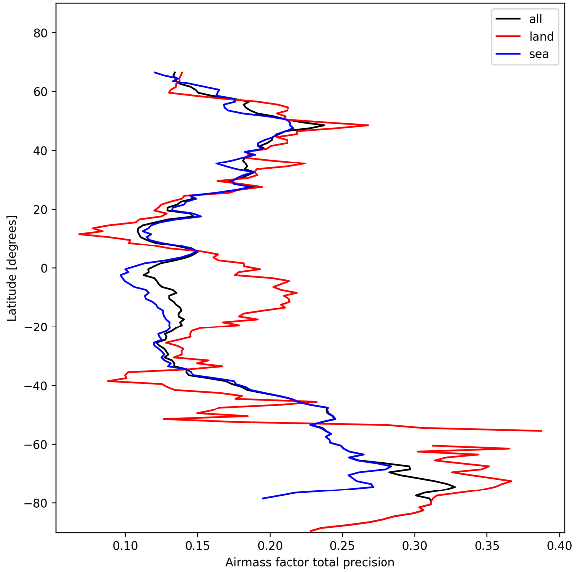
Figure 27: Zonal average of “Airmass factor total precision” for 2025-01-26 to 2025-01-28.
