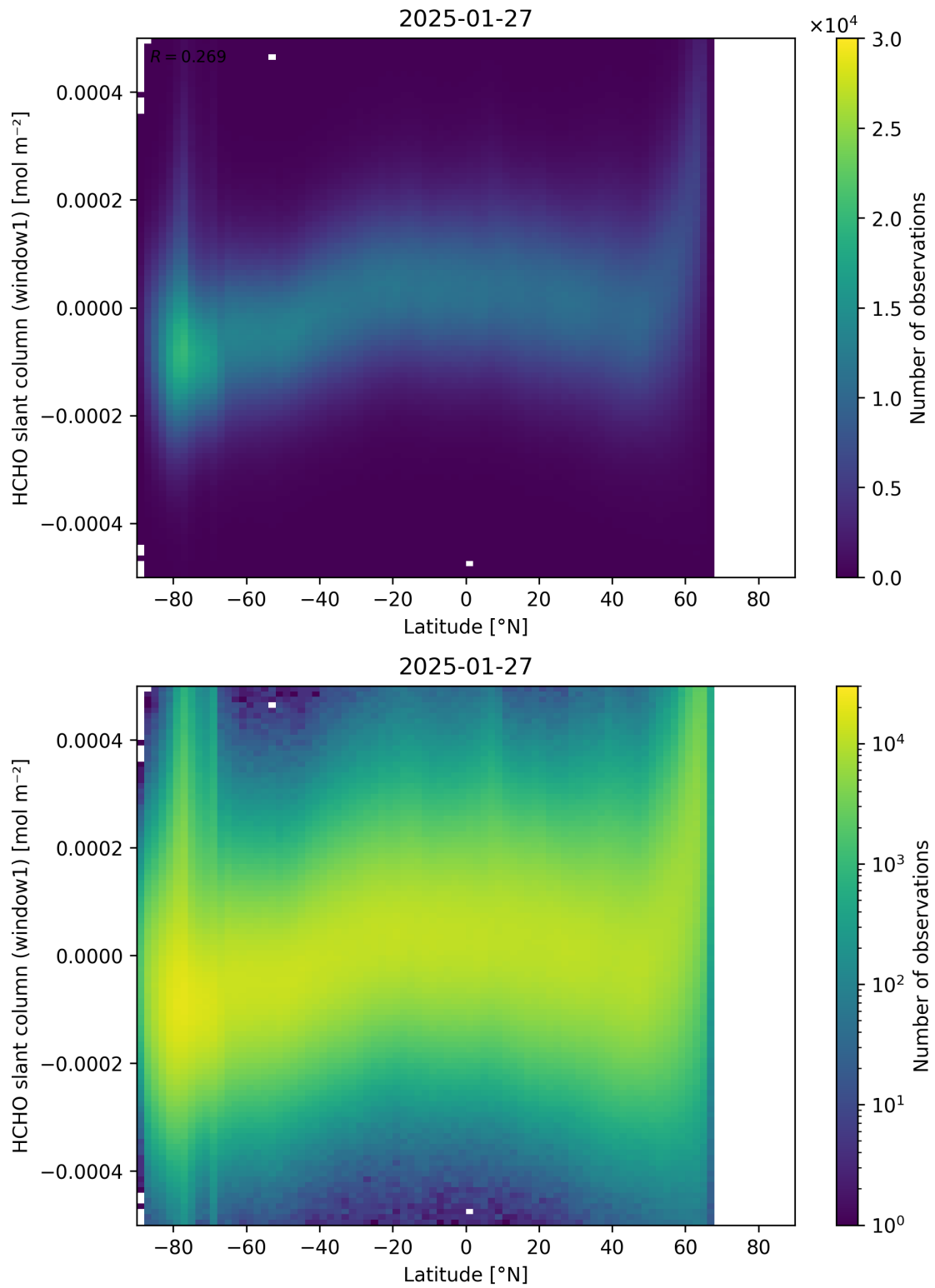
Figure 159: Scatter density plot of “Latitude” against “HCHO slant column (window1)” for 2025-01-26 to 2025-01-28.
