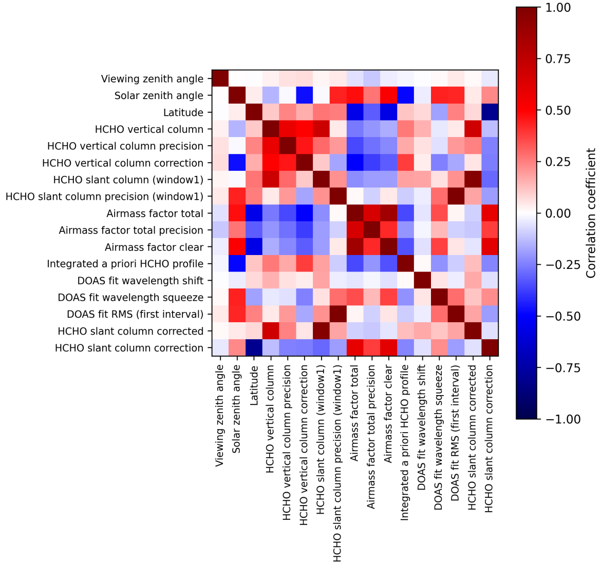
Figure 2: Map of correlation matrix for 2025-01-26 to 2025-01-28.
