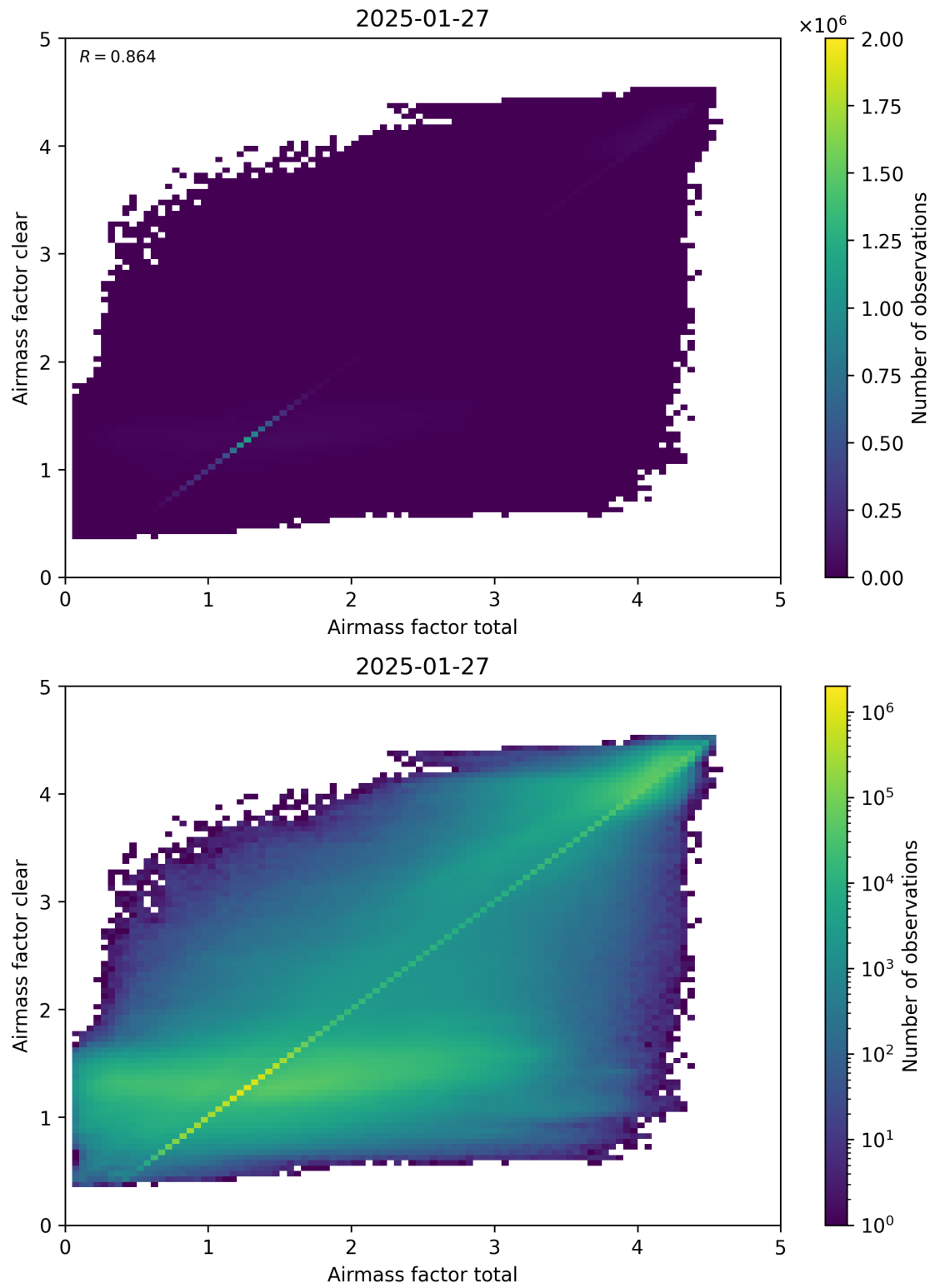
Figure 100: Scatter density plot of “Airmass factor total” against “Airmass factor clear” for 2025-01-26 to 2025-01-28.
