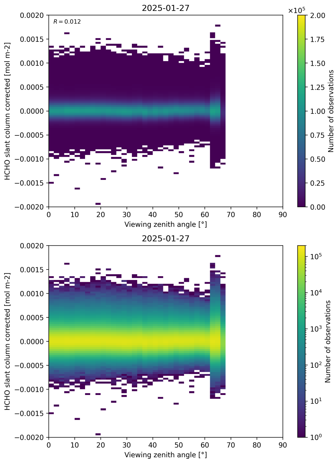
Figure 186: Scatter density plot of “Viewing zenith angle” against “HCHO slant column corrected” for 2025-01-26 to 2025-01-28.
