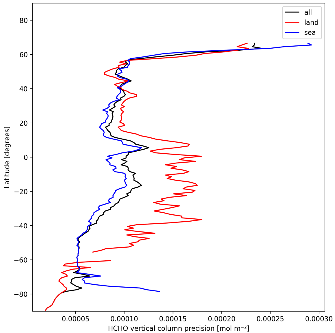
Figure 22: Zonal average of “HCHO vertical column precision” for 2025-01-26 to 2025-01-28.
