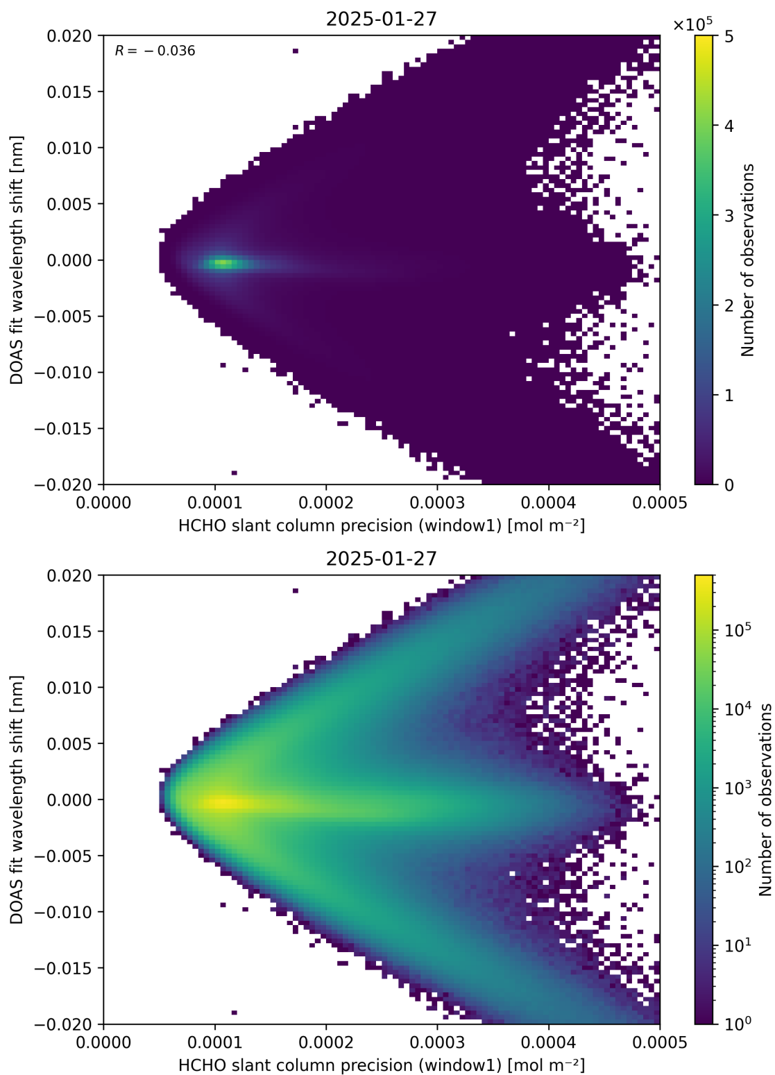
Figure 89: Scatter density plot of “HCHO slant column precision (window1)” against “DOAS fit wavelength shift” for 2025-01-26 to 2025-01-28.
