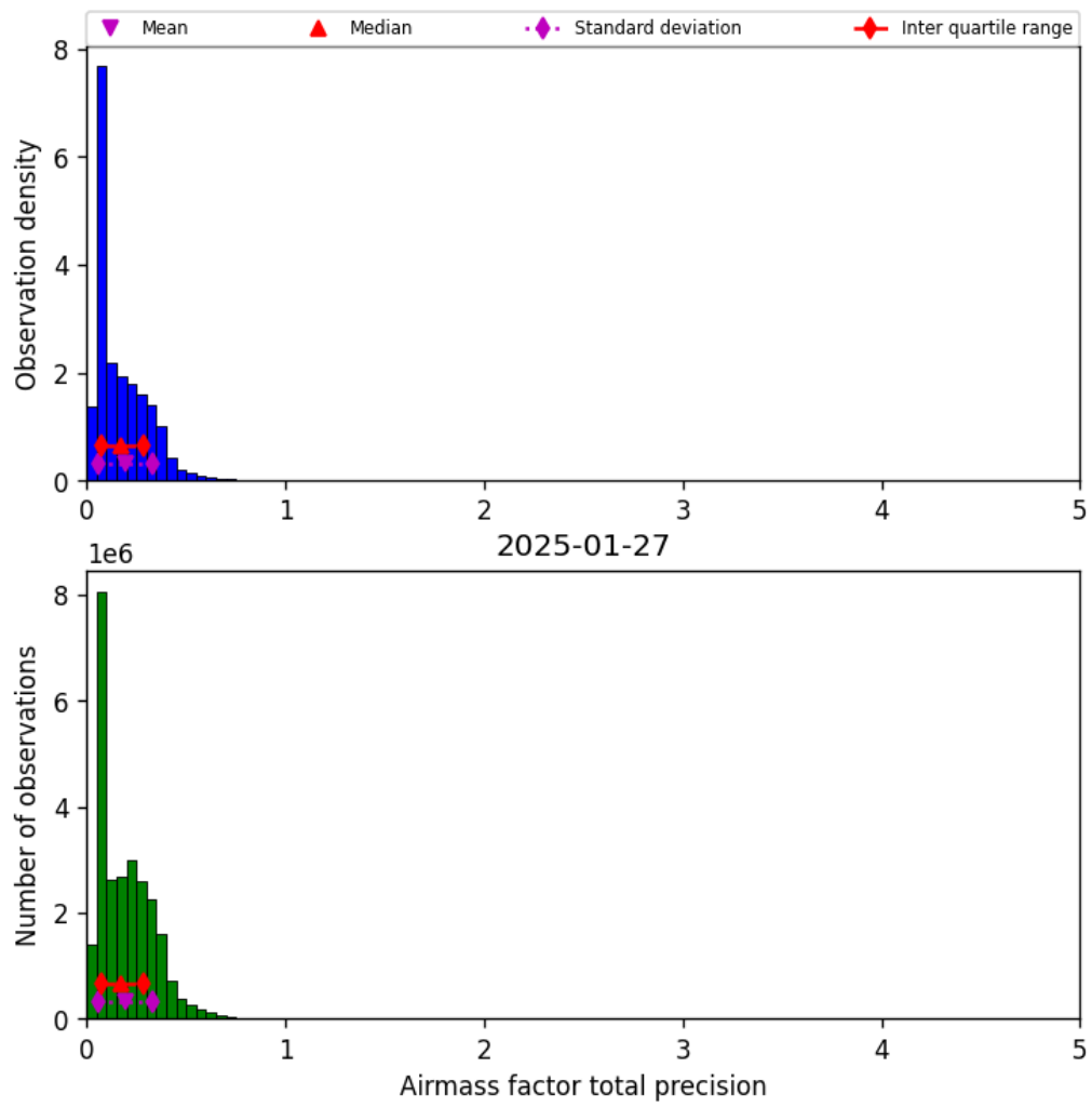
Figure 41: Histogram of “Airmass factor total precision” for 2025-01-26 to 2025-01-28
