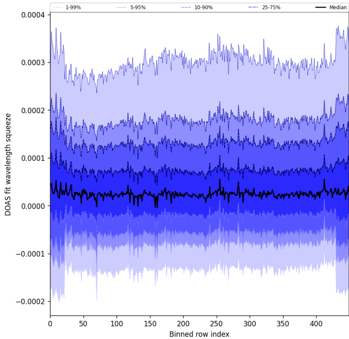
Figure 59: Along track statistics of “DOAS fit wavelength squeeze” for 2025-01-26 to 2025-01-28
