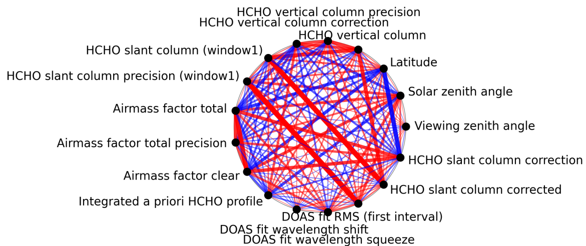
Figure 1: Map of correlation graph for 2025-01-26 to 2025-01-28.
