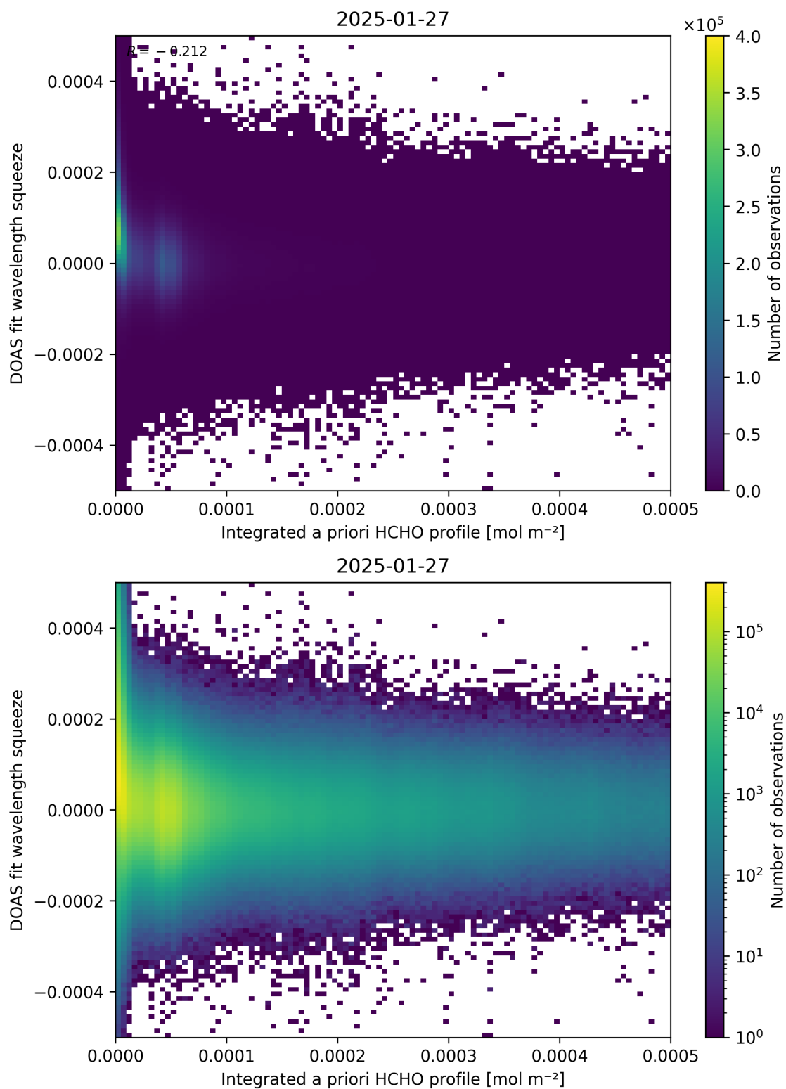
Figure 150: Scatter density plot of “Integrated a priori HCHO profile” against “DOAS fit wavelength squeeze” for 2025-01-26 to 2025-01-28.
