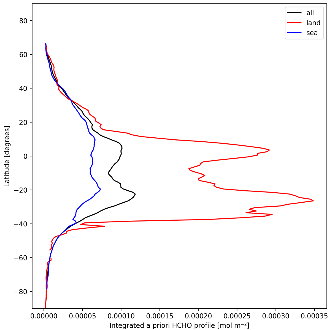
Figure 29: Zonal average of “Integrated a priori HCHO profile” for 2025-01-26 to 2025-01-28.
