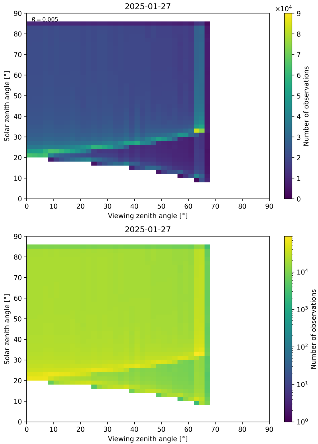
Figure 197: Scatter density plot of “Viewing zenith angle” against “Solar zenith angle” for 2025-01-26 to 2025-01-28.
