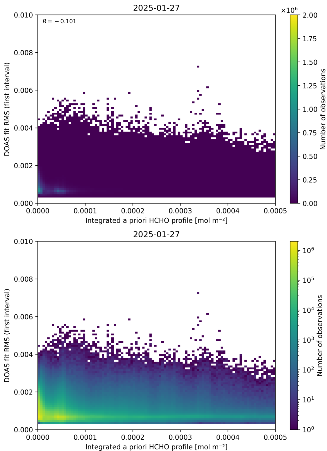
Figure 148: Scatter density plot of “Integrated a priori HCHO profile” against “DOAS fit RMS (first interval)” for 2025-01-26 to 2025-01-28.
