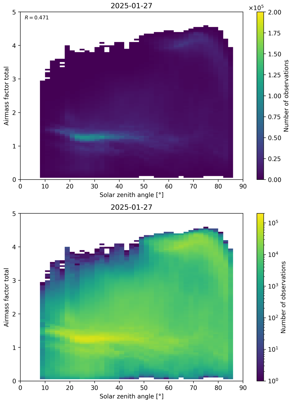
Figure 175: Scatter density plot of “Solar zenith angle” against “Airmass factor total” for 2025-01-26 to 2025-01-28.
