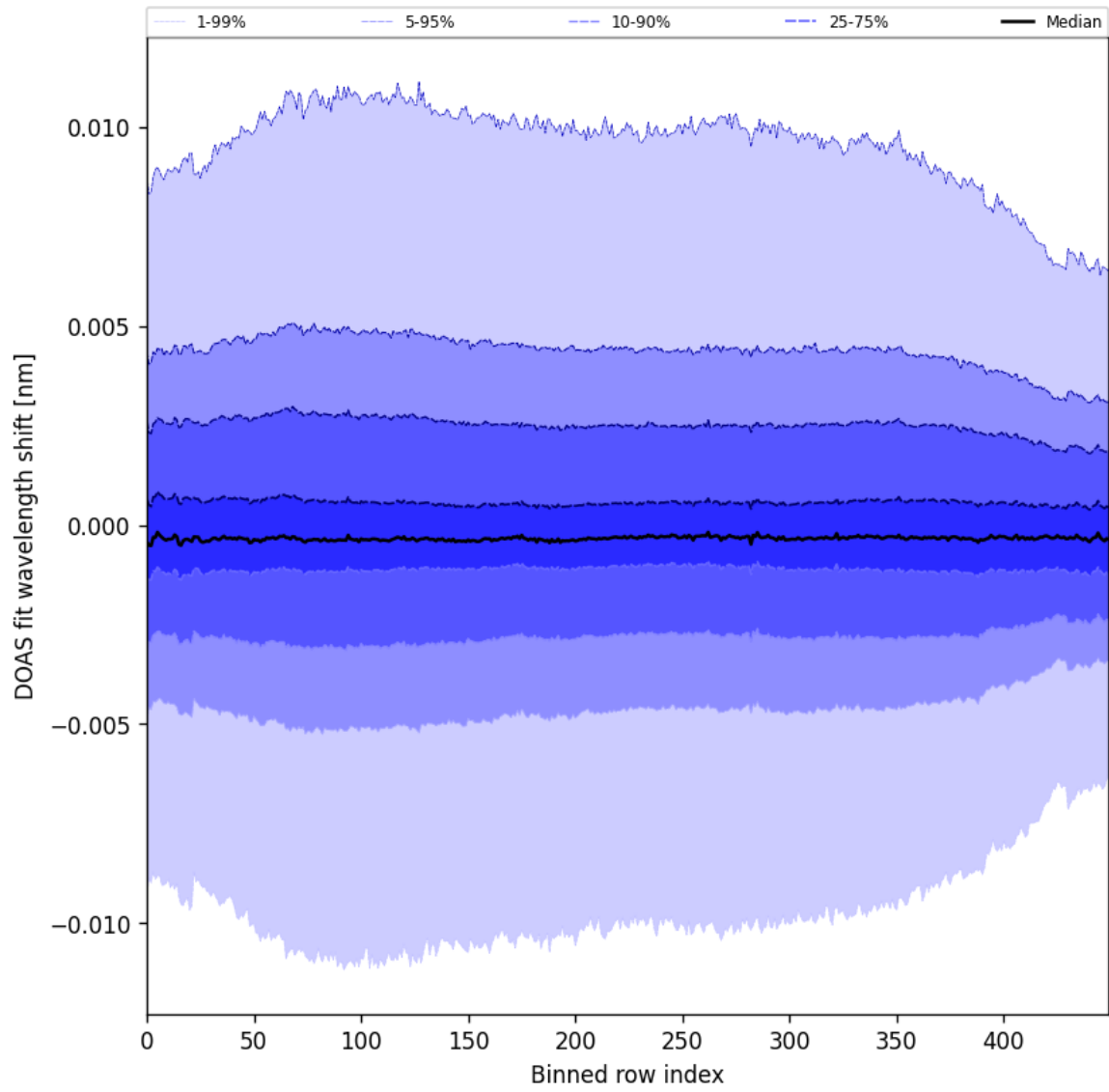
Figure 58: Along track statistics of “DOAS fit wavelength shift” for 2025-01-26 to 2025-01-28
