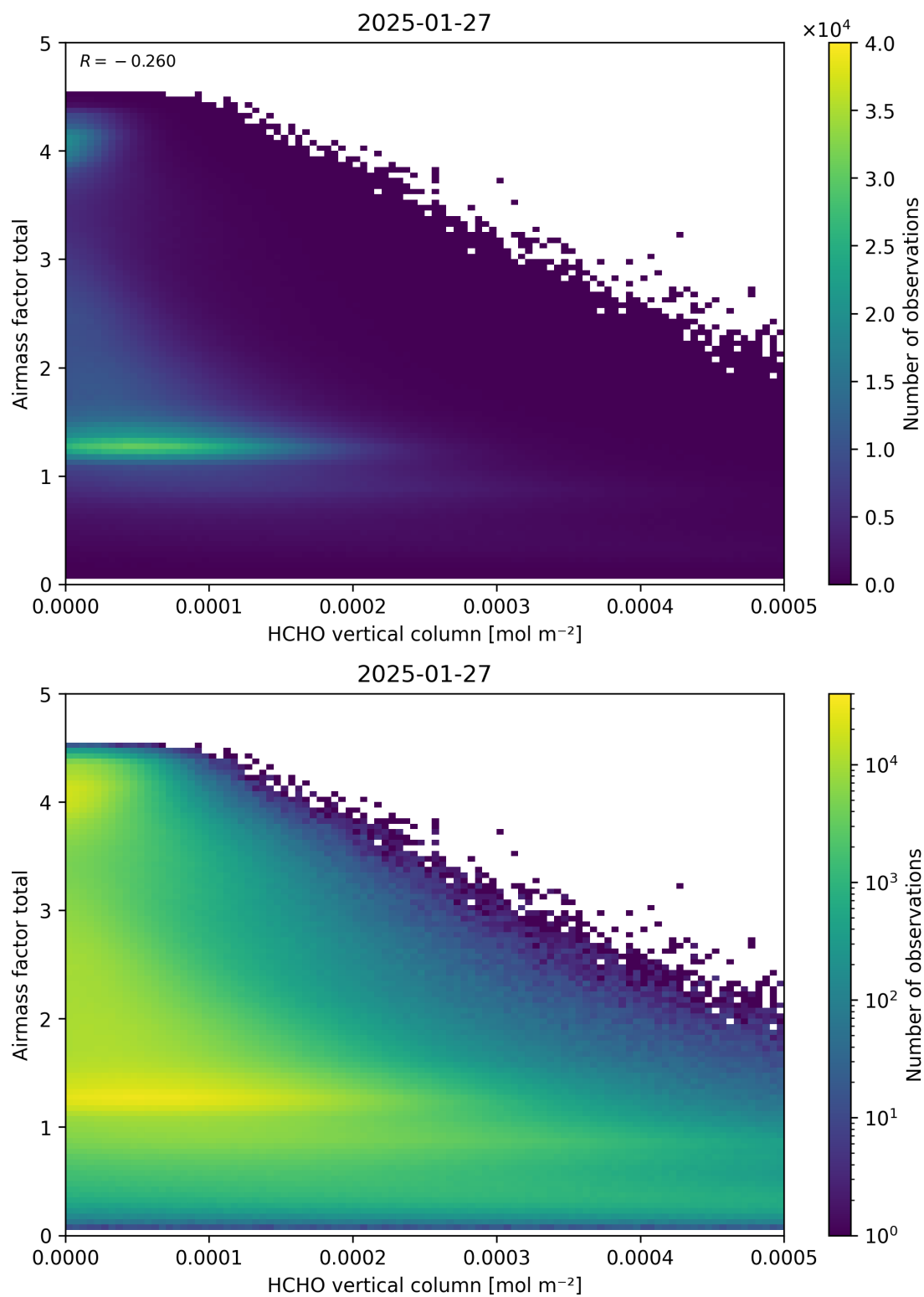
Figure 131: Scatter density plot of “HCHO vertical column” against “Airmass factor total” for 2025-01-26 to 2025-01-28.
