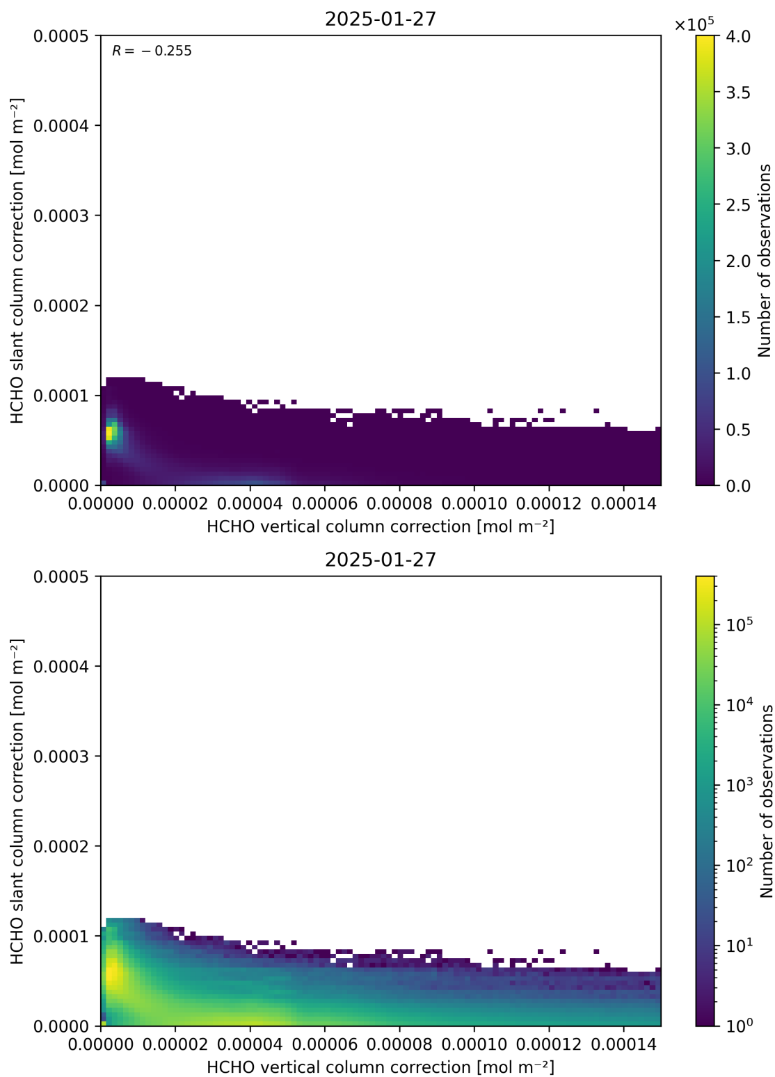
Figure 117: Scatter density plot of “HCHO vertical column correction” against “HCHO slant column correction” for 2025-01-26 to 2025-01-28.
