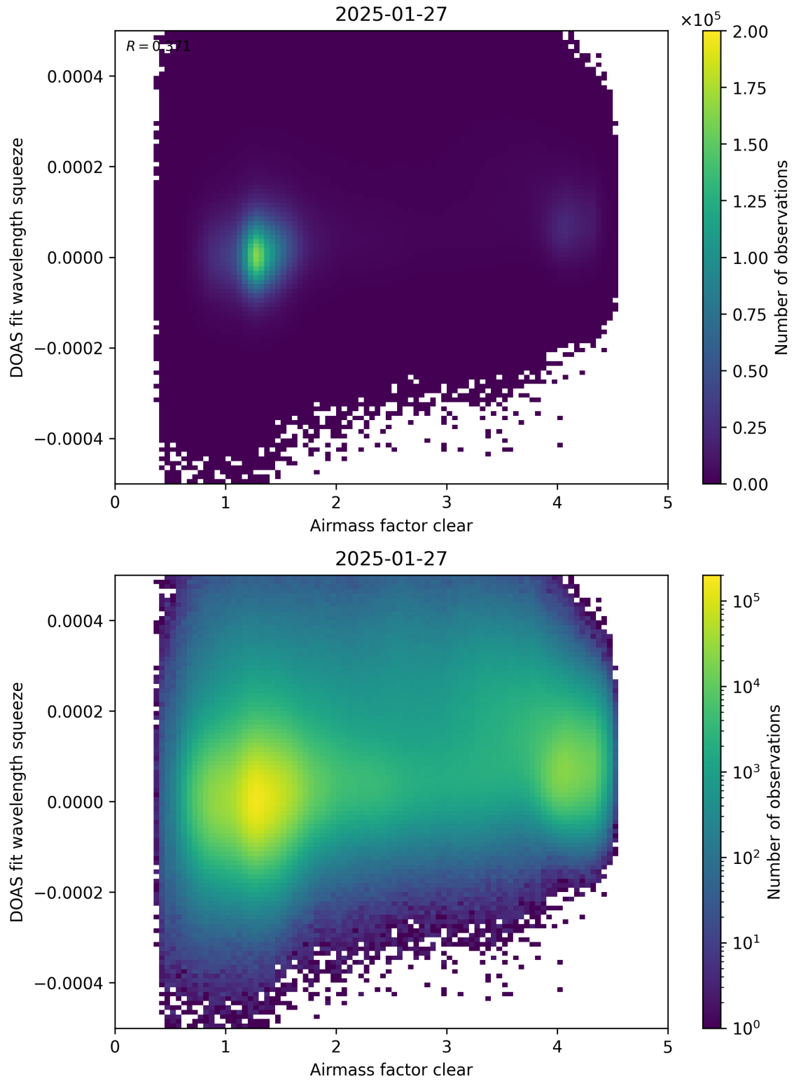
Figure 73: Scatter density plot of “Airmass factor clear” against “DOAS fit wavelength squeeze” for 2025-01-26 to 2025-01-28.
