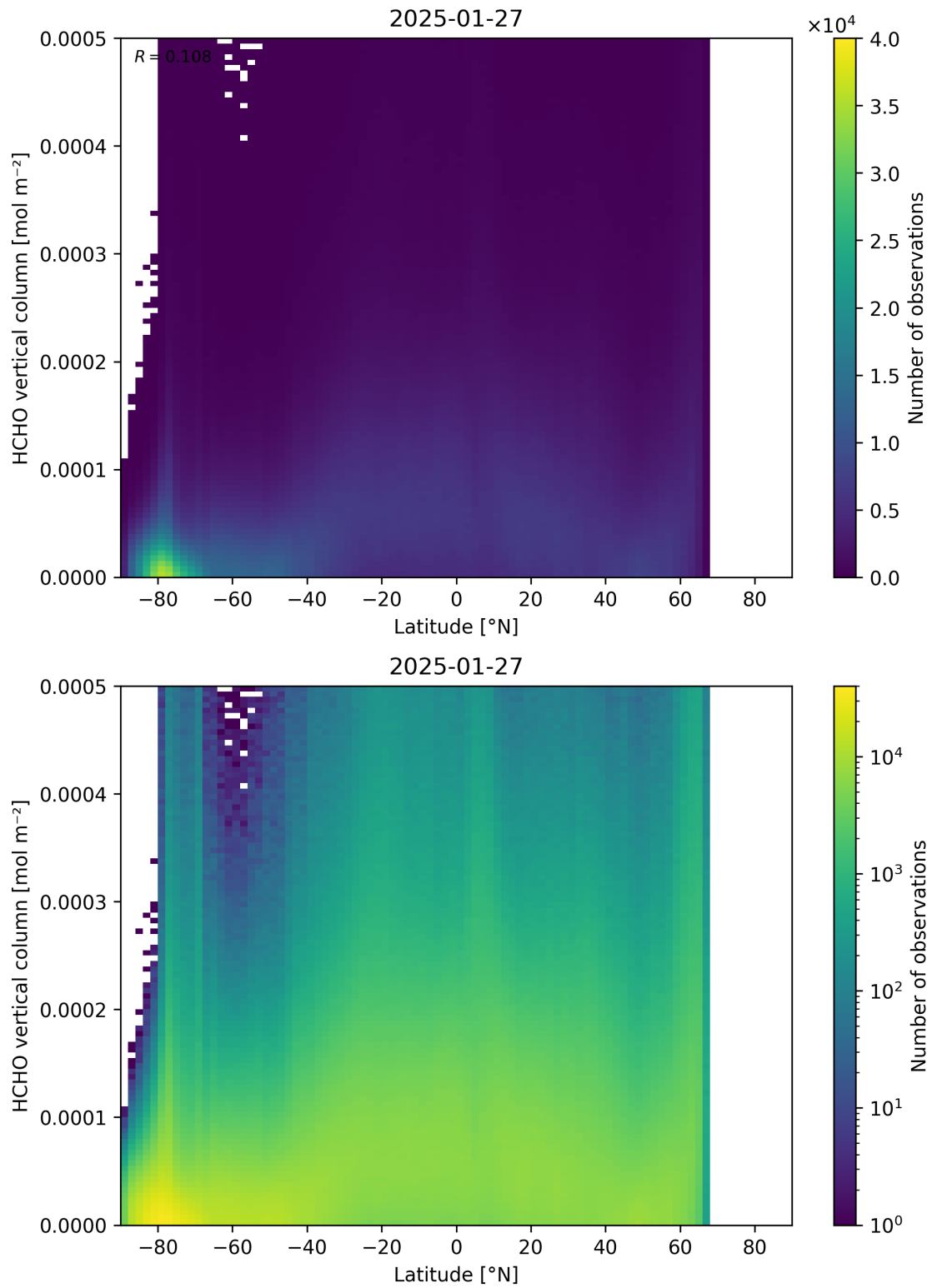
Figure 163: Scatter density plot of “Latitude” against “HCHO vertical column” for 2025-01-26 to 2025-01-28.
