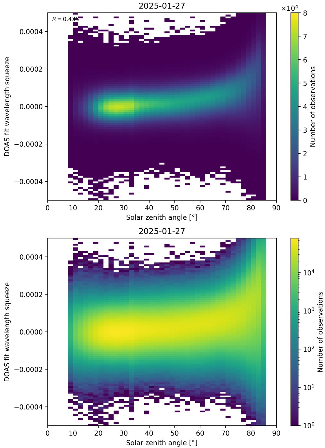
Figure 169: Scatter density plot of “Solar zenith angle” against “DOAS fit wavelength squeeze” for 2025-01-26 to 2025-01-28.
