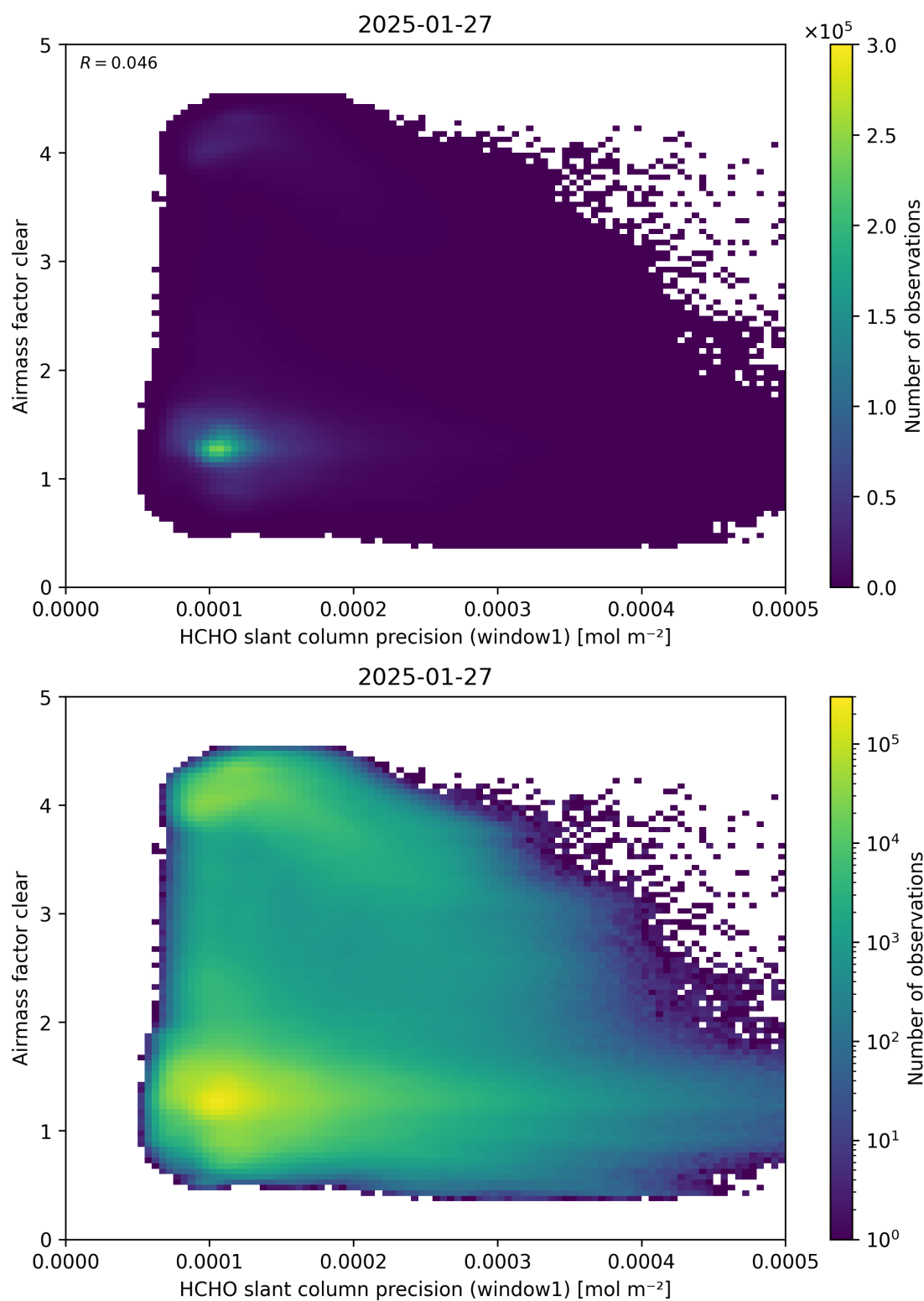
Figure 91: Scatter density plot of “HCHO slant column precision (window1)” against “Airmass factor clear” for 2025-01-26 to 2025-01-28.
