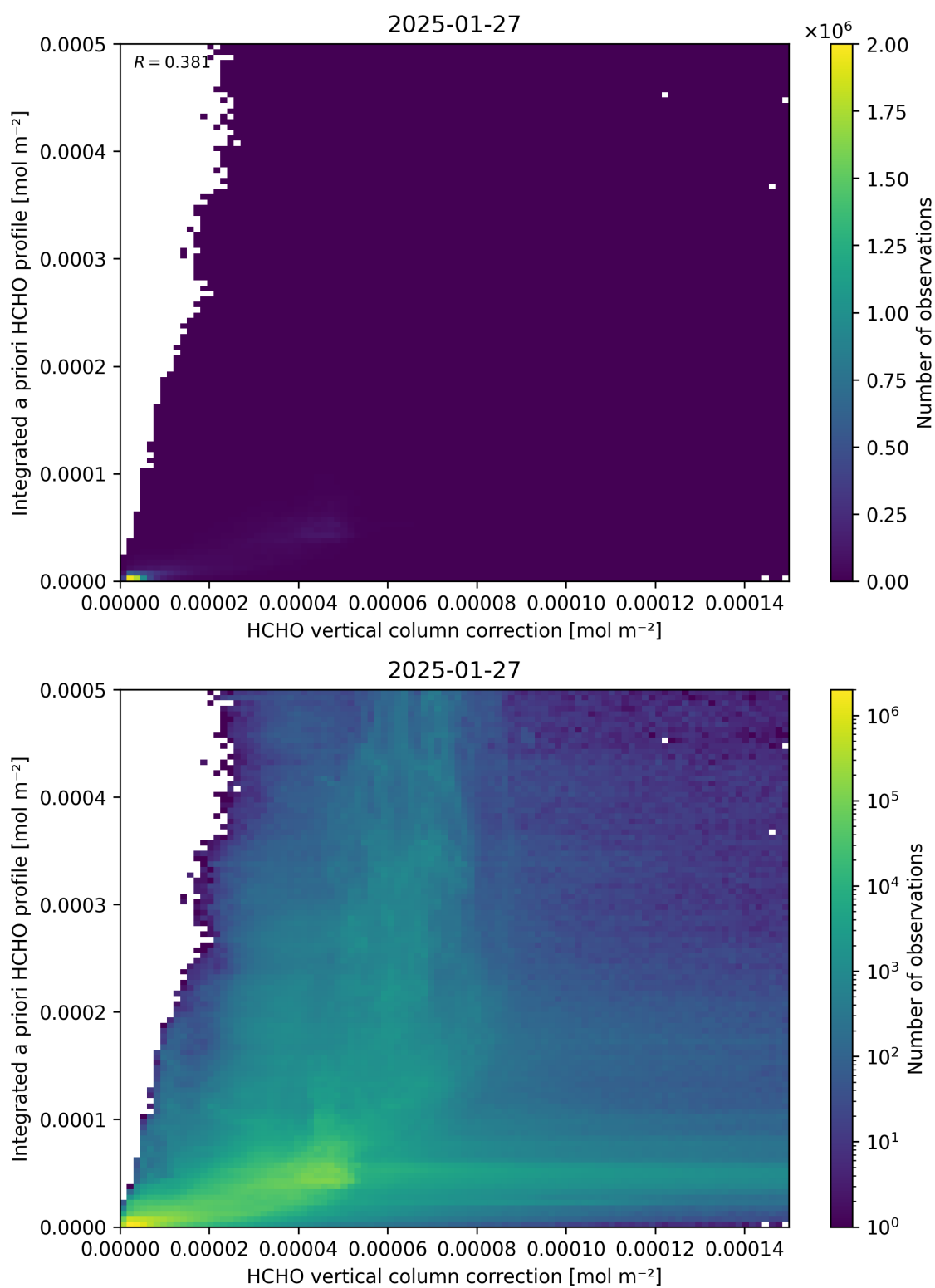
Figure 122: Scatter density plot of “HCHO vertical column correction” against “Integrated a priori HCHO profile” for 2025-01-26 to 2025-01-28.
