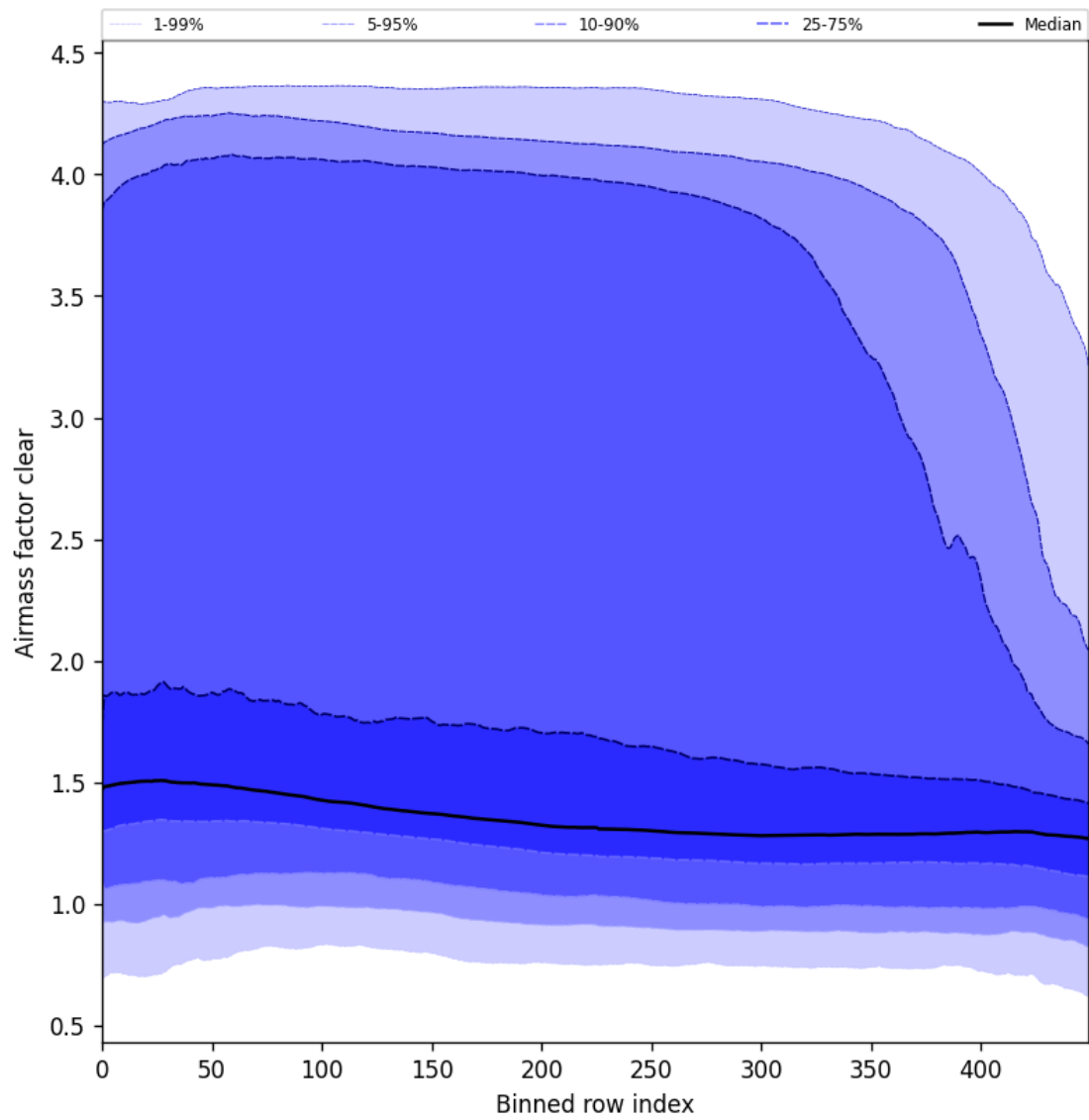
Figure 56: Along track statistics of “Airmass factor clear” for 2025-01-26 to 2025-01-28
