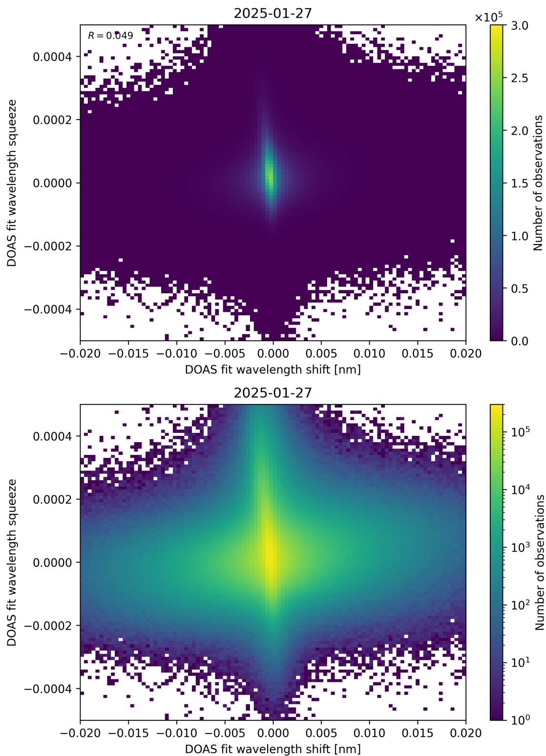
Figure 65: Scatter density plot of “DOAS fit wavelength shift” against “DOAS fit wavelength squeeze” for 2025-01-26 to 2025-01-28.
