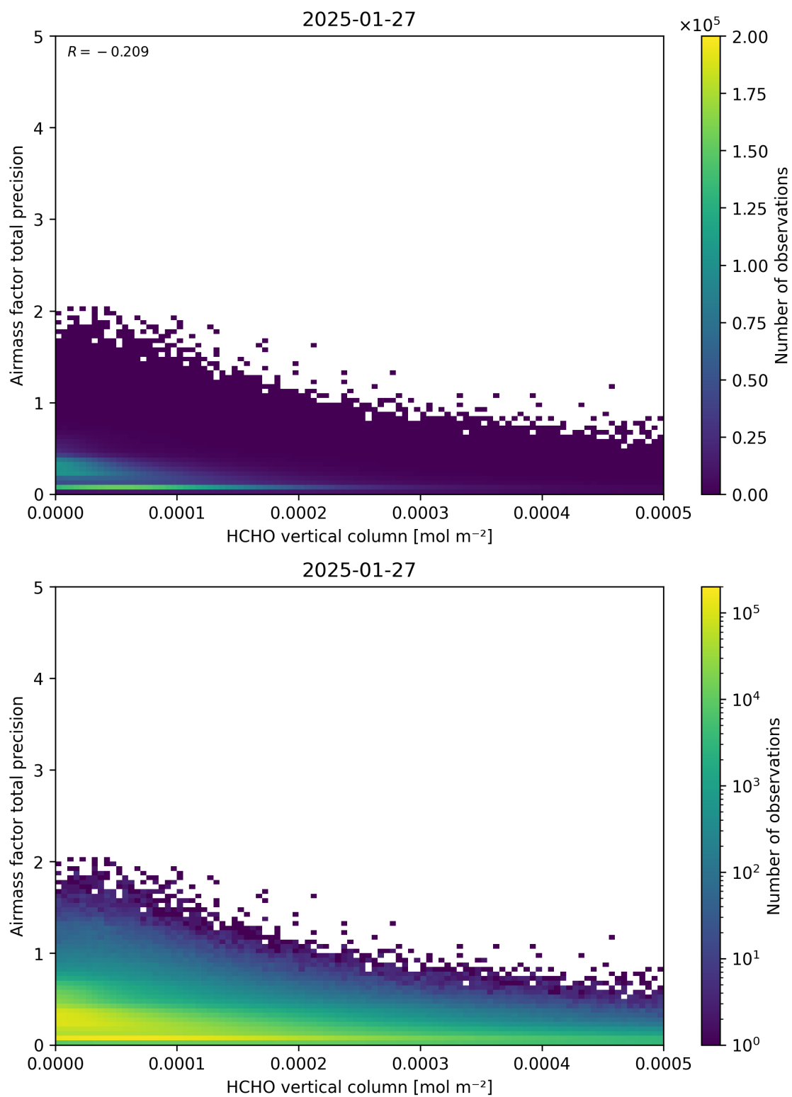
Figure 132: Scatter density plot of “HCHO vertical column” against “Airmass factor total precision” for 2025-01-26 to 2025-01-28.
