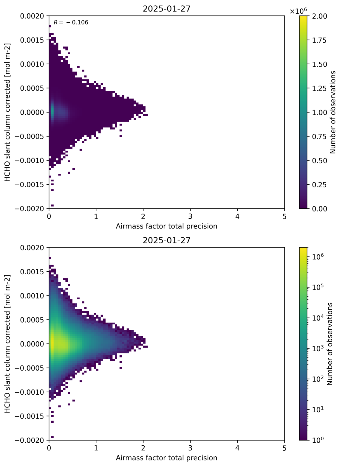
Figure 109: Scatter density plot of “Airmass factor total precision” against “HCHO slant column corrected” for 2025-01-26 to 2025-01-28.
