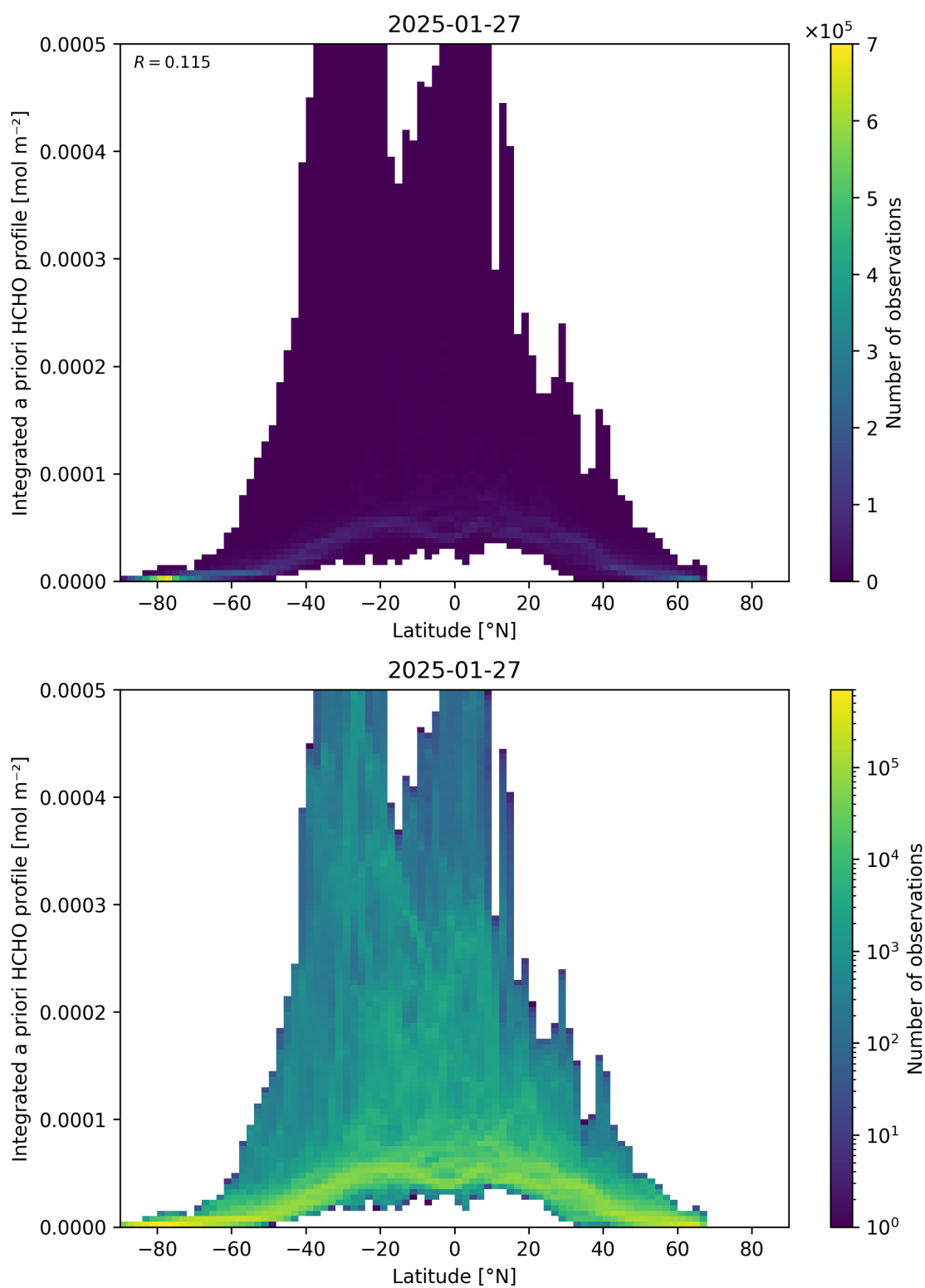
Figure 166: Scatter density plot of “Latitude” against “Integrated a priori HCHO profile” for 2025-01-26 to 2025-01-28.
