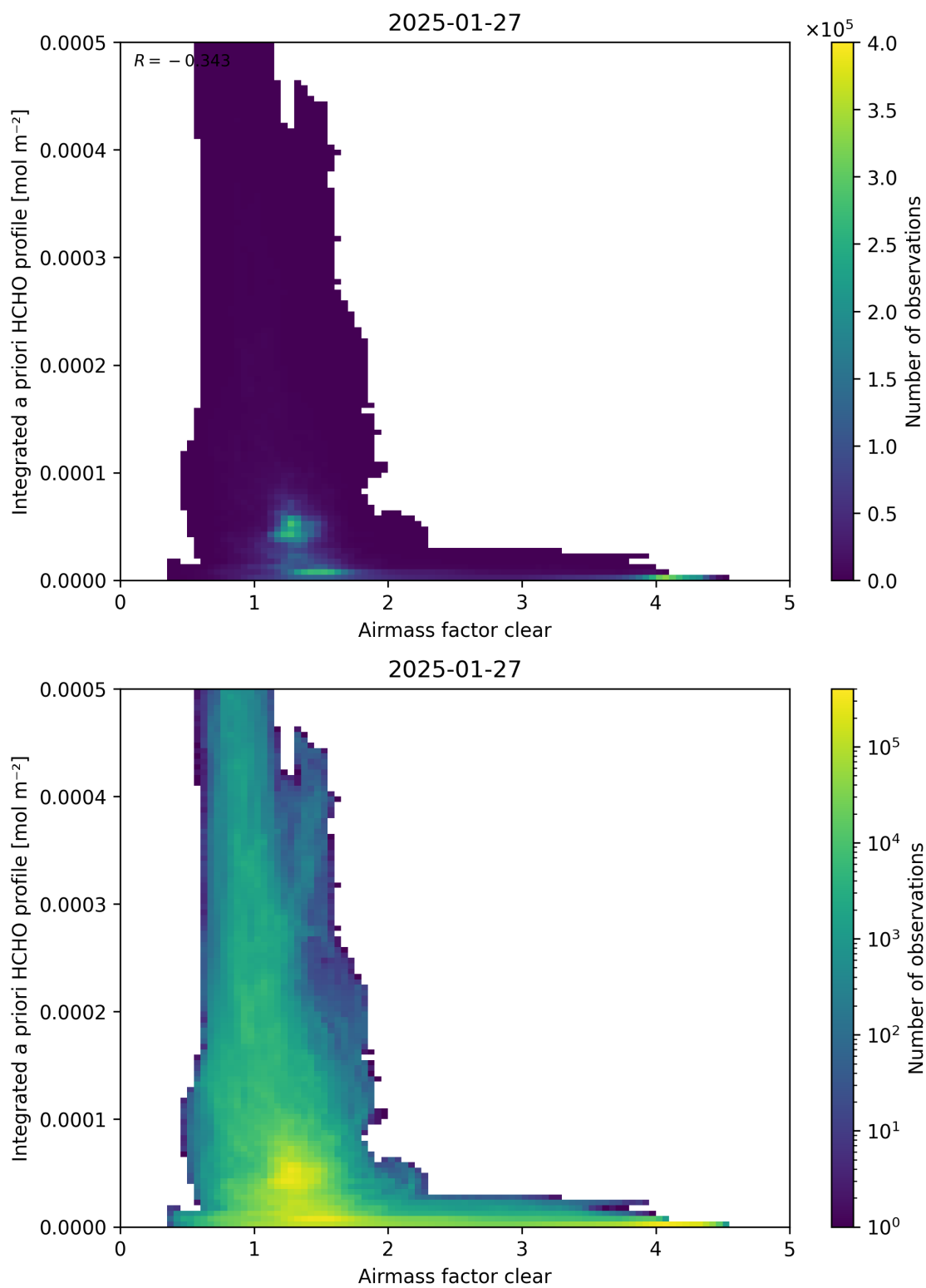
Figure 76: Scatter density plot of “Airmass factor clear” against “Integrated a priori HCHO profile” for 2025-01-26 to 2025-01-28.
