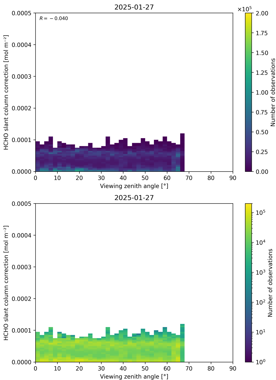
Figure 187: Scatter density plot of “Viewing zenith angle” against “HCHO slant column correction” for 2025-01-26 to 2025-01-28.
