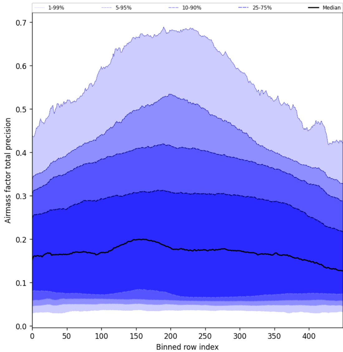
Figure 55: Along track statistics of “Airmass factor total precision” for 2025-01-26 to 2025-01-28
