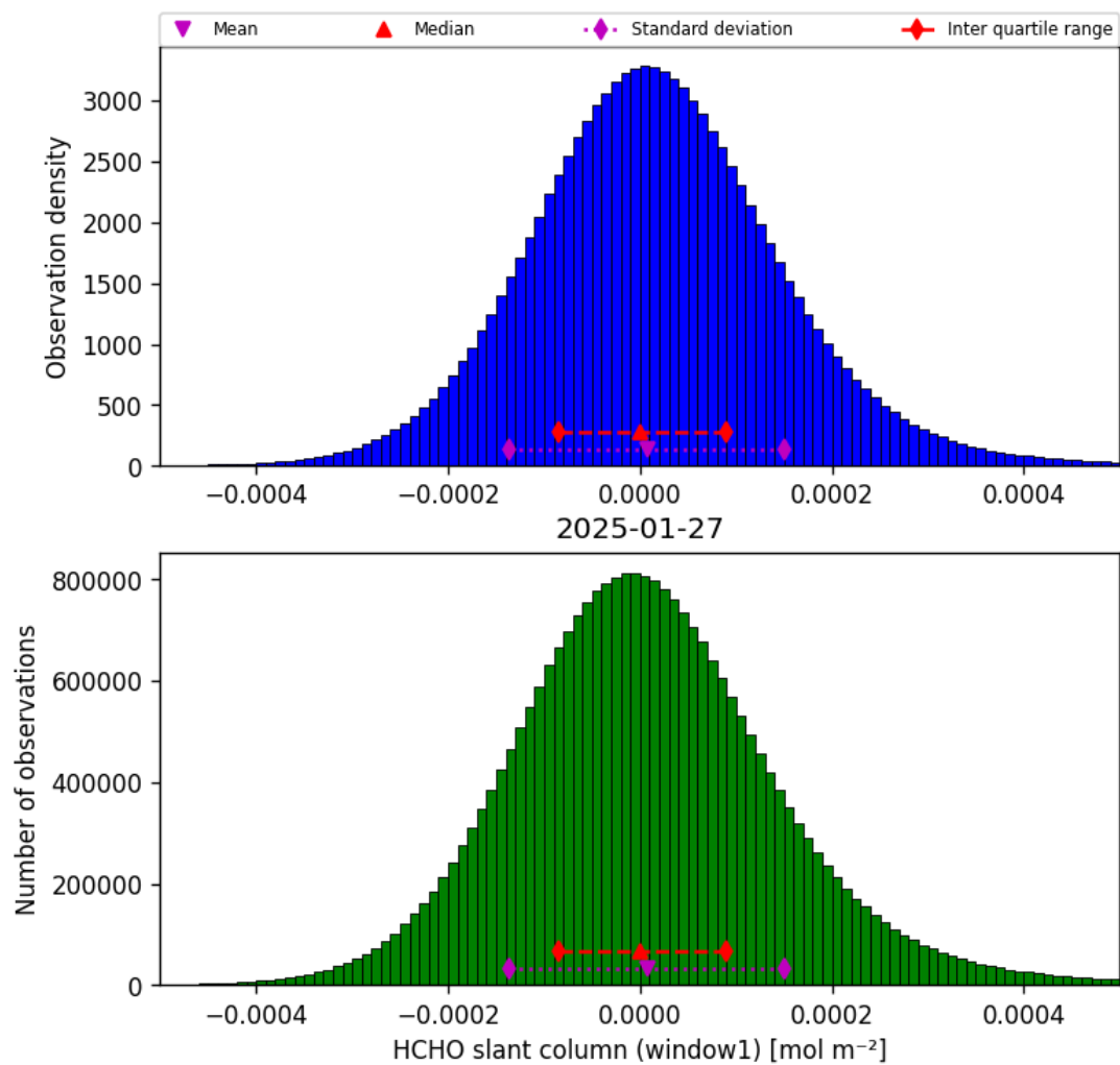
Figure 38: Histogram of “HCHO slant column (window1)” for 2025-01-26 to 2025-01-28
