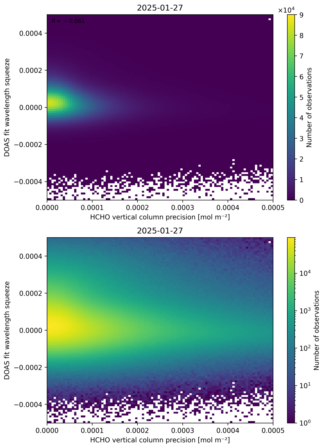
Figure 138: Scatter density plot of “HCHO vertical column precision” against “DOAS fit wavelength squeeze” for 2025-01-26 to 2025-01-28.
