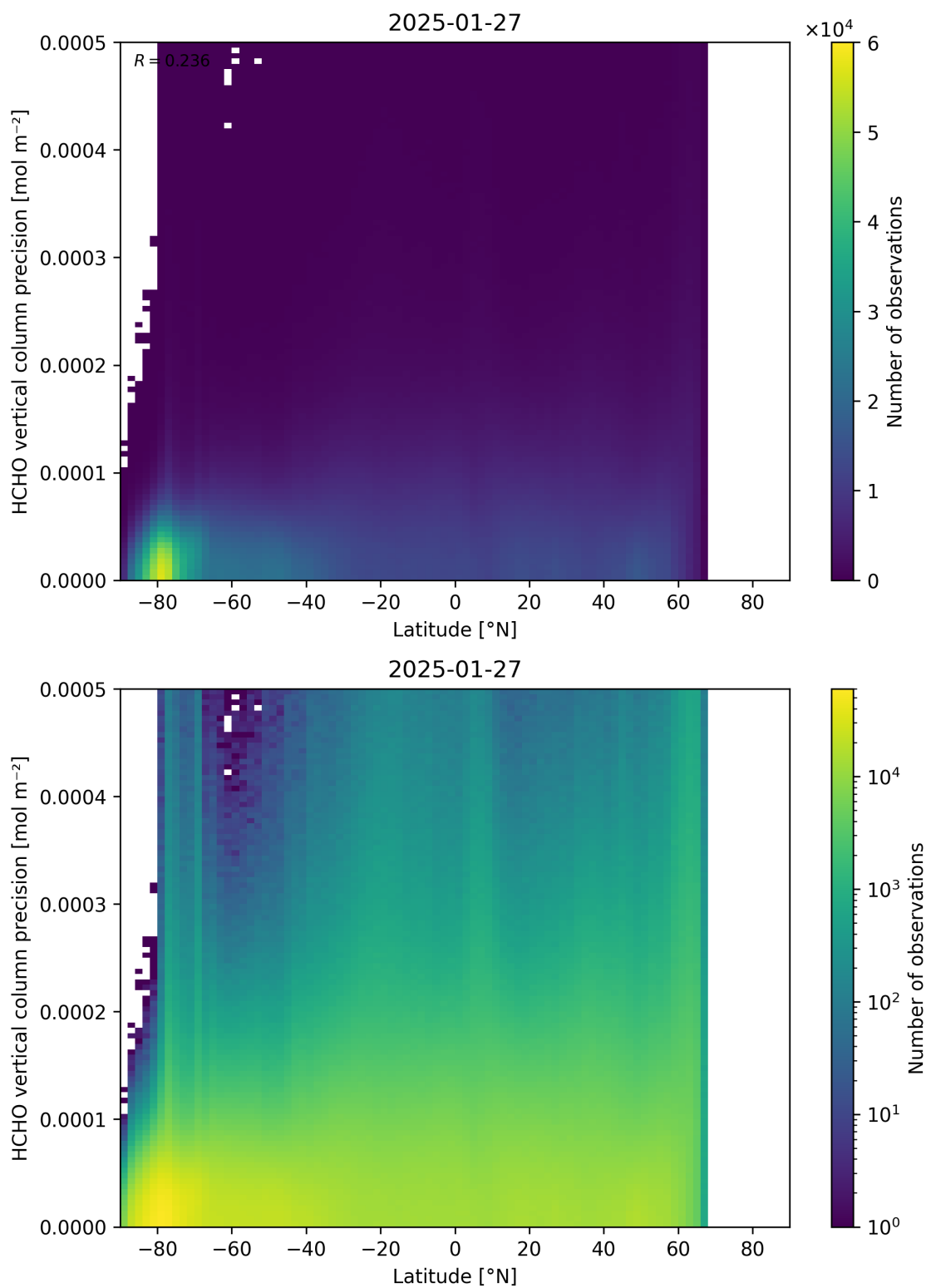
Figure 165: Scatter density plot of “Latitude” against “HCHO vertical column precision” for 2025-01-26 to 2025-01-28.
