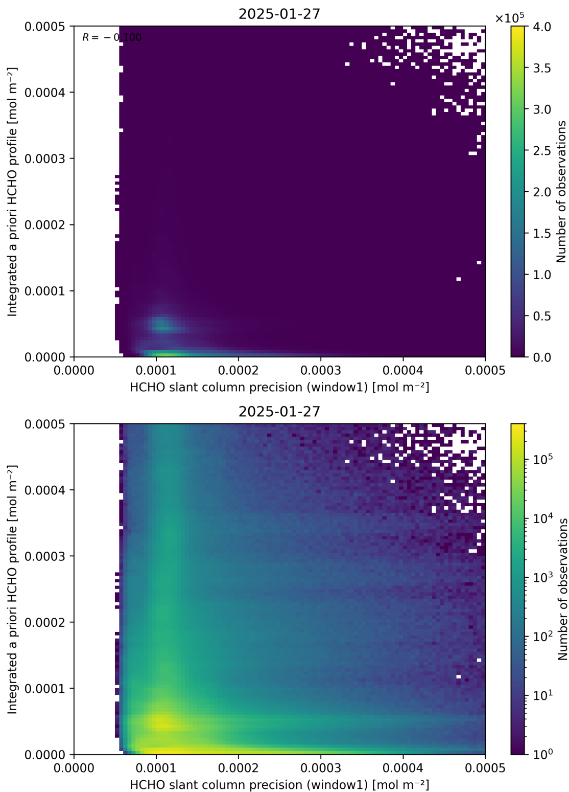
Figure 96: Scatter density plot of “HCHO slant column precision (window1)” against “Integrated a priori HCHO profile” for 2025-01-26 to 2025-01-28.
