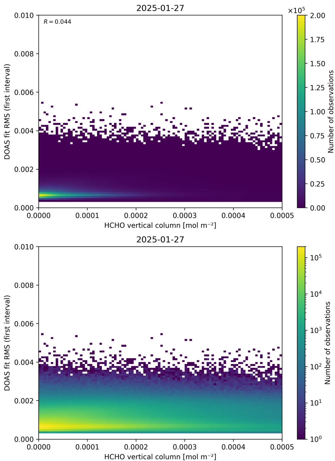
Figure 123: Scatter density plot of “HCHO vertical column” against “DOAS fit RMS (first interval)” for 2025-01-26 to 2025-01-28.
