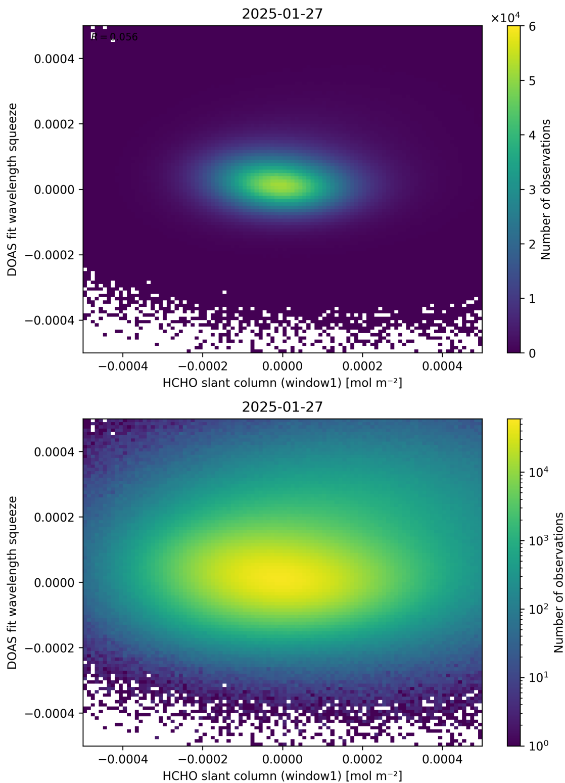
Figure 80: Scatter density plot of “HCHO slant column (window1)” against “DOAS fit wavelength squeeze” for 2025-01-26 to 2025-01-28.
