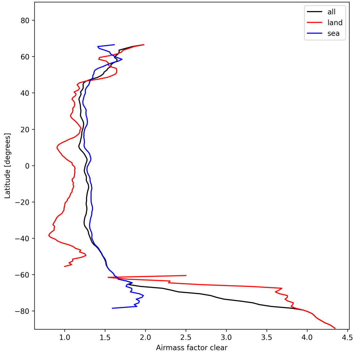
Figure 28: Zonal average of “Airmass factor clear” for 2025-01-26 to 2025-01-28.
