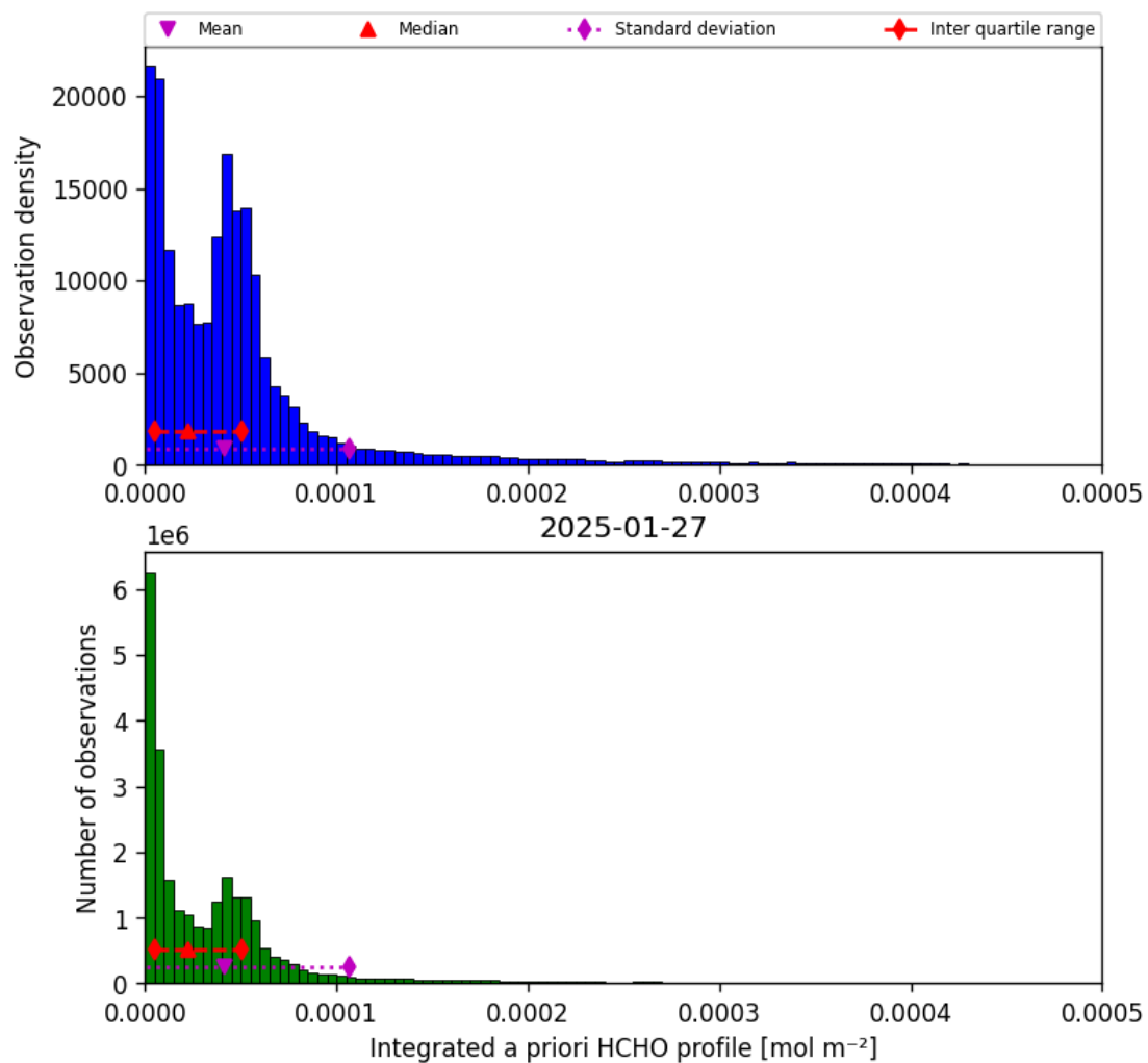
Figure 43: Histogram of “Integrated a priori HCHO profile” for 2025-01-26 to 2025-01-28
