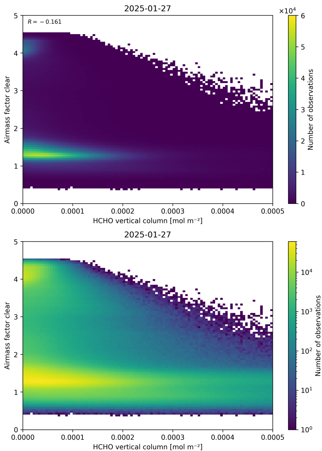
Figure 126: Scatter density plot of “HCHO vertical column” against “Airmass factor clear” for 2025-01-26 to 2025-01-28.
