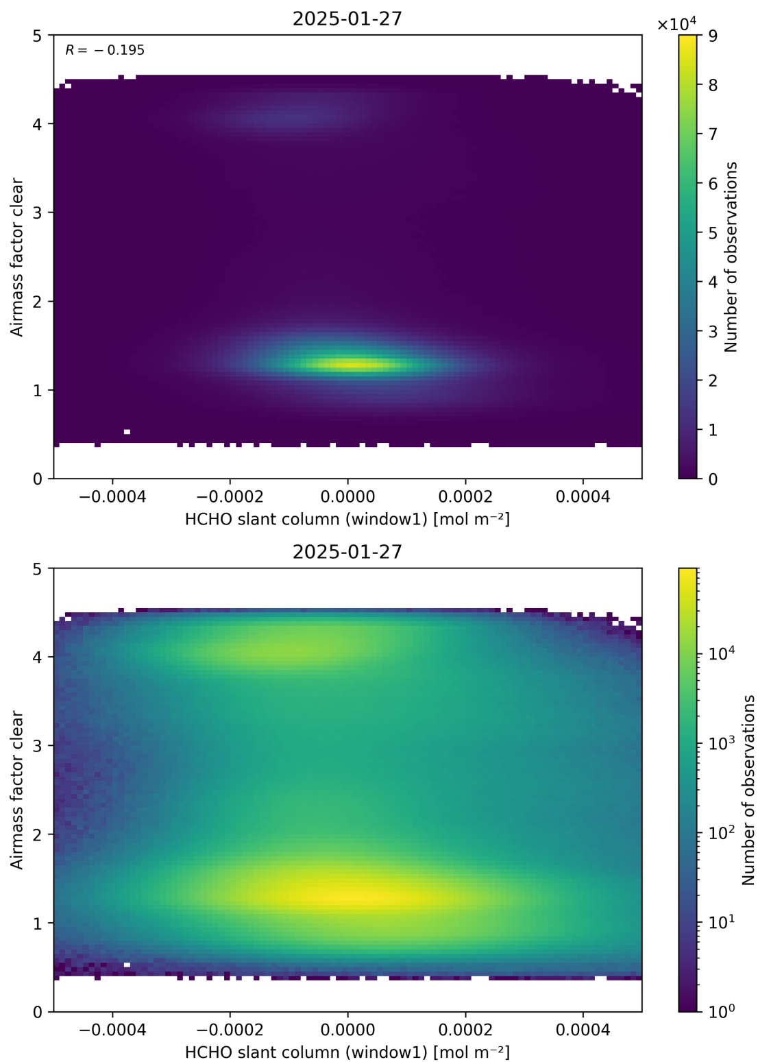
Figure 81: Scatter density plot of “HCHO slant column (window1)” against “Airmass factor clear” for 2025-01-26 to 2025-01-28.
