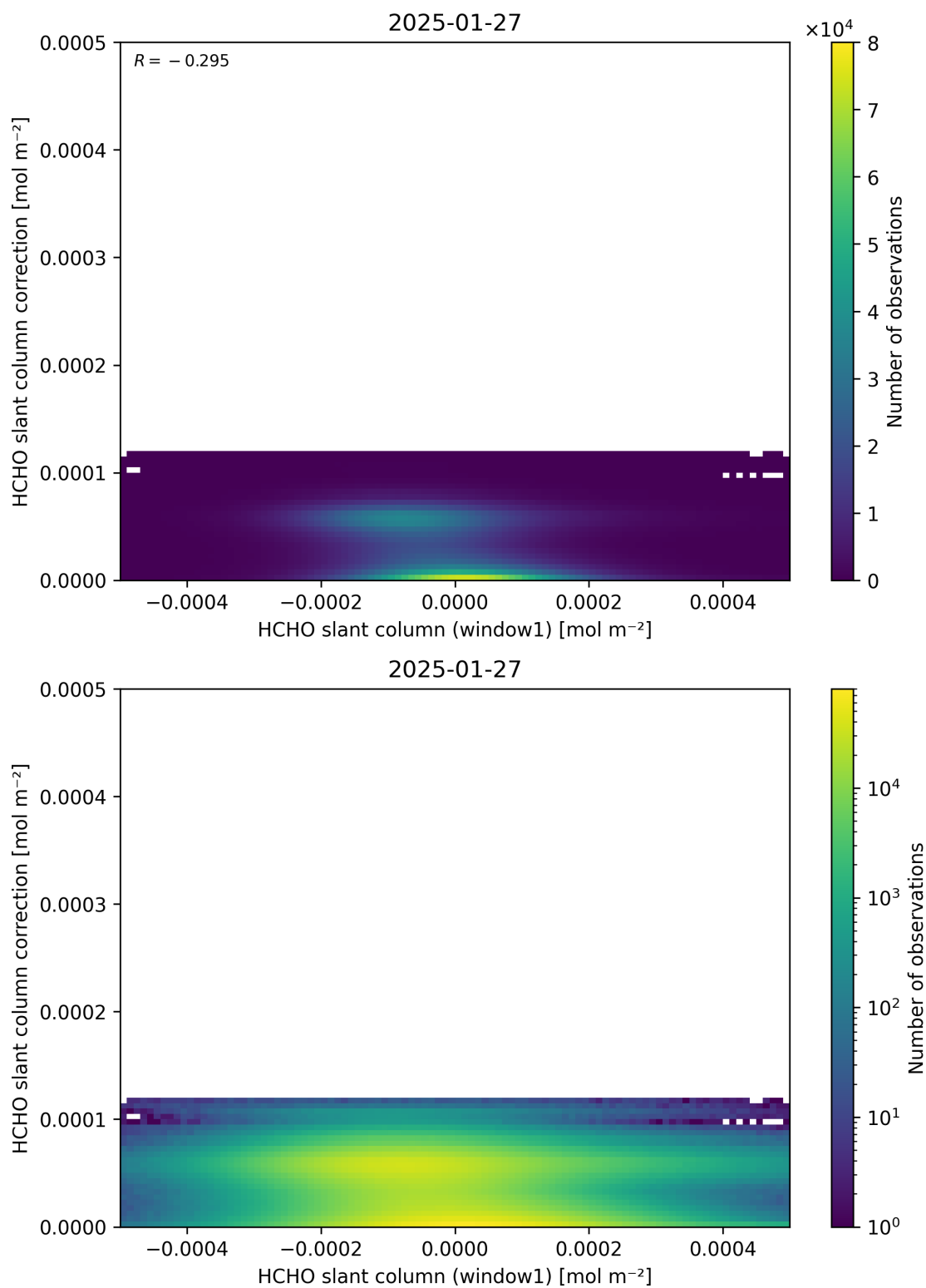
Figure 83: Scatter density plot of “HCHO slant column (window1)” against “HCHO slant column correction” for 2025-01-26 to 2025-01-28.
