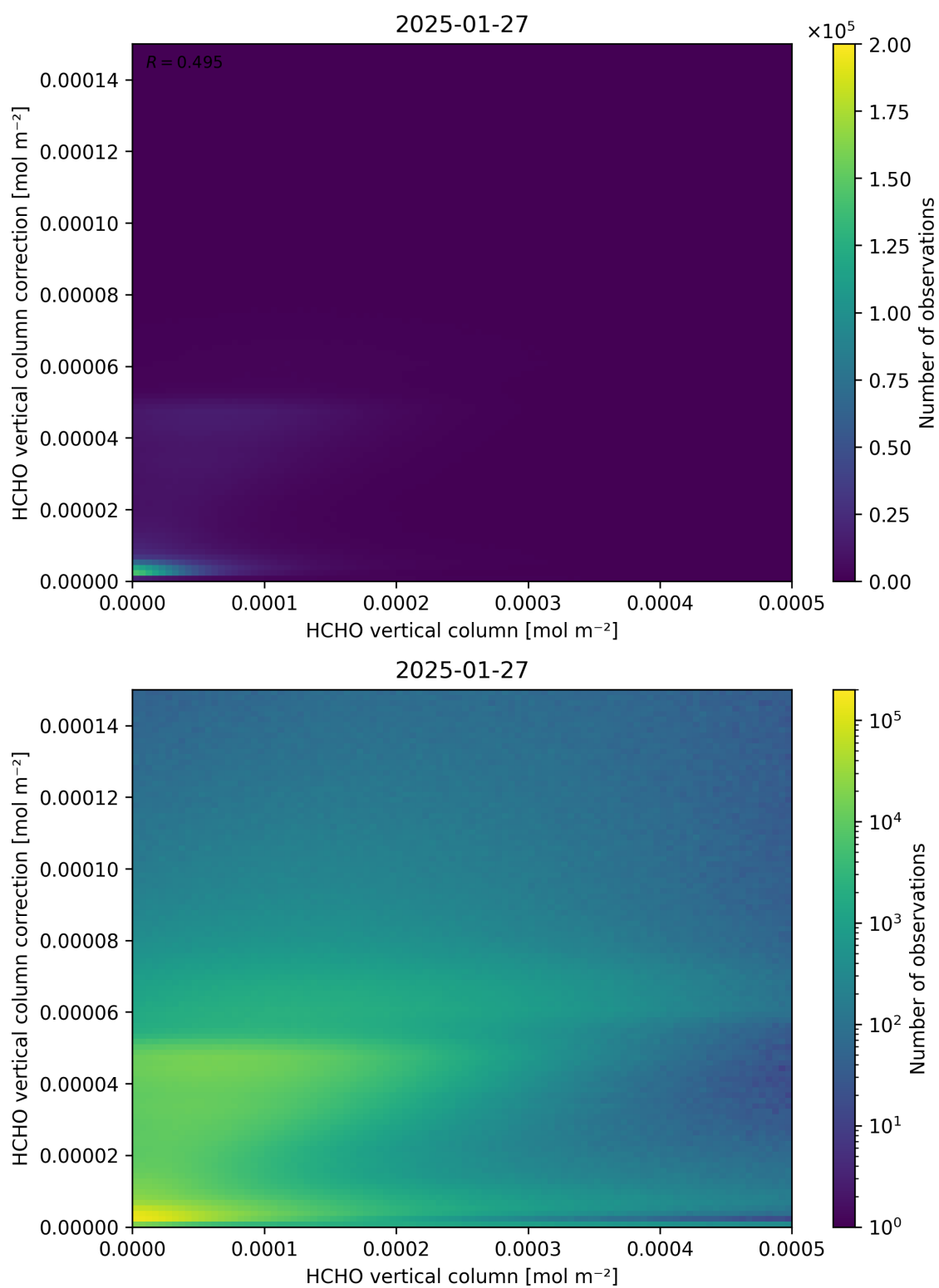
Figure 133: Scatter density plot of “HCHO vertical column” against “HCHO vertical column correction” for 2025-01-26 to 2025-01-28.
