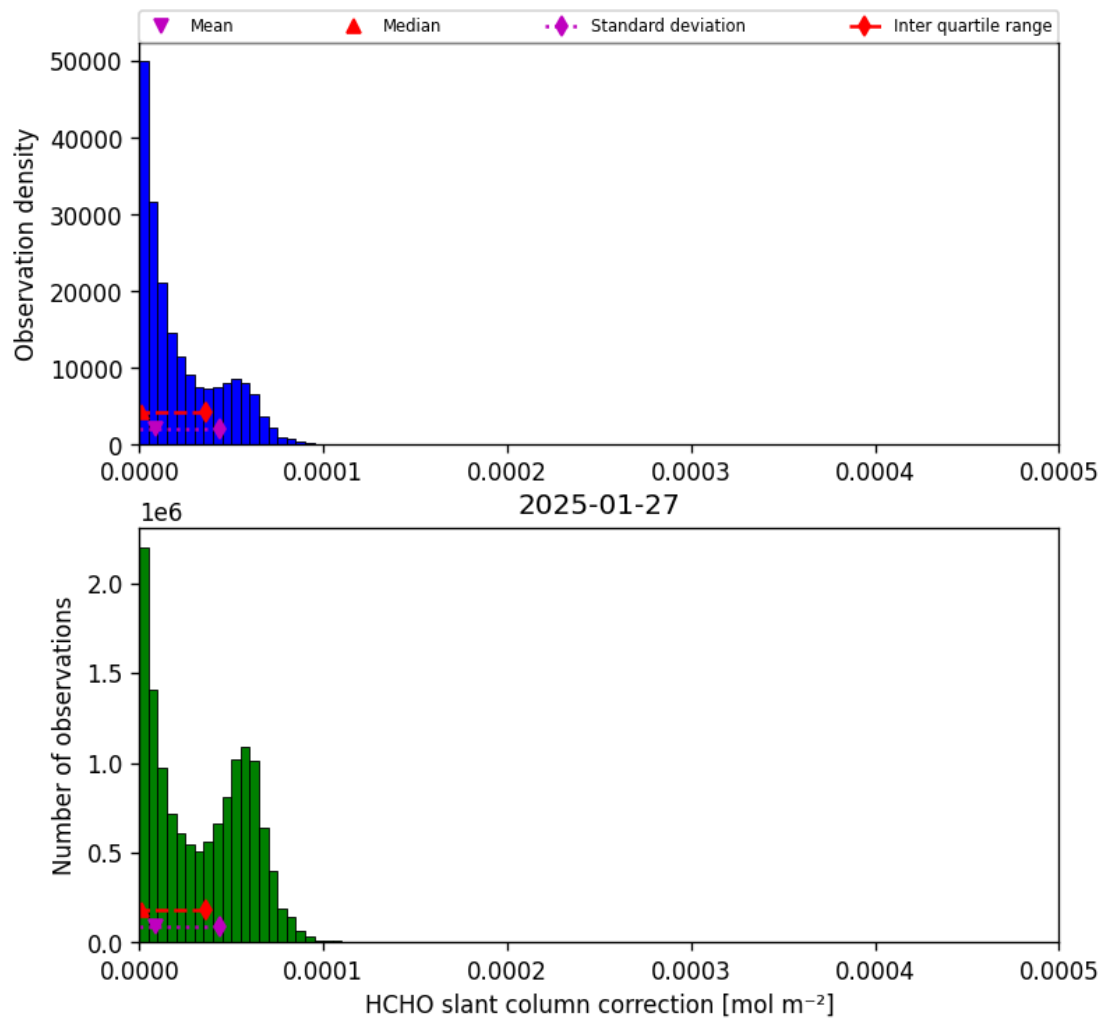
Figure 47: Histogram of “HCHO slant column correction” for 2025-01-26 to 2025-01-28
