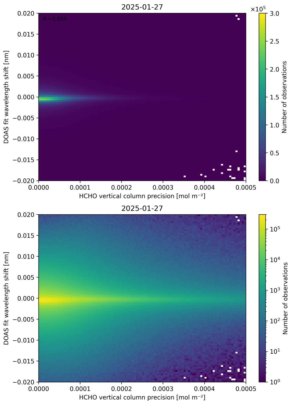
Figure 137: Scatter density plot of “HCHO vertical column precision” against “DOAS fit wavelength shift” for 2025-01-26 to 2025-01-28.
