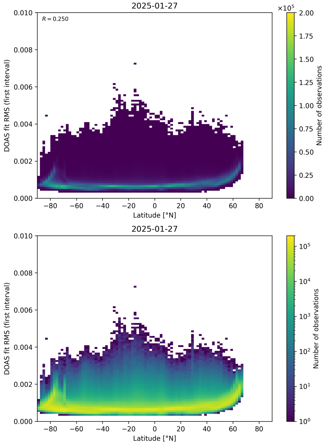
Figure 153: Scatter density plot of “Latitude” against “DOAS fit RMS (first interval)” for 2025-01-26 to 2025-01-28.
