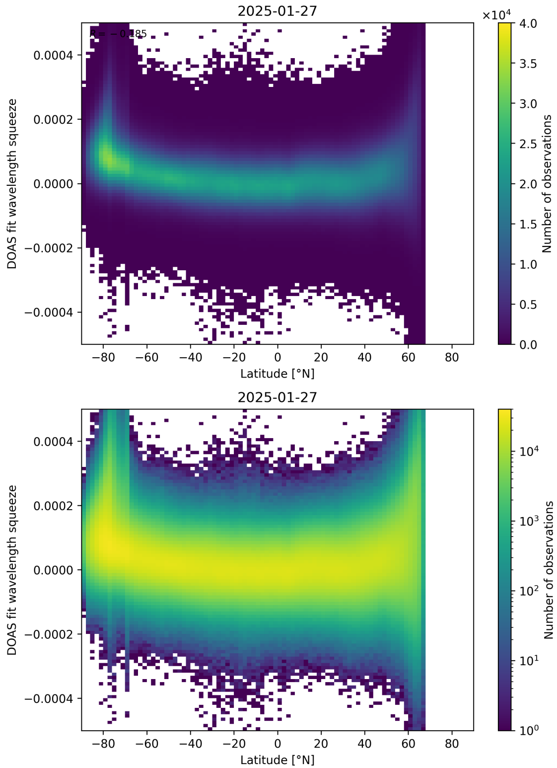
Figure 155: Scatter density plot of “Latitude” against “DOAS fit wavelength squeeze” for 2025-01-26 to 2025-01-28.
