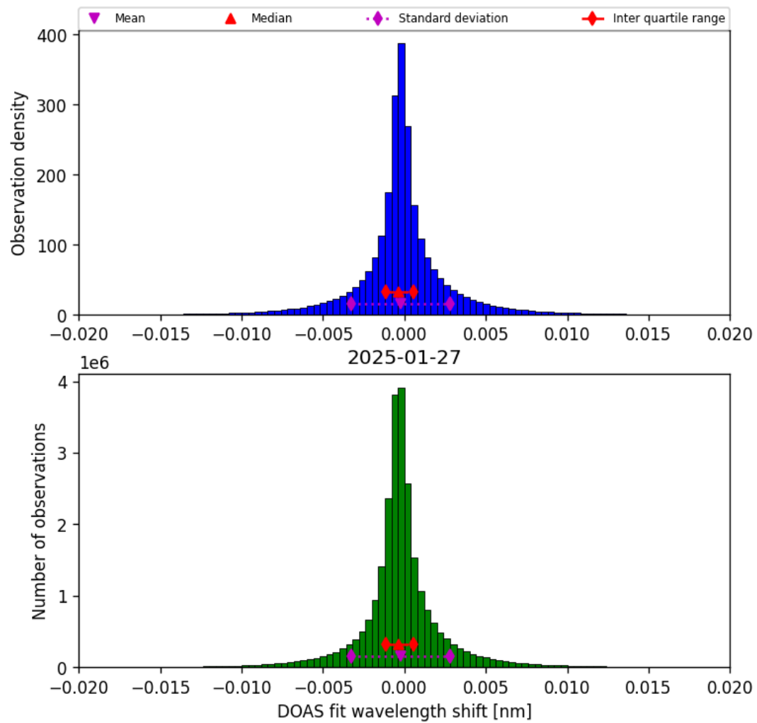
Figure 44: Histogram of “DOAS fit wavelength shift” for 2025-01-26 to 2025-01-28
