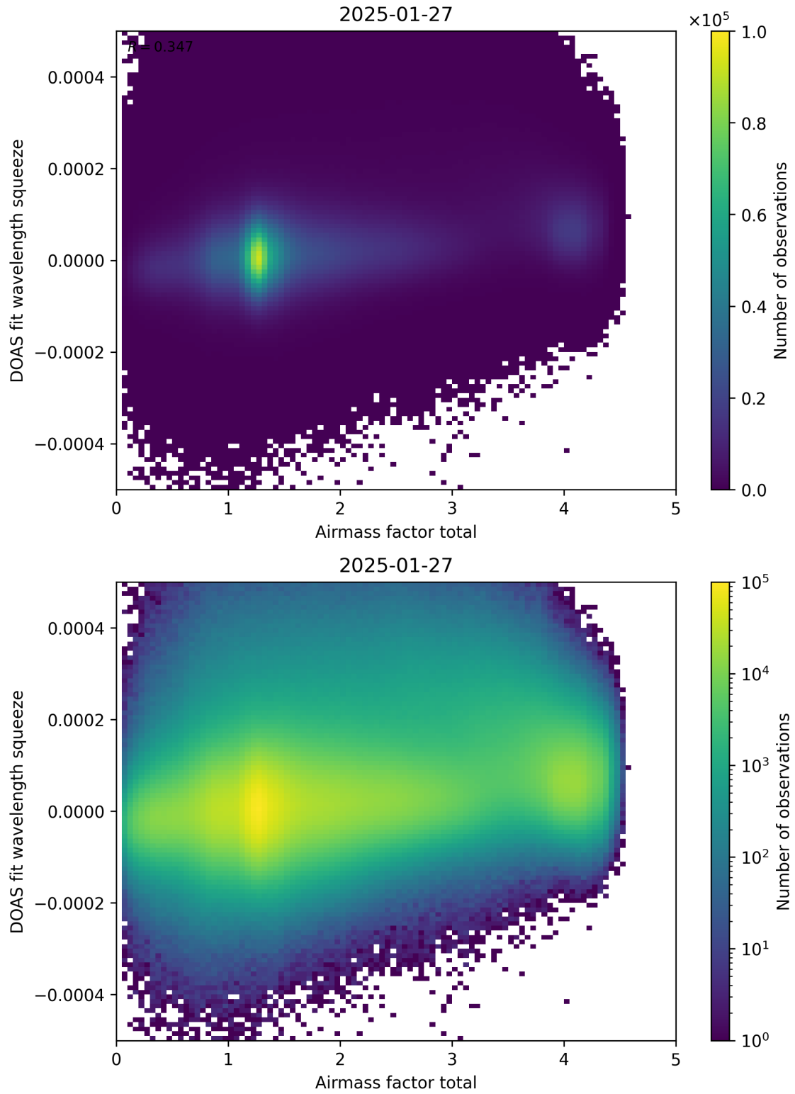
Figure 99: Scatter density plot of “Airmass factor total” against “DOAS fit wavelength squeeze” for 2025-01-26 to 2025-01-28.
