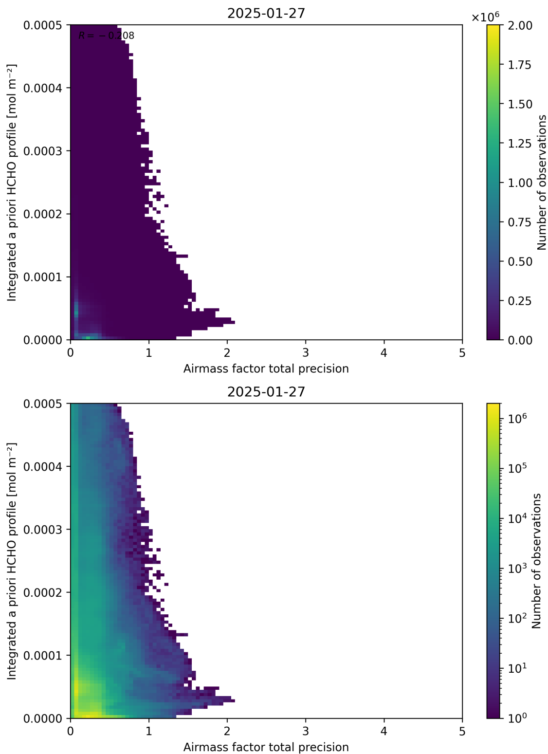
Figure 111: Scatter density plot of “Airmass factor total precision” against “Integrated a priori HCHO profile” for 2025-01-26 to 2025-01-28.
