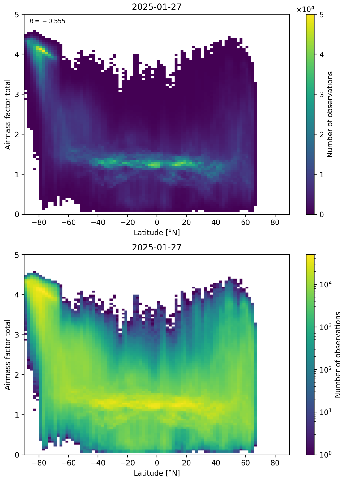
Figure 161: Scatter density plot of “Latitude” against “Airmass factor total” for 2025-01-26 to 2025-01-28.
