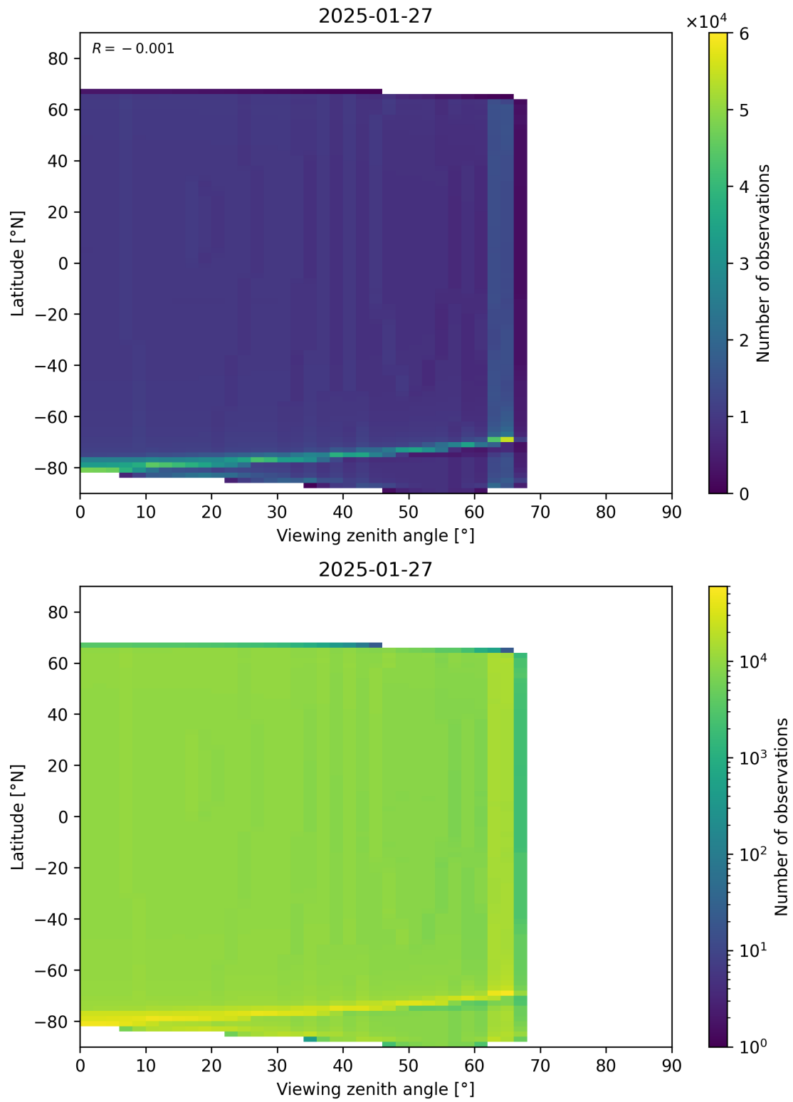
Figure 196: Scatter density plot of “Viewing zenith angle” against “Latitude” for 2025-01-26 to 2025-01-28.
