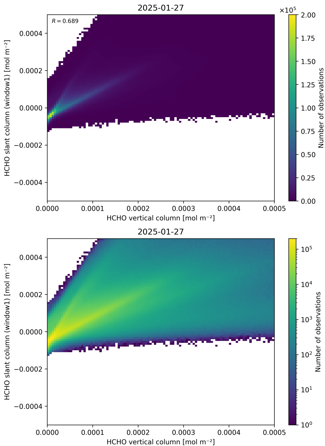
Figure 129: Scatter density plot of “HCHO vertical column” against “HCHO slant column (window1)” for 2025-01-26 to 2025-01-28.
