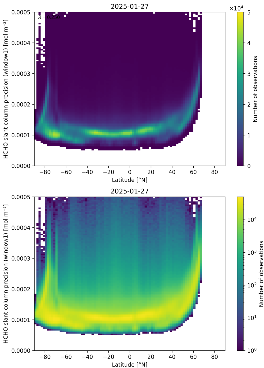
Figure 160: Scatter density plot of “Latitude” against “HCHO slant column precision (window1)” for 2025-01-26 to 2025-01-28.
