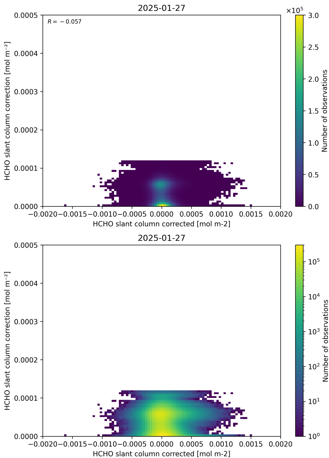
Figure 77: Scatter density plot of “HCHO slant column corrected” against “HCHO slant column correction” for 2025-01-26 to 2025-01-28.
