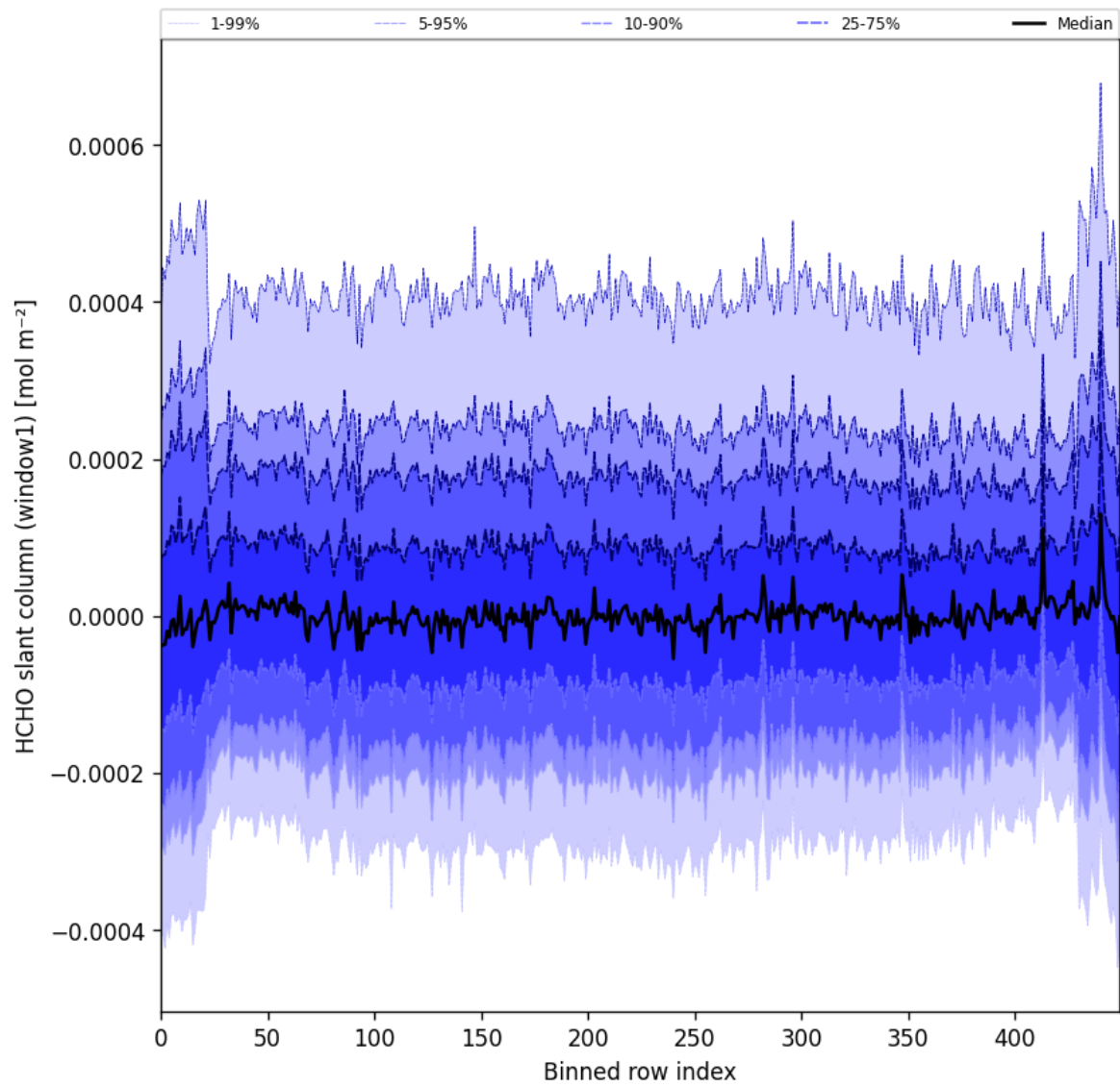
Figure 52: Along track statistics of “HCHO slant column (window1)” for 2025-01-26 to 2025-01-28
