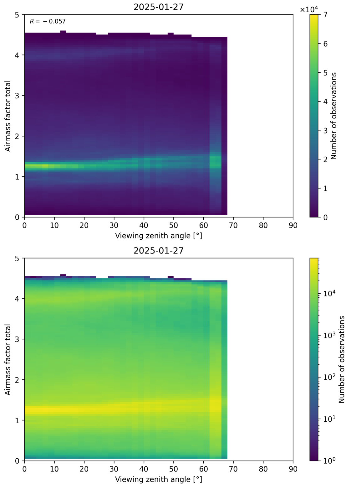
Figure 190: Scatter density plot of “Viewing zenith angle” against “Airmass factor total” for 2025-01-26 to 2025-01-28.
