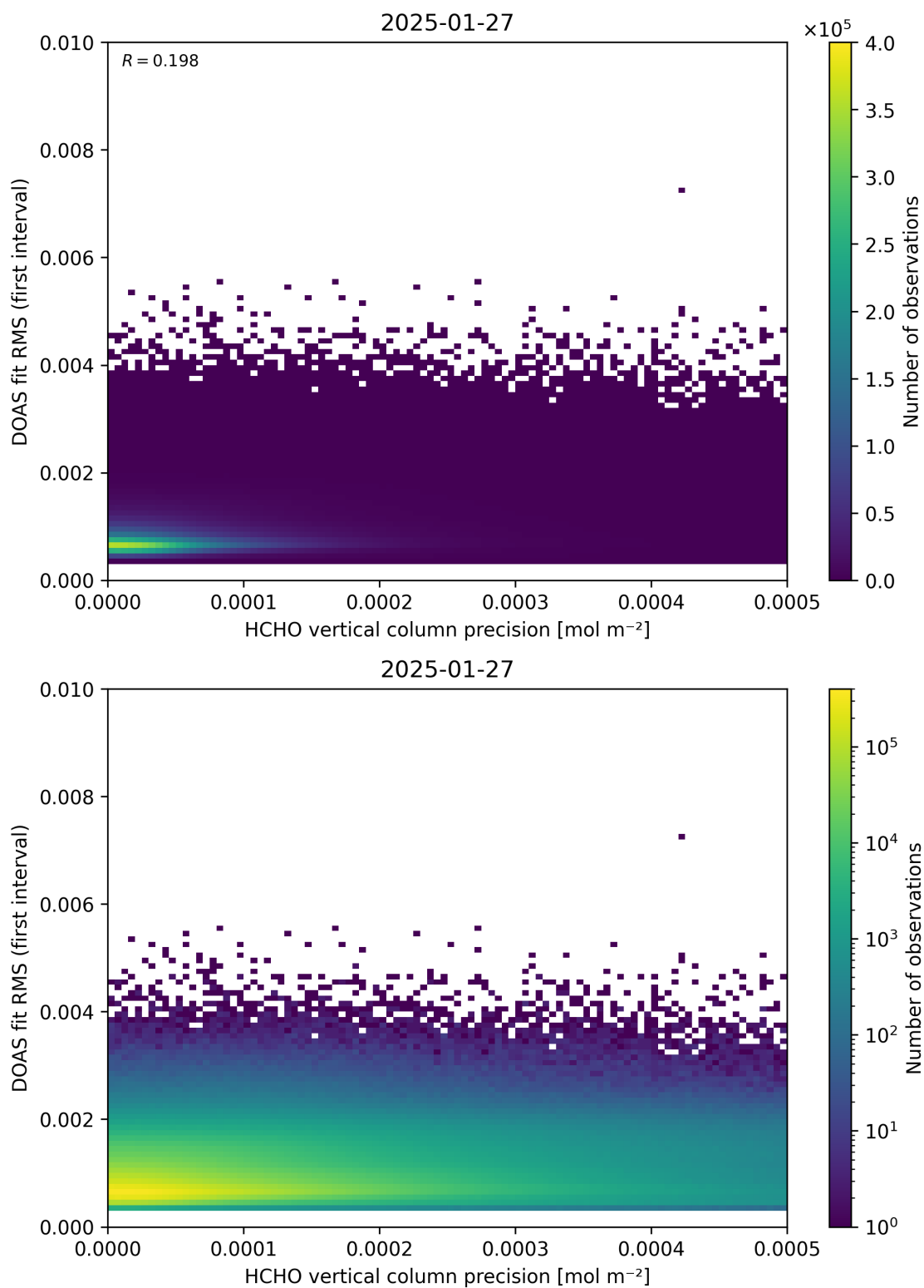
Figure 136: Scatter density plot of “HCHO vertical column precision” against “DOAS fit RMS (first interval)” for 2025-01-26 to 2025-01-28.
