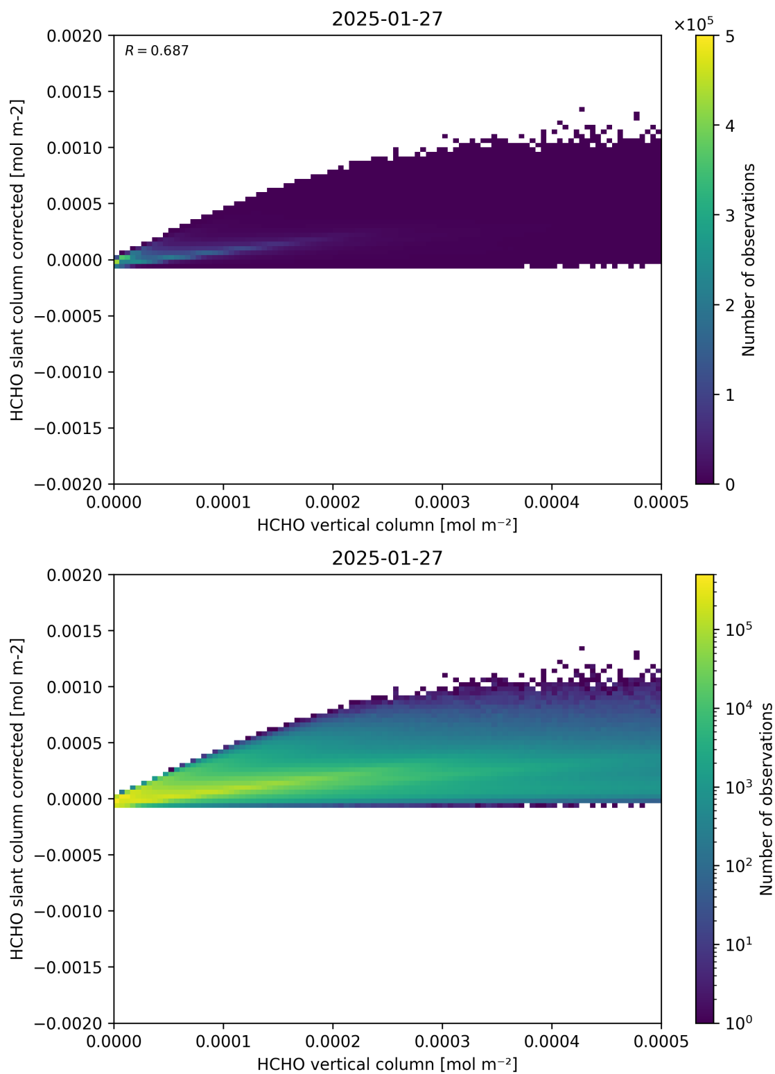
Figure 127: Scatter density plot of “HCHO vertical column” against “HCHO slant column corrected” for 2025-01-26 to 2025-01-28.
