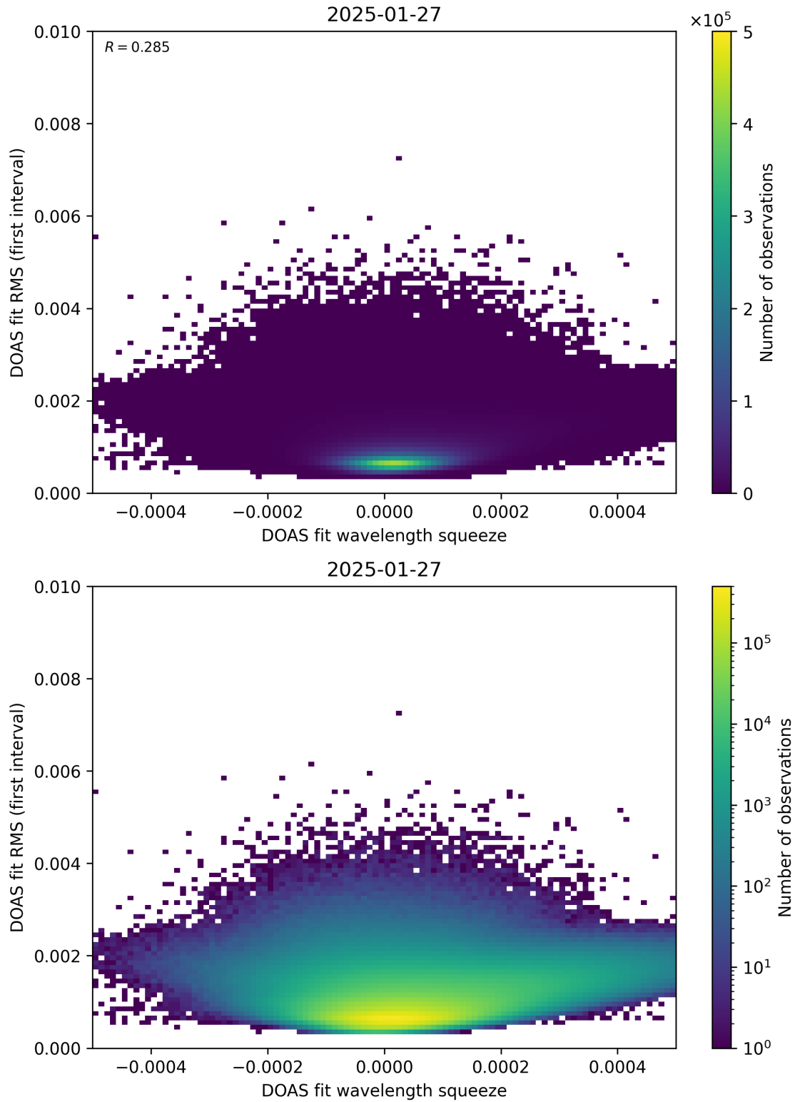
Figure 68: Scatter density plot of “DOAS fit wavelength squeeze” against “DOAS fit RMS (first interval)” for 2025-01-26 to 2025-01-28.
