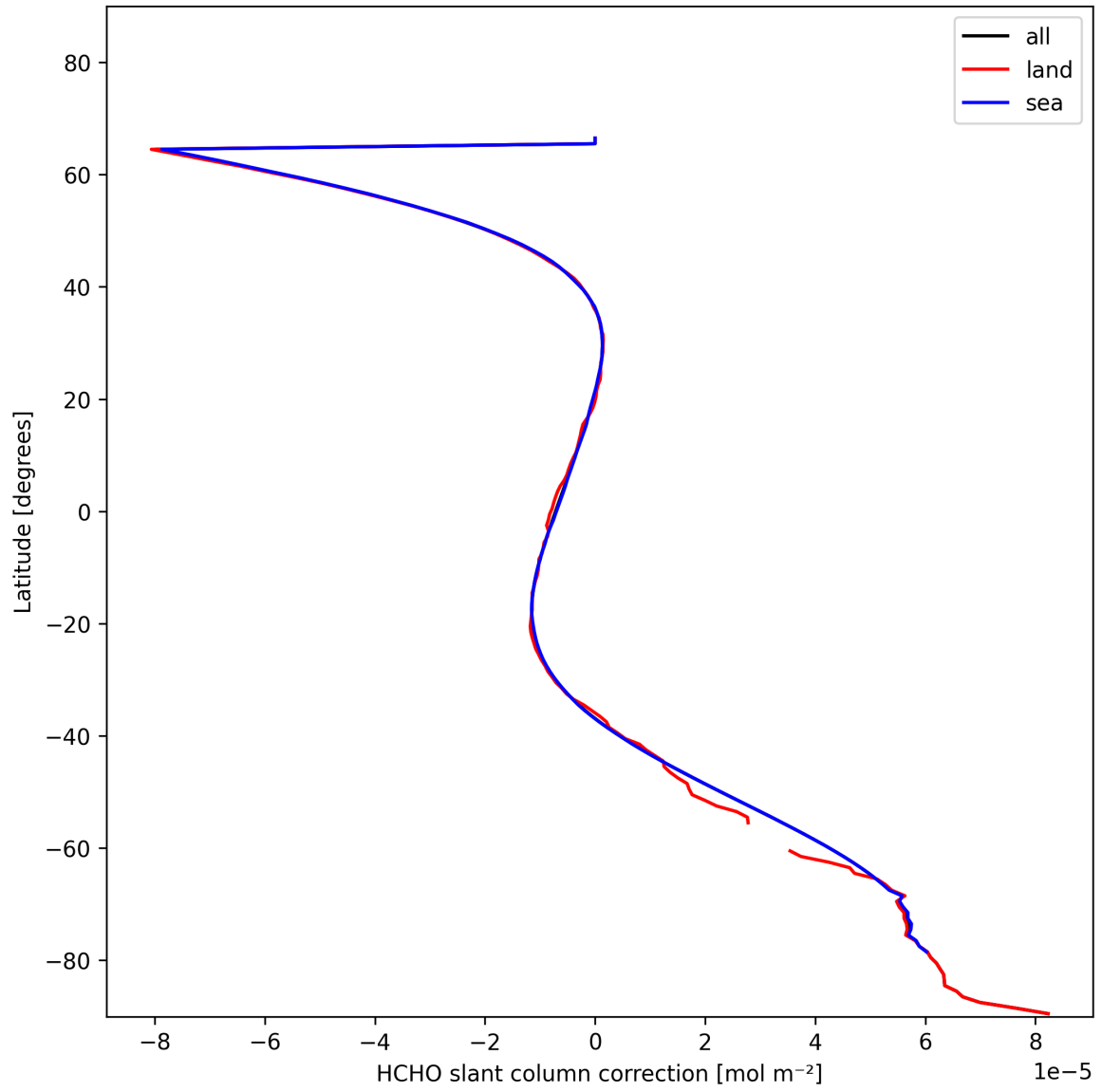
Figure 33: Zonal average of “HCHO slant column correction” for 2025-01-26 to 2025-01-28.
