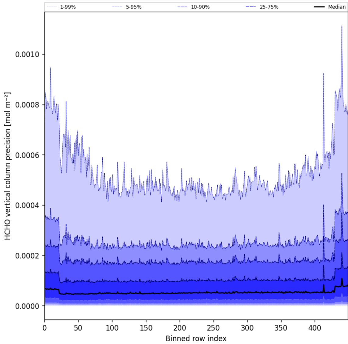
Figure 50: Along track statistics of “HCHO vertical column precision” for 2025-01-26 to 2025-01-28
