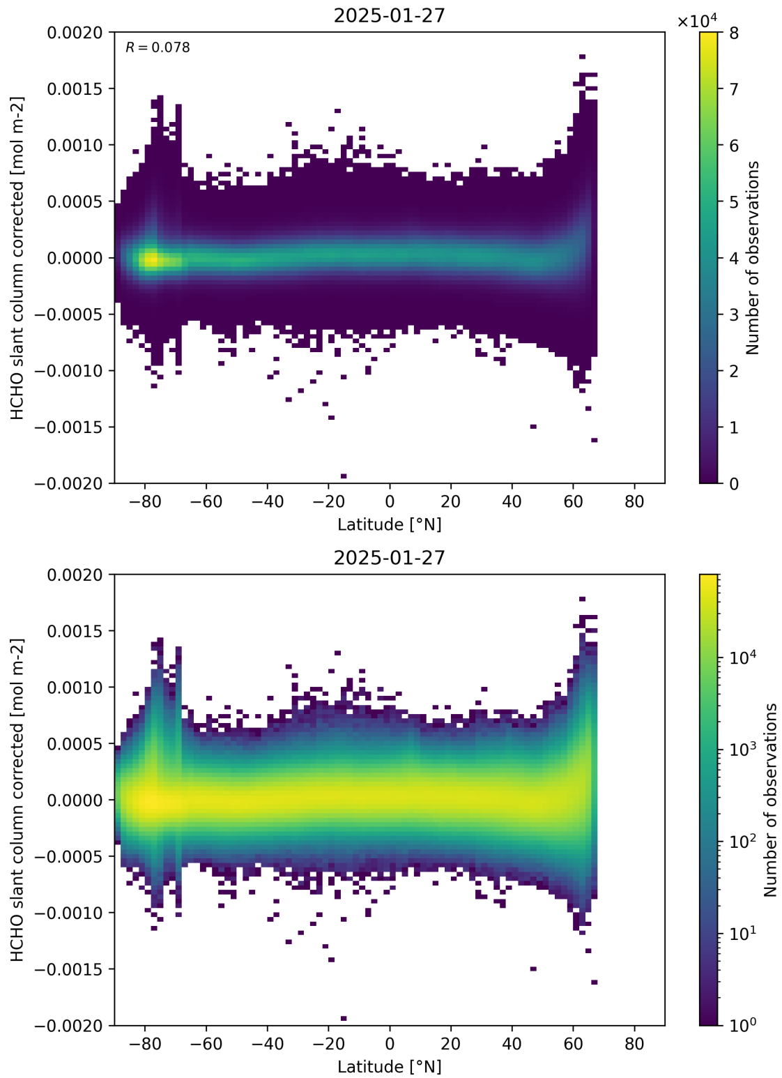
Figure 157: Scatter density plot of “Latitude” against “HCHO slant column corrected” for 2025-01-26 to 2025-01-28.
