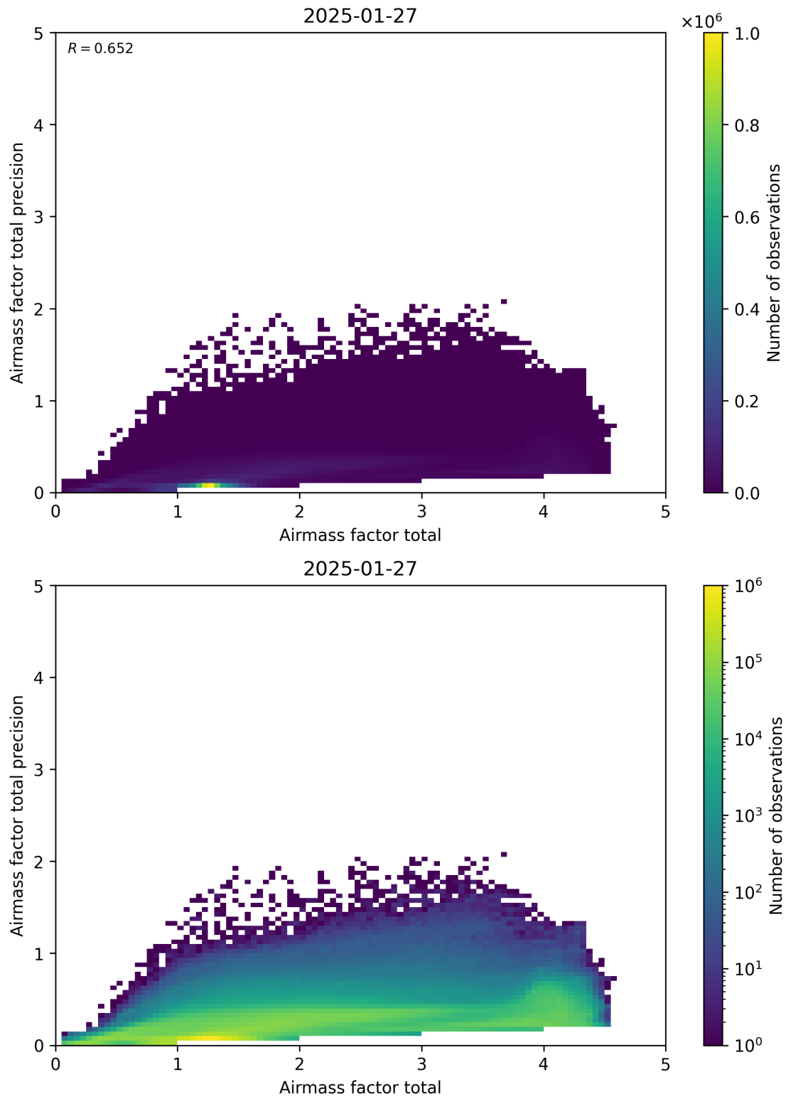
Figure 103: Scatter density plot of “Airmass factor total” against “Airmass factor total precision” for 2025-01-26 to 2025-01-28.
