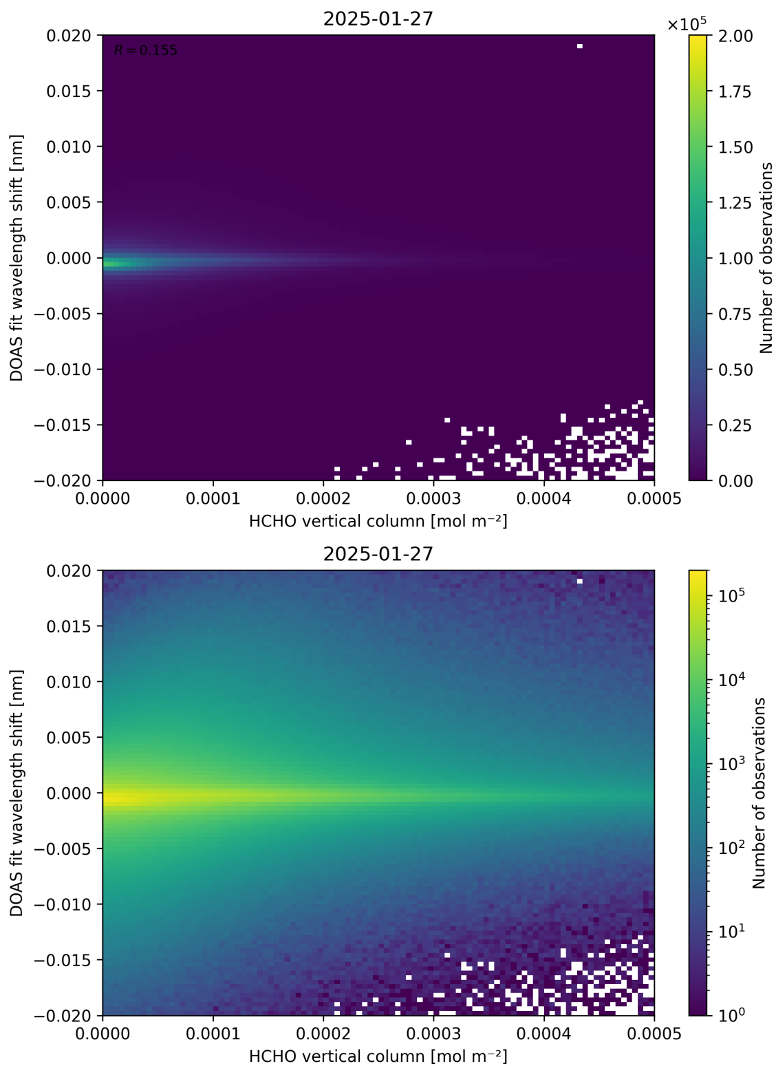
Figure 124: Scatter density plot of “HCHO vertical column” against “DOAS fit wavelength shift” for 2025-01-26 to 2025-01-28.
