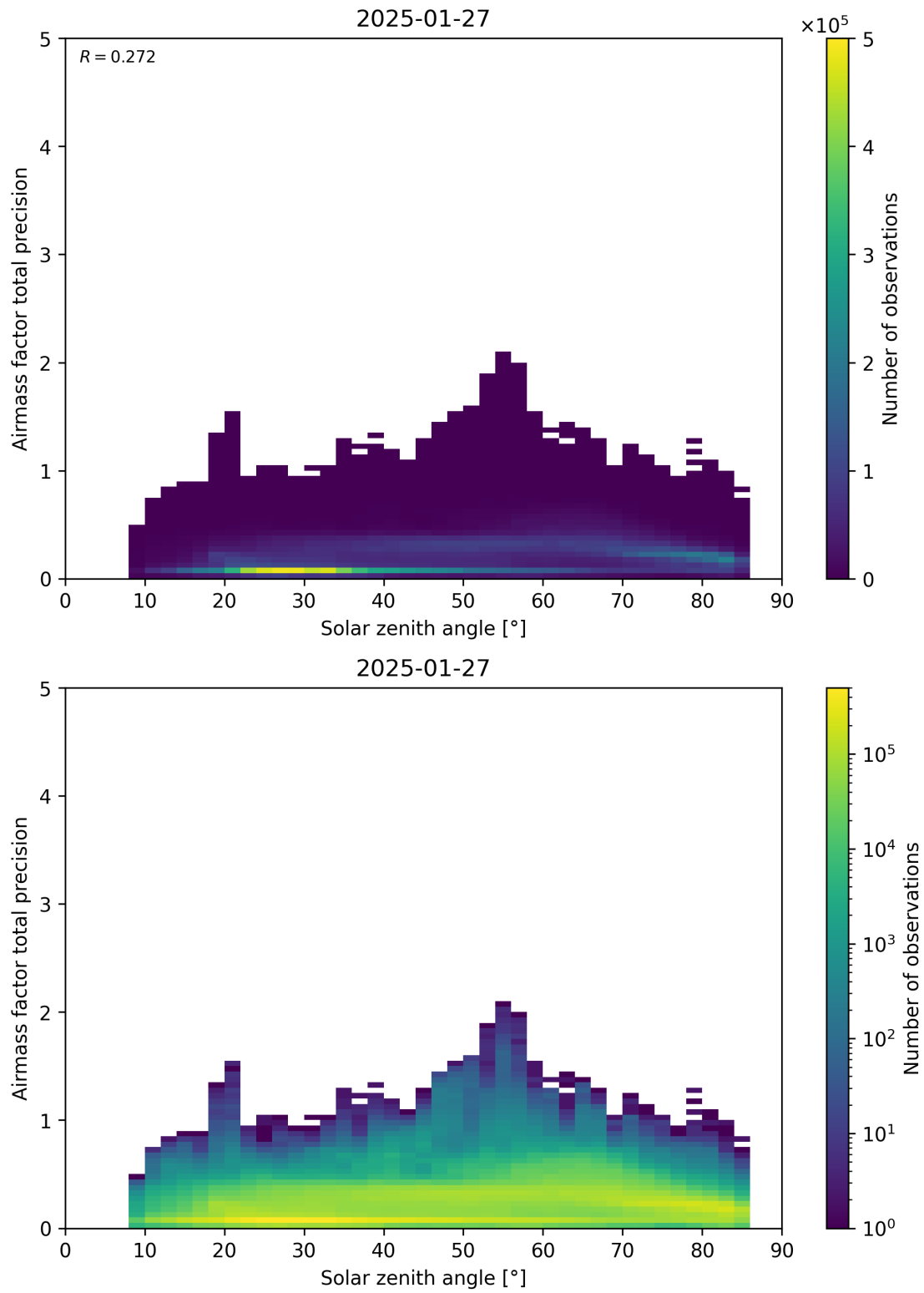
Figure 176: Scatter density plot of “Solar zenith angle” against “Airmass factor total precision” for 2025-01-26 to 2025-01-28.
