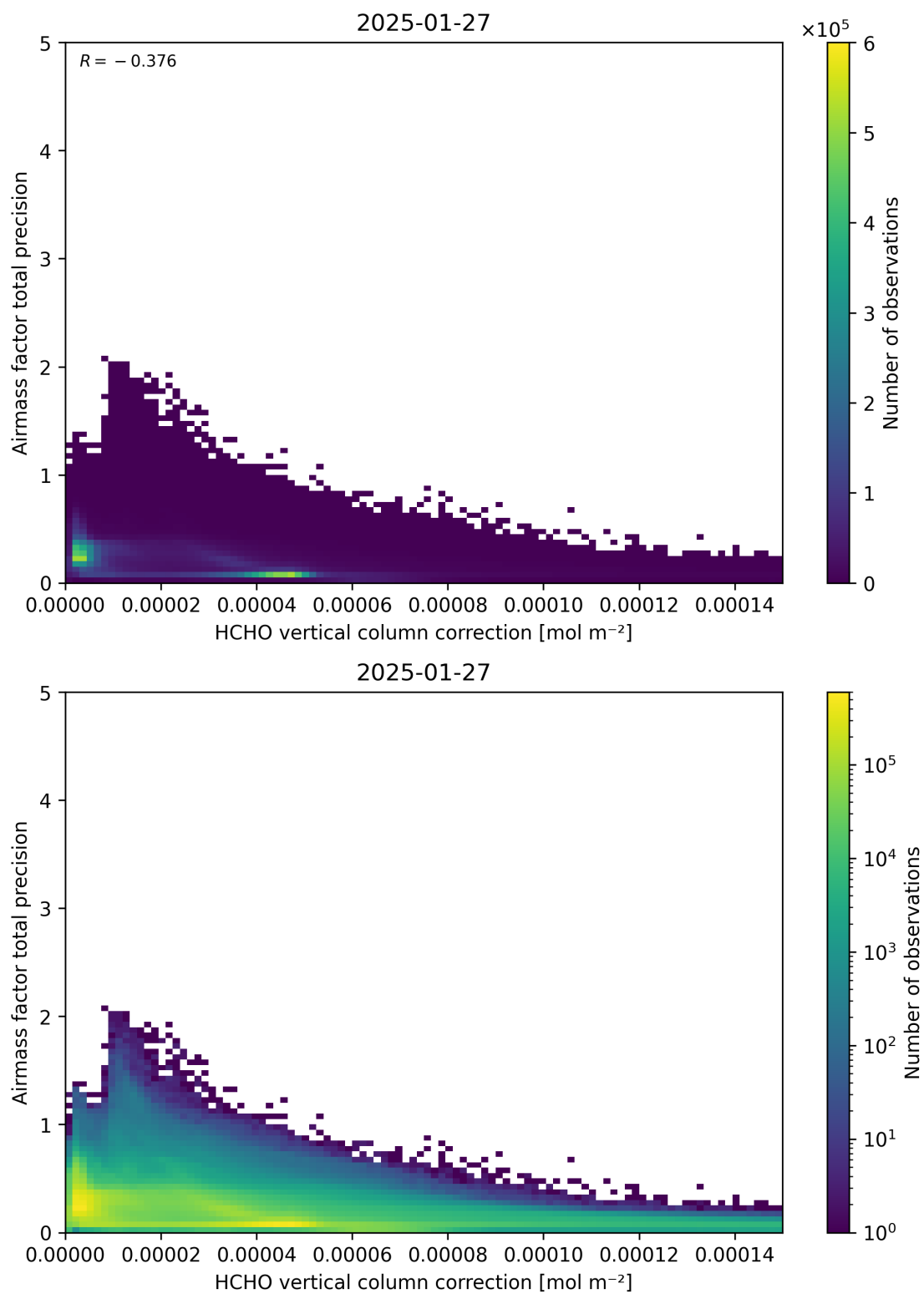
Figure 121: Scatter density plot of “HCHO vertical column correction” against “Airmass factor total precision” for 2025-01-26 to 2025-01-28.
