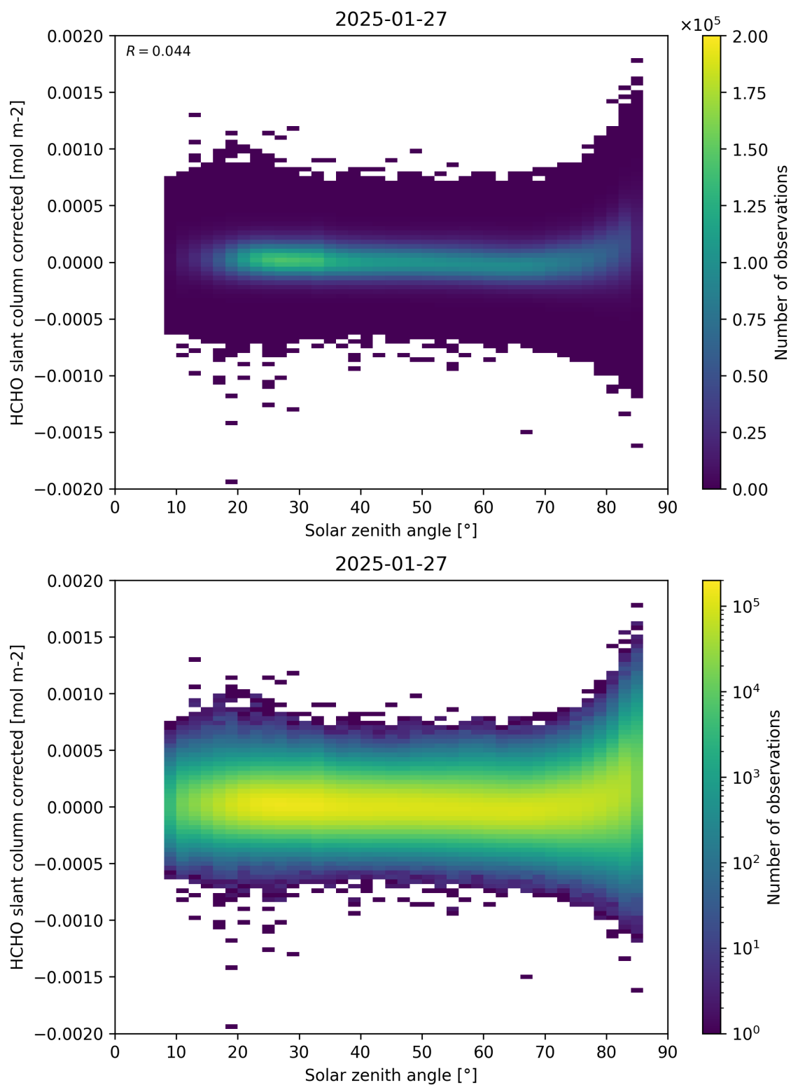
Figure 171: Scatter density plot of “Solar zenith angle” against “HCHO slant column corrected” for 2025-01-26 to 2025-01-28.
