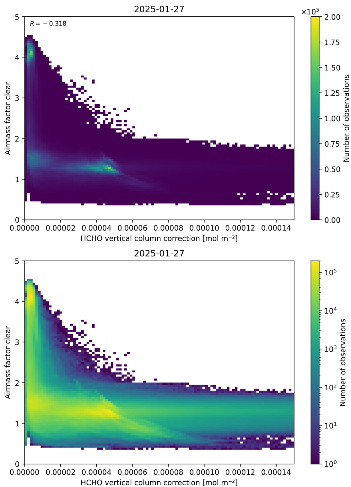
Figure 115: Scatter density plot of “HCHO vertical column correction” against “Airmass factor clear” for 2025-01-26 to 2025-01-28.
