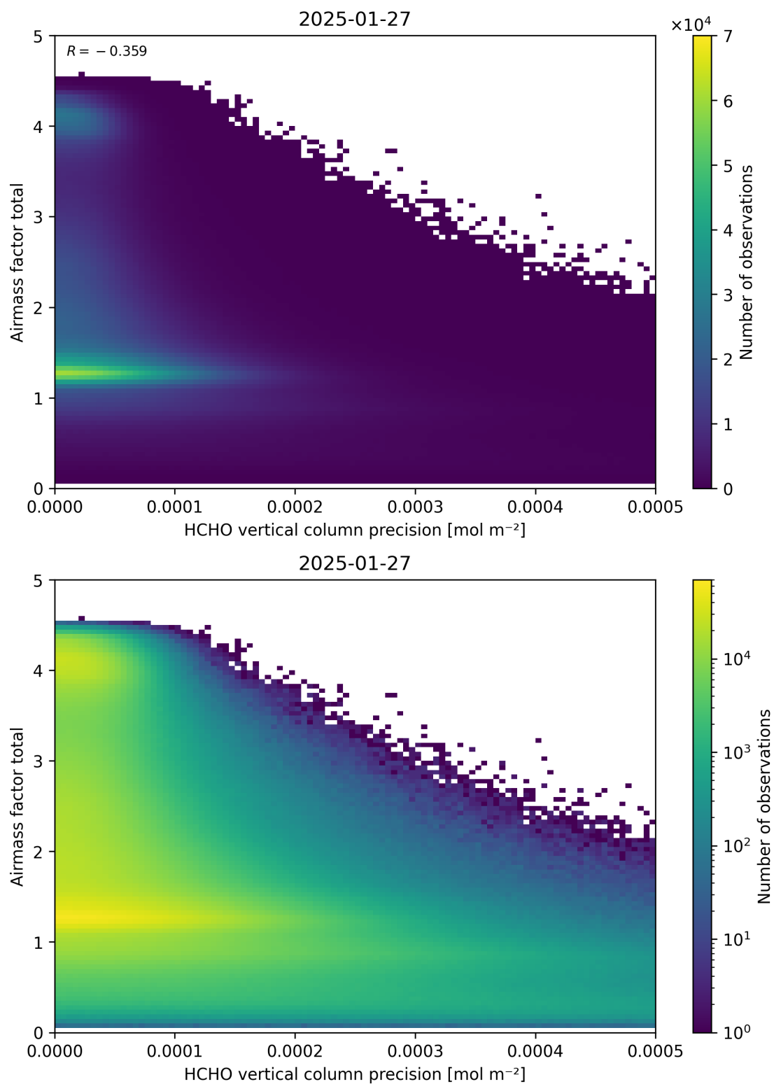
Figure 144: Scatter density plot of “HCHO vertical column precision” against “Airmass factor total” for 2025-01-26 to 2025-01-28.
