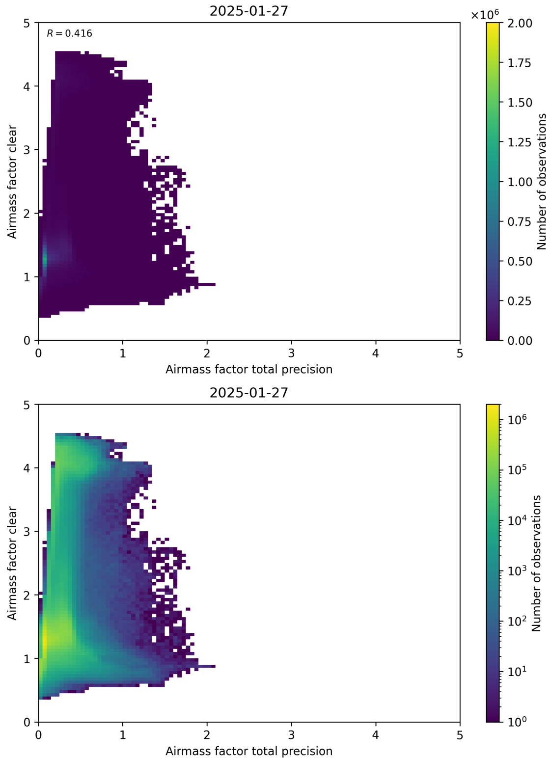
Figure 108: Scatter density plot of “Airmass factor total precision” against “Airmass factor clear” for 2025-01-26 to 2025-01-28.
