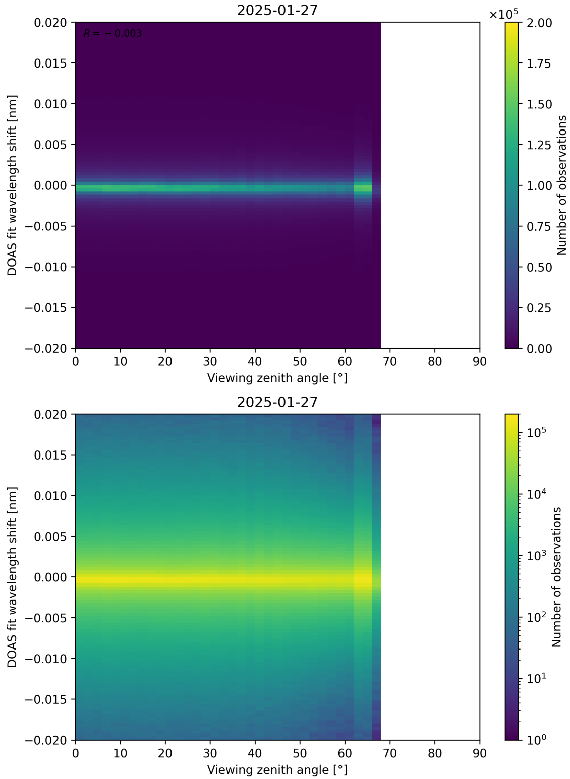
Figure 183: Scatter density plot of “Viewing zenith angle” against “DOAS fit wavelength shift” for 2025-01-26 to 2025-01-28.
