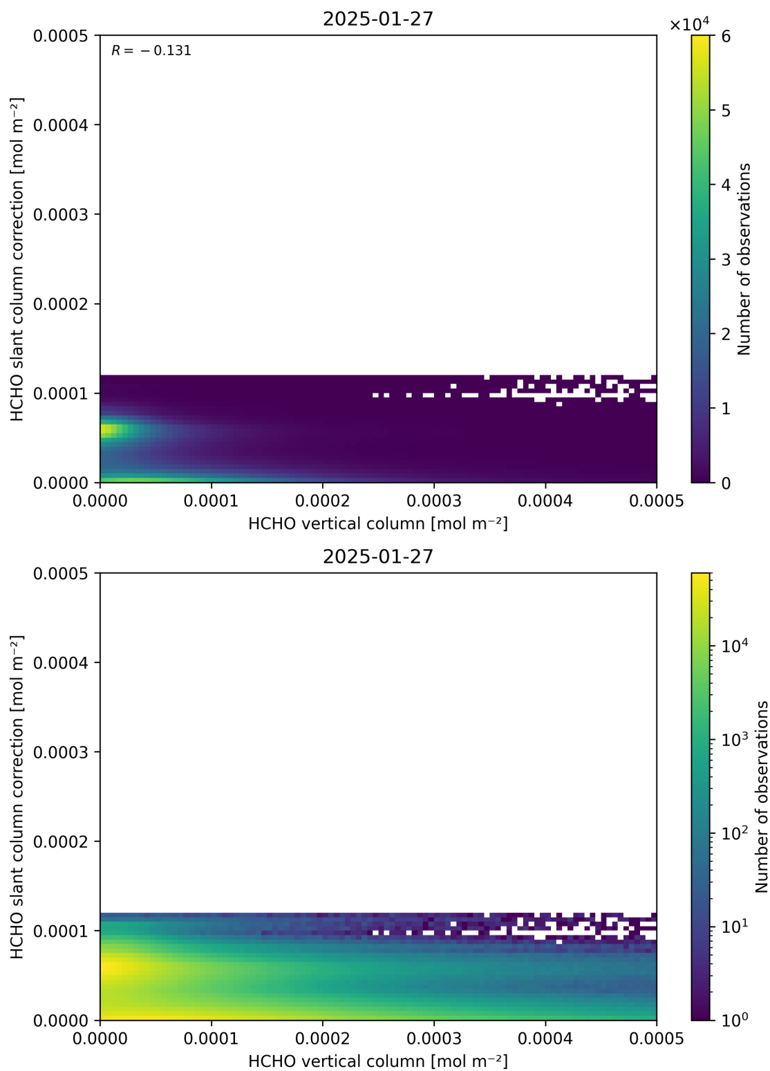
Figure 128: Scatter density plot of “HCHO vertical column” against “HCHO slant column correction” for 2025-01-26 to 2025-01-28.
