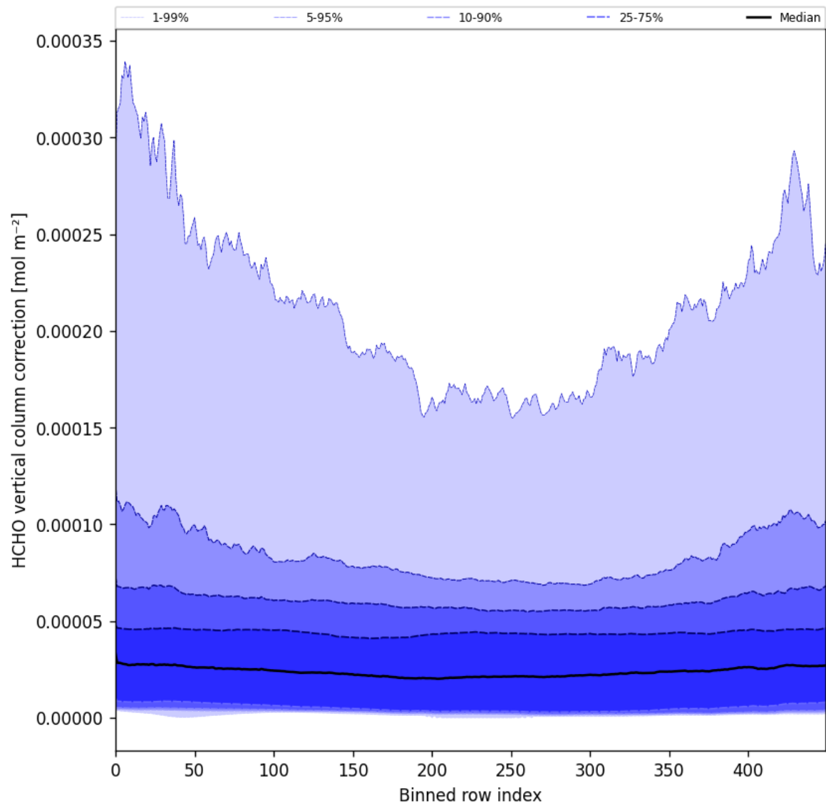
Figure 51: Along track statistics of “HCHO vertical column correction” for 2025-01-26 to 2025-01-28
