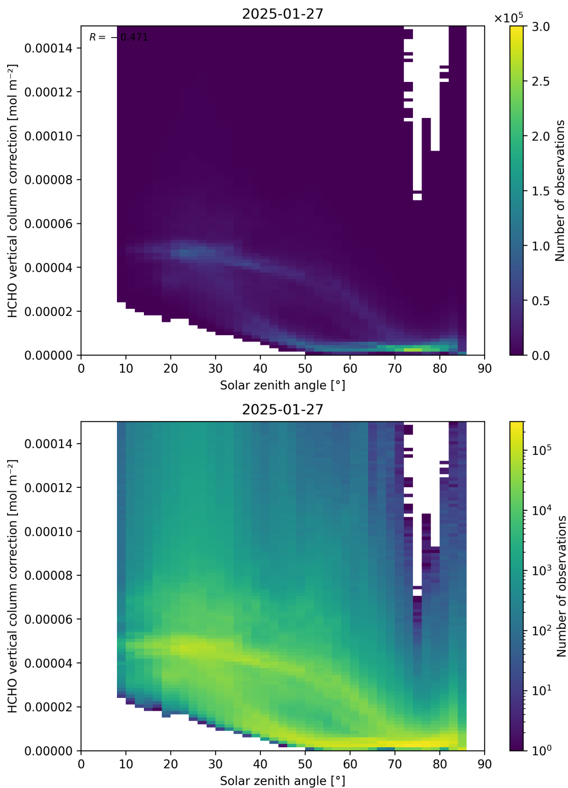
Figure 178: Scatter density plot of “Solar zenith angle” against “HCHO vertical column correction” for 2025-01-26 to 2025-01-28.
