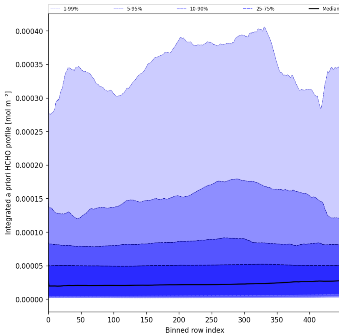
Figure 57: Along track statistics of “Integrated a priori HCHO profile” for 2025-01-26 to 2025-01-28
