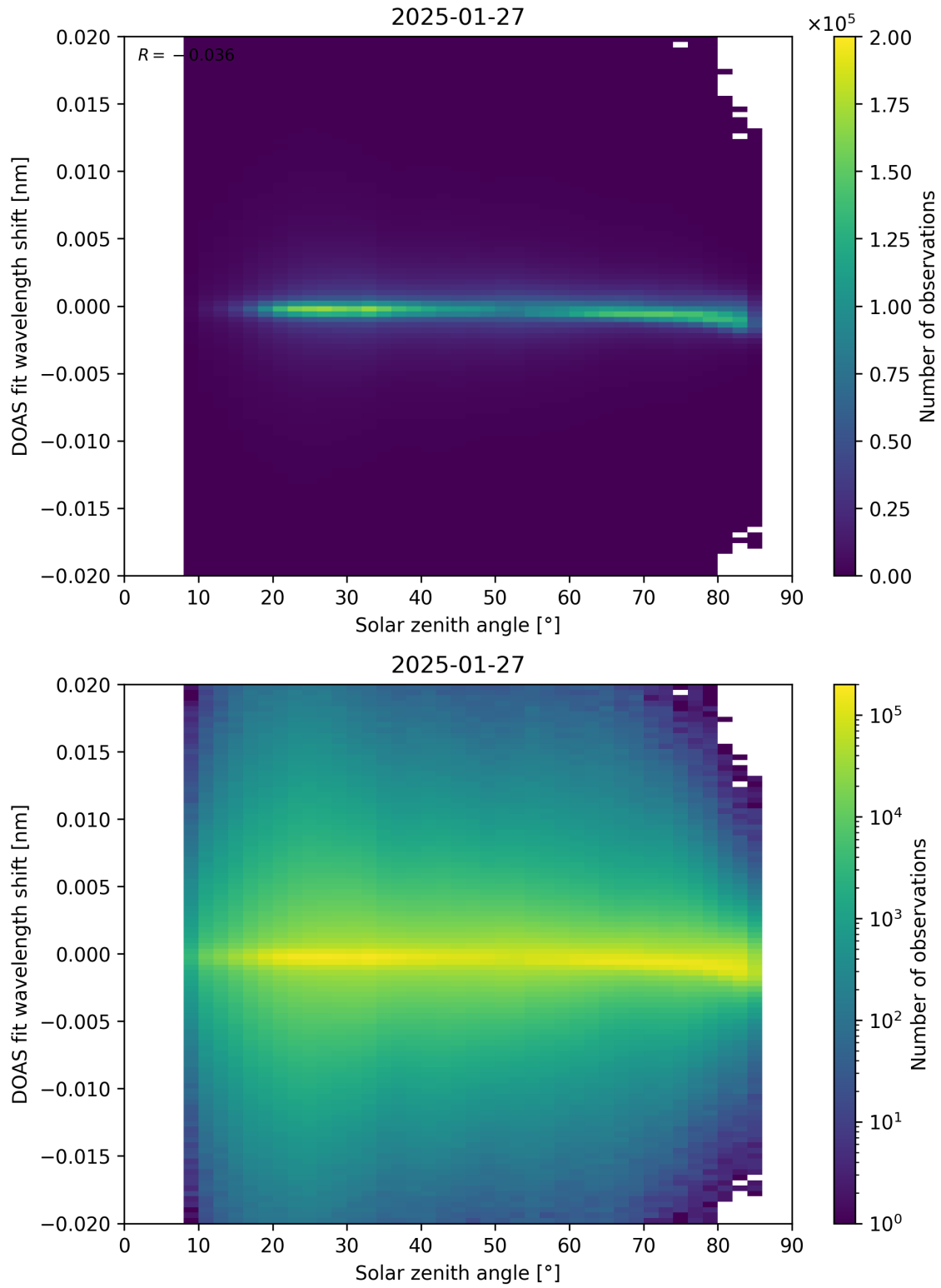
Figure 168: Scatter density plot of “Solar zenith angle” against “DOAS fit wavelength shift” for 2025-01-26 to 2025-01-28.
