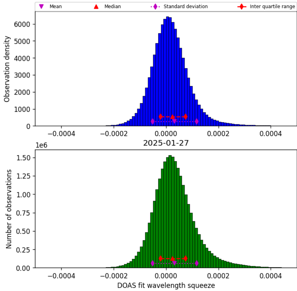
Figure 45: Histogram of “DOAS fit wavelength squeeze” for 2025-01-26 to 2025-01-28
