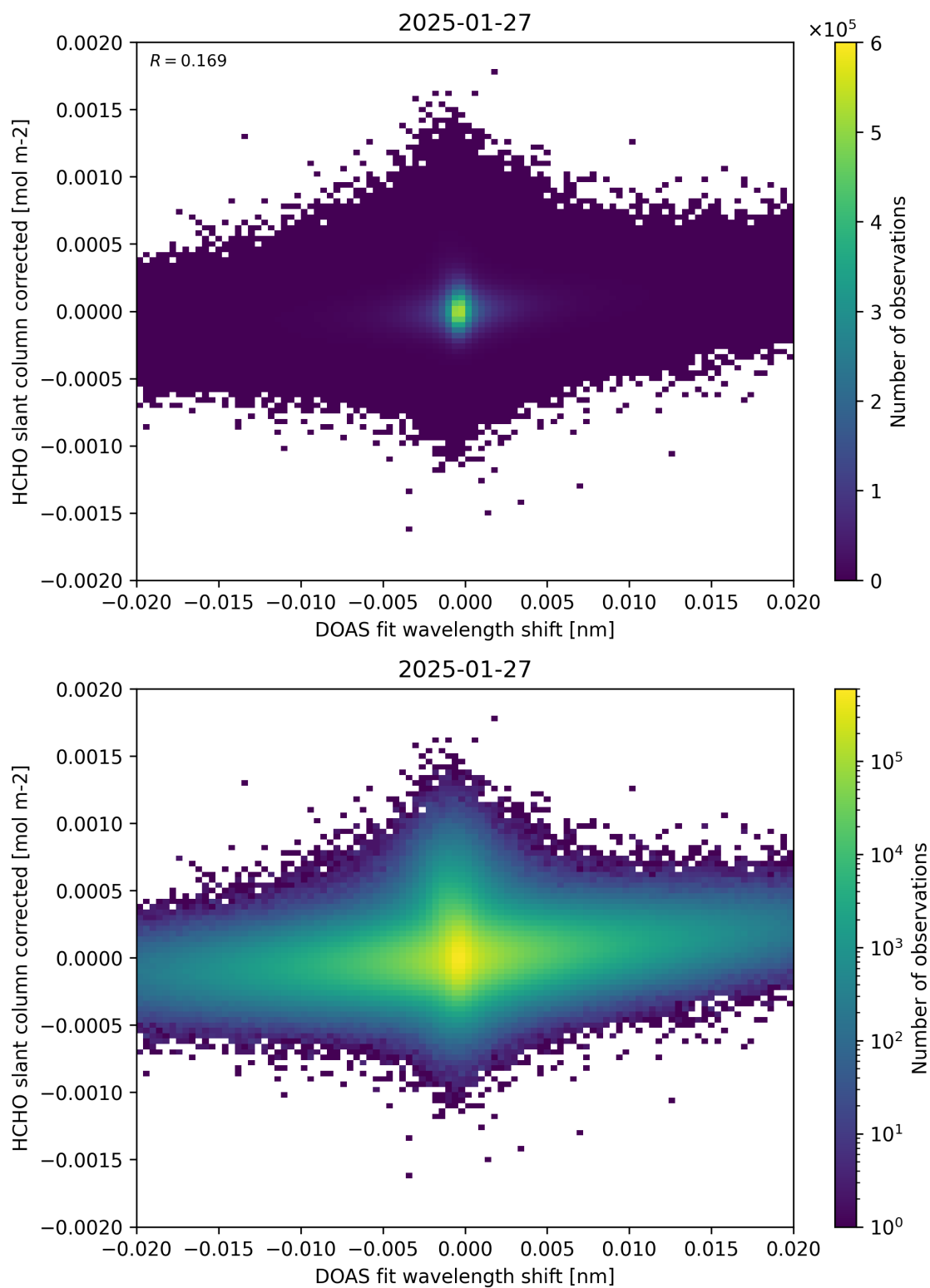
Figure 66: Scatter density plot of “DOAS fit wavelength shift” against “HCHO slant column corrected” for 2025-01-26 to 2025-01-28.
