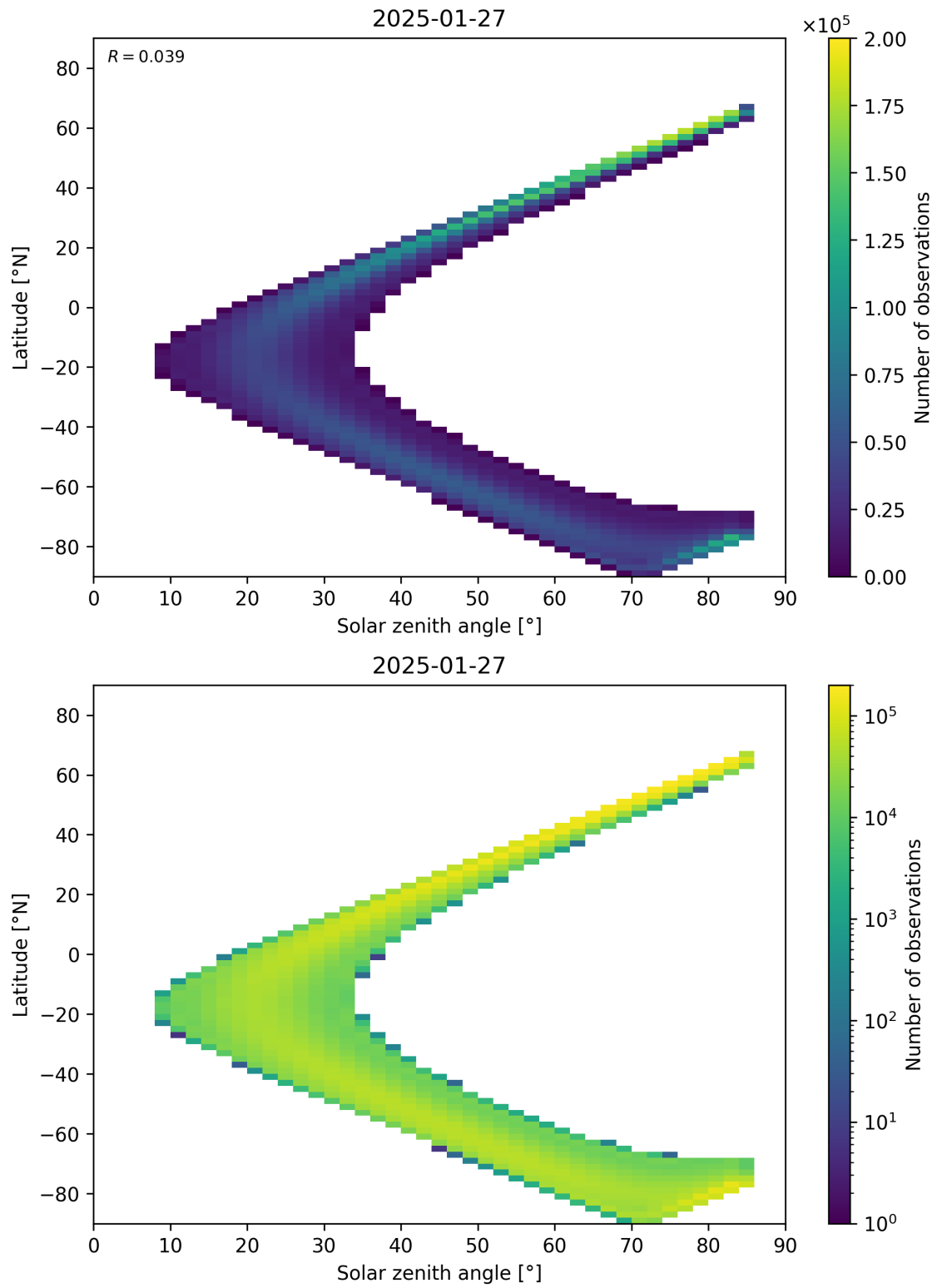
Figure 181: Scatter density plot of “Solar zenith angle” against “Latitude” for 2025-01-26 to 2025-01-28.
