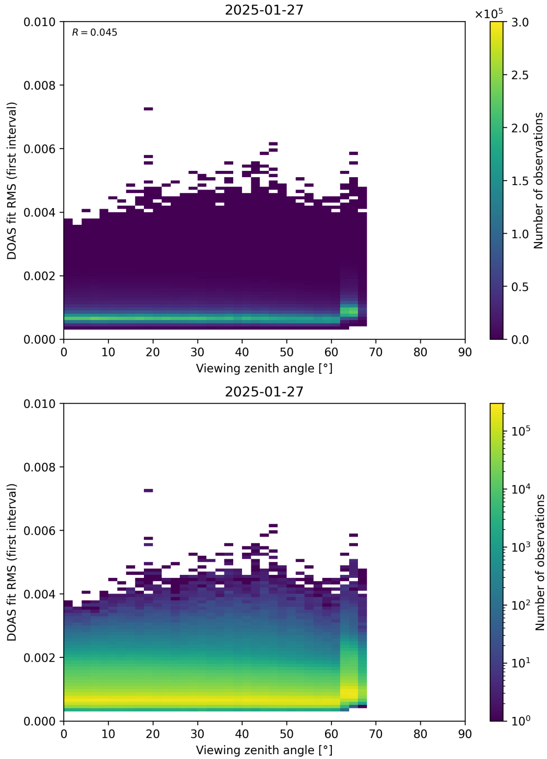
Figure 182: Scatter density plot of “Viewing zenith angle” against “DOAS fit RMS (first interval)” for 2025-01-26 to 2025-01-28.
