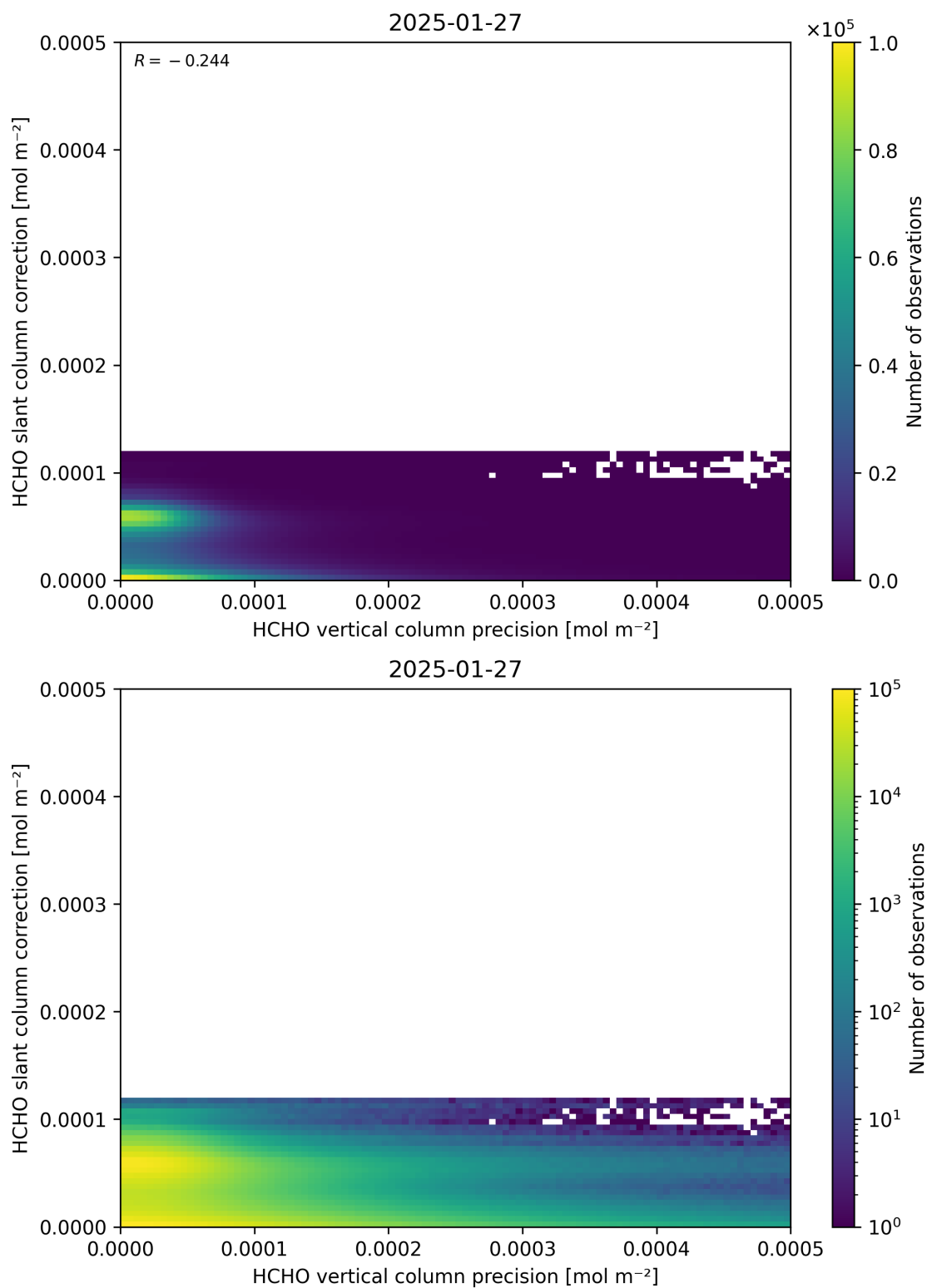
Figure 141: Scatter density plot of “HCHO vertical column precision” against “HCHO slant column correction” for 2025-01-26 to 2025-01-28.
