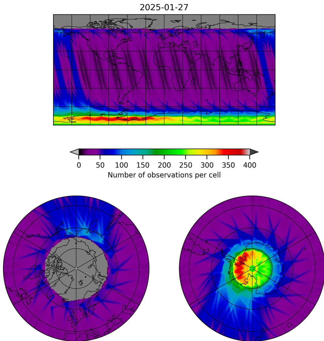
Figure 19: Map of the number of observations for 2025-01-26 to 2025-01-28
