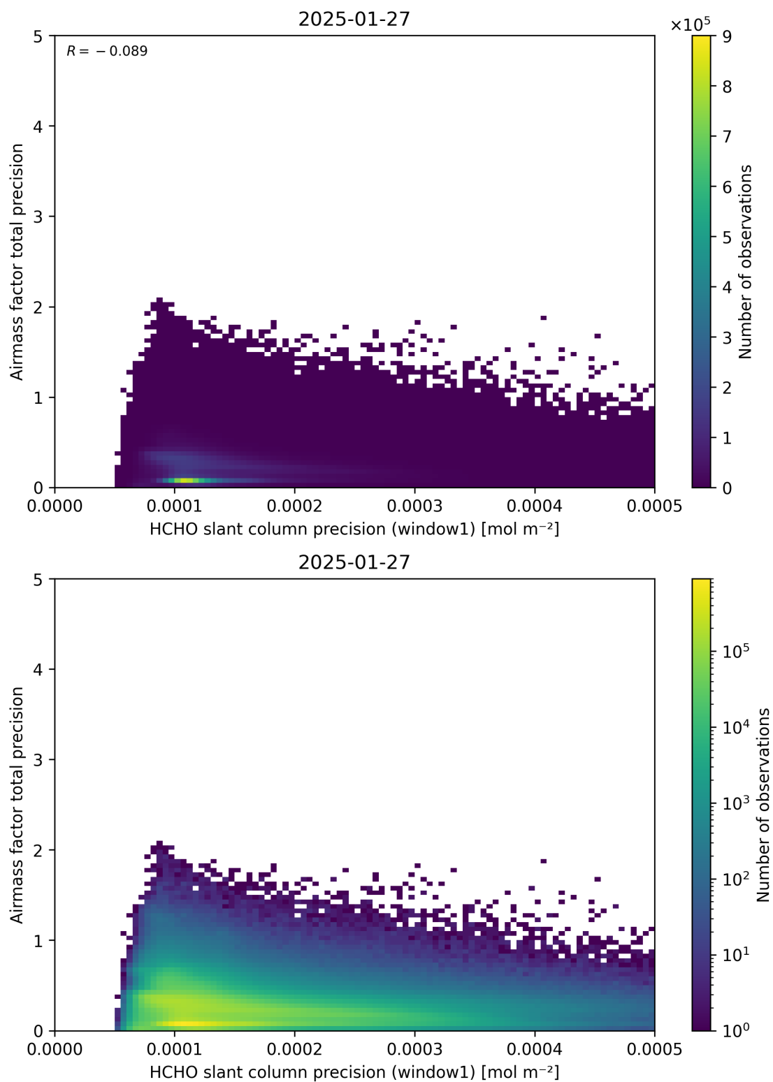
Figure 95: Scatter density plot of “HCHO slant column precision (window1)” against “Airmass factor total precision” for 2025-01-26 to 2025-01-28.
