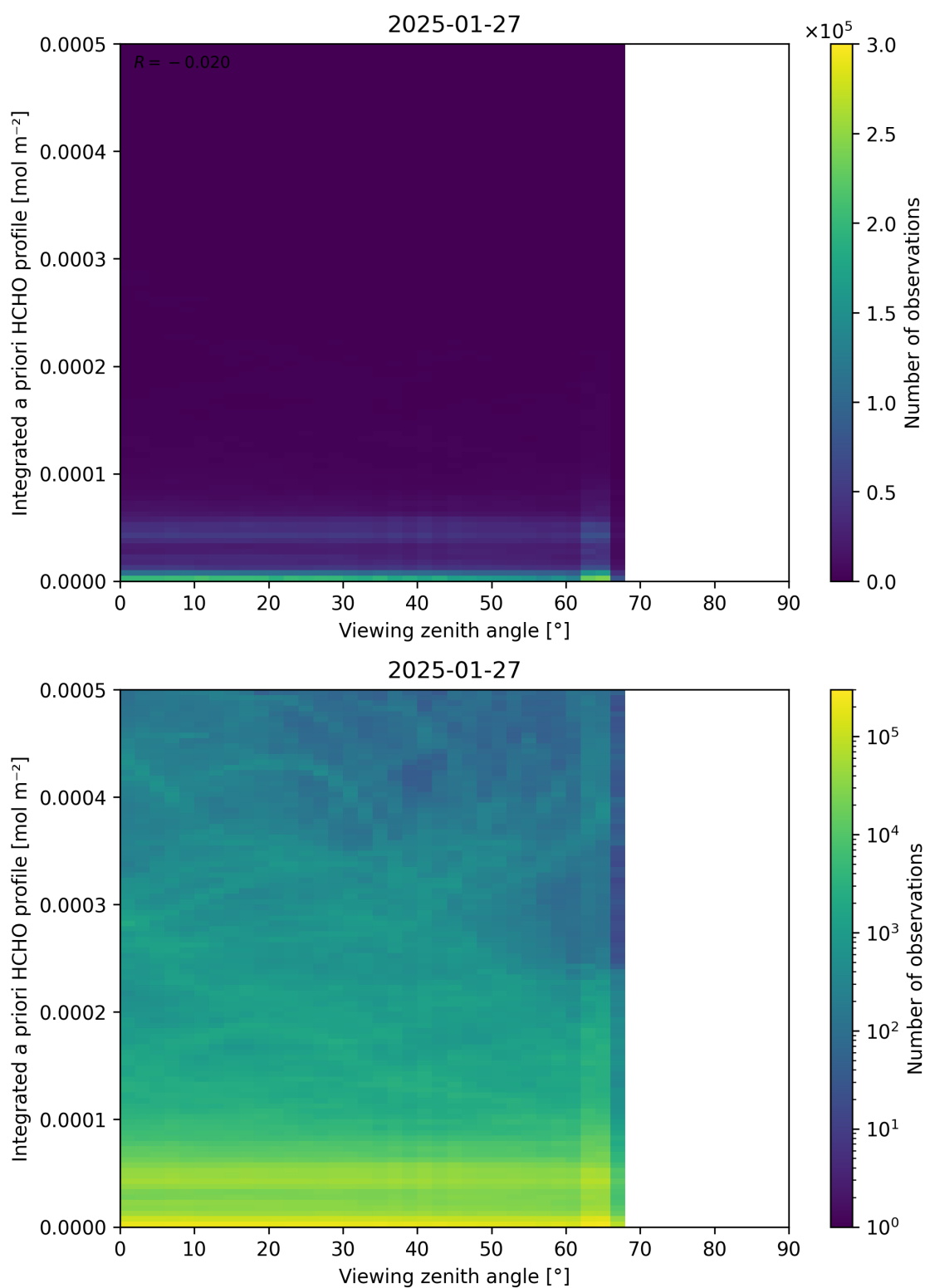
Figure 195: Scatter density plot of “Viewing zenith angle” against “Integrated a priori HCHO profile” for 2025-01-26 to 2025-01-28.
