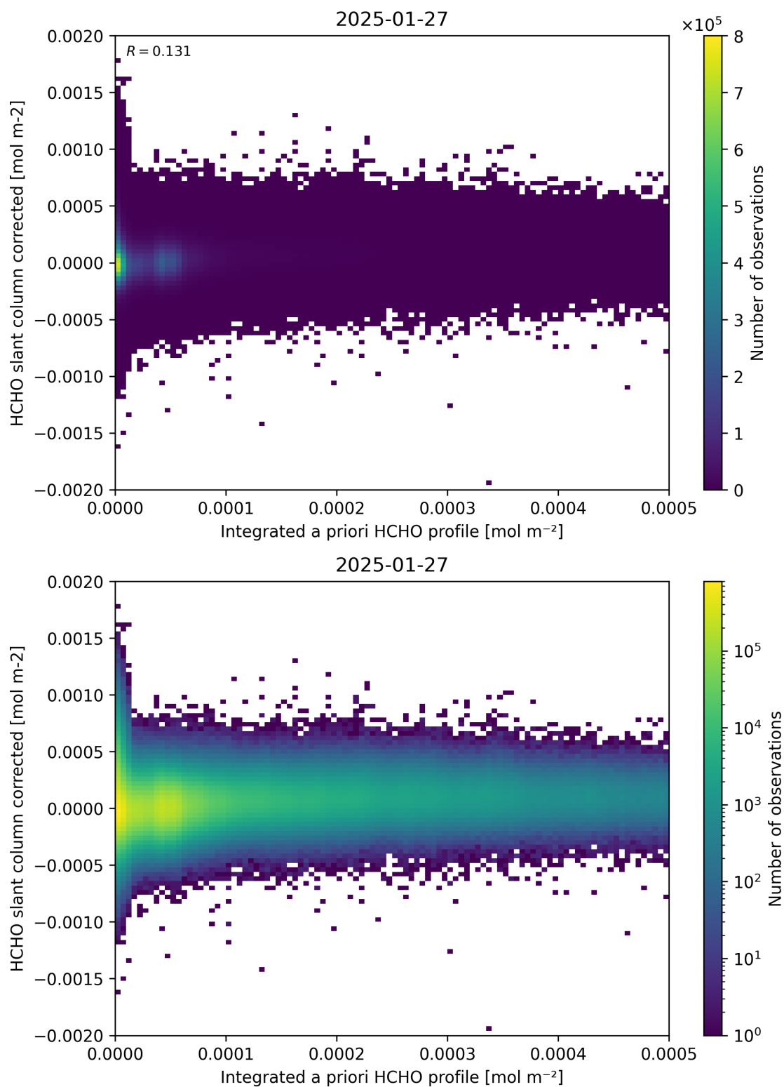
Figure 151: Scatter density plot of “Integrated a priori HCHO profile” against “HCHO slant column corrected” for 2025-01-26 to 2025-01-28.
