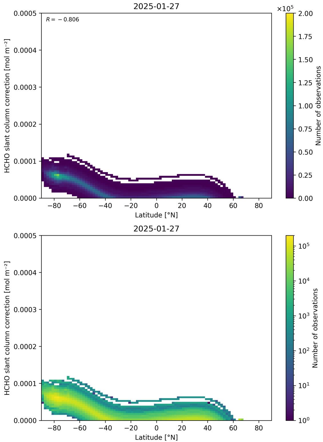
Figure 158: Scatter density plot of “Latitude” against “HCHO slant column correction” for 2025-01-26 to 2025-01-28.
