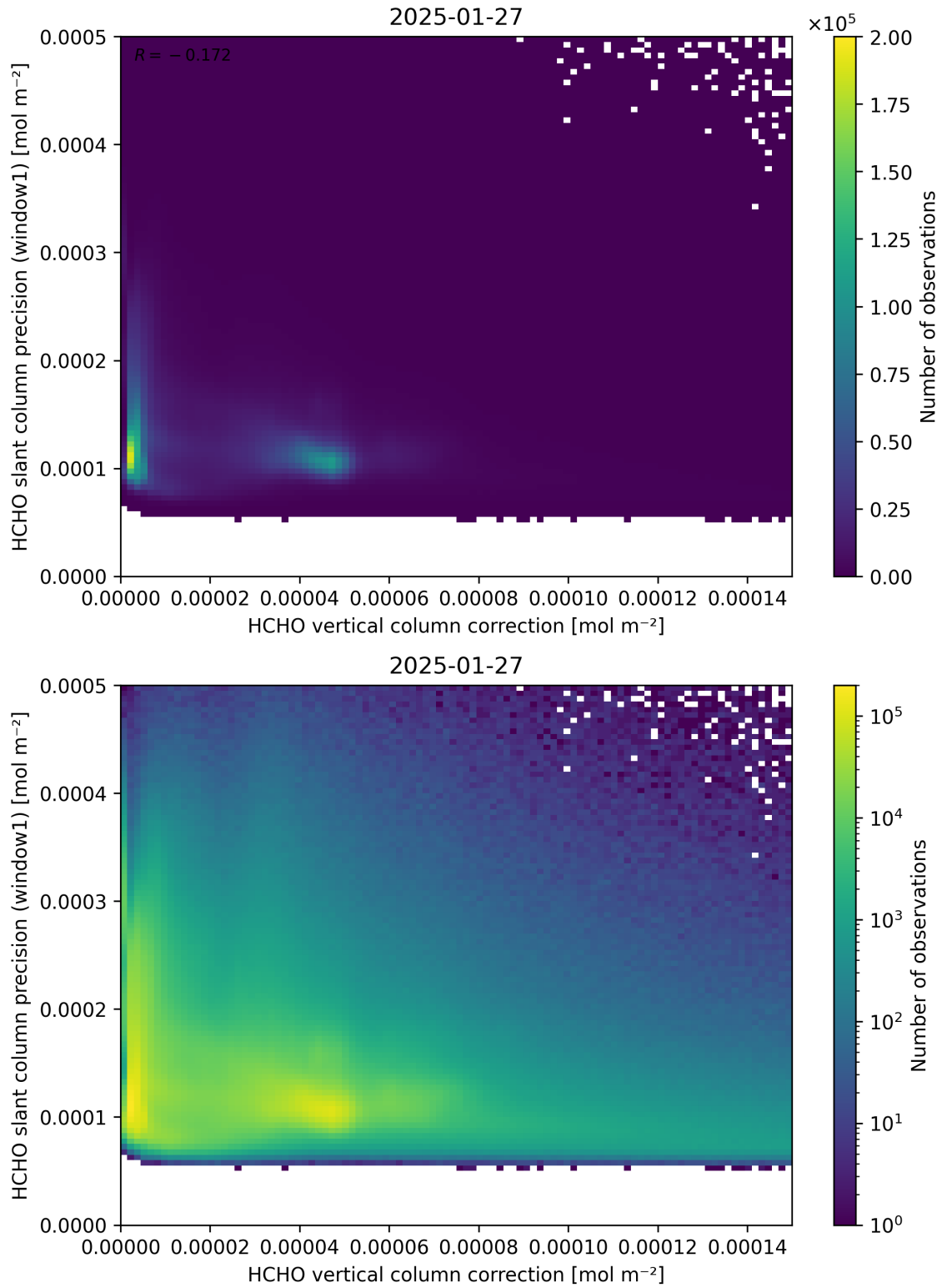
Figure 119: Scatter density plot of “HCHO vertical column correction” against “HCHO slant column precision (window1)” for 2025-01-26 to 2025-01-28.
