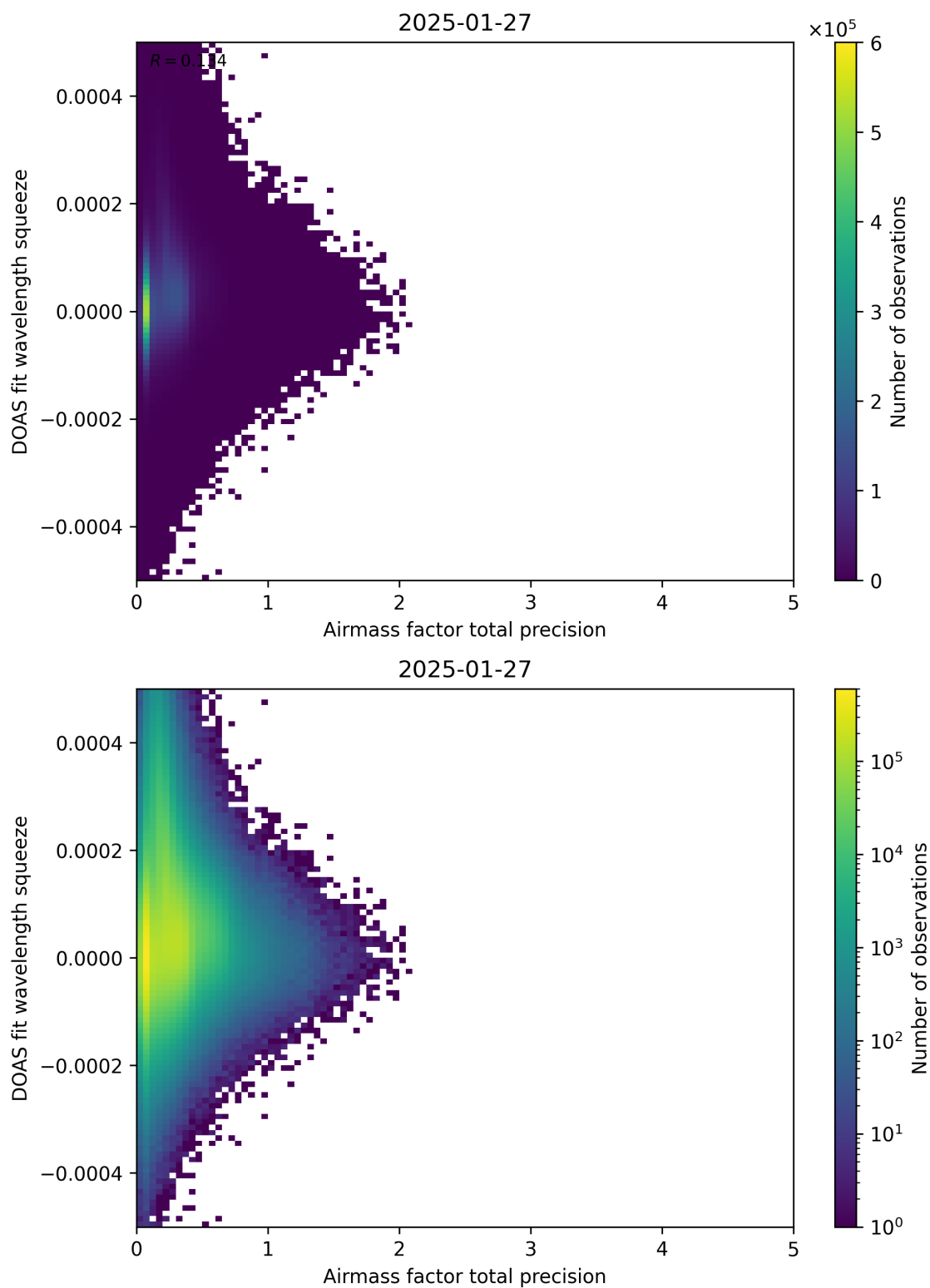
Figure 107: Scatter density plot of “Airmass factor total precision” against “DOAS fit wavelength squeeze” for 2025-01-26 to 2025-01-28.
