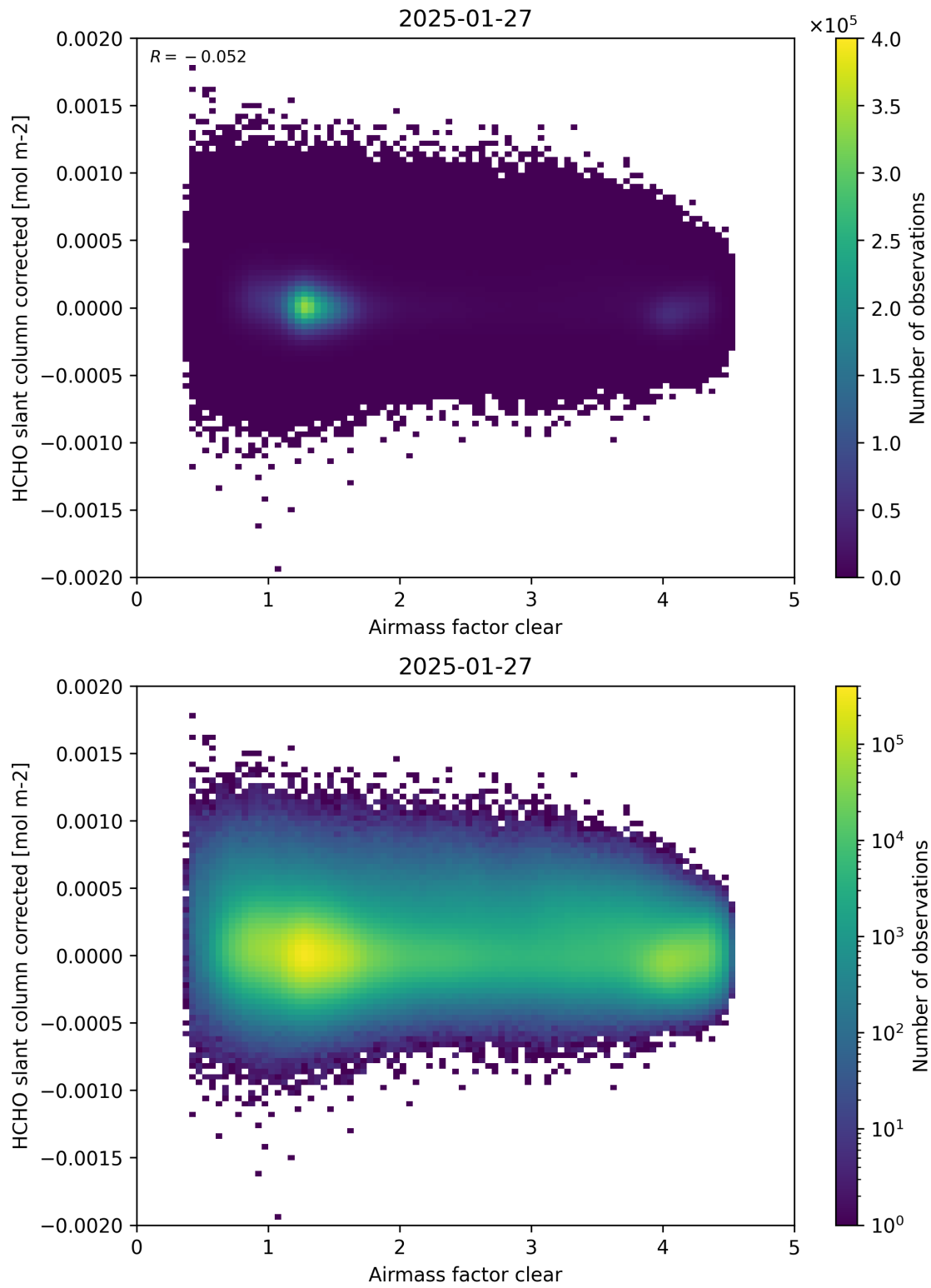
Figure 74: Scatter density plot of “Airmass factor clear” against “HCHO slant column corrected” for 2025-01-26 to 2025-01-28.
