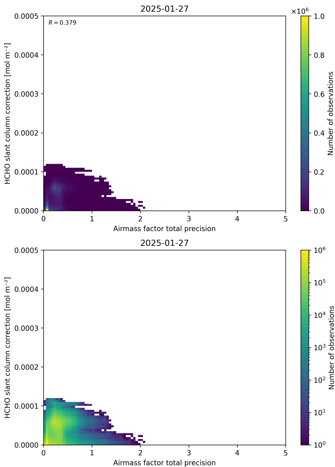
Figure 110: Scatter density plot of “Airmass factor total precision” against “HCHO slant column correction” for 2025-01-26 to 2025-01-28.
