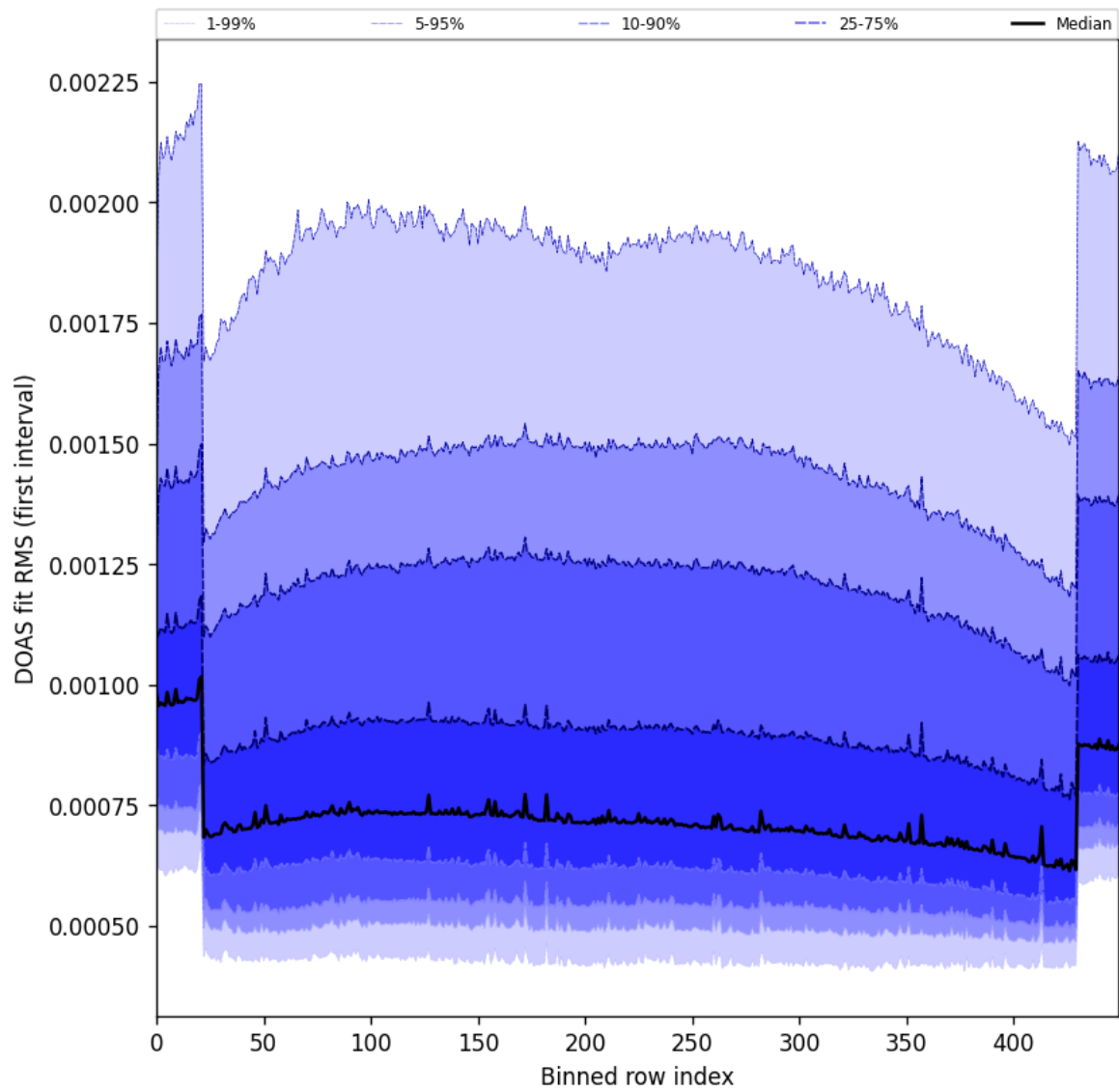
Figure 60: Along track statistics of “DOAS fit RMS (first interval)” for 2025-01-26 to 2025-01-28
