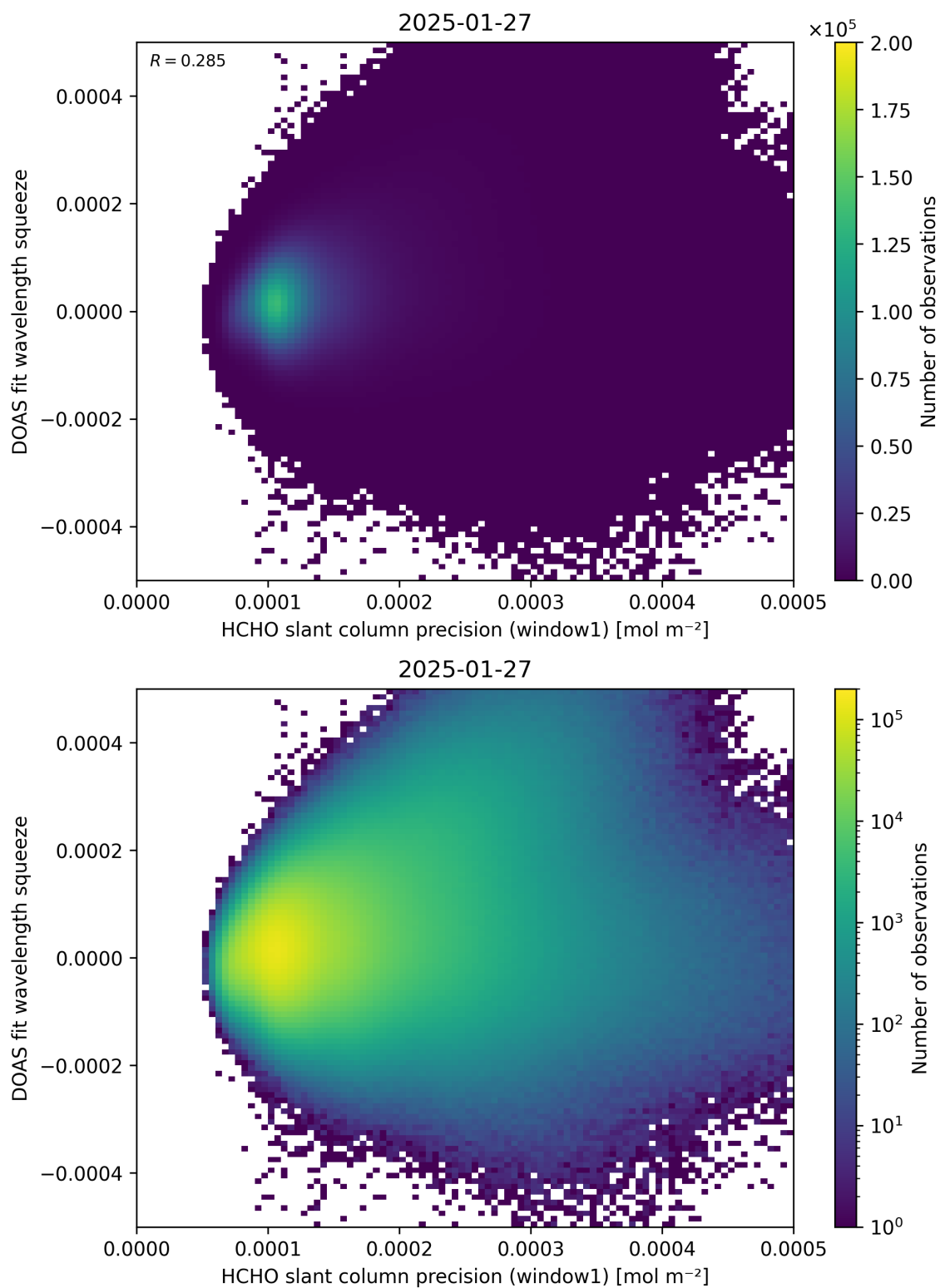
Figure 90: Scatter density plot of “HCHO slant column precision (window1)” against “DOAS fit wavelength squeeze” for 2025-01-26 to 2025-01-28.
