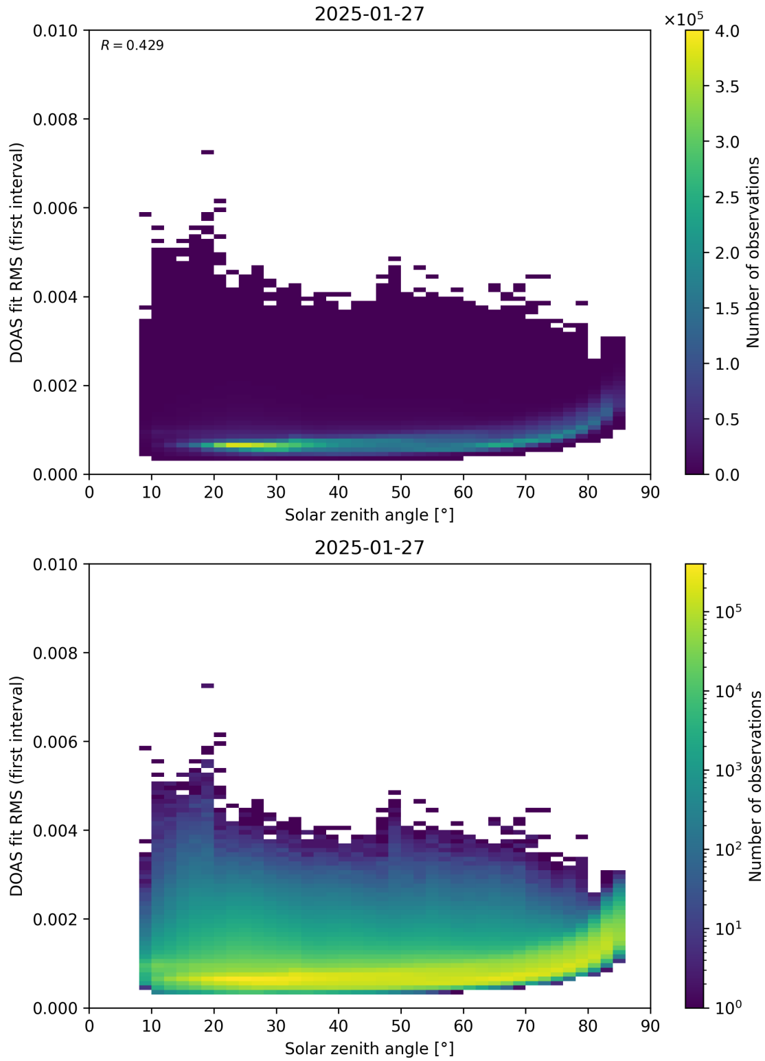
Figure 167: Scatter density plot of “Solar zenith angle” against “DOAS fit RMS (first interval)” for 2025-01-26 to 2025-01-28.
