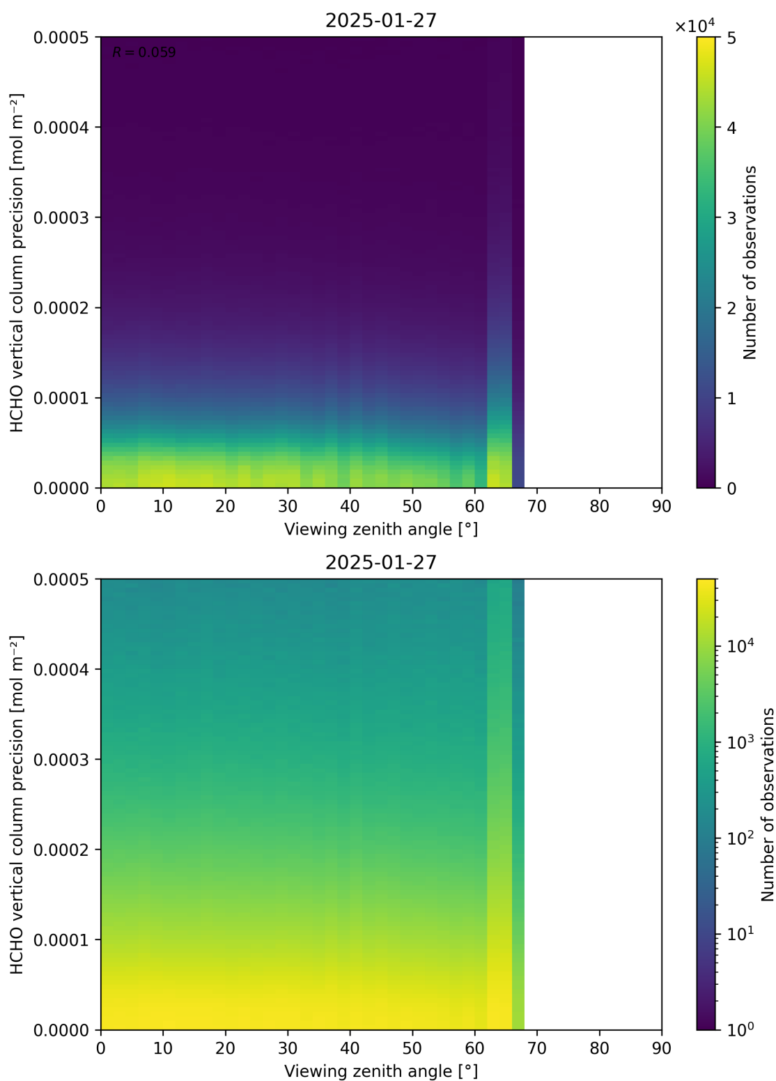
Figure 194: Scatter density plot of “Viewing zenith angle” against “HCHO vertical column precision” for 2025-01-26 to 2025-01-28.
