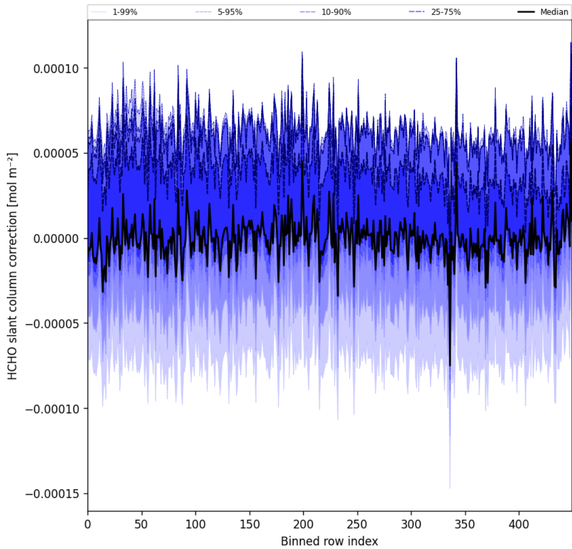
Figure 61: Along track statistics of “HCHO slant column correction” for 2025-01-26 to 2025-01-28
