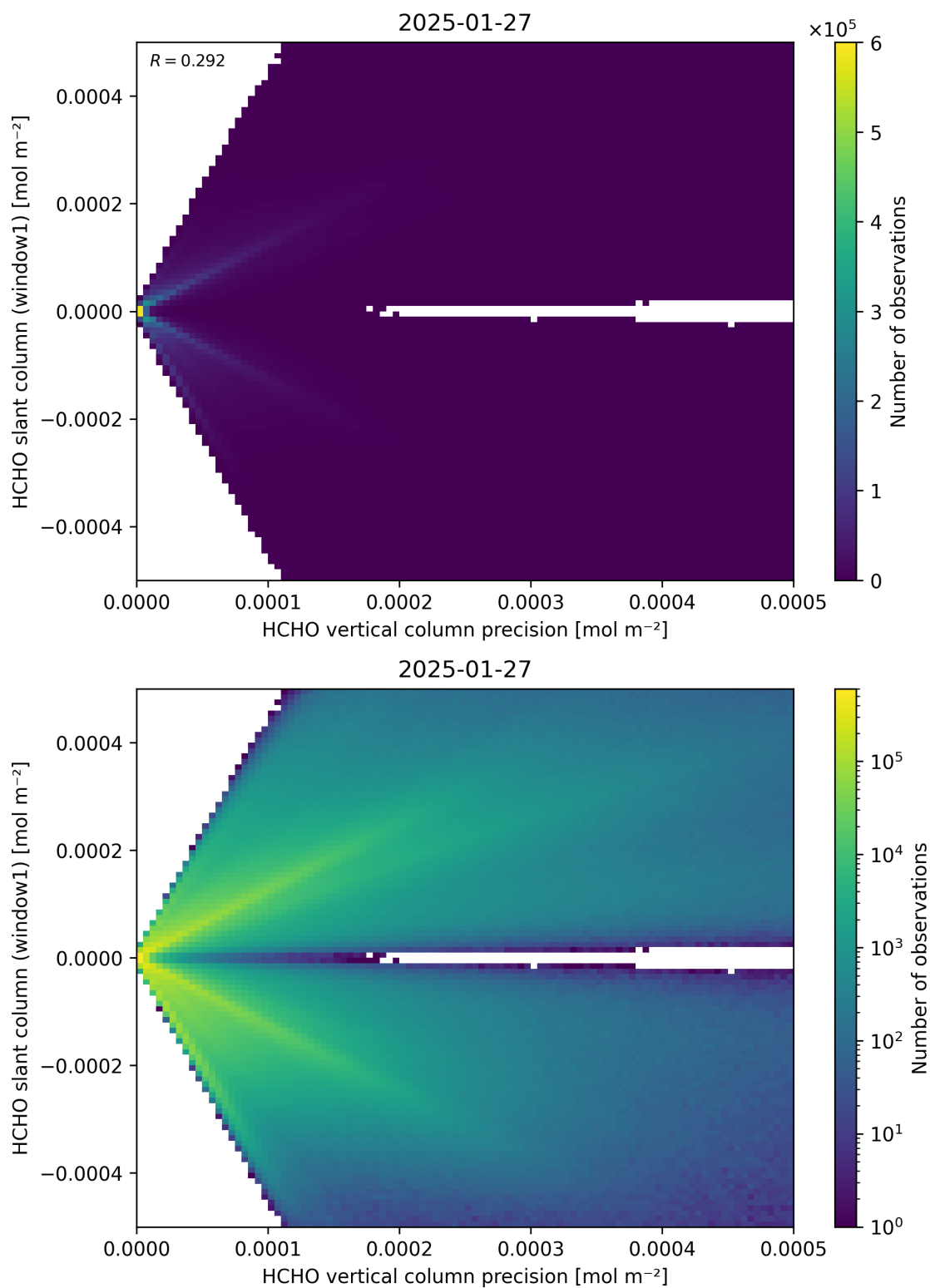
Figure 142: Scatter density plot of “HCHO vertical column precision” against “HCHO slant column (window1)” for 2025-01-26 to 2025-01-28.
