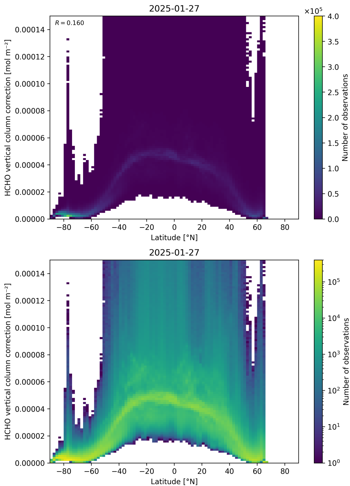
Figure 164: Scatter density plot of “Latitude” against “HCHO vertical column correction” for 2025-01-26 to 2025-01-28.
