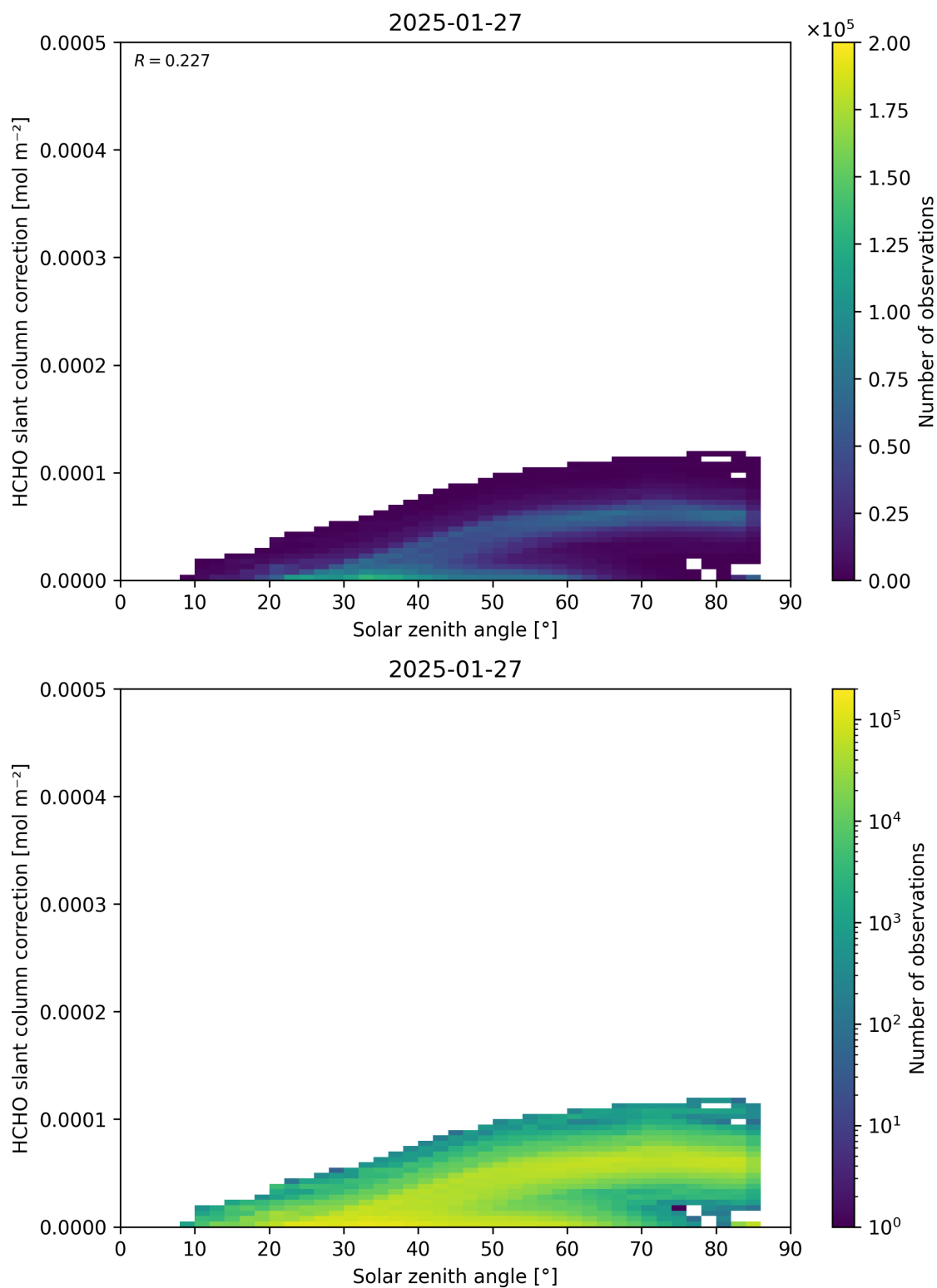
Figure 172: Scatter density plot of “Solar zenith angle” against “HCHO slant column correction” for 2025-01-26 to 2025-01-28.
