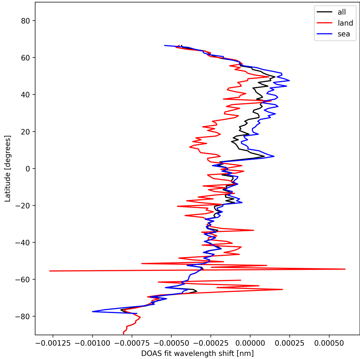
Figure 30: Zonal average of “DOAS fit wavelength shift” for 2025-01-26 to 2025-01-28.
