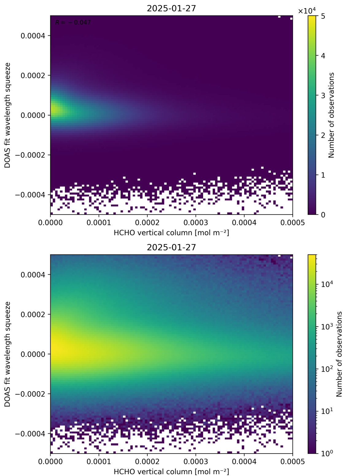
Figure 125: Scatter density plot of “HCHO vertical column” against “DOAS fit wavelength squeeze” for 2025-01-26 to 2025-01-28.
