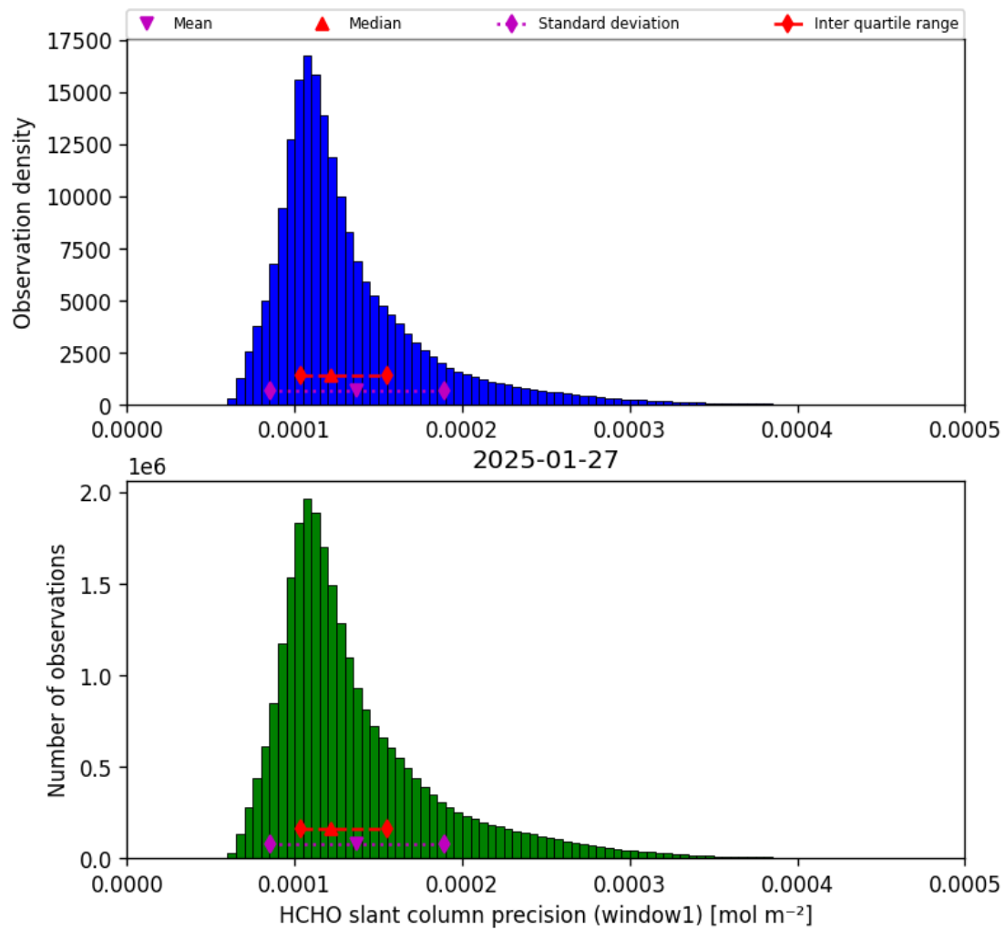
Figure 39: Histogram of “HCHO slant column precision (window1)” for 2025-01-26 to 2025-01-28
