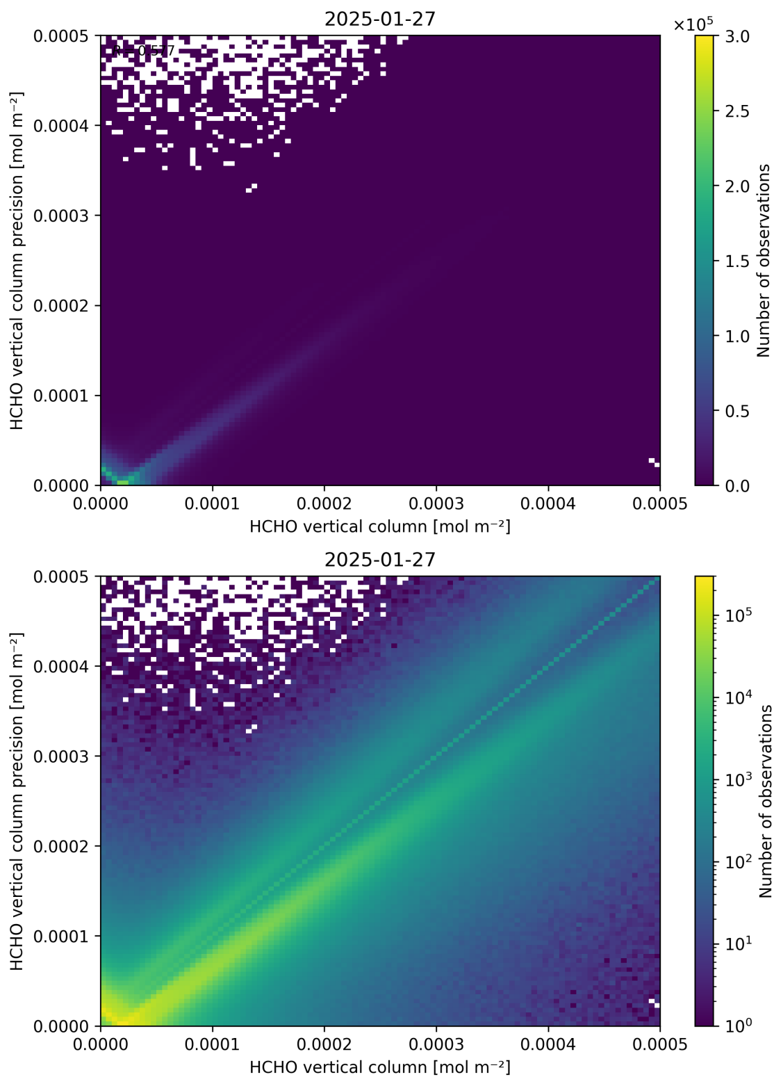
Figure 134: Scatter density plot of “HCHO vertical column” against “HCHO vertical column precision” for 2025-01-26 to 2025-01-28.
