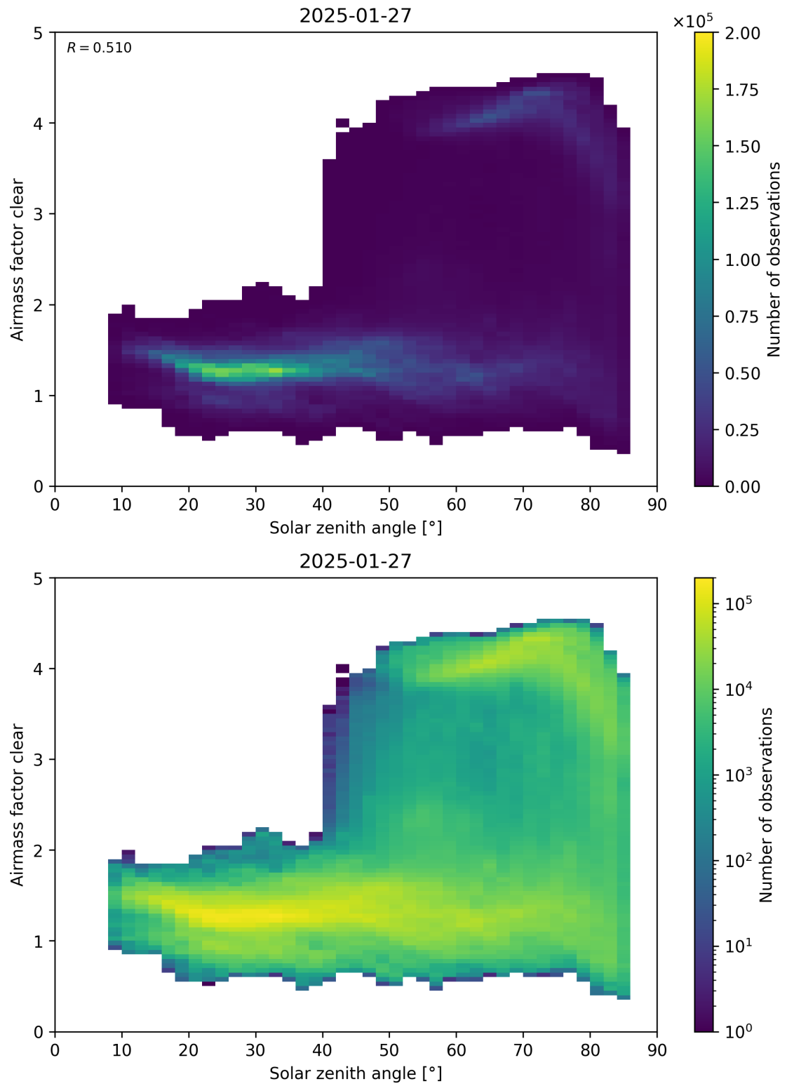
Figure 170: Scatter density plot of “Solar zenith angle” against “Airmass factor clear” for 2025-01-26 to 2025-01-28.
