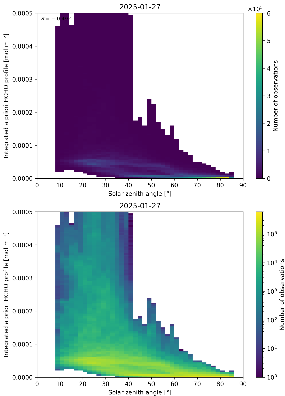
Figure 180: Scatter density plot of “Solar zenith angle” against “Integrated a priori HCHO profile” for 2025-01-26 to 2025-01-28.
