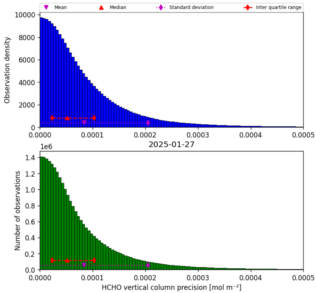
Figure 36: Histogram of “HCHO vertical column precision” for 2025-01-26 to 2025-01-28
