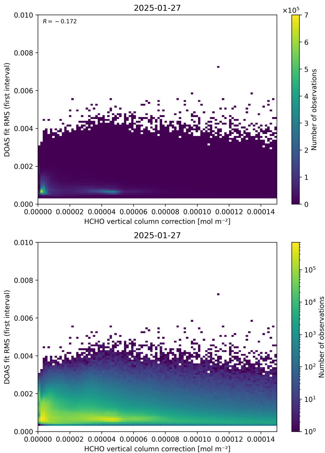
Figure 112: Scatter density plot of “HCHO vertical column correction” against “DOAS fit RMS (first interval)” for 2025-01-26 to 2025-01-28.
