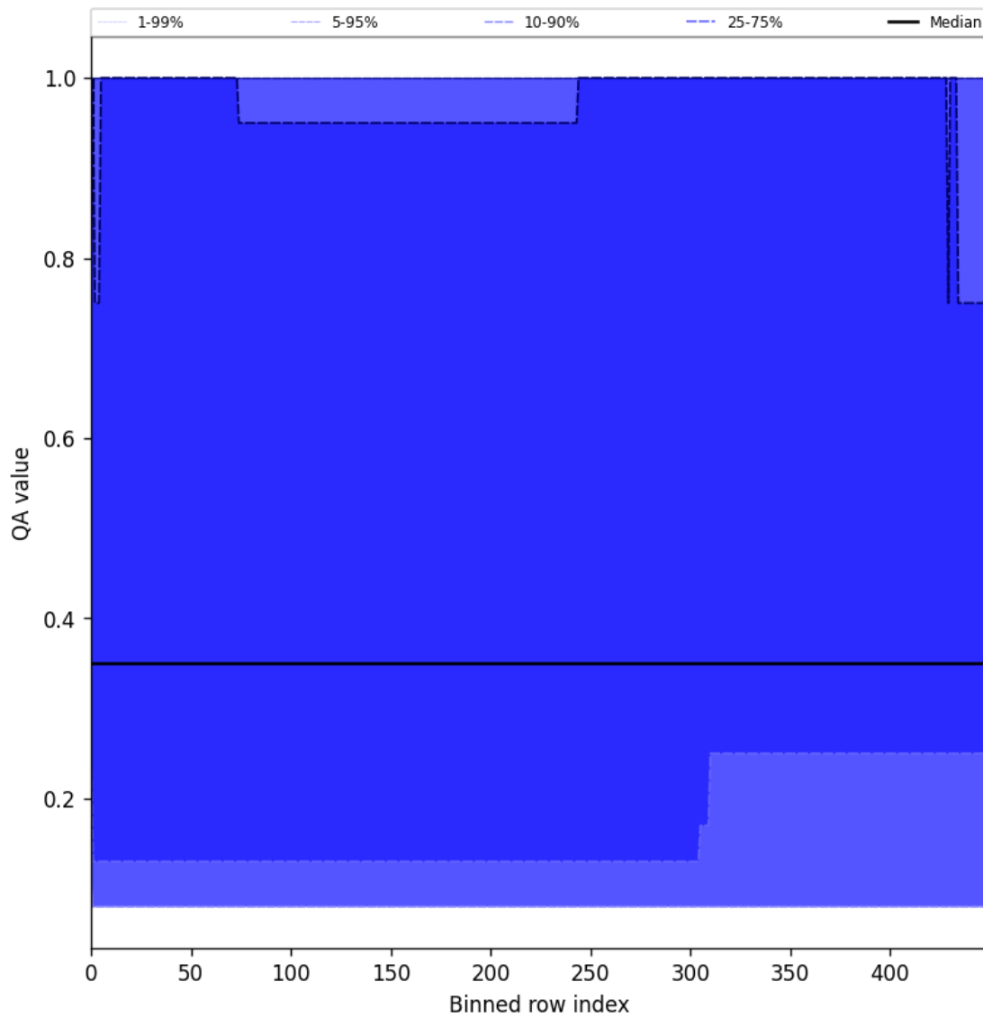
Figure 48: Along track statistics of “QA value” for 2025-01-26 to 2025-01-28
