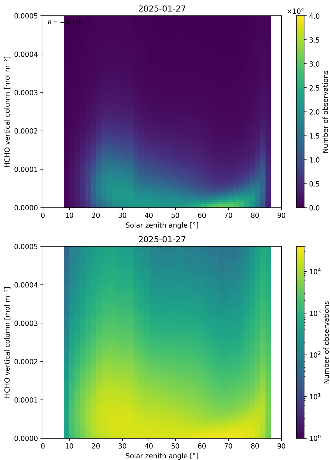
Figure 177: Scatter density plot of “Solar zenith angle” against “HCHO vertical column” for 2025-01-26 to 2025-01-28.
