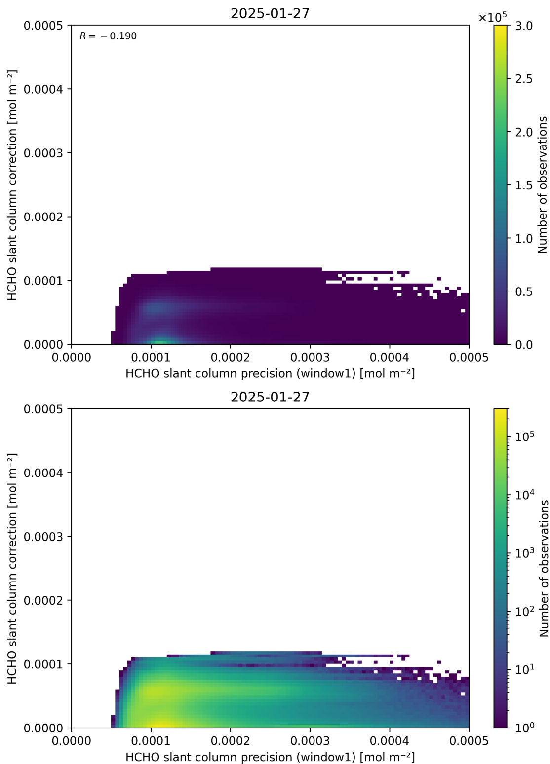
Figure 93: Scatter density plot of “HCHO slant column precision (window1)” against “HCHO slant column correction” for 2025-01-26 to 2025-01-28.
