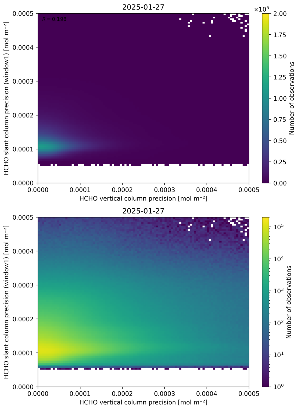
Figure 143: Scatter density plot of “HCHO vertical column precision” against “HCHO slant column precision (window1)” for 2025-01-26 to 2025-01-28.
