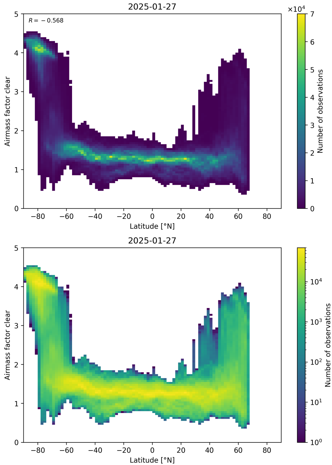
Figure 156: Scatter density plot of “Latitude” against “Airmass factor clear” for 2025-01-26 to 2025-01-28.
