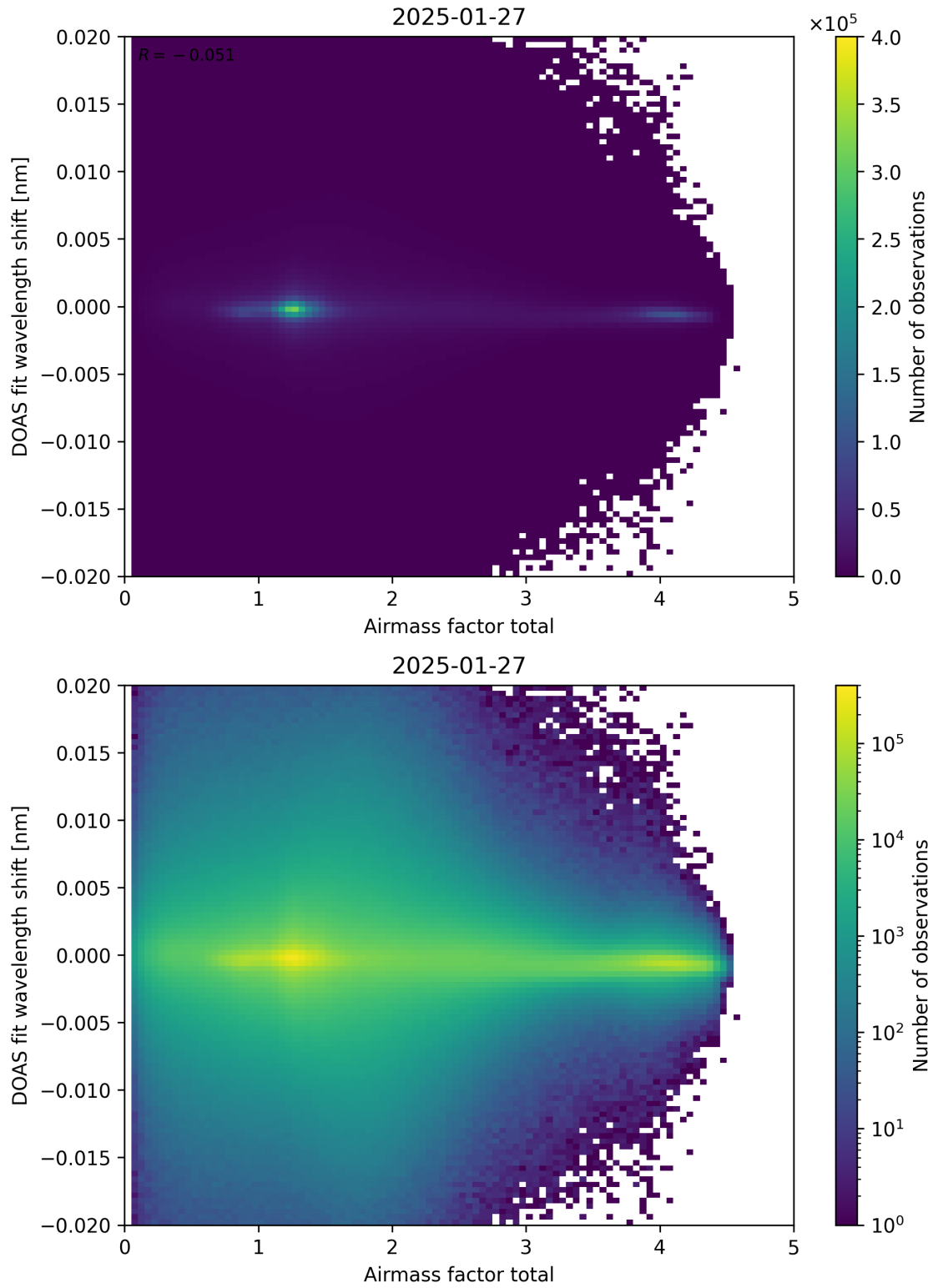
Figure 98: Scatter density plot of “Airmass factor total” against “DOAS fit wavelength shift” for 2025-01-26 to 2025-01-28.
