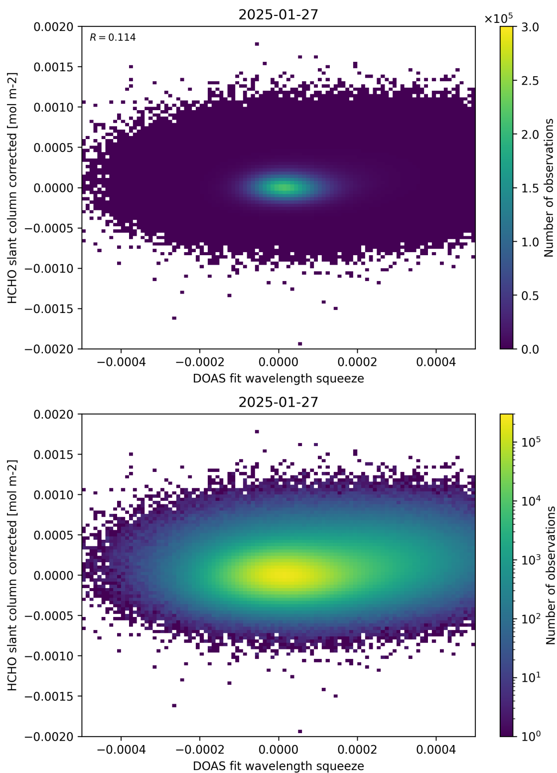
Figure 69: Scatter density plot of “DOAS fit wavelength squeeze” against “HCHO slant column corrected” for 2025-01-26 to 2025-01-28.
