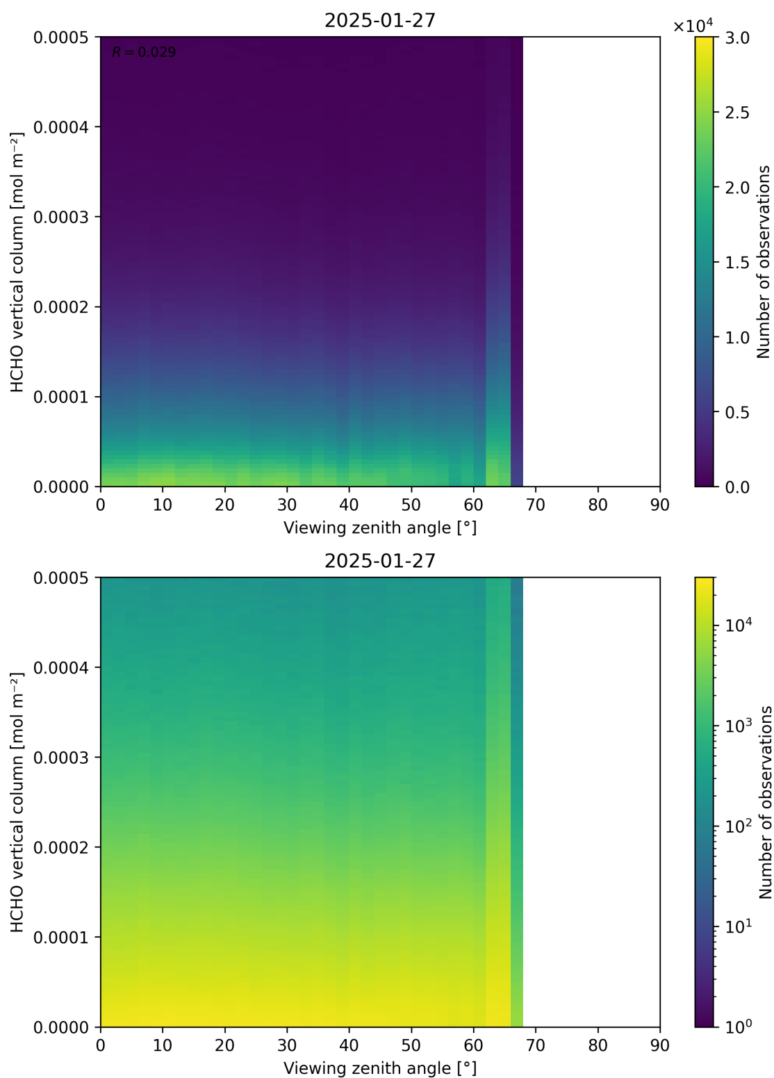
Figure 192: Scatter density plot of “Viewing zenith angle” against “HCHO vertical column” for 2025-01-26 to 2025-01-28.
