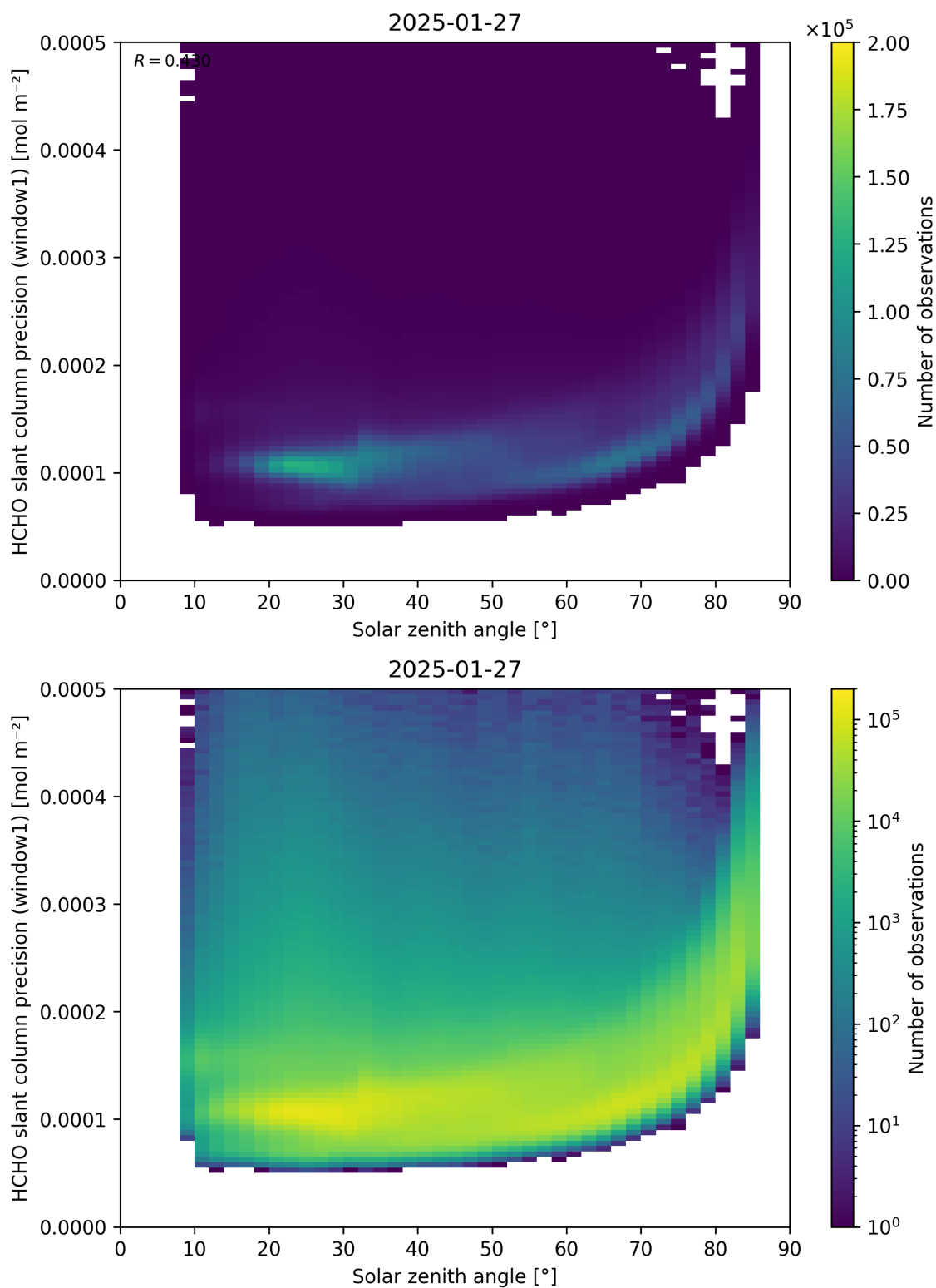
Figure 174: Scatter density plot of “Solar zenith angle” against “HCHO slant column precision (window1)” for 2025-01-26 to 2025-01-28.
