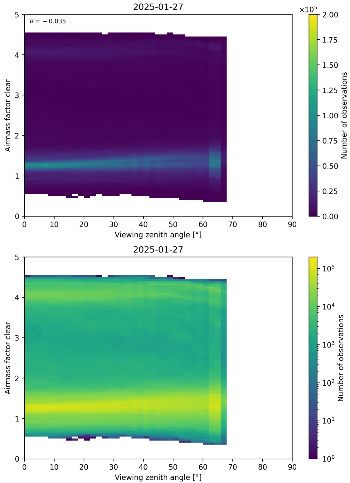
Figure 185: Scatter density plot of “Viewing zenith angle” against “Airmass factor clear” for 2025-01-26 to 2025-01-28.
