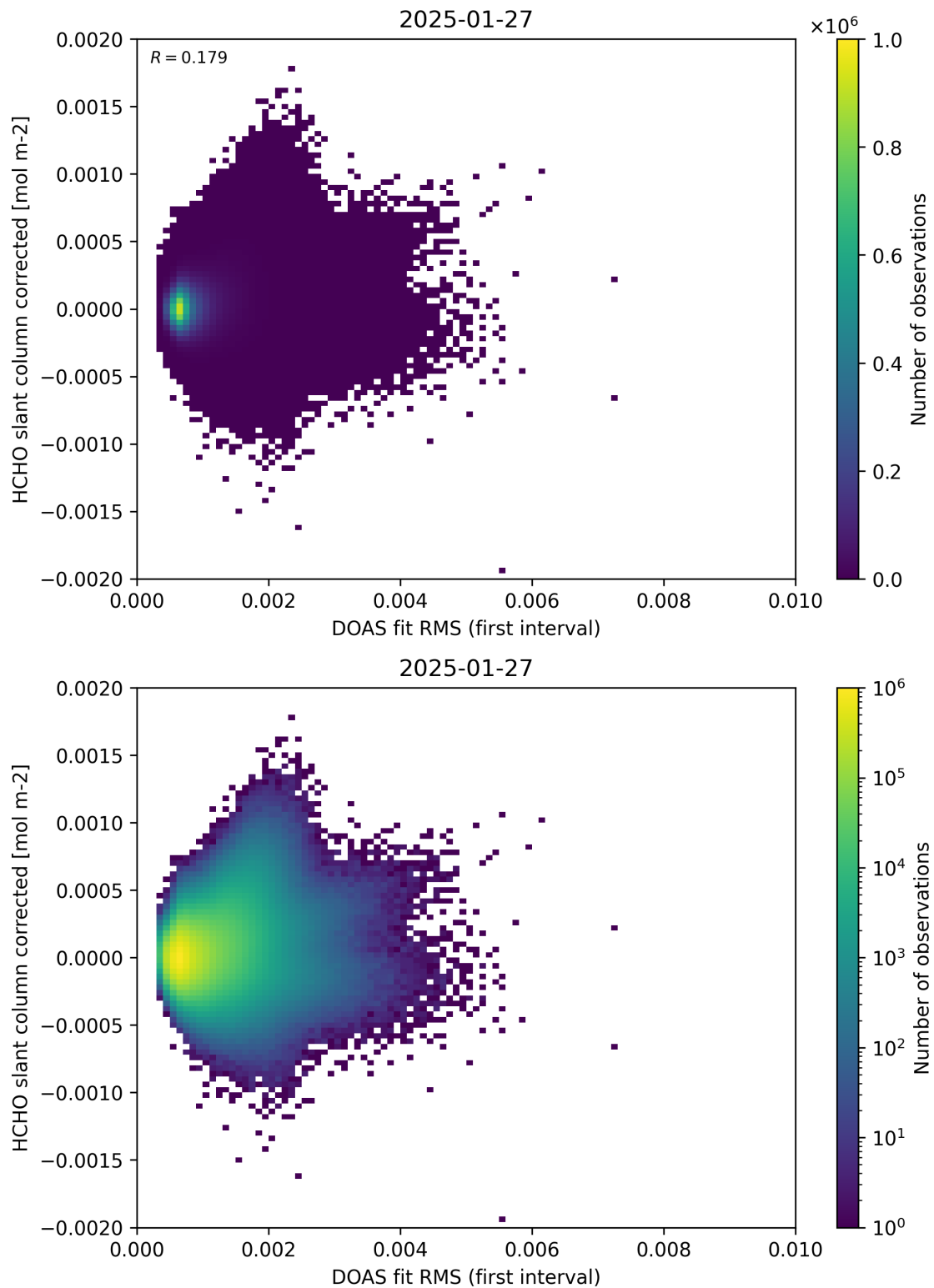
Figure 62: Scatter density plot of “DOAS fit RMS (first interval)” against “HCHO slant column corrected” for 2025-01-26 to 2025-01-28.
