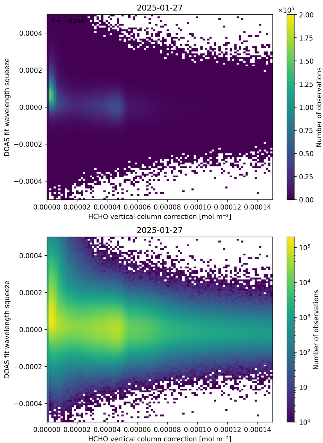
Figure 114: Scatter density plot of “HCHO vertical column correction” against “DOAS fit wavelength squeeze” for 2025-01-26 to 2025-01-28.
