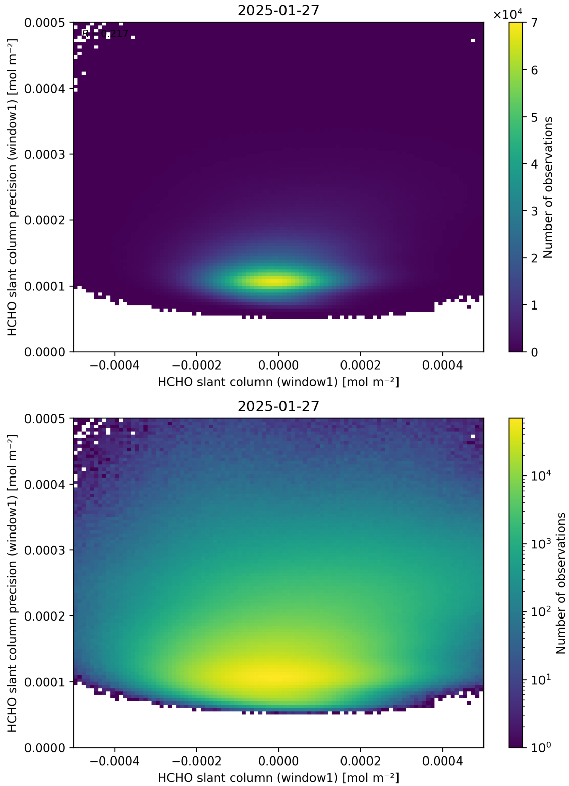
Figure 84: Scatter density plot of “HCHO slant column (window1)” against “HCHO slant column precision (window1)” for 2025-01-26 to 2025-01-28.
