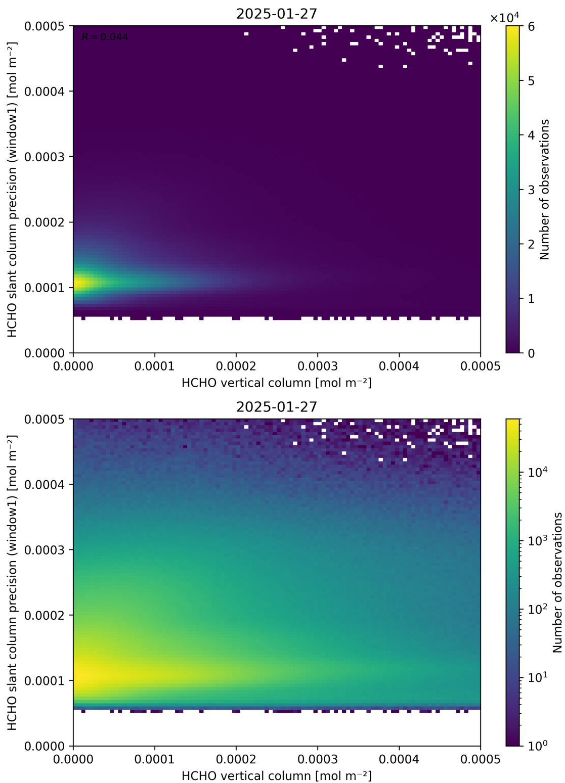
Figure 130: Scatter density plot of “HCHO vertical column” against “HCHO slant column precision (window1)” for 2025-01-26 to 2025-01-28.
