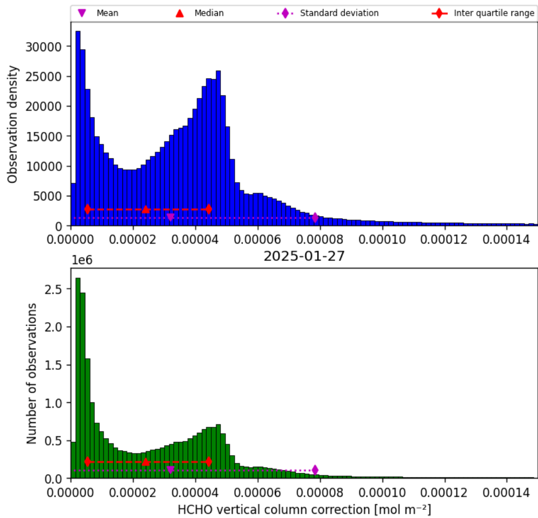
Figure 37: Histogram of “HCHO vertical column correction” for 2025-01-26 to 2025-01-28
