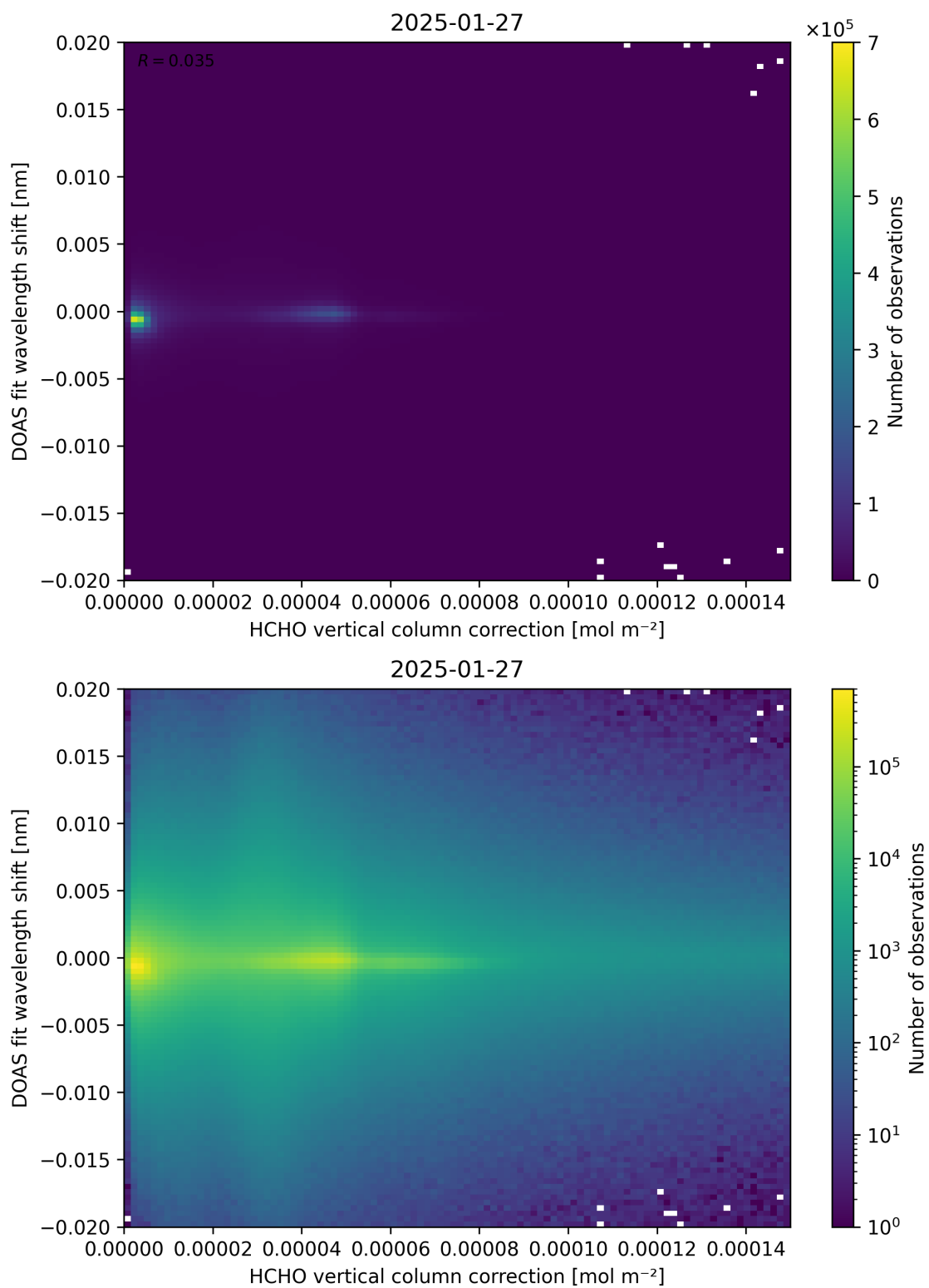
Figure 113: Scatter density plot of “HCHO vertical column correction” against “DOAS fit wavelength shift” for 2025-01-26 to 2025-01-28.
