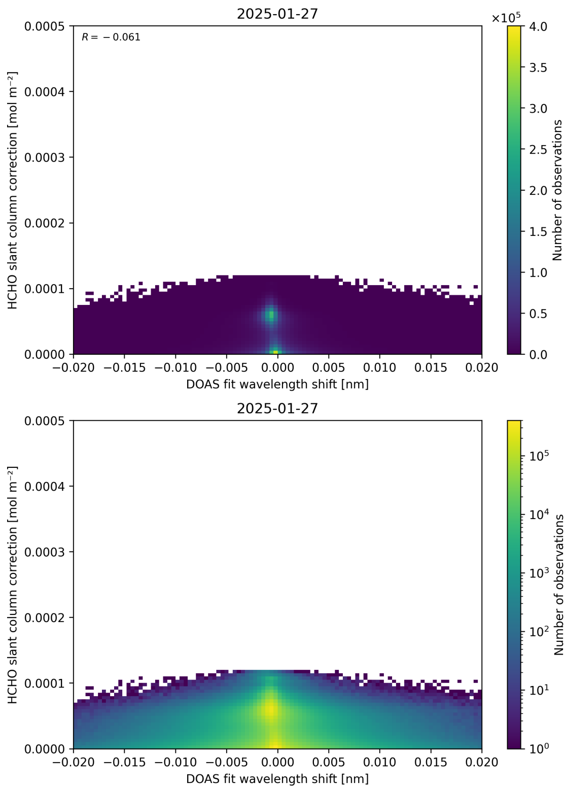
Figure 67: Scatter density plot of “DOAS fit wavelength shift” against “HCHO slant column correction” for 2025-01-26 to 2025-01-28.
