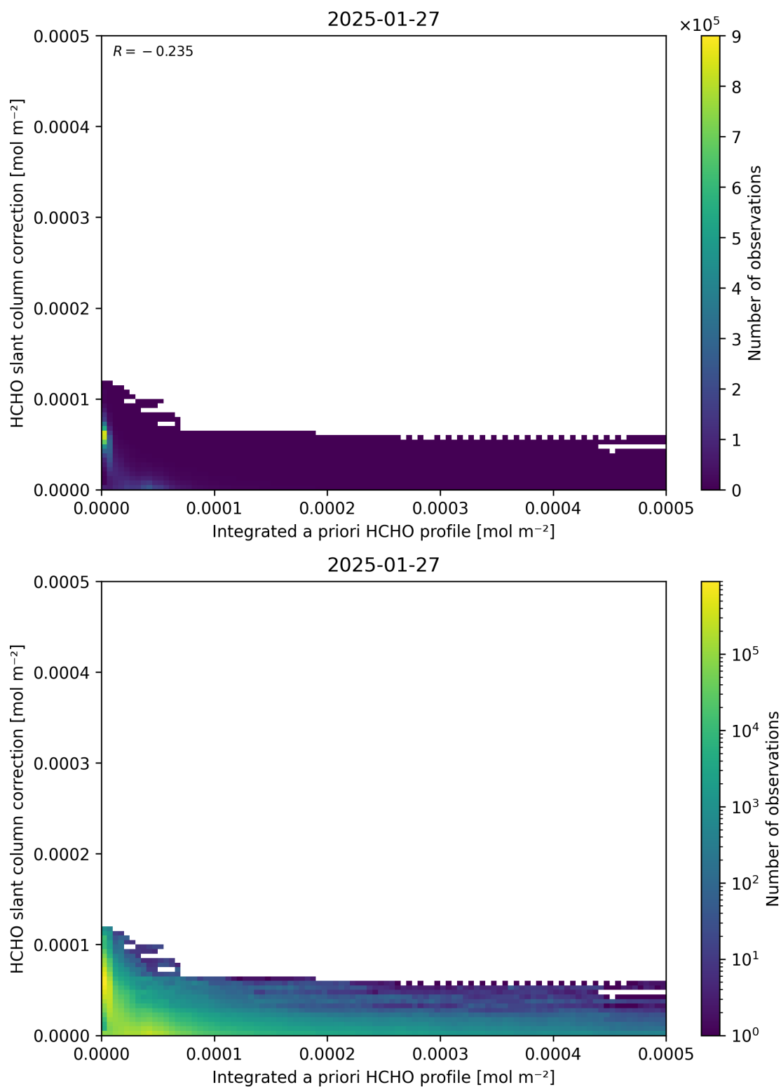
Figure 152: Scatter density plot of “Integrated a priori HCHO profile” against “HCHO slant column correction” for 2025-01-26 to 2025-01-28.
