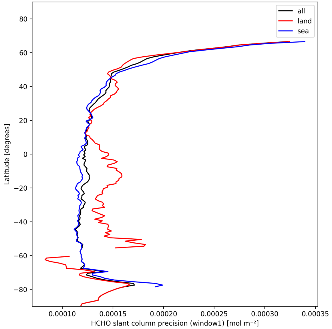
Figure 25: Zonal average of “HCHO slant column precision (window1)” for 2025-01-26 to 2025-01-28.
