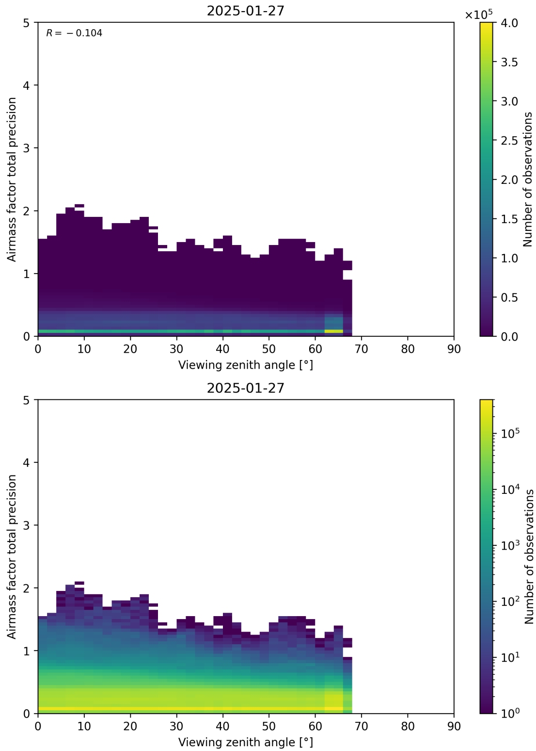
Figure 191: Scatter density plot of “Viewing zenith angle” against “Airmass factor total precision” for 2025-01-26 to 2025-01-28.
