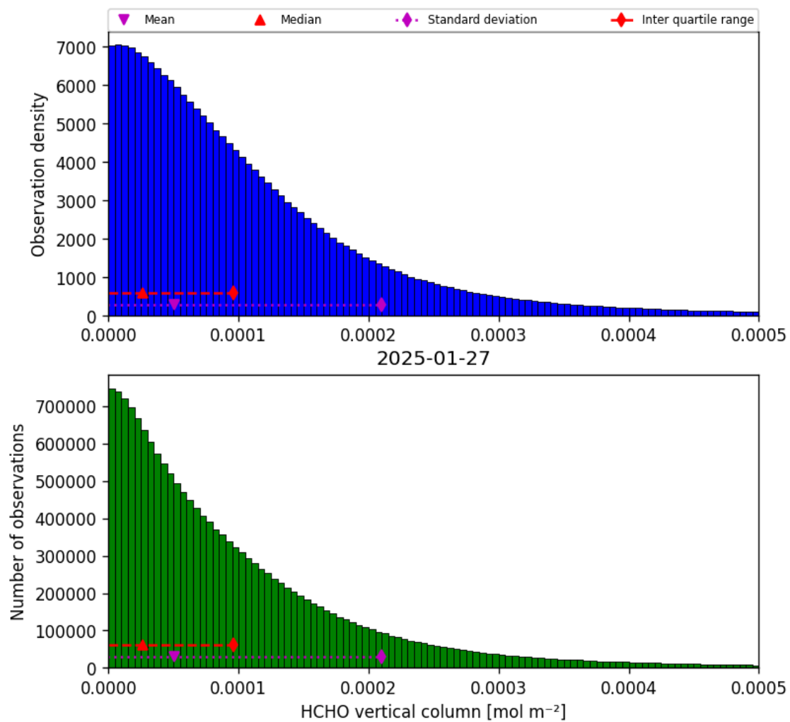
Figure 35: Histogram of “HCHO vertical column” for 2025-01-26 to 2025-01-28
