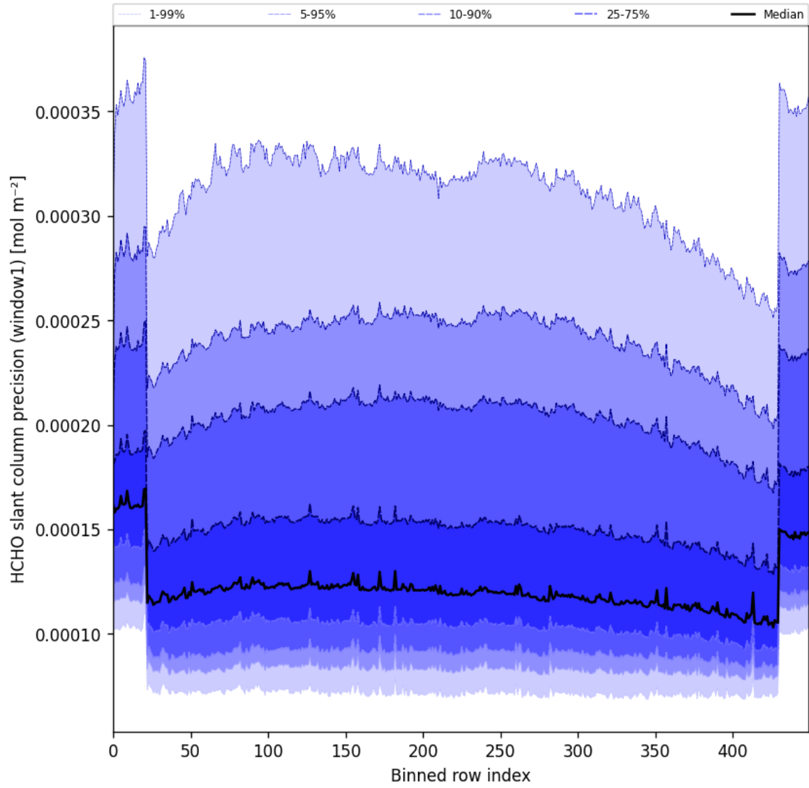
Figure 53: Along track statistics of “HCHO slant column precision (window1)” for 2025-01-26 to 2025-01-28
