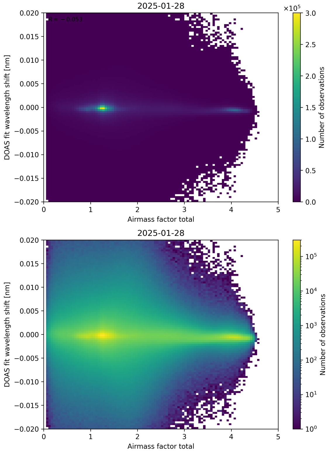
Figure 98: Scatter density plot of “Airmass factor total” against “DOAS fit wavelength shift” for 2025-01-28 to 2025-01-29.
