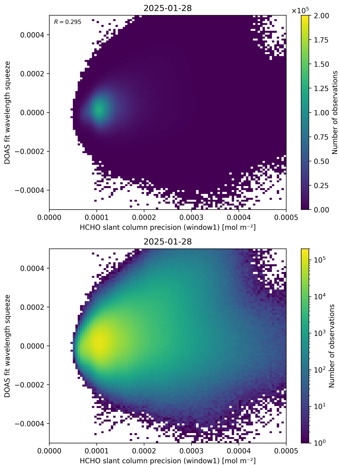
Figure 90: Scatter density plot of “HCHO slant column precision (window1)” against “DOAS fit wavelength squeeze” for 2025-01-28 to 2025-01-29.
