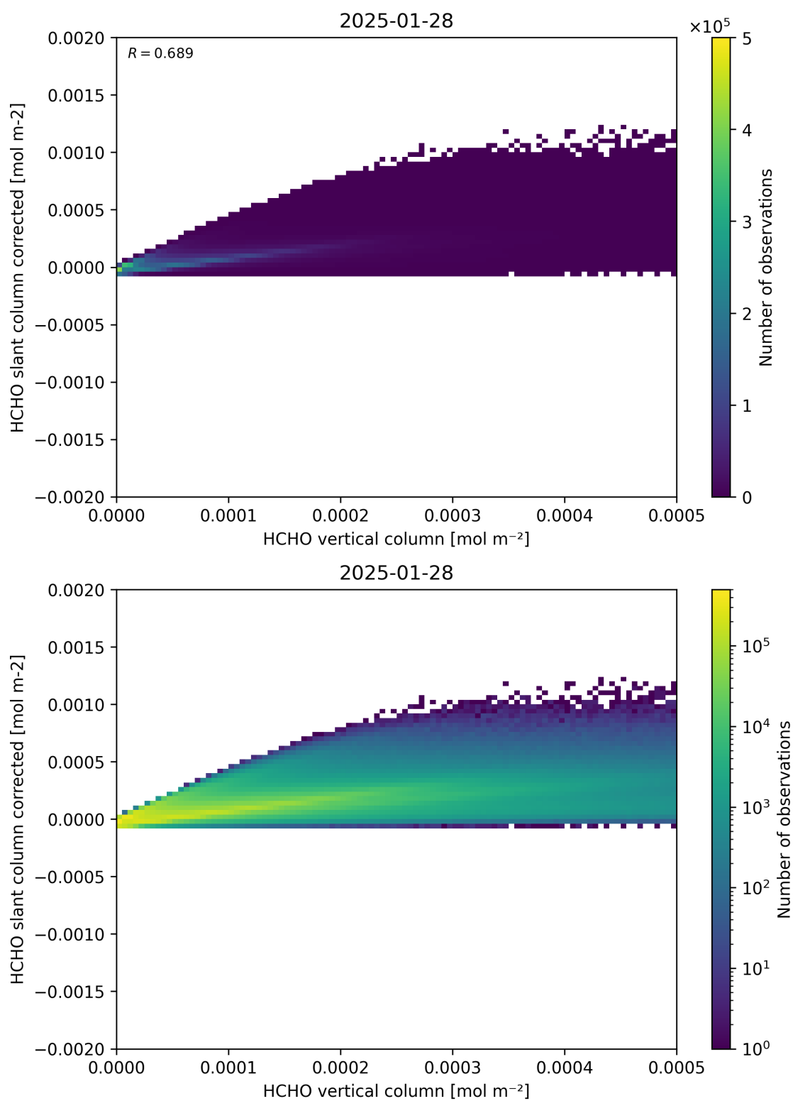
Figure 127: Scatter density plot of “HCHO vertical column” against “HCHO slant column corrected” for 2025-01-28 to 2025-01-29.
