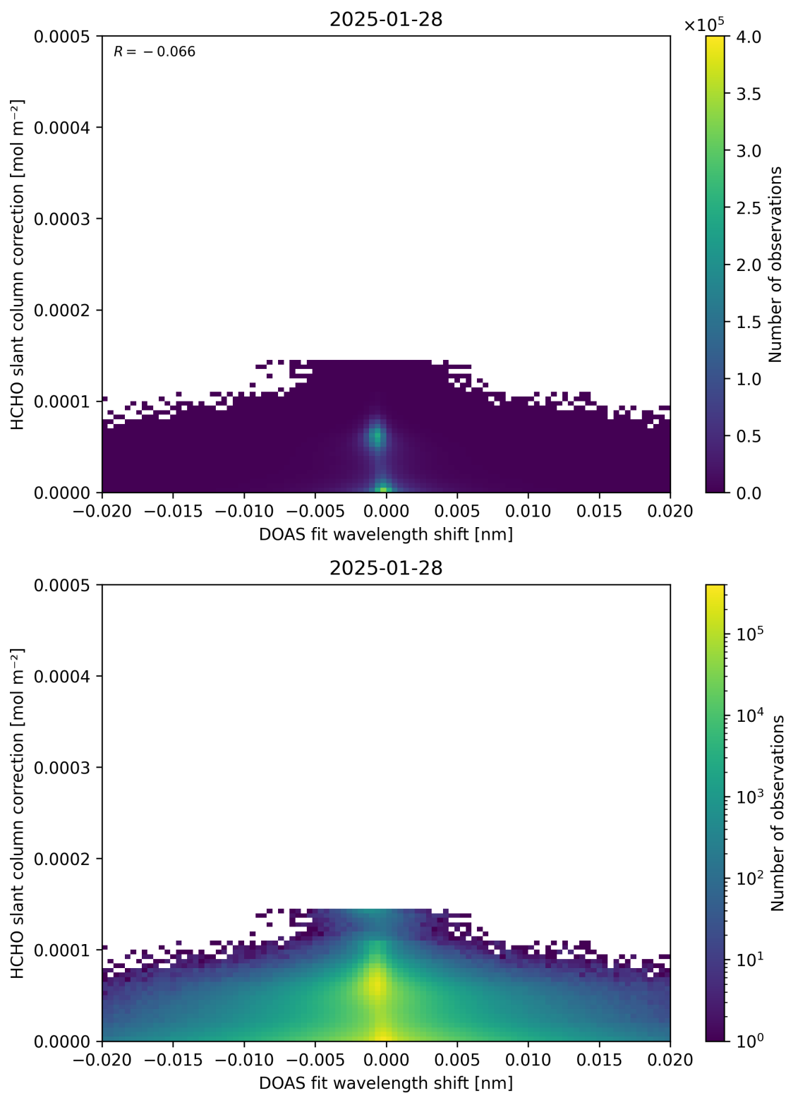
Figure 67: Scatter density plot of “DOAS fit wavelength shift” against “HCHO slant column correction” for 2025-01-28 to 2025-01-29.
