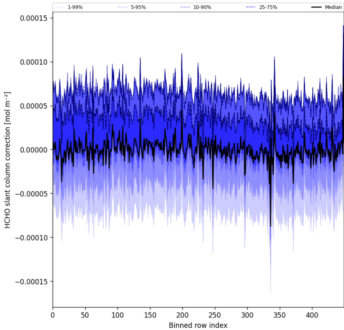
Figure 61: Along track statistics of “HCHO slant column correction” for 2025-01-28 to 2025-01-29
