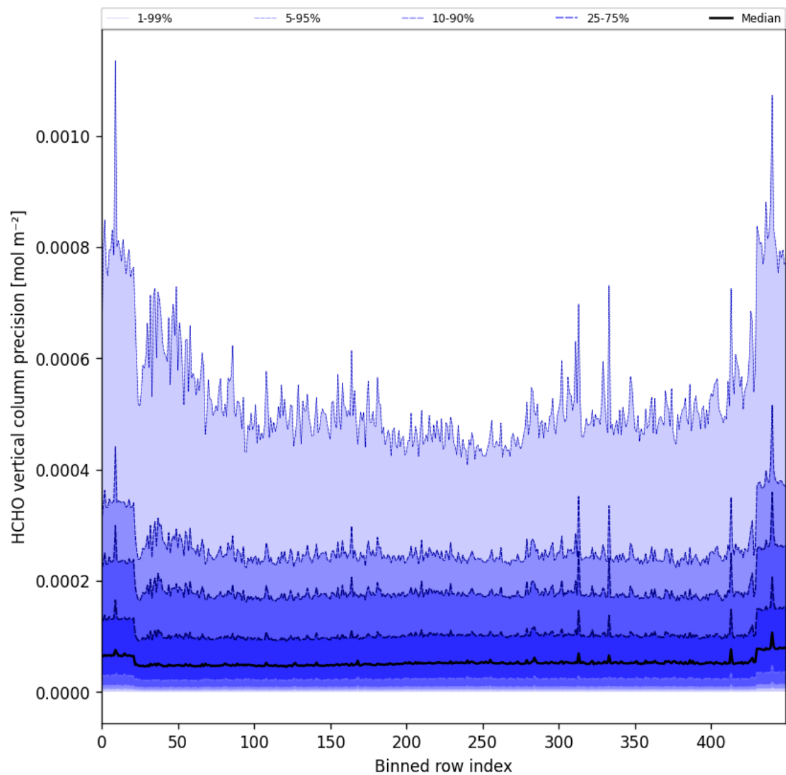
Figure 50: Along track statistics of “HCHO vertical column precision” for 2025-01-28 to 2025-01-29
