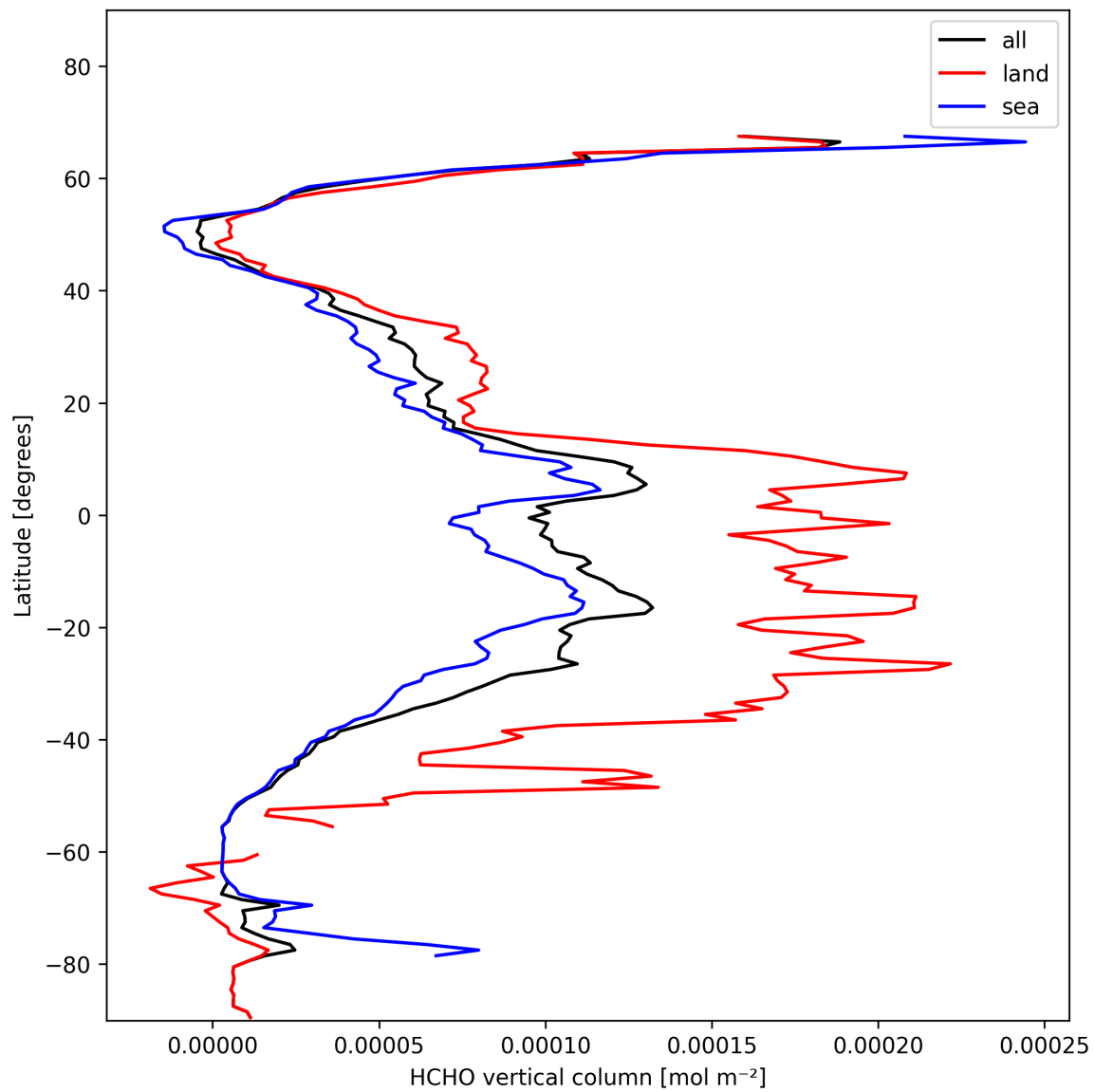
Figure 21: Zonal average of “HCHO vertical column” for 2025-01-28 to 2025-01-29.
