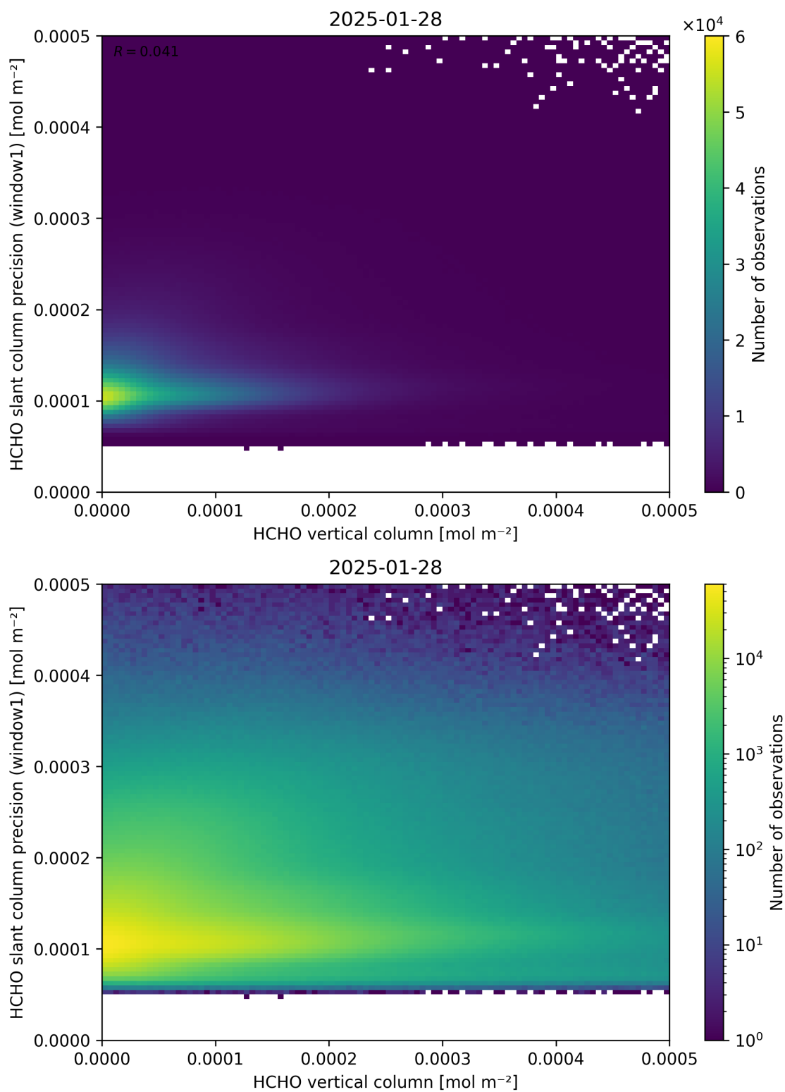
Figure 130: Scatter density plot of “HCHO vertical column” against “HCHO slant column precision (window1)” for 2025-01-28 to 2025-01-29.
