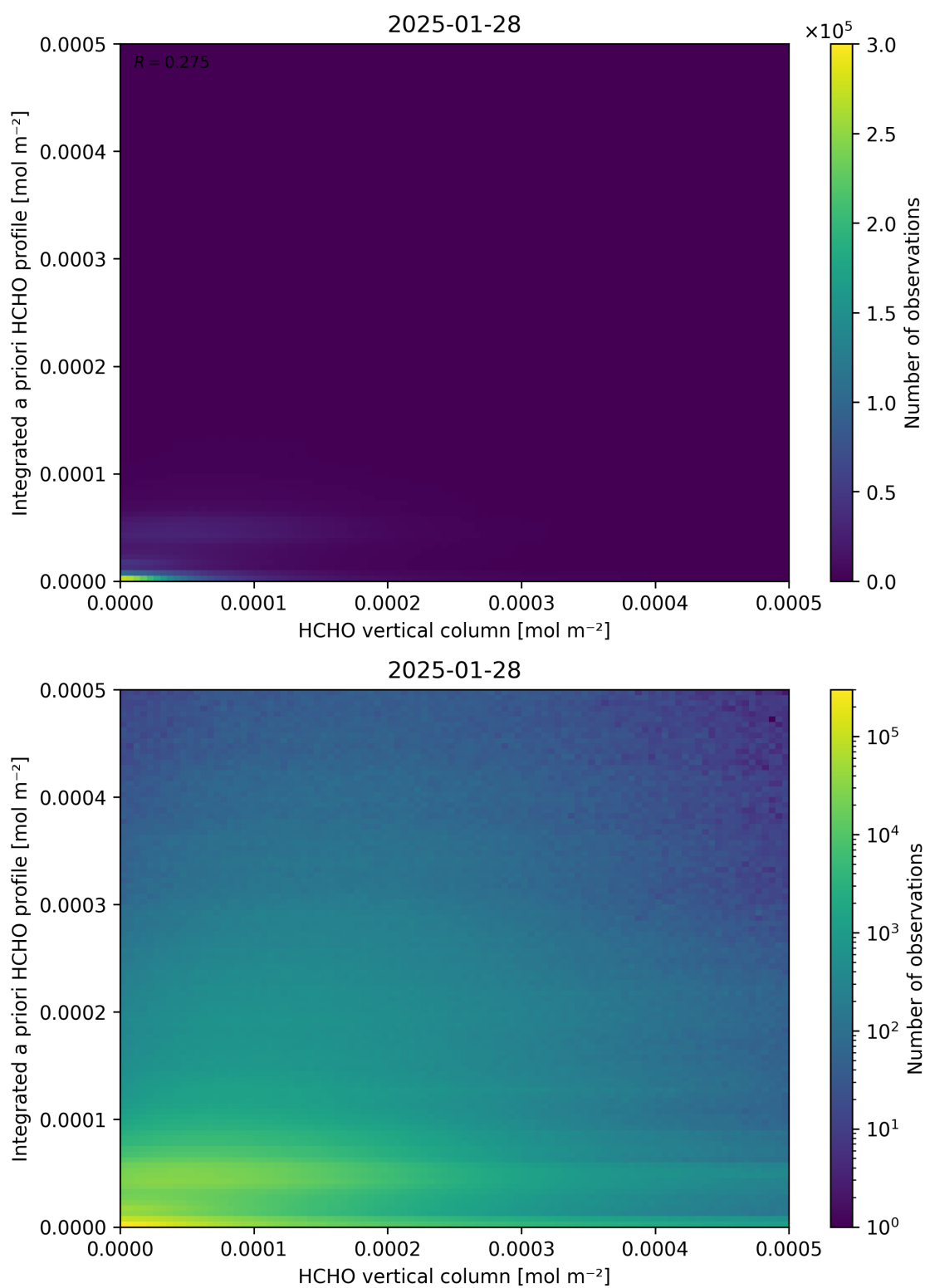
Figure 135: Scatter density plot of “HCHO vertical column” against “Integrated a priori HCHO profile” for 2025-01-28 to 2025-01-29.
