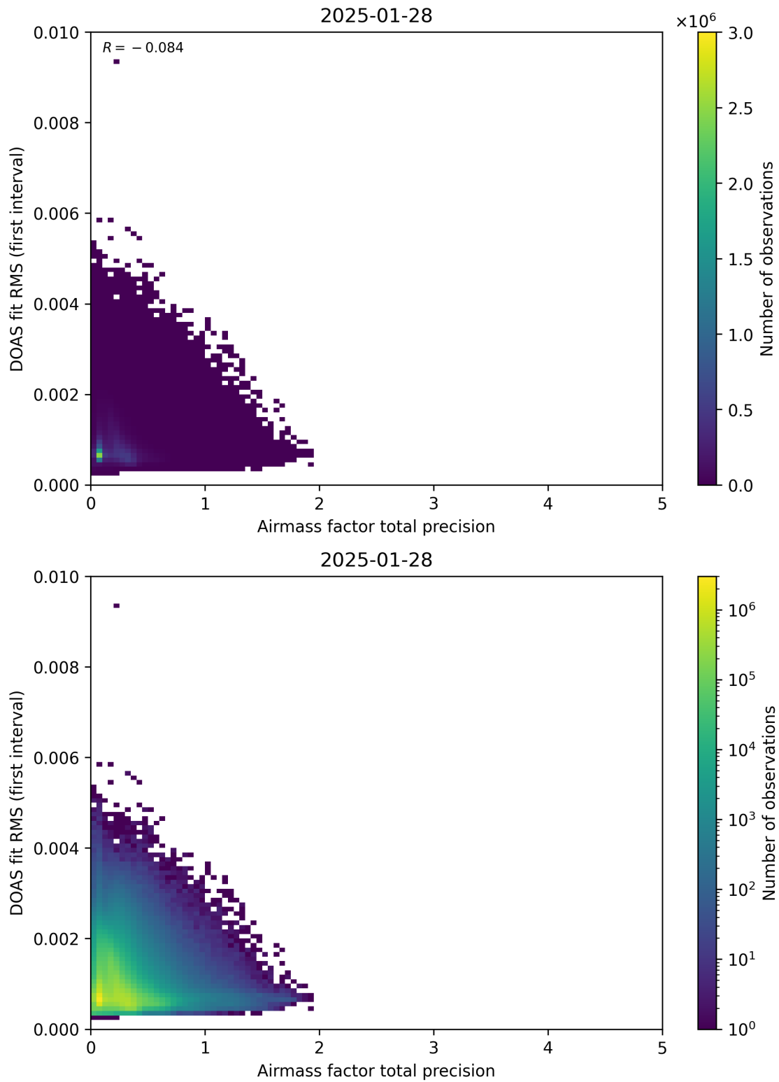
Figure 105: Scatter density plot of “Airmass factor total precision” against “DOAS fit RMS (first interval)” for 2025-01-28 to 2025-01-29.
