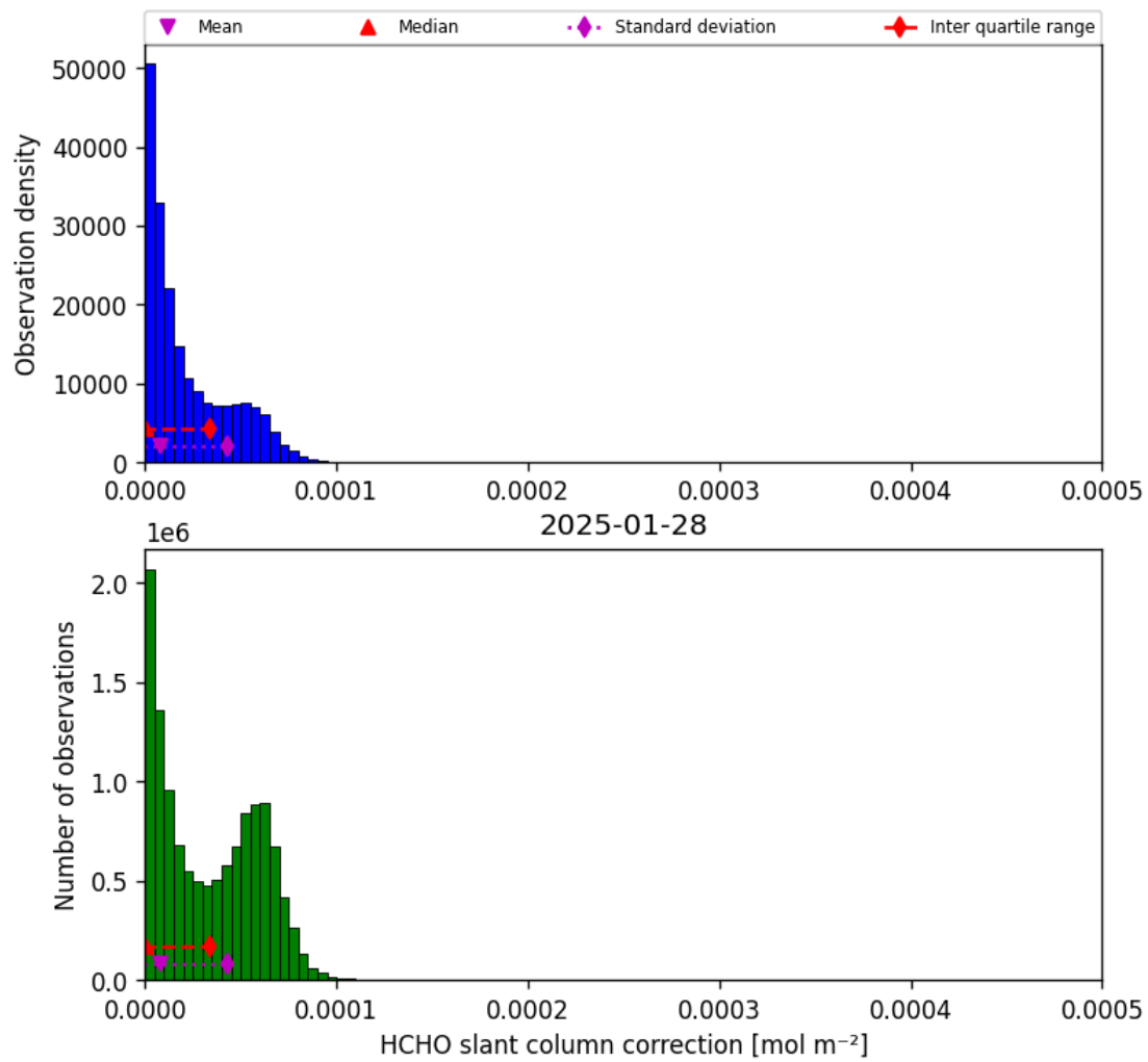
Figure 47: Histogram of “HCHO slant column correction” for 2025-01-28 to 2025-01-29
