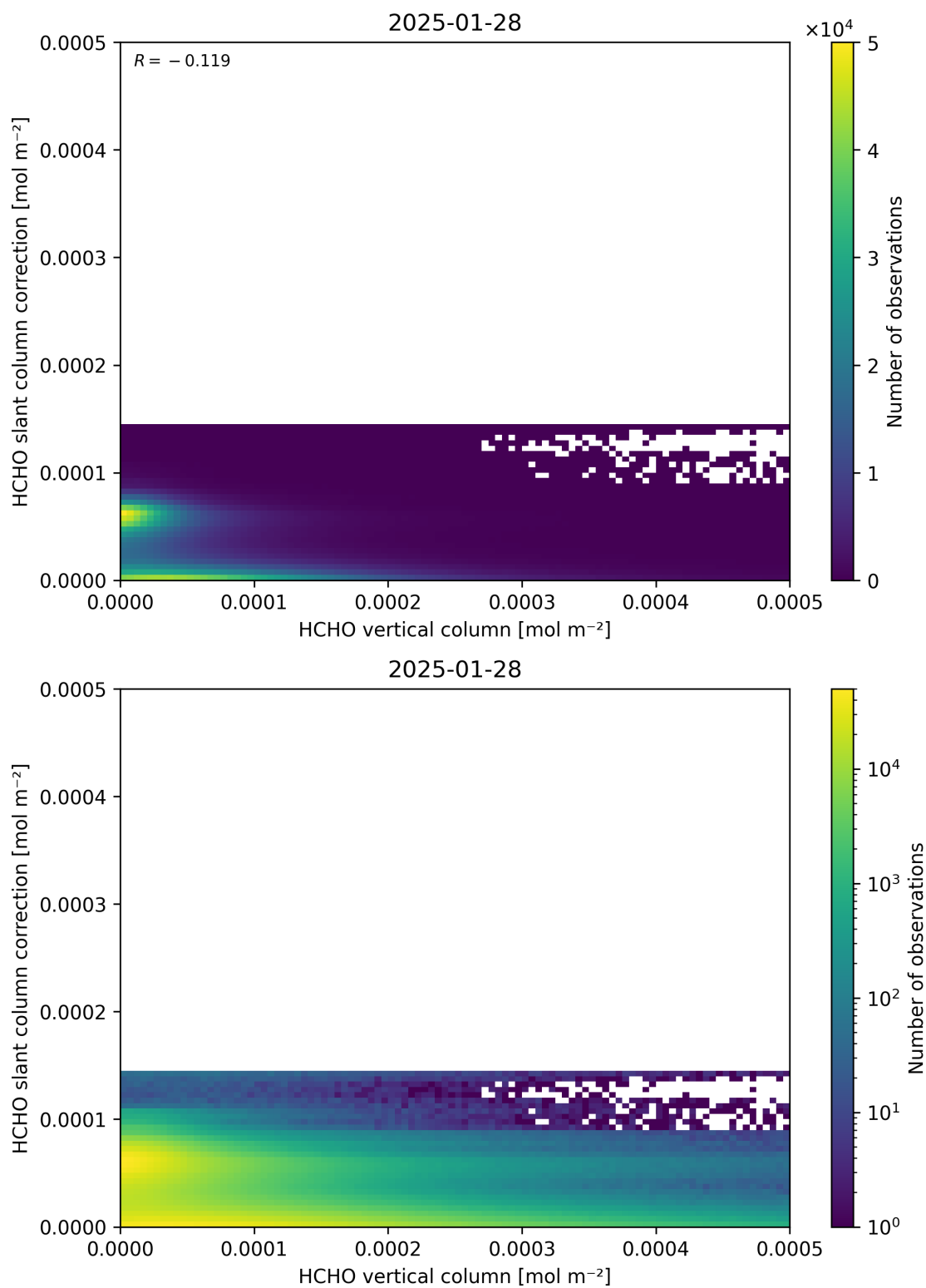
Figure 128: Scatter density plot of “HCHO vertical column” against “HCHO slant column correction” for 2025-01-28 to 2025-01-29.
