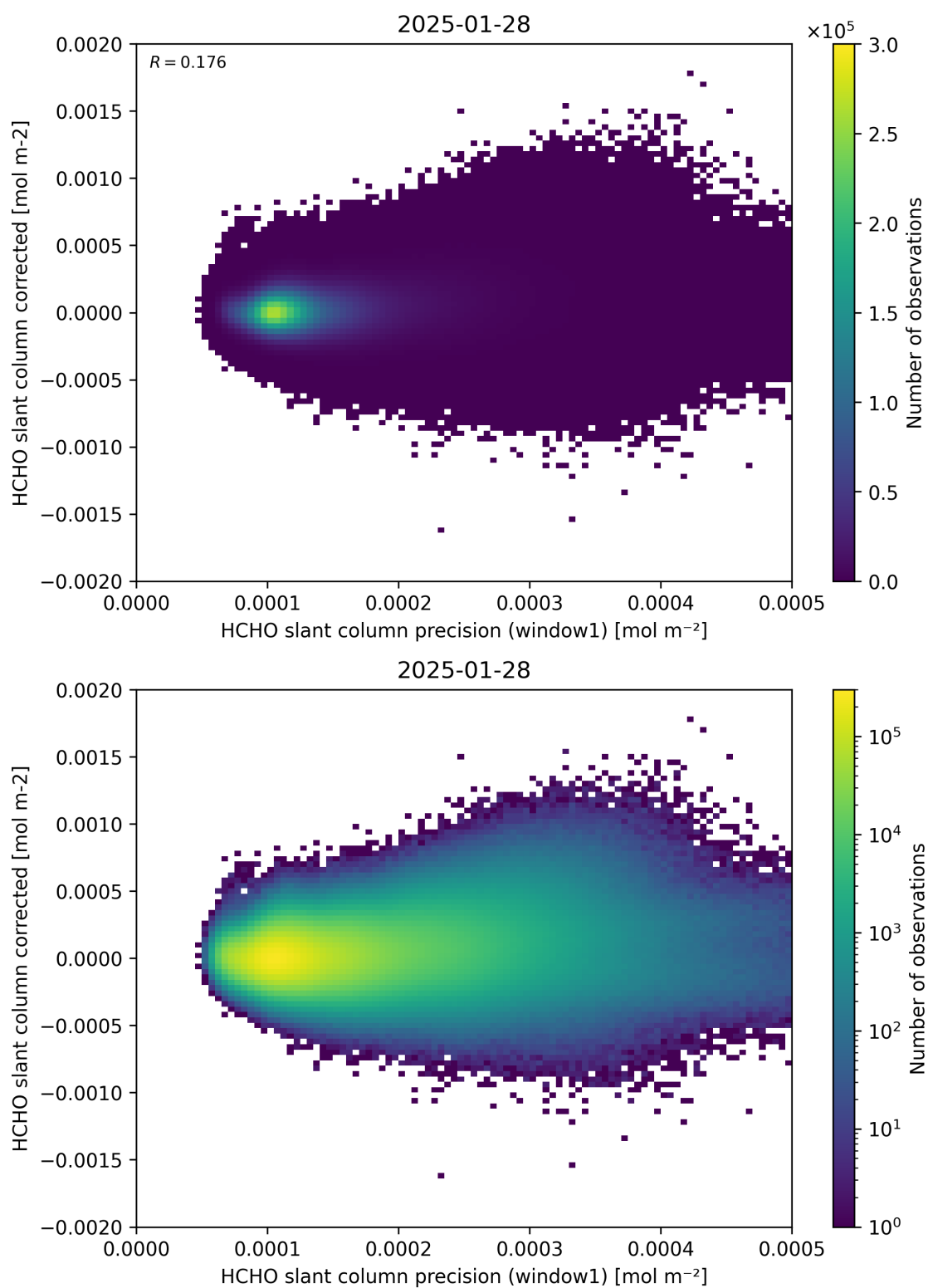
Figure 92: Scatter density plot of “HCHO slant column precision (window1)” against “HCHO slant column corrected” for 2025-01-28 to 2025-01-29.
