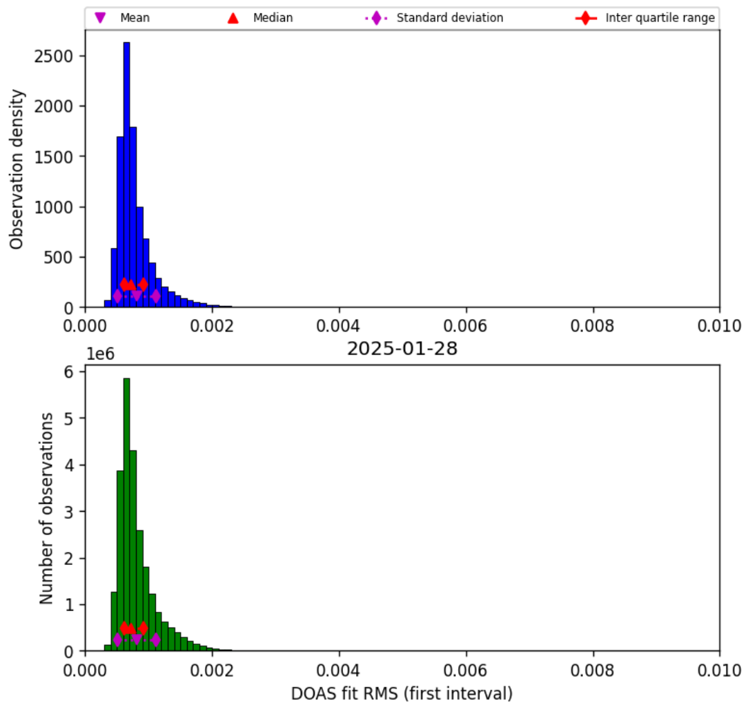
Figure 46: Histogram of "DOAS fit RMS (first interval)" for 2025-01-28 to 2025-01-29
