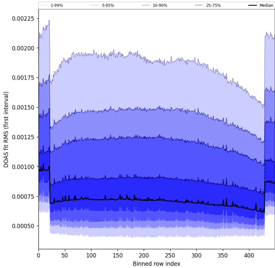
Figure 60: Along track statistics of “DOAS fit RMS (first interval)” for 2025-01-28 to 2025-01-29
