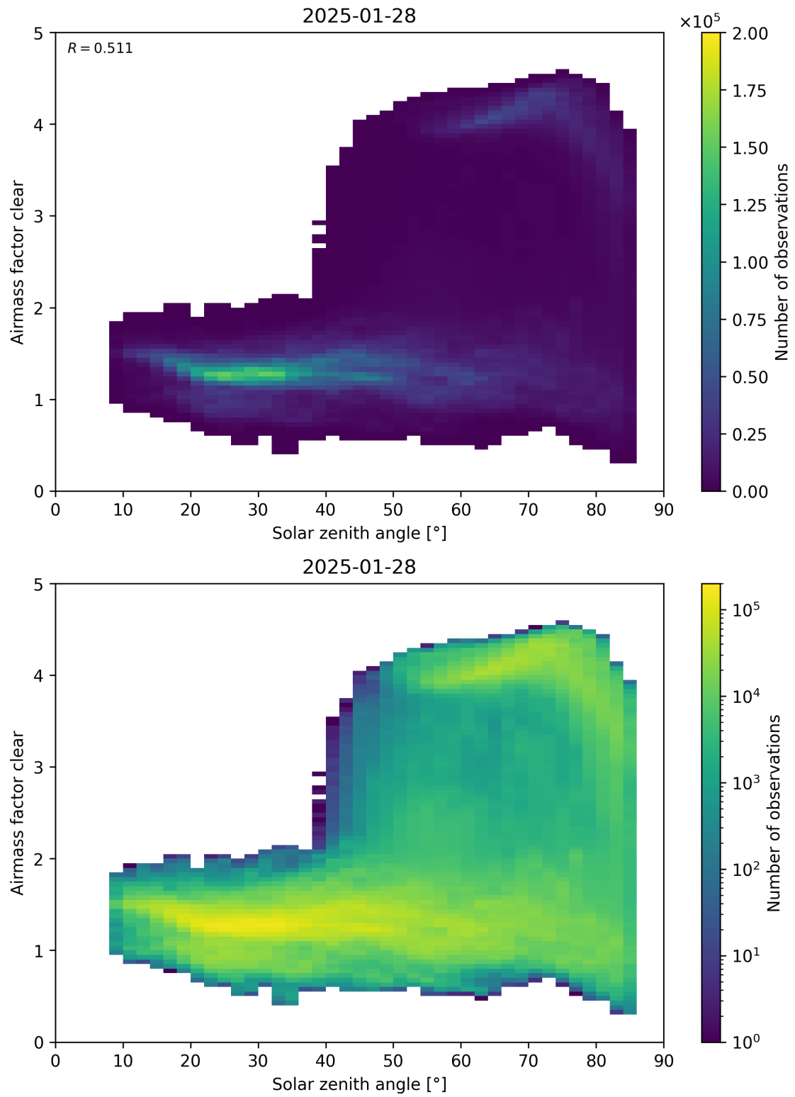
Figure 170: Scatter density plot of “Solar zenith angle” against “Airmass factor clear” for 2025-01-28 to 2025-01-29.
