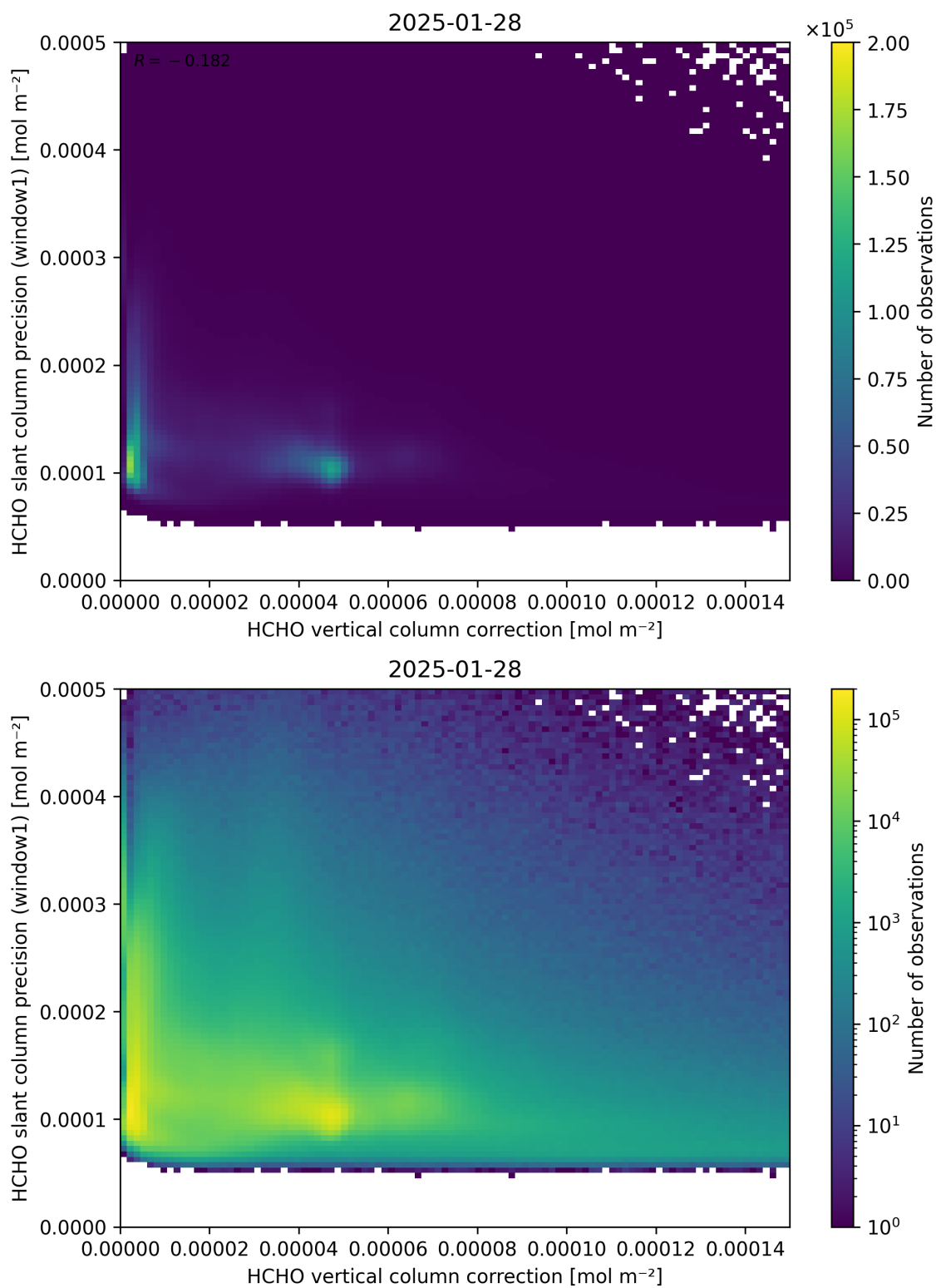
Figure 119: Scatter density plot of “HCHO vertical column correction” against “HCHO slant column precision (window1)” for 2025-01-28 to 2025-01-29.
