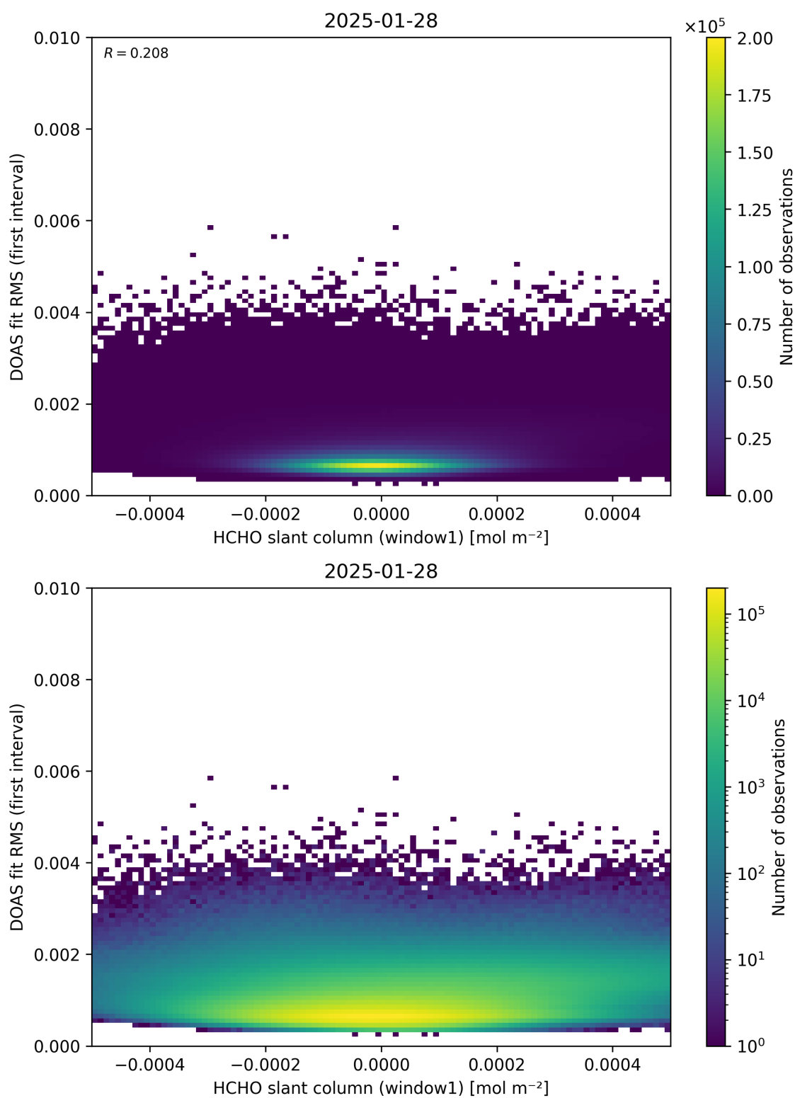
Figure 78: Scatter density plot of “HCHO slant column (window1)” against “DOAS fit RMS (first interval)” for 2025-01-28 to 2025-01-29.
