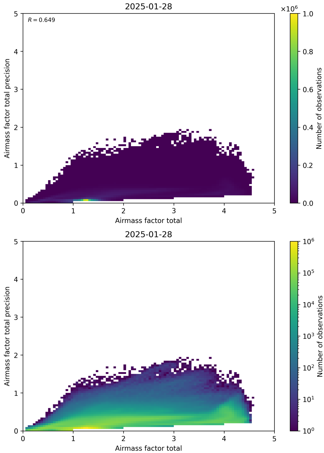
Figure 103: Scatter density plot of “Airmass factor total” against “Airmass factor total precision” for 2025-01-28 to 2025-01-29.
