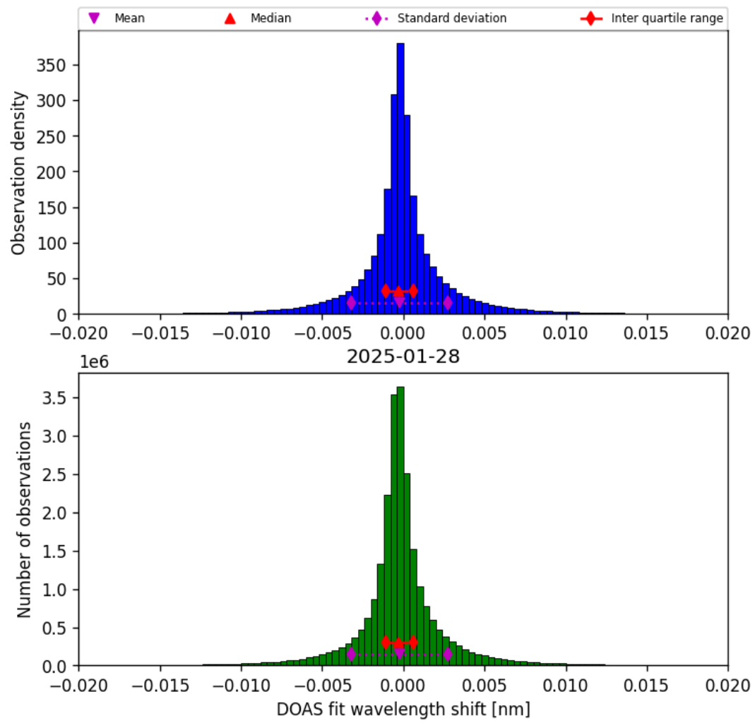
Figure 44: Histogram of “DOAS fit wavelength shift” for 2025-01-28 to 2025-01-29
