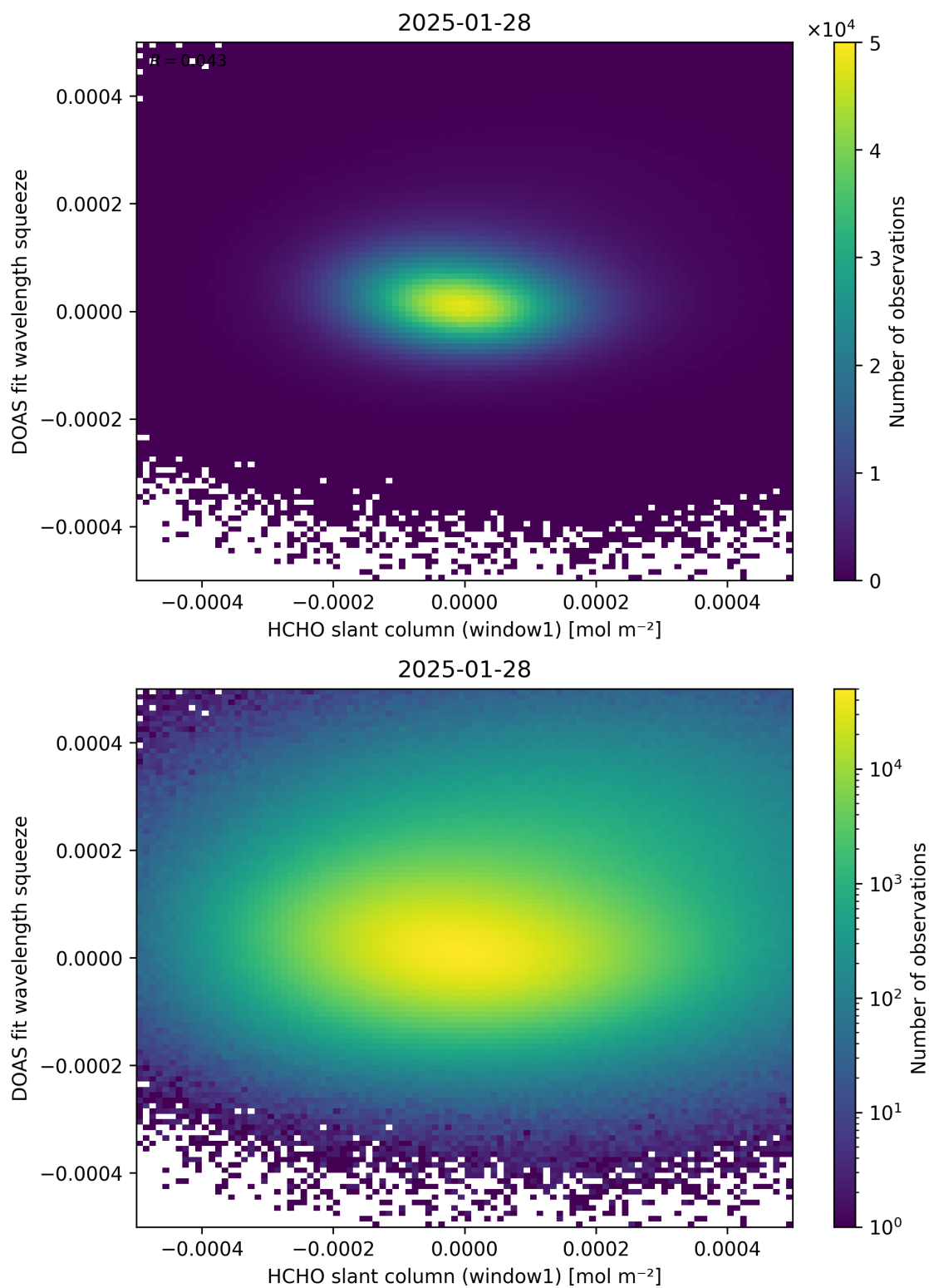
Figure 80: Scatter density plot of “HCHO slant column (window1)” against “DOAS fit wavelength squeeze” for 2025-01-28 to 2025-01-29.
