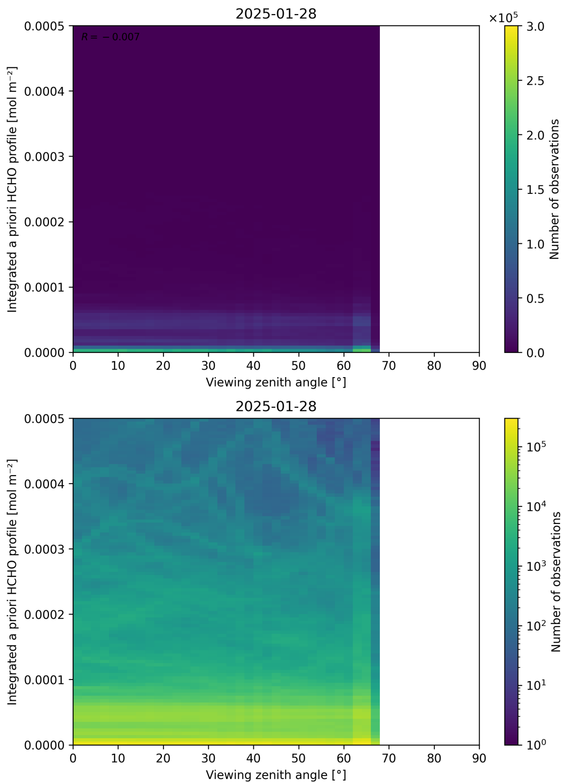
Figure 195: Scatter density plot of “Viewing zenith angle” against “Integrated a priori HCHO profile” for 2025-01-28 to 2025-01-29.
