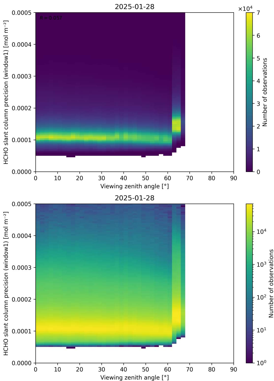
Figure 189: Scatter density plot of “Viewing zenith angle” against “HCHO slant column precision (window1)” for 2025-01-28 to 2025-01-29.
