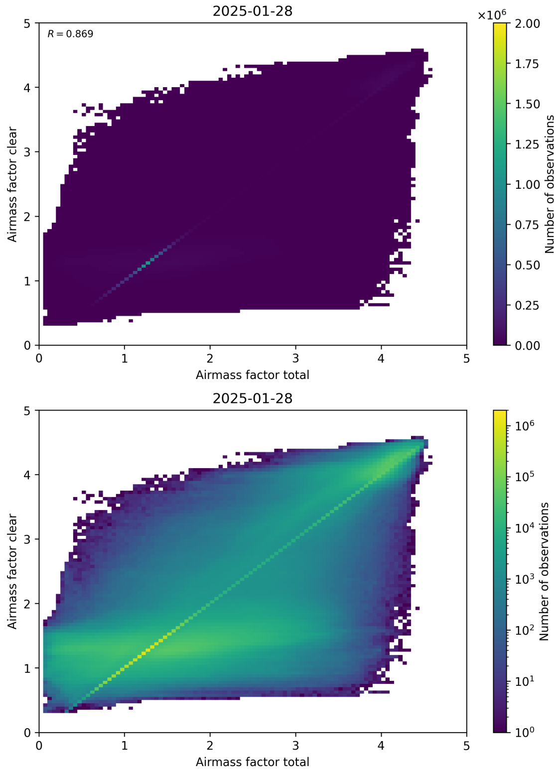
Figure 100: Scatter density plot of “Airmass factor total” against “Airmass factor clear” for 2025-01-28 to 2025-01-29.
