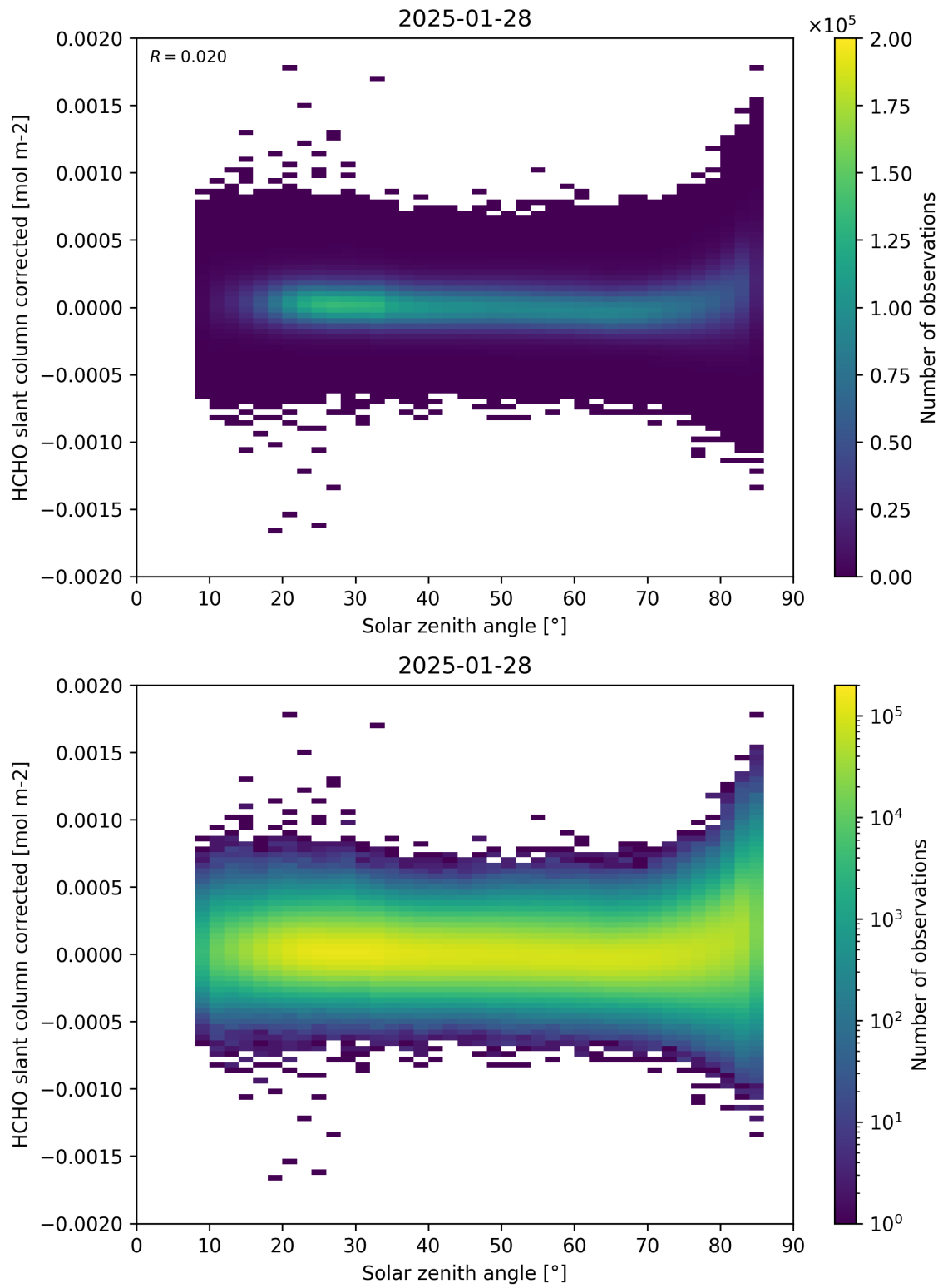
Figure 171: Scatter density plot of “Solar zenith angle” against “HCHO slant column corrected” for 2025-01-28 to 2025-01-29.
