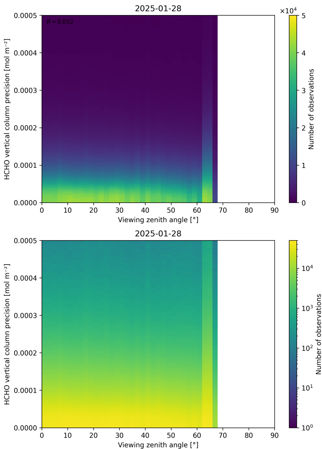
Figure 194: Scatter density plot of “Viewing zenith angle” against “HCHO vertical column precision” for 2025-01-28 to 2025-01-29.
