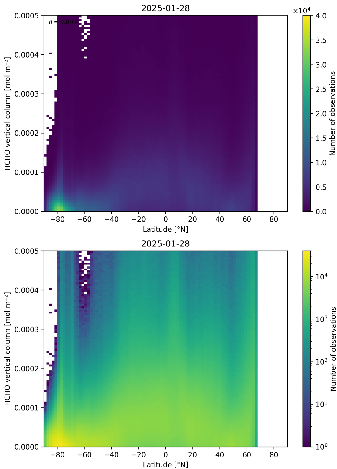
Figure 163: Scatter density plot of “Latitude” against “HCHO vertical column” for 2025-01-28 to 2025-01-29.
