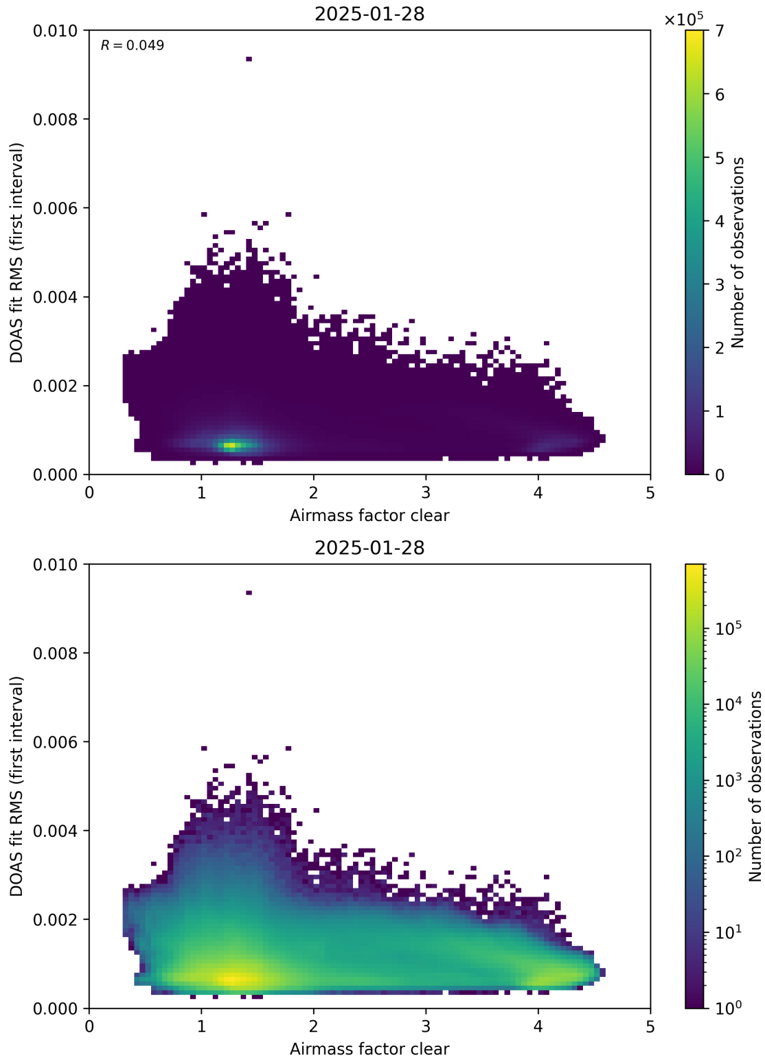
Figure 71: Scatter density plot of “Airmass factor clear” against “DOAS fit RMS (first interval)” for 2025-01-28 to 2025-01-29.
