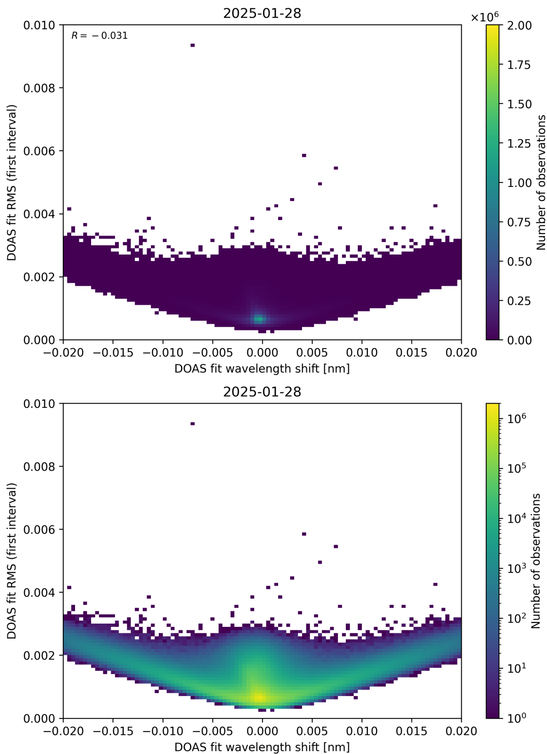
Figure 64: Scatter density plot of “DOAS fit wavelength shift” against “DOAS fit RMS (first interval)” for 2025-01-28 to 2025-01-29.
