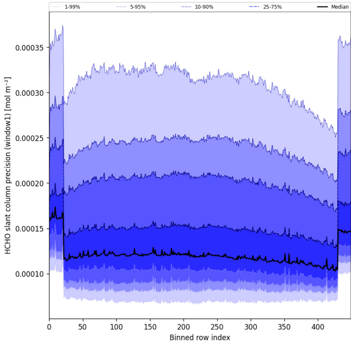
Figure 53: Along track statistics of “HCHO slant column precision (window1)” for 2025-01-28 to 2025-01-29
