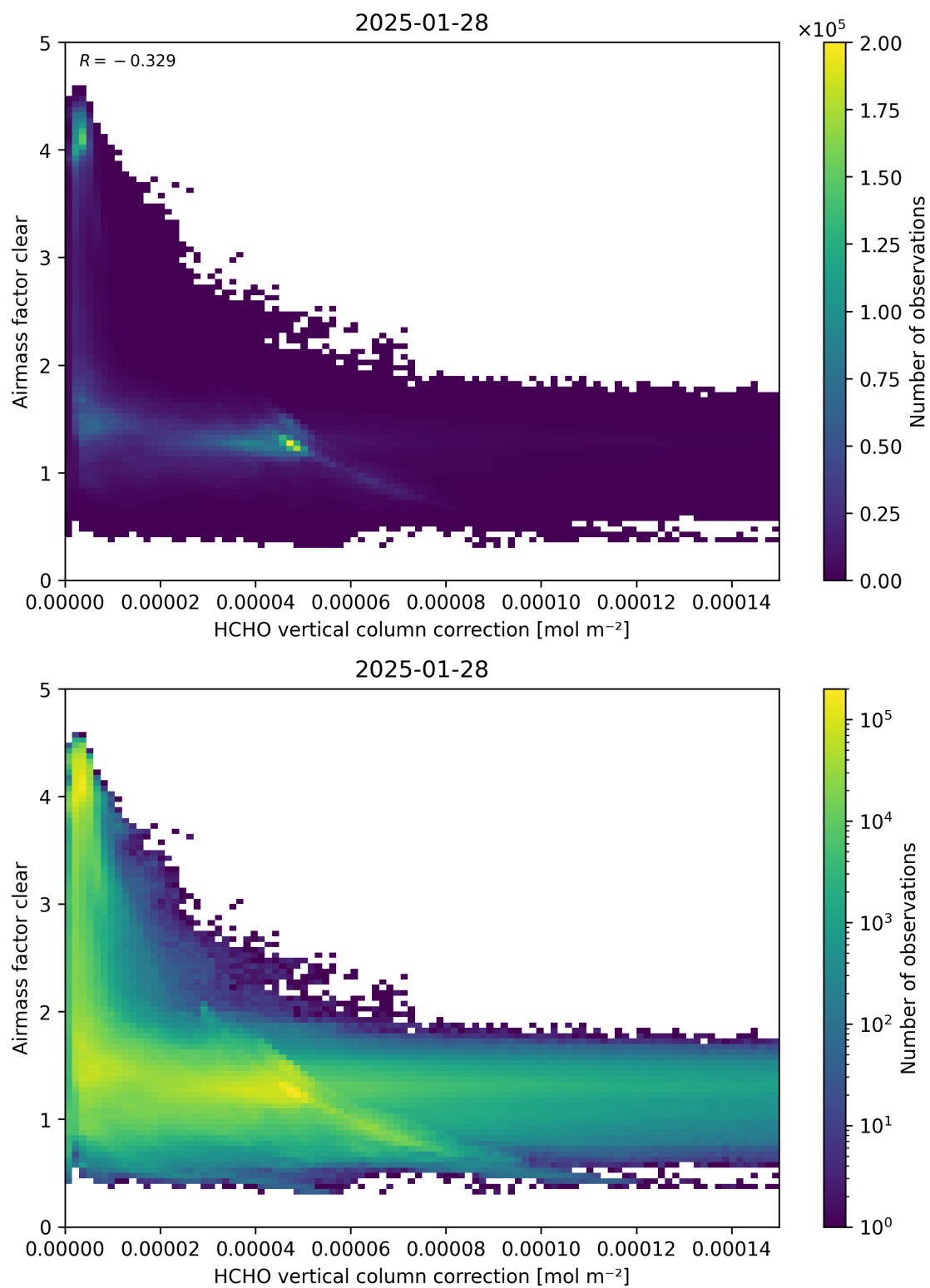
Figure 115: Scatter density plot of “HCHO vertical column correction” against “Airmass factor clear” for 2025-01-28 to 2025-01-29.
