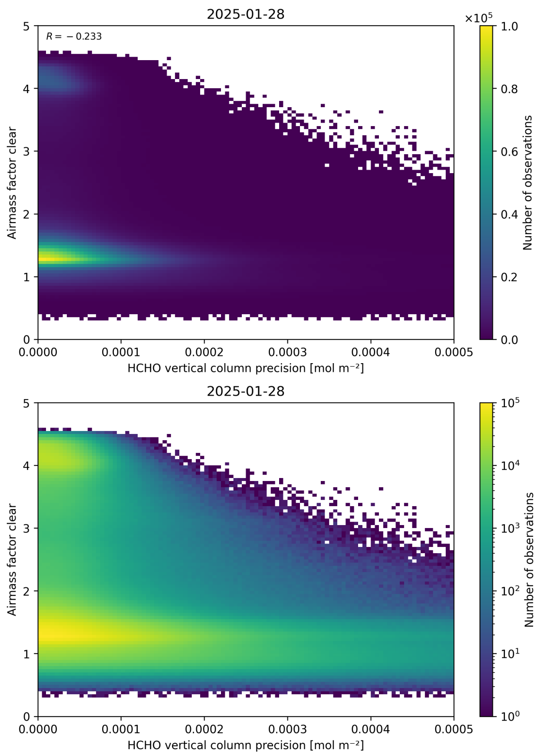
Figure 139: Scatter density plot of “HCHO vertical column precision” against “Airmass factor clear” for 2025-01-28 to 2025-01-29.
