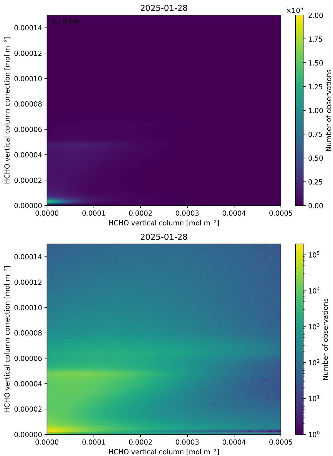
Figure 133: Scatter density plot of “HCHO vertical column” against “HCHO vertical column correction” for 2025-01-28 to 2025-01-29.
