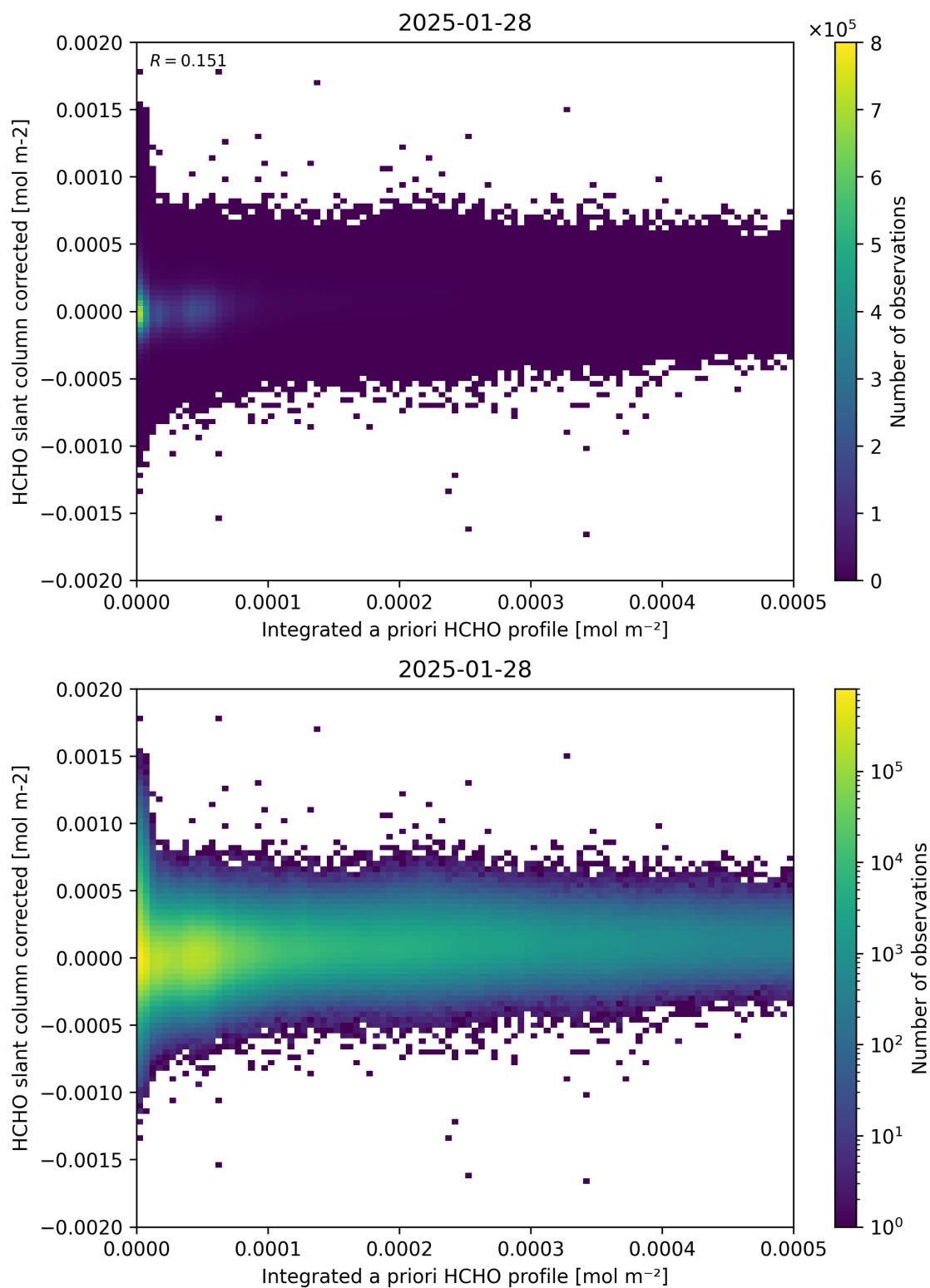
Figure 151: Scatter density plot of “Integrated a priori HCHO profile” against “HCHO slant column corrected” for 2025-01-28 to 2025-01-29.
