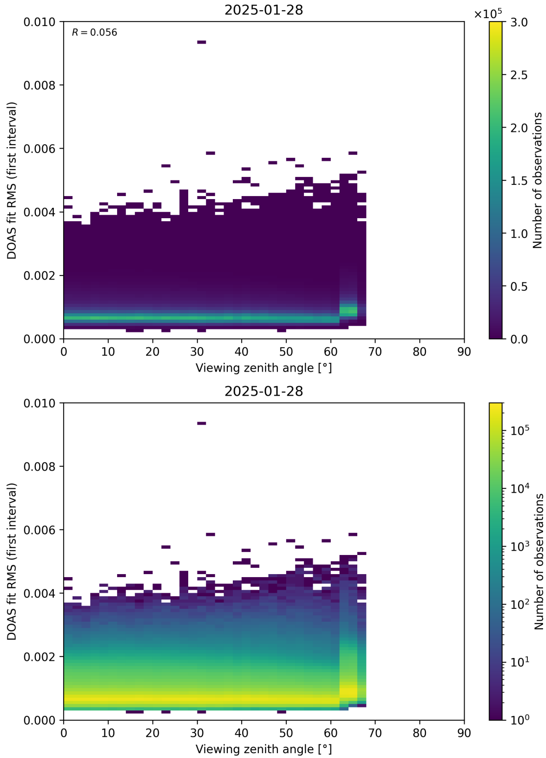
Figure 182: Scatter density plot of “Viewing zenith angle” against “DOAS fit RMS (first interval)” for 2025-01-28 to 2025-01-29.
