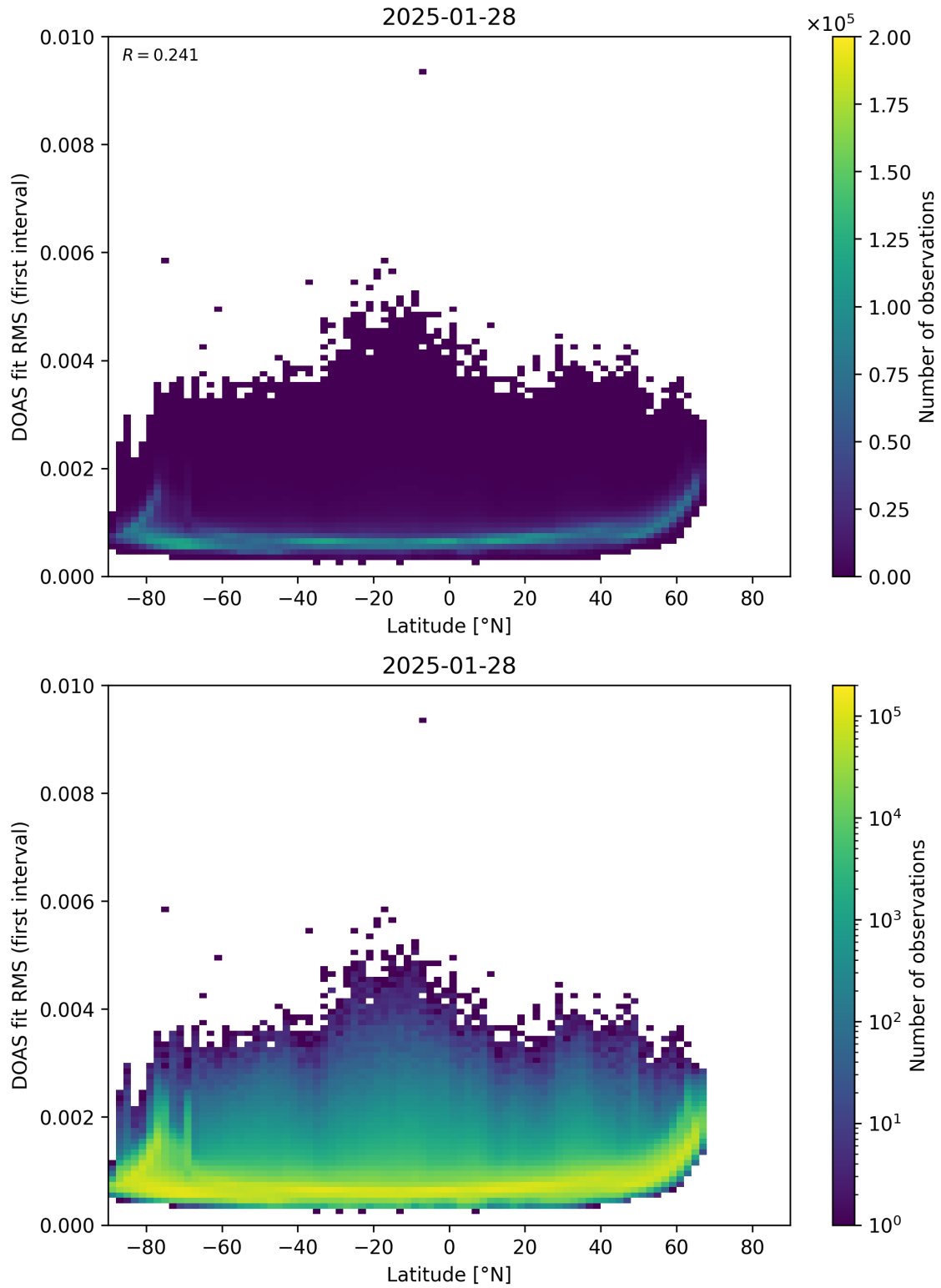
Figure 153: Scatter density plot of “Latitude” against “DOAS fit RMS (first interval)” for 2025-01-28 to 2025-01-29.
