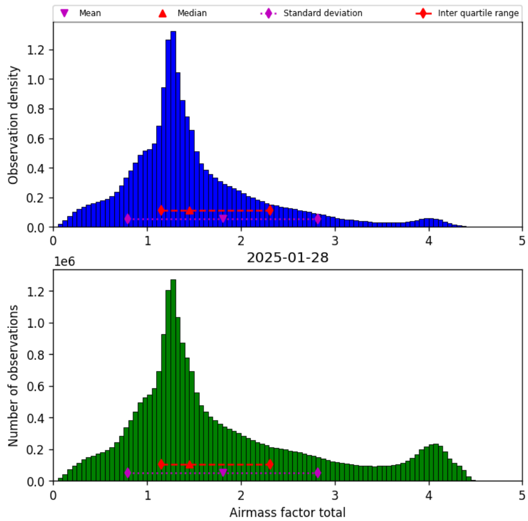
Figure 40: Histogram of “Airmass factor total” for 2025-01-28 to 2025-01-29
