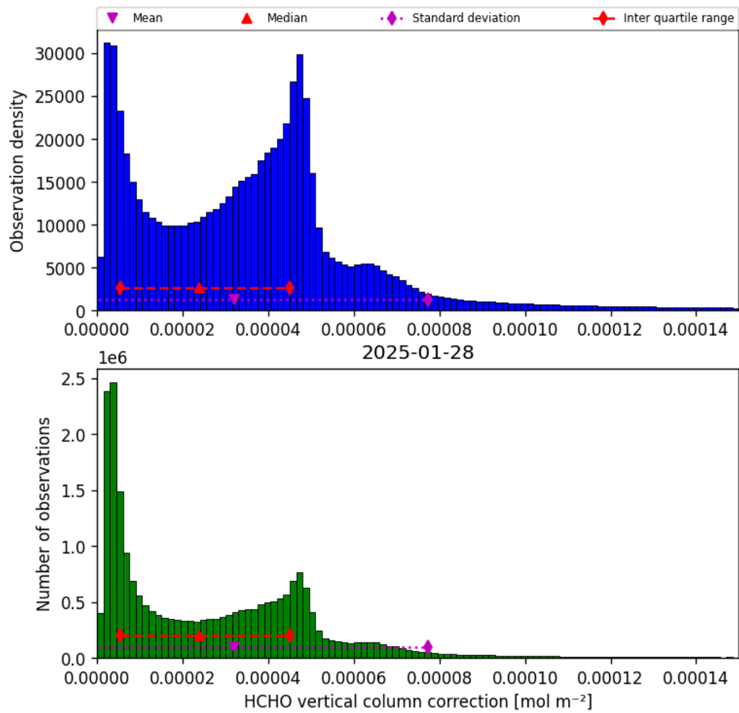
Figure 37: Histogram of “HCHO vertical column correction” for 2025-01-28 to 2025-01-29
