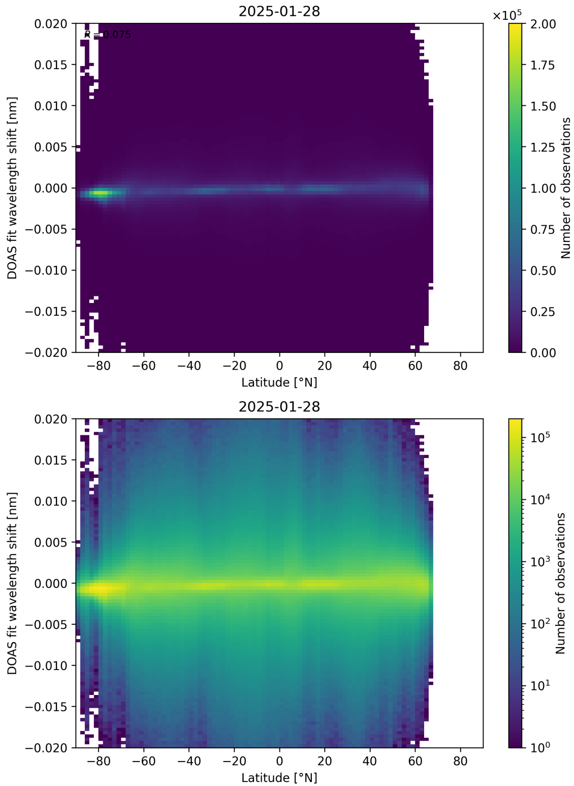
Figure 154: Scatter density plot of “Latitude” against “DOAS fit wavelength shift” for 2025-01-28 to 2025-01-29.
