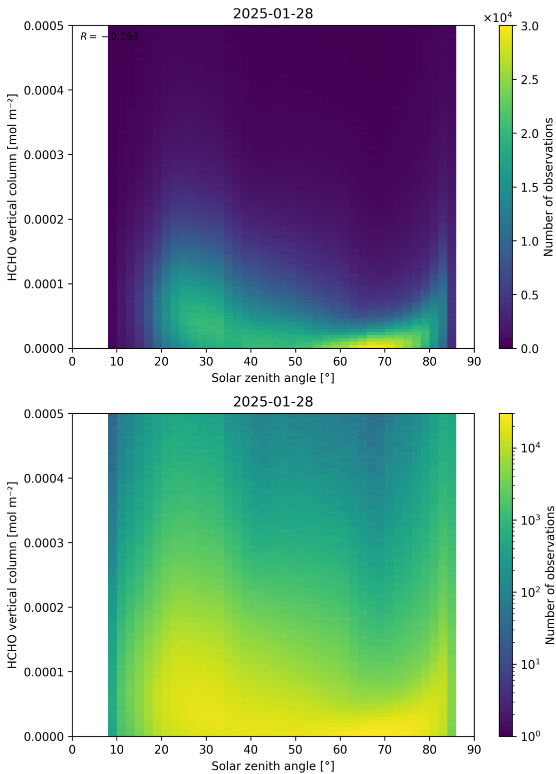
Figure 177: Scatter density plot of “Solar zenith angle” against “HCHO vertical column” for 2025-01-28 to 2025-01-29.
