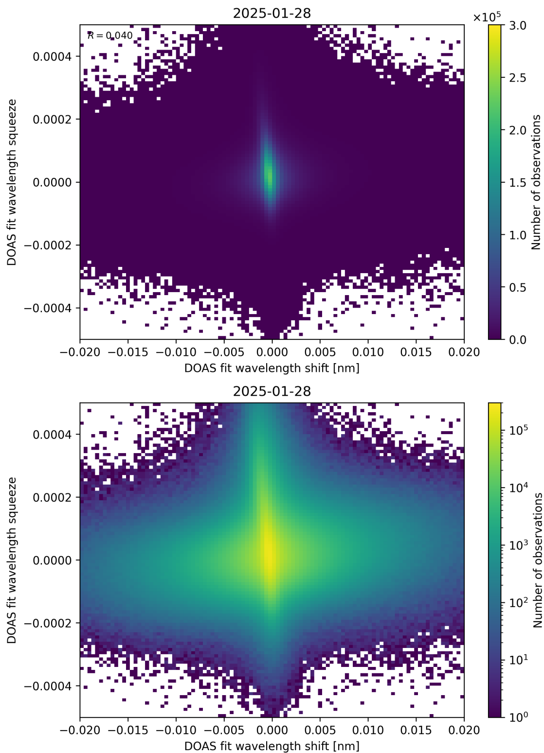
Figure 65: Scatter density plot of “DOAS fit wavelength shift” against “DOAS fit wavelength squeeze” for 2025-01-28 to 2025-01-29.
