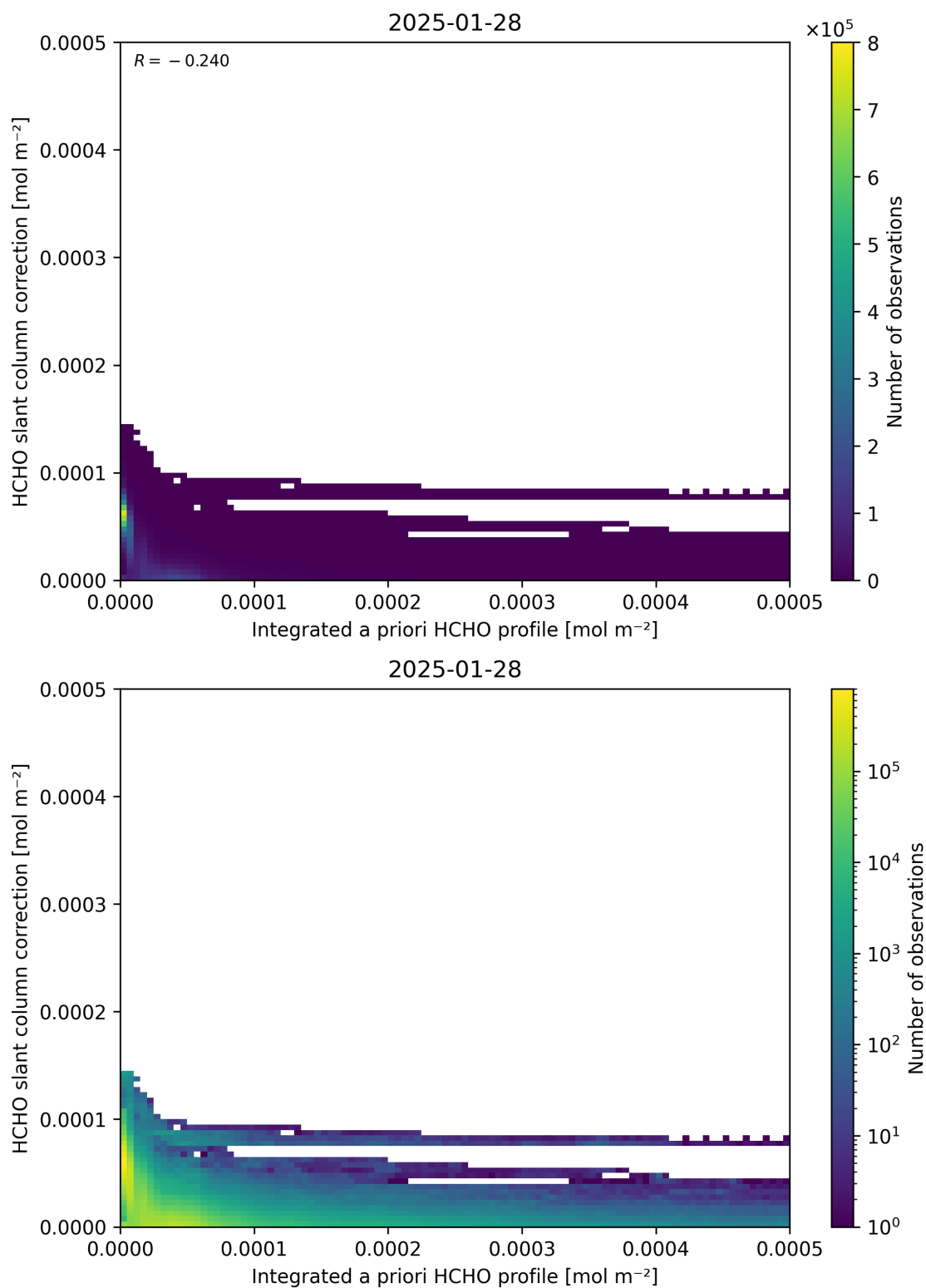
Figure 152: Scatter density plot of “Integrated a priori HCHO profile” against “HCHO slant column correction” for 2025-01-28 to 2025-01-29.
