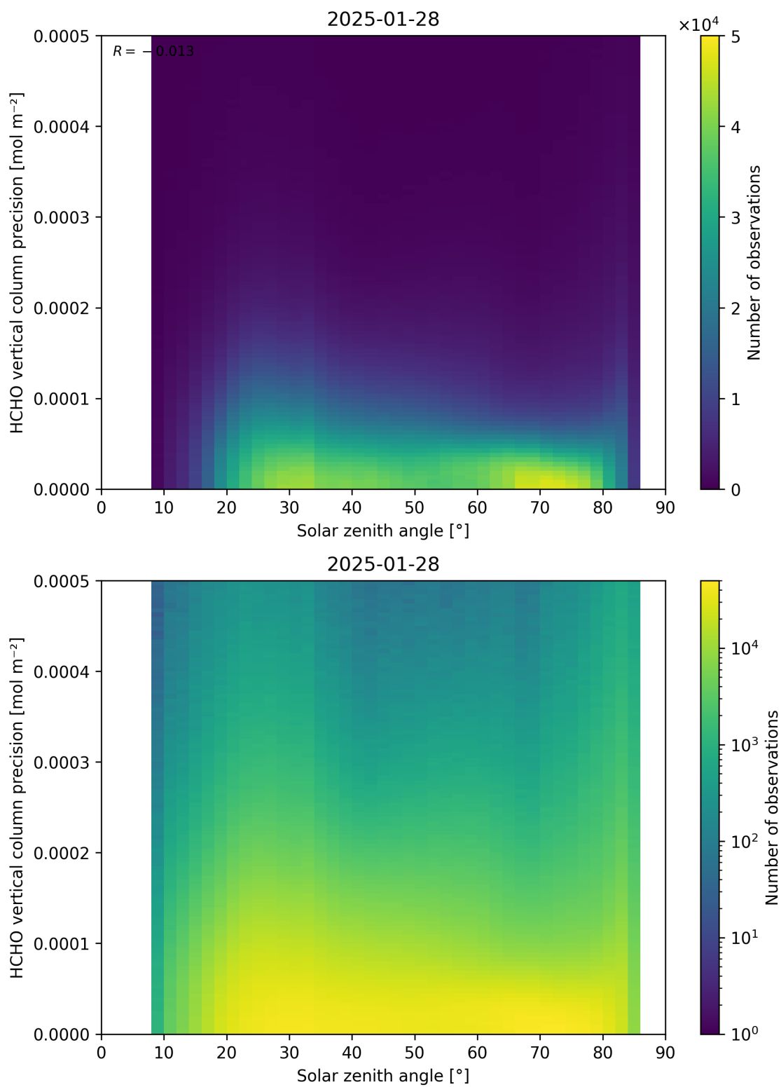
Figure 179: Scatter density plot of “Solar zenith angle” against “HCHO vertical column precision” for 2025-01-28 to 2025-01-29.
