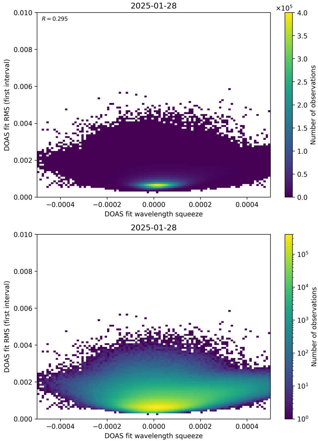
Figure 68: Scatter density plot of “DOAS fit wavelength squeeze” against “DOAS fit RMS (first interval)” for 2025-01-28 to 2025-01-29.
