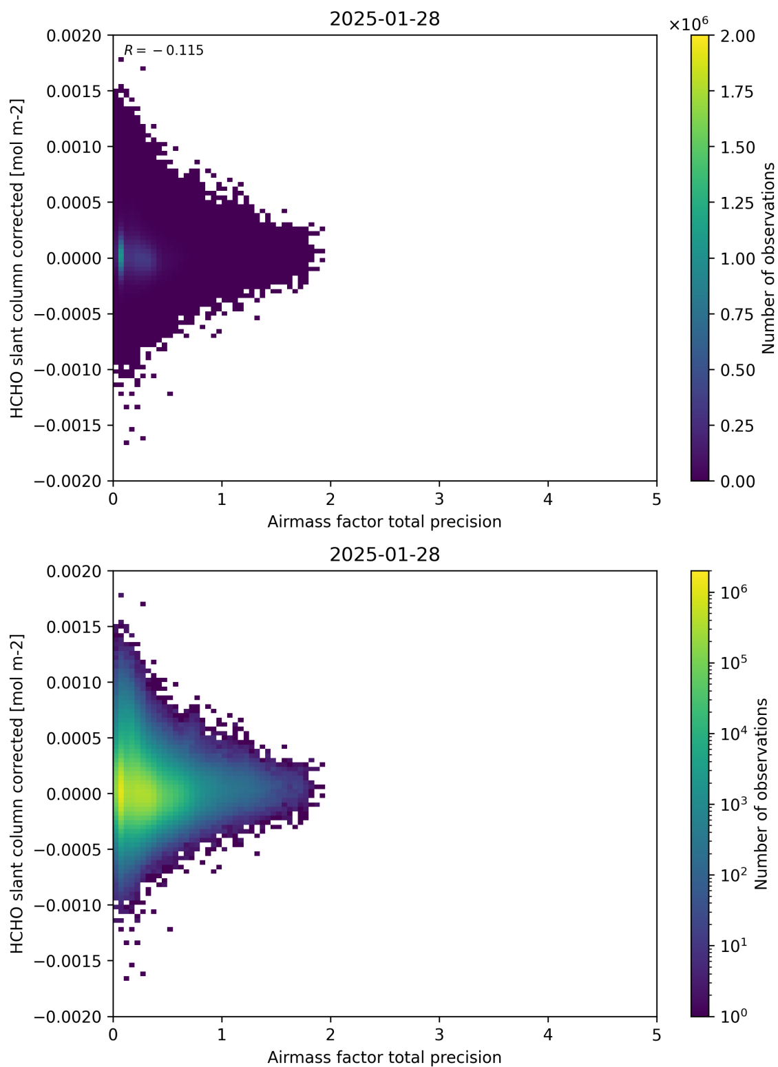
Figure 109: Scatter density plot of “Airmass factor total precision” against “HCHO slant column corrected” for 2025-01-28 to 2025-01-29.
