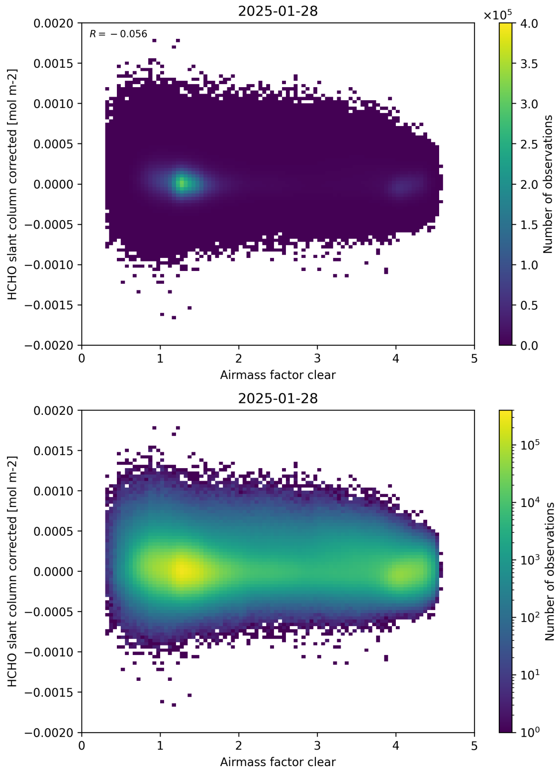
Figure 74: Scatter density plot of “Airmass factor clear” against “HCHO slant column corrected” for 2025-01-28 to 2025-01-29.
