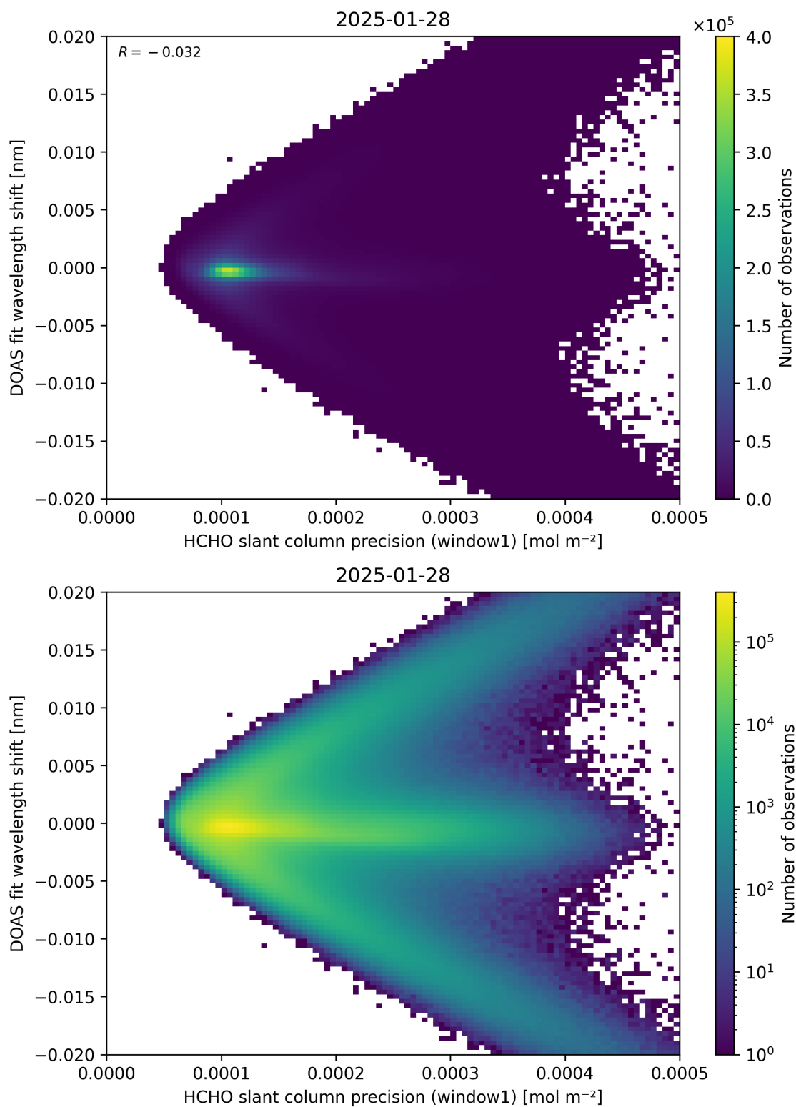
Figure 89: Scatter density plot of “HCHO slant column precision (window1)” against “DOAS fit wavelength shift” for 2025-01-28 to 2025-01-29.
