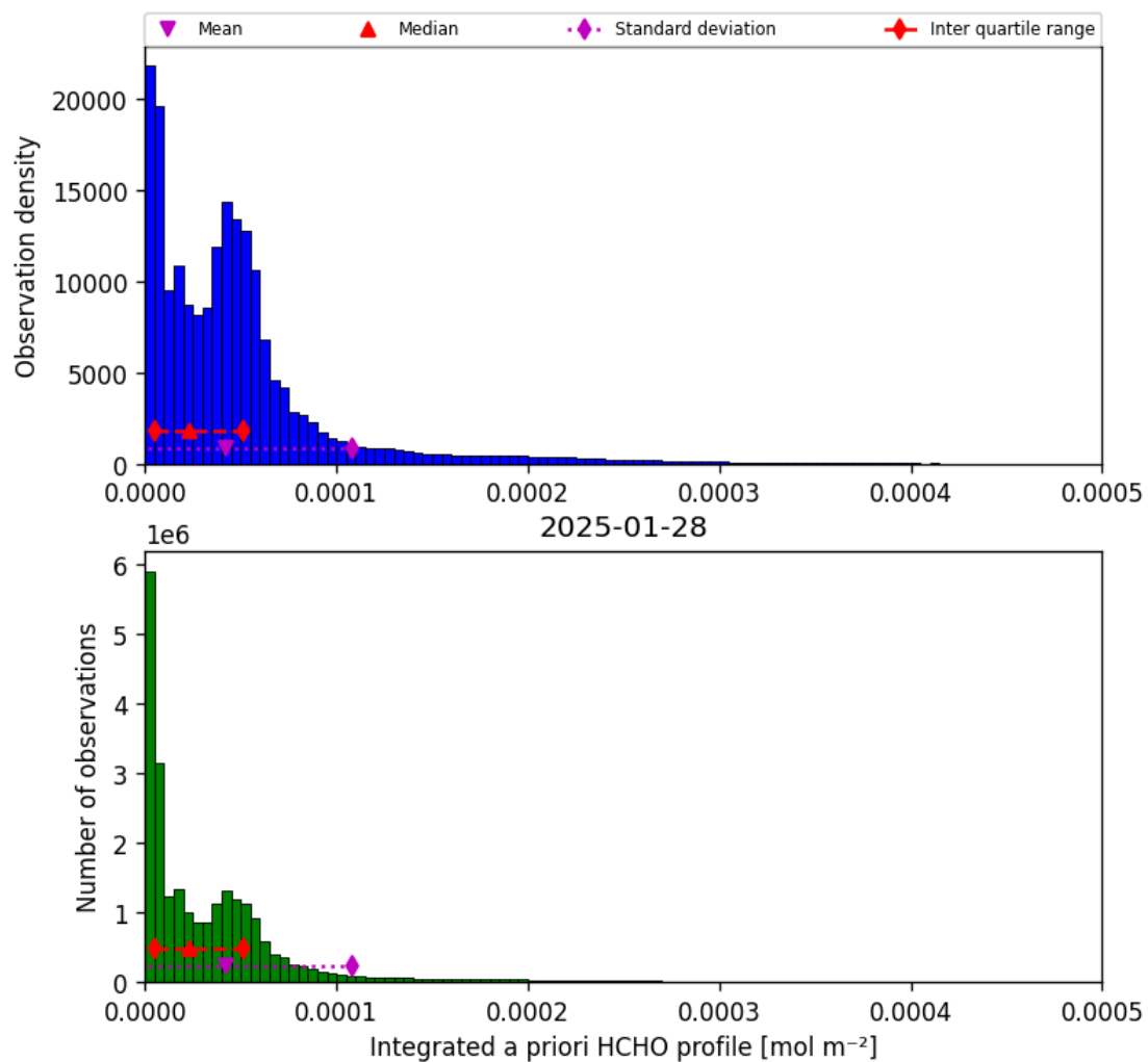
Figure 43: Histogram of “Integrated a priori HCHO profile” for 2025-01-28 to 2025-01-29
