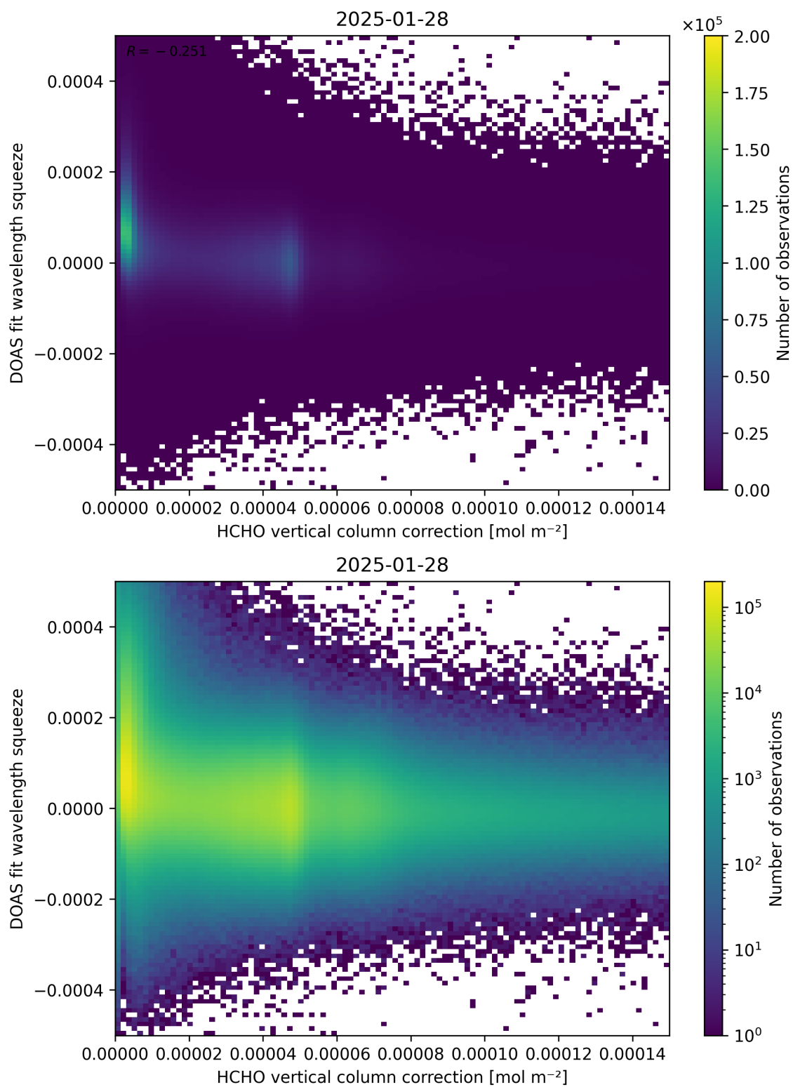
Figure 114: Scatter density plot of “HCHO vertical column correction” against “DOAS fit wavelength squeeze” for 2025-01-28 to 2025-01-29.
