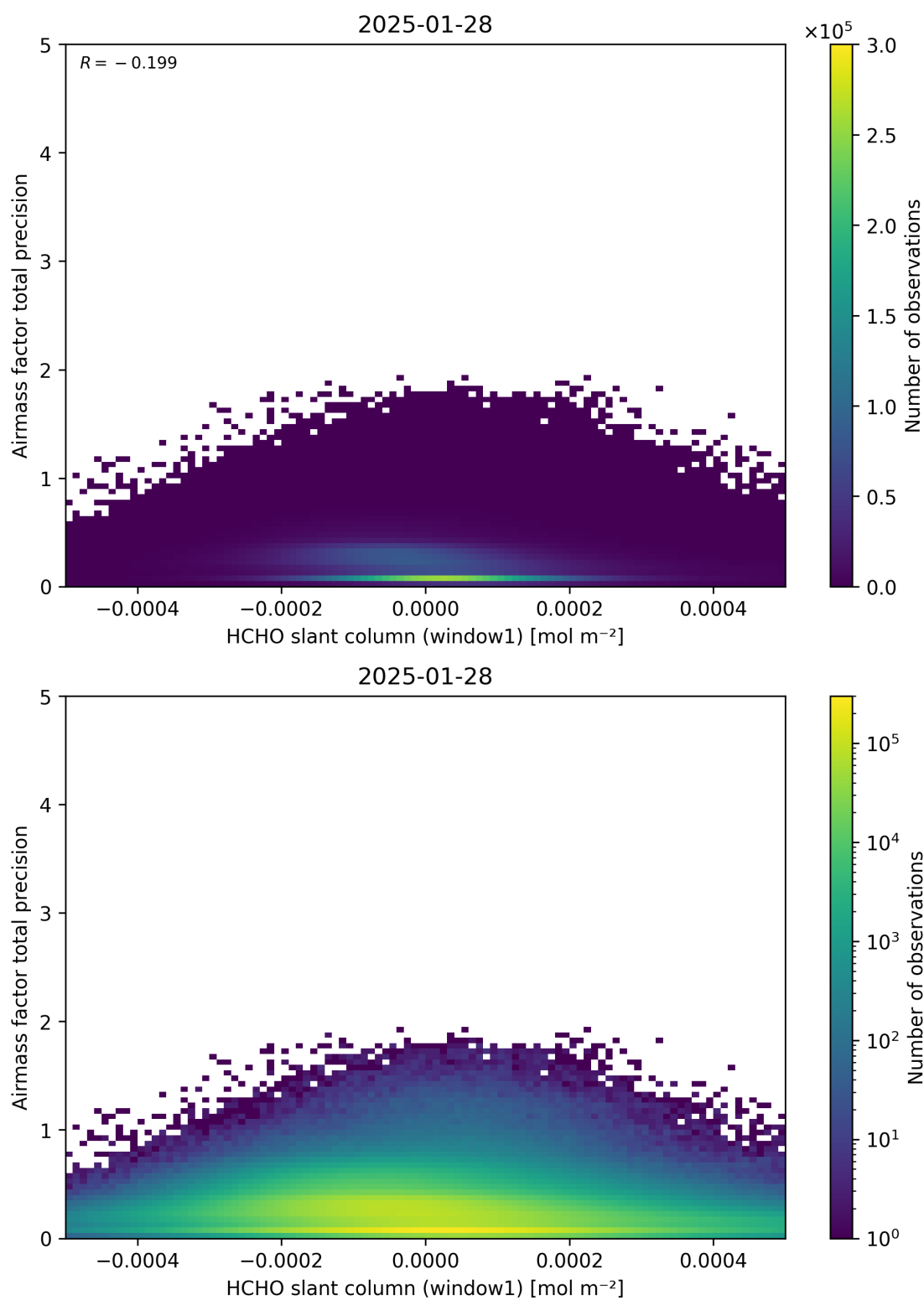
Figure 86: Scatter density plot of “HCHO slant column (window1)” against “Airmass factor total precision” for 2025-01-28 to 2025-01-29.
