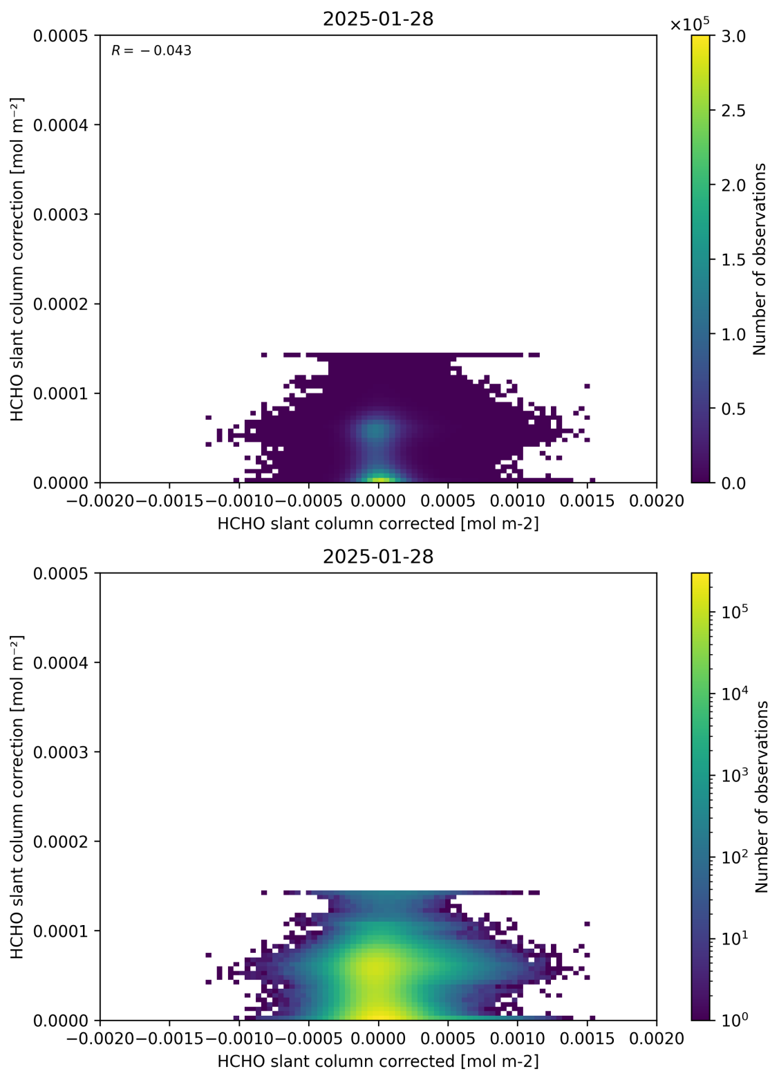
Figure 77: Scatter density plot of “HCHO slant column corrected” against “HCHO slant column correction” for 2025-01-28 to 2025-01-29.
