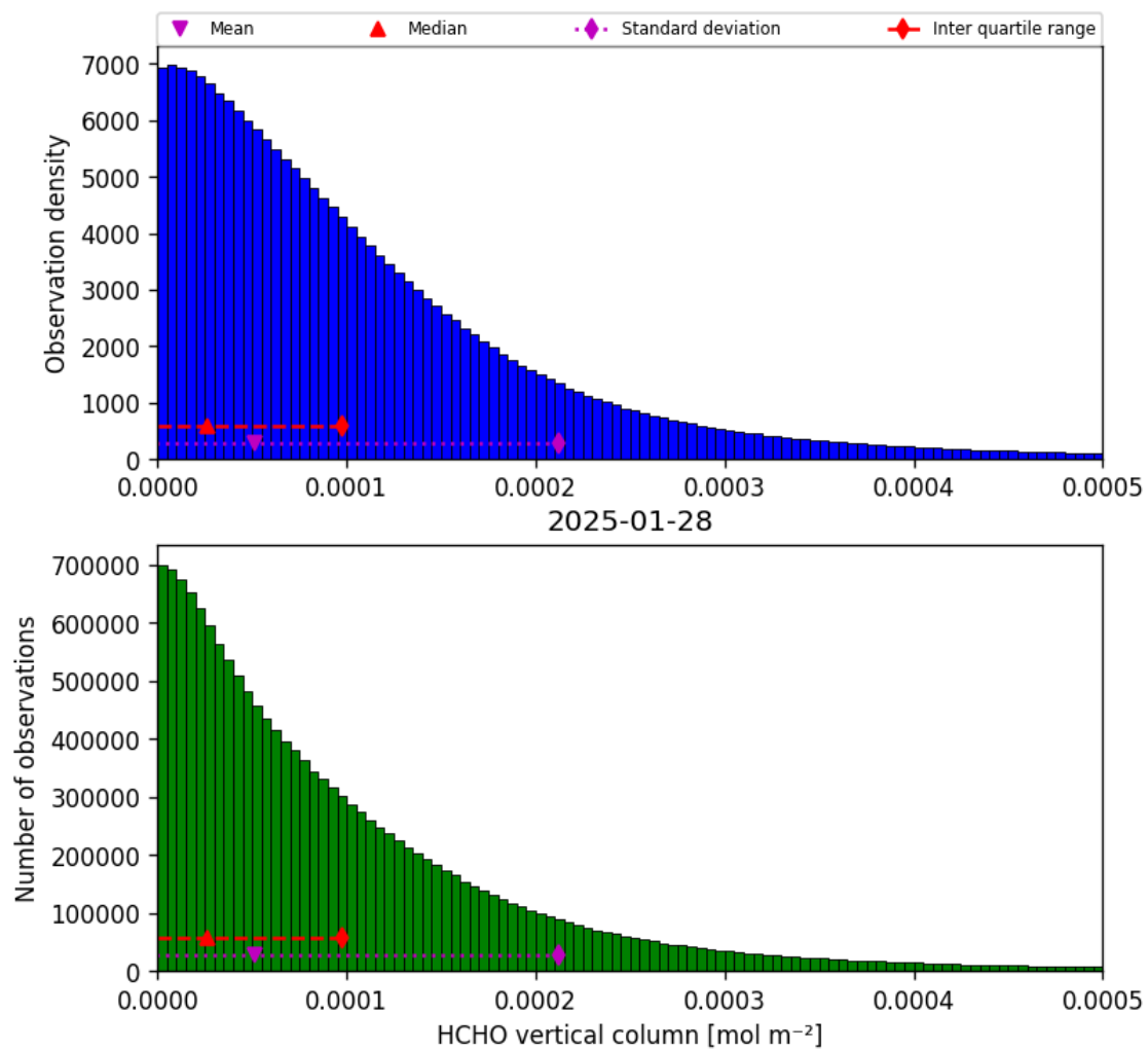
Figure 35: Histogram of “HCHO vertical column” for 2025-01-28 to 2025-01-29
