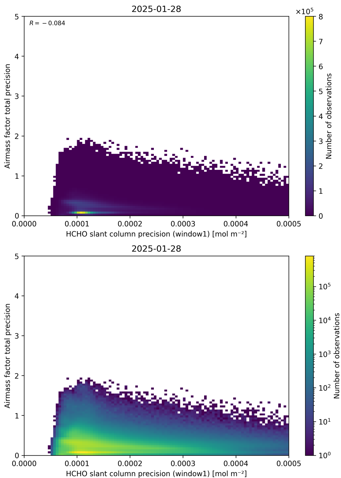
Figure 95: Scatter density plot of “HCHO slant column precision (window1)” against “Airmass factor total precision” for 2025-01-28 to 2025-01-29.
