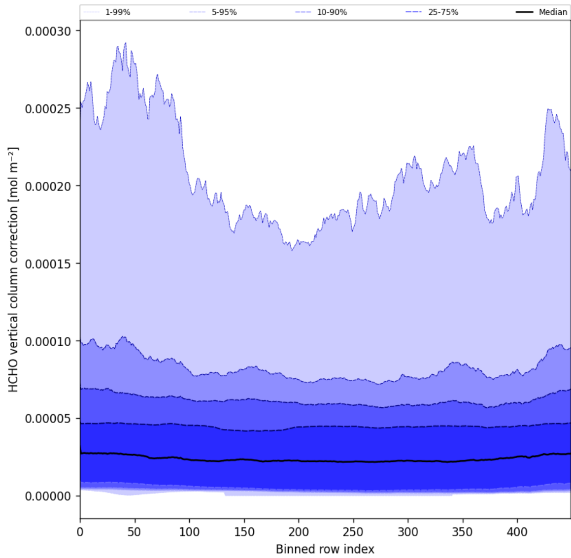
Figure 51: Along track statistics of “HCHO vertical column correction” for 2025-01-28 to 2025-01-29
