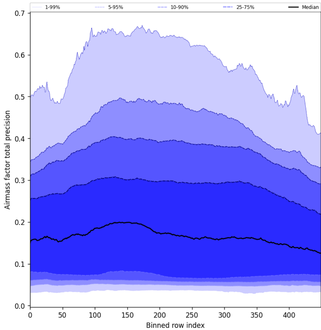
Figure 55: Along track statistics of “Airmass factor total precision” for 2025-01-28 to 2025-01-29
