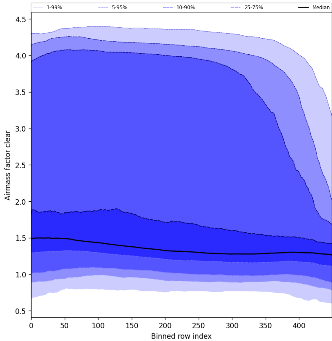
Figure 56: Along track statistics of “Airmass factor clear” for 2025-01-28 to 2025-01-29
