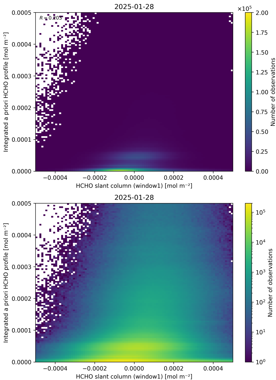
Figure 87: Scatter density plot of “HCHO slant column (window1)” against “Integrated a priori HCHO profile” for 2025-01-28 to 2025-01-29.
