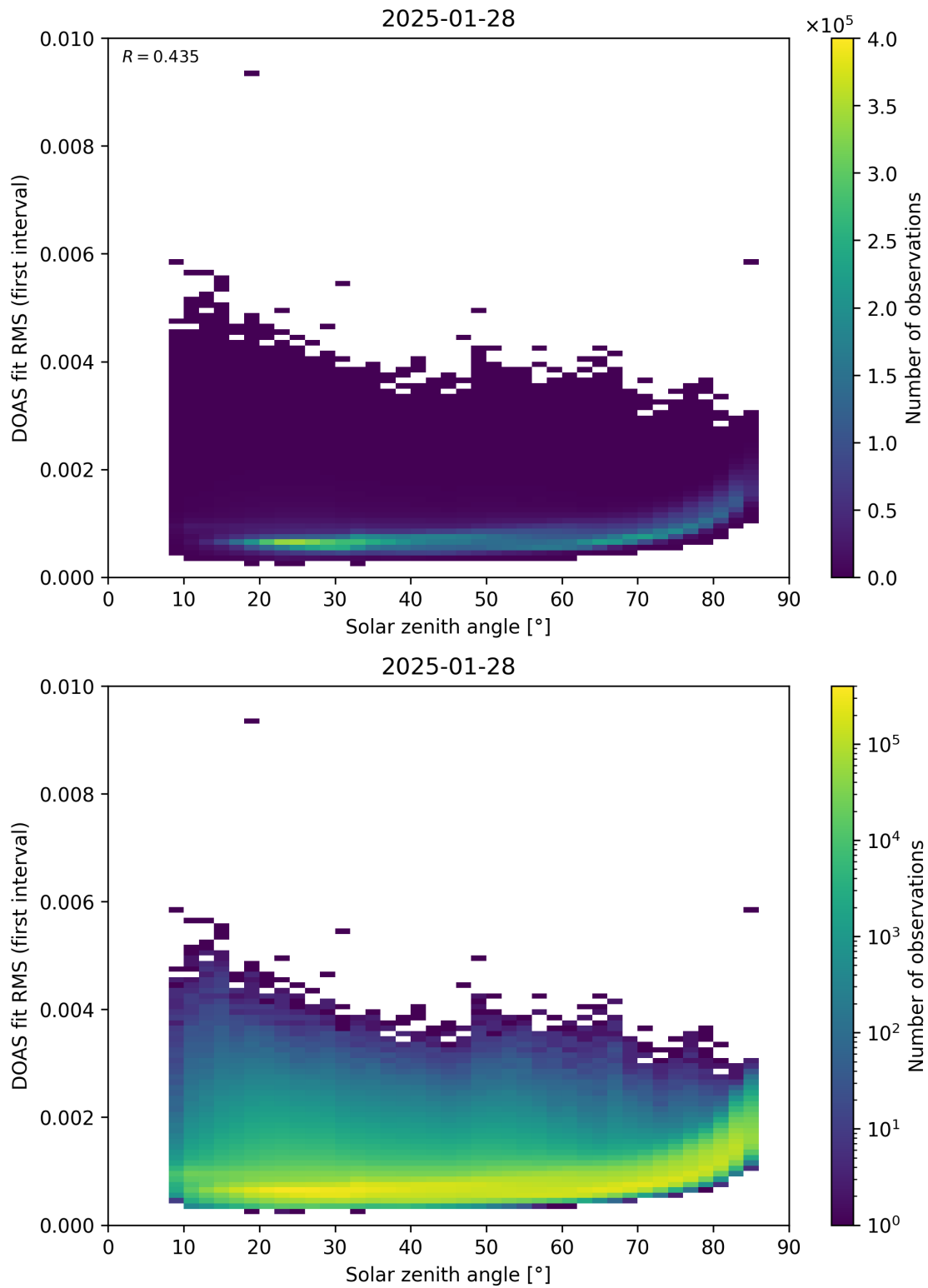
Figure 167: Scatter density plot of “Solar zenith angle” against “DOAS fit RMS (first interval)” for 2025-01-28 to 2025-01-29.
