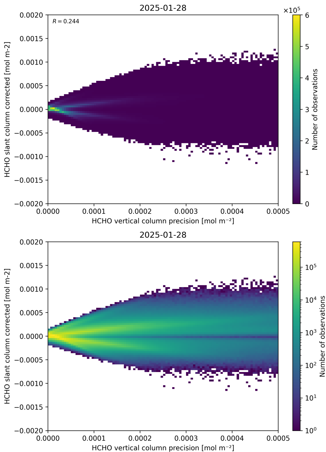
Figure 140: Scatter density plot of “HCHO vertical column precision” against “HCHO slant column corrected” for 2025-01-28 to 2025-01-29.
