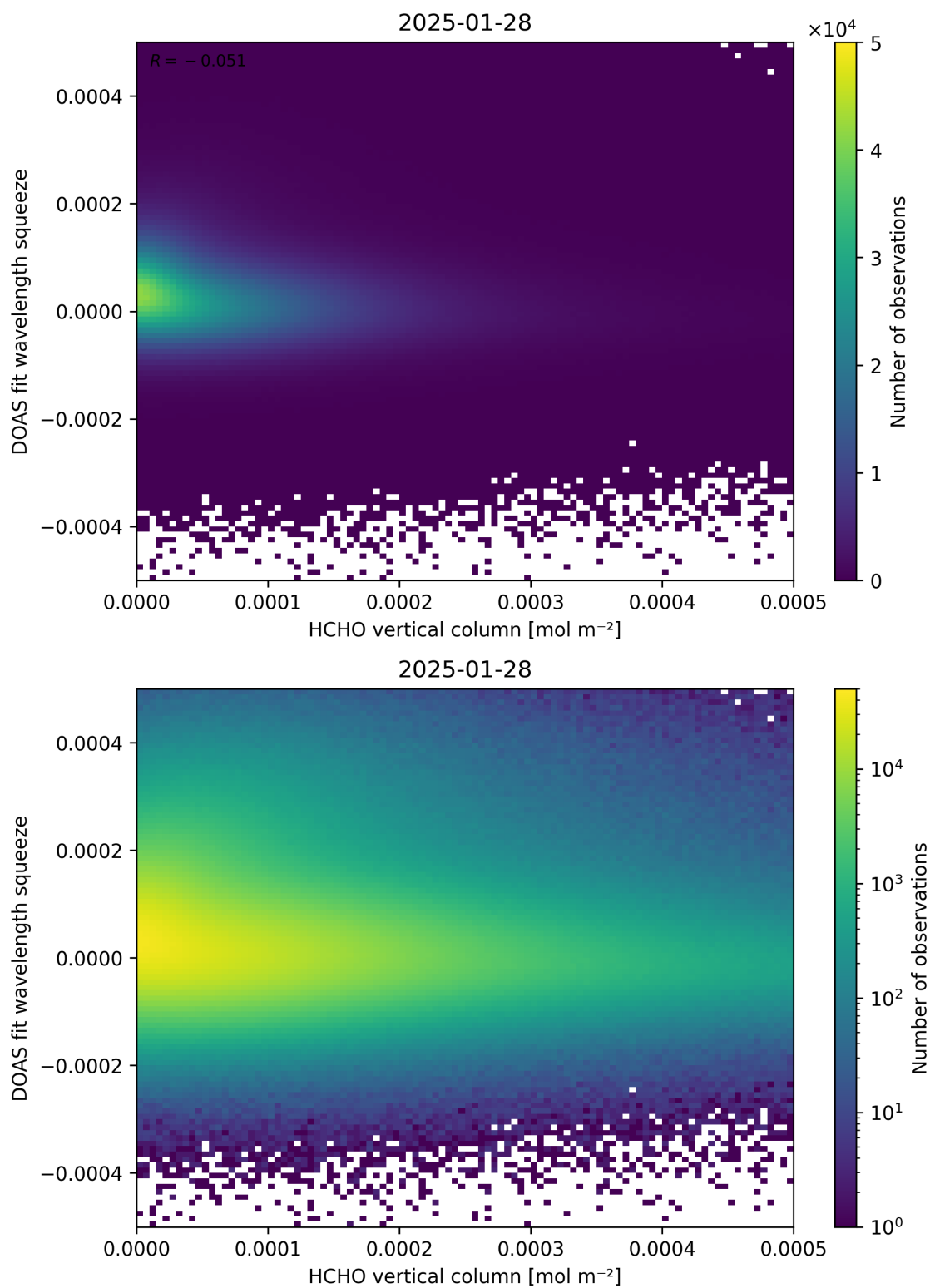
Figure 125: Scatter density plot of “HCHO vertical column” against “DOAS fit wavelength squeeze” for 2025-01-28 to 2025-01-29.
