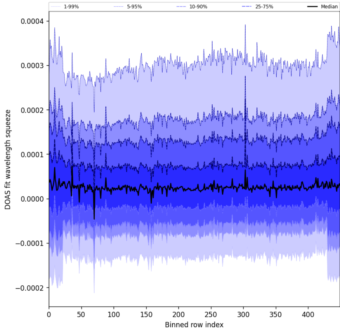
Figure 59: Along track statistics of “DOAS fit wavelength squeeze” for 2025-01-28 to 2025-01-29
