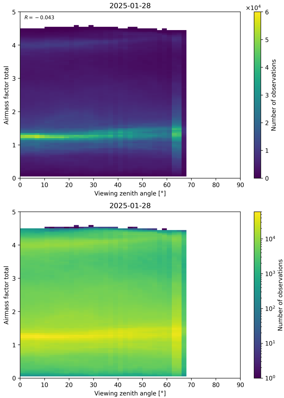
Figure 190: Scatter density plot of “Viewing zenith angle” against “Airmass factor total” for 2025-01-28 to 2025-01-29.
