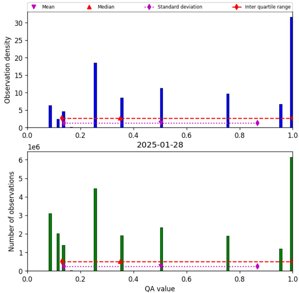
Figure 34: Histogram of “QA value” for 2025-01-28 to 2025-01-29
