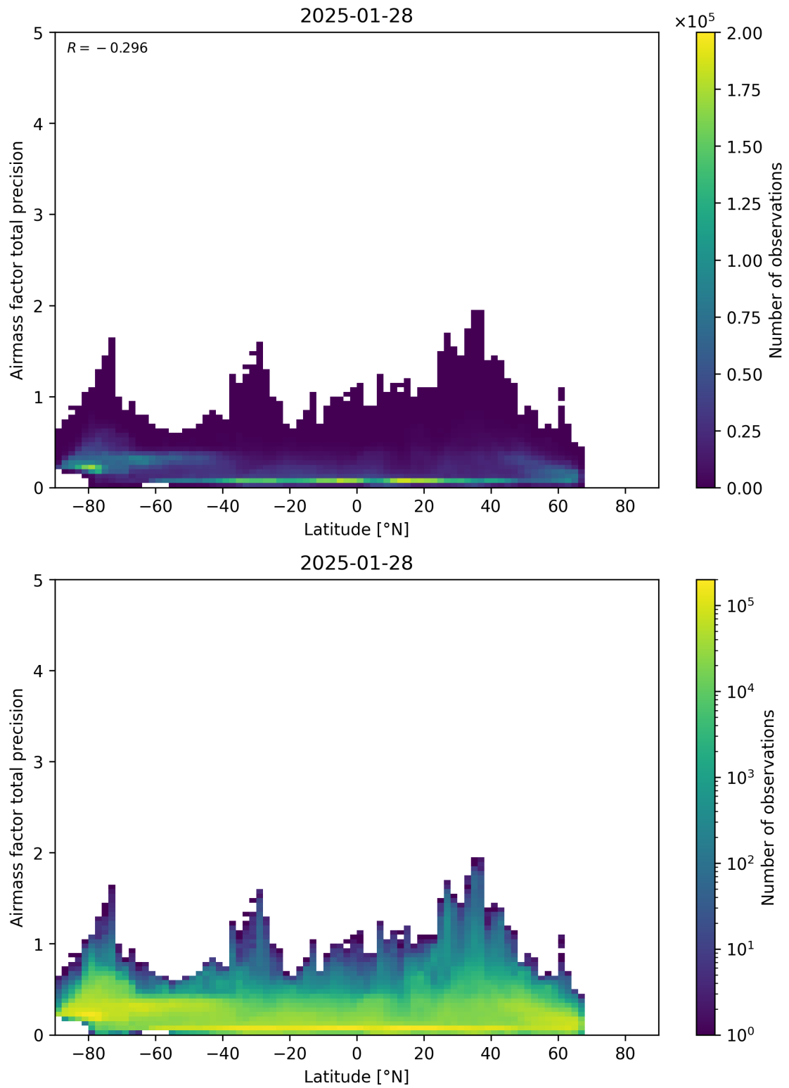
Figure 162: Scatter density plot of “Latitude” against “Airmass factor total precision” for 2025-01-28 to 2025-01-29.
