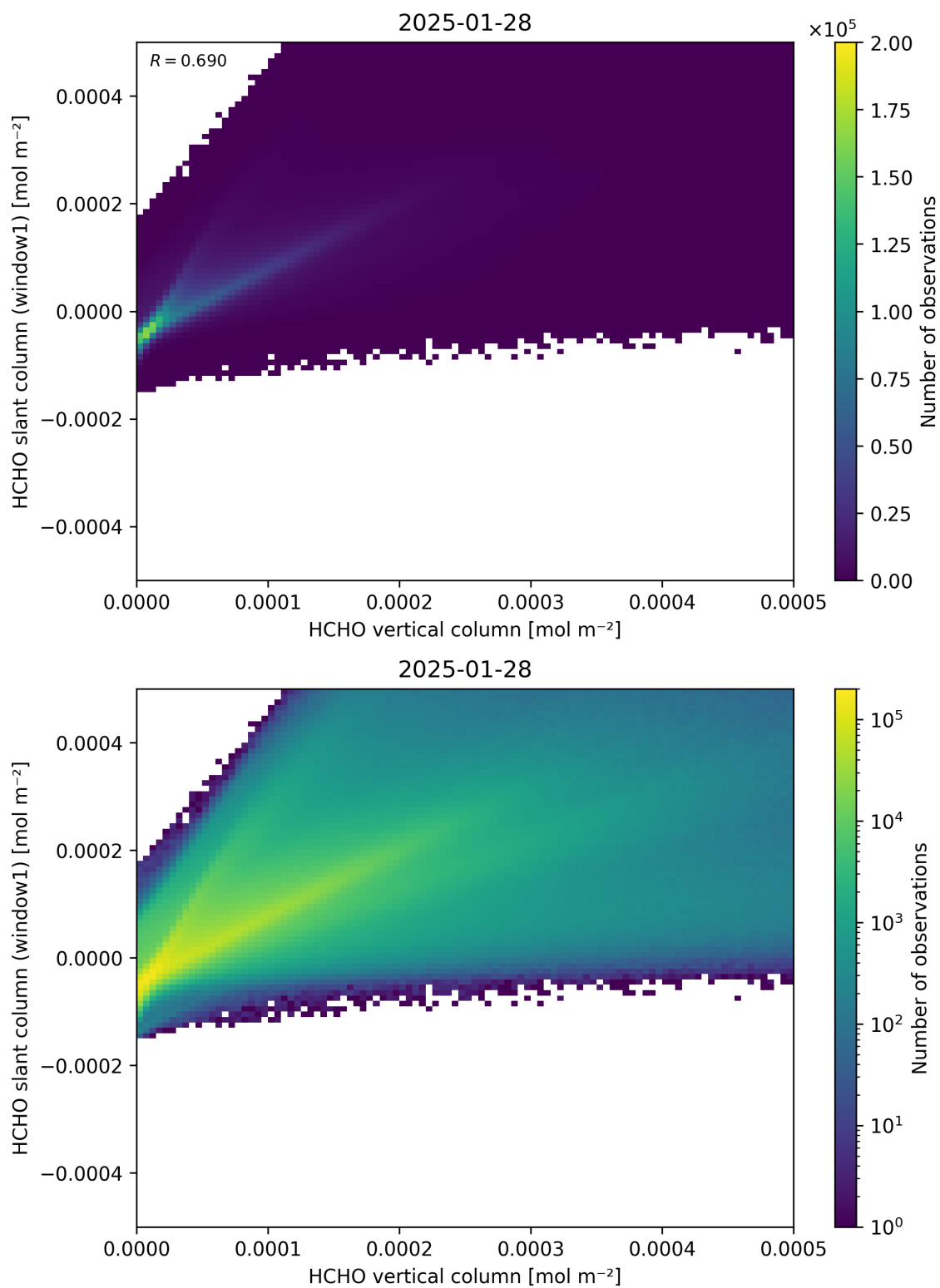
Figure 129: Scatter density plot of “HCHO vertical column” against “HCHO slant column (window1)” for 2025-01-28 to 2025-01-29.
