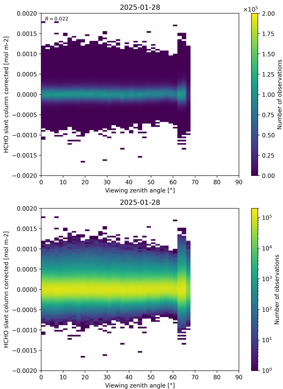
Figure 186: Scatter density plot of “Viewing zenith angle” against “HCHO slant column corrected” for 2025-01-28 to 2025-01-29.
