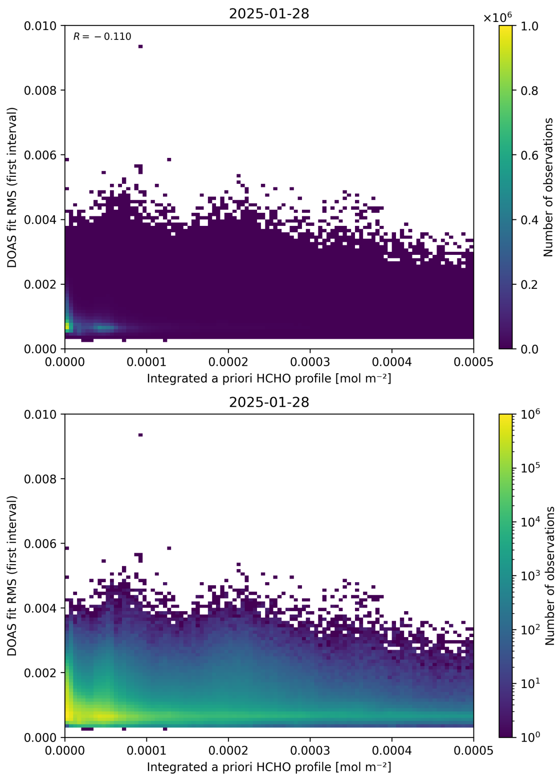
Figure 148: Scatter density plot of “Integrated a priori HCHO profile” against “DOAS fit RMS (first interval)” for 2025-01-28 to 2025-01-29.
