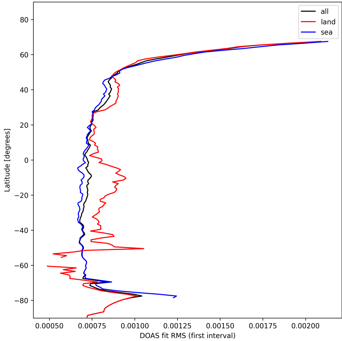
Figure 32: Zonal average of “DOAS fit RMS (first interval)” for 2025-01-28 to 2025-01-29.
