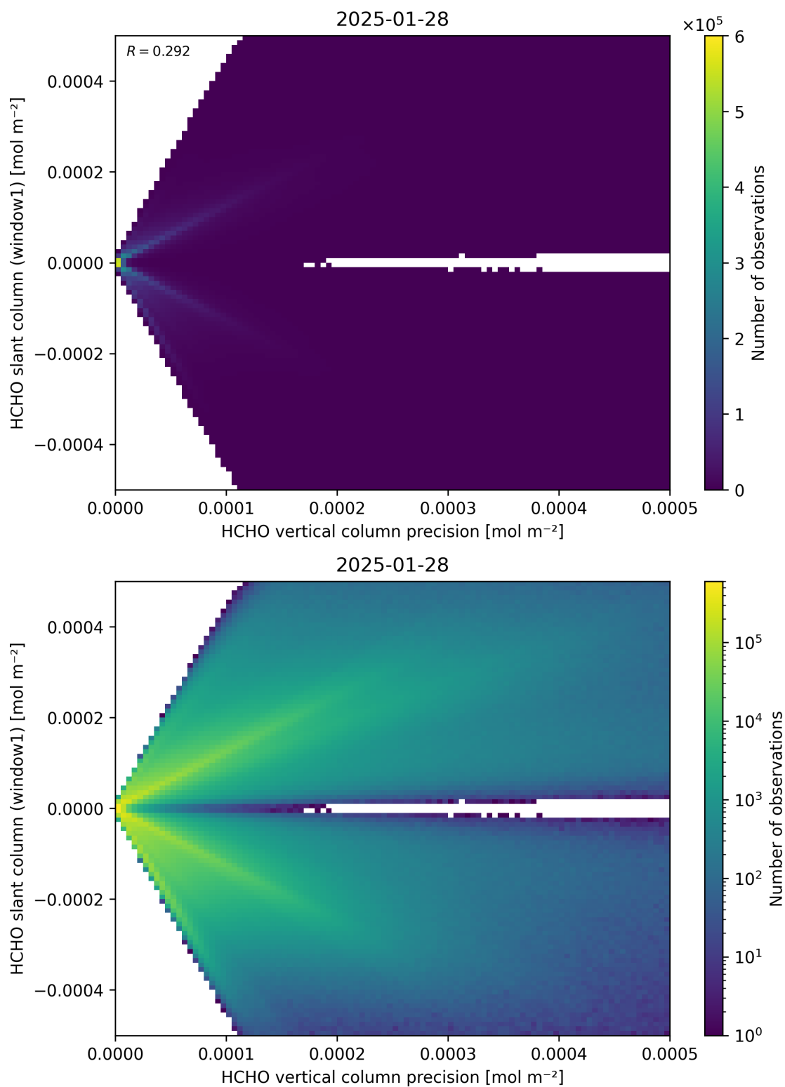
Figure 142: Scatter density plot of “HCHO vertical column precision” against “HCHO slant column (window1)” for 2025-01-28 to 2025-01-29.
