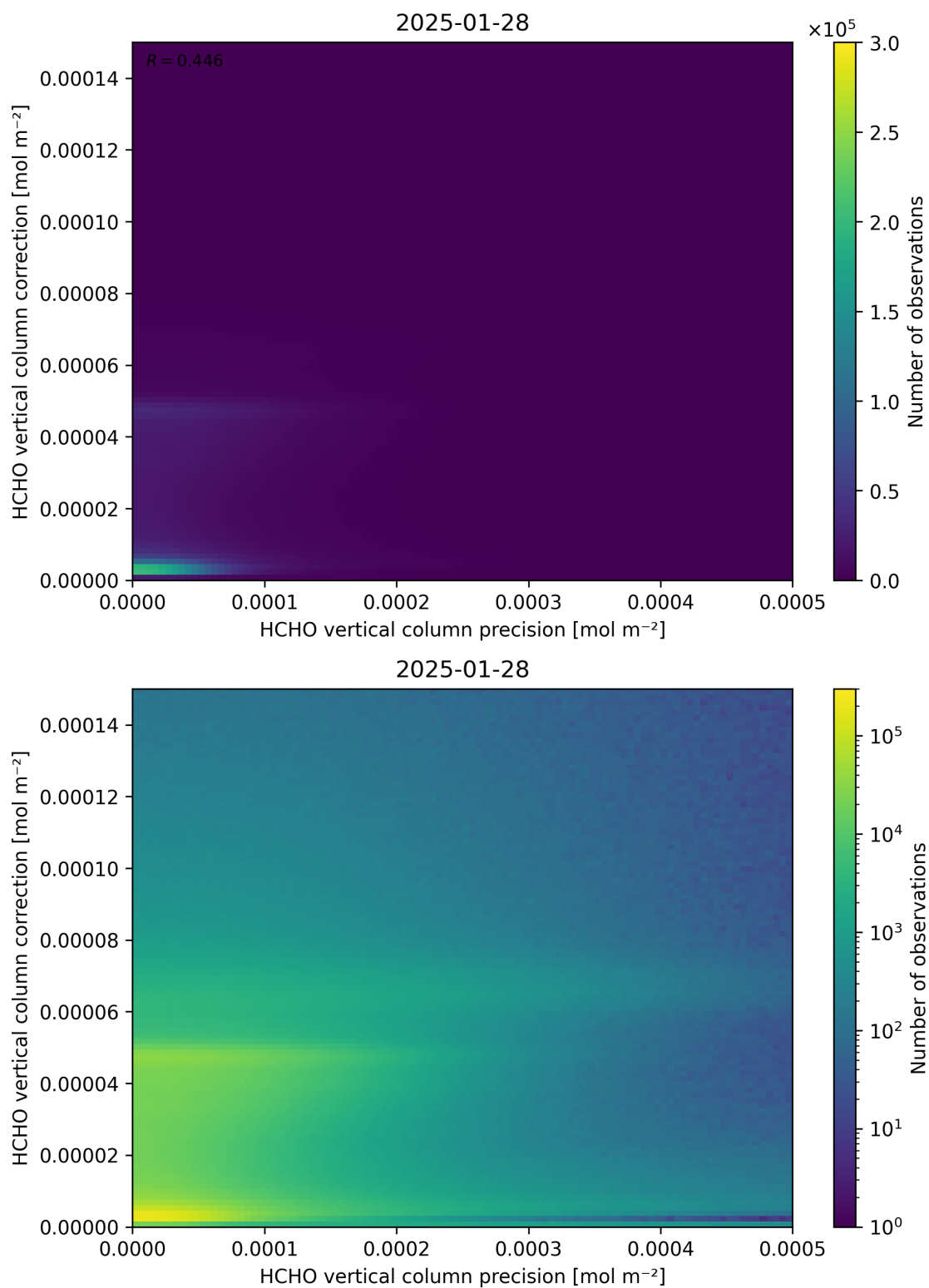
Figure 146: Scatter density plot of “HCHO vertical column precision” against “HCHO vertical column correction” for 2025-01-28 to 2025-01-29.
