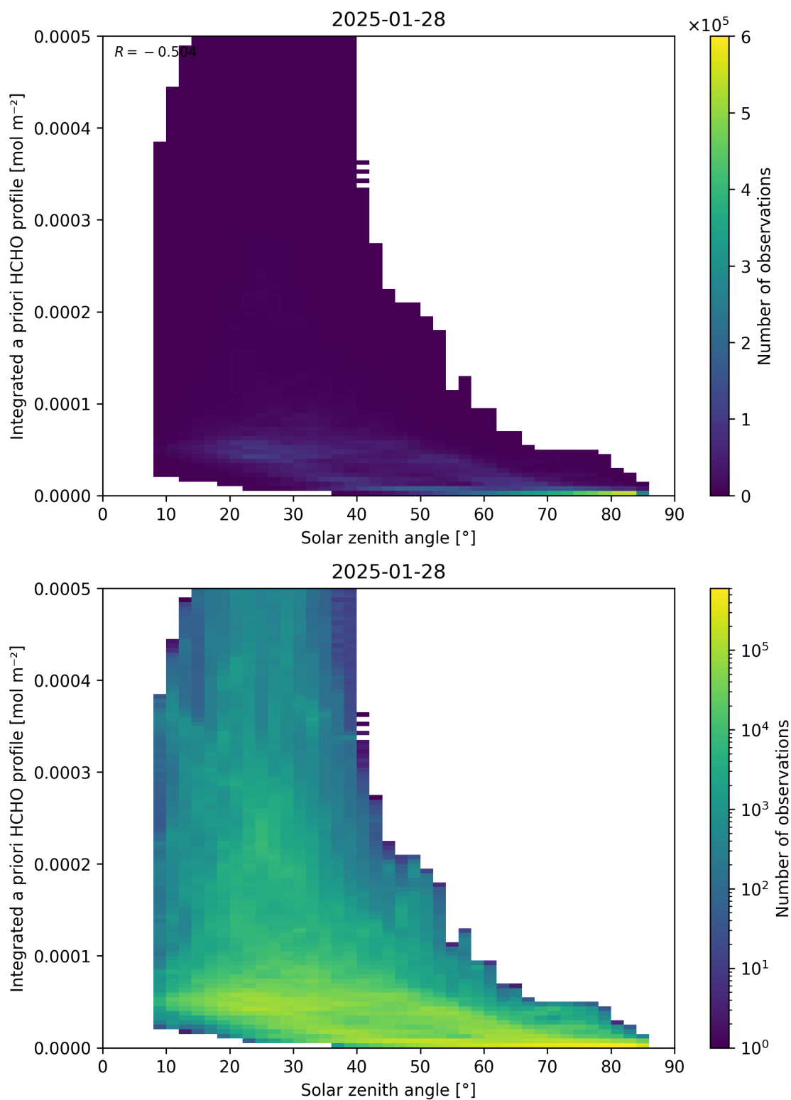
Figure 180: Scatter density plot of “Solar zenith angle” against “Integrated a priori HCHO profile” for 2025-01-28 to 2025-01-29.
