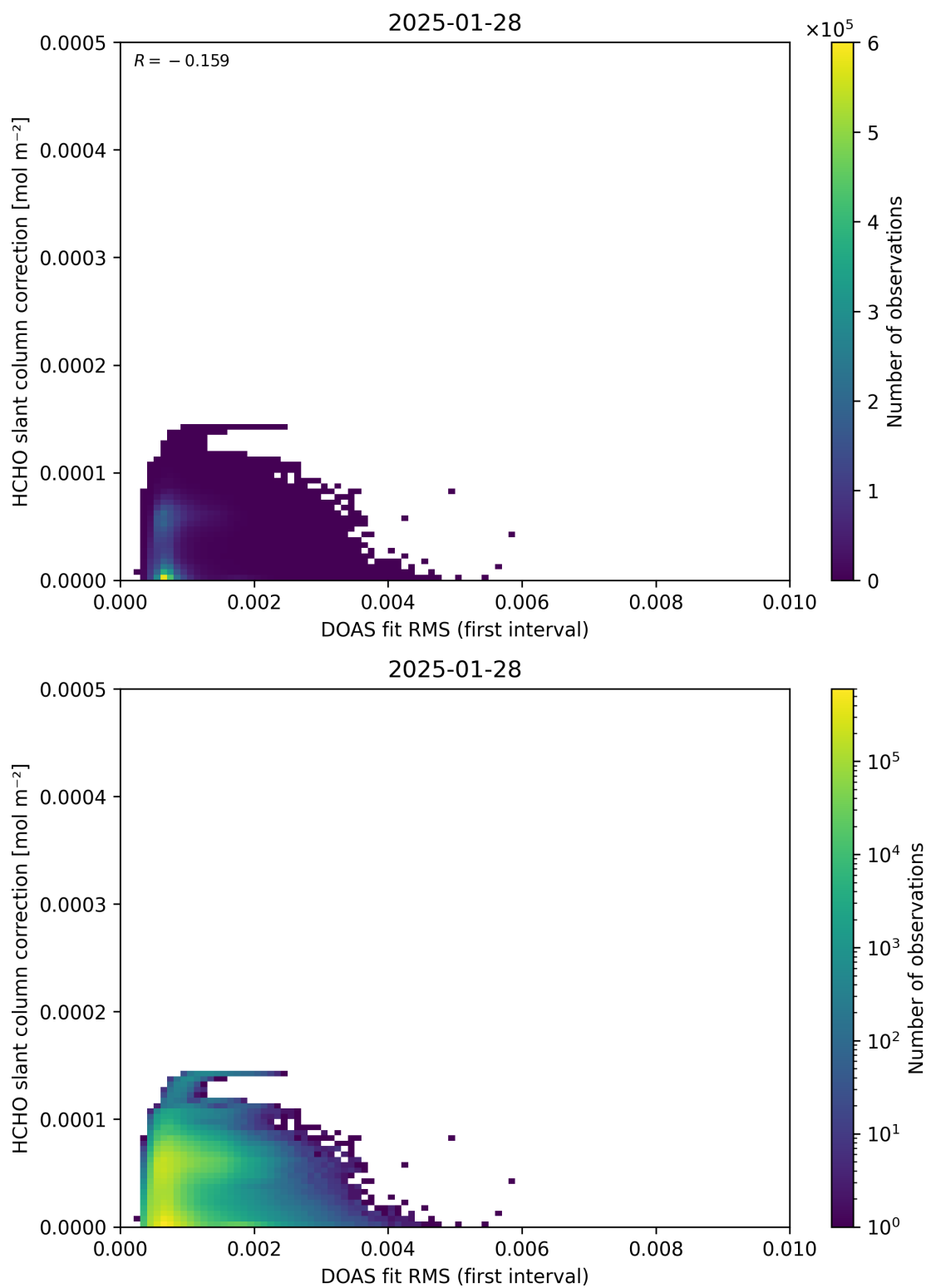
Figure 63: Scatter density plot of “DOAS fit RMS (first interval)” against “HCHO slant column correction” for 2025-01-28 to 2025-01-29.
