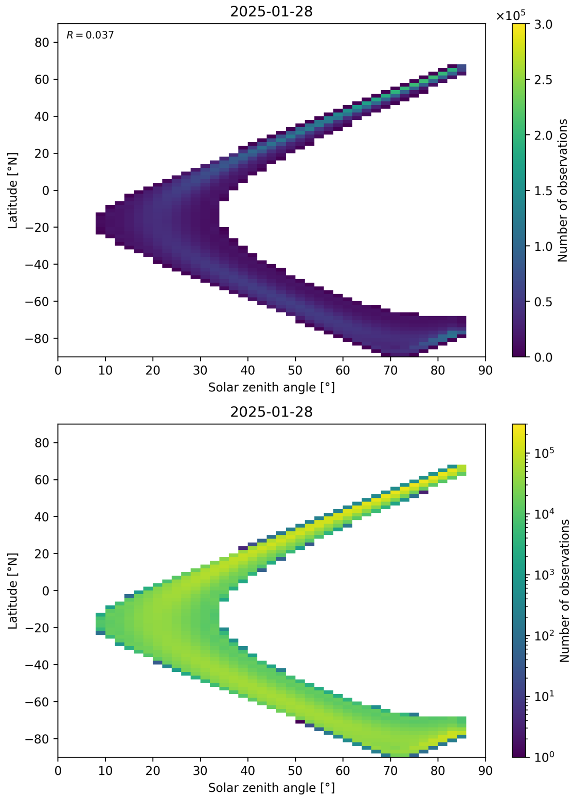
Figure 181: Scatter density plot of “Solar zenith angle” against “Latitude” for 2025-01-28 to 2025-01-29.
