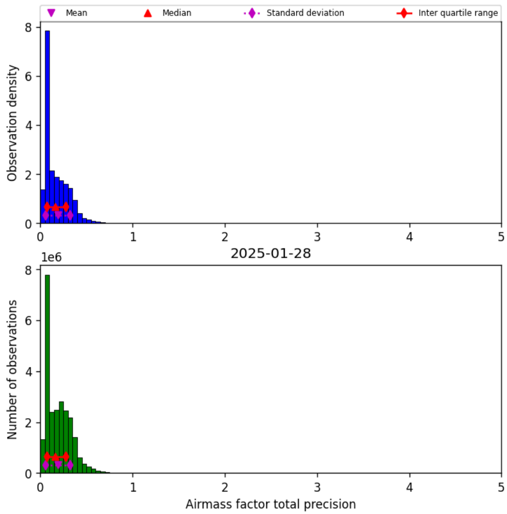
Figure 41: Histogram of “Airmass factor total precision” for 2025-01-28 to 2025-01-29
