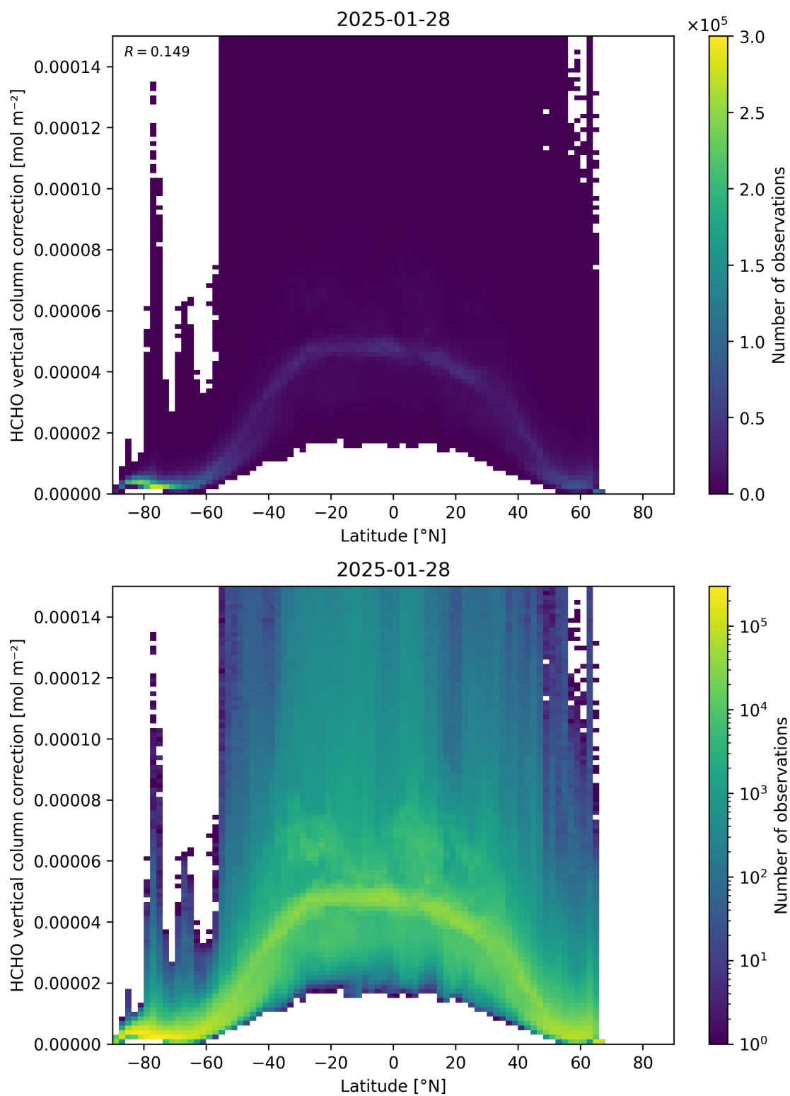
Figure 164: Scatter density plot of “Latitude” against “HCHO vertical column correction” for 2025-01-28 to 2025-01-29.
