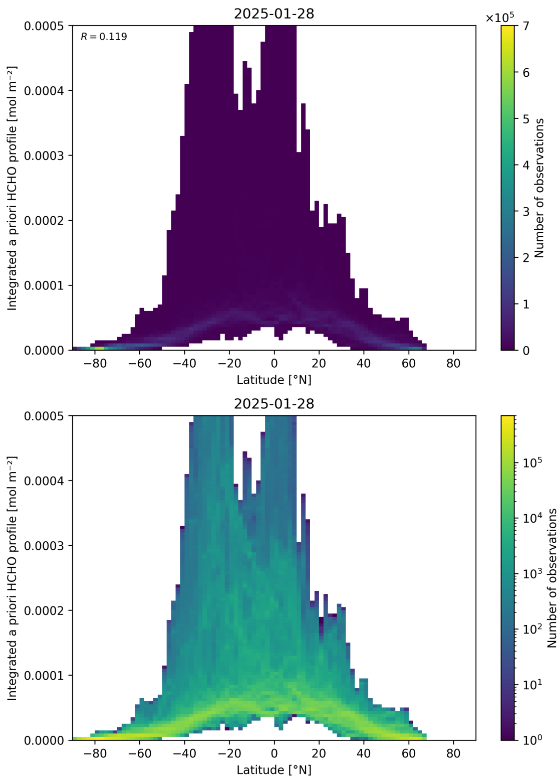
Figure 166: Scatter density plot of “Latitude” against “Integrated a priori HCHO profile” for 2025-01-28 to 2025-01-29.
