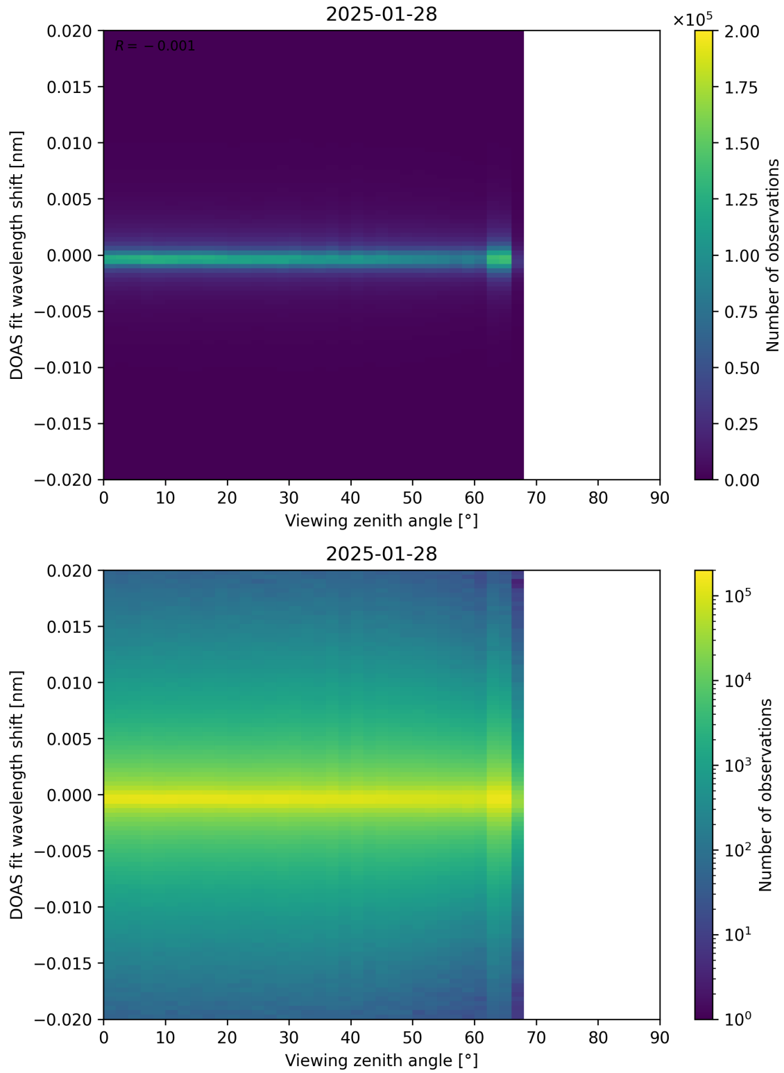
Figure 183: Scatter density plot of “Viewing zenith angle” against “DOAS fit wavelength shift” for 2025-01-28 to 2025-01-29.
