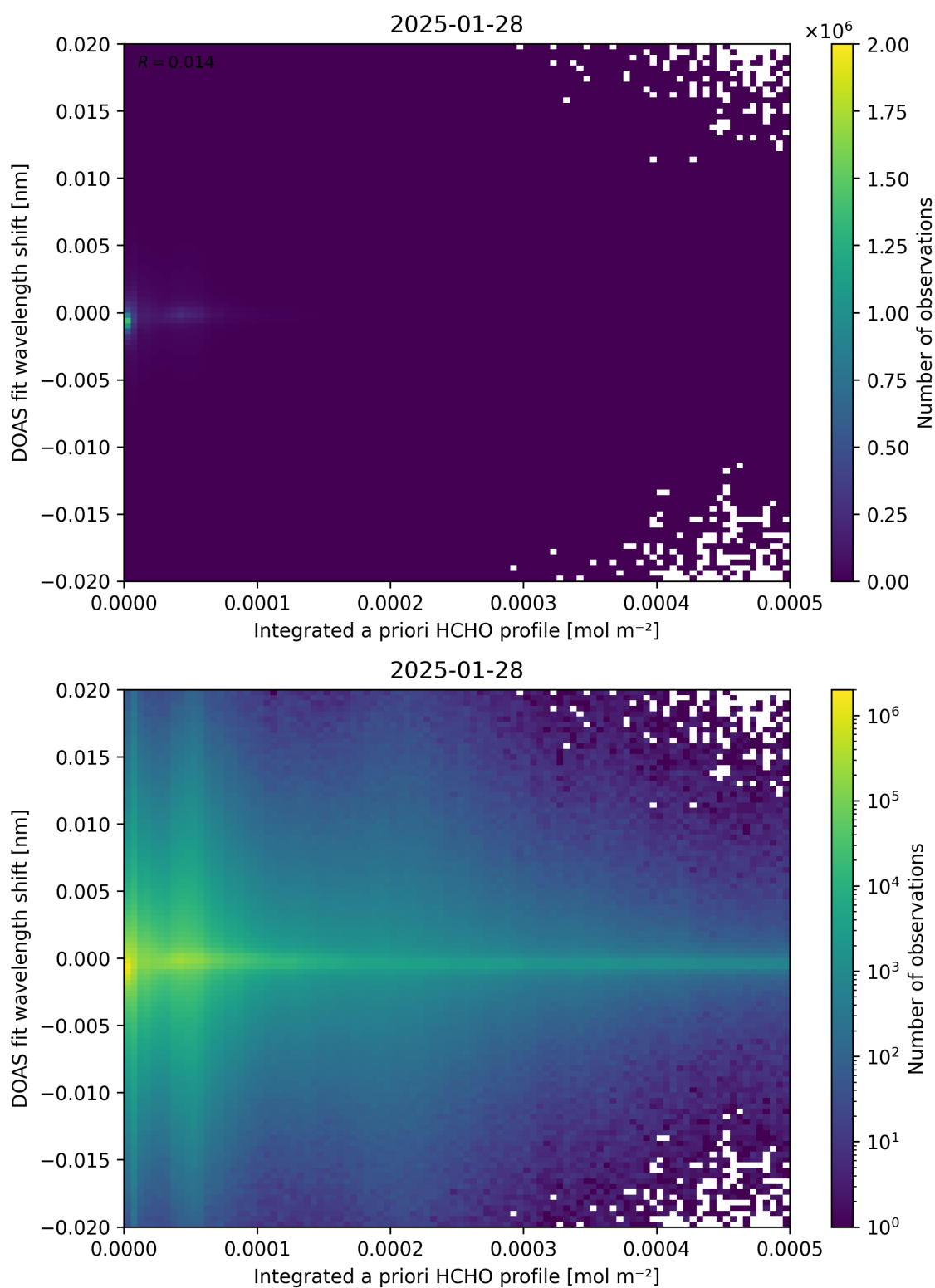
Figure 149: Scatter density plot of “Integrated a priori HCHO profile” against “DOAS fit wavelength shift” for 2025-01-28 to 2025-01-29.
