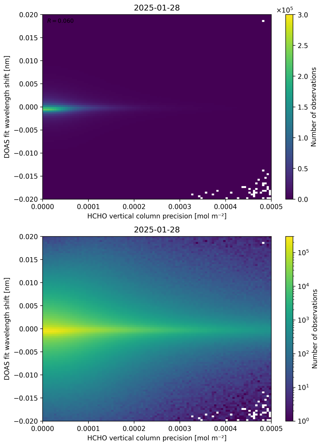
Figure 137: Scatter density plot of “HCHO vertical column precision” against “DOAS fit wavelength shift” for 2025-01-28 to 2025-01-29.
