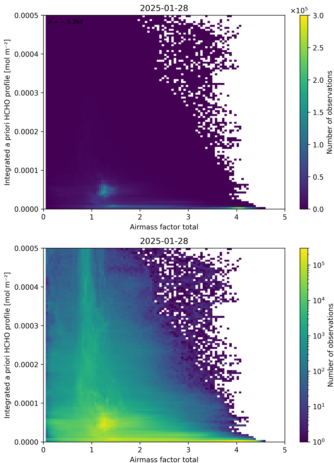
Figure 104: Scatter density plot of “Airmass factor total” against “Integrated a priori HCHO profile” for 2025-01-28 to 2025-01-29.
