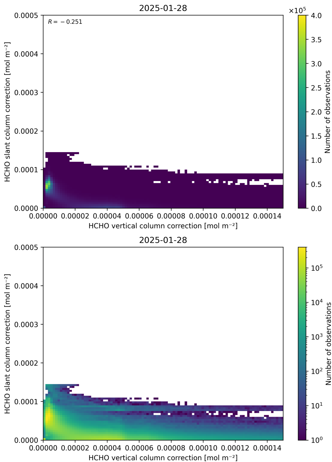
Figure 117: Scatter density plot of “HCHO vertical column correction” against “HCHO slant column correction” for 2025-01-28 to 2025-01-29.
