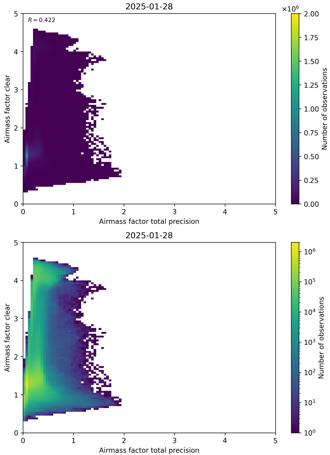
Figure 108: Scatter density plot of “Airmass factor total precision” against “Airmass factor clear” for 2025-01-28 to 2025-01-29.
