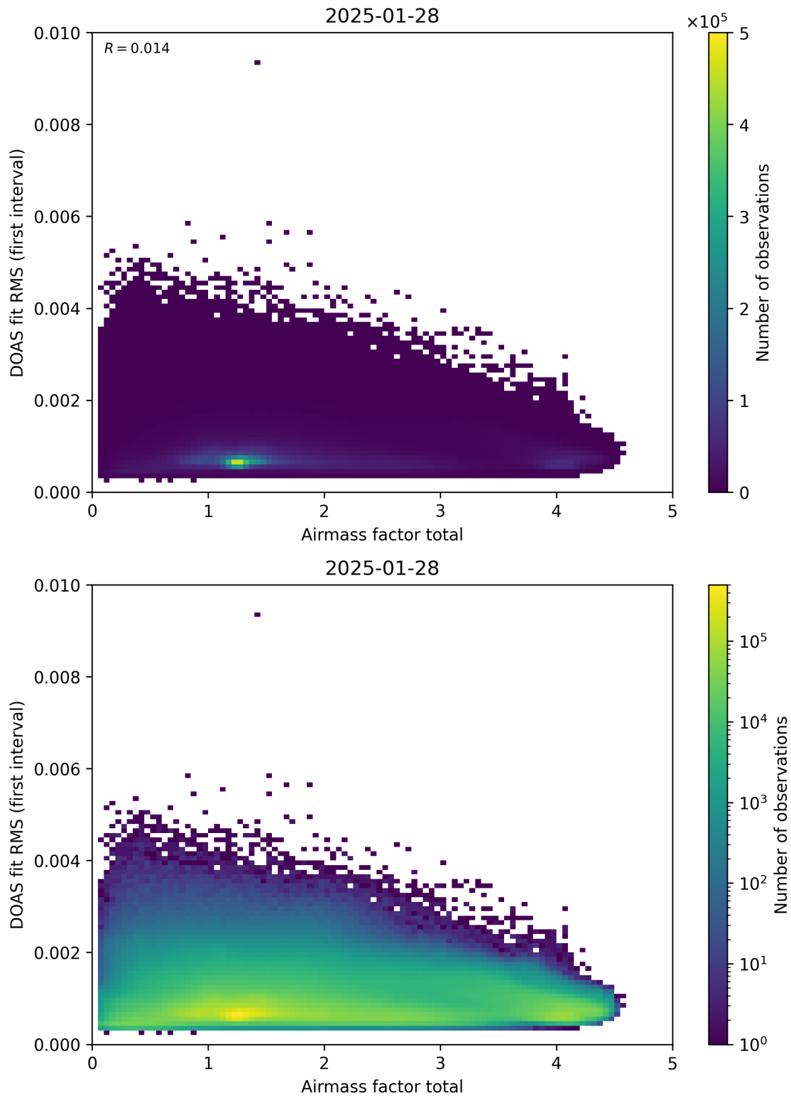
Figure 97: Scatter density plot of “Airmass factor total” against “DOAS fit RMS (first interval)” for 2025-01-28 to 2025-01-29.
