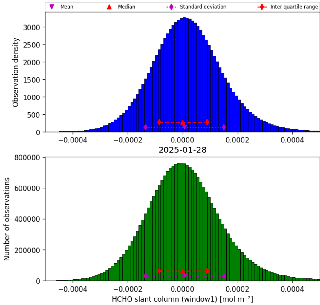
Figure 38: Histogram of “HCHO slant column (window1)” for 2025-01-28 to 2025-01-29
