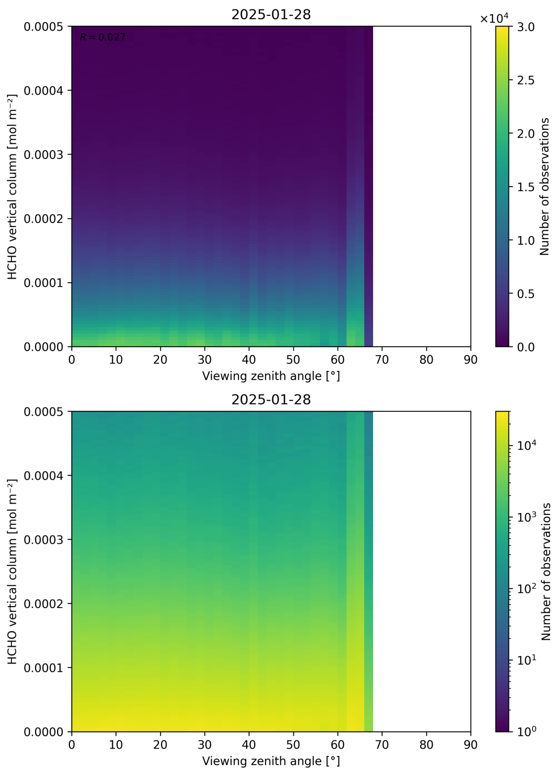
Figure 192: Scatter density plot of “Viewing zenith angle” against “HCHO vertical column” for 2025-01-28 to 2025-01-29.
