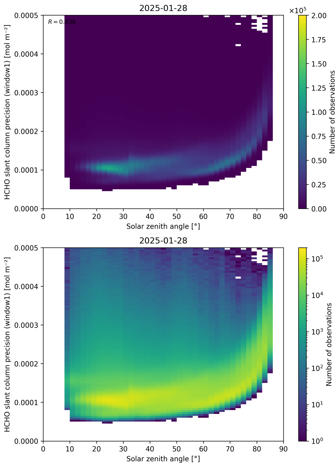
Figure 174: Scatter density plot of “Solar zenith angle” against “HCHO slant column precision (window1)” for 2025-01-28 to 2025-01-29.
