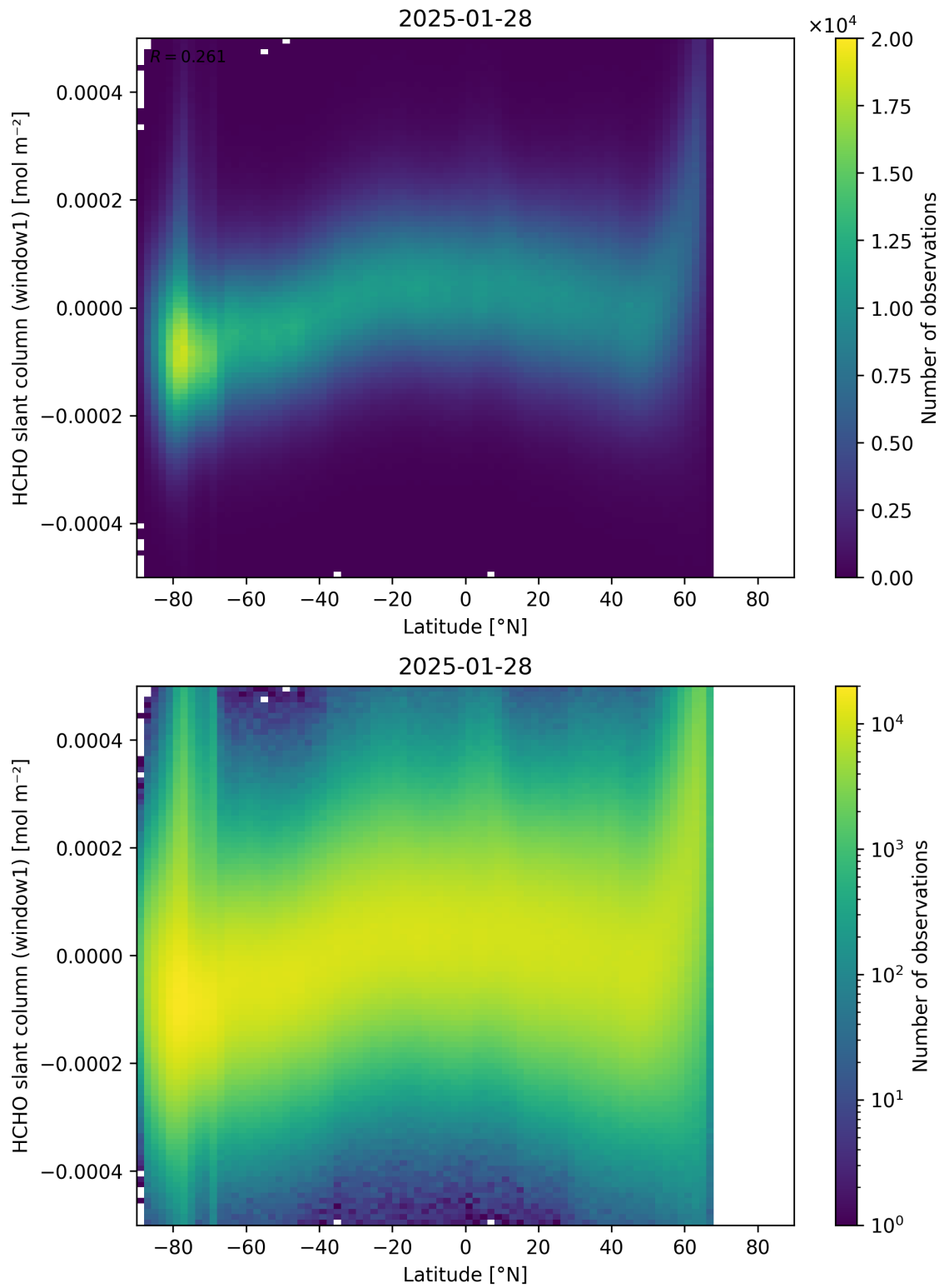
Figure 159: Scatter density plot of “Latitude” against “HCHO slant column (window1)” for 2025-01-28 to 2025-01-29.
