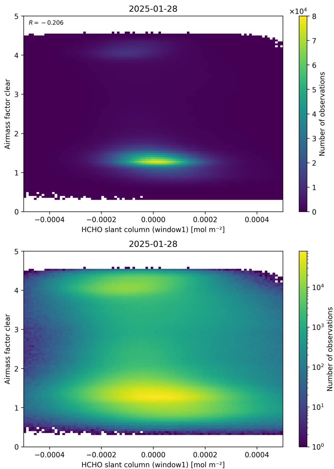
Figure 81: Scatter density plot of “HCHO slant column (window1)” against “Airmass factor clear” for 2025-01-28 to 2025-01-29.
