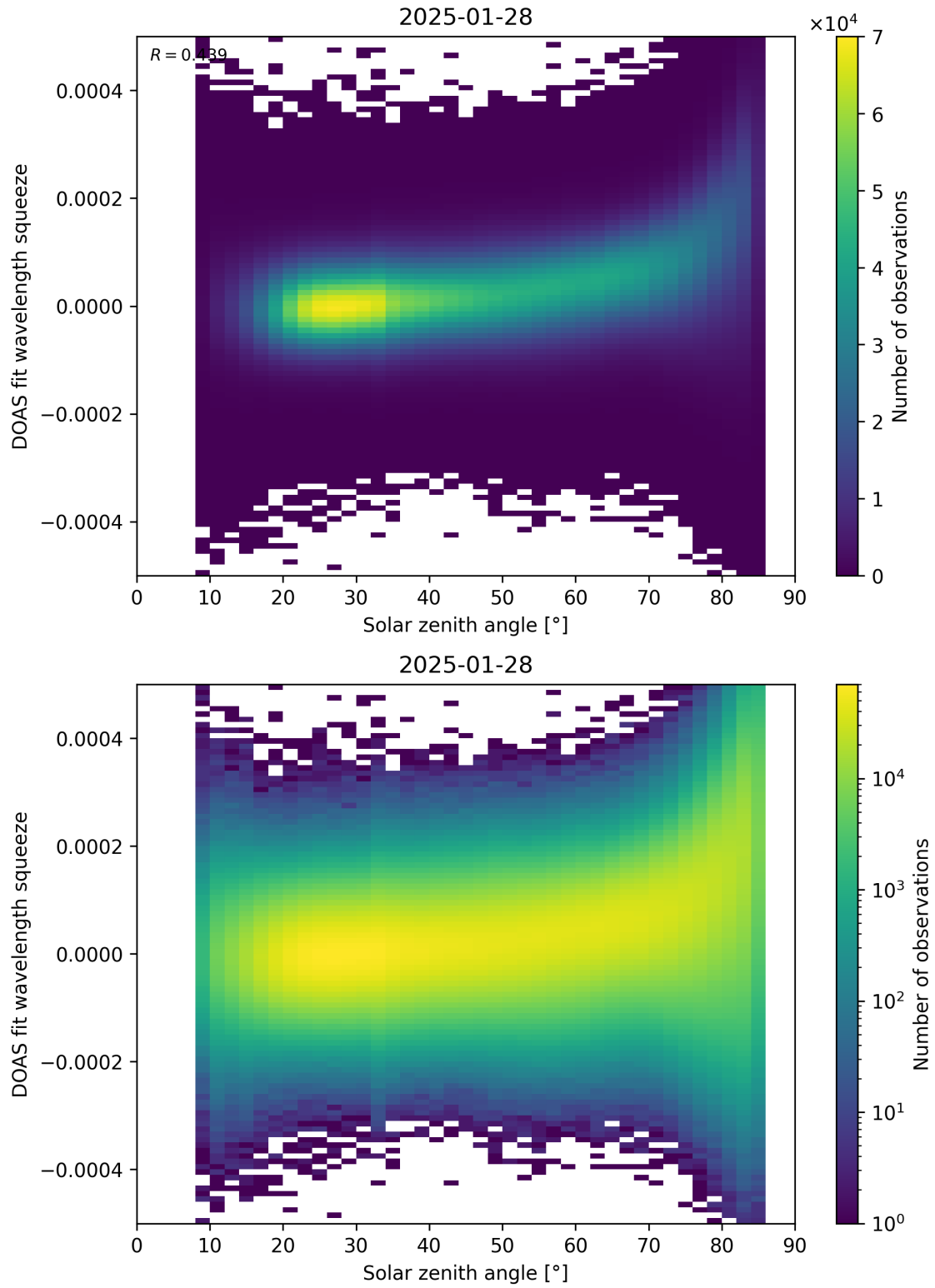
Figure 169: Scatter density plot of “Solar zenith angle” against “DOAS fit wavelength squeeze” for 2025-01-28 to 2025-01-29.
