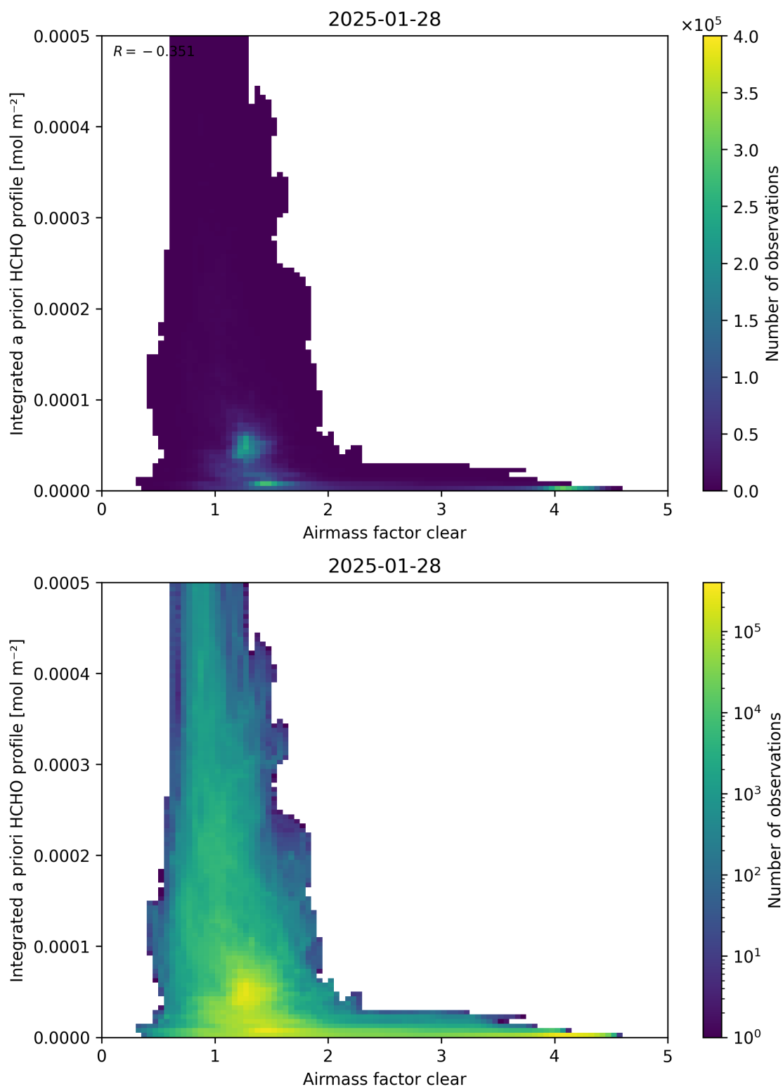
Figure 76: Scatter density plot of “Airmass factor clear” against “Integrated a priori HCHO profile” for 2025-01-28 to 2025-01-29.
