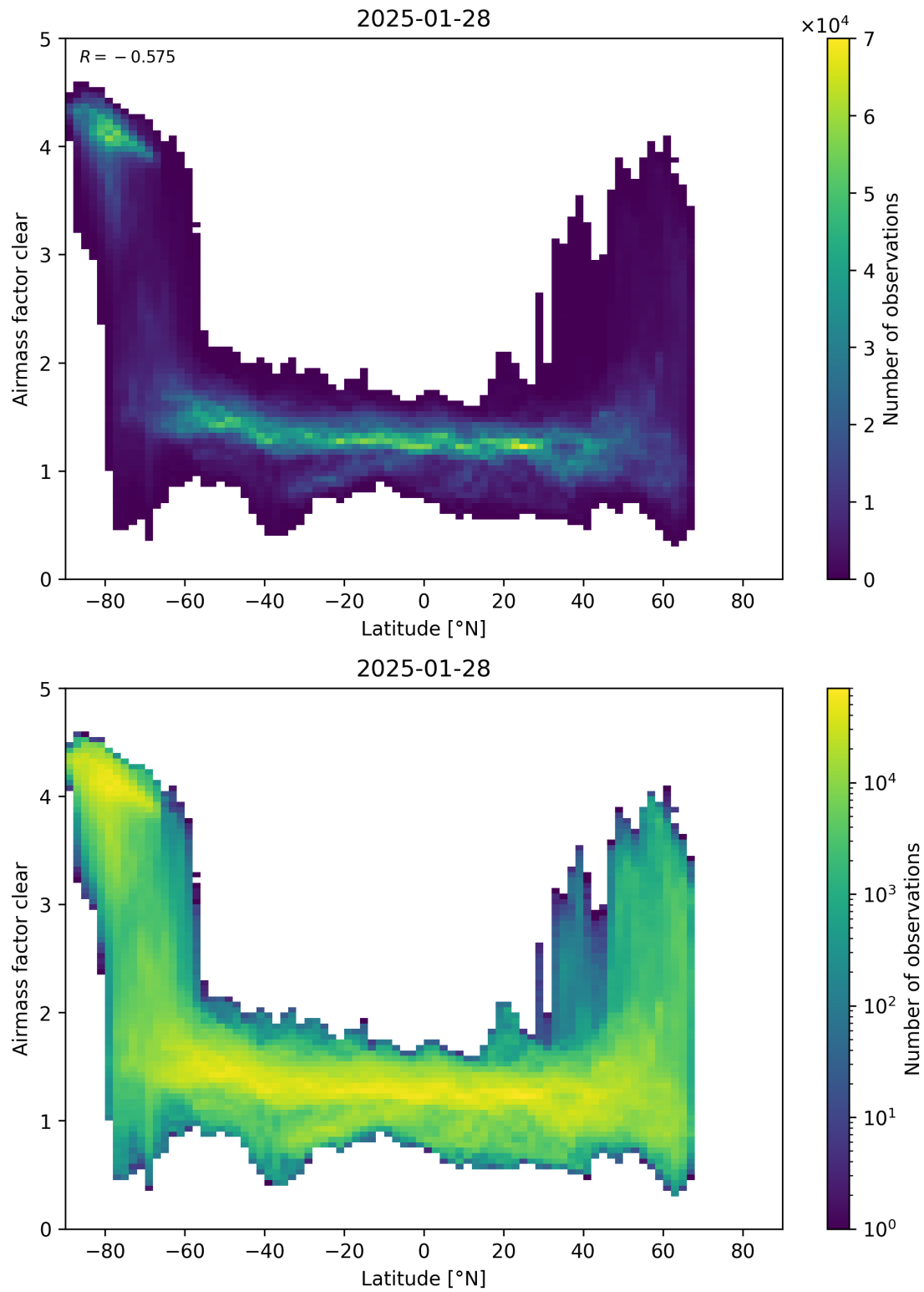
Figure 156: Scatter density plot of “Latitude” against “Airmass factor clear” for 2025-01-28 to 2025-01-29.
