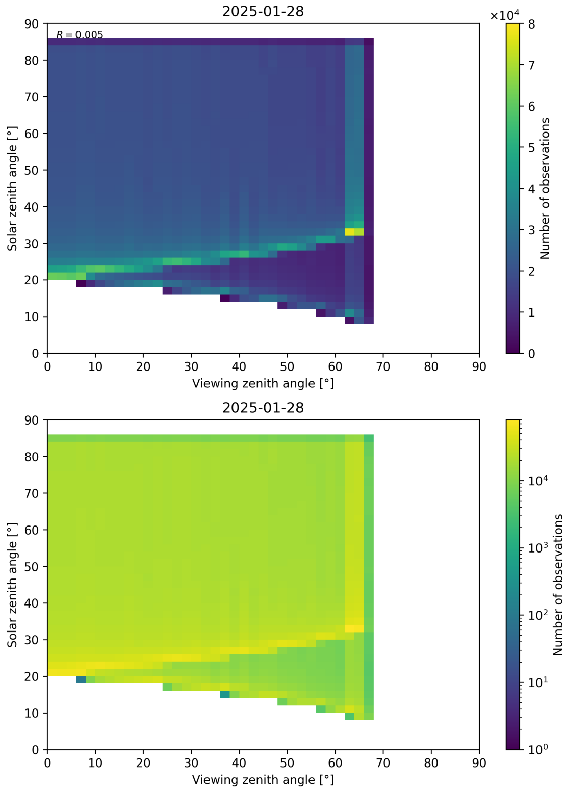
Figure 197: Scatter density plot of “Viewing zenith angle” against “Solar zenith angle” for 2025-01-28 to 2025-01-29.
