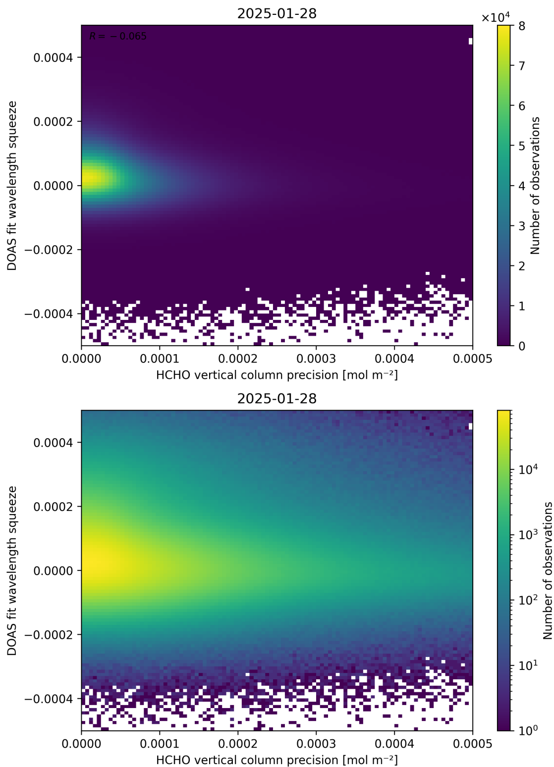
Figure 138: Scatter density plot of “HCHO vertical column precision” against “DOAS fit wavelength squeeze” for 2025-01-28 to 2025-01-29.
