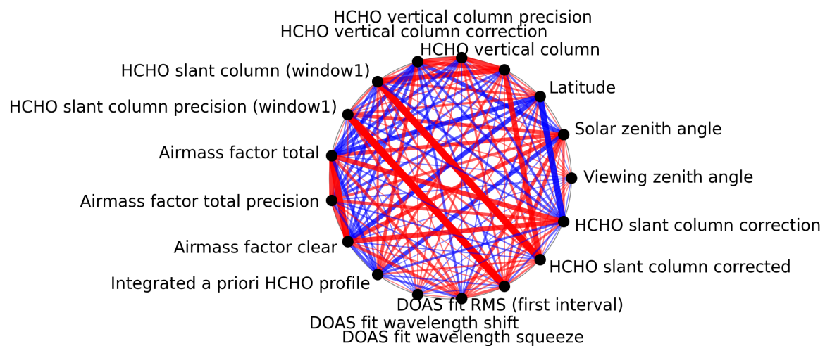
Figure 1: Map of correlation graph for 2025-01-28 to 2025-01-29.
