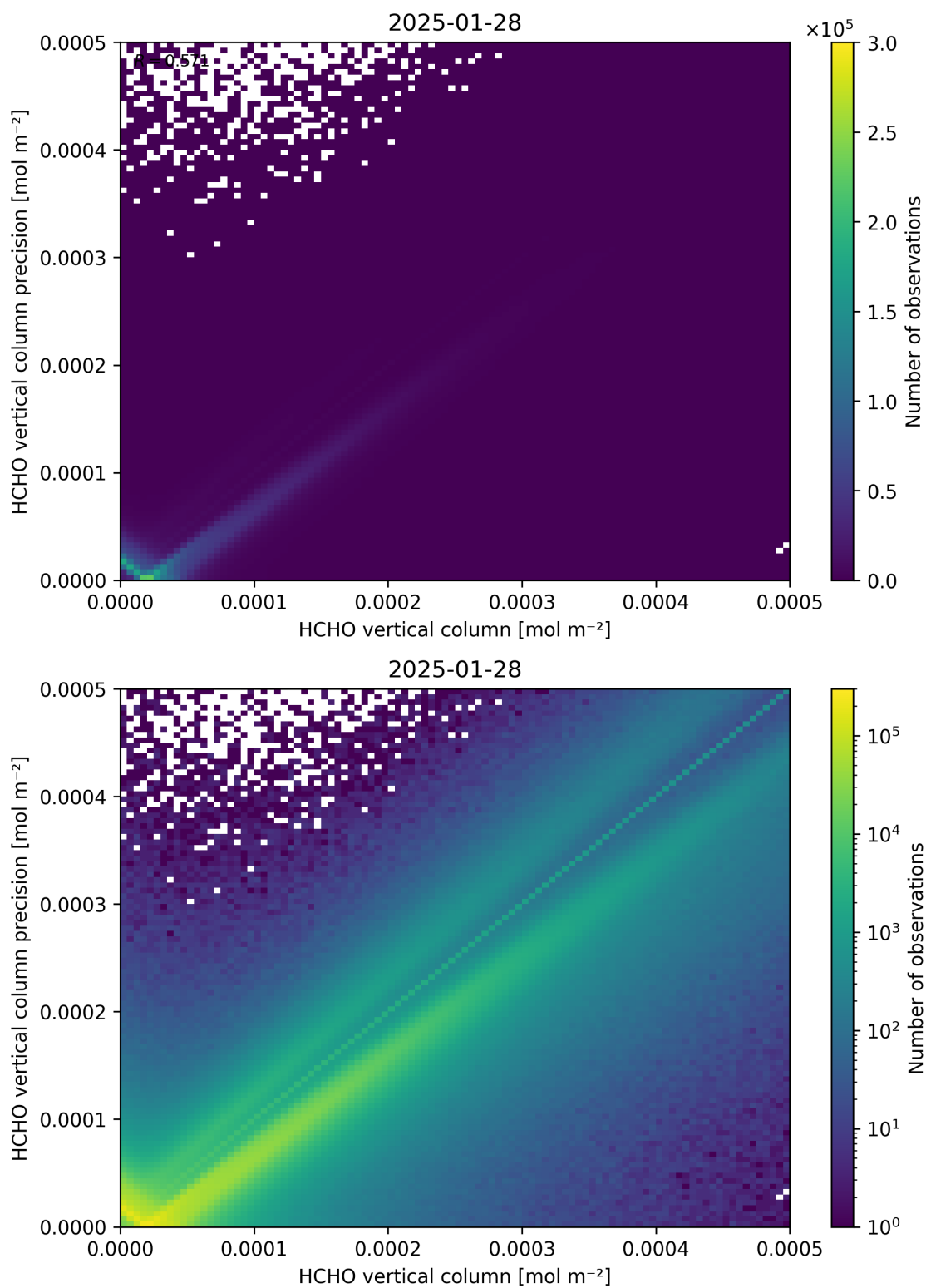
Figure 134: Scatter density plot of “HCHO vertical column” against “HCHO vertical column precision” for 2025-01-28 to 2025-01-29.
