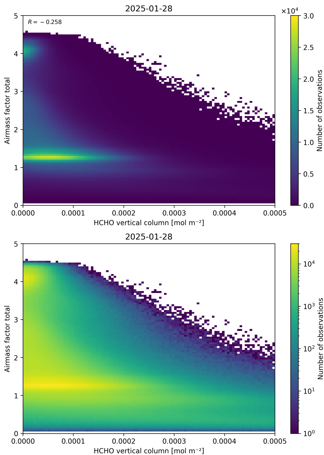
Figure 131: Scatter density plot of “HCHO vertical column” against “Airmass factor total” for 2025-01-28 to 2025-01-29.
