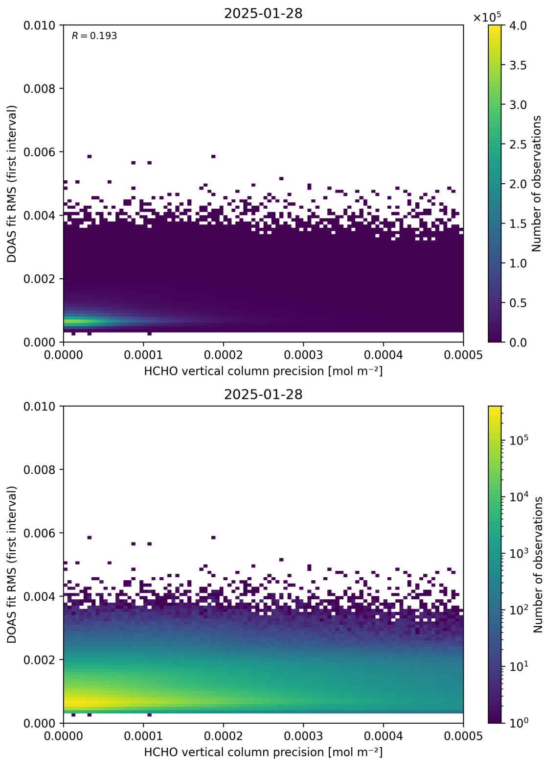
Figure 136: Scatter density plot of “HCHO vertical column precision” against “DOAS fit RMS (first interval)” for 2025-01-28 to 2025-01-29.
