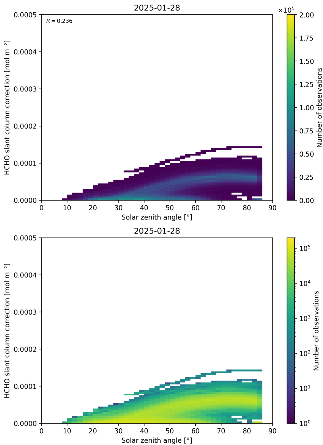
Figure 172: Scatter density plot of “Solar zenith angle” against “HCHO slant column correction” for 2025-01-28 to 2025-01-29.
