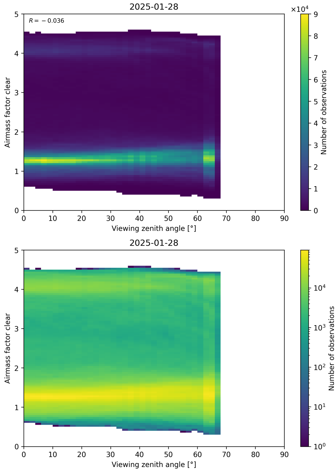
Figure 185: Scatter density plot of “Viewing zenith angle” against “Airmass factor clear” for 2025-01-28 to 2025-01-29.
