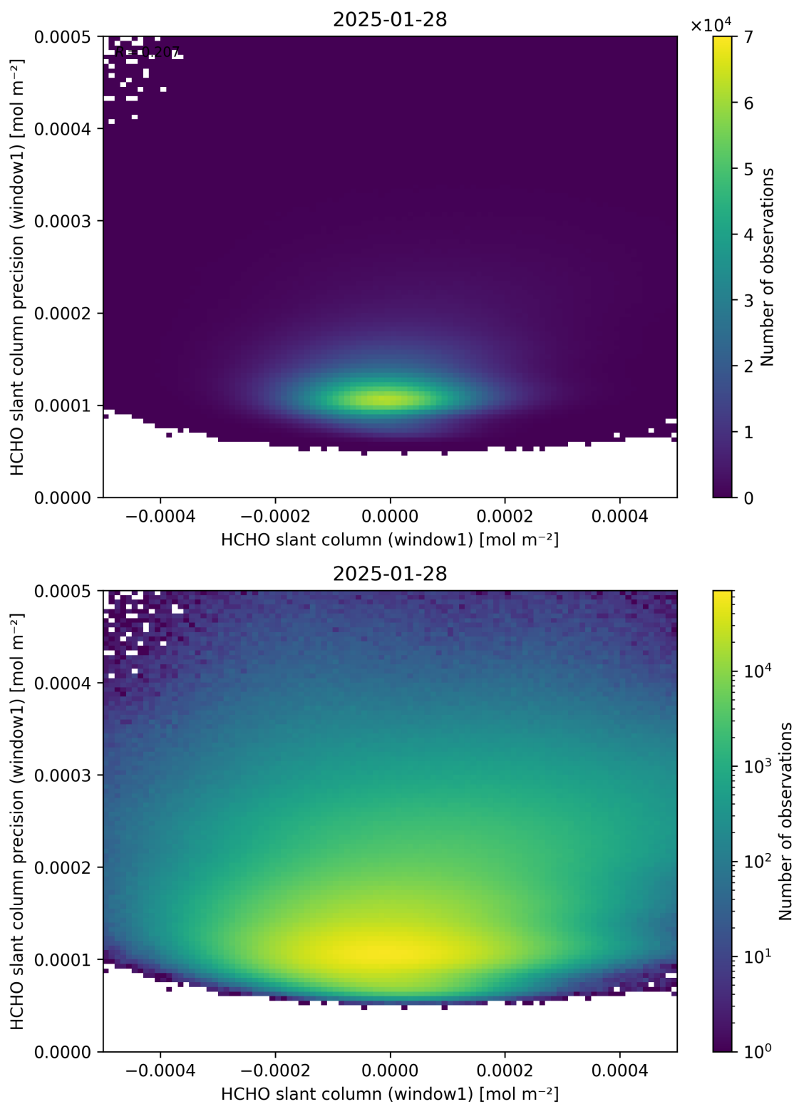
Figure 84: Scatter density plot of “HCHO slant column (window1)” against “HCHO slant column precision (window1)” for 2025-01-28 to 2025-01-29.
