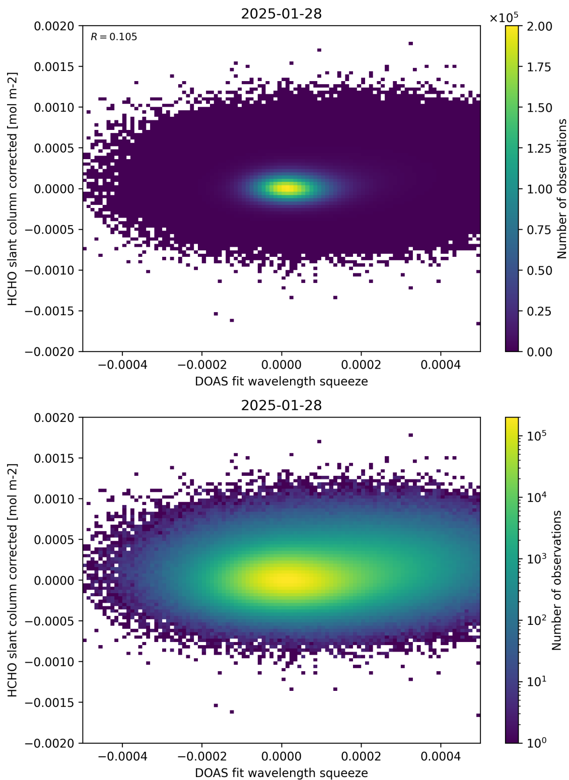
Figure 69: Scatter density plot of “DOAS fit wavelength squeeze” against “HCHO slant column corrected” for 2025-01-28 to 2025-01-29.
