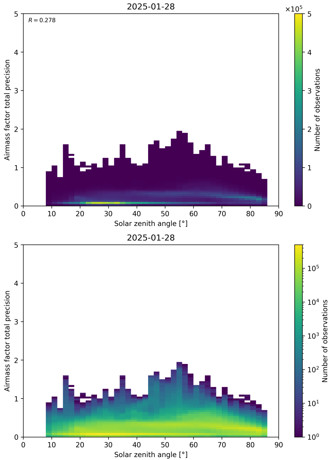
Figure 176: Scatter density plot of “Solar zenith angle” against “Airmass factor total precision” for 2025-01-28 to 2025-01-29.
