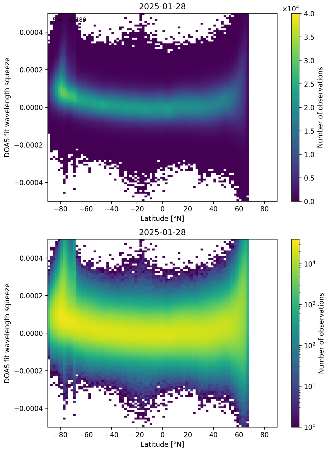
Figure 155: Scatter density plot of “Latitude” against “DOAS fit wavelength squeeze” for 2025-01-28 to 2025-01-29.
