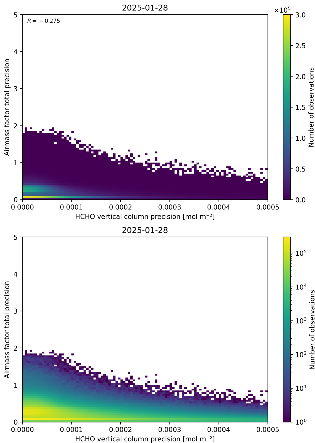
Figure 145: Scatter density plot of “HCHO vertical column precision” against “Airmass factor total precision” for 2025-01-28 to 2025-01-29.
