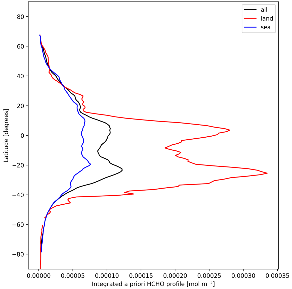
Figure 29: Zonal average of “Integrated a priori HCHO profile” for 2025-01-28 to 2025-01-29.
