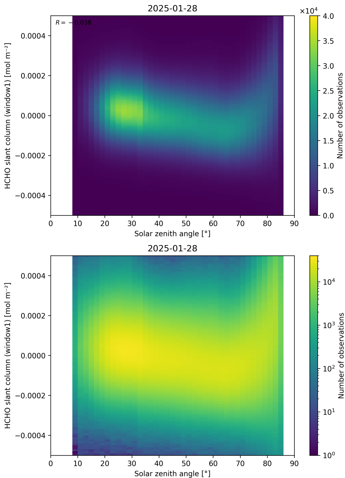
Figure 173: Scatter density plot of “Solar zenith angle” against “HCHO slant column (window1)” for 2025-01-28 to 2025-01-29.
