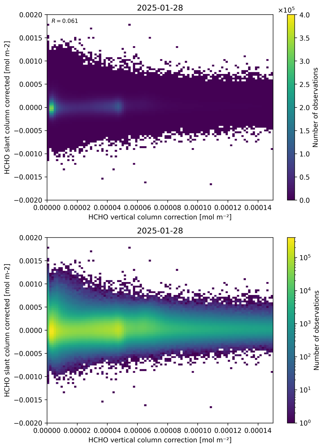
Figure 116: Scatter density plot of “HCHO vertical column correction” against “HCHO slant column corrected” for 2025-01-28 to 2025-01-29.
