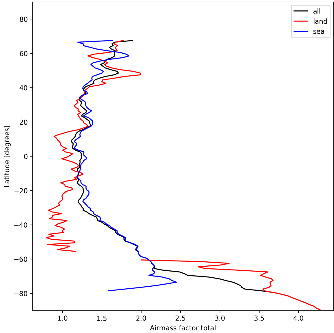
Figure 26: Zonal average of “Airmass factor total” for 2025-01-28 to 2025-01-29.
