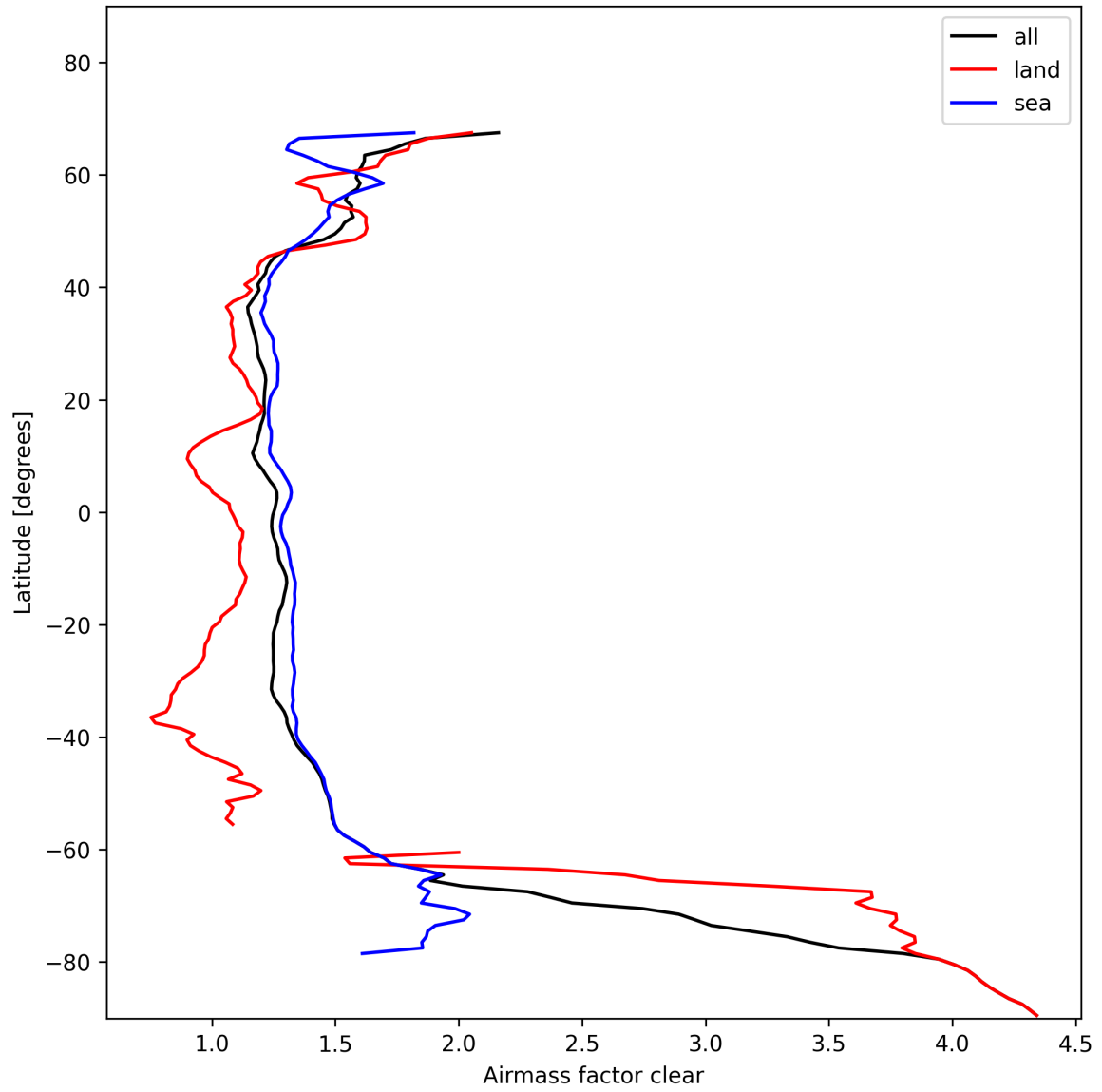
Figure 28: Zonal average of “Airmass factor clear” for 2025-01-28 to 2025-01-29.
