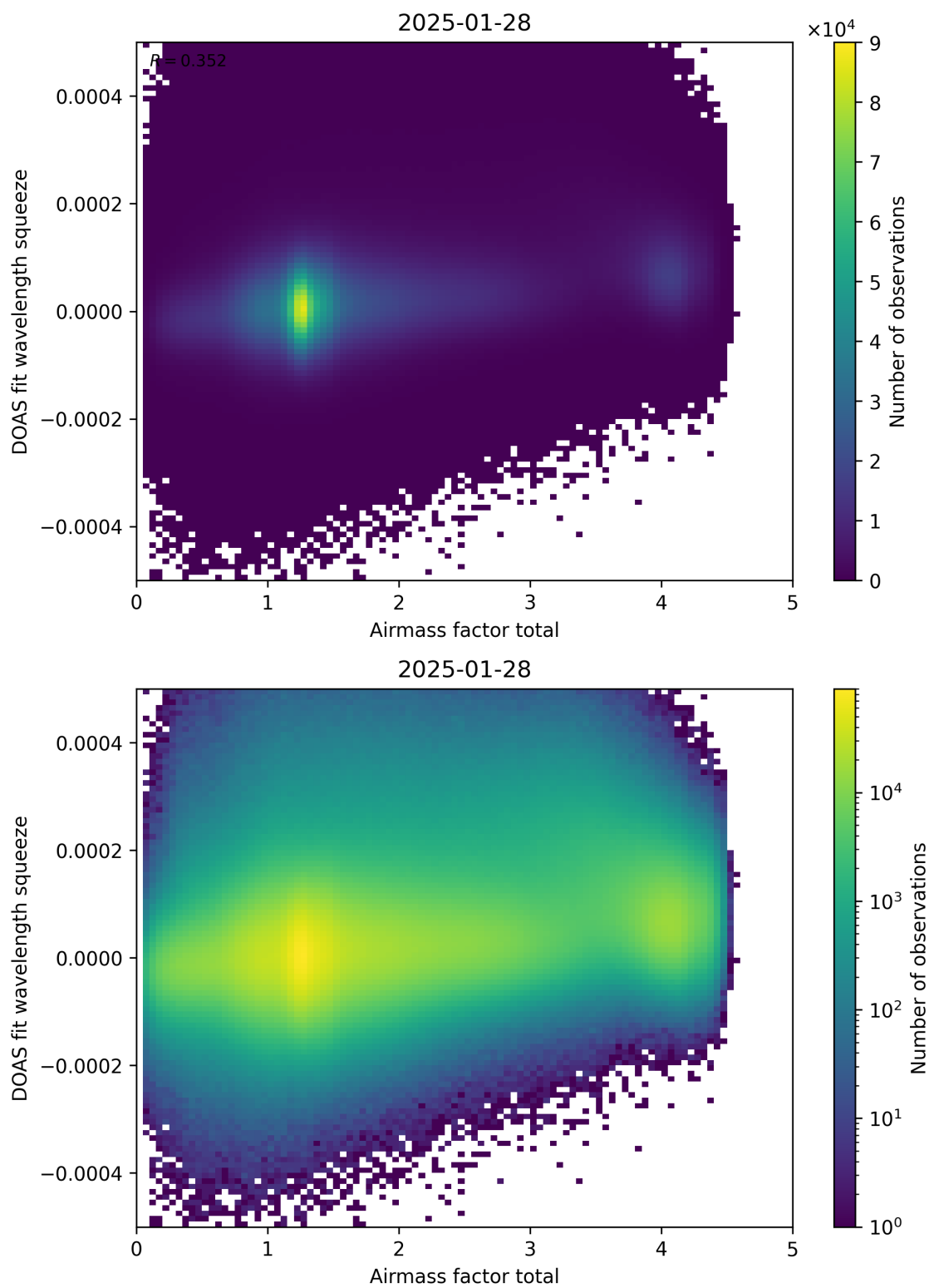
Figure 99: Scatter density plot of “Airmass factor total” against “DOAS fit wavelength squeeze” for 2025-01-28 to 2025-01-29.
