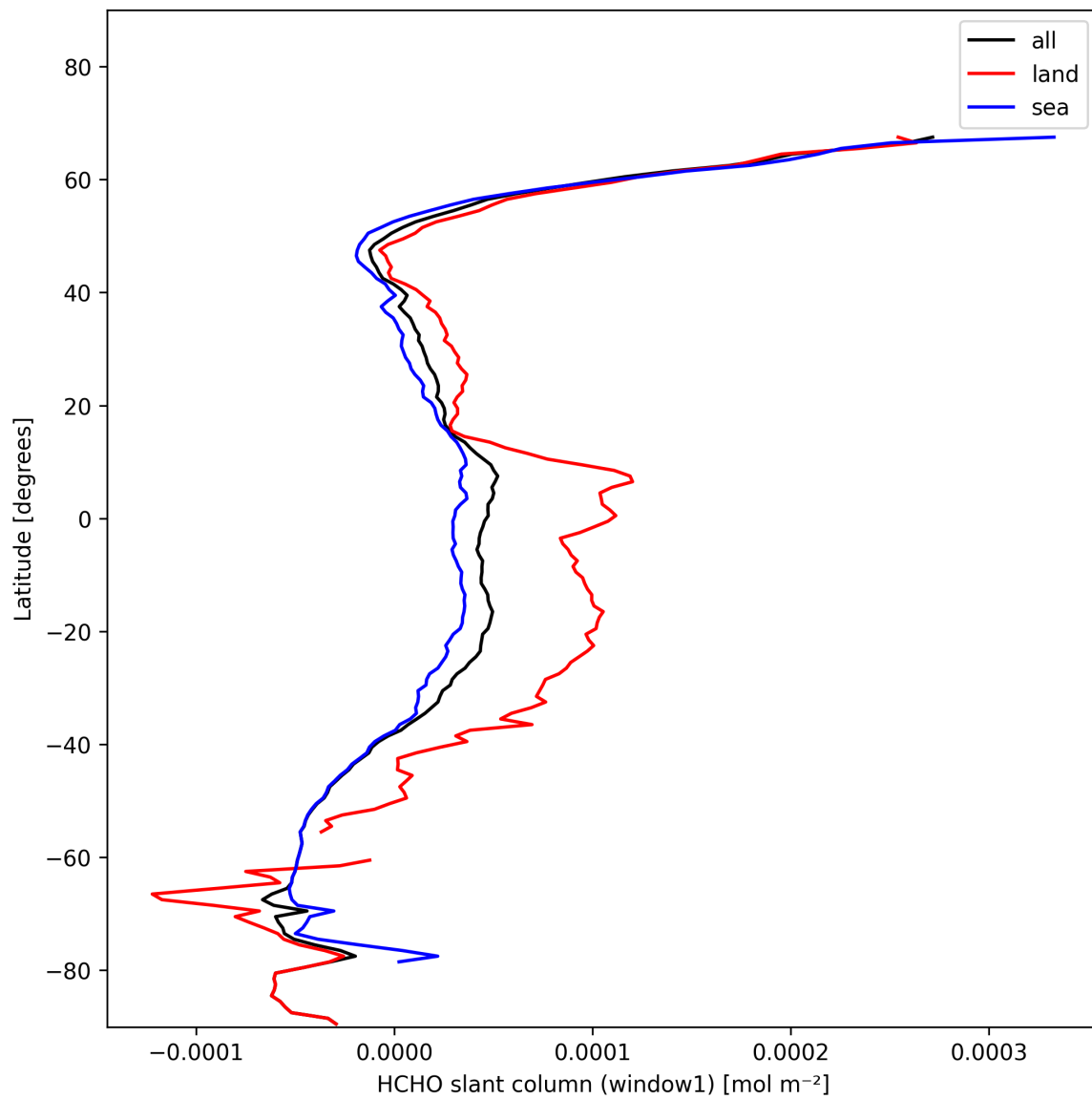
Figure 24: Zonal average of “HCHO slant column (window1)” for 2025-01-28 to 2025-01-29.
