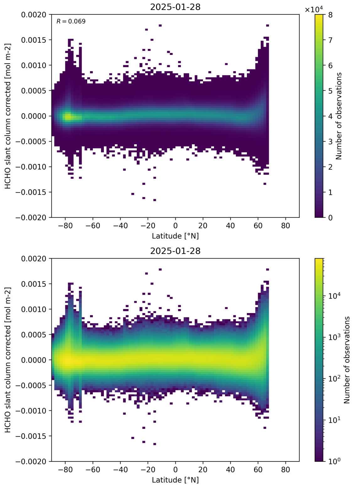
Figure 157: Scatter density plot of “Latitude” against “HCHO slant column corrected” for 2025-01-28 to 2025-01-29.
