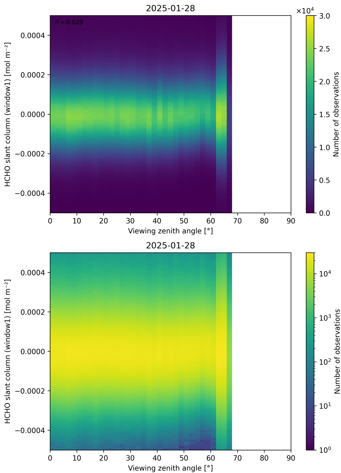
Figure 188: Scatter density plot of “Viewing zenith angle” against “HCHO slant column (window1)” for 2025-01-28 to 2025-01-29.
