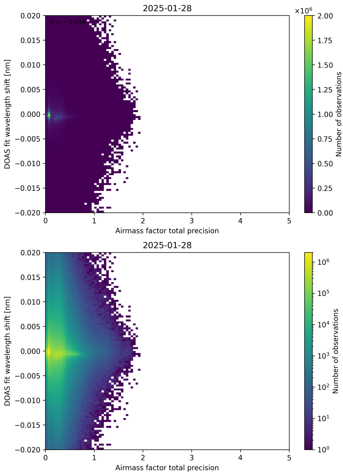
Figure 106: Scatter density plot of “Airmass factor total precision” against “DOAS fit wavelength shift” for 2025-01-28 to 2025-01-29.
