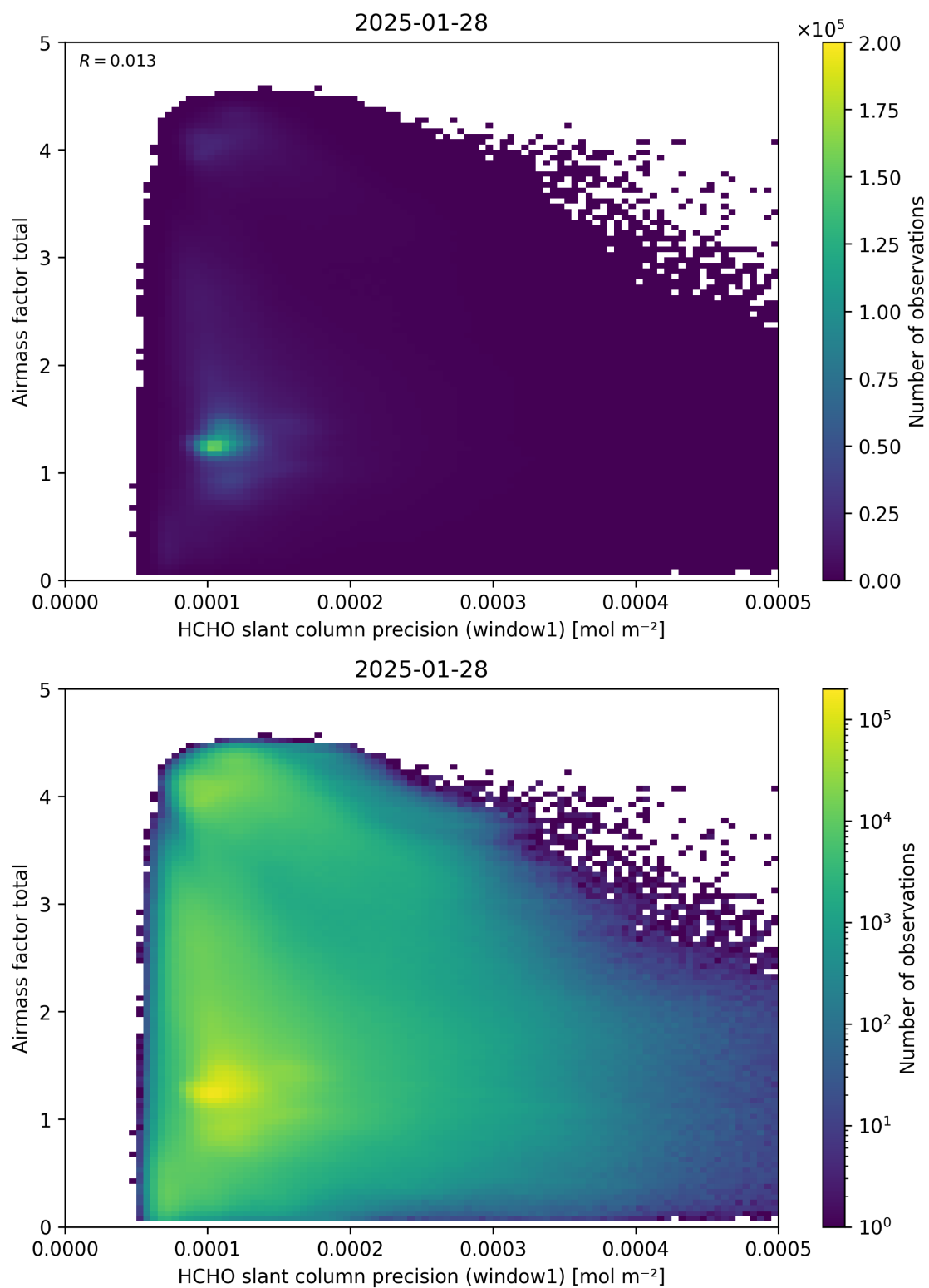
Figure 94: Scatter density plot of “HCHO slant column precision (window1)” against “Airmass factor total” for 2025-01-28 to 2025-01-29.
