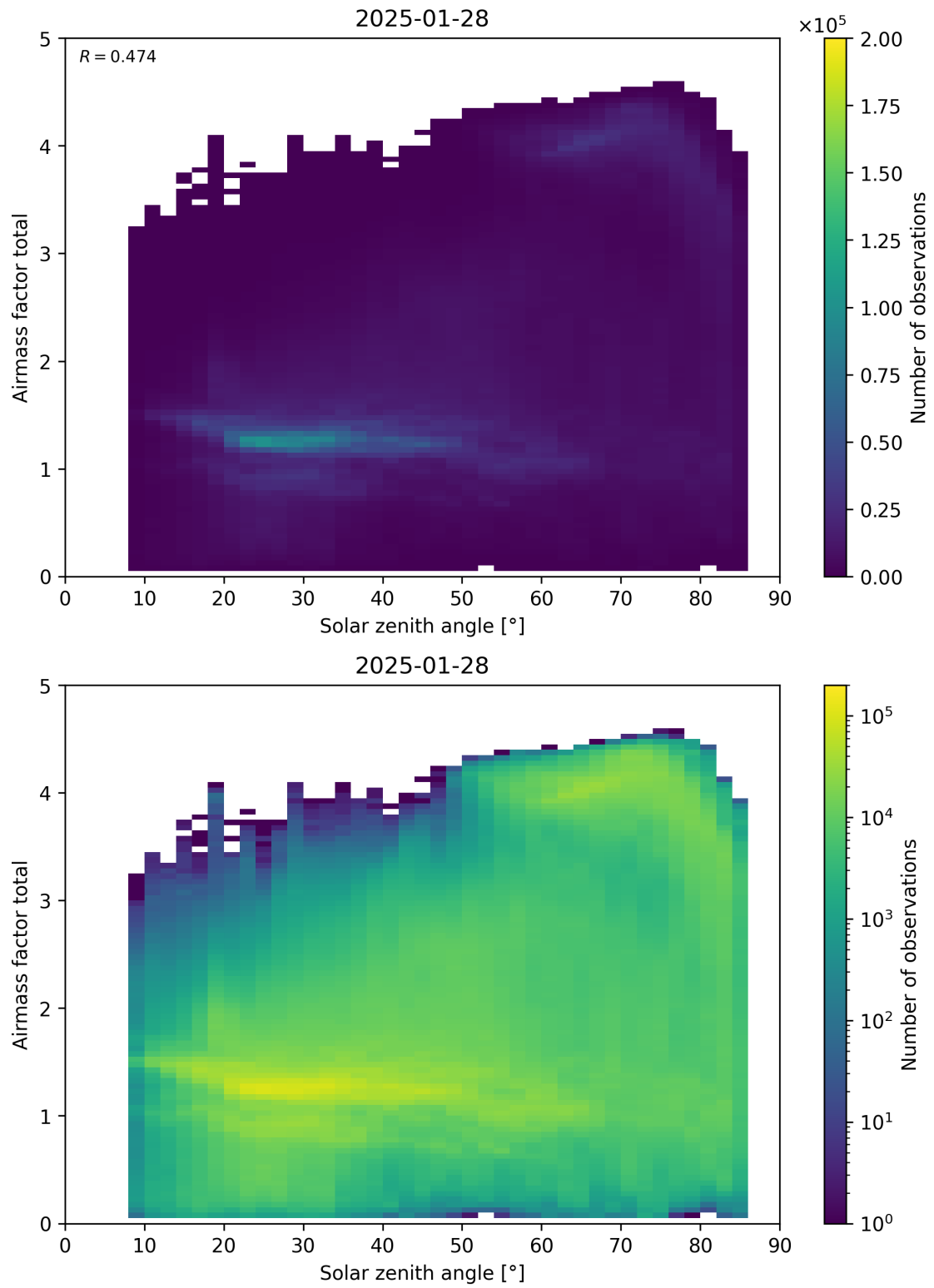
Figure 175: Scatter density plot of “Solar zenith angle” against “Airmass factor total” for 2025-01-28 to 2025-01-29.
