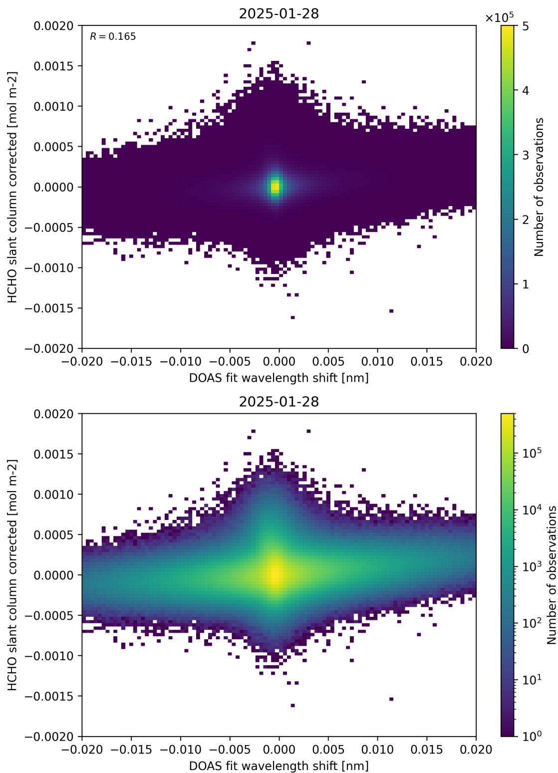
Figure 66: Scatter density plot of “DOAS fit wavelength shift” against “HCHO slant column corrected” for 2025-01-28 to 2025-01-29.
