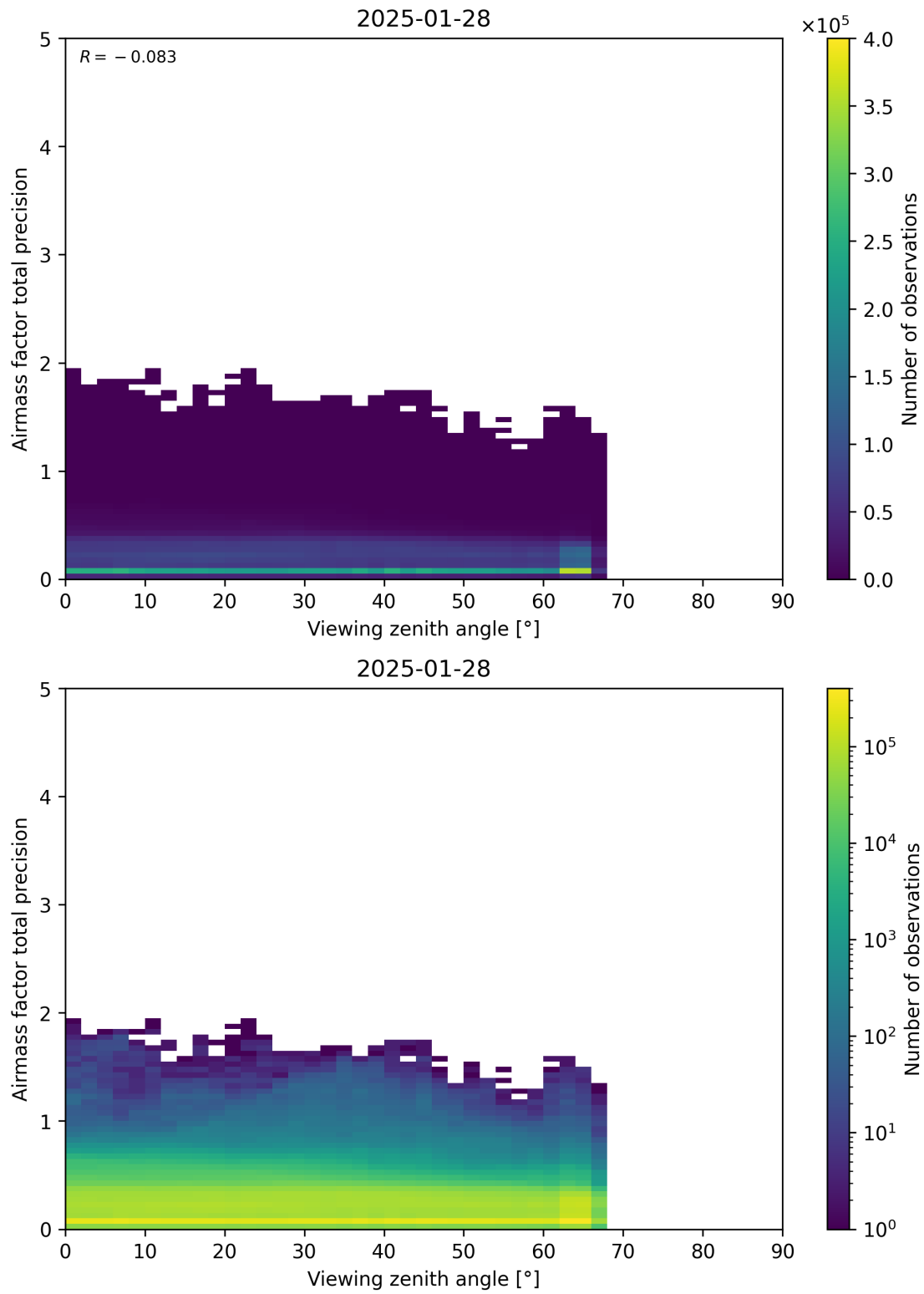
Figure 191: Scatter density plot of “Viewing zenith angle” against “Airmass factor total precision” for 2025-01-28 to 2025-01-29.
