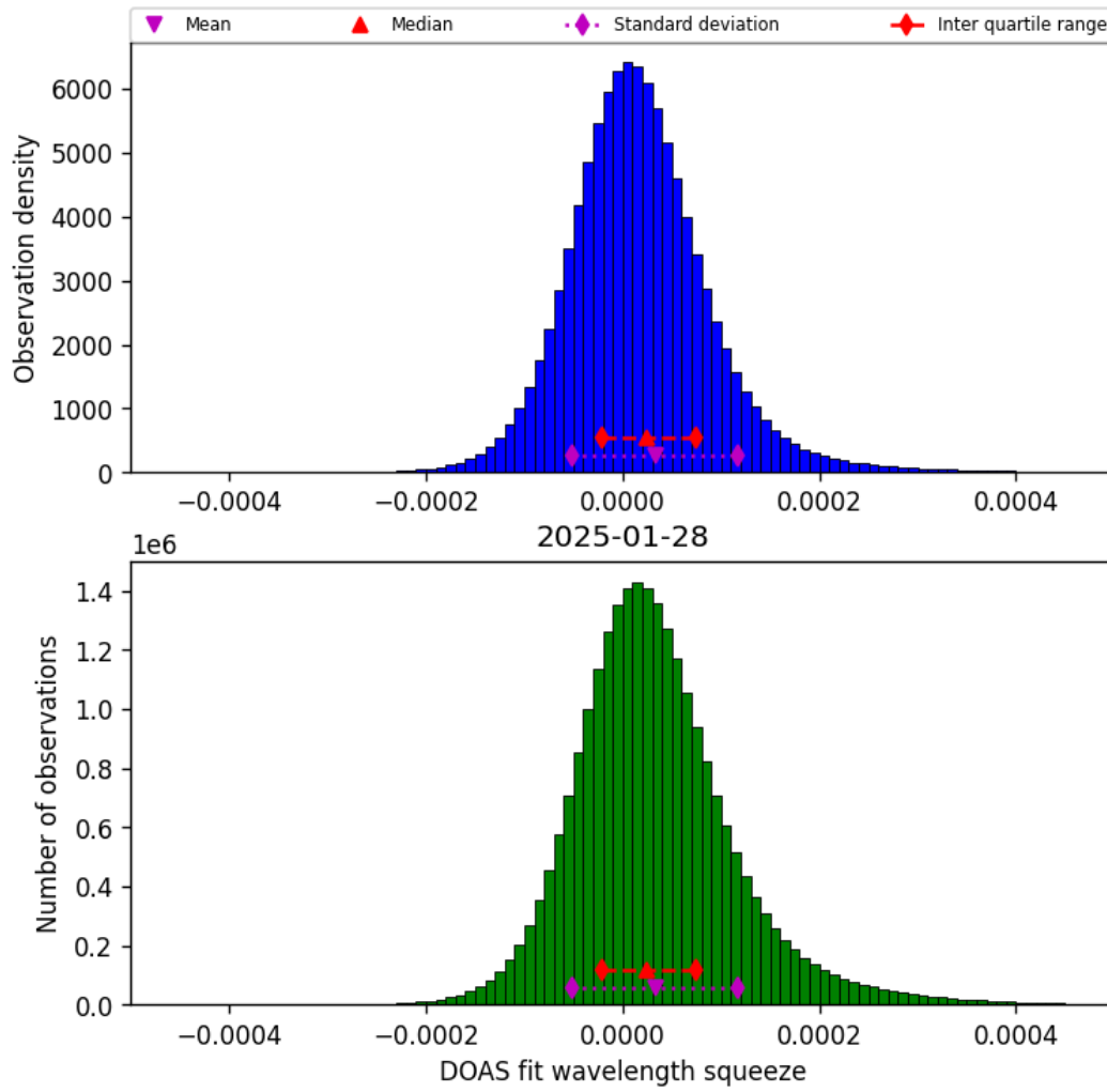
Figure 45: Histogram of “DOAS fit wavelength squeeze” for 2025-01-28 to 2025-01-29
