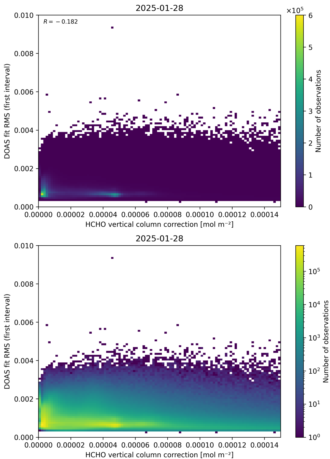
Figure 112: Scatter density plot of “HCHO vertical column correction” against “DOAS fit RMS (first interval)” for 2025-01-28 to 2025-01-29.
