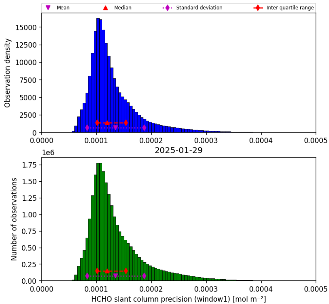
Figure 39: Histogram of “HCHO slant column precision (window1)” for 2025-01-28 to 2025-01-30
