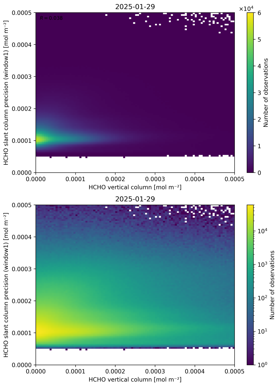
Figure 130: Scatter density plot of “HCHO vertical column” against “HCHO slant column precision (window1)” for 2025-01-28 to 2025-01-30.
