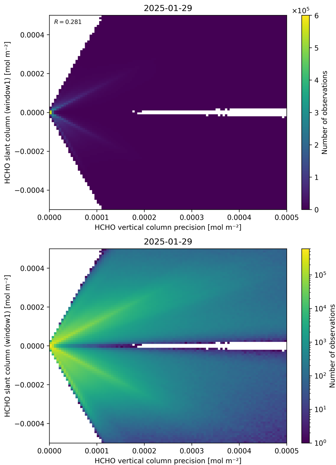
Figure 142: Scatter density plot of “HCHO vertical column precision” against “HCHO slant column (window1)” for 2025-01-28 to 2025-01-30.
