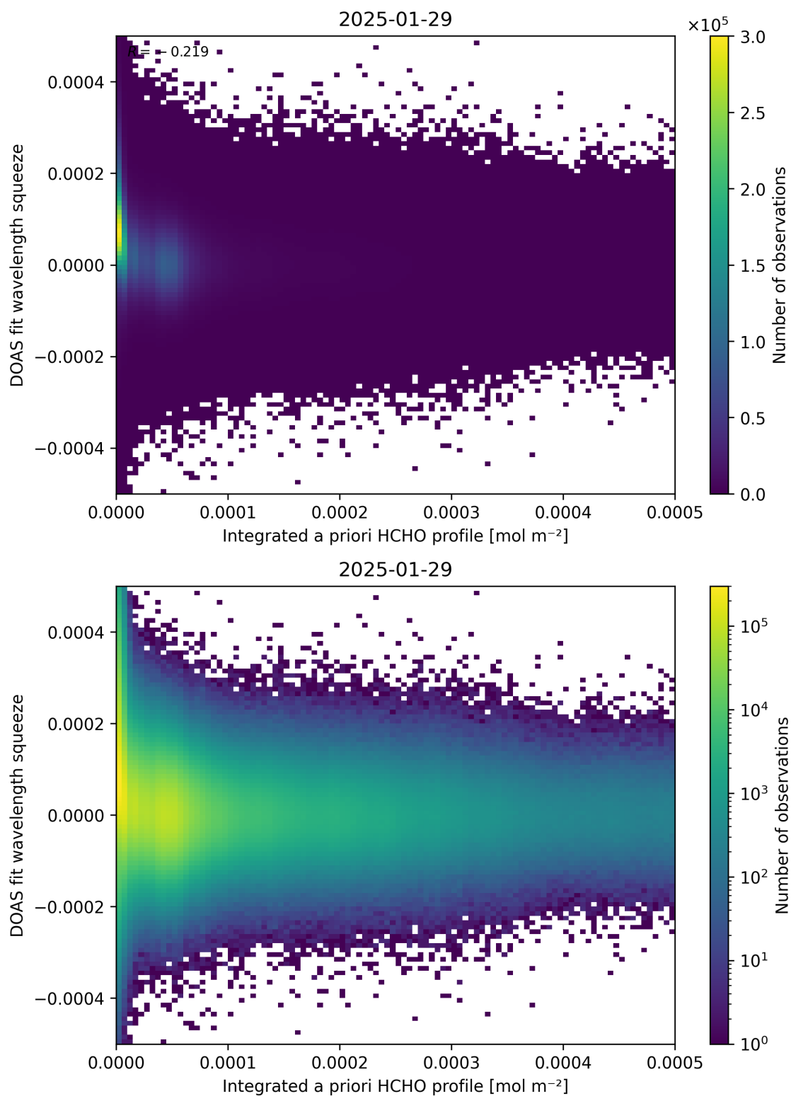
Figure 150: Scatter density plot of “Integrated a priori HCHO profile” against “DOAS fit wavelength squeeze” for 2025-01-28 to 2025-01-30.
