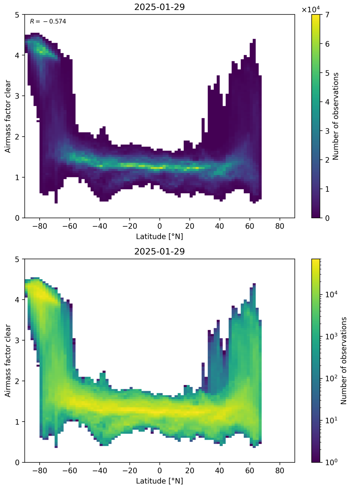
Figure 156: Scatter density plot of “Latitude” against “Airmass factor clear” for 2025-01-28 to 2025-01-30.
