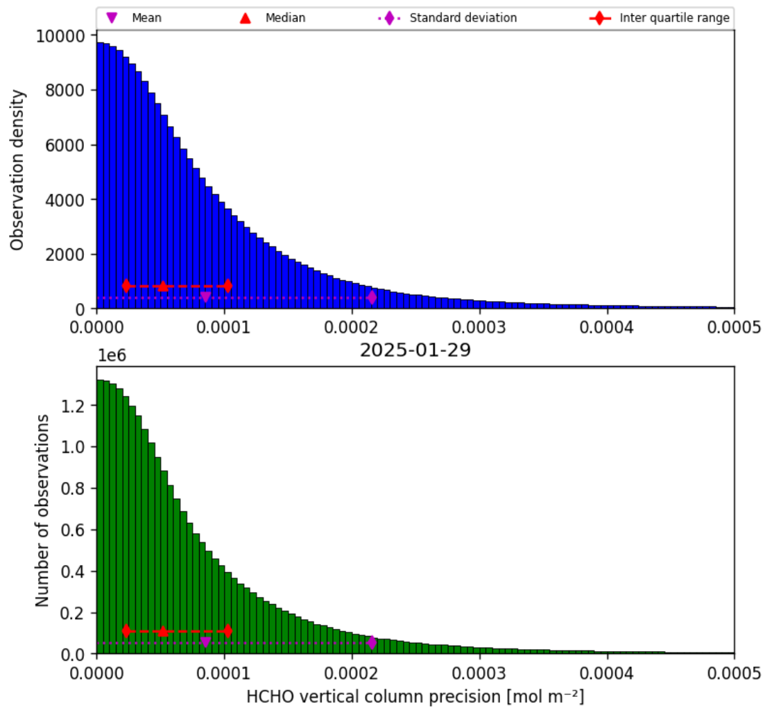
Figure 36: Histogram of “HCHO vertical column precision” for 2025-01-28 to 2025-01-30
