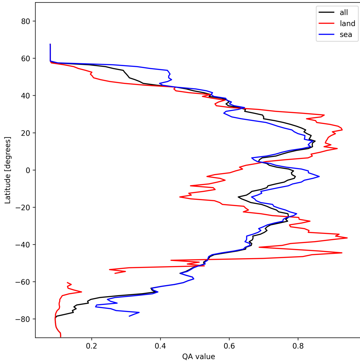
Figure 20: Zonal average of “QA value” for 2025-01-28 to 2025-01-30.
