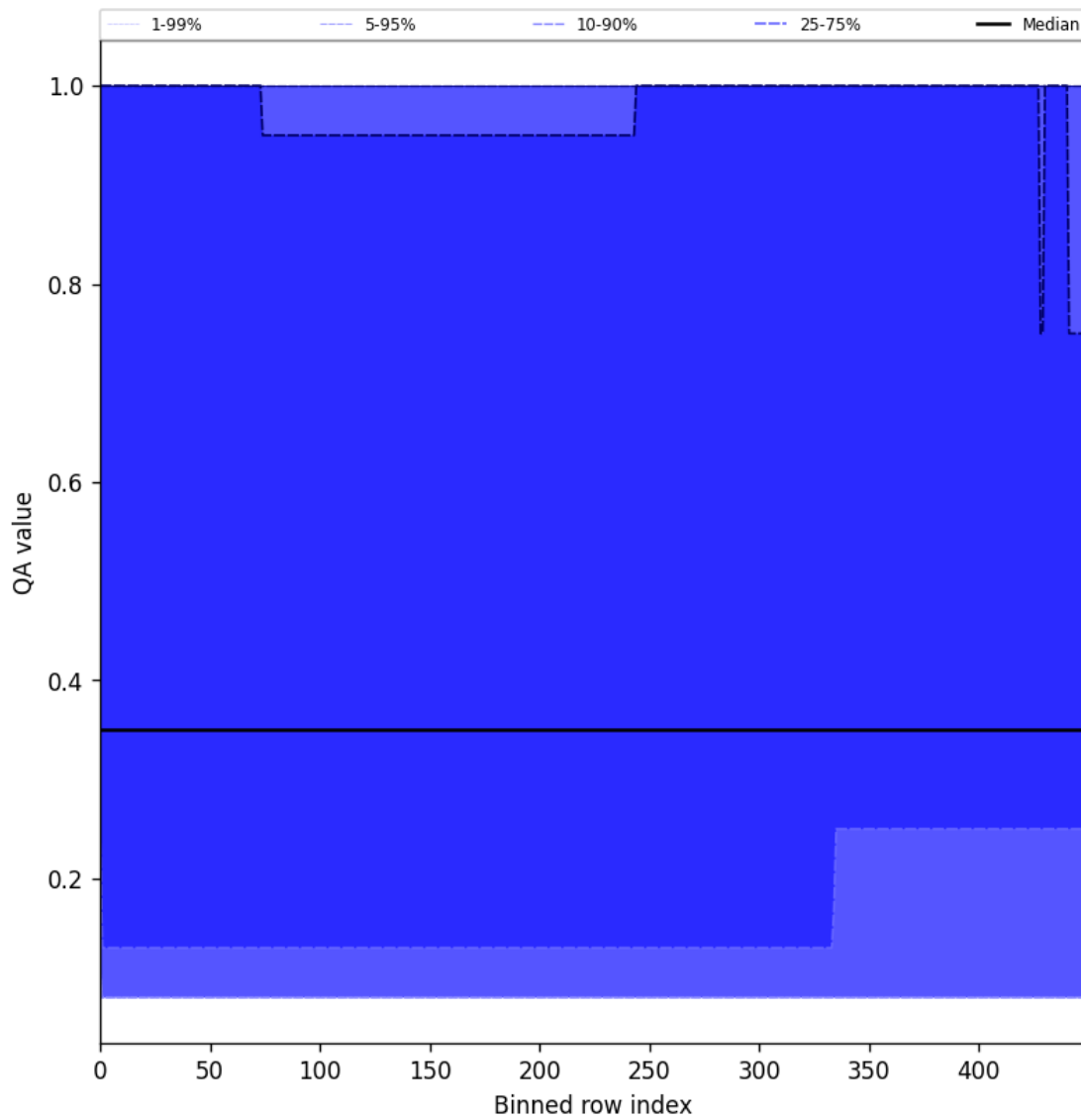
Figure 48: Along track statistics of “QA value” for 2025-01-28 to 2025-01-30
