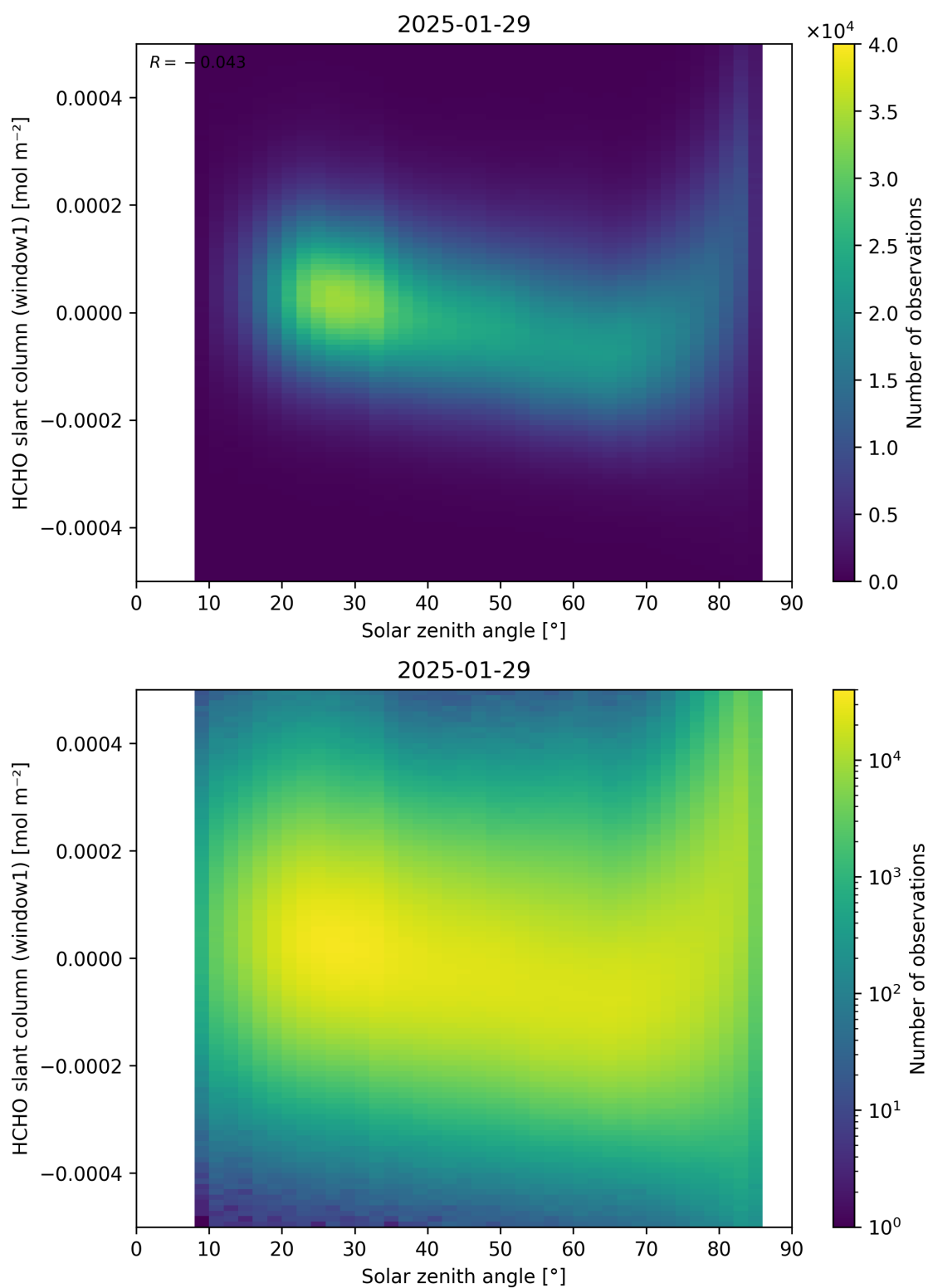
Figure 173: Scatter density plot of “Solar zenith angle” against “HCHO slant column (window1)” for 2025-01-28 to 2025-01-30.
