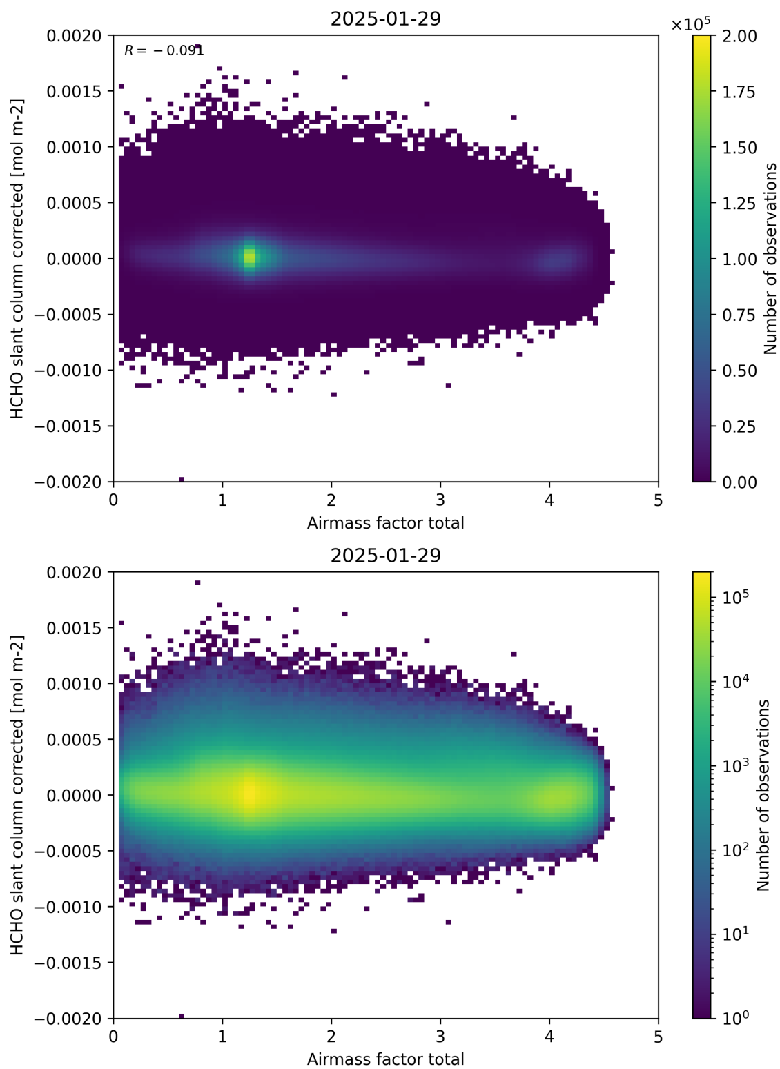
Figure 101: Scatter density plot of “Airmass factor total” against “HCHO slant column corrected” for 2025-01-28 to 2025-01-30.
