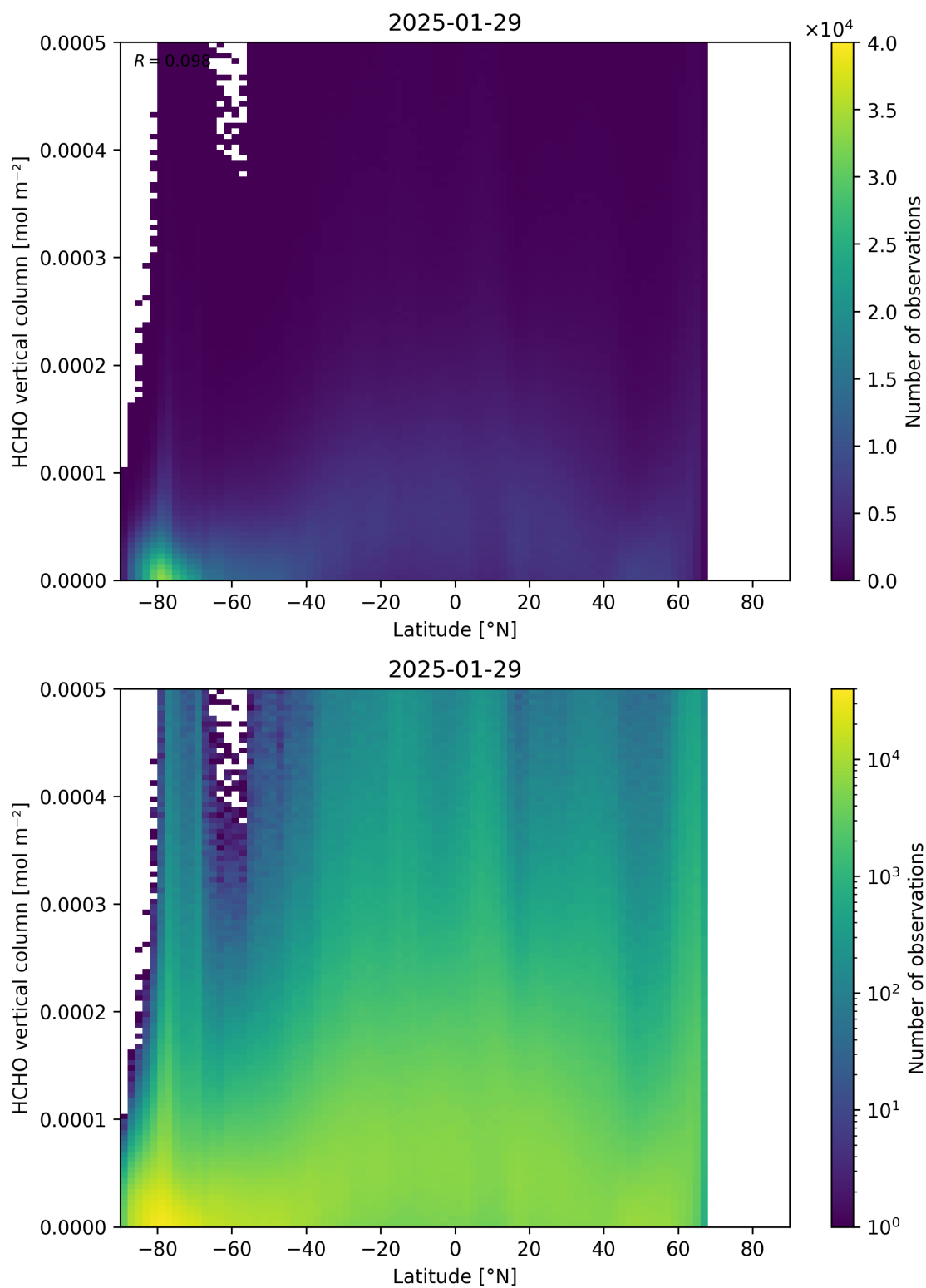
Figure 163: Scatter density plot of “Latitude” against “HCHO vertical column” for 2025-01-28 to 2025-01-30.
