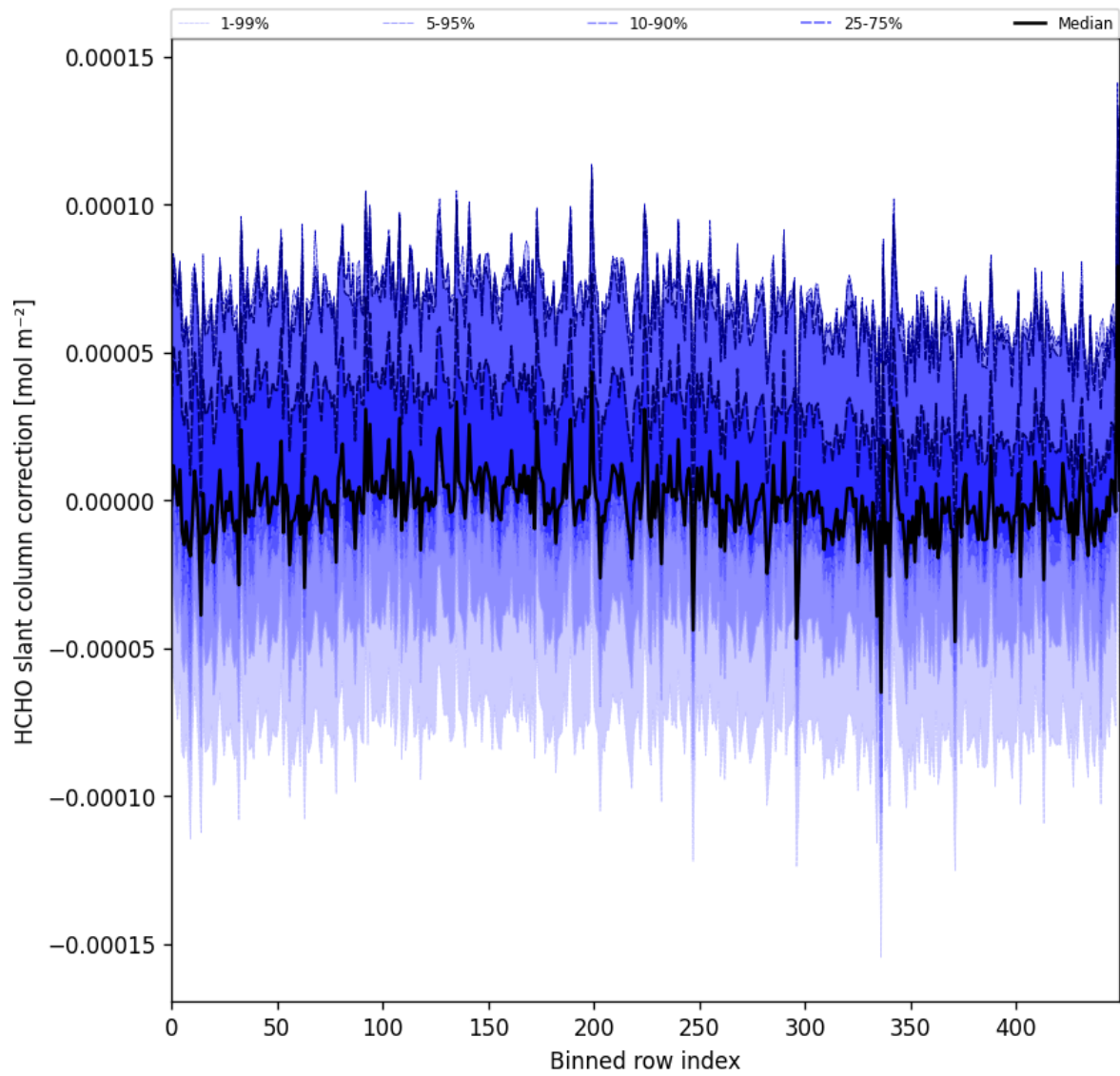
Figure 61: Along track statistics of “HCHO slant column correction” for 2025-01-28 to 2025-01-30
