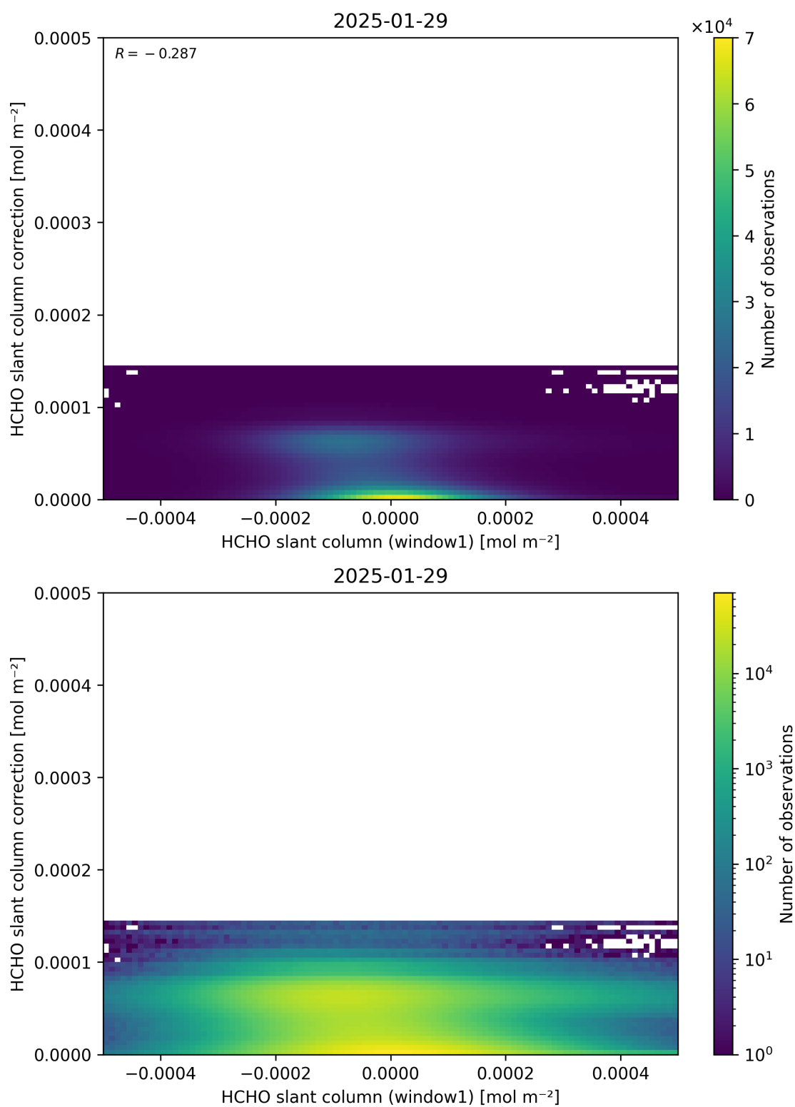
Figure 83: Scatter density plot of “HCHO slant column (window1)” against “HCHO slant column correction” for 2025-01-28 to 2025-01-30.
