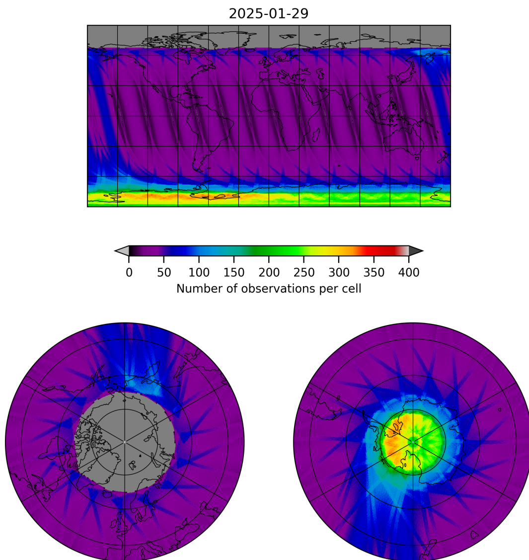
Figure 19: Map of the number of observations for 2025-01-28 to 2025-01-30
