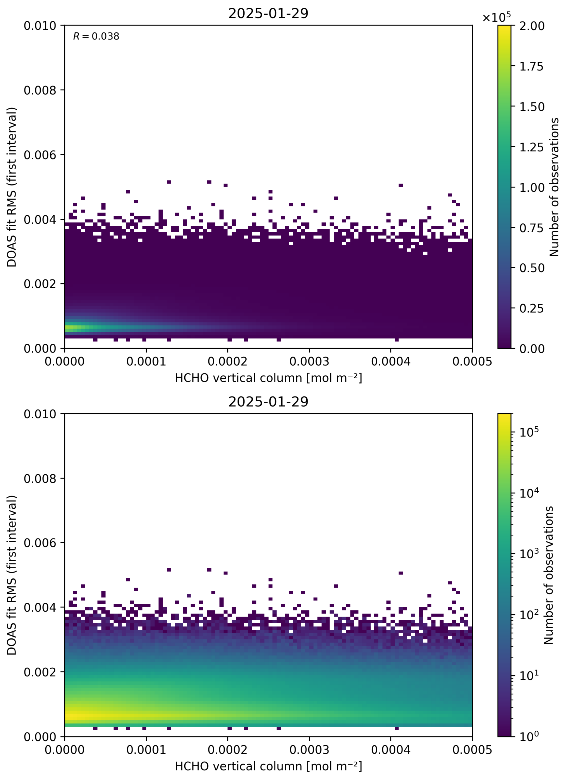
Figure 123: Scatter density plot of “HCHO vertical column” against “DOAS fit RMS (first interval)” for 2025-01-28 to 2025-01-30.
