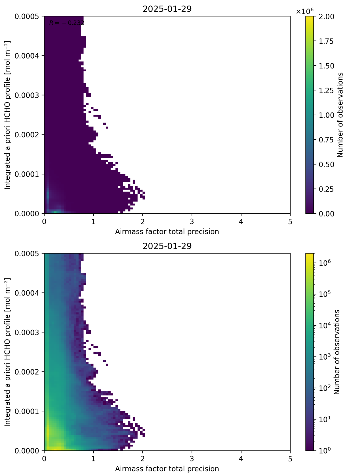
Figure 111: Scatter density plot of “Airmass factor total precision” against “Integrated a priori HCHO profile” for 2025-01-28 to 2025-01-30.
