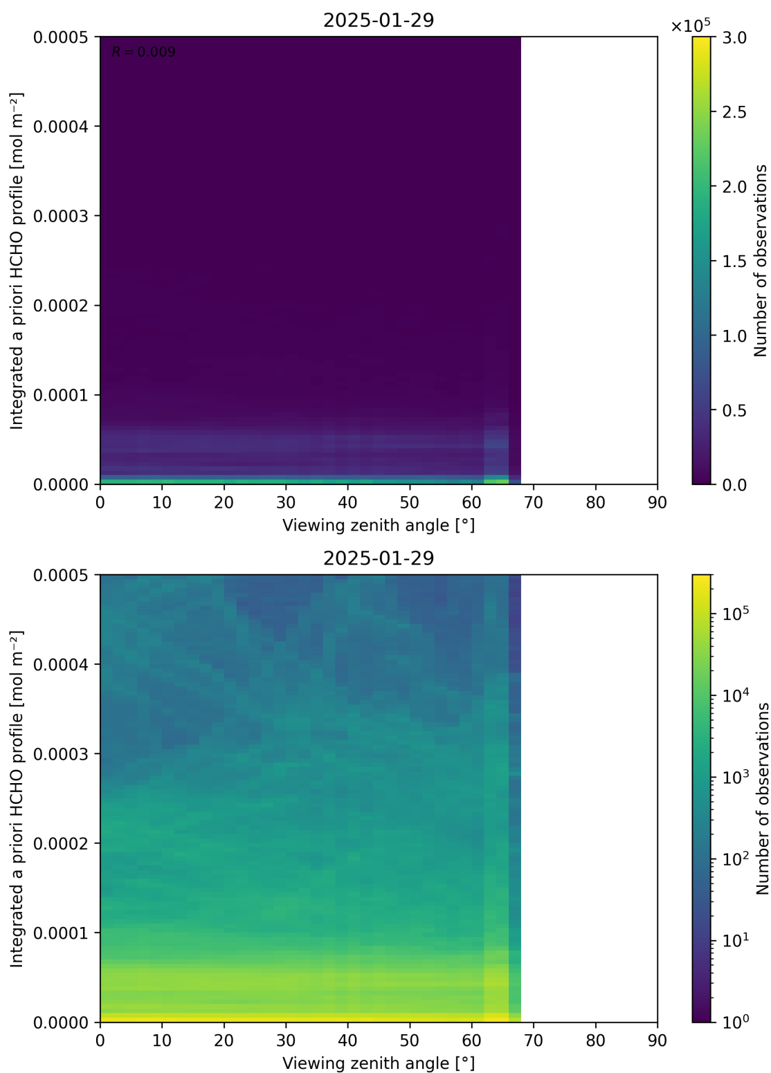
Figure 195: Scatter density plot of “Viewing zenith angle” against “Integrated a priori HCHO profile” for 2025-01-28 to 2025-01-30.
