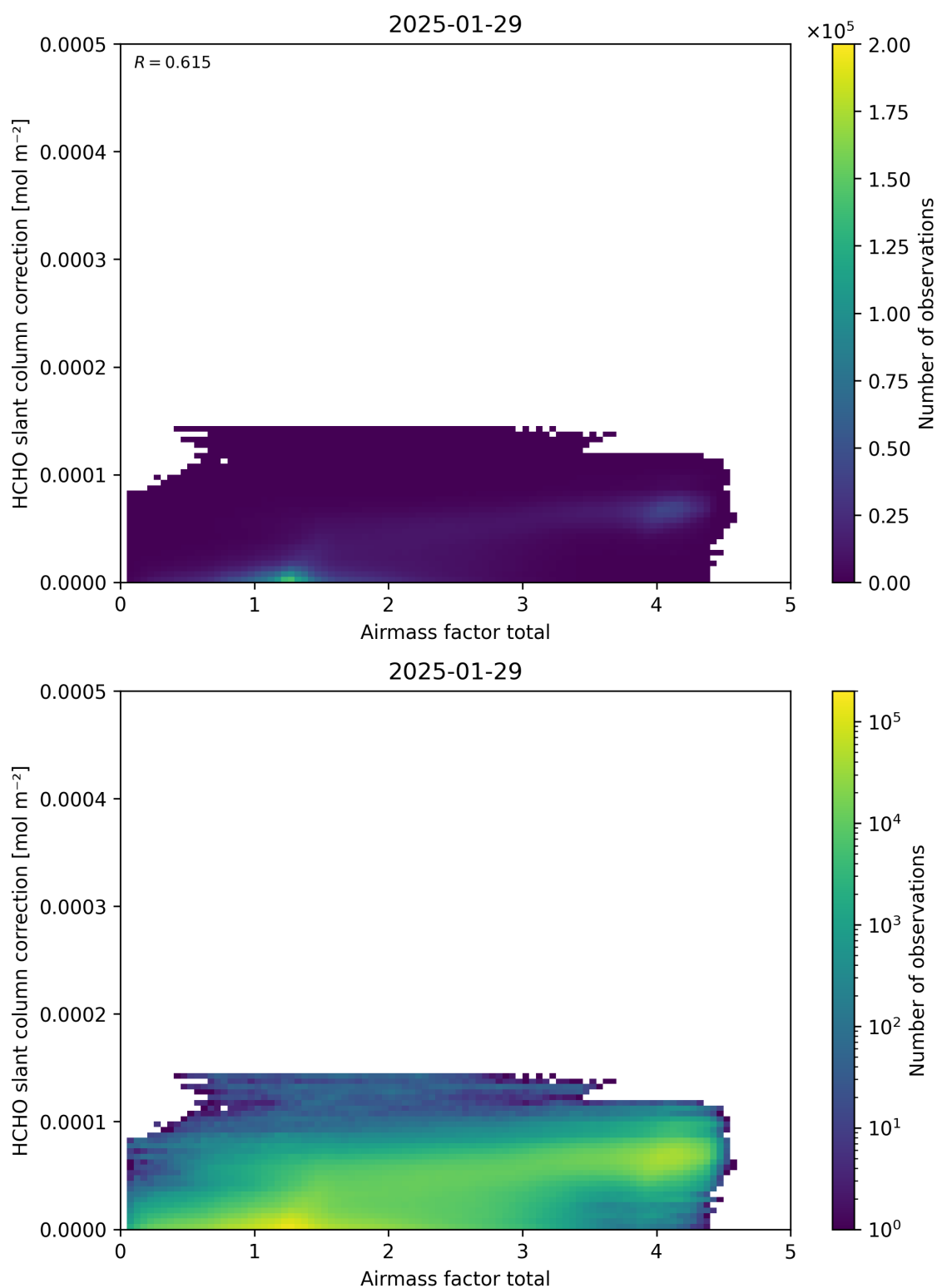
Figure 102: Scatter density plot of “Airmass factor total” against “HCHO slant column correction” for 2025-01-28 to 2025-01-30.
