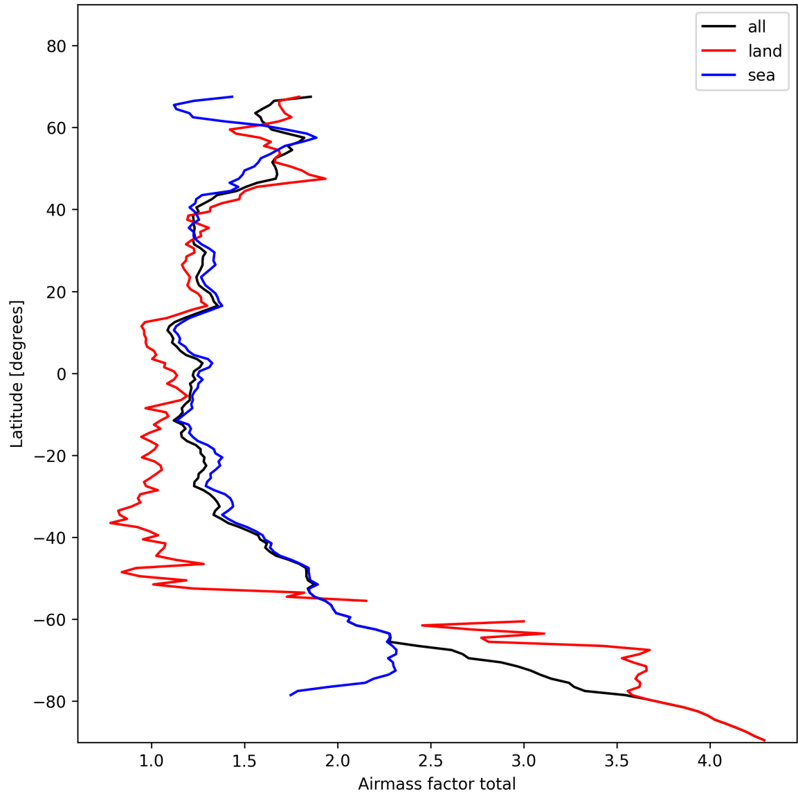
Figure 26: Zonal average of “Airmass factor total” for 2025-01-28 to 2025-01-30.
