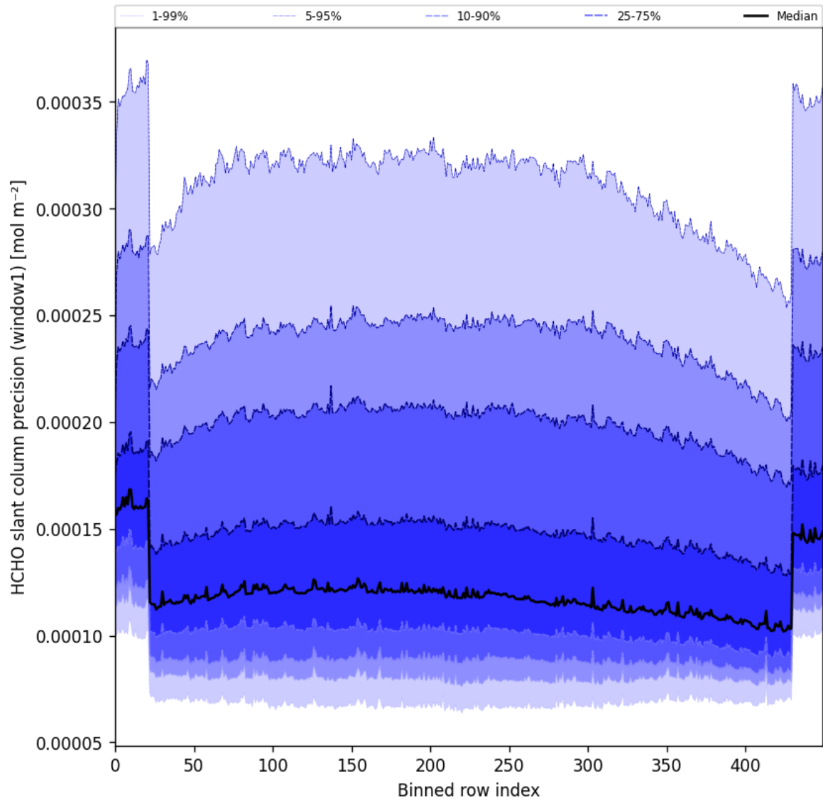
Figure 53: Along track statistics of “HCHO slant column precision (window1)” for 2025-01-28 to 2025-01-30
