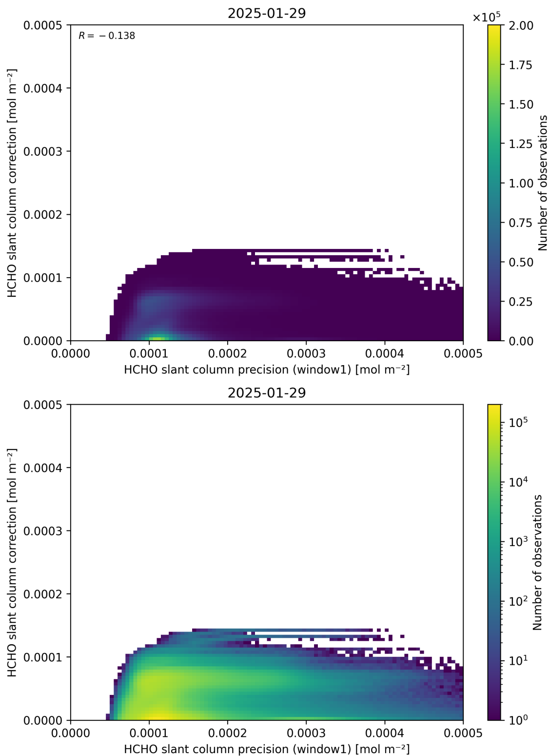
Figure 93: Scatter density plot of “HCHO slant column precision (window1)” against “HCHO slant column correction” for 2025-01-28 to 2025-01-30.
