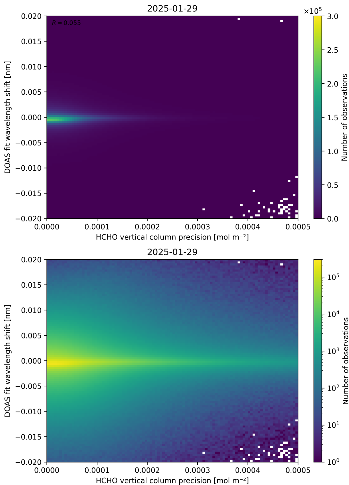
Figure 137: Scatter density plot of “HCHO vertical column precision” against “DOAS fit wavelength shift” for 2025-01-28 to 2025-01-30.
