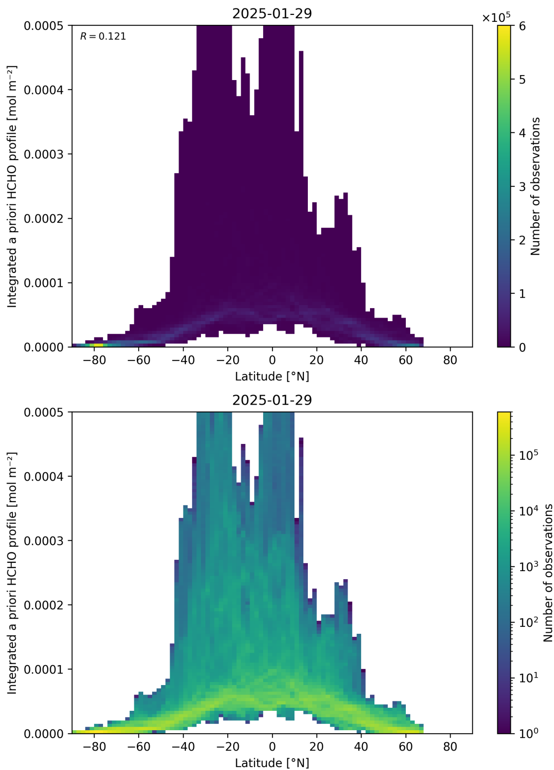
Figure 166: Scatter density plot of “Latitude” against “Integrated a priori HCHO profile” for 2025-01-28 to 2025-01-30.
