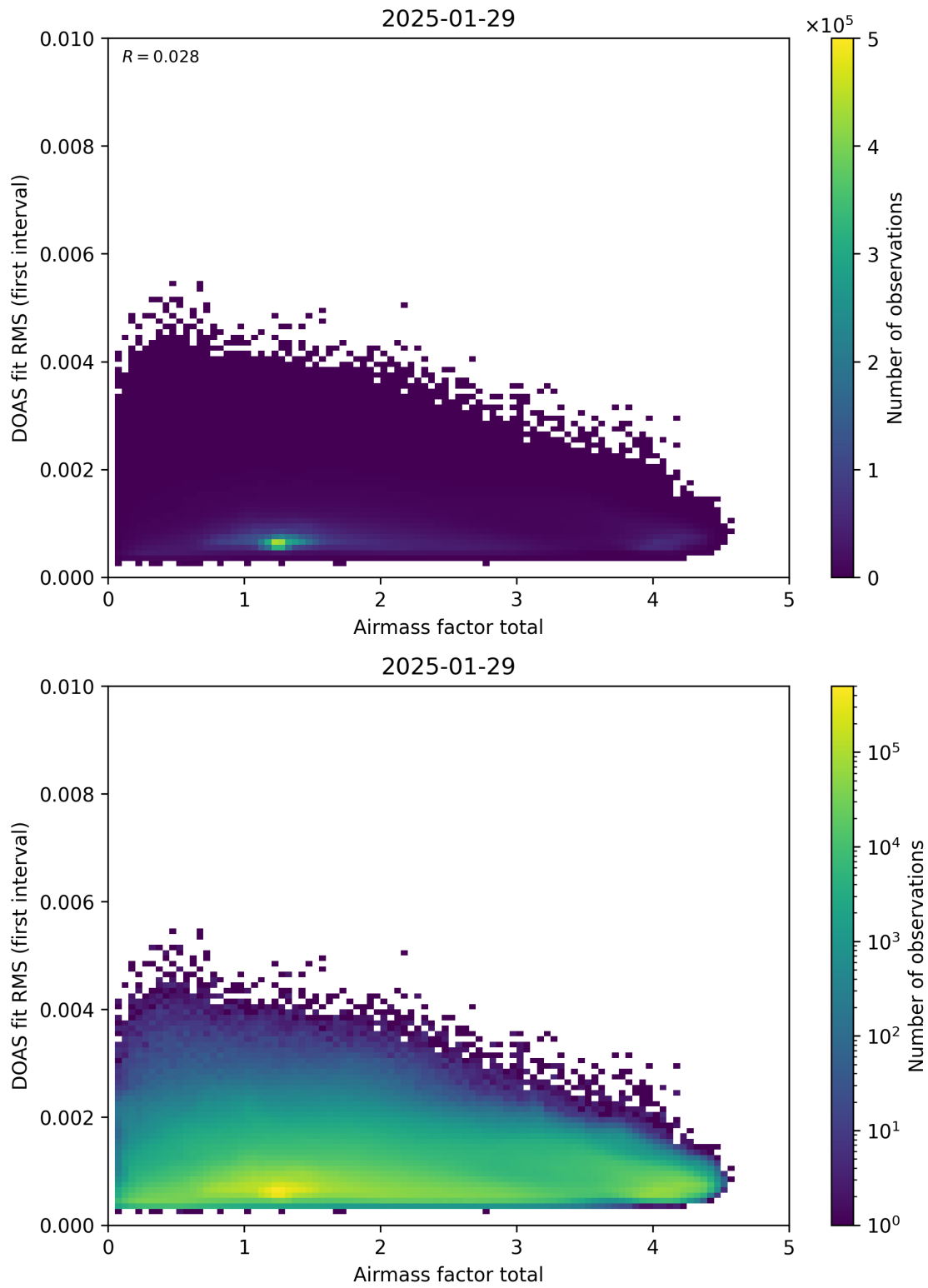
Figure 97: Scatter density plot of “Airmass factor total” against “DOAS fit RMS (first interval)” for 2025-01-28 to 2025-01-30.
