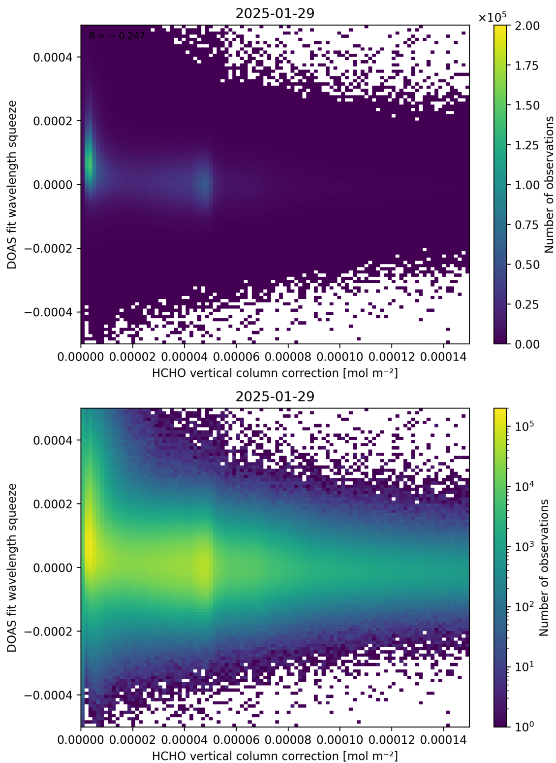
Figure 114: Scatter density plot of “HCHO vertical column correction” against “DOAS fit wavelength squeeze” for 2025-01-28 to 2025-01-30.
