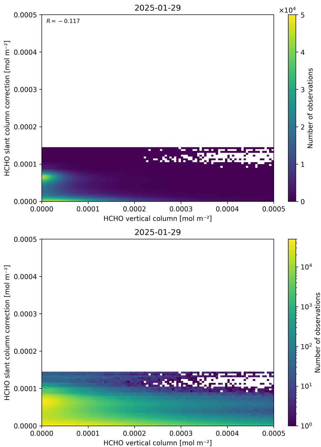
Figure 128: Scatter density plot of “HCHO vertical column” against “HCHO slant column correction” for 2025-01-28 to 2025-01-30.
