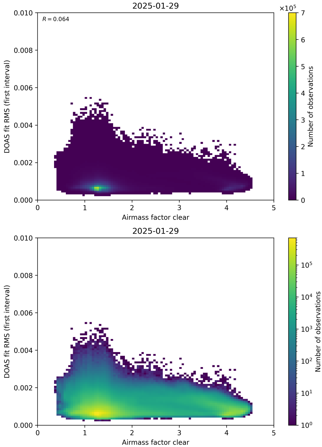
Figure 71: Scatter density plot of “Airmass factor clear” against “DOAS fit RMS (first interval)” for 2025-01-28 to 2025-01-30.
