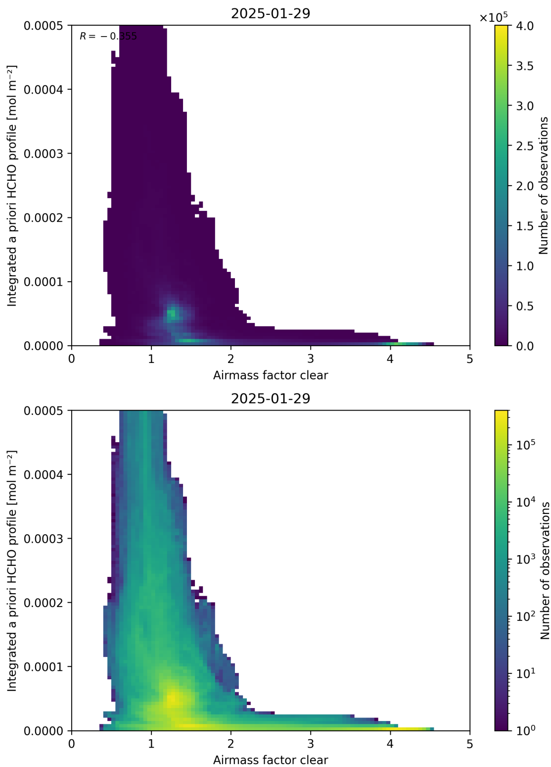
Figure 76: Scatter density plot of “Airmass factor clear” against “Integrated a priori HCHO profile” for 2025-01-28 to 2025-01-30.
