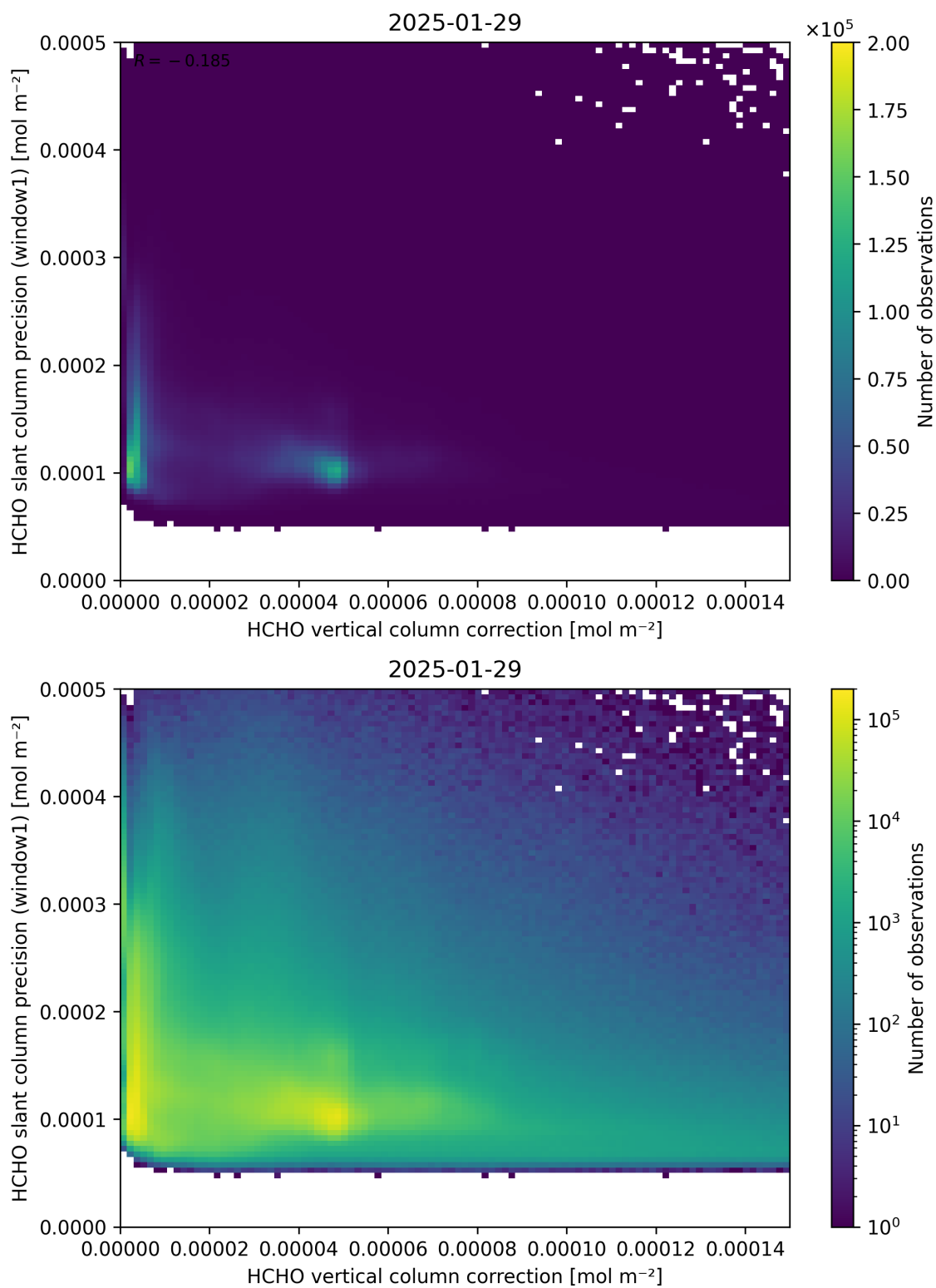
Figure 119: Scatter density plot of “HCHO vertical column correction” against “HCHO slant column precision (window1)” for 2025-01-28 to 2025-01-30.
