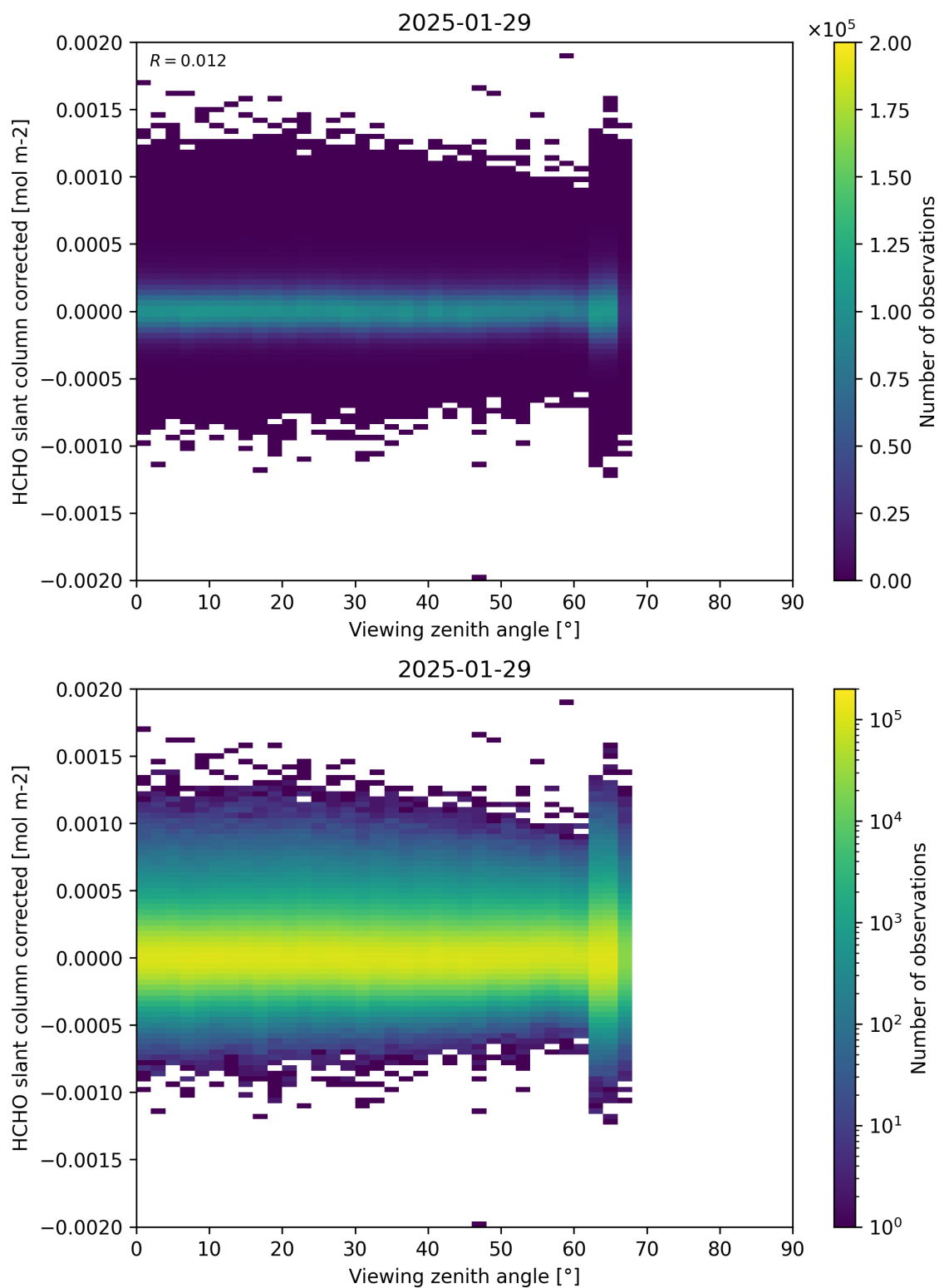
Figure 186: Scatter density plot of “Viewing zenith angle” against “HCHO slant column corrected” for 2025-01-28 to 2025-01-30.
