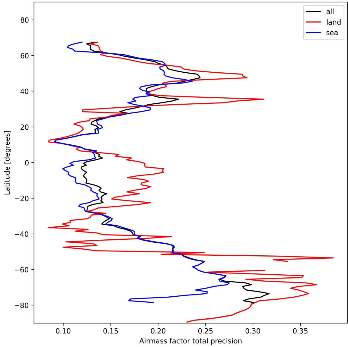
Figure 27: Zonal average of “Airmass factor total precision” for 2025-01-28 to 2025-01-30.
