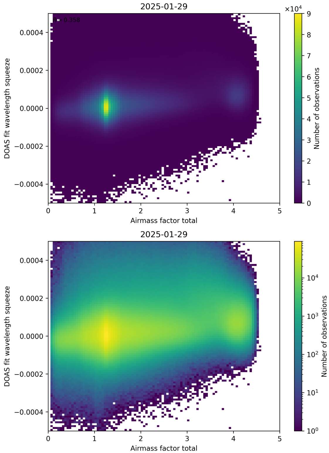
Figure 99: Scatter density plot of “Airmass factor total” against “DOAS fit wavelength squeeze” for 2025-01-28 to 2025-01-30.
