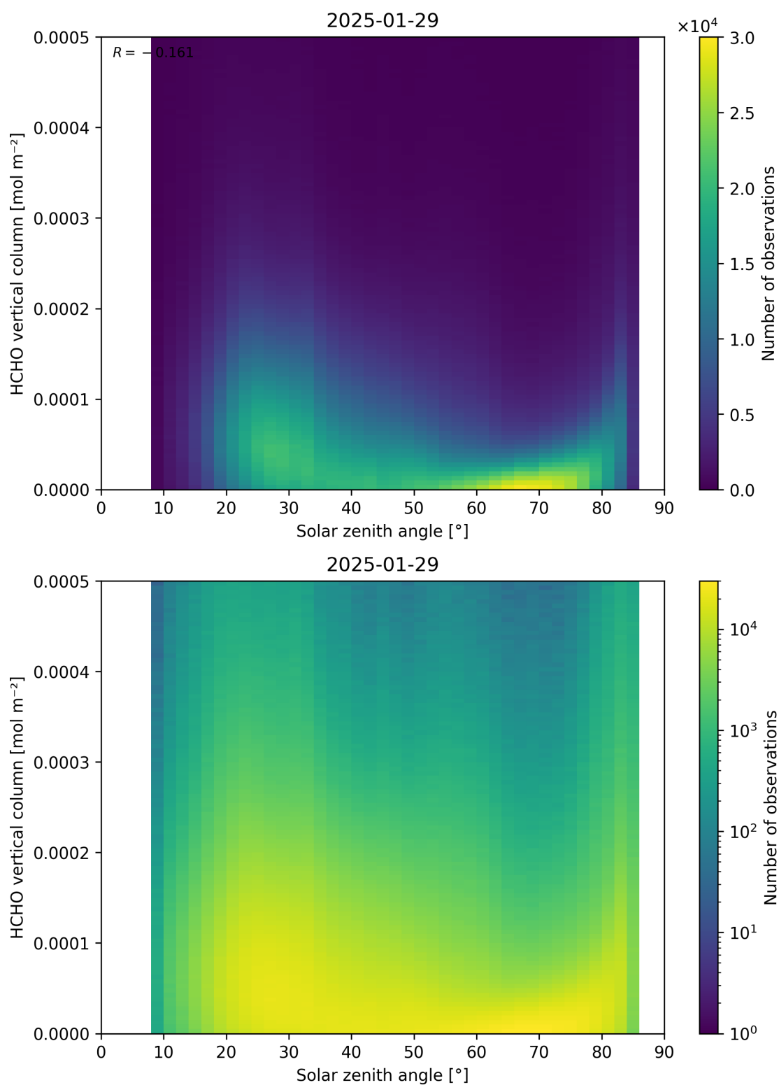
Figure 177: Scatter density plot of “Solar zenith angle” against “HCHO vertical column” for 2025-01-28 to 2025-01-30.
