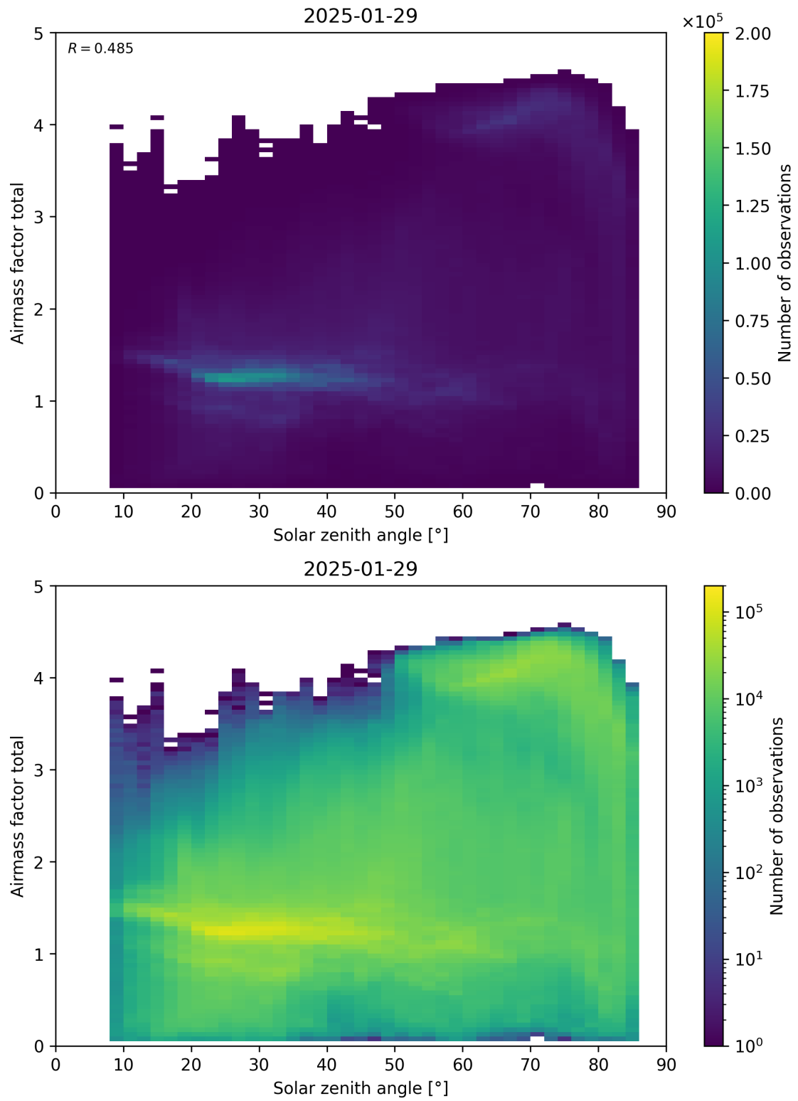
Figure 175: Scatter density plot of “Solar zenith angle” against “Airmass factor total” for 2025-01-28 to 2025-01-30.
