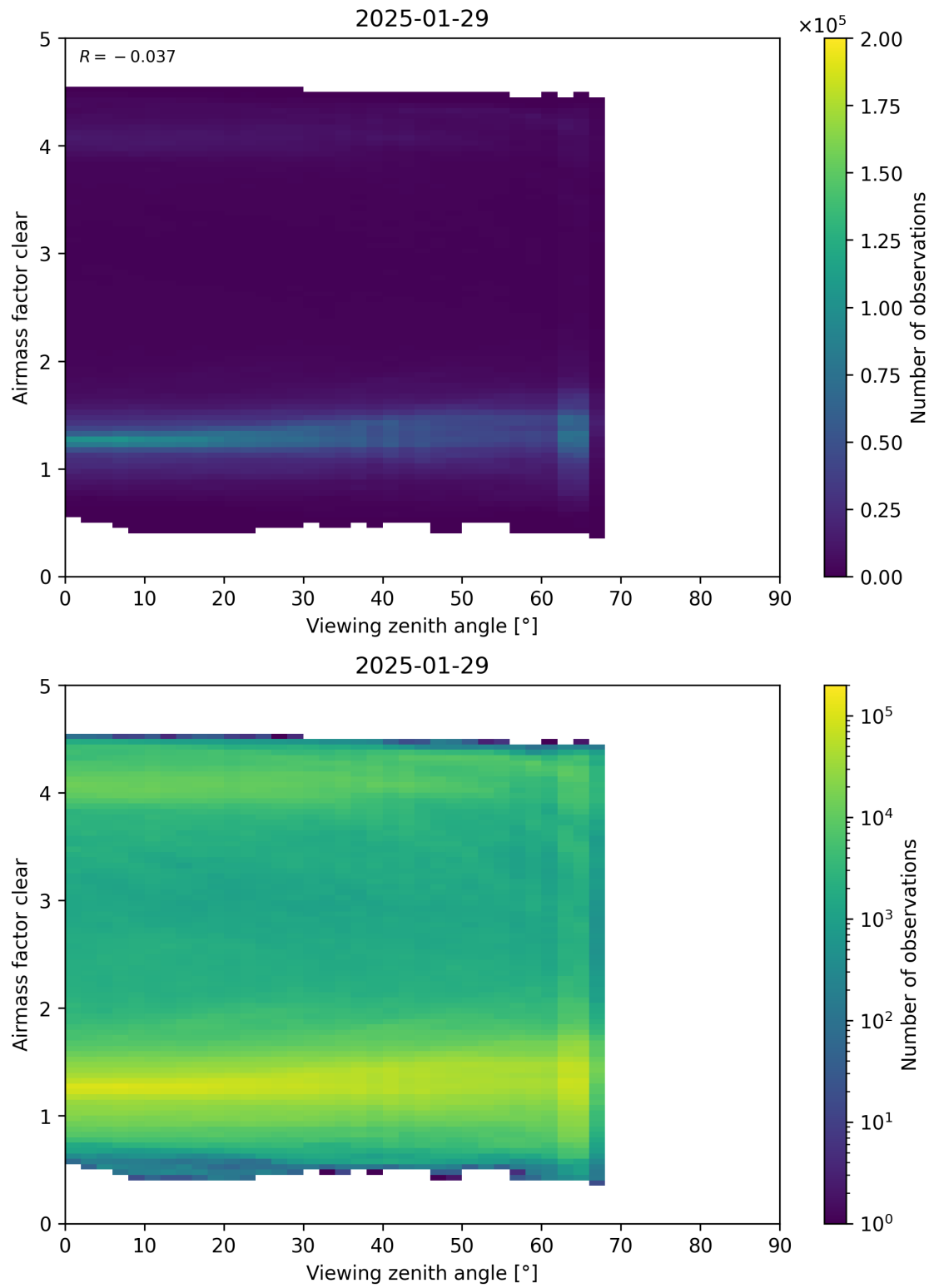
Figure 185: Scatter density plot of “Viewing zenith angle” against “Airmass factor clear” for 2025-01-28 to 2025-01-30.
