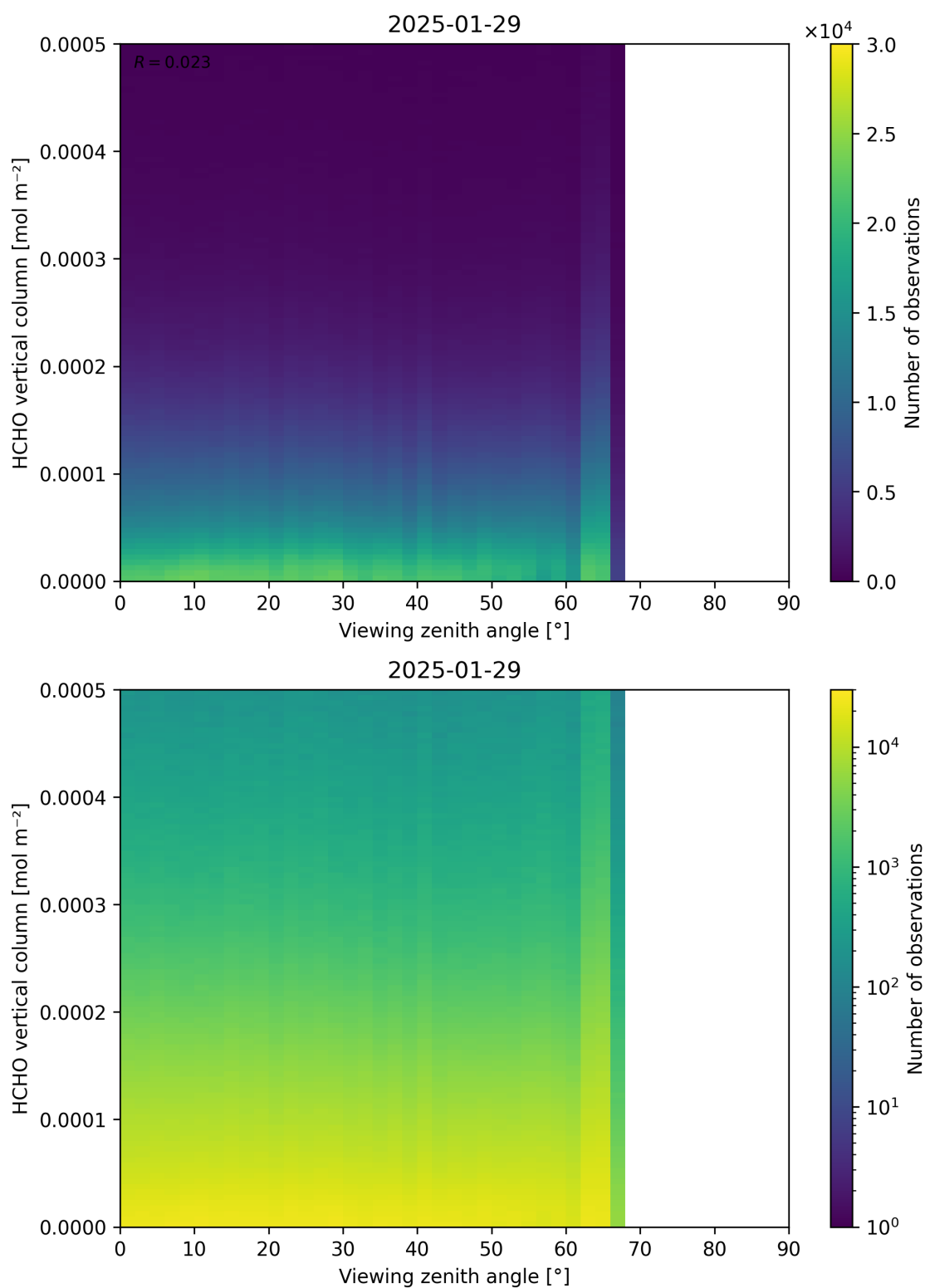
Figure 192: Scatter density plot of “Viewing zenith angle” against “HCHO vertical column” for 2025-01-28 to 2025-01-30.
