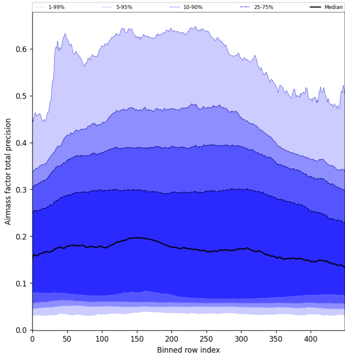
Figure 55: Along track statistics of “Airmass factor total precision” for 2025-01-28 to 2025-01-30
