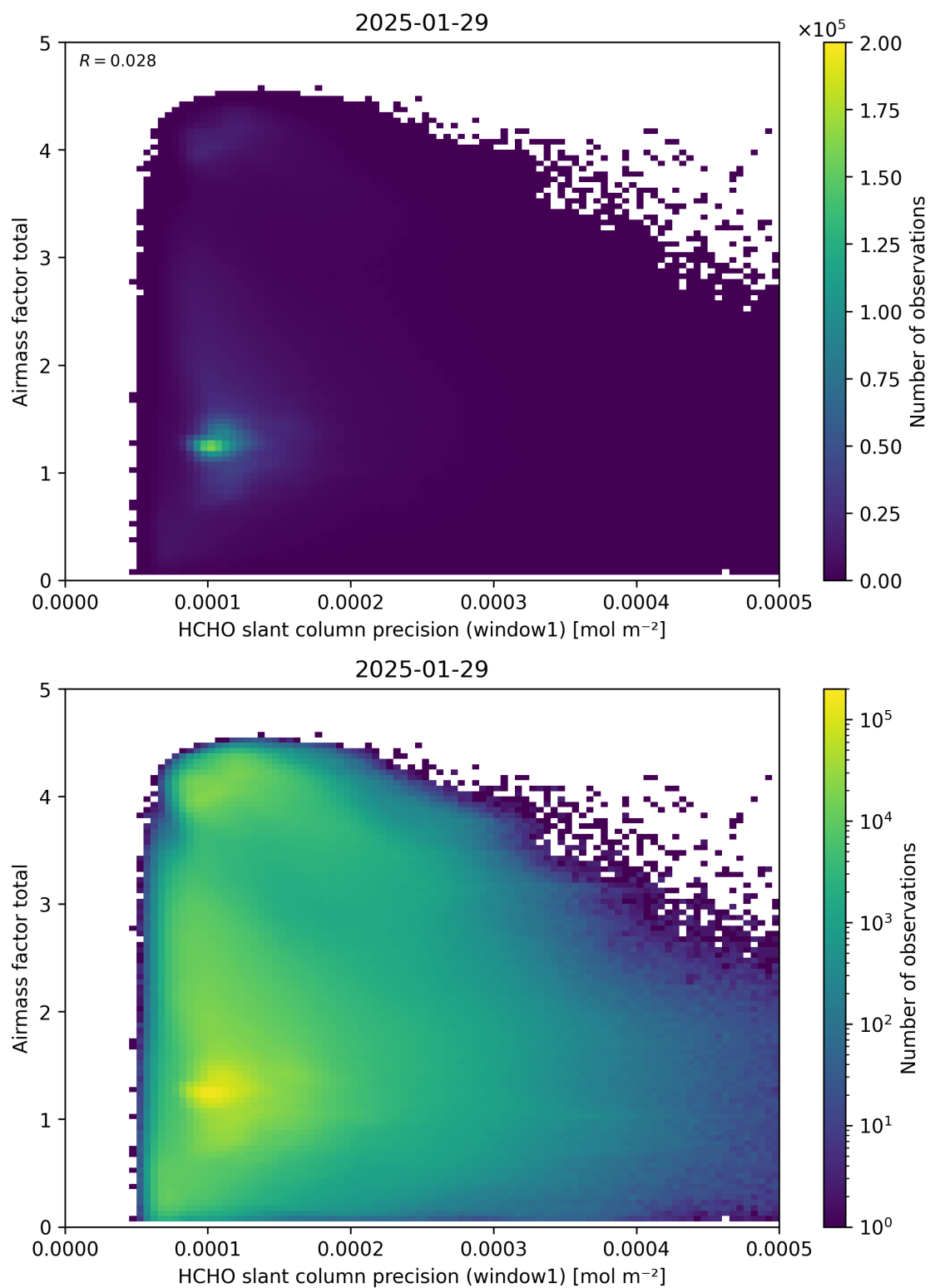
Figure 94: Scatter density plot of “HCHO slant column precision (window1)” against “Airmass factor total” for 2025-01-28 to 2025-01-30.
