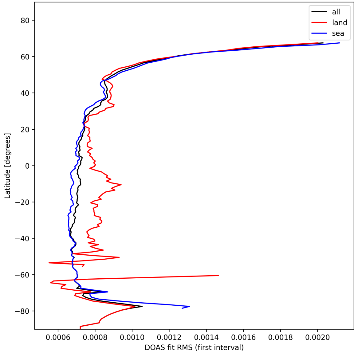
Figure 32: Zonal average of "DOAS fit RMS (first interval)" for 2025-01-28 to 2025-01-30.
