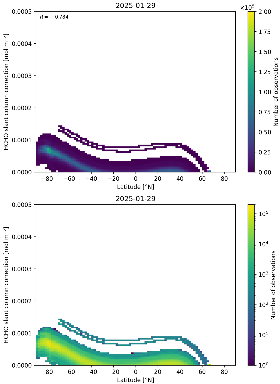
Figure 158: Scatter density plot of “Latitude” against “HCHO slant column correction” for 2025-01-28 to 2025-01-30.
