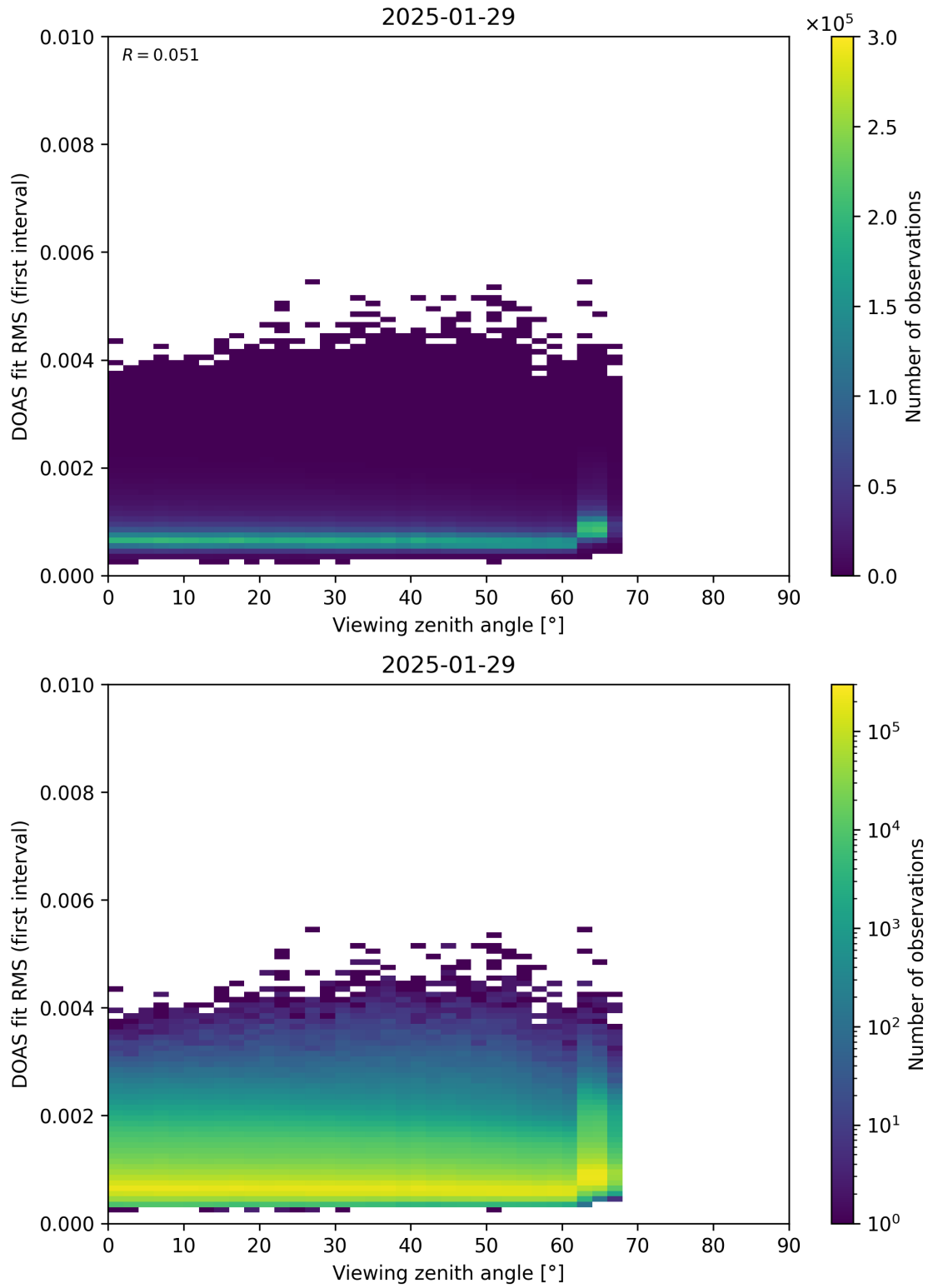
Figure 182: Scatter density plot of “Viewing zenith angle” against “DOAS fit RMS (first interval)” for 2025-01-28 to 2025-01-30.
