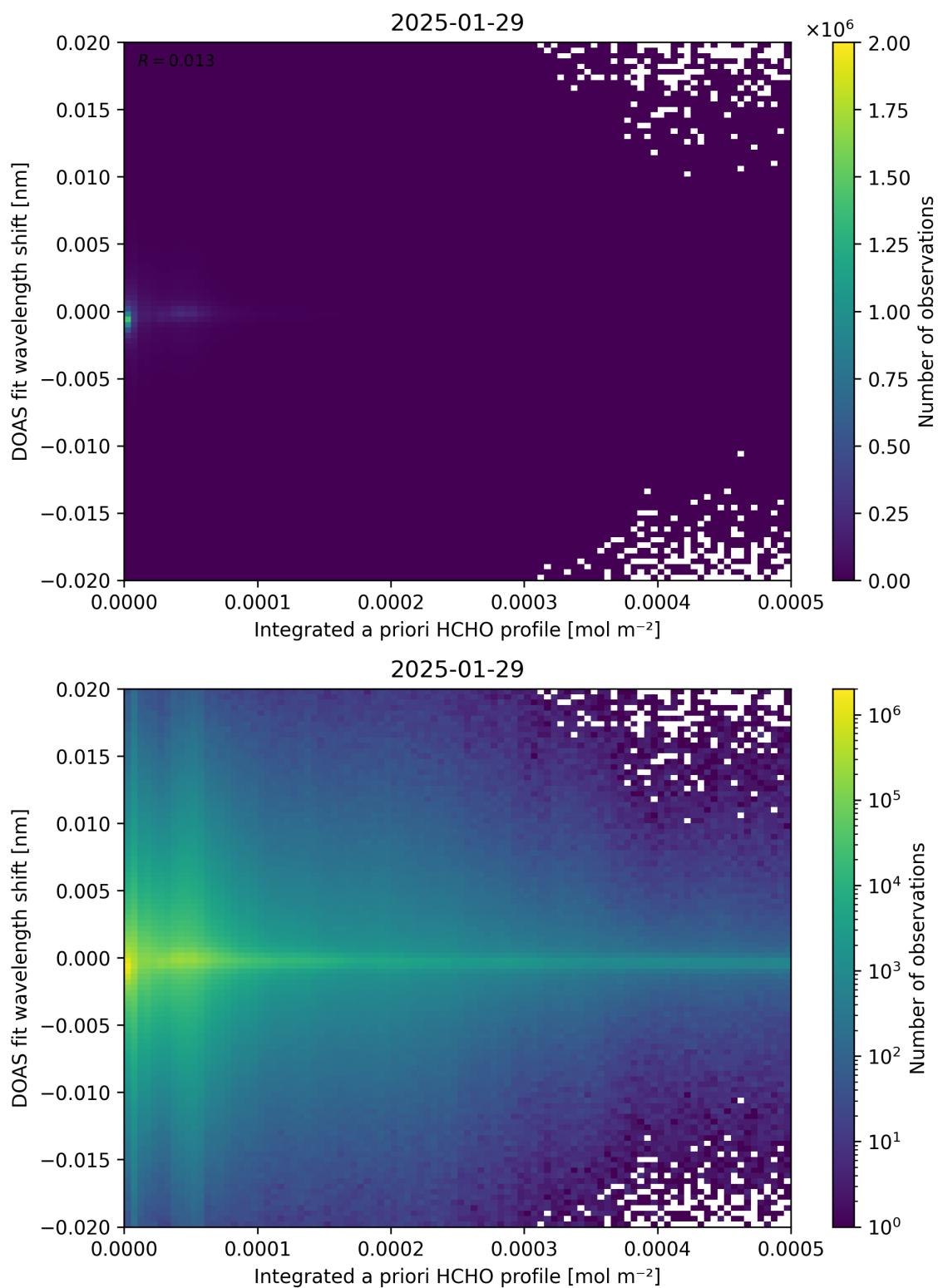
Figure 149: Scatter density plot of “Integrated a priori HCHO profile” against “DOAS fit wavelength shift” for 2025-01-28 to 2025-01-30.
