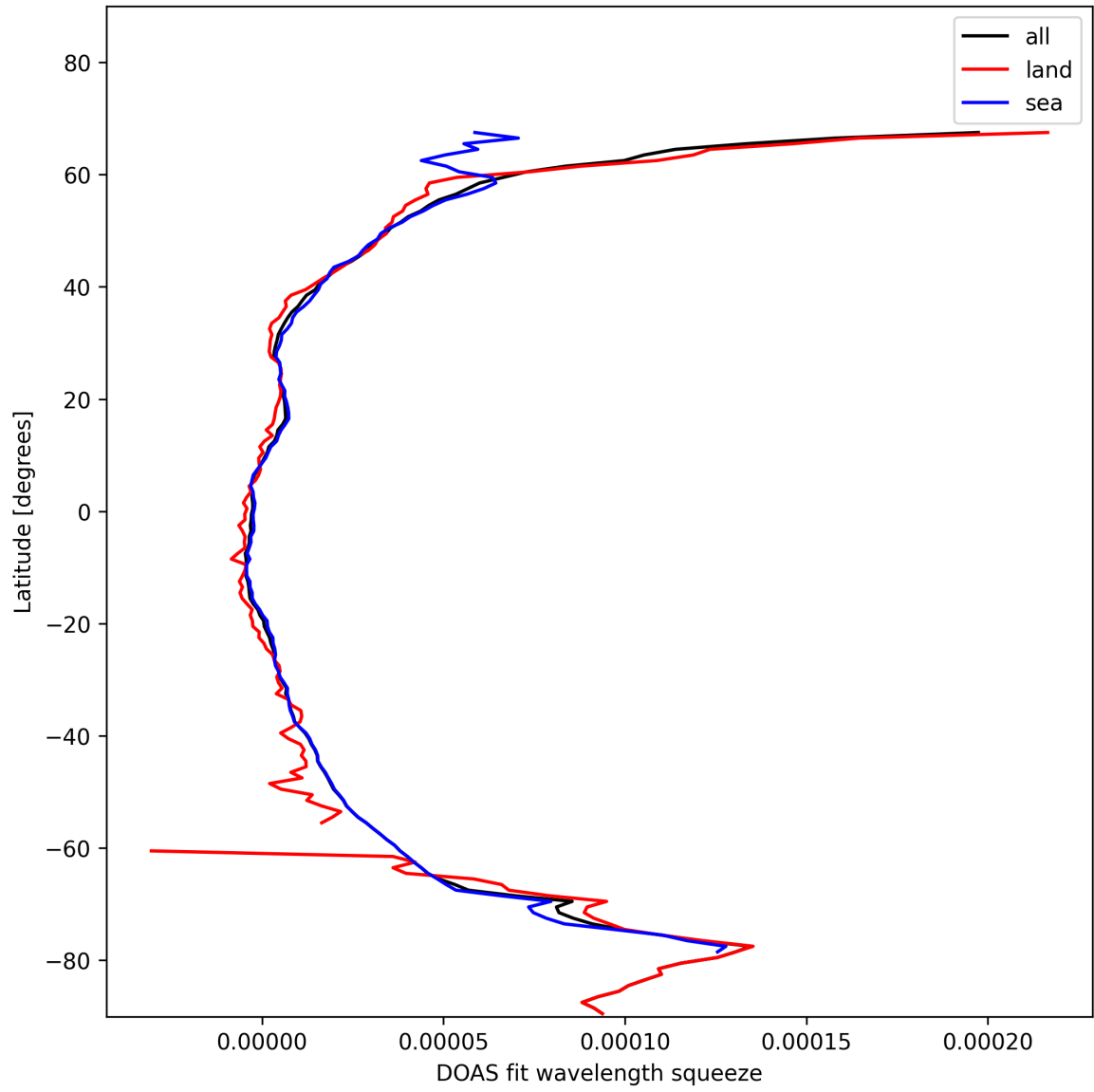
Figure 31: Zonal average of “DOAS fit wavelength squeeze” for 2025-01-28 to 2025-01-30.
