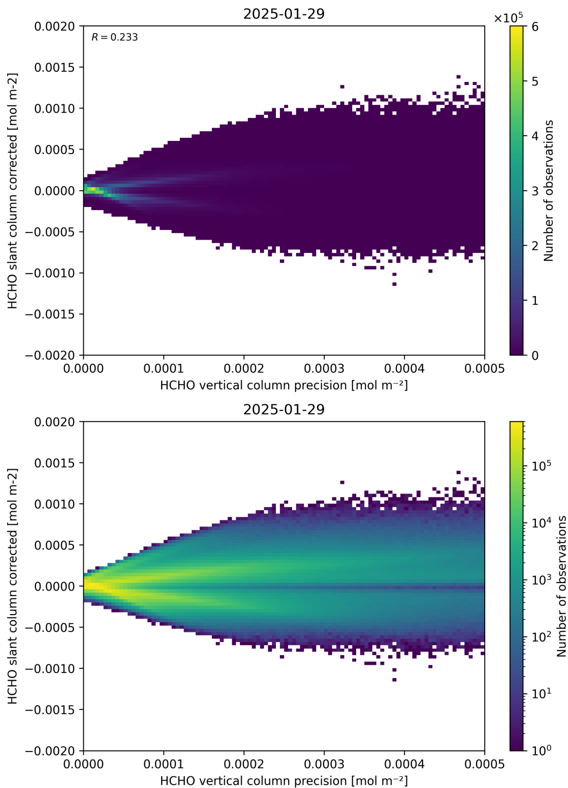
Figure 140: Scatter density plot of “HCHO vertical column precision” against “HCHO slant column corrected” for 2025-01-28 to 2025-01-30.
