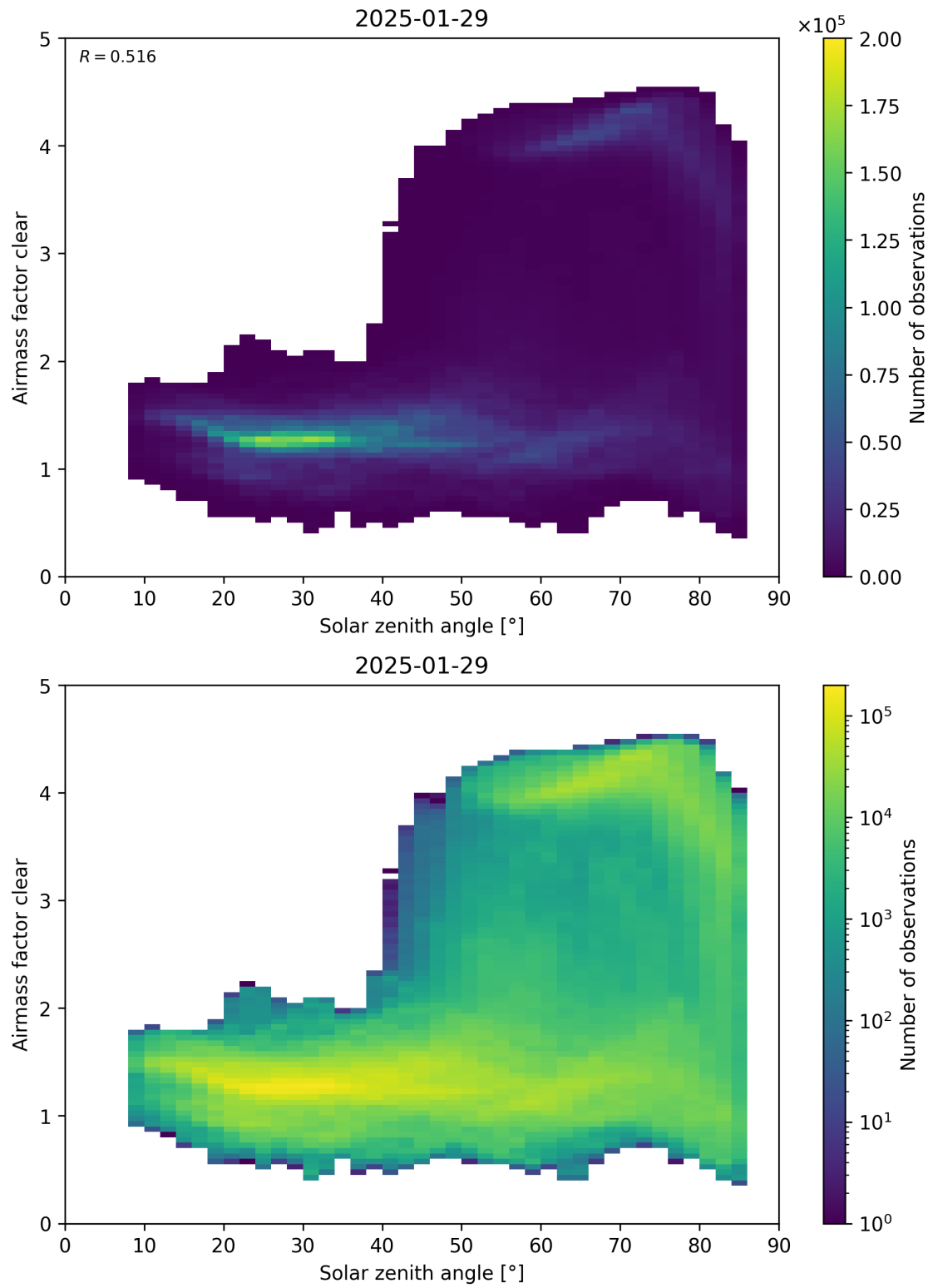
Figure 170: Scatter density plot of “Solar zenith angle” against “Airmass factor clear” for 2025-01-28 to 2025-01-30.
