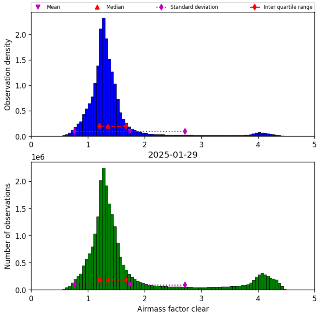
Figure 42: Histogram of “Airmass factor clear” for 2025-01-28 to 2025-01-30
