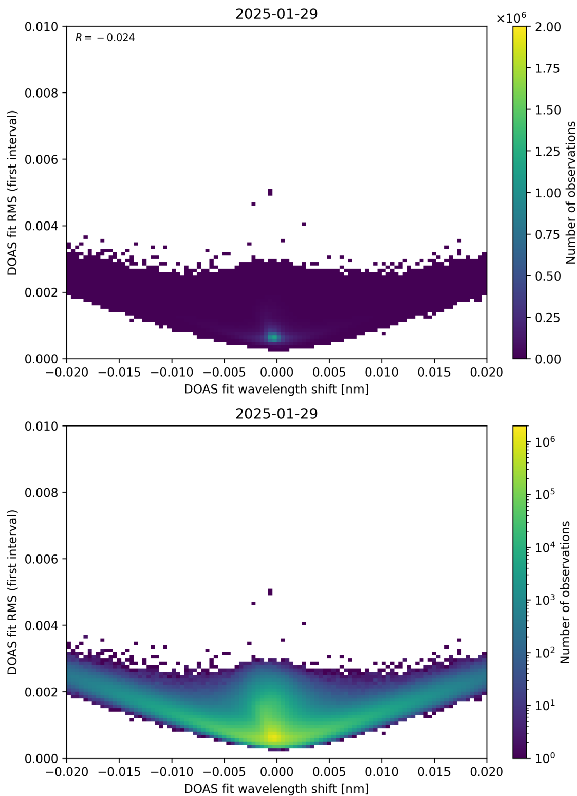
Figure 64: Scatter density plot of “DOAS fit wavelength shift” against “DOAS fit RMS (first interval)” for 2025-01-28 to 2025-01-30.
