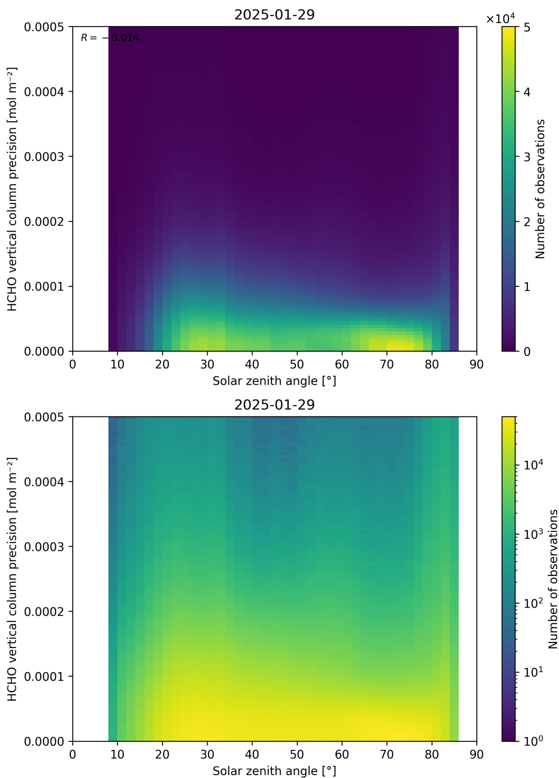
Figure 179: Scatter density plot of “Solar zenith angle” against “HCHO vertical column precision” for 2025-01-28 to 2025-01-30.
