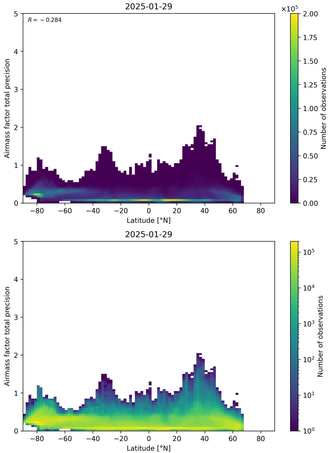
Figure 162: Scatter density plot of “Latitude” against “Airmass factor total precision” for 2025-01-28 to 2025-01-30.
