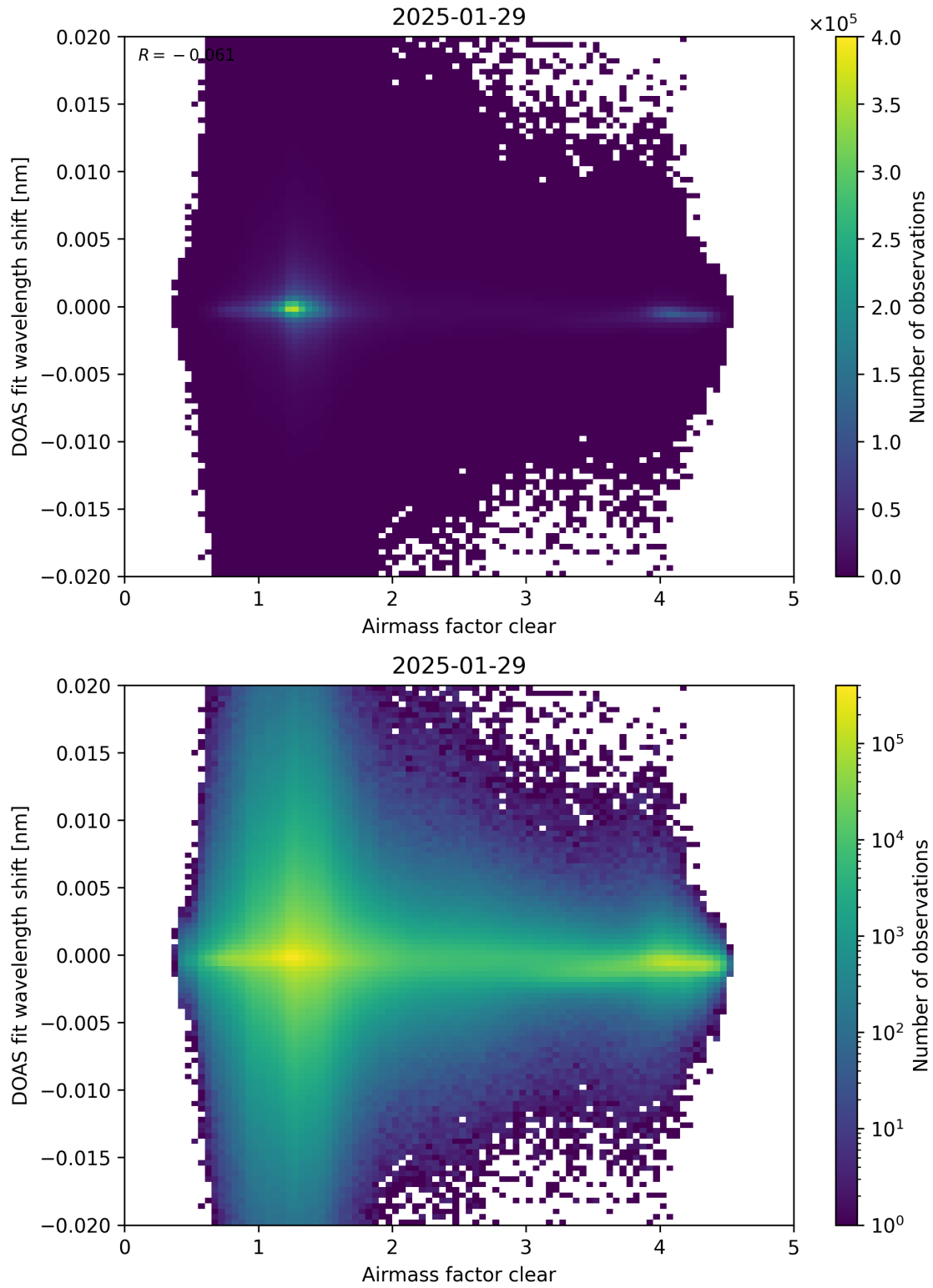
Figure 72: Scatter density plot of “Airmass factor clear” against “DOAS fit wavelength shift” for 2025-01-28 to 2025-01-30.
