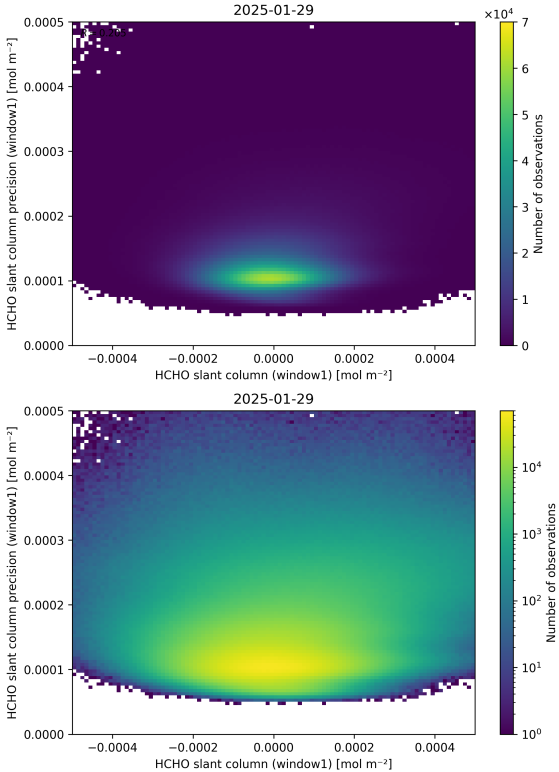
Figure 84: Scatter density plot of “HCHO slant column (window1)” against “HCHO slant column precision (window1)” for 2025-01-28 to 2025-01-30.
