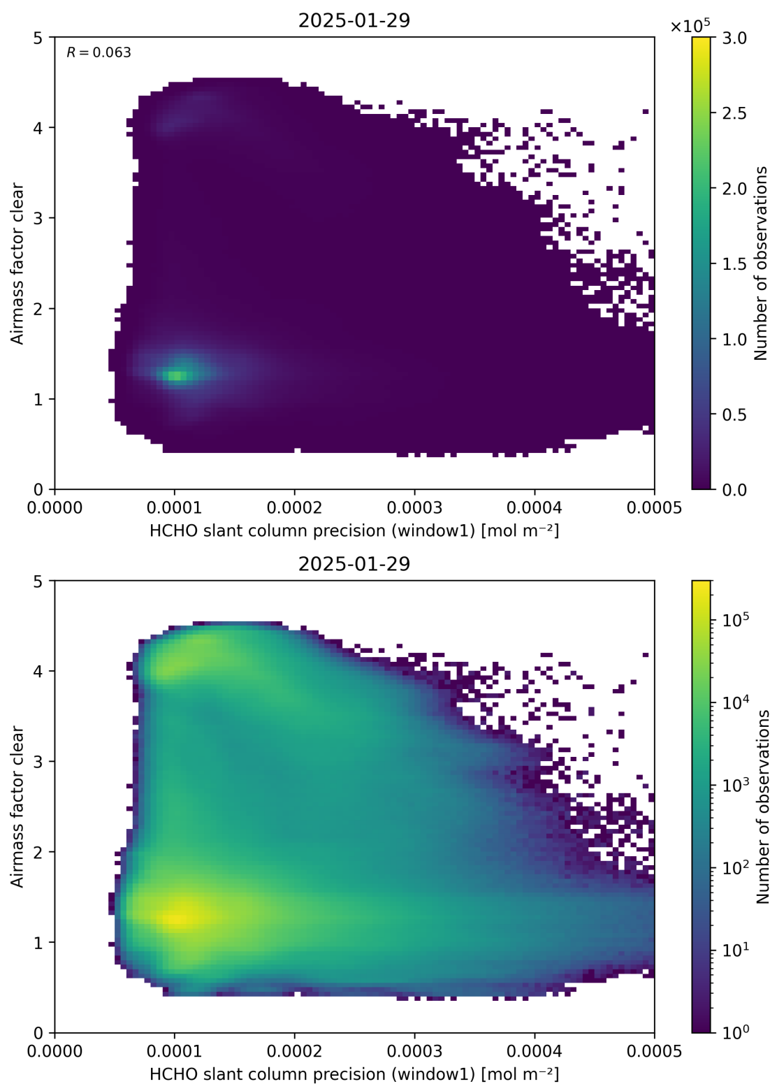
Figure 91: Scatter density plot of “HCHO slant column precision (window1)” against “Airmass factor clear” for 2025-01-28 to 2025-01-30.
