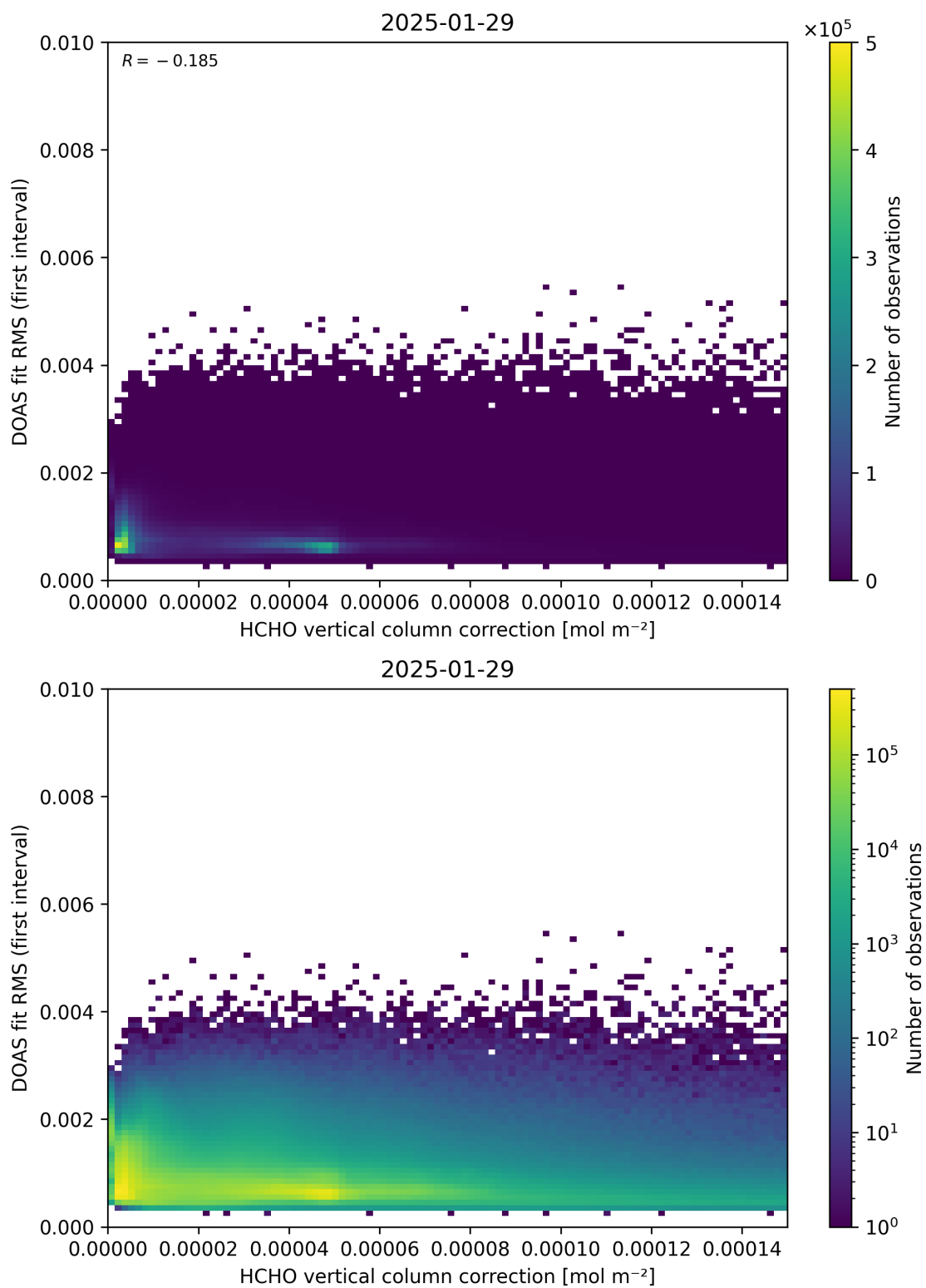
Figure 112: Scatter density plot of “HCHO vertical column correction” against “DOAS fit RMS (first interval)” for 2025-01-28 to 2025-01-30.
