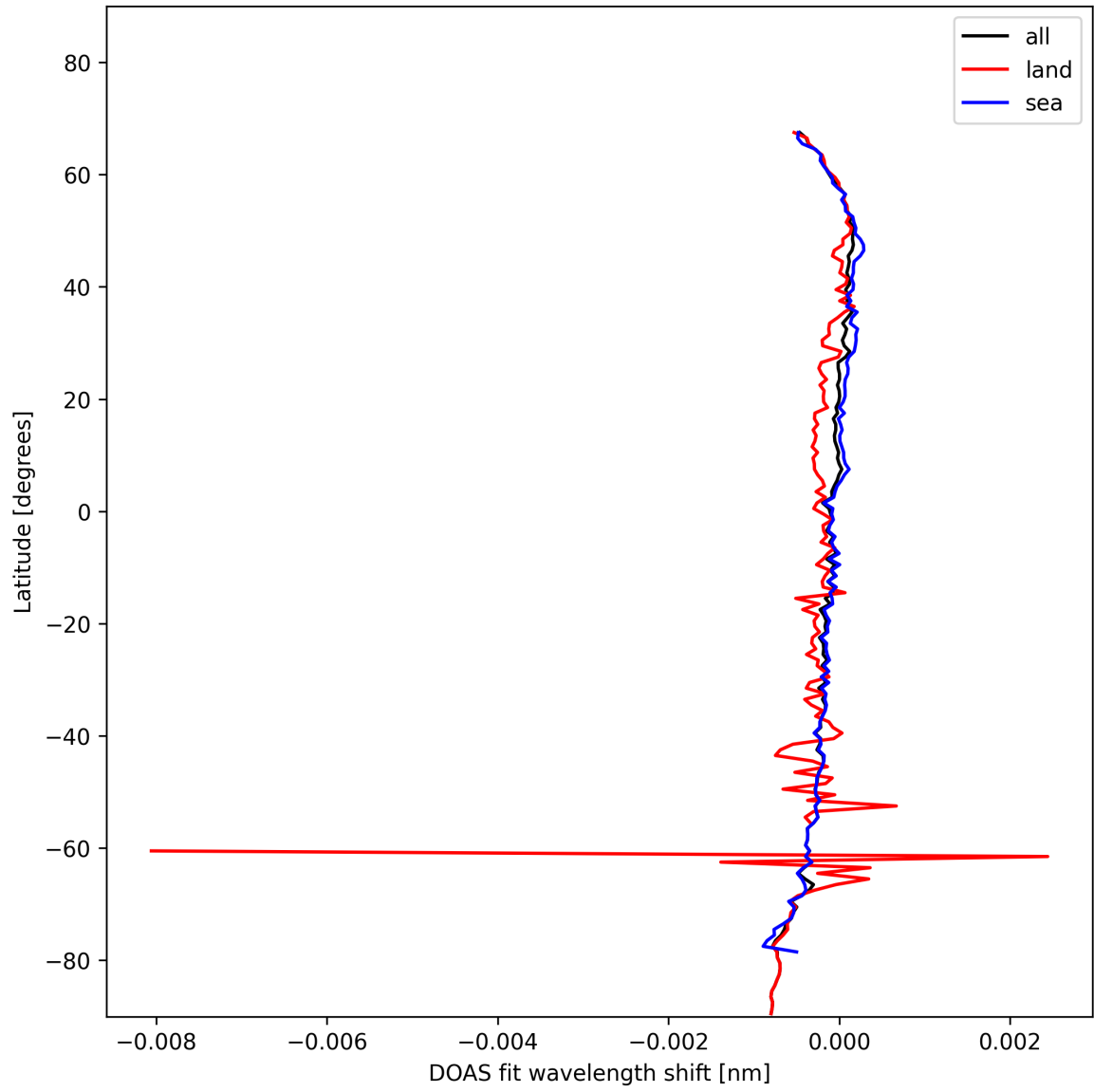
Figure 30: Zonal average of "DOAS fit wavelength shift" for 2025-01-28 to 2025-01-30.
