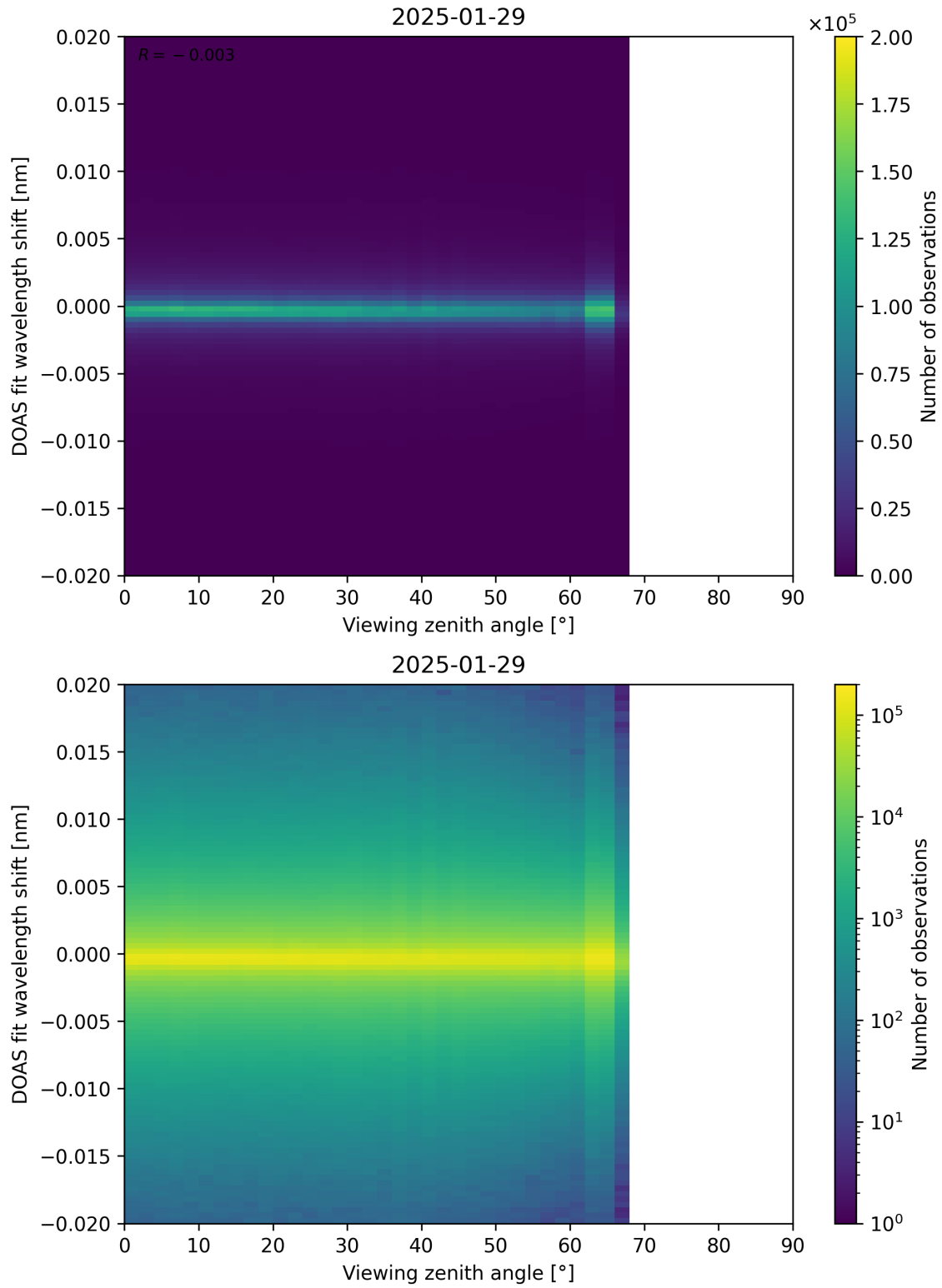
Figure 183: Scatter density plot of “Viewing zenith angle” against “DOAS fit wavelength shift” for 2025-01-28 to 2025-01-30.
