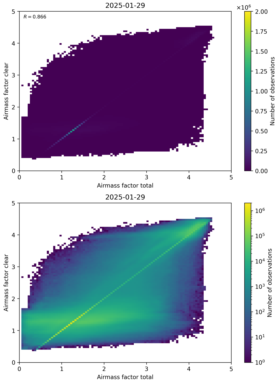
Figure 100: Scatter density plot of “Airmass factor total” against “Airmass factor clear” for 2025-01-28 to 2025-01-30.
