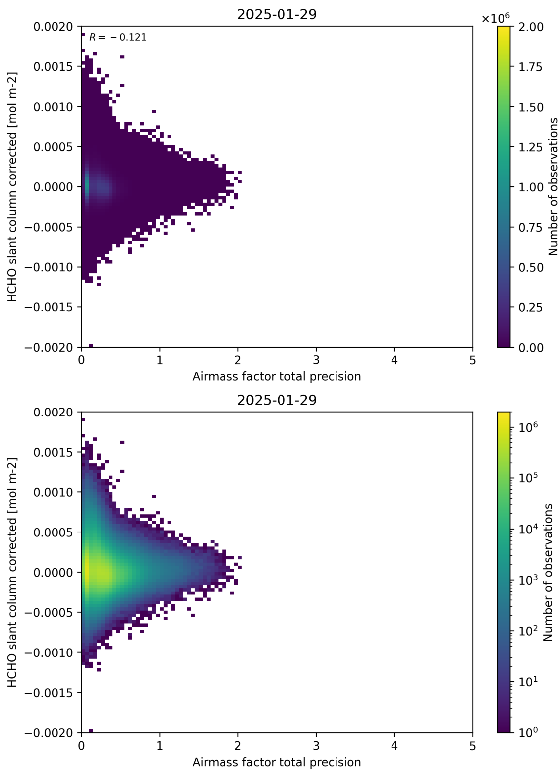
Figure 109: Scatter density plot of “Airmass factor total precision” against “HCHO slant column corrected” for 2025-01-28 to 2025-01-30.
