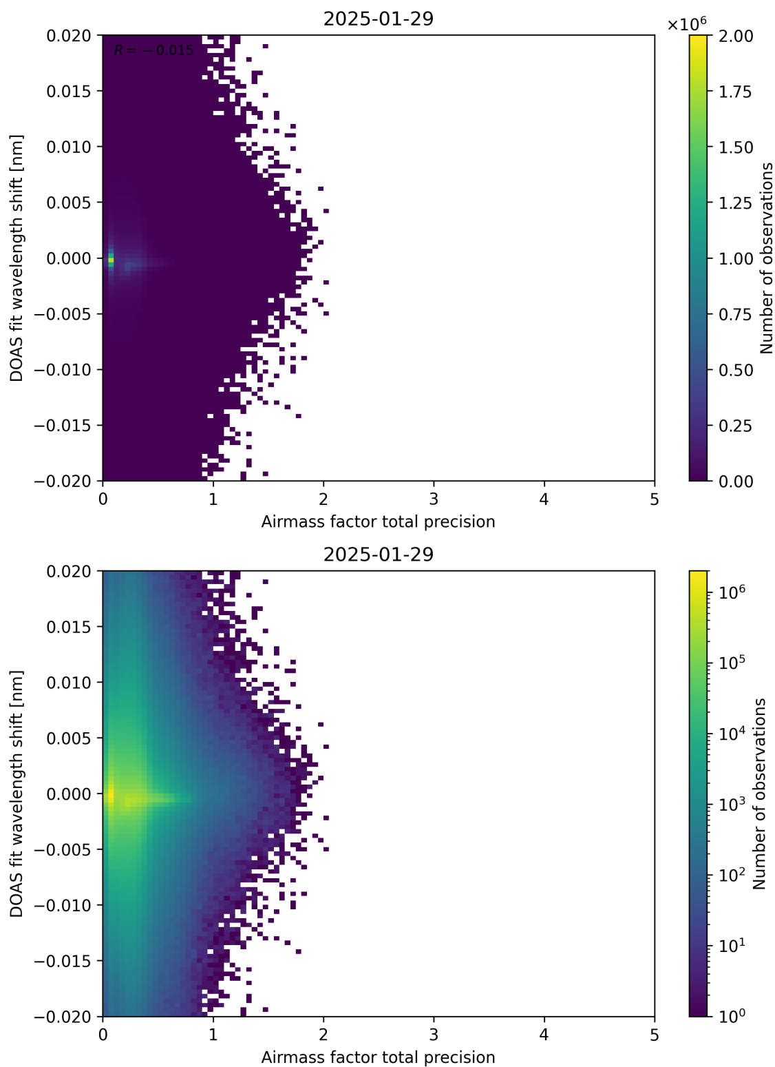
Figure 106: Scatter density plot of “Airmass factor total precision” against “DOAS fit wavelength shift” for 2025-01-28 to 2025-01-30.
