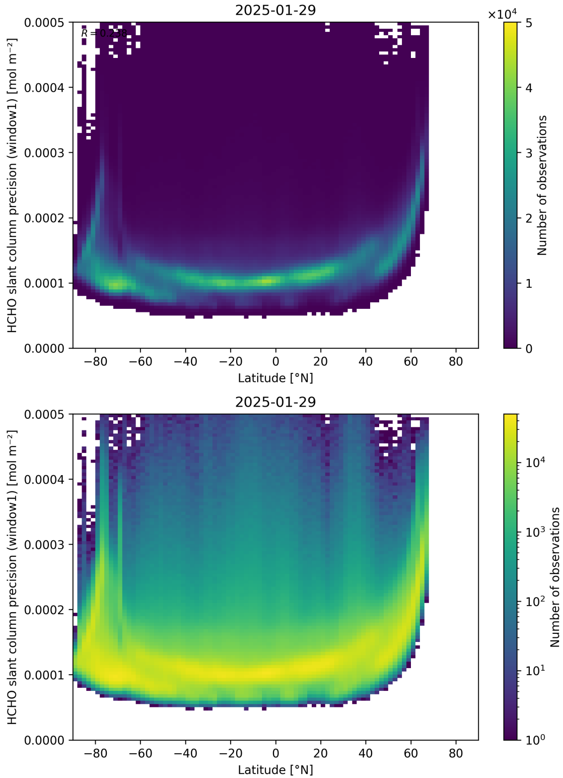
Figure 160: Scatter density plot of “Latitude” against “HCHO slant column precision (window1)” for 2025-01-28 to 2025-01-30.
