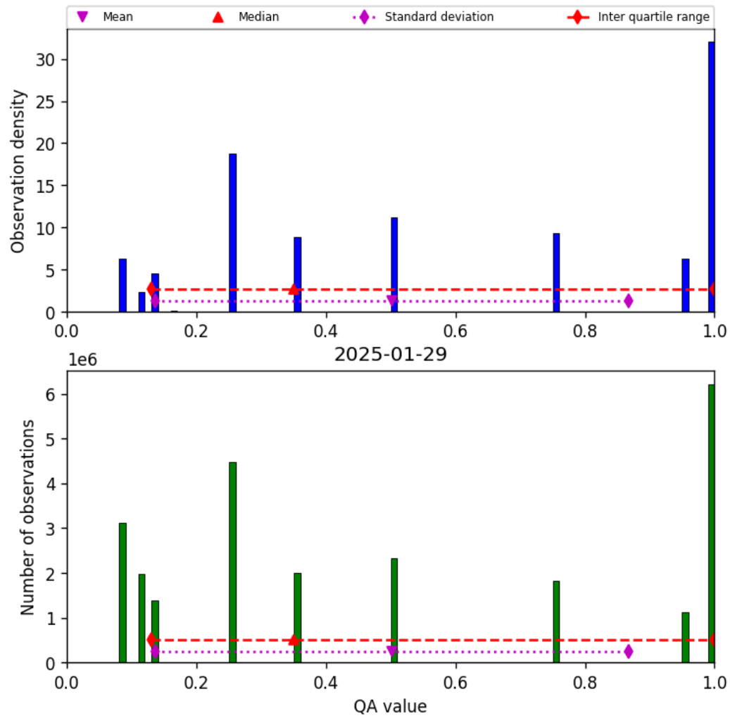
Figure 34: Histogram of “QA value” for 2025-01-28 to 2025-01-30
