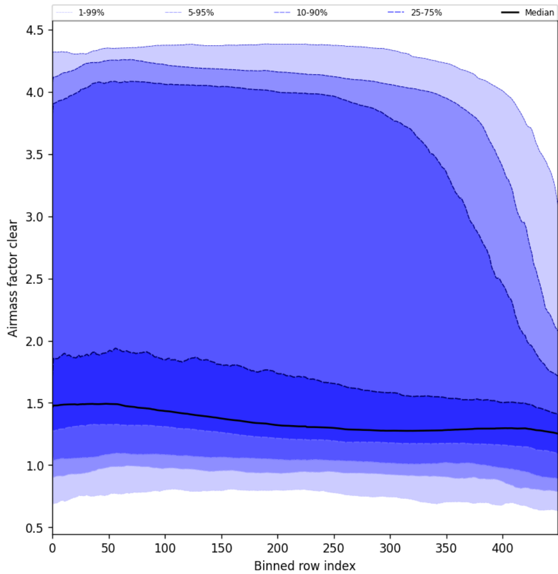
Figure 56: Along track statistics of “Airmass factor clear” for 2025-01-28 to 2025-01-30
