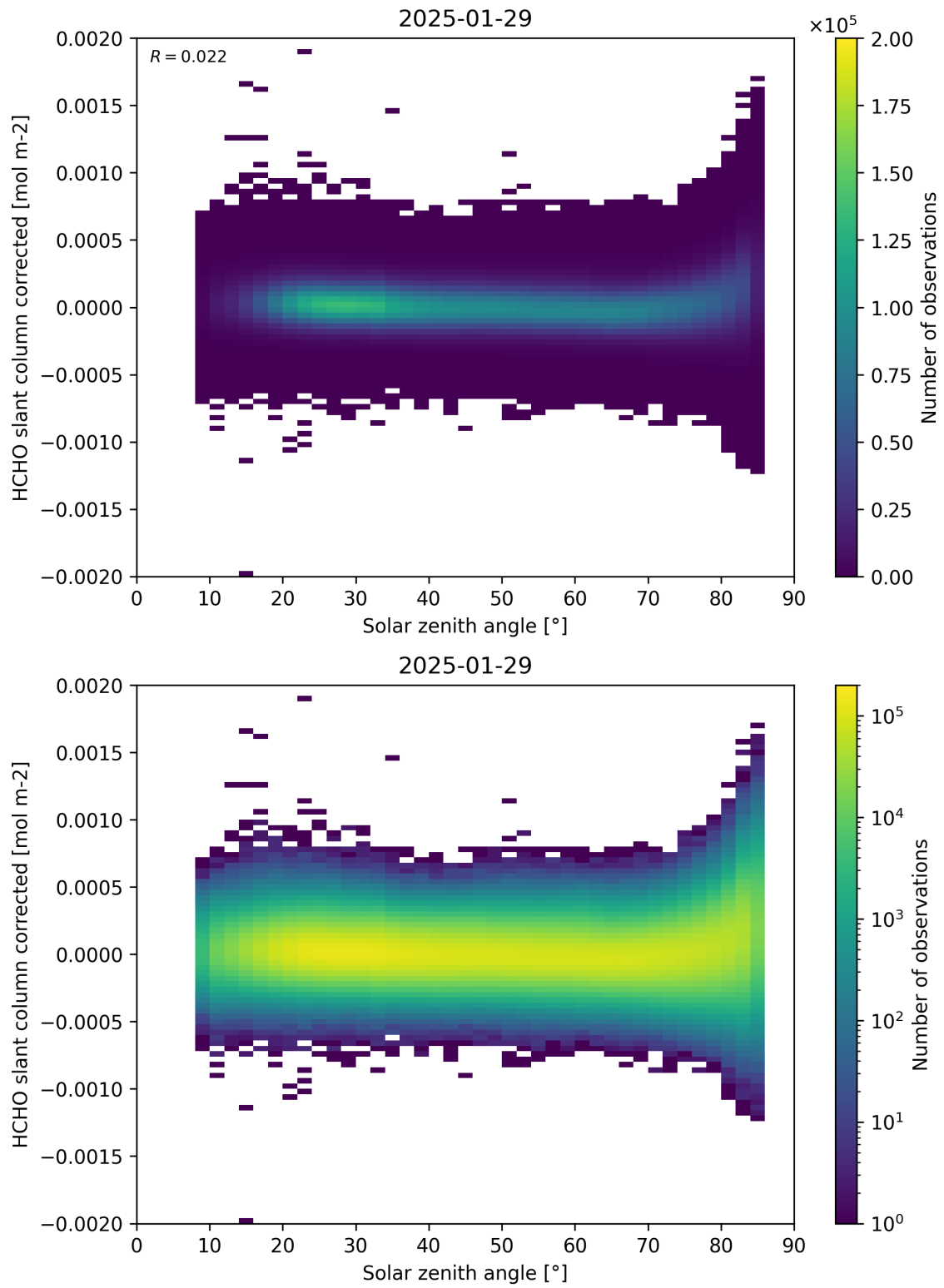
Figure 171: Scatter density plot of “Solar zenith angle” against “HCHO slant column corrected” for 2025-01-28 to 2025-01-30.
