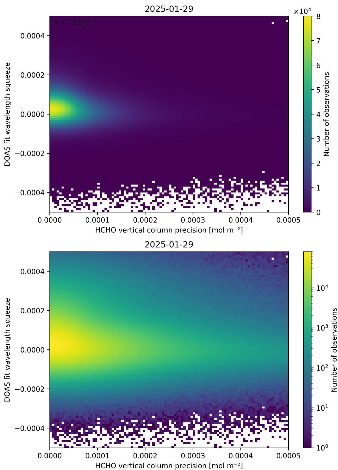
Figure 138: Scatter density plot of “HCHO vertical column precision” against “DOAS fit wavelength squeeze” for 2025-01-28 to 2025-01-30.
