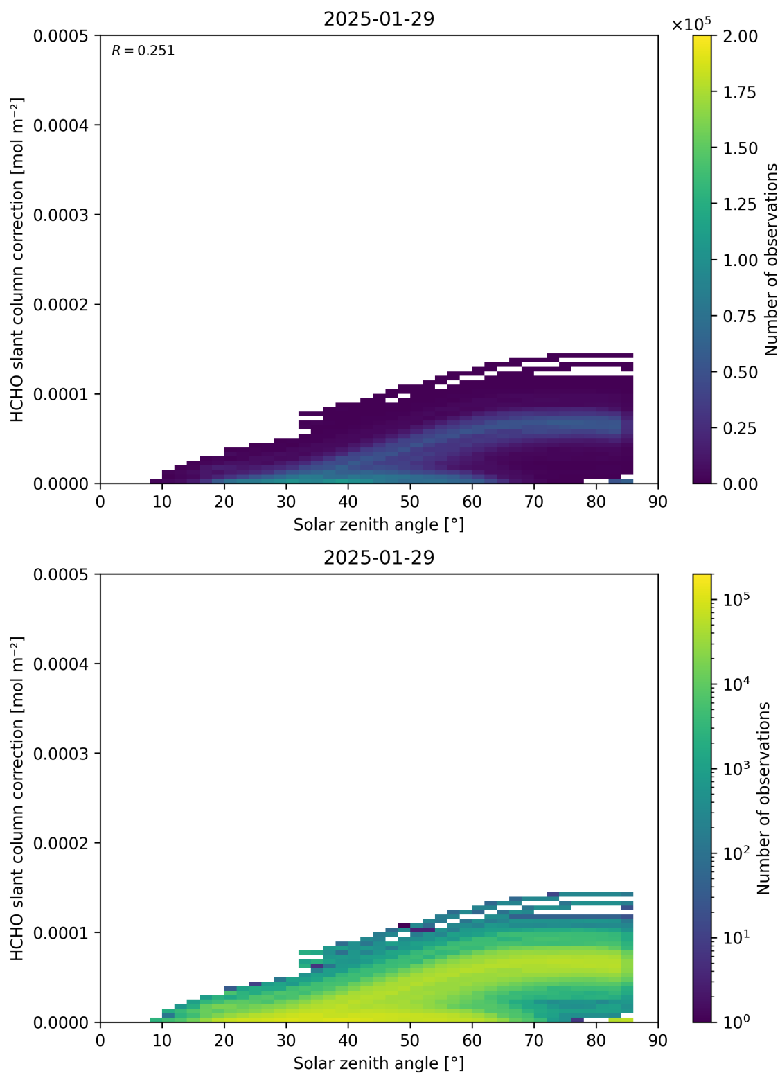
Figure 172: Scatter density plot of “Solar zenith angle” against “HCHO slant column correction” for 2025-01-28 to 2025-01-30.
