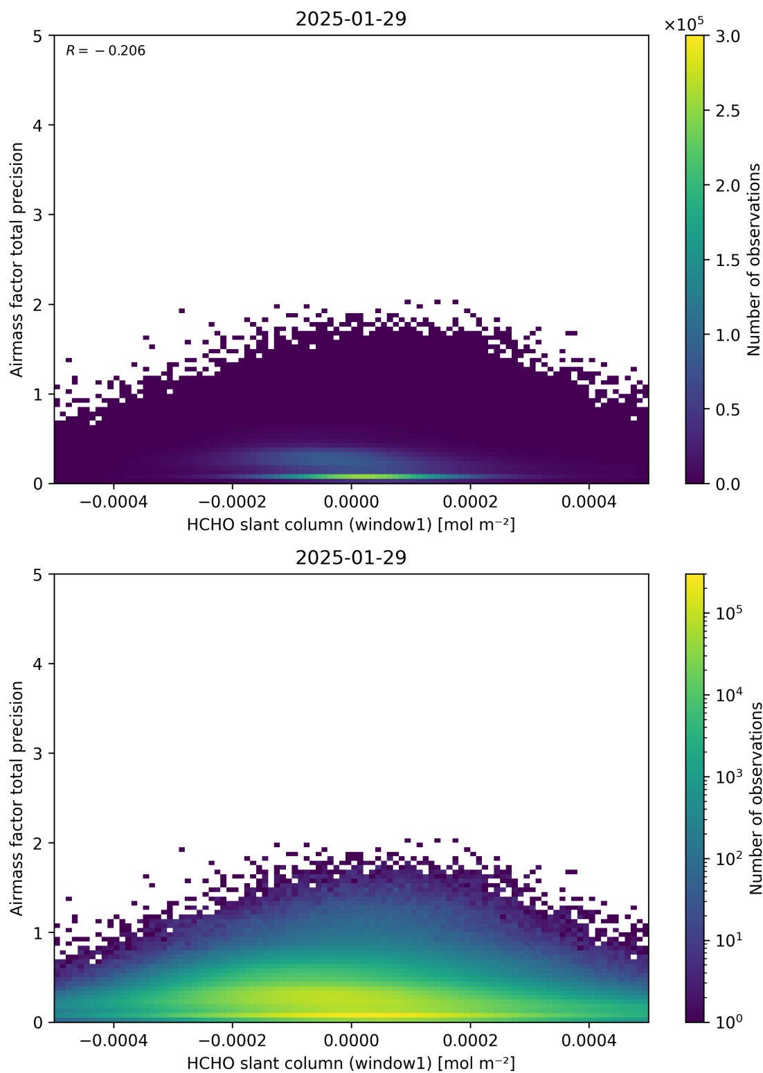
Figure 86: Scatter density plot of “HCHO slant column (window1)” against “Airmass factor total precision” for 2025-01-28 to 2025-01-30.
