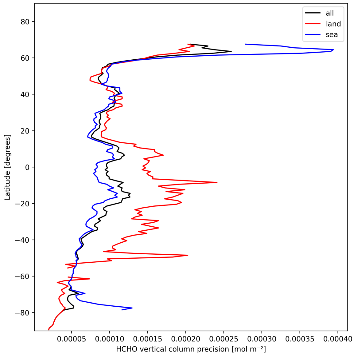
Figure 22: Zonal average of “HCHO vertical column precision” for 2025-01-28 to 2025-01-30.
