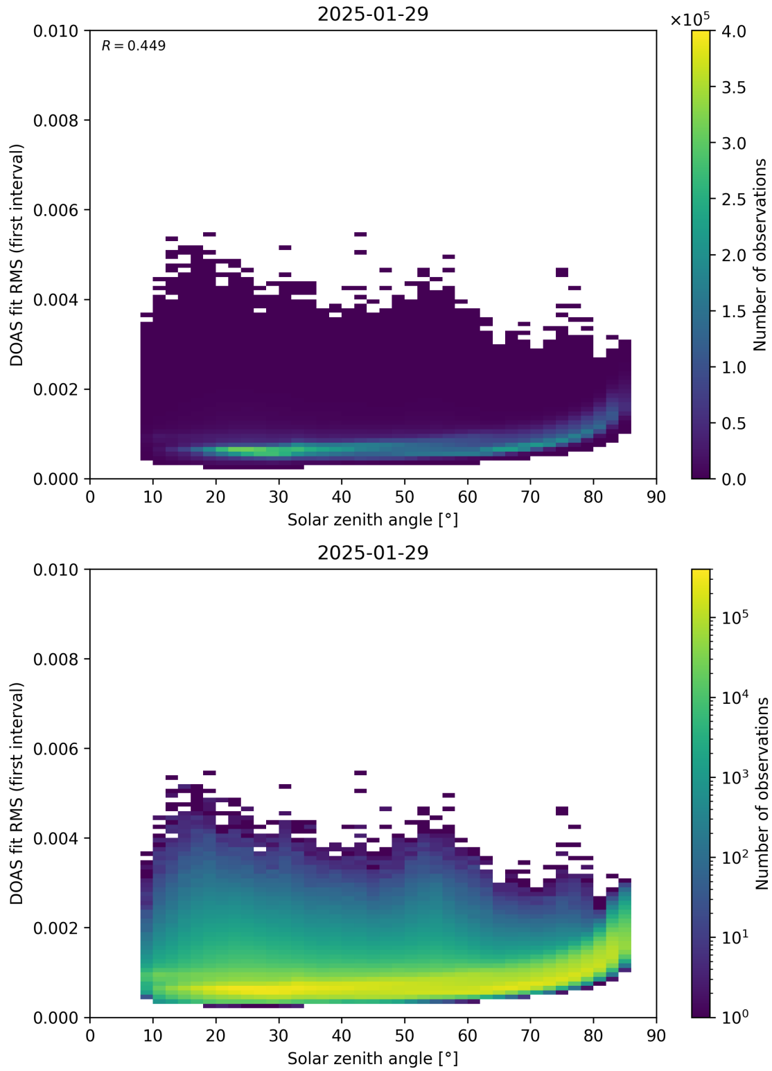
Figure 167: Scatter density plot of “Solar zenith angle” against “DOAS fit RMS (first interval)” for 2025-01-28 to 2025-01-30.
