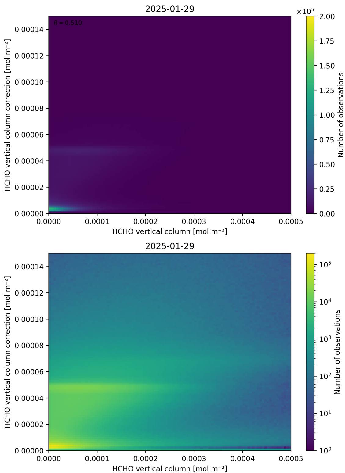
Figure 133: Scatter density plot of “HCHO vertical column” against “HCHO vertical column correction” for 2025-01-28 to 2025-01-30.
