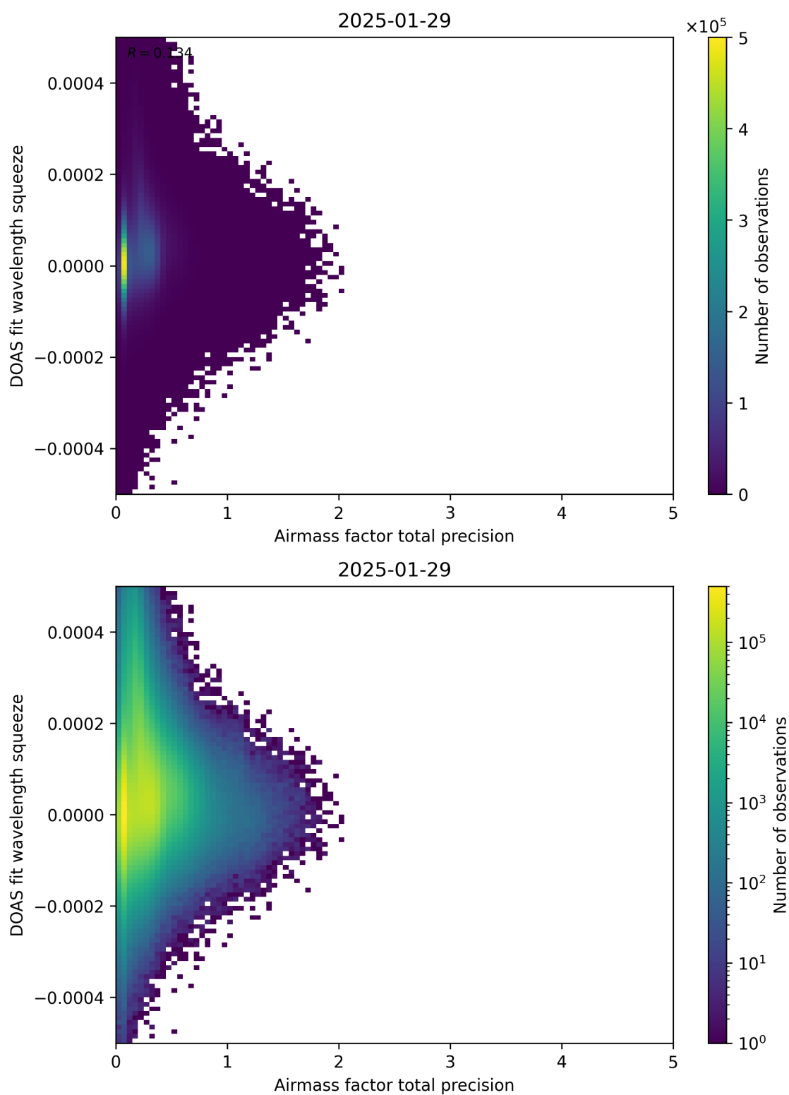
Figure 107: Scatter density plot of “Airmass factor total precision” against “DOAS fit wavelength squeeze” for 2025-01-28 to 2025-01-30.
