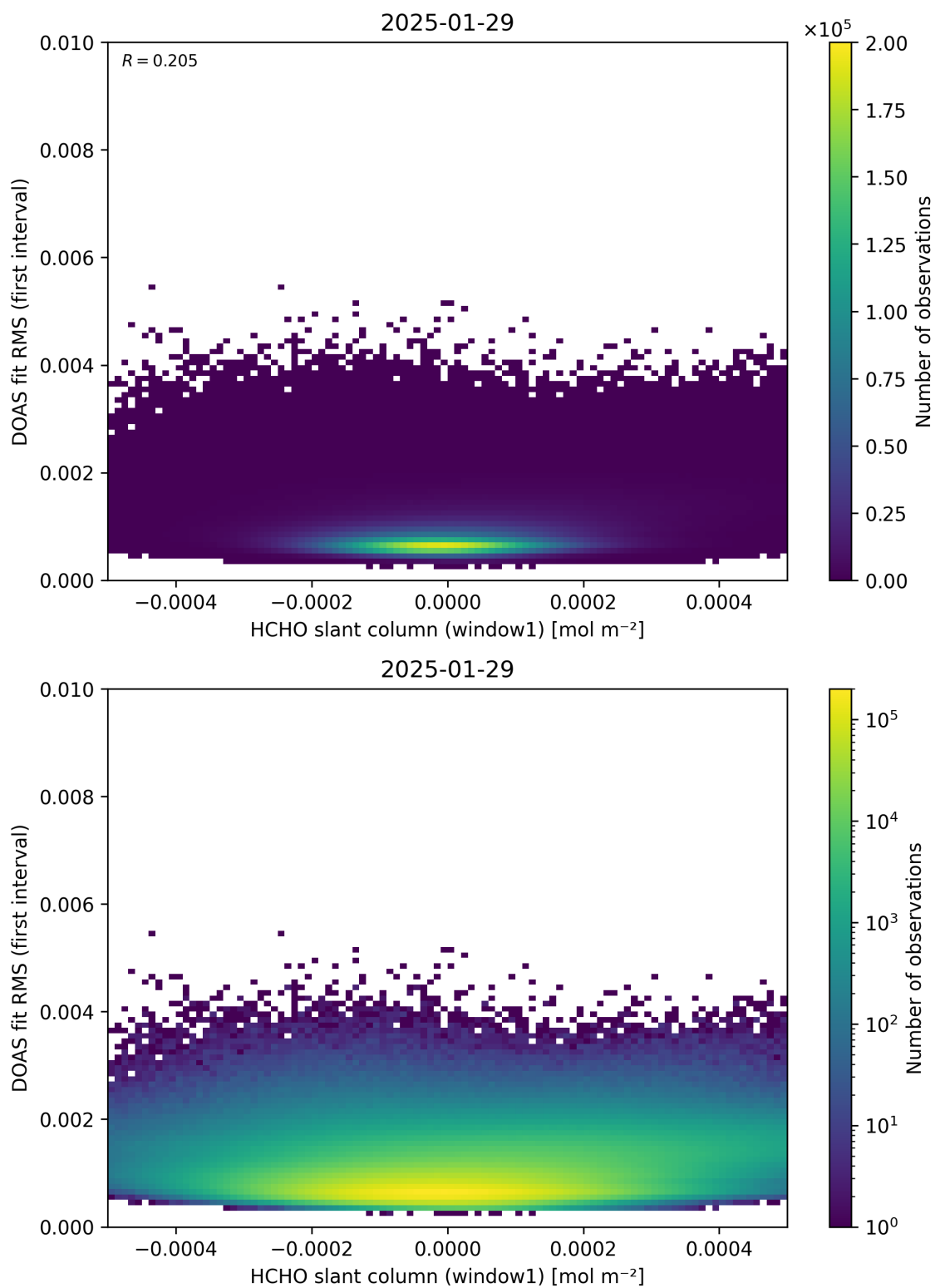
Figure 78: Scatter density plot of “HCHO slant column (window1)” against “DOAS fit RMS (first interval)” for 2025-01-28 to 2025-01-30.
