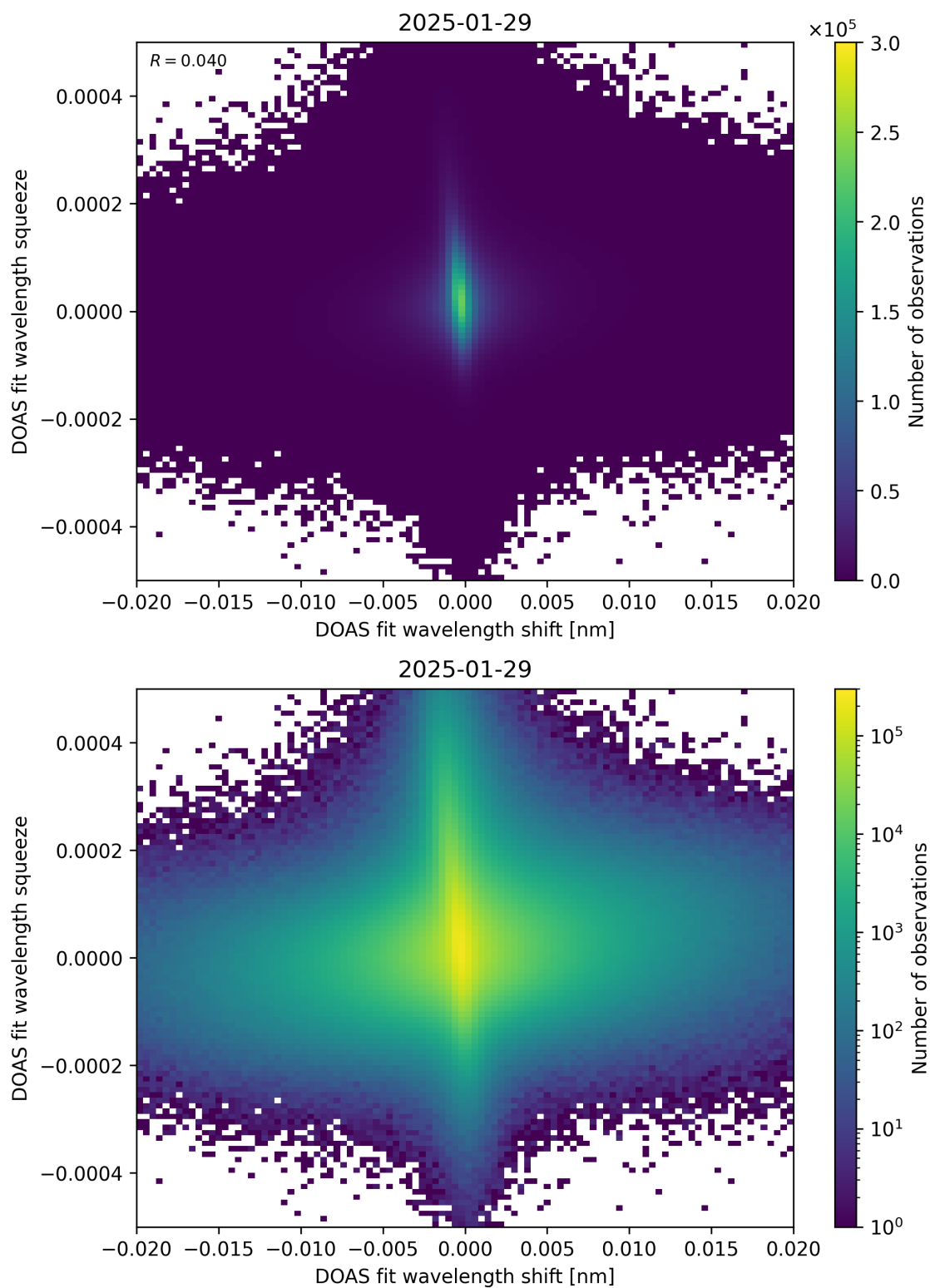
Figure 65: Scatter density plot of “DOAS fit wavelength shift” against “DOAS fit wavelength squeeze” for 2025-01-28 to 2025-01-30.
