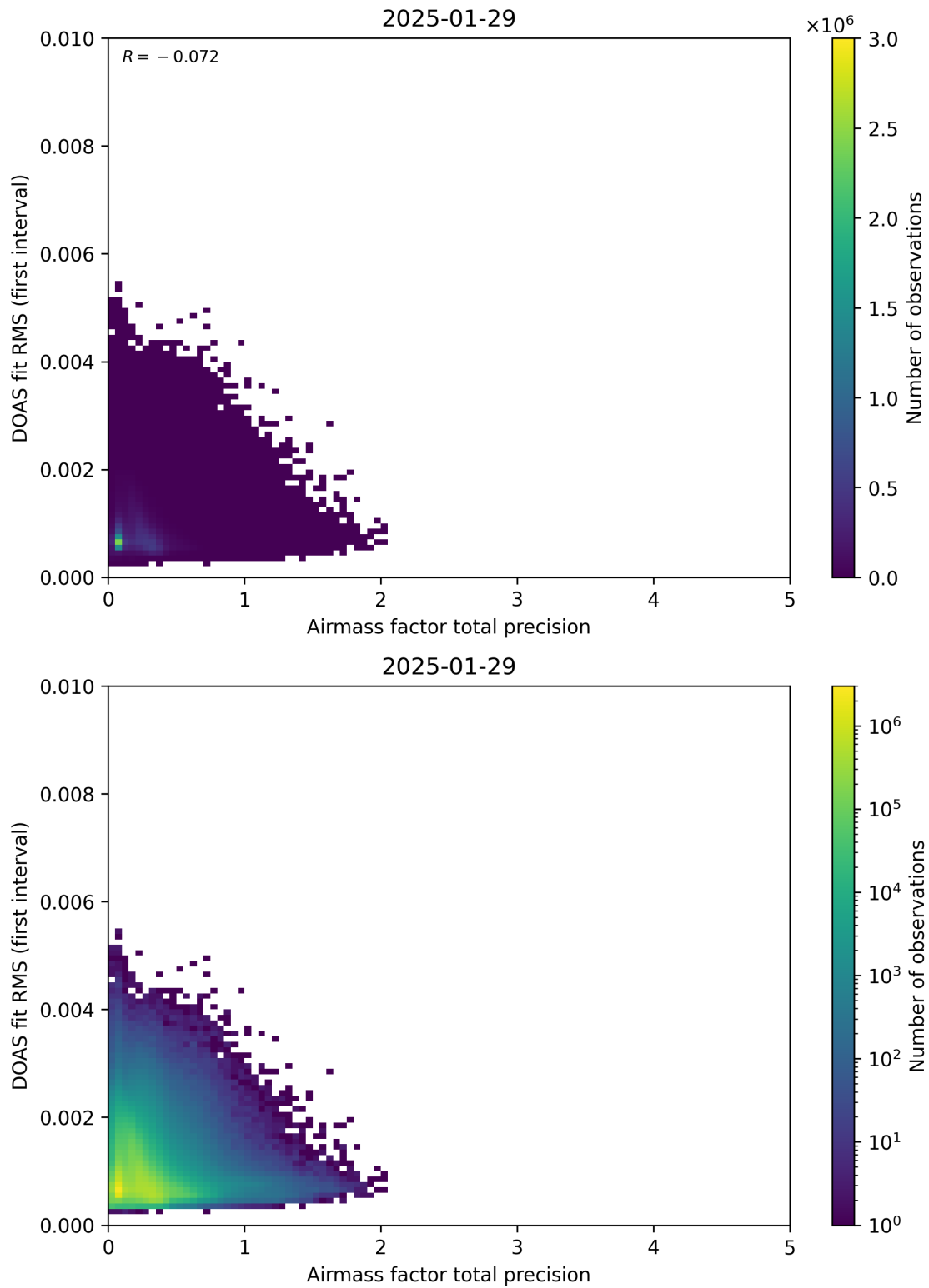
Figure 105: Scatter density plot of “Airmass factor total precision” against “DOAS fit RMS (first interval)” for 2025-01-28 to 2025-01-30.
