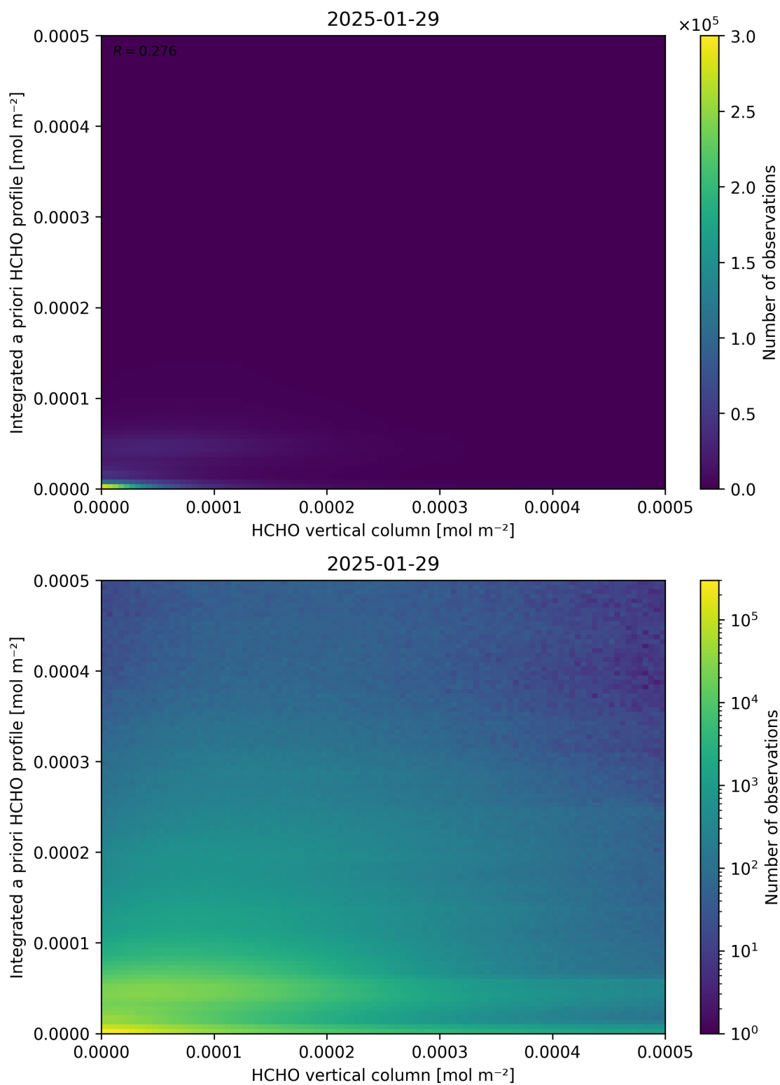
Figure 135: Scatter density plot of “HCHO vertical column” against “Integrated a priori HCHO profile” for 2025-01-28 to 2025-01-30.
