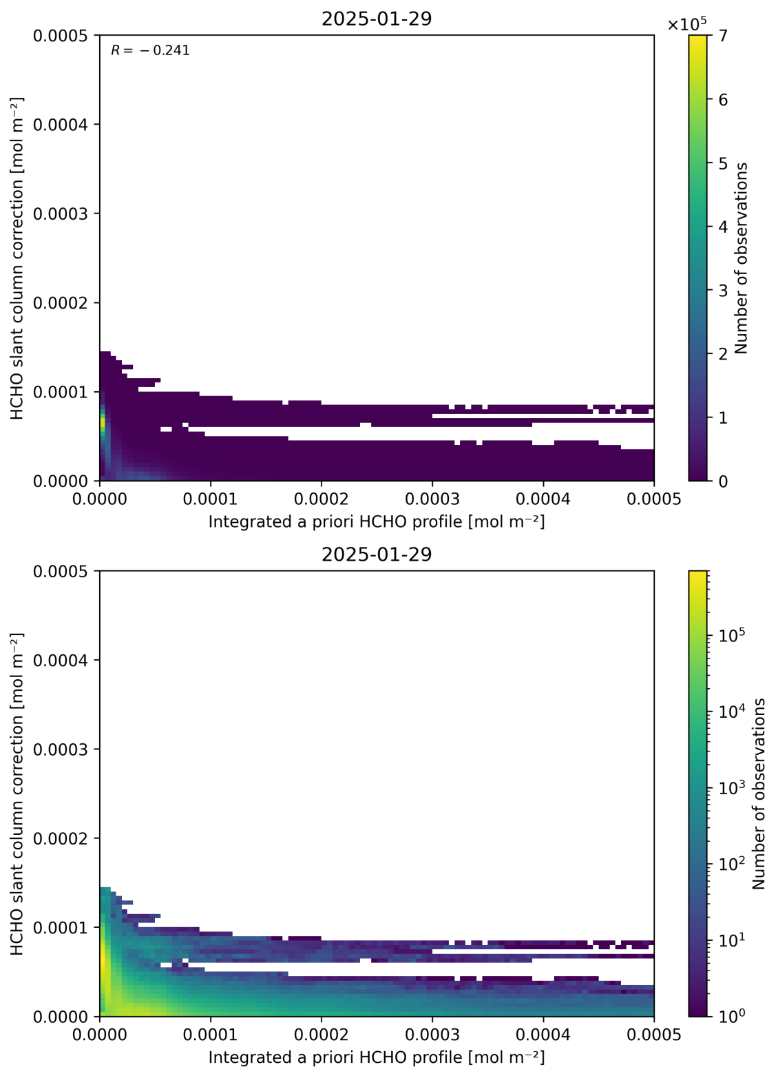
Figure 152: Scatter density plot of “Integrated a priori HCHO profile” against “HCHO slant column correction” for 2025-01-28 to 2025-01-30.
