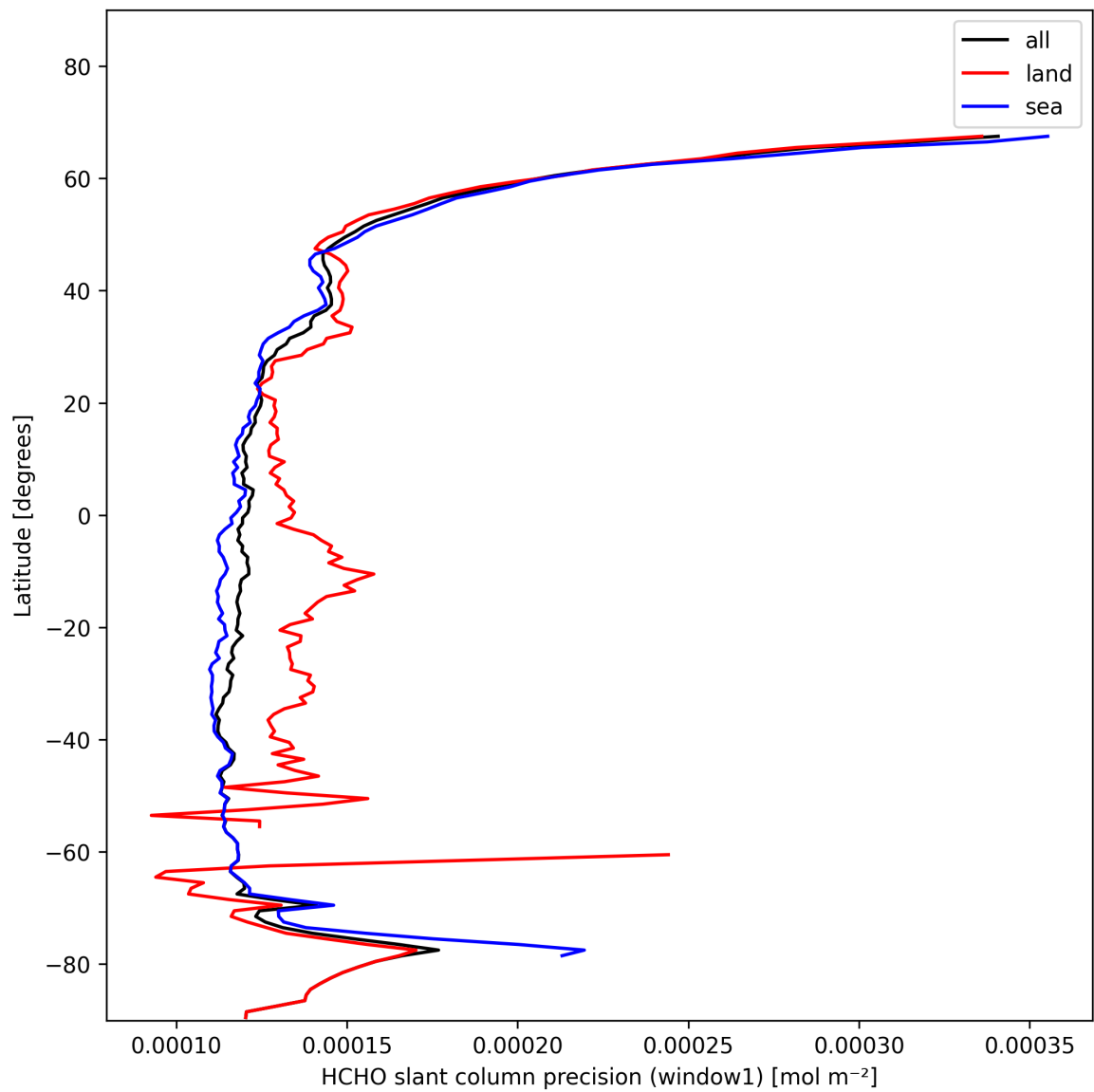
Figure 25: Zonal average of “HCHO slant column precision (window1)” for 2025-01-28 to 2025-01-30.
