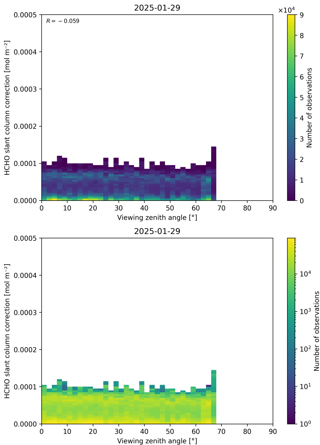
Figure 187: Scatter density plot of “Viewing zenith angle” against “HCHO slant column correction” for 2025-01-28 to 2025-01-30.
