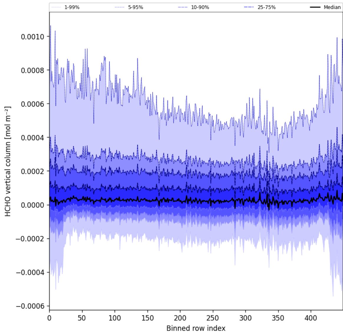
Figure 49: Along track statistics of “HCHO vertical column” for 2025-01-28 to 2025-01-30
