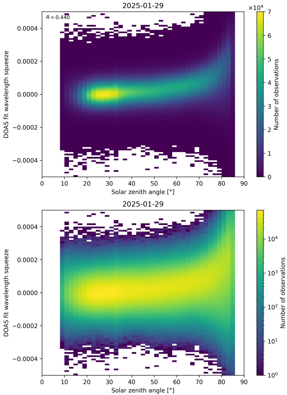
Figure 169: Scatter density plot of “Solar zenith angle” against “DOAS fit wavelength squeeze” for 2025-01-28 to 2025-01-30.
