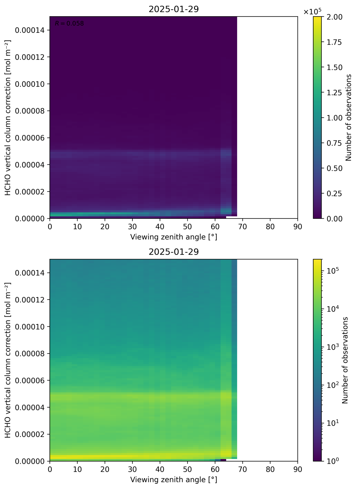
Figure 193: Scatter density plot of “Viewing zenith angle” against “HCHO vertical column correction” for 2025-01-28 to 2025-01-30.
