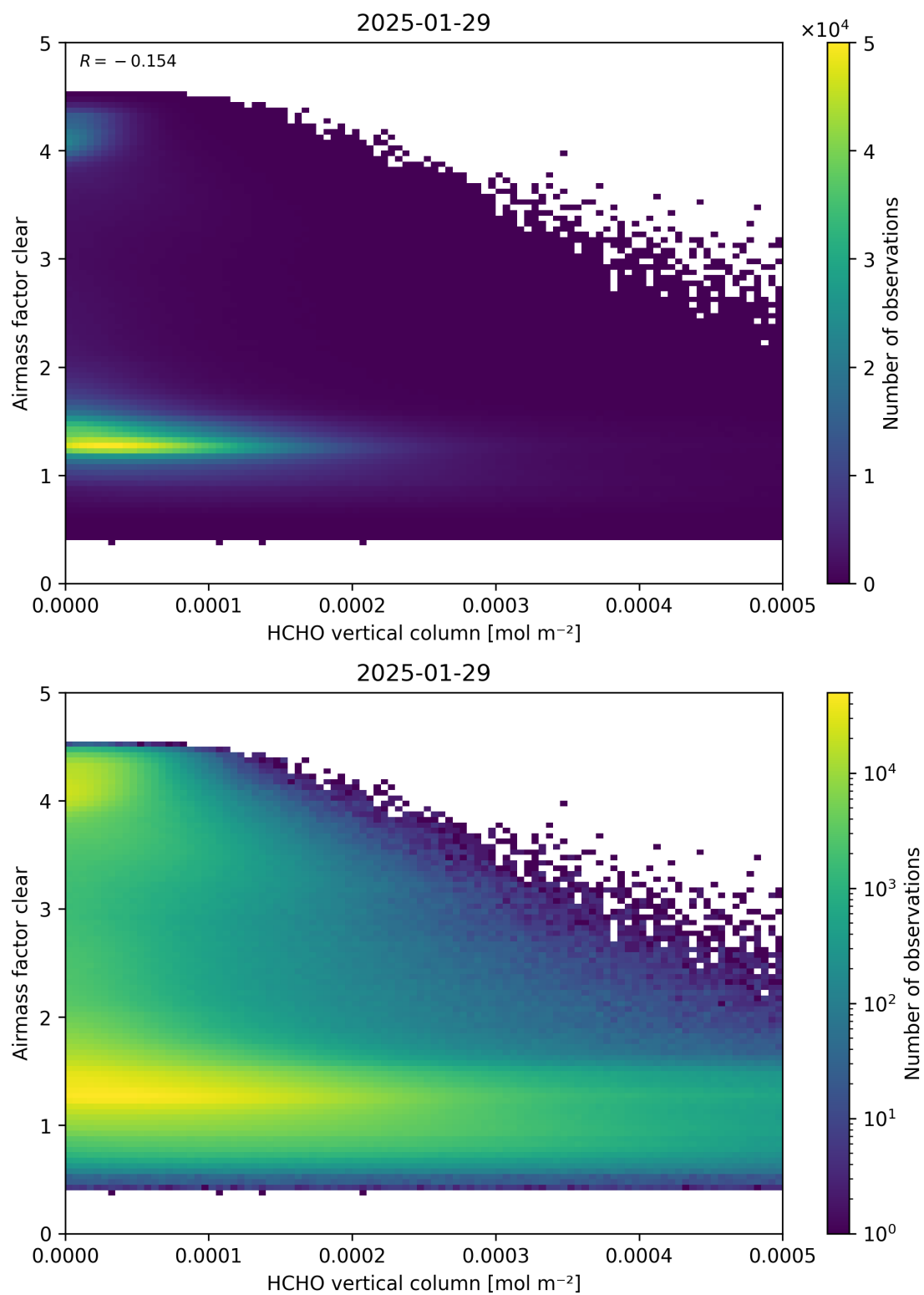
Figure 126: Scatter density plot of “HCHO vertical column” against “Airmass factor clear” for 2025-01-28 to 2025-01-30.
