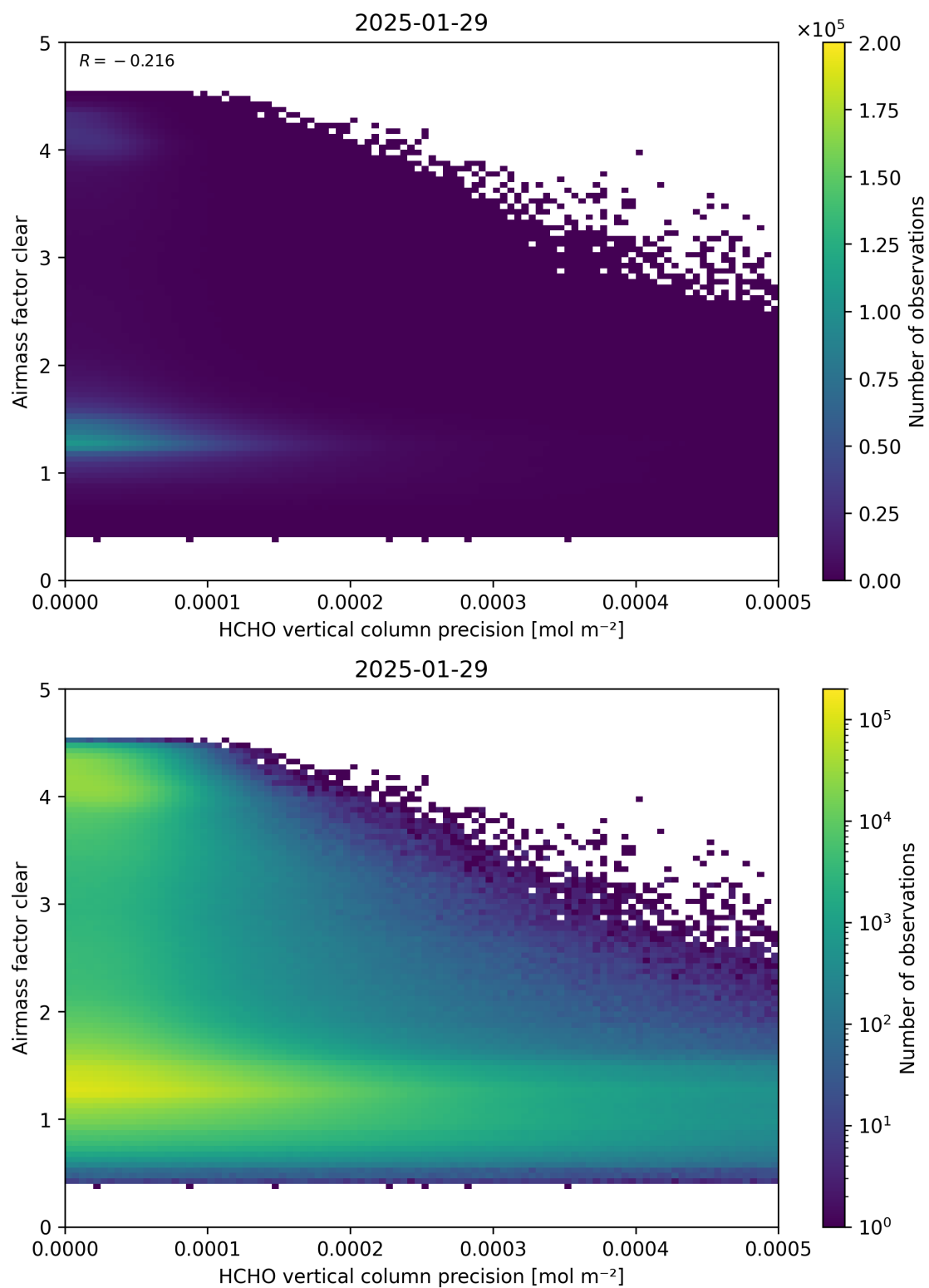
Figure 139: Scatter density plot of “HCHO vertical column precision” against “Airmass factor clear” for 2025-01-28 to 2025-01-30.
