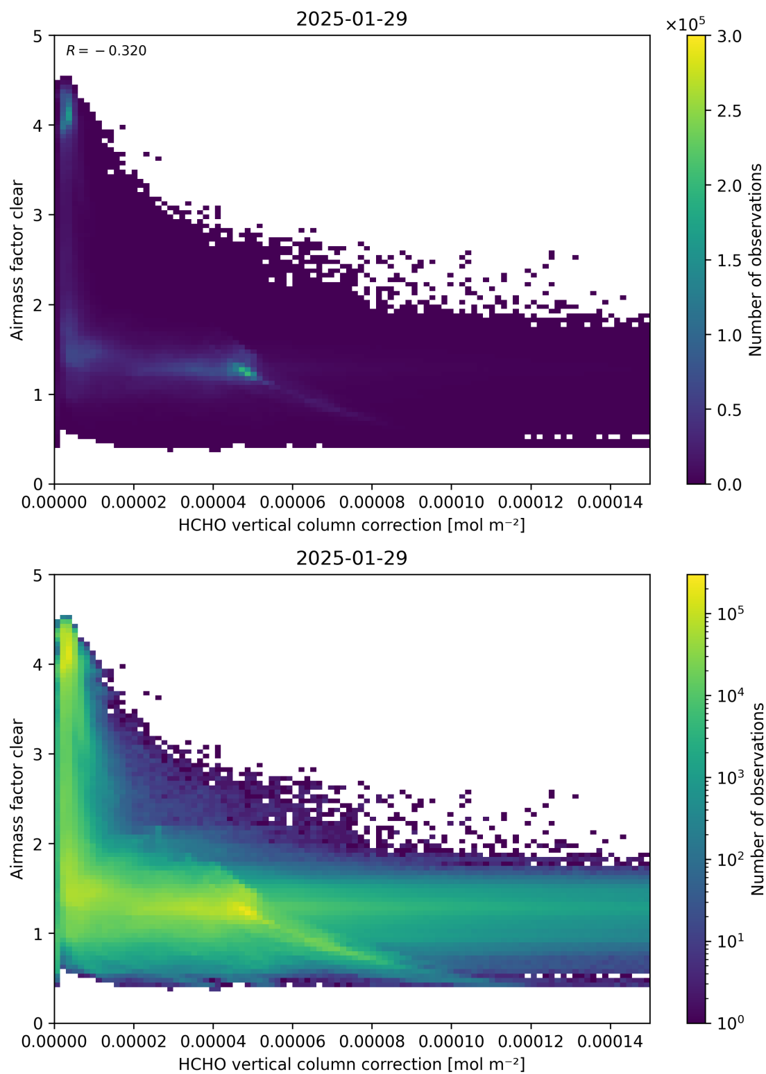
Figure 115: Scatter density plot of “HCHO vertical column correction” against “Airmass factor clear” for 2025-01-28 to 2025-01-30.
