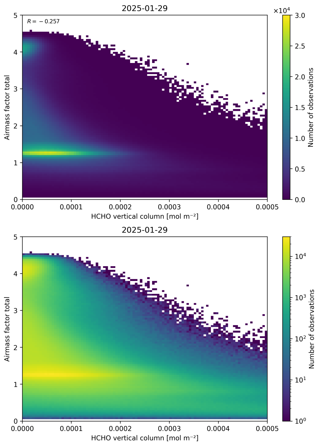
Figure 131: Scatter density plot of “HCHO vertical column” against “Airmass factor total” for 2025-01-28 to 2025-01-30.
