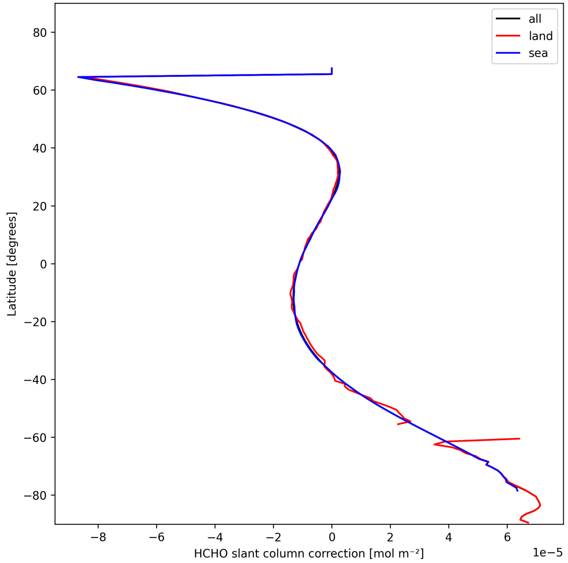
Figure 33: Zonal average of "HCHO slant column correction" for 2025-01-28 to 2025-01-30.
