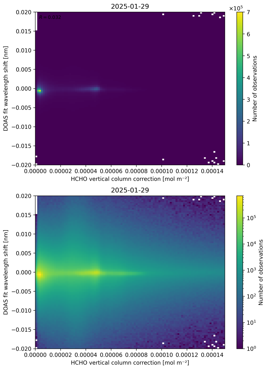
Figure 113: Scatter density plot of “HCHO vertical column correction” against “DOAS fit wavelength shift” for 2025-01-28 to 2025-01-30.
