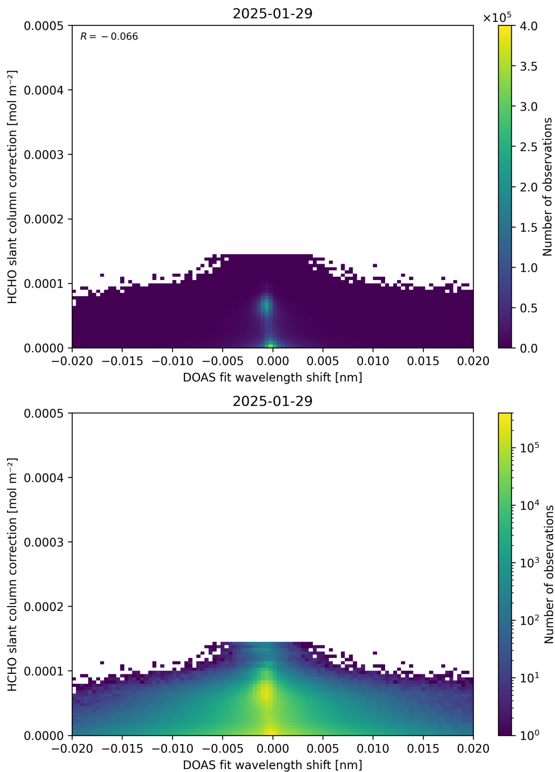
Figure 67: Scatter density plot of “DOAS fit wavelength shift” against “HCHO slant column correction” for 2025-01-28 to 2025-01-30.
