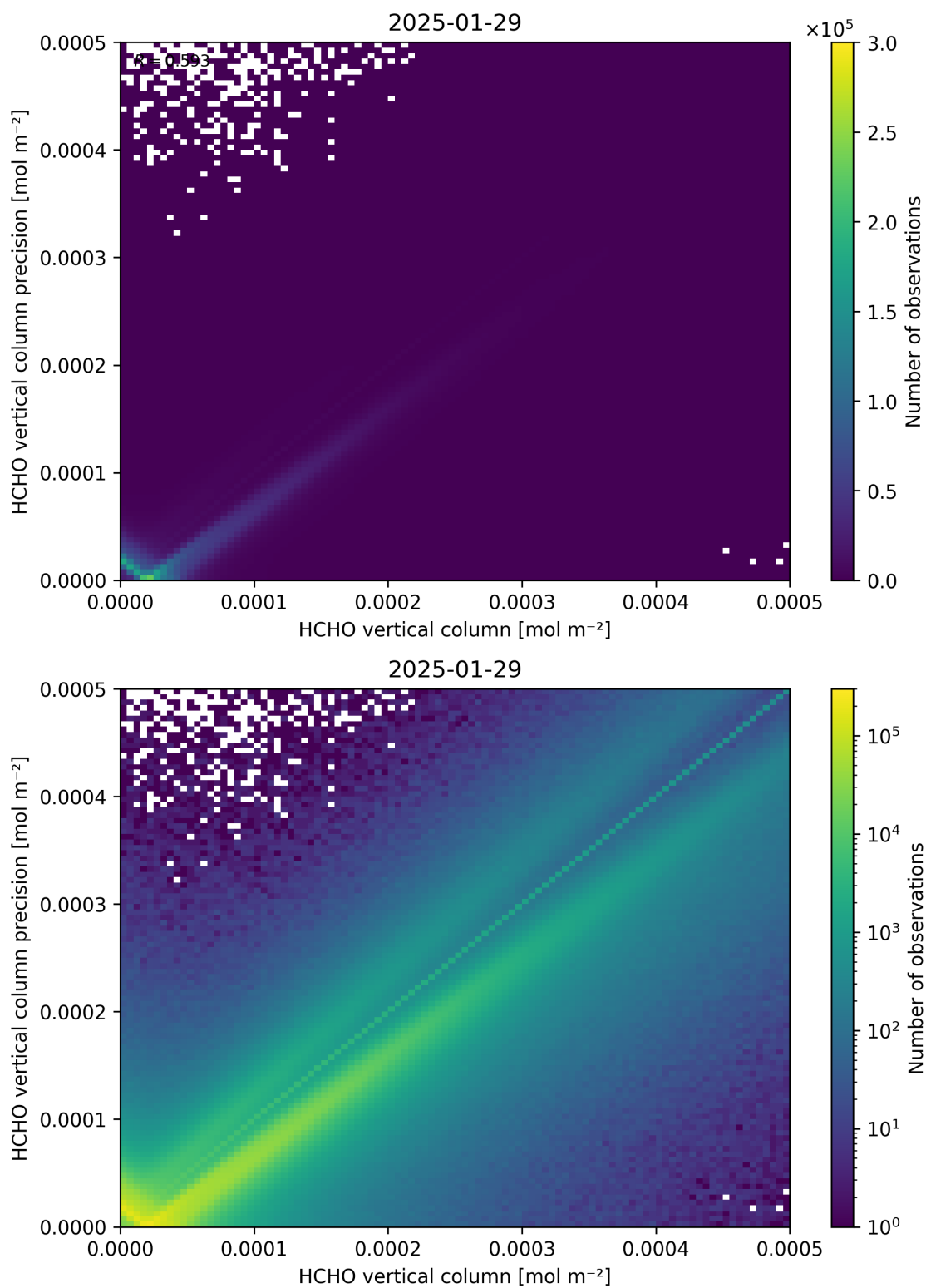
Figure 134: Scatter density plot of “HCHO vertical column” against “HCHO vertical column precision” for 2025-01-28 to 2025-01-30.
