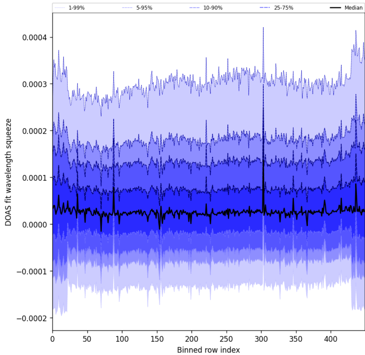
Figure 59: Along track statistics of “DOAS fit wavelength squeeze” for 2025-01-28 to 2025-01-30
