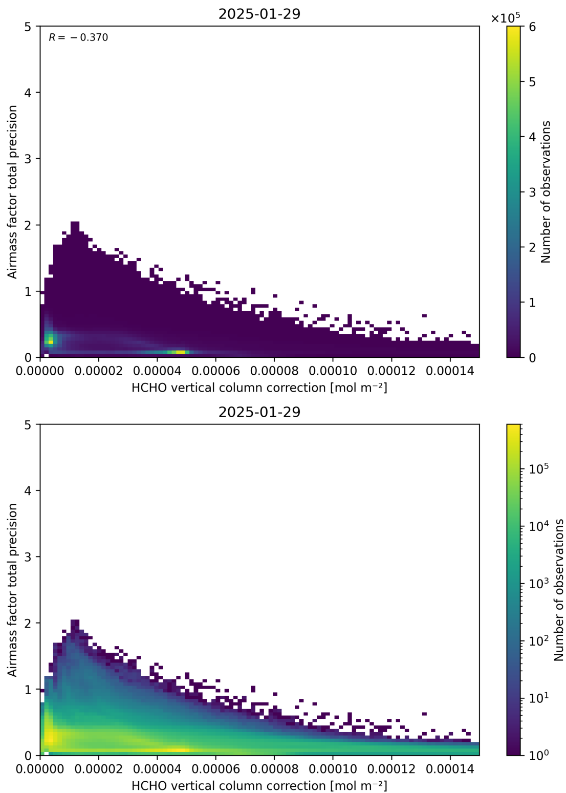
Figure 121: Scatter density plot of “HCHO vertical column correction” against “Airmass factor total precision” for 2025-01-28 to 2025-01-30.
