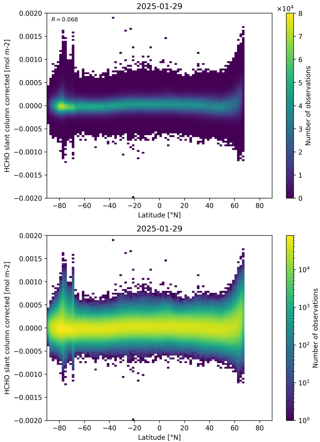
Figure 157: Scatter density plot of “Latitude” against “HCHO slant column corrected” for 2025-01-28 to 2025-01-30.
