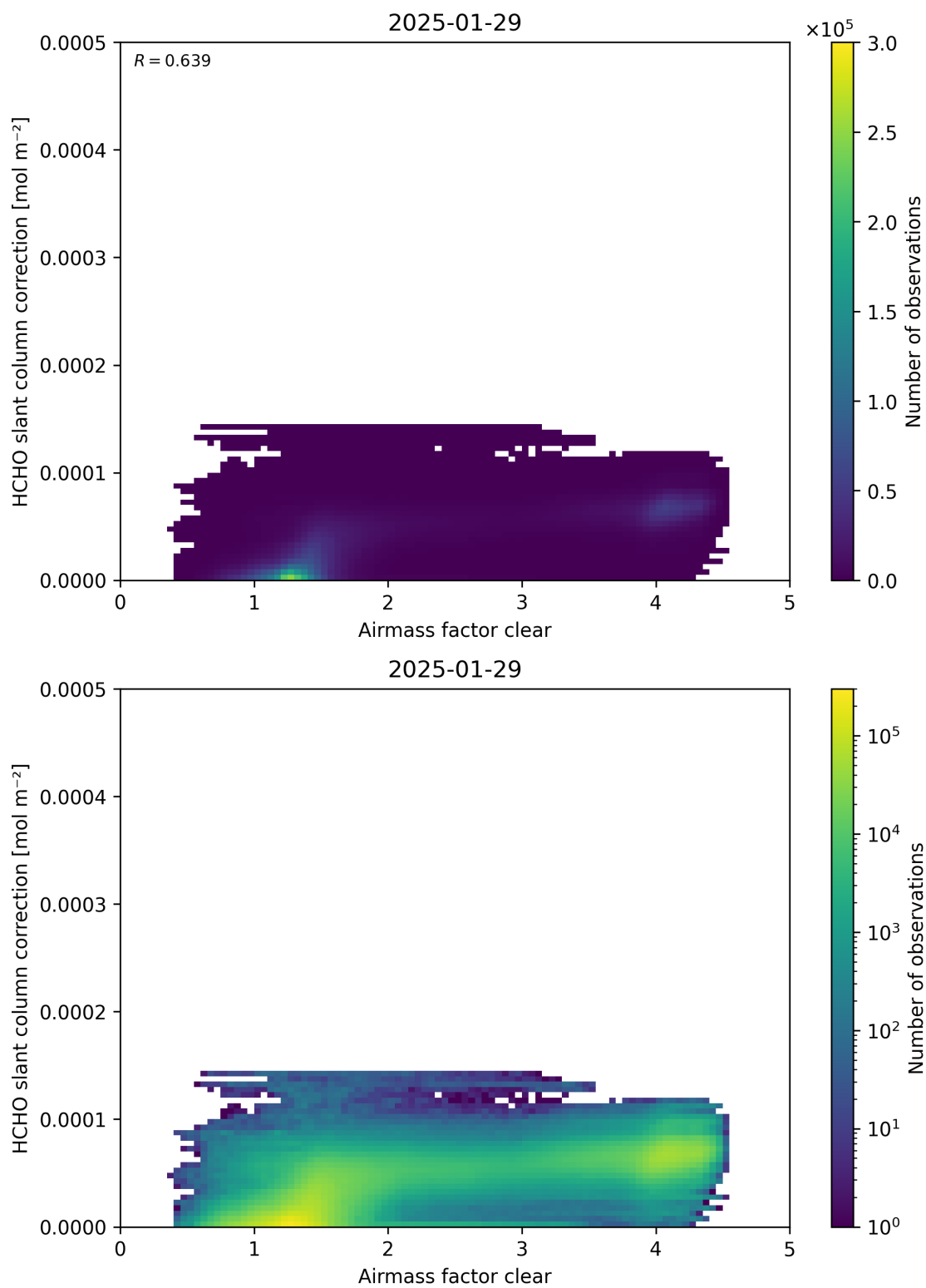
Figure 75: Scatter density plot of “Airmass factor clear” against “HCHO slant column correction” for 2025-01-28 to 2025-01-30.
