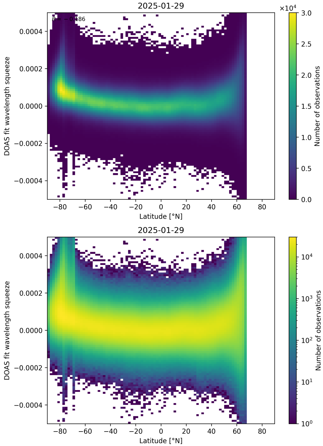
Figure 155: Scatter density plot of “Latitude” against “DOAS fit wavelength squeeze” for 2025-01-28 to 2025-01-30.
