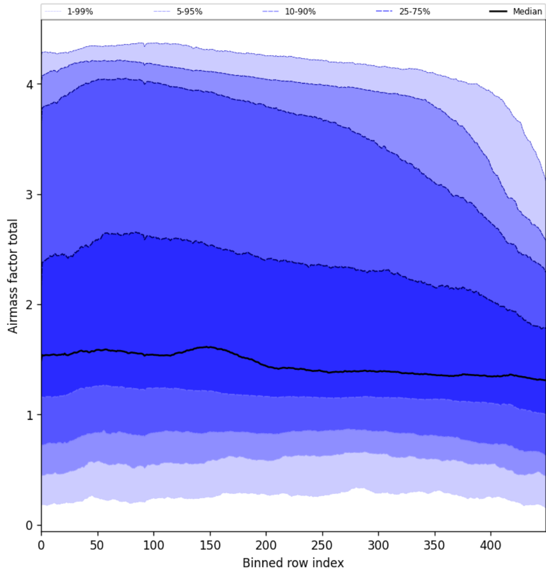
Figure 54: Along track statistics of “Airmass factor total” for 2025-01-28 to 2025-01-30
