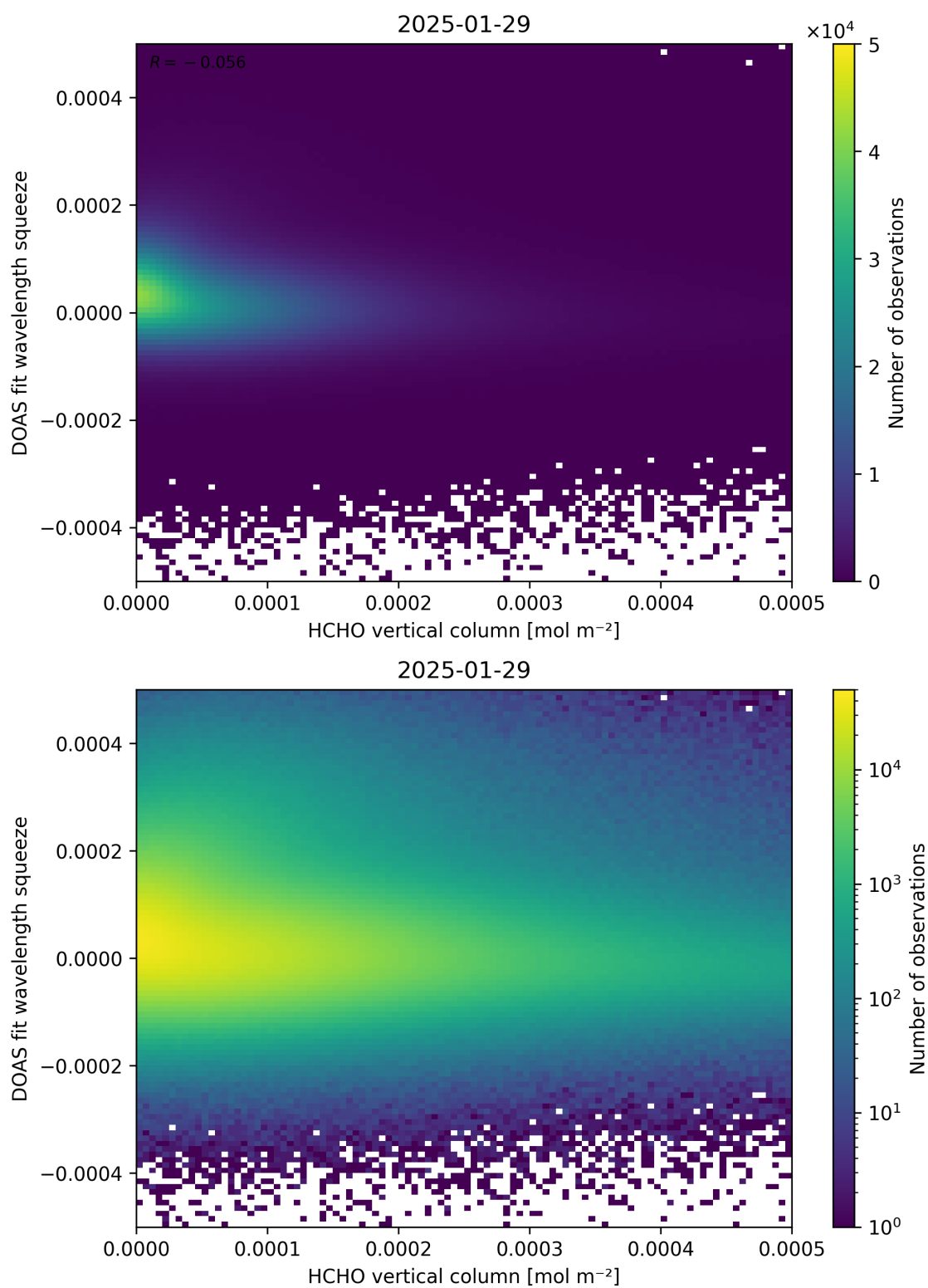
Figure 125: Scatter density plot of “HCHO vertical column” against “DOAS fit wavelength squeeze” for 2025-01-28 to 2025-01-30.
