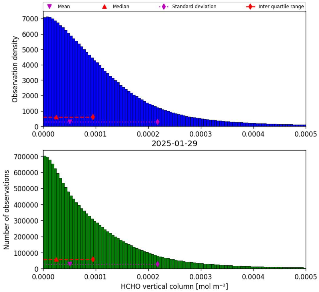
Figure 35: Histogram of “HCHO vertical column” for 2025-01-28 to 2025-01-30
