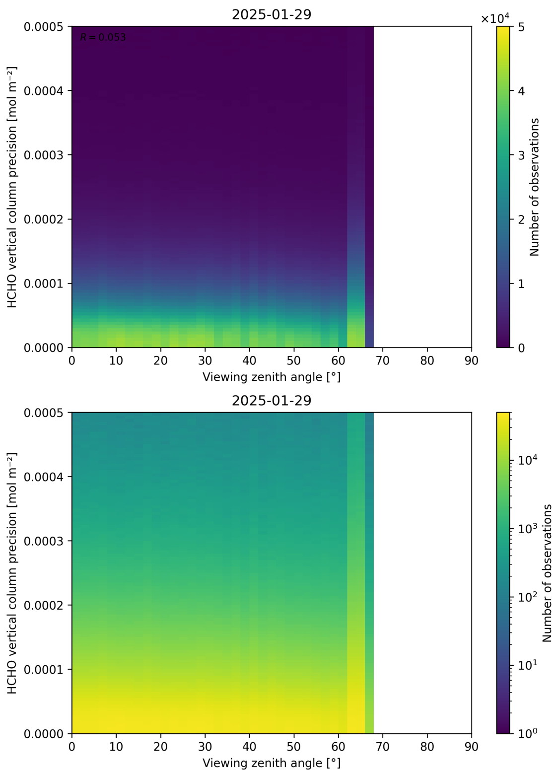
Figure 194: Scatter density plot of “Viewing zenith angle” against “HCHO vertical column precision” for 2025-01-28 to 2025-01-30.
