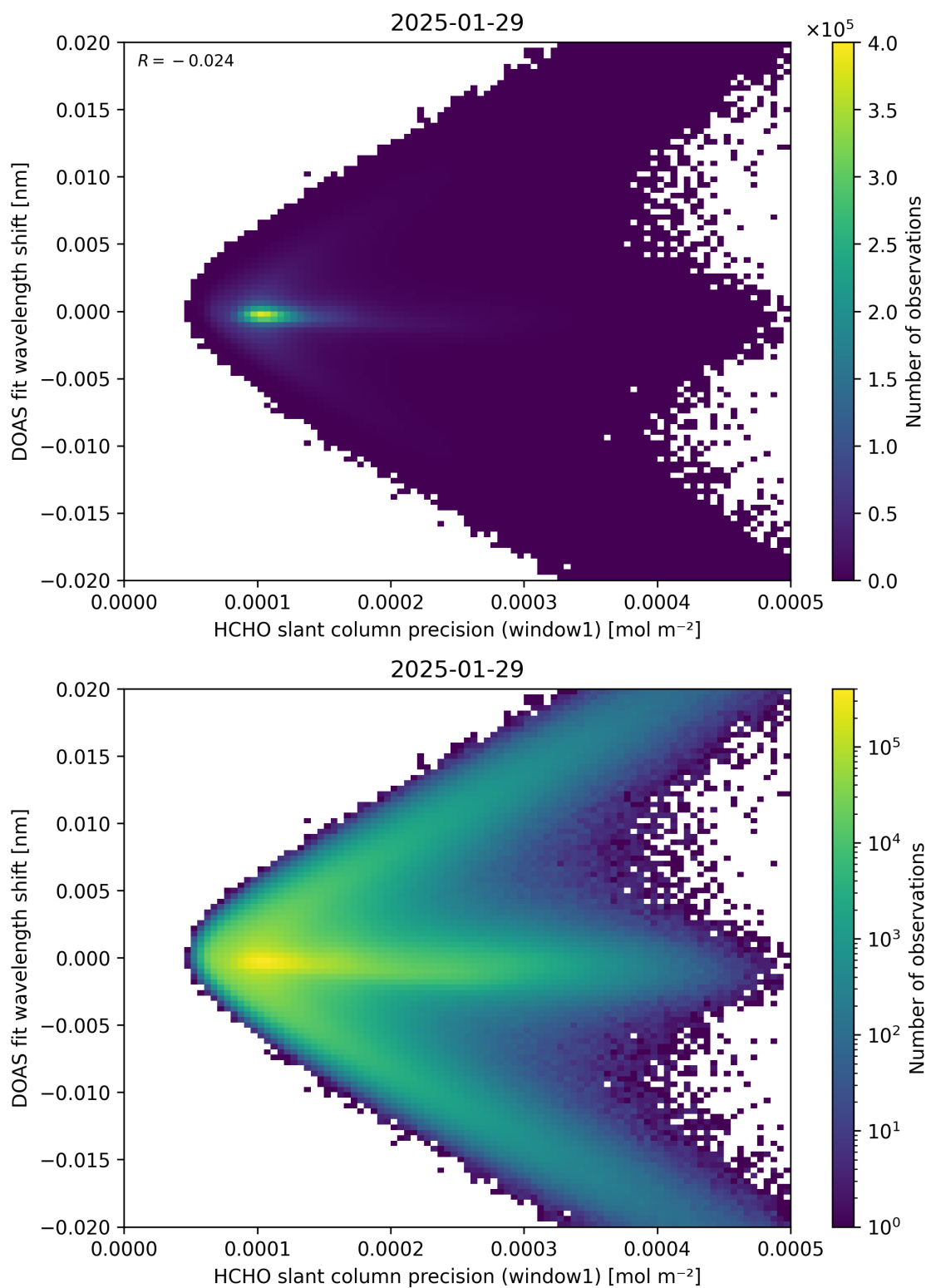
Figure 89: Scatter density plot of “HCHO slant column precision (window1)” against “DOAS fit wavelength shift” for 2025-01-28 to 2025-01-30.
