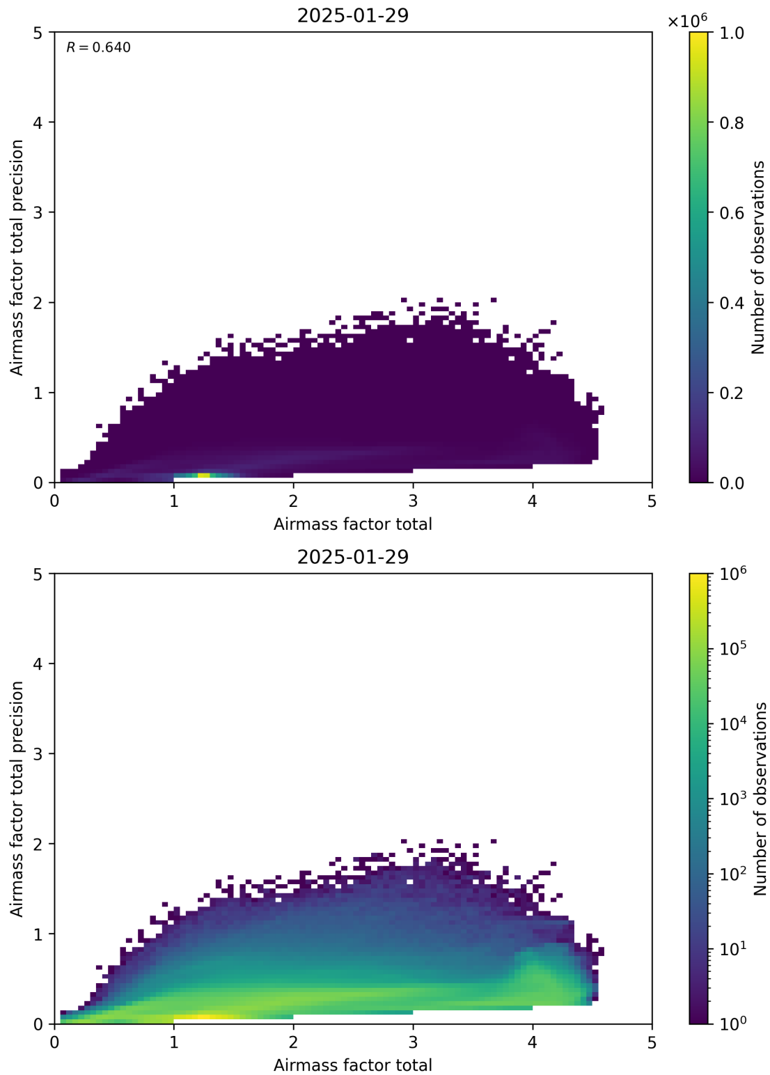
Figure 103: Scatter density plot of “Airmass factor total” against “Airmass factor total precision” for 2025-01-28 to 2025-01-30.
