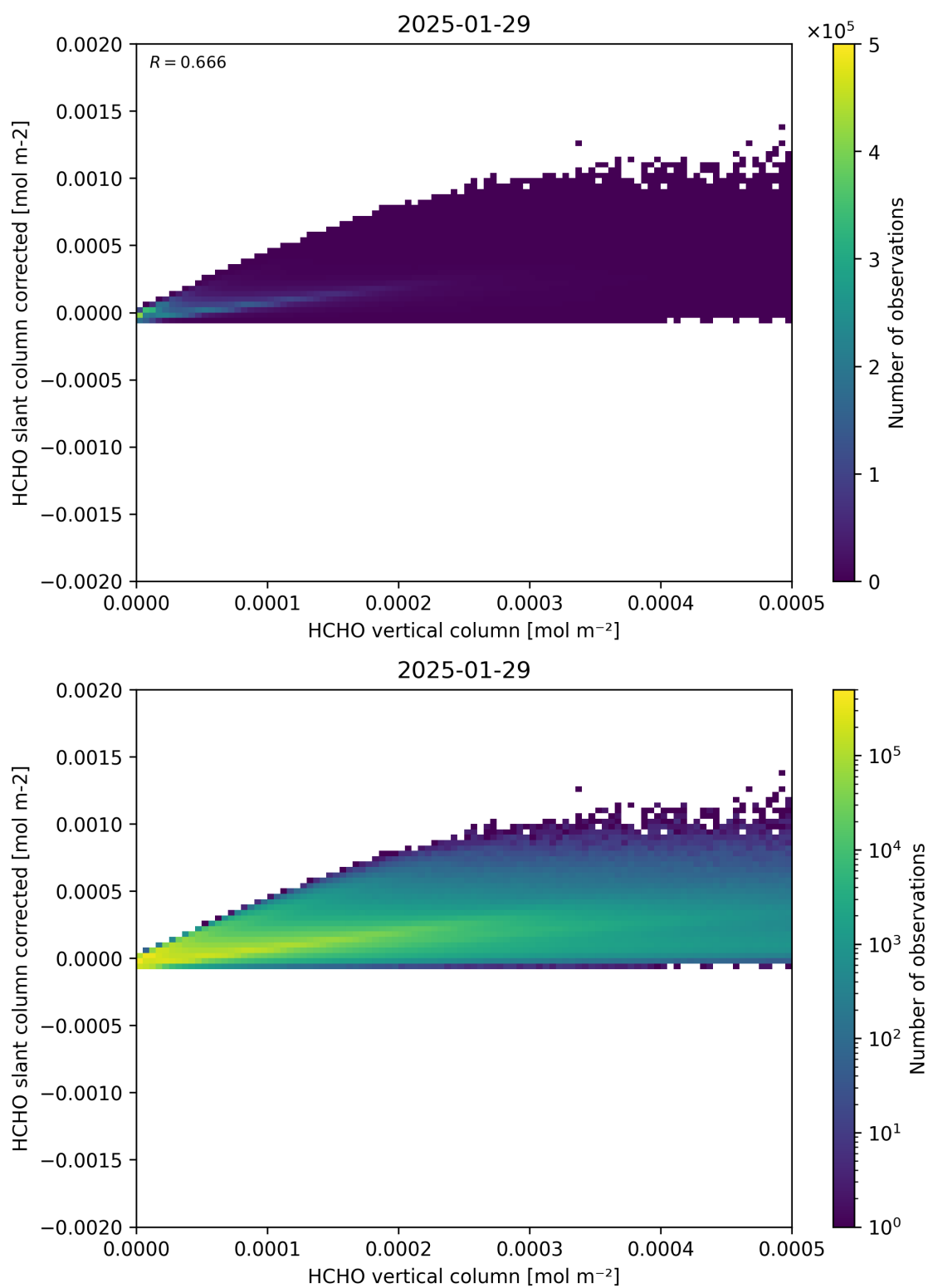
Figure 127: Scatter density plot of “HCHO vertical column” against “HCHO slant column corrected” for 2025-01-28 to 2025-01-30.
