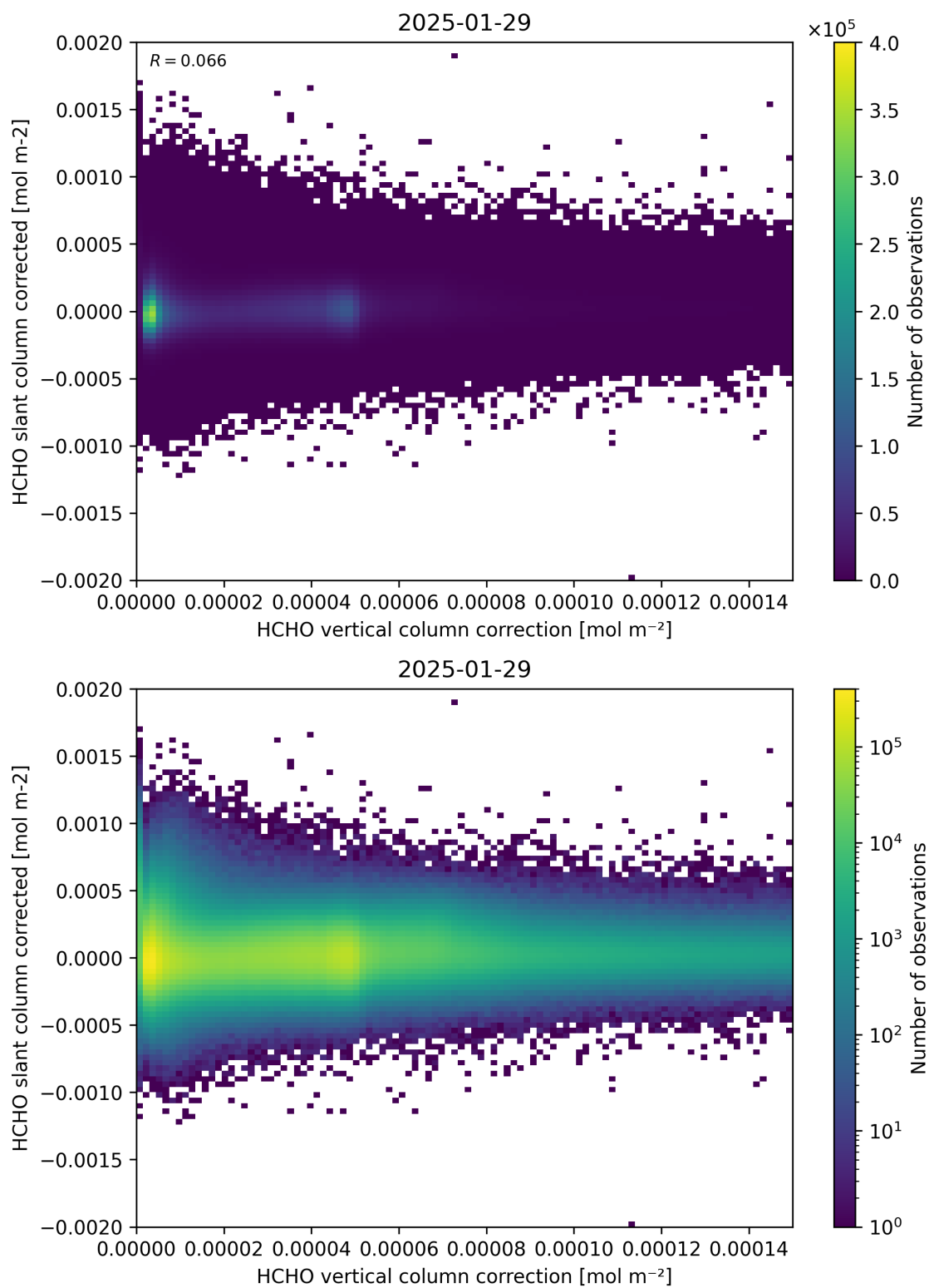
Figure 116: Scatter density plot of “HCHO vertical column correction” against “HCHO slant column corrected” for 2025-01-28 to 2025-01-30.
