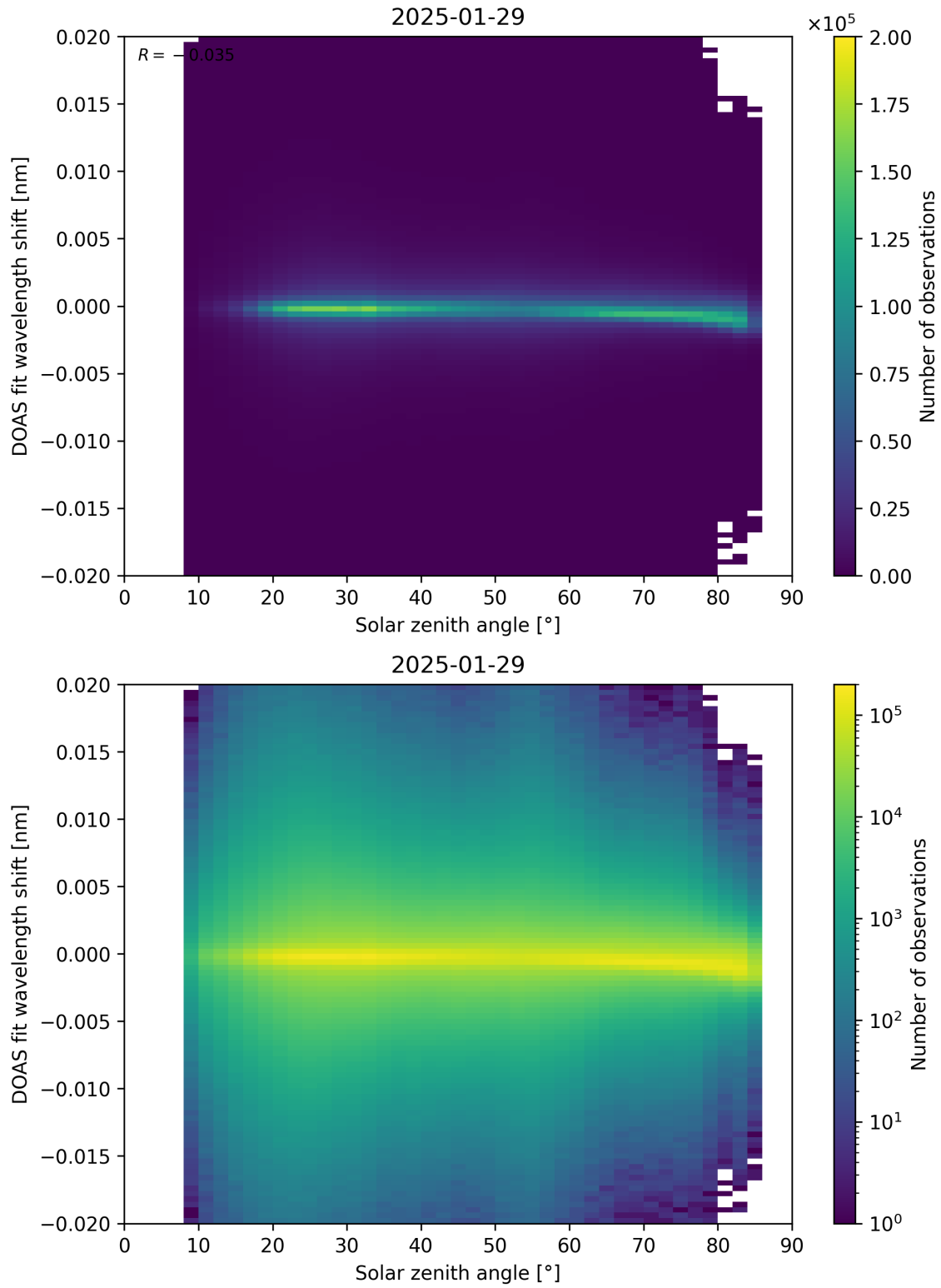
Figure 168: Scatter density plot of “Solar zenith angle” against “DOAS fit wavelength shift” for 2025-01-28 to 2025-01-30.
