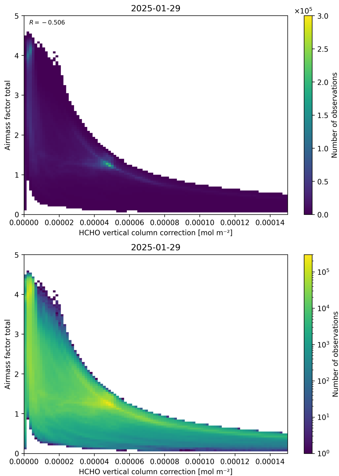
Figure 120: Scatter density plot of “HCHO vertical column correction” against “Airmass factor total” for 2025-01-28 to 2025-01-30.
