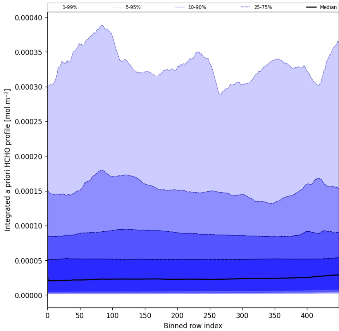
Figure 57: Along track statistics of “Integrated a priori HCHO profile” for 2025-01-28 to 2025-01-30
