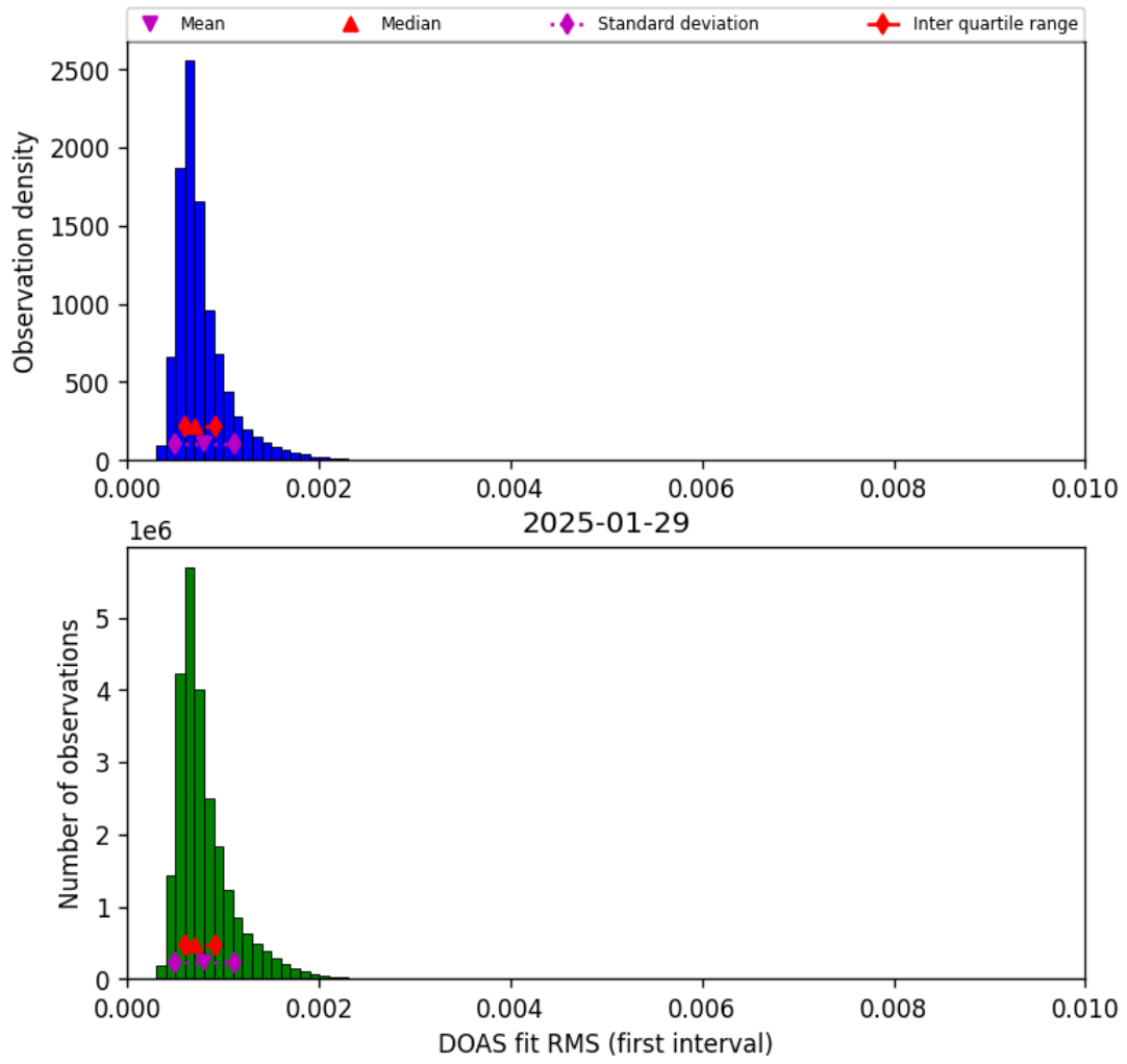
Figure 46: Histogram of “DOAS fit RMS (first interval)” for 2025-01-28 to 2025-01-30
