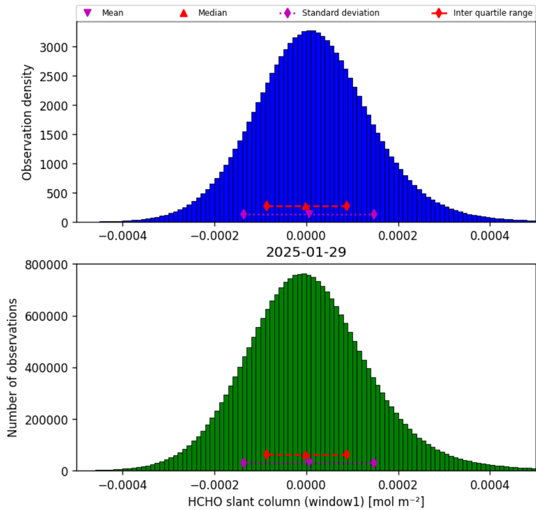
Figure 38: Histogram of “HCHO slant column (window1)” for 2025-01-28 to 2025-01-30
