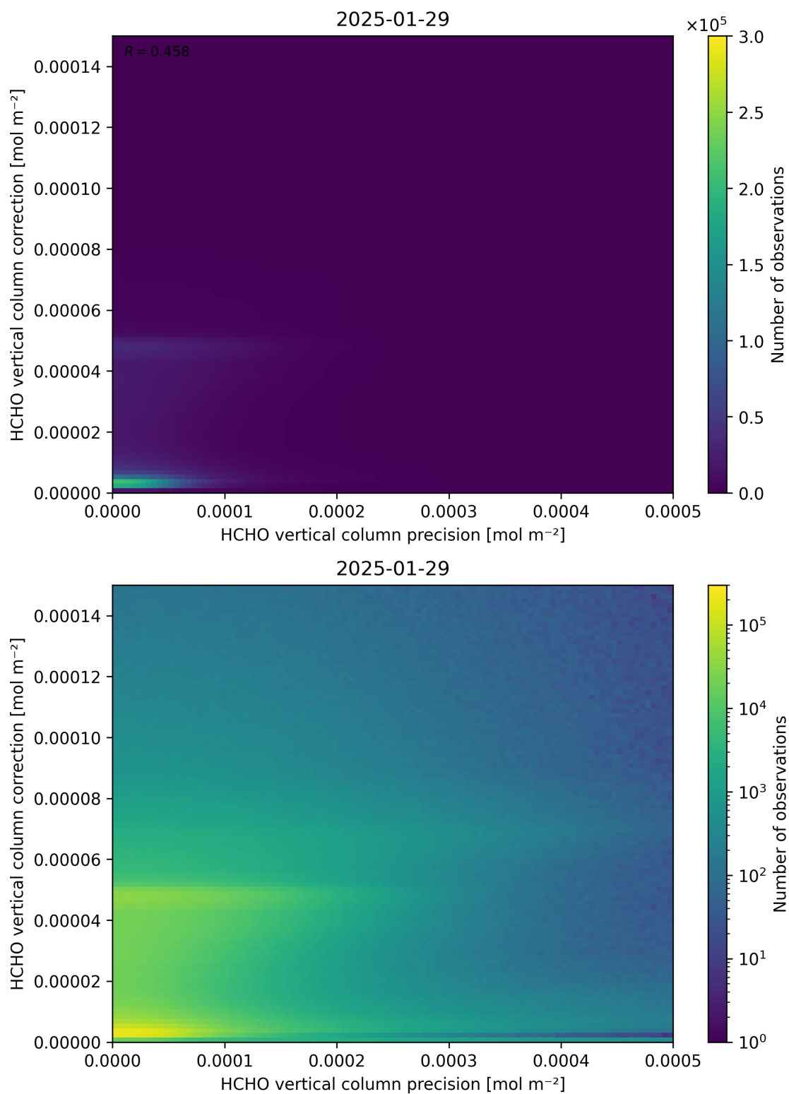
Figure 146: Scatter density plot of “HCHO vertical column precision” against “HCHO vertical column correction” for 2025-01-28 to 2025-01-30.
