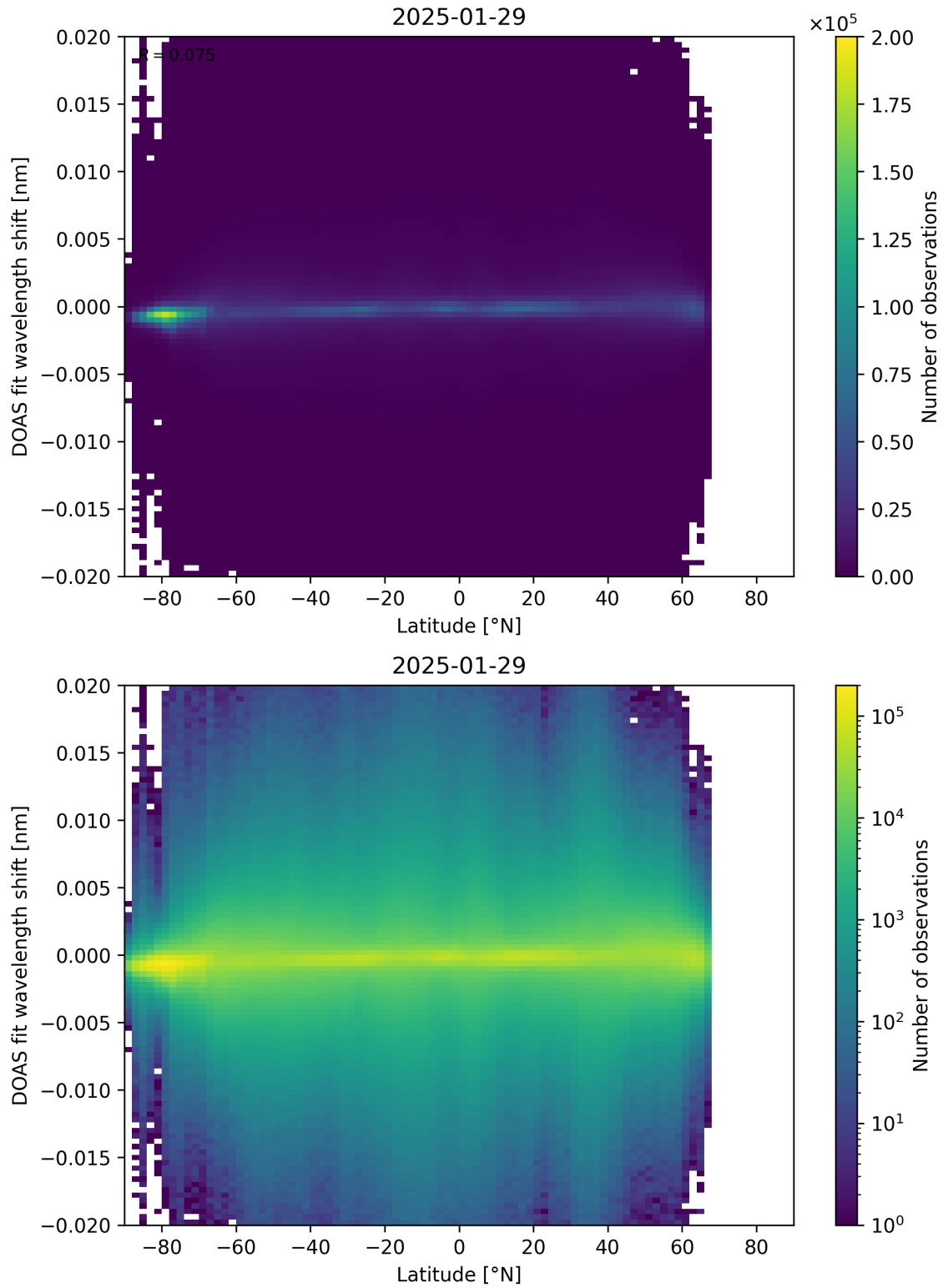
Figure 154: Scatter density plot of “Latitude” against “DOAS fit wavelength shift” for 2025-01-28 to 2025-01-30.
