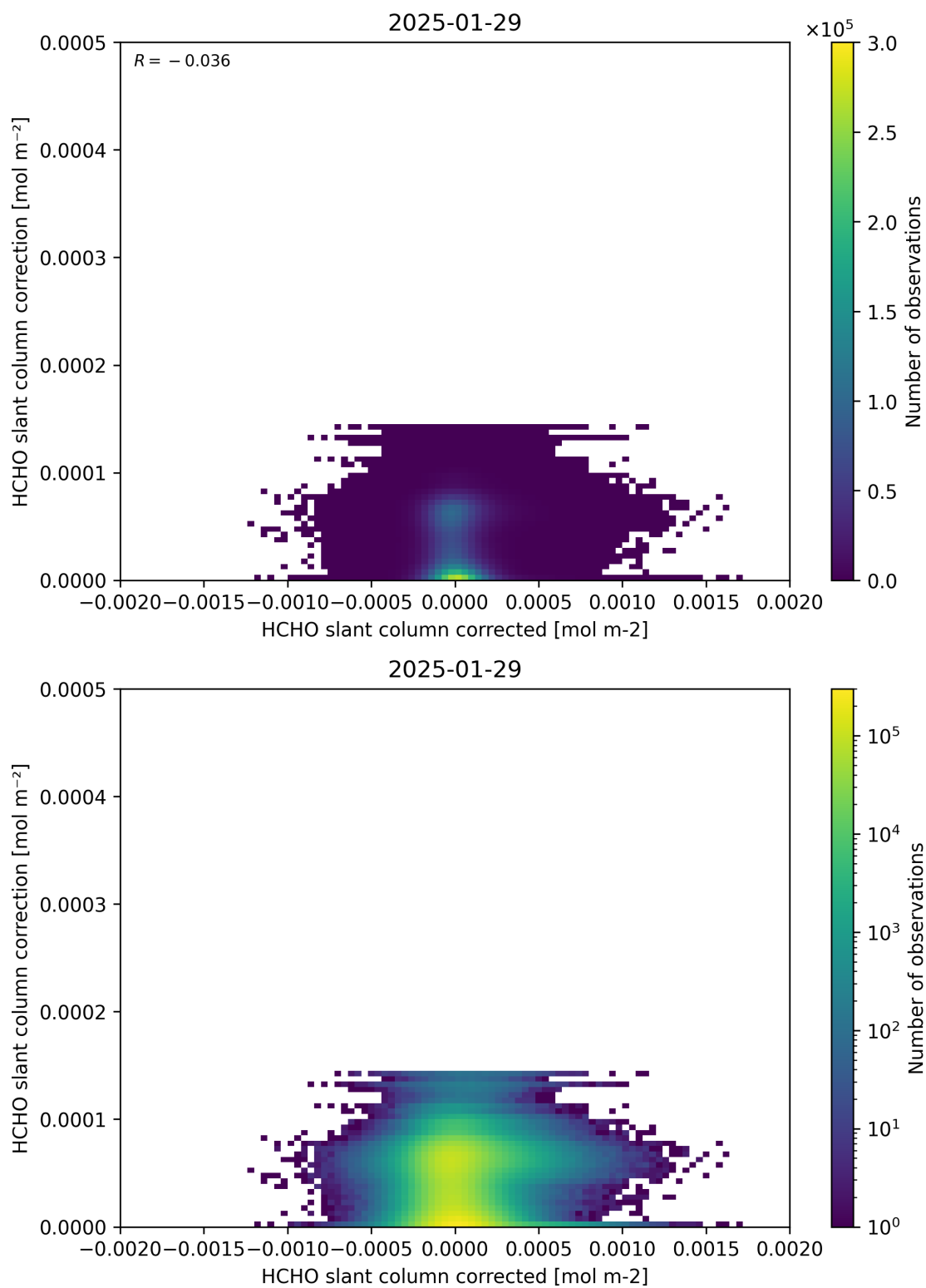
Figure 77: Scatter density plot of “HCHO slant column corrected” against “HCHO slant column correction” for 2025-01-28 to 2025-01-30.
