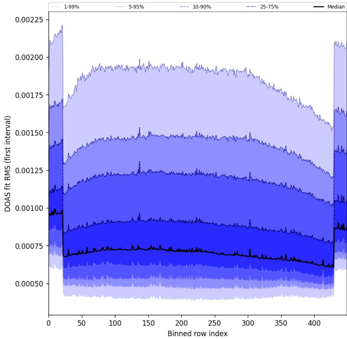
Figure 60: Along track statistics of “DOAS fit RMS (first interval)” for 2025-01-28 to 2025-01-30
