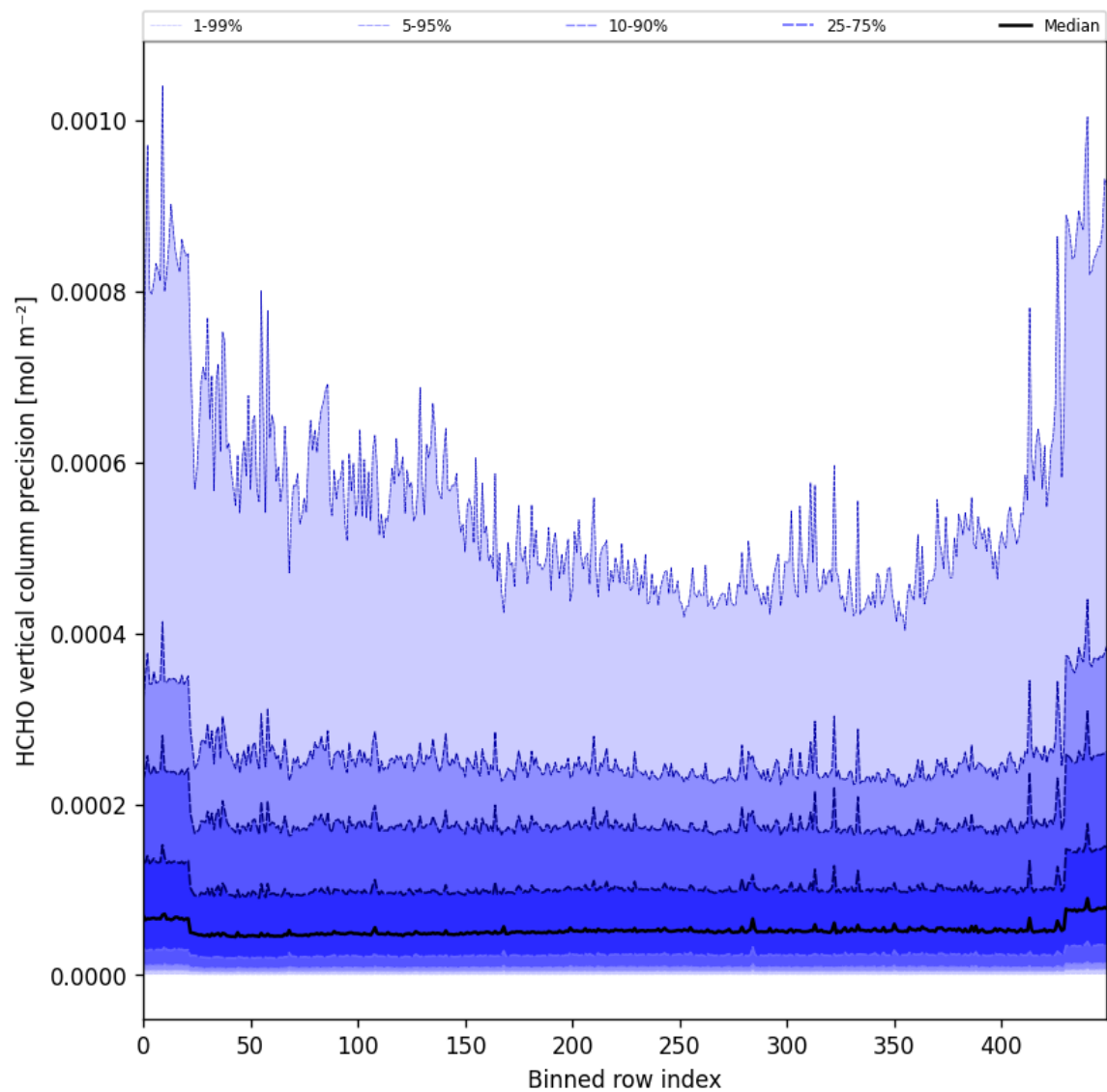
Figure 50: Along track statistics of “HCHO vertical column precision” for 2025-01-28 to 2025-01-30
