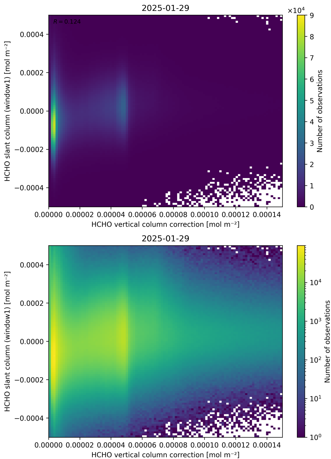
Figure 118: Scatter density plot of “HCHO vertical column correction” against “HCHO slant column (window1)” for 2025-01-28 to 2025-01-30.
