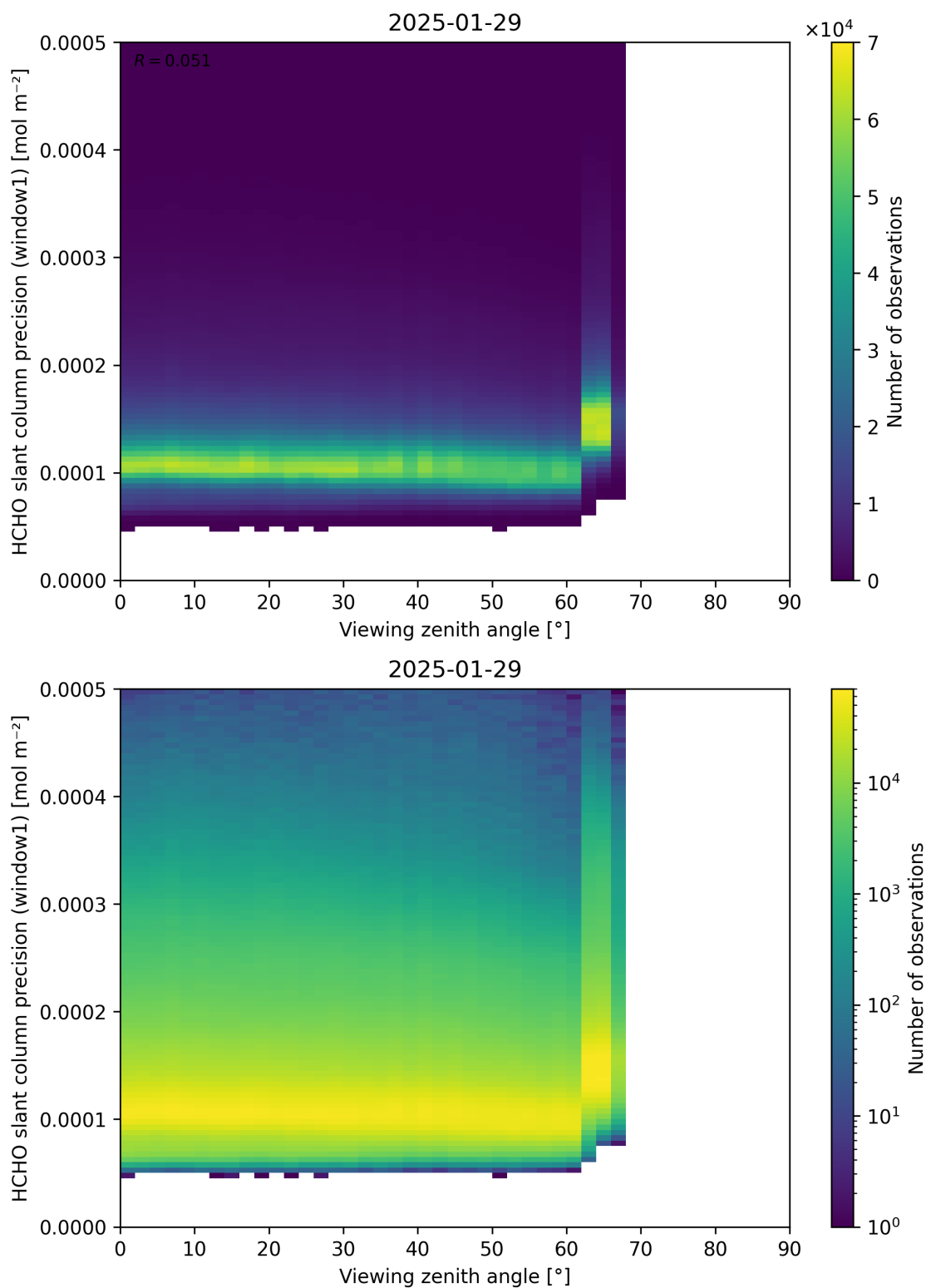
Figure 189: Scatter density plot of “Viewing zenith angle” against “HCHO slant column precision (window1)” for 2025-01-28 to 2025-01-30.
