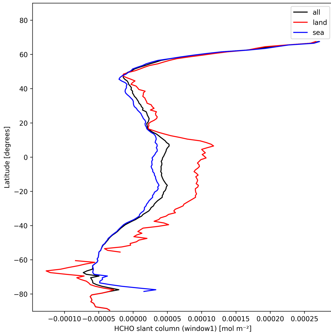
Figure 24: Zonal average of “HCHO slant column (window1)” for 2025-01-28 to 2025-01-30.
