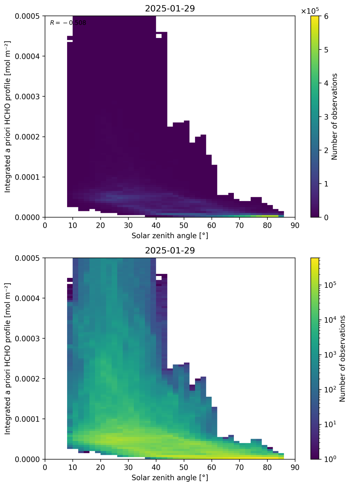
Figure 180: Scatter density plot of “Solar zenith angle” against “Integrated a priori HCHO profile” for 2025-01-28 to 2025-01-30.
