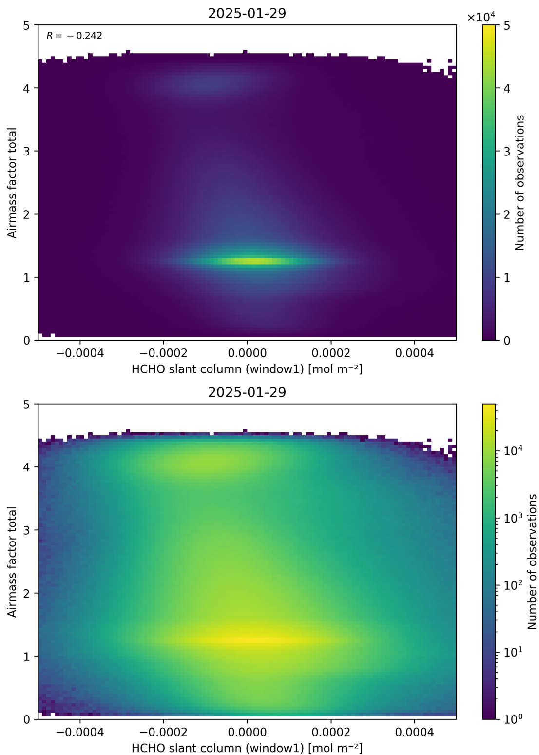
Figure 85: Scatter density plot of “HCHO slant column (window1)” against “Airmass factor total” for 2025-01-28 to 2025-01-30.
