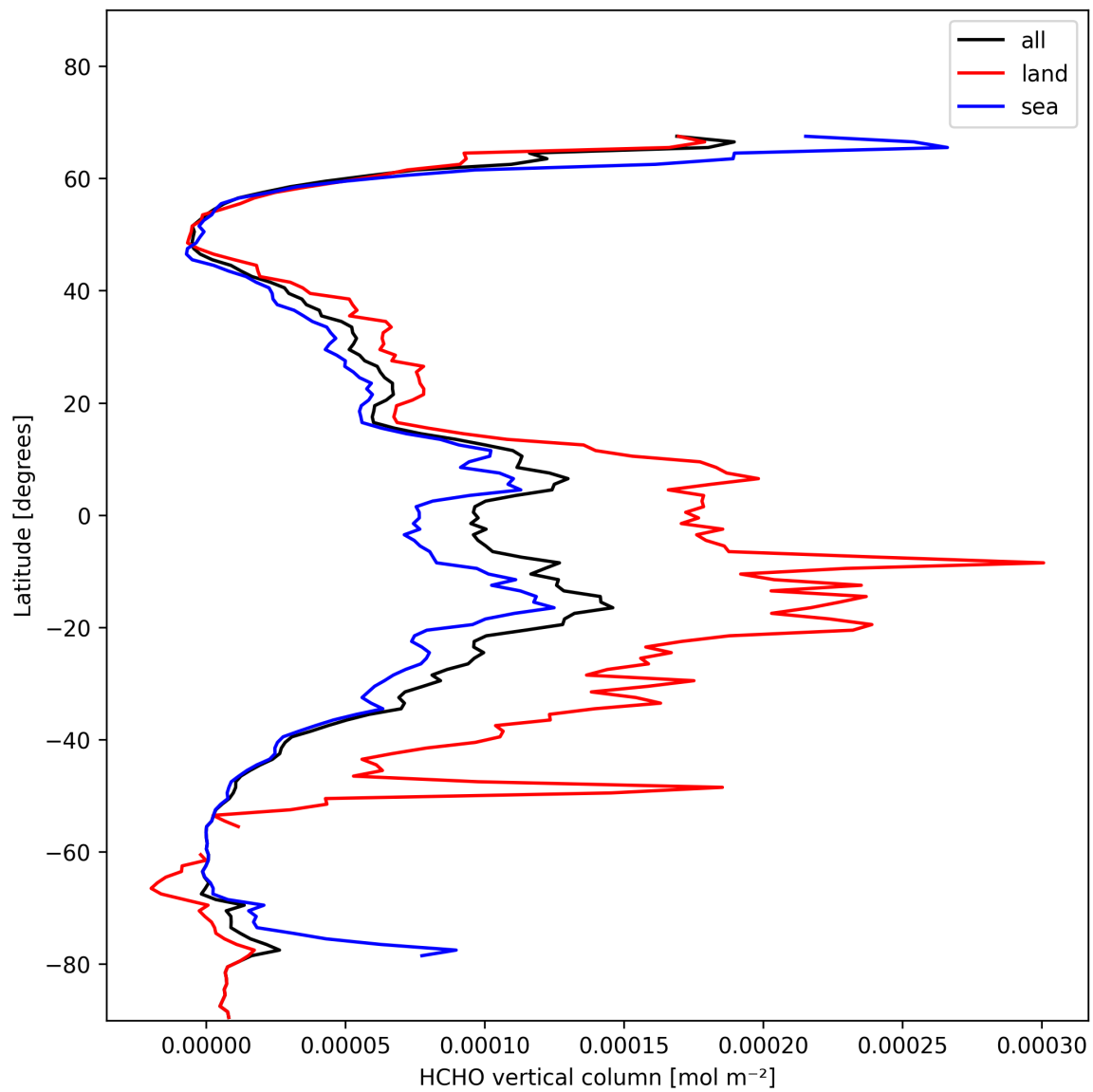
Figure 21: Zonal average of “HCHO vertical column” for 2025-01-28 to 2025-01-30.
