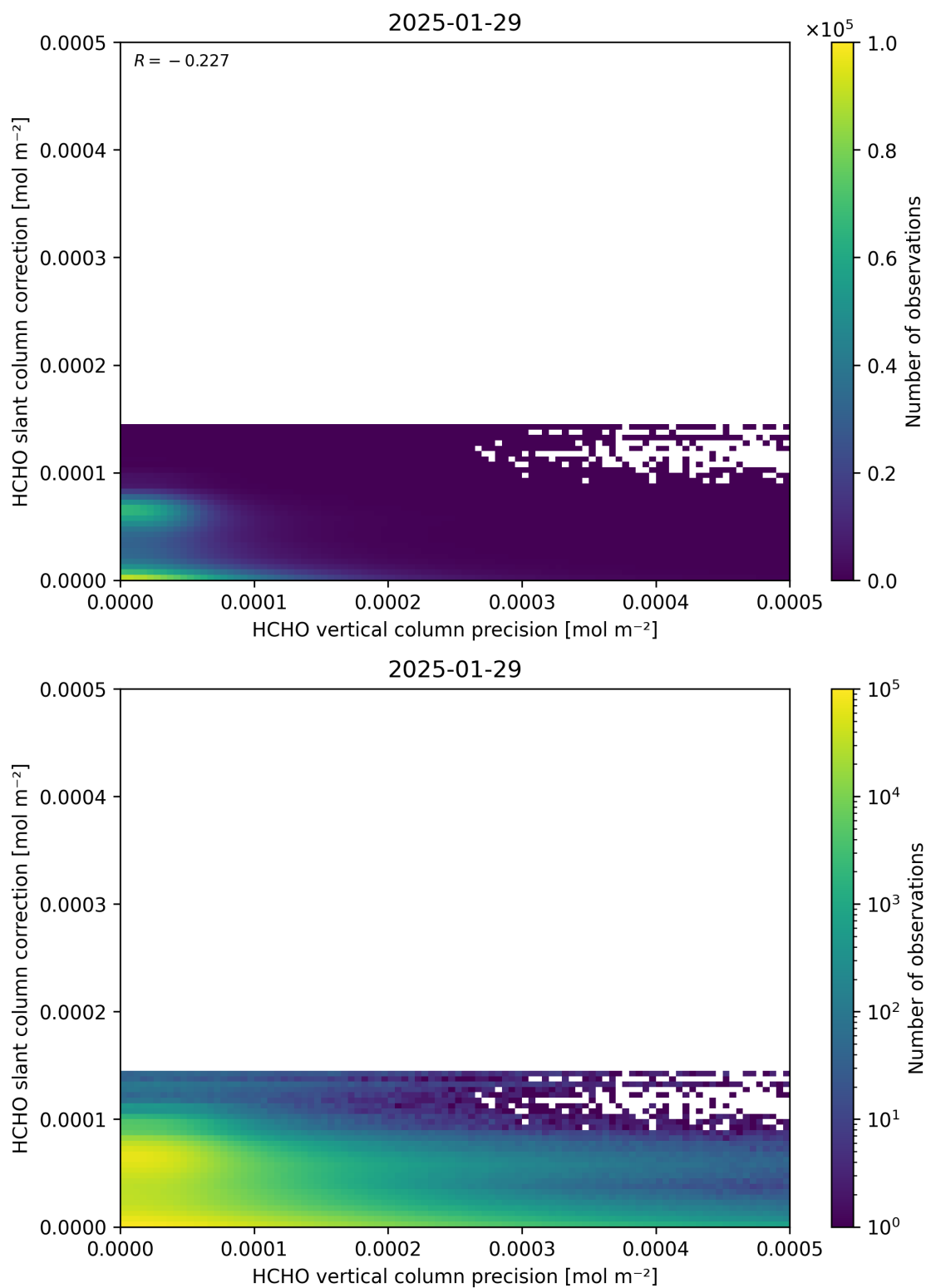
Figure 141: Scatter density plot of “HCHO vertical column precision” against “HCHO slant column correction” for 2025-01-28 to 2025-01-30.
