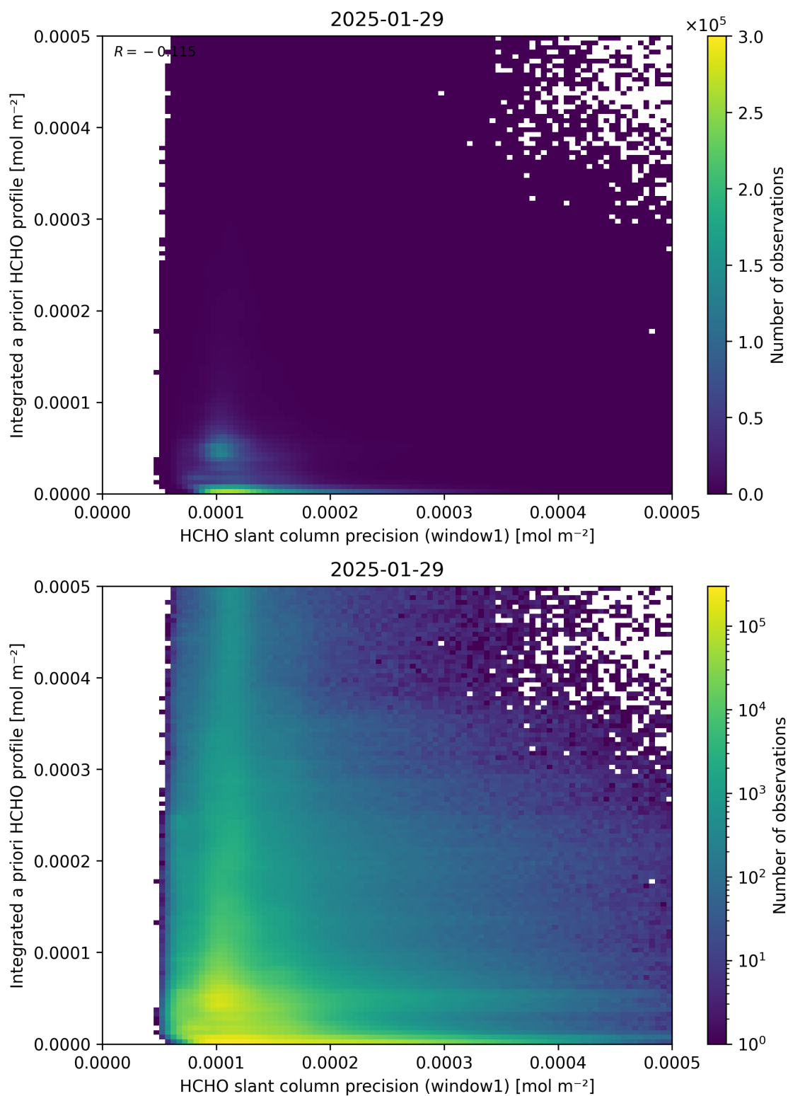
Figure 96: Scatter density plot of “HCHO slant column precision (window1)” against “Integrated a priori HCHO profile” for 2025-01-28 to 2025-01-30.
