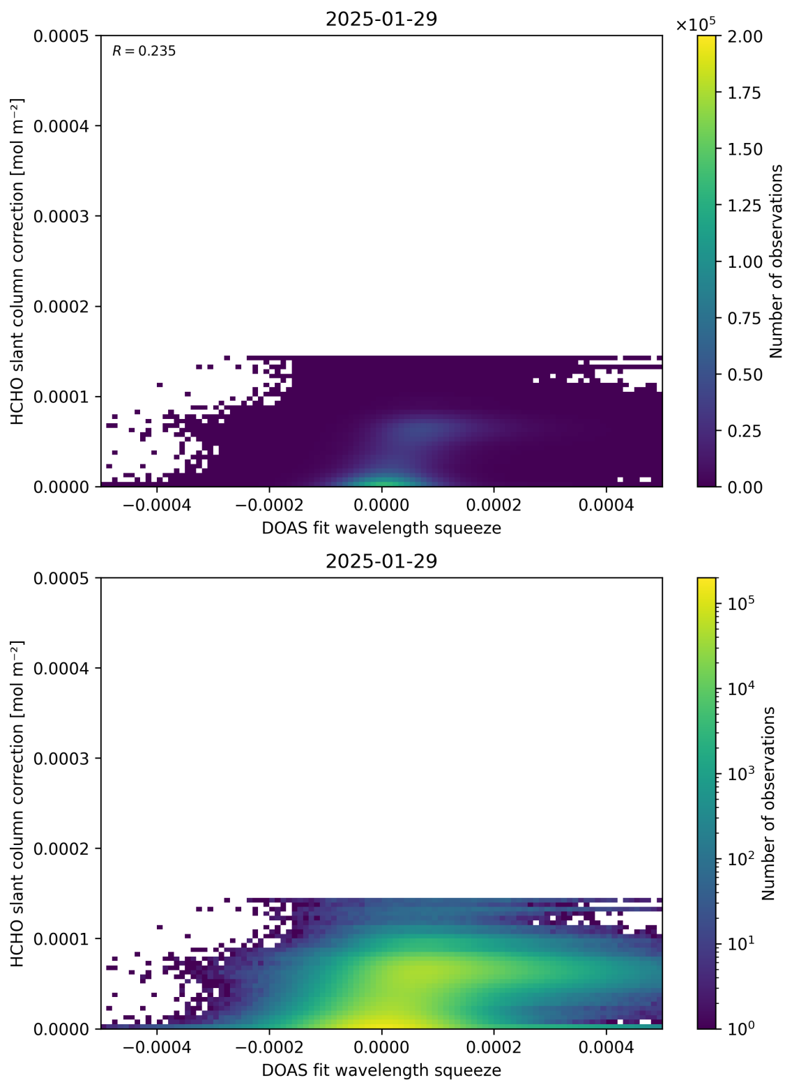
Figure 70: Scatter density plot of “DOAS fit wavelength squeeze” against “HCHO slant column correction” for 2025-01-28 to 2025-01-30.
