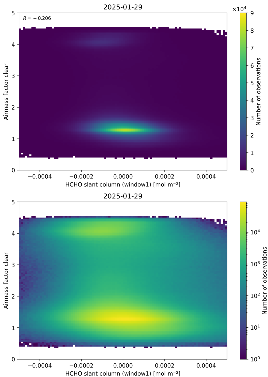
Figure 81: Scatter density plot of “HCHO slant column (window1)” against “Airmass factor clear” for 2025-01-28 to 2025-01-30.
