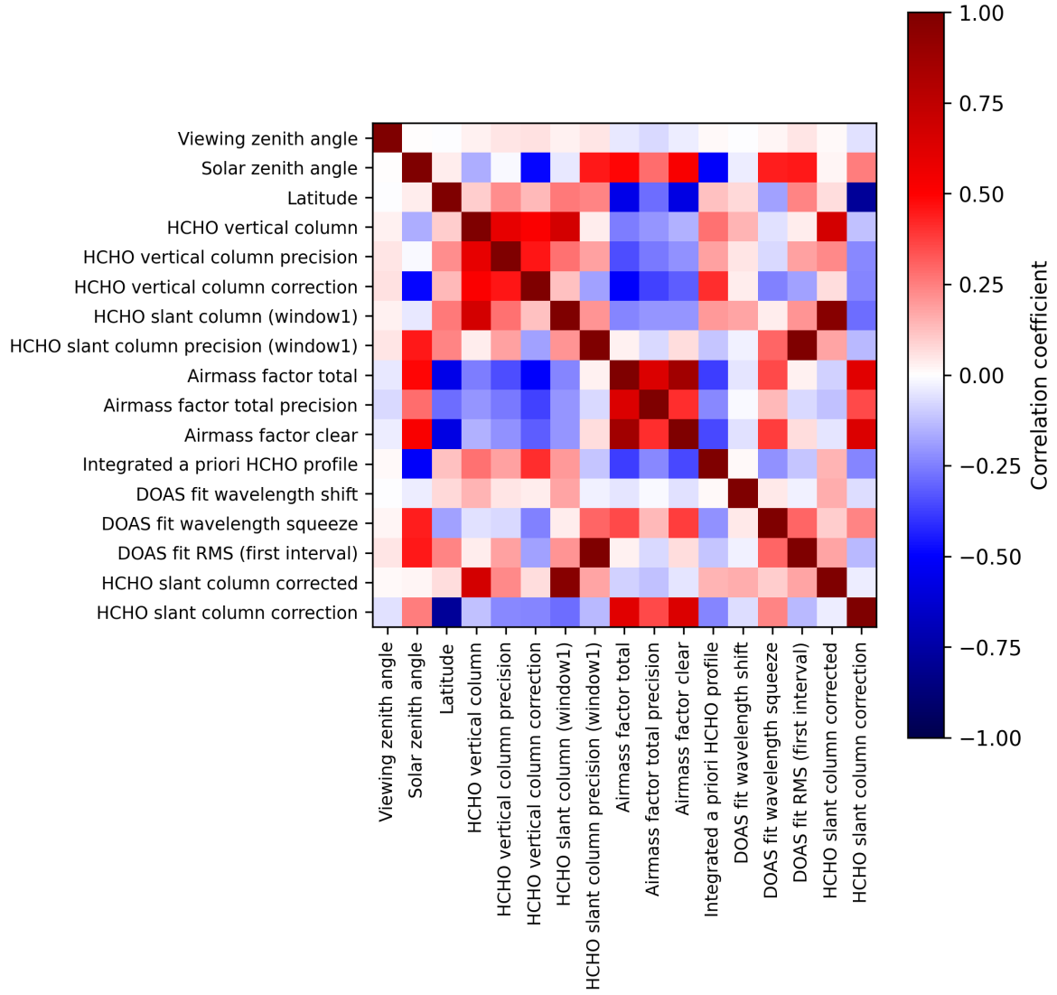
Figure 2: Map of correlation matrix for 2025-01-28 to 2025-01-30.
