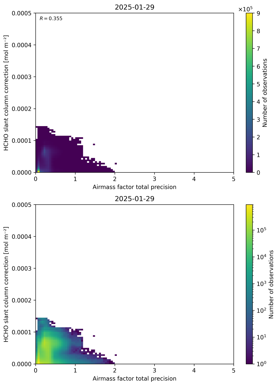
Figure 110: Scatter density plot of “Airmass factor total precision” against “HCHO slant column correction” for 2025-01-28 to 2025-01-30.
