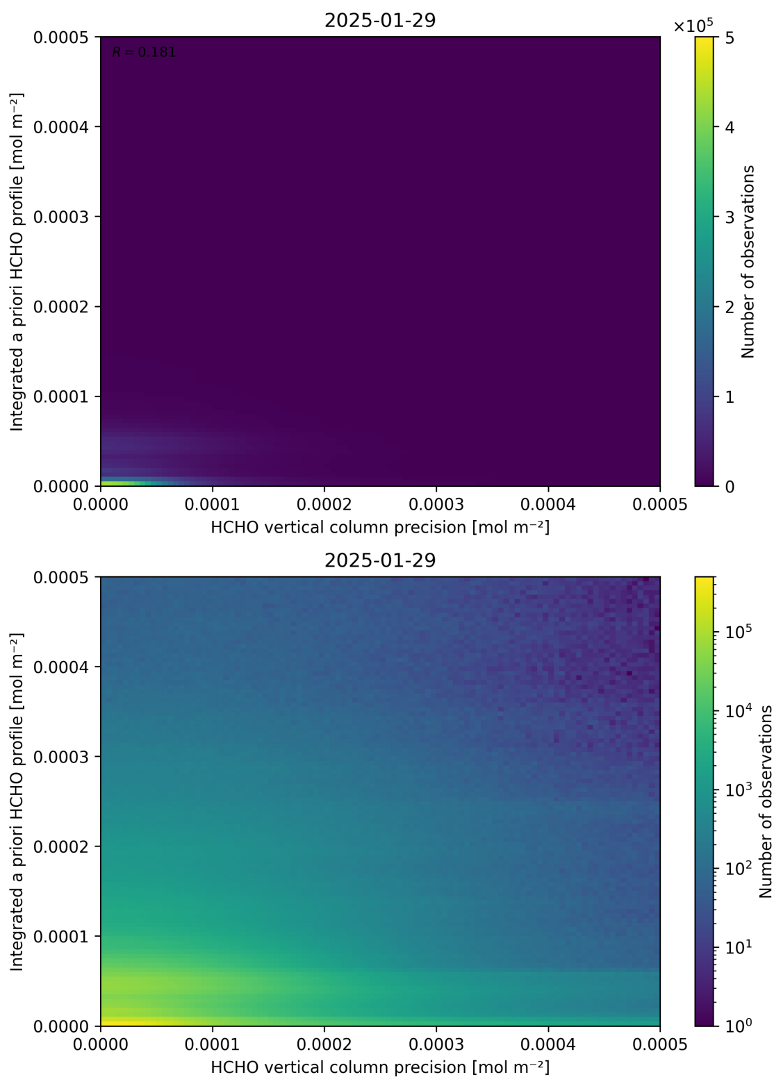
Figure 147: Scatter density plot of “HCHO vertical column precision” against “Integrated a priori HCHO profile” for 2025-01-28 to 2025-01-30.
