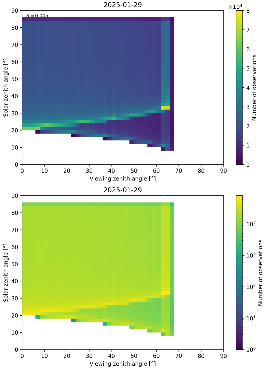
Figure 197: Scatter density plot of “Viewing zenith angle” against “Solar zenith angle” for 2025-01-28 to 2025-01-30.
