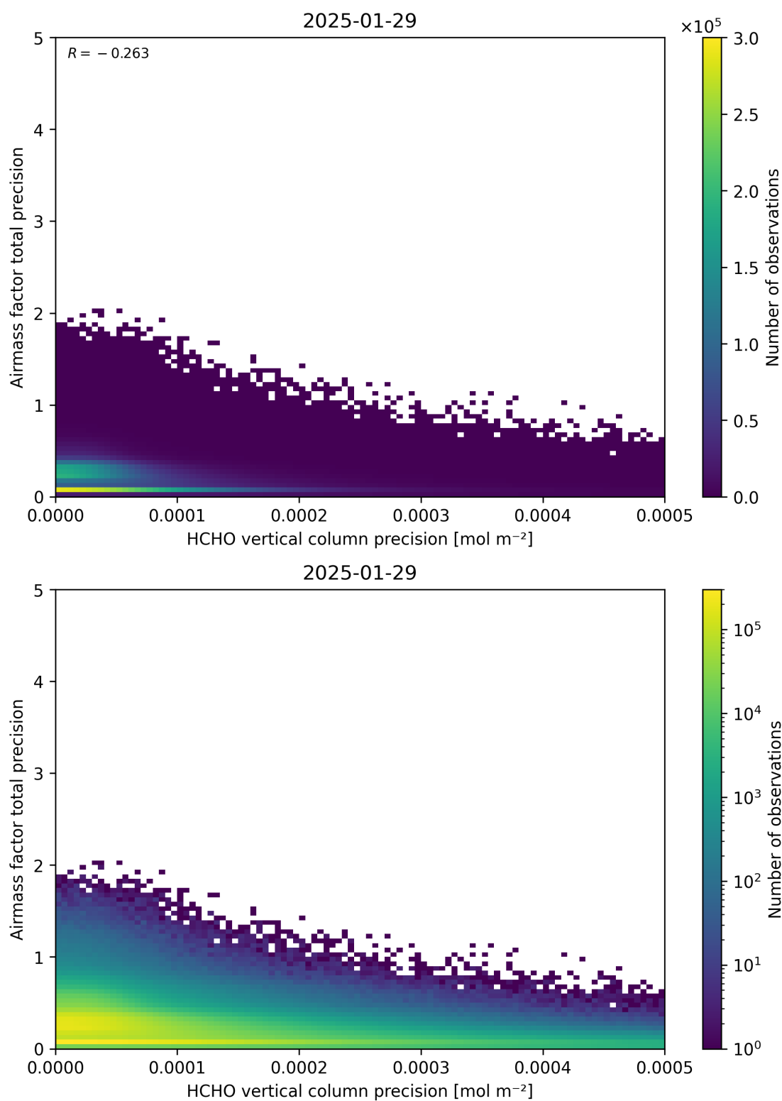
Figure 145: Scatter density plot of “HCHO vertical column precision” against “Airmass factor total precision” for 2025-01-28 to 2025-01-30.
