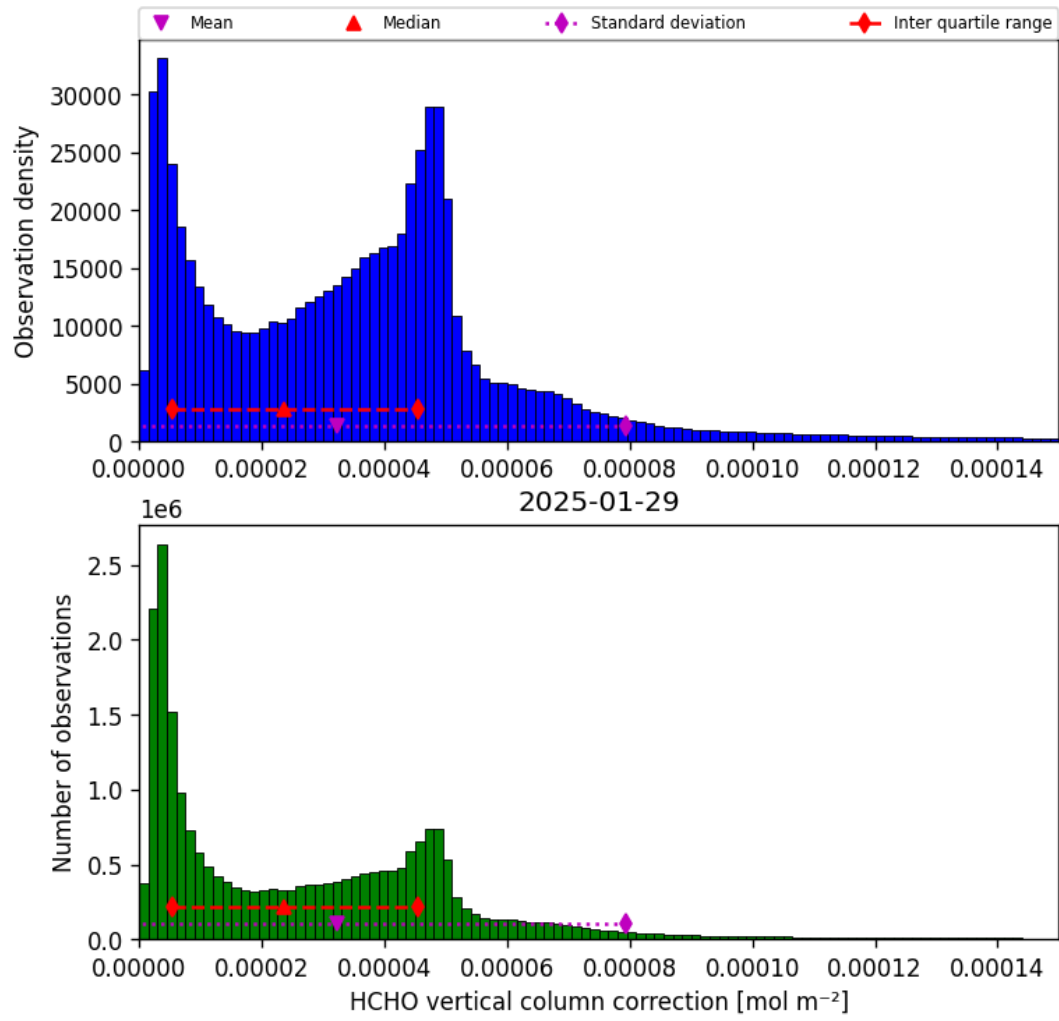
Figure 37: Histogram of “HCHO vertical column correction” for 2025-01-28 to 2025-01-30
