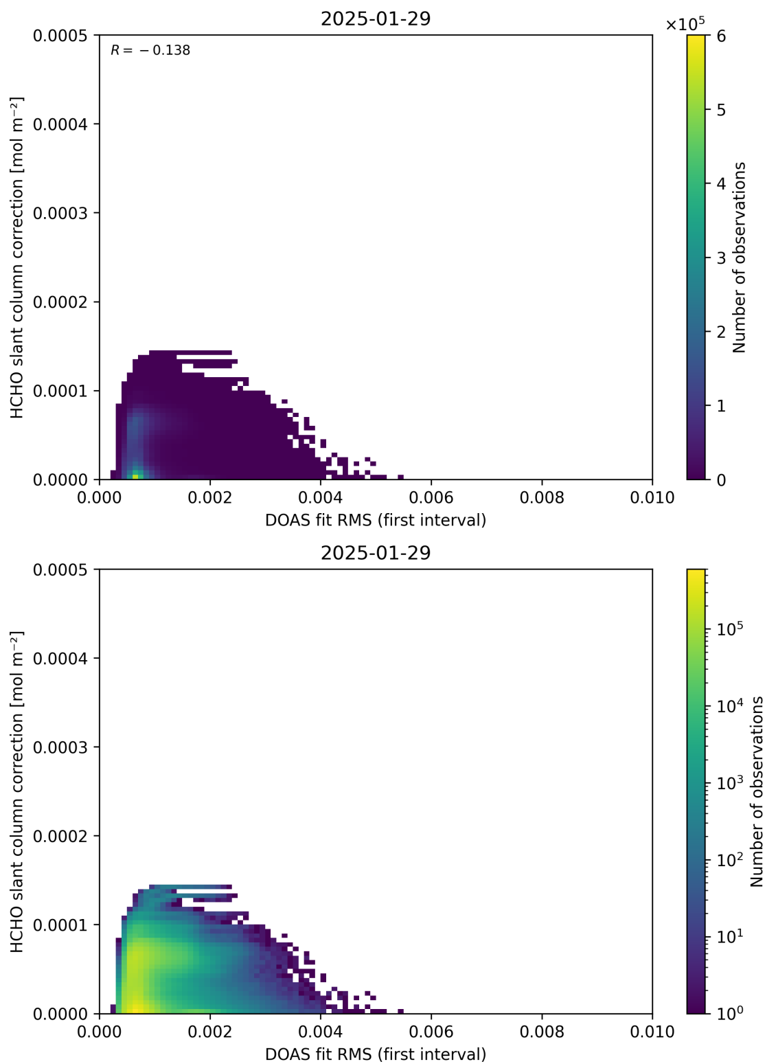
Figure 63: Scatter density plot of “DOAS fit RMS (first interval)” against “HCHO slant column correction” for 2025-01-28 to 2025-01-30.
