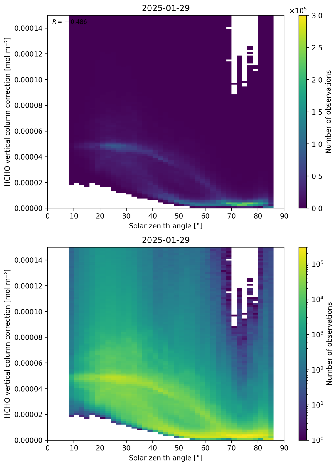
Figure 178: Scatter density plot of “Solar zenith angle” against “HCHO vertical column correction” for 2025-01-28 to 2025-01-30.
