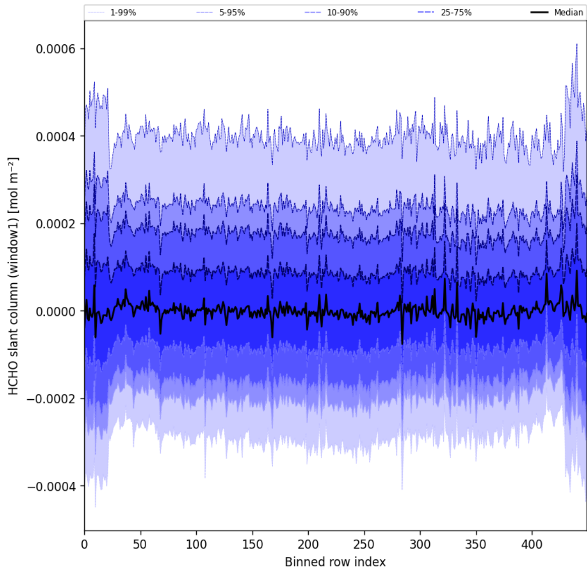
Figure 52: Along track statistics of “HCHO slant column (window1)” for 2025-01-28 to 2025-01-30
