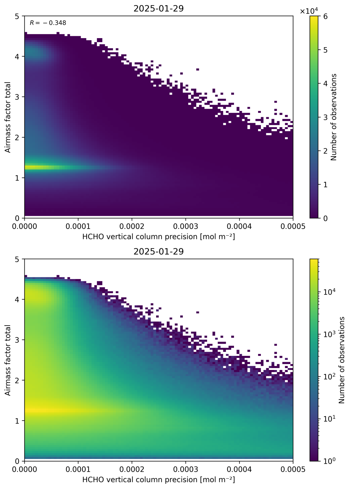
Figure 144: Scatter density plot of “HCHO vertical column precision” against “Airmass factor total” for 2025-01-28 to 2025-01-30.
