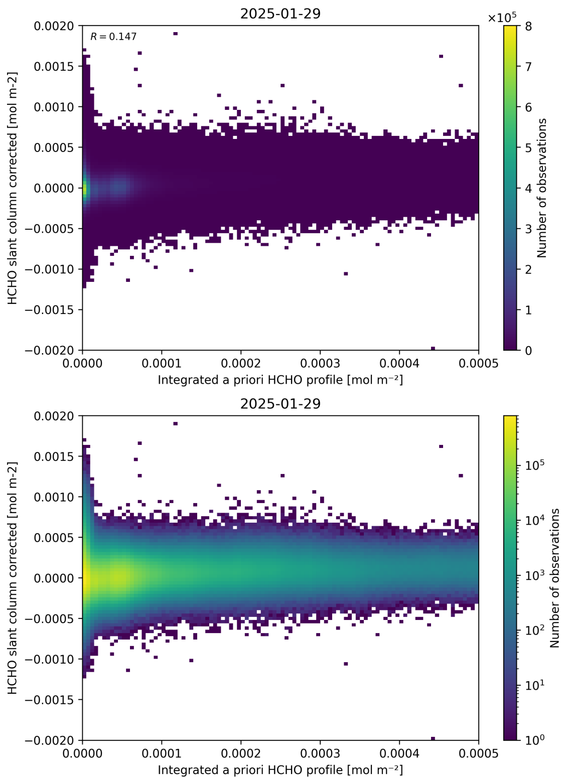
Figure 151: Scatter density plot of “Integrated a priori HCHO profile” against “HCHO slant column corrected” for 2025-01-28 to 2025-01-30.
