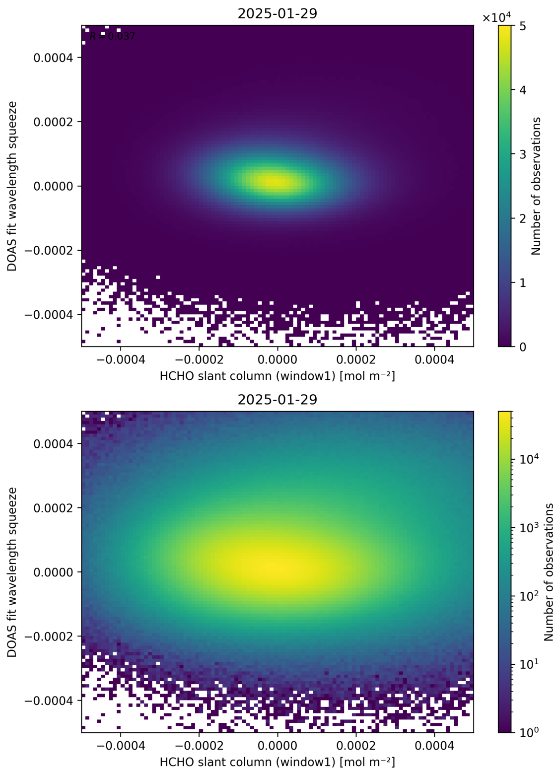
Figure 80: Scatter density plot of “HCHO slant column (window1)” against “DOAS fit wavelength squeeze” for 2025-01-28 to 2025-01-30.
