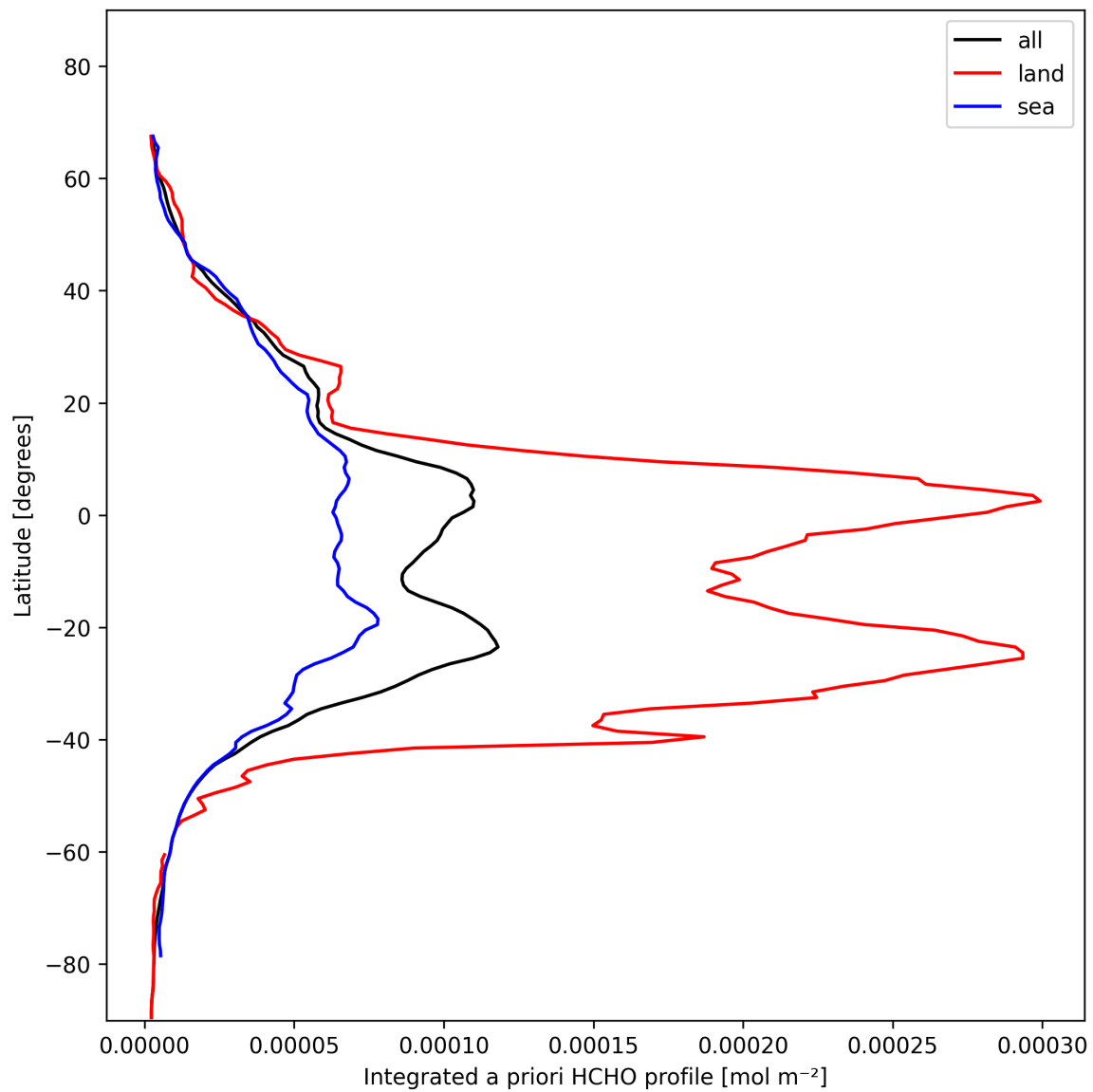
Figure 29: Zonal average of “Integrated a priori HCHO profile” for 2025-01-28 to 2025-01-30.
