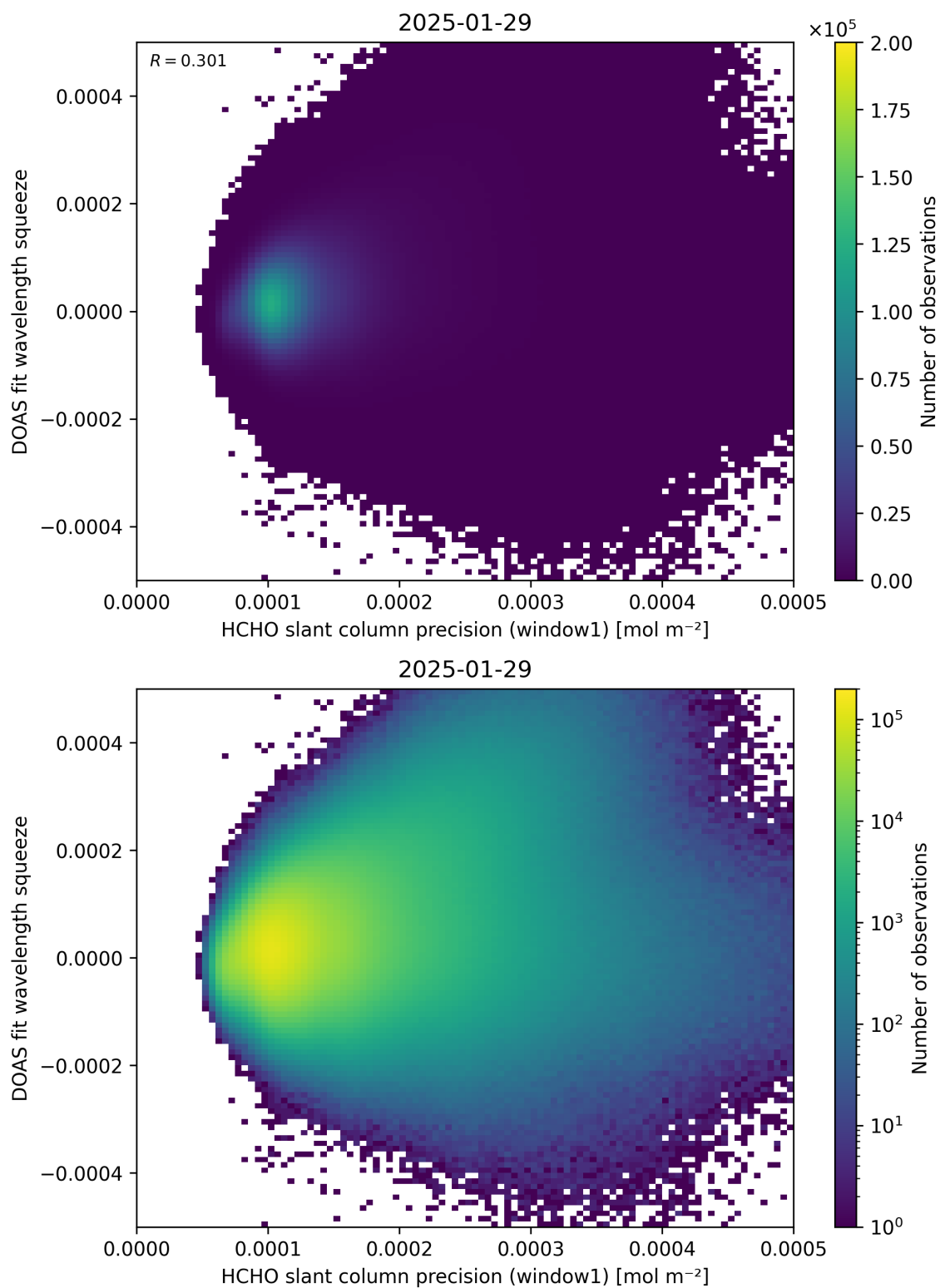
Figure 90: Scatter density plot of “HCHO slant column precision (window1)” against “DOAS fit wavelength squeeze” for 2025-01-28 to 2025-01-30.
