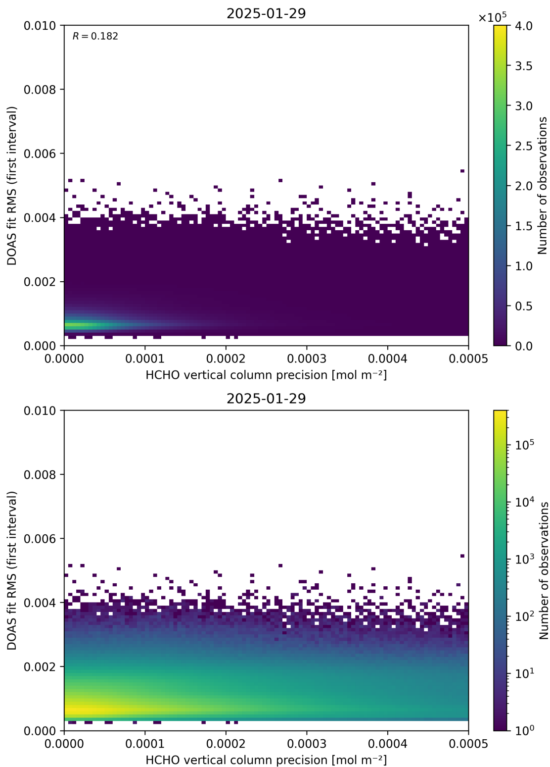
Figure 136: Scatter density plot of “HCHO vertical column precision” against “DOAS fit RMS (first interval)” for 2025-01-28 to 2025-01-30.
