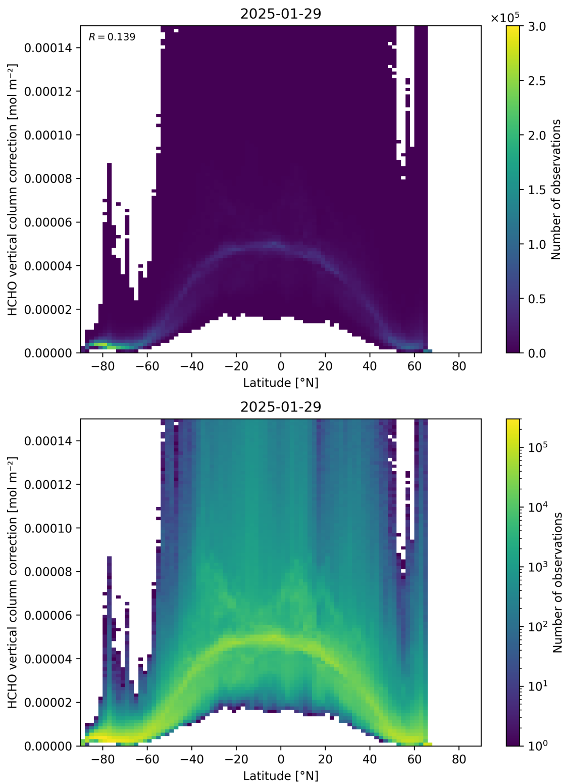
Figure 164: Scatter density plot of “Latitude” against “HCHO vertical column correction” for 2025-01-28 to 2025-01-30.
