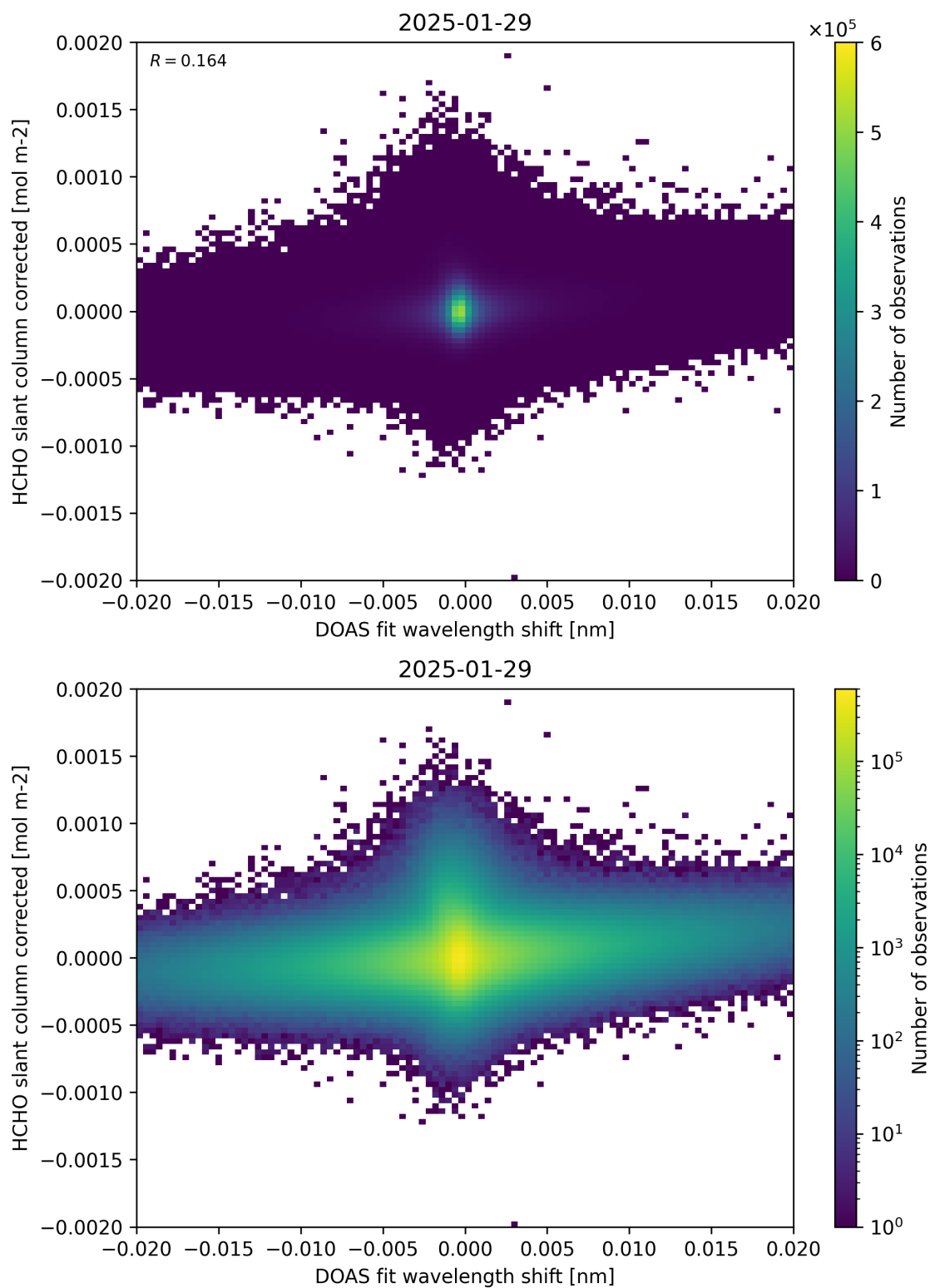
Figure 66: Scatter density plot of “DOAS fit wavelength shift” against “HCHO slant column corrected” for 2025-01-28 to 2025-01-30.
