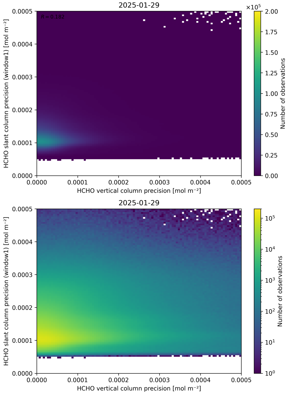
Figure 143: Scatter density plot of “HCHO vertical column precision” against “HCHO slant column precision (window1)” for 2025-01-28 to 2025-01-30.
