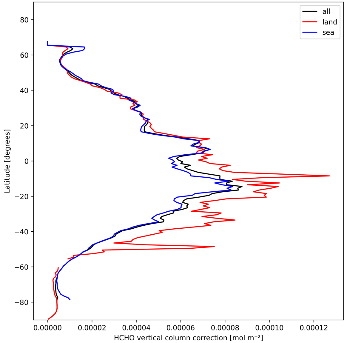
Figure 23: Zonal average of “HCHO vertical column correction” for 2025-01-28 to 2025-01-30.
