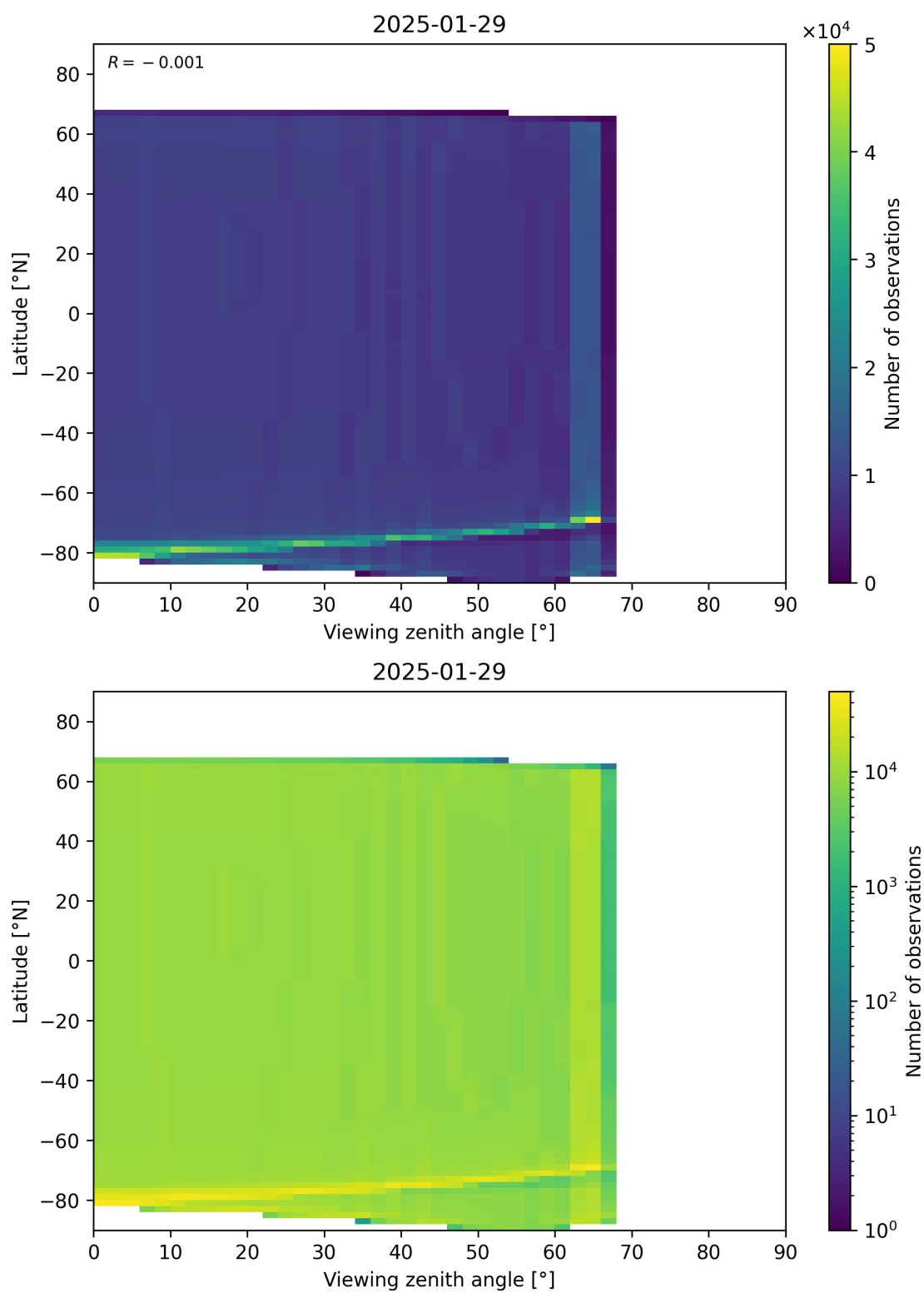
Figure 196: Scatter density plot of “Viewing zenith angle” against “Latitude” for 2025-01-28 to 2025-01-30.
