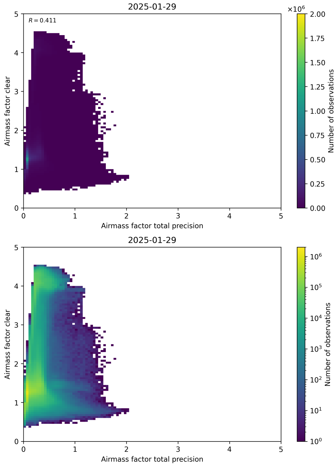
Figure 108: Scatter density plot of “Airmass factor total precision” against “Airmass factor clear” for 2025-01-28 to 2025-01-30.
