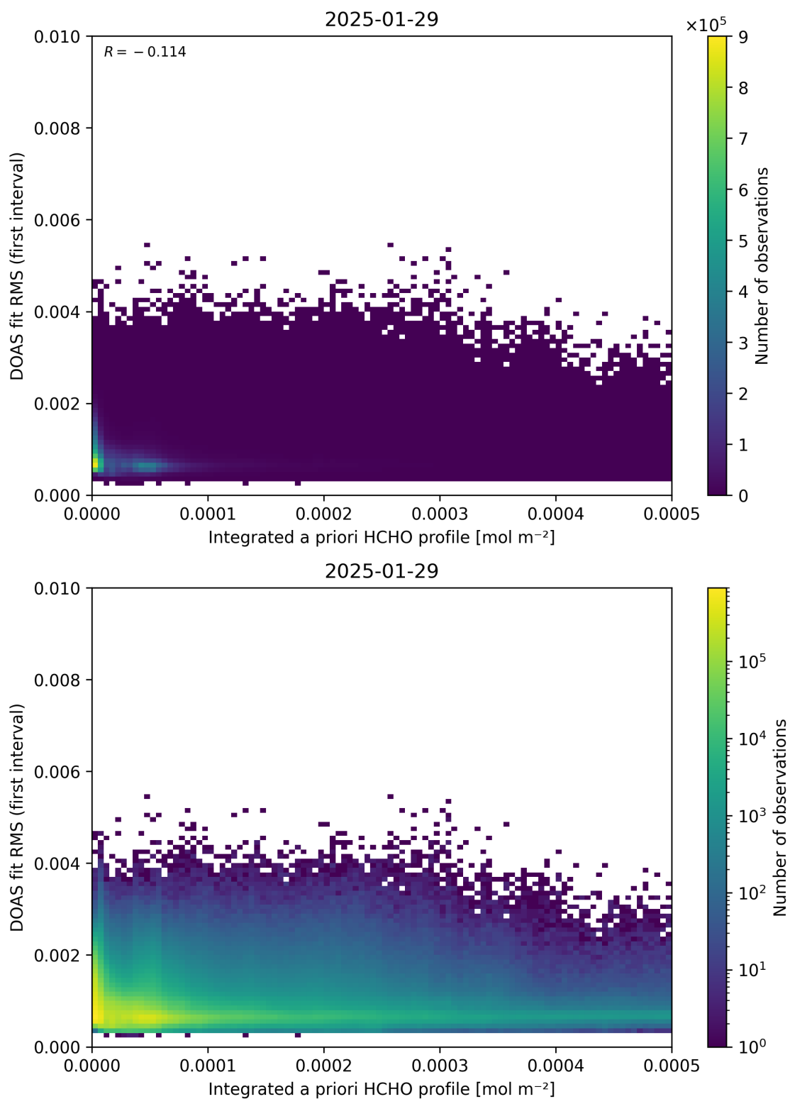
Figure 148: Scatter density plot of “Integrated a priori HCHO profile” against “DOAS fit RMS (first interval)” for 2025-01-28 to 2025-01-30.
