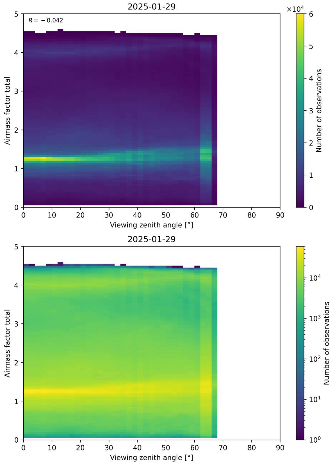
Figure 190: Scatter density plot of “Viewing zenith angle” against “Airmass factor total” for 2025-01-28 to 2025-01-30.
