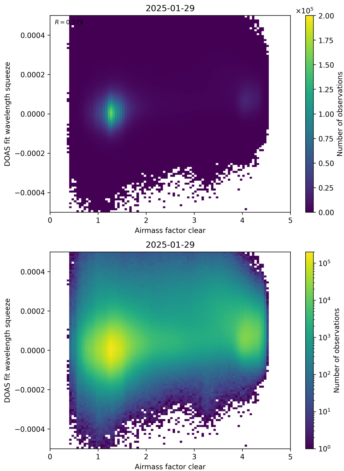
Figure 73: Scatter density plot of “Airmass factor clear” against “DOAS fit wavelength squeeze” for 2025-01-28 to 2025-01-30.
