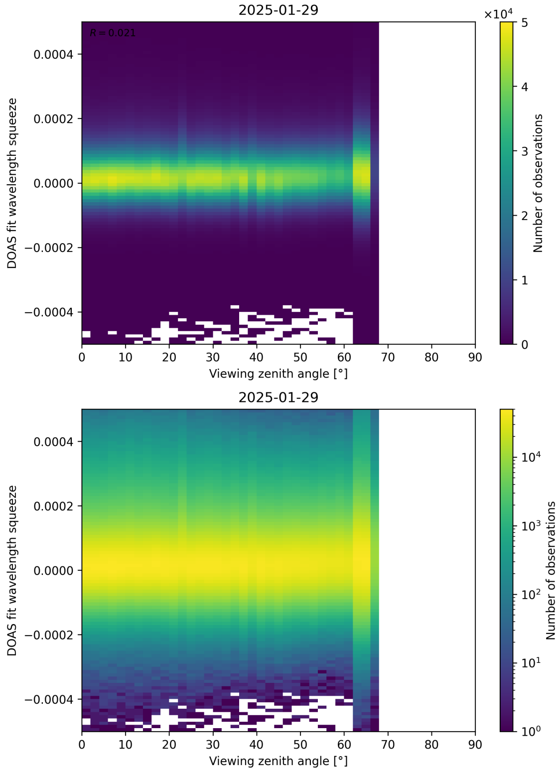
Figure 184: Scatter density plot of “Viewing zenith angle” against “DOAS fit wavelength squeeze” for 2025-01-28 to 2025-01-30.
