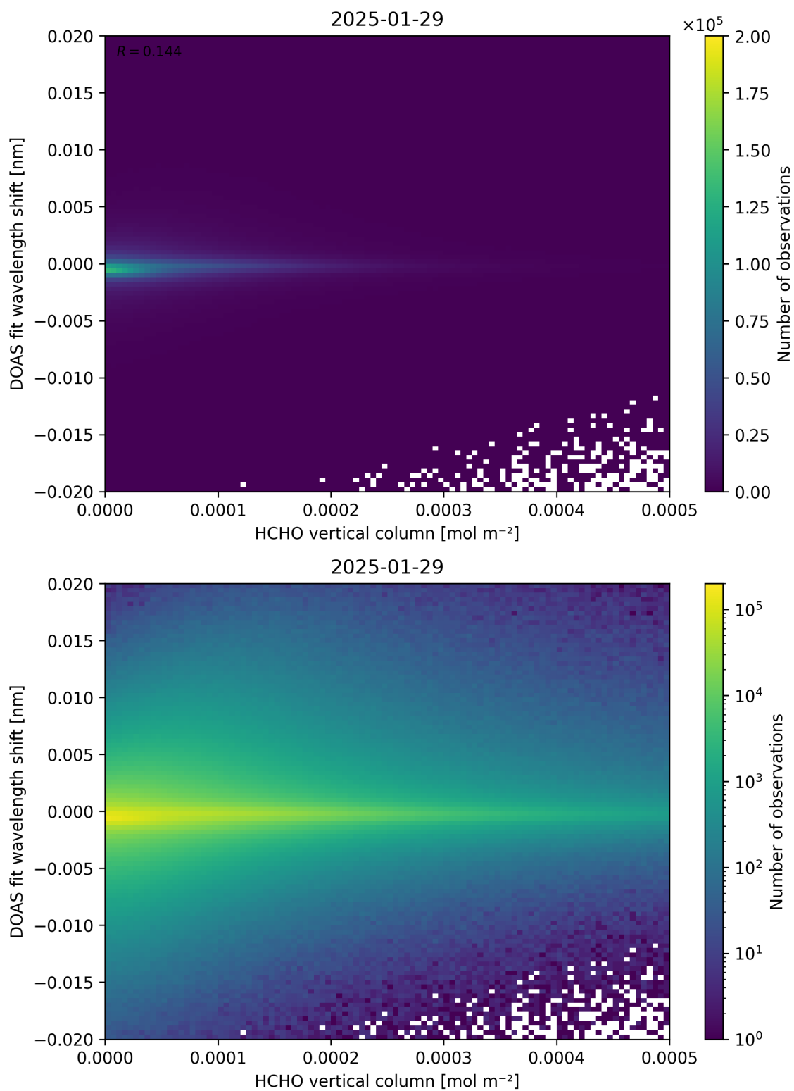
Figure 124: Scatter density plot of “HCHO vertical column” against “DOAS fit wavelength shift” for 2025-01-28 to 2025-01-30.
