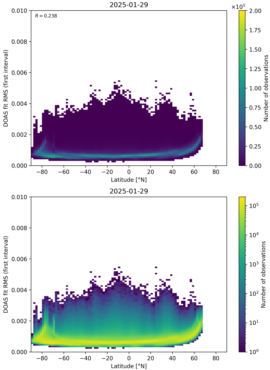
Figure 153: Scatter density plot of “Latitude” against “DOAS fit RMS (first interval)” for 2025-01-28 to 2025-01-30.
