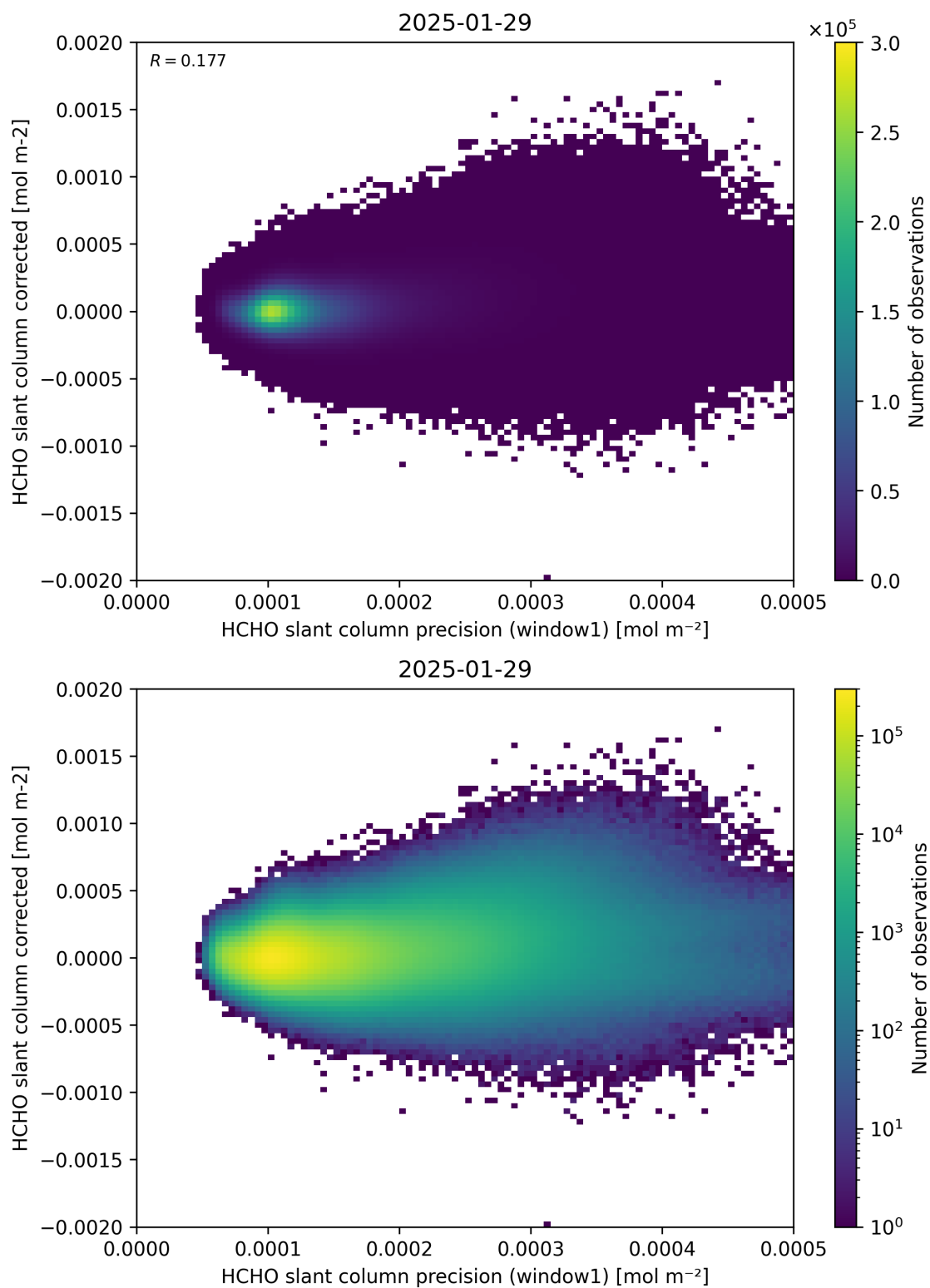
Figure 92: Scatter density plot of “HCHO slant column precision (window1)” against “HCHO slant column corrected” for 2025-01-28 to 2025-01-30.
