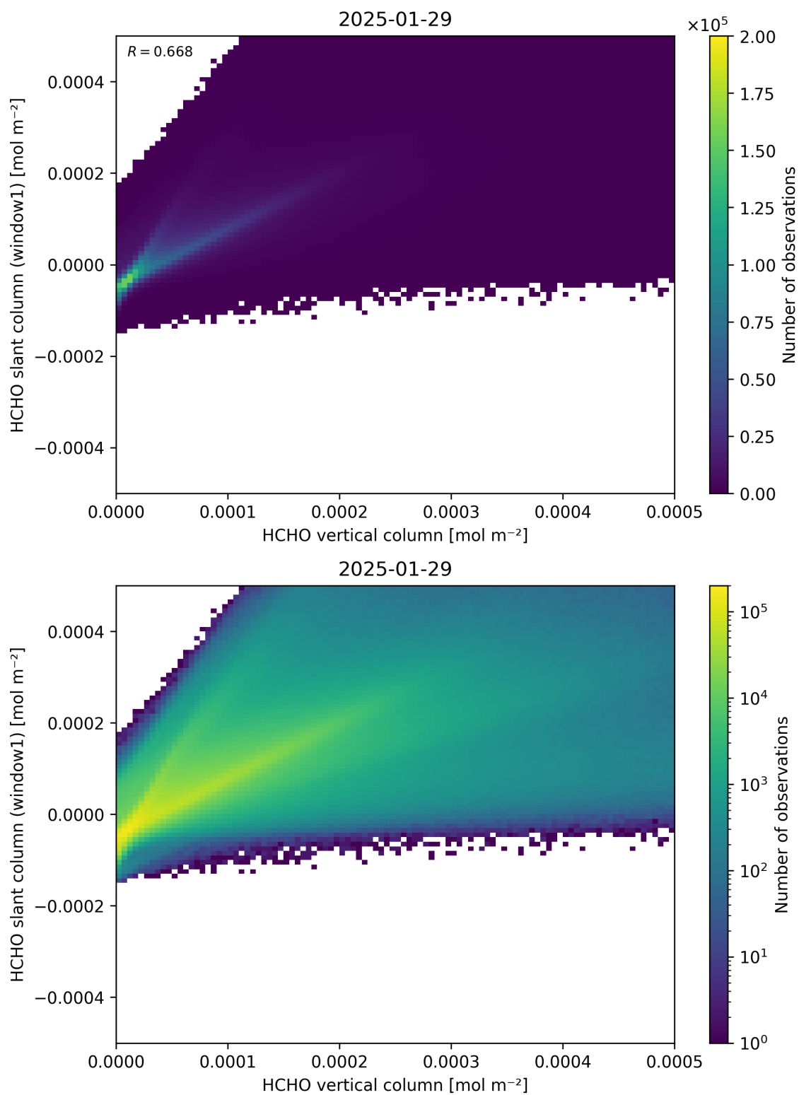
Figure 129: Scatter density plot of “HCHO vertical column” against “HCHO slant column (window1)” for 2025-01-28 to 2025-01-30.
