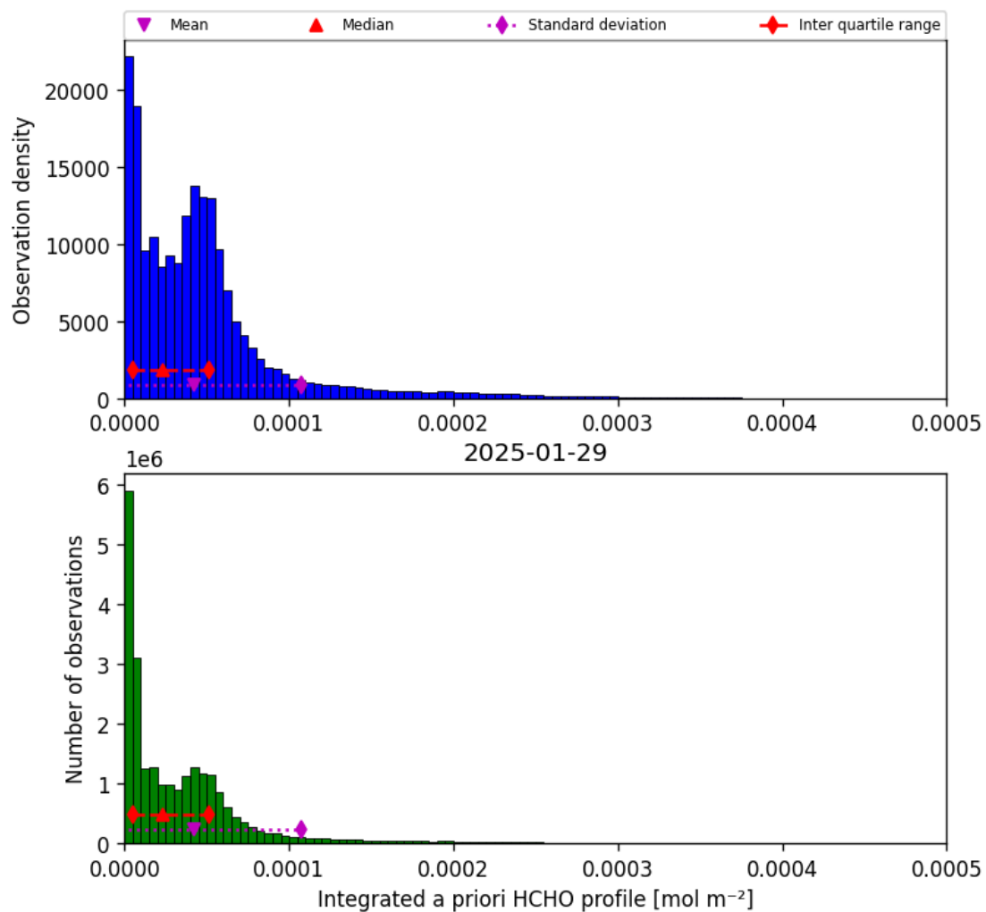
Figure 43: Histogram of “Integrated a priori HCHO profile” for 2025-01-28 to 2025-01-30
