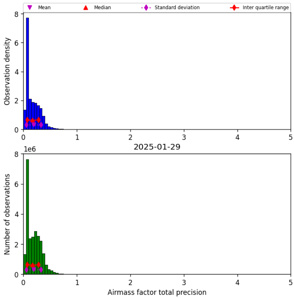
Figure 41: Histogram of “Airmass factor total precision” for 2025-01-28 to 2025-01-30
