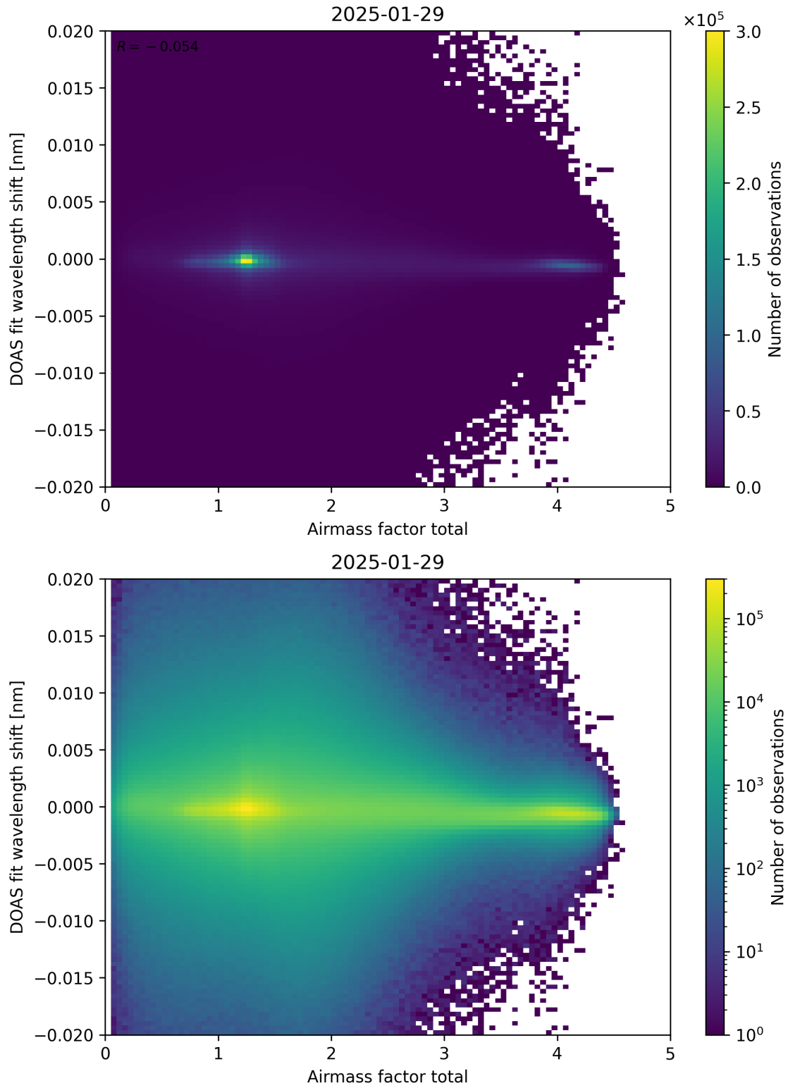
Figure 98: Scatter density plot of “Airmass factor total” against “DOAS fit wavelength shift” for 2025-01-28 to 2025-01-30.
