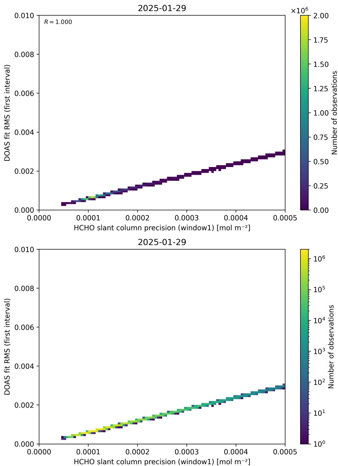
Figure 88: Scatter density plot of “HCHO slant column precision (window1)” against “DOAS fit RMS (first interval)” for 2025-01-28 to 2025-01-30.
