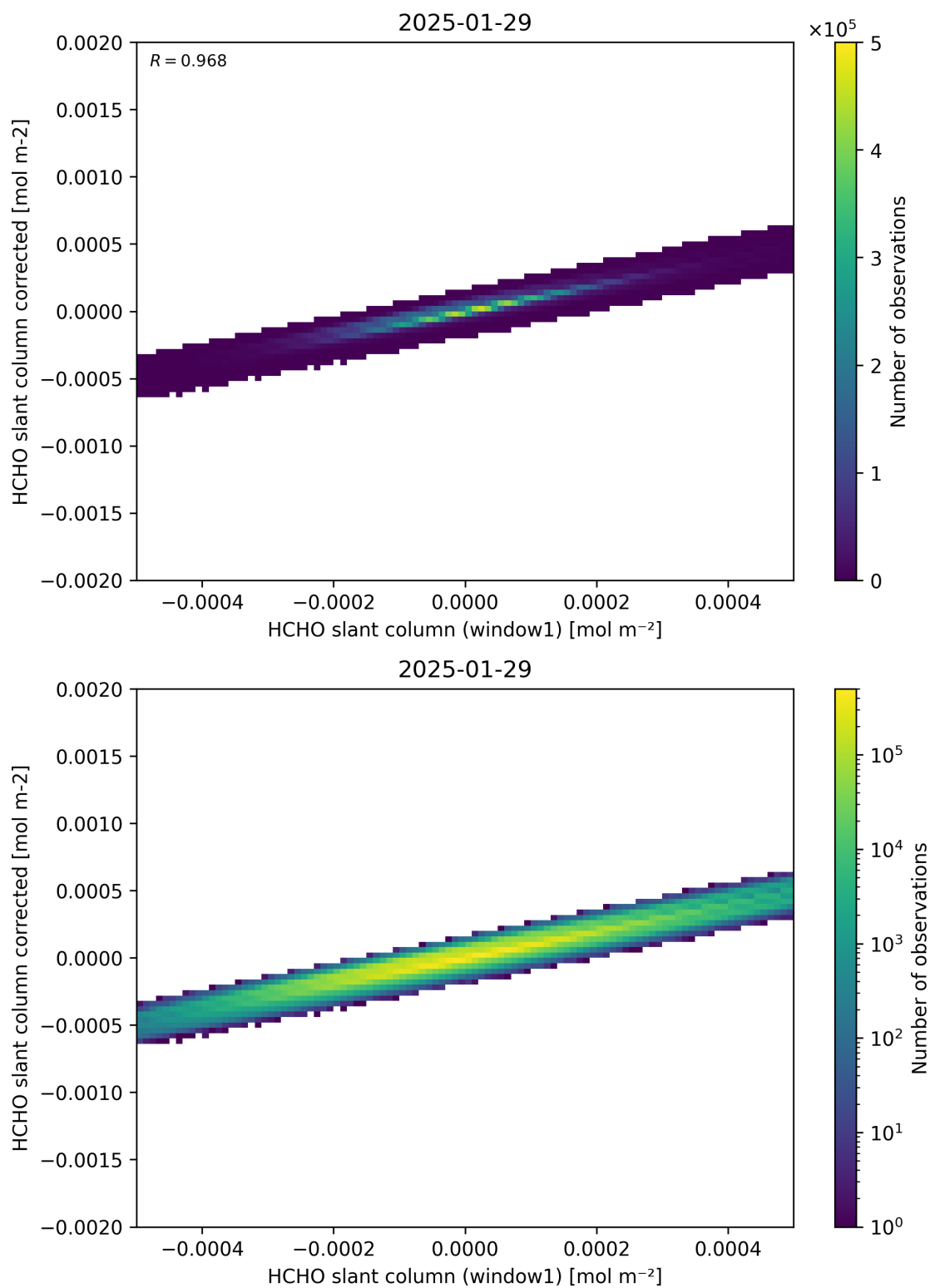
Figure 82: Scatter density plot of “HCHO slant column (window1)” against “HCHO slant column corrected” for 2025-01-28 to 2025-01-30.
