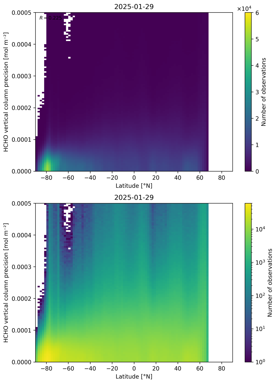
Figure 165: Scatter density plot of “Latitude” against “HCHO vertical column precision” for 2025-01-28 to 2025-01-30.
