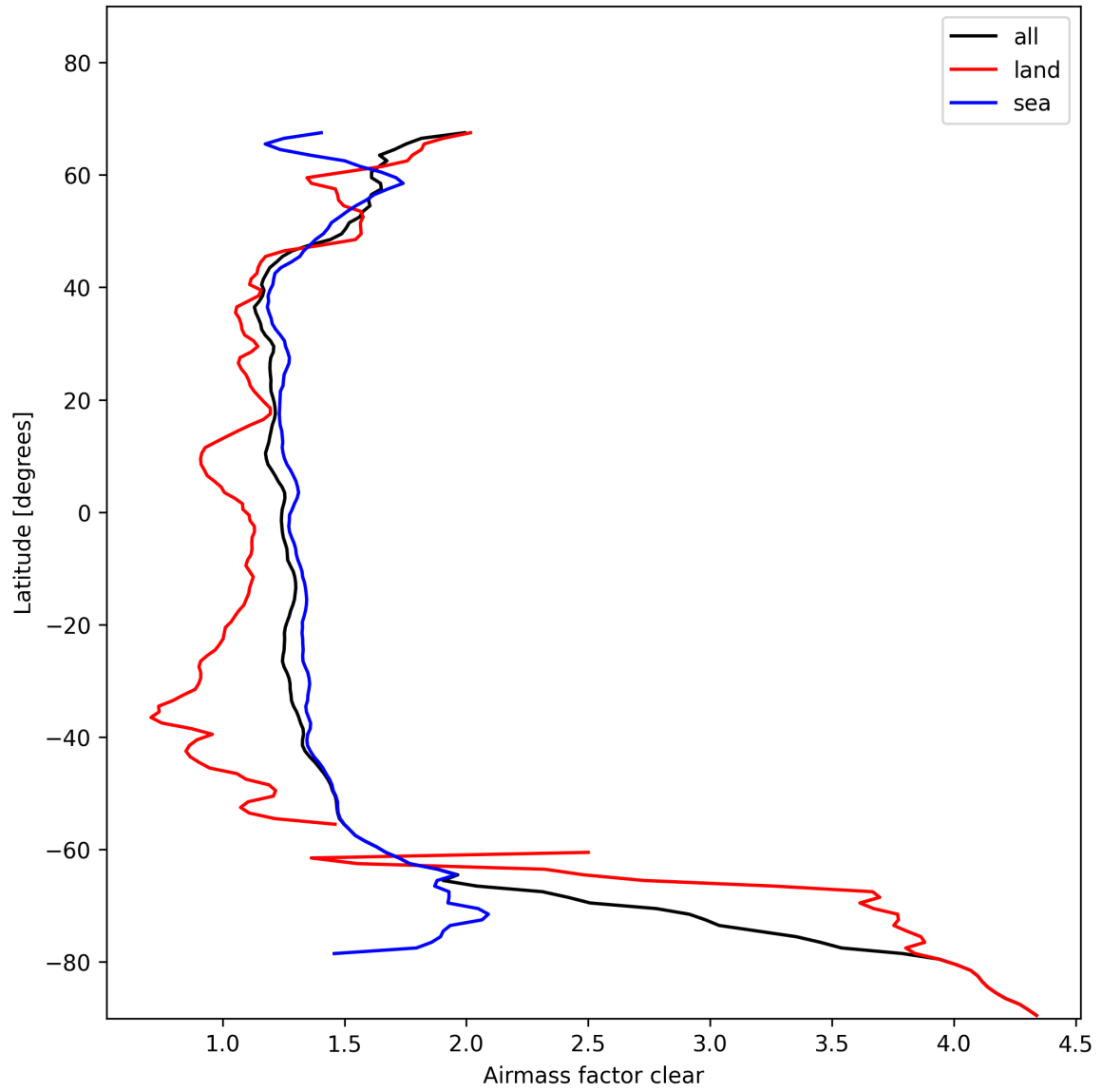
Figure 28: Zonal average of “Airmass factor clear” for 2025-01-28 to 2025-01-30.
