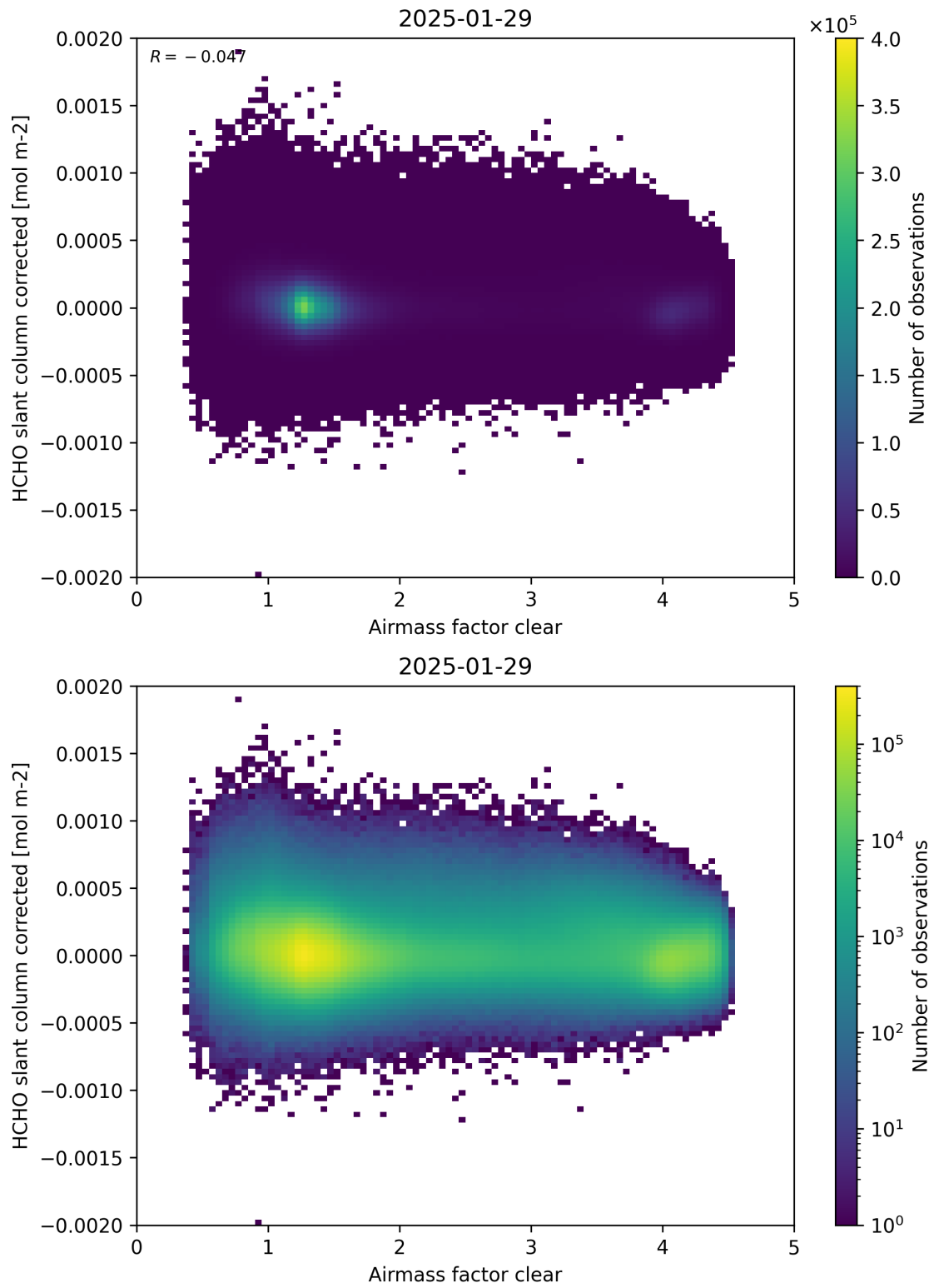
Figure 74: Scatter density plot of “Airmass factor clear” against “HCHO slant column corrected” for 2025-01-28 to 2025-01-30.
