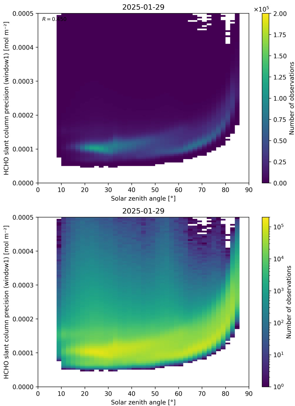
Figure 174: Scatter density plot of “Solar zenith angle” against “HCHO slant column precision (window1)” for 2025-01-28 to 2025-01-30.
