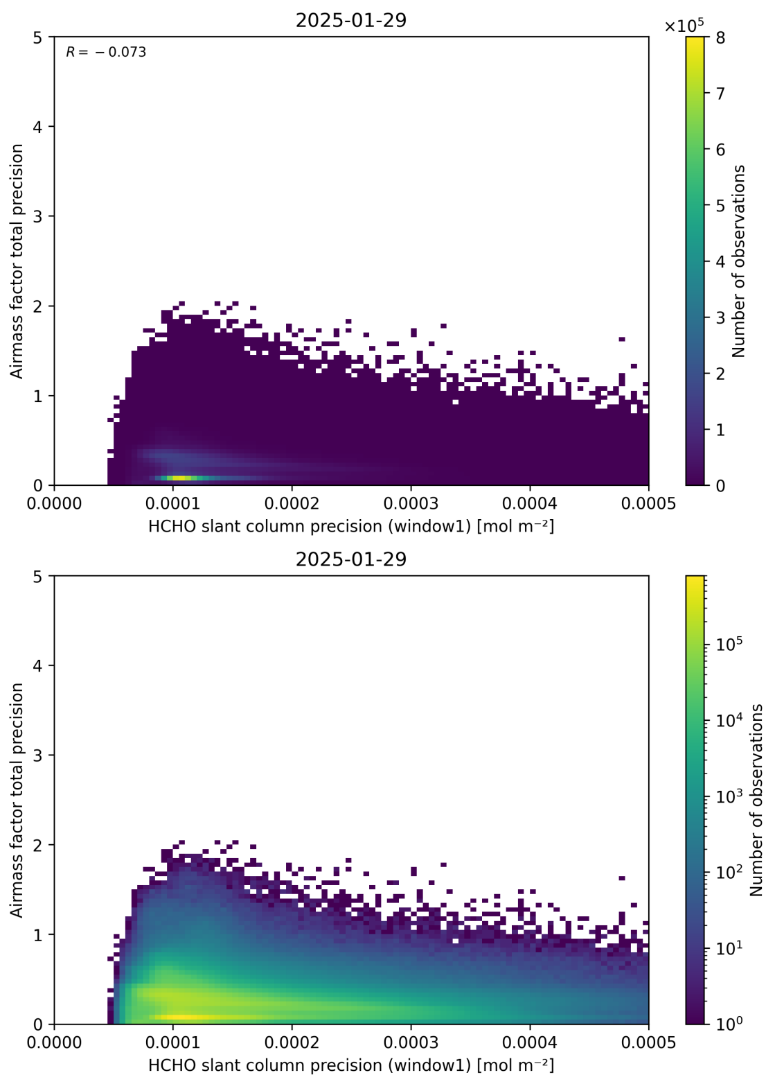
Figure 95: Scatter density plot of “HCHO slant column precision (window1)” against “Airmass factor total precision” for 2025-01-28 to 2025-01-30.
