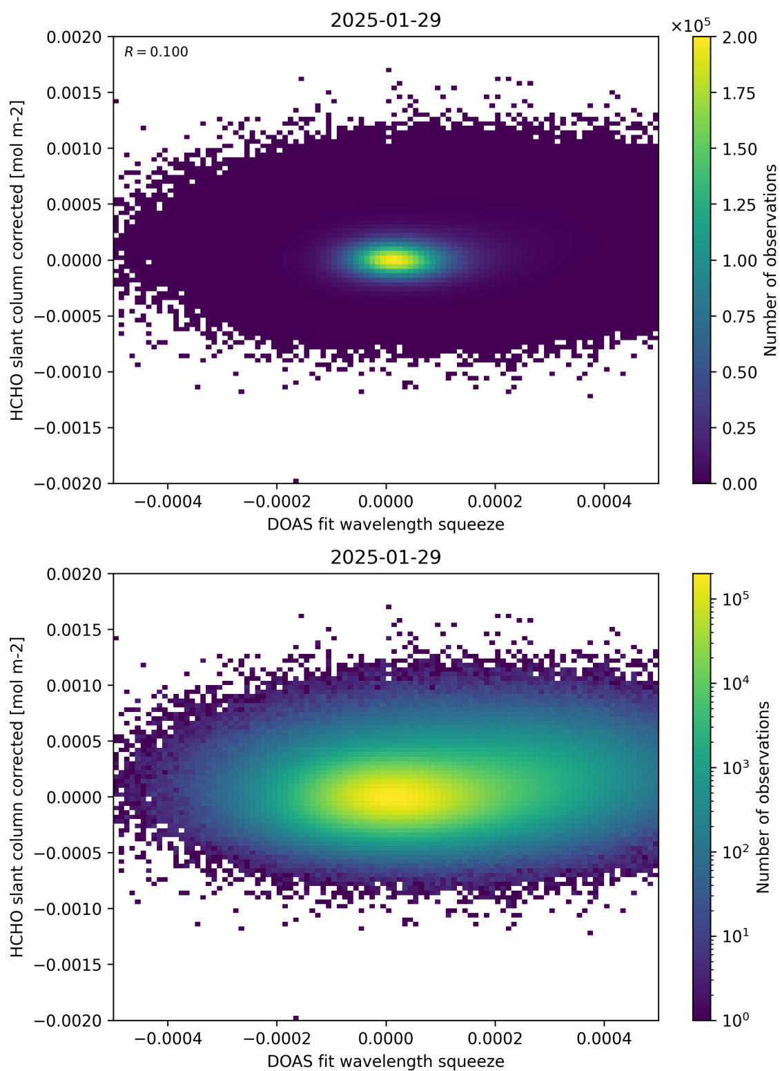
Figure 69: Scatter density plot of “DOAS fit wavelength squeeze” against “HCHO slant column corrected” for 2025-01-28 to 2025-01-30.
