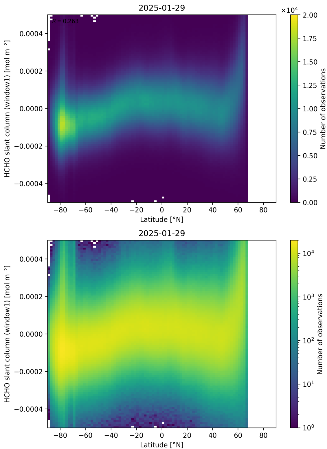
Figure 159: Scatter density plot of “Latitude” against “HCHO slant column (window1)” for 2025-01-28 to 2025-01-30.
