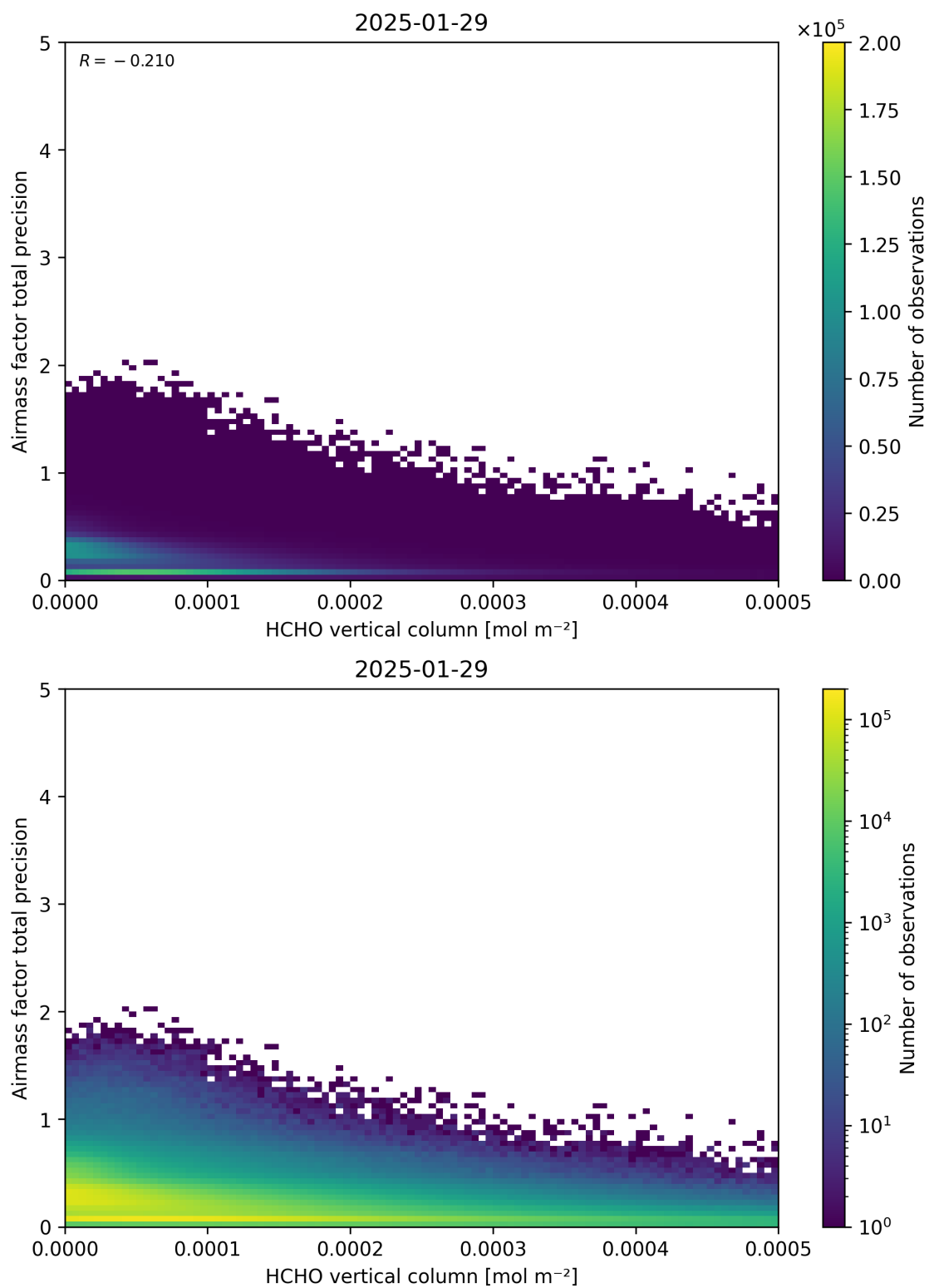
Figure 132: Scatter density plot of “HCHO vertical column” against “Airmass factor total precision” for 2025-01-28 to 2025-01-30.
