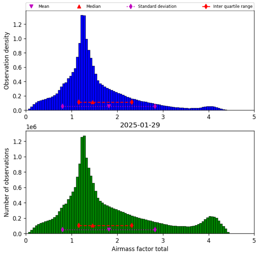
Figure 40: Histogram of “Airmass factor total” for 2025-01-28 to 2025-01-30
