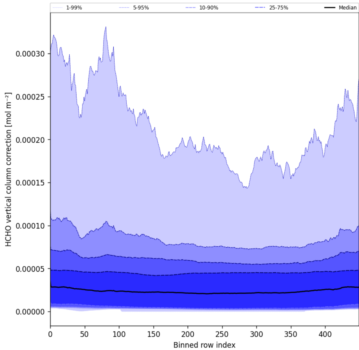
Figure 51: Along track statistics of “HCHO vertical column correction” for 2025-01-28 to 2025-01-30
