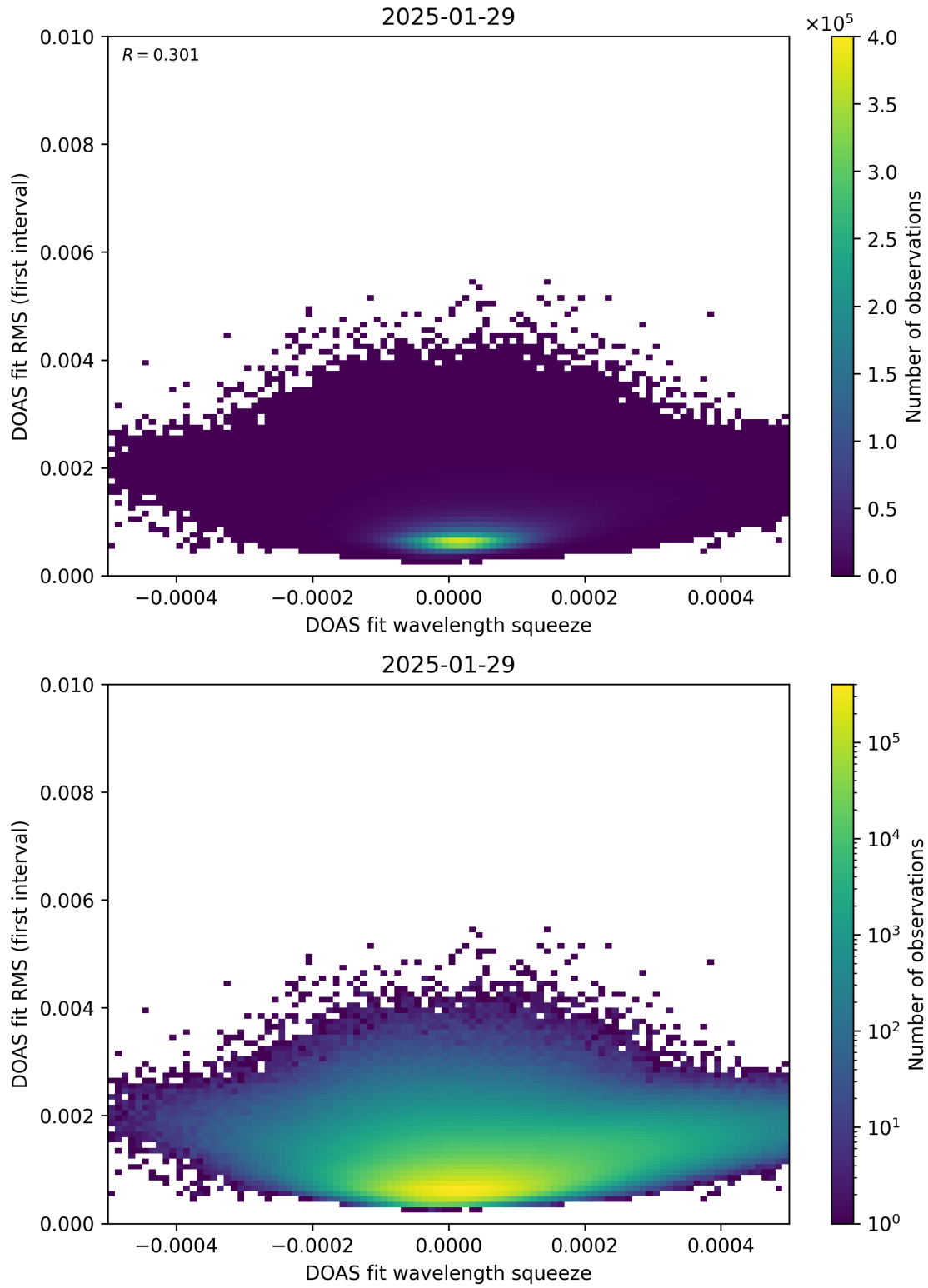
Figure 68: Scatter density plot of “DOAS fit wavelength squeeze” against “DOAS fit RMS (first interval)” for 2025-01-28 to 2025-01-30.
