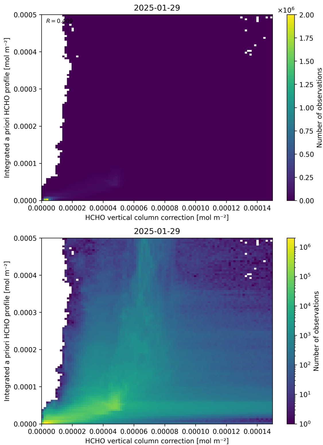
Figure 122: Scatter density plot of “HCHO vertical column correction” against “Integrated a priori HCHO profile” for 2025-01-28 to 2025-01-30.
