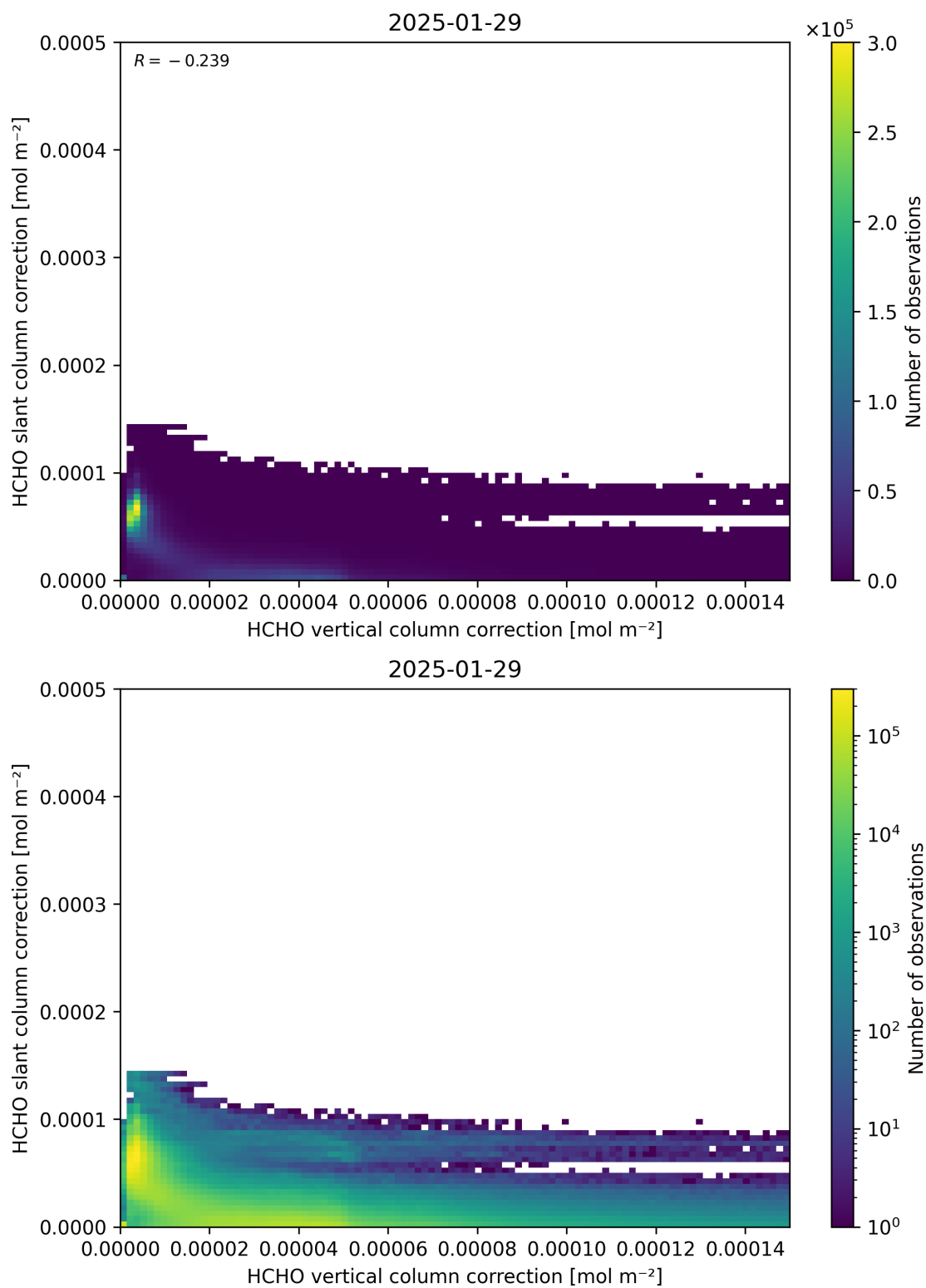
Figure 117: Scatter density plot of “HCHO vertical column correction” against “HCHO slant column correction” for 2025-01-28 to 2025-01-30.
