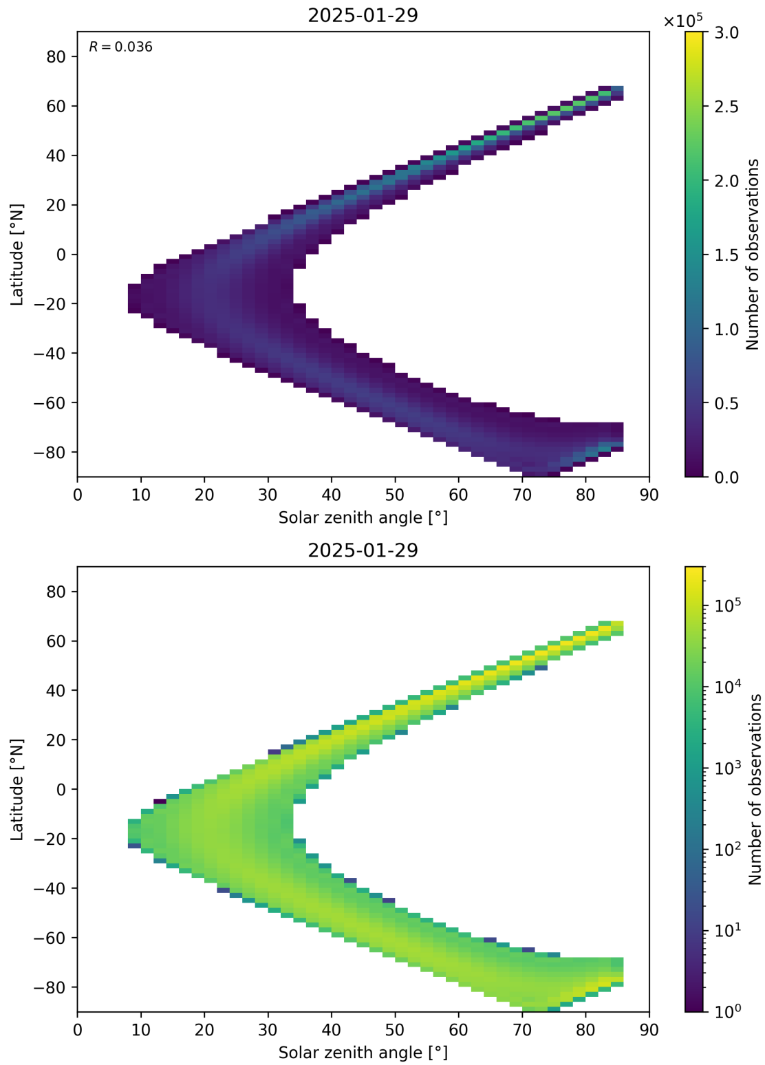
Figure 181: Scatter density plot of “Solar zenith angle” against “Latitude” for 2025-01-28 to 2025-01-30.
