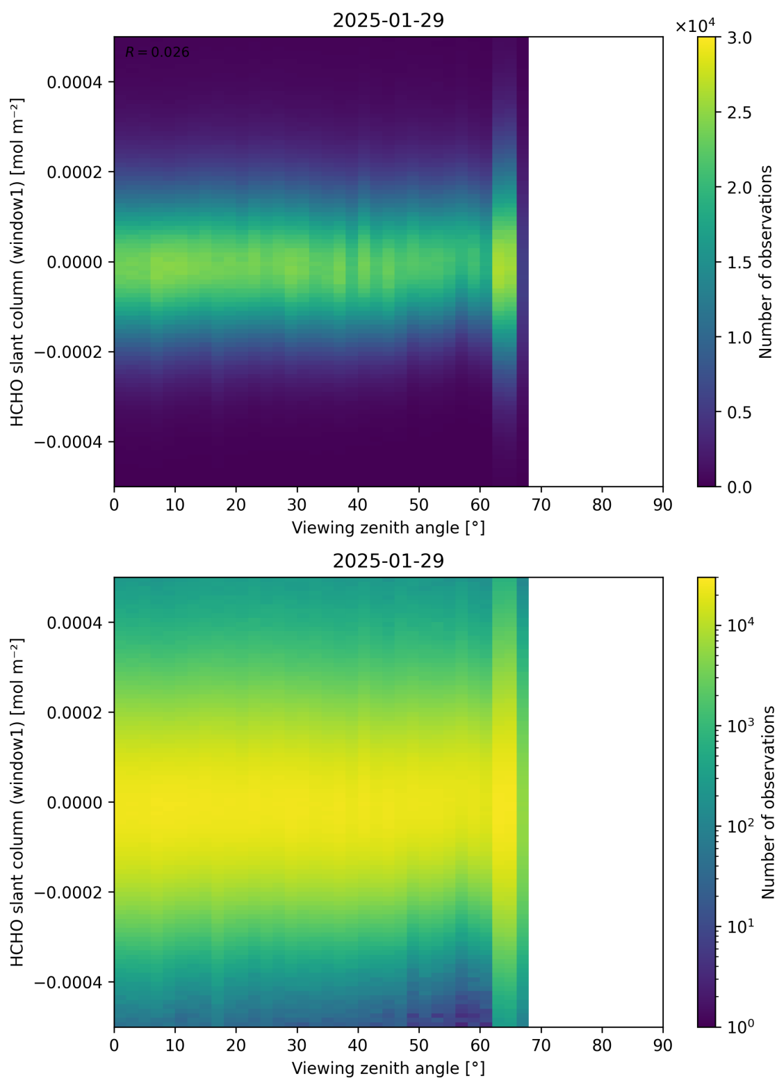
Figure 188: Scatter density plot of “Viewing zenith angle” against “HCHO slant column (window1)” for 2025-01-28 to 2025-01-30.
