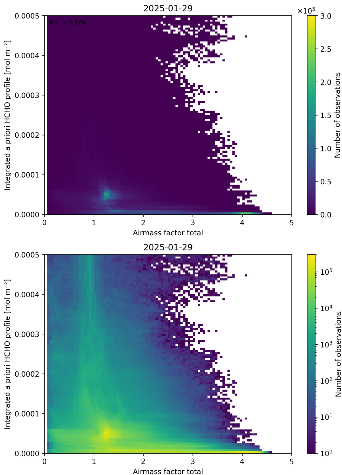
Figure 104: Scatter density plot of “Airmass factor total” against “Integrated a priori HCHO profile” for 2025-01-28 to 2025-01-30.
