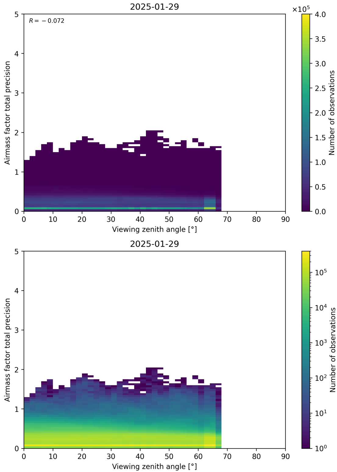
Figure 191: Scatter density plot of “Viewing zenith angle” against “Airmass factor total precision” for 2025-01-28 to 2025-01-30.
