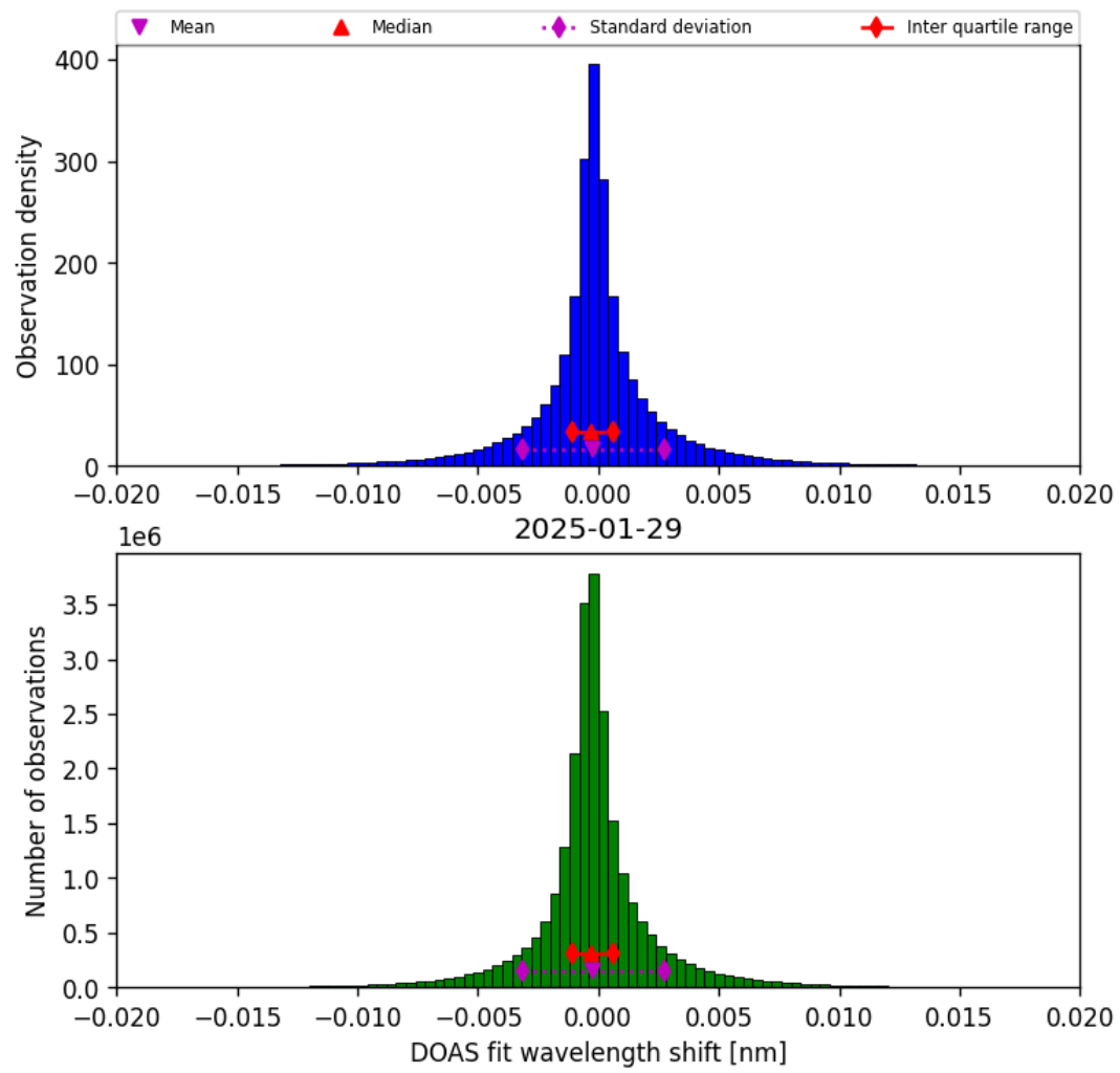
Figure 44: Histogram of “DOAS fit wavelength shift” for 2025-01-28 to 2025-01-30
