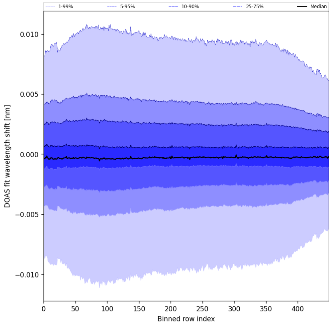
Figure 58: Along track statistics of “DOAS fit wavelength shift” for 2025-01-28 to 2025-01-30
