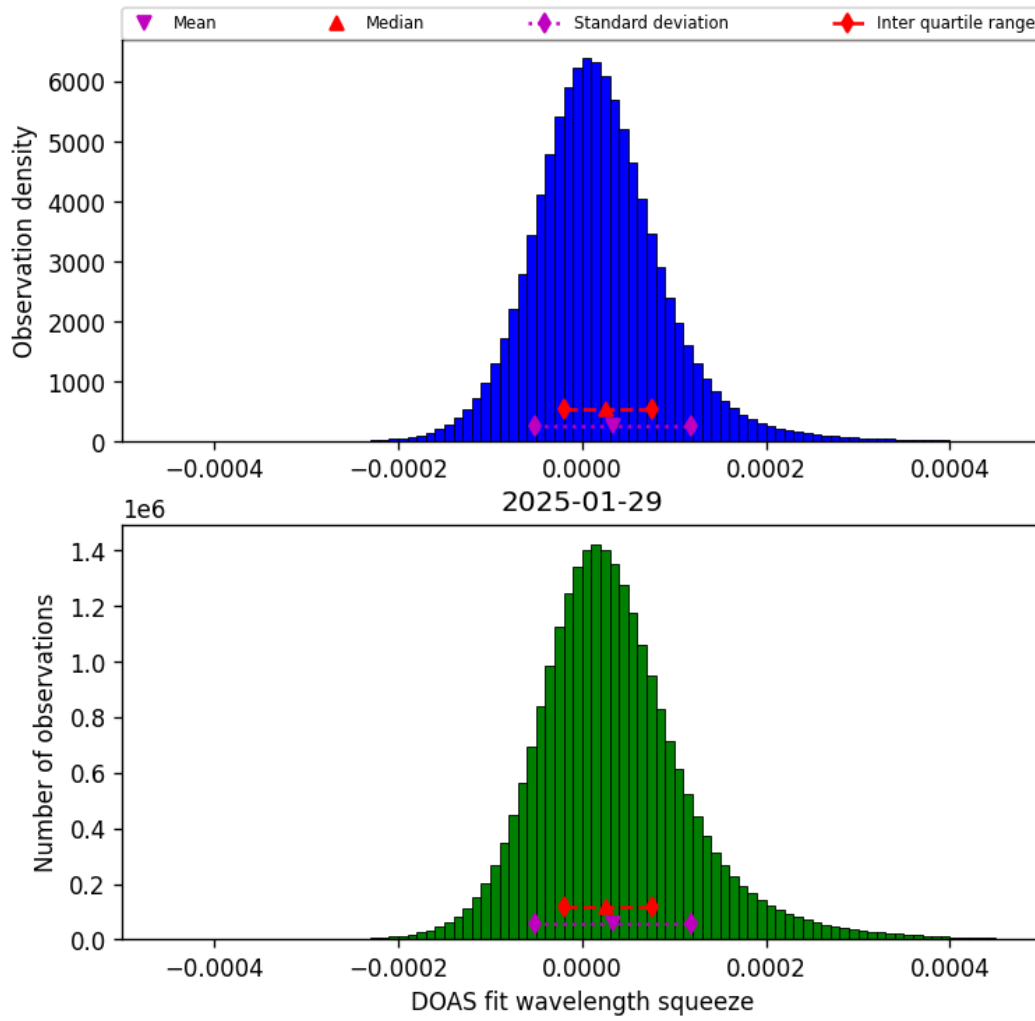
Figure 45: Histogram of “DOAS fit wavelength squeeze” for 2025-01-28 to 2025-01-30
