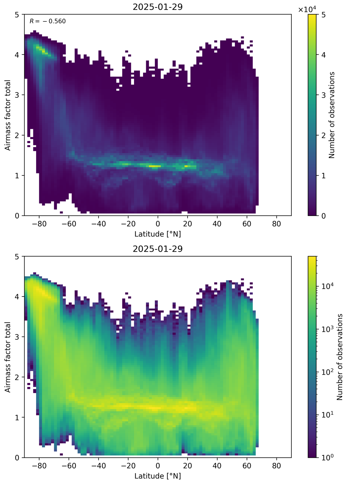
Figure 161: Scatter density plot of “Latitude” against “Airmass factor total” for 2025-01-28 to 2025-01-30.
