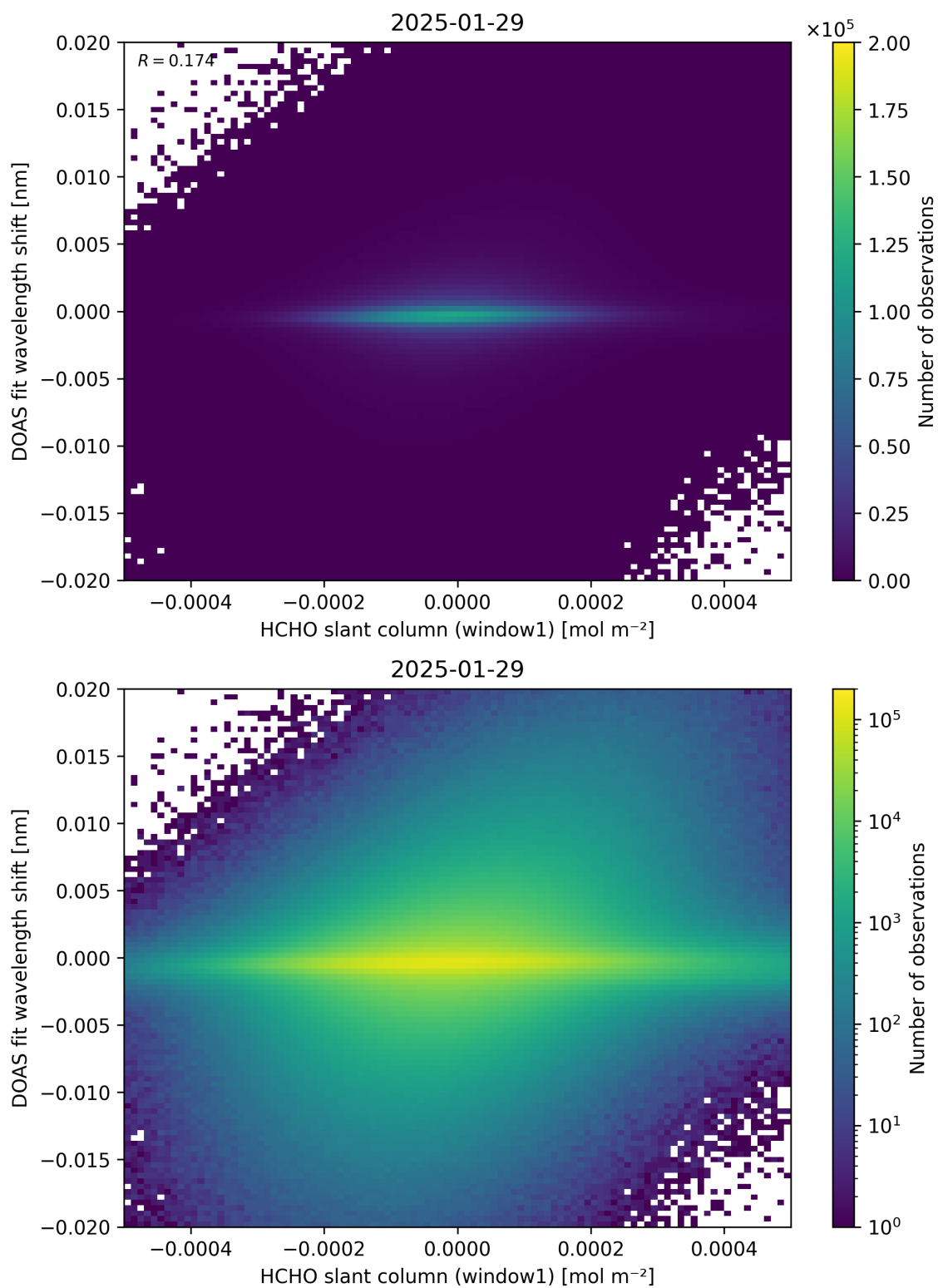
Figure 79: Scatter density plot of “HCHO slant column (window1)” against “DOAS fit wavelength shift” for 2025-01-28 to 2025-01-30.
