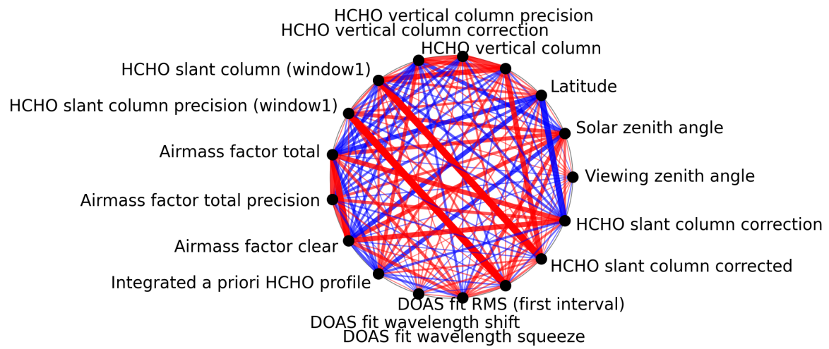
Figure 1: Map of correlation graph for 2025-01-28 to 2025-01-30.
