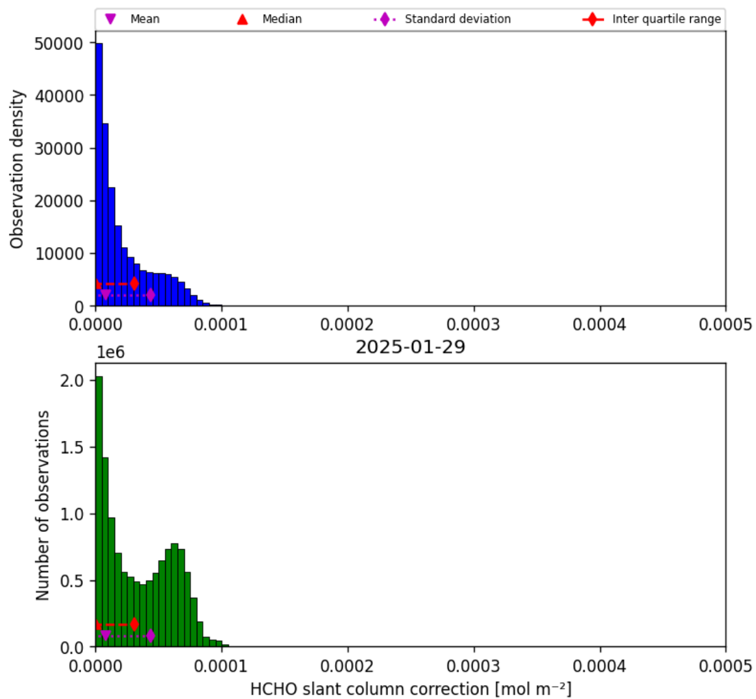
Figure 47: Histogram of “HCHO slant column correction” for 2025-01-28 to 2025-01-30
