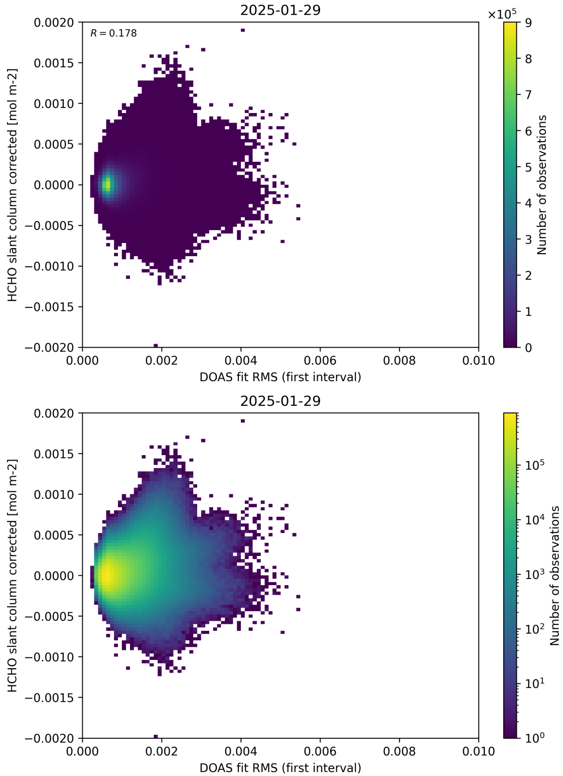
Figure 62: Scatter density plot of “DOAS fit RMS (first interval)” against “HCHO slant column corrected” for 2025-01-28 to 2025-01-30.
