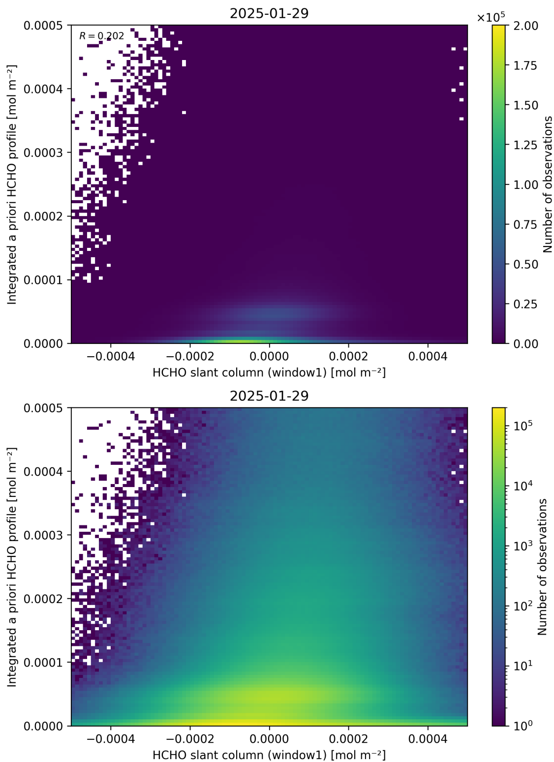
Figure 87: Scatter density plot of “HCHO slant column (window1)” against “Integrated a priori HCHO profile” for 2025-01-28 to 2025-01-30.
