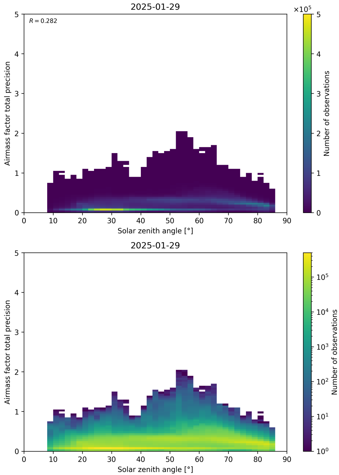
Figure 176: Scatter density plot of “Solar zenith angle” against “Airmass factor total precision” for 2025-01-28 to 2025-01-30.
