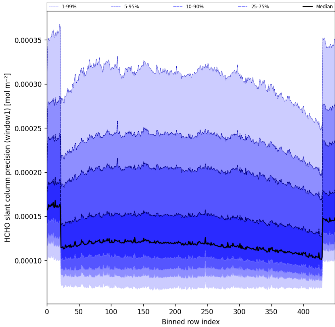
Figure 53: Along track statistics of "HCHO slant column precision (window1)" for 2025-01-30 to 2025-02-01
