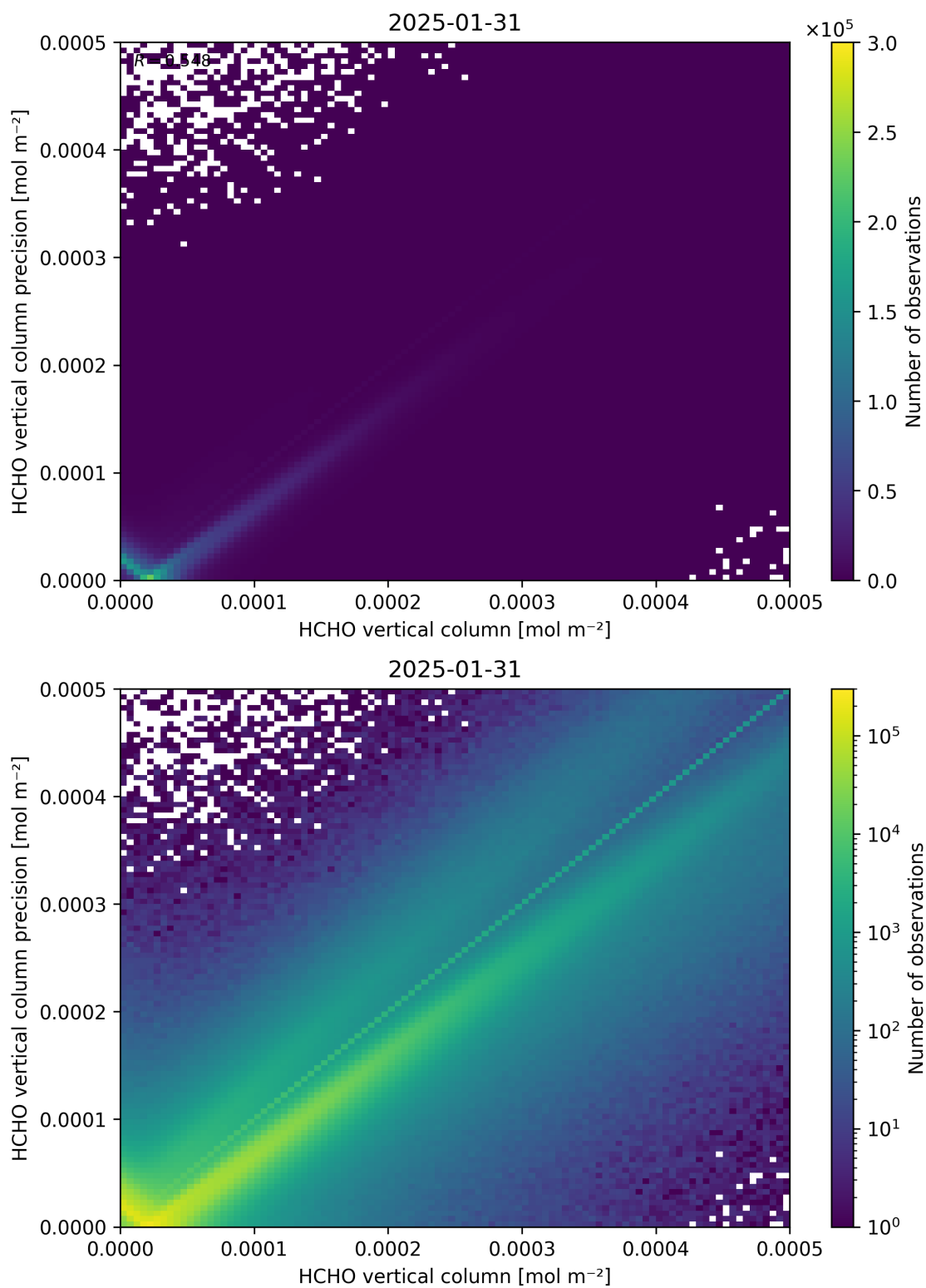
Figure 134: Scatter density plot of “HCHO vertical column” against “HCHO vertical column precision” for 2025-01-30 to 2025-02-01.
