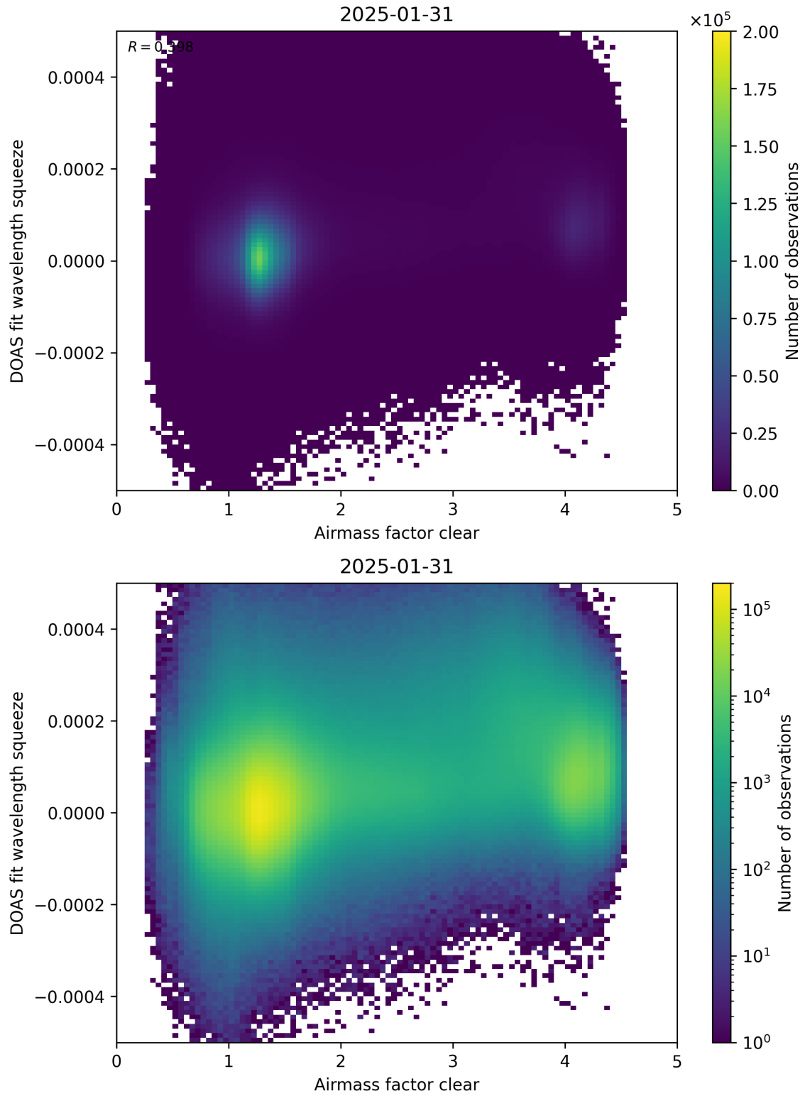
Figure 73: Scatter density plot of “Airmass factor clear” against “DOAS fit wavelength squeeze” for 2025-01-30 to 2025-02-01.
