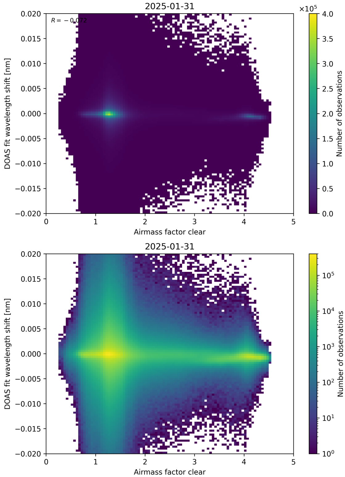
Figure 72: Scatter density plot of “Airmass factor clear” against “DOAS fit wavelength shift” for 2025-01-30 to 2025-02-01.
