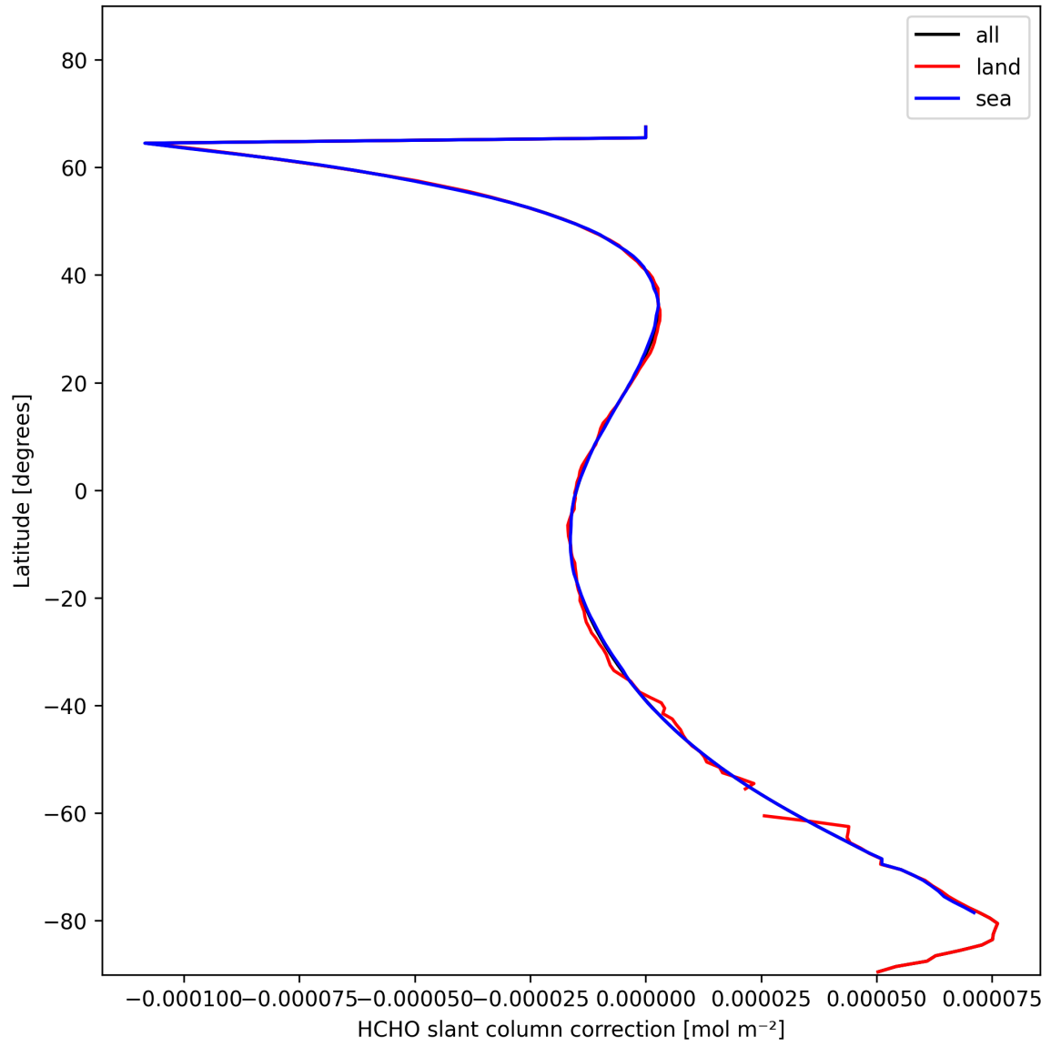
Figure 33: Zonal average of “HCHO slant column correction” for 2025-01-30 to 2025-02-01.
