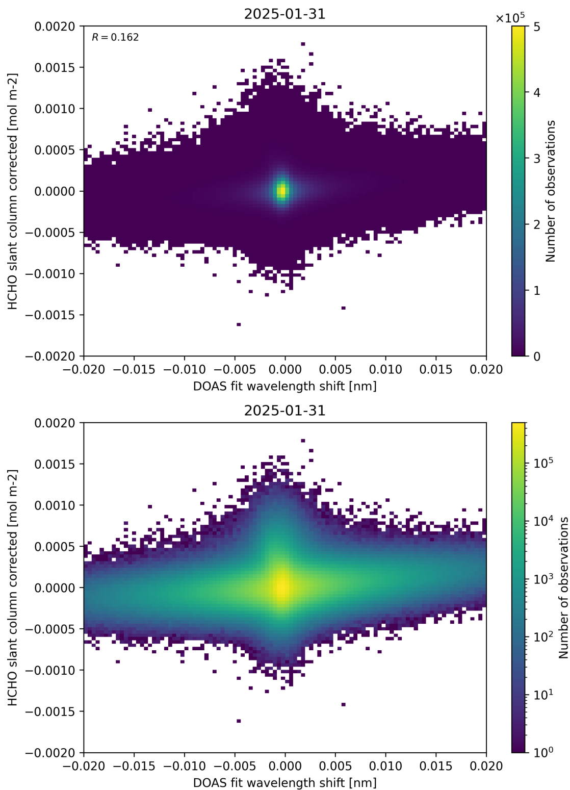
Figure 66: Scatter density plot of “DOAS fit wavelength shift” against “HCHO slant column corrected” for 2025-01-30 to 2025-02-01.
