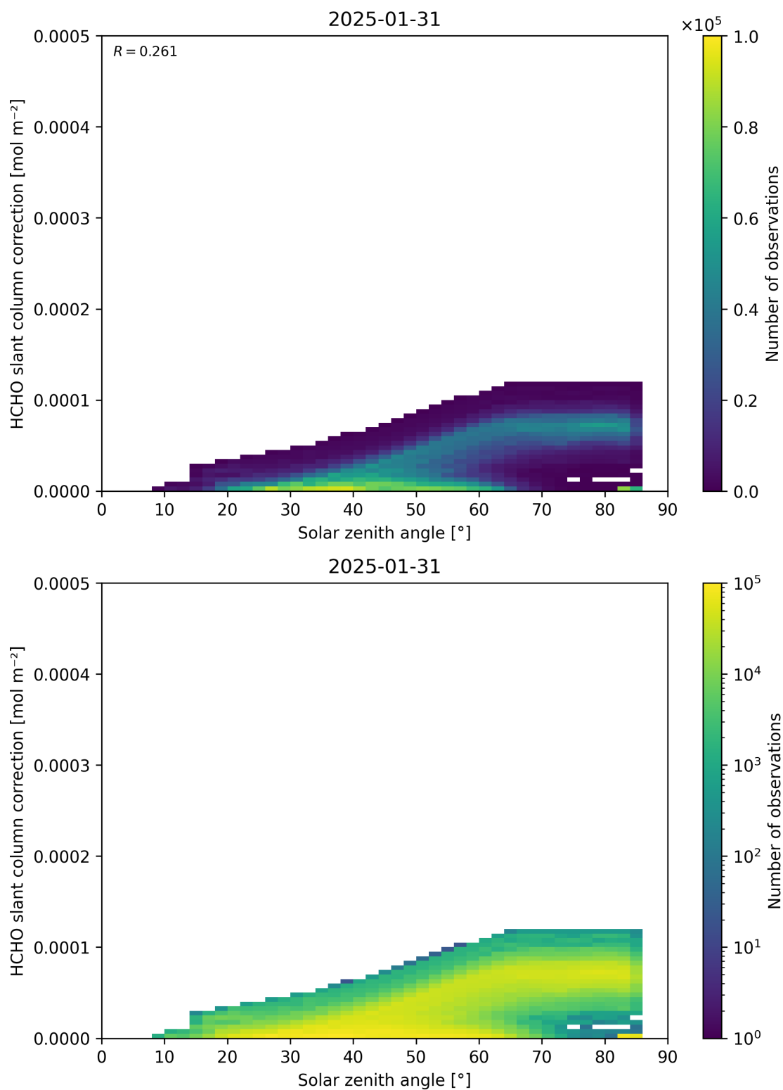
Figure 172: Scatter density plot of “Solar zenith angle” against “HCHO slant column correction” for 2025-01-30 to 2025-02-01.
