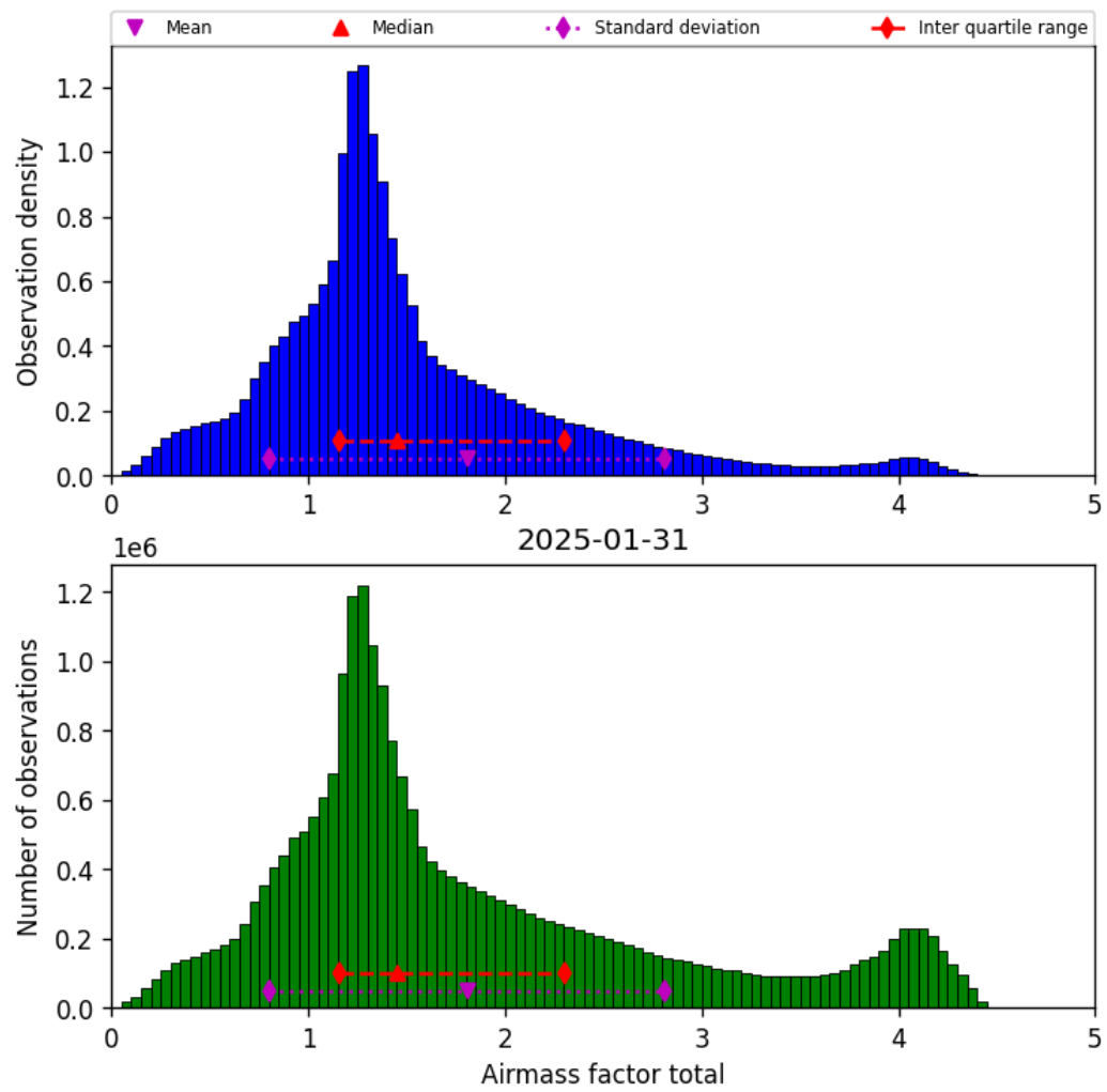
Figure 40: Histogram of “Airmass factor total” for 2025-01-30 to 2025-02-01
