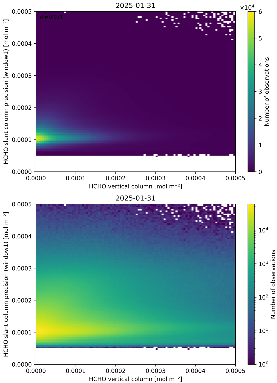
Figure 130: Scatter density plot of “HCHO vertical column” against “HCHO slant column precision (window1)” for 2025-01-30 to 2025-02-01.
