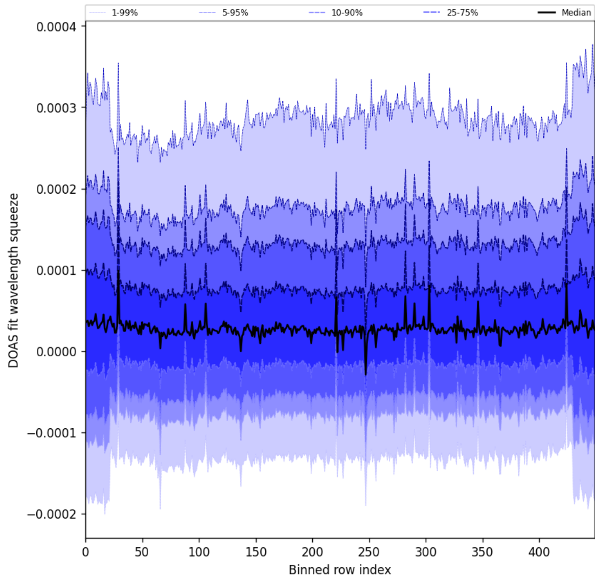
Figure 59: Along track statistics of “DOAS fit wavelength squeeze” for 2025-01-30 to 2025-02-01
