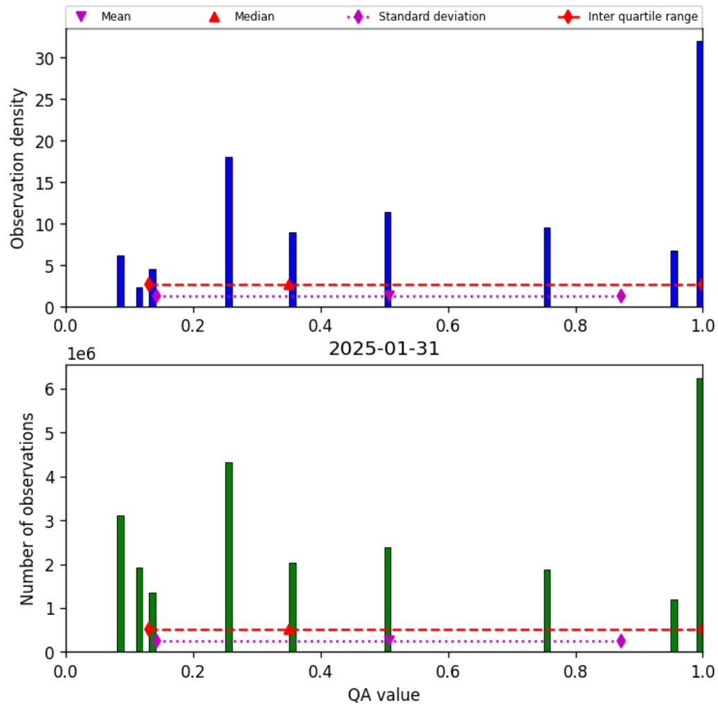
Figure 34: Histogram of “QA value” for 2025-01-30 to 2025-02-01
