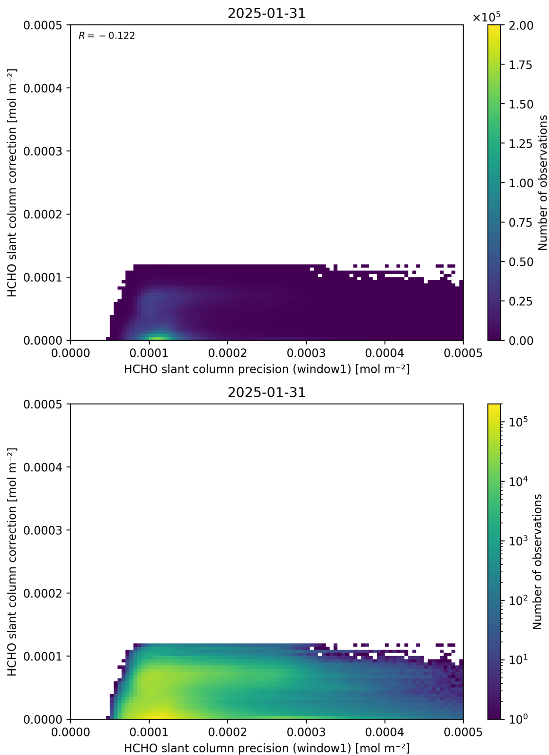
Figure 93: Scatter density plot of “HCHO slant column precision (window1)” against “HCHO slant column correction” for 2025-01-30 to 2025-02-01.
