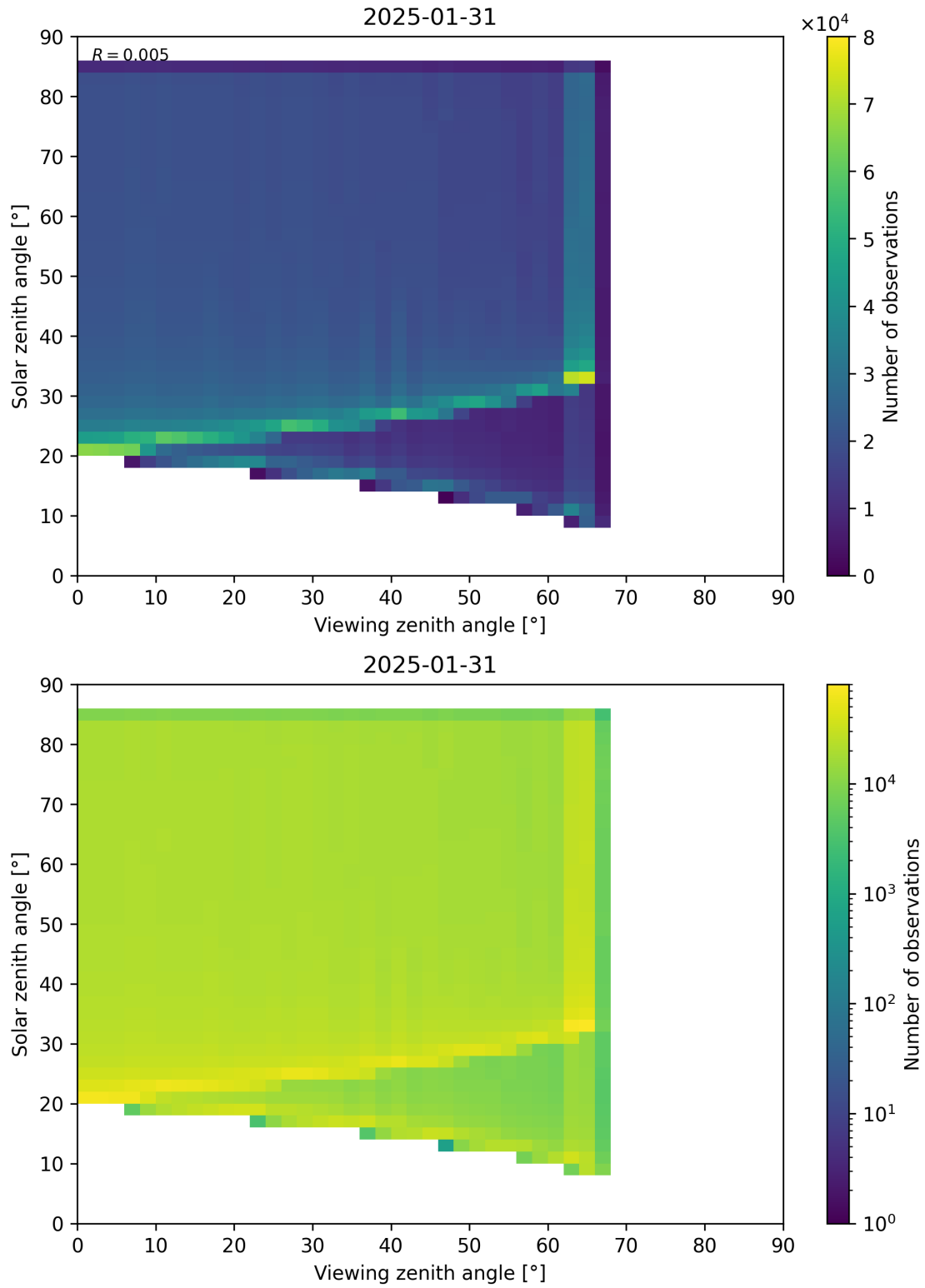
Figure 197: Scatter density plot of “Viewing zenith angle” against “Solar zenith angle” for 2025-01-30 to 2025-02-01.
