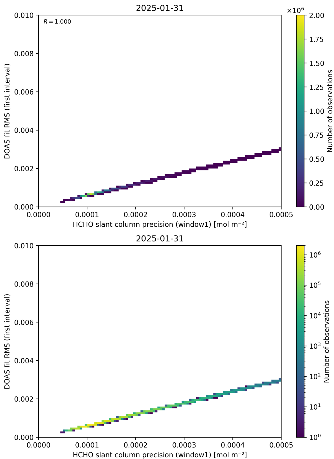
Figure 88: Scatter density plot of “HCHO slant column precision (window1)” against “DOAS fit RMS (first interval)” for 2025-01-30 to 2025-02-01.
