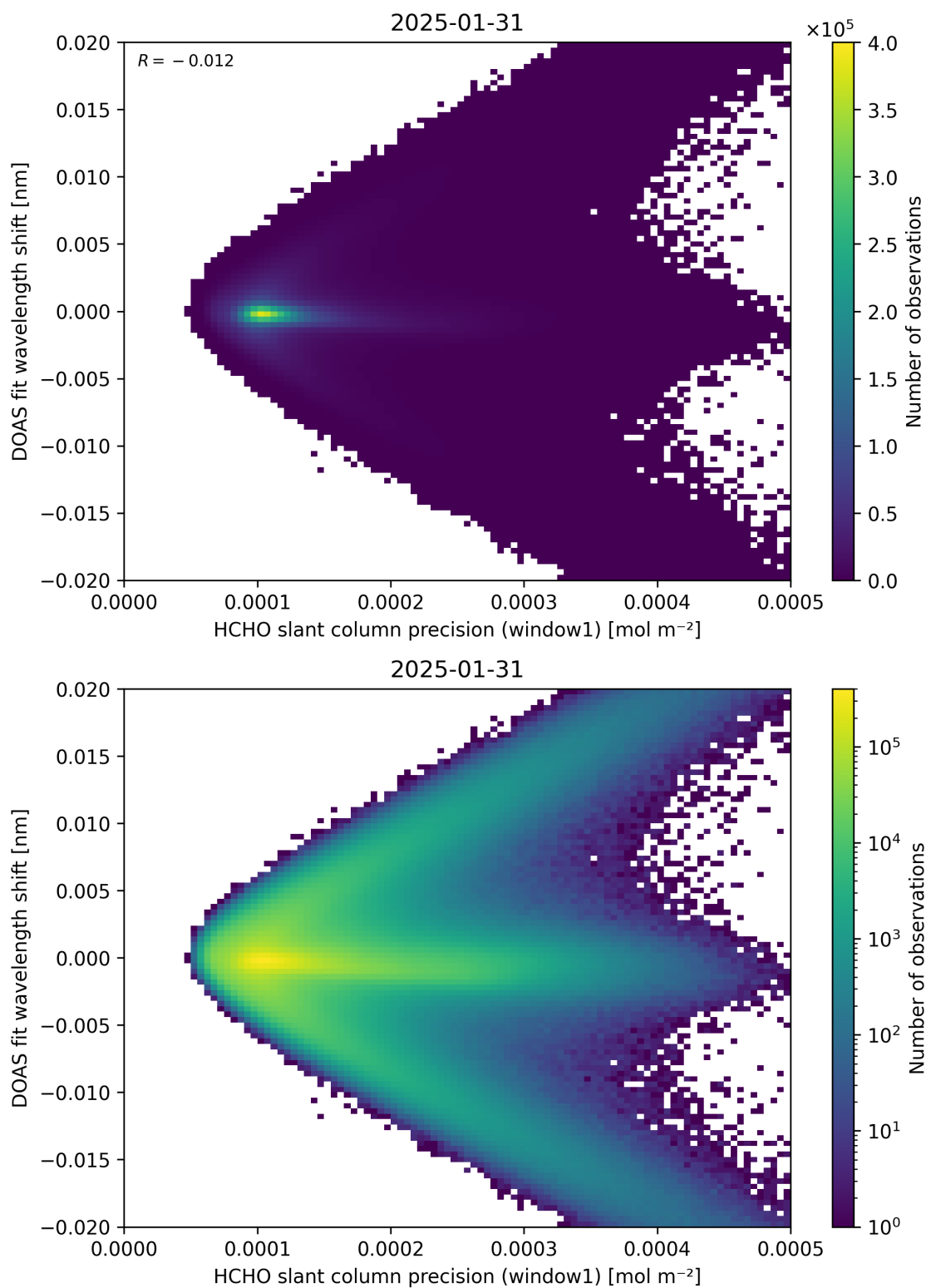
Figure 89: Scatter density plot of “HCHO slant column precision (window1)” against “DOAS fit wavelength shift” for 2025-01-30 to 2025-02-01.
