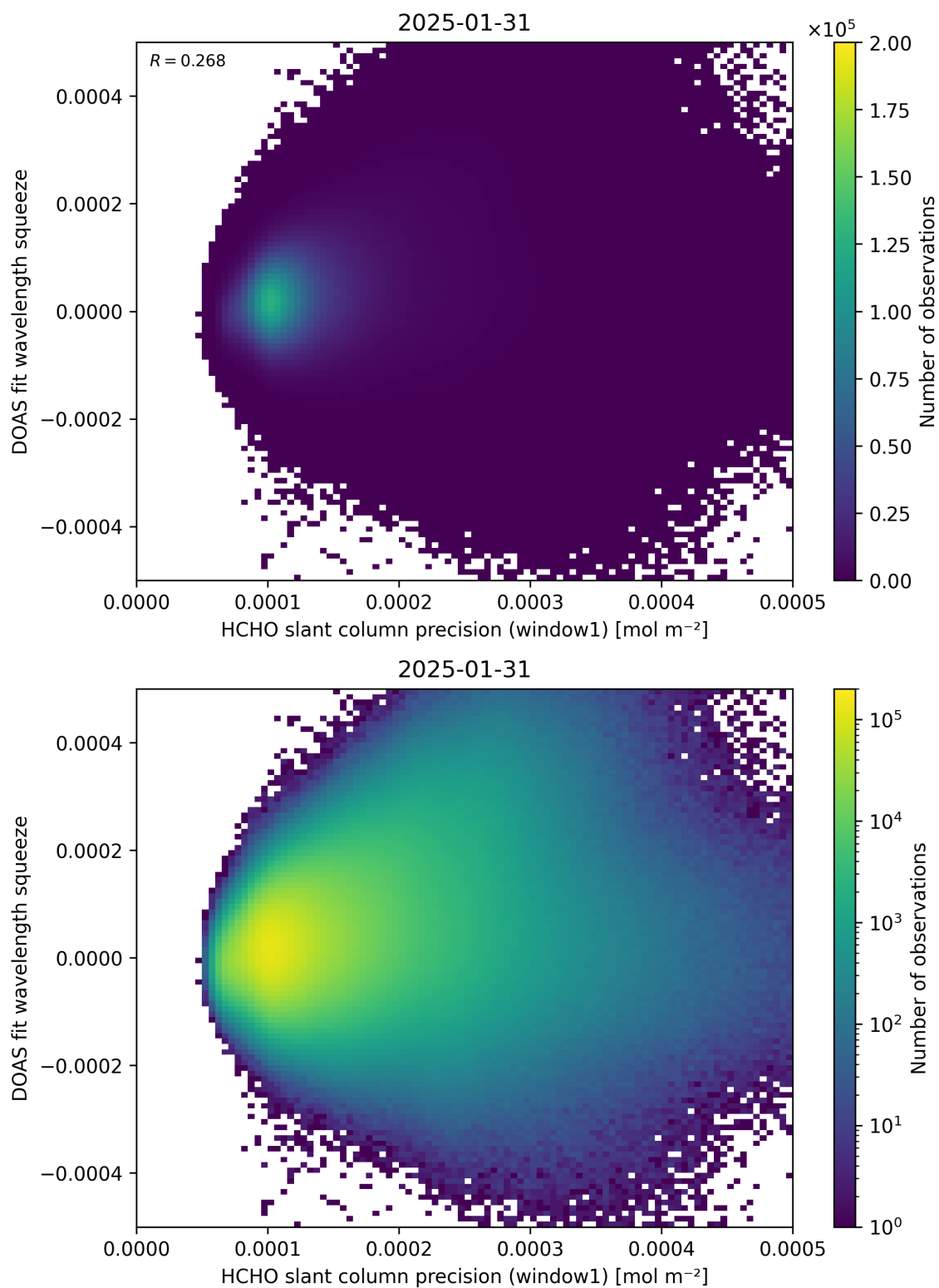
Figure 90: Scatter density plot of “HCHO slant column precision (window1)” against “DOAS fit wavelength squeeze” for 2025-01-30 to 2025-02-01.
