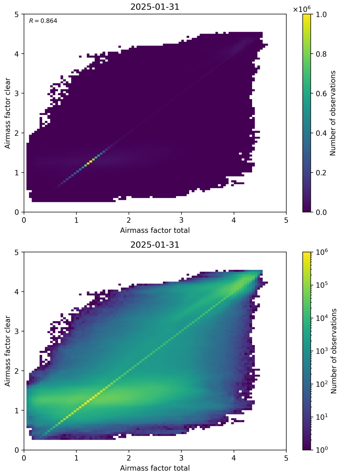
Figure 100: Scatter density plot of “Airmass factor total” against “Airmass factor clear” for 2025-01-30 to 2025-02-01.
