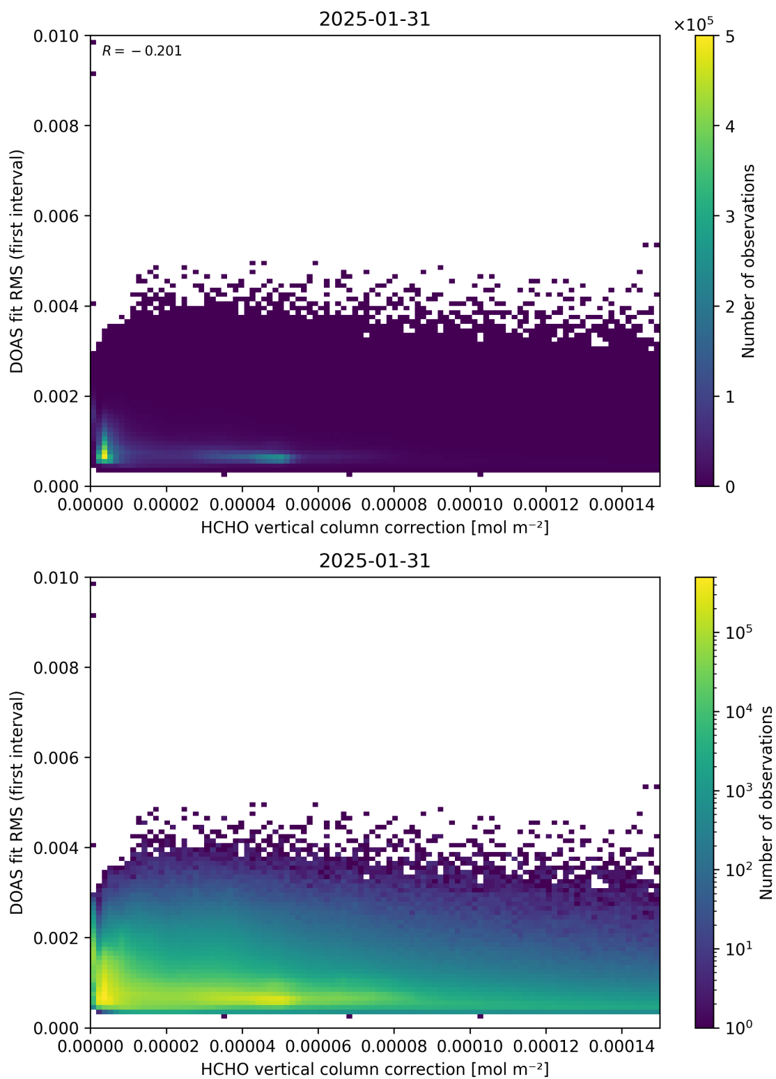
Figure 112: Scatter density plot of “HCHO vertical column correction” against “DOAS fit RMS (first interval)” for 2025-01-30 to 2025-02-01.
