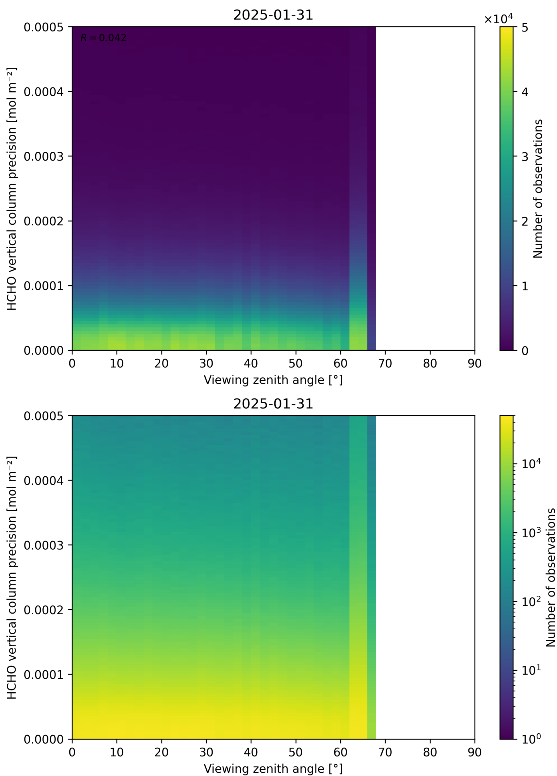
Figure 194: Scatter density plot of “Viewing zenith angle” against “HCHO vertical column precision” for 2025-01-30 to 2025-02-01.
