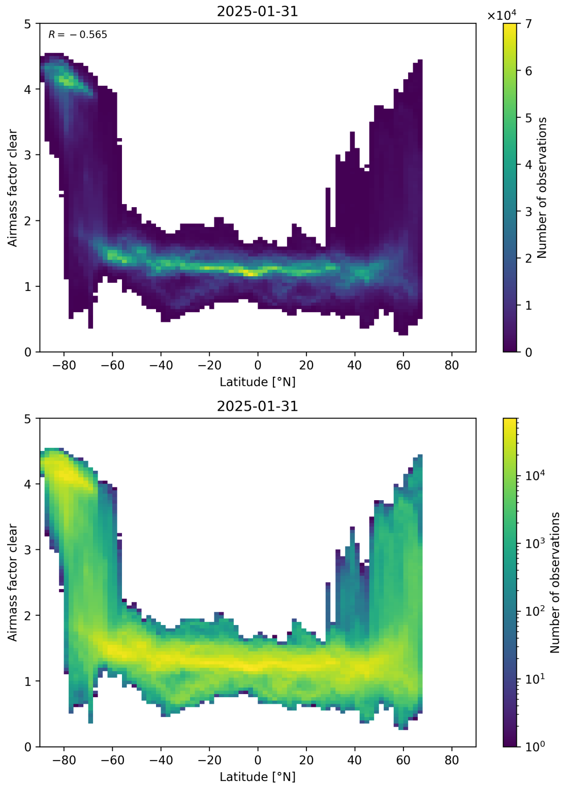
Figure 156: Scatter density plot of “Latitude” against “Airmass factor clear” for 2025-01-30 to 2025-02-01.
