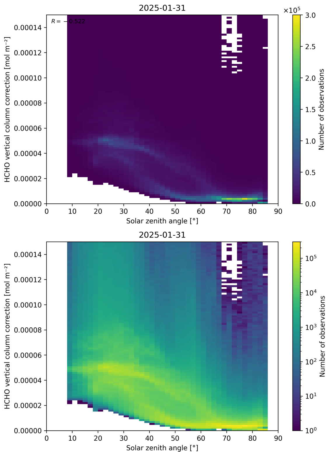
Figure 178: Scatter density plot of “Solar zenith angle” against “HCHO vertical column correction” for 2025-01-30 to 2025-02-01.
