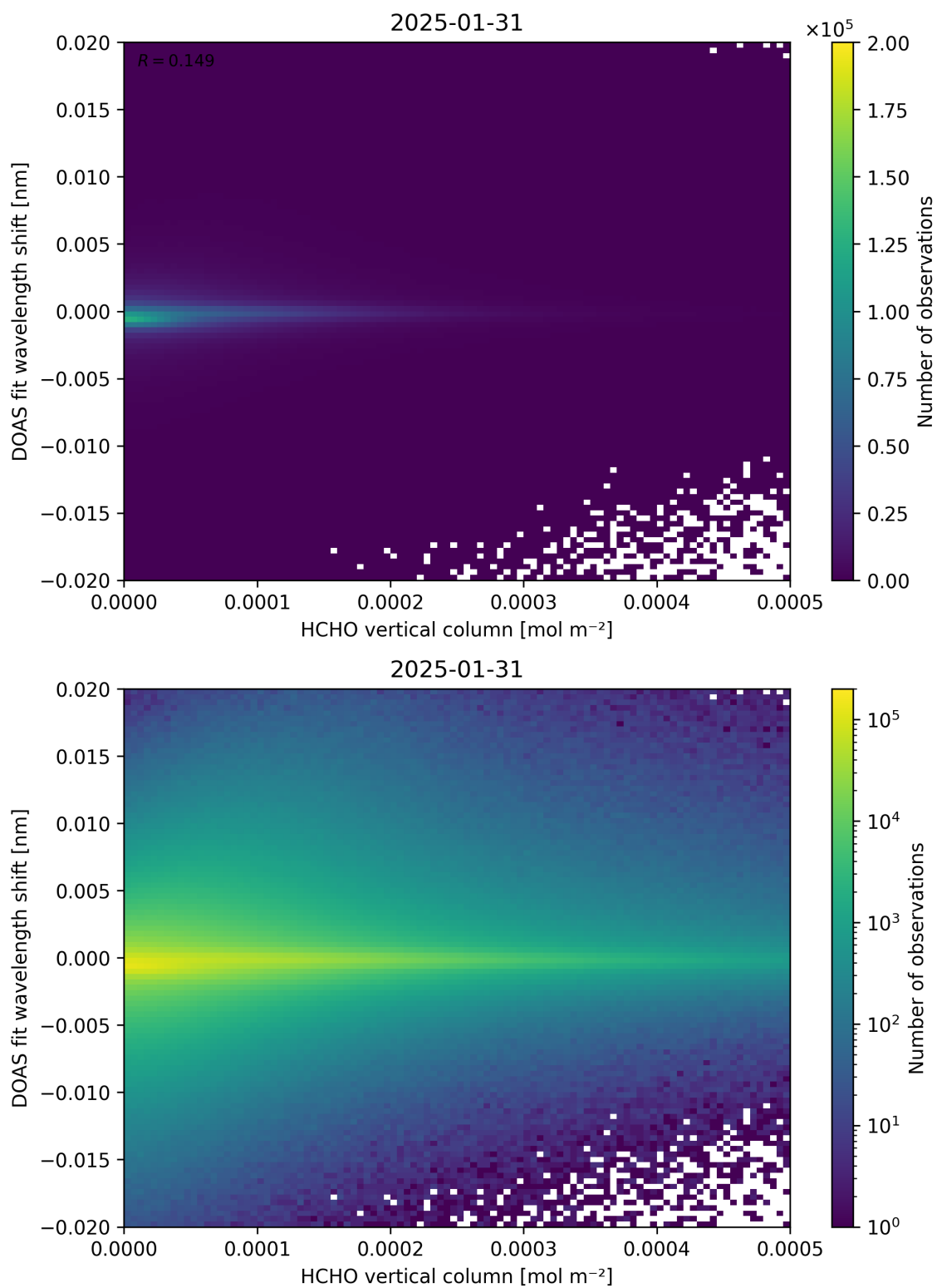
Figure 124: Scatter density plot of “HCHO vertical column” against “DOAS fit wavelength shift” for 2025-01-30 to 2025-02-01.
