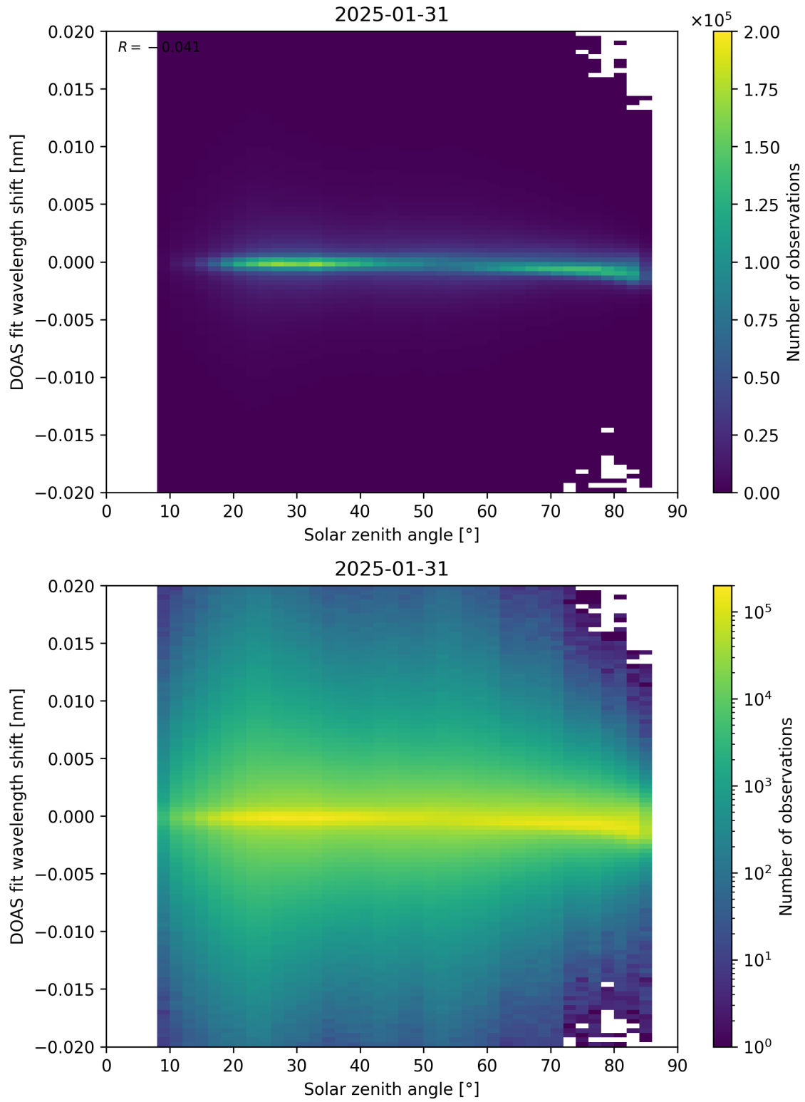
Figure 168: Scatter density plot of “Solar zenith angle” against “DOAS fit wavelength shift” for 2025-01-30 to 2025-02-01.
