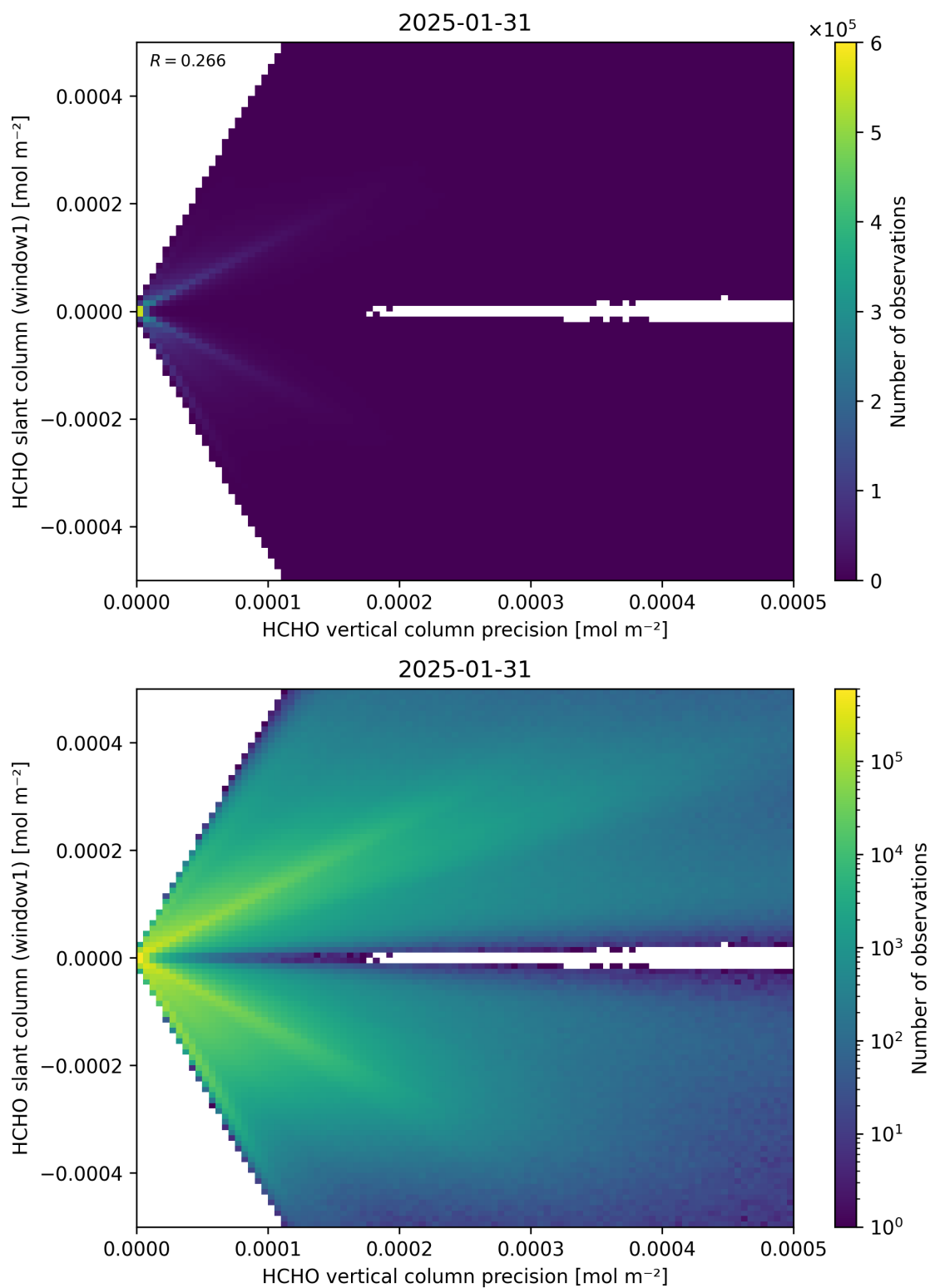
Figure 142: Scatter density plot of “HCHO vertical column precision” against “HCHO slant column (window1)” for 2025-01-30 to 2025-02-01.
