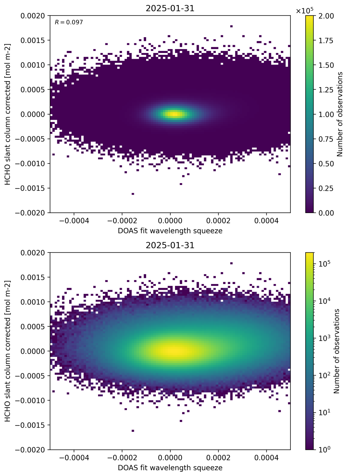
Figure 69: Scatter density plot of “DOAS fit wavelength squeeze” against “HCHO slant column corrected” for 2025-01-30 to 2025-02-01.
