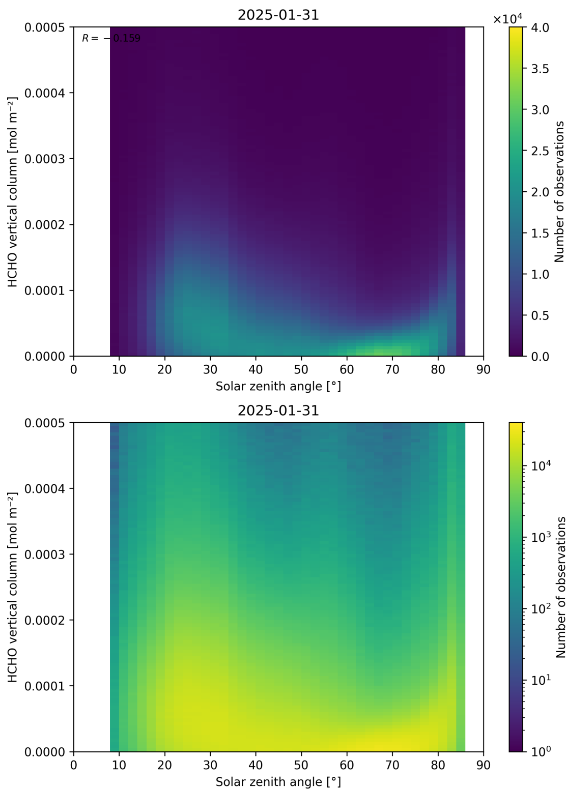
Figure 177: Scatter density plot of “Solar zenith angle” against “HCHO vertical column” for 2025-01-30 to 2025-02-01.
