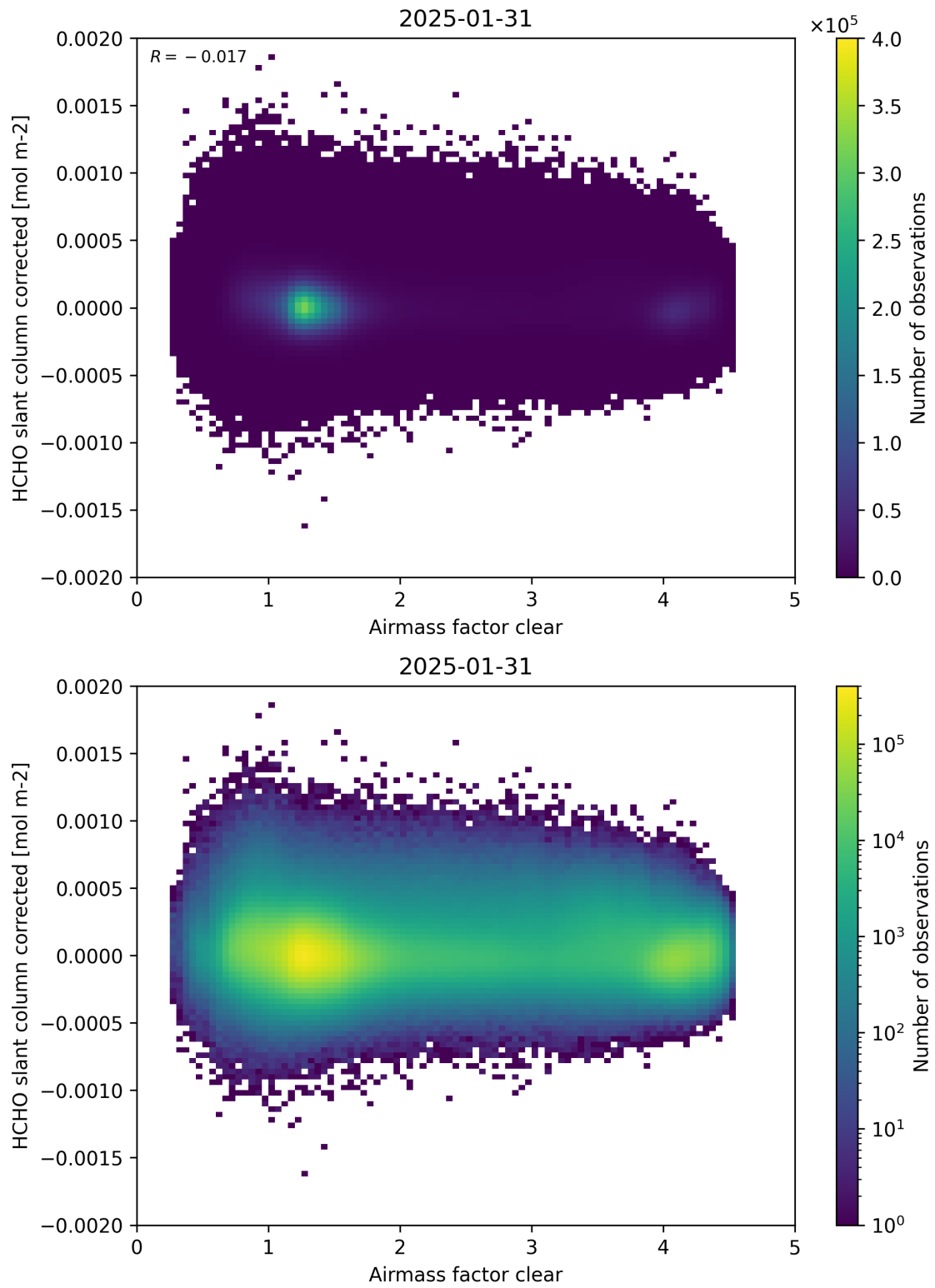
Figure 74: Scatter density plot of “Airmass factor clear” against “HCHO slant column corrected” for 2025-01-30 to 2025-02-01.
