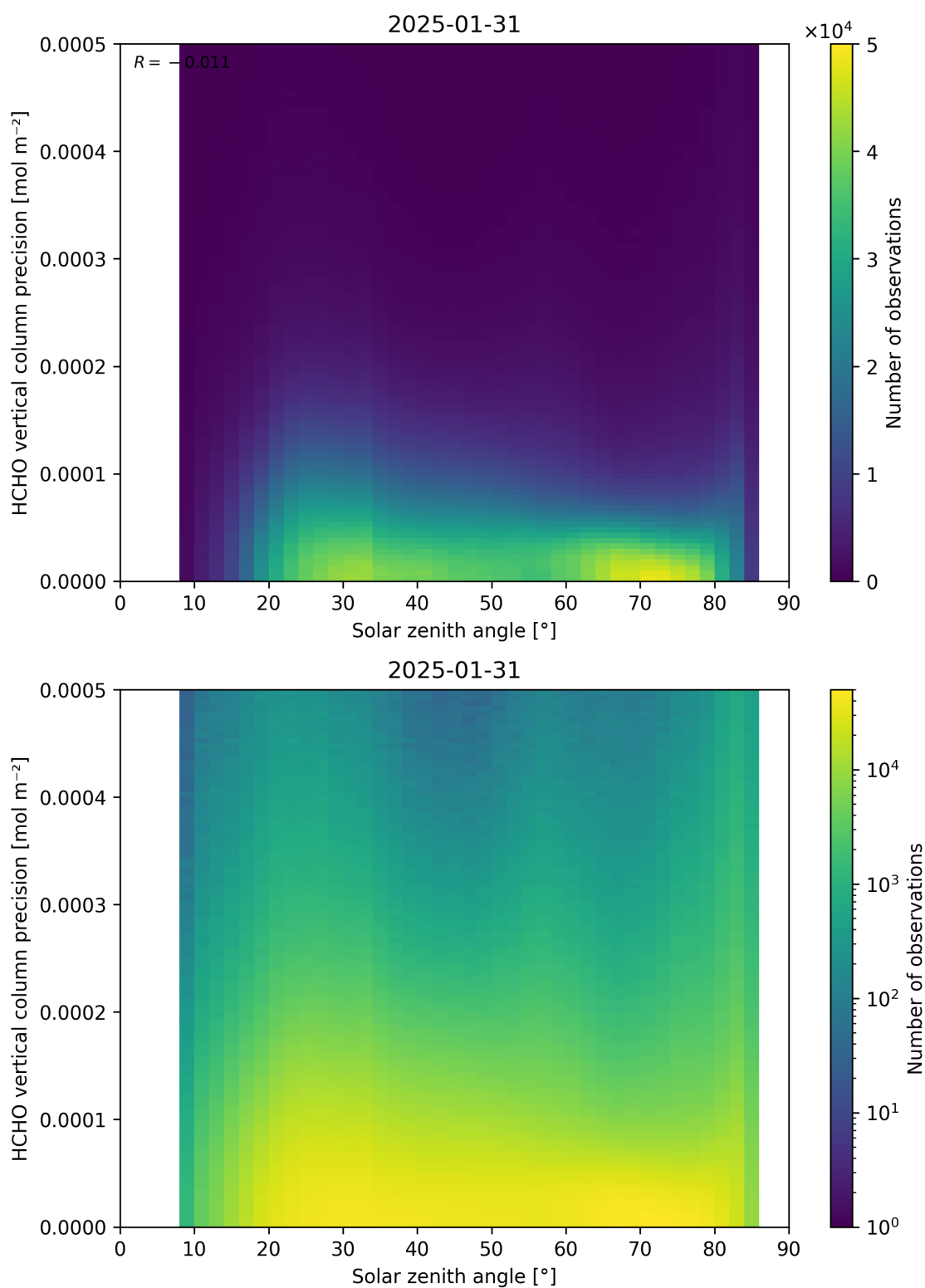
Figure 179: Scatter density plot of “Solar zenith angle” against “HCHO vertical column precision” for 2025-01-30 to 2025-02-01.
