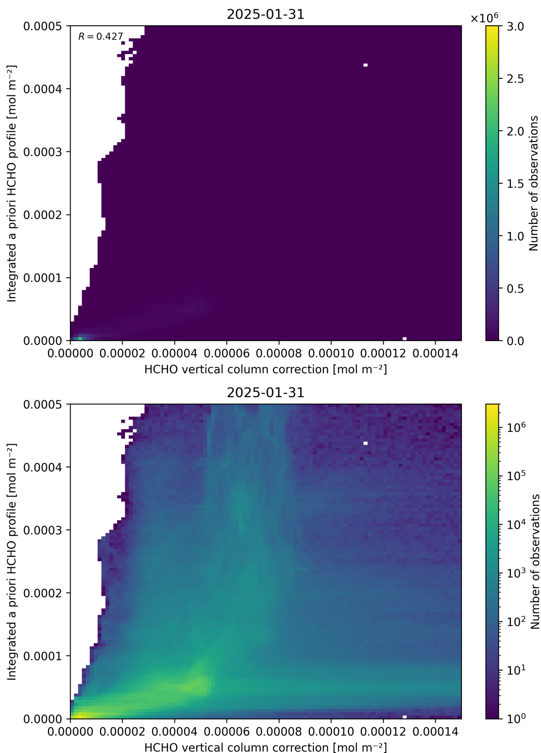
Figure 122: Scatter density plot of “HCHO vertical column correction” against “Integrated a priori HCHO profile” for 2025-01-30 to 2025-02-01.
