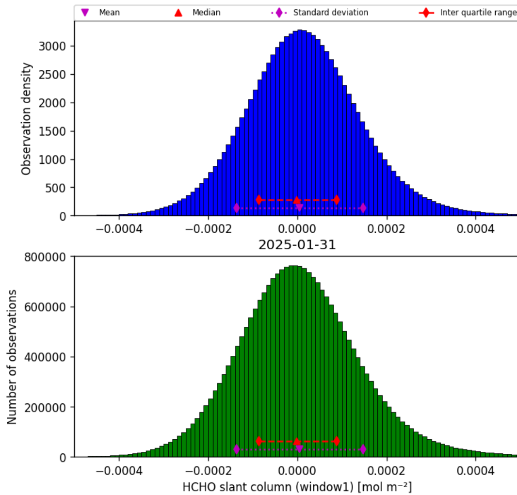
Figure 38: Histogram of “HCHO slant column (window1)” for 2025-01-30 to 2025-02-01
