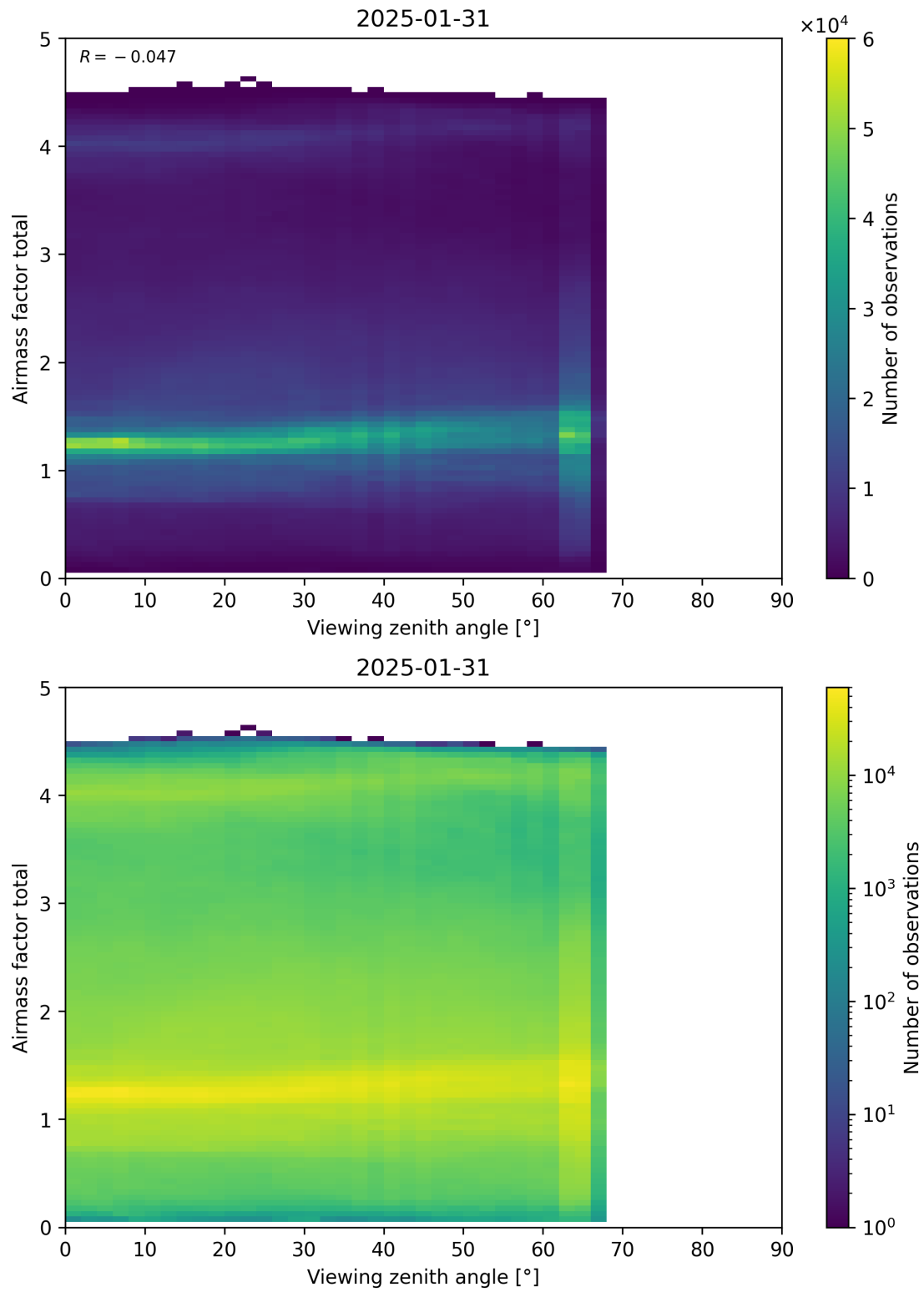
Figure 190: Scatter density plot of “Viewing zenith angle” against “Airmass factor total” for 2025-01-30 to 2025-02-01.
