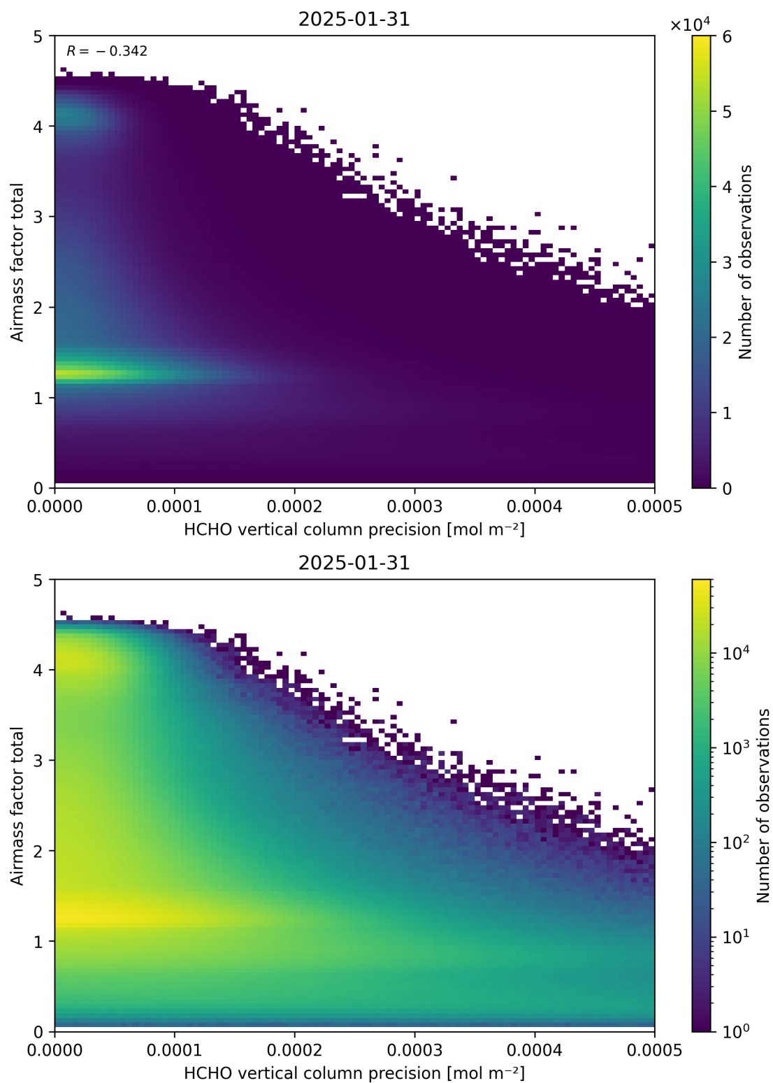
Figure 144: Scatter density plot of “HCHO vertical column precision” against “Airmass factor total” for 2025-01-30 to 2025-02-01.
