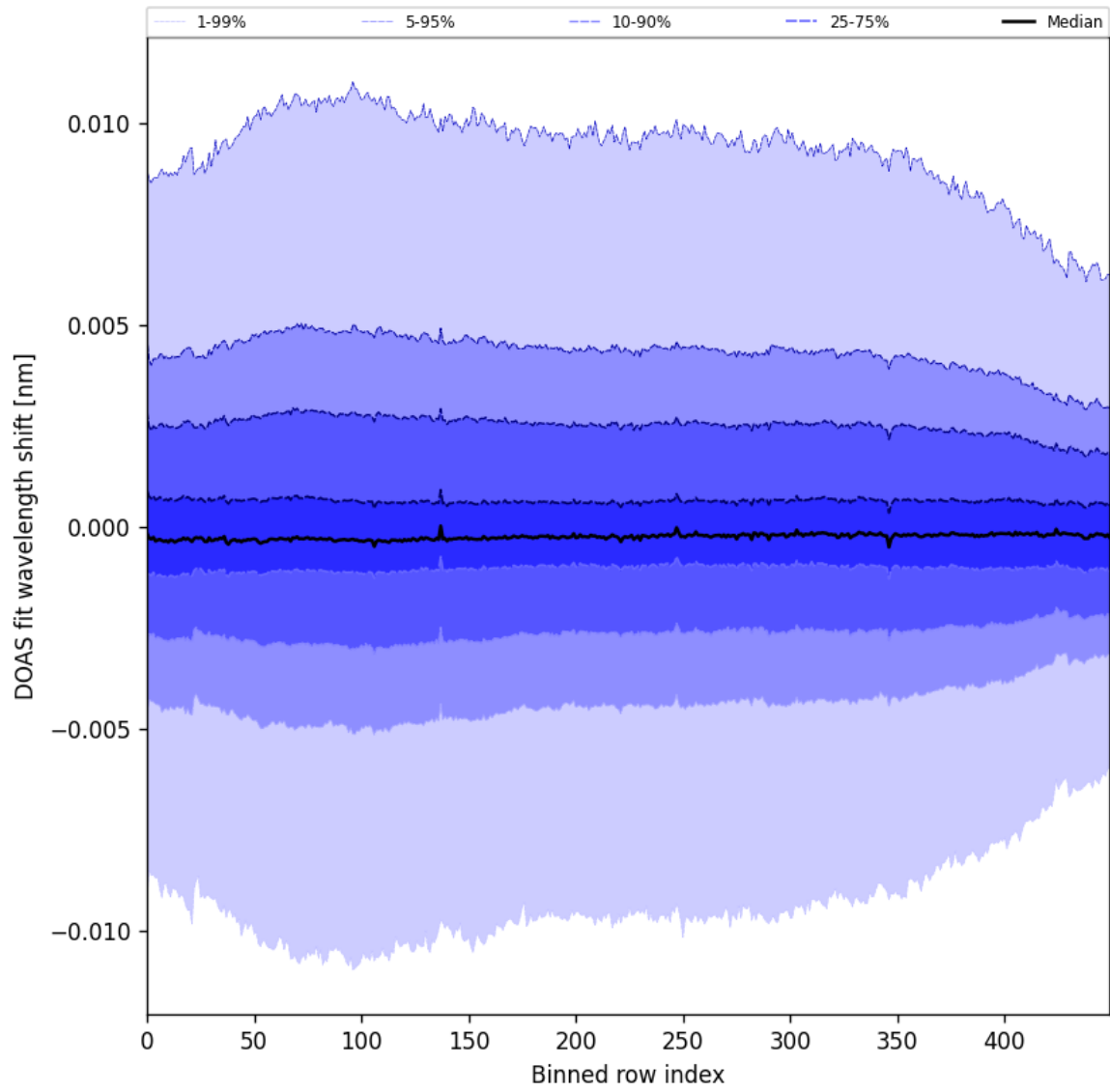
Figure 58: Along track statistics of “DOAS fit wavelength shift” for 2025-01-30 to 2025-02-01
