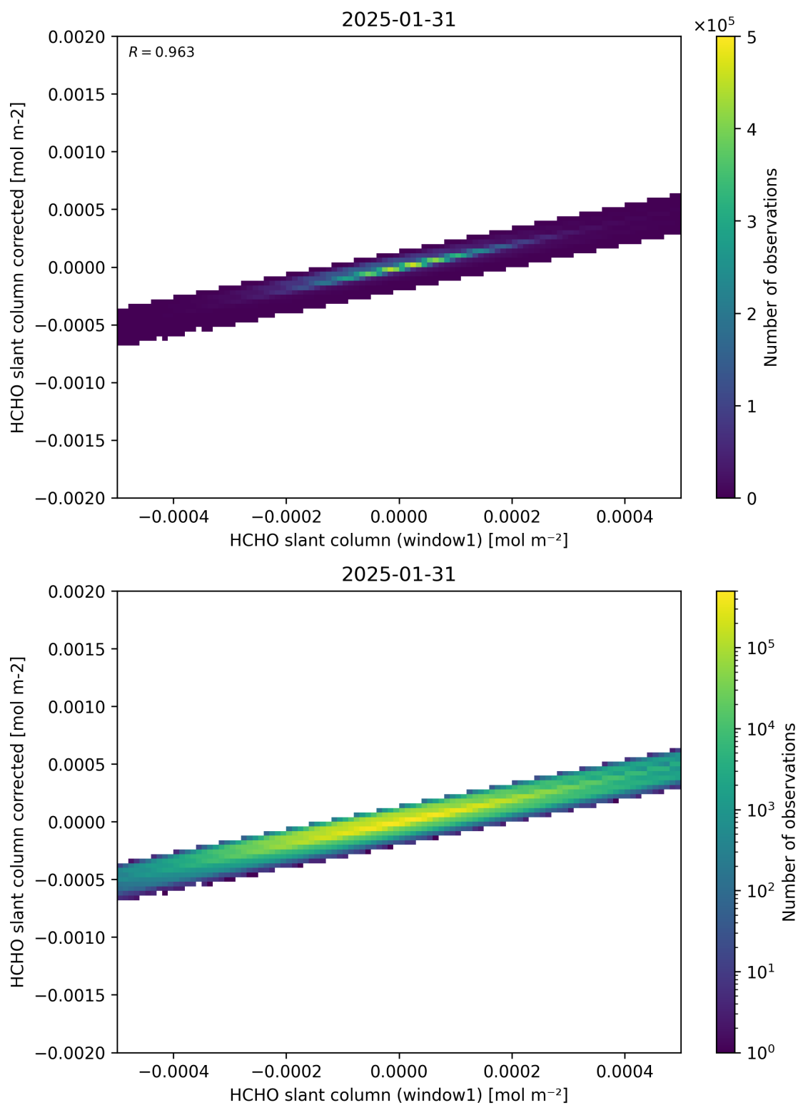
Figure 82: Scatter density plot of “HCHO slant column (window1)” against “HCHO slant column corrected” for 2025-01-30 to 2025-02-01.
