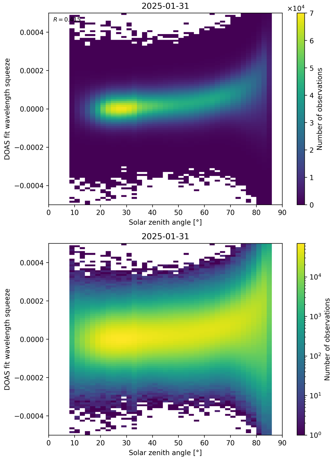
Figure 169: Scatter density plot of “Solar zenith angle” against “DOAS fit wavelength squeeze” for 2025-01-30 to 2025-02-01.
