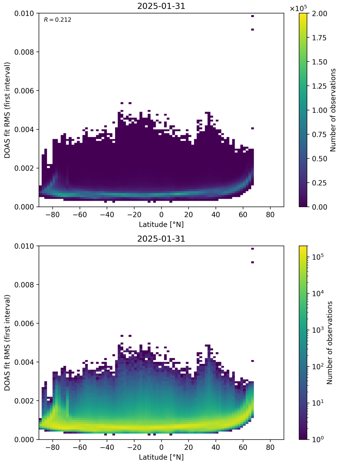
Figure 153: Scatter density plot of “Latitude” against “DOAS fit RMS (first interval)” for 2025-01-30 to 2025-02-01.
