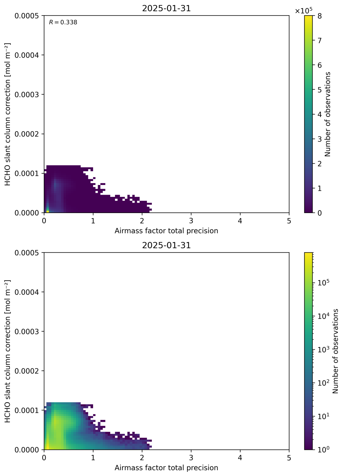
Figure 110: Scatter density plot of “Airmass factor total precision” against “HCHO slant column correction” for 2025-01-30 to 2025-02-01.
