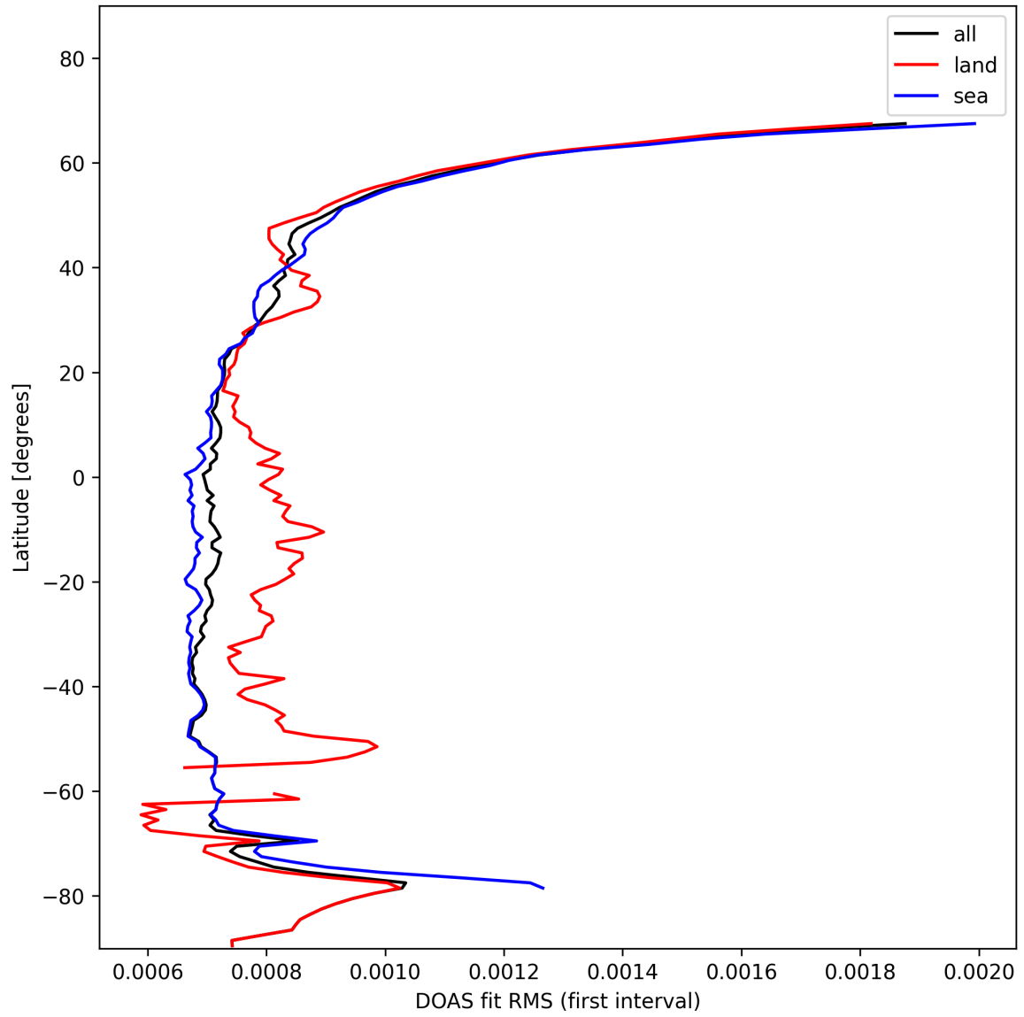
Figure 32: Zonal average of "DOAS fit RMS (first interval)" for 2025-01-30 to 2025-02-01.
