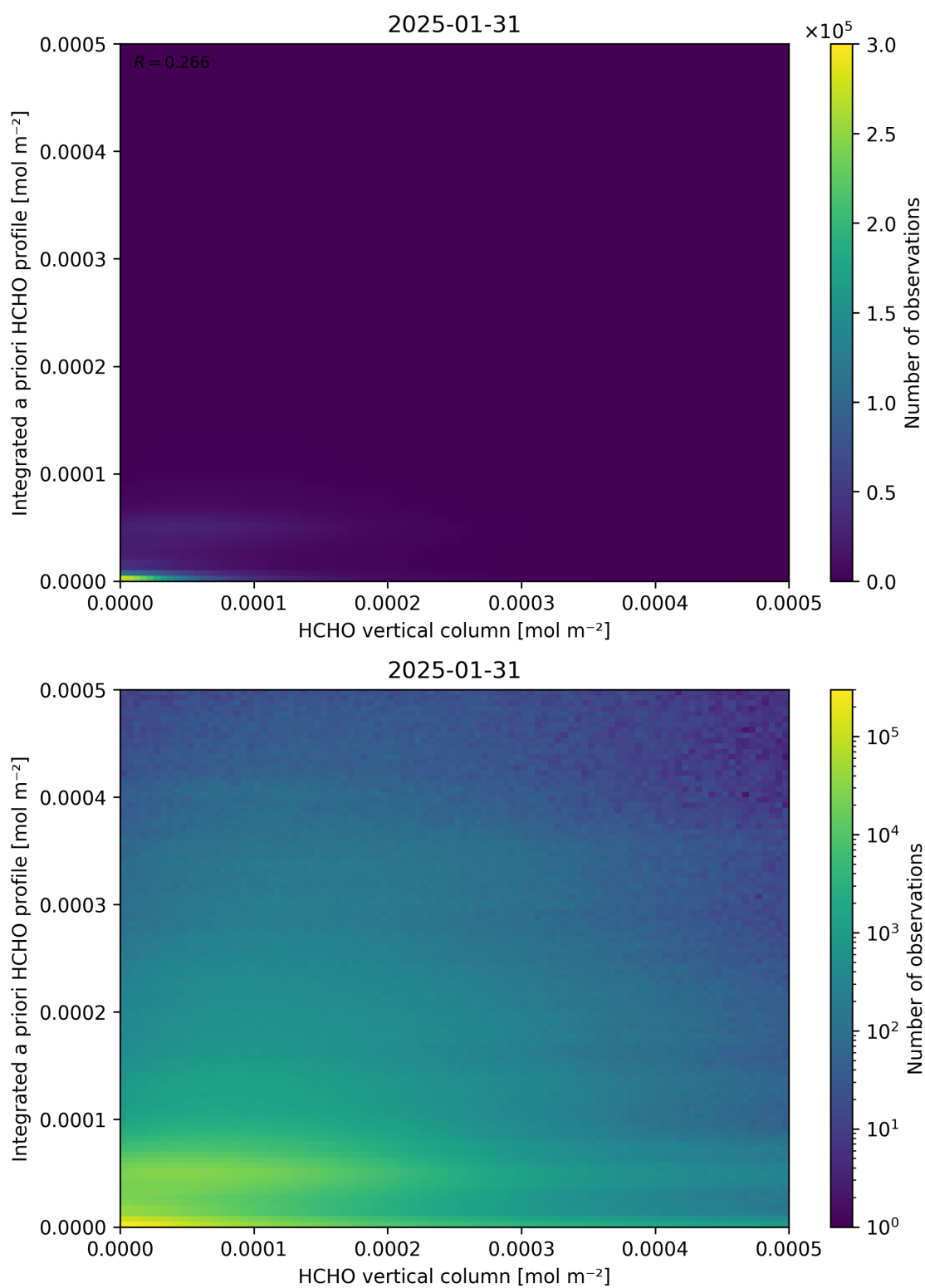
Figure 135: Scatter density plot of “HCHO vertical column” against “Integrated a priori HCHO profile” for 2025-01-30 to 2025-02-01.
