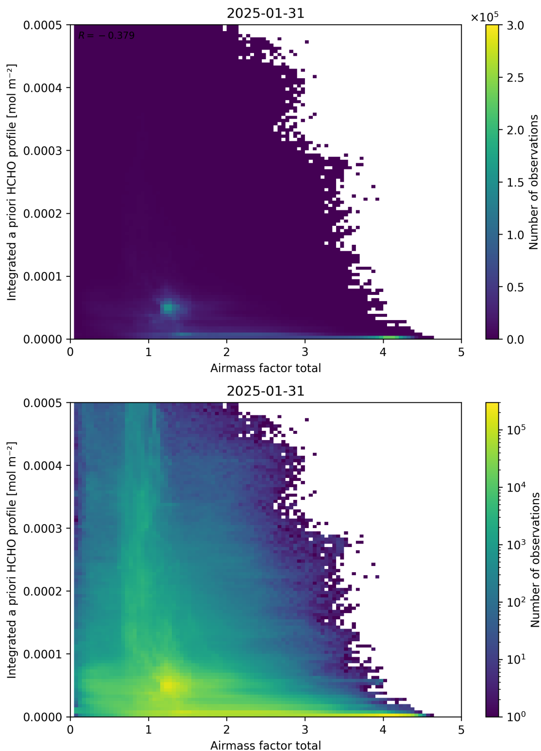
Figure 104: Scatter density plot of “Airmass factor total” against “Integrated a priori HCHO profile” for 2025-01-30 to 2025-02-01.
