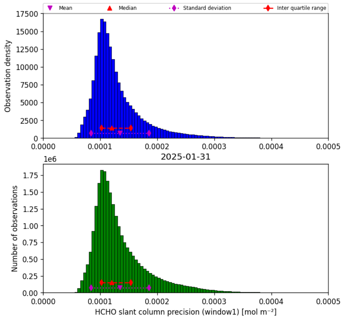
Figure 39: Histogram of “HCHO slant column precision (window1)” for 2025-01-30 to 2025-02-01
