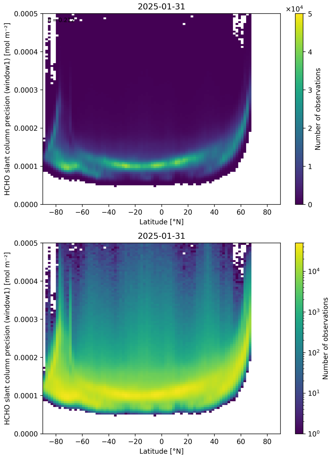
Figure 160: Scatter density plot of “Latitude” against “HCHO slant column precision (window1)” for 2025-01-30 to 2025-02-01.
