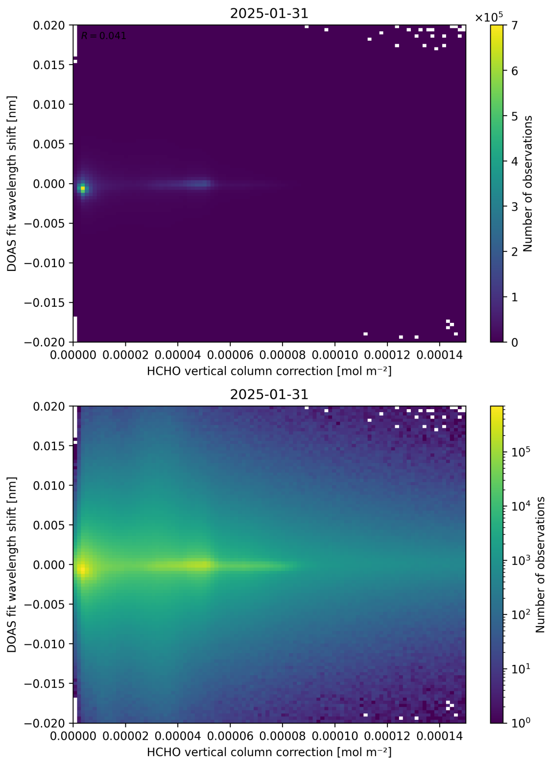
Figure 113: Scatter density plot of “HCHO vertical column correction” against “DOAS fit wavelength shift” for 2025-01-30 to 2025-02-01.
