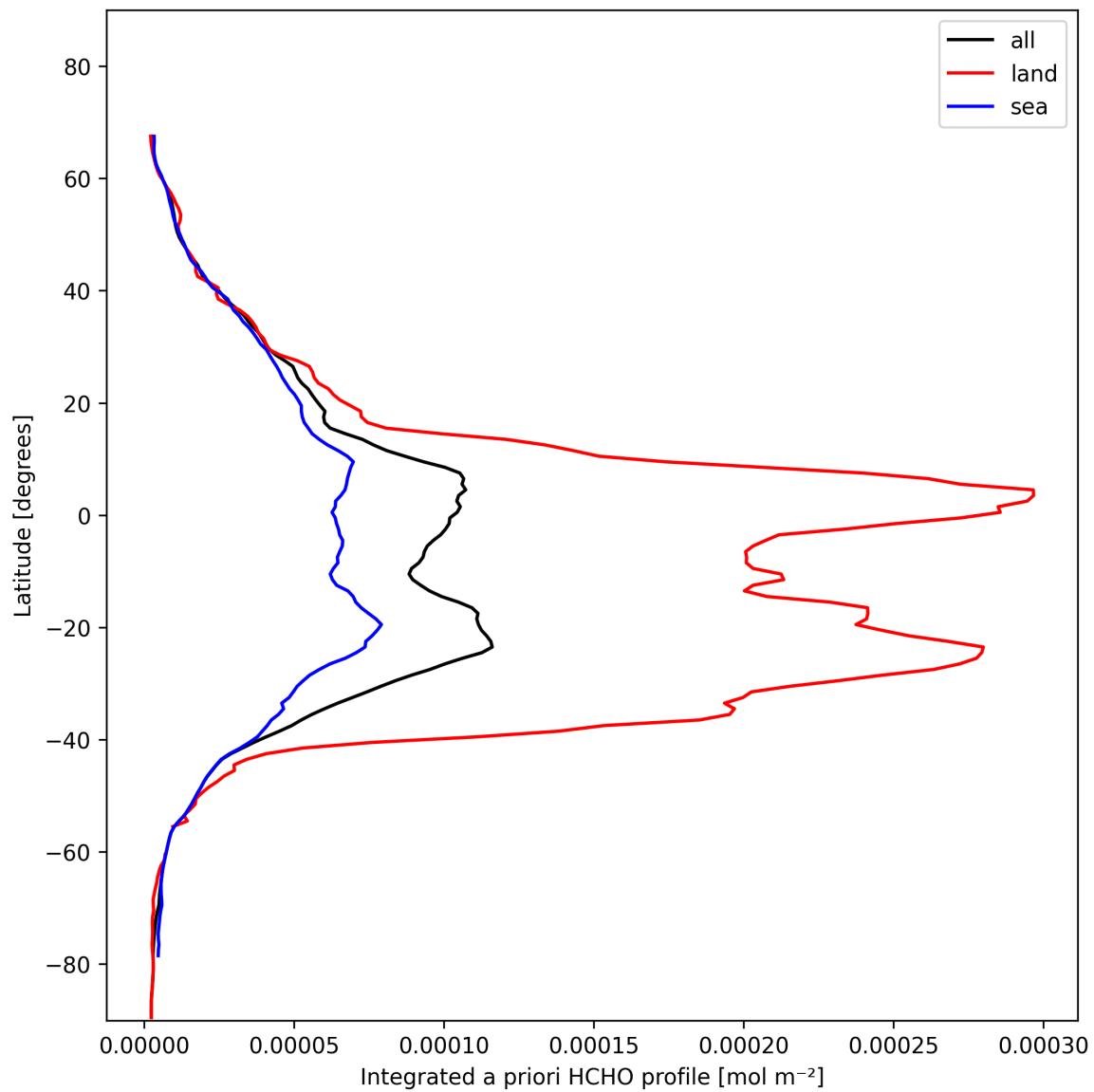
Figure 29: Zonal average of “Integrated a priori HCHO profile” for 2025-01-30 to 2025-02-01.
