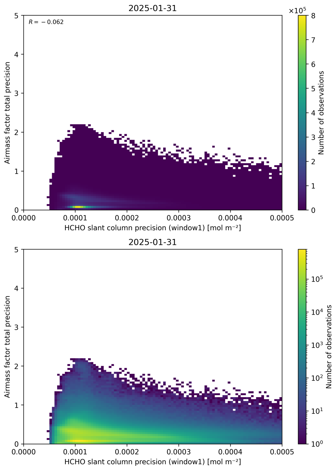
Figure 95: Scatter density plot of “HCHO slant column precision (window1)” against “Airmass factor total precision” for 2025-01-30 to 2025-02-01.
