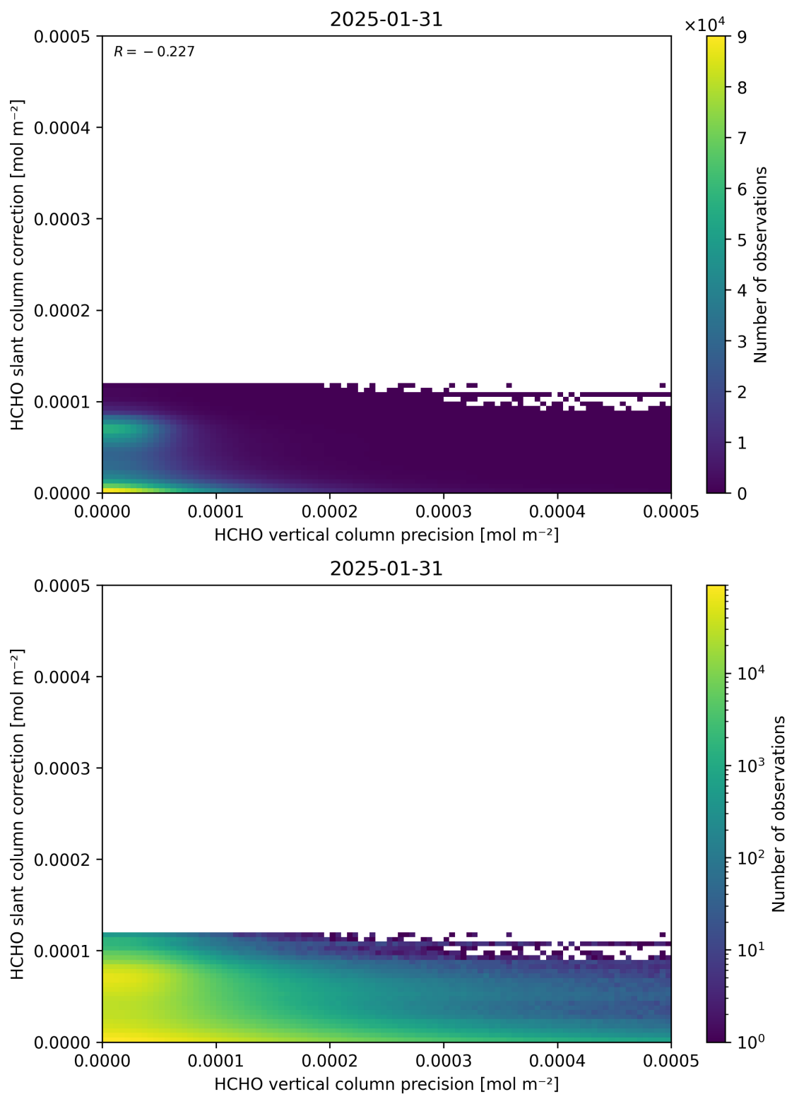
Figure 141: Scatter density plot of “HCHO vertical column precision” against “HCHO slant column correction” for 2025-01-30 to 2025-02-01.
