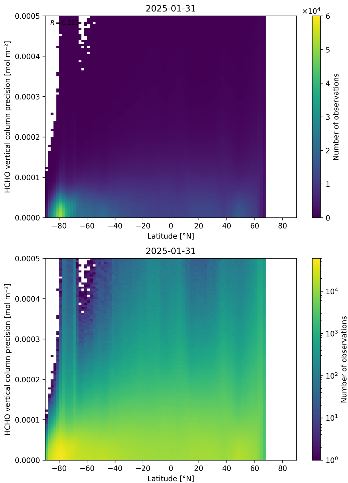
Figure 165: Scatter density plot of “Latitude” against “HCHO vertical column precision” for 2025-01-30 to 2025-02-01.
