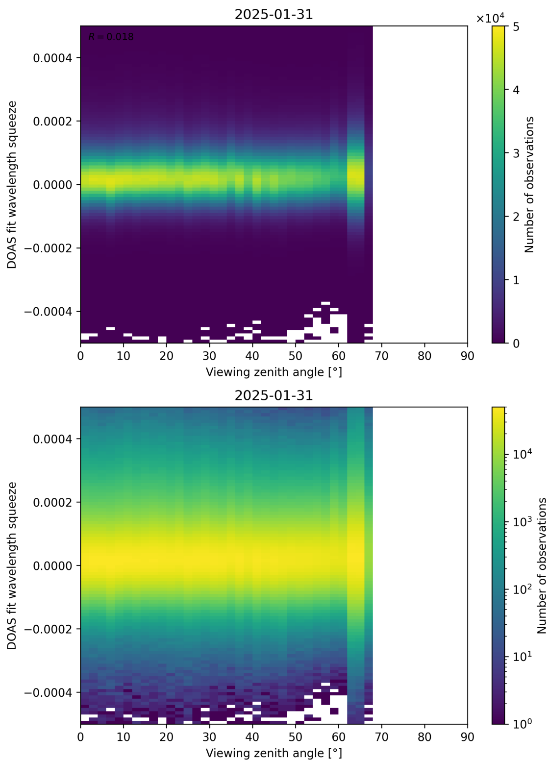
Figure 184: Scatter density plot of “Viewing zenith angle” against “DOAS fit wavelength squeeze” for 2025-01-30 to 2025-02-01.
