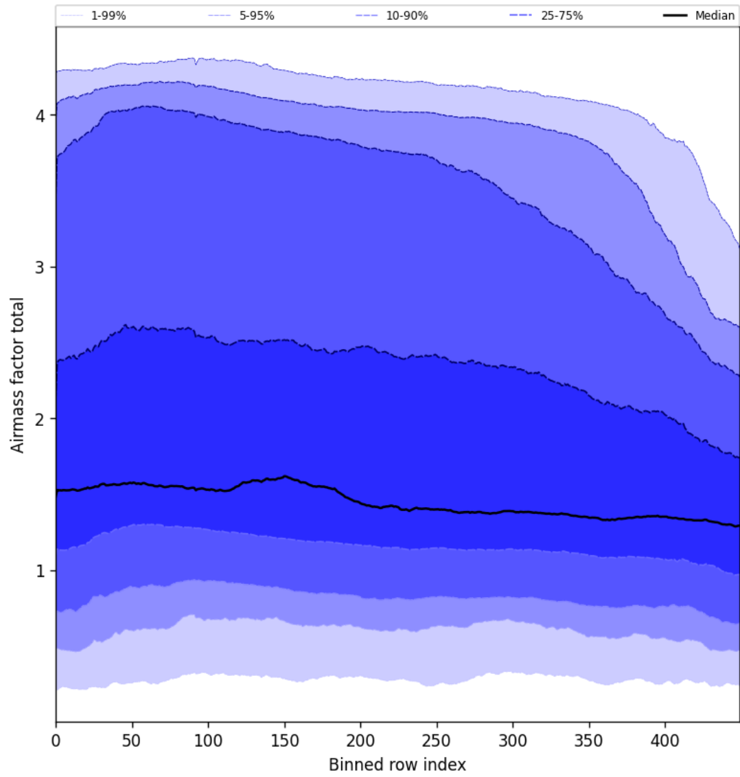
Figure 54: Along track statistics of “Airmass factor total” for 2025-01-30 to 2025-02-01
