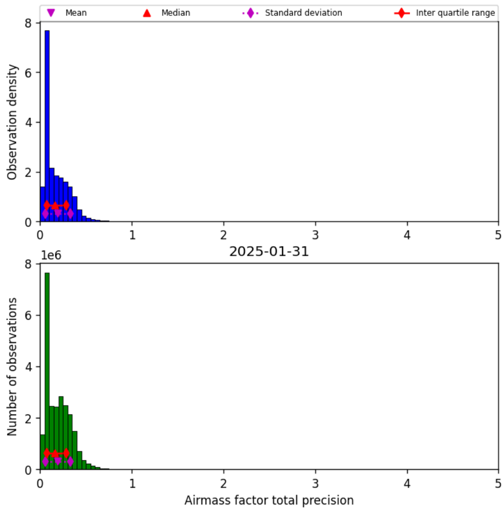
Figure 41: Histogram of “Airmass factor total precision” for 2025-01-30 to 2025-02-01
