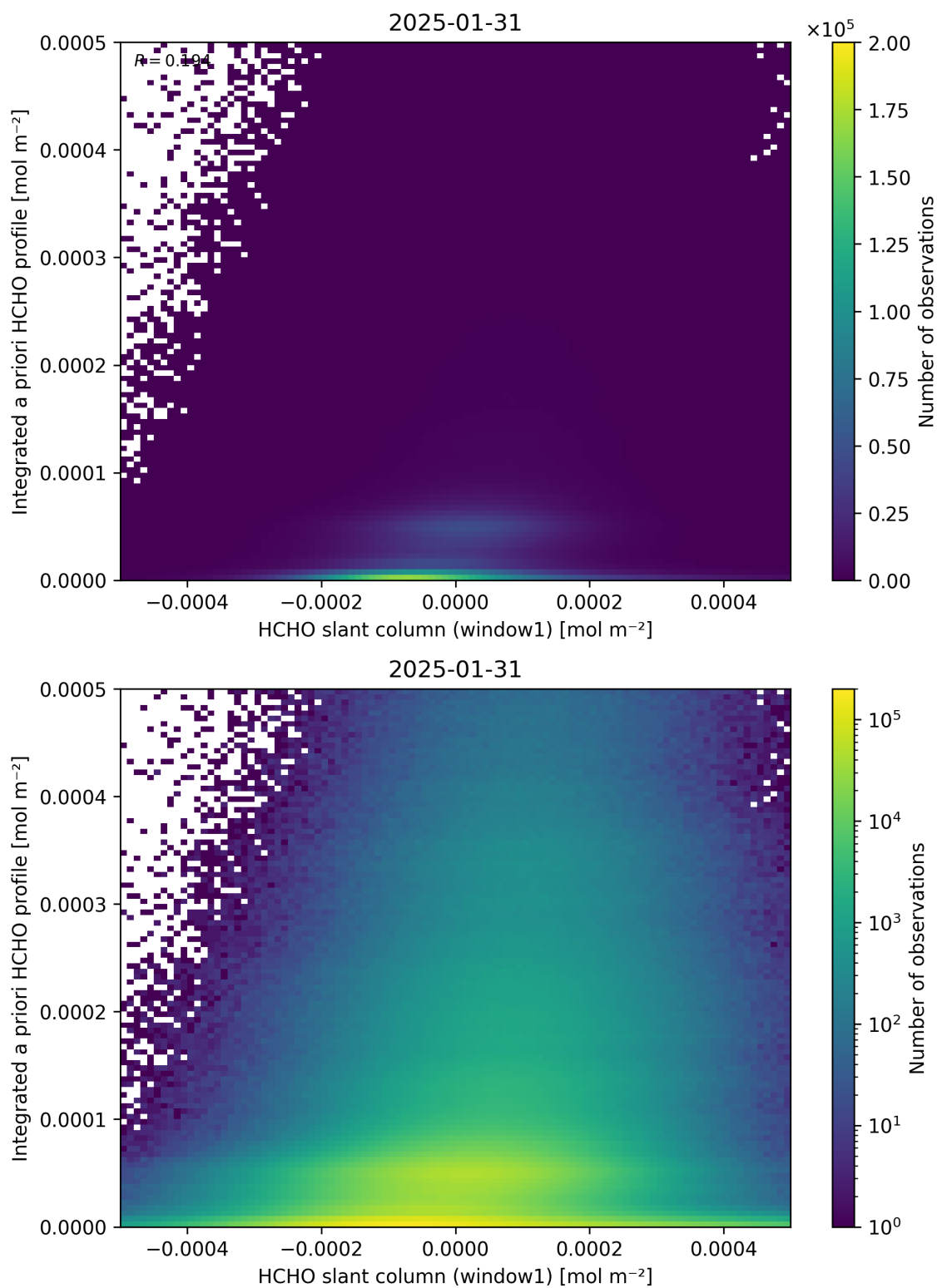
Figure 87: Scatter density plot of “HCHO slant column (window1)” against “Integrated a priori HCHO profile” for 2025-01-30 to 2025-02-01.
