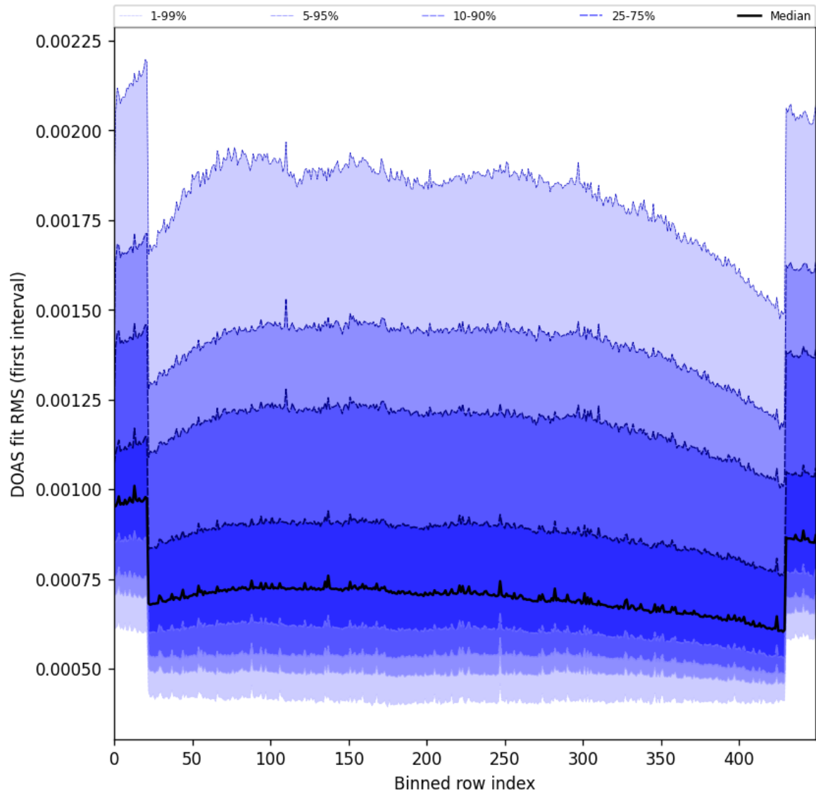
Figure 60: Along track statistics of “DOAS fit RMS (first interval)” for 2025-01-30 to 2025-02-01
