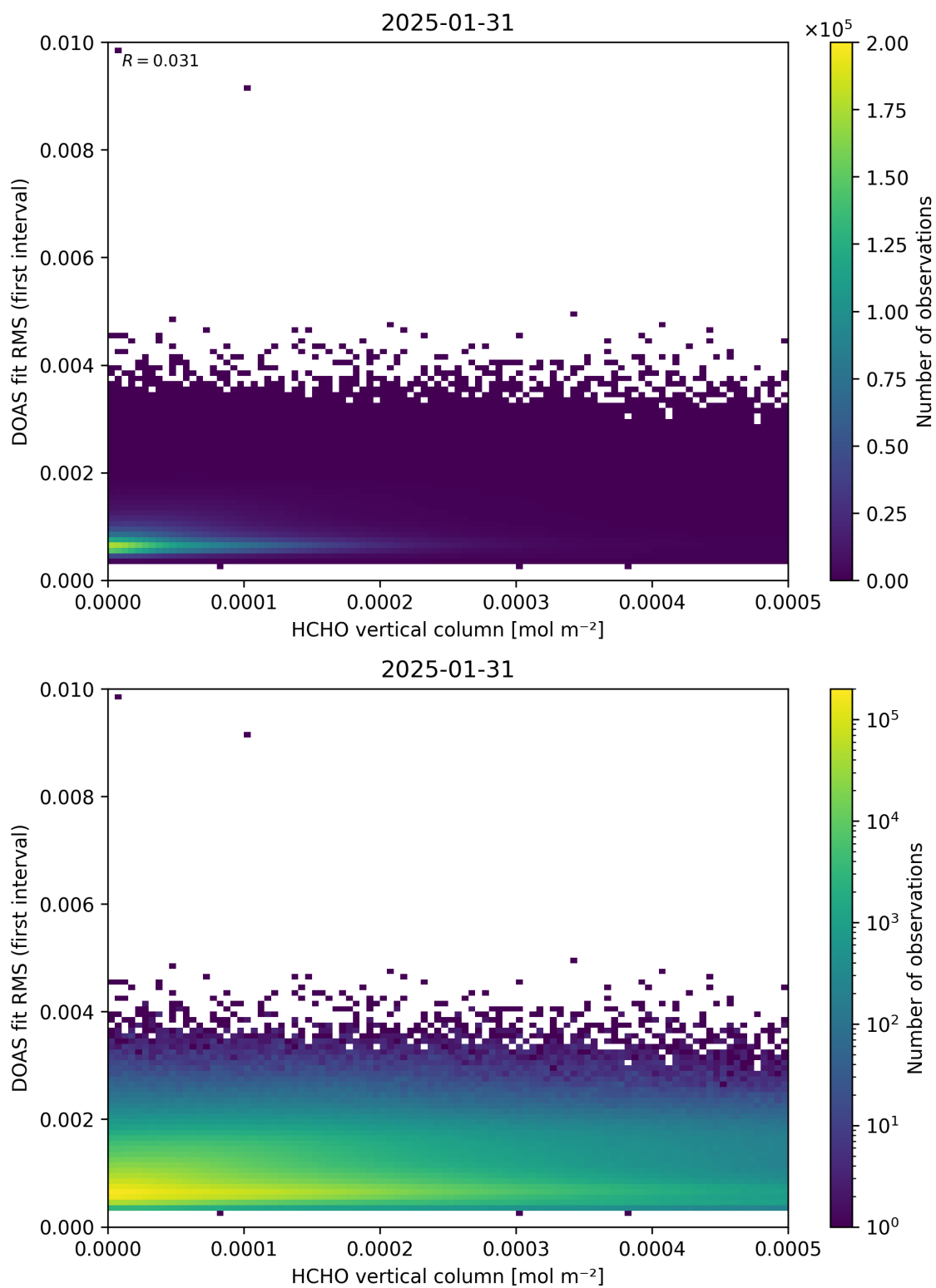
Figure 123: Scatter density plot of “HCHO vertical column” against “DOAS fit RMS (first interval)” for 2025-01-30 to 2025-02-01.
