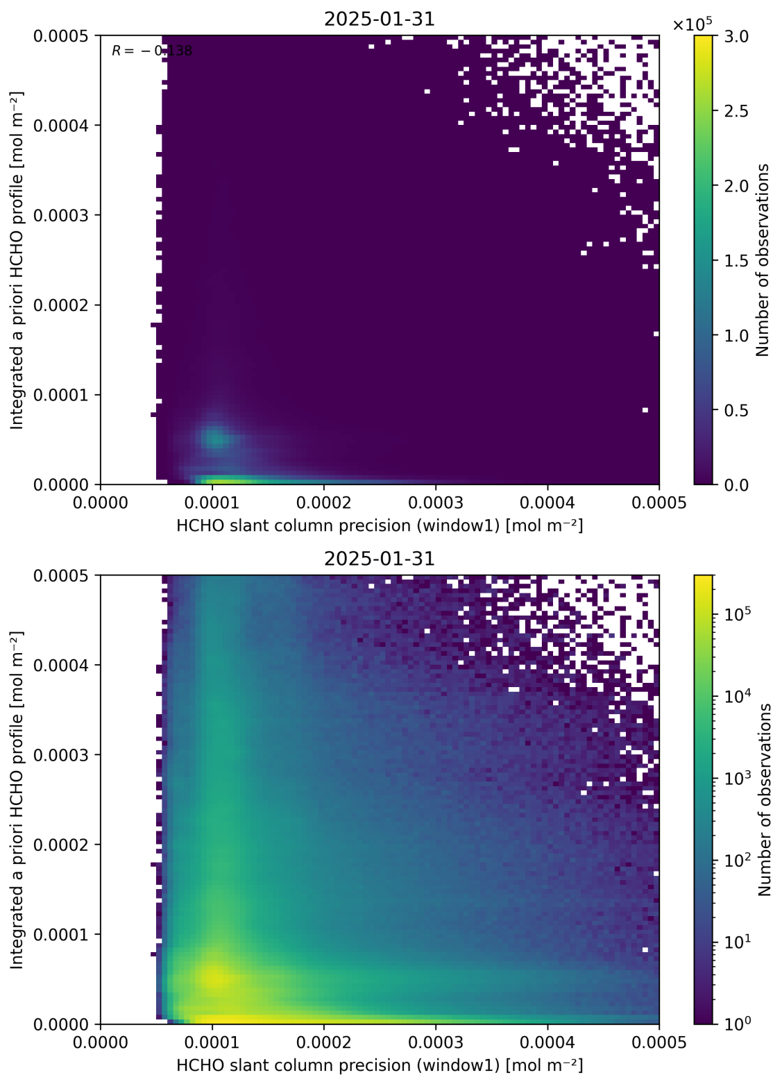
Figure 96: Scatter density plot of “HCHO slant column precision (window1)” against “Integrated a priori HCHO profile” for 2025-01-30 to 2025-02-01.
