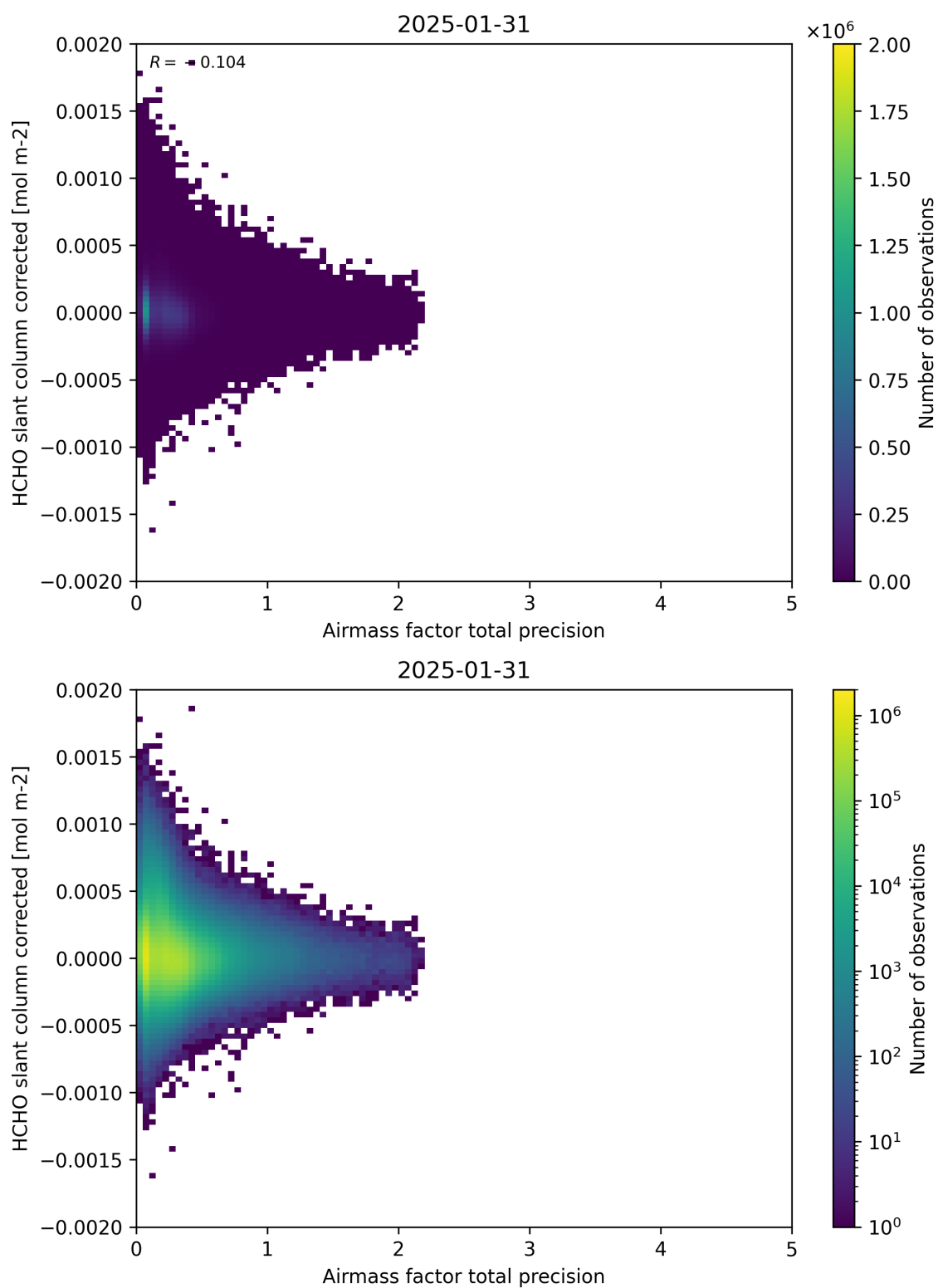
Figure 109: Scatter density plot of “Airmass factor total precision” against “HCHO slant column corrected” for 2025-01-30 to 2025-02-01.
