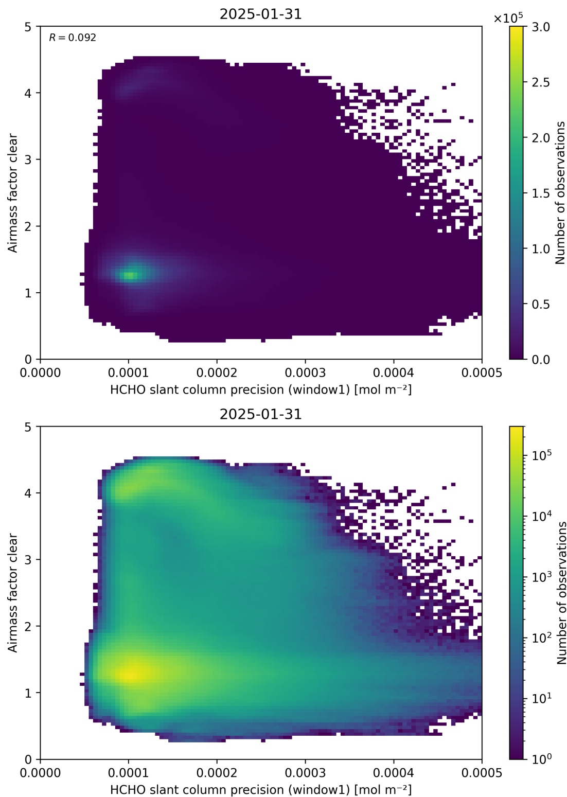
Figure 91: Scatter density plot of “HCHO slant column precision (window1)” against “Airmass factor clear” for 2025-01-30 to 2025-02-01.
