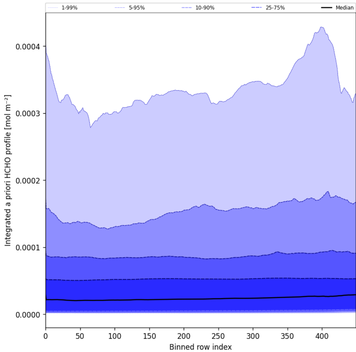
Figure 57: Along track statistics of "Integrated a priori HCHO profile" for 2025-01-30 to 2025-02-01
