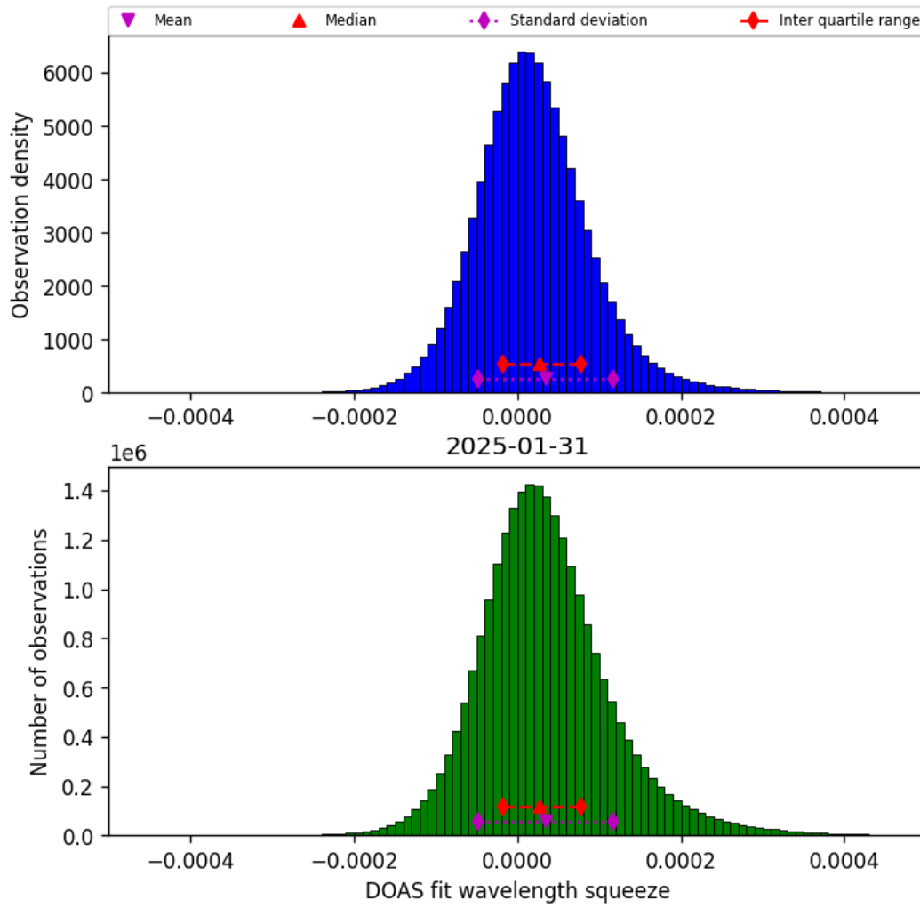
Figure 45: Histogram of “DOAS fit wavelength squeeze” for 2025-01-30 to 2025-02-01
