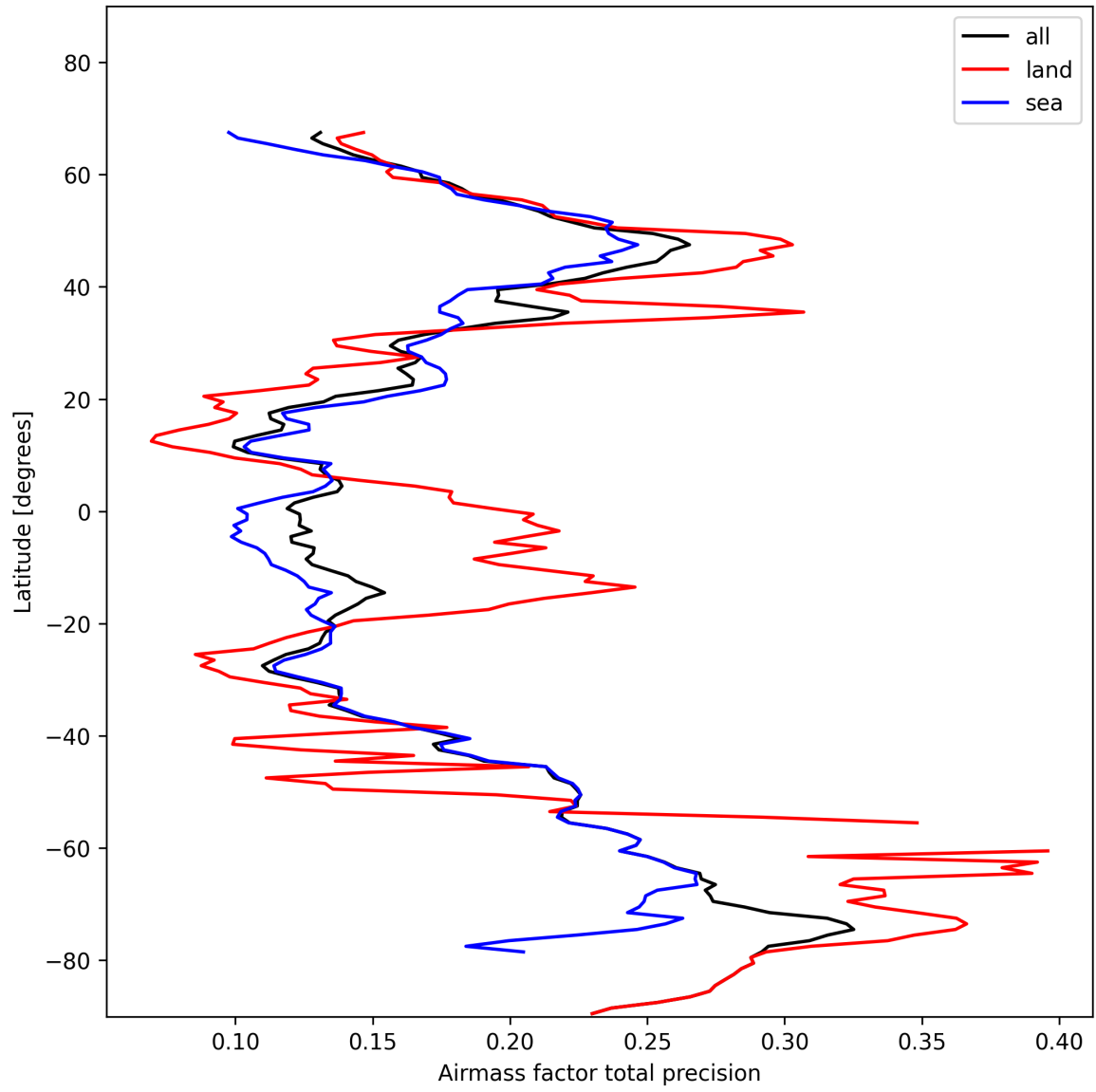
Figure 27: Zonal average of “Airmass factor total precision” for 2025-01-30 to 2025-02-01.
