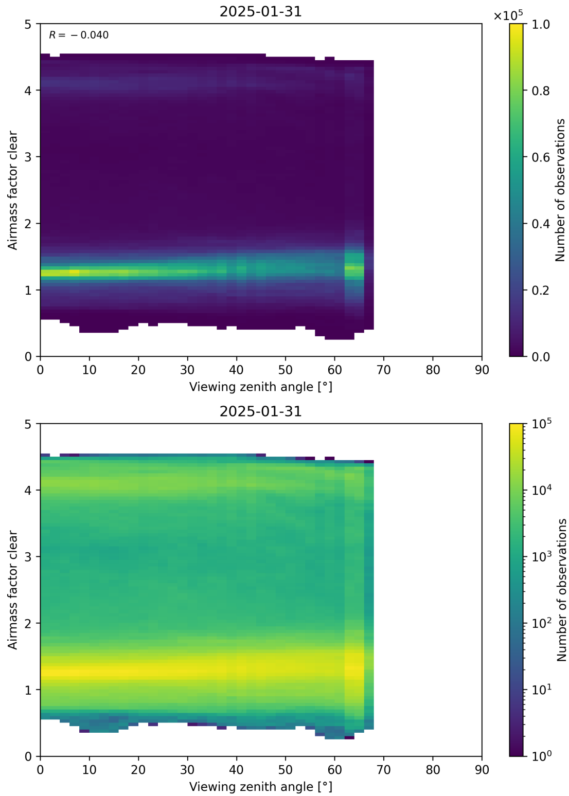
Figure 185: Scatter density plot of “Viewing zenith angle” against “Airmass factor clear” for 2025-01-30 to 2025-02-01.
