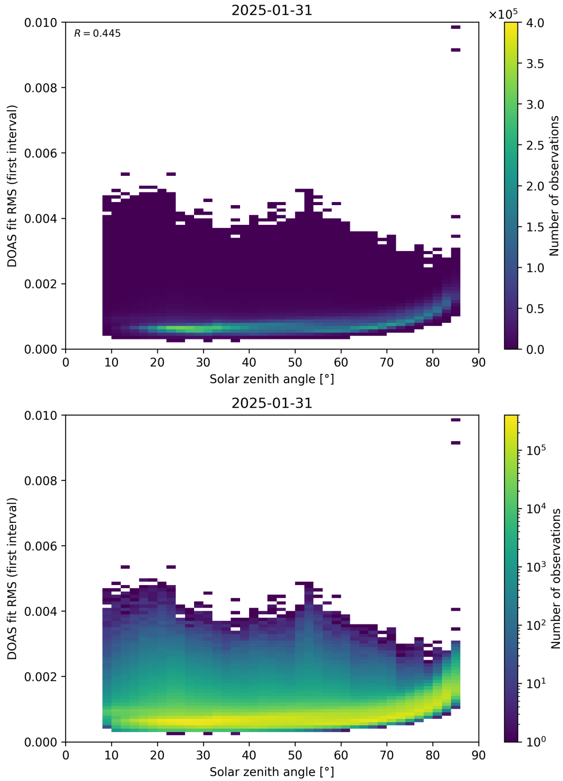
Figure 167: Scatter density plot of “Solar zenith angle” against “DOAS fit RMS (first interval)” for 2025-01-30 to 2025-02-01.
