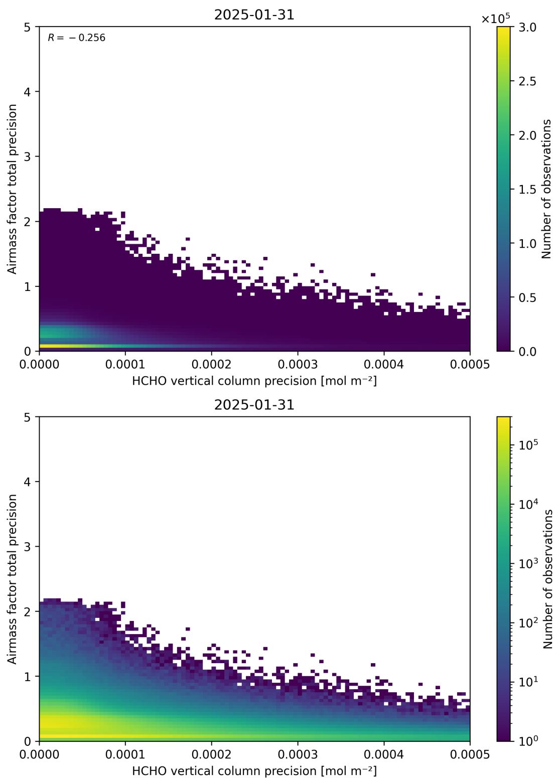
Figure 145: Scatter density plot of “HCHO vertical column precision” against “Airmass factor total precision” for 2025-01-30 to 2025-02-01.
