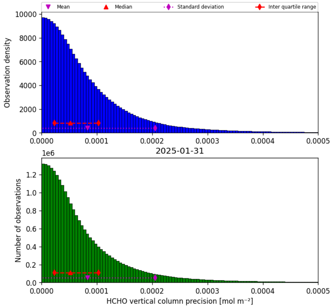
Figure 36: Histogram of “HCHO vertical column precision” for 2025-01-30 to 2025-02-01
