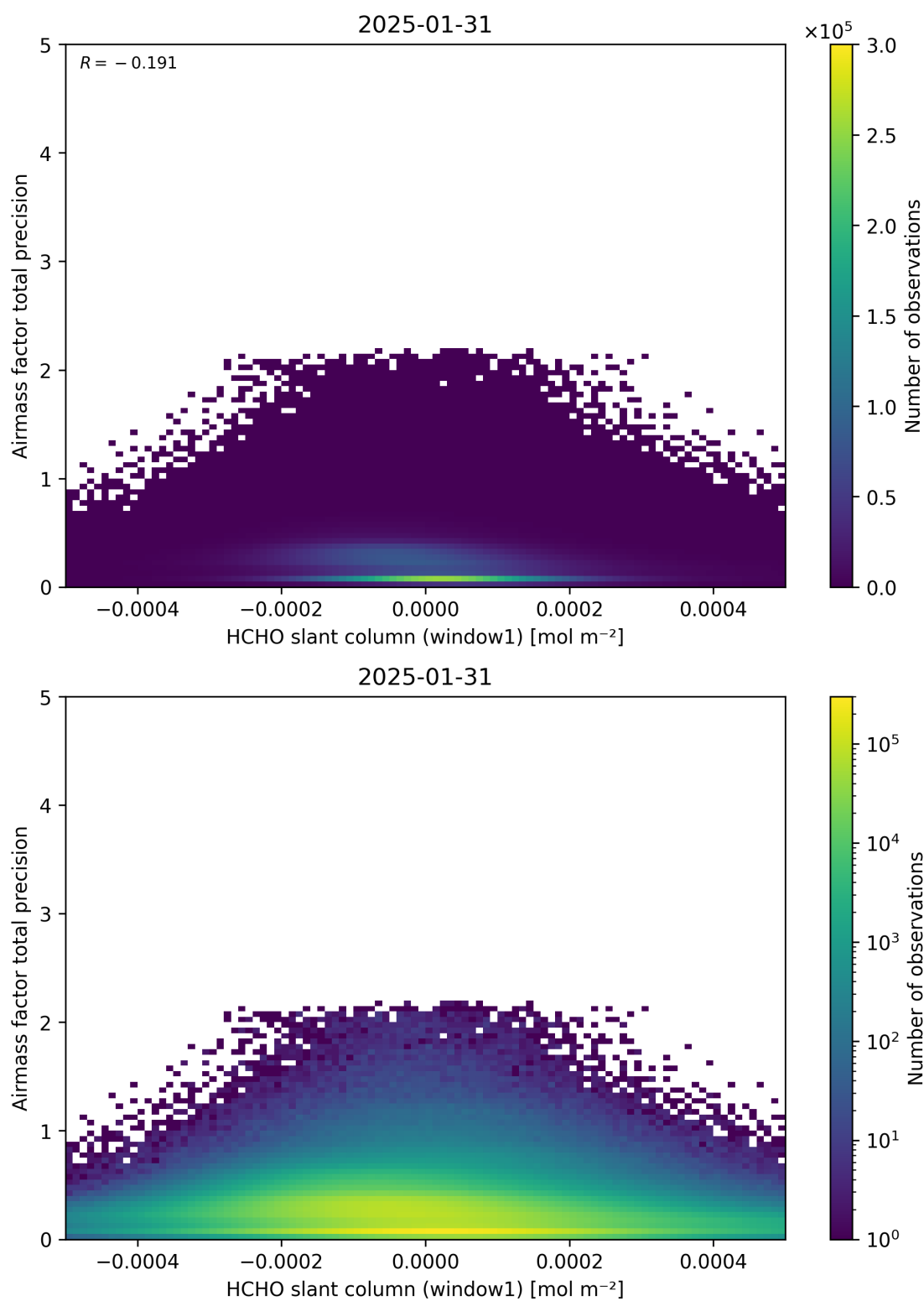
Figure 86: Scatter density plot of “HCHO slant column (window1)” against “Airmass factor total precision” for 2025-01-30 to 2025-02-01.
