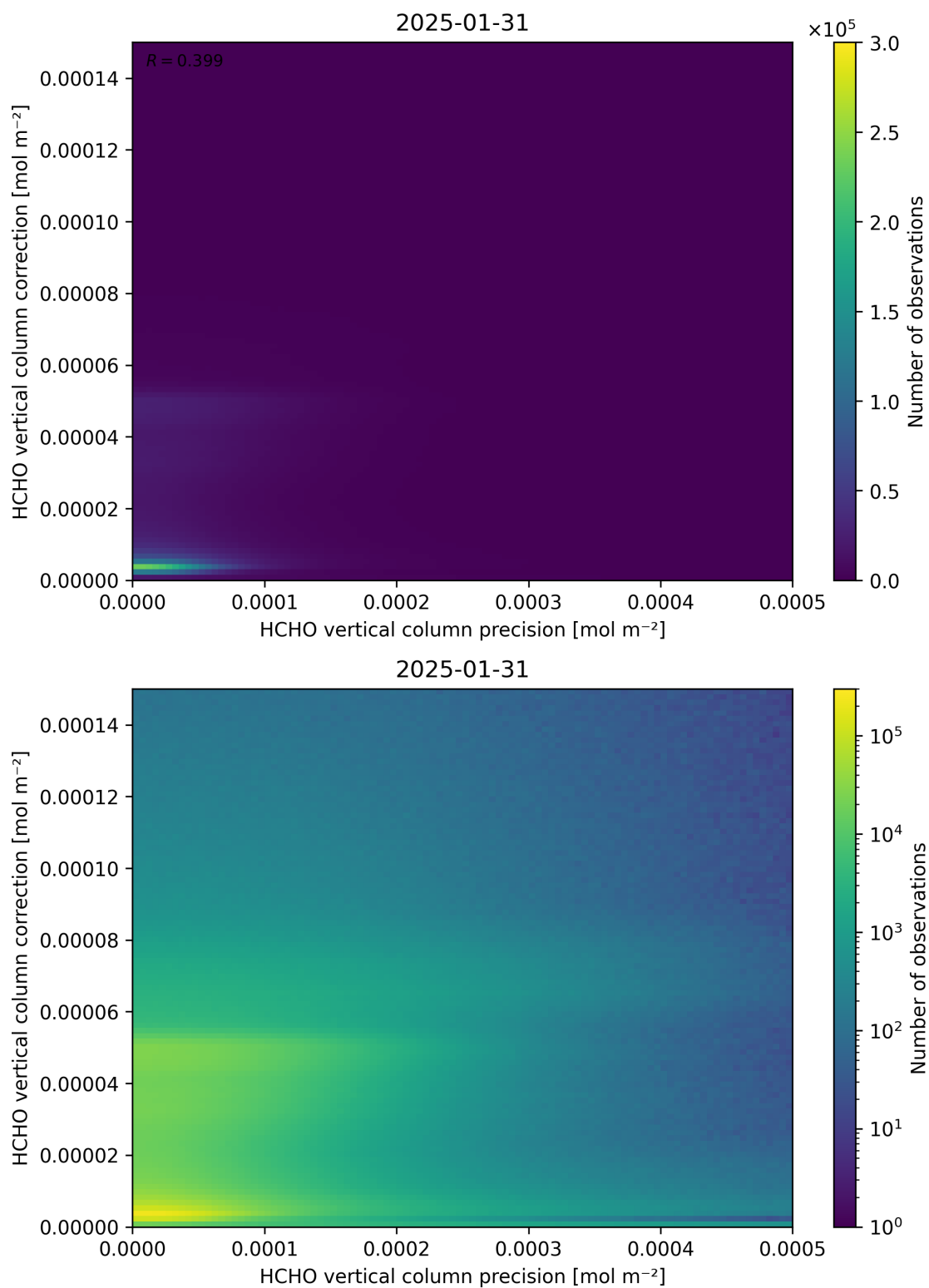
Figure 146: Scatter density plot of “HCHO vertical column precision” against “HCHO vertical column correction” for 2025-01-30 to 2025-02-01.
