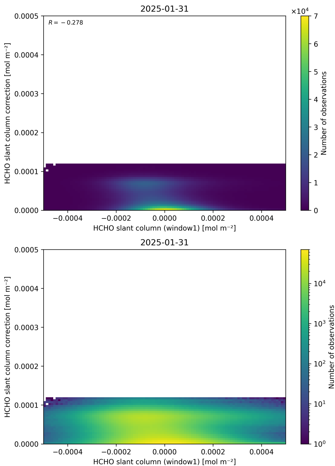
Figure 83: Scatter density plot of “HCHO slant column (window1)” against “HCHO slant column correction” for 2025-01-30 to 2025-02-01.
