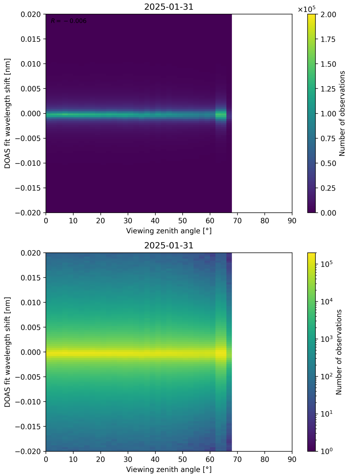
Figure 183: Scatter density plot of “Viewing zenith angle” against “DOAS fit wavelength shift” for 2025-01-30 to 2025-02-01.
