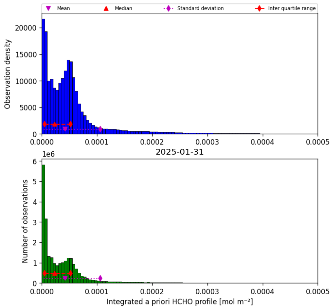
Figure 43: Histogram of “Integrated a priori HCHO profile” for 2025-01-30 to 2025-02-01
