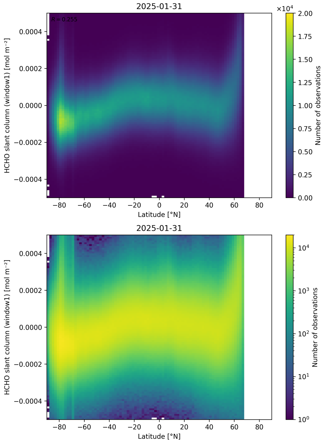
Figure 159: Scatter density plot of “Latitude” against “HCHO slant column (window1)” for 2025-01-30 to 2025-02-01.
