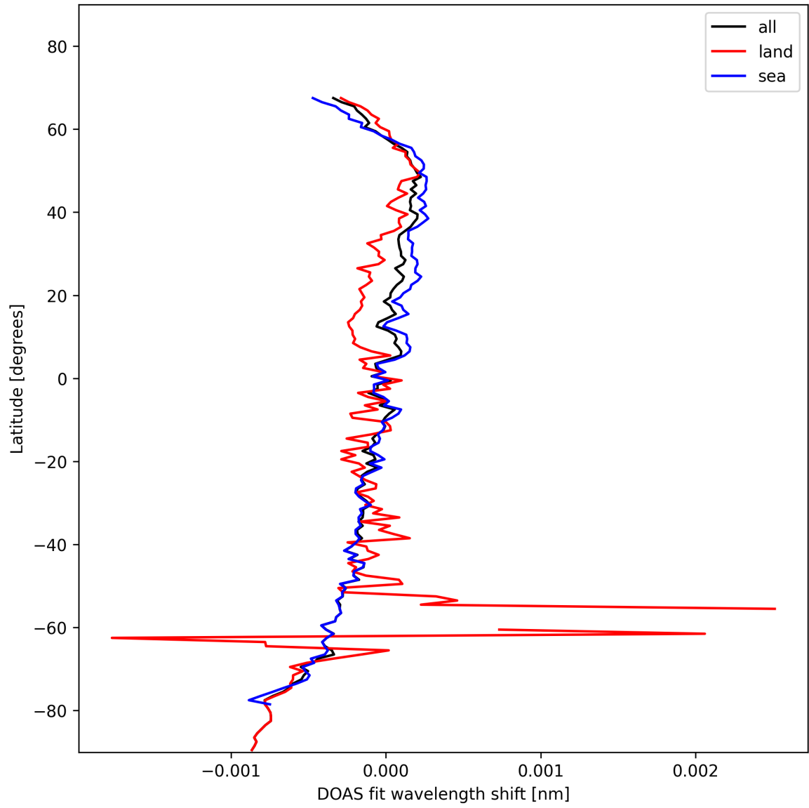
Figure 30: Zonal average of “DOAS fit wavelength shift” for 2025-01-30 to 2025-02-01.
