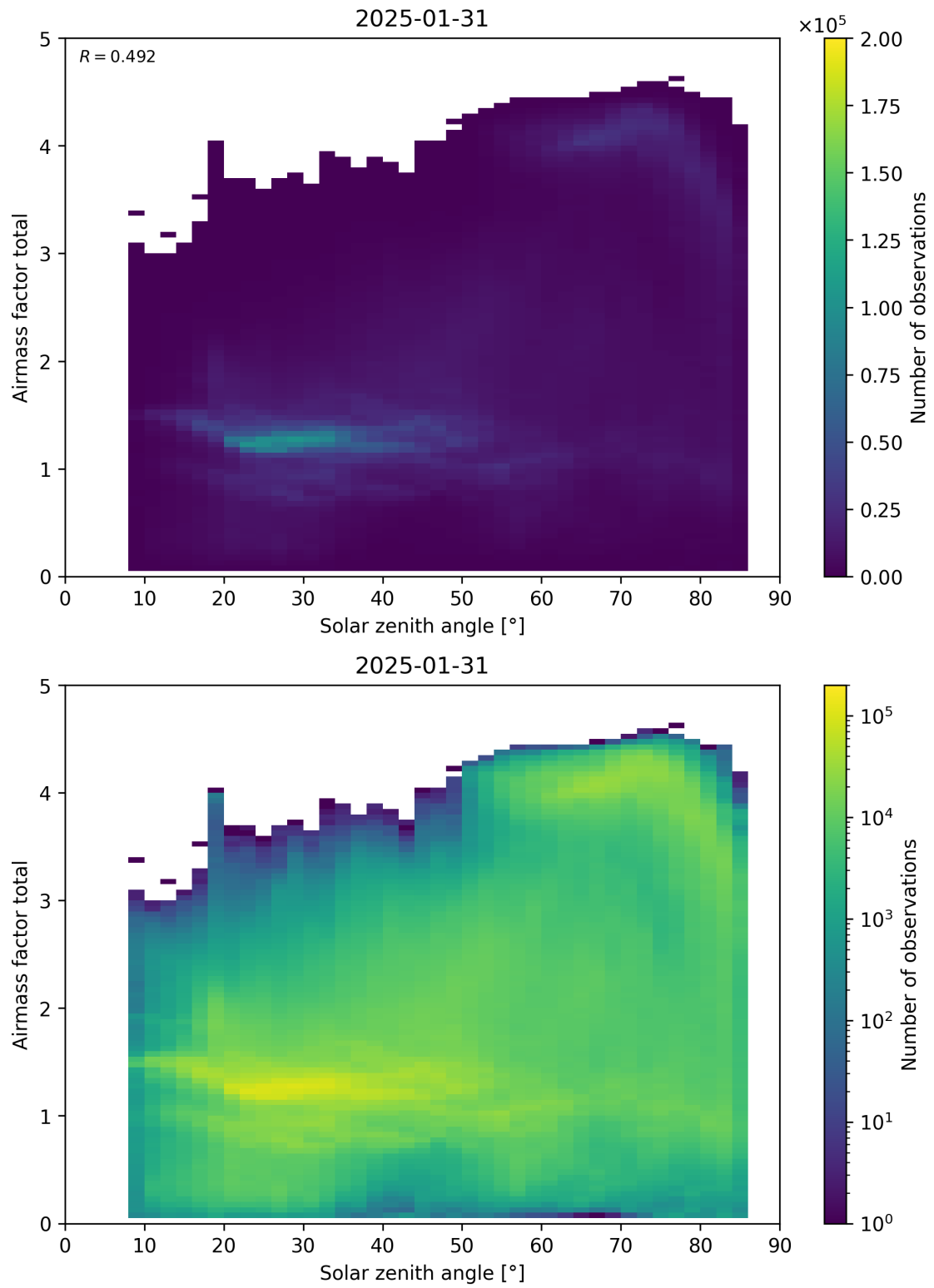
Figure 175: Scatter density plot of “Solar zenith angle” against “Airmass factor total” for 2025-01-30 to 2025-02-01.
