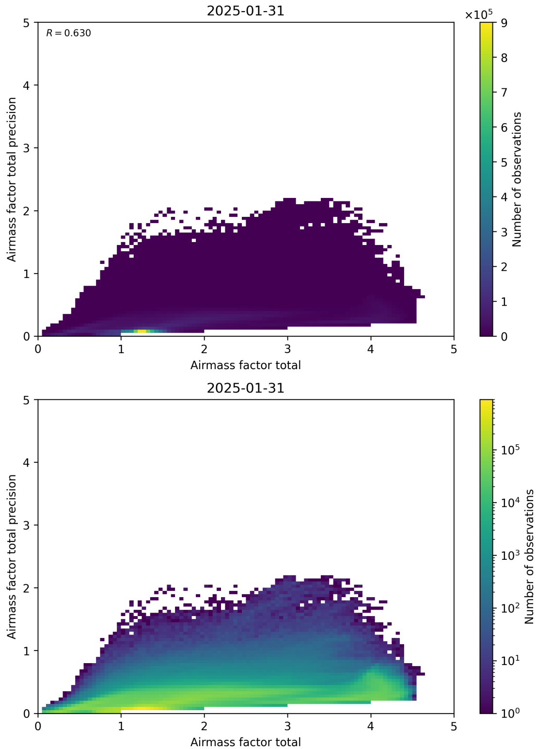
Figure 103: Scatter density plot of “Airmass factor total” against “Airmass factor total precision” for 2025-01-30 to 2025-02-01.
