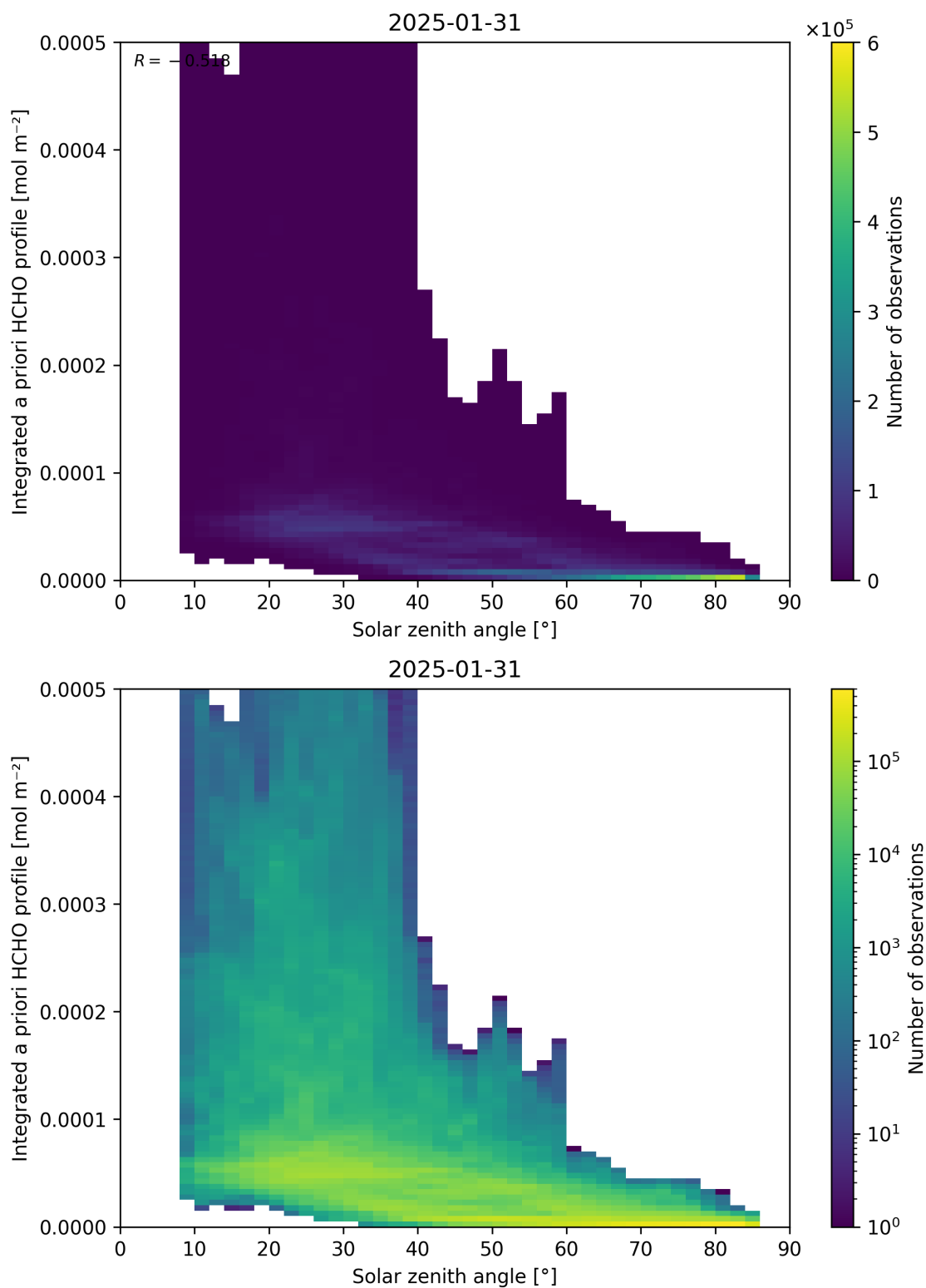
Figure 180: Scatter density plot of “Solar zenith angle” against “Integrated a priori HCHO profile” for 2025-01-30 to 2025-02-01.
