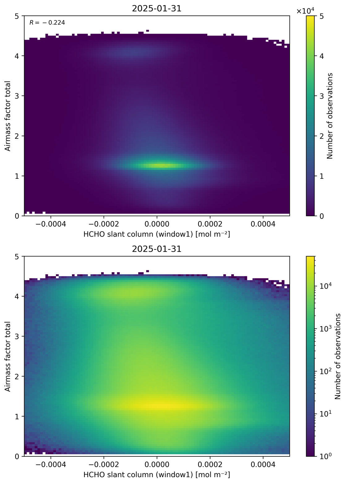
Figure 85: Scatter density plot of “HCHO slant column (window1)” against “Airmass factor total” for 2025-01-30 to 2025-02-01.
