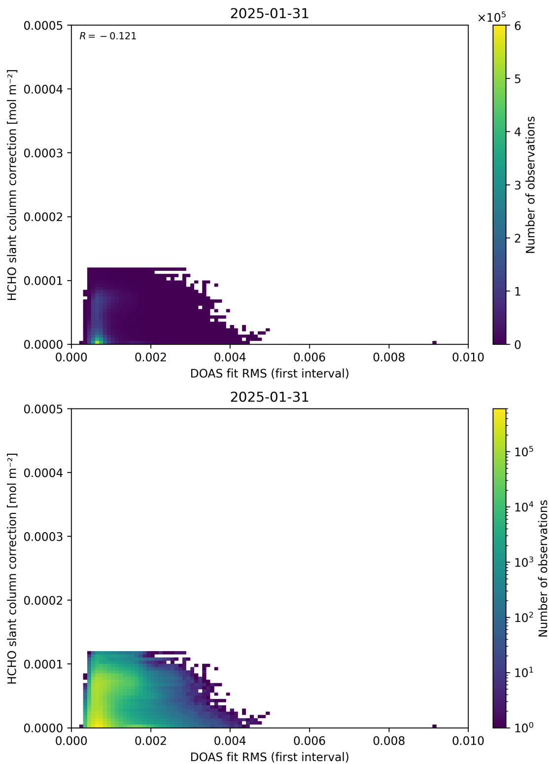
Figure 63: Scatter density plot of “DOAS fit RMS (first interval)” against “HCHO slant column correction” for 2025-01-30 to 2025-02-01.
