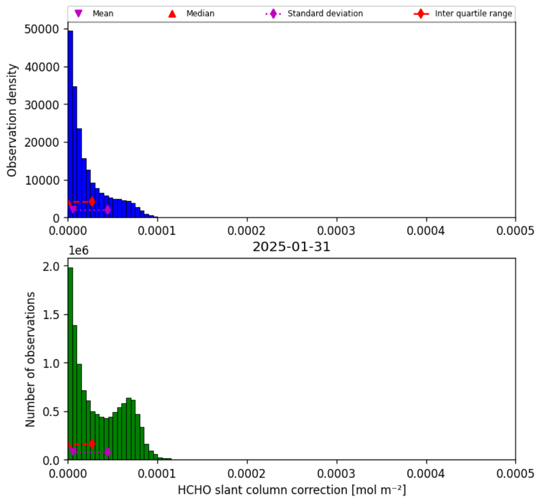
Figure 47: Histogram of “HCHO slant column correction” for 2025-01-30 to 2025-02-01
