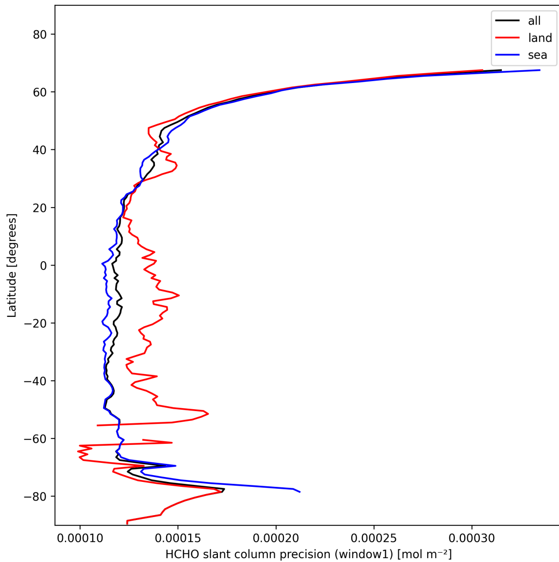
Figure 25: Zonal average of “HCHO slant column precision (window1)” for 2025-01-30 to 2025-02-01.
