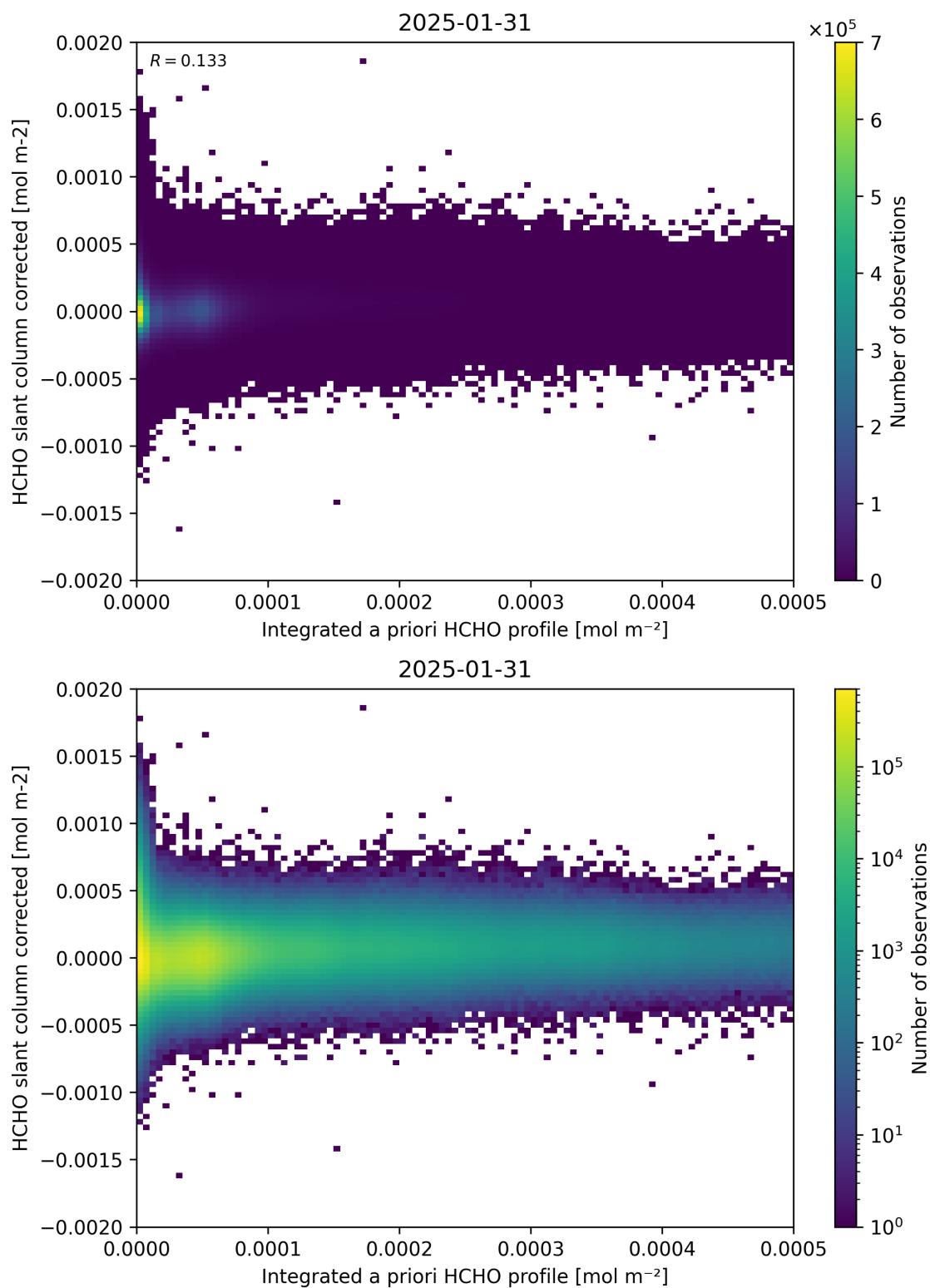
Figure 151: Scatter density plot of “Integrated a priori HCHO profile” against “HCHO slant column corrected” for 2025-01-30 to 2025-02-01.
