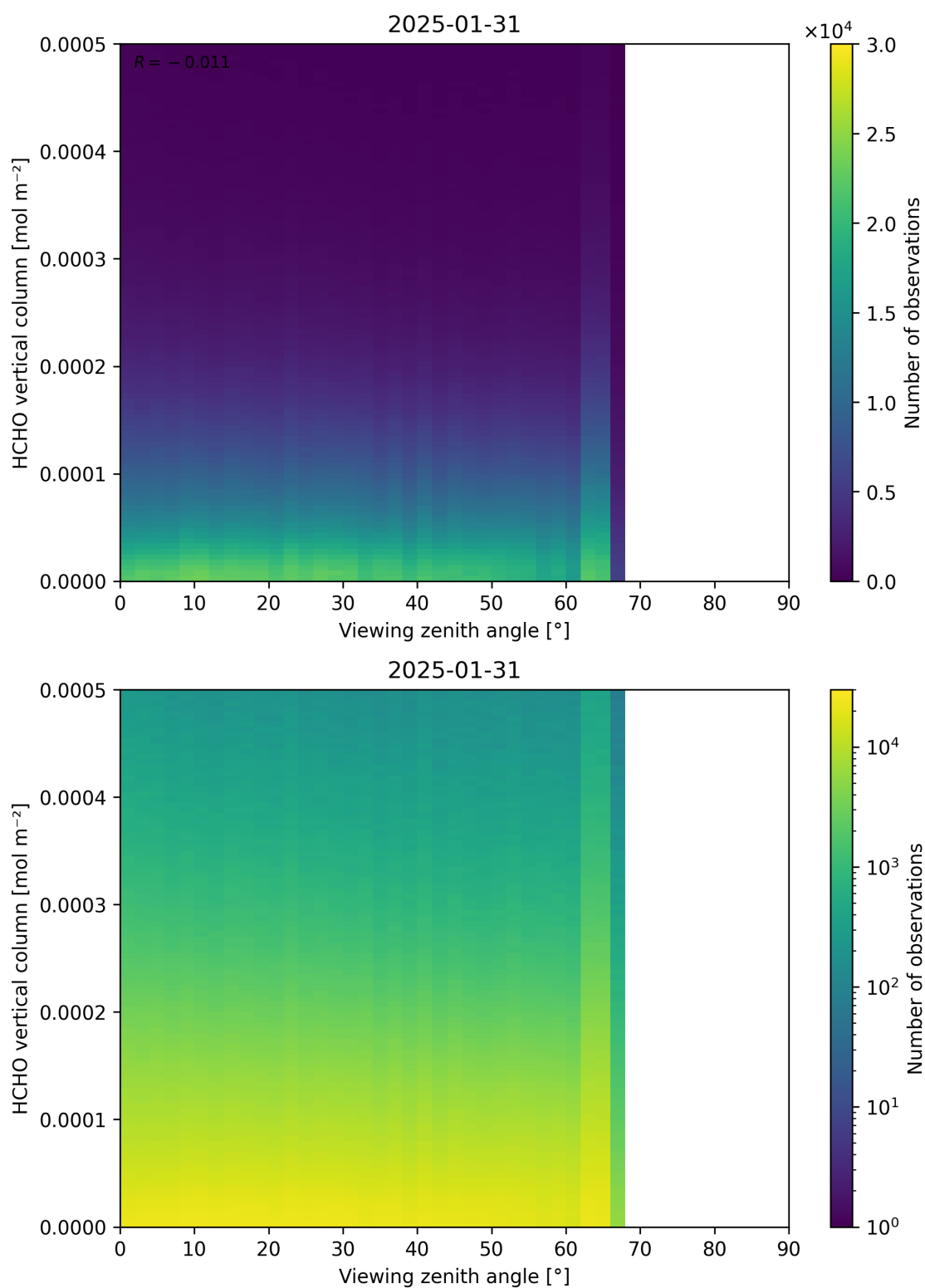
Figure 192: Scatter density plot of “Viewing zenith angle” against “HCHO vertical column” for 2025-01-30 to 2025-02-01.
