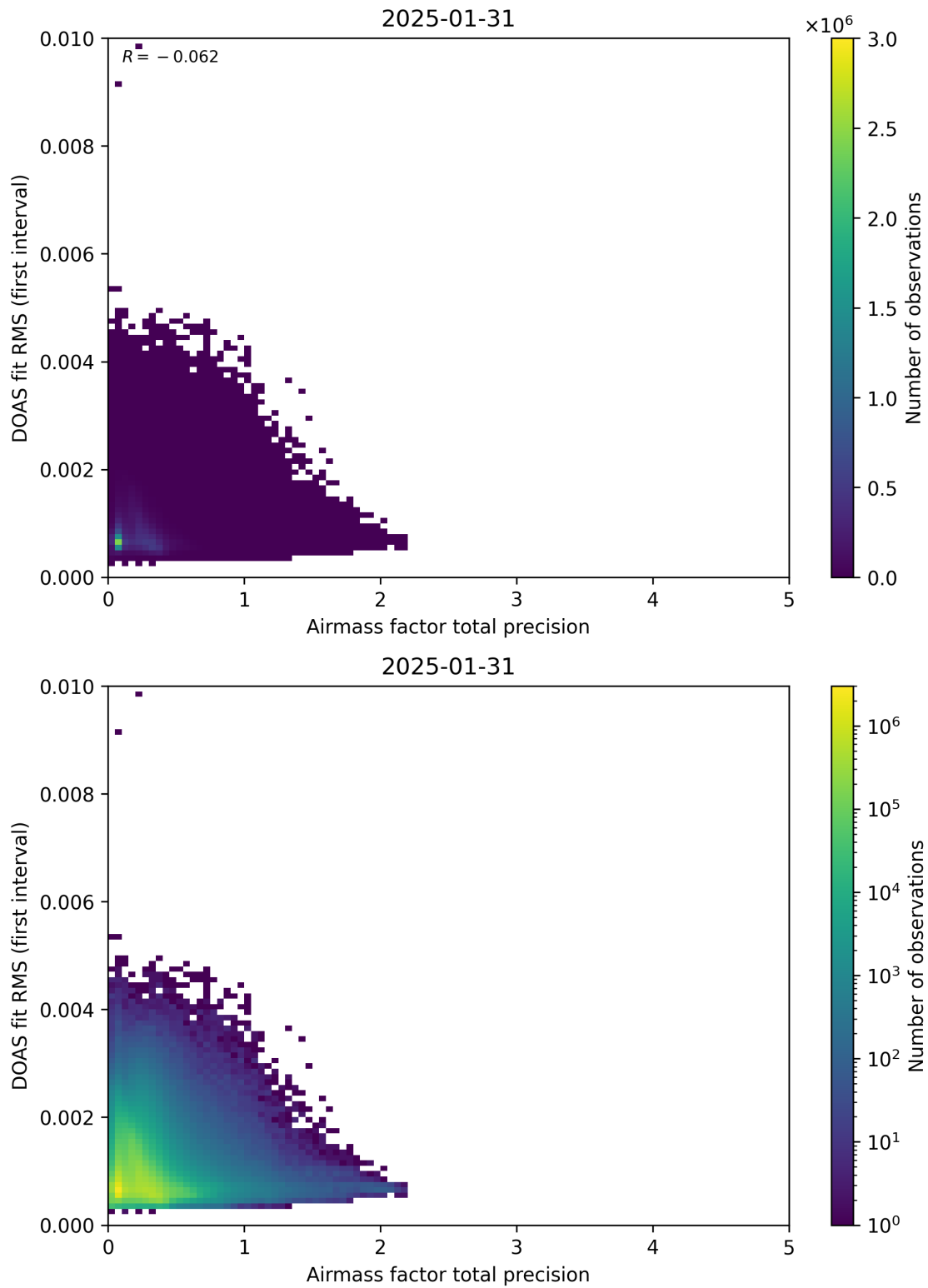
Figure 105: Scatter density plot of “Airmass factor total precision” against “DOAS fit RMS (first interval)” for 2025-01-30 to 2025-02-01.
