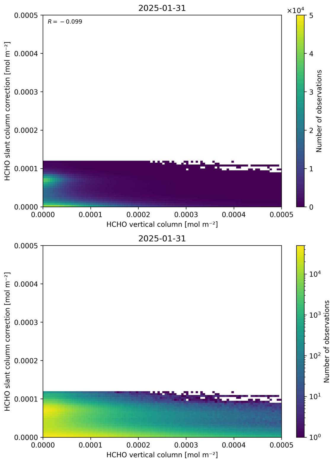
Figure 128: Scatter density plot of “HCHO vertical column” against “HCHO slant column correction” for 2025-01-30 to 2025-02-01.
