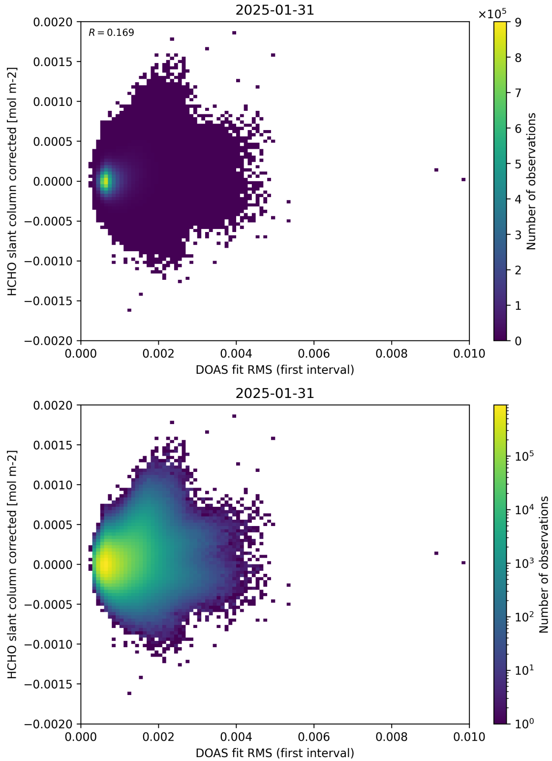
Figure 62: Scatter density plot of “DOAS fit RMS (first interval)” against “HCHO slant column corrected” for 2025-01-30 to 2025-02-01.
