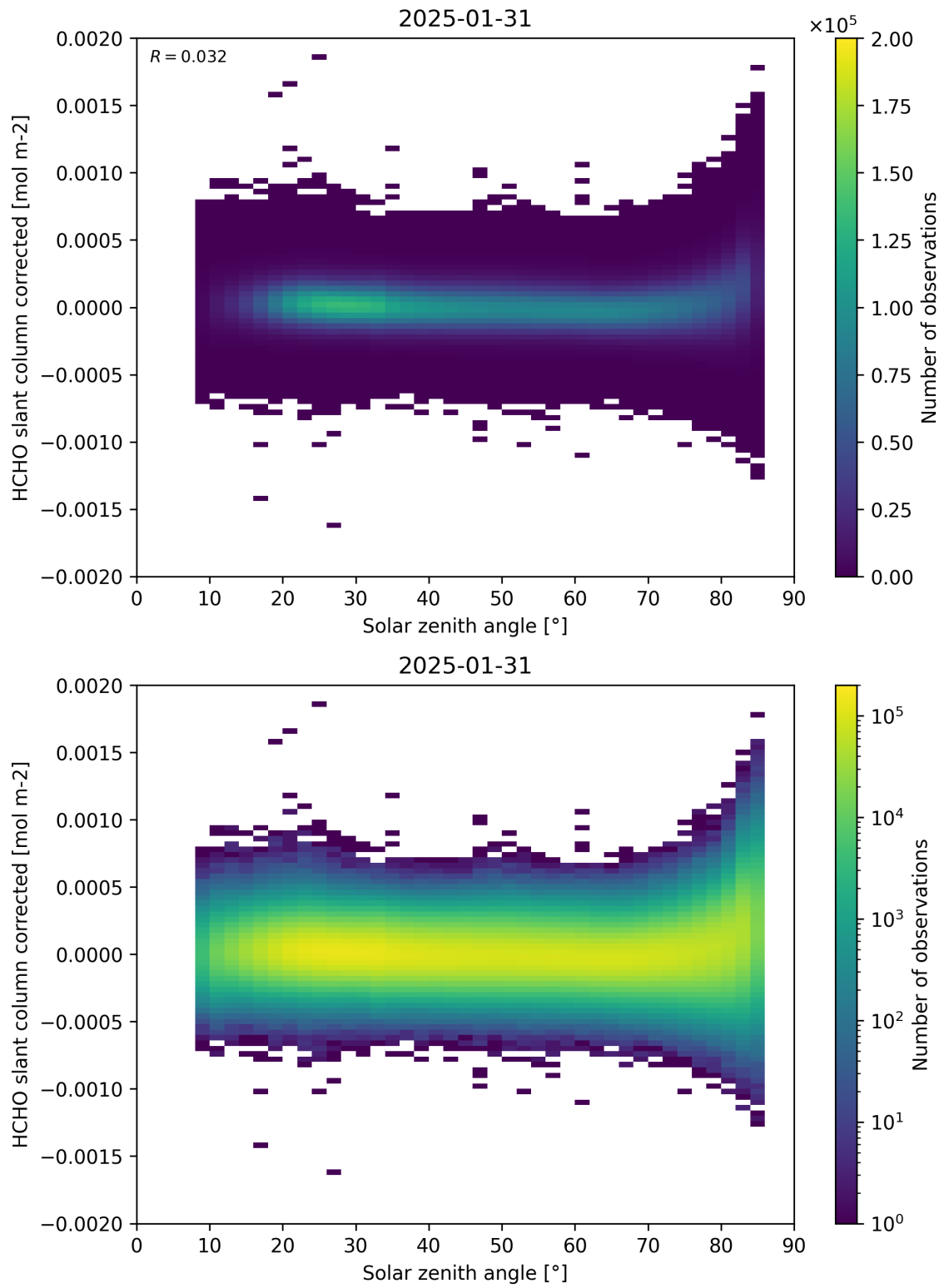
Figure 171: Scatter density plot of “Solar zenith angle” against “HCHO slant column corrected” for 2025-01-30 to 2025-02-01.
