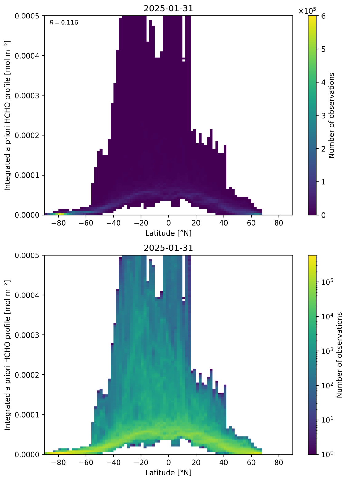
Figure 166: Scatter density plot of “Latitude” against “Integrated a priori HCHO profile” for 2025-01-30 to 2025-02-01.
