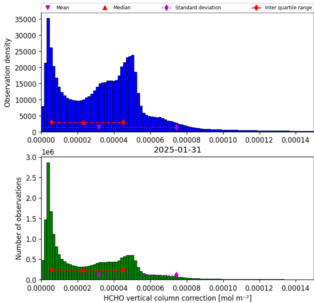
Figure 37: Histogram of “HCHO vertical column correction” for 2025-01-30 to 2025-02-01
