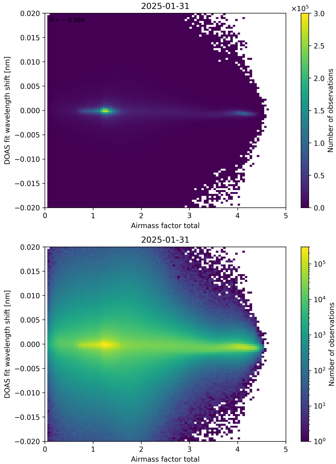
Figure 98: Scatter density plot of “Airmass factor total” against “DOAS fit wavelength shift” for 2025-01-30 to 2025-02-01.
