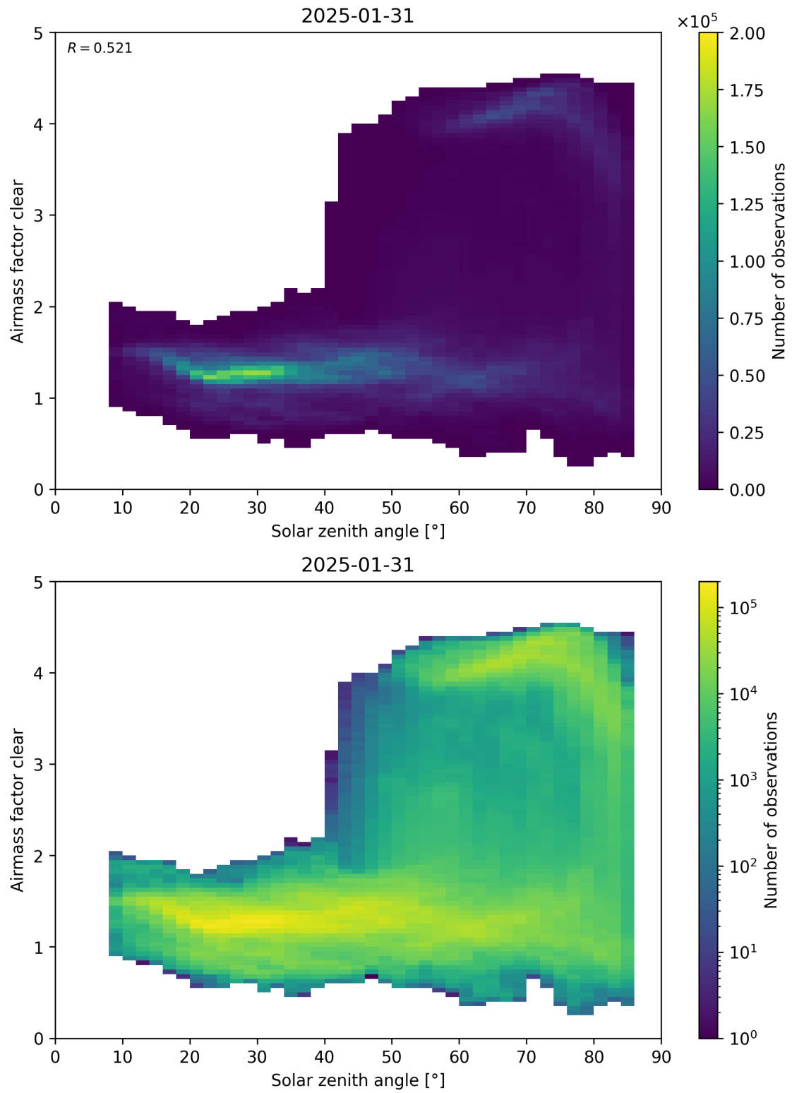
Figure 170: Scatter density plot of “Solar zenith angle” against “Airmass factor clear” for 2025-01-30 to 2025-02-01.
