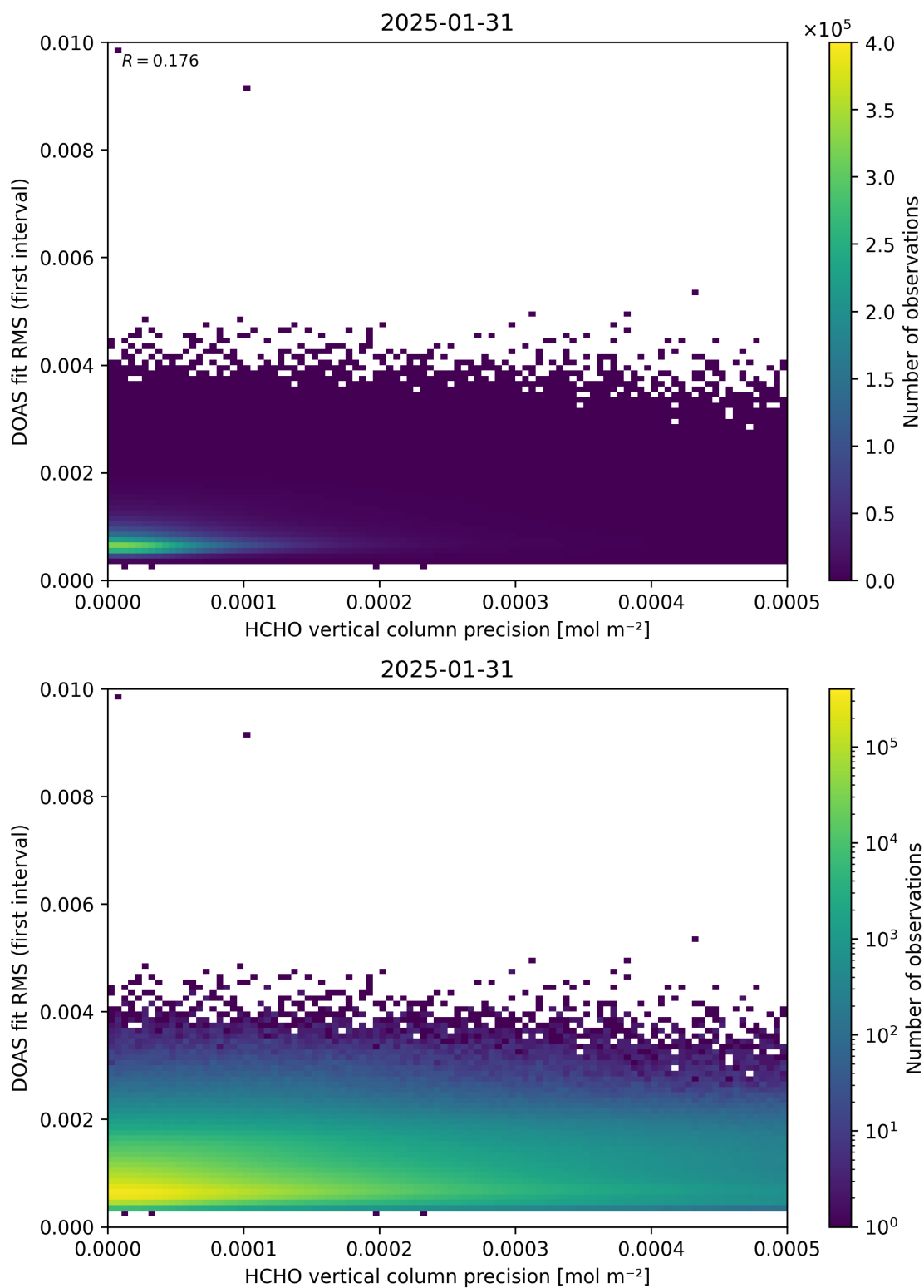
Figure 136: Scatter density plot of “HCHO vertical column precision” against “DOAS fit RMS (first interval)” for 2025-01-30 to 2025-02-01.
