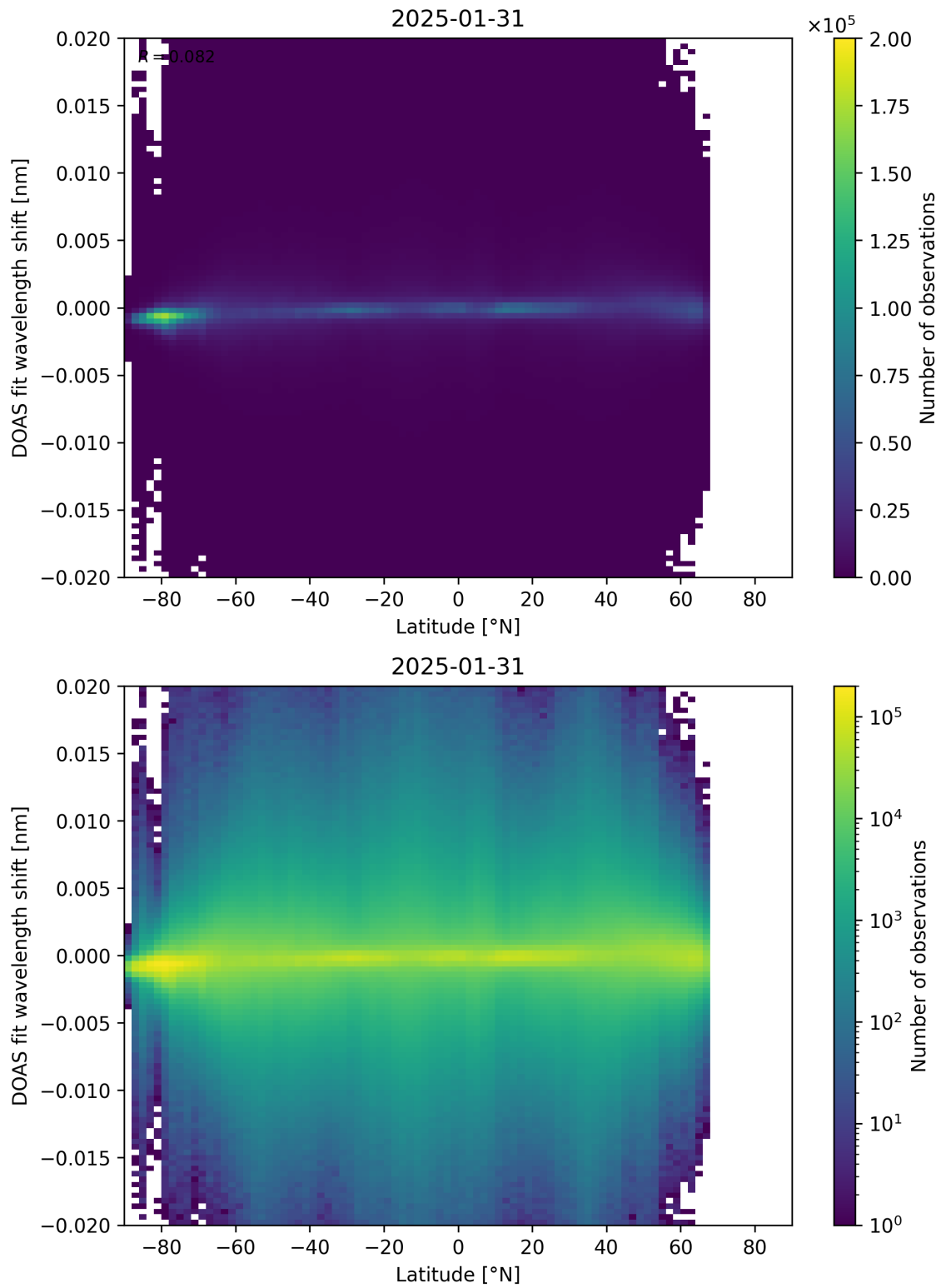
Figure 154: Scatter density plot of “Latitude” against “DOAS fit wavelength shift” for 2025-01-30 to 2025-02-01.
