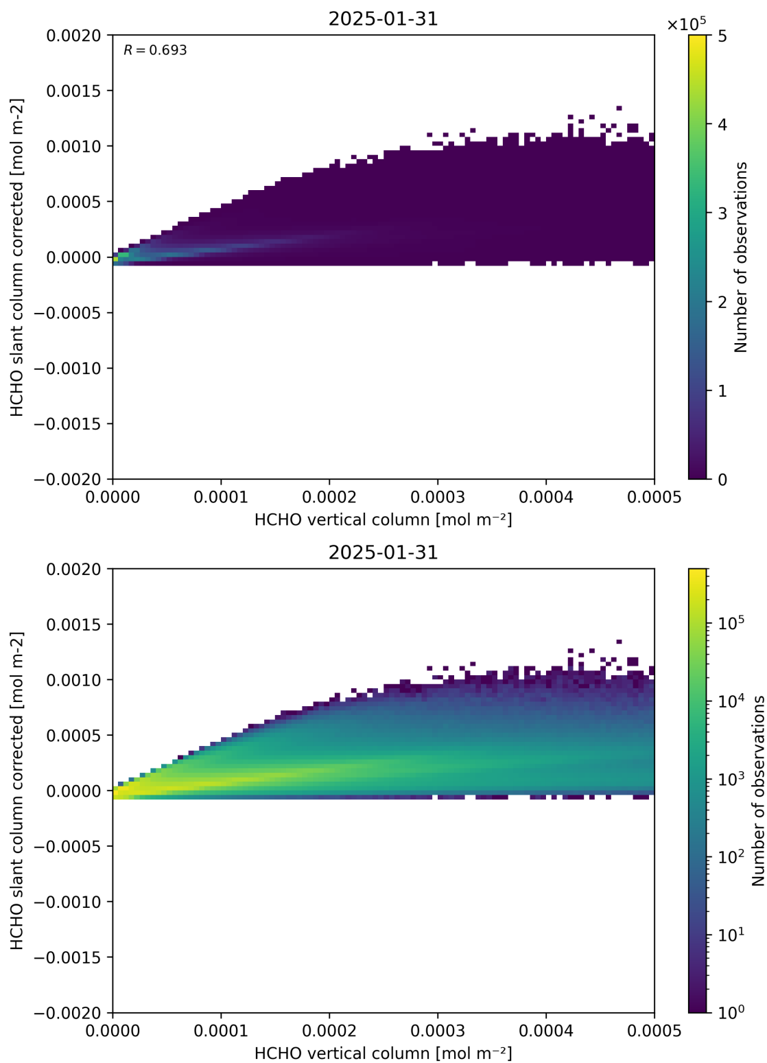
Figure 127: Scatter density plot of “HCHO vertical column” against “HCHO slant column corrected” for 2025-01-30 to 2025-02-01.
