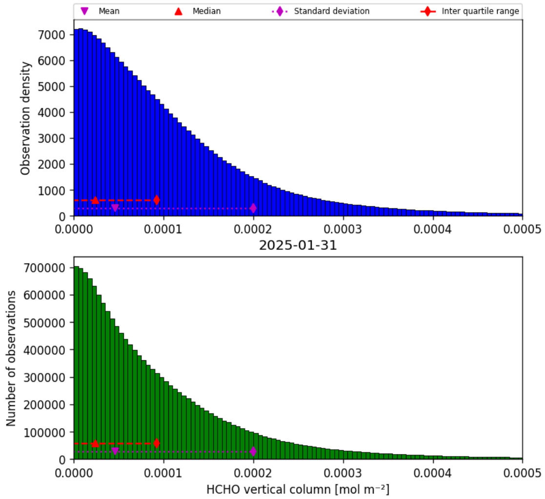
Figure 35: Histogram of “HCHO vertical column” for 2025-01-30 to 2025-02-01
