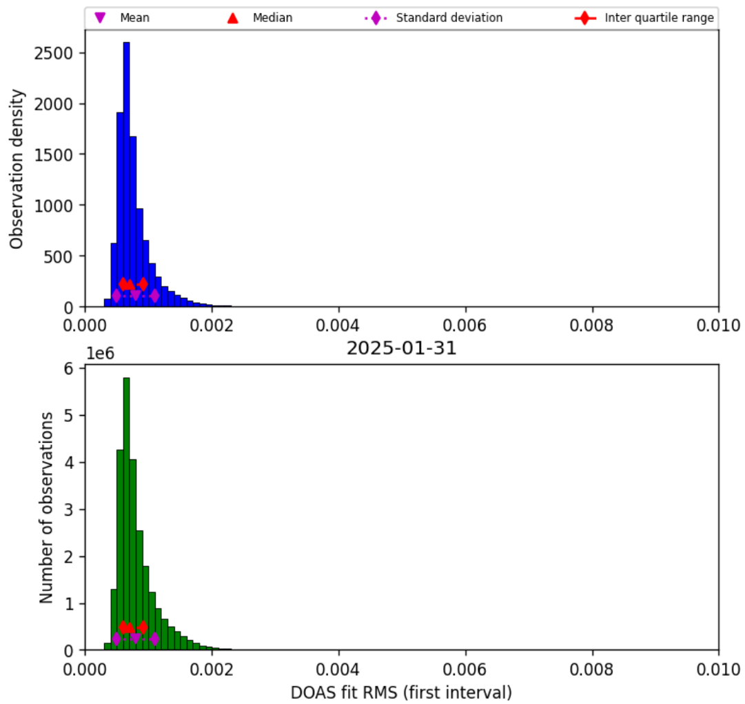
Figure 46: Histogram of “DOAS fit RMS (first interval)” for 2025-01-30 to 2025-02-01
