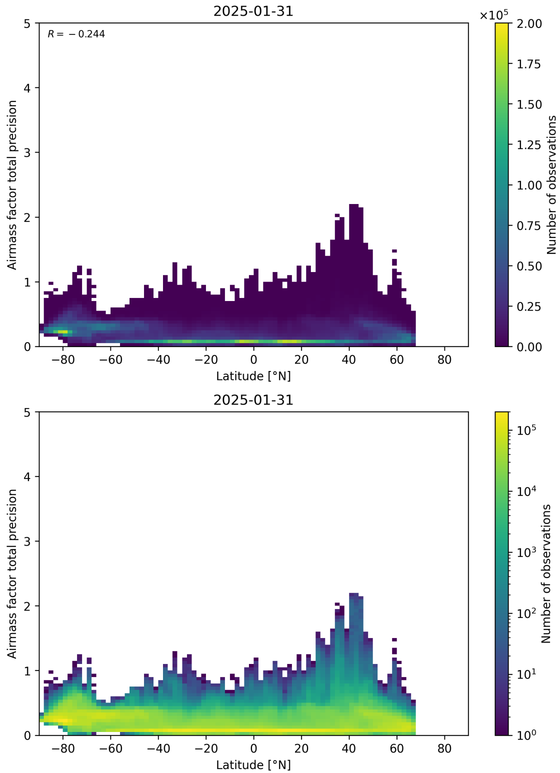
Figure 162: Scatter density plot of “Latitude” against “Airmass factor total precision” for 2025-01-30 to 2025-02-01.
