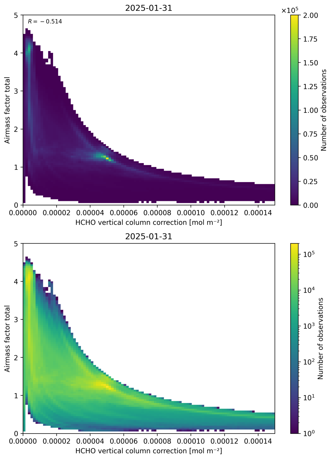
Figure 120: Scatter density plot of “HCHO vertical column correction” against “Airmass factor total” for 2025-01-30 to 2025-02-01.
