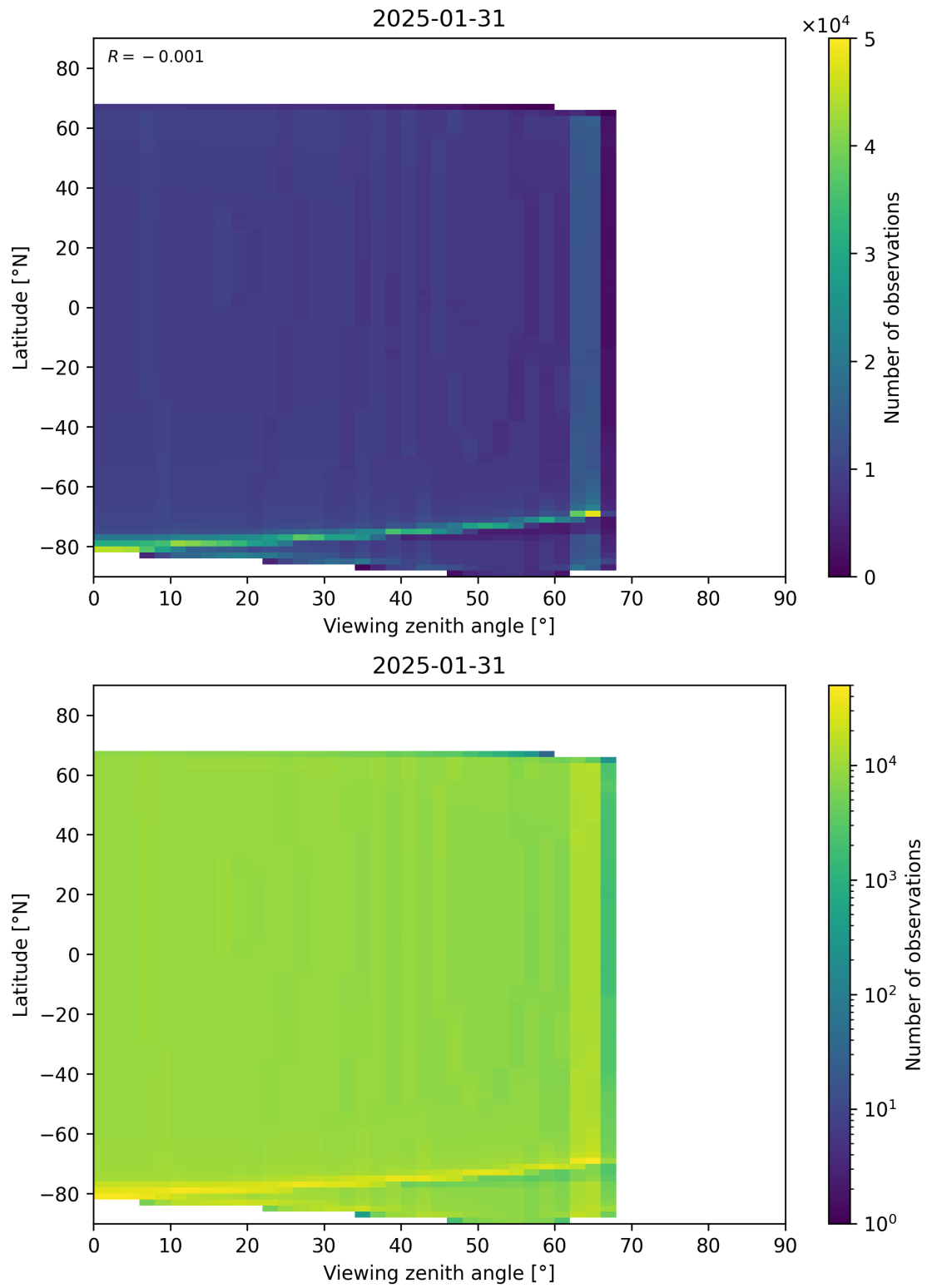
Figure 196: Scatter density plot of “Viewing zenith angle” against “Latitude” for 2025-01-30 to 2025-02-01.
