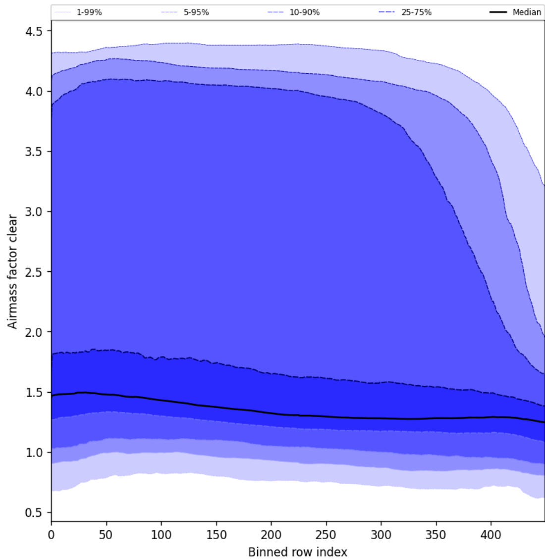
Figure 56: Along track statistics of “Airmass factor clear” for 2025-01-30 to 2025-02-01
