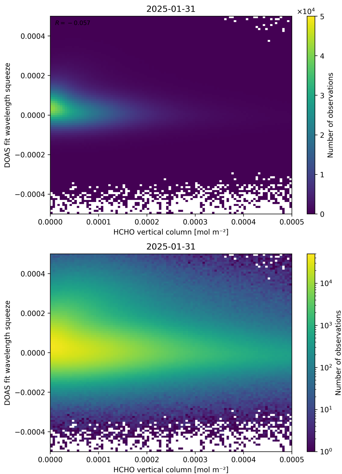
Figure 125: Scatter density plot of “HCHO vertical column” against “DOAS fit wavelength squeeze” for 2025-01-30 to 2025-02-01.
