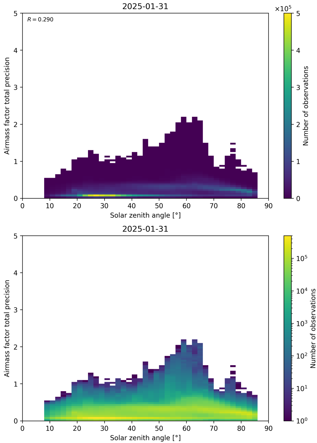
Figure 176: Scatter density plot of “Solar zenith angle” against “Airmass factor total precision” for 2025-01-30 to 2025-02-01.
