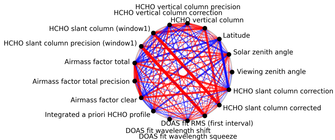
Figure 1: Map of correlation graph for 2025-01-30 to 2025-02-01.
