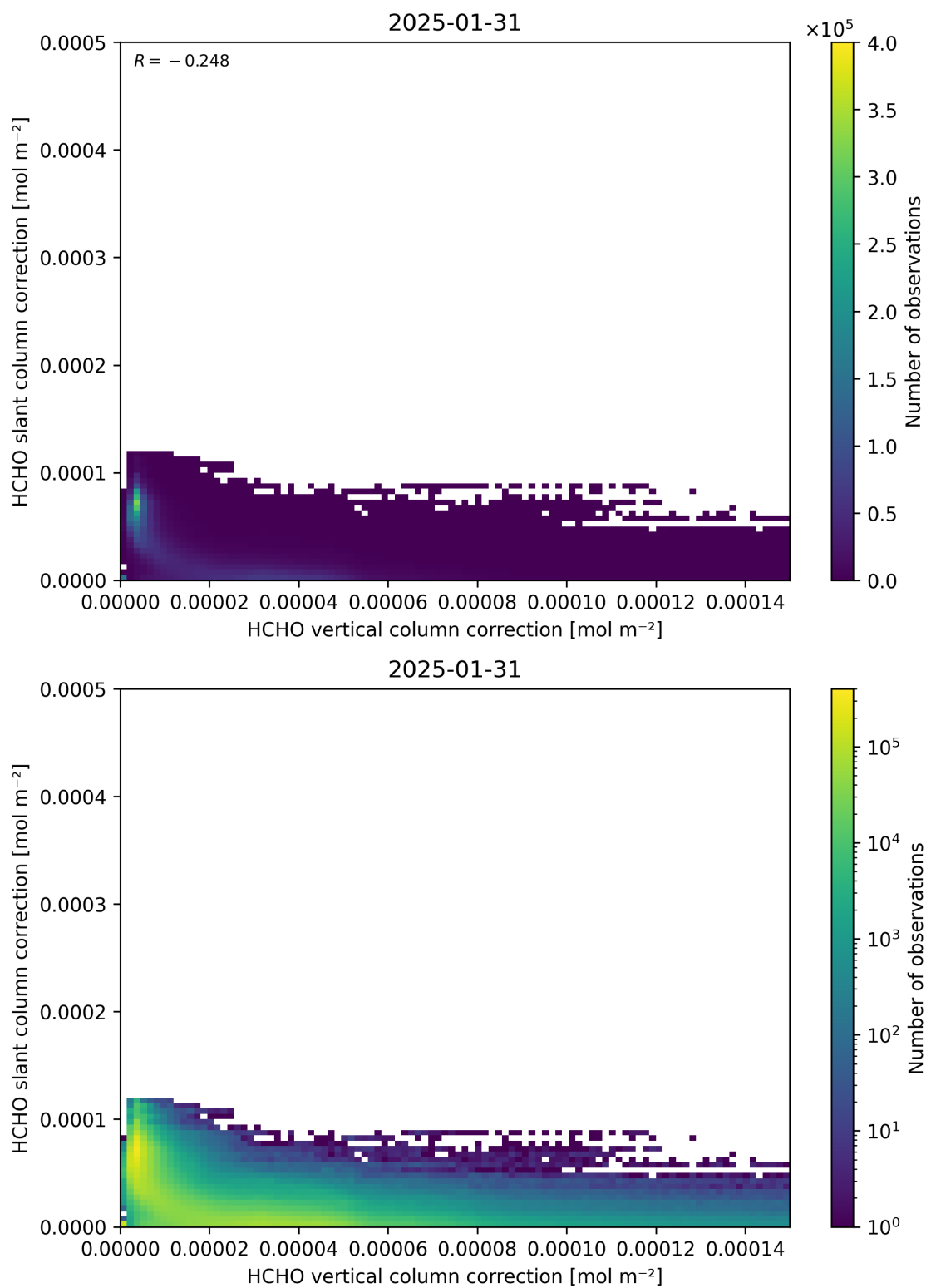
Figure 117: Scatter density plot of “HCHO vertical column correction” against “HCHO slant column correction” for 2025-01-30 to 2025-02-01.
