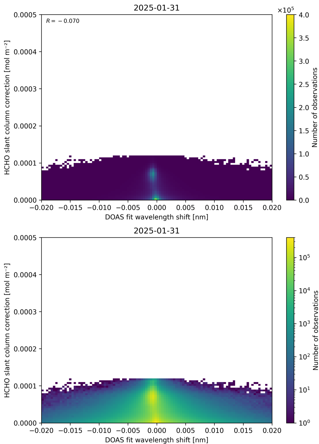
Figure 67: Scatter density plot of “DOAS fit wavelength shift” against “HCHO slant column correction” for 2025-01-30 to 2025-02-01.
