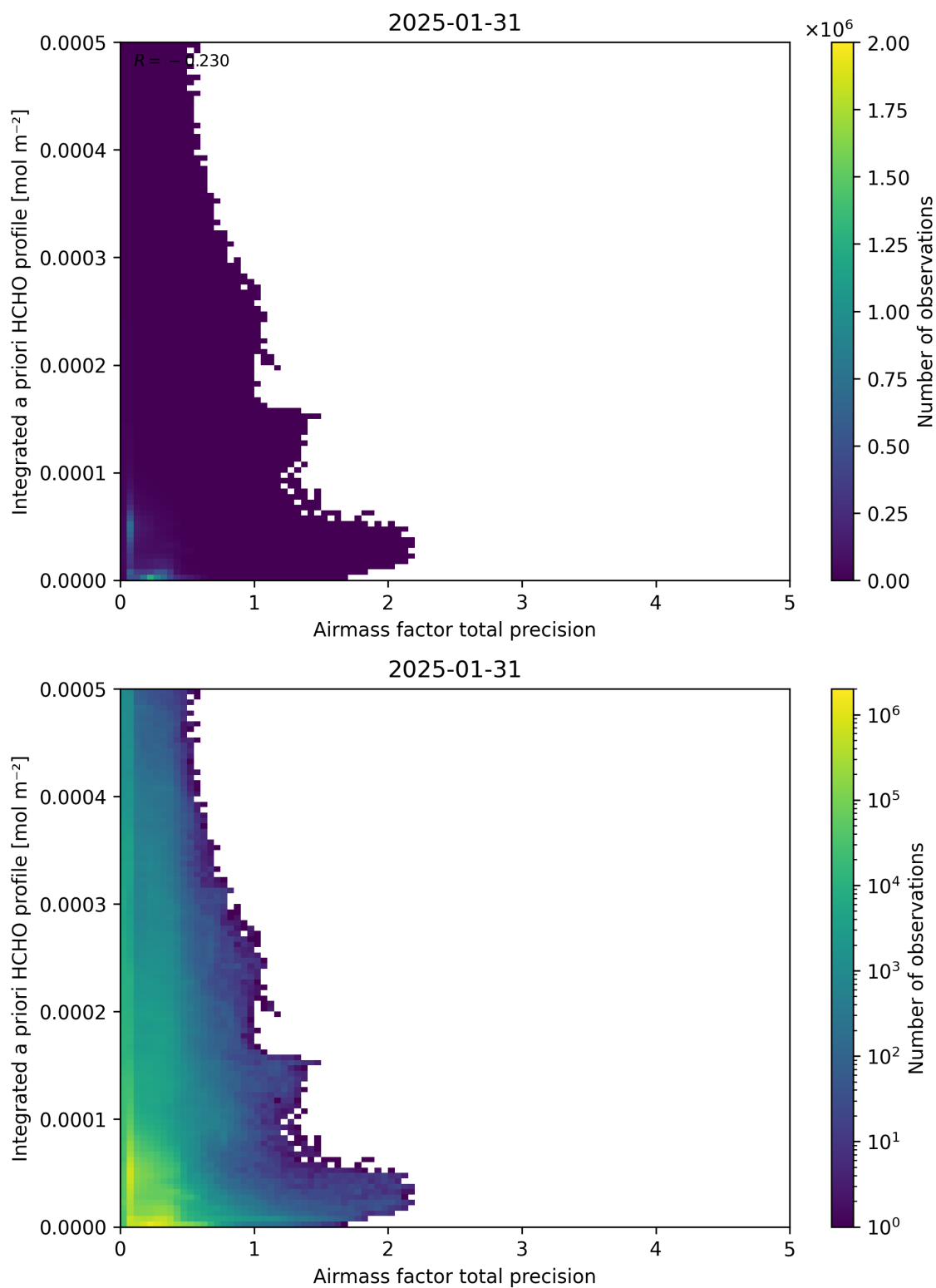
Figure 111: Scatter density plot of “Airmass factor total precision” against “Integrated a priori HCHO profile” for 2025-01-30 to 2025-02-01.
