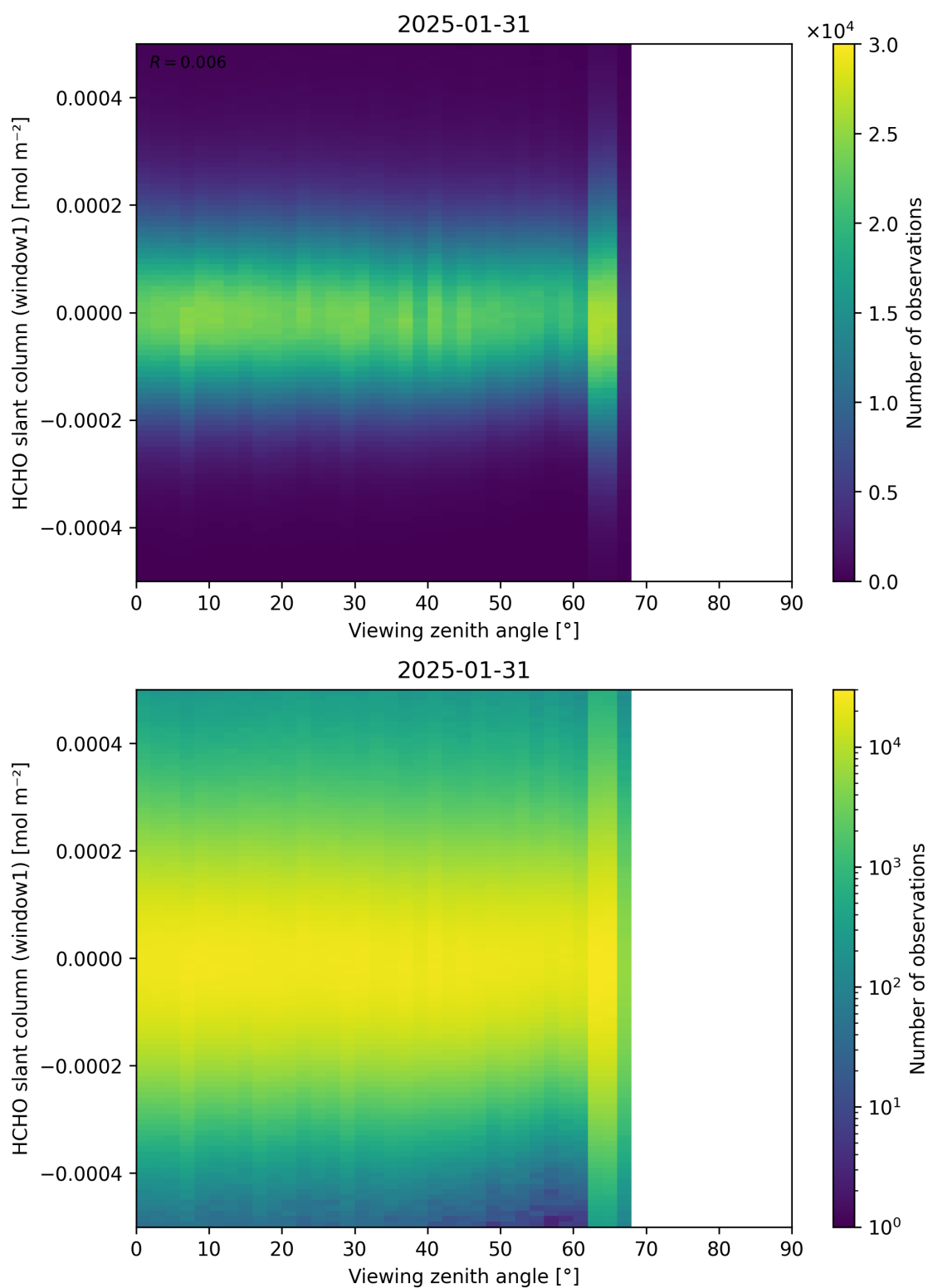
Figure 188: Scatter density plot of “Viewing zenith angle” against “HCHO slant column (window1)” for 2025-01-30 to 2025-02-01.
