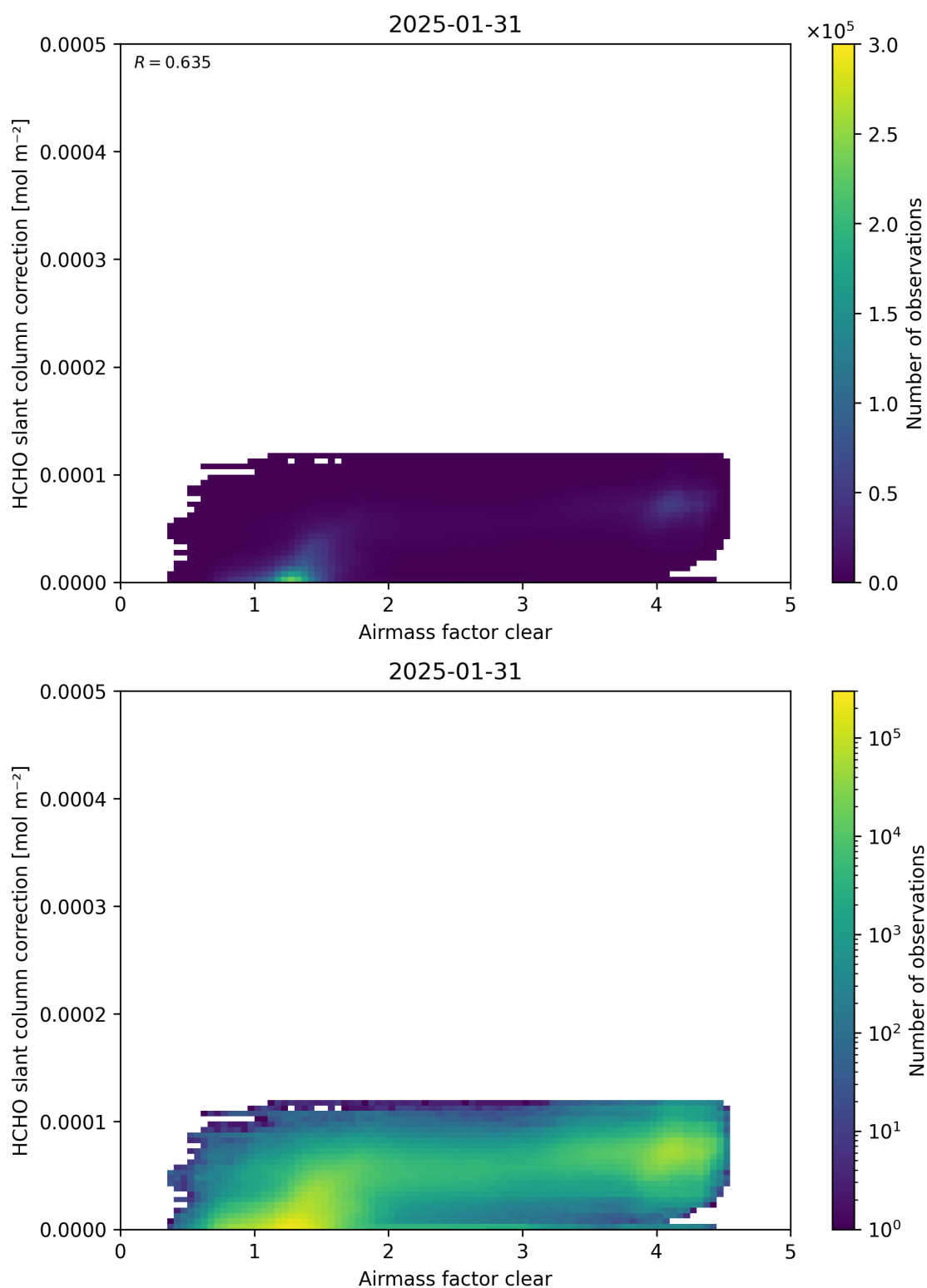
Figure 75: Scatter density plot of “Airmass factor clear” against “HCHO slant column correction” for 2025-01-30 to 2025-02-01.
