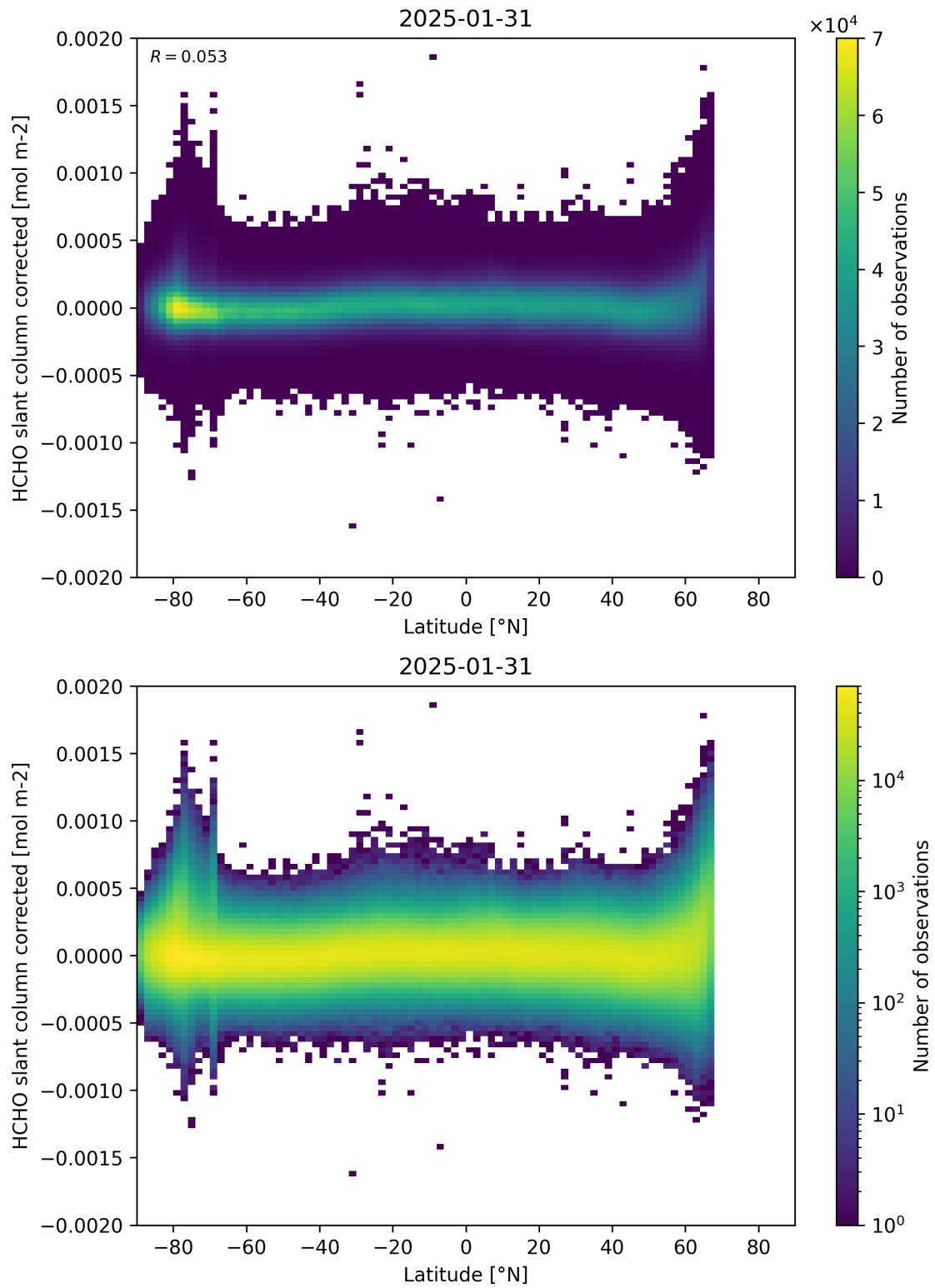
Figure 157: Scatter density plot of “Latitude” against “HCHO slant column corrected” for 2025-01-30 to 2025-02-01.
