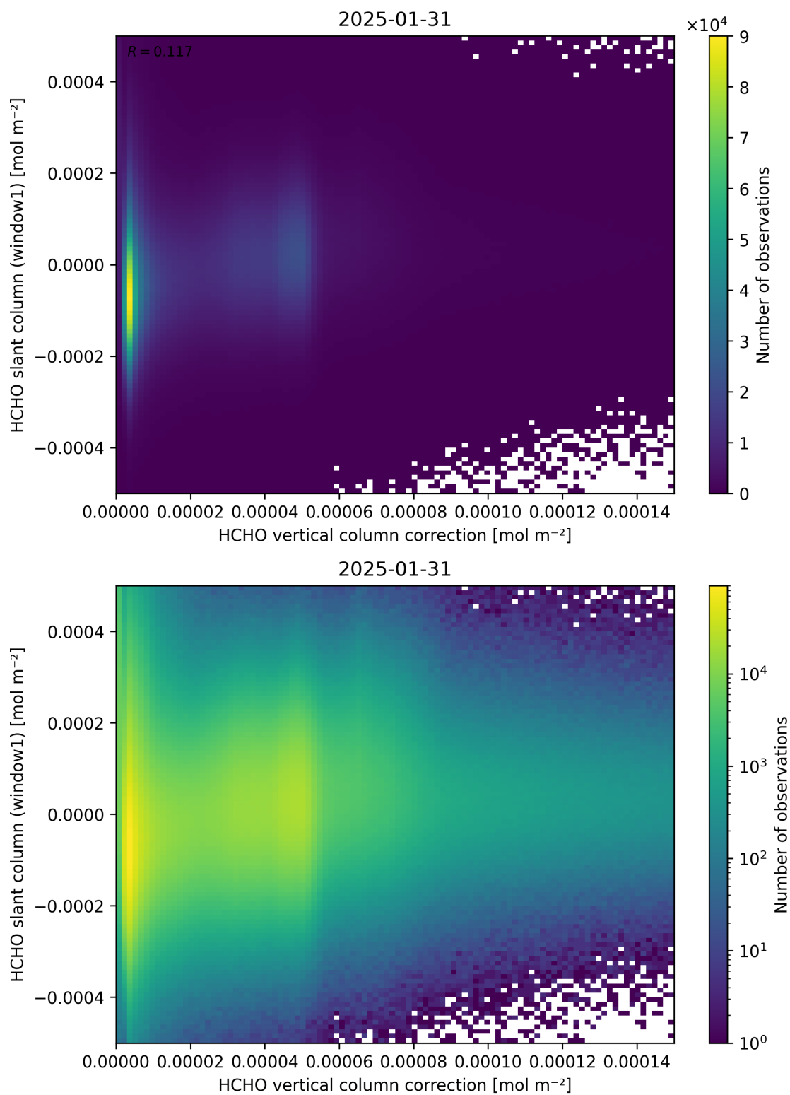
Figure 118: Scatter density plot of “HCHO vertical column correction” against “HCHO slant column (window1)” for 2025-01-30 to 2025-02-01.
