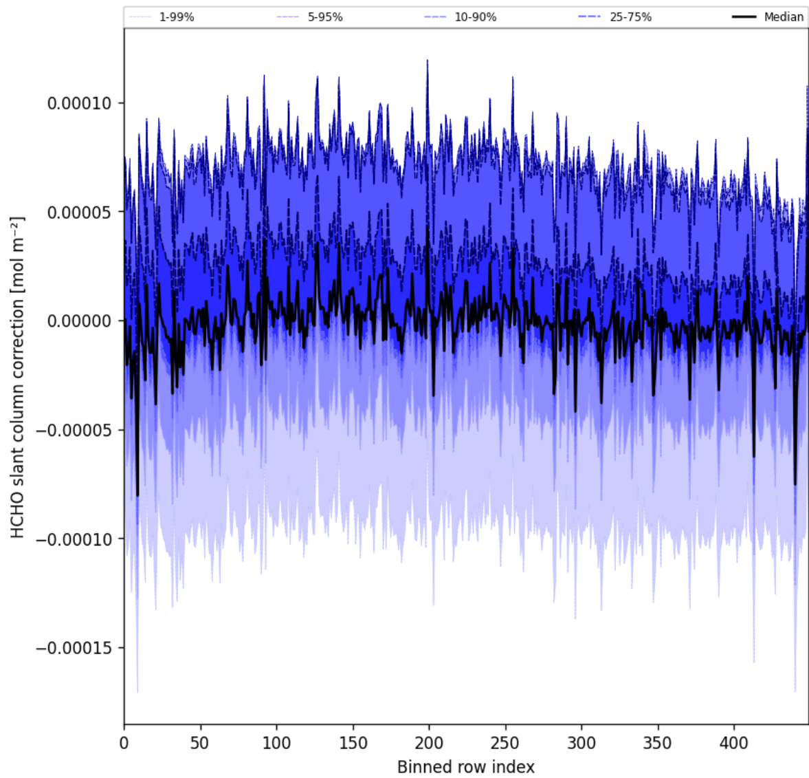
Figure 61: Along track statistics of “HCHO slant column correction” for 2025-01-30 to 2025-02-01
