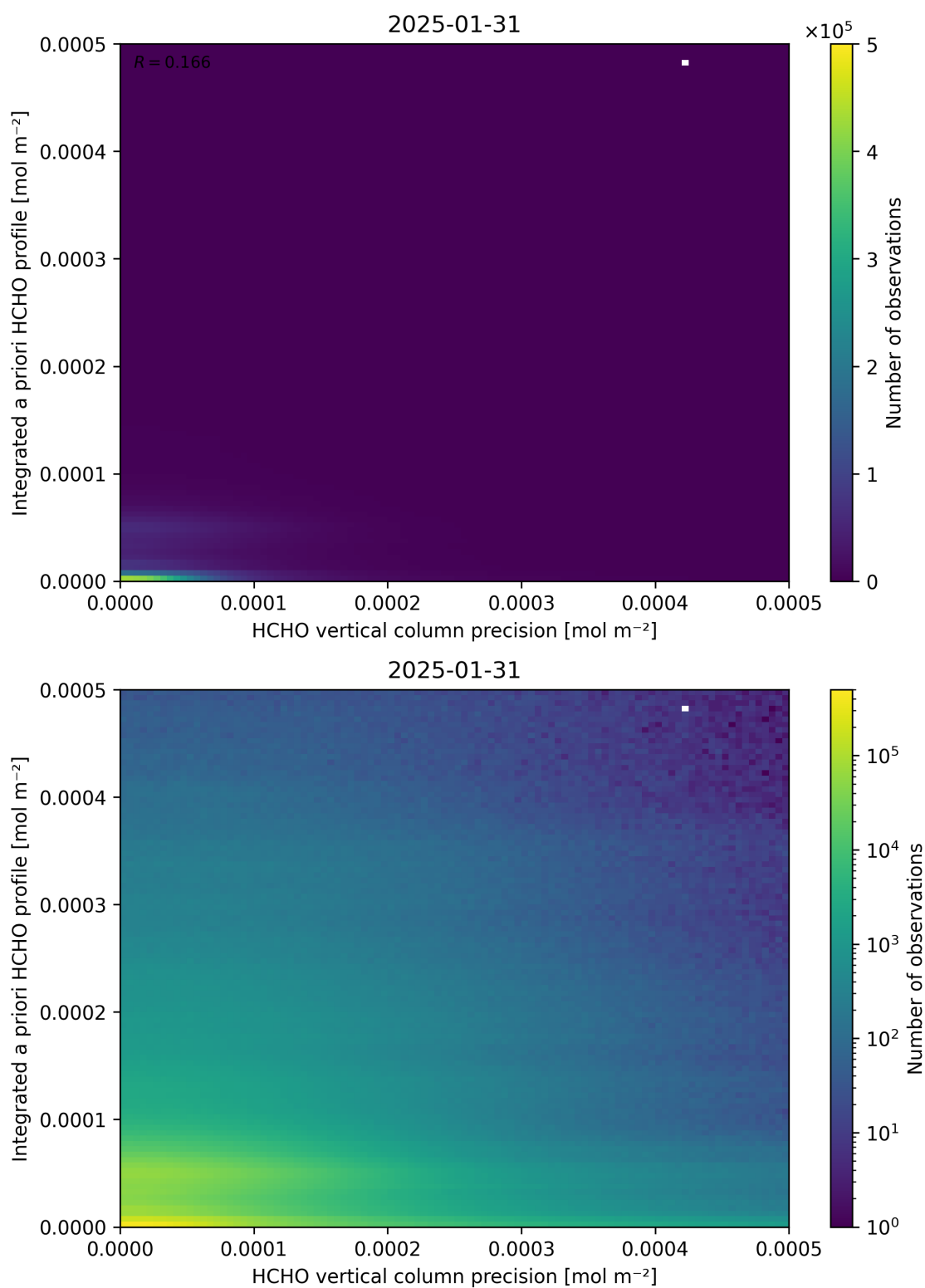
Figure 147: Scatter density plot of “HCHO vertical column precision” against “Integrated a priori HCHO profile” for 2025-01-30 to 2025-02-01.
