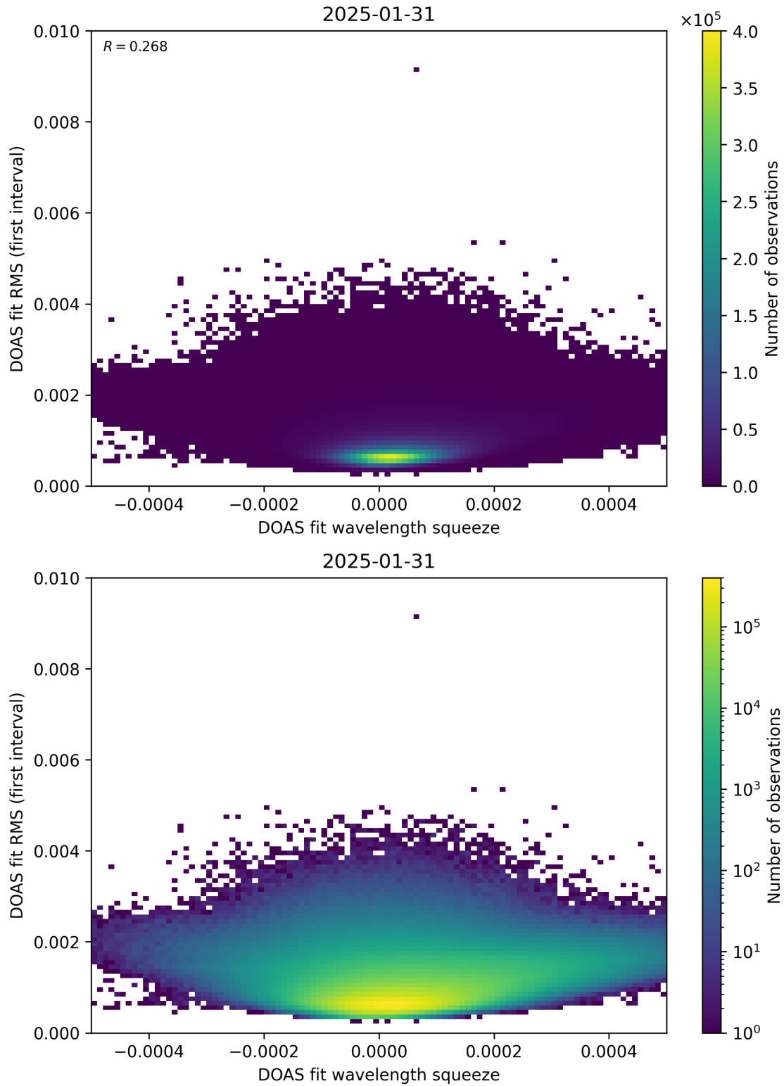
Figure 68: Scatter density plot of “DOAS fit wavelength squeeze” against “DOAS fit RMS (first interval)” for 2025-01-30 to 2025-02-01.
