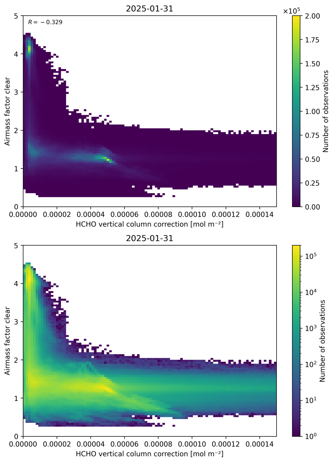
Figure 115: Scatter density plot of “HCHO vertical column correction” against “Airmass factor clear” for 2025-01-30 to 2025-02-01.
