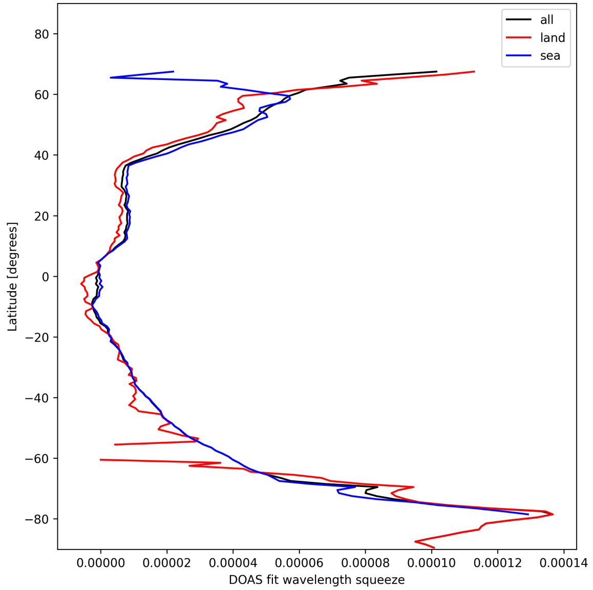
Figure 31: Zonal average of “DOAS fit wavelength squeeze” for 2025-01-30 to 2025-02-01.
