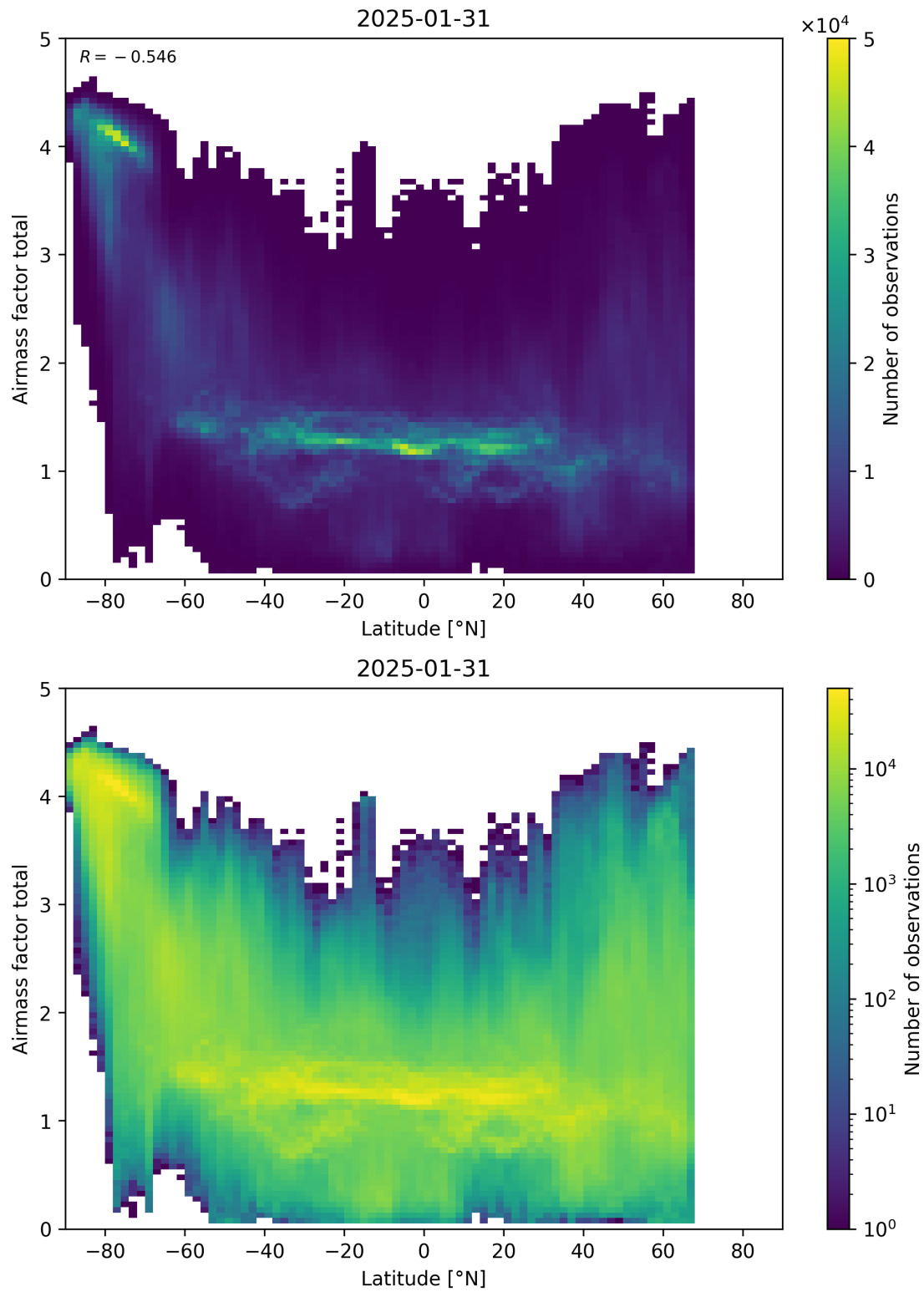
Figure 161: Scatter density plot of “Latitude” against “Airmass factor total” for 2025-01-30 to 2025-02-01.
