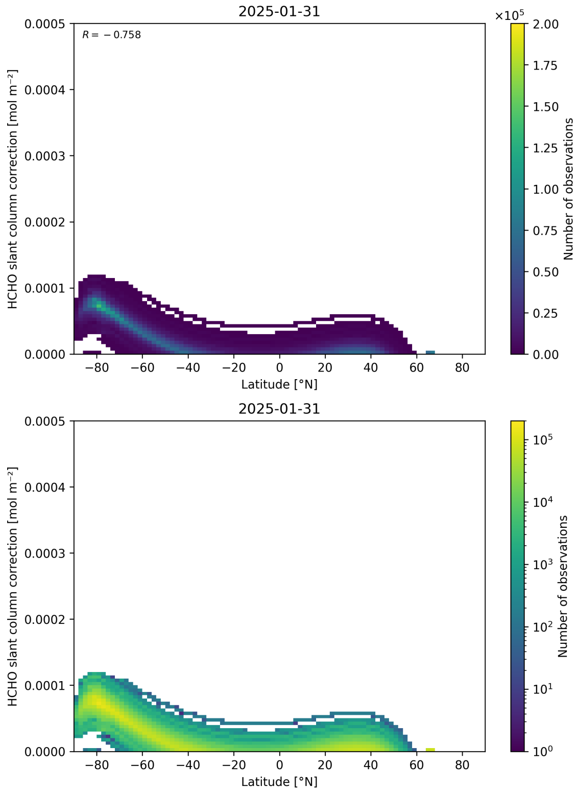
Figure 158: Scatter density plot of “Latitude” against “HCHO slant column correction” for 2025-01-30 to 2025-02-01.
