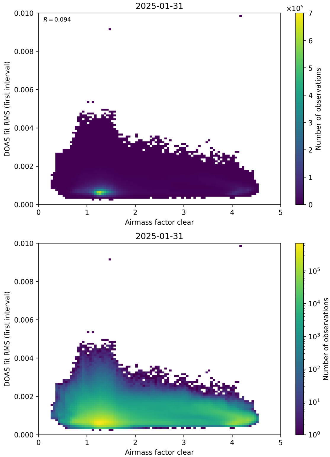
Figure 71: Scatter density plot of “Airmass factor clear” against “DOAS fit RMS (first interval)” for 2025-01-30 to 2025-02-01.
