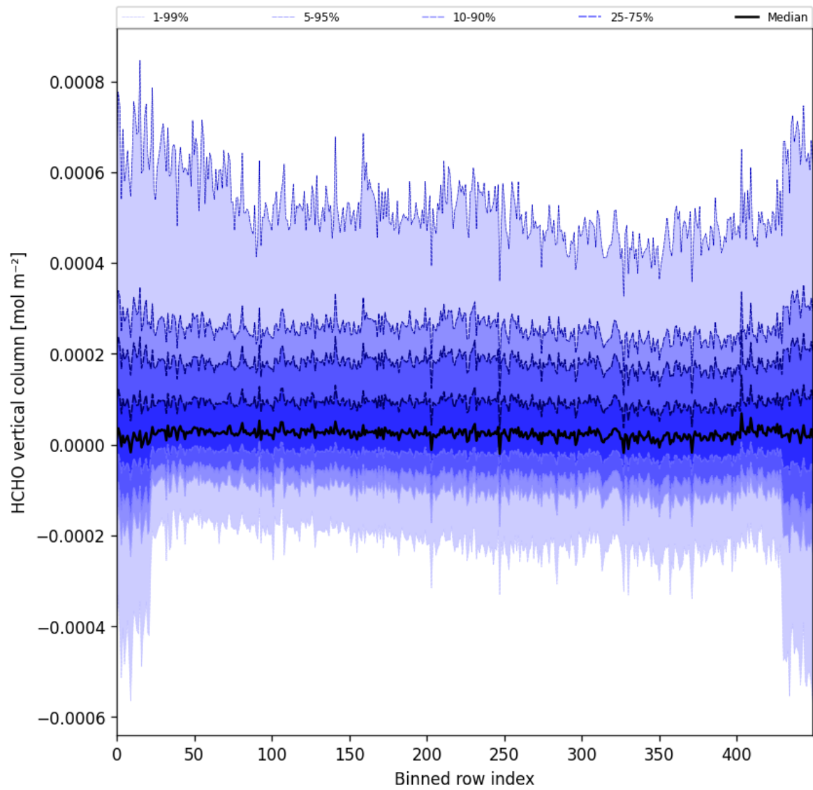
Figure 49: Along track statistics of “HCHO vertical column” for 2025-01-30 to 2025-02-01
