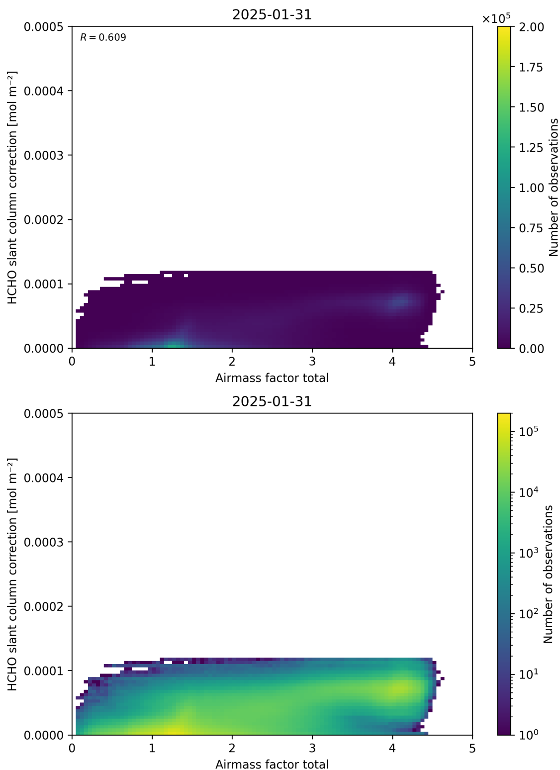
Figure 102: Scatter density plot of “Airmass factor total” against “HCHO slant column correction” for 2025-01-30 to 2025-02-01.
