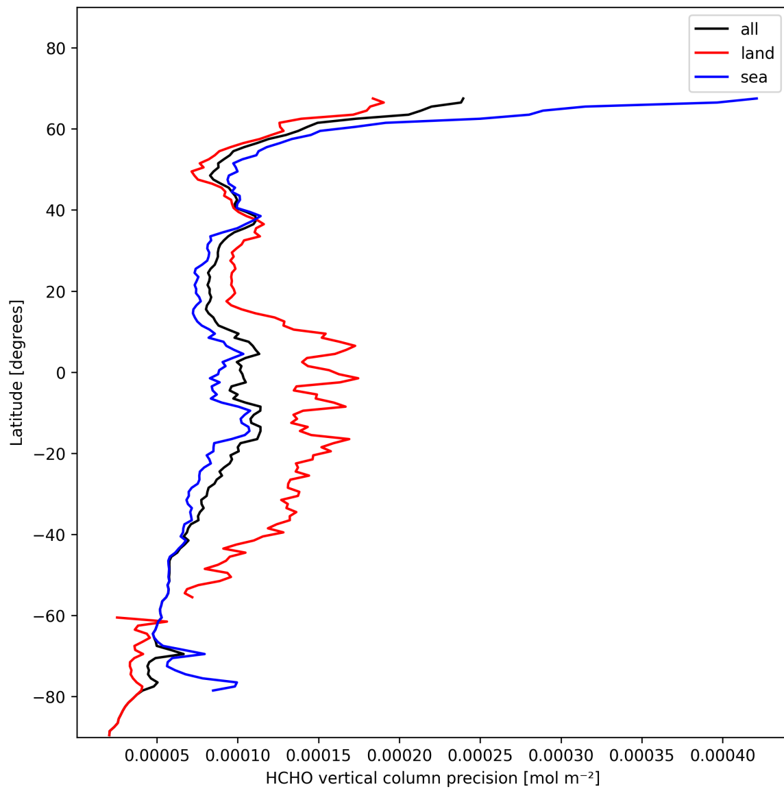
Figure 22: Zonal average of “HCHO vertical column precision” for 2025-01-30 to 2025-02-01.
