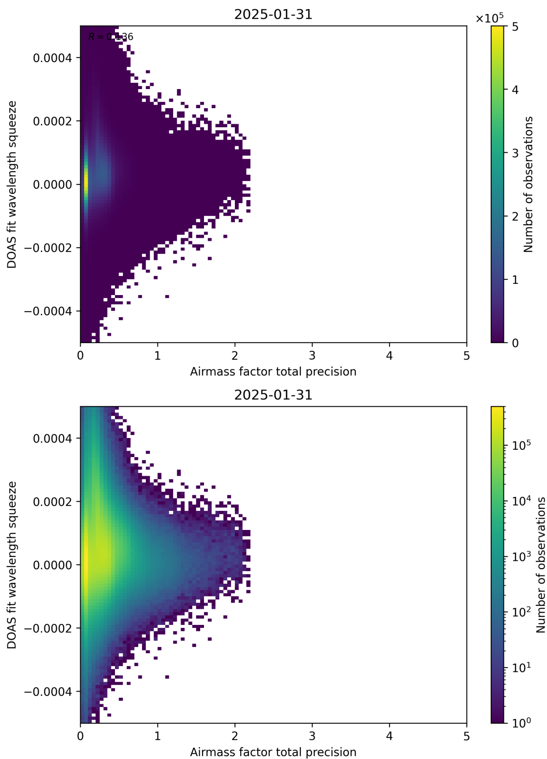
Figure 107: Scatter density plot of “Airmass factor total precision” against “DOAS fit wavelength squeeze” for 2025-01-30 to 2025-02-01.
