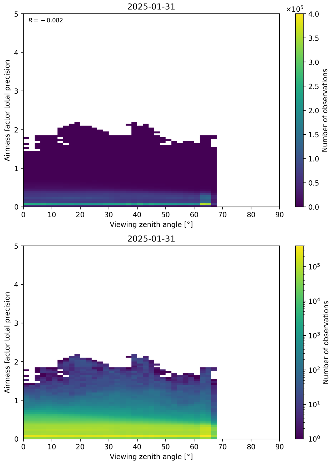
Figure 191: Scatter density plot of “Viewing zenith angle” against “Airmass factor total precision” for 2025-01-30 to 2025-02-01.
