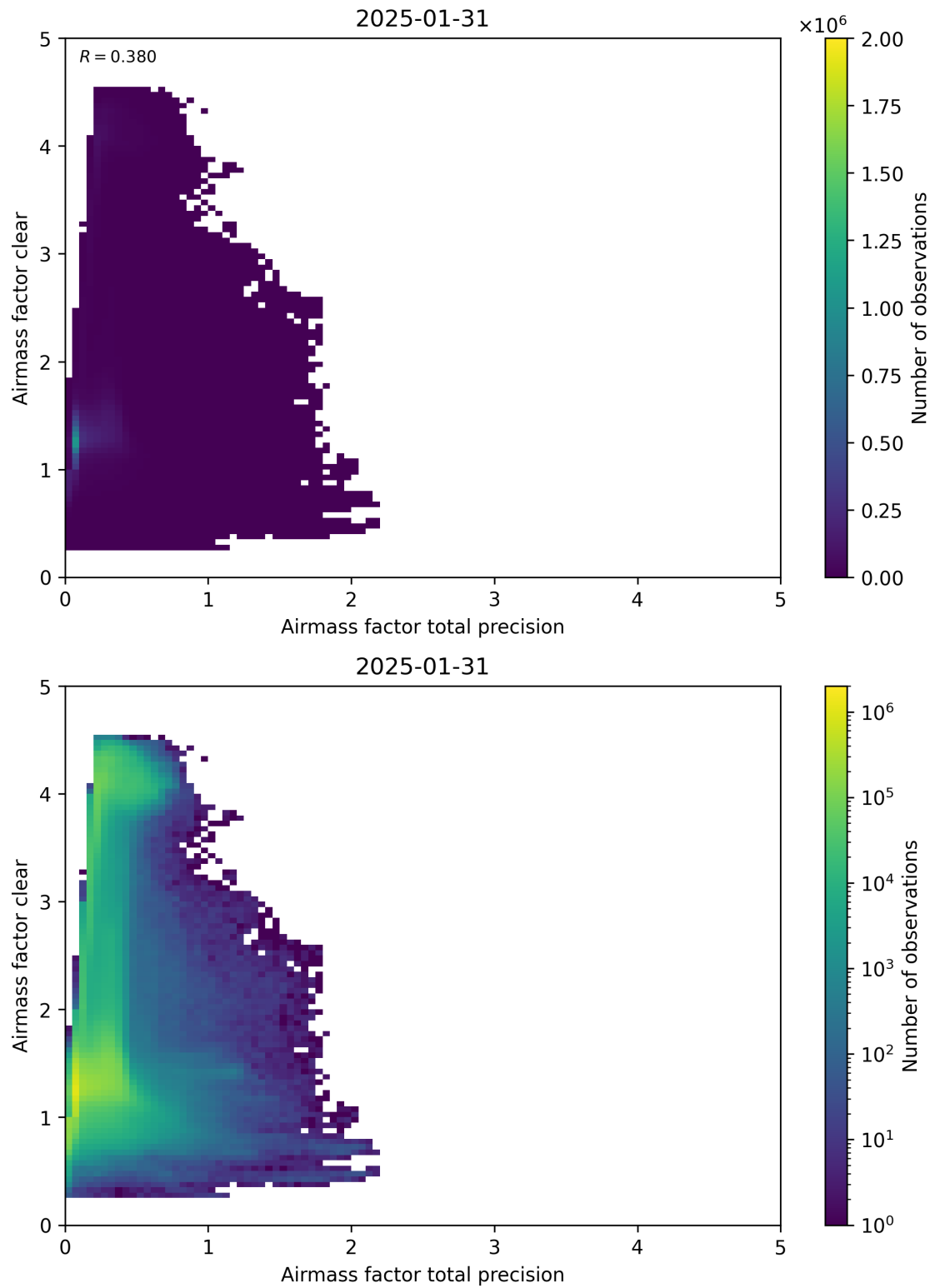
Figure 108: Scatter density plot of “Airmass factor total precision” against “Airmass factor clear” for 2025-01-30 to 2025-02-01.
