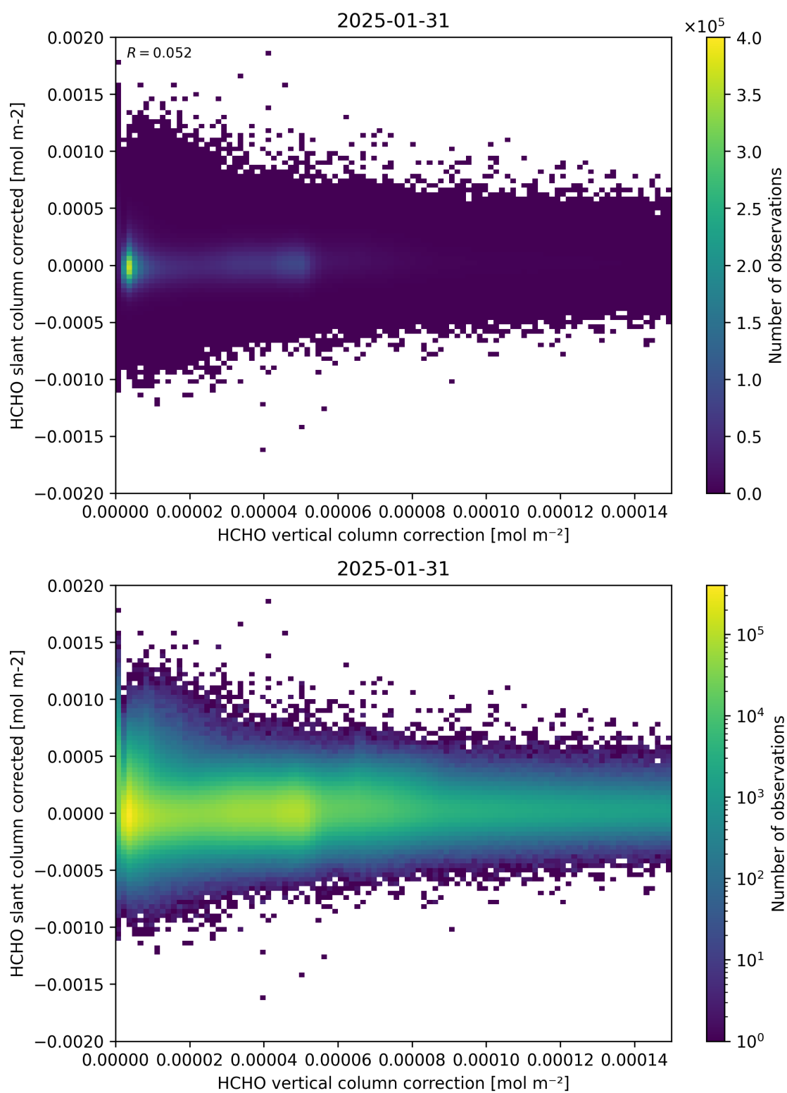
Figure 116: Scatter density plot of “HCHO vertical column correction” against “HCHO slant column corrected” for 2025-01-30 to 2025-02-01.
