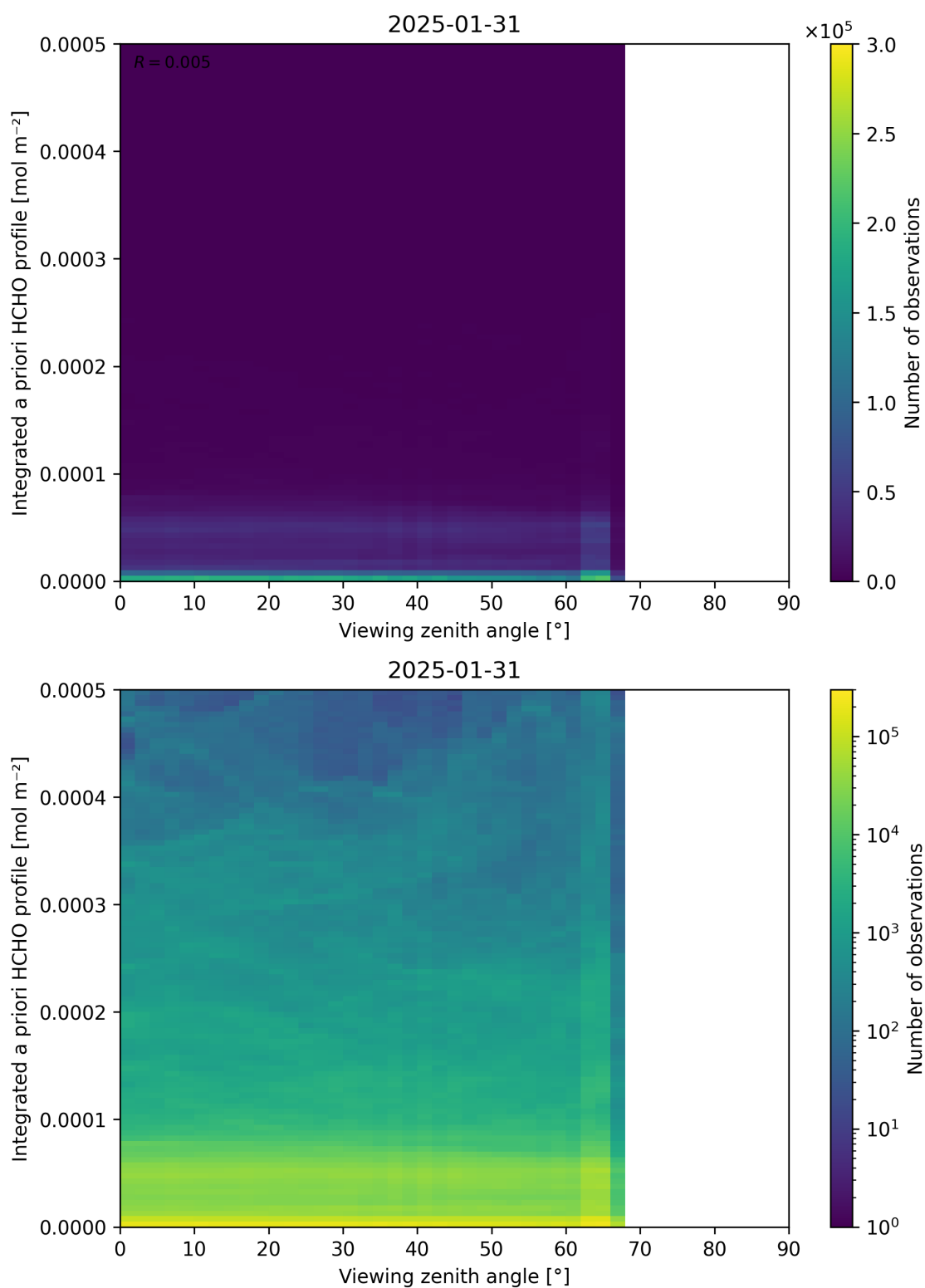
Figure 195: Scatter density plot of “Viewing zenith angle” against “Integrated a priori HCHO profile” for 2025-01-30 to 2025-02-01.
