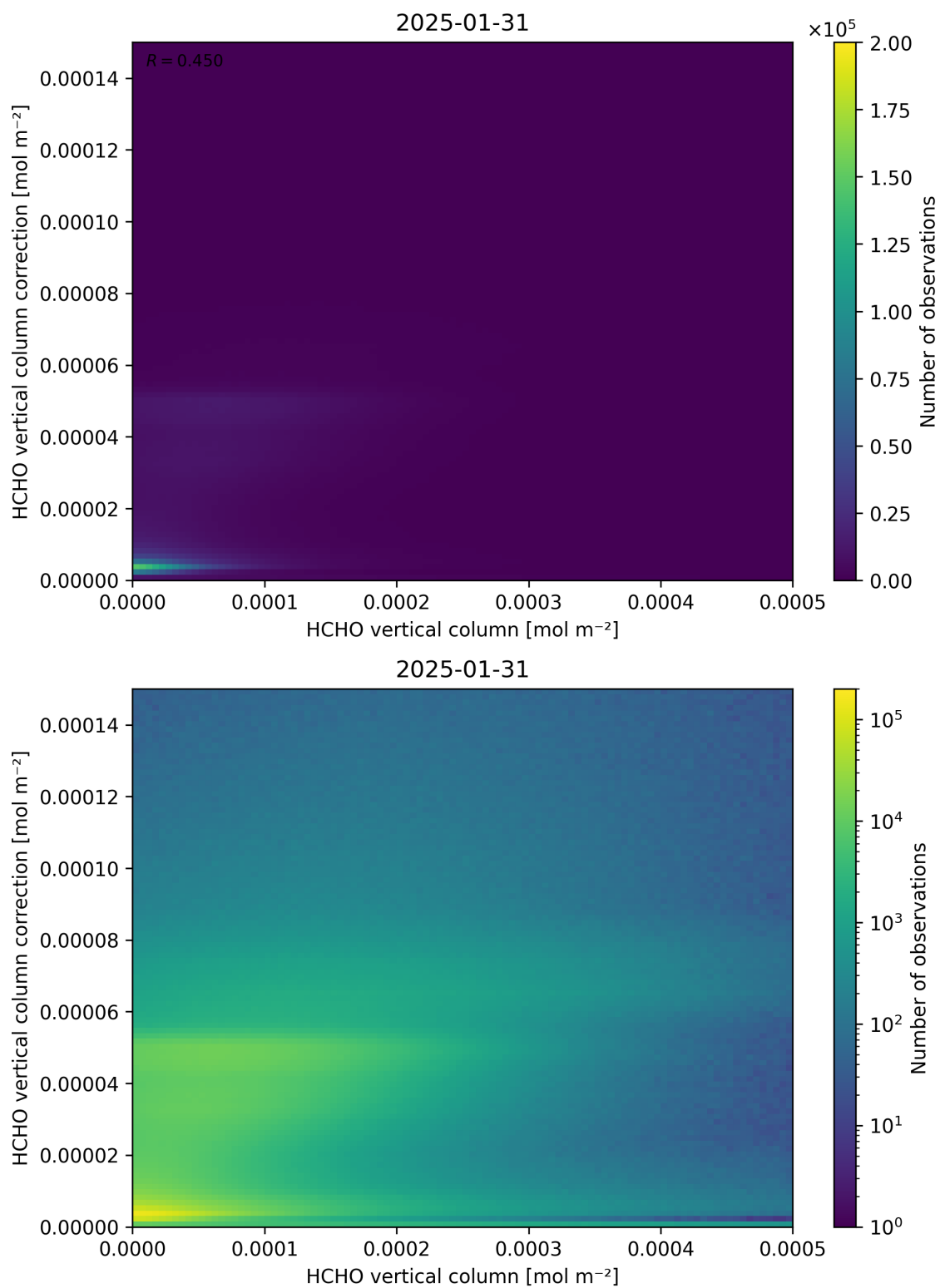
Figure 133: Scatter density plot of “HCHO vertical column” against “HCHO vertical column correction” for 2025-01-30 to 2025-02-01.
