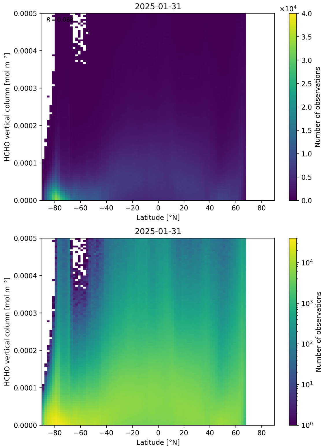
Figure 163: Scatter density plot of “Latitude” against “HCHO vertical column” for 2025-01-30 to 2025-02-01.
