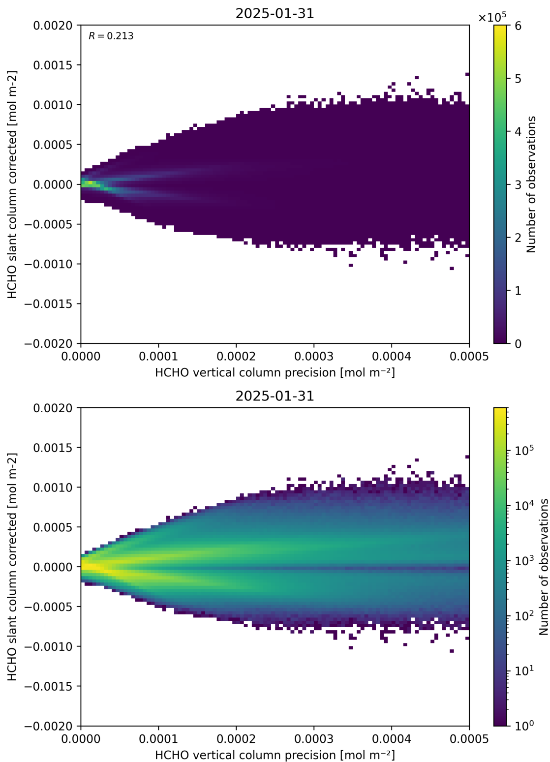
Figure 140: Scatter density plot of “HCHO vertical column precision” against “HCHO slant column corrected” for 2025-01-30 to 2025-02-01.
