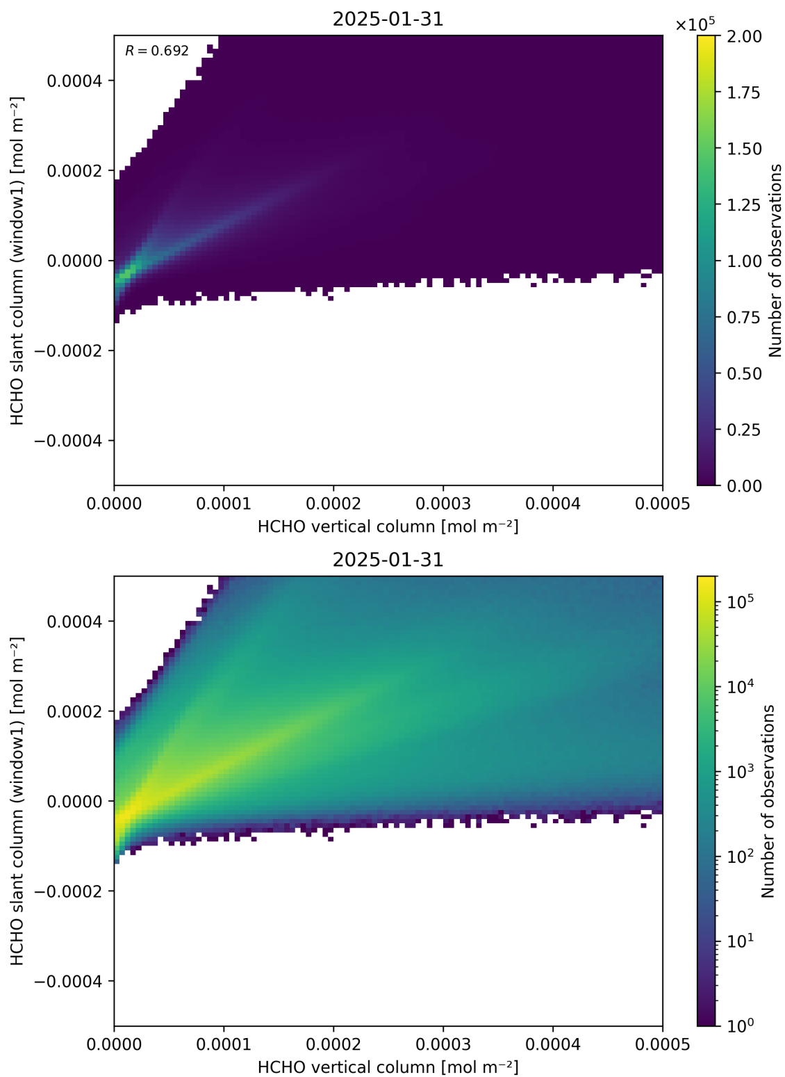
Figure 129: Scatter density plot of “HCHO vertical column” against “HCHO slant column (window1)” for 2025-01-30 to 2025-02-01.
