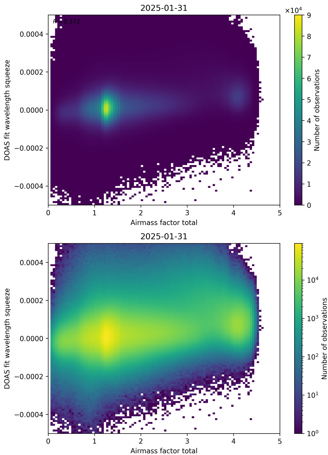
Figure 99: Scatter density plot of “Airmass factor total” against “DOAS fit wavelength squeeze” for 2025-01-30 to 2025-02-01.
