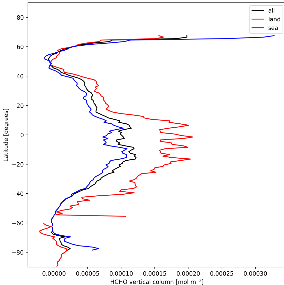
Figure 21: Zonal average of “HCHO vertical column” for 2025-01-30 to 2025-02-01.
