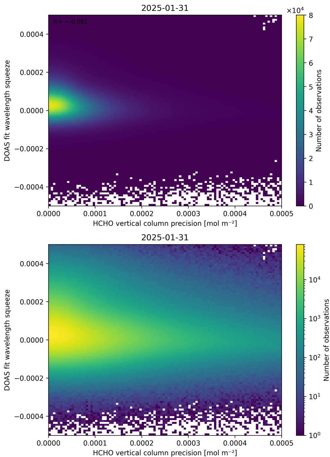
Figure 138: Scatter density plot of “HCHO vertical column precision” against “DOAS fit wavelength squeeze” for 2025-01-30 to 2025-02-01.
