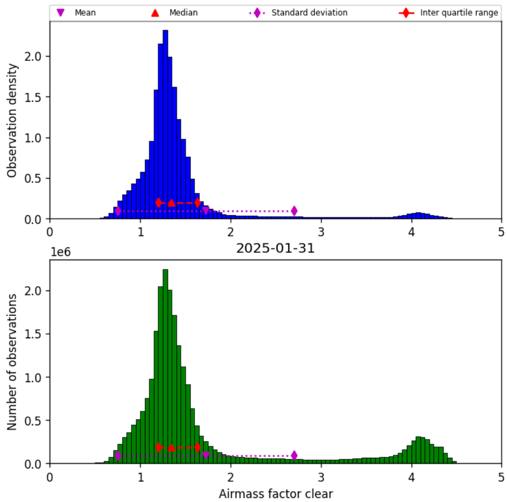
Figure 42: Histogram of “Airmass factor clear” for 2025-01-30 to 2025-02-01
