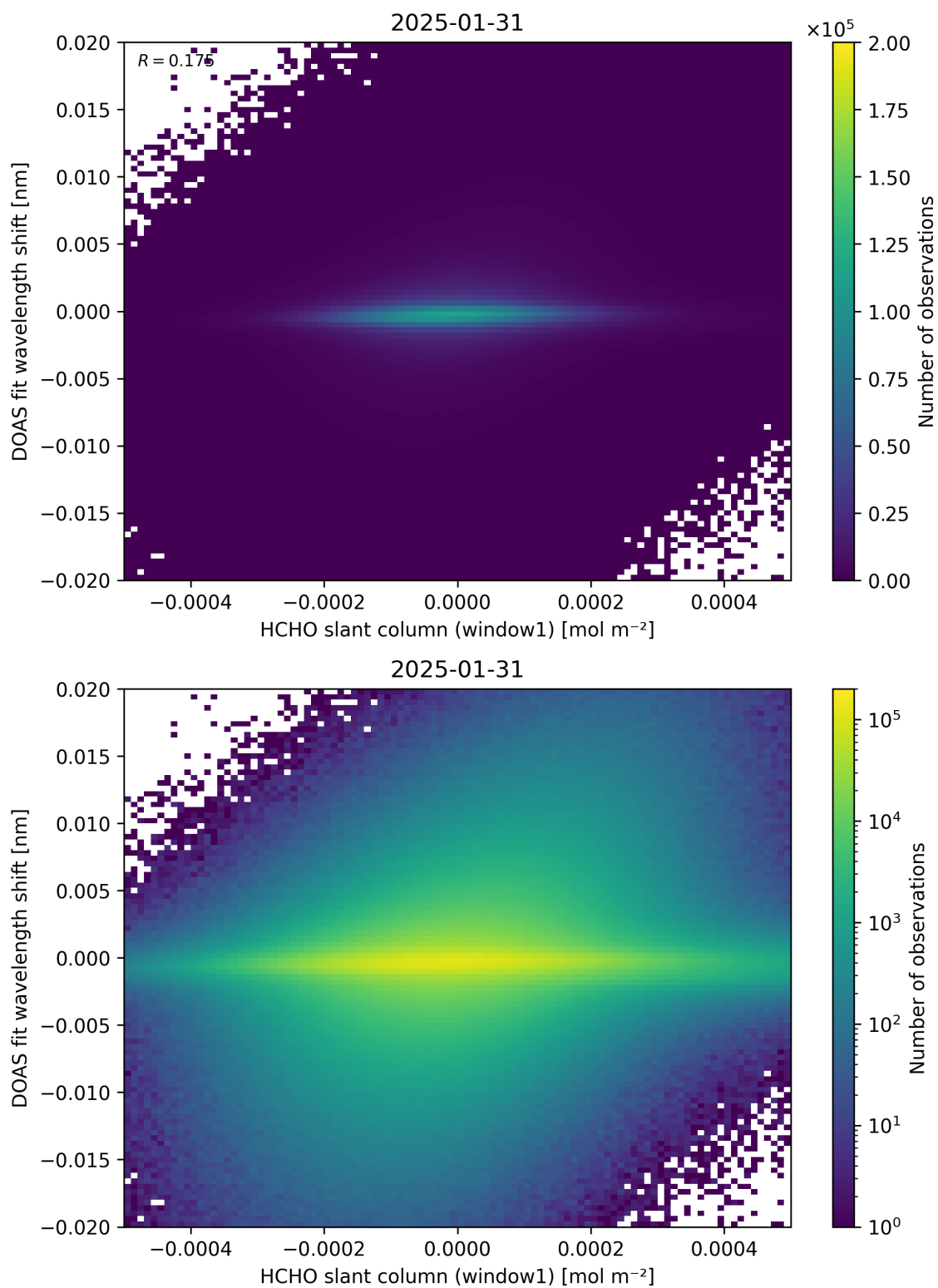
Figure 79: Scatter density plot of “HCHO slant column (window1)” against “DOAS fit wavelength shift” for 2025-01-30 to 2025-02-01.
