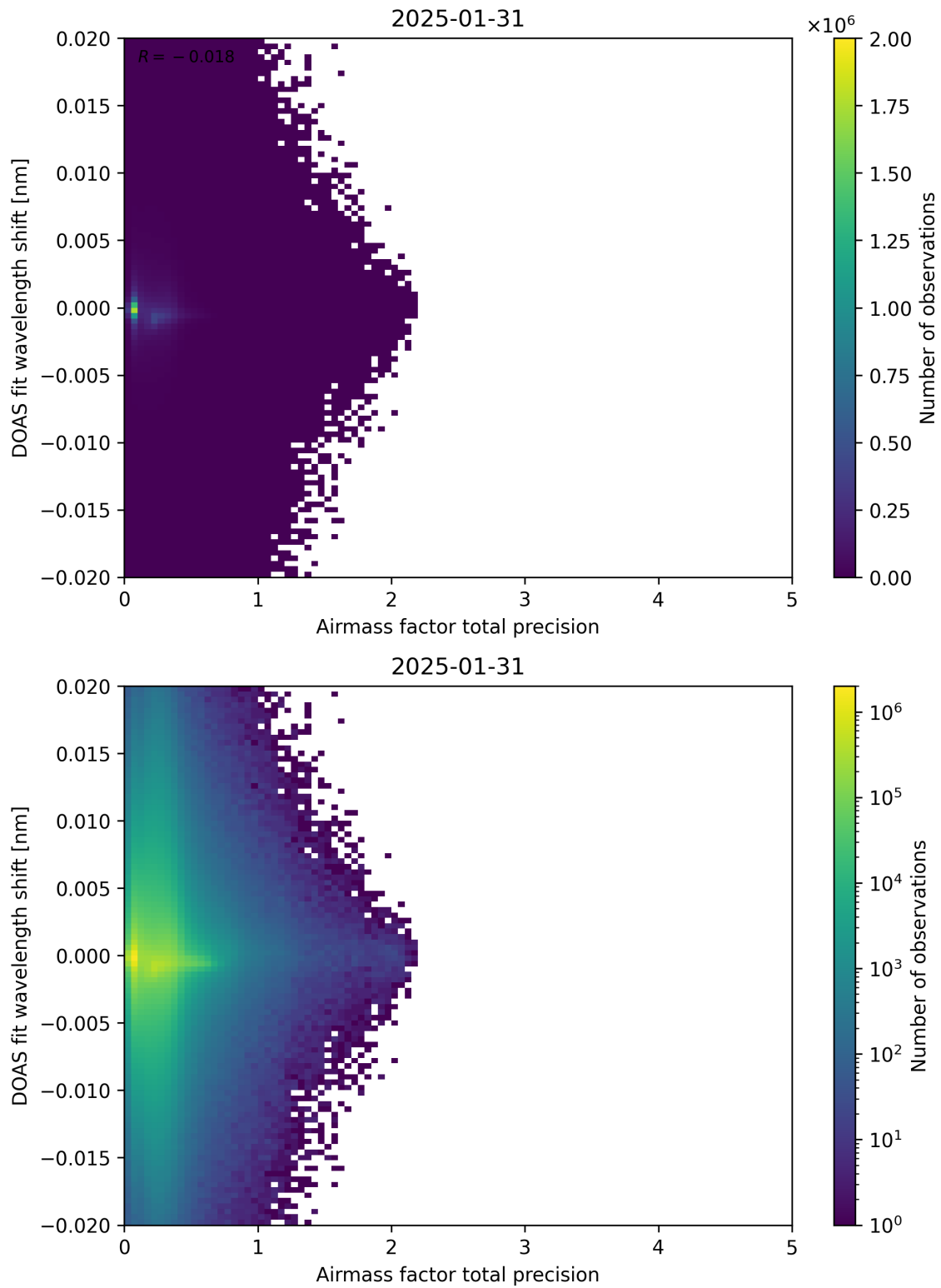
Figure 106: Scatter density plot of “Airmass factor total precision” against “DOAS fit wavelength shift” for 2025-01-30 to 2025-02-01.
