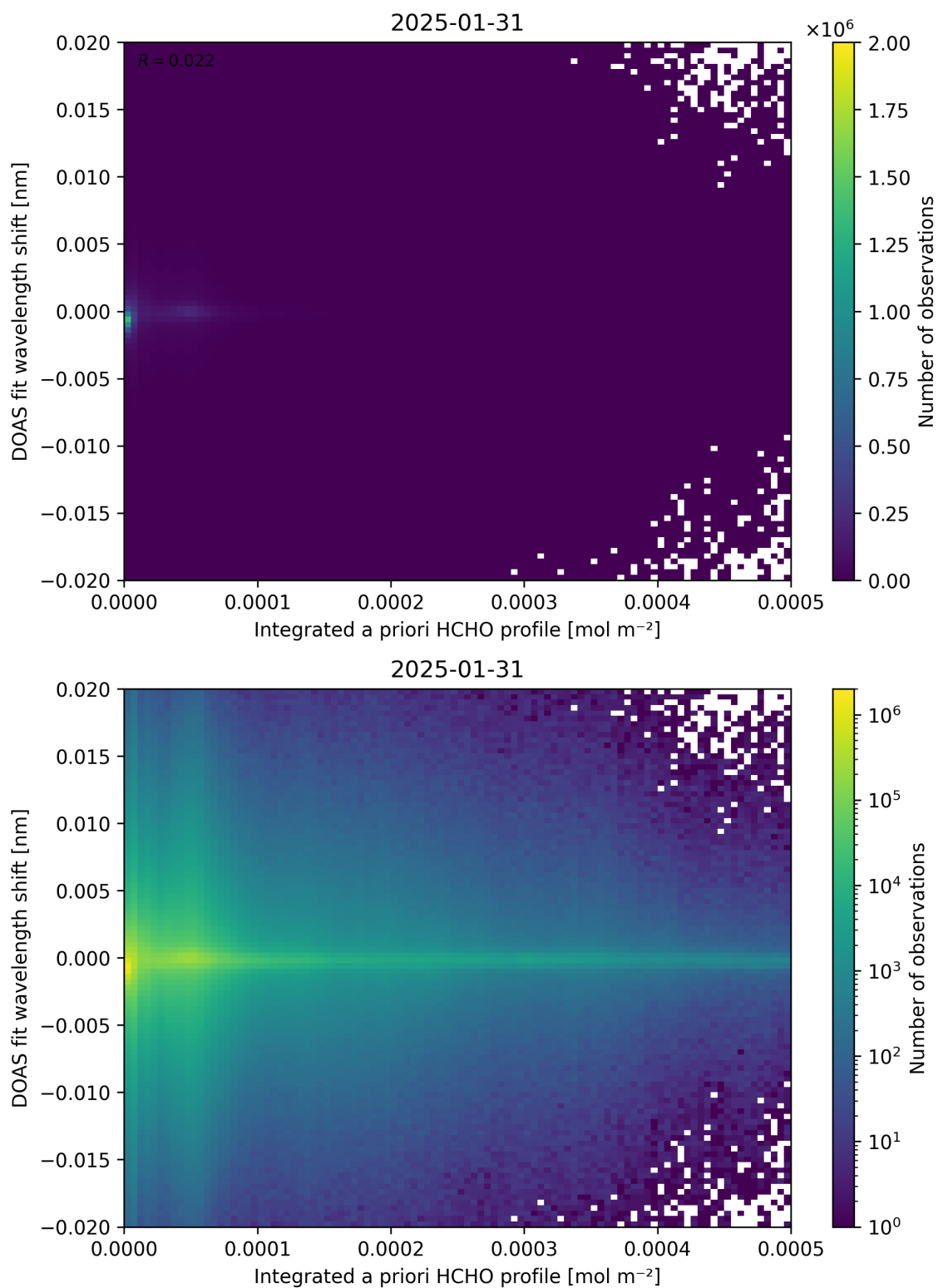
Figure 149: Scatter density plot of “Integrated a priori HCHO profile” against “DOAS fit wavelength shift” for 2025-01-30 to 2025-02-01.
