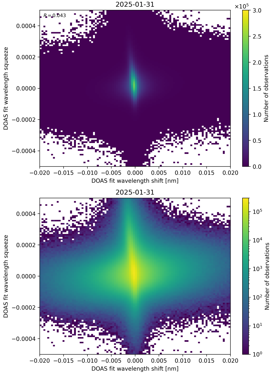
Figure 65: Scatter density plot of “DOAS fit wavelength shift” against “DOAS fit wavelength squeeze” for 2025-01-30 to 2025-02-01.
