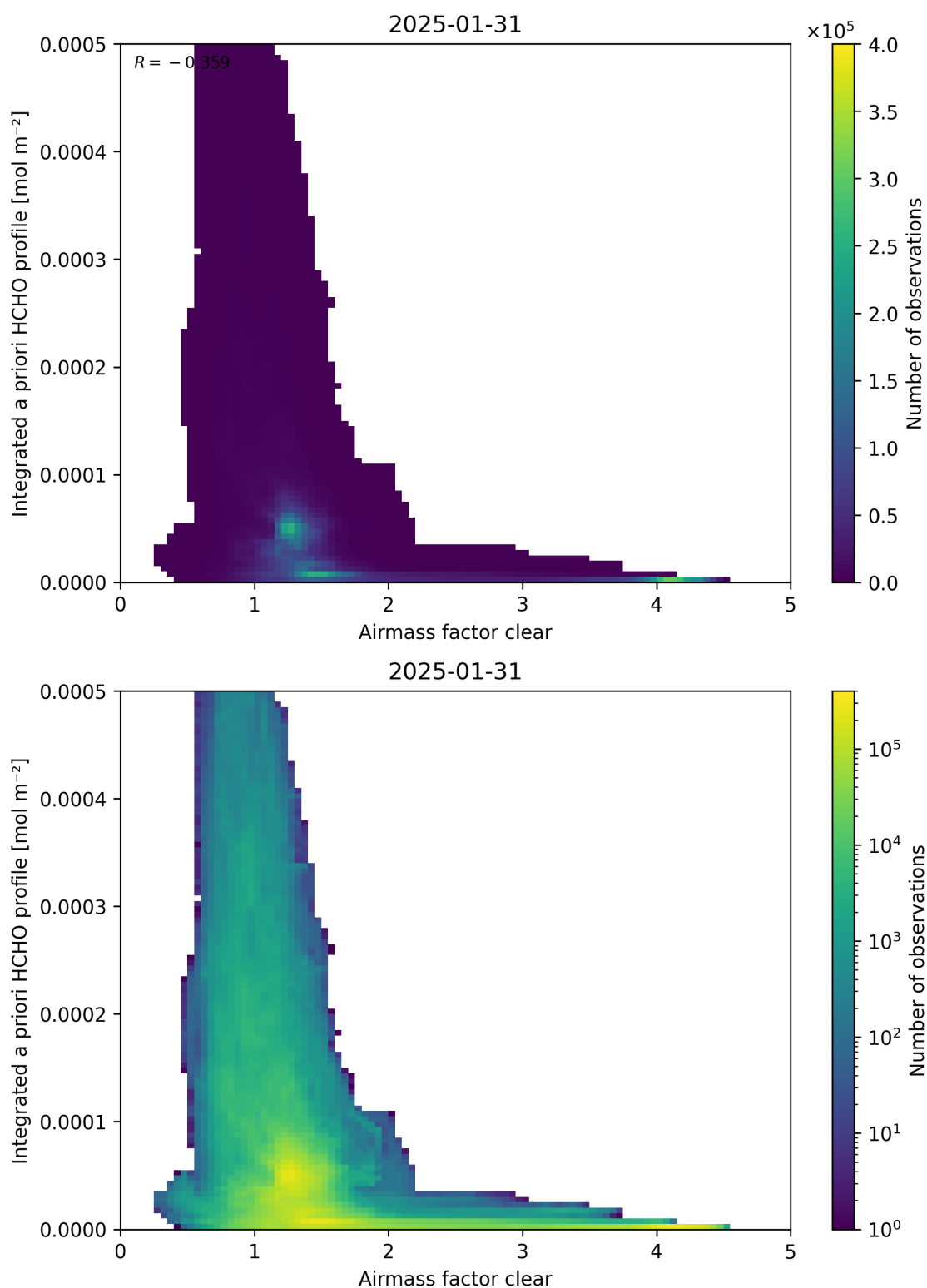
Figure 76: Scatter density plot of “Airmass factor clear” against “Integrated a priori HCHO profile” for 2025-01-30 to 2025-02-01.
