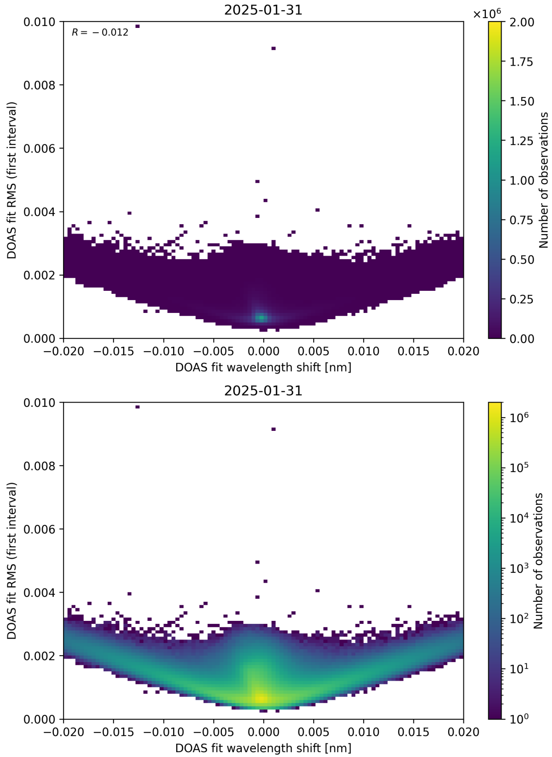
Figure 64: Scatter density plot of “DOAS fit wavelength shift” against “DOAS fit RMS (first interval)” for 2025-01-30 to 2025-02-01.
