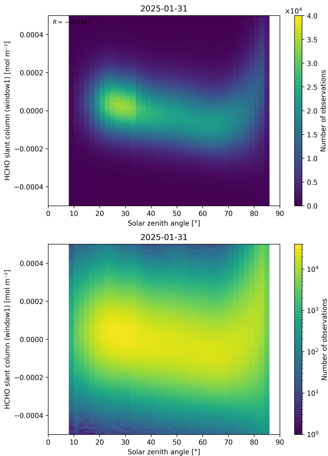
Figure 173: Scatter density plot of “Solar zenith angle” against “HCHO slant column (window1)” for 2025-01-30 to 2025-02-01.
