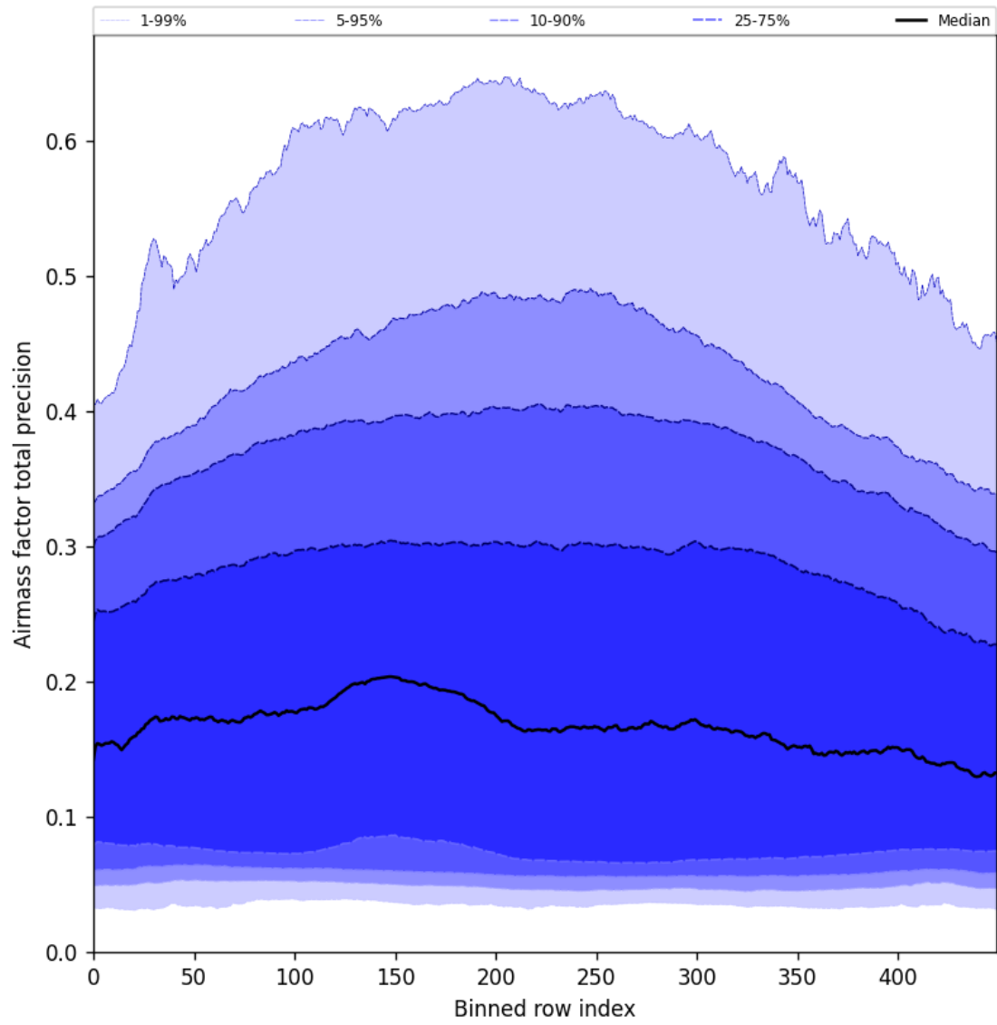
Figure 55: Along track statistics of “Airmass factor total precision” for 2025-01-30 to 2025-02-01
