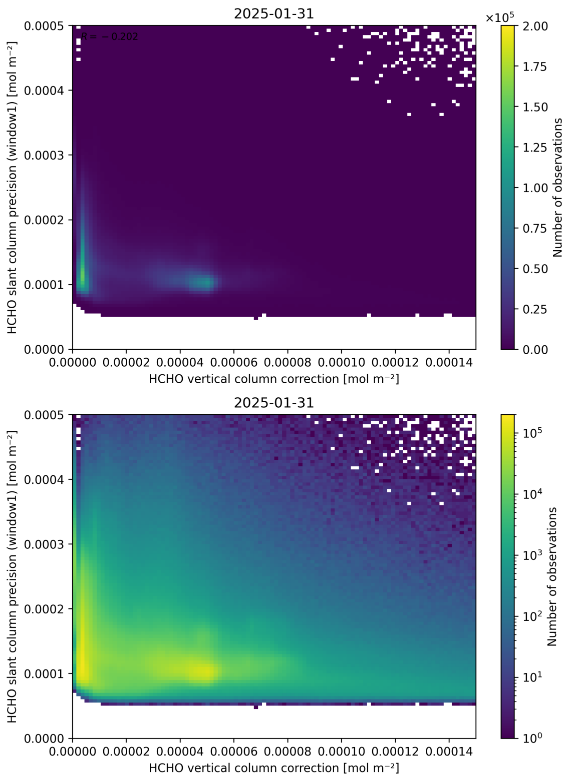
Figure 119: Scatter density plot of “HCHO vertical column correction” against “HCHO slant column precision (window1)” for 2025-01-30 to 2025-02-01.
