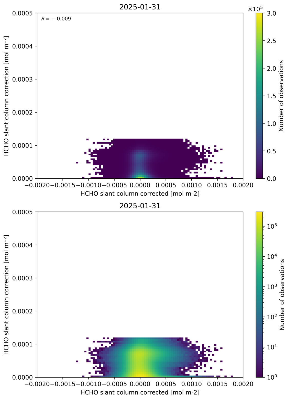
Figure 77: Scatter density plot of “HCHO slant column corrected” against “HCHO slant column correction” for 2025-01-30 to 2025-02-01.
