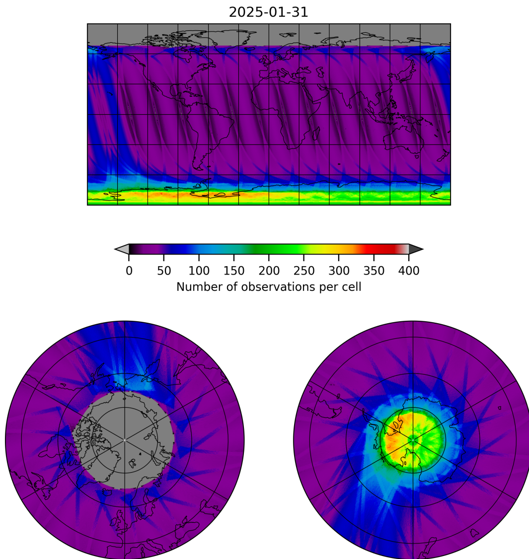
Figure 19: Map of the number of observations for 2025-01-30 to 2025-02-01
