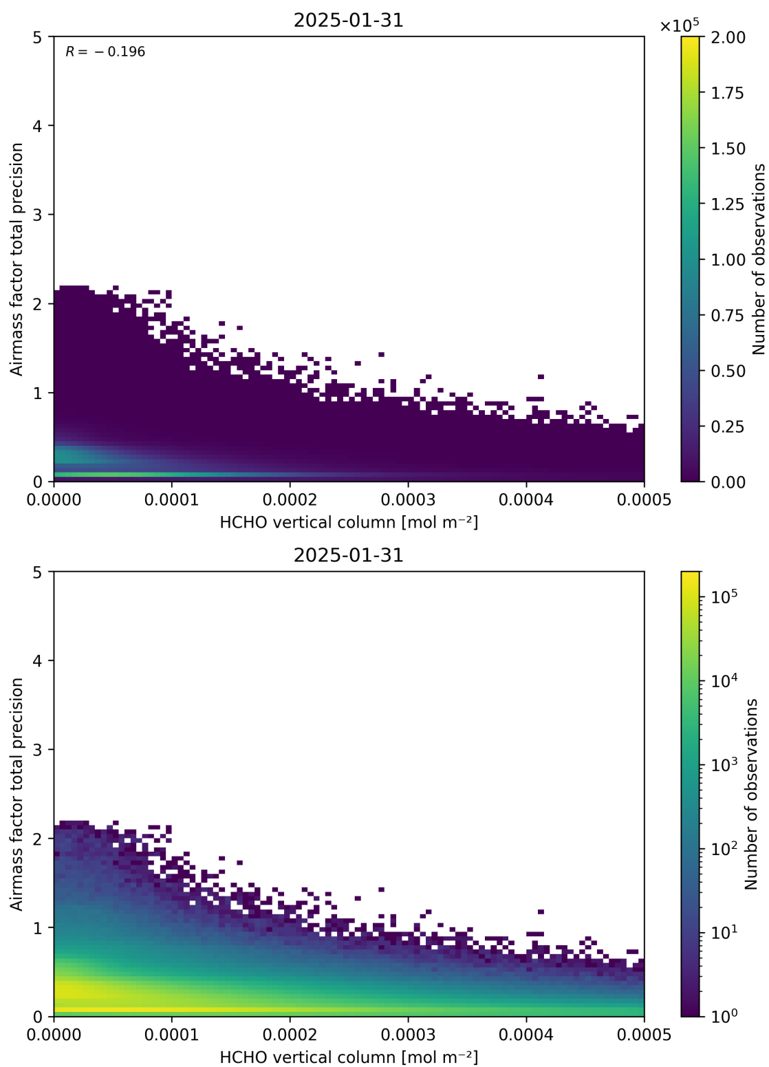
Figure 132: Scatter density plot of “HCHO vertical column” against “Airmass factor total precision” for 2025-01-30 to 2025-02-01.
