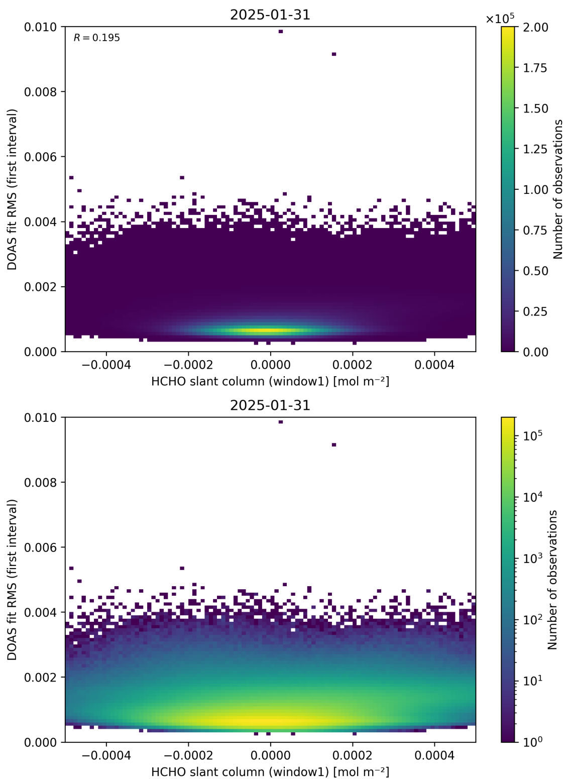
Figure 78: Scatter density plot of “HCHO slant column (window1)” against “DOAS fit RMS (first interval)” for 2025-01-30 to 2025-02-01.
