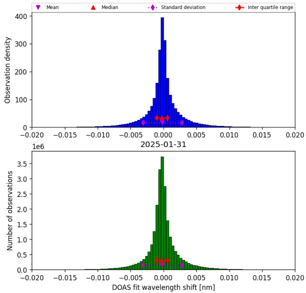
Figure 44: Histogram of “DOAS fit wavelength shift” for 2025-01-30 to 2025-02-01
