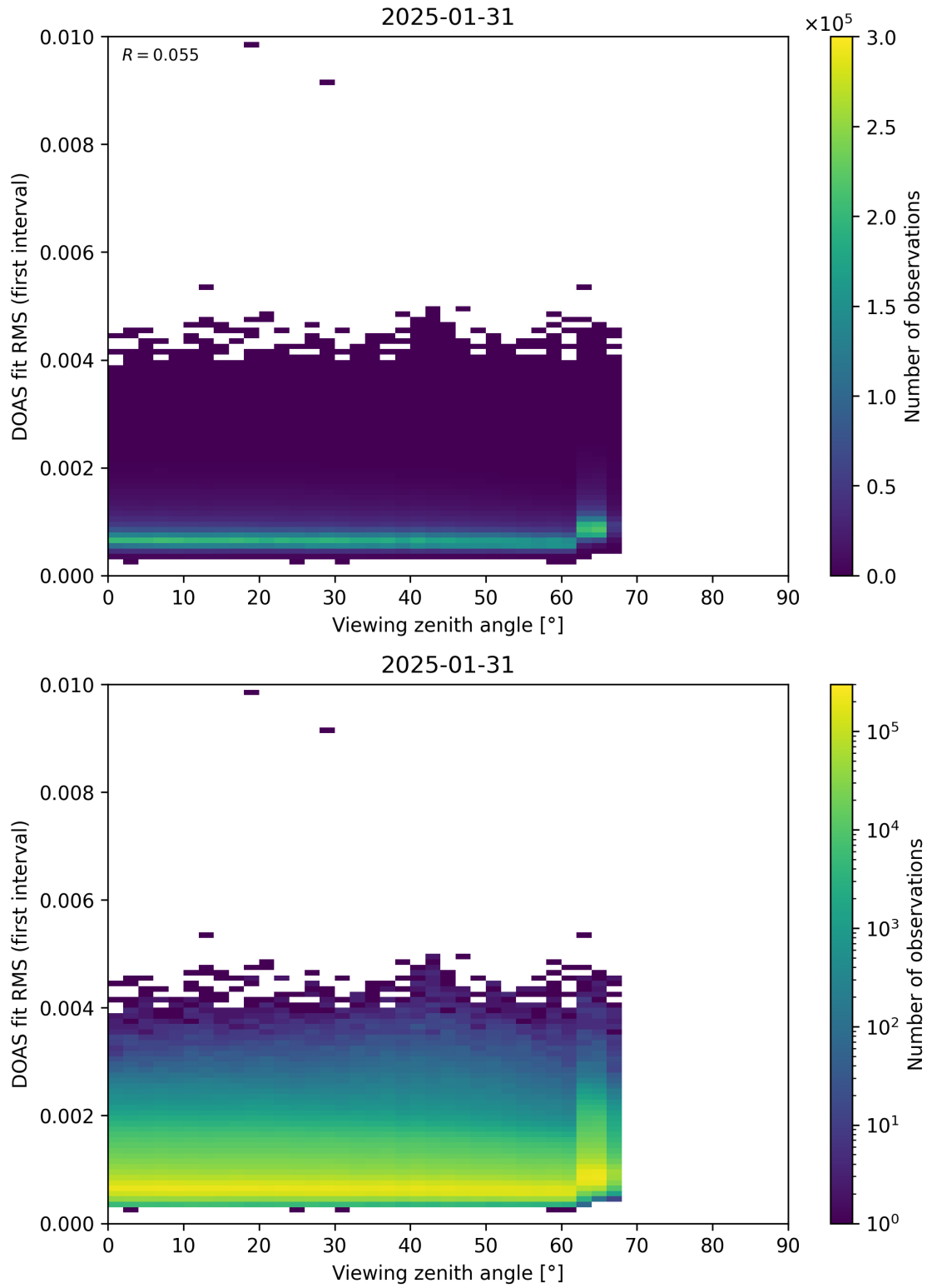
Figure 182: Scatter density plot of “Viewing zenith angle” against “DOAS fit RMS (first interval)” for 2025-01-30 to 2025-02-01.
