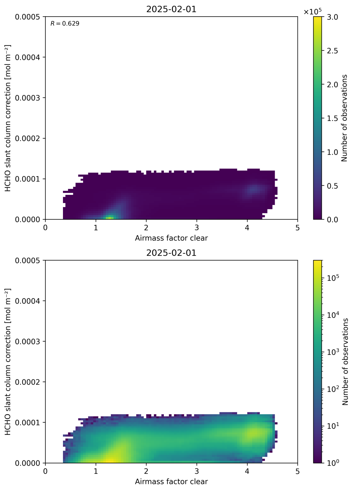
Figure 75: Scatter density plot of “Air mass factor clear” against “HCHO slant column correction” for 2025-01-31 to 2025-02-02.
