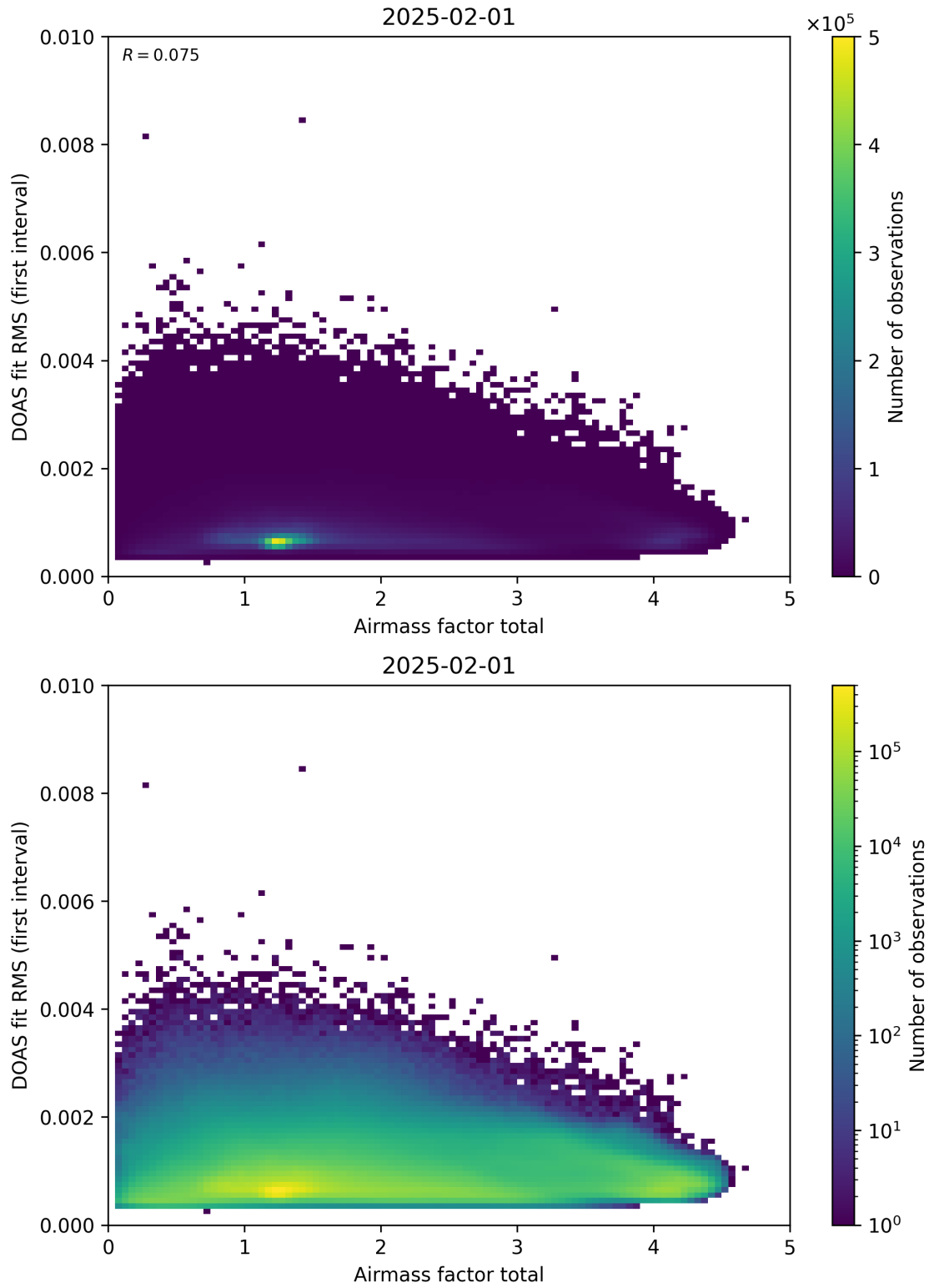
Figure 97: Scatter density plot of “Airmass factor total” against “DOAS fit RMS (first interval)” for 2025-01-31 to 2025-02-02.
