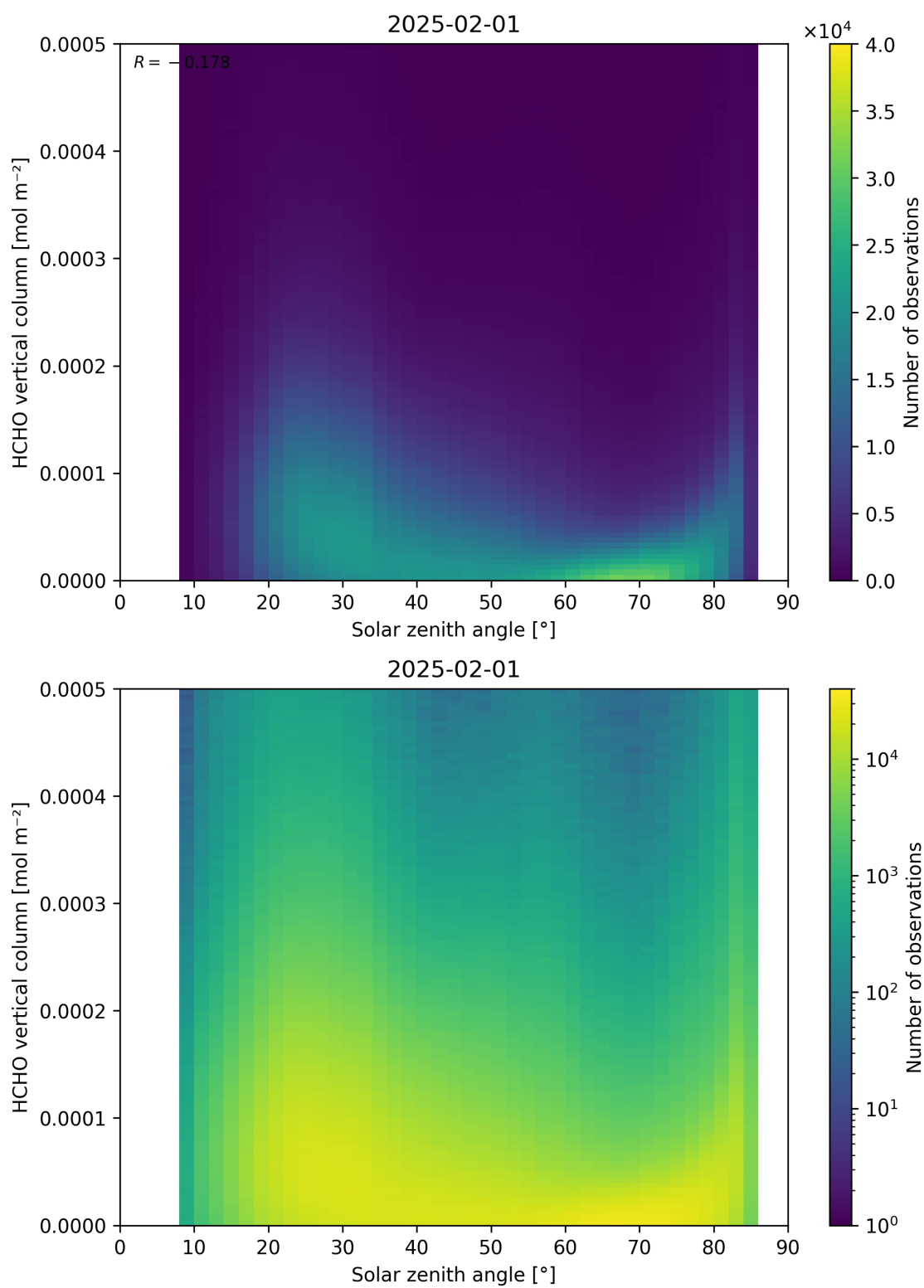
Figure 177: Scatter density plot of “Solar zenith angle” against “HCHO vertical column” for 2025-01-31 to 2025-02-02.
