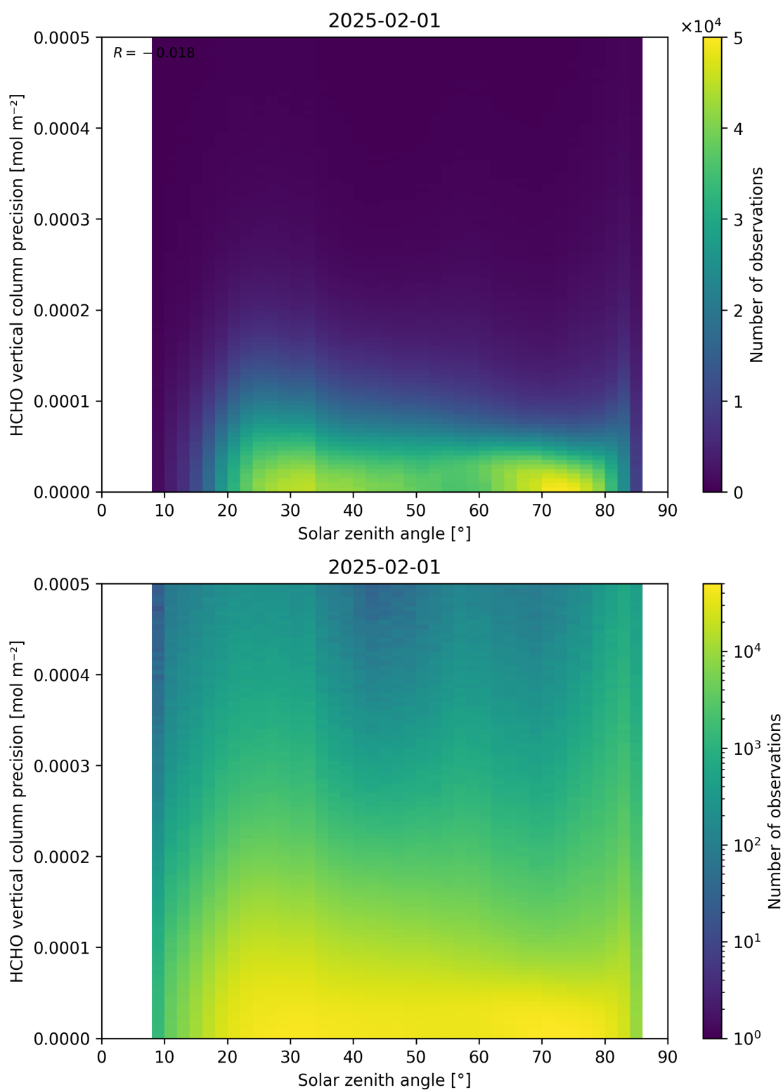
Figure 179: Scatter density plot of “Solar zenith angle” against “HCHO vertical column precision” for 2025-01-31 to 2025-02-02.
