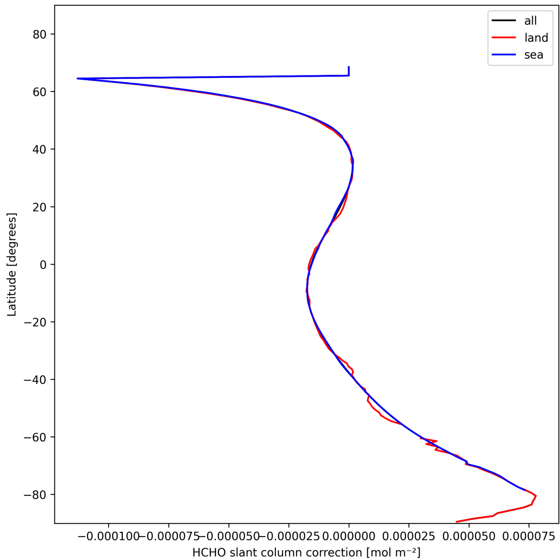
Figure 33: Zonal average of “HCHO slant column correction” for 2025-01-31 to 2025-02-02.
