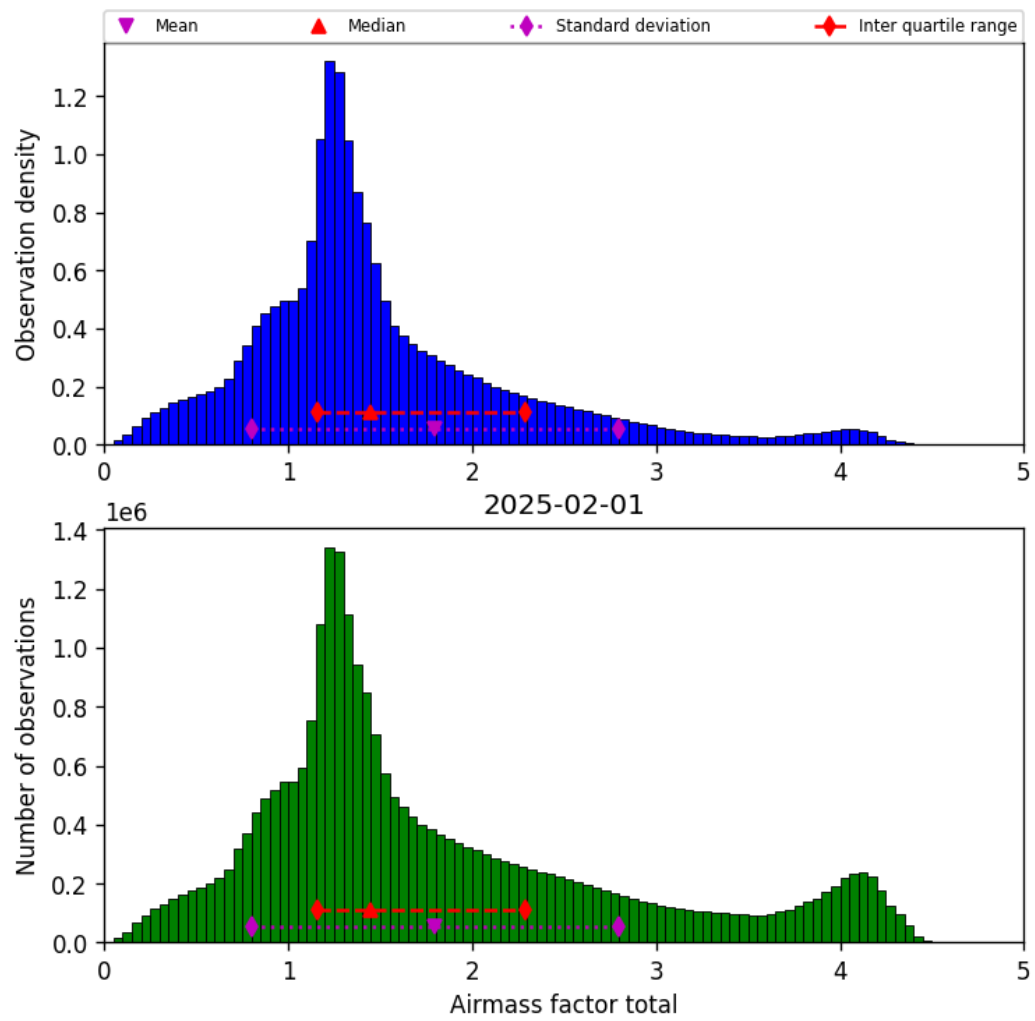
Figure 40: Histogram of “Airmass factor total” for 2025-01-31 to 2025-02-02
