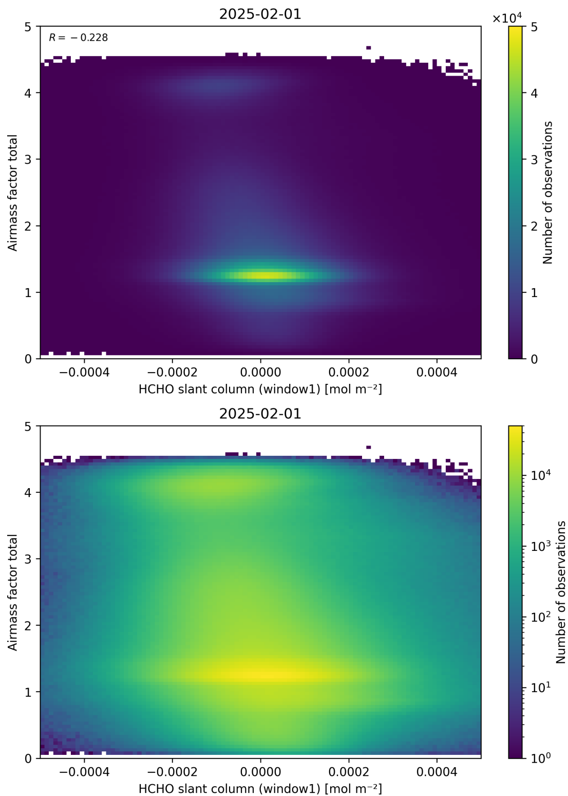
Figure 85: Scatter density plot of “HCHO slant column (window1)” against “Airmass factor total” for 2025-01-31 to 2025-02-02.
