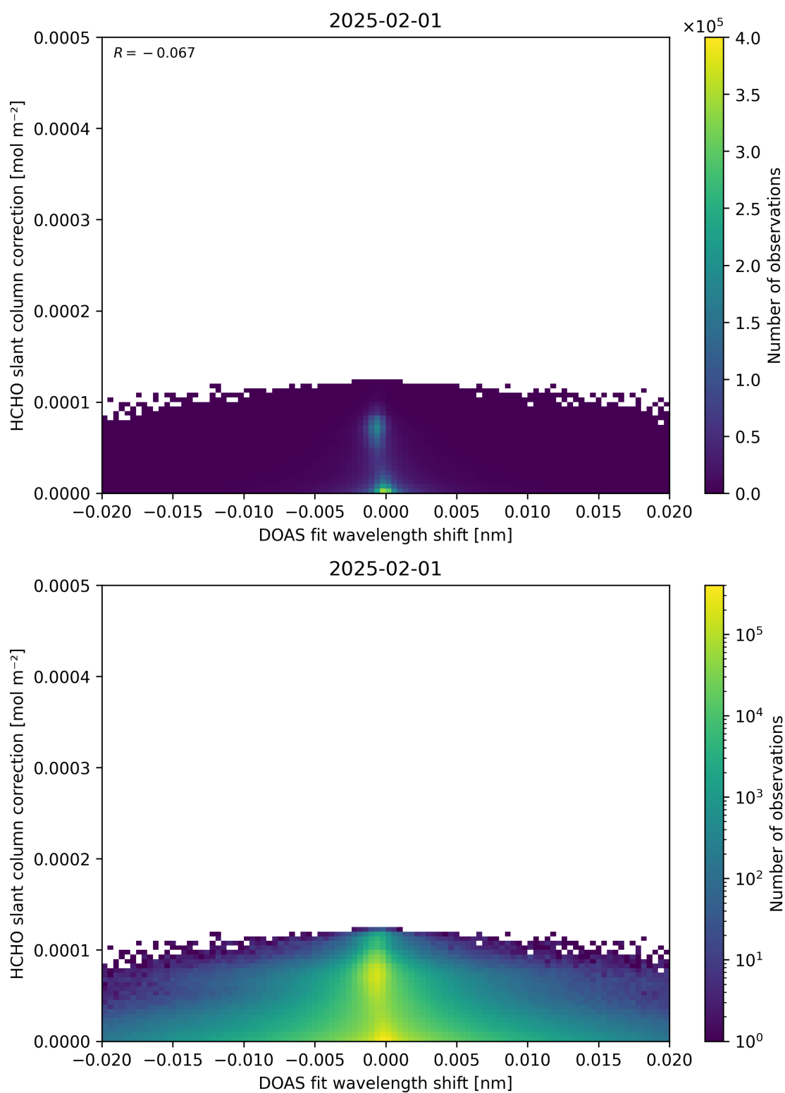
Figure 67: Scatter density plot of “DOAS fit wavelength shift” against “HCHO slant column correction” for 2025-01-31 to 2025-02-02.
