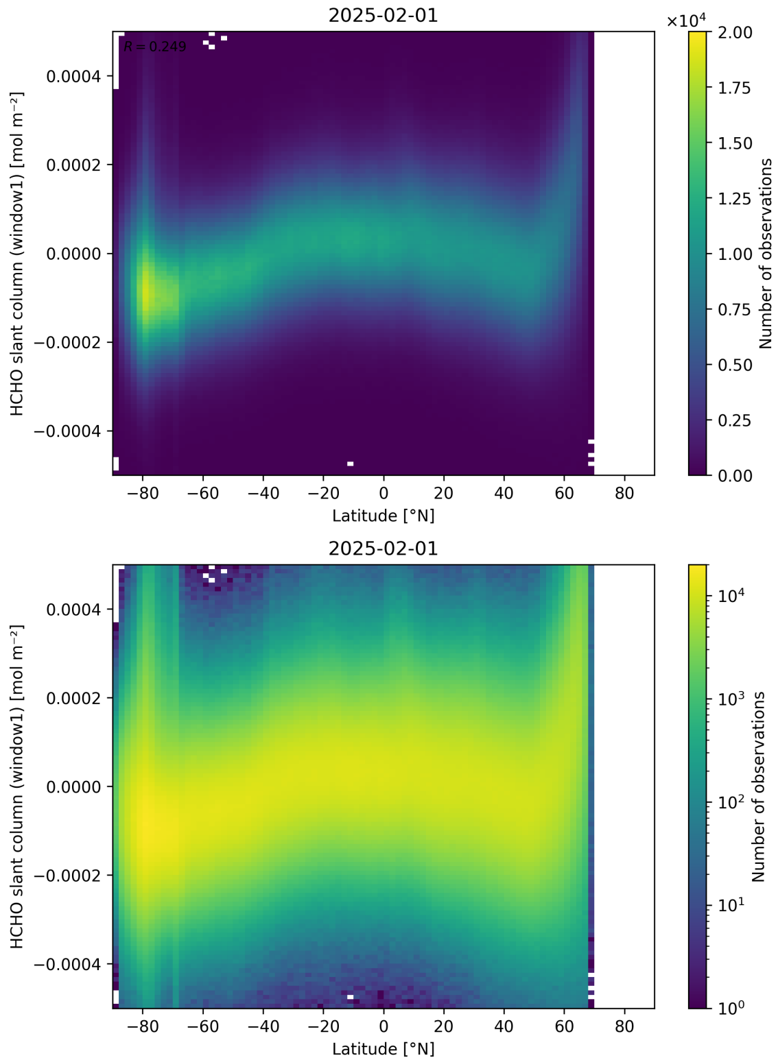
Figure 159: Scatter density plot of “Latitude” against “HCHO slant column (window1)” for 2025-01-31 to 2025-02-02.
