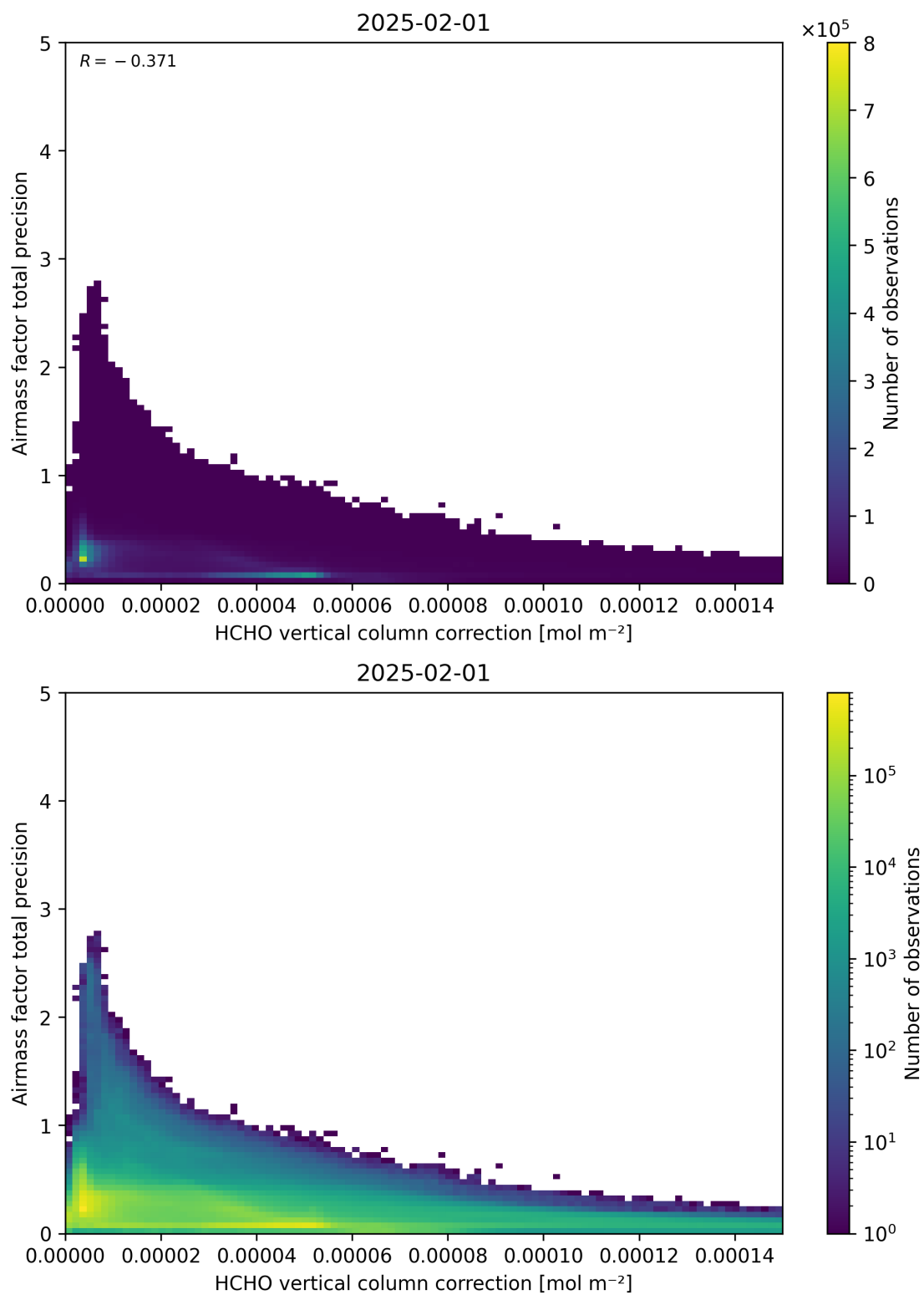
Figure 121: Scatter density plot of “HCHO vertical column correction” against “Airmass factor total precision” for 2025-01-31 to 2025-02-02.
