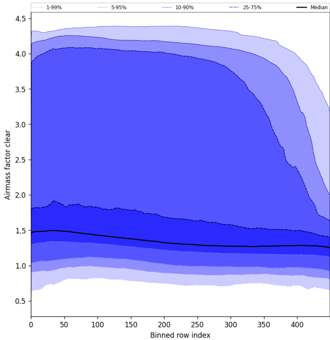
Figure 56: Along track statistics of “Airmass factor clear” for 2025-01-31 to 2025-02-02
