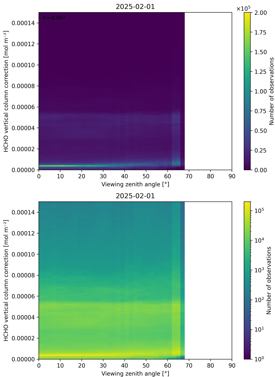
Figure 193: Scatter density plot of “Viewing zenith angle” against “HCHO vertical column correction” for 2025-01-31 to 2025-02-02.
