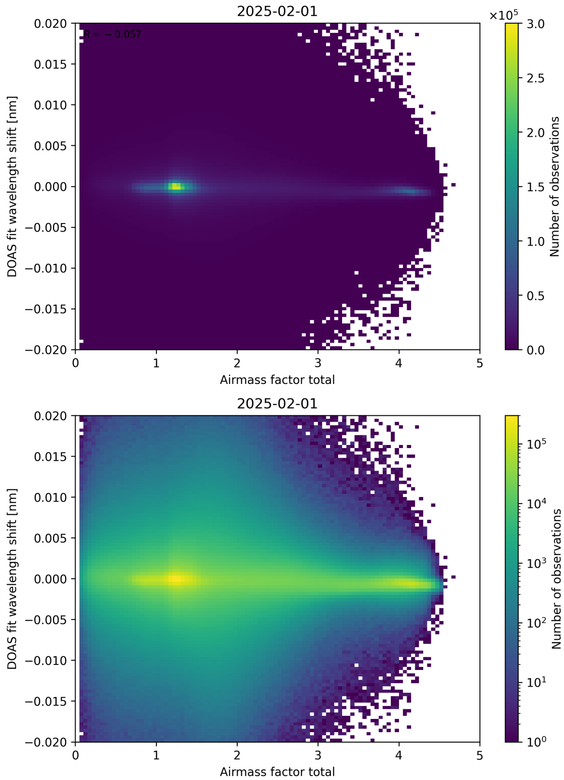
Figure 98: Scatter density plot of “Airmass factor total” against “DOAS fit wavelength shift” for 2025-01-31 to 2025-02-02.
