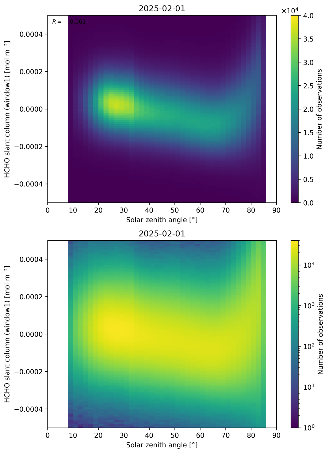
Figure 173: Scatter density plot of “Solar zenith angle” against “HCHO slant column (window1)” for 2025-01-31 to 2025-02-02.
