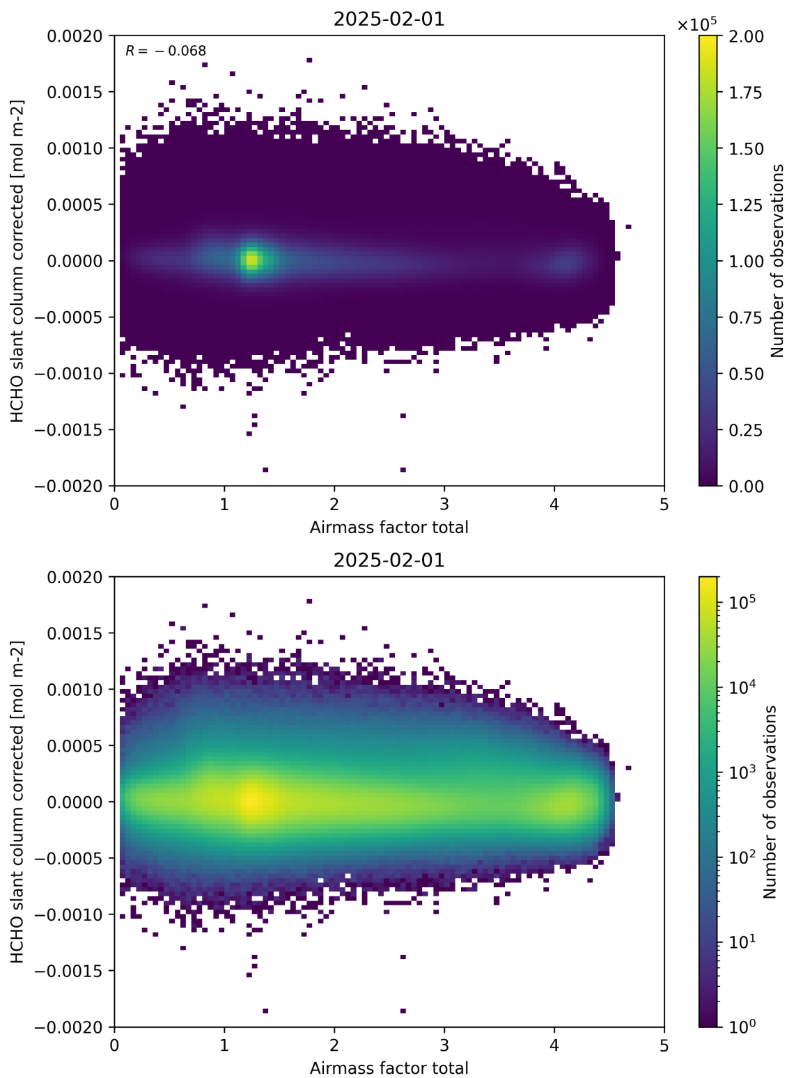
Figure 101: Scatter density plot of “Airmass factor total” against “HCHO slant column corrected” for 2025-01-31 to 2025-02-02.
