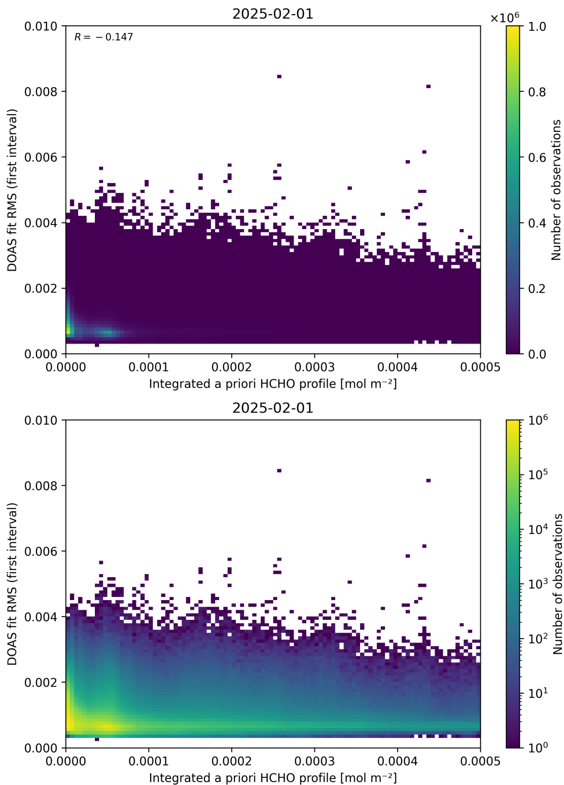
Figure 148: Scatter density plot of “Integrated a priori HCHO profile” against “DOAS fit RMS (first interval)” for 2025-01-31 to 2025-02-02.
