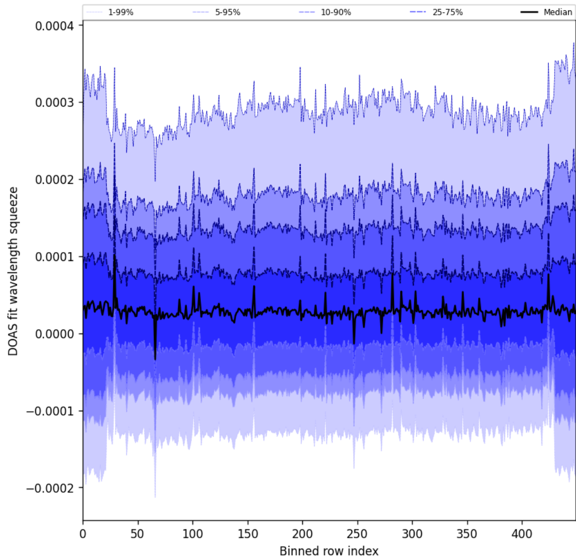
Figure 59: Along track statistics of “DOAS fit wavelength squeeze” for 2025-01-31 to 2025-02-02
