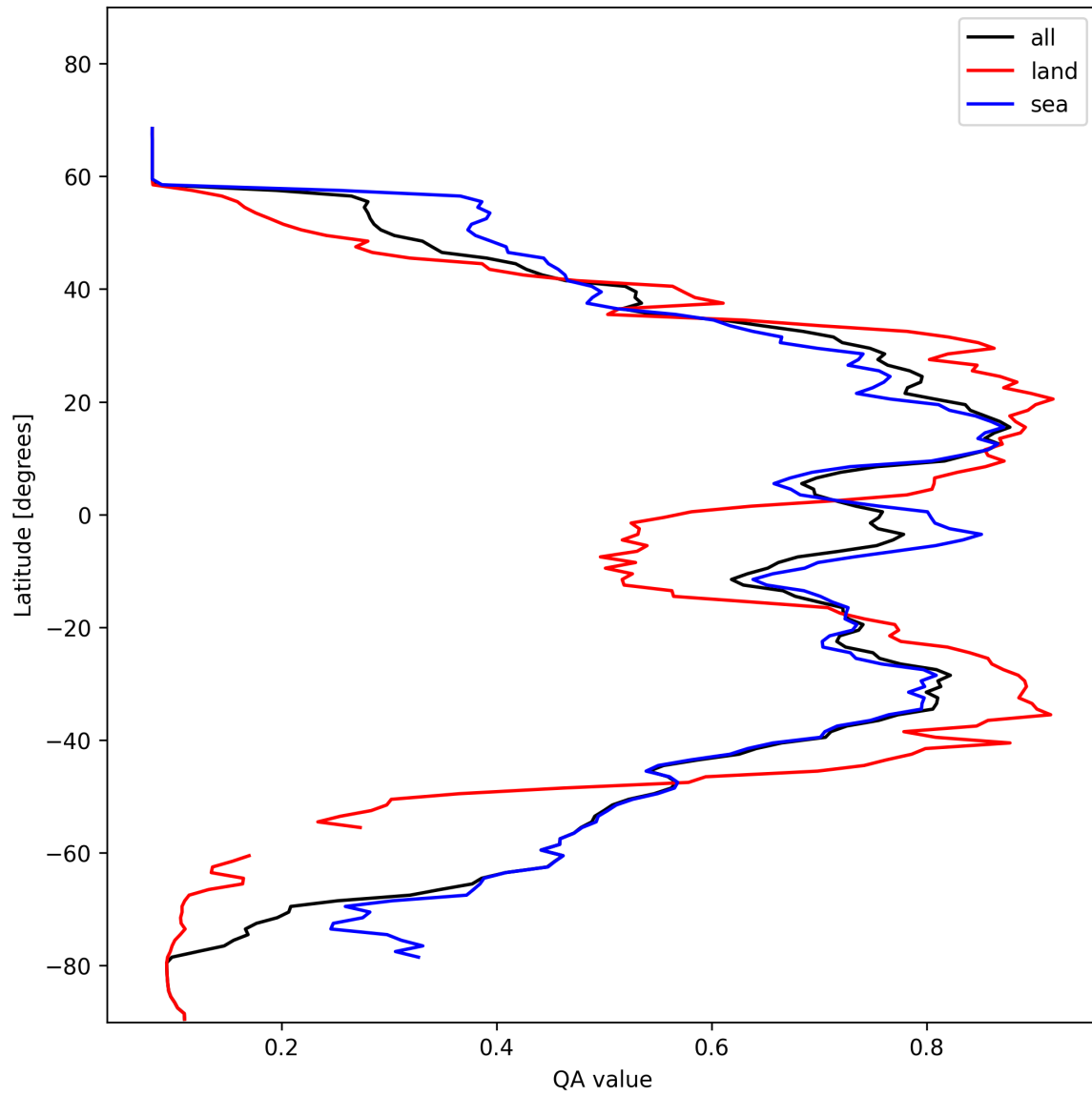
Figure 20: Zonal average of “QA value” for 2025-01-31 to 2025-02-02.
