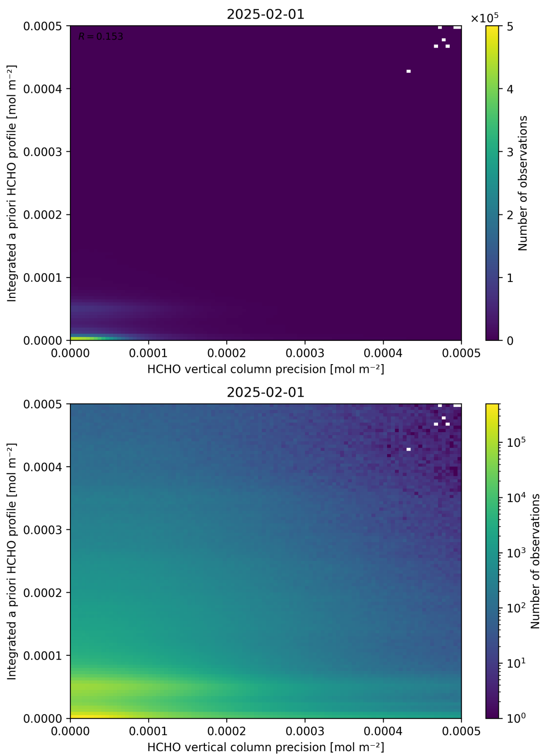
Figure 147: Scatter density plot of “HCHO vertical column precision” against “Integrated a priori HCHO profile” for 2025-01-31 to 2025-02-02.
