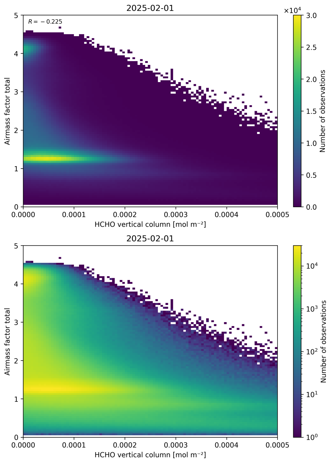
Figure 131: Scatter density plot of “HCHO vertical column” against “Airmass factor total” for 2025-01-31 to 2025-02-02.
