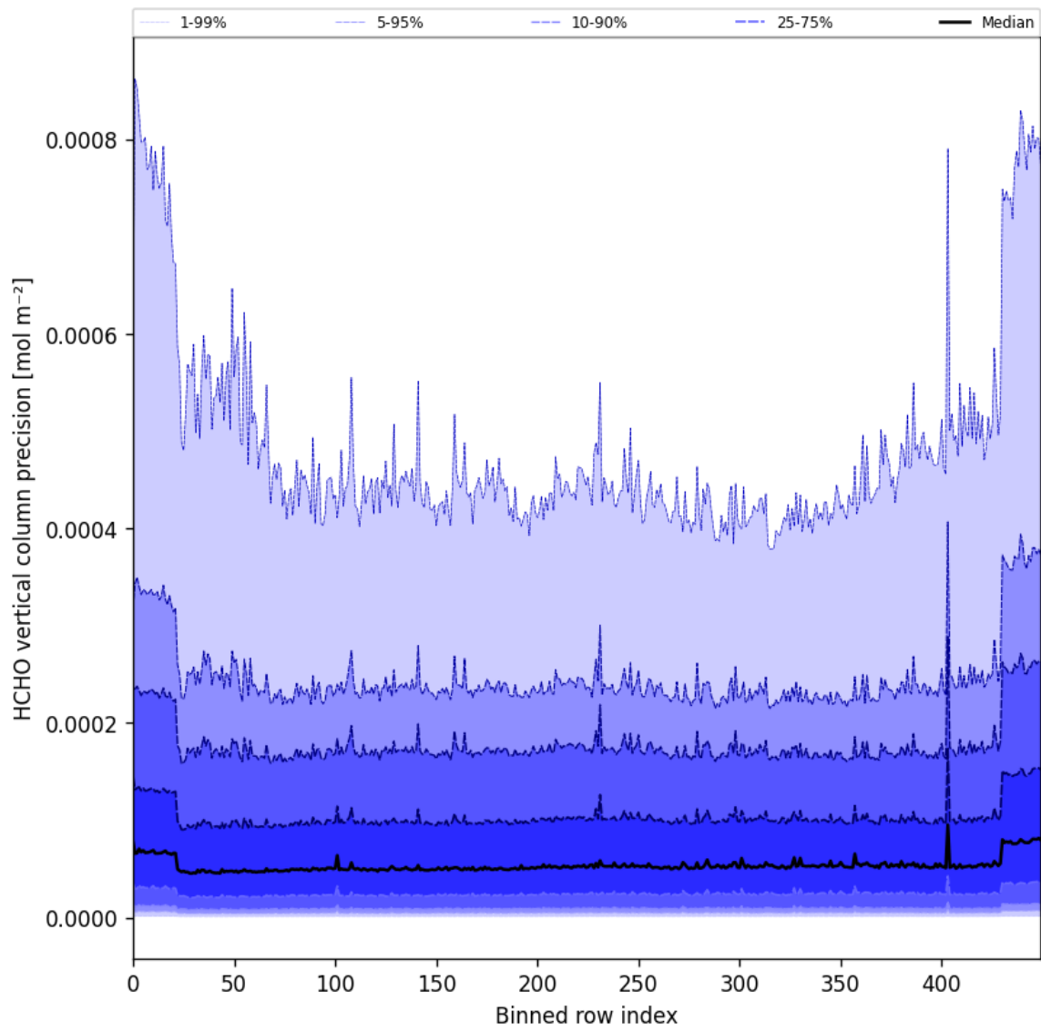
Figure 50: Along track statistics of “HCHO vertical column precision” for 2025-01-31 to 2025-02-02
