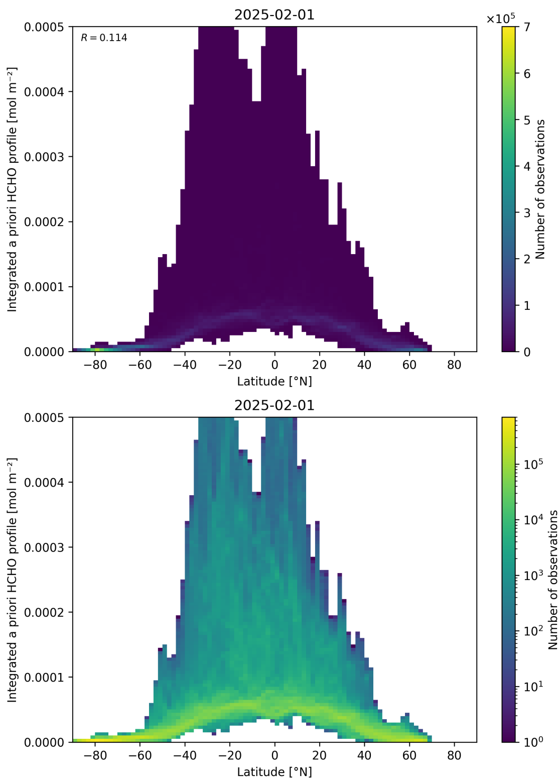
Figure 166: Scatter density plot of “Latitude” against “Integrated a priori HCHO profile” for 2025-01-31 to 2025-02-02.
