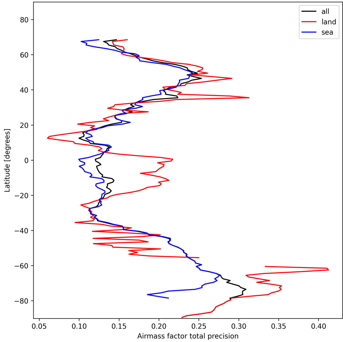
Figure 27: Zonal average of “Airmass factor total precision” for 2025-01-31 to 2025-02-02.
