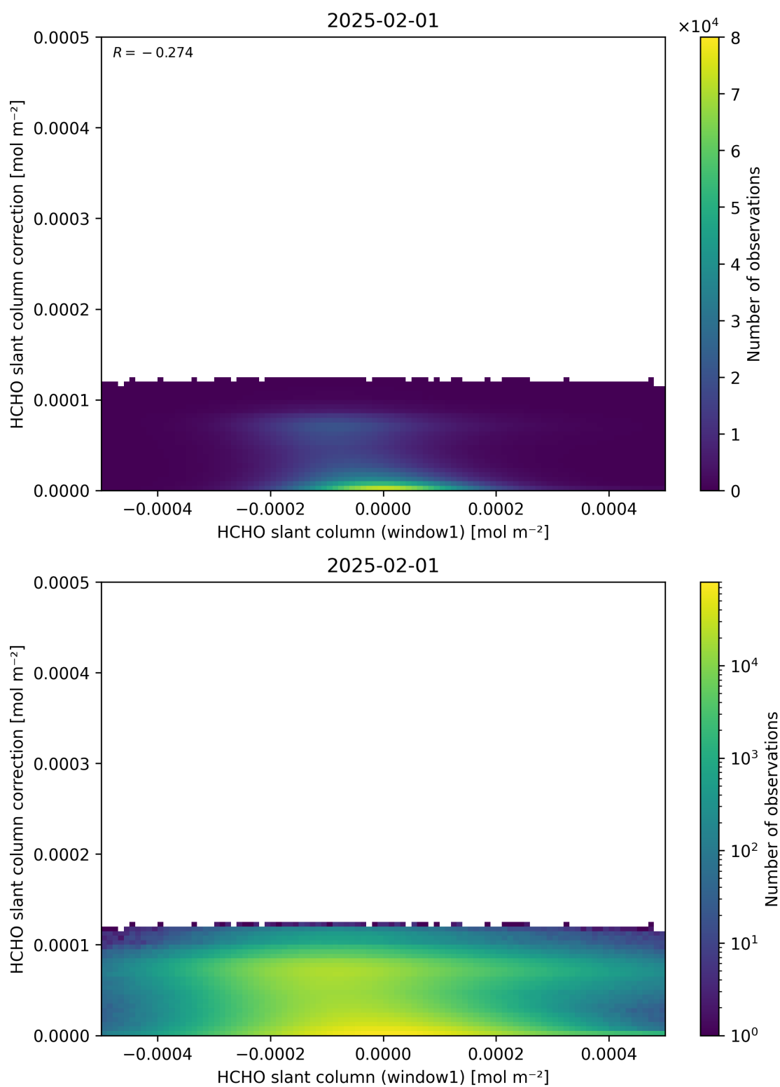
Figure 83: Scatter density plot of “HCHO slant column (window1)” against “HCHO slant column correction” for 2025-01-31 to 2025-02-02.
