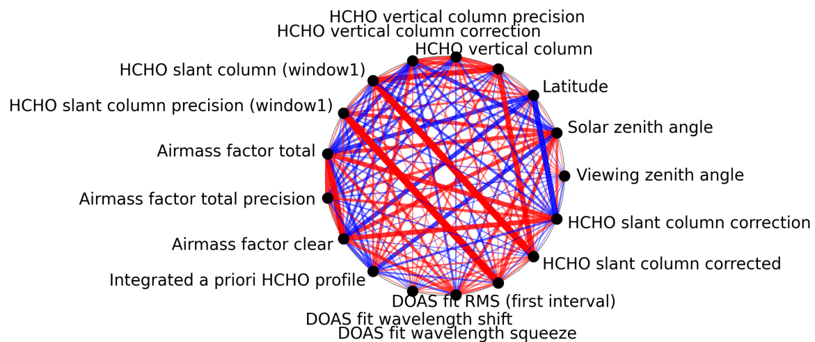
Figure 1: Map of correlation graph for 2025-01-31 to 2025-02-02.
