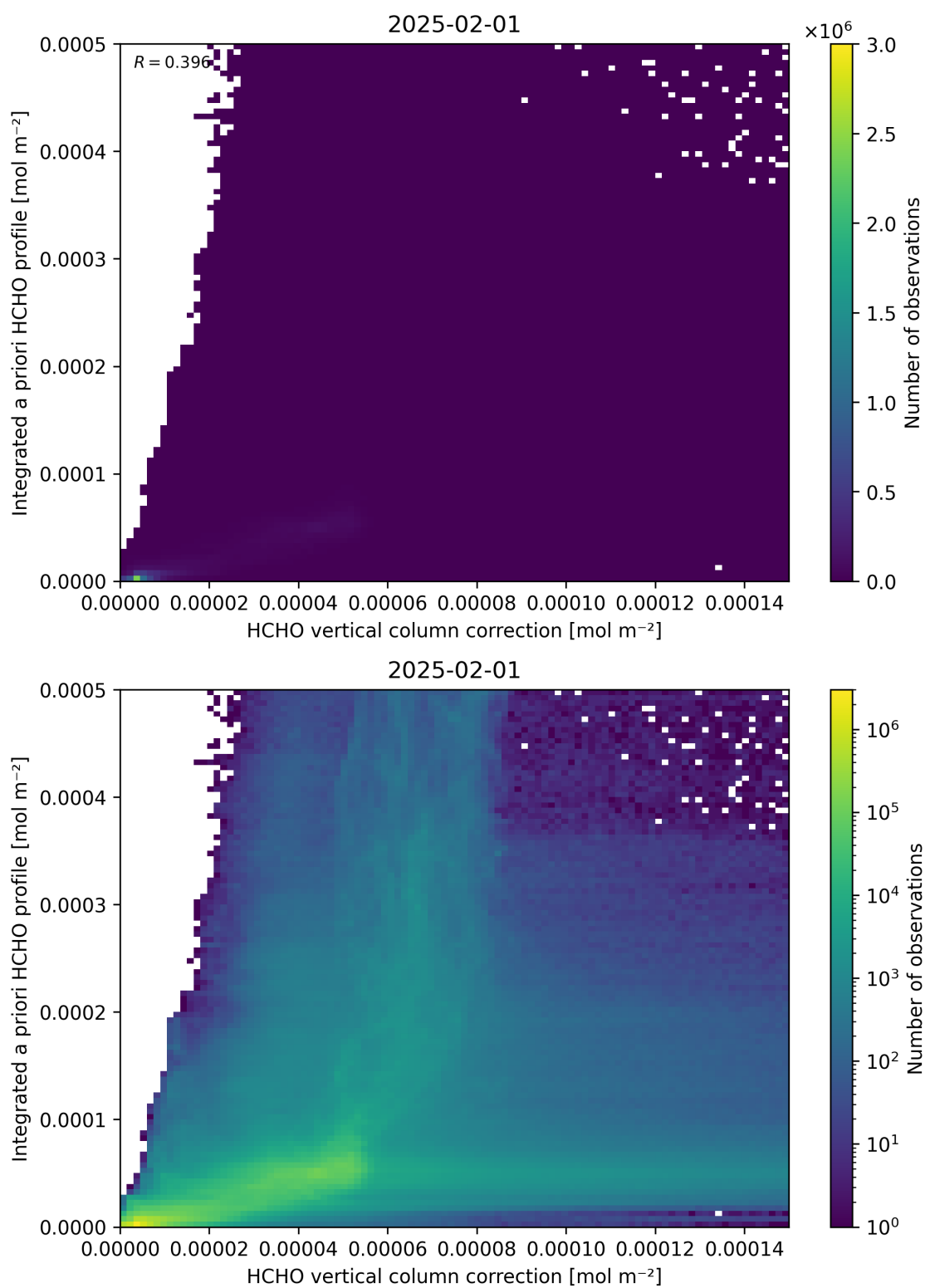
Figure 122: Scatter density plot of “HCHO vertical column correction” against “Integrated a priori HCHO profile” for 2025-01-31 to 2025-02-02.
