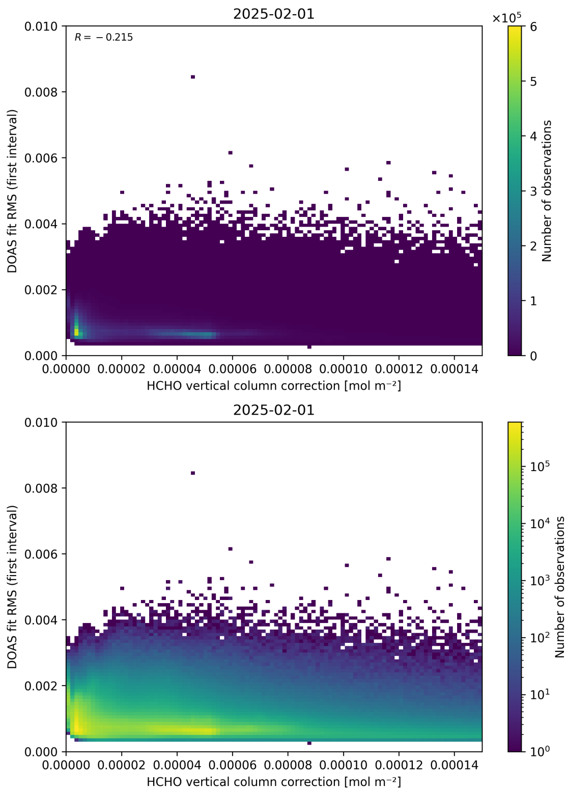
Figure 112: Scatter density plot of “HCHO vertical column correction” against “DOAS fit RMS (first interval)” for 2025-01-31 to 2025-02-02.
