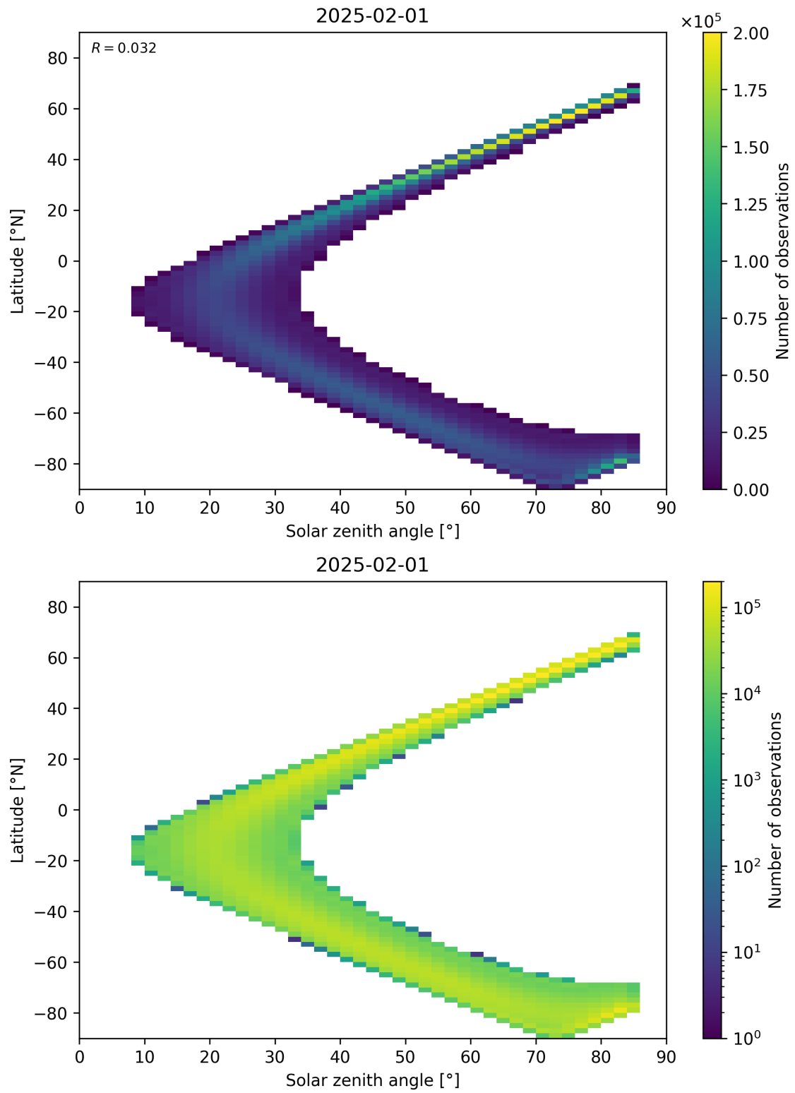
Figure 181: Scatter density plot of “Solar zenith angle” against “Latitude” for 2025-01-31 to 2025-02-02.
