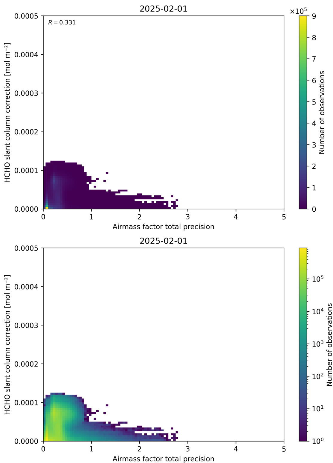
Figure 110: Scatter density plot of “Airmass factor total precision” against “HCHO slant column correction” for 2025-01-31 to 2025-02-02.
