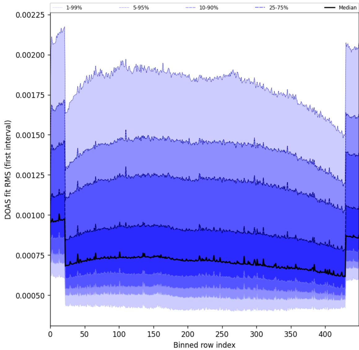
Figure 60: Along track statistics of “DOAS fit RMS (first interval)” for 2025-01-31 to 2025-02-02
