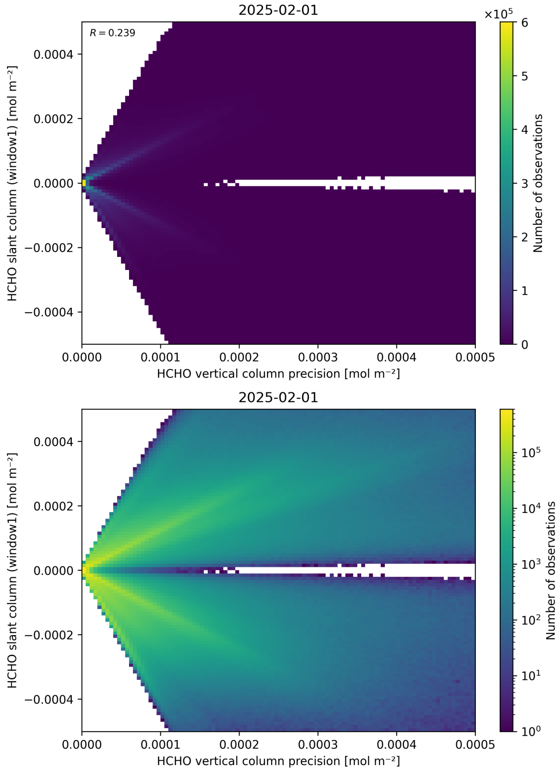
Figure 142: Scatter density plot of “HCHO vertical column precision” against “HCHO slant column (window1)” for 2025-01-31 to 2025-02-02.
