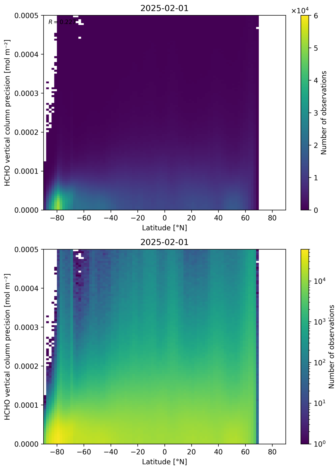
Figure 165: Scatter density plot of “Latitude” against “HCHO vertical column precision” for 2025-01-31 to 2025-02-02.
