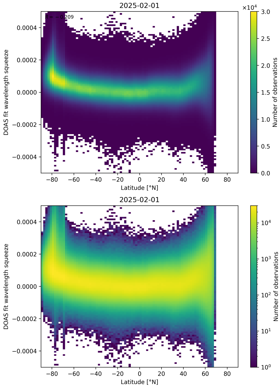
Figure 155: Scatter density plot of “Latitude” against “DOAS fit wavelength squeeze” for 2025-01-31 to 2025-02-02.
