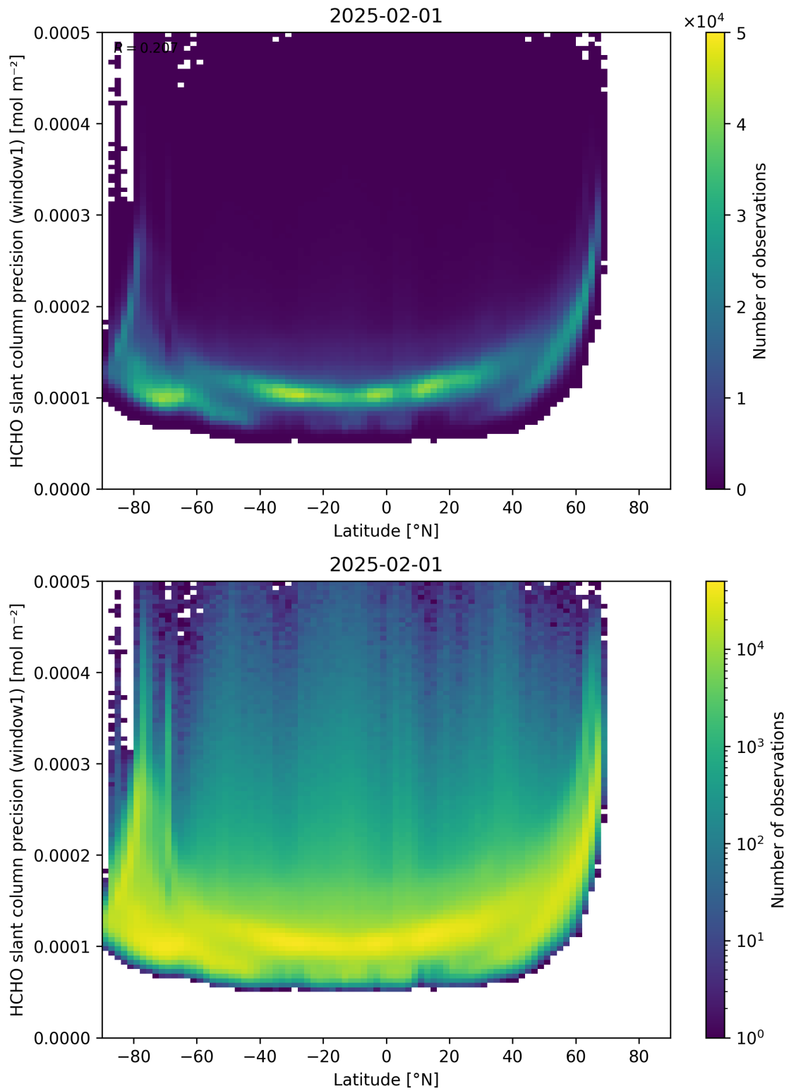
Figure 160: Scatter density plot of “Latitude” against “HCHO slant column precision (window1)” for 2025-01-31 to 2025-02-02.
