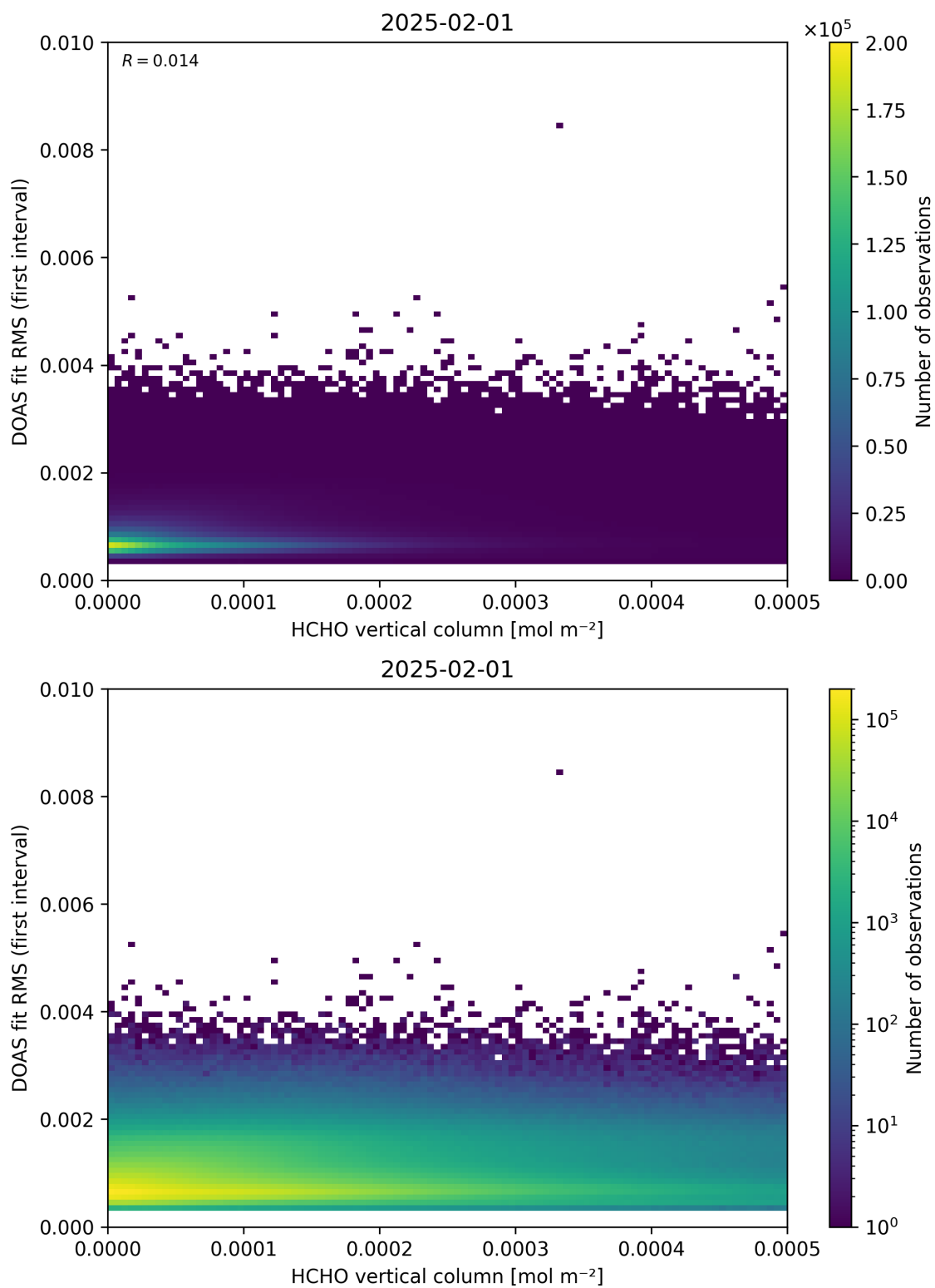
Figure 123: Scatter density plot of “HCHO vertical column” against “DOAS fit RMS (first interval)” for 2025-01-31 to 2025-02-02.
