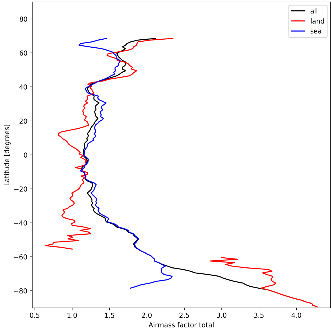
Figure 26: Zonal average of “Airmass factor total” for 2025-01-31 to 2025-02-02.
