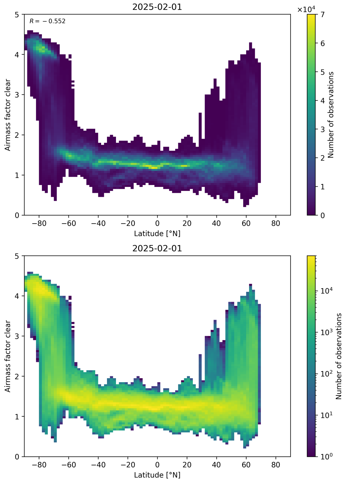
Figure 156: Scatter density plot of “Latitude” against “Airmass factor clear” for 2025-01-31 to 2025-02-02.
