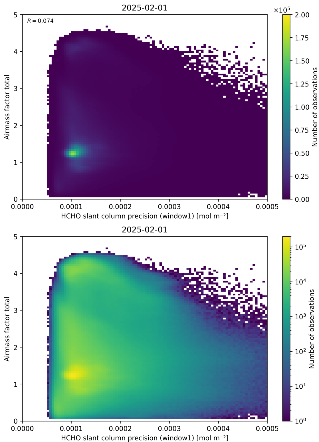
Figure 94: Scatter density plot of “HCHO slant column precision (window1)” against “Airmass factor total” for 2025-01-31 to 2025-02-02.
