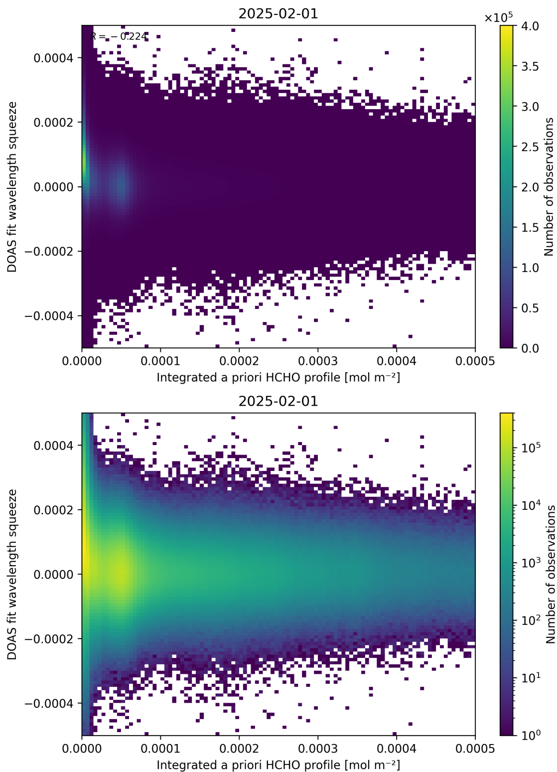
Figure 150: Scatter density plot of “Integrated a priori HCHO profile” against “DOAS fit wavelength squeeze” for 2025-01-31 to 2025-02-02.
