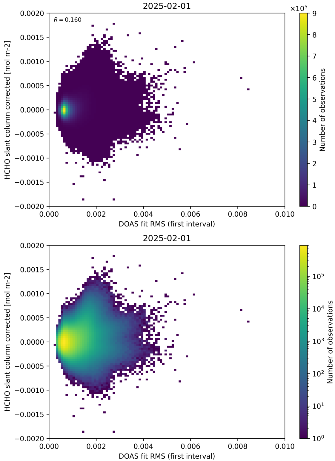
Figure 62: Scatter density plot of “DOAS fit RMS (first interval)” against “HCHO slant column corrected” for 2025-01-31 to 2025-02-02.
