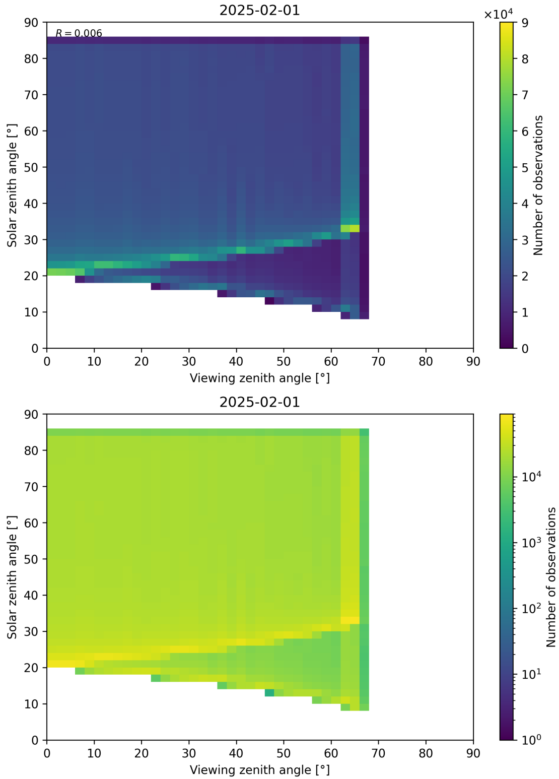
Figure 197: Scatter density plot of “Viewing zenith angle” against “Solar zenith angle” for 2025-01-31 to 2025-02-02.
