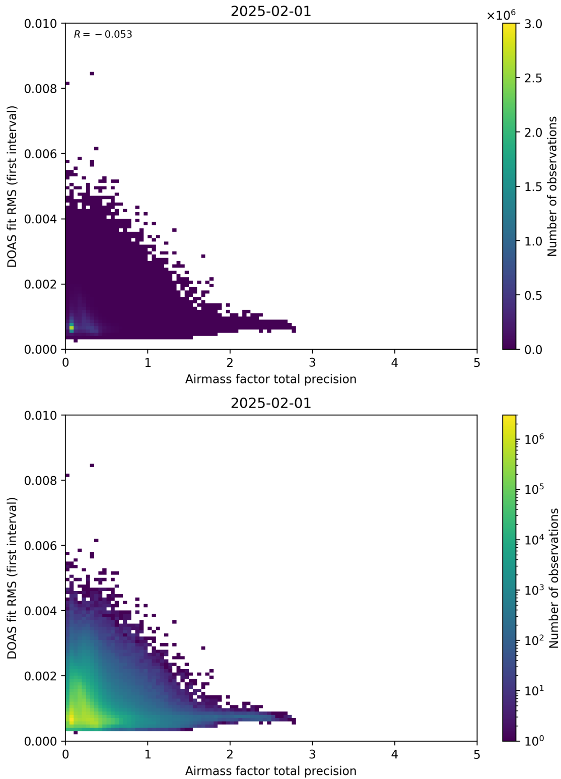
Figure 105: Scatter density plot of “Airmass factor total precision” against “DOAS fit RMS (first interval)” for 2025-01-31 to 2025-02-02.
