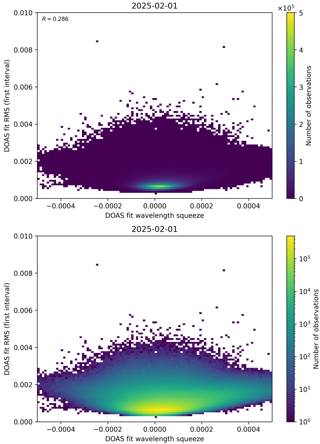
Figure 68: Scatter density plot of “DOAS fit wavelength squeeze” against “DOAS fit RMS (first interval)” for 2025-01-31 to 2025-02-02.
