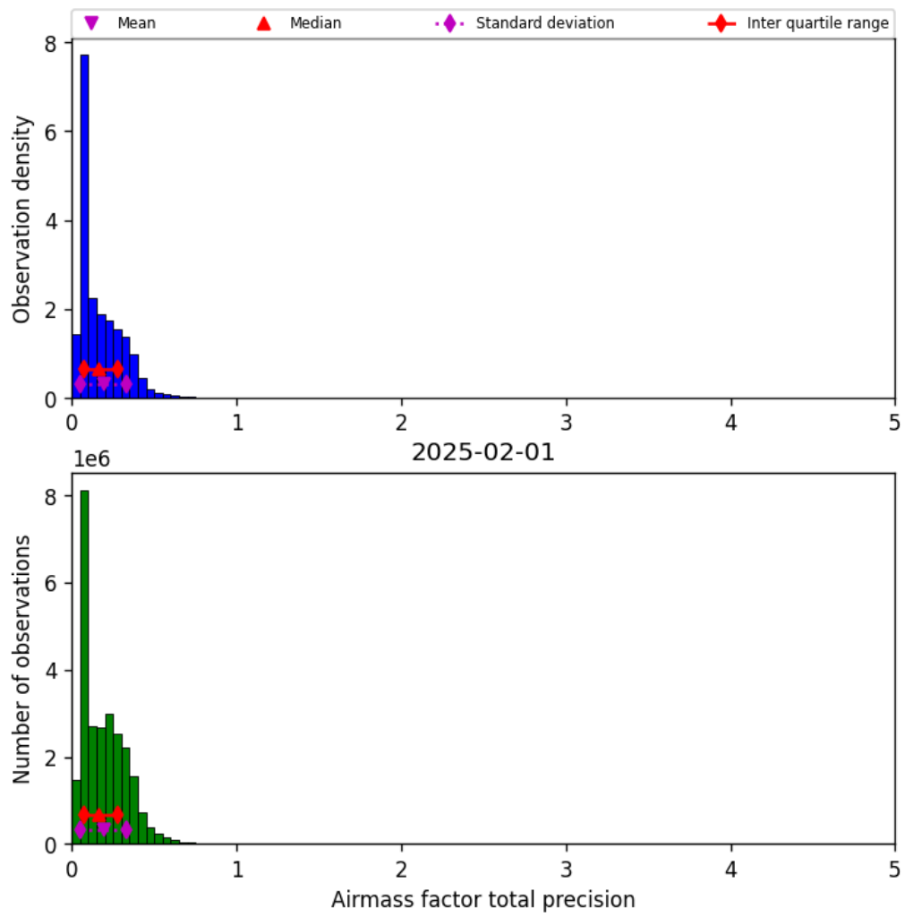
Figure 41: Histogram of “Airmass factor total precision” for 2025-01-31 to 2025-02-02
