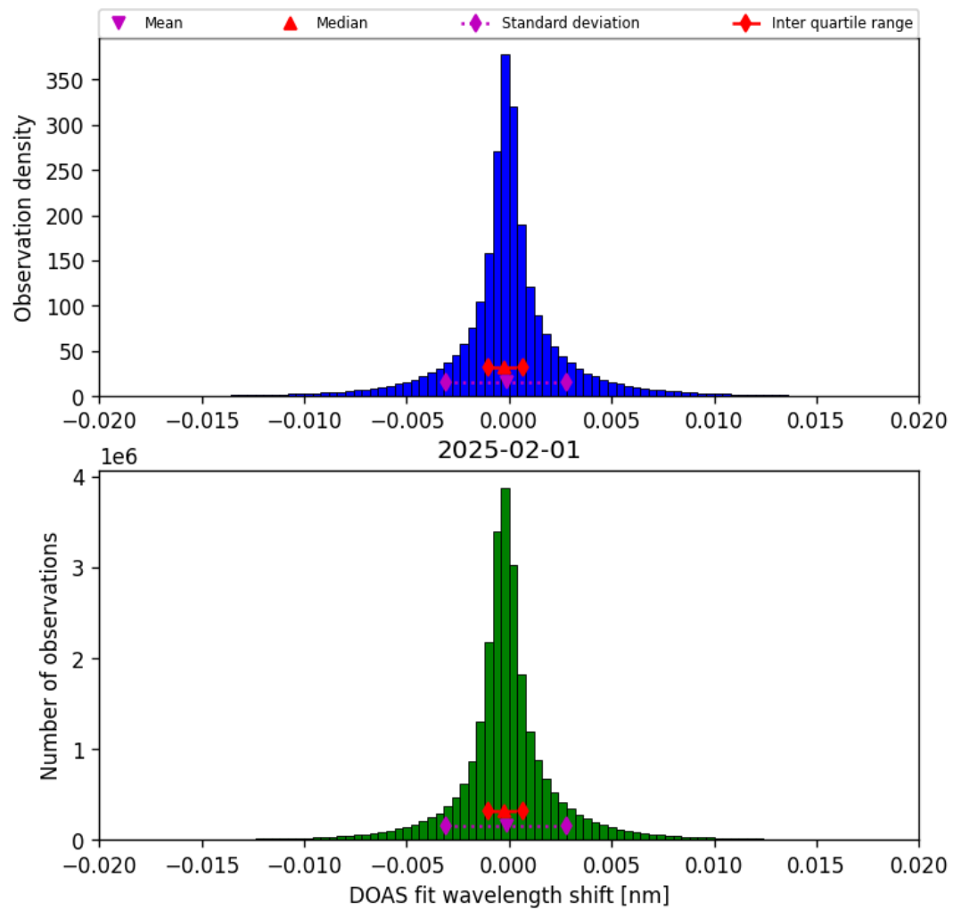
Figure 44: Histogram of “DOAS fit wavelength shift” for 2025-01-31 to 2025-02-02
