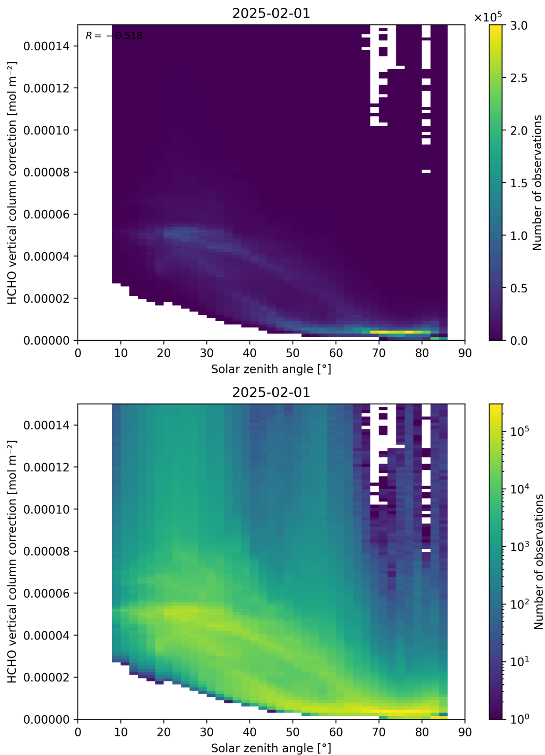
Figure 178: Scatter density plot of “Solar zenith angle” against “HCHO vertical column correction” for 2025-01-31 to 2025-02-02.
