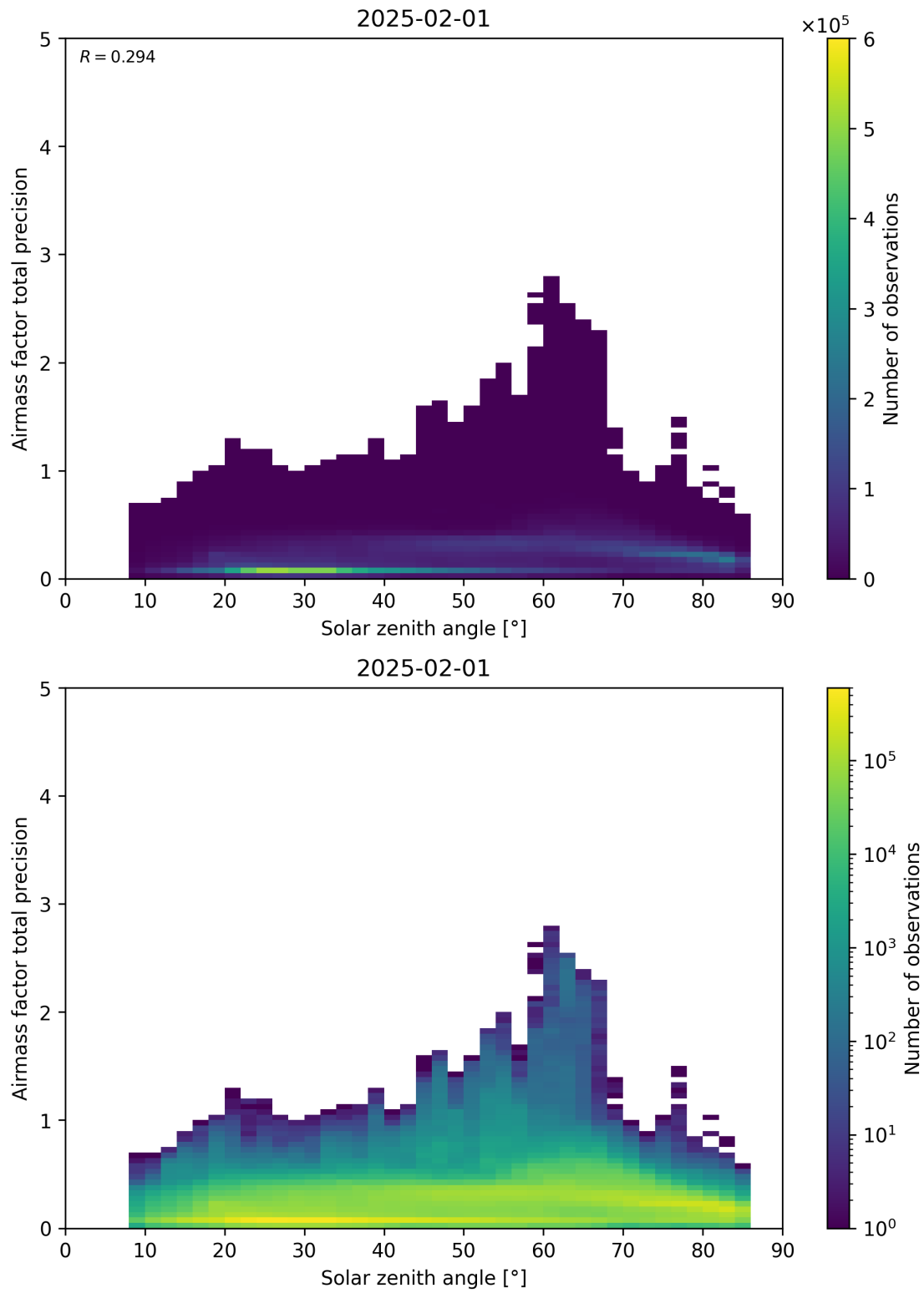
Figure 176: Scatter density plot of “Solar zenith angle” against “Airmass factor total precision” for 2025-01-31 to 2025-02-02.
