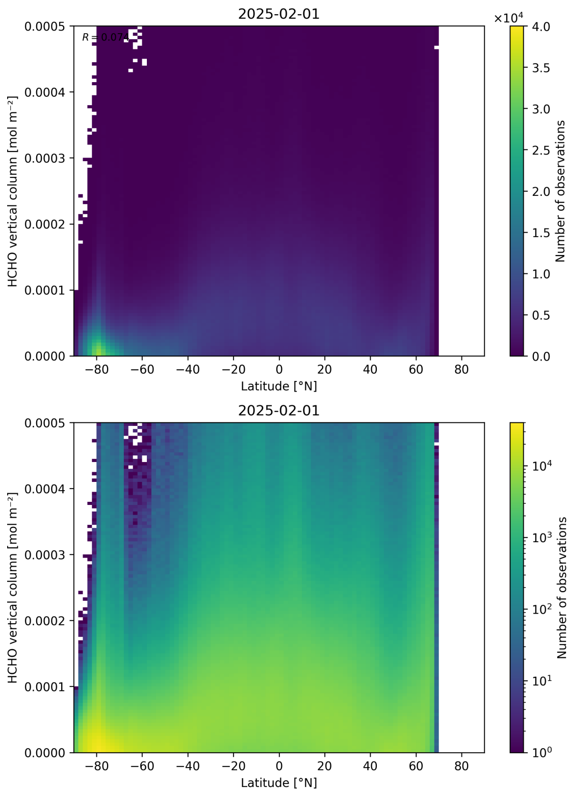
Figure 163: Scatter density plot of “Latitude” against “HCHO vertical column” for 2025-01-31 to 2025-02-02.
