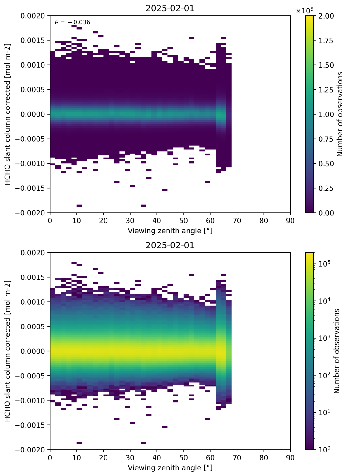
Figure 186: Scatter density plot of “Viewing zenith angle” against “HCHO slant column corrected” for 2025-01-31 to 2025-02-02.
