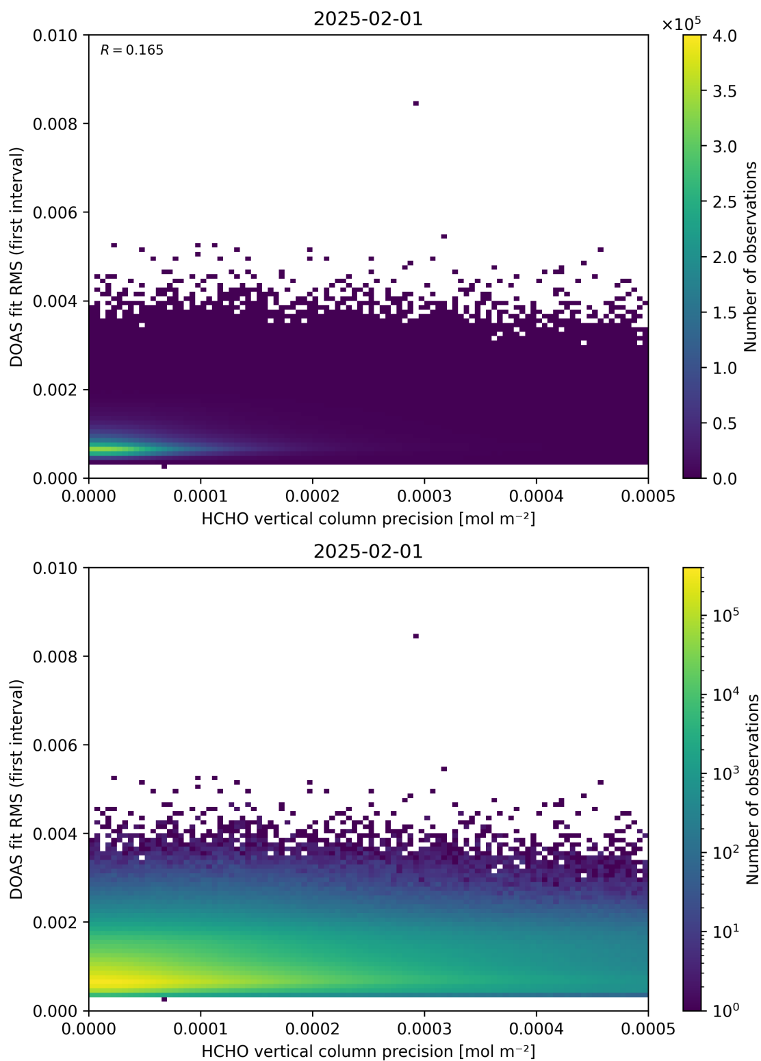
Figure 136: Scatter density plot of “HCHO vertical column precision” against “DOAS fit RMS (first interval)” for 2025-01-31 to 2025-02-02.
