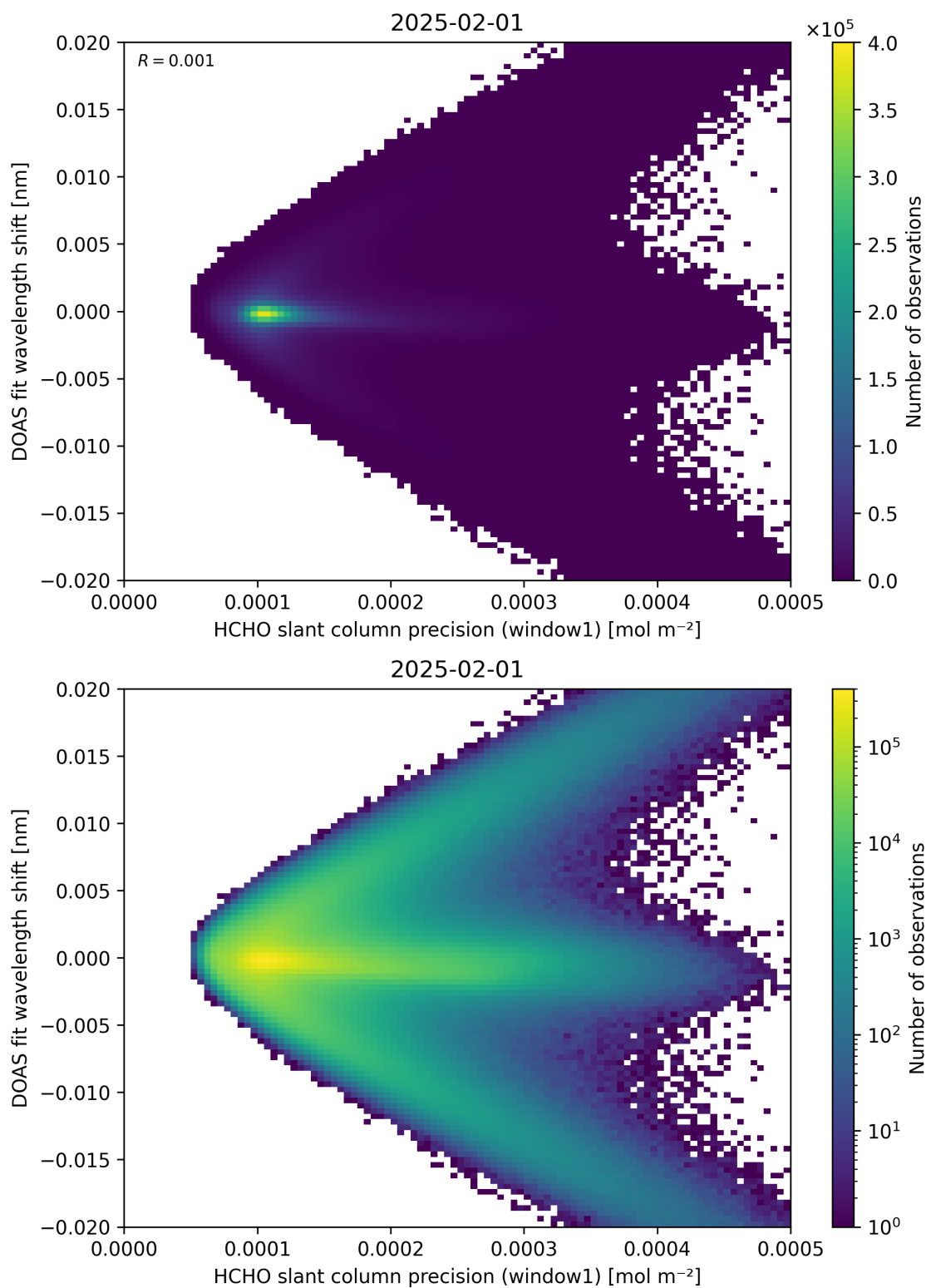
Figure 89: Scatter density plot of “HCHO slant column precision (window1)” against “DOAS fit wavelength shift” for 2025-01-31 to 2025-02-02.
