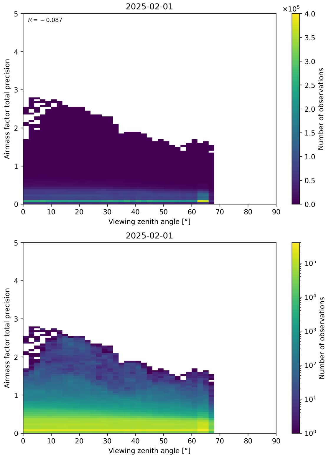
Figure 191: Scatter density plot of “Viewing zenith angle” against “Airmass factor total precision” for 2025-01-31 to 2025-02-02.
