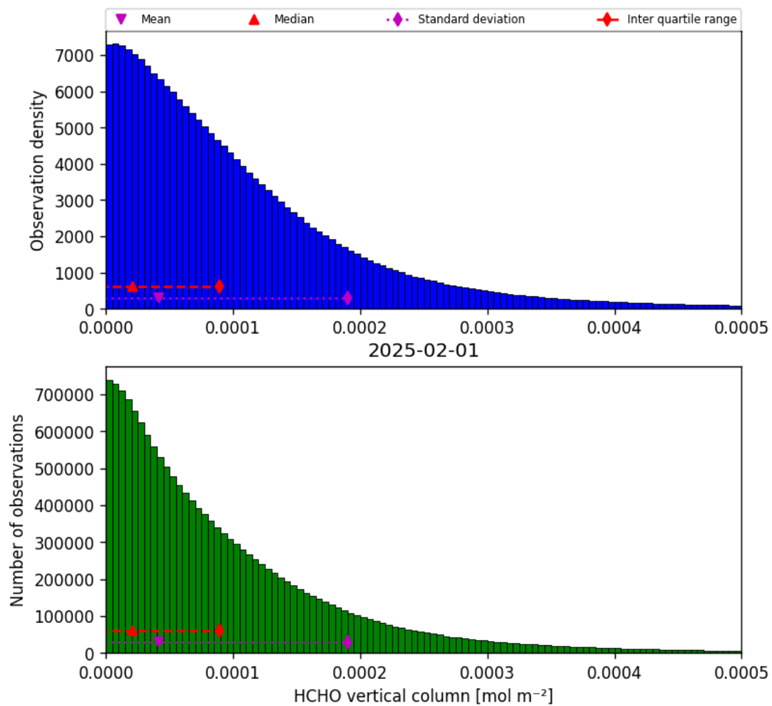
Figure 35: Histogram of “HCHO vertical column” for 2025-01-31 to 2025-02-02
