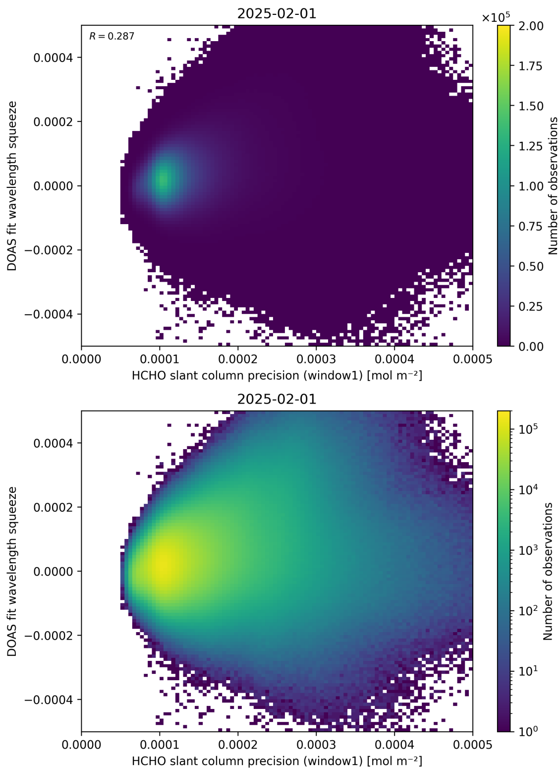
Figure 90: Scatter density plot of “HCHO slant column precision (window1)” against “DOAS fit wavelength squeeze” for 2025-01-31 to 2025-02-02.
