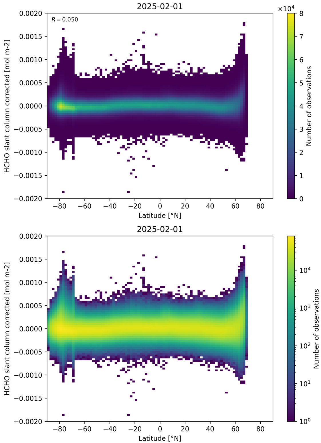
Figure 157: Scatter density plot of “Latitude” against “HCHO slant column corrected” for 2025-01-31 to 2025-02-02.
