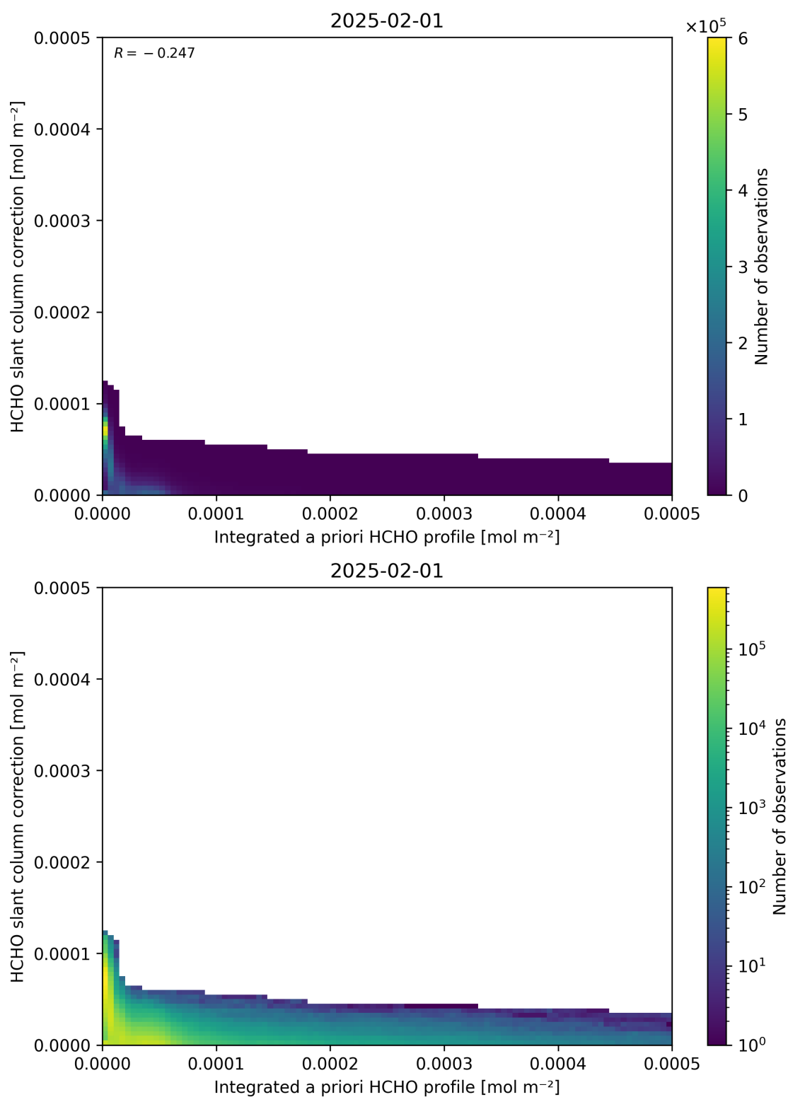
Figure 152: Scatter density plot of “Integrated a priori HCHO profile” against “HCHO slant column correction” for 2025-01-31 to 2025-02-02.
