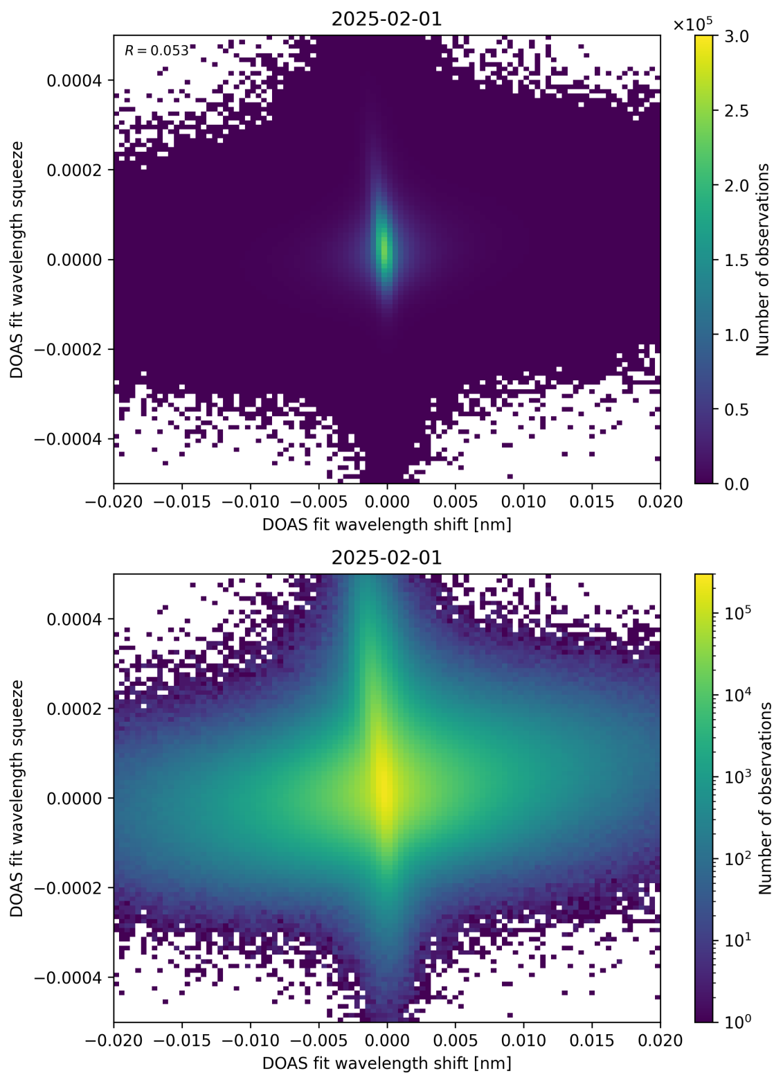
Figure 65: Scatter density plot of “DOAS fit wavelength shift” against “DOAS fit wavelength squeeze” for 2025-01-31 to 2025-02-02.
