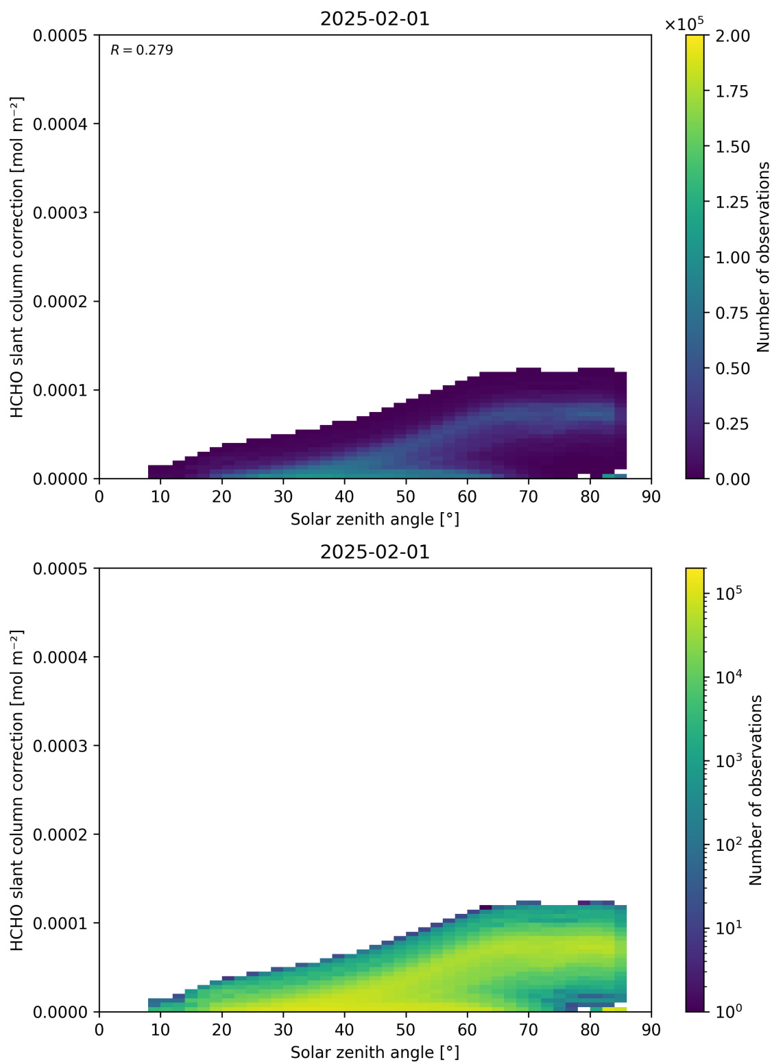
Figure 172: Scatter density plot of “Solar zenith angle” against “HCHO slant column correction” for 2025-01-31 to 2025-02-02.
