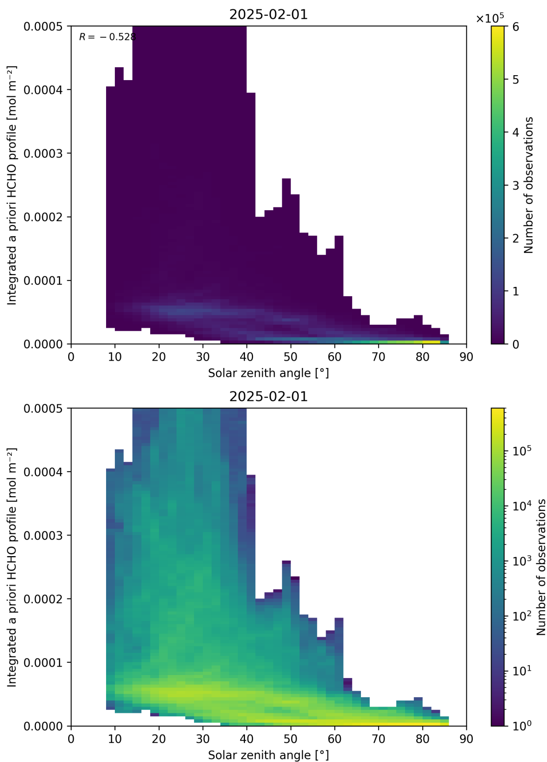
Figure 180: Scatter density plot of “Solar zenith angle” against “Integrated a priori HCHO profile” for 2025-01-31 to 2025-02-02.
