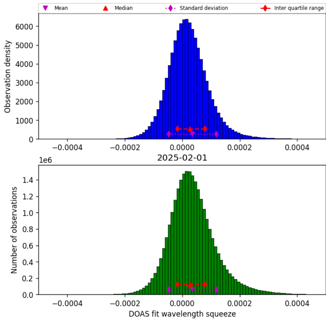
Figure 45: Histogram of “DOAS fit wavelength squeeze” for 2025-01-31 to 2025-02-02
