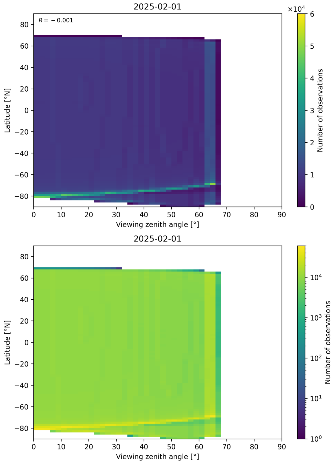
Figure 196: Scatter density plot of “Viewing zenith angle” against “Latitude” for 2025-01-31 to 2025-02-02.
