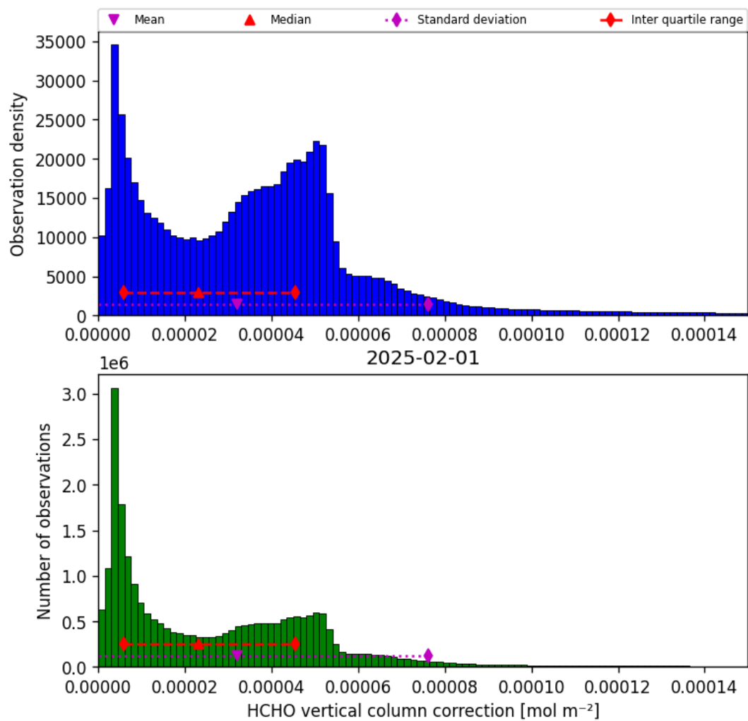
Figure 37: Histogram of “HCHO vertical column correction” for 2025-01-31 to 2025-02-02
