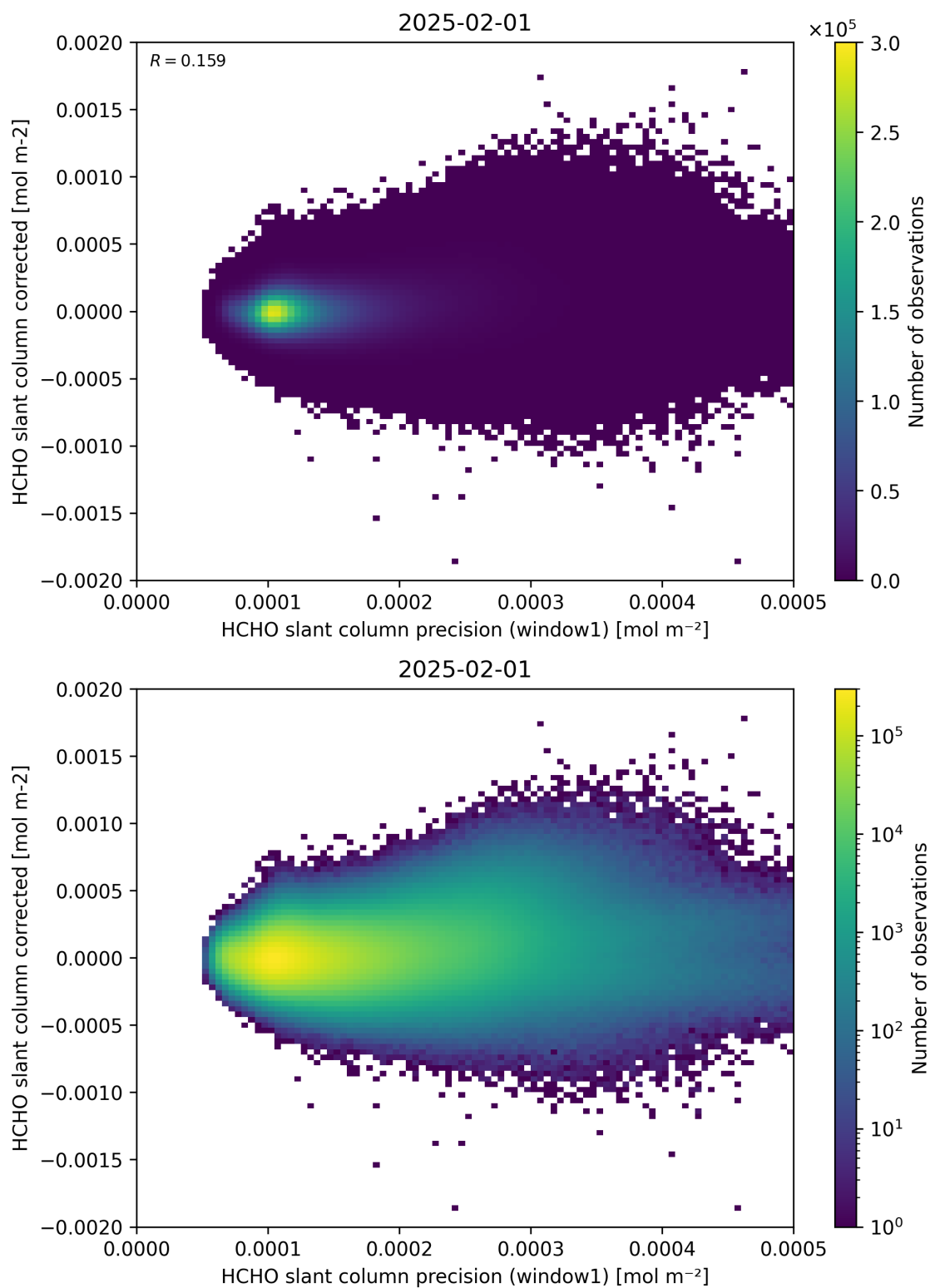
Figure 92: Scatter density plot of “HCHO slant column precision (window1)” against “HCHO slant column corrected” for 2025-01-31 to 2025-02-02.
