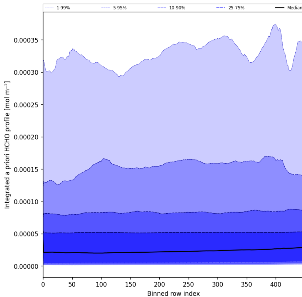
Figure 57: Along track statistics of “Integrated a priori HCHO profile” for 2025-01-31 to 2025-02-02
