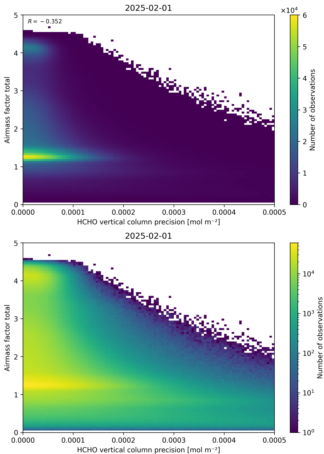
Figure 144: Scatter density plot of “HCHO vertical column precision” against “Airmass factor total” for 2025-01-31 to 2025-02-02.
