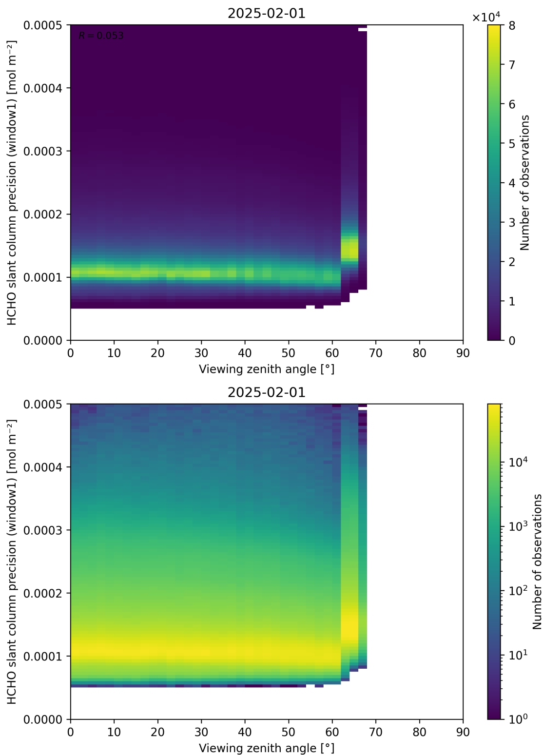
Figure 189: Scatter density plot of “Viewing zenith angle” against “HCHO slant column precision (window1)” for 2025-01-31 to 2025-02-02.
