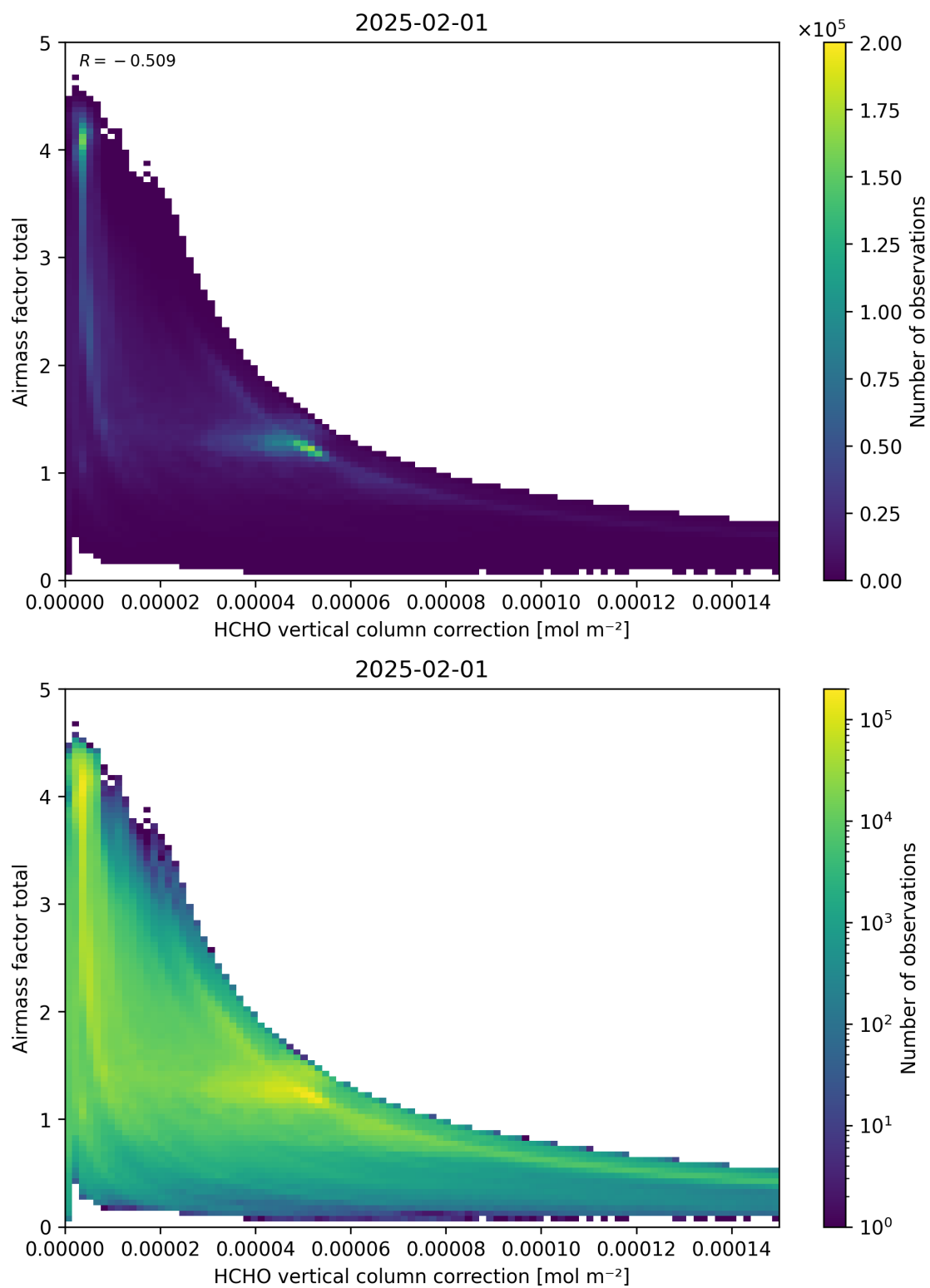
Figure 120: Scatter density plot of “HCHO vertical column correction” against “Airmass factor total” for 2025-01-31 to 2025-02-02.
