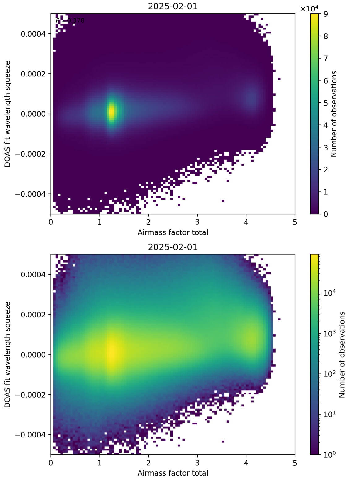
Figure 99: Scatter density plot of “Airmass factor total” against “DOAS fit wavelength squeeze” for 2025-01-31 to 2025-02-02.
