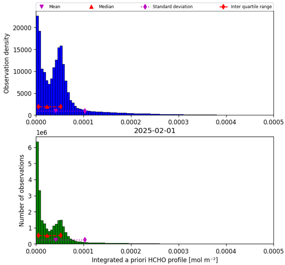
Figure 43: Histogram of “Integrated a priori HCHO profile” for 2025-01-31 to 2025-02-02
