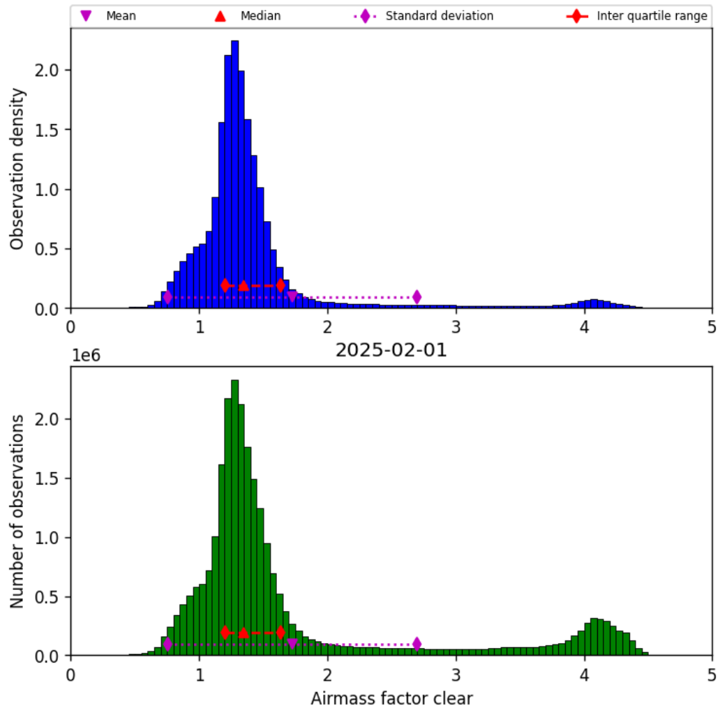
Figure 42: Histogram of “Airmass factor clear” for 2025-01-31 to 2025-02-02
