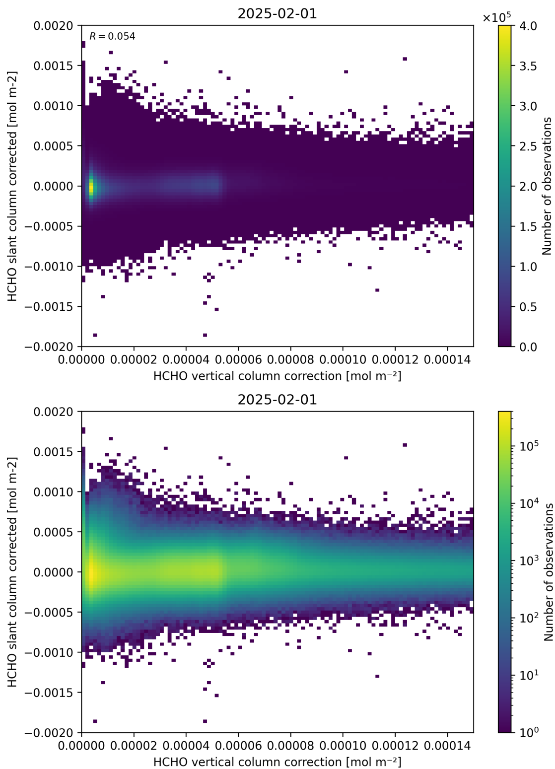
Figure 116: Scatter density plot of “HCHO vertical column correction” against “HCHO slant column corrected” for 2025-01-31 to 2025-02-02.
