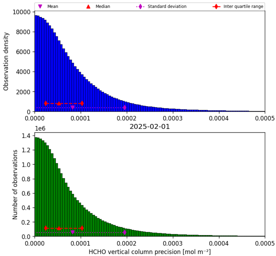
Figure 36: Histogram of “HCHO vertical column precision” for 2025-01-31 to 2025-02-02
