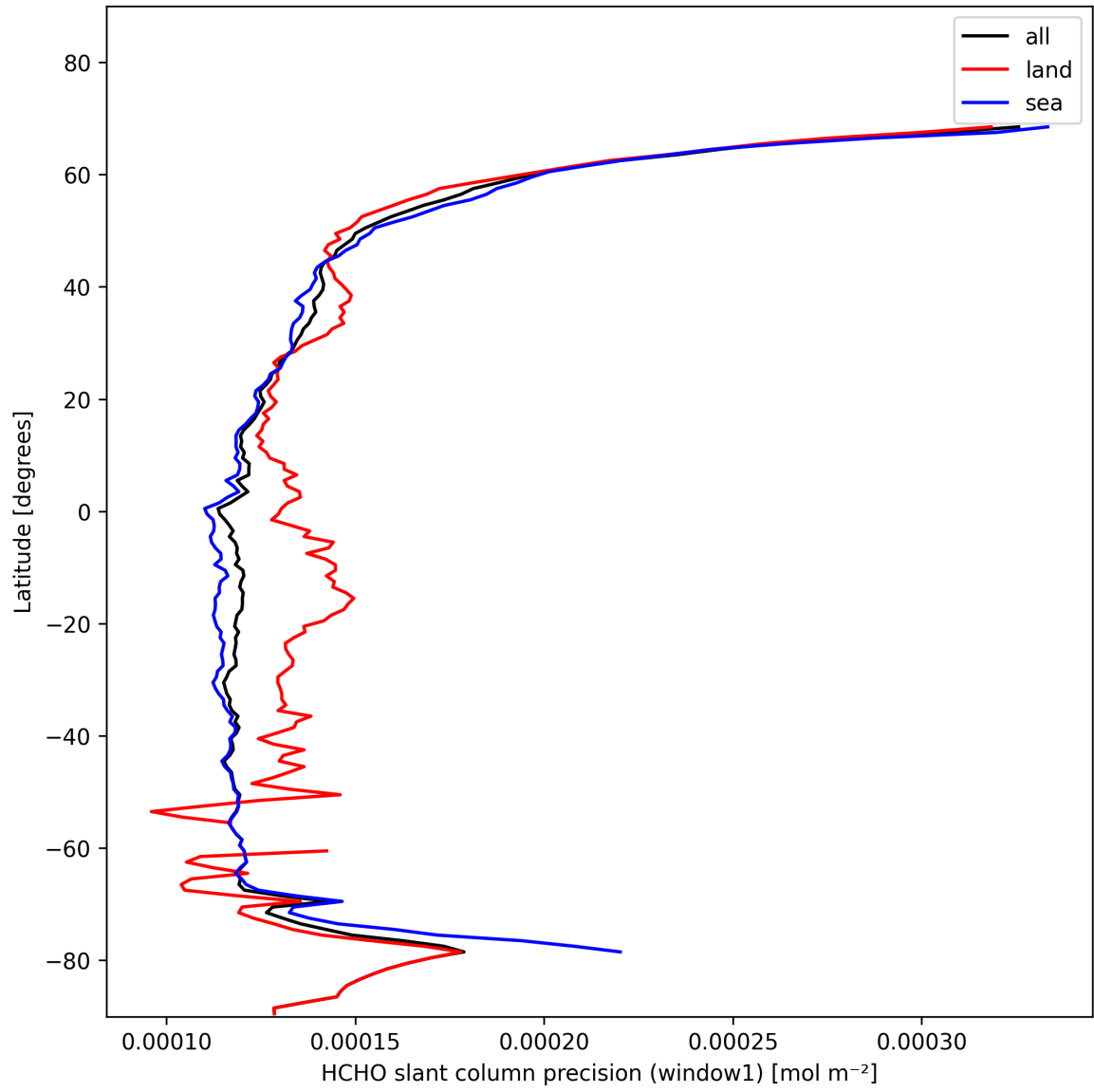
Figure 25: Zonal average of “HCHO slant column precision (window1)” for 2025-01-31 to 2025-02-02.
