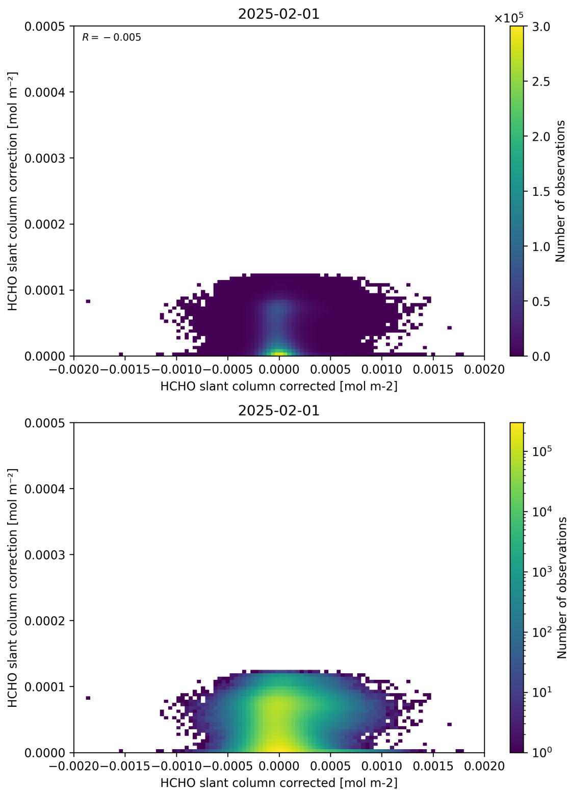
Figure 77: Scatter density plot of “HCHO slant column corrected” against “HCHO slant column correction” for 2025-01-31 to 2025-02-02.
