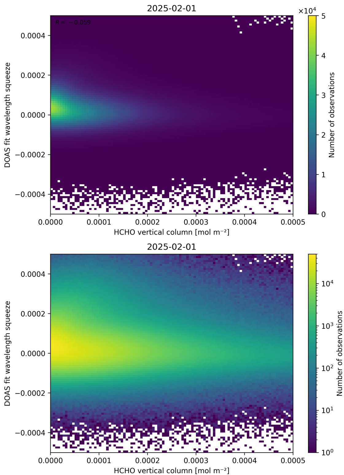
Figure 125: Scatter density plot of “HCHO vertical column” against “DOAS fit wavelength squeeze” for 2025-01-31 to 2025-02-02.
