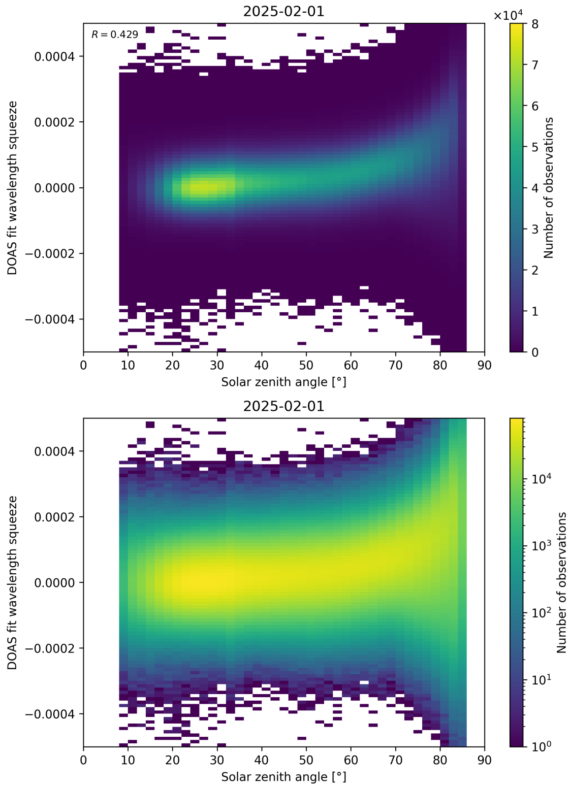
Figure 169: Scatter density plot of “Solar zenith angle” against “DOAS fit wavelength squeeze” for 2025-01-31 to 2025-02-02.
