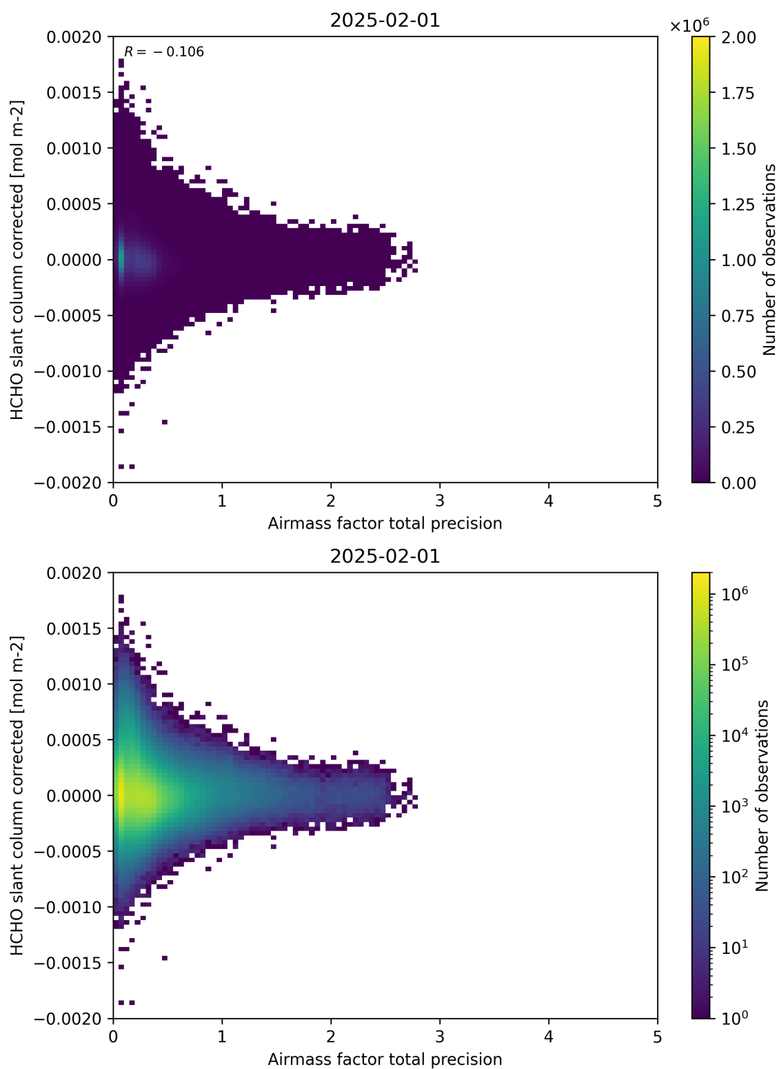
Figure 109: Scatter density plot of “Airmass factor total precision” against “HCHO slant column corrected” for 2025-01-31 to 2025-02-02.
