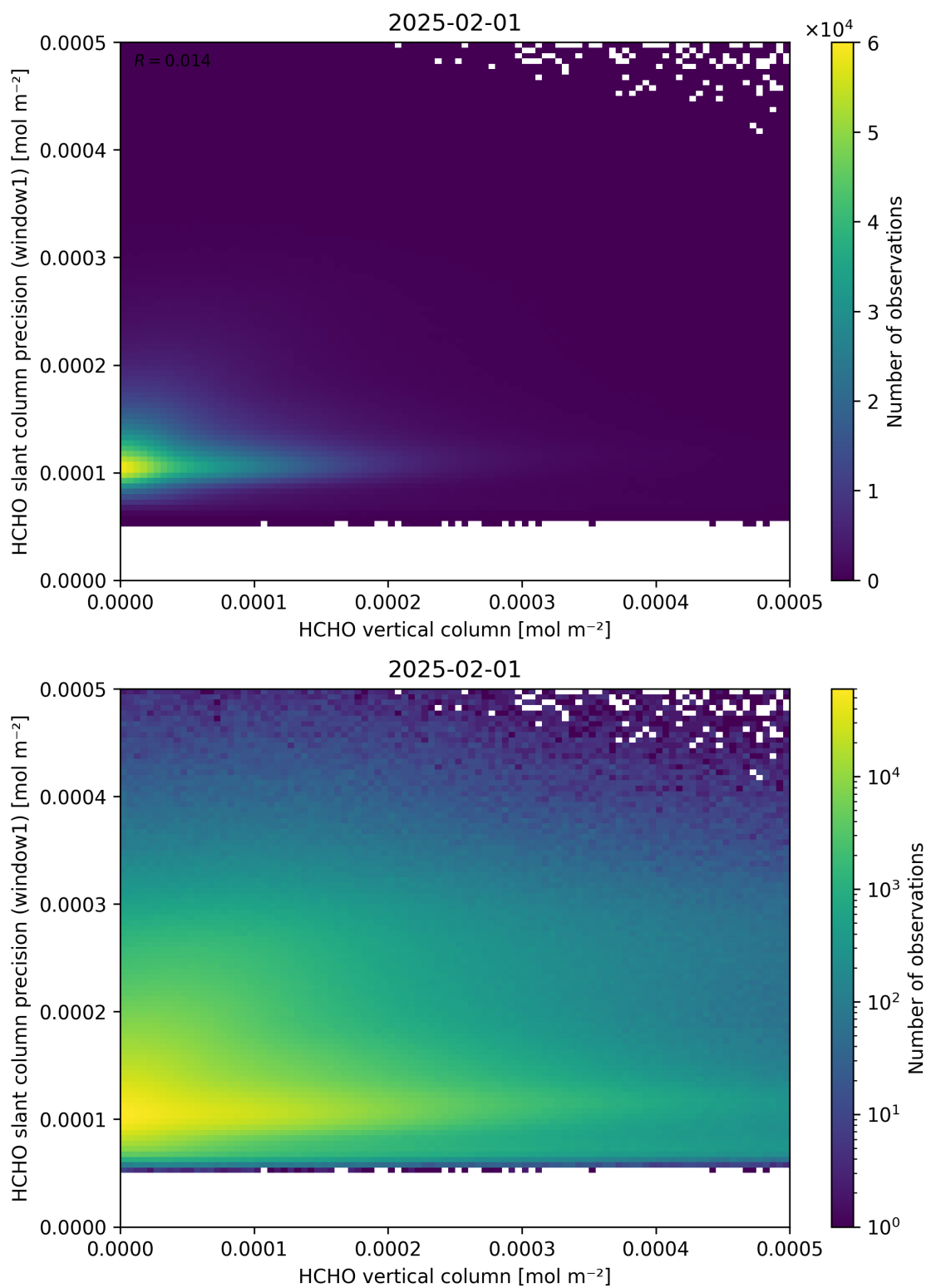
Figure 130: Scatter density plot of “HCHO vertical column” against “HCHO slant column precision (window1)” for 2025-01-31 to 2025-02-02.
