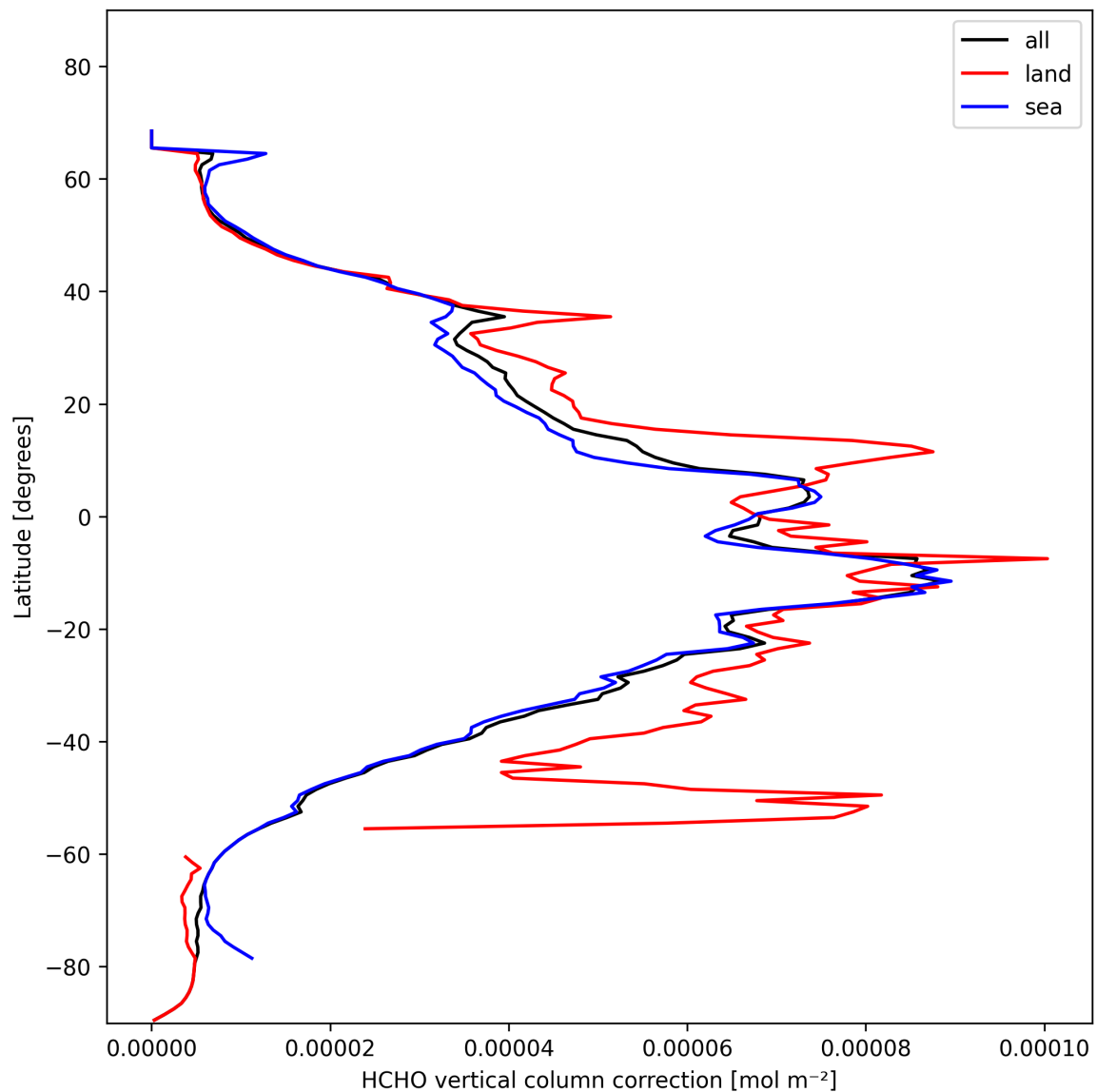
Figure 23: Zonal average of “HCHO vertical column correction” for 2025-01-31 to 2025-02-02.
