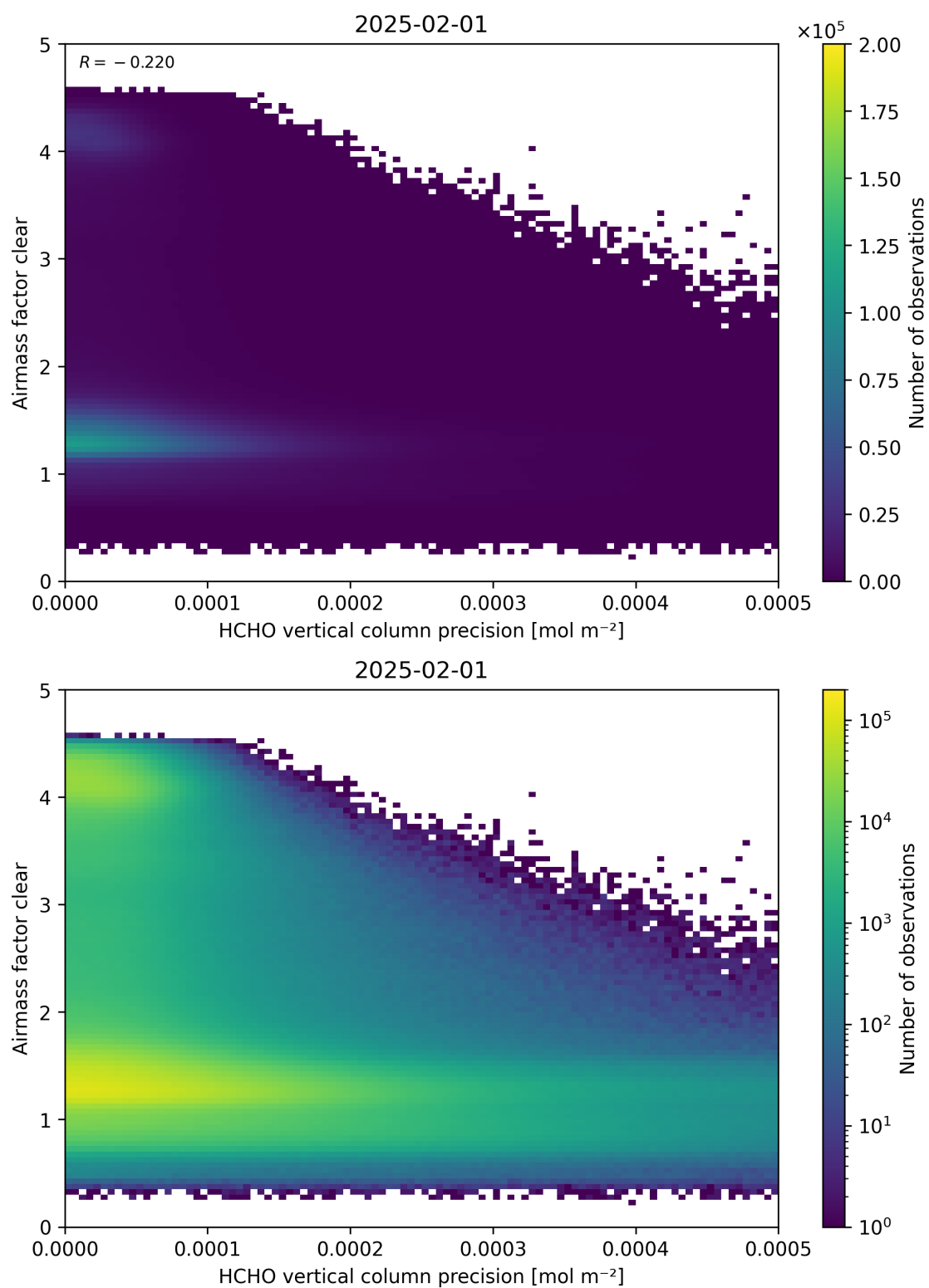
Figure 139: Scatter density plot of “HCHO vertical column precision” against “Airmass factor clear” for 2025-01-31 to 2025-02-02.
