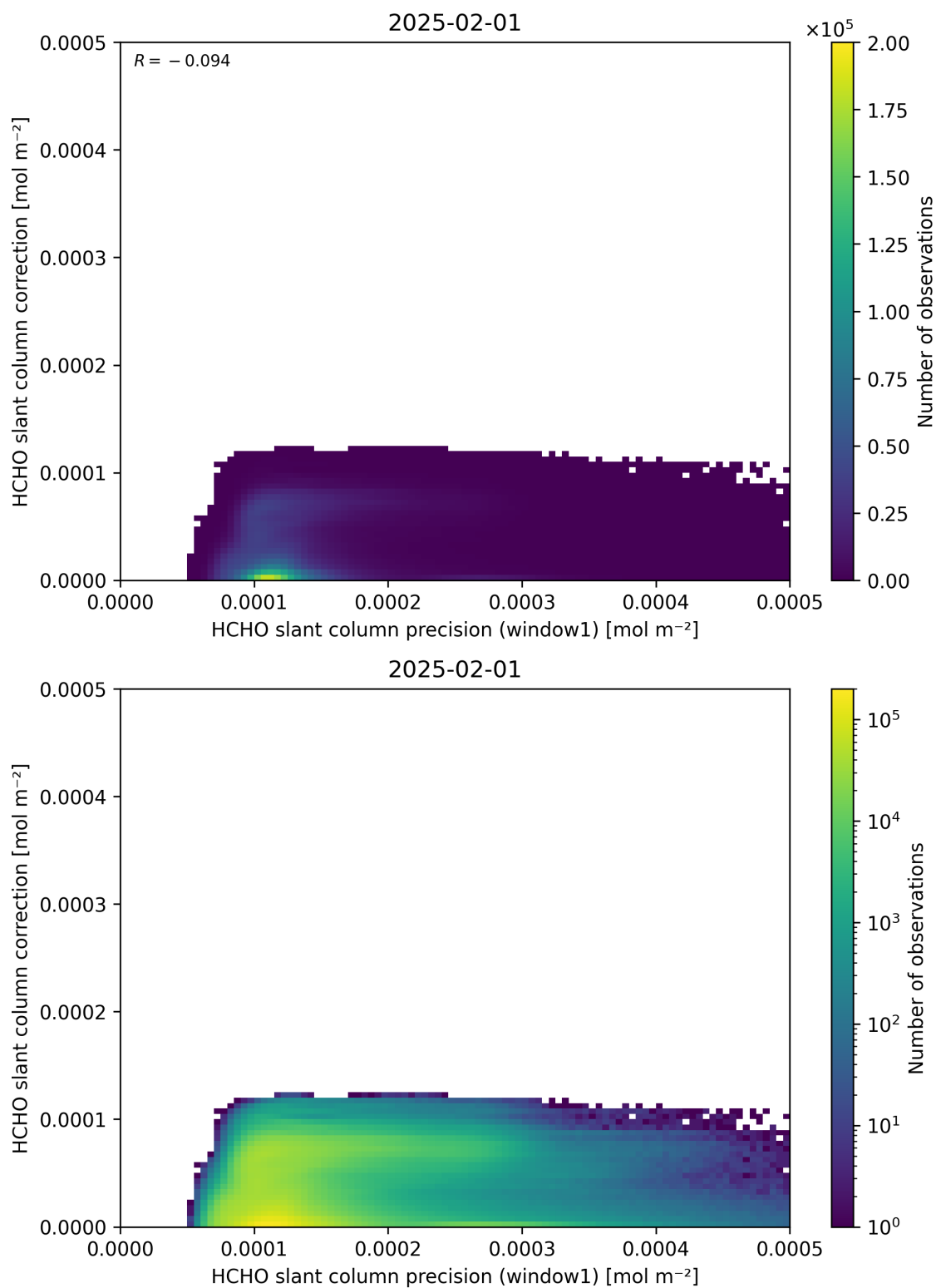
Figure 93: Scatter density plot of “HCHO slant column precision (window1)” against “HCHO slant column correction” for 2025-01-31 to 2025-02-02.
