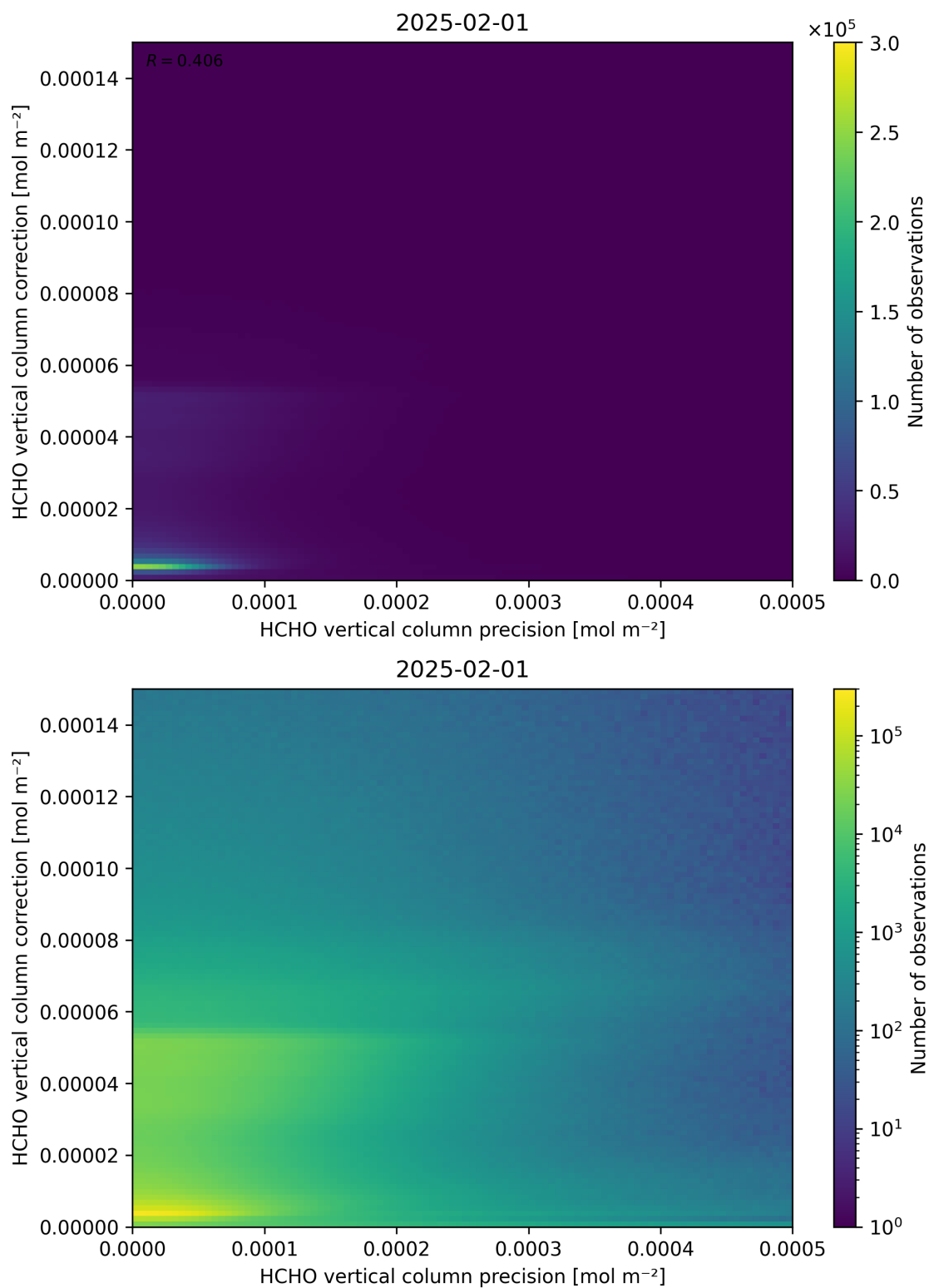
Figure 146: Scatter density plot of “HCHO vertical column precision” against “HCHO vertical column correction” for 2025-01-31 to 2025-02-02.
