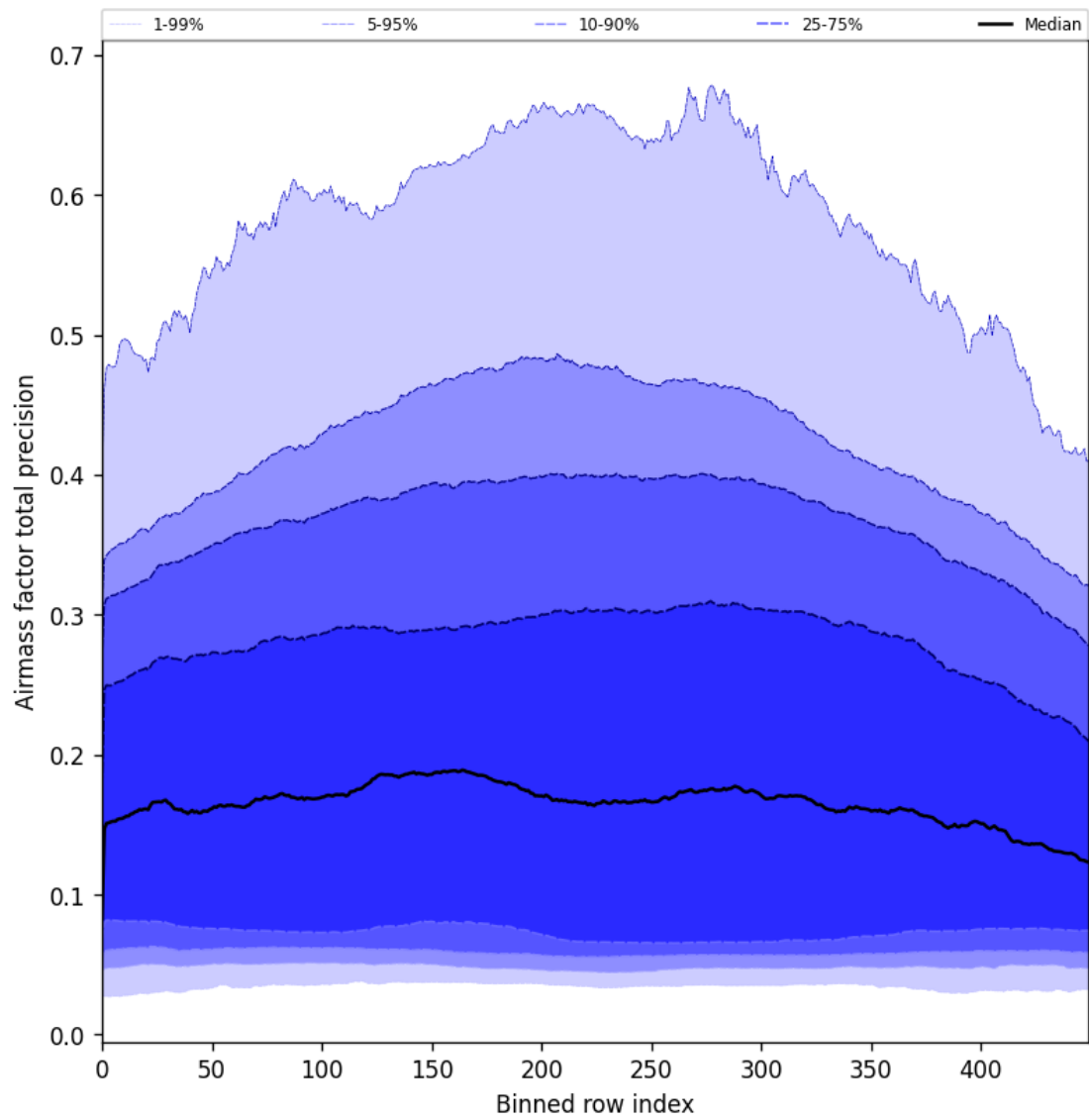
Figure 55: Along track statistics of “Airmass factor total precision” for 2025-01-31 to 2025-02-02
