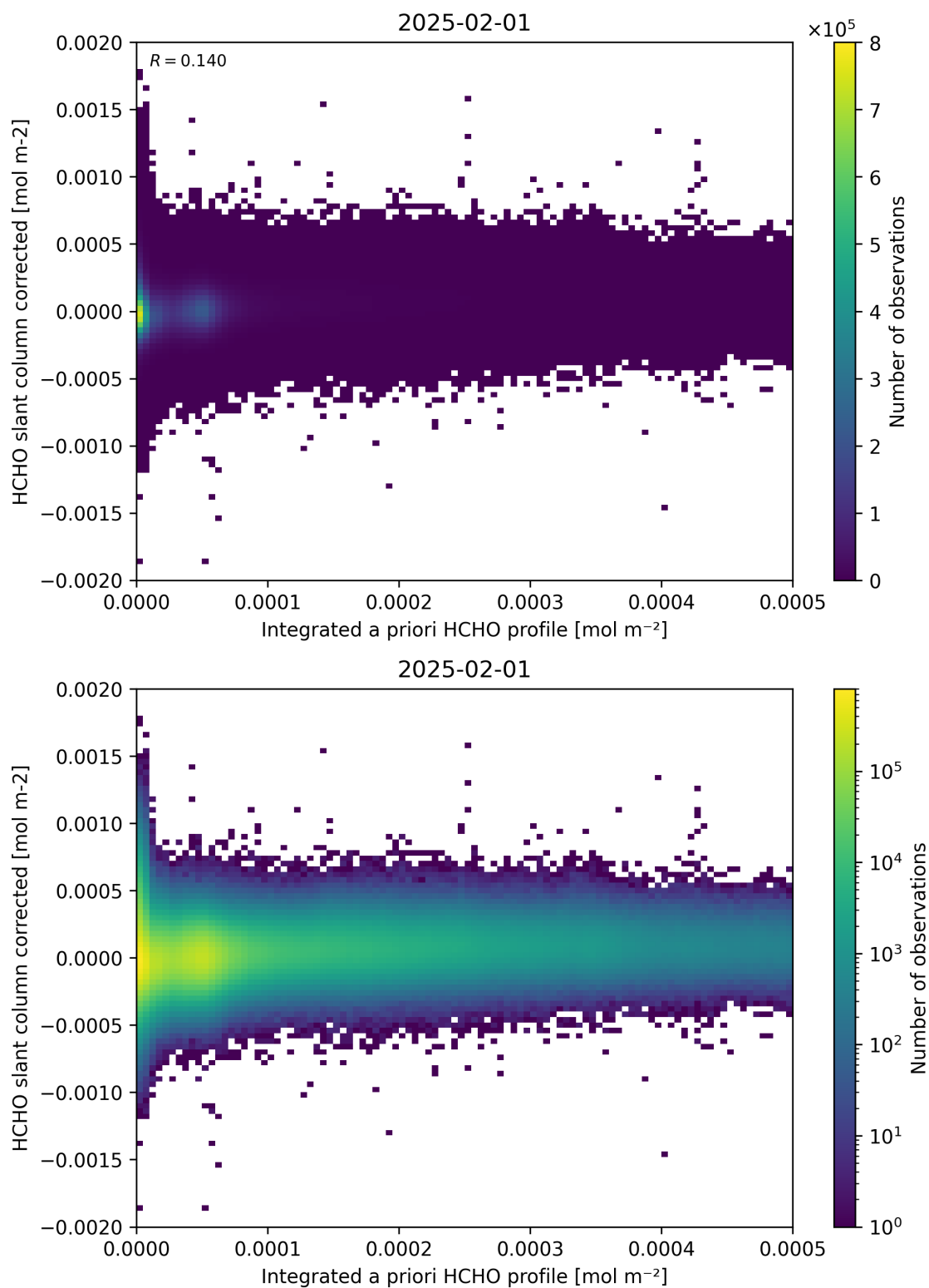
Figure 151: Scatter density plot of “Integrated a priori HCHO profile” against “HCHO slant column corrected” for 2025-01-31 to 2025-02-02.
