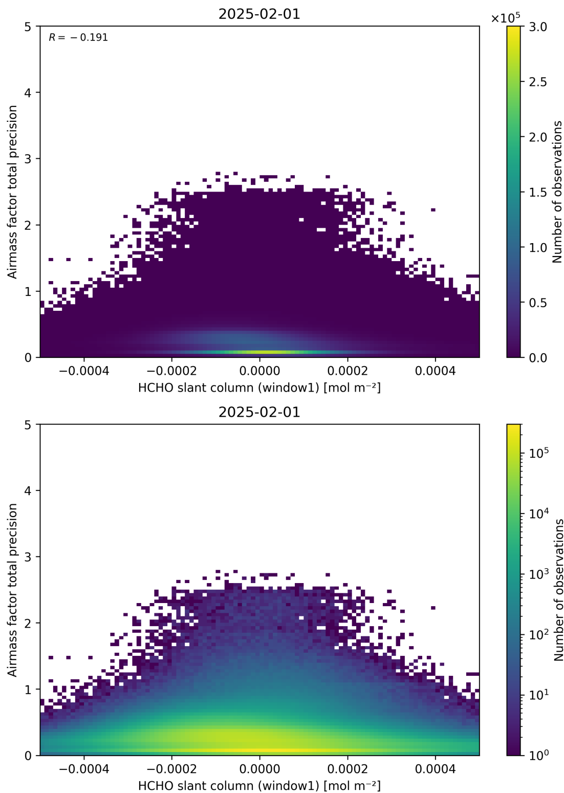
Figure 86: Scatter density plot of “HCHO slant column (window1)” against “Airmass factor total precision” for 2025-01-31 to 2025-02-02.
