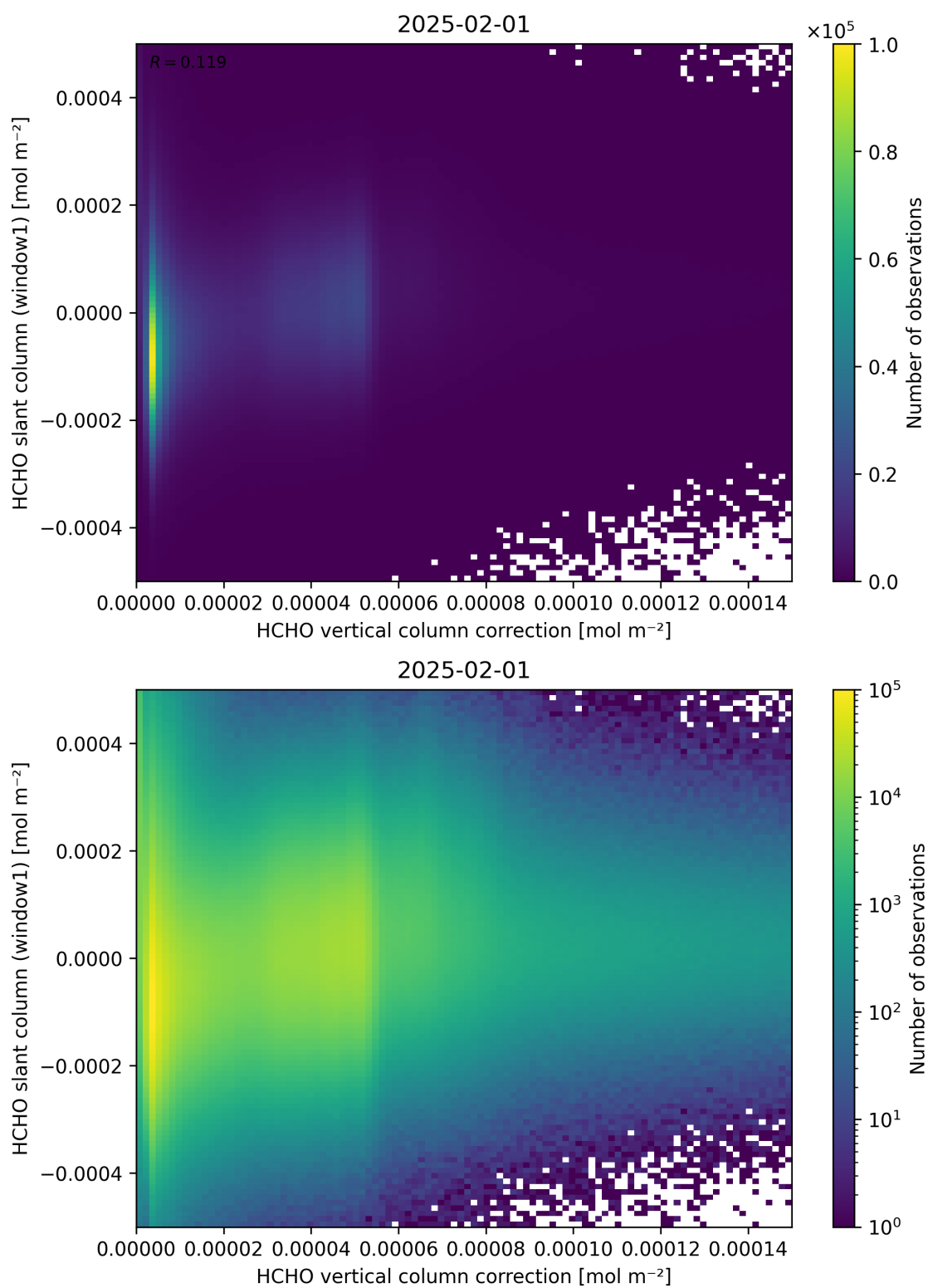
Figure 118: Scatter density plot of “HCHO vertical column correction” against “HCHO slant column (window1)” for 2025-01-31 to 2025-02-02.
