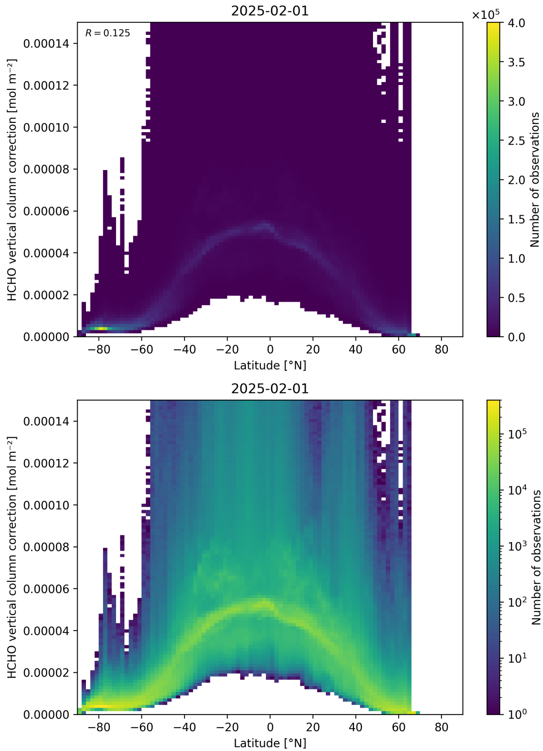
Figure 164: Scatter density plot of “Latitude” against “HCHO vertical column correction” for 2025-01-31 to 2025-02-02.
