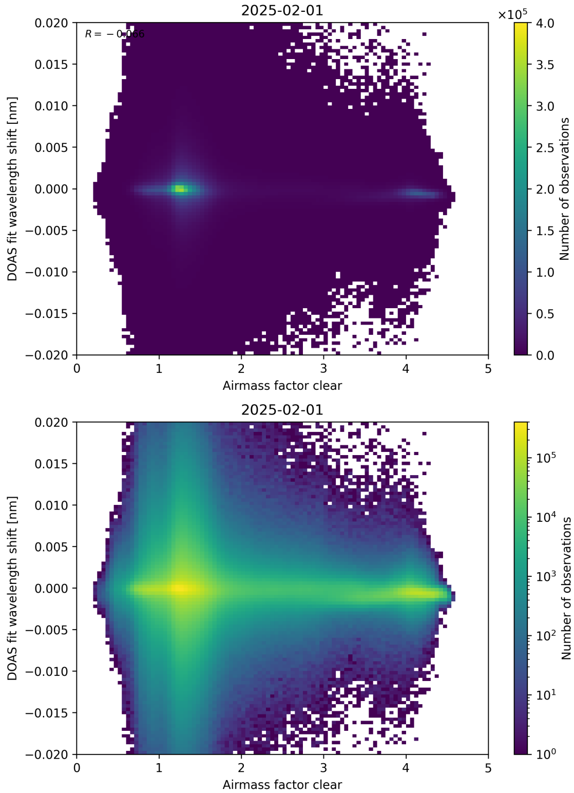
Figure 72: Scatter density plot of “Airmass factor clear” against “DOAS fit wavelength shift” for 2025-01-31 to 2025-02-02.
