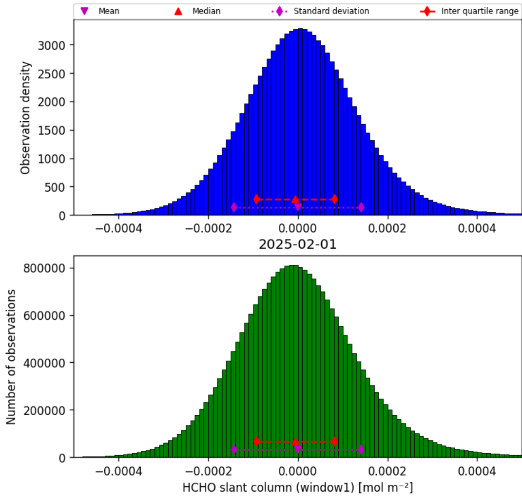
Figure 38: Histogram of “HCHO slant column (window1)” for 2025-01-31 to 2025-02-02
