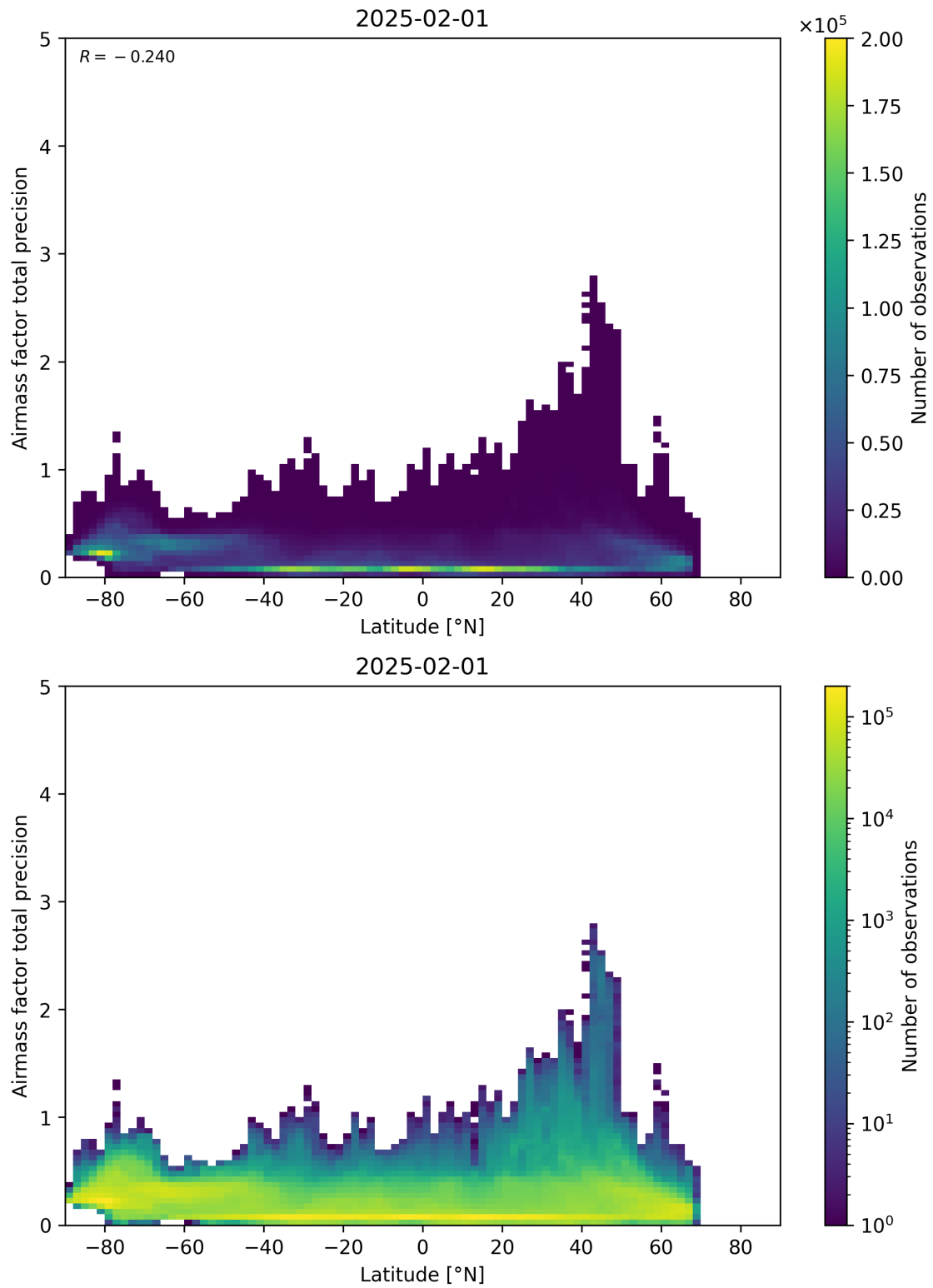
Figure 162: Scatter density plot of “Latitude” against “Airmass factor total precision” for 2025-01-31 to 2025-02-02.
