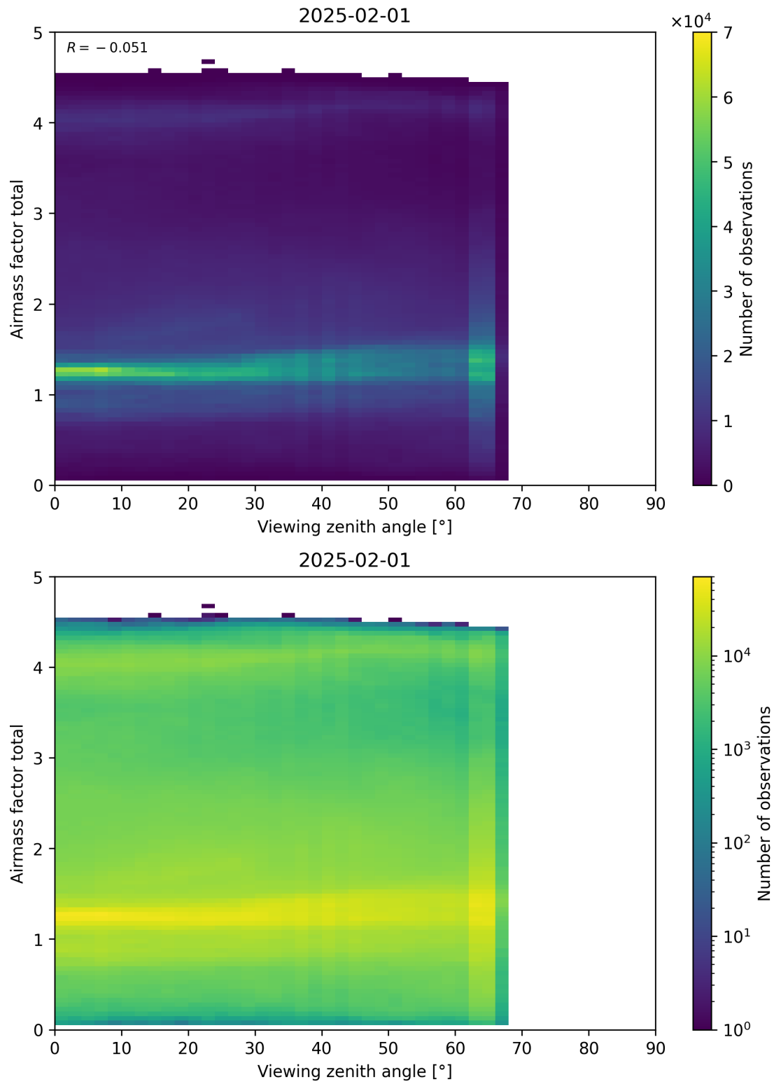
Figure 190: Scatter density plot of “Viewing zenith angle” against “Airmass factor total” for 2025-01-31 to 2025-02-02.
