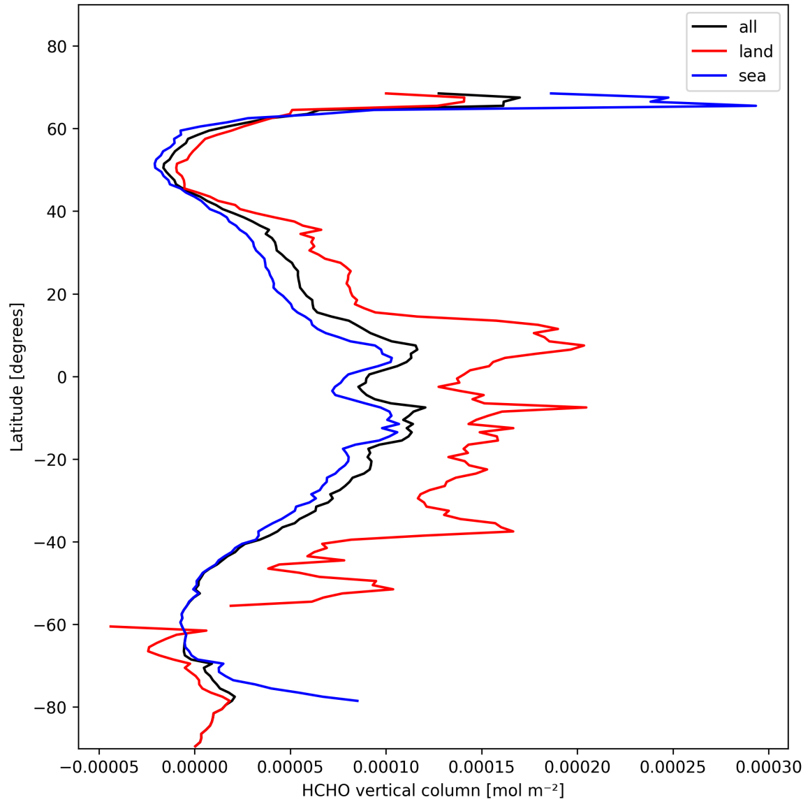
Figure 21: Zonal average of “HCHO vertical column” for 2025-01-31 to 2025-02-02.
