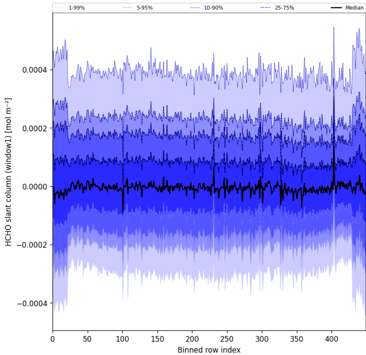
Figure 52: Along track statistics of “HCHO slant column (window1)” for 2025-01-31 to 2025-02-02
