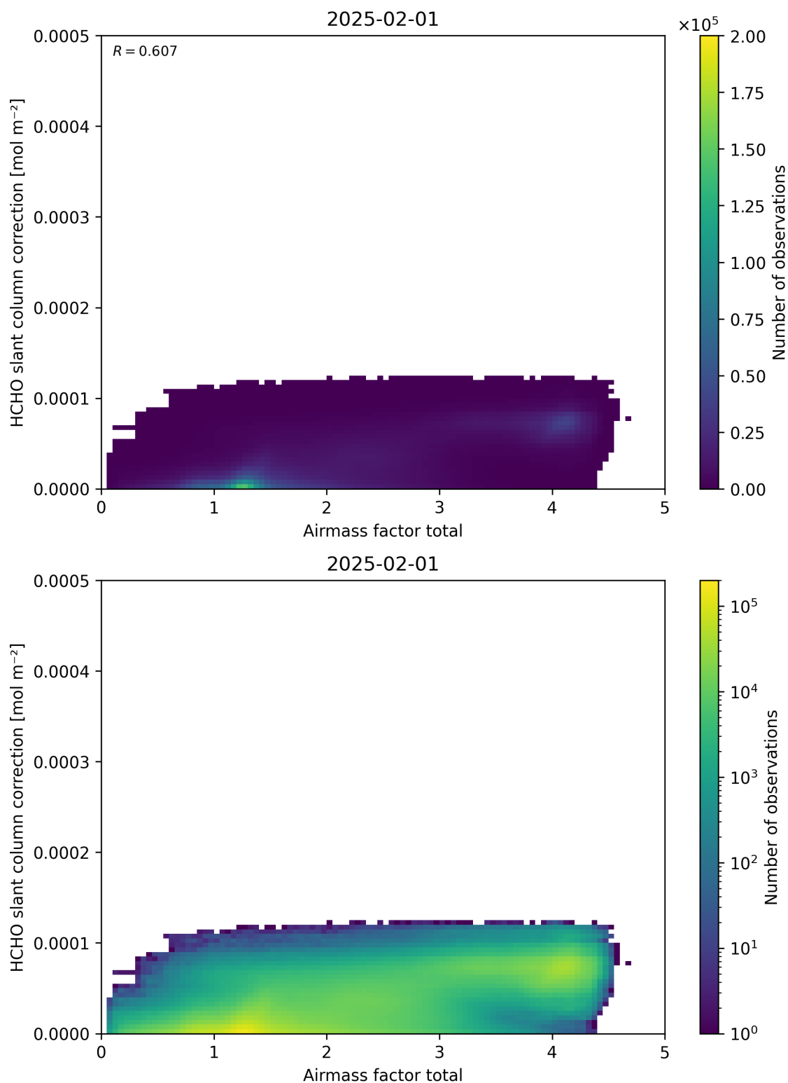
Figure 102: Scatter density plot of “Airmass factor total” against “HCHO slant column correction” for 2025-01-31 to 2025-02-02.
