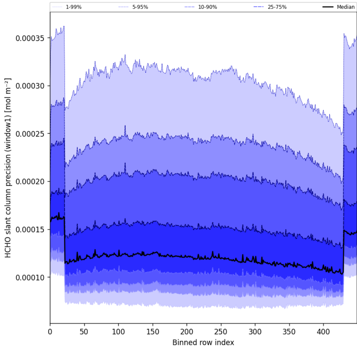
Figure 53: Along track statistics of “HCHO slant column precision (window1)” for 2025-01-31 to 2025-02-02
