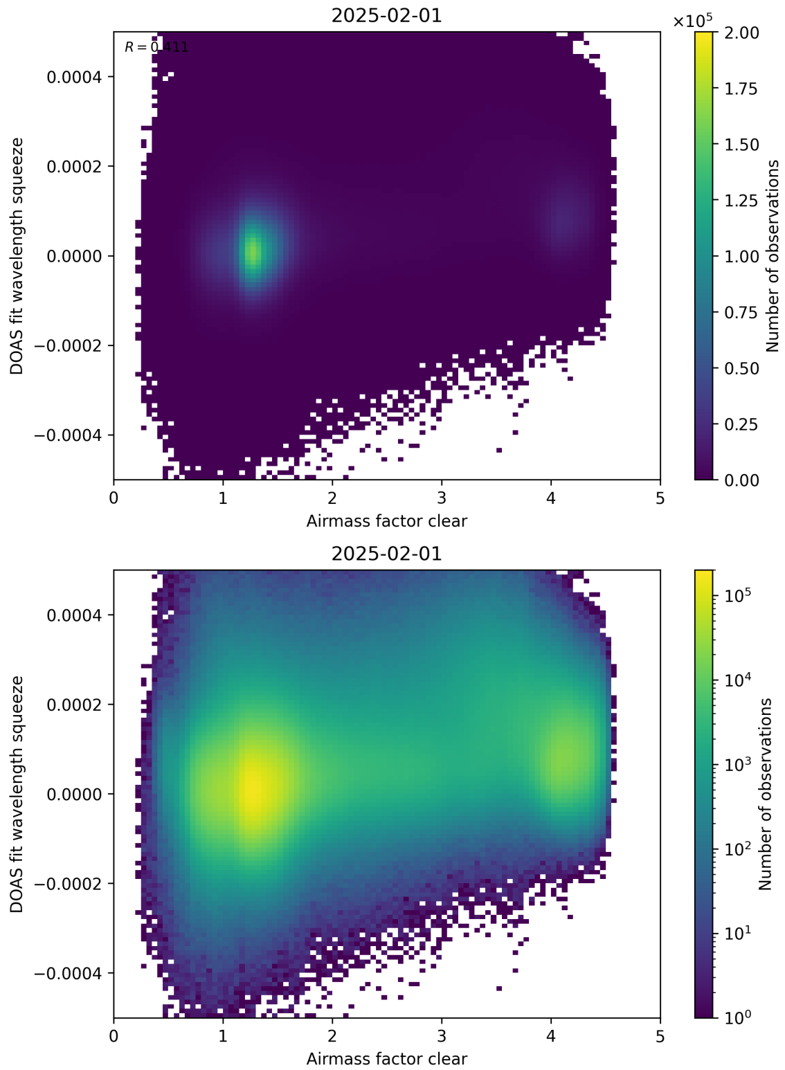
Figure 73: Scatter density plot of “Airmass factor clear” against “DOAS fit wavelength squeeze” for 2025-01-31 to 2025-02-02.
