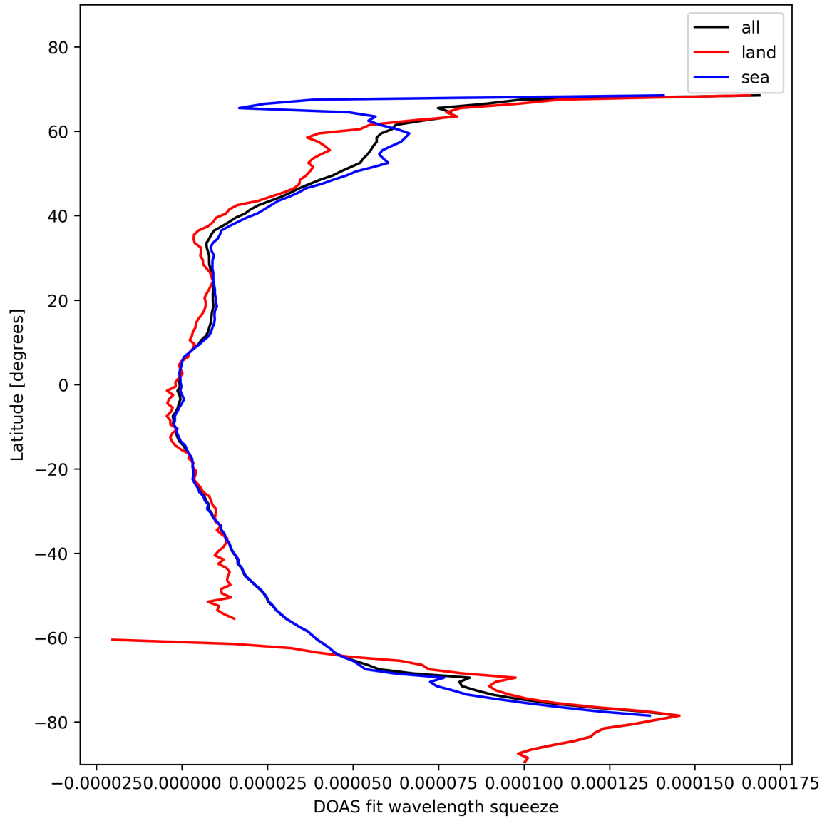
Figure 31: Zonal average of “DOAS fit wavelength squeeze” for 2025-01-31 to 2025-02-02.
