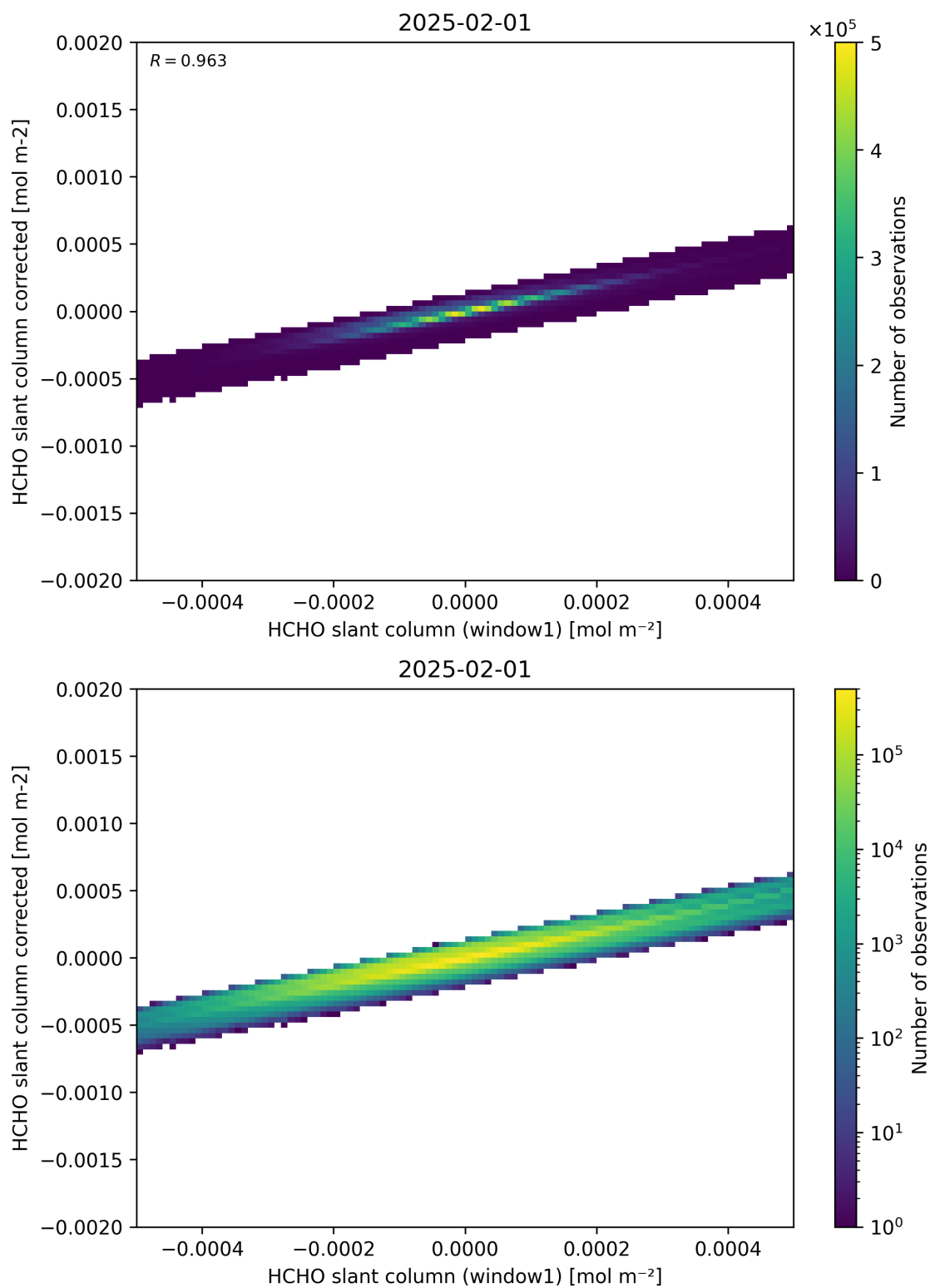
Figure 82: Scatter density plot of “HCHO slant column (window1)” against “HCHO slant column corrected” for 2025-01-31 to 2025-02-02.
