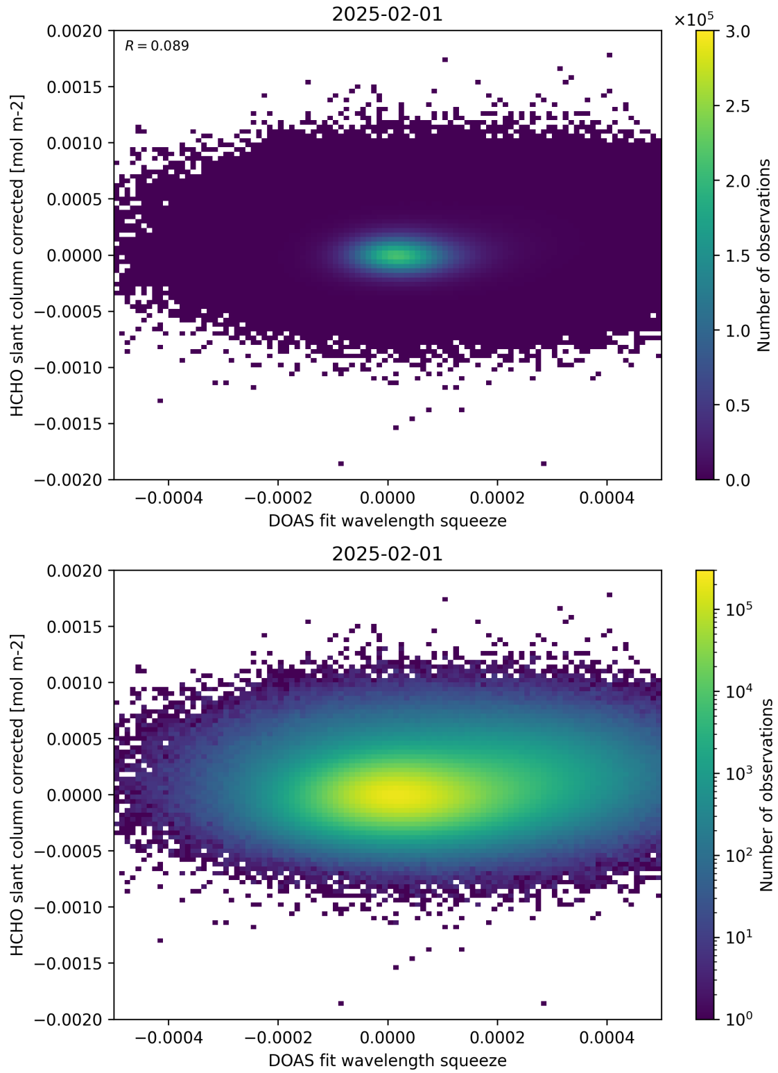
Figure 69: Scatter density plot of “DOAS fit wavelength squeeze” against “HCHO slant column corrected” for 2025-01-31 to 2025-02-02.
