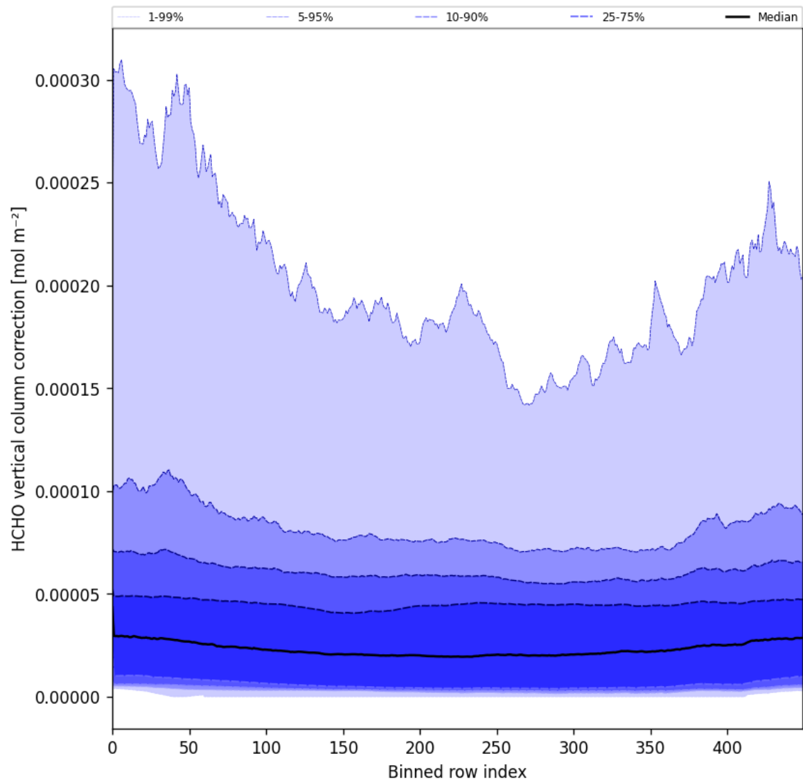
Figure 51: Along track statistics of “HCHO vertical column correction” for 2025-01-31 to 2025-02-02
