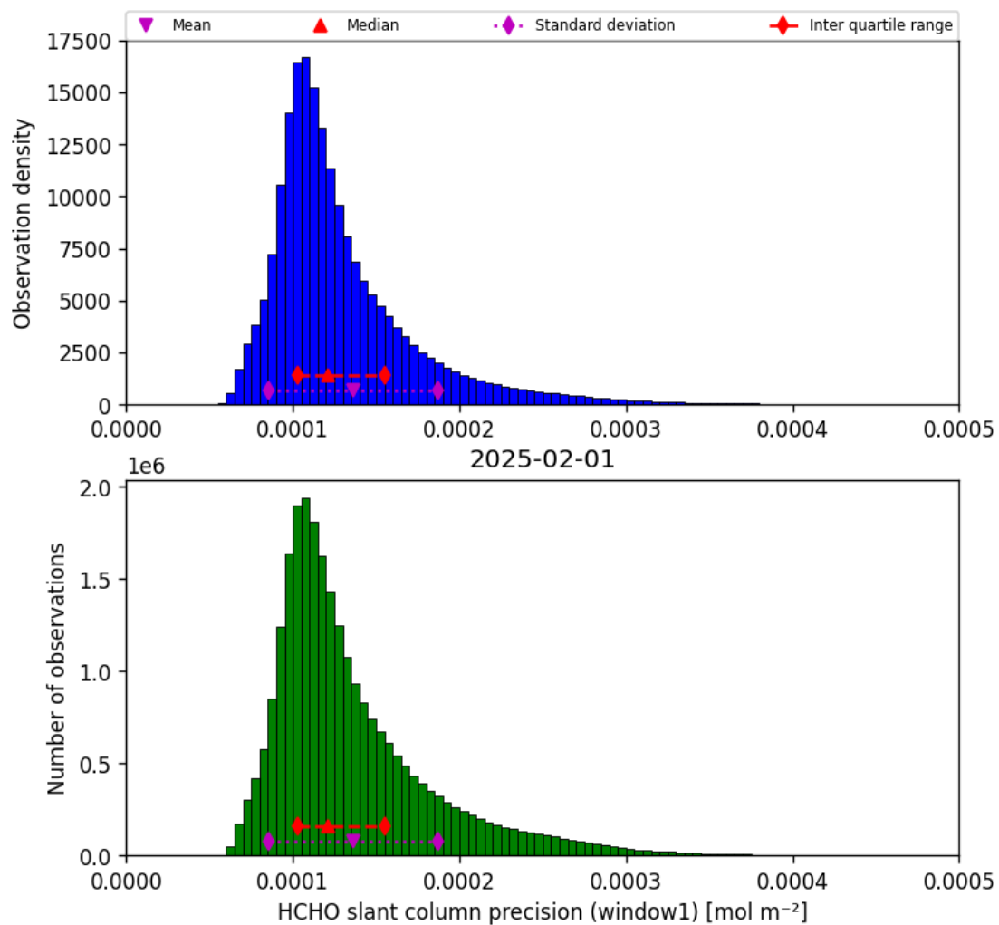
Figure 39: Histogram of “HCHO slant column precision (window1)” for 2025-01-31 to 2025-02-02
