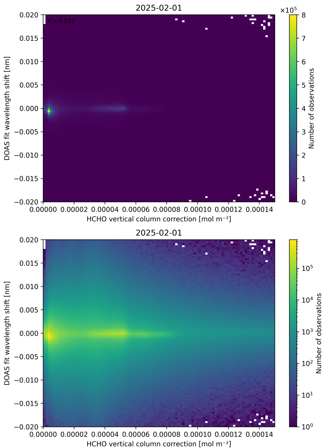
Figure 113: Scatter density plot of “HCHO vertical column correction” against “DOAS fit wavelength shift” for 2025-01-31 to 2025-02-02.
