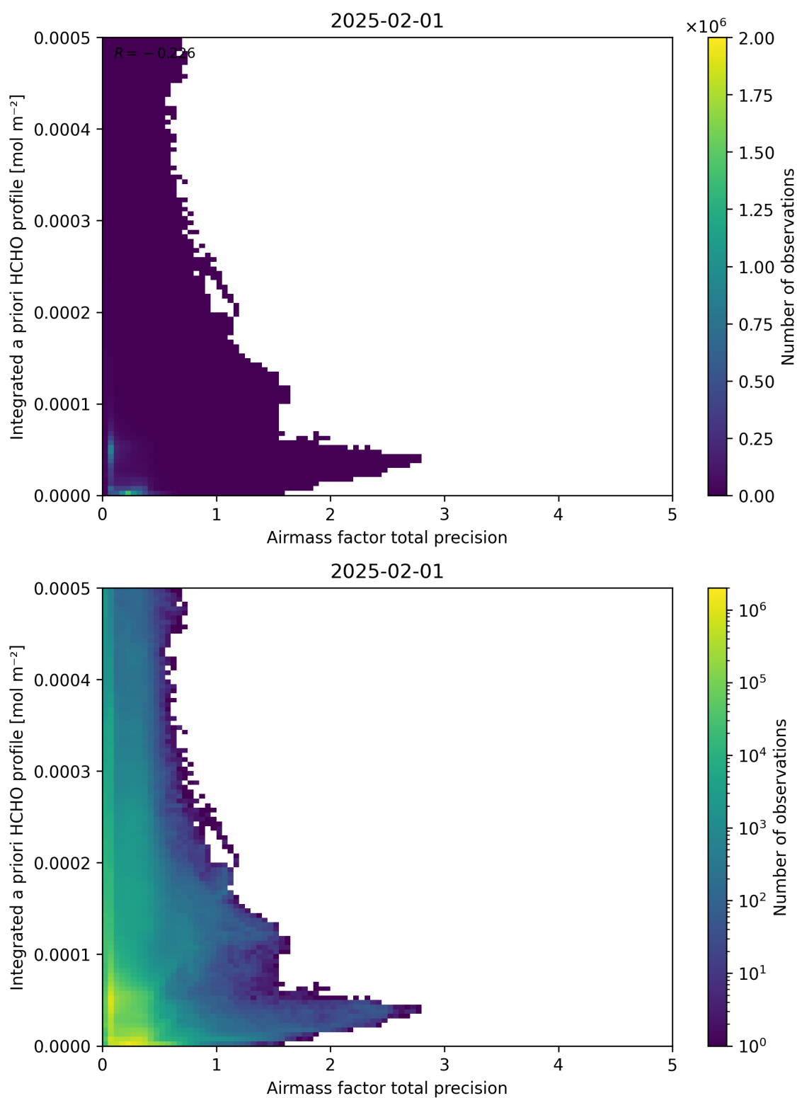
Figure 111: Scatter density plot of “Airmass factor total precision” against “Integrated a priori HCHO profile” for 2025-01-31 to 2025-02-02.
