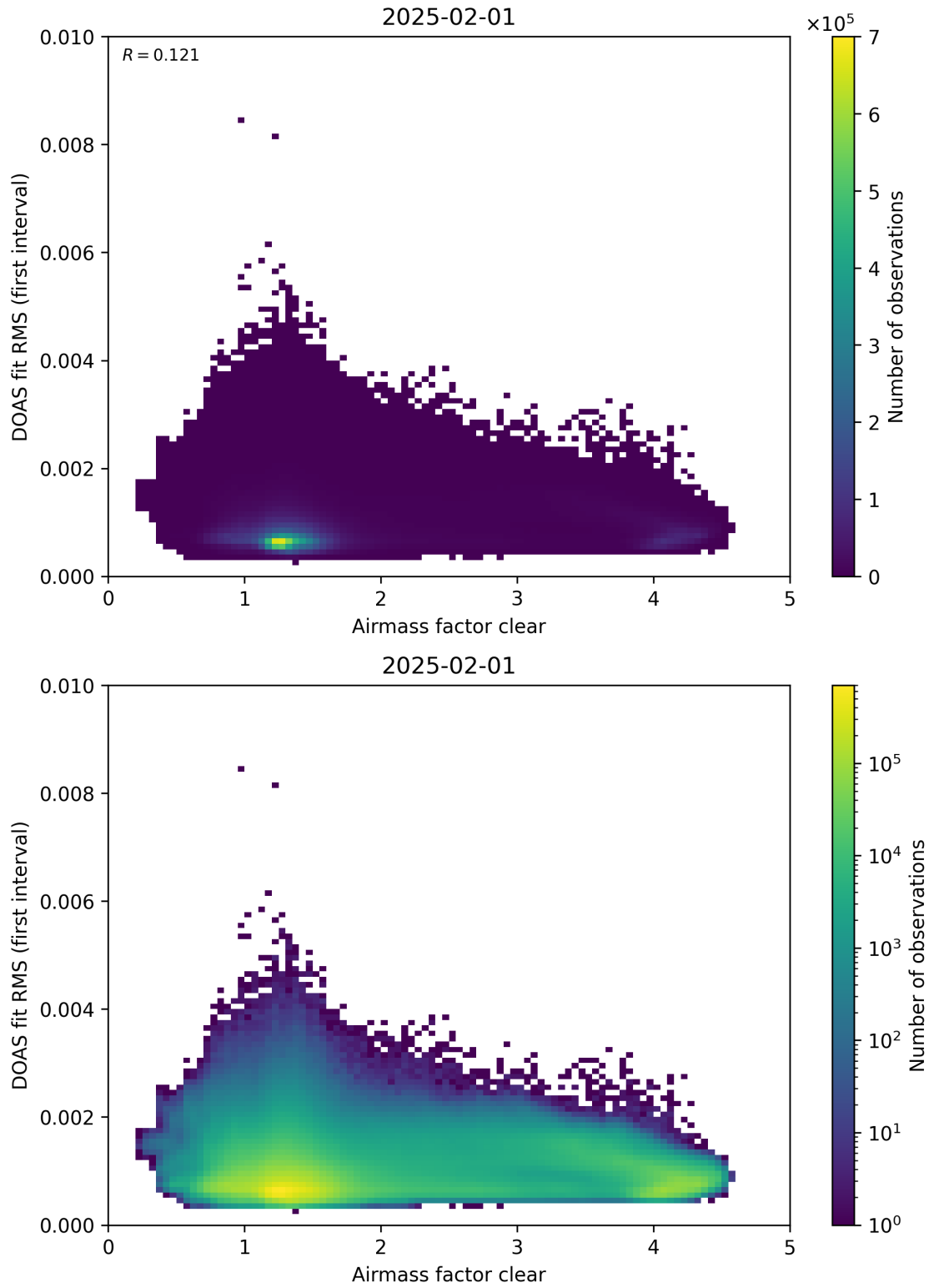
Figure 71: Scatter density plot of “Airmass factor clear” against “DOAS fit RMS (first interval)” for 2025-01-31 to 2025-02-02.
