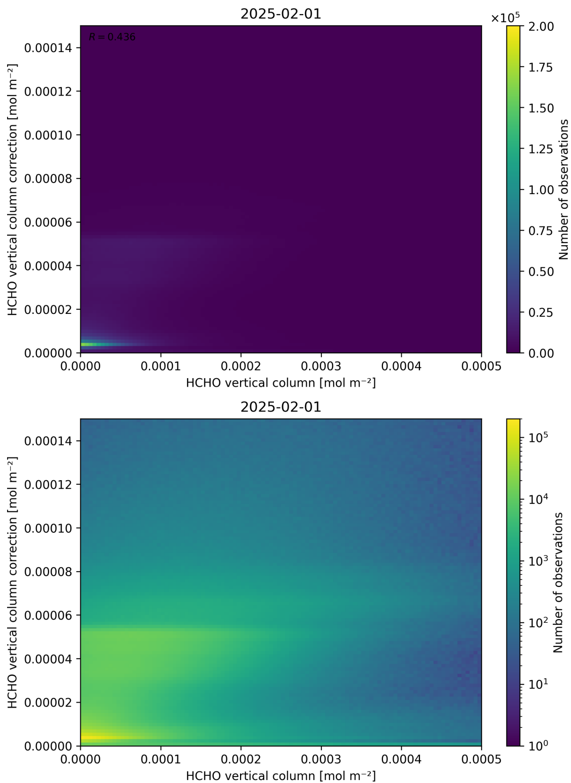
Figure 133: Scatter density plot of “HCHO vertical column” against “HCHO vertical column correction” for 2025-01-31 to 2025-02-02.
