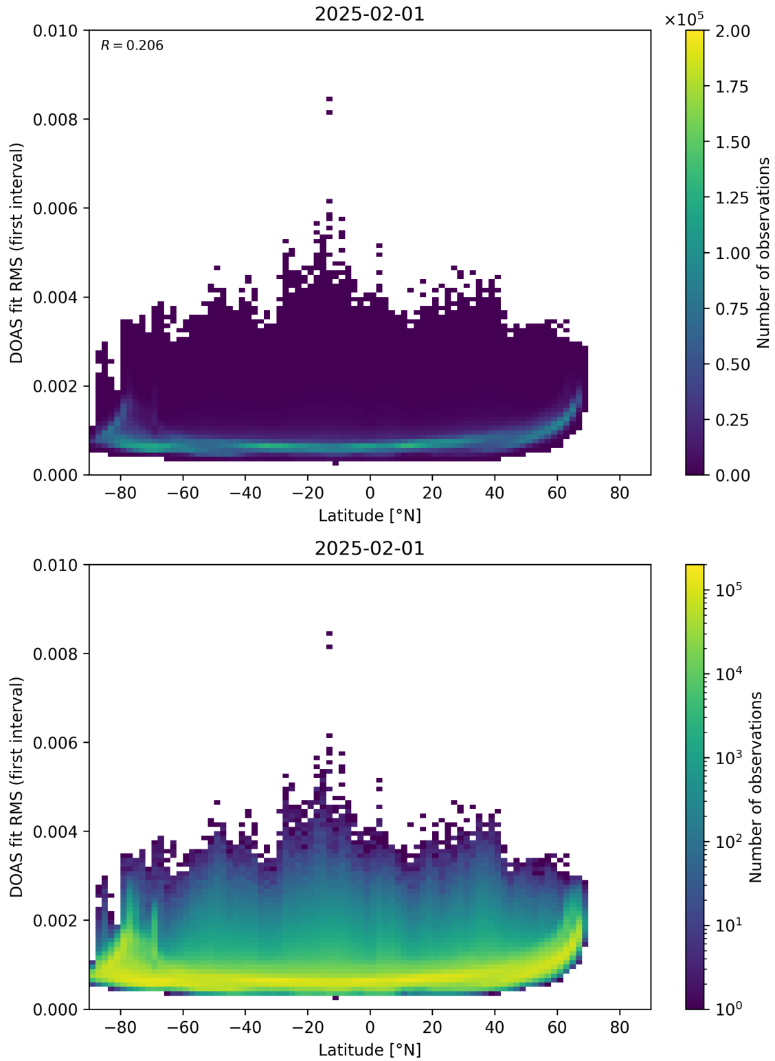
Figure 153: Scatter density plot of “Latitude” against “DOAS fit RMS (first interval)” for 2025-01-31 to 2025-02-02.
