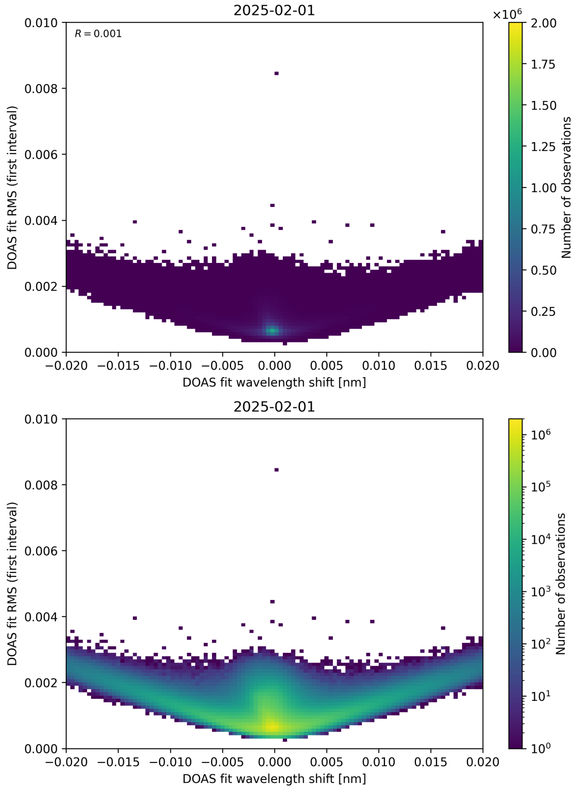
Figure 64: Scatter density plot of “DOAS fit wavelength shift” against “DOAS fit RMS (first interval)” for 2025-01-31 to 2025-02-02.
