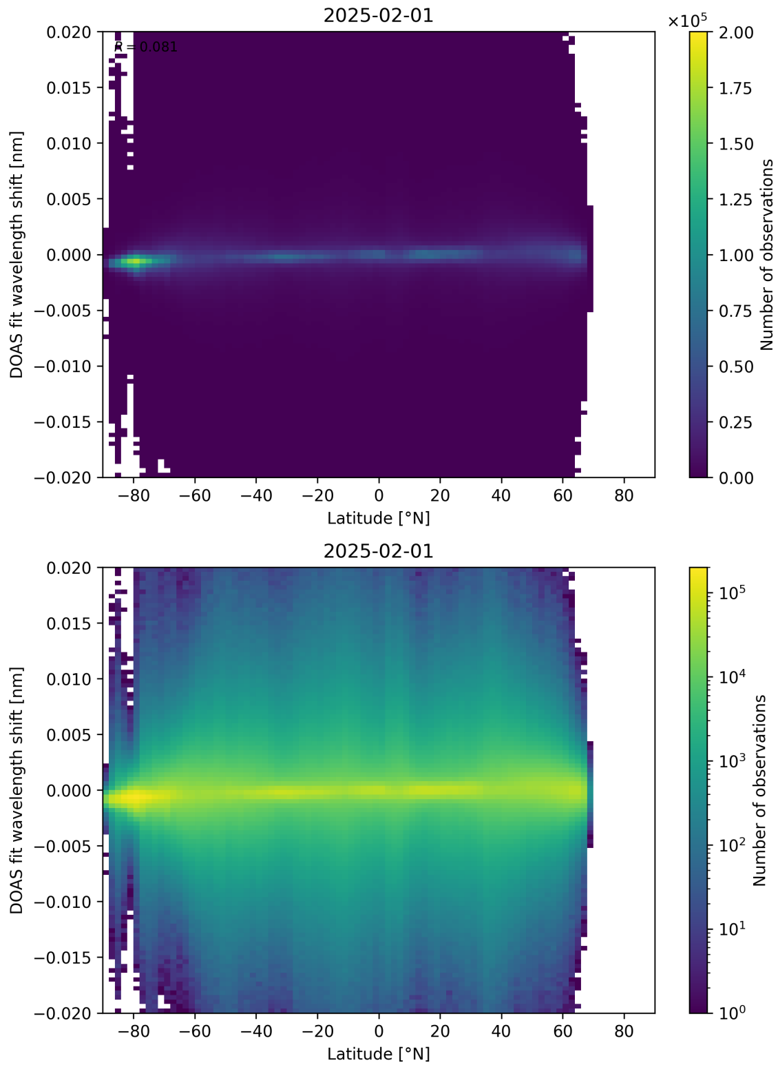
Figure 154: Scatter density plot of “Latitude” against “DOAS fit wavelength shift” for 2025-01-31 to 2025-02-02.
