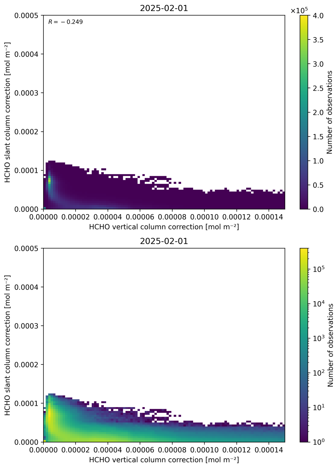
Figure 117: Scatter density plot of “HCHO vertical column correction” against “HCHO slant column correction” for 2025-01-31 to 2025-02-02.
