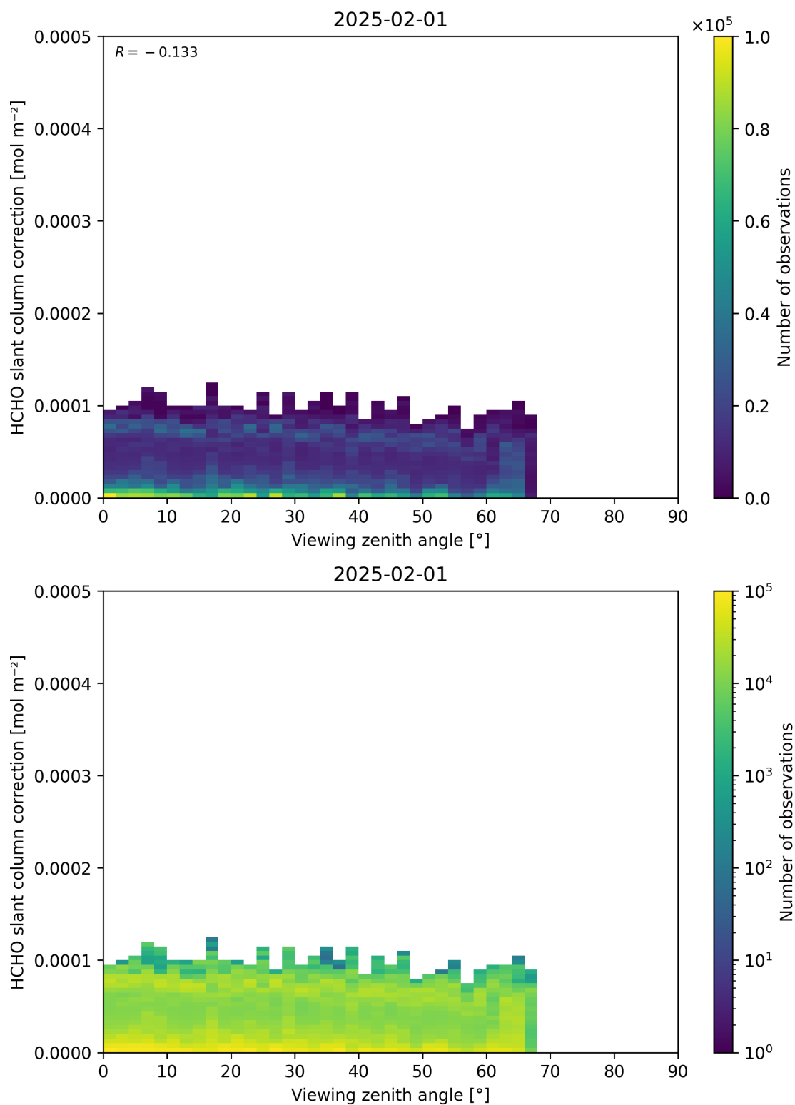
Figure 187: Scatter density plot of “Viewing zenith angle” against “HCHO slant column correction” for 2025-01-31 to 2025-02-02.
