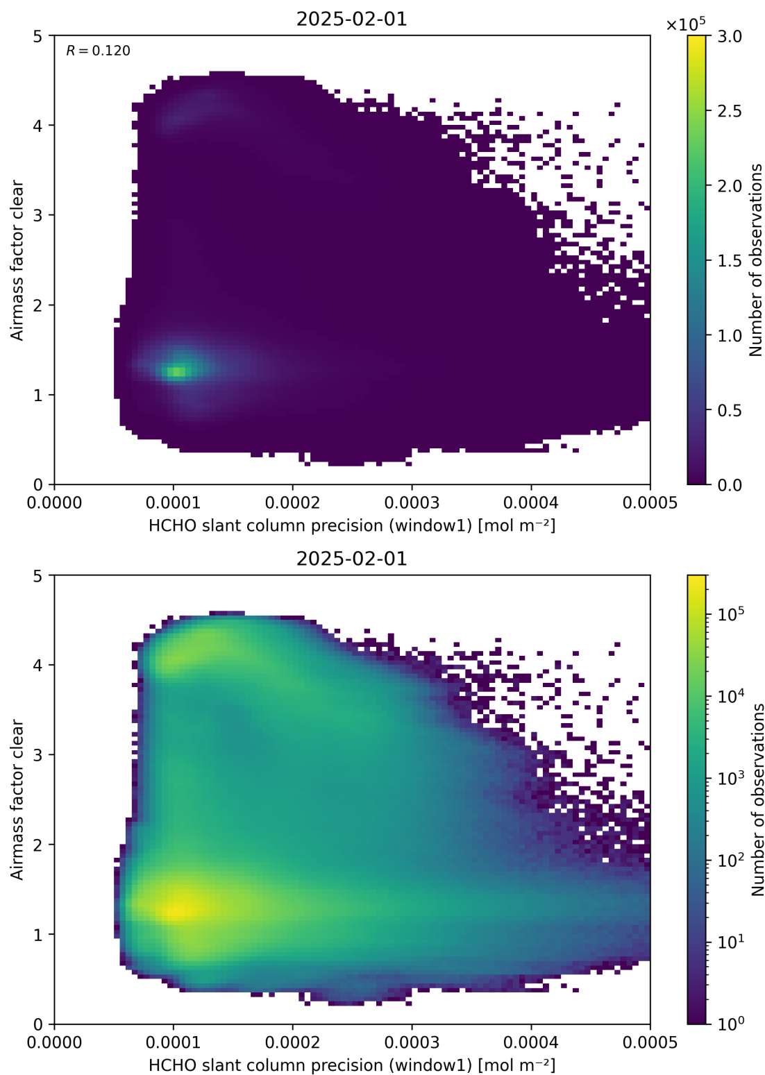
Figure 91: Scatter density plot of “HCHO slant column precision (window1)” against “Airmass factor clear” for 2025-01-31 to 2025-02-02.
