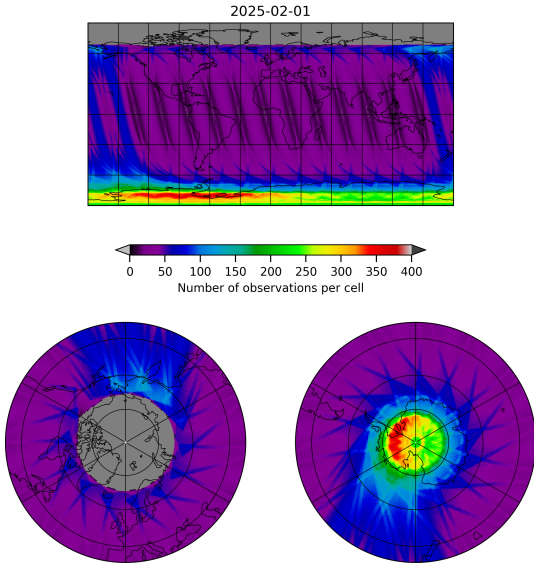
Figure 19: Map of the number of observations for 2025-01-31 to 2025-02-02
