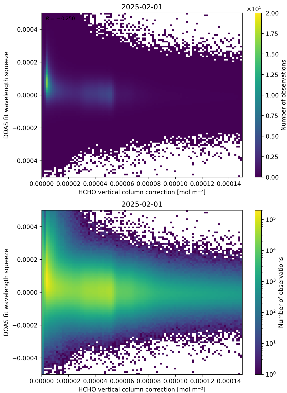
Figure 114: Scatter density plot of “HCHO vertical column correction” against “DOAS fit wavelength squeeze” for 2025-01-31 to 2025-02-02.
