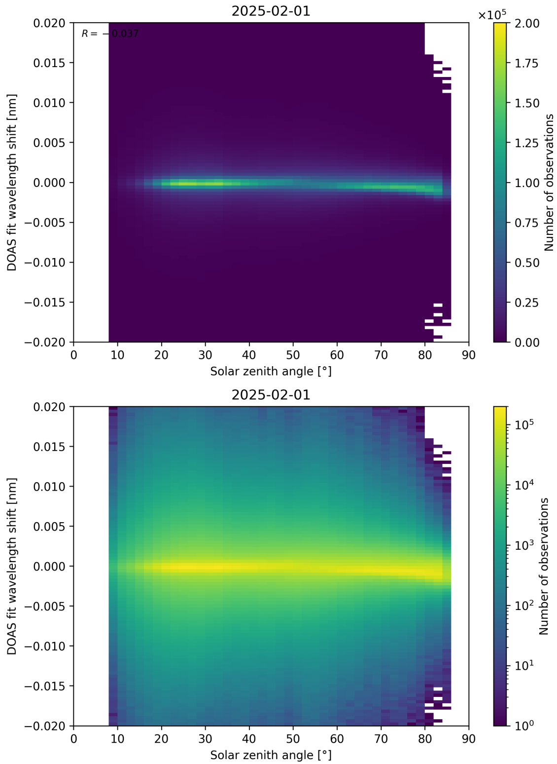
Figure 168: Scatter density plot of “Solar zenith angle” against “DOAS fit wavelength shift” for 2025-01-31 to 2025-02-02.
