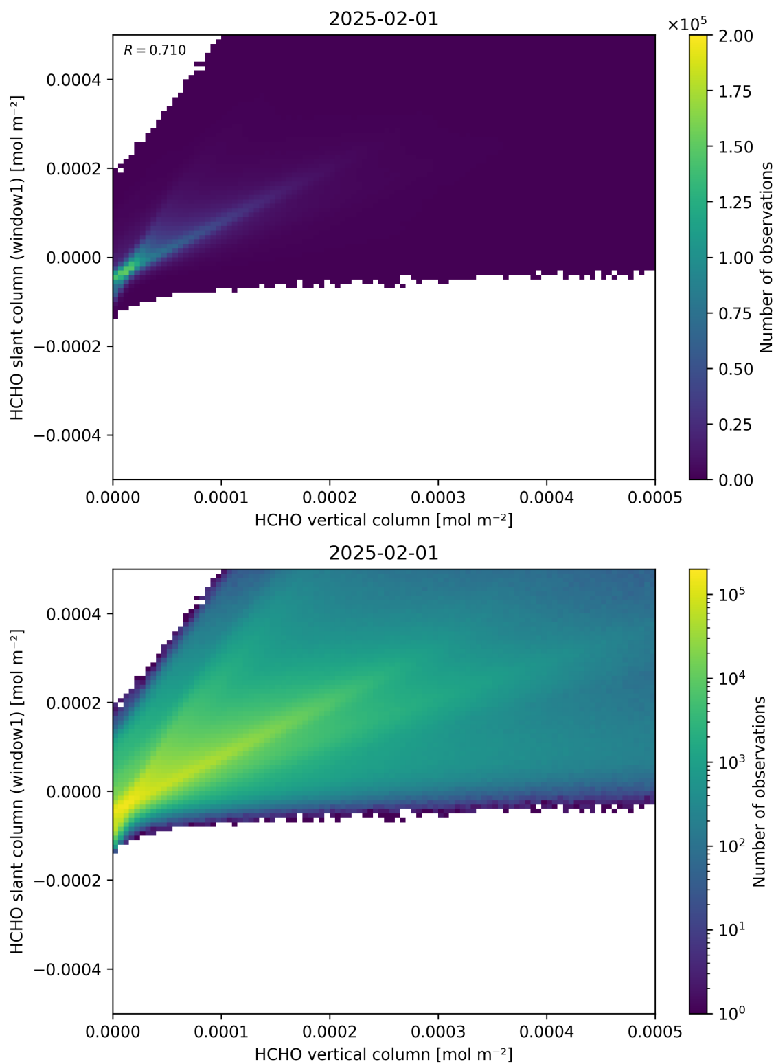
Figure 129: Scatter density plot of “HCHO vertical column” against “HCHO slant column (window1)” for 2025-01-31 to 2025-02-02.
