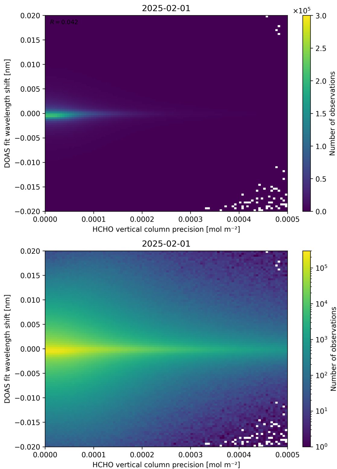
Figure 137: Scatter density plot of “HCHO vertical column precision” against “DOAS fit wavelength shift” for 2025-01-31 to 2025-02-02.
