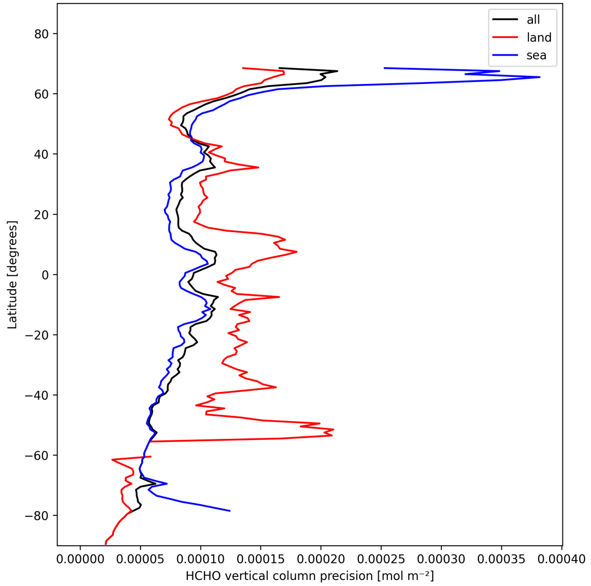
Figure 22: Zonal average of “HCHO vertical column precision” for 2025-01-31 to 2025-02-02.
