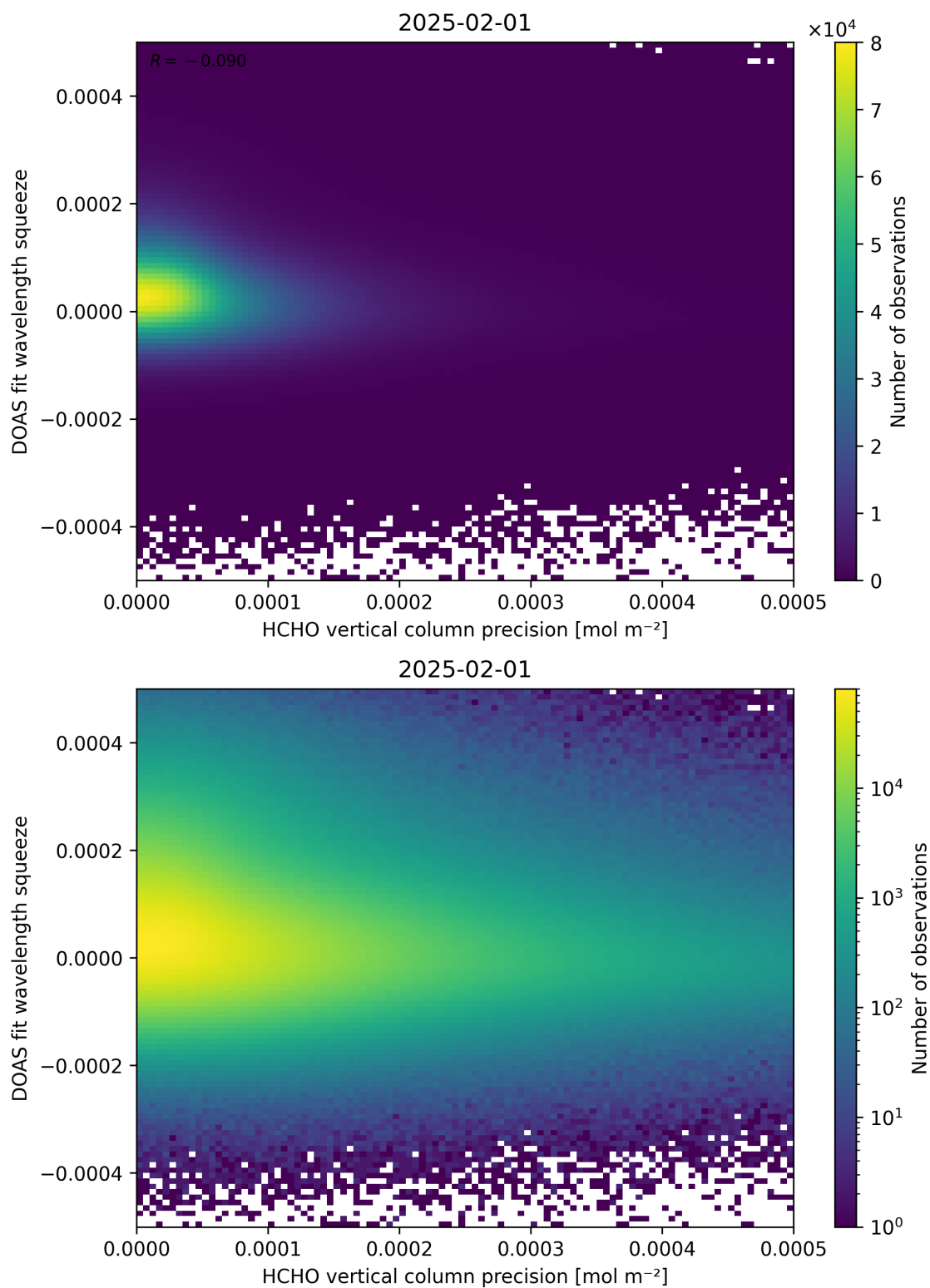
Figure 138: Scatter density plot of “HCHO vertical column precision” against “DOAS fit wavelength squeeze” for 2025-01-31 to 2025-02-02.
