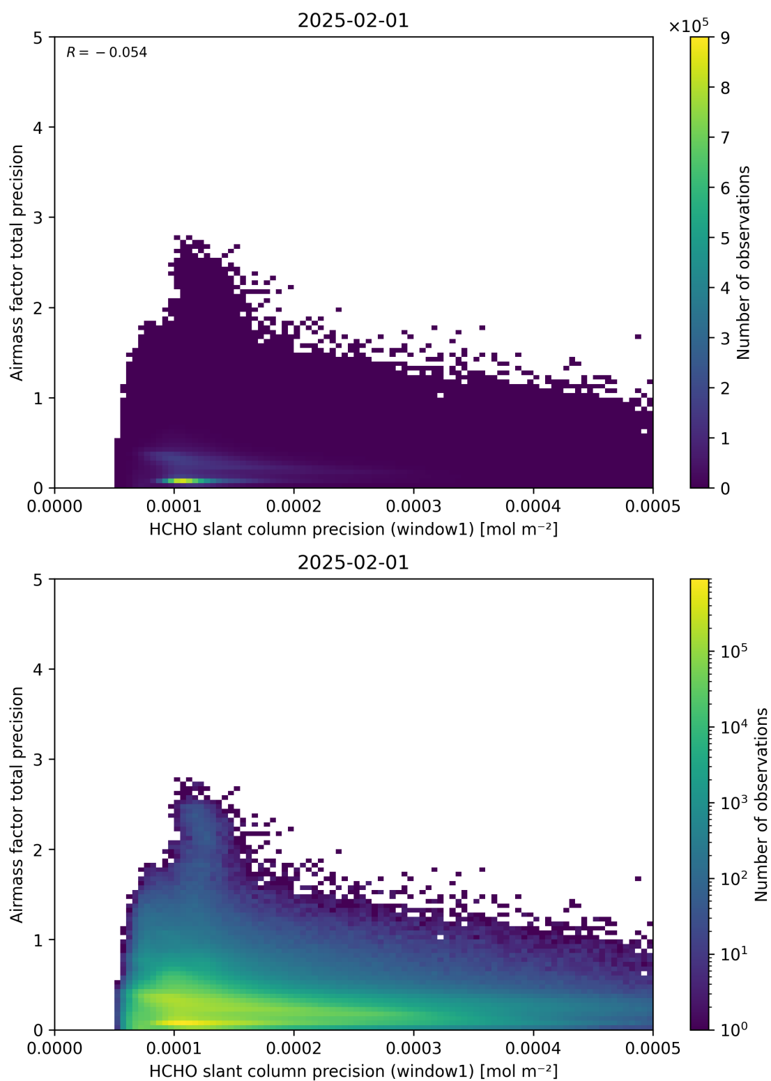
Figure 95: Scatter density plot of “HCHO slant column precision (window1)” against “Airmass factor total precision” for 2025-01-31 to 2025-02-02.
