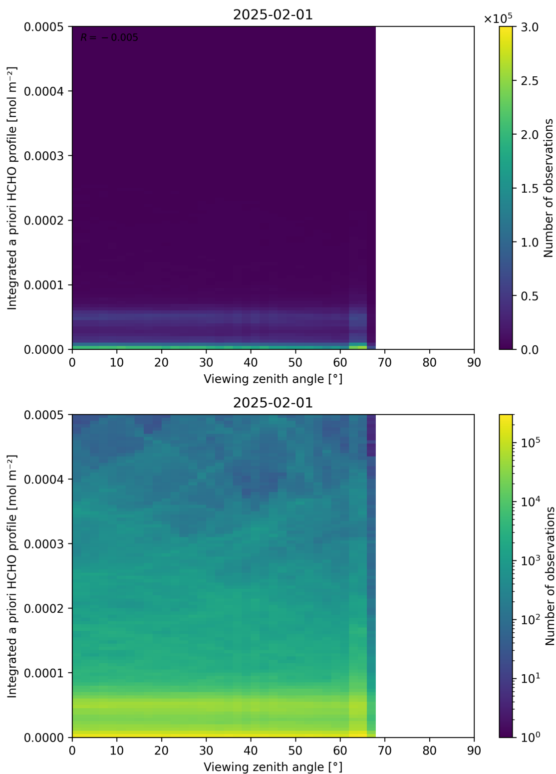
Figure 195: Scatter density plot of “Viewing zenith angle” against “Integrated a priori HCHO profile” for 2025-01-31 to 2025-02-02.
