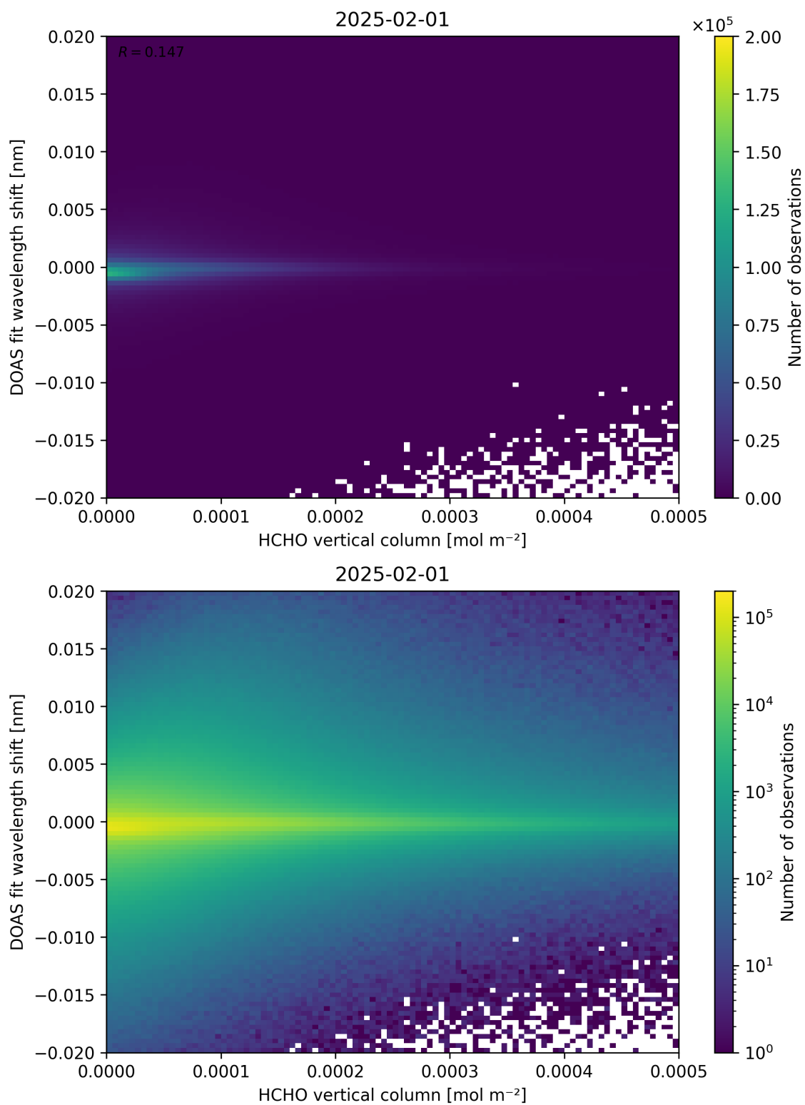
Figure 124: Scatter density plot of “HCHO vertical column” against “DOAS fit wavelength shift” for 2025-01-31 to 2025-02-02.
