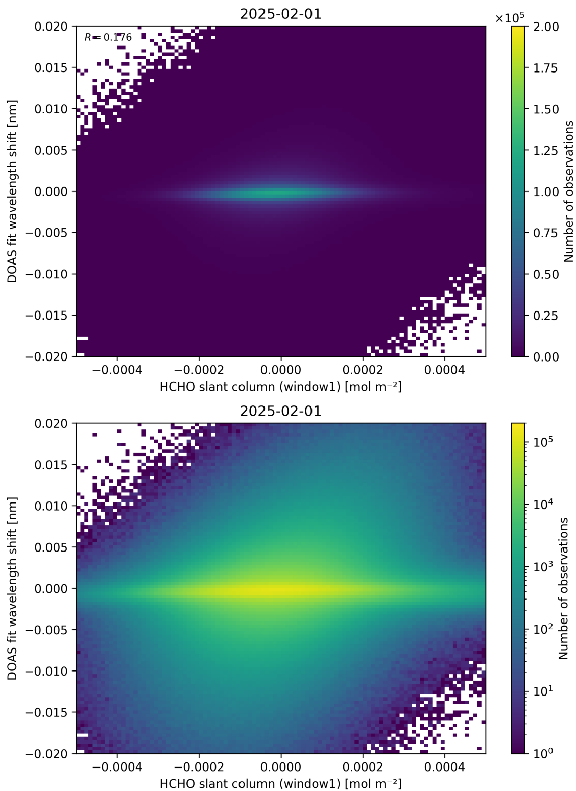
Figure 79: Scatter density plot of “HCHO slant column (window1)” against “DOAS fit wavelength shift” for 2025-01-31 to 2025-02-02.
