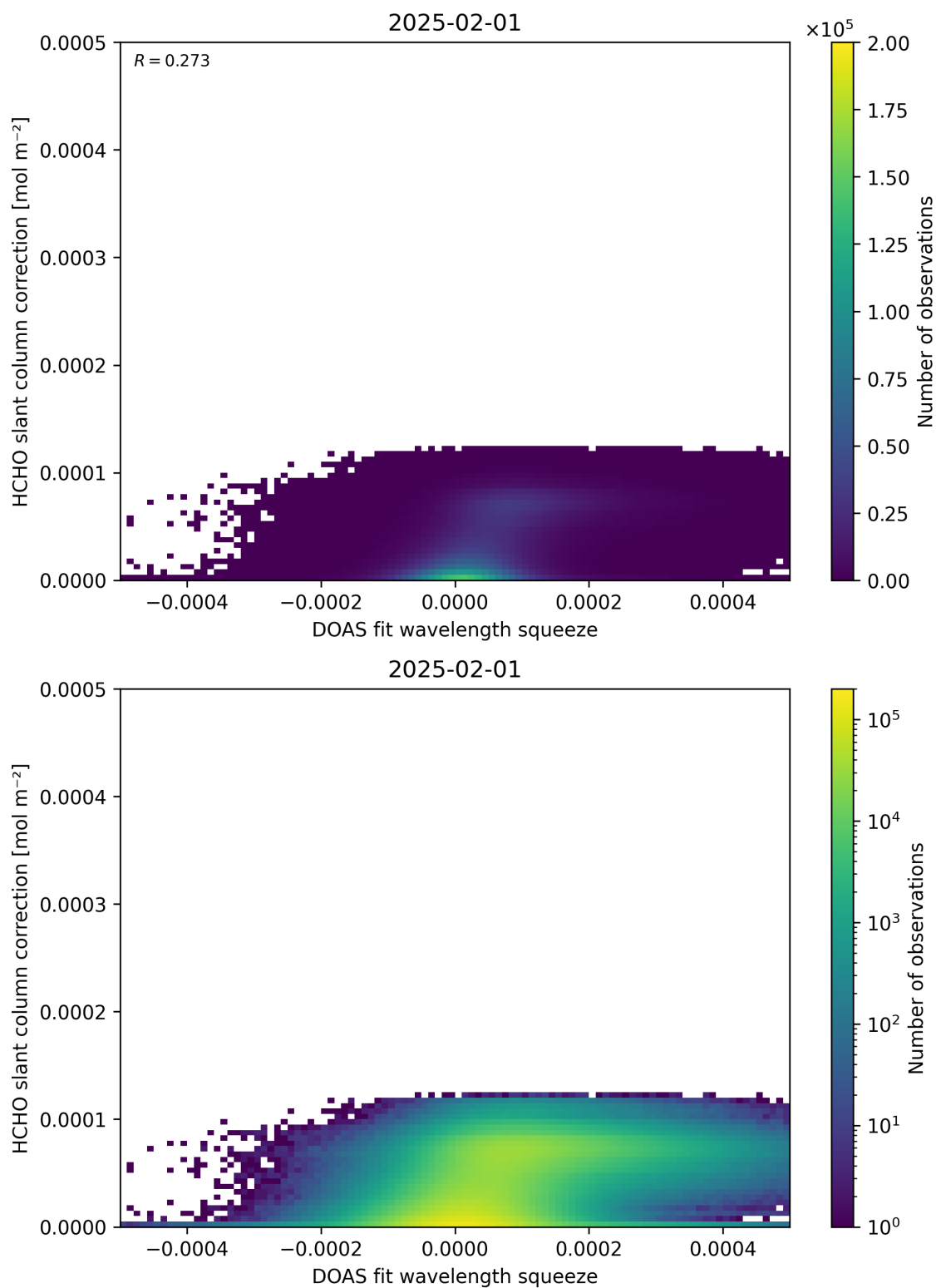
Figure 70: Scatter density plot of “DOAS fit wavelength squeeze” against “HCHO slant column correction” for 2025-01-31 to 2025-02-02.
