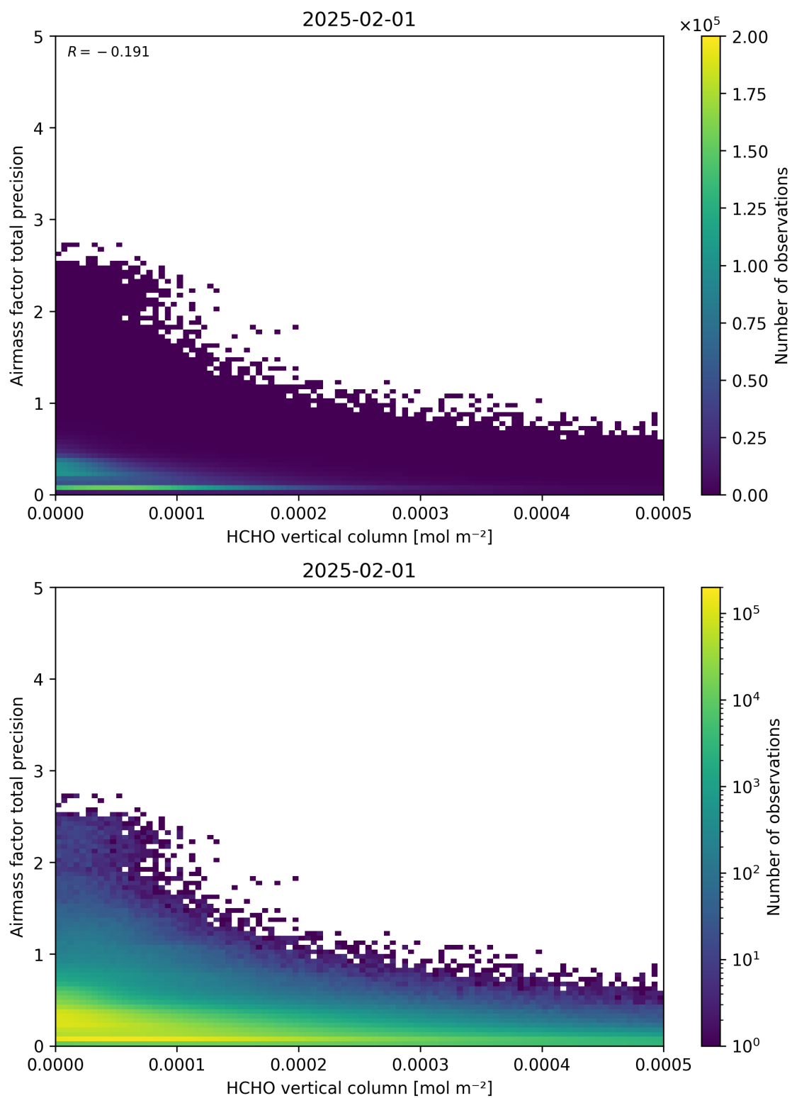
Figure 132: Scatter density plot of “HCHO vertical column” against “Airmass factor total precision” for 2025-01-31 to 2025-02-02.
