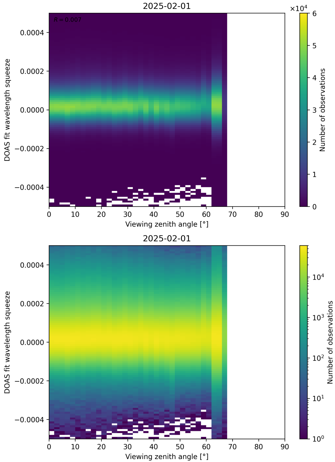
Figure 184: Scatter density plot of “Viewing zenith angle” against “DOAS fit wavelength squeeze” for 2025-01-31 to 2025-02-02.
