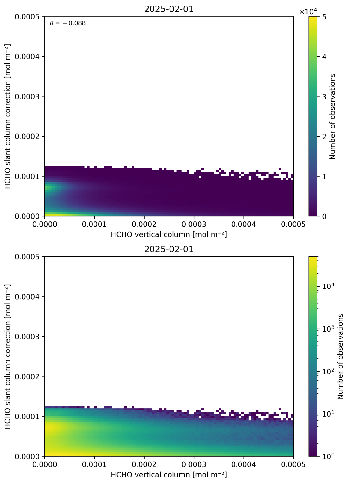
Figure 128: Scatter density plot of “HCHO vertical column” against “HCHO slant column correction” for 2025-01-31 to 2025-02-02.
