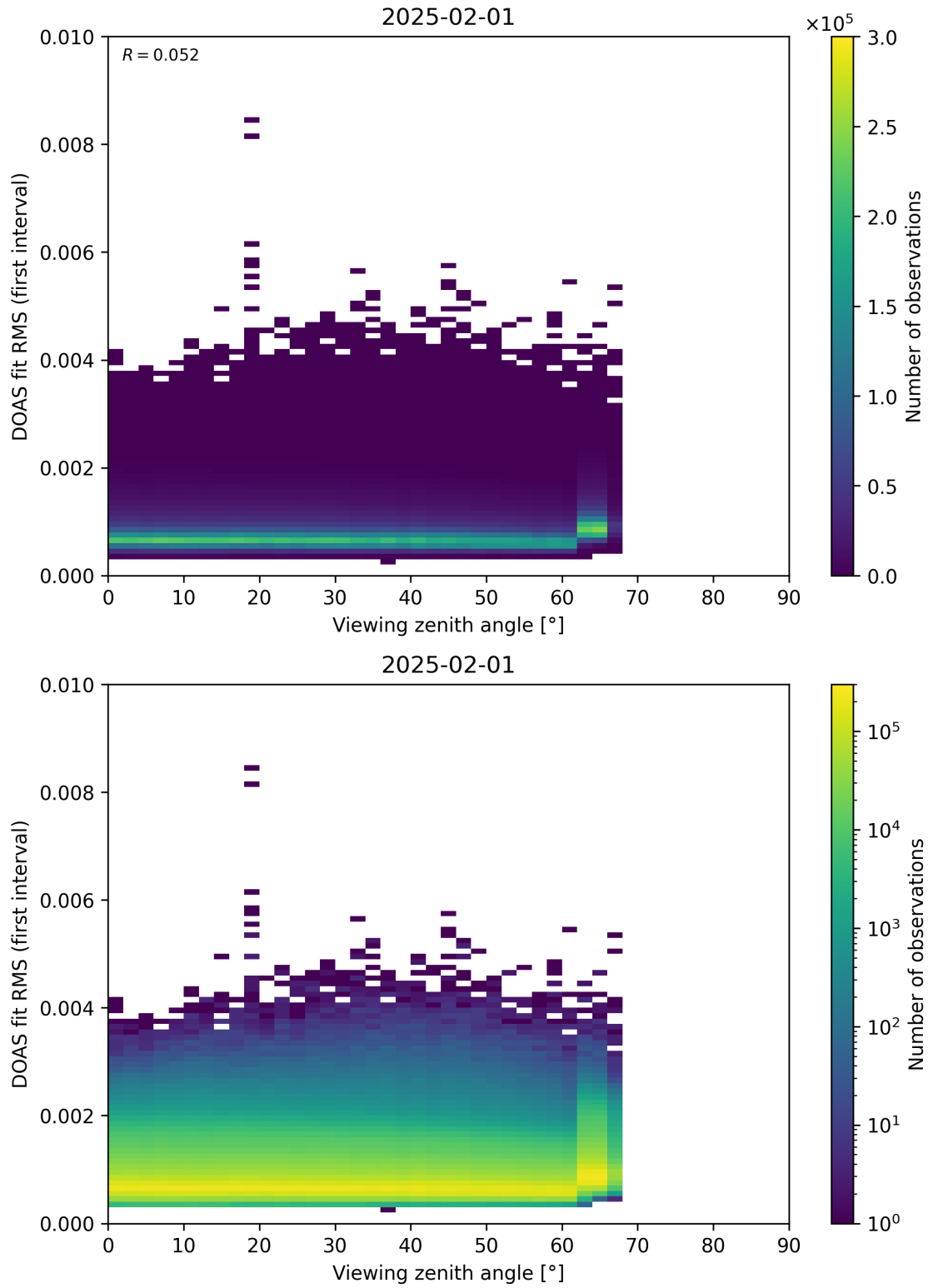
Figure 182: Scatter density plot of “Viewing zenith angle” against “DOAS fit RMS (first interval)” for 2025-01-31 to 2025-02-02.
