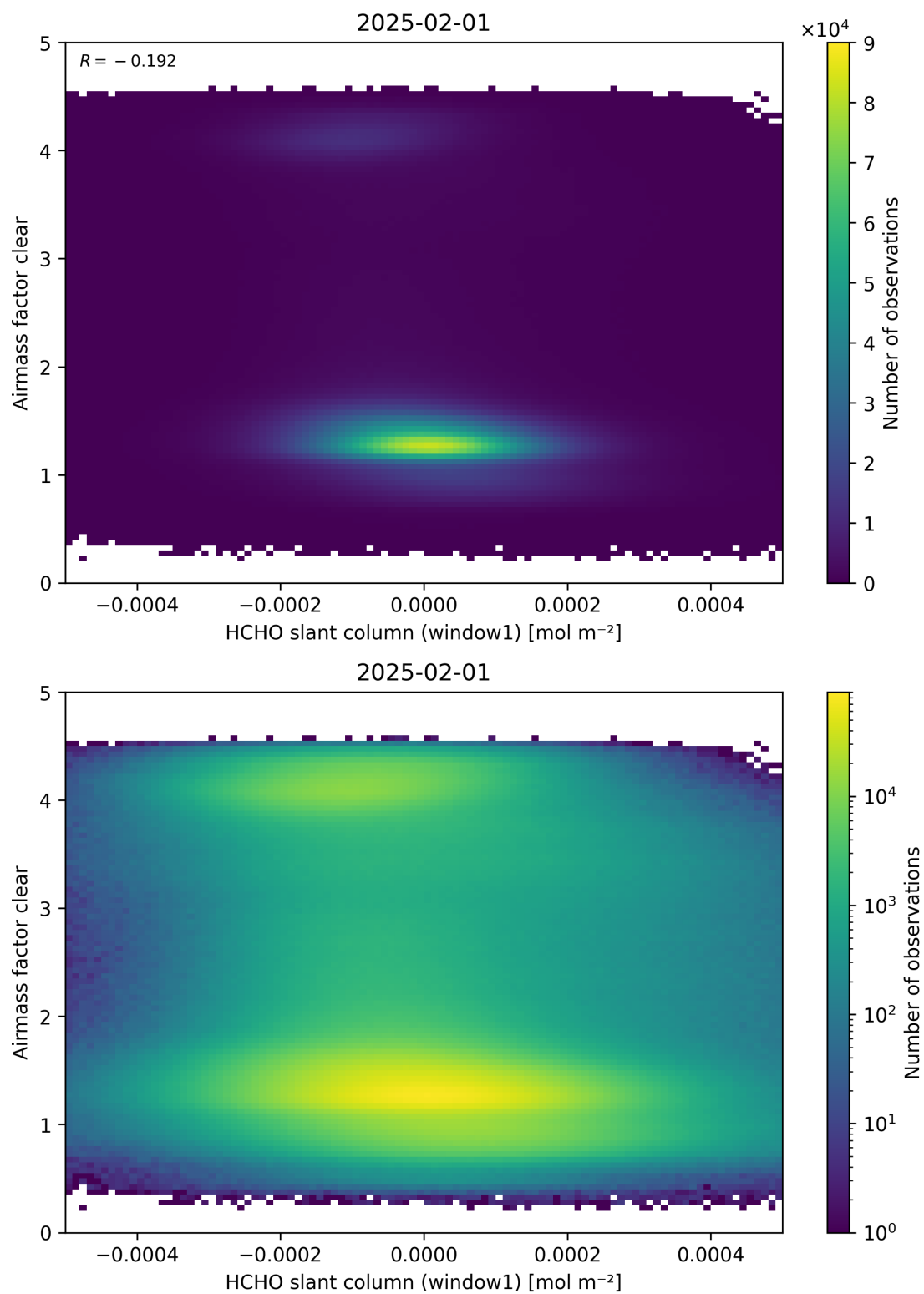
Figure 81: Scatter density plot of “HCHO slant column (window1)” against “Airmass factor clear” for 2025-01-31 to 2025-02-02.
