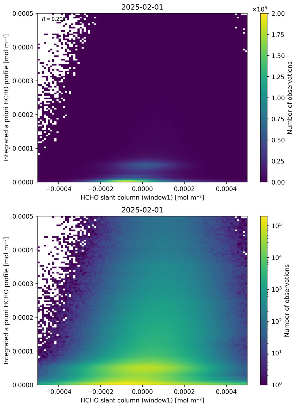
Figure 87: Scatter density plot of “HCHO slant column (window1)” against “Integrated a priori HCHO profile” for 2025-01-31 to 2025-02-02.
