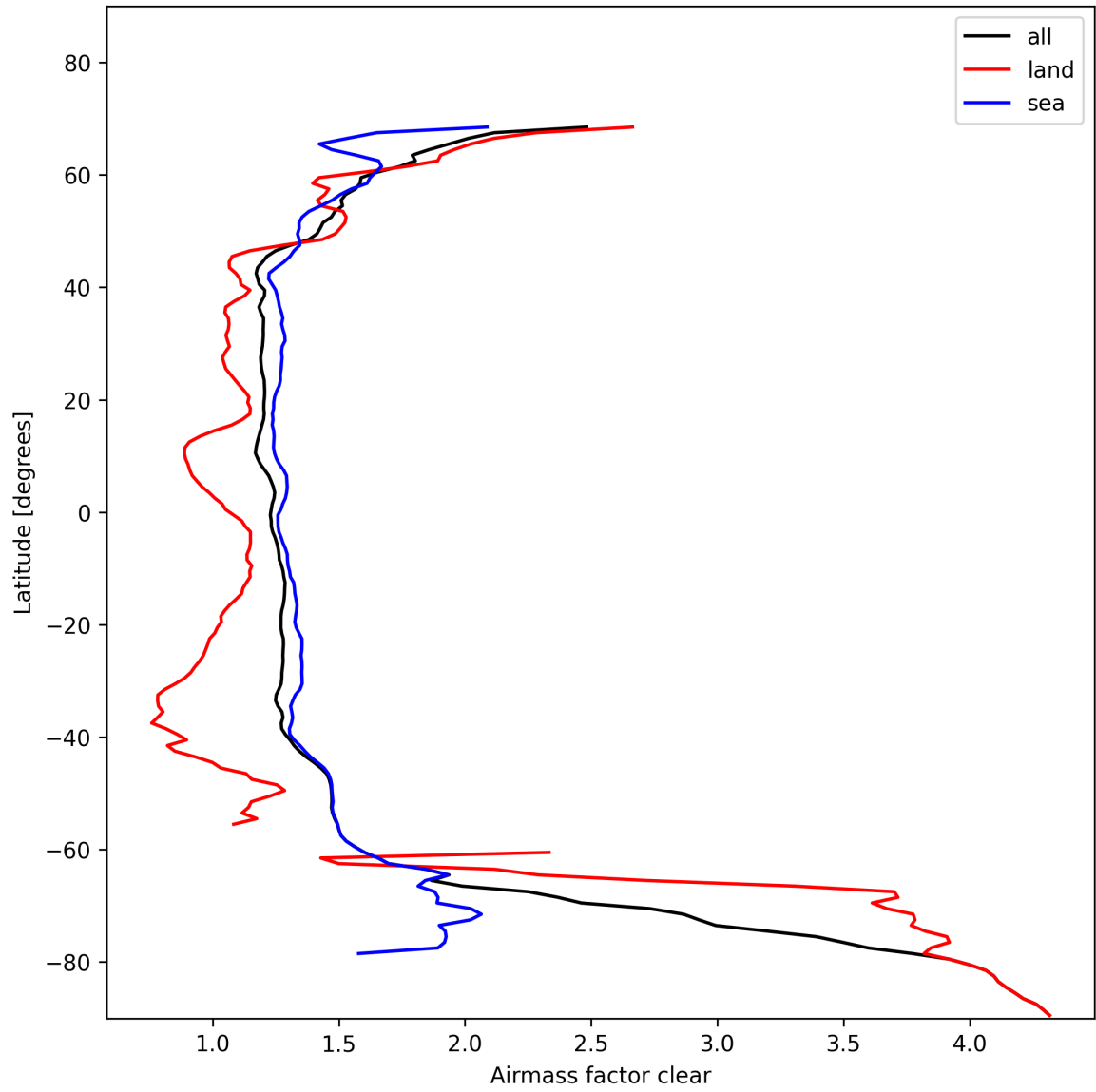
Figure 28: Zonal average of “Airmass factor clear” for 2025-01-31 to 2025-02-02.
