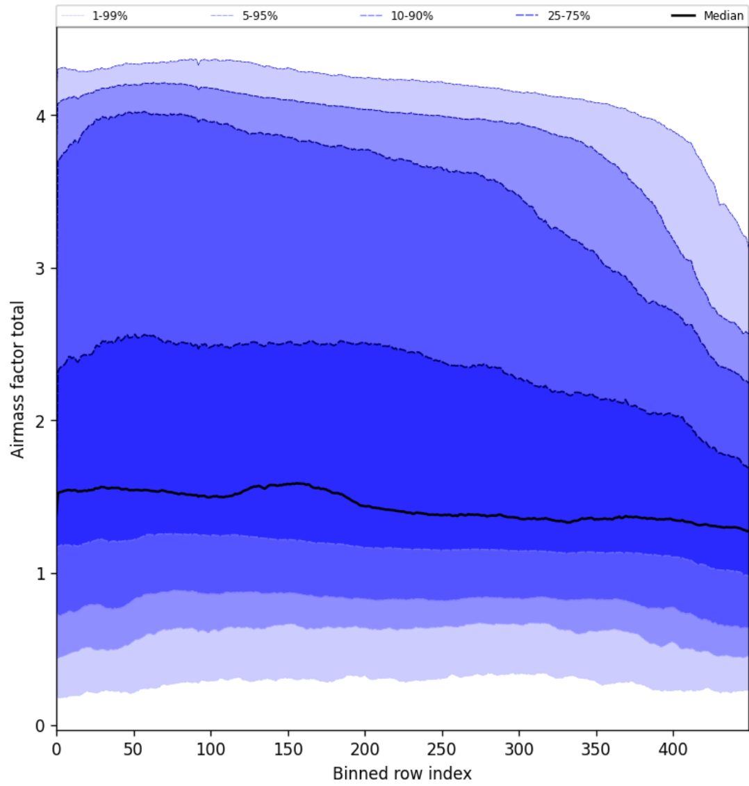
Figure 54: Along track statistics of “Airmass factor total” for 2025-01-31 to 2025-02-02
