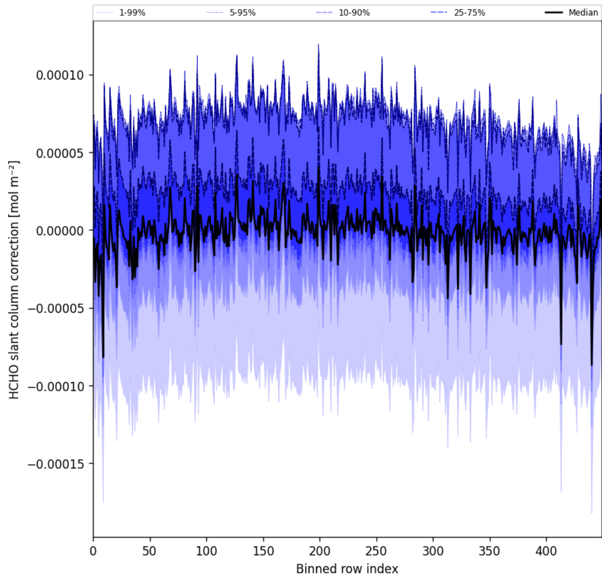
Figure 61: Along track statistics of “HCHO slant column correction” for 2025-01-31 to 2025-02-02
