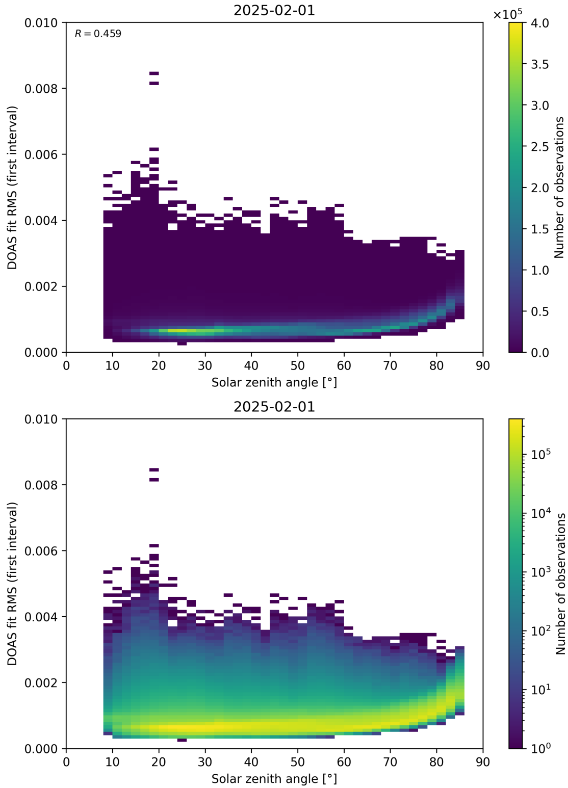
Figure 167: Scatter density plot of “Solar zenith angle” against “DOAS fit RMS (first interval)” for 2025-01-31 to 2025-02-02.
