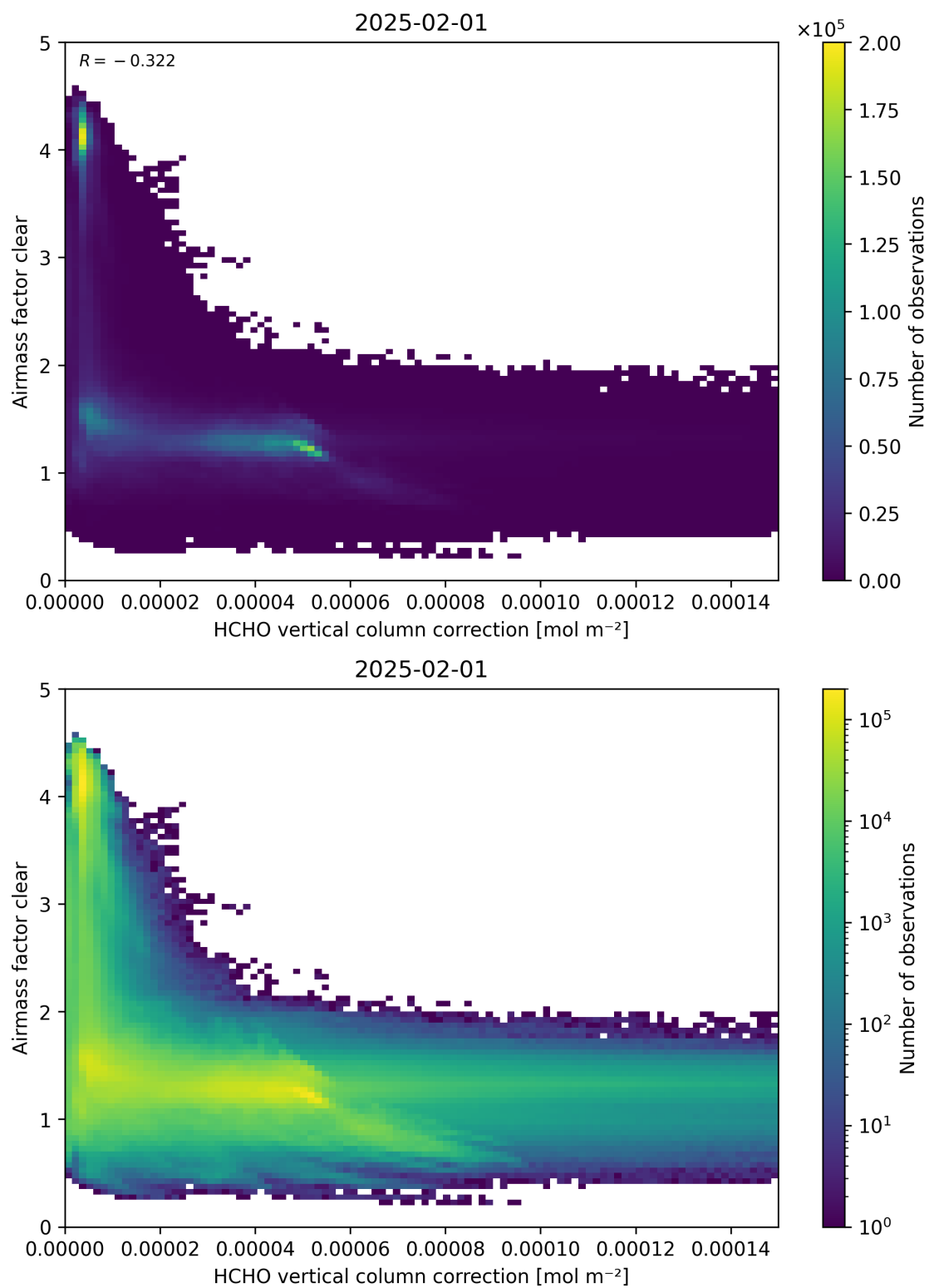
Figure 115: Scatter density plot of “HCHO vertical column correction” against “Airmass factor clear” for 2025-01-31 to 2025-02-02.
