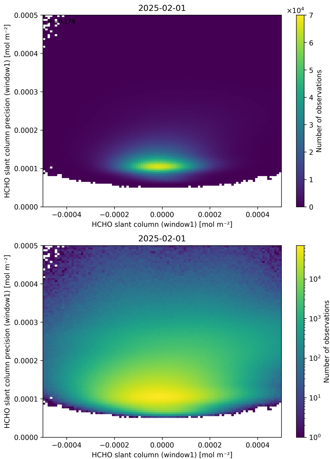
Figure 84: Scatter density plot of “HCHO slant column (window1)” against “HCHO slant column precision (window1)” for 2025-01-31 to 2025-02-02.
