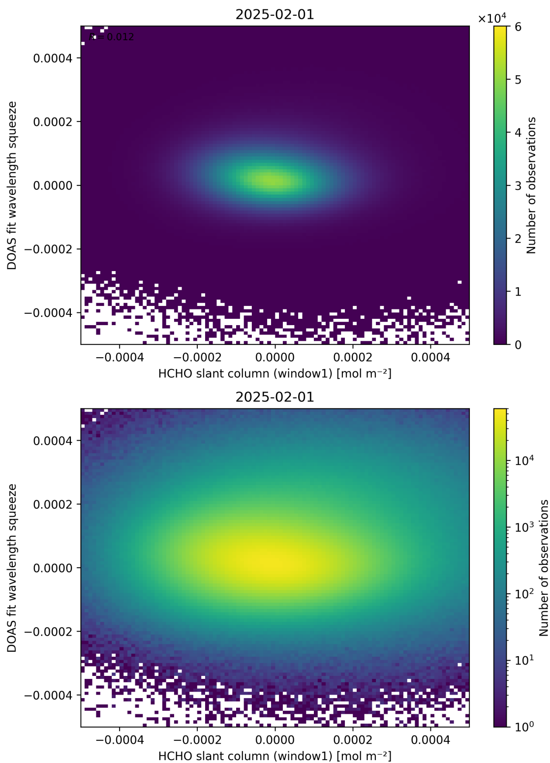
Figure 80: Scatter density plot of “HCHO slant column (window1)” against “DOAS fit wavelength squeeze” for 2025-01-31 to 2025-02-02.
