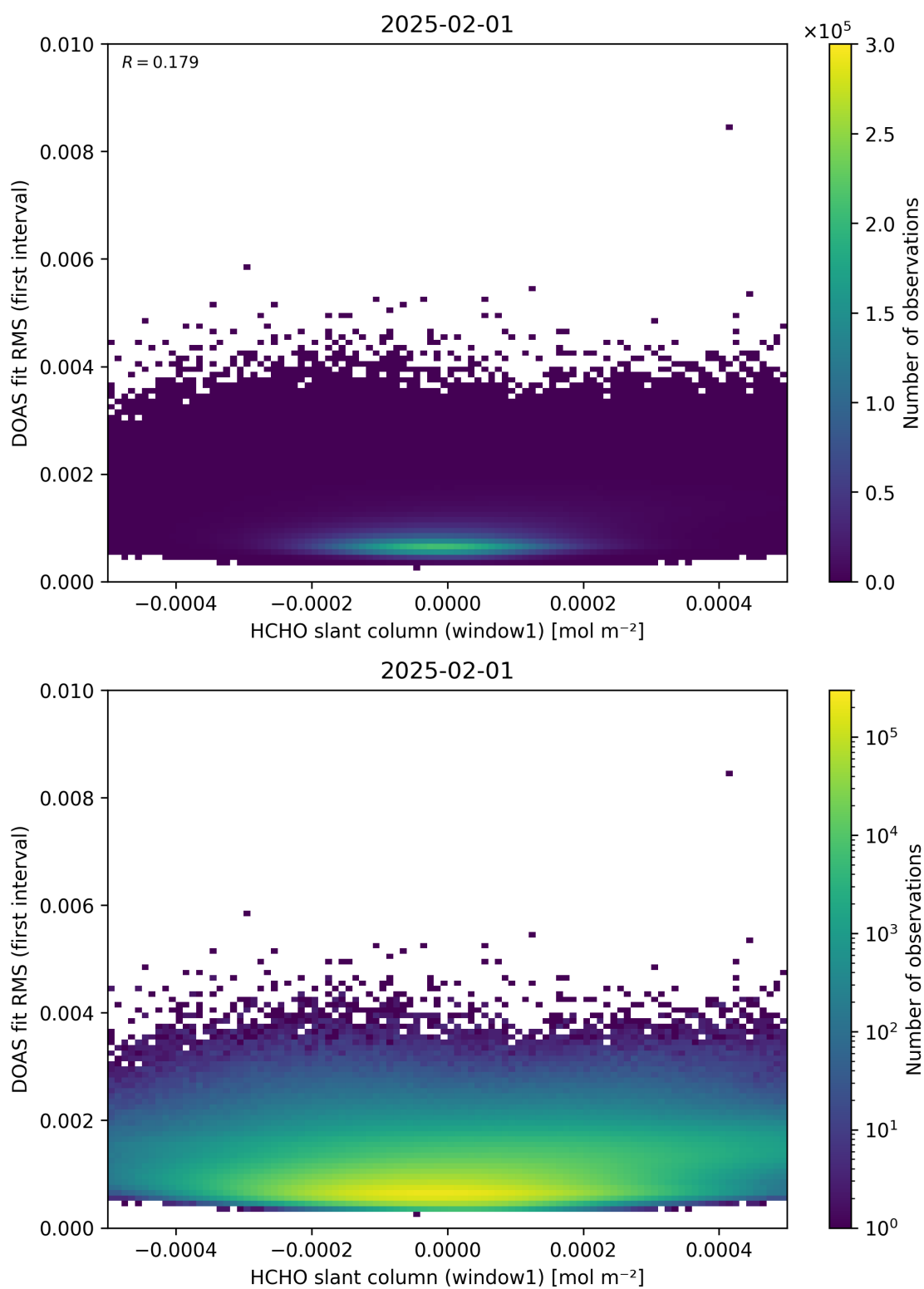
Figure 78: Scatter density plot of “HCHO slant column (window1)” against “DOAS fit RMS (first interval)” for 2025-01-31 to 2025-02-02.
