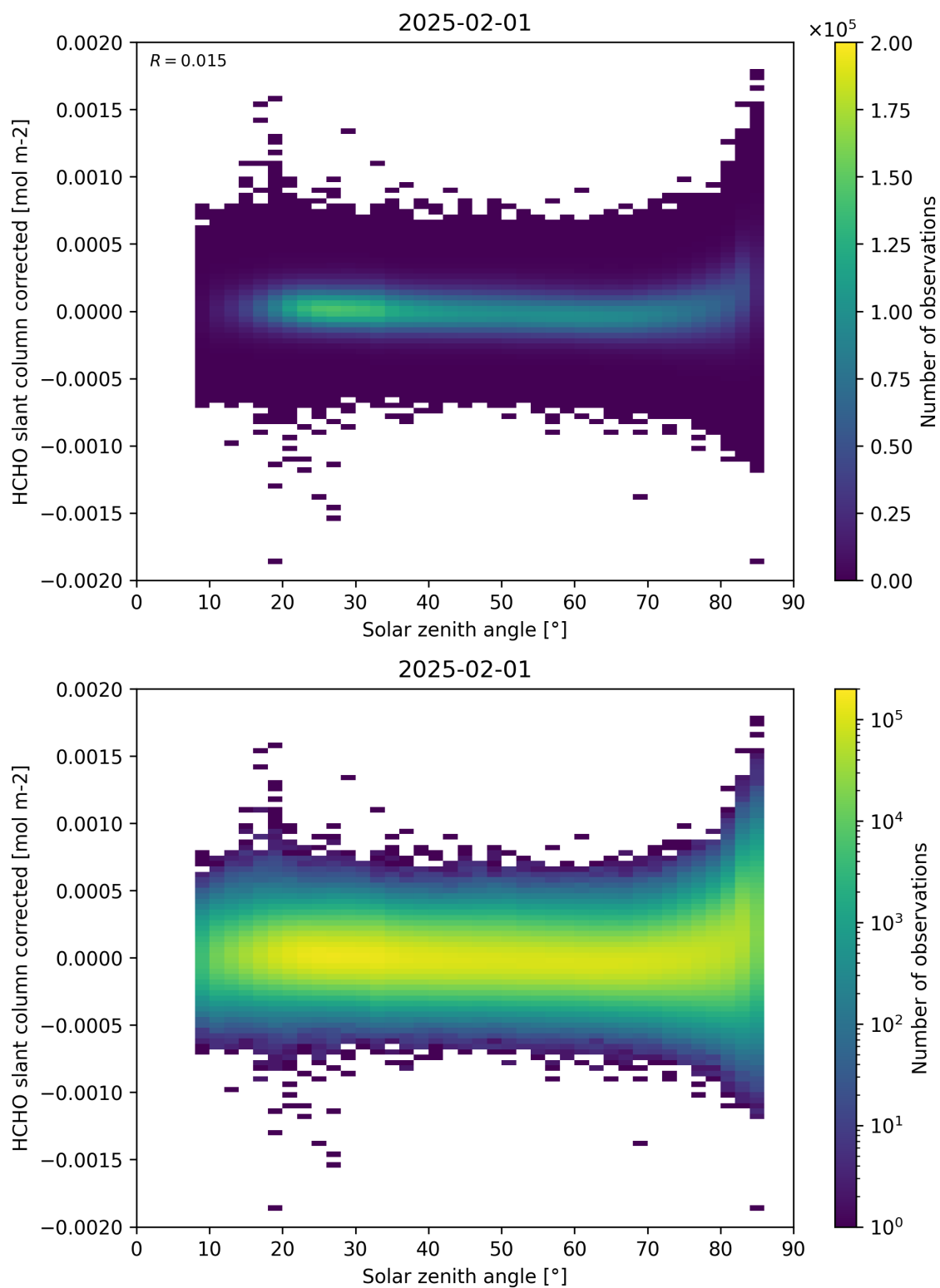
Figure 171: Scatter density plot of “Solar zenith angle” against “HCHO slant column corrected” for 2025-01-31 to 2025-02-02.
