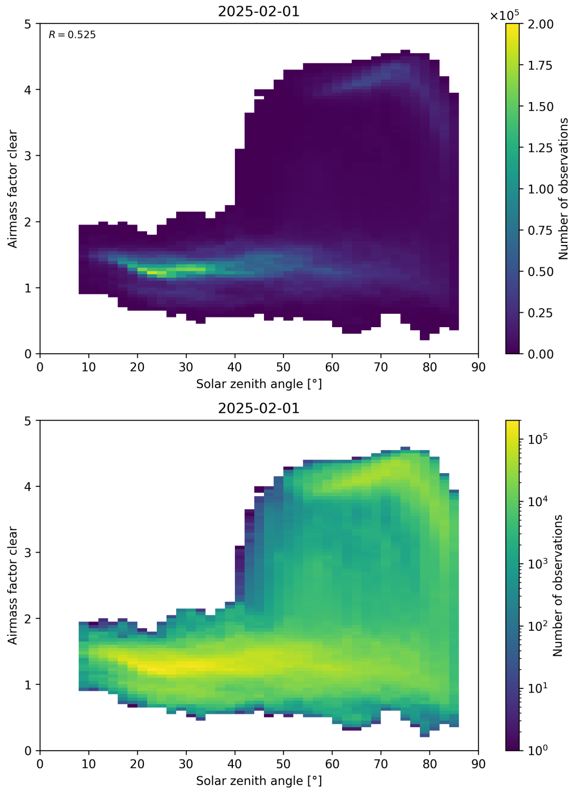
Figure 170: Scatter density plot of “Solar zenith angle” against “Airmass factor clear” for 2025-01-31 to 2025-02-02.
