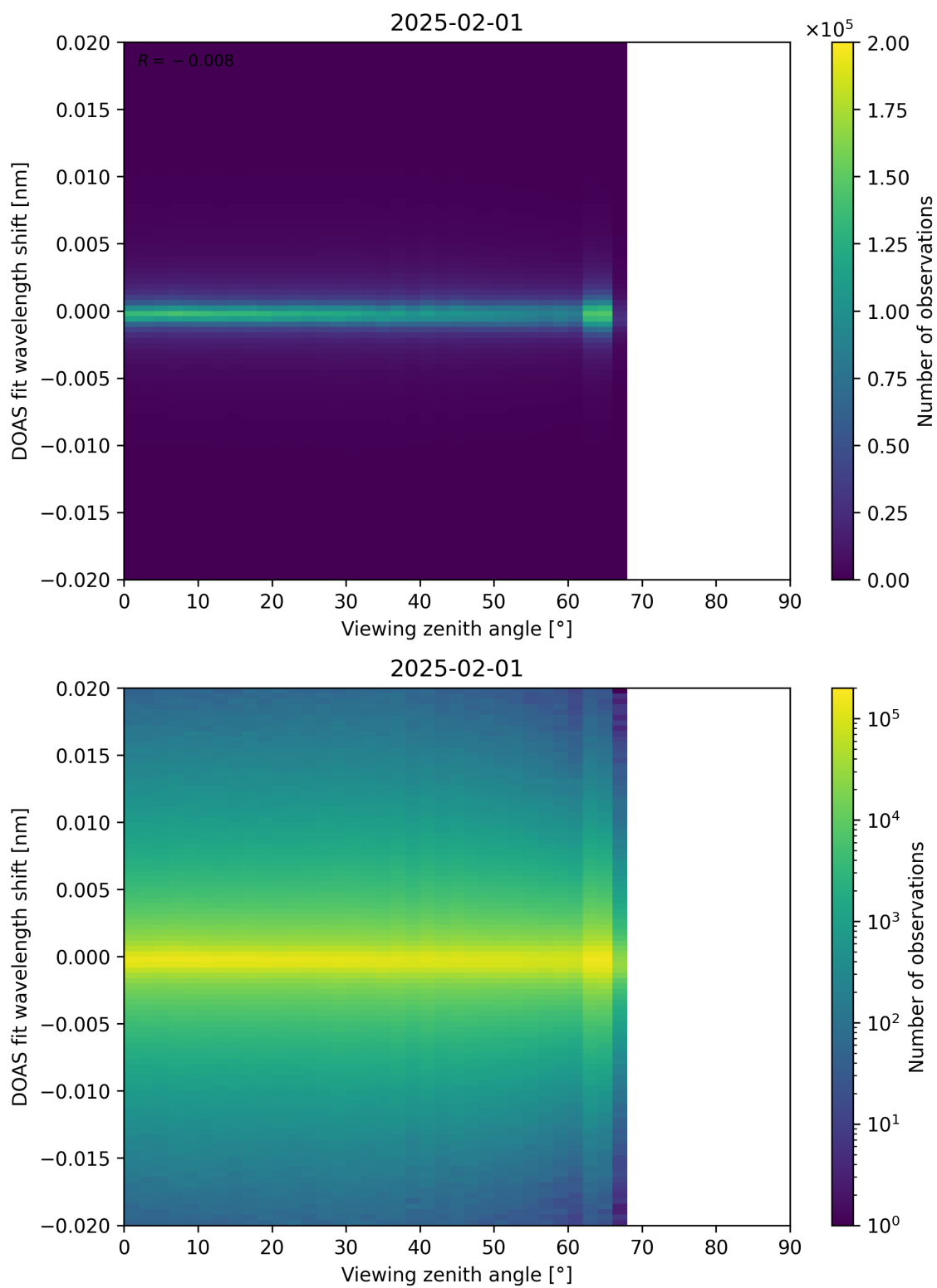
Figure 183: Scatter density plot of “Viewing zenith angle” against “DOAS fit wavelength shift” for 2025-01-31 to 2025-02-02.
