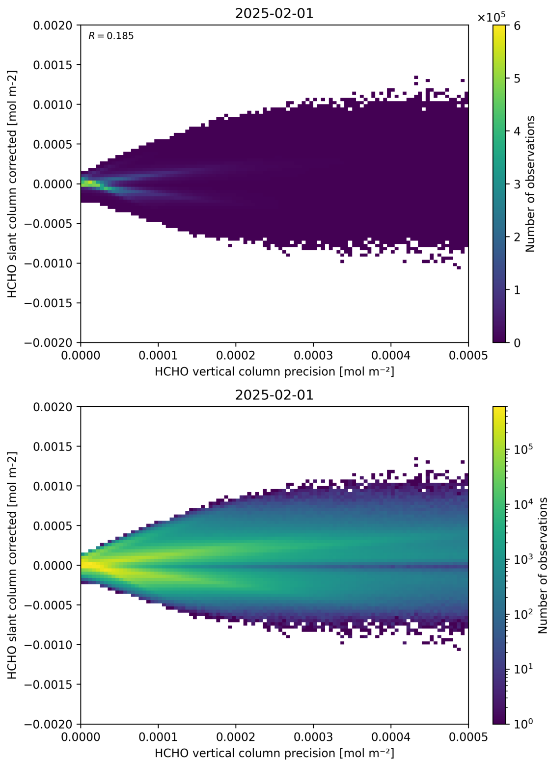
Figure 140: Scatter density plot of “HCHO vertical column precision” against “HCHO slant column corrected” for 2025-01-31 to 2025-02-02.
