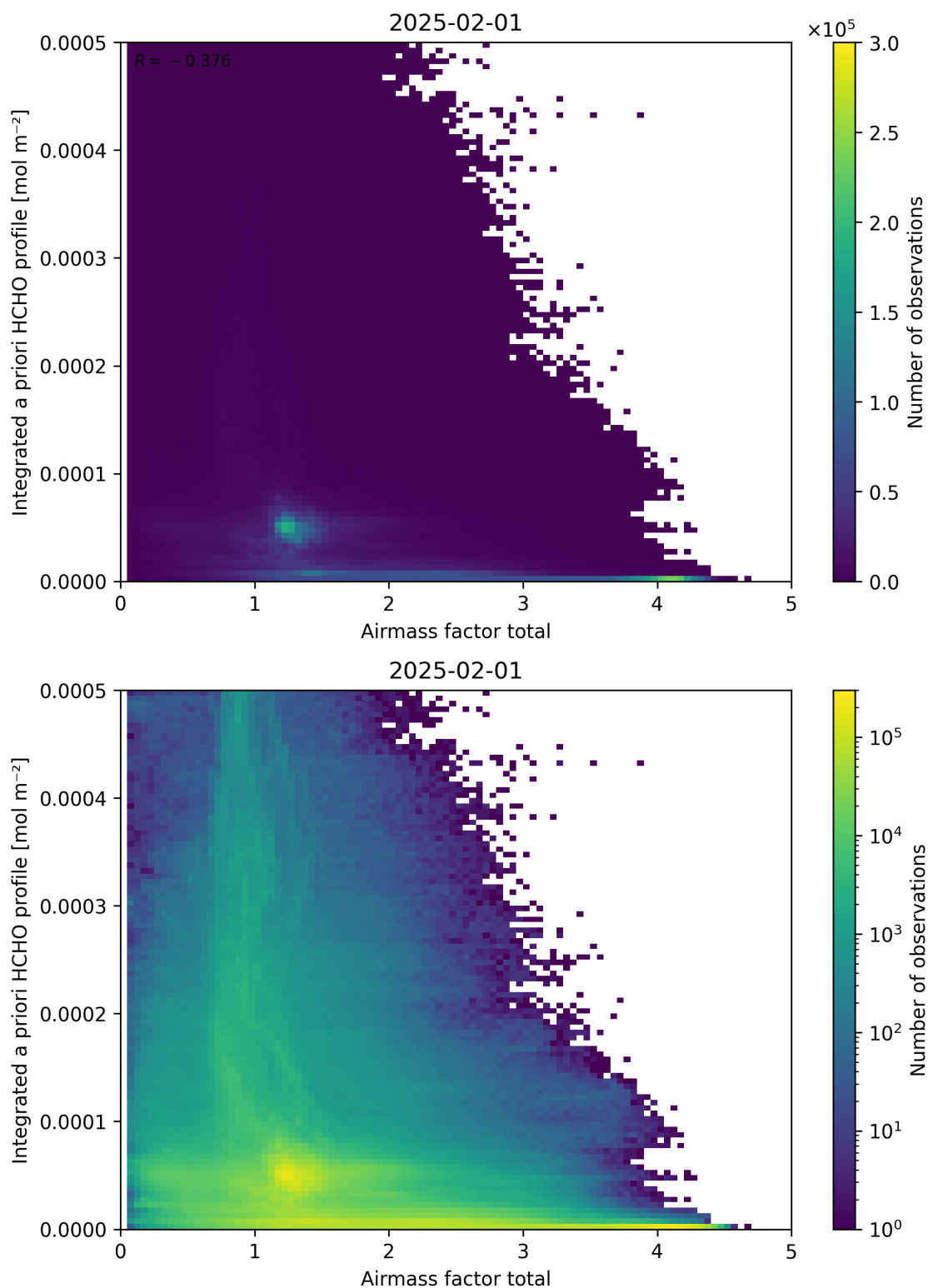
Figure 104: Scatter density plot of “Airmass factor total” against “Integrated a priori HCHO profile” for 2025-01-31 to 2025-02-02.
