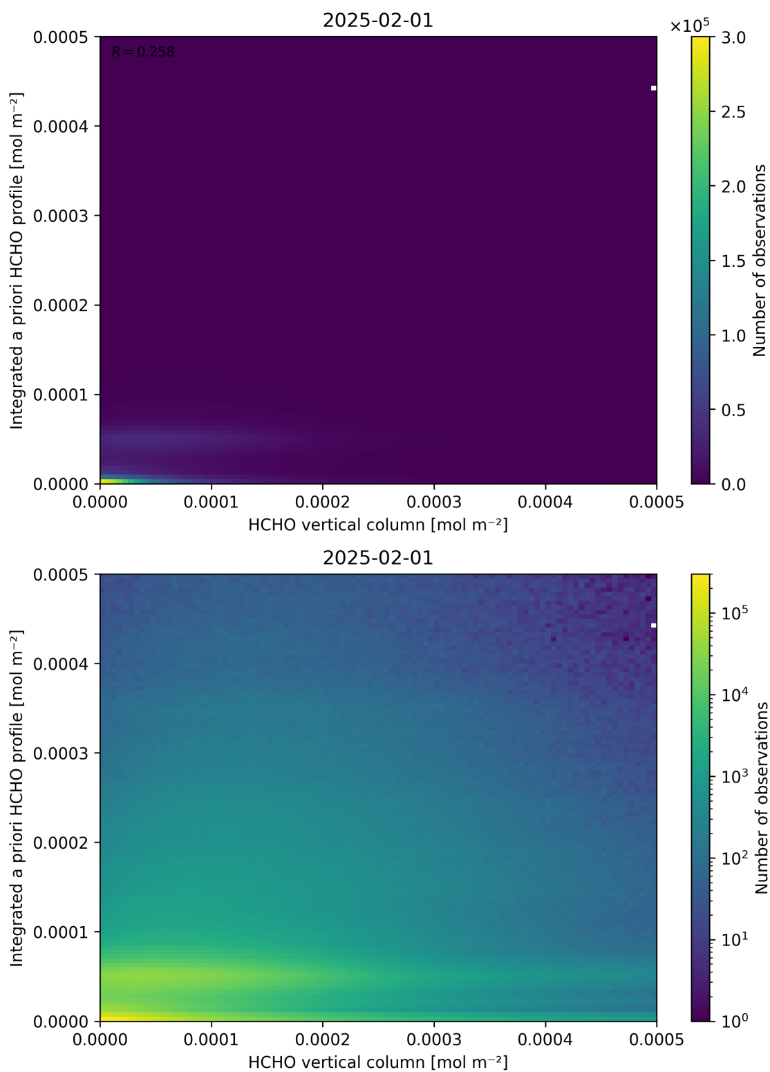
Figure 135: Scatter density plot of “HCHO vertical column” against “Integrated a priori HCHO profile” for 2025-01-31 to 2025-02-02.
