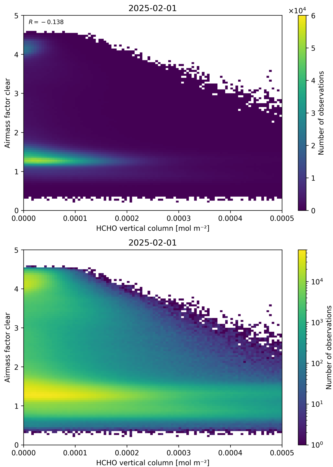
Figure 126: Scatter density plot of “HCHO vertical column” against “Airmass factor clear” for 2025-01-31 to 2025-02-02.
