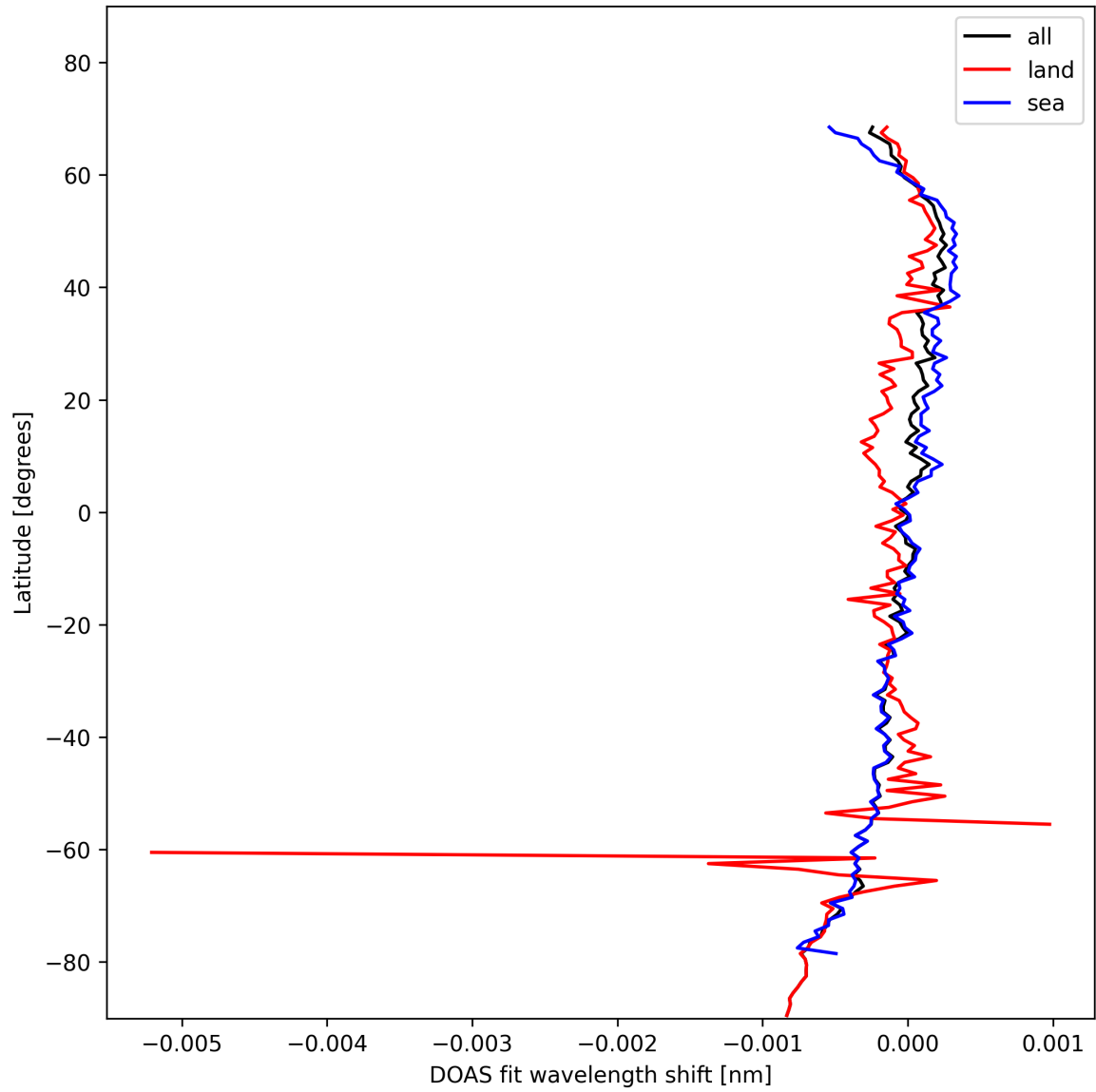
Figure 30: Zonal average of “DOAS fit wavelength shift” for 2025-01-31 to 2025-02-02.
