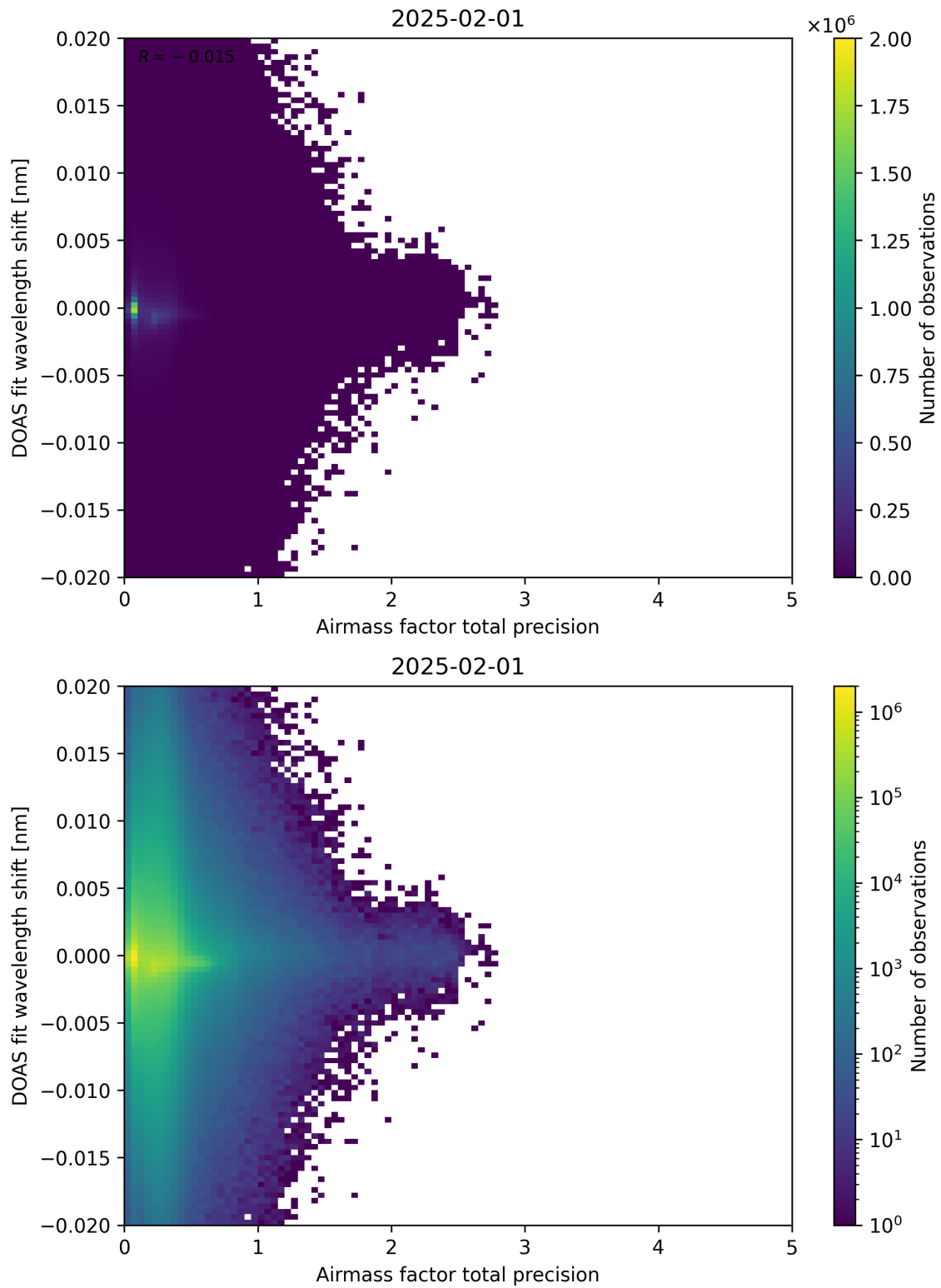
Figure 106: Scatter density plot of “Airmass factor total precision” against “DOAS fit wavelength shift” for 2025-01-31 to 2025-02-02.
