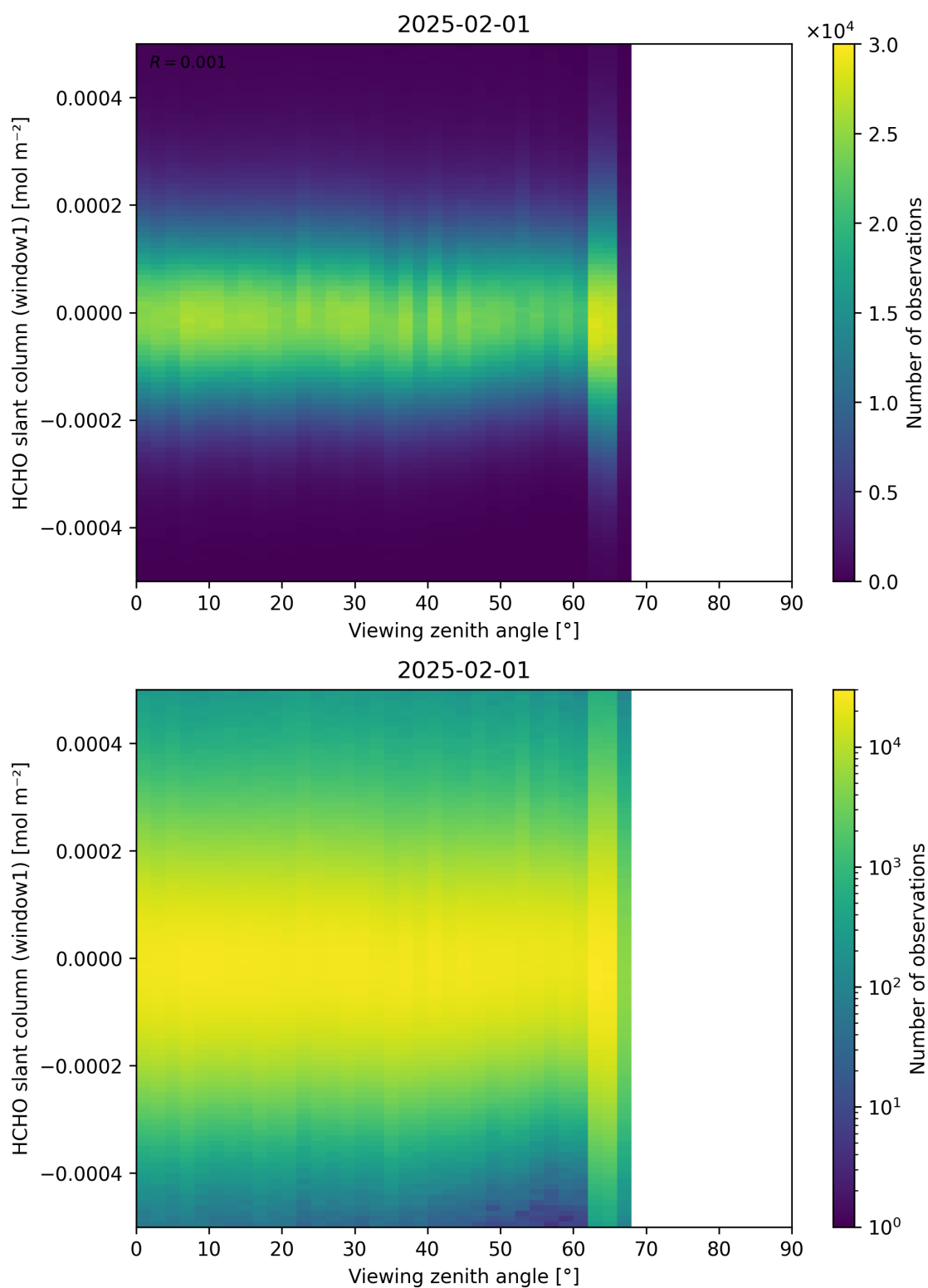
Figure 188: Scatter density plot of “Viewing zenith angle” against “HCHO slant column (window1)” for 2025-01-31 to 2025-02-02.
