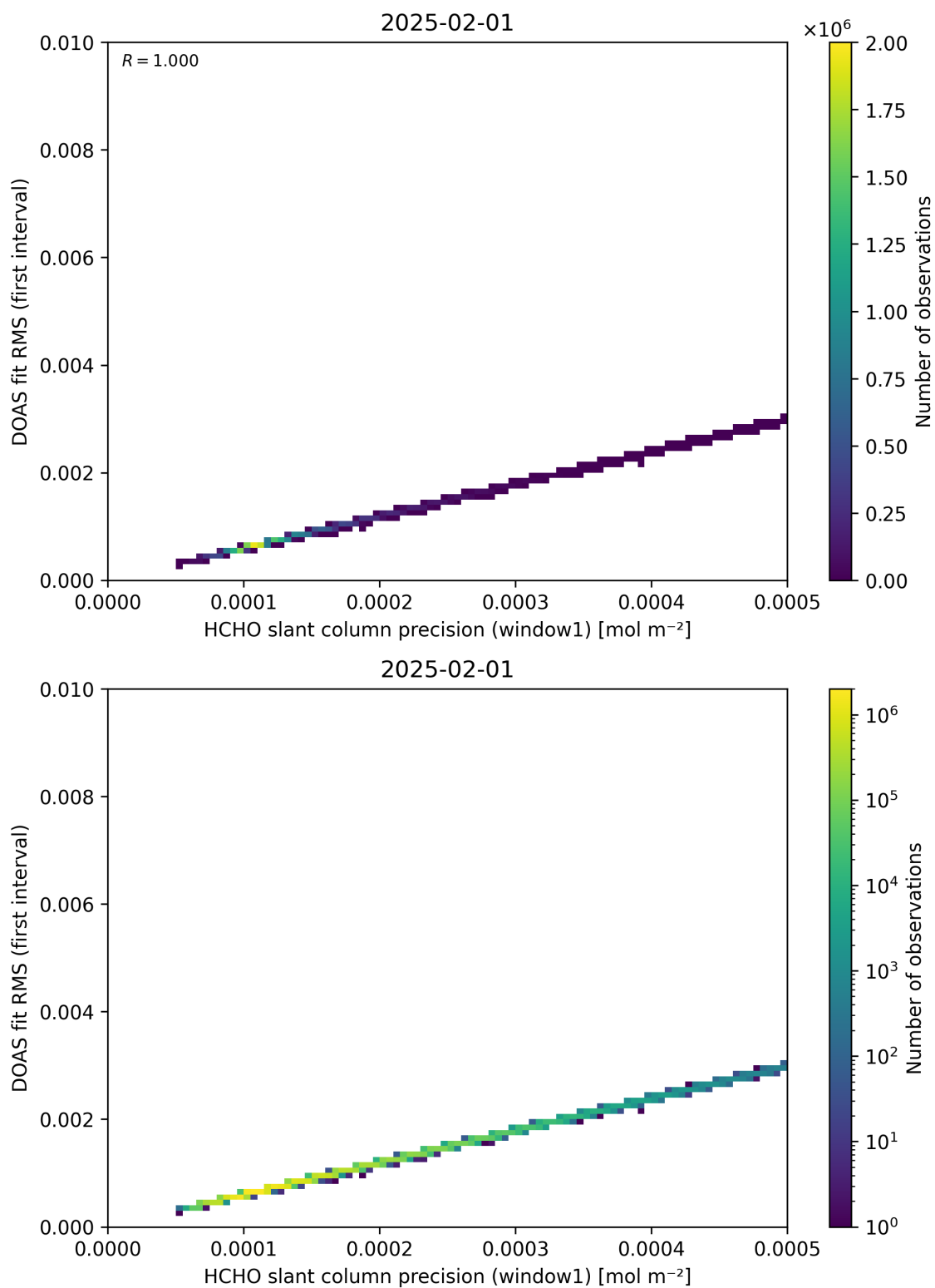
Figure 88: Scatter density plot of “HCHO slant column precision (window1)” against “DOAS fit RMS (first interval)” for 2025-01-31 to 2025-02-02.
