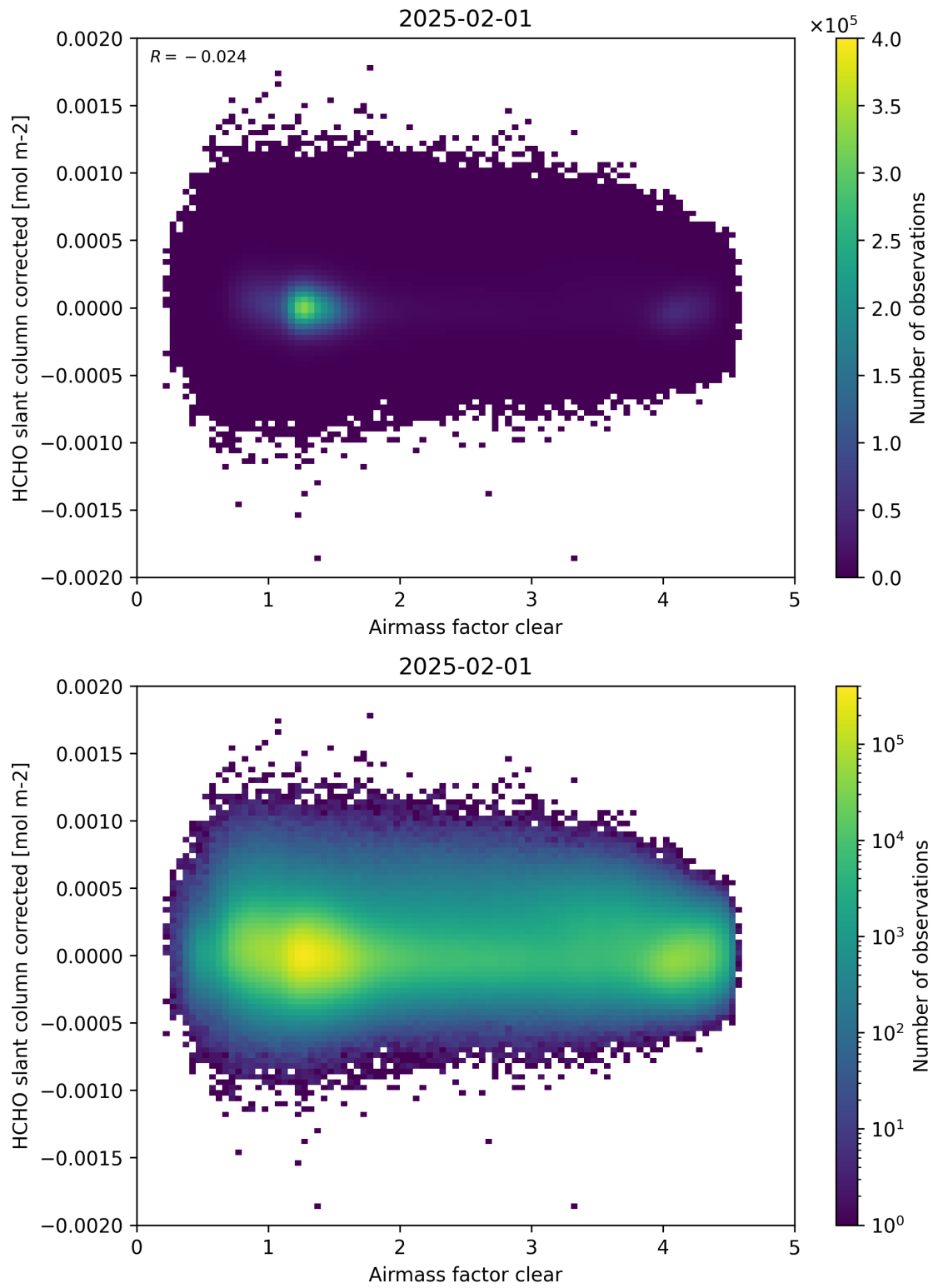
Figure 74: Scatter density plot of “Airmass factor clear” against “HCHO slant column corrected” for 2025-01-31 to 2025-02-02.
