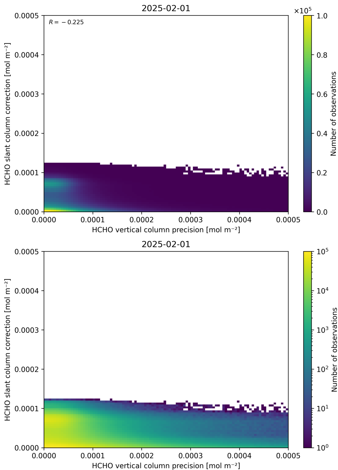
Figure 141: Scatter density plot of “HCHO vertical column precision” against “HCHO slant column correction” for 2025-01-31 to 2025-02-02.
