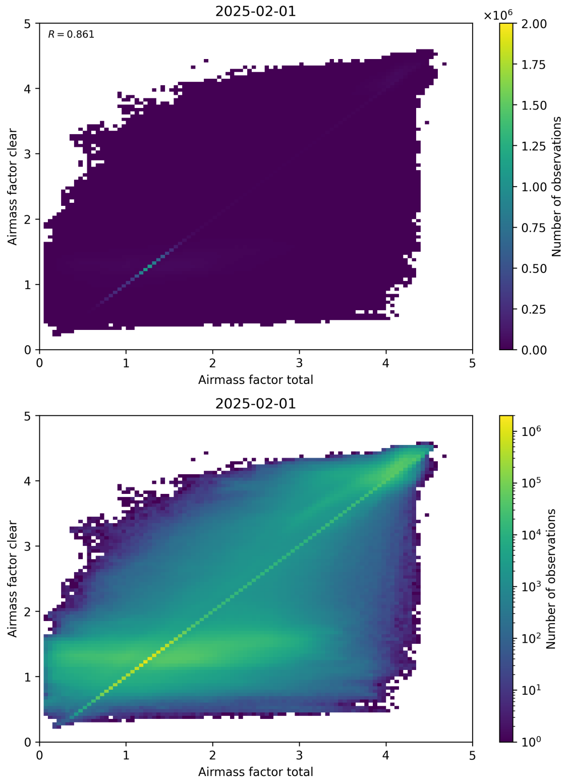
Figure 100: Scatter density plot of “Airmass factor total” against “Airmass factor clear” for 2025-01-31 to 2025-02-02.
