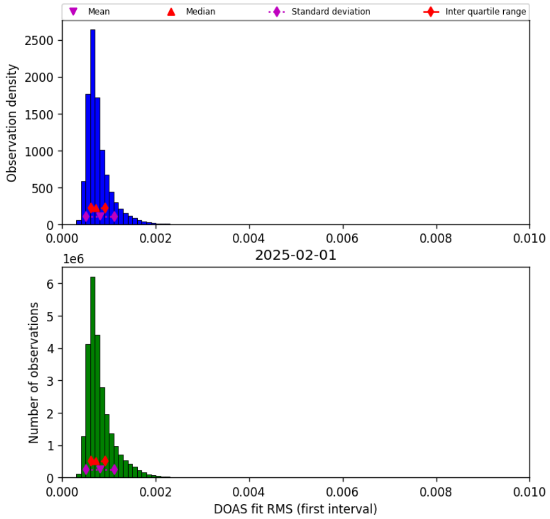
Figure 46: Histogram of “DOAS fit RMS (first interval)” for 2025-01-31 to 2025-02-02
