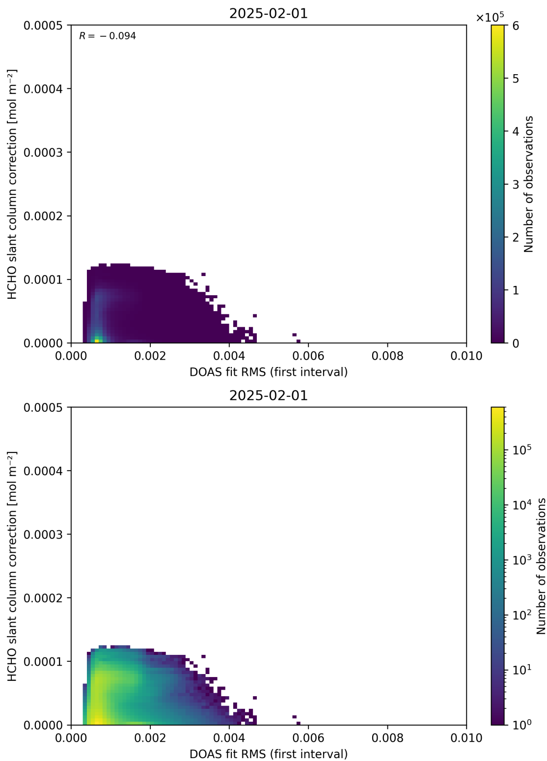
Figure 63: Scatter density plot of “DOAS fit RMS (first interval)” against “HCHO slant column correction” for 2025-01-31 to 2025-02-02.
