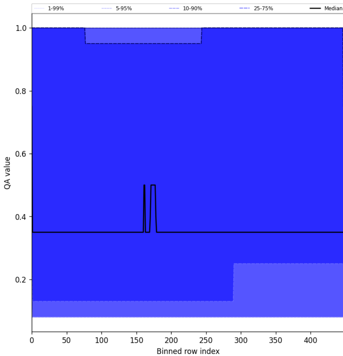
Figure 48: Along track statistics of “QA value” for 2025-01-31 to 2025-02-02
