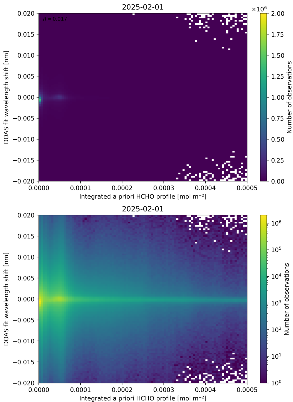
Figure 149: Scatter density plot of “Integrated a priori HCHO profile” against “DOAS fit wavelength shift” for 2025-01-31 to 2025-02-02.
