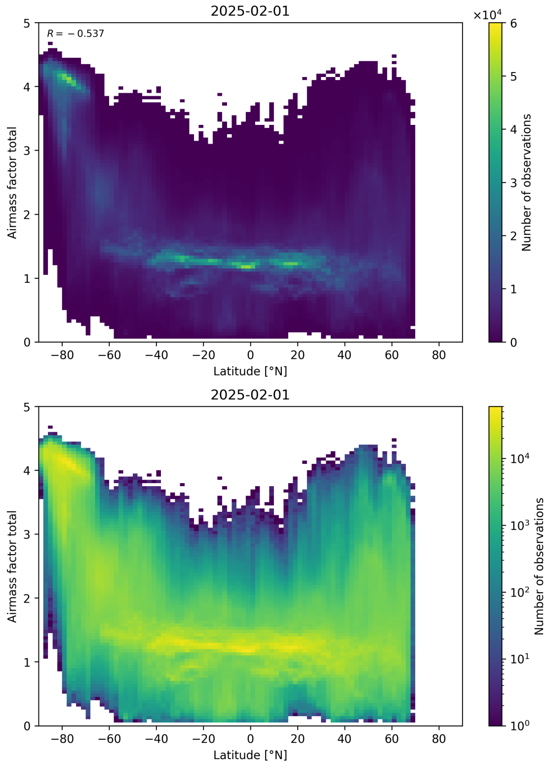
Figure 161: Scatter density plot of “Latitude” against “Airmass factor total” for 2025-01-31 to 2025-02-02.
