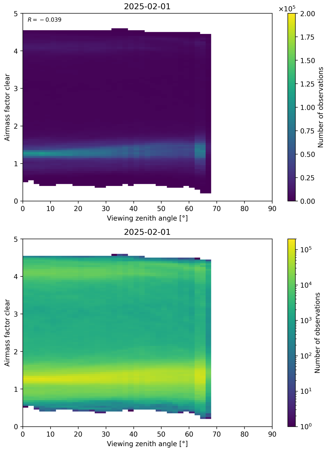
Figure 185: Scatter density plot of “Viewing zenith angle” against “Airmass factor clear” for 2025-01-31 to 2025-02-02.
