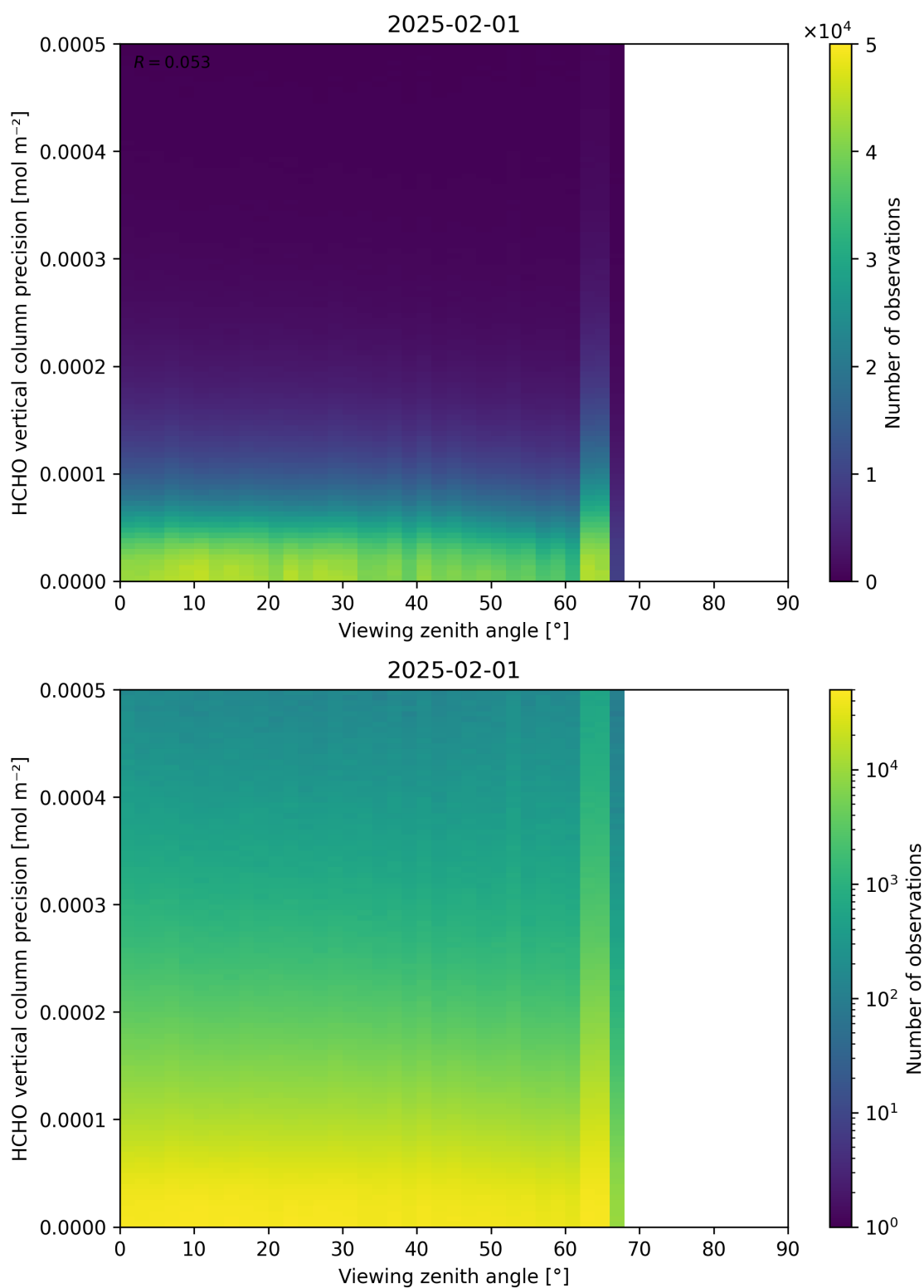
Figure 194: Scatter density plot of “Viewing zenith angle” against “HCHO vertical column precision” for 2025-01-31 to 2025-02-02.
