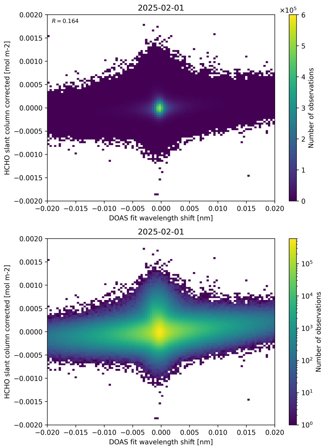
Figure 66: Scatter density plot of “DOAS fit wavelength shift” against “HCHO slant column corrected” for 2025-01-31 to 2025-02-02.
