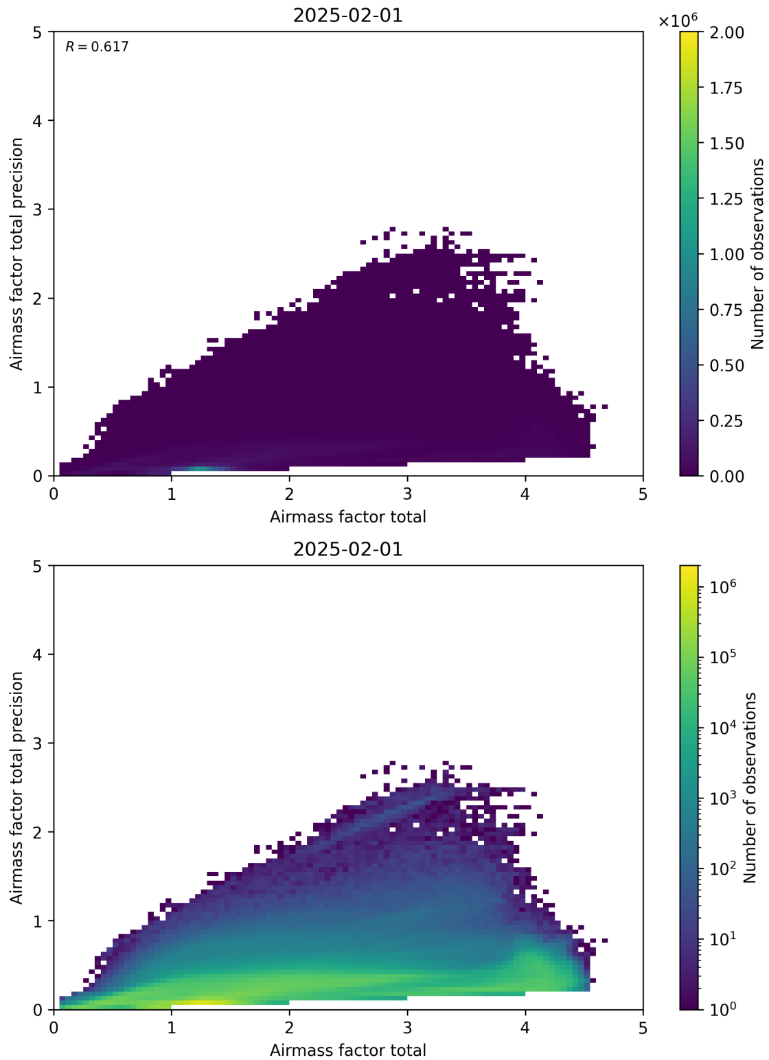
Figure 103: Scatter density plot of “Airmass factor total” against “Airmass factor total precision” for 2025-01-31 to 2025-02-02.
