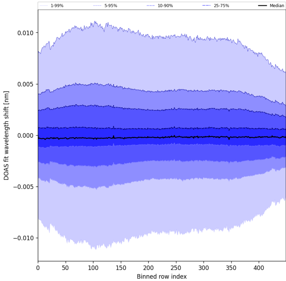
Figure 58: Along track statistics of “DOAS fit wavelength shift” for 2025-01-31 to 2025-02-02
