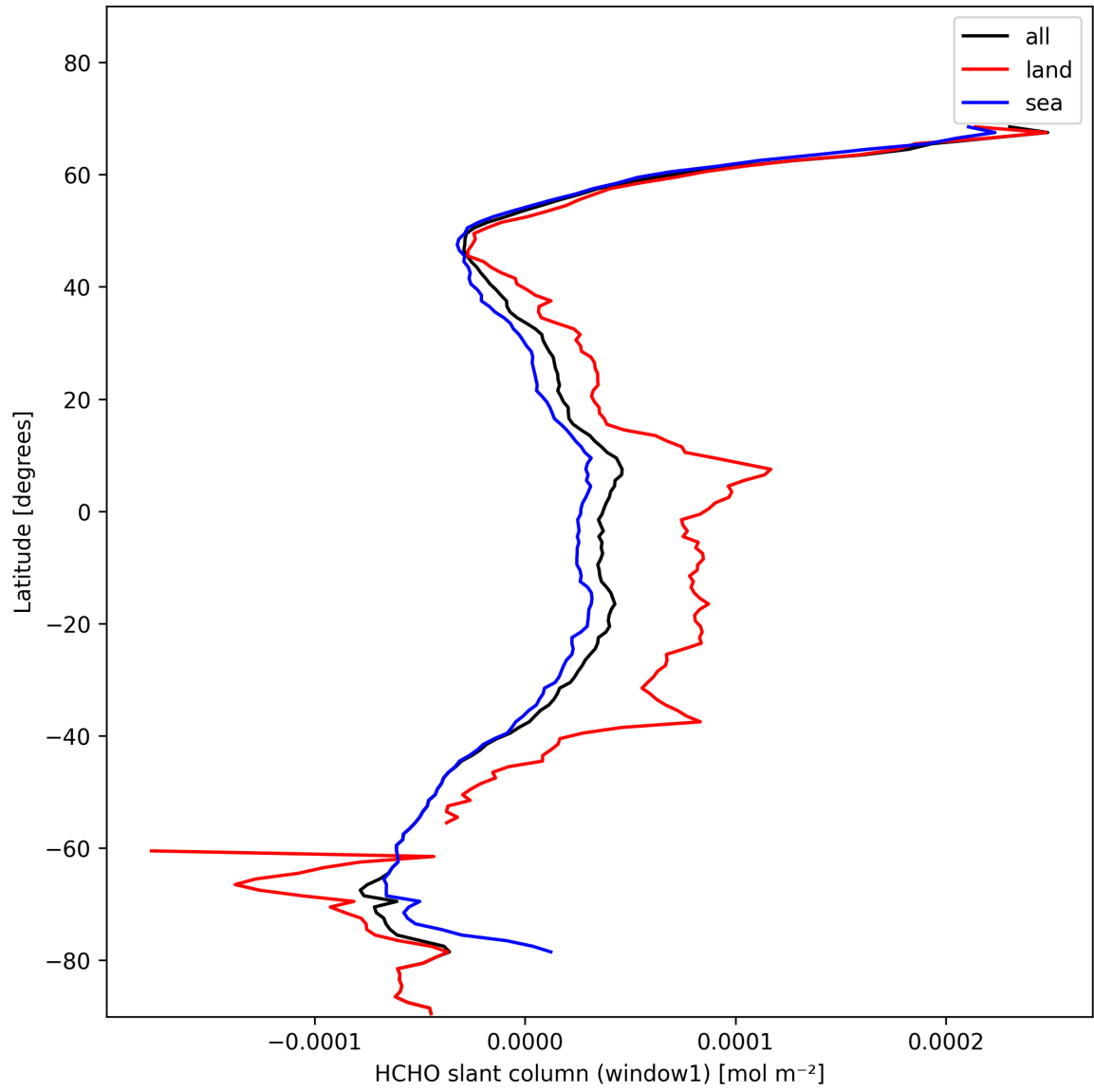
Figure 24: Zonal average of “HCHO slant column (window1)” for 2025-01-31 to 2025-02-02.
