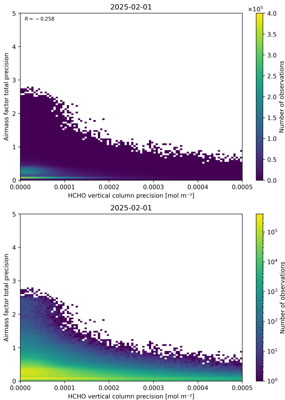
Figure 145: Scatter density plot of “HCHO vertical column precision” against “Airmass factor total precision” for 2025-01-31 to 2025-02-02.
