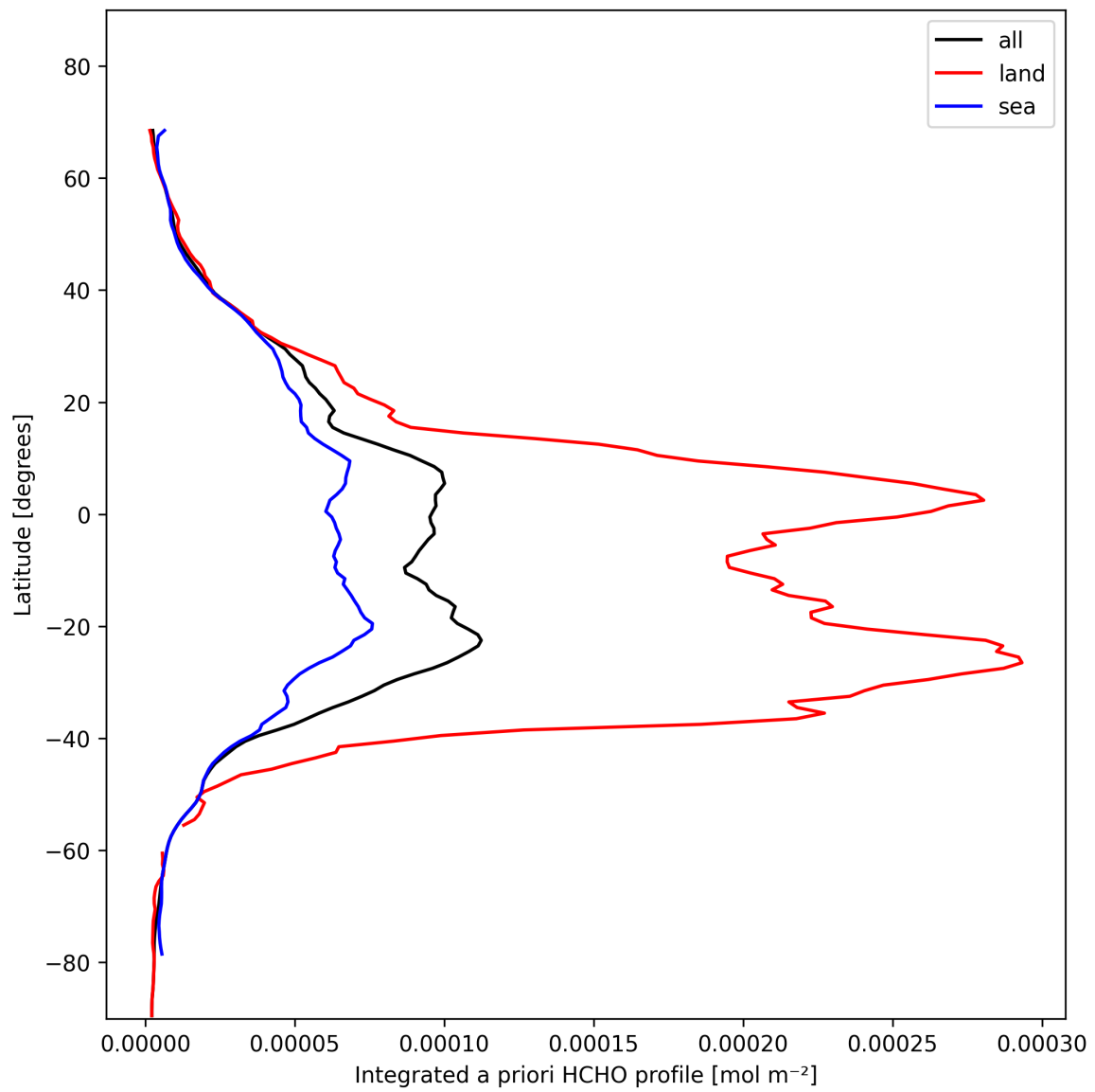
Figure 29: Zonal average of “Integrated a priori HCHO profile” for 2025-01-31 to 2025-02-02.
