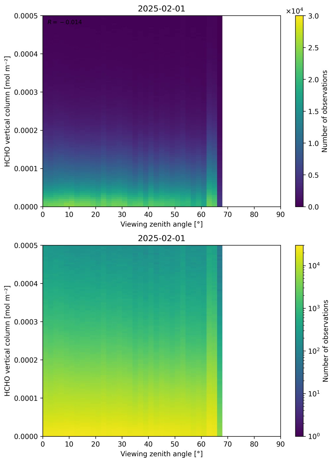
Figure 192: Scatter density plot of “Viewing zenith angle” against “HCHO vertical column” for 2025-01-31 to 2025-02-02.
