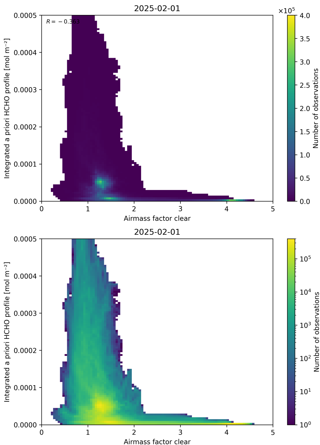
Figure 76: Scatter density plot of “Airmass factor clear” against “Integrated a priori HCHO profile” for 2025-01-31 to 2025-02-02.
