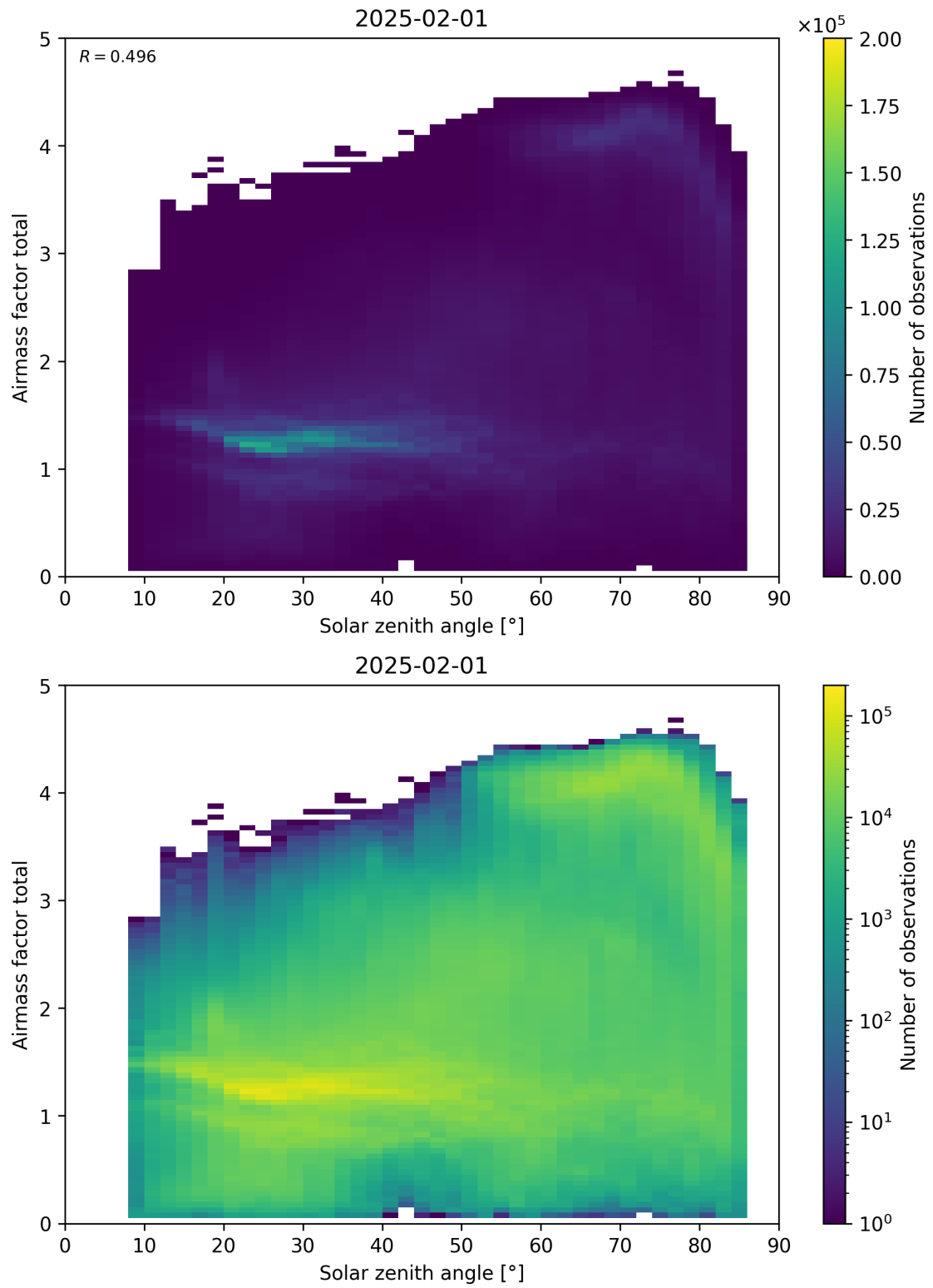
Figure 175: Scatter density plot of “Solar zenith angle” against “Airmass factor total” for 2025-01-31 to 2025-02-02.
