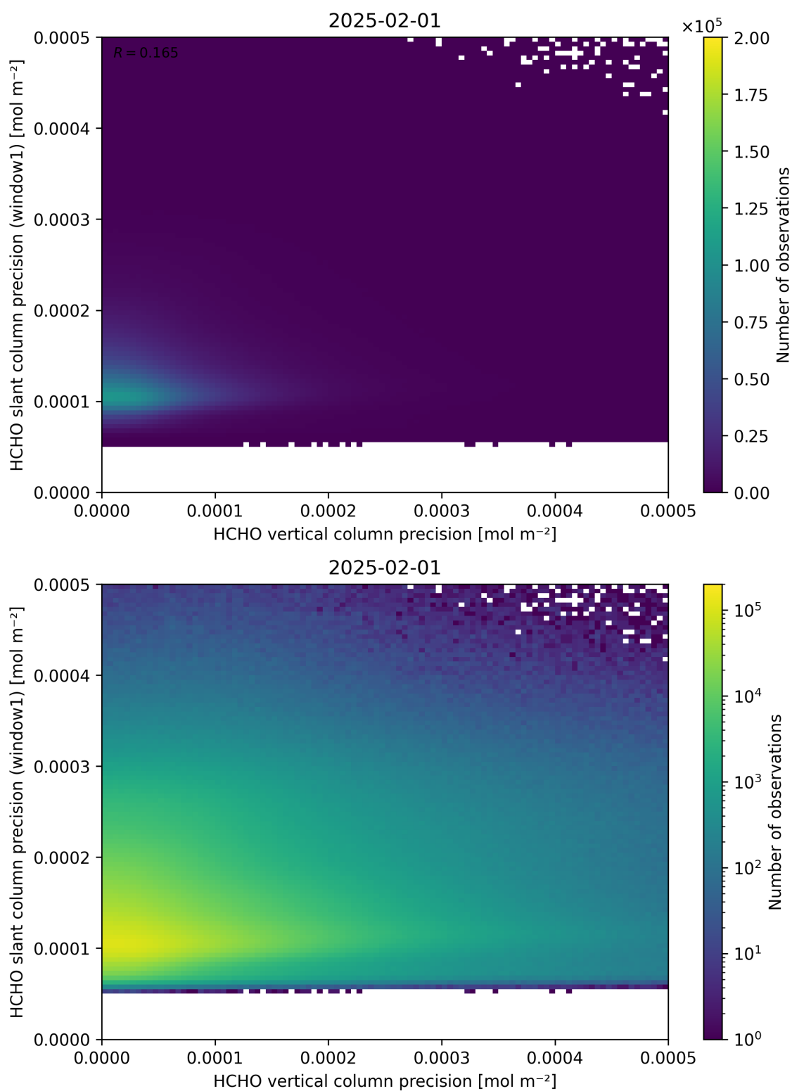
Figure 143: Scatter density plot of “HCHO vertical column precision” against “HCHO slant column precision (window1)” for 2025-01-31 to 2025-02-02.
