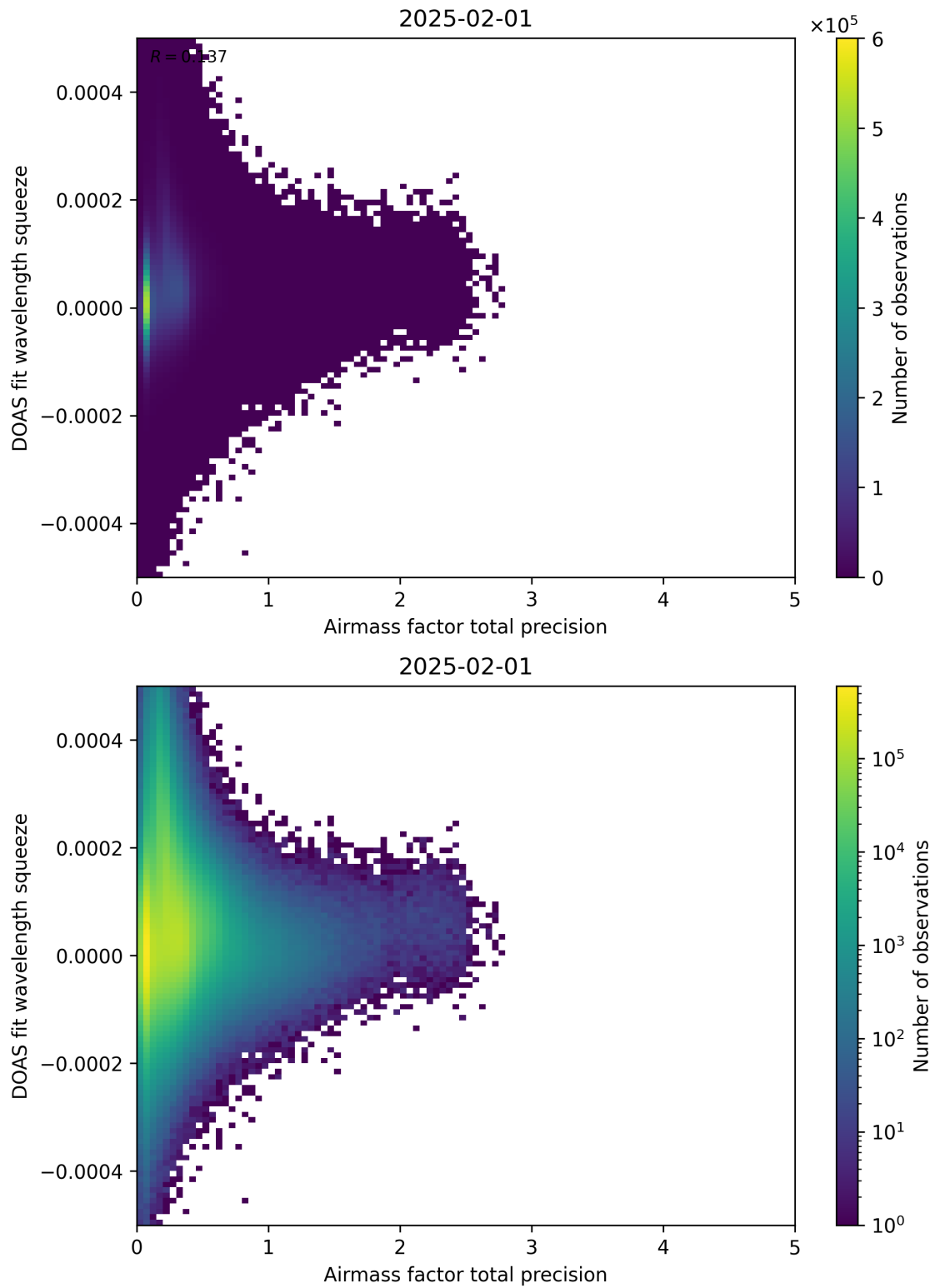
Figure 107: Scatter density plot of “Airmass factor total precision” against “DOAS fit wavelength squeeze” for 2025-01-31 to 2025-02-02.
