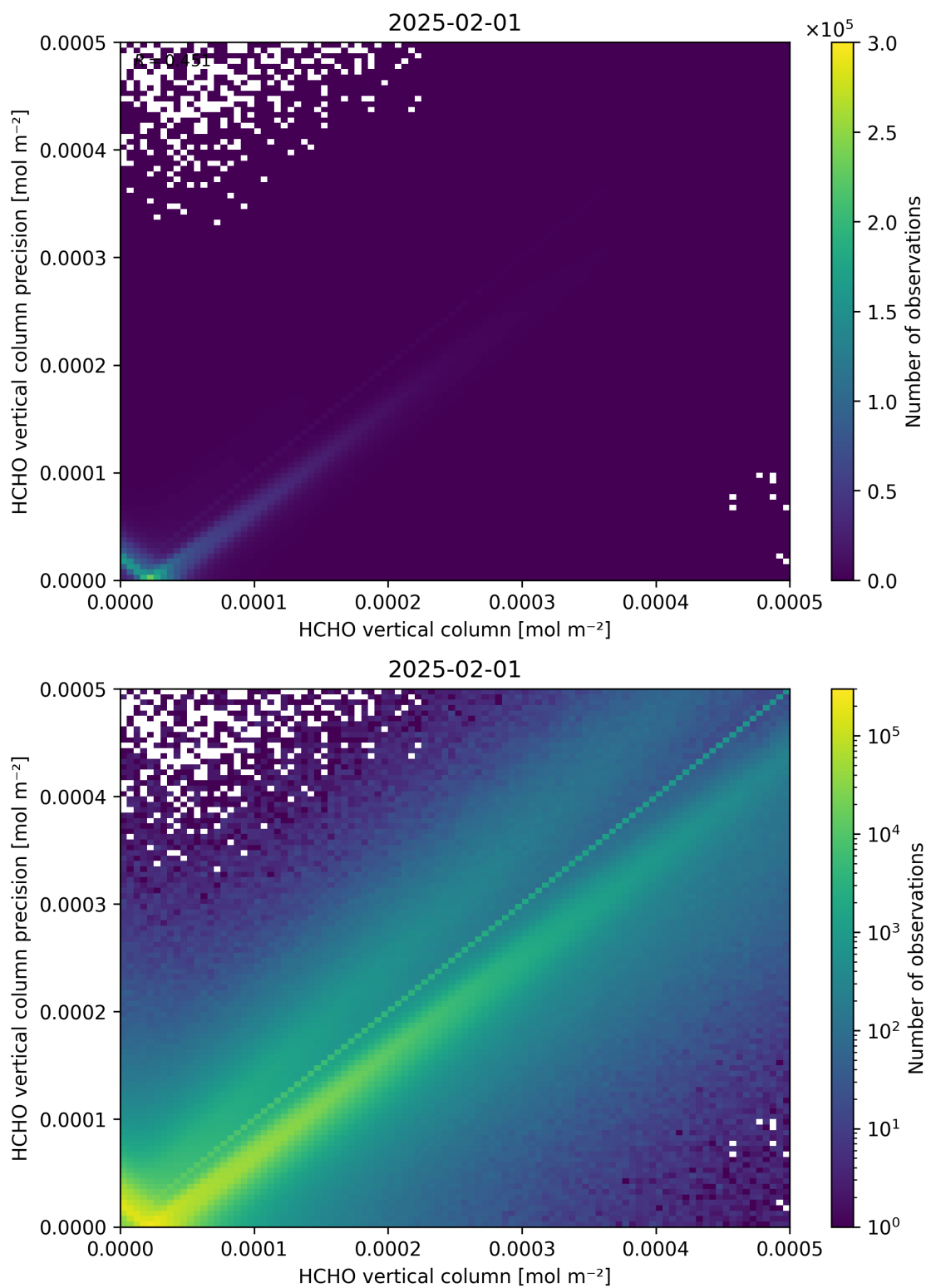
Figure 134: Scatter density plot of “HCHO vertical column” against “HCHO vertical column precision” for 2025-01-31 to 2025-02-02.
