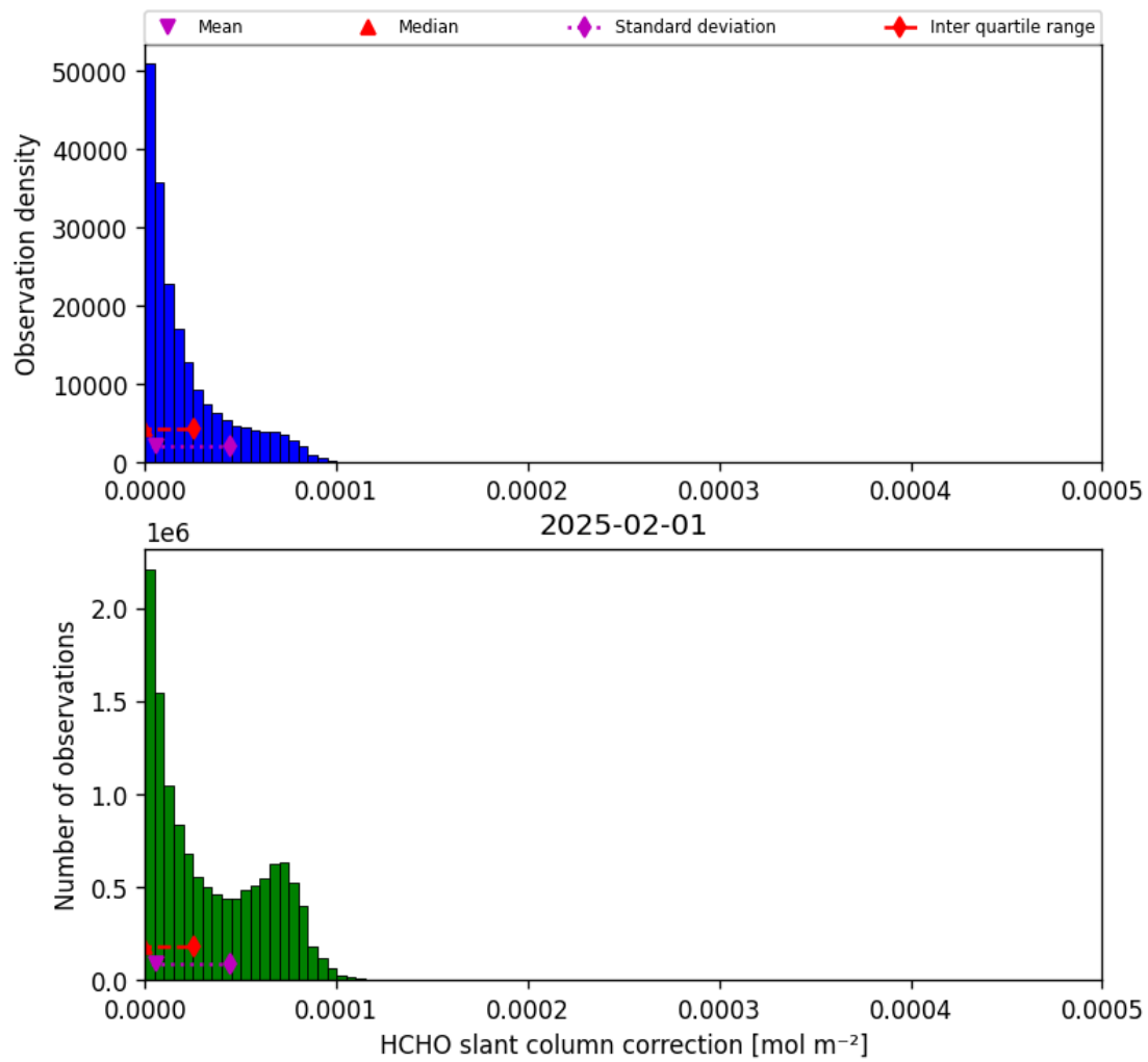
Figure 47: Histogram of “HCHO slant column correction” for 2025-01-31 to 2025-02-02
