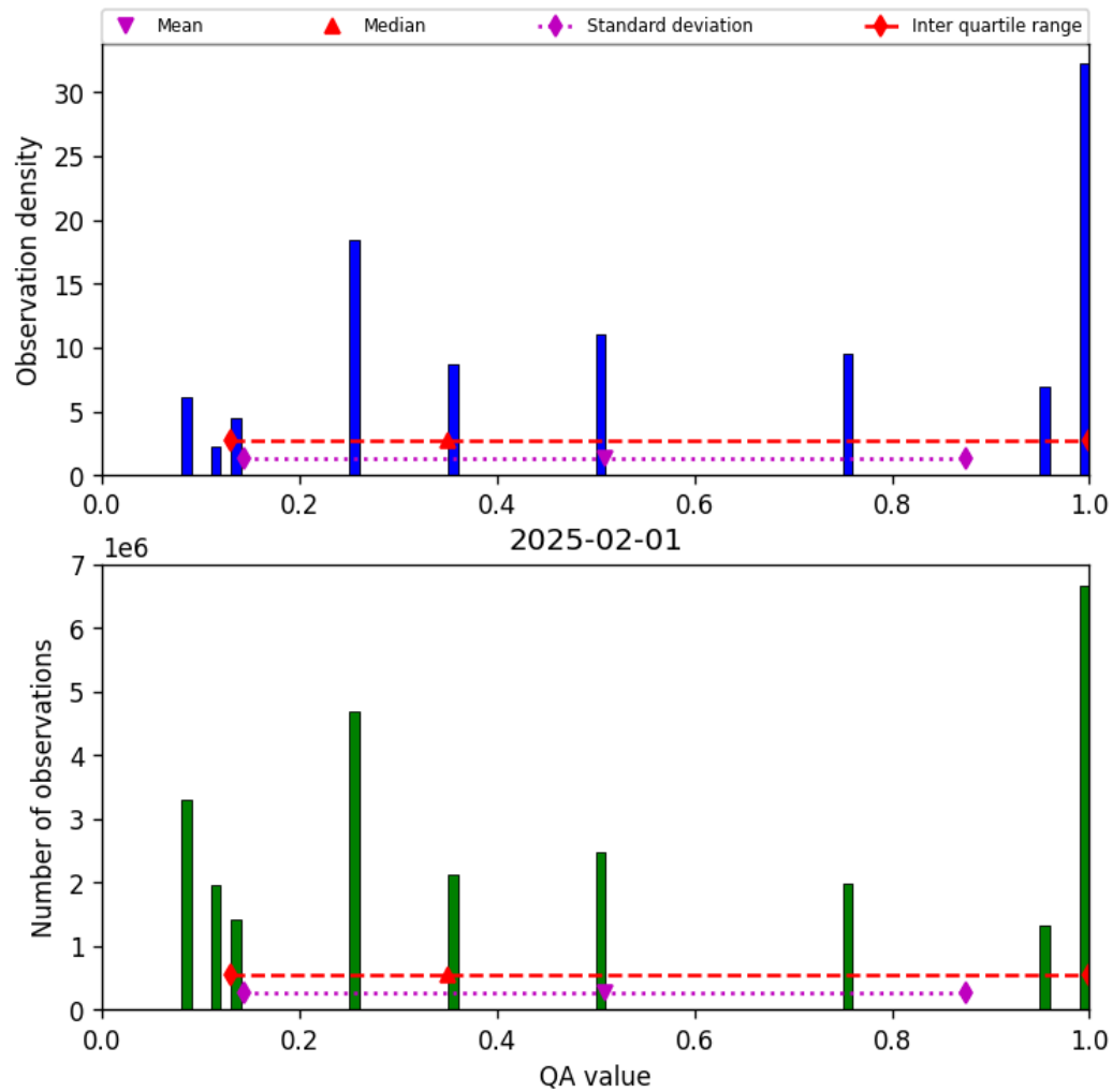
Figure 34: Histogram of “QA value” for 2025-01-31 to 2025-02-02
