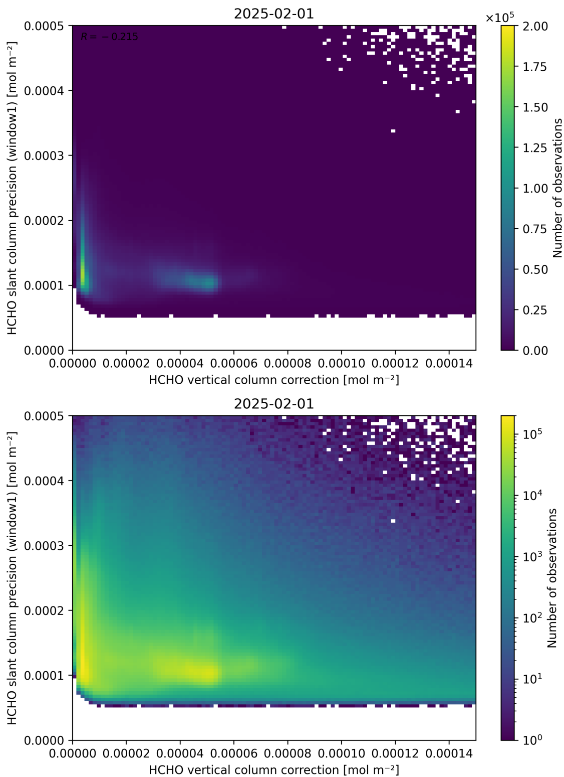
Figure 119: Scatter density plot of “HCHO vertical column correction” against “HCHO slant column precision (window1)” for 2025-01-31 to 2025-02-02.
