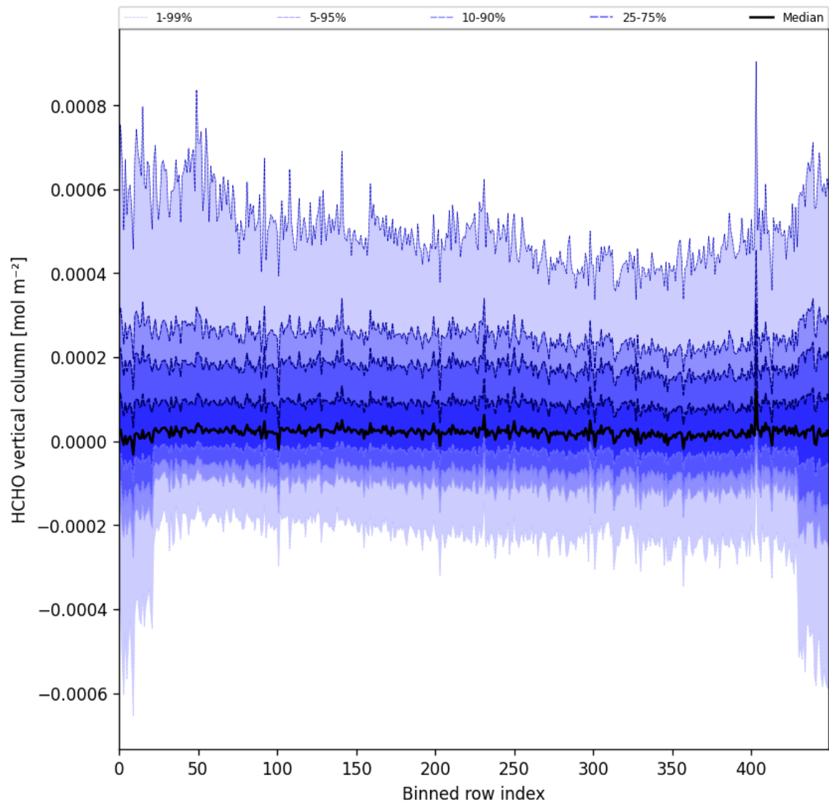
Figure 49: Along track statistics of “HCHO vertical column” for 2025-01-31 to 2025-02-02
