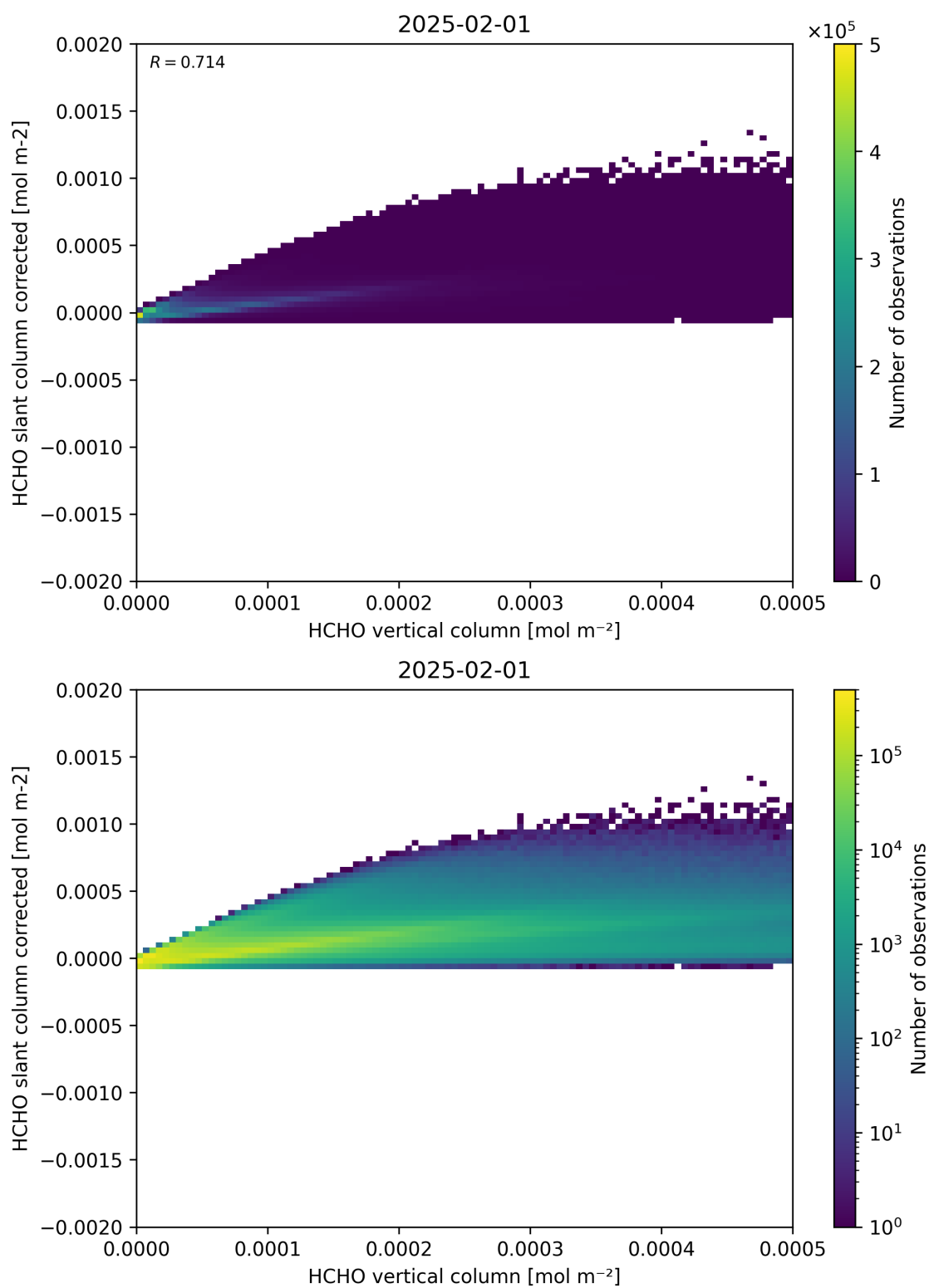
Figure 127: Scatter density plot of “HCHO vertical column” against “HCHO slant column corrected” for 2025-01-31 to 2025-02-02.
