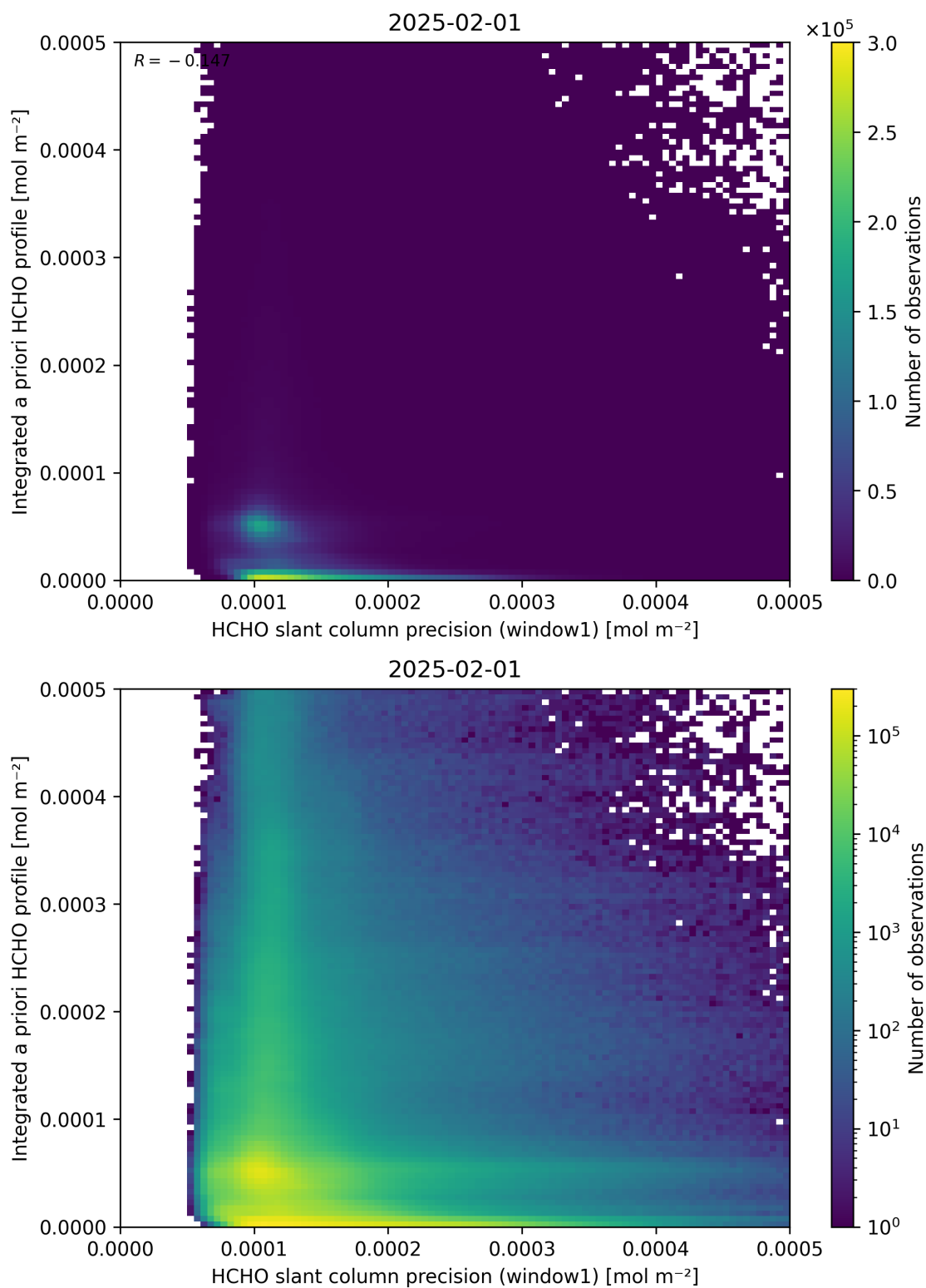
Figure 96: Scatter density plot of “HCHO slant column precision (window1)” against “Integrated a priori HCHO profile” for 2025-01-31 to 2025-02-02.
