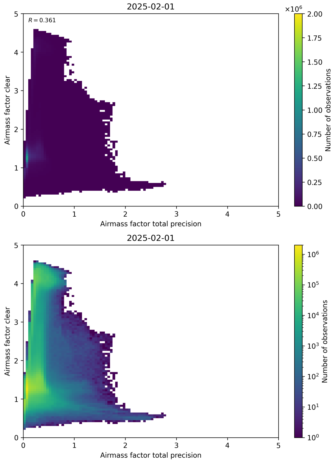
Figure 108: Scatter density plot of “Airmass factor total precision” against “Airmass factor clear” for 2025-01-31 to 2025-02-02.
