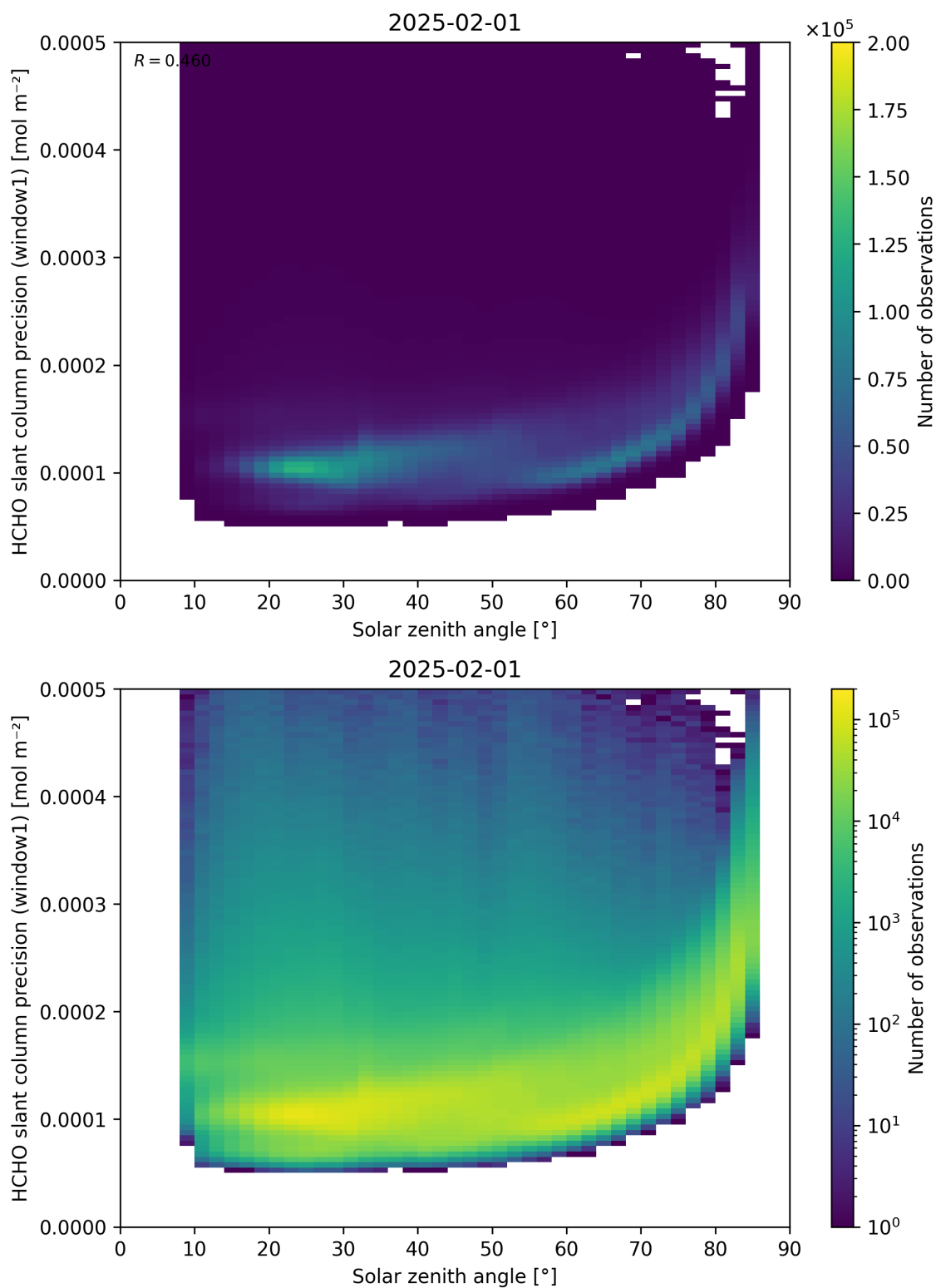
Figure 174: Scatter density plot of “Solar zenith angle” against “HCHO slant column precision (window1)” for 2025-01-31 to 2025-02-02.
