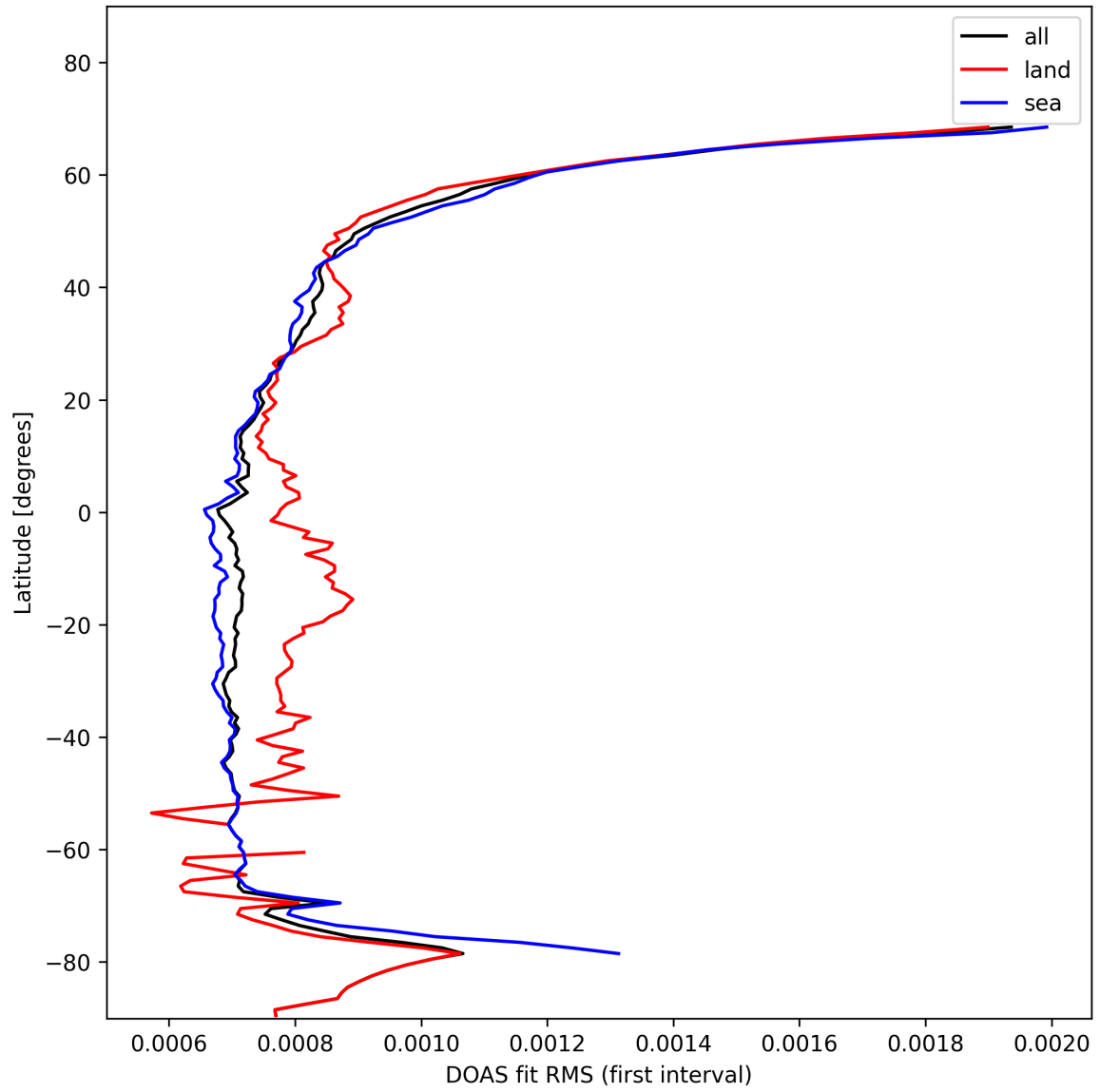
Figure 32: Zonal average of “DOAS fit RMS (first interval)” for 2025-01-31 to 2025-02-02.
