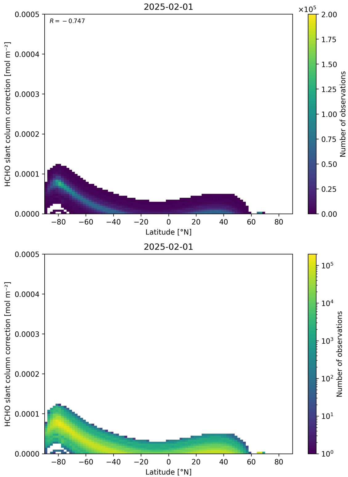
Figure 158: Scatter density plot of “Latitude” against “HCHO slant column correction” for 2025-01-31 to 2025-02-02.
