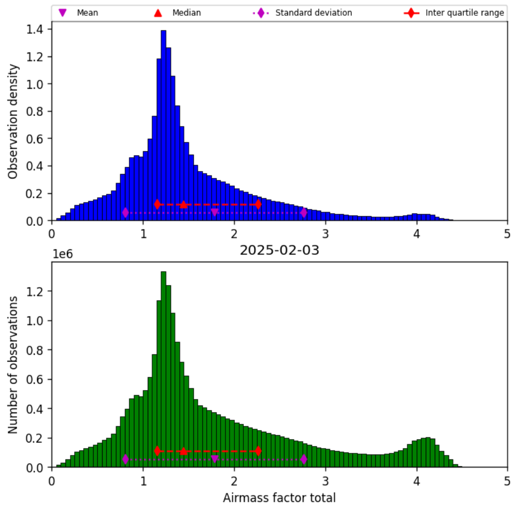
Figure 40: Histogram of “Airmass factor total” for 2025-02-03 to 2025-02-04
