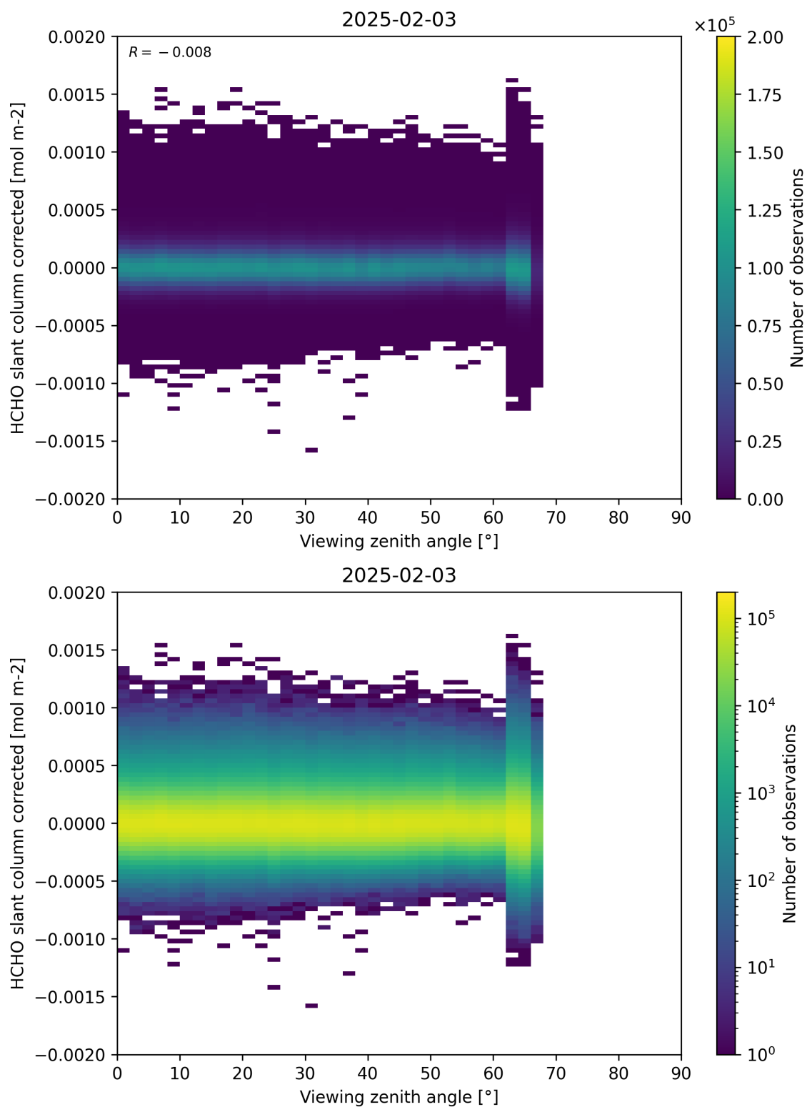
Figure 186: Scatter density plot of “Viewing zenith angle” against “HCHO slant column corrected” for 2025-02-03 to 2025-02-04.
