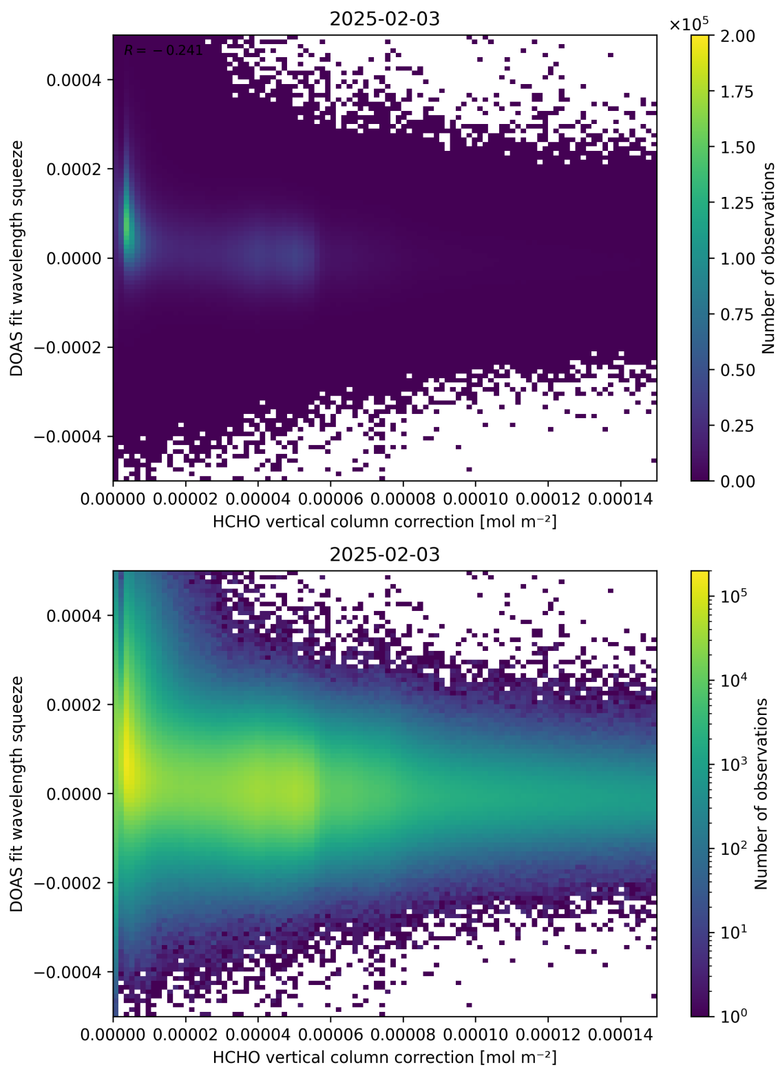
Figure 114: Scatter density plot of “HCHO vertical column correction” against “DOAS fit wavelength squeeze” for 2025-02-03 to 2025-02-04.
