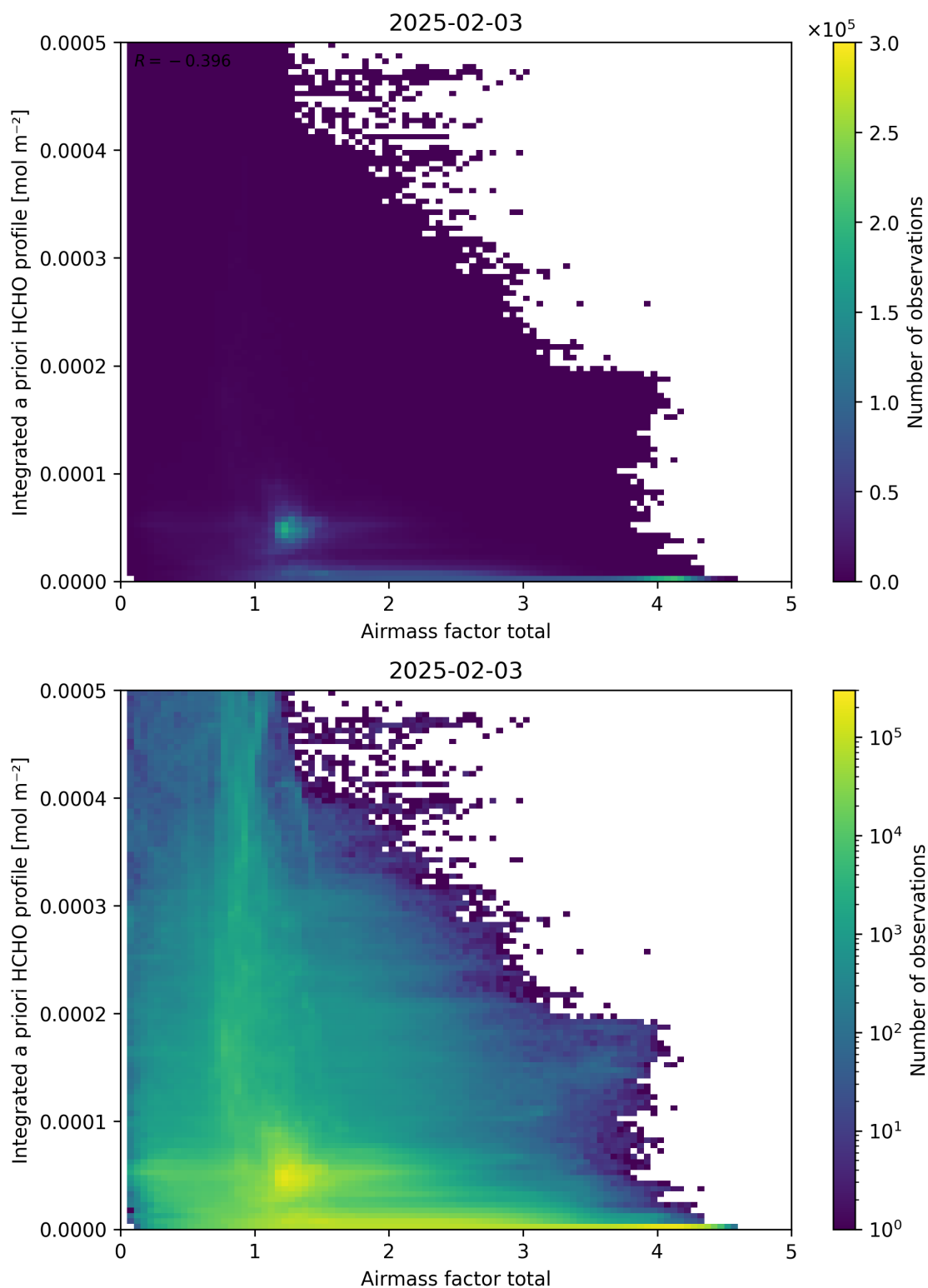
Figure 104: Scatter density plot of “Airmass factor total” against “Integrated a priori HCHO profile” for 2025-02-03 to 2025-02-04.
