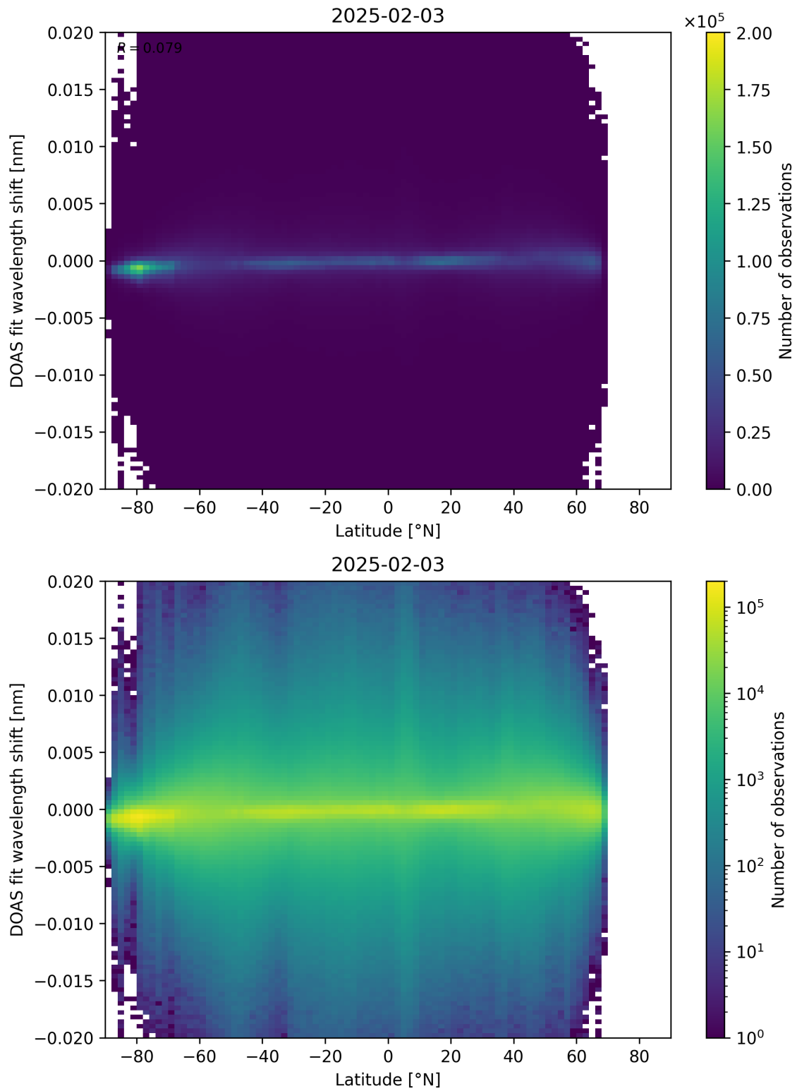
Figure 154: Scatter density plot of “Latitude” against “DOAS fit wavelength shift” for 2025-02-03 to 2025-02-04.
