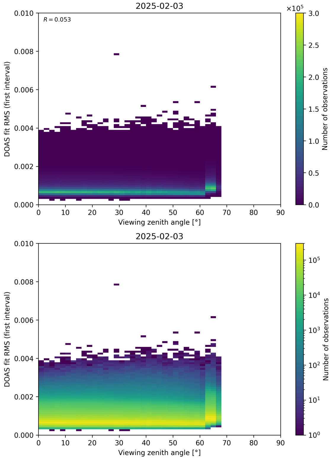
Figure 182: Scatter density plot of “Viewing zenith angle” against “DOAS fit RMS (first interval)” for 2025-02-03 to 2025-02-04.
