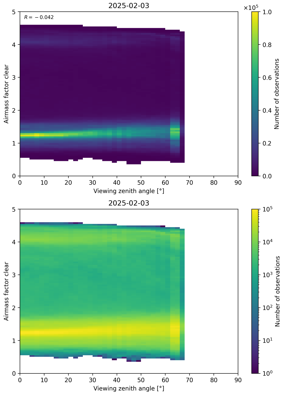
Figure 185: Scatter density plot of “Viewing zenith angle” against “Airmass factor clear” for 2025-02-03 to 2025-02-04.
