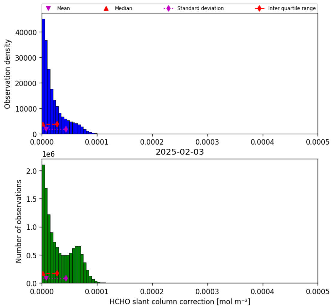
Figure 47: Histogram of “HCHO slant column correction” for 2025-02-03 to 2025-02-04
