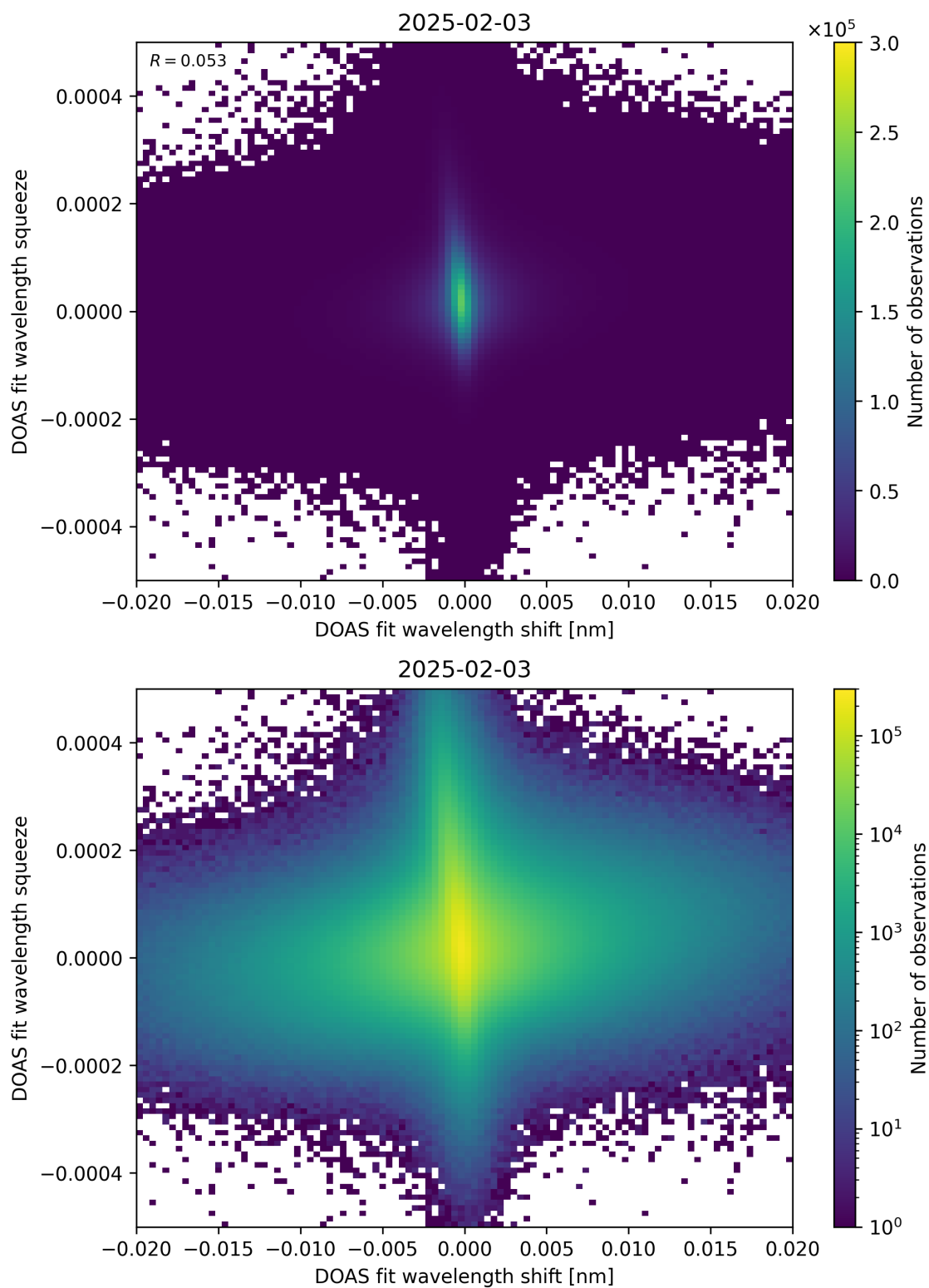
Figure 65: Scatter density plot of “DOAS fit wavelength shift” against “DOAS fit wavelength squeeze” for 2025-02-03 to 2025-02-04.
