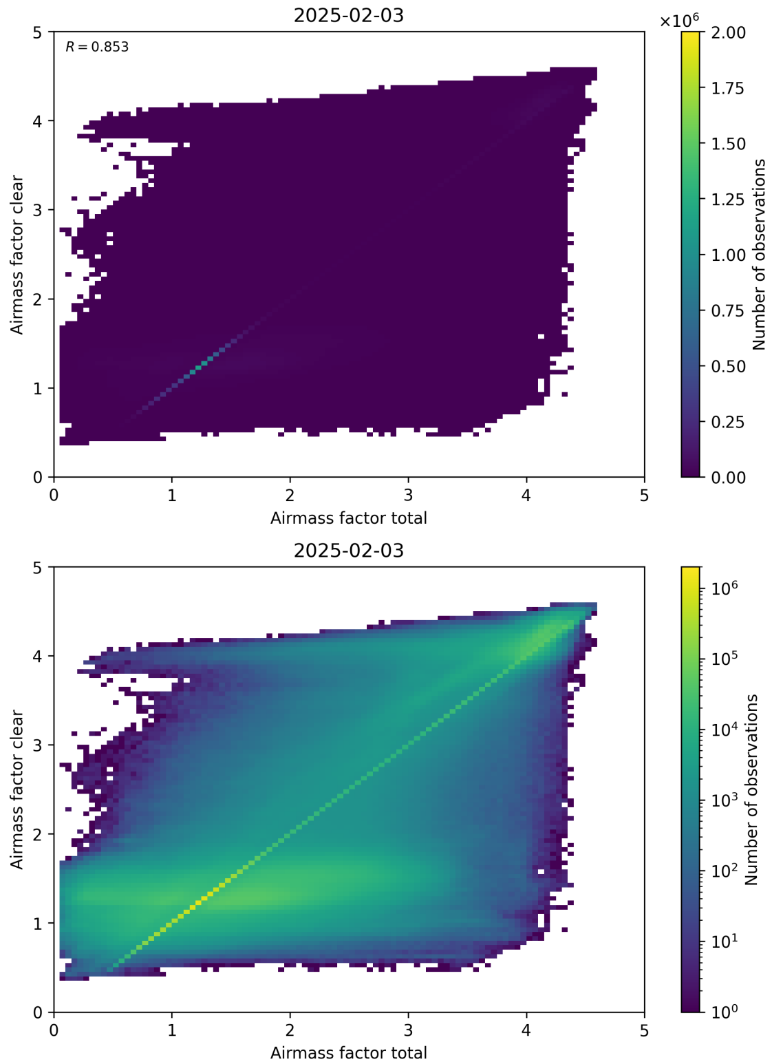
Figure 100: Scatter density plot of “Airmass factor total” against “Airmass factor clear” for 2025-02-03 to 2025-02-04.
