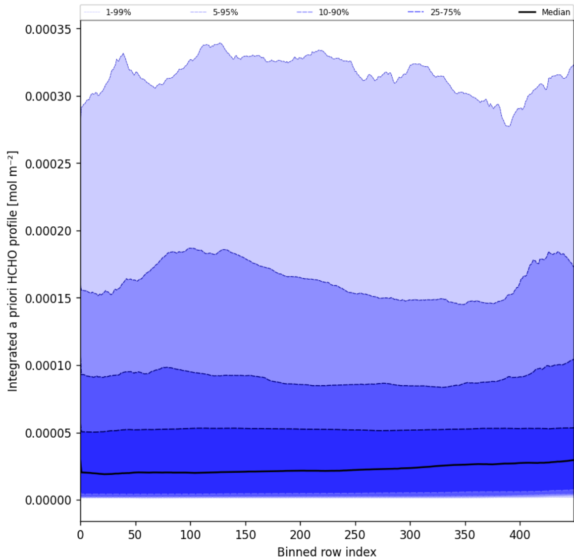
Figure 57: Along track statistics of “Integrated a priori HCHO profile” for 2025-02-03 to 2025-02-04
