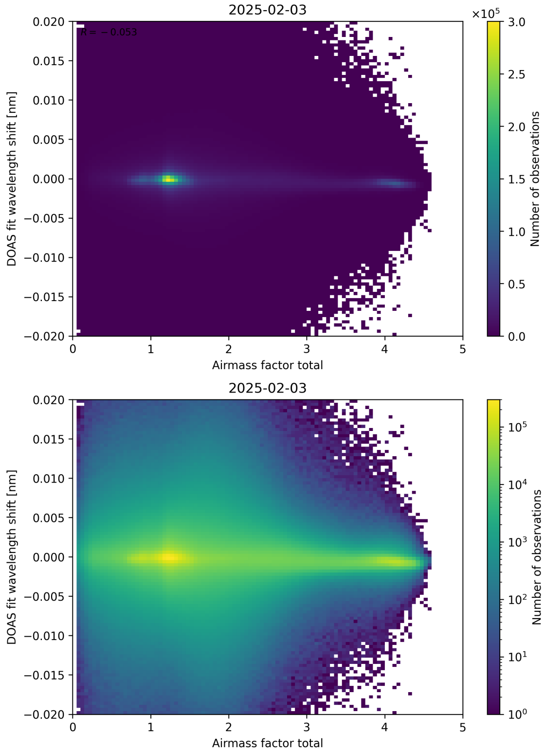
Figure 98: Scatter density plot of “Airmass factor total” against “DOAS fit wavelength shift” for 2025-02-03 to 2025-02-04.
