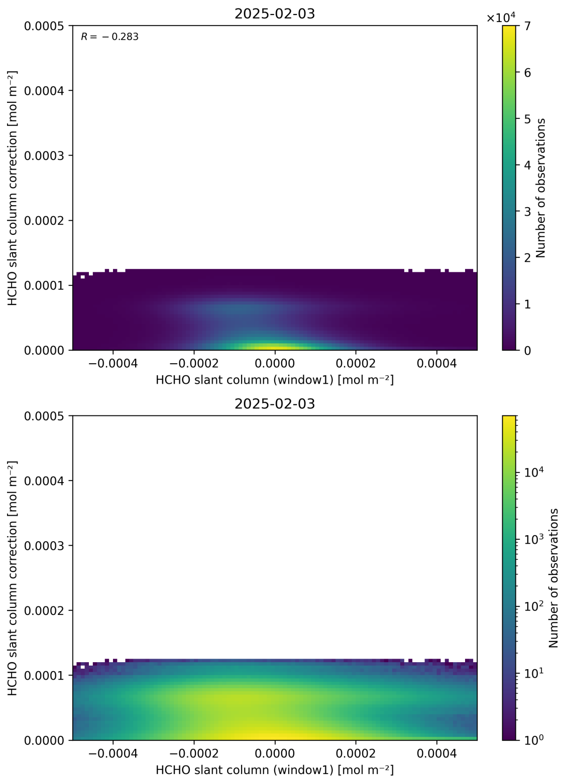
Figure 83: Scatter density plot of “HCHO slant column (window1)” against “HCHO slant column correction” for 2025-02-03 to 2025-02-04.
