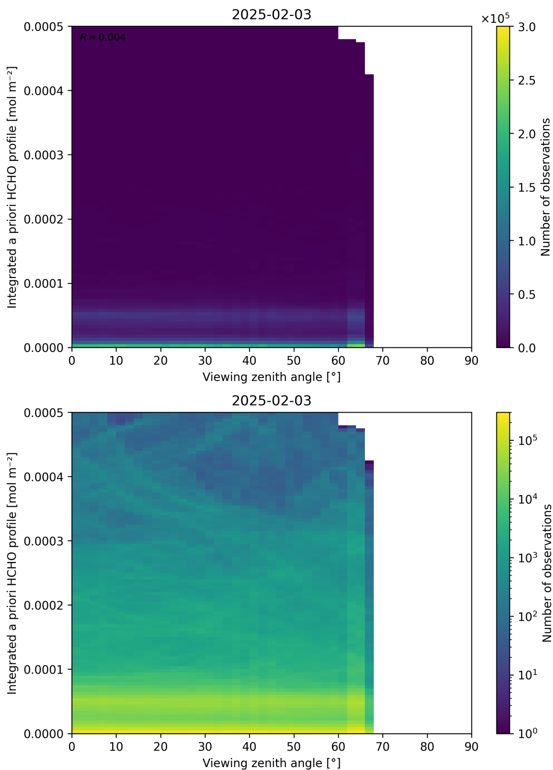
Figure 195: Scatter density plot of “Viewing zenith angle” against “Integrated a priori HCHO profile” for 2025-02-03 to 2025-02-04.
