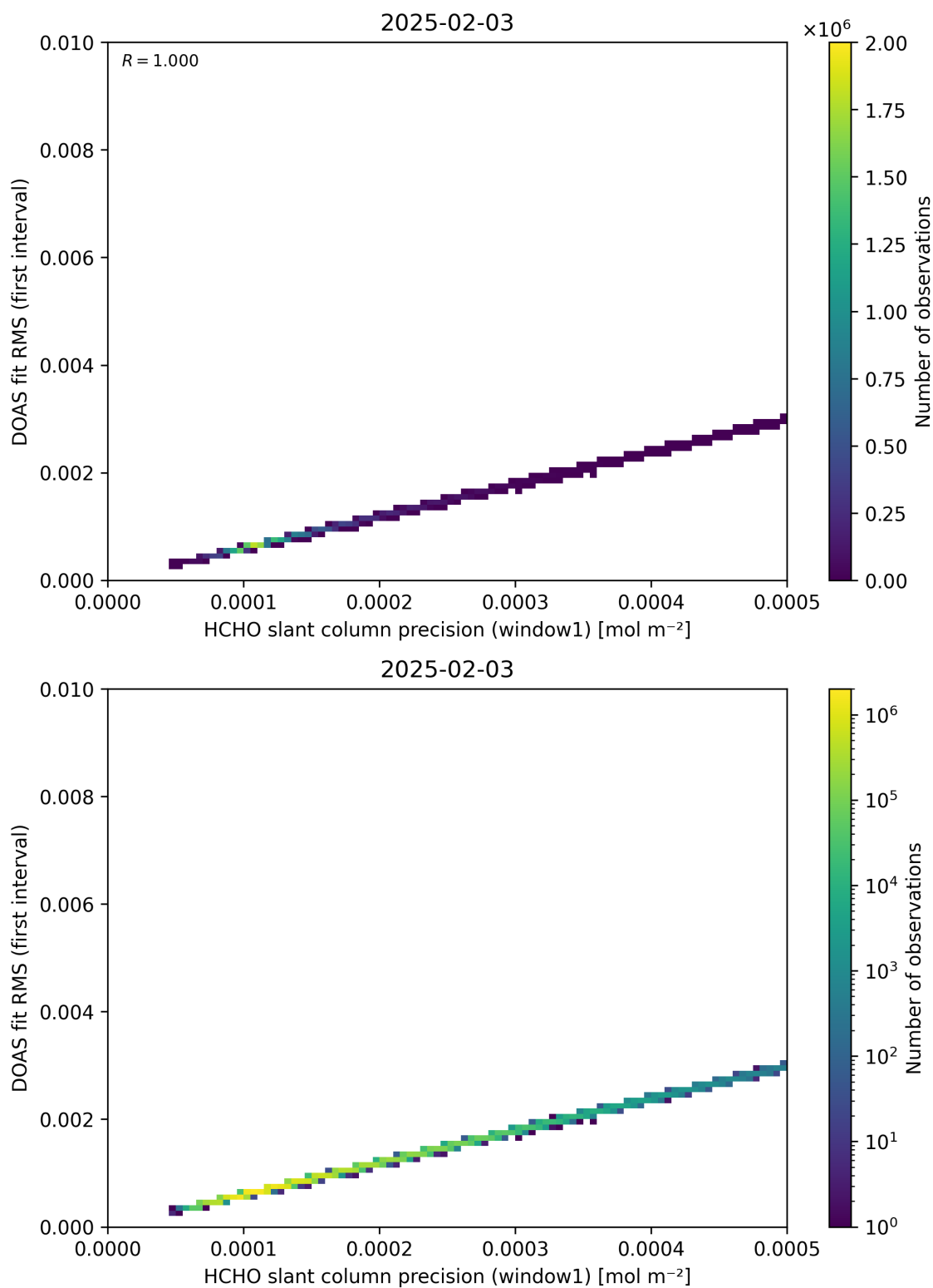
Figure 88: Scatter density plot of “HCHO slant column precision (window1)” against “DOAS fit RMS (first interval)” for 2025-02-03 to 2025-02-04.
