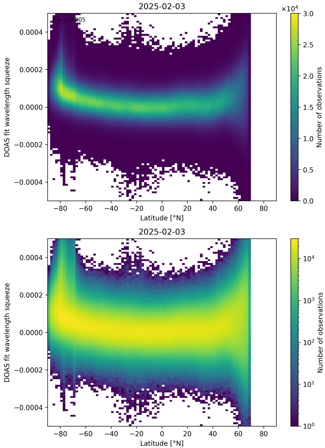
Figure 155: Scatter density plot of “Latitude” against “DOAS fit wavelength squeeze” for 2025-02-03 to 2025-02-04.
