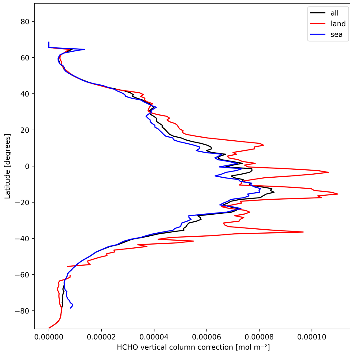
Figure 23: Zonal average of “HCHO vertical column correction” for 2025-02-03 to 2025-02-04.
