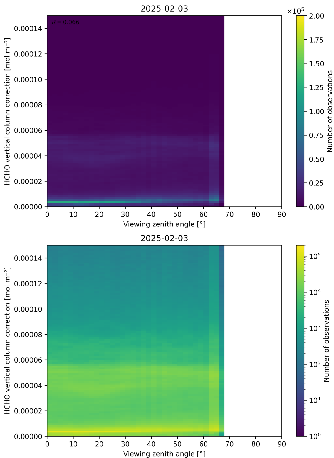
Figure 193: Scatter density plot of “Viewing zenith angle” against “HCHO vertical column correction” for 2025-02-03 to 2025-02-04.
