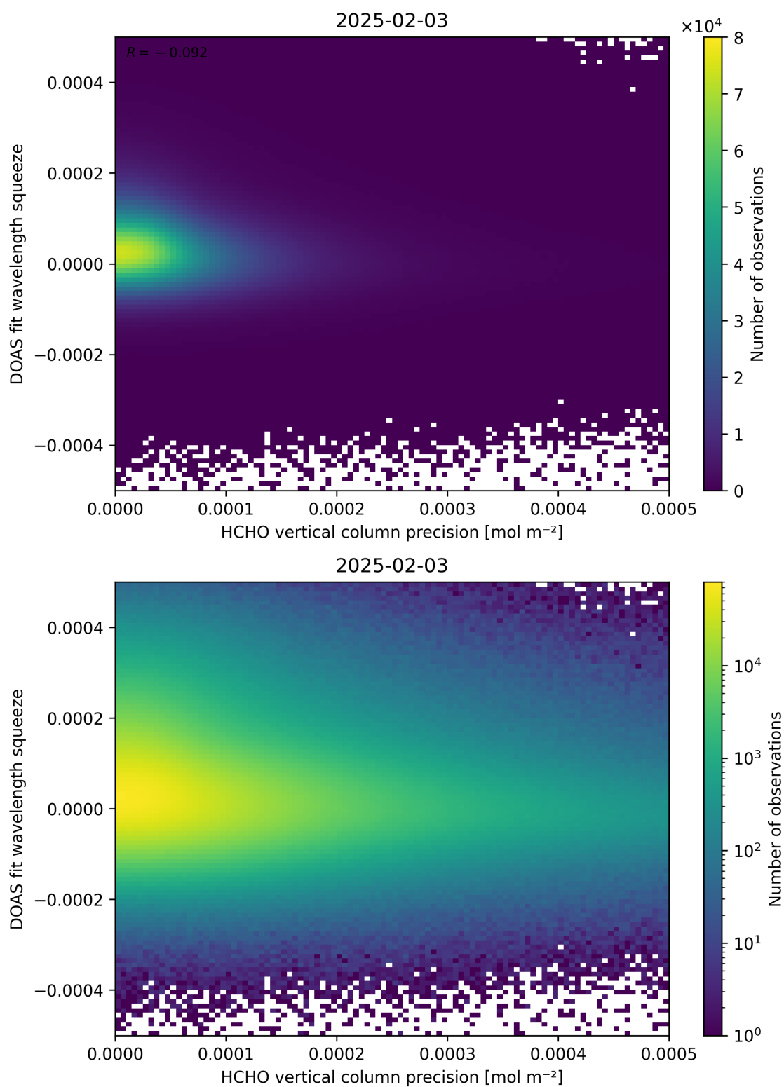
Figure 138: Scatter density plot of “HCHO vertical column precision” against “DOAS fit wavelength squeeze” for 2025-02-03 to 2025-02-04.
