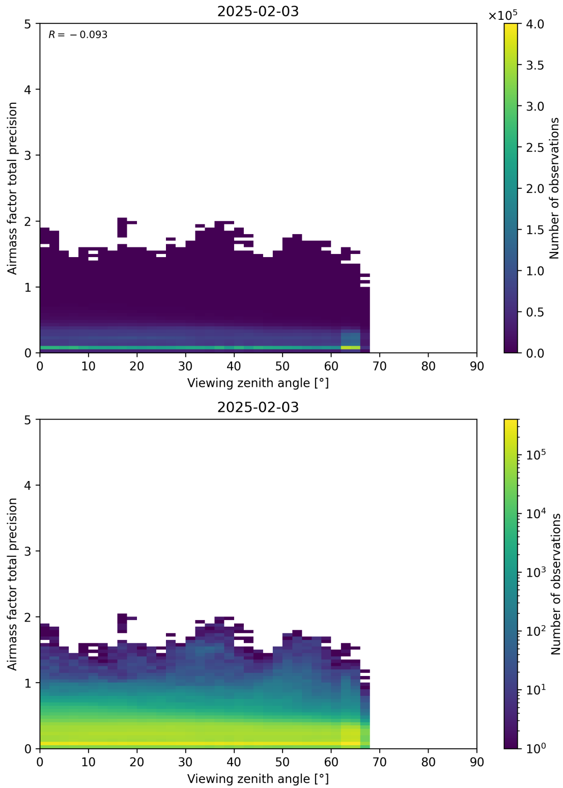
Figure 191: Scatter density plot of “Viewing zenith angle” against “Airmass factor total precision” for 2025-02-03 to 2025-02-04.
