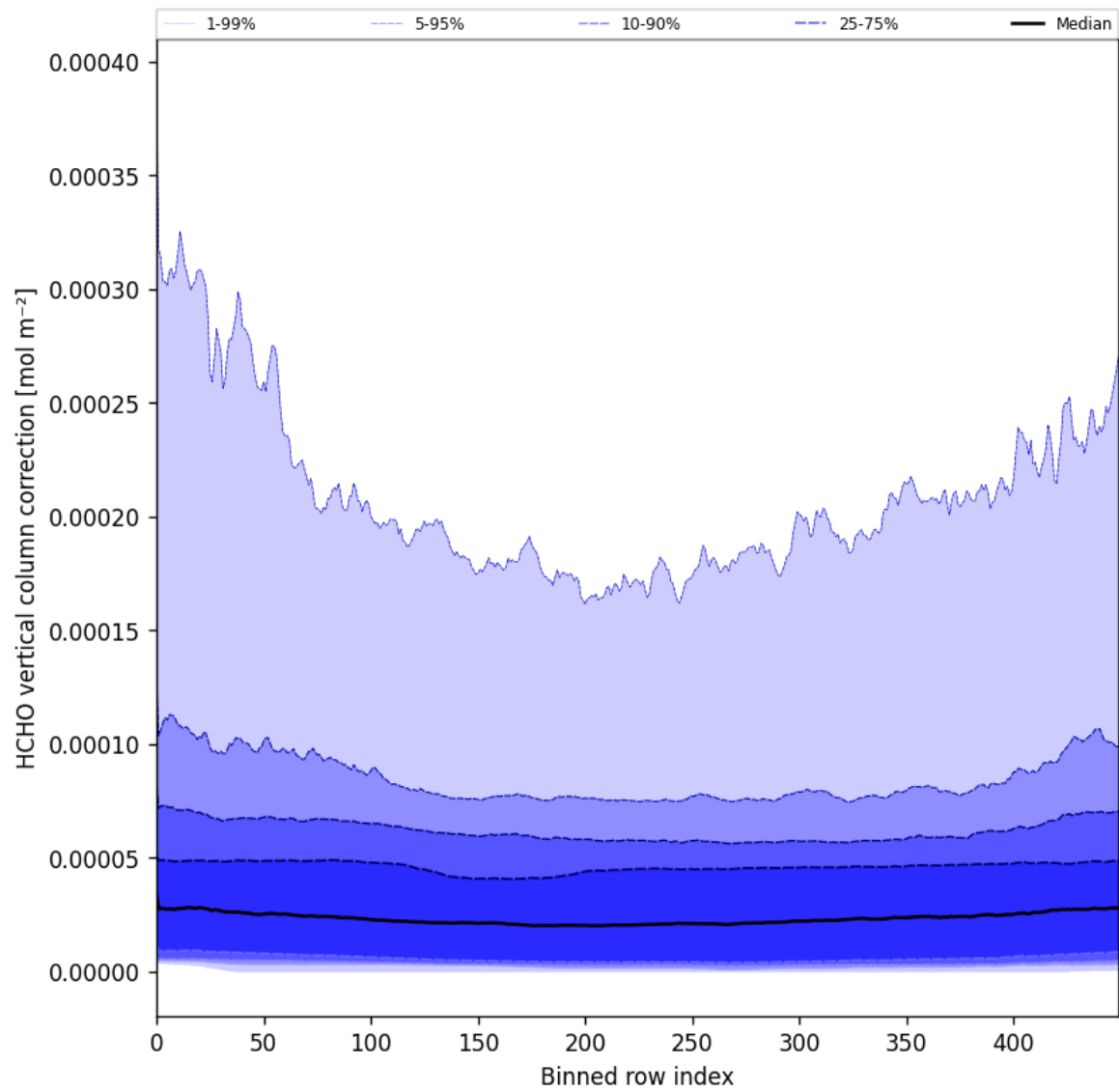
Figure 51: Along track statistics of “HCHO vertical column correction” for 2025-02-03 to 2025-02-04
