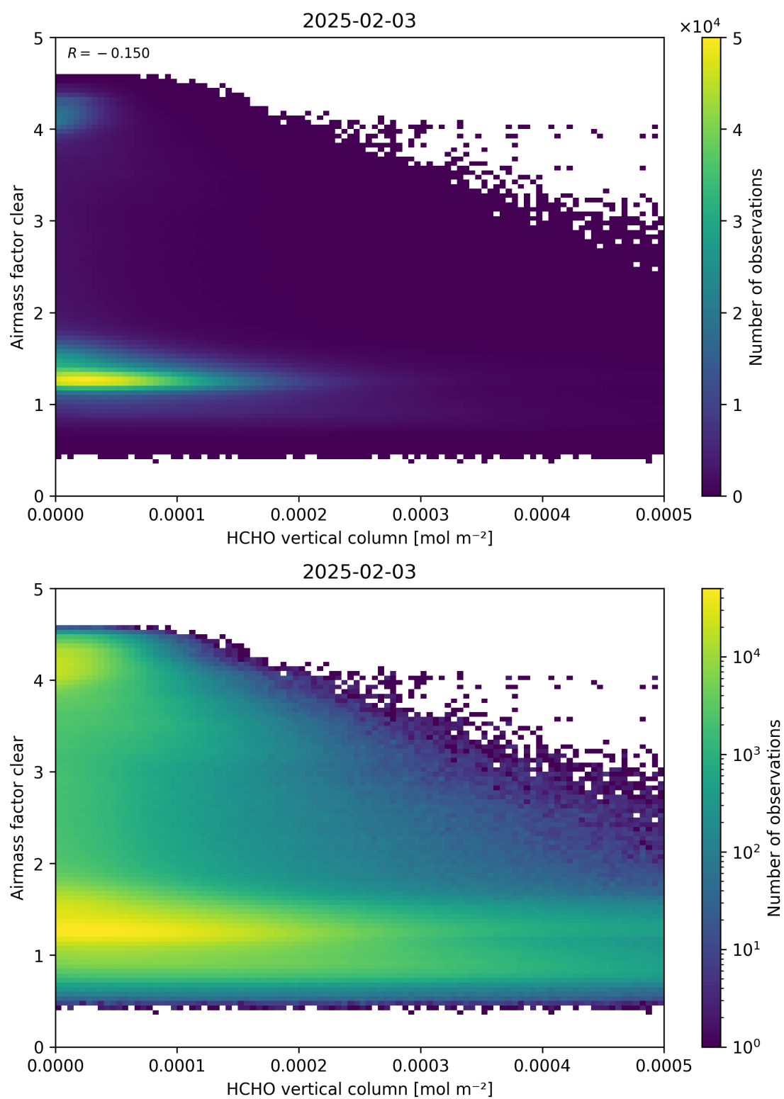
Figure 126: Scatter density plot of “HCHO vertical column” against “Airmass factor clear” for 2025-02-03 to 2025-02-04.
