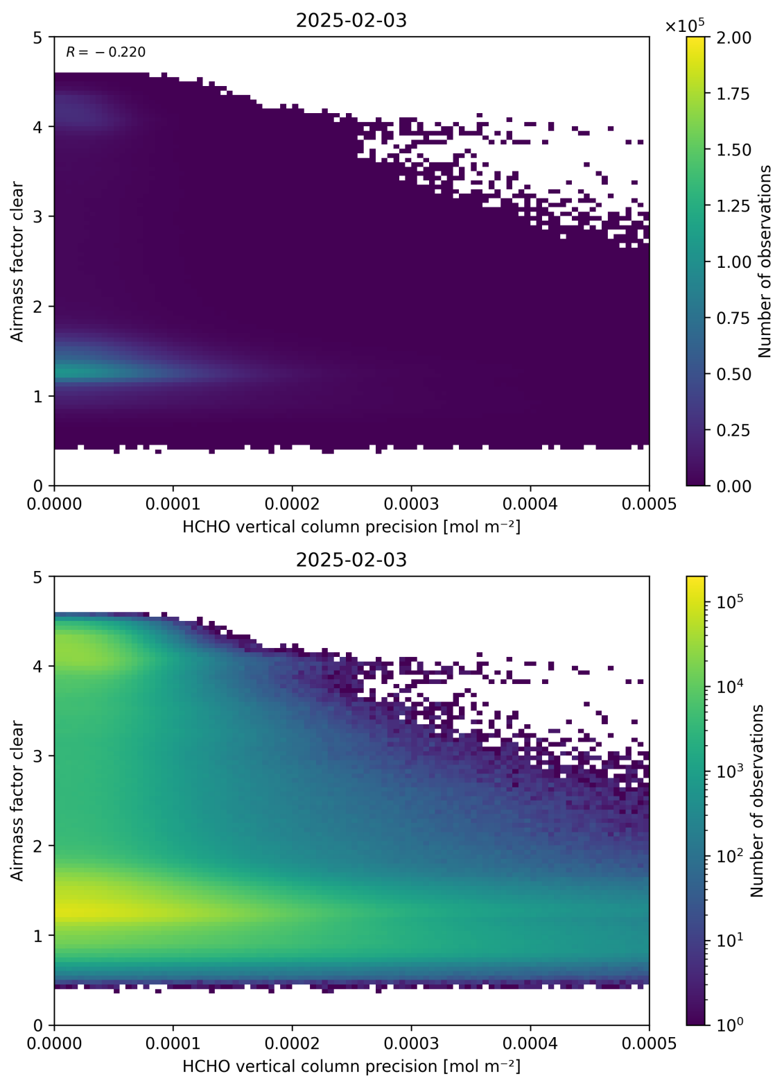
Figure 139: Scatter density plot of “HCHO vertical column precision” against “Airmass factor clear” for 2025-02-03 to 2025-02-04.
