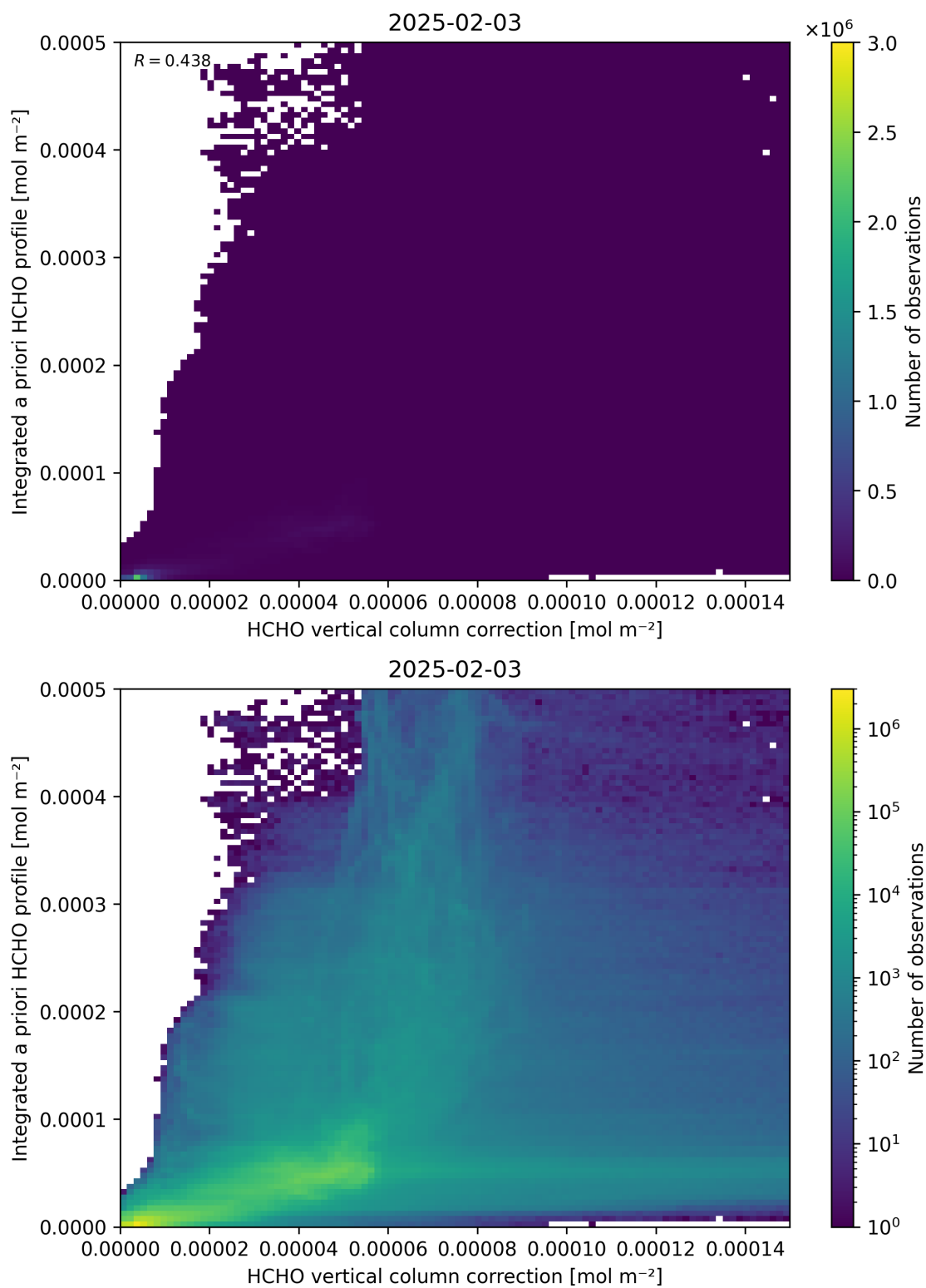
Figure 122: Scatter density plot of “HCHO vertical column correction” against “Integrated a priori HCHO profile” for 2025-02-03 to 2025-02-04.
