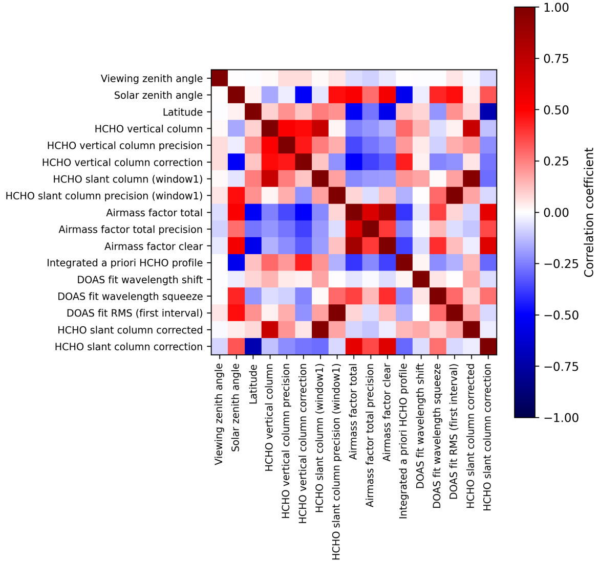
Figure 2: Map of correlation matrix for 2025-02-03 to 2025-02-04.
