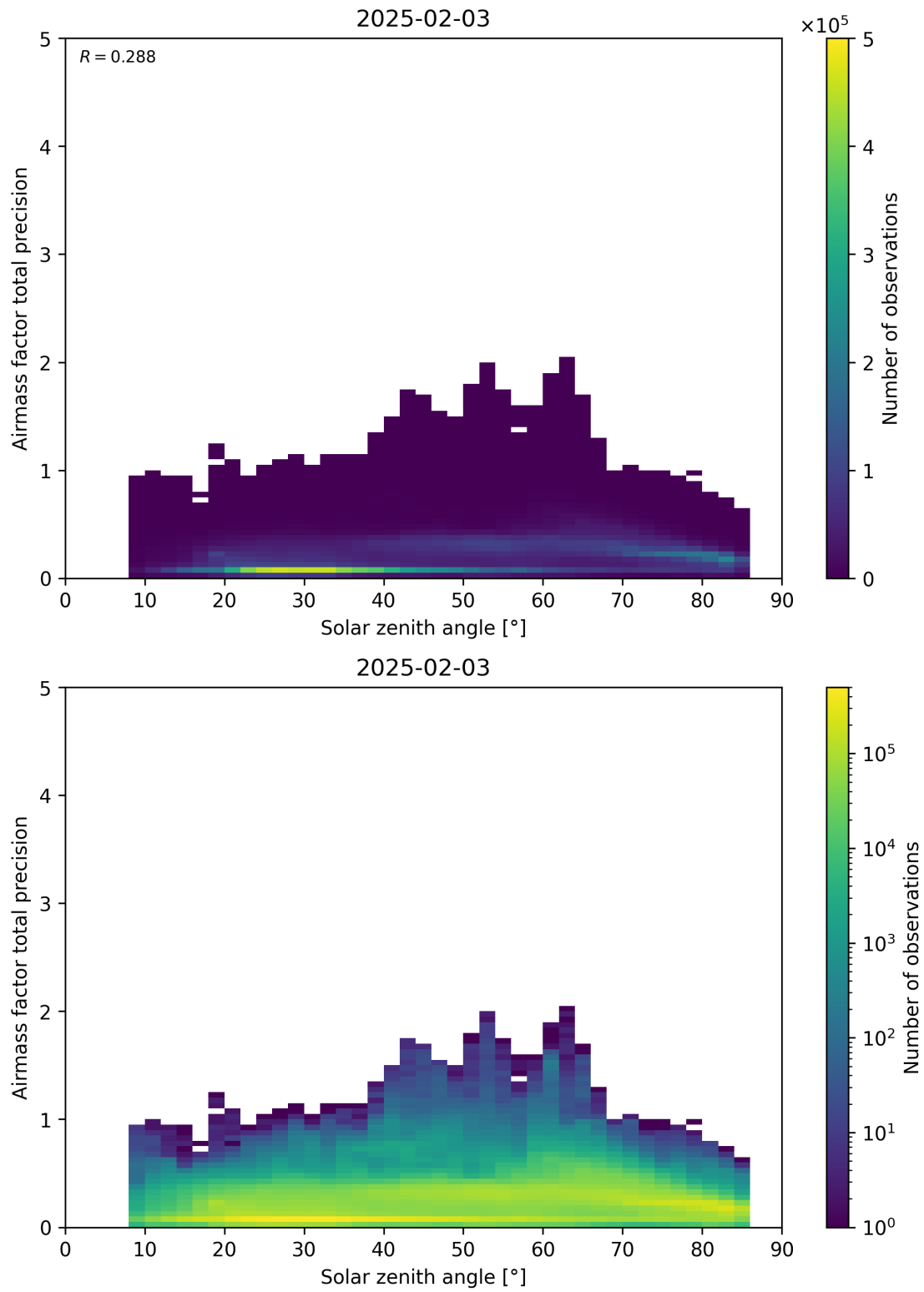
Figure 176: Scatter density plot of “Solar zenith angle” against “Airmass factor total precision” for 2025-02-03 to 2025-02-04.
