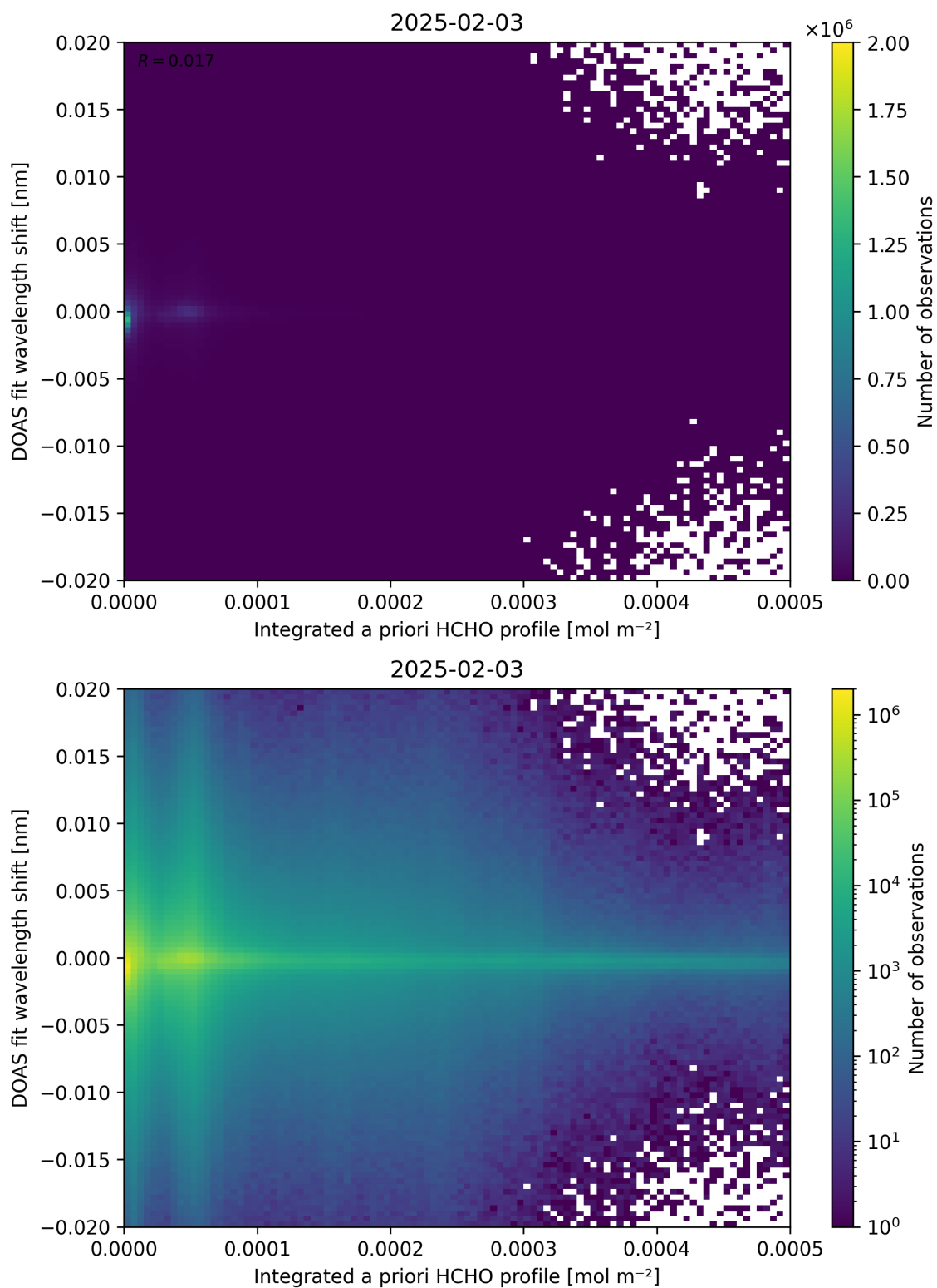
Figure 149: Scatter density plot of “Integrated a priori HCHO profile” against “DOAS fit wavelength shift” for 2025-02-03 to 2025-02-04.
