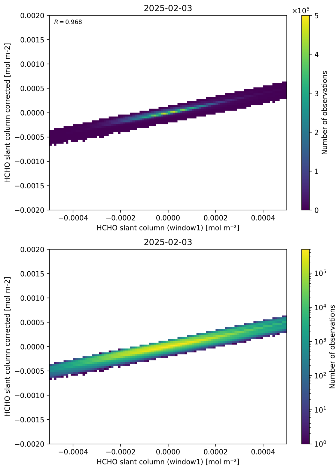
Figure 82: Scatter density plot of “HCHO slant column (window1)” against “HCHO slant column corrected” for 2025-02-03 to 2025-02-04.
