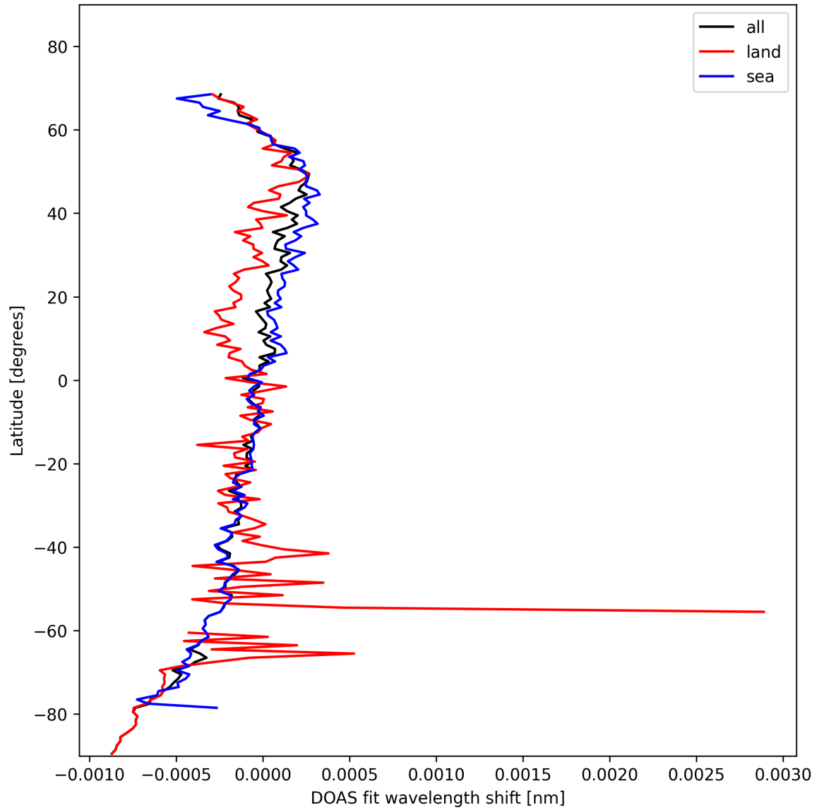
Figure 30: Zonal average of “DOAS fit wavelength shift” for 2025-02-03 to 2025-02-04.
