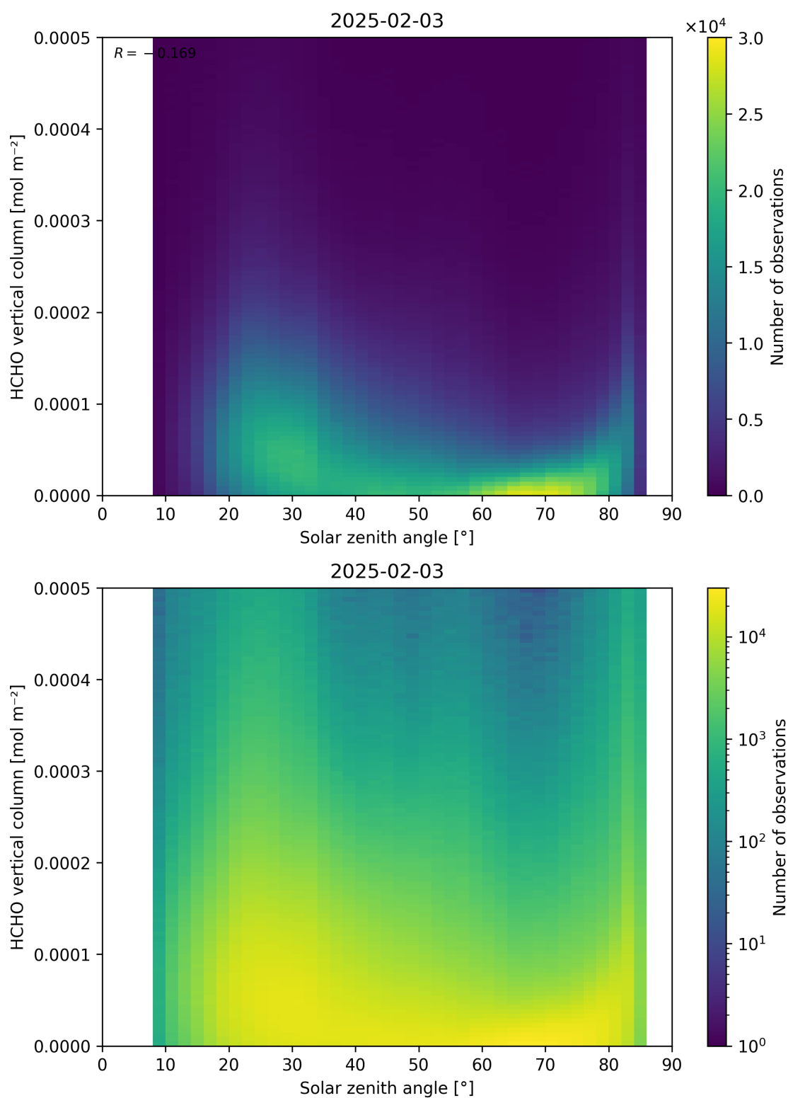
Figure 177: Scatter density plot of “Solar zenith angle” against “HCHO vertical column” for 2025-02-03 to 2025-02-04.
