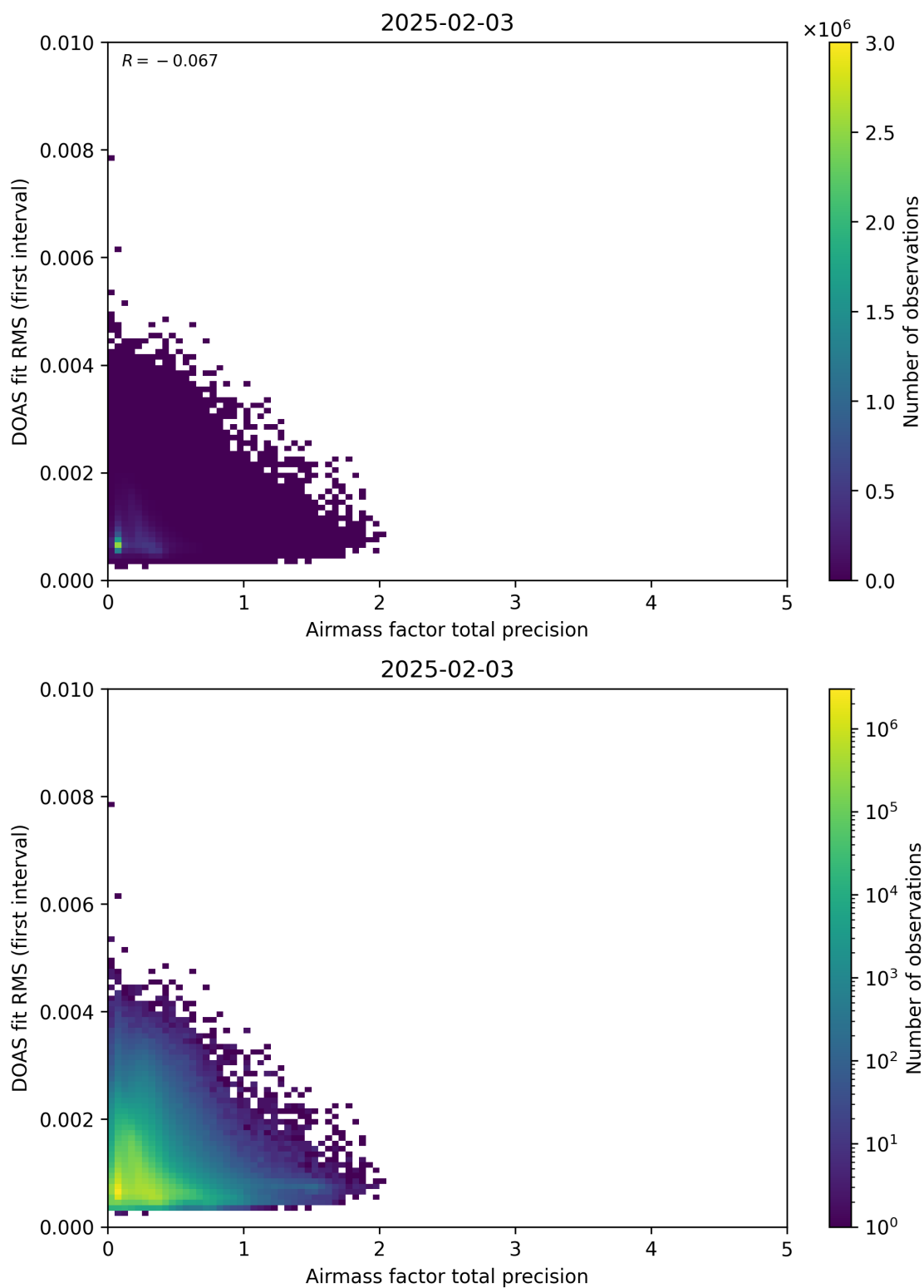
Figure 105: Scatter density plot of “Airmass factor total precision” against “DOAS fit RMS (first interval)” for 2025-02-03 to 2025-02-04.
