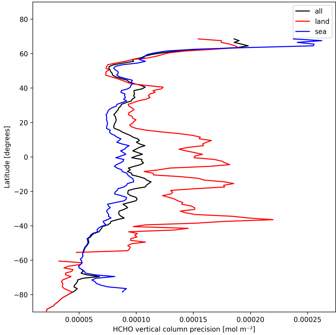
Figure 22: Zonal average of "HCHO vertical column precision" for 2025-02-03 to 2025-02-04.
