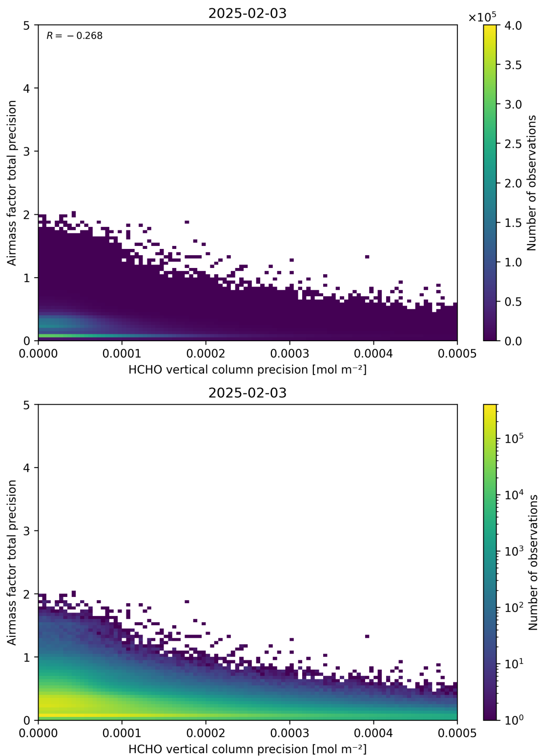
Figure 145: Scatter density plot of “HCHO vertical column precision” against “Airmass factor total precision” for 2025-02-03 to 2025-02-04.
