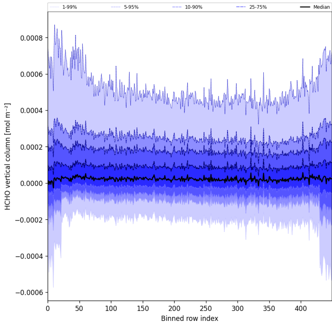
Figure 49: Along track statistics of “HCHO vertical column” for 2025-02-03 to 2025-02-04
