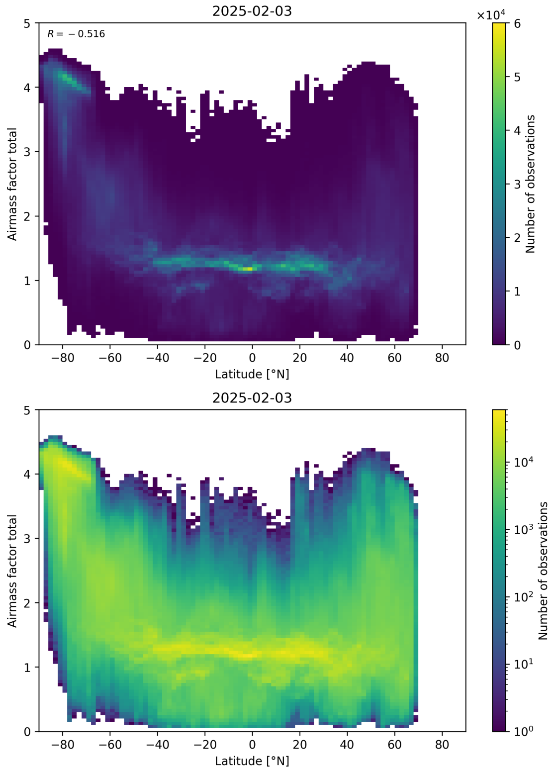
Figure 161: Scatter density plot of “Latitude” against “Airmass factor total” for 2025-02-03 to 2025-02-04.
