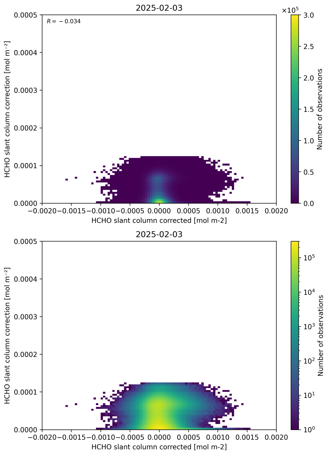
Figure 77: Scatter density plot of “HCHO slant column corrected” against “HCHO slant column correction” for 2025-02-03 to 2025-02-04.
