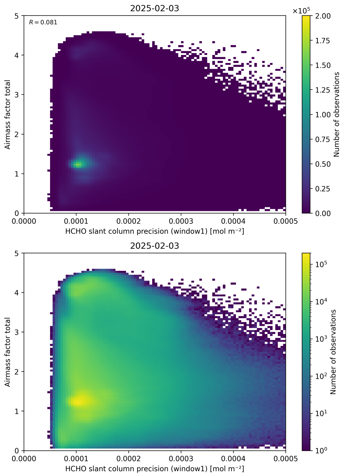
Figure 94: Scatter density plot of “HCHO slant column precision (window1)” against “Airmass factor total” for 2025-02-03 to 2025-02-04.
