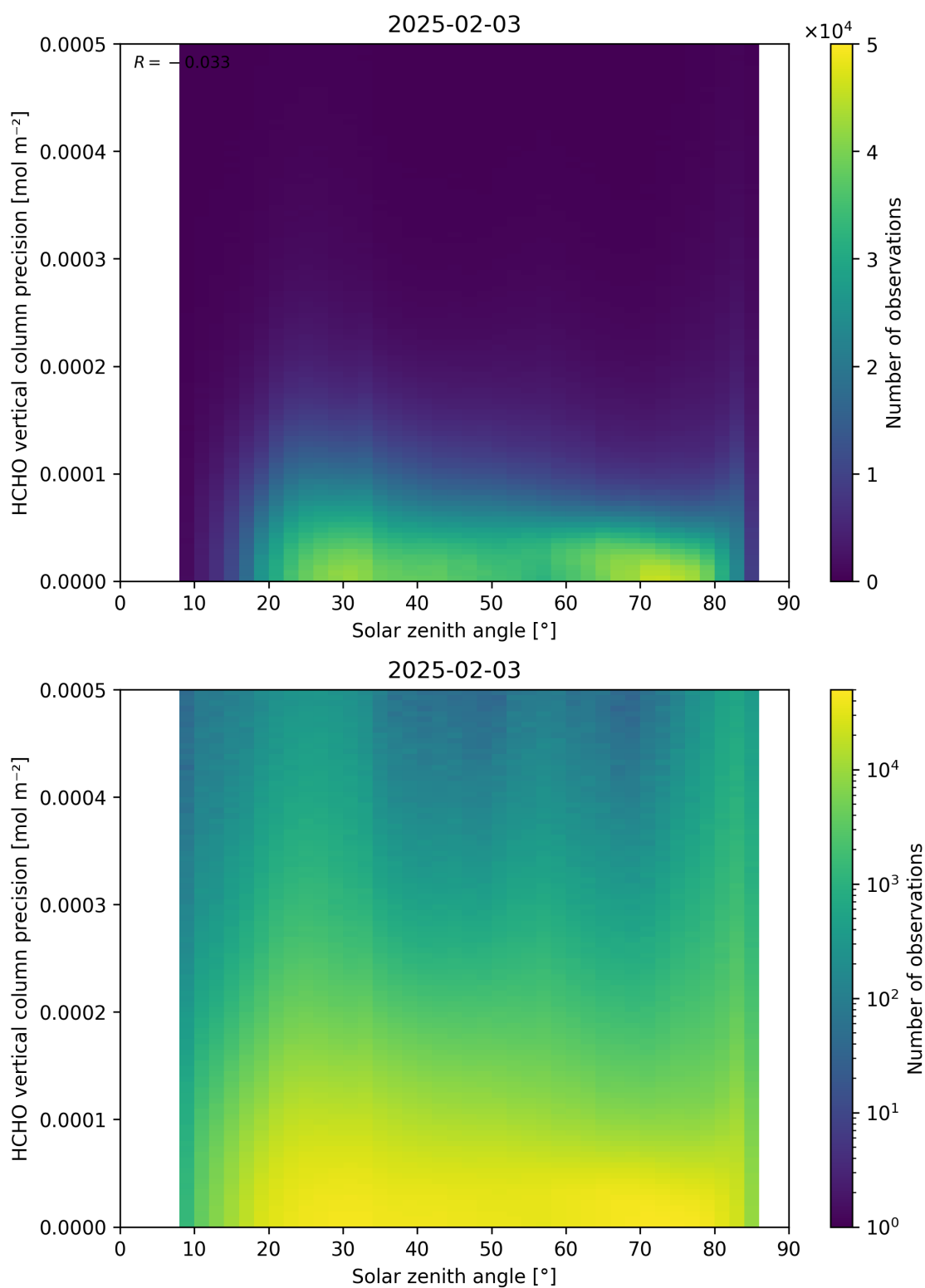
Figure 179: Scatter density plot of “Solar zenith angle” against “HCHO vertical column precision” for 2025-02-03 to 2025-02-04.
