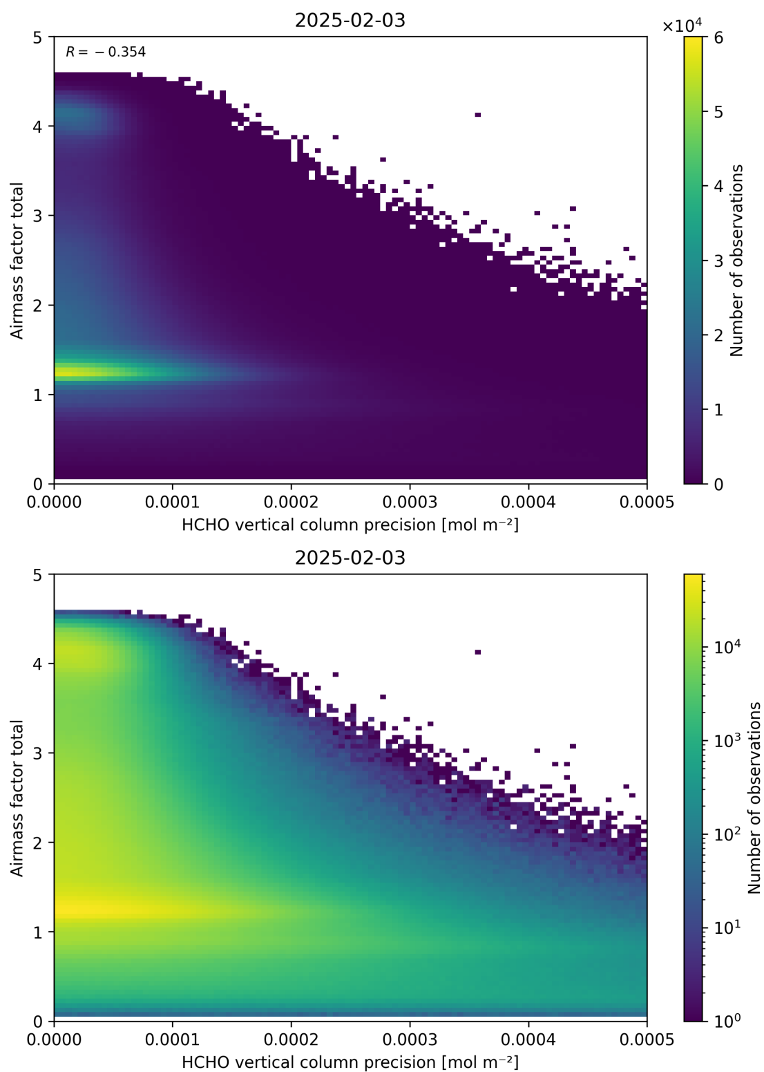
Figure 144: Scatter density plot of “HCHO vertical column precision” against “Airmass factor total” for 2025-02-03 to 2025-02-04.
