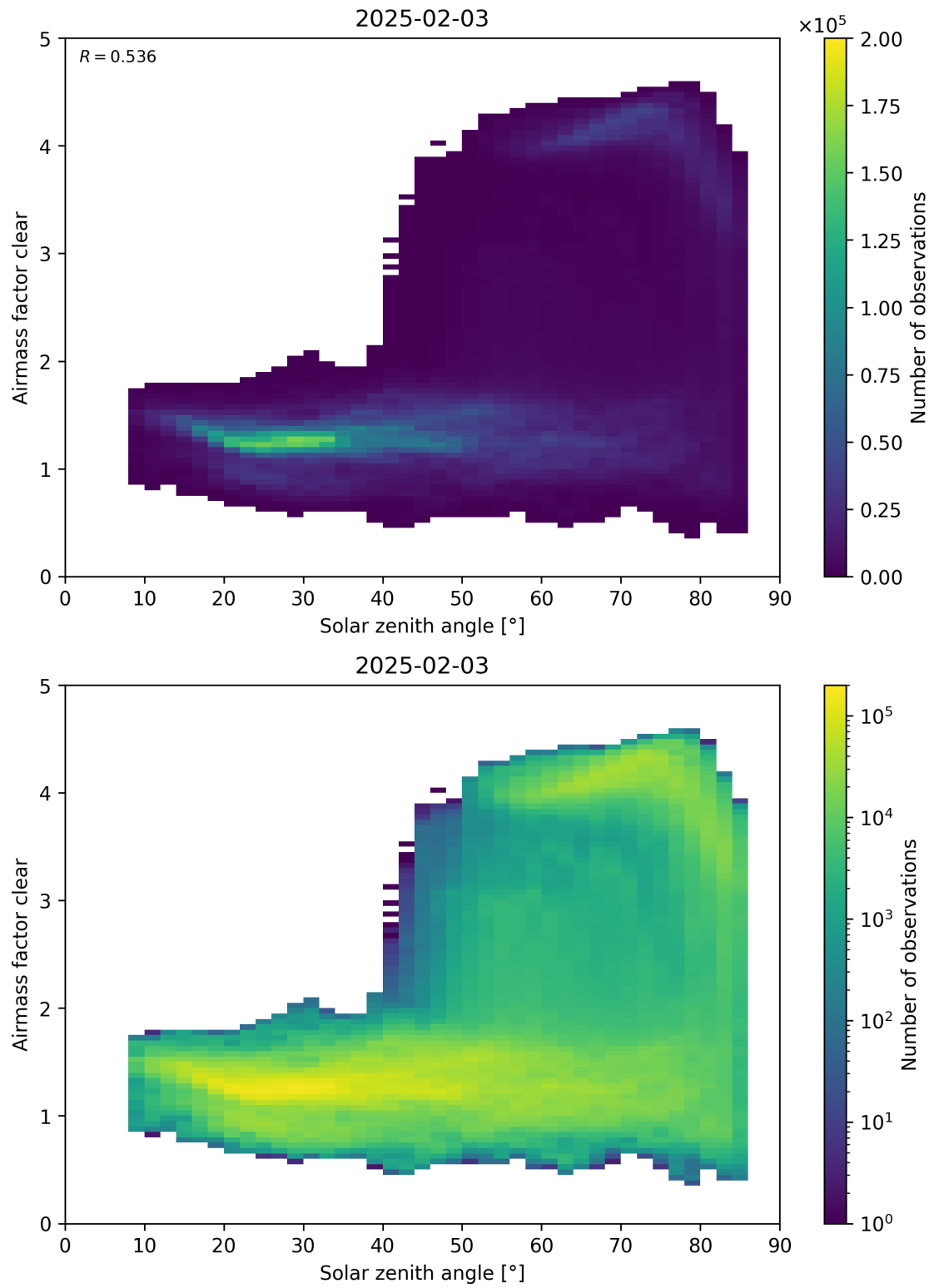
Figure 170: Scatter density plot of “Solar zenith angle” against “Airmass factor clear” for 2025-02-03 to 2025-02-04.
