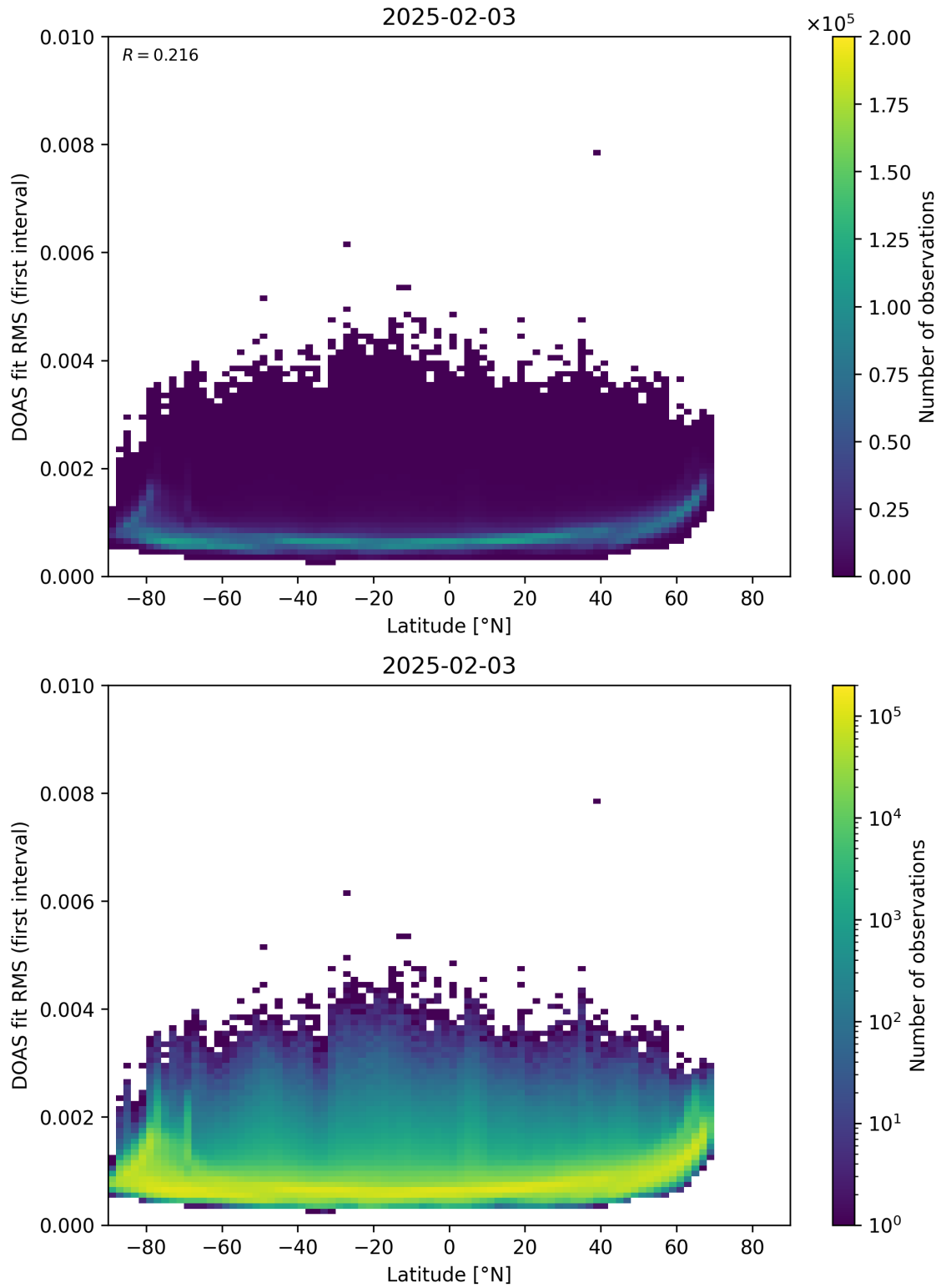
Figure 153: Scatter density plot of “Latitude” against “DOAS fit RMS (first interval)” for 2025-02-03 to 2025-02-04.
