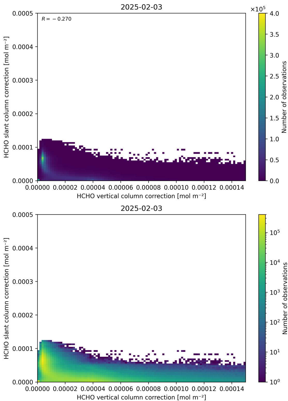
Figure 117: Scatter density plot of “HCHO vertical column correction” against “HCHO slant column correction” for 2025-02-03 to 2025-02-04.
