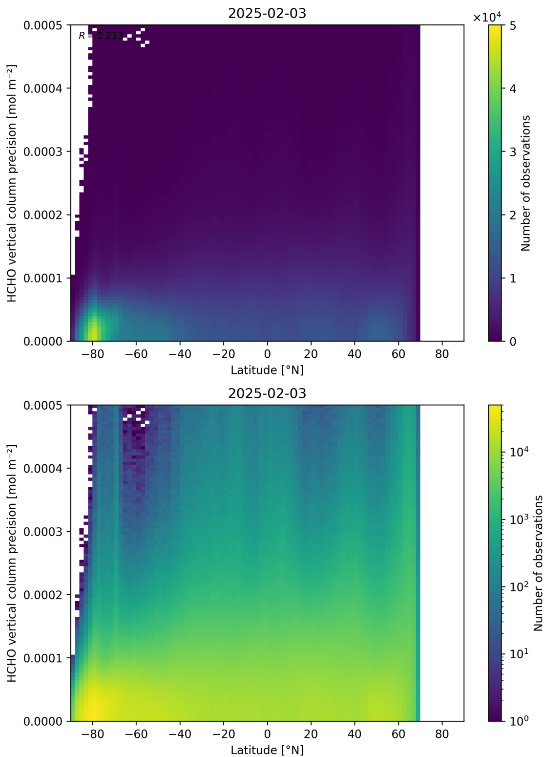
Figure 165: Scatter density plot of “Latitude” against “HCHO vertical column precision” for 2025-02-03 to 2025-02-04.
