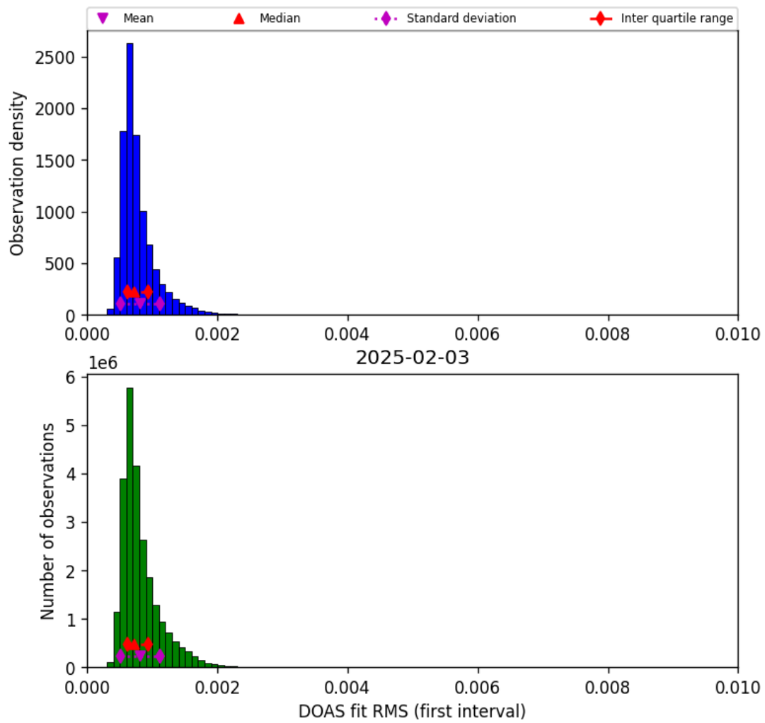
Figure 46: Histogram of “DOAS fit RMS (first interval)” for 2025-02-03 to 2025-02-04
