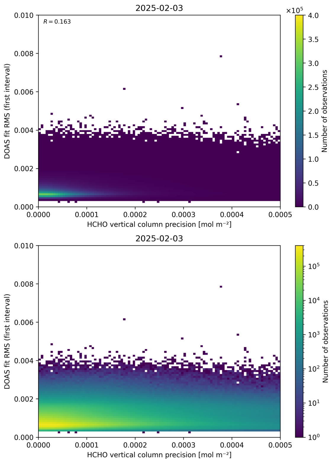
Figure 136: Scatter density plot of “HCHO vertical column precision” against “DOAS fit RMS (first interval)” for 2025-02-03 to 2025-02-04.
