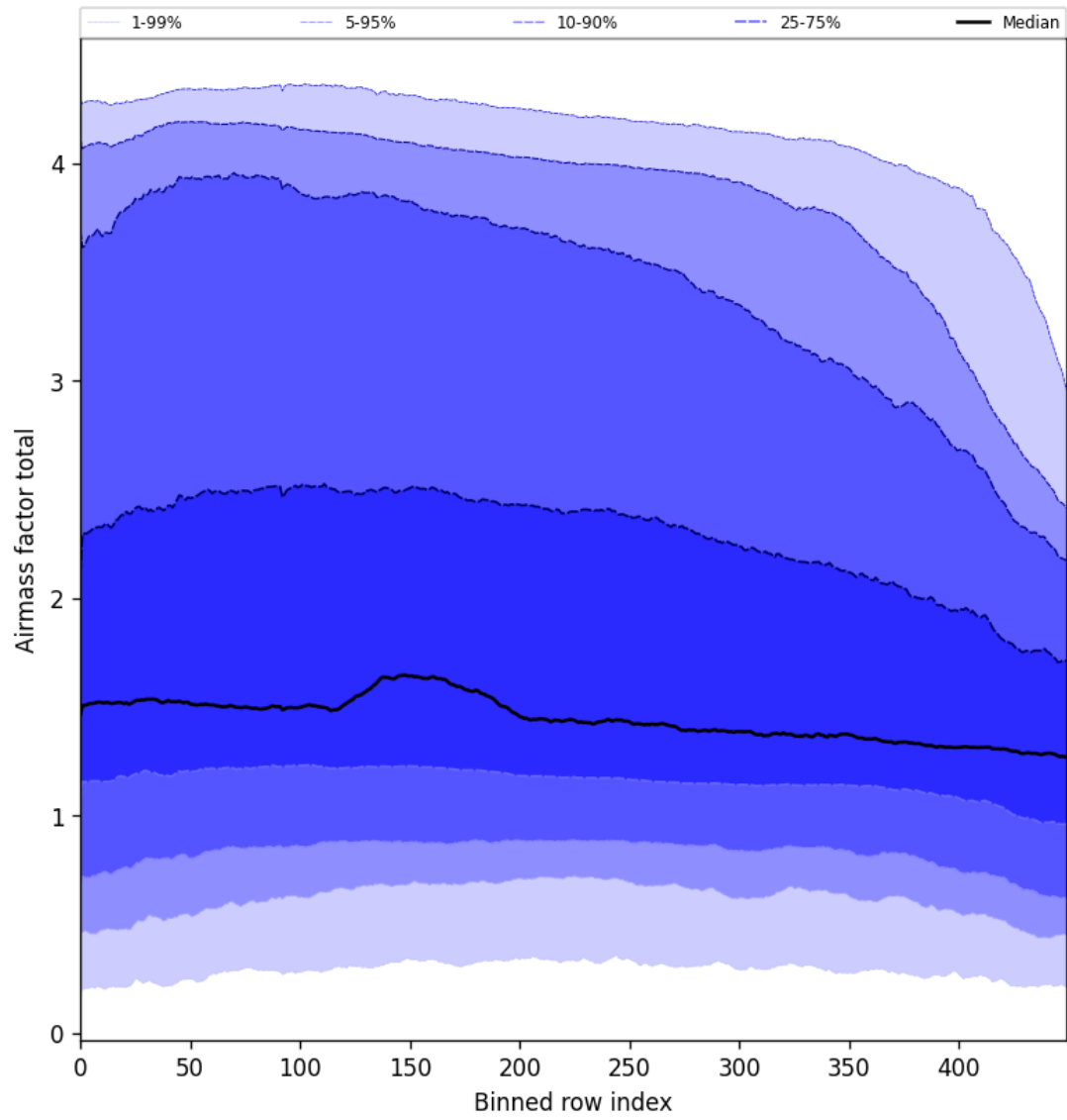
Figure 54: Along track statistics of “Airmass factor total” for 2025-02-03 to 2025-02-04
