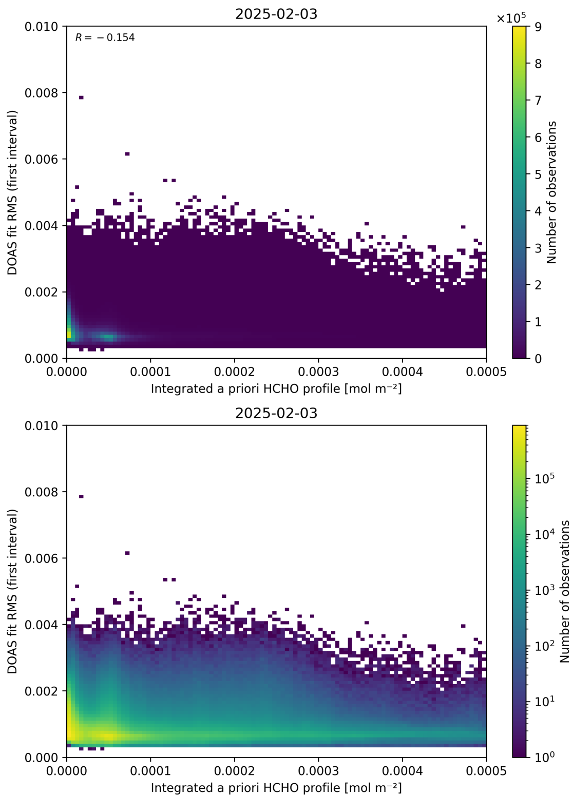
Figure 148: Scatter density plot of “Integrated a priori HCHO profile” against “DOAS fit RMS (first interval)” for 2025-02-03 to 2025-02-04.
