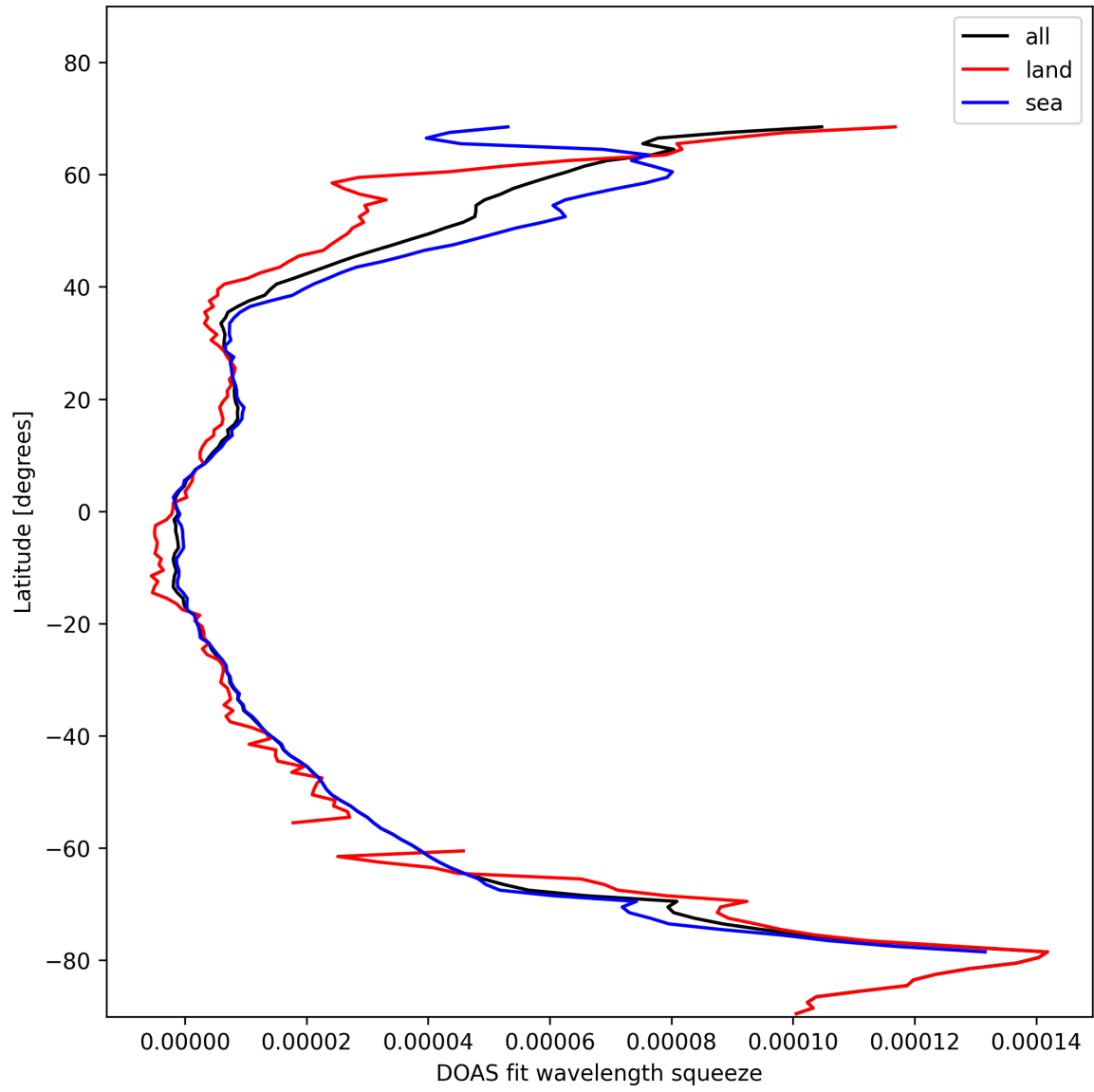
Figure 31: Zonal average of “DOAS fit wavelength squeeze” for 2025-02-03 to 2025-02-04.
