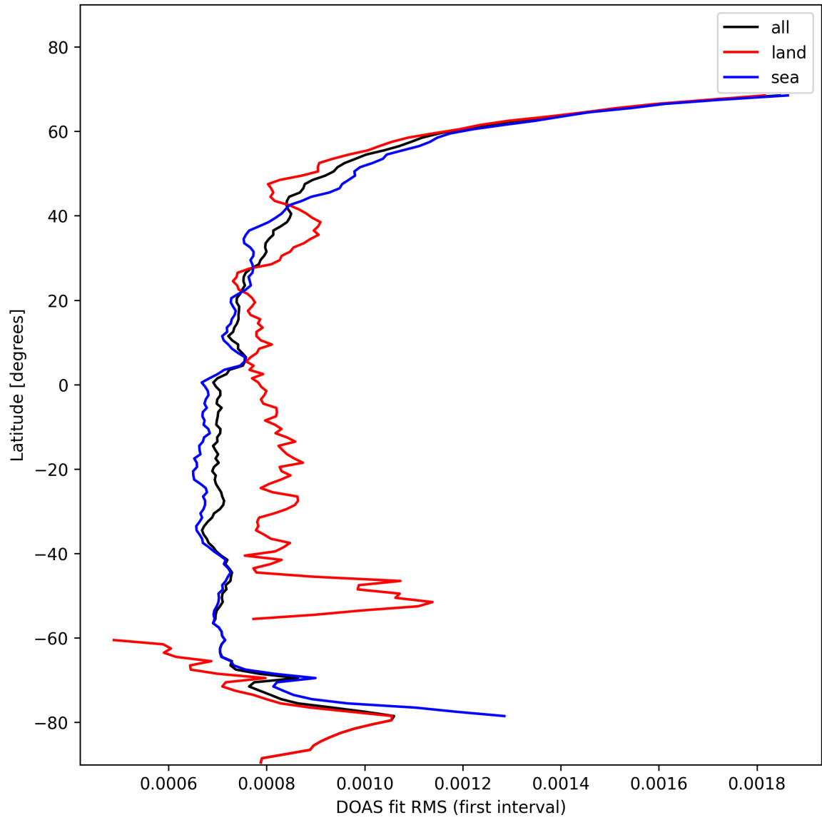
Figure 32: Zonal average of "DOAS fit RMS (first interval)" for 2025-02-03 to 2025-02-04.
