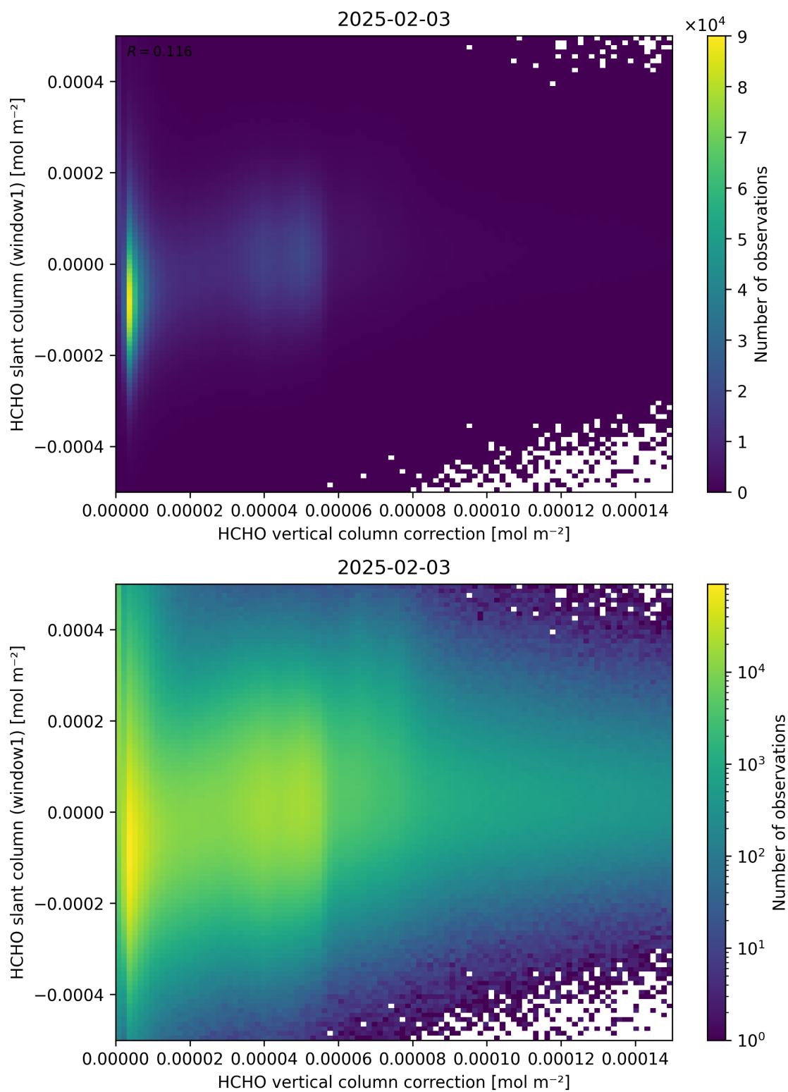
Figure 118: Scatter density plot of “HCHO vertical column correction” against “HCHO slant column (window1)” for 2025-02-03 to 2025-02-04.
