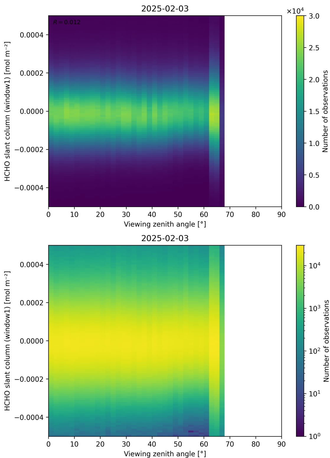
Figure 188: Scatter density plot of “Viewing zenith angle” against “HCHO slant column (window1)” for 2025-02-03 to 2025-02-04.
