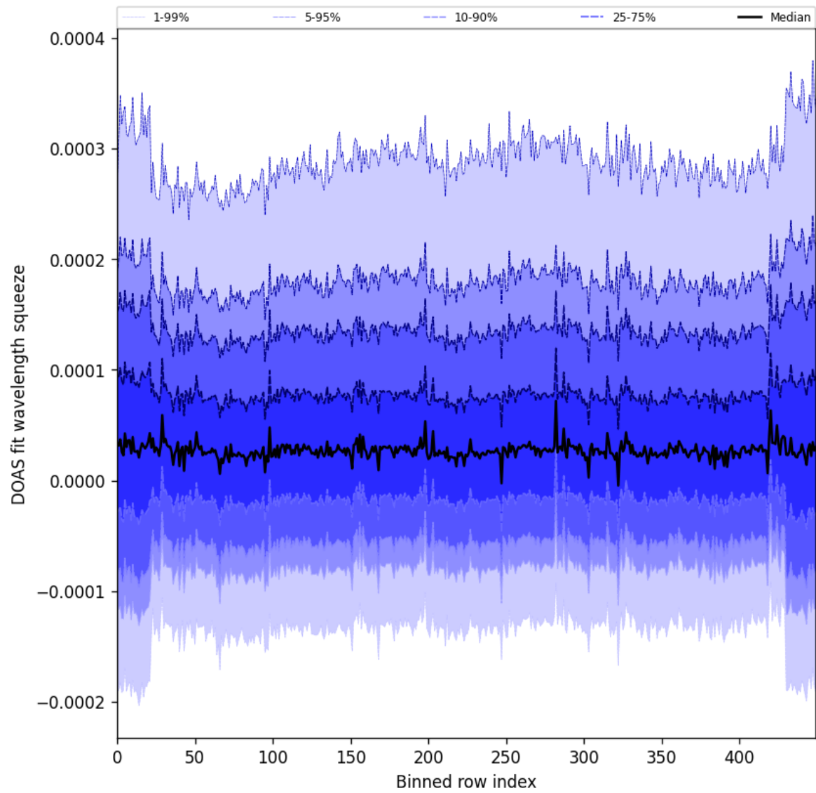
Figure 59: Along track statistics of “DOAS fit wavelength squeeze” for 2025-02-03 to 2025-02-04
