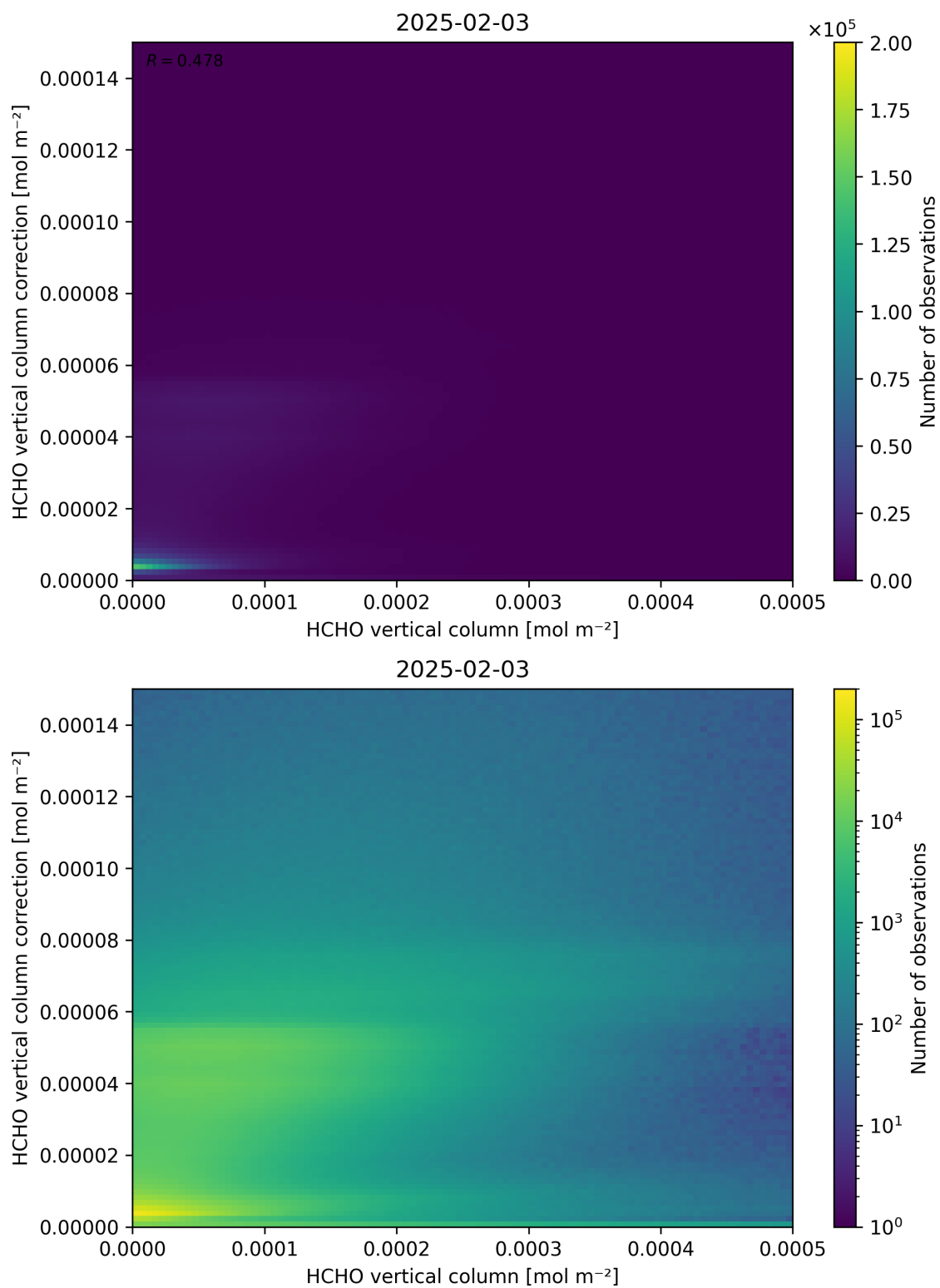
Figure 133: Scatter density plot of “HCHO vertical column” against “HCHO vertical column correction” for 2025-02-03 to 2025-02-04.
