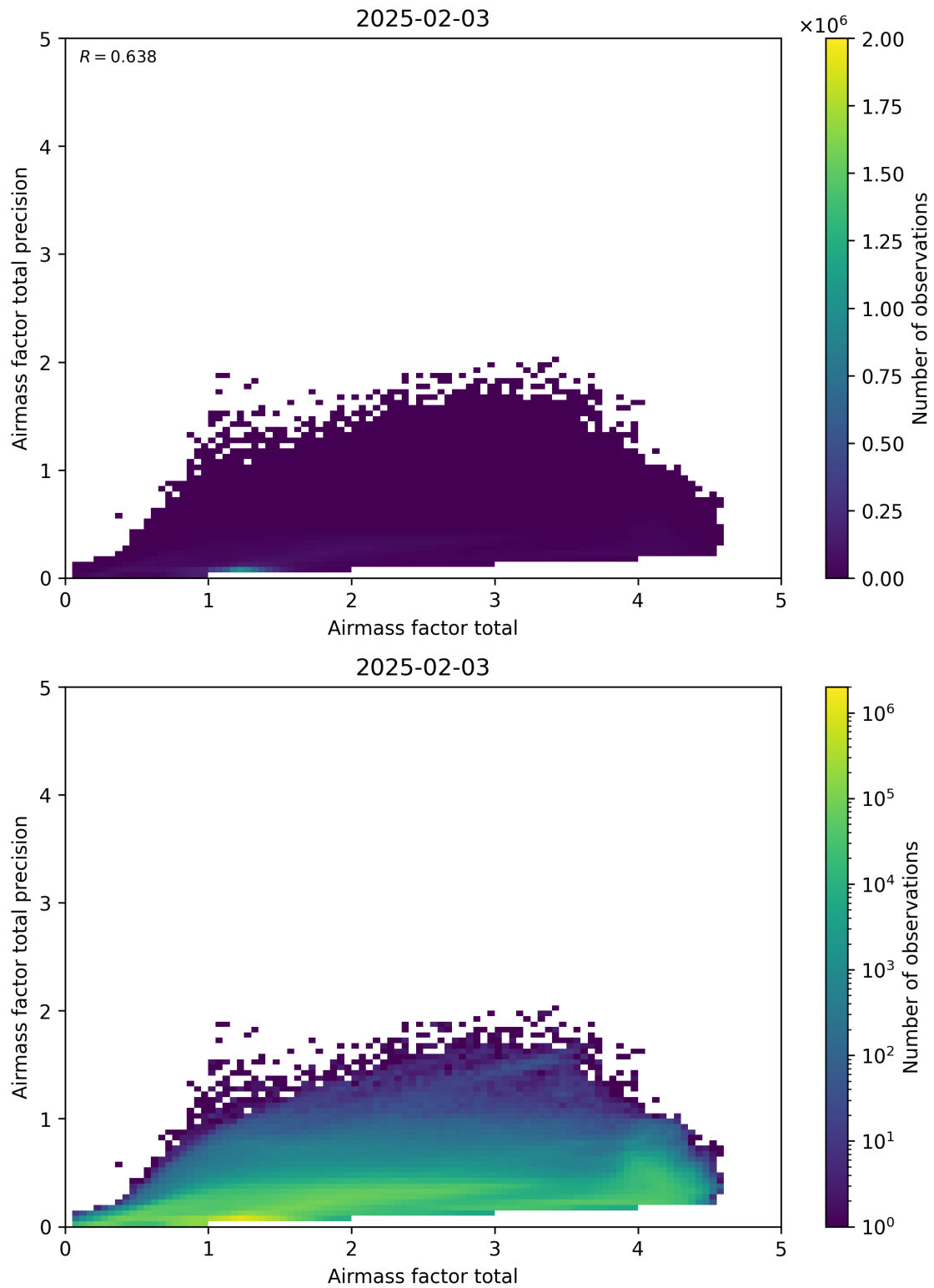
Figure 103: Scatter density plot of “Airmass factor total” against “Airmass factor total precision” for 2025-02-03 to 2025-02-04.
