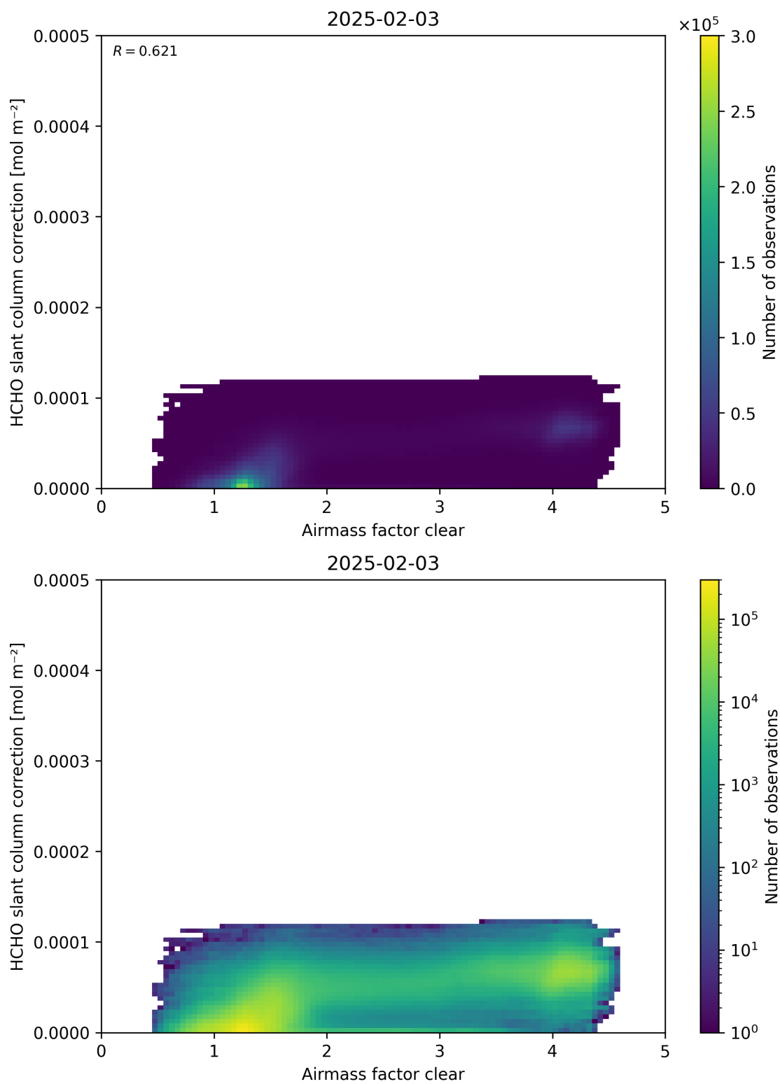
Figure 75: Scatter density plot of “Airmass factor clear” against “HCHO slant column correction” for 2025-02-03 to 2025-02-04.
