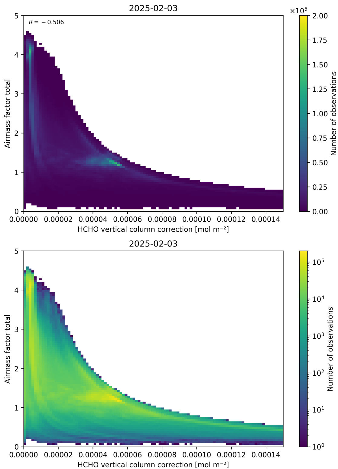
Figure 120: Scatter density plot of “HCHO vertical column correction” against “Airmass factor total” for 2025-02-03 to 2025-02-04.
