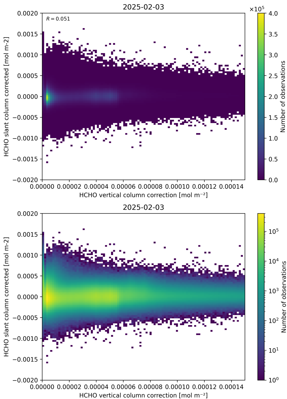
Figure 116: Scatter density plot of “HCHO vertical column correction” against “HCHO slant column corrected” for 2025-02-03 to 2025-02-04.
