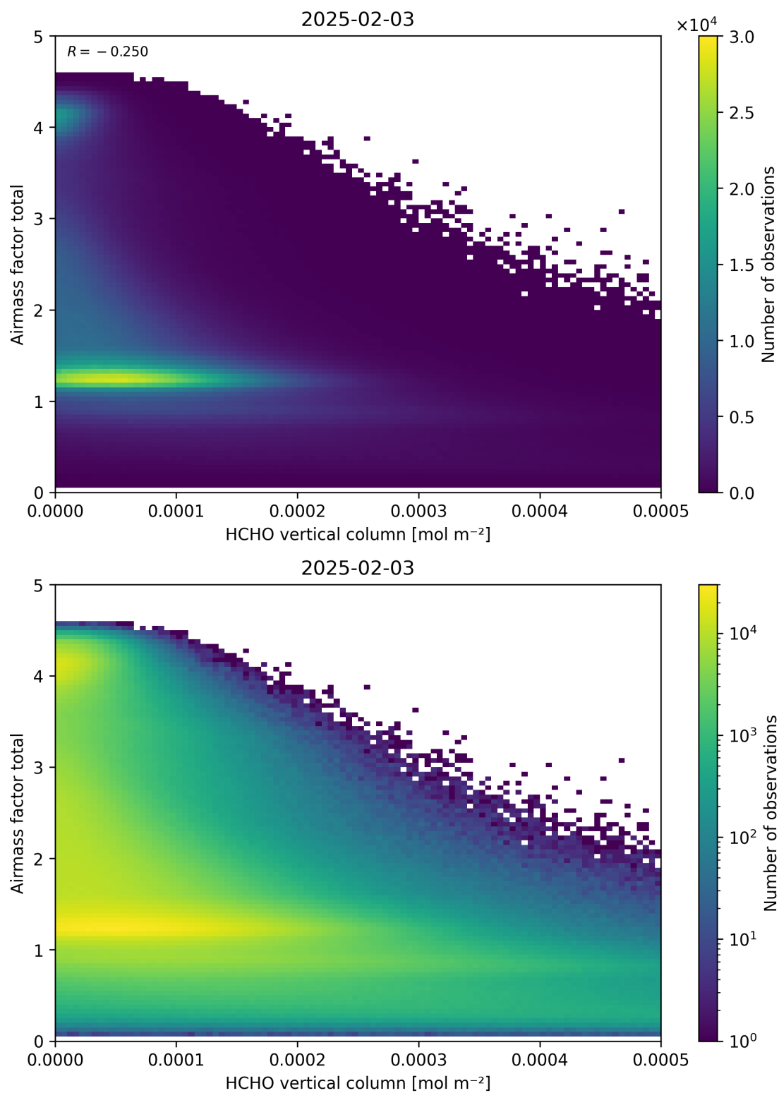
Figure 131: Scatter density plot of “HCHO vertical column” against “Airmass factor total” for 2025-02-03 to 2025-02-04.
