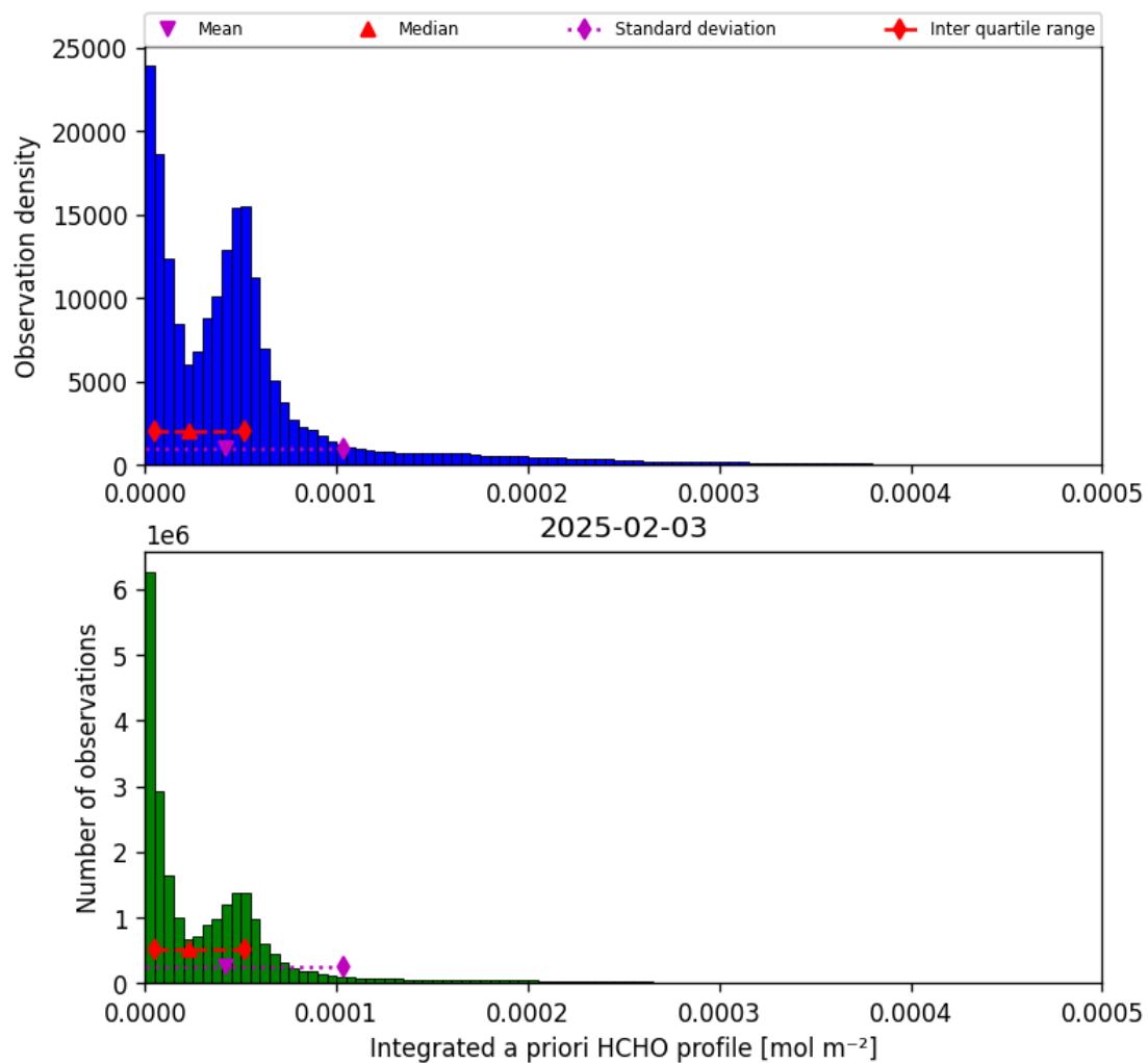
Figure 43: Histogram of “Integrated a priori HCHO profile” for 2025-02-03 to 2025-02-04
