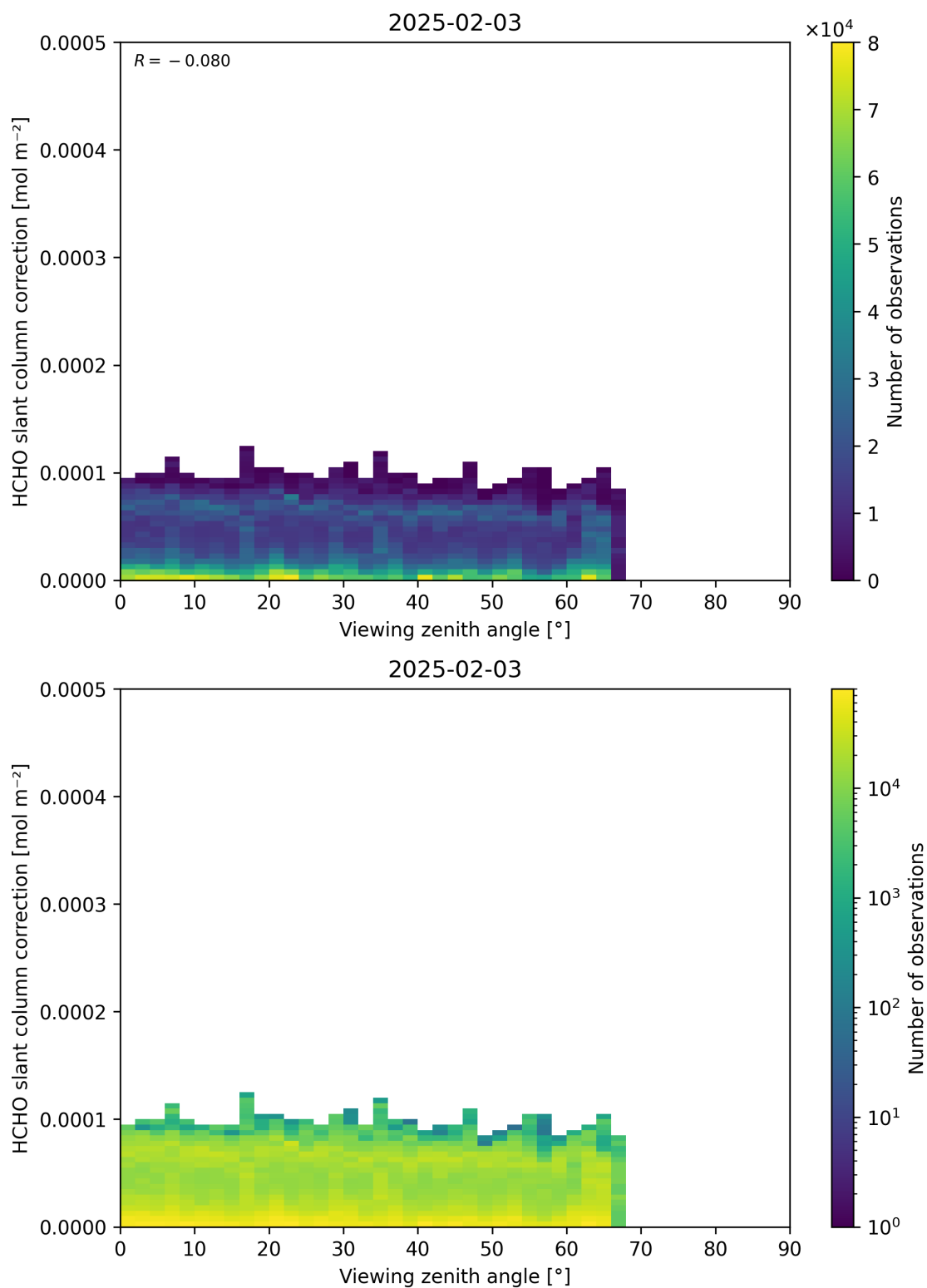
Figure 187: Scatter density plot of “Viewing zenith angle” against “HCHO slant column correction” for 2025-02-03 to 2025-02-04.
