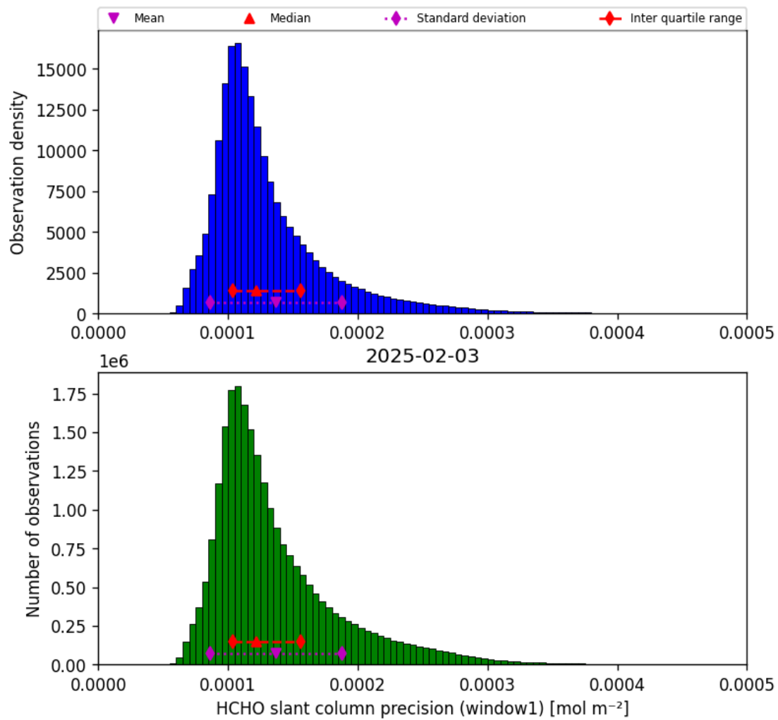
Figure 39: Histogram of “HCHO slant column precision (window1)” for 2025-02-03 to 2025-02-04
