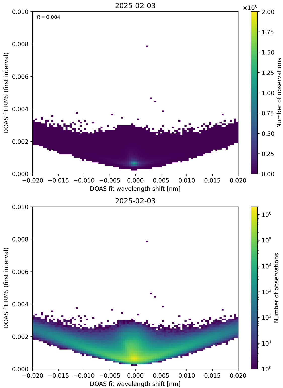
Figure 64: Scatter density plot of “DOAS fit wavelength shift” against “DOAS fit RMS (first interval)” for 2025-02-03 to 2025-02-04.
