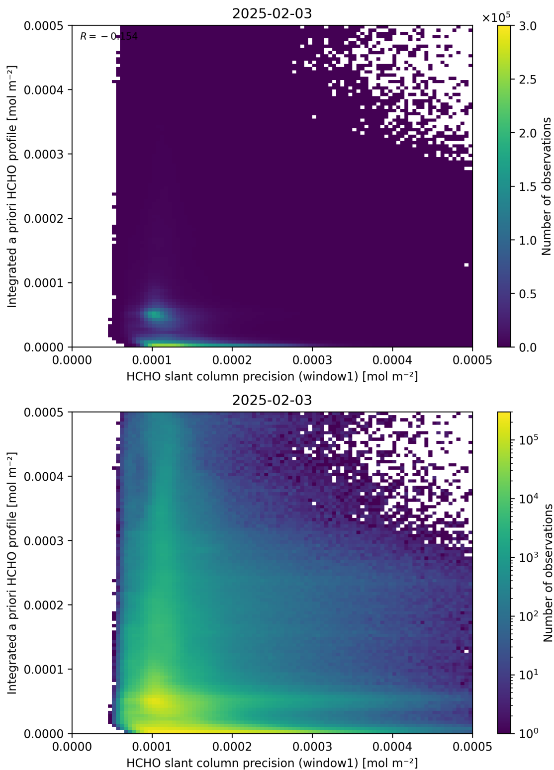
Figure 96: Scatter density plot of “HCHO slant column precision (window1)” against “Integrated a priori HCHO profile” for 2025-02-03 to 2025-02-04.
