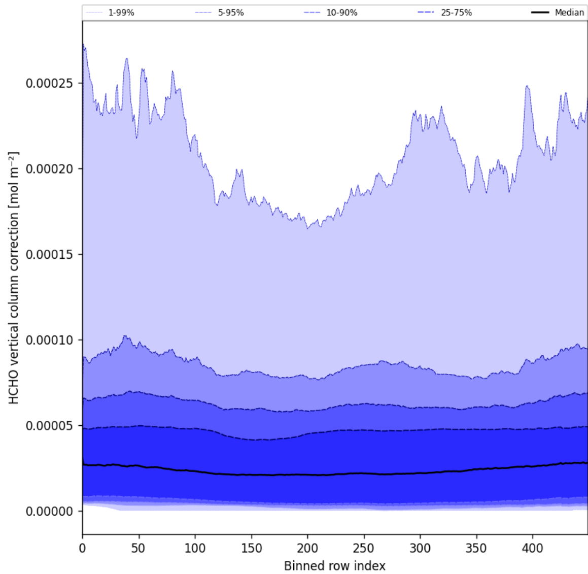
Figure 51: Along track statistics of “HCHO vertical column correction” for 2025-02-03 to 2025-02-05
