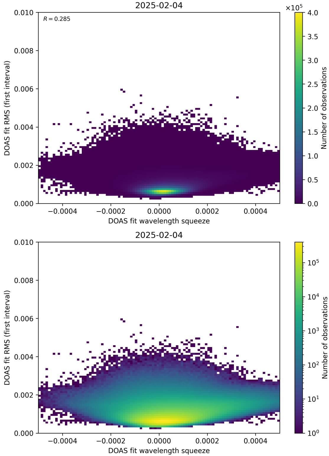
Figure 68: Scatter density plot of “DOAS fit wavelength squeeze” against “DOAS fit RMS (first interval)” for 2025-02-03 to 2025-02-05.
