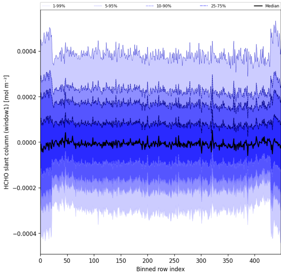
Figure 52: Along track statistics of "HCHO slant column (window1)" for 2025-02-03 to 2025-02-05
