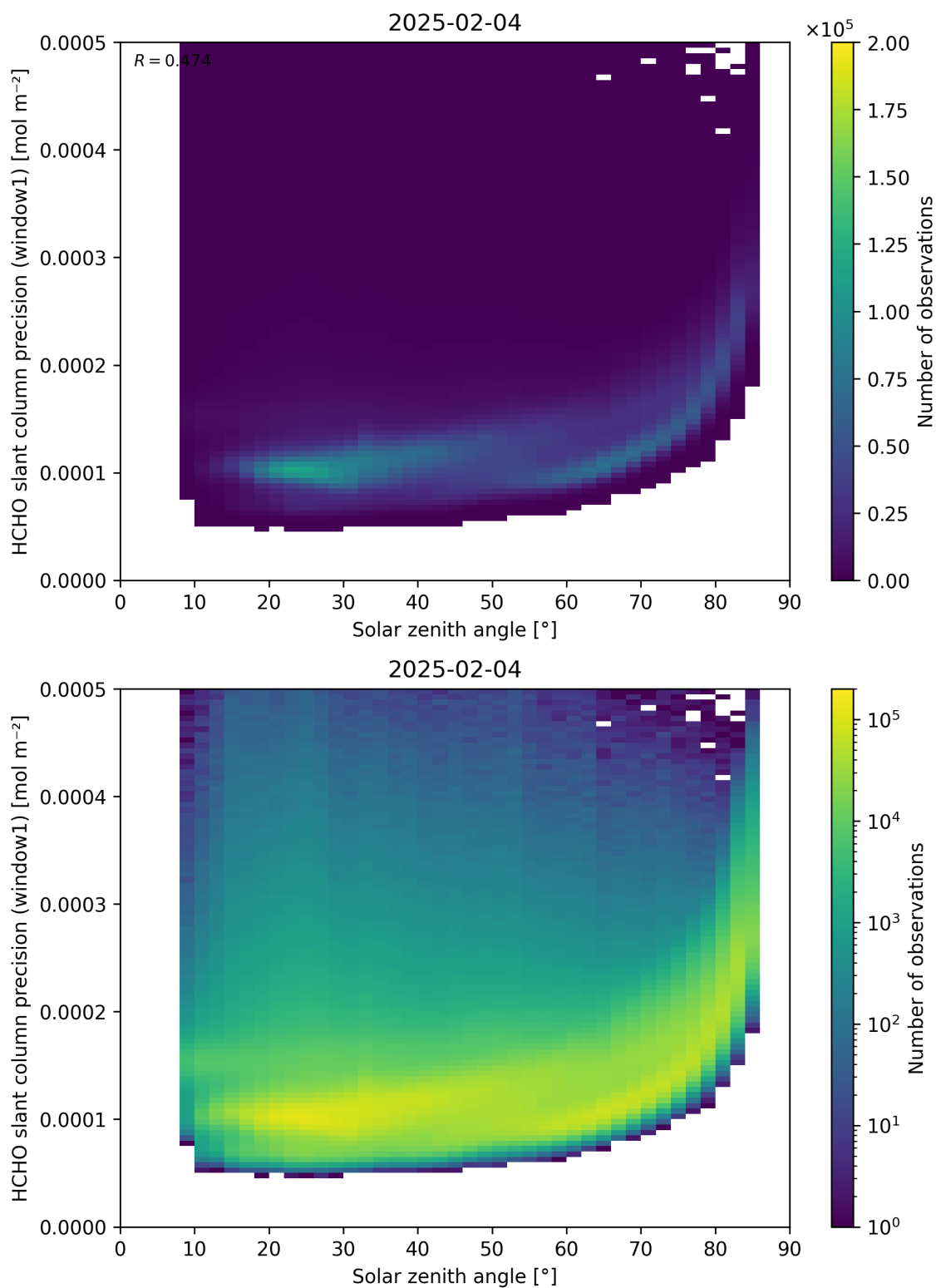
Figure 174: Scatter density plot of “Solar zenith angle” against “HCHO slant column precision (window1)” for 2025-02-03 to 2025-02-05.
