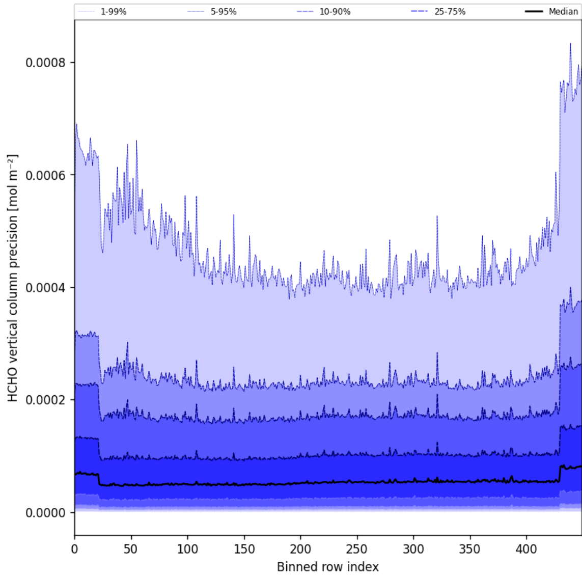
Figure 50: Along track statistics of “HCHO vertical column precision” for 2025-02-03 to 2025-02-05
