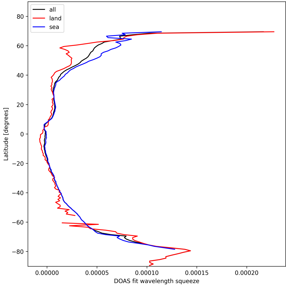
Figure 31: Zonal average of “DOAS fit wavelength squeeze” for 2025-02-03 to 2025-02-05.
