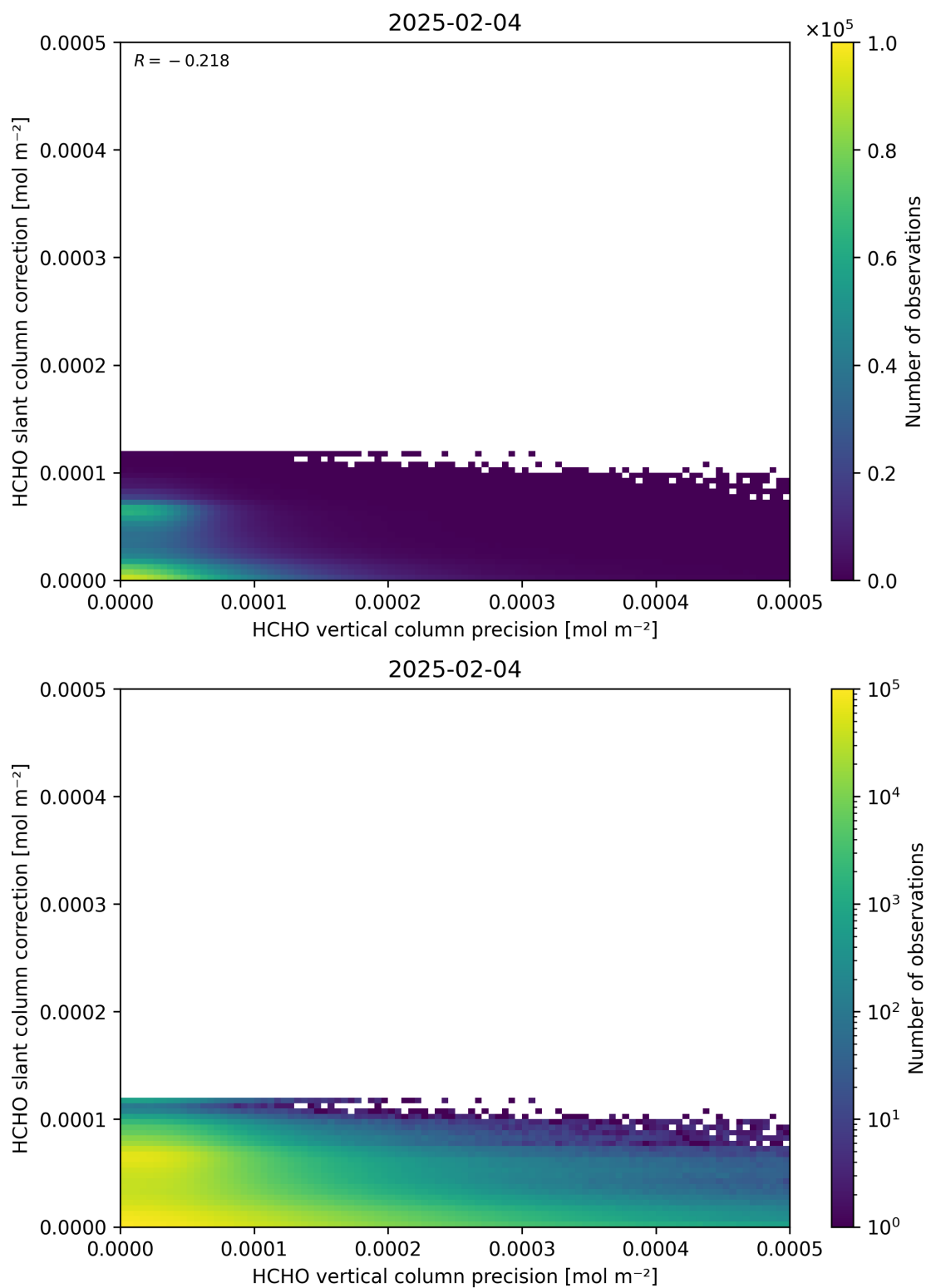
Figure 141: Scatter density plot of “HCHO vertical column precision” against “HCHO slant column correction” for 2025-02-03 to 2025-02-05.
