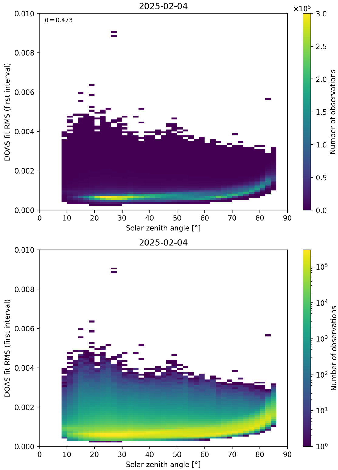
Figure 167: Scatter density plot of “Solar zenith angle” against “DOAS fit RMS (first interval)” for 2025-02-03 to 2025-02-05.
