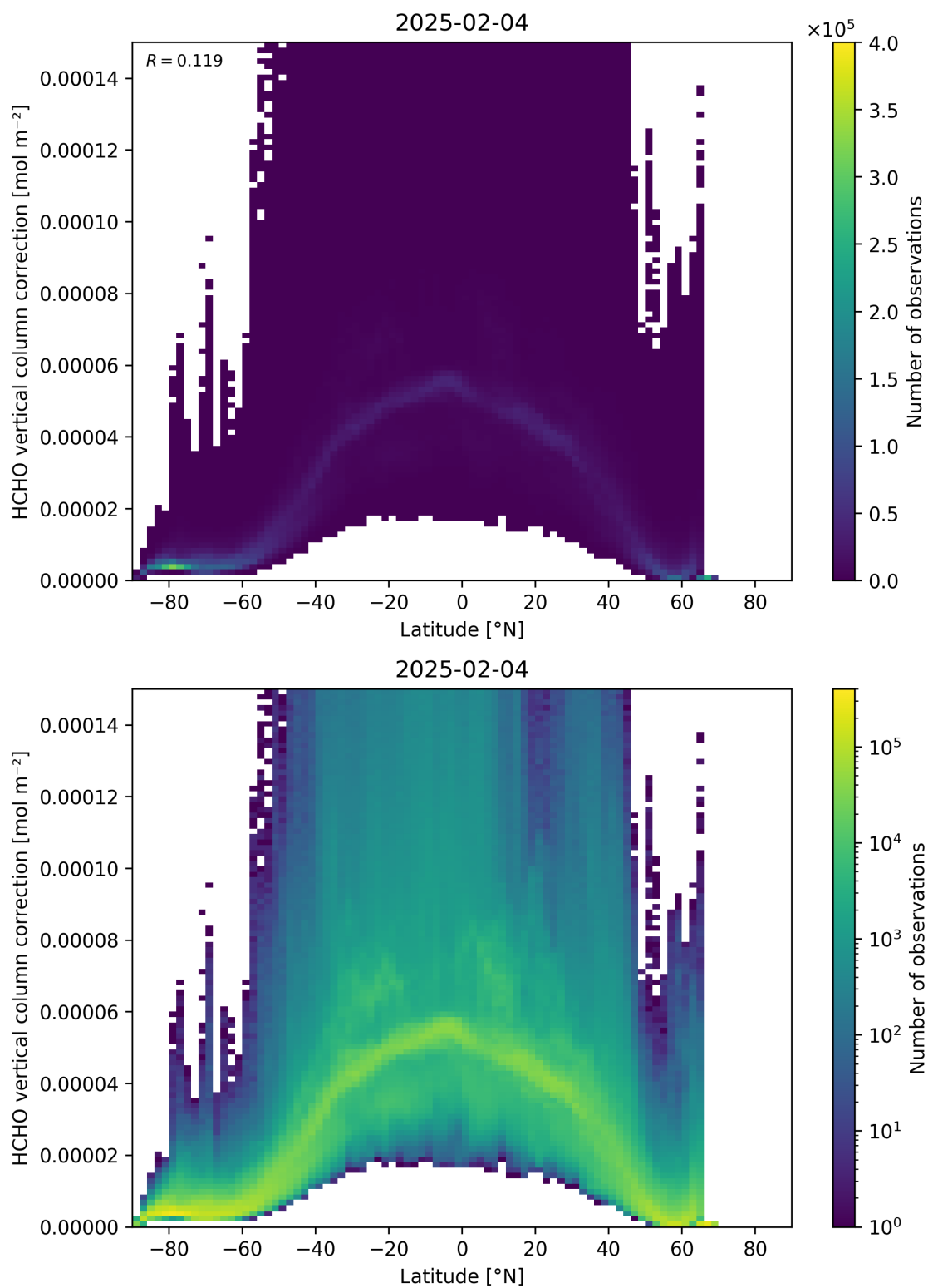
Figure 164: Scatter density plot of “Latitude” against “HCHO vertical column correction” for 2025-02-03 to 2025-02-05.
