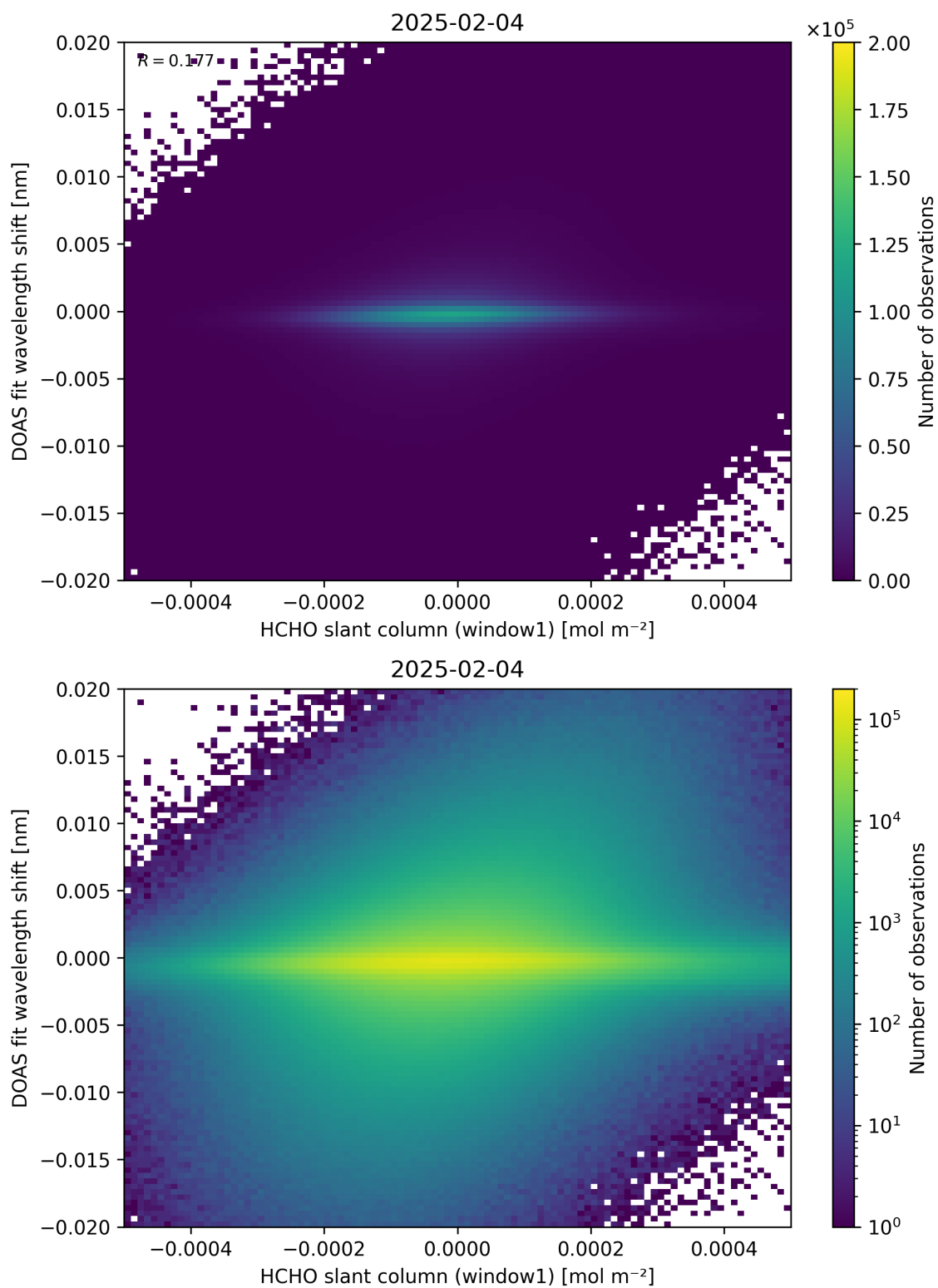
Figure 79: Scatter density plot of “HCHO slant column (window1)” against “DOAS fit wavelength shift” for 2025-02-03 to 2025-02-05.
