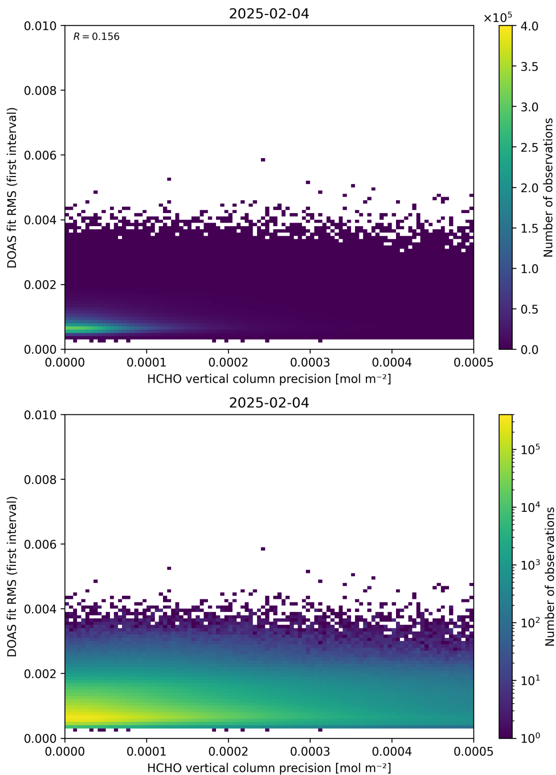
Figure 136: Scatter density plot of “HCHO vertical column precision” against “DOAS fit RMS (first interval)” for 2025-02-03 to 2025-02-05.
