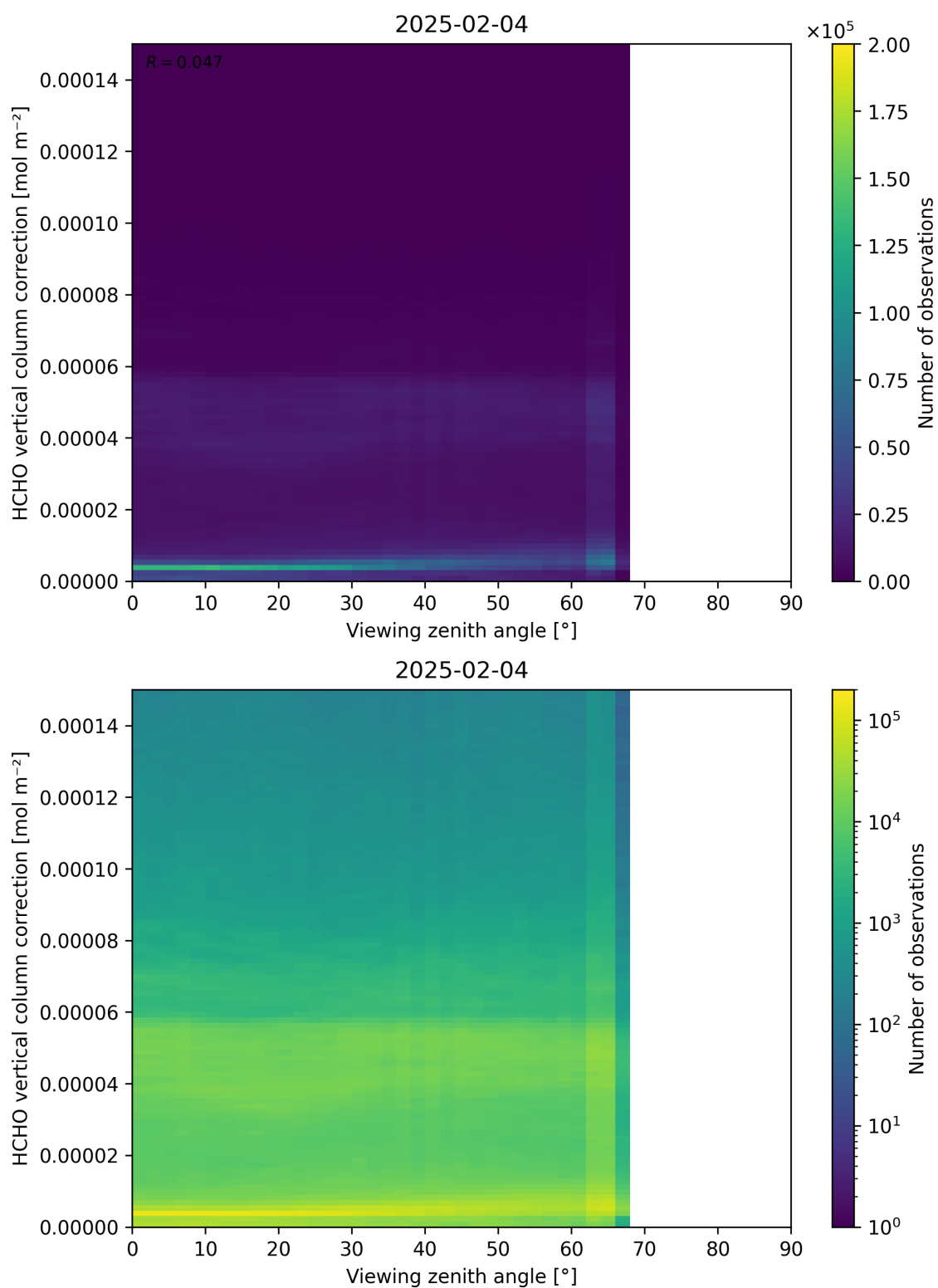
Figure 193: Scatter density plot of “Viewing zenith angle” against “HCHO vertical column correction” for 2025-02-03 to 2025-02-05.
