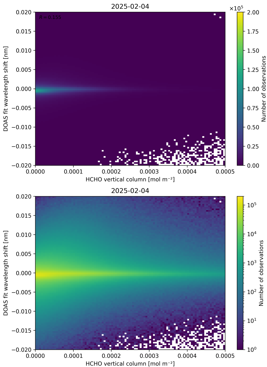
Figure 124: Scatter density plot of “HCHO vertical column” against “DOAS fit wavelength shift” for 2025-02-03 to 2025-02-05.
