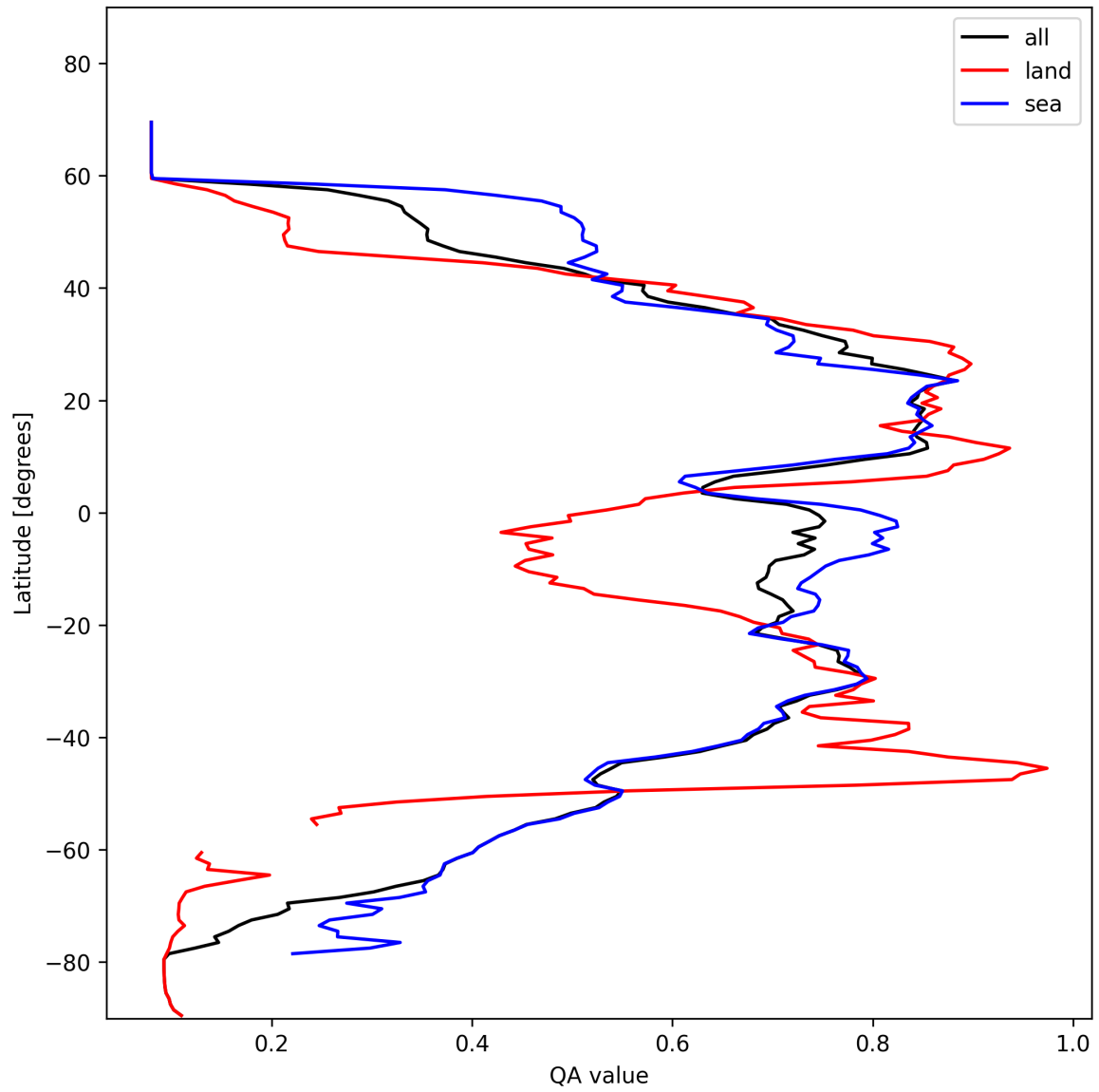
Figure 20: Zonal average of “QA value” for 2025-02-03 to 2025-02-05.
