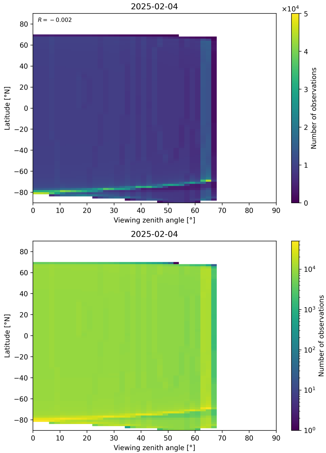
Figure 196: Scatter density plot of “Viewing zenith angle” against “Latitude” for 2025-02-03 to 2025-02-05.
