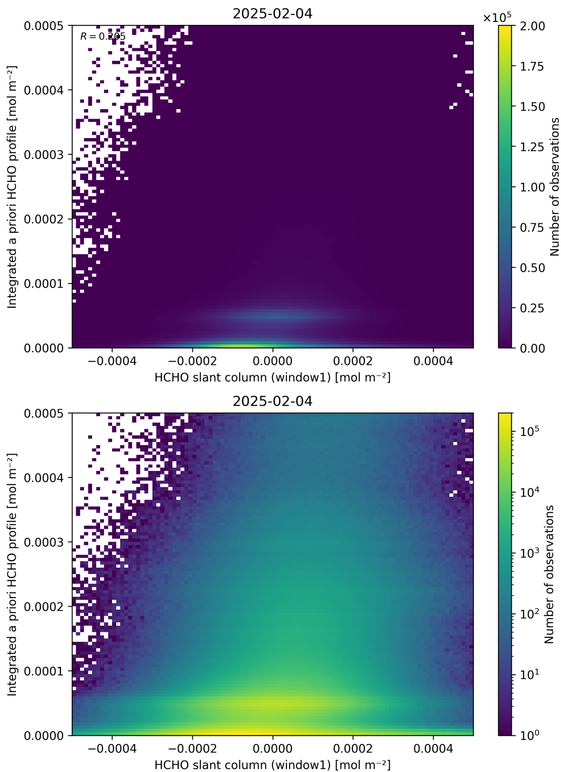
Figure 87: Scatter density plot of “HCHO slant column (window1)” against “Integrated a priori HCHO profile” for 2025-02-03 to 2025-02-05.
