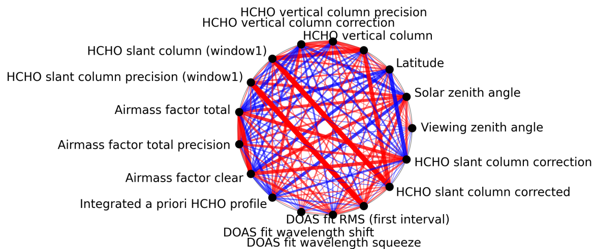
Figure 1: Map of correlation graph for 2025-02-03 to 2025-02-05.
