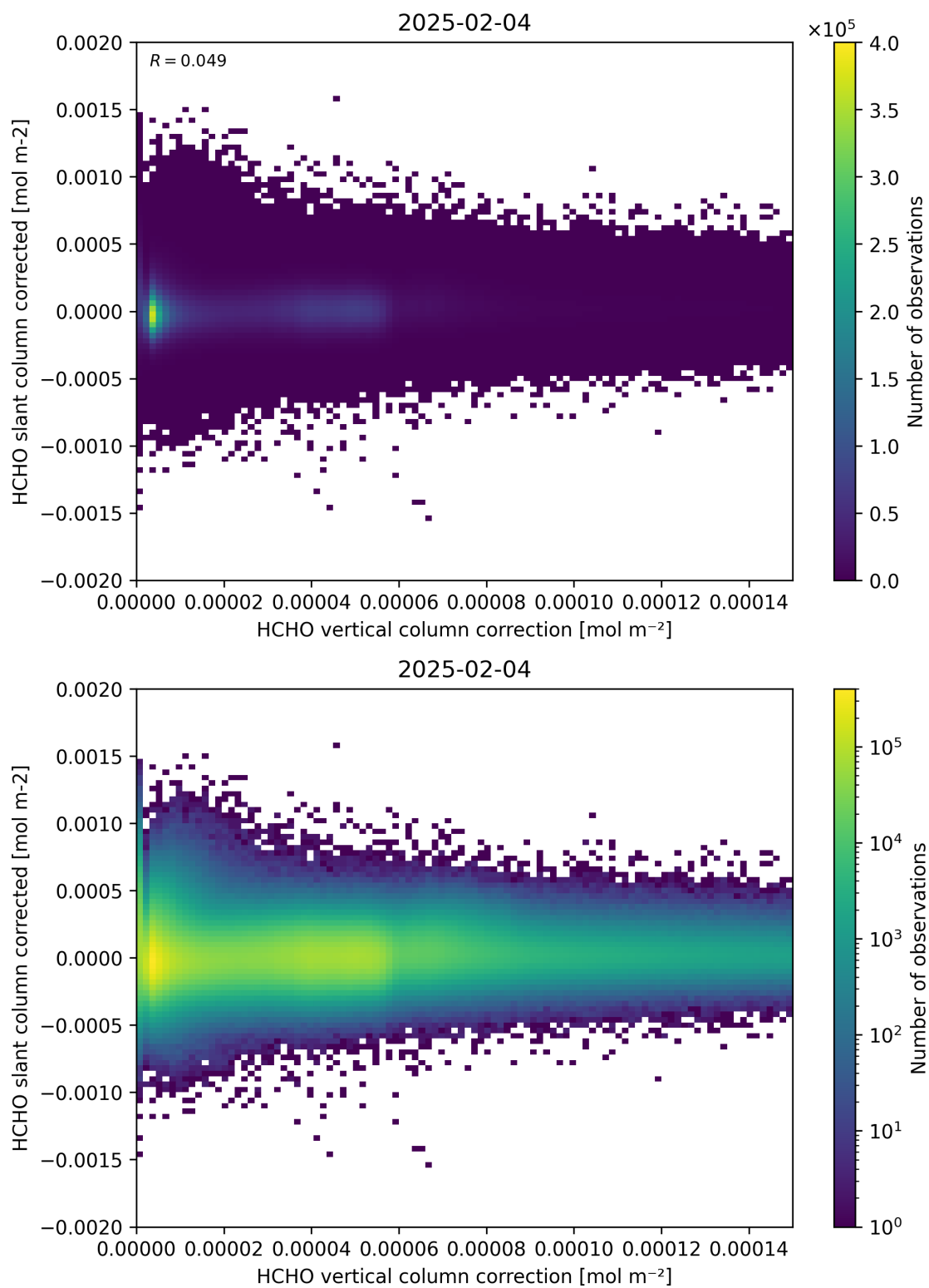
Figure 116: Scatter density plot of “HCHO vertical column correction” against “HCHO slant column corrected” for 2025-02-03 to 2025-02-05.
