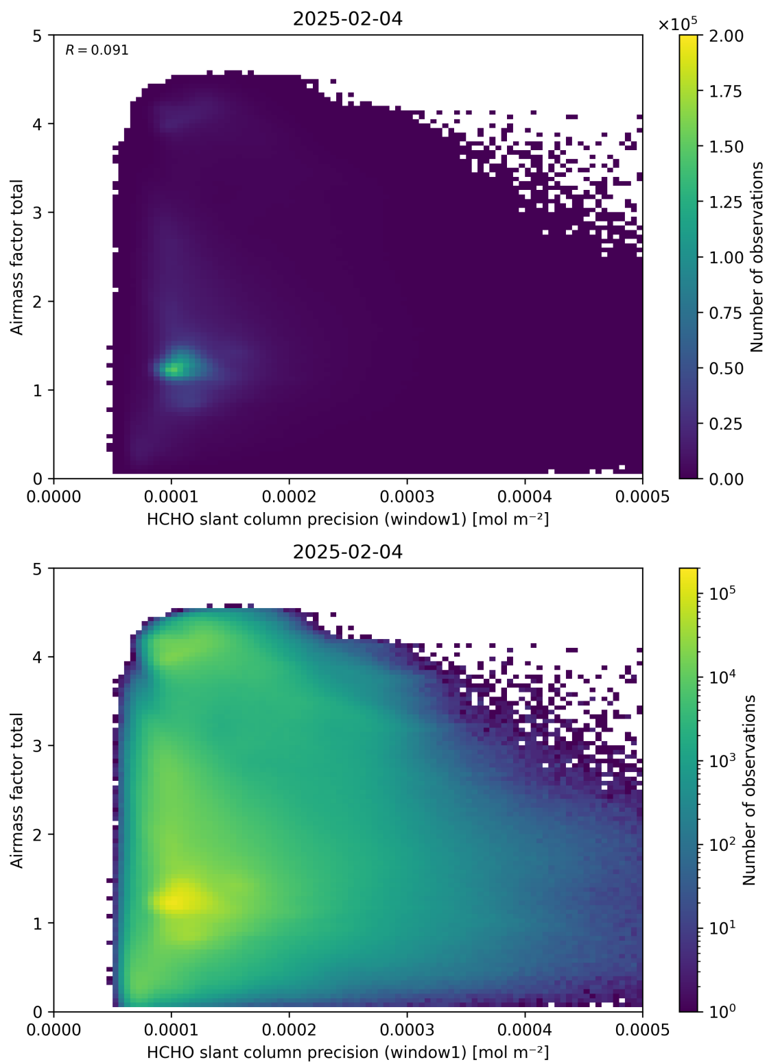
Figure 94: Scatter density plot of “HCHO slant column precision (window1)” against “Airmass factor total” for 2025-02-03 to 2025-02-05.
