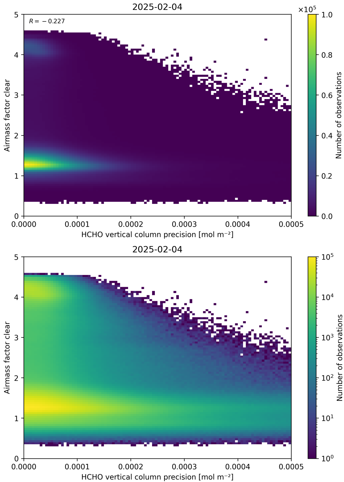
Figure 139: Scatter density plot of “HCHO vertical column precision” against “Airmass factor clear” for 2025-02-03 to 2025-02-05.
