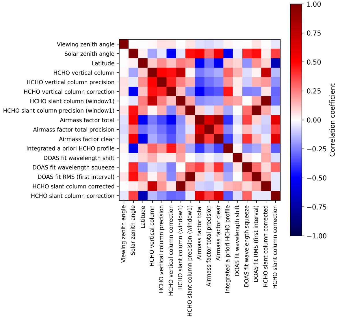
Figure 2: Map of correlation matrix for 2025-02-03 to 2025-02-05.
