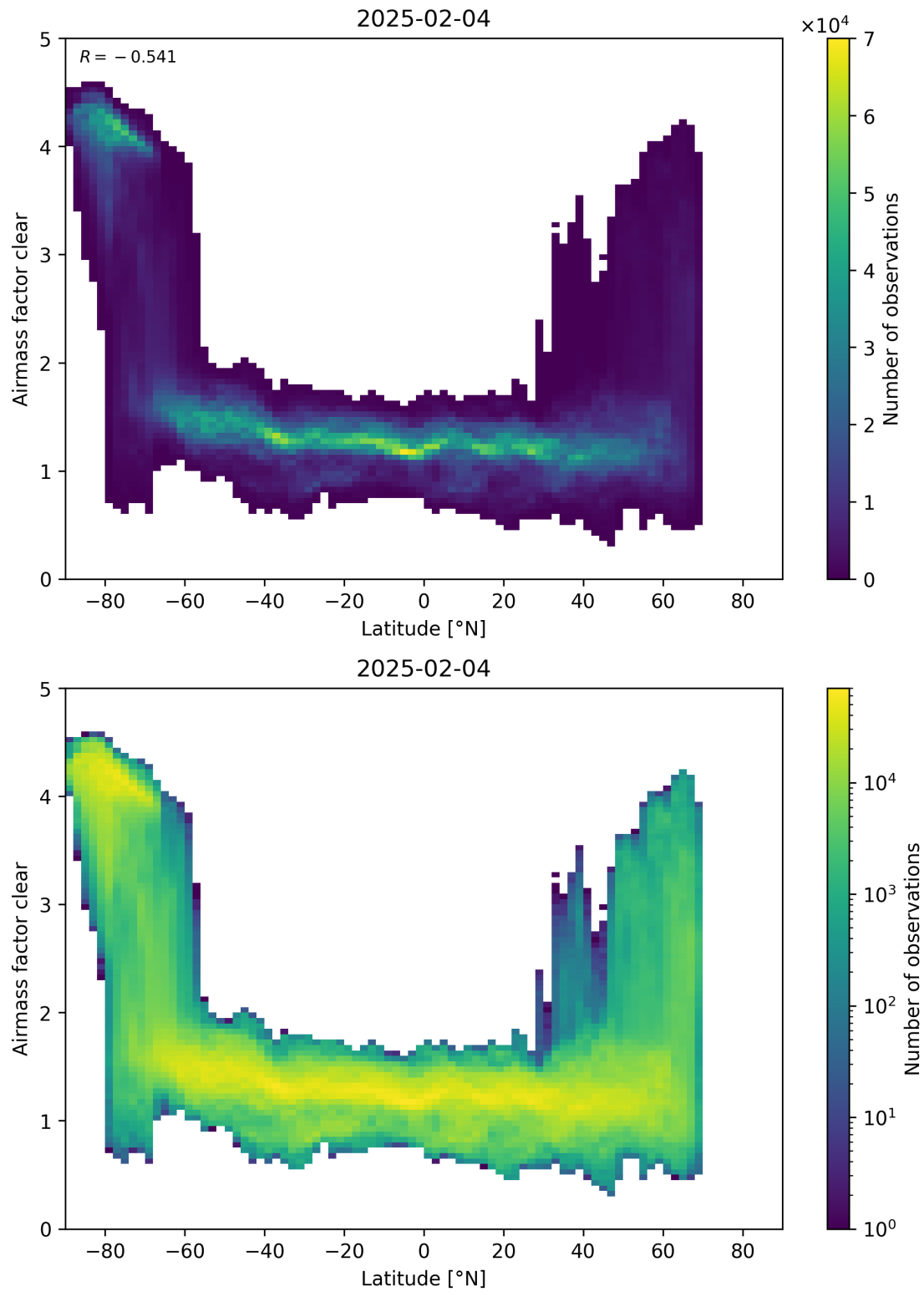
Figure 156: Scatter density plot of “Latitude” against “Airmass factor clear” for 2025-02-03 to 2025-02-05.
