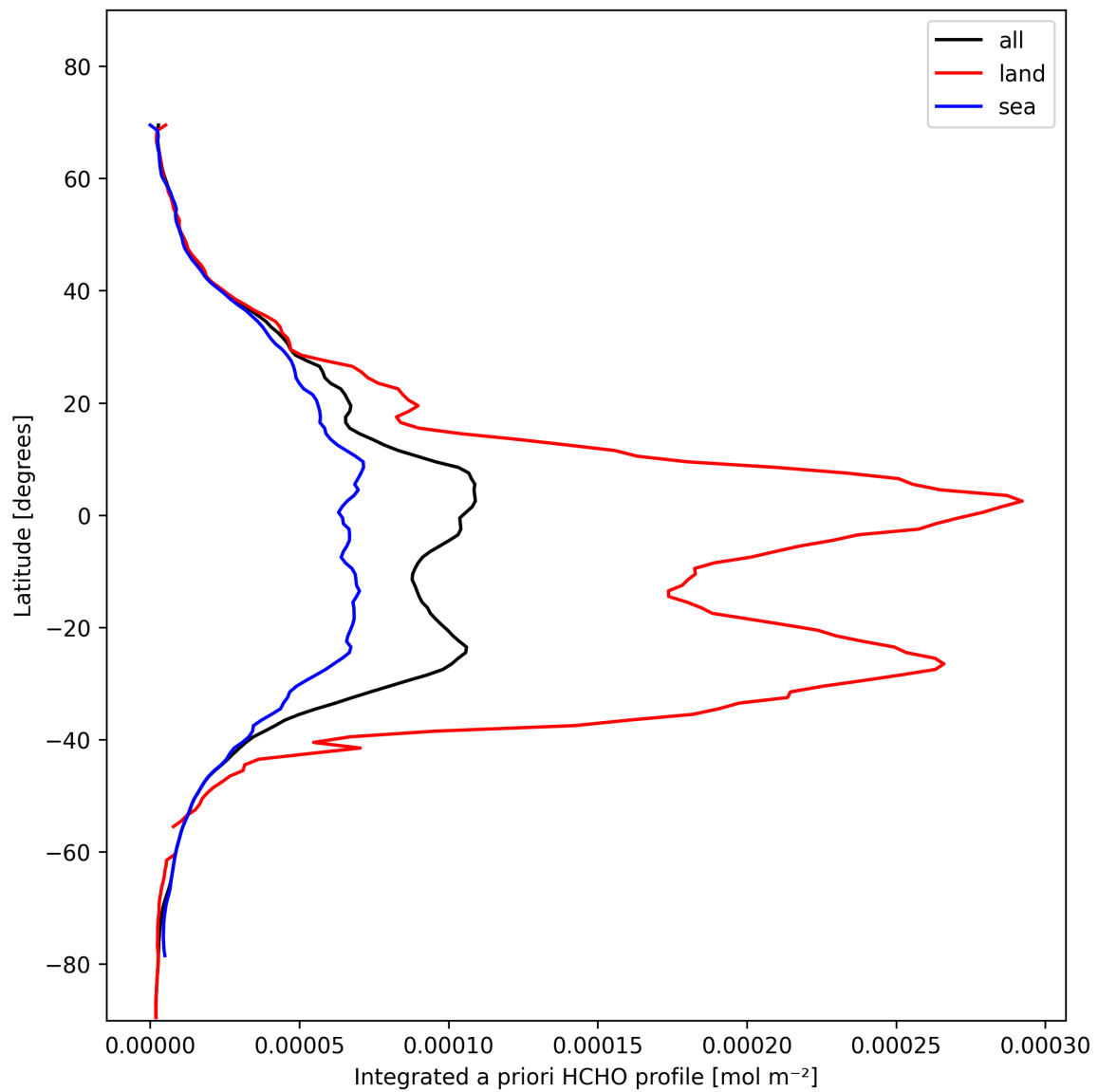
Figure 29: Zonal average of “Integrated a priori HCHO profile” for 2025-02-03 to 2025-02-05.
