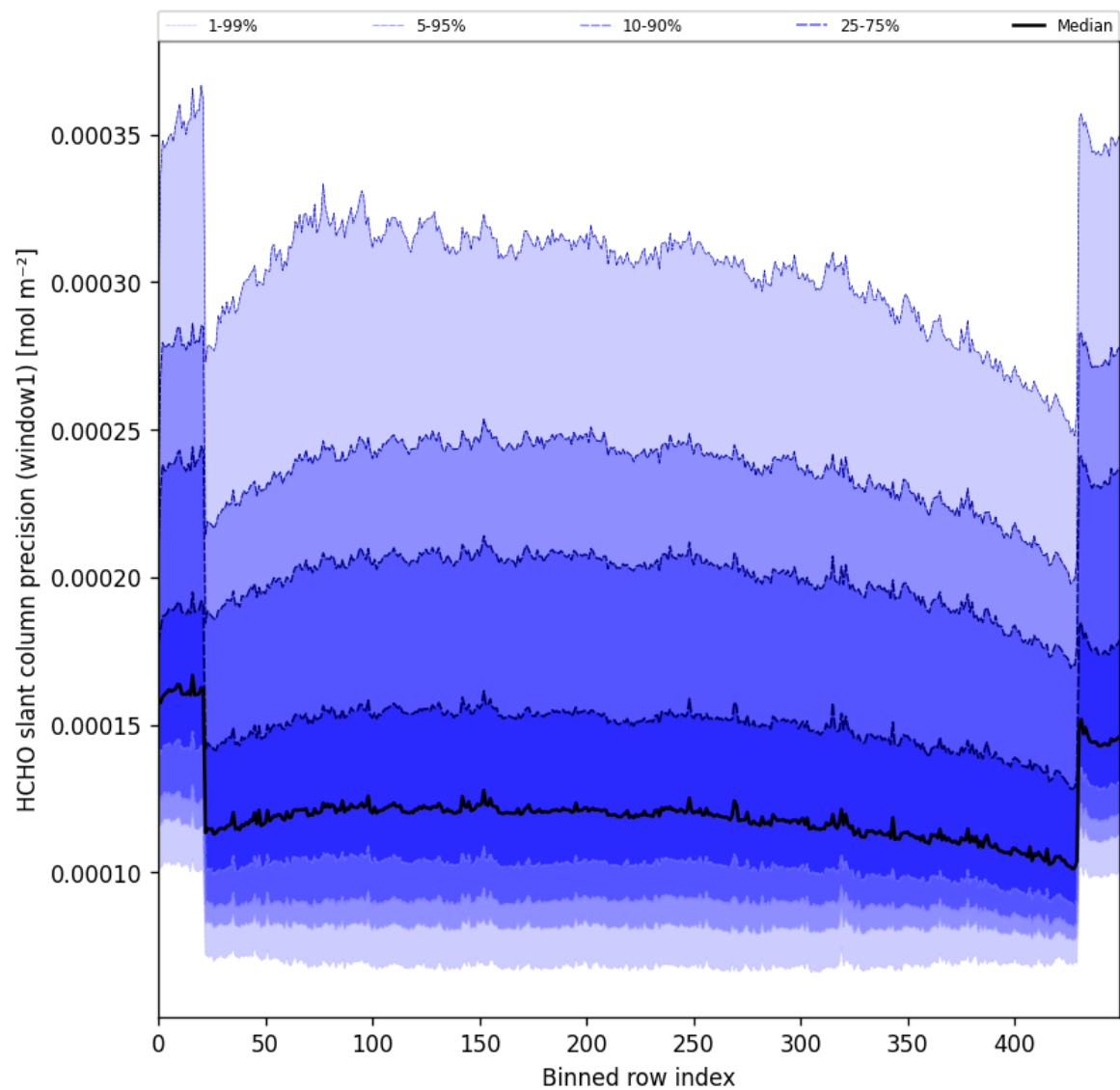
Figure 53: Along track statistics of “HCHO slant column precision (window1)” for 2025-02-03 to 2025-02-05
