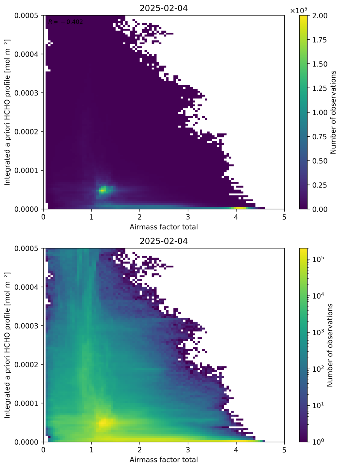
Figure 104: Scatter density plot of “Airmass factor total” against “Integrated a priori HCHO profile” for 2025-02-03 to 2025-02-05.
