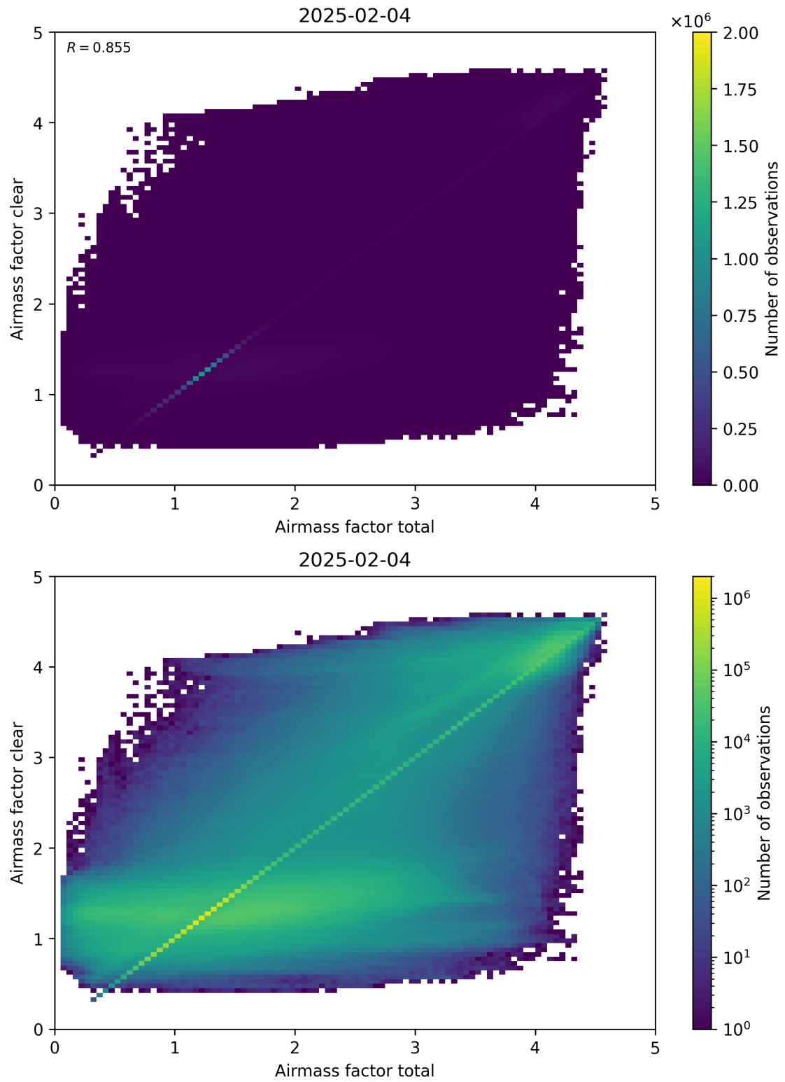
Figure 100: Scatter density plot of “Airmass factor total” against “Airmass factor clear” for 2025-02-03 to 2025-02-05.
