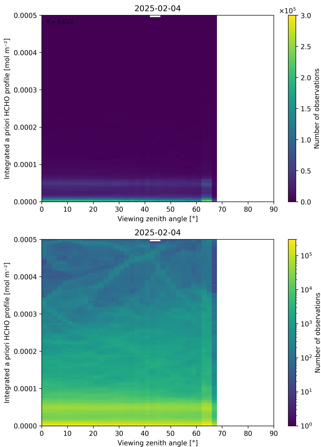
Figure 195: Scatter density plot of “Viewing zenith angle” against “Integrated a priori HCHO profile” for 2025-02-03 to 2025-02-05.
