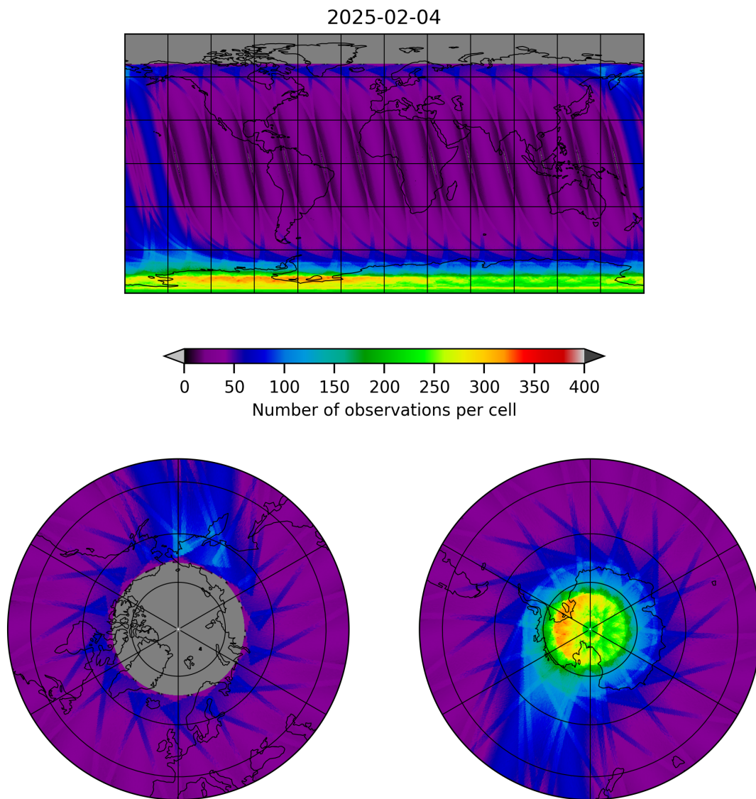
Figure 19: Map of the number of observations for 2025-02-03 to 2025-02-05
