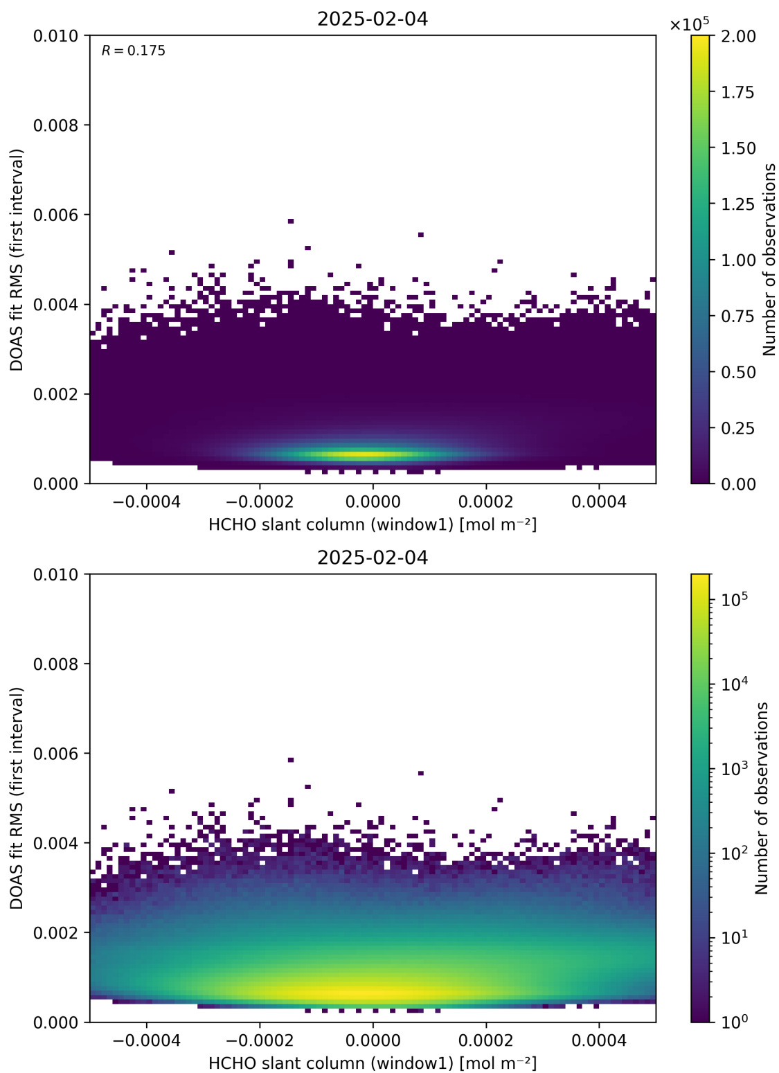
Figure 78: Scatter density plot of “HCHO slant column (window1)” against “DOAS fit RMS (first interval)” for 2025-02-03 to 2025-02-05.
