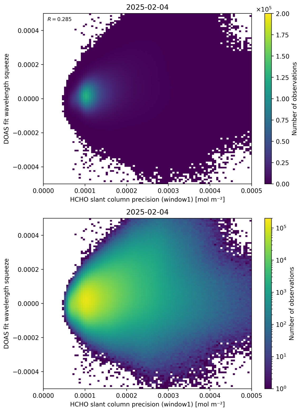
Figure 90: Scatter density plot of “HCHO slant column precision (window1)” against “DOAS fit wavelength squeeze” for 2025-02-03 to 2025-02-05.
