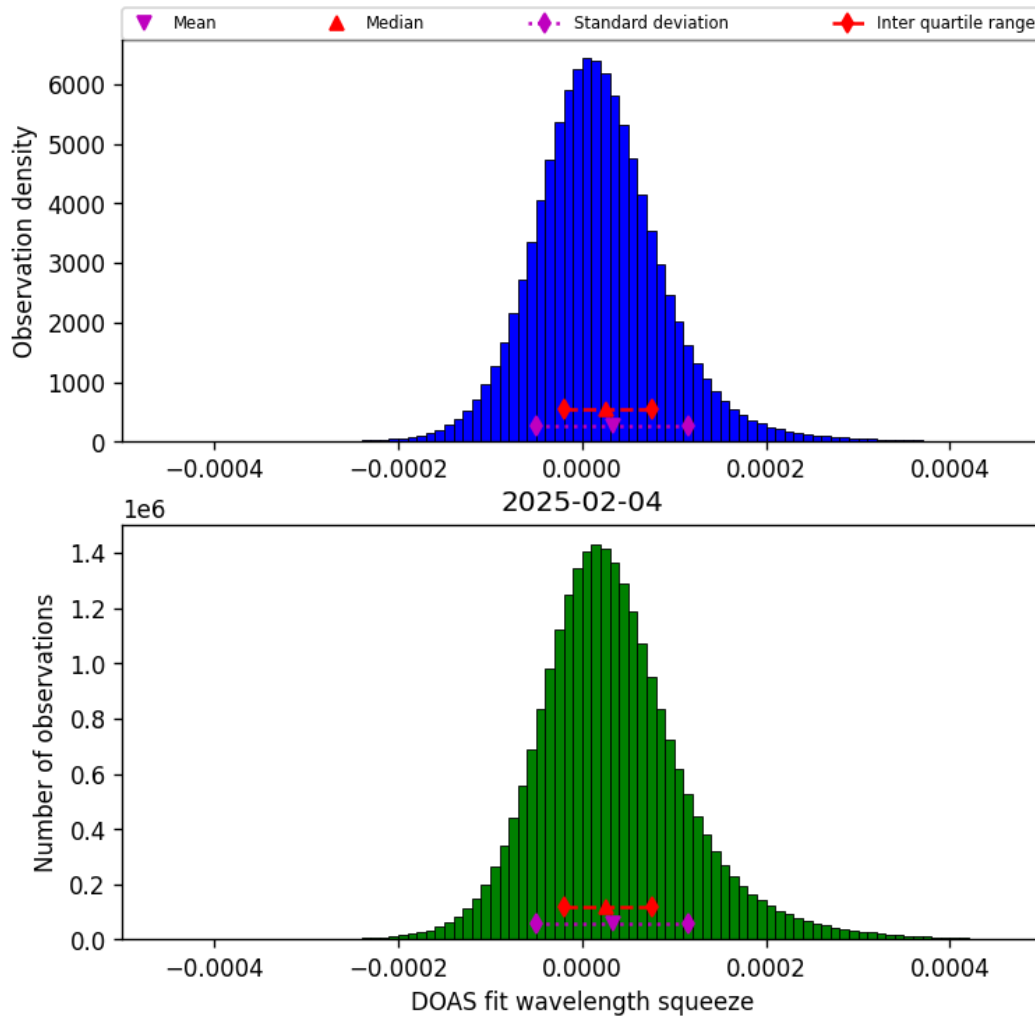
Figure 45: Histogram of “DOAS fit wavelength squeeze” for 2025-02-03 to 2025-02-05
