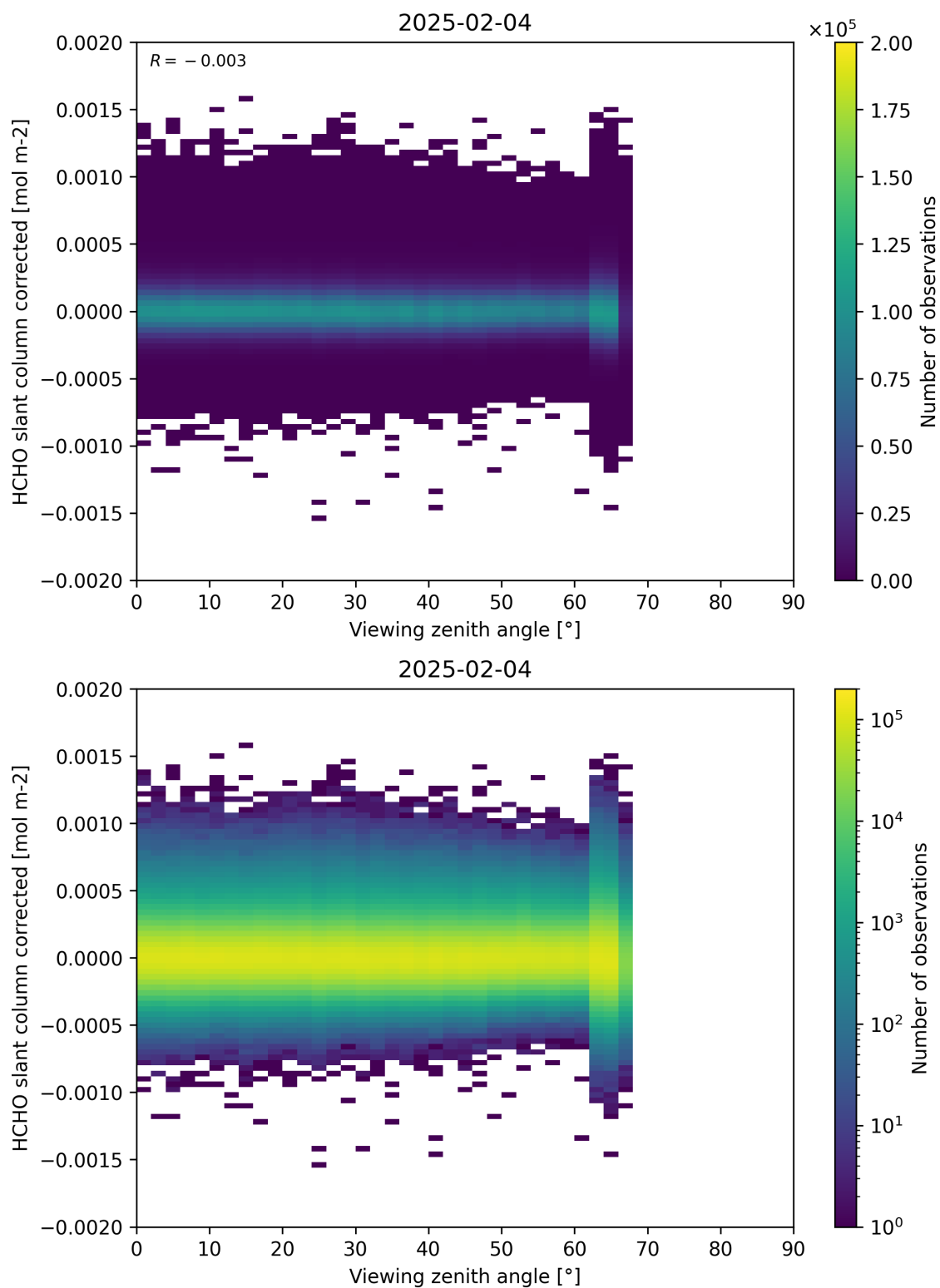
Figure 186: Scatter density plot of “Viewing zenith angle” against “HCHO slant column corrected” for 2025-02-03 to 2025-02-05.
