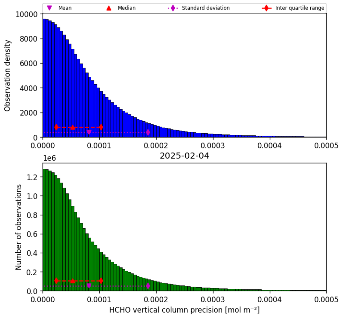
Figure 36: Histogram of “HCHO vertical column precision” for 2025-02-03 to 2025-02-05
