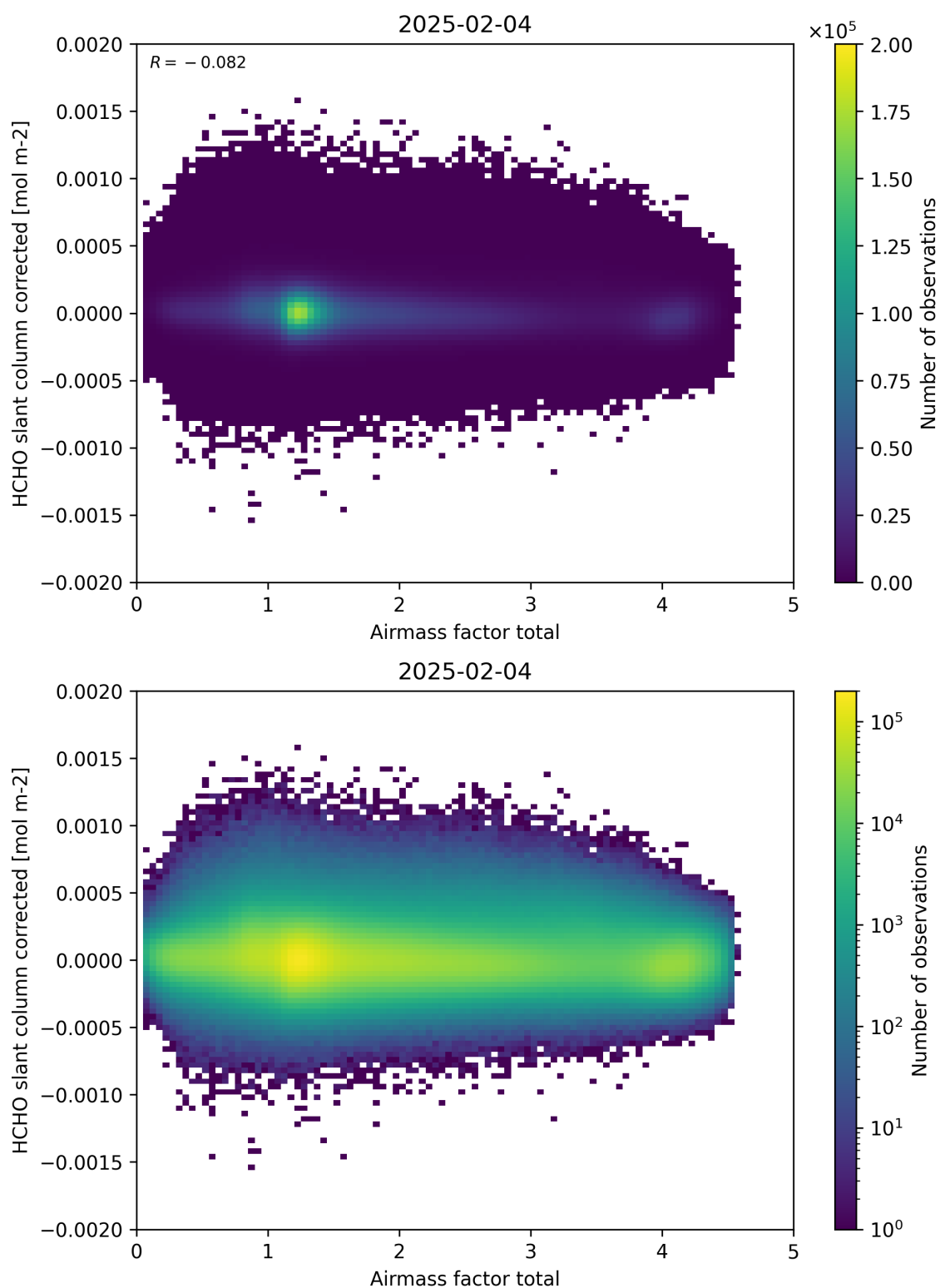
Figure 101: Scatter density plot of “Airmass factor total” against “HCHO slant column corrected” for 2025-02-03 to 2025-02-05.
