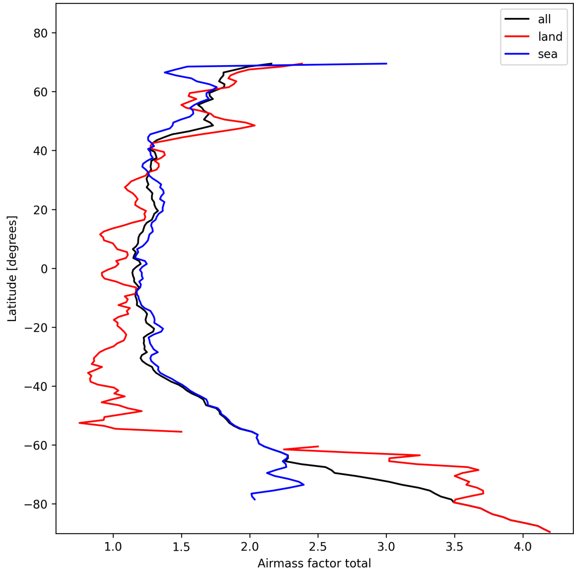
Figure 26: Zonal average of “Airmass factor total” for 2025-02-03 to 2025-02-05.
