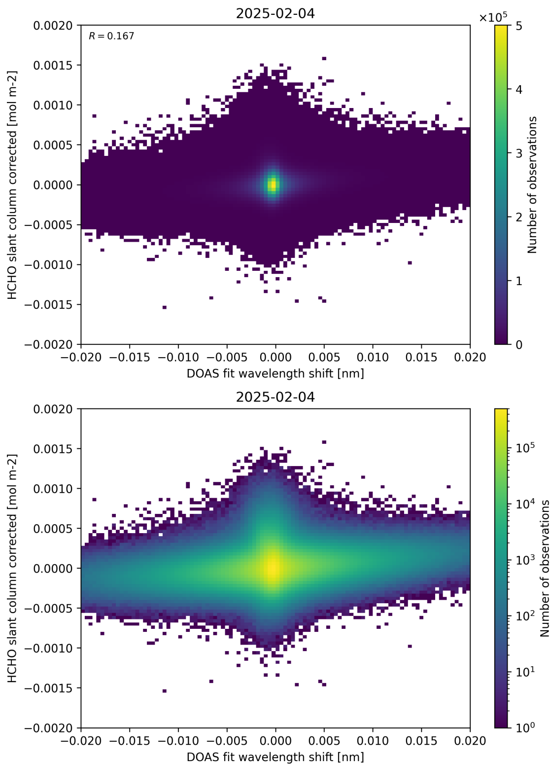
Figure 66: Scatter density plot of “DOAS fit wavelength shift” against “HCHO slant column corrected” for 2025-02-03 to 2025-02-05.
