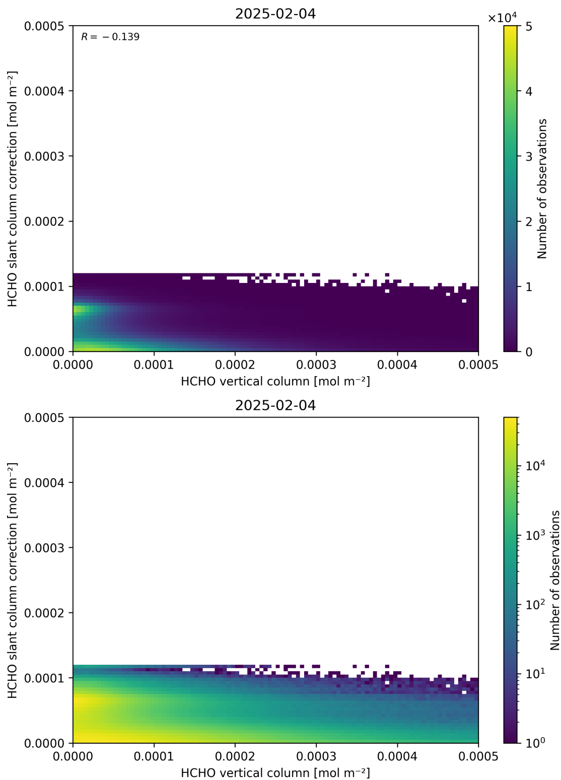
Figure 128: Scatter density plot of “HCHO vertical column” against “HCHO slant column correction” for 2025-02-03 to 2025-02-05.
