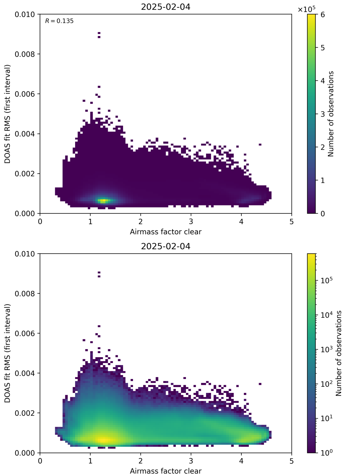
Figure 71: Scatter density plot of “Airmass factor clear” against “DOAS fit RMS (first interval)” for 2025-02-03 to 2025-02-05.
