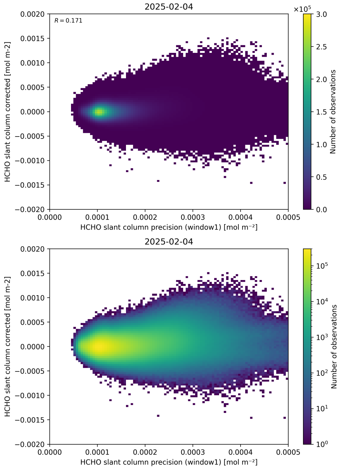
Figure 92: Scatter density plot of “HCHO slant column precision (window1)” against “HCHO slant column corrected” for 2025-02-03 to 2025-02-05.
