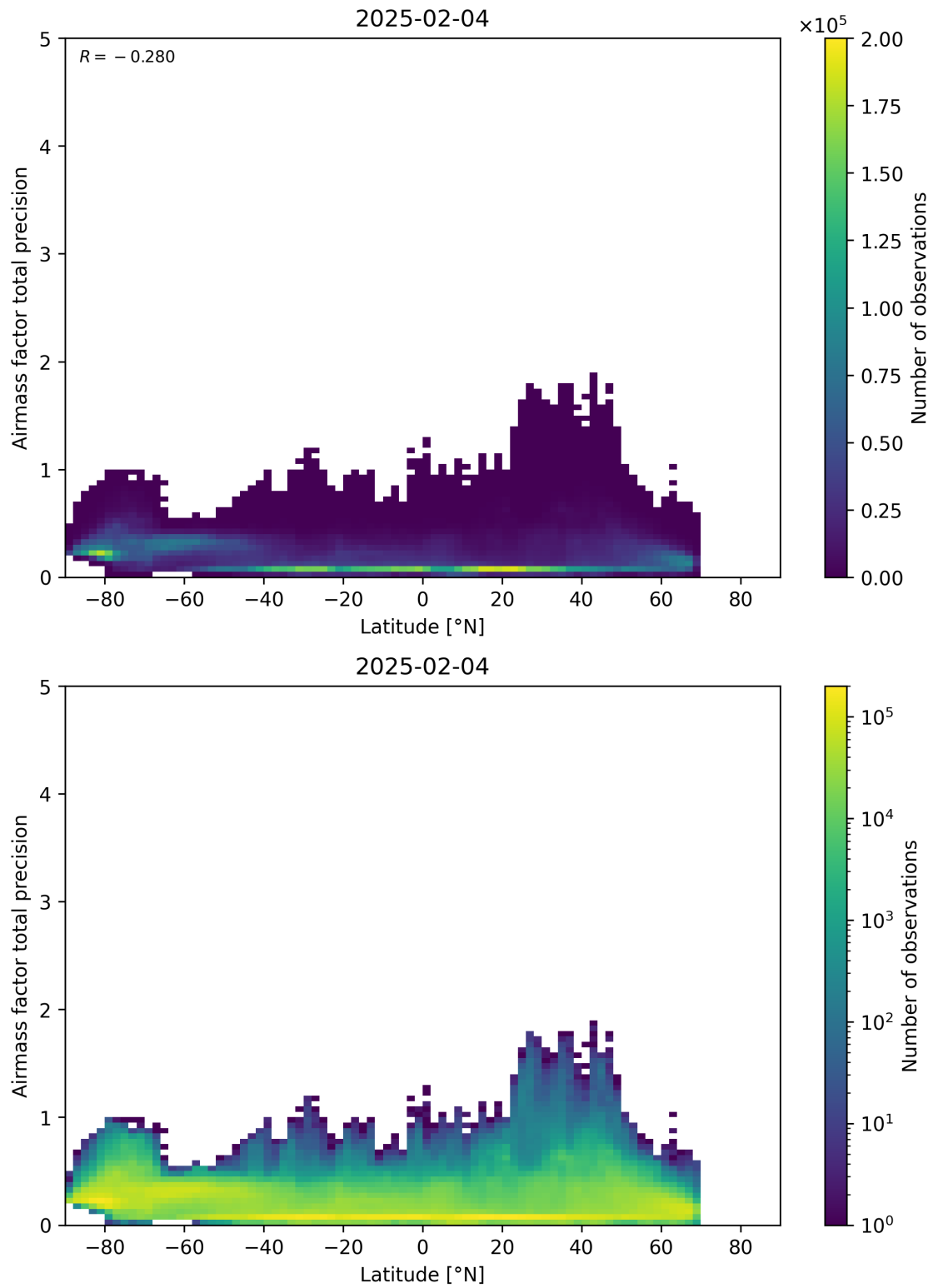
Figure 162: Scatter density plot of “Latitude” against “Airmass factor total precision” for 2025-02-03 to 2025-02-05.
