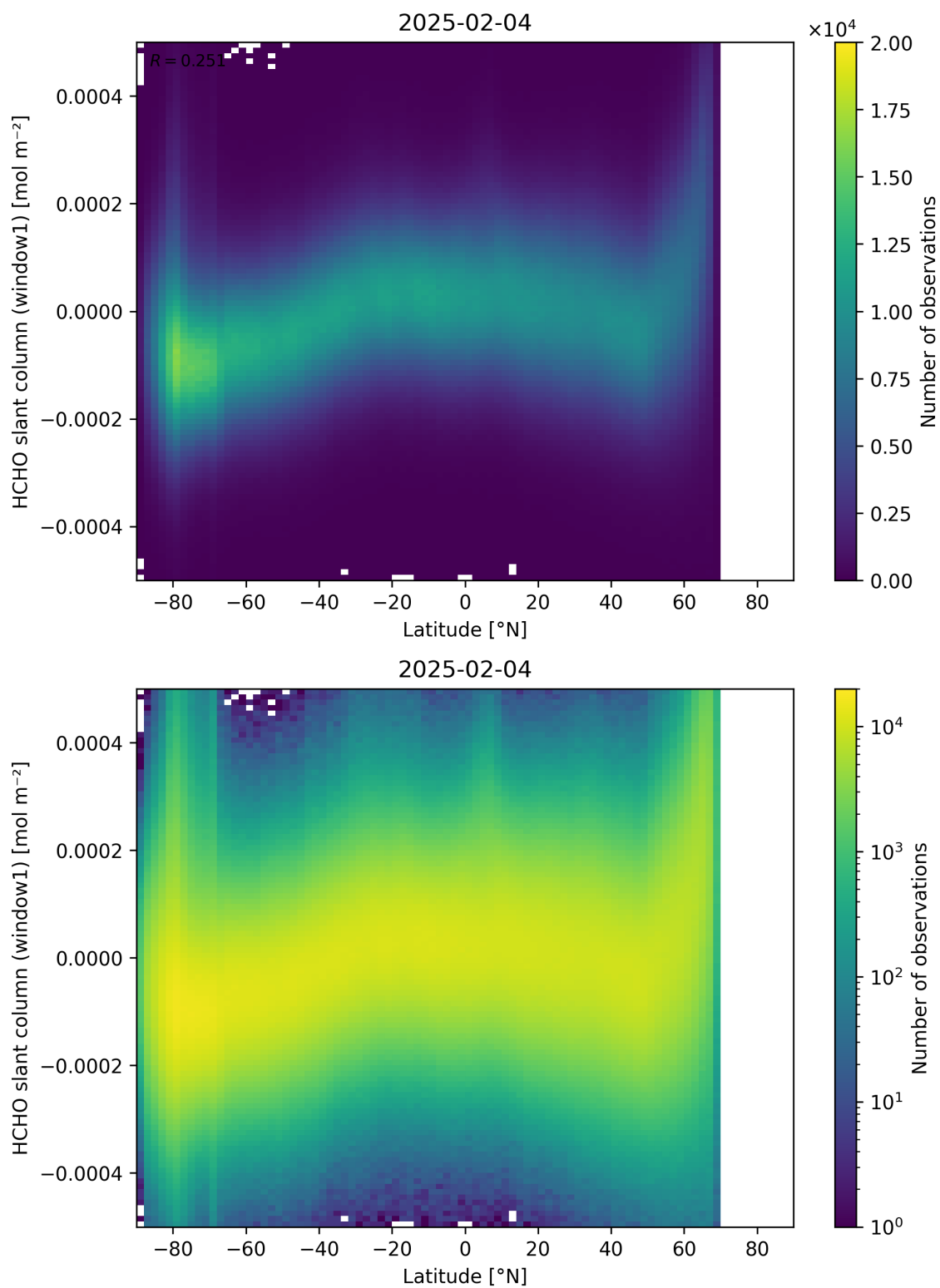
Figure 159: Scatter density plot of “Latitude” against “HCHO slant column (window1)” for 2025-02-03 to 2025-02-05.
