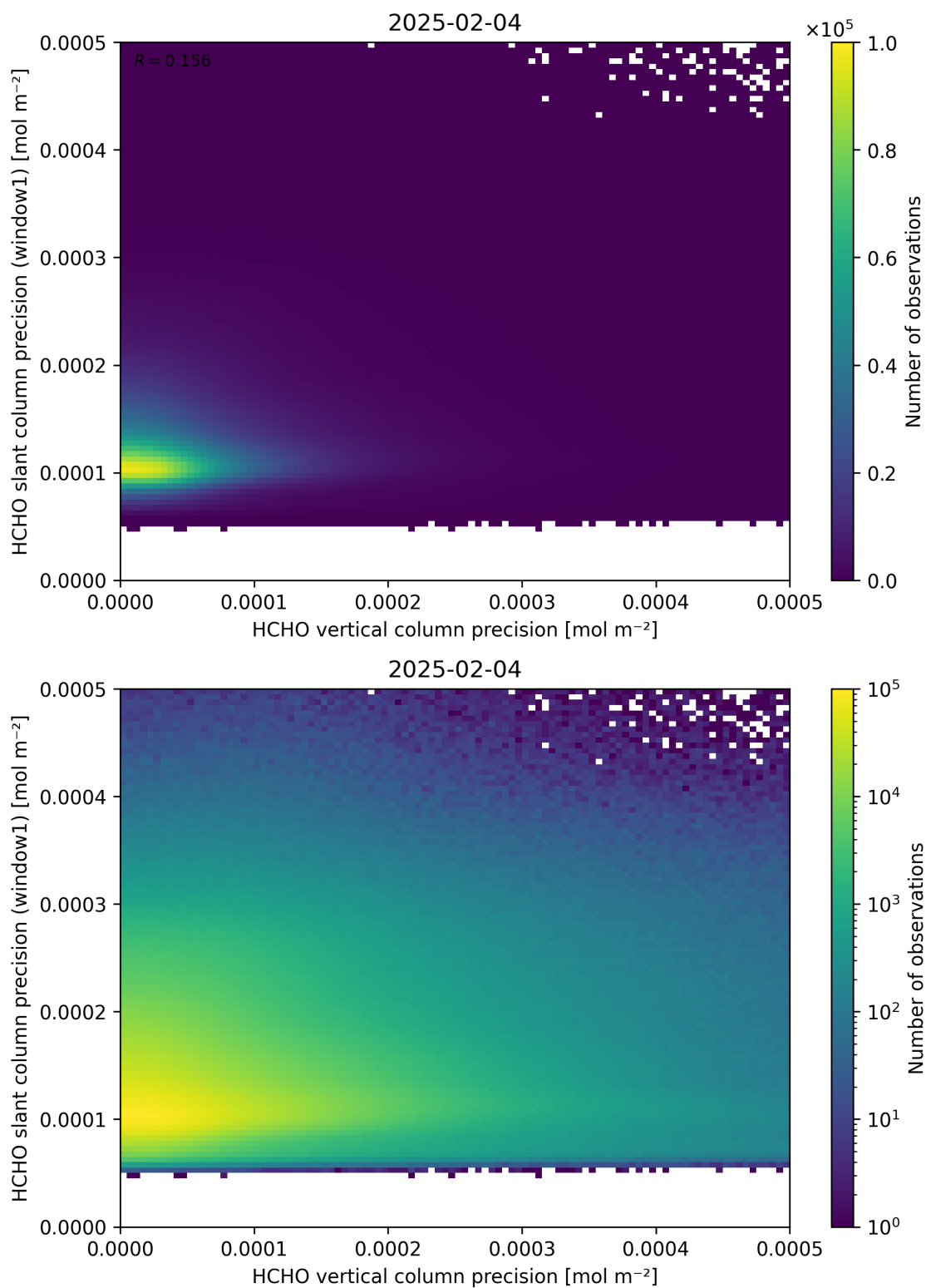
Figure 143: Scatter density plot of “HCHO vertical column precision” against “HCHO slant column precision (window1)” for 2025-02-03 to 2025-02-05.
