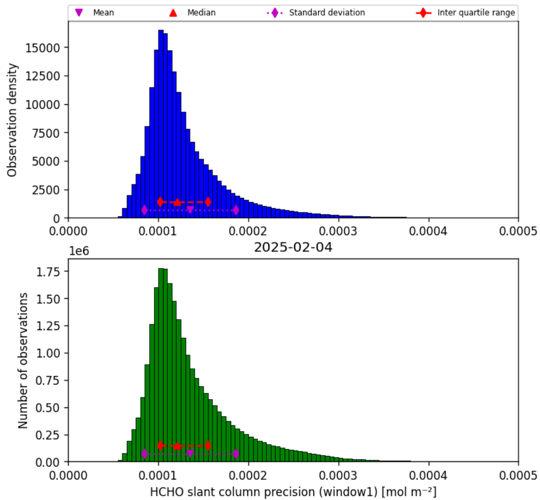
Figure 39: Histogram of “HCHO slant column precision (window1)” for 2025-02-03 to 2025-02-05
