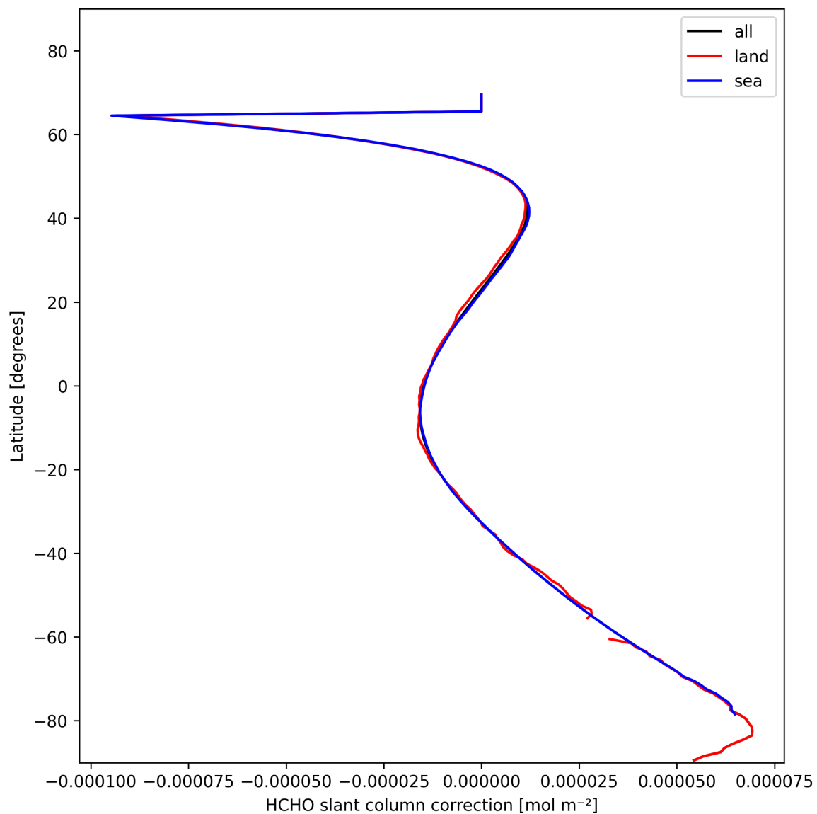
Figure 33: Zonal average of “HCHO slant column correction” for 2025-02-03 to 2025-02-05.
