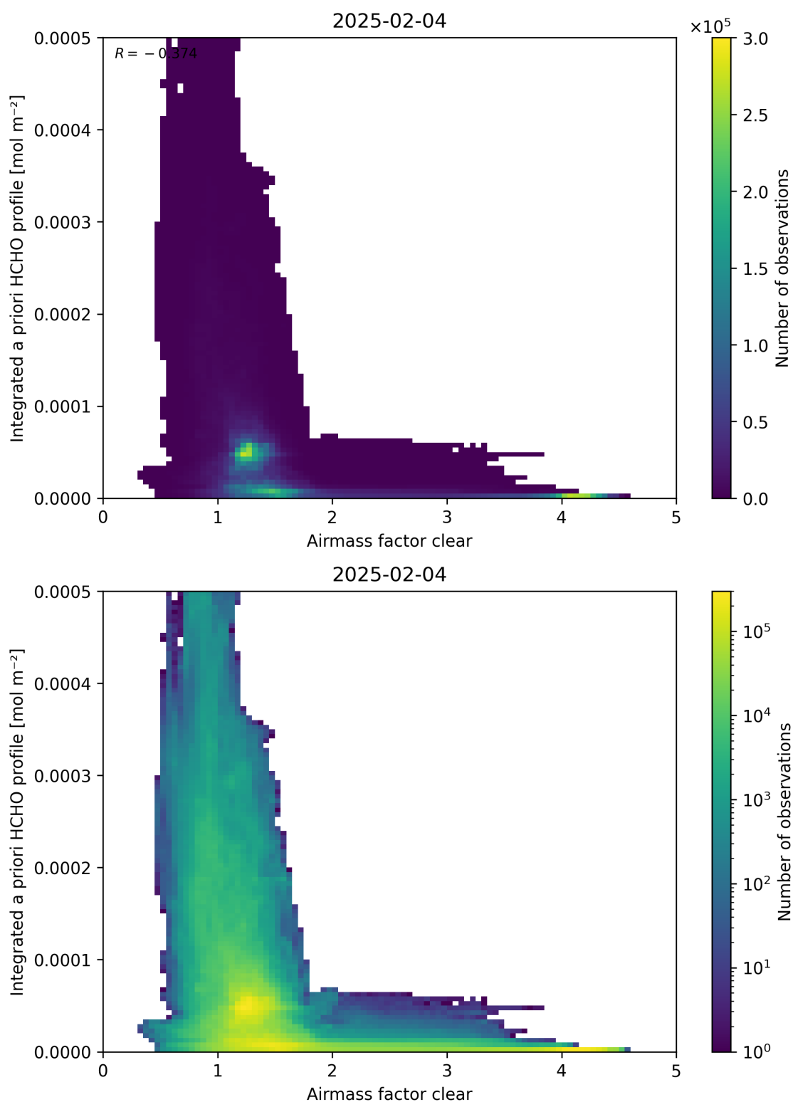
Figure 76: Scatter density plot of “Airmass factor clear” against “Integrated a priori HCHO profile” for 2025-02-03 to 2025-02-05.
