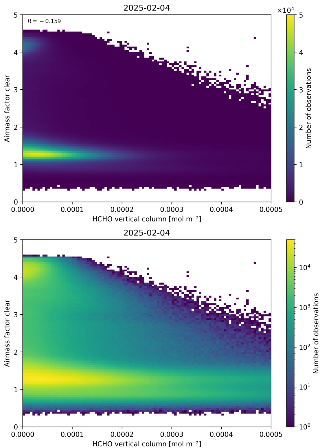
Figure 126: Scatter density plot of “HCHO vertical column” against “Airmass factor clear” for 2025-02-03 to 2025-02-05.
