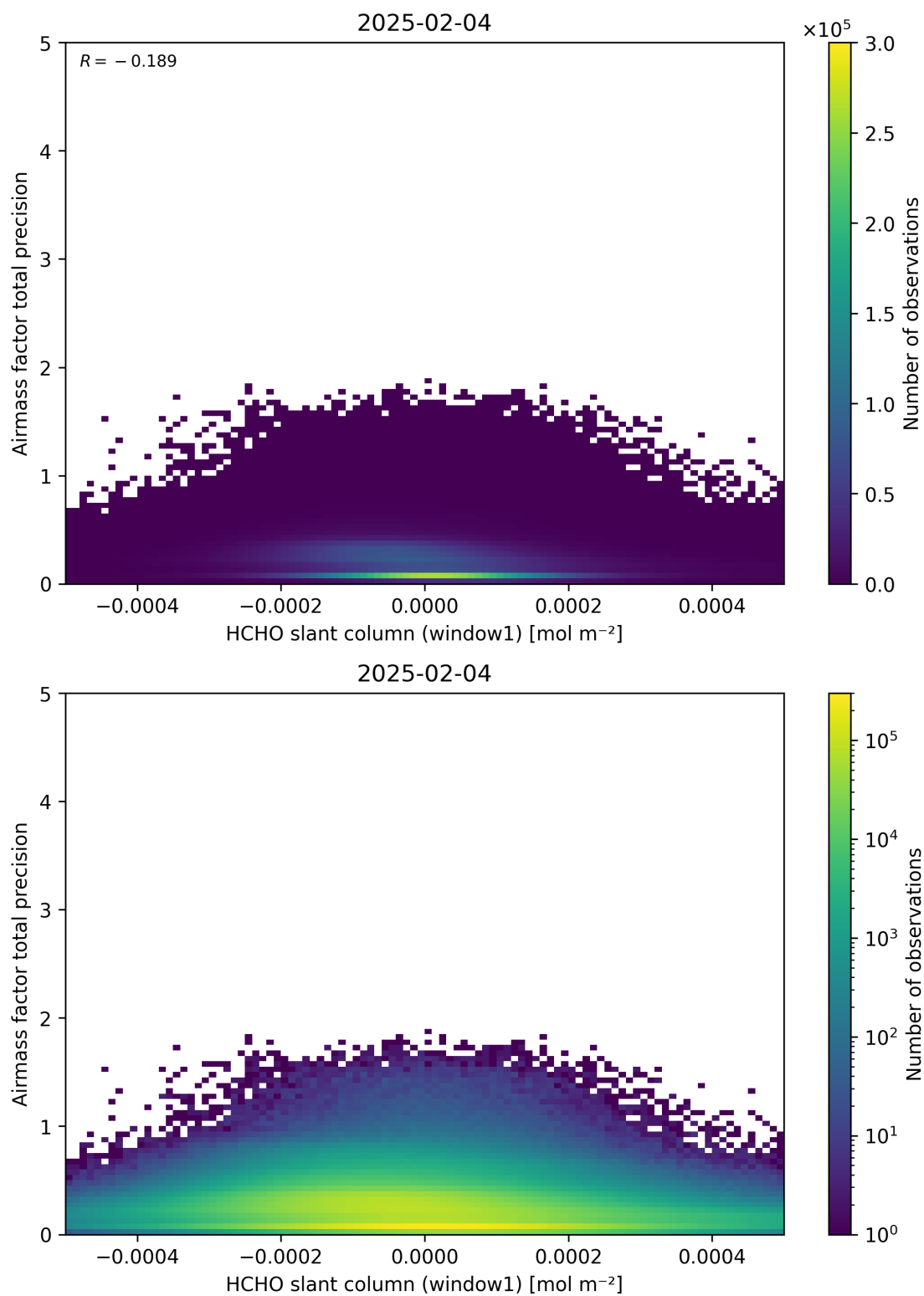
Figure 86: Scatter density plot of “HCHO slant column (window1)” against “Airmass factor total precision” for 2025-02-03 to 2025-02-05.
