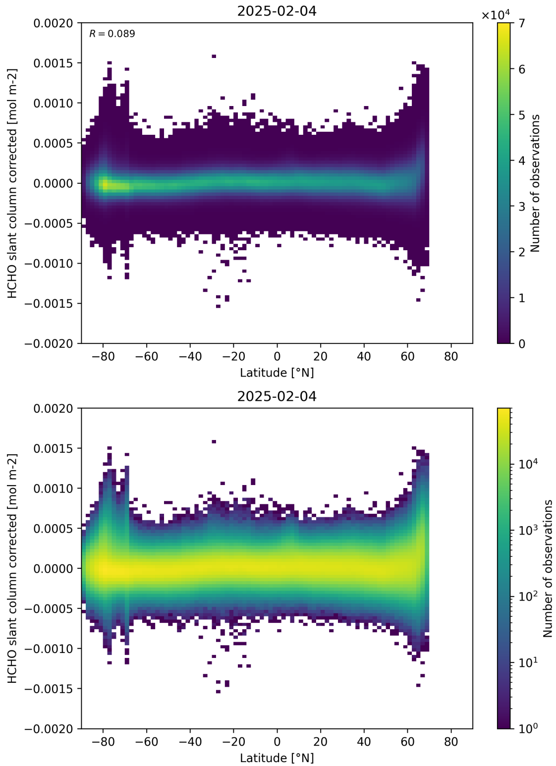
Figure 157: Scatter density plot of “Latitude” against “HCHO slant column corrected” for 2025-02-03 to 2025-02-05.
