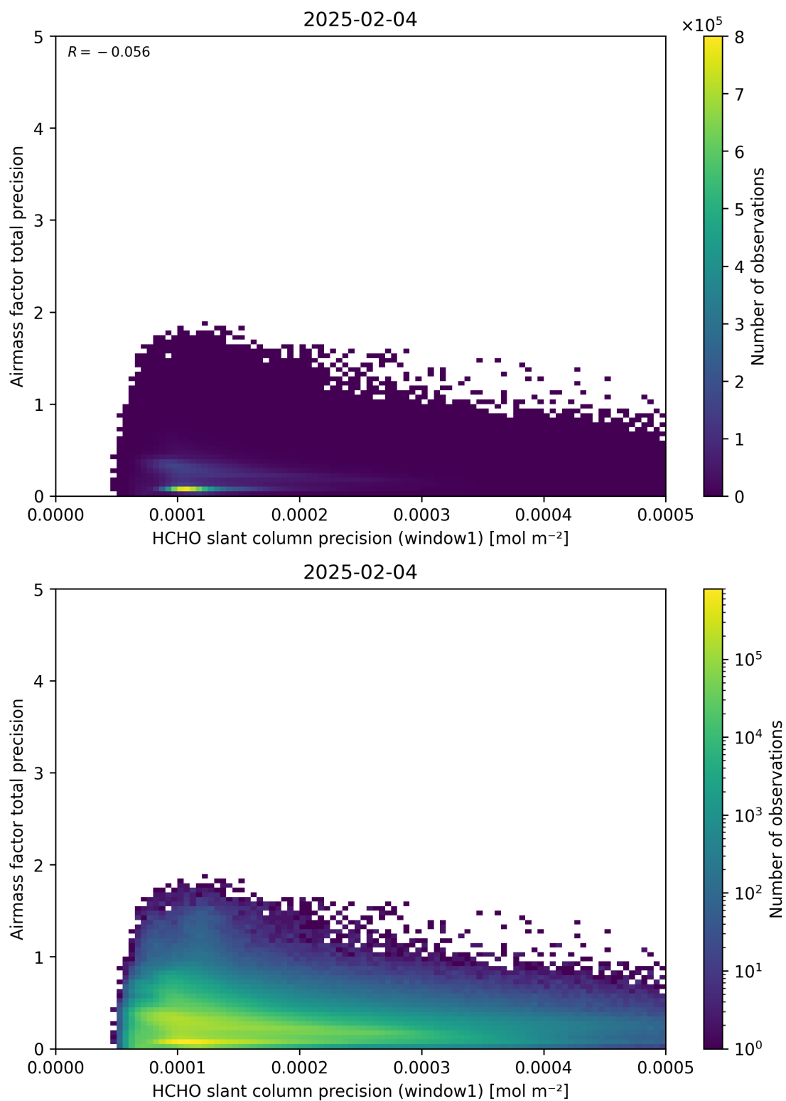
Figure 95: Scatter density plot of “HCHO slant column precision (window1)” against “Airmass factor total precision” for 2025-02-03 to 2025-02-05.
