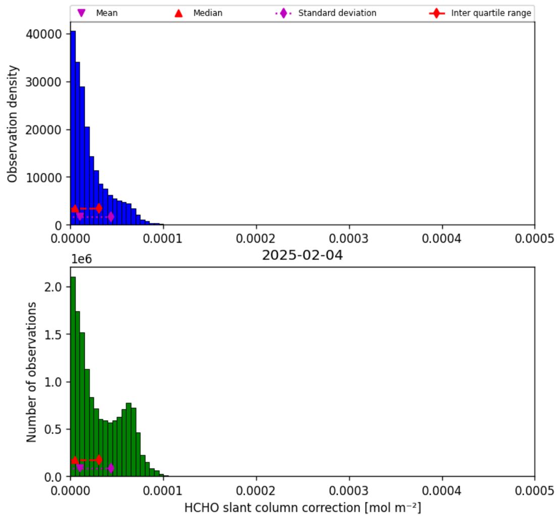
Figure 47: Histogram of “HCHO slant column correction” for 2025-02-03 to 2025-02-05
