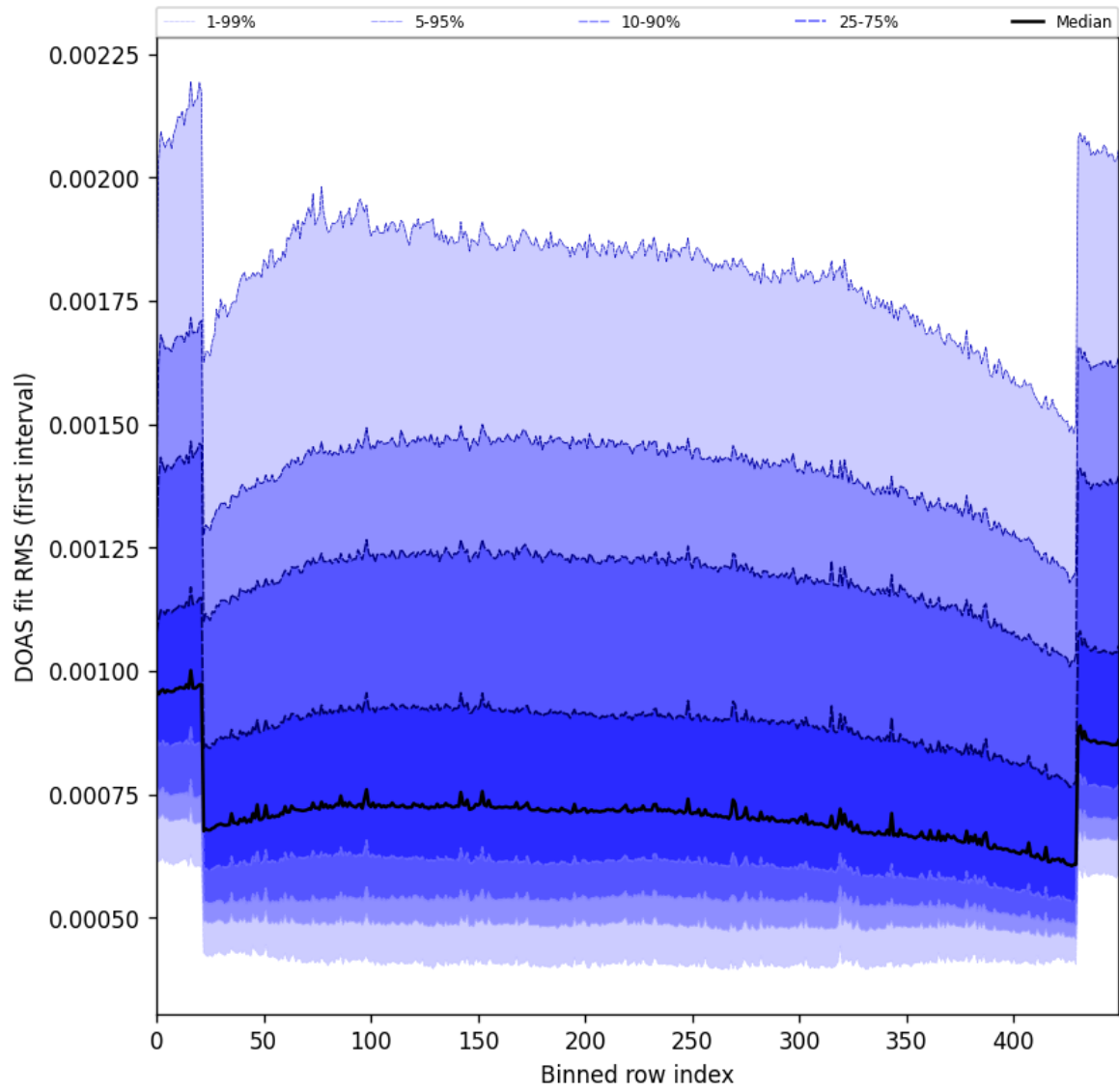
Figure 60: Along track statistics of “DOAS fit RMS (first interval)” for 2025-02-03 to 2025-02-05
