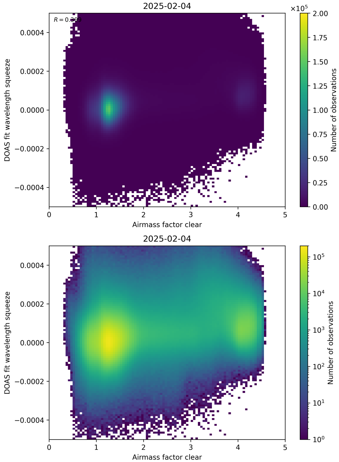
Figure 73: Scatter density plot of “Airmass factor clear” against “DOAS fit wavelength squeeze” for 2025-02-03 to 2025-02-05.
