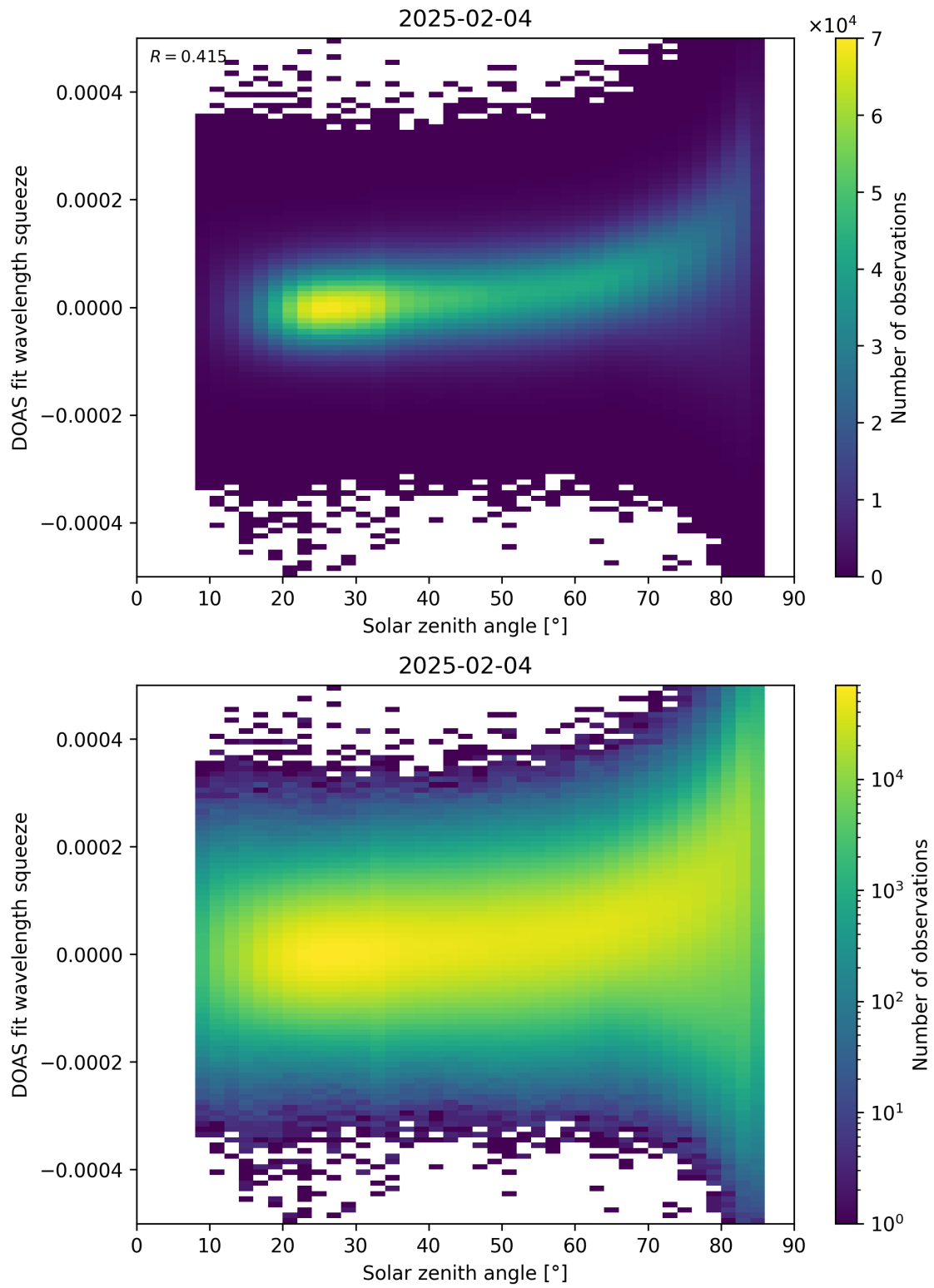
Figure 169: Scatter density plot of “Solar zenith angle” against “DOAS fit wavelength squeeze” for 2025-02-03 to 2025-02-05.
