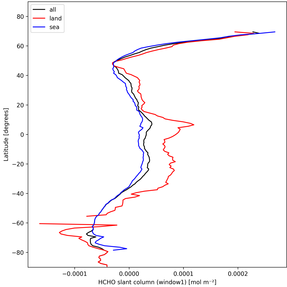
Figure 24: Zonal average of “HCHO slant column (window1)” for 2025-02-03 to 2025-02-05.
