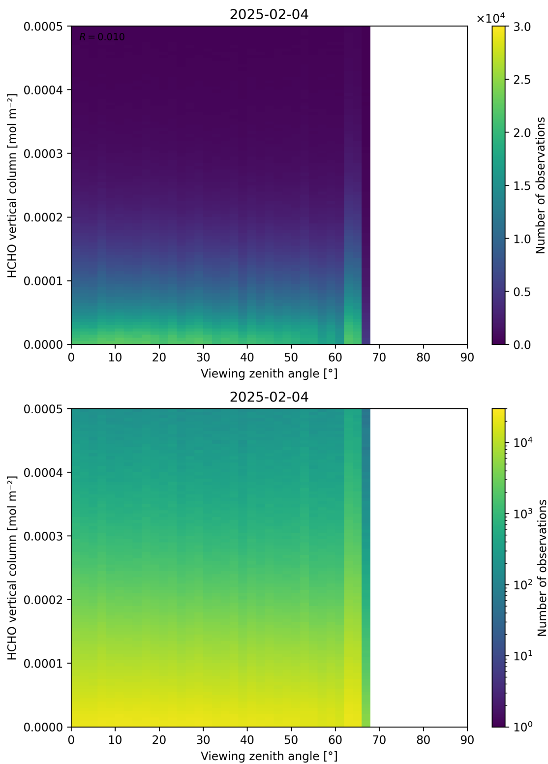
Figure 192: Scatter density plot of “Viewing zenith angle” against “HCHO vertical column” for 2025-02-03 to 2025-02-05.
