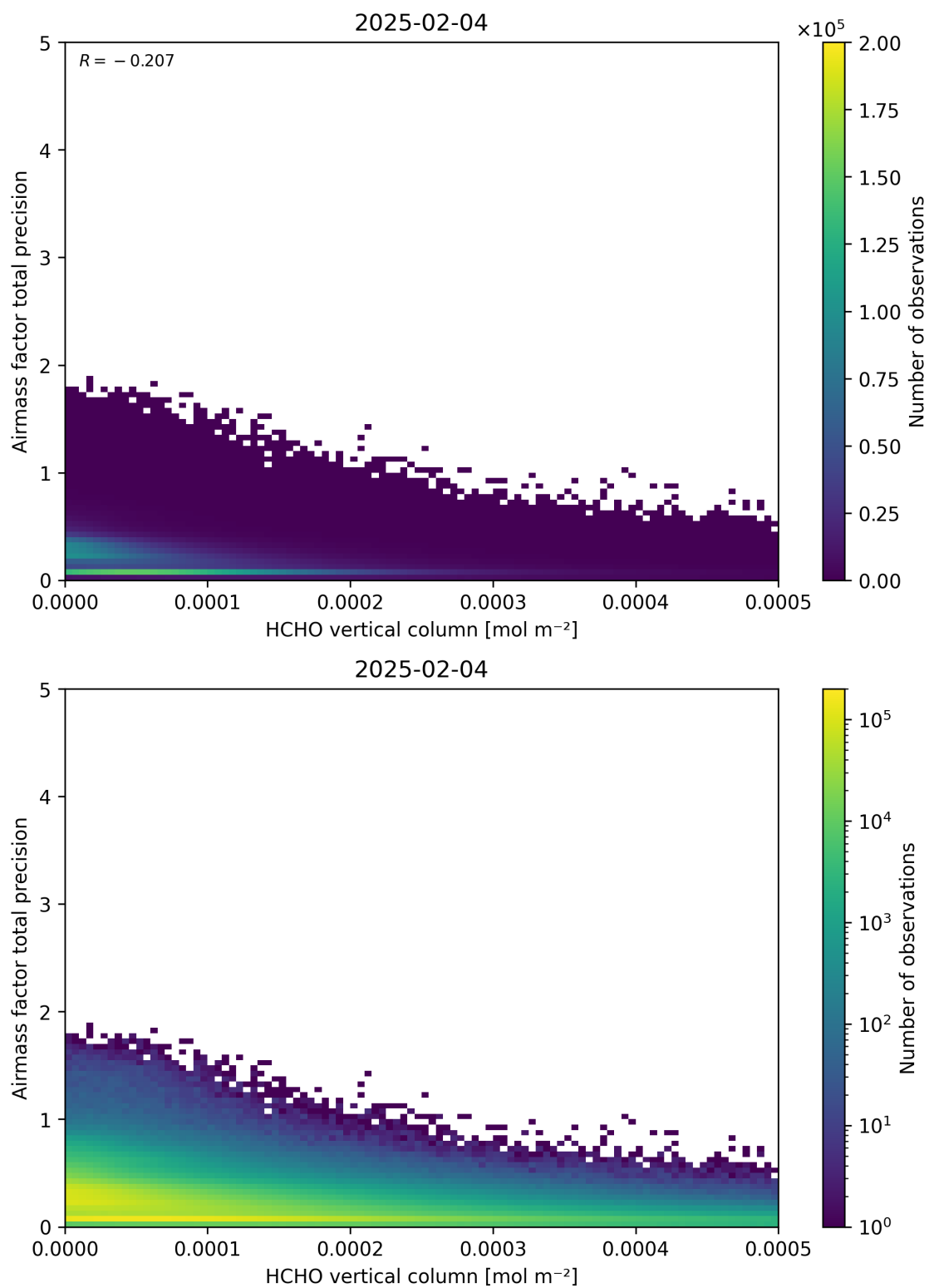
Figure 132: Scatter density plot of “HCHO vertical column” against “Airmass factor total precision” for 2025-02-03 to 2025-02-05.
