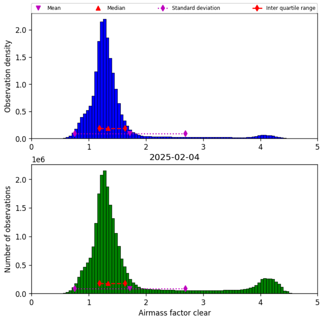
Figure 42: Histogram of “Airmass factor clear” for 2025-02-03 to 2025-02-05
