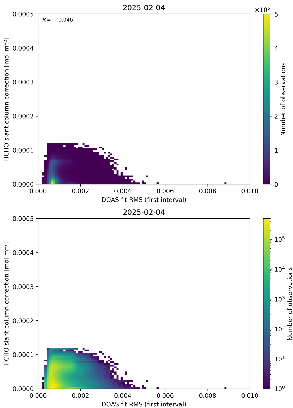
Figure 63: Scatter density plot of “DOAS fit RMS (first interval)” against “HCHO slant column correction” for 2025-02-03 to 2025-02-05.
