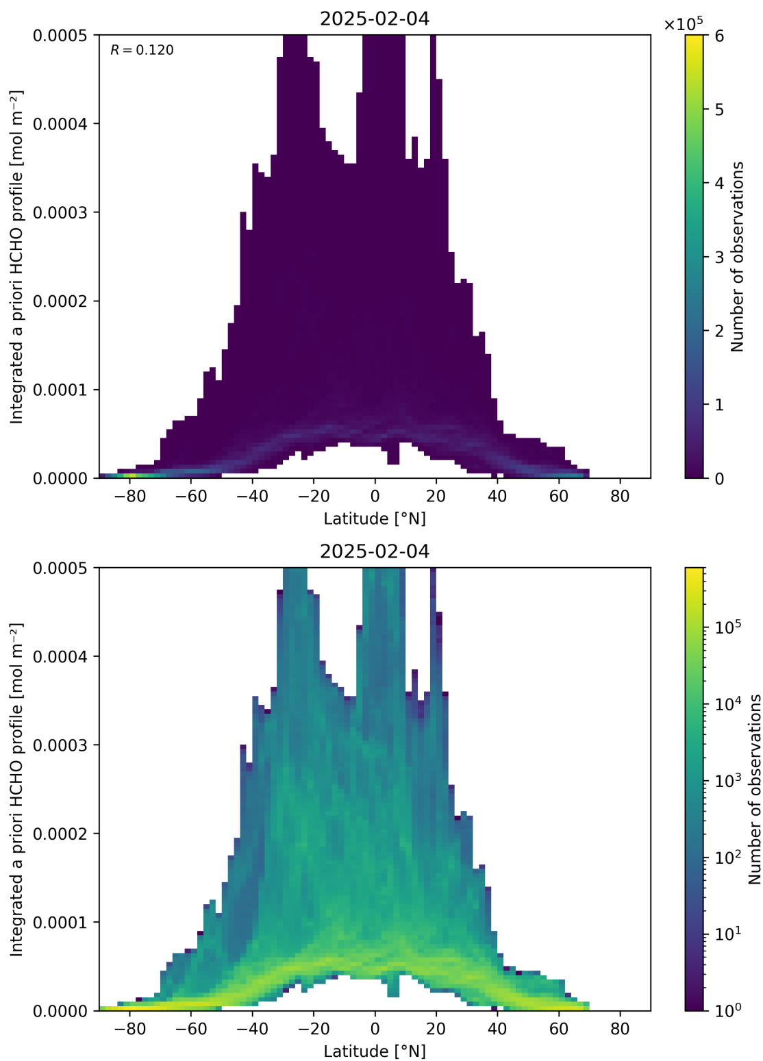
Figure 166: Scatter density plot of “Latitude” against “Integrated a priori HCHO profile” for 2025-02-03 to 2025-02-05.
