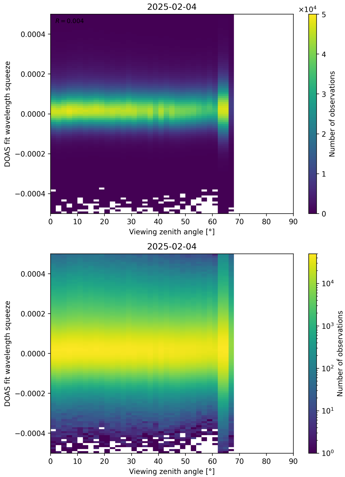
Figure 184: Scatter density plot of “Viewing zenith angle” against “DOAS fit wavelength squeeze” for 2025-02-03 to 2025-02-05.
