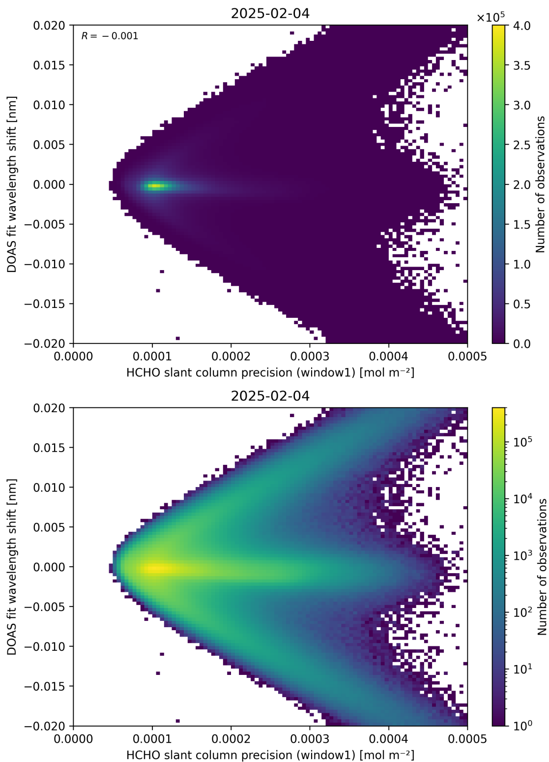
Figure 89: Scatter density plot of “HCHO slant column precision (window1)” against “DOAS fit wavelength shift” for 2025-02-03 to 2025-02-05.
