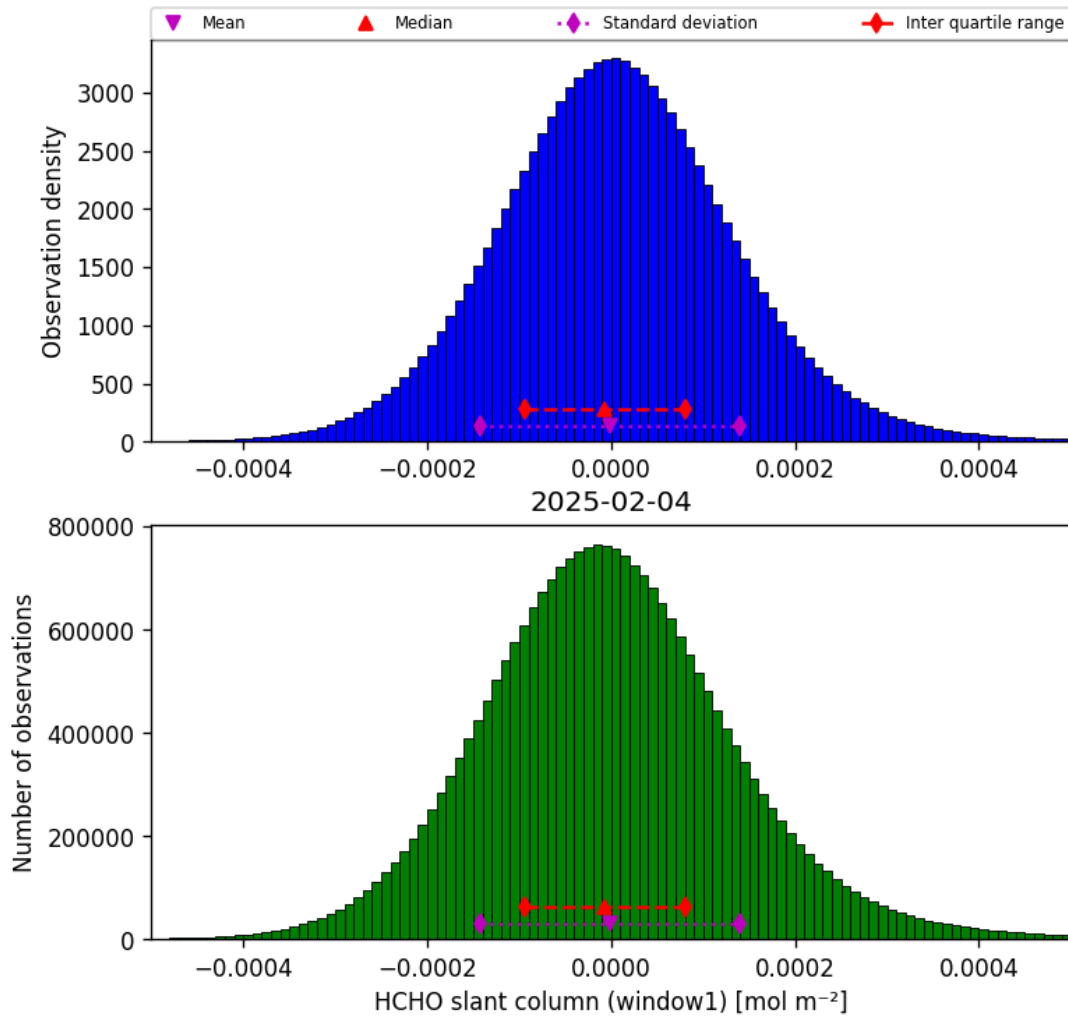
Figure 38: Histogram of “HCHO slant column (window1)” for 2025-02-03 to 2025-02-05
