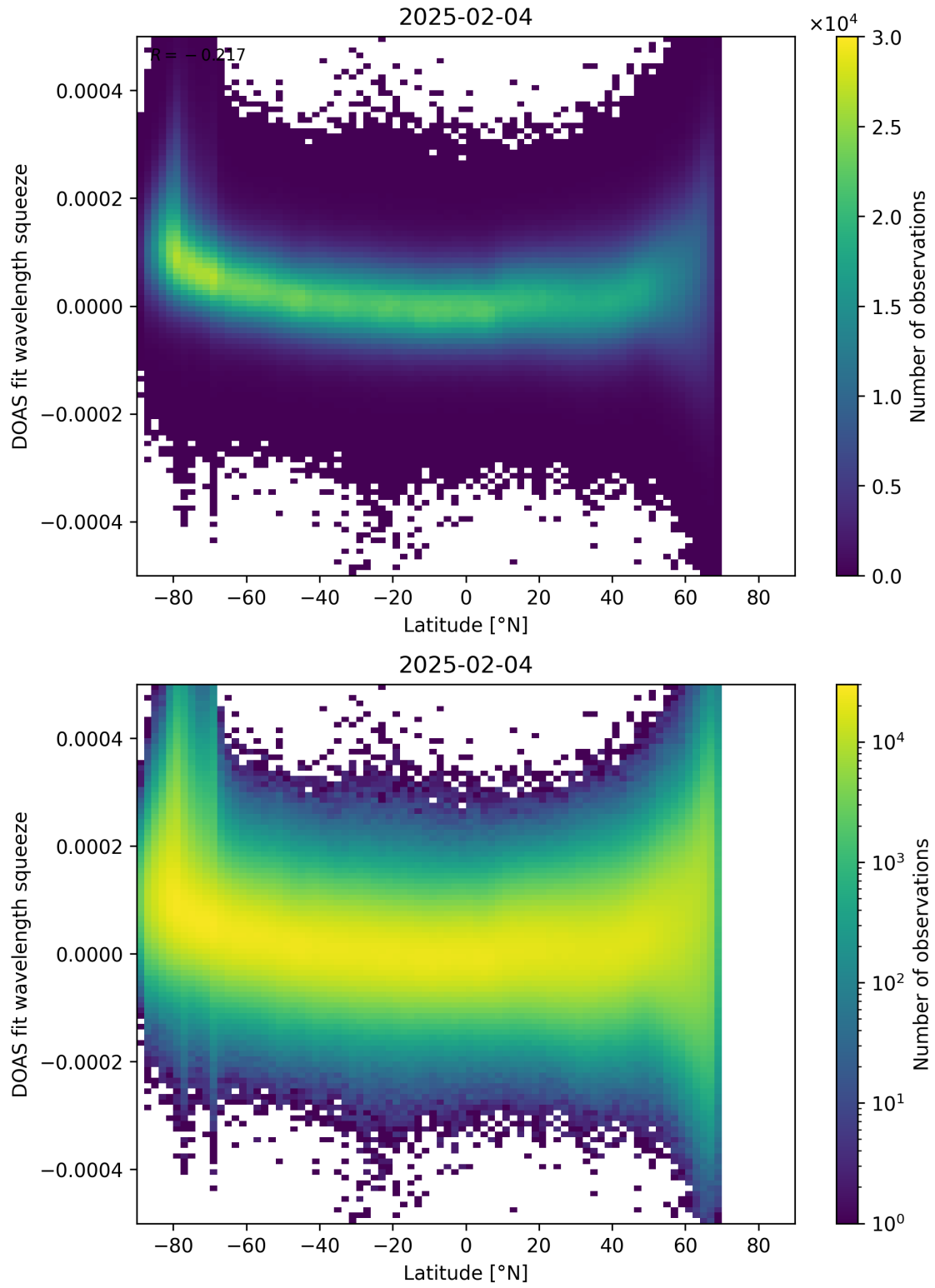
Figure 155: Scatter density plot of “Latitude” against “DOAS fit wavelength squeeze” for 2025-02-03 to 2025-02-05.
