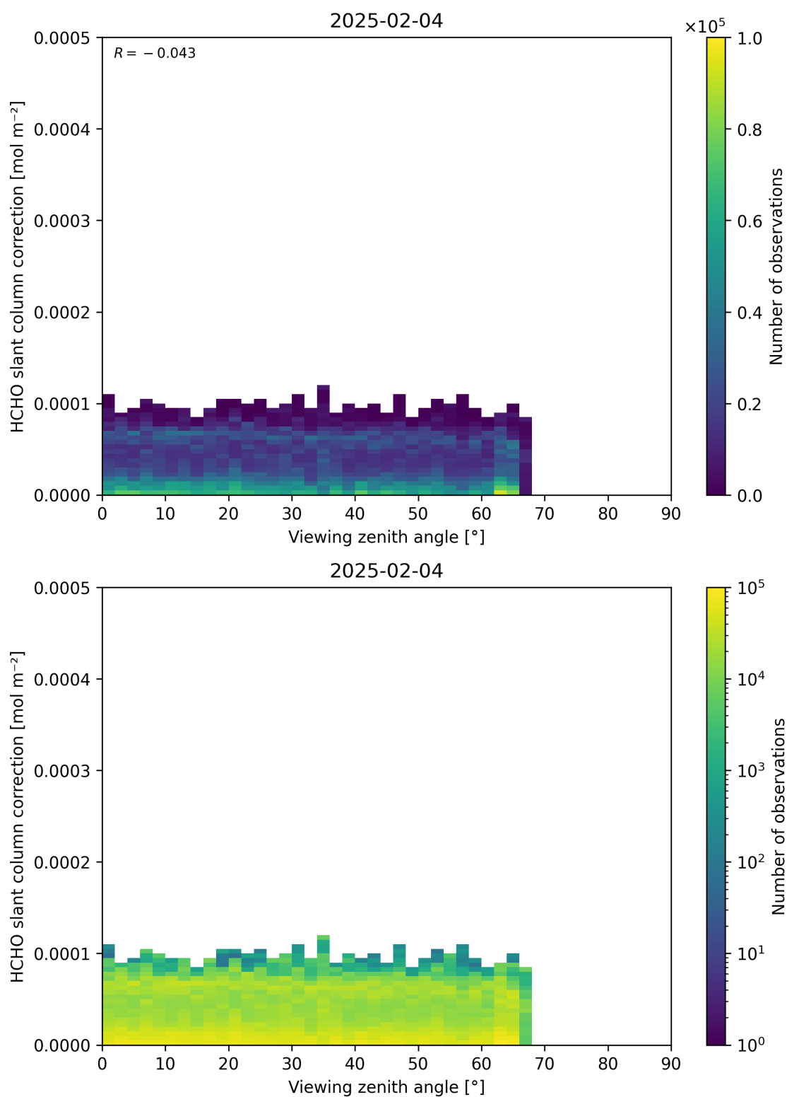
Figure 187: Scatter density plot of “Viewing zenith angle” against “HCHO slant column correction” for 2025-02-03 to 2025-02-05.
