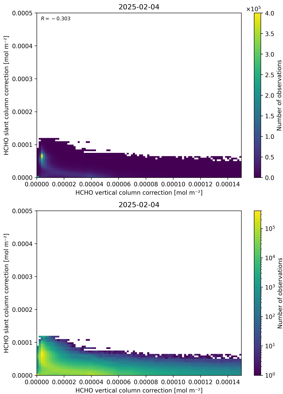
Figure 117: Scatter density plot of “HCHO vertical column correction” against “HCHO slant column correction” for 2025-02-03 to 2025-02-05.
