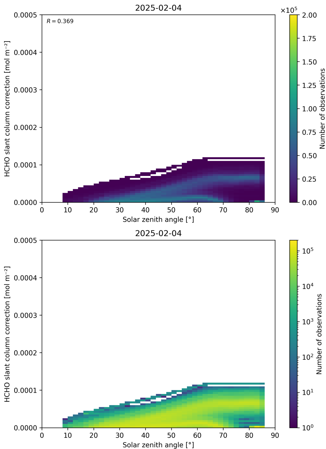
Figure 172: Scatter density plot of “Solar zenith angle” against “HCHO slant column correction” for 2025-02-03 to 2025-02-05.
