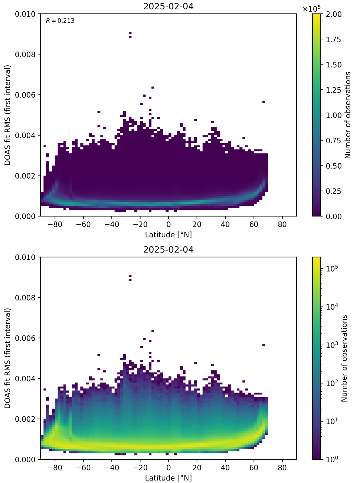
Figure 153: Scatter density plot of “Latitude” against “DOAS fit RMS (first interval)” for 2025-02-03 to 2025-02-05.
