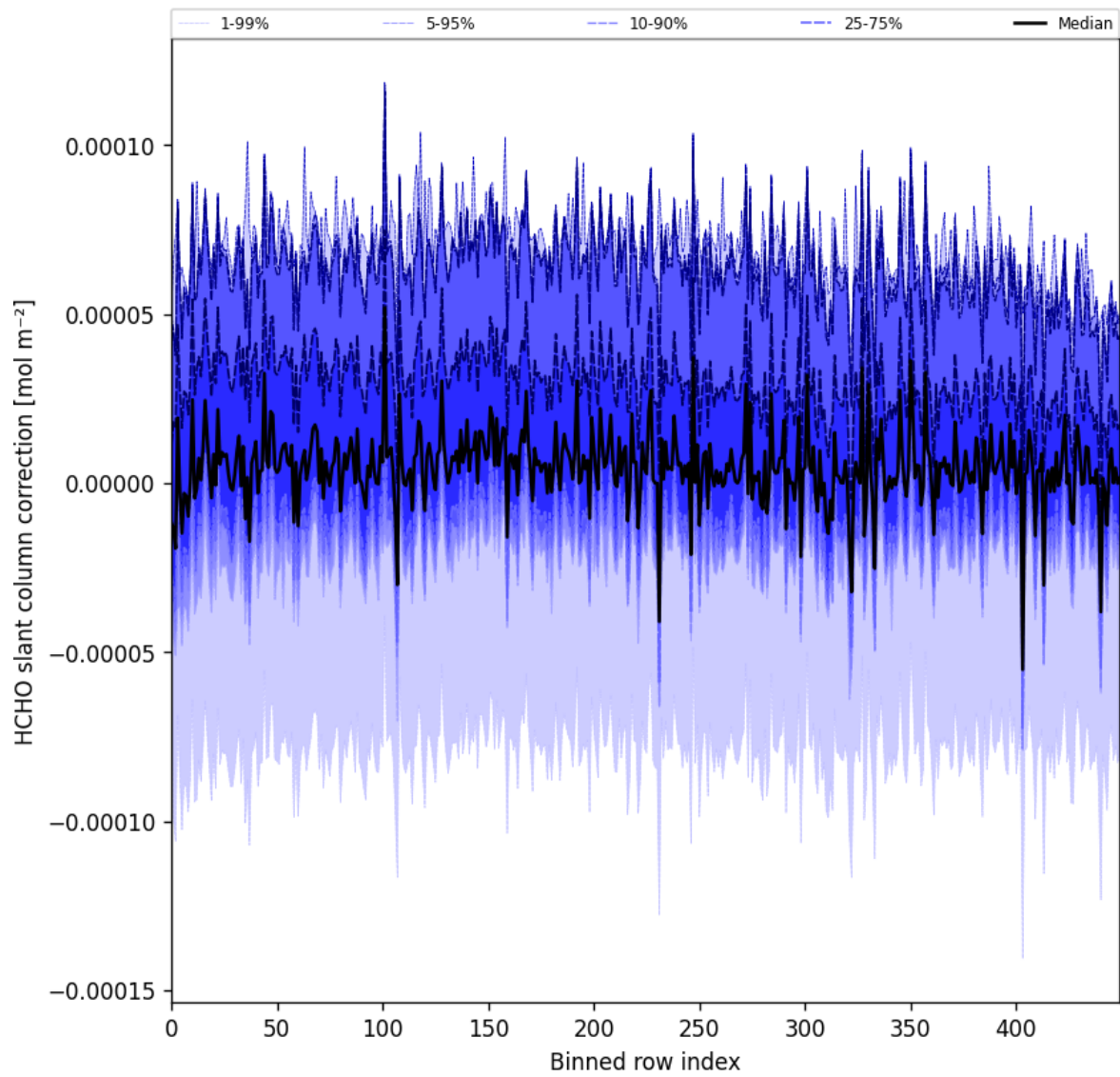
Figure 61: Along track statistics of “HCHO slant column correction” for 2025-02-03 to 2025-02-05
