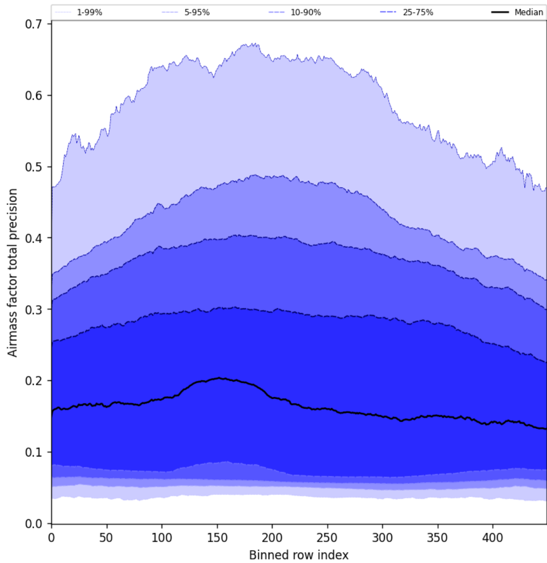
Figure 55: Along track statistics of “Airmass factor total precision” for 2025-02-03 to 2025-02-05
