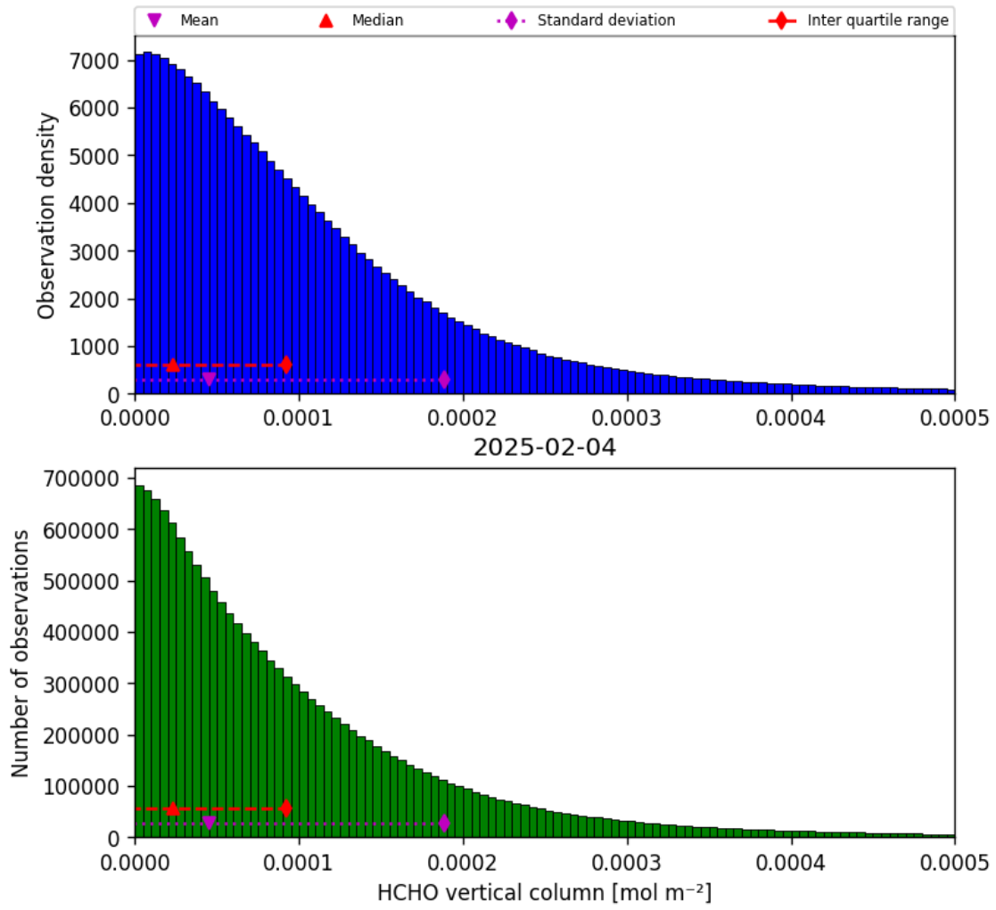
Figure 35: Histogram of “HCHO vertical column” for 2025-02-03 to 2025-02-05
