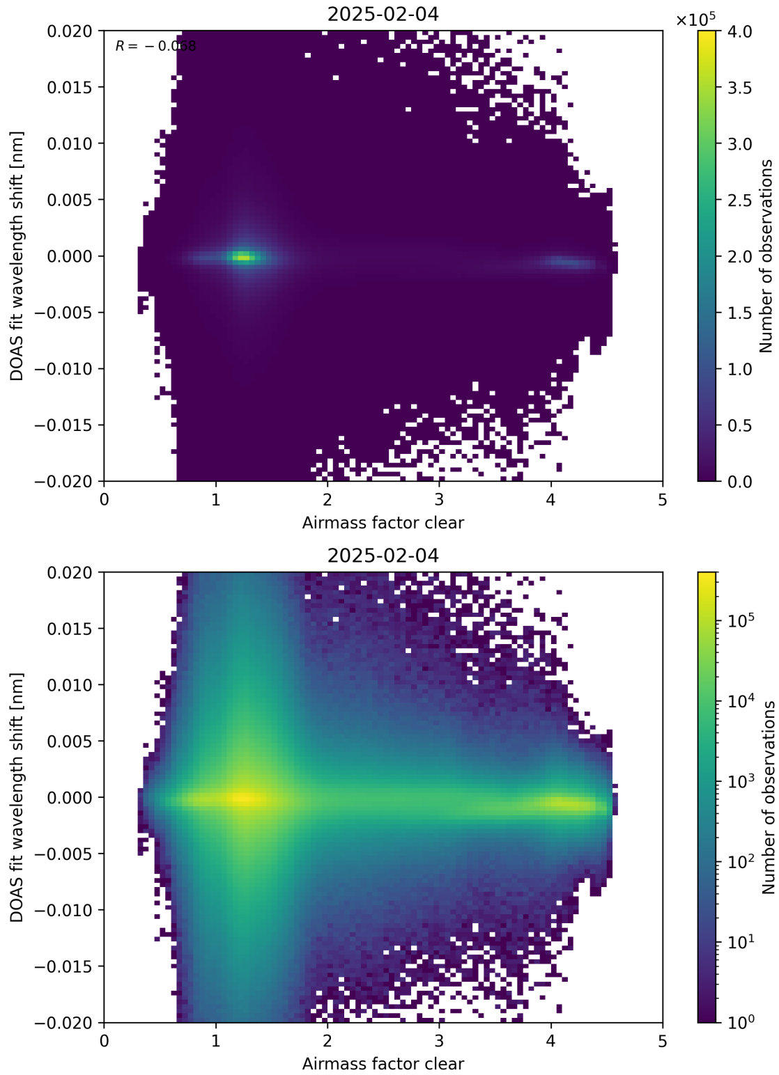
Figure 72: Scatter density plot of “Airmass factor clear” against “DOAS fit wavelength shift” for 2025-02-03 to 2025-02-05.
