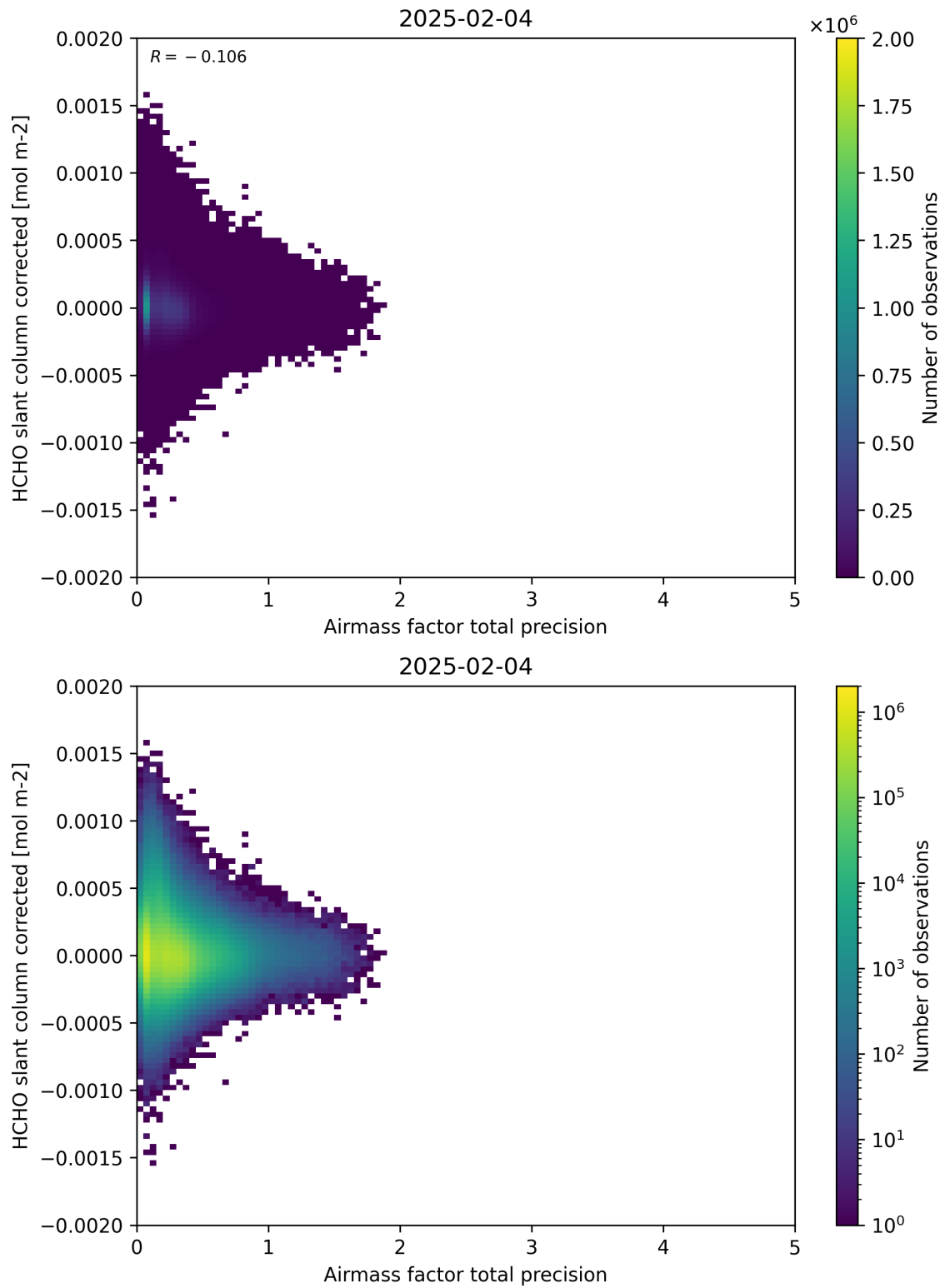
Figure 109: Scatter density plot of “Airmass factor total precision” against “HCHO slant column corrected” for 2025-02-03 to 2025-02-05.
