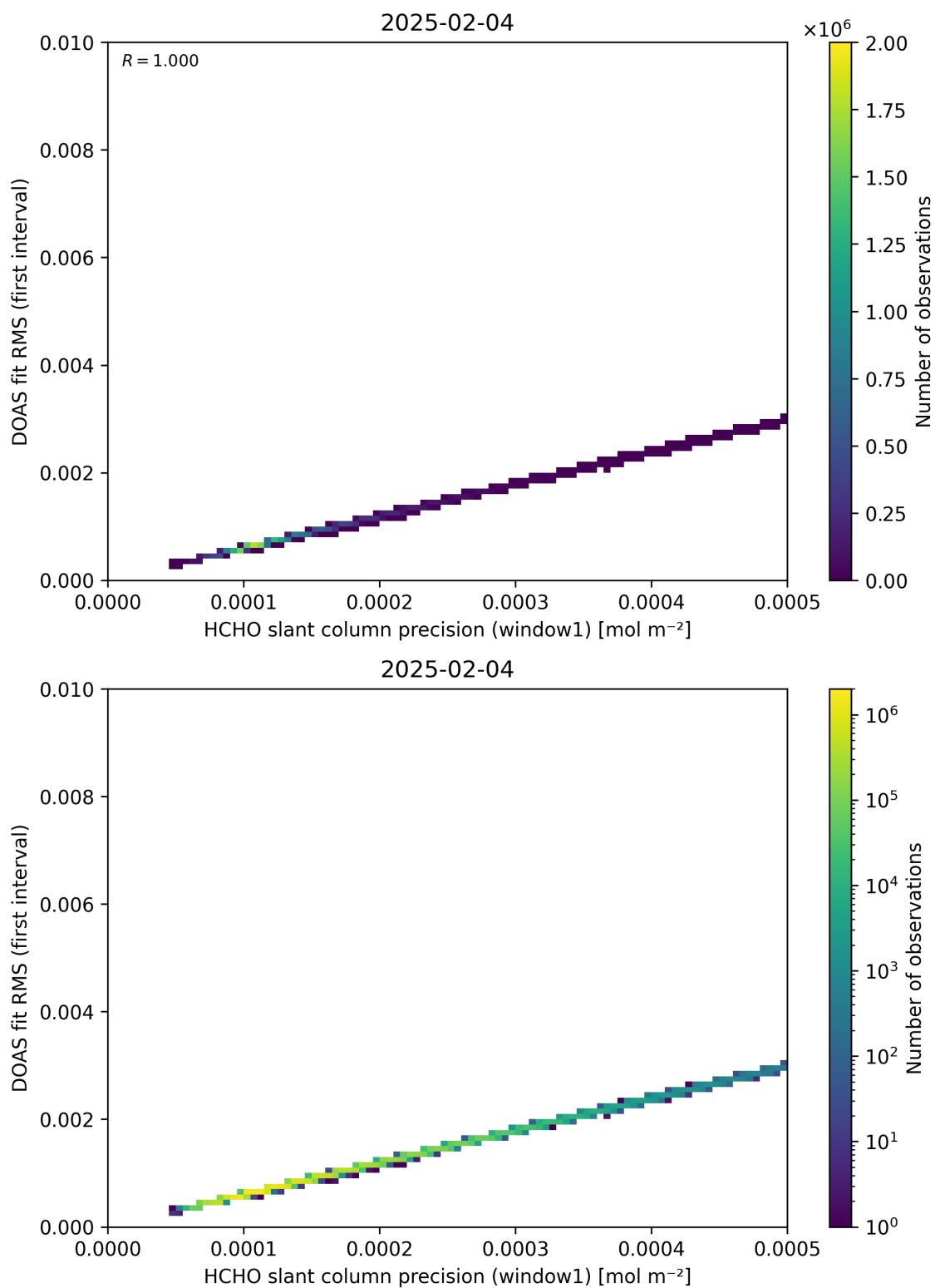
Figure 88: Scatter density plot of “HCHO slant column precision (window1)” against “DOAS fit RMS (first interval)” for 2025-02-03 to 2025-02-05.
