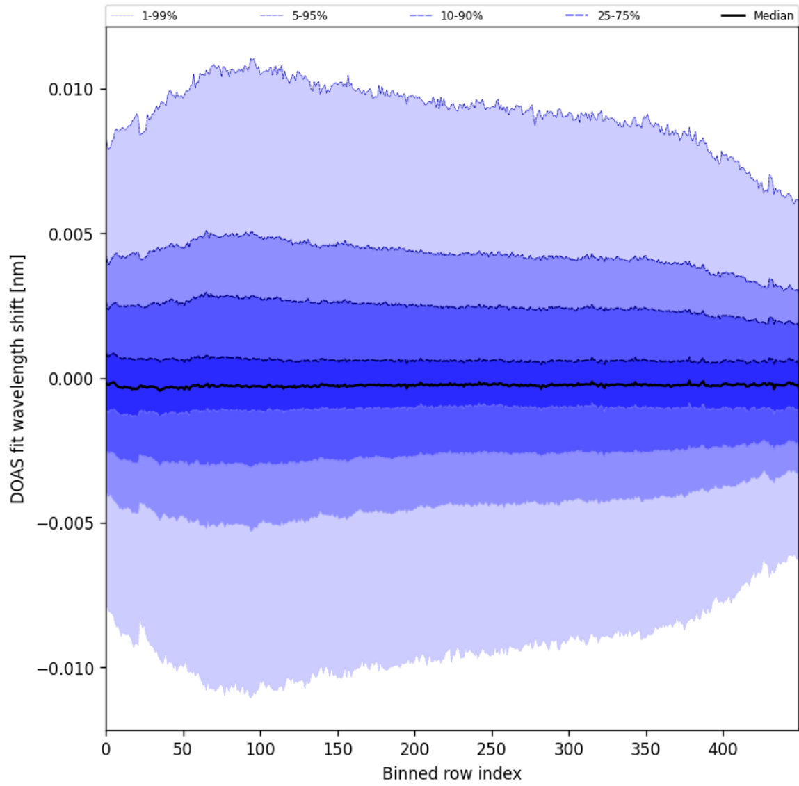
Figure 58: Along track statistics of “DOAS fit wavelength shift” for 2025-02-03 to 2025-02-05
