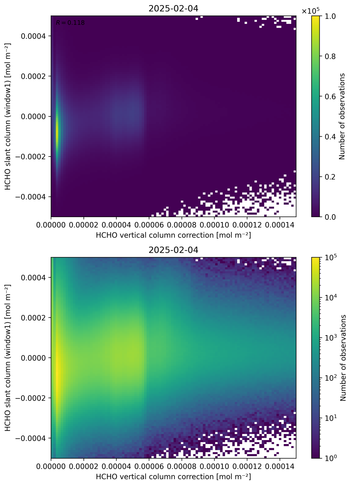
Figure 118: Scatter density plot of “HCHO vertical column correction” against “HCHO slant column (window1)” for 2025-02-03 to 2025-02-05.
