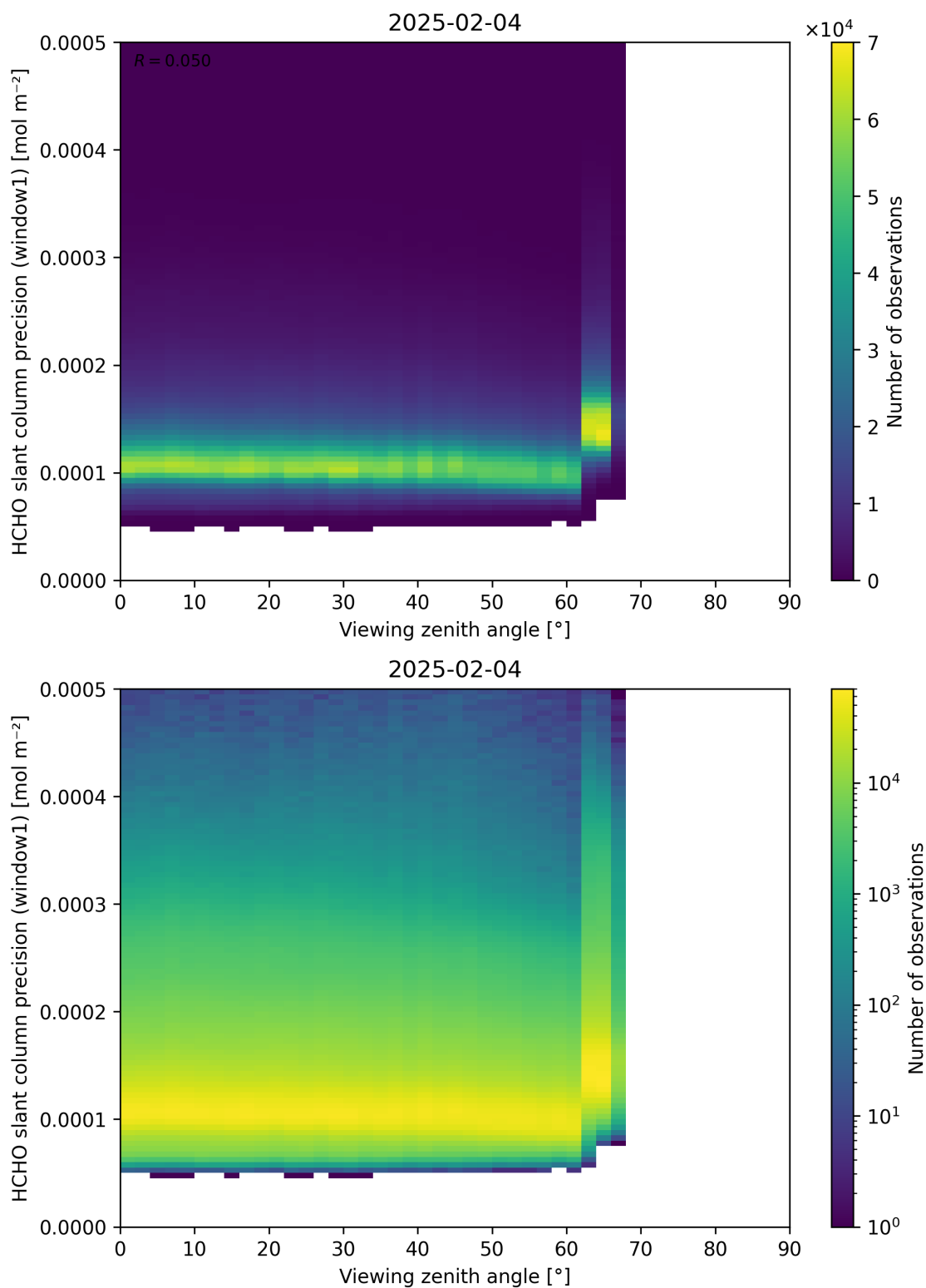
Figure 189: Scatter density plot of “Viewing zenith angle” against “HCHO slant column precision (window1)” for 2025-02-03 to 2025-02-05.
