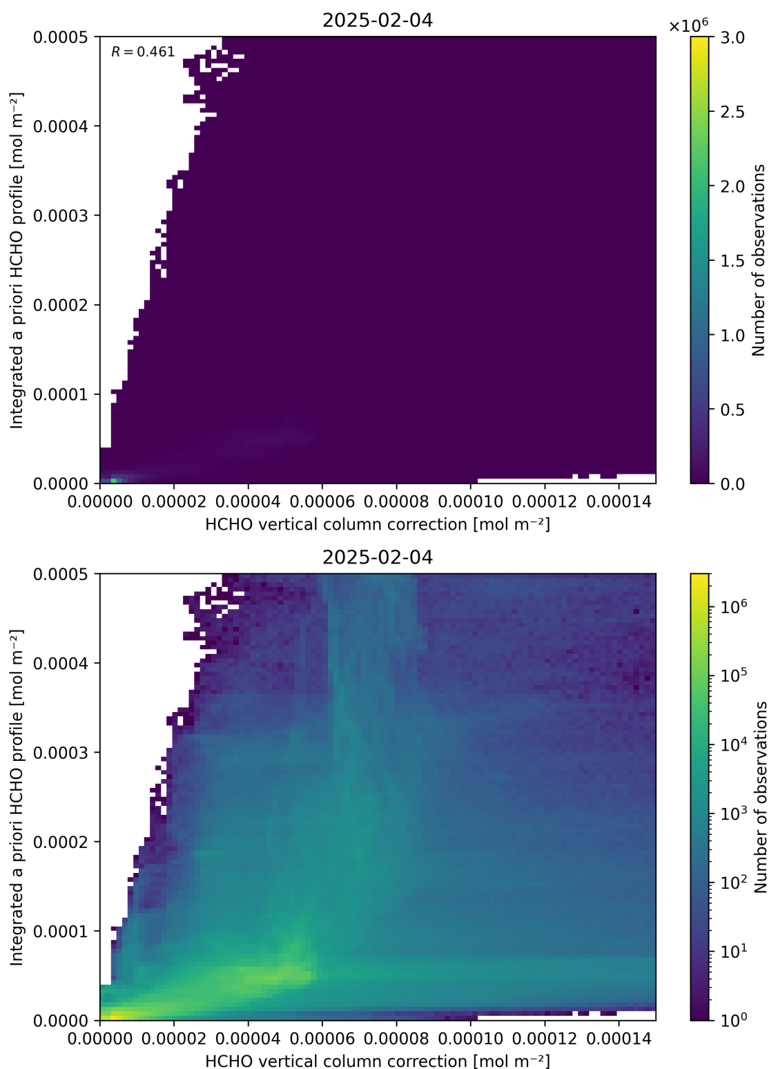
Figure 122: Scatter density plot of “HCHO vertical column correction” against “Integrated a priori HCHO profile” for 2025-02-03 to 2025-02-05.
