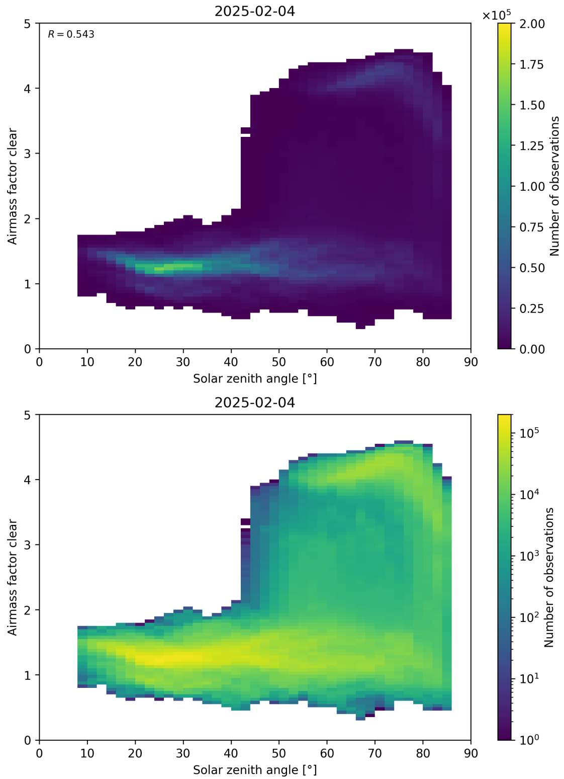
Figure 170: Scatter density plot of “Solar zenith angle” against “Airmass factor clear” for 2025-02-03 to 2025-02-05.
