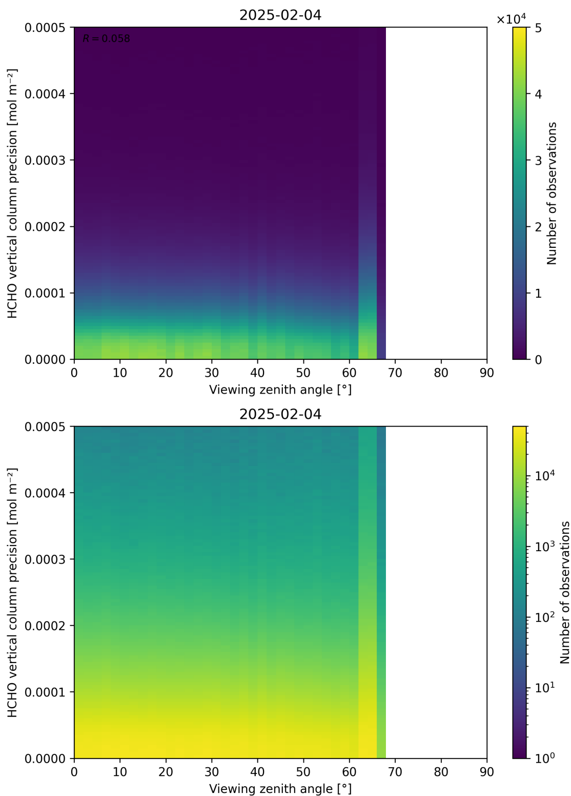
Figure 194: Scatter density plot of “Viewing zenith angle” against “HCHO vertical column precision” for 2025-02-03 to 2025-02-05.
