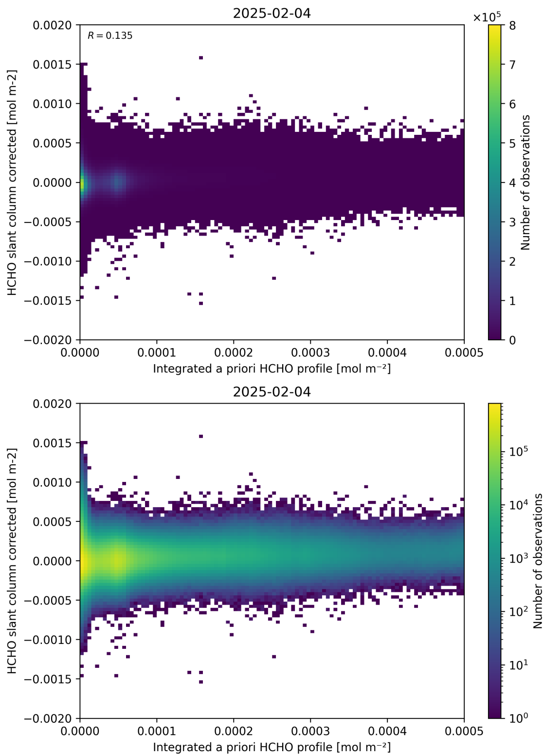
Figure 151: Scatter density plot of “Integrated a priori HCHO profile” against “HCHO slant column corrected” for 2025-02-03 to 2025-02-05.
