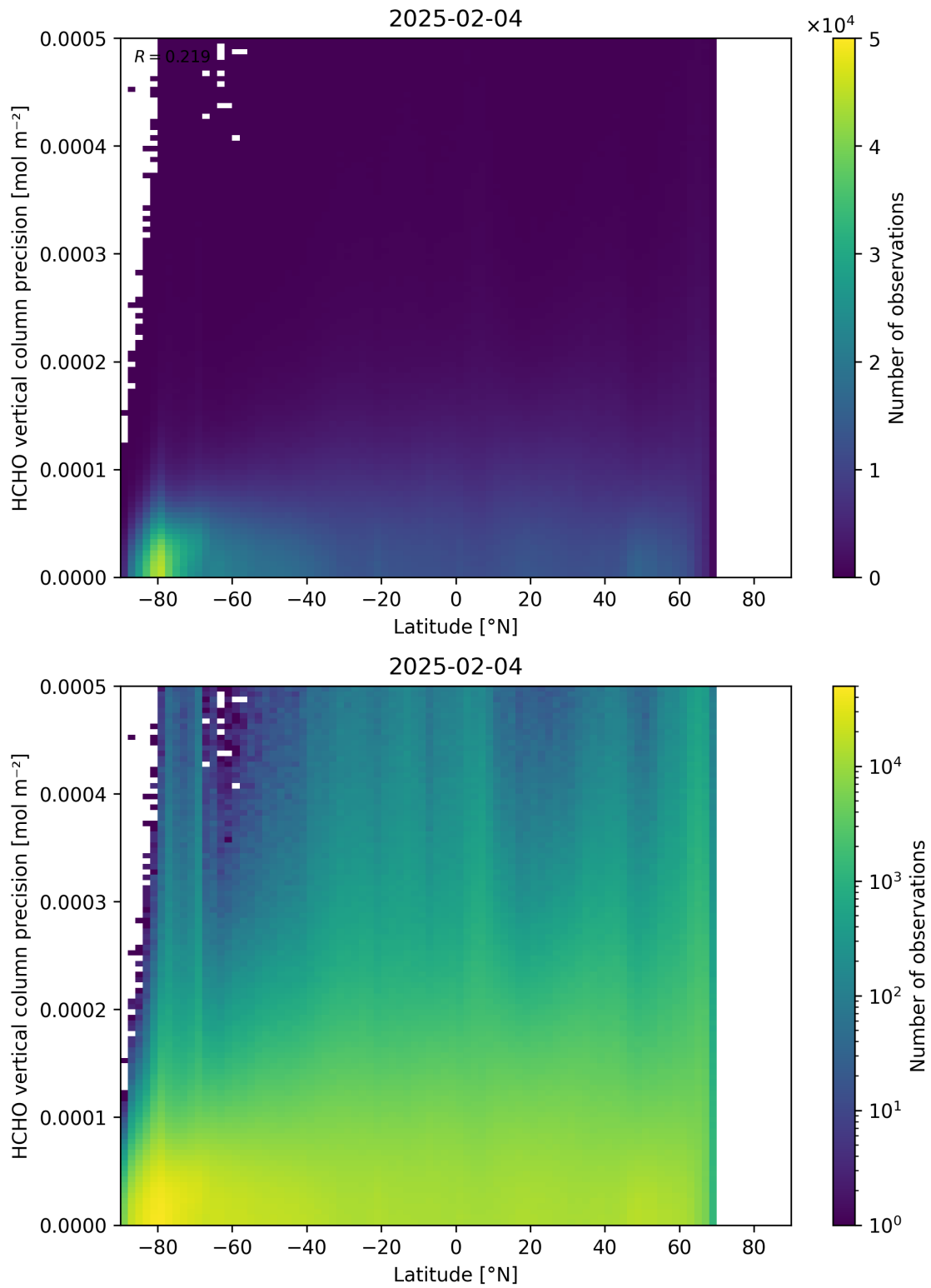
Figure 165: Scatter density plot of “Latitude” against “HCHO vertical column precision” for 2025-02-03 to 2025-02-05.
