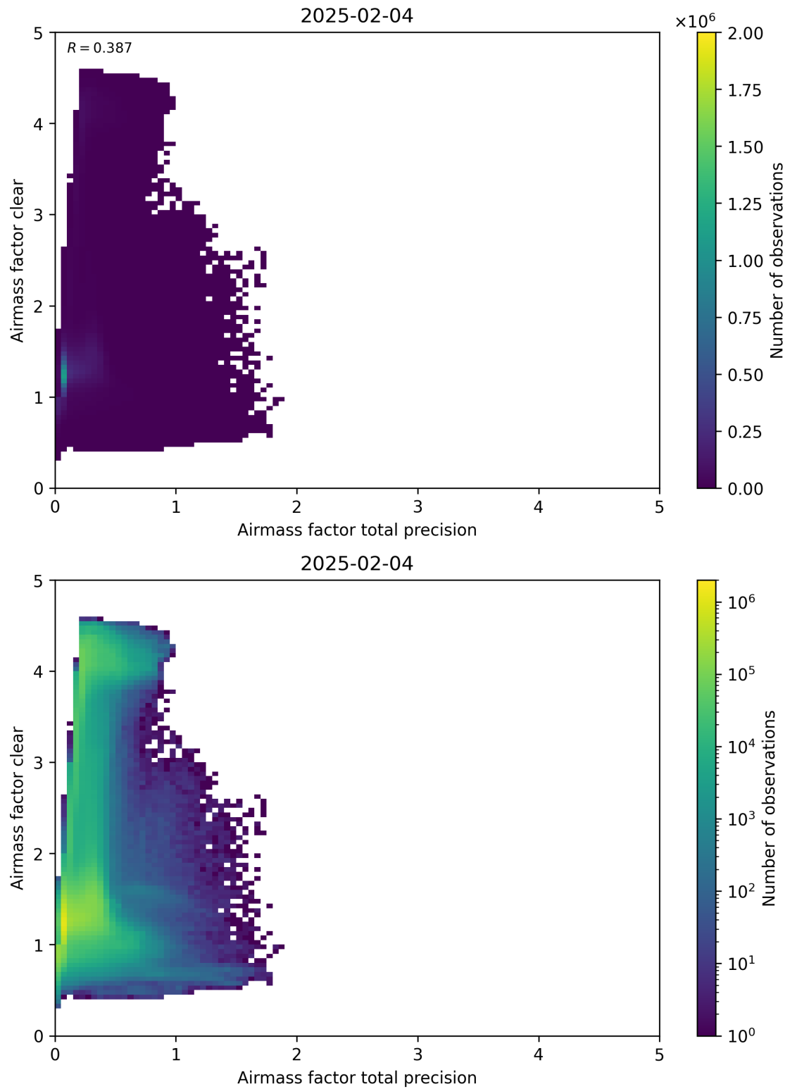
Figure 108: Scatter density plot of “Airmass factor total precision” against “Airmass factor clear” for 2025-02-03 to 2025-02-05.
