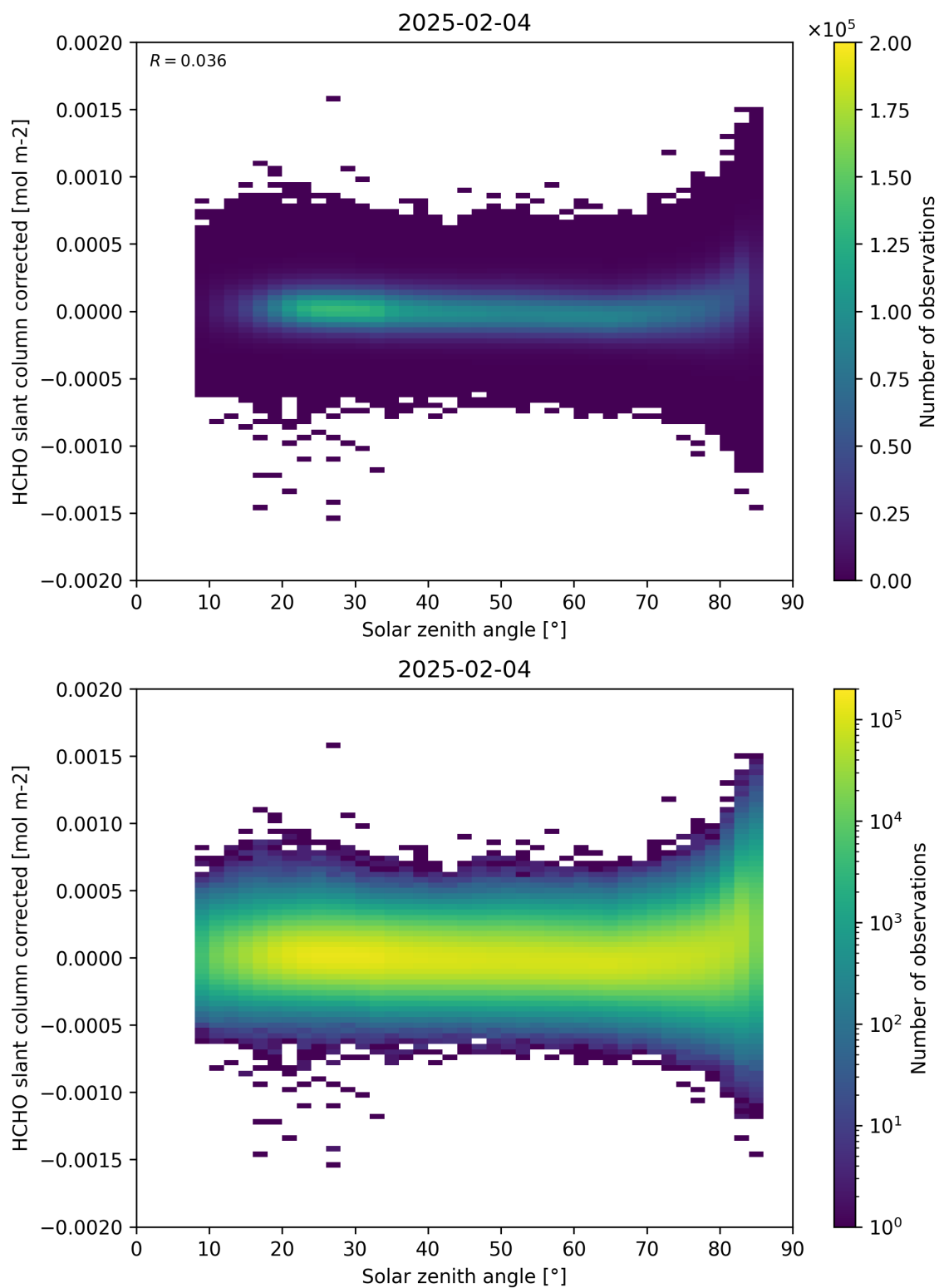
Figure 171: Scatter density plot of “Solar zenith angle” against “HCHO slant column corrected” for 2025-02-03 to 2025-02-05.
