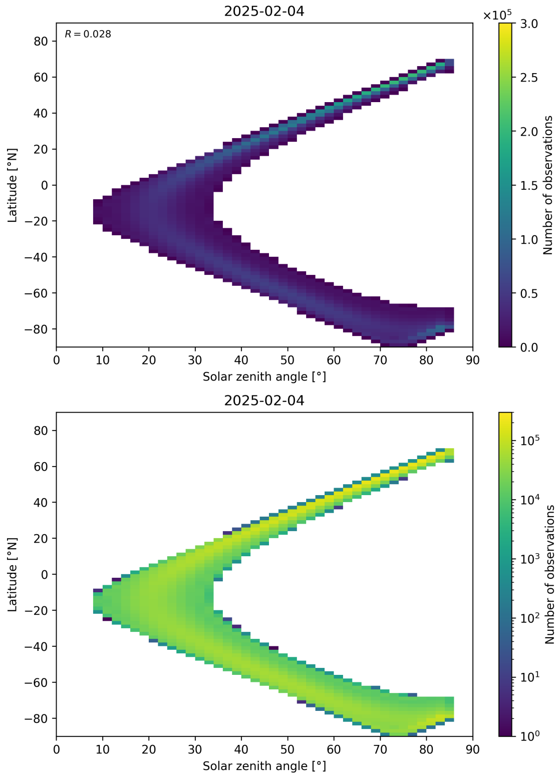
Figure 181: Scatter density plot of “Solar zenith angle” against “Latitude” for 2025-02-03 to 2025-02-05.
