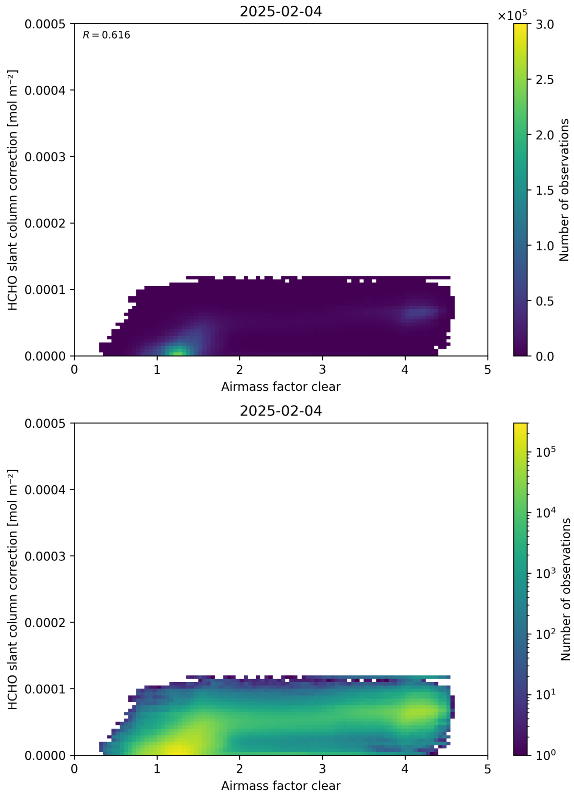
Figure 75: Scatter density plot of “Airmass factor clear” against “HCHO slant column correction” for 2025-02-03 to 2025-02-05.
