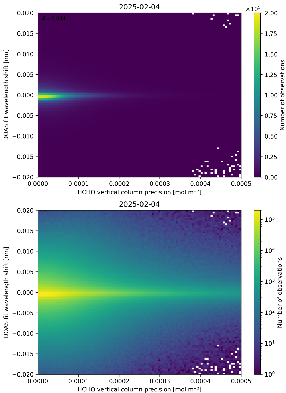
Figure 137: Scatter density plot of “HCHO vertical column precision” against “DOAS fit wavelength shift” for 2025-02-03 to 2025-02-05.
