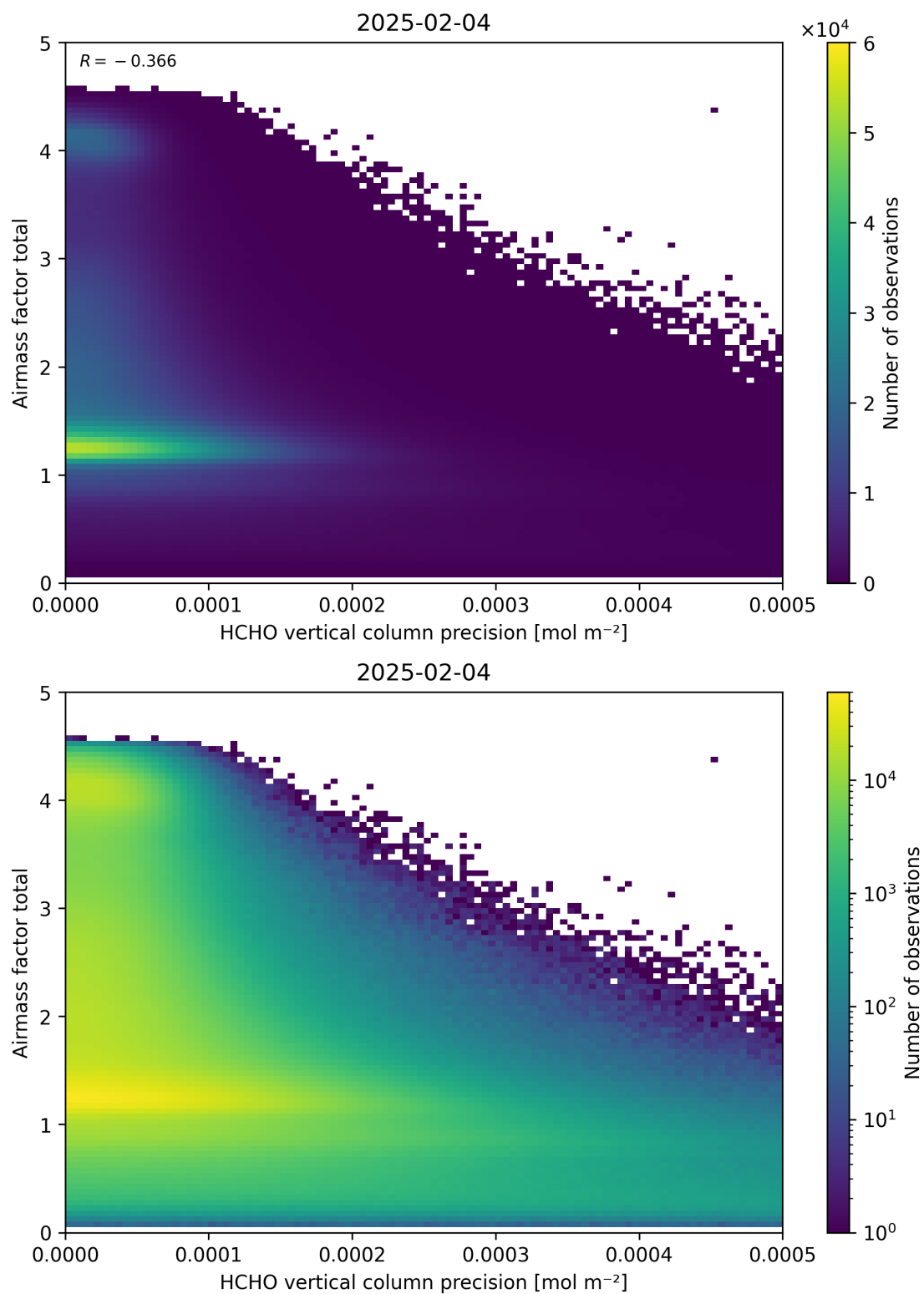
Figure 144: Scatter density plot of “HCHO vertical column precision” against “Airmass factor total” for 2025-02-03 to 2025-02-05.
