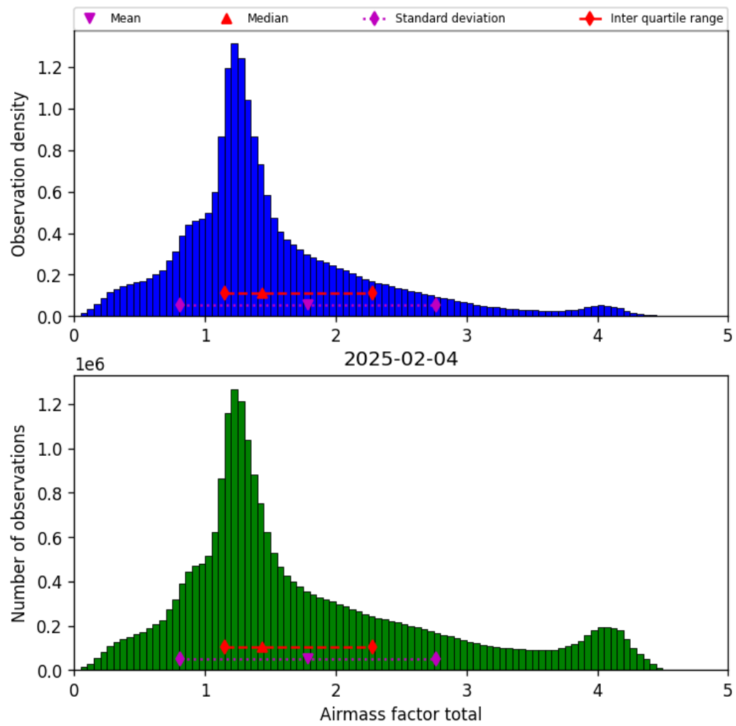
Figure 40: Histogram of “Airmass factor total” for 2025-02-03 to 2025-02-05
