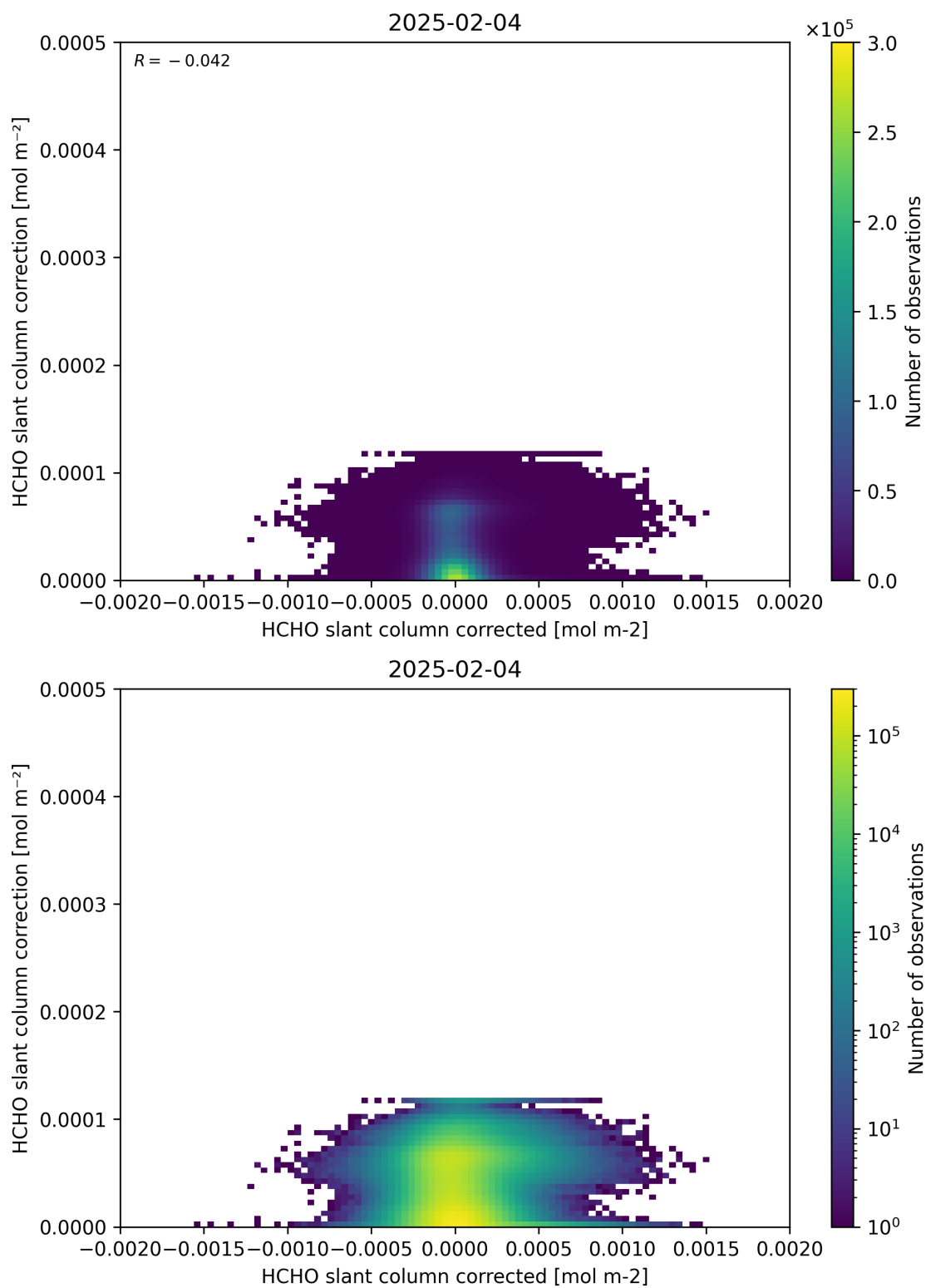
Figure 77: Scatter density plot of “HCHO slant column corrected” against “HCHO slant column correction” for 2025-02-03 to 2025-02-05.
