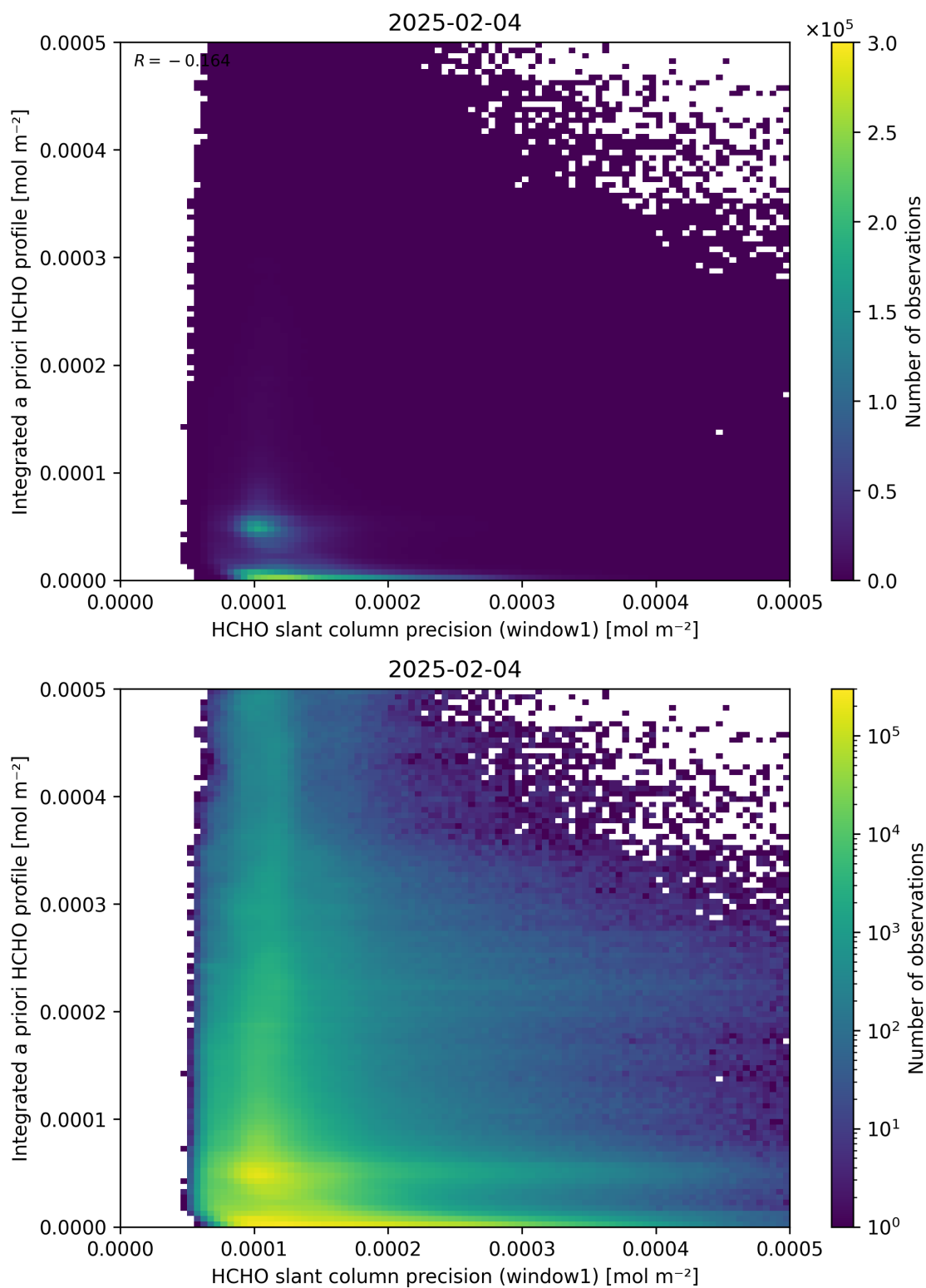
Figure 96: Scatter density plot of “HCHO slant column precision (window1)” against “Integrated a priori HCHO profile” for 2025-02-03 to 2025-02-05.
