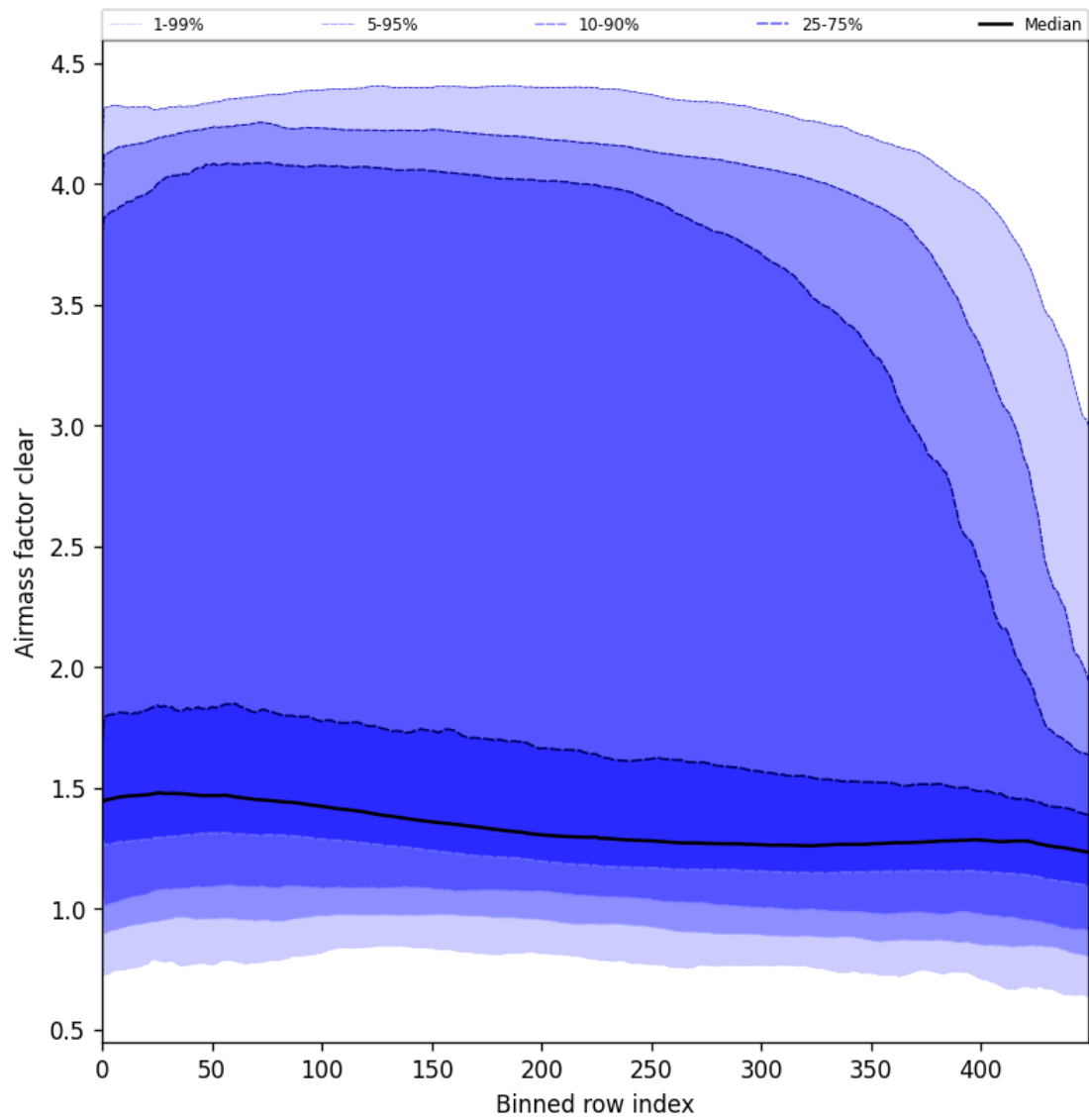
Figure 56: Along track statistics of “Airmass factor clear” for 2025-02-03 to 2025-02-05
