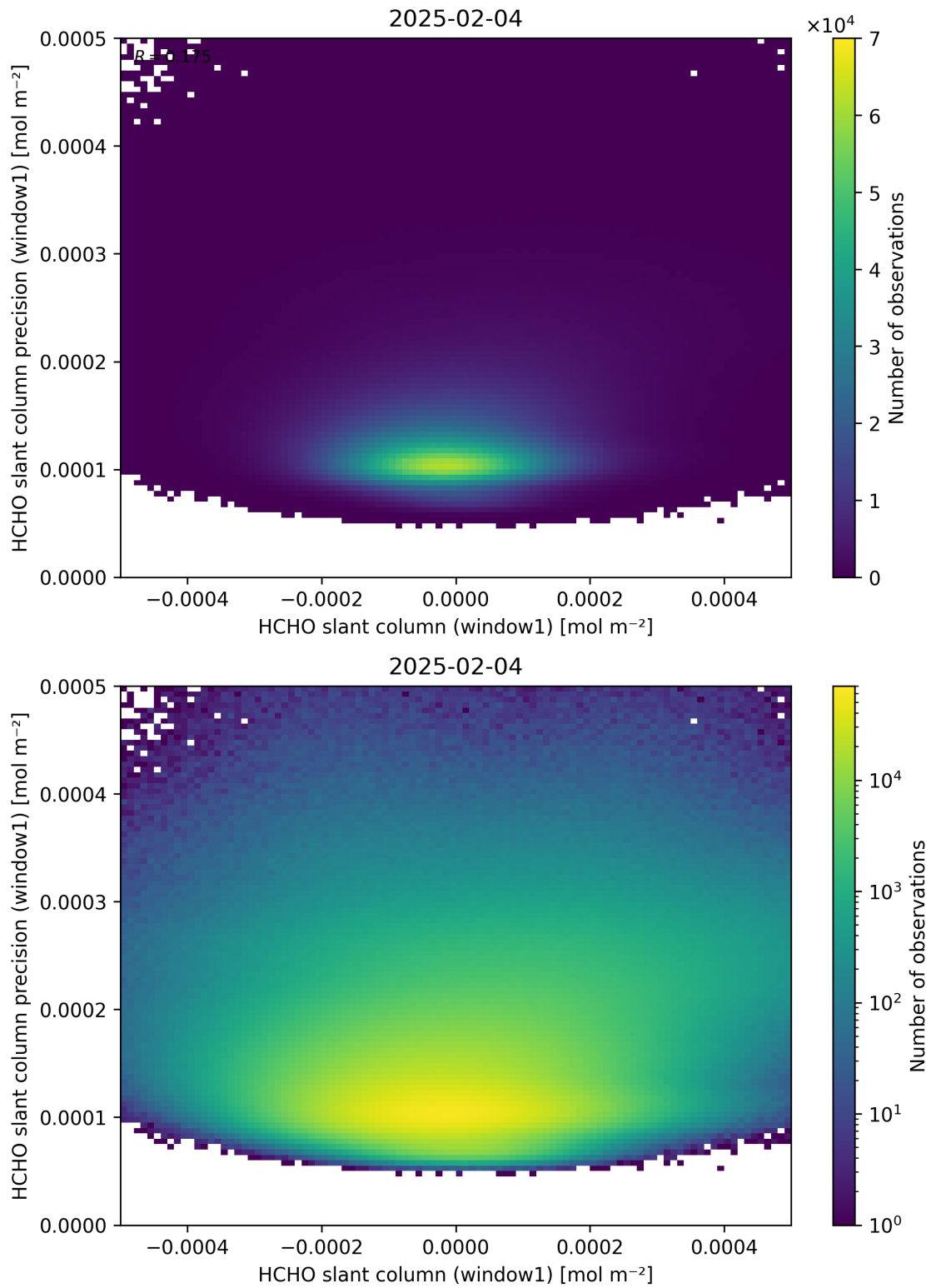
Figure 84: Scatter density plot of “HCHO slant column (window1)” against “HCHO slant column precision (window1)” for 2025-02-03 to 2025-02-05.
