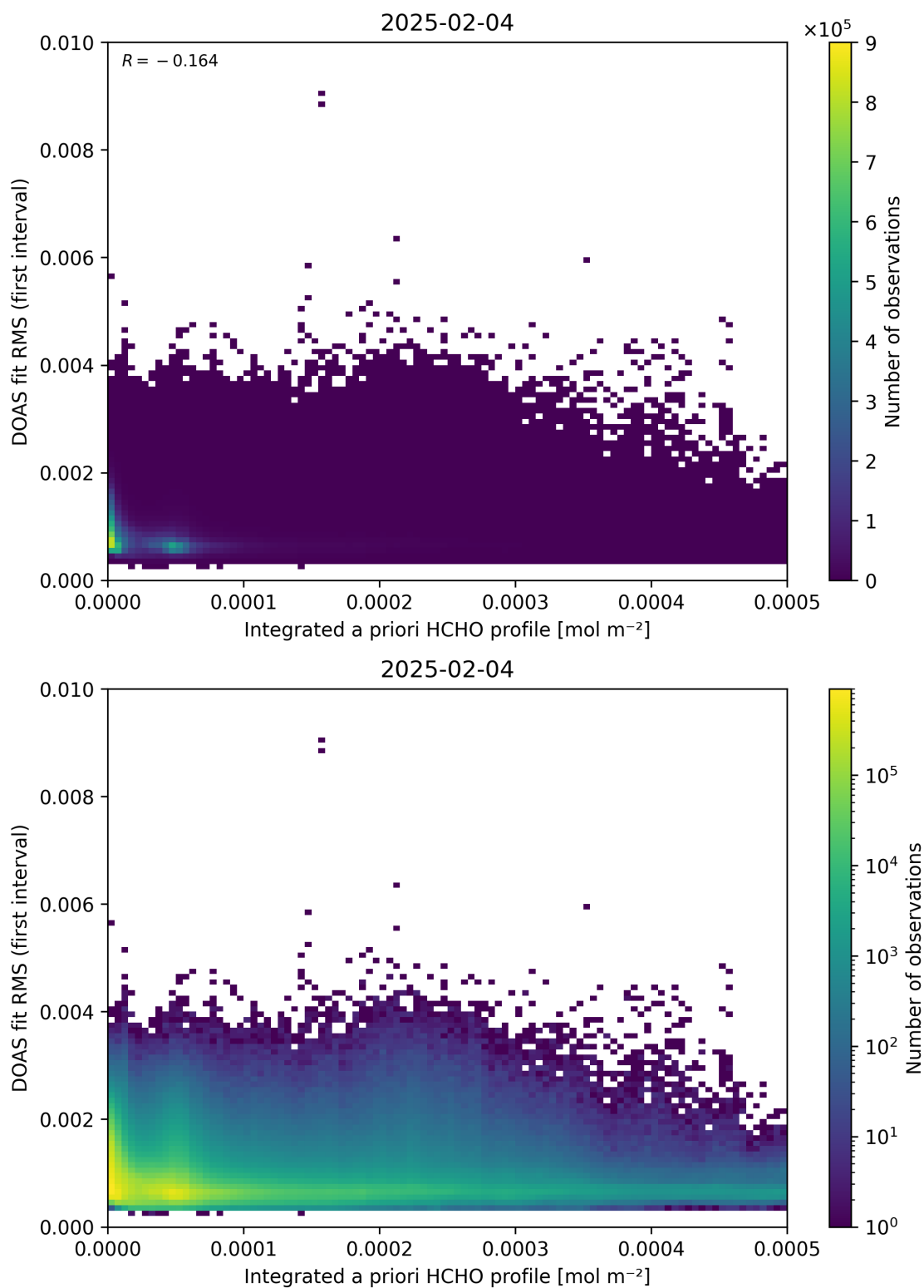
Figure 148: Scatter density plot of “Integrated a priori HCHO profile” against “DOAS fit RMS (first interval)” for 2025-02-03 to 2025-02-05.
