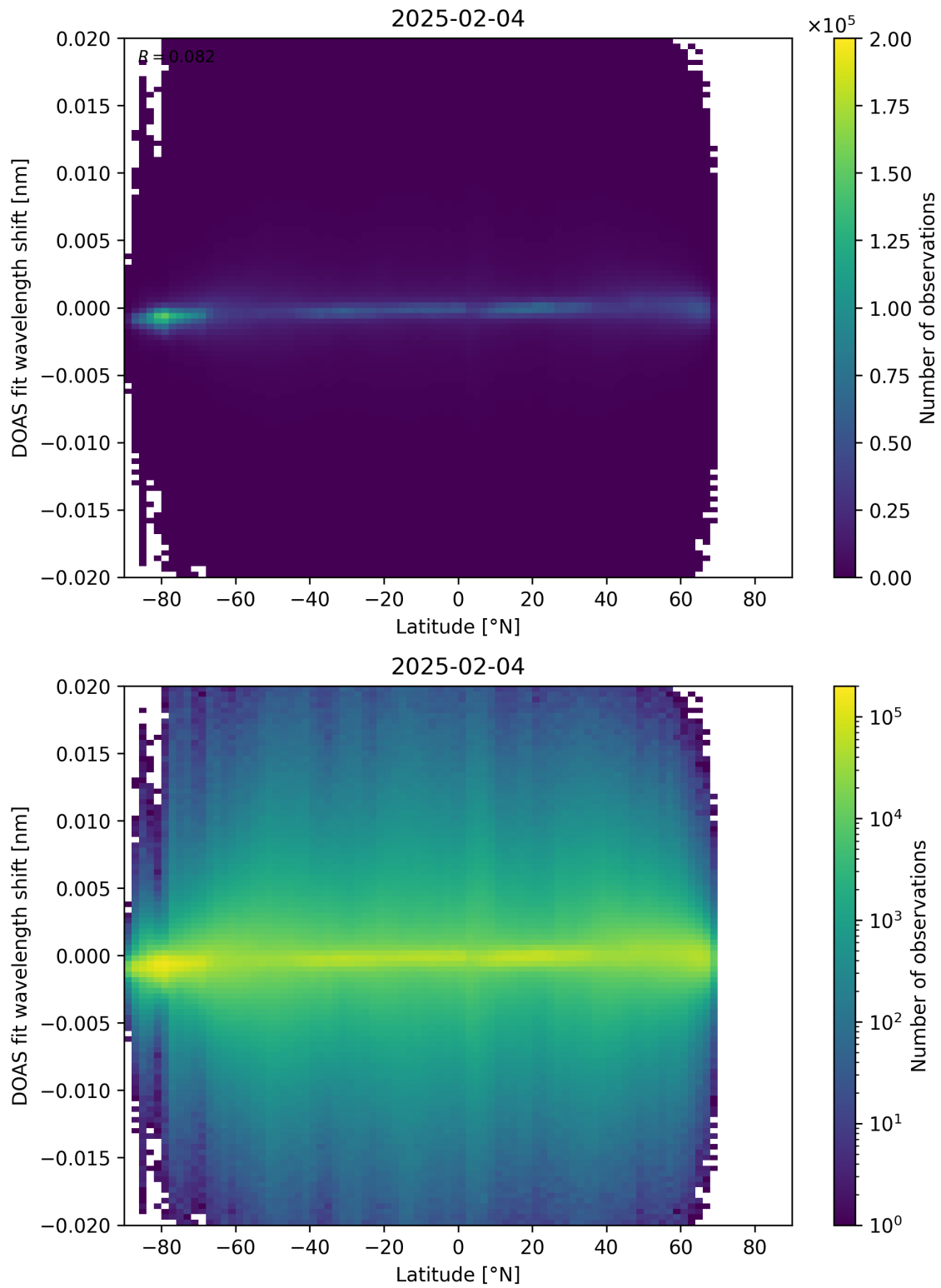
Figure 154: Scatter density plot of “Latitude” against “DOAS fit wavelength shift” for 2025-02-03 to 2025-02-05.
