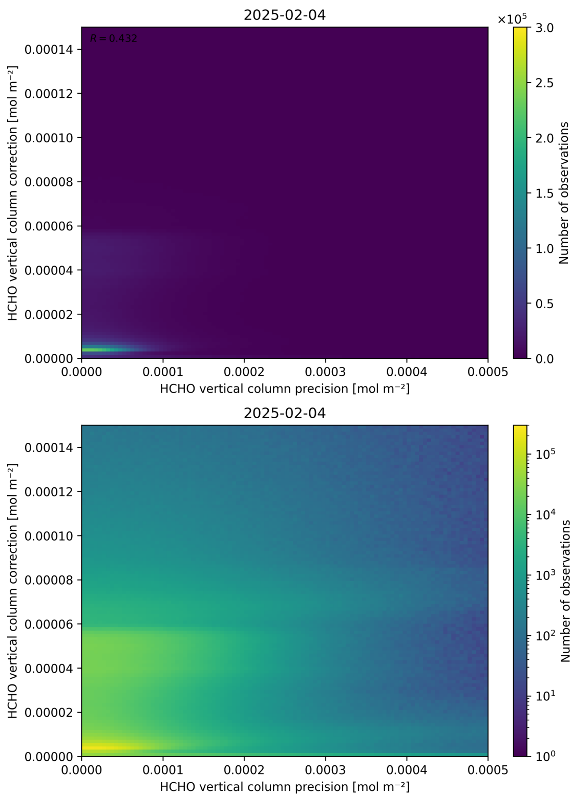
Figure 146: Scatter density plot of “HCHO vertical column precision” against “HCHO vertical column correction” for 2025-02-03 to 2025-02-05.
