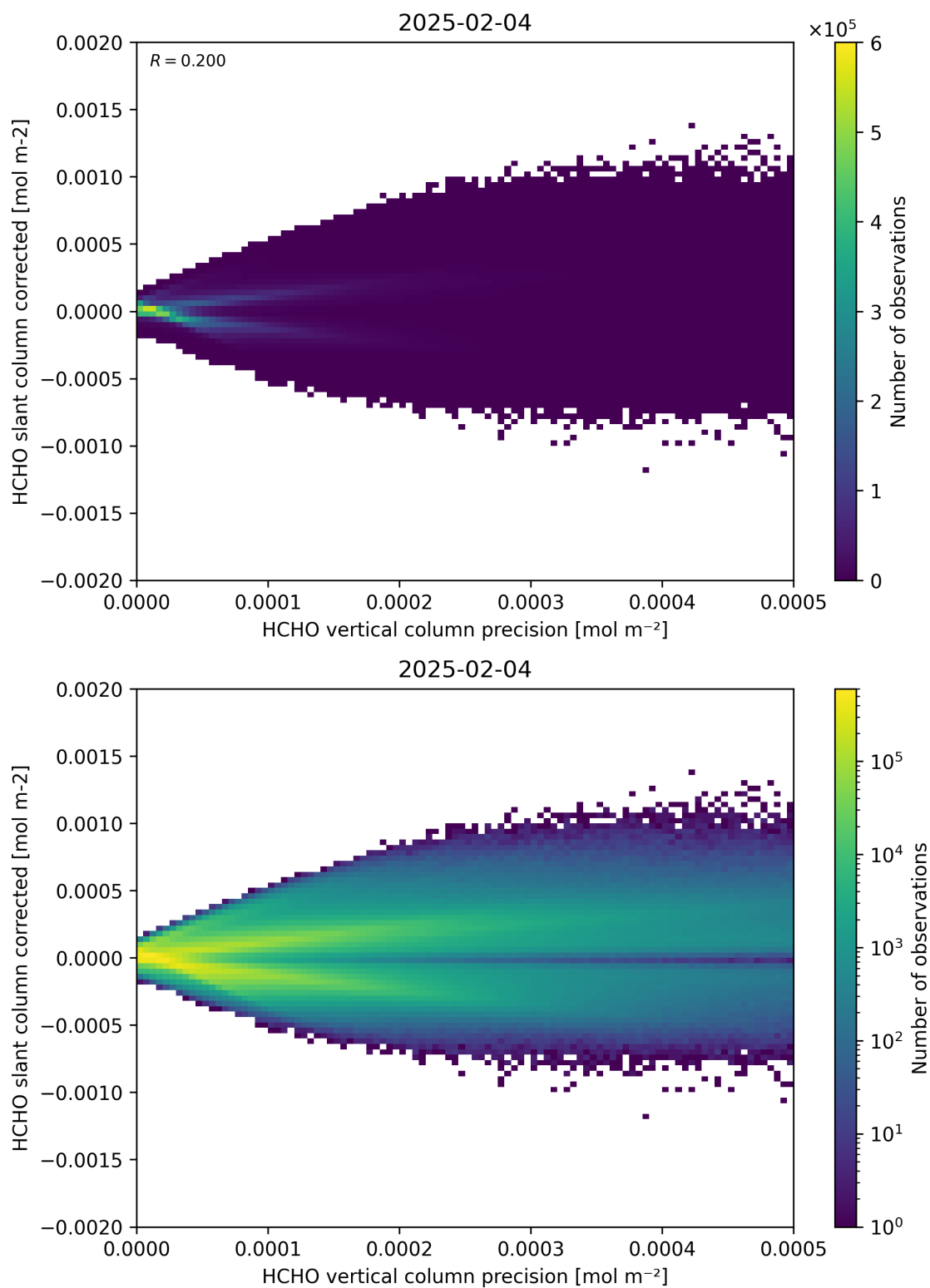
Figure 140: Scatter density plot of “HCHO vertical column precision” against “HCHO slant column corrected” for 2025-02-03 to 2025-02-05.
