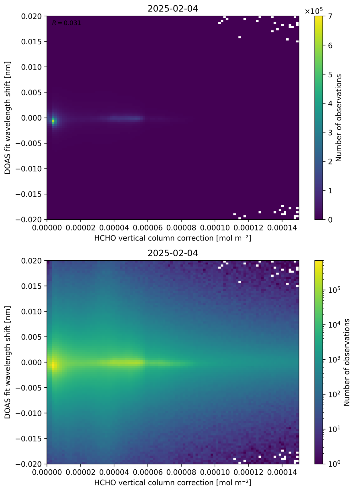
Figure 113: Scatter density plot of “HCHO vertical column correction” against “DOAS fit wavelength shift” for 2025-02-03 to 2025-02-05.
