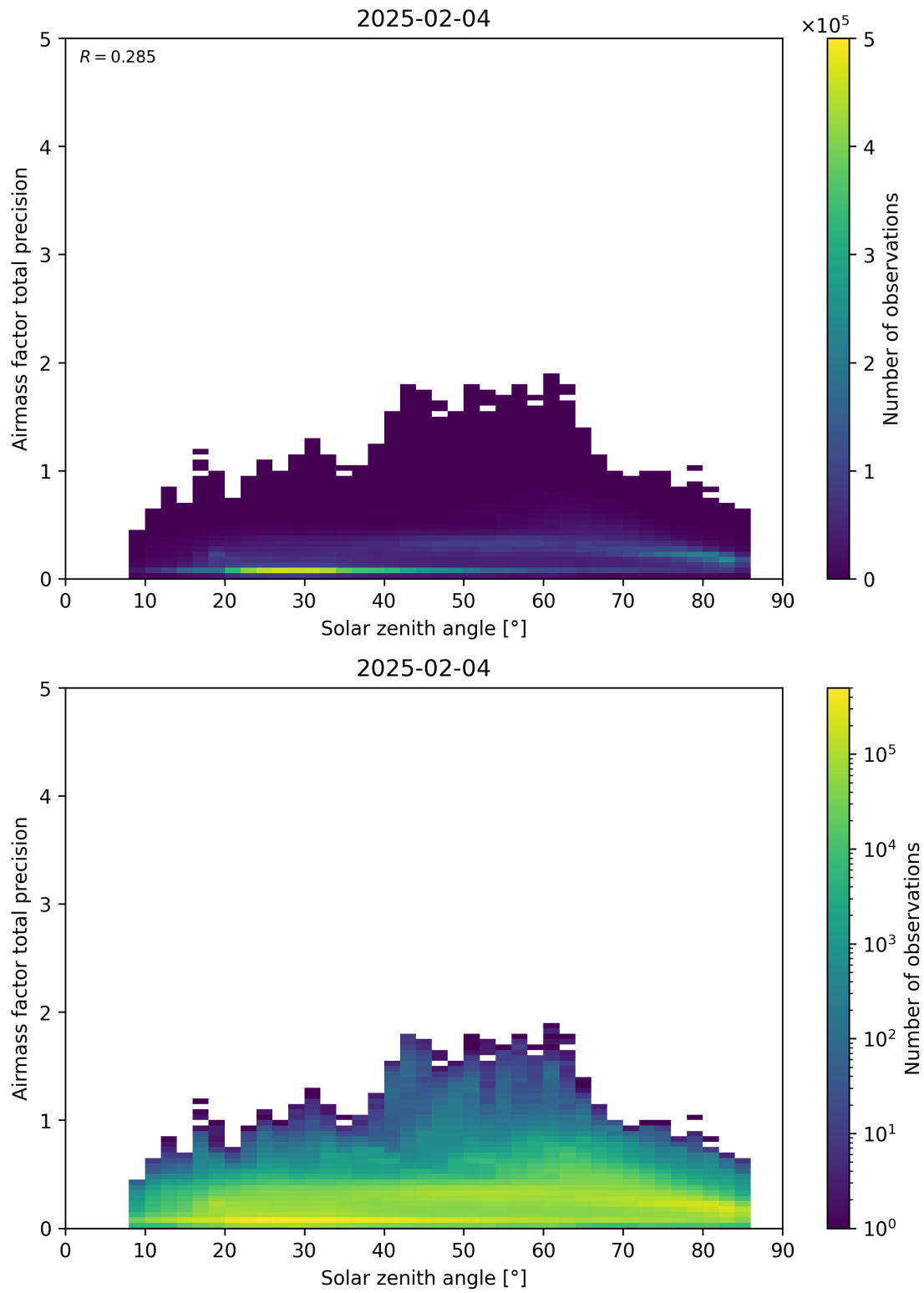
Figure 176: Scatter density plot of “Solar zenith angle” against “Airmass factor total precision” for 2025-02-03 to 2025-02-05.
