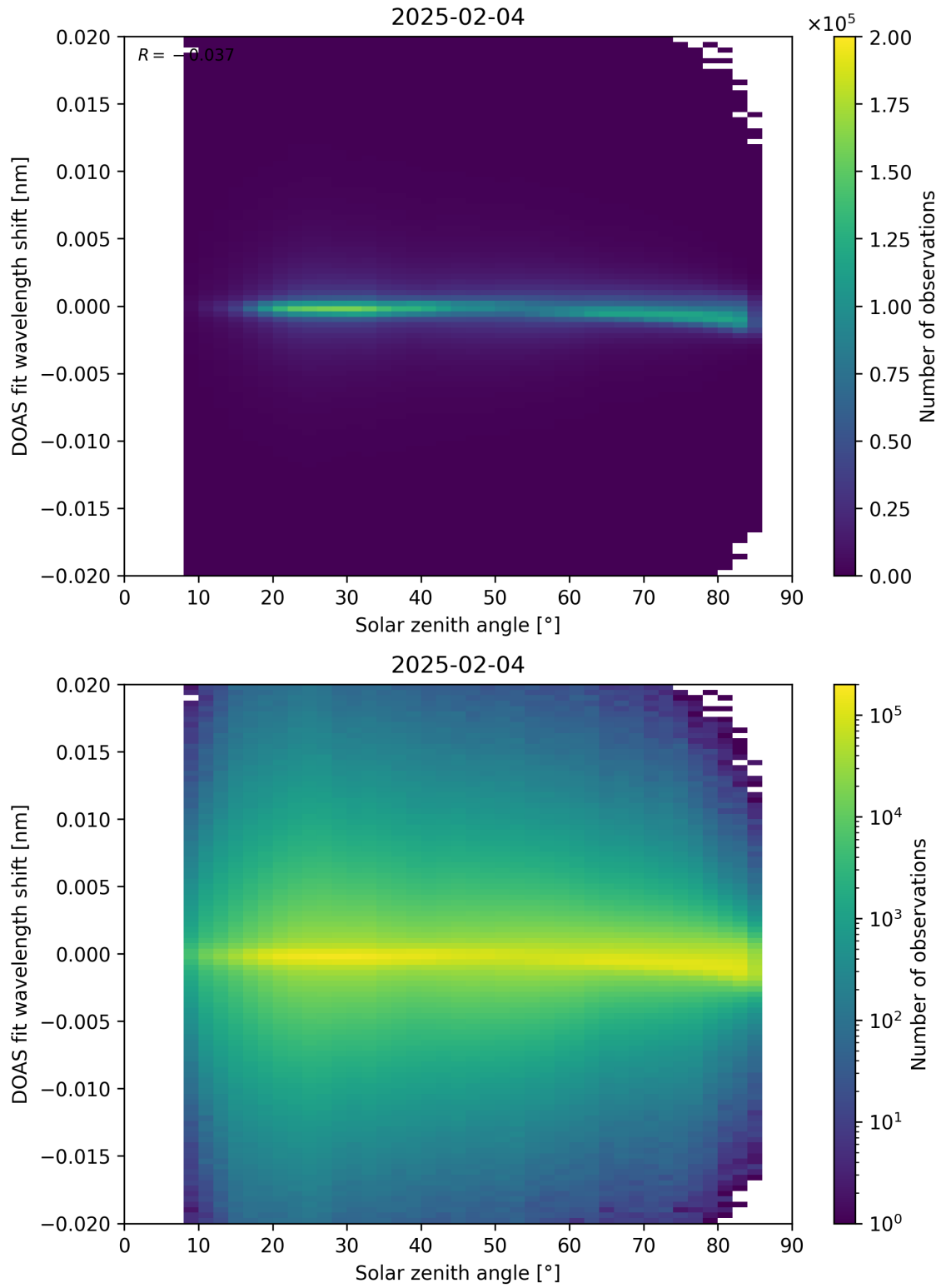
Figure 168: Scatter density plot of “Solar zenith angle” against “DOAS fit wavelength shift” for 2025-02-03 to 2025-02-05.
