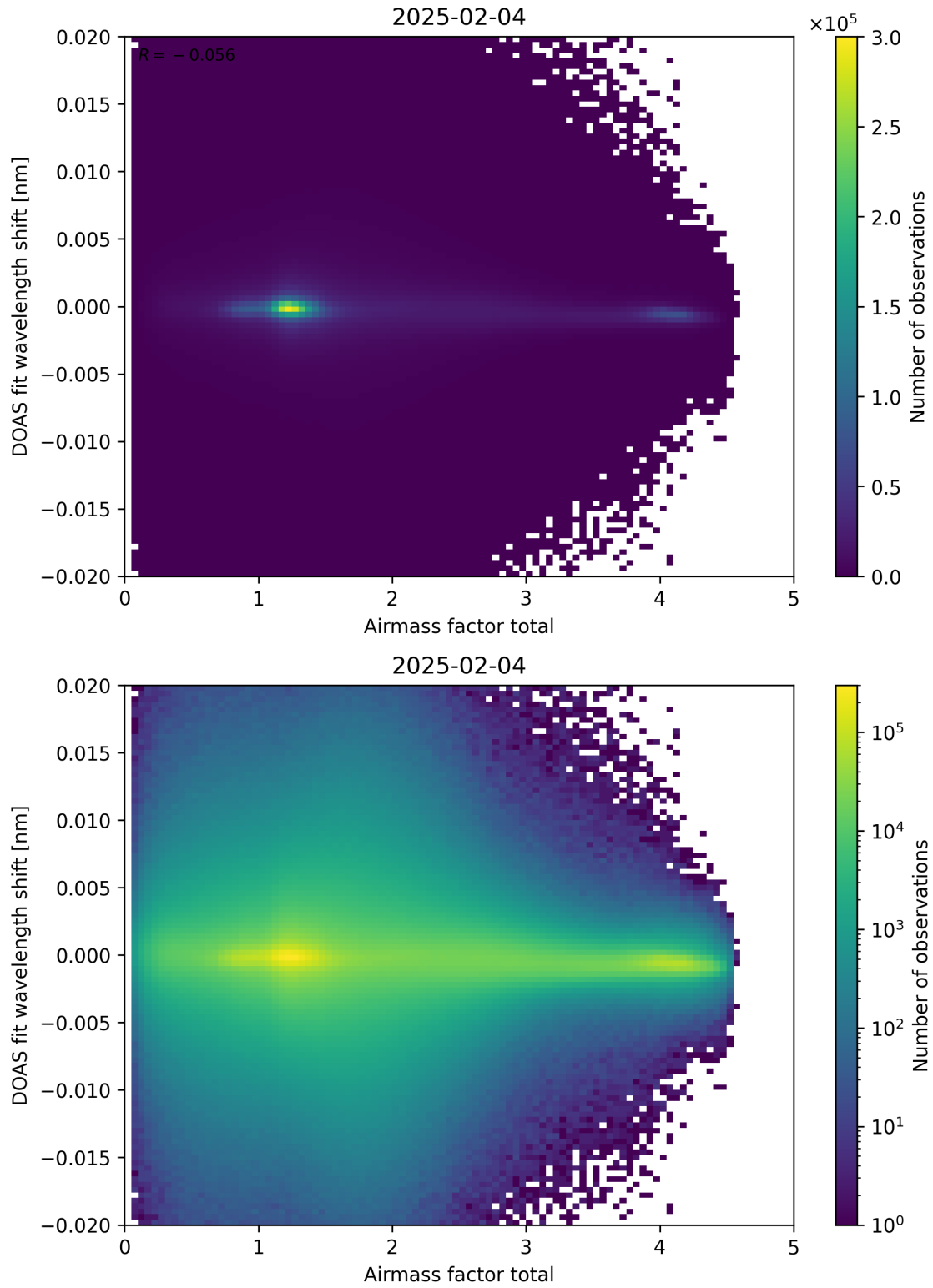
Figure 98: Scatter density plot of “Airmass factor total” against “DOAS fit wavelength shift” for 2025-02-03 to 2025-02-05.
