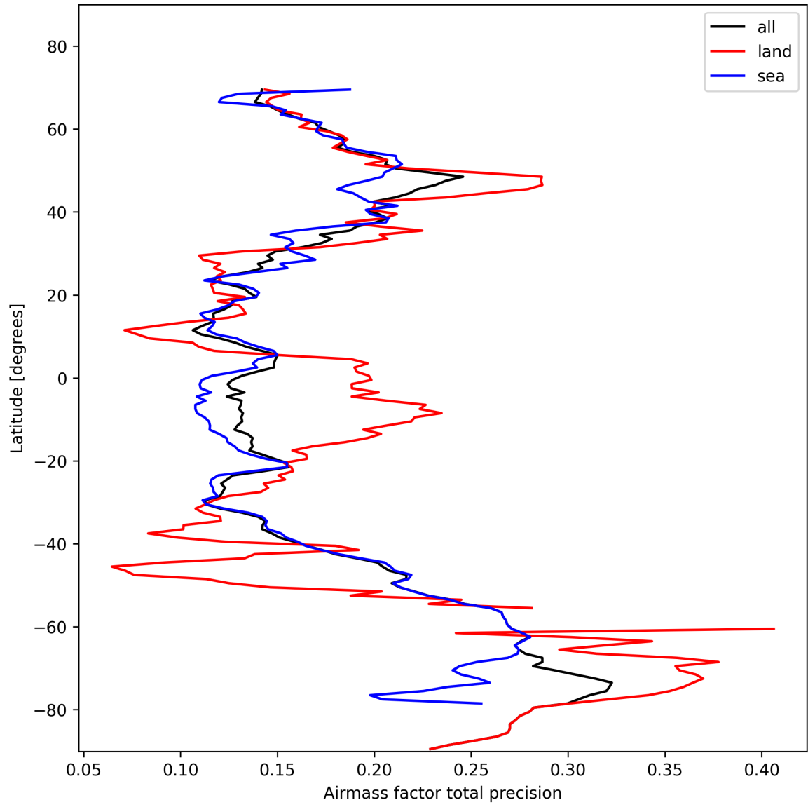
Figure 27: Zonal average of “Airmass factor total precision” for 2025-02-03 to 2025-02-05.
