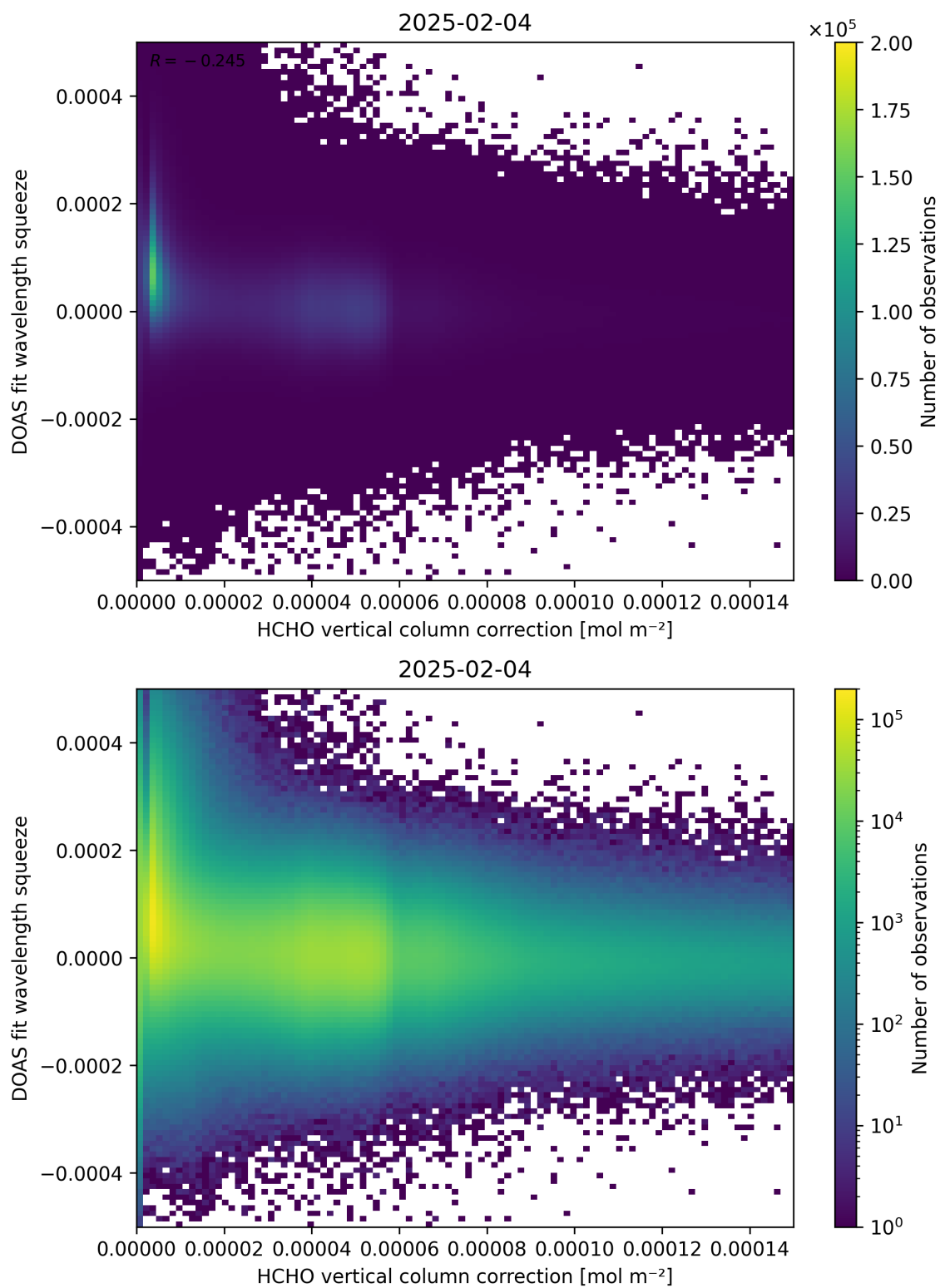
Figure 114: Scatter density plot of “HCHO vertical column correction” against “DOAS fit wavelength squeeze” for 2025-02-03 to 2025-02-05.
