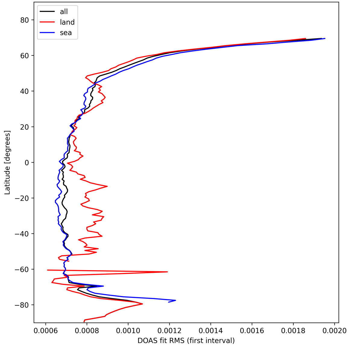
Figure 32: Zonal average of “DOAS fit RMS (first interval)” for 2025-02-03 to 2025-02-05.
