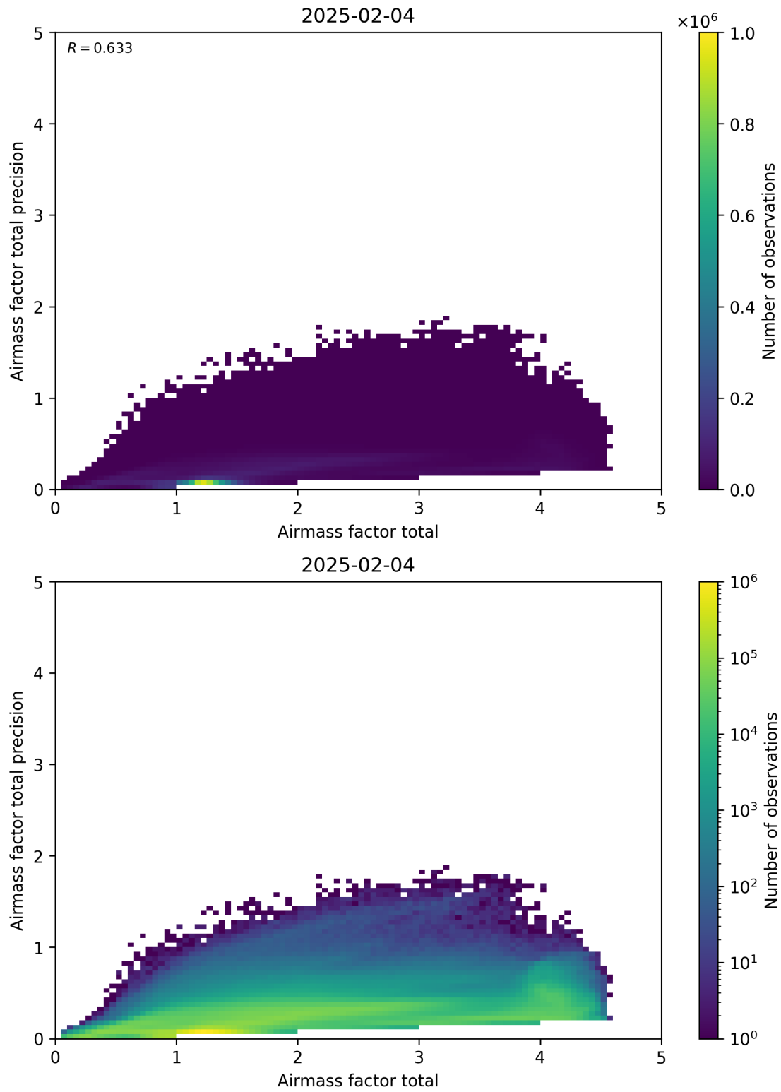
Figure 103: Scatter density plot of “Airmass factor total” against “Airmass factor total precision” for 2025-02-03 to 2025-02-05.
