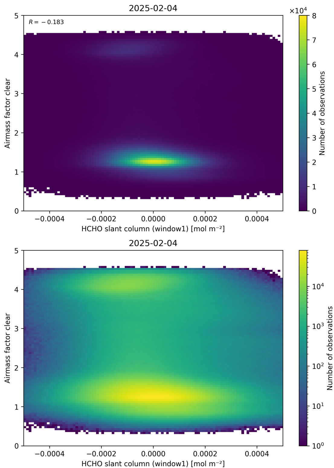
Figure 81: Scatter density plot of “HCHO slant column (window1)” against “Airmass factor clear” for 2025-02-03 to 2025-02-05.
