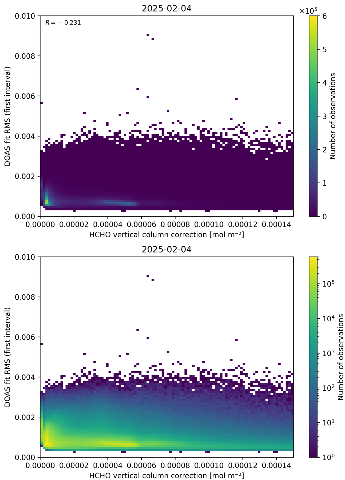
Figure 112: Scatter density plot of “HCHO vertical column correction” against “DOAS fit RMS (first interval)” for 2025-02-03 to 2025-02-05.
