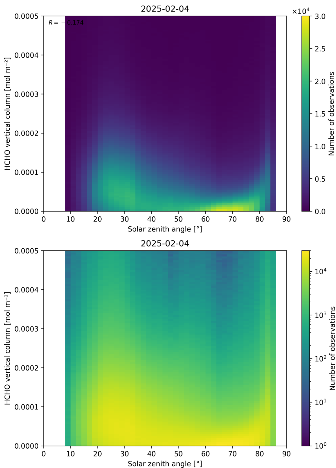
Figure 177: Scatter density plot of “Solar zenith angle” against “HCHO vertical column” for 2025-02-03 to 2025-02-05.
