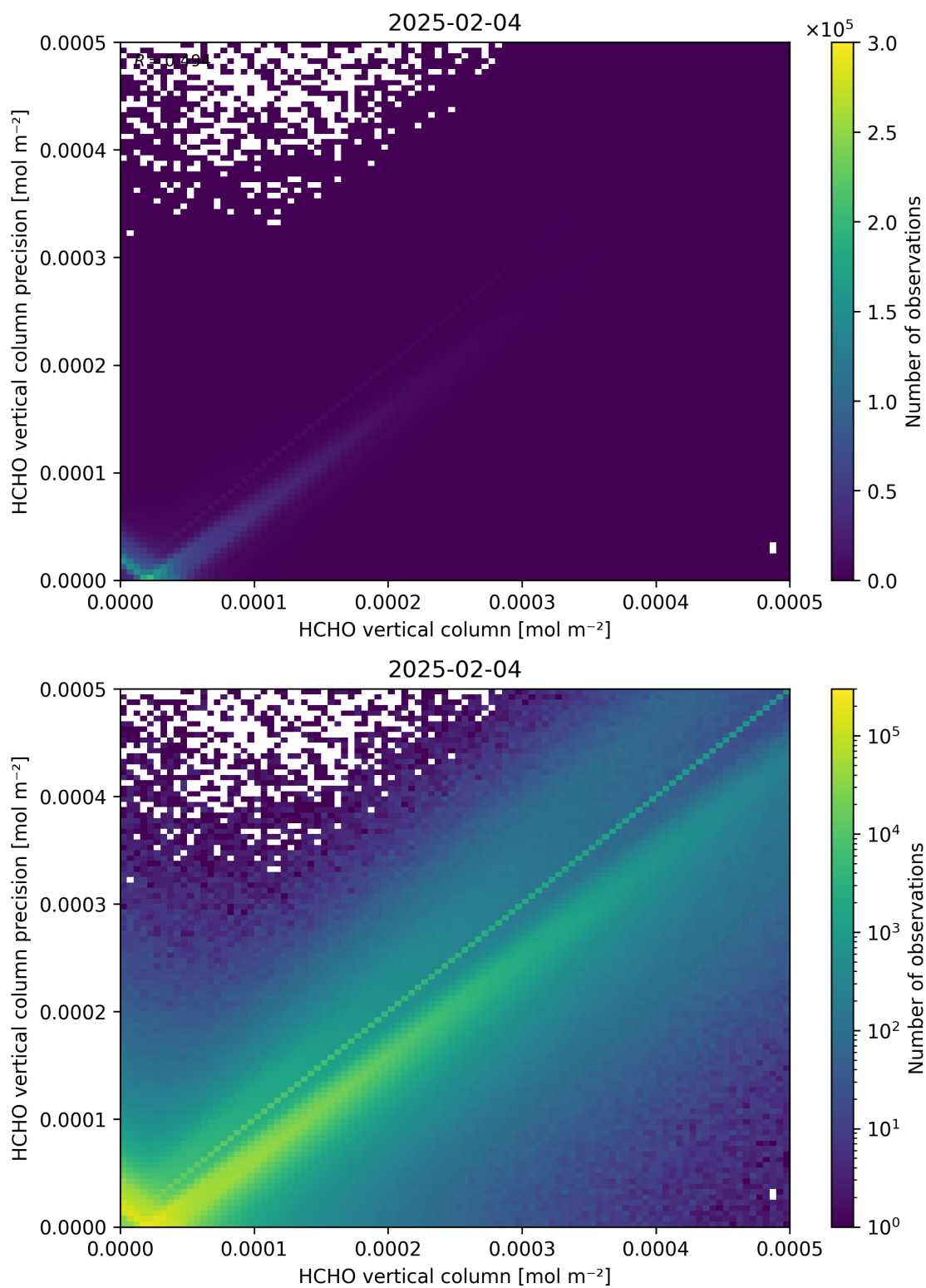
Figure 134: Scatter density plot of “HCHO vertical column” against “HCHO vertical column precision” for 2025-02-03 to 2025-02-05.
