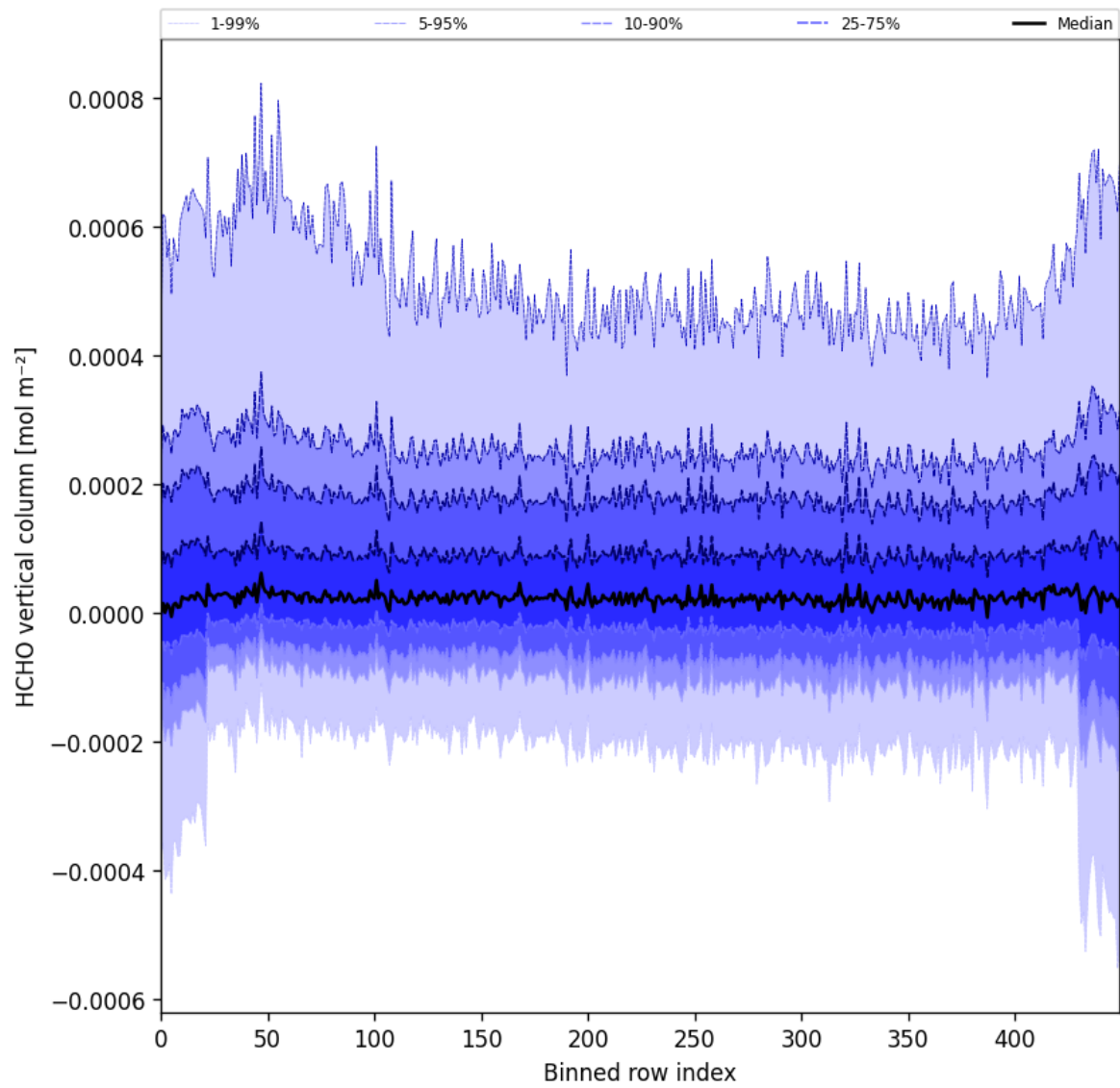
Figure 49: Along track statistics of “HCHO vertical column” for 2025-02-03 to 2025-02-05
