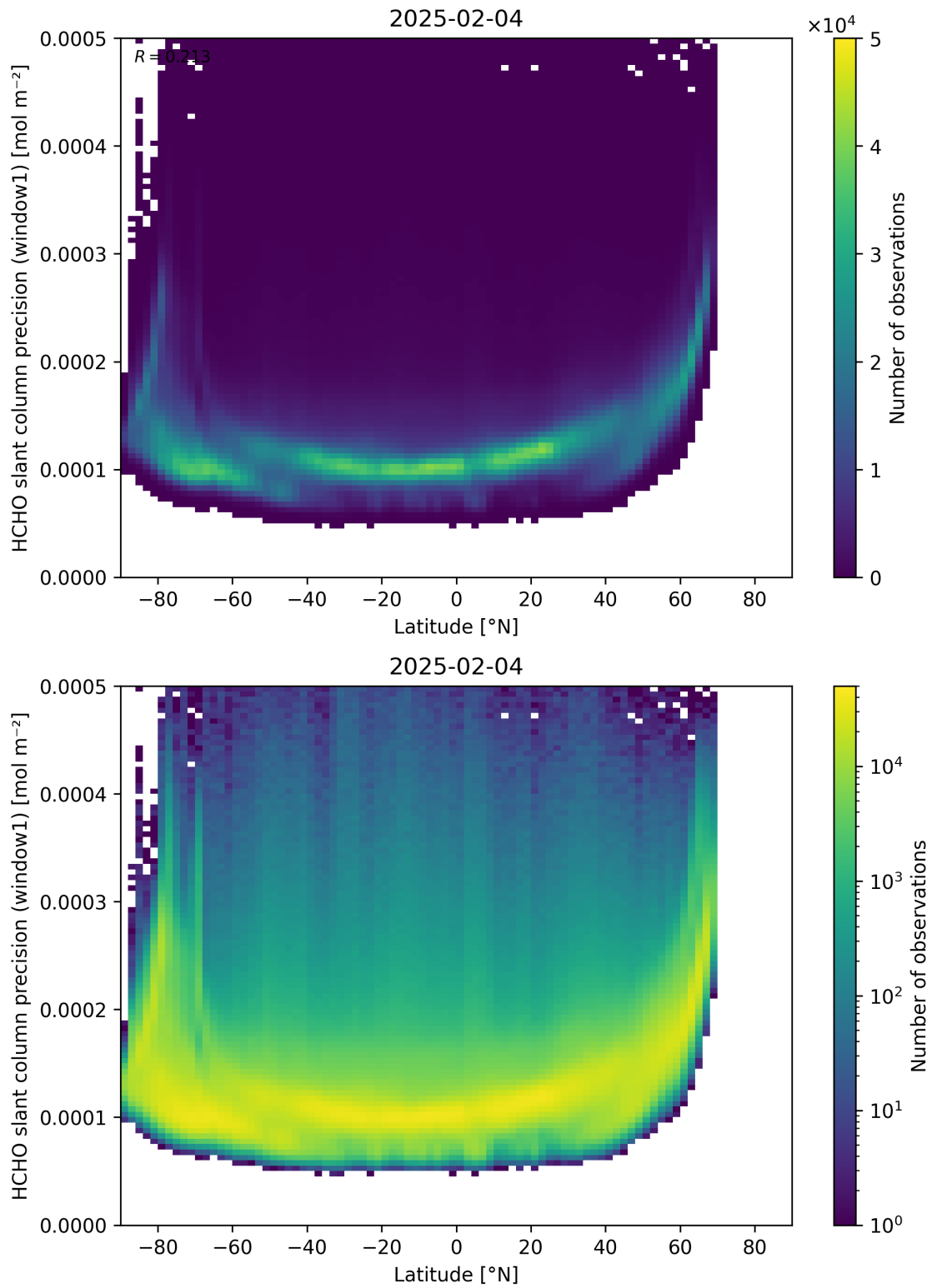
Figure 160: Scatter density plot of “Latitude” against “HCHO slant column precision (window1)” for 2025-02-03 to 2025-02-05.
