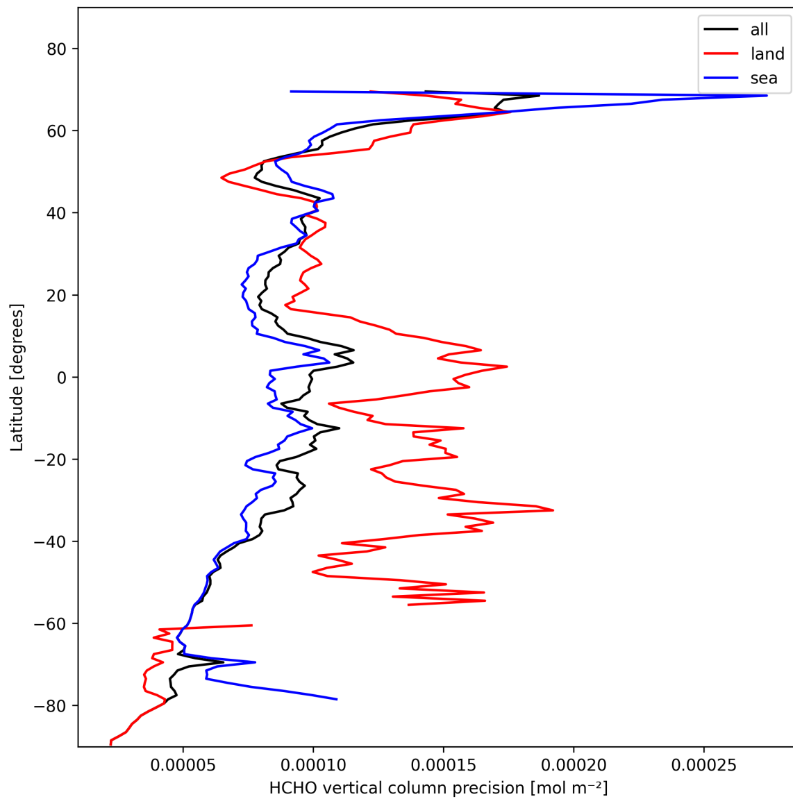
Figure 22: Zonal average of “HCHO vertical column precision” for 2025-02-03 to 2025-02-05.
