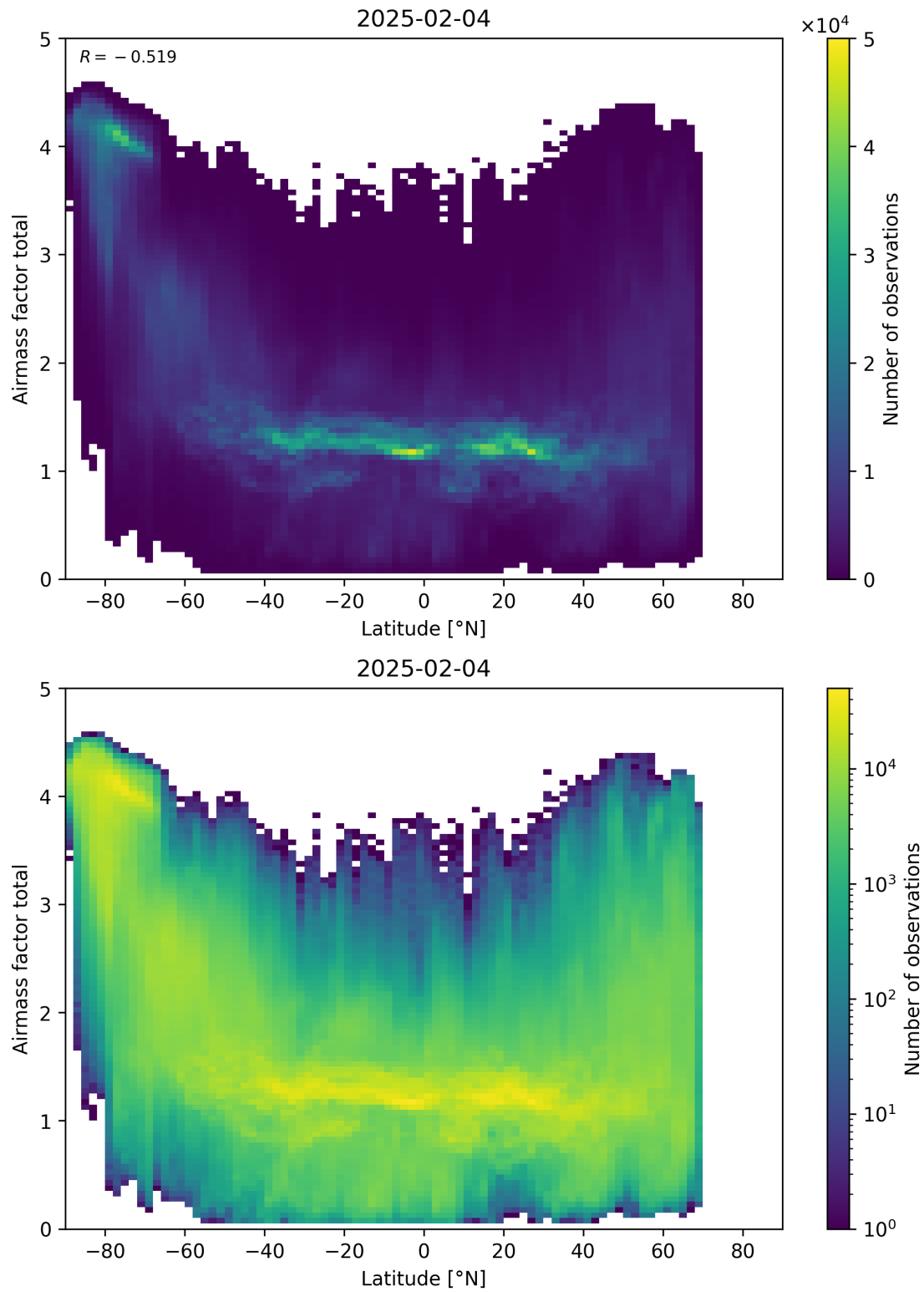
Figure 161: Scatter density plot of “Latitude” against “Airmass factor total” for 2025-02-03 to 2025-02-05.
