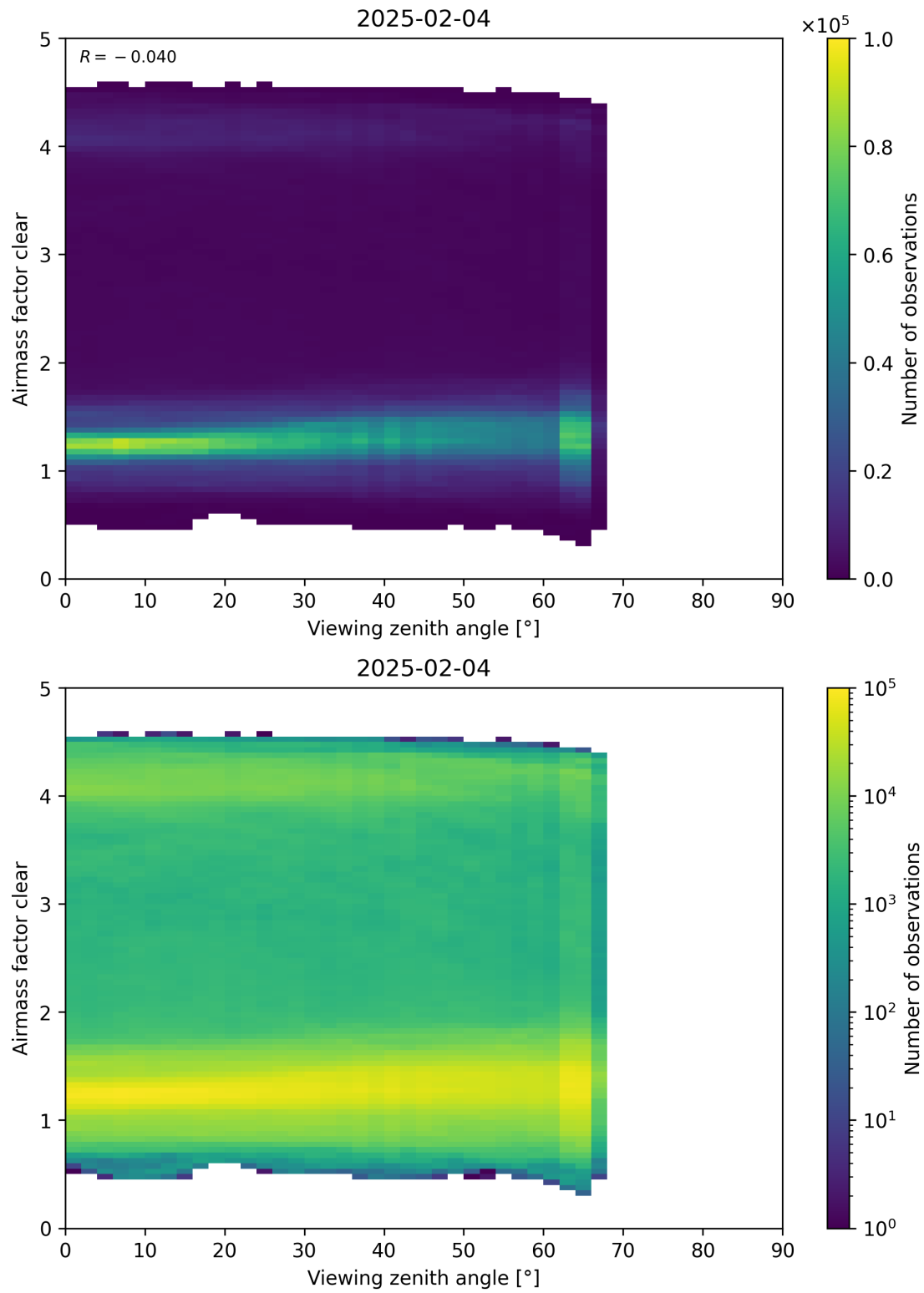
Figure 185: Scatter density plot of “Viewing zenith angle” against “Airmass factor clear” for 2025-02-03 to 2025-02-05.
