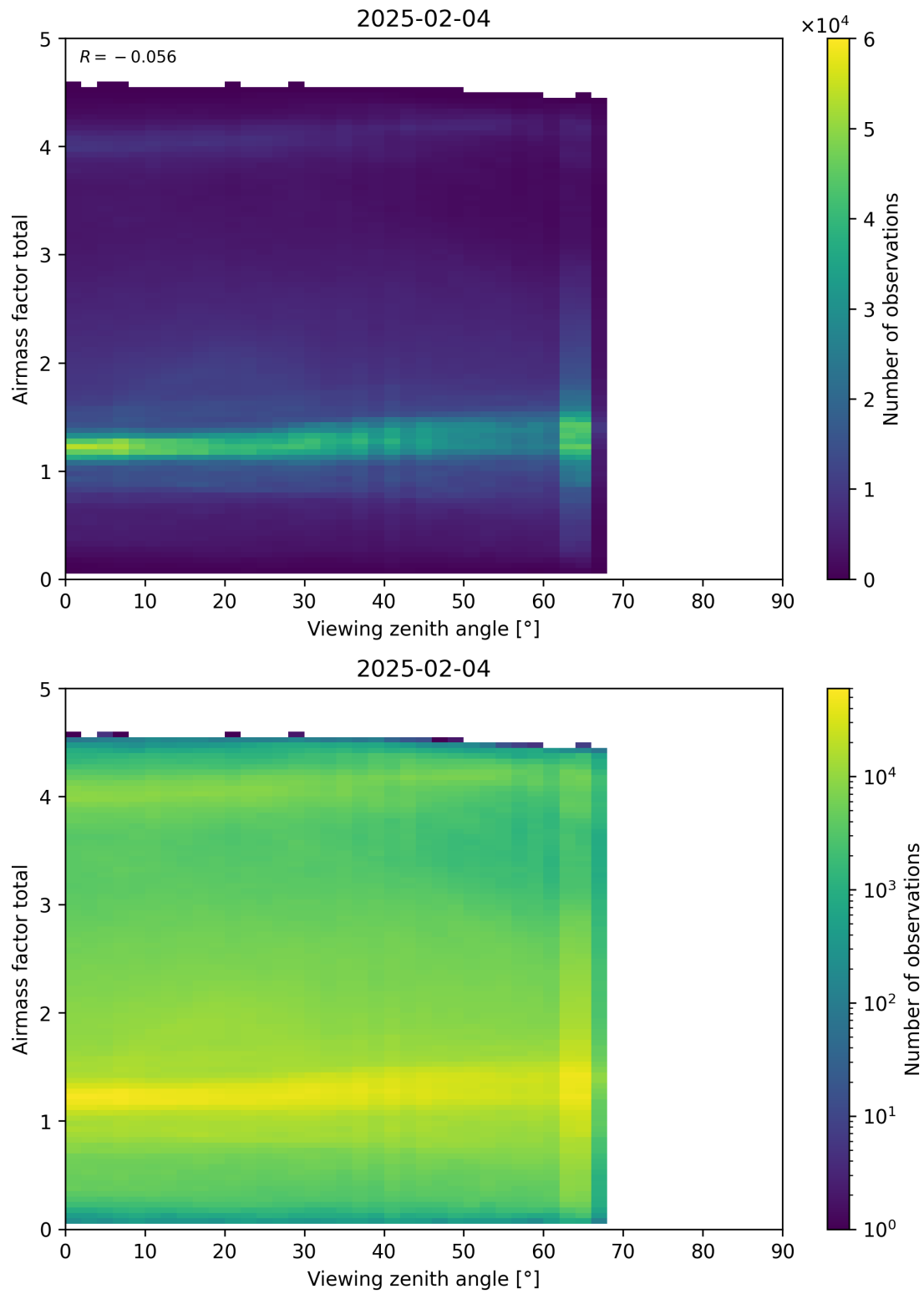
Figure 190: Scatter density plot of “Viewing zenith angle” against “Airmass factor total” for 2025-02-03 to 2025-02-05.
