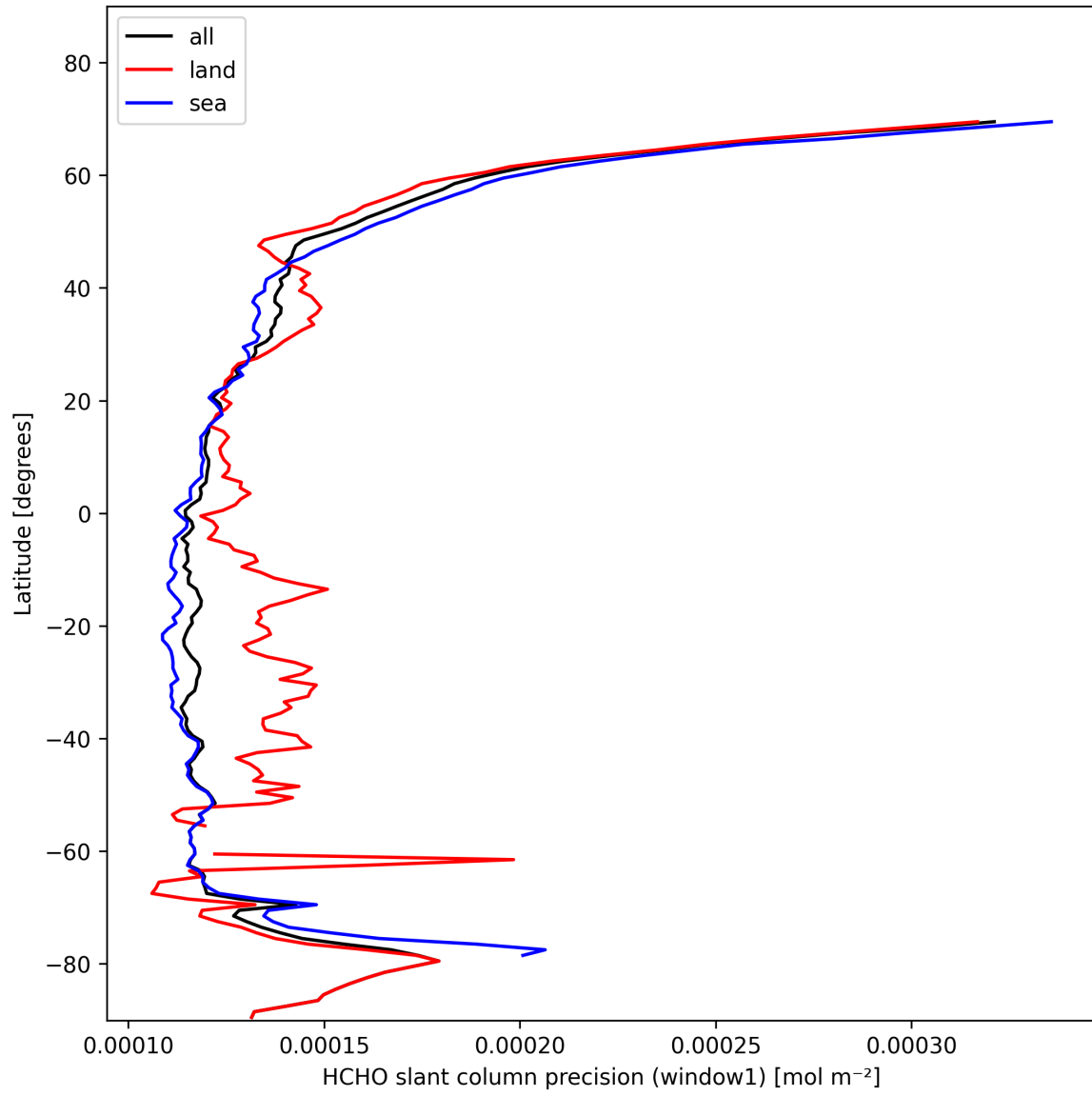
Figure 25: Zonal average of “HCHO slant column precision (window1)” for 2025-02-03 to 2025-02-05.
