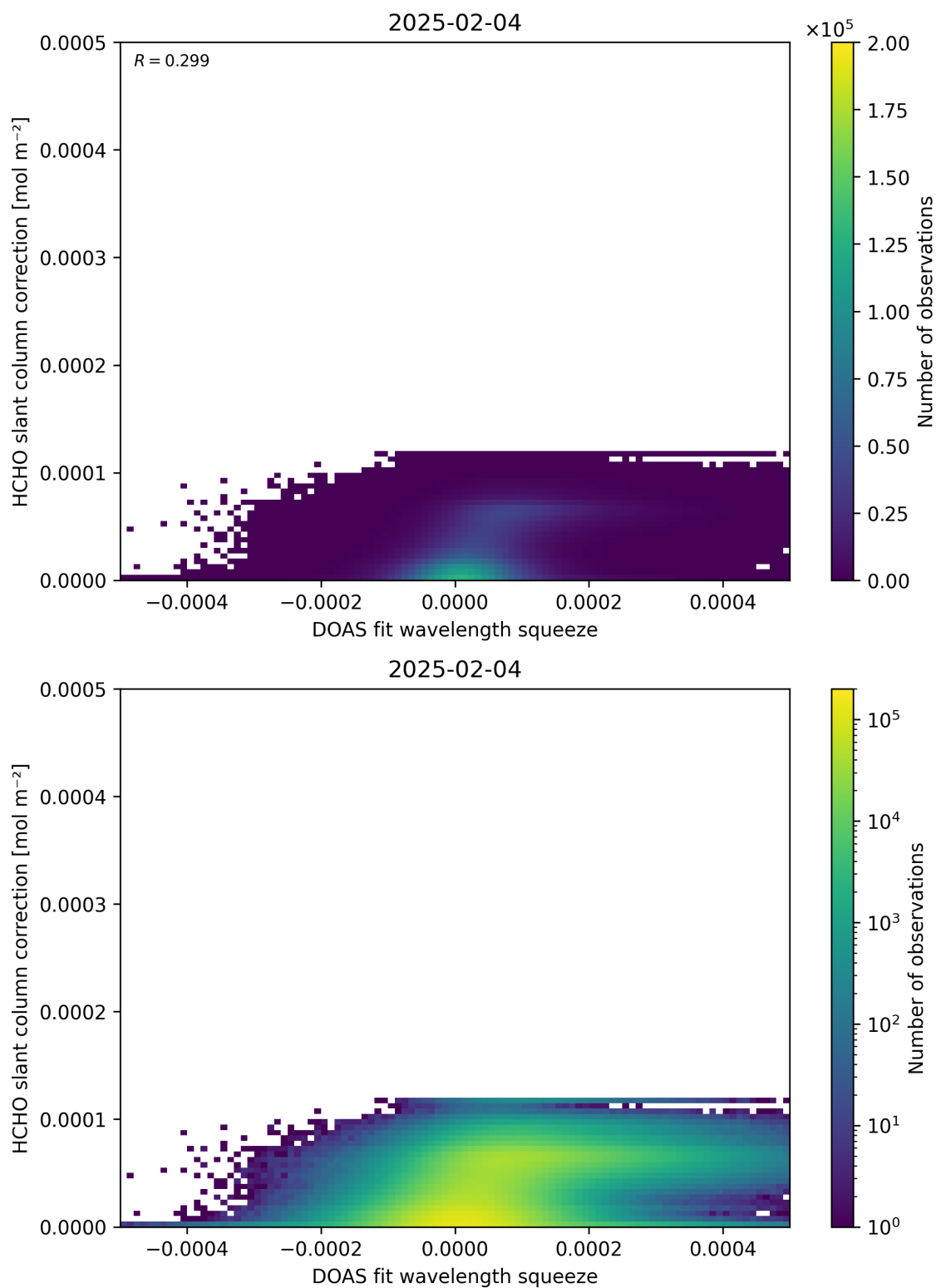
Figure 70: Scatter density plot of “DOAS fit wavelength squeeze” against “HCHO slant column correction” for 2025-02-03 to 2025-02-05.
