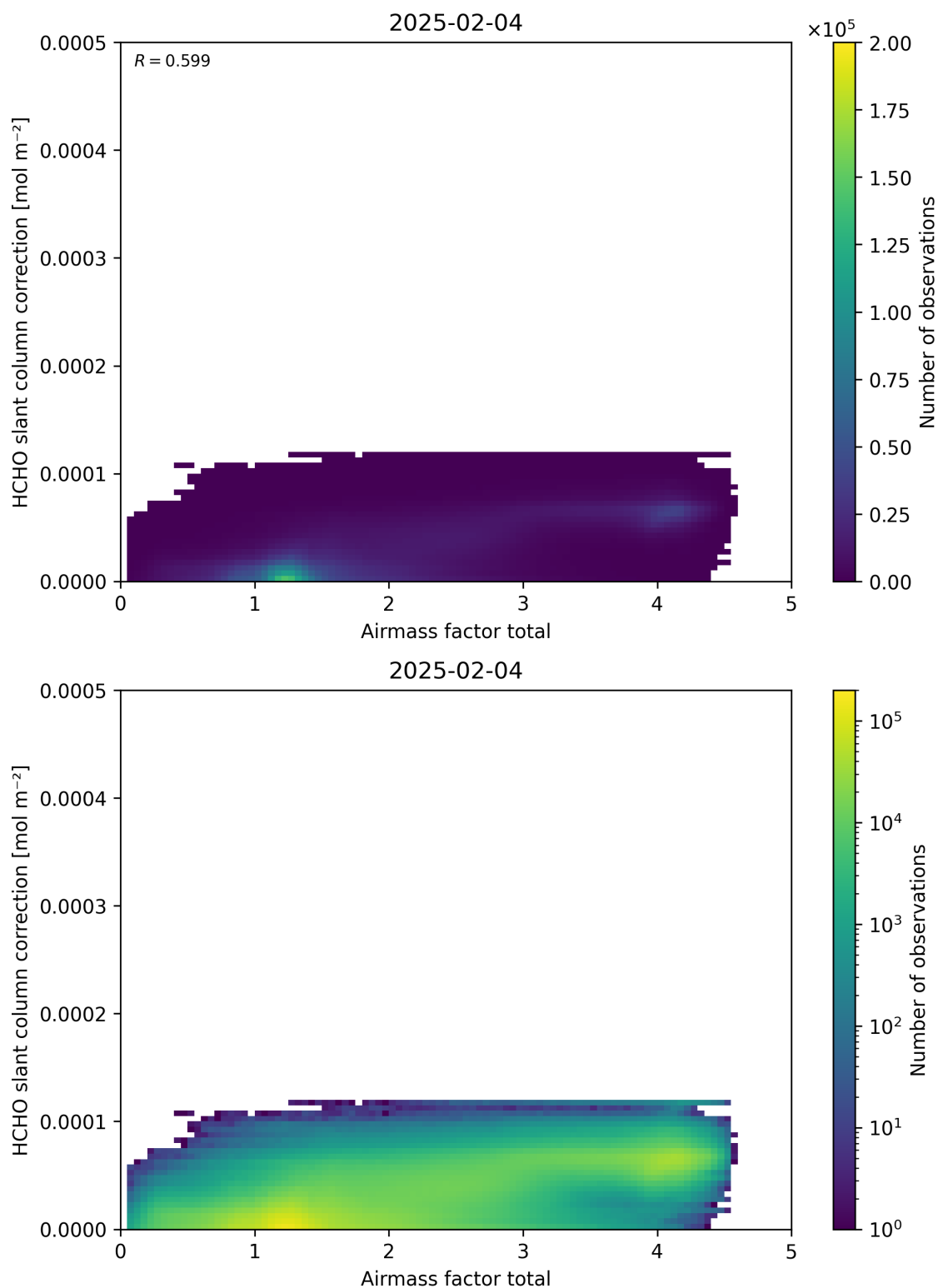
Figure 102: Scatter density plot of “Airmass factor total” against “HCHO slant column correction” for 2025-02-03 to 2025-02-05.
