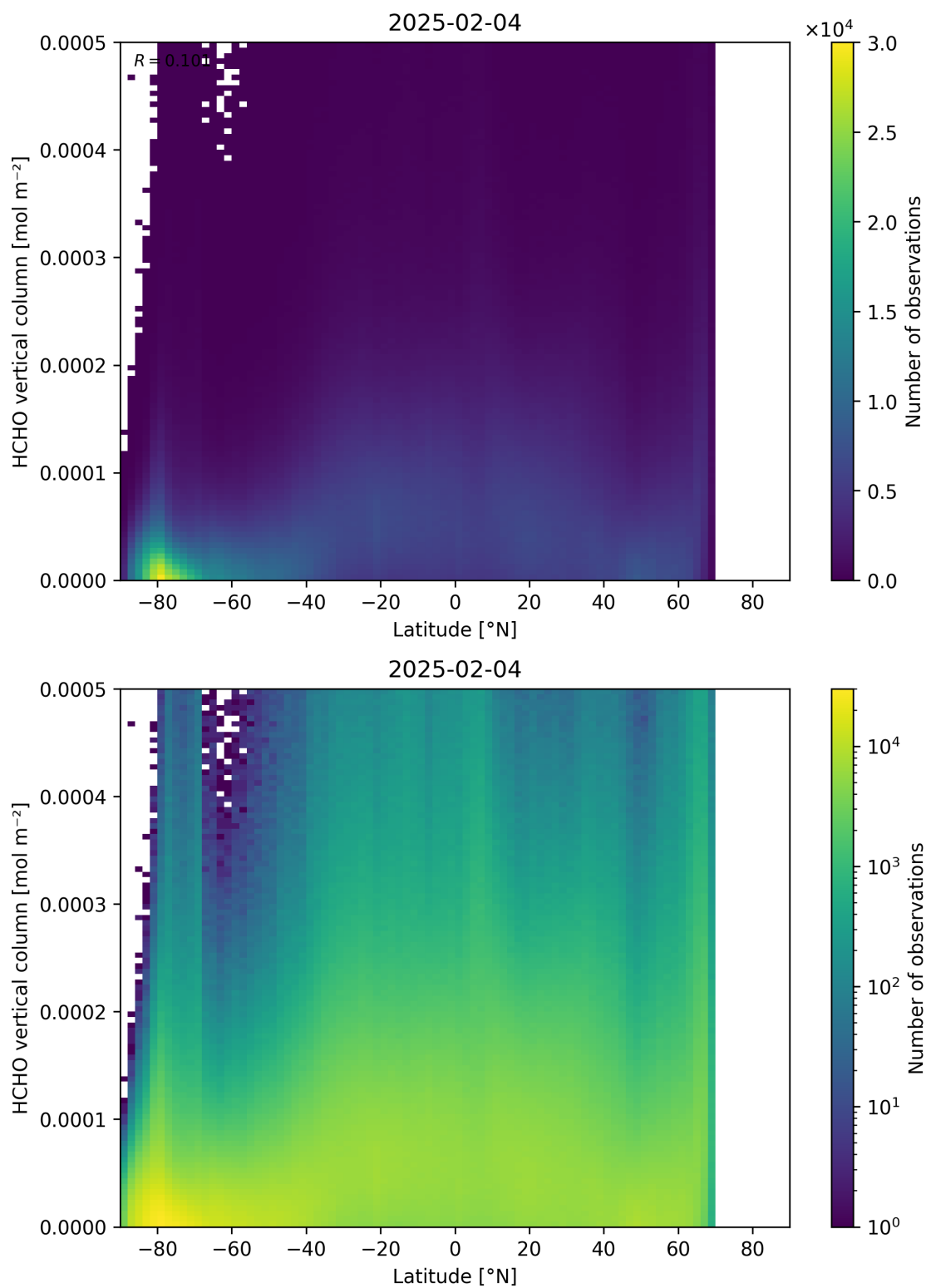
Figure 163: Scatter density plot of “Latitude” against “HCHO vertical column” for 2025-02-03 to 2025-02-05.
