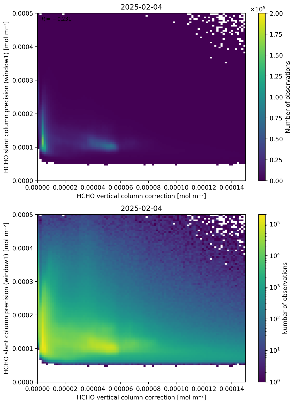
Figure 119: Scatter density plot of “HCHO vertical column correction” against “HCHO slant column precision (window1)” for 2025-02-03 to 2025-02-05.
