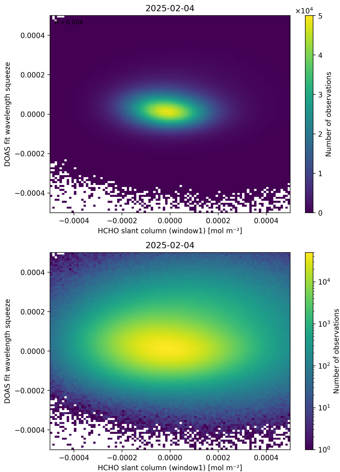
Figure 80: Scatter density plot of “HCHO slant column (window1)” against “DOAS fit wavelength squeeze” for 2025-02-03 to 2025-02-05.
