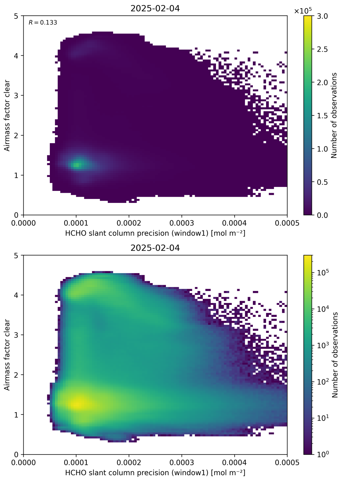
Figure 91: Scatter density plot of “HCHO slant column precision (window1)” against “Airmass factor clear” for 2025-02-03 to 2025-02-05.
