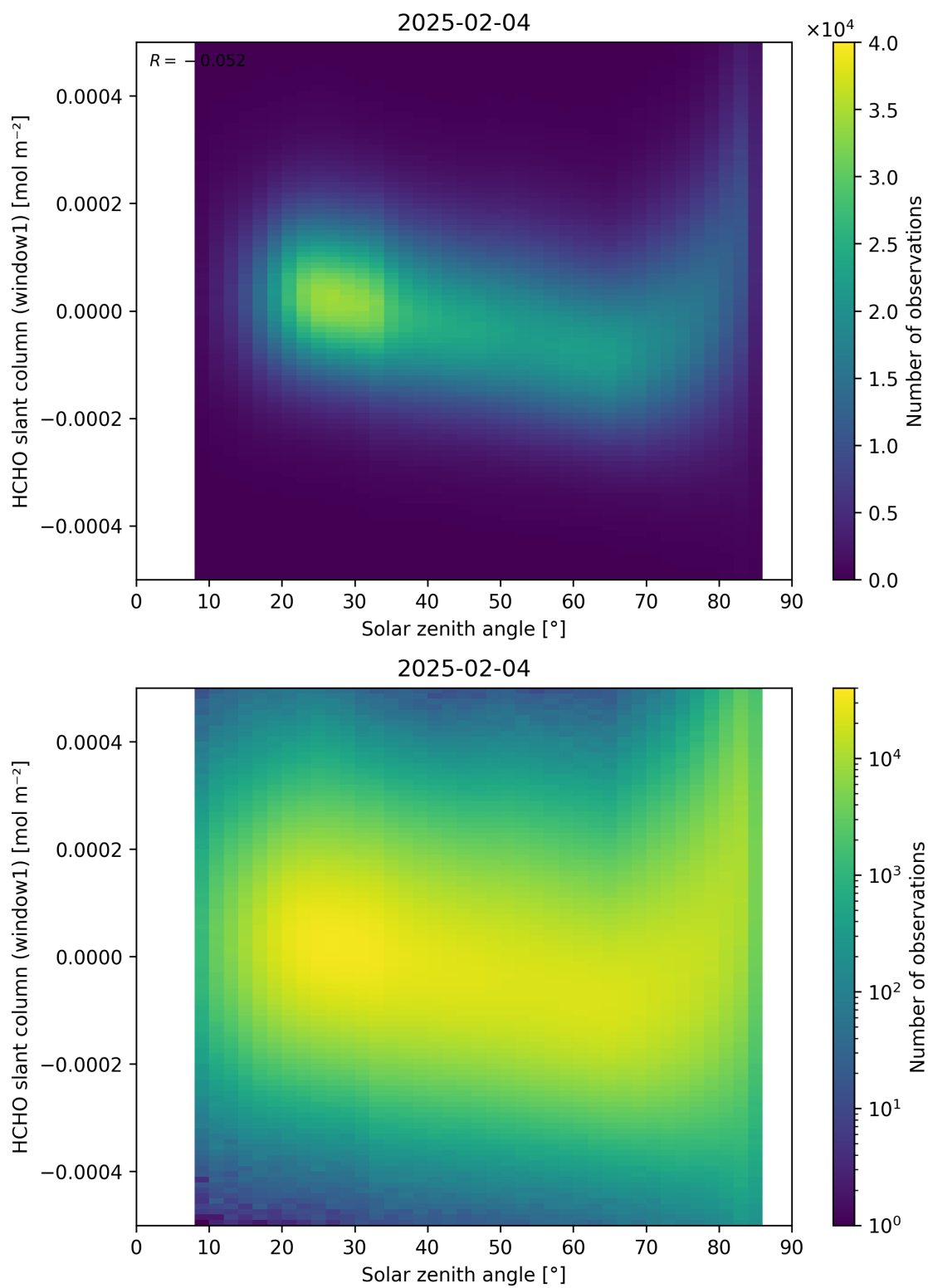
Figure 173: Scatter density plot of “Solar zenith angle” against “HCHO slant column (window1)” for 2025-02-03 to 2025-02-05.
