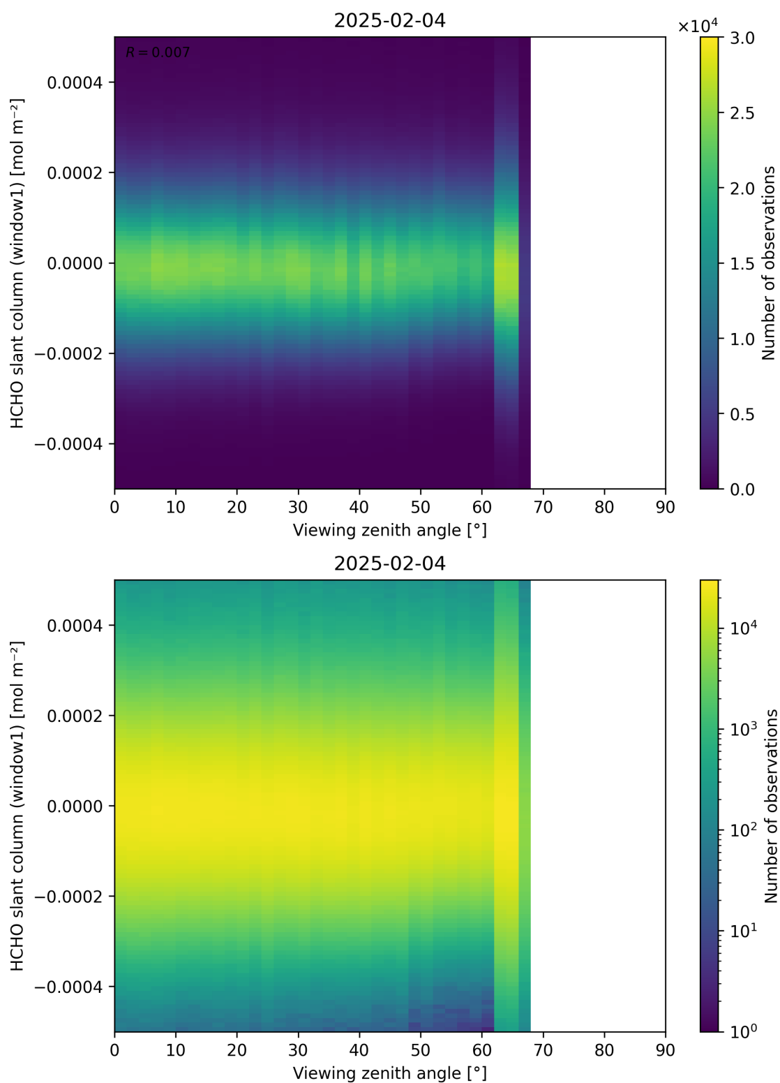
Figure 188: Scatter density plot of “Viewing zenith angle” against “HCHO slant column (window1)” for 2025-02-03 to 2025-02-05.
