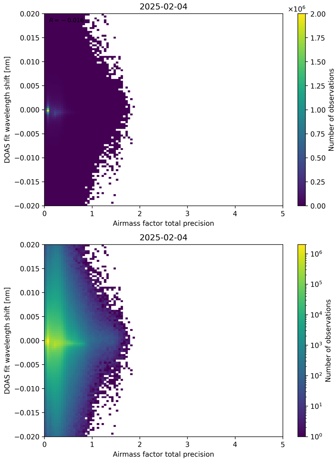
Figure 106: Scatter density plot of “Airmass factor total precision” against “DOAS fit wavelength shift” for 2025-02-03 to 2025-02-05.
