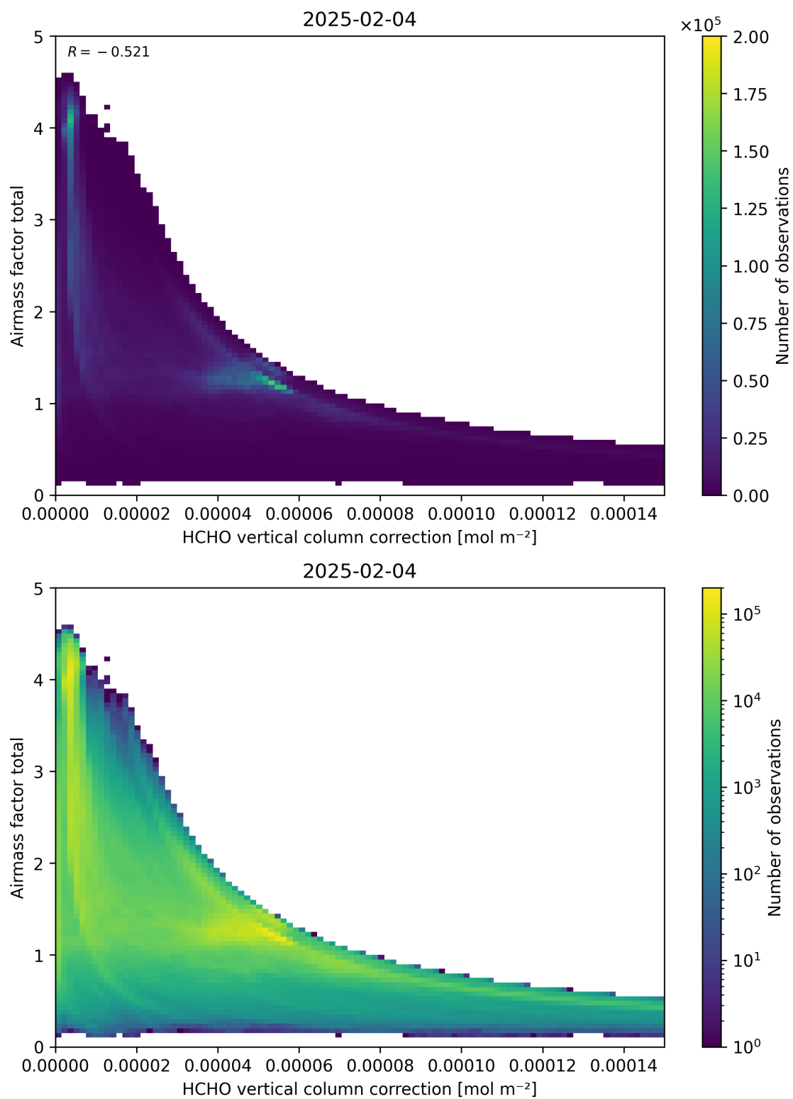
Figure 120: Scatter density plot of “HCHO vertical column correction” against “Airmass factor total” for 2025-02-03 to 2025-02-05.
