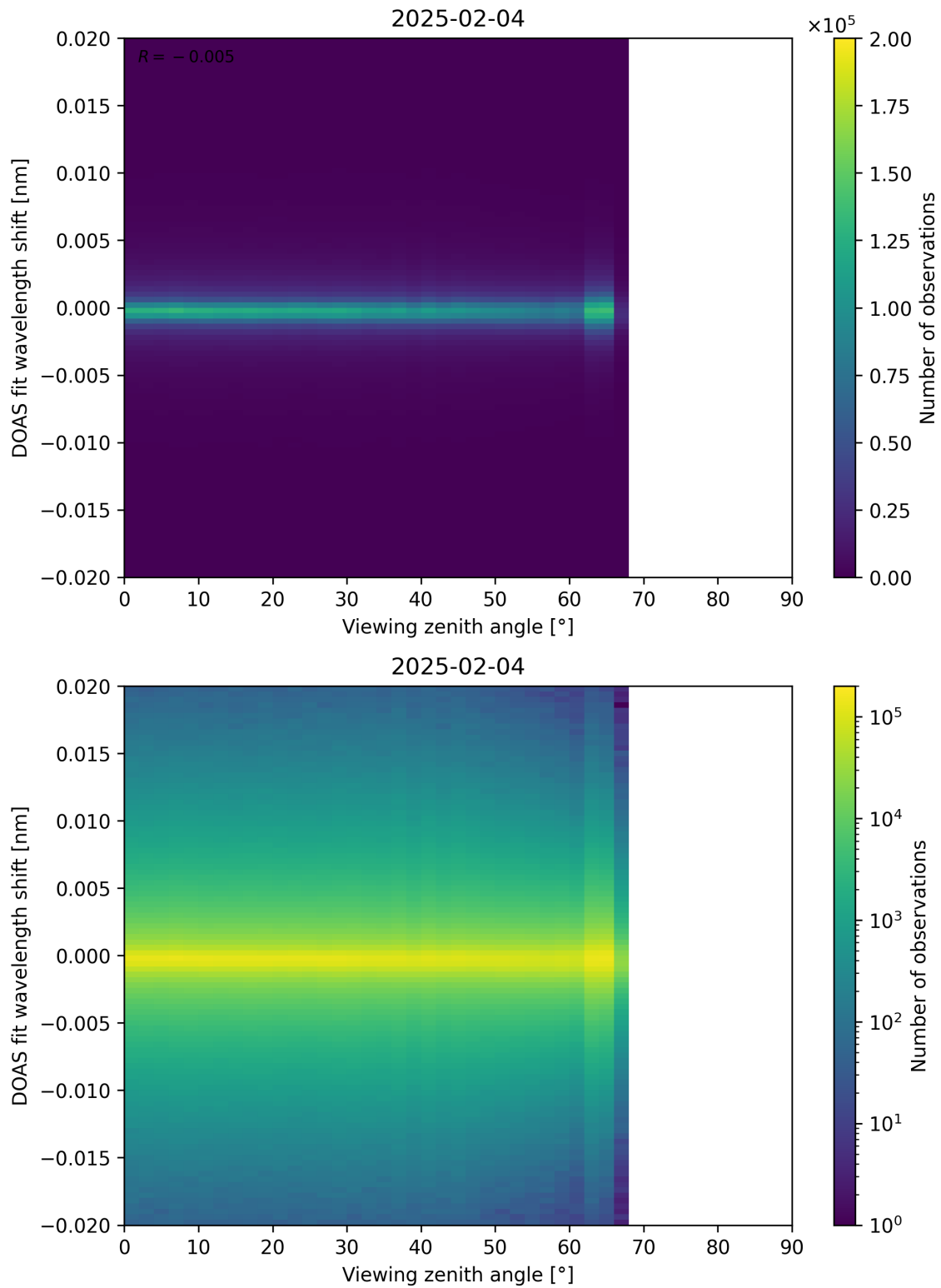
Figure 183: Scatter density plot of “Viewing zenith angle” against “DOAS fit wavelength shift” for 2025-02-03 to 2025-02-05.
