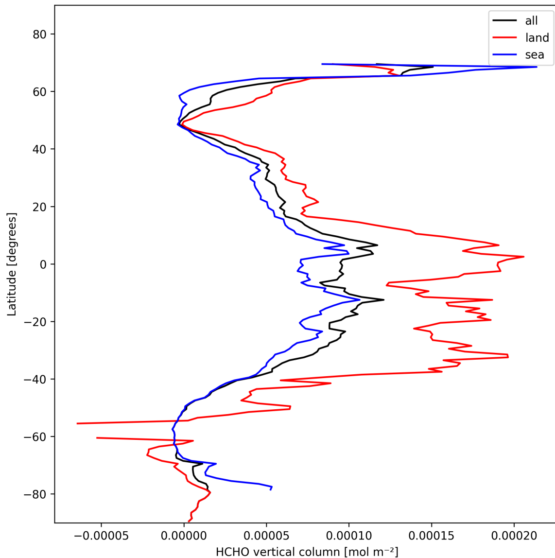
Figure 21: Zonal average of “HCHO vertical column” for 2025-02-03 to 2025-02-05.
