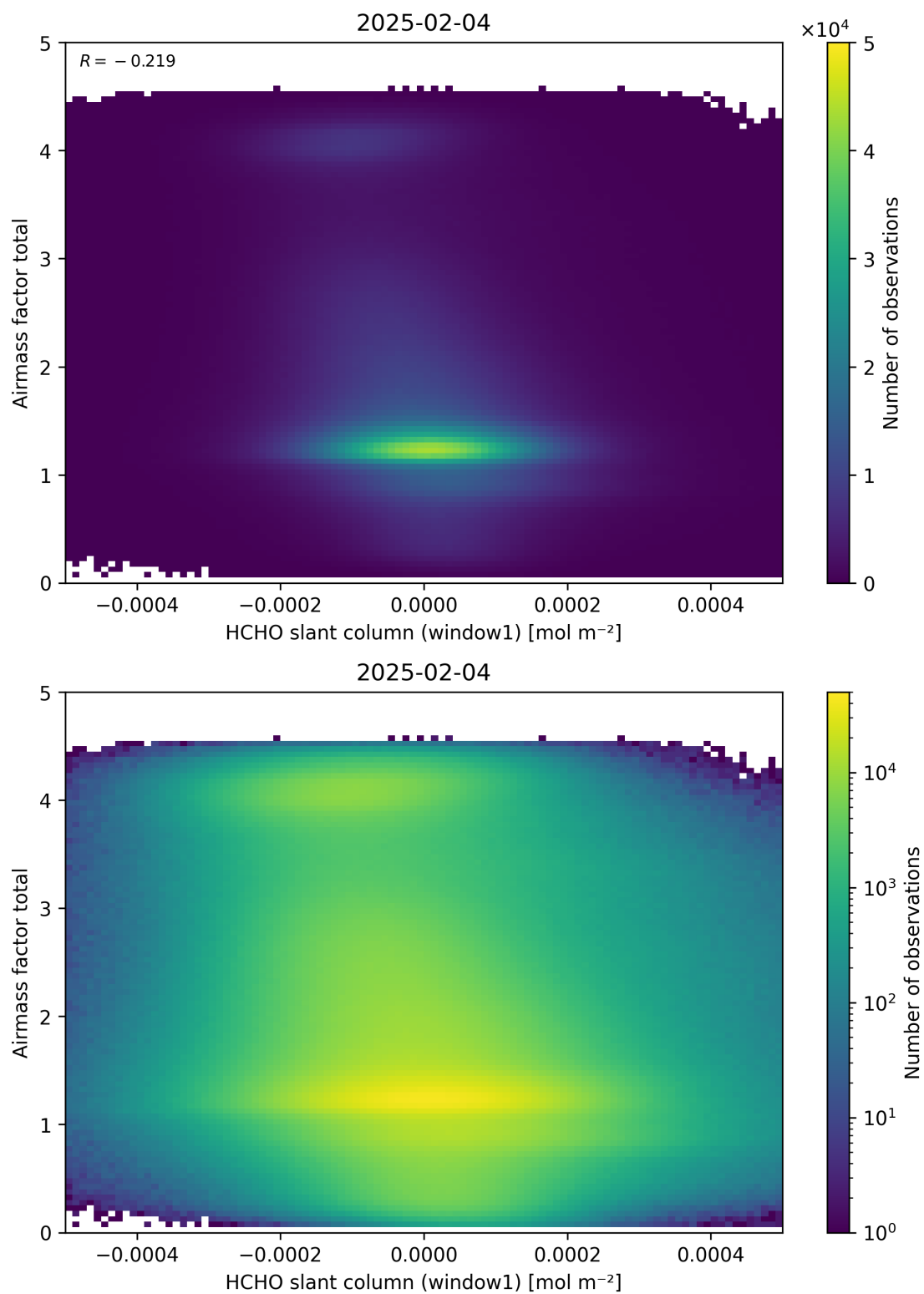
Figure 85: Scatter density plot of “HCHO slant column (window1)” against “Airmass factor total” for 2025-02-03 to 2025-02-05.
