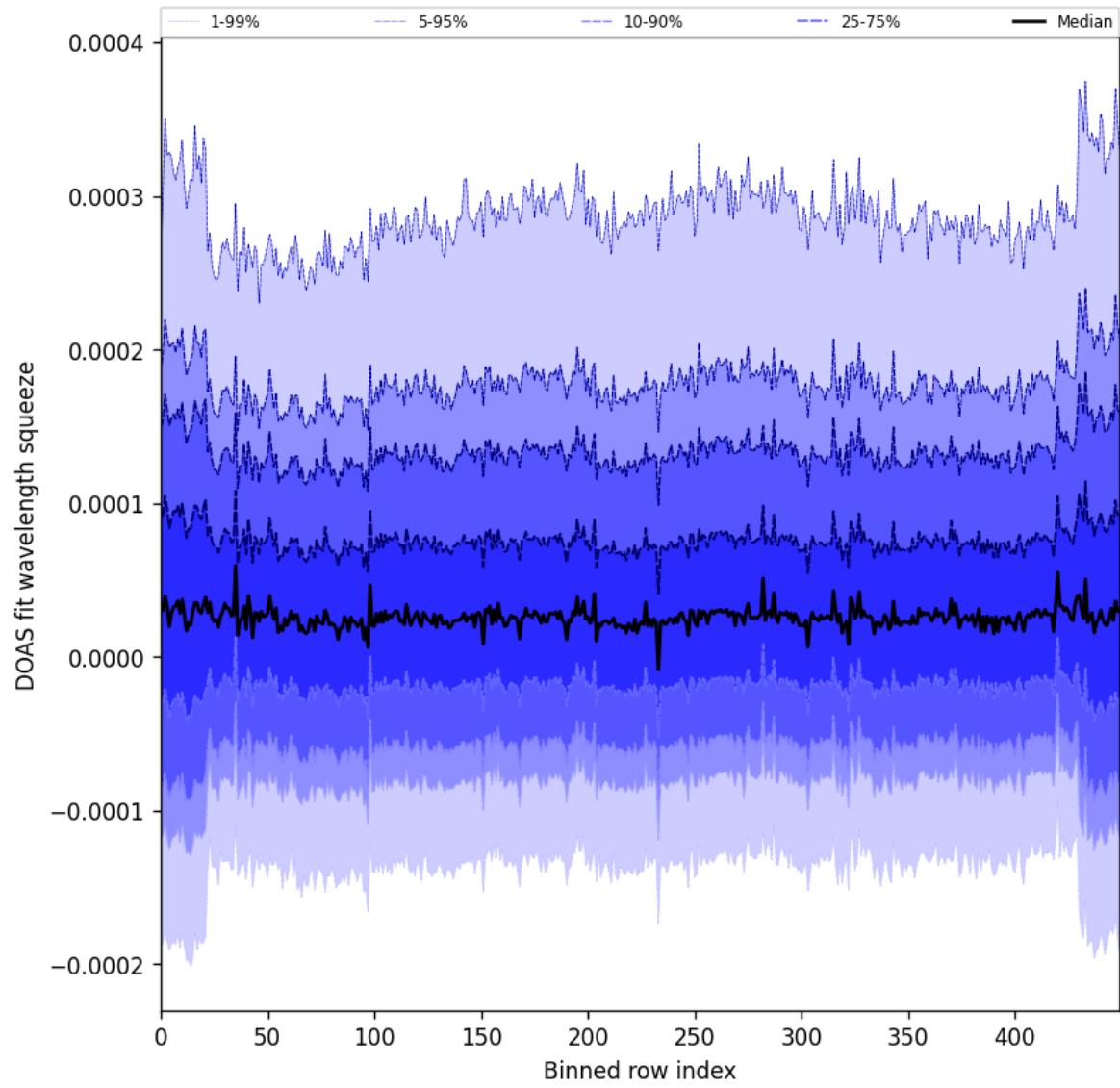
Figure 59: Along track statistics of “DOAS fit wavelength squeeze” for 2025-02-03 to 2025-02-05
