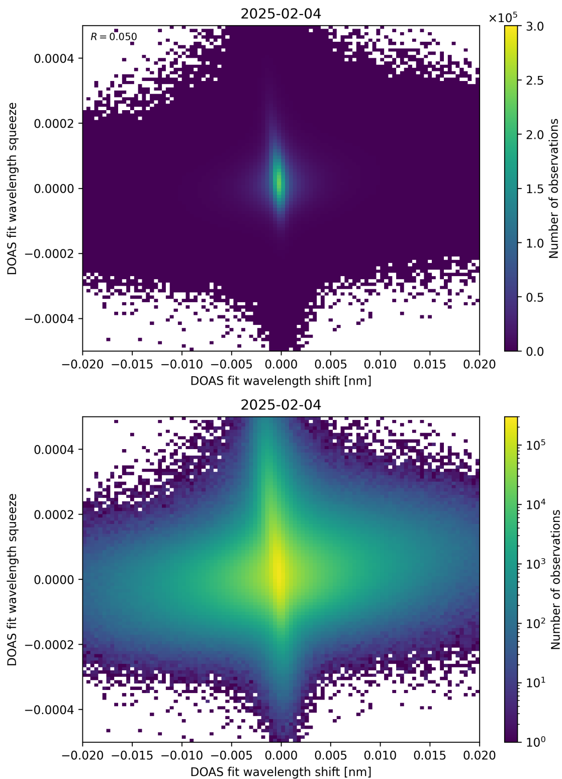
Figure 65: Scatter density plot of “DOAS fit wavelength shift” against “DOAS fit wavelength squeeze” for 2025-02-03 to 2025-02-05.
