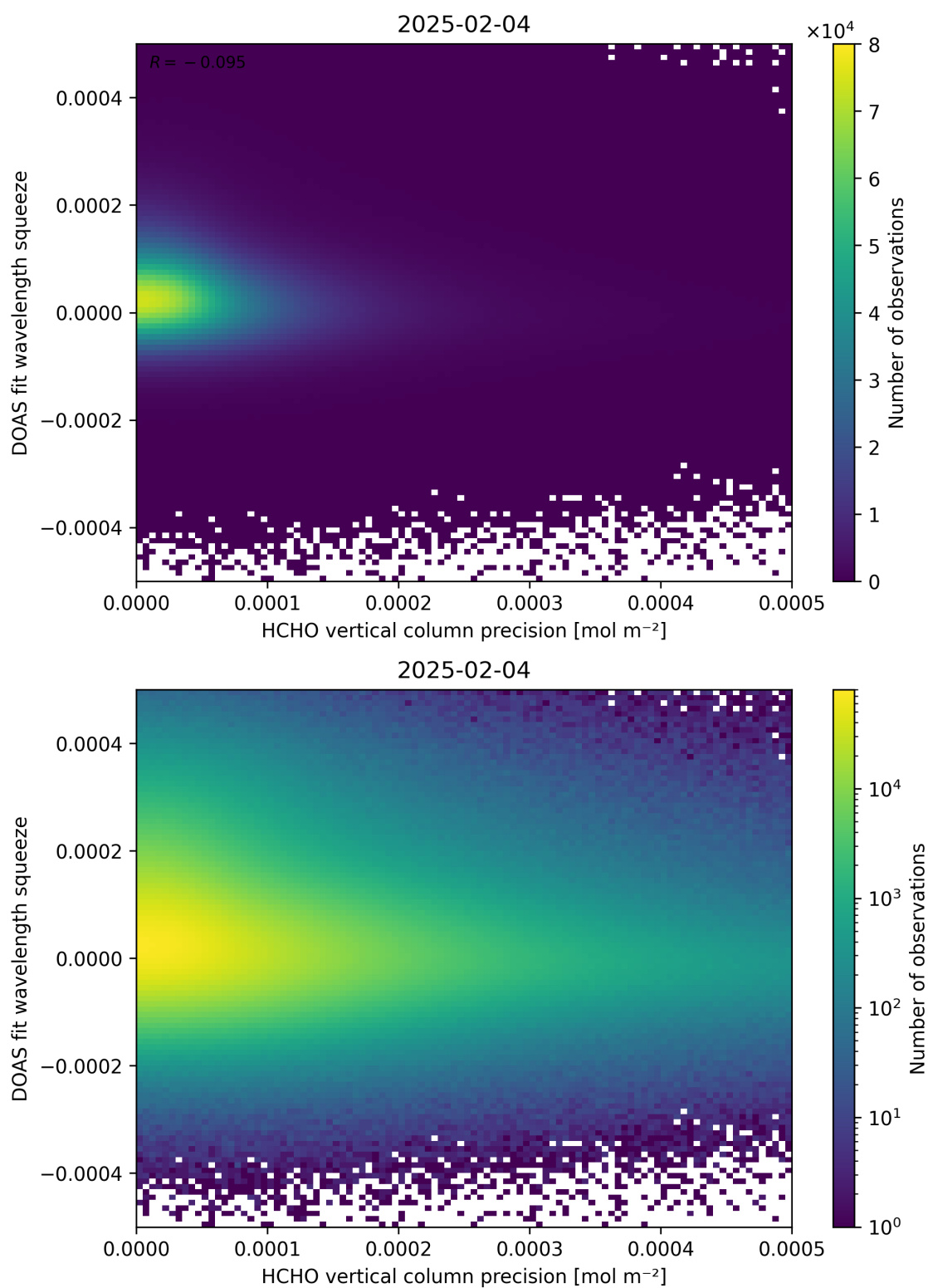
Figure 138: Scatter density plot of “HCHO vertical column precision” against “DOAS fit wavelength squeeze” for 2025-02-03 to 2025-02-05.
