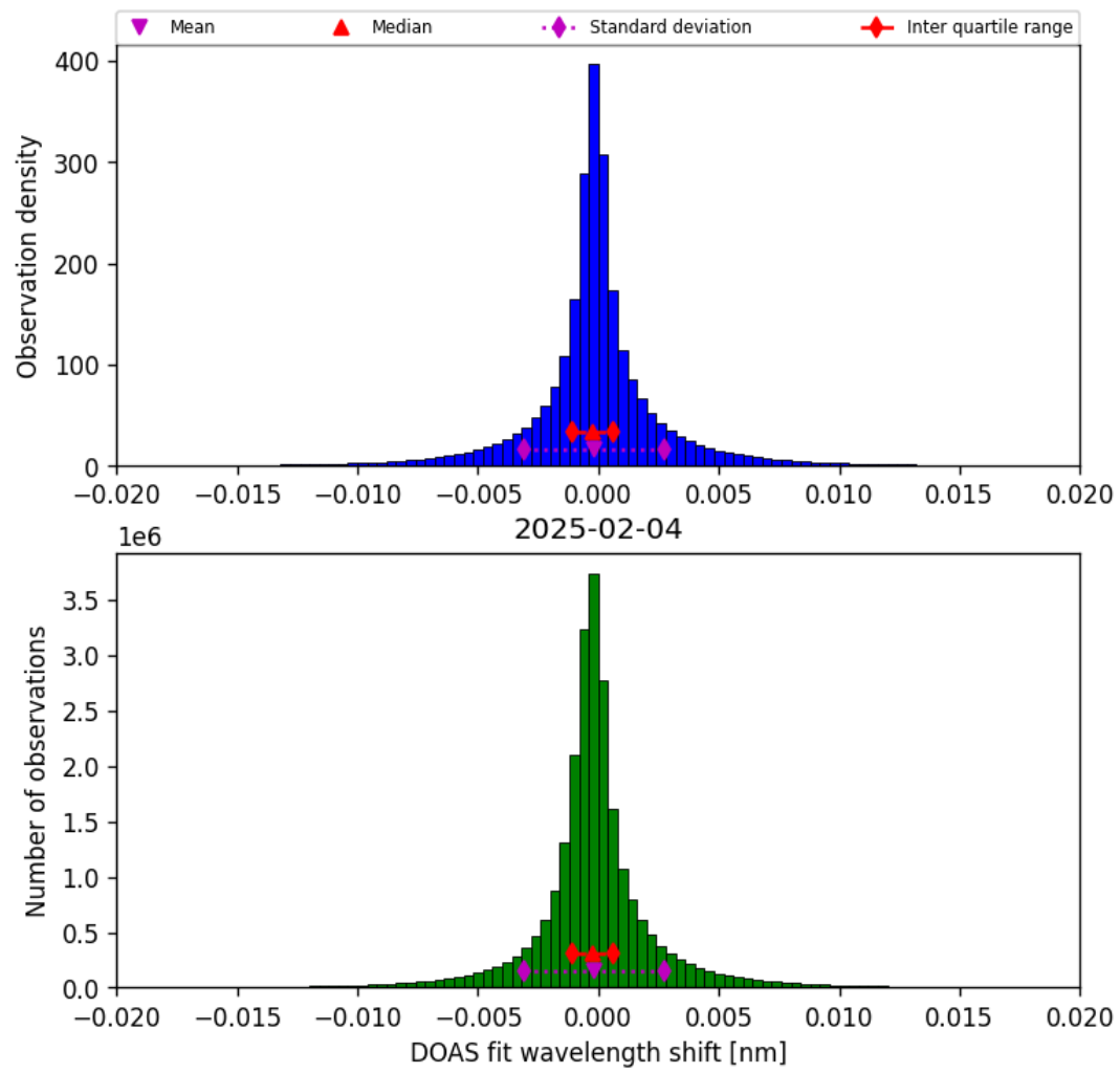
Figure 44: Histogram of “DOAS fit wavelength shift” for 2025-02-03 to 2025-02-05
