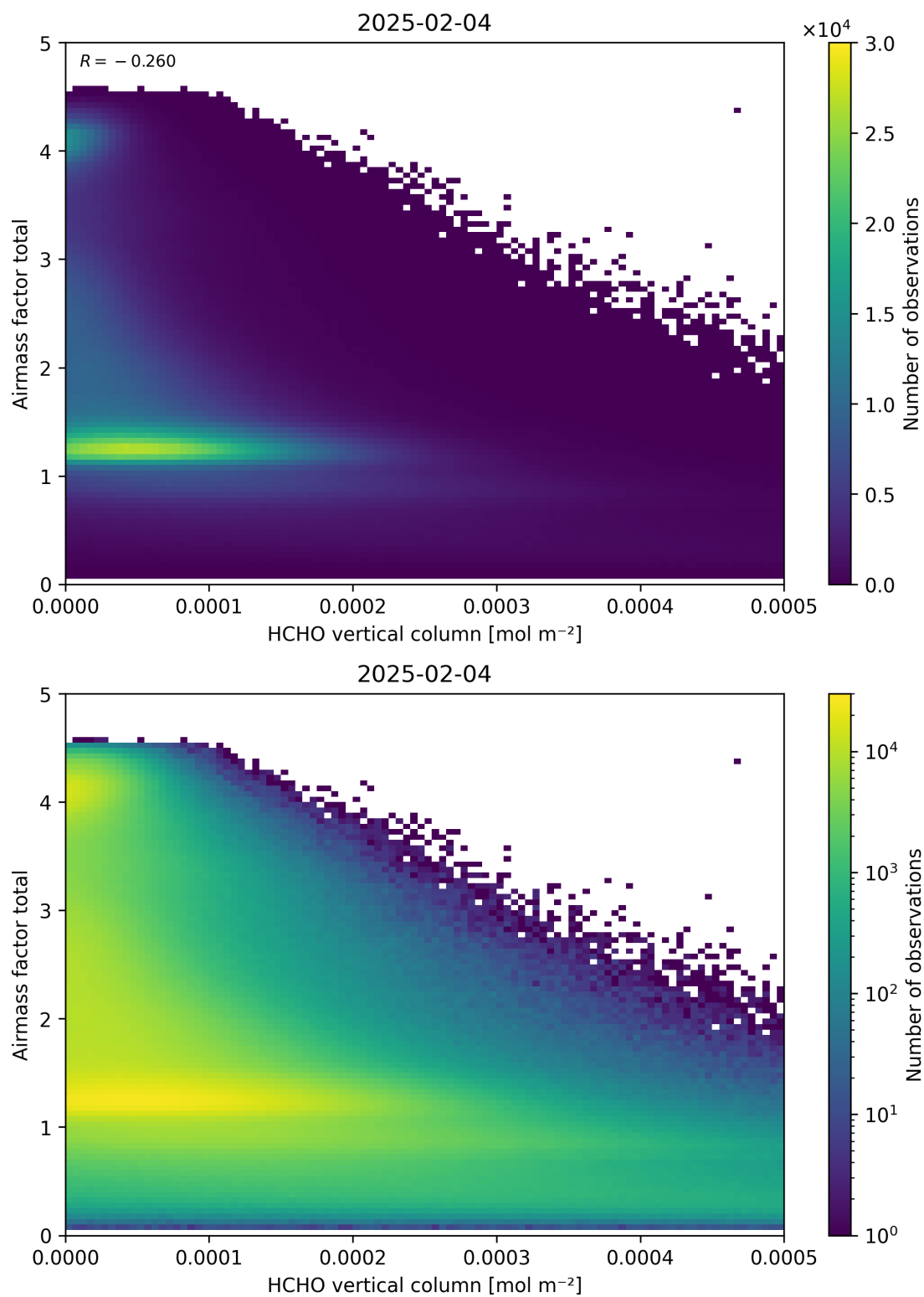
Figure 131: Scatter density plot of “HCHO vertical column” against “Airmass factor total” for 2025-02-03 to 2025-02-05.
