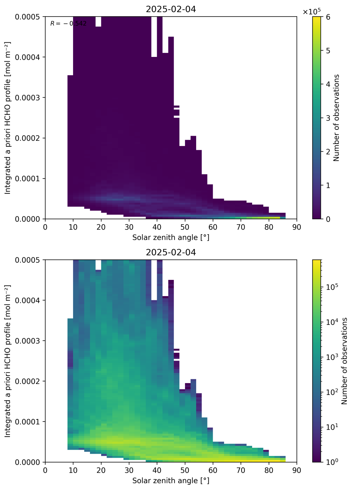
Figure 180: Scatter density plot of “Solar zenith angle” against “Integrated a priori HCHO profile” for 2025-02-03 to 2025-02-05.
