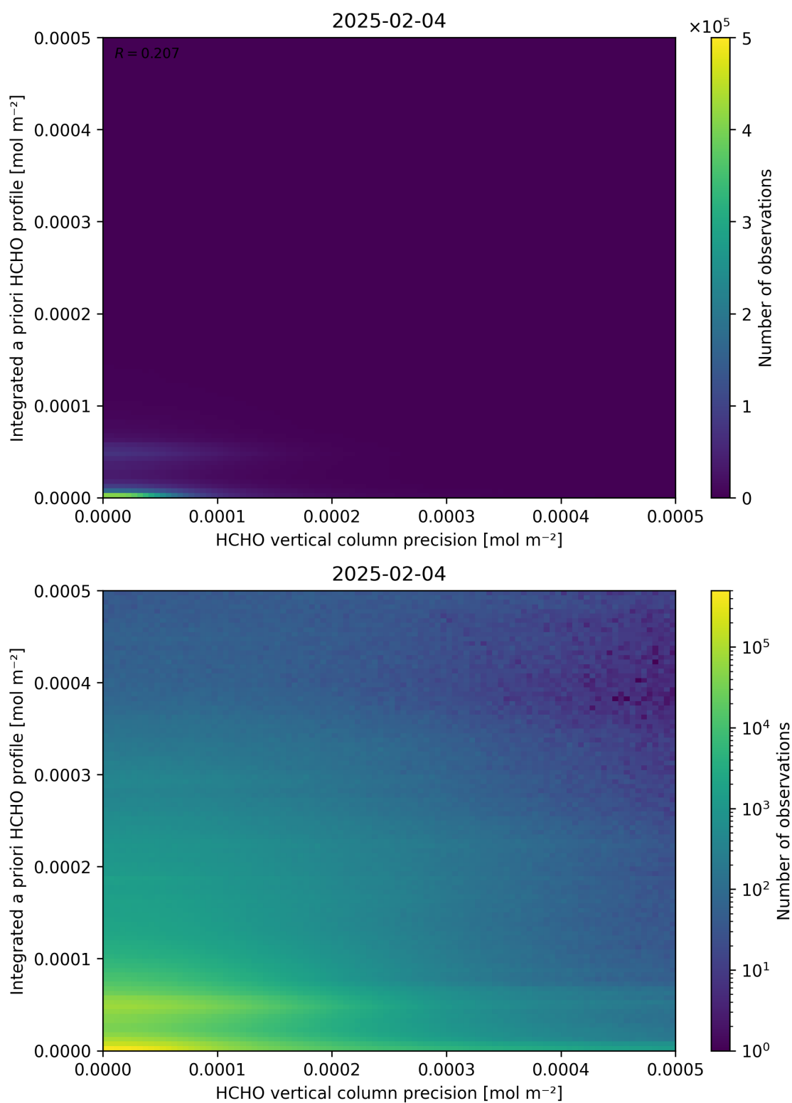
Figure 147: Scatter density plot of “HCHO vertical column precision” against “Integrated a priori HCHO profile” for 2025-02-03 to 2025-02-05.
