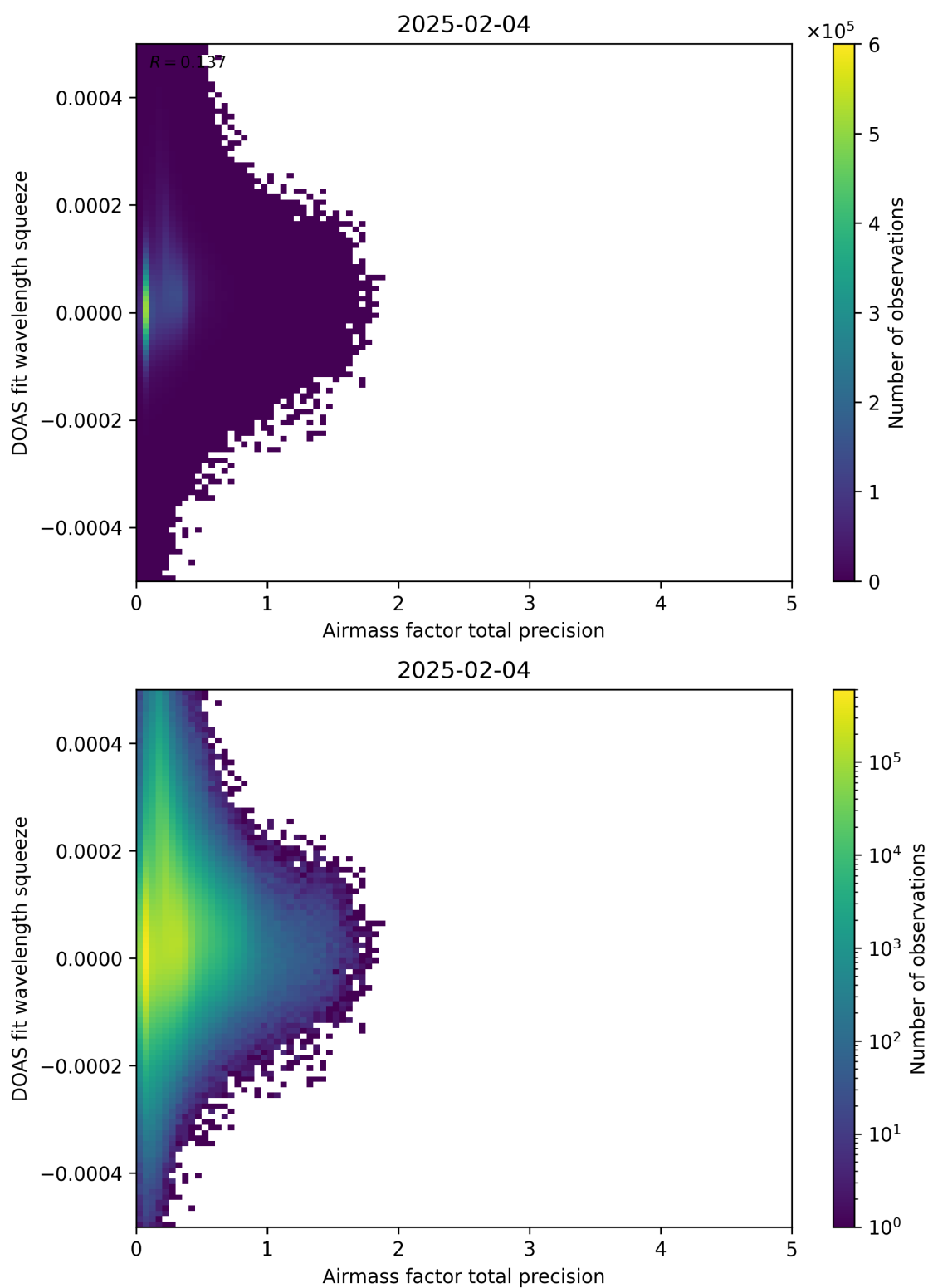
Figure 107: Scatter density plot of “Airmass factor total precision” against “DOAS fit wavelength squeeze” for 2025-02-03 to 2025-02-05.
