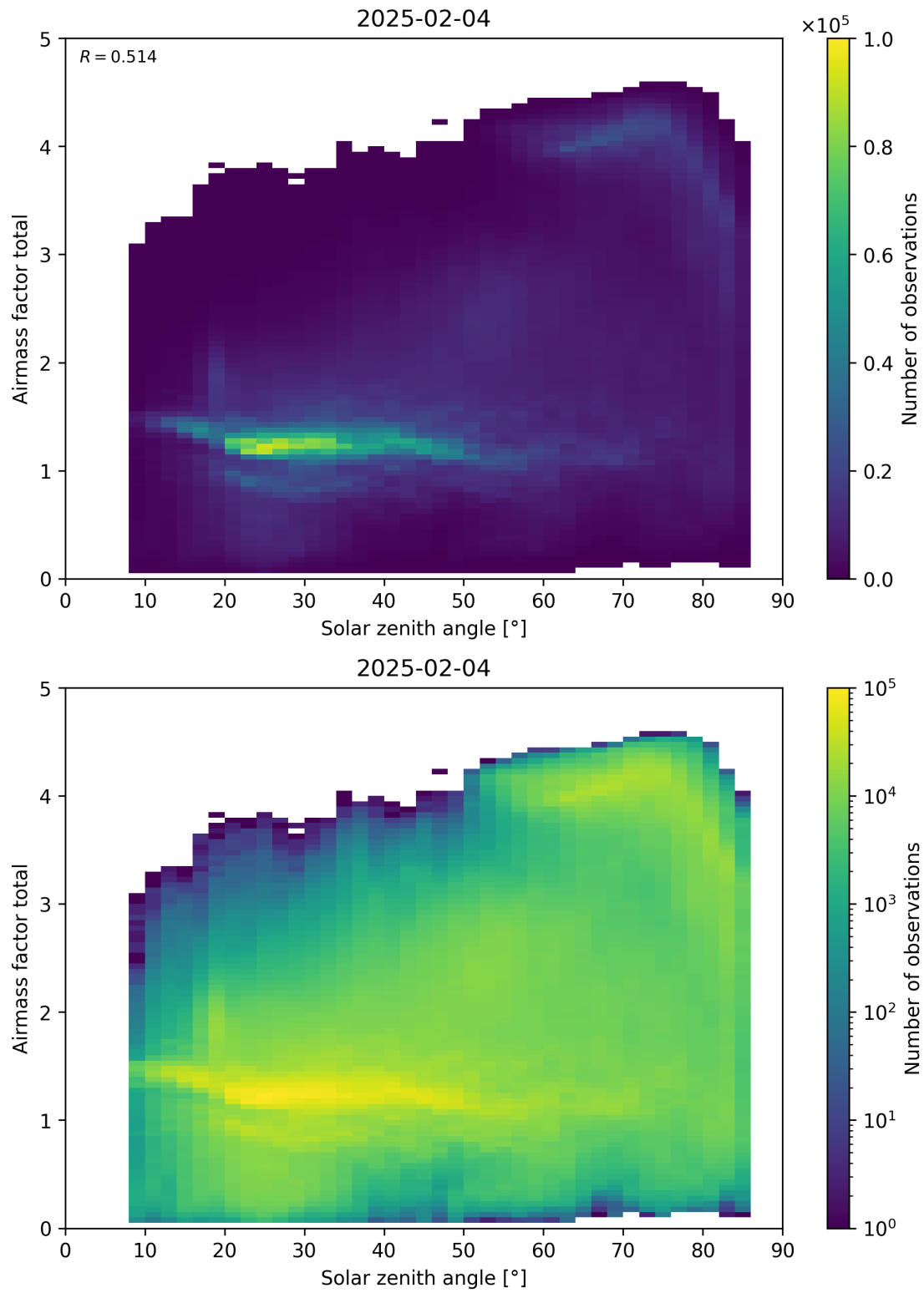
Figure 175: Scatter density plot of “Solar zenith angle” against “Airmass factor total” for 2025-02-03 to 2025-02-05.
