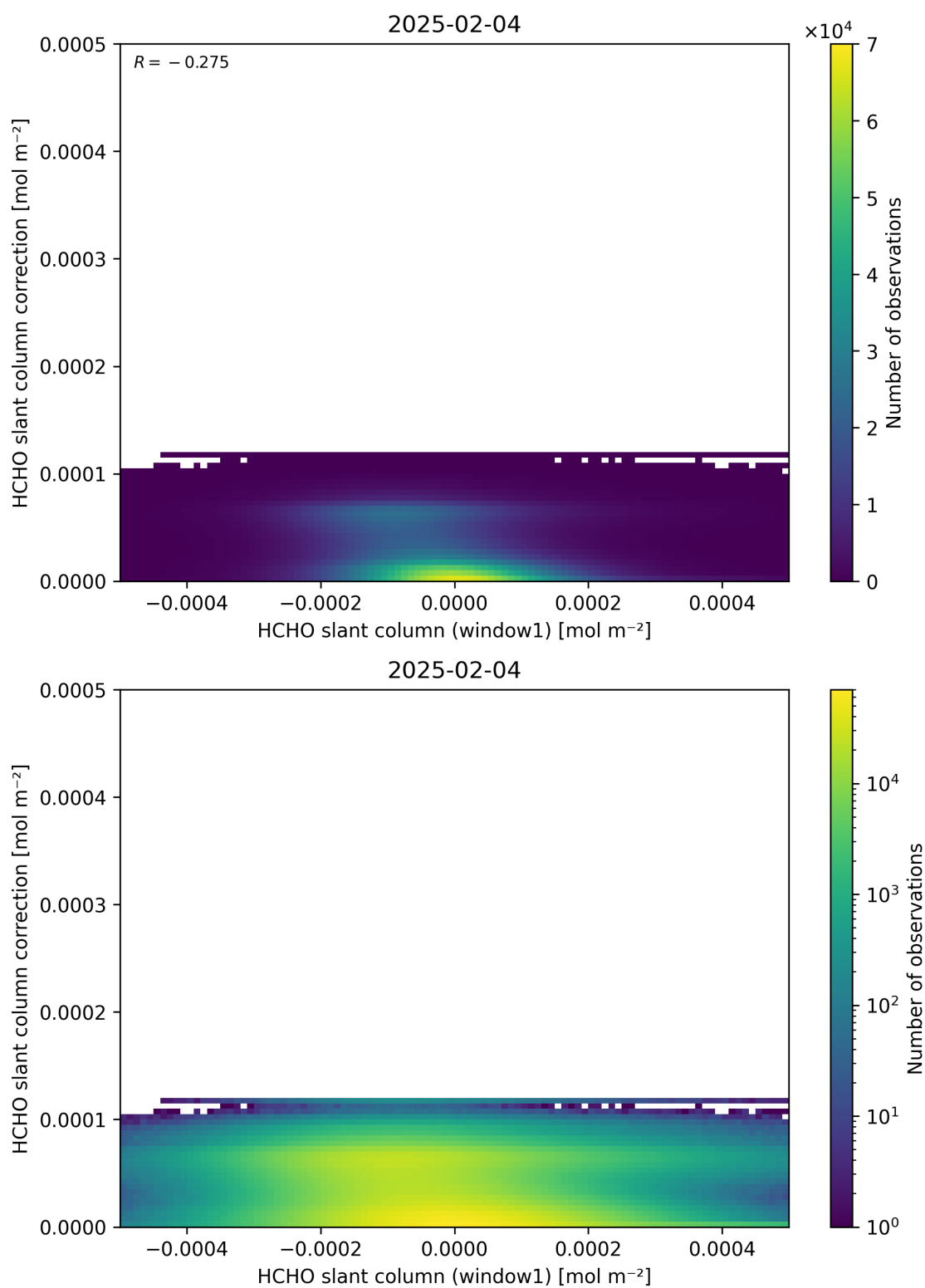
Figure 83: Scatter density plot of “HCHO slant column (window1)” against “HCHO slant column correction” for 2025-02-03 to 2025-02-05.
