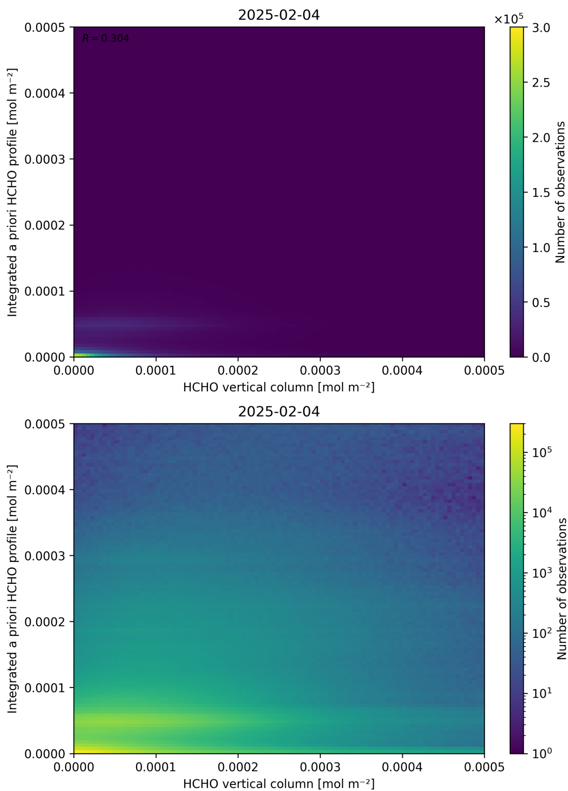
Figure 135: Scatter density plot of “HCHO vertical column” against “Integrated a priori HCHO profile” for 2025-02-03 to 2025-02-05.
