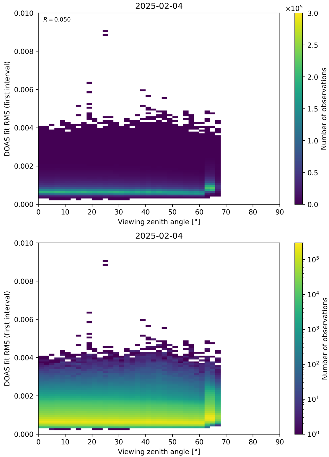
Figure 182: Scatter density plot of “Viewing zenith angle” against “DOAS fit RMS (first interval)” for 2025-02-03 to 2025-02-05.
