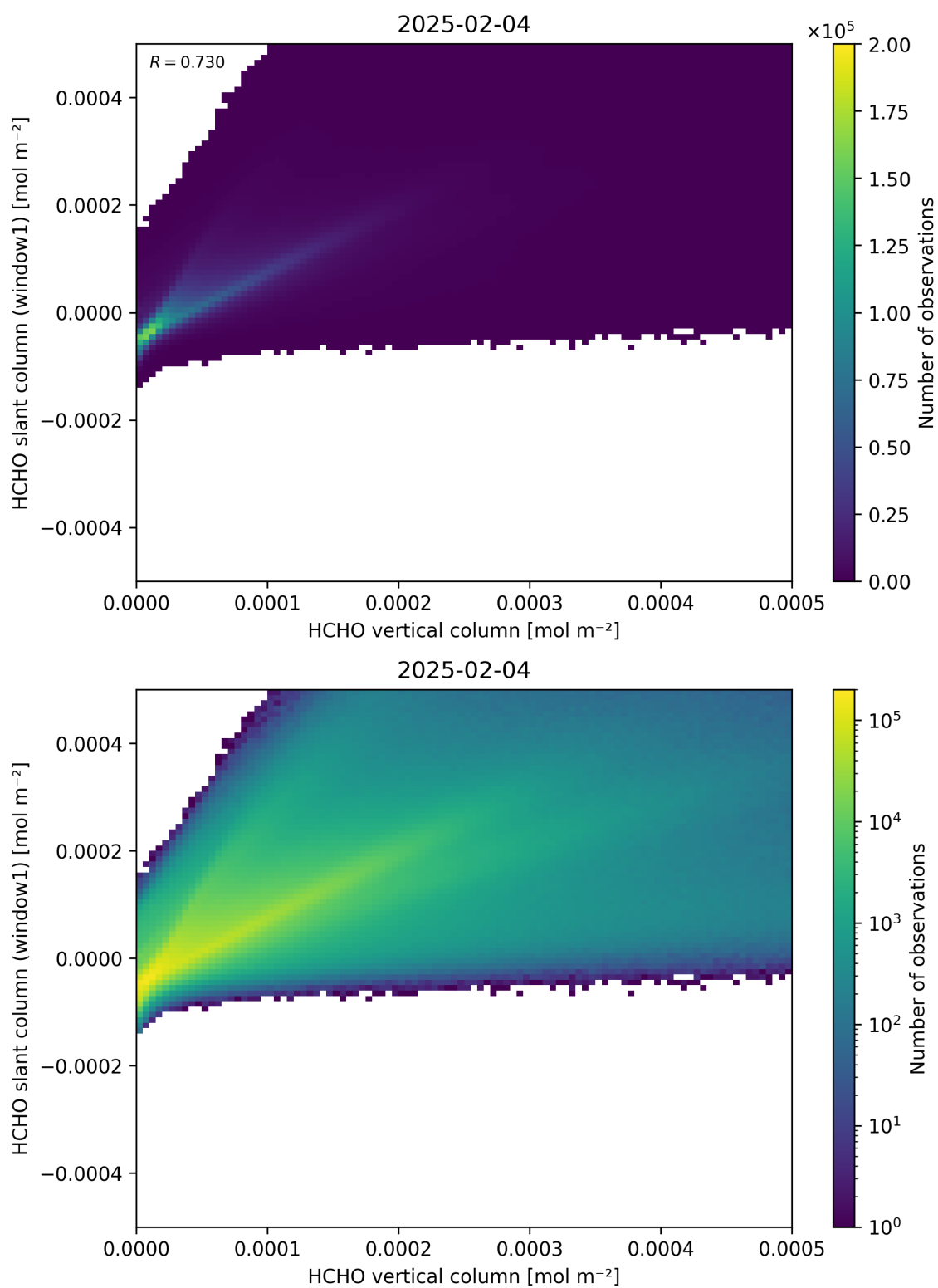
Figure 129: Scatter density plot of “HCHO vertical column” against “HCHO slant column (window1)” for 2025-02-03 to 2025-02-05.
