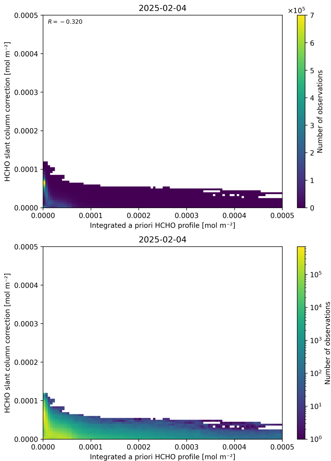
Figure 152: Scatter density plot of “Integrated a priori HCHO profile” against “HCHO slant column correction” for 2025-02-03 to 2025-02-05.
