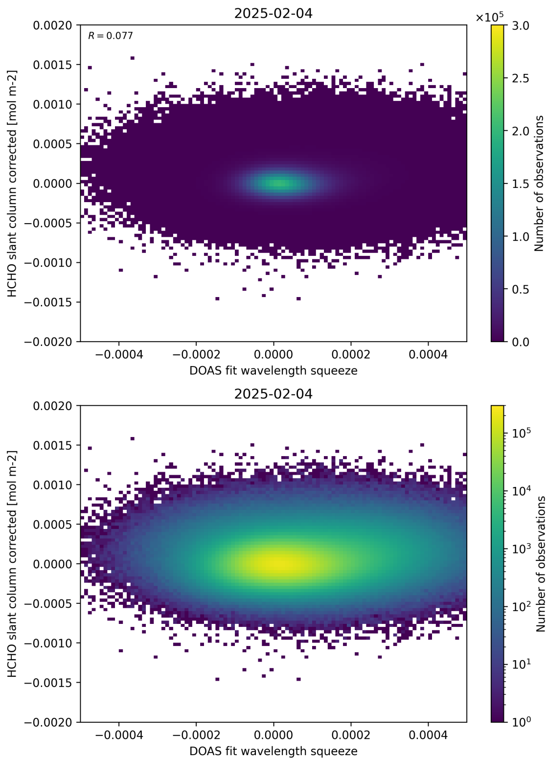
Figure 69: Scatter density plot of “DOAS fit wavelength squeeze” against “HCHO slant column corrected” for 2025-02-03 to 2025-02-05.
