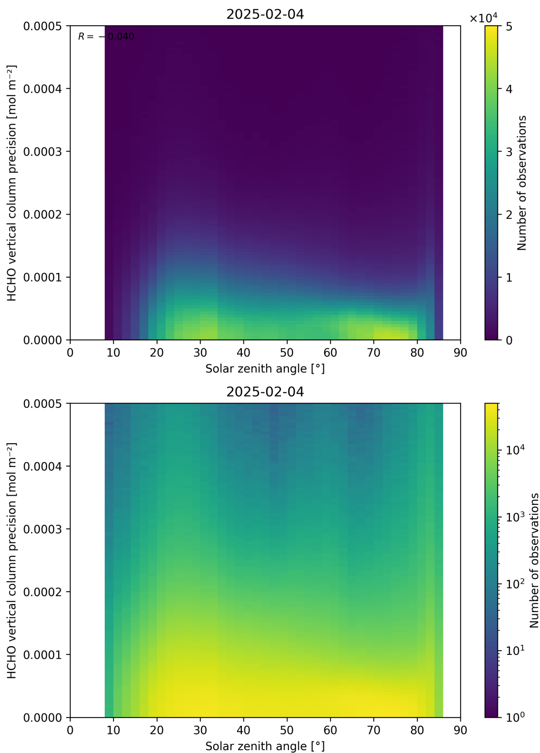
Figure 179: Scatter density plot of “Solar zenith angle” against “HCHO vertical column precision” for 2025-02-03 to 2025-02-05.
