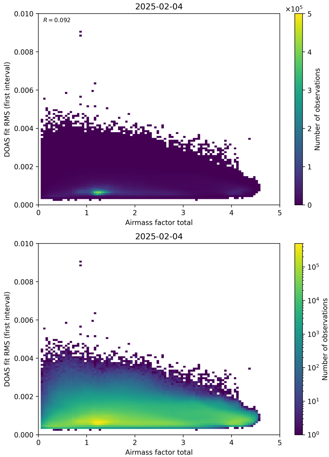
Figure 97: Scatter density plot of “Airmass factor total” against “DOAS fit RMS (first interval)” for 2025-02-03 to 2025-02-05.
