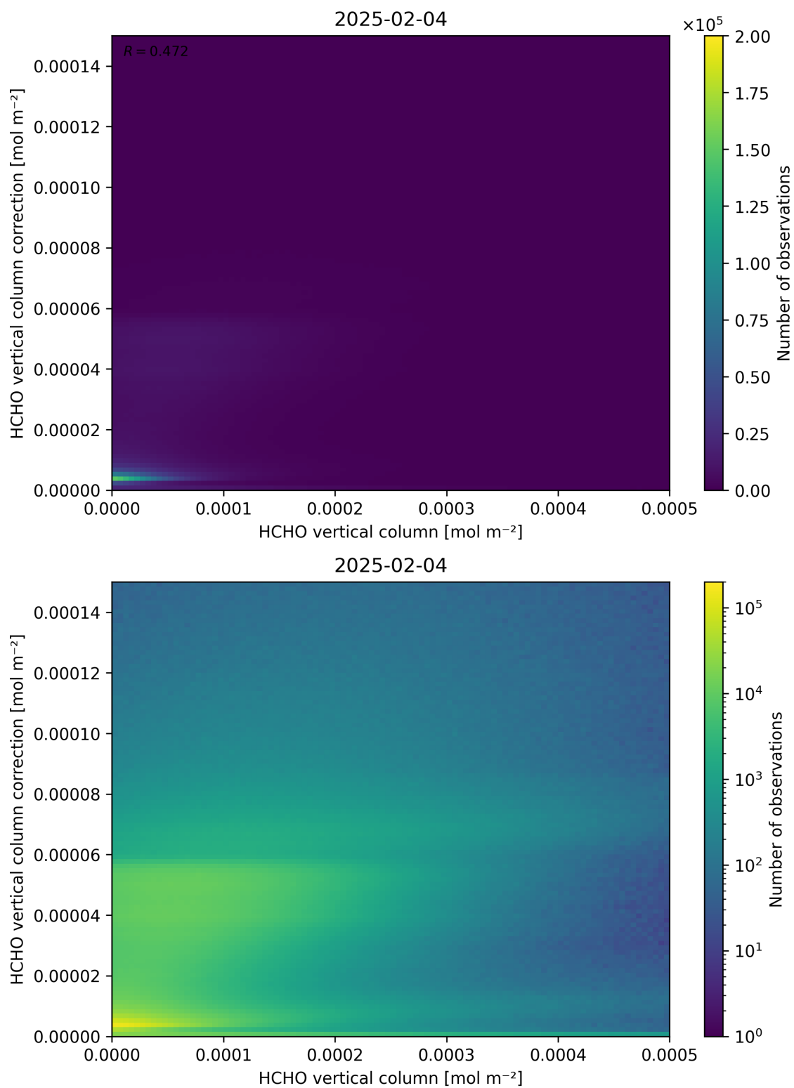
Figure 133: Scatter density plot of “HCHO vertical column” against “HCHO vertical column correction” for 2025-02-03 to 2025-02-05.
