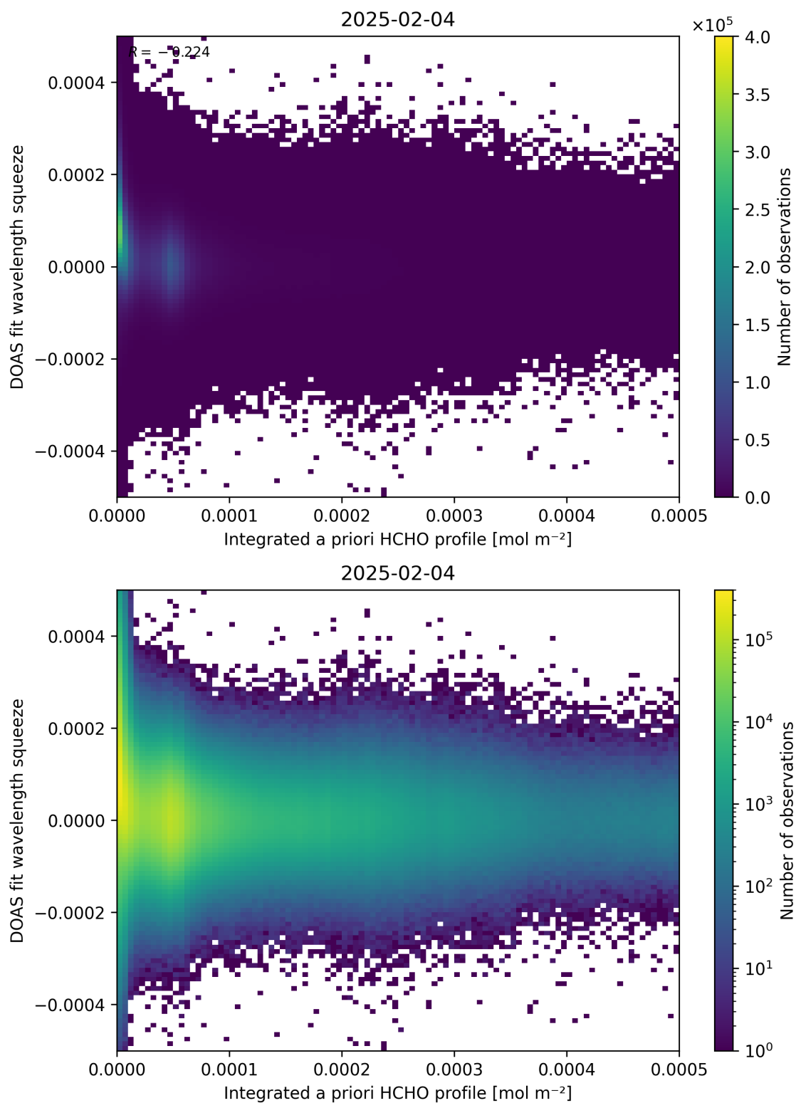
Figure 150: Scatter density plot of “Integrated a priori HCHO profile” against “DOAS fit wavelength squeeze” for 2025-02-03 to 2025-02-05.
