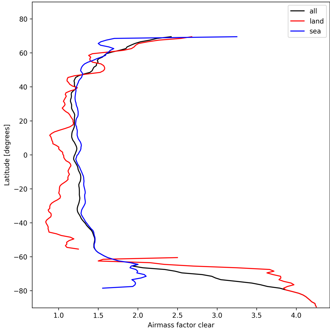
Figure 28: Zonal average of “Airmass factor clear” for 2025-02-03 to 2025-02-05.
