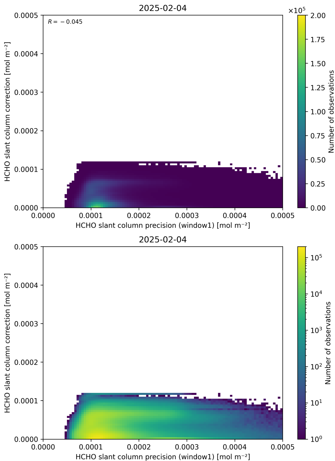
Figure 93: Scatter density plot of “HCHO slant column precision (window1)” against “HCHO slant column correction” for 2025-02-03 to 2025-02-05.
