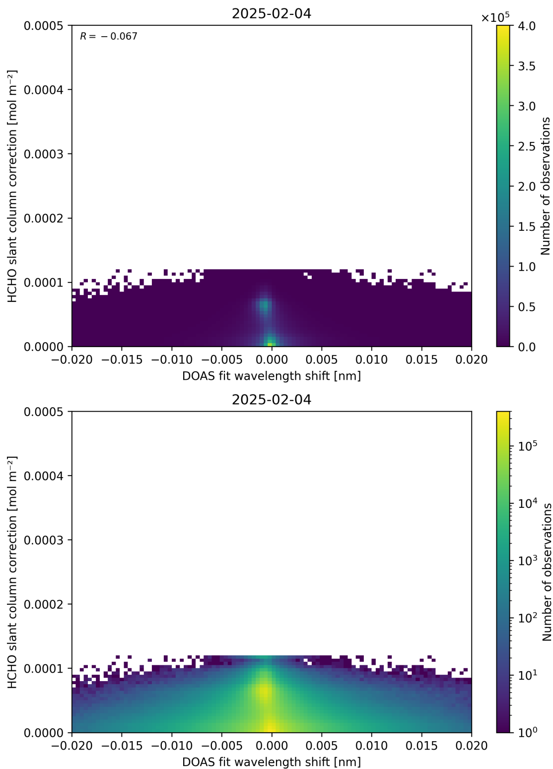
Figure 67: Scatter density plot of “DOAS fit wavelength shift” against “HCHO slant column correction” for 2025-02-03 to 2025-02-05.
