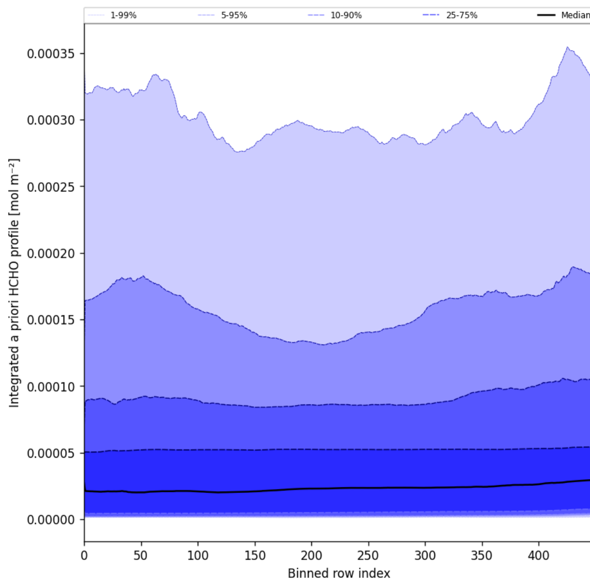
Figure 57: Along track statistics of “Integrated a priori HCHO profile” for 2025-02-03 to 2025-02-05
