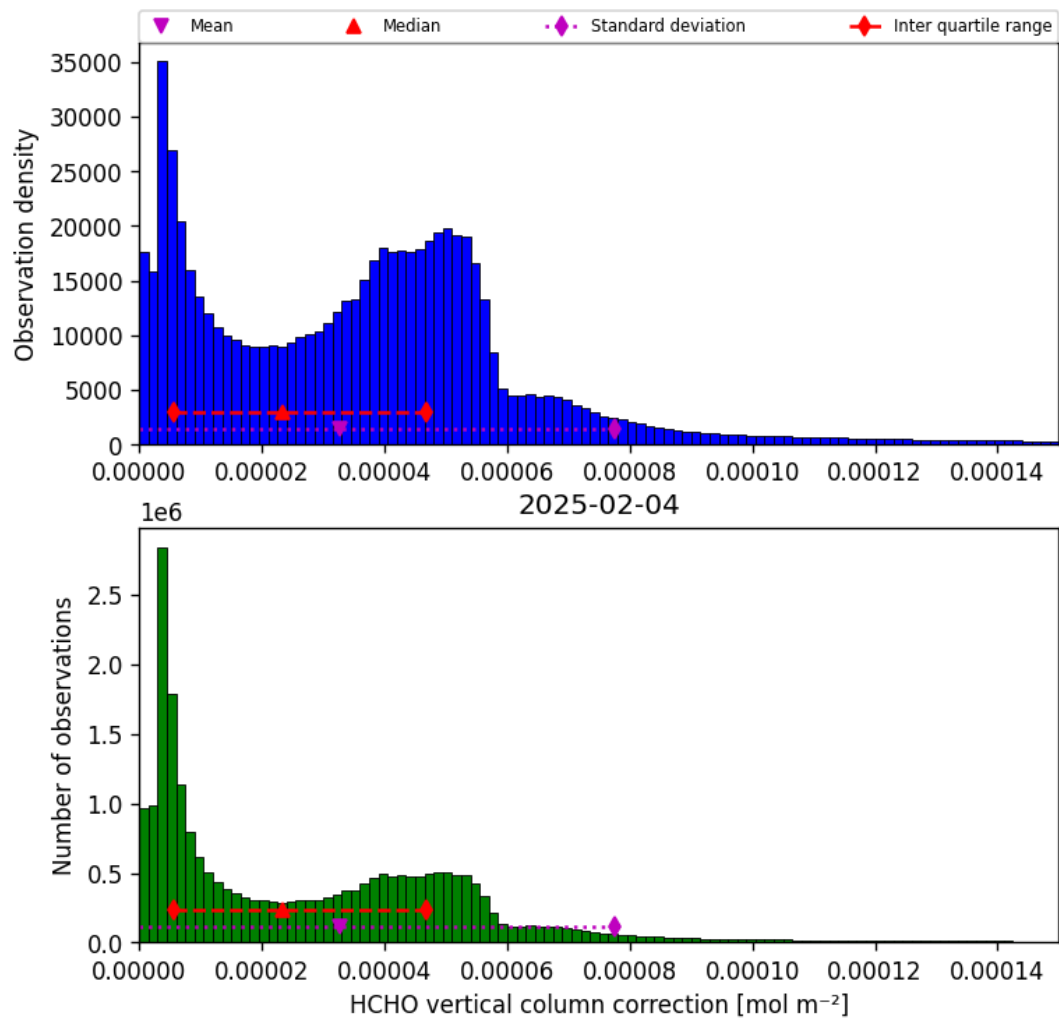
Figure 37: Histogram of “HCHO vertical column correction” for 2025-02-03 to 2025-02-05
