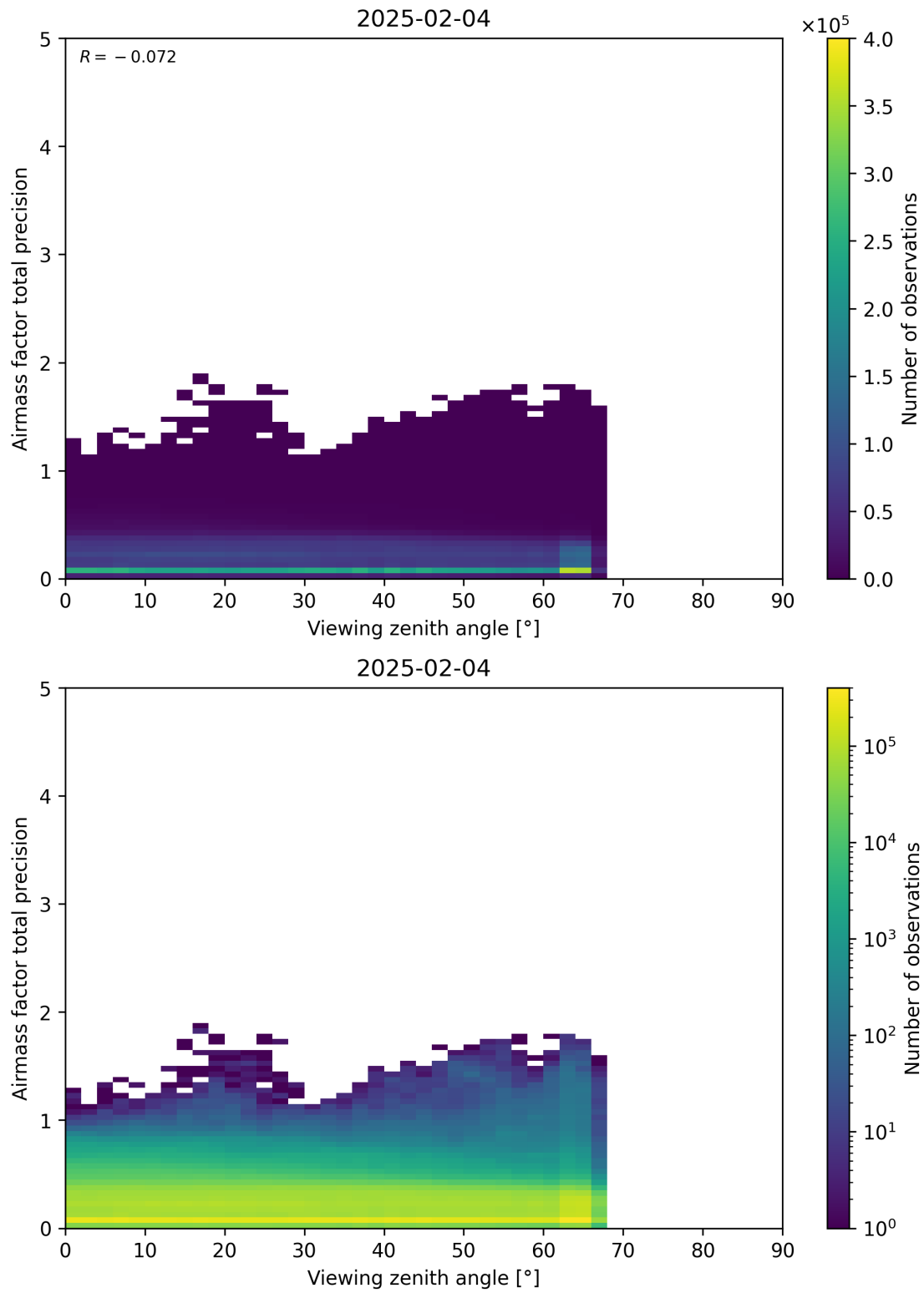
Figure 191: Scatter density plot of “Viewing zenith angle” against “Airmass factor total precision” for 2025-02-03 to 2025-02-05.
