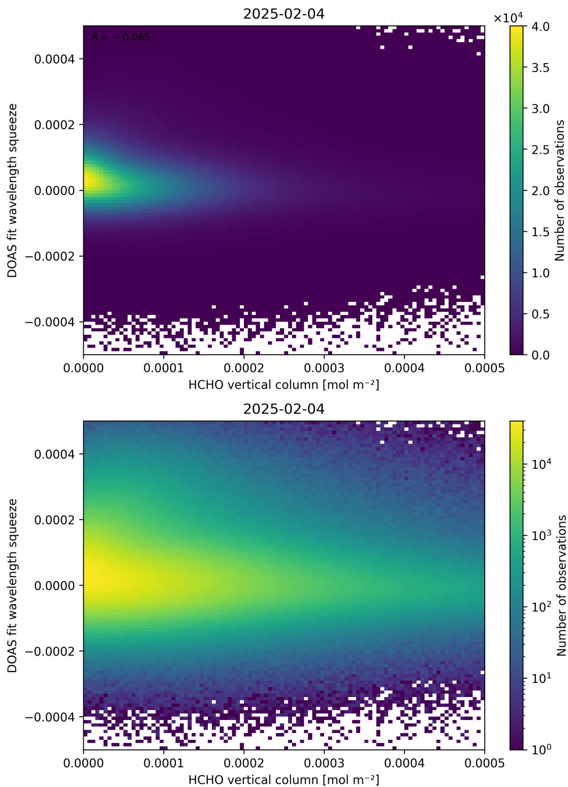
Figure 125: Scatter density plot of “HCHO vertical column” against “DOAS fit wavelength squeeze” for 2025-02-03 to 2025-02-05.
