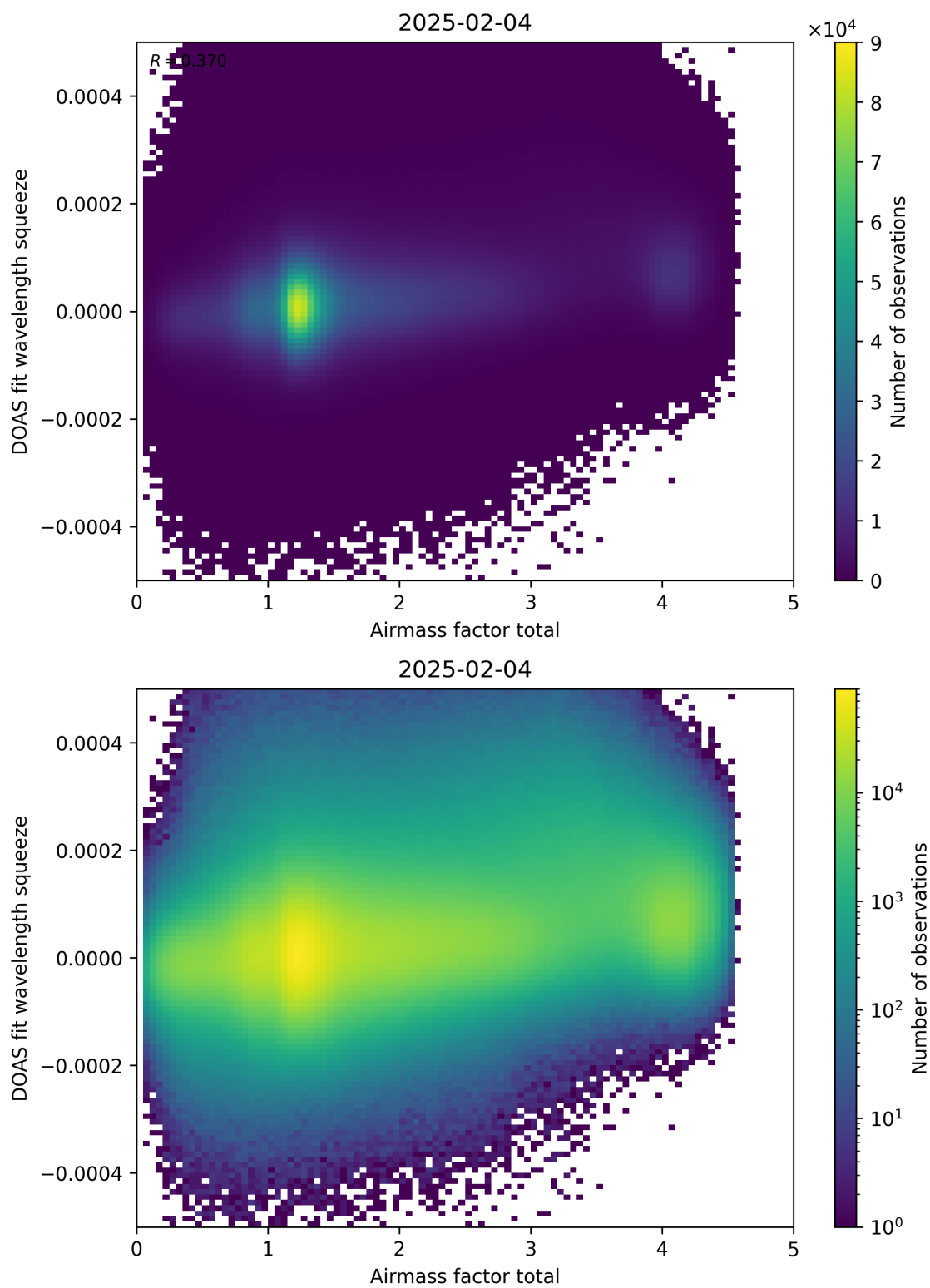
Figure 99: Scatter density plot of “Airmass factor total” against “DOAS fit wavelength squeeze” for 2025-02-03 to 2025-02-05.
