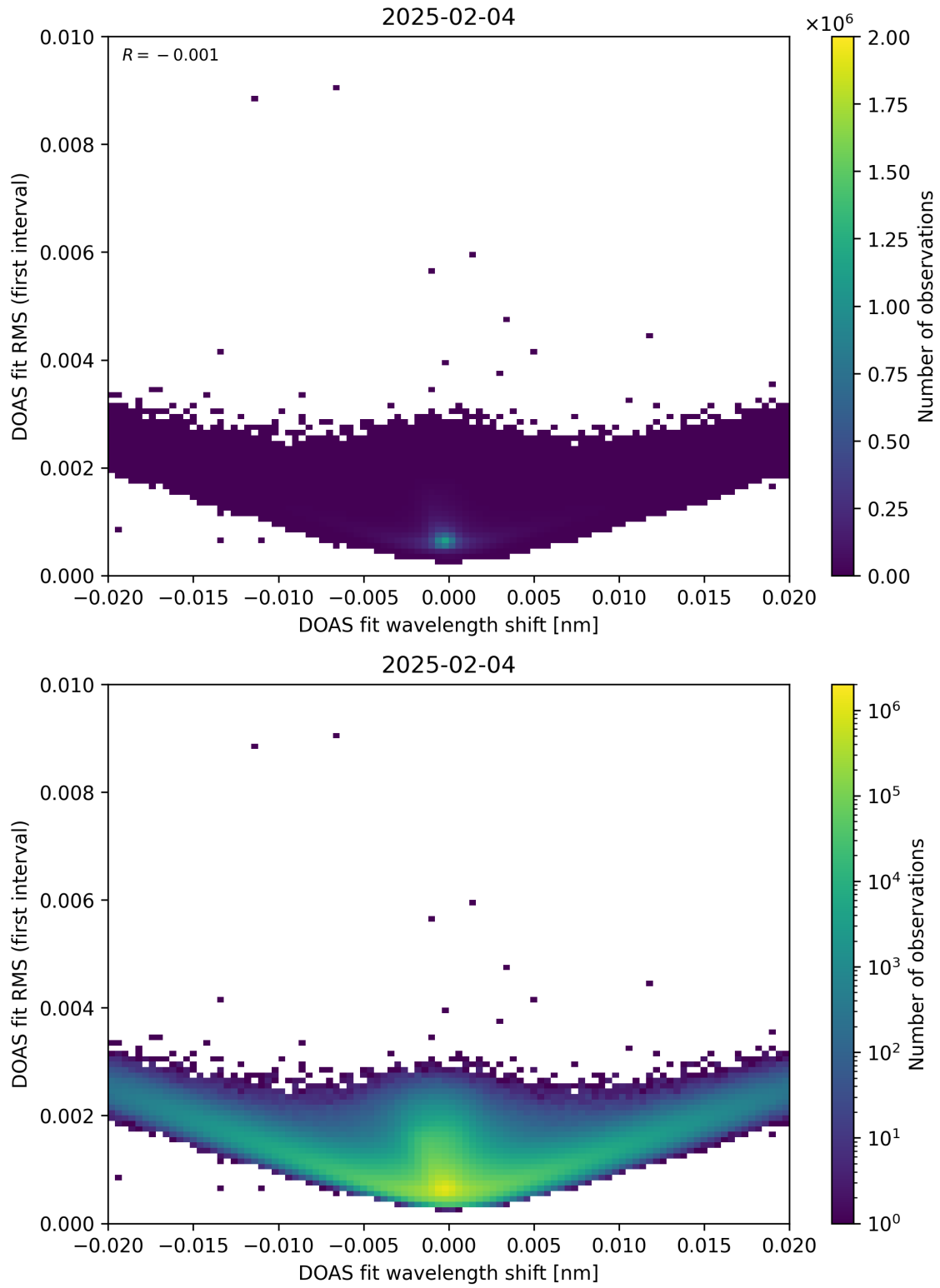
Figure 64: Scatter density plot of “DOAS fit wavelength shift” against “DOAS fit RMS (first interval)” for 2025-02-03 to 2025-02-05.
