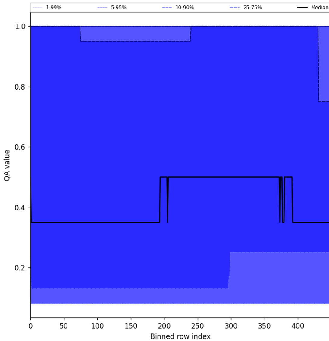
Figure 48: Along track statistics of “QA value” for 2025-02-03 to 2025-02-05
