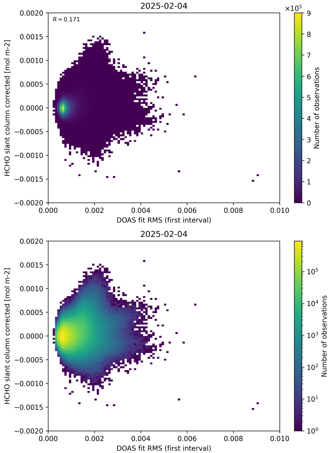
Figure 62: Scatter density plot of “DOAS fit RMS (first interval)” against “HCHO slant column corrected” for 2025-02-03 to 2025-02-05.
