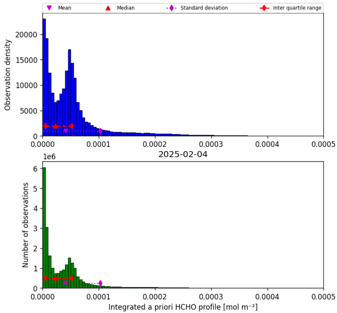
Figure 43: Histogram of “Integrated a priori HCHO profile” for 2025-02-03 to 2025-02-05
