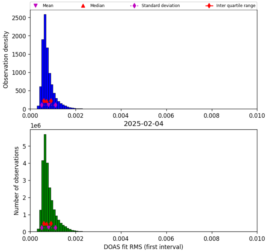
Figure 46: Histogram of “DOAS fit RMS (first interval)” for 2025-02-03 to 2025-02-05
