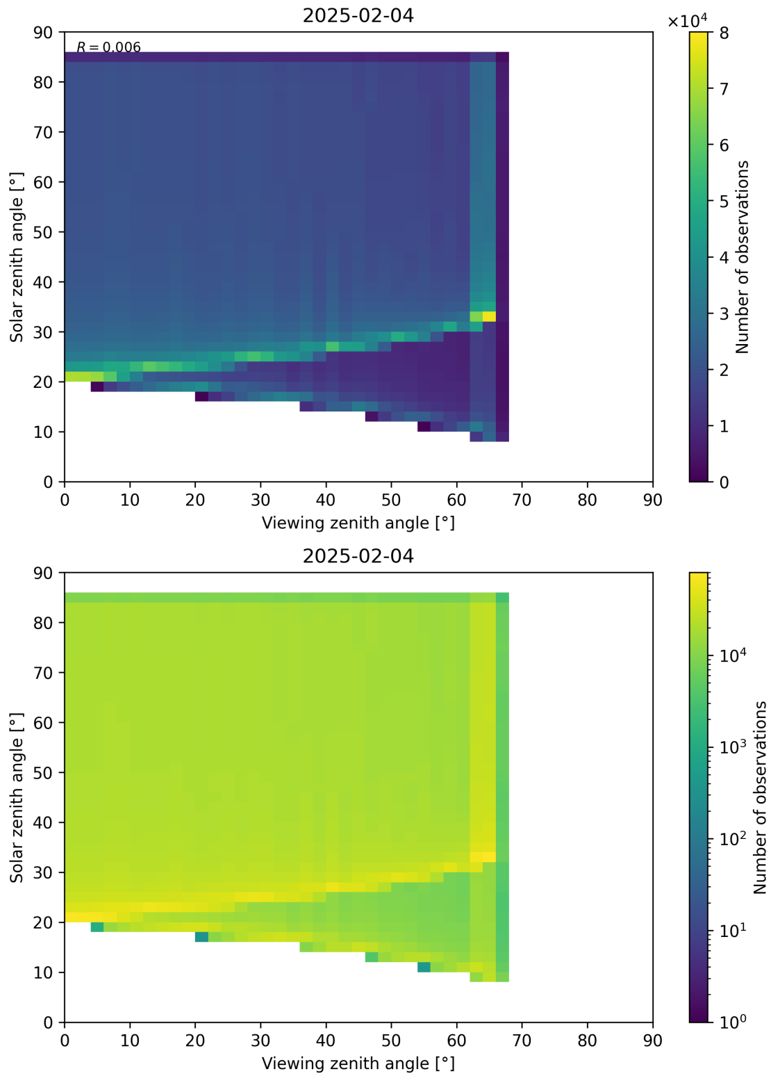
Figure 197: Scatter density plot of “Viewing zenith angle” against “Solar zenith angle” for 2025-02-03 to 2025-02-05.
