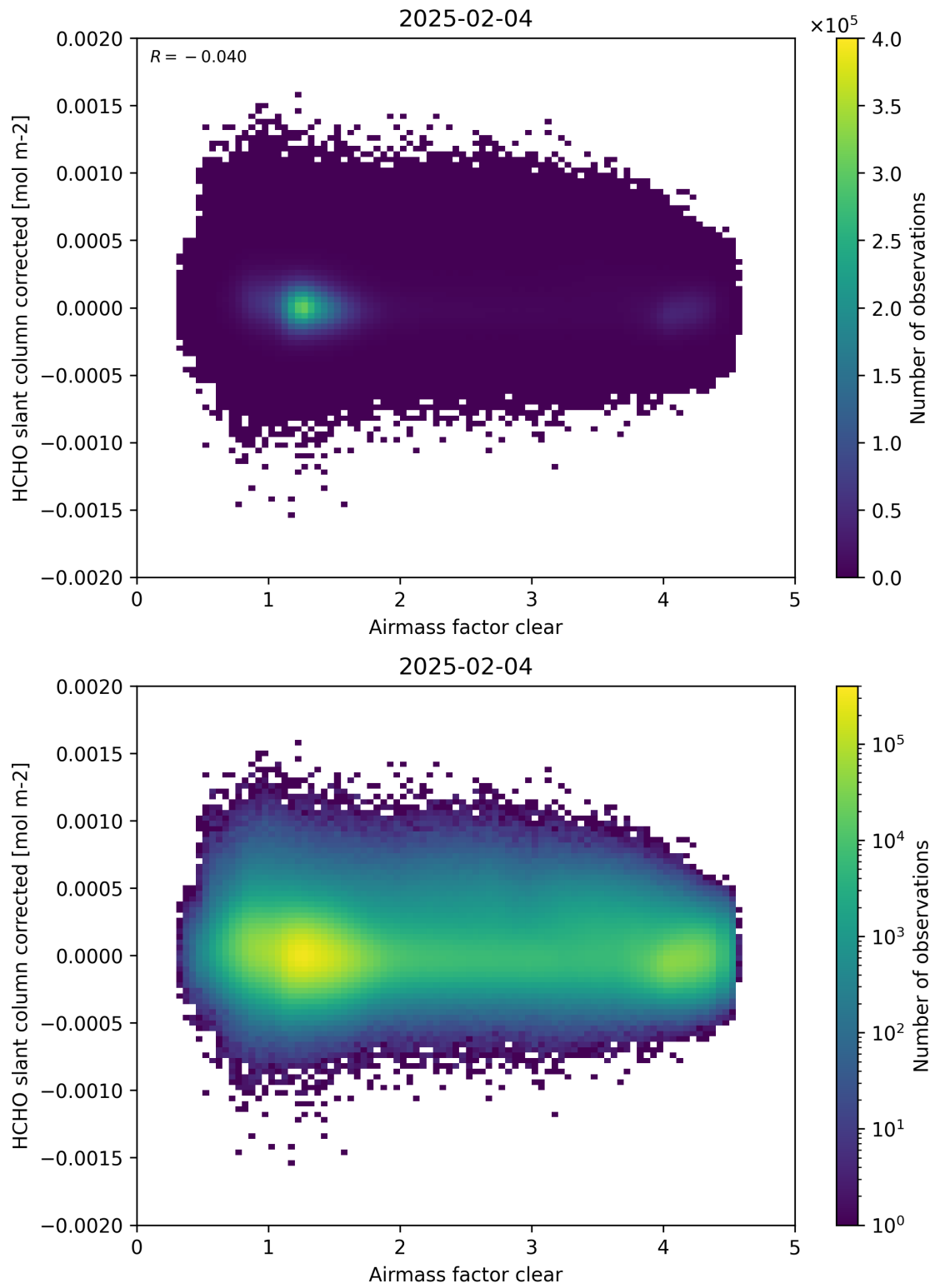
Figure 74: Scatter density plot of “Airmass factor clear” against “HCHO slant column corrected” for 2025-02-03 to 2025-02-05.
