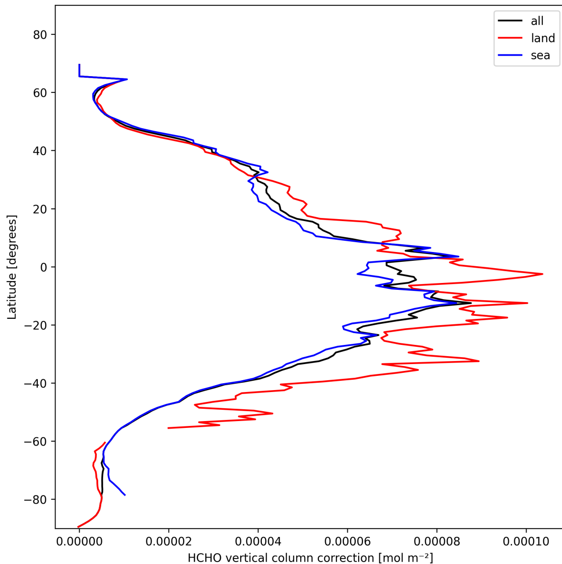
Figure 23: Zonal average of “HCHO vertical column correction” for 2025-02-03 to 2025-02-05.
