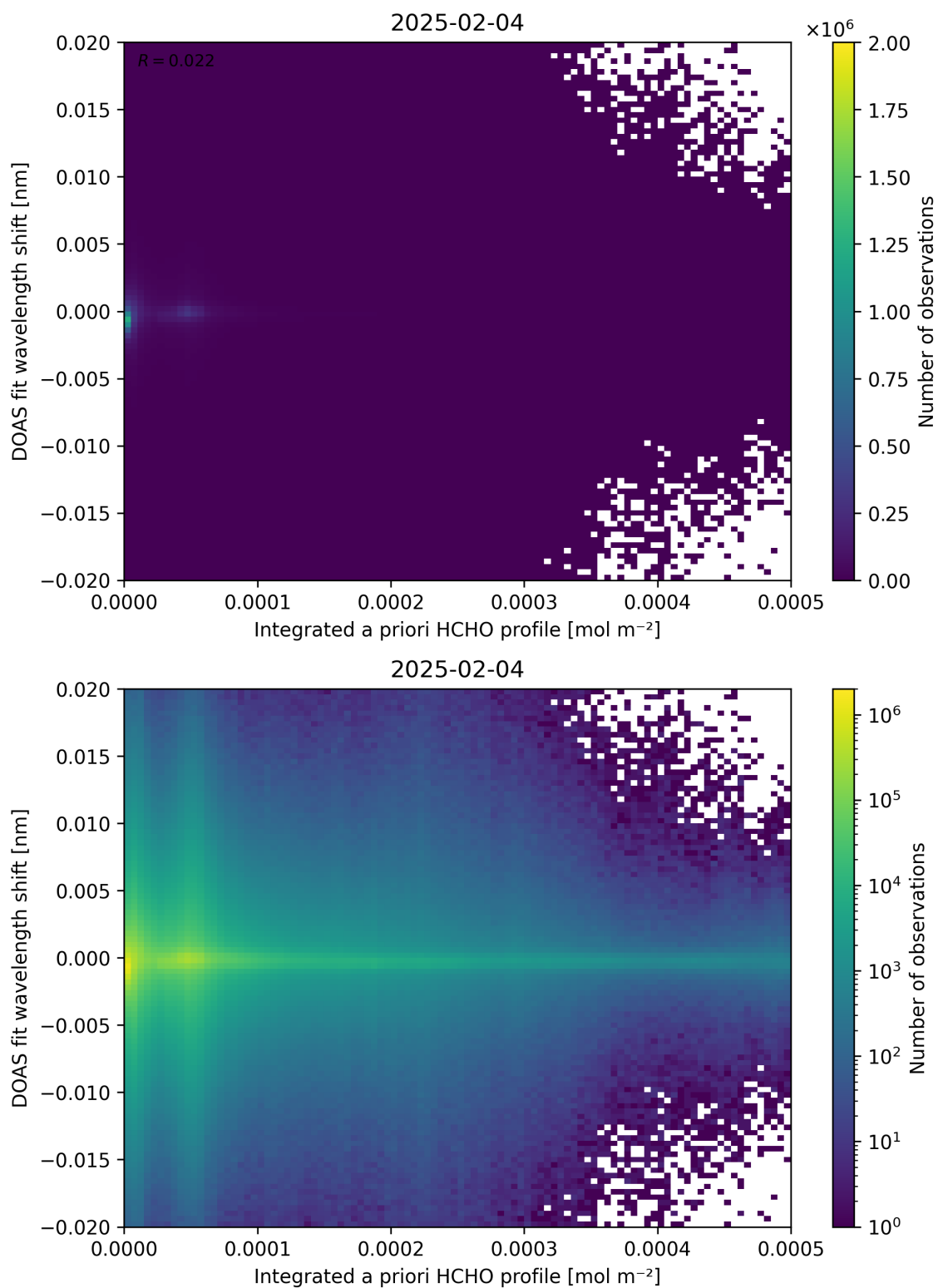
Figure 149: Scatter density plot of “Integrated a priori HCHO profile” against “DOAS fit wavelength shift” for 2025-02-03 to 2025-02-05.
