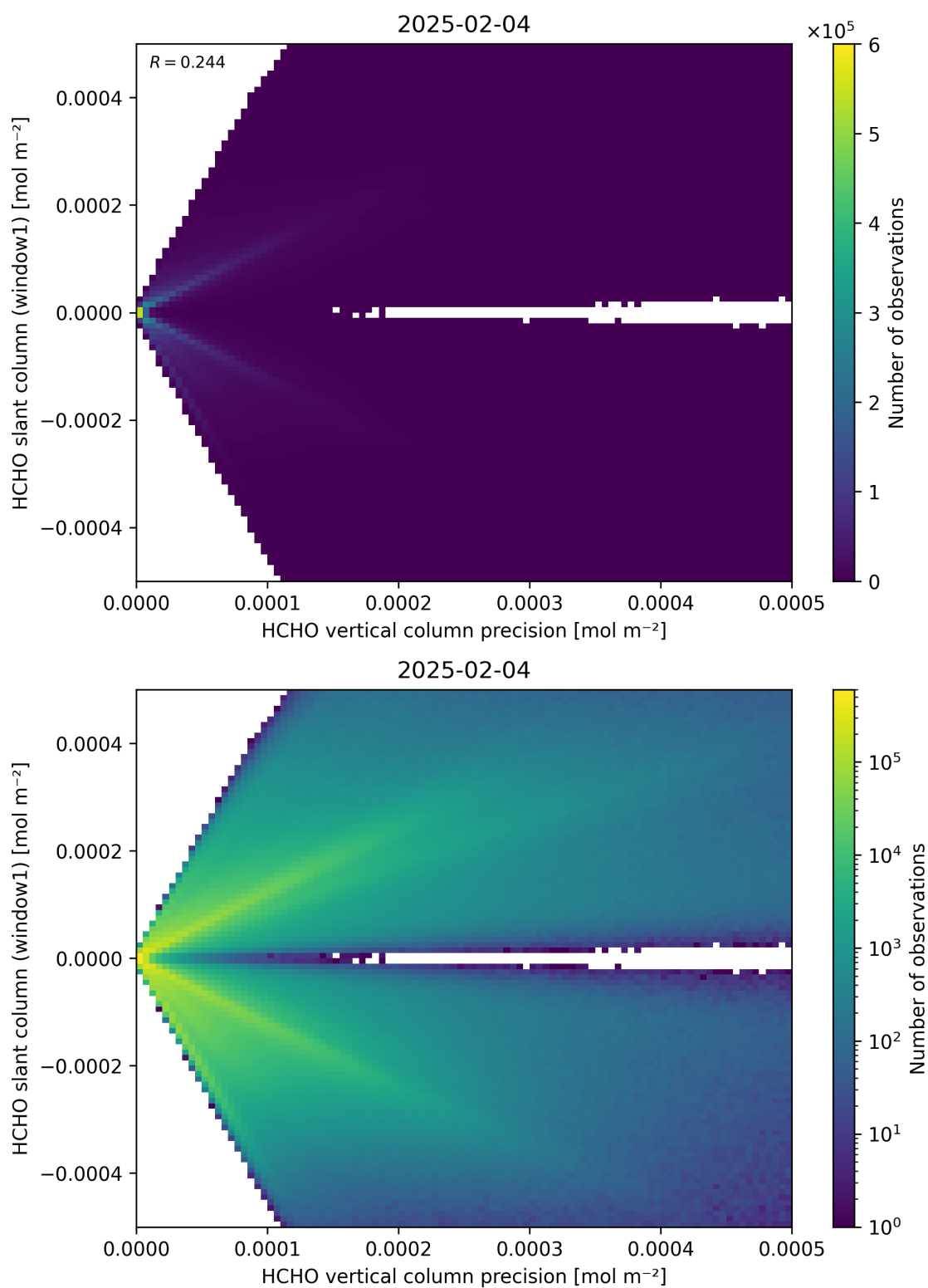
Figure 142: Scatter density plot of “HCHO vertical column precision” against “HCHO slant column (window1)” for 2025-02-03 to 2025-02-05.
