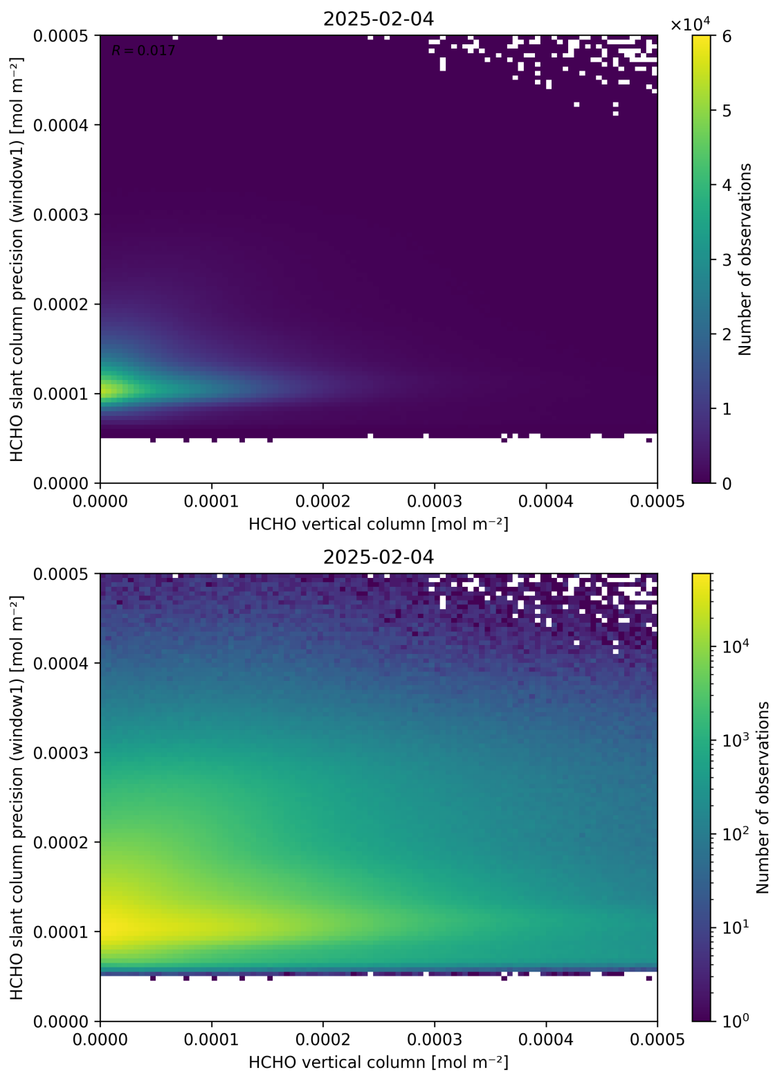
Figure 130: Scatter density plot of “HCHO vertical column” against “HCHO slant column precision (window1)” for 2025-02-03 to 2025-02-05.
