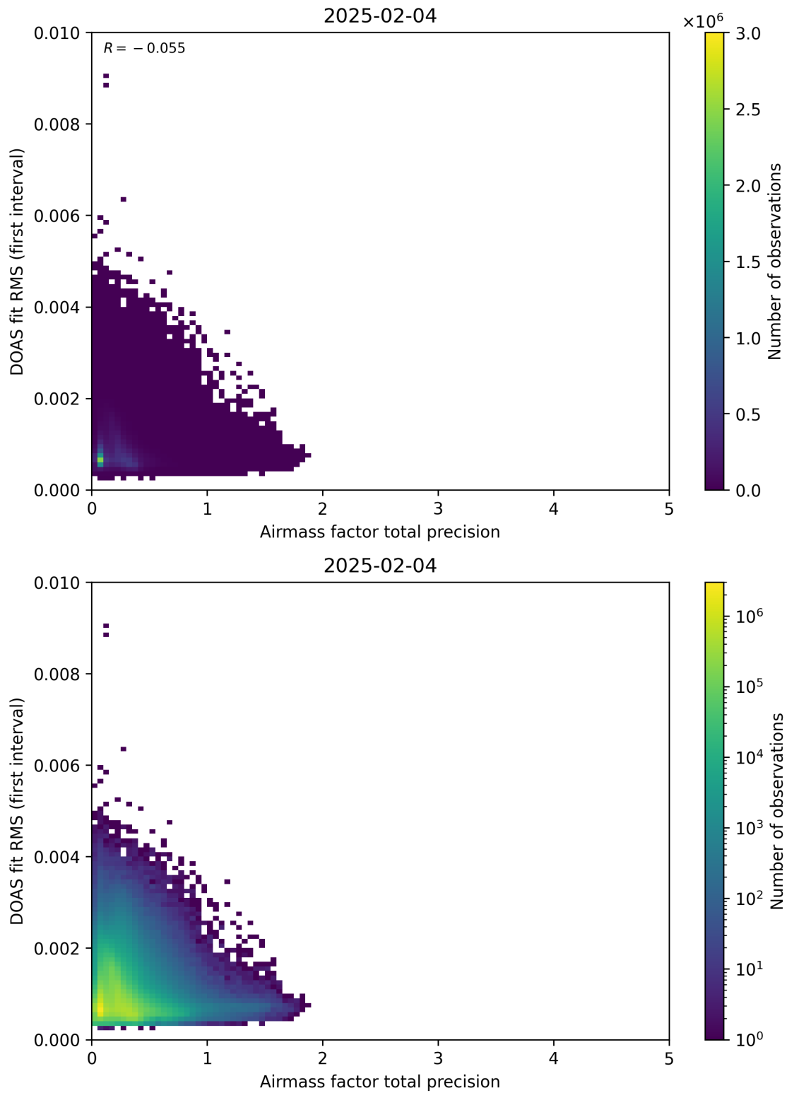
Figure 105: Scatter density plot of “Airmass factor total precision” against “DOAS fit RMS (first interval)” for 2025-02-03 to 2025-02-05.
