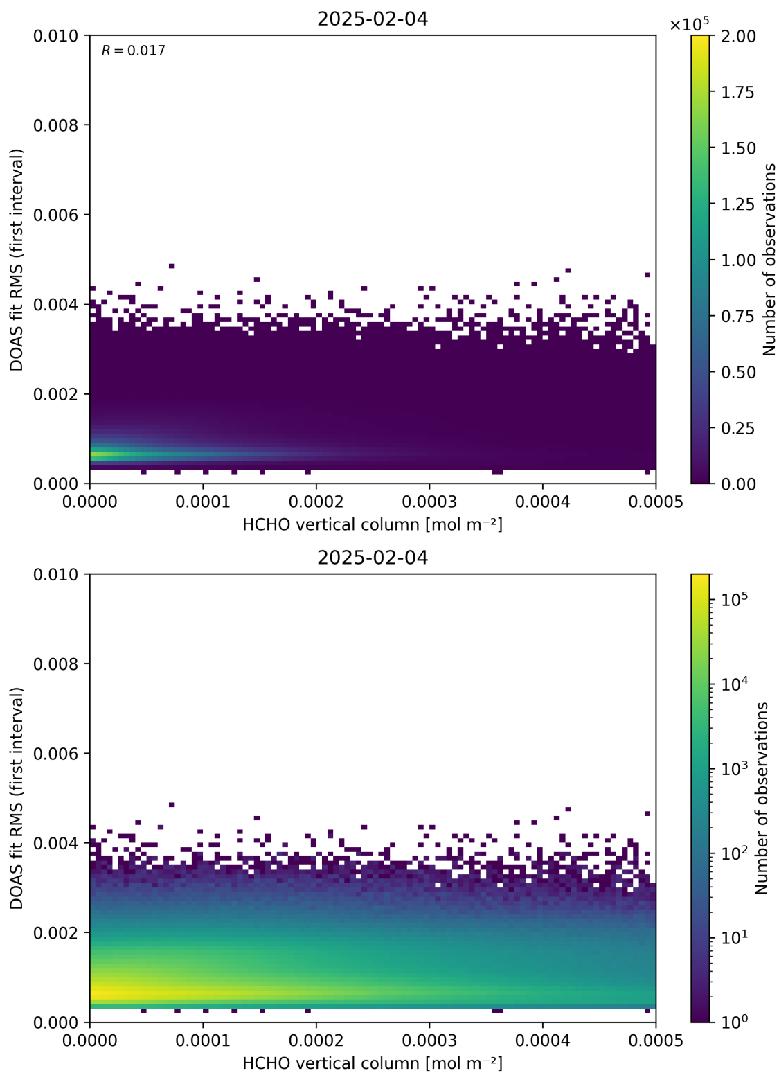
Figure 123: Scatter density plot of “HCHO vertical column” against “DOAS fit RMS (first interval)” for 2025-02-03 to 2025-02-05.
