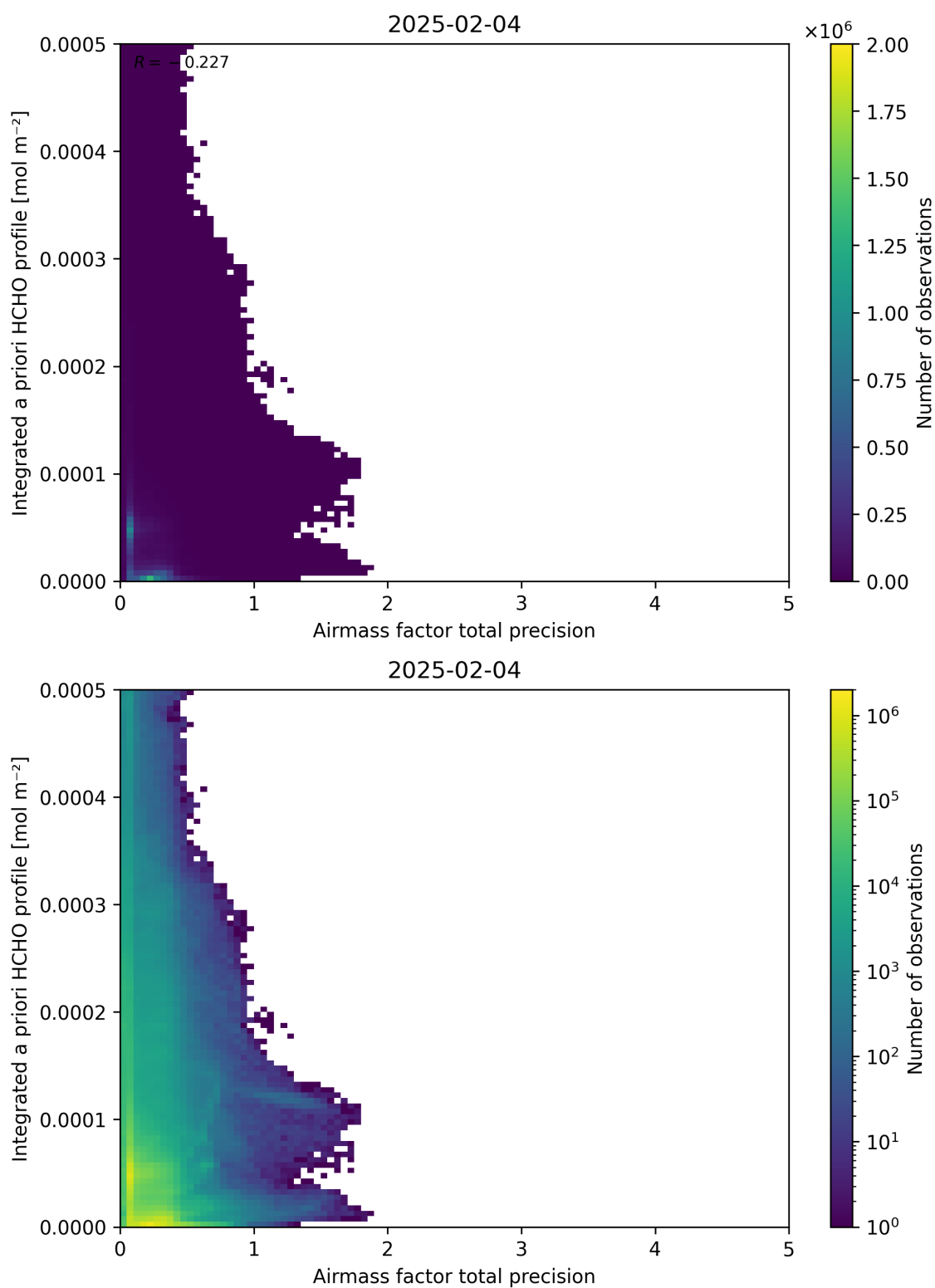
Figure 111: Scatter density plot of “Airmass factor total precision” against “Integrated a priori HCHO profile” for 2025-02-03 to 2025-02-05.
