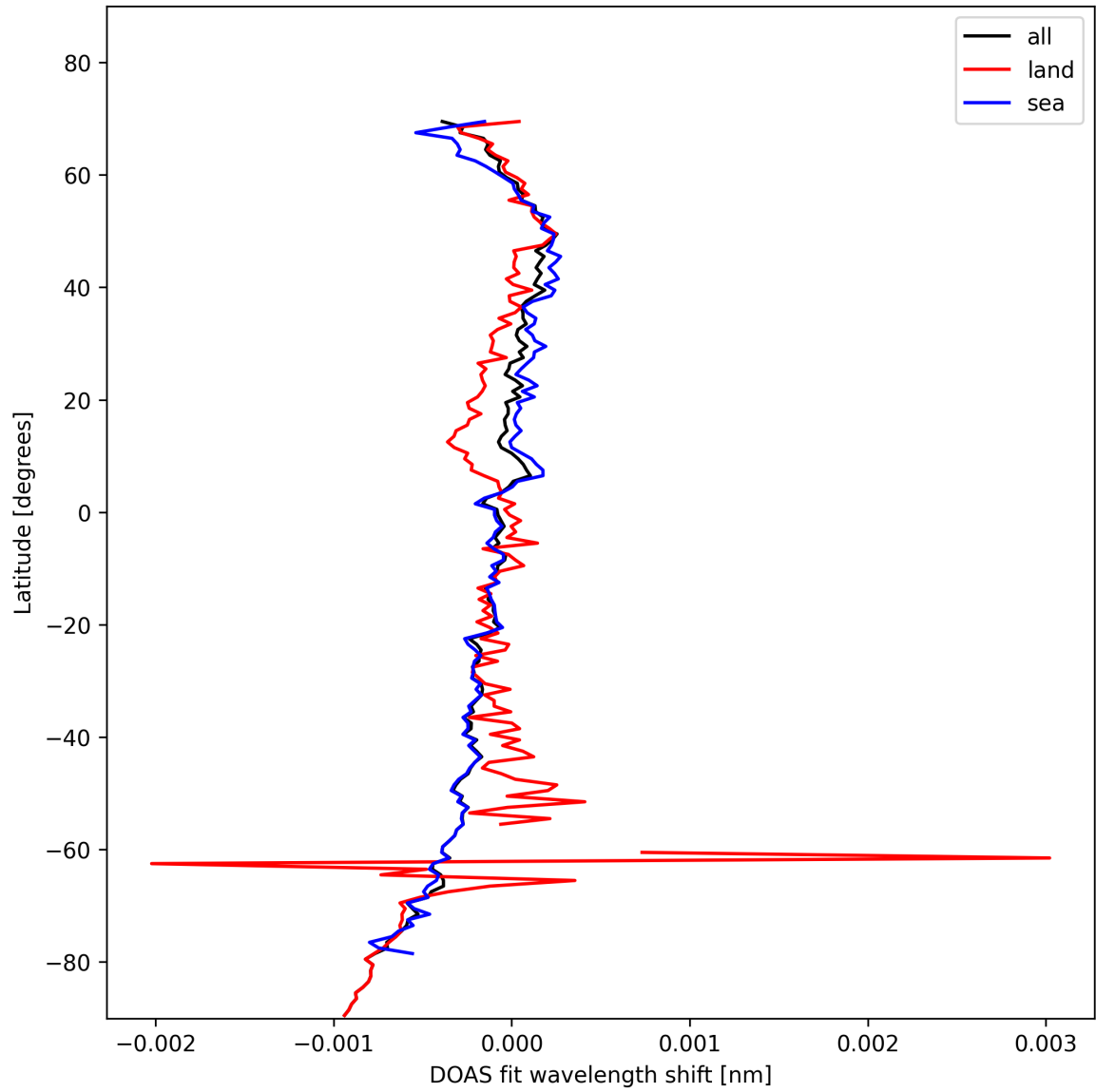
Figure 30: Zonal average of “DOAS fit wavelength shift” for 2025-02-03 to 2025-02-05.
