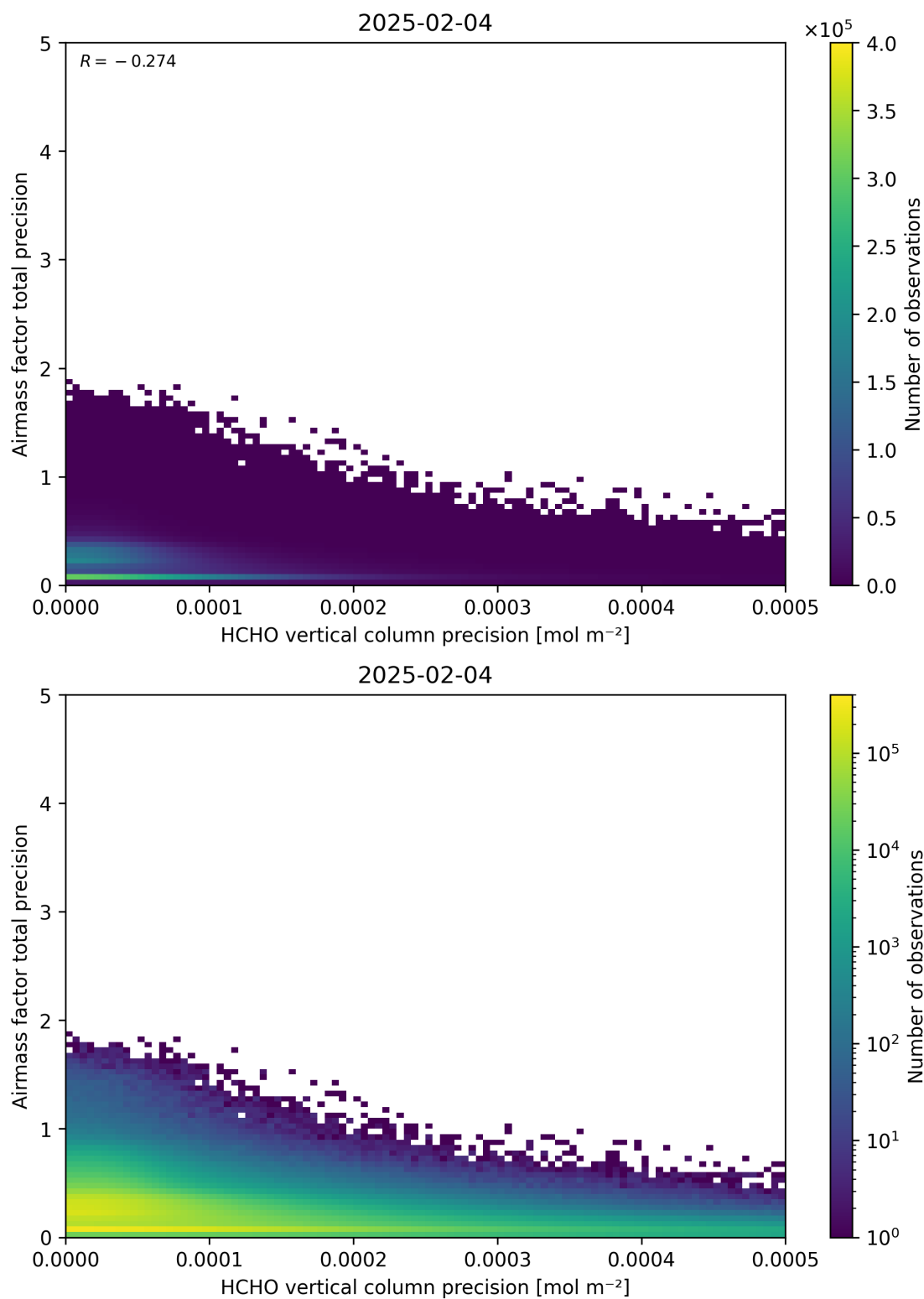
Figure 145: Scatter density plot of “HCHO vertical column precision” against “Airmass factor total precision” for 2025-02-03 to 2025-02-05.
