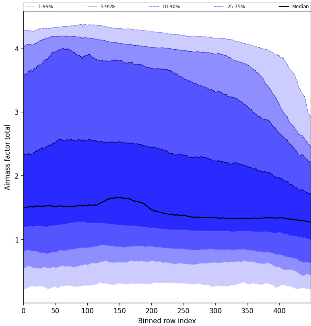
Figure 54: Along track statistics of “Airmass factor total” for 2025-02-03 to 2025-02-05
