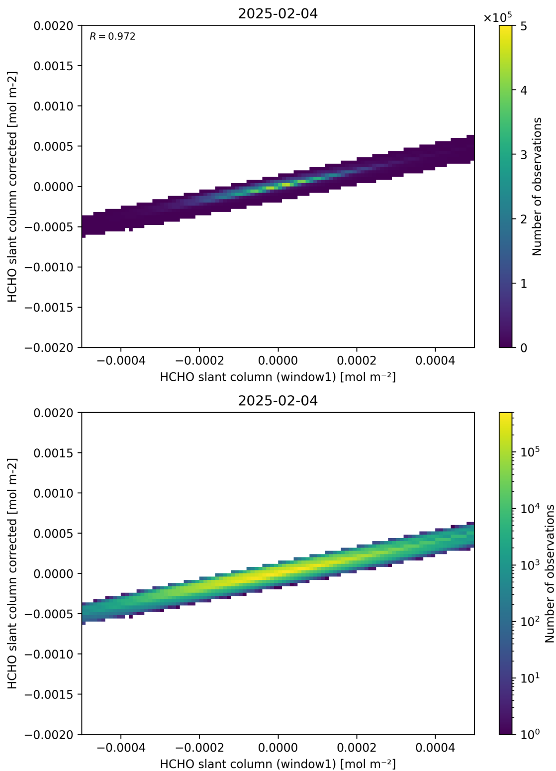
Figure 82: Scatter density plot of “HCHO slant column (window1)” against “HCHO slant column corrected” for 2025-02-03 to 2025-02-05.
