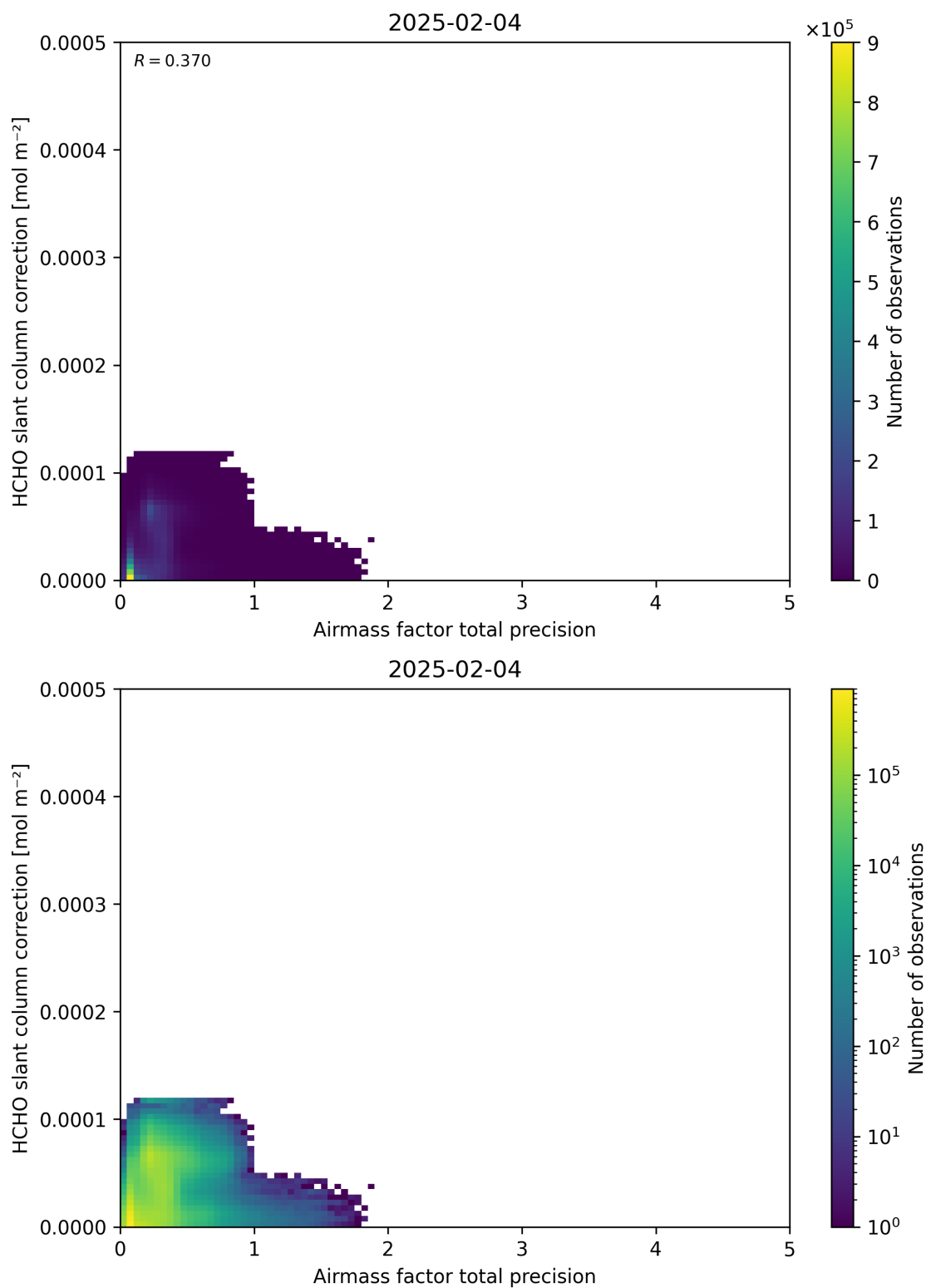
Figure 110: Scatter density plot of “Airmass factor total precision” against “HCHO slant column correction” for 2025-02-03 to 2025-02-05.
