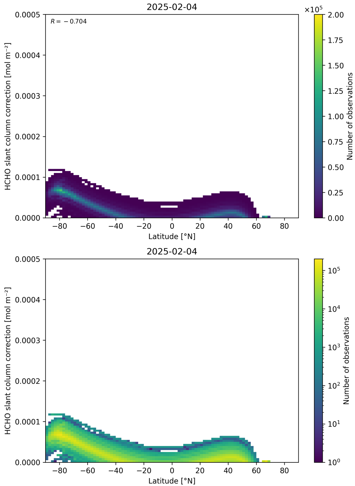
Figure 158: Scatter density plot of “Latitude” against “HCHO slant column correction” for 2025-02-03 to 2025-02-05.
