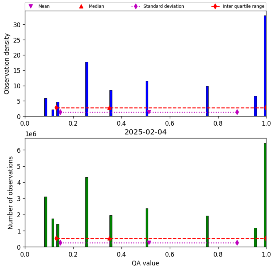
Figure 34: Histogram of “QA value” for 2025-02-03 to 2025-02-05
