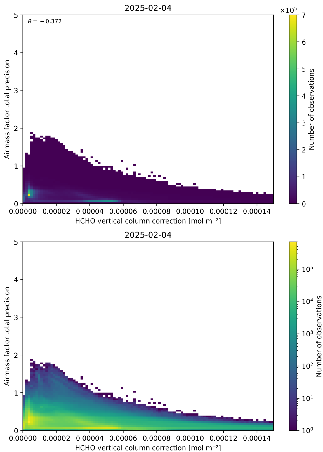
Figure 121: Scatter density plot of “HCHO vertical column correction” against “Airmass factor total precision” for 2025-02-03 to 2025-02-05.
