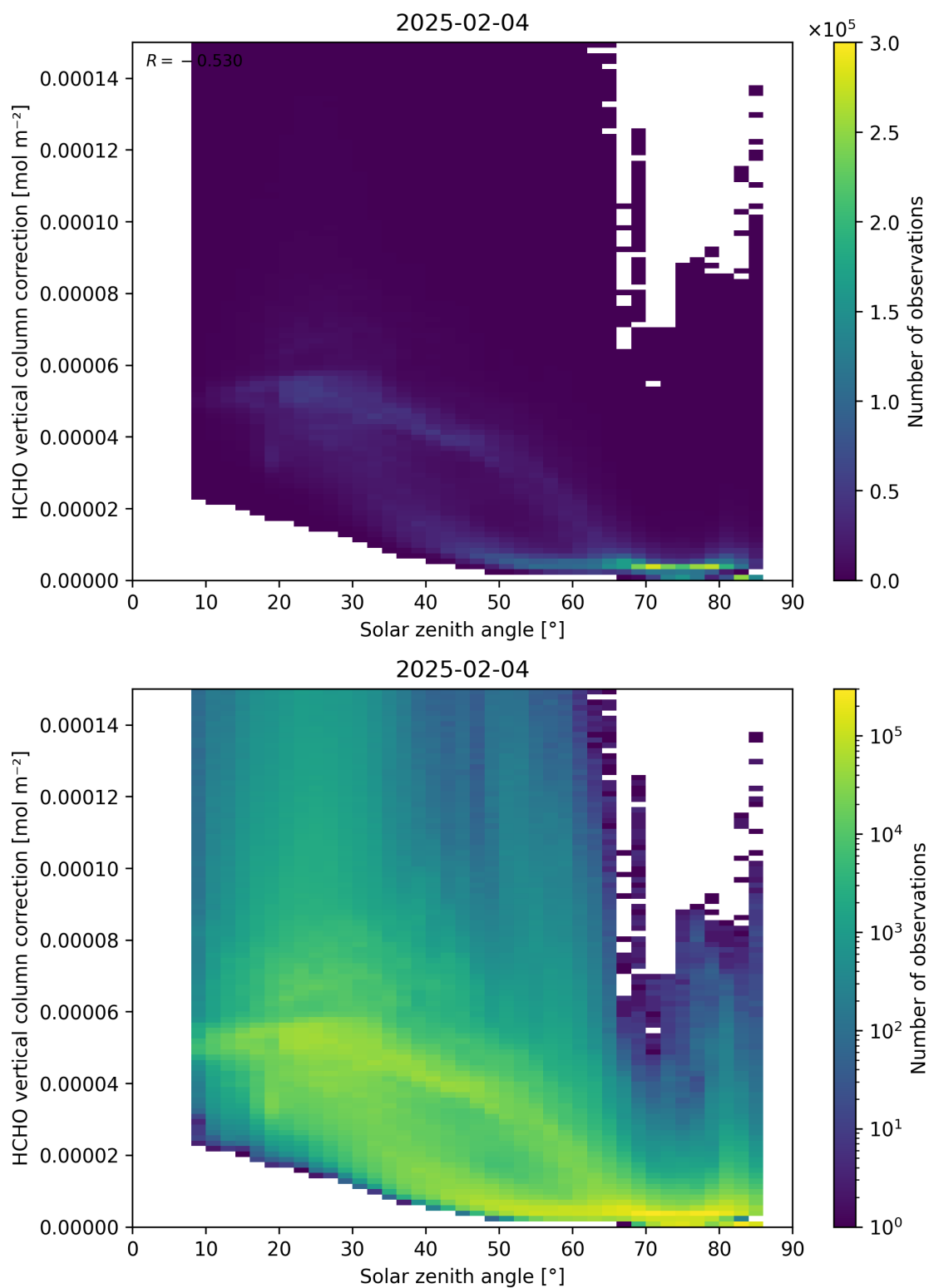
Figure 178: Scatter density plot of “Solar zenith angle” against “HCHO vertical column correction” for 2025-02-03 to 2025-02-05.
