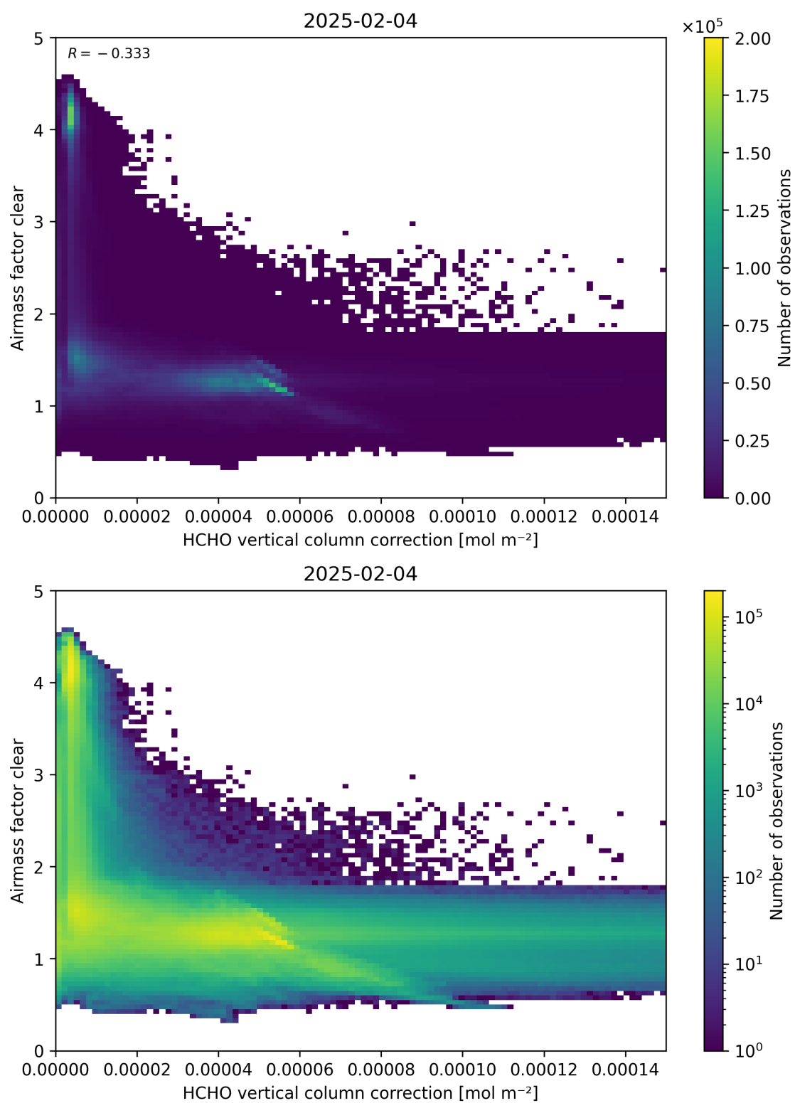
Figure 115: Scatter density plot of “HCHO vertical column correction” against “Airmass factor clear” for 2025-02-03 to 2025-02-05.
