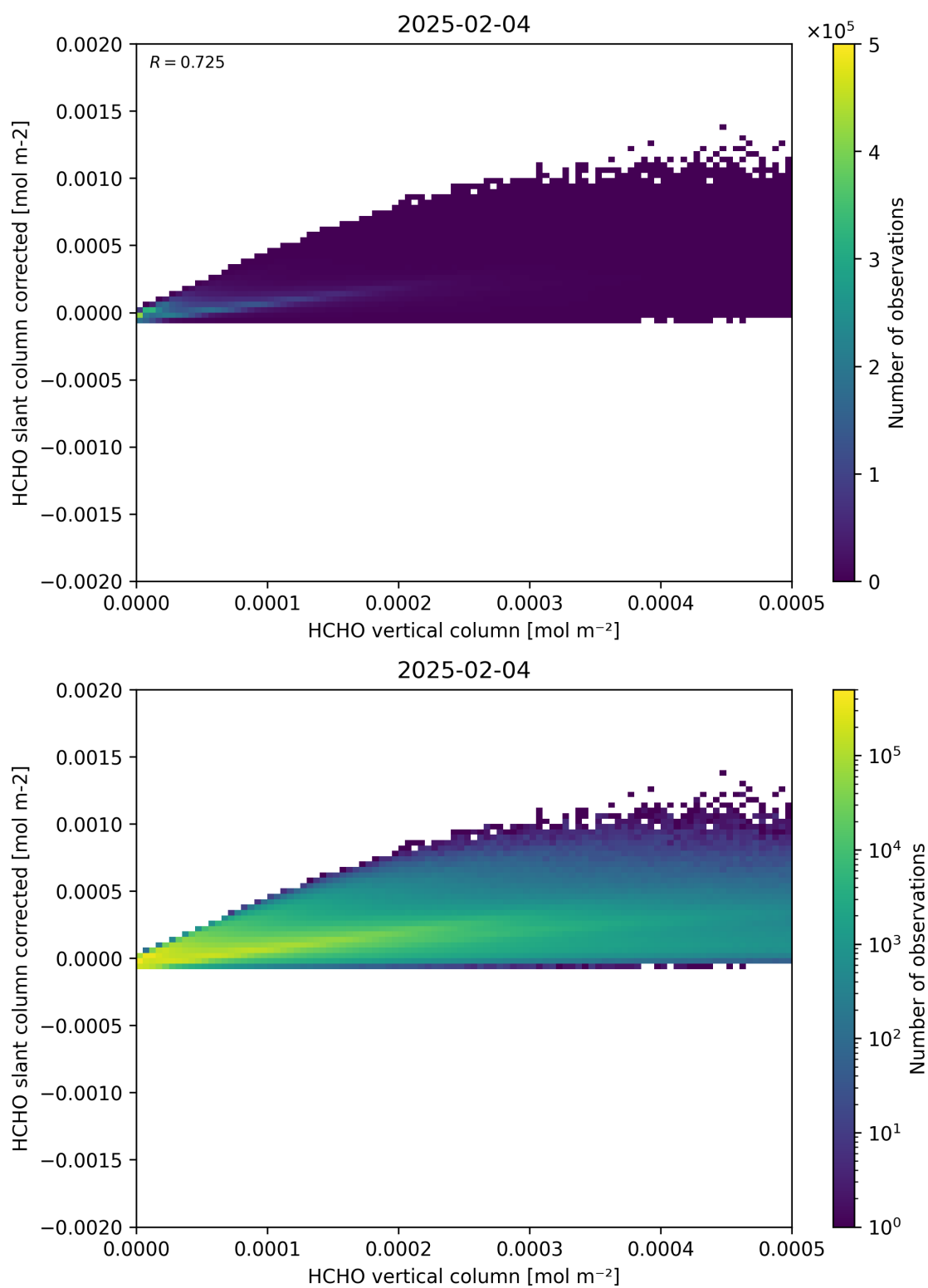
Figure 127: Scatter density plot of “HCHO vertical column” against “HCHO slant column corrected” for 2025-02-03 to 2025-02-05.
