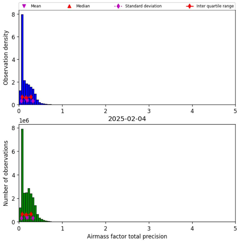
Figure 41: Histogram of “Airmass factor total precision” for 2025-02-03 to 2025-02-05
