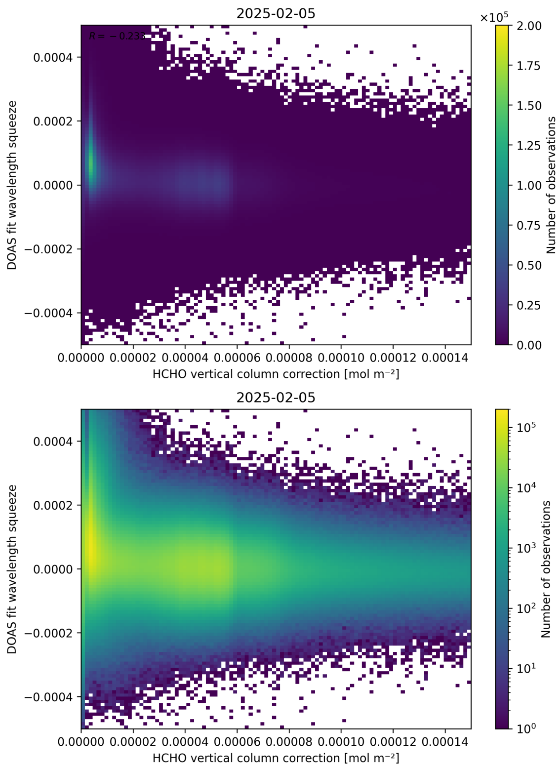
Figure 114: Scatter density plot of “HCHO vertical column correction” against “DOAS fit wavelength squeeze” for 2025-02-04 to 2025-02-06.
