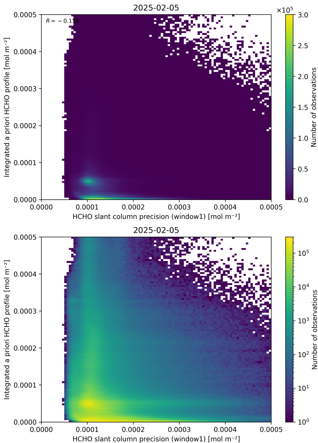
Figure 96: Scatter density plot of “HCHO slant column precision (window1)” against “Integrated a priori HCHO profile” for 2025-02-04 to 2025-02-06.
