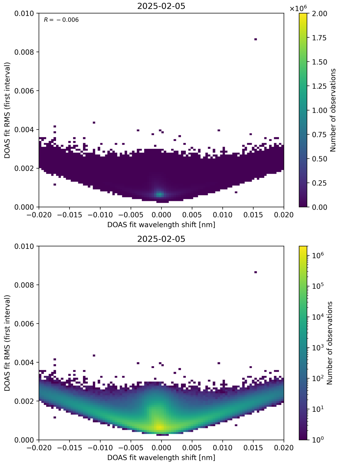
Figure 64: Scatter density plot of “DOAS fit wavelength shift” against “DOAS fit RMS (first interval)” for 2025-02-04 to 2025-02-06.
