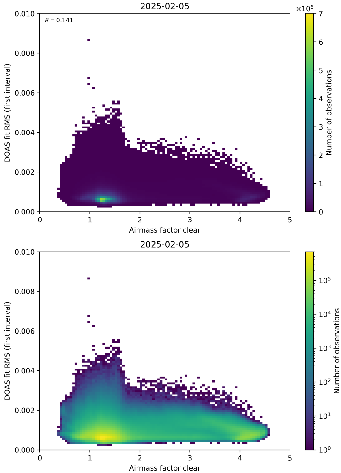
Figure 71: Scatter density plot of “Airmass factor clear” against “DOAS fit RMS (first interval)” for 2025-02-04 to 2025-02-06.
