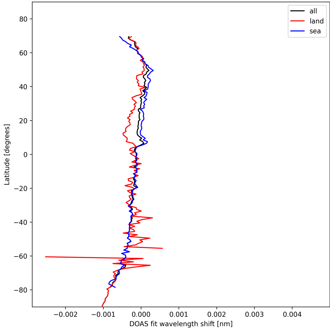
Figure 30: Zonal average of “DOAS fit wavelength shift” for 2025-02-04 to 2025-02-06.
