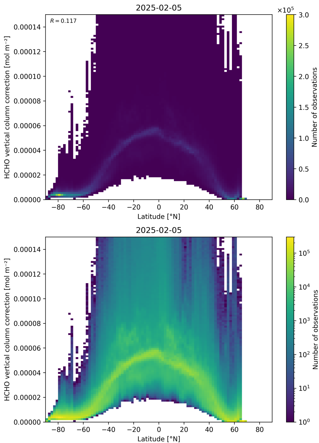
Figure 164: Scatter density plot of “Latitude” against “HCHO vertical column correction” for 2025-02-04 to 2025-02-06.
