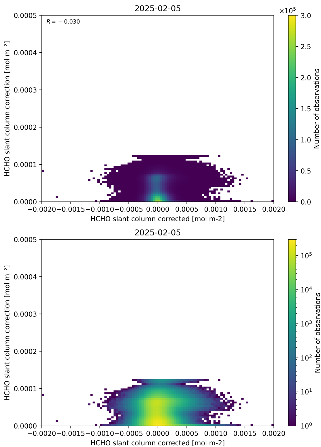
Figure 77: Scatter density plot of “HCHO slant column corrected” against “HCHO slant column correction” for 2025-02-04 to 2025-02-06.
