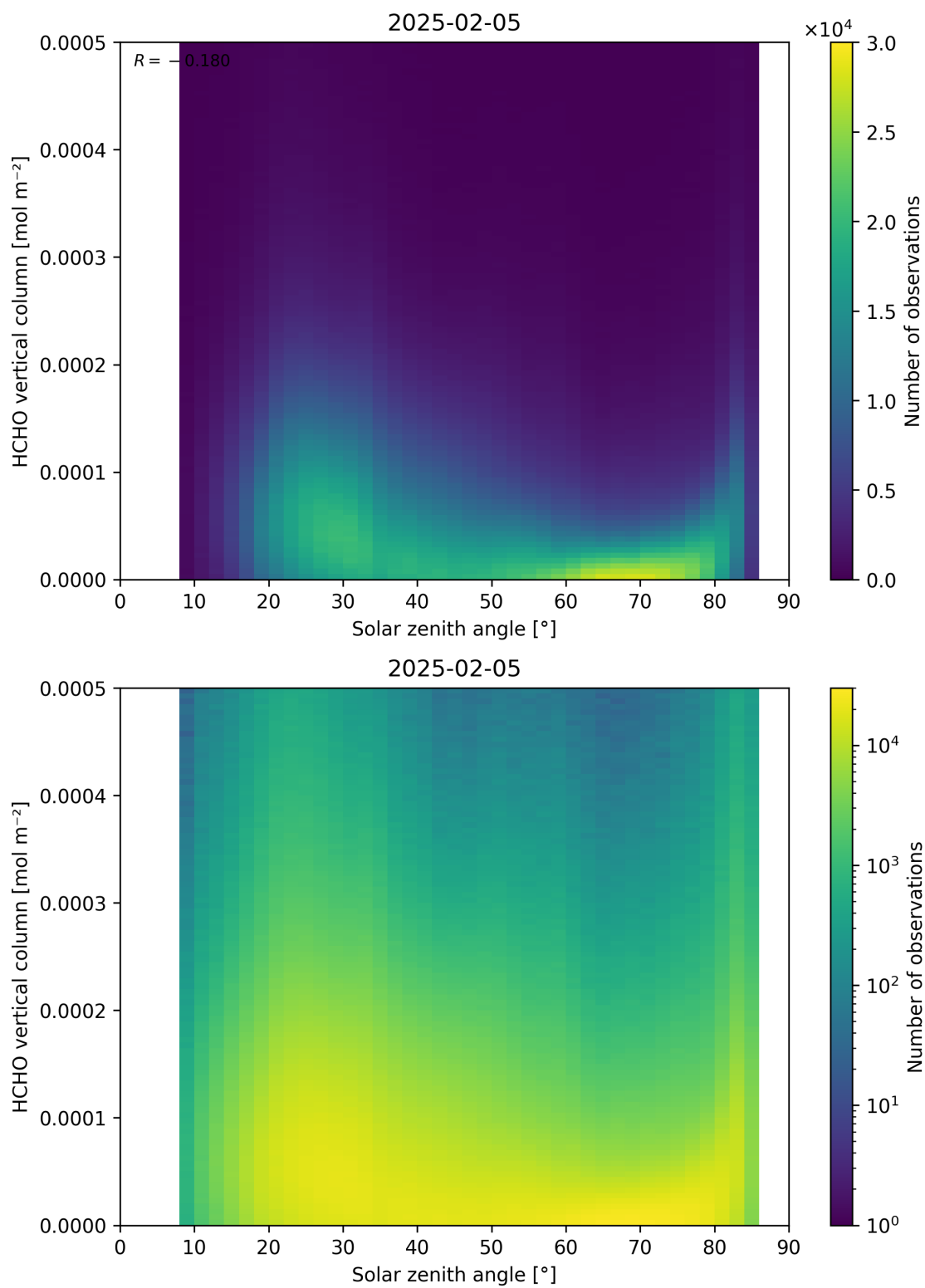
Figure 177: Scatter density plot of “Solar zenith angle” against “HCHO vertical column” for 2025-02-04 to 2025-02-06.
