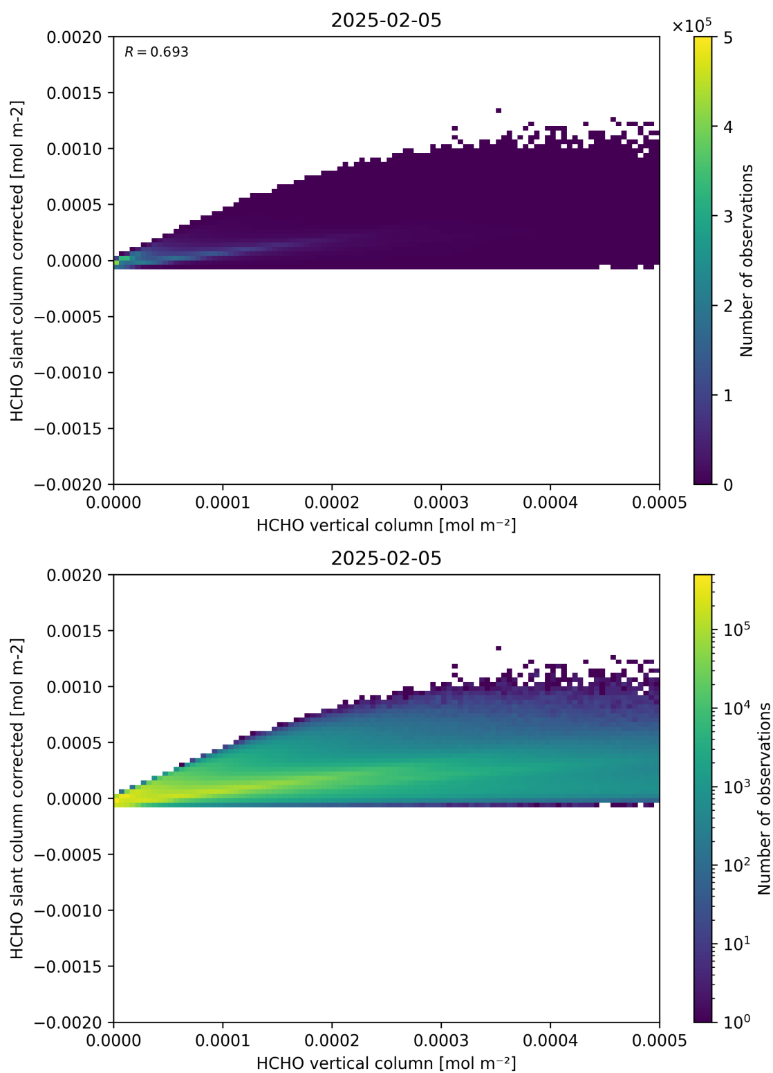
Figure 127: Scatter density plot of “HCHO vertical column” against “HCHO slant column corrected” for 2025-02-04 to 2025-02-06.
