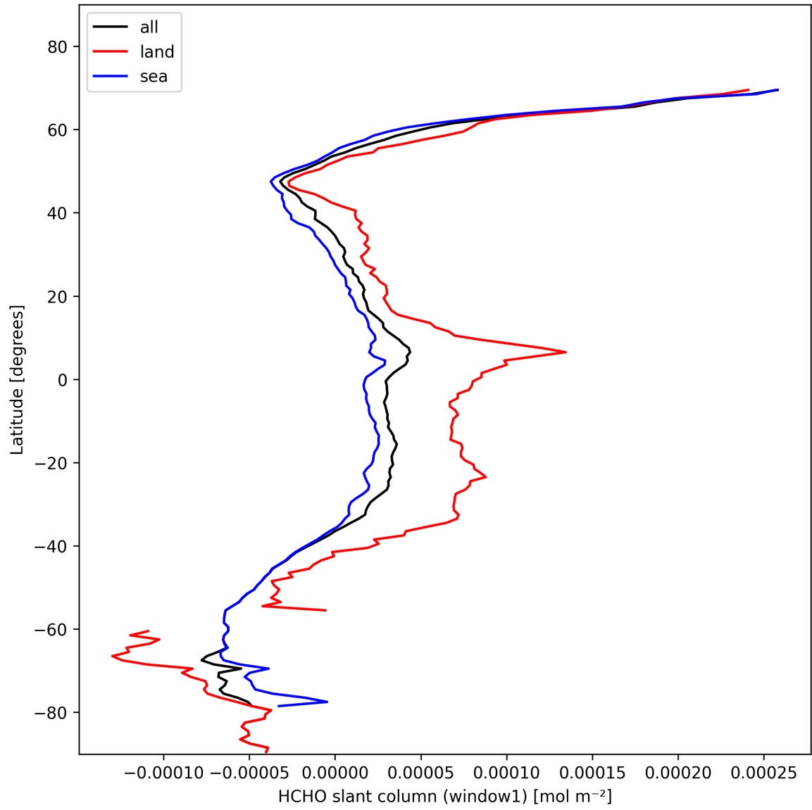
Figure 24: Zonal average of “HCHO slant column (window1)” for 2025-02-04 to 2025-02-06.
