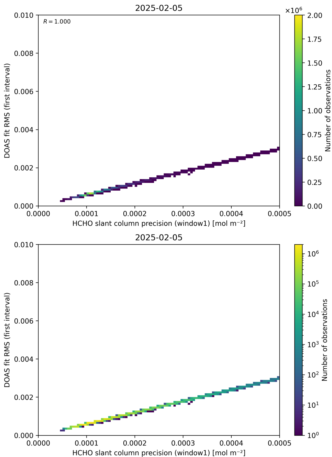
Figure 88: Scatter density plot of “HCHO slant column precision (window1)” against “DOAS fit RMS (first interval)” for 2025-02-04 to 2025-02-06.
