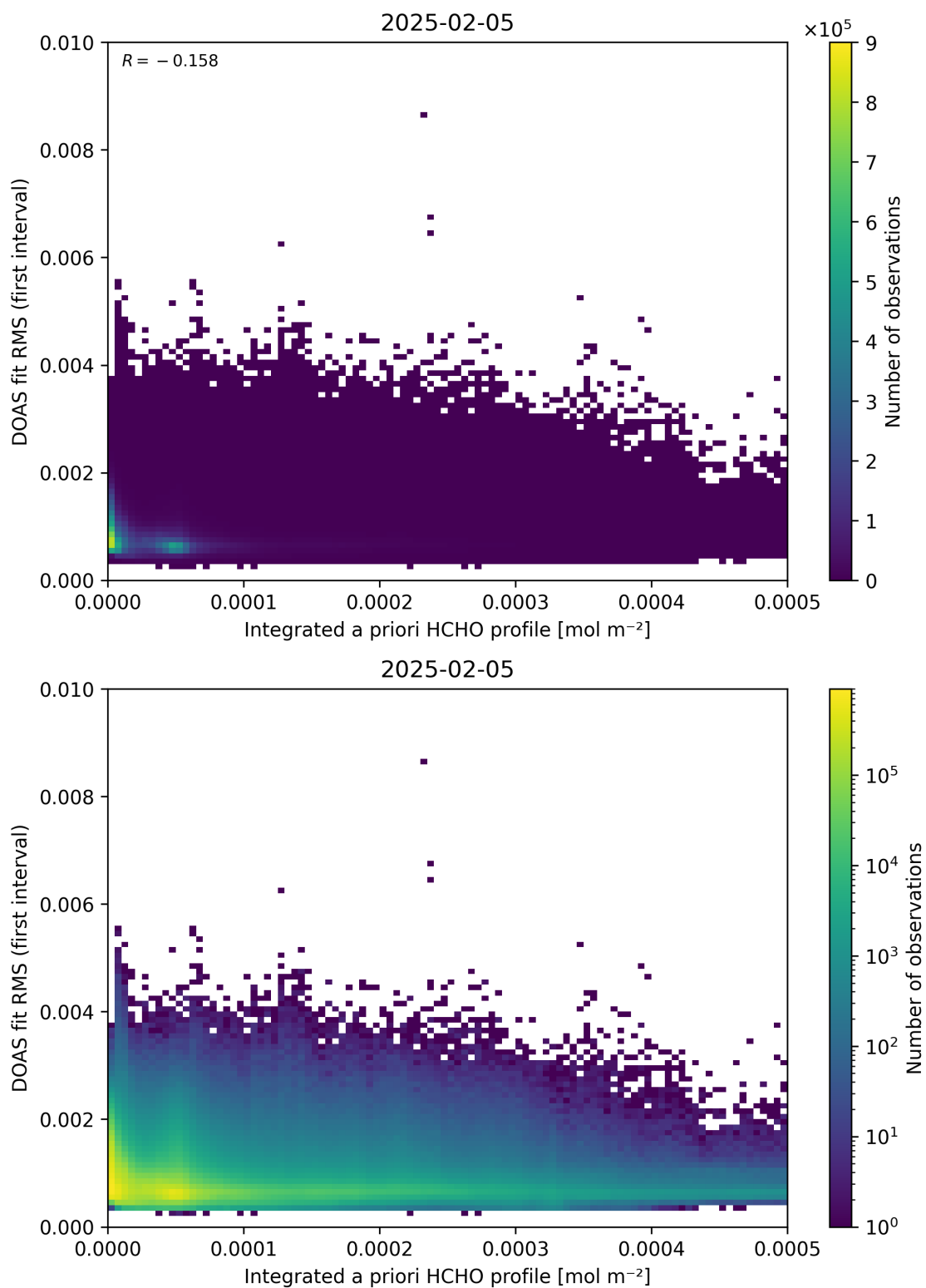
Figure 148: Scatter density plot of “Integrated a priori HCHO profile” against “DOAS fit RMS (first interval)” for 2025-02-04 to 2025-02-06.
