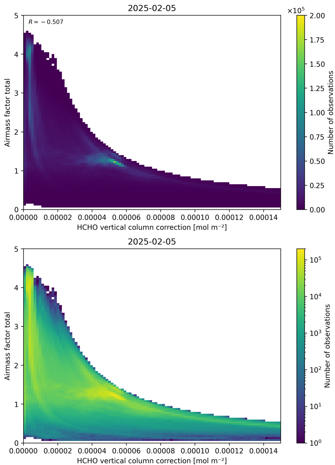
Figure 120: Scatter density plot of “HCHO vertical column correction” against “Airmass factor total” for 2025-02-04 to 2025-02-06.
