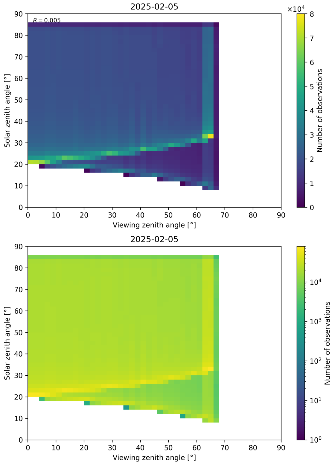
Figure 197: Scatter density plot of “Viewing zenith angle” against “Solar zenith angle” for 2025-02-04 to 2025-02-06.
