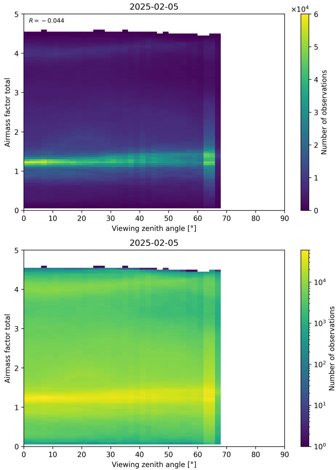
Figure 190: Scatter density plot of “Viewing zenith angle” against “Airmass factor total” for 2025-02-04 to 2025-02-06.
