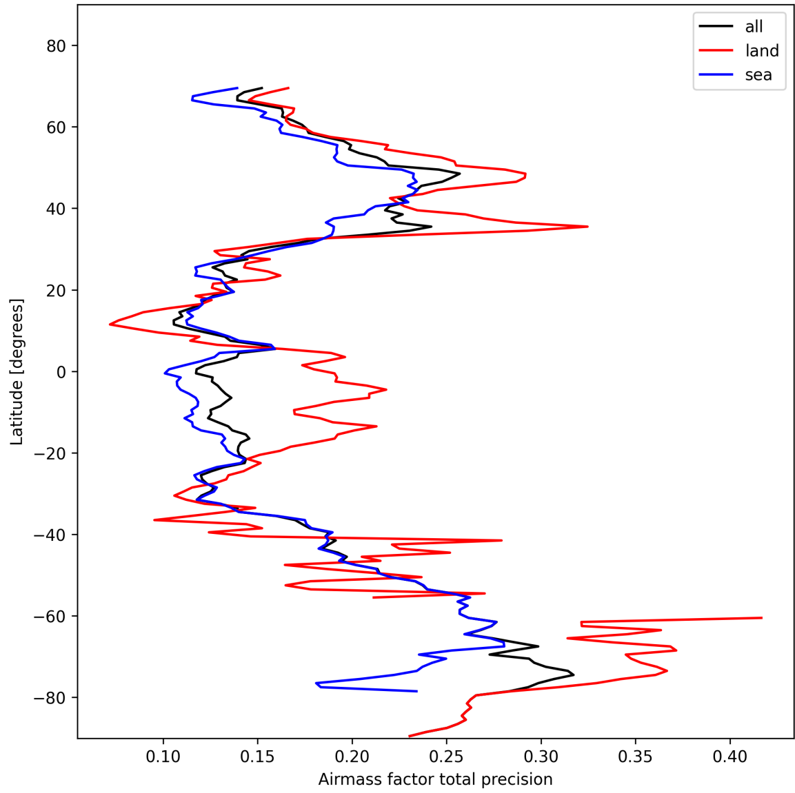
Figure 27: Zonal average of “Airmass factor total precision” for 2025-02-04 to 2025-02-06.
