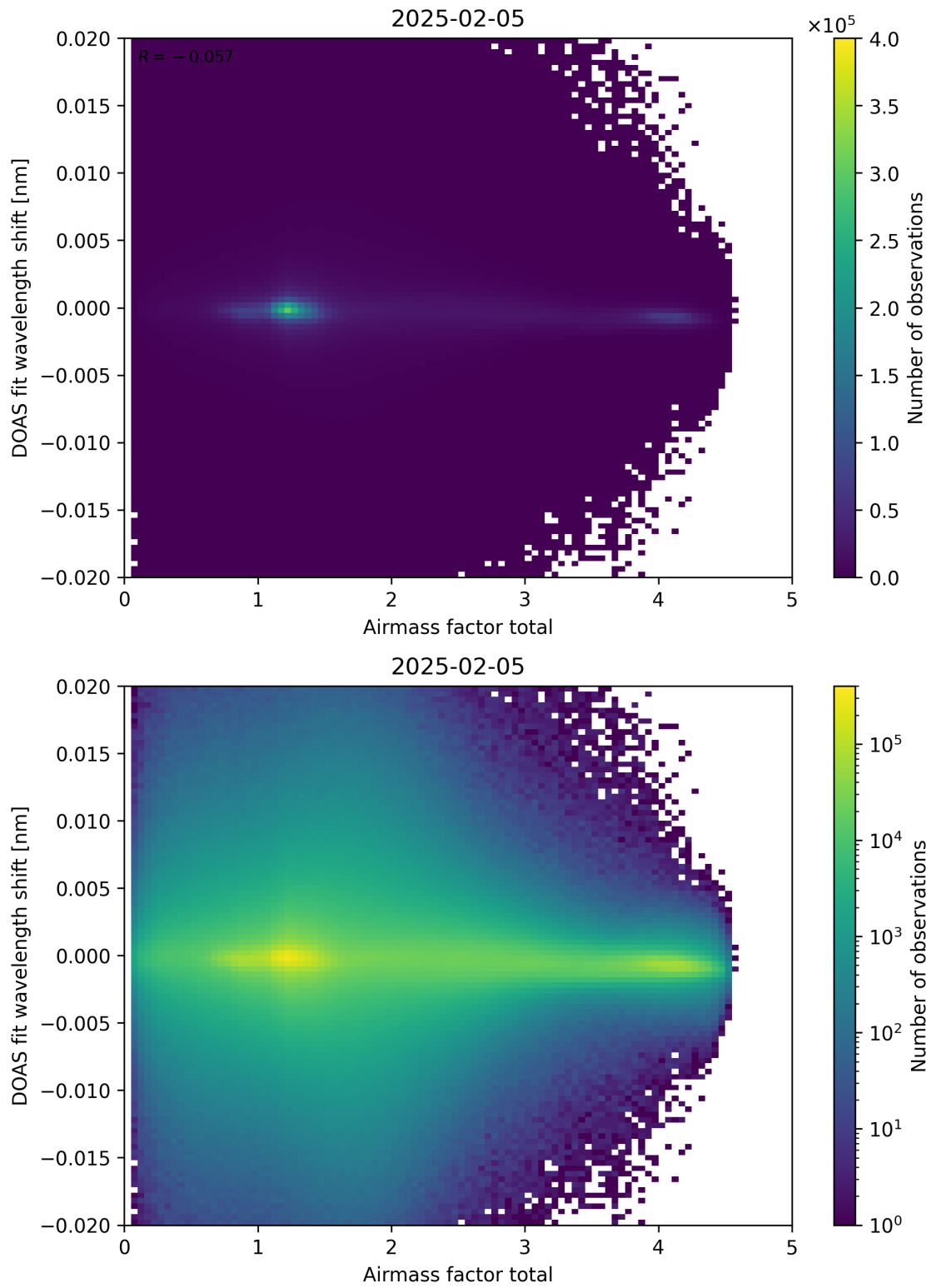
Figure 98: Scatter density plot of “Airmass factor total” against “DOAS fit wavelength shift” for 2025-02-04 to 2025-02-06.
