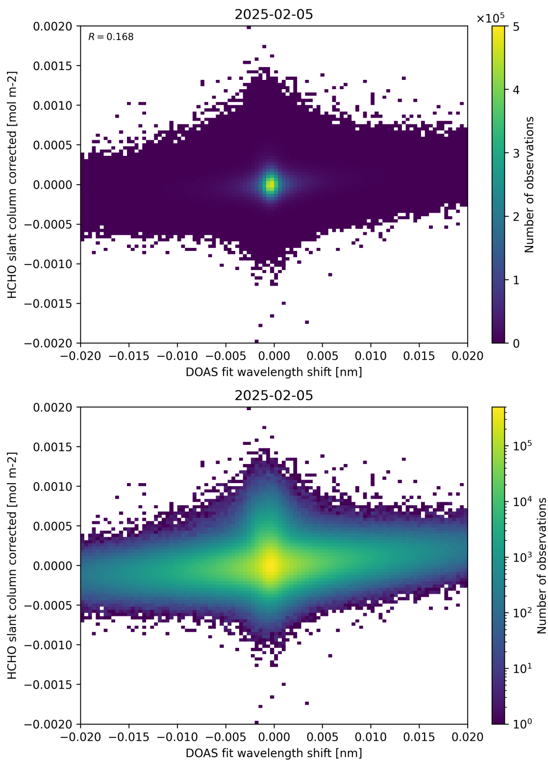
Figure 66: Scatter density plot of “DOAS fit wavelength shift” against “HCHO slant column corrected” for 2025-02-04 to 2025-02-06.
