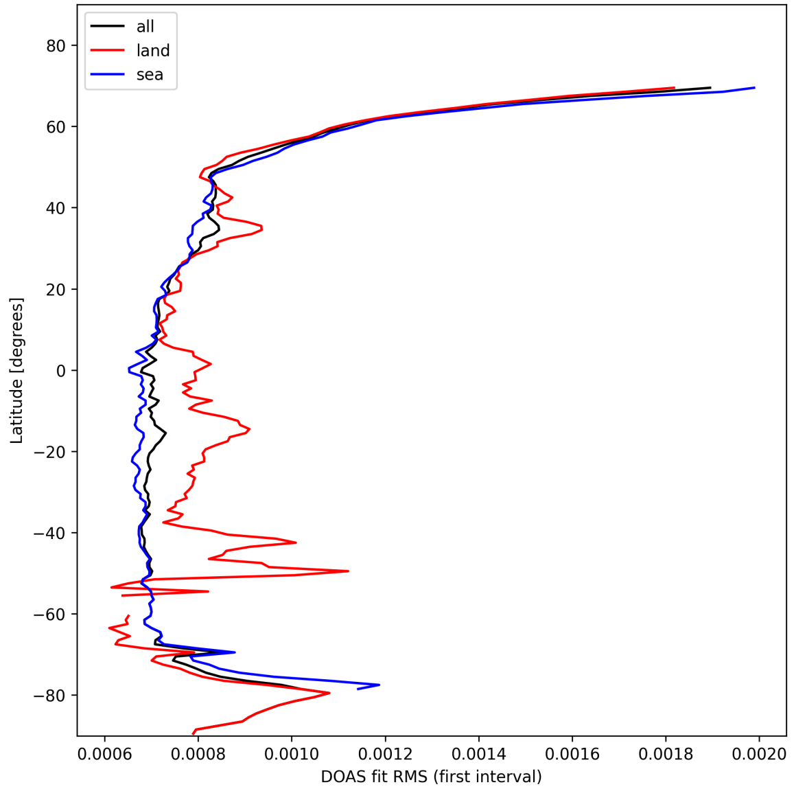
Figure 32: Zonal average of "DOAS fit RMS (first interval)" for 2025-02-04 to 2025-02-06.
