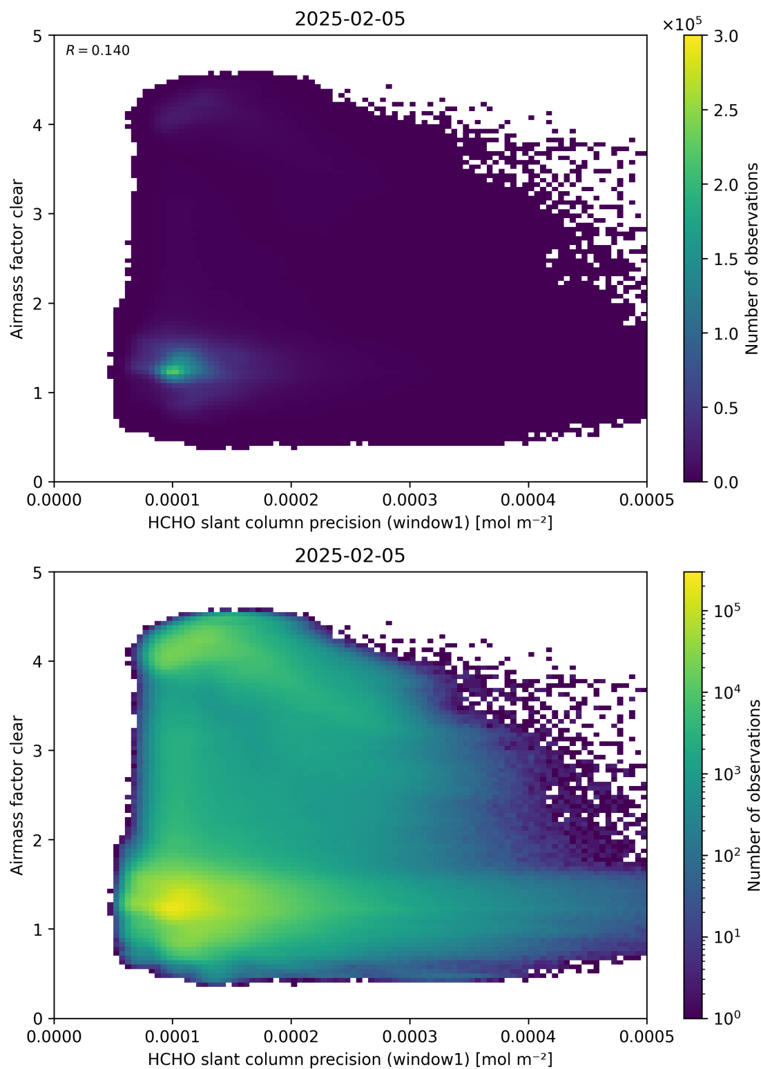
Figure 91: Scatter density plot of “HCHO slant column precision (window1)” against “Airmass factor clear” for 2025-02-04 to 2025-02-06.
