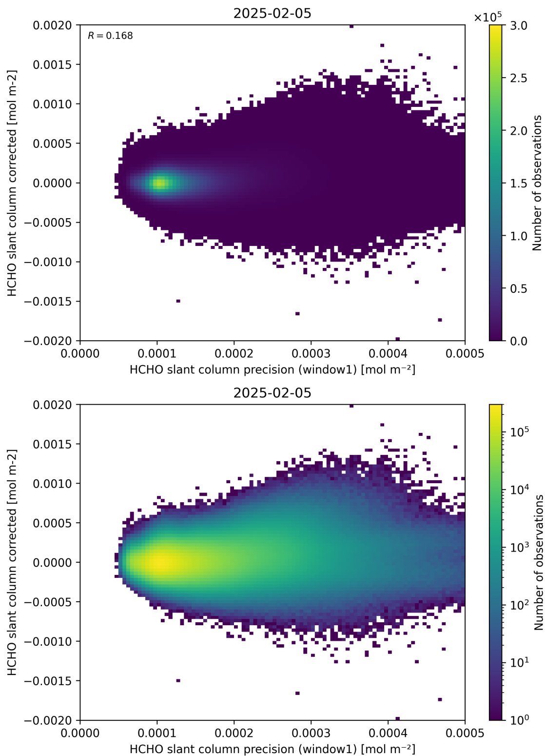
Figure 92: Scatter density plot of “HCHO slant column precision (window1)” against “HCHO slant column corrected” for 2025-02-04 to 2025-02-06.
