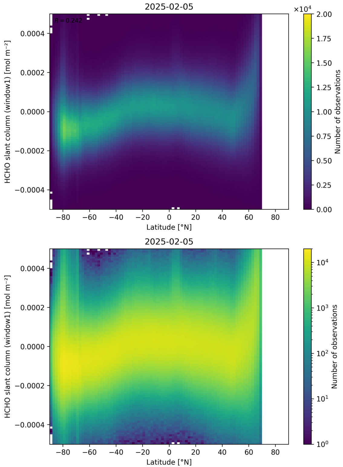
Figure 159: Scatter density plot of “Latitude” against “HCHO slant column (window1)” for 2025-02-04 to 2025-02-06.
