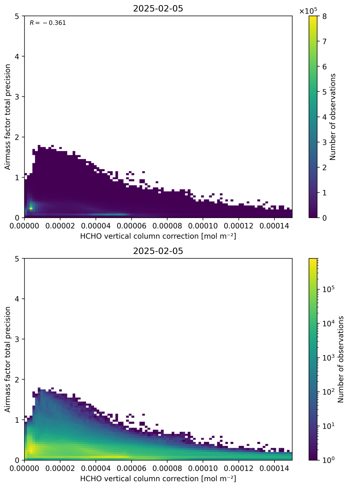
Figure 121: Scatter density plot of “HCHO vertical column correction” against “Airmass factor total precision” for 2025-02-04 to 2025-02-06.
