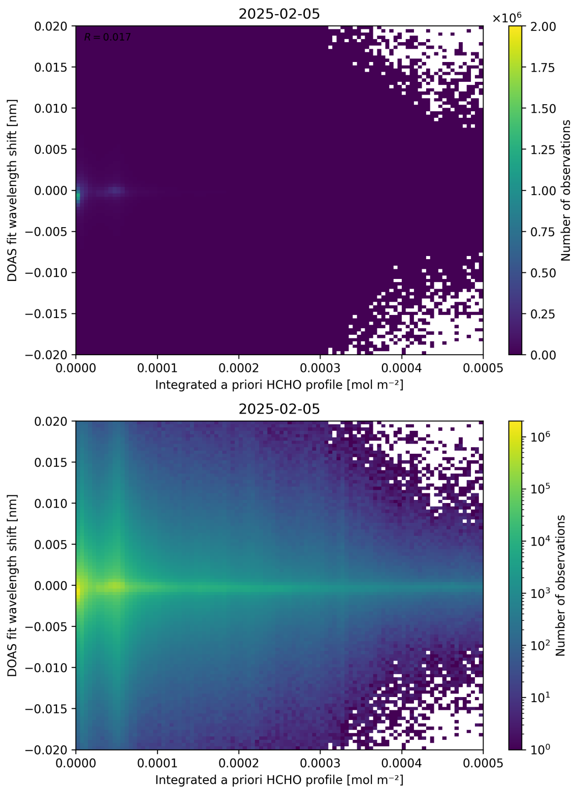
Figure 149: Scatter density plot of “Integrated a priori HCHO profile” against “DOAS fit wavelength shift” for 2025-02-04 to 2025-02-06.
