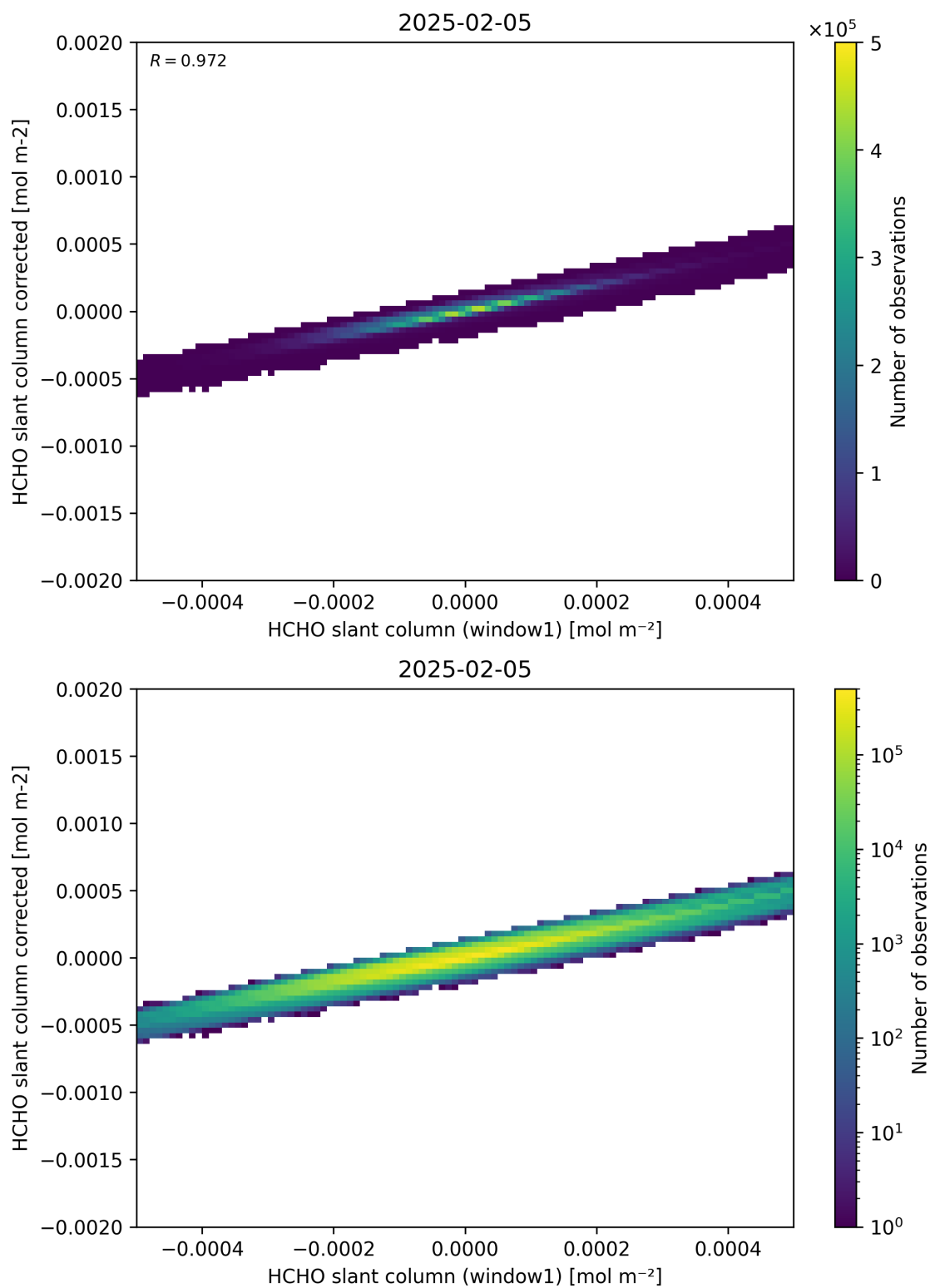
Figure 82: Scatter density plot of “HCHO slant column (window1)” against “HCHO slant column corrected” for 2025-02-04 to 2025-02-06.
