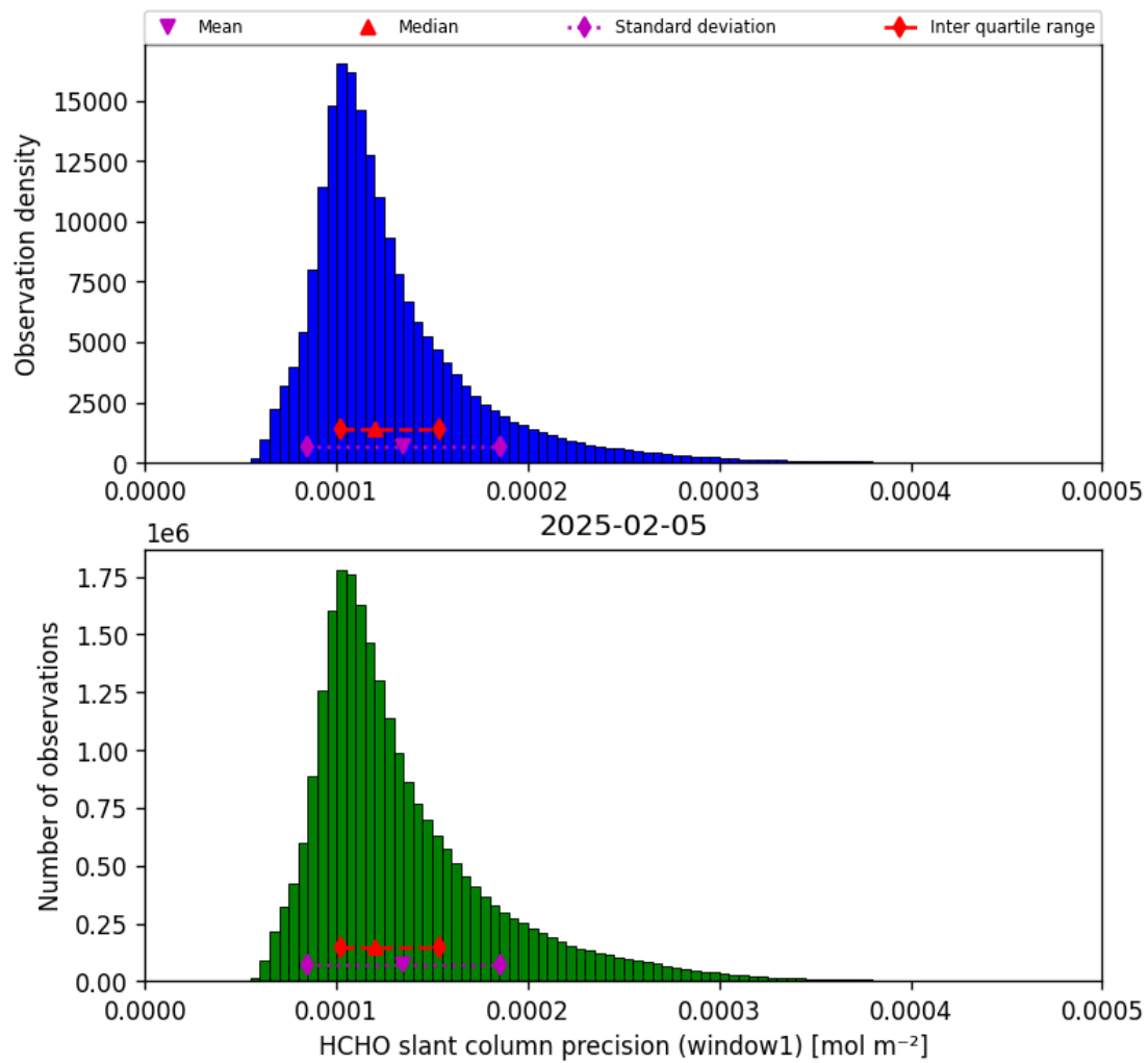
Figure 39: Histogram of “HCHO slant column precision (window1)” for 2025-02-04 to 2025-02-06
