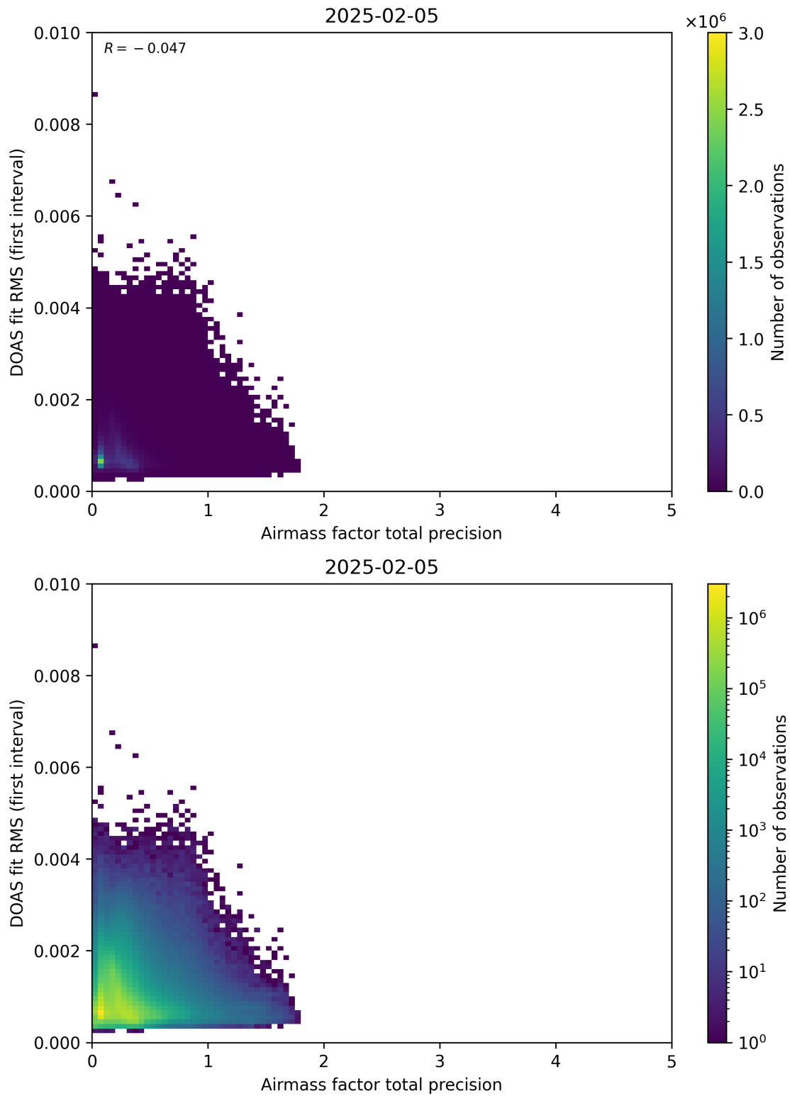
Figure 105: Scatter density plot of “Airmass factor total precision” against “DOAS fit RMS (first interval)” for 2025-02-04 to 2025-02-06.
