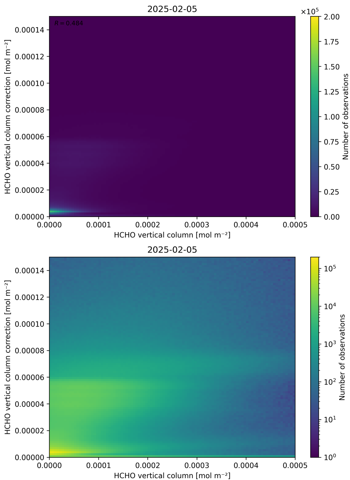
Figure 133: Scatter density plot of “HCHO vertical column” against “HCHO vertical column correction” for 2025-02-04 to 2025-02-06.
