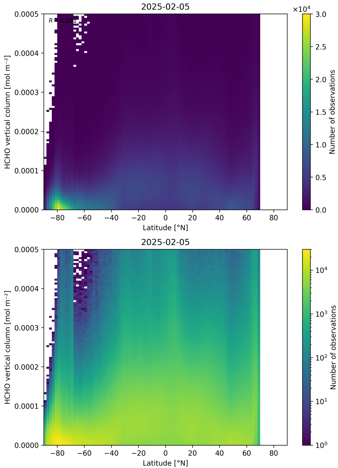
Figure 163: Scatter density plot of “Latitude” against “HCHO vertical column” for 2025-02-04 to 2025-02-06.
