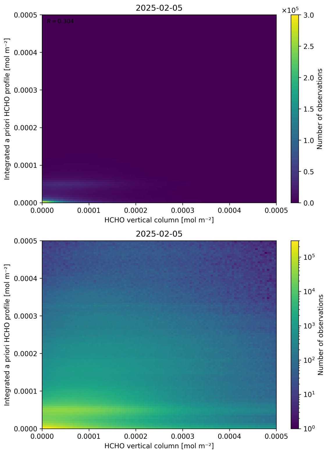
Figure 135: Scatter density plot of “HCHO vertical column” against “Integrated a priori HCHO profile” for 2025-02-04 to 2025-02-06.
