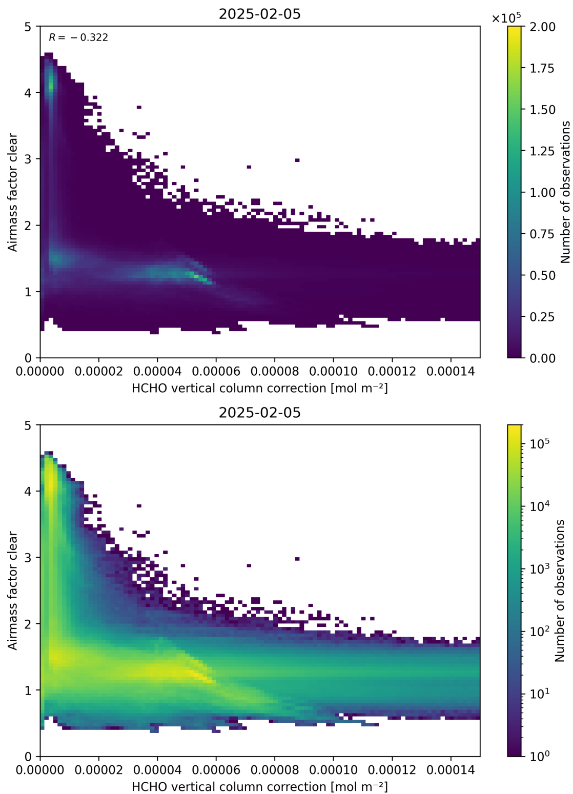
Figure 115: Scatter density plot of “HCHO vertical column correction” against “Airmass factor clear” for 2025-02-04 to 2025-02-06.
