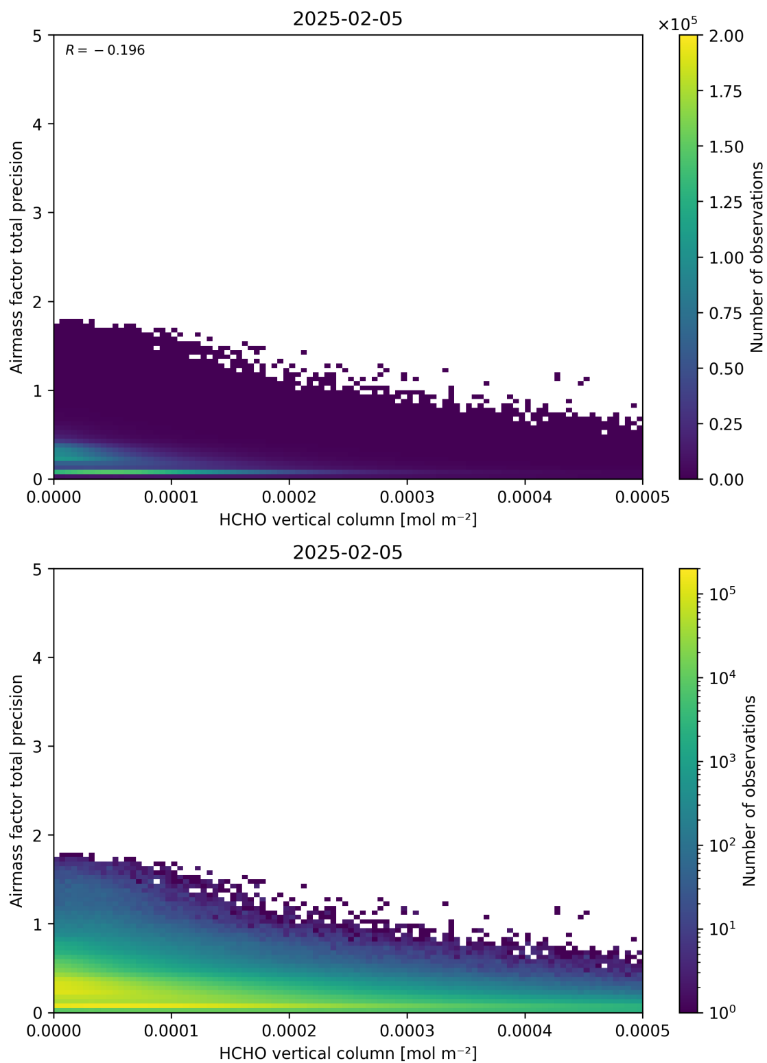
Figure 132: Scatter density plot of “HCHO vertical column” against “Airmass factor total precision” for 2025-02-04 to 2025-02-06.
