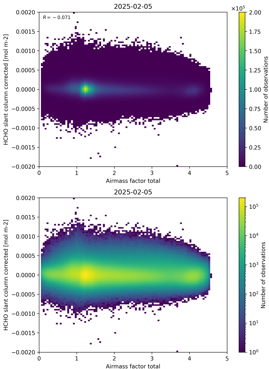
Figure 101: Scatter density plot of “Airmass factor total” against “HCHO slant column corrected” for 2025-02-04 to 2025-02-06.
