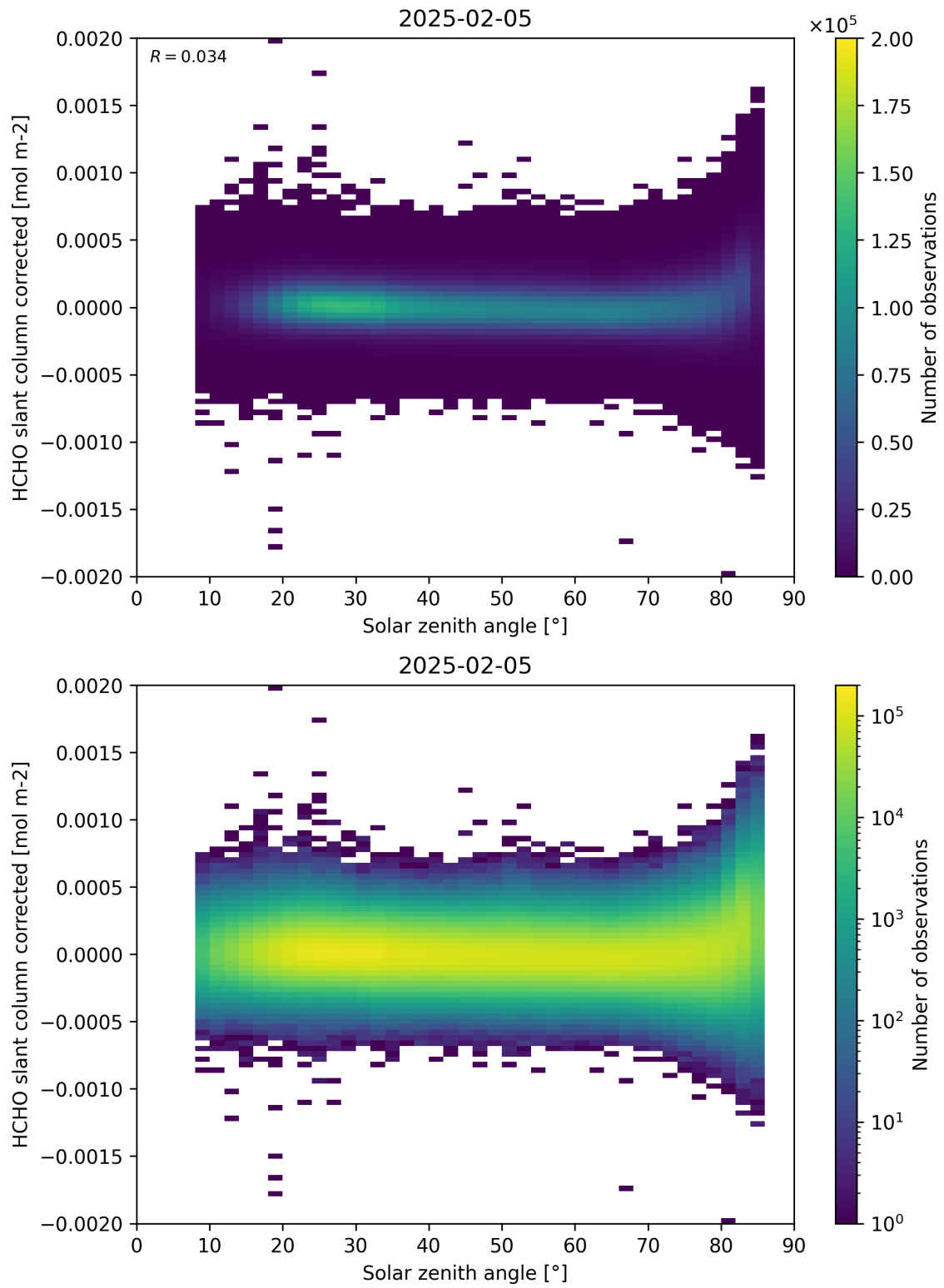
Figure 171: Scatter density plot of “Solar zenith angle” against “HCHO slant column corrected” for 2025-02-04 to 2025-02-06.
