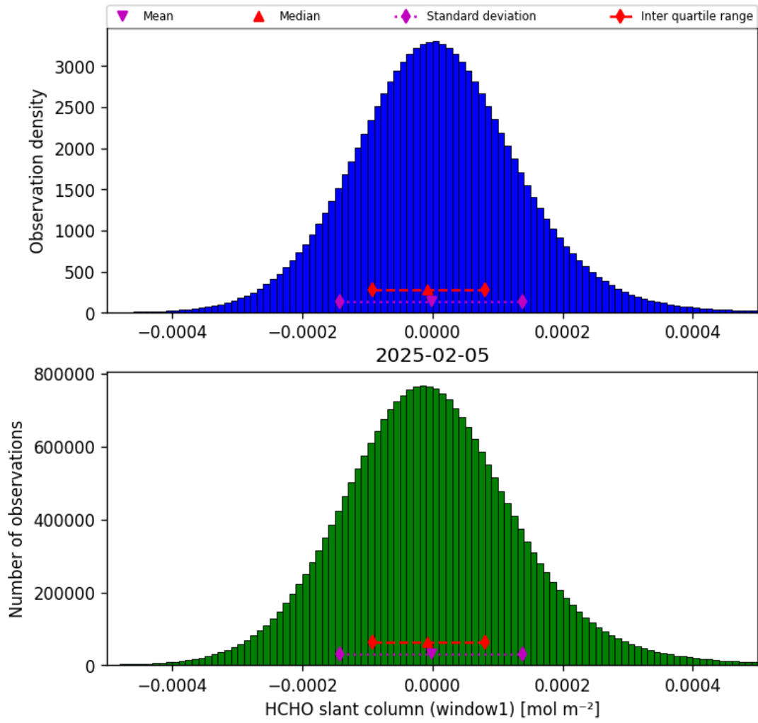
Figure 38: Histogram of “HCHO slant column (window1)” for 2025-02-04 to 2025-02-06
