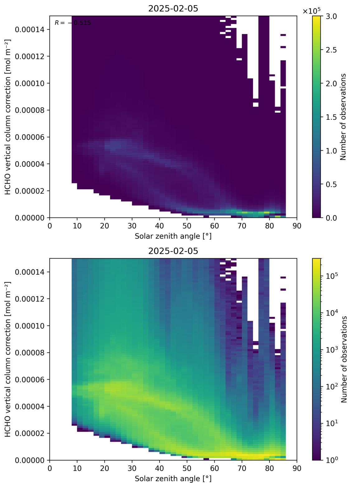
Figure 178: Scatter density plot of “Solar zenith angle” against “HCHO vertical column correction” for 2025-02-04 to 2025-02-06.
