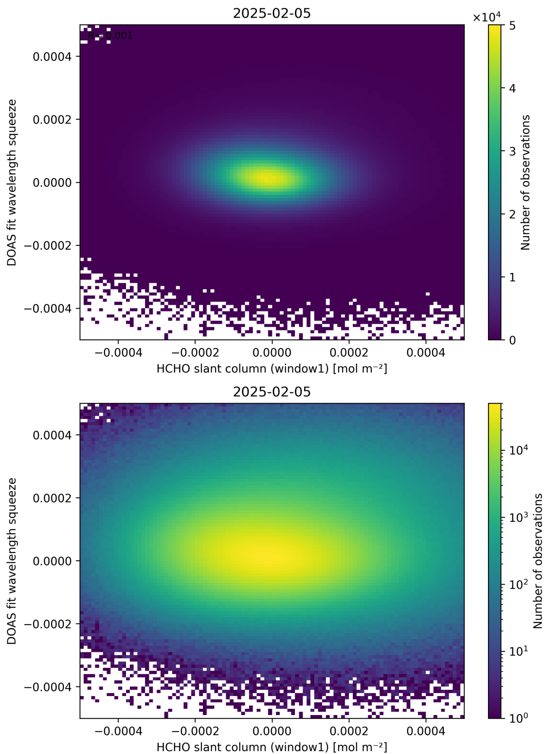
Figure 80: Scatter density plot of “HCHO slant column (window1)” against “DOAS fit wavelength squeeze” for 2025-02-04 to 2025-02-06.
