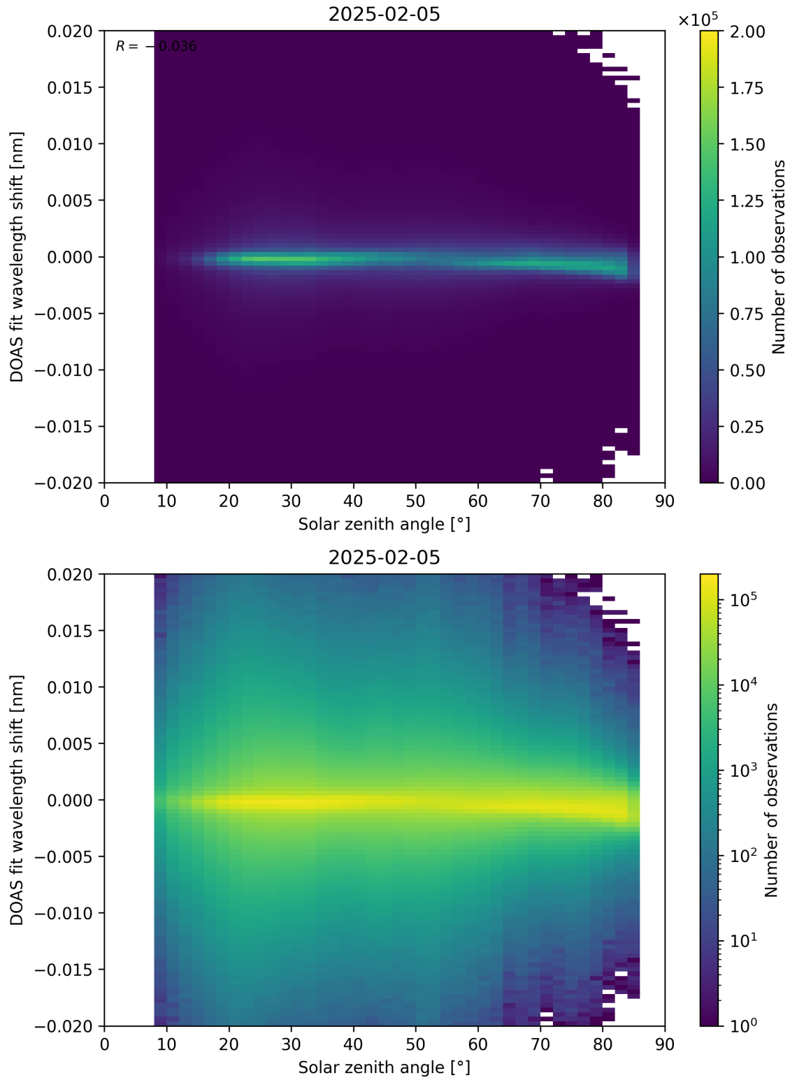
Figure 168: Scatter density plot of “Solar zenith angle” against “DOAS fit wavelength shift” for 2025-02-04 to 2025-02-06.
