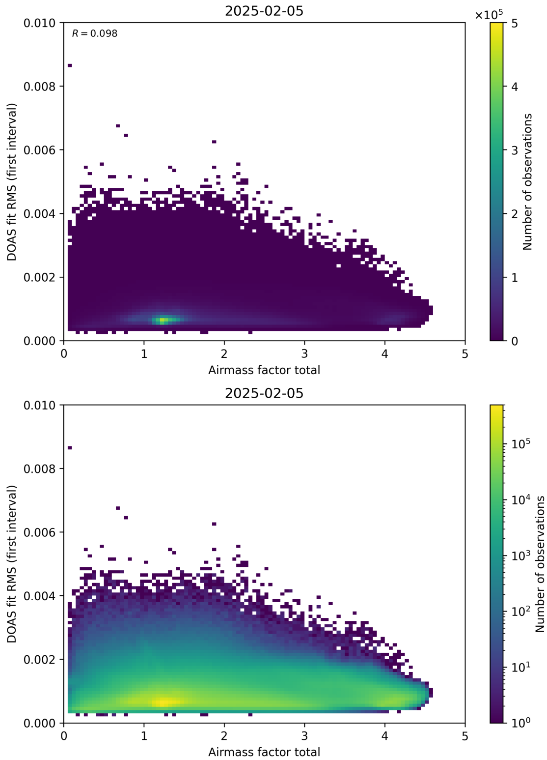
Figure 97: Scatter density plot of “Airmass factor total” against “DOAS fit RMS (first interval)” for 2025-02-04 to 2025-02-06.
