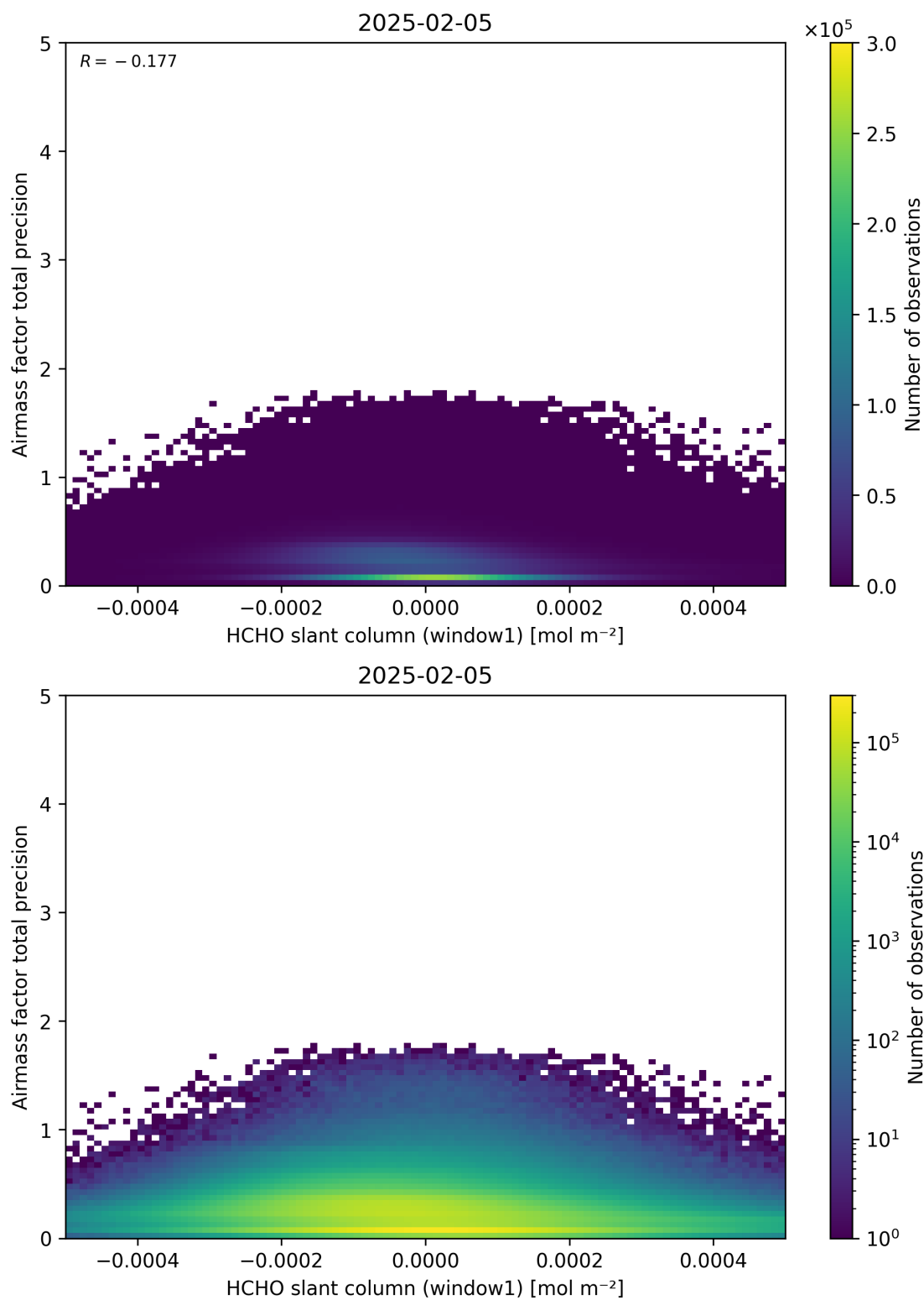
Figure 86: Scatter density plot of “HCHO slant column (window1)” against “Airmass factor total precision” for 2025-02-04 to 2025-02-06.
