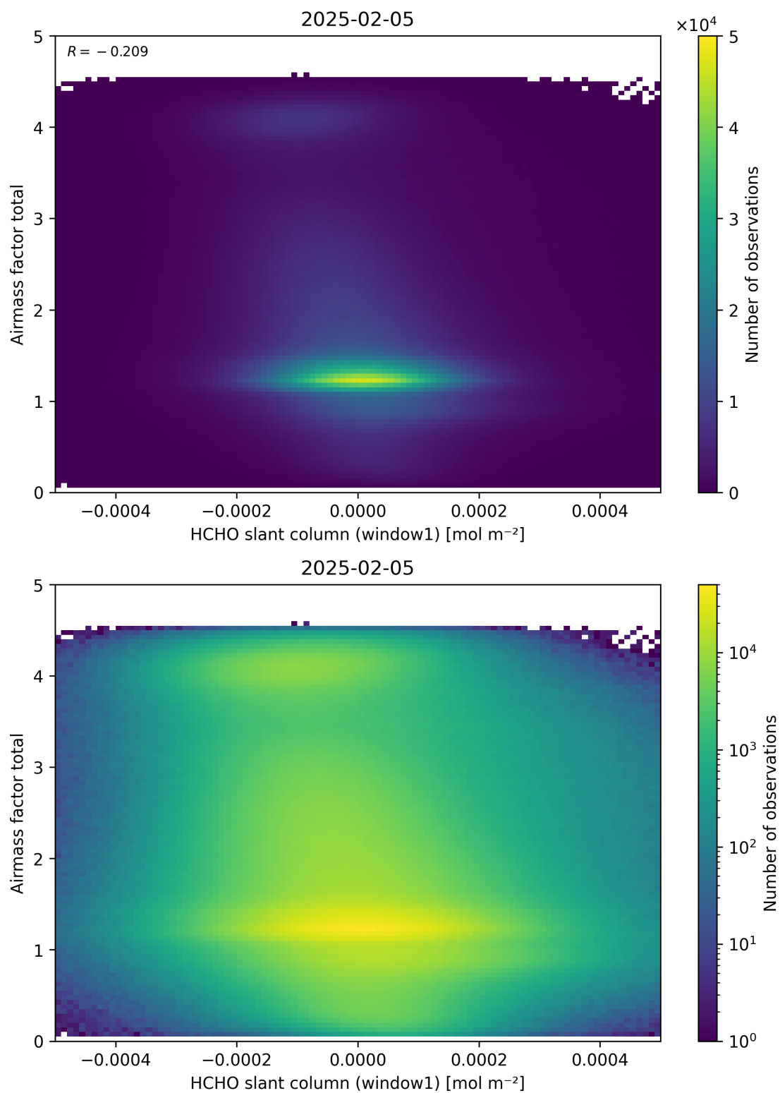
Figure 85: Scatter density plot of “HCHO slant column (window1)” against “Airmass factor total” for 2025-02-04 to 2025-02-06.
