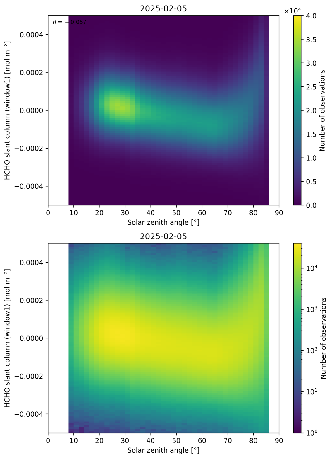
Figure 173: Scatter density plot of “Solar zenith angle” against “HCHO slant column (window1)” for 2025-02-04 to 2025-02-06.
