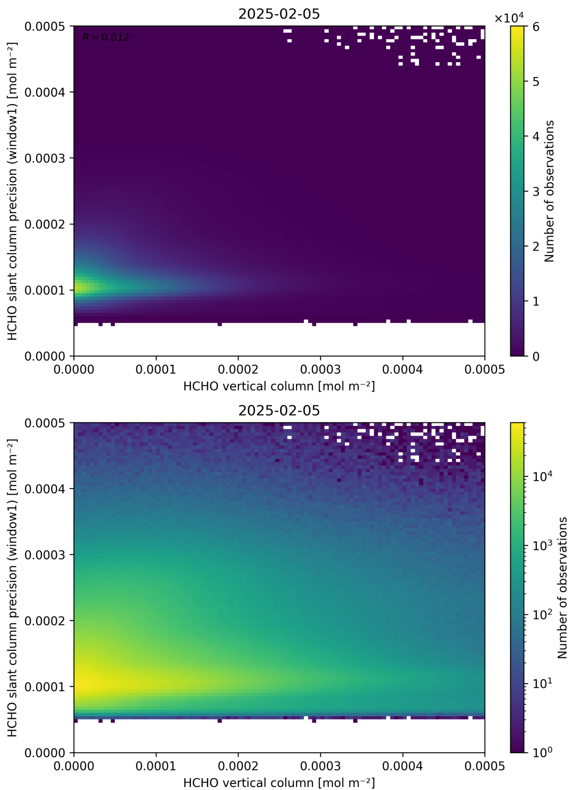
Figure 130: Scatter density plot of “HCHO vertical column” against “HCHO slant column precision (window1)” for 2025-02-04 to 2025-02-06.
