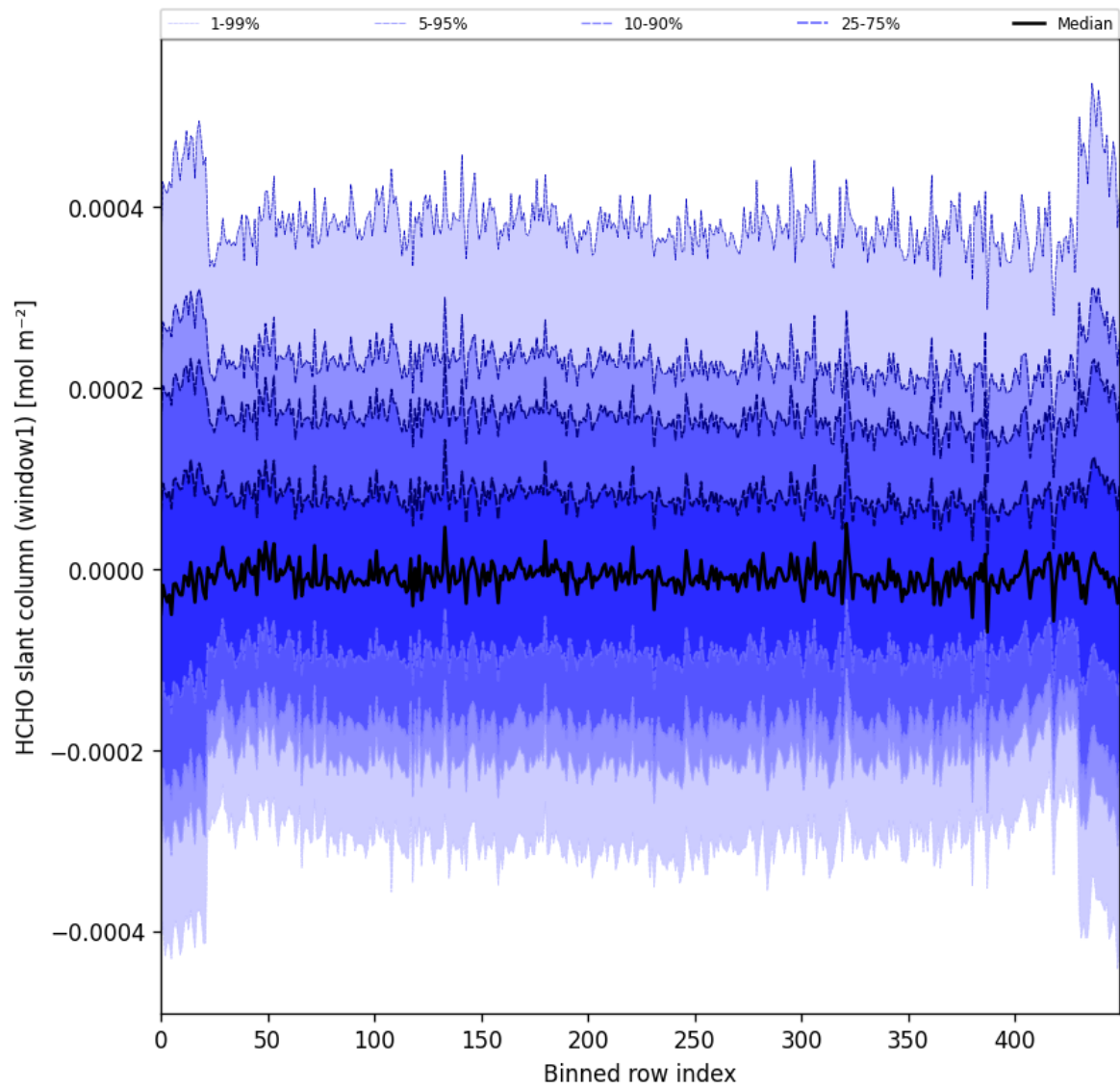
Figure 52: Along track statistics of “HCHO slant column (window1)” for 2025-02-04 to 2025-02-06
