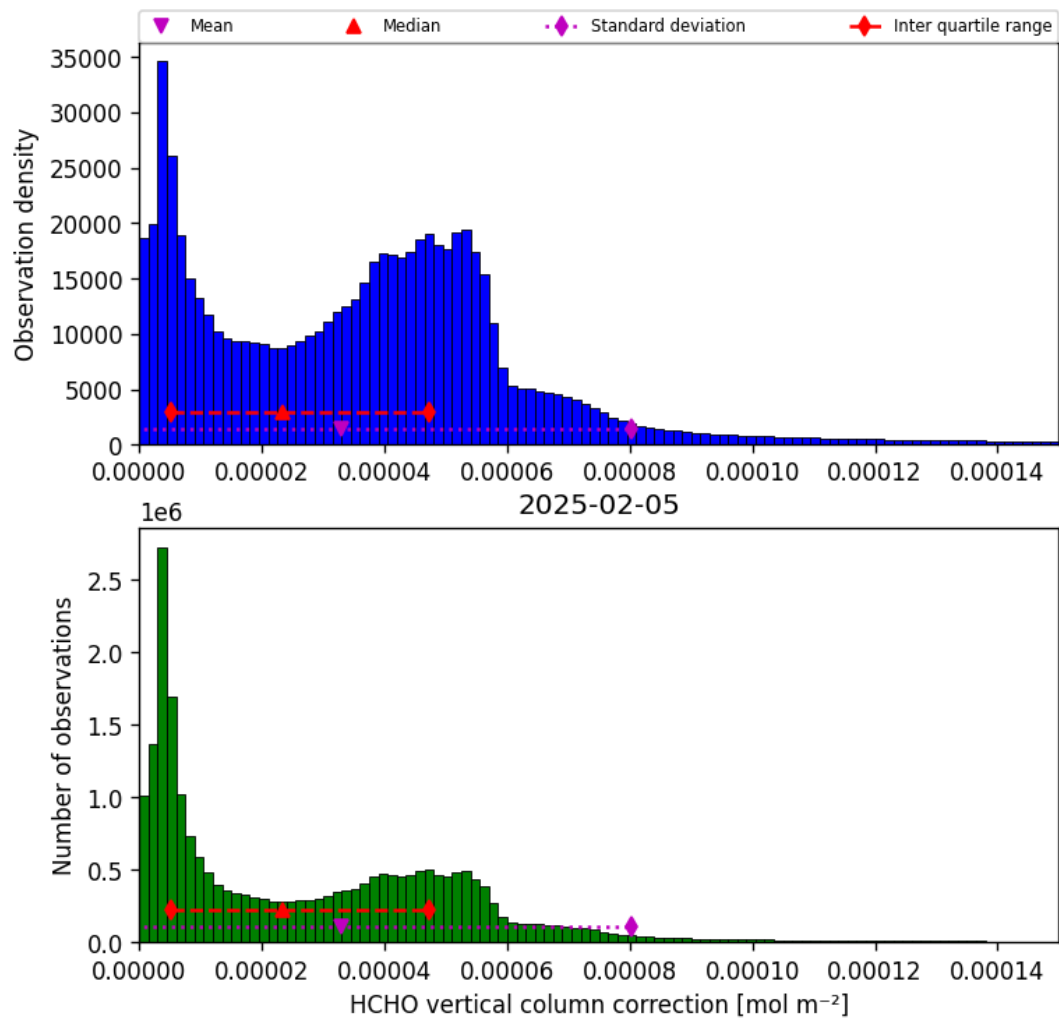
Figure 37: Histogram of “HCHO vertical column correction” for 2025-02-04 to 2025-02-06
