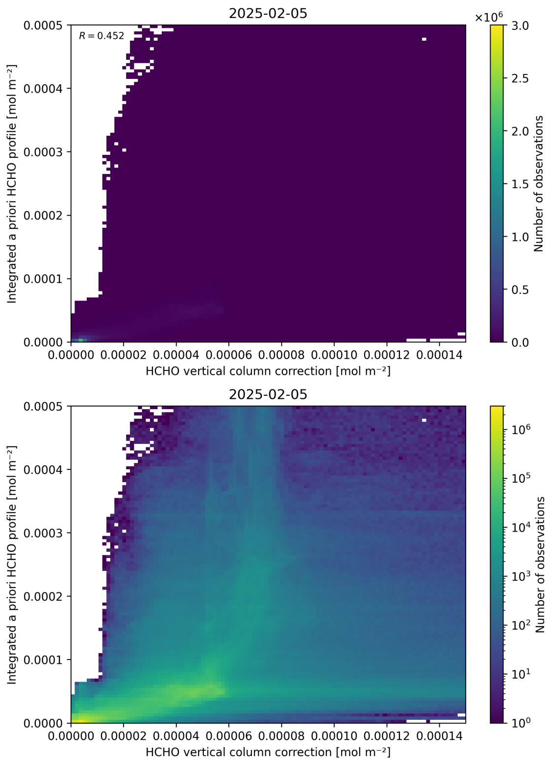
Figure 122: Scatter density plot of “HCHO vertical column correction” against “Integrated a priori HCHO profile” for 2025-02-04 to 2025-02-06.
