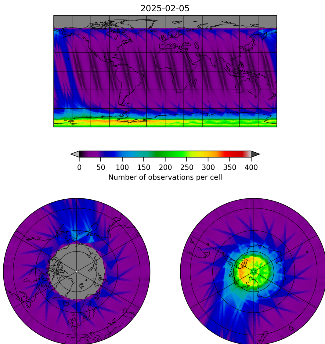
Figure 19: Map of the number of observations for 2025-02-04 to 2025-02-06
