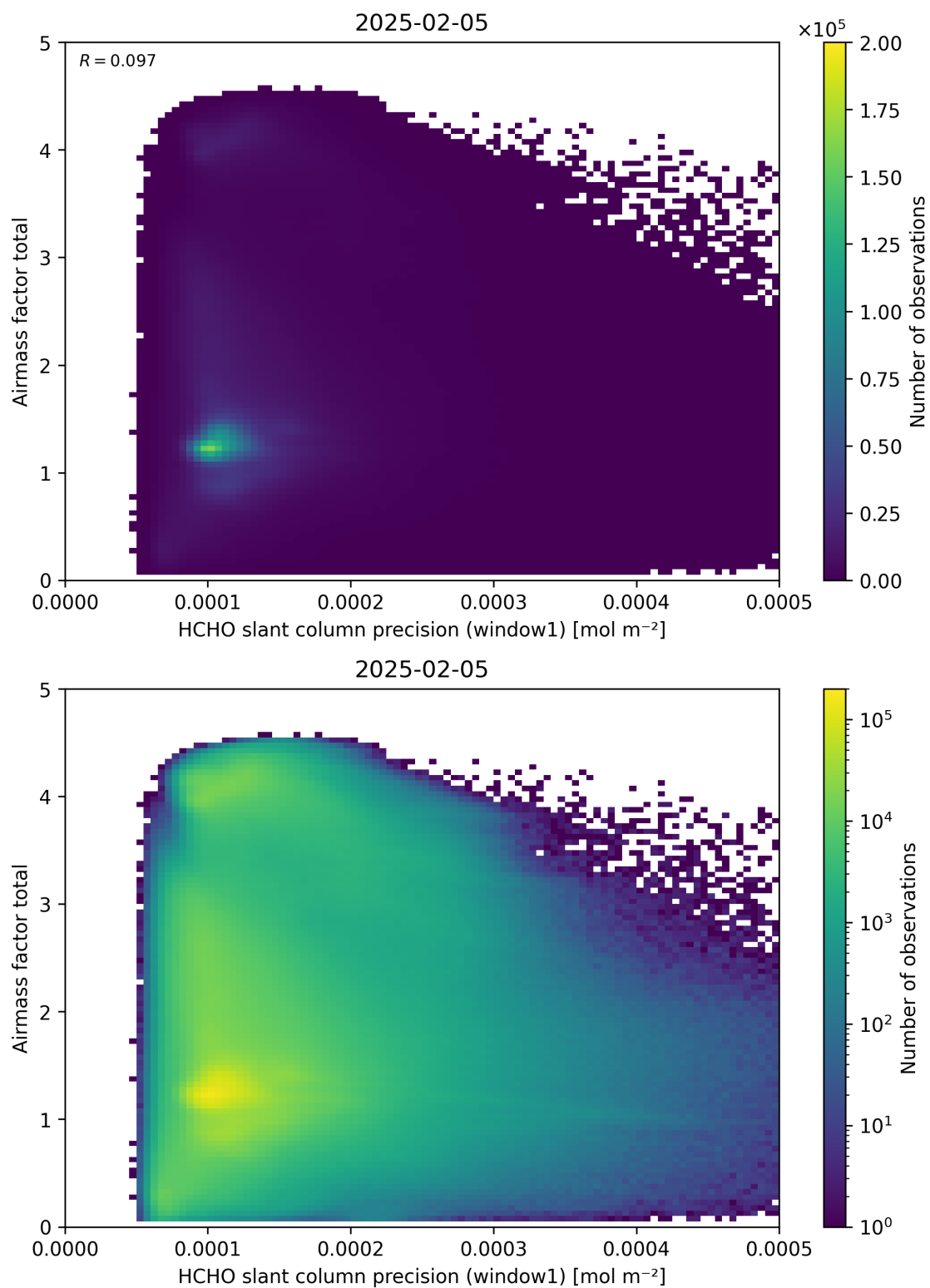
Figure 94: Scatter density plot of “HCHO slant column precision (window1)” against “Airmass factor total” for 2025-02-04 to 2025-02-06.
