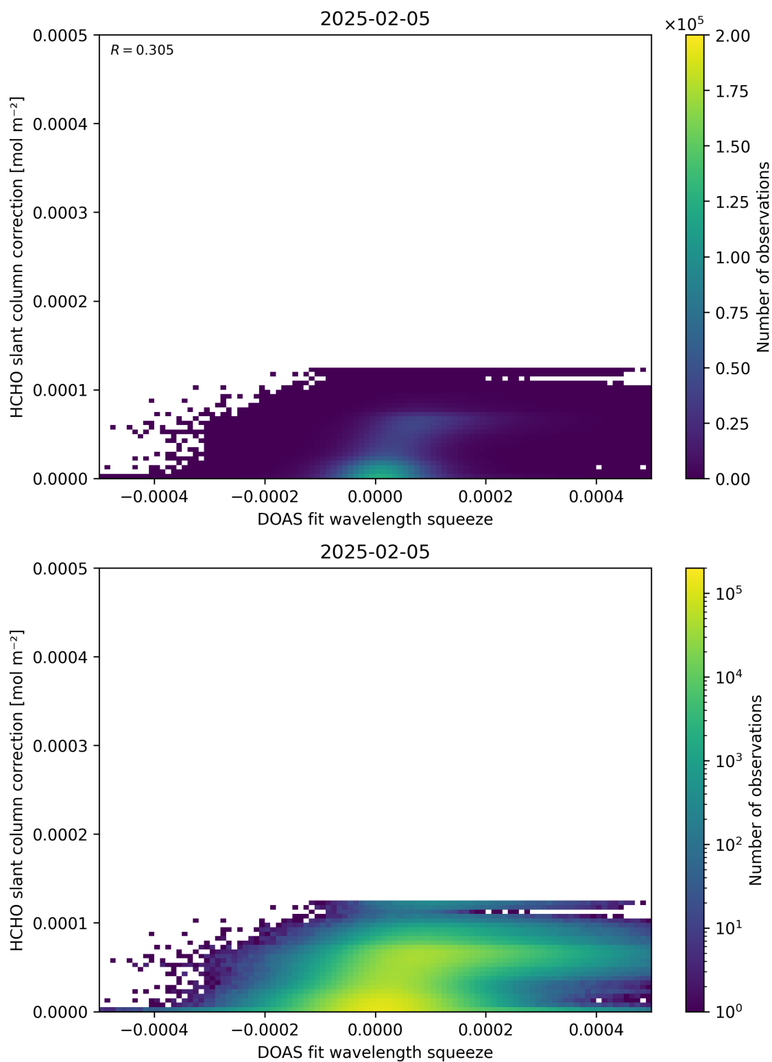
Figure 70: Scatter density plot of “DOAS fit wavelength squeeze” against “HCHO slant column correction” for 2025-02-04 to 2025-02-06.
