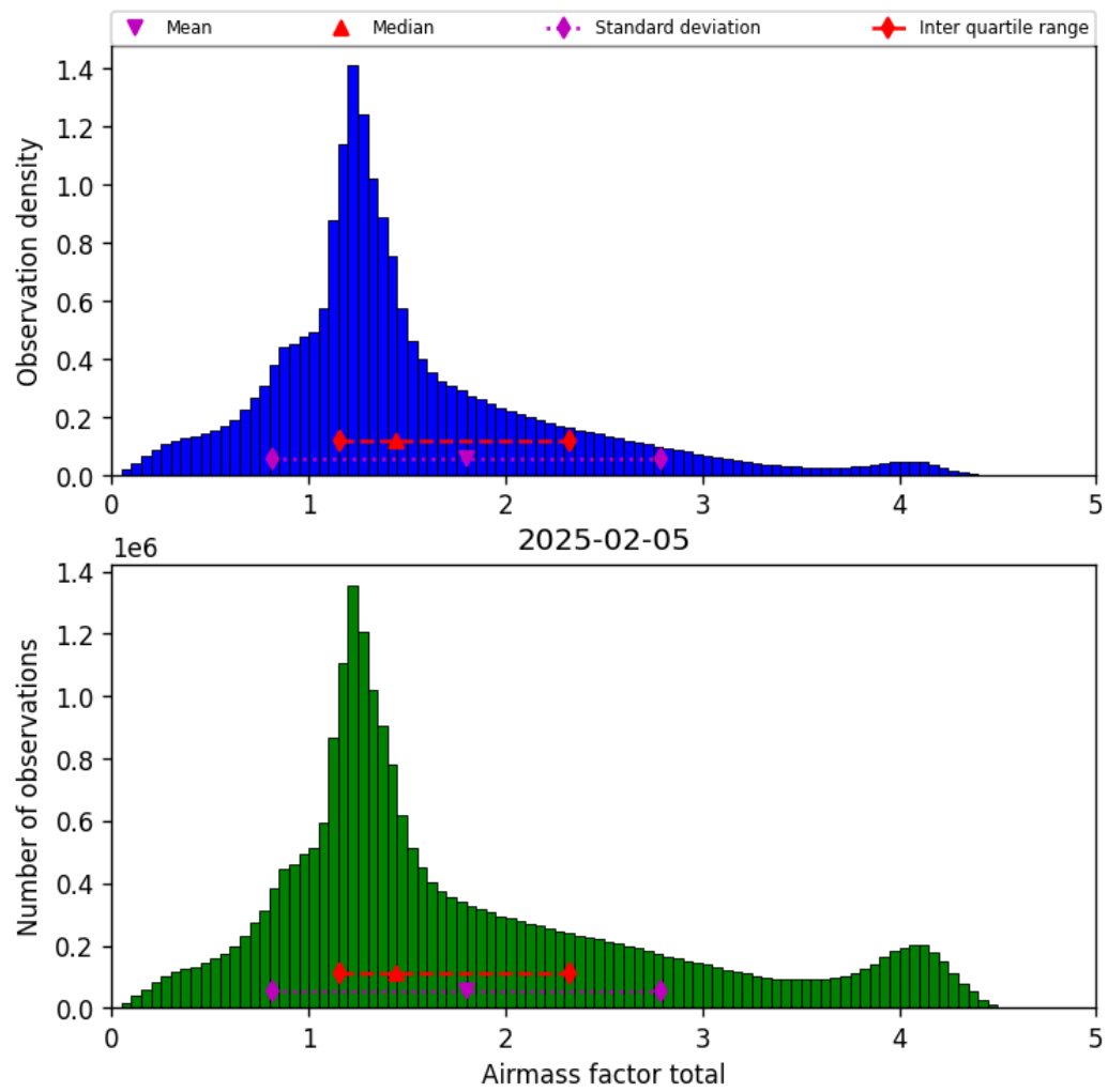
Figure 40: Histogram of “Airmass factor total” for 2025-02-04 to 2025-02-06
