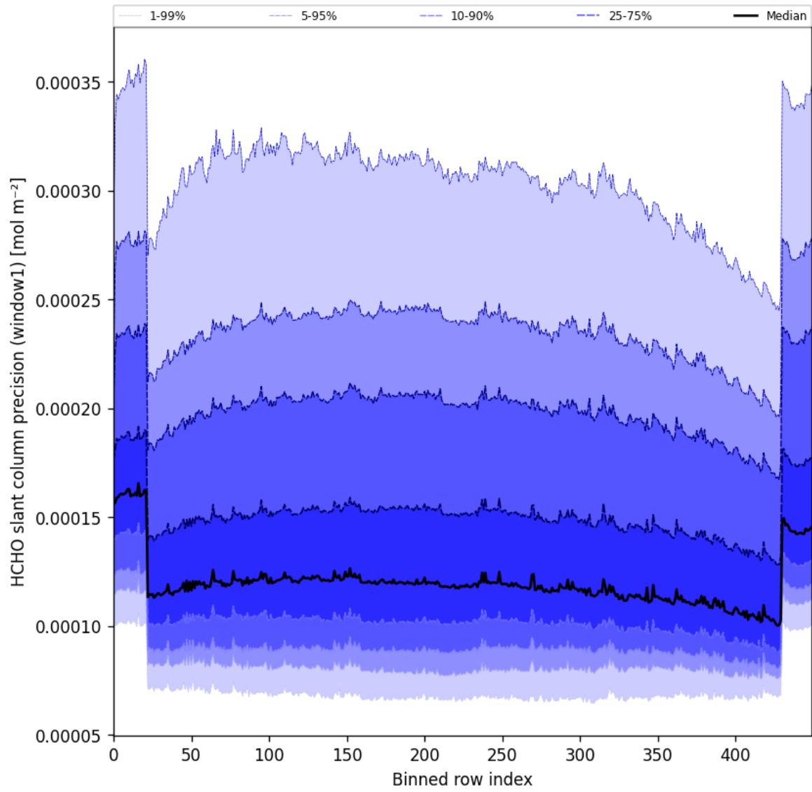
Figure 53: Along track statistics of “HCHO slant column precision (window1)” for 2025-02-04 to 2025-02-06
