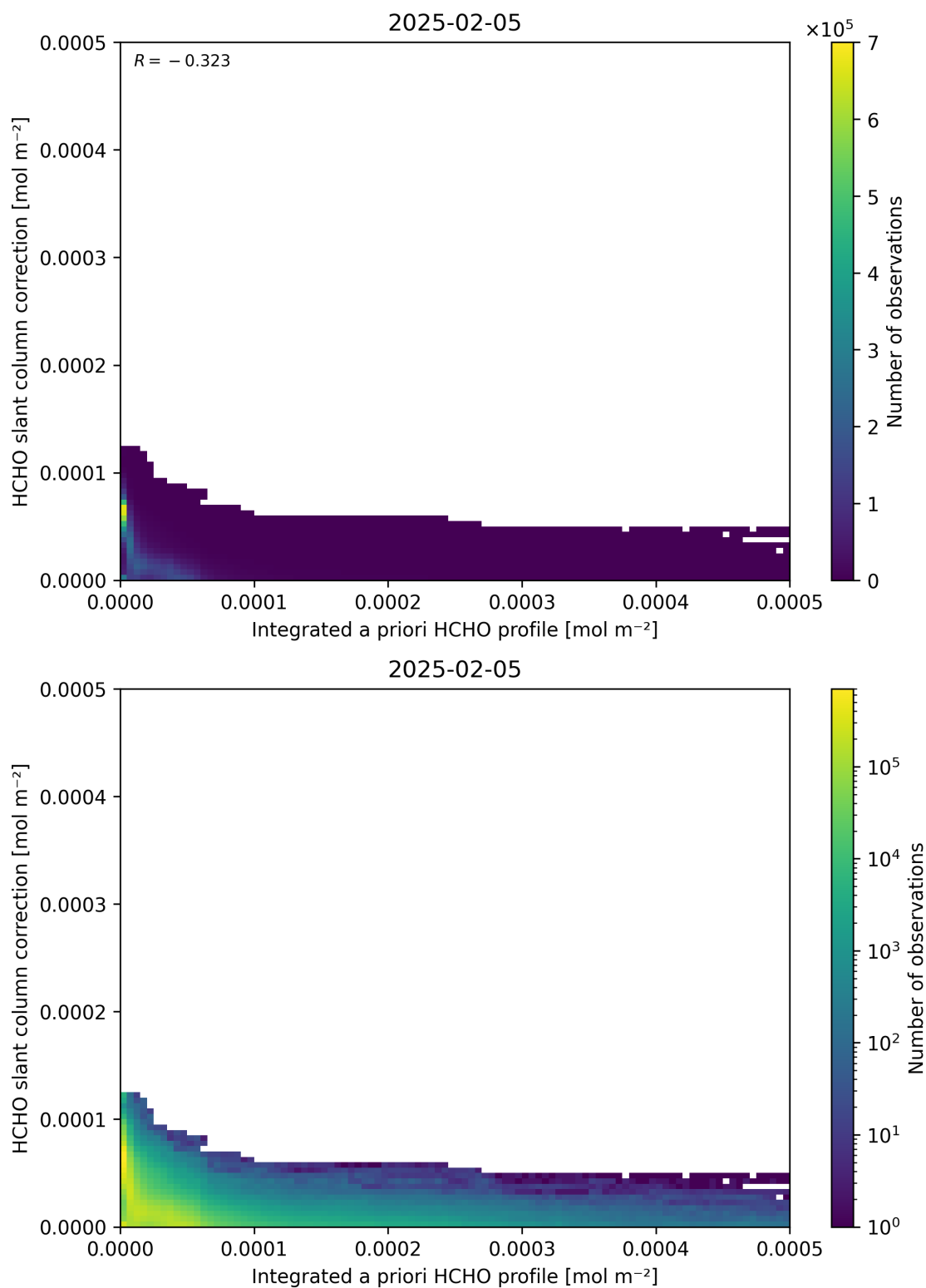
Figure 152: Scatter density plot of “Integrated a priori HCHO profile” against “HCHO slant column correction” for 2025-02-04 to 2025-02-06.
