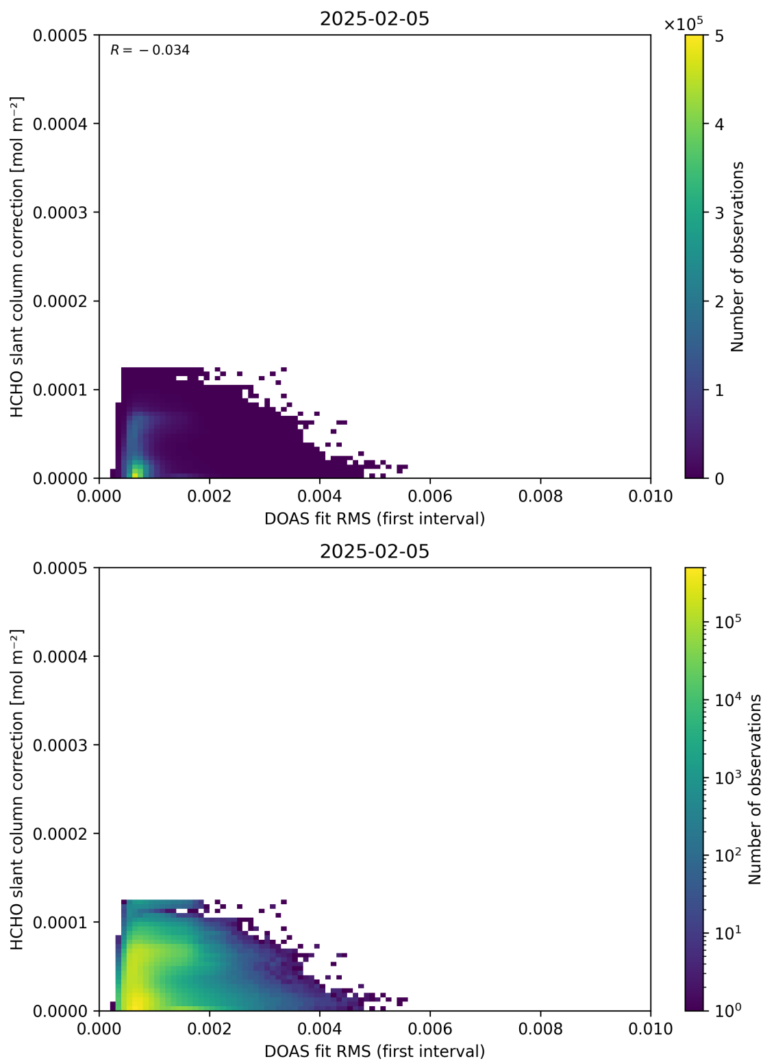
Figure 63: Scatter density plot of “DOAS fit RMS (first interval)” against “HCHO slant column correction” for 2025-02-04 to 2025-02-06.
