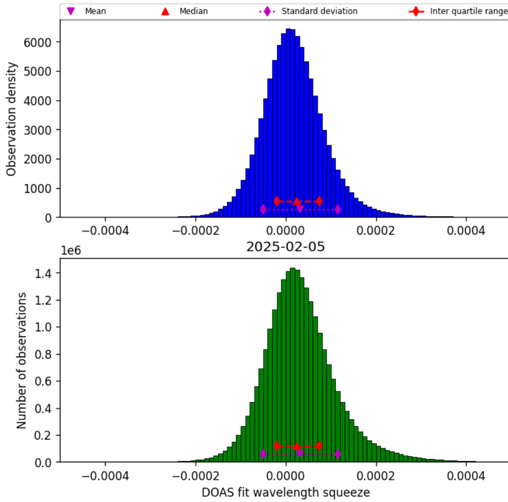
Figure 45: Histogram of “DOAS fit wavelength squeeze” for 2025-02-04 to 2025-02-06
