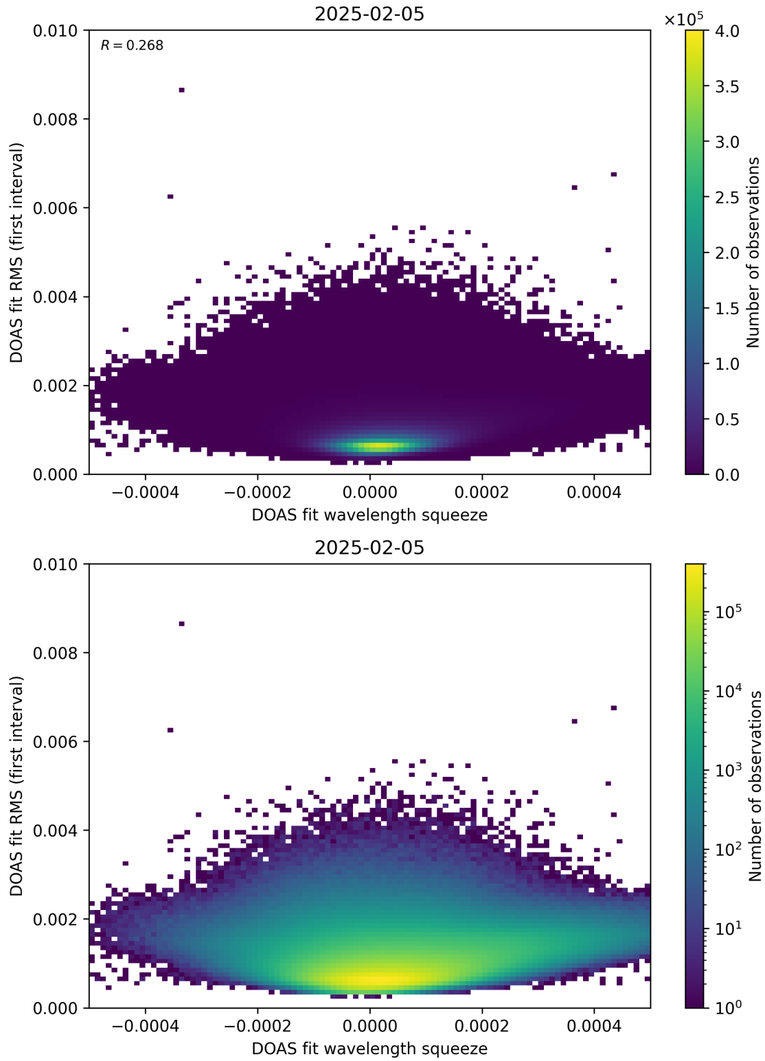
Figure 68: Scatter density plot of “DOAS fit wavelength squeeze” against “DOAS fit RMS (first interval)” for 2025-02-04 to 2025-02-06.
