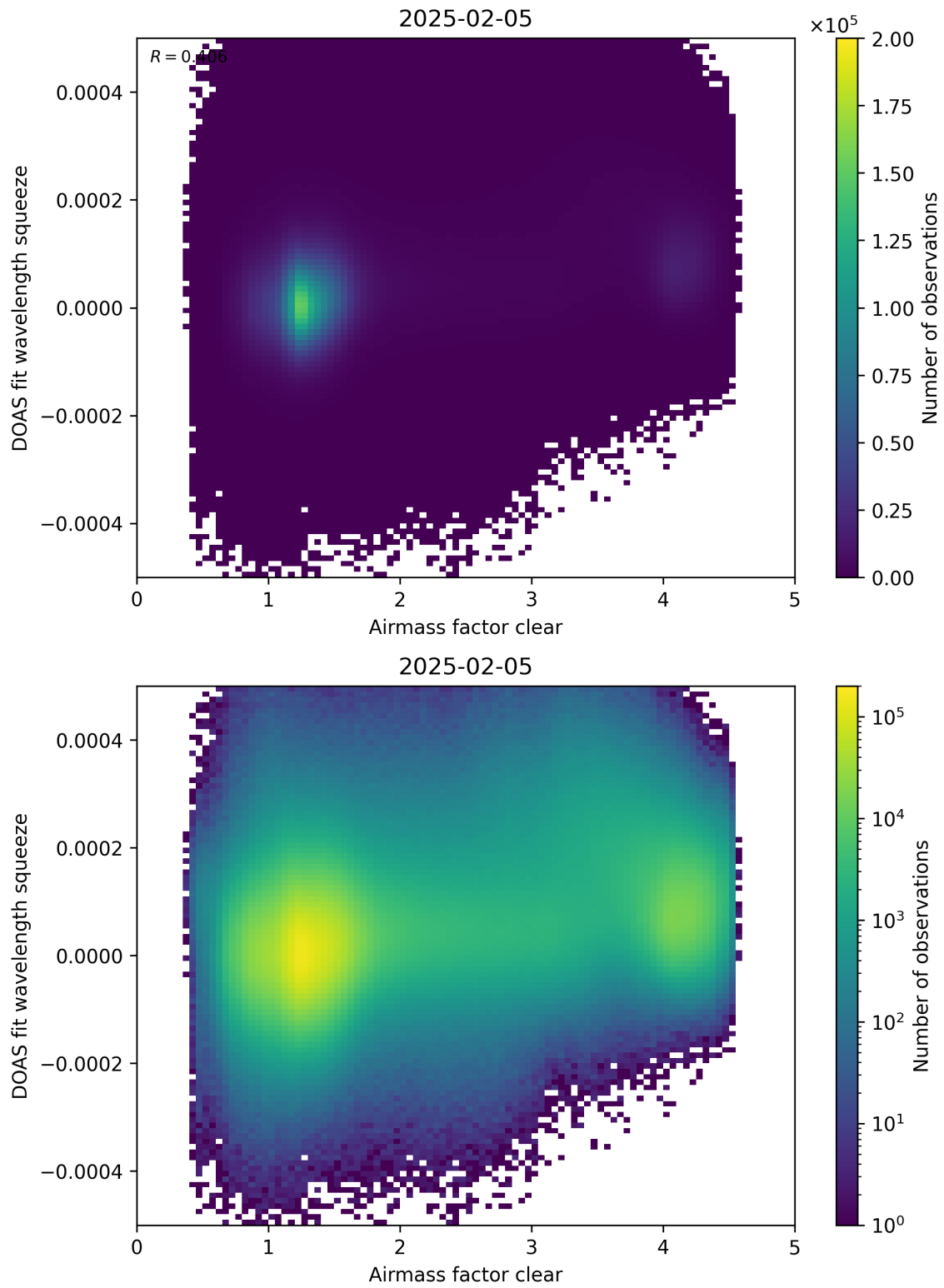
Figure 73: Scatter density plot of “Airmass factor clear” against “DOAS fit wavelength squeeze” for 2025-02-04 to 2025-02-06.
