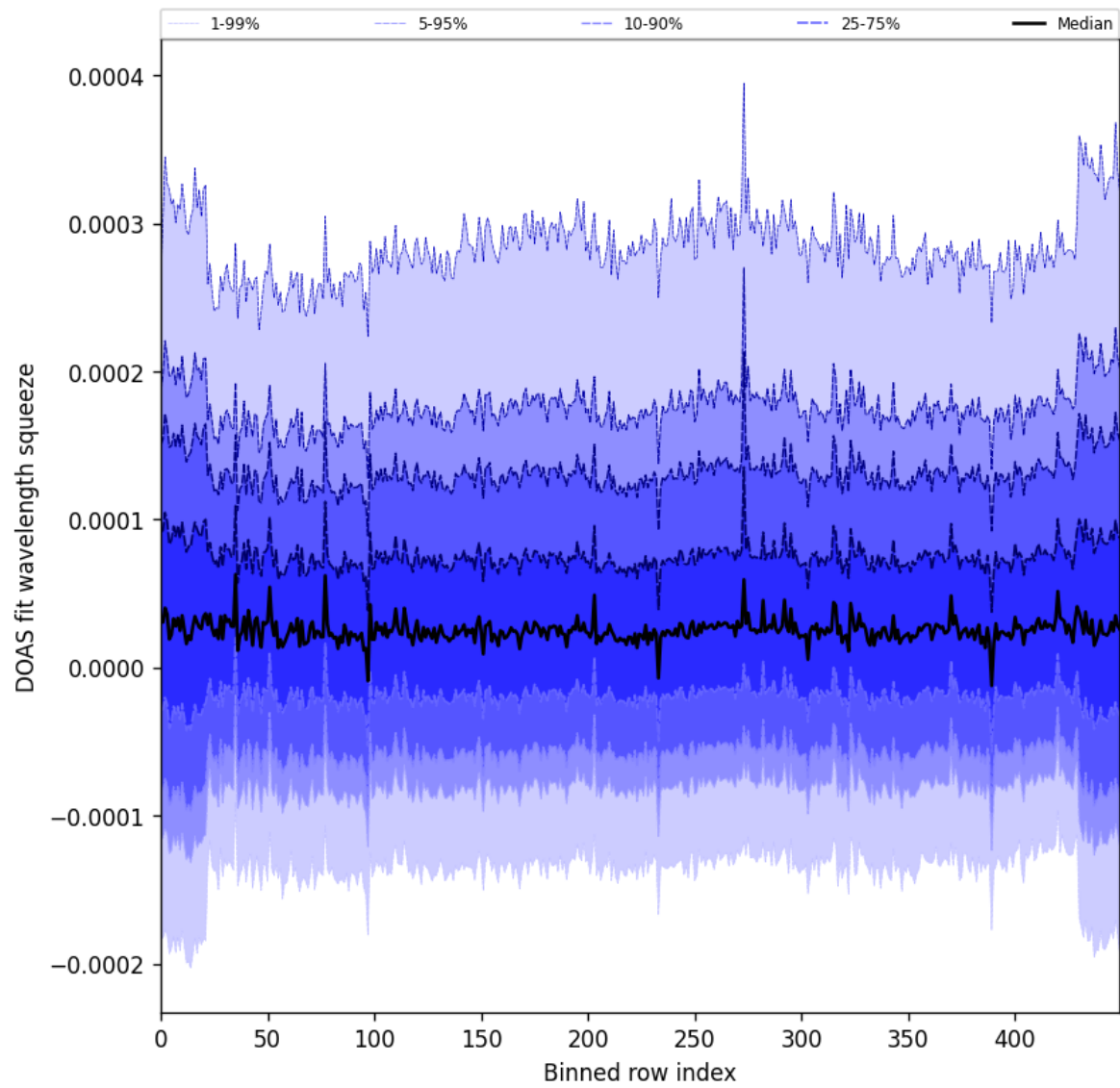
Figure 59: Along track statistics of “DOAS fit wavelength squeeze” for 2025-02-04 to 2025-02-06
