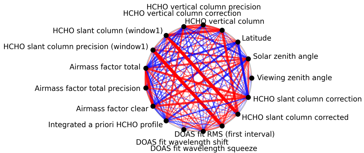
Figure 1: Map of correlation graph for 2025-02-04 to 2025-02-06.
