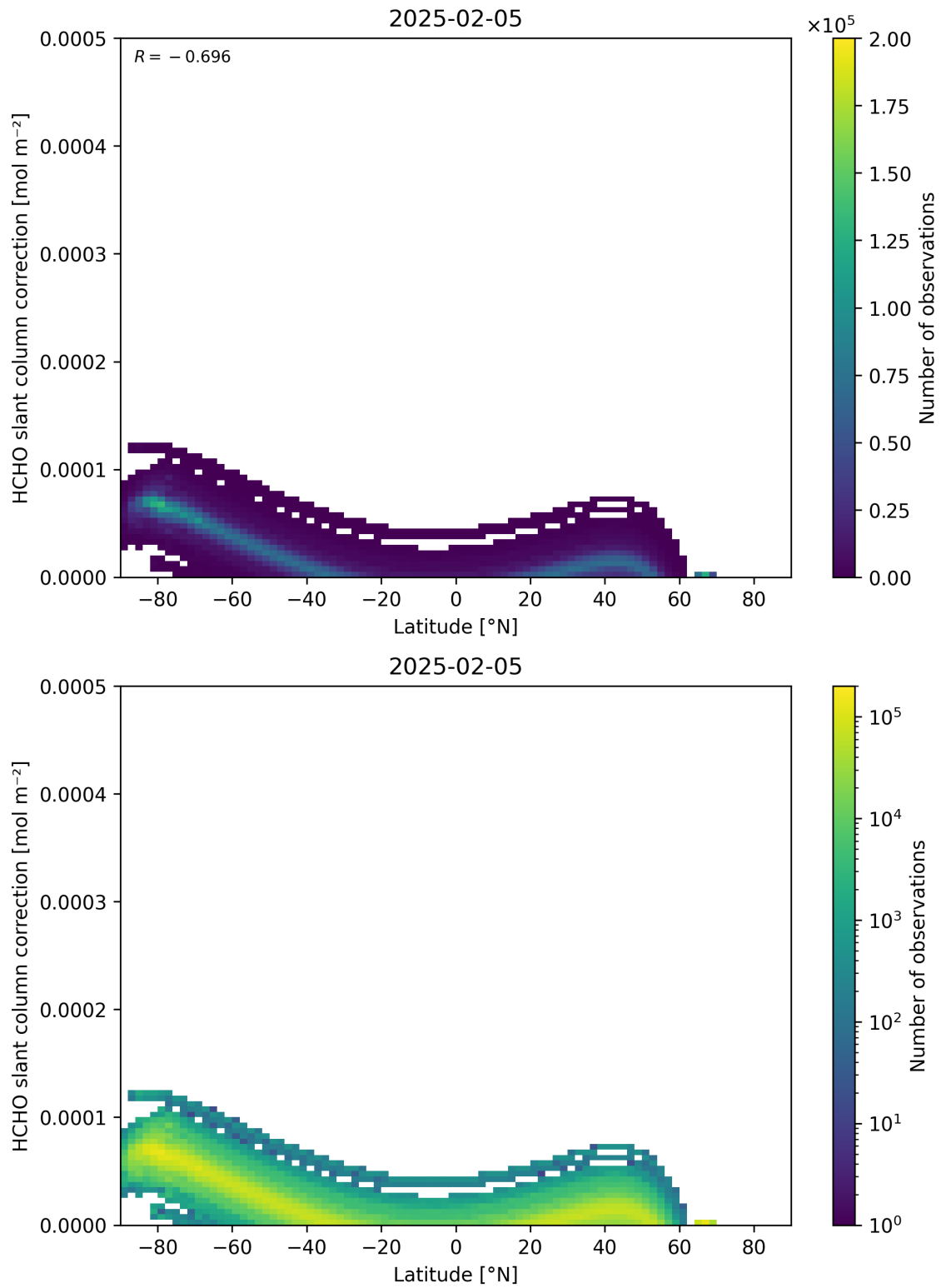
Figure 158: Scatter density plot of “Latitude” against “HCHO slant column correction” for 2025-02-04 to 2025-02-06.
