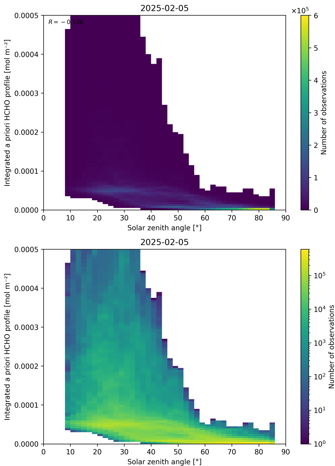
Figure 180: Scatter density plot of “Solar zenith angle” against “Integrated a priori HCHO profile” for 2025-02-04 to 2025-02-06.
