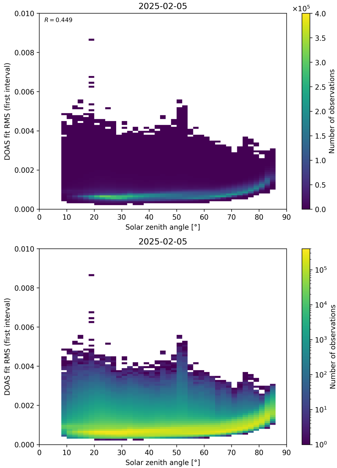
Figure 167: Scatter density plot of “Solar zenith angle” against “DOAS fit RMS (first interval)” for 2025-02-04 to 2025-02-06.
