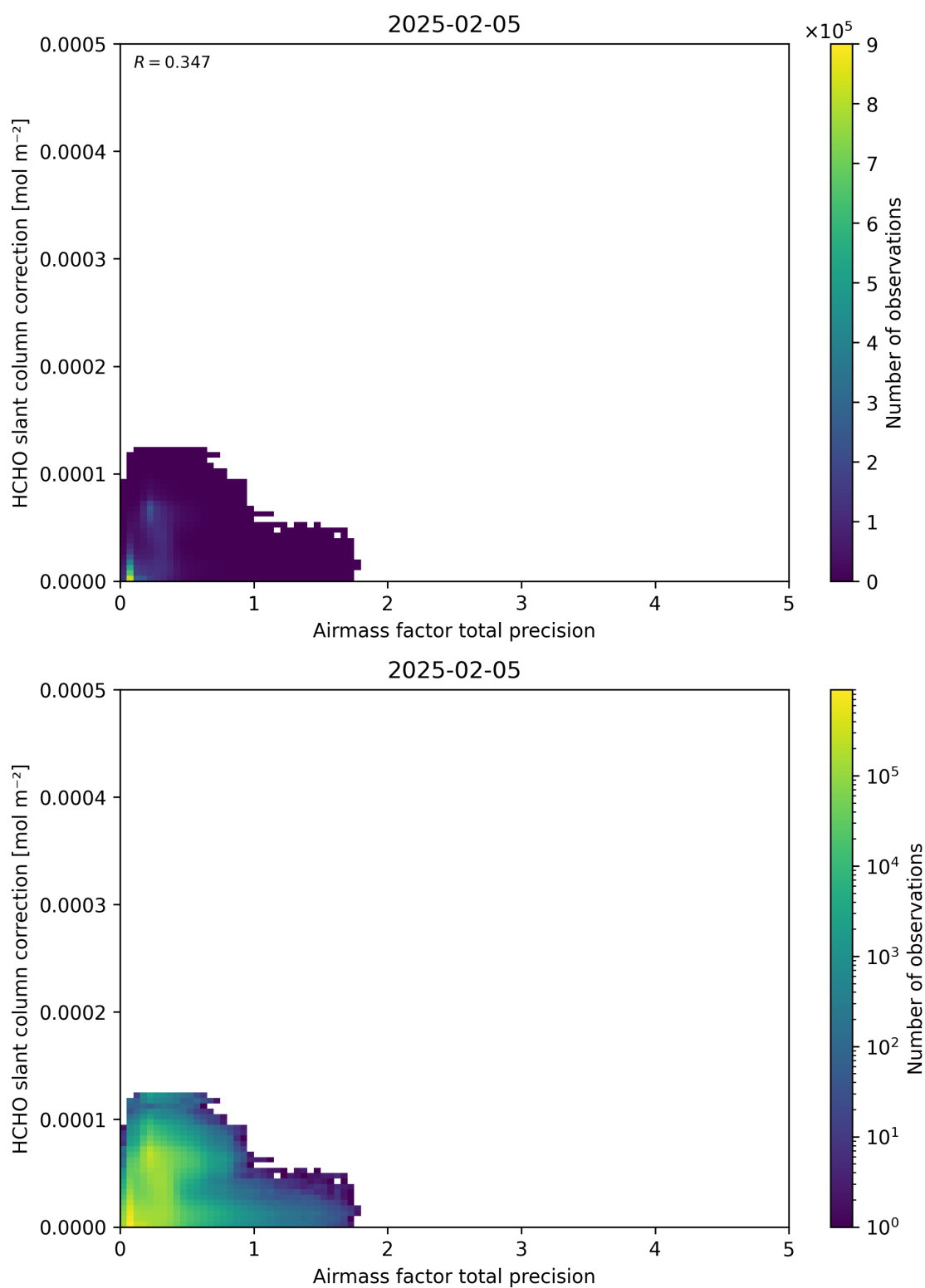
Figure 110: Scatter density plot of “Airmass factor total precision” against “HCHO slant column correction” for 2025-02-04 to 2025-02-06.
