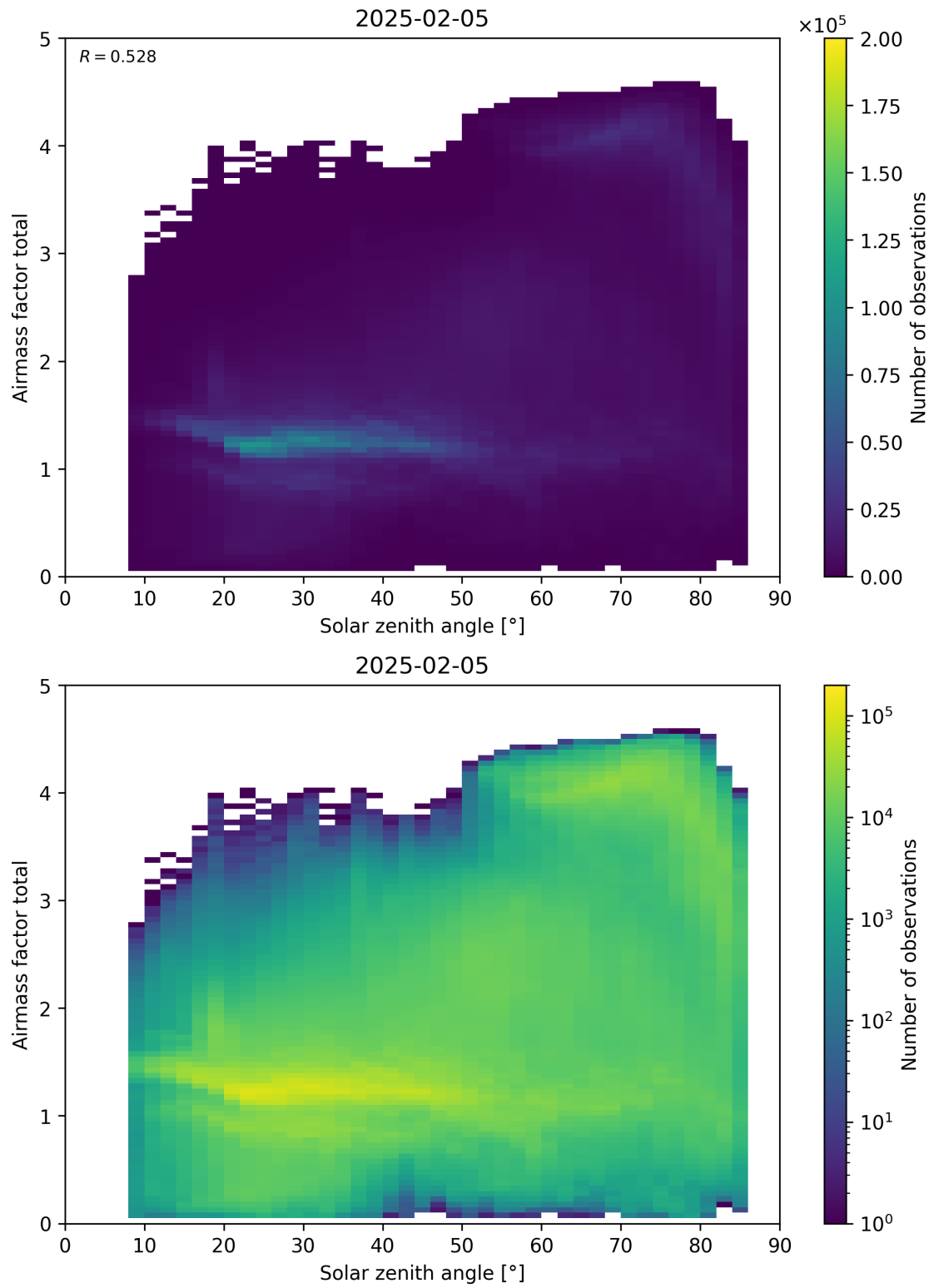
Figure 175: Scatter density plot of “Solar zenith angle” against “Airmass factor total” for 2025-02-04 to 2025-02-06.
