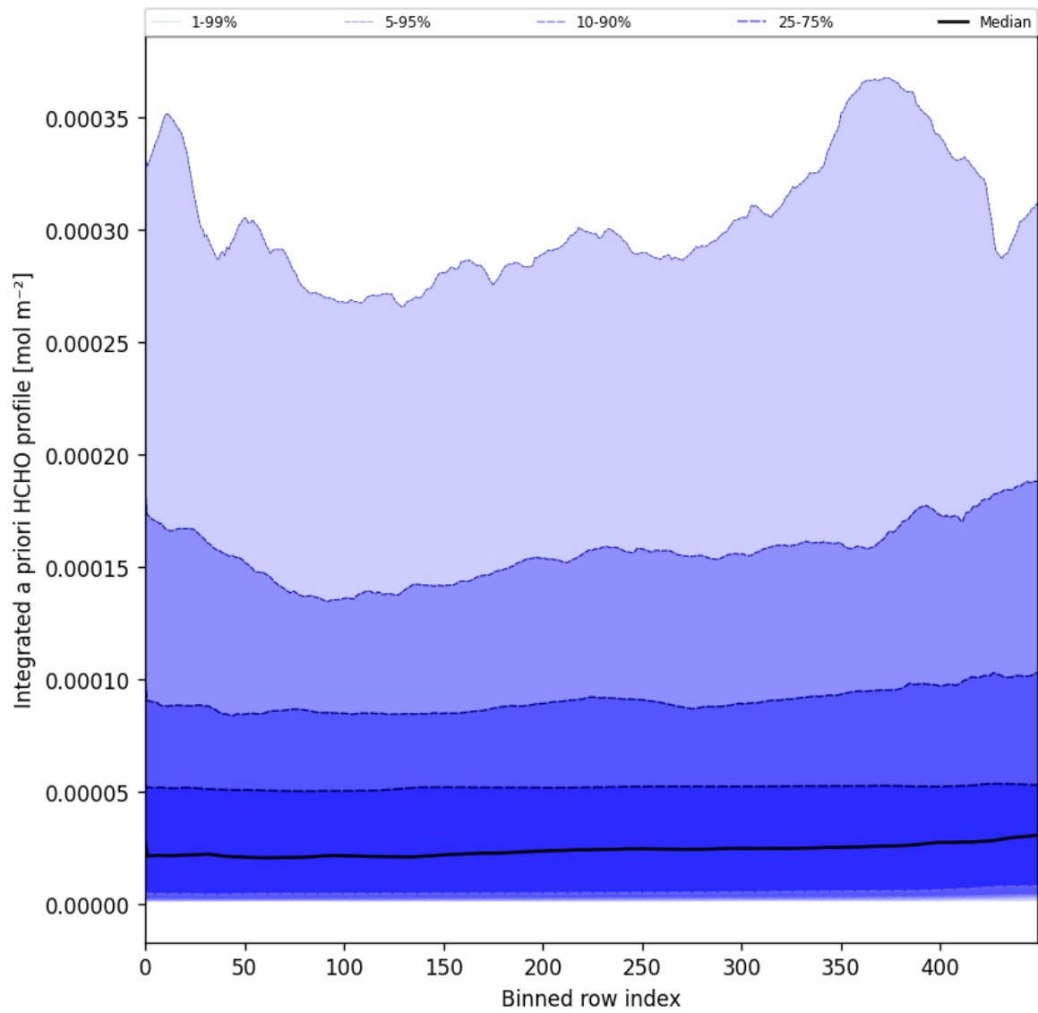
Figure 57: Along track statistics of “Integrated a priori HCHO profile” for 2025-02-04 to 2025-02-06
