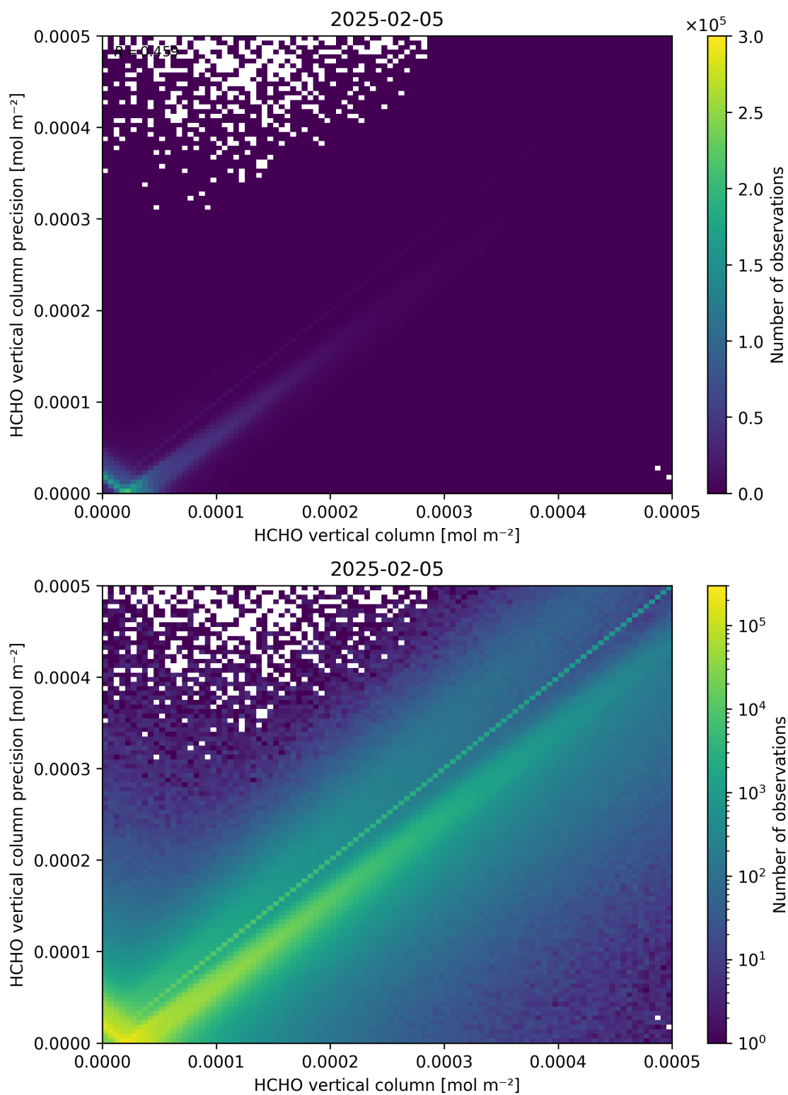
Figure 134: Scatter density plot of “HCHO vertical column” against “HCHO vertical column precision” for 2025-02-04 to 2025-02-06.
