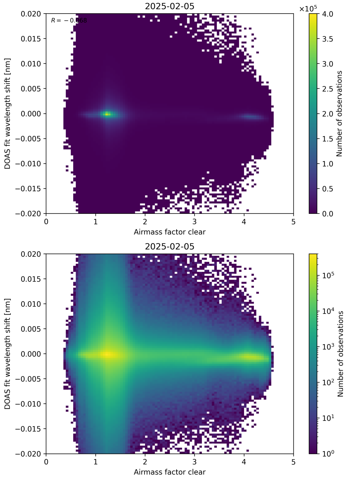
Figure 72: Scatter density plot of “Airmass factor clear” against “DOAS fit wavelength shift” for 2025-02-04 to 2025-02-06.
