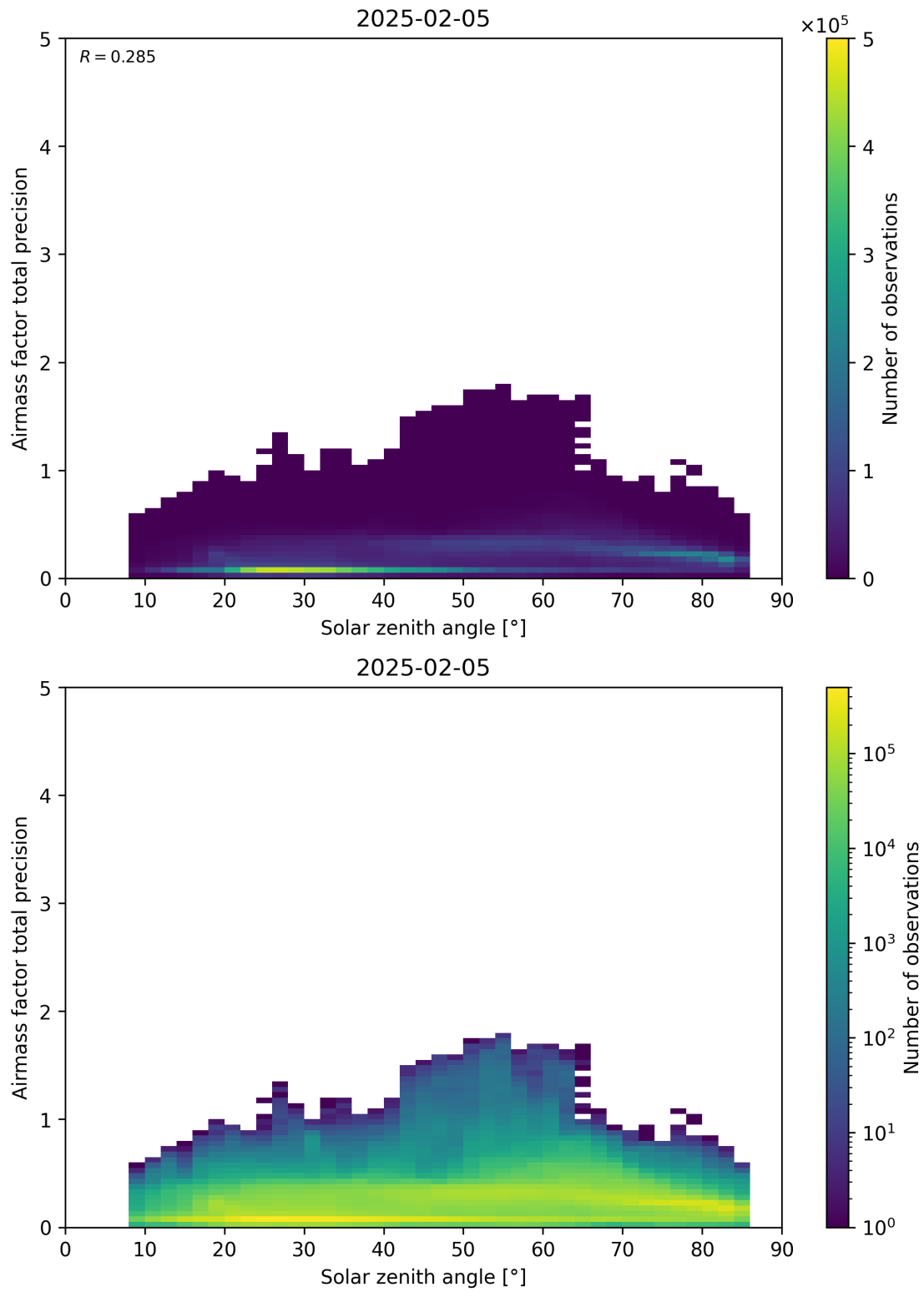
Figure 176: Scatter density plot of “Solar zenith angle” against “Airmass factor total precision” for 2025-02-04 to 2025-02-06.
