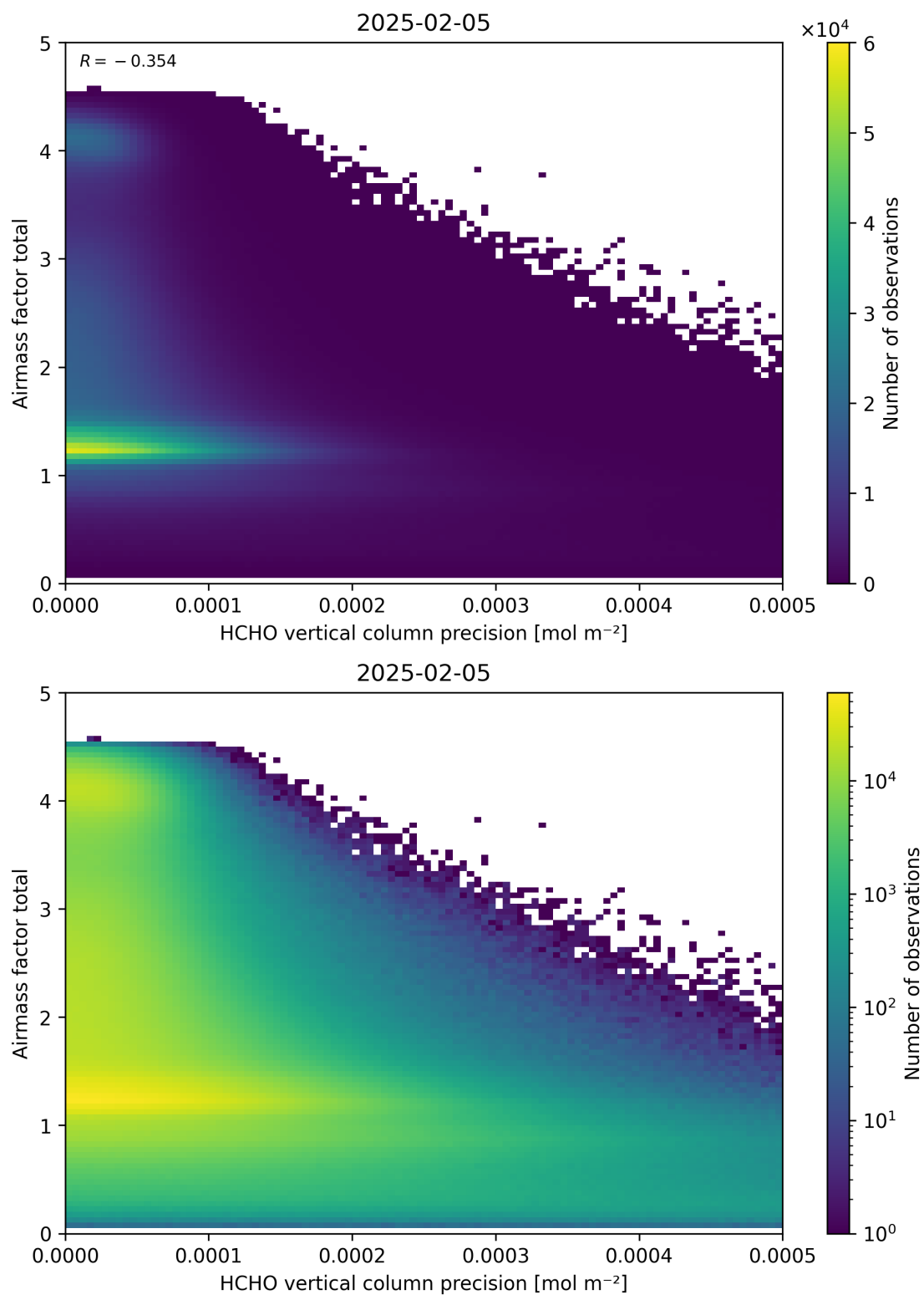
Figure 144: Scatter density plot of “HCHO vertical column precision” against “Airmass factor total” for 2025-02-04 to 2025-02-06.
