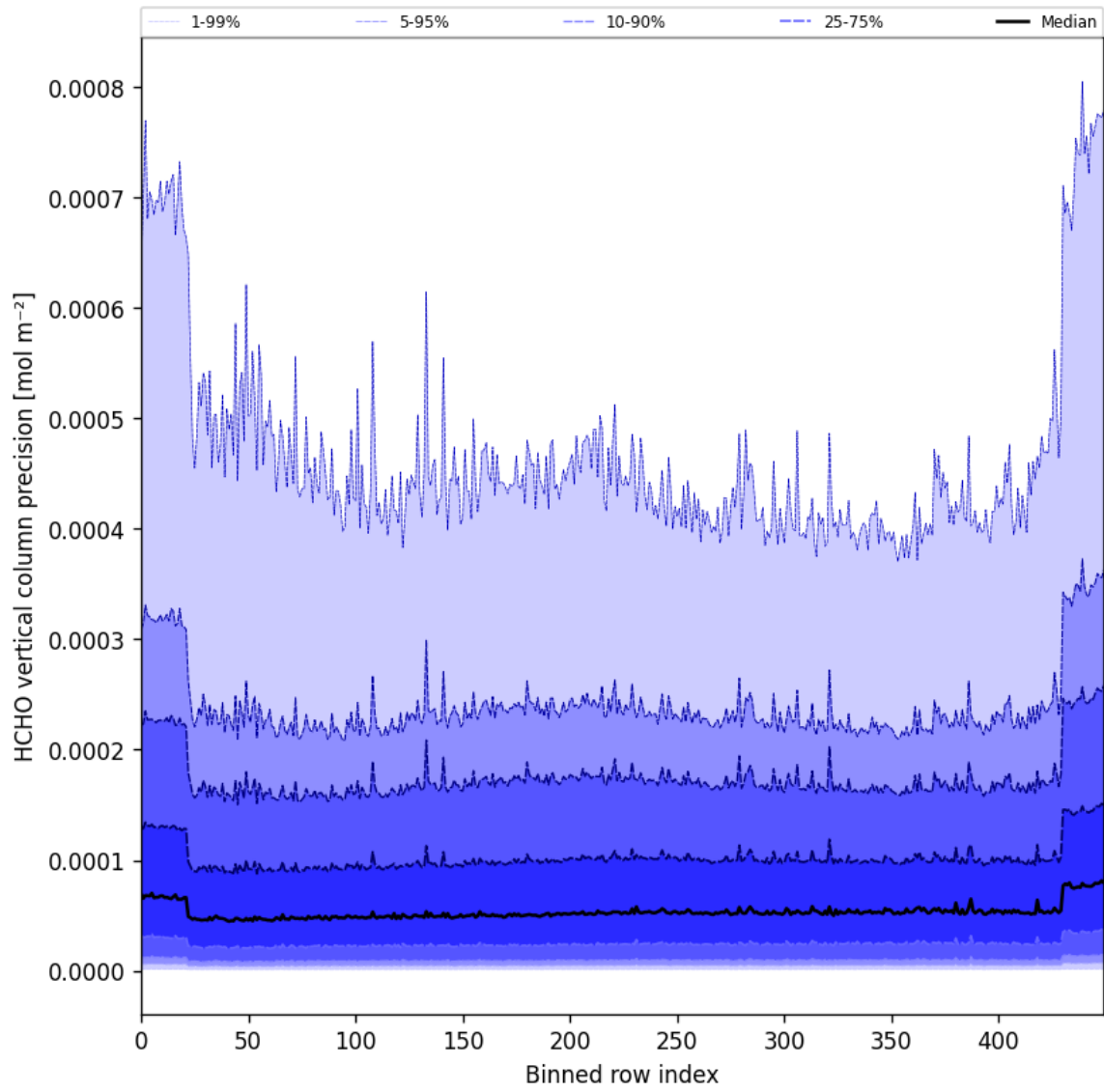
Figure 50: Along track statistics of “HCHO vertical column precision” for 2025-02-04 to 2025-02-06
