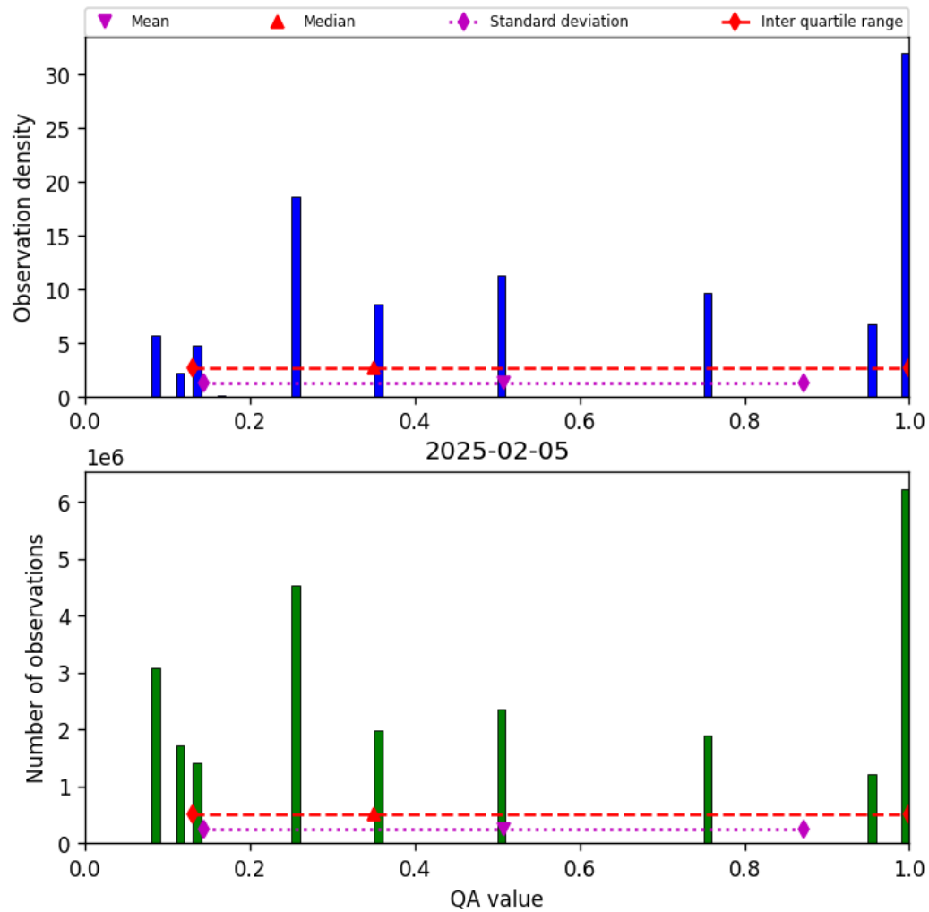
Figure 34: Histogram of “QA value” for 2025-02-04 to 2025-02-06
