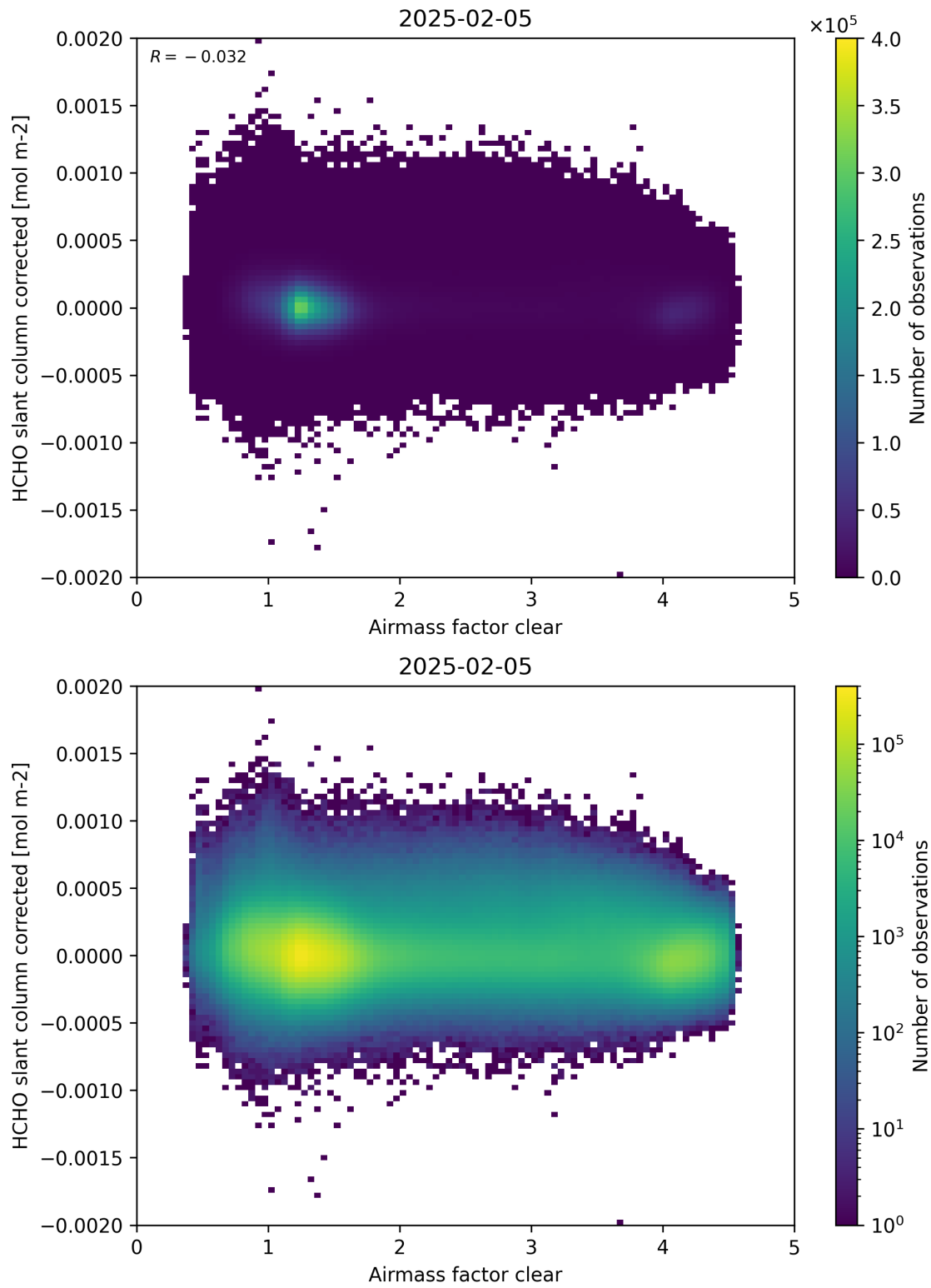
Figure 74: Scatter density plot of “Airmass factor clear” against “HCHO slant column corrected” for 2025-02-04 to 2025-02-06.
