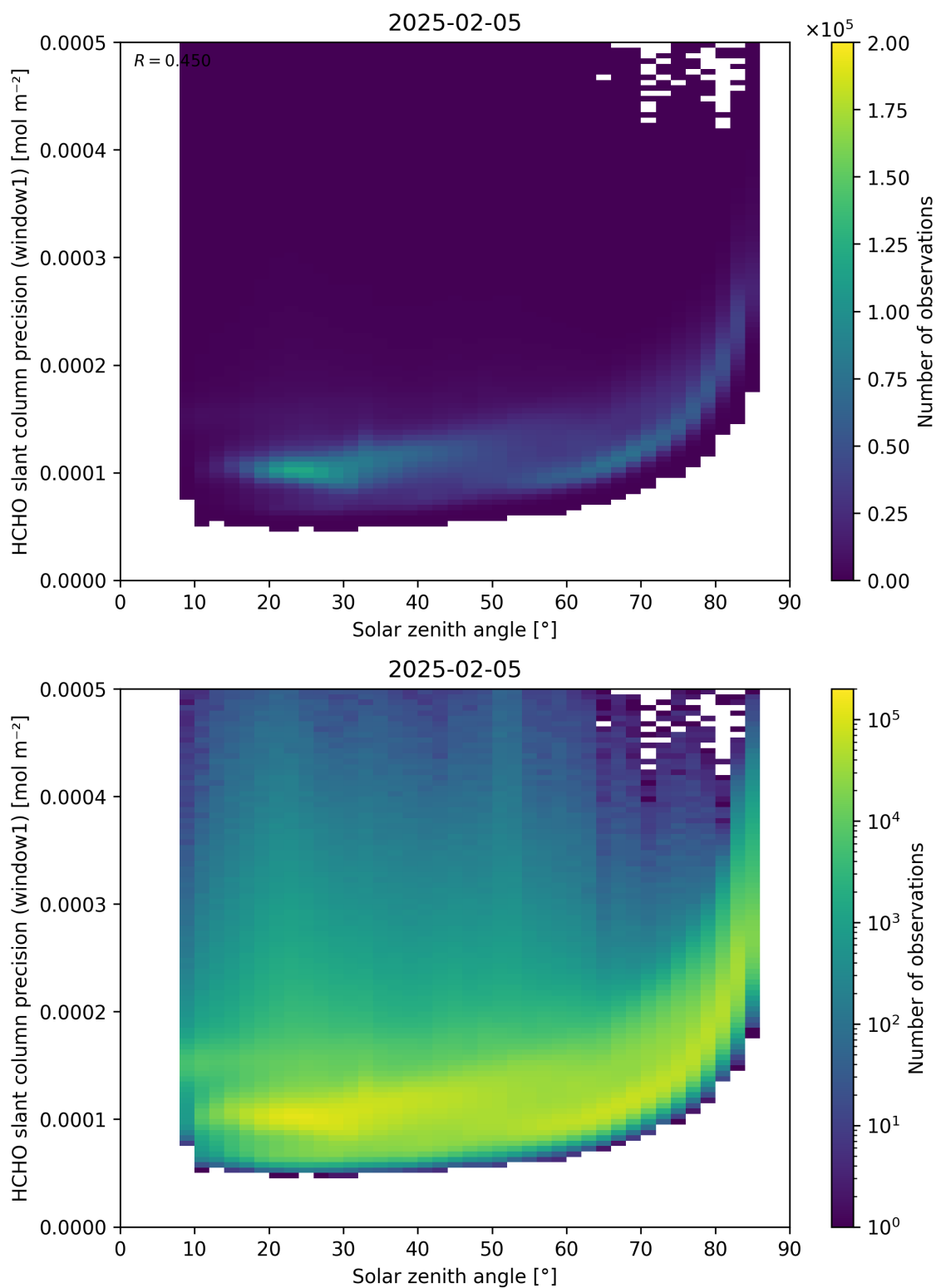
Figure 174: Scatter density plot of “Solar zenith angle” against “HCHO slant column precision (window1)” for 2025-02-04 to 2025-02-06.
