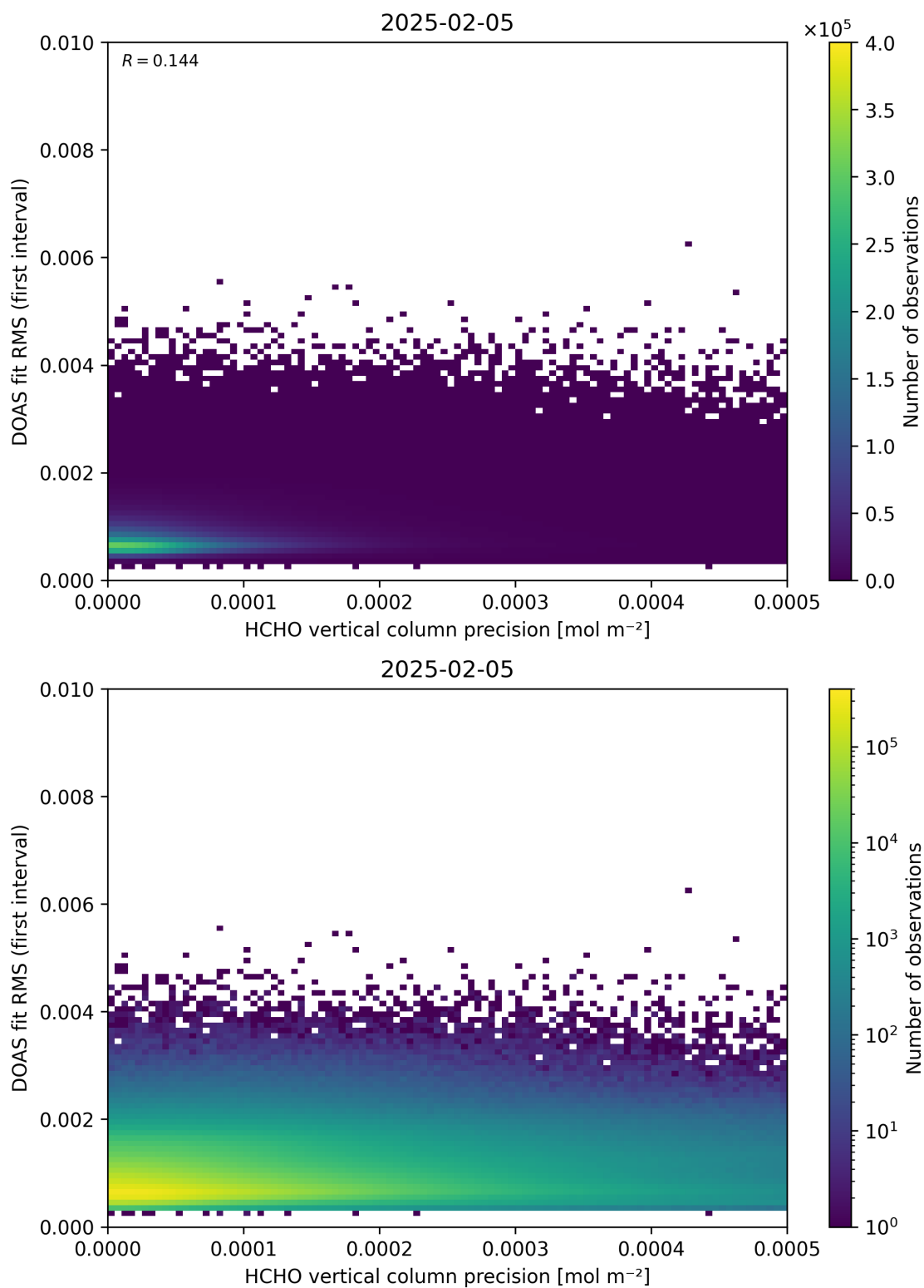
Figure 136: Scatter density plot of “HCHO vertical column precision” against “DOAS fit RMS (first interval)” for 2025-02-04 to 2025-02-06.
