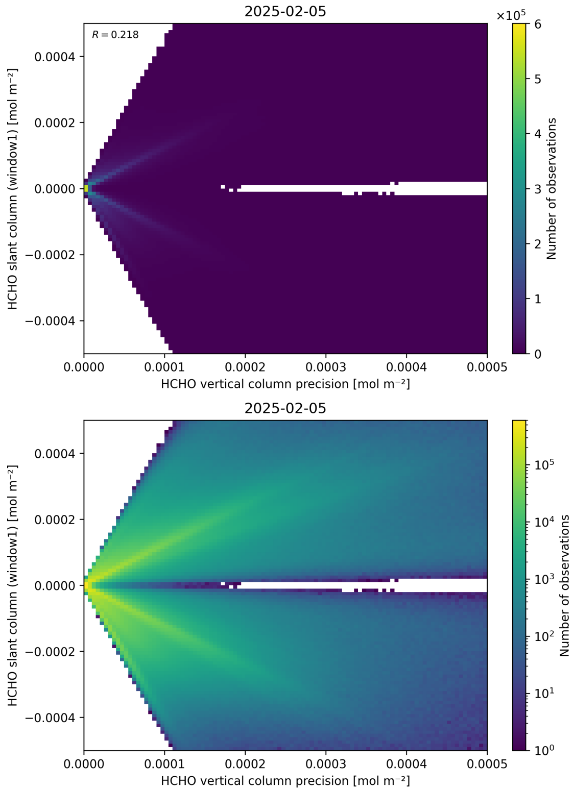
Figure 142: Scatter density plot of “HCHO vertical column precision” against “HCHO slant column (window1)” for 2025-02-04 to 2025-02-06.
