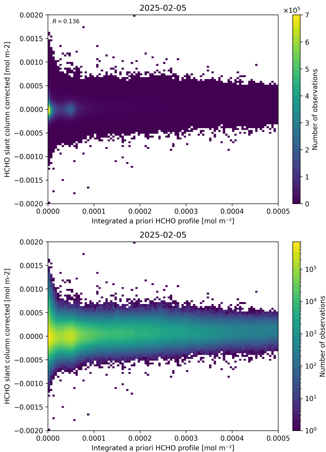
Figure 151: Scatter density plot of “Integrated a priori HCHO profile” against “HCHO slant column corrected” for 2025-02-04 to 2025-02-06.
