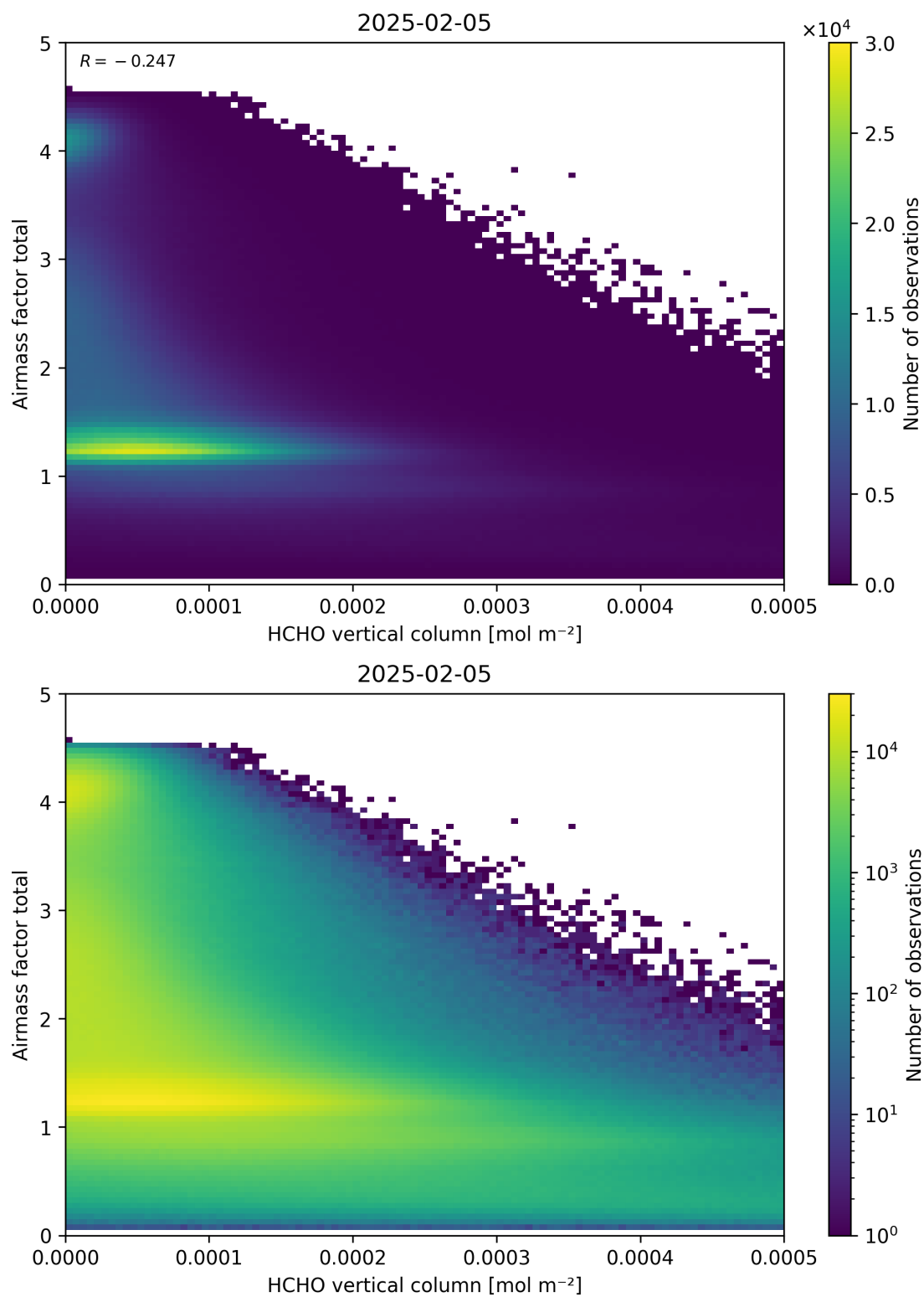
Figure 131: Scatter density plot of “HCHO vertical column” against “Airmass factor total” for 2025-02-04 to 2025-02-06.
