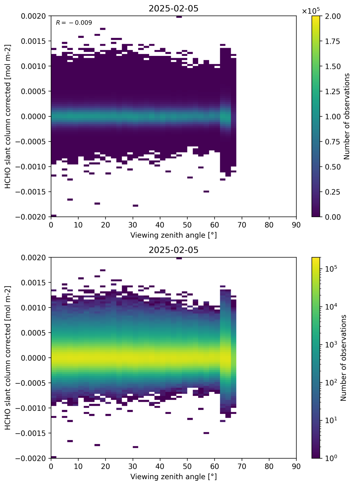
Figure 186: Scatter density plot of “Viewing zenith angle” against “HCHO slant column corrected” for 2025-02-04 to 2025-02-06.
