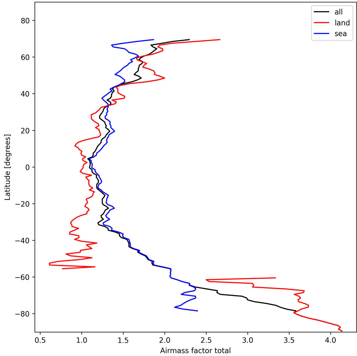
Figure 26: Zonal average of “Airmass factor total” for 2025-02-04 to 2025-02-06.
