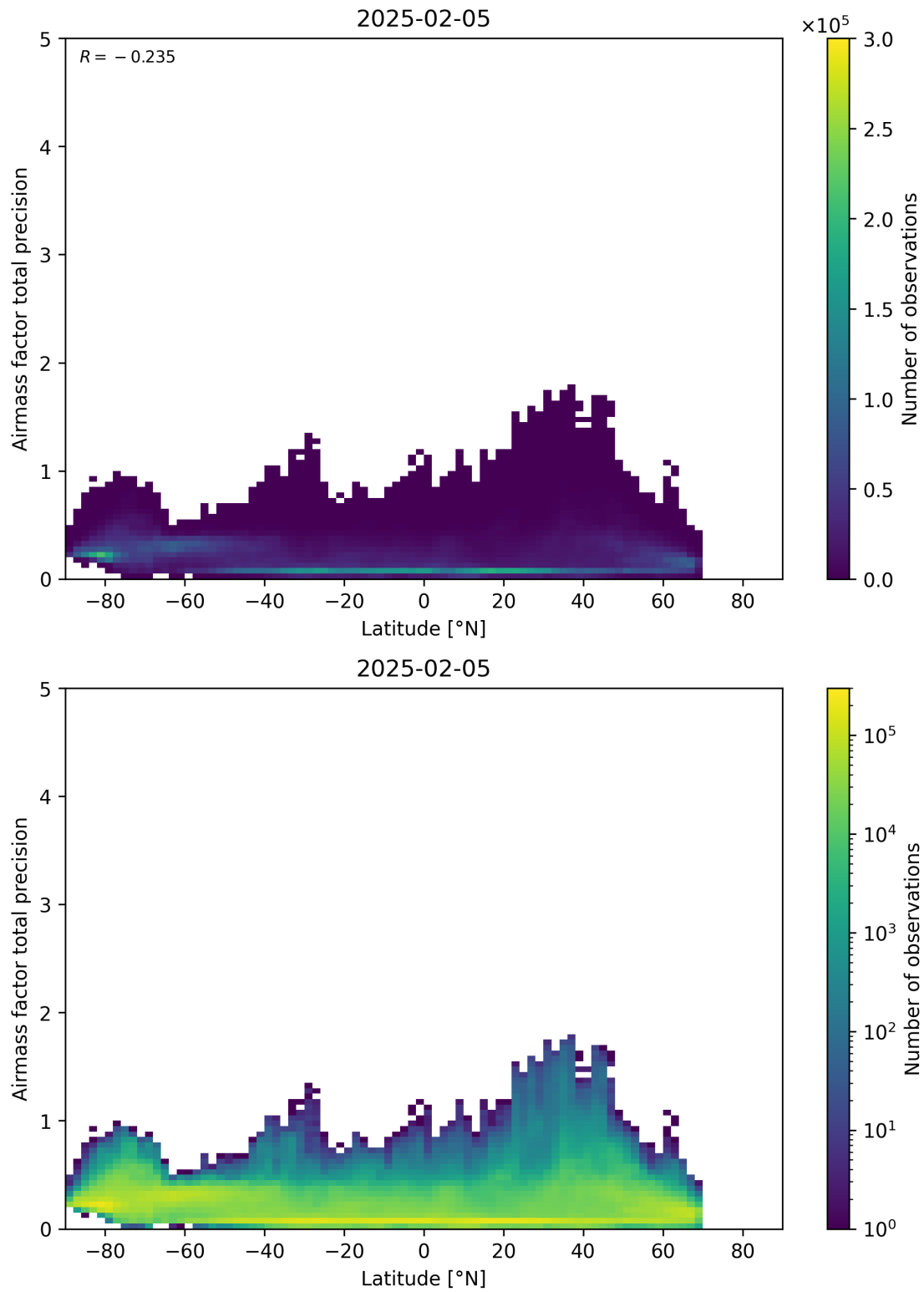
Figure 162: Scatter density plot of “Latitude” against “Airmass factor total precision” for 2025-02-04 to 2025-02-06.
