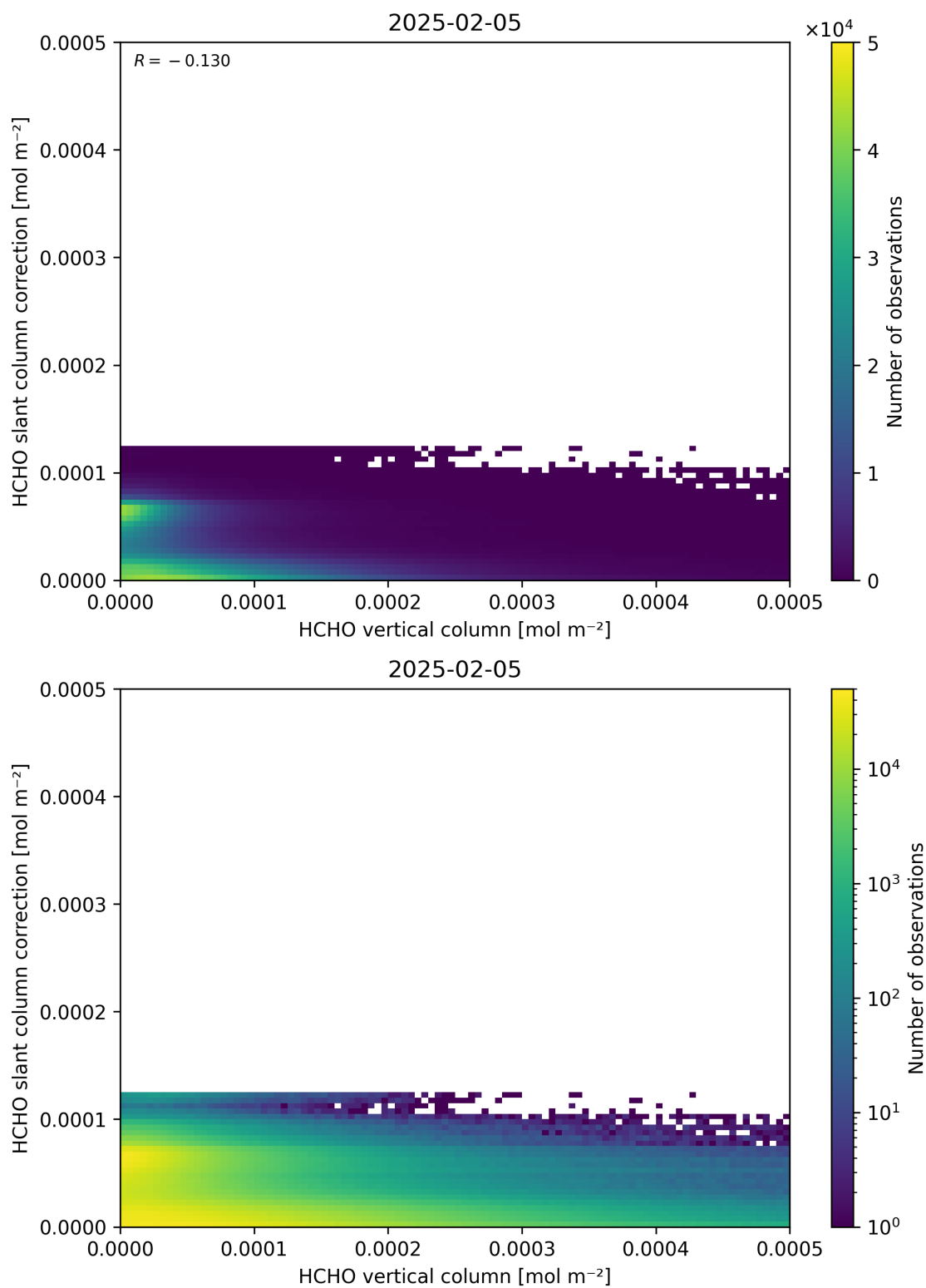
Figure 128: Scatter density plot of “HCHO vertical column” against “HCHO slant column correction” for 2025-02-04 to 2025-02-06.
