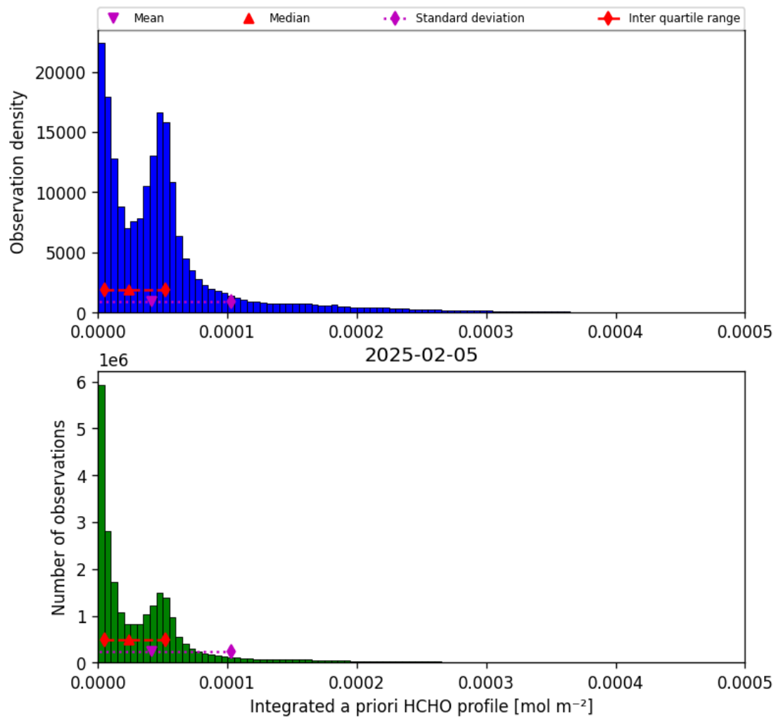
Figure 43: Histogram of “Integrated a priori HCHO profile” for 2025-02-04 to 2025-02-06
