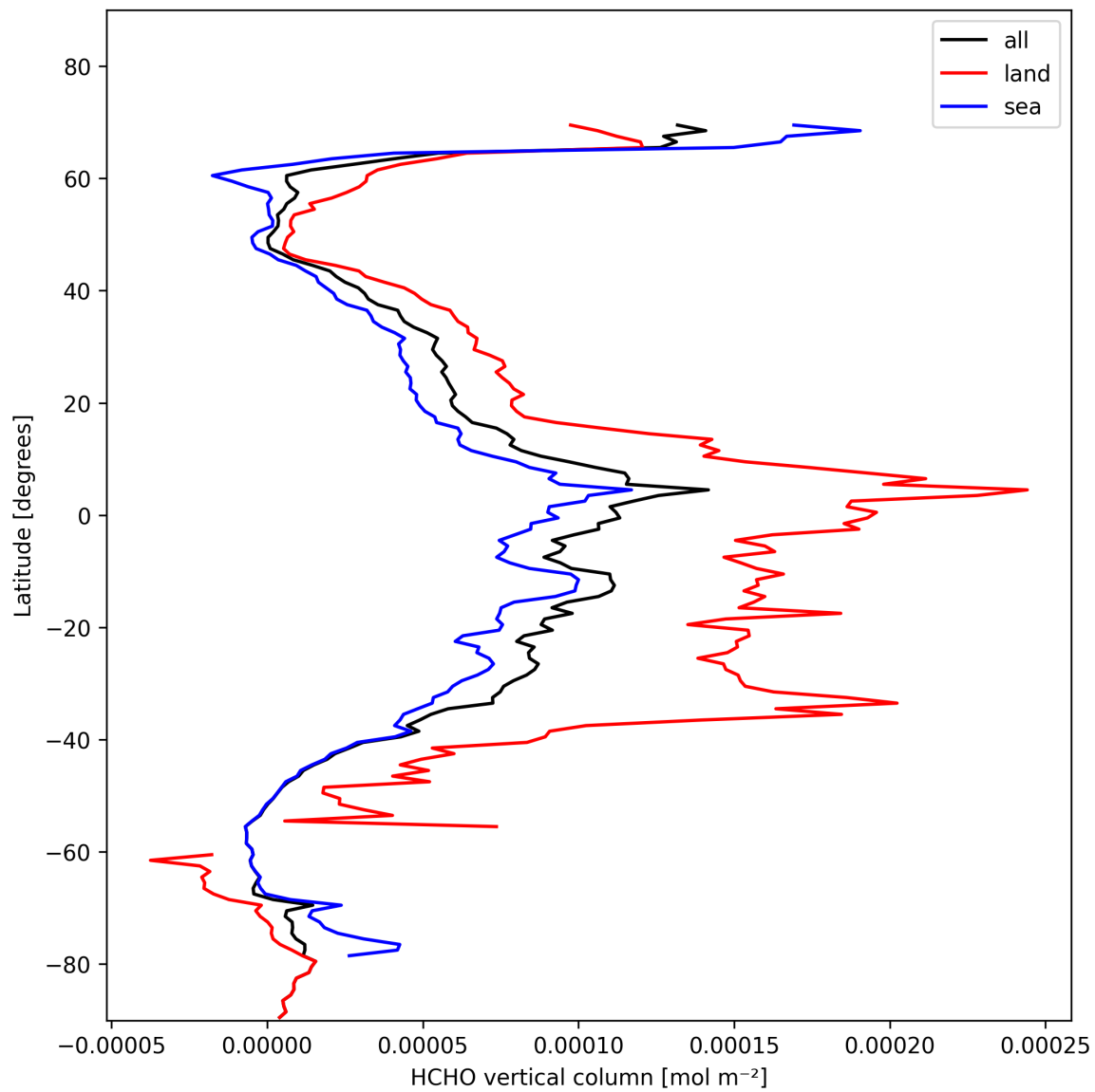
Figure 21: Zonal average of “HCHO vertical column” for 2025-02-04 to 2025-02-06.
