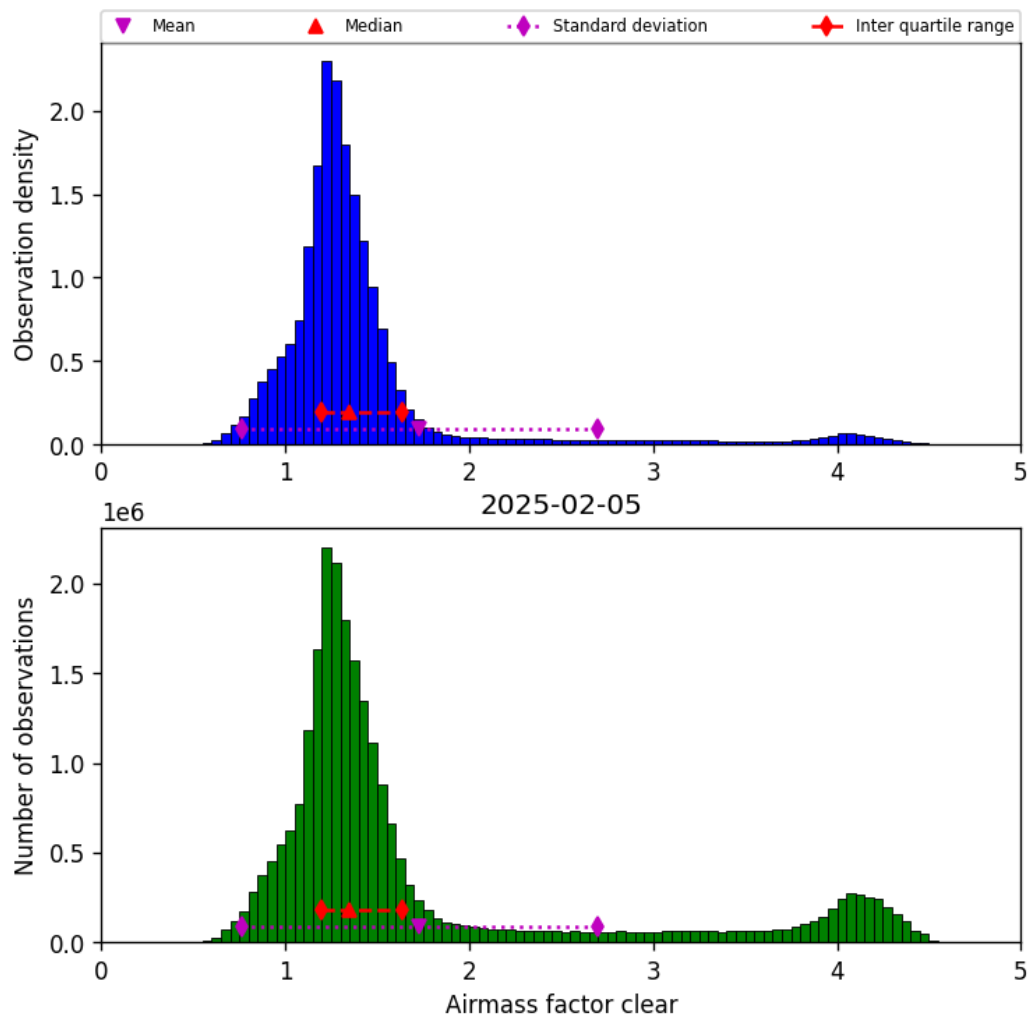
Figure 42: Histogram of “Airmass factor clear” for 2025-02-04 to 2025-02-06
