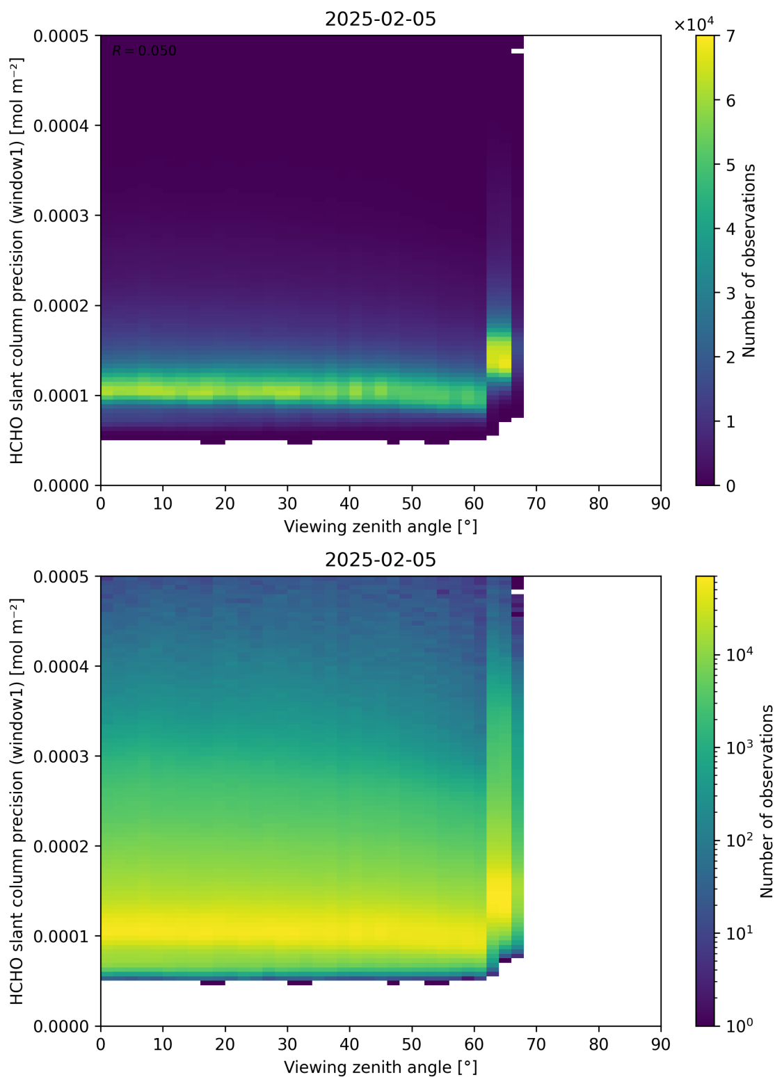
Figure 189: Scatter density plot of “Viewing zenith angle” against “HCHO slant column precision (window1)” for 2025-02-04 to 2025-02-06.
