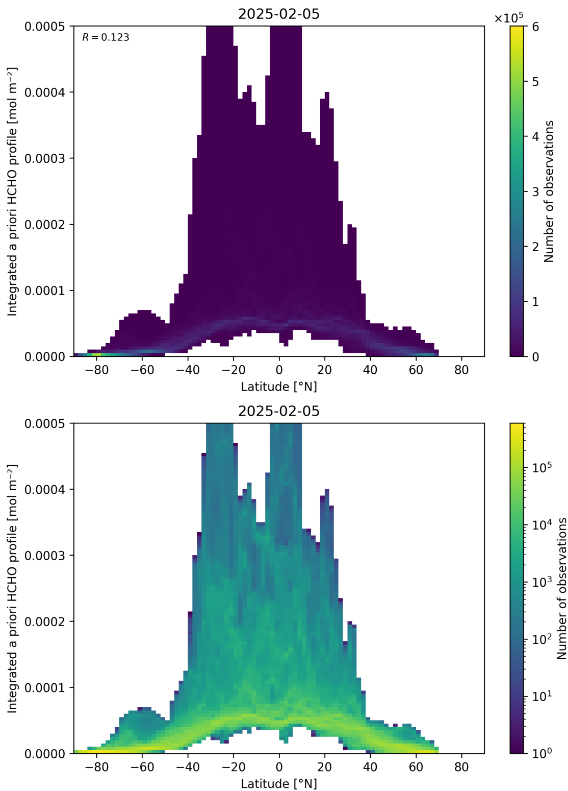
Figure 166: Scatter density plot of “Latitude” against “Integrated a priori HCHO profile” for 2025-02-04 to 2025-02-06.
