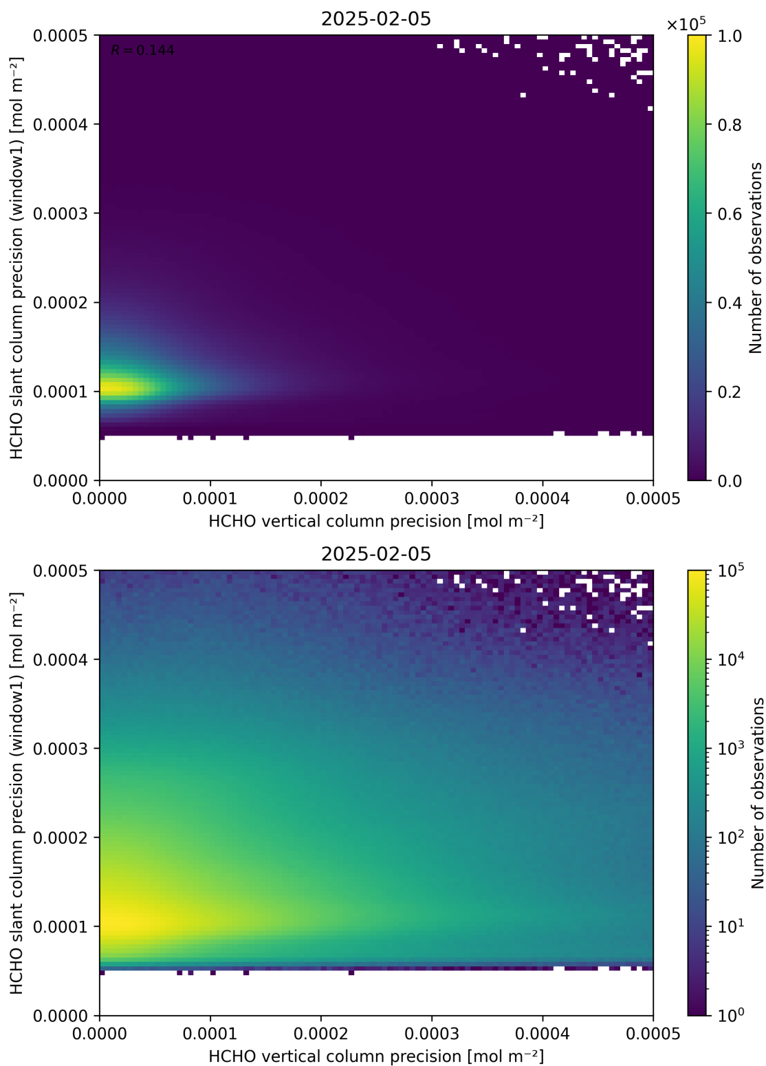
Figure 143: Scatter density plot of “HCHO vertical column precision” against “HCHO slant column precision (window1)” for 2025-02-04 to 2025-02-06.
