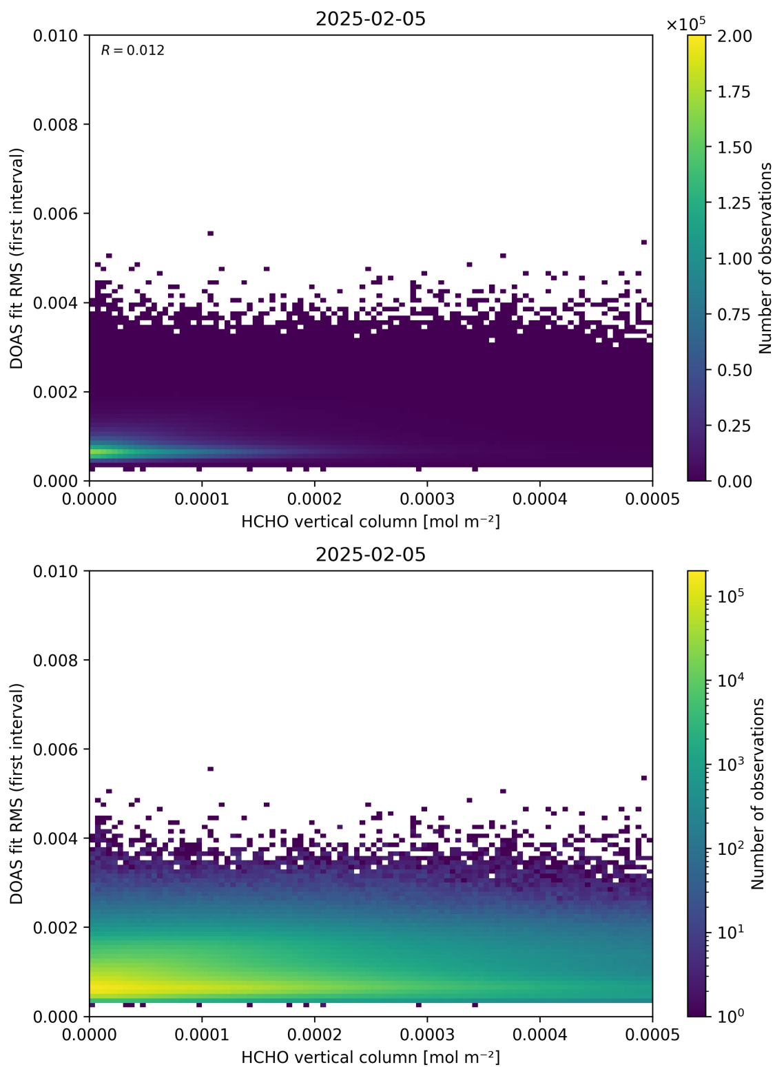
Figure 123: Scatter density plot of “HCHO vertical column” against “DOAS fit RMS (first interval)” for 2025-02-04 to 2025-02-06.
