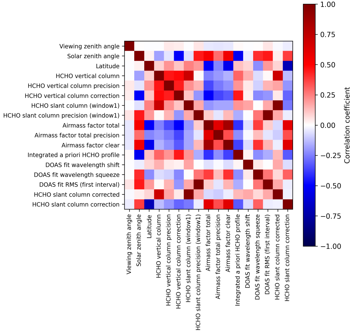
Figure 2: Map of correlation matrix for 2025-02-04 to 2025-02-06.
