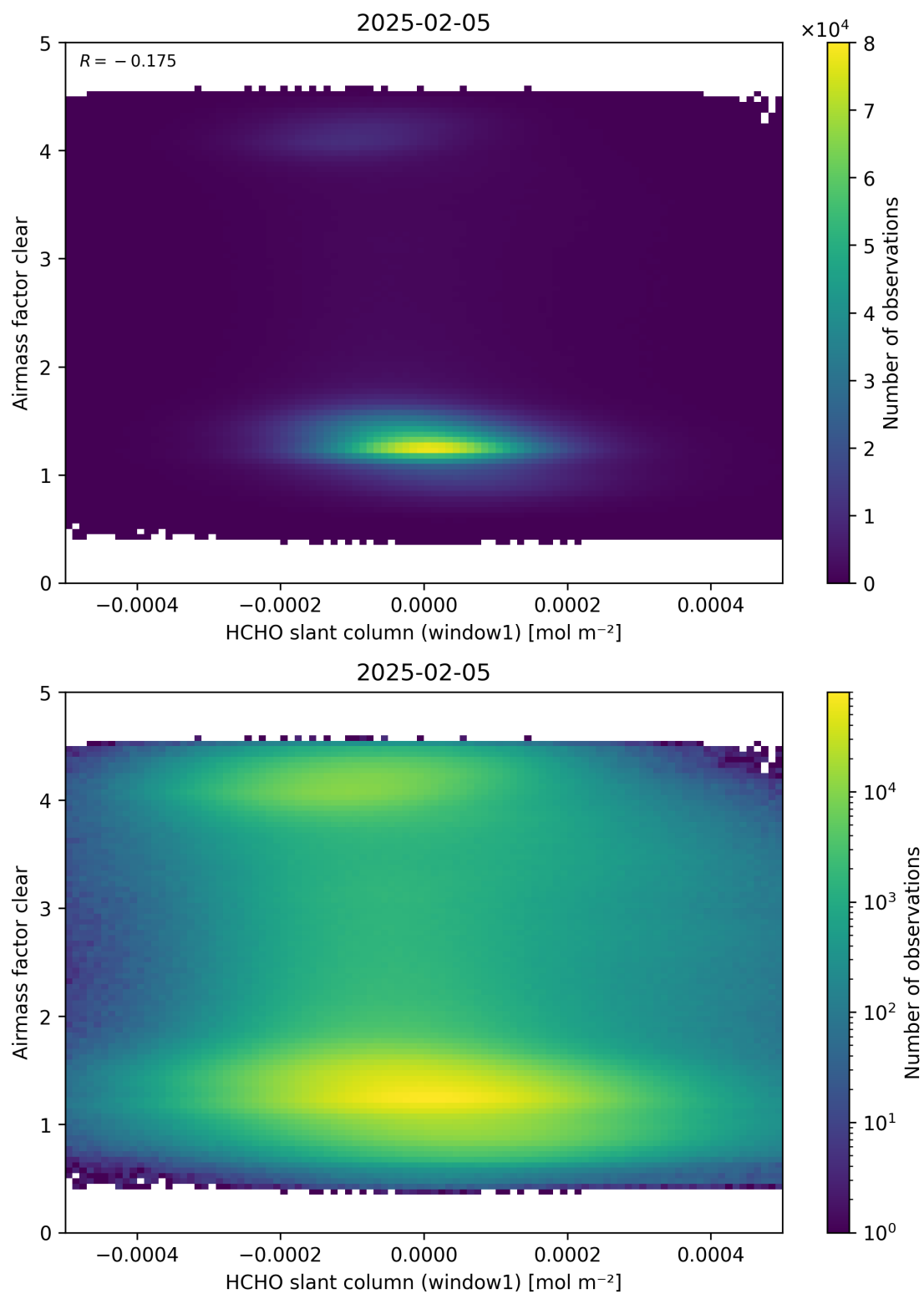
Figure 81: Scatter density plot of “HCHO slant column (window1)” against “Airmass factor clear” for 2025-02-04 to 2025-02-06.
