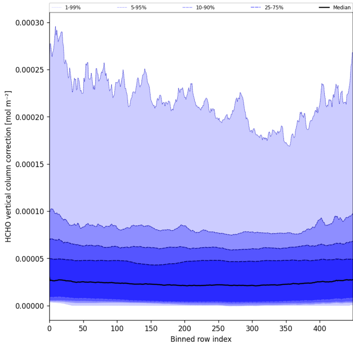
Figure 51: Along track statistics of “HCHO vertical column correction” for 2025-02-04 to 2025-02-06
