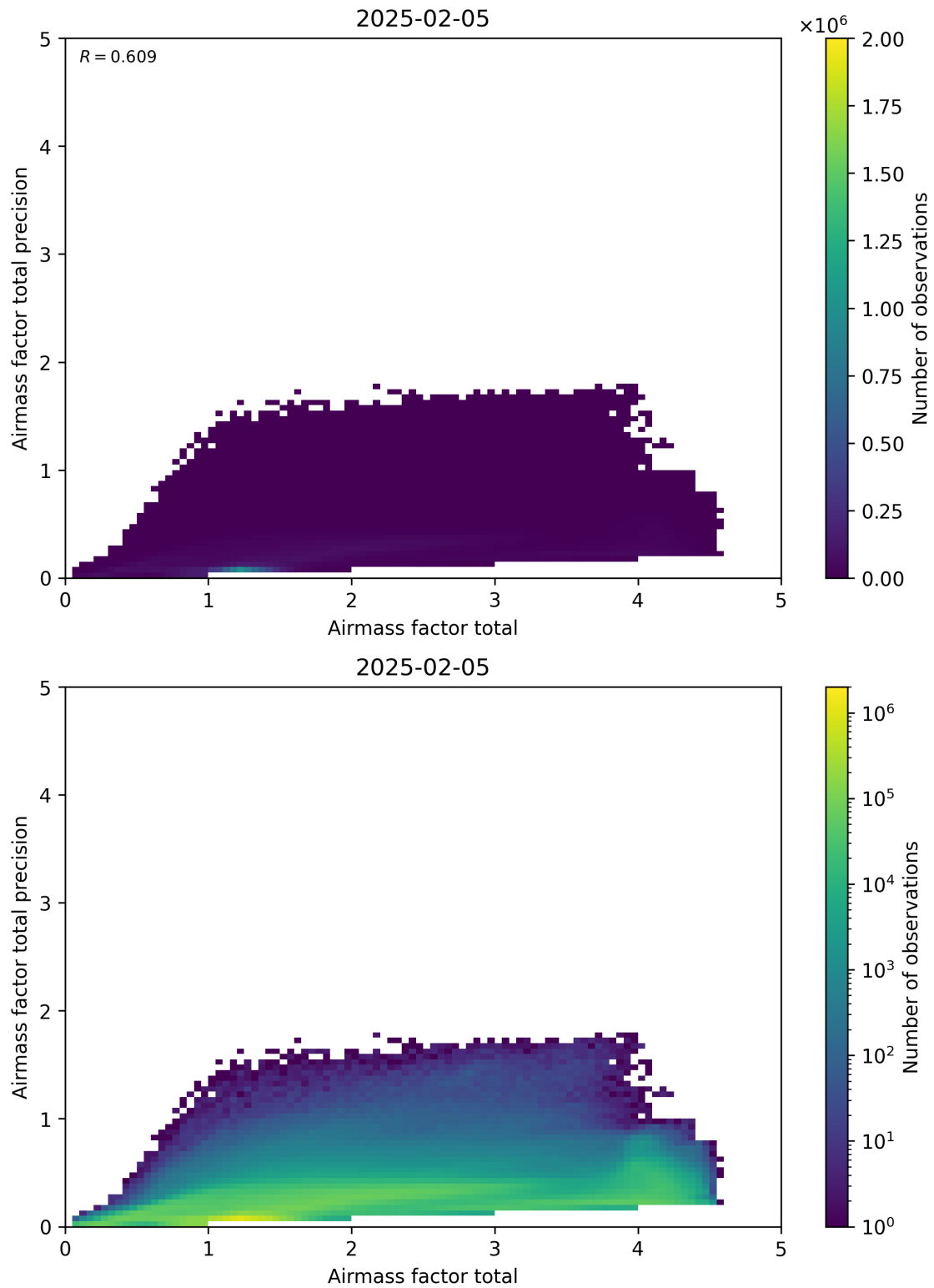
Figure 103: Scatter density plot of “Airmass factor total” against “Airmass factor total precision” for 2025-02-04 to 2025-02-06.
