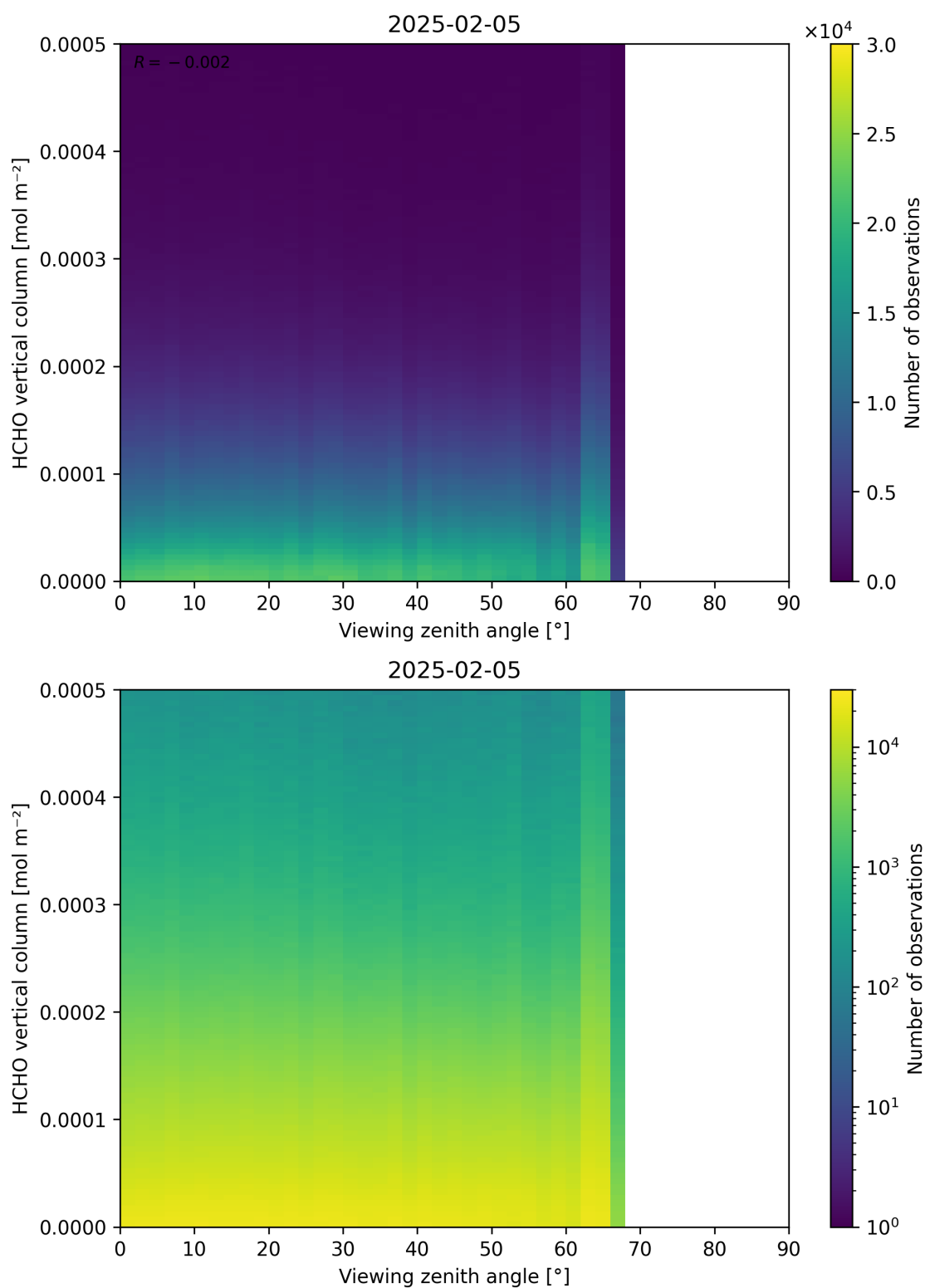
Figure 192: Scatter density plot of “Viewing zenith angle” against “HCHO vertical column” for 2025-02-04 to 2025-02-06.
