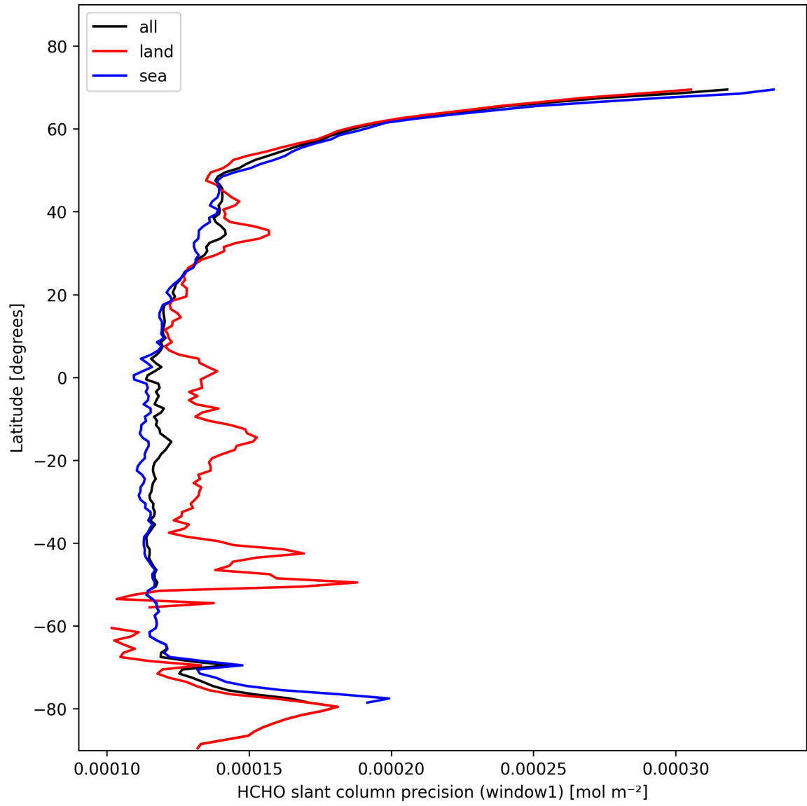
Figure 25: Zonal average of "HCHO slant column precision (window1)" for 2025-02-04 to 2025-02-06.
