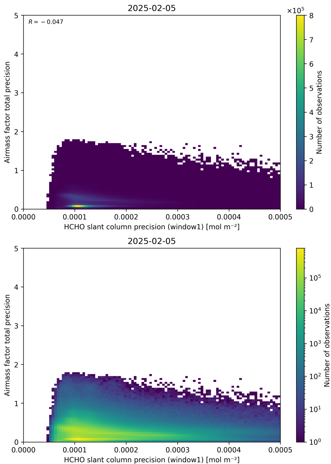
Figure 95: Scatter density plot of “HCHO slant column precision (window1)” against “Airmass factor total precision” for 2025-02-04 to 2025-02-06.
