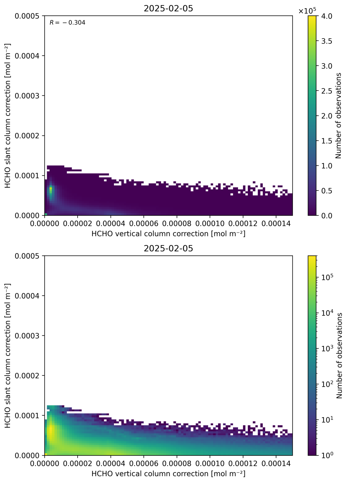
Figure 117: Scatter density plot of “HCHO vertical column correction” against “HCHO slant column correction” for 2025-02-04 to 2025-02-06.
