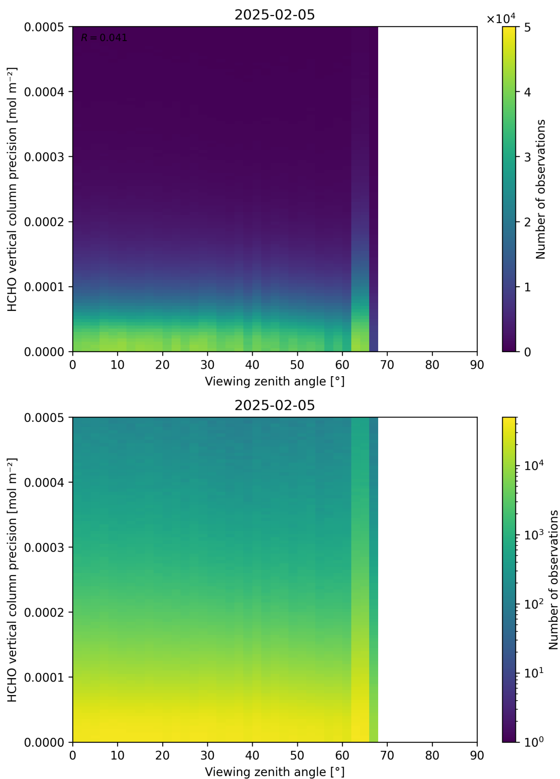
Figure 194: Scatter density plot of “Viewing zenith angle” against “HCHO vertical column precision” for 2025-02-04 to 2025-02-06.
