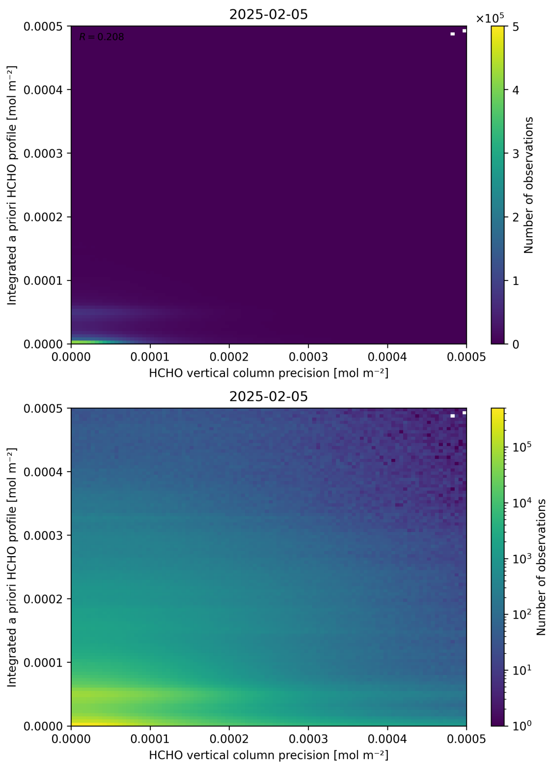
Figure 147: Scatter density plot of “HCHO vertical column precision” against “Integrated a priori HCHO profile” for 2025-02-04 to 2025-02-06.
