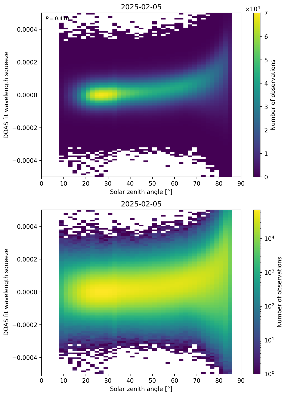
Figure 169: Scatter density plot of “Solar zenith angle” against “DOAS fit wavelength squeeze” for 2025-02-04 to 2025-02-06.
