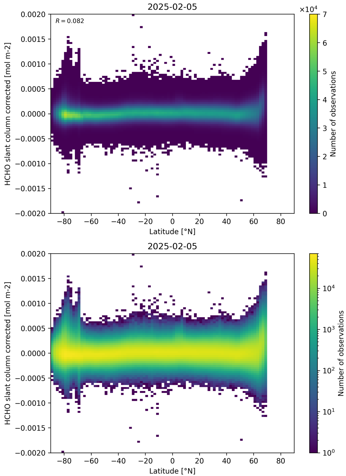
Figure 157: Scatter density plot of “Latitude” against “HCHO slant column corrected” for 2025-02-04 to 2025-02-06.
