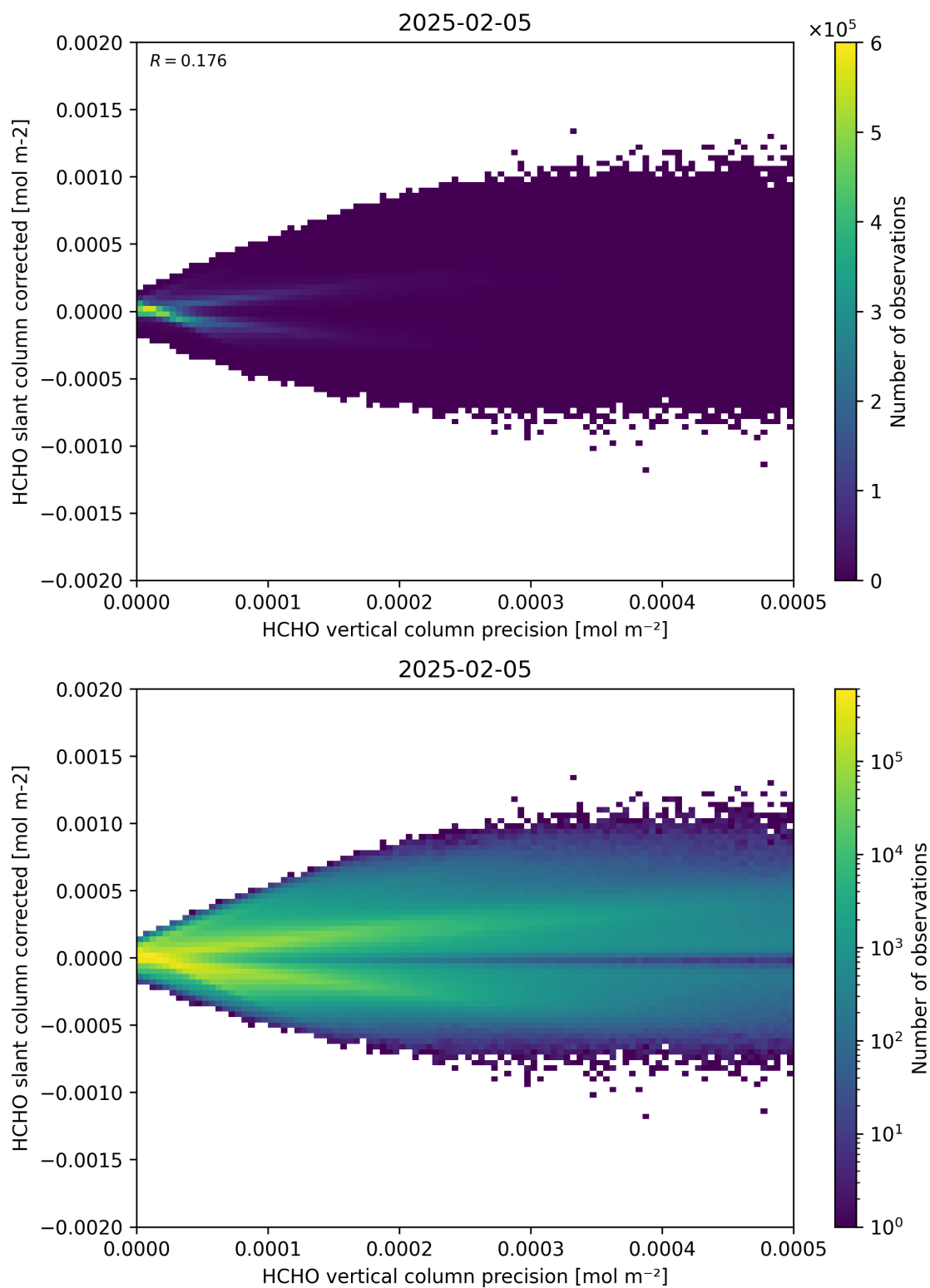
Figure 140: Scatter density plot of “HCHO vertical column precision” against “HCHO slant column corrected” for 2025-02-04 to 2025-02-06.
