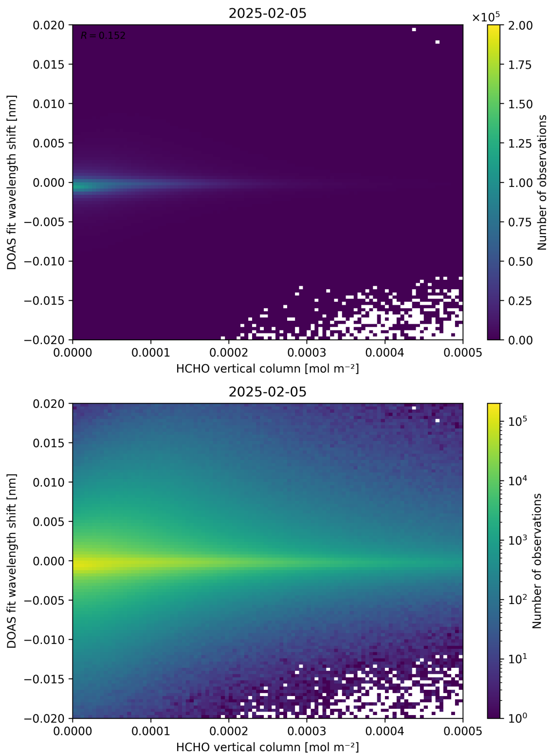
Figure 124: Scatter density plot of “HCHO vertical column” against “DOAS fit wavelength shift” for 2025-02-04 to 2025-02-06.
