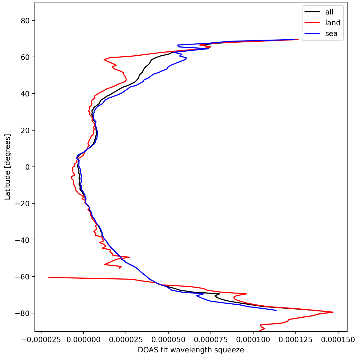
Figure 31: Zonal average of “DOAS fit wavelength squeeze” for 2025-02-04 to 2025-02-06.
