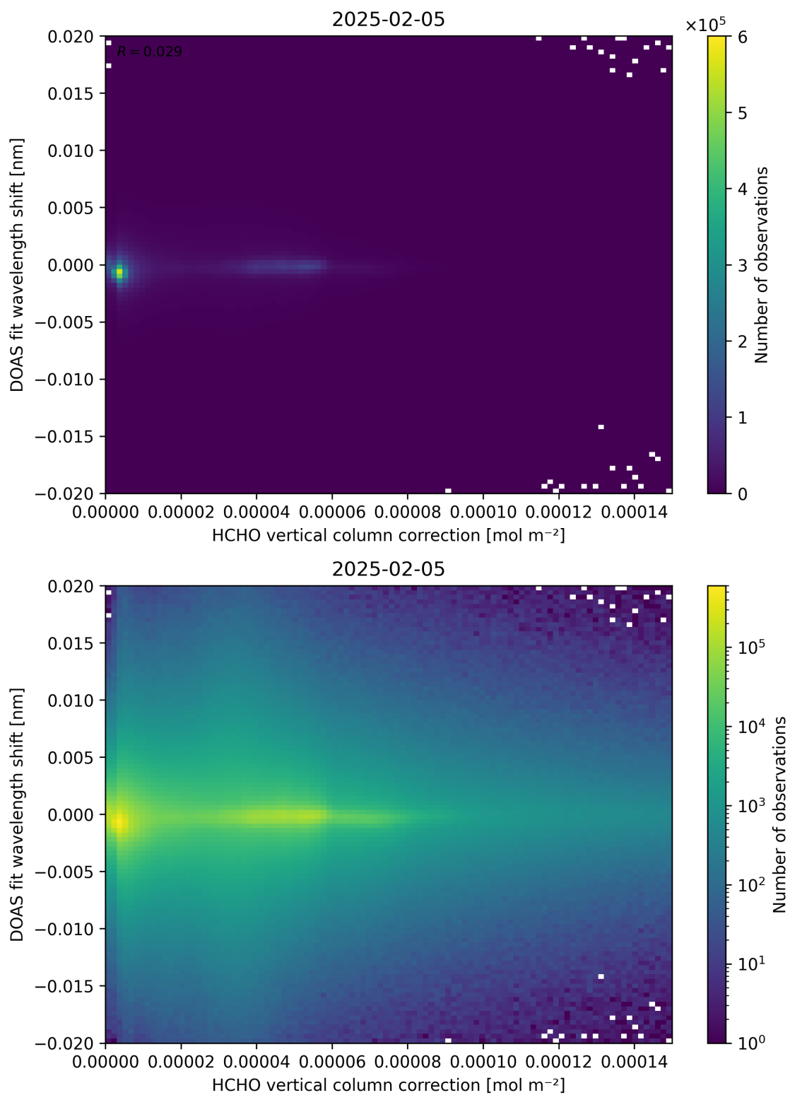
Figure 113: Scatter density plot of “HCHO vertical column correction” against “DOAS fit wavelength shift” for 2025-02-04 to 2025-02-06.
