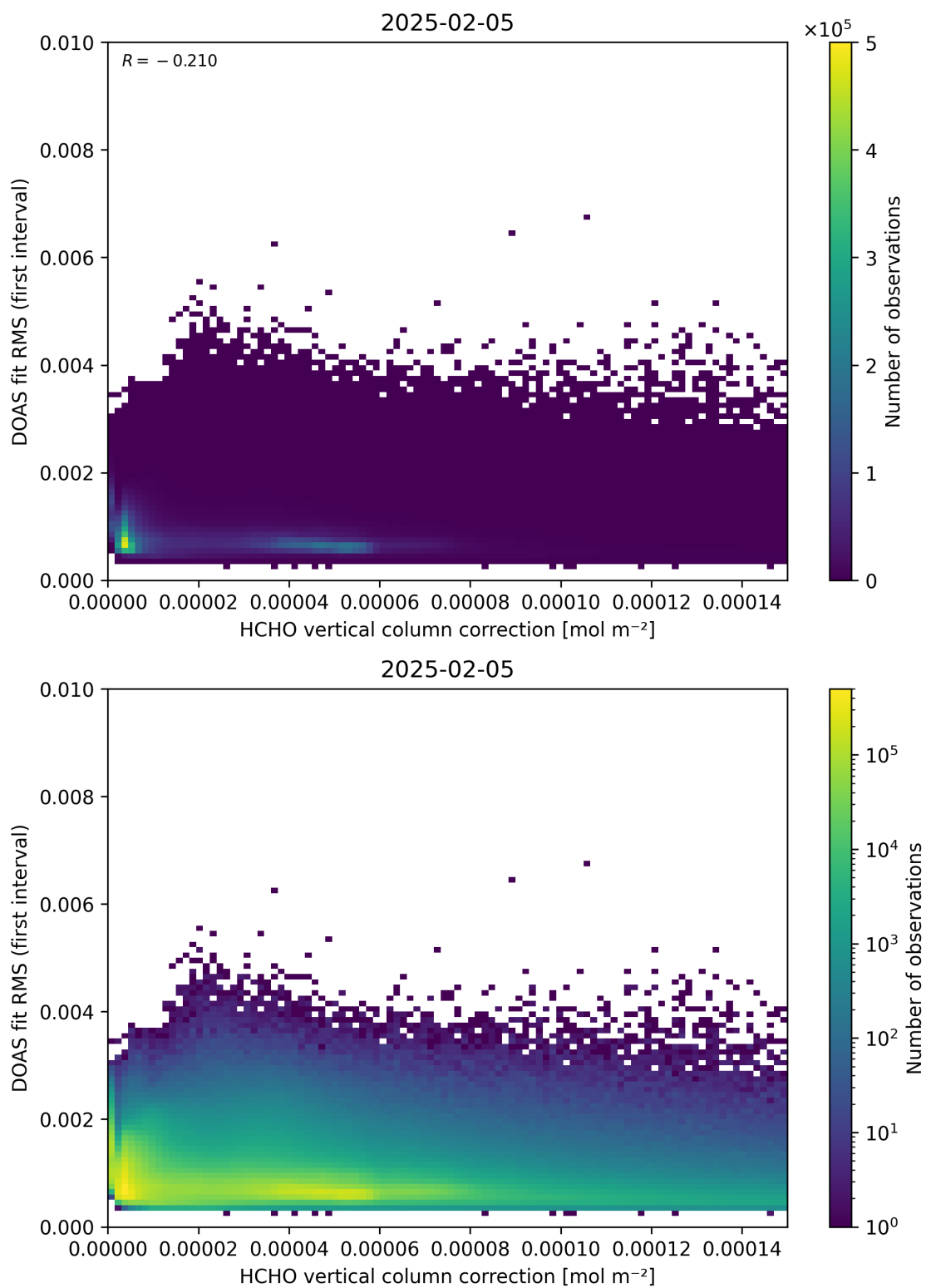
Figure 112: Scatter density plot of “HCHO vertical column correction” against “DOAS fit RMS (first interval)” for 2025-02-04 to 2025-02-06.
