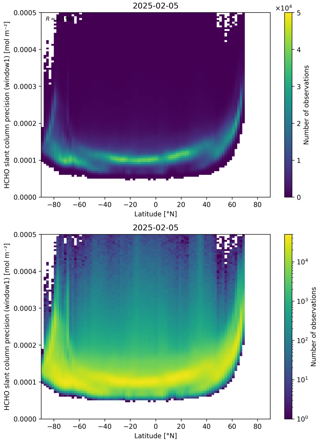
Figure 160: Scatter density plot of “Latitude” against “HCHO slant column precision (window1)” for 2025-02-04 to 2025-02-06.
