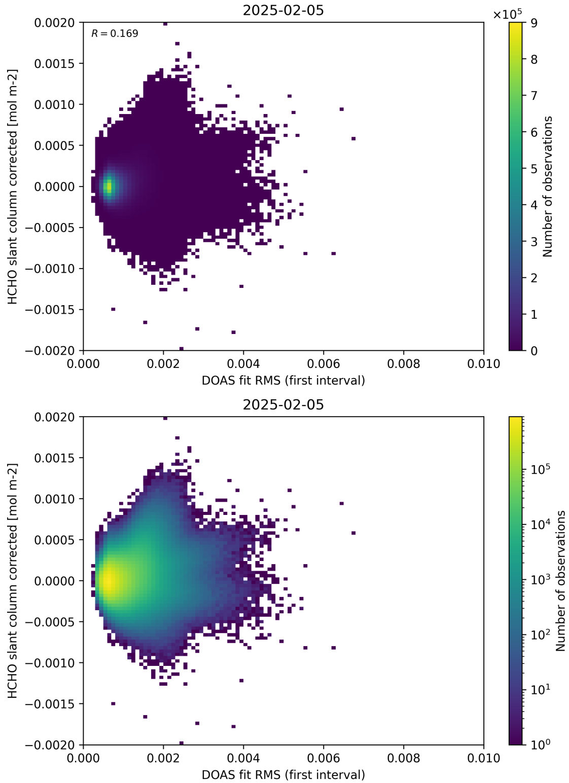
Figure 62: Scatter density plot of “DOAS fit RMS (first interval)” against “HCHO slant column corrected” for 2025-02-04 to 2025-02-06.
