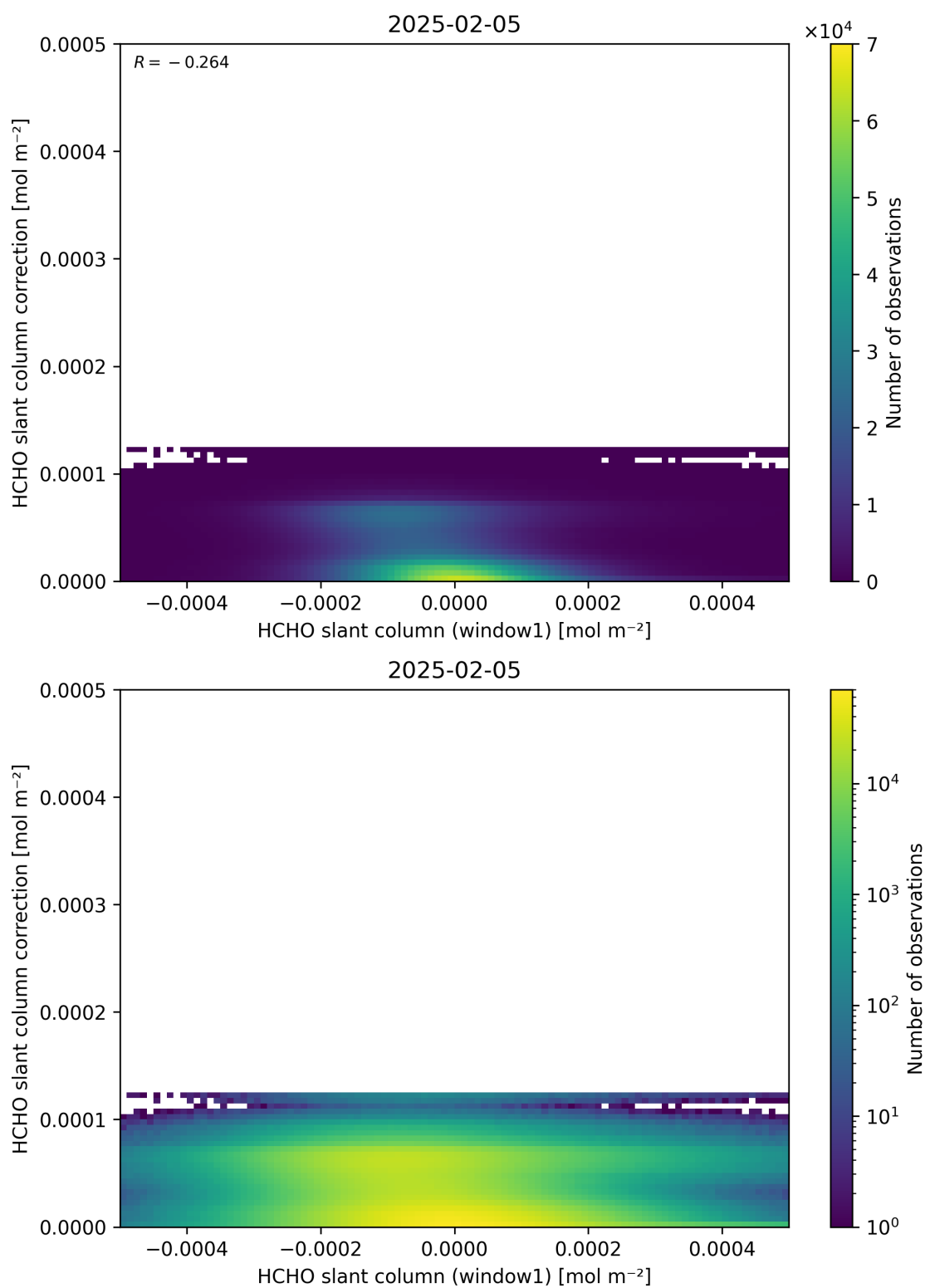
Figure 83: Scatter density plot of “HCHO slant column (window1)” against “HCHO slant column correction” for 2025-02-04 to 2025-02-06.
