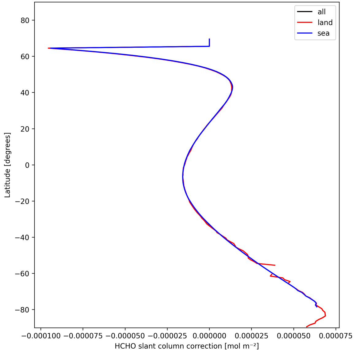
Figure 33: Zonal average of “HCHO slant column correction” for 2025-02-04 to 2025-02-06.
