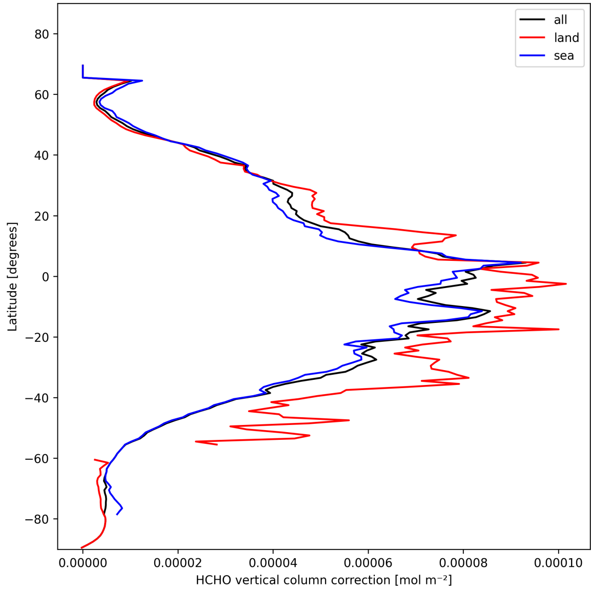
Figure 23: Zonal average of “HCHO vertical column correction” for 2025-02-04 to 2025-02-06.
