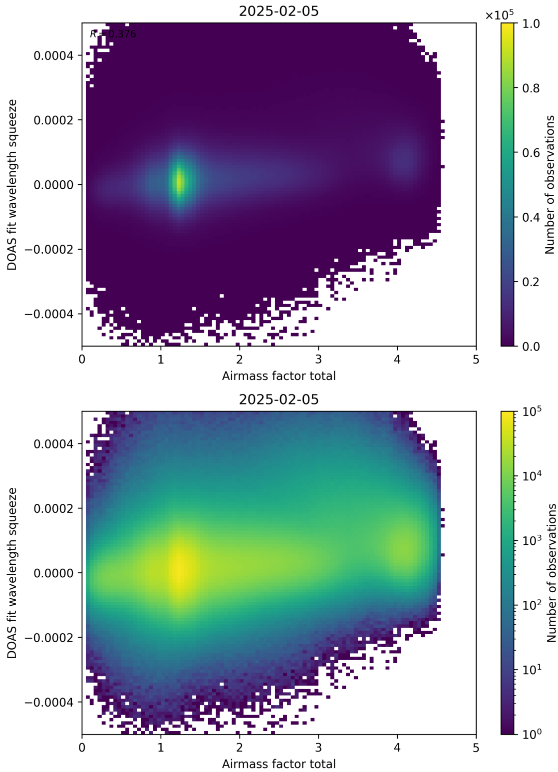
Figure 99: Scatter density plot of “Airmass factor total” against “DOAS fit wavelength squeeze” for 2025-02-04 to 2025-02-06.
