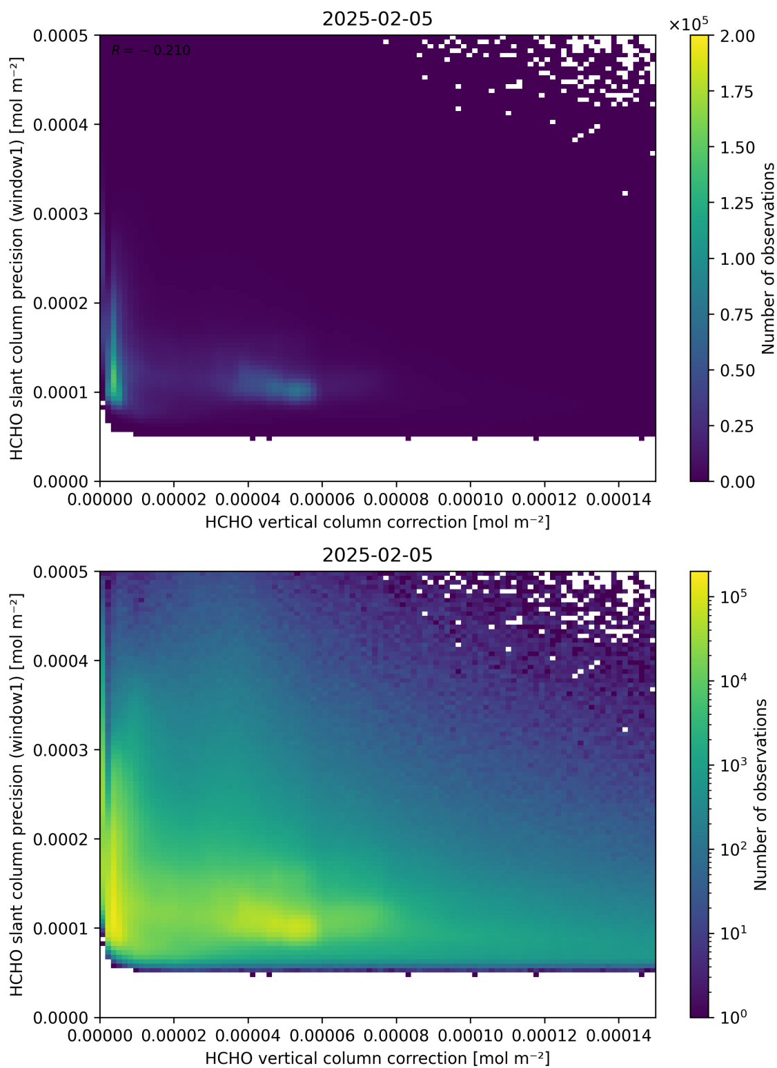
Figure 119: Scatter density plot of “HCHO vertical column correction” against “HCHO slant column precision (window1)” for 2025-02-04 to 2025-02-06.
