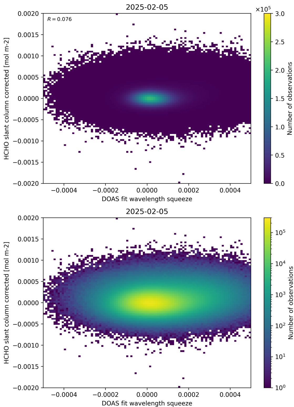
Figure 69: Scatter density plot of “DOAS fit wavelength squeeze” against “HCHO slant column corrected” for 2025-02-04 to 2025-02-06.
