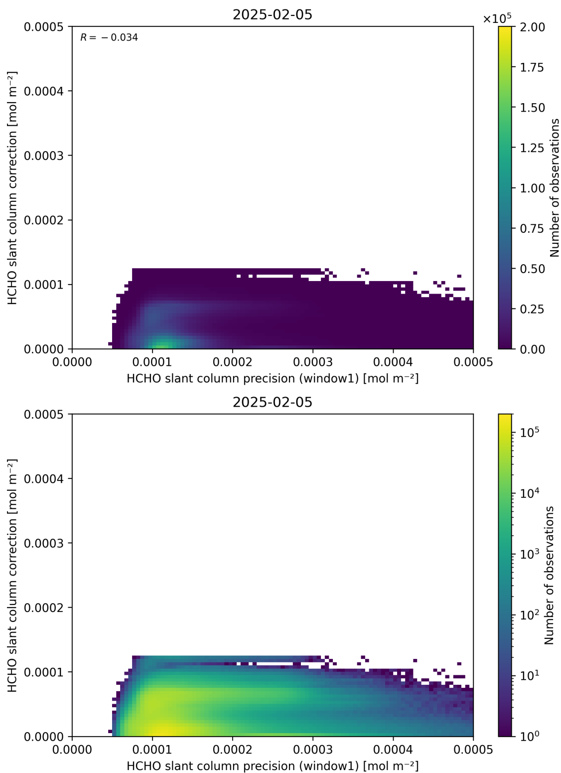
Figure 93: Scatter density plot of “HCHO slant column precision (window1)” against “HCHO slant column correction” for 2025-02-04 to 2025-02-06.
