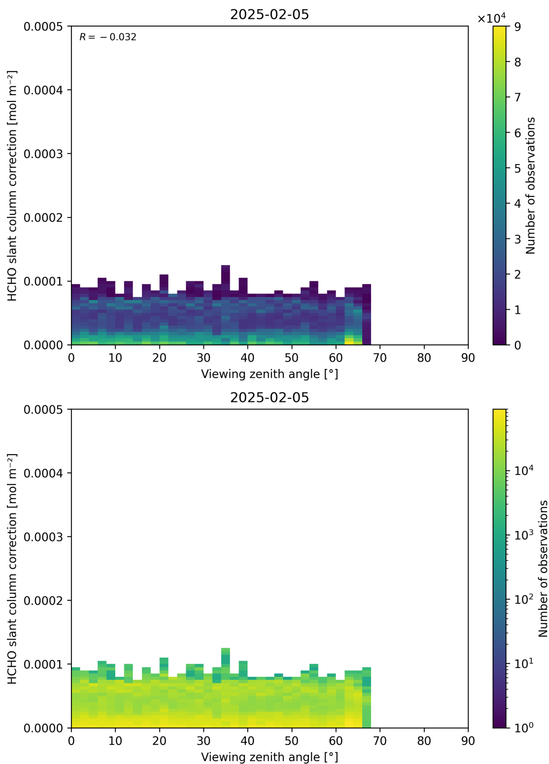
Figure 187: Scatter density plot of “Viewing zenith angle” against “HCHO slant column correction” for 2025-02-04 to 2025-02-06.
