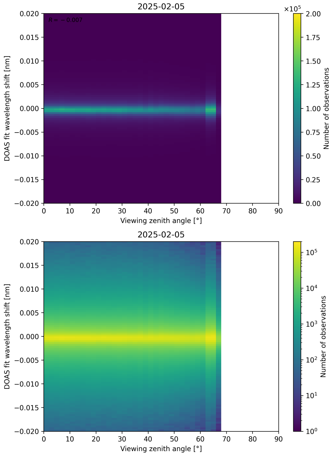
Figure 183: Scatter density plot of “Viewing zenith angle” against “DOAS fit wavelength shift” for 2025-02-04 to 2025-02-06.
