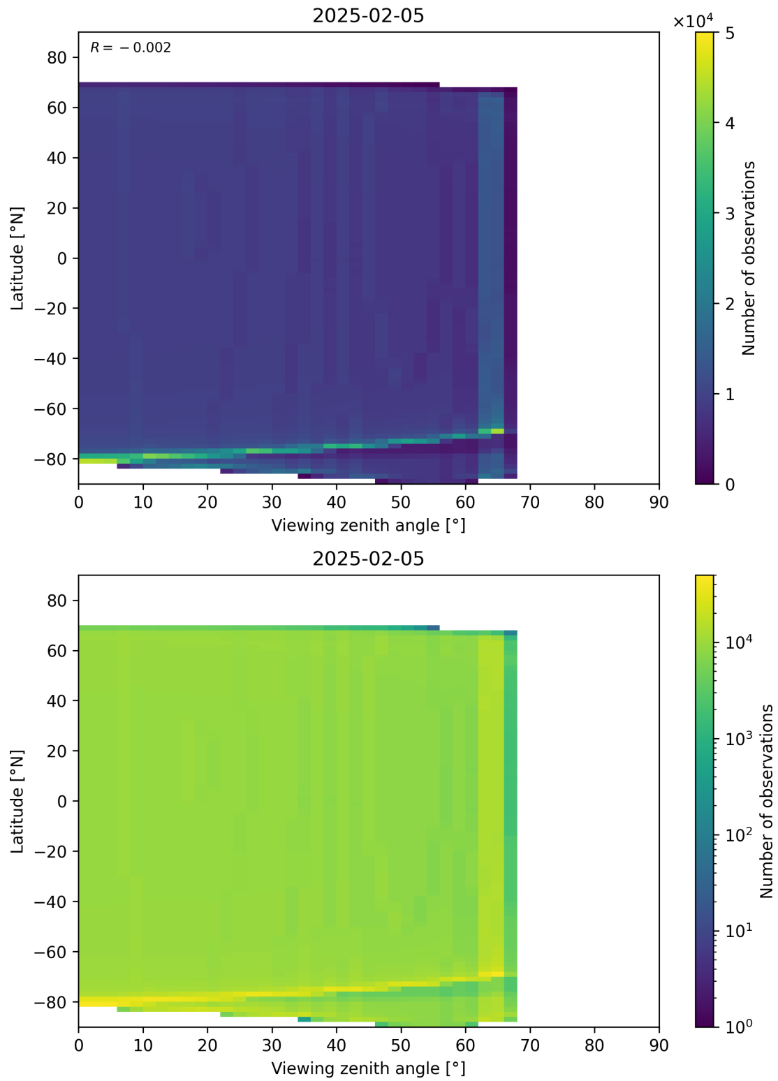
Figure 196: Scatter density plot of “Viewing zenith angle” against “Latitude” for 2025-02-04 to 2025-02-06.
