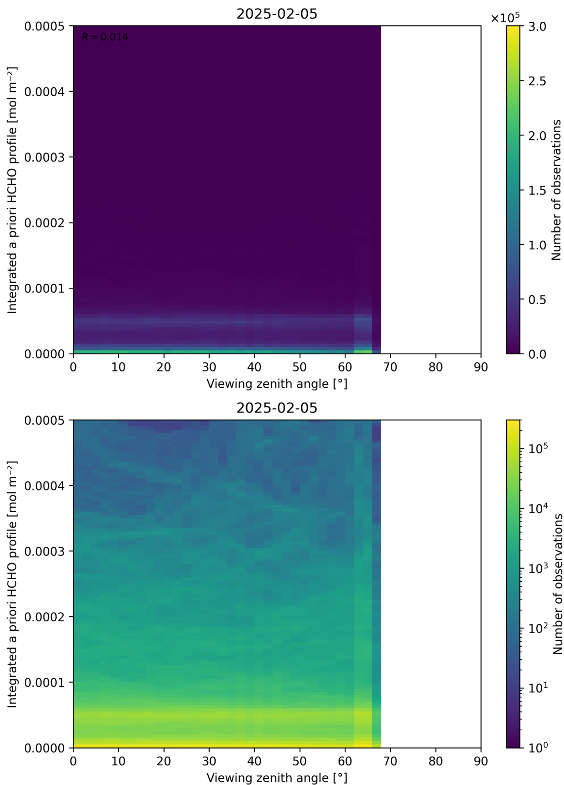
Figure 195: Scatter density plot of “Viewing zenith angle” against “Integrated a priori HCHO profile” for 2025-02-04 to 2025-02-06.
