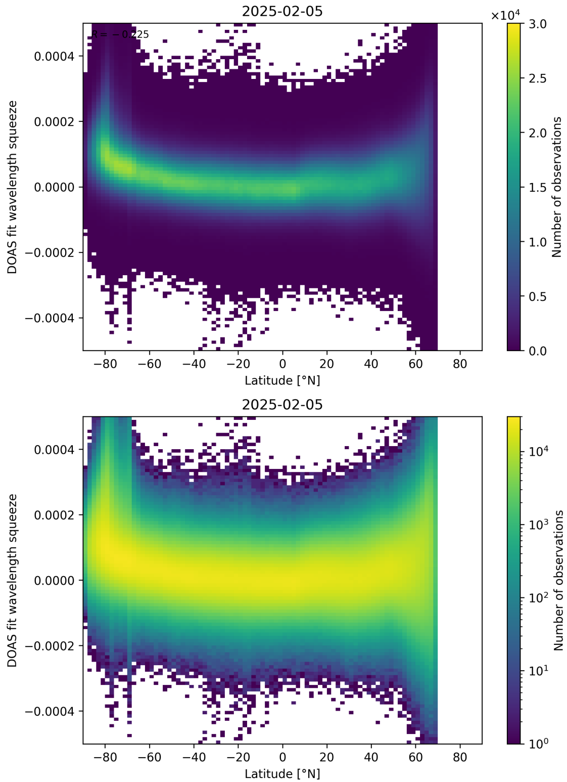
Figure 155: Scatter density plot of “Latitude” against “DOAS fit wavelength squeeze” for 2025-02-04 to 2025-02-06.
