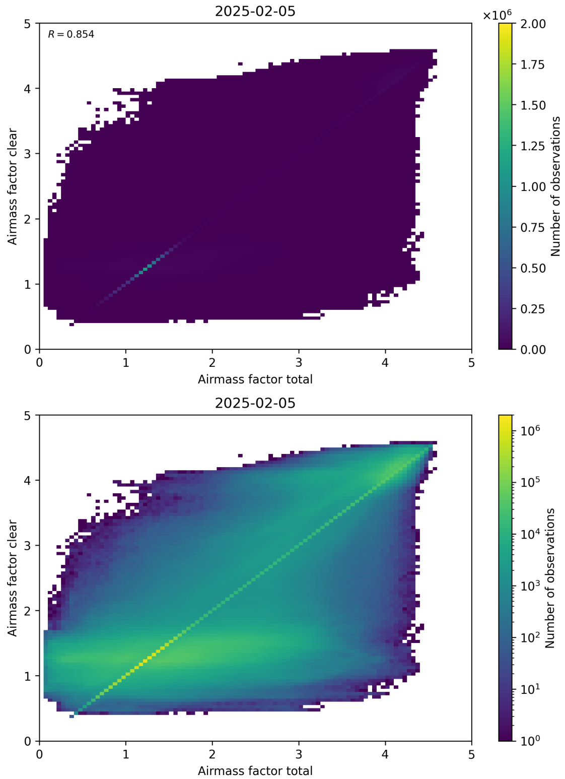
Figure 100: Scatter density plot of “Airmass factor total” against “Airmass factor clear” for 2025-02-04 to 2025-02-06.
