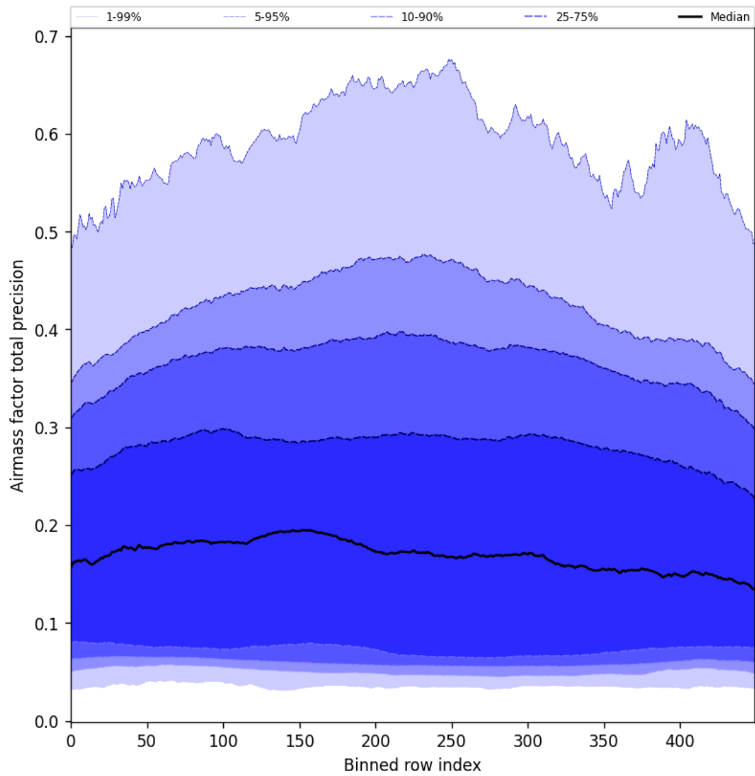
Figure 55: Along track statistics of “Airmass factor total precision” for 2025-02-04 to 2025-02-06
