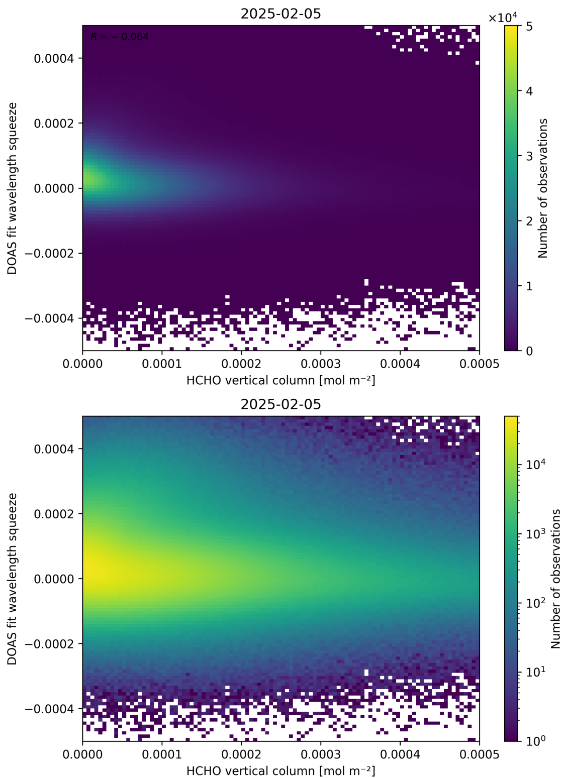
Figure 125: Scatter density plot of “HCHO vertical column” against “DOAS fit wavelength squeeze” for 2025-02-04 to 2025-02-06.
