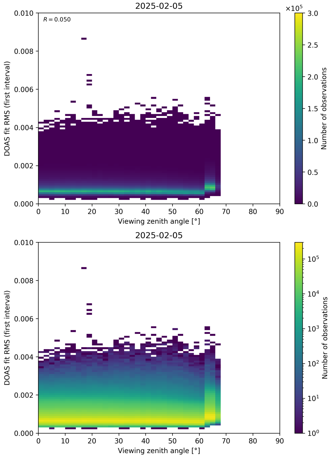
Figure 182: Scatter density plot of “Viewing zenith angle” against “DOAS fit RMS (first interval)” for 2025-02-04 to 2025-02-06.
