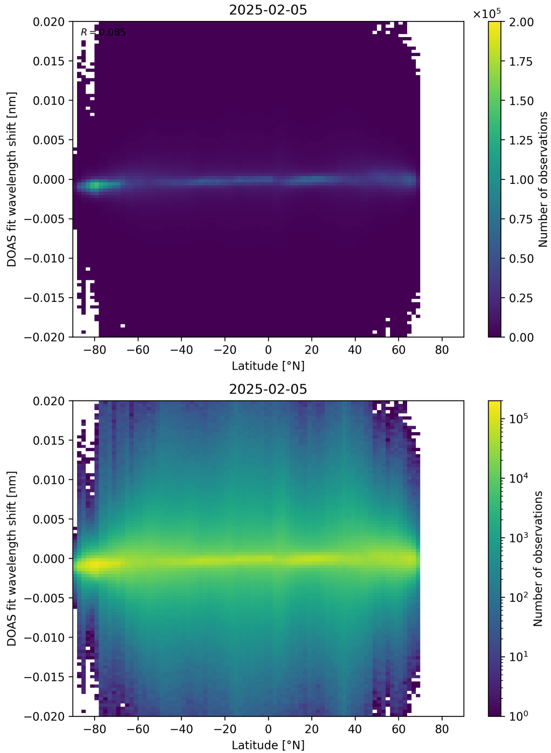
Figure 154: Scatter density plot of “Latitude” against “DOAS fit wavelength shift” for 2025-02-04 to 2025-02-06.
