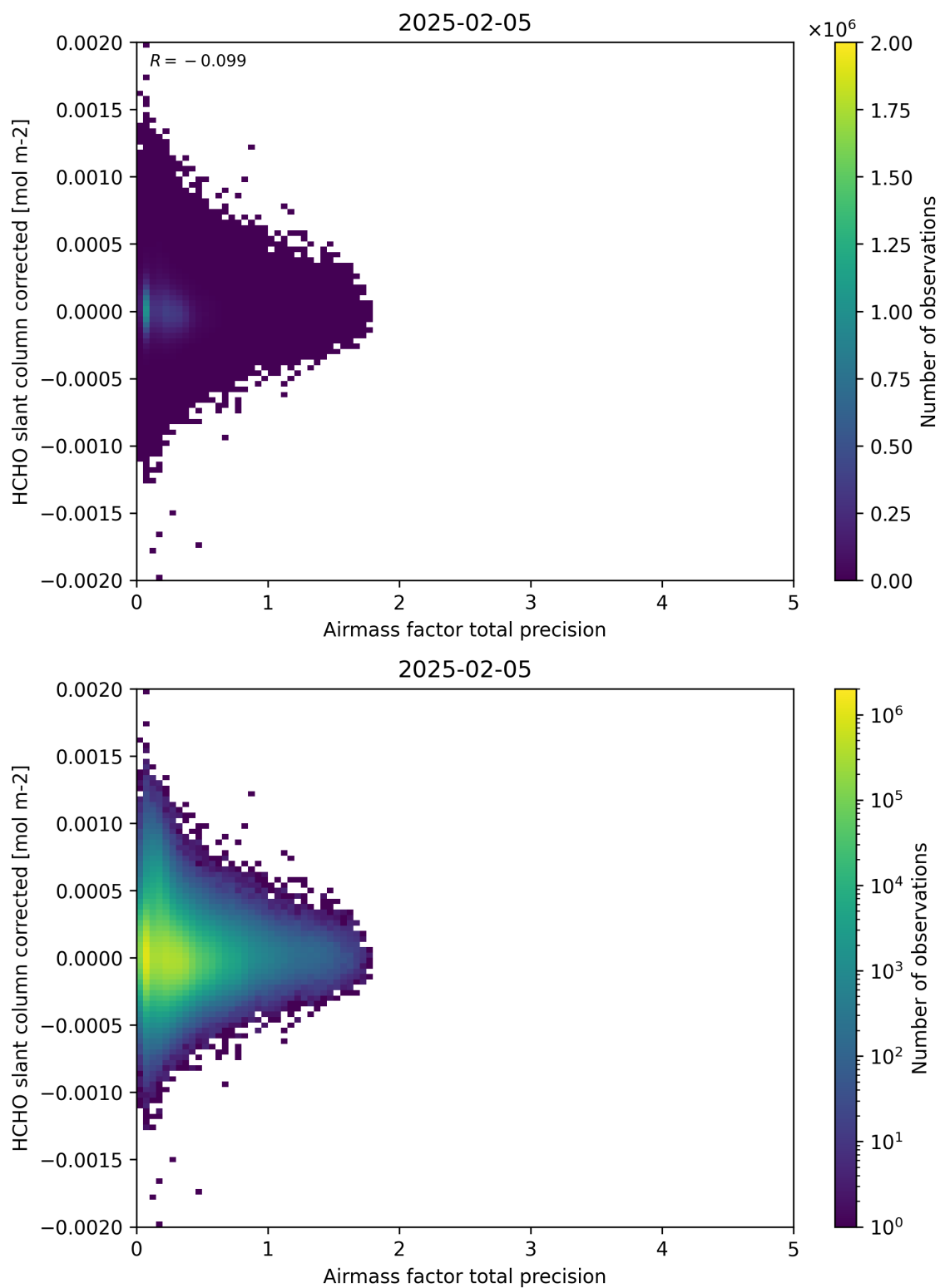
Figure 109: Scatter density plot of “Airmass factor total precision” against “HCHO slant column corrected” for 2025-02-04 to 2025-02-06.
