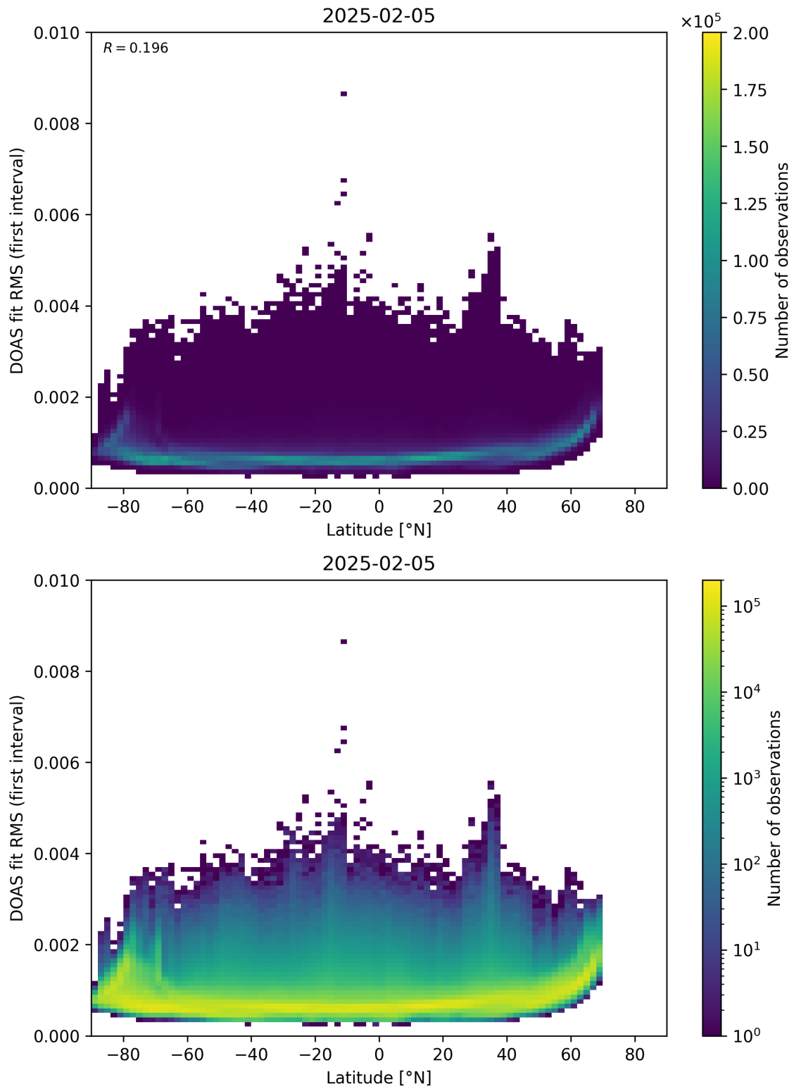
Figure 153: Scatter density plot of “Latitude” against “DOAS fit RMS (first interval)” for 2025-02-04 to 2025-02-06.
