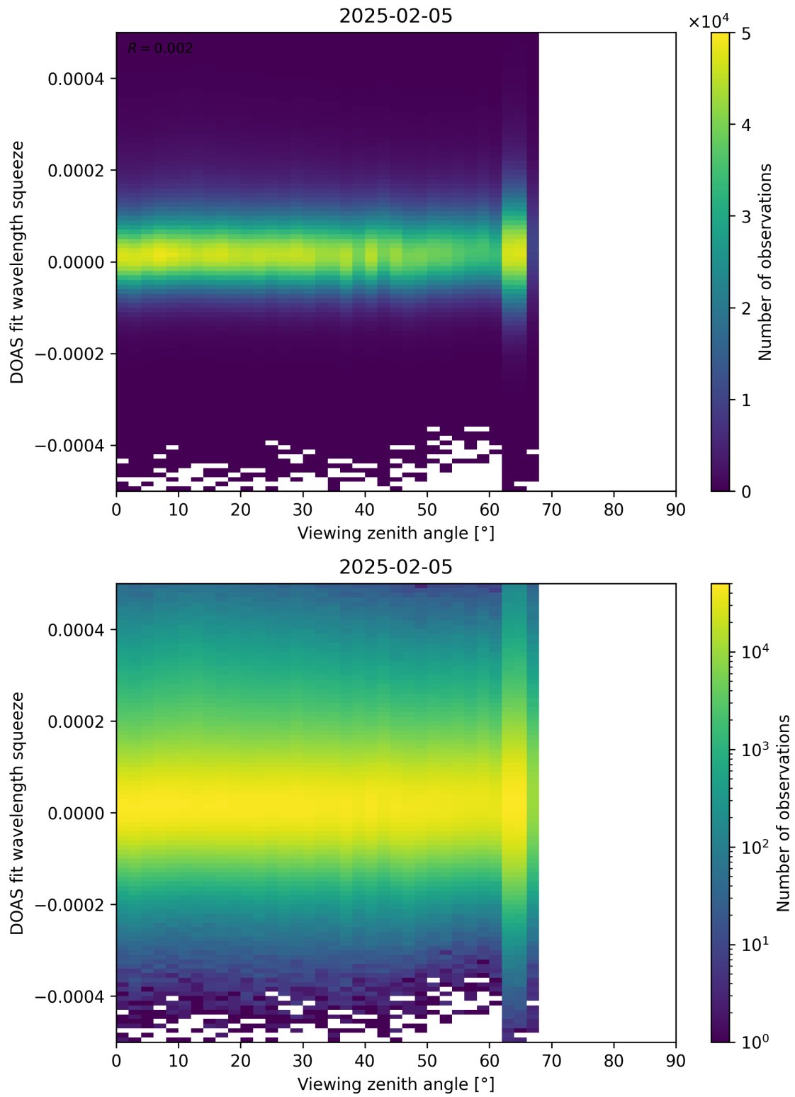
Figure 184: Scatter density plot of “Viewing zenith angle” against “DOAS fit wavelength squeeze” for 2025-02-04 to 2025-02-06.
