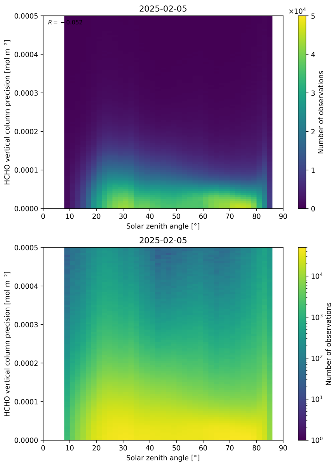
Figure 179: Scatter density plot of “Solar zenith angle” against “HCHO vertical column precision” for 2025-02-04 to 2025-02-06.
