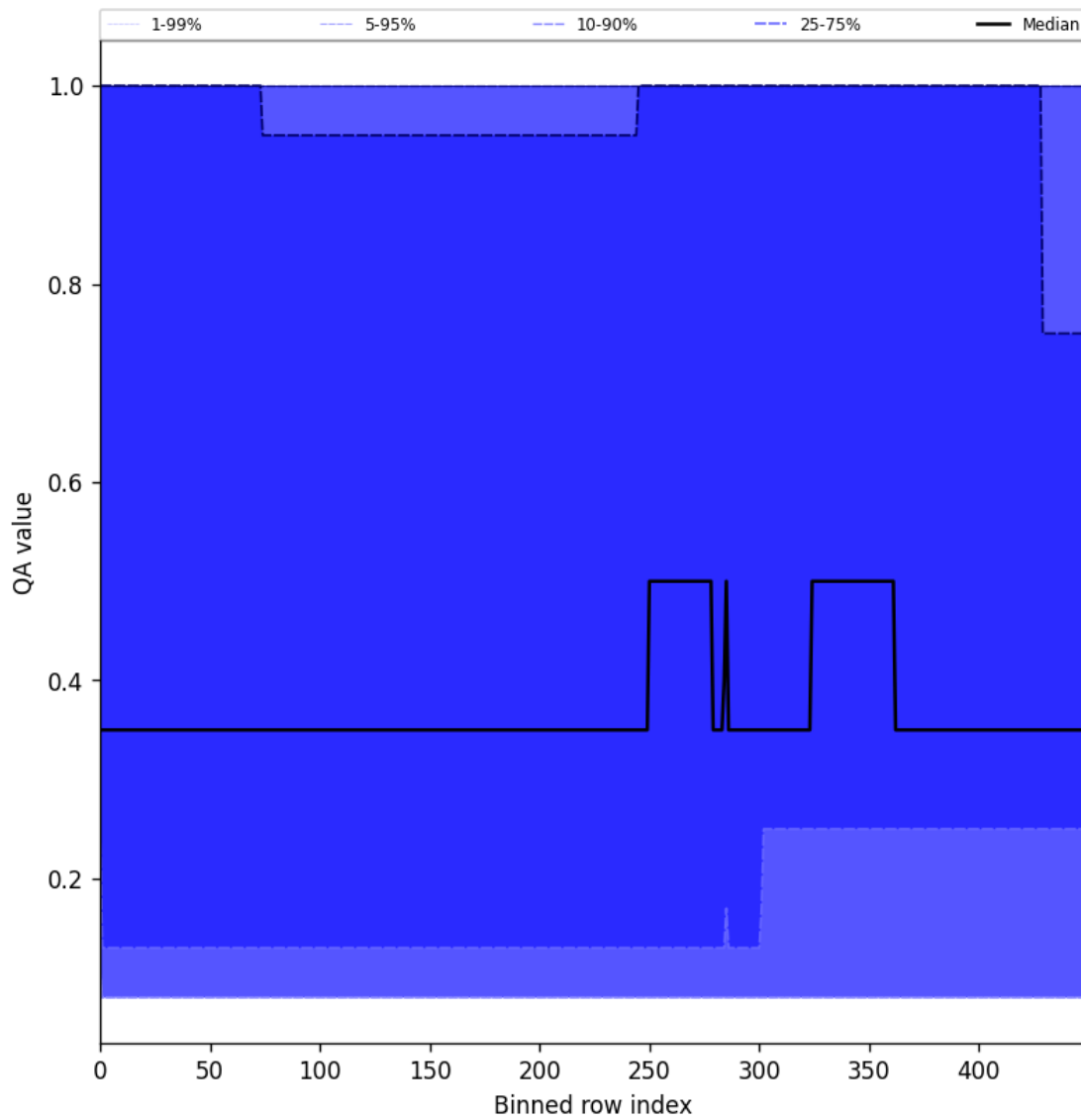
Figure 48: Along track statistics of “QA value” for 2025-02-04 to 2025-02-06
