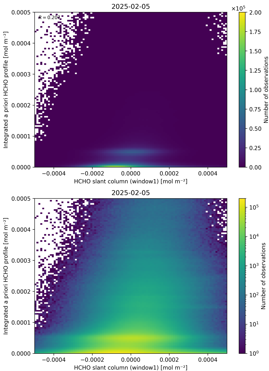
Figure 87: Scatter density plot of “HCHO slant column (window1)” against “Integrated a priori HCHO profile” for 2025-02-04 to 2025-02-06.
