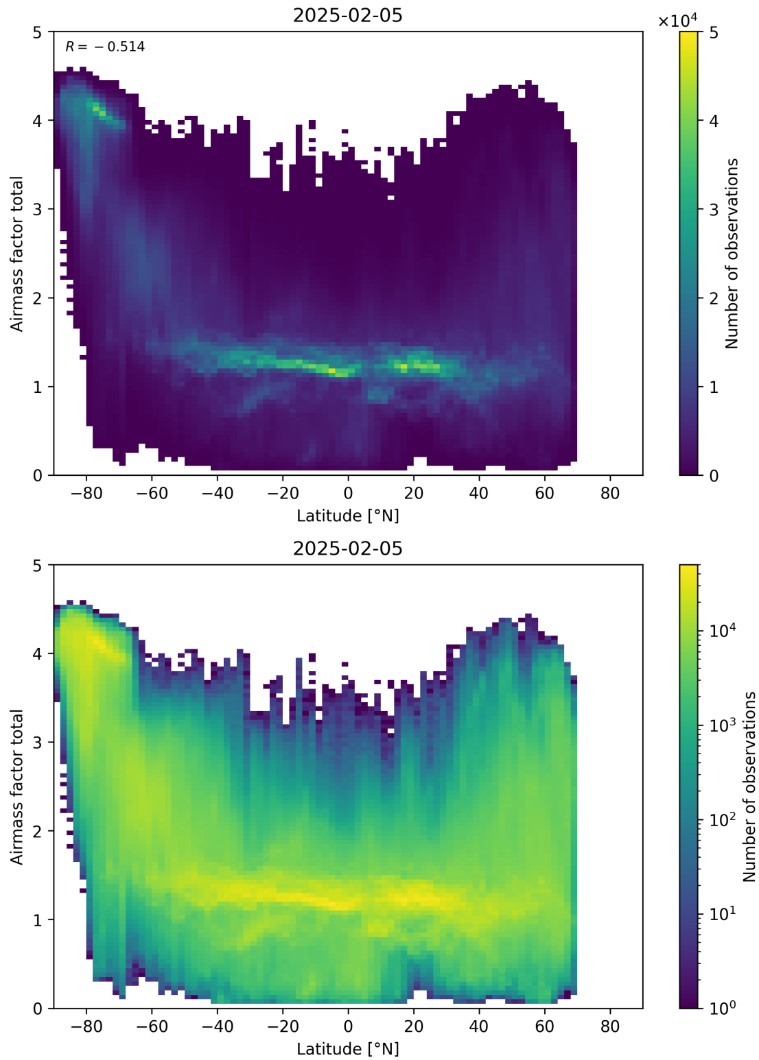
Figure 161: Scatter density plot of “Latitude” against “Airmass factor total” for 2025-02-04 to 2025-02-06.
