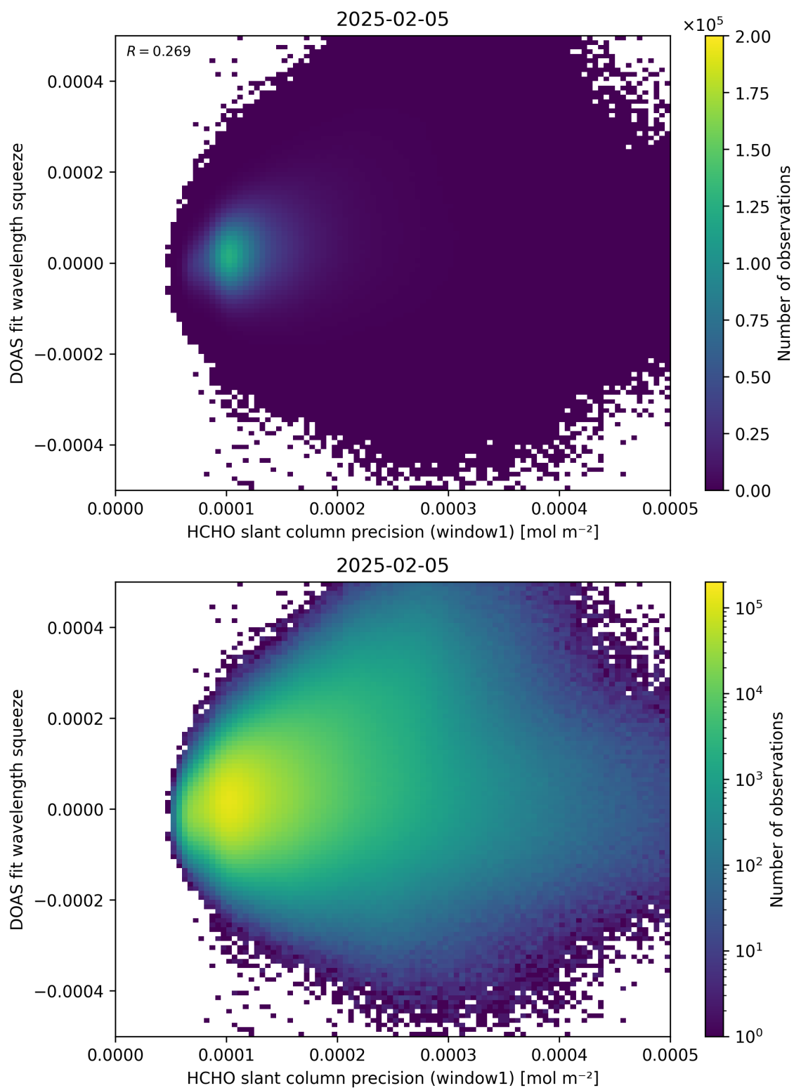
Figure 90: Scatter density plot of “HCHO slant column precision (window1)” against “DOAS fit wavelength squeeze” for 2025-02-04 to 2025-02-06.
