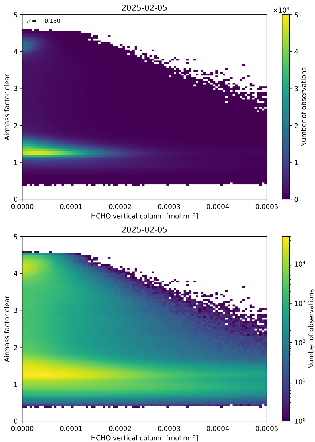
Figure 126: Scatter density plot of “HCHO vertical column” against “Airmass factor clear” for 2025-02-04 to 2025-02-06.
