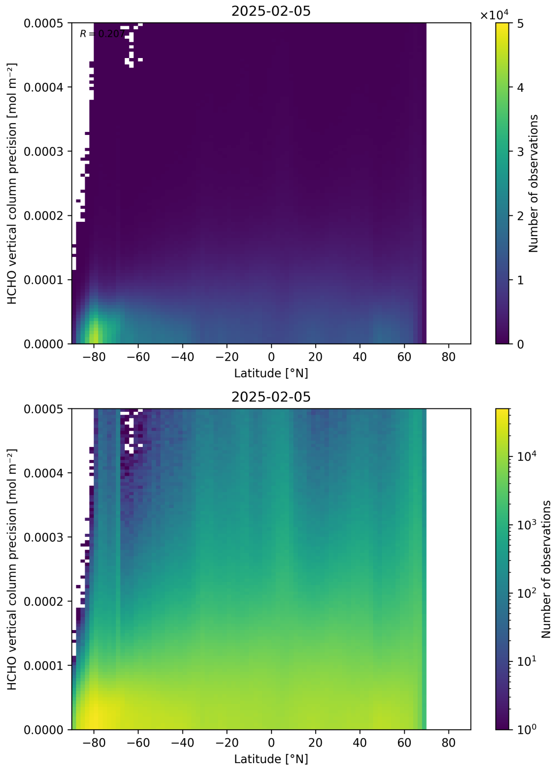
Figure 165: Scatter density plot of “Latitude” against “HCHO vertical column precision” for 2025-02-04 to 2025-02-06.
