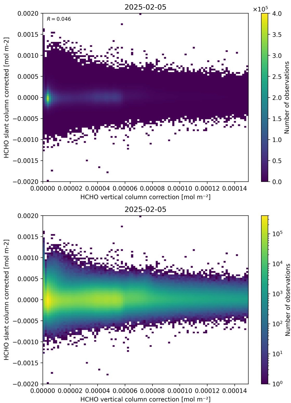
Figure 116: Scatter density plot of “HCHO vertical column correction” against “HCHO slant column corrected” for 2025-02-04 to 2025-02-06.
