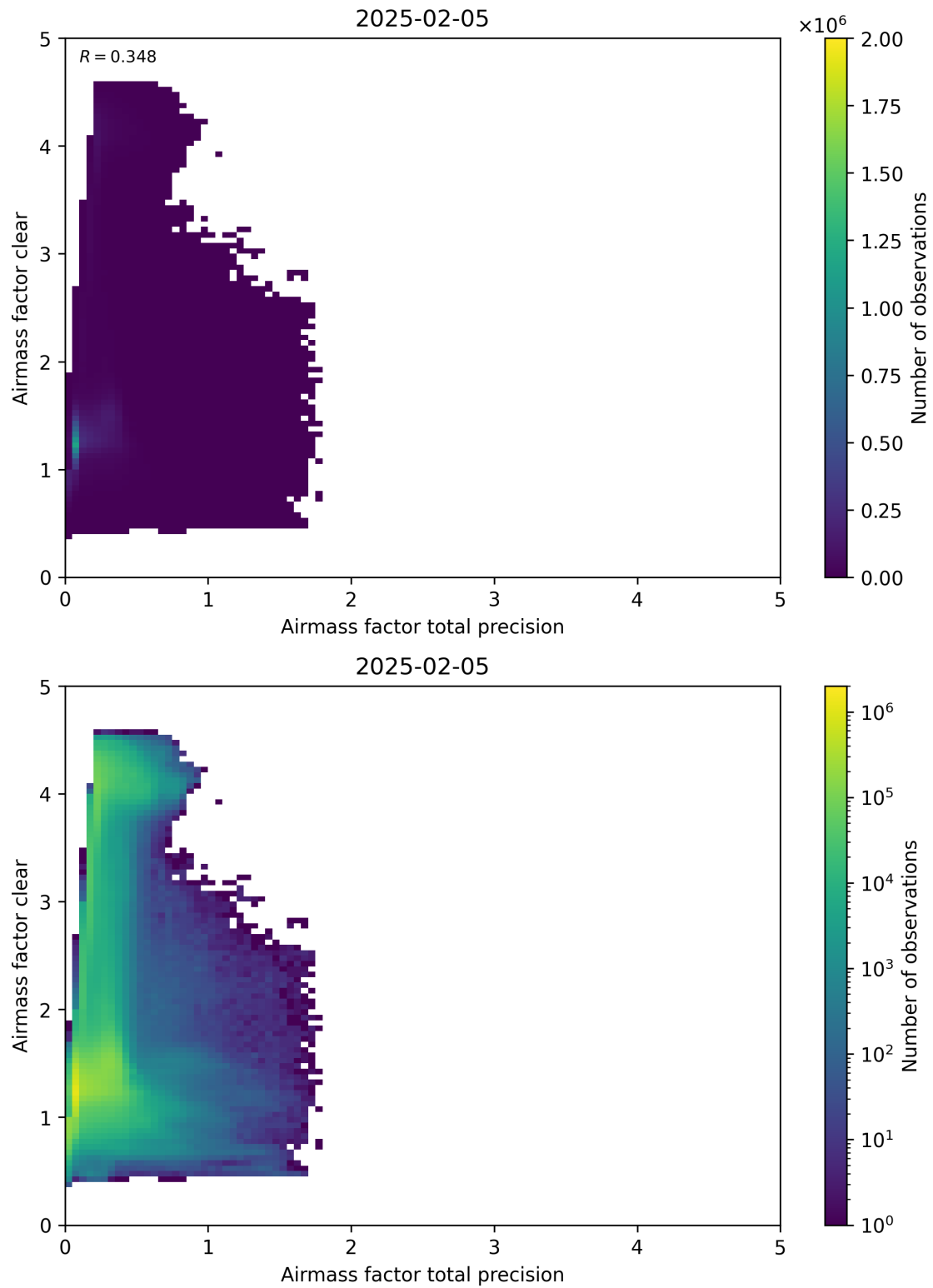
Figure 108: Scatter density plot of “Airmass factor total precision” against “Airmass factor clear” for 2025-02-04 to 2025-02-06.
