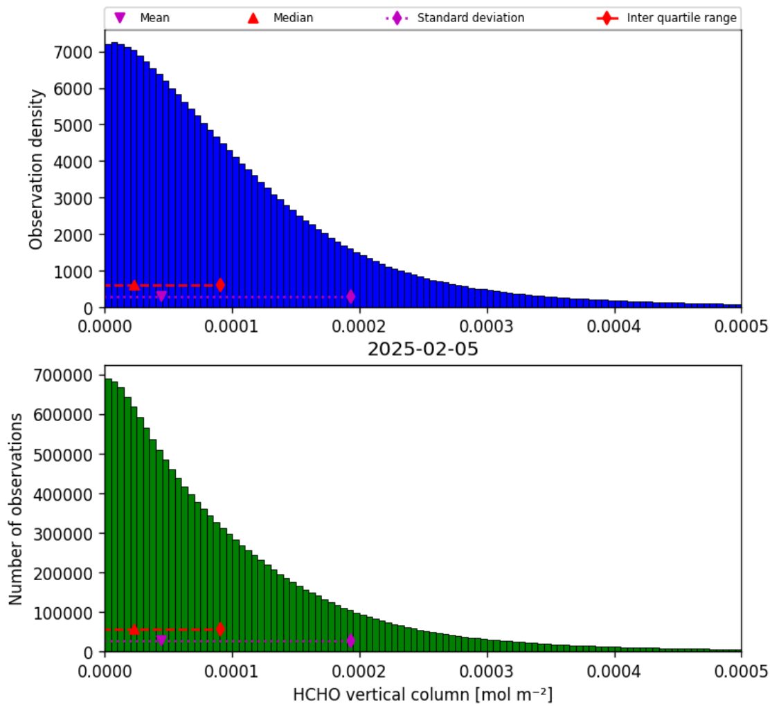
Figure 35: Histogram of “HCHO vertical column” for 2025-02-04 to 2025-02-06
