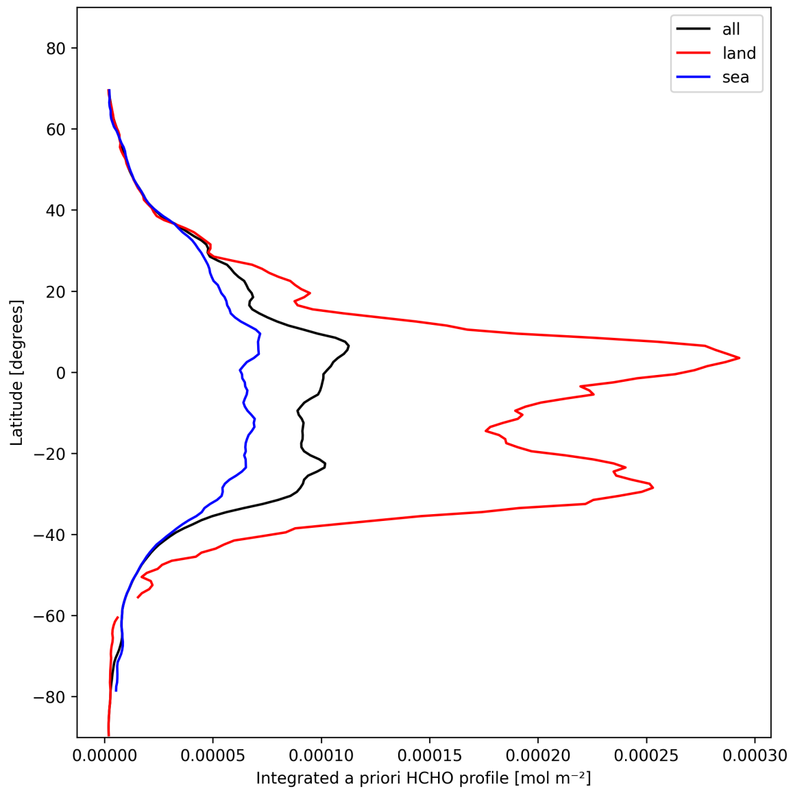
Figure 29: Zonal average of “Integrated a priori HCHO profile” for 2025-02-04 to 2025-02-06.
