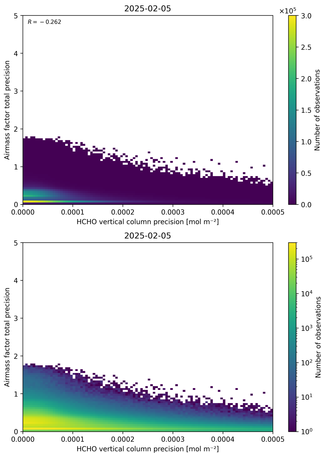
Figure 145: Scatter density plot of “HCHO vertical column precision” against “Airmass factor total precision” for 2025-02-04 to 2025-02-06.
