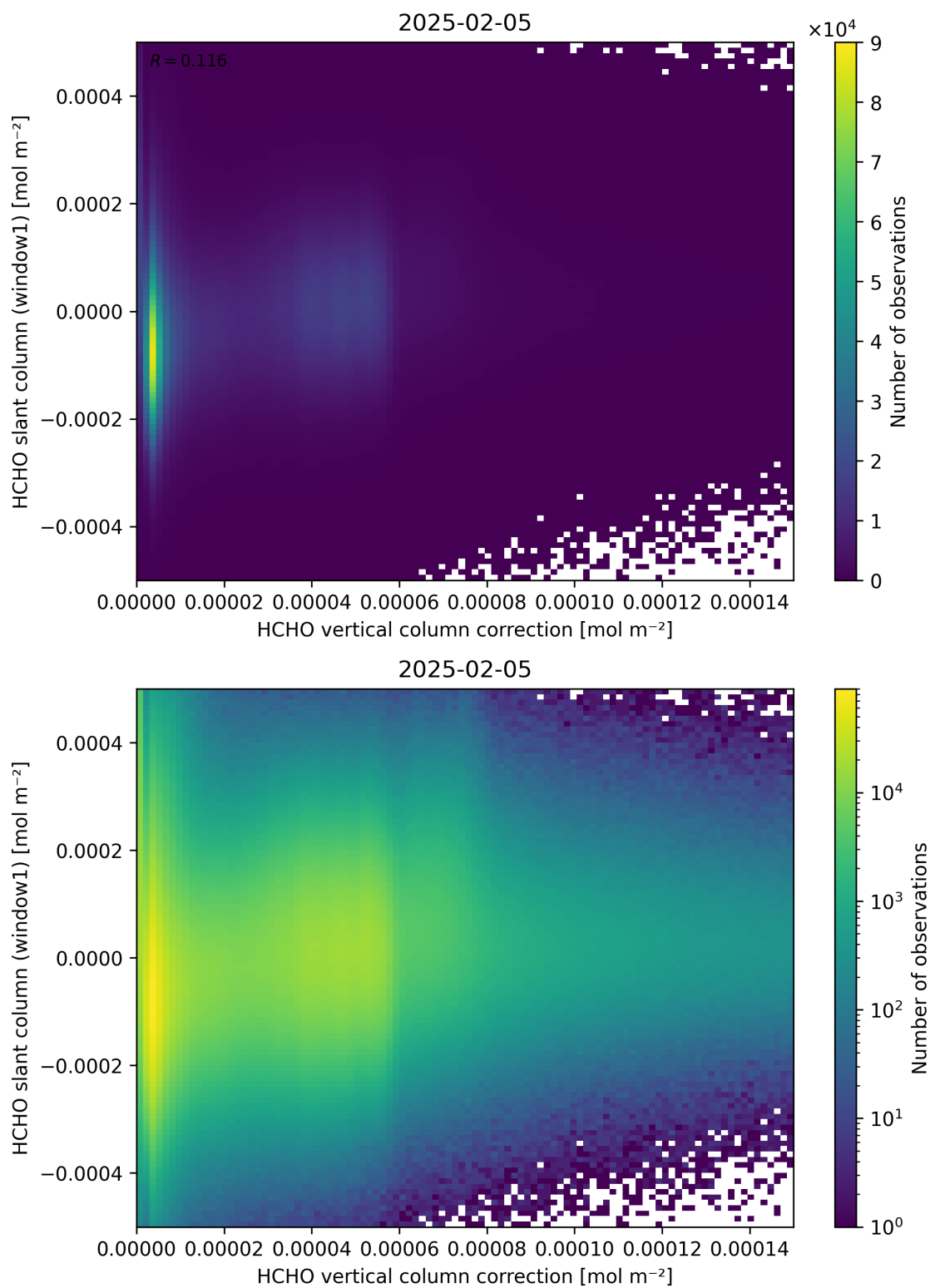
Figure 118: Scatter density plot of “HCHO vertical column correction” against “HCHO slant column (window1)” for 2025-02-04 to 2025-02-06.
