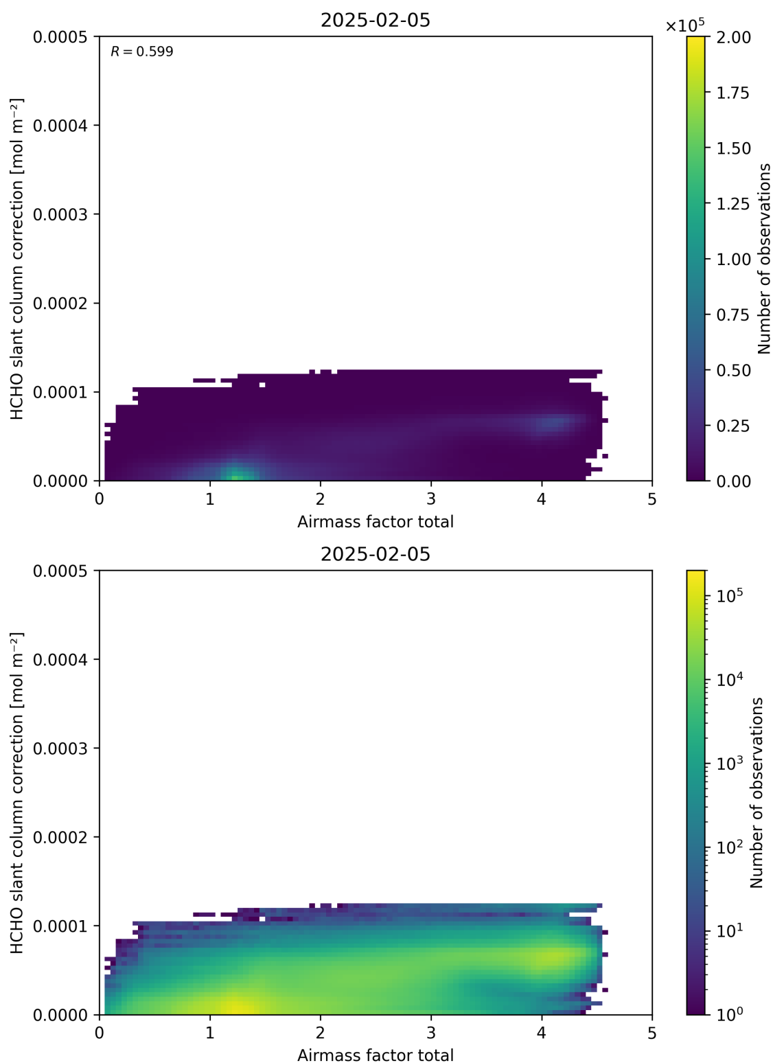
Figure 102: Scatter density plot of “Airmass factor total” against “HCHO slant column correction” for 2025-02-04 to 2025-02-06.
