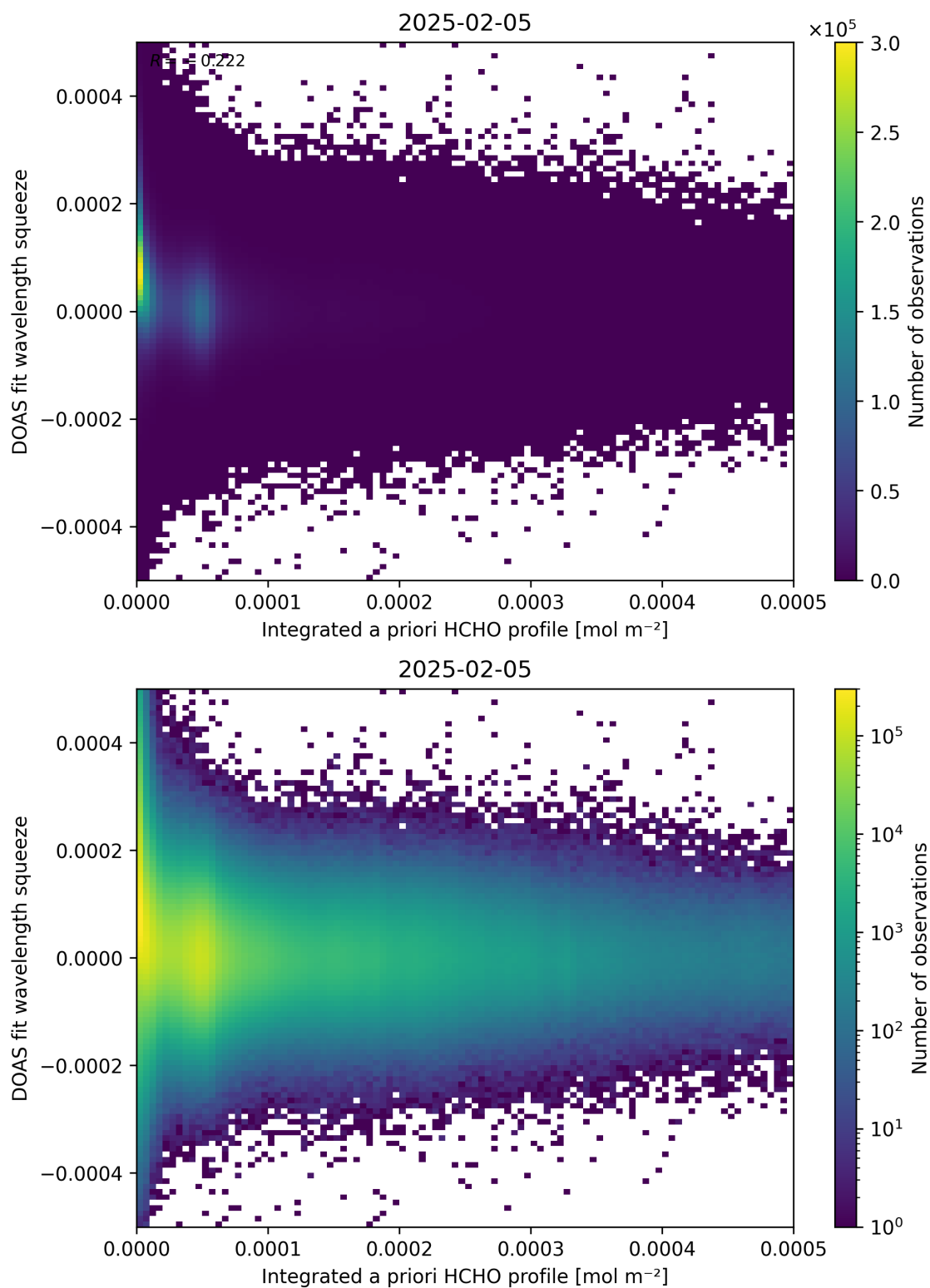
Figure 150: Scatter density plot of “Integrated a priori HCHO profile” against “DOAS fit wavelength squeeze” for 2025-02-04 to 2025-02-06.
