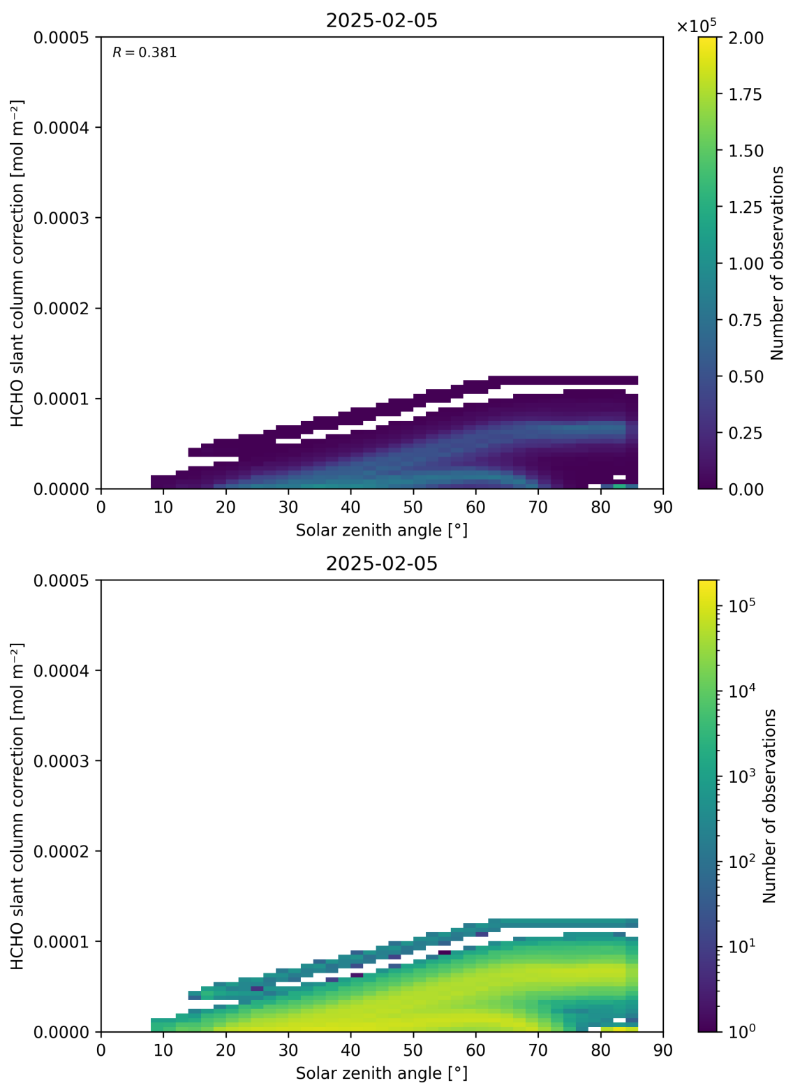
Figure 172: Scatter density plot of “Solar zenith angle” against “HCHO slant column correction” for 2025-02-04 to 2025-02-06.
