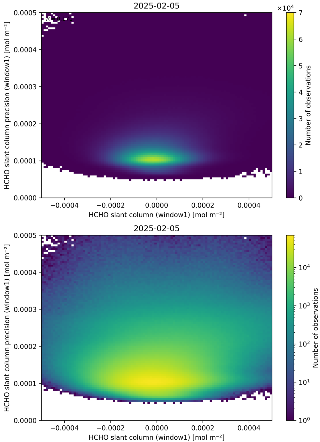
Figure 84: Scatter density plot of “HCHO slant column (window1)” against “HCHO slant column precision (window1)” for 2025-02-04 to 2025-02-06.
