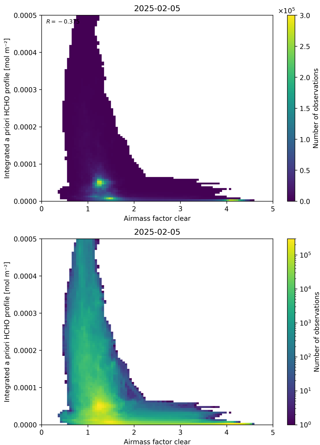
Figure 76: Scatter density plot of “Airmass factor clear” against “Integrated a priori HCHO profile” for 2025-02-04 to 2025-02-06.
