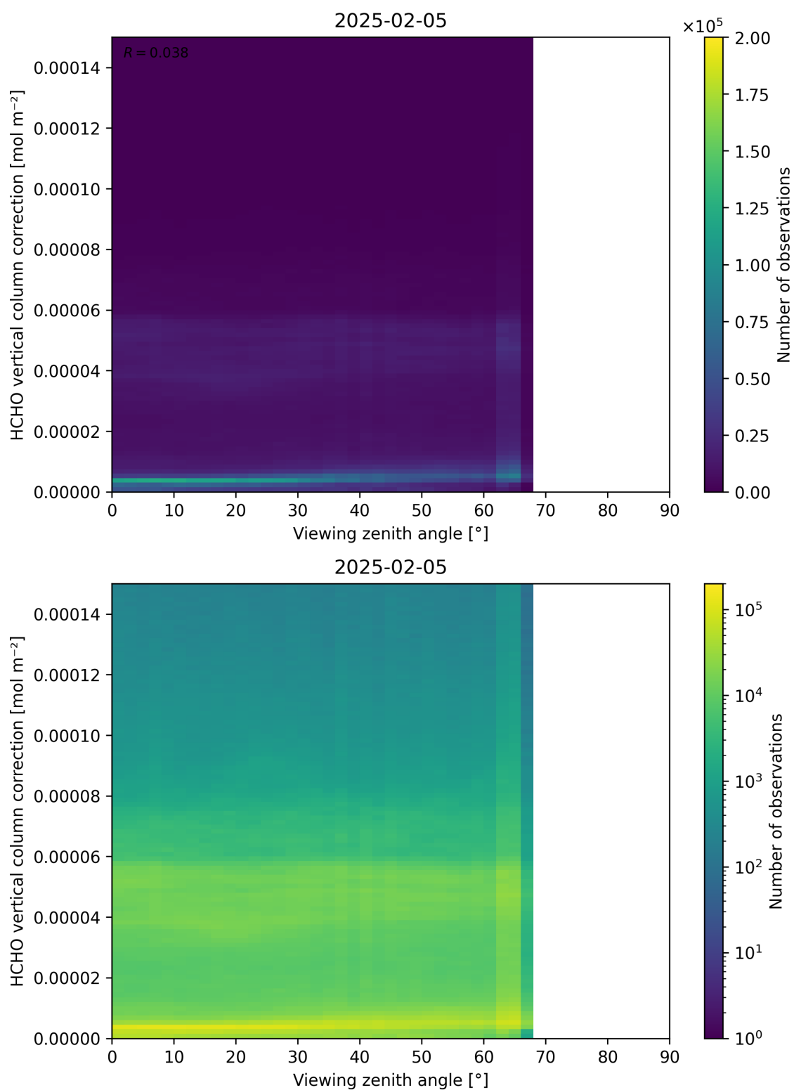
Figure 193: Scatter density plot of “Viewing zenith angle” against “HCHO vertical column correction” for 2025-02-04 to 2025-02-06.
