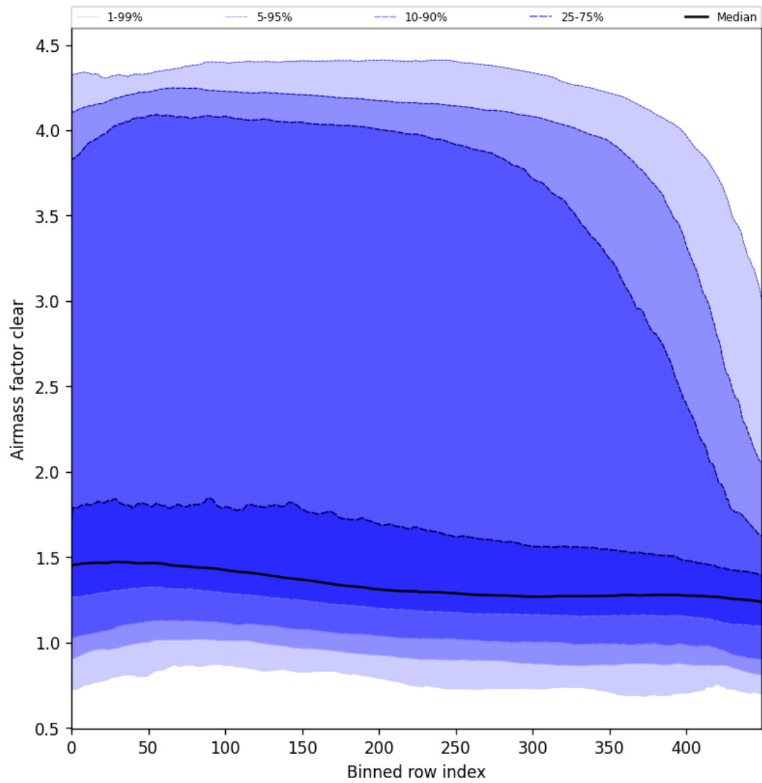
Figure 56: Along track statistics of “Airmass factor clear” for 2025-02-04 to 2025-02-06
