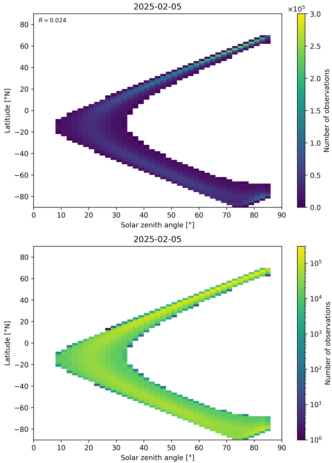
Figure 181: Scatter density plot of “Solar zenith angle” against “Latitude” for 2025-02-04 to 2025-02-06.
