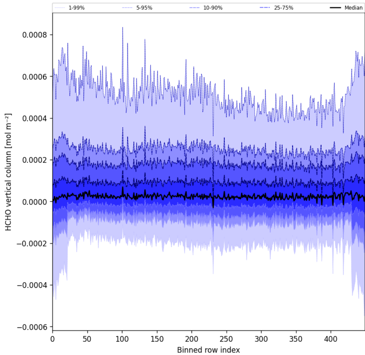
Figure 49: Along track statistics of “HCHO vertical column” for 2025-02-04 to 2025-02-06
