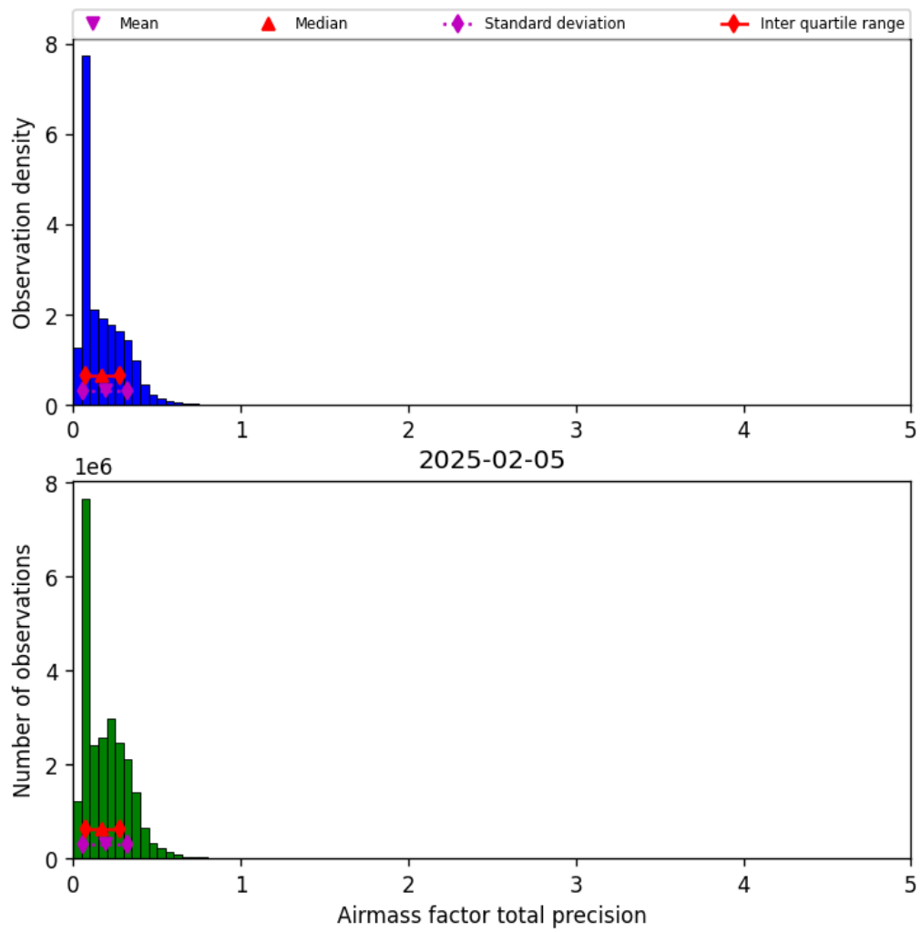
Figure 41: Histogram of “Airmass factor total precision” for 2025-02-04 to 2025-02-06
