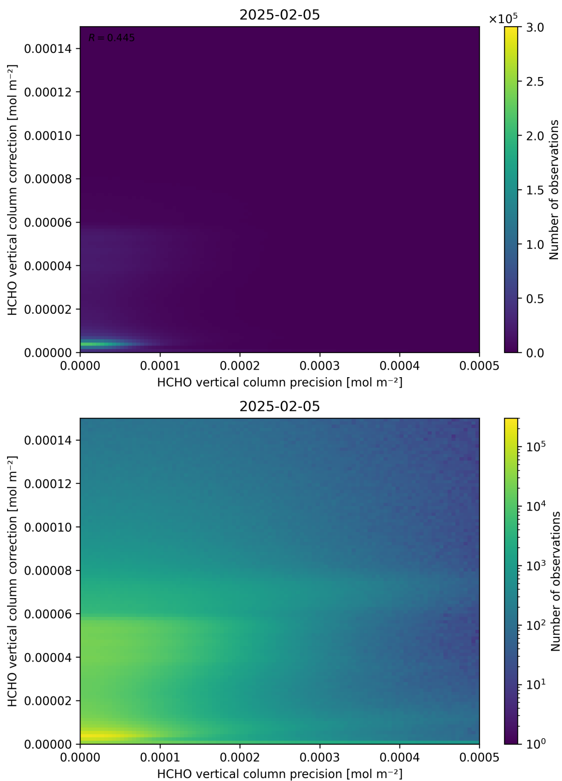
Figure 146: Scatter density plot of “HCHO vertical column precision” against “HCHO vertical column correction” for 2025-02-04 to 2025-02-06.
