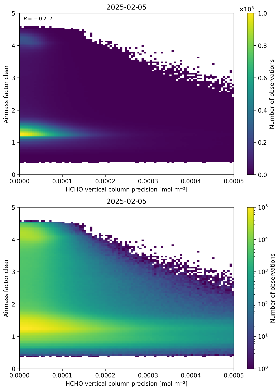
Figure 139: Scatter density plot of “HCHO vertical column precision” against “Airmass factor clear” for 2025-02-04 to 2025-02-06.
