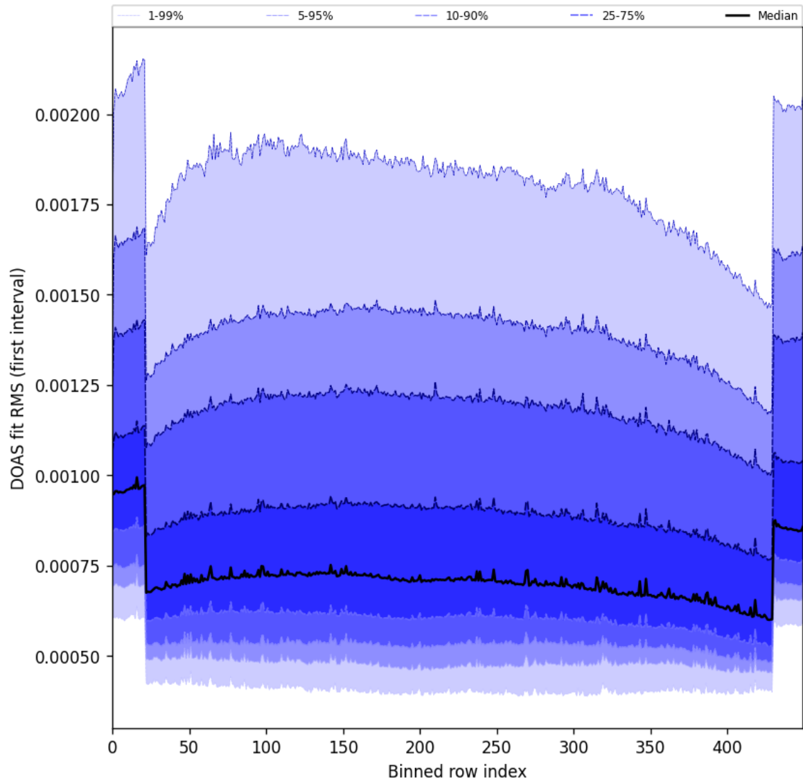
Figure 60: Along track statistics of “DOAS fit RMS (first interval)” for 2025-02-04 to 2025-02-06
