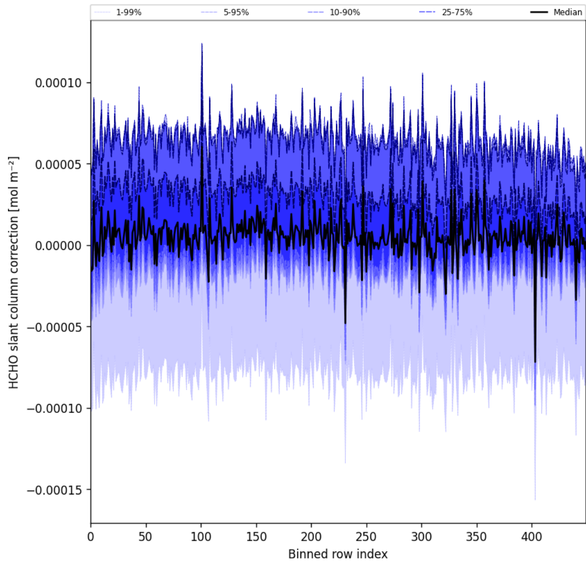
Figure 61: Along track statistics of “HCHO slant column correction” for 2025-02-04 to 2025-02-06
