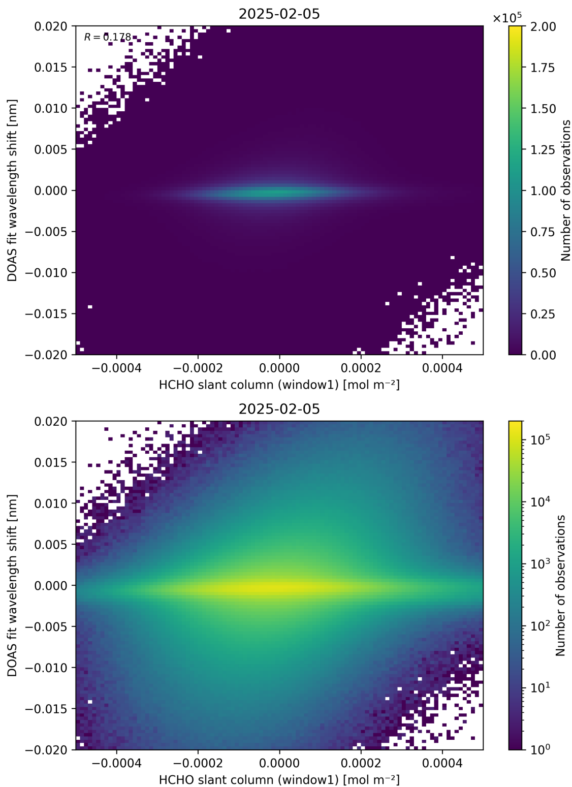
Figure 79: Scatter density plot of “HCHO slant column (window1)” against “DOAS fit wavelength shift” for 2025-02-04 to 2025-02-06.
