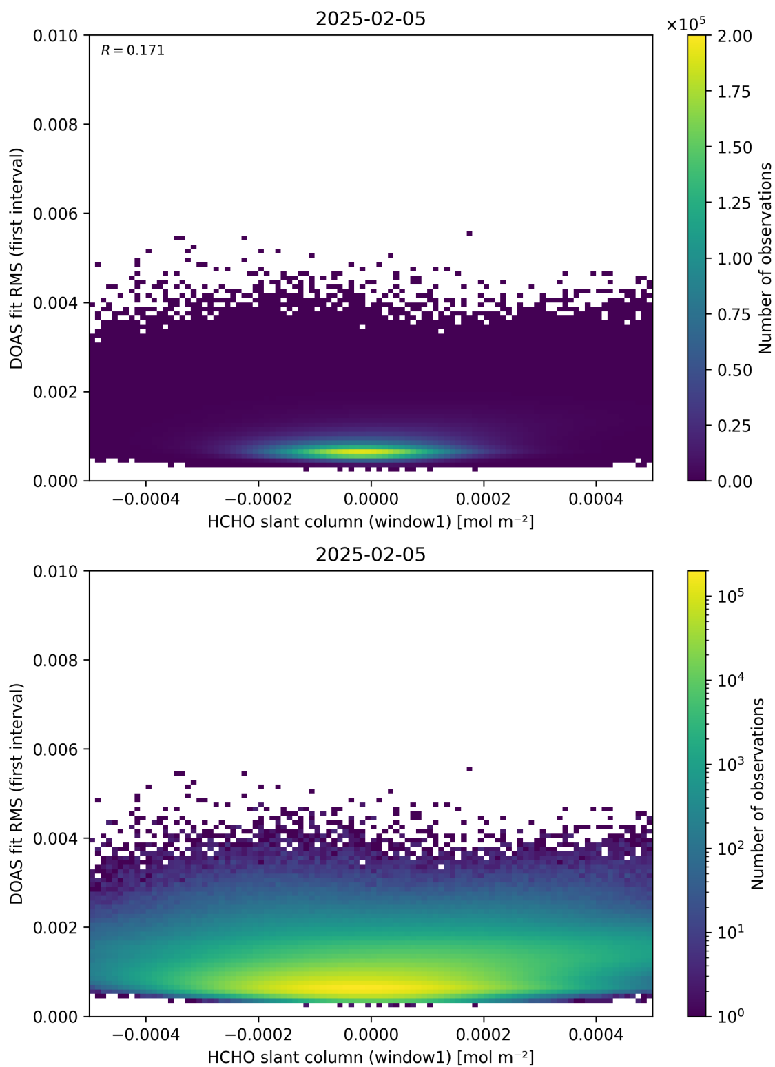
Figure 78: Scatter density plot of “HCHO slant column (window1)” against “DOAS fit RMS (first interval)” for 2025-02-04 to 2025-02-06.
