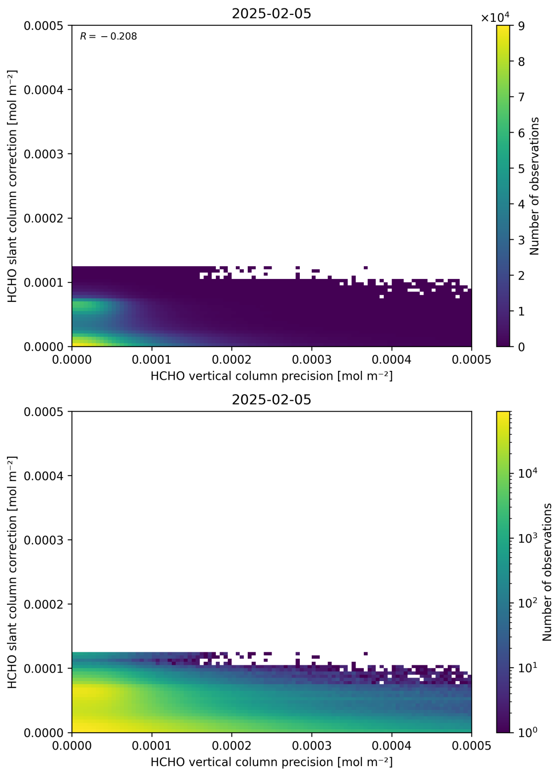
Figure 141: Scatter density plot of “HCHO vertical column precision” against “HCHO slant column correction” for 2025-02-04 to 2025-02-06.
