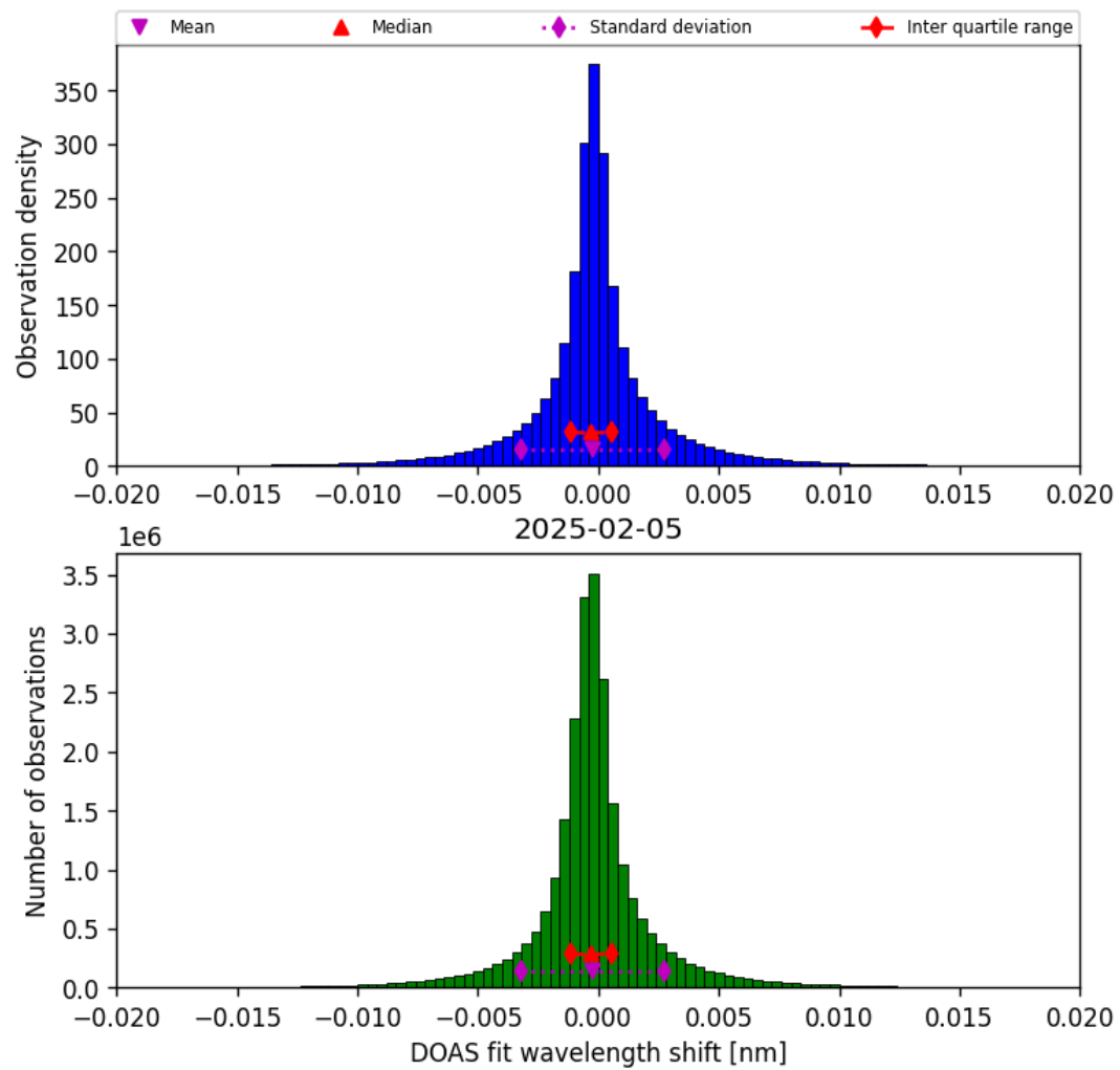
Figure 44: Histogram of “DOAS fit wavelength shift” for 2025-02-04 to 2025-02-06
