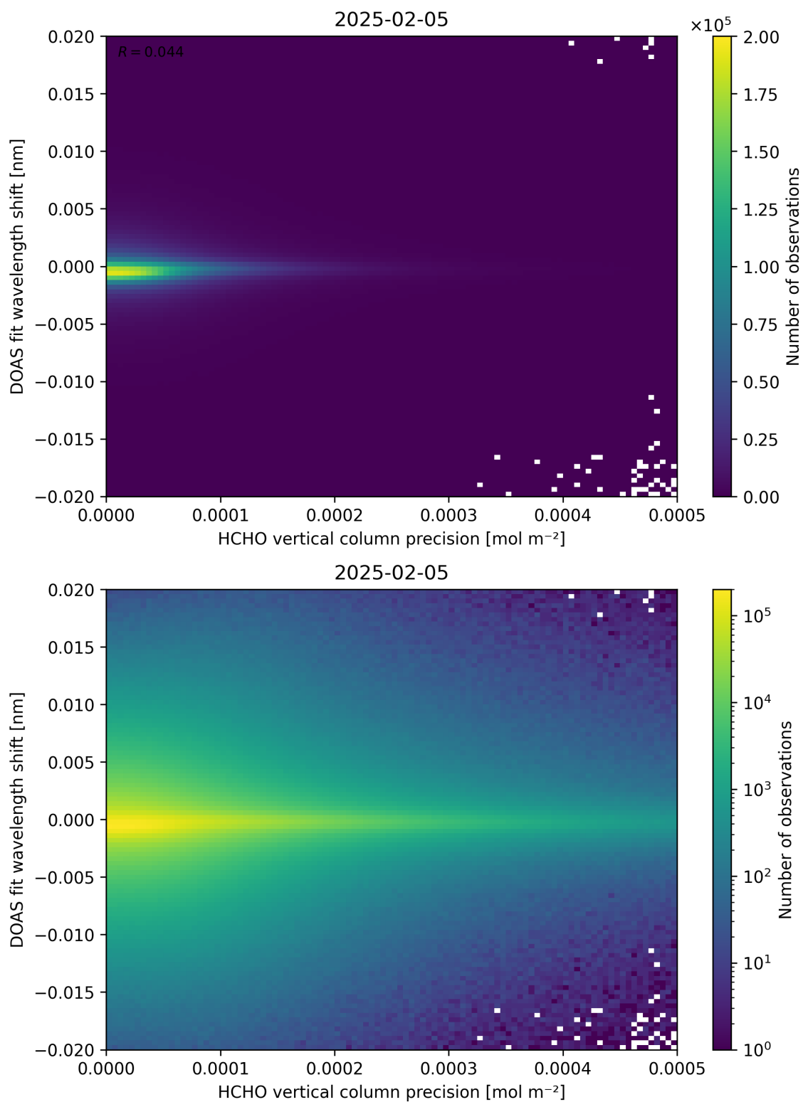
Figure 137: Scatter density plot of “HCHO vertical column precision” against “DOAS fit wavelength shift” for 2025-02-04 to 2025-02-06.
