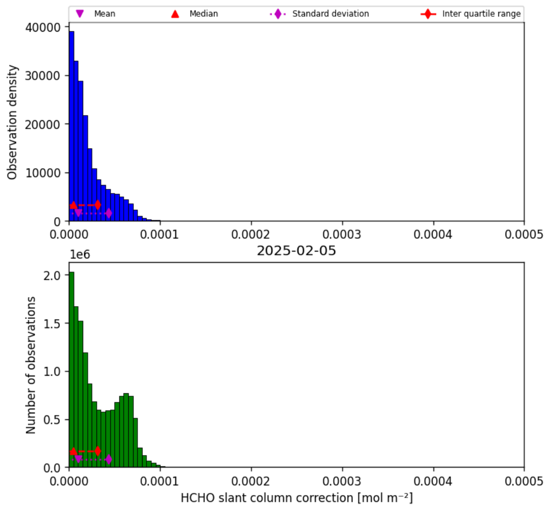
Figure 47: Histogram of “HCHO slant column correction” for 2025-02-04 to 2025-02-06
