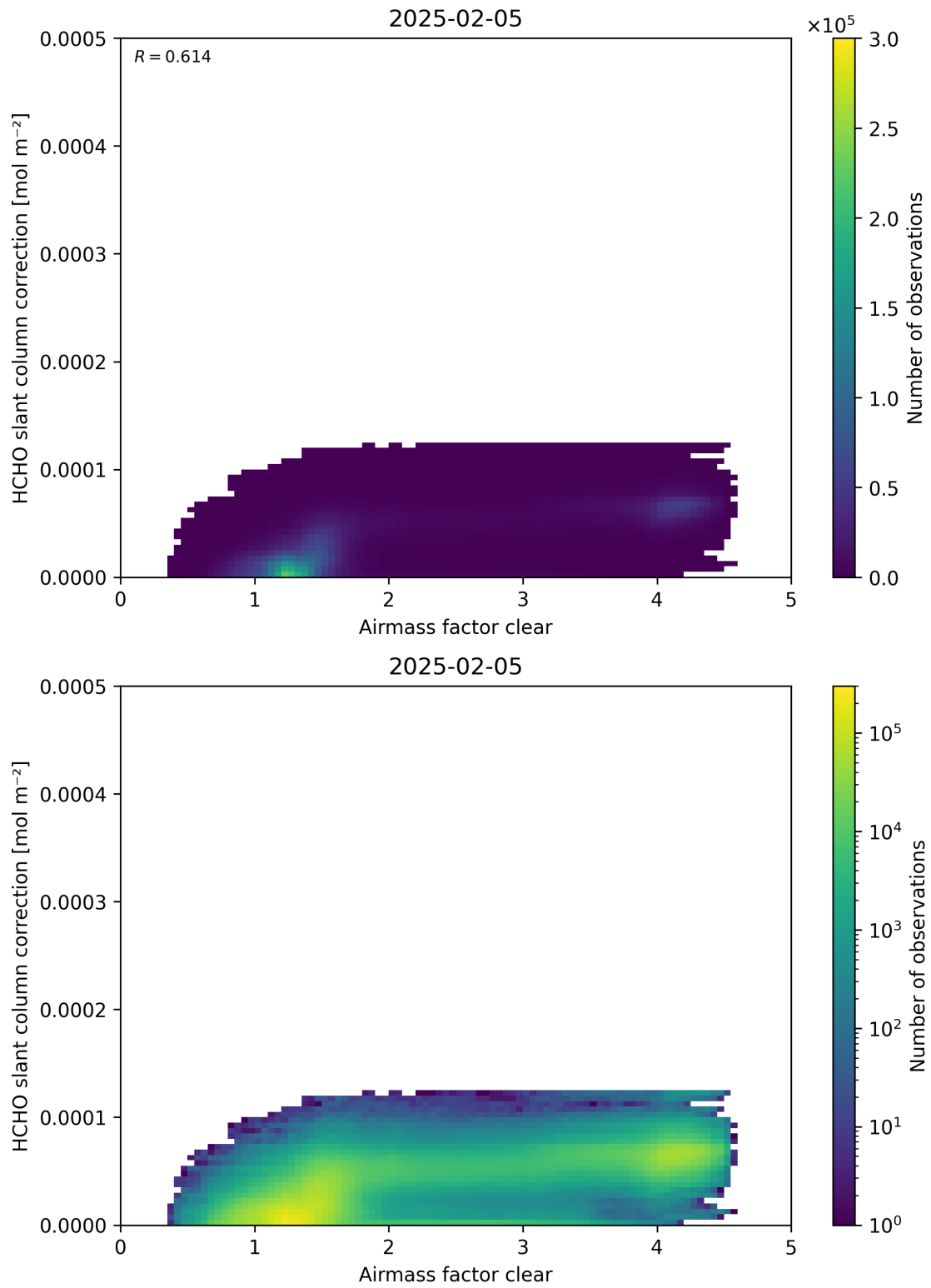
Figure 75: Scatter density plot of “Airmass factor clear” against “HCHO slant column correction” for 2025-02-04 to 2025-02-06.
