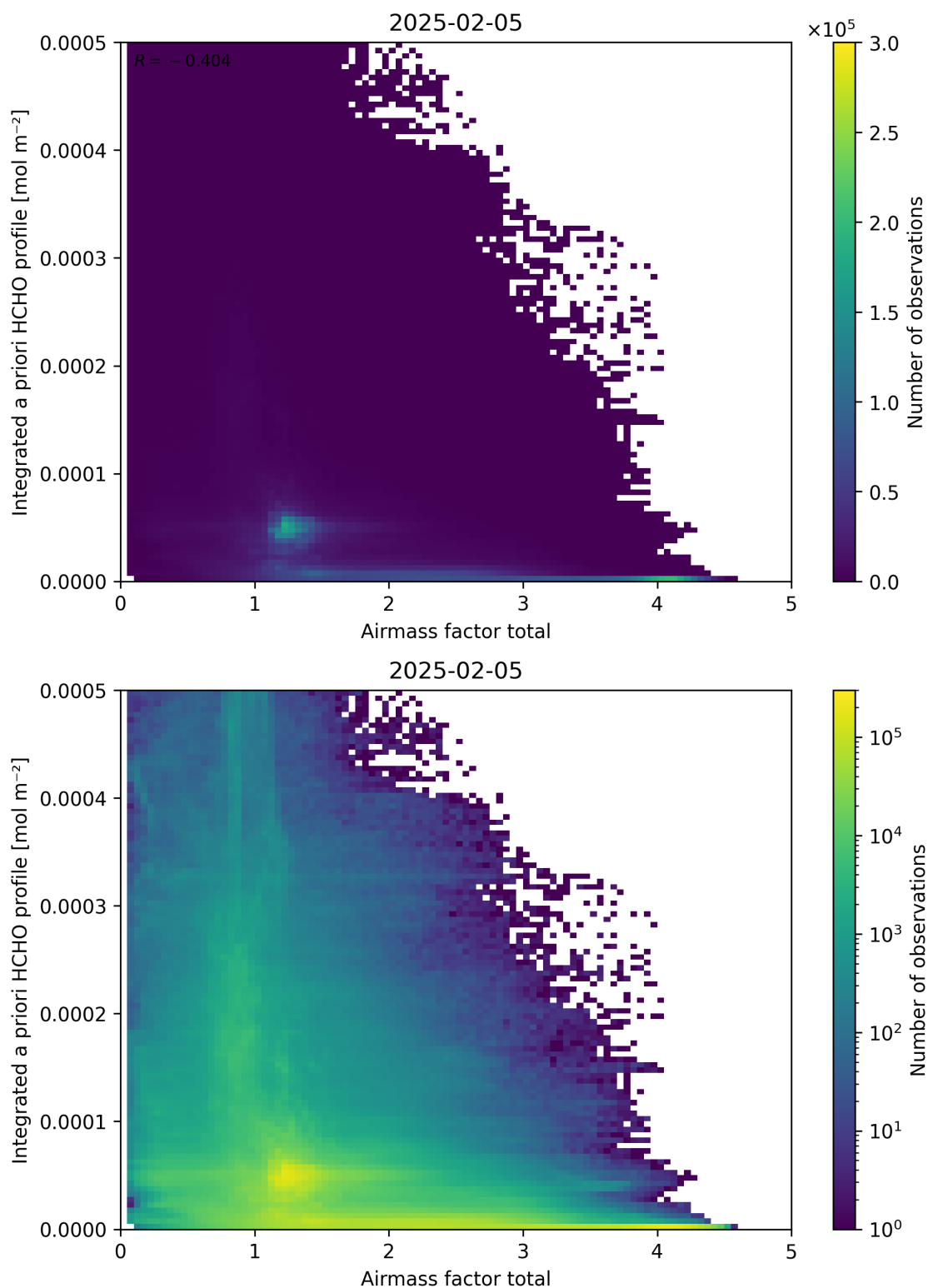
Figure 104: Scatter density plot of “Airmass factor total” against “Integrated a priori HCHO profile” for 2025-02-04 to 2025-02-06.
