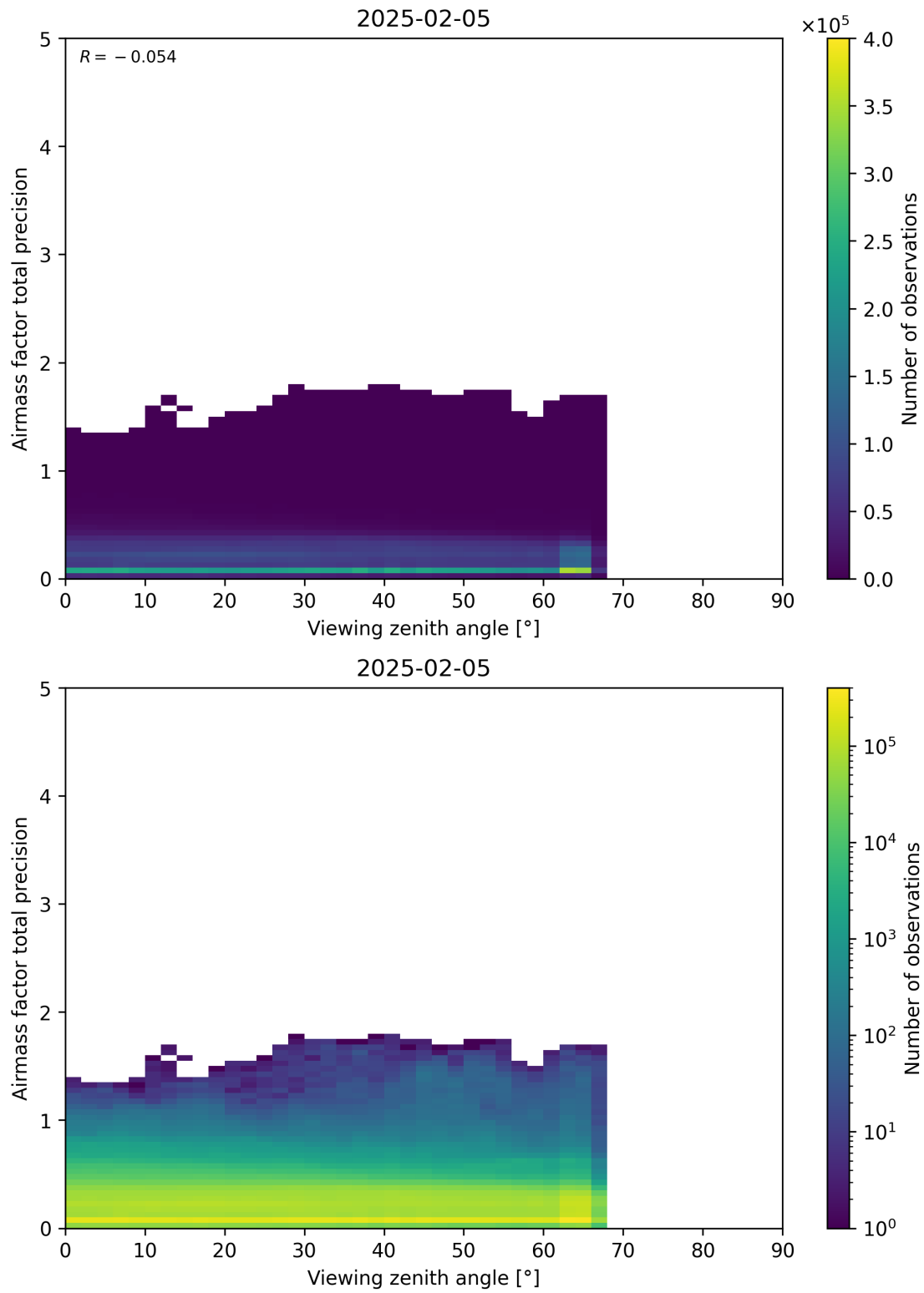
Figure 191: Scatter density plot of “Viewing zenith angle” against “Airmass factor total precision” for 2025-02-04 to 2025-02-06.
