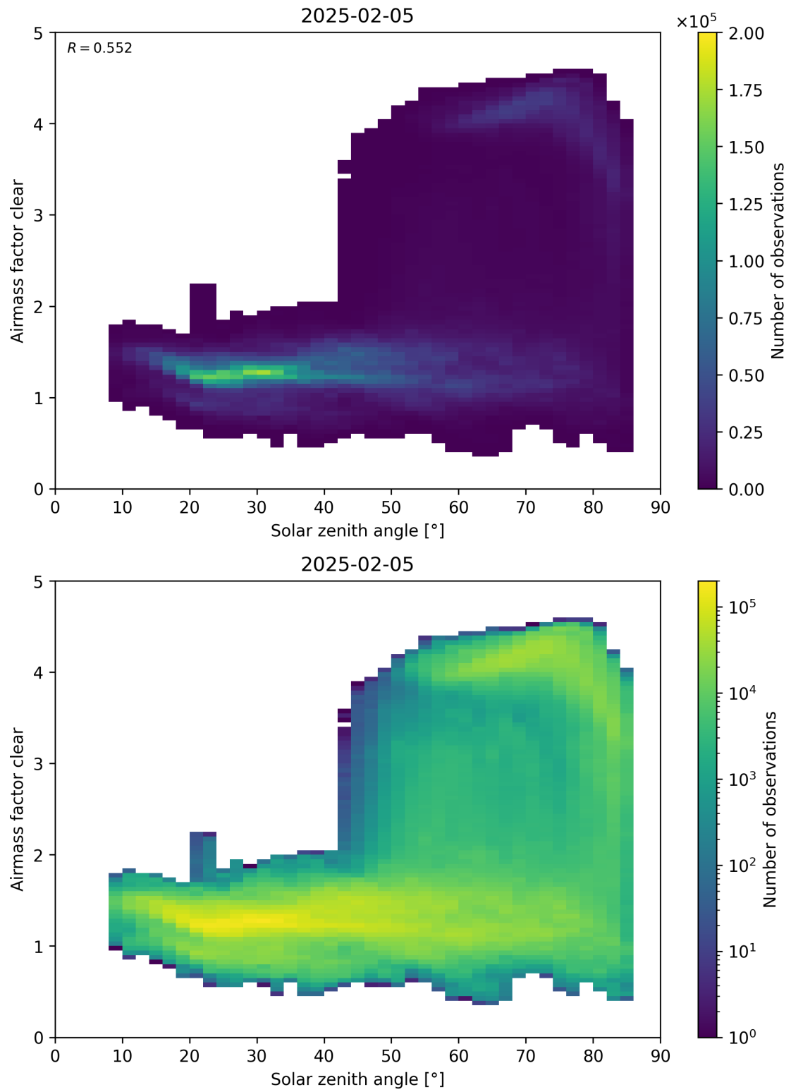
Figure 170: Scatter density plot of “Solar zenith angle” against “Airmass factor clear” for 2025-02-04 to 2025-02-06.
