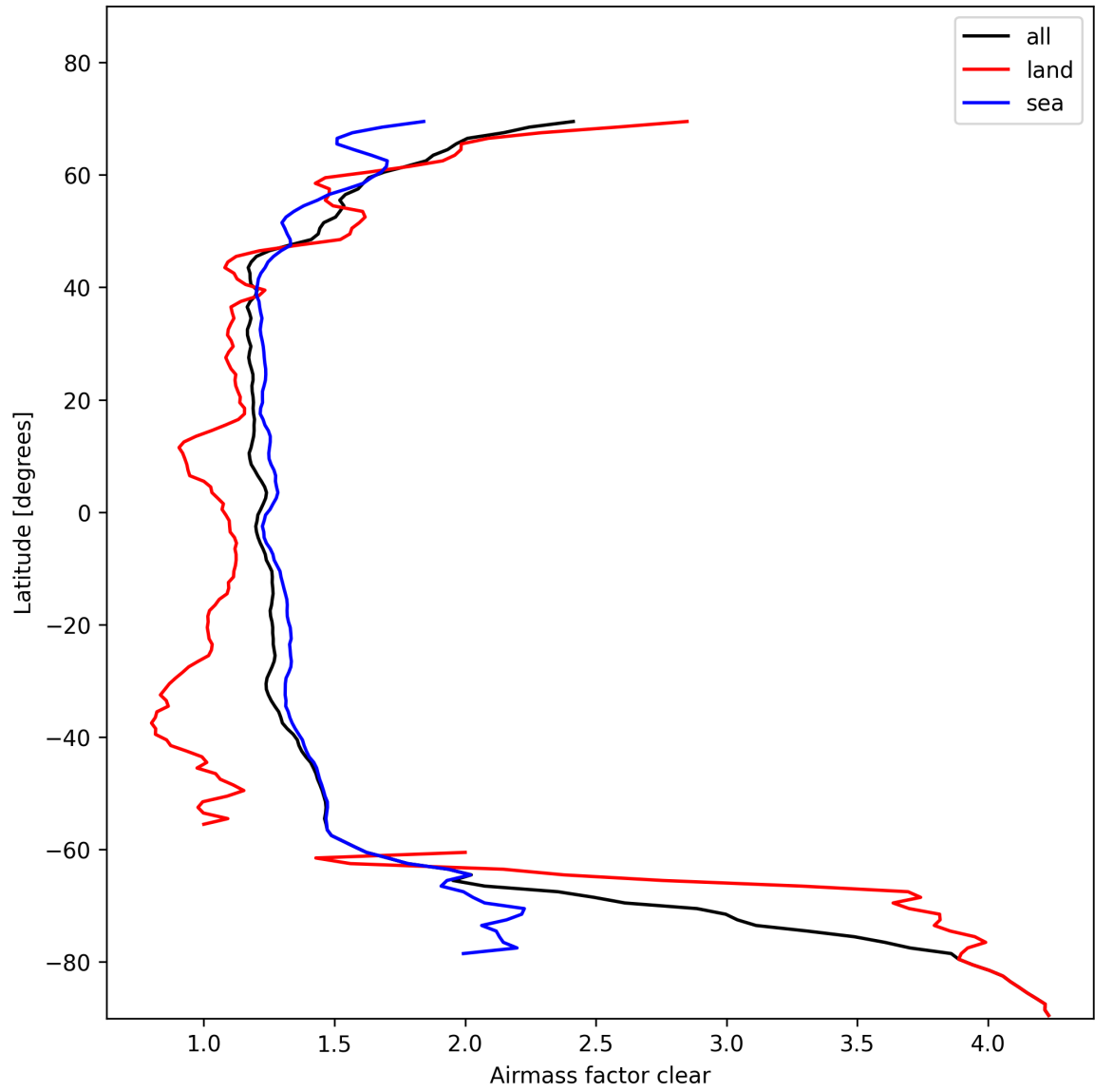
Figure 28: Zonal average of “Airmass factor clear” for 2025-02-04 to 2025-02-06.
