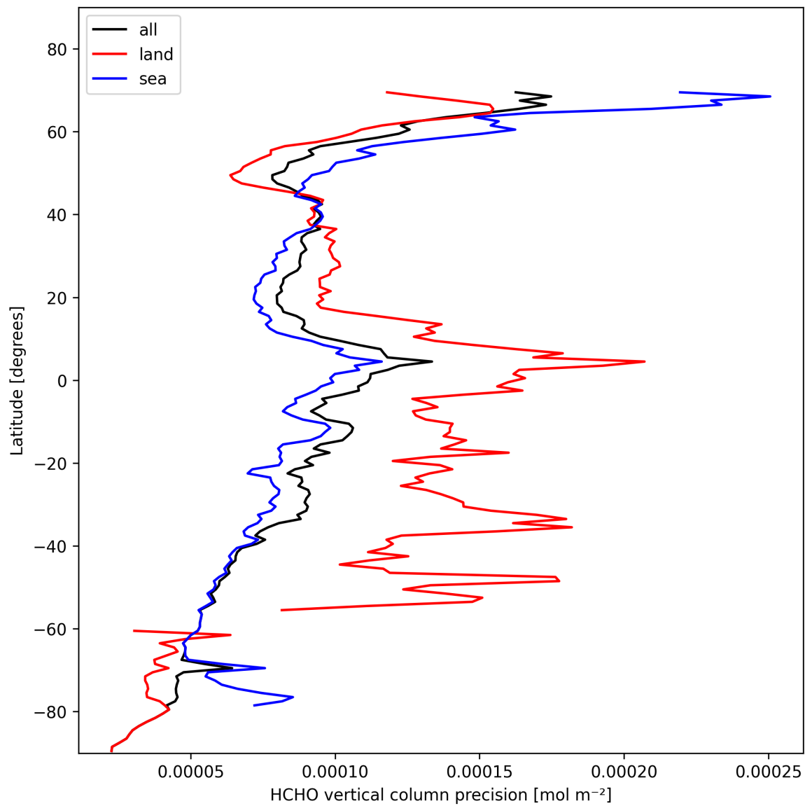
Figure 22: Zonal average of “HCHO vertical column precision” for 2025-02-04 to 2025-02-06.
