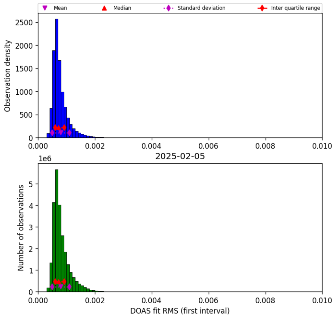
Figure 46: Histogram of “DOAS fit RMS (first interval)” for 2025-02-04 to 2025-02-06
