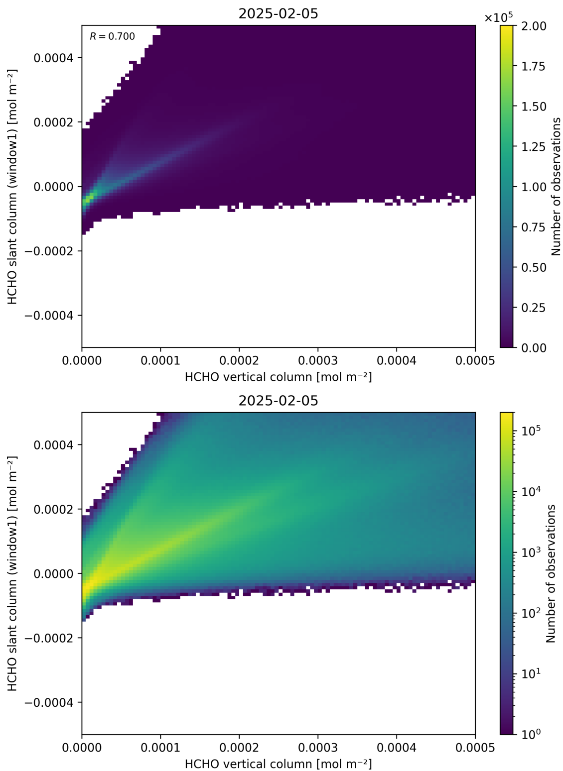
Figure 129: Scatter density plot of “HCHO vertical column” against “HCHO slant column (window1)” for 2025-02-04 to 2025-02-06.
