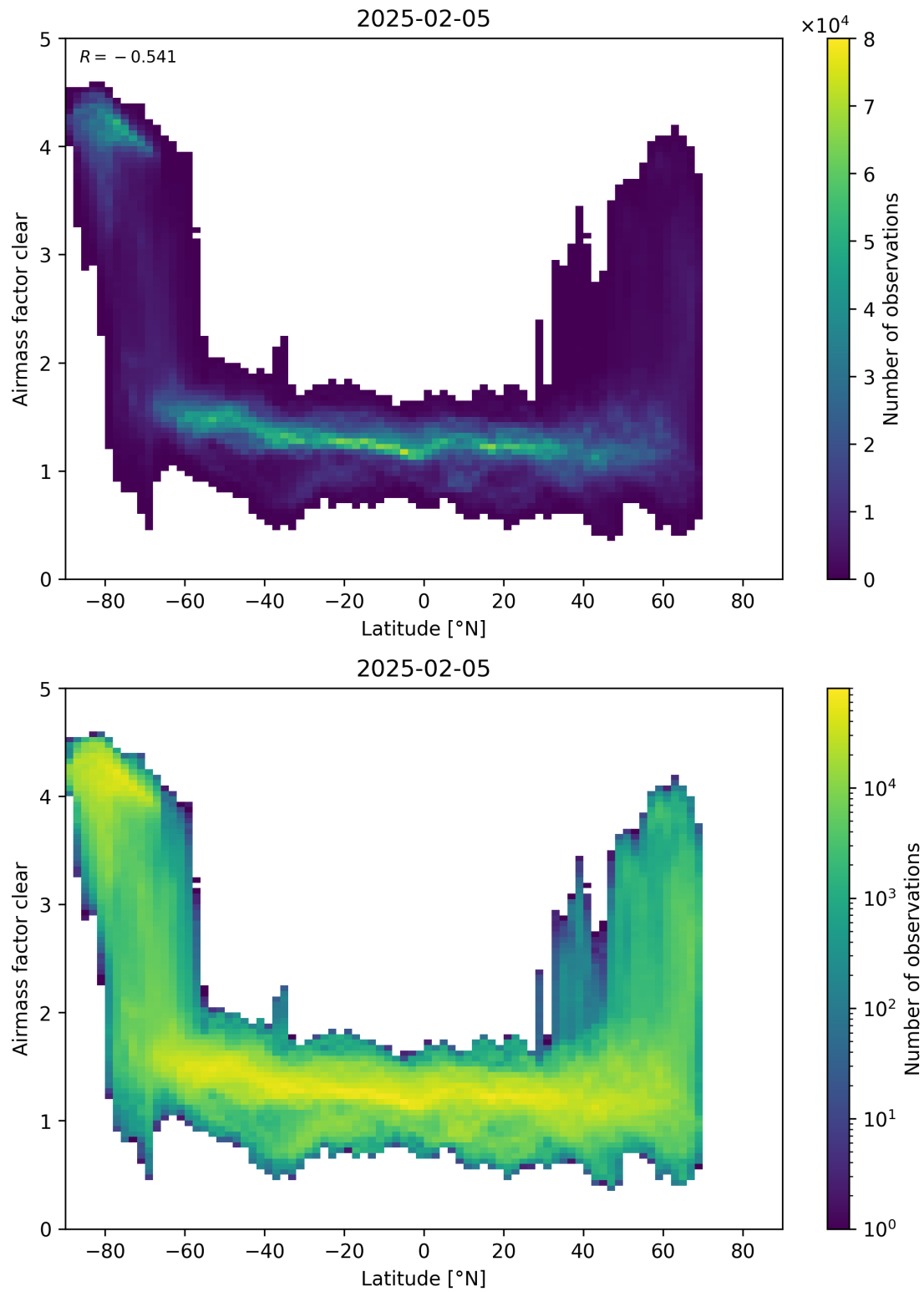
Figure 156: Scatter density plot of “Latitude” against “Airmass factor clear” for 2025-02-04 to 2025-02-06.
