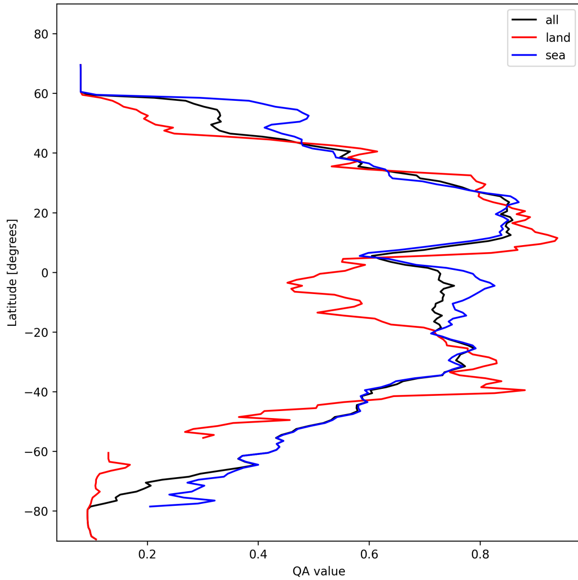
Figure 20: Zonal average of “QA value” for 2025-02-04 to 2025-02-06.
