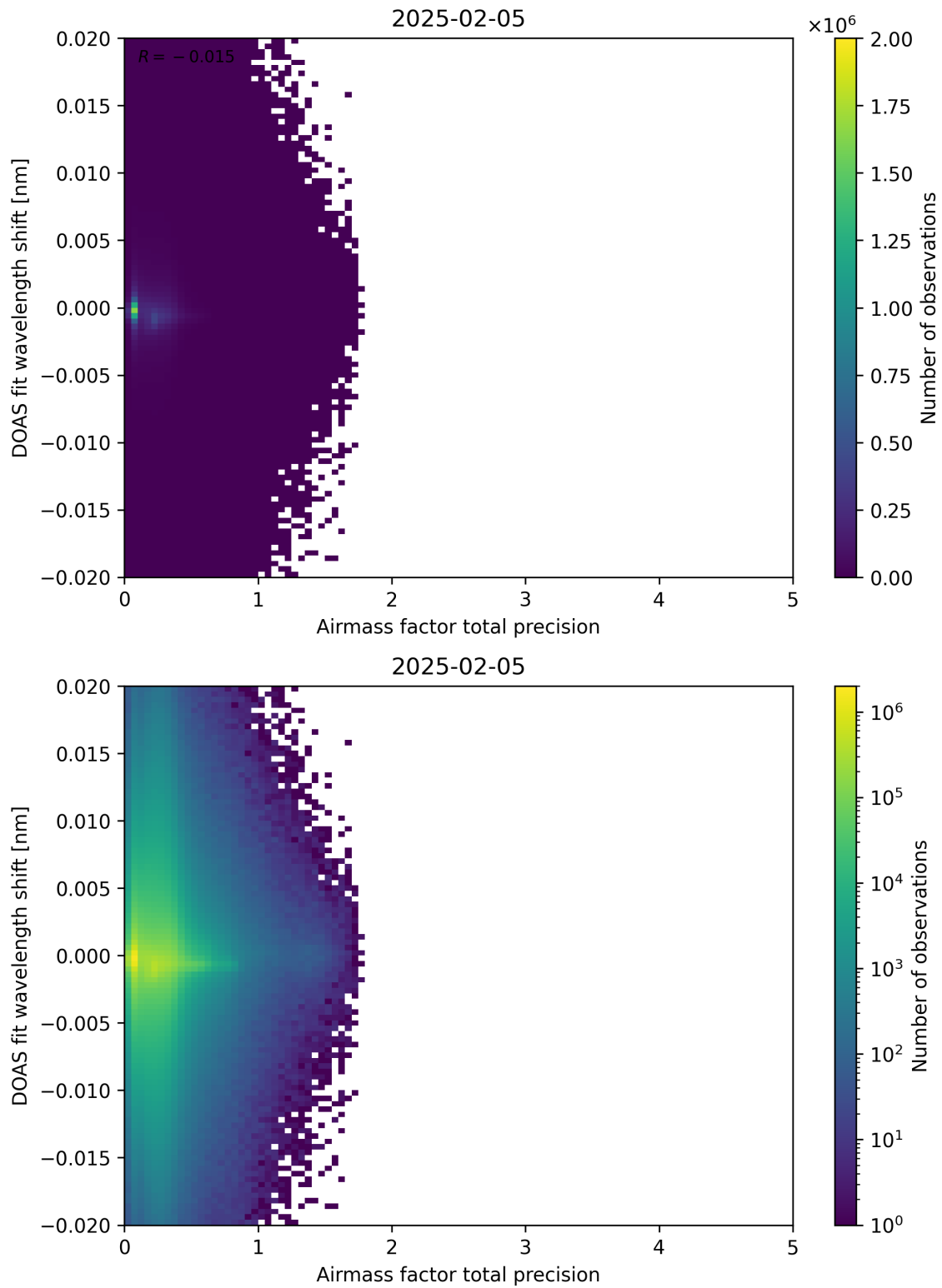
Figure 106: Scatter density plot of “Airmass factor total precision” against “DOAS fit wavelength shift” for 2025-02-04 to 2025-02-06.
