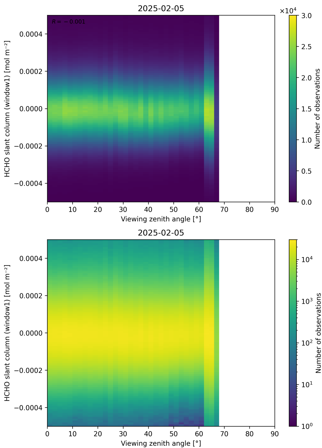
Figure 188: Scatter density plot of “Viewing zenith angle” against “HCHO slant column (window1)” for 2025-02-04 to 2025-02-06.
