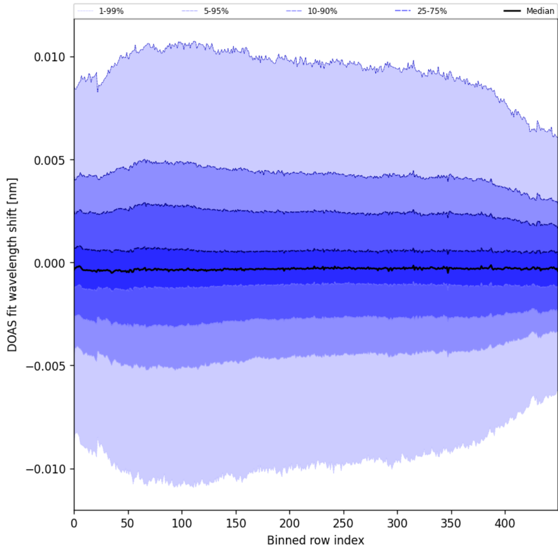
Figure 58: Along track statistics of “DOAS fit wavelength shift” for 2025-02-04 to 2025-02-06
