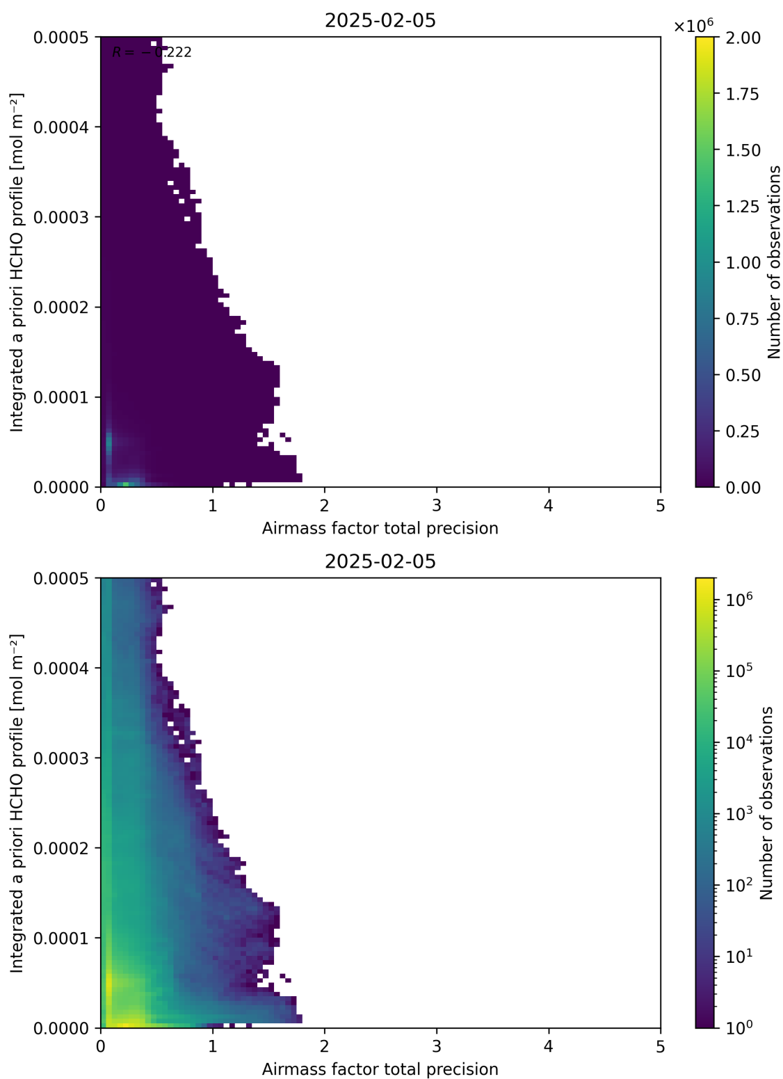
Figure 111: Scatter density plot of “Airmass factor total precision” against “Integrated a priori HCHO profile” for 2025-02-04 to 2025-02-06.
