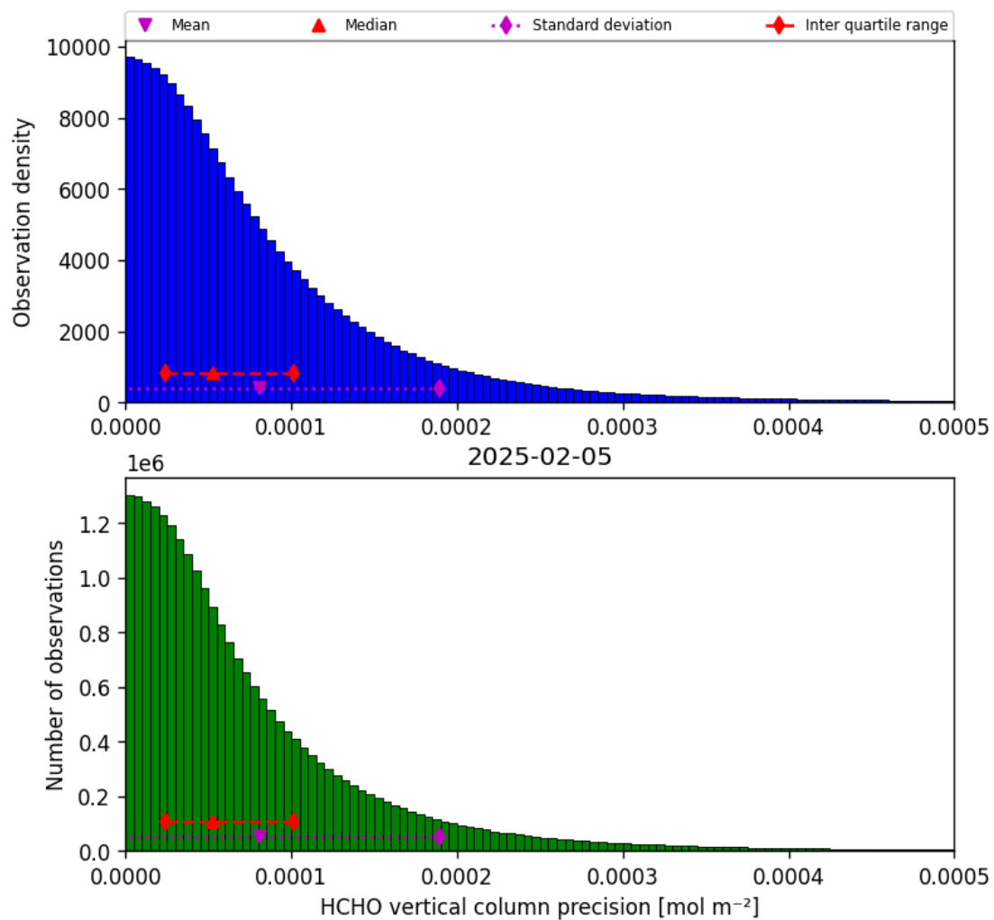
Figure 36: Histogram of “HCHO vertical column precision” for 2025-02-04 to 2025-02-06
