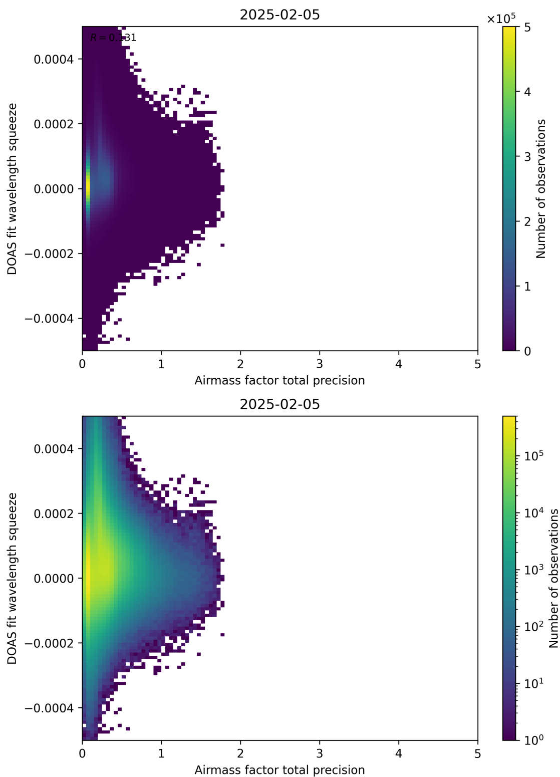
Figure 107: Scatter density plot of “Airmass factor total precision” against “DOAS fit wavelength squeeze” for 2025-02-04 to 2025-02-06.
