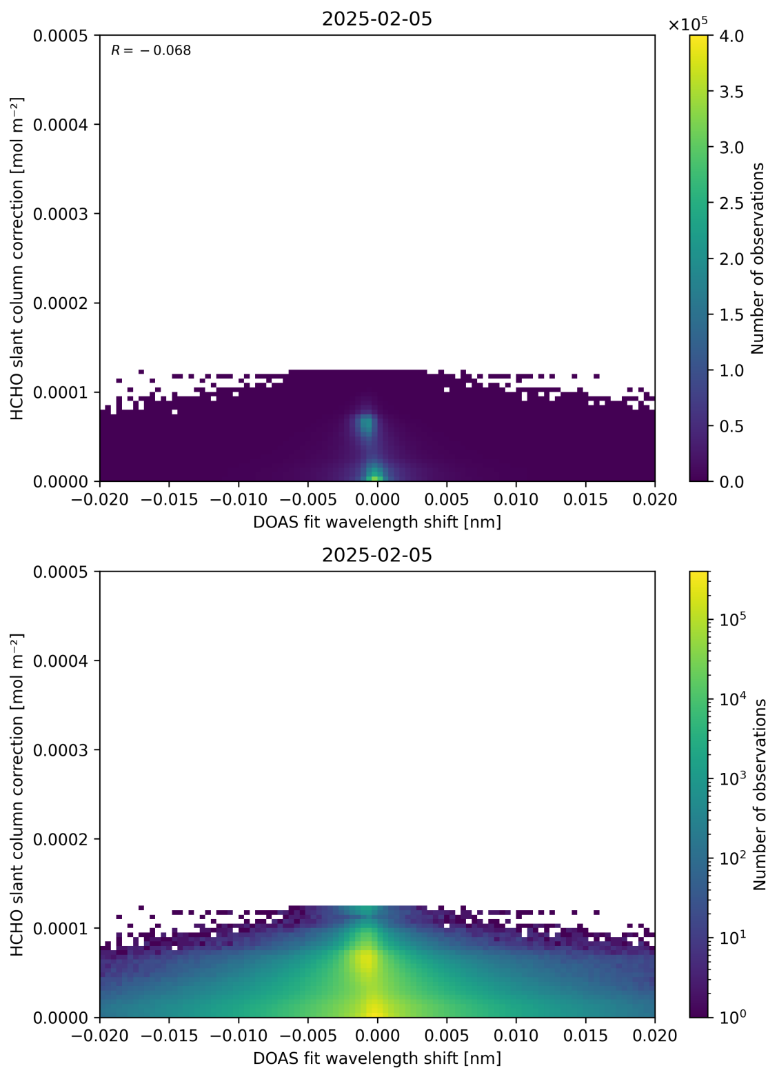
Figure 67: Scatter density plot of “DOAS fit wavelength shift” against “HCHO slant column correction” for 2025-02-04 to 2025-02-06.
