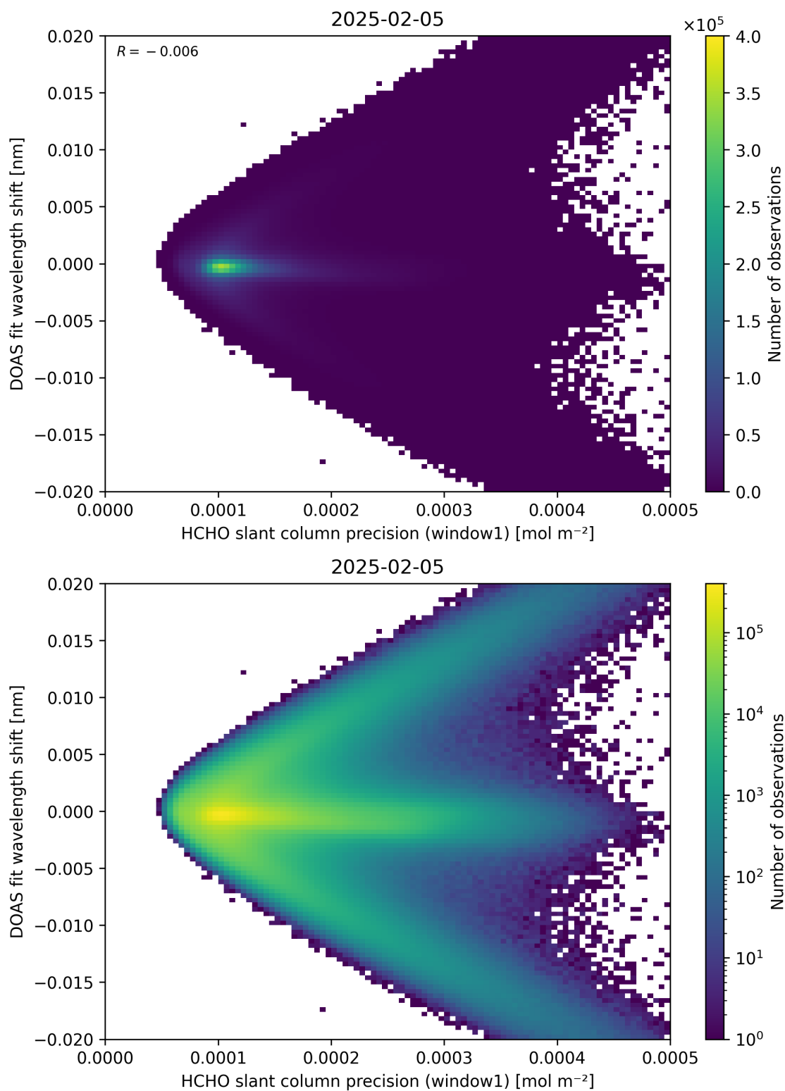
Figure 89: Scatter density plot of “HCHO slant column precision (window1)” against “DOAS fit wavelength shift” for 2025-02-04 to 2025-02-06.
