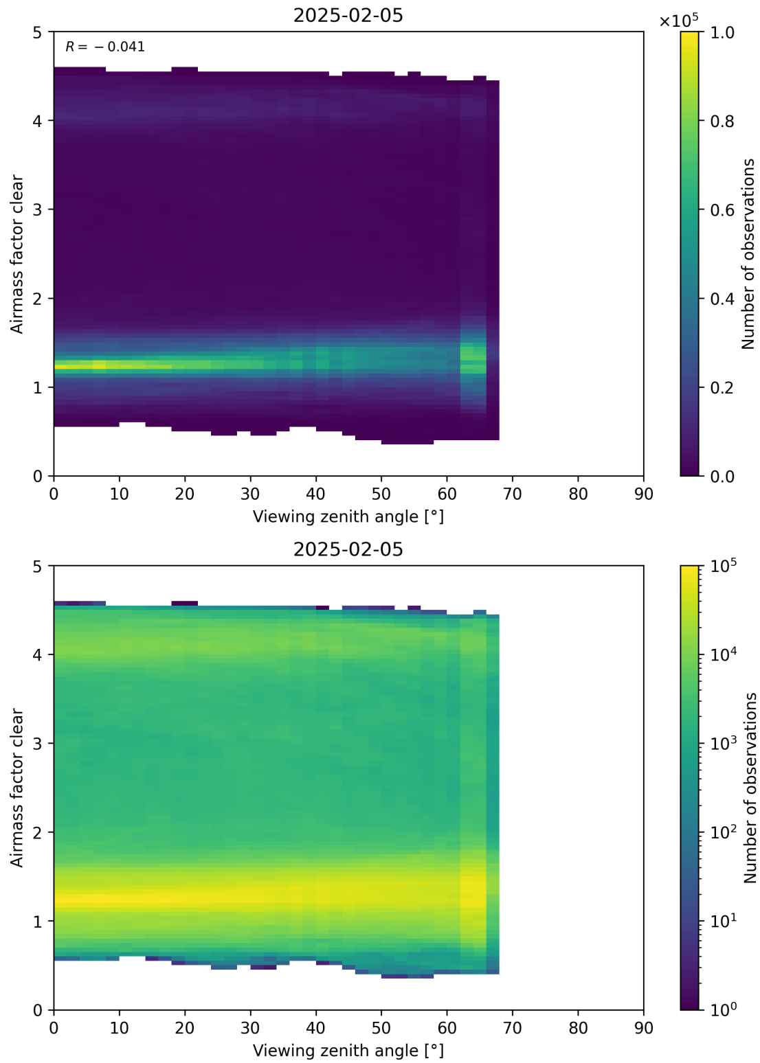
Figure 185: Scatter density plot of “Viewing zenith angle” against “Airmass factor clear” for 2025-02-04 to 2025-02-06.
