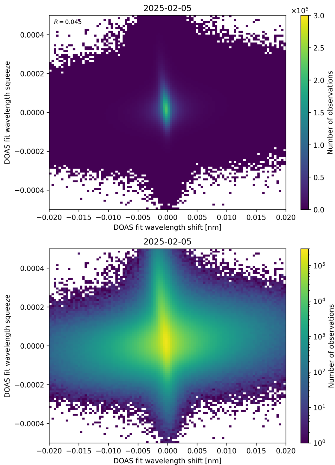
Figure 65: Scatter density plot of “DOAS fit wavelength shift” against “DOAS fit wavelength squeeze” for 2025-02-04 to 2025-02-06.
