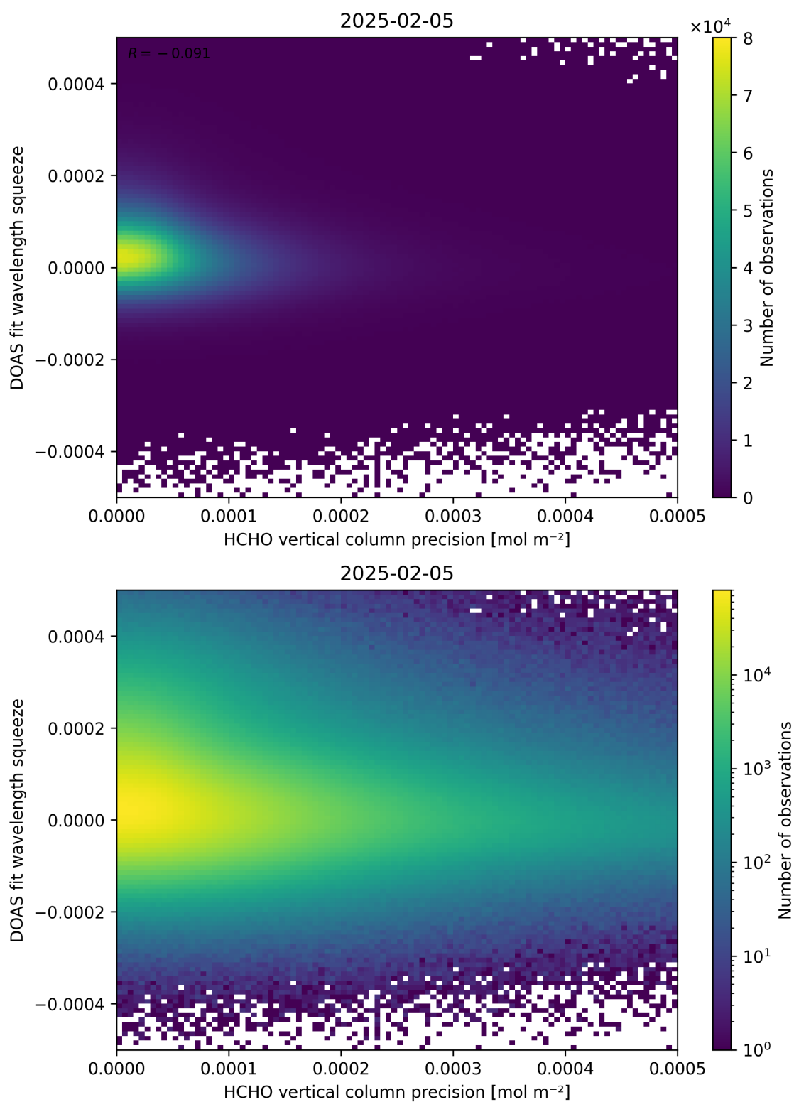
Figure 138: Scatter density plot of “HCHO vertical column precision” against “DOAS fit wavelength squeeze” for 2025-02-04 to 2025-02-06.
