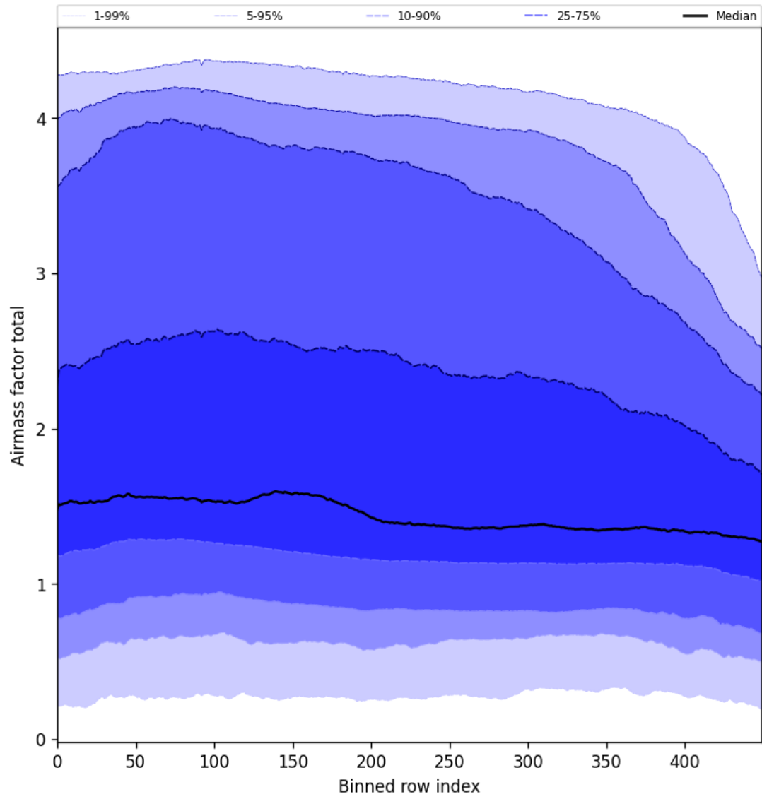
Figure 54: Along track statistics of “Airmass factor total” for 2025-02-04 to 2025-02-06
