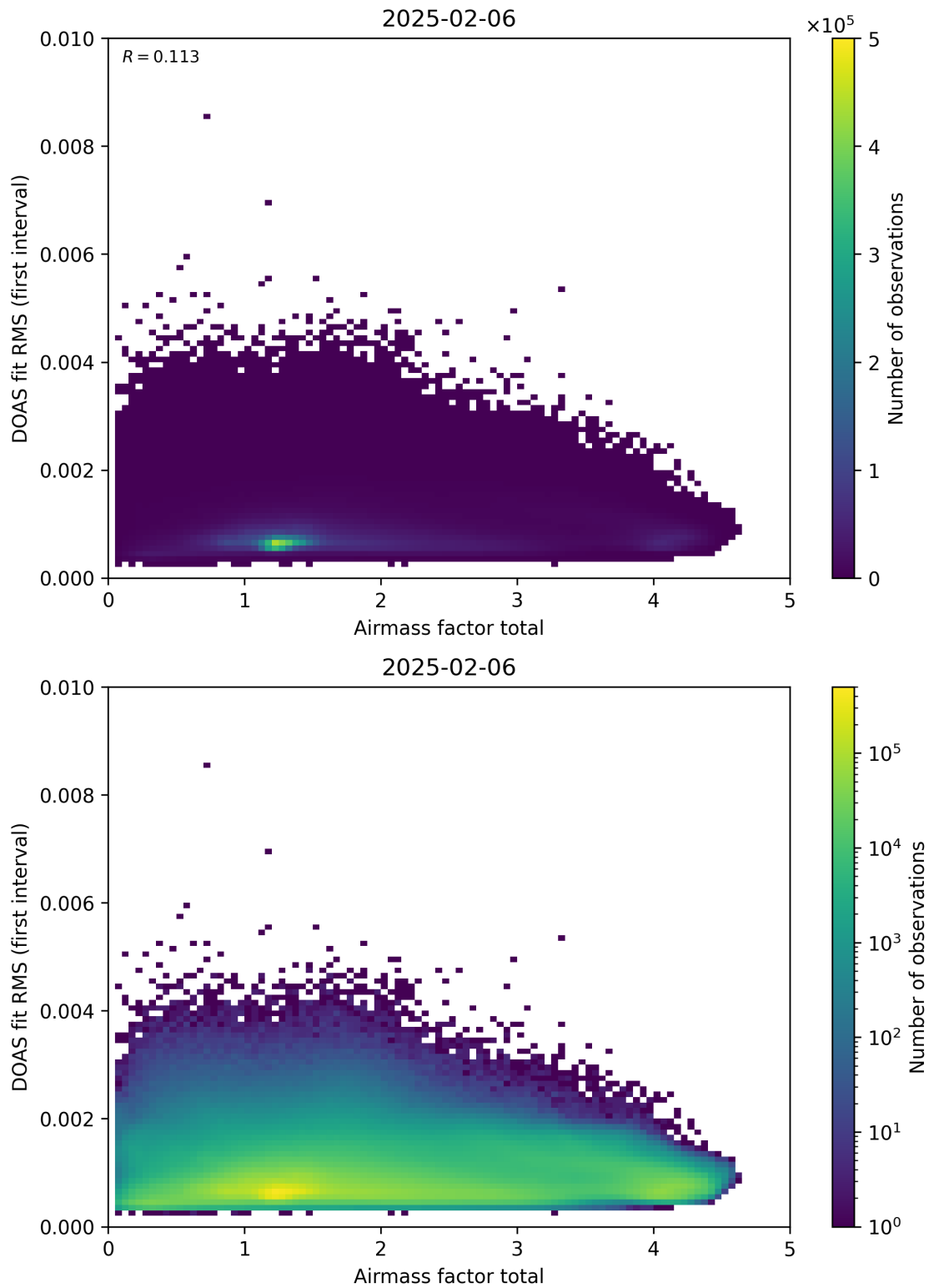
Figure 97: Scatter density plot of “Airmass factor total” against “DOAS fit RMS (first interval)” for 2025-02-05 to 2025-02-07.
