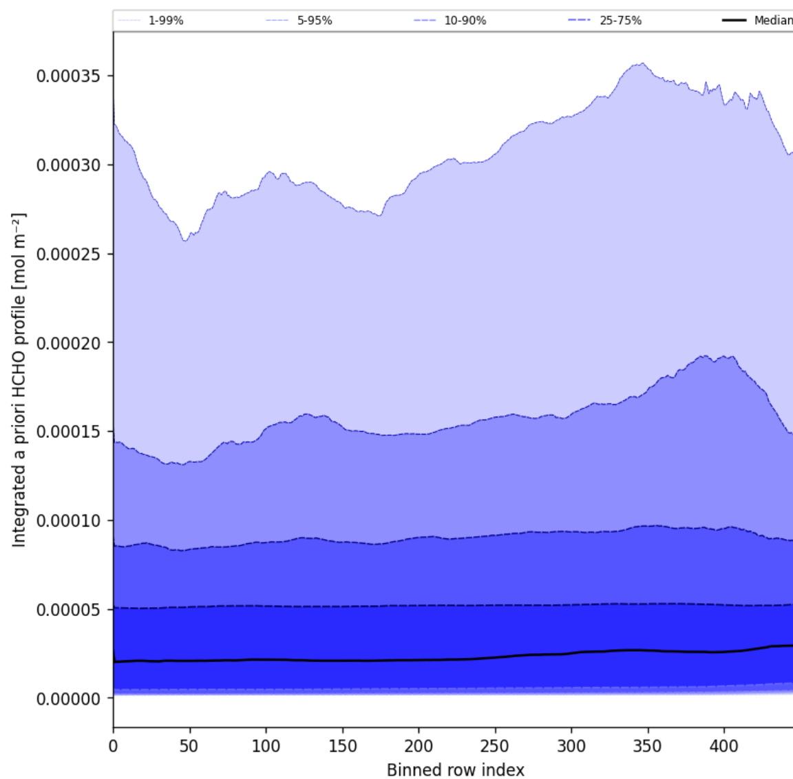
Figure 57: Along track statistics of “Integrated a priori HCHO profile” for 2025-02-05 to 2025-02-07
