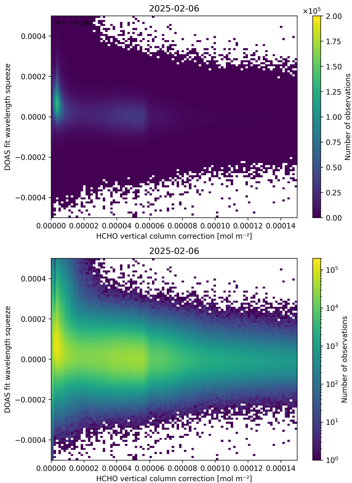
Figure 114: Scatter density plot of “HCHO vertical column correction” against “DOAS fit wavelength squeeze” for 2025-02-05 to 2025-02-07.
