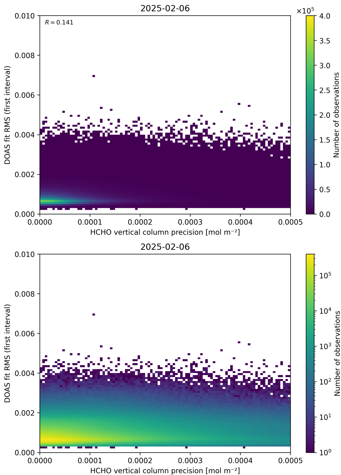
Figure 136: Scatter density plot of “HCHO vertical column precision” against “DOAS fit RMS (first interval)” for 2025-02-05 to 2025-02-07.
