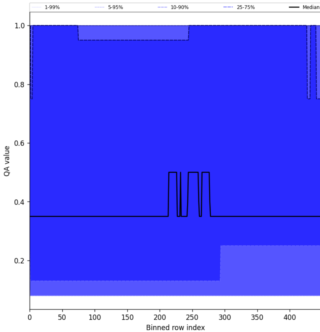
Figure 48: Along track statistics of “QA value” for 2025-02-05 to 2025-02-07
