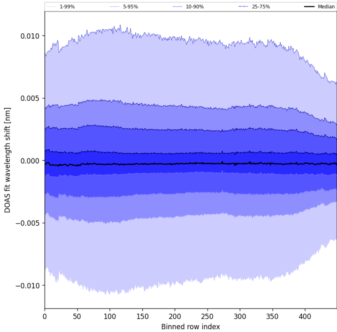
Figure 58: Along track statistics of “DOAS fit wavelength shift” for 2025-02-05 to 2025-02-07
