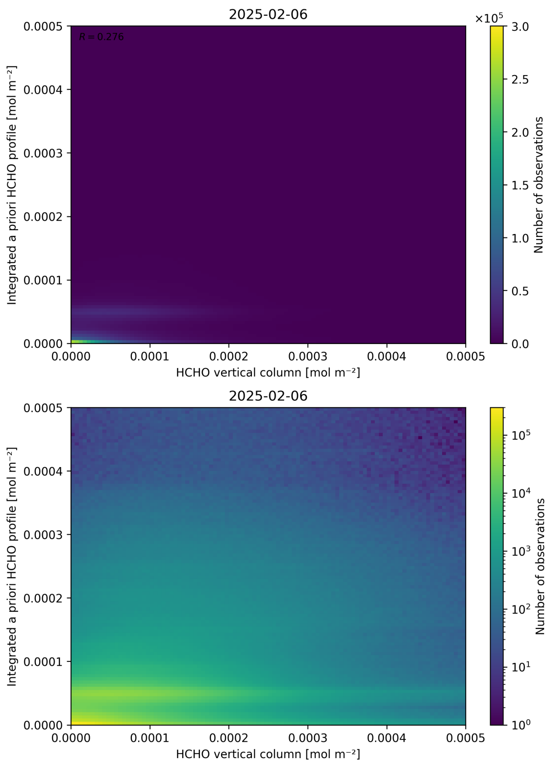
Figure 135: Scatter density plot of “HCHO vertical column” against “Integrated a priori HCHO profile” for 2025-02-05 to 2025-02-07.
