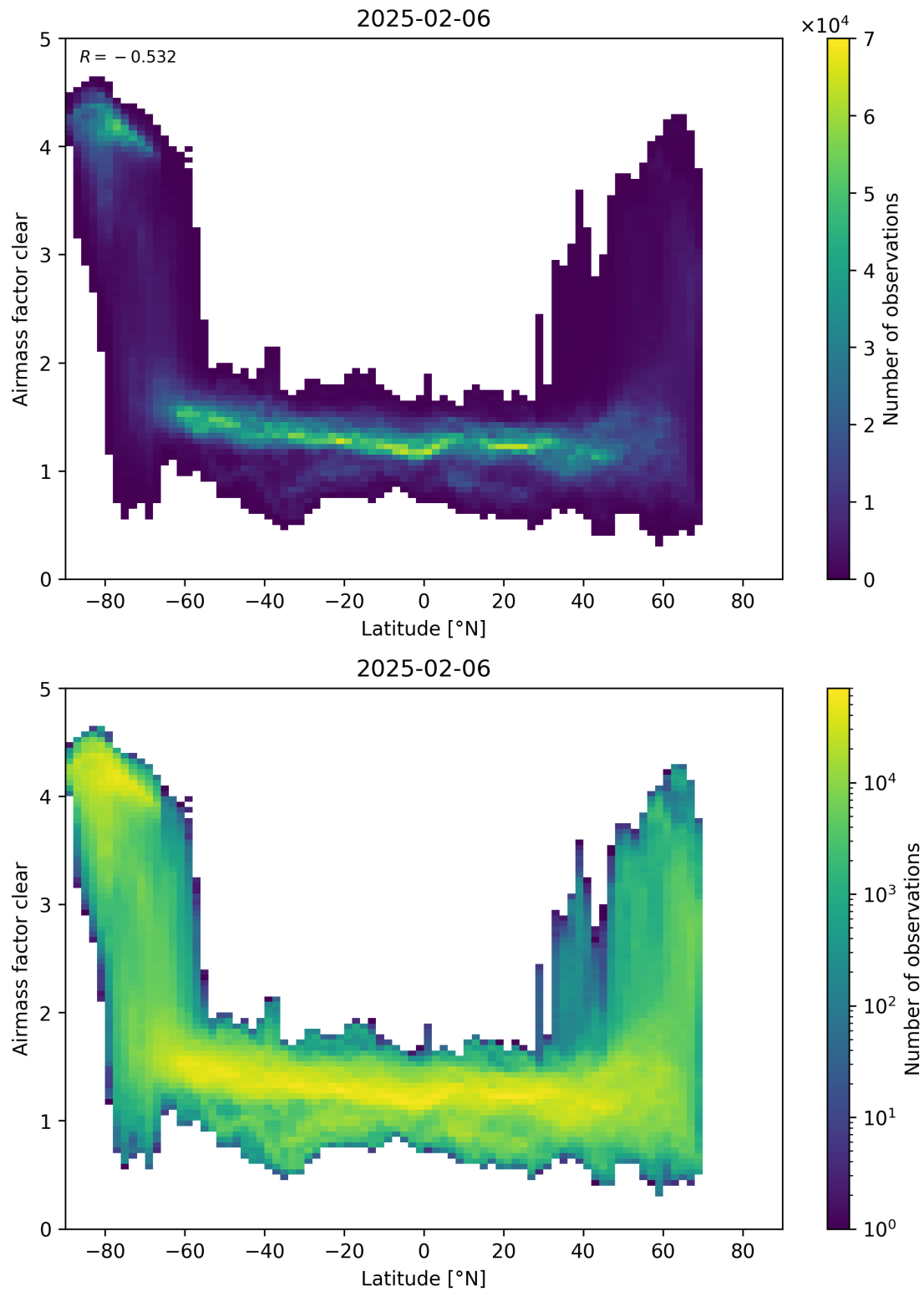
Figure 156: Scatter density plot of “Latitude” against “Airmass factor clear” for 2025-02-05 to 2025-02-07.
