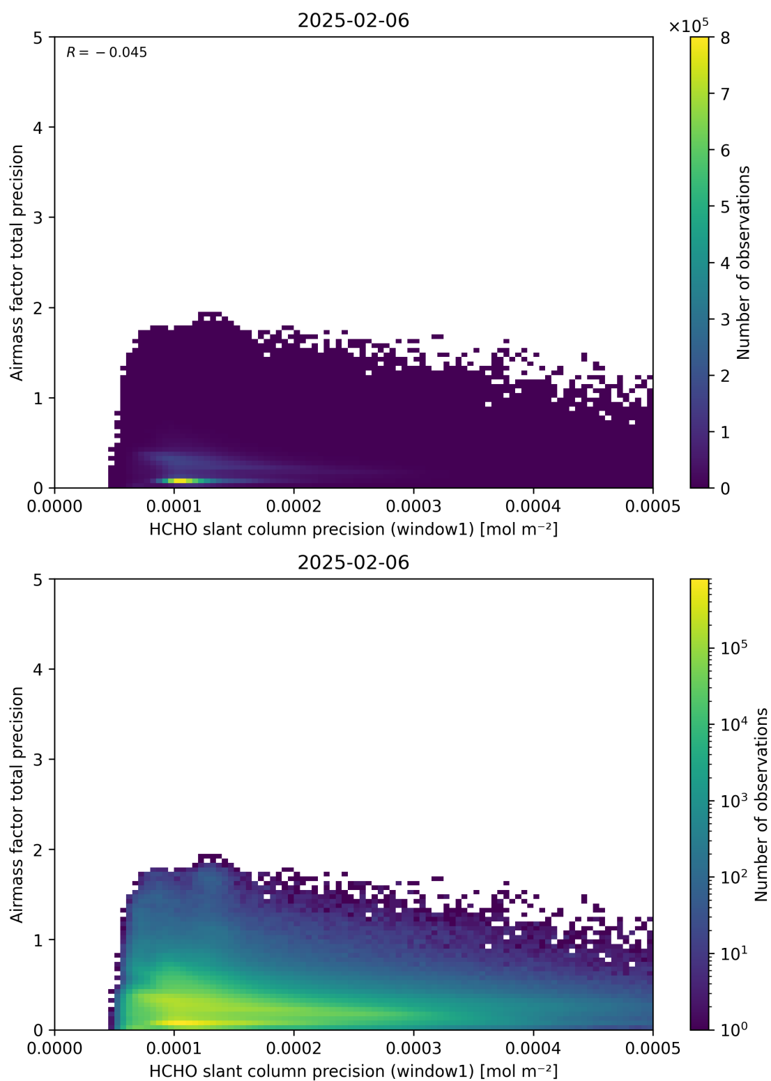
Figure 95: Scatter density plot of “HCHO slant column precision (window1)” against “Airmass factor total precision” for 2025-02-05 to 2025-02-07.
