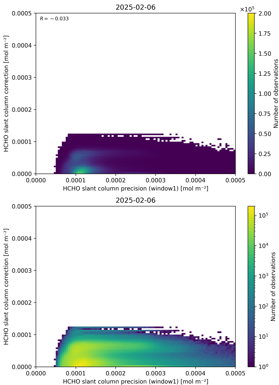
Figure 93: Scatter density plot of “HCHO slant column precision (window1)” against “HCHO slant column correction” for 2025-02-05 to 2025-02-07.
