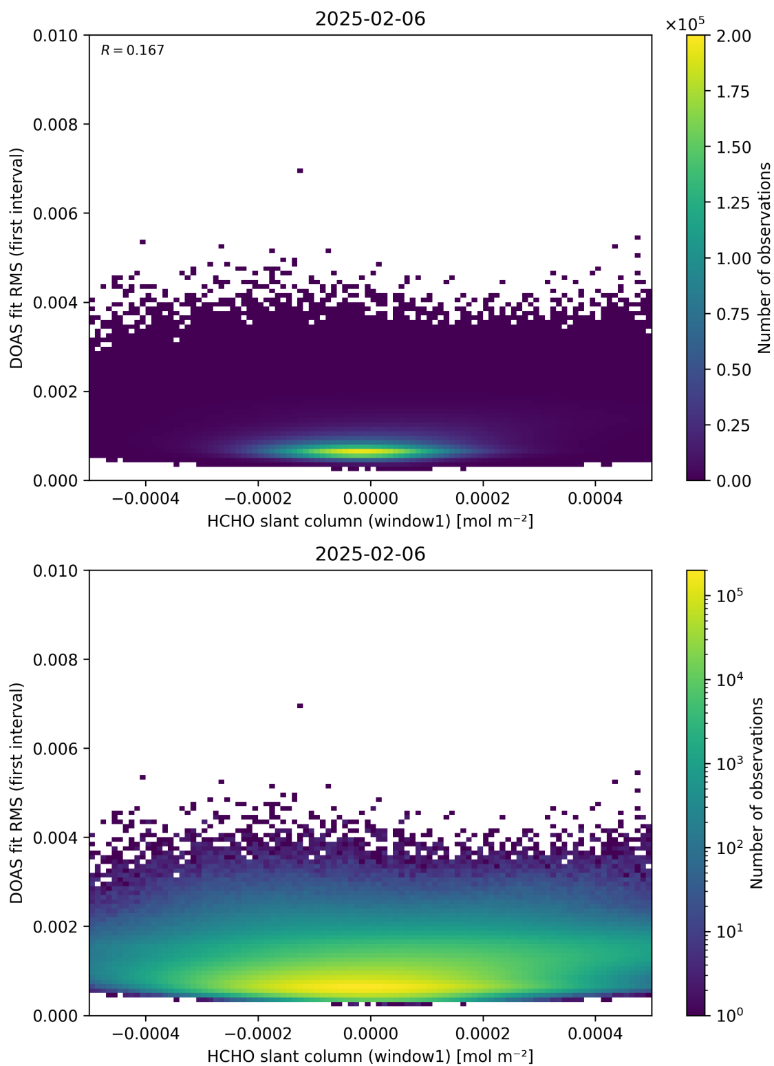
Figure 78: Scatter density plot of “HCHO slant column (window1)” against “DOAS fit RMS (first interval)” for 2025-02-05 to 2025-02-07.
