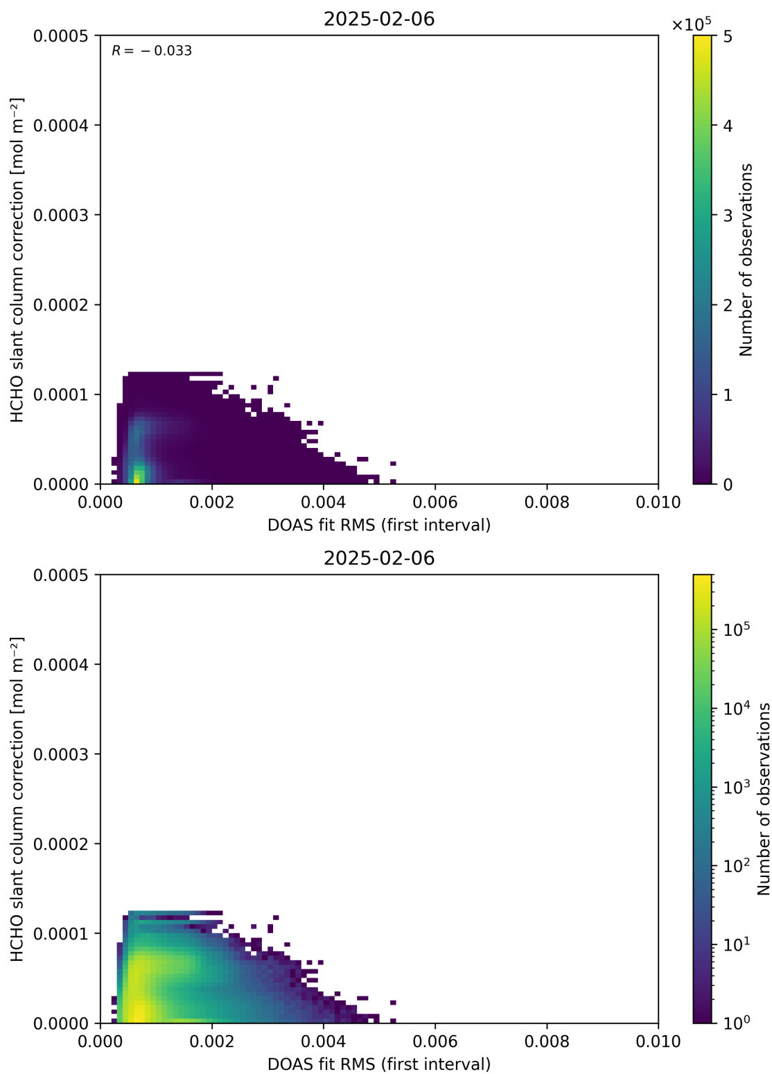
Figure 63: Scatter density plot of “DOAS fit RMS (first interval)” against “HCHO slant column correction” for 2025-02-05 to 2025-02-07.
