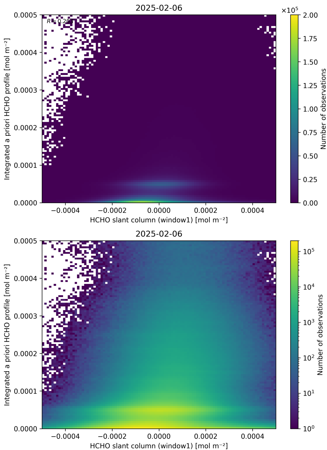
Figure 87: Scatter density plot of “HCHO slant column (window1)” against “Integrated a priori HCHO profile” for 2025-02-05 to 2025-02-07.
