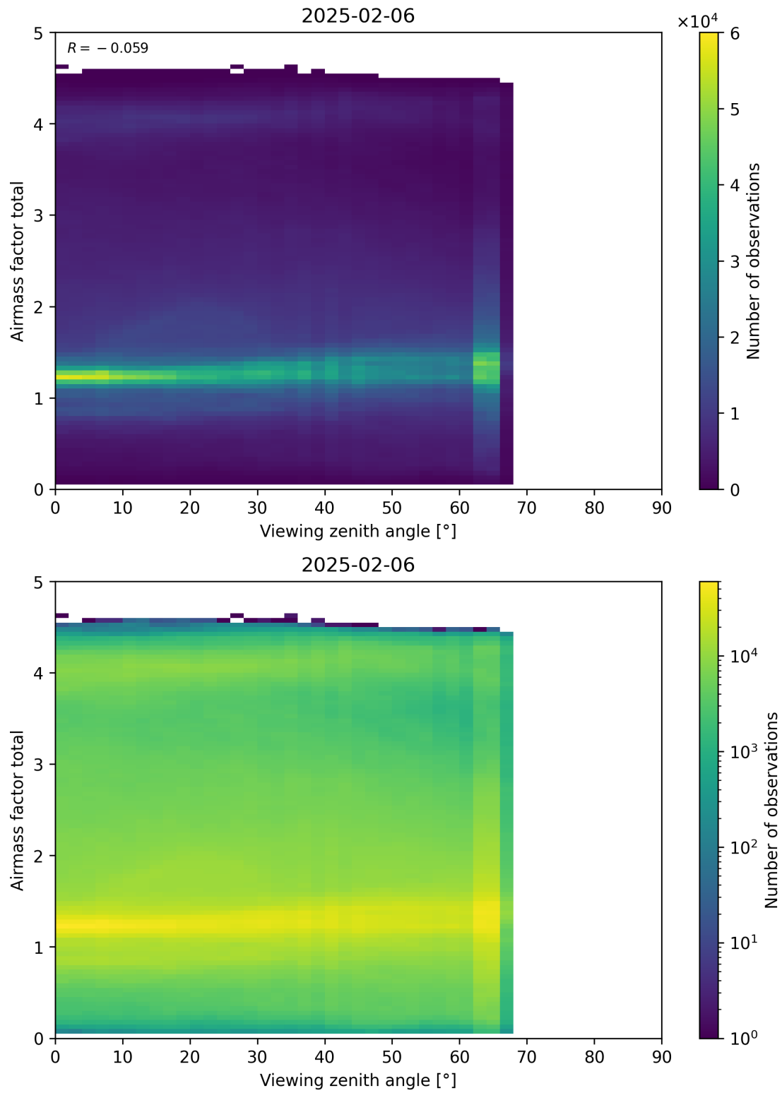
Figure 190: Scatter density plot of “Viewing zenith angle” against “Airmass factor total” for 2025-02-05 to 2025-02-07.
