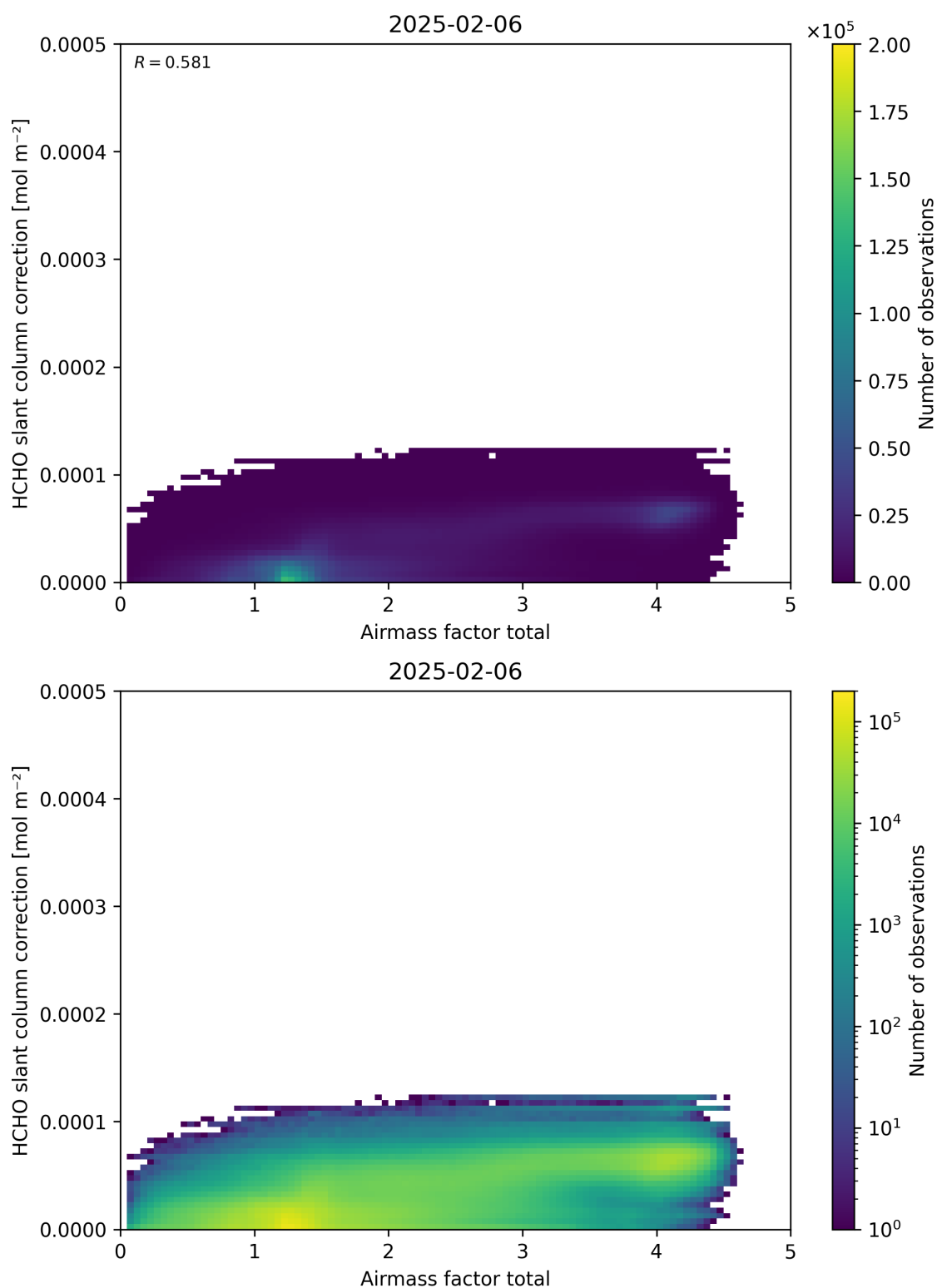
Figure 102: Scatter density plot of “Airmass factor total” against “HCHO slant column correction” for 2025-02-05 to 2025-02-07.
