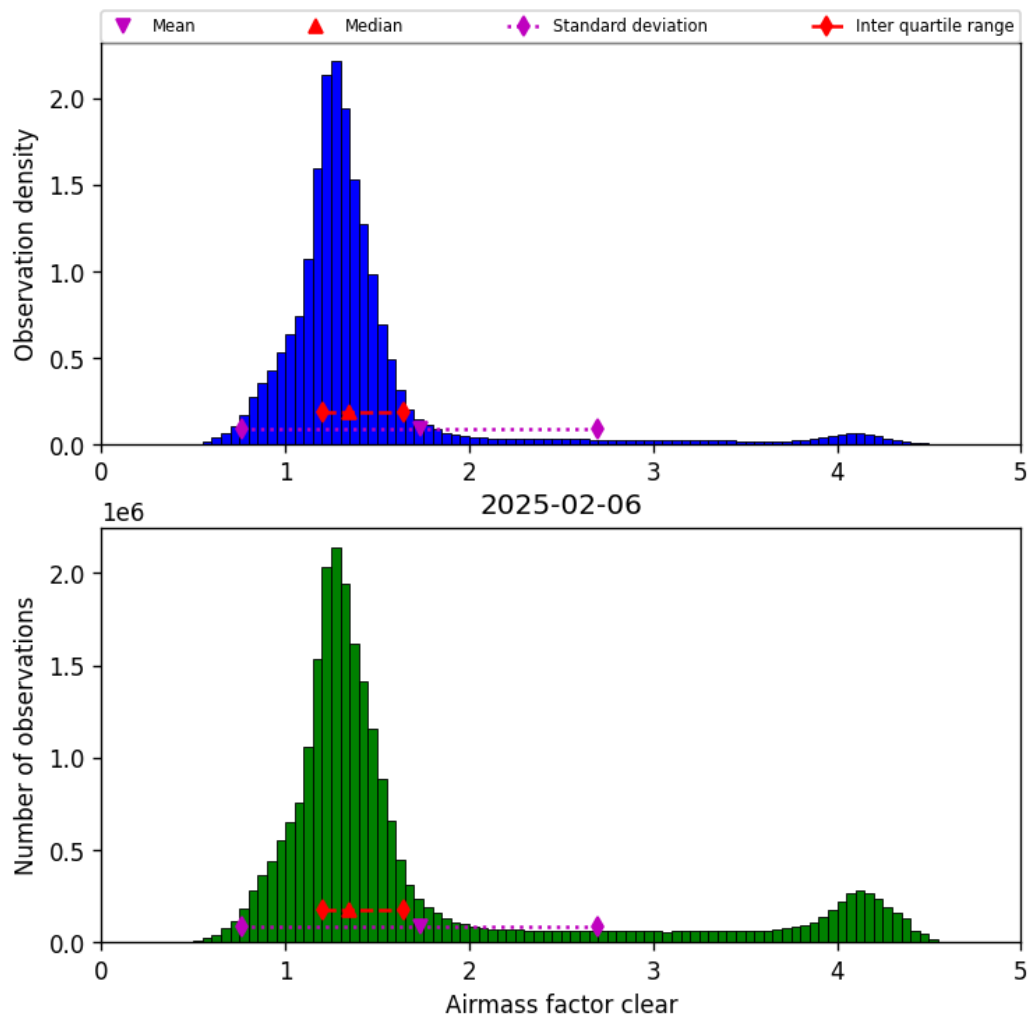
Figure 42: Histogram of “Airmass factor clear” for 2025-02-05 to 2025-02-07
