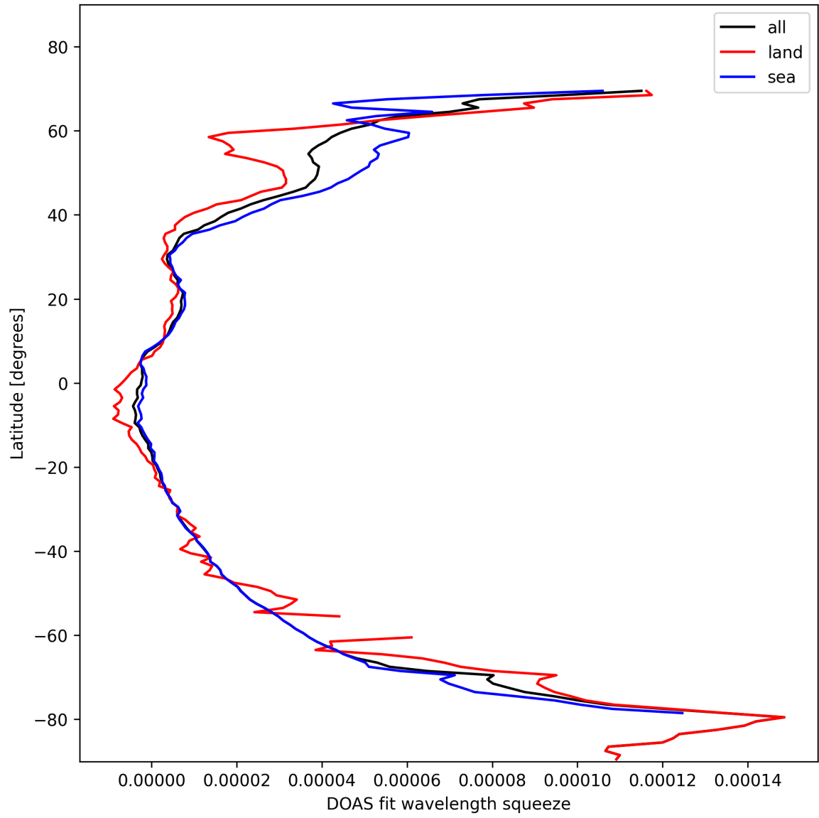
Figure 31: Zonal average of “DOAS fit wavelength squeeze” for 2025-02-05 to 2025-02-07.
