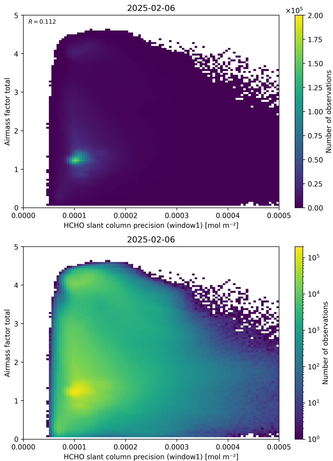
Figure 94: Scatter density plot of “HCHO slant column precision (window1)” against “Airmass factor total” for 2025-02-05 to 2025-02-07.
