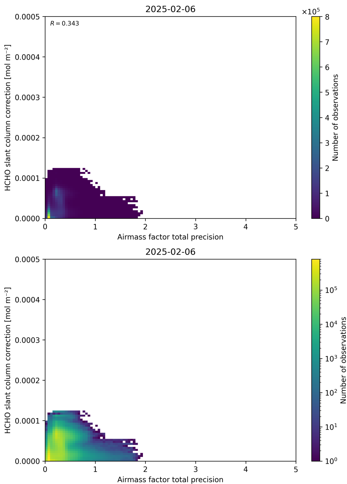
Figure 110: Scatter density plot of “Airmass factor total precision” against “HCHO slant column correction” for 2025-02-05 to 2025-02-07.
