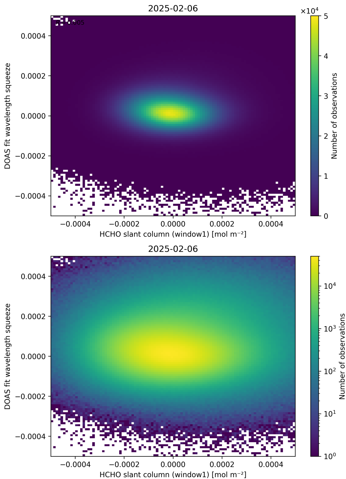
Figure 80: Scatter density plot of “HCHO slant column (window1)” against “DOAS fit wavelength squeeze” for 2025-02-05 to 2025-02-07.
