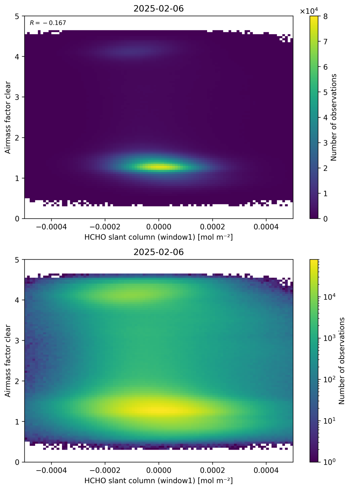
Figure 81: Scatter density plot of “HCHO slant column (window1)” against “Airmass factor clear” for 2025-02-05 to 2025-02-07.
