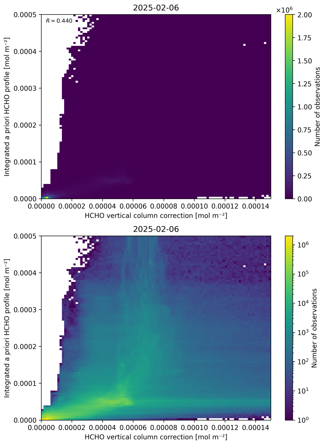
Figure 122: Scatter density plot of “HCHO vertical column correction” against “Integrated a priori HCHO profile” for 2025-02-05 to 2025-02-07.
