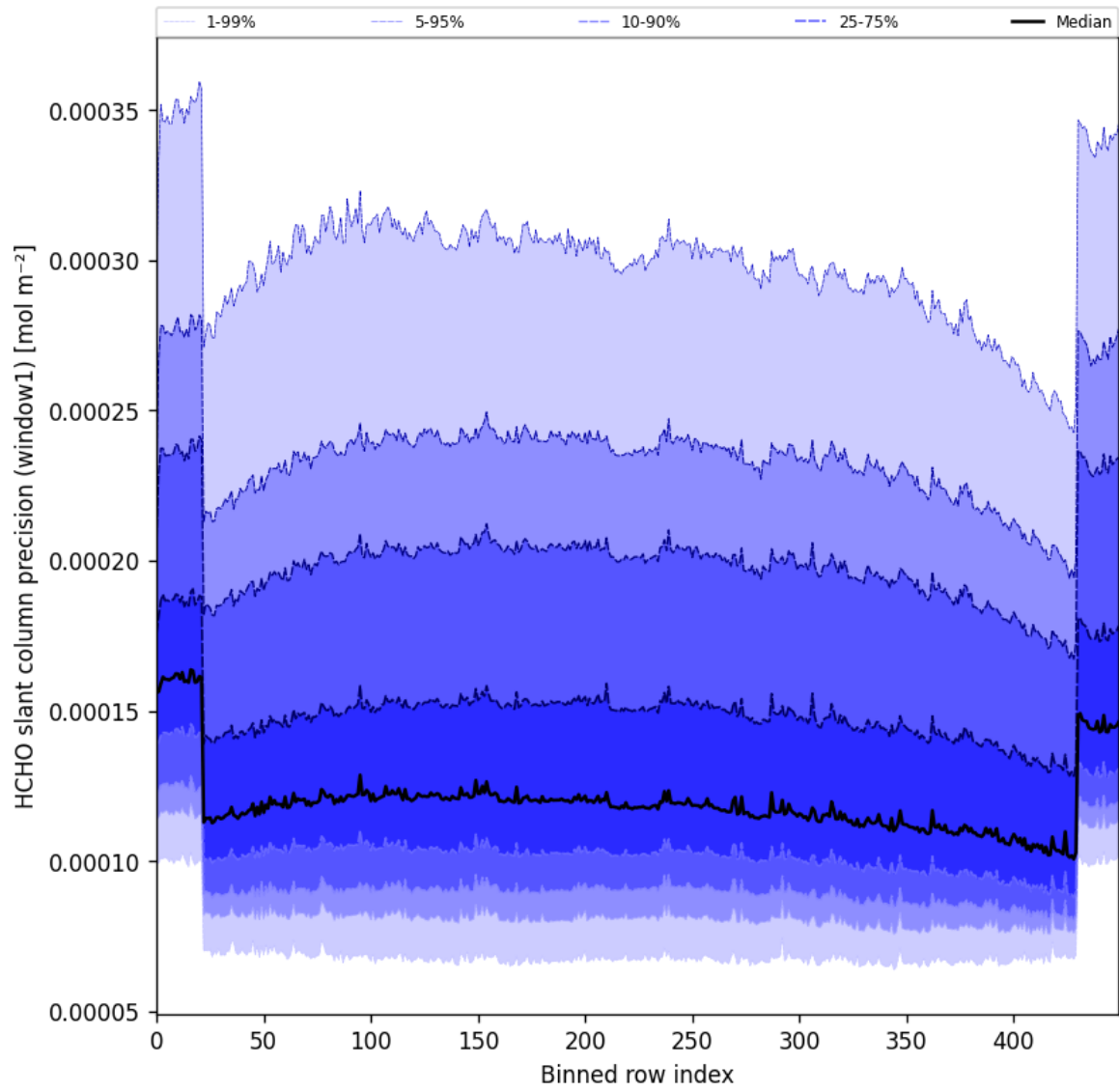
Figure 53: Along track statistics of “HCHO slant column precision (window1)” for 2025-02-05 to 2025-02-07
