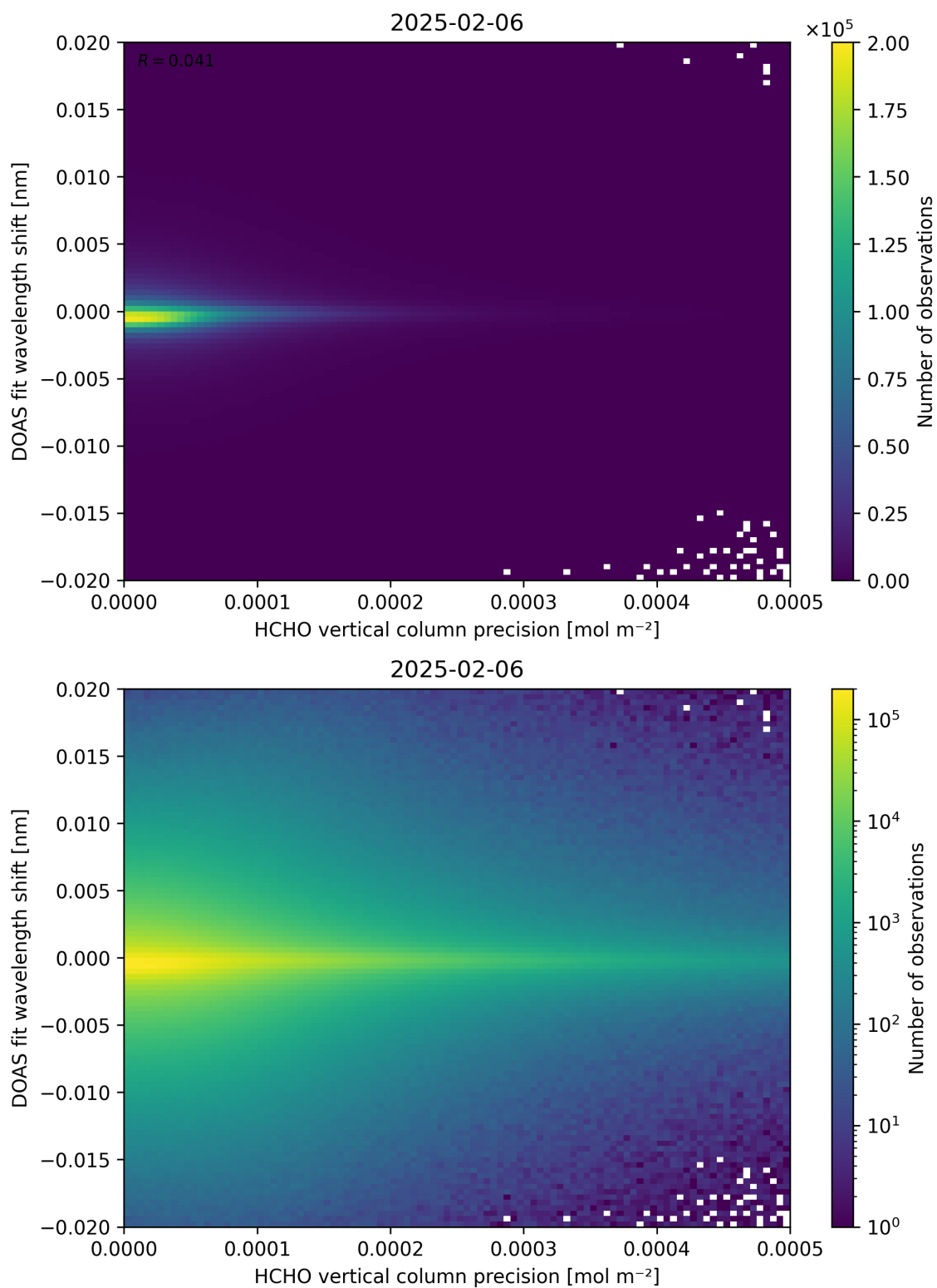
Figure 137: Scatter density plot of “HCHO vertical column precision” against “DOAS fit wavelength shift” for 2025-02-05 to 2025-02-07.
