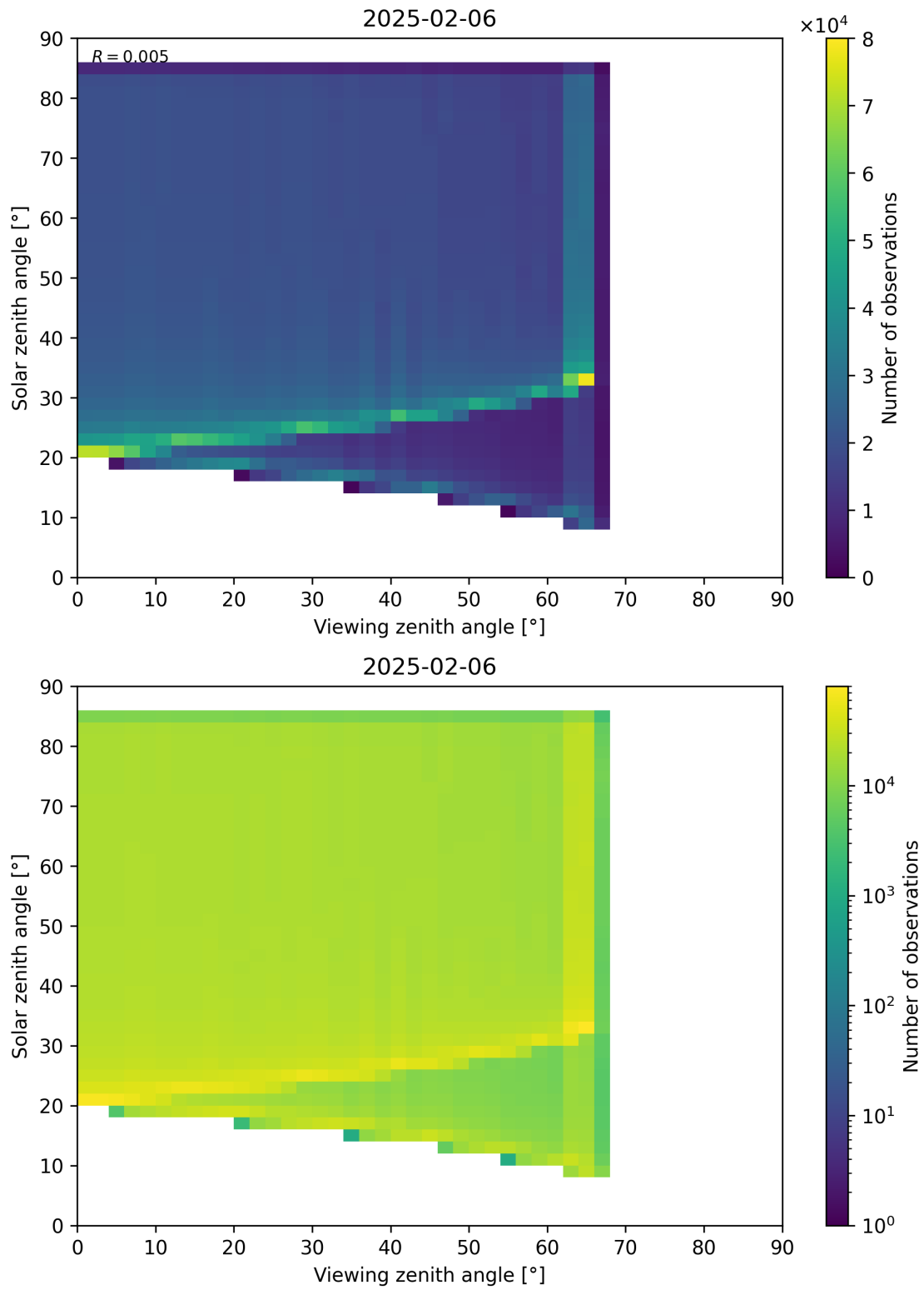
Figure 197: Scatter density plot of “Viewing zenith angle” against “Solar zenith angle” for 2025-02-05 to 2025-02-07.
