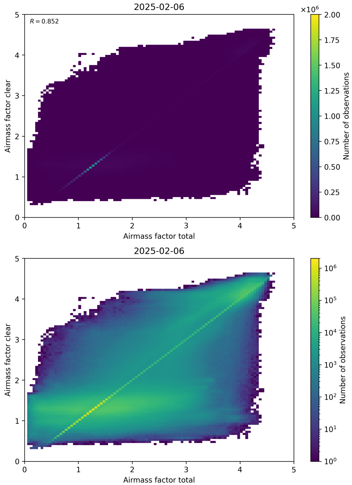
Figure 100: Scatter density plot of “Airmass factor total” against “Airmass factor clear” for 2025-02-05 to 2025-02-07.
