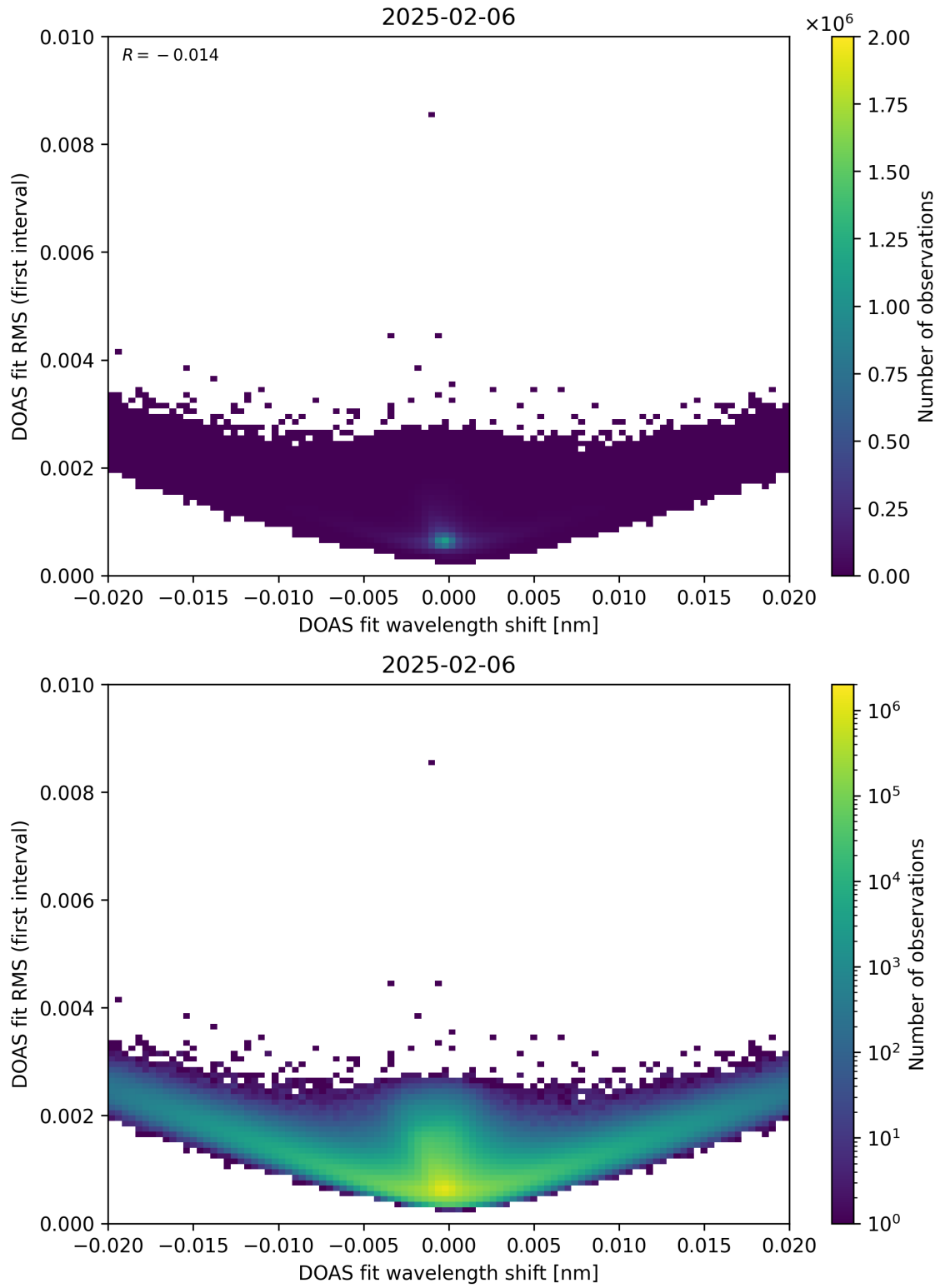
Figure 64: Scatter density plot of “DOAS fit wavelength shift” against “DOAS fit RMS (first interval)” for 2025-02-05 to 2025-02-07.
