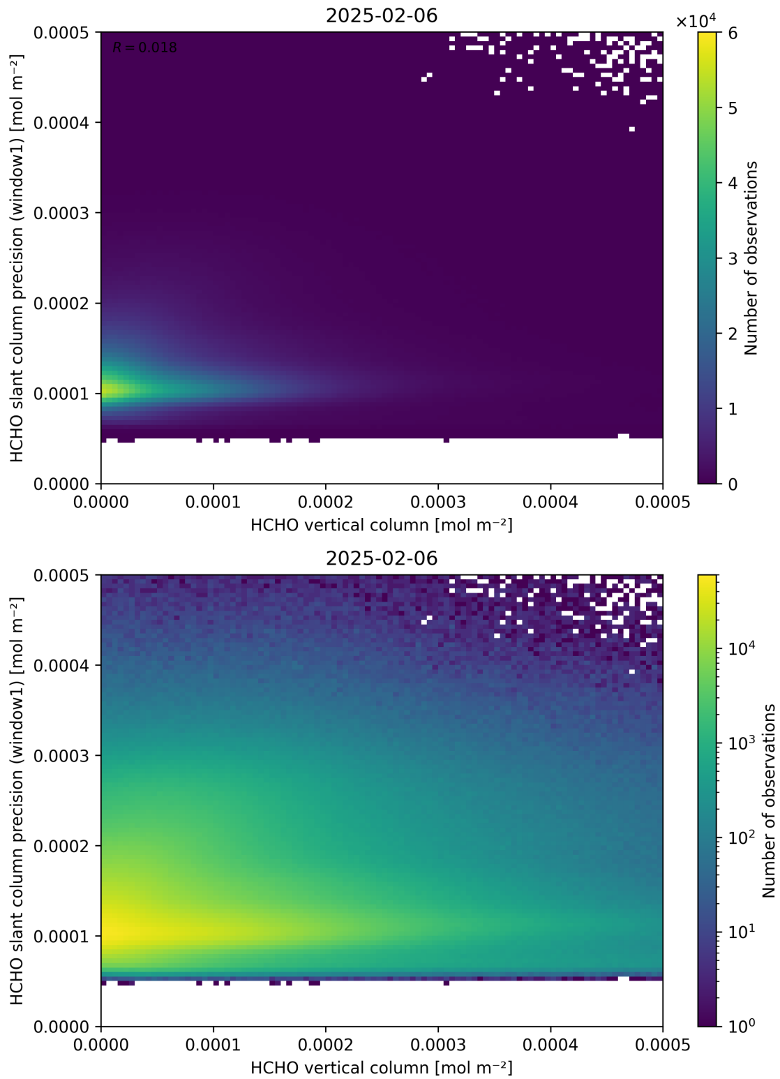
Figure 130: Scatter density plot of “HCHO vertical column” against “HCHO slant column precision (window1)” for 2025-02-05 to 2025-02-07.
