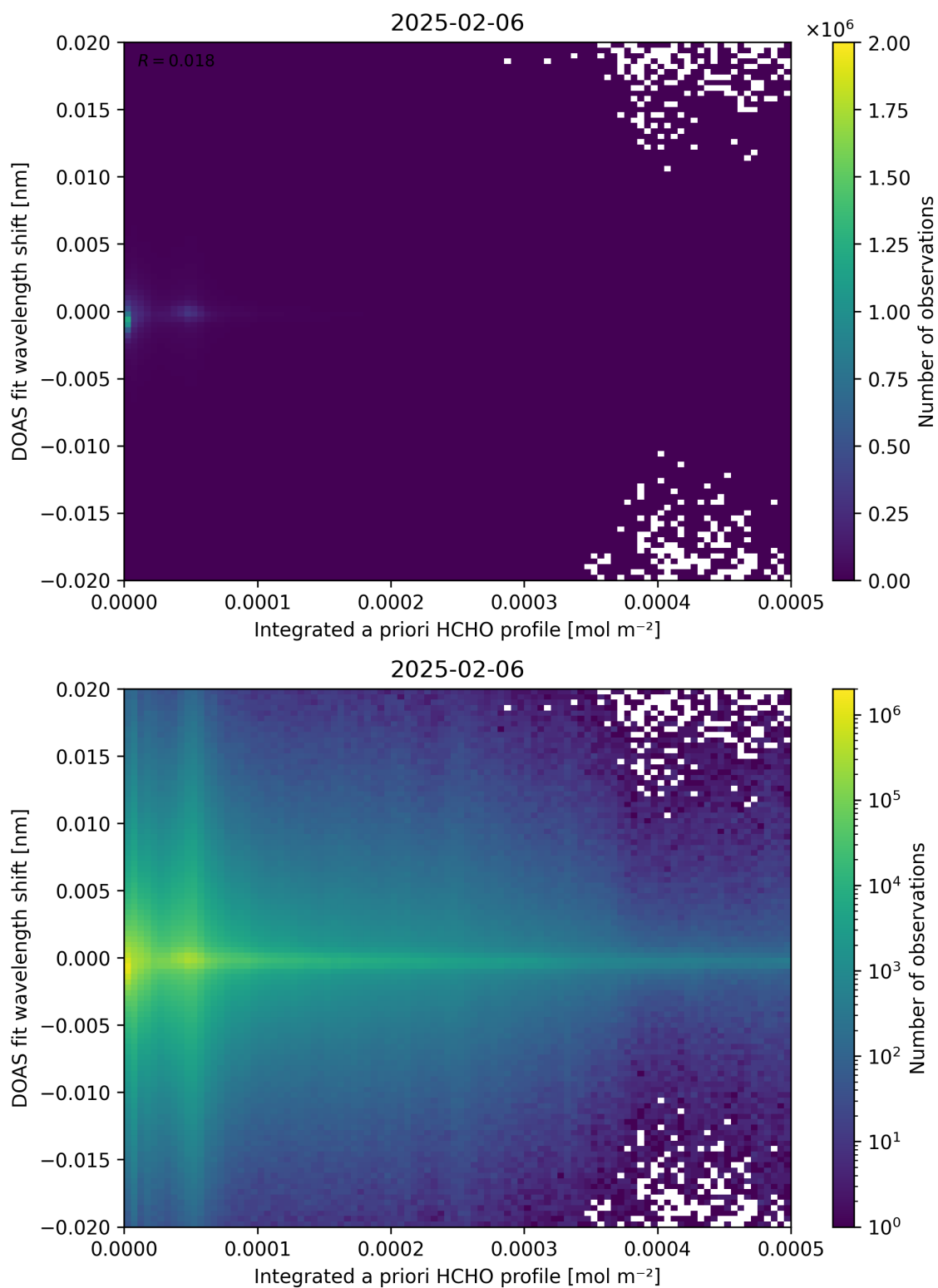
Figure 149: Scatter density plot of “Integrated a priori HCHO profile” against “DOAS fit wavelength shift” for 2025-02-05 to 2025-02-07.
