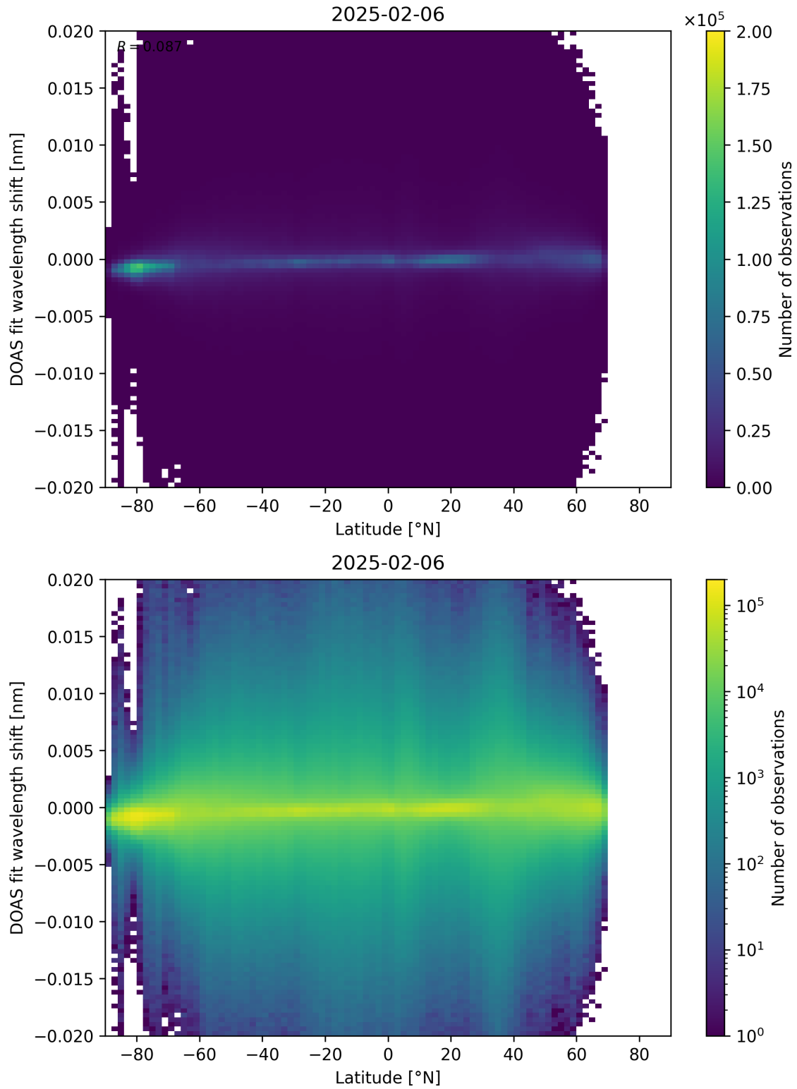
Figure 154: Scatter density plot of “Latitude” against “DOAS fit wavelength shift” for 2025-02-05 to 2025-02-07.
