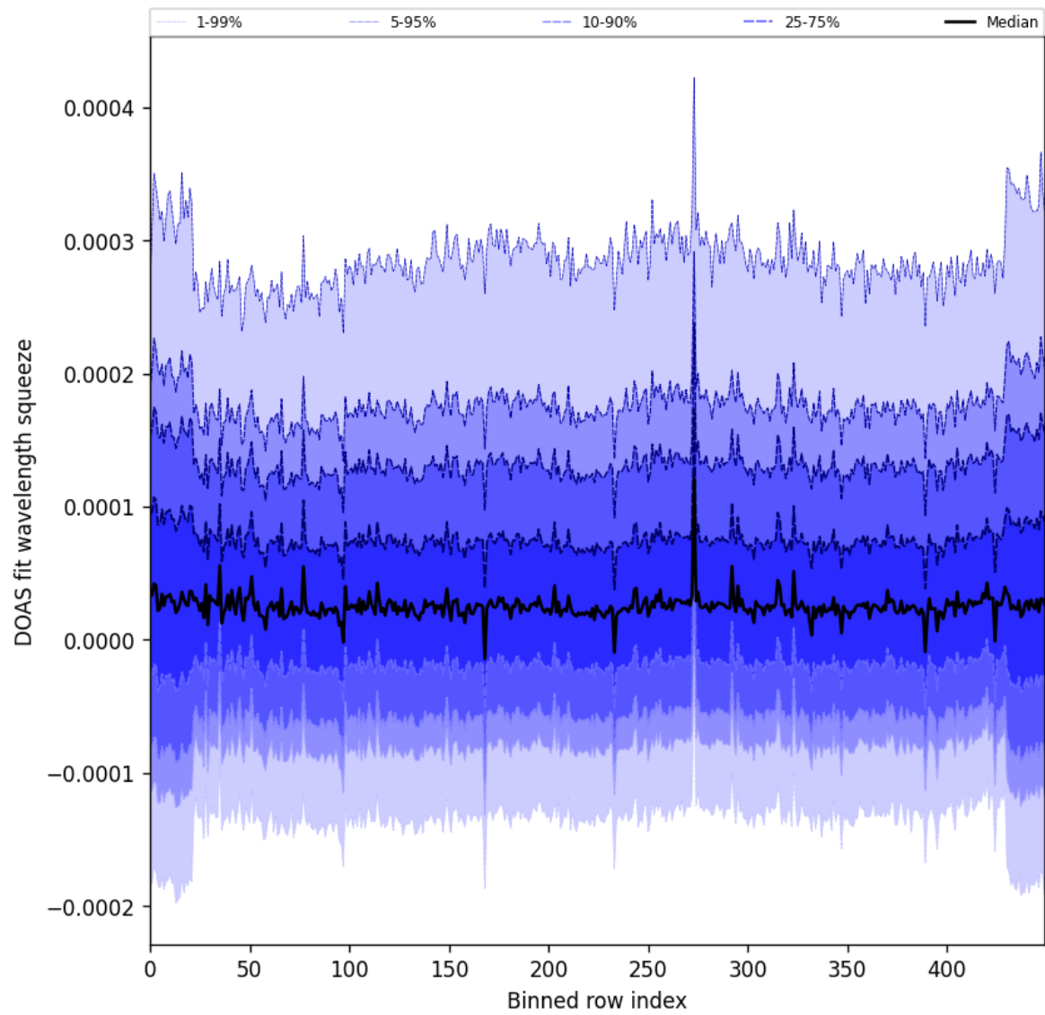
Figure 59: Along track statistics of “DOAS fit wavelength squeeze” for 2025-02-05 to 2025-02-07
