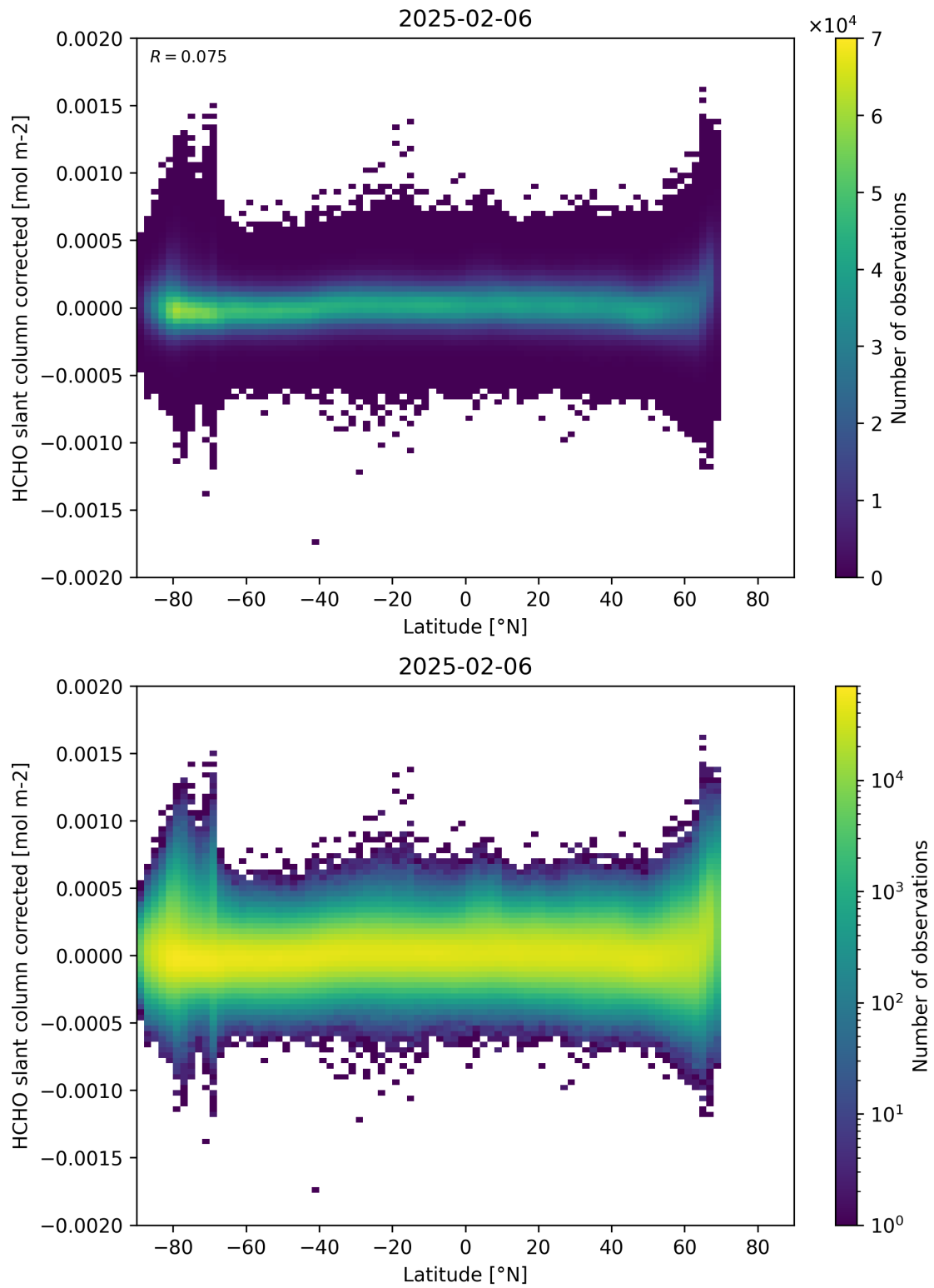
Figure 157: Scatter density plot of “Latitude” against “HCHO slant column corrected” for 2025-02-05 to 2025-02-07.
