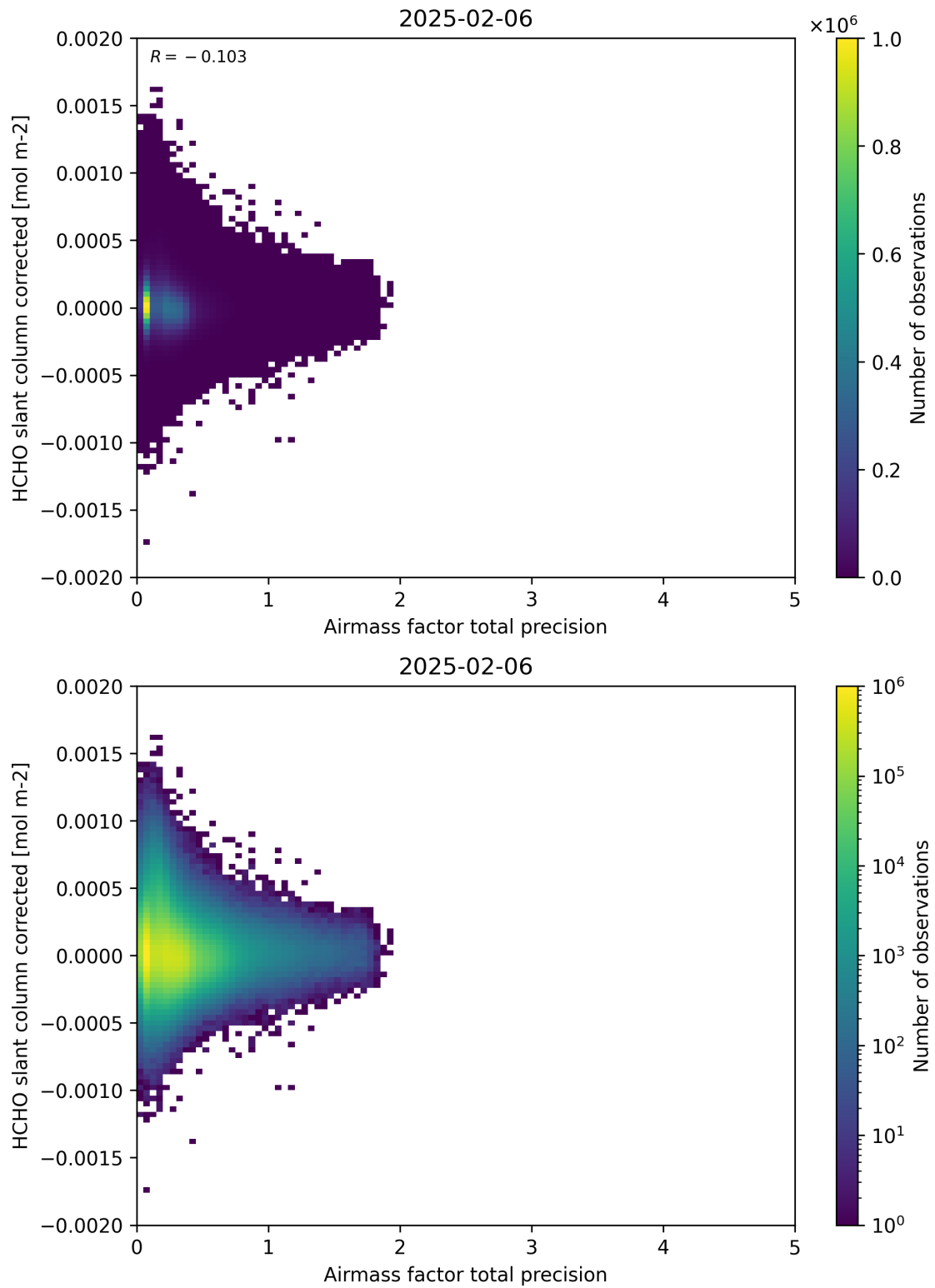
Figure 109: Scatter density plot of “Airmass factor total precision” against “HCHO slant column corrected” for 2025-02-05 to 2025-02-07.
