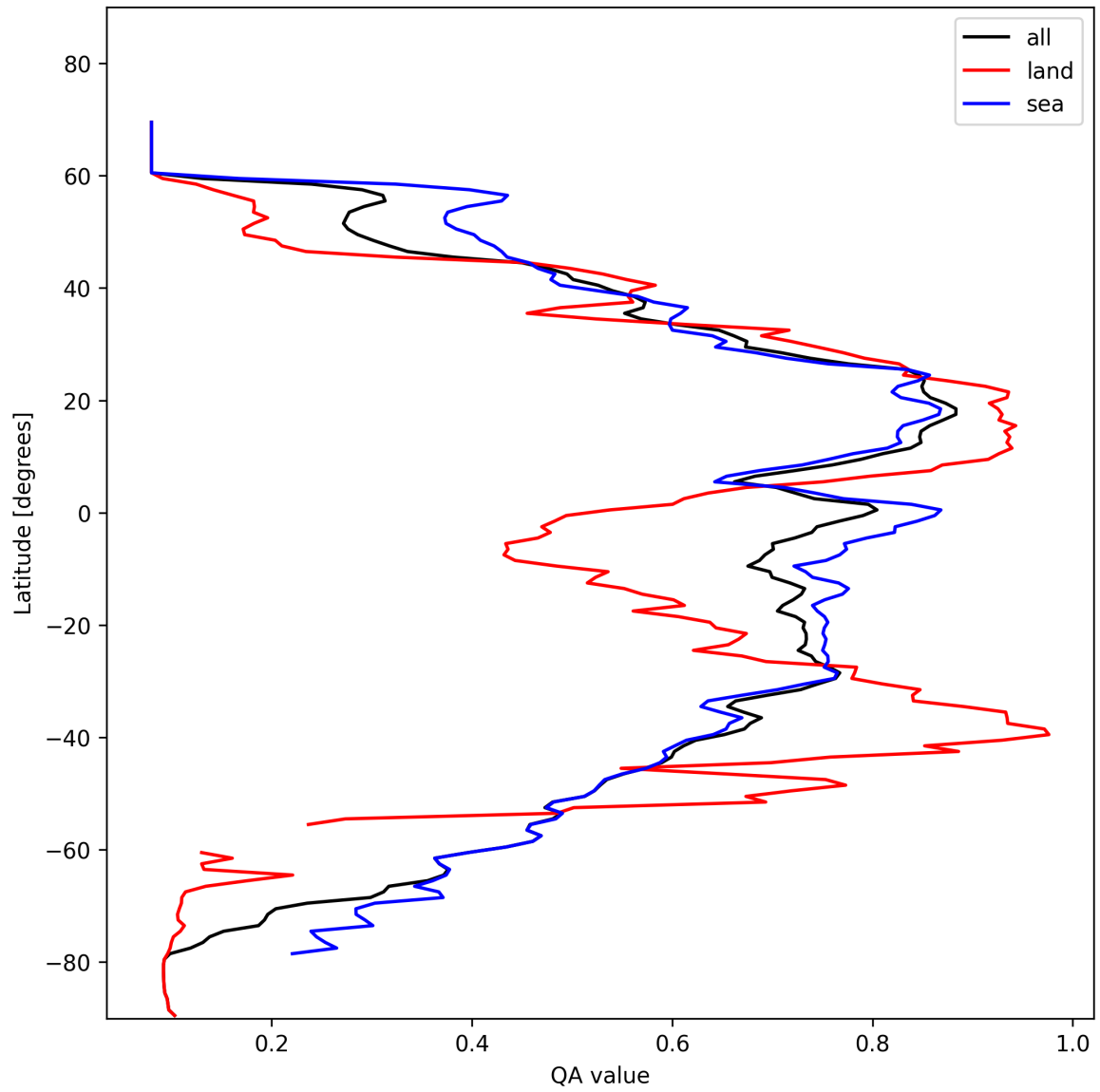
Figure 20: Zonal average of “QA value” for 2025-02-05 to 2025-02-07.
