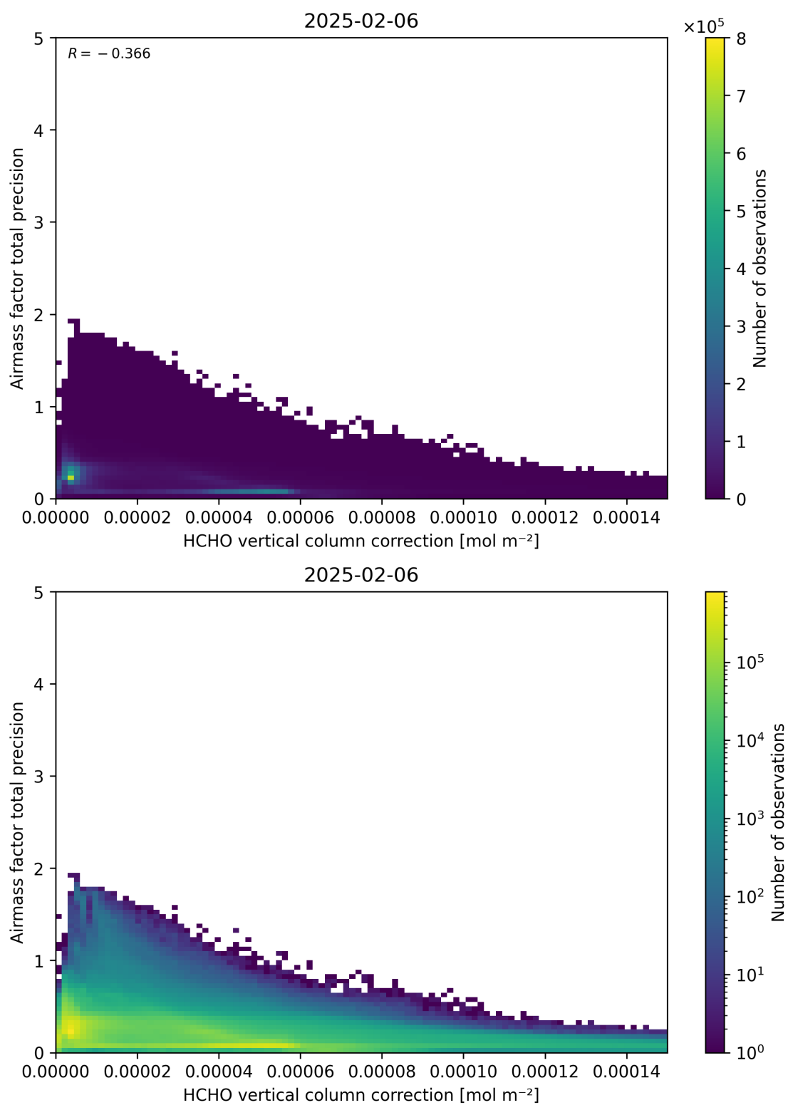
Figure 121: Scatter density plot of “HCHO vertical column correction” against “Airmass factor total precision” for 2025-02-05 to 2025-02-07.
