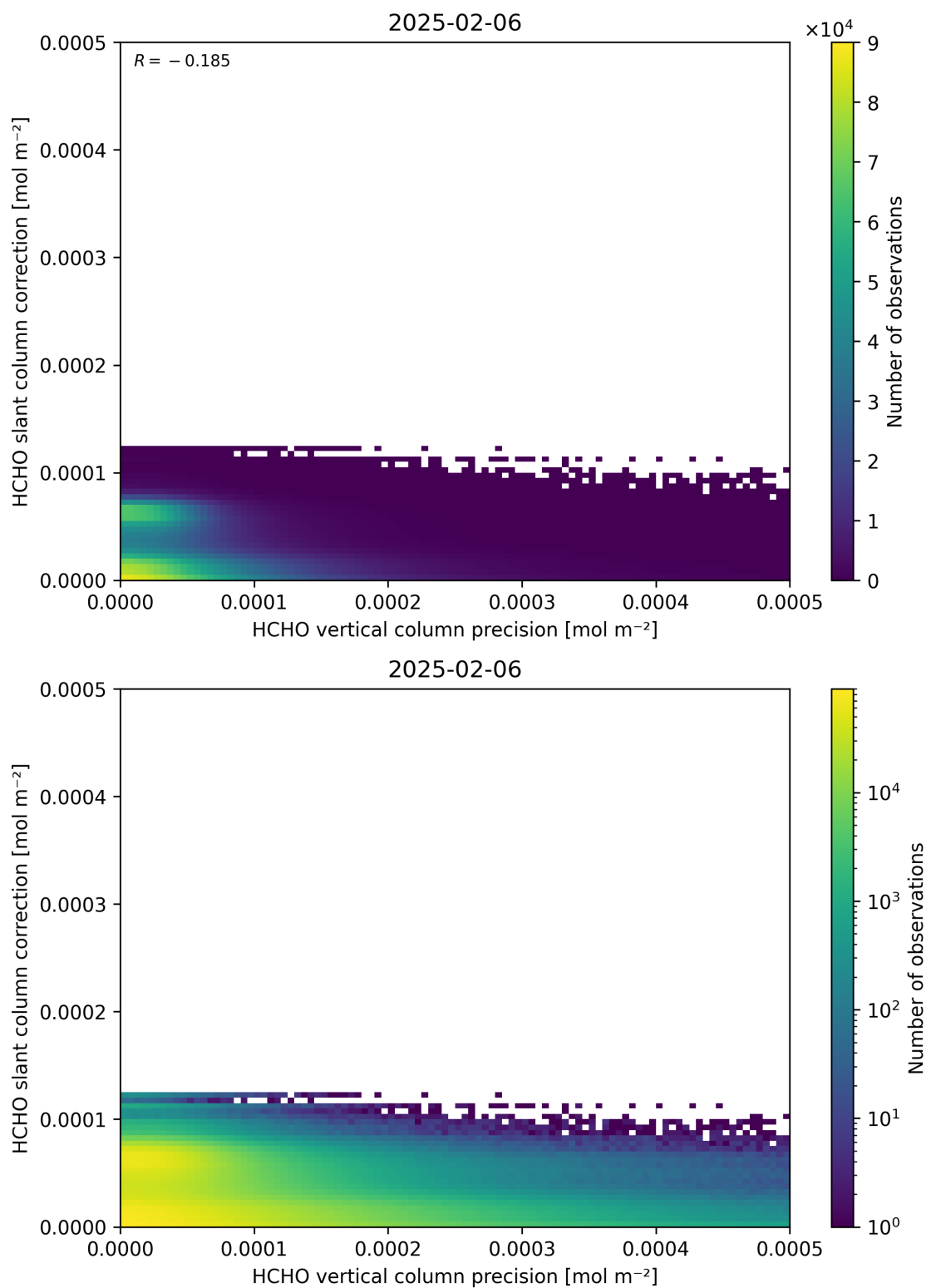
Figure 141: Scatter density plot of “HCHO vertical column precision” against “HCHO slant column correction” for 2025-02-05 to 2025-02-07.
