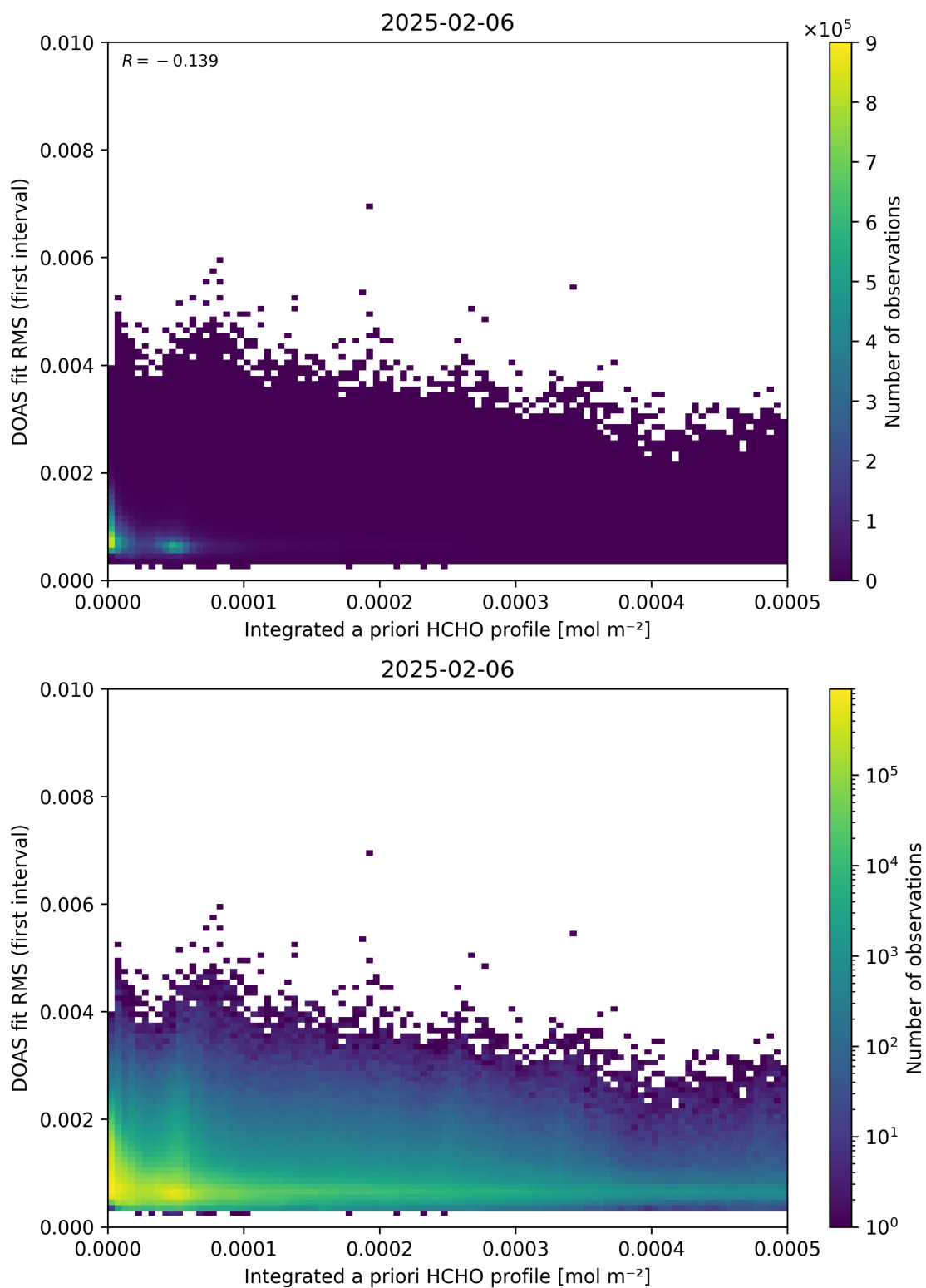
Figure 148: Scatter density plot of “Integrated a priori HCHO profile” against “DOAS fit RMS (first interval)” for 2025-02-05 to 2025-02-07.
