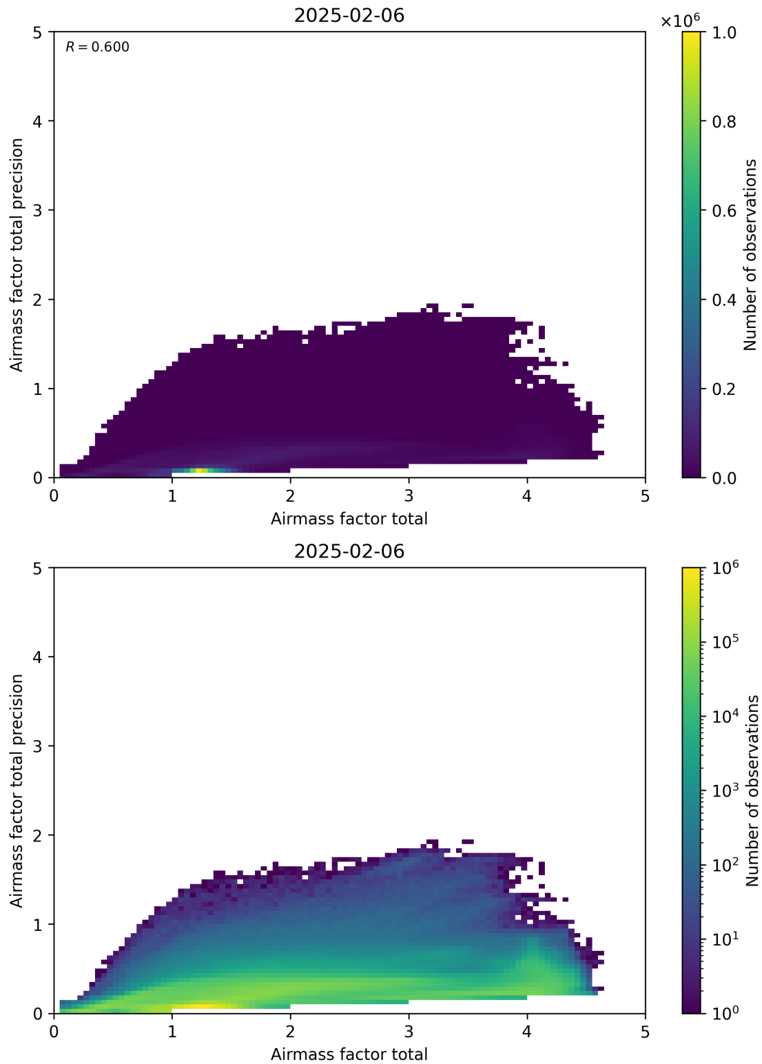
Figure 103: Scatter density plot of “Airmass factor total” against “Airmass factor total precision” for 2025-02-05 to 2025-02-07.
