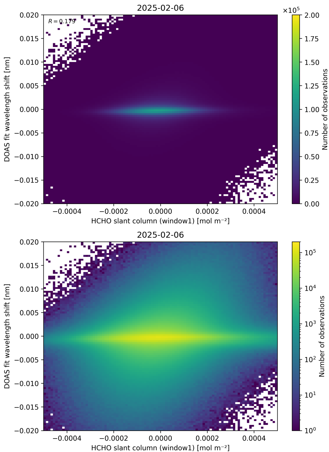
Figure 79: Scatter density plot of “HCHO slant column (window1)” against “DOAS fit wavelength shift” for 2025-02-05 to 2025-02-07.
