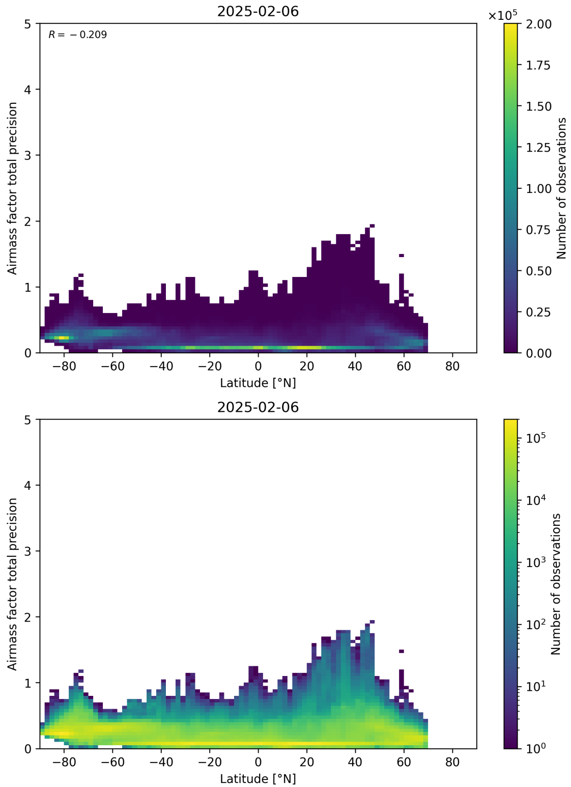
Figure 162: Scatter density plot of “Latitude” against “Airmass factor total precision” for 2025-02-05 to 2025-02-07.
