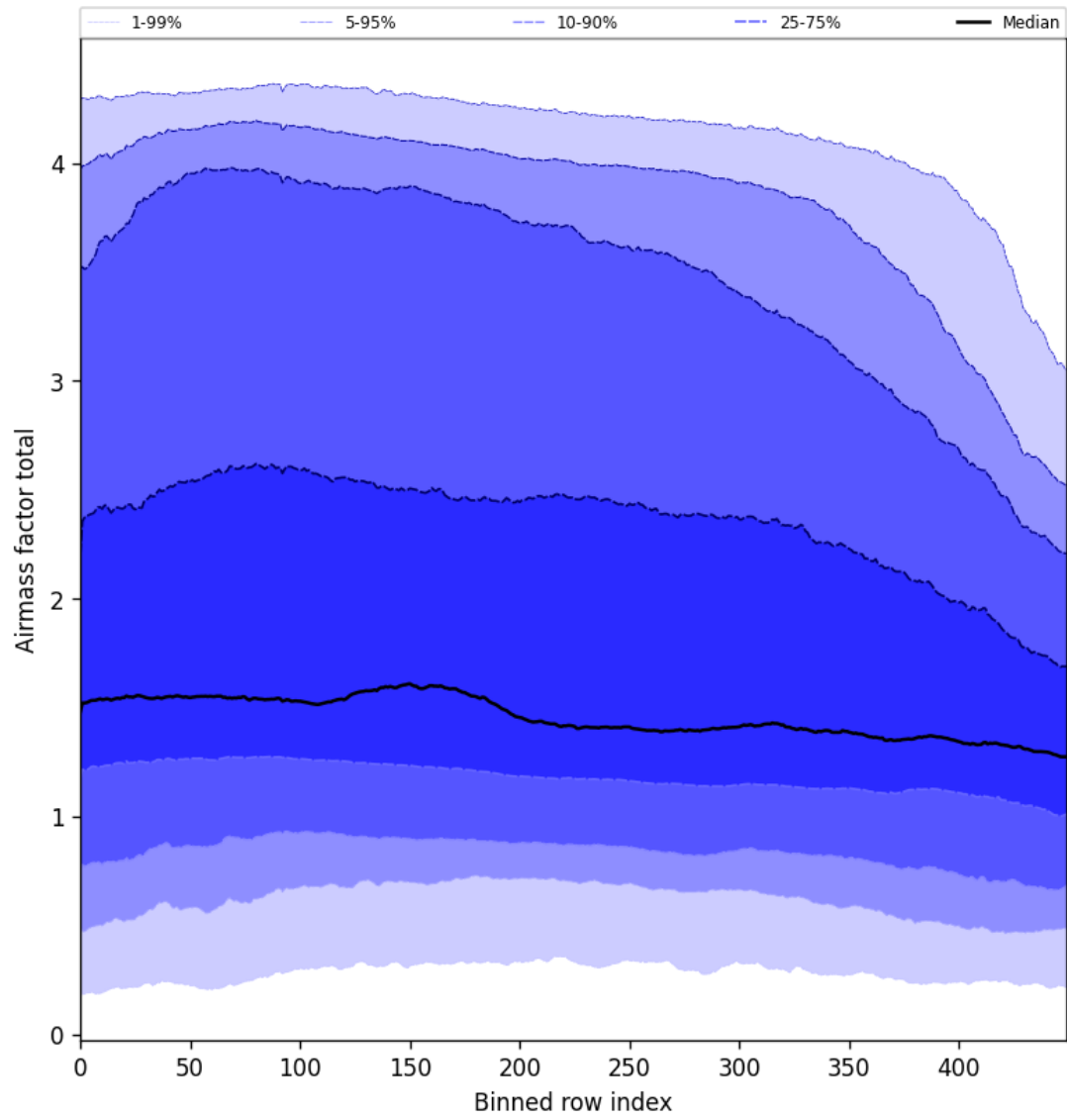
Figure 54: Along track statistics of “Airmass factor total” for 2025-02-05 to 2025-02-07
