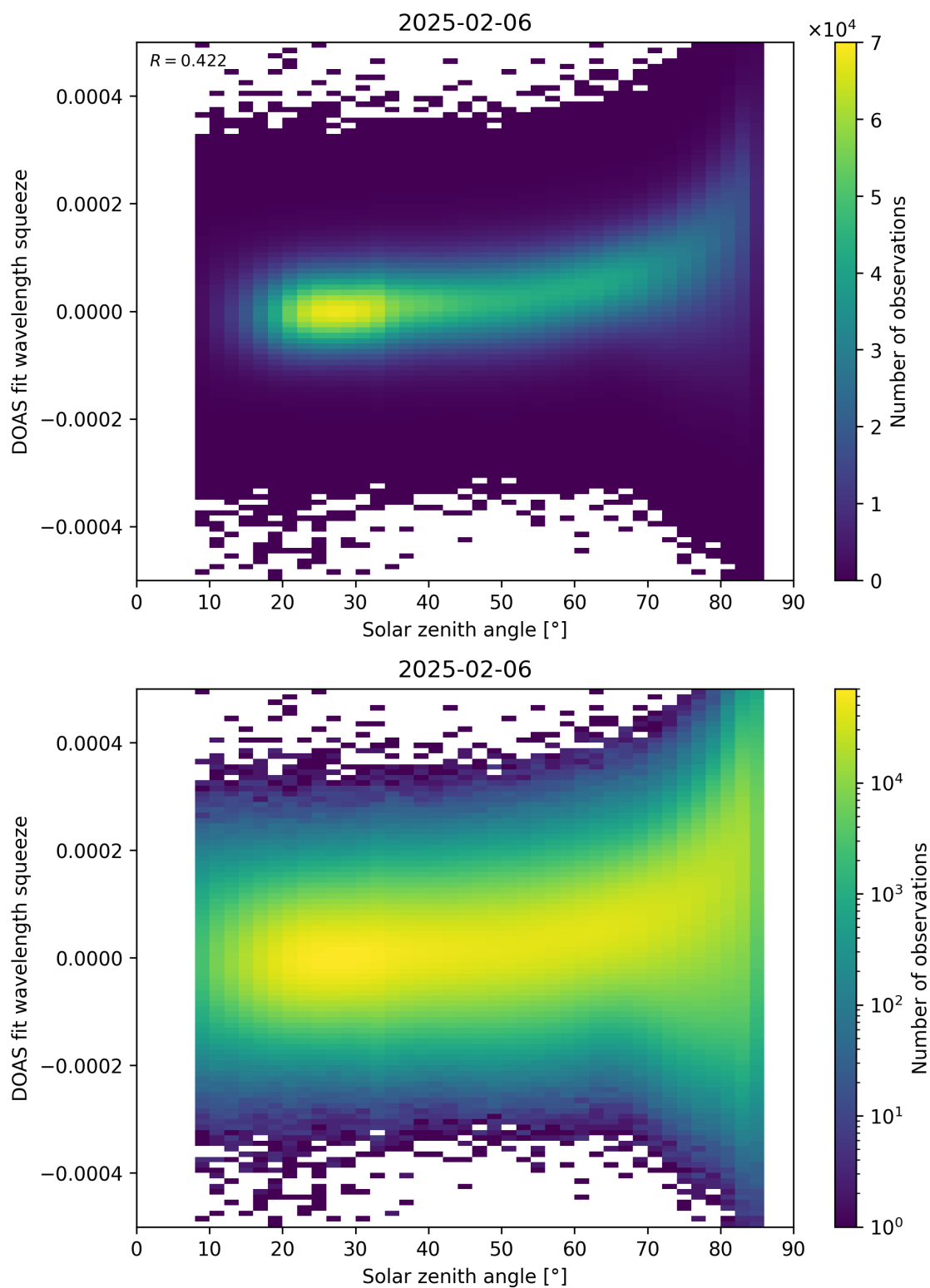
Figure 169: Scatter density plot of “Solar zenith angle” against “DOAS fit wavelength squeeze” for 2025-02-05 to 2025-02-07.
