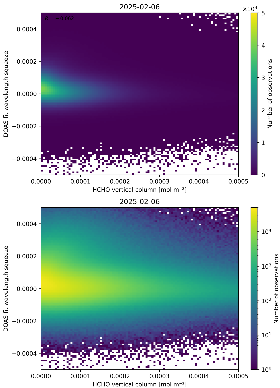
Figure 125: Scatter density plot of “HCHO vertical column” against “DOAS fit wavelength squeeze” for 2025-02-05 to 2025-02-07.
