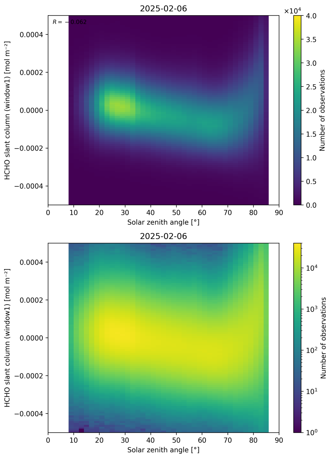
Figure 173: Scatter density plot of “Solar zenith angle” against “HCHO slant column (window1)” for 2025-02-05 to 2025-02-07.
