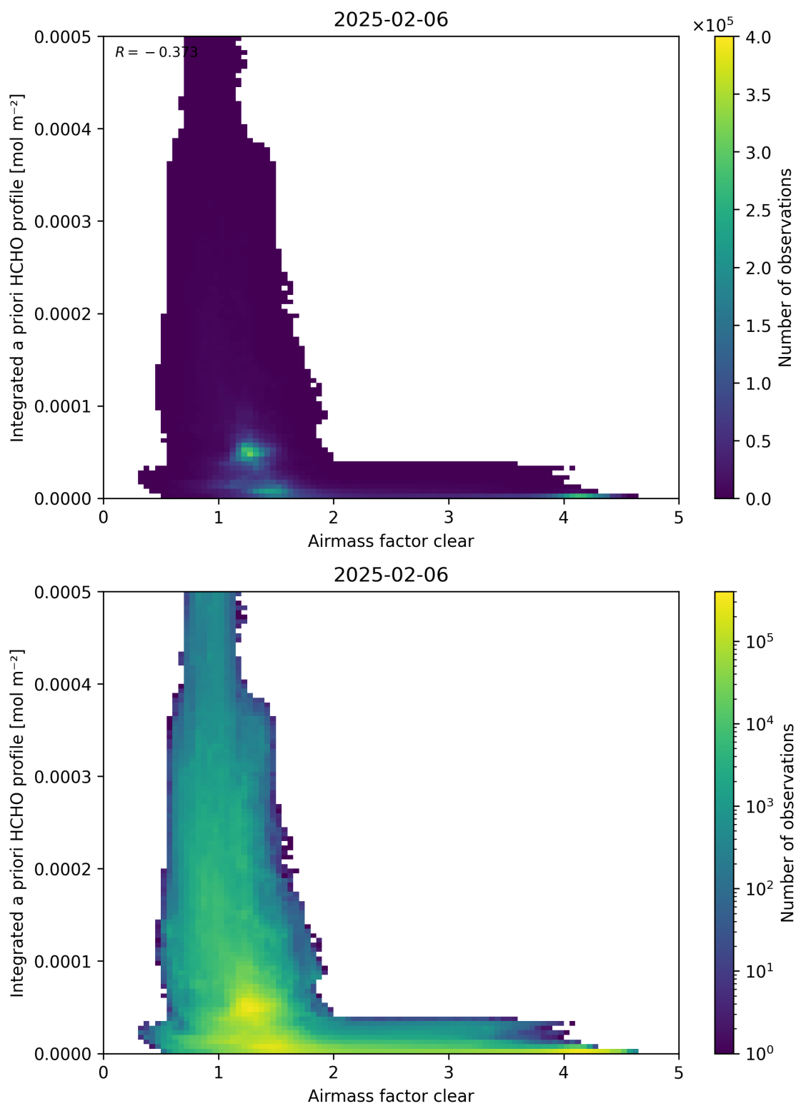
Figure 76: Scatter density plot of “Airmass factor clear” against “Integrated a priori HCHO profile” for 2025-02-05 to 2025-02-07.
