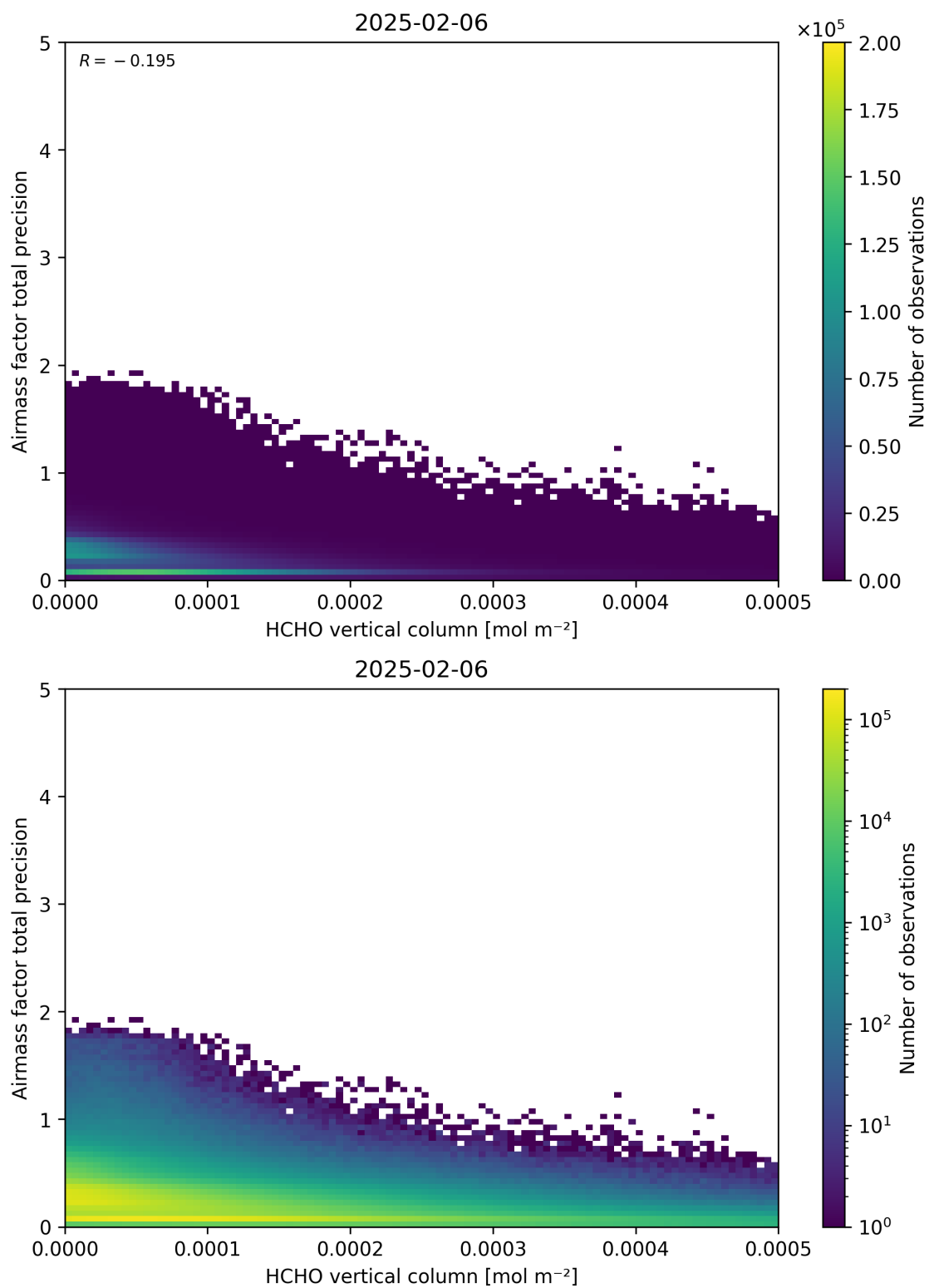
Figure 132: Scatter density plot of “HCHO vertical column” against “Airmass factor total precision” for 2025-02-05 to 2025-02-07.
