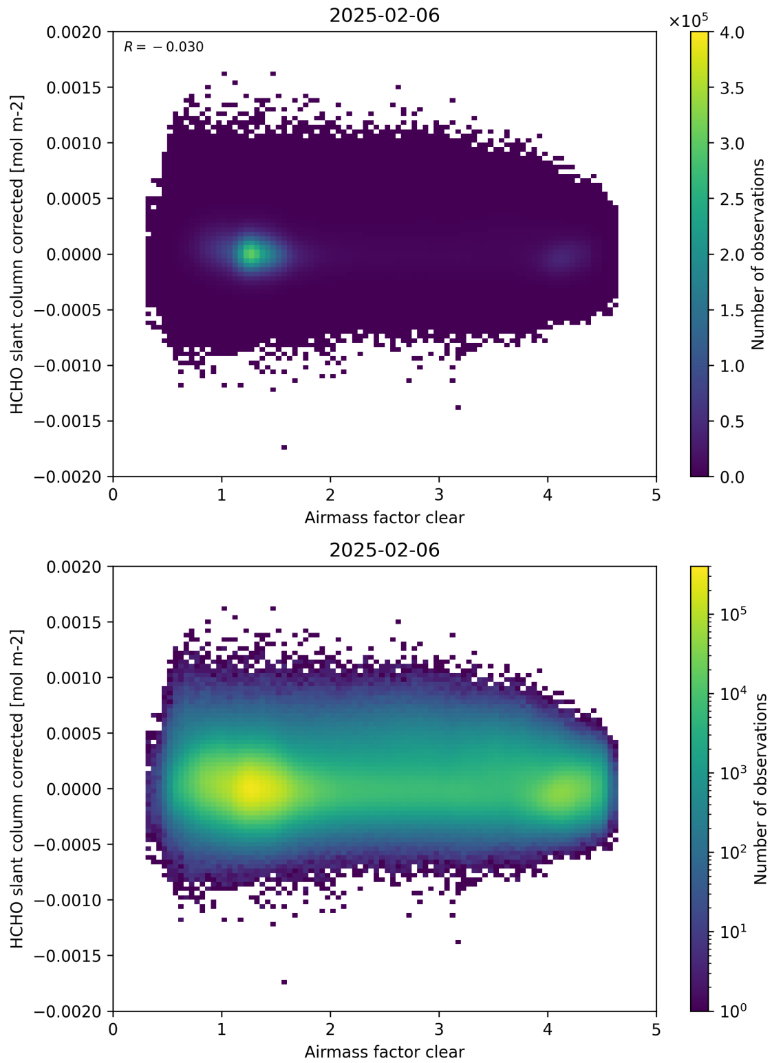
Figure 74: Scatter density plot of “Airmass factor clear” against “HCHO slant column corrected” for 2025-02-05 to 2025-02-07.
