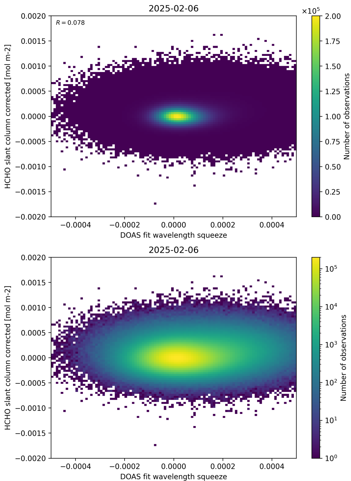
Figure 69: Scatter density plot of “DOAS fit wavelength squeeze” against “HCHO slant column corrected” for 2025-02-05 to 2025-02-07.
