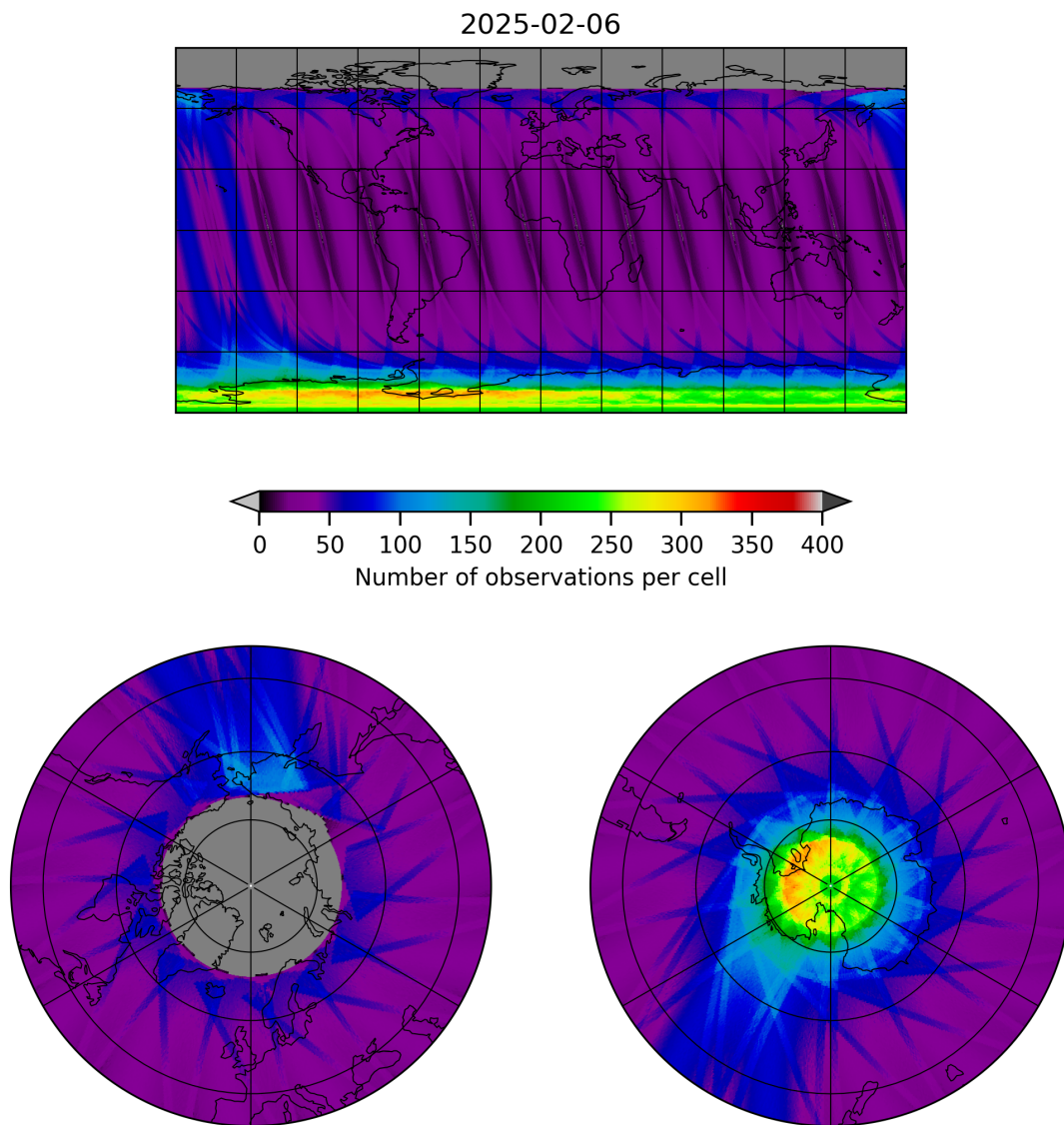
Figure 19: Map of the number of observations for 2025-02-05 to 2025-02-07
