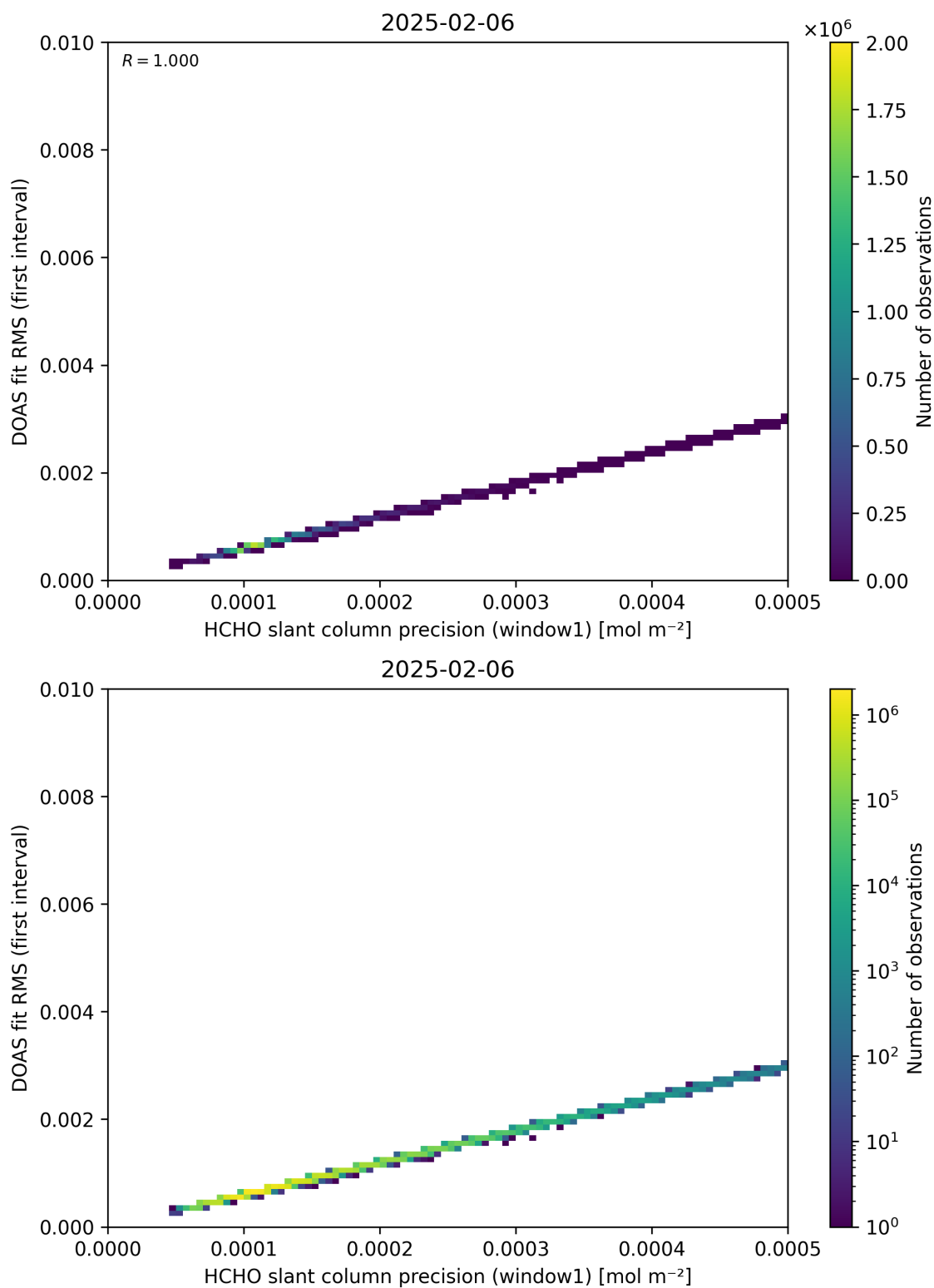
Figure 88: Scatter density plot of “HCHO slant column precision (window1)” against “DOAS fit RMS (first interval)” for 2025-02-05 to 2025-02-07.
