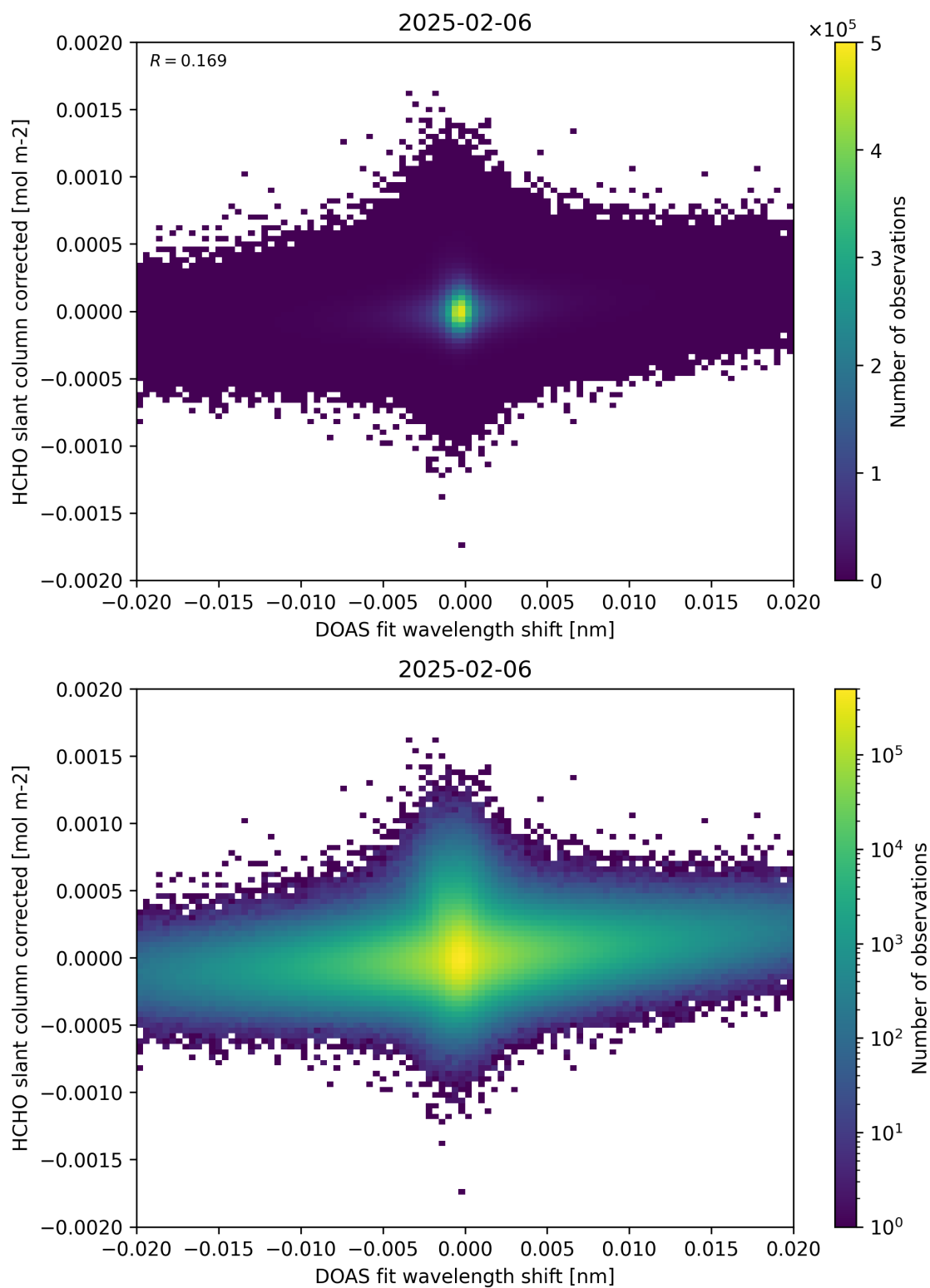
Figure 66: Scatter density plot of “DOAS fit wavelength shift” against “HCHO slant column corrected” for 2025-02-05 to 2025-02-07.
