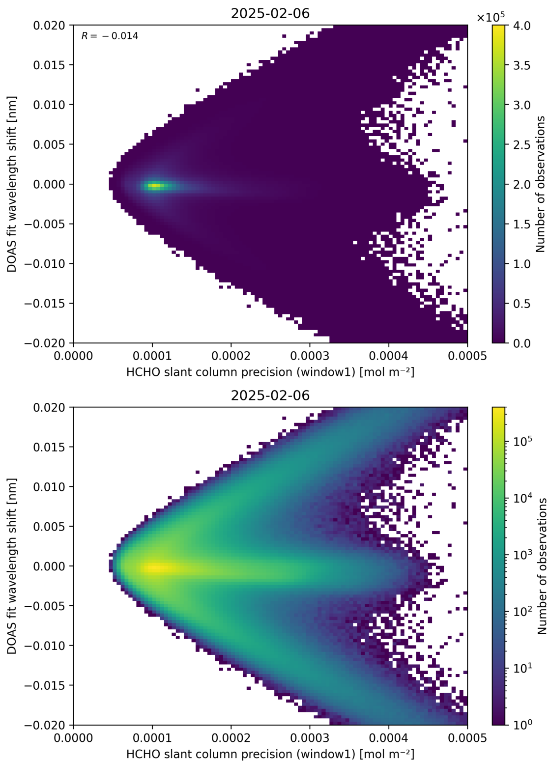
Figure 89: Scatter density plot of “HCHO slant column precision (window1)” against “DOAS fit wavelength shift” for 2025-02-05 to 2025-02-07.
