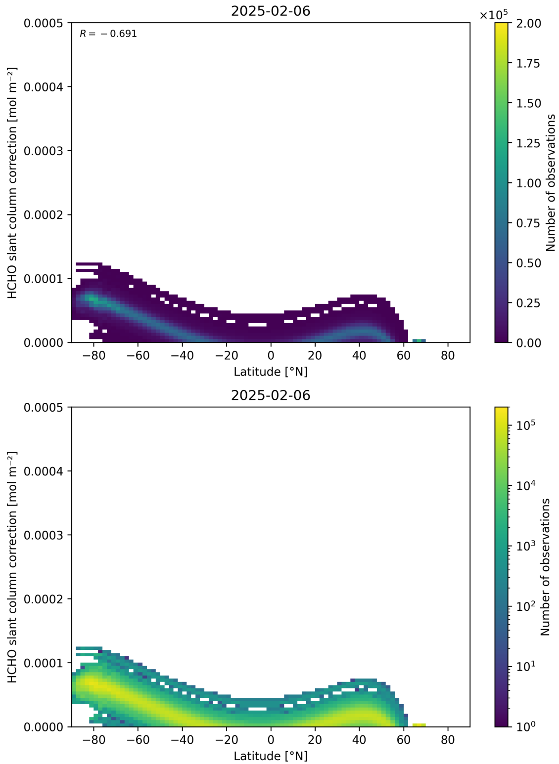
Figure 158: Scatter density plot of “Latitude” against “HCHO slant column correction” for 2025-02-05 to 2025-02-07.
