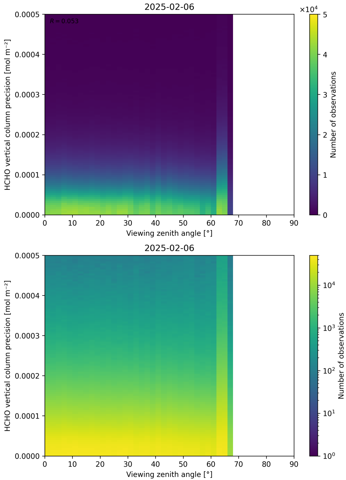
Figure 194: Scatter density plot of “Viewing zenith angle” against “HCHO vertical column precision” for 2025-02-05 to 2025-02-07.
