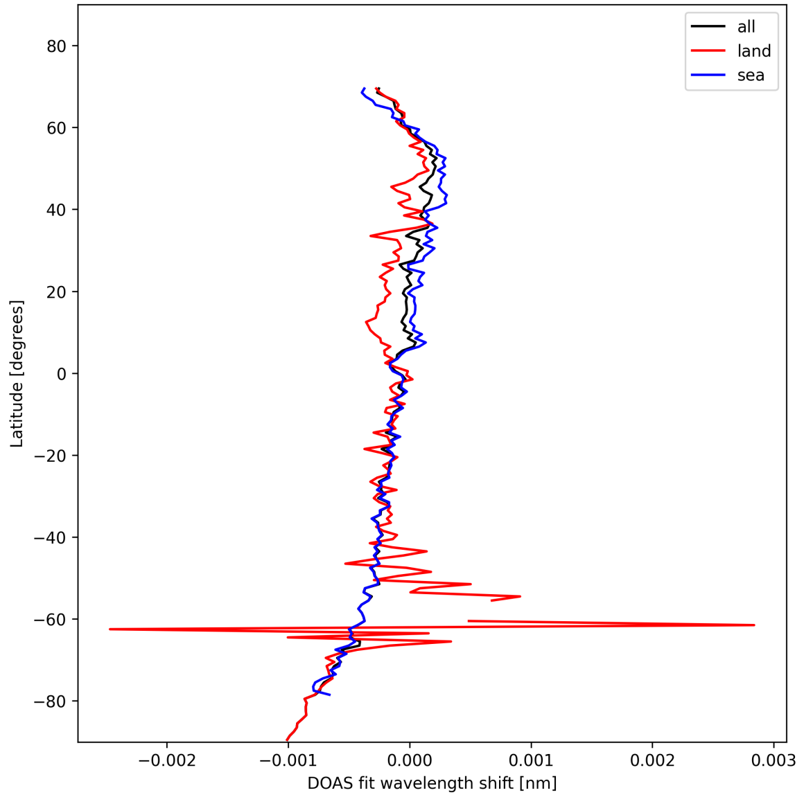
Figure 30: Zonal average of “DOAS fit wavelength shift” for 2025-02-05 to 2025-02-07.
