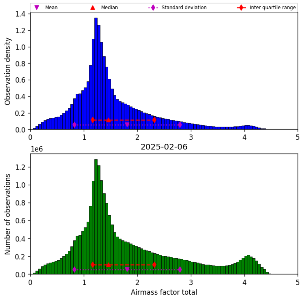
Figure 40: Histogram of “Airmass factor total” for 2025-02-05 to 2025-02-07
