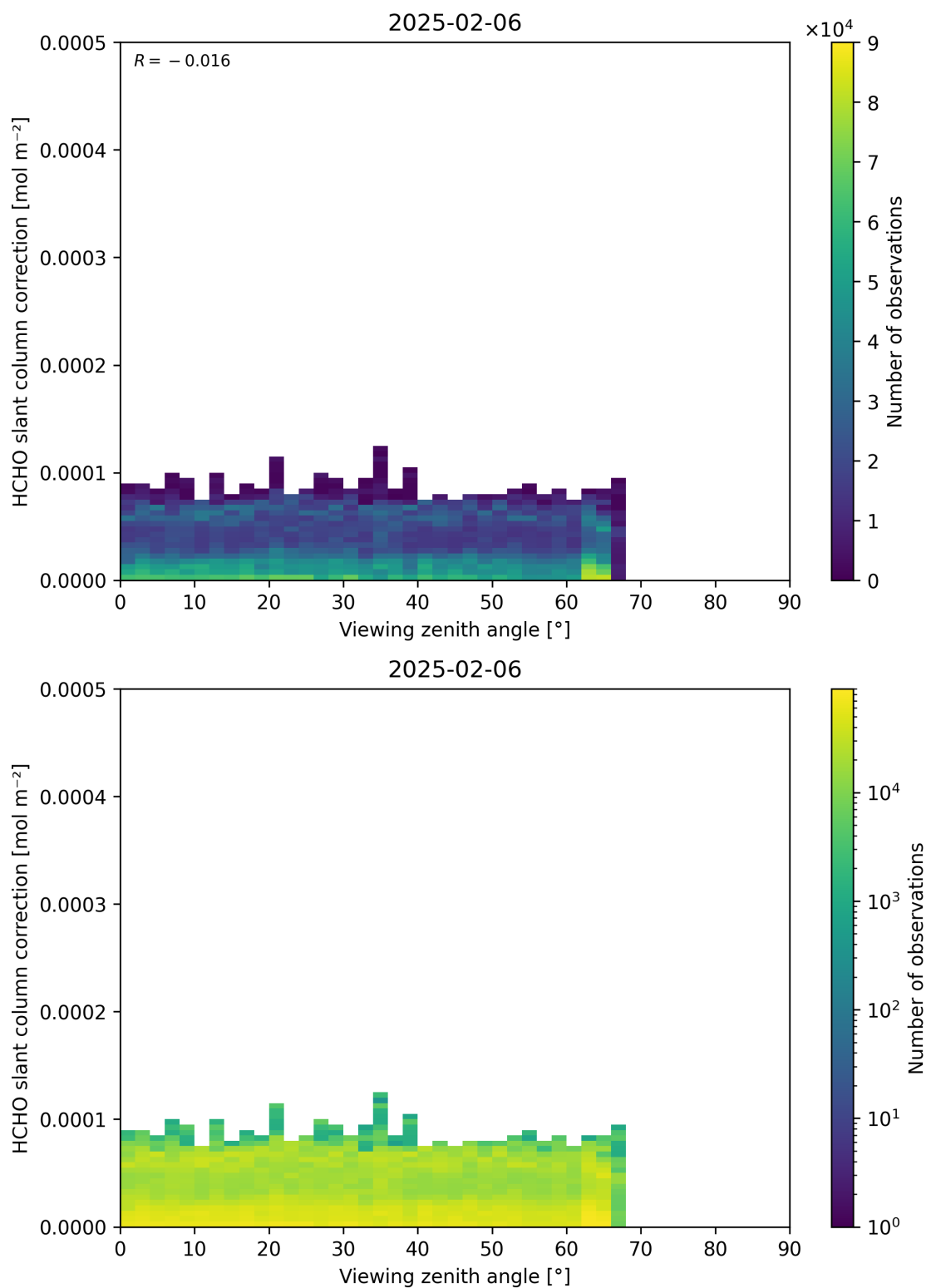
Figure 187: Scatter density plot of “Viewing zenith angle” against “HCHO slant column correction” for 2025-02-05 to 2025-02-07.
