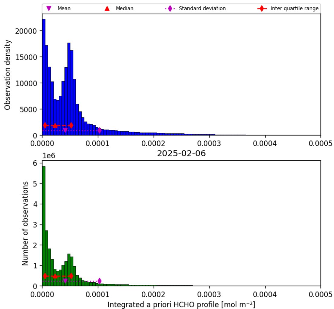
Figure 43: Histogram of “Integrated a priori HCHO profile” for 2025-02-05 to 2025-02-07
