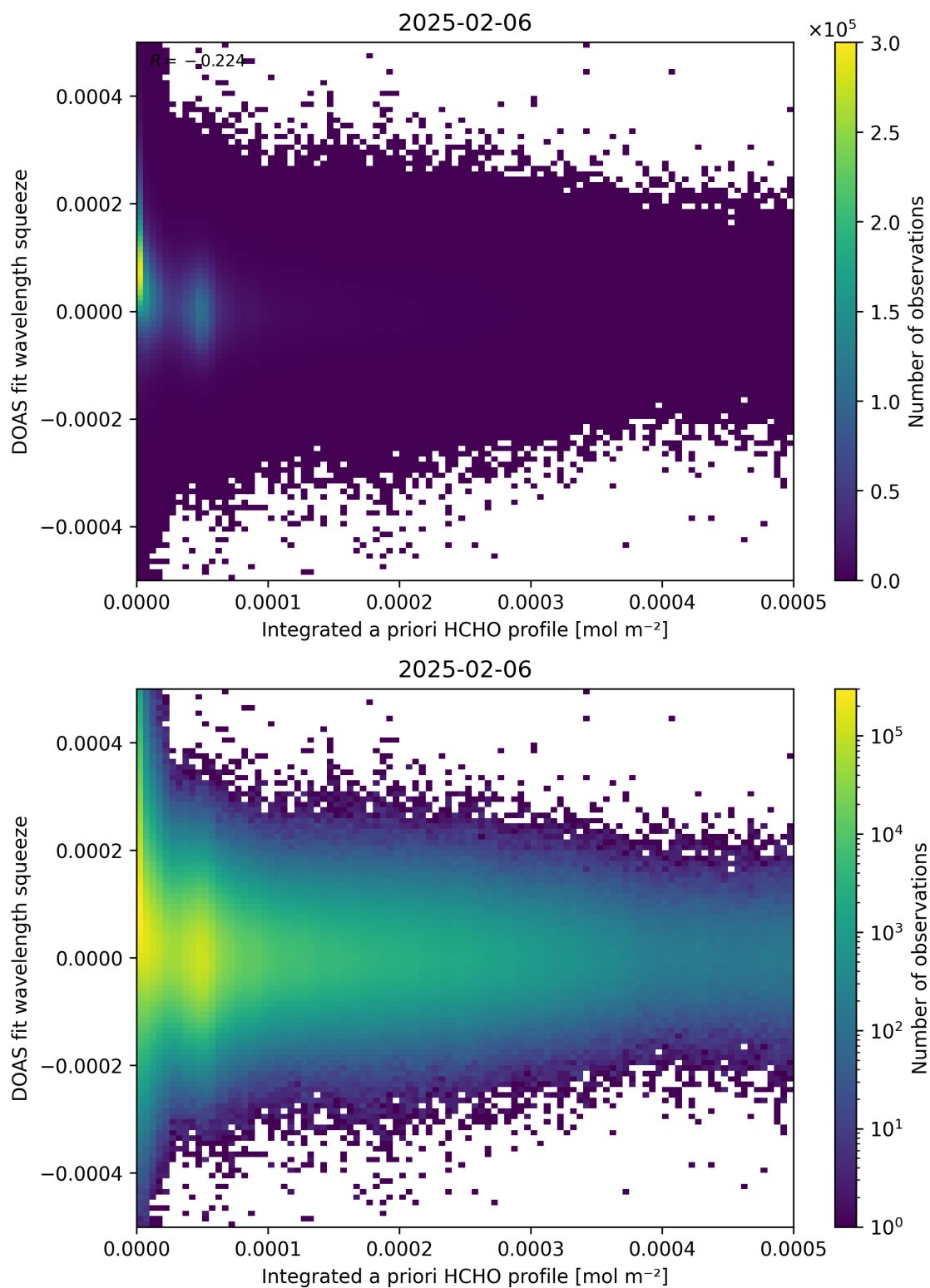
Figure 150: Scatter density plot of “Integrated a priori HCHO profile” against “DOAS fit wavelength squeeze” for 2025-02-05 to 2025-02-07.
