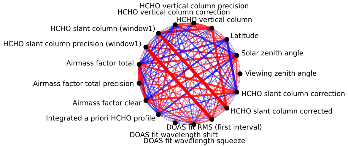
Figure 1: Map of correlation graph for 2025-02-05 to 2025-02-07.
