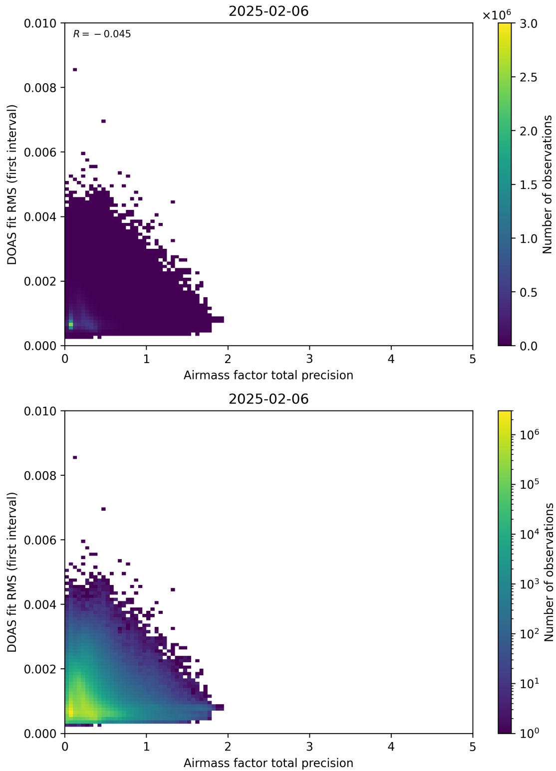
Figure 105: Scatter density plot of “Airmass factor total precision” against “DOAS fit RMS (first interval)” for 2025-02-05 to 2025-02-07.
