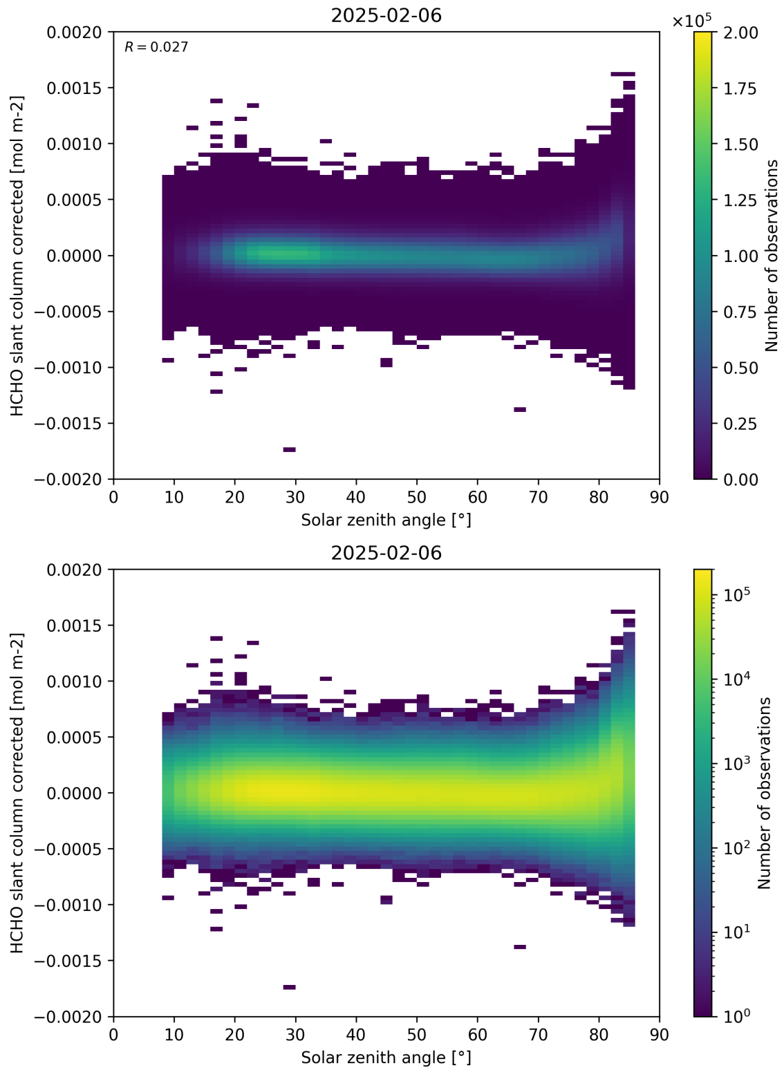
Figure 171: Scatter density plot of “Solar zenith angle” against “HCHO slant column corrected” for 2025-02-05 to 2025-02-07.
