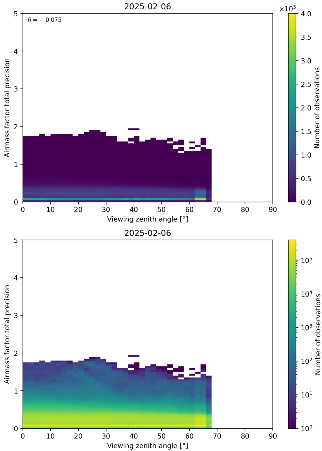
Figure 191: Scatter density plot of “Viewing zenith angle” against “Airmass factor total precision” for 2025-02-05 to 2025-02-07.
