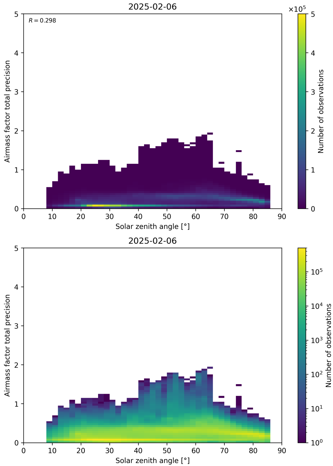
Figure 176: Scatter density plot of “Solar zenith angle” against “Airmass factor total precision” for 2025-02-05 to 2025-02-07.
