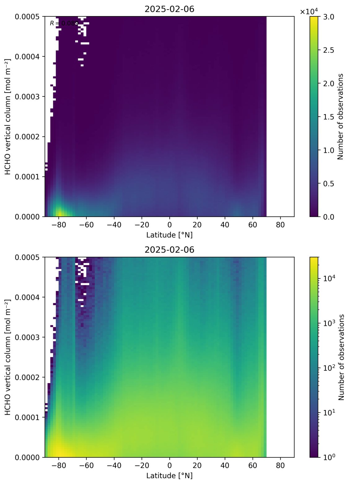
Figure 163: Scatter density plot of “Latitude” against “HCHO vertical column” for 2025-02-05 to 2025-02-07.
