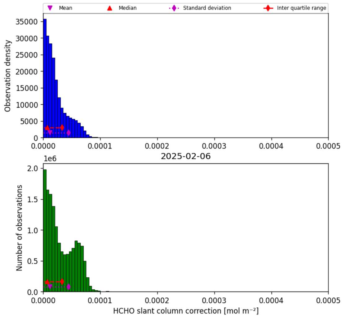
Figure 47: Histogram of “HCHO slant column correction” for 2025-02-05 to 2025-02-07
