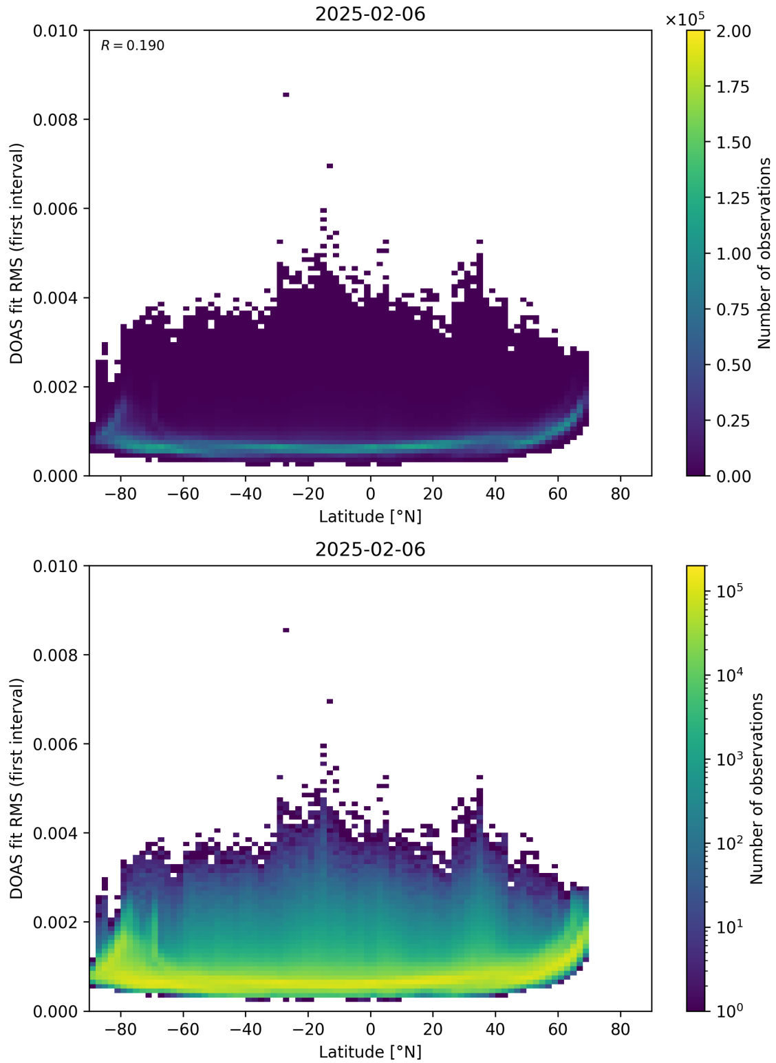
Figure 153: Scatter density plot of “Latitude” against “DOAS fit RMS (first interval)” for 2025-02-05 to 2025-02-07.
