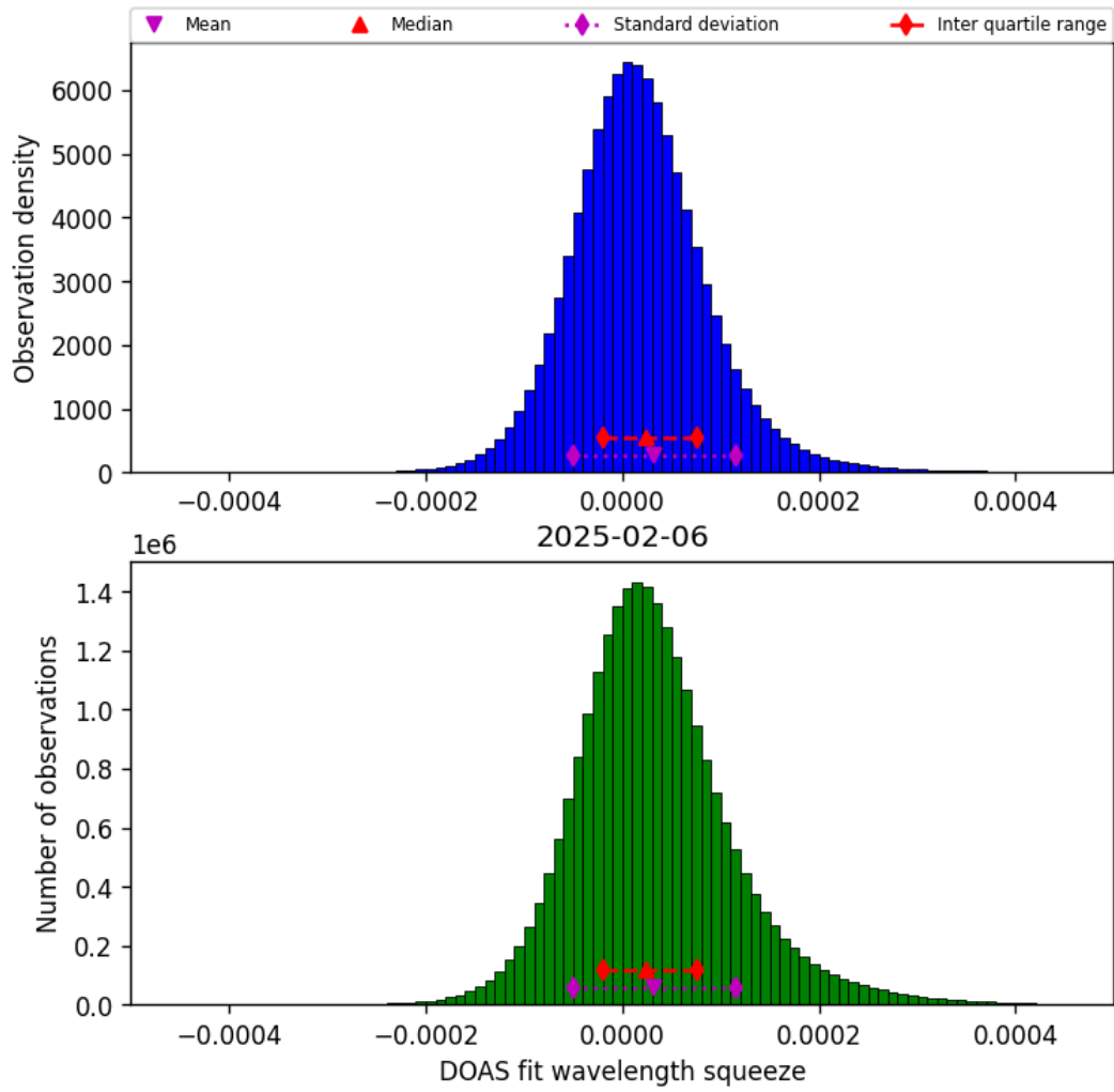
Figure 45: Histogram of “DOAS fit wavelength squeeze” for 2025-02-05 to 2025-02-07
