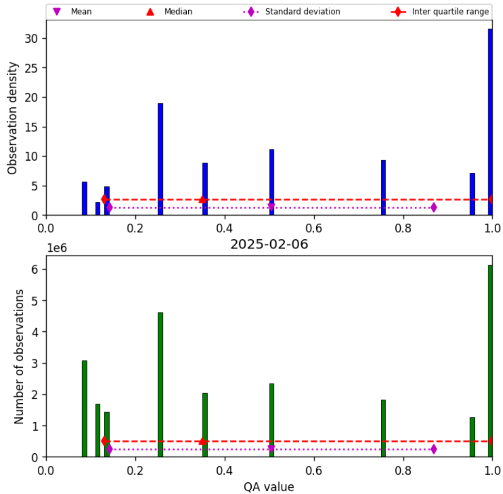
Figure 34: Histogram of “QA value” for 2025-02-05 to 2025-02-07
