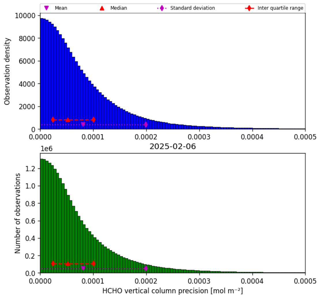
Figure 36: Histogram of “HCHO vertical column precision” for 2025-02-05 to 2025-02-07
