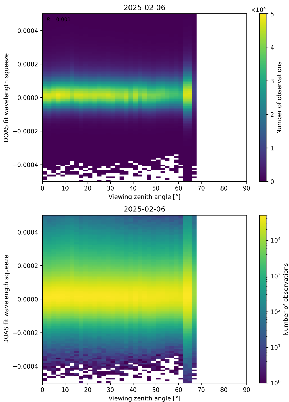
Figure 184: Scatter density plot of “Viewing zenith angle” against “DOAS fit wavelength squeeze” for 2025-02-05 to 2025-02-07.
