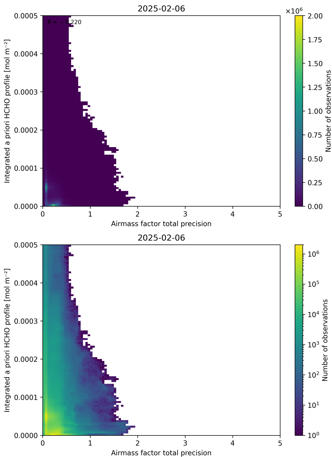
Figure 111: Scatter density plot of “Airmass factor total precision” against “Integrated a priori HCHO profile” for 2025-02-05 to 2025-02-07.
