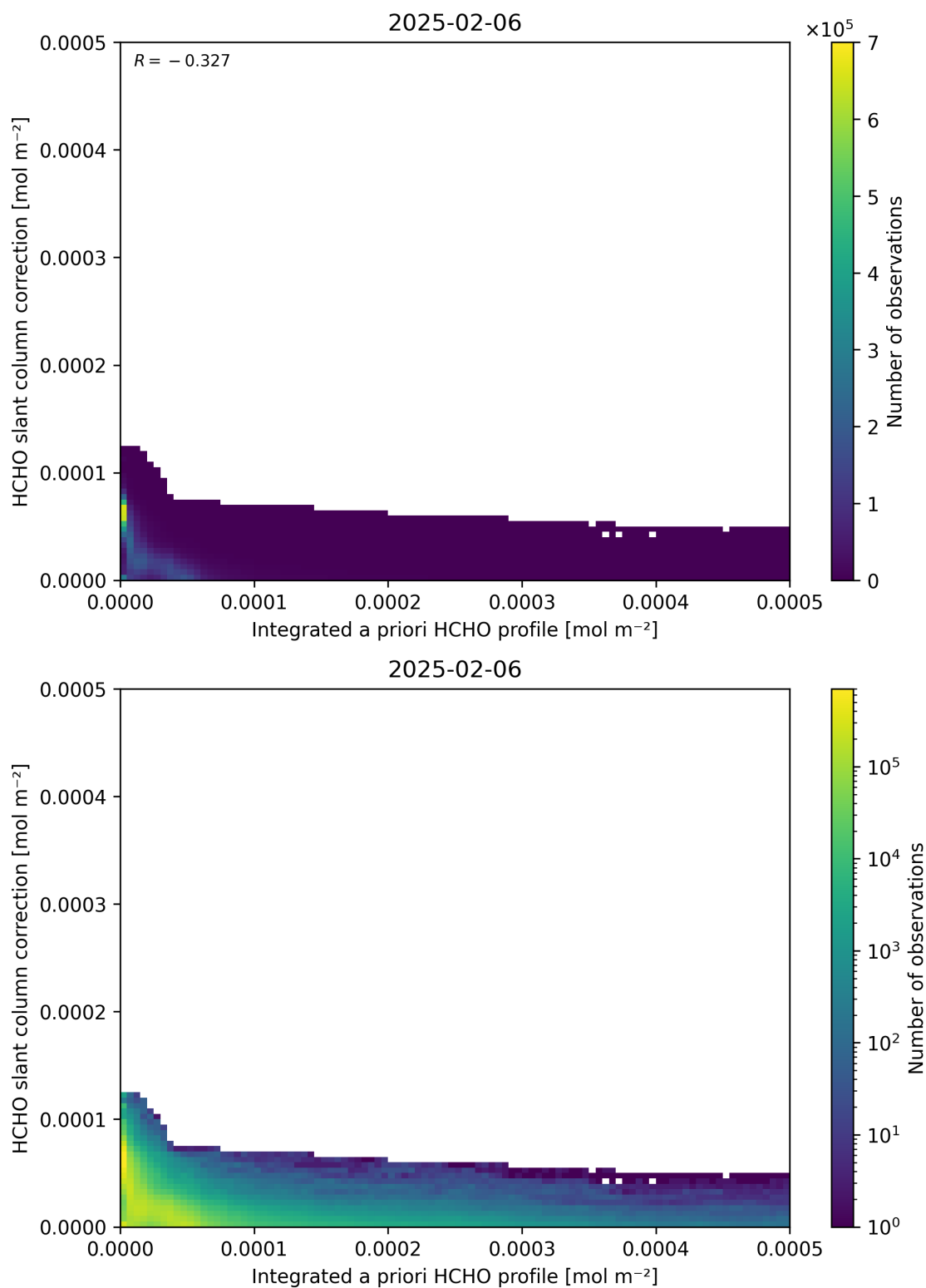
Figure 152: Scatter density plot of “Integrated a priori HCHO profile” against “HCHO slant column correction” for 2025-02-05 to 2025-02-07.
