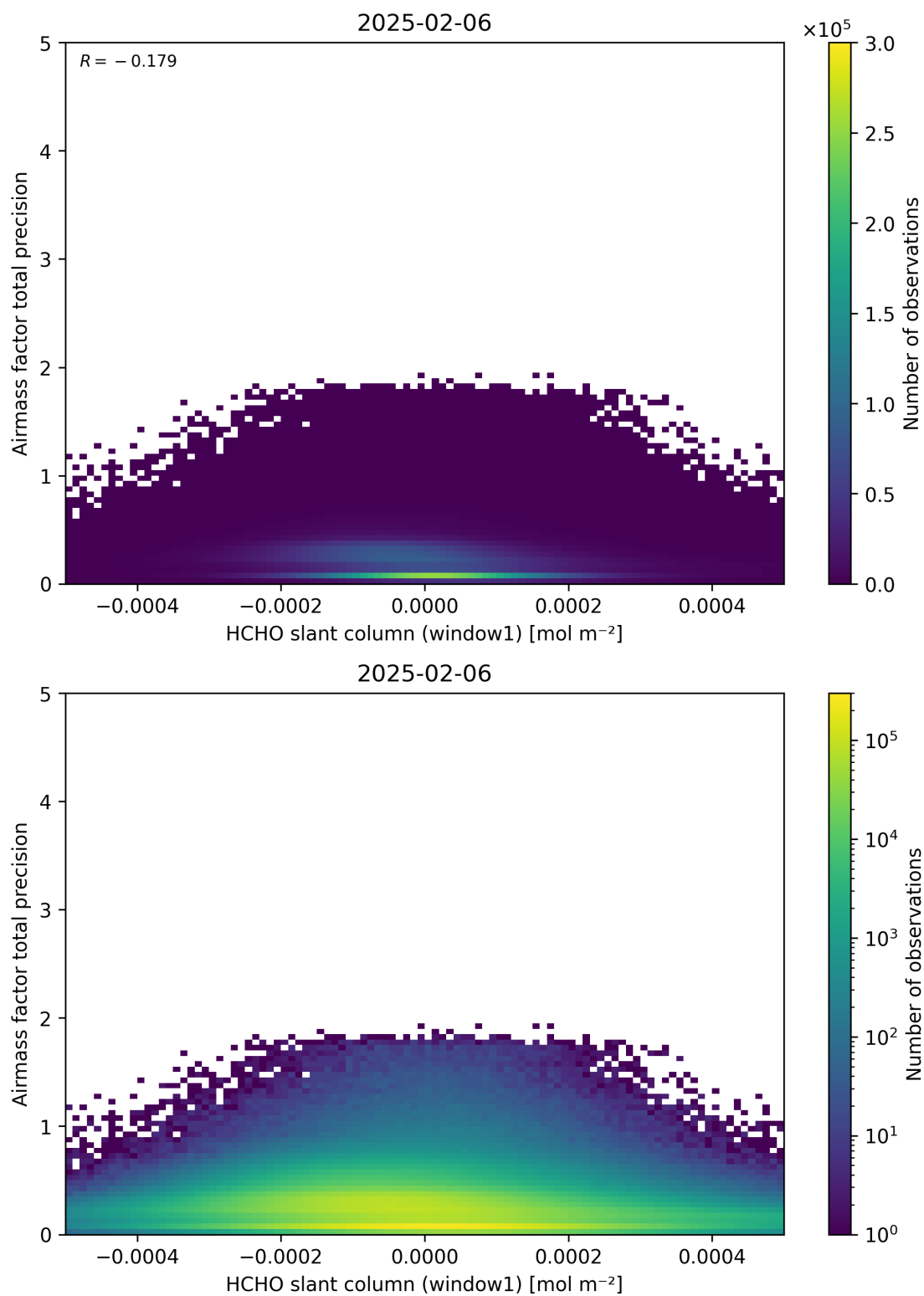
Figure 86: Scatter density plot of “HCHO slant column (window1)” against “Airmass factor total precision” for 2025-02-05 to 2025-02-07.
