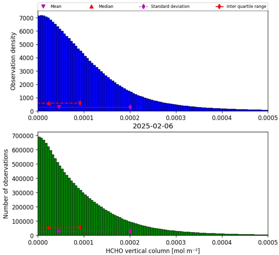
Figure 35: Histogram of “HCHO vertical column” for 2025-02-05 to 2025-02-07
