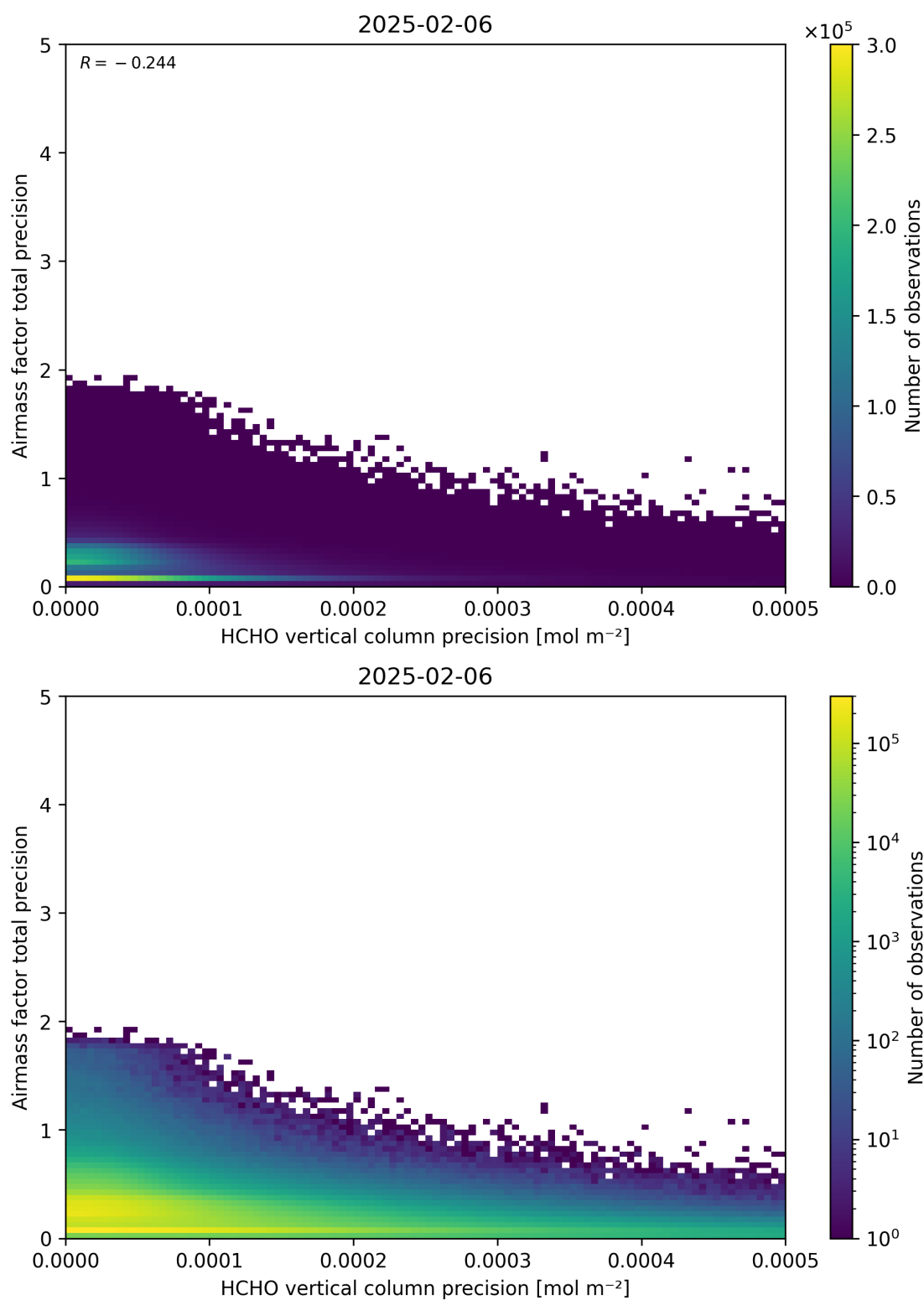
Figure 145: Scatter density plot of “HCHO vertical column precision” against “Airmass factor total precision” for 2025-02-05 to 2025-02-07.
