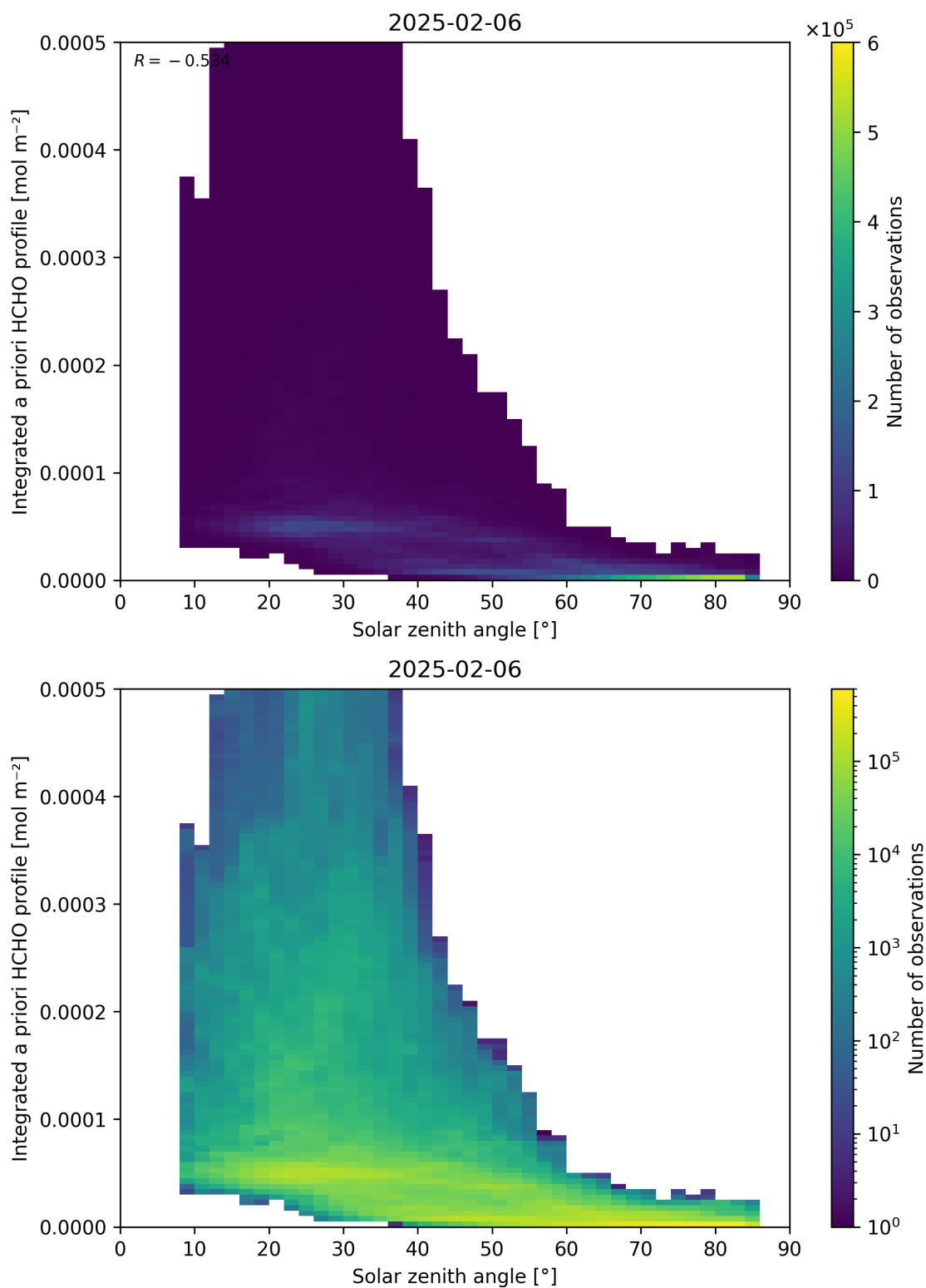
Figure 180: Scatter density plot of “Solar zenith angle” against “Integrated a priori HCHO profile” for 2025-02-05 to 2025-02-07.
