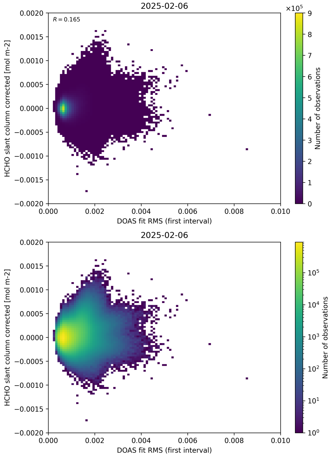
Figure 62: Scatter density plot of “DOAS fit RMS (first interval)” against “HCHO slant column corrected” for 2025-02-05 to 2025-02-07.
