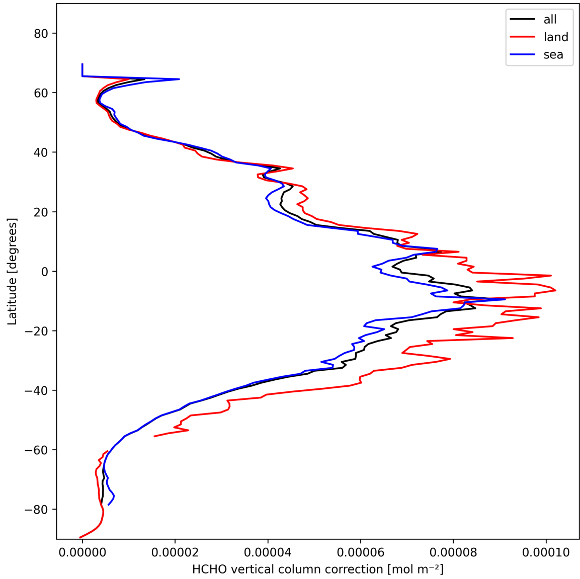
Figure 23: Zonal average of “HCHO vertical column correction” for 2025-02-05 to 2025-02-07.
