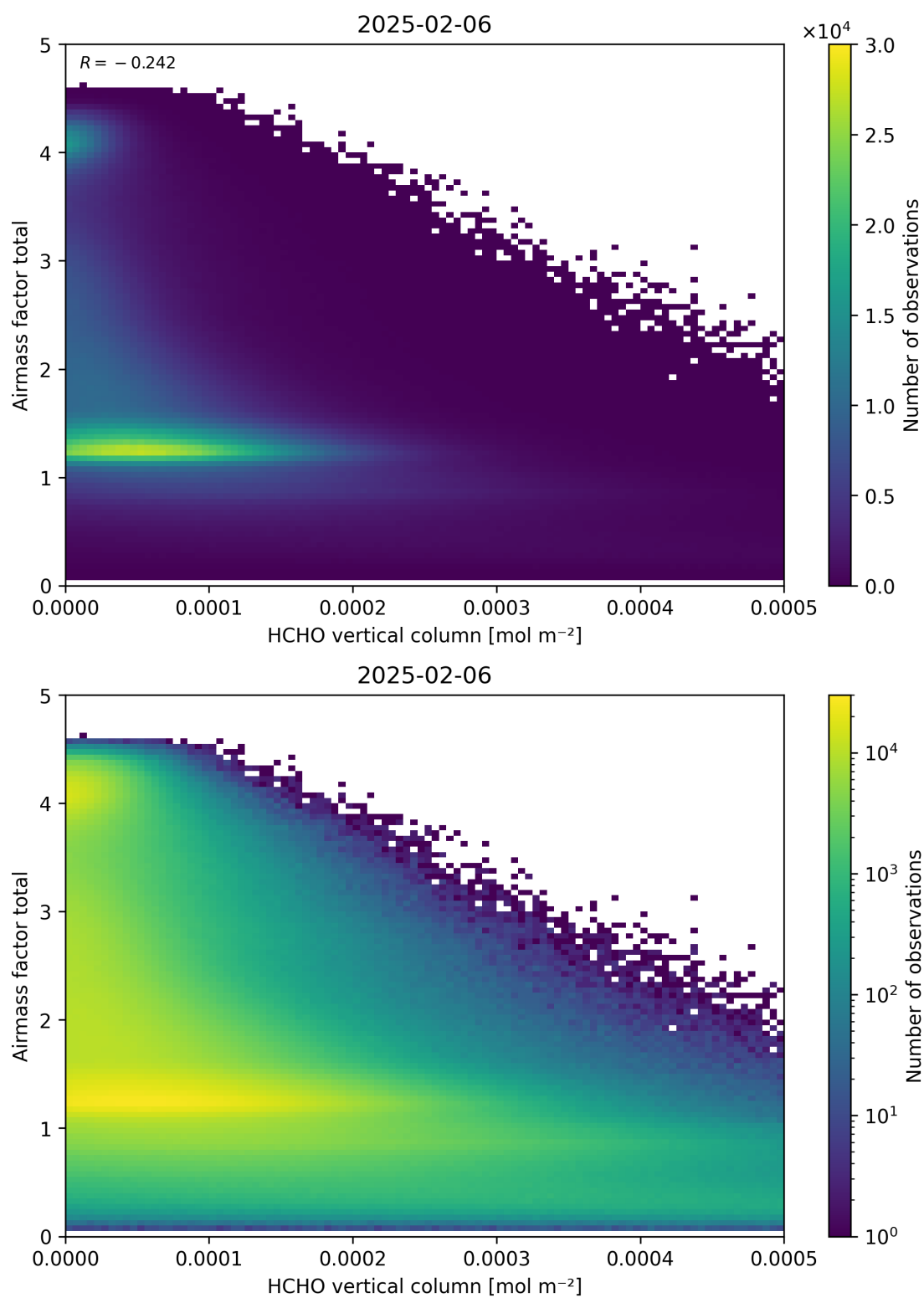
Figure 131: Scatter density plot of “HCHO vertical column” against “Airmass factor total” for 2025-02-05 to 2025-02-07.
