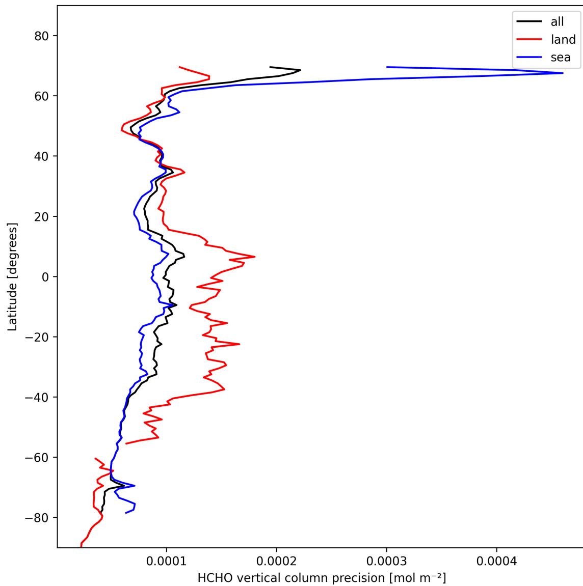
Figure 22: Zonal average of “HCHO vertical column precision” for 2025-02-05 to 2025-02-07.
