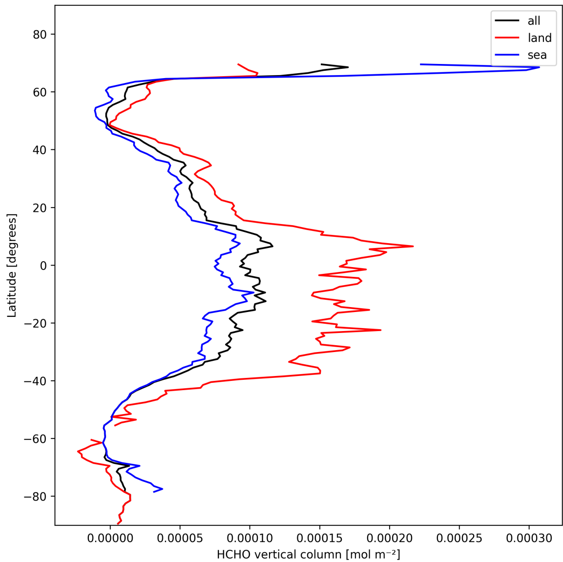
Figure 21: Zonal average of “HCHO vertical column” for 2025-02-05 to 2025-02-07.
