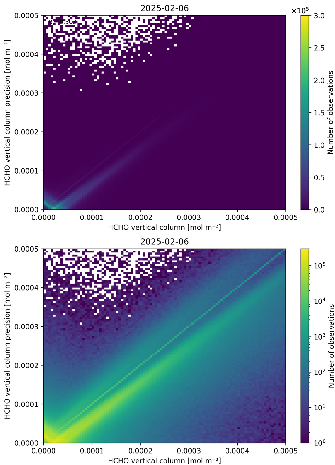
Figure 134: Scatter density plot of “HCHO vertical column” against “HCHO vertical column precision” for 2025-02-05 to 2025-02-07.
