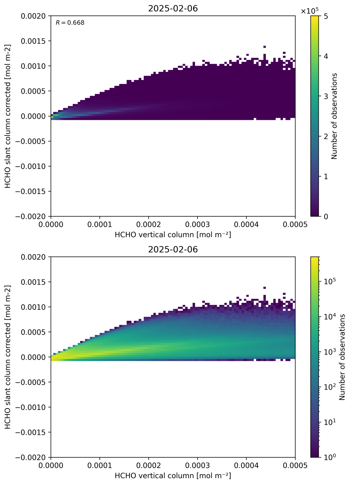
Figure 127: Scatter density plot of “HCHO vertical column” against “HCHO slant column corrected” for 2025-02-05 to 2025-02-07.
