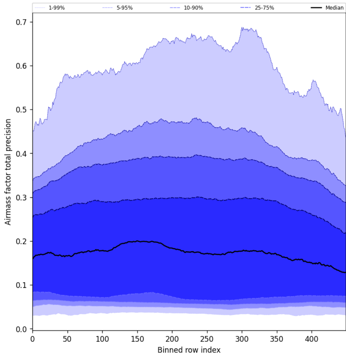
Figure 55: Along track statistics of “Airmass factor total precision” for 2025-02-05 to 2025-02-07
