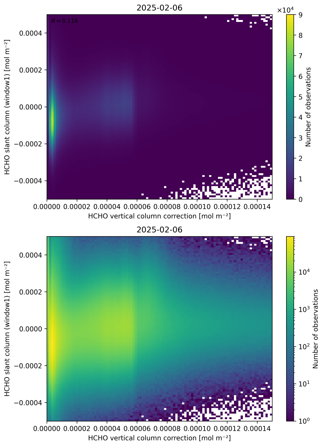
Figure 118: Scatter density plot of “HCHO vertical column correction” against “HCHO slant column (window1)” for 2025-02-05 to 2025-02-07.
