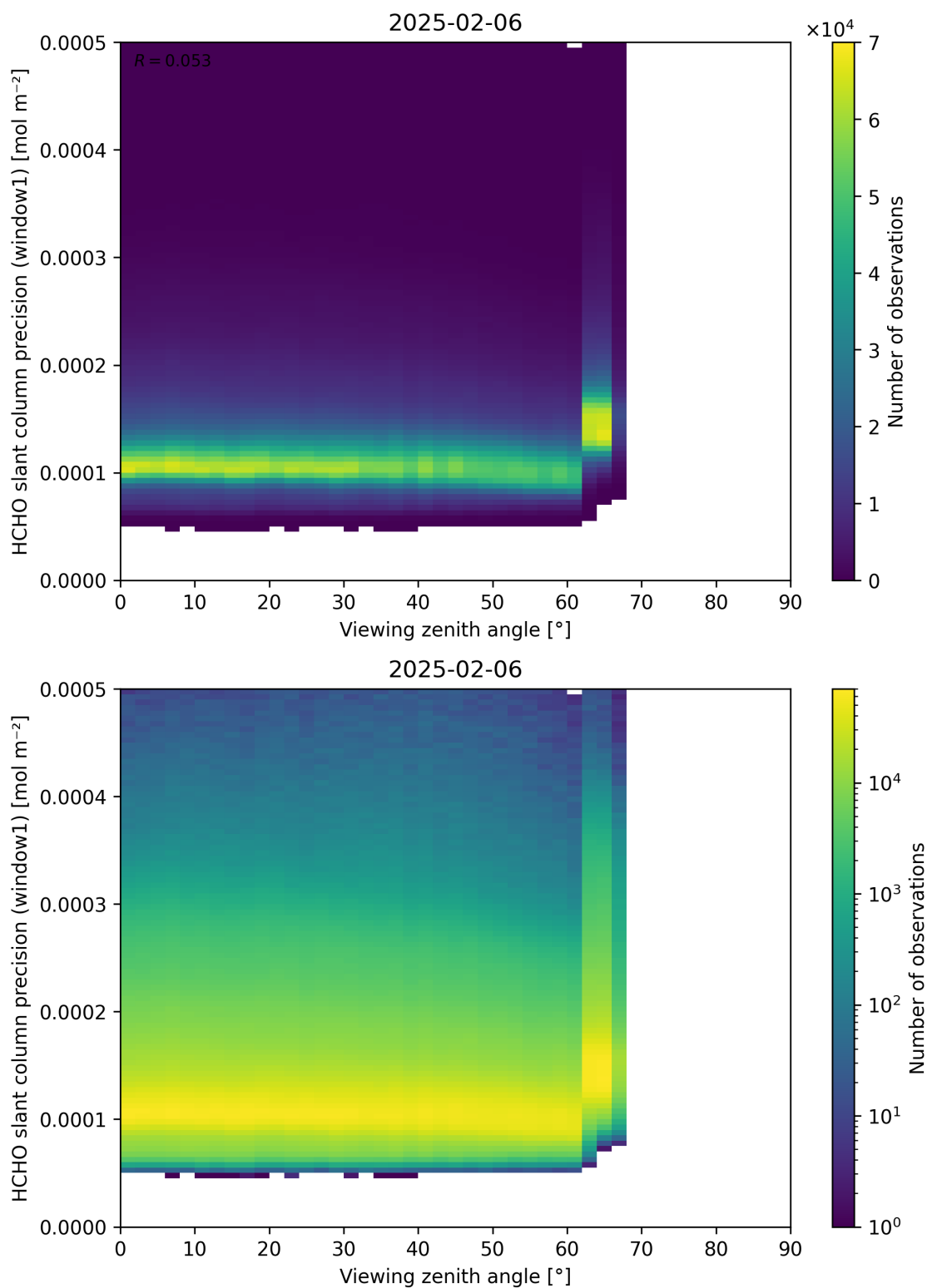
Figure 189: Scatter density plot of “Viewing zenith angle” against “HCHO slant column precision (window1)” for 2025-02-05 to 2025-02-07.
