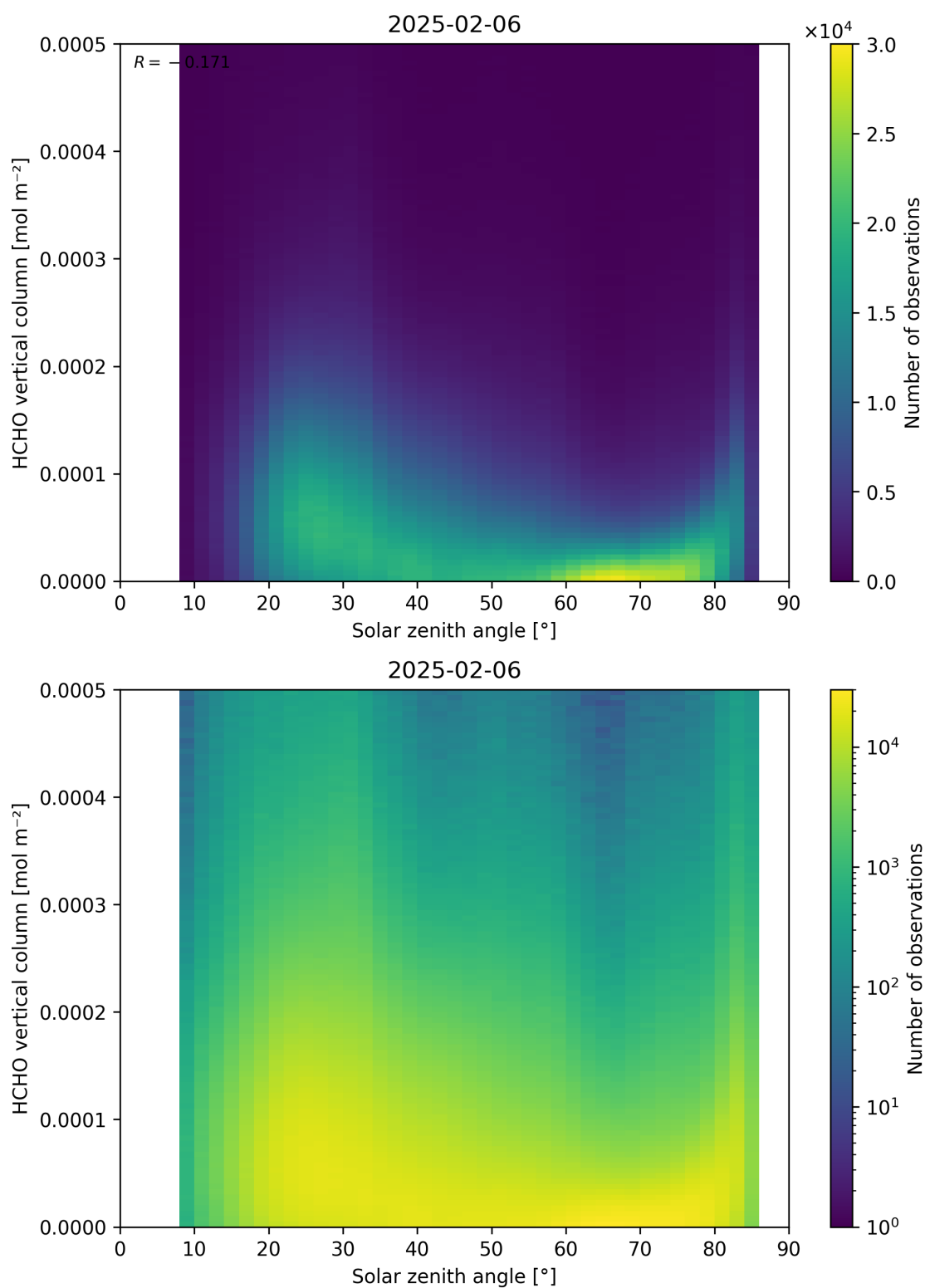
Figure 177: Scatter density plot of “Solar zenith angle” against “HCHO vertical column” for 2025-02-05 to 2025-02-07.
