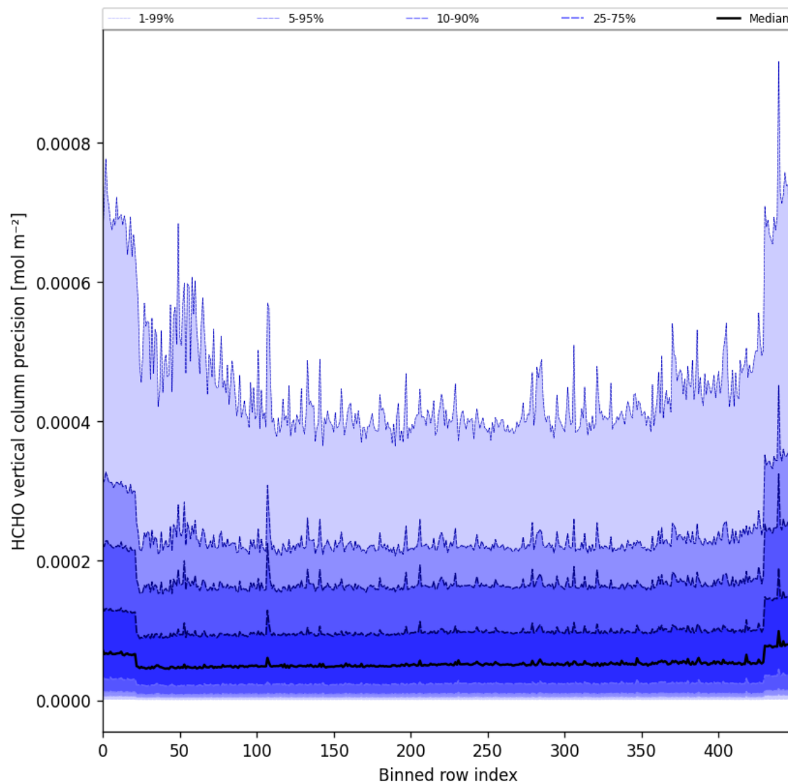
Figure 50: Along track statistics of “HCHO vertical column precision” for 2025-02-05 to 2025-02-07
