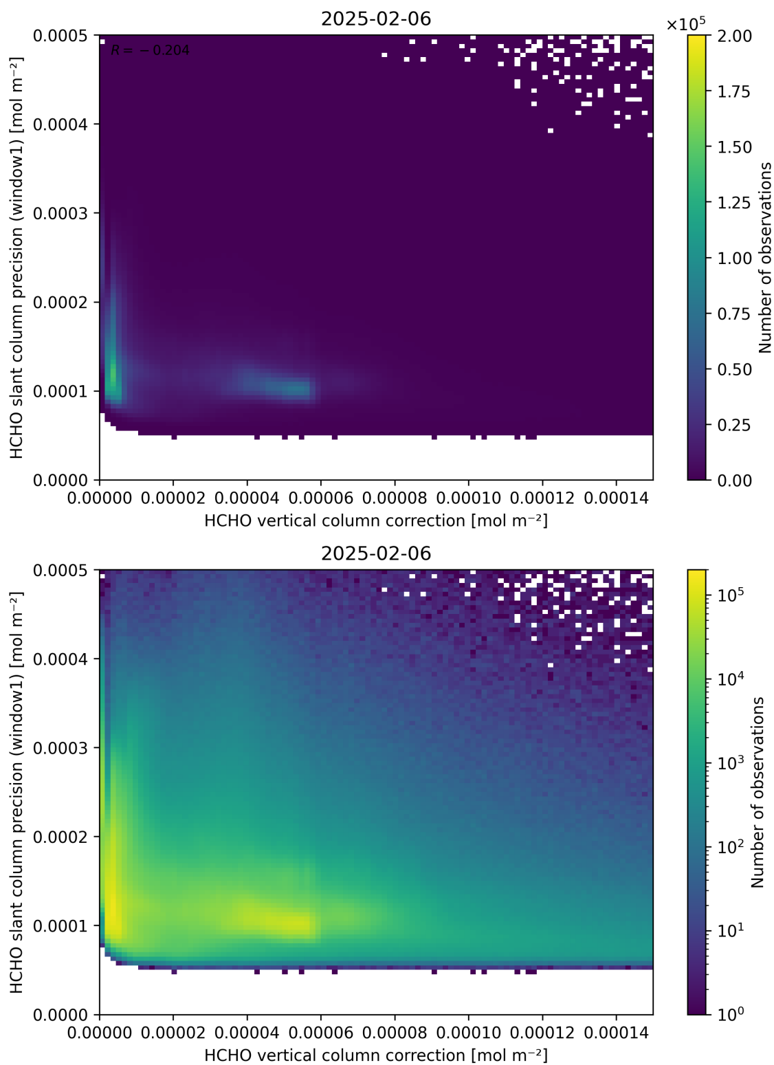
Figure 119: Scatter density plot of “HCHO vertical column correction” against “HCHO slant column precision (window1)” for 2025-02-05 to 2025-02-07.
