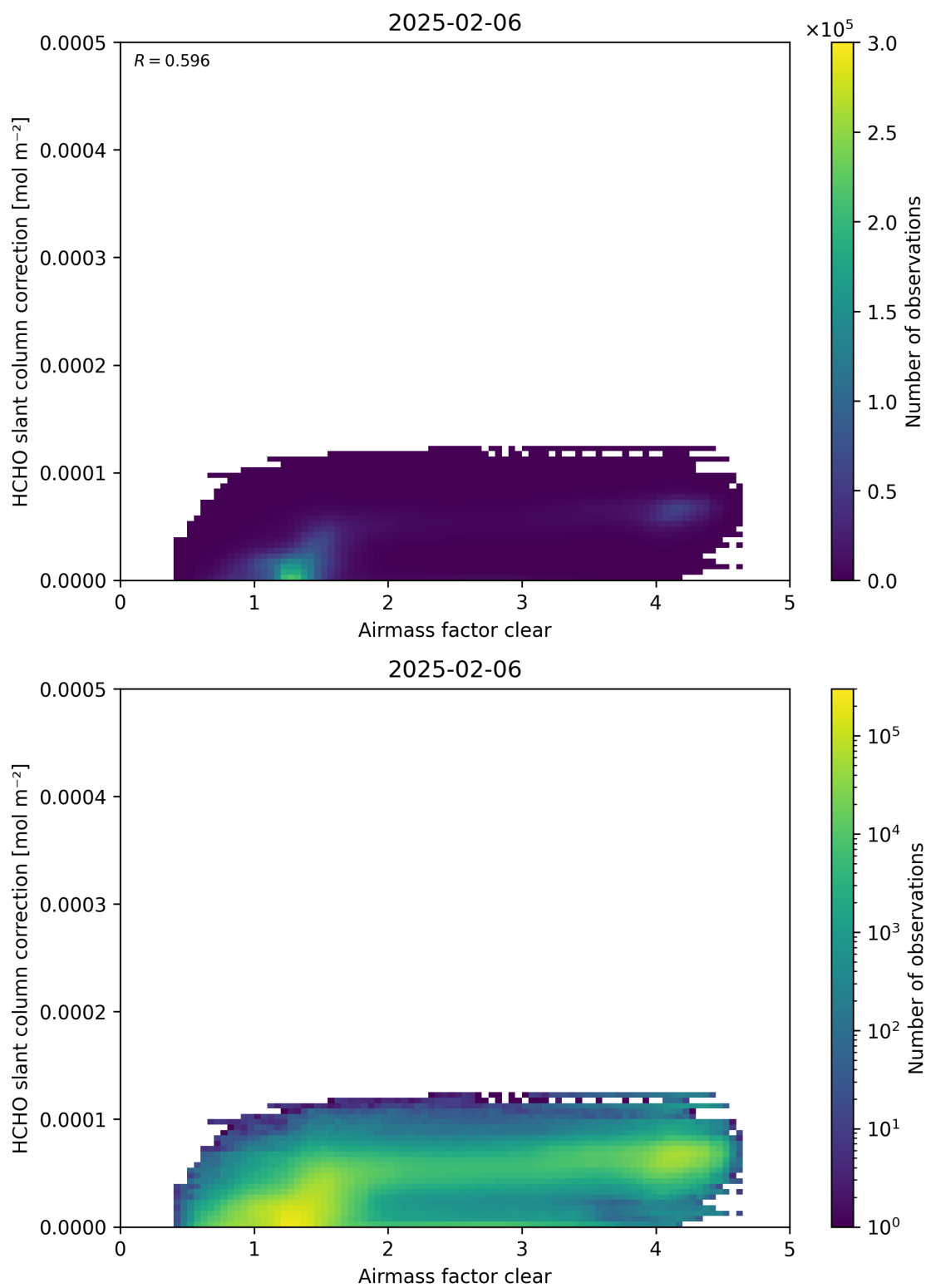
Figure 75: Scatter density plot of “Airmass factor clear” against “HCHO slant column correction” for 2025-02-05 to 2025-02-07.
