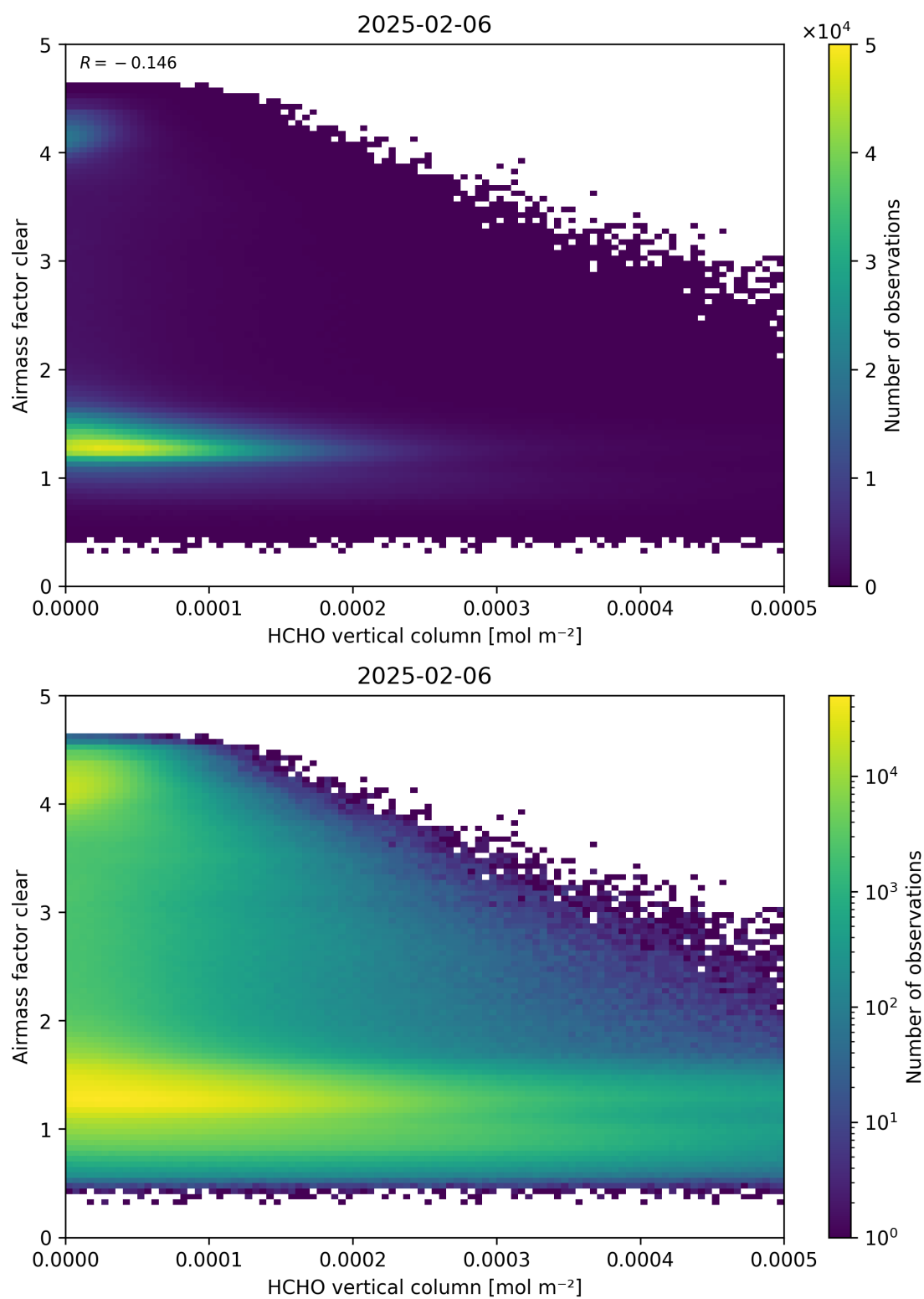
Figure 126: Scatter density plot of “HCHO vertical column” against “Airmass factor clear” for 2025-02-05 to 2025-02-07.
