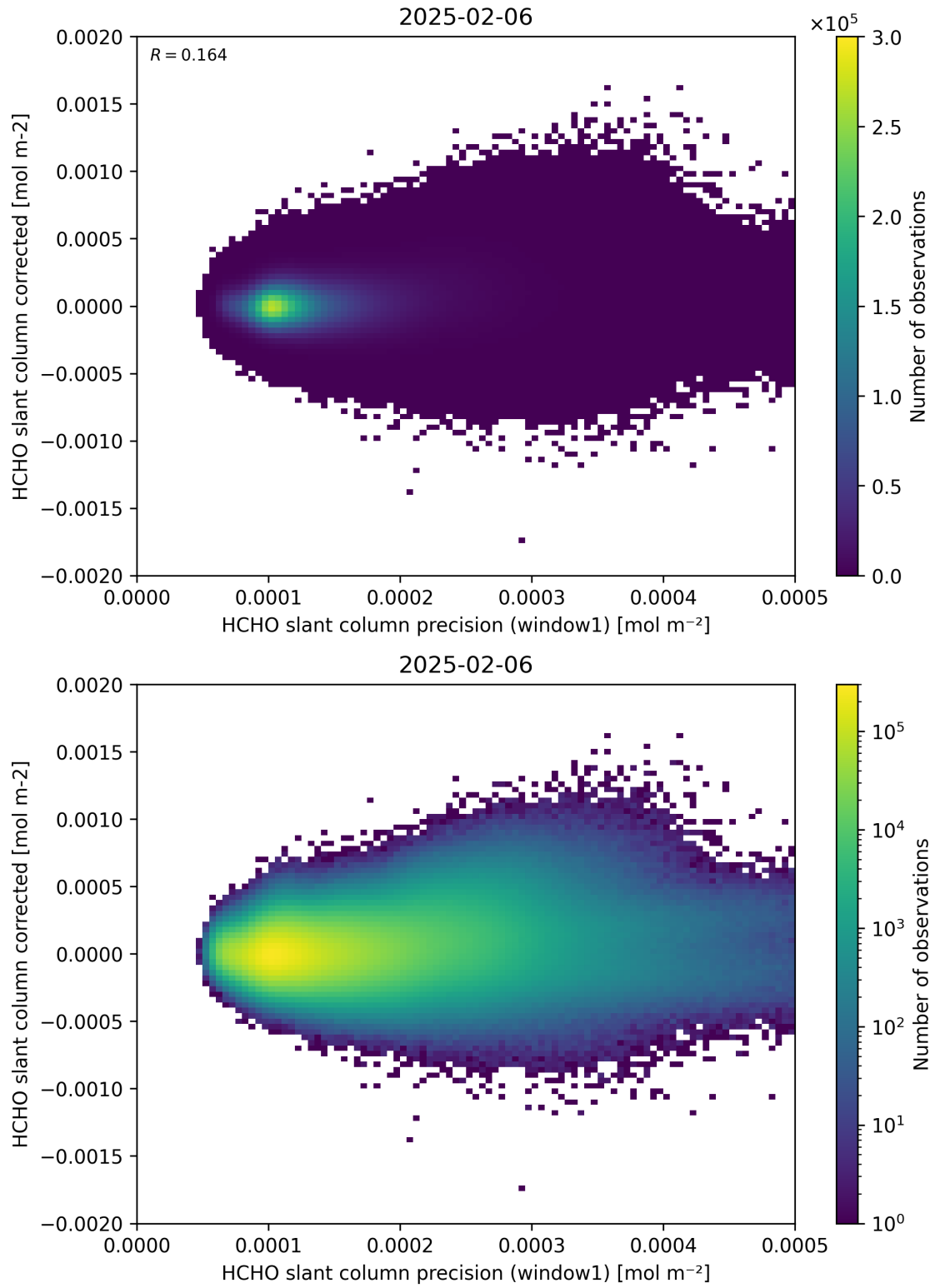
Figure 92: Scatter density plot of “HCHO slant column precision (window1)” against “HCHO slant column corrected” for 2025-02-05 to 2025-02-07.
