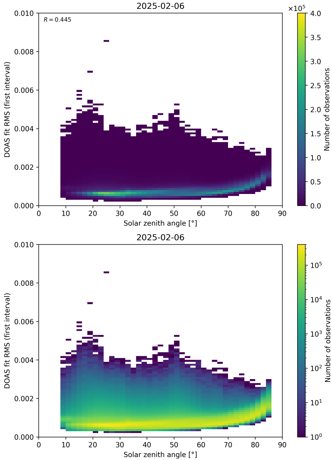
Figure 167: Scatter density plot of “Solar zenith angle” against “DOAS fit RMS (first interval)” for 2025-02-05 to 2025-02-07.
