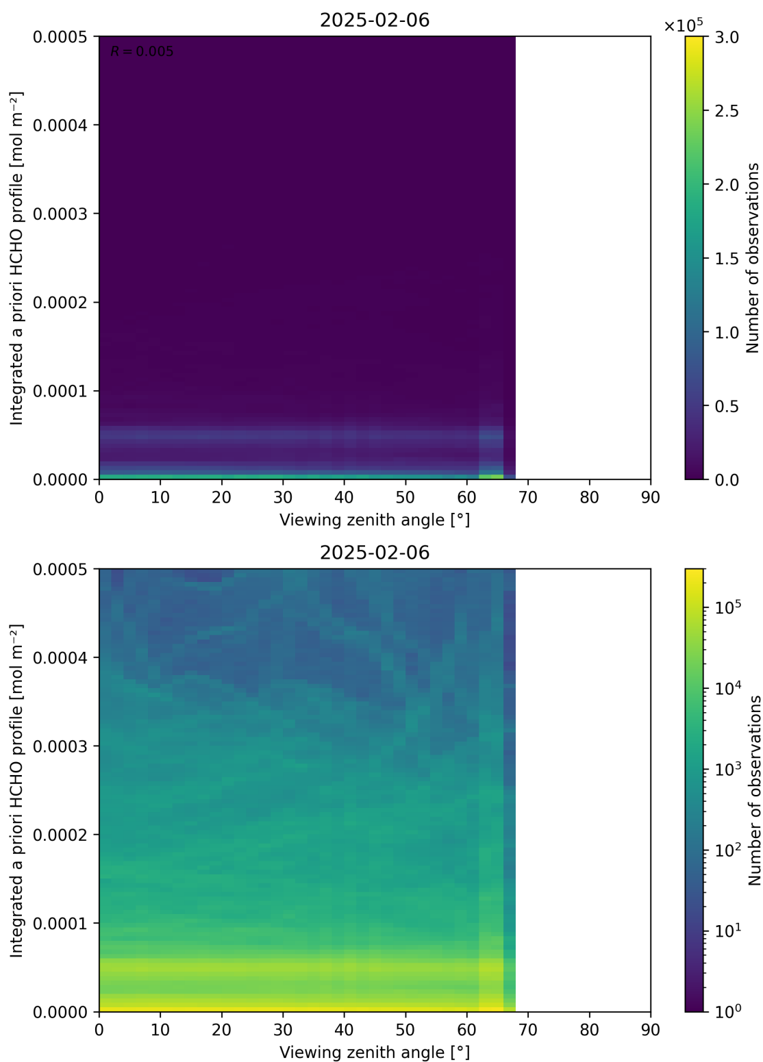
Figure 195: Scatter density plot of “Viewing zenith angle” against “Integrated a priori HCHO profile” for 2025-02-05 to 2025-02-07.
