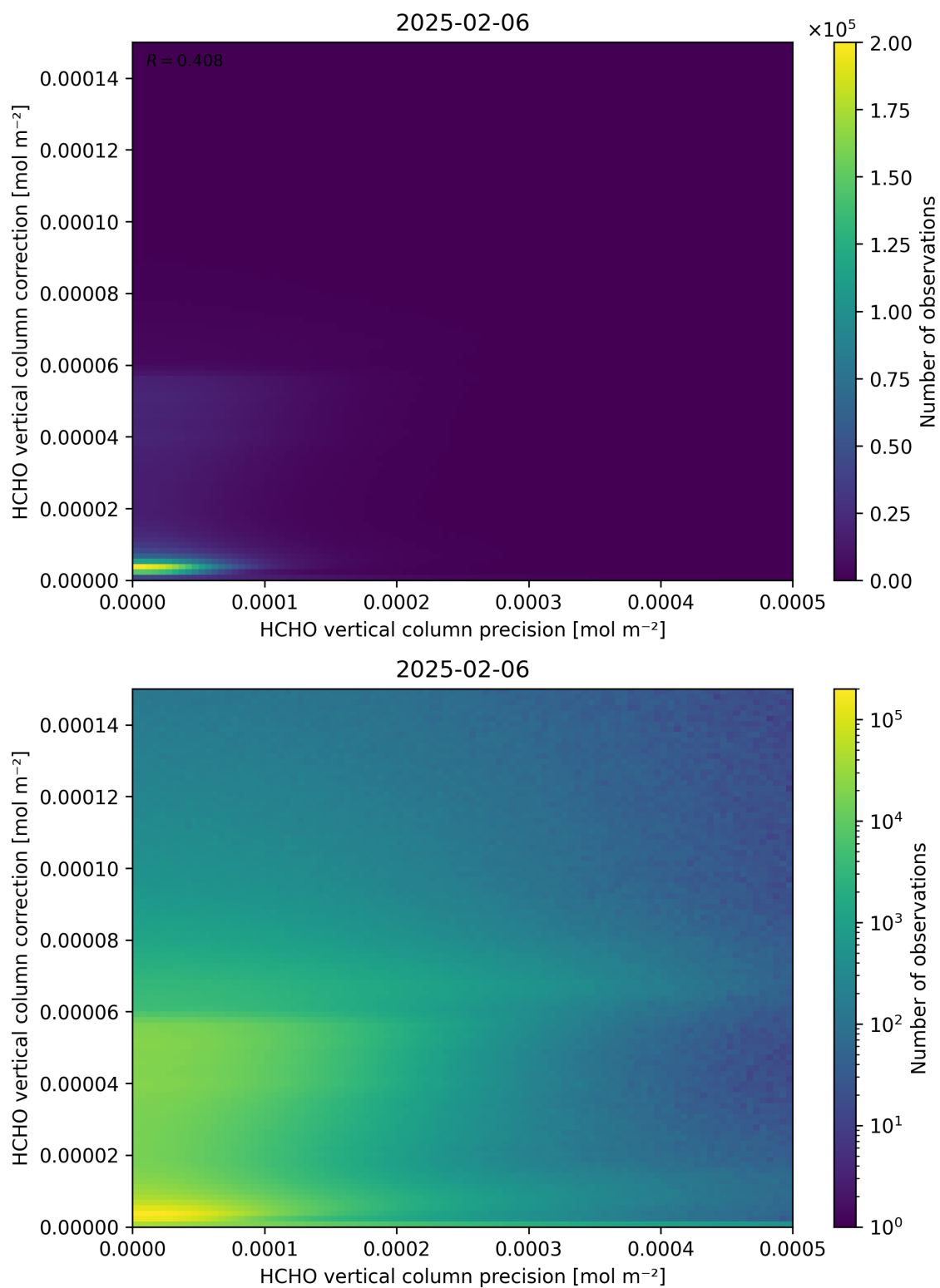
Figure 146: Scatter density plot of “HCHO vertical column precision” against “HCHO vertical column correction” for 2025-02-05 to 2025-02-07.
