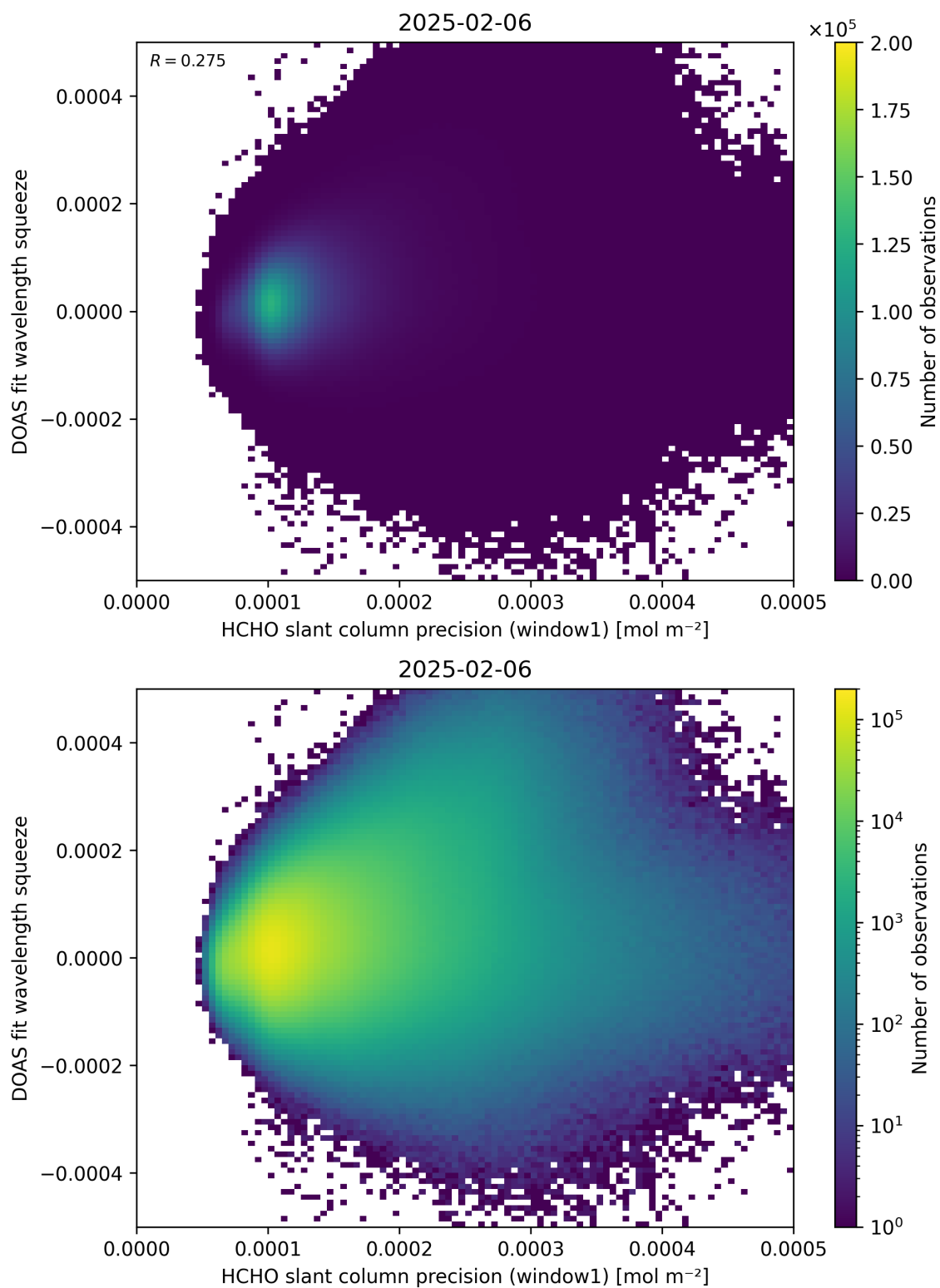
Figure 90: Scatter density plot of “HCHO slant column precision (window1)” against “DOAS fit wavelength squeeze” for 2025-02-05 to 2025-02-07.
