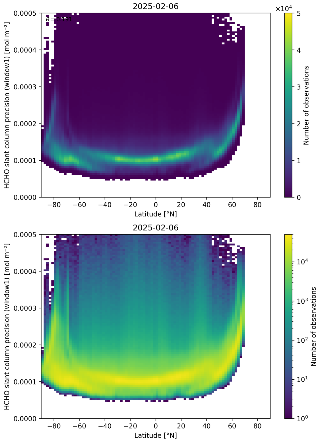
Figure 160: Scatter density plot of “Latitude” against “HCHO slant column precision (window1)” for 2025-02-05 to 2025-02-07.
