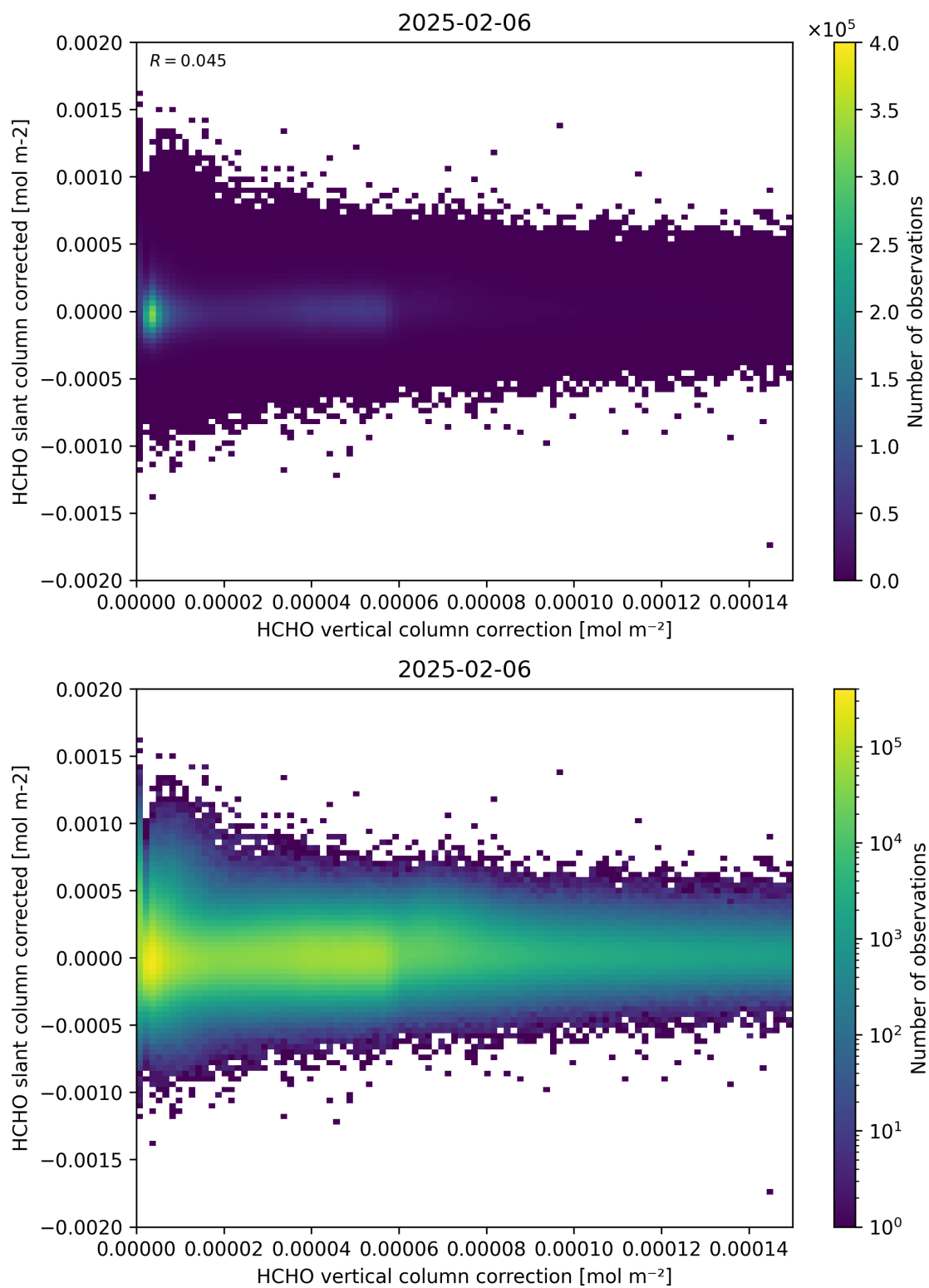
Figure 116: Scatter density plot of “HCHO vertical column correction” against “HCHO slant column corrected” for 2025-02-05 to 2025-02-07.
