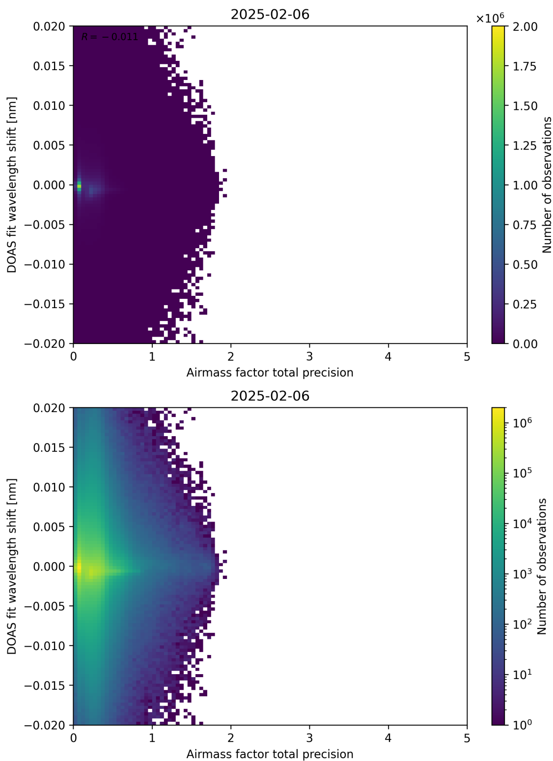
Figure 106: Scatter density plot of “Airmass factor total precision” against “DOAS fit wavelength shift” for 2025-02-05 to 2025-02-07.
