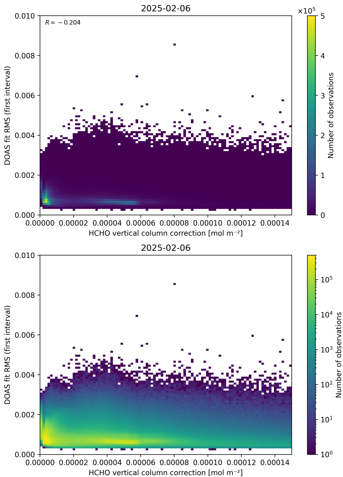
Figure 112: Scatter density plot of “HCHO vertical column correction” against “DOAS fit RMS (first interval)” for 2025-02-05 to 2025-02-07.
