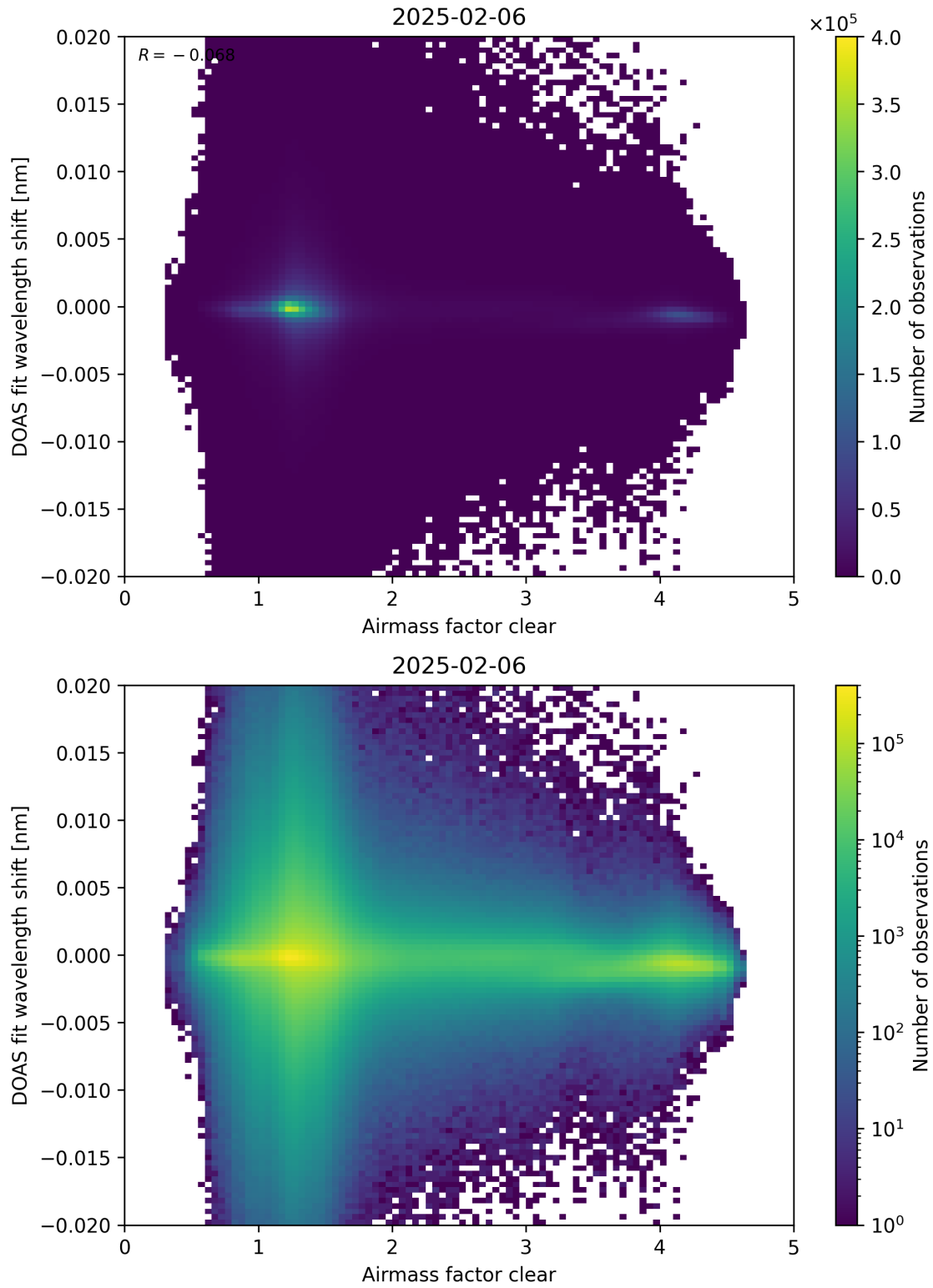
Figure 72: Scatter density plot of “Airmass factor clear” against “DOAS fit wavelength shift” for 2025-02-05 to 2025-02-07.
