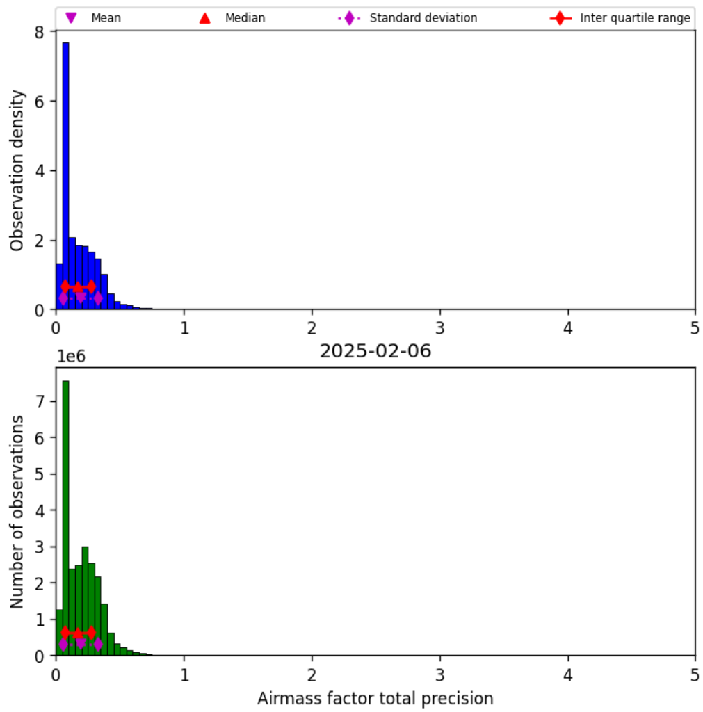
Figure 41: Histogram of “Airmass factor total precision” for 2025-02-05 to 2025-02-07
