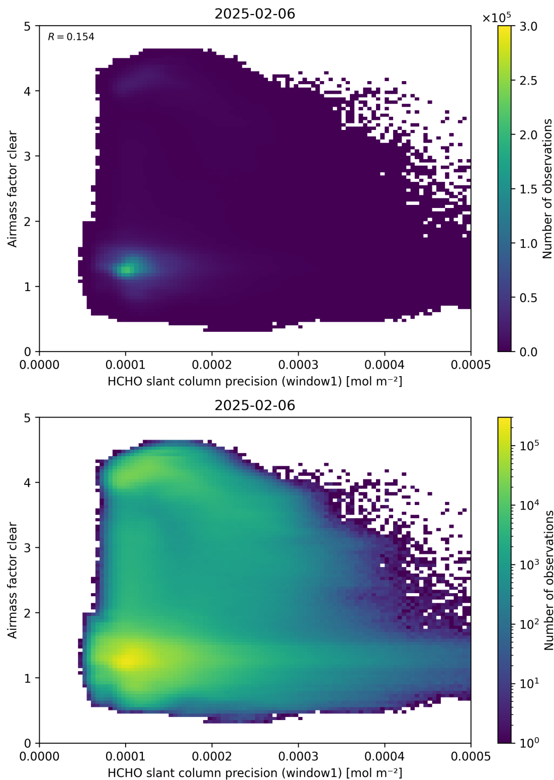
Figure 91: Scatter density plot of “HCHO slant column precision (window1)” against “Airmass factor clear” for 2025-02-05 to 2025-02-07.
