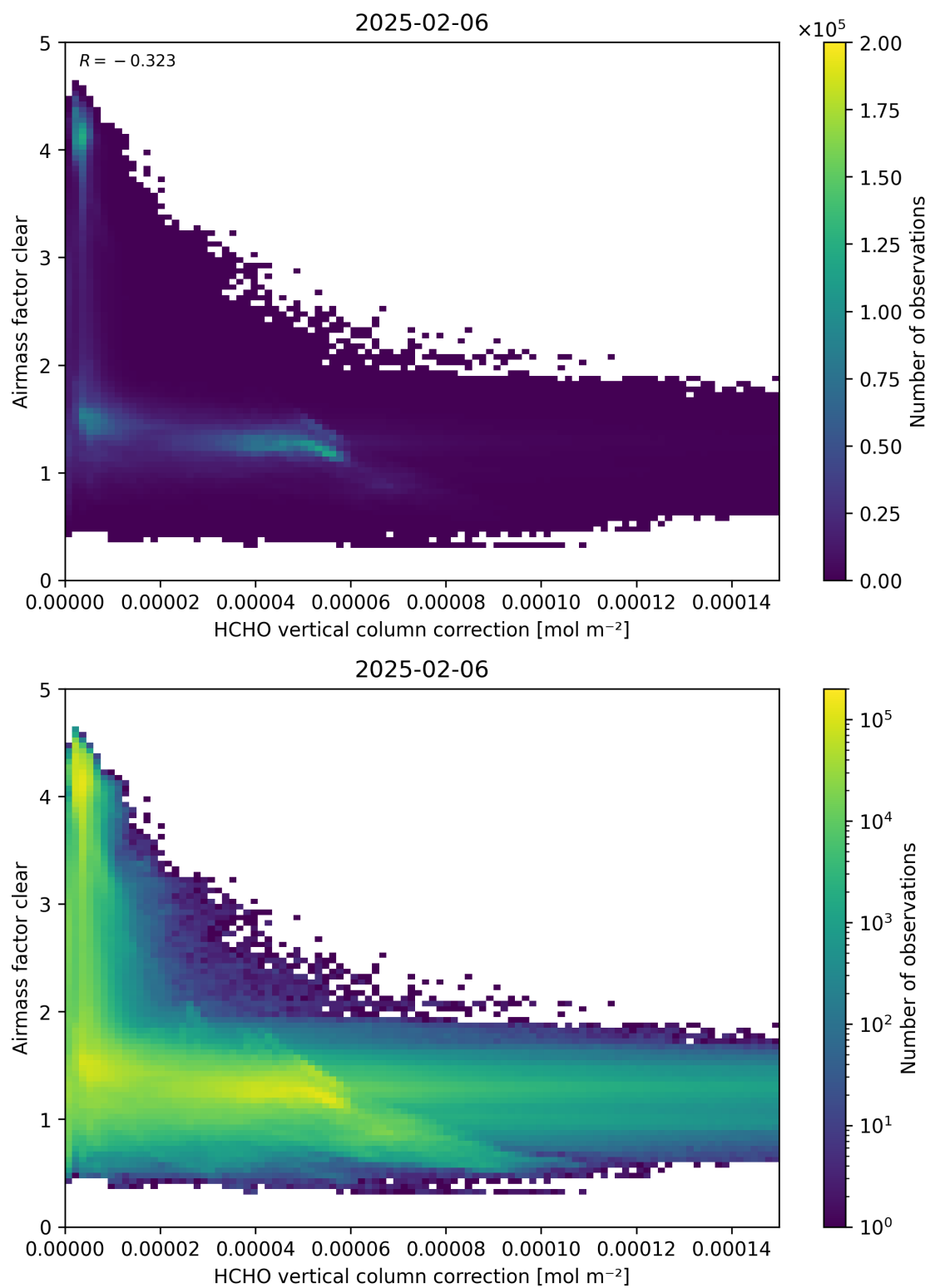
Figure 115: Scatter density plot of “HCHO vertical column correction” against “Airmass factor clear” for 2025-02-05 to 2025-02-07.
