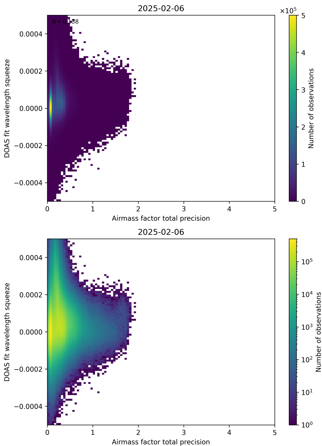
Figure 107: Scatter density plot of “Airmass factor total precision” against “DOAS fit wavelength squeeze” for 2025-02-05 to 2025-02-07.
