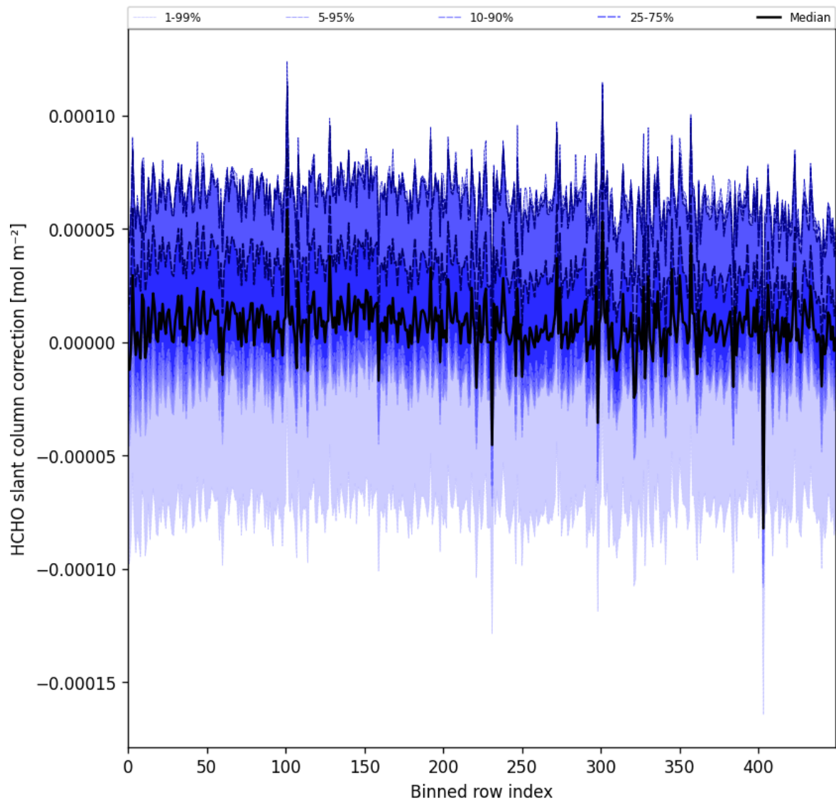
Figure 61: Along track statistics of “HCHO slant column correction” for 2025-02-05 to 2025-02-07
