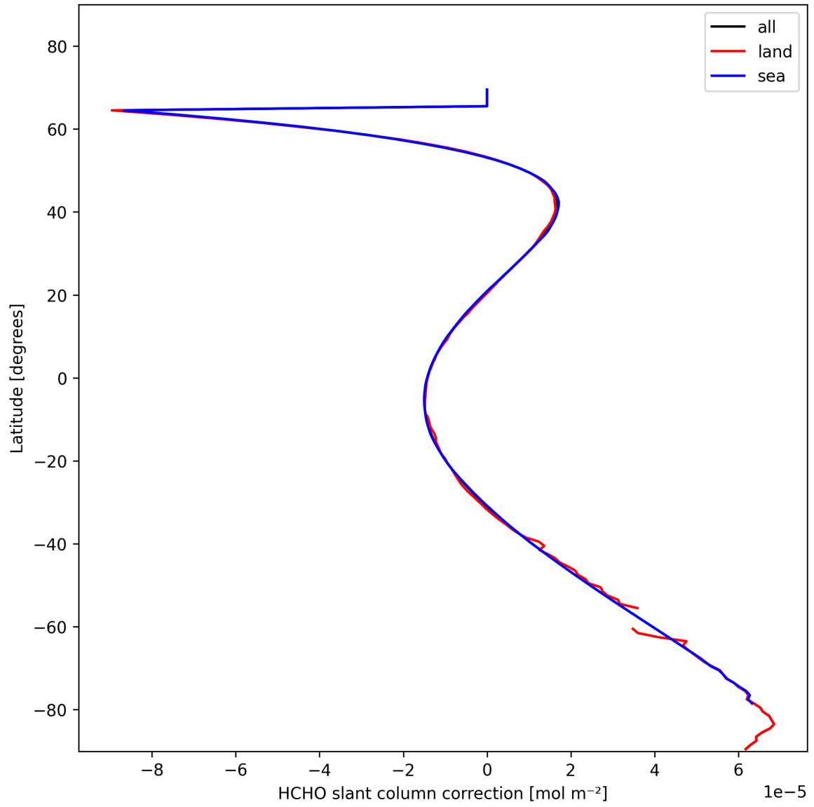
Figure 33: Zonal average of “HCHO slant column correction” for 2025-02-05 to 2025-02-07.
