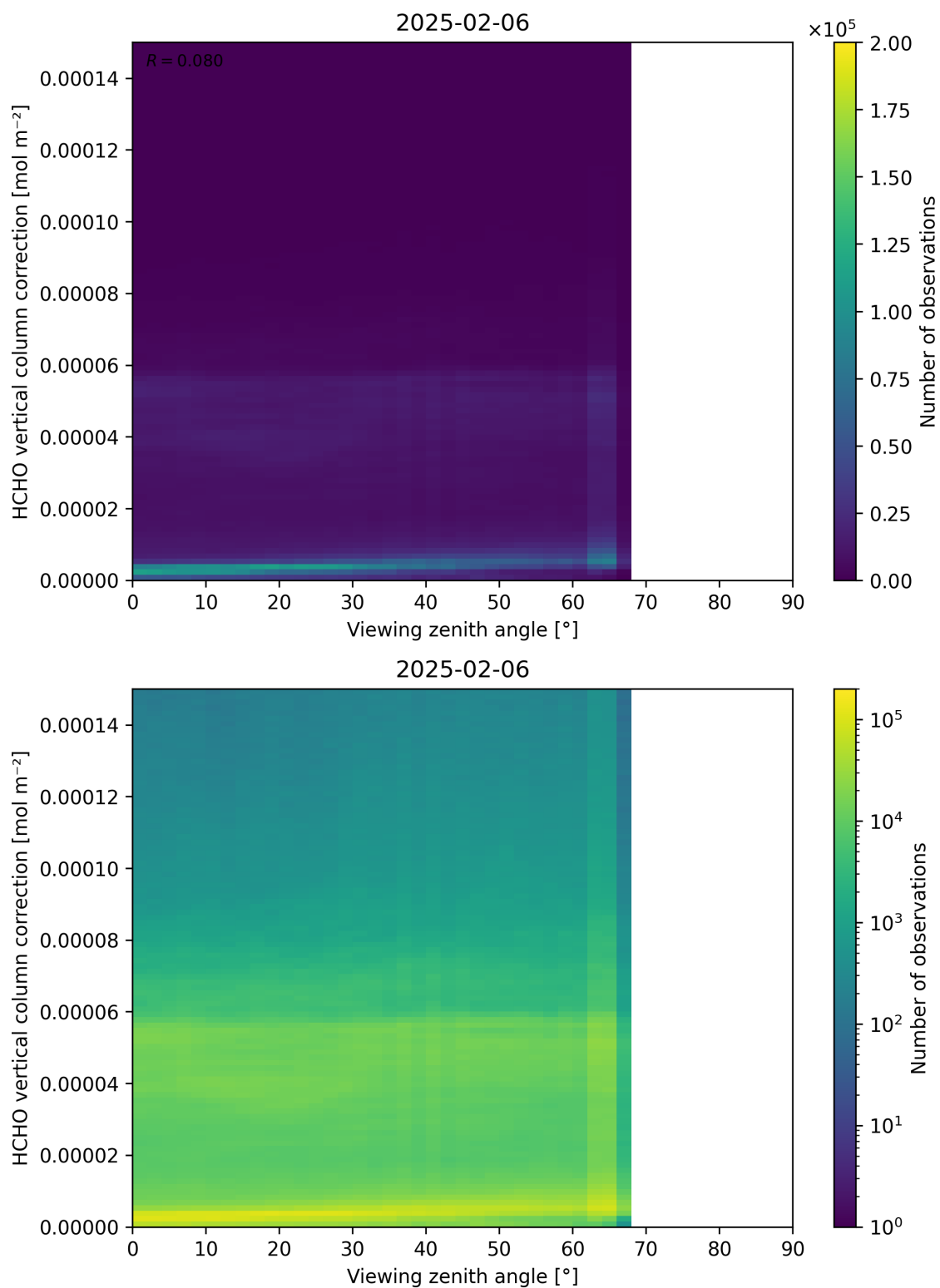
Figure 193: Scatter density plot of “Viewing zenith angle” against “HCHO vertical column correction” for 2025-02-05 to 2025-02-07.
