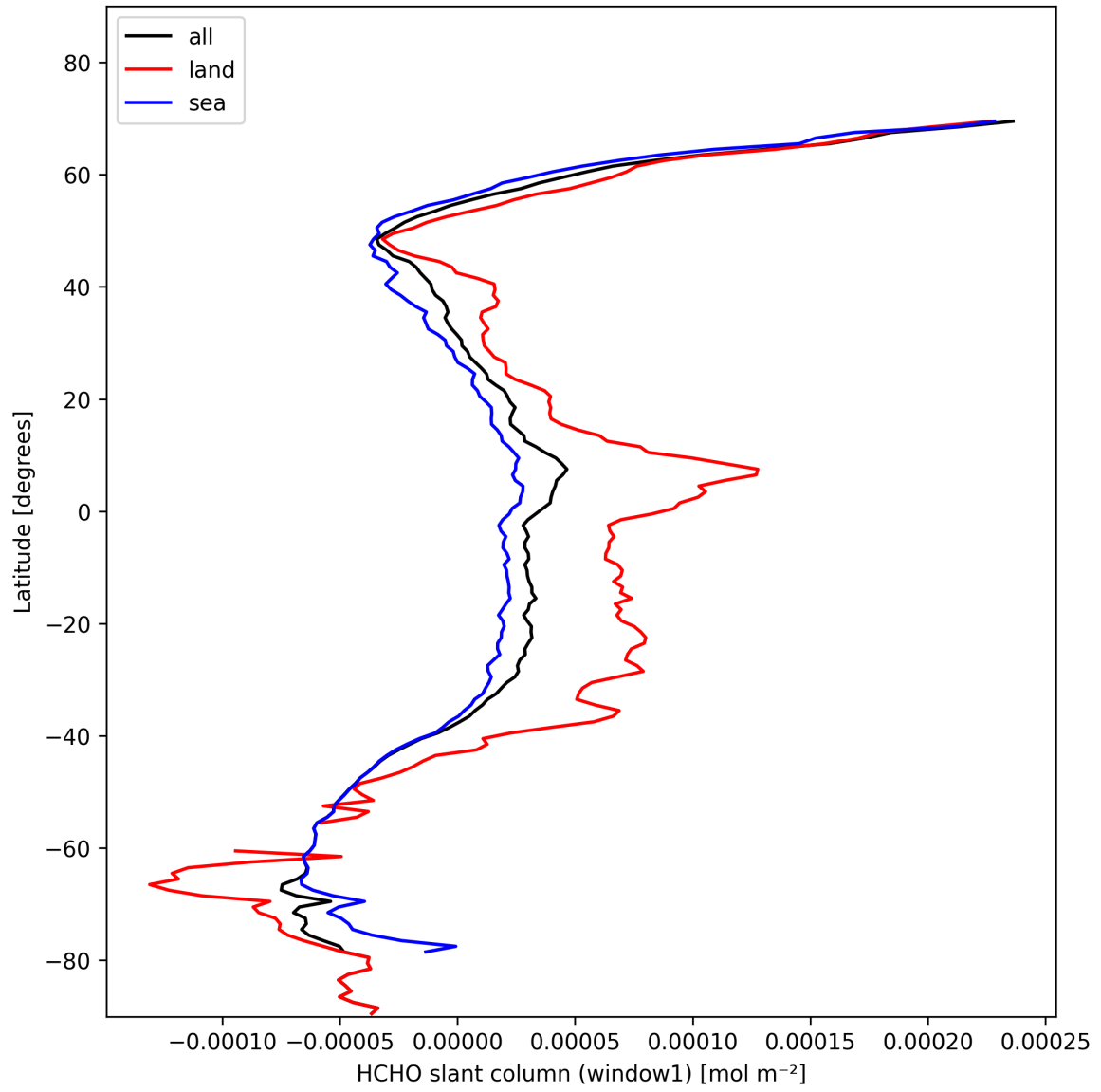
Figure 24: Zonal average of “HCHO slant column (window1)” for 2025-02-05 to 2025-02-07.
