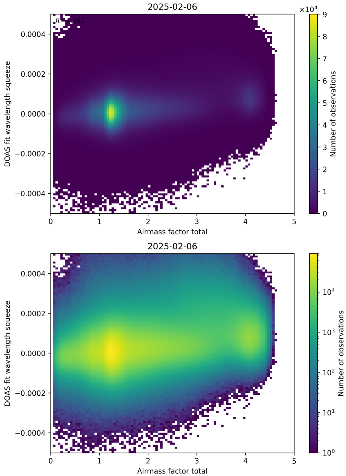
Figure 99: Scatter density plot of “Airmass factor total” against “DOAS fit wavelength squeeze” for 2025-02-05 to 2025-02-07.
