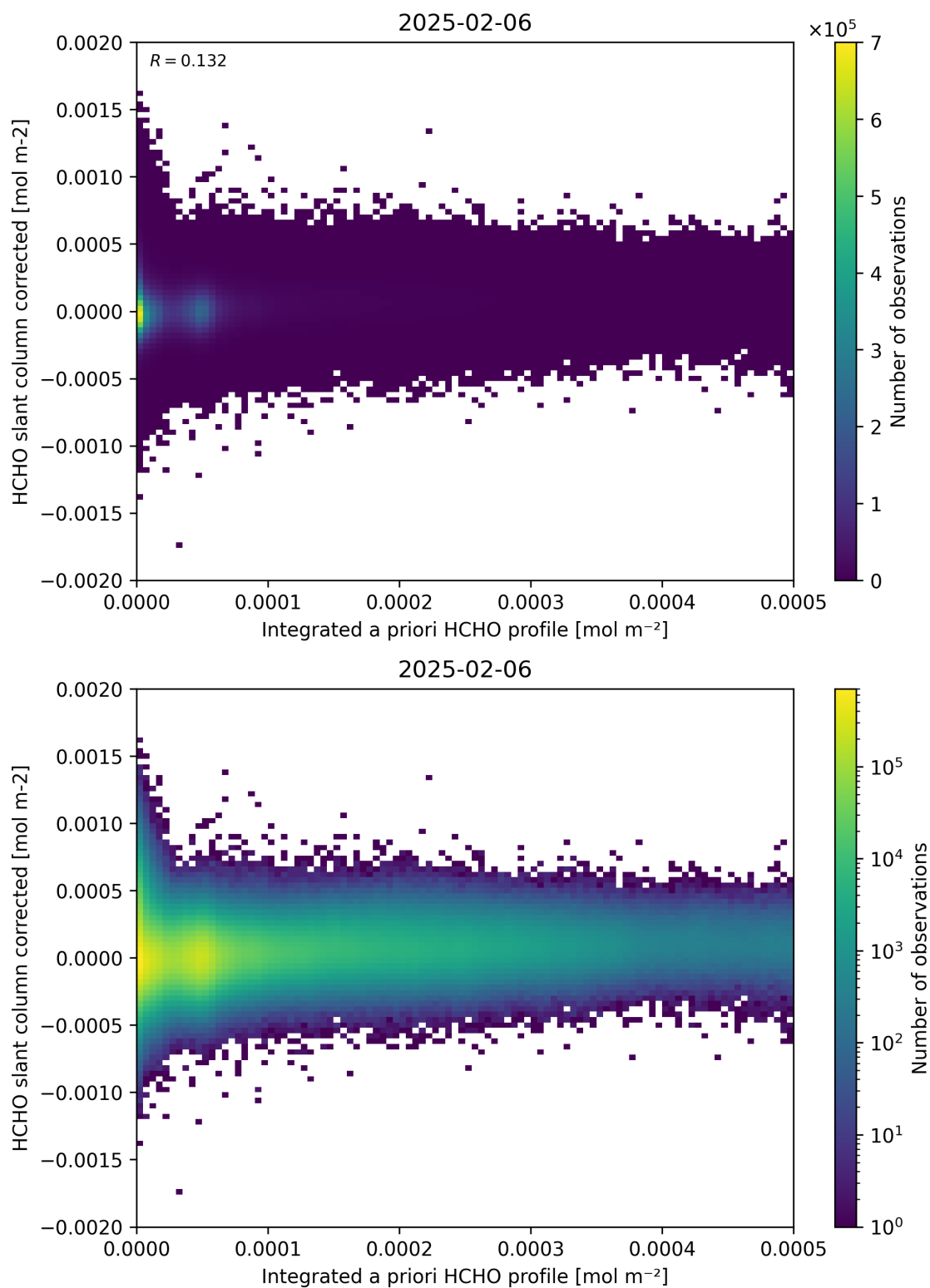
Figure 151: Scatter density plot of “Integrated a priori HCHO profile” against “HCHO slant column corrected” for 2025-02-05 to 2025-02-07.
