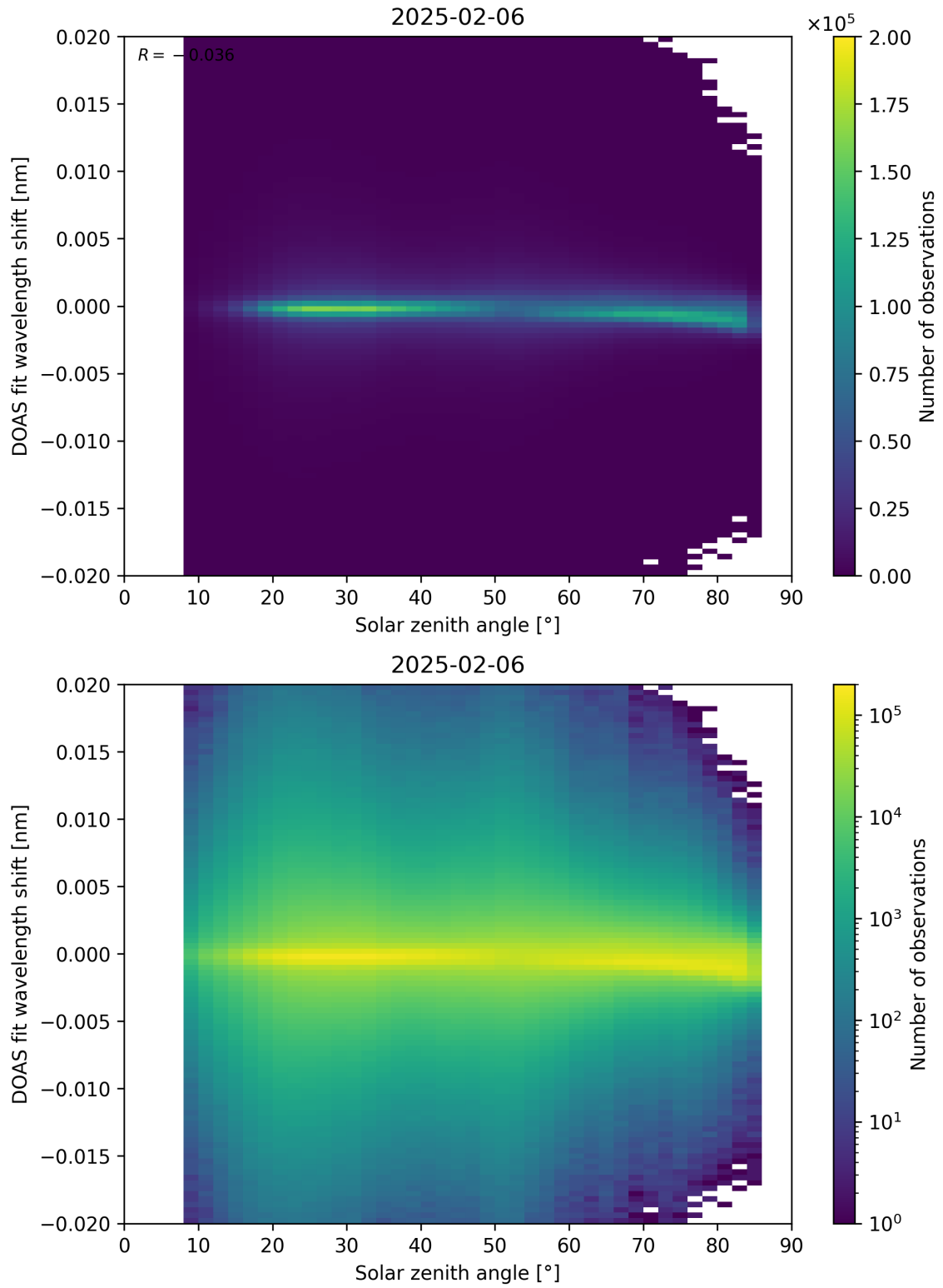
Figure 168: Scatter density plot of “Solar zenith angle” against “DOAS fit wavelength shift” for 2025-02-05 to 2025-02-07.
