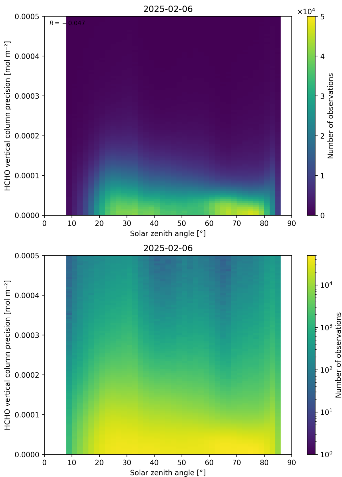
Figure 179: Scatter density plot of “Solar zenith angle” against “HCHO vertical column precision” for 2025-02-05 to 2025-02-07.
