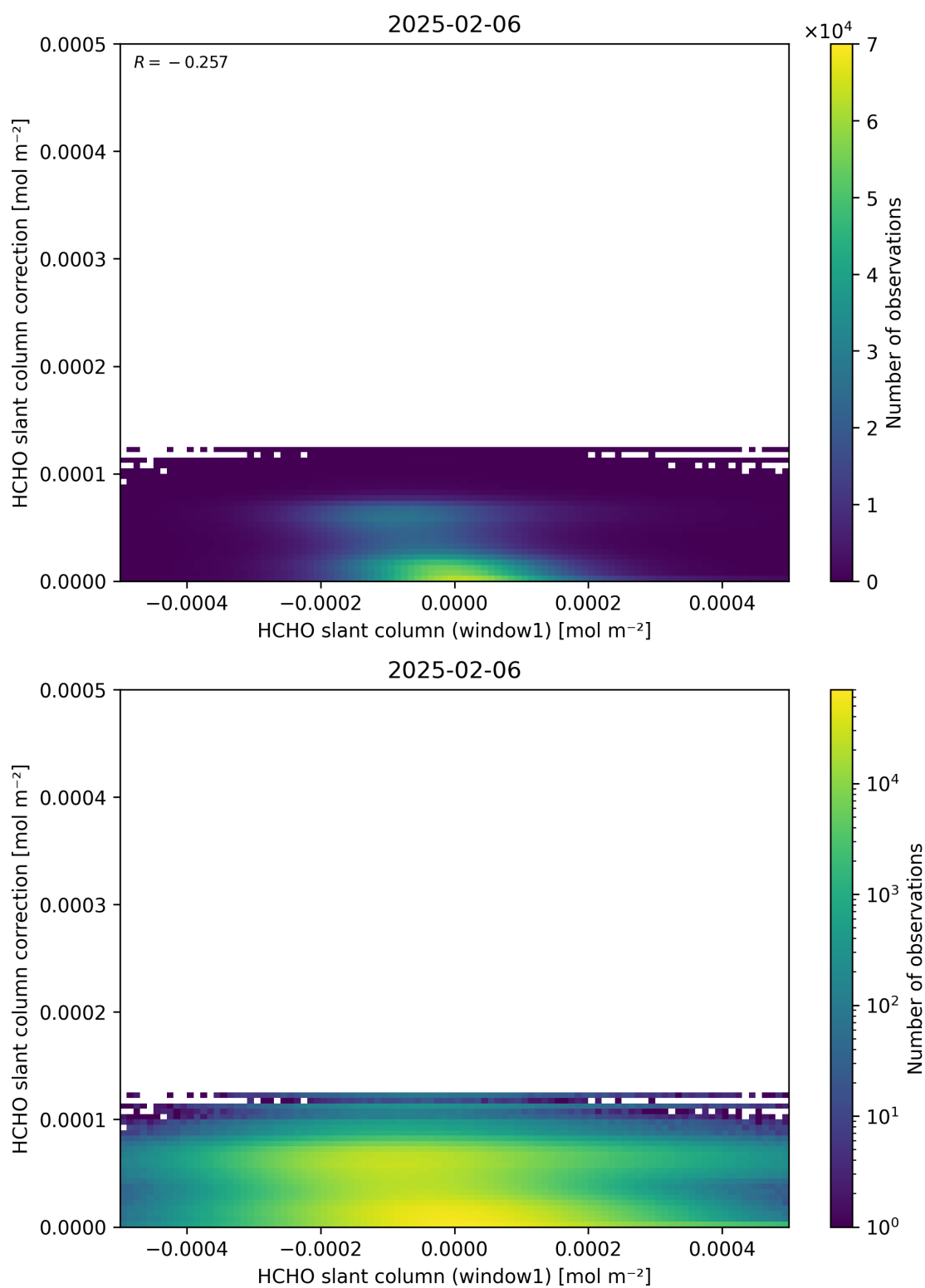
Figure 83: Scatter density plot of “HCHO slant column (window1)” against “HCHO slant column correction” for 2025-02-05 to 2025-02-07.
