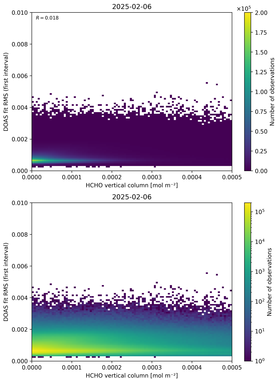
Figure 123: Scatter density plot of “HCHO vertical column” against “DOAS fit RMS (first interval)” for 2025-02-05 to 2025-02-07.
