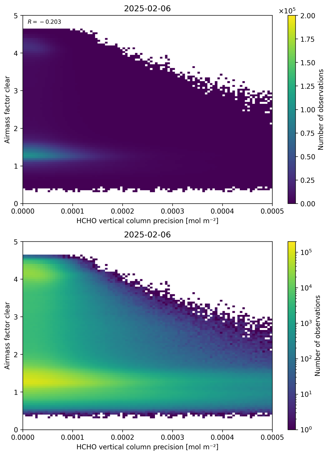
Figure 139: Scatter density plot of “HCHO vertical column precision” against “Airmass factor clear” for 2025-02-05 to 2025-02-07.
