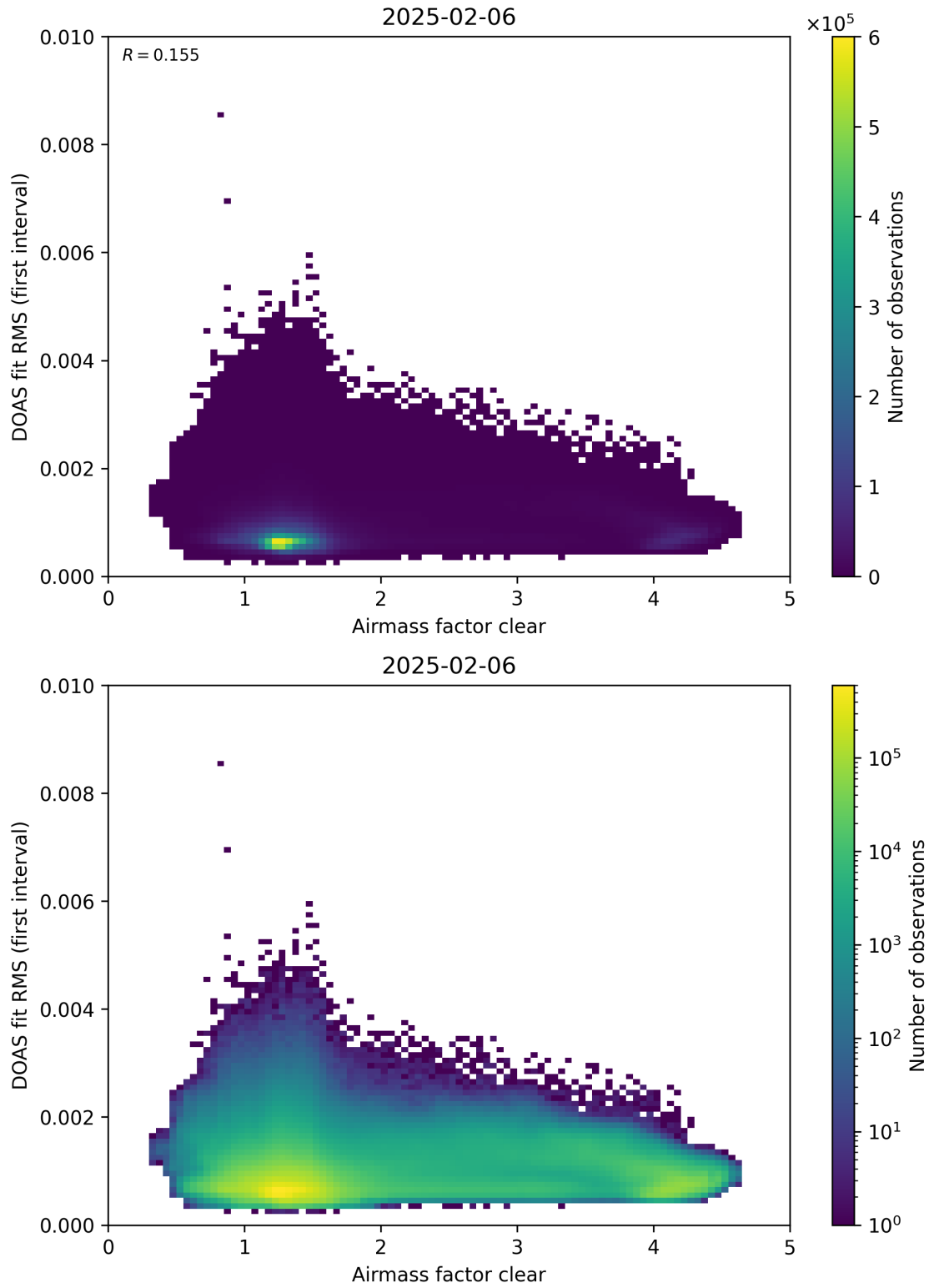
Figure 71: Scatter density plot of “Airmass factor clear” against “DOAS fit RMS (first interval)” for 2025-02-05 to 2025-02-07.
