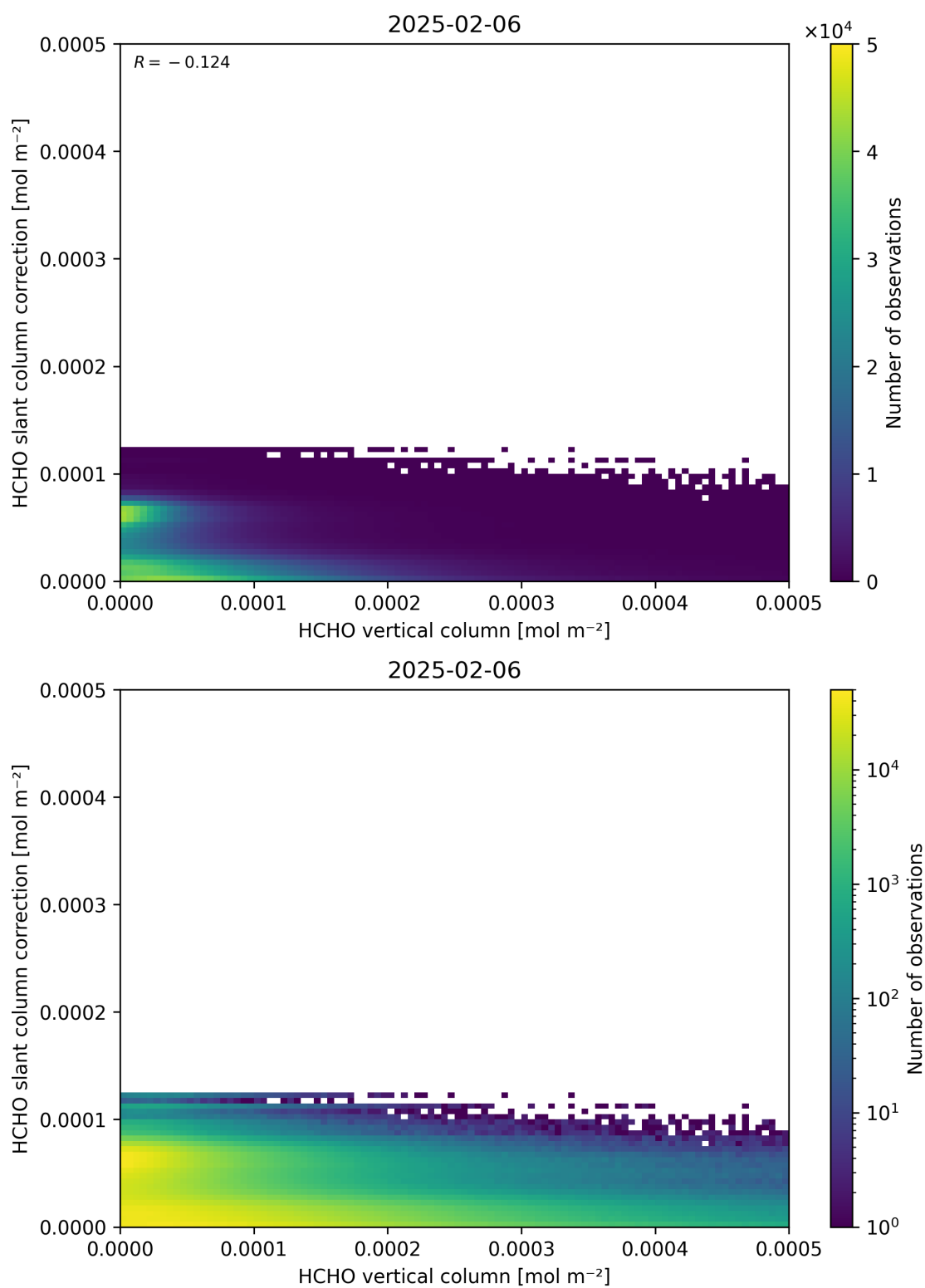
Figure 128: Scatter density plot of “HCHO vertical column” against “HCHO slant column correction” for 2025-02-05 to 2025-02-07.
