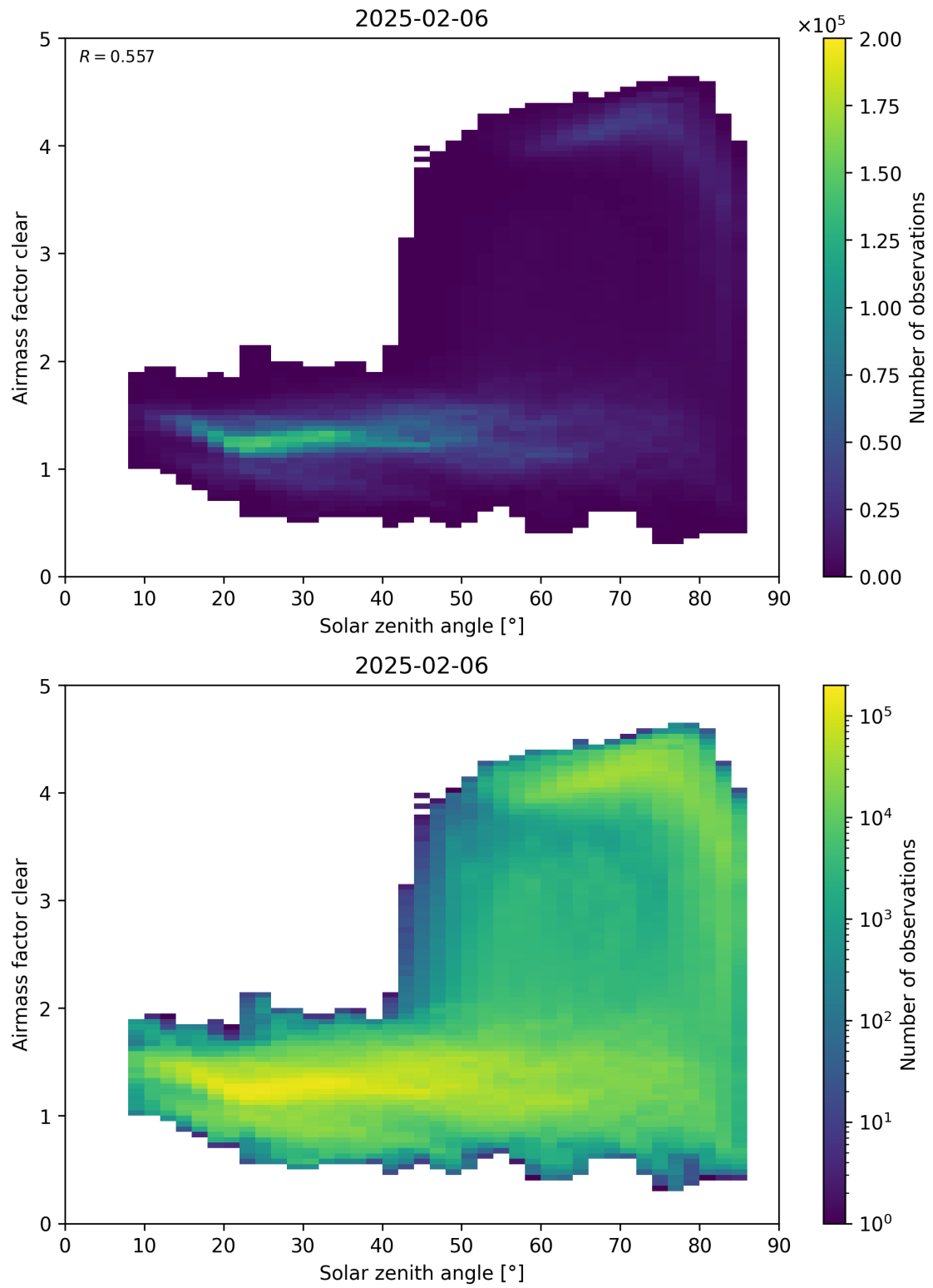
Figure 170: Scatter density plot of “Solar zenith angle” against “Airmass factor clear” for 2025-02-05 to 2025-02-07.
