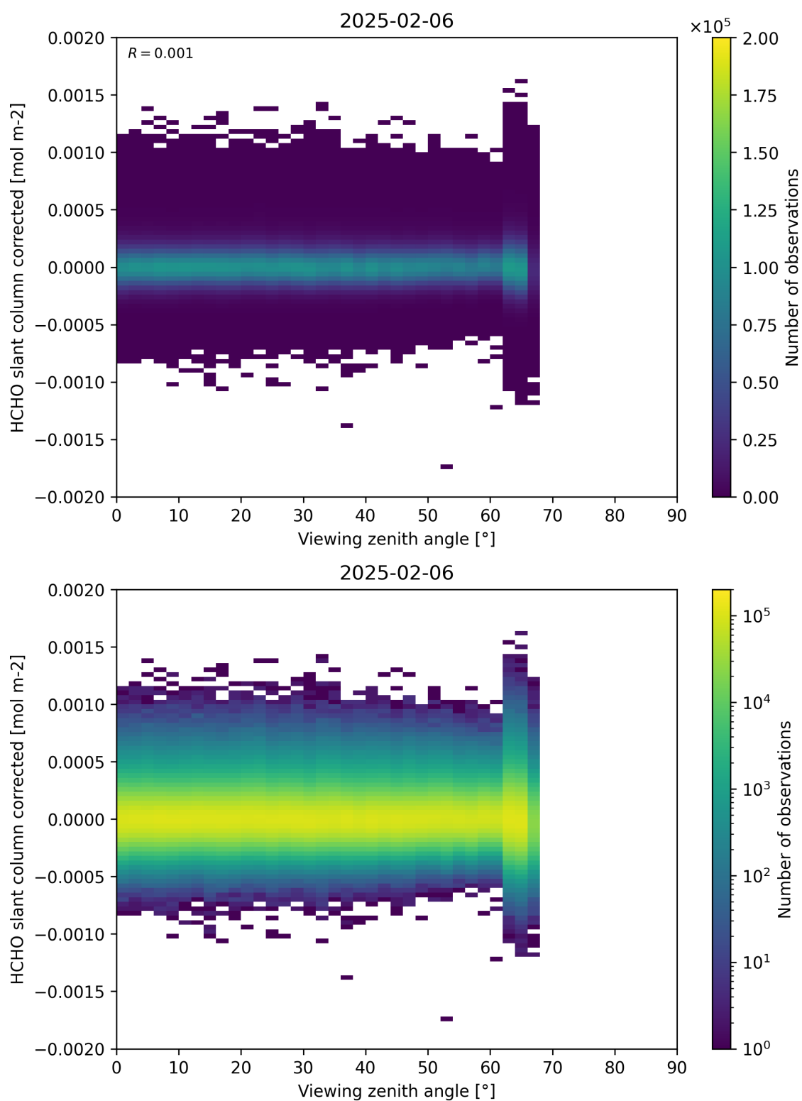
Figure 186: Scatter density plot of “Viewing zenith angle” against “HCHO slant column corrected” for 2025-02-05 to 2025-02-07.
