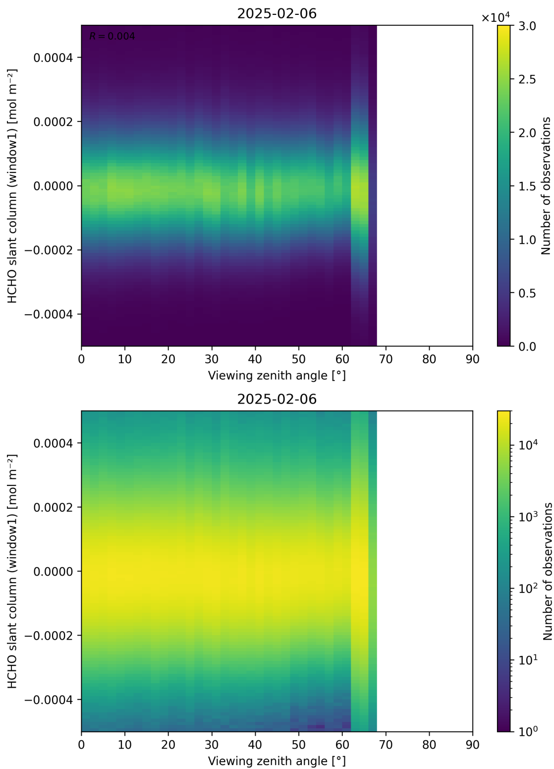
Figure 188: Scatter density plot of “Viewing zenith angle” against “HCHO slant column (window1)” for 2025-02-05 to 2025-02-07.
