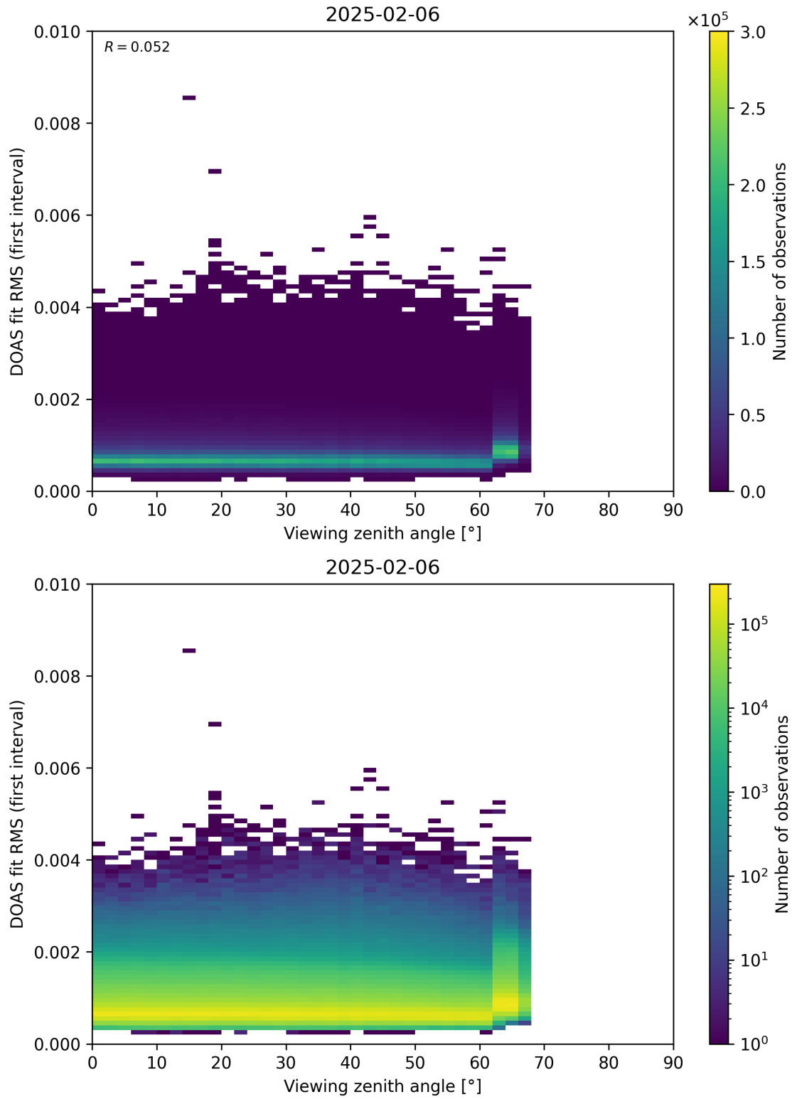
Figure 182: Scatter density plot of “Viewing zenith angle” against “DOAS fit RMS (first interval)” for 2025-02-05 to 2025-02-07.
