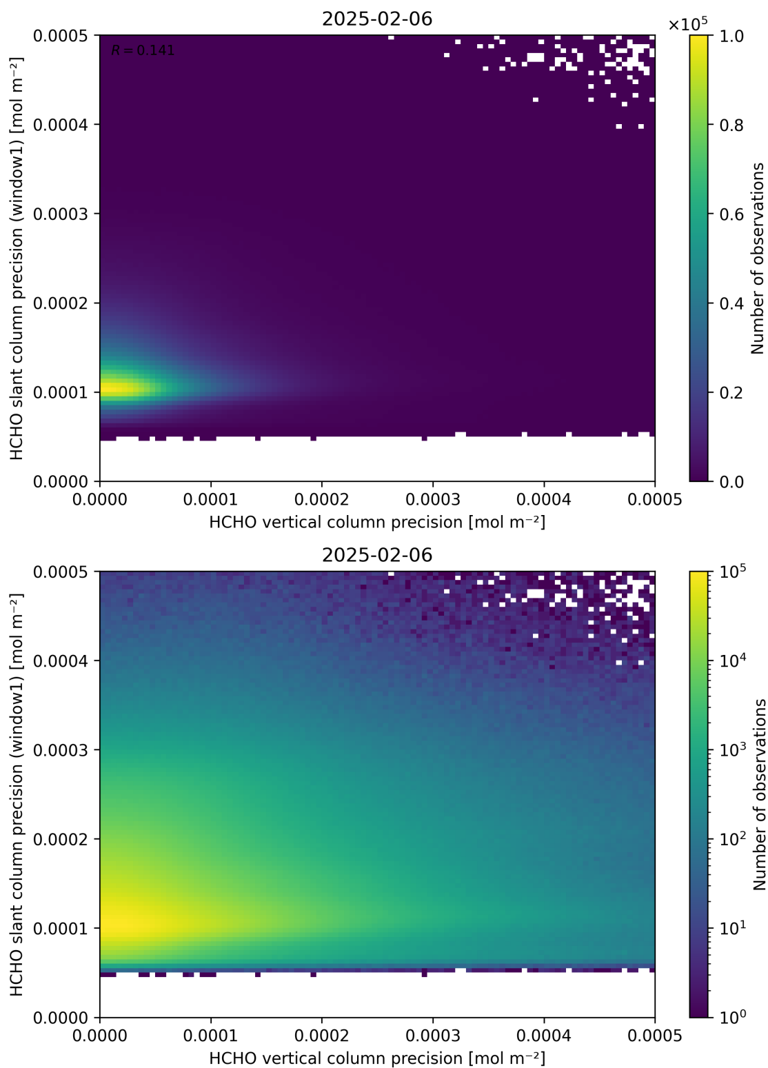
Figure 143: Scatter density plot of “HCHO vertical column precision” against “HCHO slant column precision (window1)” for 2025-02-05 to 2025-02-07.
