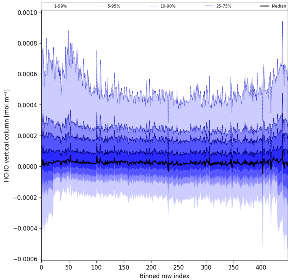
Figure 49: Along track statistics of “HCHO vertical column” for 2025-02-05 to 2025-02-07
