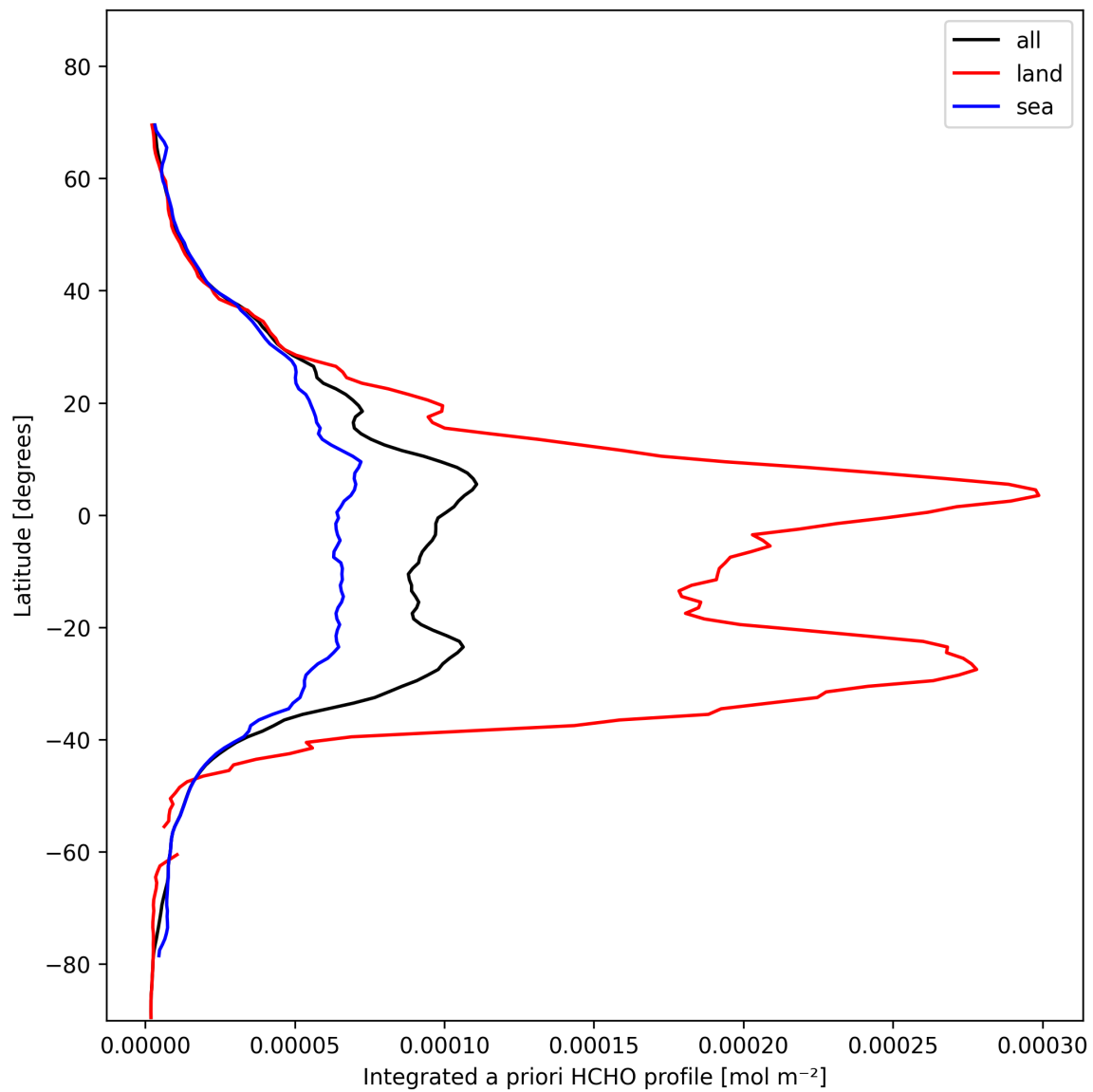
Figure 29: Zonal average of “Integrated a priori HCHO profile” for 2025-02-05 to 2025-02-07.
