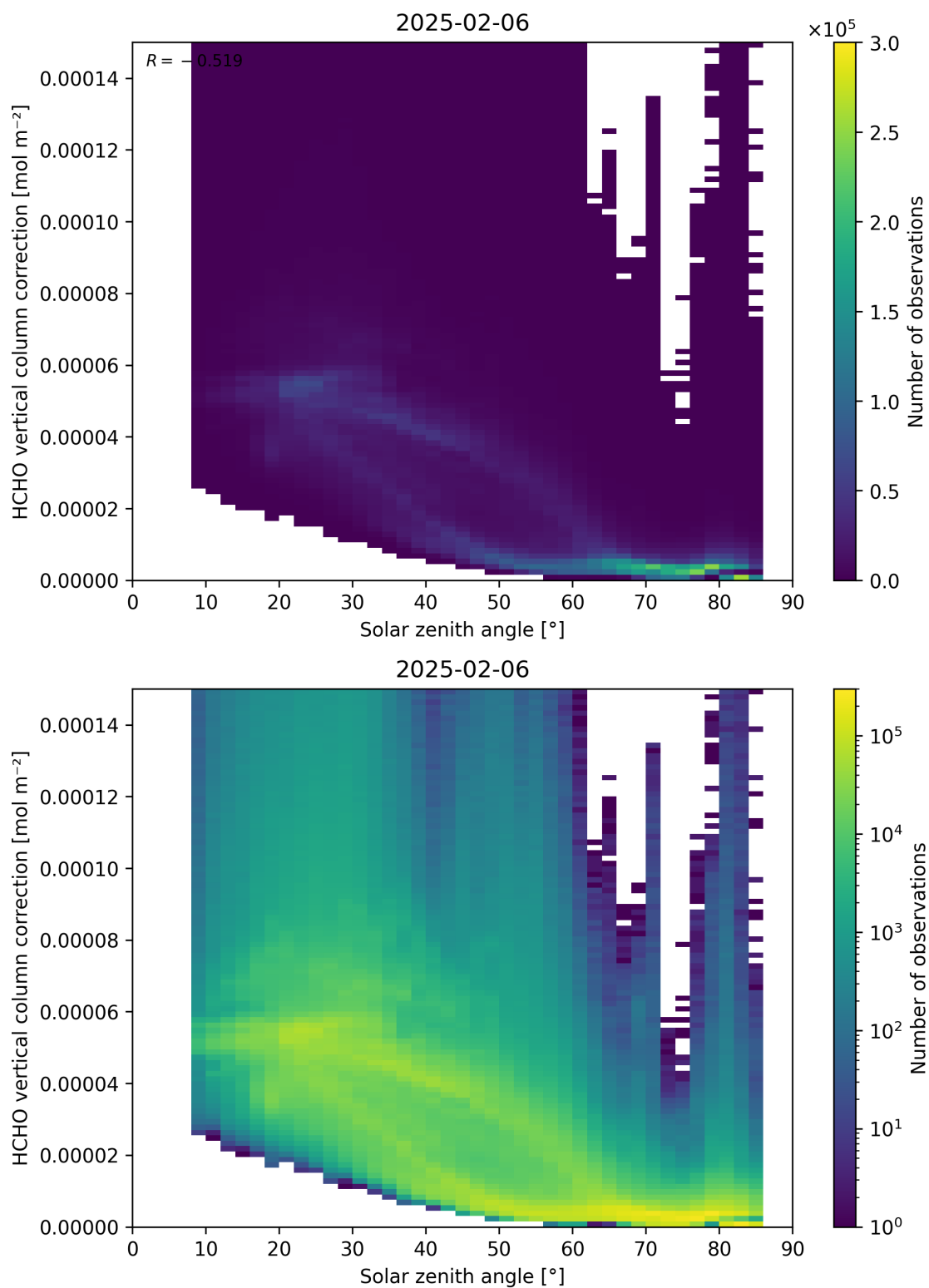
Figure 178: Scatter density plot of “Solar zenith angle” against “HCHO vertical column correction” for 2025-02-05 to 2025-02-07.
