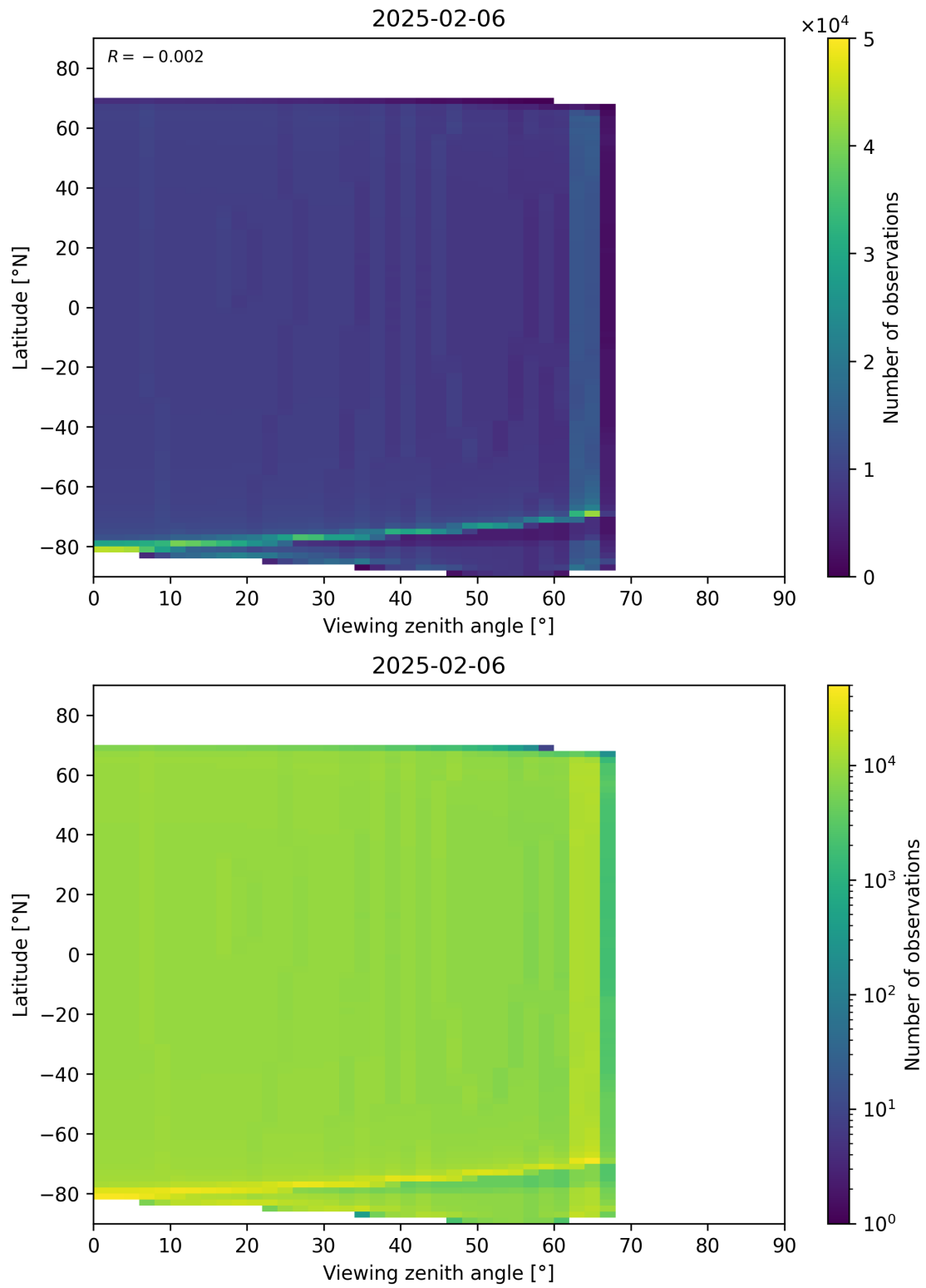
Figure 196: Scatter density plot of “Viewing zenith angle” against “Latitude” for 2025-02-05 to 2025-02-07.
