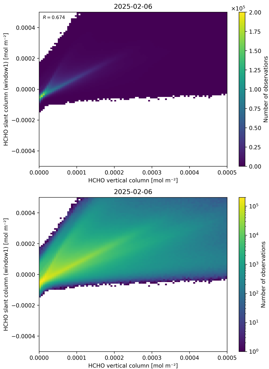
Figure 129: Scatter density plot of “HCHO vertical column” against “HCHO slant column (window1)” for 2025-02-05 to 2025-02-07.
