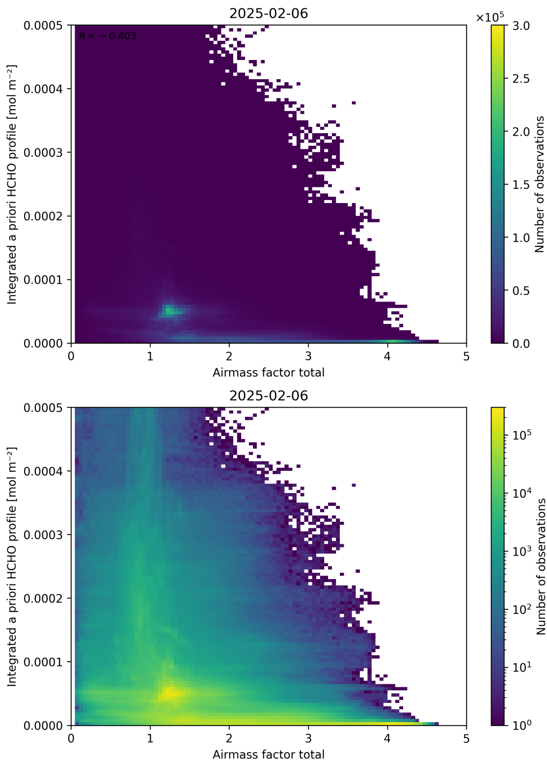
Figure 104: Scatter density plot of “Airmass factor total” against “Integrated a priori HCHO profile” for 2025-02-05 to 2025-02-07.
