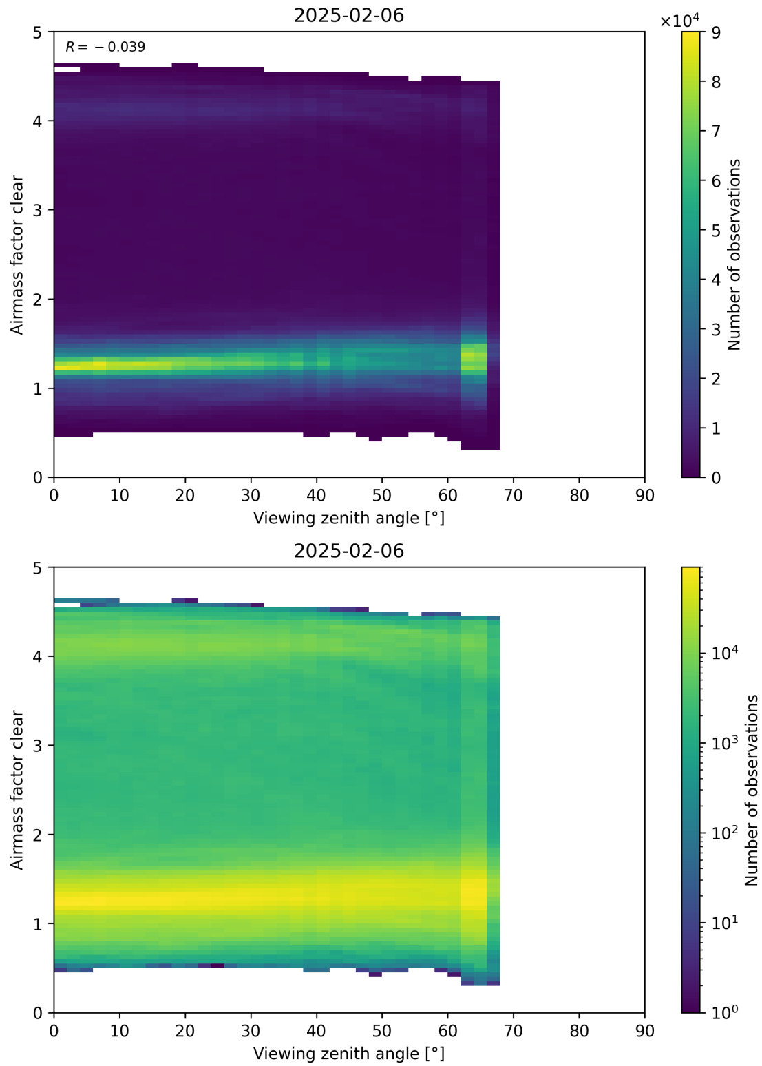
Figure 185: Scatter density plot of “Viewing zenith angle” against “Airmass factor clear” for 2025-02-05 to 2025-02-07.
