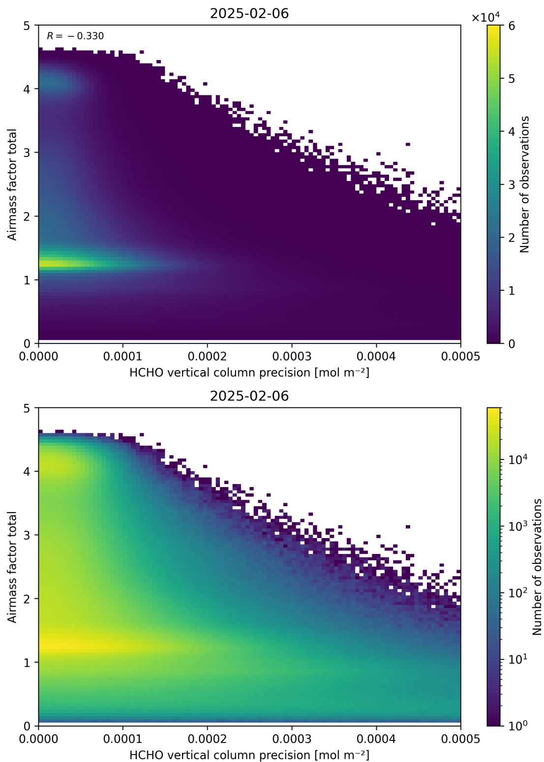
Figure 144: Scatter density plot of “HCHO vertical column precision” against “Airmass factor total” for 2025-02-05 to 2025-02-07.
