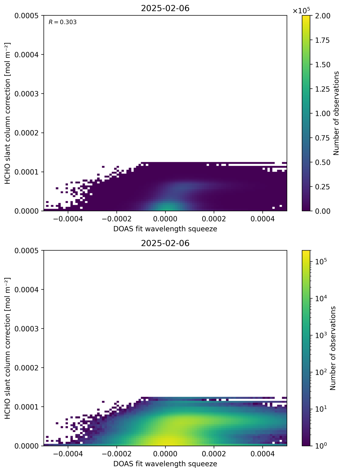
Figure 70: Scatter density plot of “DOAS fit wavelength squeeze” against “HCHO slant column correction” for 2025-02-05 to 2025-02-07.
