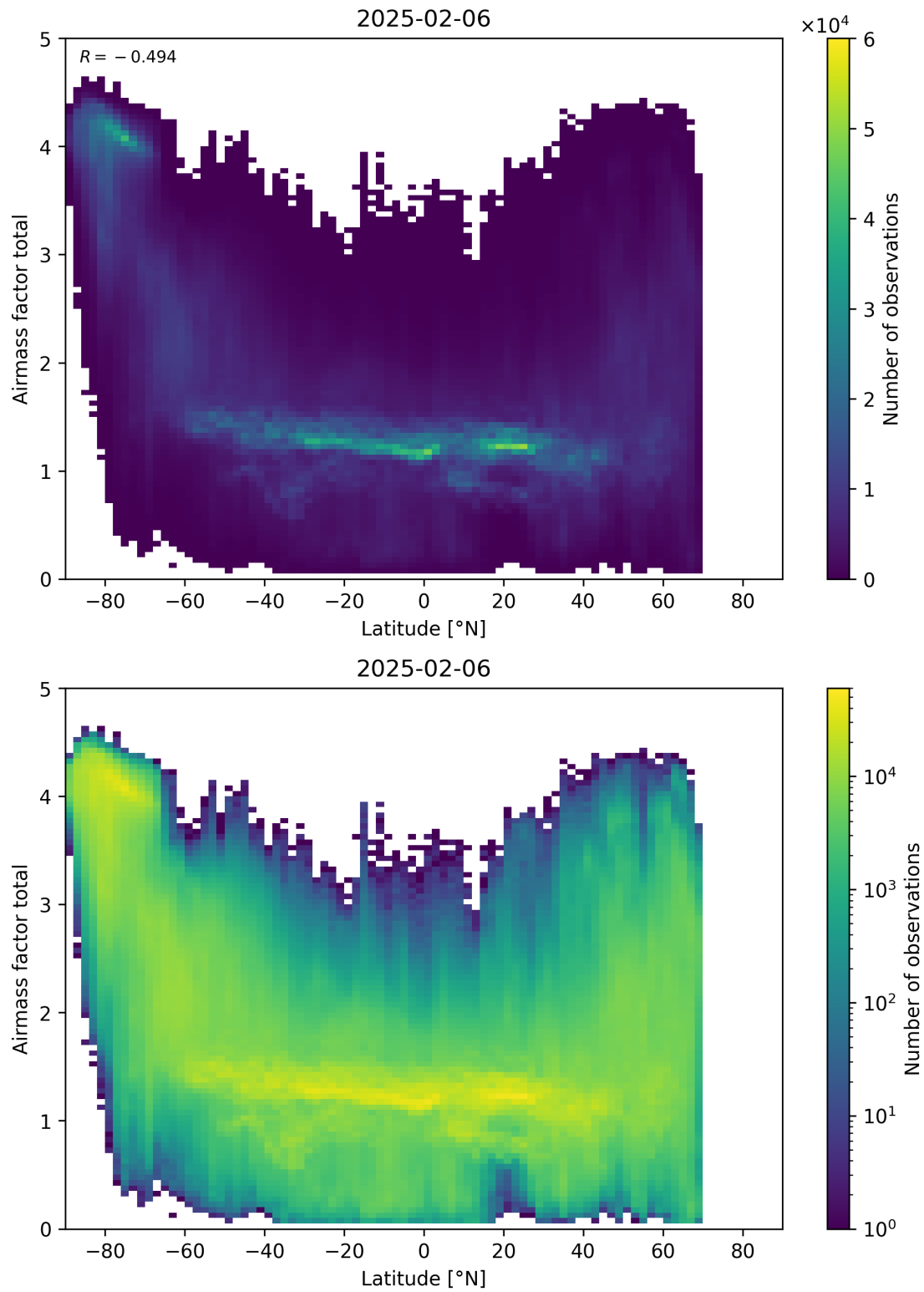
Figure 161: Scatter density plot of “Latitude” against “Airmass factor total” for 2025-02-05 to 2025-02-07.
