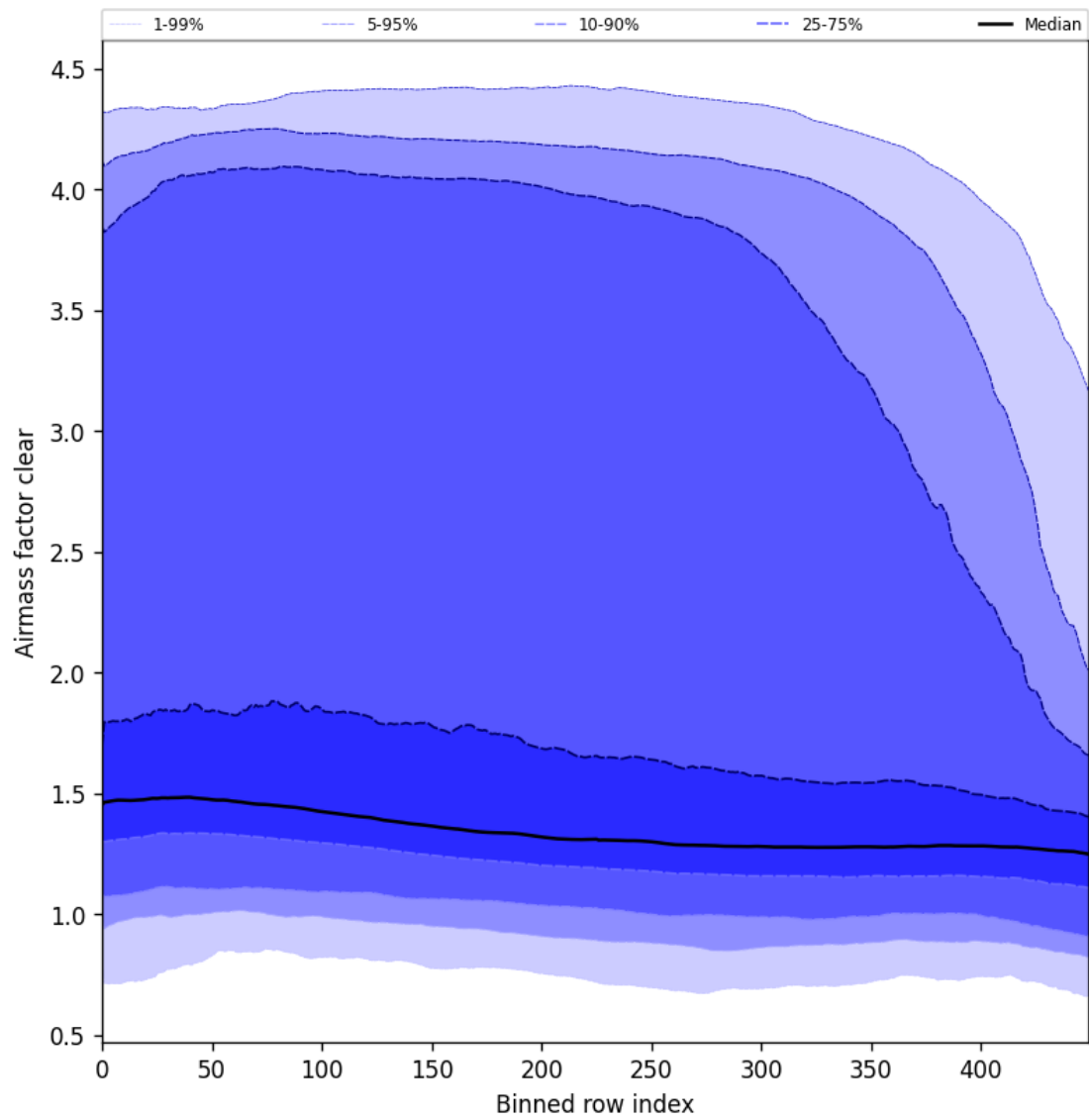
Figure 56: Along track statistics of “Air mass factor clear” for 2025-02-05 to 2025-02-07
