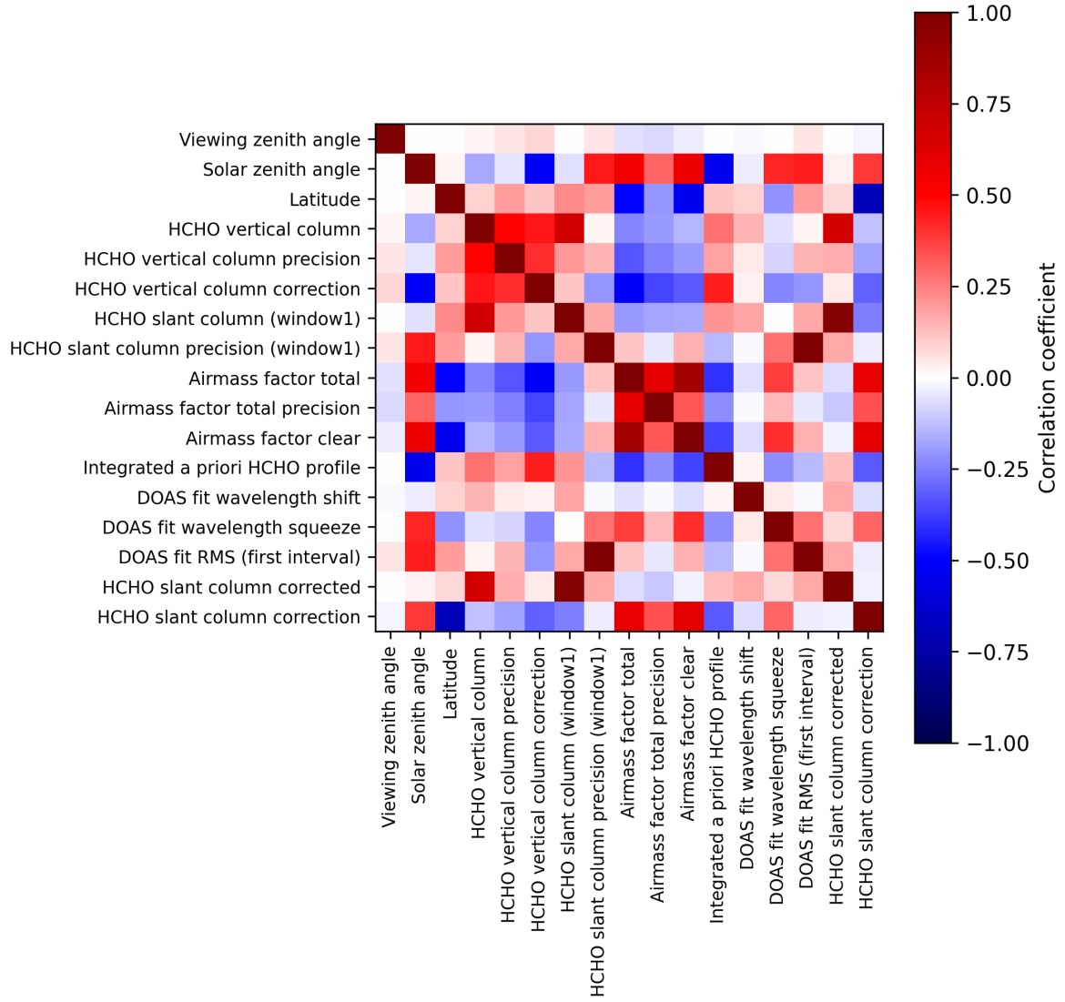
Figure 2: Map of correlation matrix for 2025-02-05 to 2025-02-07.
