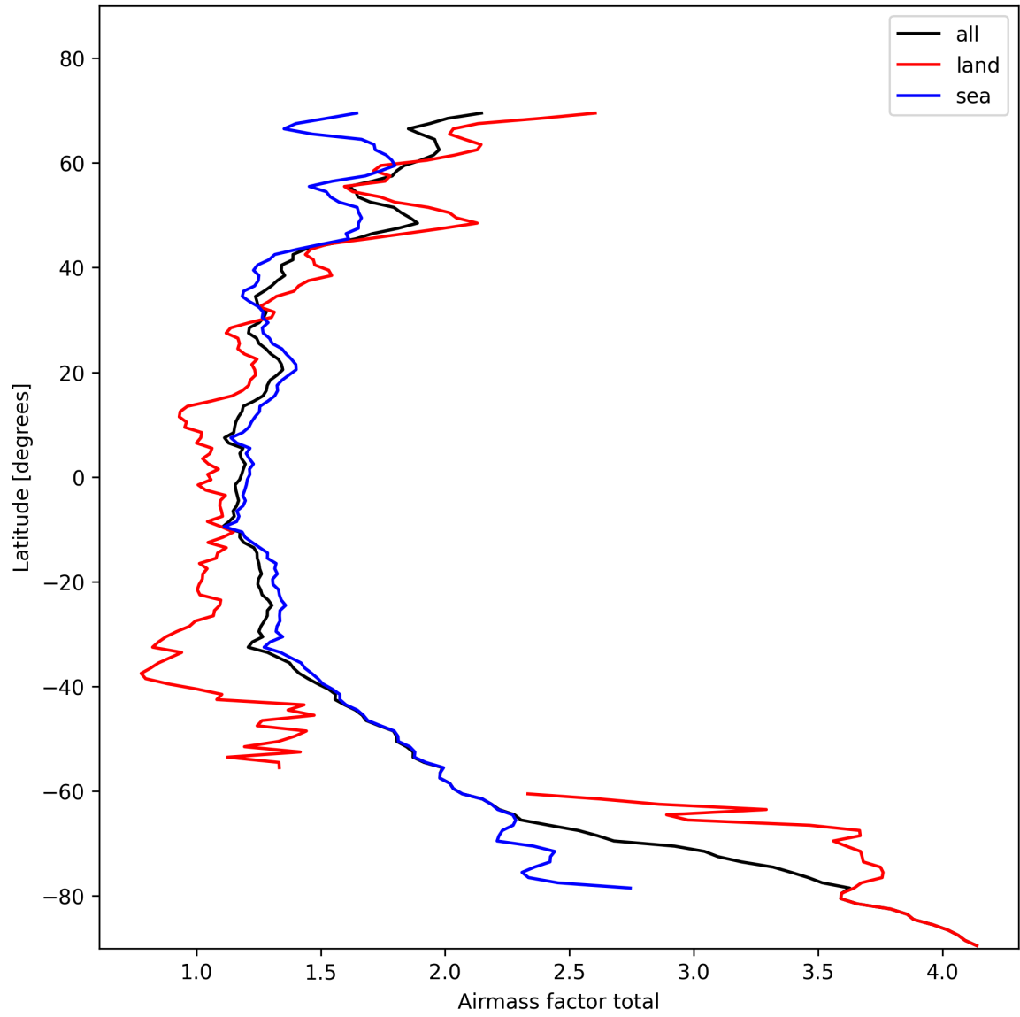
Figure 26: Zonal average of “Airmass factor total” for 2025-02-05 to 2025-02-07.
