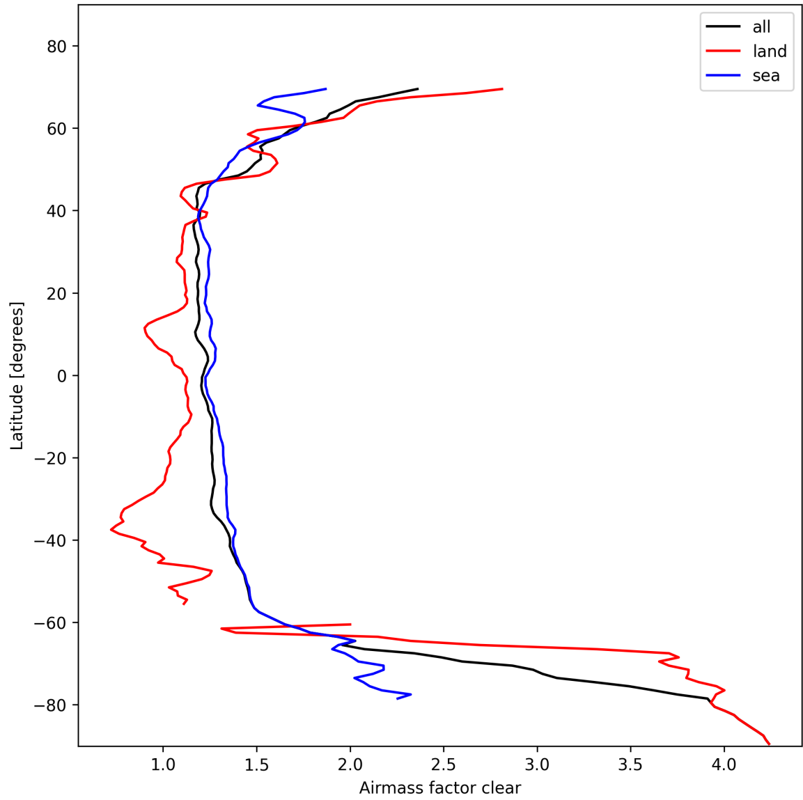
Figure 28: Zonal average of “Airmass factor clear” for 2025-02-05 to 2025-02-07.
