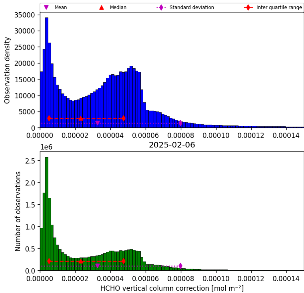
Figure 37: Histogram of “HCHO vertical column correction” for 2025-02-05 to 2025-02-07
