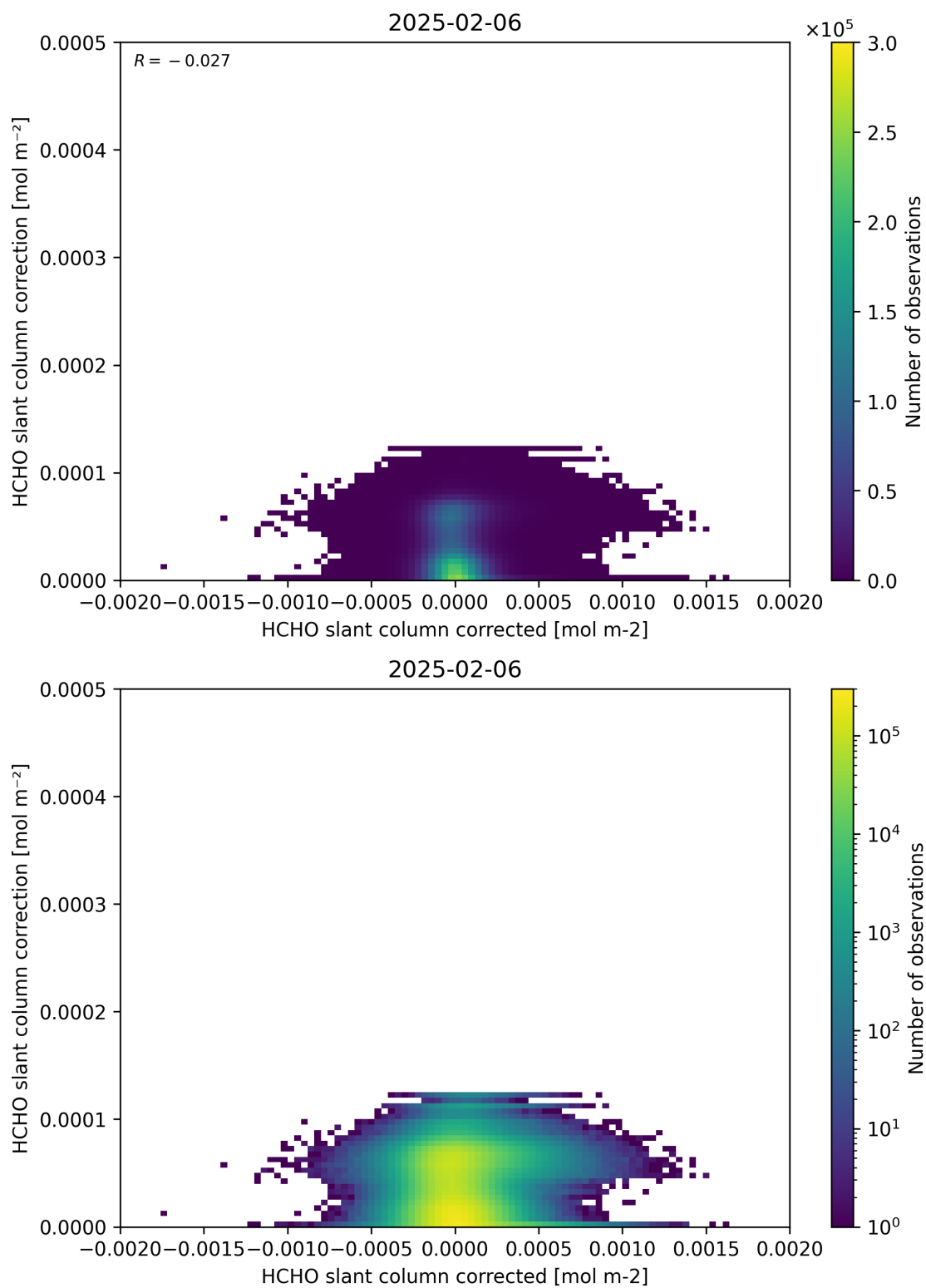
Figure 77: Scatter density plot of “HCHO slant column corrected” against “HCHO slant column correction” for 2025-02-05 to 2025-02-07.
