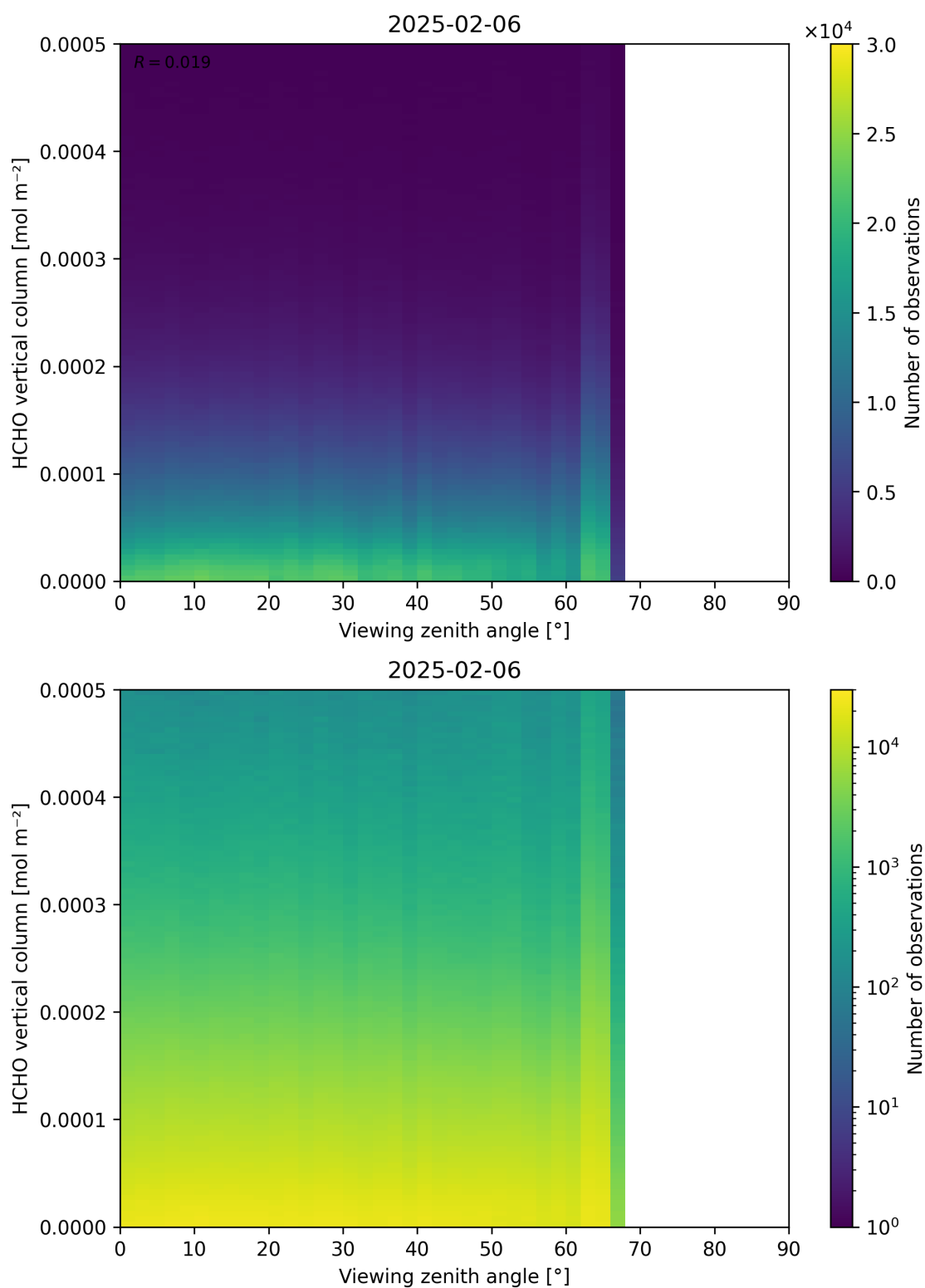
Figure 192: Scatter density plot of “Viewing zenith angle” against “HCHO vertical column” for 2025-02-05 to 2025-02-07.
