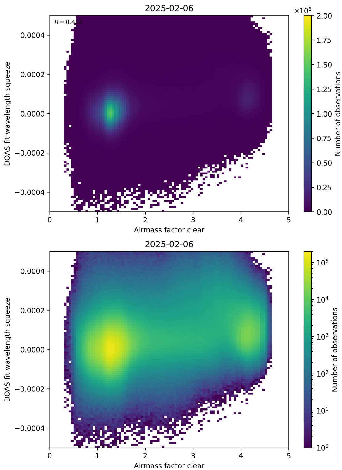
Figure 73: Scatter density plot of “Airmass factor clear” against “DOAS fit wavelength squeeze” for 2025-02-05 to 2025-02-07.
