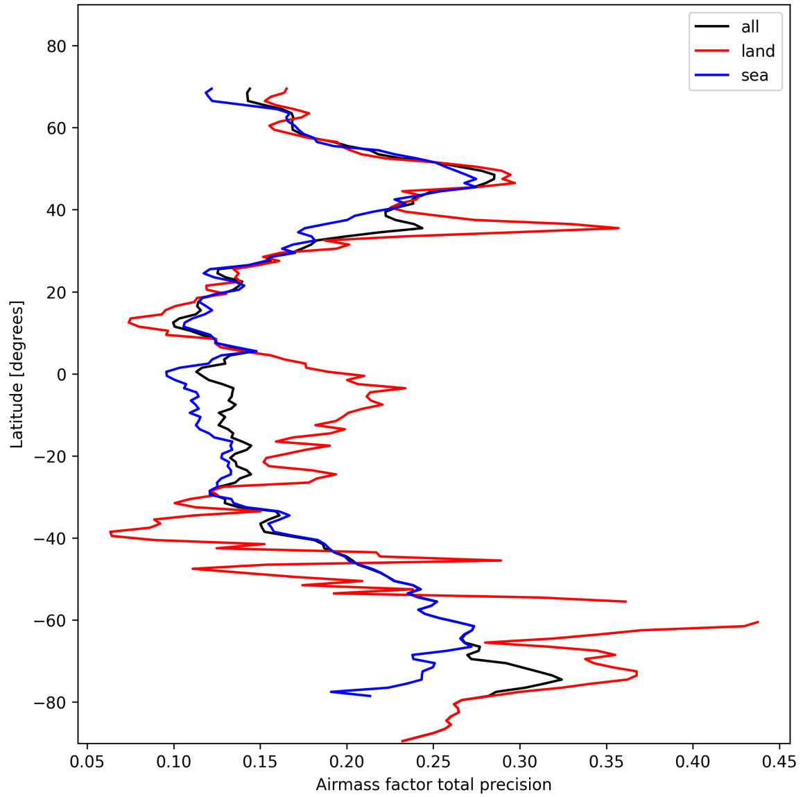
Figure 27: Zonal average of “Airmass factor total precision” for 2025-02-05 to 2025-02-07.
