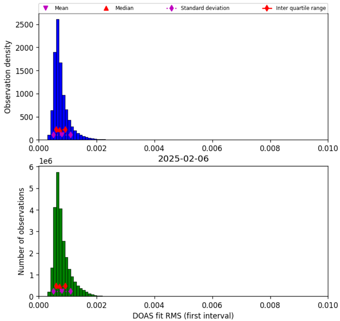
Figure 46: Histogram of “DOAS fit RMS (first interval)” for 2025-02-05 to 2025-02-07
