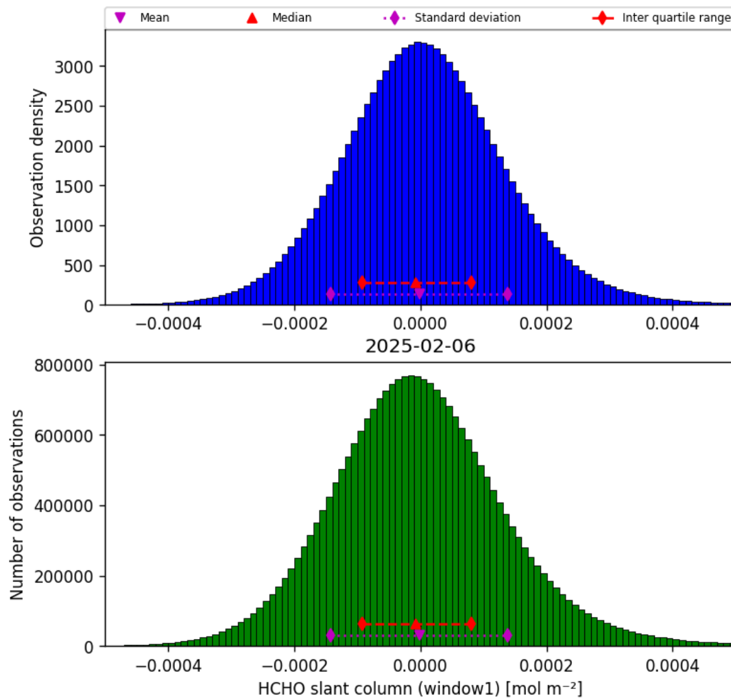
Figure 38: Histogram of “HCHO slant column (window1)” for 2025-02-05 to 2025-02-07
