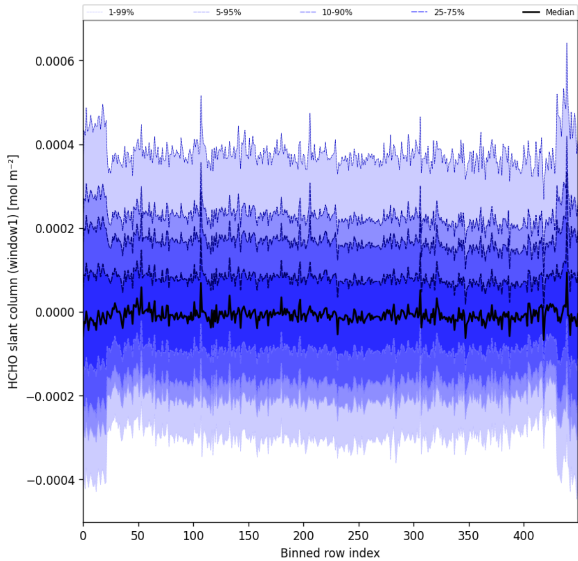
Figure 52: Along track statistics of “HCHO slant column (window1)” for 2025-02-05 to 2025-02-07
