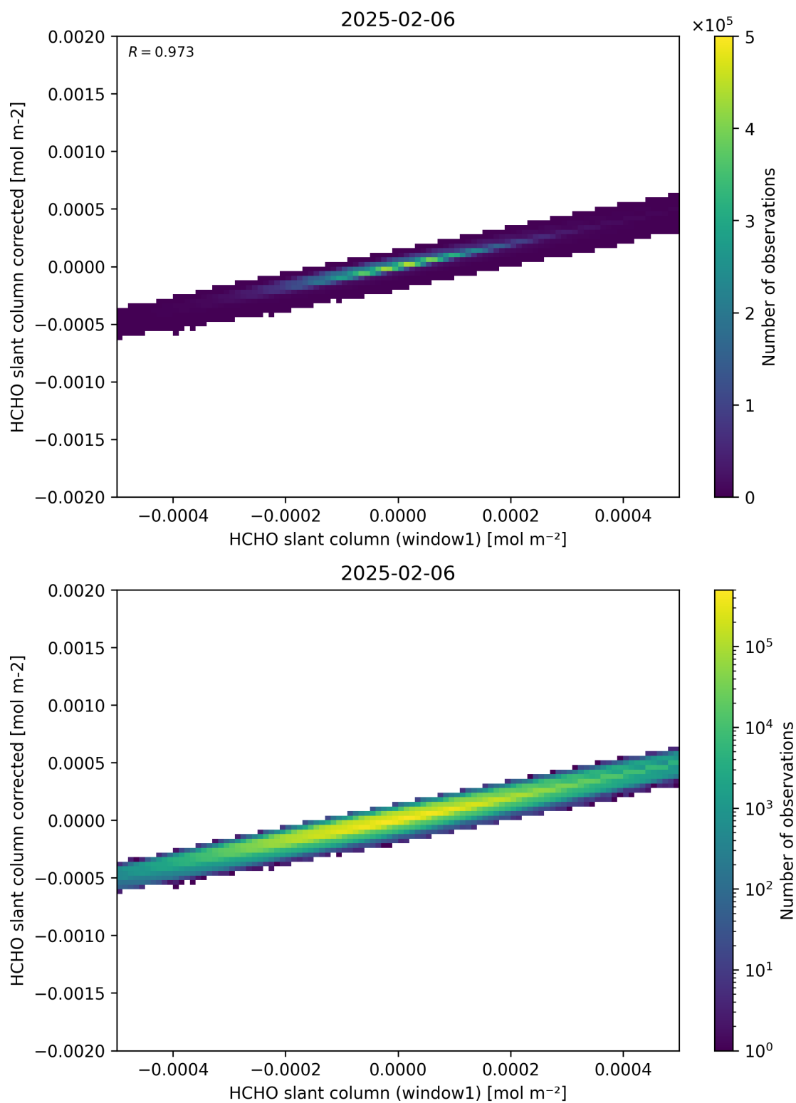
Figure 82: Scatter density plot of “HCHO slant column (window1)” against “HCHO slant column corrected” for 2025-02-05 to 2025-02-07.
