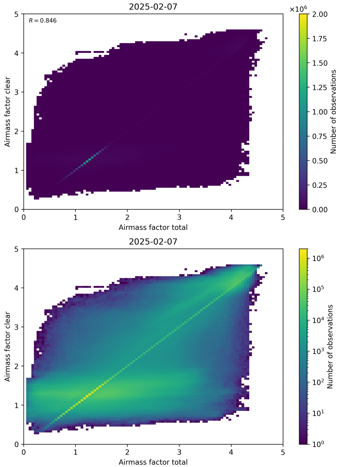
Figure 100: Scatter density plot of “Airmass factor total” against “Airmass factor clear” for 2025-02-06 to 2025-02-08.
