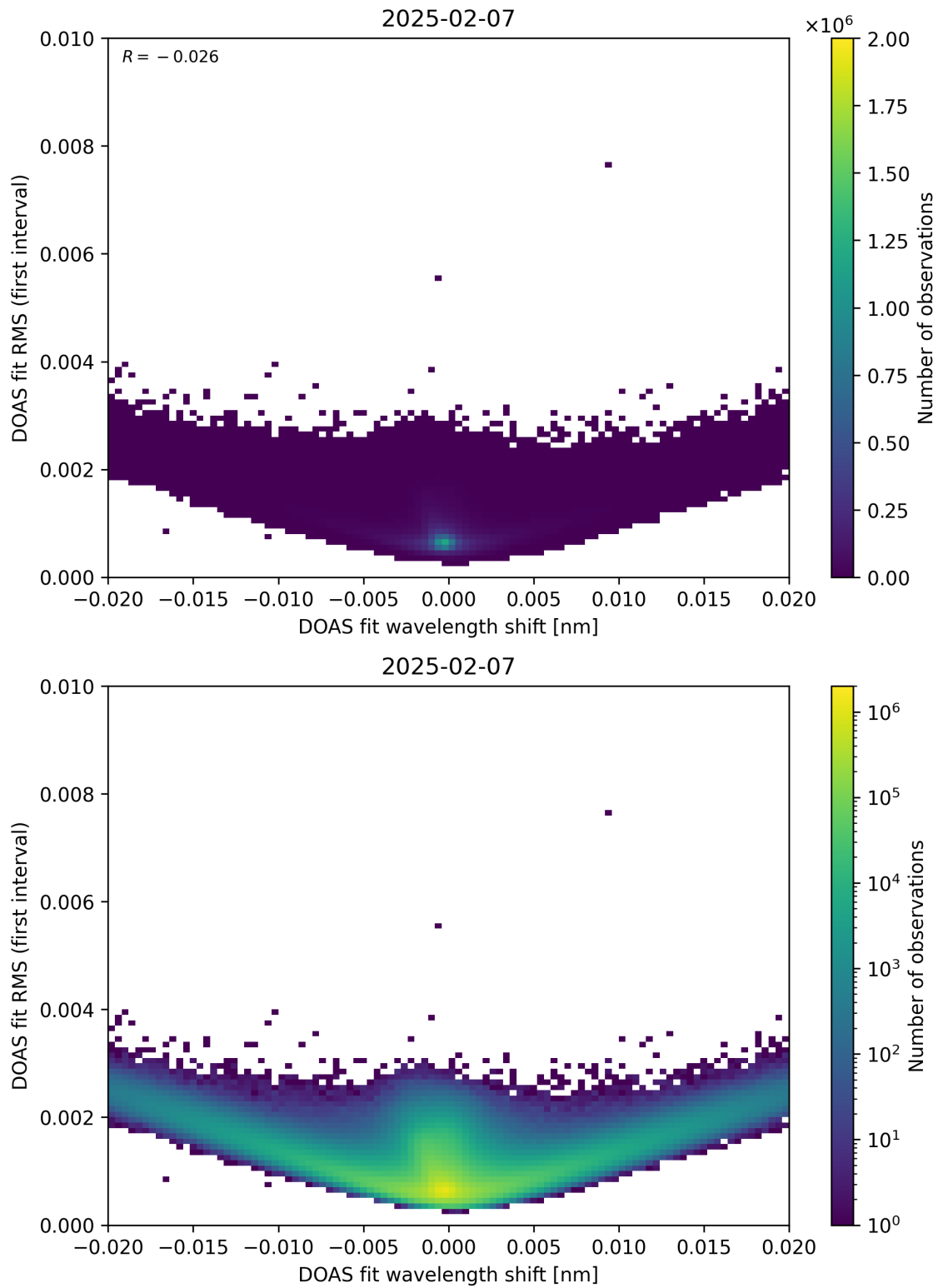
Figure 64: Scatter density plot of “DOAS fit wavelength shift” against “DOAS fit RMS (first interval)” for 2025-02-06 to 2025-02-08.
