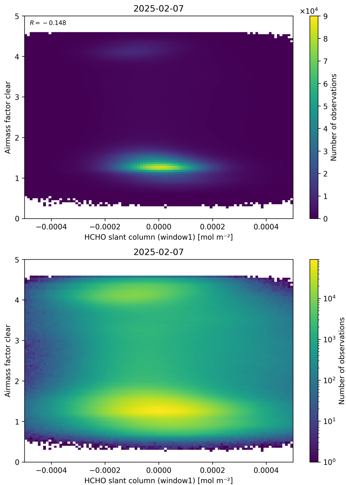
Figure 81: Scatter density plot of “HCHO slant column (window1)” against “Airmass factor clear” for 2025-02-06 to 2025-02-08.
