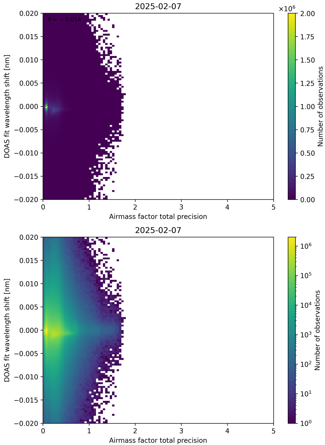
Figure 106: Scatter density plot of “Airmass factor total precision” against “DOAS fit wavelength shift” for 2025-02-06 to 2025-02-08.
