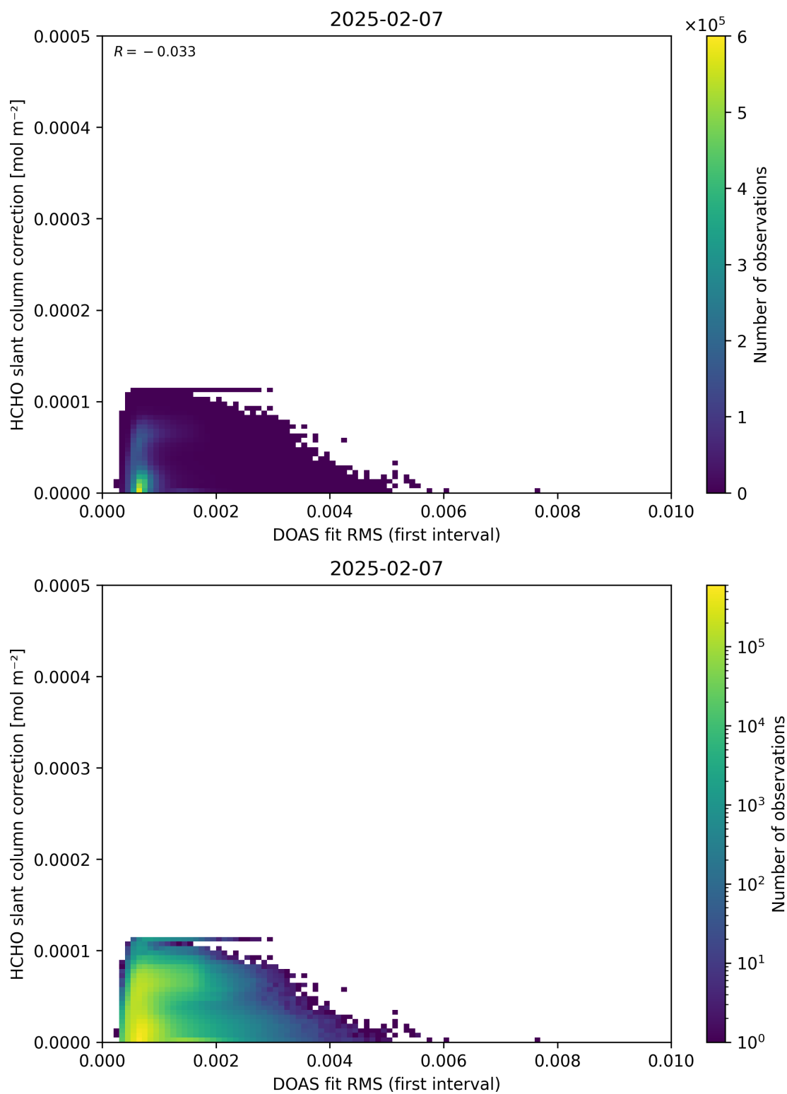
Figure 63: Scatter density plot of “DOAS fit RMS (first interval)” against “HCHO slant column correction” for 2025-02-06 to 2025-02-08.
