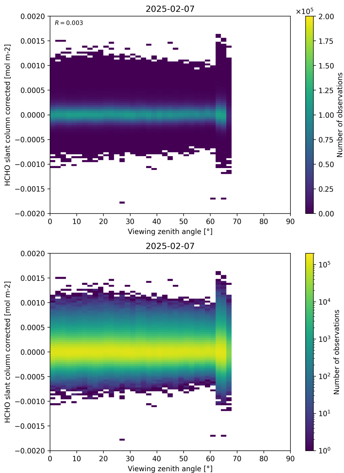
Figure 186: Scatter density plot of “Viewing zenith angle” against “HCHO slant column corrected” for 2025-02-06 to 2025-02-08.
