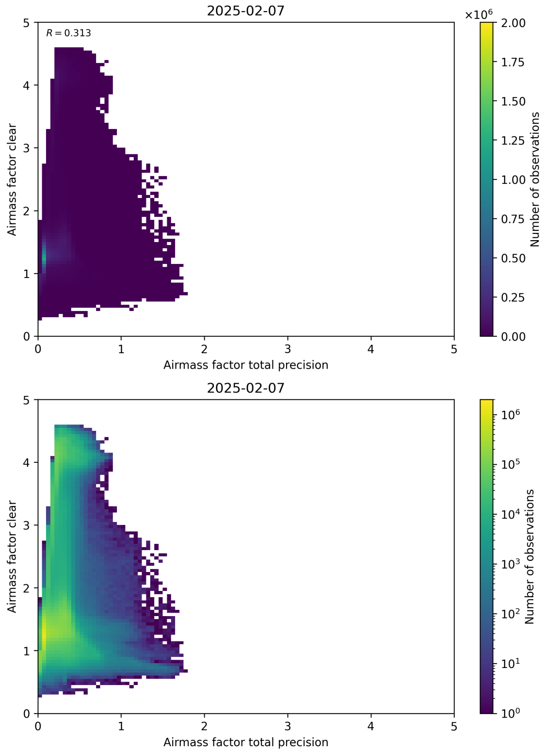
Figure 108: Scatter density plot of “Airmass factor total precision” against “Airmass factor clear” for 2025-02-06 to 2025-02-08.
