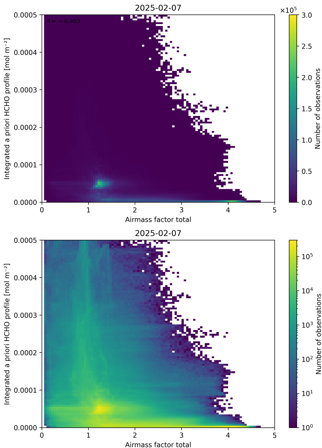
Figure 104: Scatter density plot of “Airmass factor total” against “Integrated a priori HCHO profile” for 2025-02-06 to 2025-02-08.
