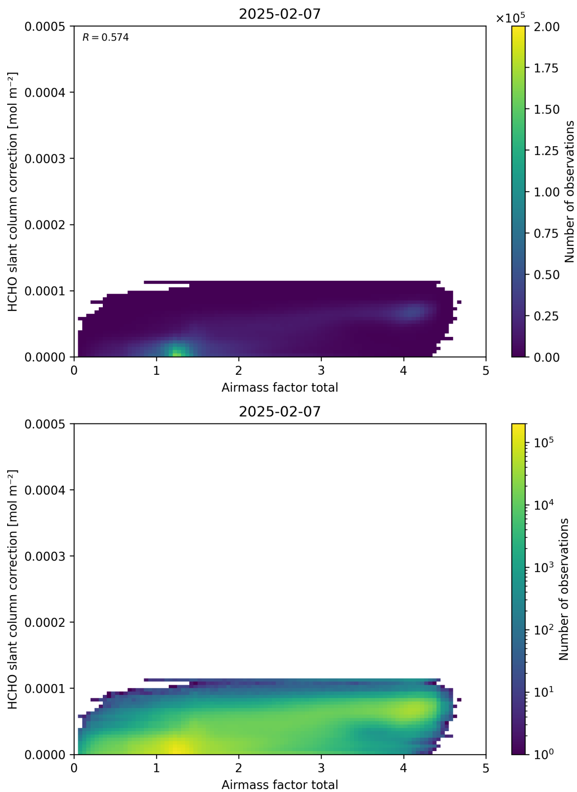
Figure 102: Scatter density plot of “Airmass factor total” against “HCHO slant column correction” for 2025-02-06 to 2025-02-08.
