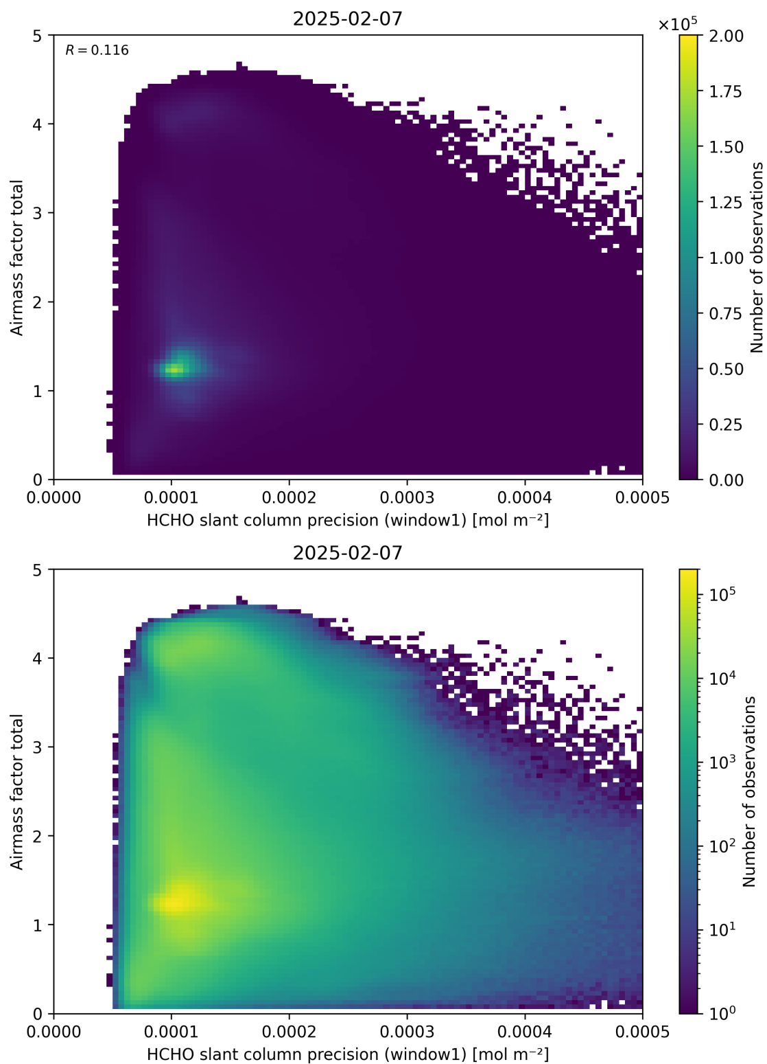
Figure 94: Scatter density plot of “HCHO slant column precision (window1)” against “Airmass factor total” for 2025-02-06 to 2025-02-08.
