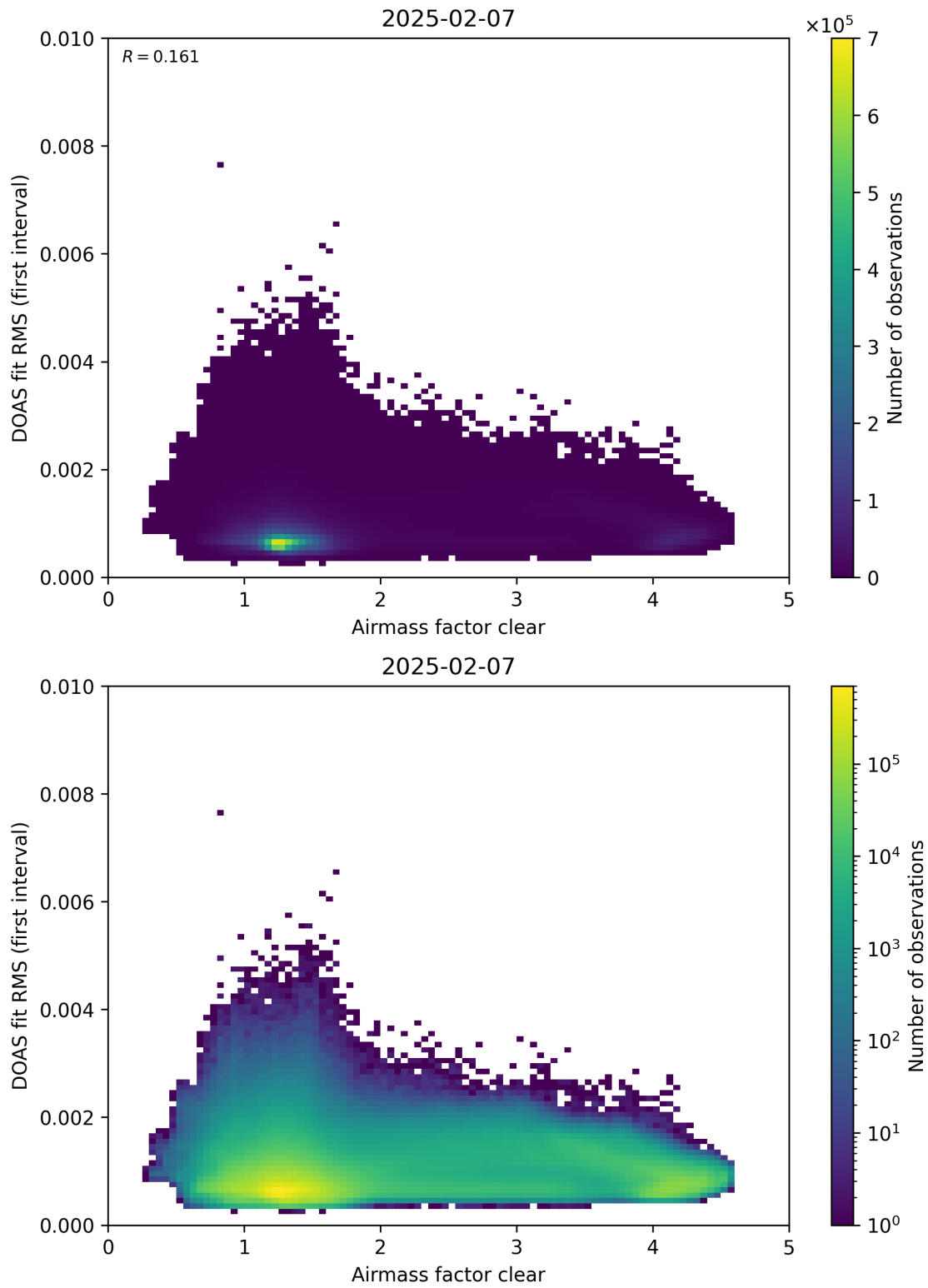
Figure 71: Scatter density plot of “Airmass factor clear” against “DOAS fit RMS (first interval)” for 2025-02-06 to 2025-02-08.
