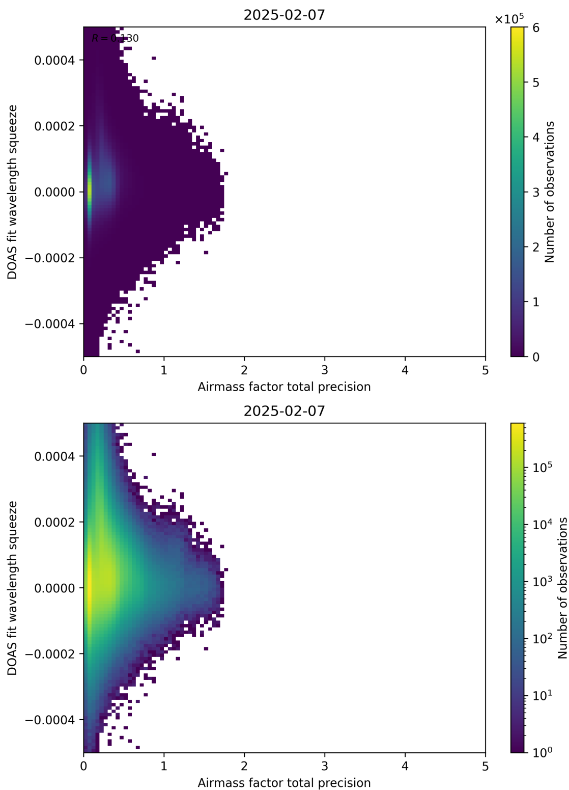
Figure 107: Scatter density plot of “Airmass factor total precision” against “DOAS fit wavelength squeeze” for 2025-02-06 to 2025-02-08.
