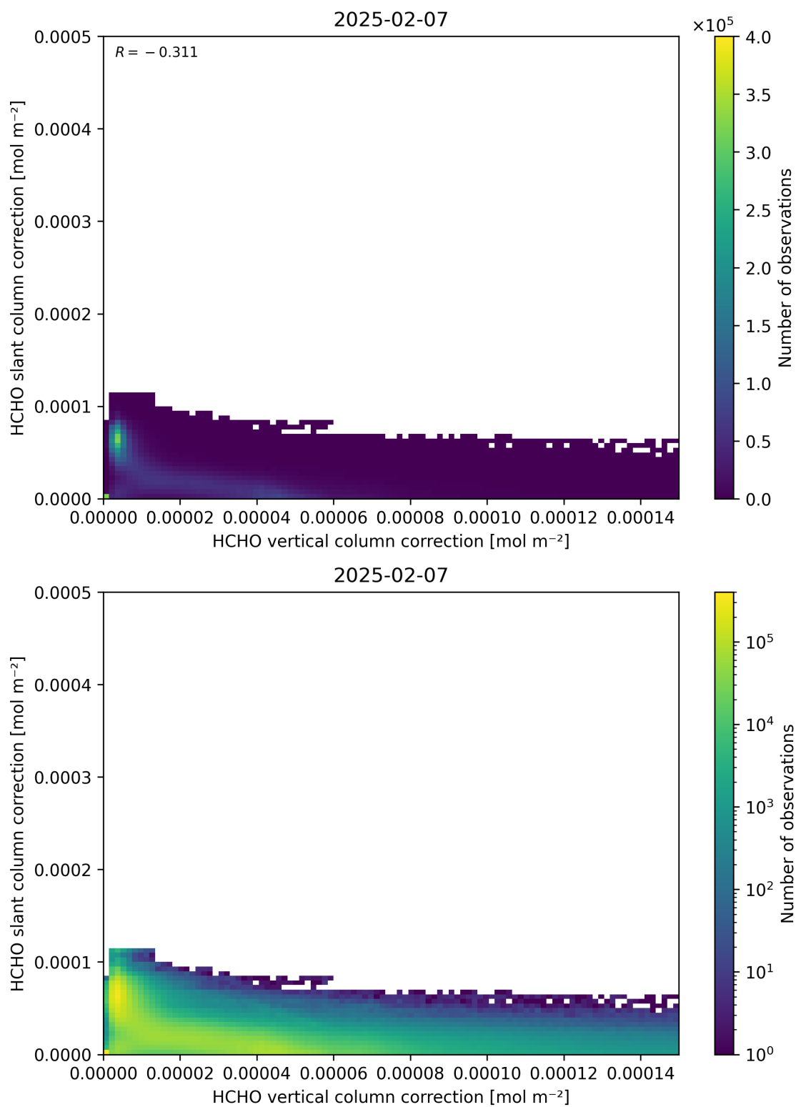
Figure 117: Scatter density plot of “HCHO vertical column correction” against “HCHO slant column correction” for 2025-02-06 to 2025-02-08.
