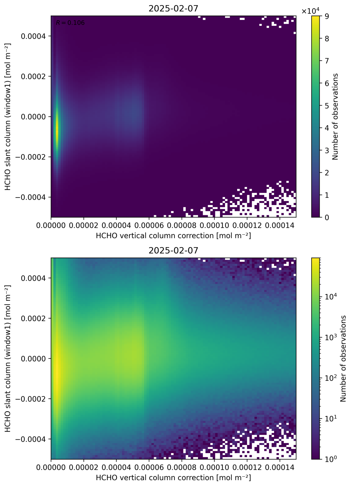
Figure 118: Scatter density plot of “HCHO vertical column correction” against “HCHO slant column (window1)” for 2025-02-06 to 2025-02-08.
