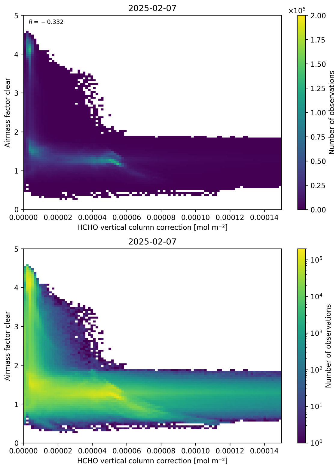
Figure 115: Scatter density plot of “HCHO vertical column correction” against “Airmass factor clear” for 2025-02-06 to 2025-02-08.
