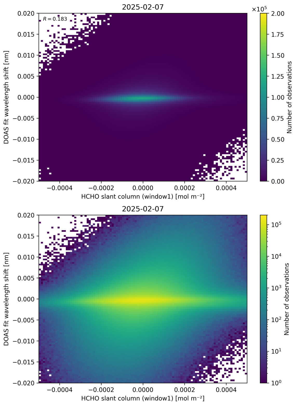
Figure 79: Scatter density plot of “HCHO slant column (window1)” against “DOAS fit wavelength shift” for 2025-02-06 to 2025-02-08.
