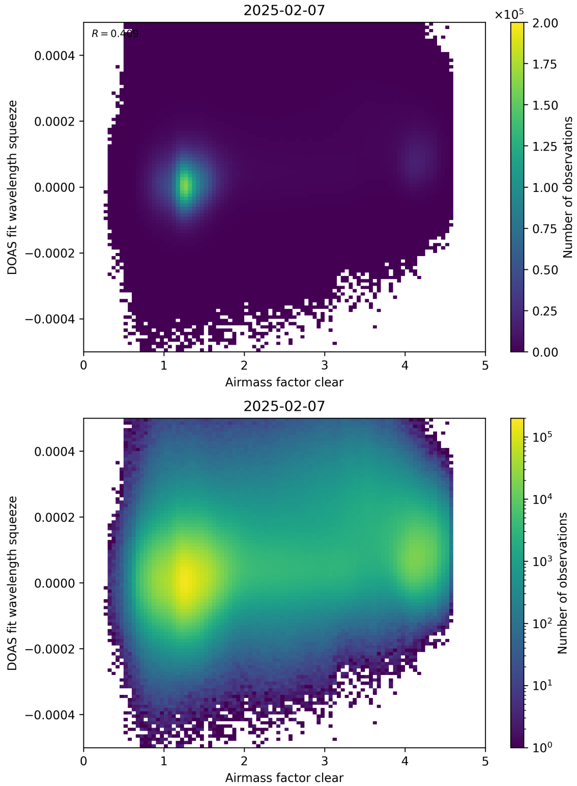
Figure 73: Scatter density plot of “Airmass factor clear” against “DOAS fit wavelength squeeze” for 2025-02-06 to 2025-02-08.
