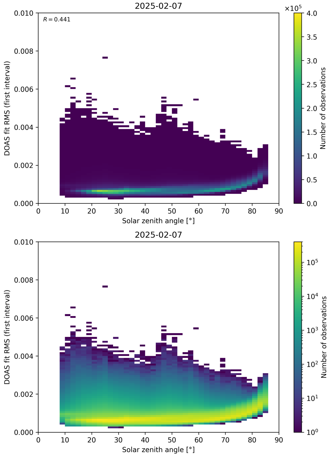
Figure 167: Scatter density plot of “Solar zenith angle” against “DOAS fit RMS (first interval)” for 2025-02-06 to 2025-02-08.
