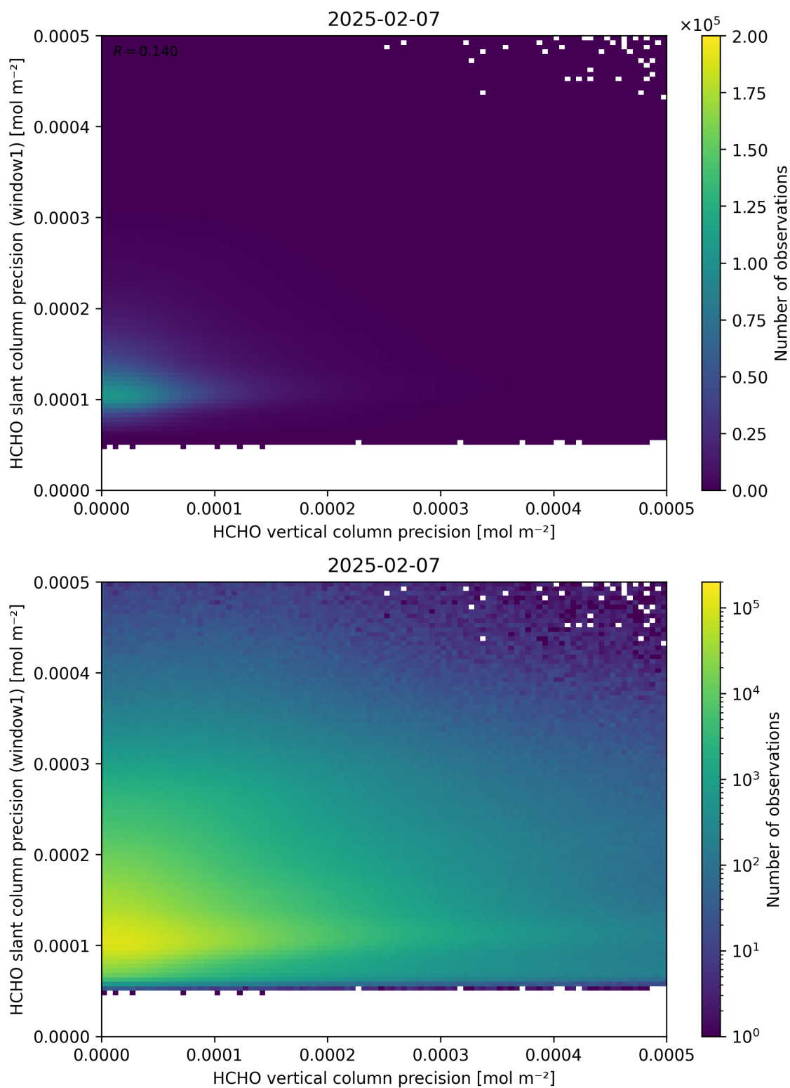
Figure 143: Scatter density plot of “HCHO vertical column precision” against “HCHO slant column precision (window1)” for 2025-02-06 to 2025-02-08.
