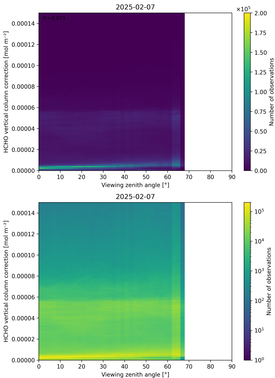
Figure 193: Scatter density plot of “Viewing zenith angle” against “HCHO vertical column correction” for 2025-02-06 to 2025-02-08.
