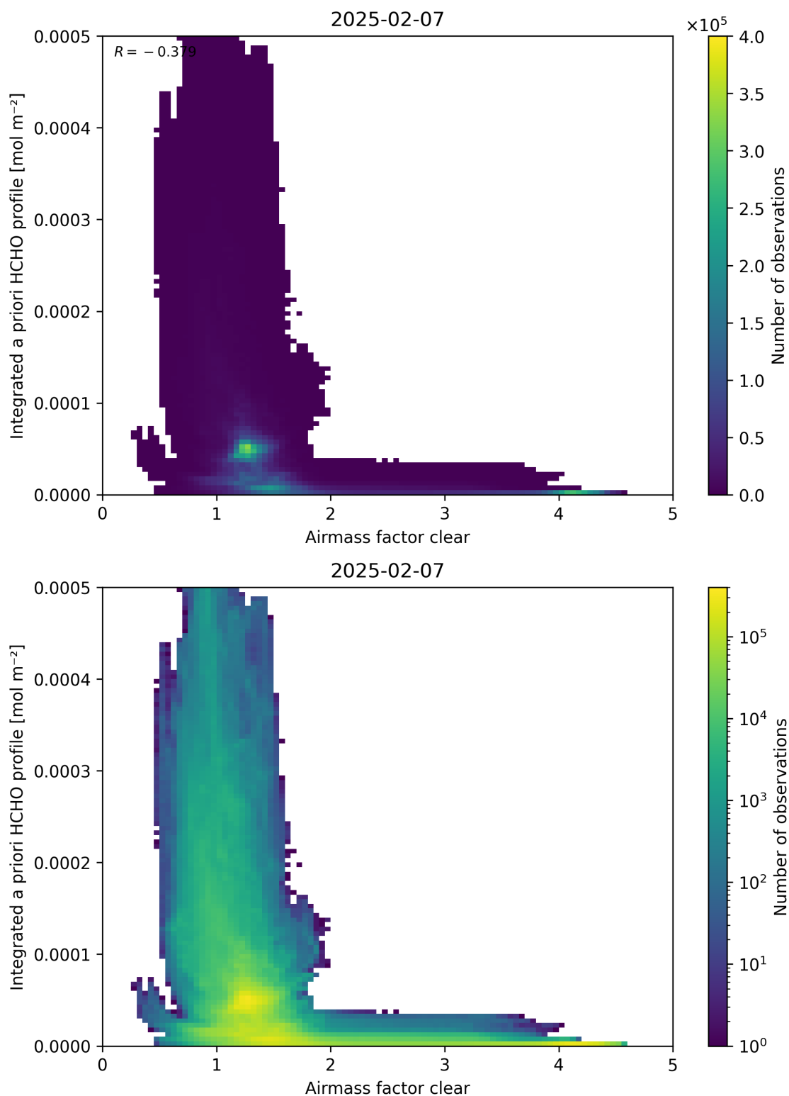
Figure 76: Scatter density plot of “Airmass factor clear” against “Integrated a priori HCHO profile” for 2025-02-06 to 2025-02-08.
