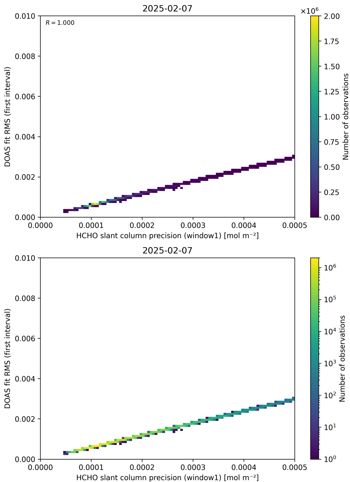
Figure 88: Scatter density plot of “HCHO slant column precision (window1)” against “DOAS fit RMS (first interval)” for 2025-02-06 to 2025-02-08.
