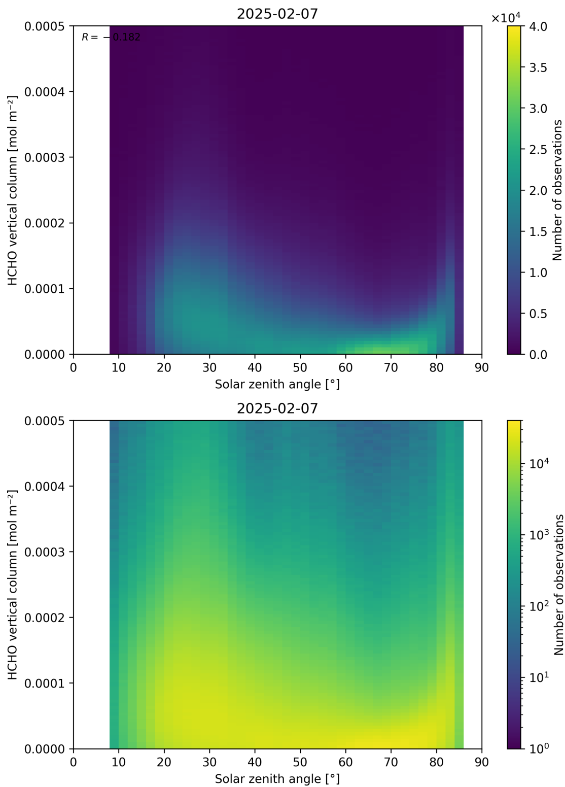
Figure 177: Scatter density plot of “Solar zenith angle” against “HCHO vertical column” for 2025-02-06 to 2025-02-08.
