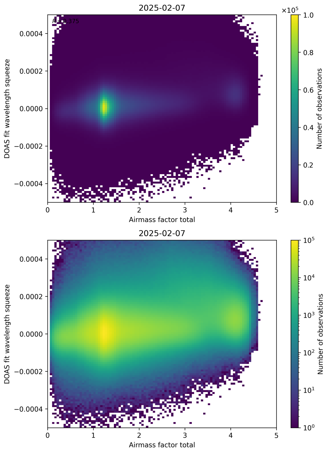
Figure 99: Scatter density plot of “Airmass factor total” against “DOAS fit wavelength squeeze” for 2025-02-06 to 2025-02-08.
