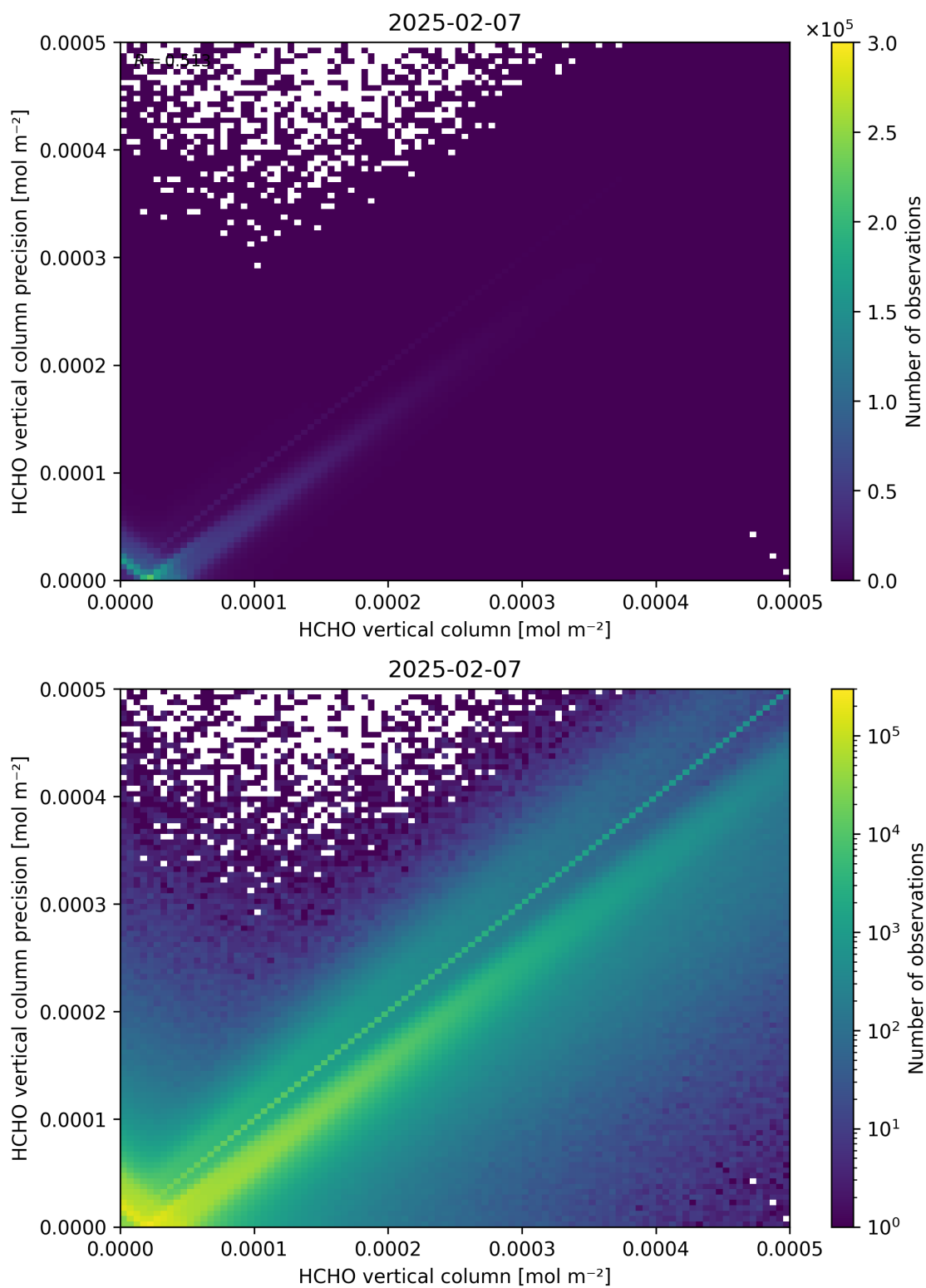
Figure 134: Scatter density plot of “HCHO vertical column” against “HCHO vertical column precision” for 2025-02-06 to 2025-02-08.
