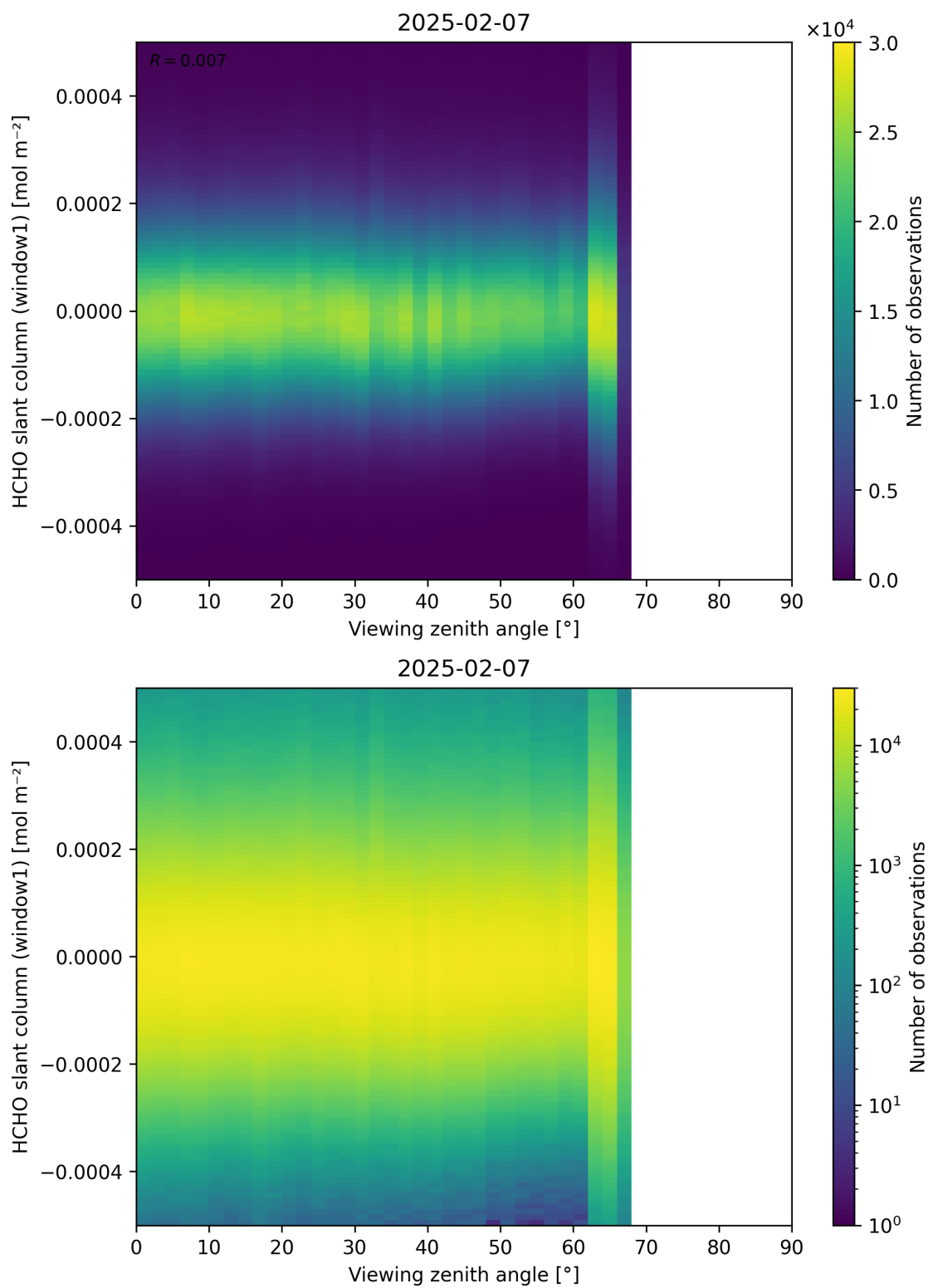
Figure 188: Scatter density plot of “Viewing zenith angle” against “HCHO slant column (window1)” for 2025-02-06 to 2025-02-08.
