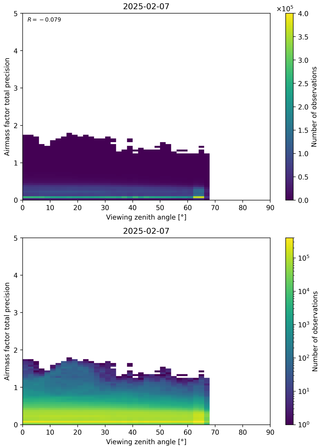
Figure 191: Scatter density plot of “Viewing zenith angle” against “Airmass factor total precision” for 2025-02-06 to 2025-02-08.
