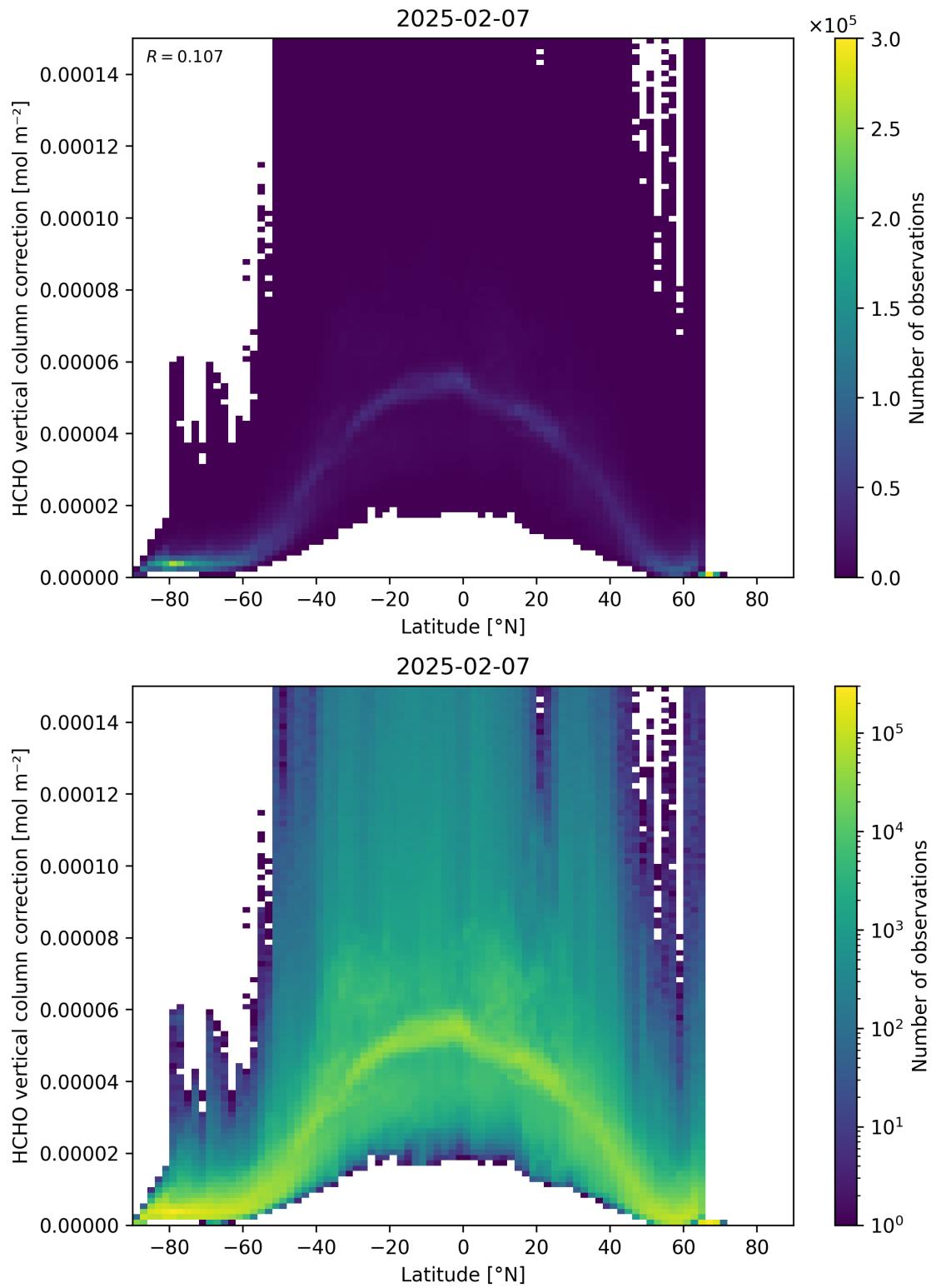
Figure 164: Scatter density plot of “Latitude” against “HCHO vertical column correction” for 2025-02-06 to 2025-02-08.
