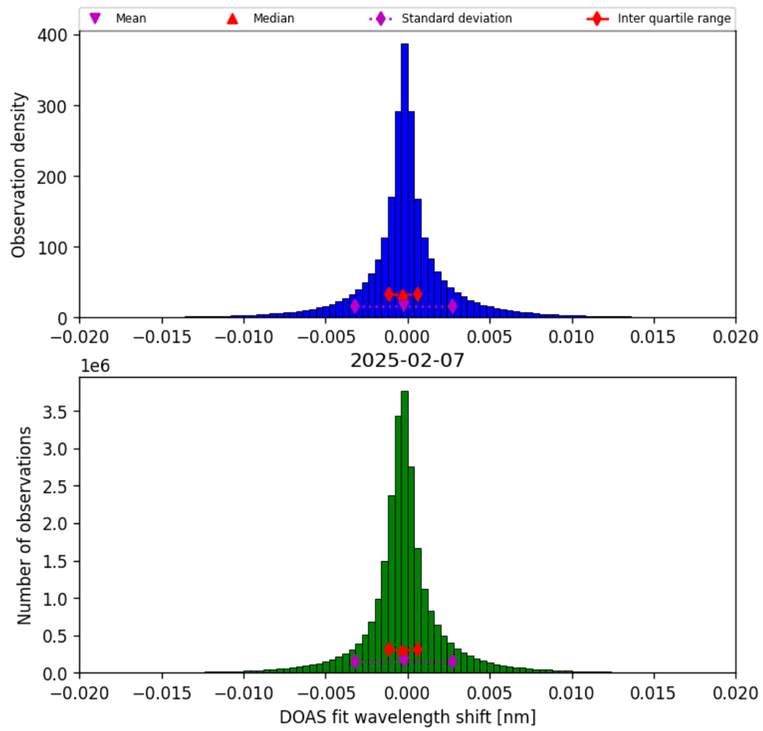
Figure 44: Histogram of “DOAS fit wavelength shift” for 2025-02-06 to 2025-02-08
