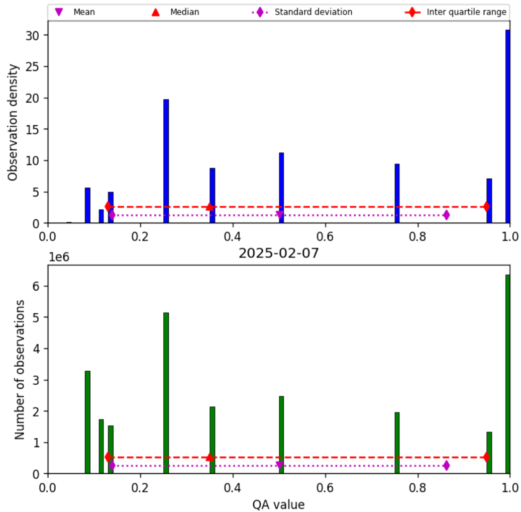
Figure 34: Histogram of “QA value” for 2025-02-06 to 2025-02-08
