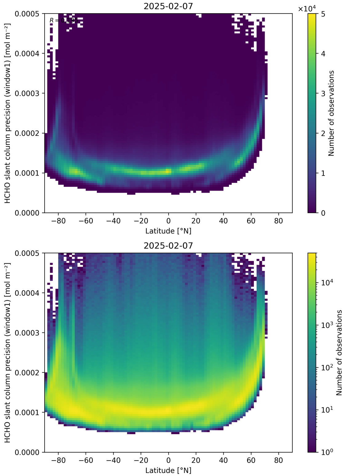
Figure 160: Scatter density plot of “Latitude” against “HCHO slant column precision (window1)” for 2025-02-06 to 2025-02-08.
