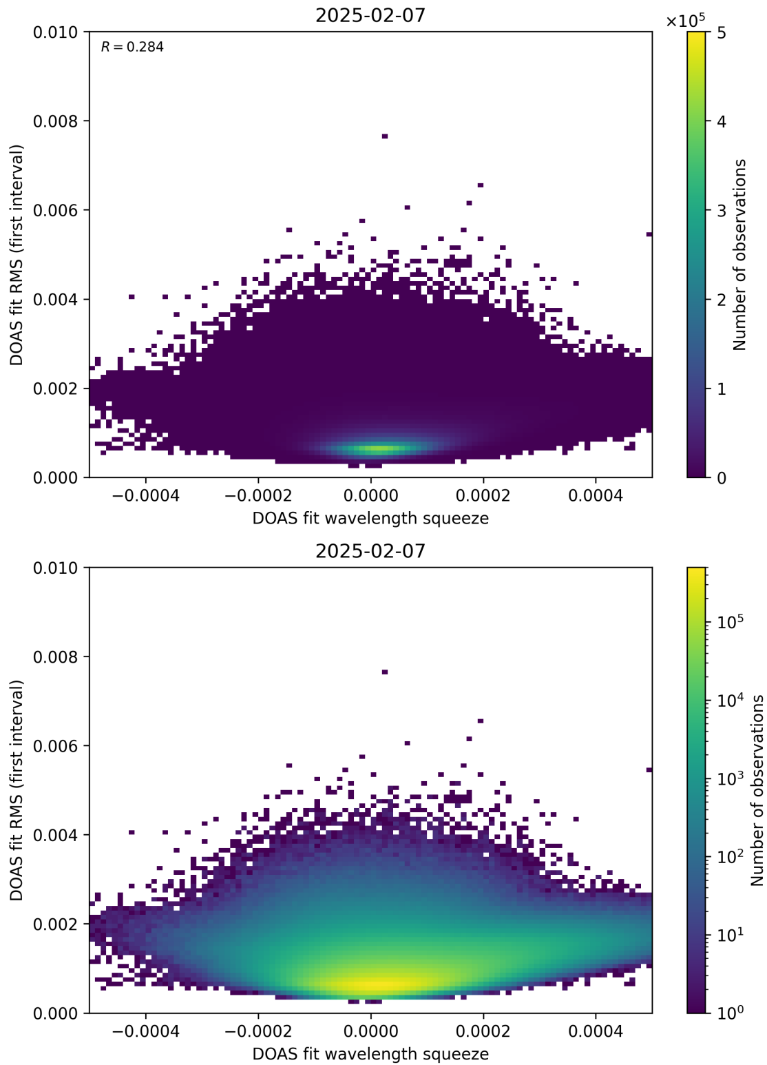
Figure 68: Scatter density plot of “DOAS fit wavelength squeeze” against “DOAS fit RMS (first interval)” for 2025-02-06 to 2025-02-08.
