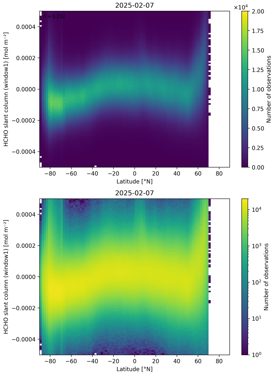
Figure 159: Scatter density plot of “Latitude” against “HCHO slant column (window1)” for 2025-02-06 to 2025-02-08.
