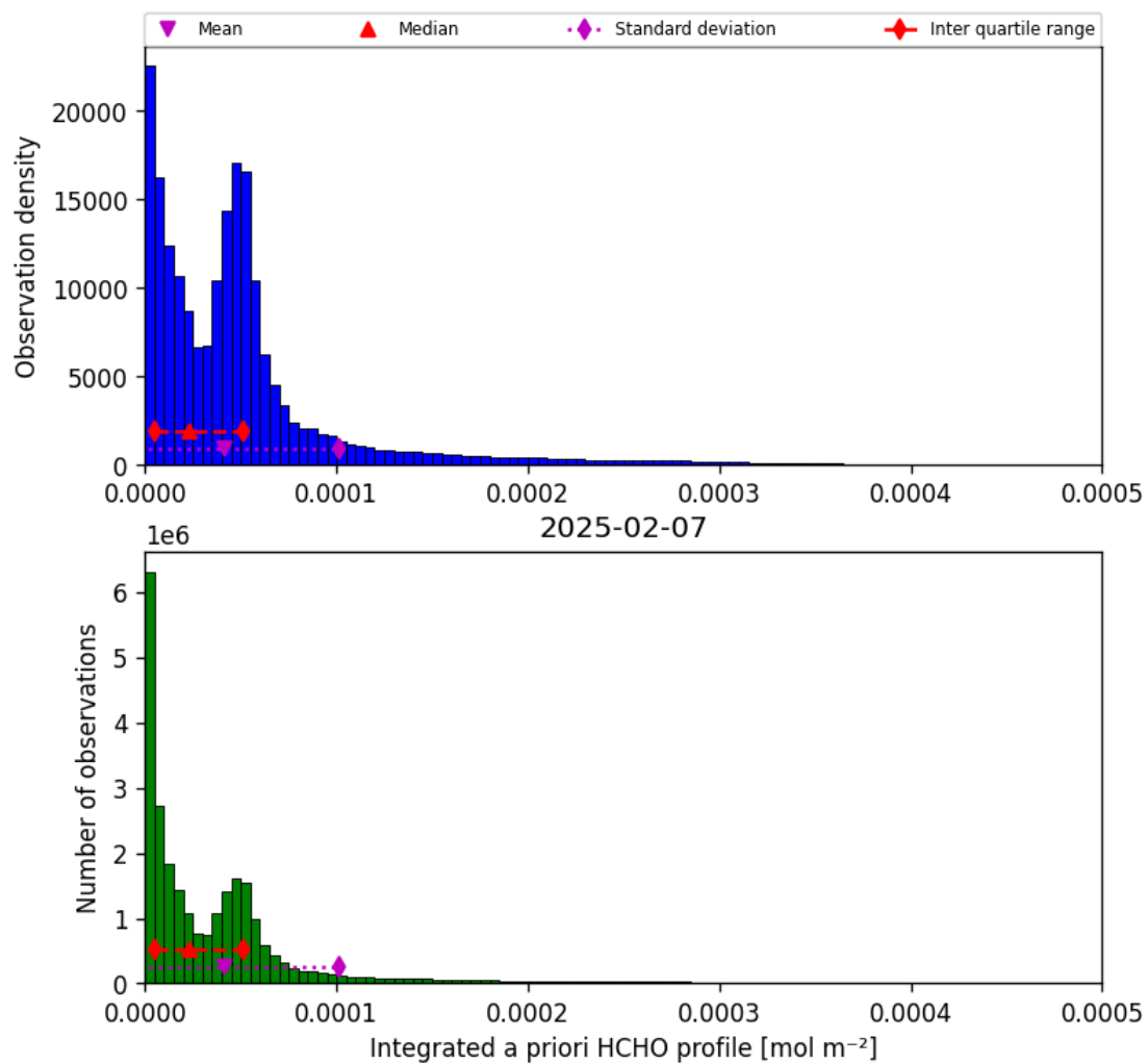
Figure 43: Histogram of “Integrated a priori HCHO profile” for 2025-02-06 to 2025-02-08
