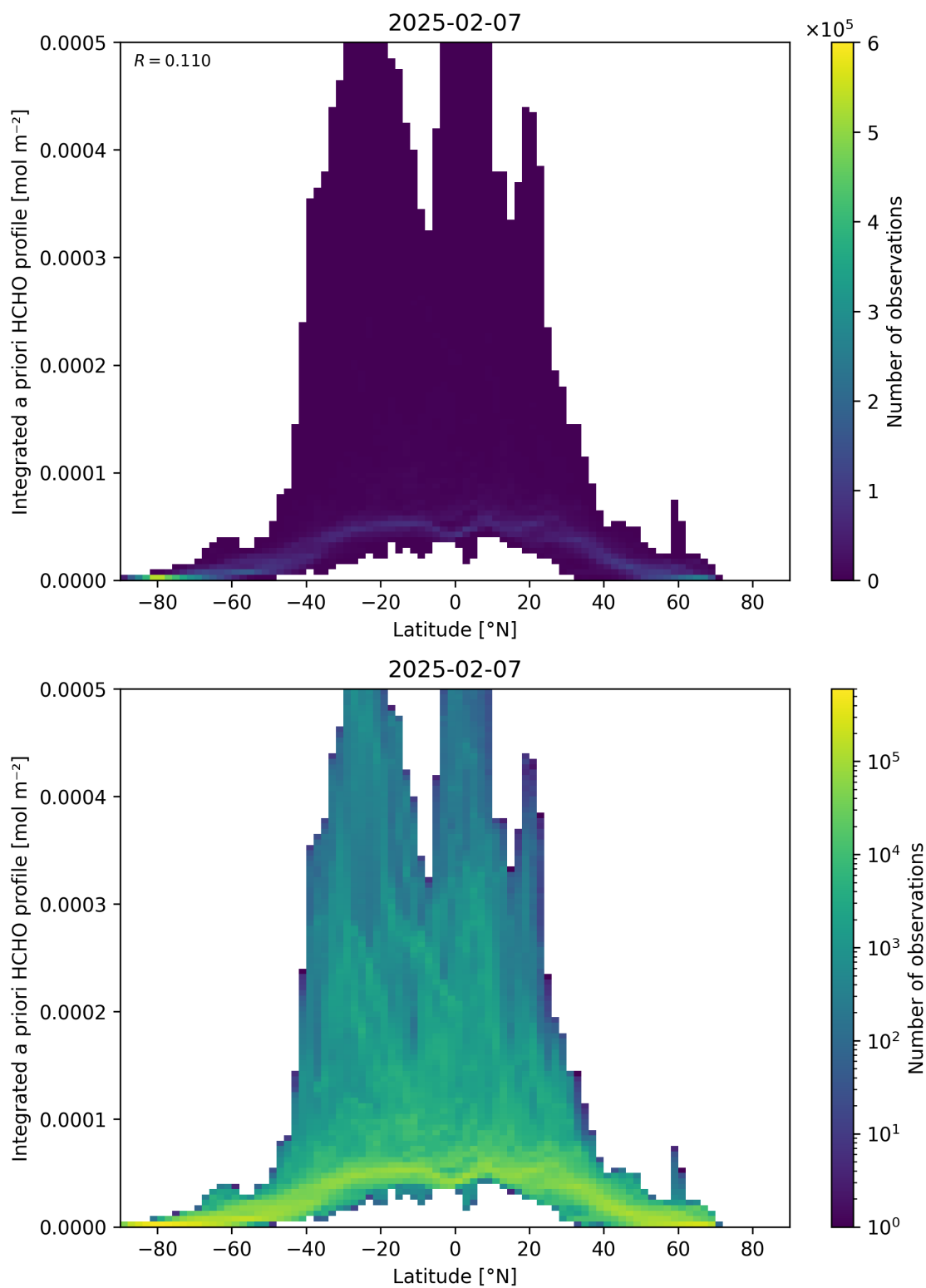
Figure 166: Scatter density plot of “Latitude” against “Integrated a priori HCHO profile” for 2025-02-06 to 2025-02-08.
