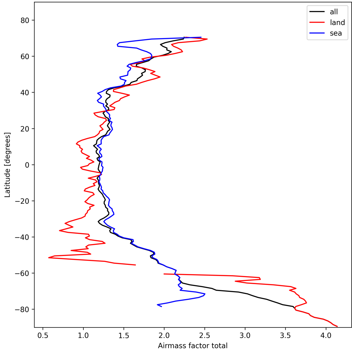
Figure 26: Zonal average of “Airmass factor total” for 2025-02-06 to 2025-02-08.
