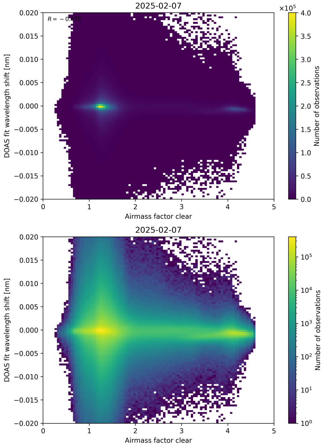
Figure 72: Scatter density plot of “Airmass factor clear” against “DOAS fit wavelength shift” for 2025-02-06 to 2025-02-08.
