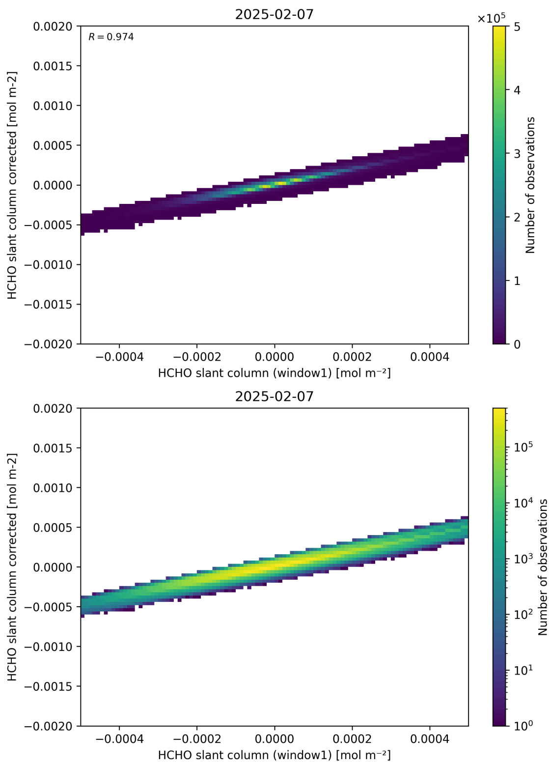
Figure 82: Scatter density plot of “HCHO slant column (window1)” against “HCHO slant column corrected” for 2025-02-06 to 2025-02-08.
