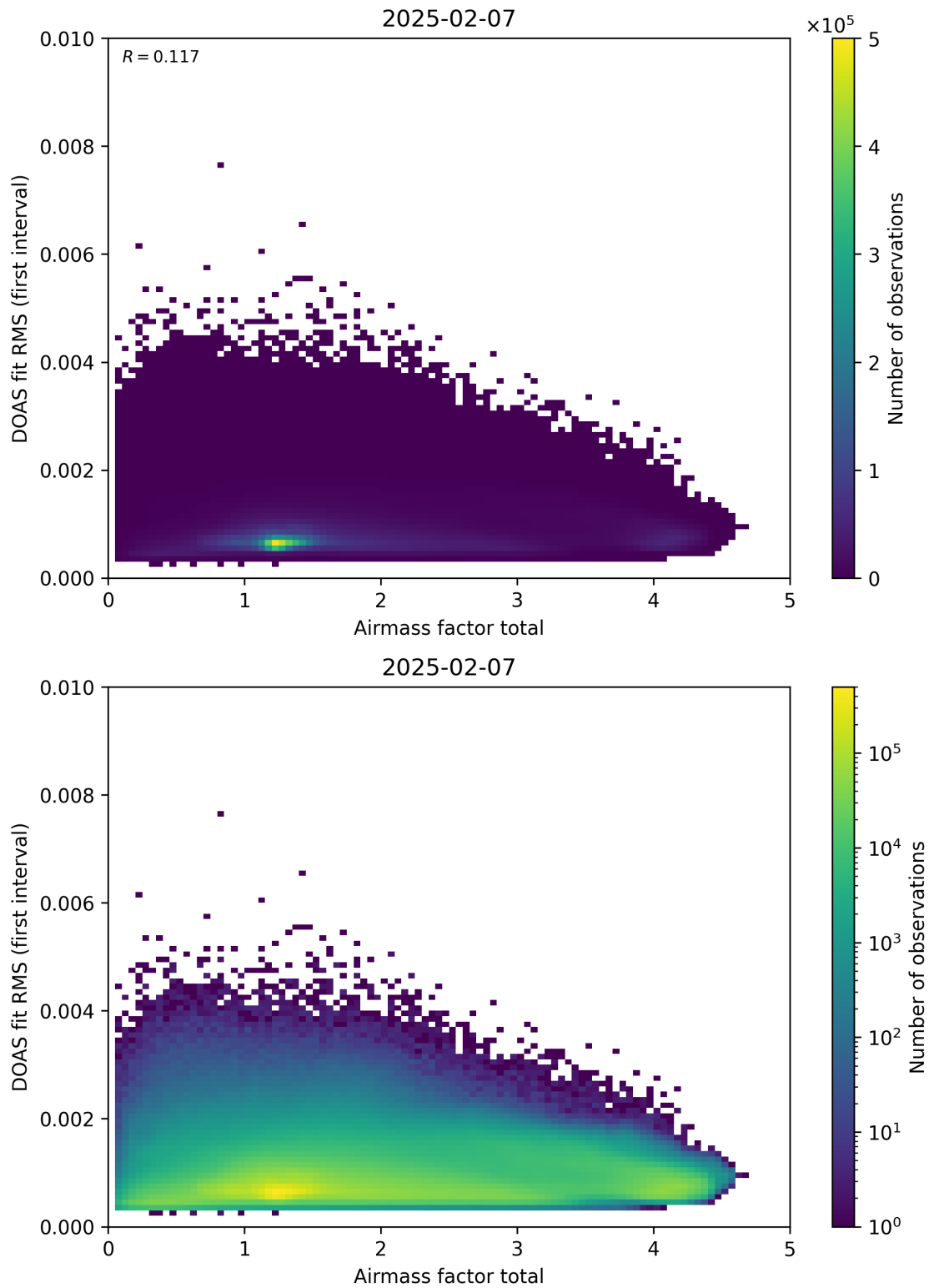
Figure 97: Scatter density plot of “Airmass factor total” against “DOAS fit RMS (first interval)” for 2025-02-06 to 2025-02-08.
