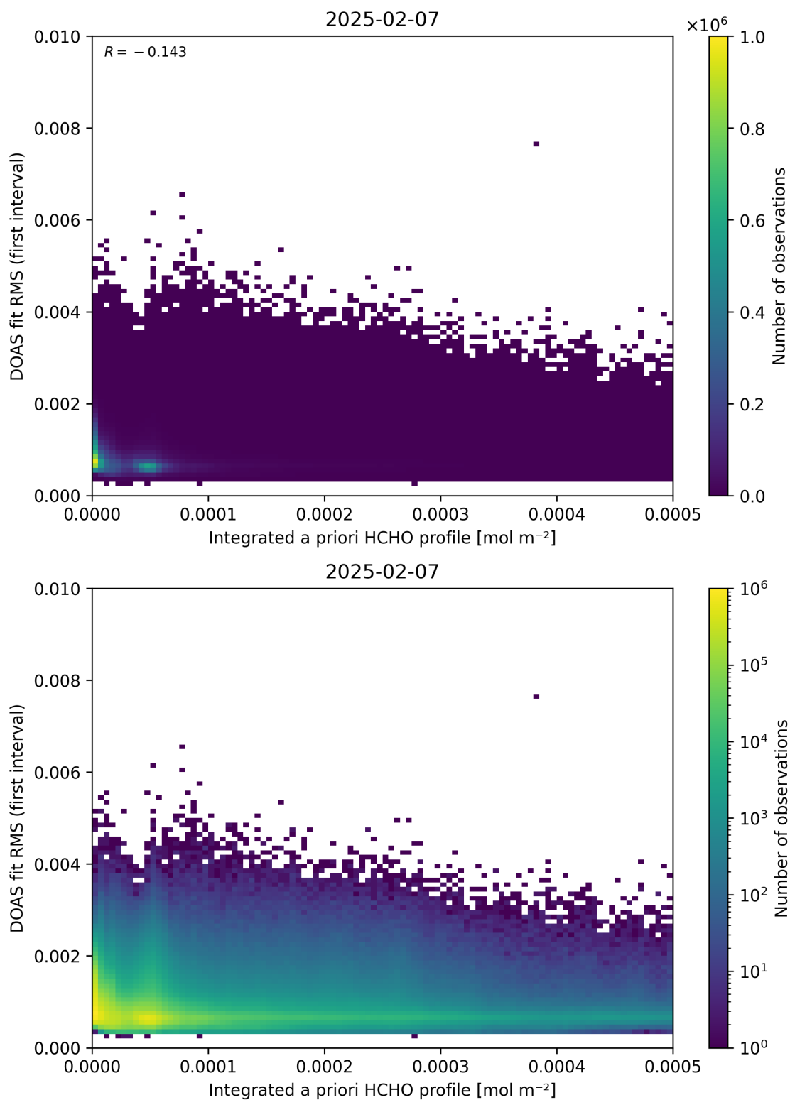
Figure 148: Scatter density plot of “Integrated a priori HCHO profile” against “DOAS fit RMS (first interval)” for 2025-02-06 to 2025-02-08.
