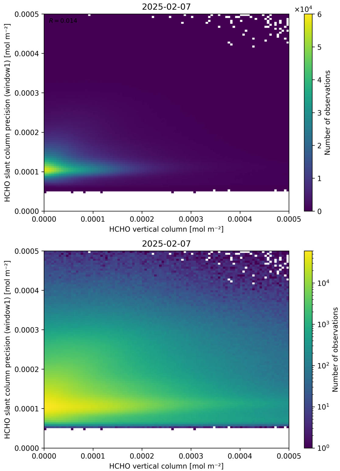
Figure 130: Scatter density plot of “HCHO vertical column” against “HCHO slant column precision (window1)” for 2025-02-06 to 2025-02-08.
