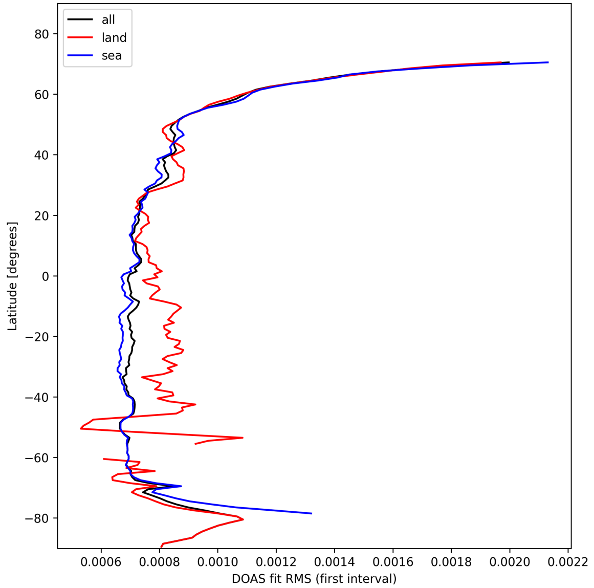
Figure 32: Zonal average of “DOAS fit RMS (first interval)” for 2025-02-06 to 2025-02-08.
