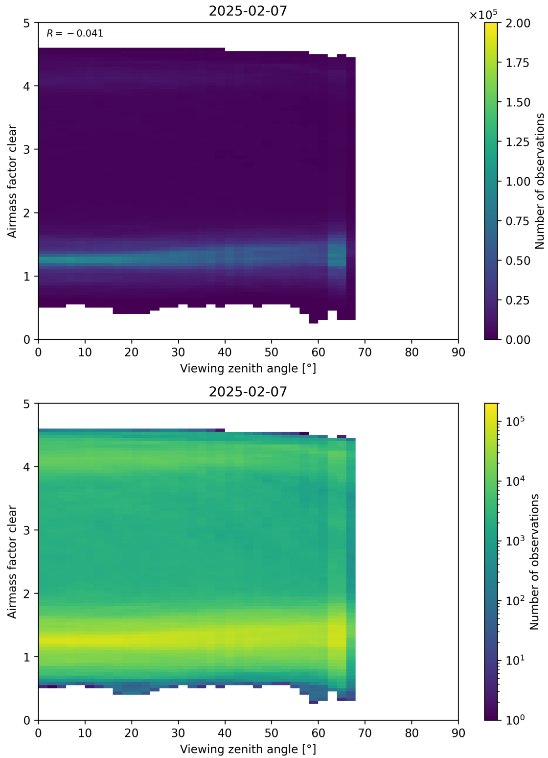
Figure 185: Scatter density plot of “Viewing zenith angle” against “Airmass factor clear” for 2025-02-06 to 2025-02-08.
