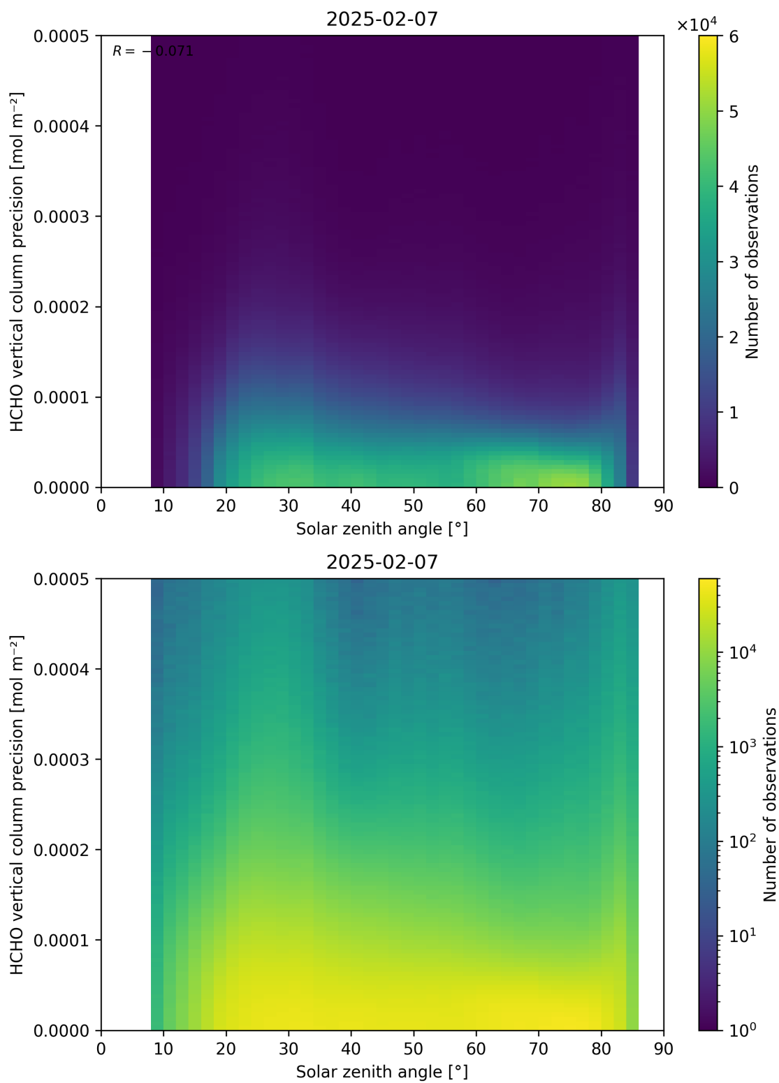
Figure 179: Scatter density plot of “Solar zenith angle” against “HCHO vertical column precision” for 2025-02-06 to 2025-02-08.
