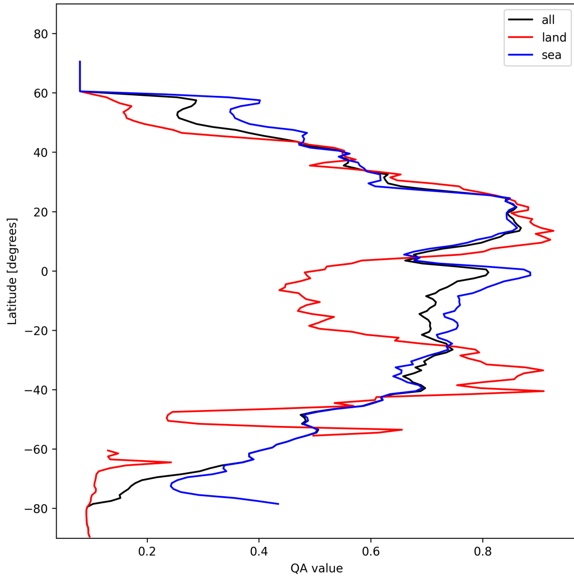
Figure 20: Zonal average of “QA value” for 2025-02-06 to 2025-02-08.
