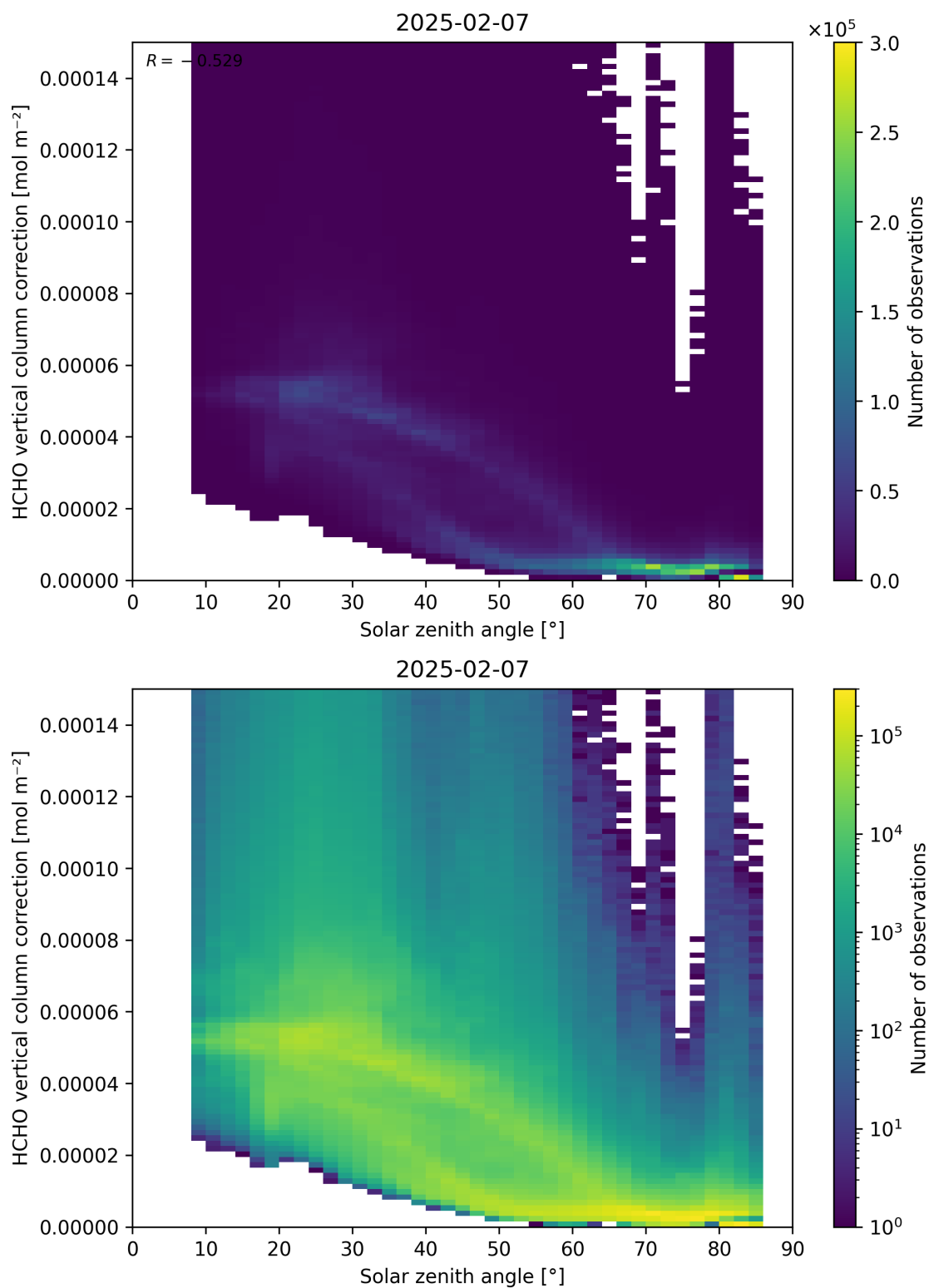
Figure 178: Scatter density plot of “Solar zenith angle” against “HCHO vertical column correction” for 2025-02-06 to 2025-02-08.
