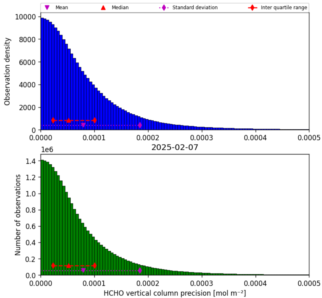
Figure 36: Histogram of “HCHO vertical column precision” for 2025-02-06 to 2025-02-08
