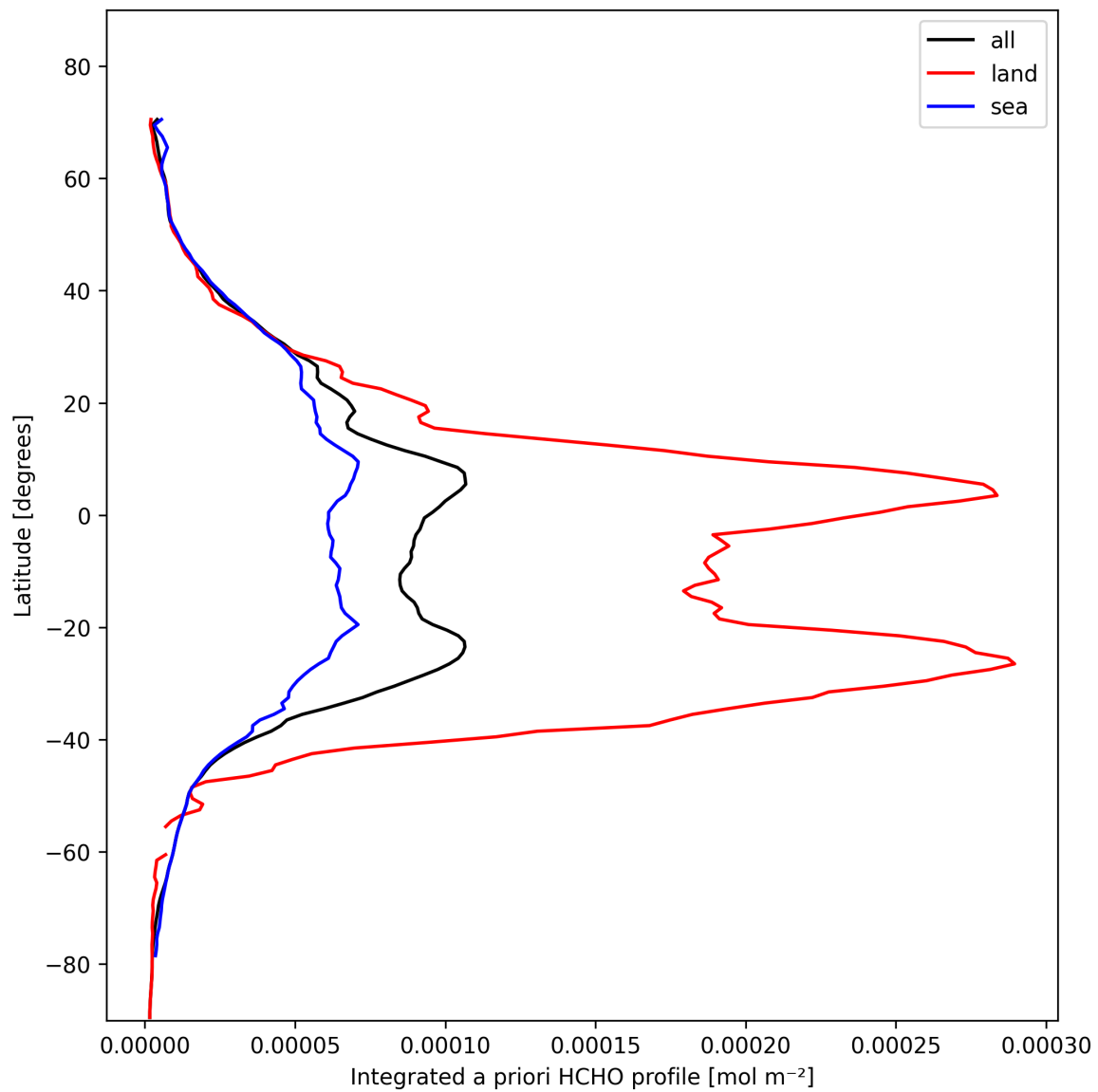
Figure 29: Zonal average of “Integrated a priori HCHO profile” for 2025-02-06 to 2025-02-08.
