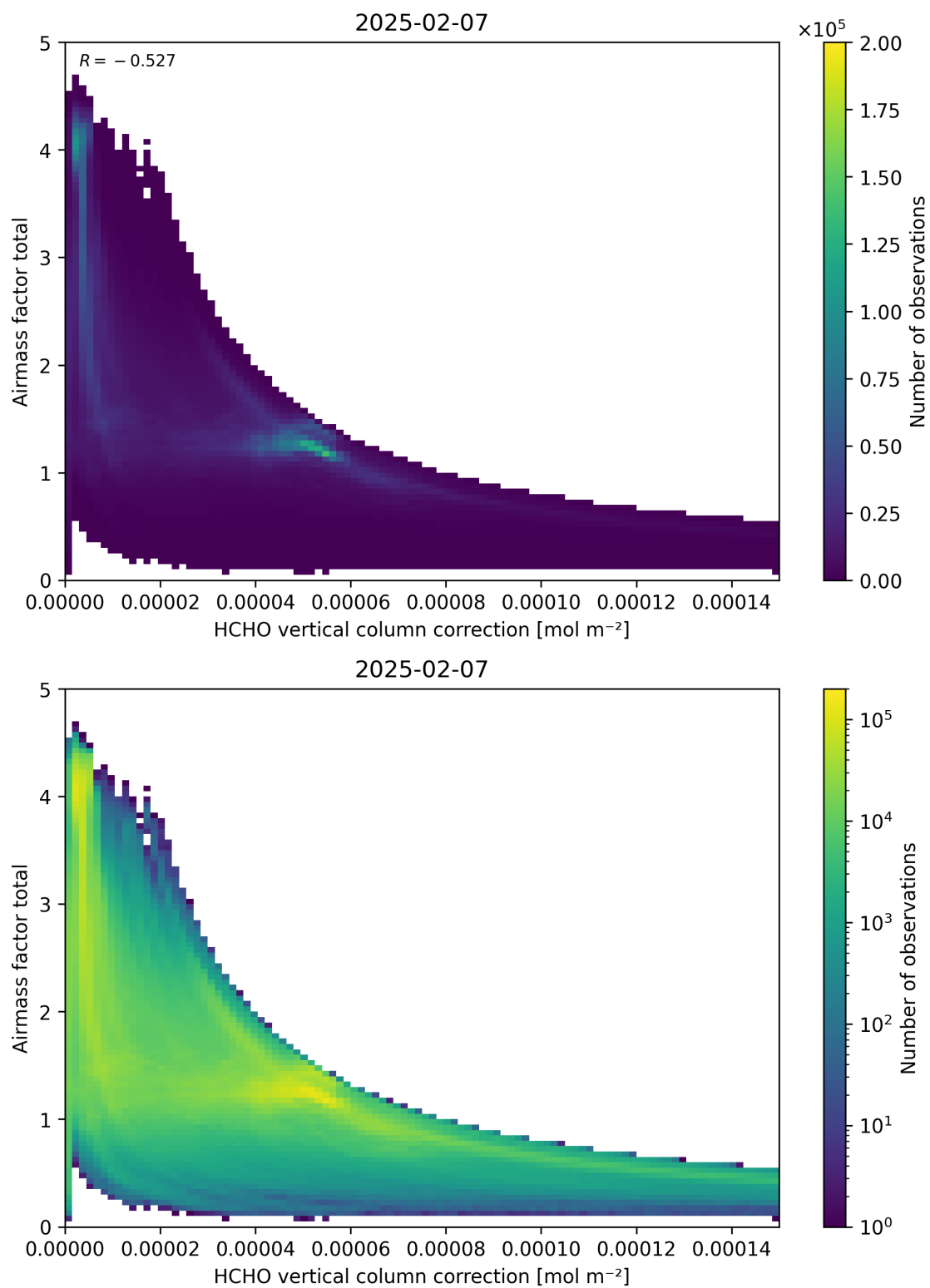
Figure 120: Scatter density plot of “HCHO vertical column correction” against “Airmass factor total” for 2025-02-06 to 2025-02-08.
