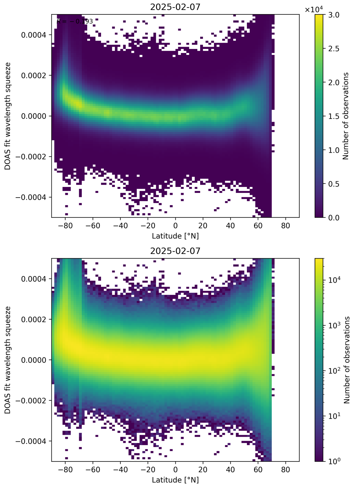
Figure 155: Scatter density plot of “Latitude” against “DOAS fit wavelength squeeze” for 2025-02-06 to 2025-02-08.
