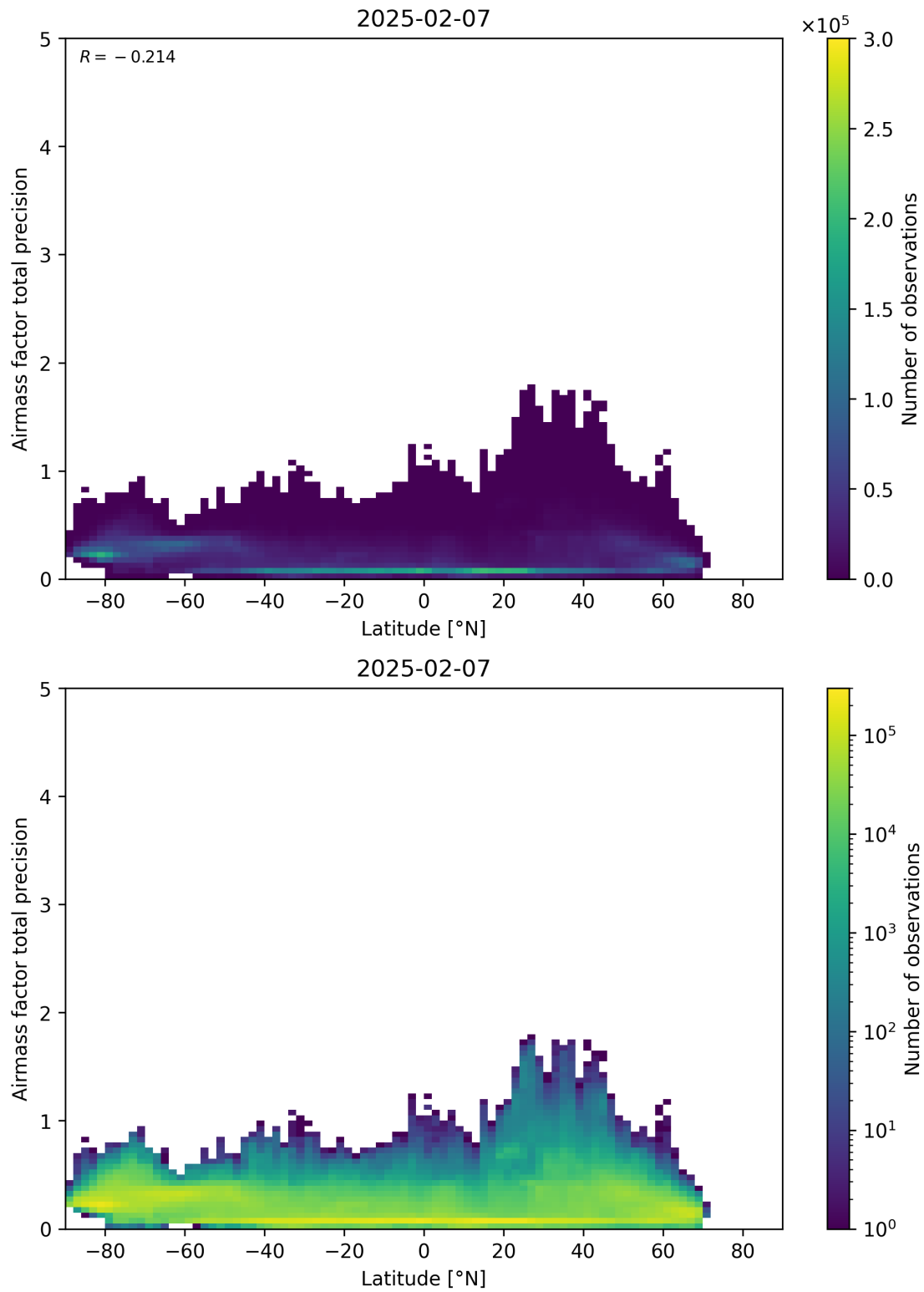
Figure 162: Scatter density plot of “Latitude” against “Airmass factor total precision” for 2025-02-06 to 2025-02-08.
