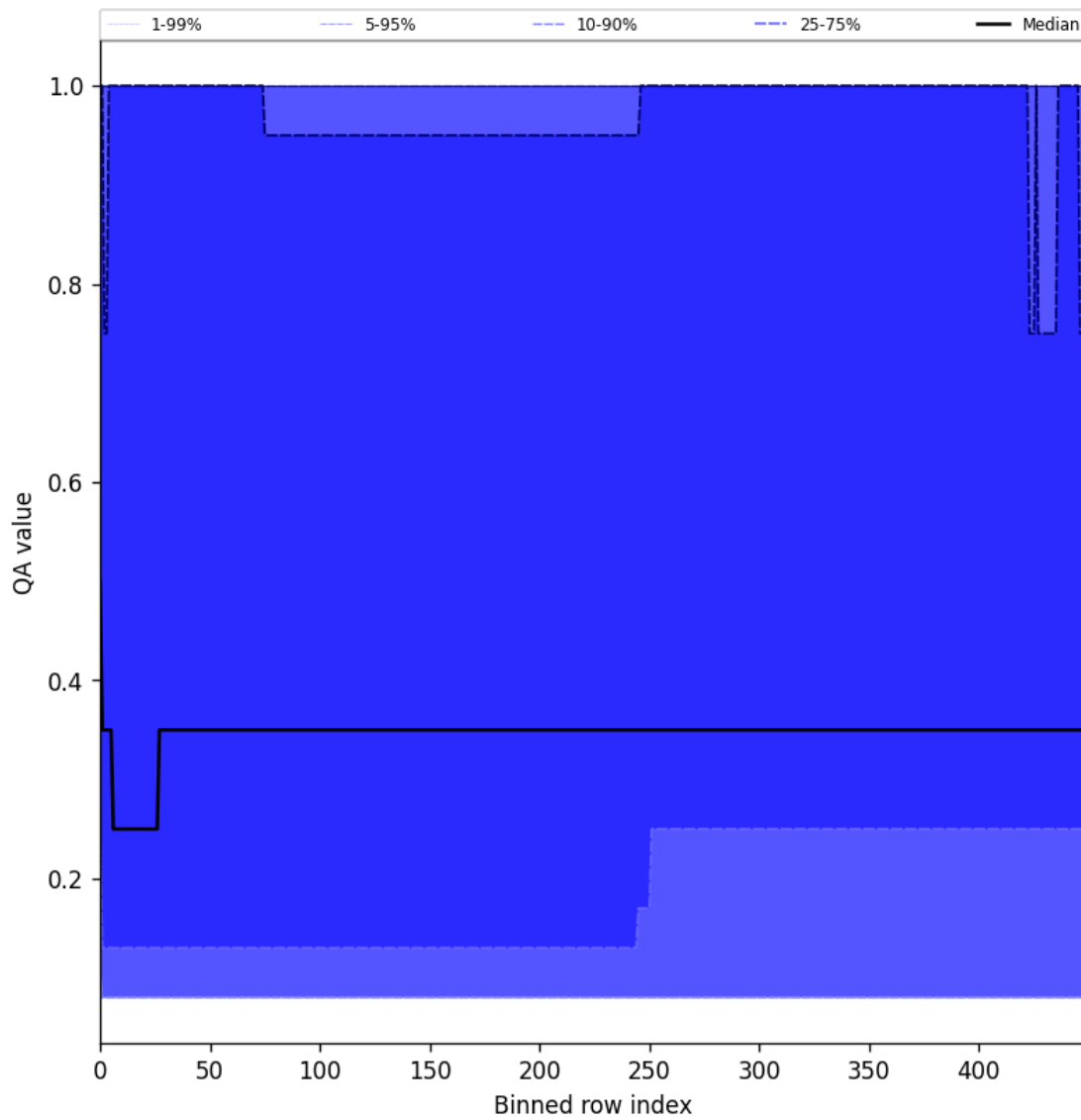
Figure 48: Along track statistics of “QA value” for 2025-02-06 to 2025-02-08
