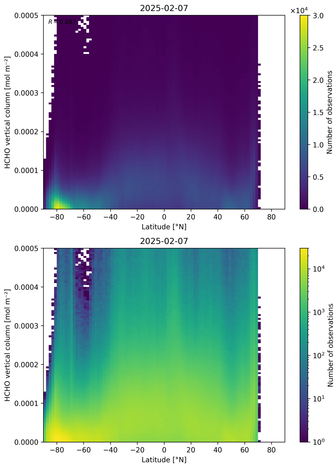
Figure 163: Scatter density plot of “Latitude” against “HCHO vertical column” for 2025-02-06 to 2025-02-08.
