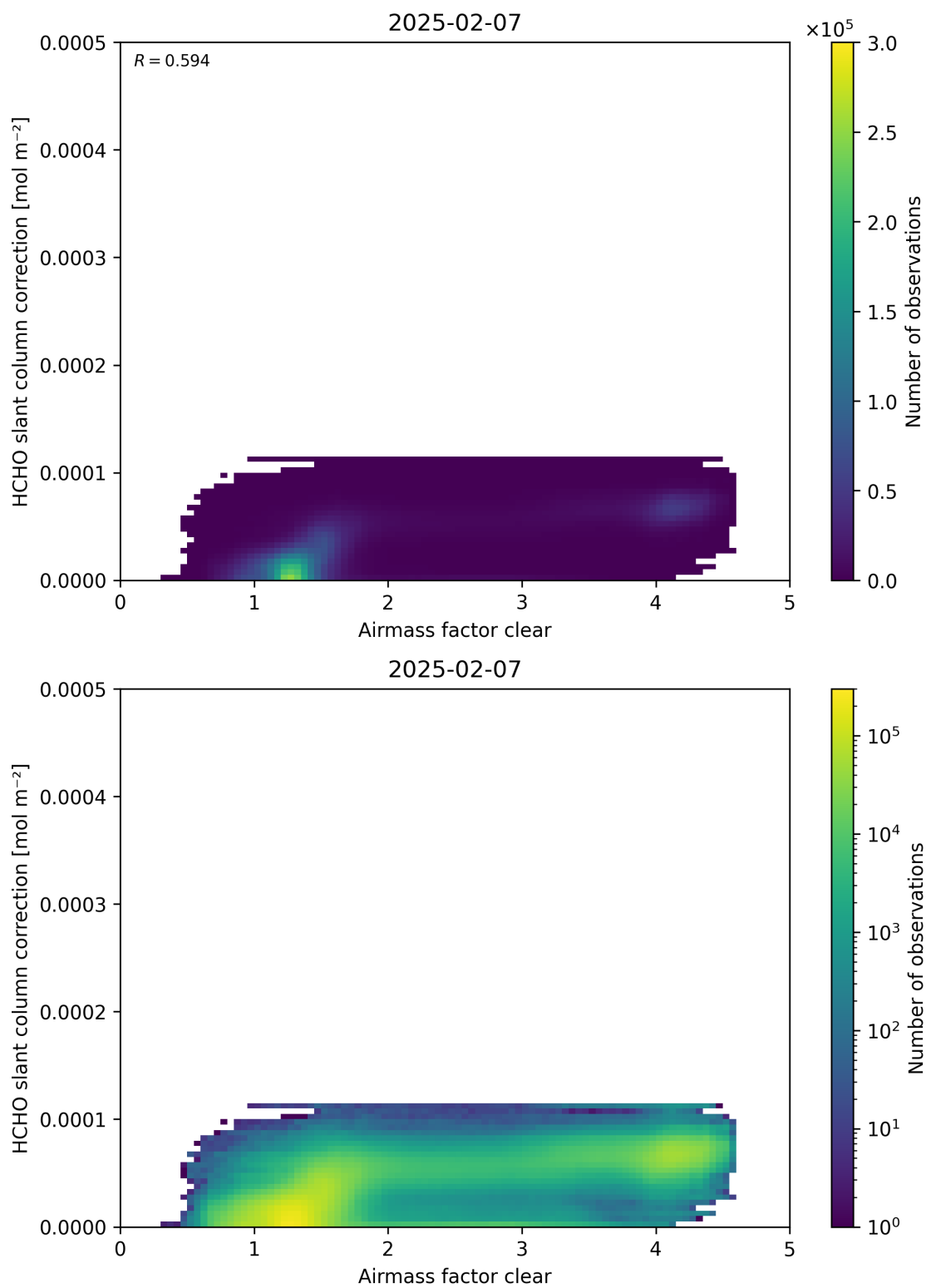
Figure 75: Scatter density plot of “Airmass factor clear” against “HCHO slant column correction” for 2025-02-06 to 2025-02-08.
