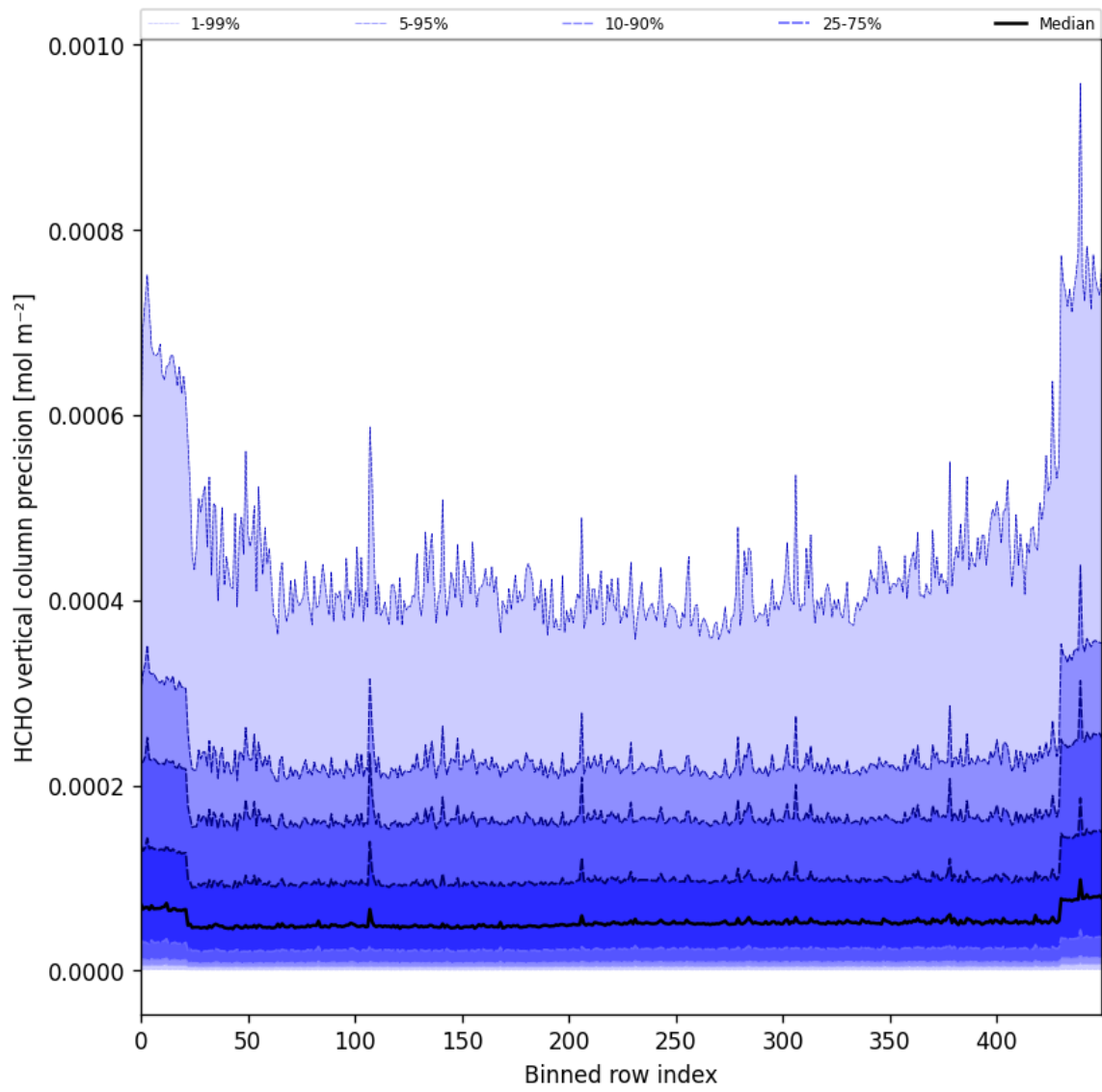
Figure 50: Along track statistics of “HCHO vertical column precision” for 2025-02-06 to 2025-02-08
