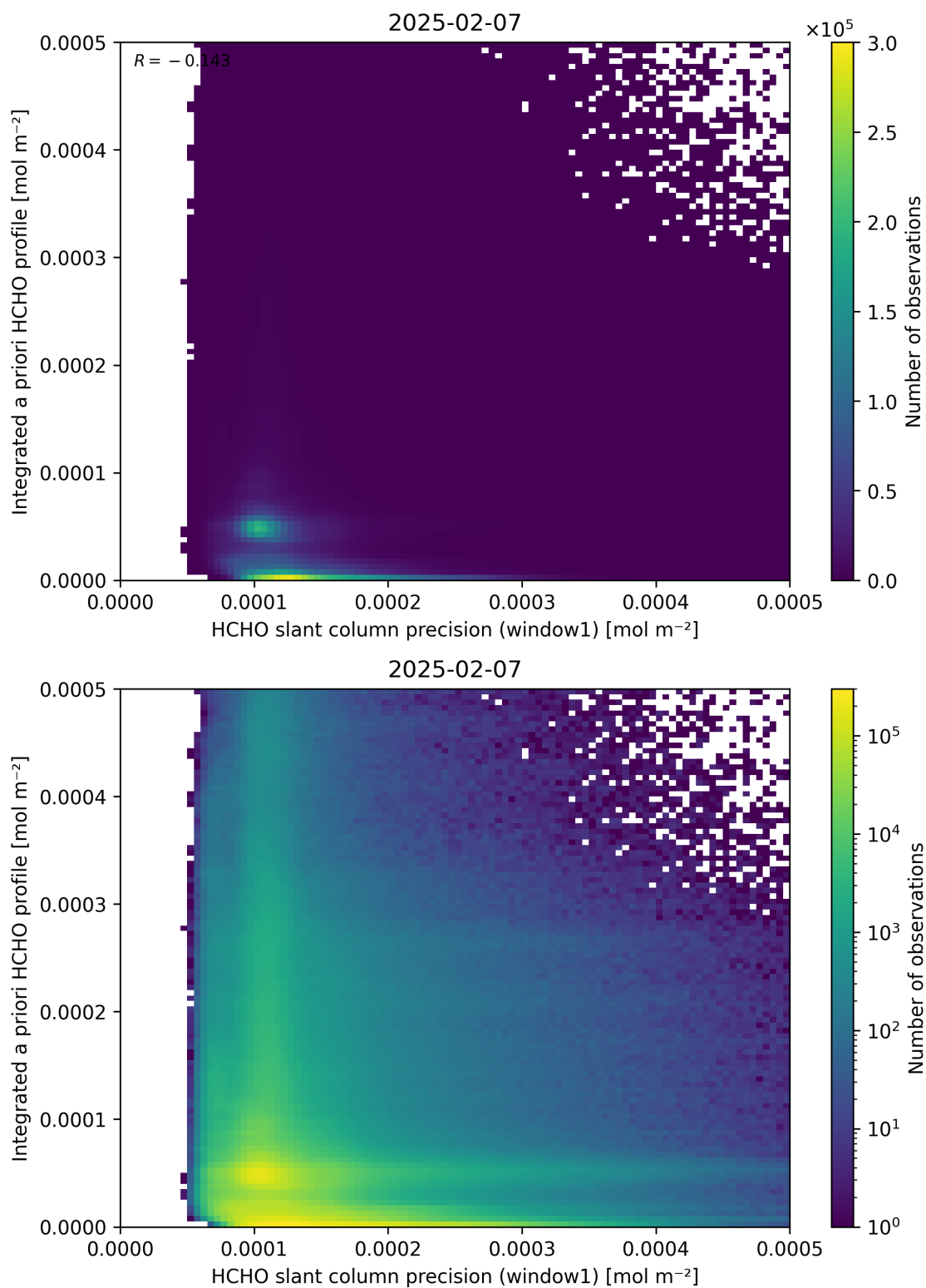
Figure 96: Scatter density plot of “HCHO slant column precision (window1)” against “Integrated a priori HCHO profile” for 2025-02-06 to 2025-02-08.
