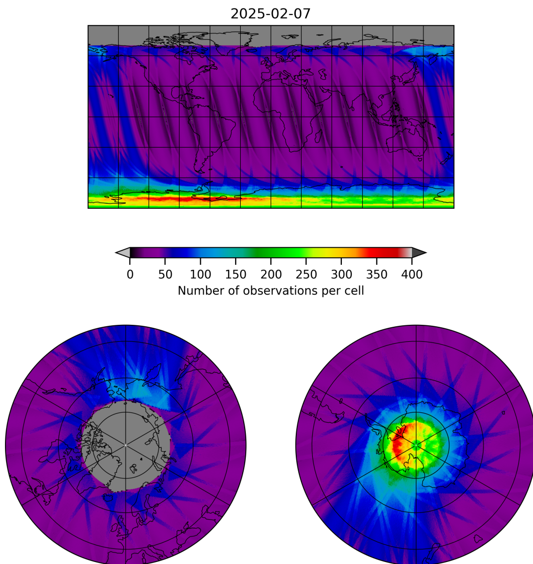
Figure 19: Map of the number of observations for 2025-02-06 to 2025-02-08
