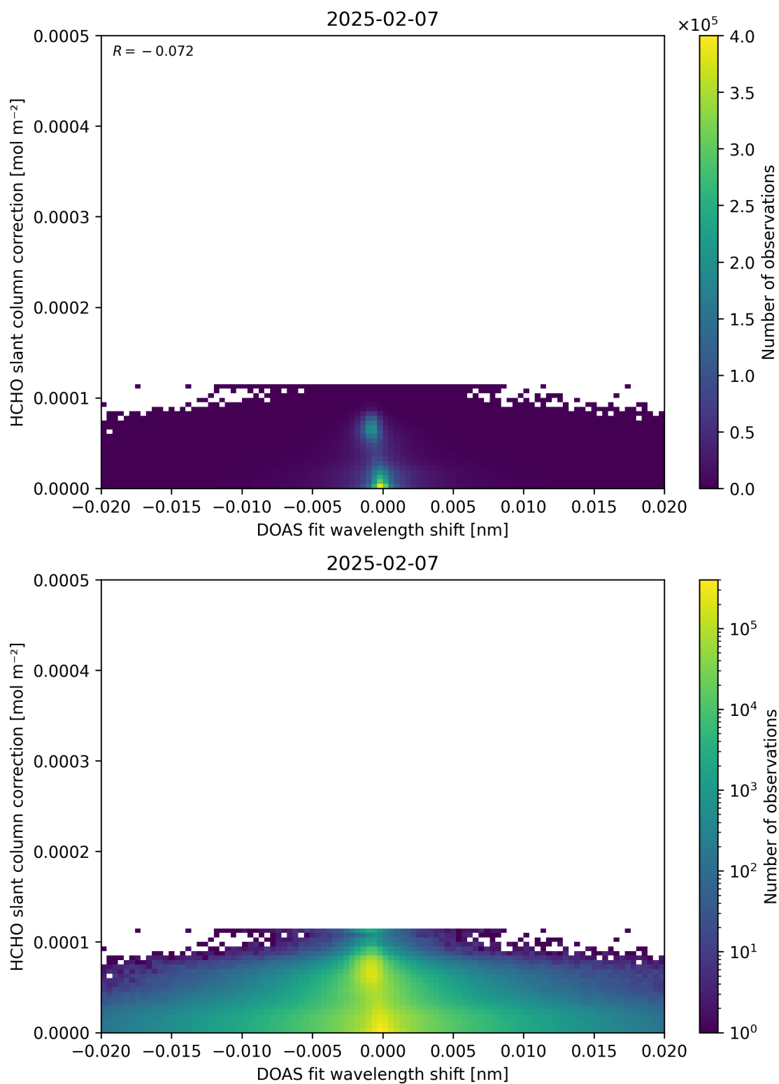
Figure 67: Scatter density plot of “DOAS fit wavelength shift” against “HCHO slant column correction” for 2025-02-06 to 2025-02-08.
