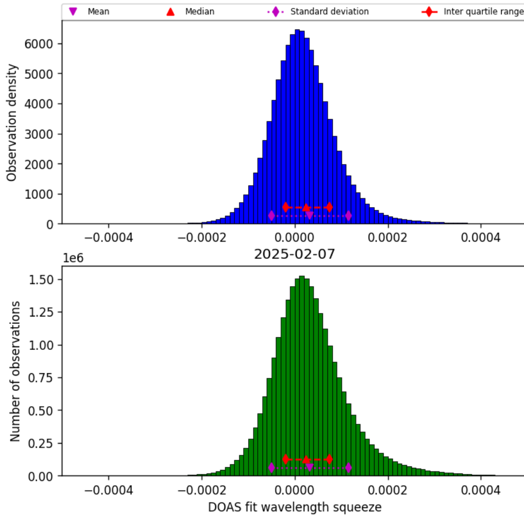
Figure 45: Histogram of “DOAS fit wavelength squeeze” for 2025-02-06 to 2025-02-08
