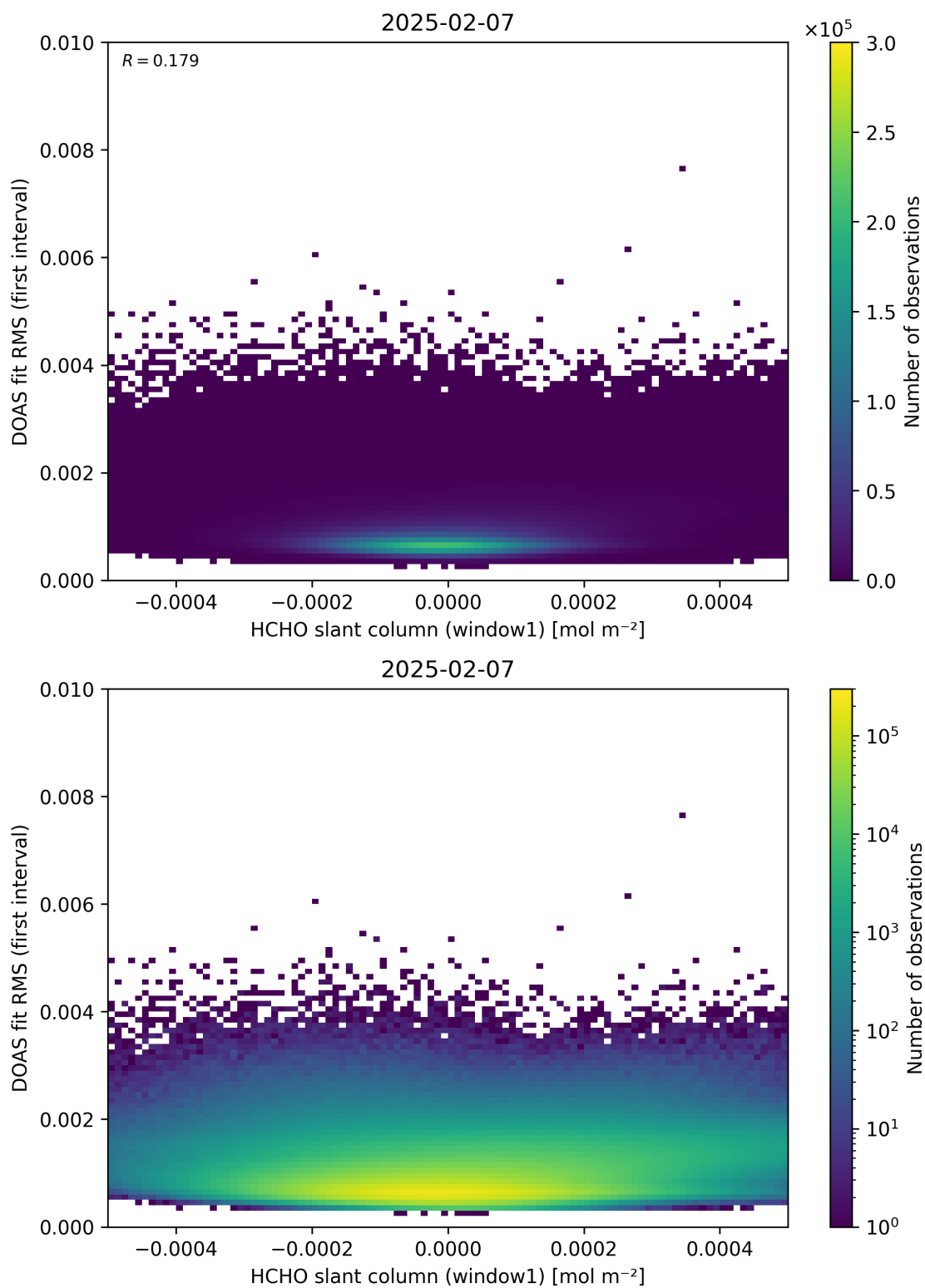
Figure 78: Scatter density plot of “HCHO slant column (window1)” against “DOAS fit RMS (first interval)” for 2025-02-06 to 2025-02-08.
