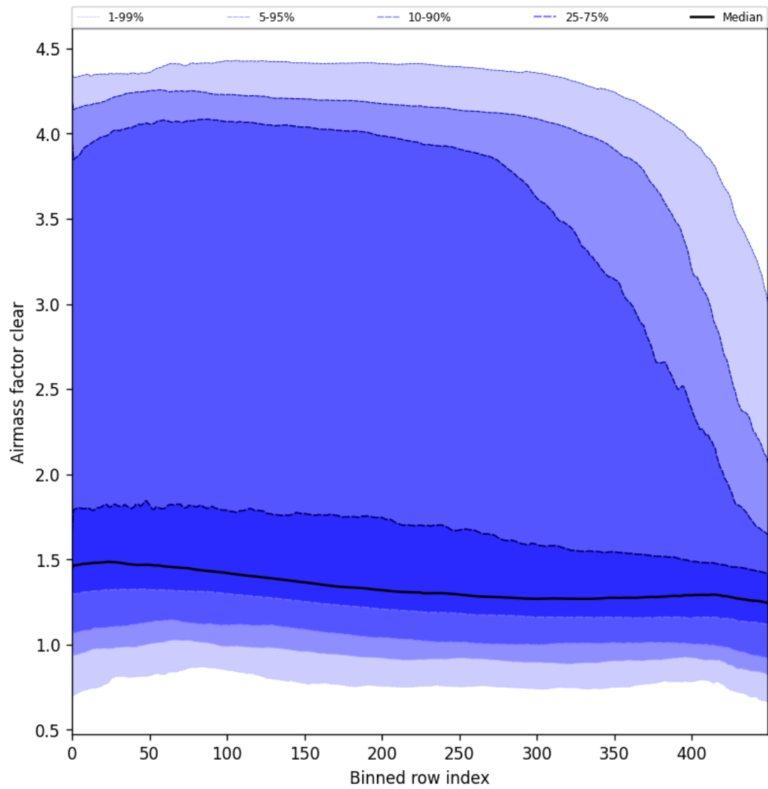
Figure 56: Along track statistics of “Airmass factor clear” for 2025-02-06 to 2025-02-08
