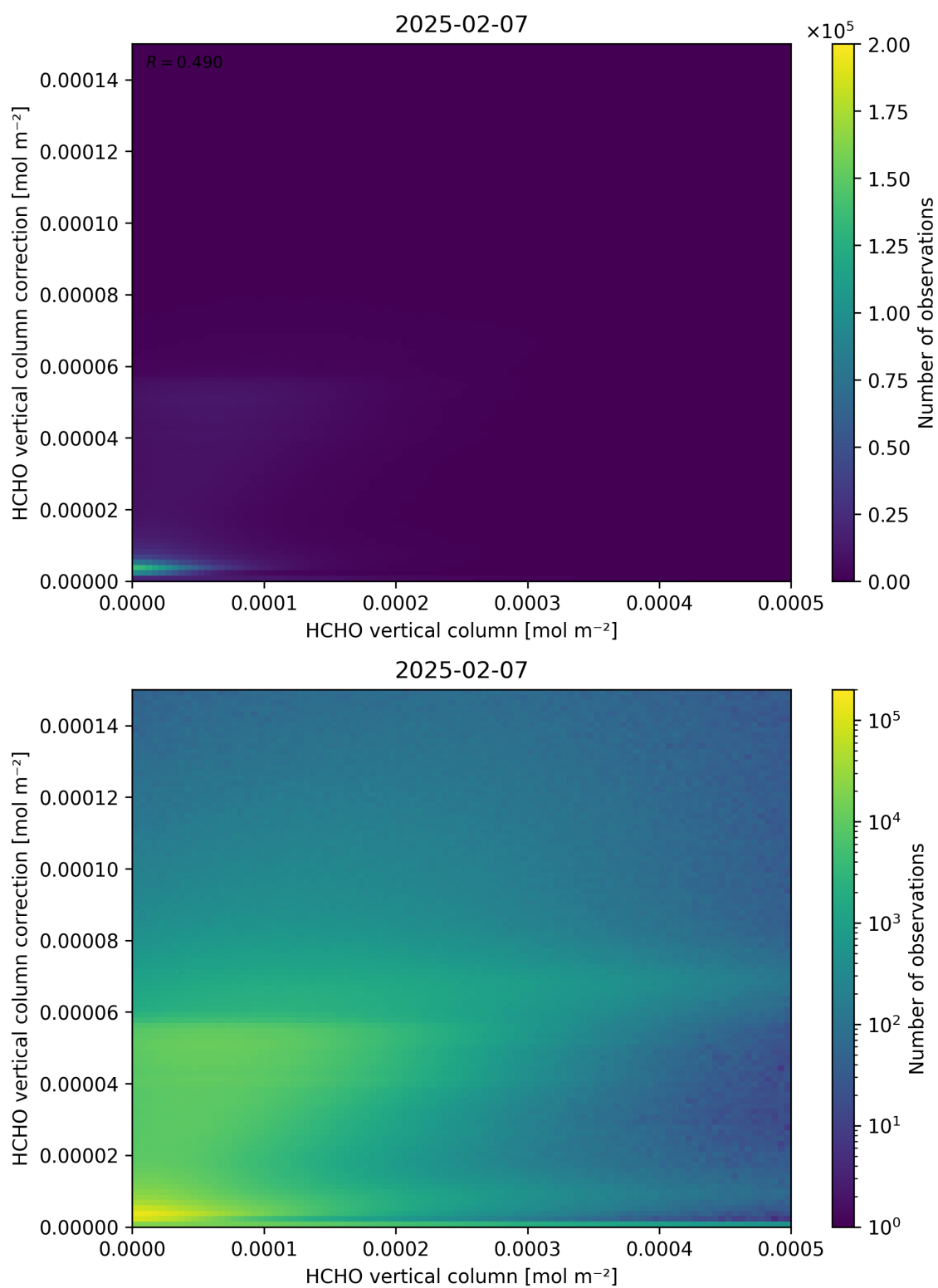
Figure 133: Scatter density plot of “HCHO vertical column” against “HCHO vertical column correction” for 2025-02-06 to 2025-02-08.
