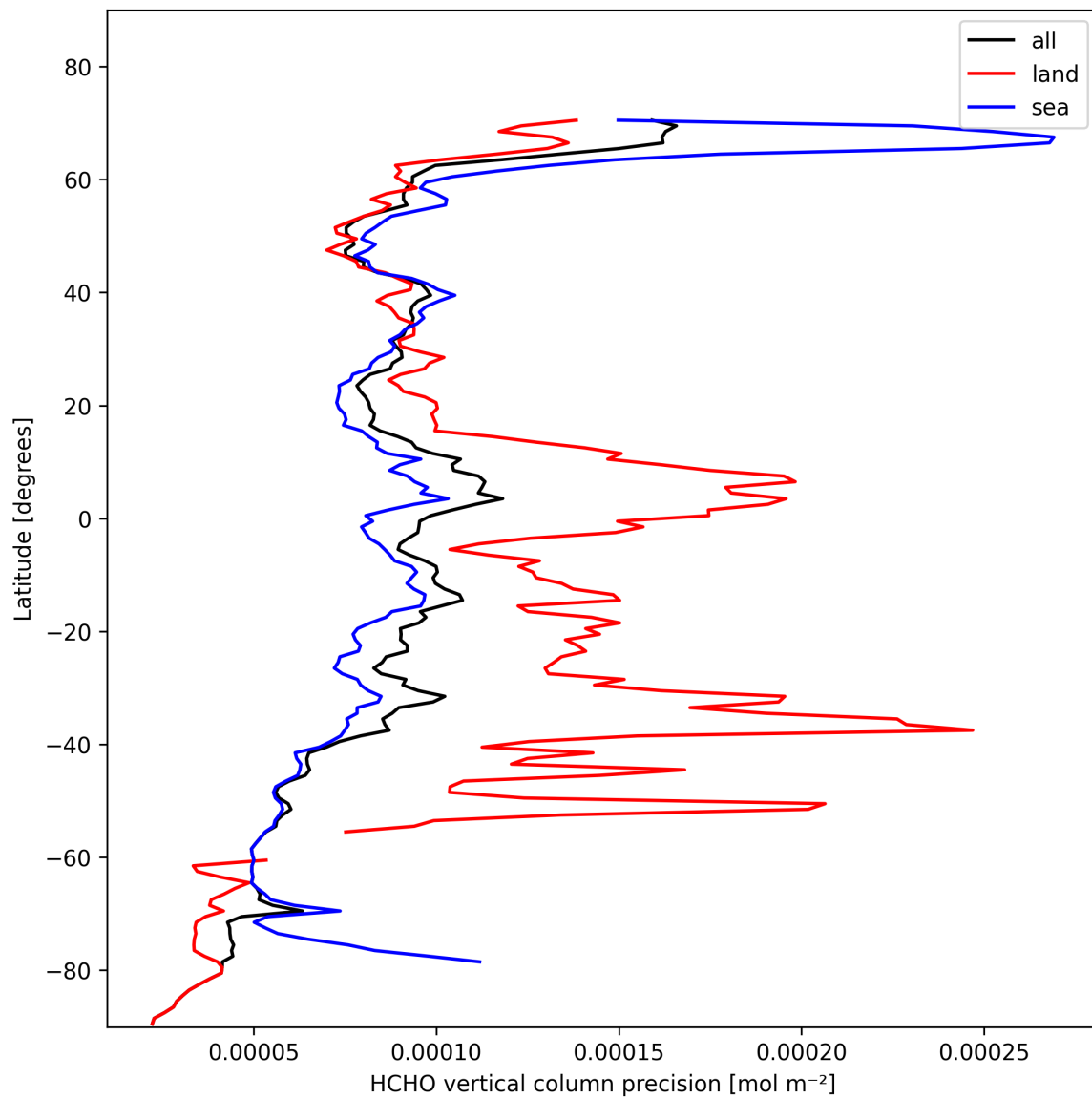
Figure 22: Zonal average of “HCHO vertical column precision” for 2025-02-06 to 2025-02-08.
