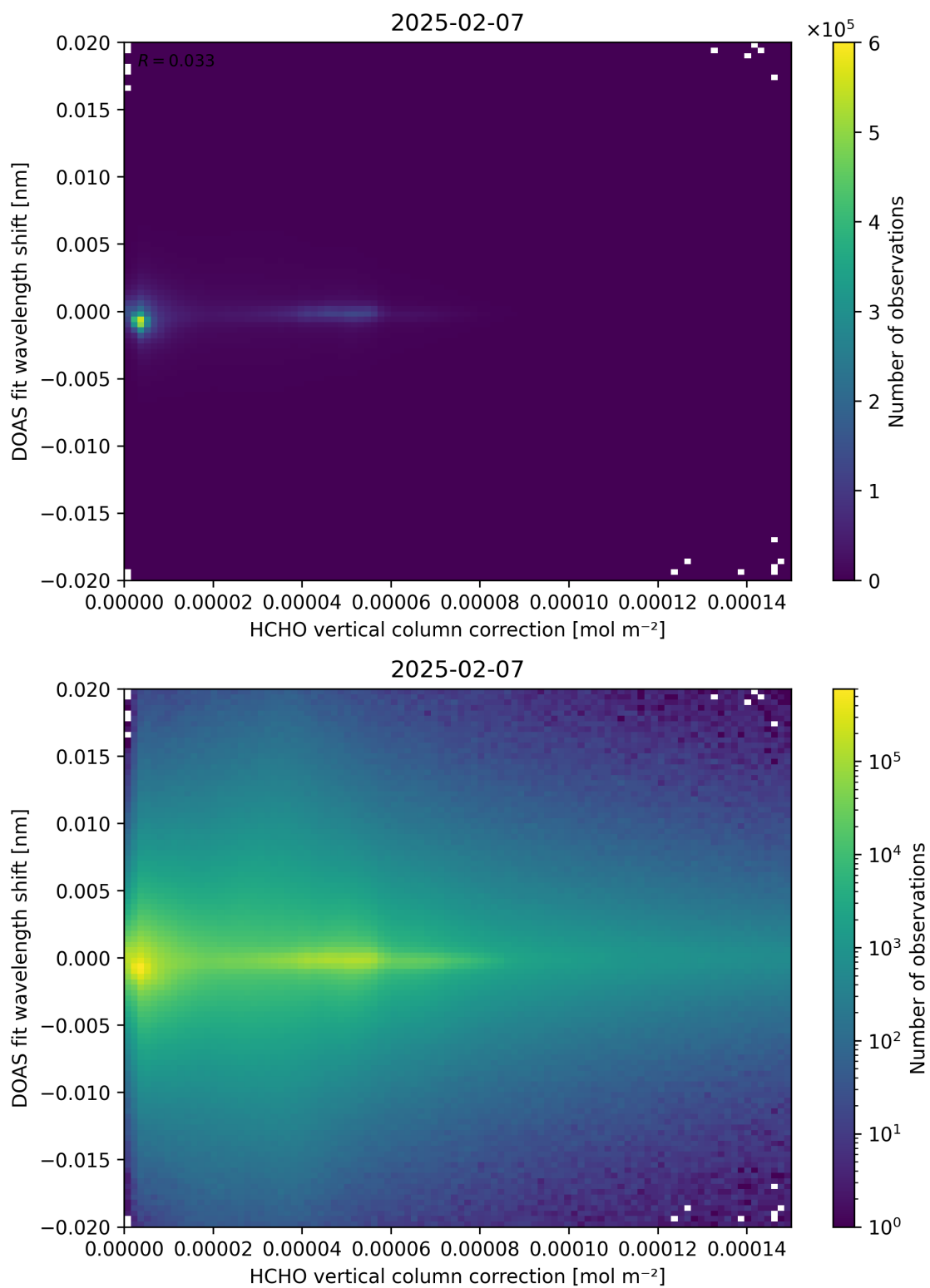
Figure 113: Scatter density plot of “HCHO vertical column correction” against “DOAS fit wavelength shift” for 2025-02-06 to 2025-02-08.
