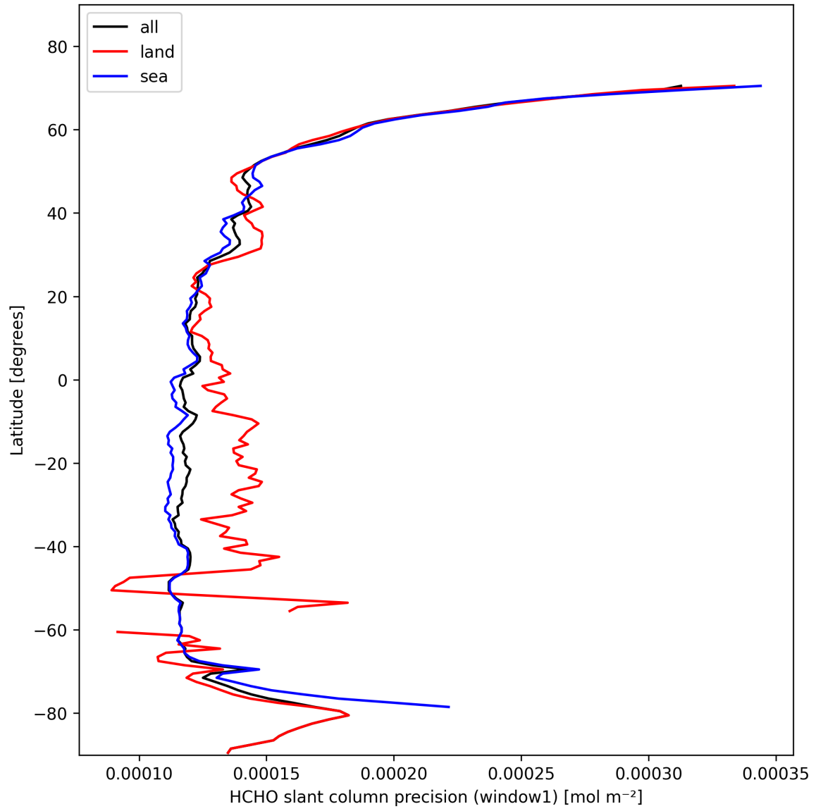
Figure 25: Zonal average of “HCHO slant column precision (window1)” for 2025-02-06 to 2025-02-08.
