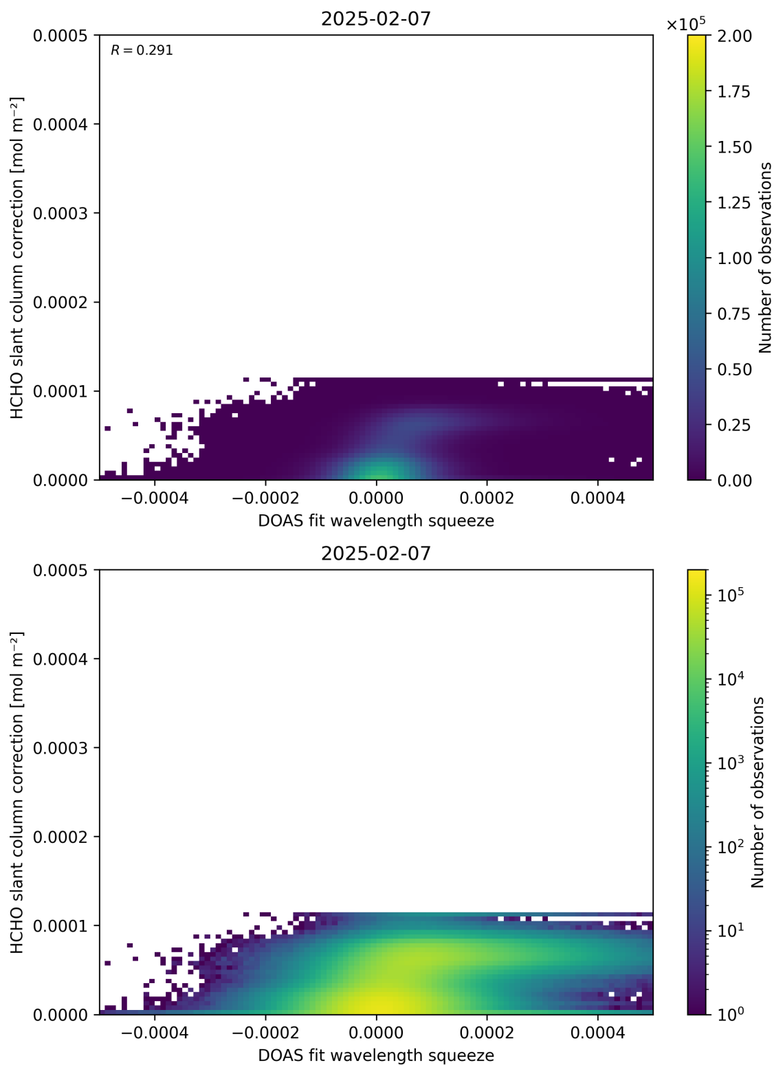
Figure 70: Scatter density plot of “DOAS fit wavelength squeeze” against “HCHO slant column correction” for 2025-02-06 to 2025-02-08.
