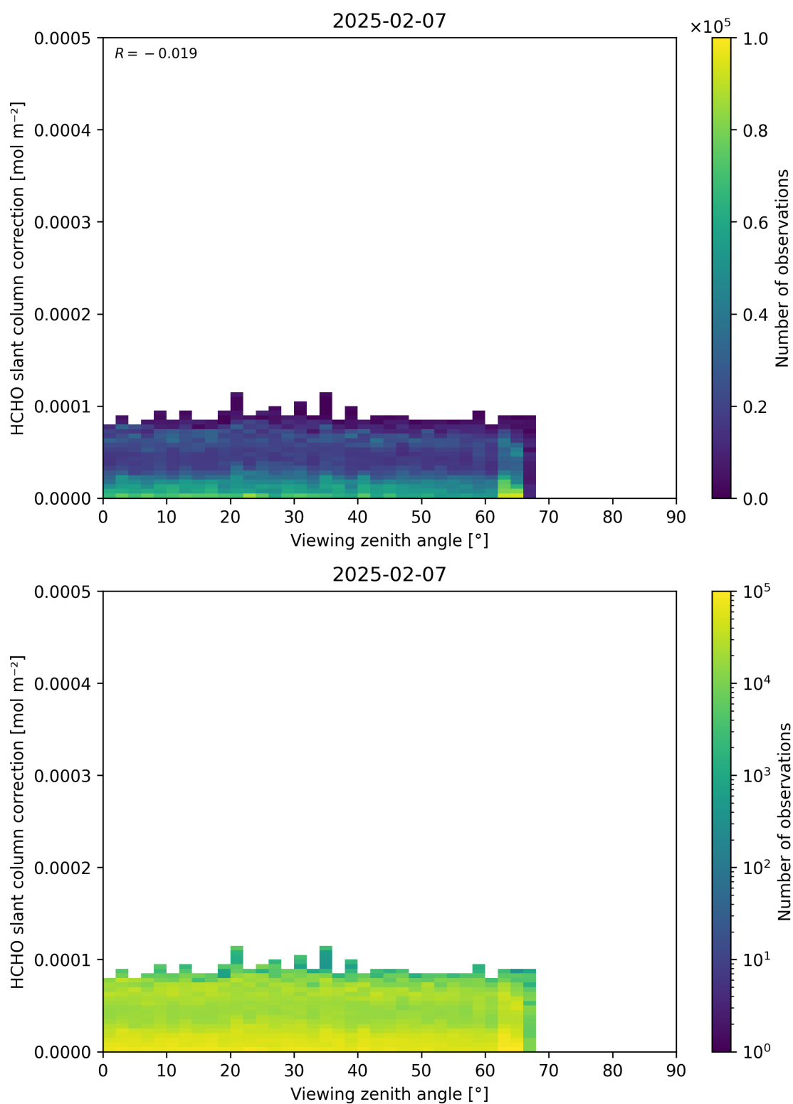
Figure 187: Scatter density plot of “Viewing zenith angle” against “HCHO slant column correction” for 2025-02-06 to 2025-02-08.
