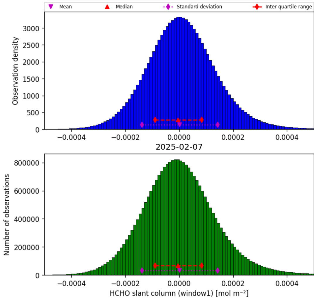
Figure 38: Histogram of “HCHO slant column (window1)” for 2025-02-06 to 2025-02-08
