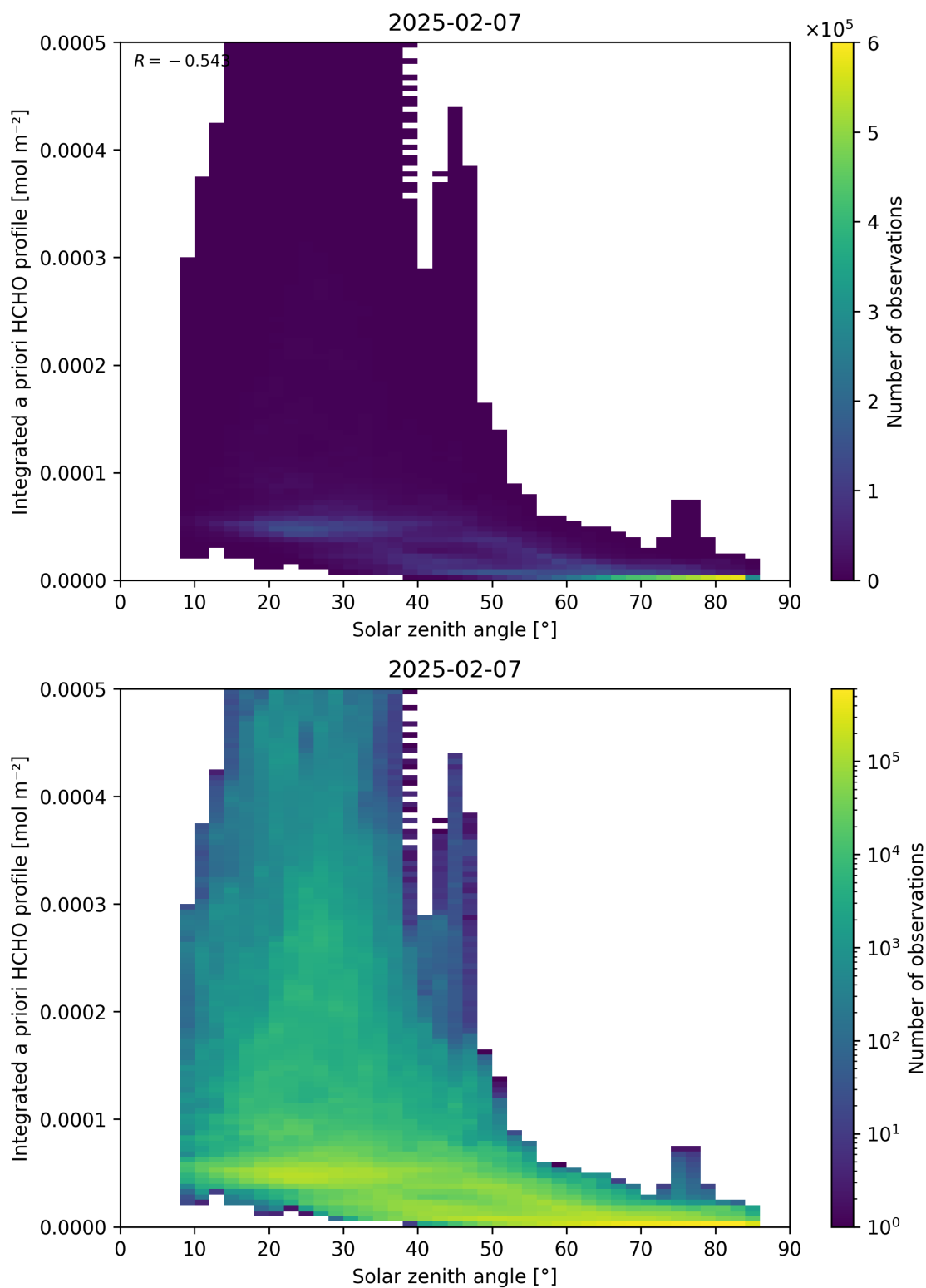
Figure 180: Scatter density plot of “Solar zenith angle” against “Integrated a priori HCHO profile” for 2025-02-06 to 2025-02-08.
