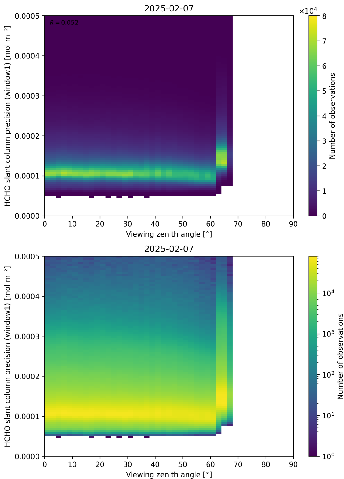
Figure 189: Scatter density plot of “Viewing zenith angle” against “HCHO slant column precision (window1)” for 2025-02-06 to 2025-02-08.
