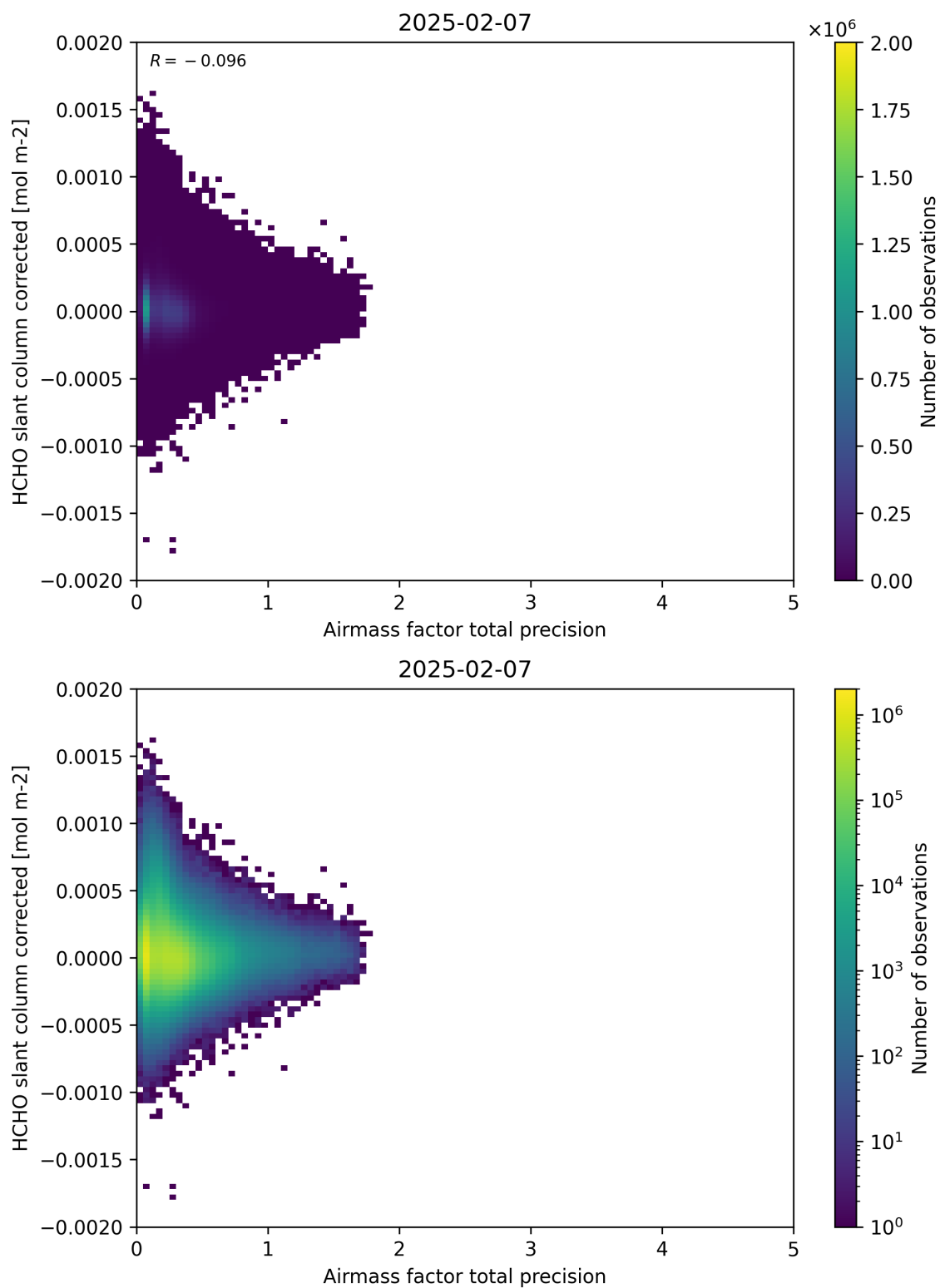
Figure 109: Scatter density plot of “Airmass factor total precision” against “HCHO slant column corrected” for 2025-02-06 to 2025-02-08.
