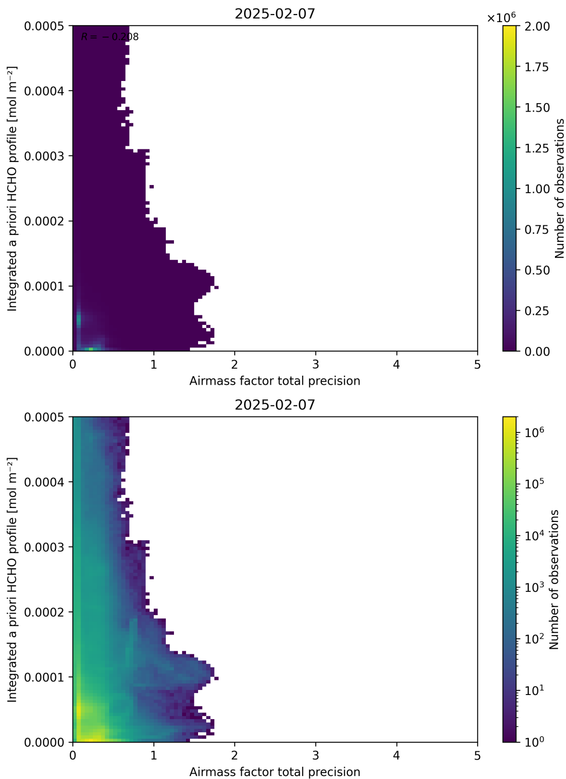
Figure 111: Scatter density plot of “Airmass factor total precision” against “Integrated a priori HCHO profile” for 2025-02-06 to 2025-02-08.
