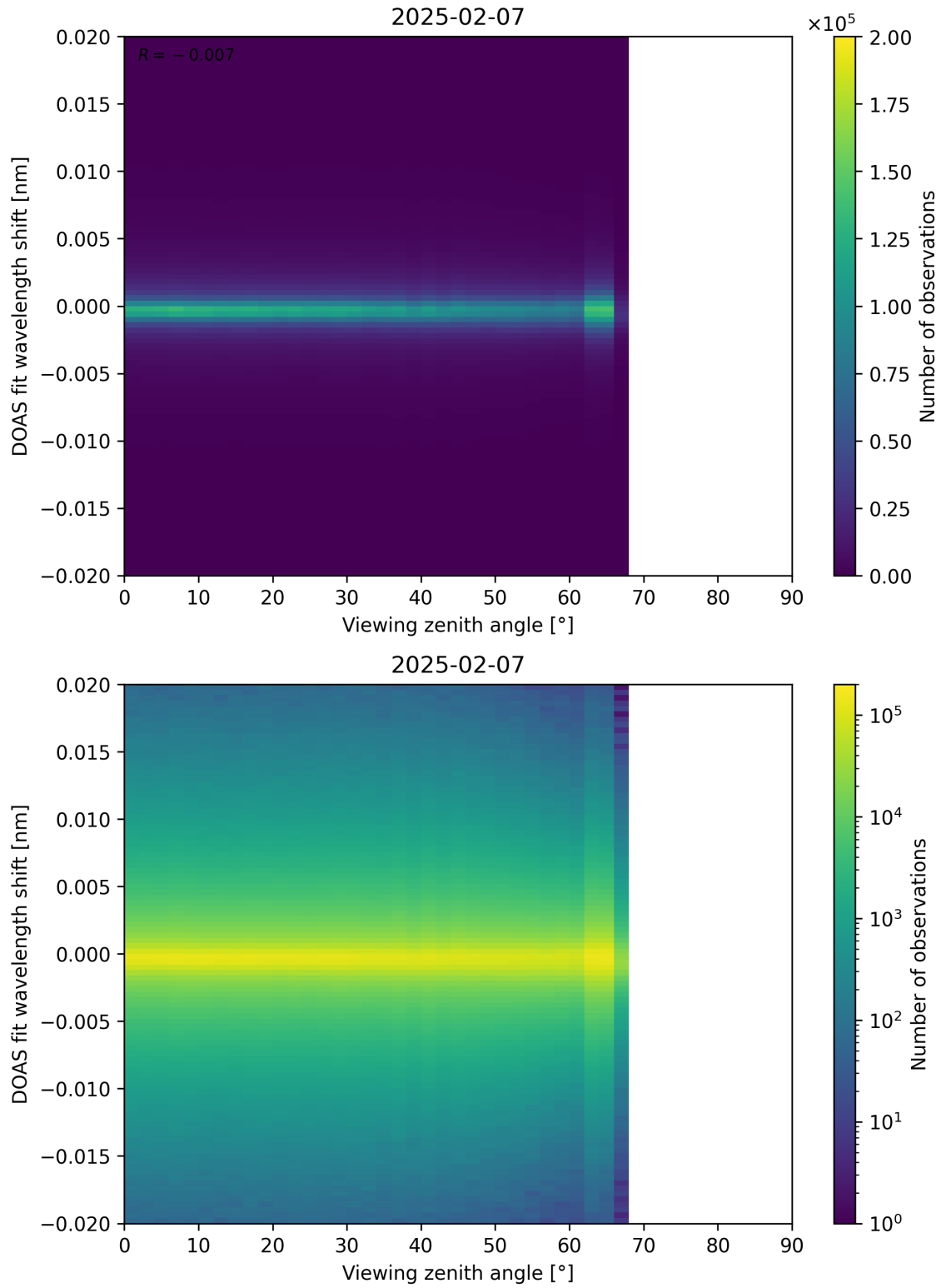
Figure 183: Scatter density plot of “Viewing zenith angle” against “DOAS fit wavelength shift” for 2025-02-06 to 2025-02-08.
