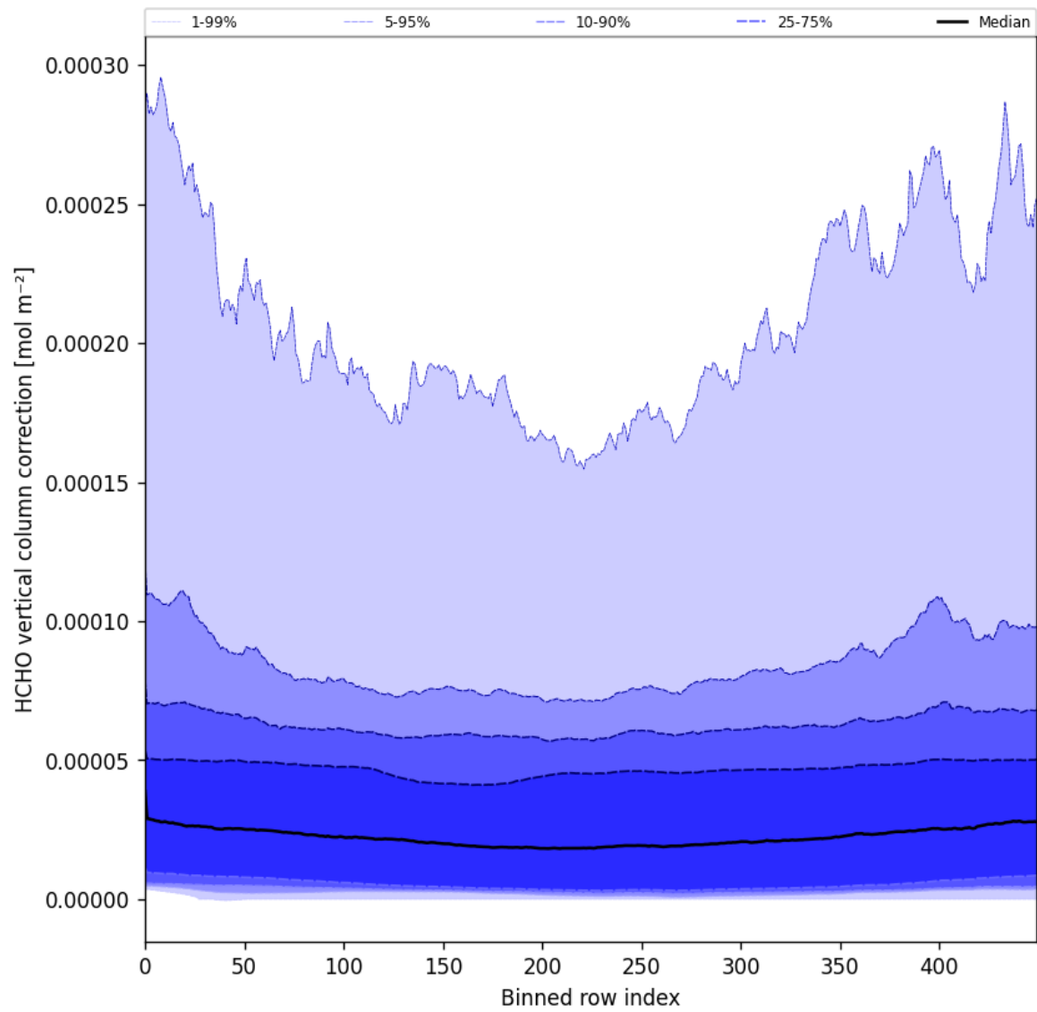
Figure 51: Along track statistics of “HCHO vertical column correction” for 2025-02-06 to 2025-02-08
