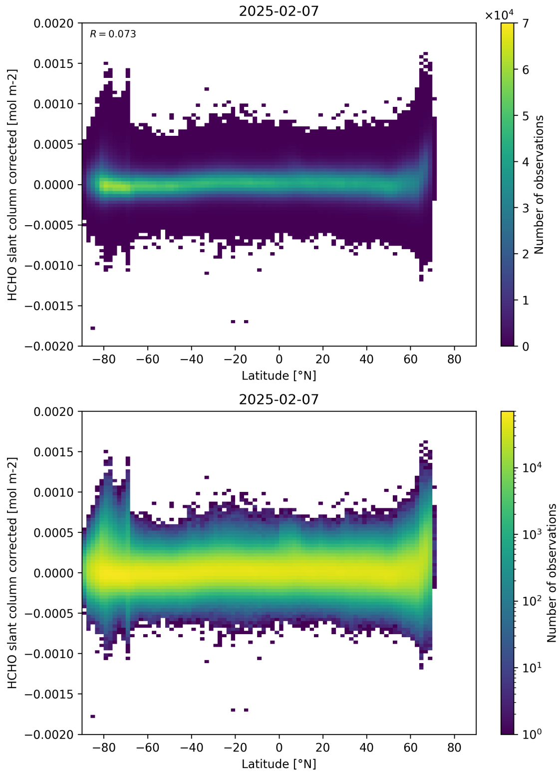
Figure 157: Scatter density plot of “Latitude” against “HCHO slant column corrected” for 2025-02-06 to 2025-02-08.
