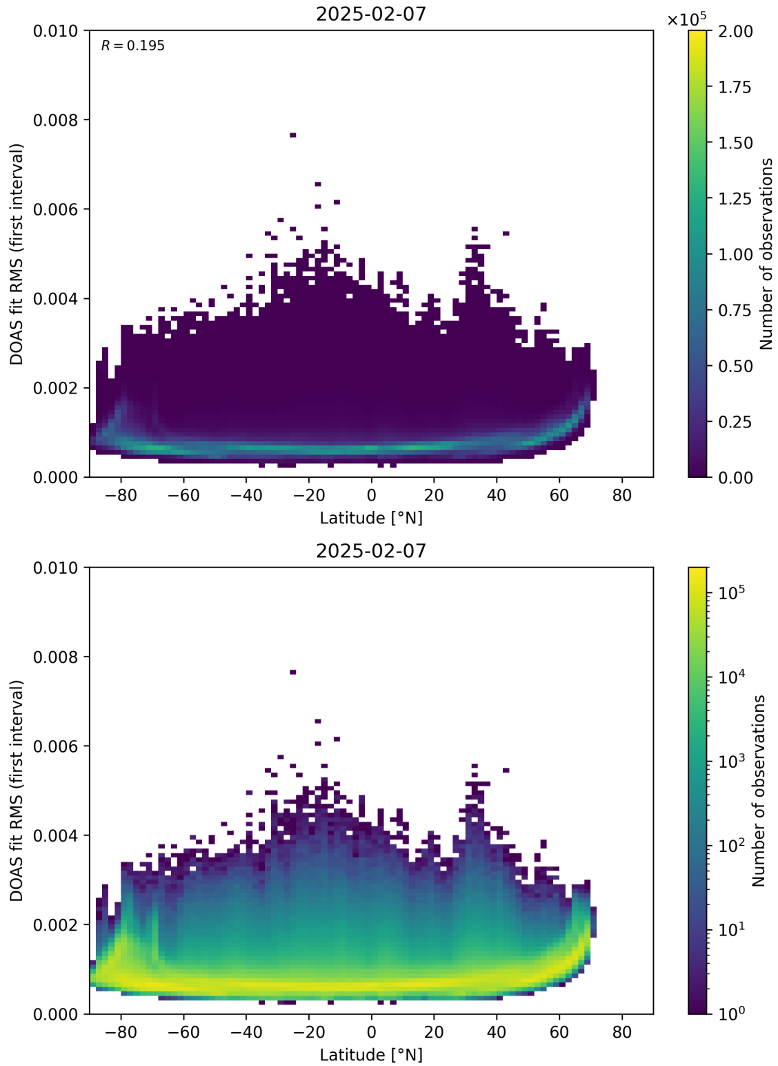
Figure 153: Scatter density plot of “Latitude” against “DOAS fit RMS (first interval)” for 2025-02-06 to 2025-02-08.
