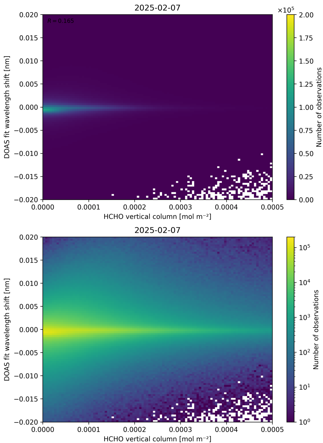
Figure 124: Scatter density plot of “HCHO vertical column” against “DOAS fit wavelength shift” for 2025-02-06 to 2025-02-08.
