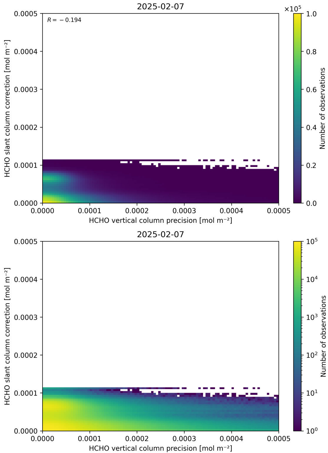
Figure 141: Scatter density plot of “HCHO vertical column precision” against “HCHO slant column correction” for 2025-02-06 to 2025-02-08.
