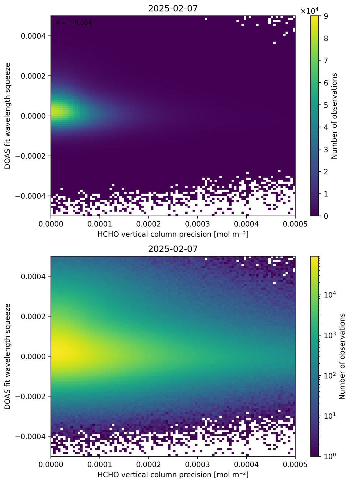
Figure 138: Scatter density plot of “HCHO vertical column precision” against “DOAS fit wavelength squeeze” for 2025-02-06 to 2025-02-08.
