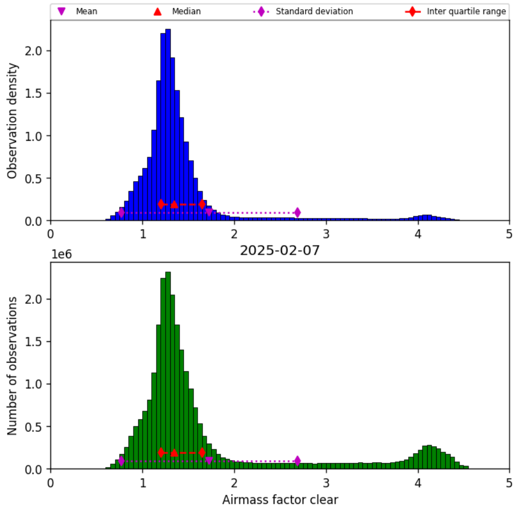
Figure 42: Histogram of “Airmass factor clear” for 2025-02-06 to 2025-02-08
