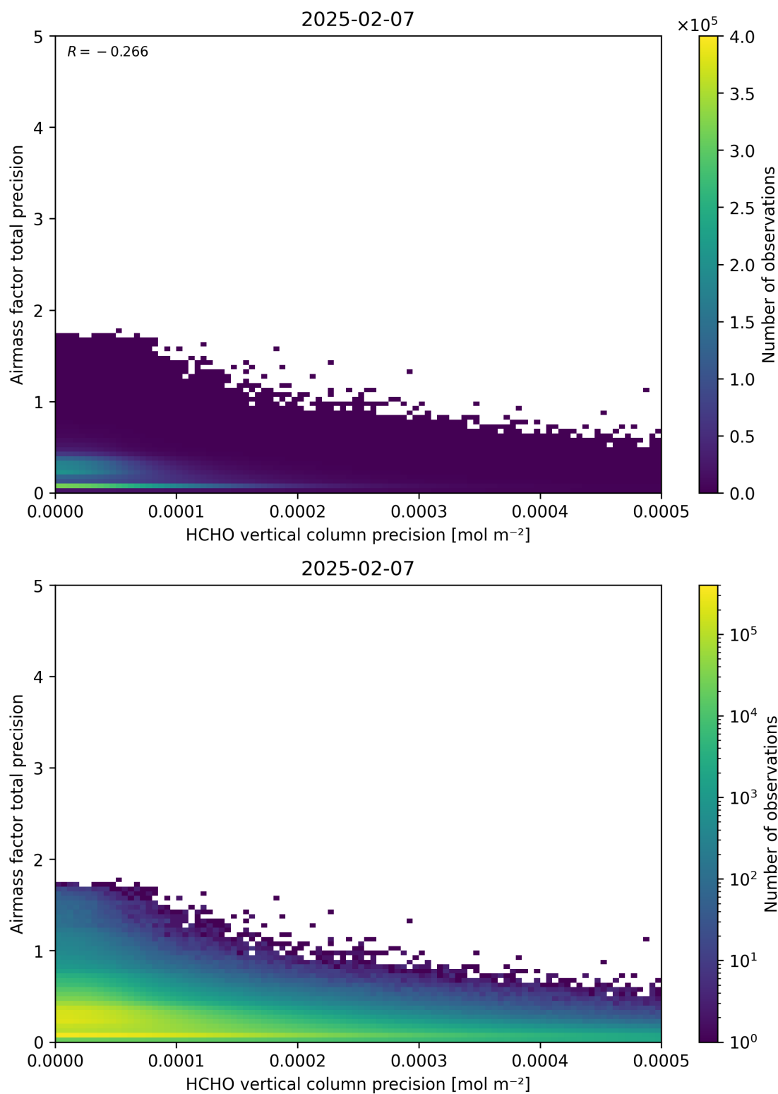
Figure 145: Scatter density plot of “HCHO vertical column precision” against “Airmass factor total precision” for 2025-02-06 to 2025-02-08.
