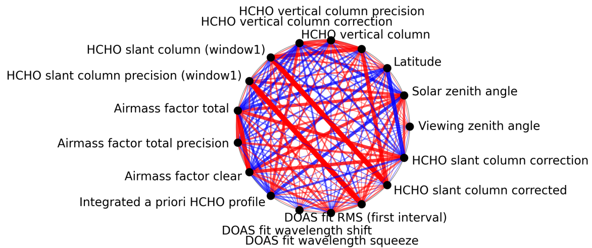
Figure 1: Map of correlation graph for 2025-02-06 to 2025-02-08.
