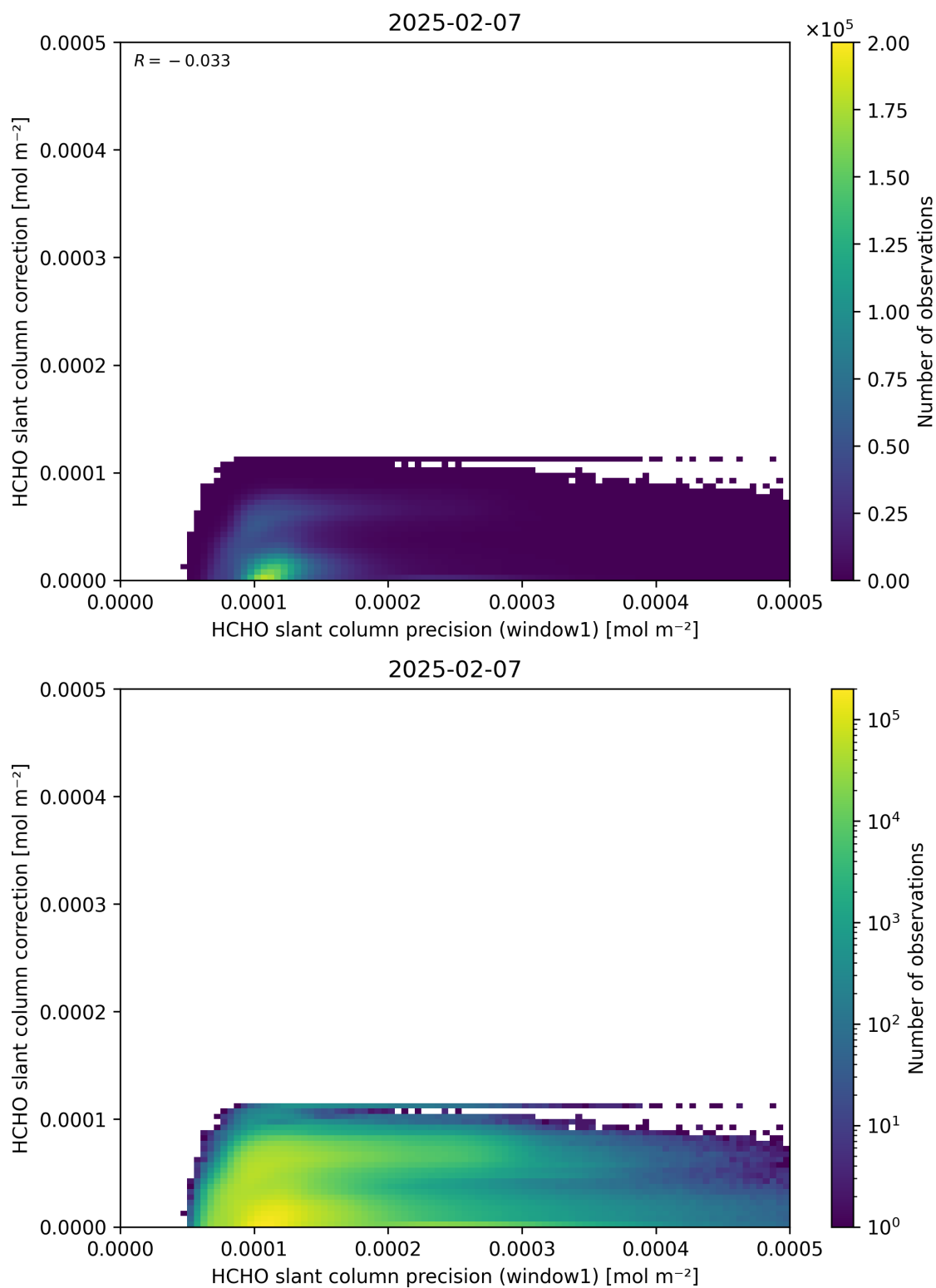
Figure 93: Scatter density plot of “HCHO slant column precision (window1)” against “HCHO slant column correction” for 2025-02-06 to 2025-02-08.
