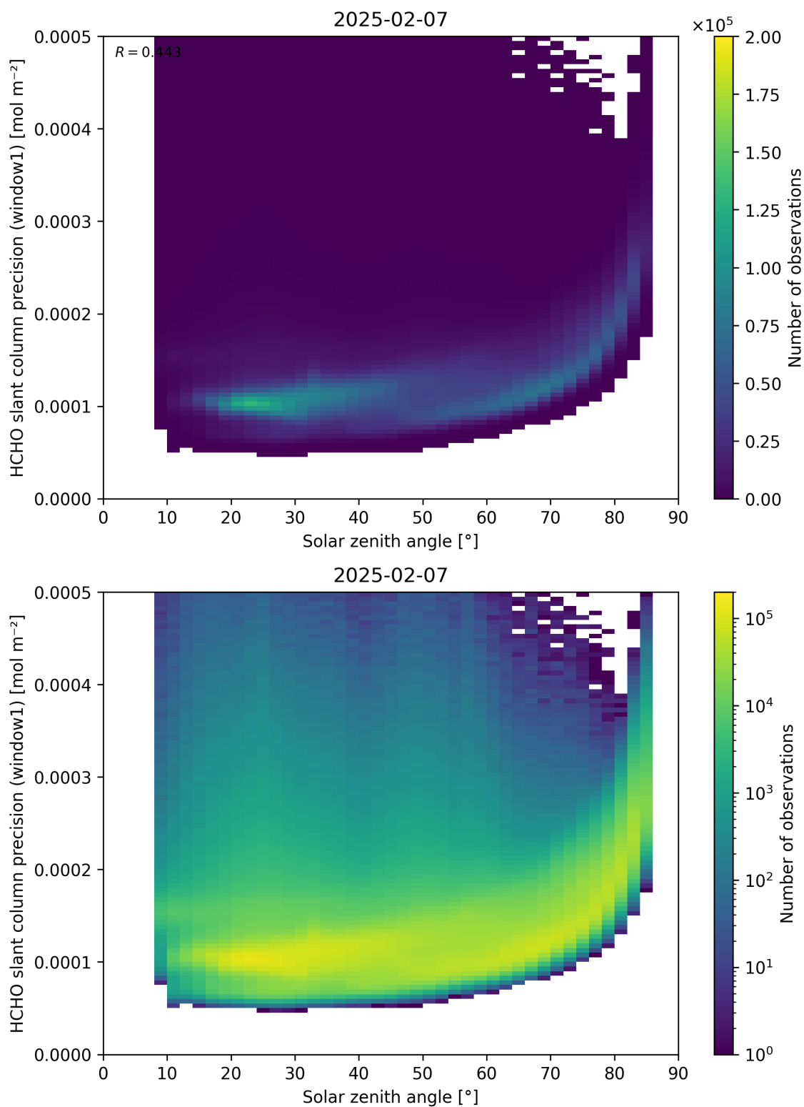
Figure 174: Scatter density plot of “Solar zenith angle” against “HCHO slant column precision (window1)” for 2025-02-06 to 2025-02-08.
