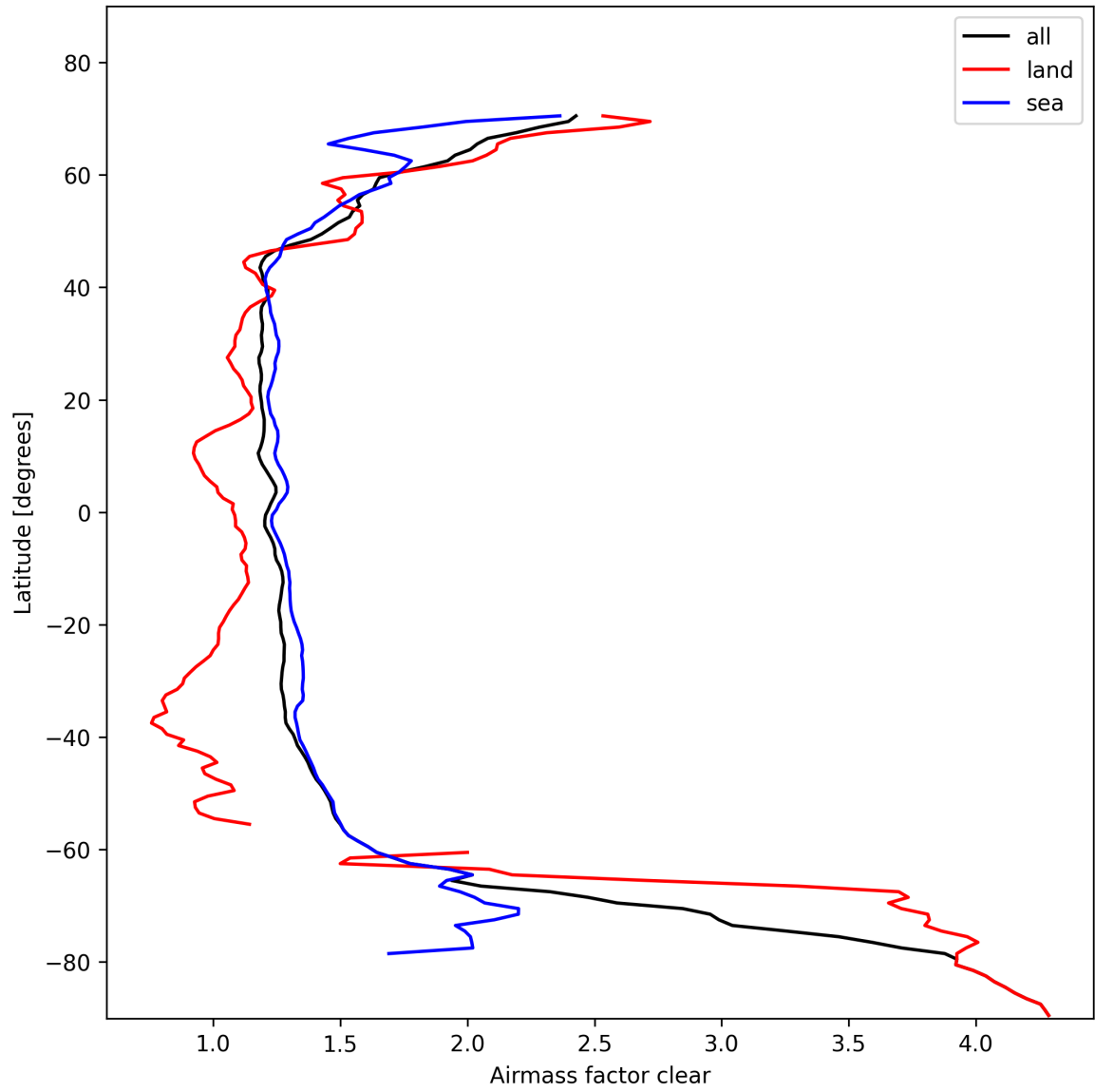
Figure 28: Zonal average of “Airmass factor clear” for 2025-02-06 to 2025-02-08.
