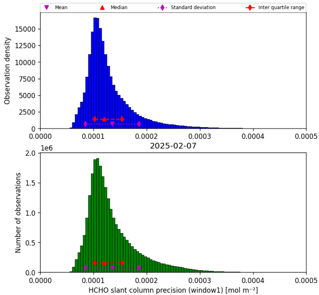
Figure 39: Histogram of “HCHO slant column precision (window1)” for 2025-02-06 to 2025-02-08
