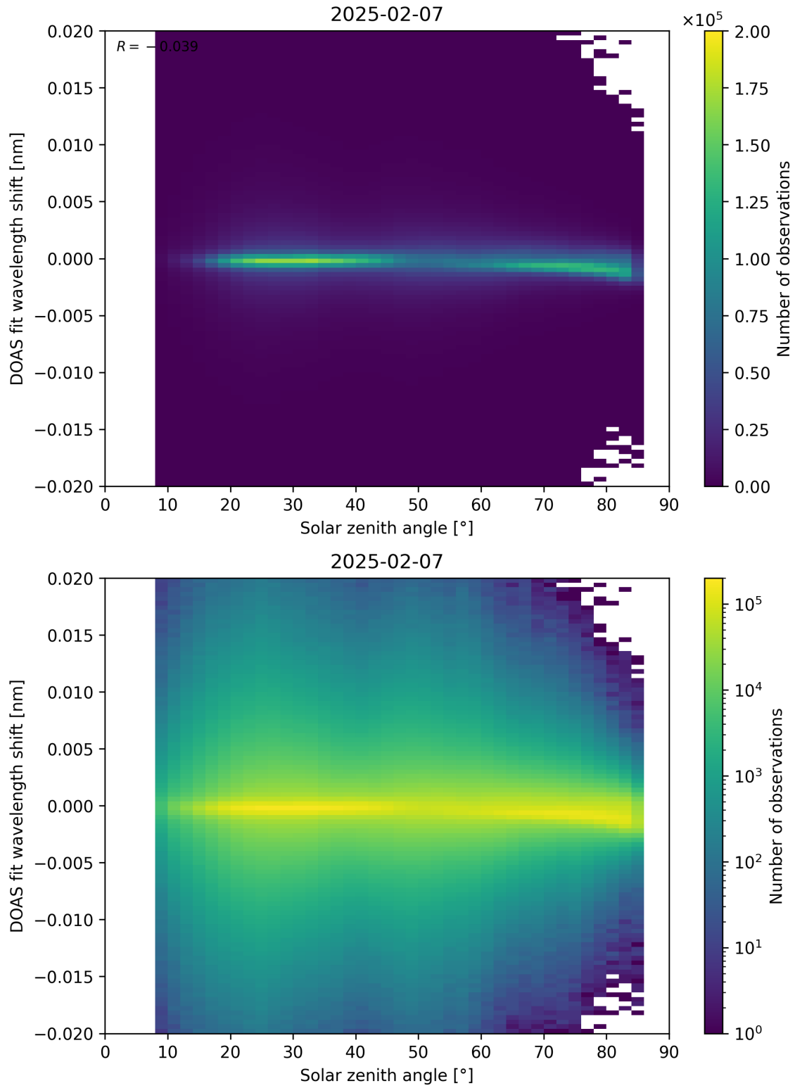
Figure 168: Scatter density plot of “Solar zenith angle” against “DOAS fit wavelength shift” for 2025-02-06 to 2025-02-08.
