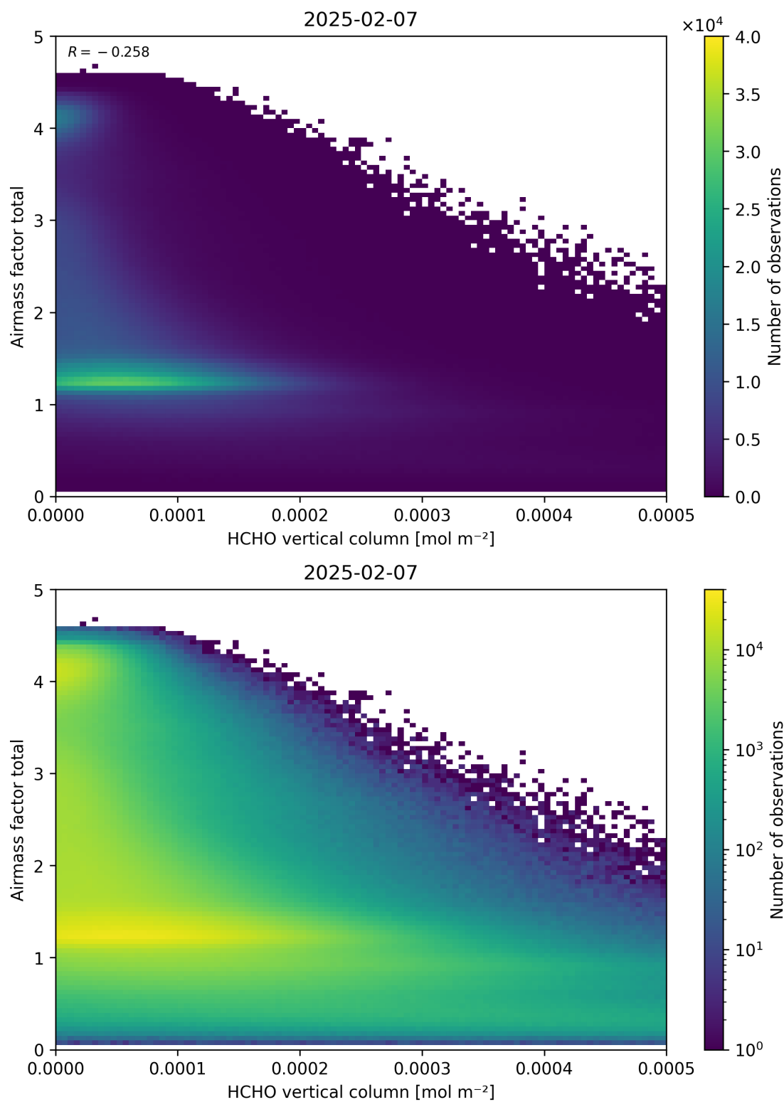
Figure 131: Scatter density plot of “HCHO vertical column” against “Airmass factor total” for 2025-02-06 to 2025-02-08.
