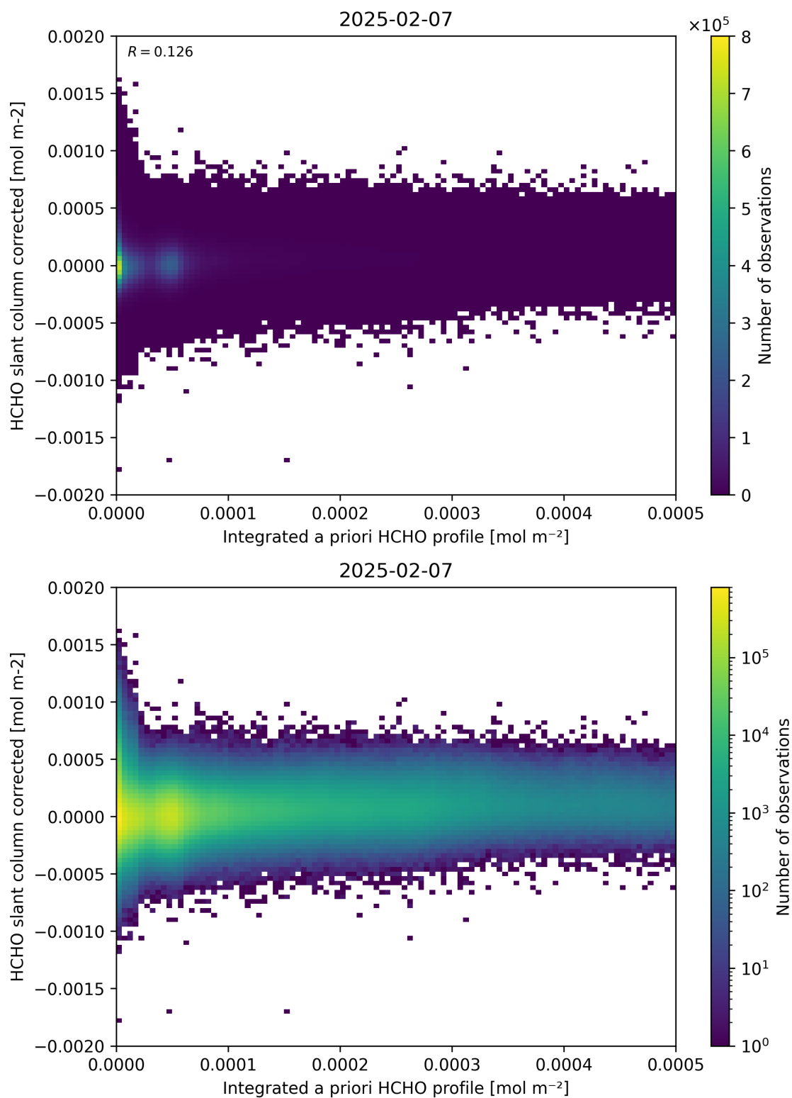
Figure 151: Scatter density plot of “Integrated a priori HCHO profile” against “HCHO slant column corrected” for 2025-02-06 to 2025-02-08.
