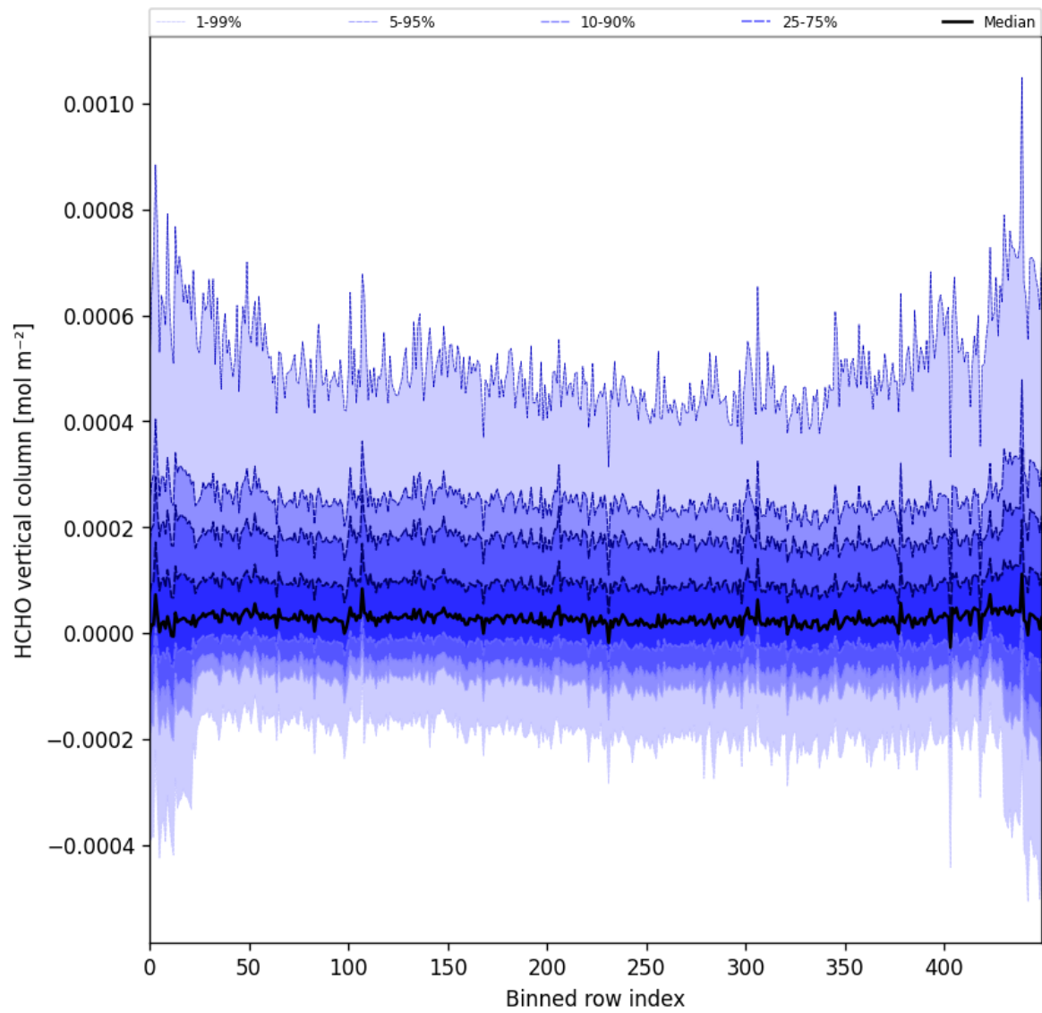
Figure 49: Along track statistics of “HCHO vertical column” for 2025-02-06 to 2025-02-08
