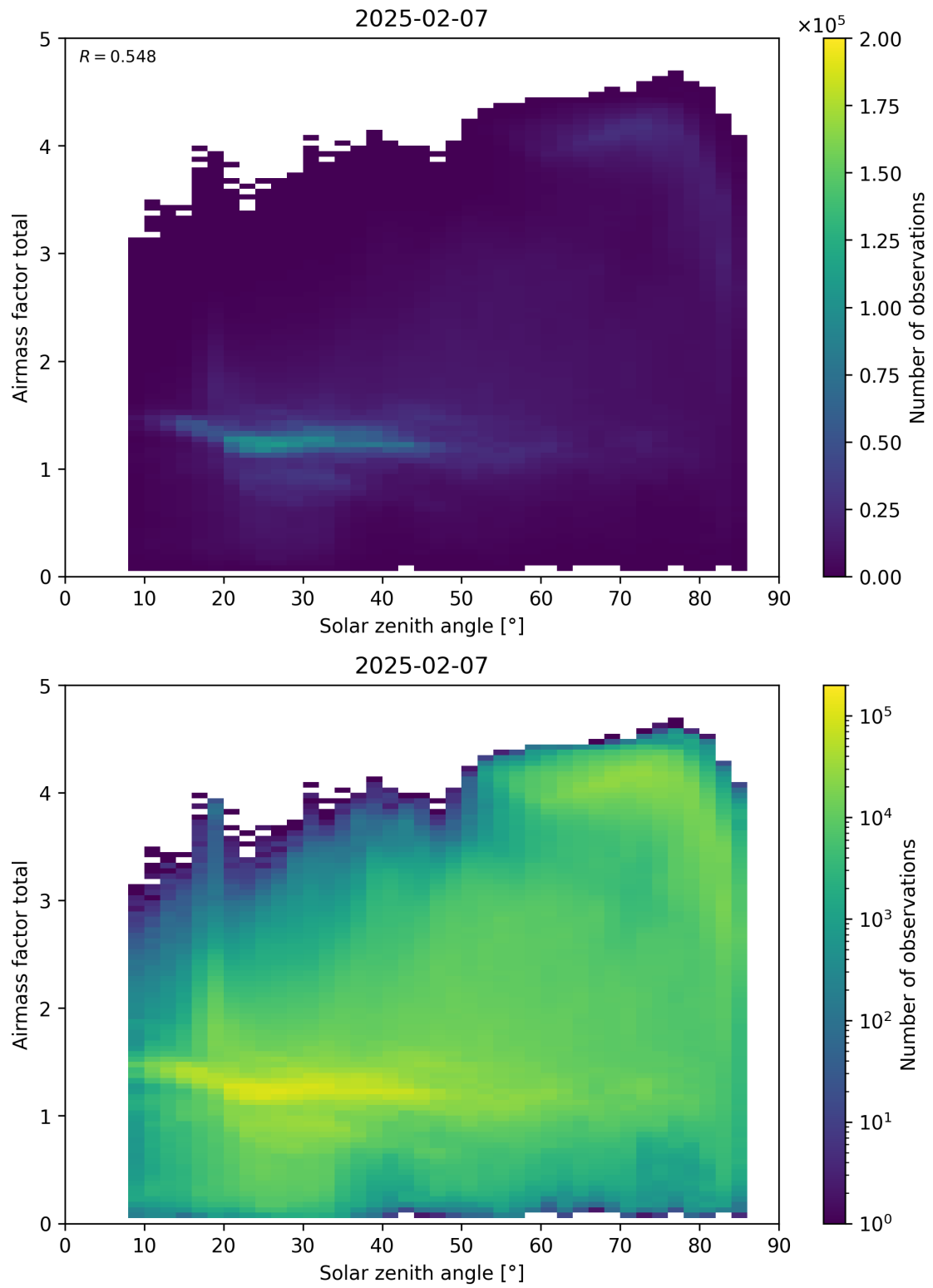
Figure 175: Scatter density plot of “Solar zenith angle” against “Airmass factor total” for 2025-02-06 to 2025-02-08.
