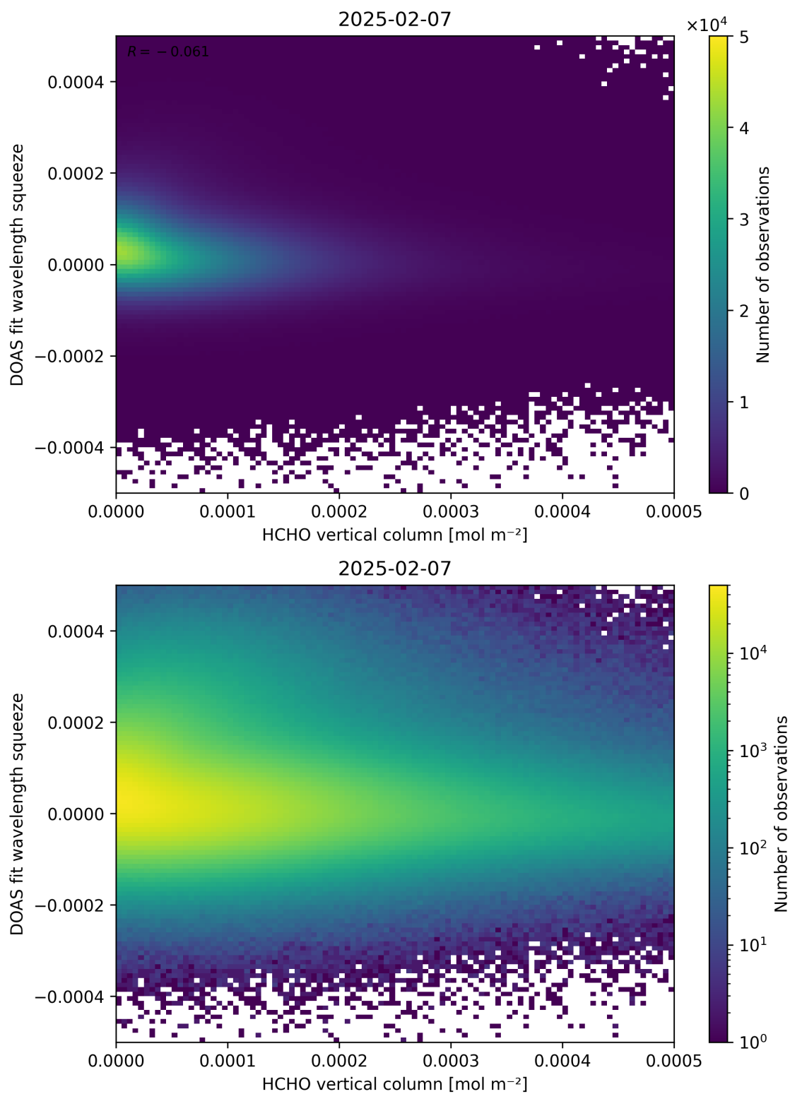
Figure 125: Scatter density plot of “HCHO vertical column” against “DOAS fit wavelength squeeze” for 2025-02-06 to 2025-02-08.
