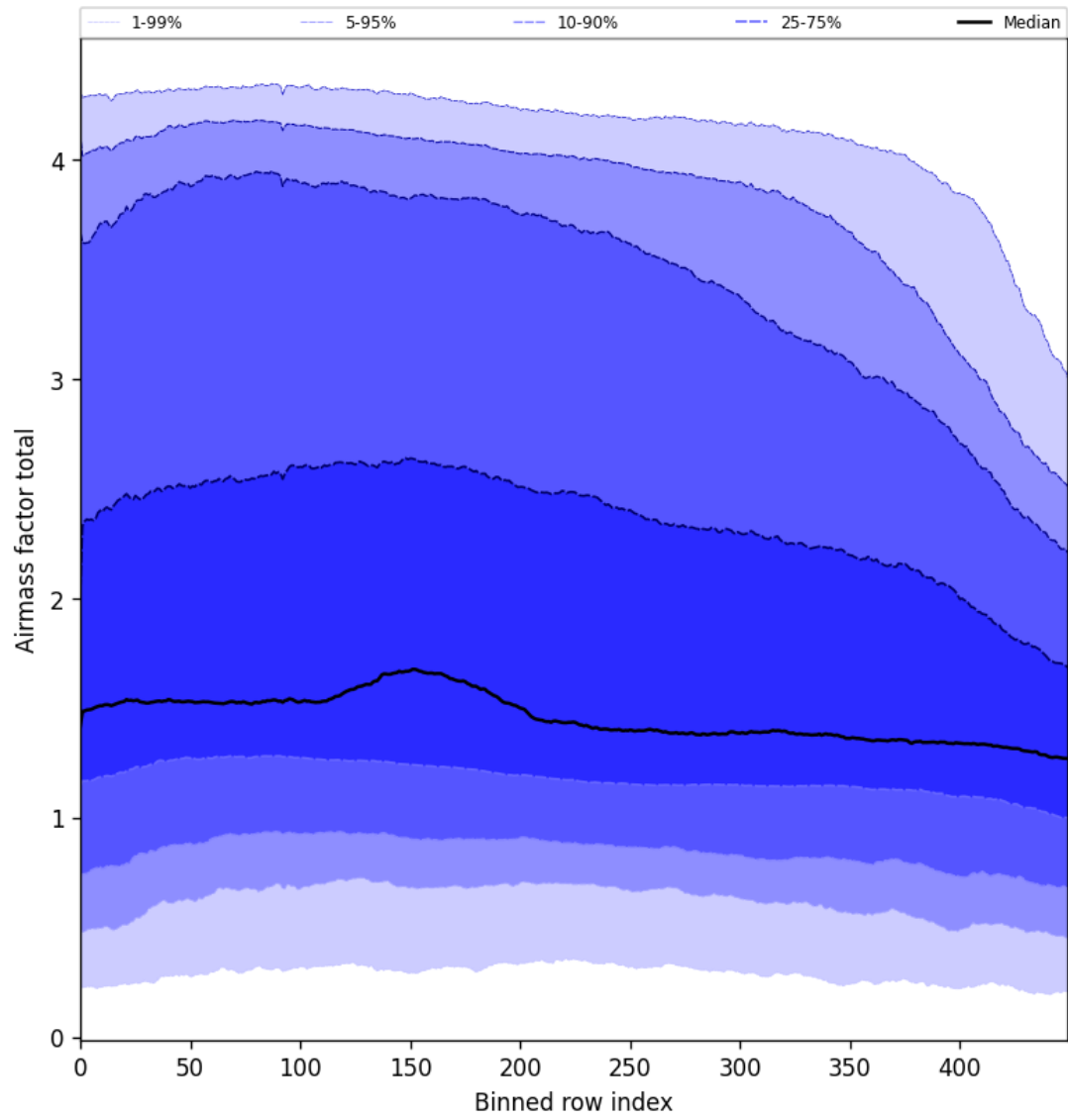
Figure 54: Along track statistics of “Airmass factor total” for 2025-02-06 to 2025-02-08
