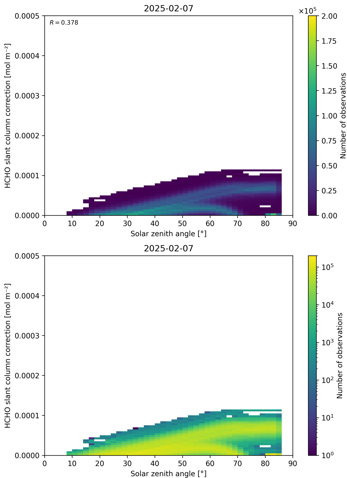
Figure 172: Scatter density plot of “Solar zenith angle” against “HCHO slant column correction” for 2025-02-06 to 2025-02-08.
