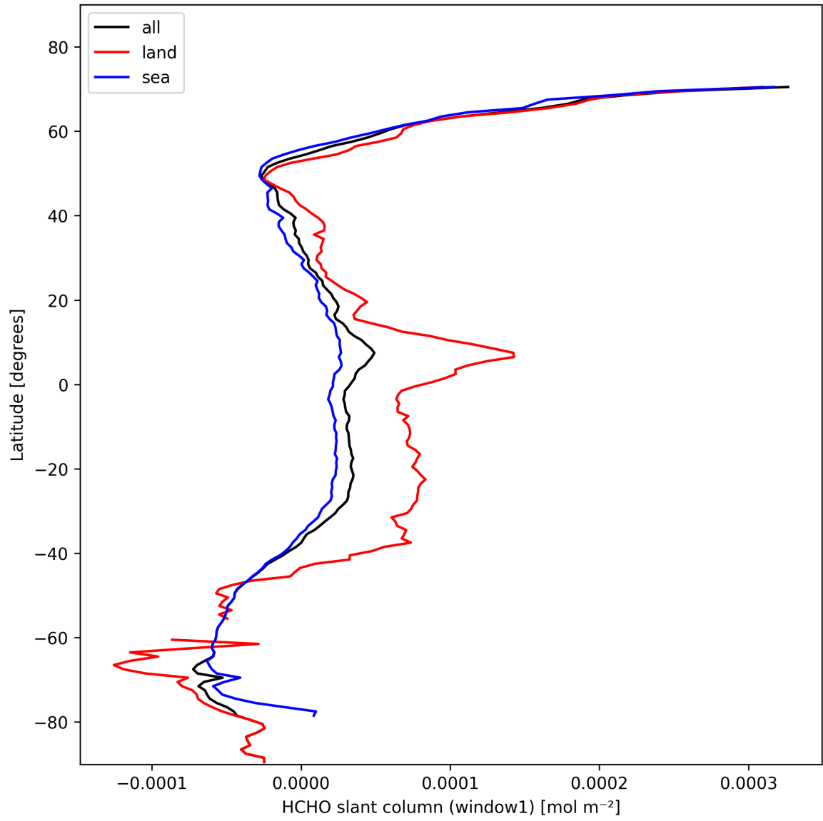
Figure 24: Zonal average of “HCHO slant column (window1)” for 2025-02-06 to 2025-02-08.
