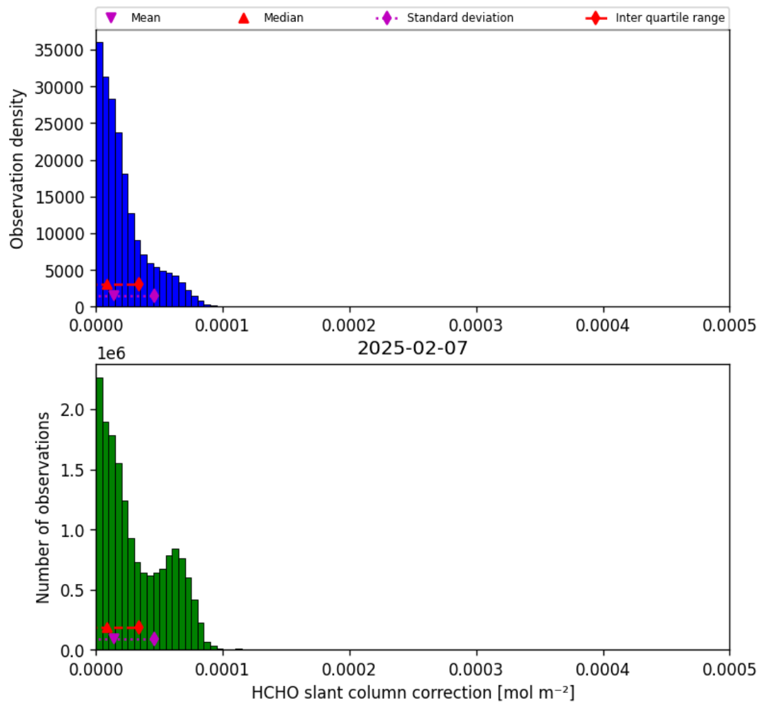
Figure 47: Histogram of “HCHO slant column correction” for 2025-02-06 to 2025-02-08
