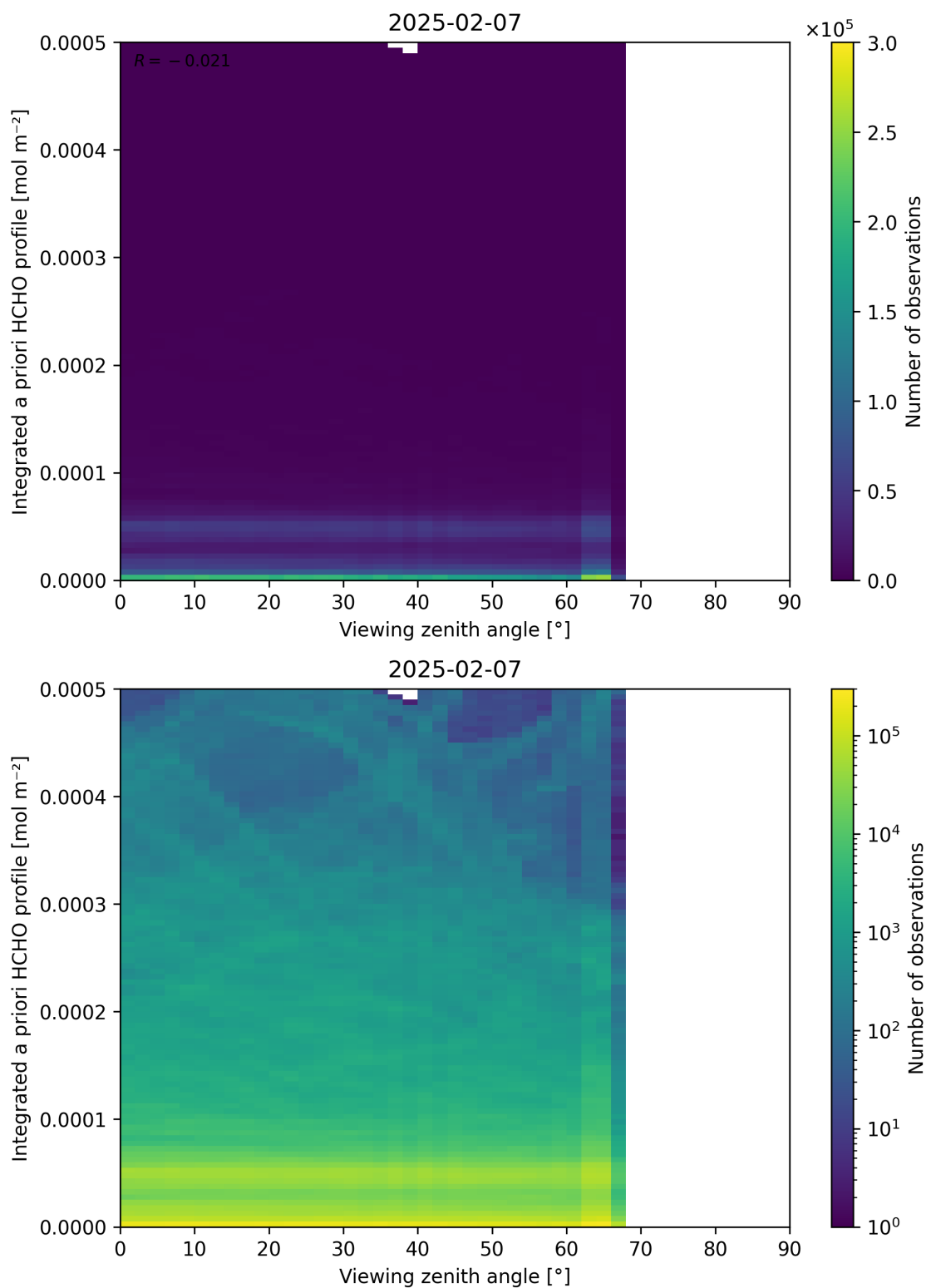
Figure 195: Scatter density plot of “Viewing zenith angle” against “Integrated a priori HCHO profile” for 2025-02-06 to 2025-02-08.
