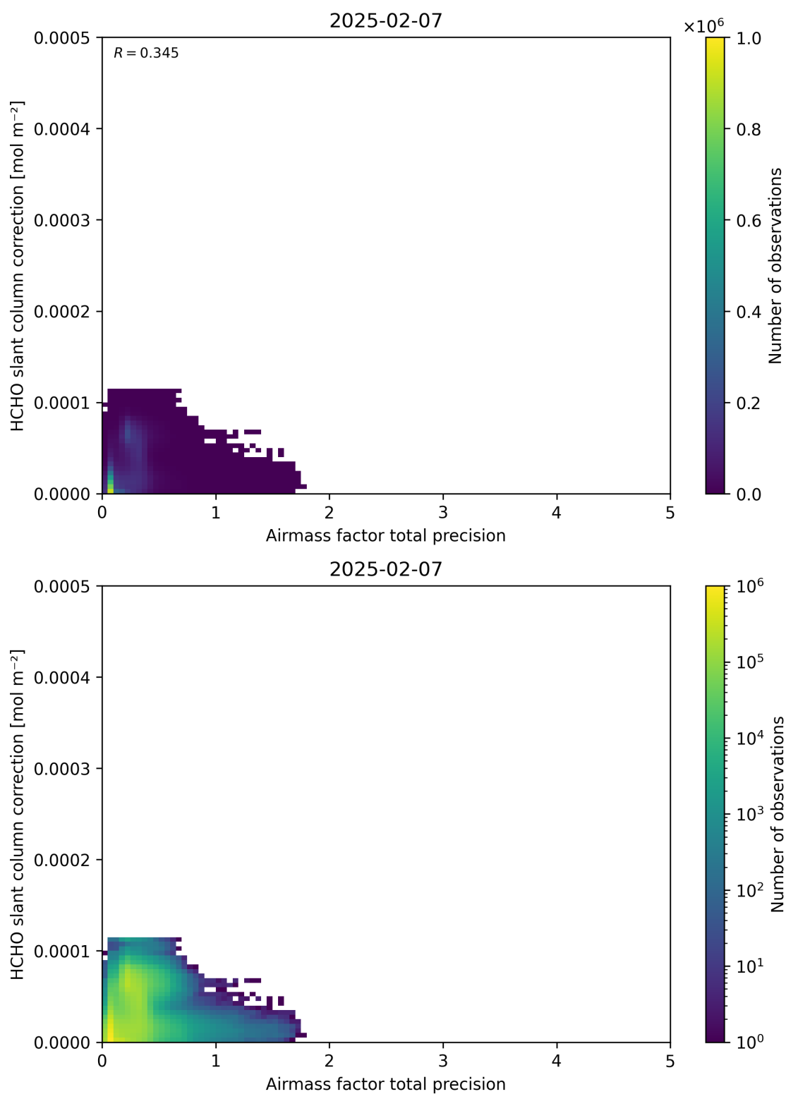
Figure 110: Scatter density plot of “Airmass factor total precision” against “HCHO slant column correction” for 2025-02-06 to 2025-02-08.
