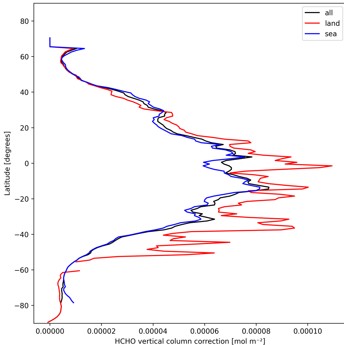
Figure 23: Zonal average of “HCHO vertical column correction” for 2025-02-06 to 2025-02-08.
