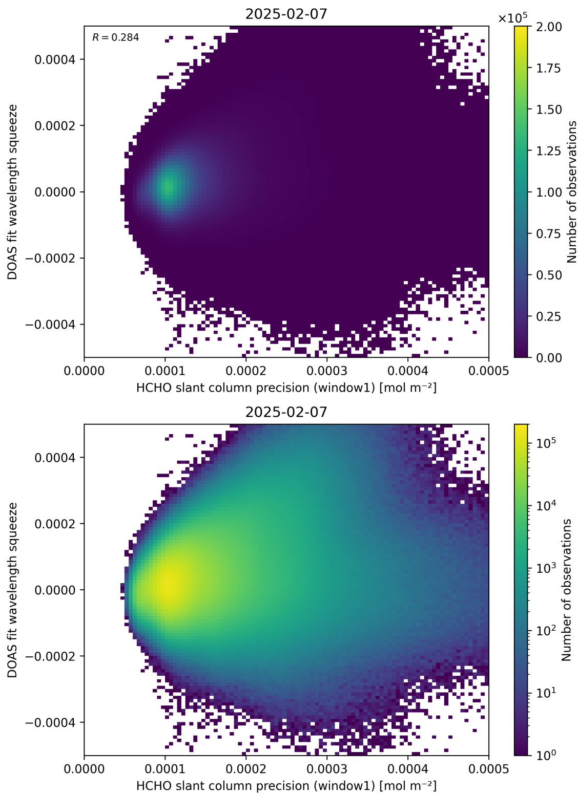
Figure 90: Scatter density plot of “HCHO slant column precision (window1)” against “DOAS fit wavelength squeeze” for 2025-02-06 to 2025-02-08.
