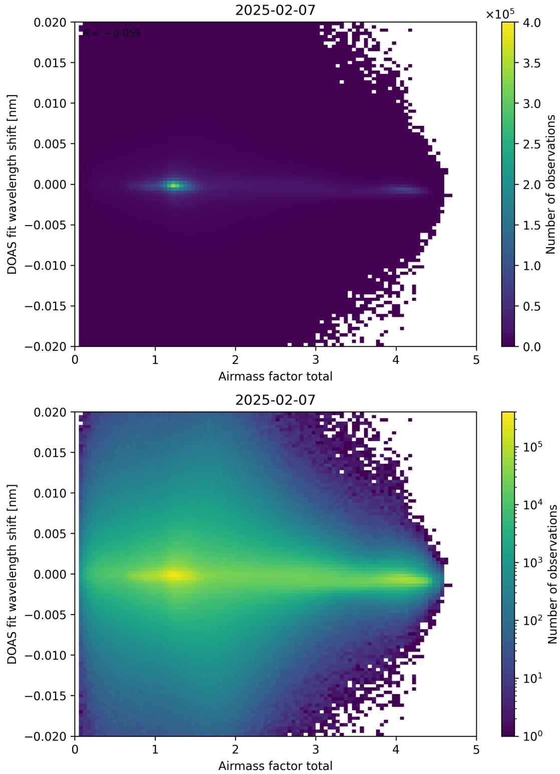
Figure 98: Scatter density plot of “Airmass factor total” against “DOAS fit wavelength shift” for 2025-02-06 to 2025-02-08.
