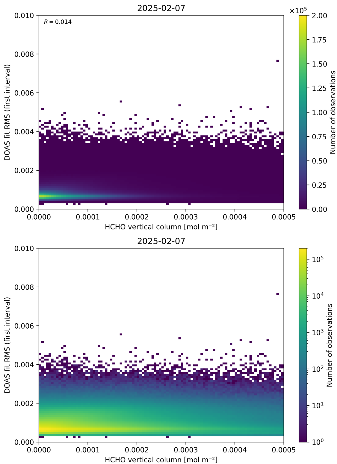
Figure 123: Scatter density plot of “HCHO vertical column” against “DOAS fit RMS (first interval)” for 2025-02-06 to 2025-02-08.
