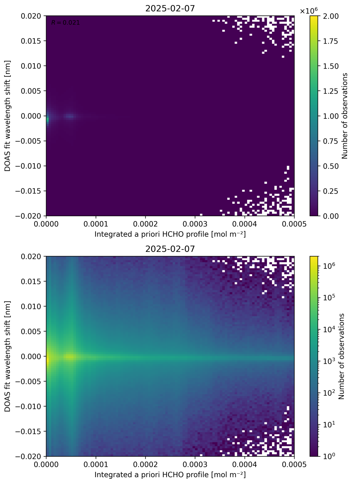
Figure 149: Scatter density plot of “Integrated a priori HCHO profile” against “DOAS fit wavelength shift” for 2025-02-06 to 2025-02-08.
