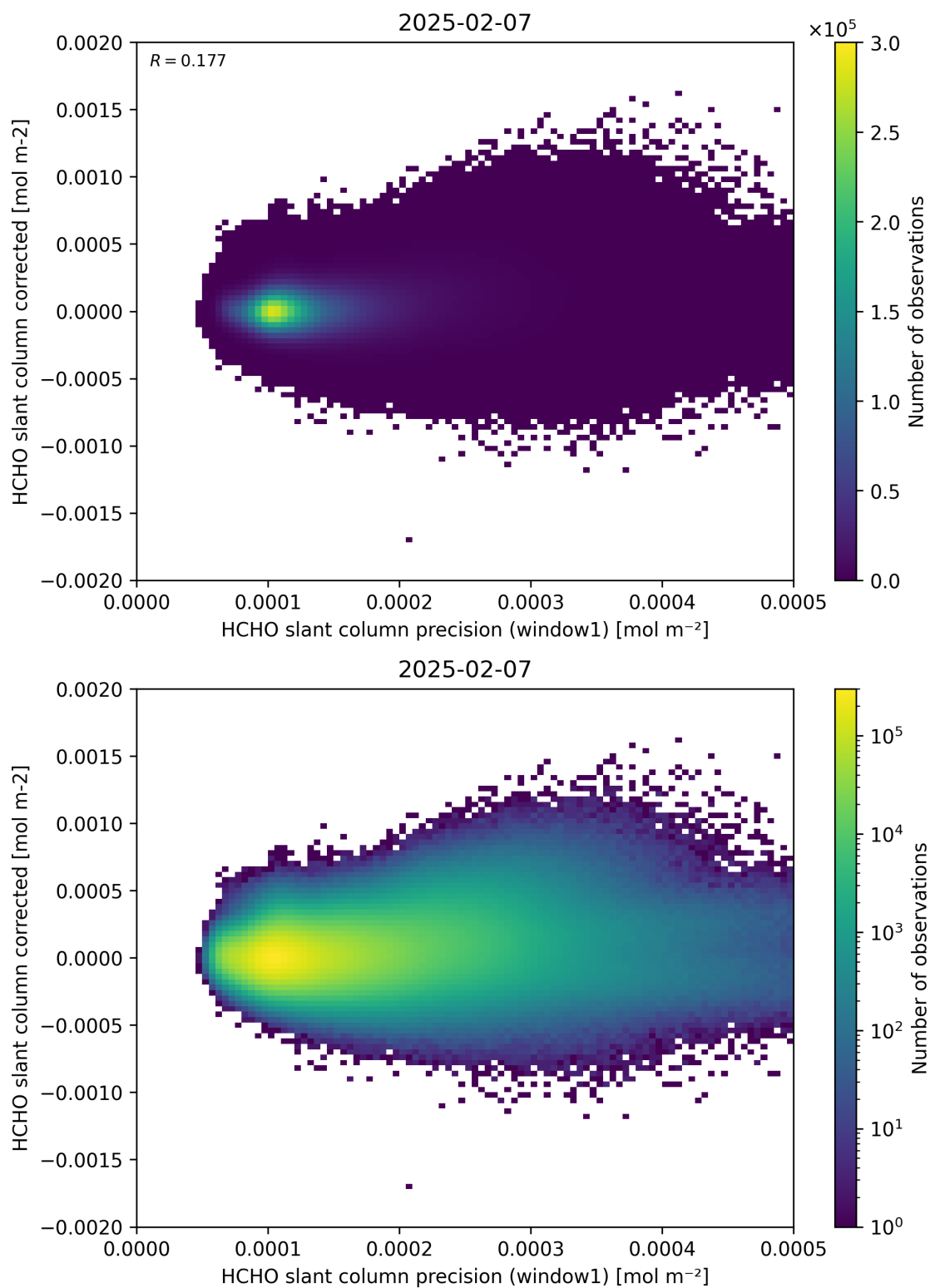
Figure 92: Scatter density plot of “HCHO slant column precision (window1)” against “HCHO slant column corrected” for 2025-02-06 to 2025-02-08.
