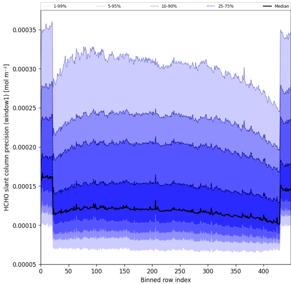
Figure 53: Along track statistics of “HCHO slant column precision (window1)” for 2025-02-06 to 2025-02-08
