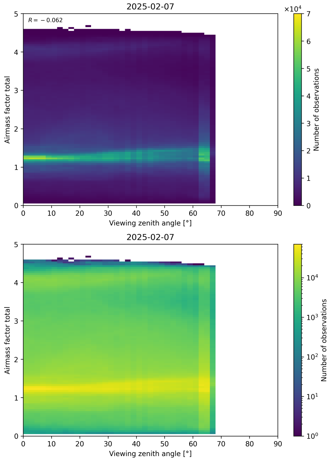
Figure 190: Scatter density plot of “Viewing zenith angle” against “Airmass factor total” for 2025-02-06 to 2025-02-08.
