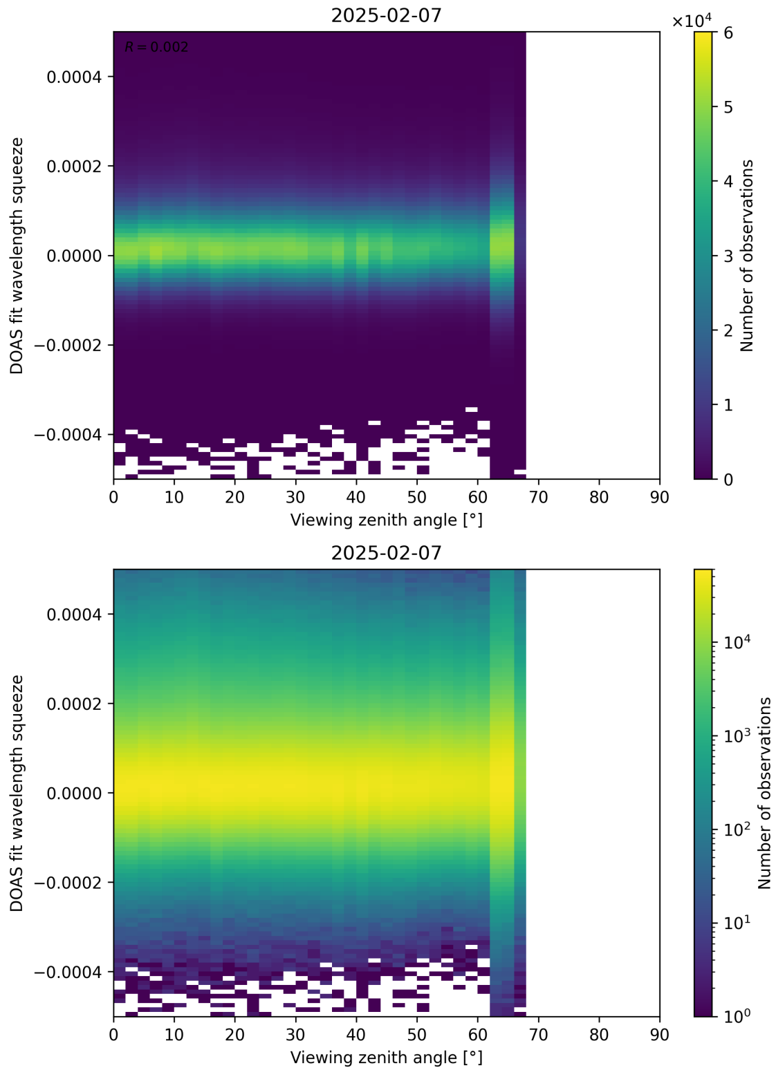
Figure 184: Scatter density plot of “Viewing zenith angle” against “DOAS fit wavelength squeeze” for 2025-02-06 to 2025-02-08.
