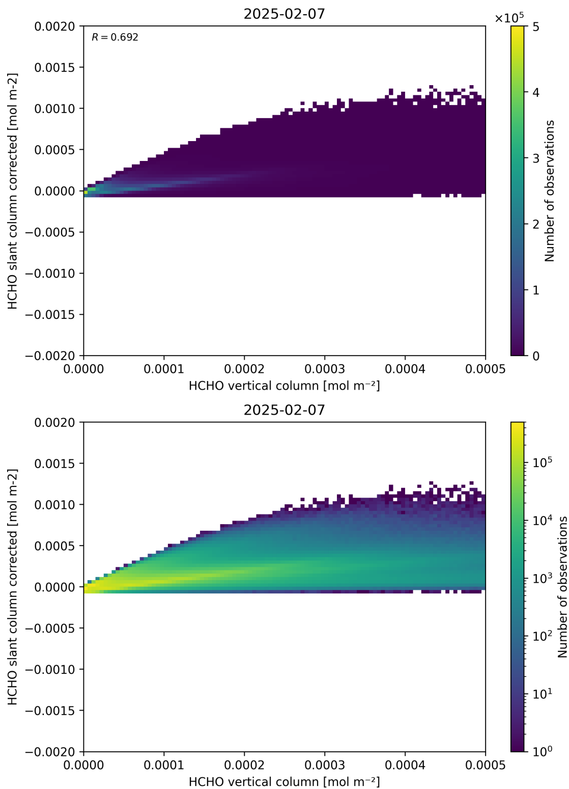
Figure 127: Scatter density plot of “HCHO vertical column” against “HCHO slant column corrected” for 2025-02-06 to 2025-02-08.
