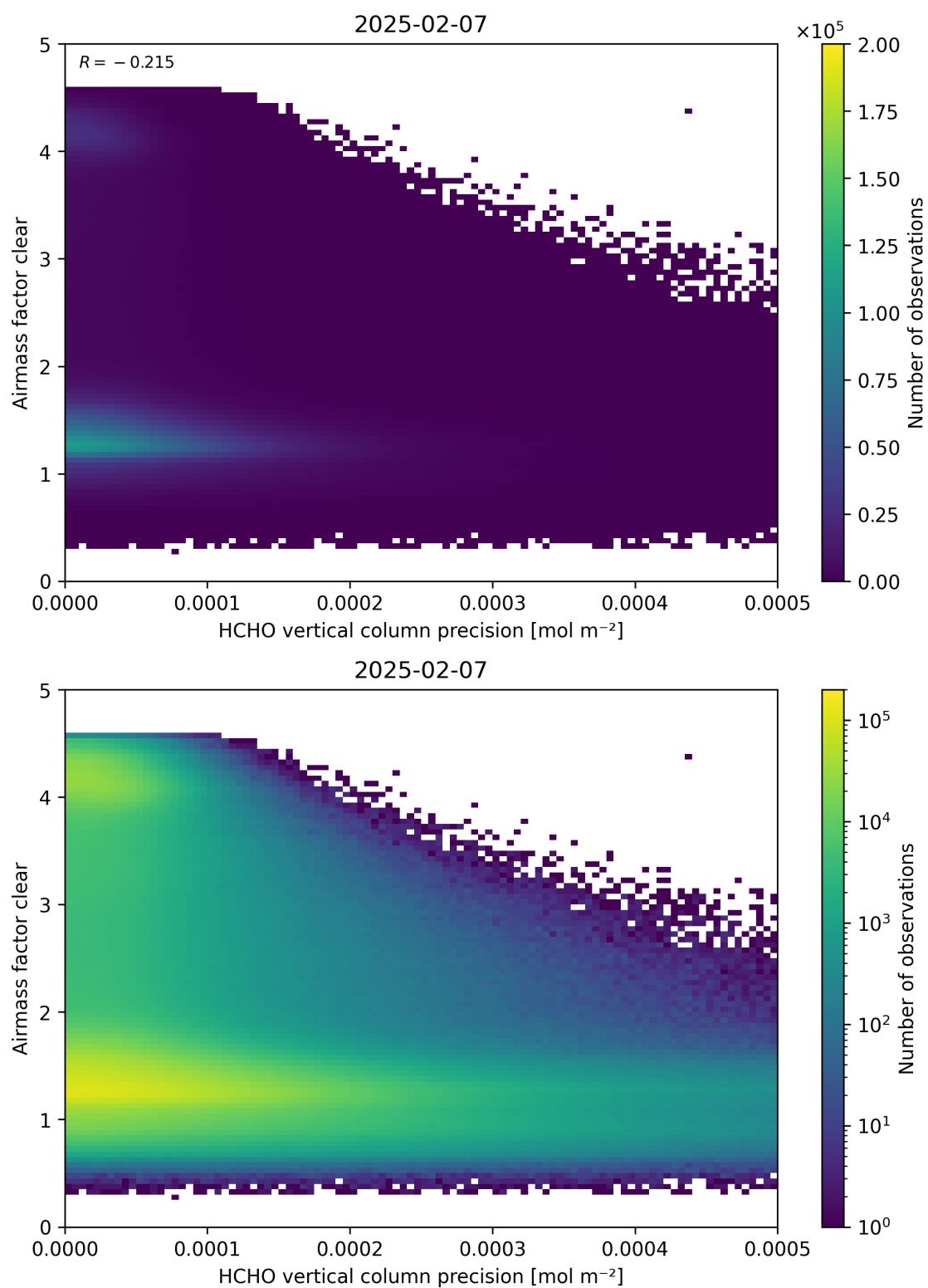
Figure 139: Scatter density plot of “HCHO vertical column precision” against “Airmass factor clear” for 2025-02-06 to 2025-02-08.
