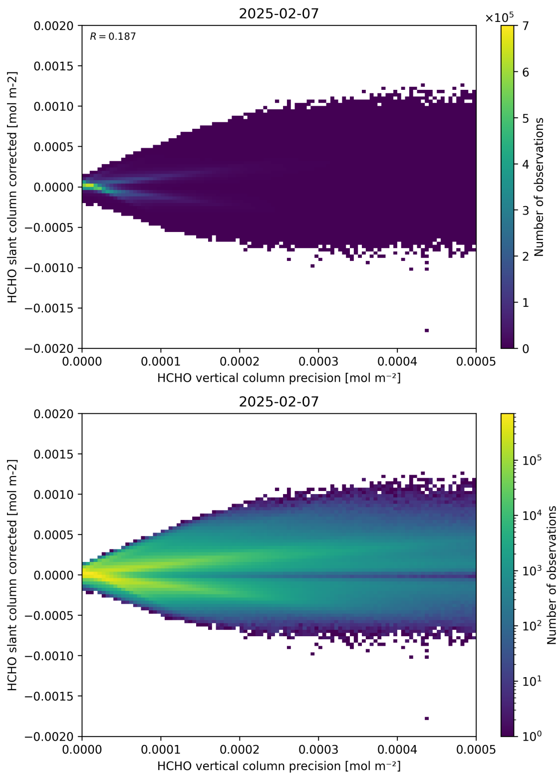
Figure 140: Scatter density plot of “HCHO vertical column precision” against “HCHO slant column corrected” for 2025-02-06 to 2025-02-08.
