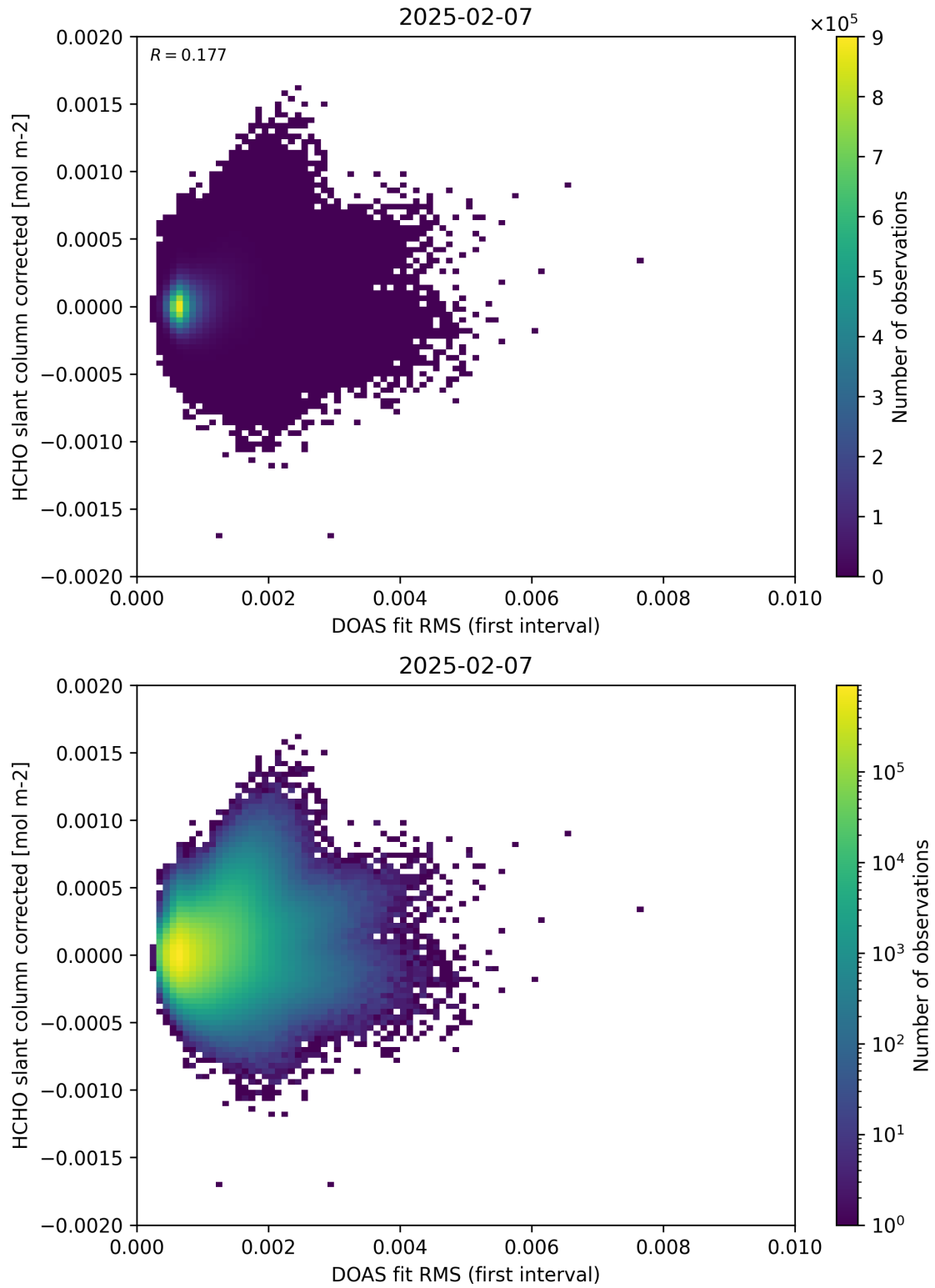
Figure 62: Scatter density plot of “DOAS fit RMS (first interval)” against “HCHO slant column corrected” for 2025-02-06 to 2025-02-08.
