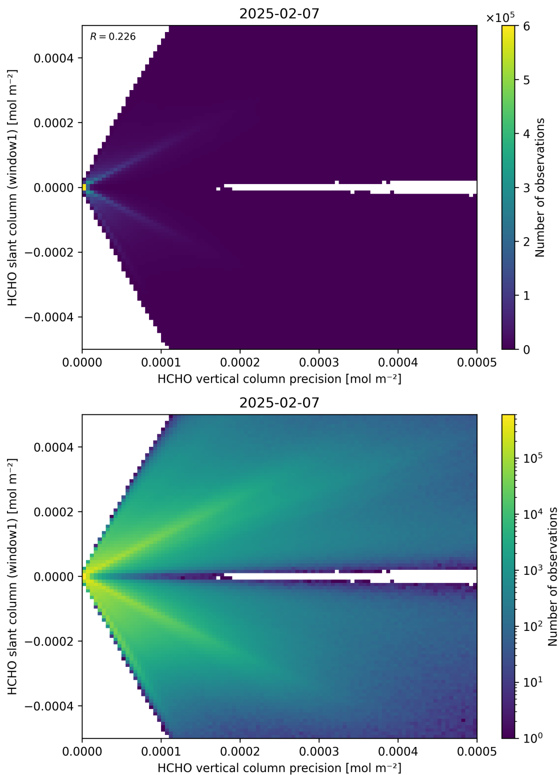
Figure 142: Scatter density plot of “HCHO vertical column precision” against “HCHO slant column (window1)” for 2025-02-06 to 2025-02-08.
