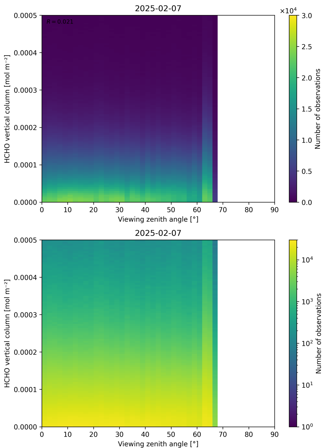
Figure 192: Scatter density plot of “Viewing zenith angle” against “HCHO vertical column” for 2025-02-06 to 2025-02-08.
