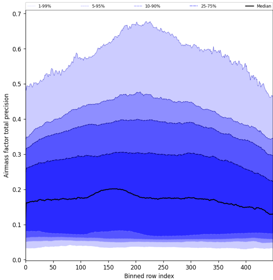
Figure 55: Along track statistics of “Airmass factor total precision” for 2025-02-06 to 2025-02-08
