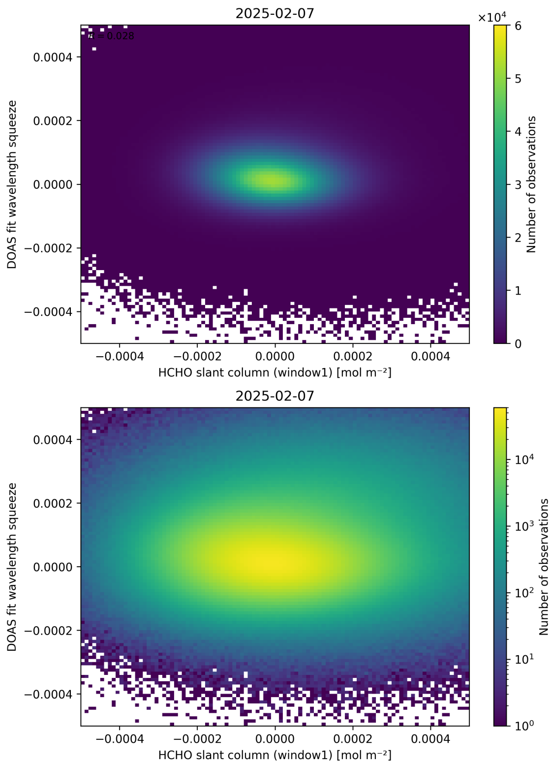
Figure 80: Scatter density plot of “HCHO slant column (window1)” against “DOAS fit wavelength squeeze” for 2025-02-06 to 2025-02-08.
