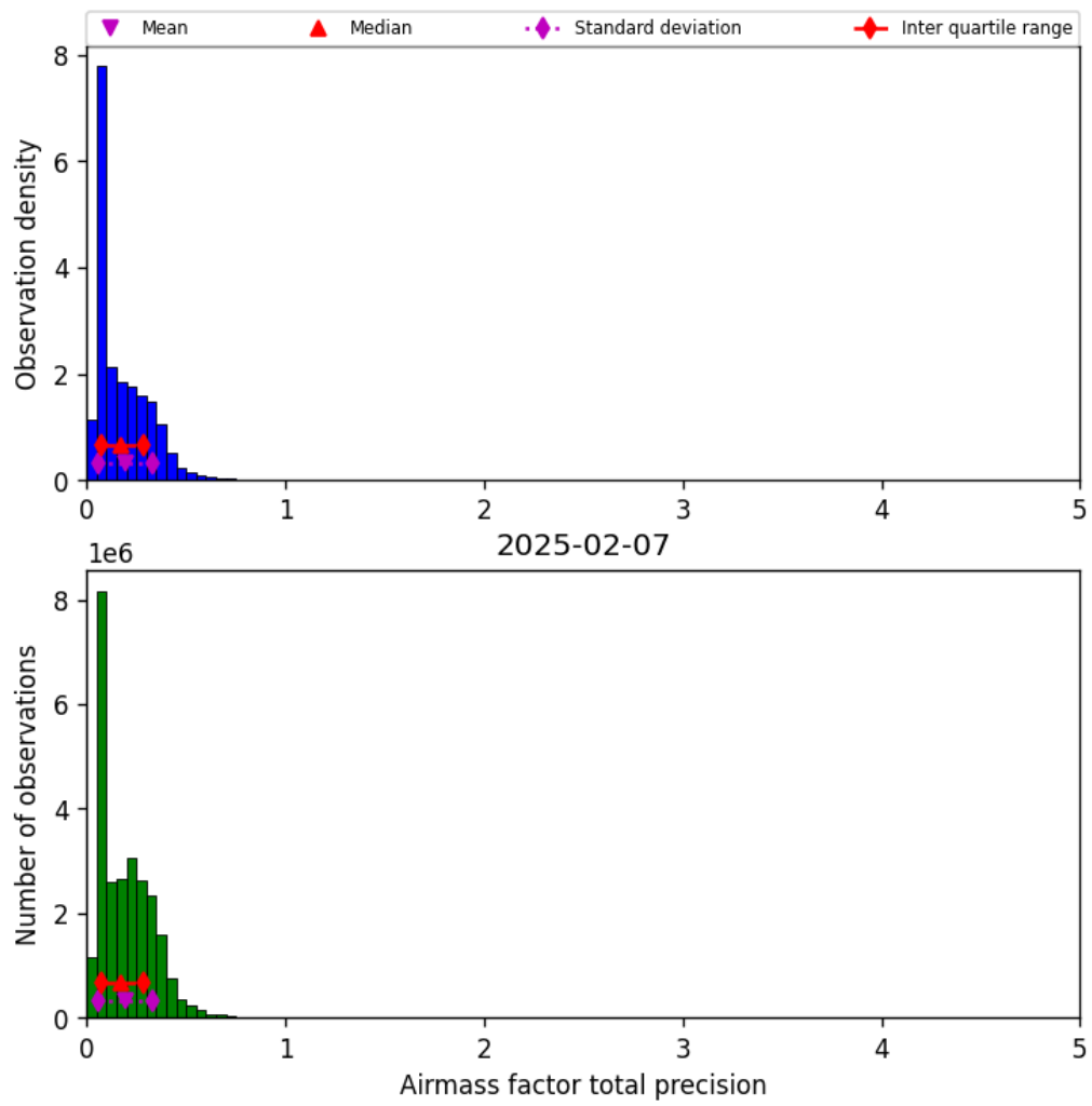
Figure 41: Histogram of “Airmass factor total precision” for 2025-02-06 to 2025-02-08
