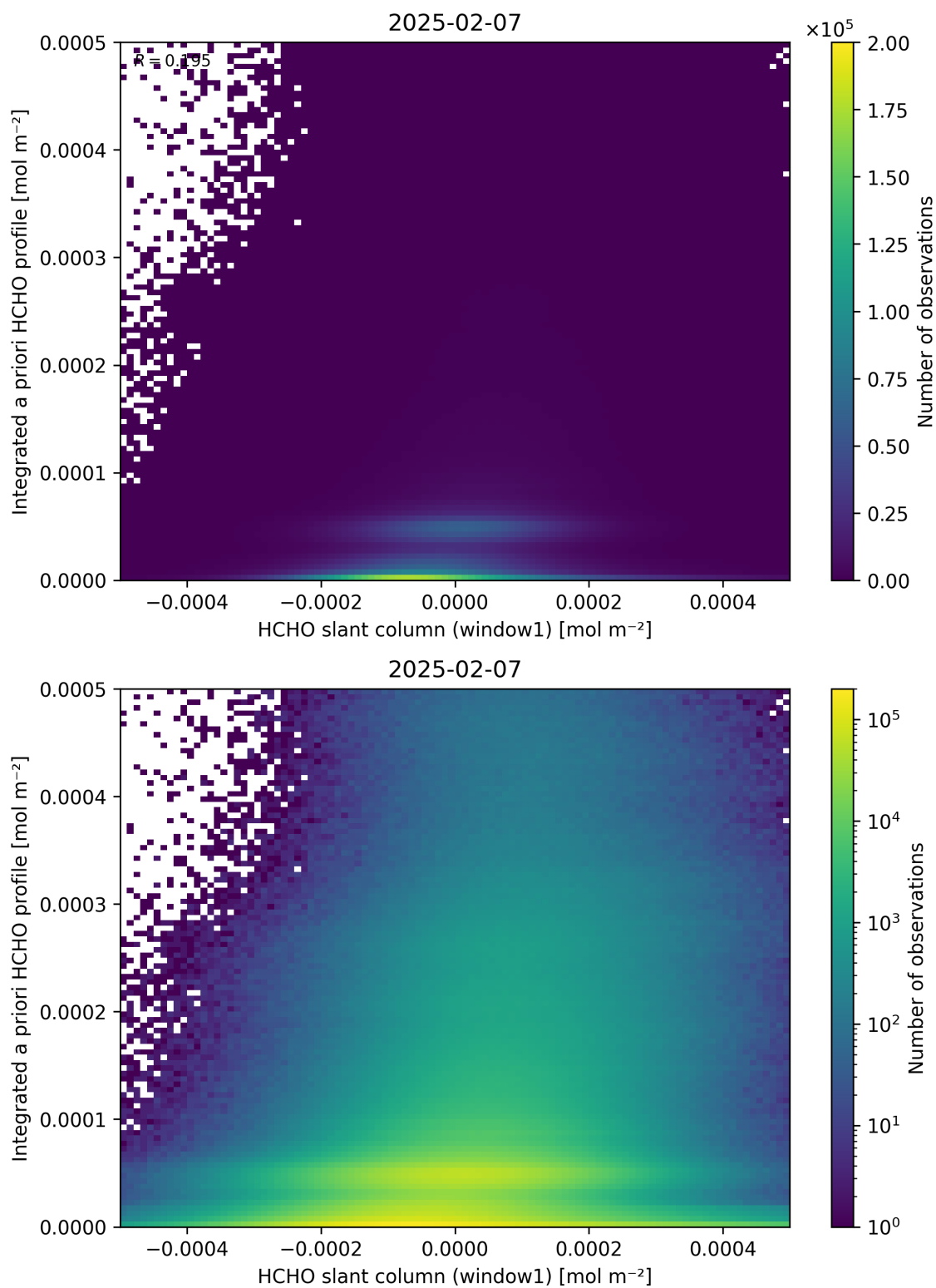
Figure 87: Scatter density plot of “HCHO slant column (window1)” against “Integrated a priori HCHO profile” for 2025-02-06 to 2025-02-08.
