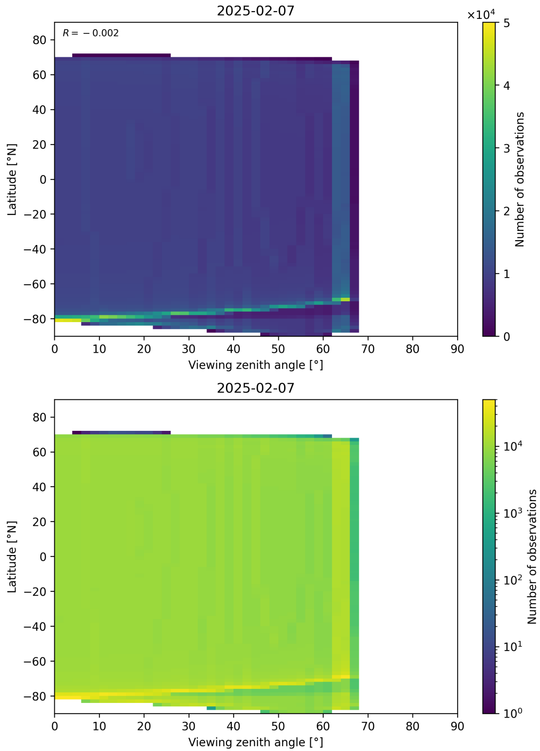
Figure 196: Scatter density plot of “Viewing zenith angle” against “Latitude” for 2025-02-06 to 2025-02-08.
