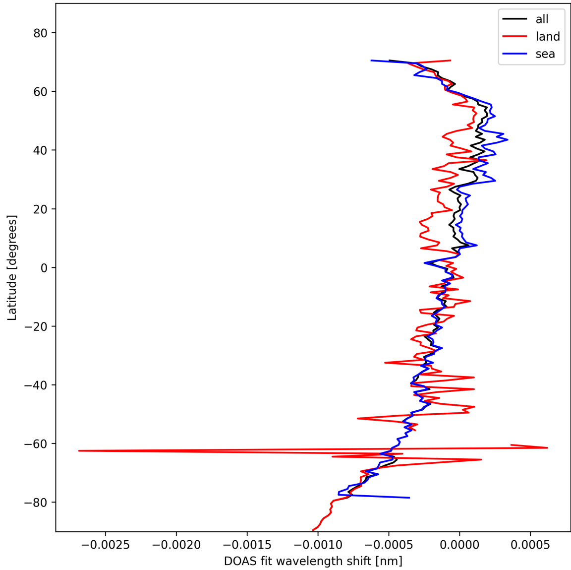
Figure 30: Zonal average of “DOAS fit wavelength shift” for 2025-02-06 to 2025-02-08.
