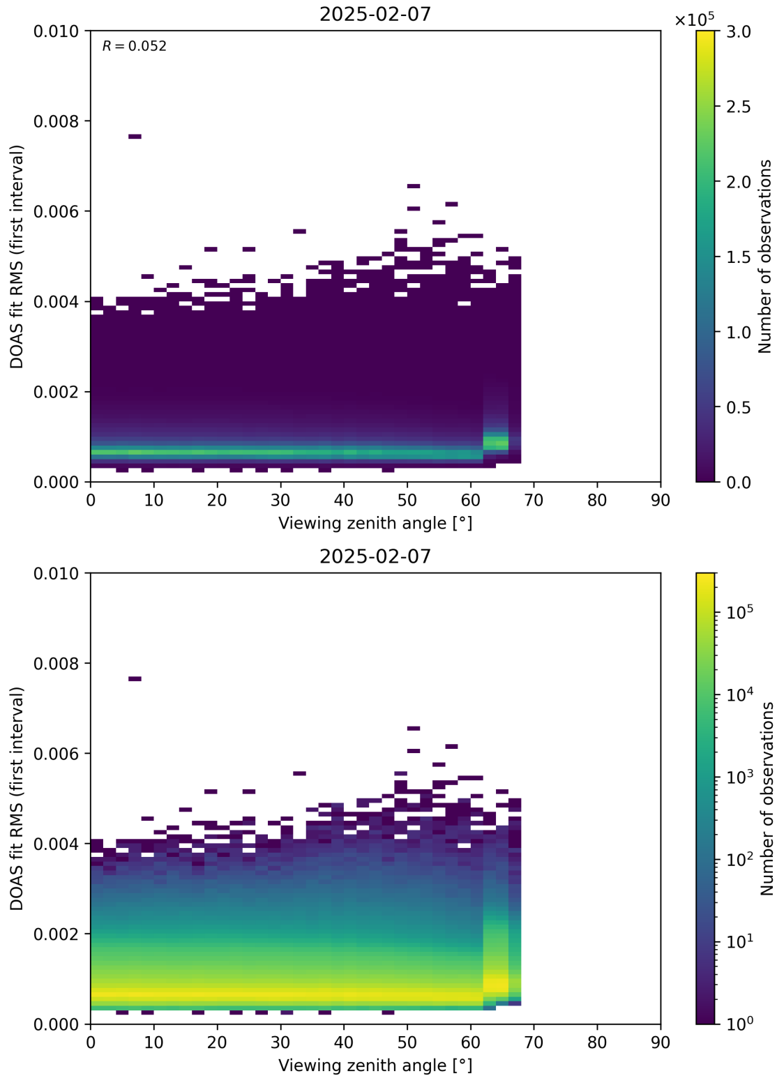
Figure 182: Scatter density plot of “Viewing zenith angle” against “DOAS fit RMS (first interval)” for 2025-02-06 to 2025-02-08.
