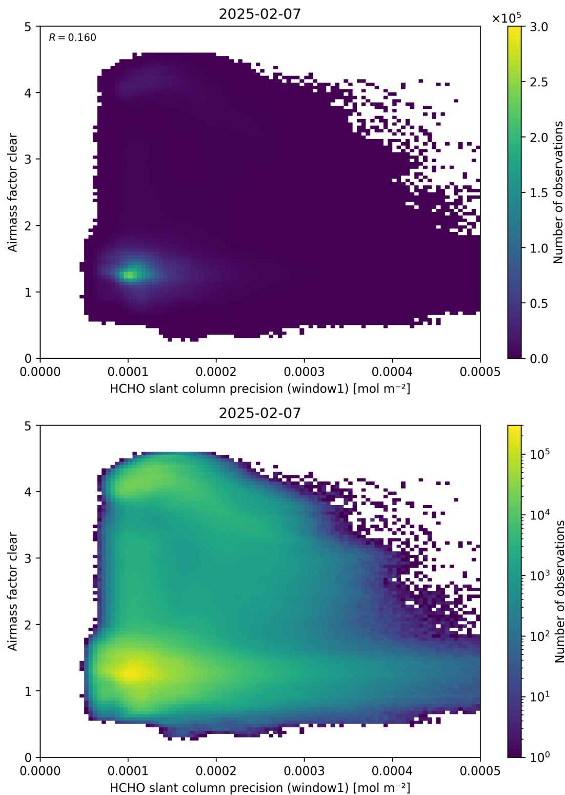
Figure 91: Scatter density plot of “HCHO slant column precision (window1)” against “Airmass factor clear” for 2025-02-06 to 2025-02-08.
