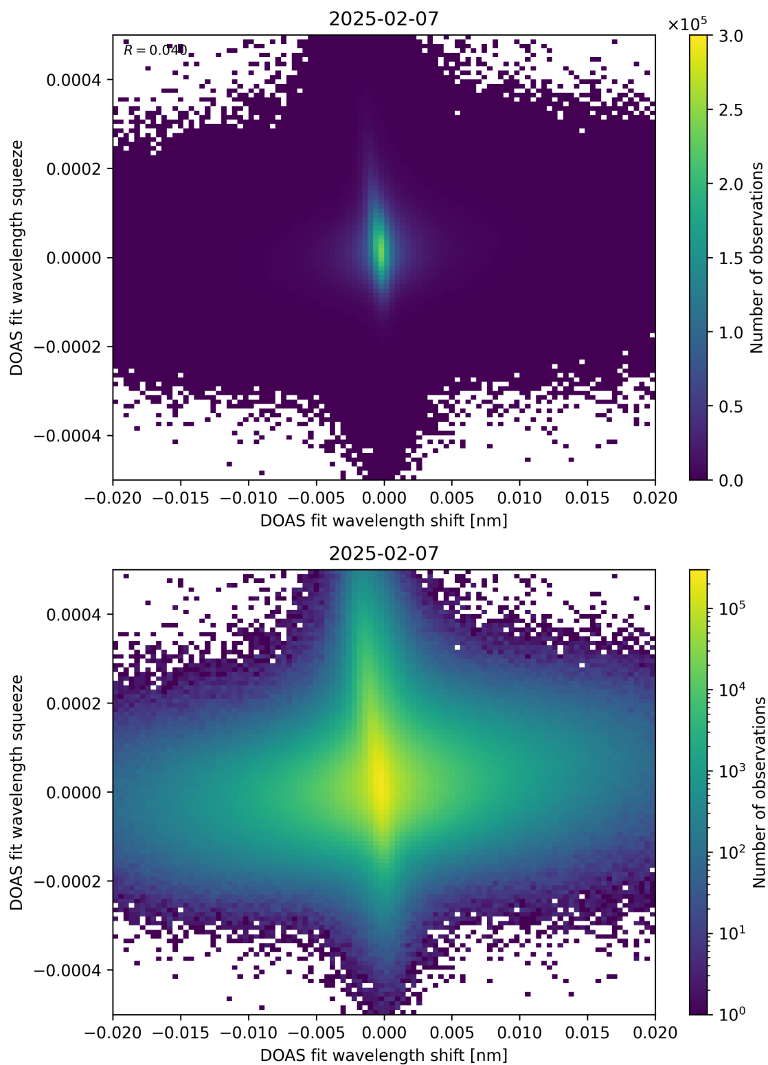
Figure 65: Scatter density plot of “DOAS fit wavelength shift” against “DOAS fit wavelength squeeze” for 2025-02-06 to 2025-02-08.
