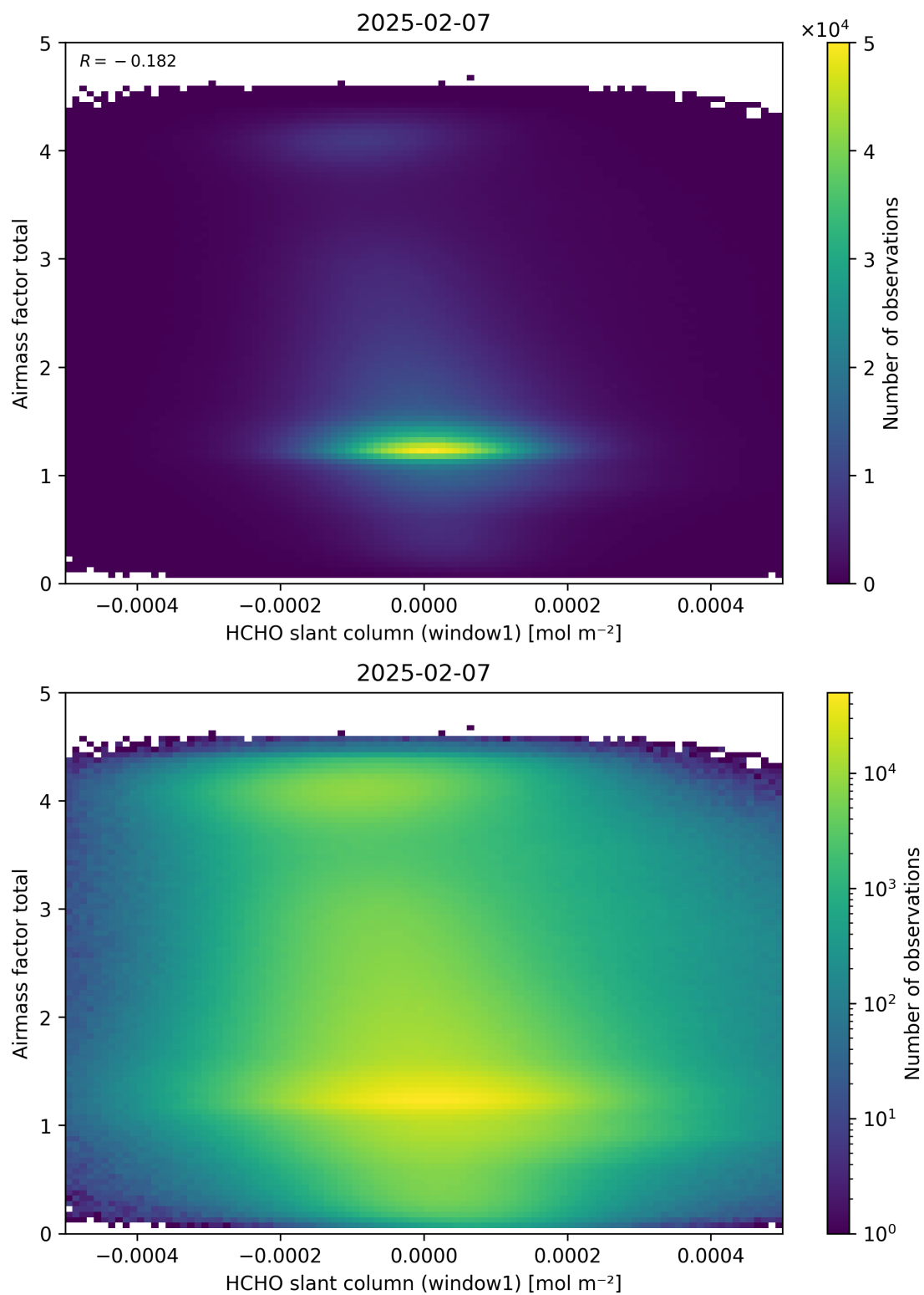
Figure 85: Scatter density plot of “HCHO slant column (window1)” against “Airmass factor total” for 2025-02-06 to 2025-02-08.
