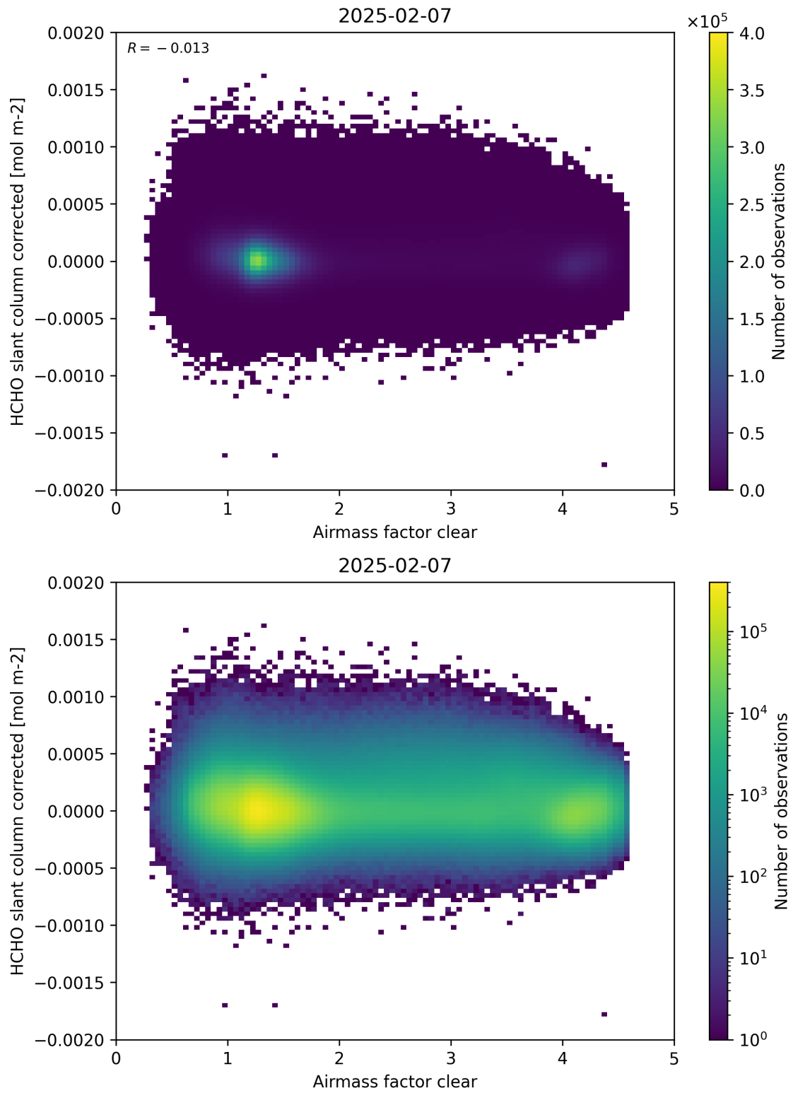
Figure 74: Scatter density plot of “Airmass factor clear” against “HCHO slant column corrected” for 2025-02-06 to 2025-02-08.
