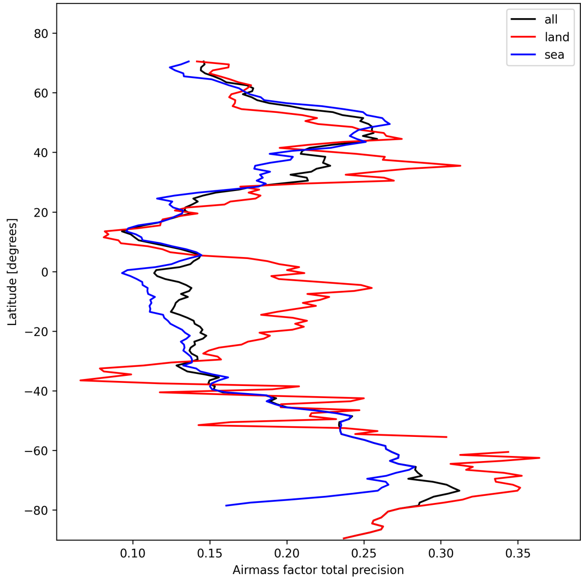
Figure 27: Zonal average of “Airmass factor total precision” for 2025-02-06 to 2025-02-08.
