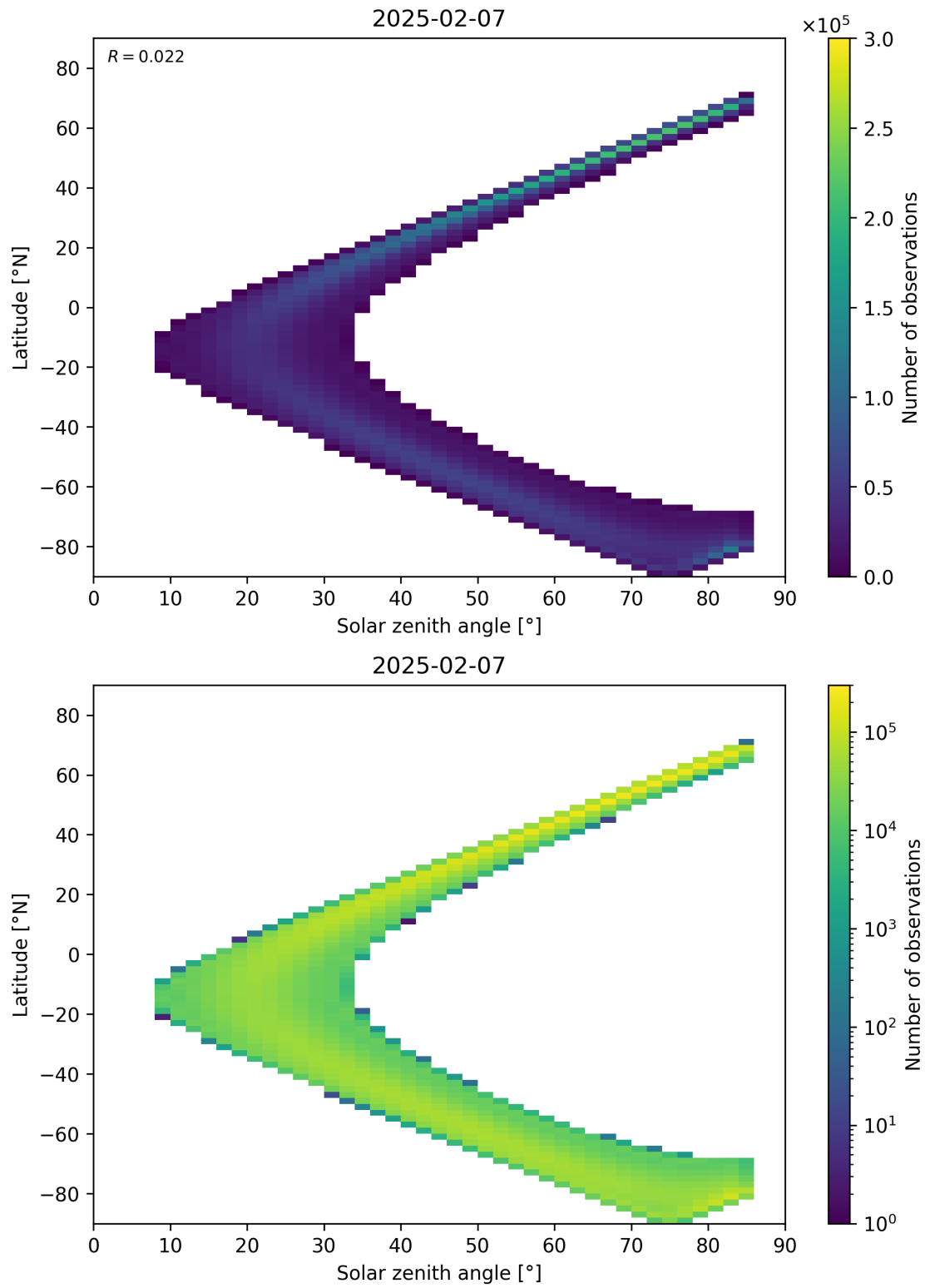
Figure 181: Scatter density plot of “Solar zenith angle” against “Latitude” for 2025-02-06 to 2025-02-08.
