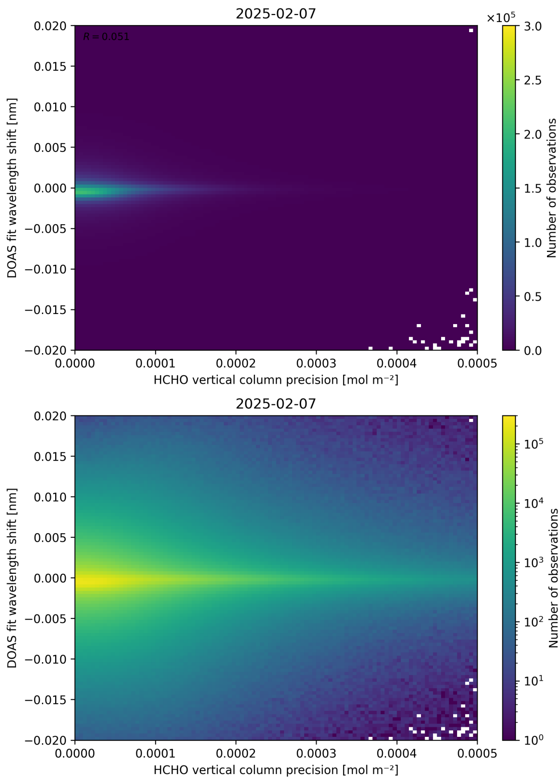
Figure 137: Scatter density plot of “HCHO vertical column precision” against “DOAS fit wavelength shift” for 2025-02-06 to 2025-02-08.
