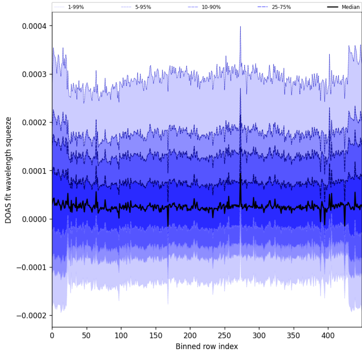
Figure 59: Along track statistics of “DOAS fit wavelength squeeze” for 2025-02-06 to 2025-02-08
