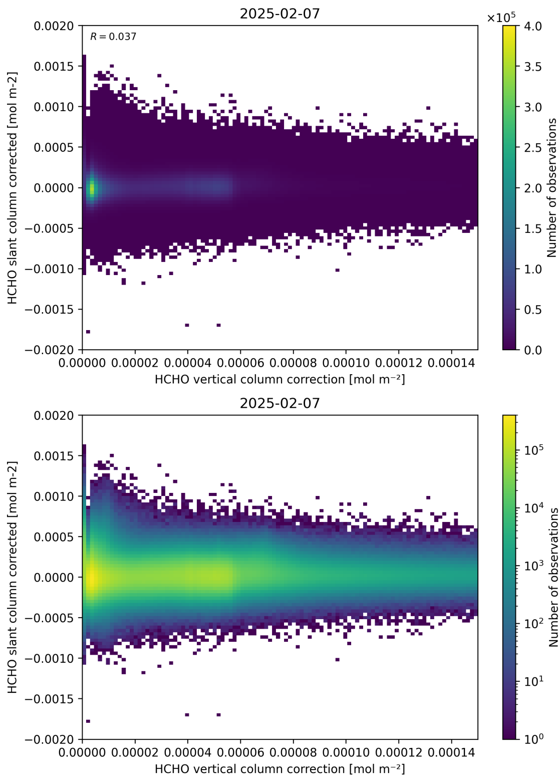
Figure 116: Scatter density plot of “HCHO vertical column correction” against “HCHO slant column corrected” for 2025-02-06 to 2025-02-08.
