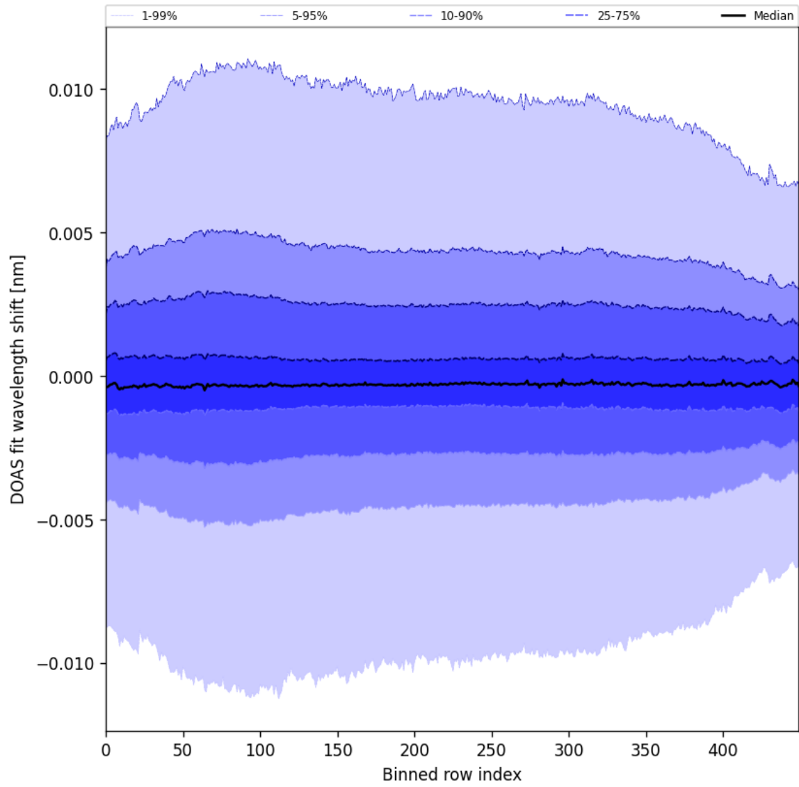
Figure 58: Along track statistics of “DOAS fit wavelength shift” for 2025-02-06 to 2025-02-08
