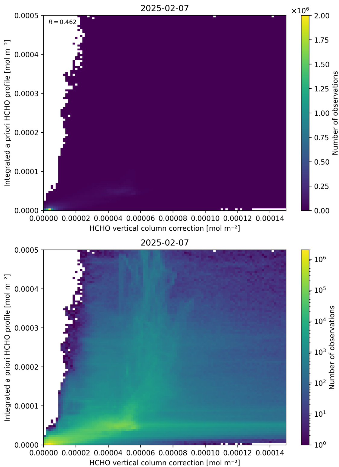
Figure 122: Scatter density plot of “HCHO vertical column correction” against “Integrated a priori HCHO profile” for 2025-02-06 to 2025-02-08.
