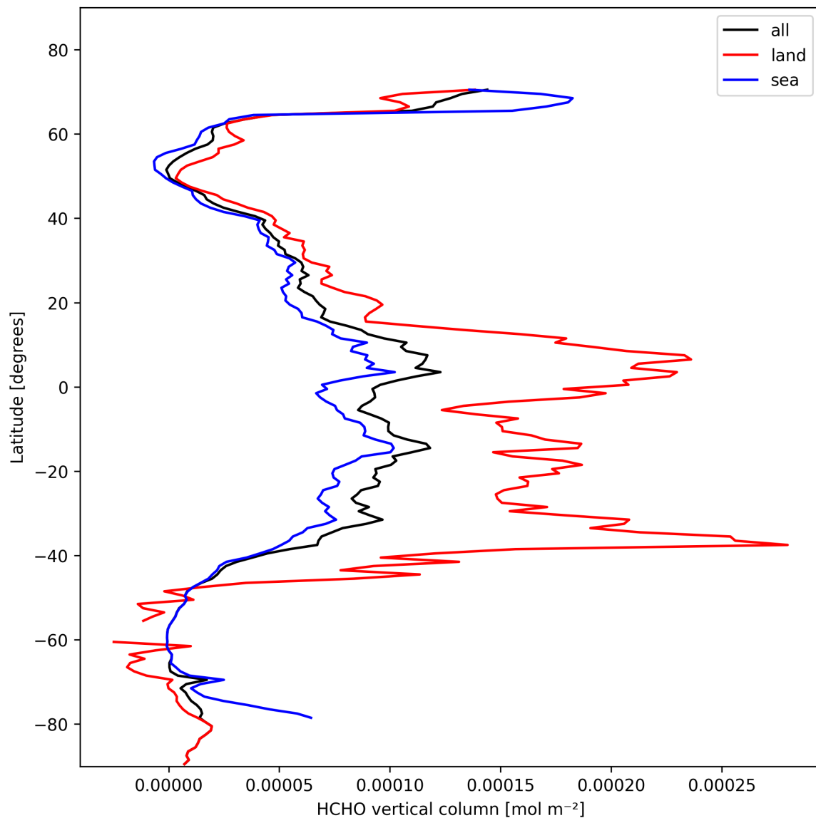
Figure 21: Zonal average of “HCHO vertical column” for 2025-02-06 to 2025-02-08.
