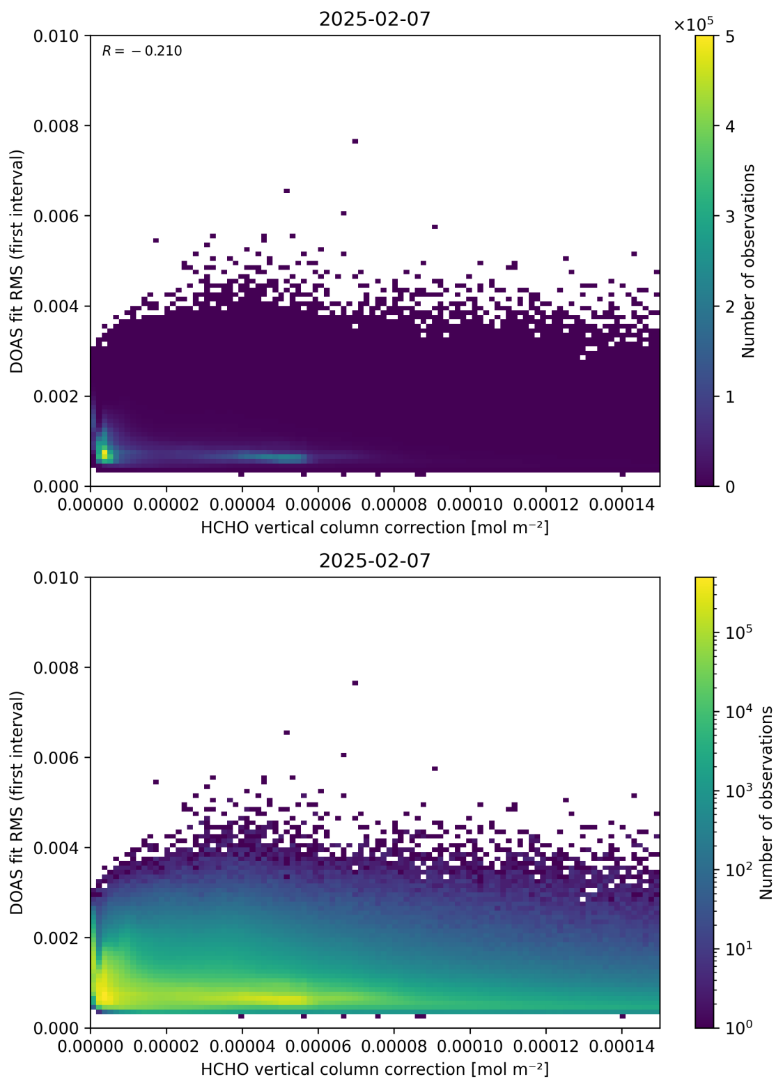
Figure 112: Scatter density plot of “HCHO vertical column correction” against “DOAS fit RMS (first interval)” for 2025-02-06 to 2025-02-08.
