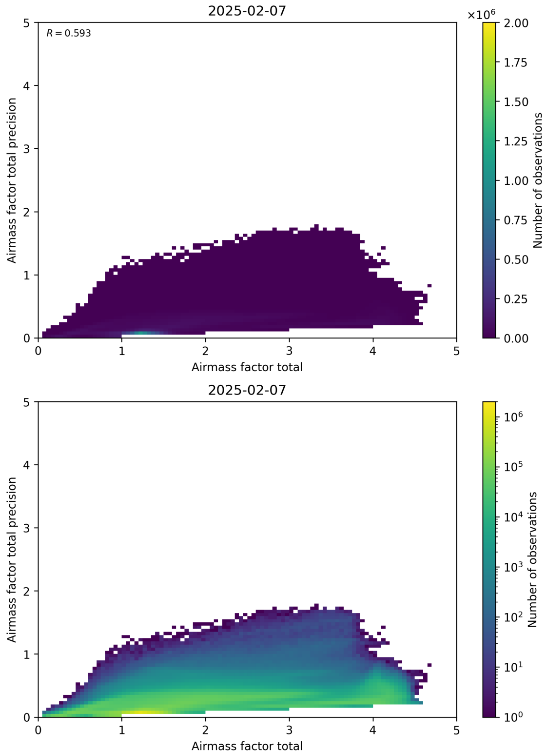
Figure 103: Scatter density plot of “Airmass factor total” against “Airmass factor total precision” for 2025-02-06 to 2025-02-08.
