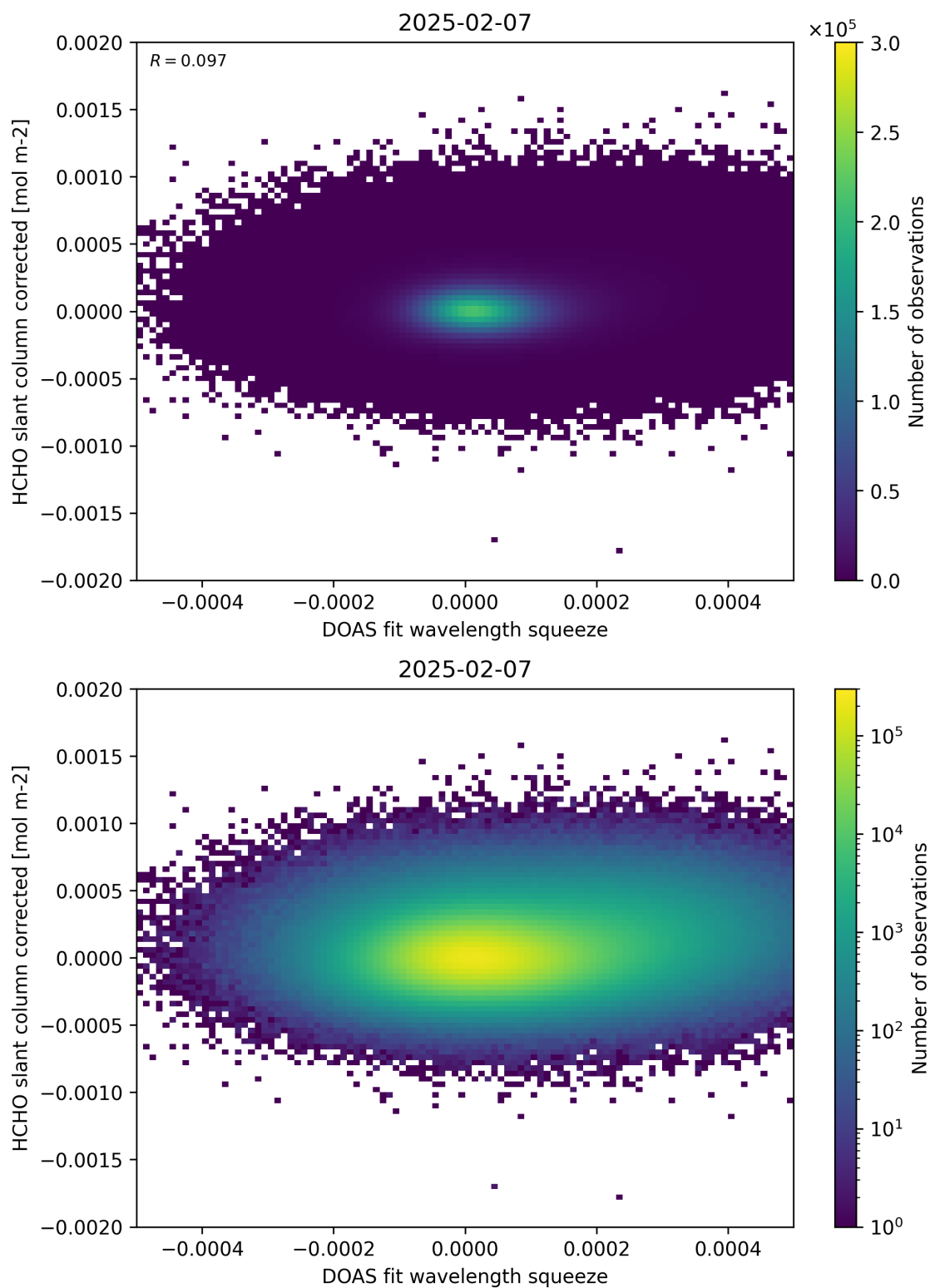
Figure 69: Scatter density plot of “DOAS fit wavelength squeeze” against “HCHO slant column corrected” for 2025-02-06 to 2025-02-08.
