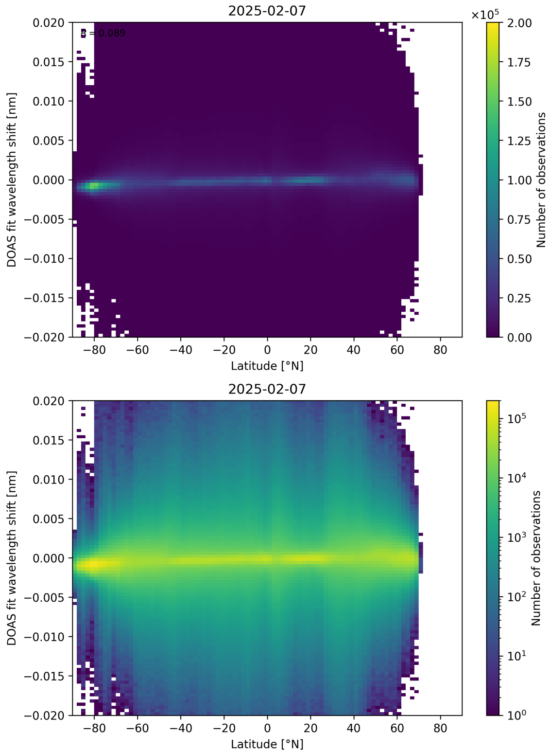
Figure 154: Scatter density plot of “Latitude” against “DOAS fit wavelength shift” for 2025-02-06 to 2025-02-08.
