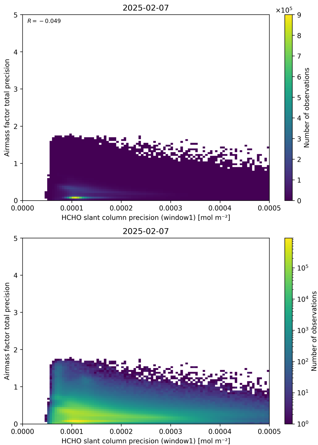
Figure 95: Scatter density plot of “HCHO slant column precision (window1)” against “Airmass factor total precision” for 2025-02-06 to 2025-02-08.
