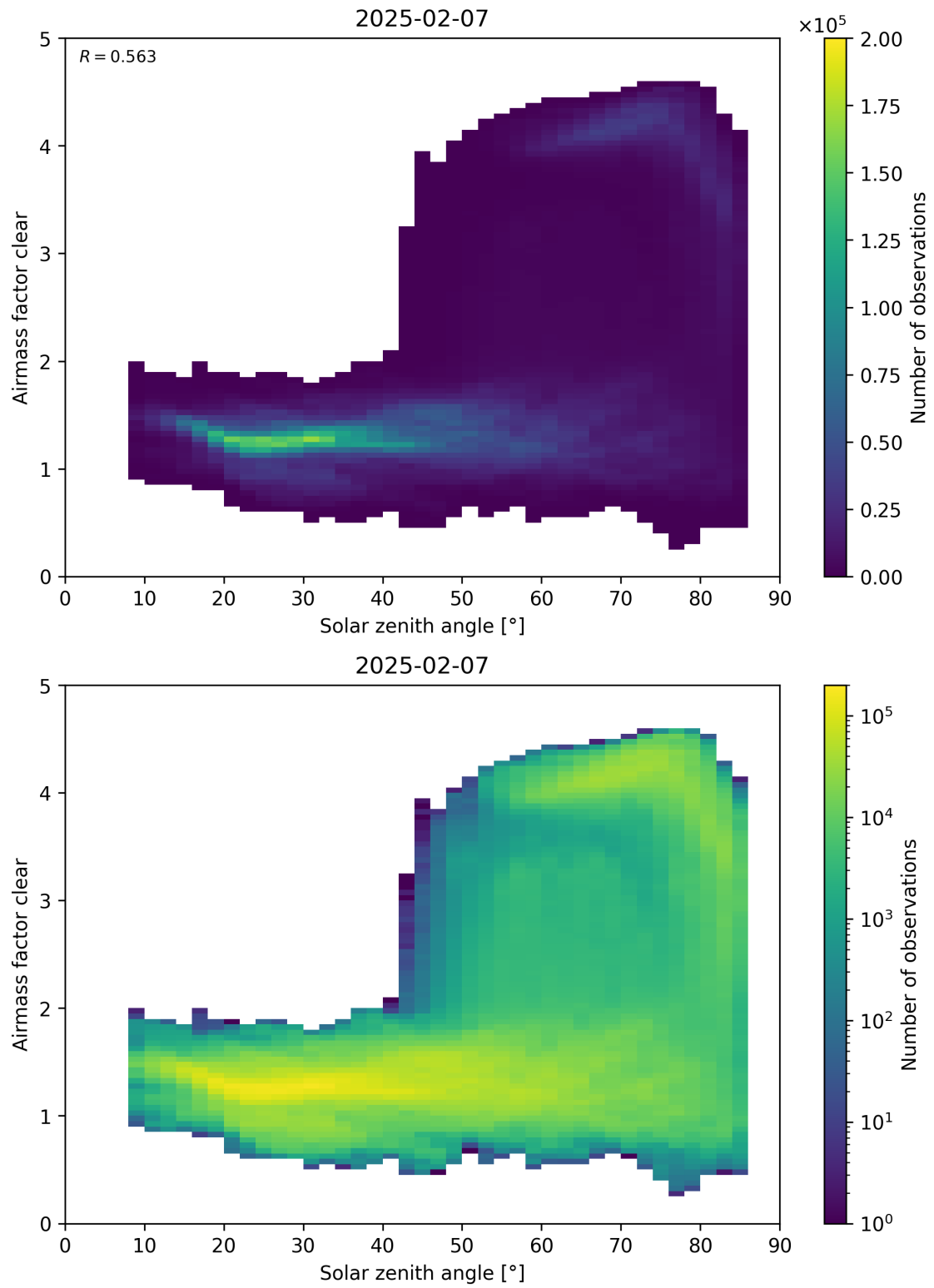
Figure 170: Scatter density plot of “Solar zenith angle” against “Airmass factor clear” for 2025-02-06 to 2025-02-08.
