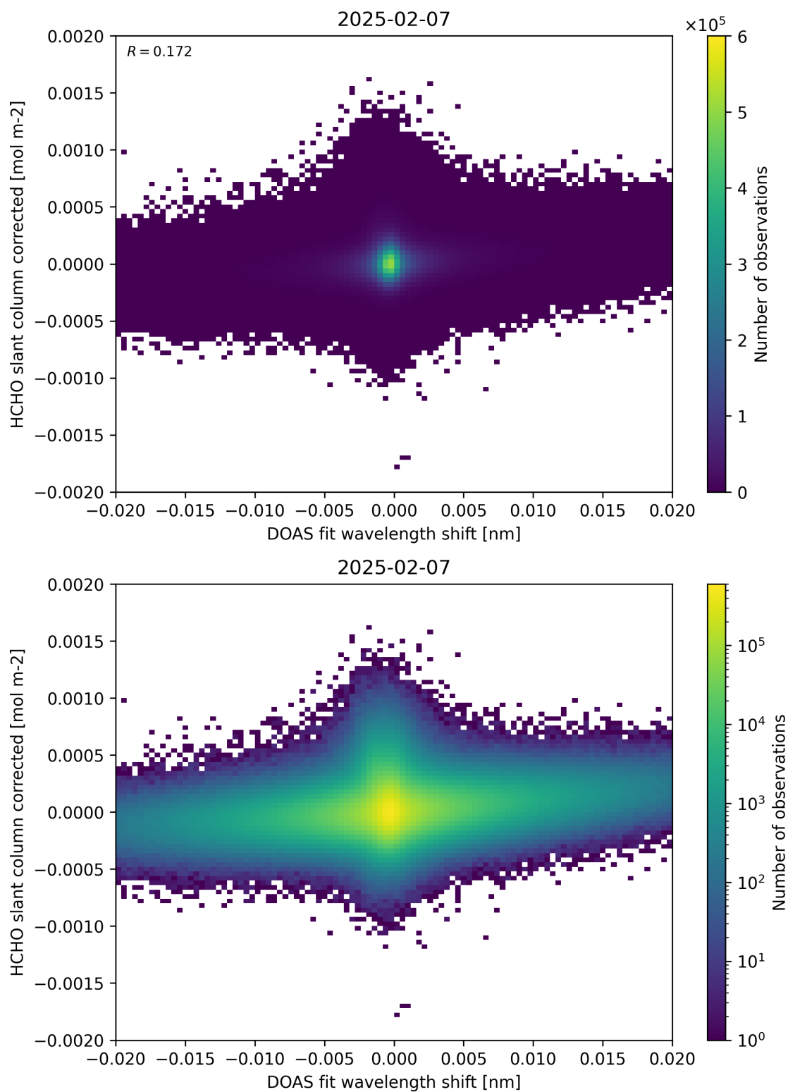
Figure 66: Scatter density plot of “DOAS fit wavelength shift” against “HCHO slant column corrected” for 2025-02-06 to 2025-02-08.
