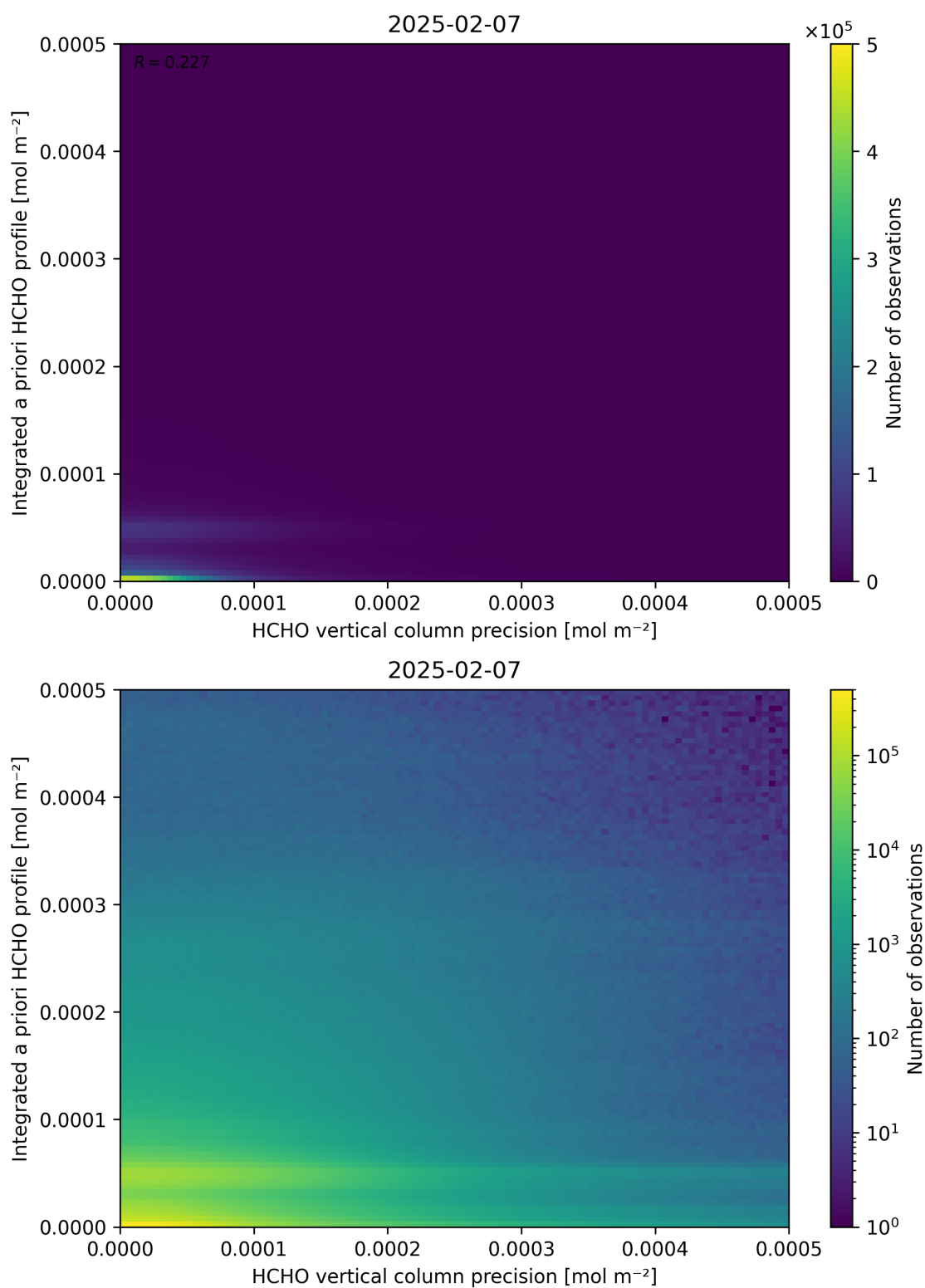
Figure 147: Scatter density plot of “HCHO vertical column precision” against “Integrated a priori HCHO profile” for 2025-02-06 to 2025-02-08.
