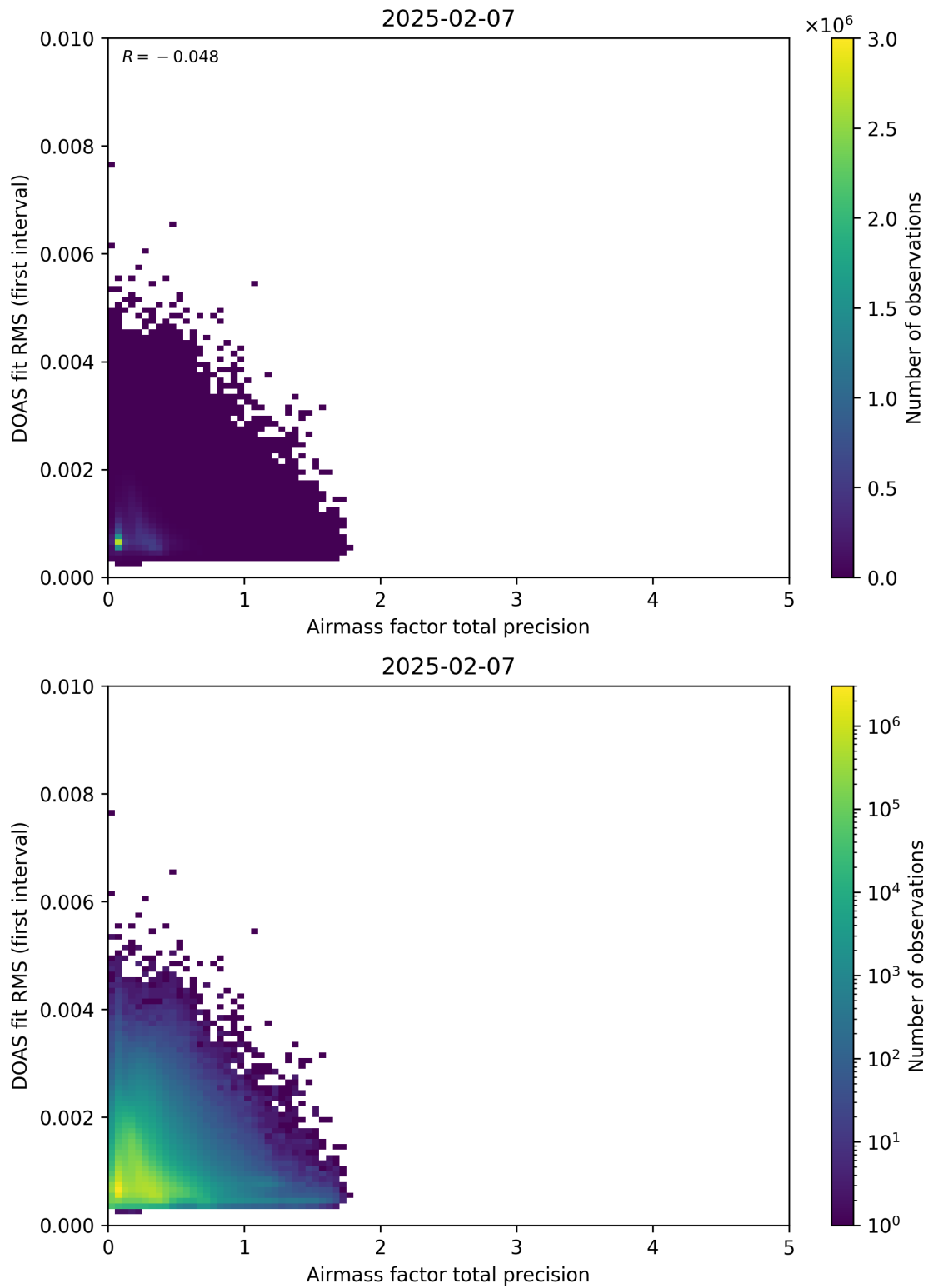
Figure 105: Scatter density plot of “Airmass factor total precision” against “DOAS fit RMS (first interval)” for 2025-02-06 to 2025-02-08.
