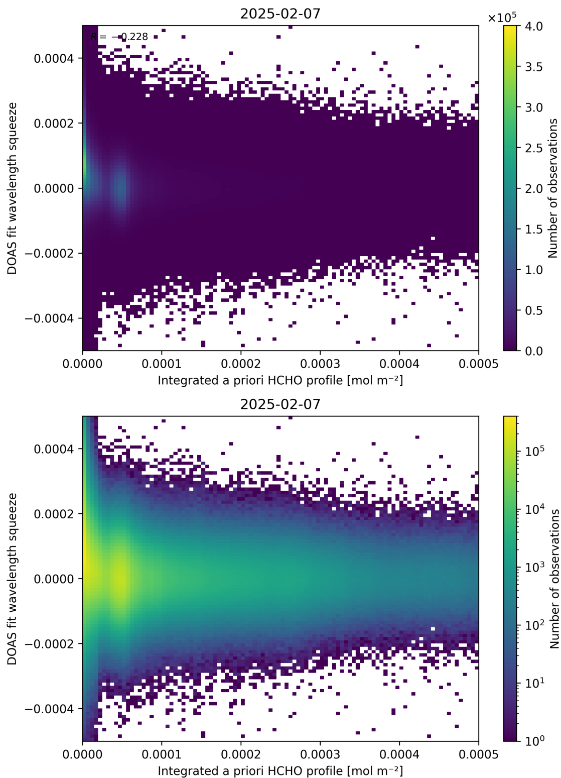
Figure 150: Scatter density plot of “Integrated a priori HCHO profile” against “DOAS fit wavelength squeeze” for 2025-02-06 to 2025-02-08.
