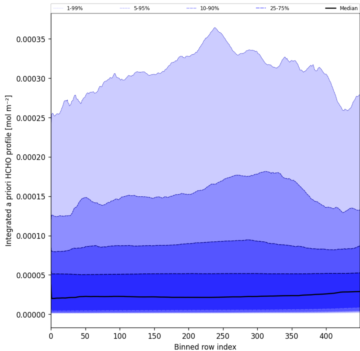
Figure 57: Along track statistics of “Integrated a priori HCHO profile” for 2025-02-06 to 2025-02-08
