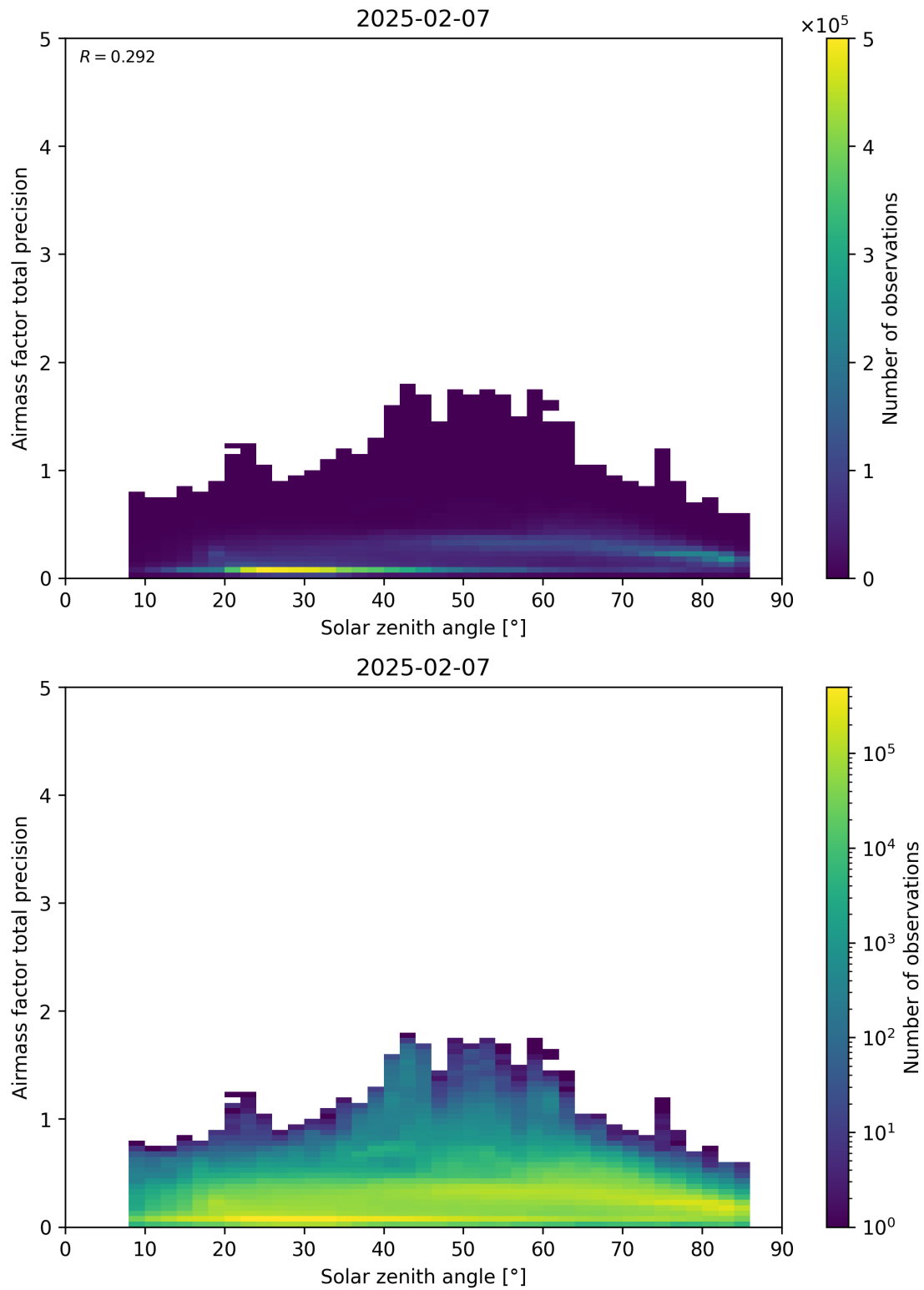
Figure 176: Scatter density plot of “Solar zenith angle” against “Airmass factor total precision” for 2025-02-06 to 2025-02-08.
