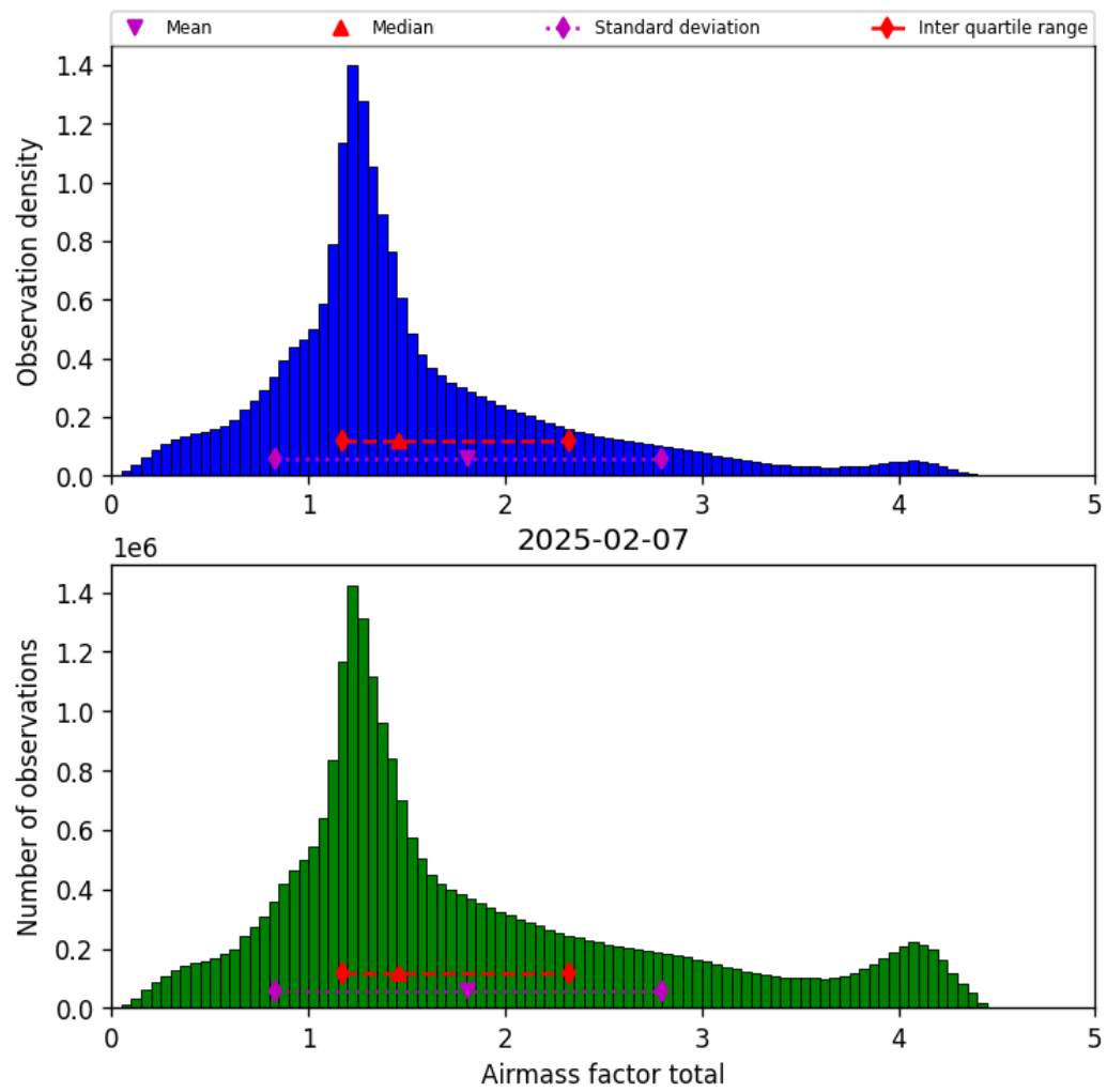
Figure 40: Histogram of “Airmass factor total” for 2025-02-06 to 2025-02-08
