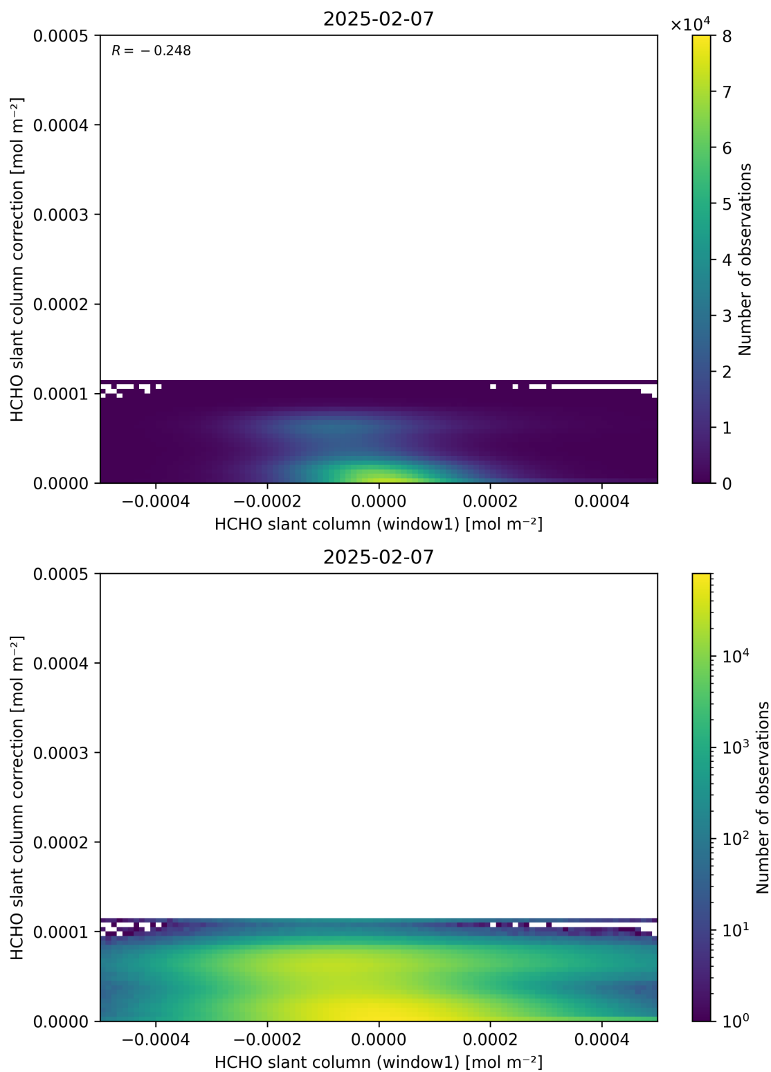
Figure 83: Scatter density plot of “HCHO slant column (window1)” against “HCHO slant column correction” for 2025-02-06 to 2025-02-08.
