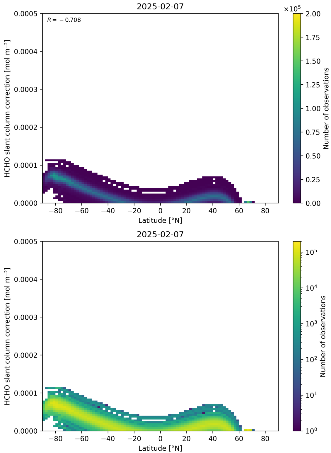
Figure 158: Scatter density plot of “Latitude” against “HCHO slant column correction” for 2025-02-06 to 2025-02-08.
