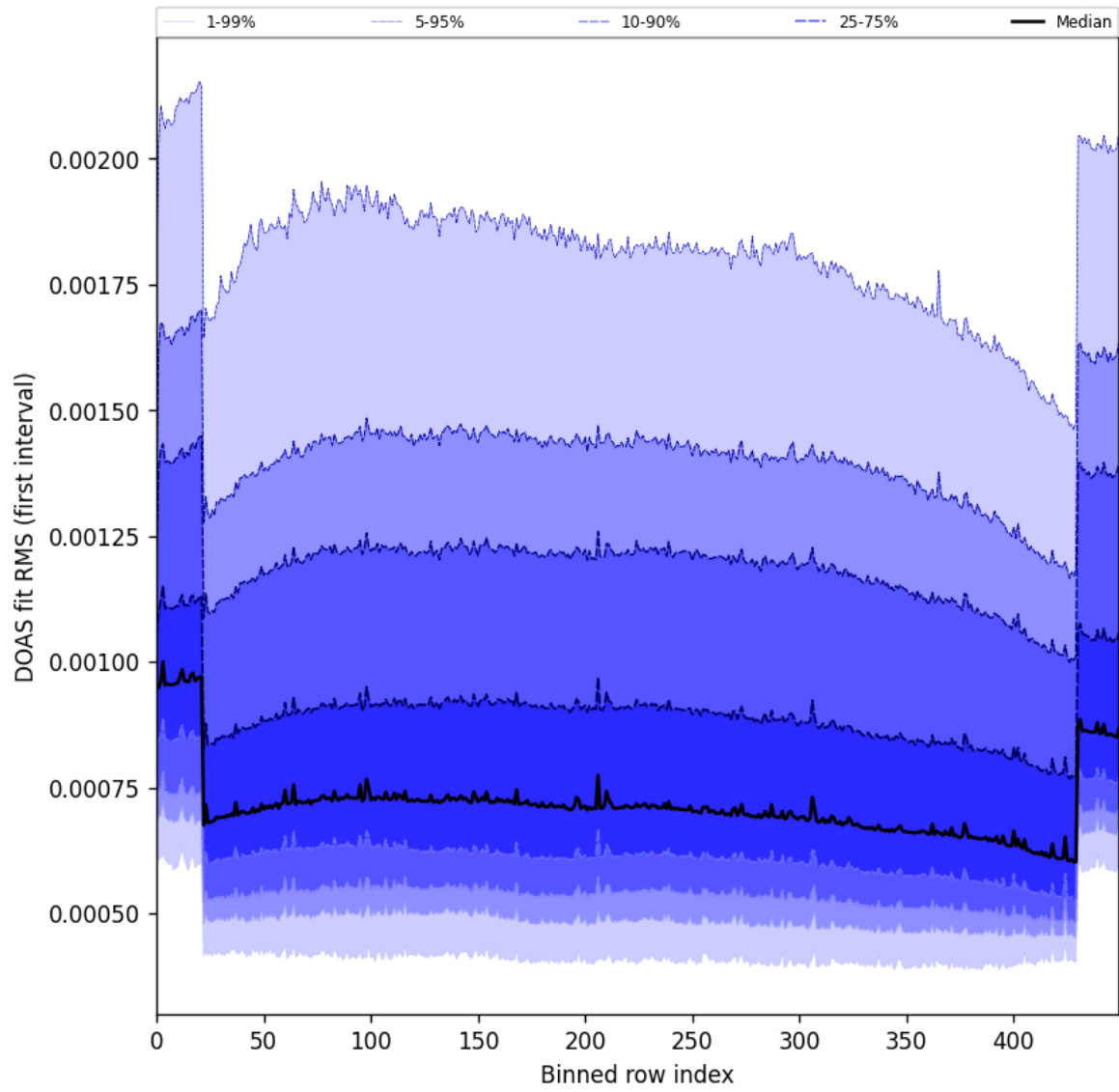
Figure 60: Along track statistics of “DOAS fit RMS (first interval)” for 2025-02-06 to 2025-02-08
