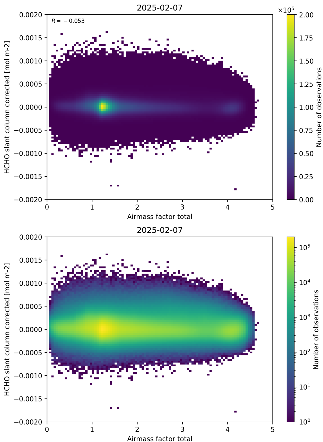
Figure 101: Scatter density plot of “Airmass factor total” against “HCHO slant column corrected” for 2025-02-06 to 2025-02-08.
