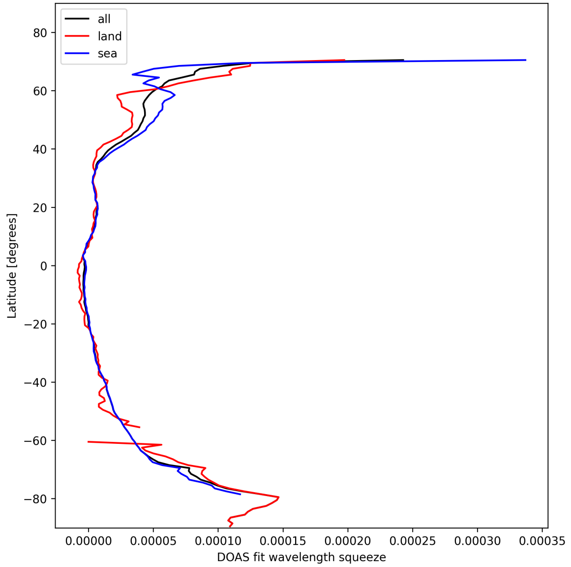
Figure 31: Zonal average of “DOAS fit wavelength squeeze” for 2025-02-06 to 2025-02-08.
