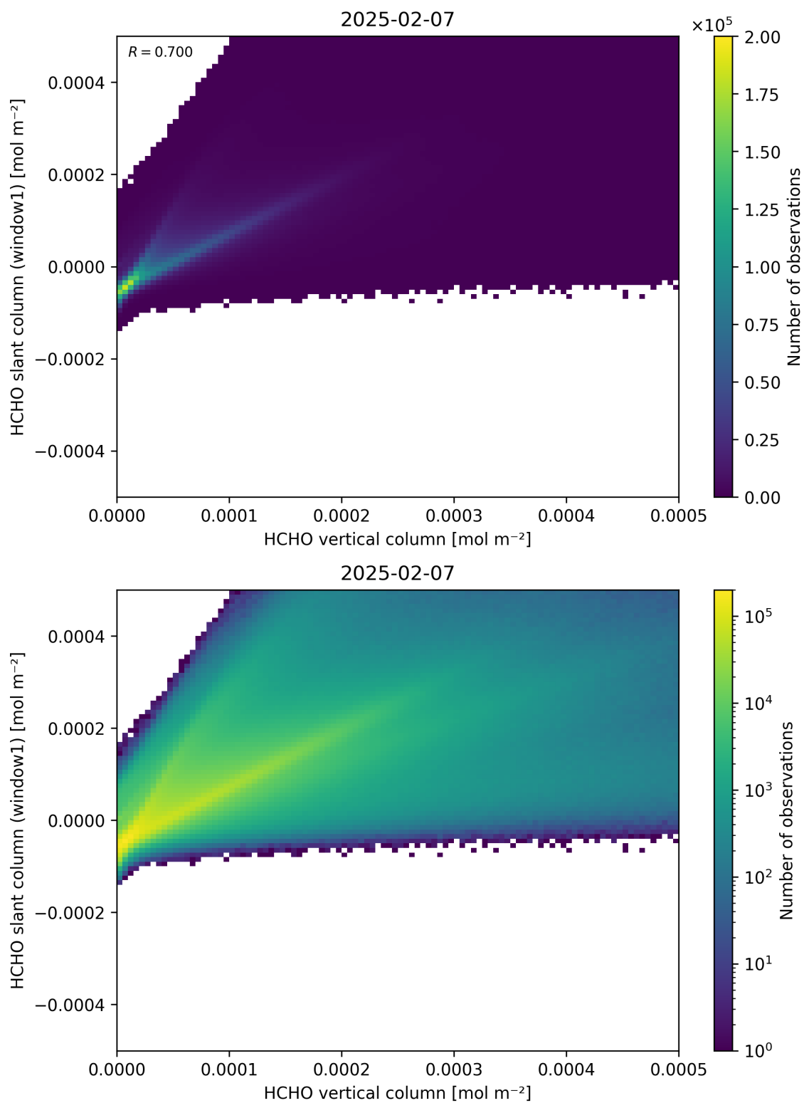
Figure 129: Scatter density plot of “HCHO vertical column” against “HCHO slant column (window1)” for 2025-02-06 to 2025-02-08.
