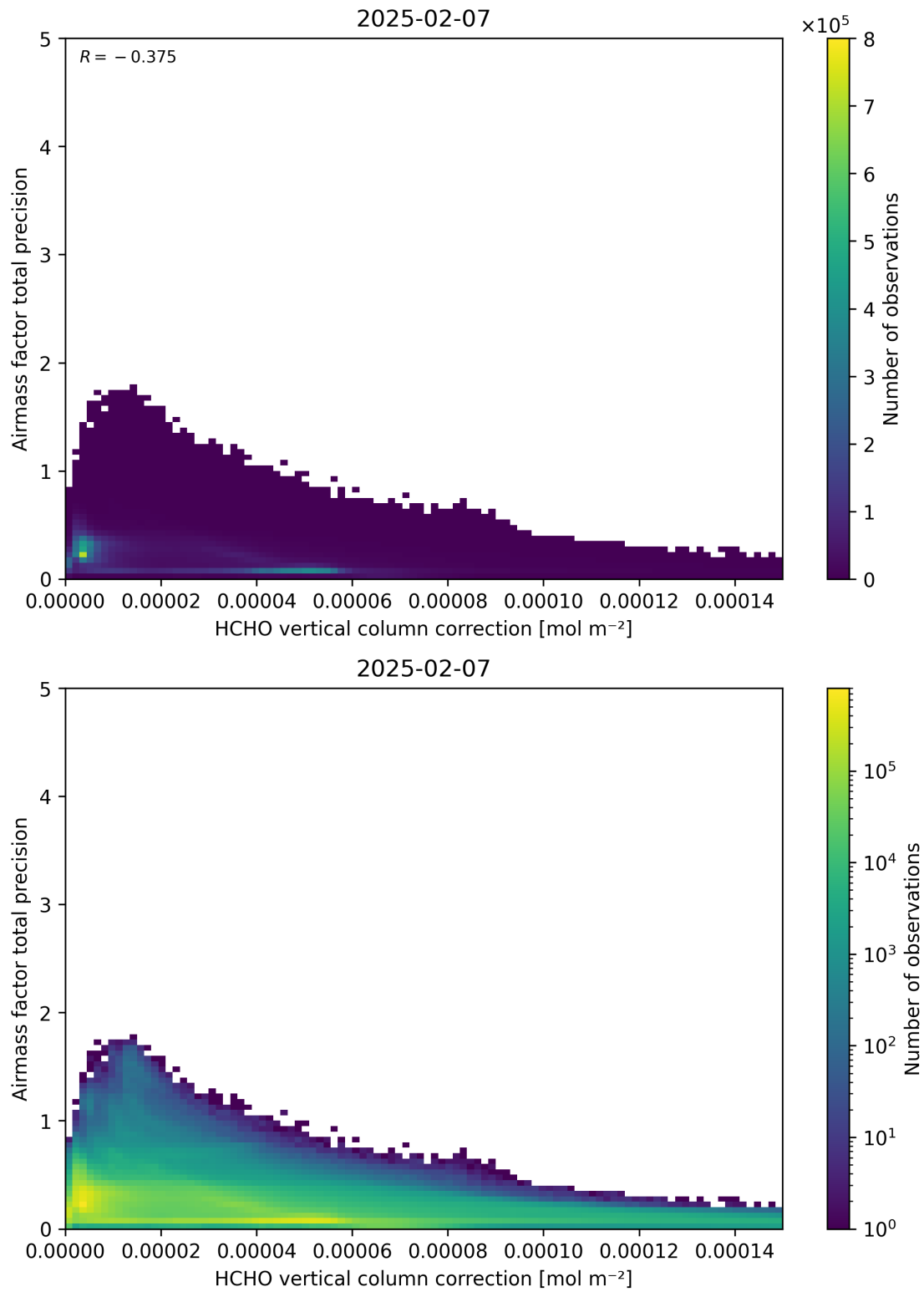
Figure 121: Scatter density plot of “HCHO vertical column correction” against “Airmass factor total precision” for 2025-02-06 to 2025-02-08.
