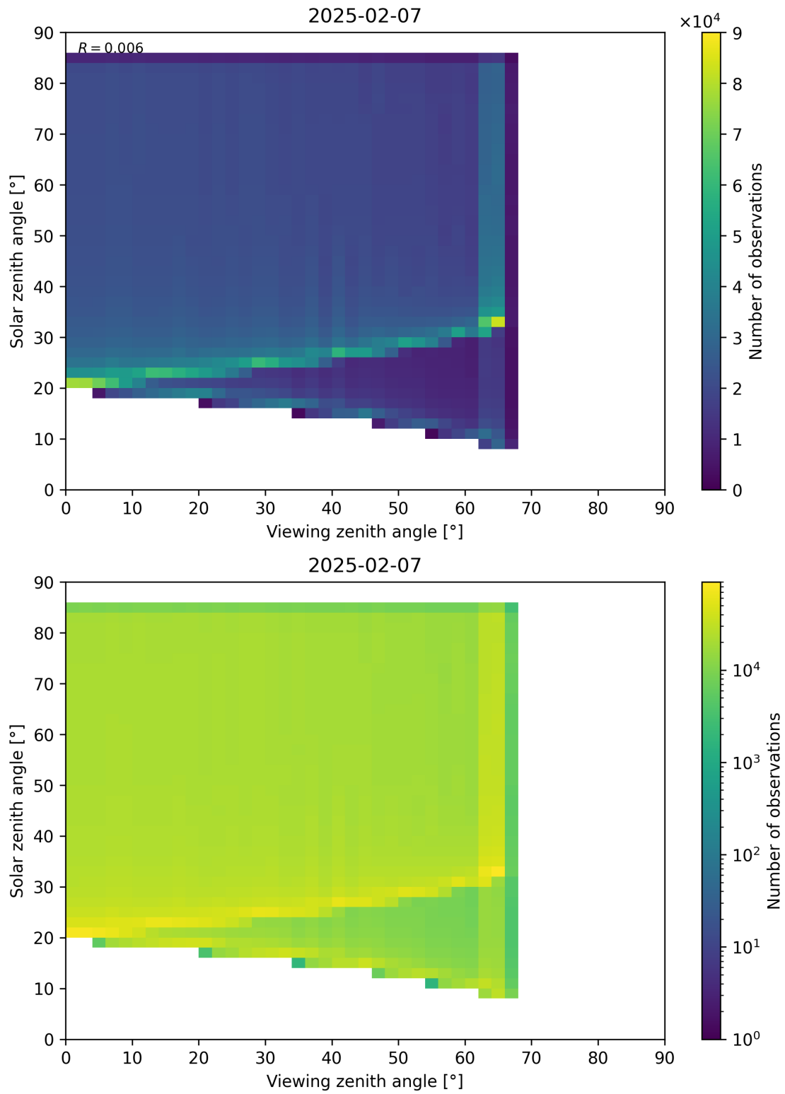
Figure 197: Scatter density plot of “Viewing zenith angle” against “Solar zenith angle” for 2025-02-06 to 2025-02-08.
