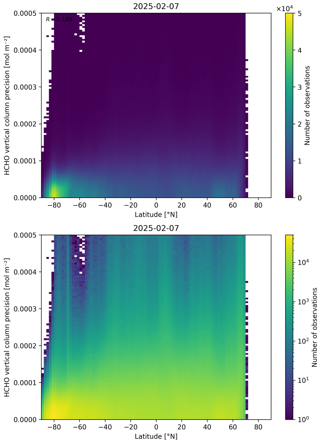
Figure 165: Scatter density plot of “Latitude” against “HCHO vertical column precision” for 2025-02-06 to 2025-02-08.
