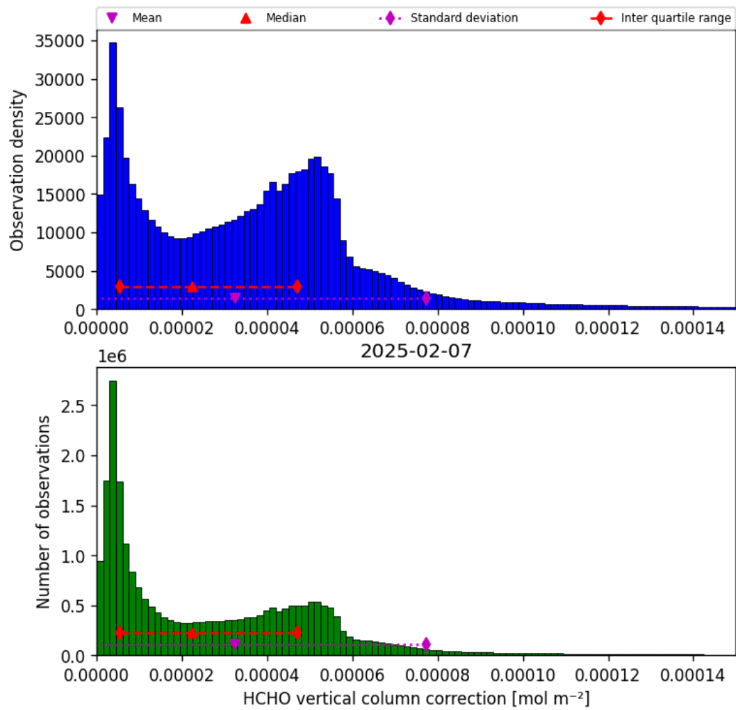
Figure 37: Histogram of “HCHO vertical column correction” for 2025-02-06 to 2025-02-08
