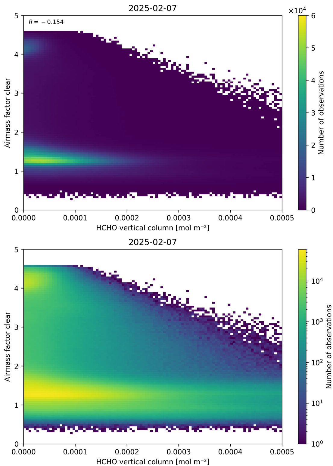
Figure 126: Scatter density plot of “HCHO vertical column” against “Airmass factor clear” for 2025-02-06 to 2025-02-08.
