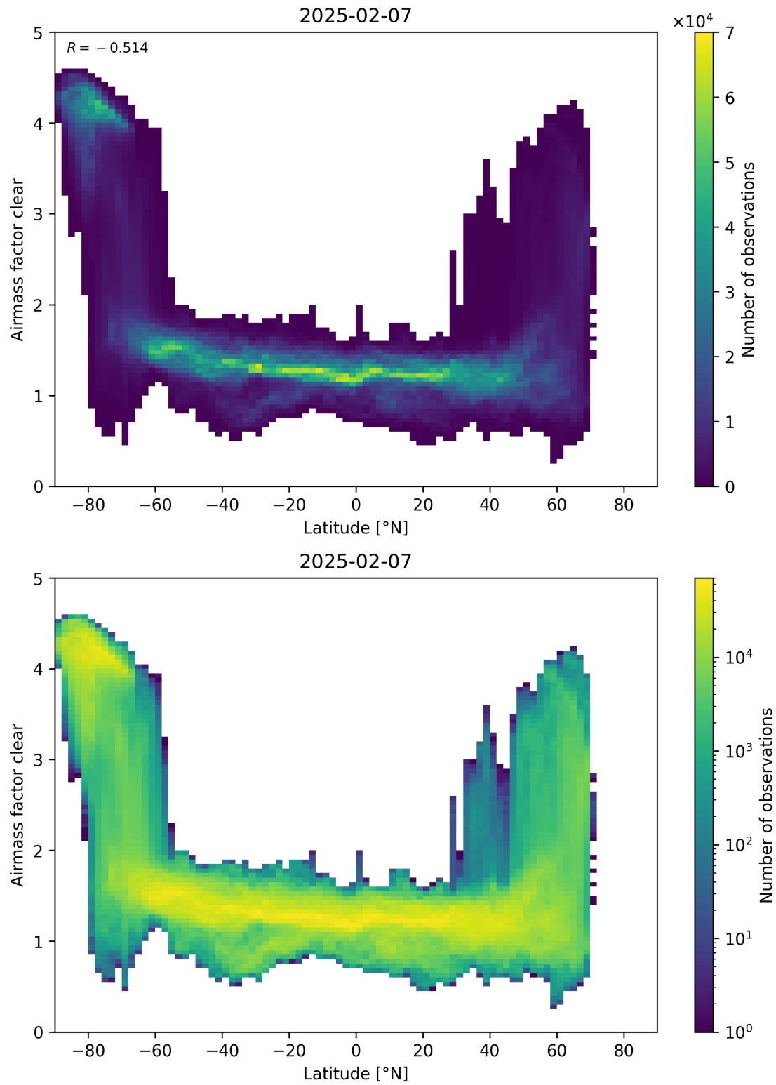
Figure 156: Scatter density plot of “Latitude” against “Airmass factor clear” for 2025-02-06 to 2025-02-08.
