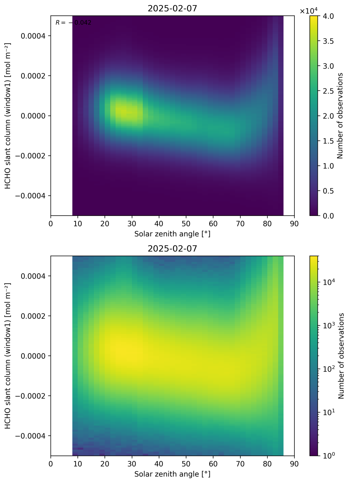
Figure 173: Scatter density plot of “Solar zenith angle” against “HCHO slant column (window1)” for 2025-02-06 to 2025-02-08.
