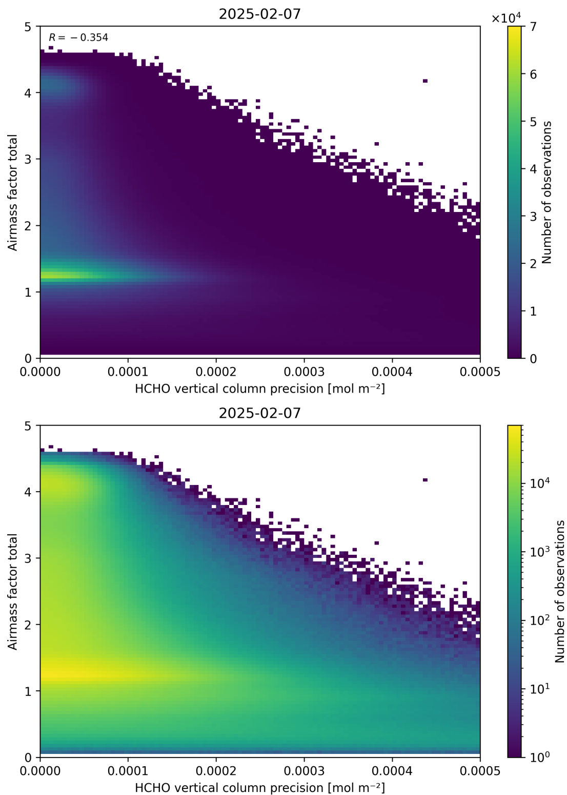
Figure 144: Scatter density plot of “HCHO vertical column precision” against “Airmass factor total” for 2025-02-06 to 2025-02-08.
