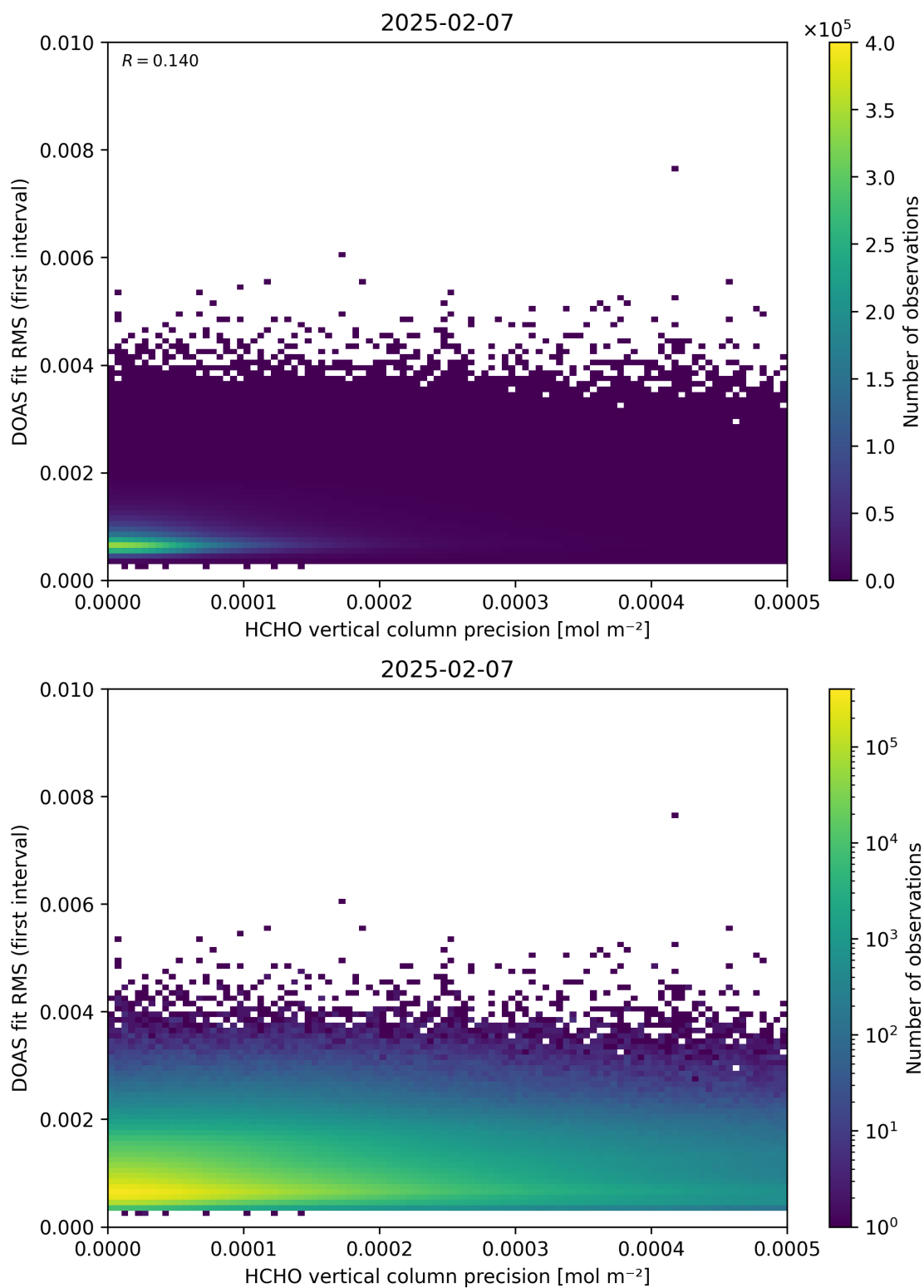
Figure 136: Scatter density plot of “HCHO vertical column precision” against “DOAS fit RMS (first interval)” for 2025-02-06 to 2025-02-08.
