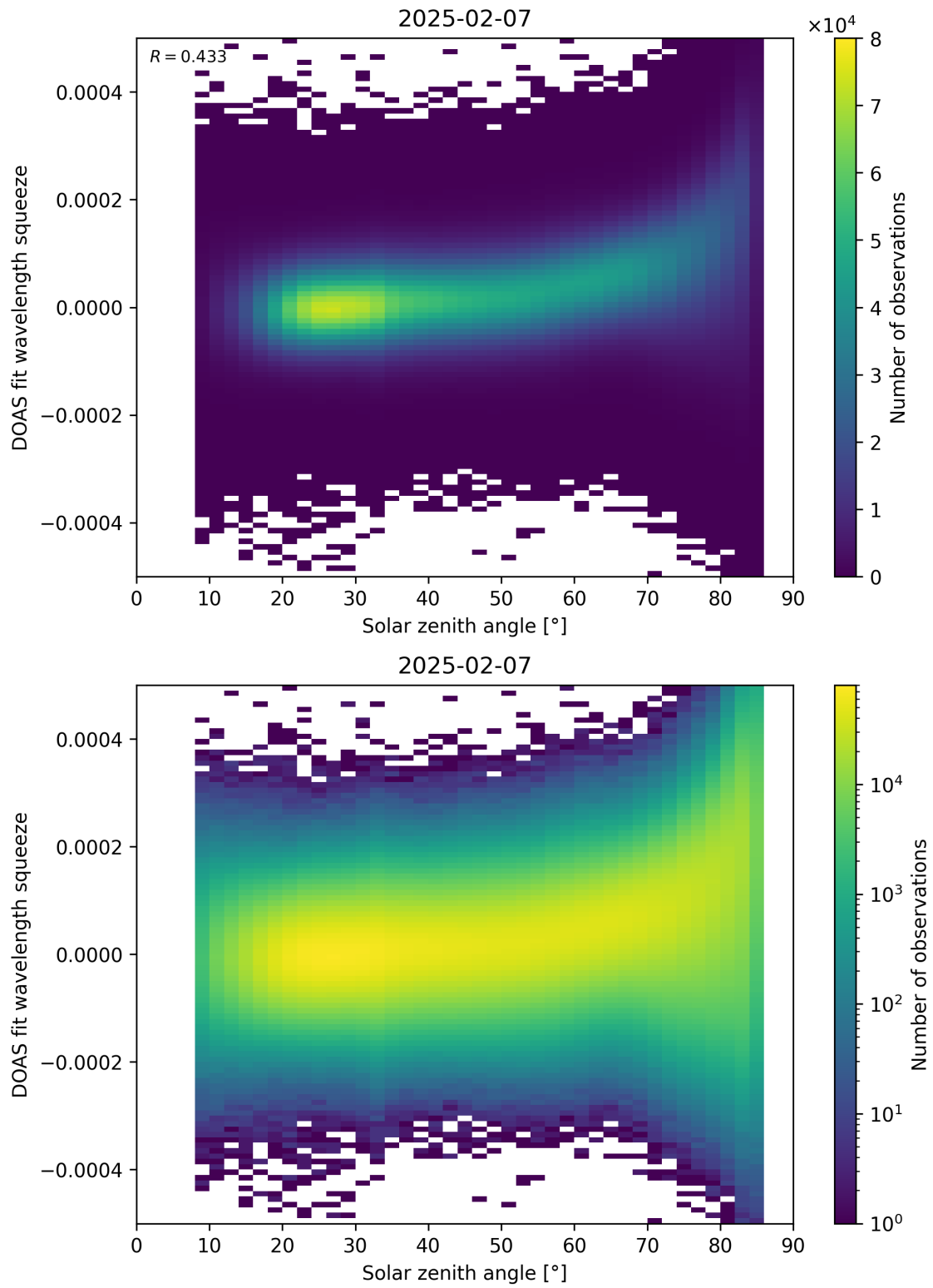
Figure 169: Scatter density plot of “Solar zenith angle” against “DOAS fit wavelength squeeze” for 2025-02-06 to 2025-02-08.
