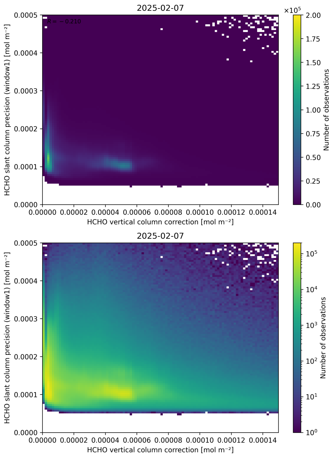
Figure 119: Scatter density plot of “HCHO vertical column correction” against “HCHO slant column precision (window1)” for 2025-02-06 to 2025-02-08.
