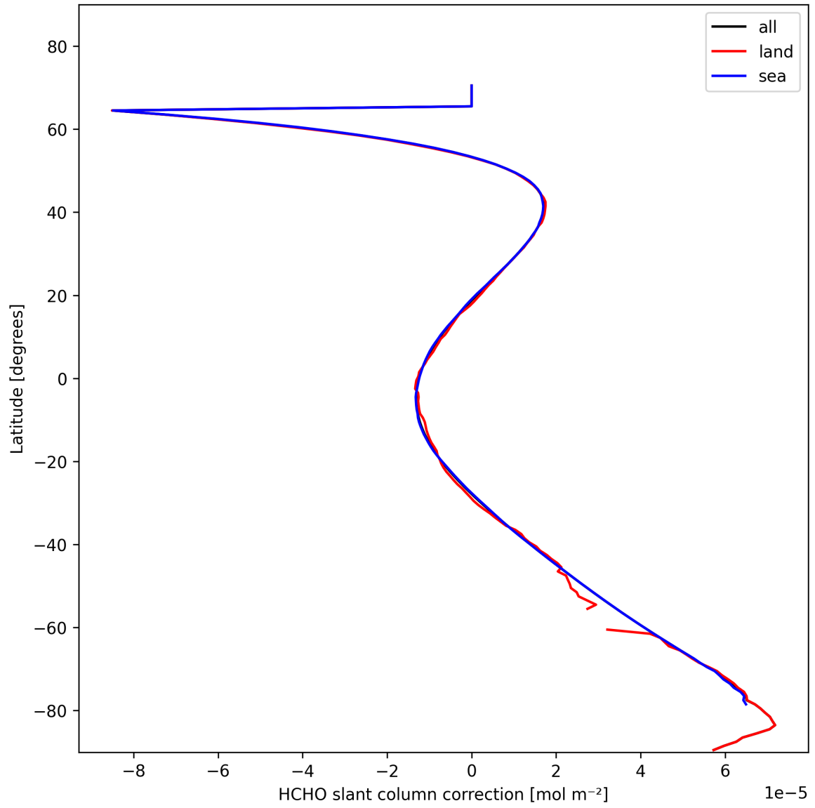
Figure 33: Zonal average of “HCHO slant column correction” for 2025-02-06 to 2025-02-08.
