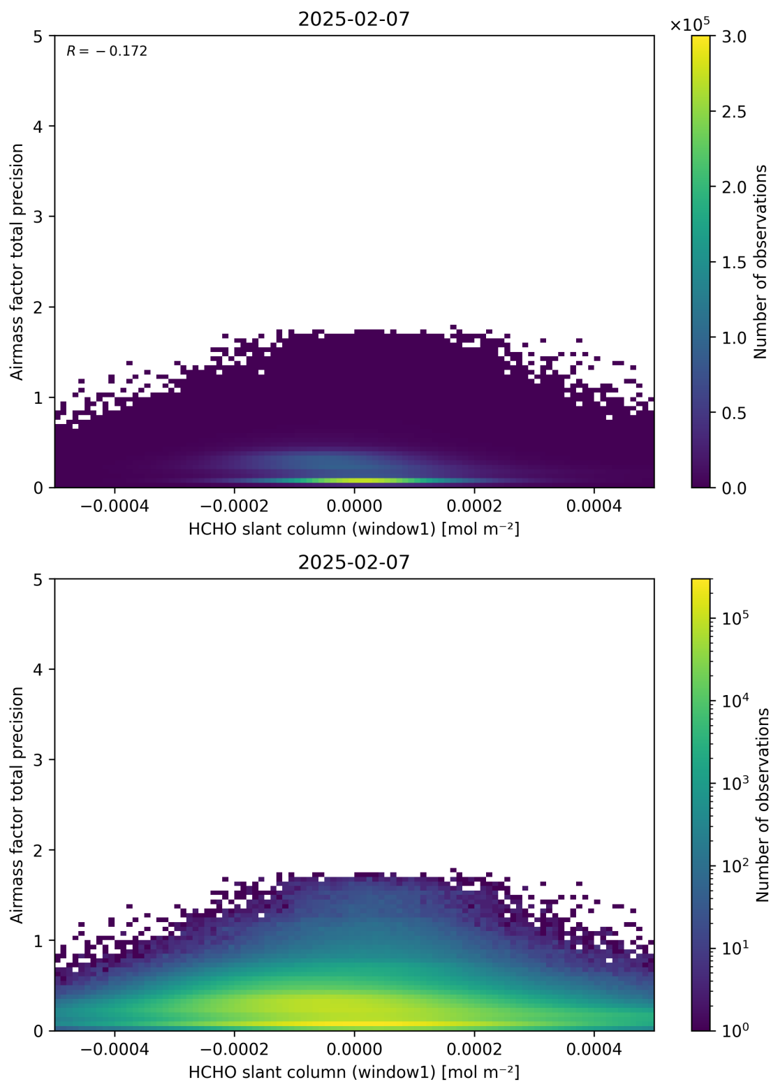
Figure 86: Scatter density plot of “HCHO slant column (window1)” against “Airmass factor total precision” for 2025-02-06 to 2025-02-08.
