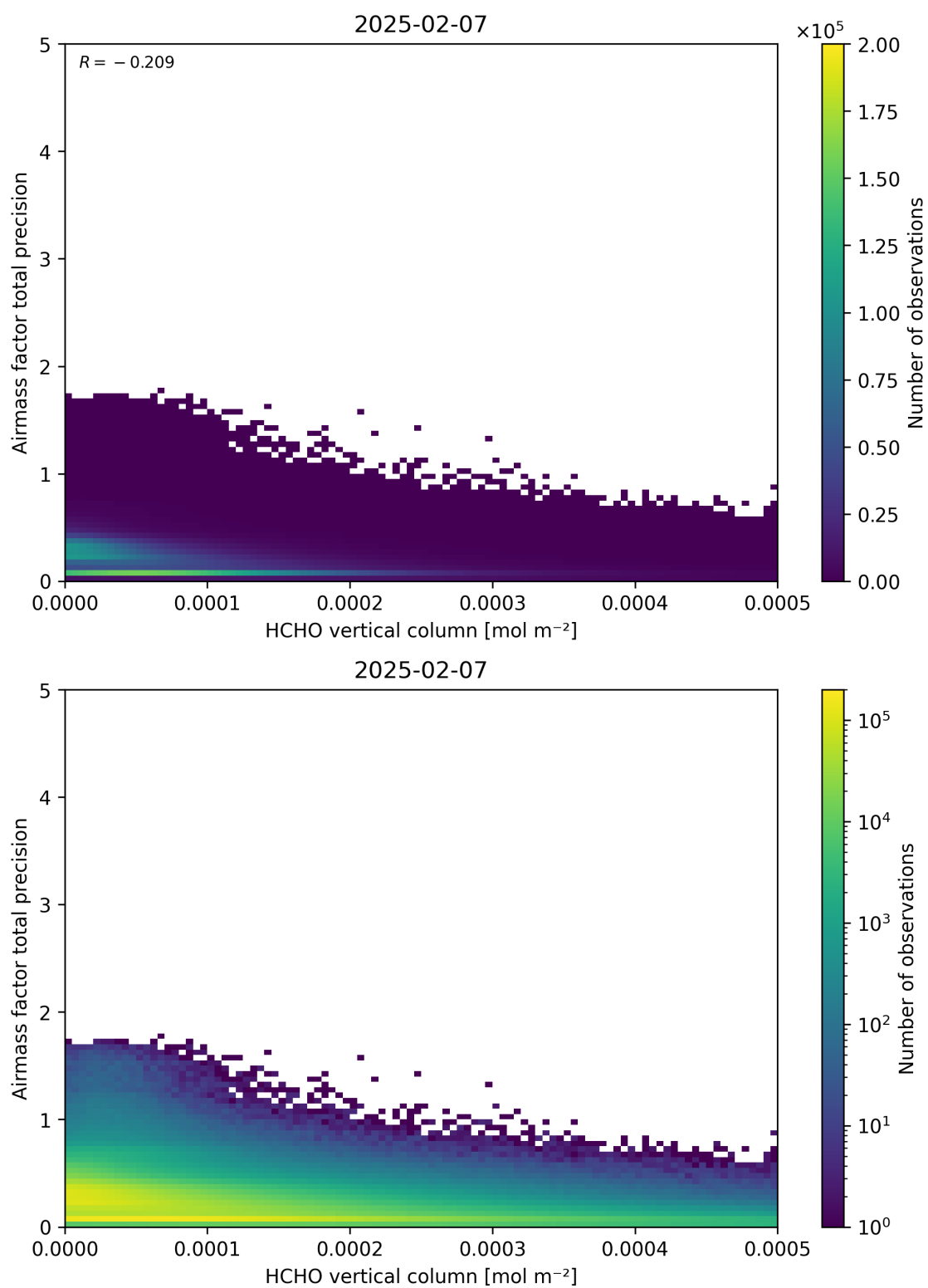
Figure 132: Scatter density plot of “HCHO vertical column” against “Airmass factor total precision” for 2025-02-06 to 2025-02-08.
