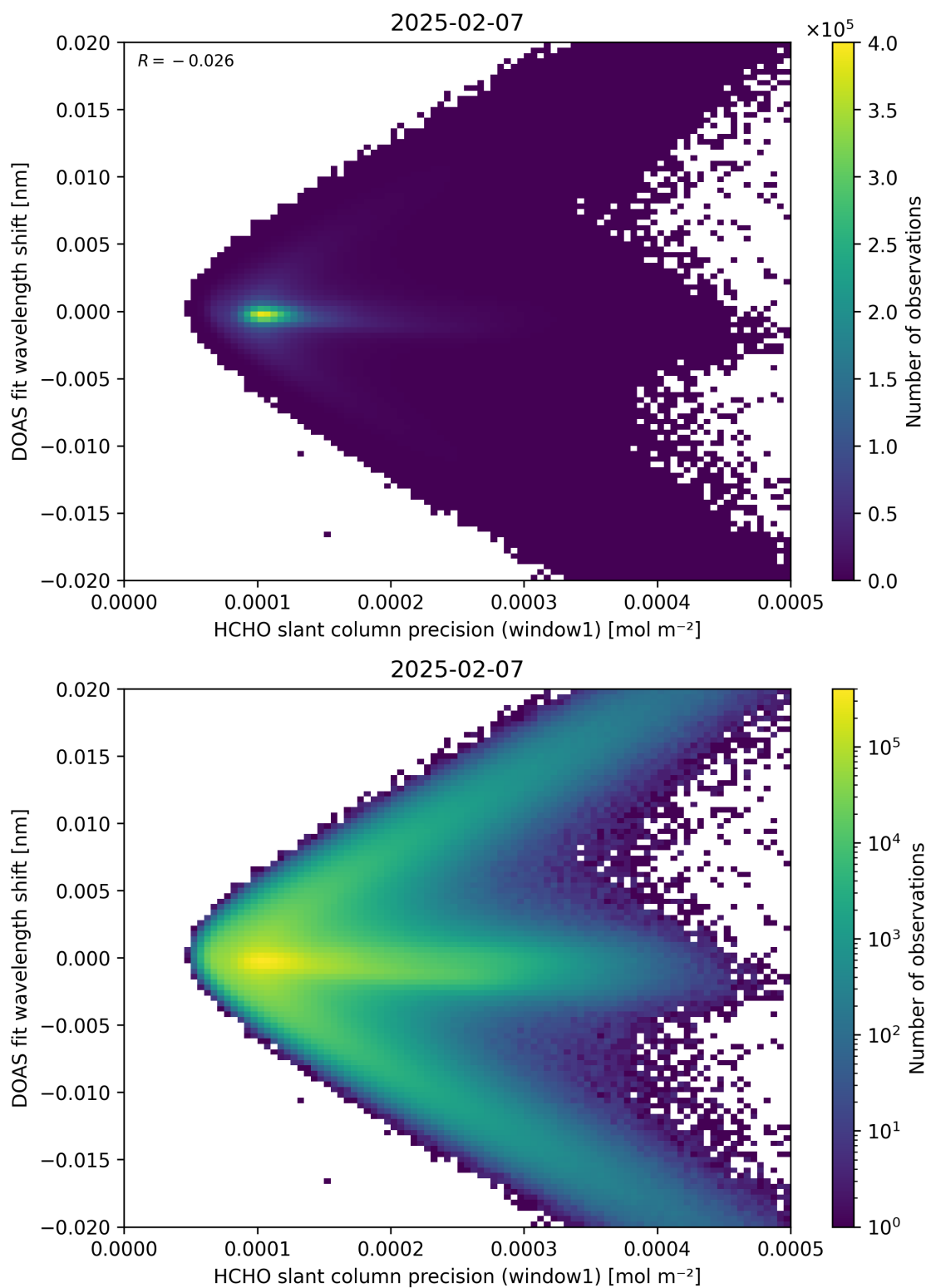
Figure 89: Scatter density plot of “HCHO slant column precision (window1)” against “DOAS fit wavelength shift” for 2025-02-06 to 2025-02-08.
