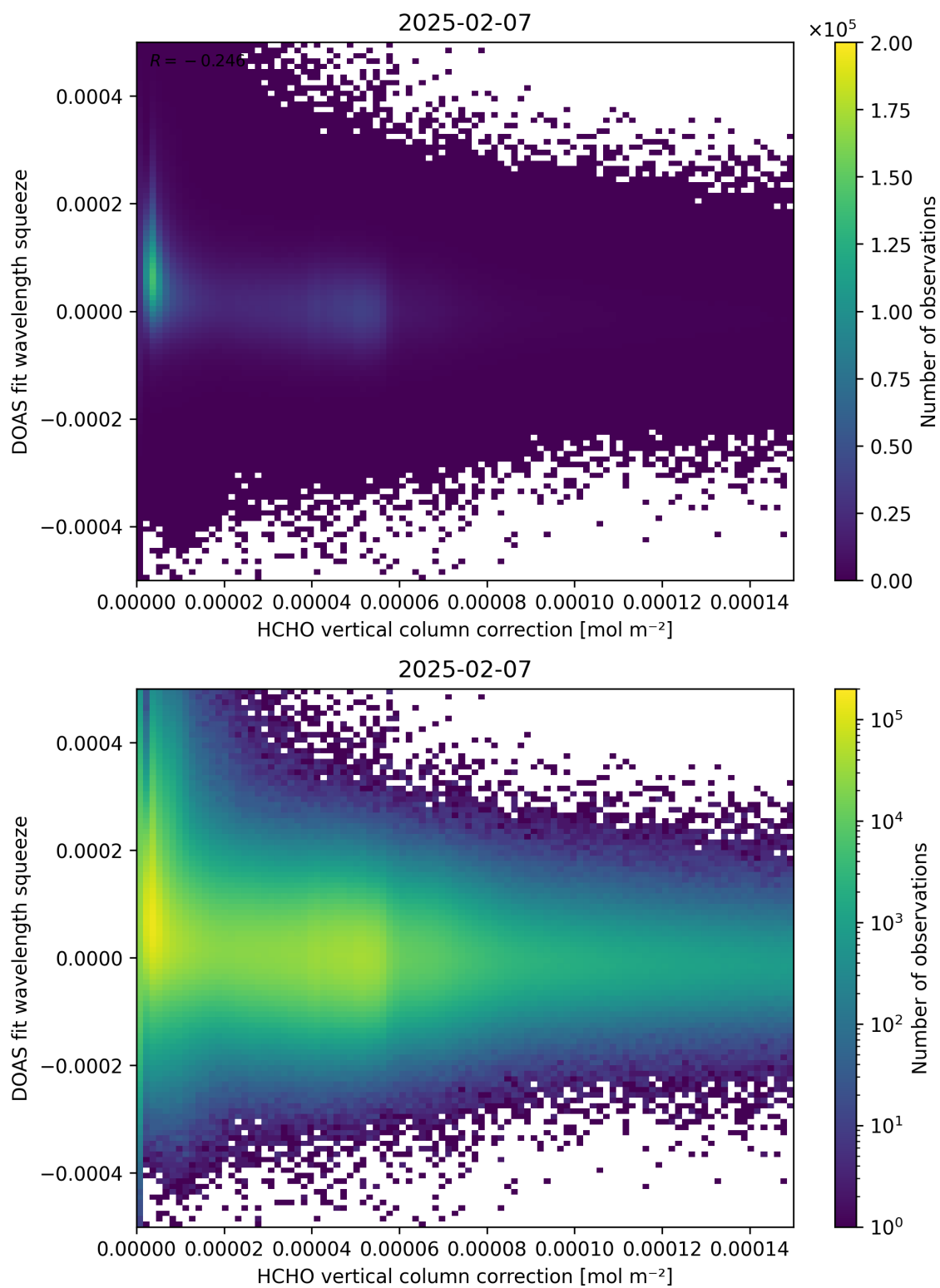
Figure 114: Scatter density plot of “HCHO vertical column correction” against “DOAS fit wavelength squeeze” for 2025-02-06 to 2025-02-08.
