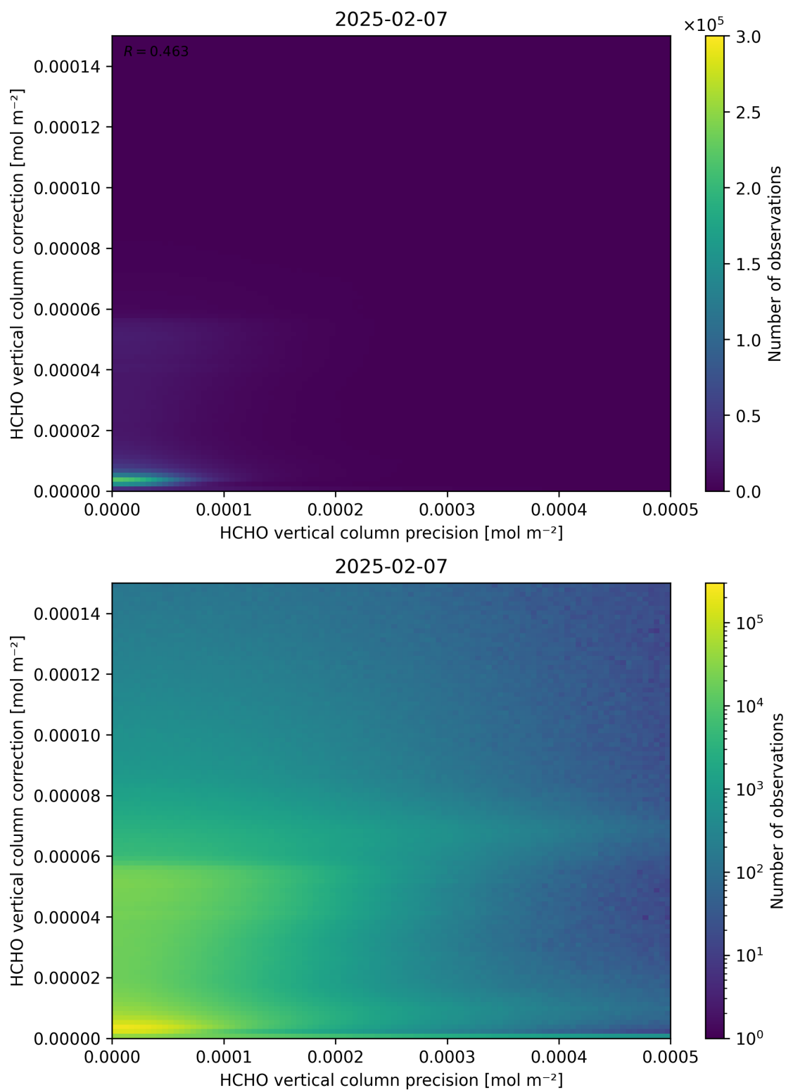
Figure 146: Scatter density plot of “HCHO vertical column precision” against “HCHO vertical column correction” for 2025-02-06 to 2025-02-08.
