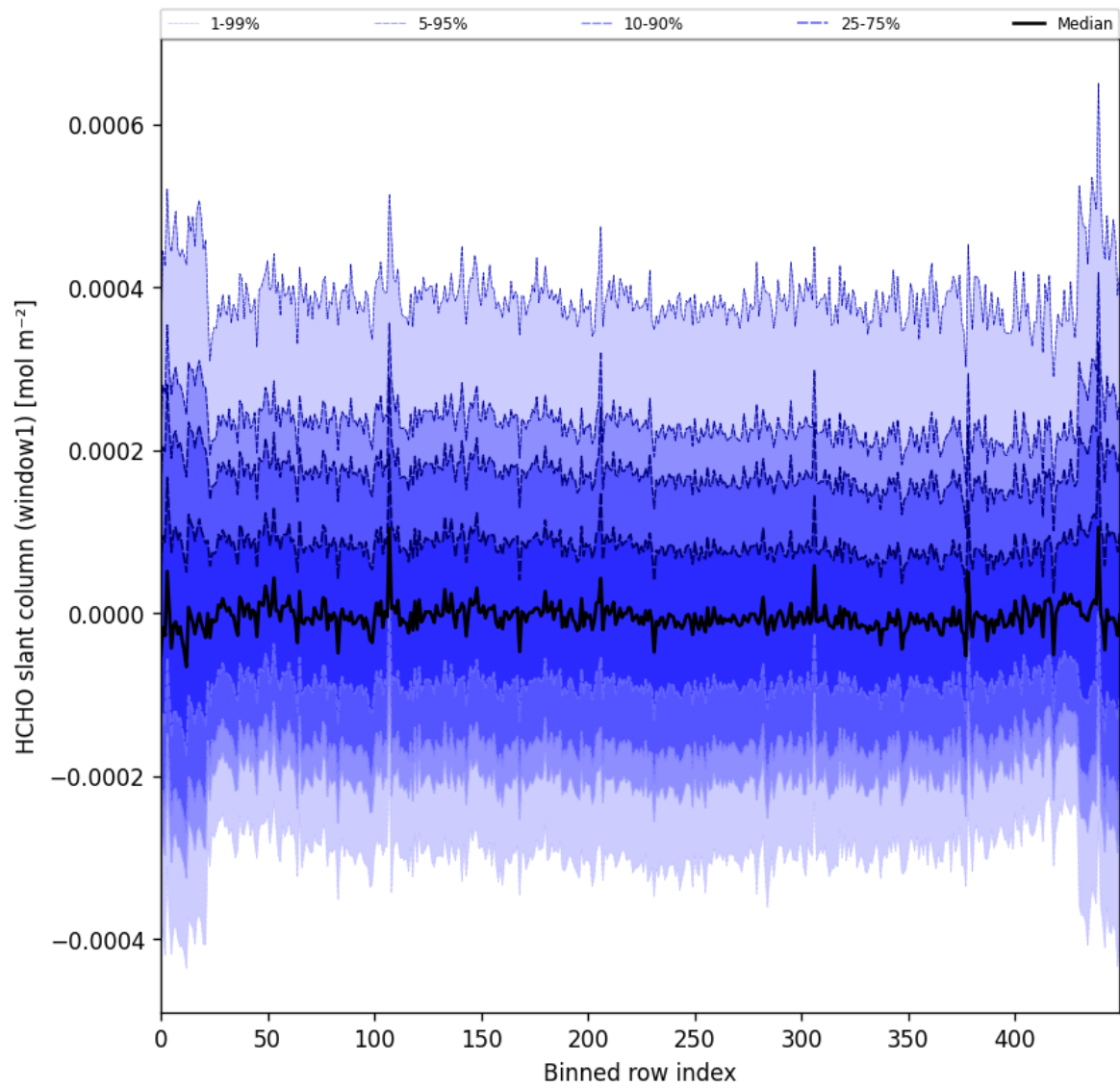
Figure 52: Along track statistics of “HCHO slant column (window1)” for 2025-02-06 to 2025-02-08
