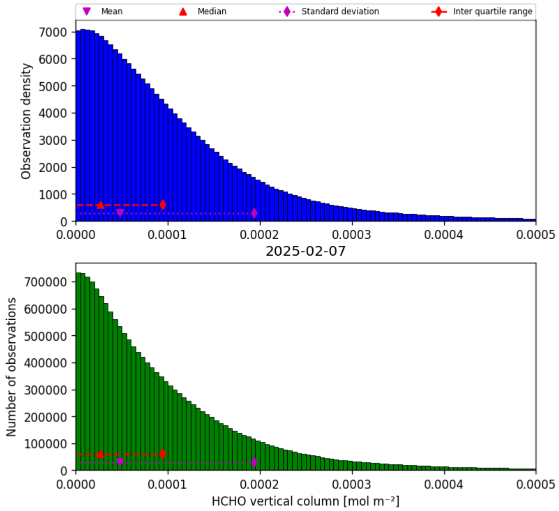
Figure 35: Histogram of “HCHO vertical column” for 2025-02-06 to 2025-02-08
