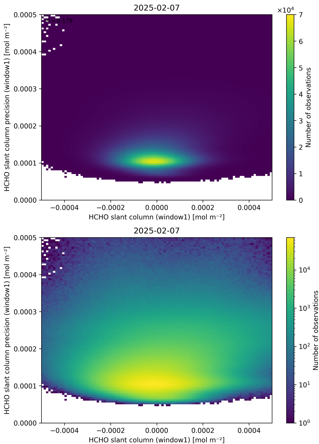
Figure 84: Scatter density plot of “HCHO slant column (window1)” against “HCHO slant column precision (window1)” for 2025-02-06 to 2025-02-08.
