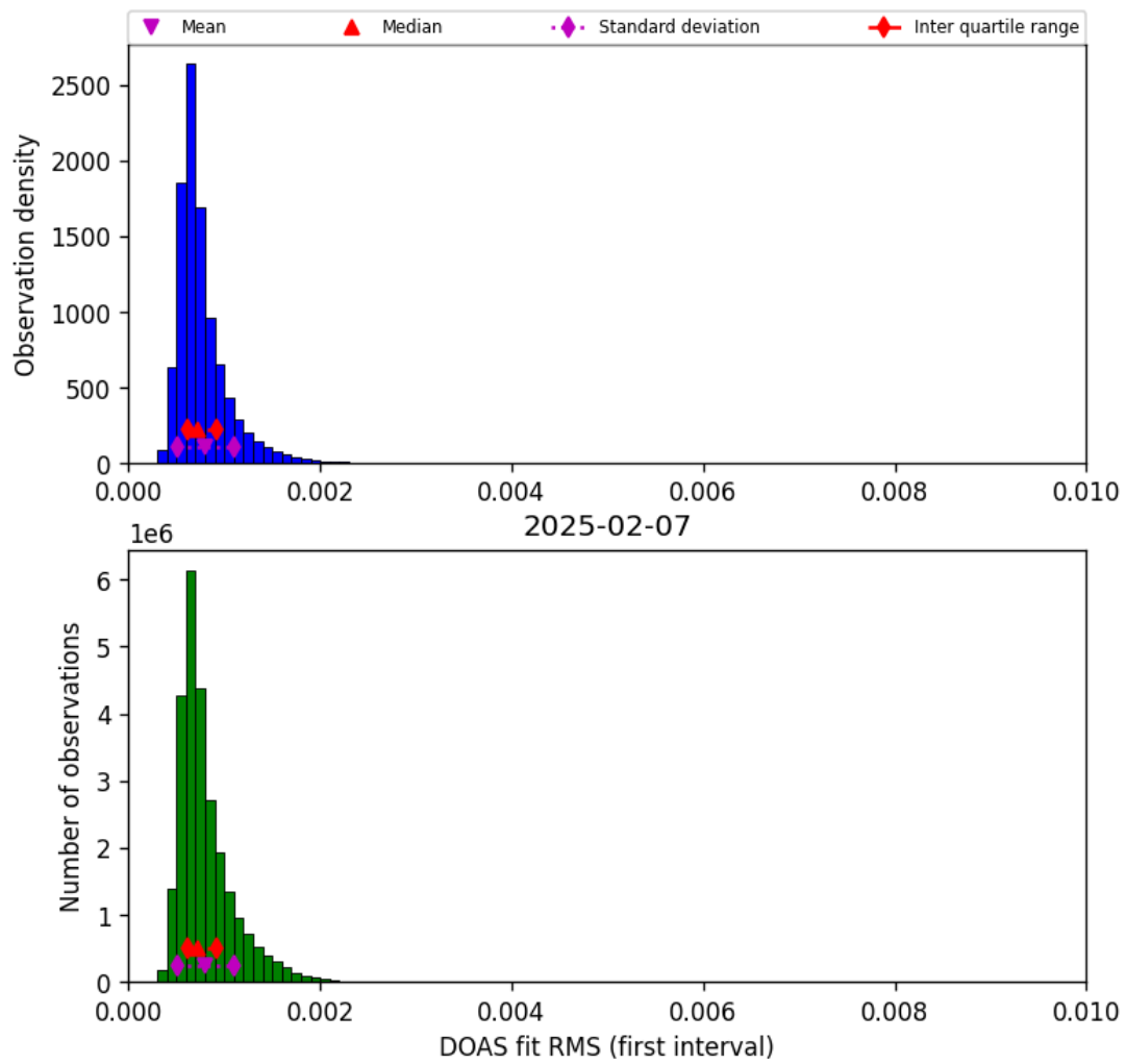
Figure 46: Histogram of “DOAS fit RMS (first interval)” for 2025-02-06 to 2025-02-08
