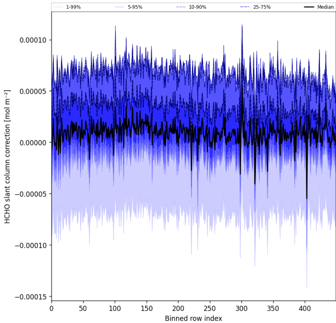
Figure 61: Along track statistics of “HCHO slant column correction” for 2025-02-06 to 2025-02-08
