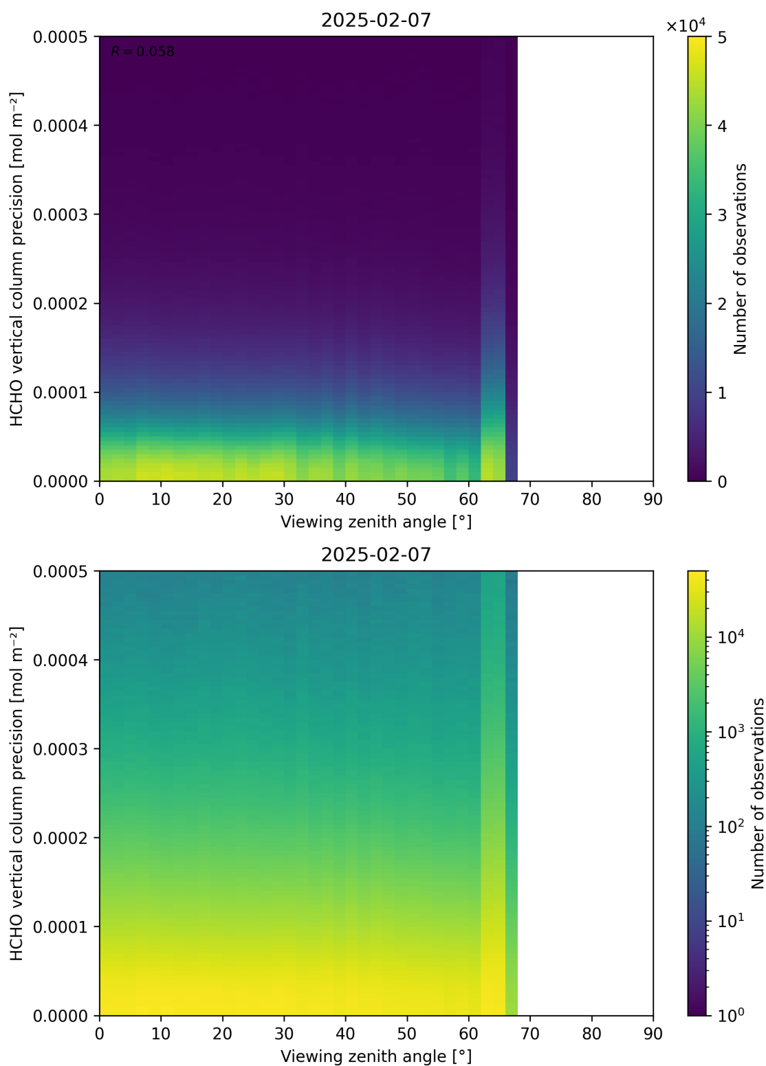
Figure 194: Scatter density plot of “Viewing zenith angle” against “HCHO vertical column precision” for 2025-02-06 to 2025-02-08.
