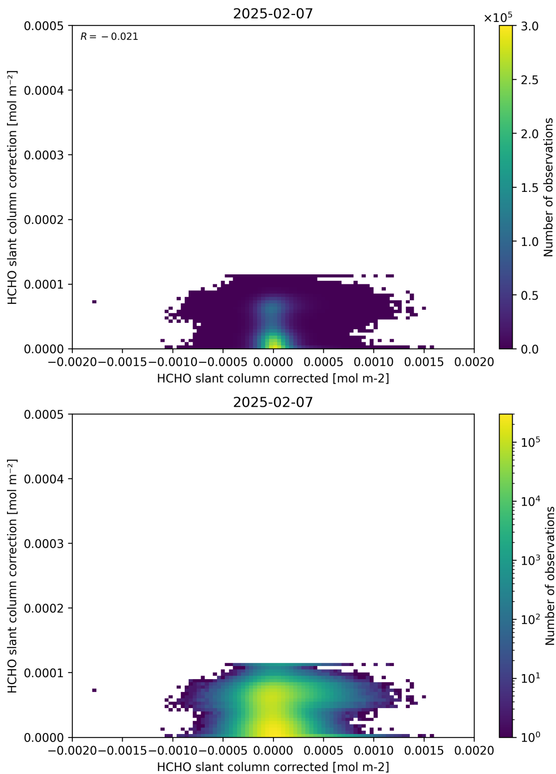
Figure 77: Scatter density plot of “HCHO slant column corrected” against “HCHO slant column correction” for 2025-02-06 to 2025-02-08.
