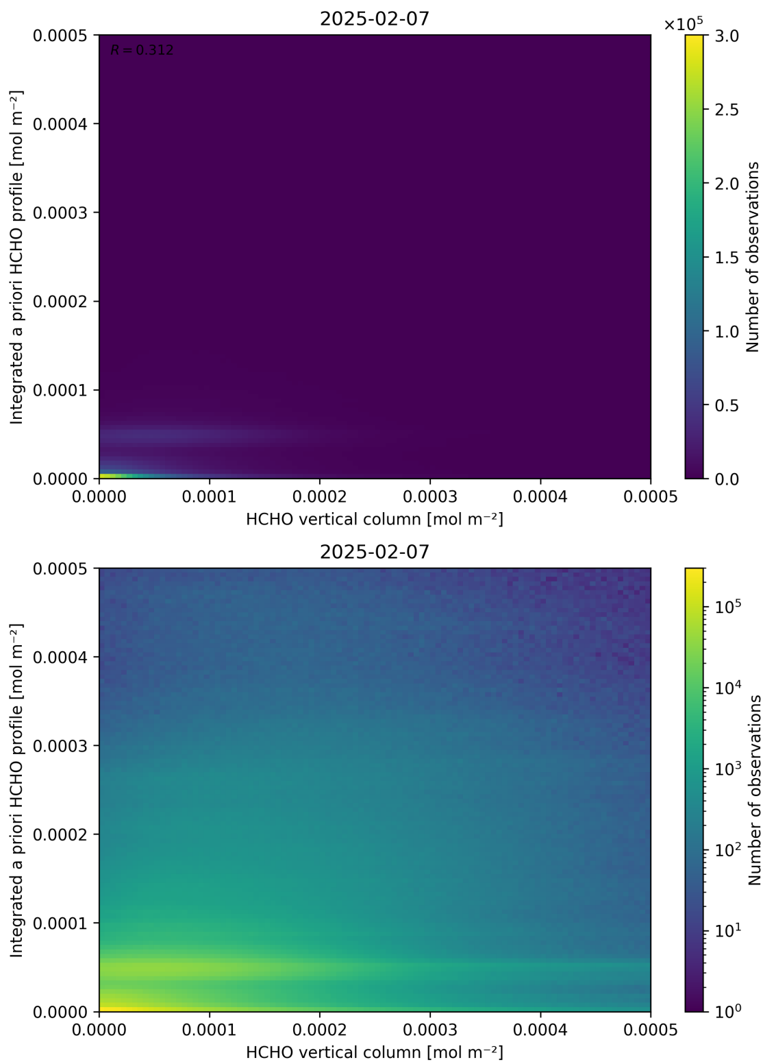
Figure 135: Scatter density plot of “HCHO vertical column” against “Integrated a priori HCHO profile” for 2025-02-06 to 2025-02-08.
