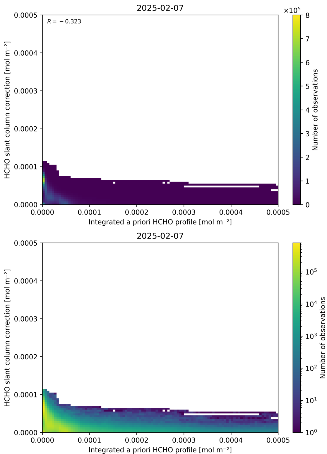
Figure 152: Scatter density plot of “Integrated a priori HCHO profile” against “HCHO slant column correction” for 2025-02-06 to 2025-02-08.
