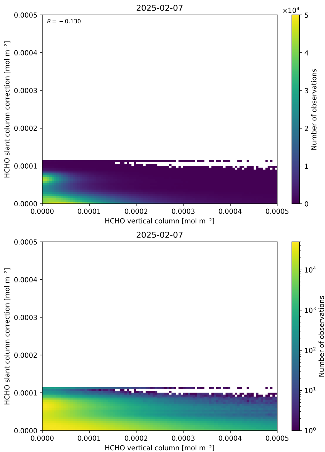
Figure 128: Scatter density plot of “HCHO vertical column” against “HCHO slant column correction” for 2025-02-06 to 2025-02-08.
