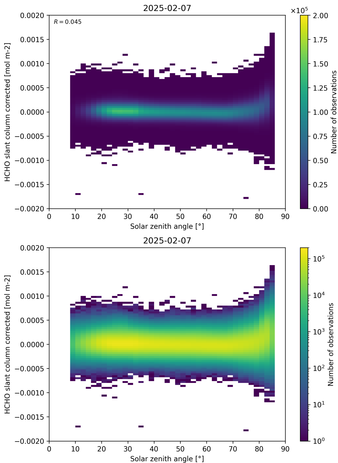
Figure 171: Scatter density plot of “Solar zenith angle” against “HCHO slant column corrected” for 2025-02-06 to 2025-02-08.
