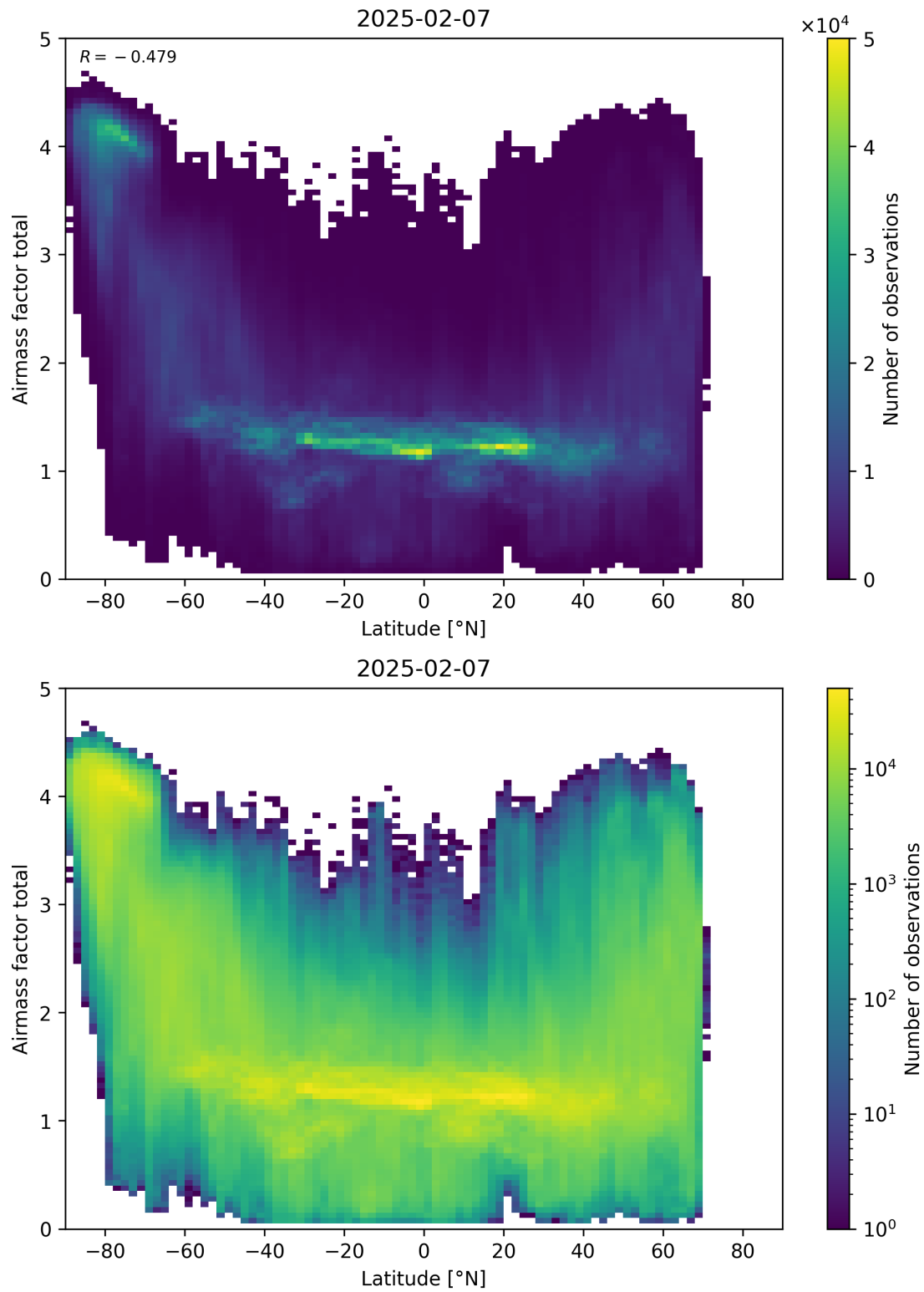
Figure 161: Scatter density plot of “Latitude” against “Airmass factor total” for 2025-02-06 to 2025-02-08.
