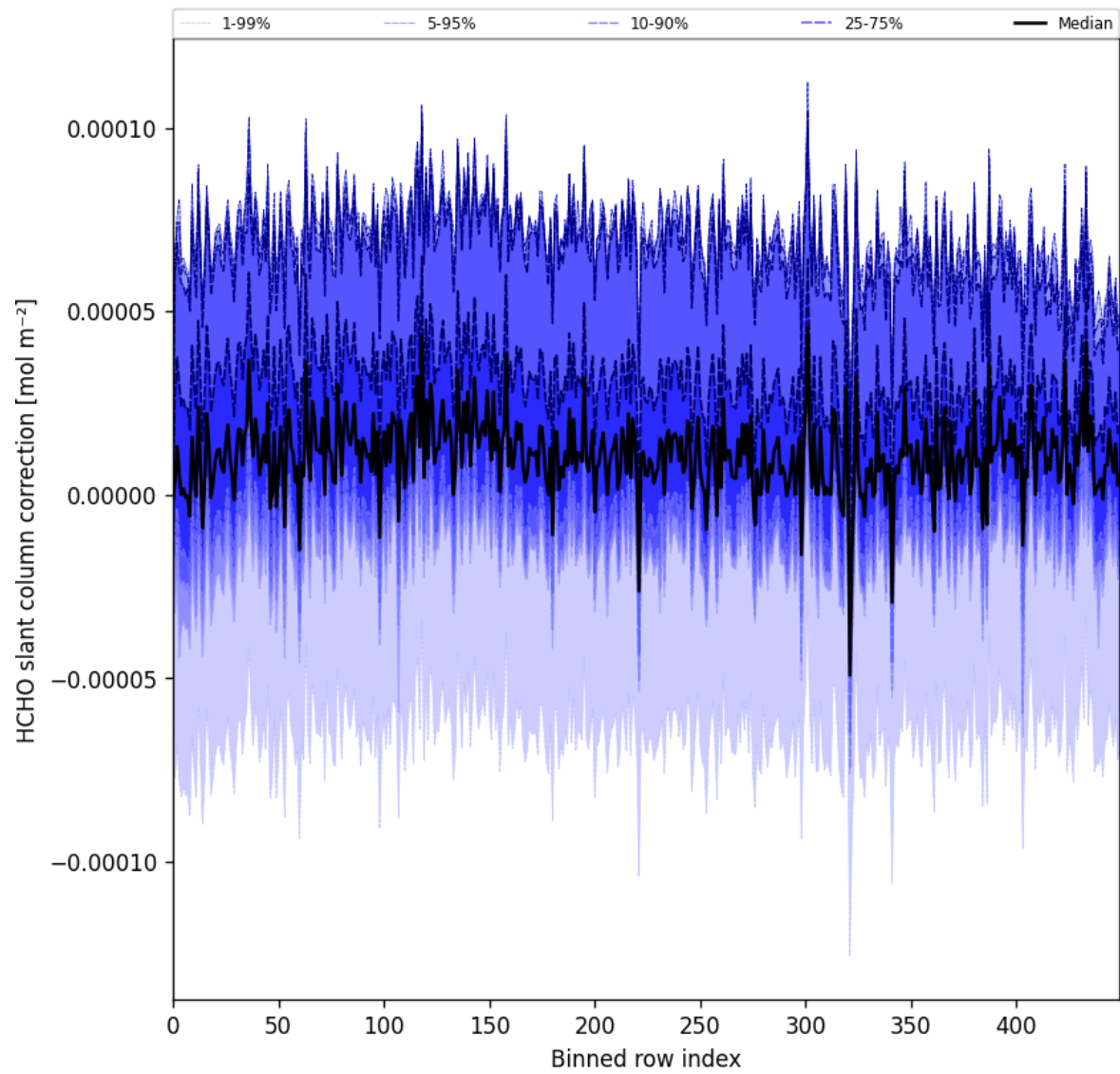
Figure 61: Along track statistics of “HCHO slant column correction” for 2025-02-08 to 2025-02-09
