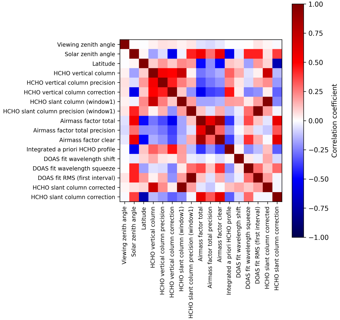
Figure 2: Map of correlation matrix for 2025-02-08 to 2025-02-09.
