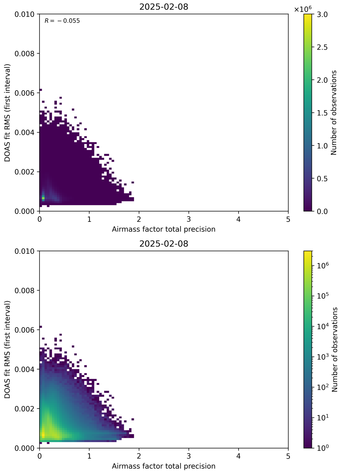
Figure 105: Scatter density plot of “Airmass factor total precision” against “DOAS fit RMS (first interval)” for 2025-02-08 to 2025-02-09.
