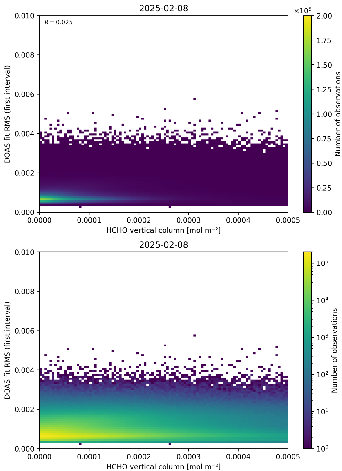
Figure 123: Scatter density plot of “HCHO vertical column” against “DOAS fit RMS (first interval)” for 2025-02-08 to 2025-02-09.
