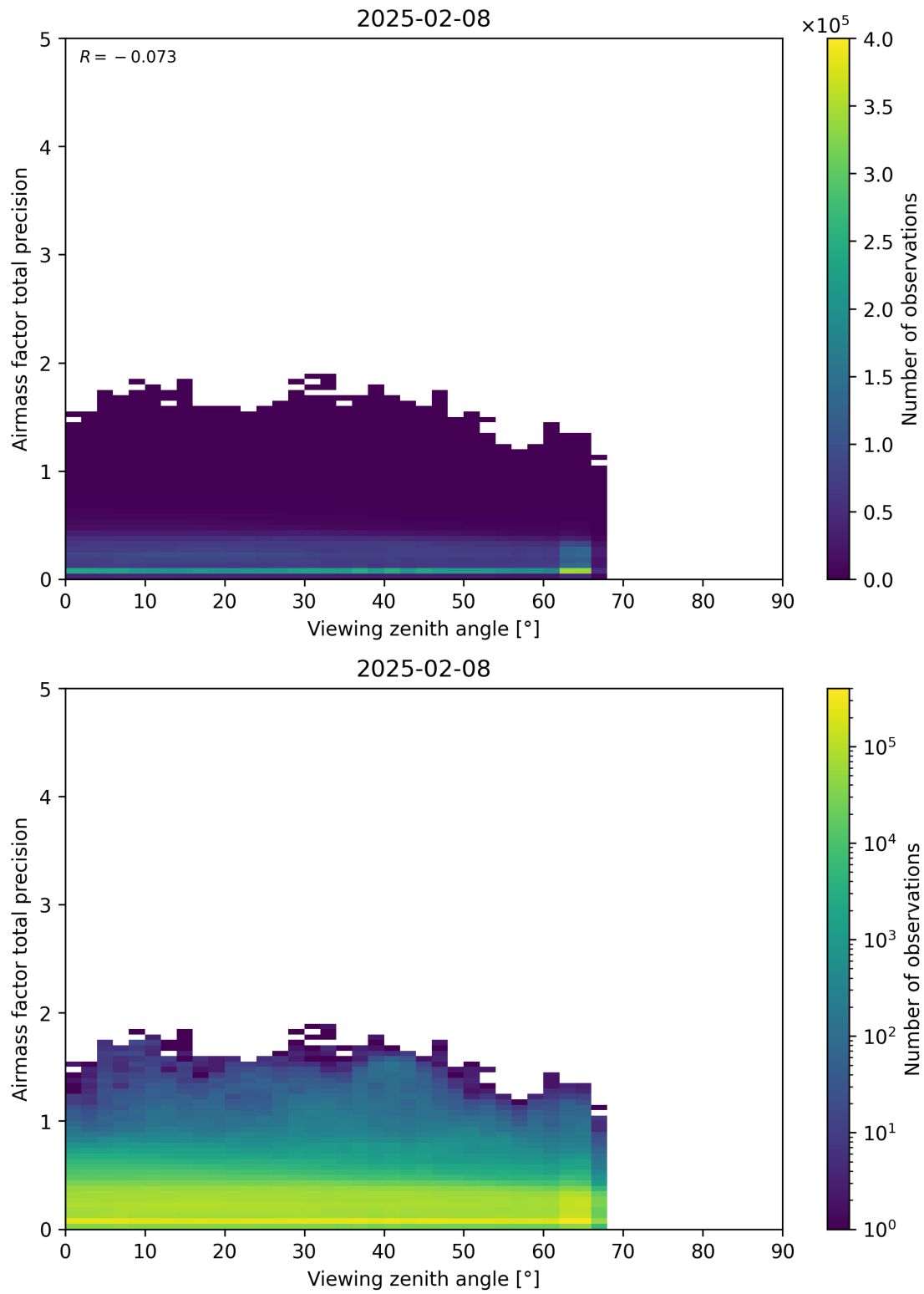
Figure 191: Scatter density plot of “Viewing zenith angle” against “Airmass factor total precision” for 2025-02-08 to 2025-02-09.
