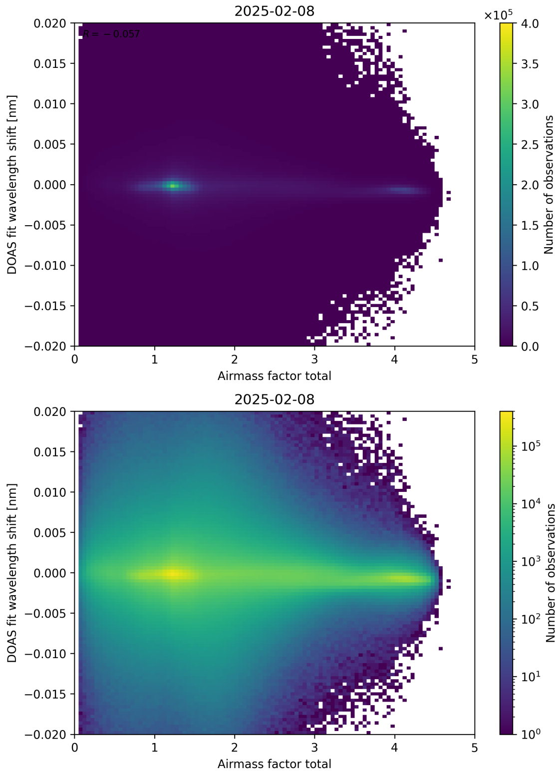
Figure 98: Scatter density plot of “Airmass factor total” against “DOAS fit wavelength shift” for 2025-02-08 to 2025-02-09.
