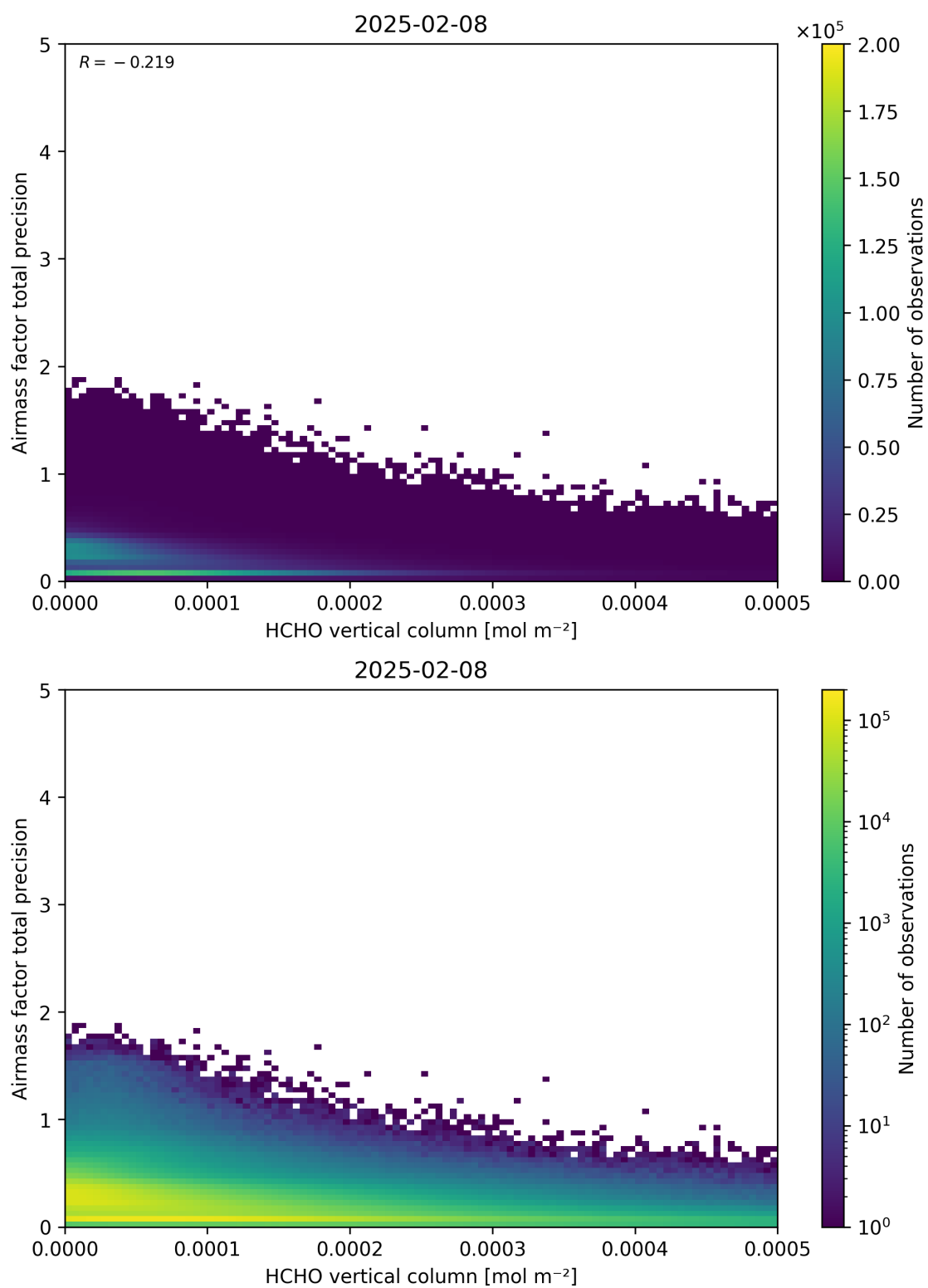
Figure 132: Scatter density plot of “HCHO vertical column” against “Airmass factor total precision” for 2025-02-08 to 2025-02-09.
