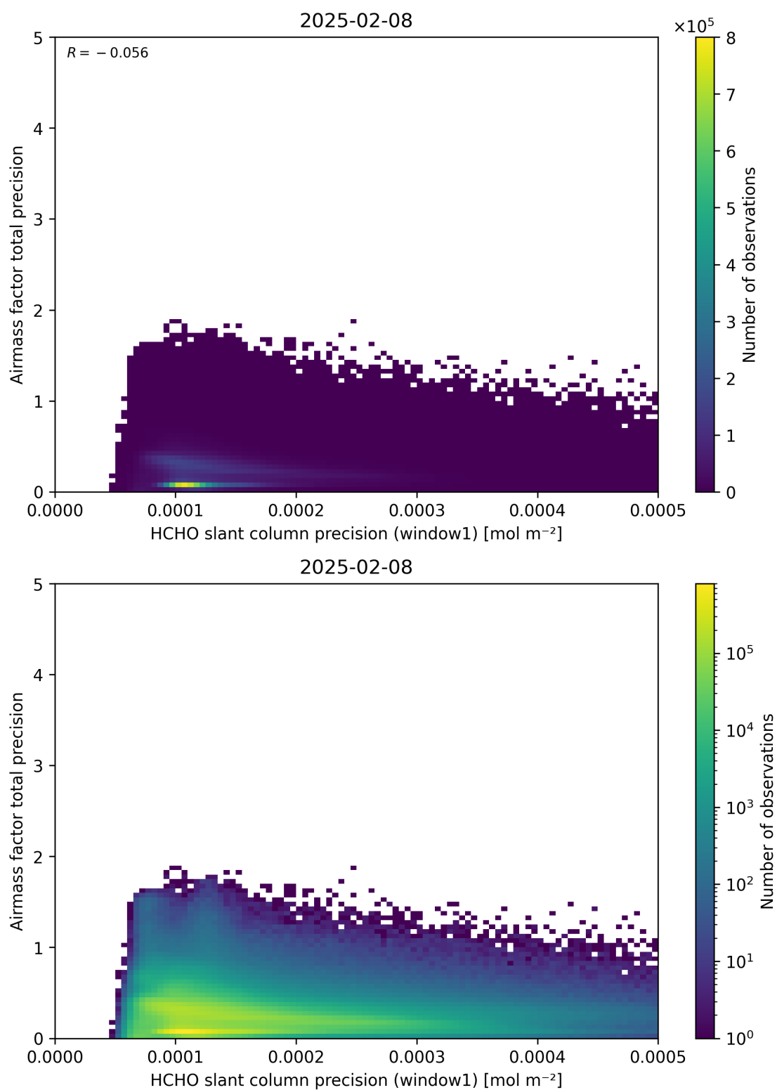
Figure 95: Scatter density plot of “HCHO slant column precision (window1)” against “Airmass factor total precision” for 2025-02-08 to 2025-02-09.
