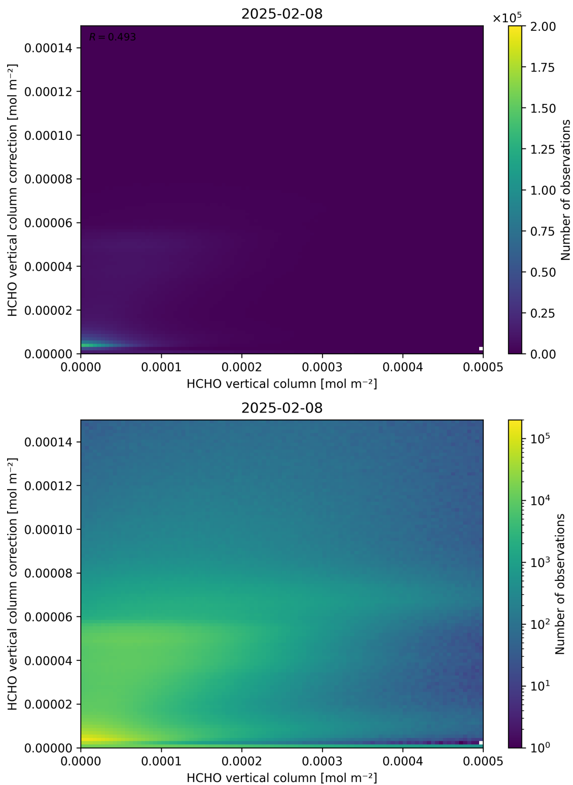
Figure 133: Scatter density plot of “HCHO vertical column” against “HCHO vertical column correction” for 2025-02-08 to 2025-02-09.
