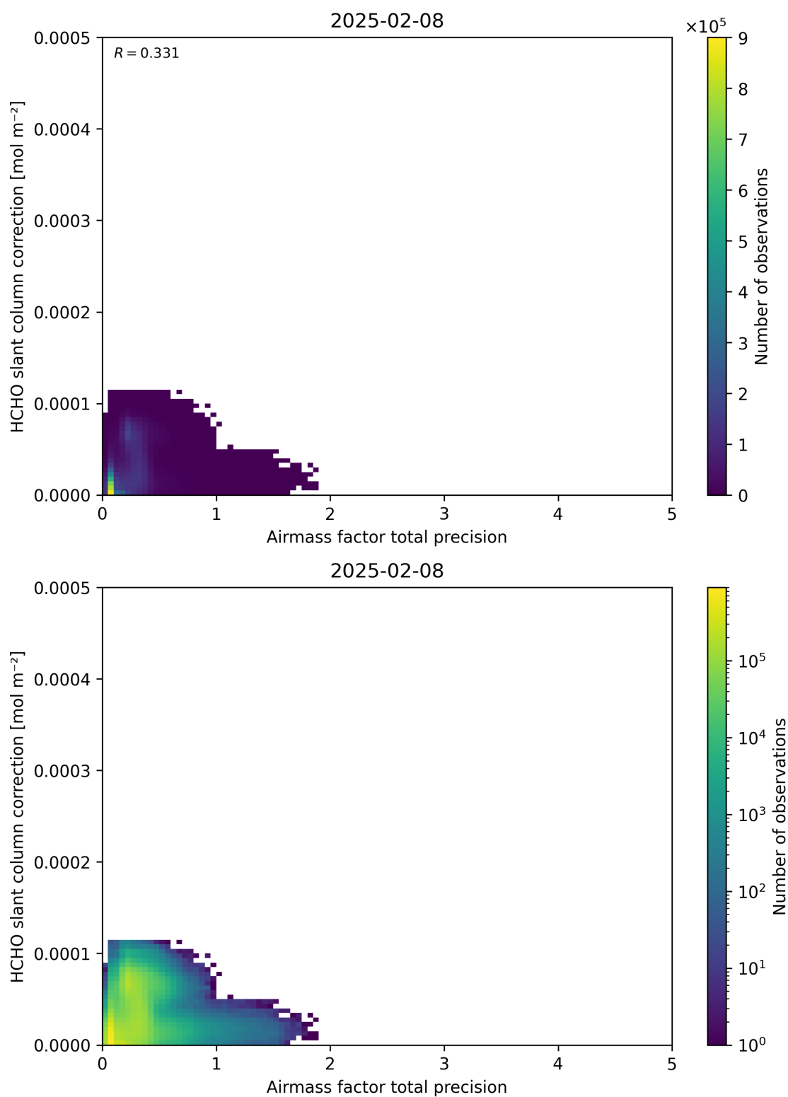
Figure 110: Scatter density plot of “Airmass factor total precision” against “HCHO slant column correction” for 2025-02-08 to 2025-02-09.
