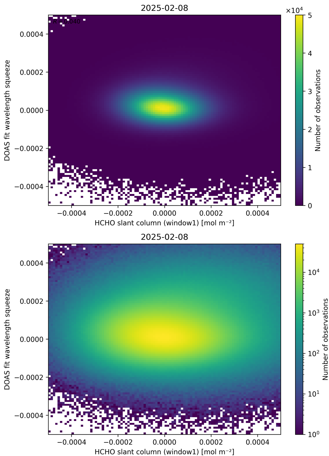
Figure 80: Scatter density plot of “HCHO slant column (window1)” against “DOAS fit wavelength squeeze” for 2025-02-08 to 2025-02-09.
