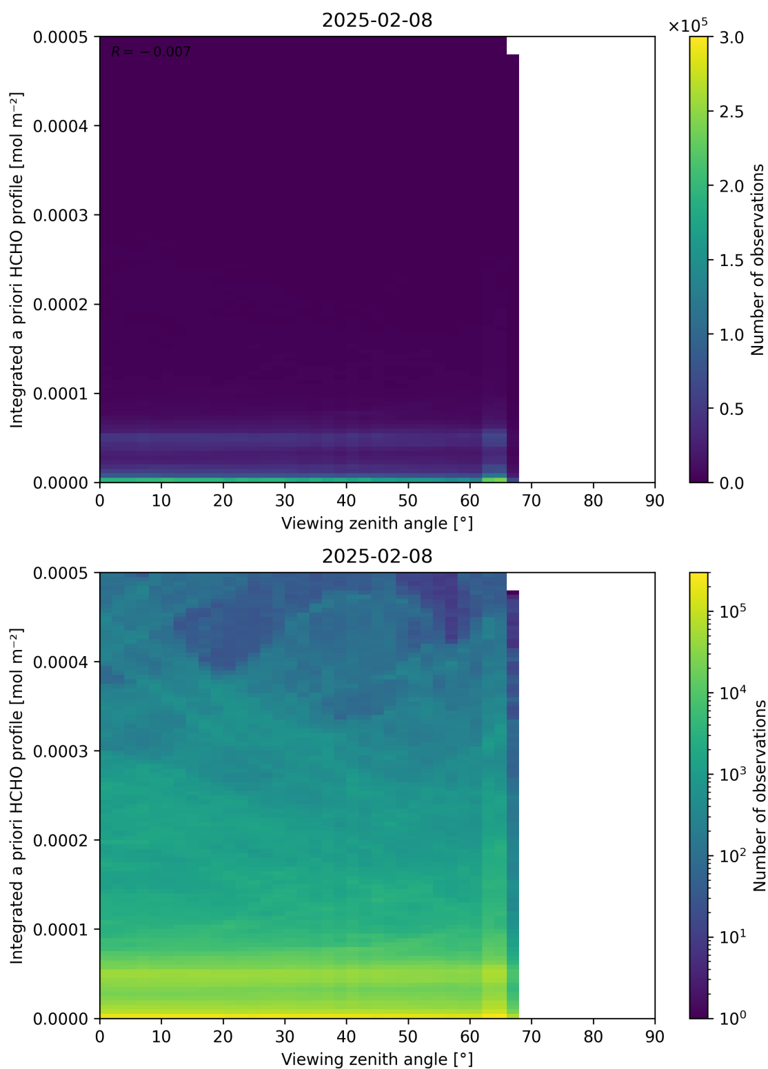
Figure 195: Scatter density plot of “Viewing zenith angle” against “Integrated a priori HCHO profile” for 2025-02-08 to 2025-02-09.
