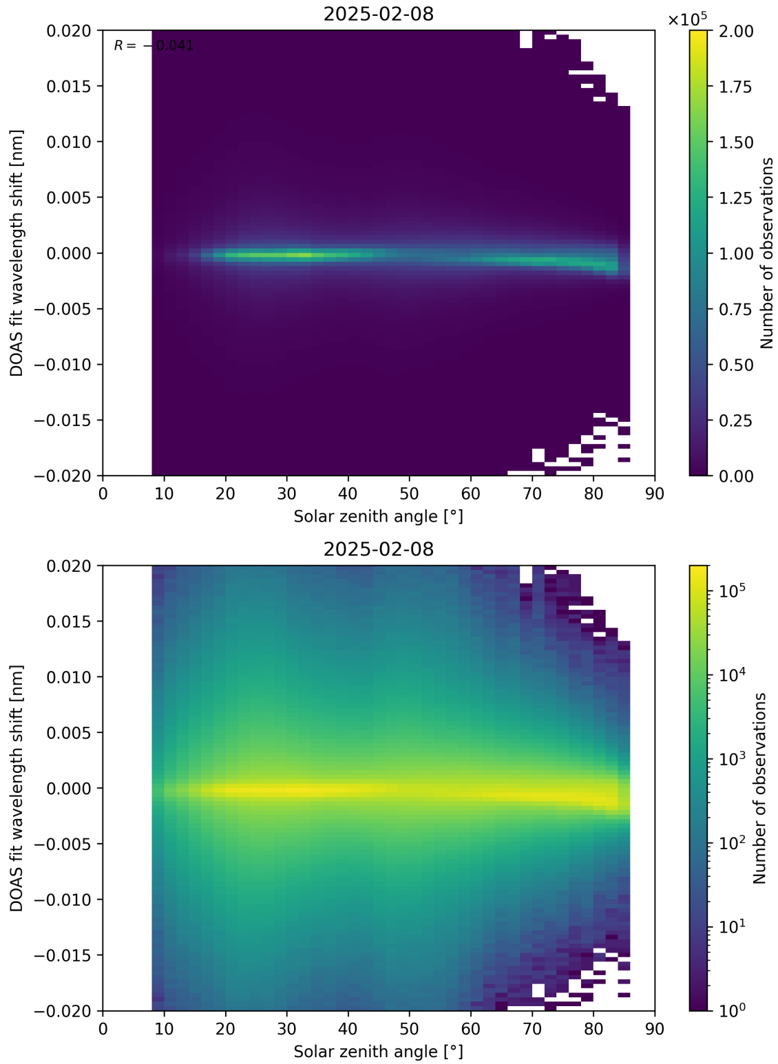
Figure 168: Scatter density plot of “Solar zenith angle” against “DOAS fit wavelength shift” for 2025-02-08 to 2025-02-09.
