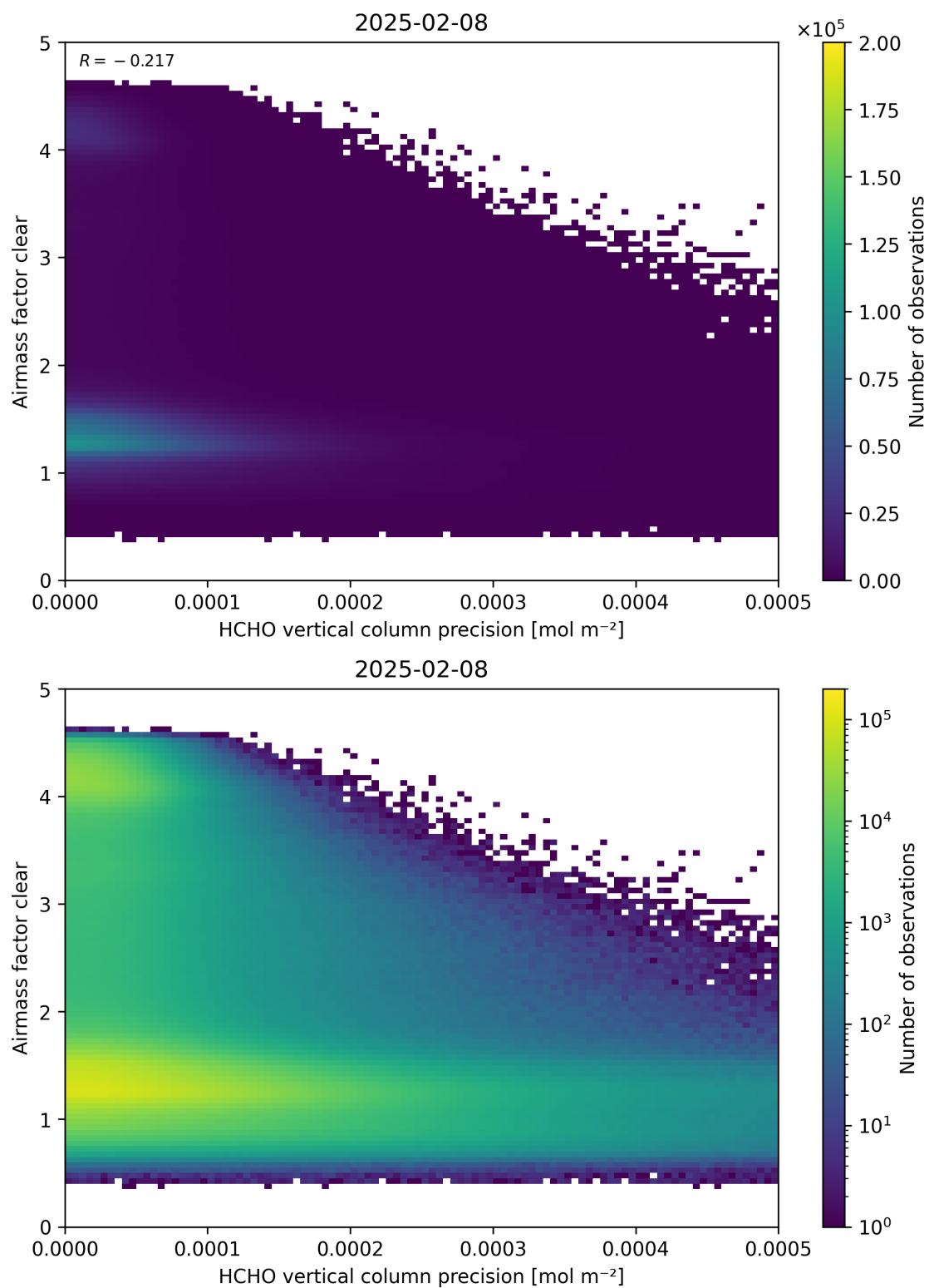
Figure 139: Scatter density plot of “HCHO vertical column precision” against “Airmass factor clear” for 2025-02-08 to 2025-02-09.
