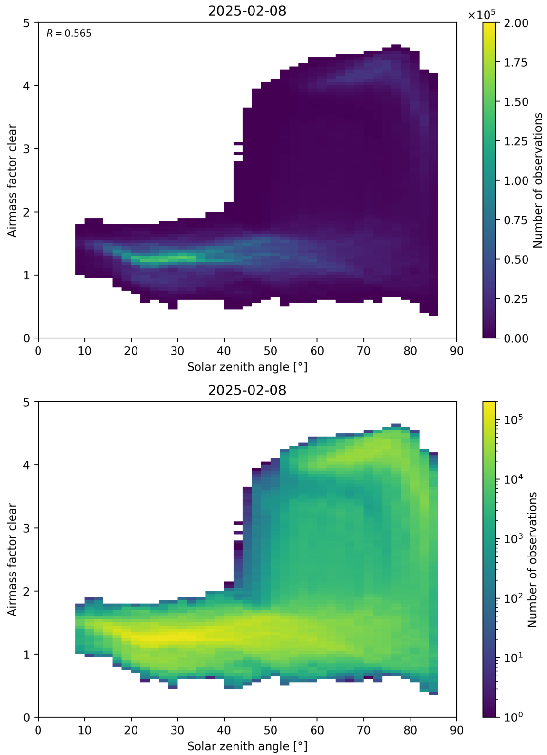
Figure 170: Scatter density plot of “Solar zenith angle” against “Airmass factor clear” for 2025-02-08 to 2025-02-09.
