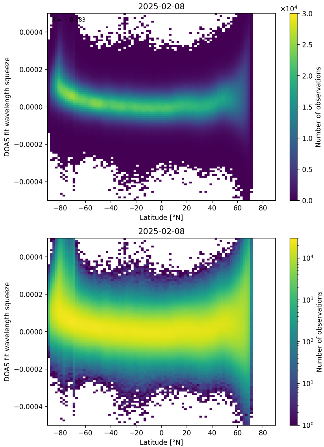
Figure 155: Scatter density plot of “Latitude” against “DOAS fit wavelength squeeze” for 2025-02-08 to 2025-02-09.
