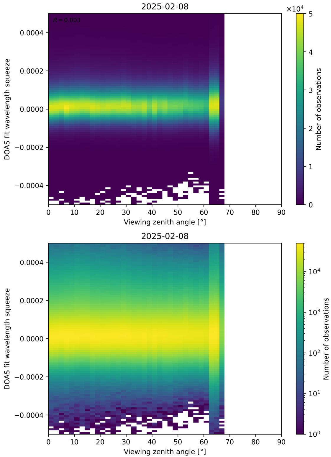
Figure 184: Scatter density plot of “Viewing zenith angle” against “DOAS fit wavelength squeeze” for 2025-02-08 to 2025-02-09.
