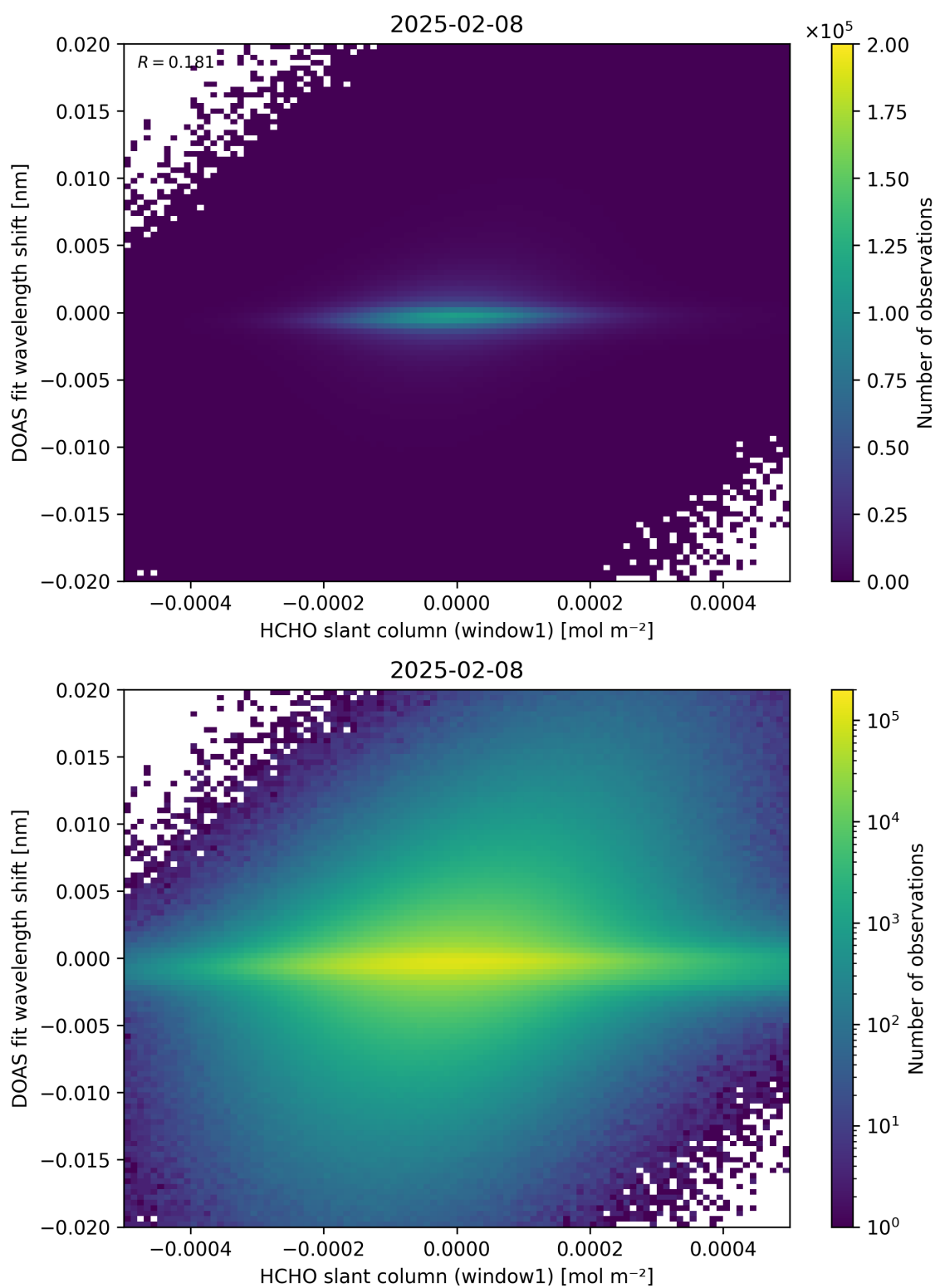
Figure 79: Scatter density plot of “HCHO slant column (window1)” against “DOAS fit wavelength shift” for 2025-02-08 to 2025-02-09.
