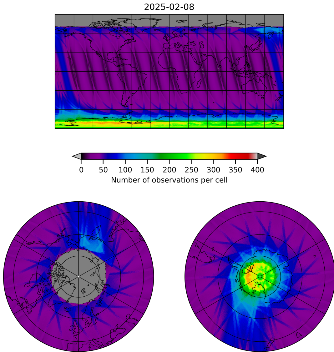
Figure 19: Map of the number of observations for 2025-02-08 to 2025-02-09
