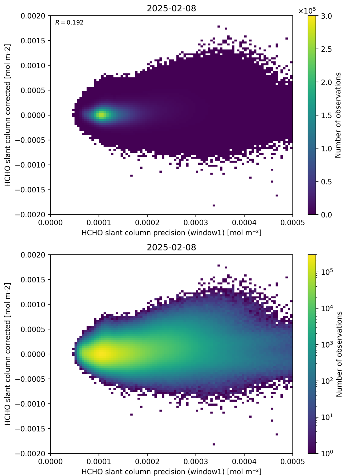
Figure 92: Scatter density plot of “HCHO slant column precision (window1)” against “HCHO slant column corrected” for 2025-02-08 to 2025-02-09.
