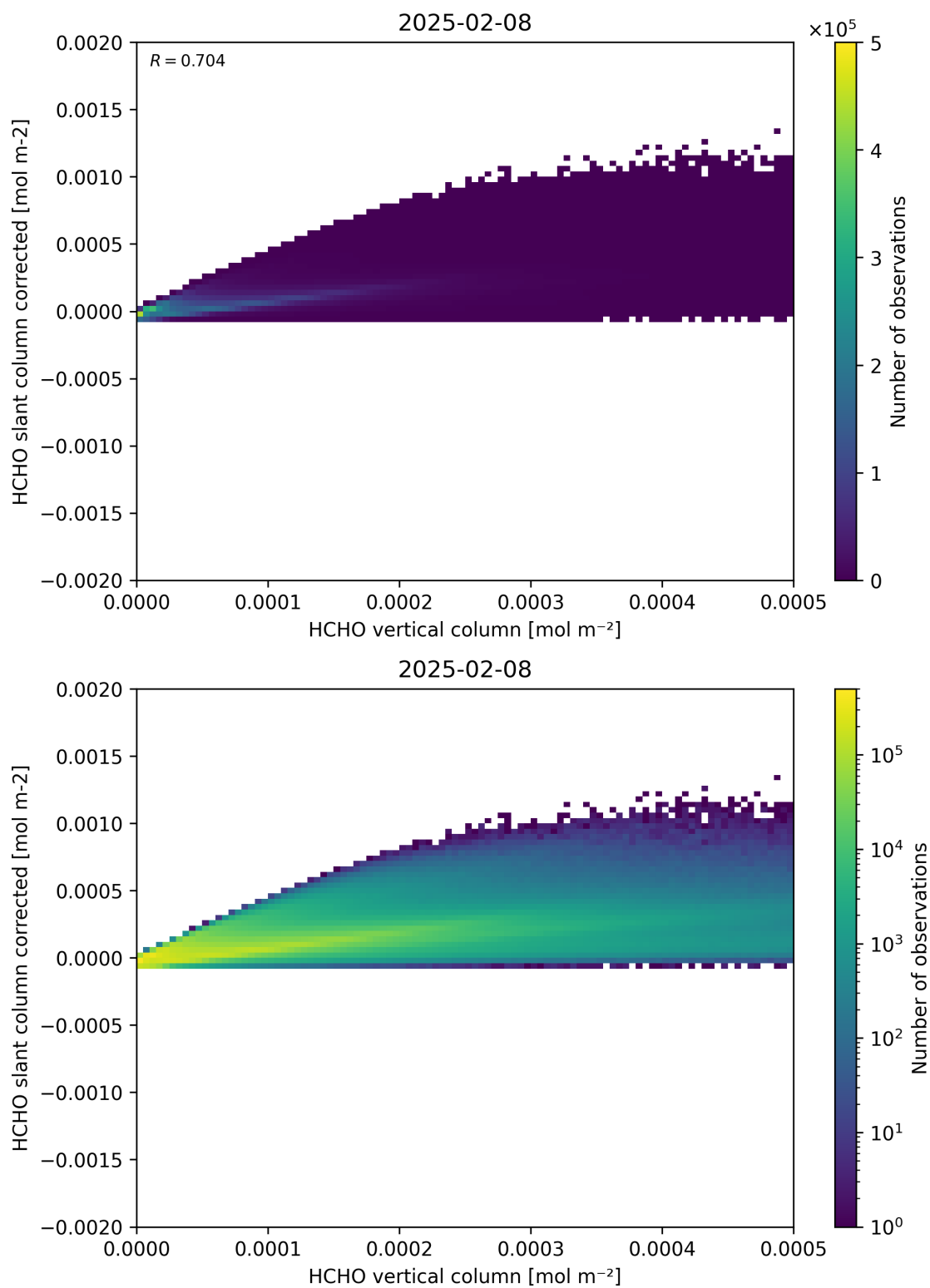
Figure 127: Scatter density plot of “HCHO vertical column” against “HCHO slant column corrected” for 2025-02-08 to 2025-02-09.
