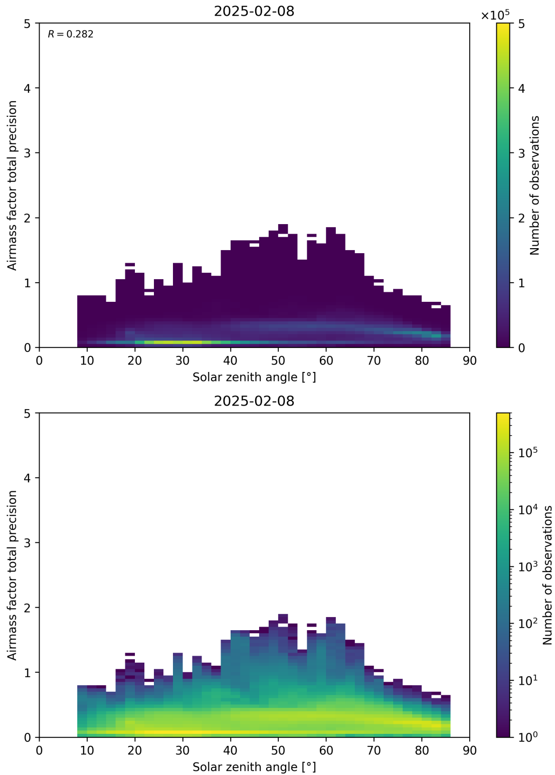
Figure 176: Scatter density plot of “Solar zenith angle” against “Airmass factor total precision” for 2025-02-08 to 2025-02-09.
