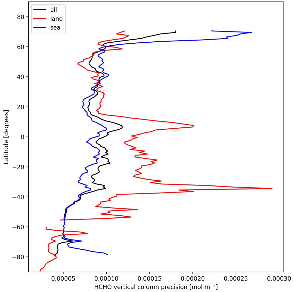
Figure 22: Zonal average of “HCHO vertical column precision” for 2025-02-08 to 2025-02-09.
