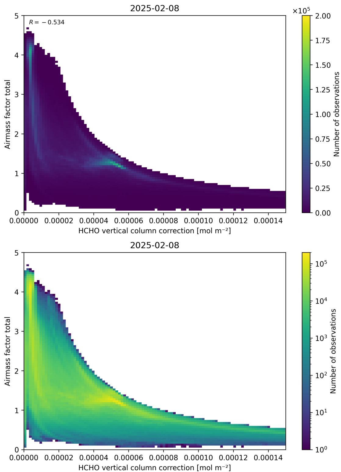
Figure 120: Scatter density plot of “HCHO vertical column correction” against “Airmass factor total” for 2025-02-08 to 2025-02-09.
