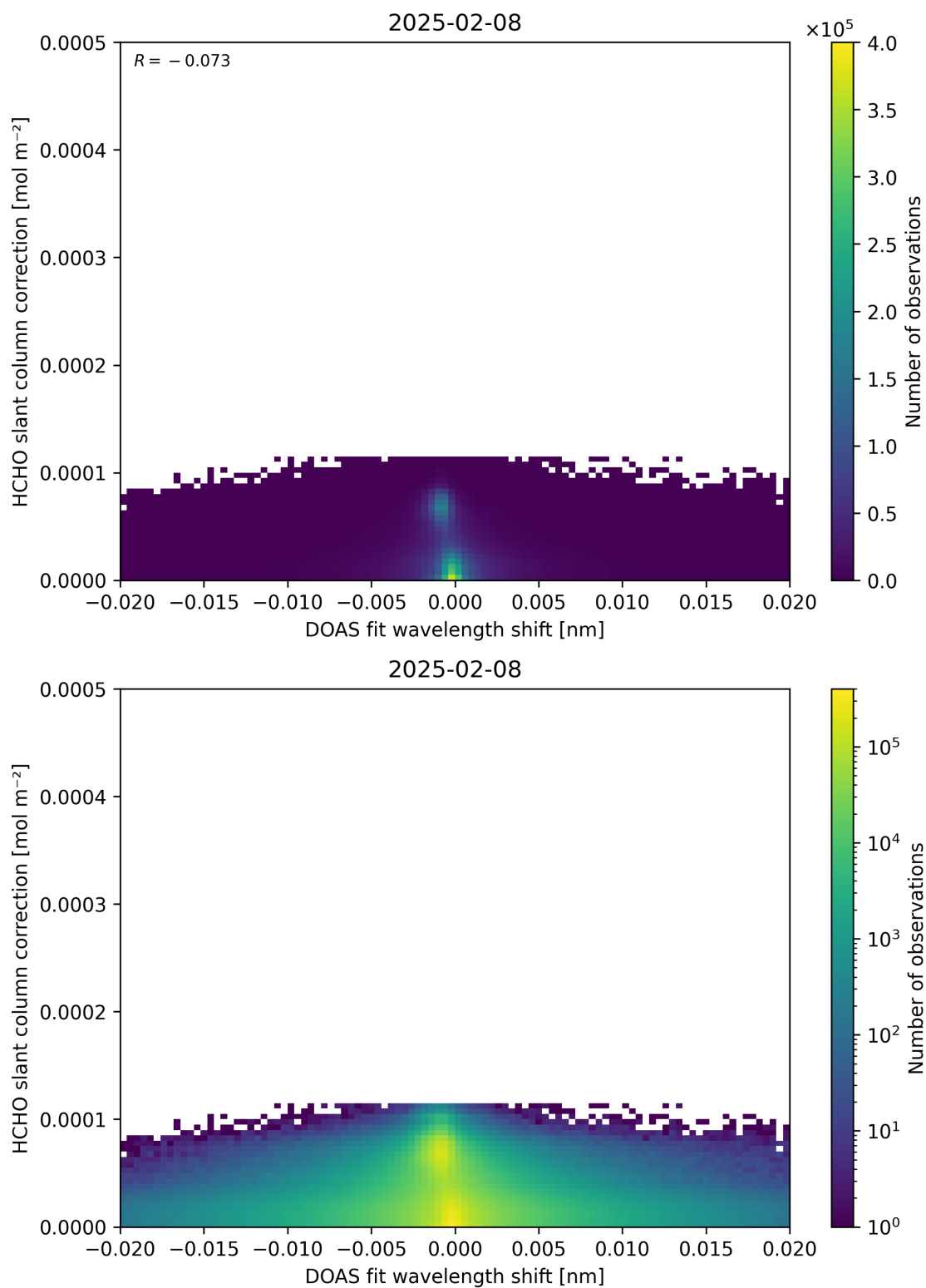
Figure 67: Scatter density plot of “DOAS fit wavelength shift” against “HCHO slant column correction” for 2025-02-08 to 2025-02-09.
