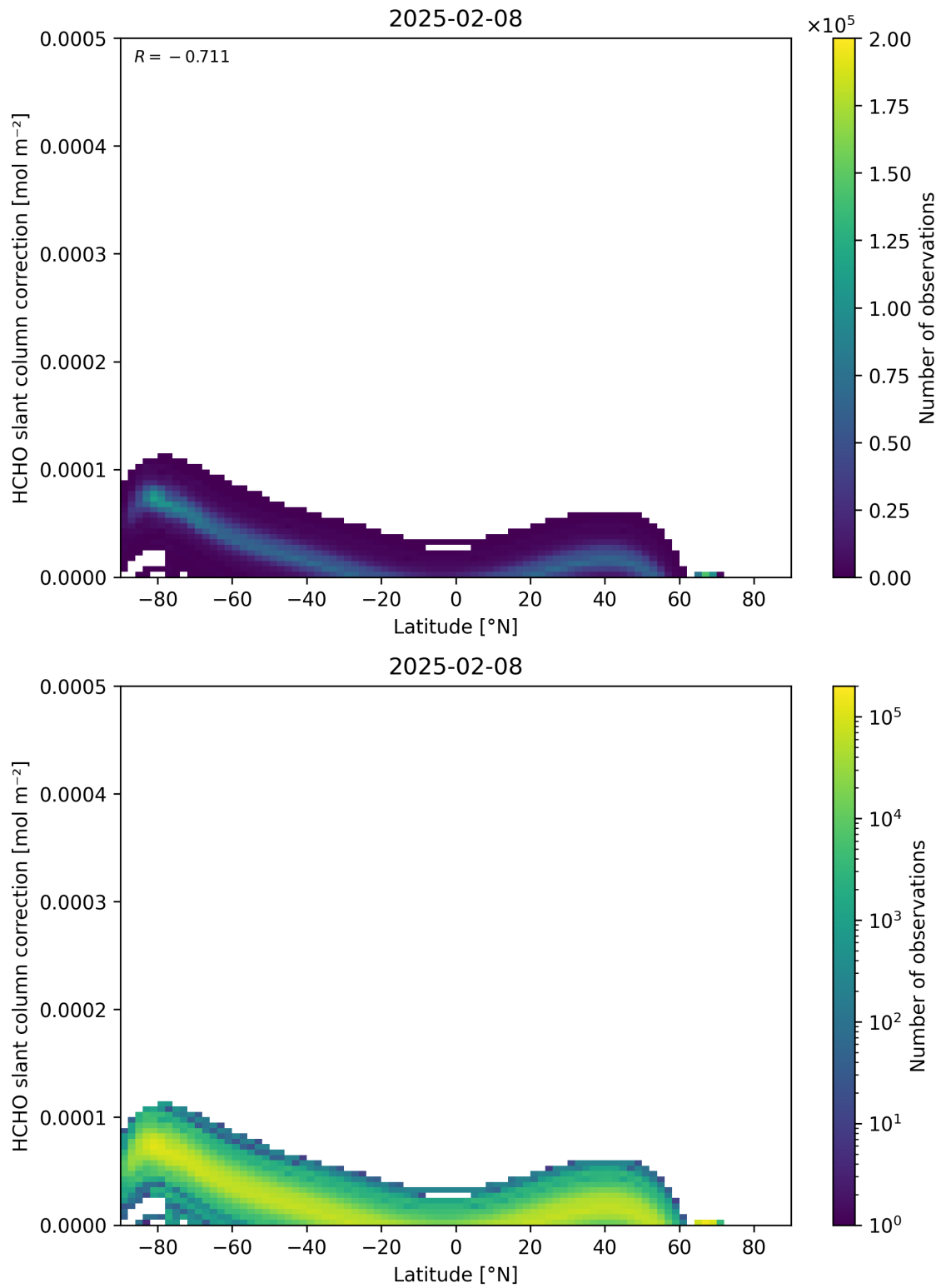
Figure 158: Scatter density plot of “Latitude” against “HCHO slant column correction” for 2025-02-08 to 2025-02-09.
