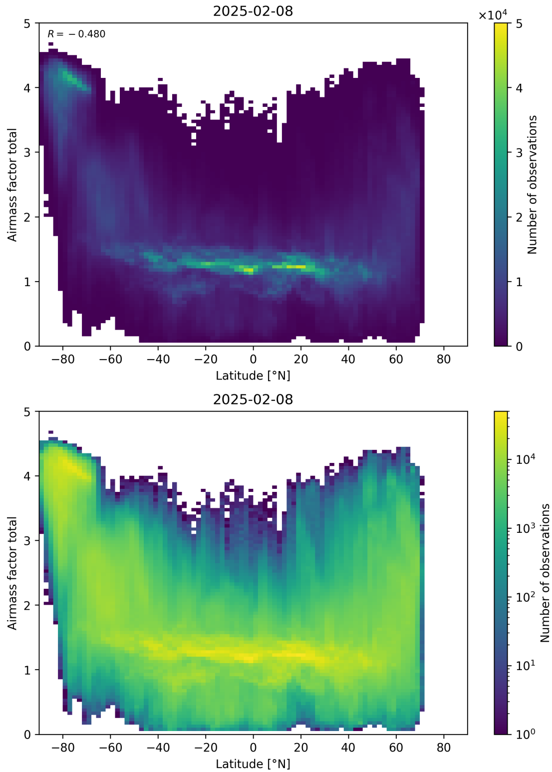
Figure 161: Scatter density plot of “Latitude” against “Airmass factor total” for 2025-02-08 to 2025-02-09.
