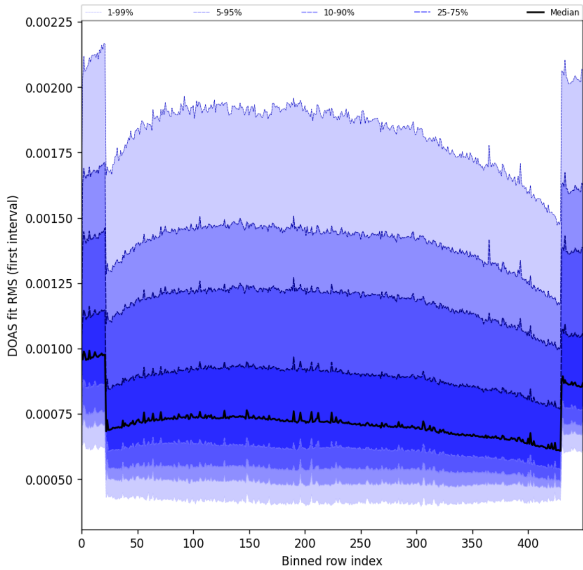
Figure 60: Along track statistics of “DOAS fit RMS (first interval)” for 2025-02-08 to 2025-02-09
