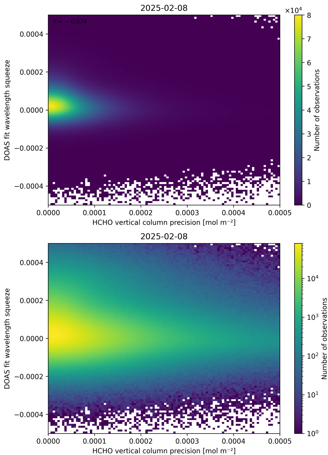
Figure 138: Scatter density plot of “HCHO vertical column precision” against “DOAS fit wavelength squeeze” for 2025-02-08 to 2025-02-09.
