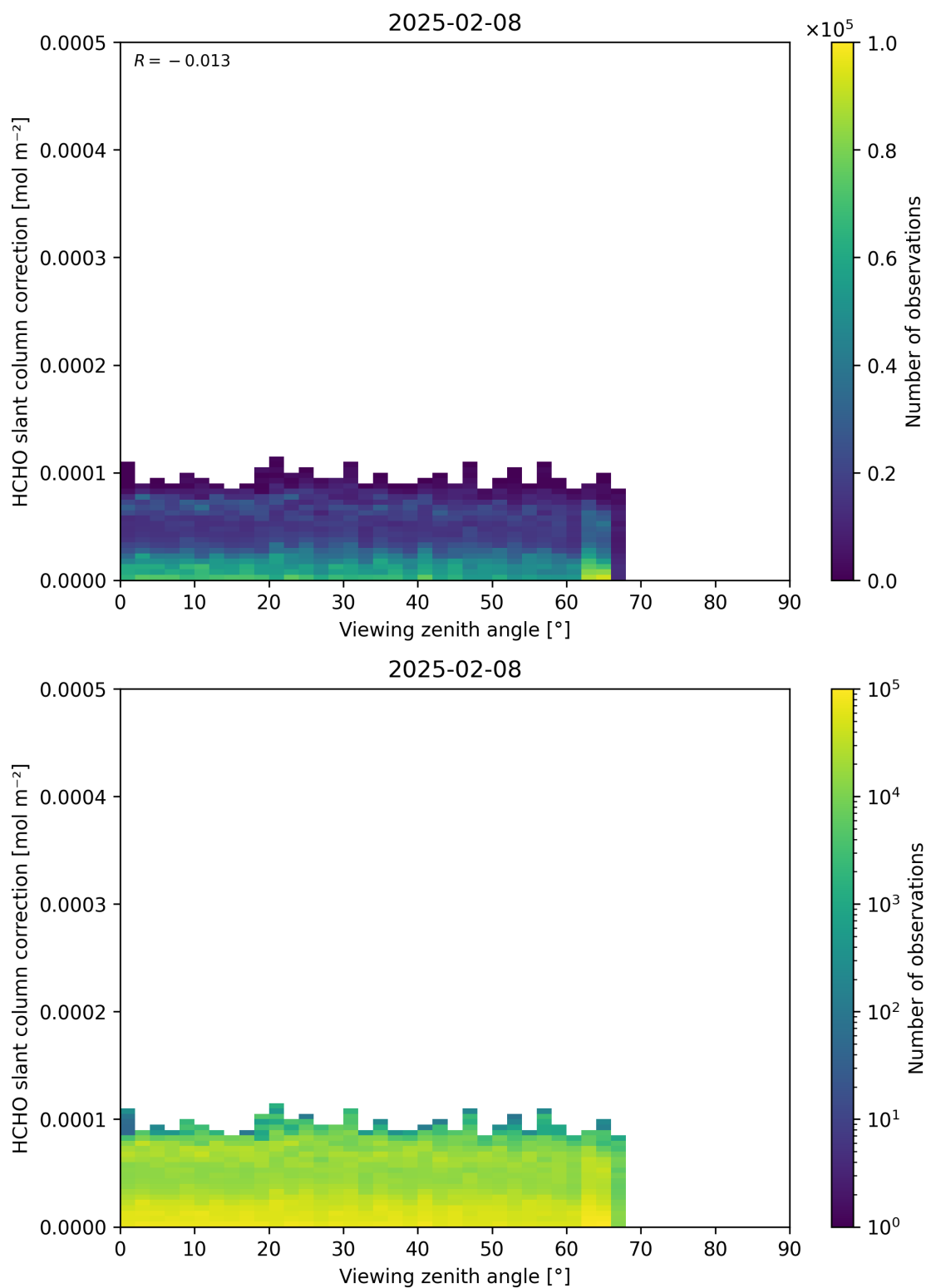
Figure 187: Scatter density plot of “Viewing zenith angle” against “HCHO slant column correction” for 2025-02-08 to 2025-02-09.
