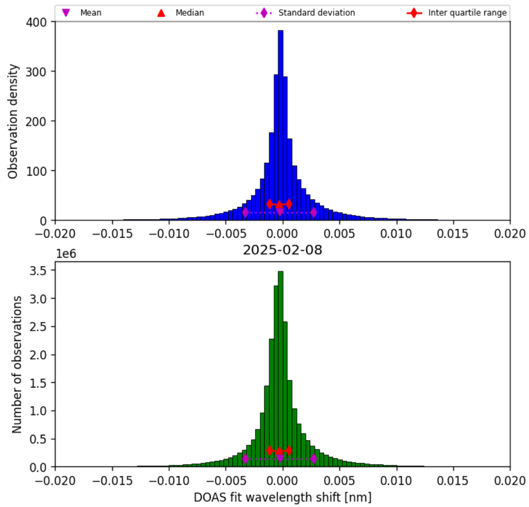
Figure 44: Histogram of “DOAS fit wavelength shift” for 2025-02-08 to 2025-02-09
