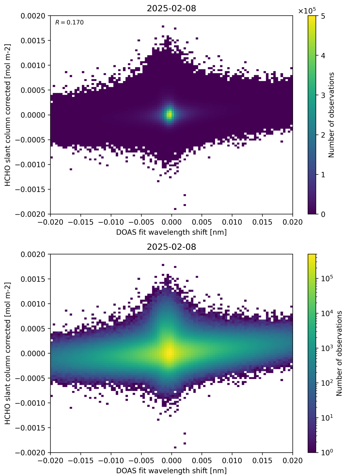
Figure 66: Scatter density plot of “DOAS fit wavelength shift” against “HCHO slant column corrected” for 2025-02-08 to 2025-02-09.
