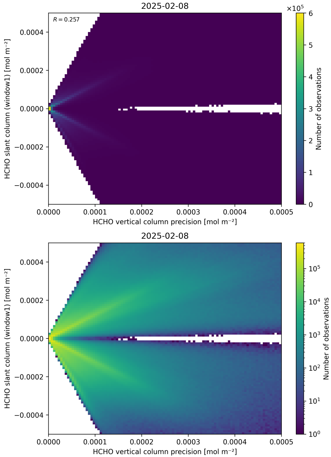
Figure 142: Scatter density plot of “HCHO vertical column precision” against “HCHO slant column (window1)” for 2025-02-08 to 2025-02-09.
