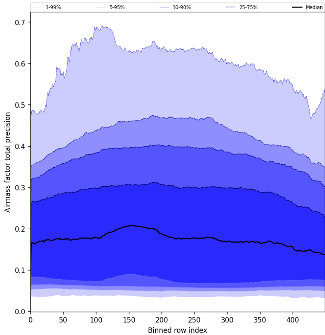
Figure 55: Along track statistics of “Airmass factor total precision” for 2025-02-08 to 2025-02-09
