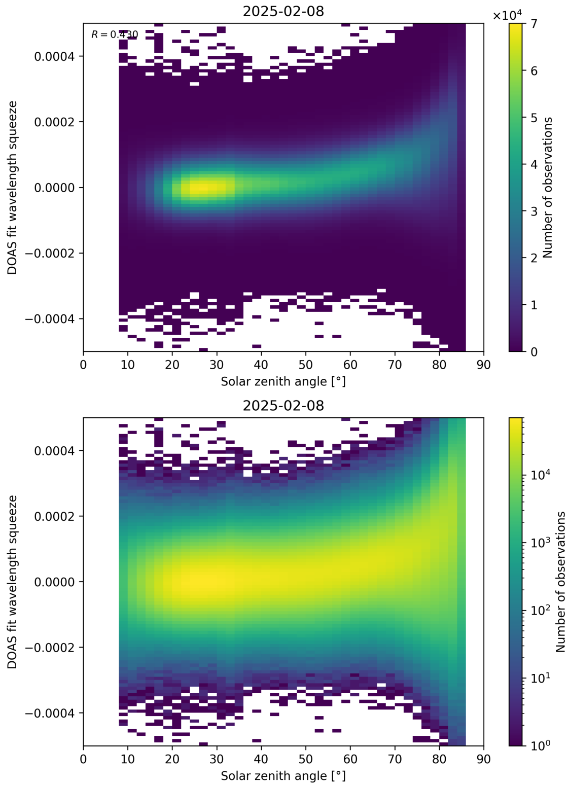
Figure 169: Scatter density plot of “Solar zenith angle” against “DOAS fit wavelength squeeze” for 2025-02-08 to 2025-02-09.
