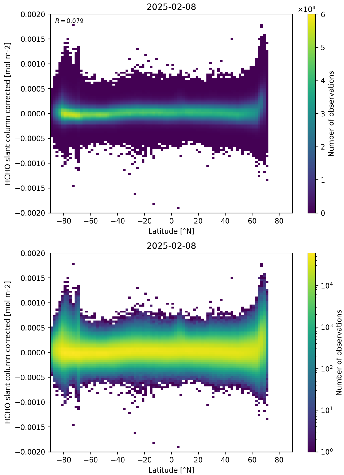
Figure 157: Scatter density plot of “Latitude” against “HCHO slant column corrected” for 2025-02-08 to 2025-02-09.
