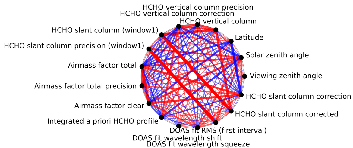
Figure 1: Map of correlation graph for 2025-02-08 to 2025-02-09.
