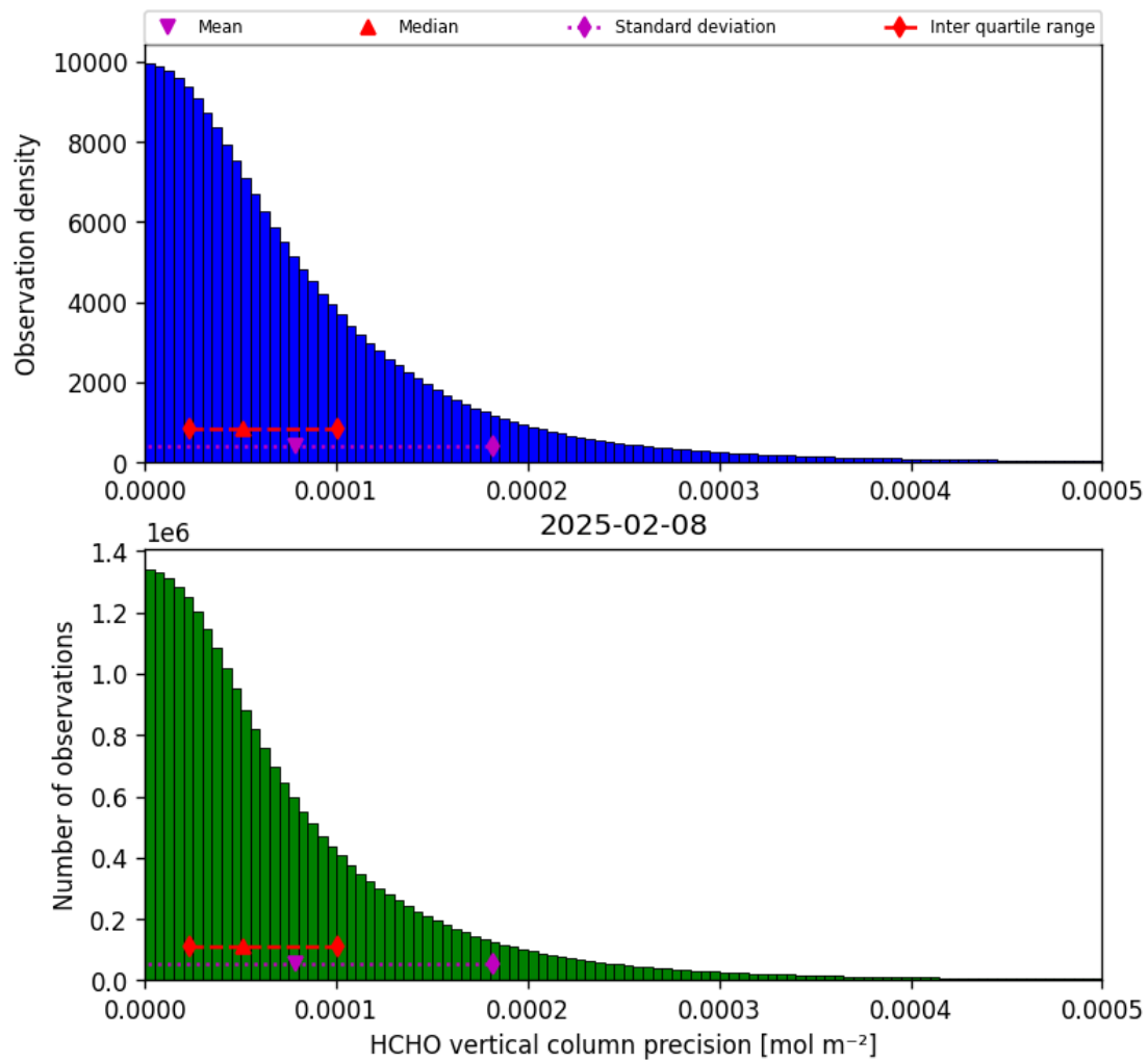
Figure 36: Histogram of “HCHO vertical column precision” for 2025-02-08 to 2025-02-09
