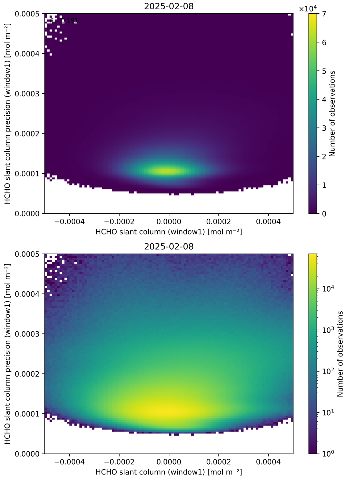
Figure 84: Scatter density plot of “HCHO slant column (window1)” against “HCHO slant column precision (window1)” for 2025-02-08 to 2025-02-09.
