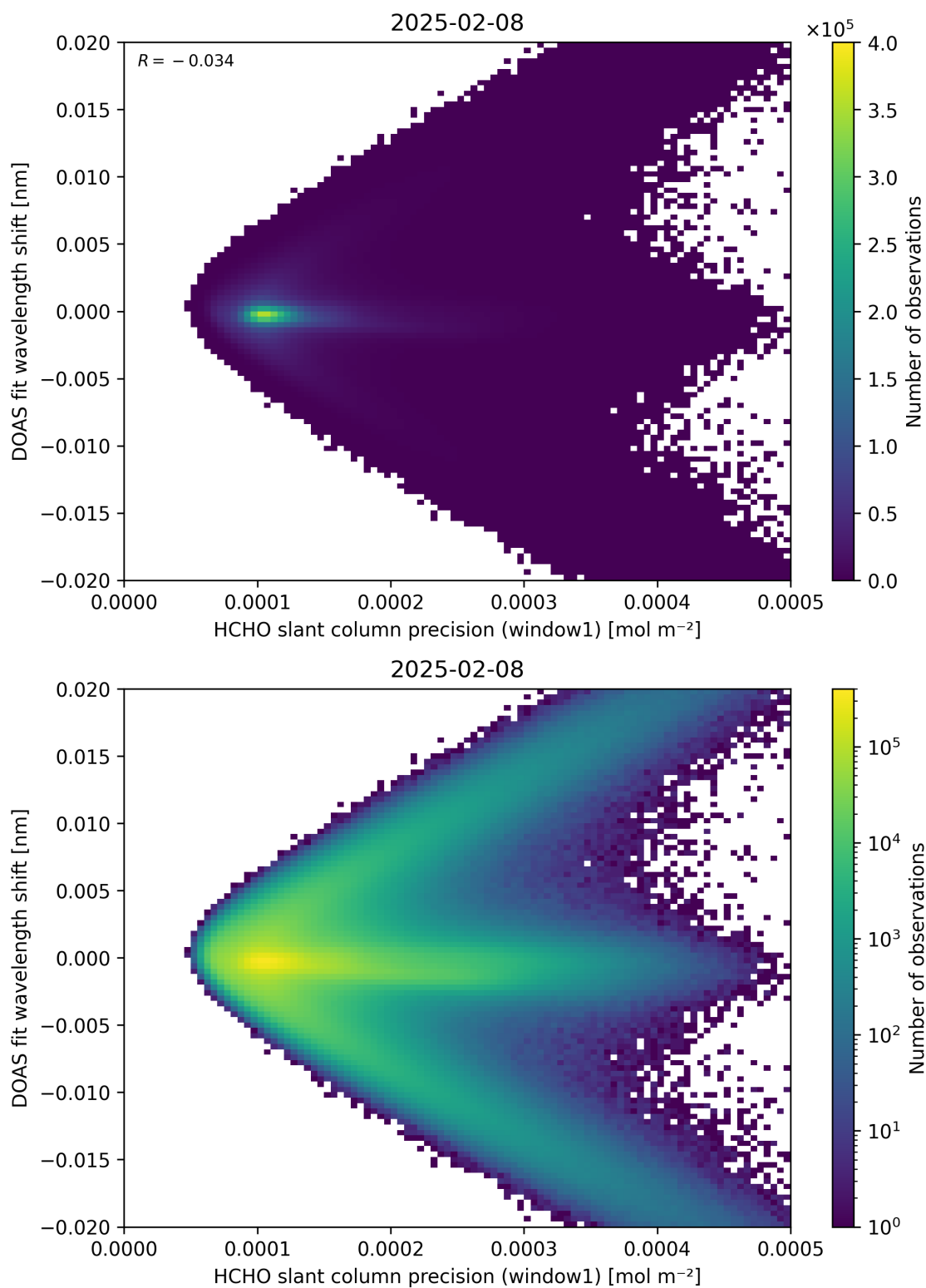
Figure 89: Scatter density plot of “HCHO slant column precision (window1)” against “DOAS fit wavelength shift” for 2025-02-08 to 2025-02-09.
