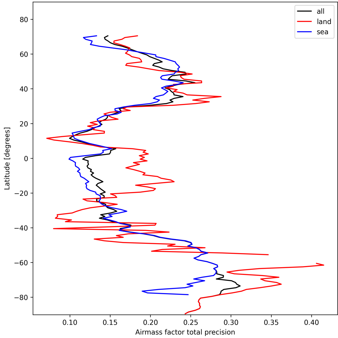
Figure 27: Zonal average of “Airmass factor total precision” for 2025-02-08 to 2025-02-09.
