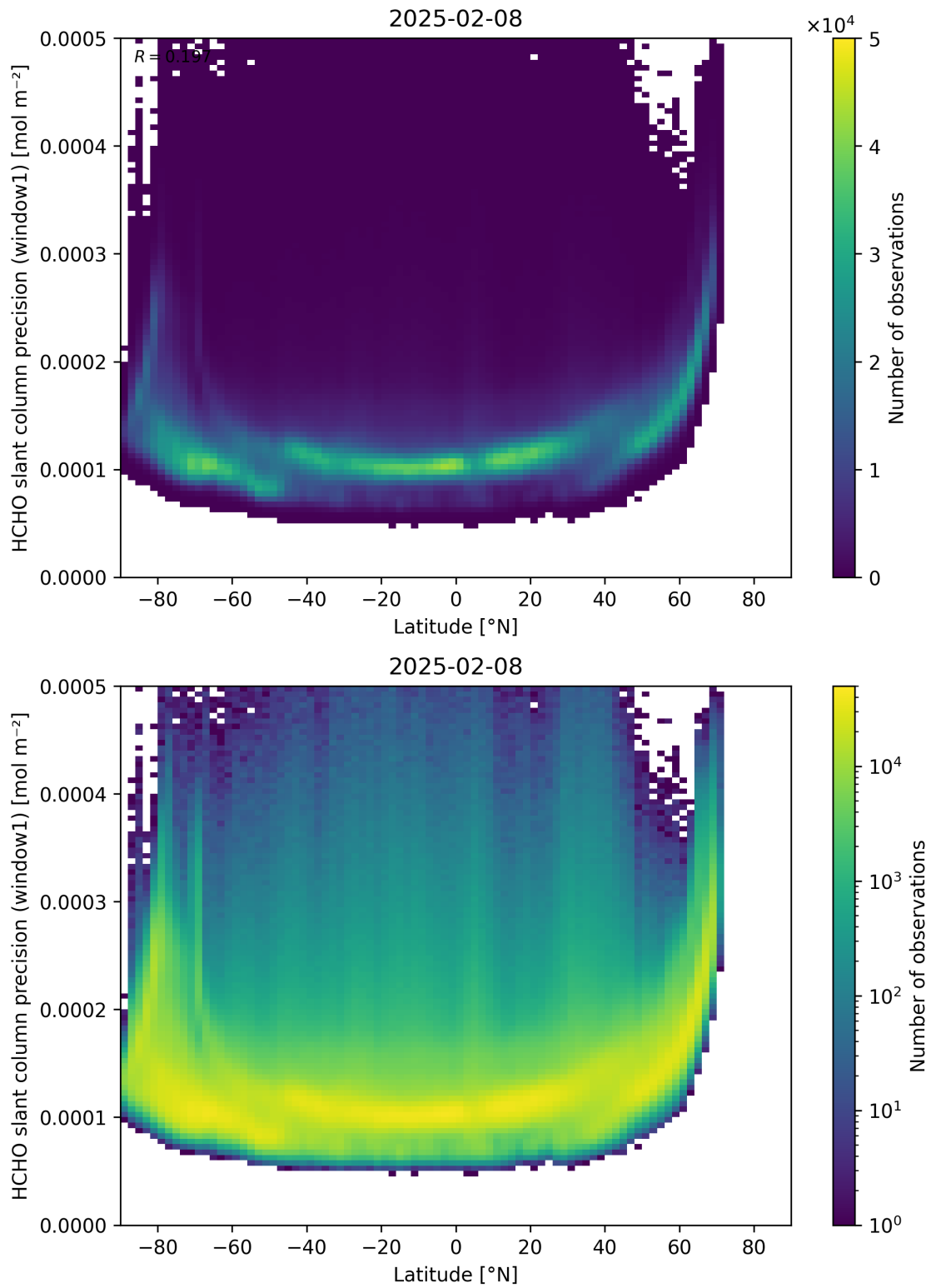
Figure 160: Scatter density plot of “Latitude” against “HCHO slant column precision (window1)” for 2025-02-08 to 2025-02-09.
