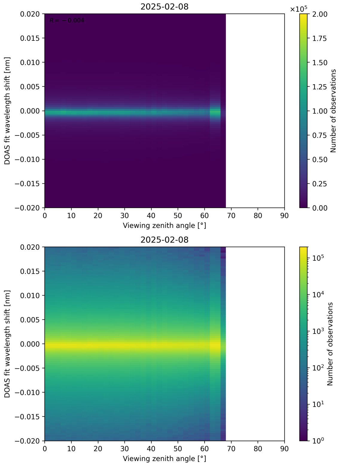
Figure 183: Scatter density plot of “Viewing zenith angle” against “DOAS fit wavelength shift” for 2025-02-08 to 2025-02-09.
