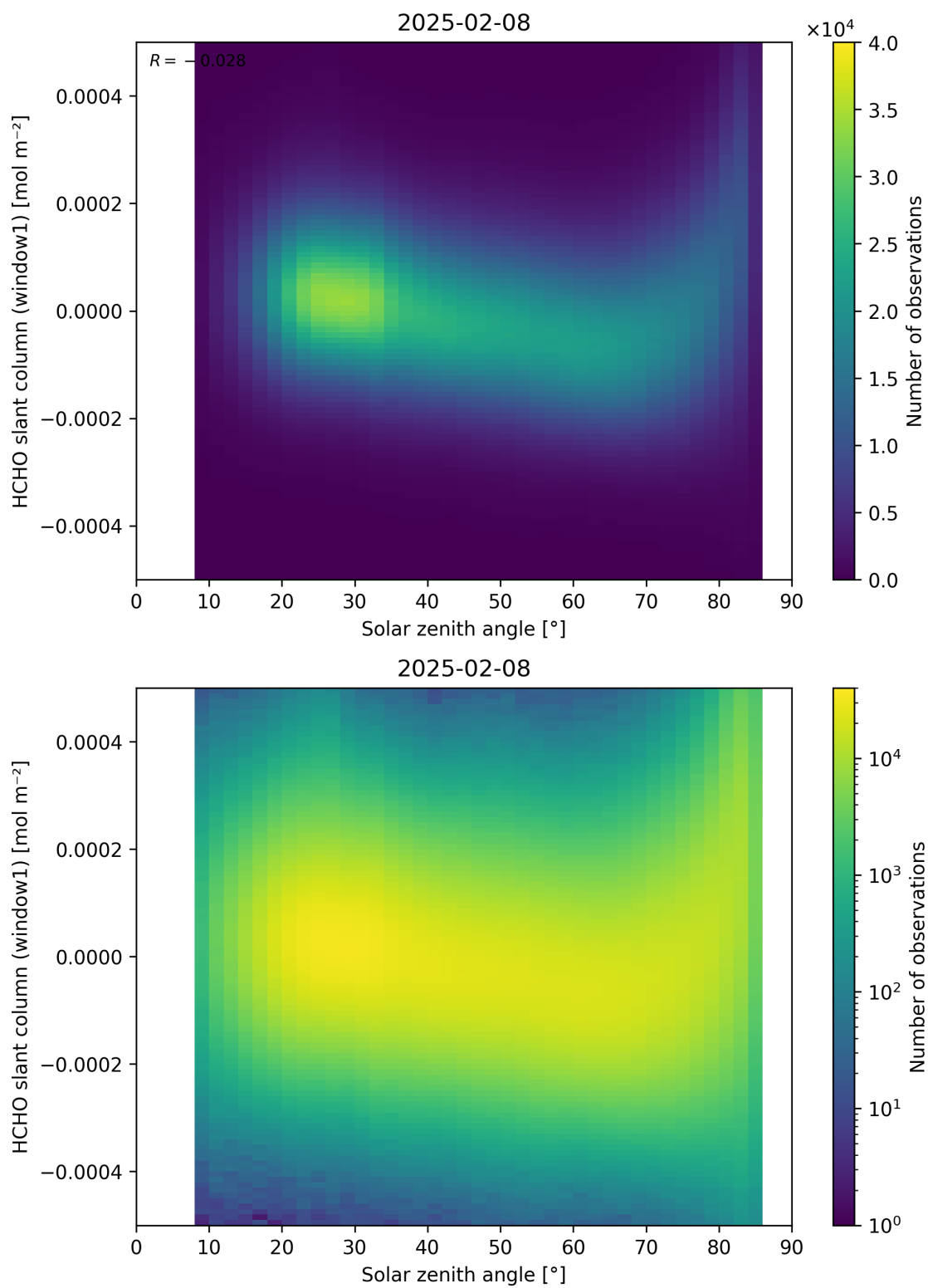
Figure 173: Scatter density plot of “Solar zenith angle” against “HCHO slant column (window1)” for 2025-02-08 to 2025-02-09.
