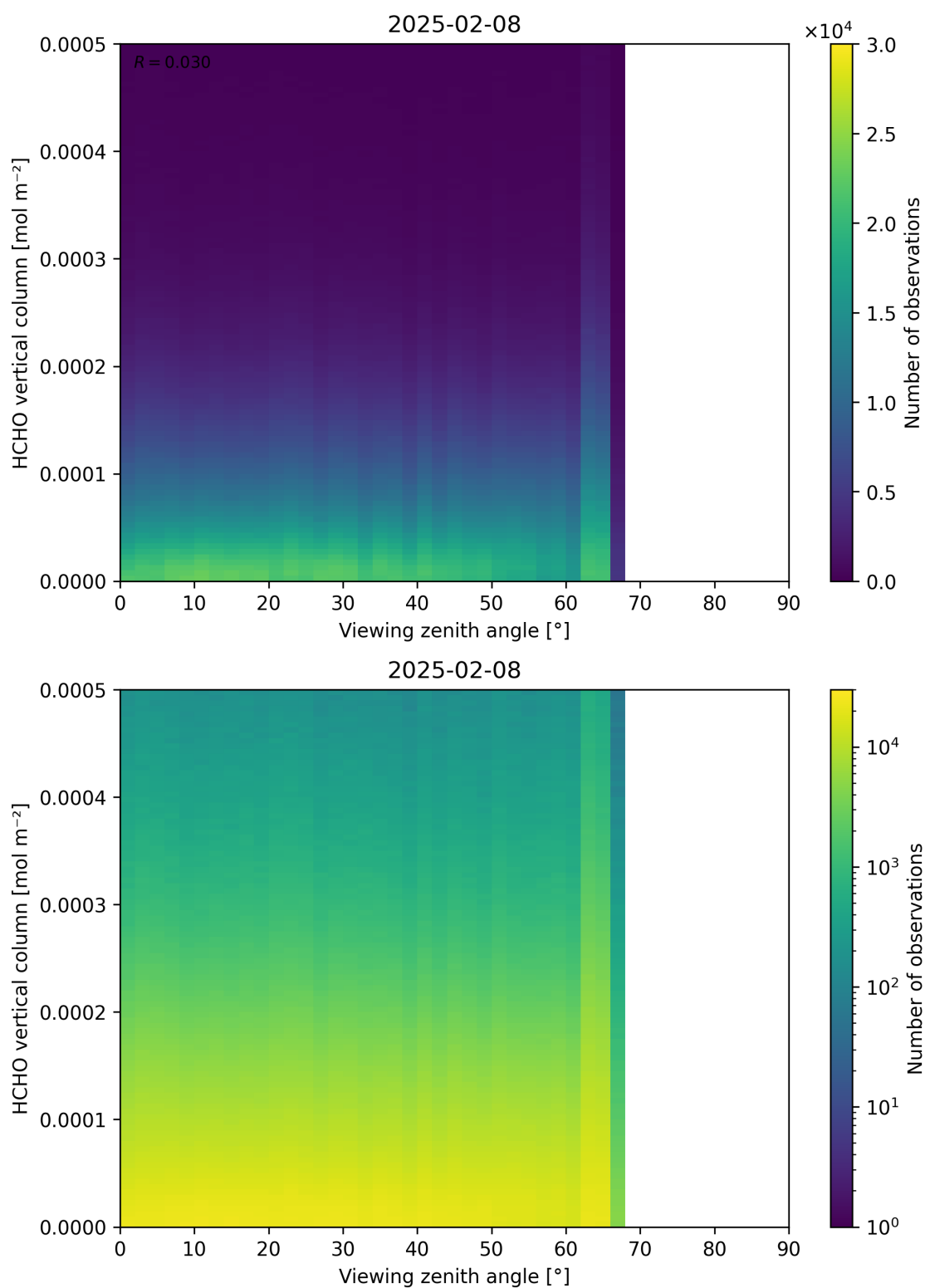
Figure 192: Scatter density plot of “Viewing zenith angle” against “HCHO vertical column” for 2025-02-08 to 2025-02-09.
