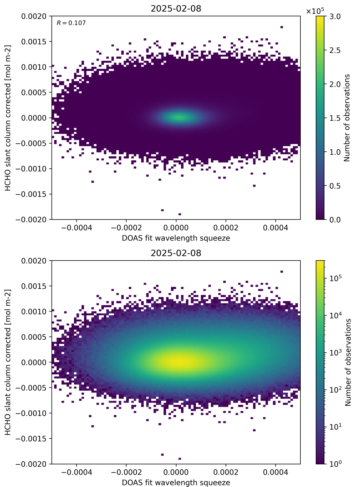
Figure 69: Scatter density plot of “DOAS fit wavelength squeeze” against “HCHO slant column corrected” for 2025-02-08 to 2025-02-09.
