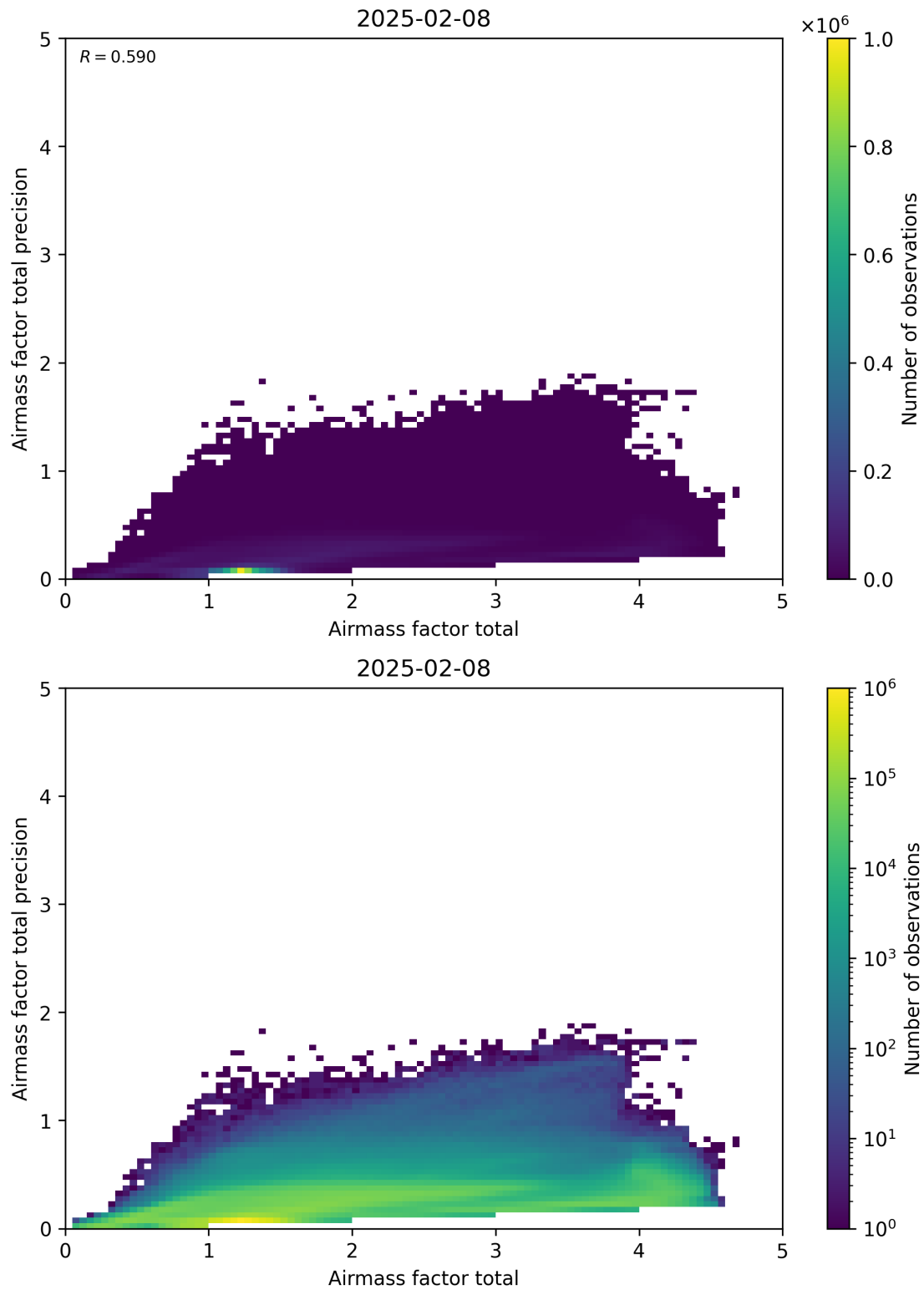
Figure 103: Scatter density plot of “Airmass factor total” against “Airmass factor total precision” for 2025-02-08 to 2025-02-09.
