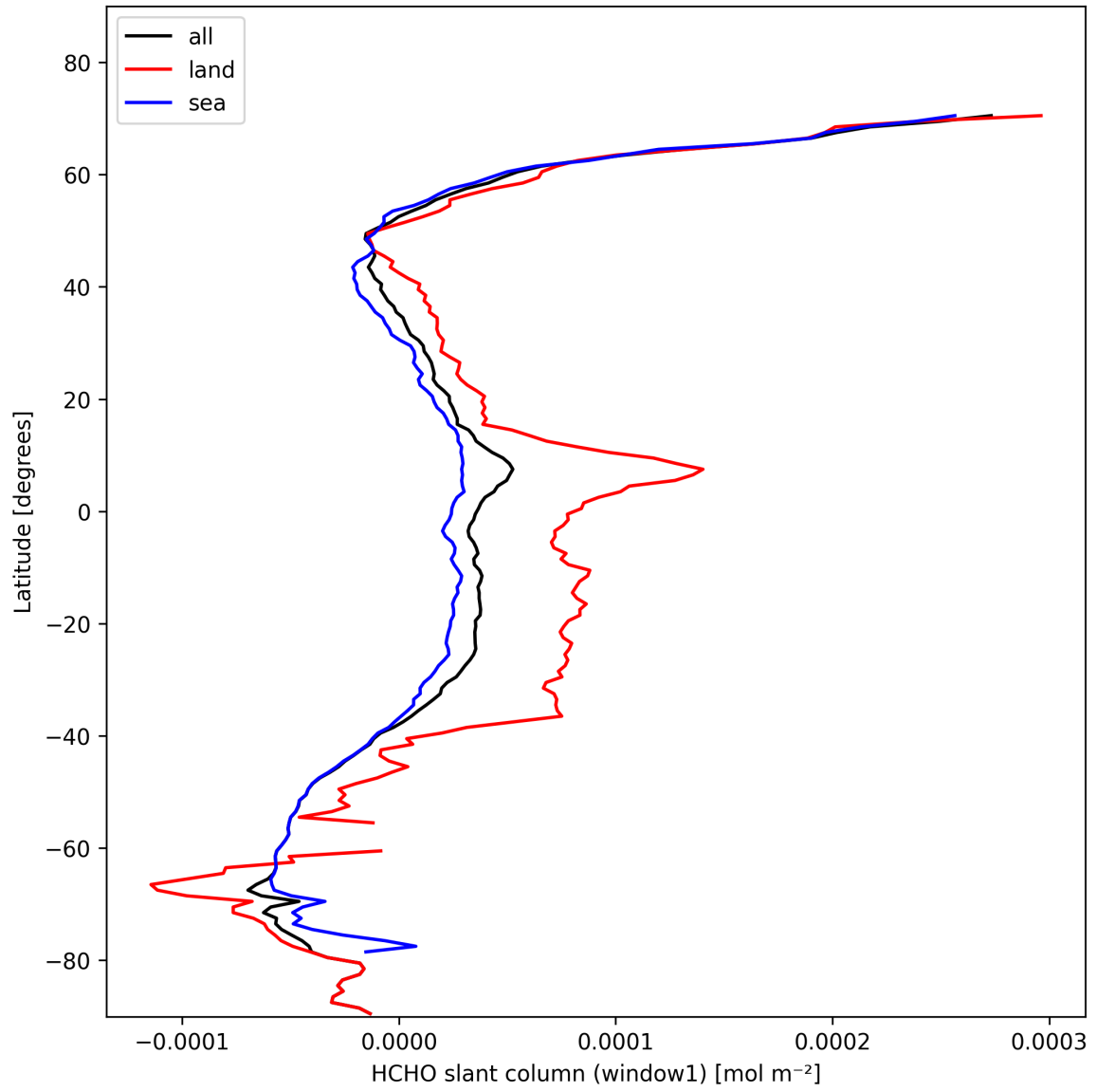
Figure 24: Zonal average of “HCHO slant column (window1)” for 2025-02-08 to 2025-02-09.
