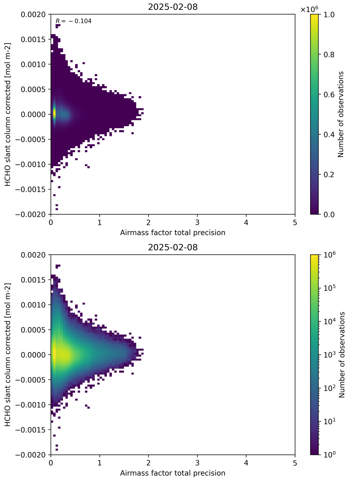
Figure 109: Scatter density plot of “Airmass factor total precision” against “HCHO slant column corrected” for 2025-02-08 to 2025-02-09.
