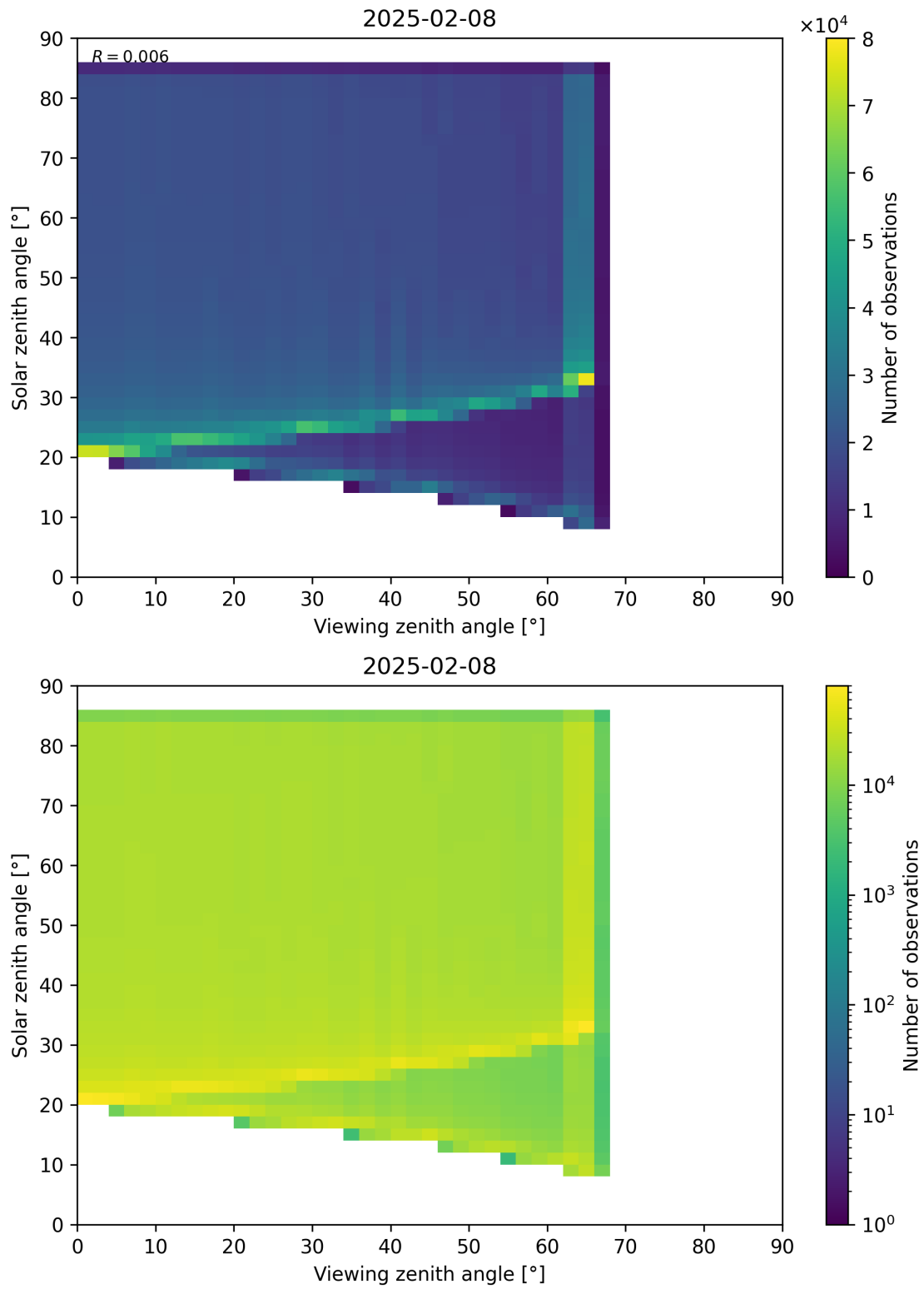
Figure 197: Scatter density plot of “Viewing zenith angle” against “Solar zenith angle” for 2025-02-08 to 2025-02-09.
