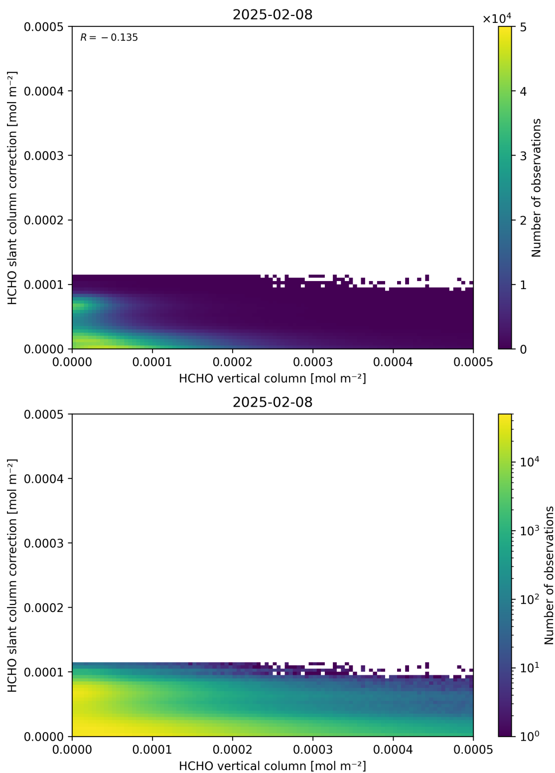
Figure 128: Scatter density plot of “HCHO vertical column” against “HCHO slant column correction” for 2025-02-08 to 2025-02-09.
