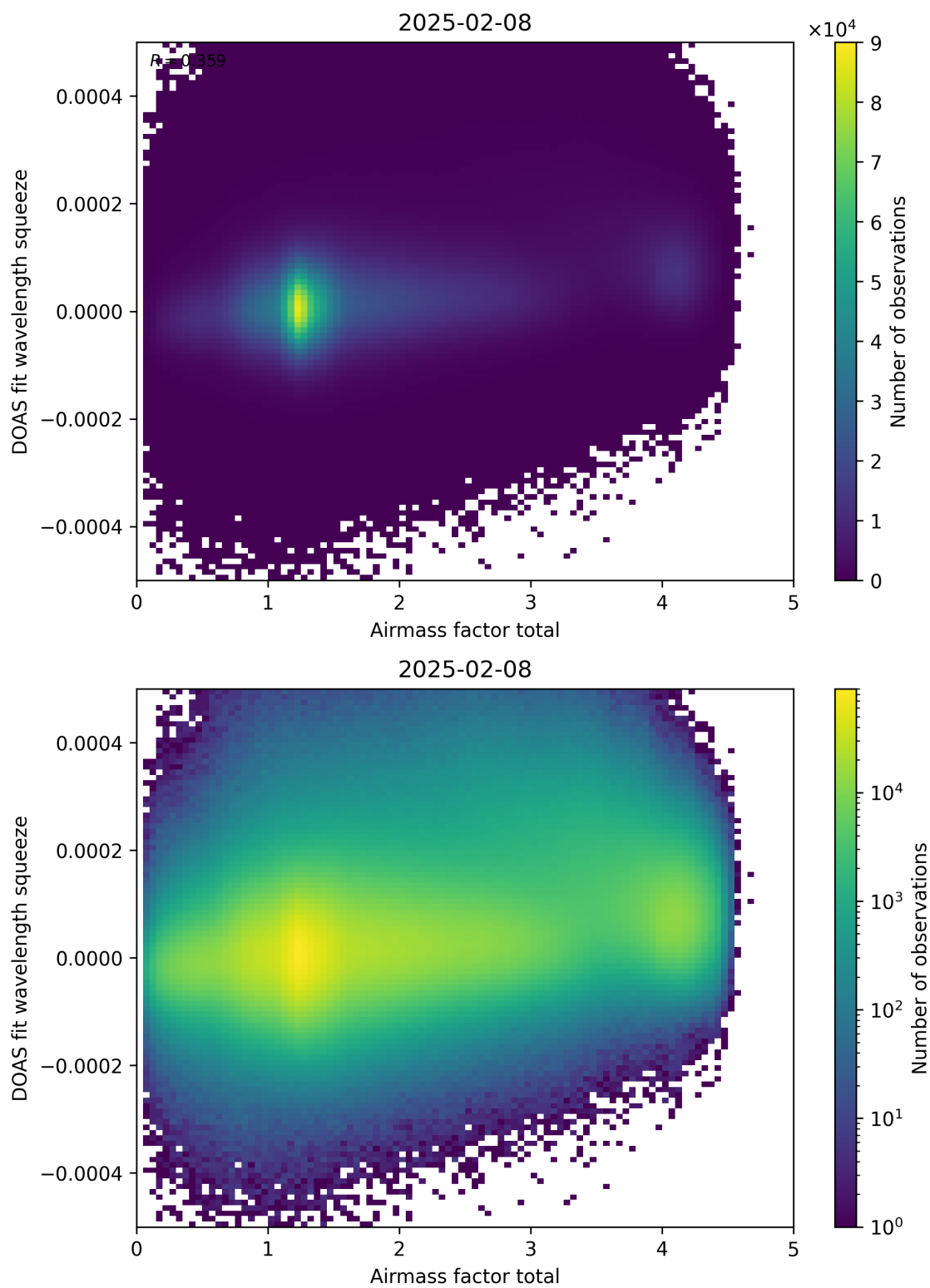
Figure 99: Scatter density plot of “Airmass factor total” against “DOAS fit wavelength squeeze” for 2025-02-08 to 2025-02-09.
