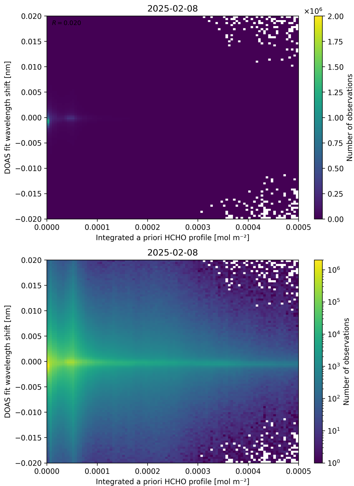
Figure 149: Scatter density plot of “Integrated a priori HCHO profile” against “DOAS fit wavelength shift” for 2025-02-08 to 2025-02-09.
