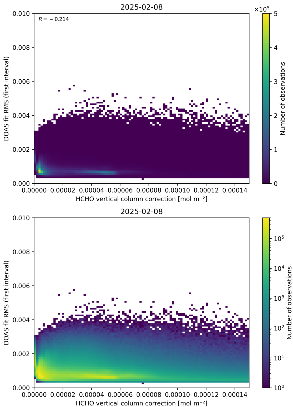
Figure 112: Scatter density plot of “HCHO vertical column correction” against “DOAS fit RMS (first interval)” for 2025-02-08 to 2025-02-09.
