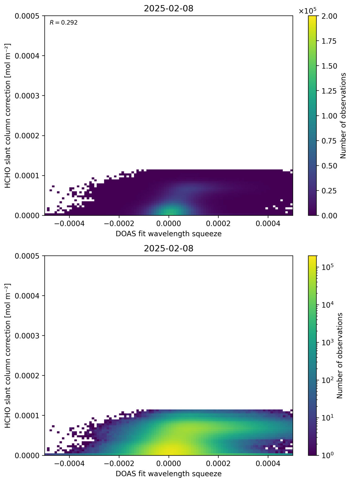
Figure 70: Scatter density plot of “DOAS fit wavelength squeeze” against “HCHO slant column correction” for 2025-02-08 to 2025-02-09.
