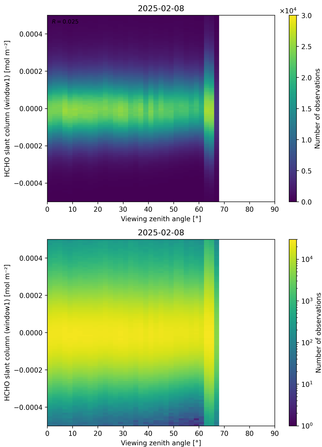
Figure 188: Scatter density plot of “Viewing zenith angle” against “HCHO slant column (window1)” for 2025-02-08 to 2025-02-09.
