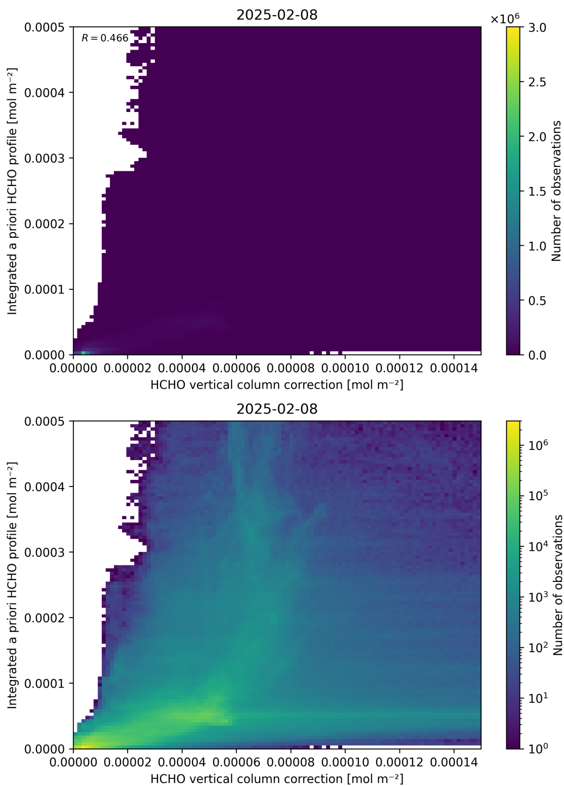
Figure 122: Scatter density plot of “HCHO vertical column correction” against “Integrated a priori HCHO profile” for 2025-02-08 to 2025-02-09.
