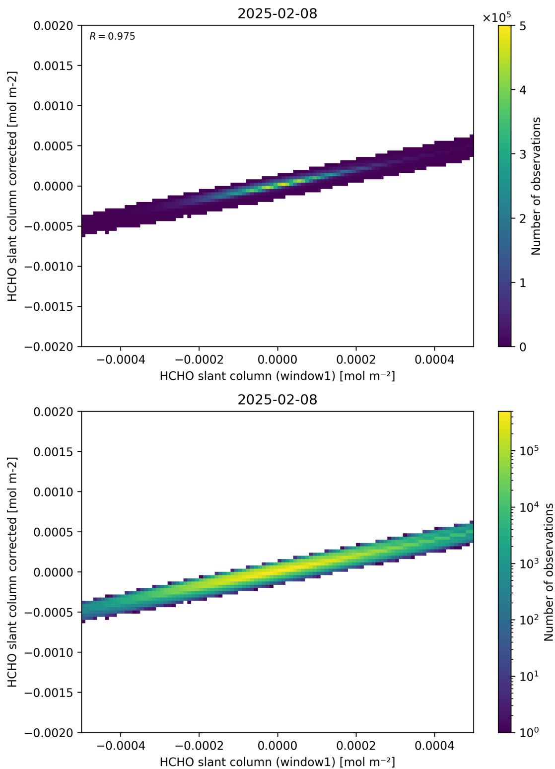
Figure 82: Scatter density plot of “HCHO slant column (window1)” against “HCHO slant column corrected” for 2025-02-08 to 2025-02-09.
