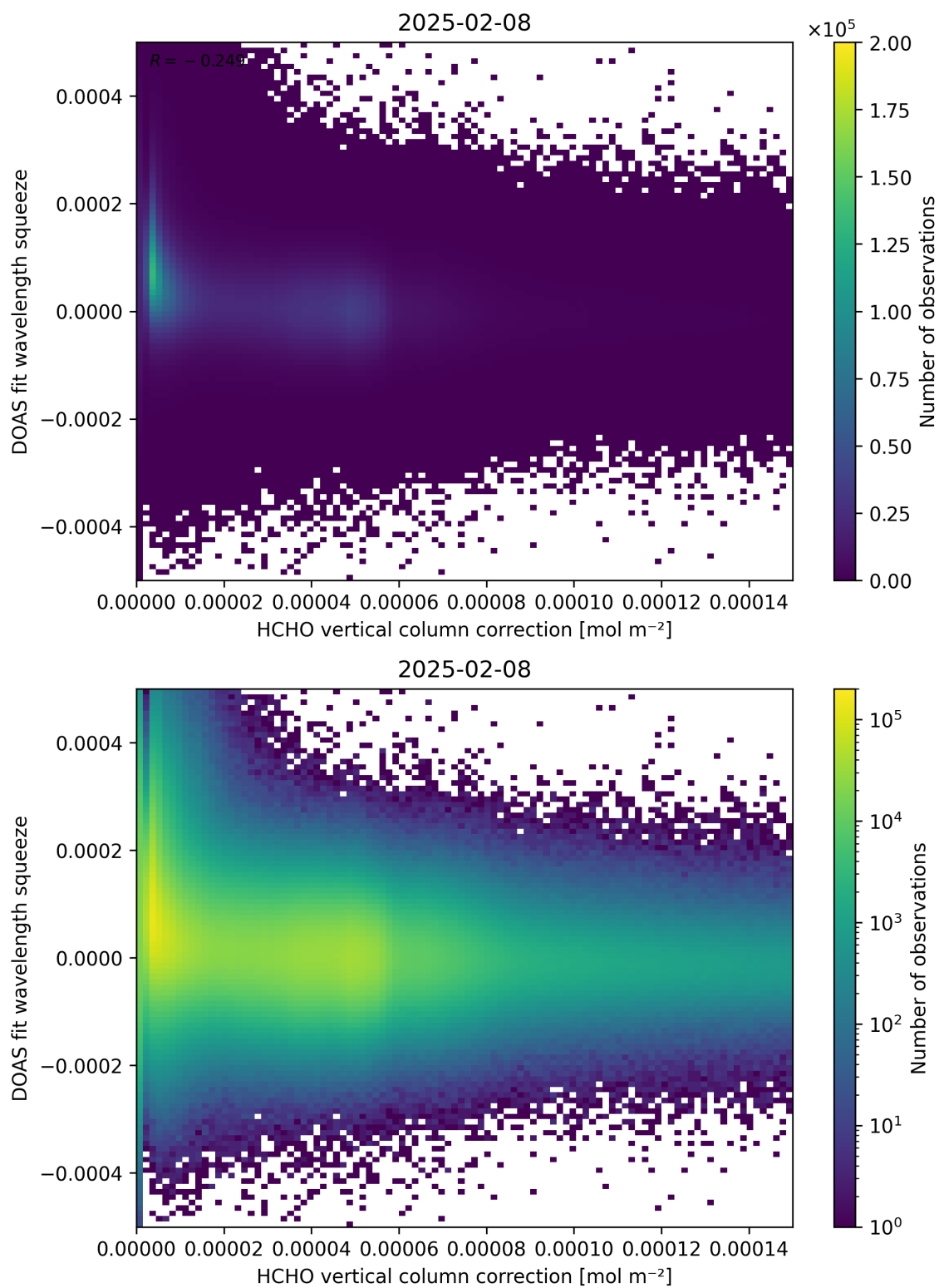
Figure 114: Scatter density plot of “HCHO vertical column correction” against “DOAS fit wavelength squeeze” for 2025-02-08 to 2025-02-09.
