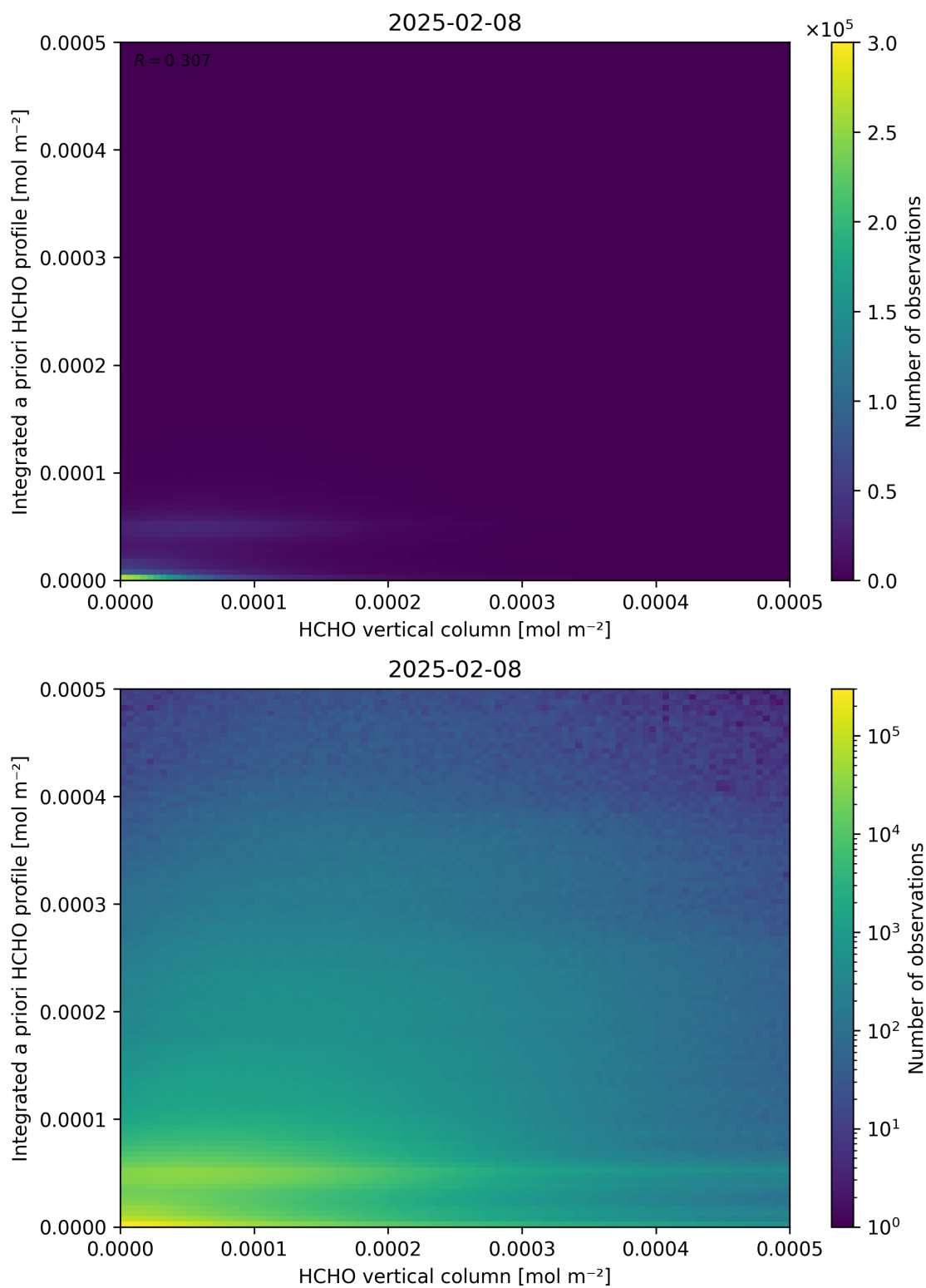
Figure 135: Scatter density plot of “HCHO vertical column” against “Integrated a priori HCHO profile” for 2025-02-08 to 2025-02-09.
