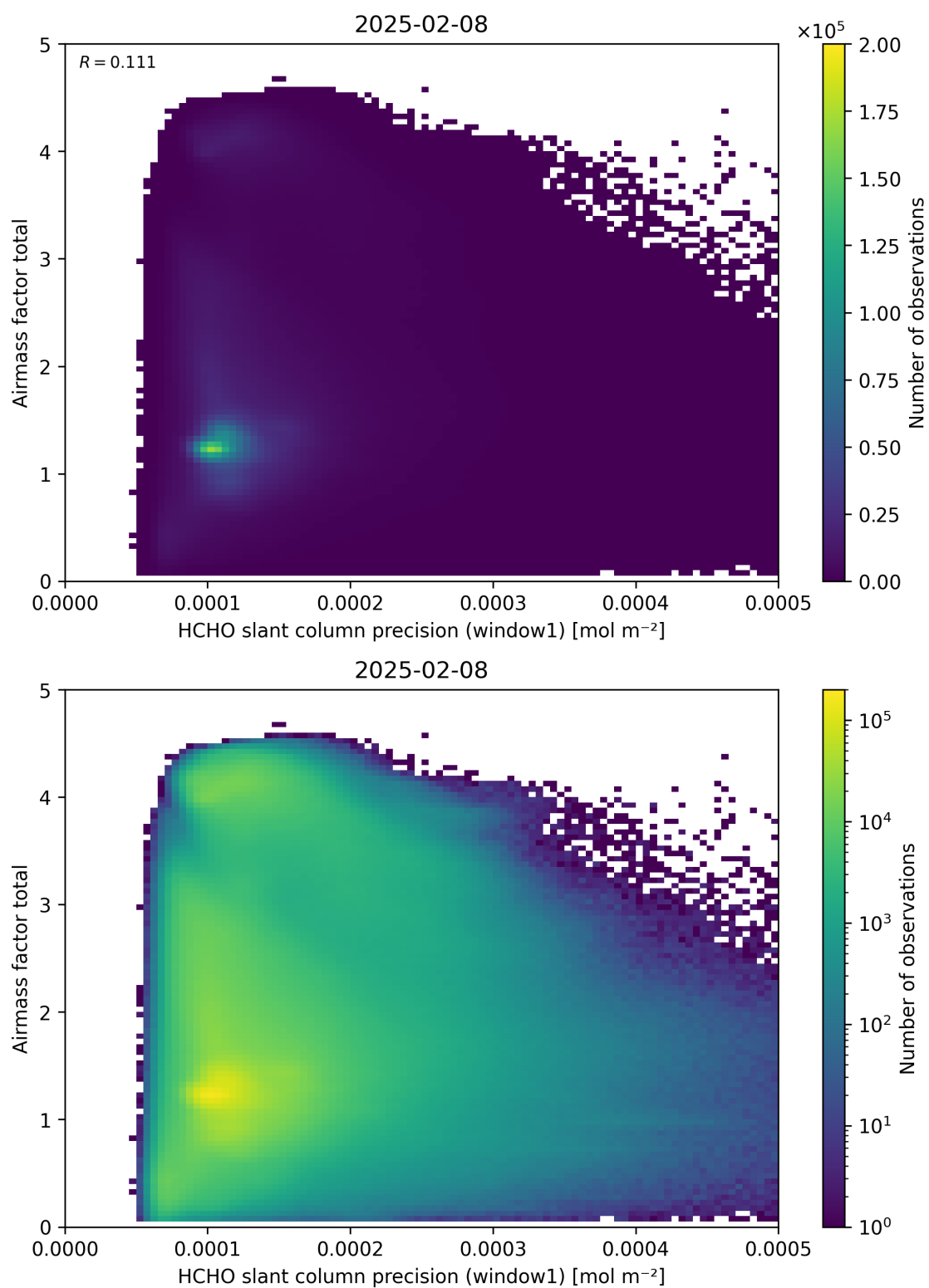
Figure 94: Scatter density plot of “HCHO slant column precision (window1)” against “Airmass factor total” for 2025-02-08 to 2025-02-09.
