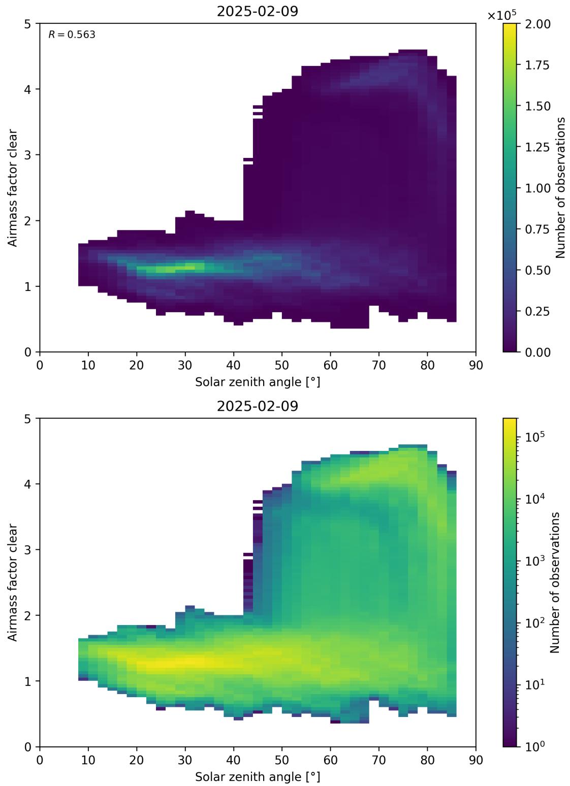
Figure 170: Scatter density plot of “Solar zenith angle” against “Airmass factor clear” for 2025-02-08 to 2025-02-10.
