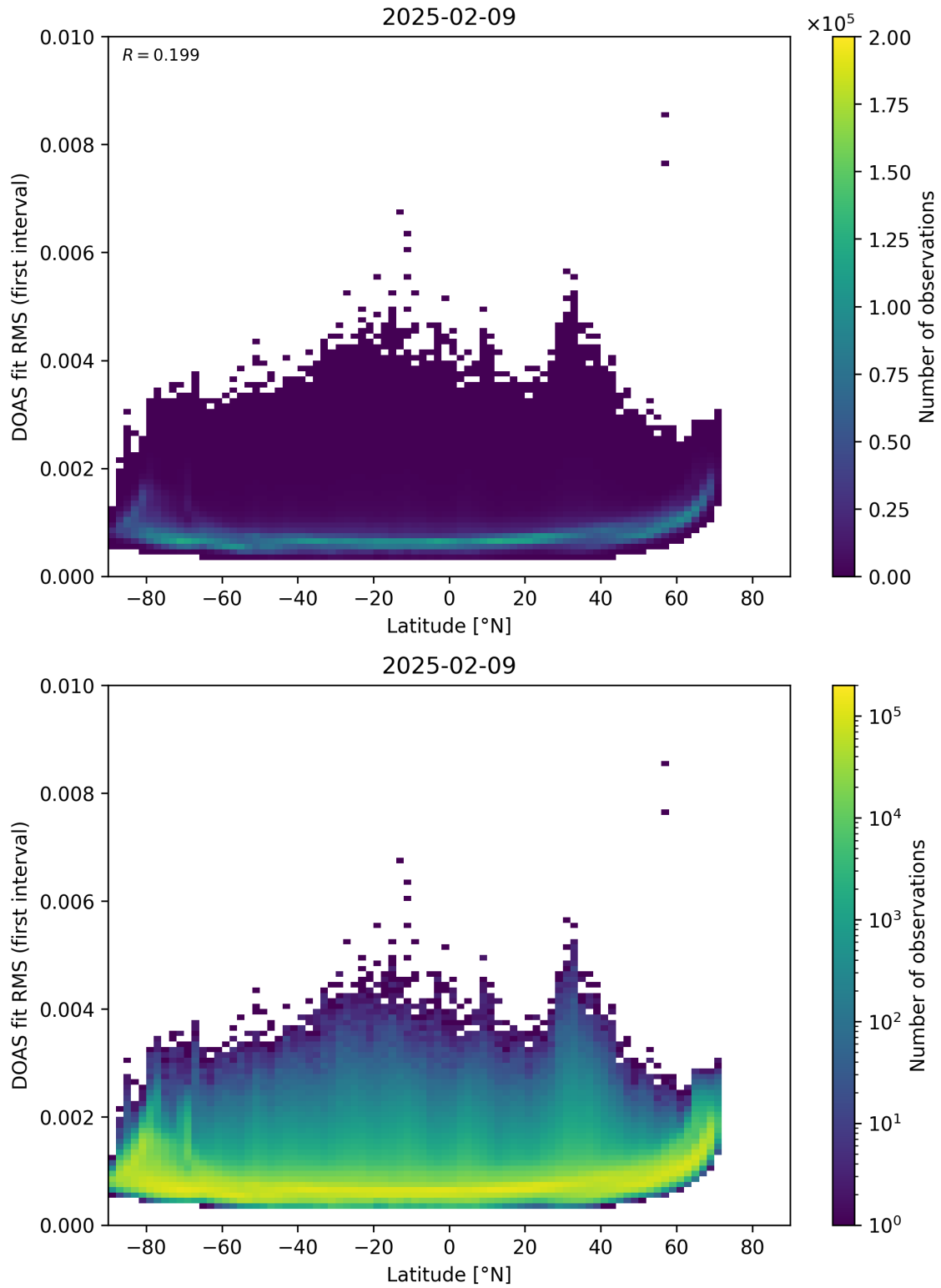
Figure 153: Scatter density plot of “Latitude” against “DOAS fit RMS (first interval)” for 2025-02-08 to 2025-02-10.
