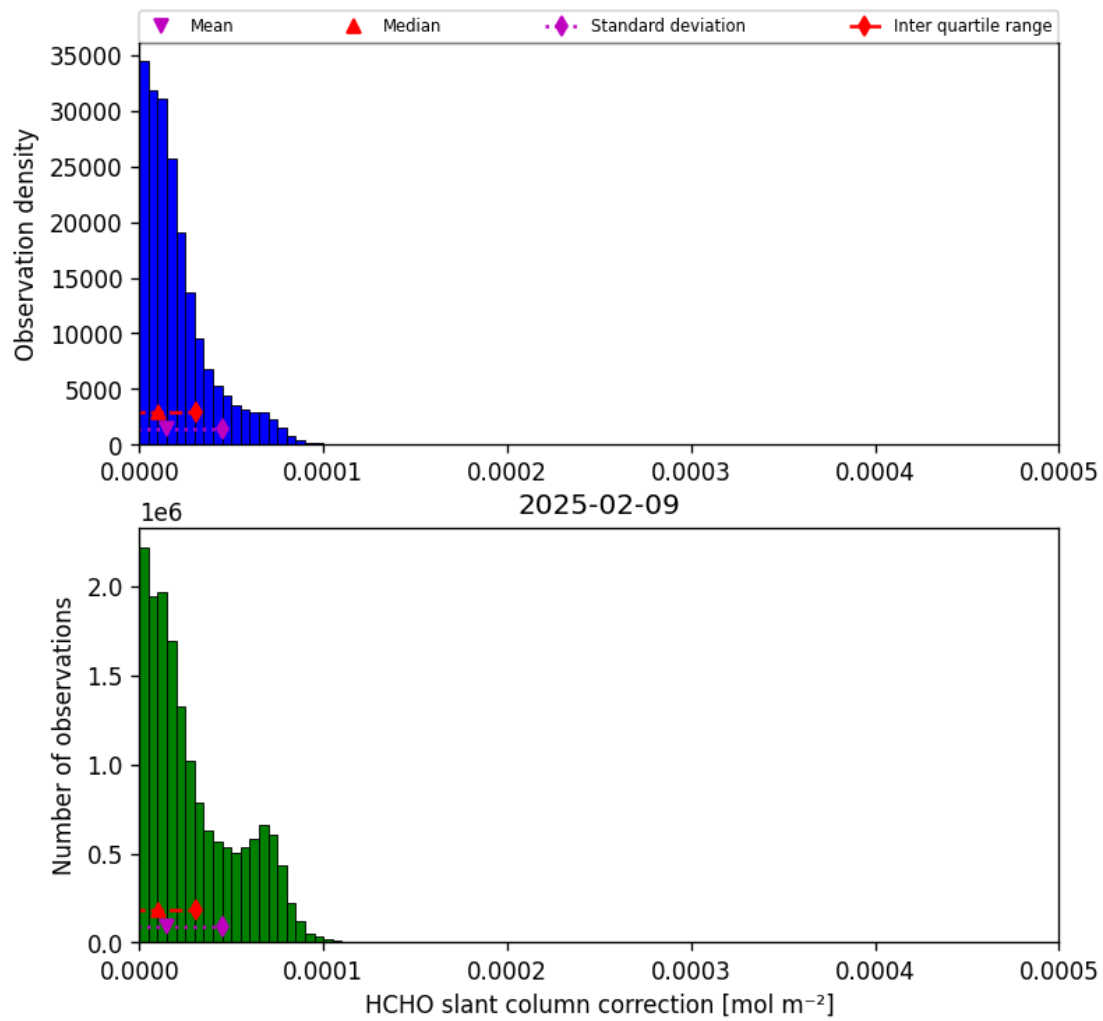
Figure 47: Histogram of “HCHO slant column correction” for 2025-02-08 to 2025-02-10
