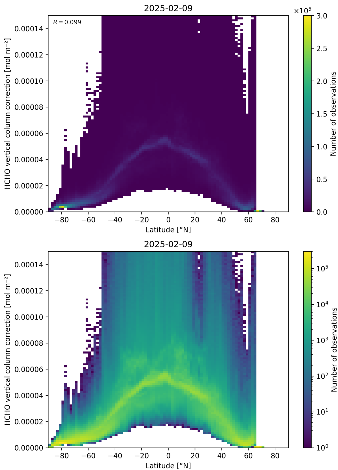
Figure 164: Scatter density plot of “Latitude” against “HCHO vertical column correction” for 2025-02-08 to 2025-02-10.
