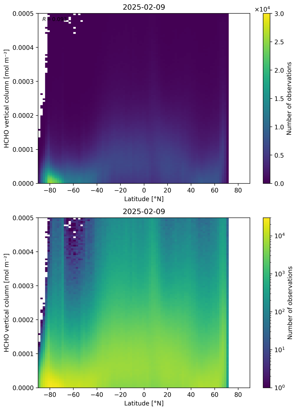
Figure 163: Scatter density plot of “Latitude” against “HCHO vertical column” for 2025-02-08 to 2025-02-10.
