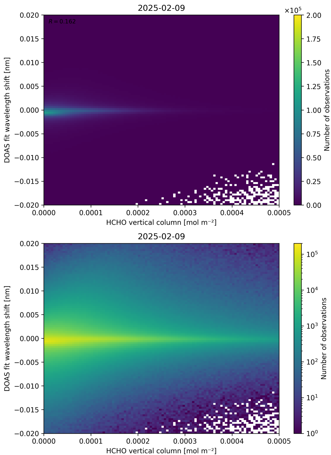
Figure 124: Scatter density plot of “HCHO vertical column” against “DOAS fit wavelength shift” for 2025-02-08 to 2025-02-10.
