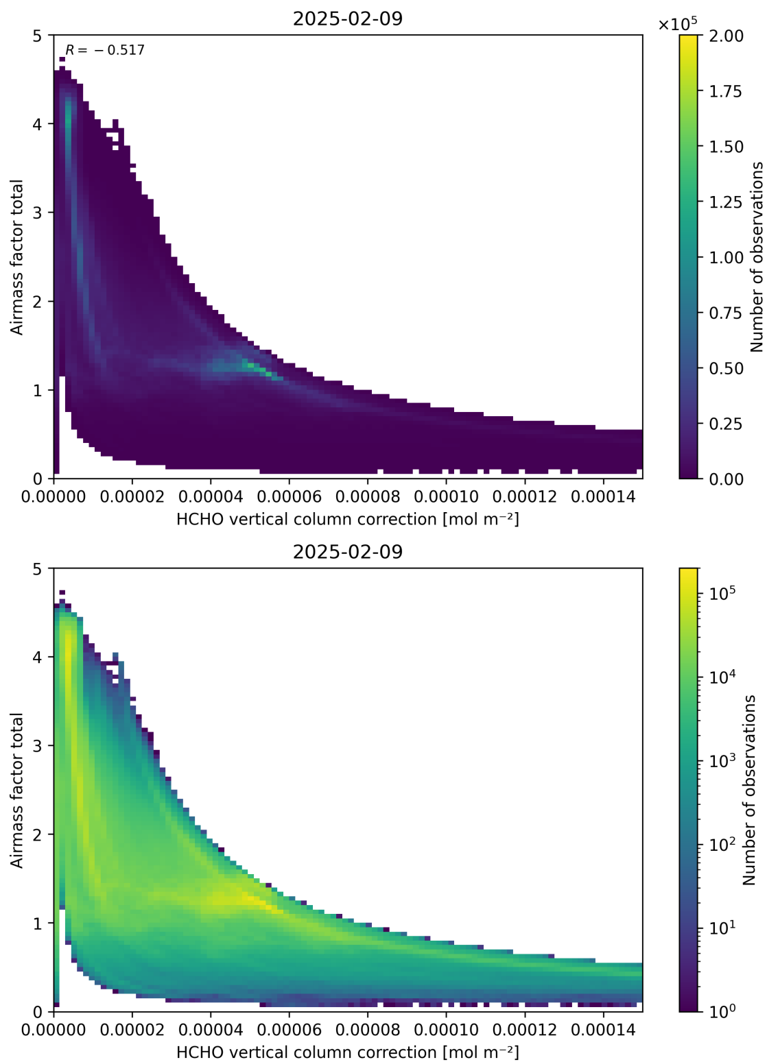
Figure 120: Scatter density plot of “HCHO vertical column correction” against “Airmass factor total” for 2025-02-08 to 2025-02-10.
