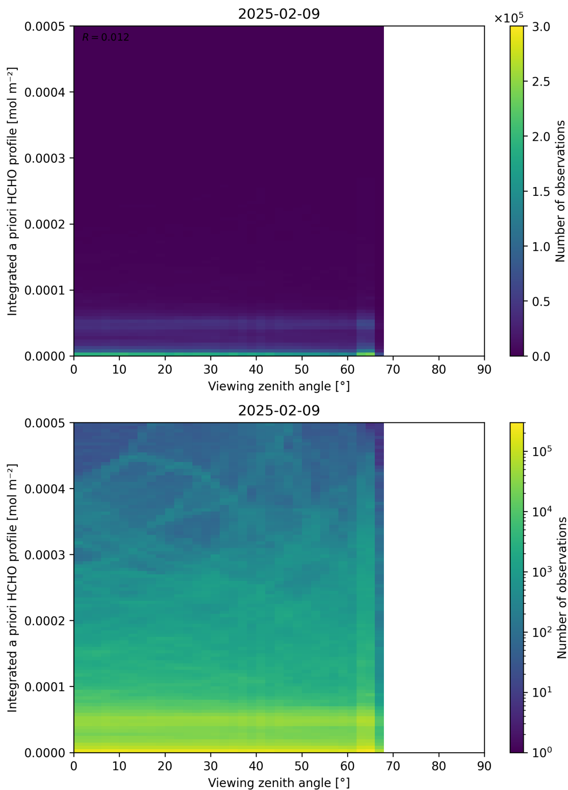
Figure 195: Scatter density plot of “Viewing zenith angle” against “Integrated a priori HCHO profile” for 2025-02-08 to 2025-02-10.
