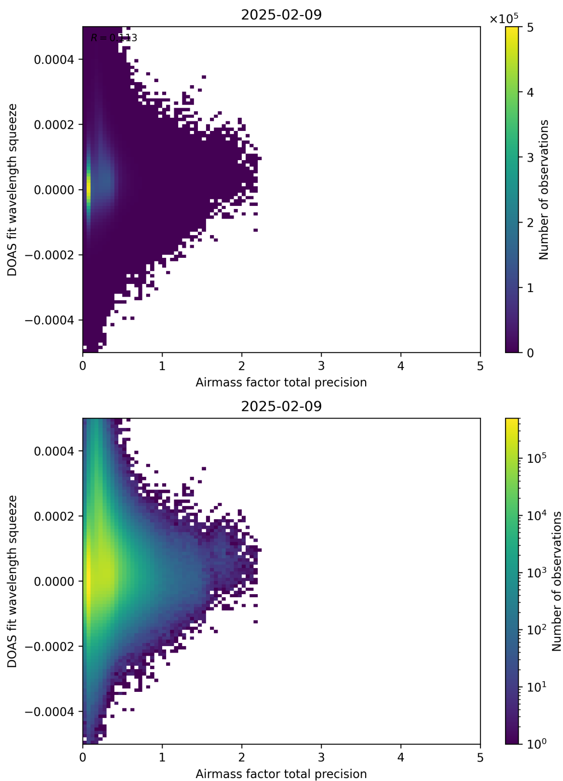
Figure 107: Scatter density plot of “Airmass factor total precision” against “DOAS fit wavelength squeeze” for 2025-02-08 to 2025-02-10.
