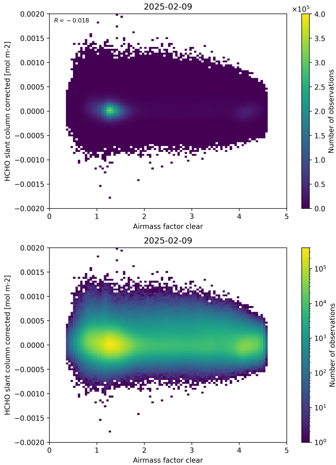
Figure 74: Scatter density plot of “Airmass factor clear” against “HCHO slant column corrected” for 2025-02-08 to 2025-02-10.
