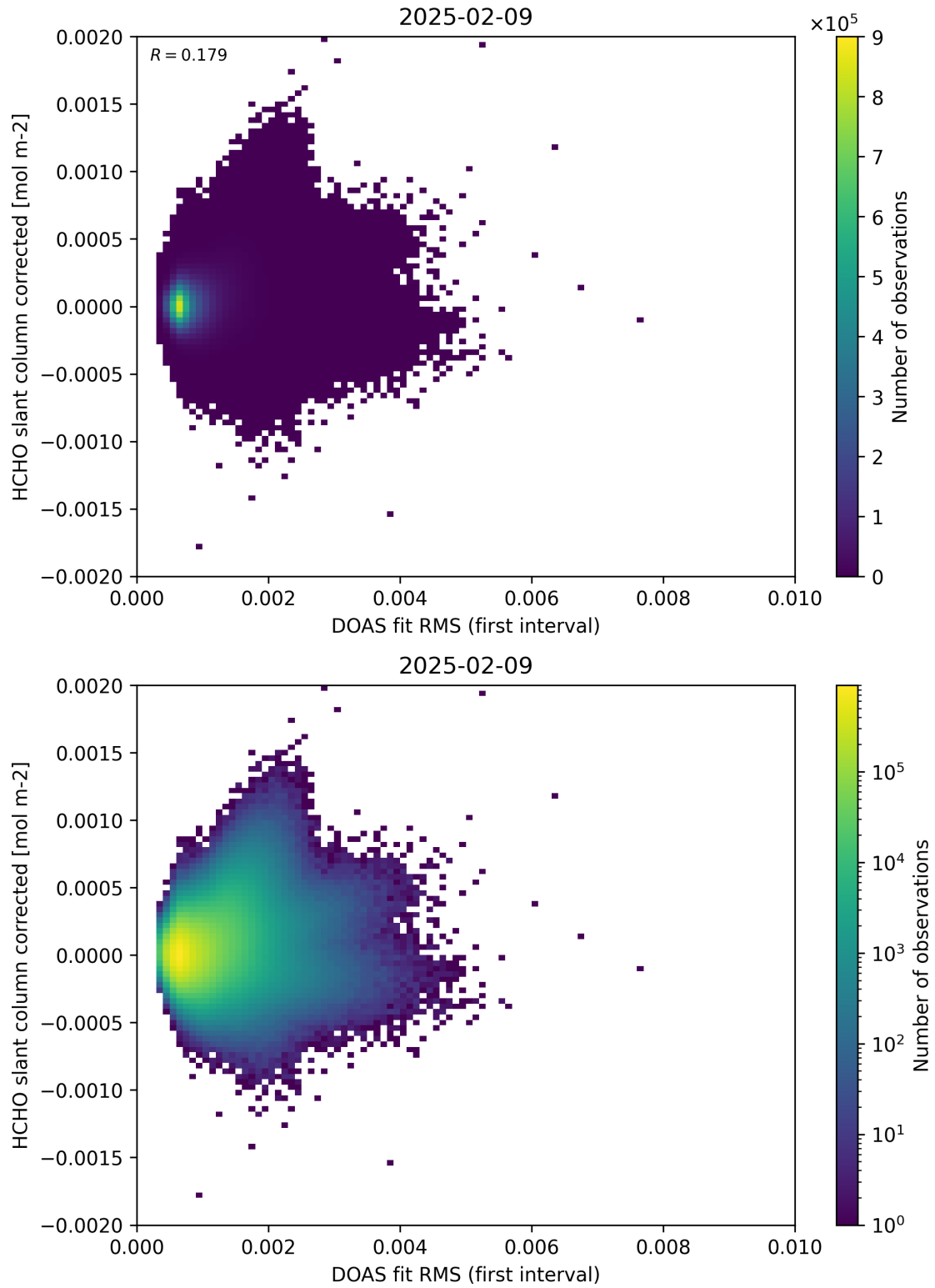
Figure 62: Scatter density plot of “DOAS fit RMS (first interval)” against “HCHO slant column corrected” for 2025-02-08 to 2025-02-10.
