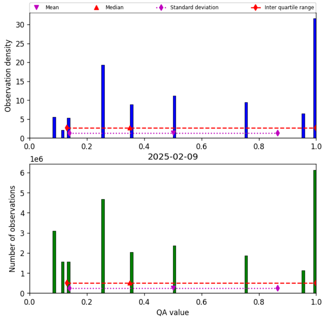
Figure 34: Histogram of “QA value” for 2025-02-08 to 2025-02-10
