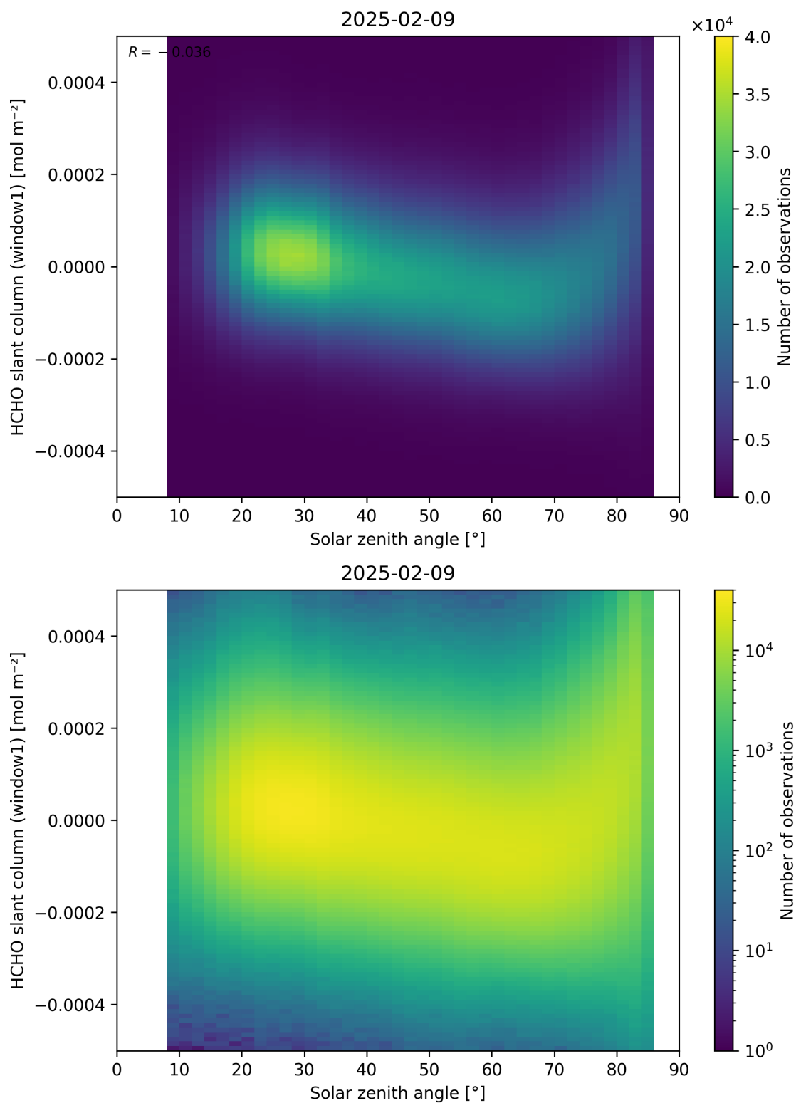
Figure 173: Scatter density plot of “Solar zenith angle” against “HCHO slant column (window1)” for 2025-02-08 to 2025-02-10.
