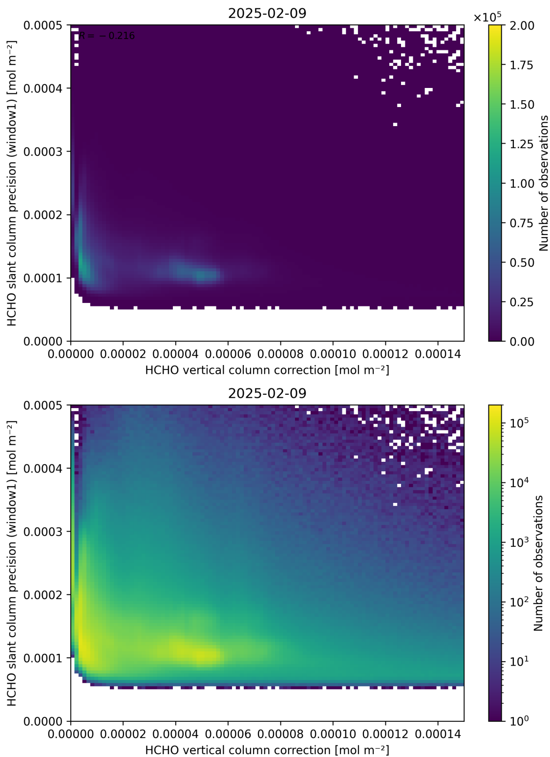
Figure 119: Scatter density plot of “HCHO vertical column correction” against “HCHO slant column precision (window1)” for 2025-02-08 to 2025-02-10.
