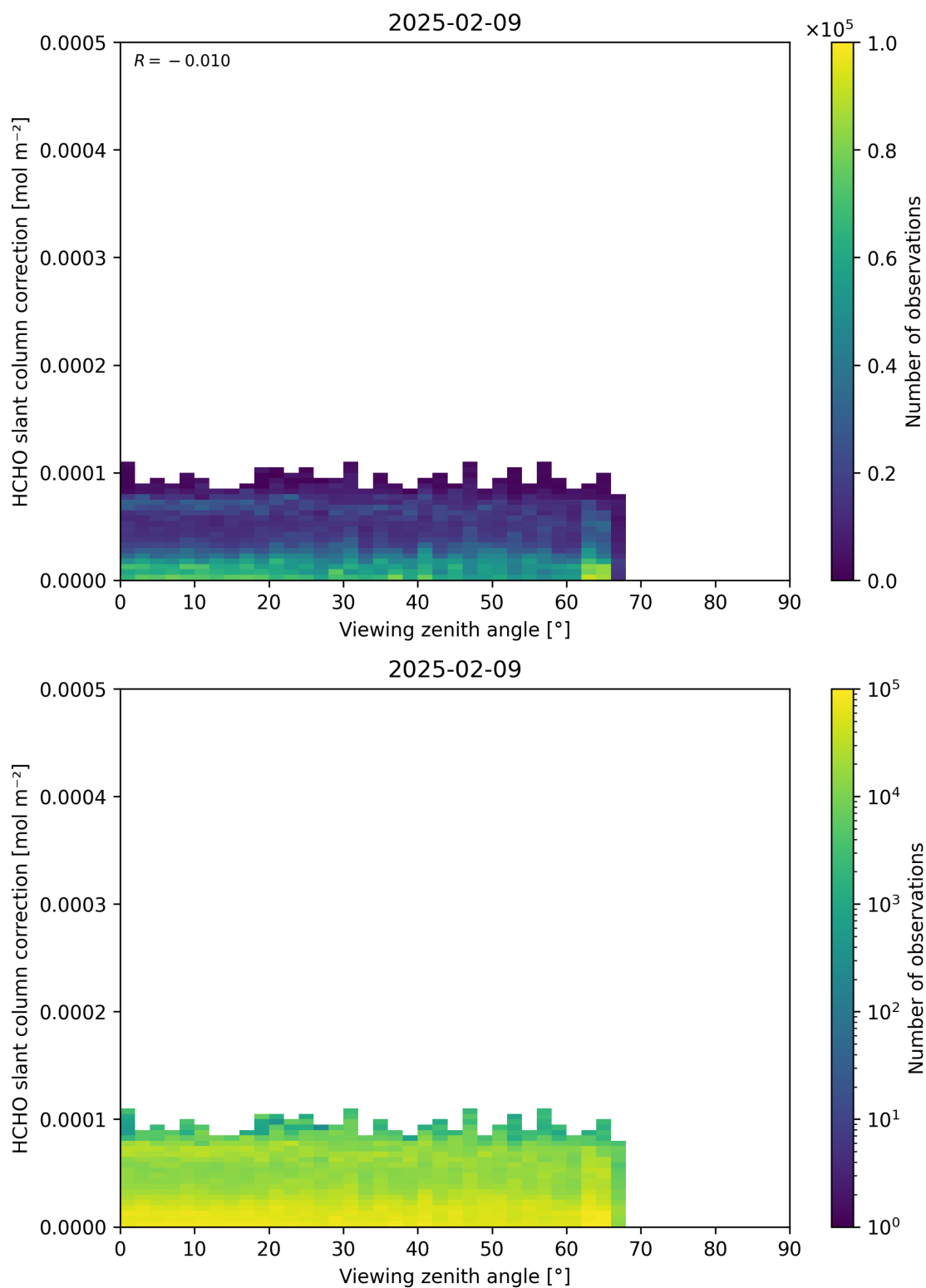
Figure 187: Scatter density plot of “Viewing zenith angle” against “HCHO slant column correction” for 2025-02-08 to 2025-02-10.
