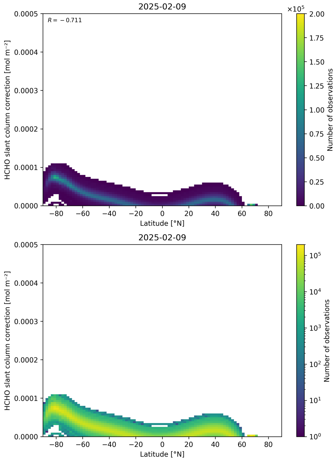
Figure 158: Scatter density plot of “Latitude” against “HCHO slant column correction” for 2025-02-08 to 2025-02-10.
