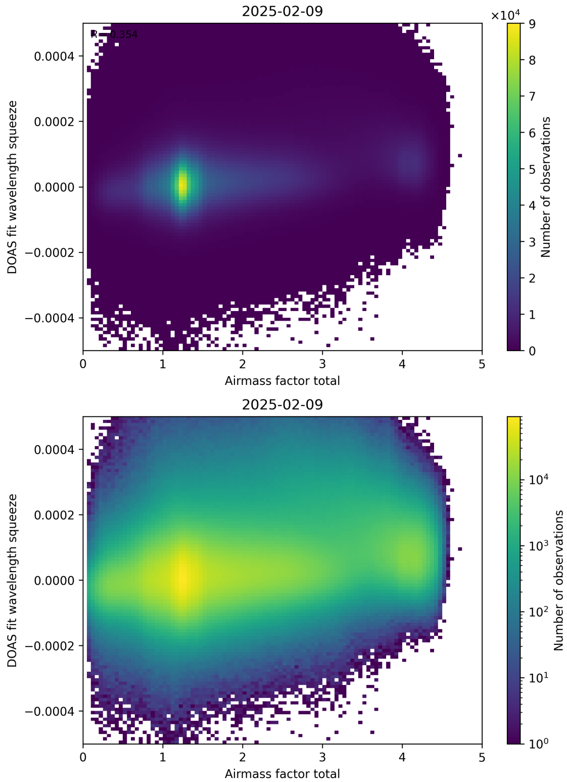
Figure 99: Scatter density plot of “Airmass factor total” against “DOAS fit wavelength squeeze” for 2025-02-08 to 2025-02-10.
