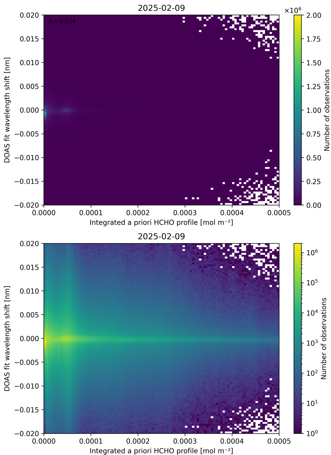
Figure 149: Scatter density plot of “Integrated a priori HCHO profile” against “DOAS fit wavelength shift” for 2025-02-08 to 2025-02-10.
