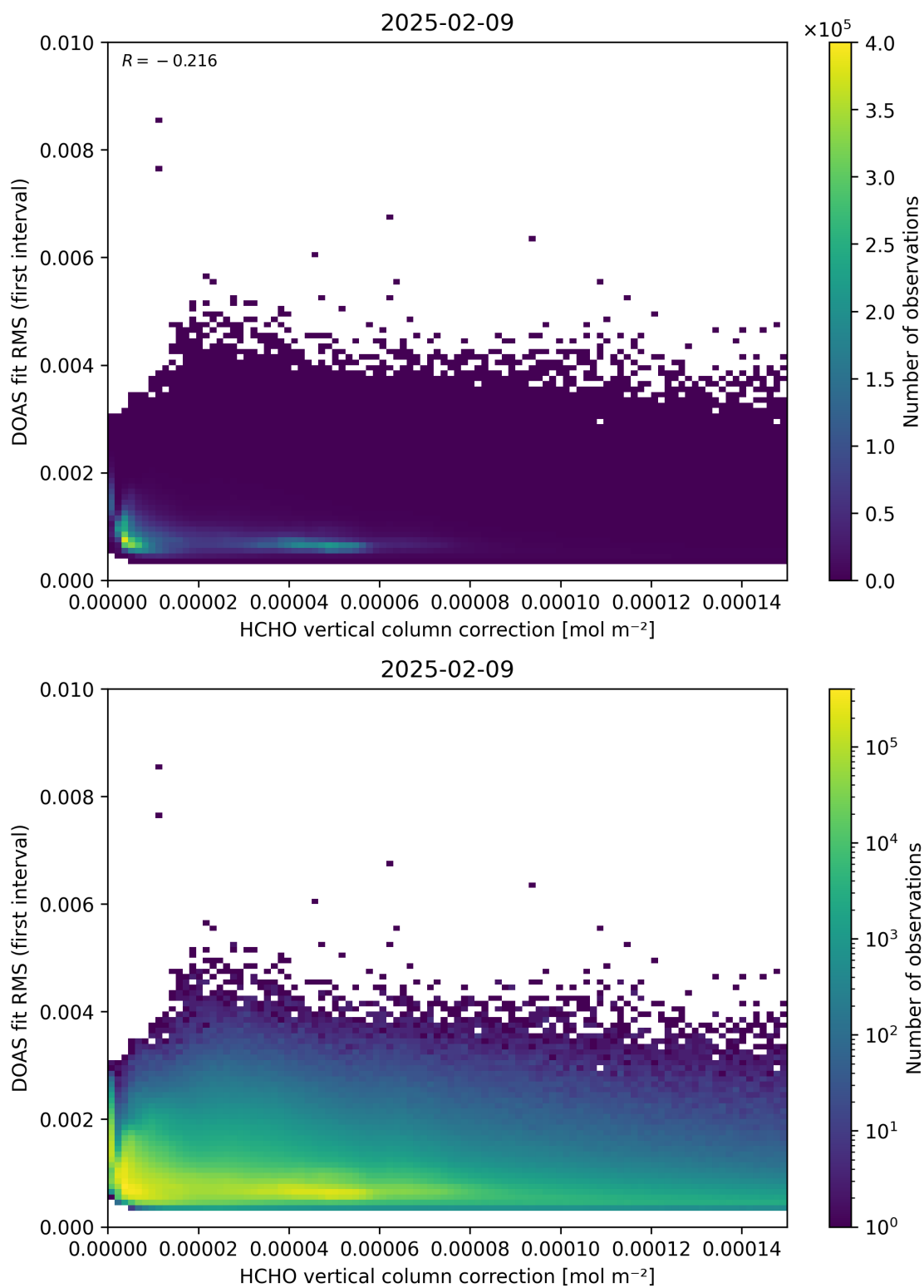
Figure 112: Scatter density plot of “HCHO vertical column correction” against “DOAS fit RMS (first interval)” for 2025-02-08 to 2025-02-10.
