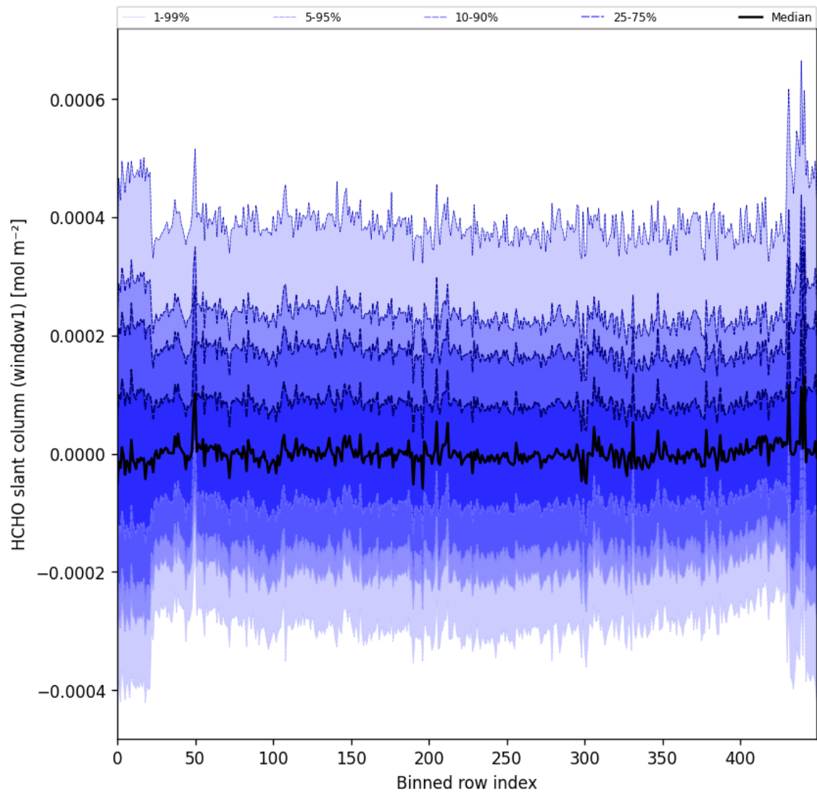
Figure 52: Along track statistics of “HCHO slant column (window1)” for 2025-02-08 to 2025-02-10
