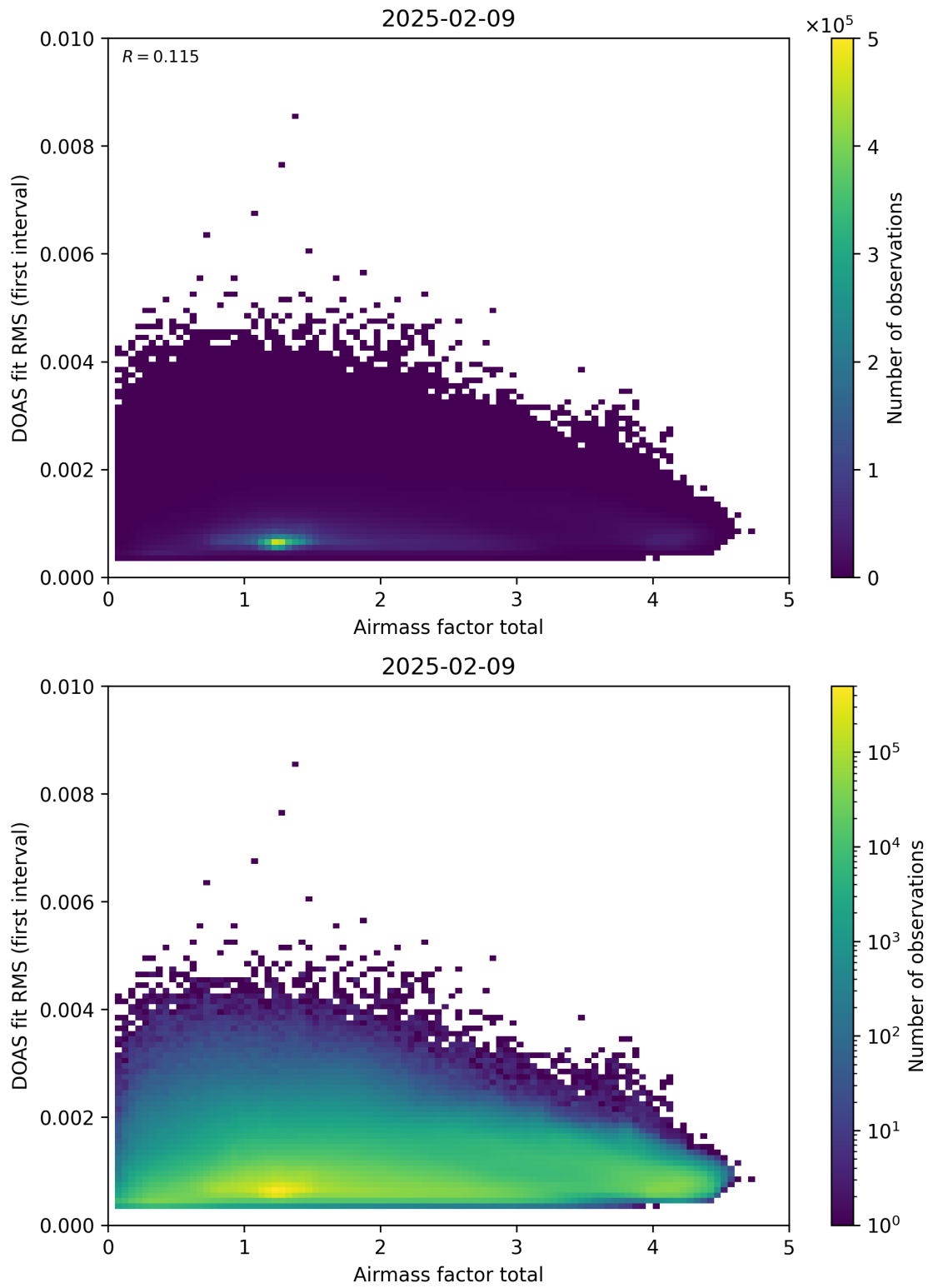
Figure 97: Scatter density plot of “Airmass factor total” against “DOAS fit RMS (first interval)” for 2025-02-08 to 2025-02-10.
