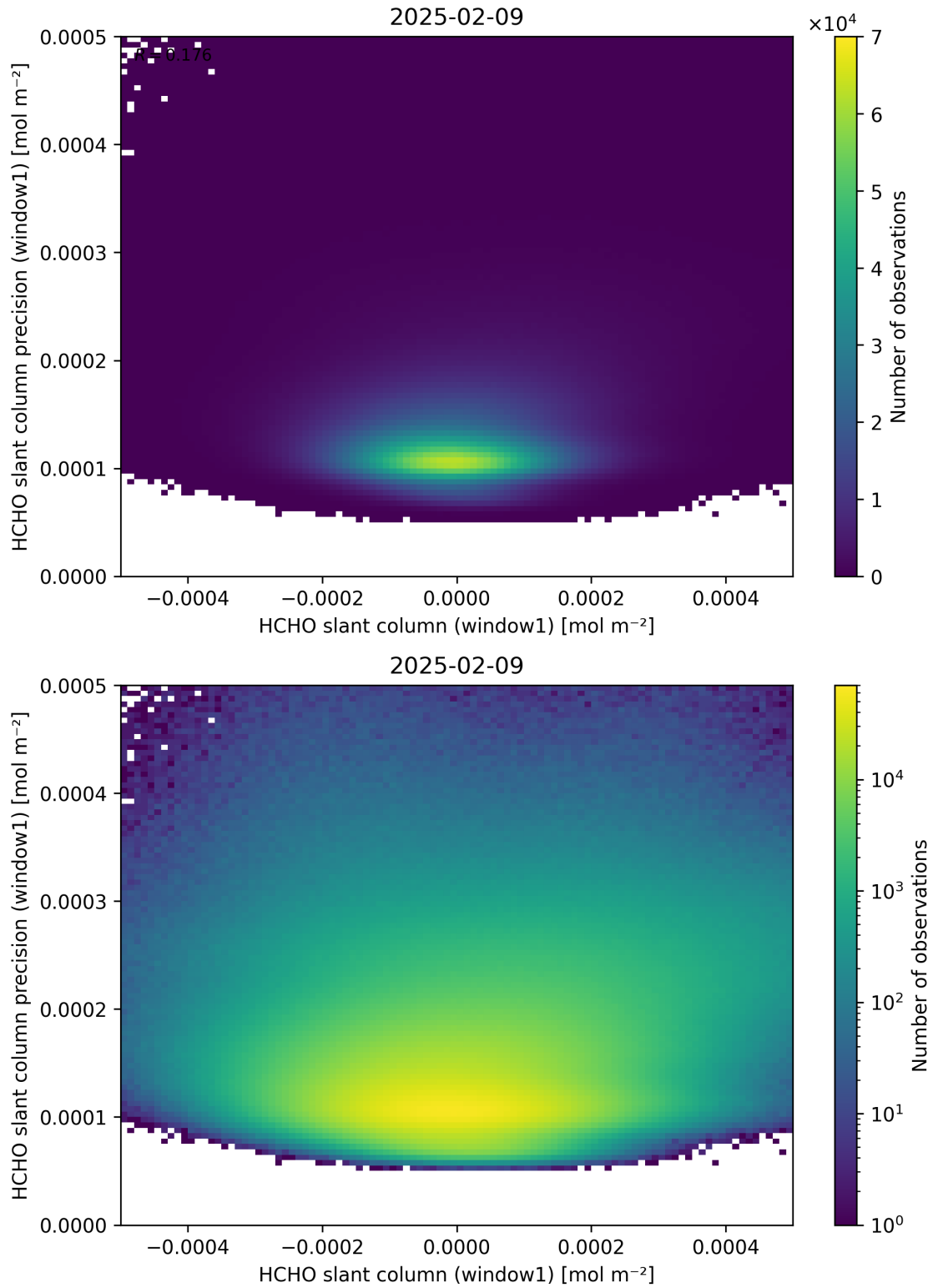
Figure 84: Scatter density plot of “HCHO slant column (window1)” against “HCHO slant column precision (window1)” for 2025-02-08 to 2025-02-10.
