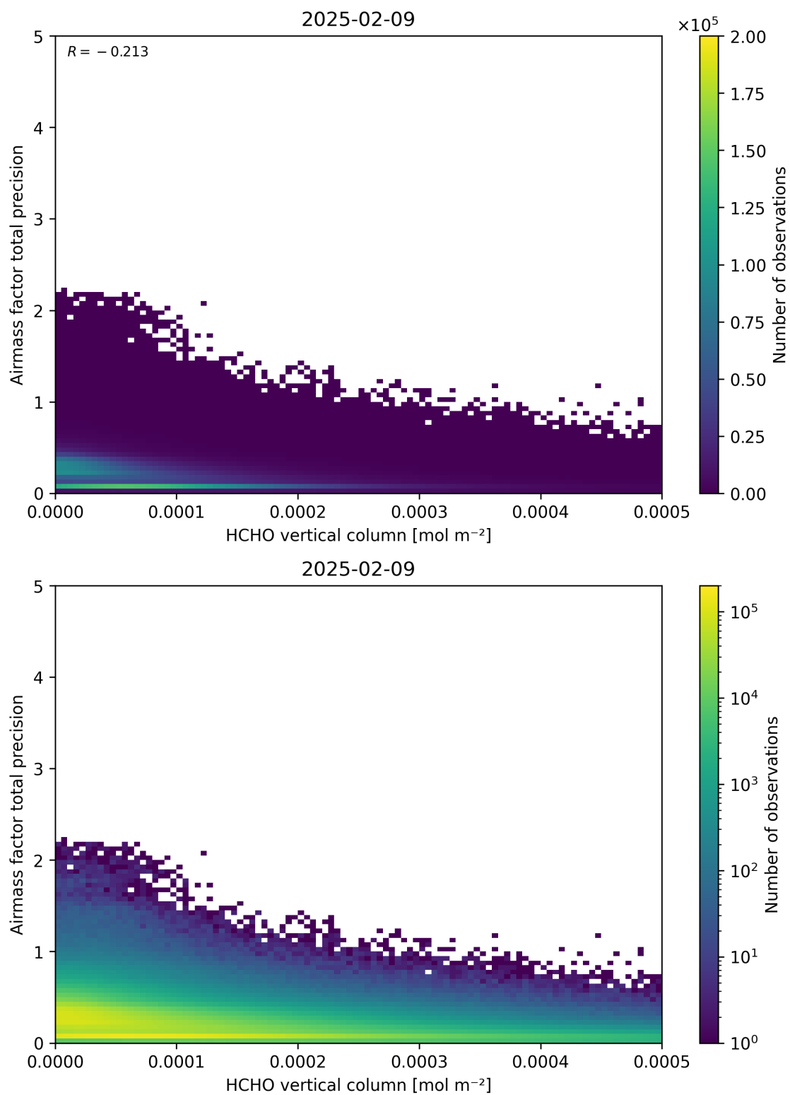
Figure 132: Scatter density plot of “HCHO vertical column” against “Airmass factor total precision” for 2025-02-08 to 2025-02-10.
