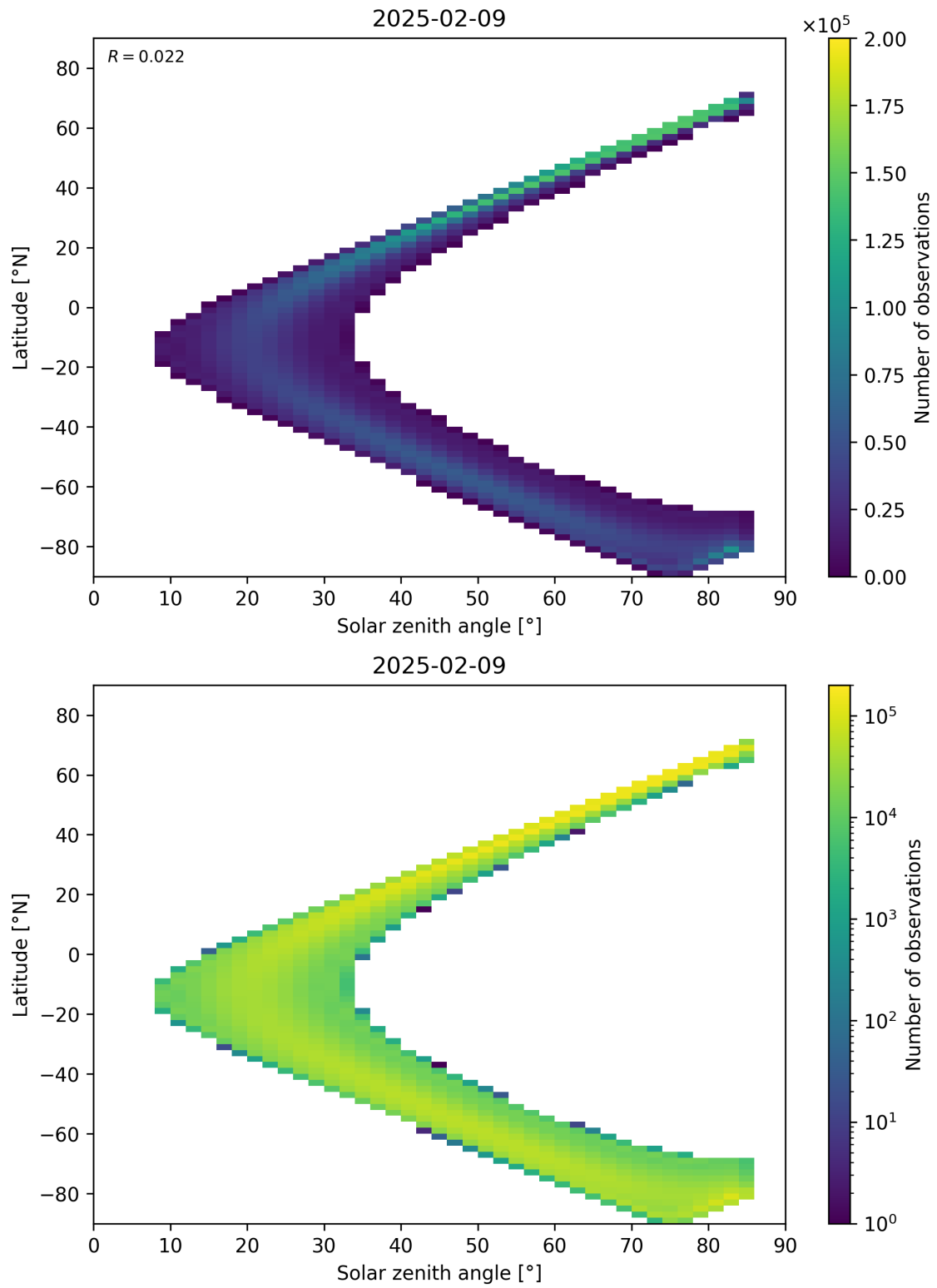
Figure 181: Scatter density plot of “Solar zenith angle” against “Latitude” for 2025-02-08 to 2025-02-10.
