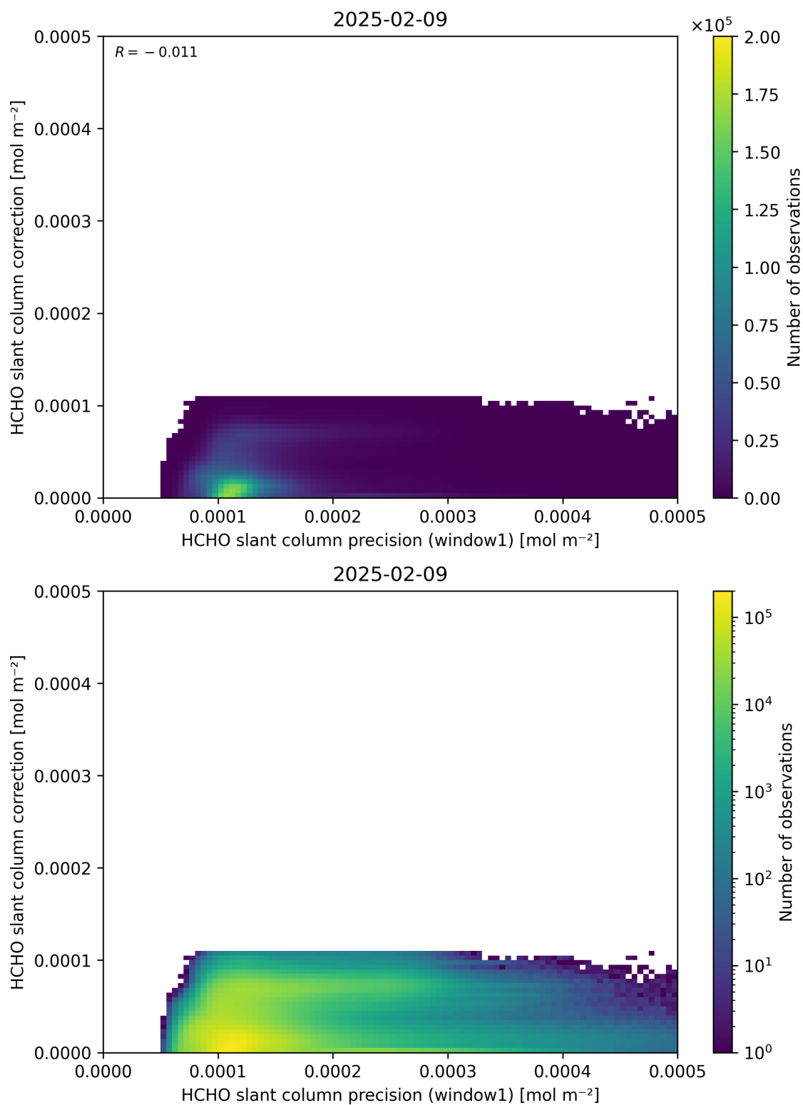
Figure 93: Scatter density plot of “HCHO slant column precision (window1)” against “HCHO slant column correction” for 2025-02-08 to 2025-02-10.
