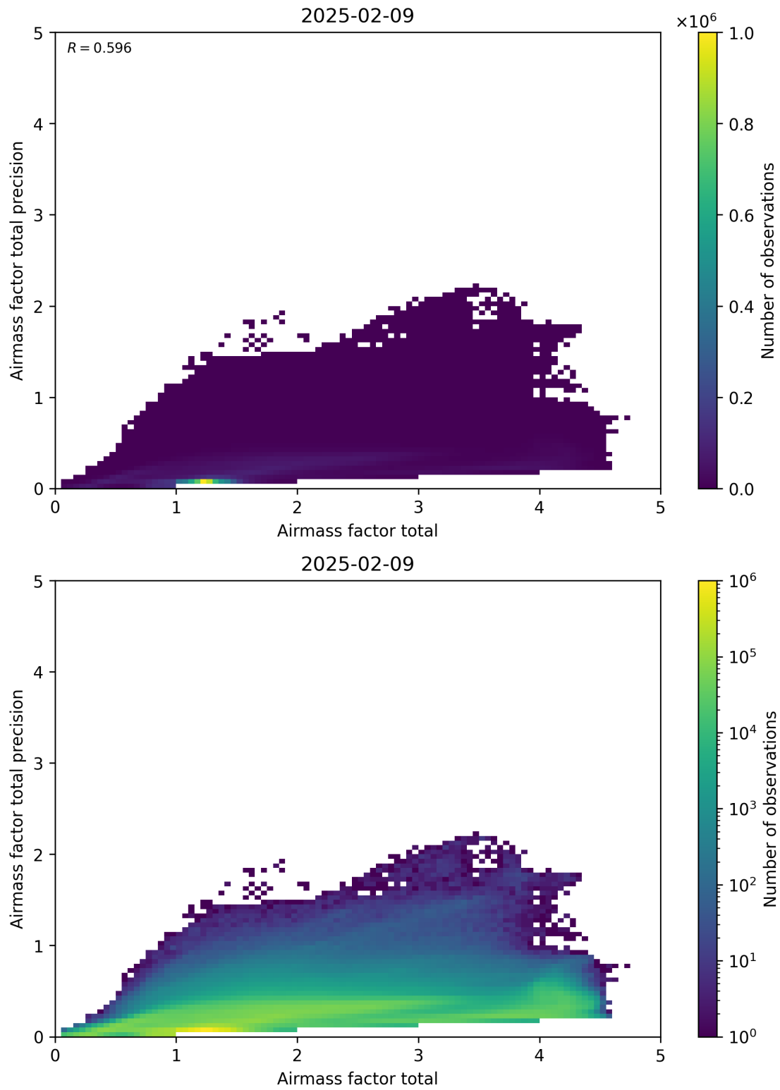
Figure 103: Scatter density plot of “Airmass factor total” against “Airmass factor total precision” for 2025-02-08 to 2025-02-10.
