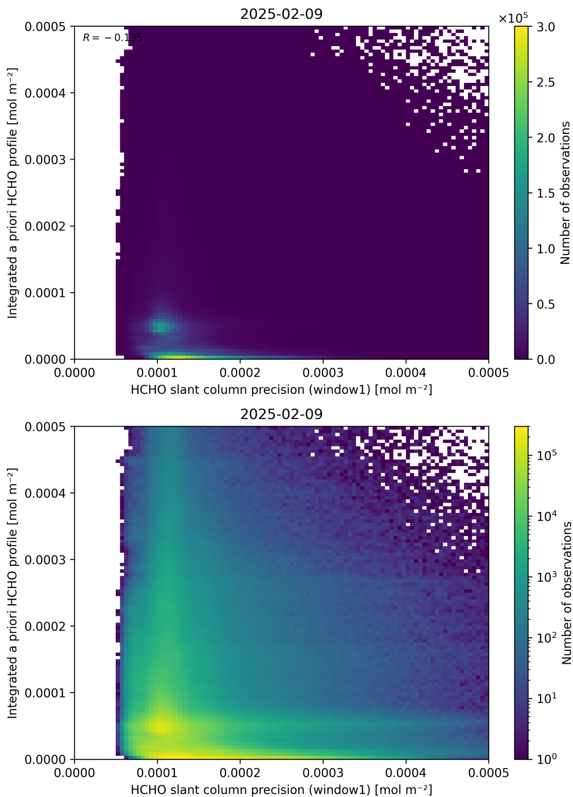
Figure 96: Scatter density plot of “HCHO slant column precision (window1)” against “Integrated a priori HCHO profile” for 2025-02-08 to 2025-02-10.
