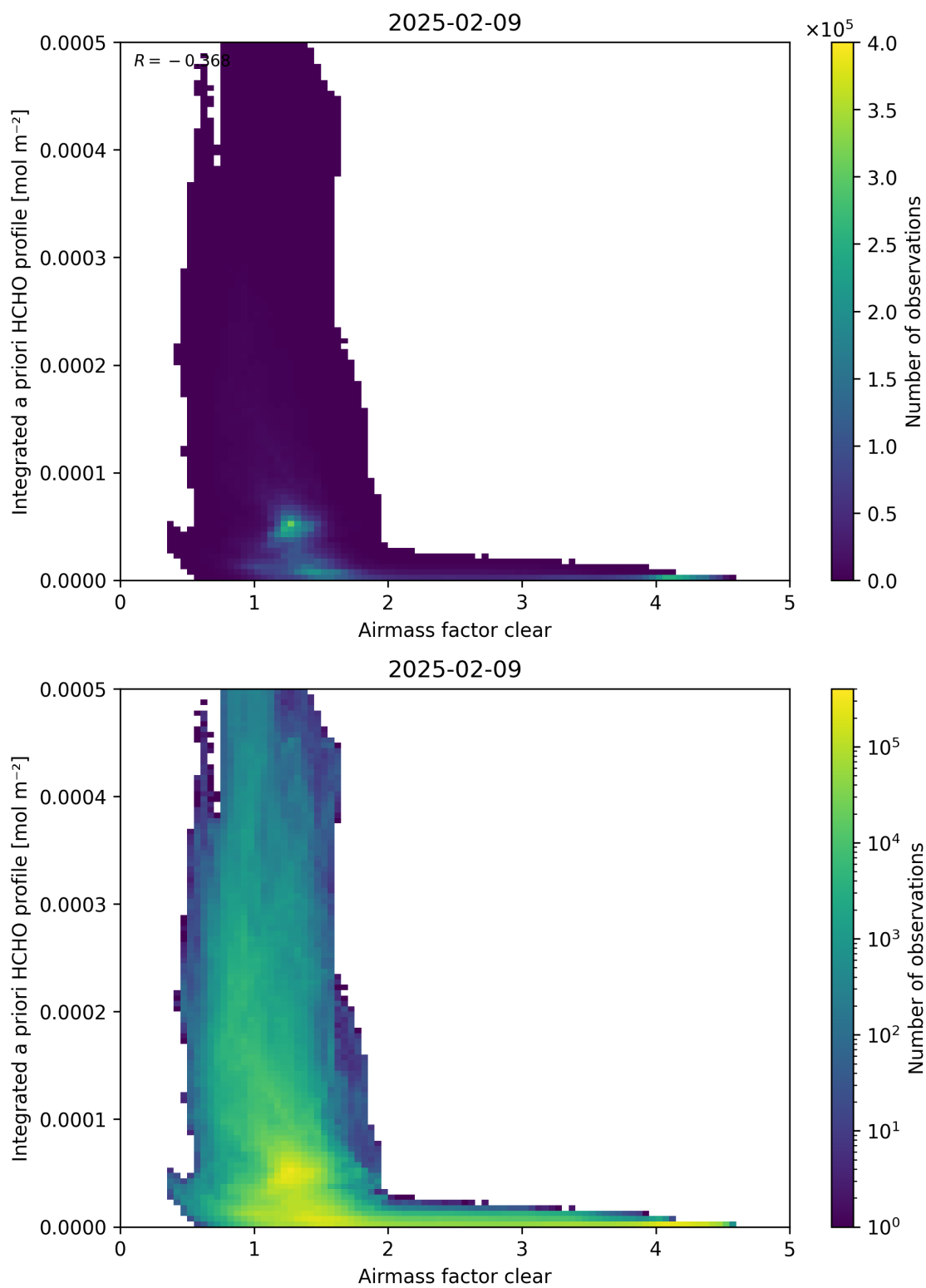
Figure 76: Scatter density plot of “Airmass factor clear” against “Integrated a priori HCHO profile” for 2025-02-08 to 2025-02-10.
