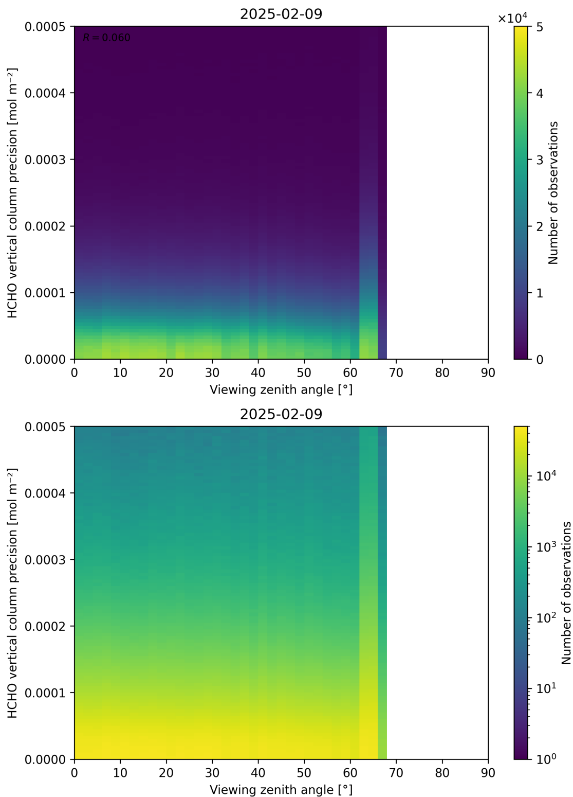
Figure 194: Scatter density plot of “Viewing zenith angle” against “HCHO vertical column precision” for 2025-02-08 to 2025-02-10.
