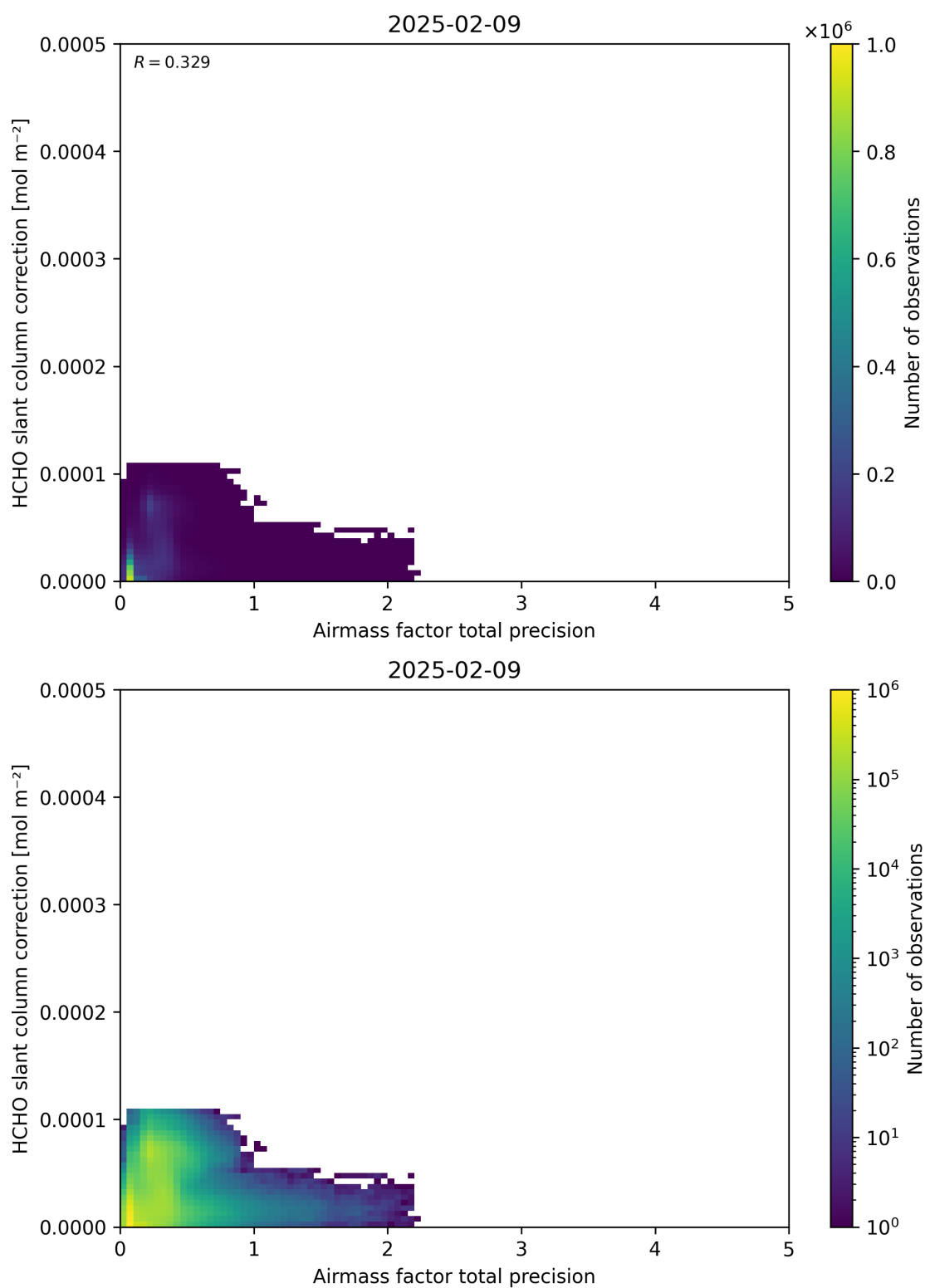
Figure 110: Scatter density plot of “Airmass factor total precision” against “HCHO slant column correction” for 2025-02-08 to 2025-02-10.
