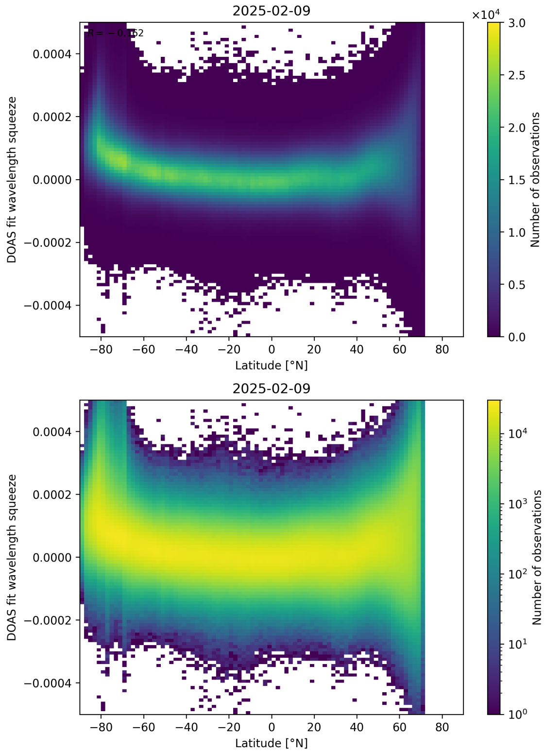
Figure 155: Scatter density plot of “Latitude” against “DOAS fit wavelength squeeze” for 2025-02-08 to 2025-02-10.
