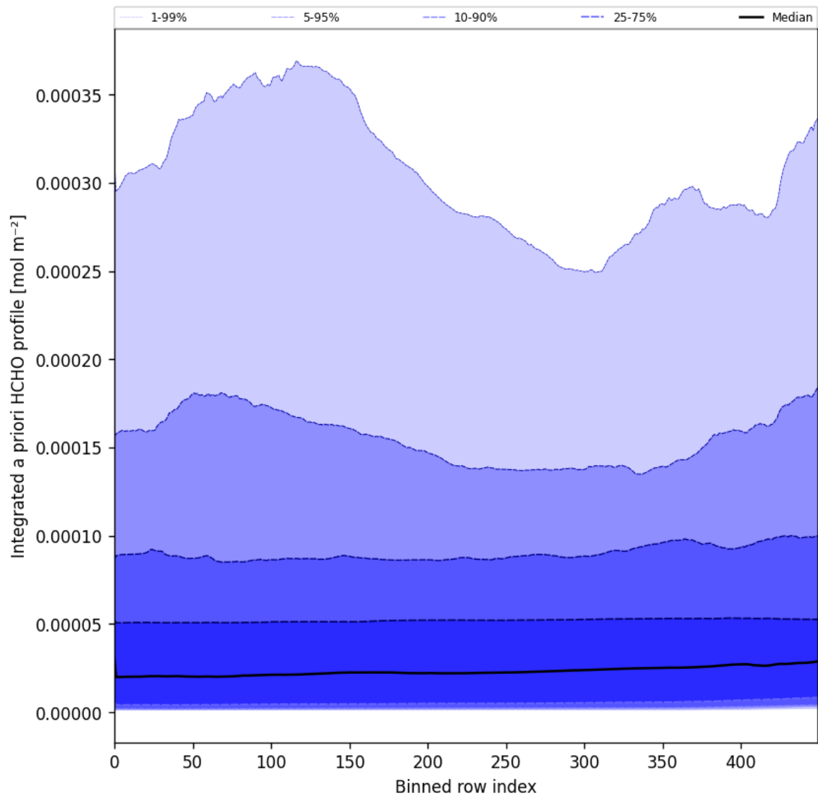
Figure 57: Along track statistics of "Integrated a priori HCHO profile" for 2025-02-08 to 2025-02-10
