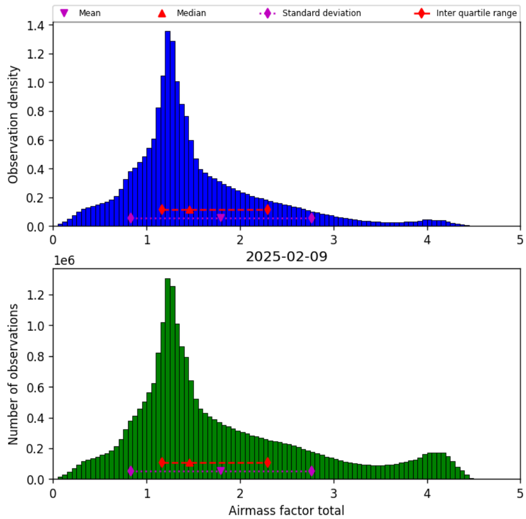
Figure 40: Histogram of “Airmass factor total” for 2025-02-08 to 2025-02-10
