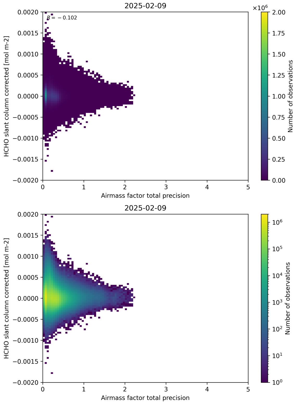
Figure 109: Scatter density plot of “Airmass factor total precision” against “HCHO slant column corrected” for 2025-02-08 to 2025-02-10.
