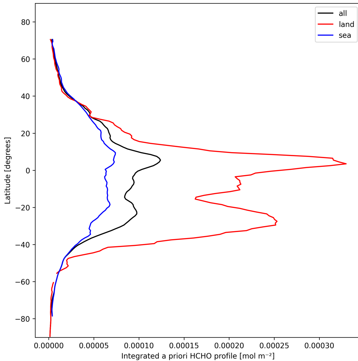
Figure 29: Zonal average of “Integrated a priori HCHO profile” for 2025-02-08 to 2025-02-10.
