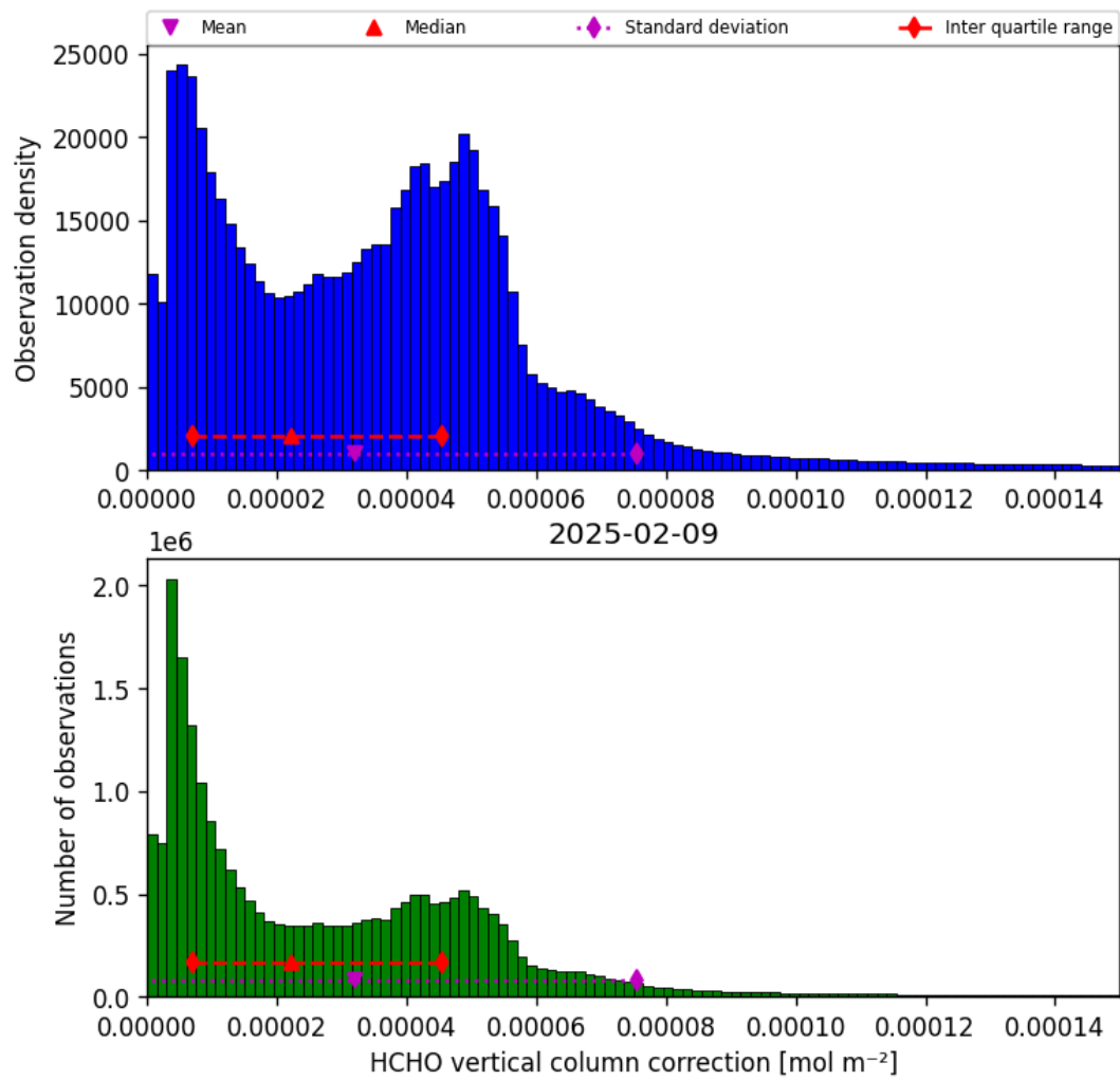
Figure 37: Histogram of “HCHO vertical column correction” for 2025-02-08 to 2025-02-10
