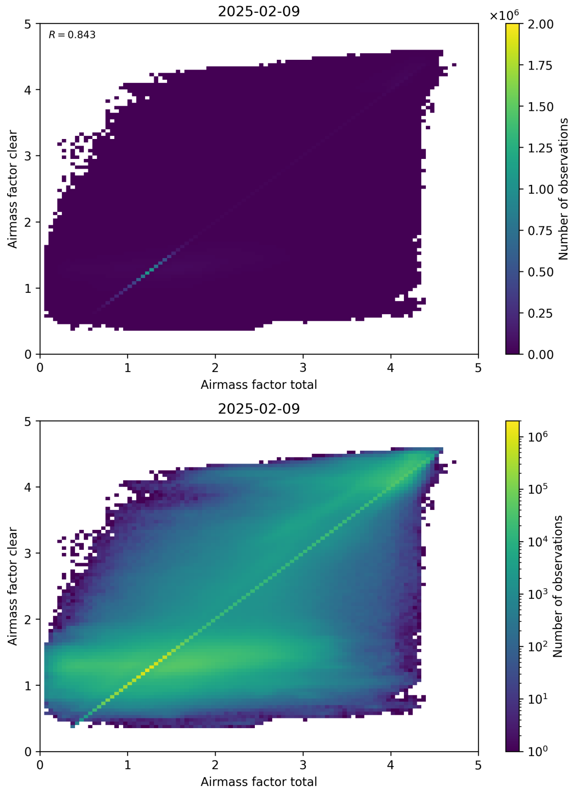
Figure 100: Scatter density plot of “Airmass factor total” against “Airmass factor clear” for 2025-02-08 to 2025-02-10.
