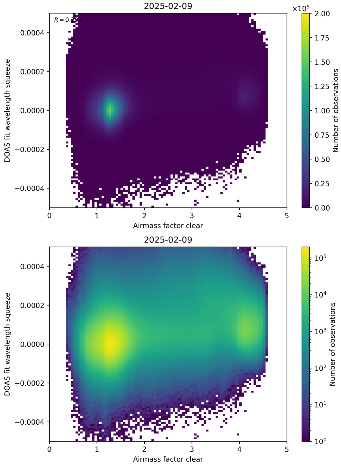
Figure 73: Scatter density plot of “Airmass factor clear” against “DOAS fit wavelength squeeze” for 2025-02-08 to 2025-02-10.
