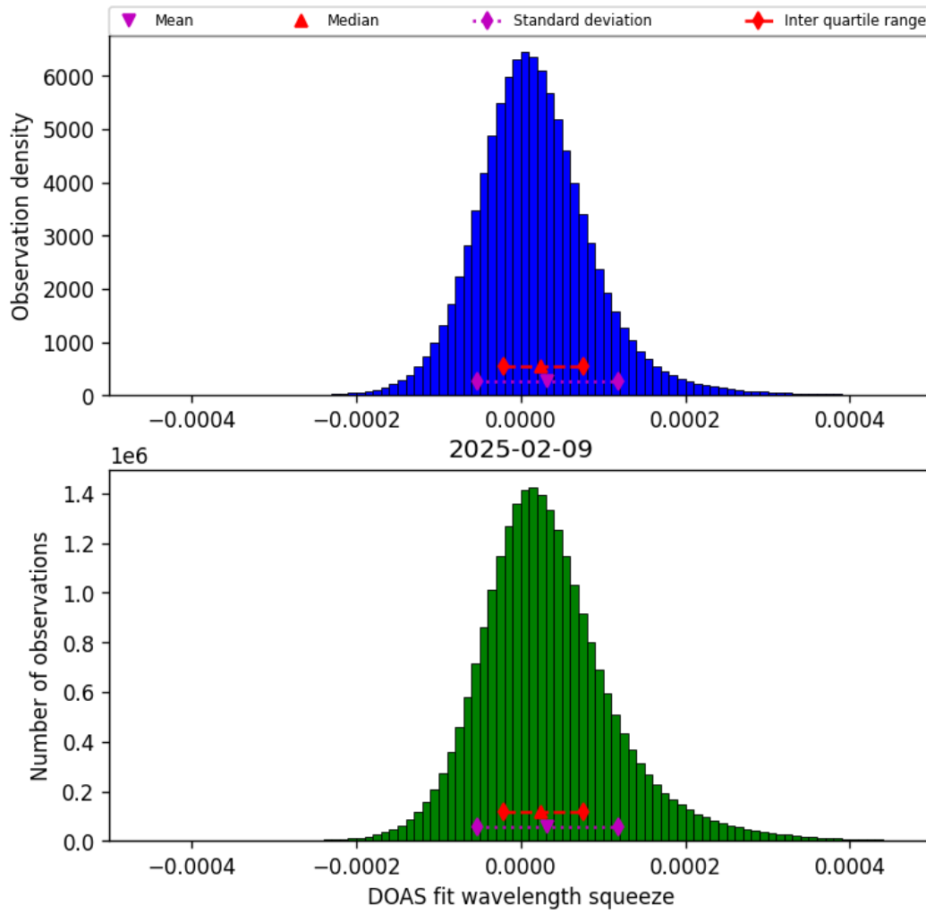
Figure 45: Histogram of “DOAS fit wavelength squeeze” for 2025-02-08 to 2025-02-10
