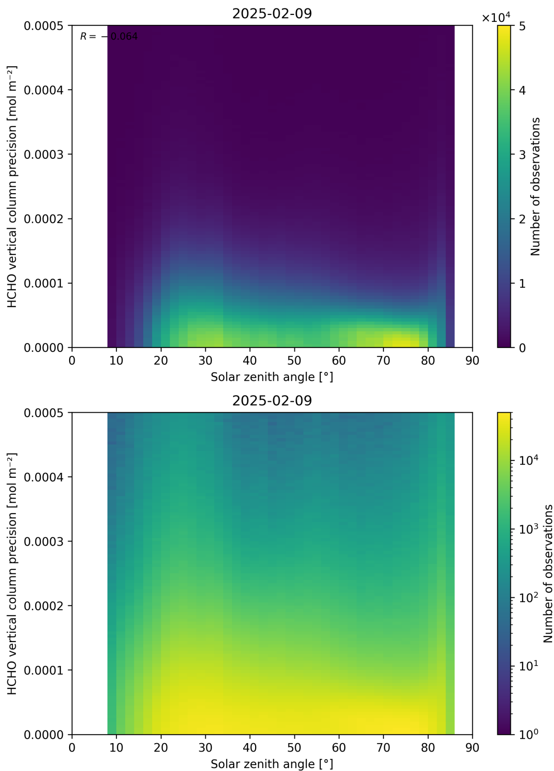
Figure 179: Scatter density plot of “Solar zenith angle” against “HCHO vertical column precision” for 2025-02-08 to 2025-02-10.
