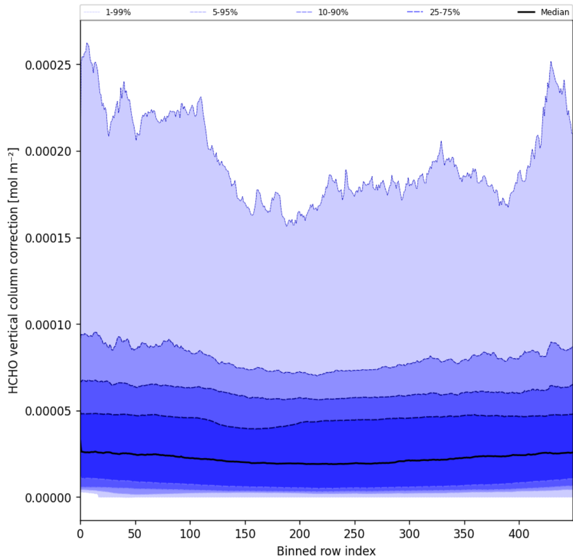
Figure 51: Along track statistics of “HCHO vertical column correction” for 2025-02-08 to 2025-02-10
