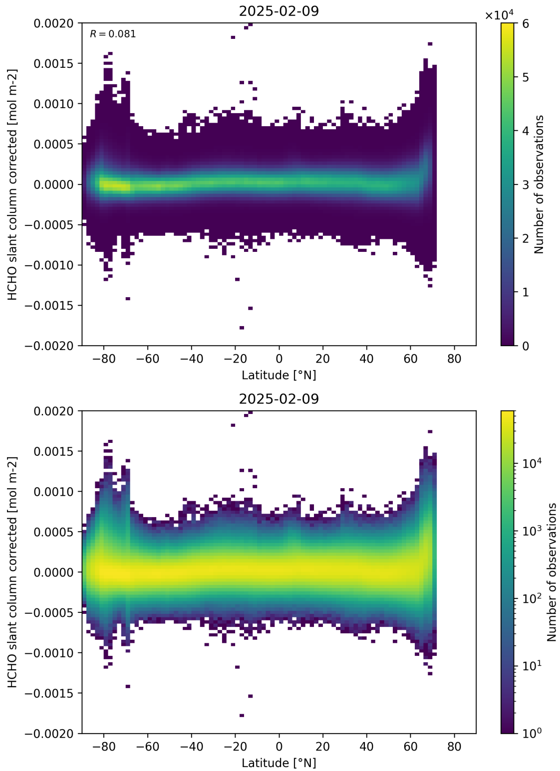
Figure 157: Scatter density plot of “Latitude” against “HCHO slant column corrected” for 2025-02-08 to 2025-02-10.
