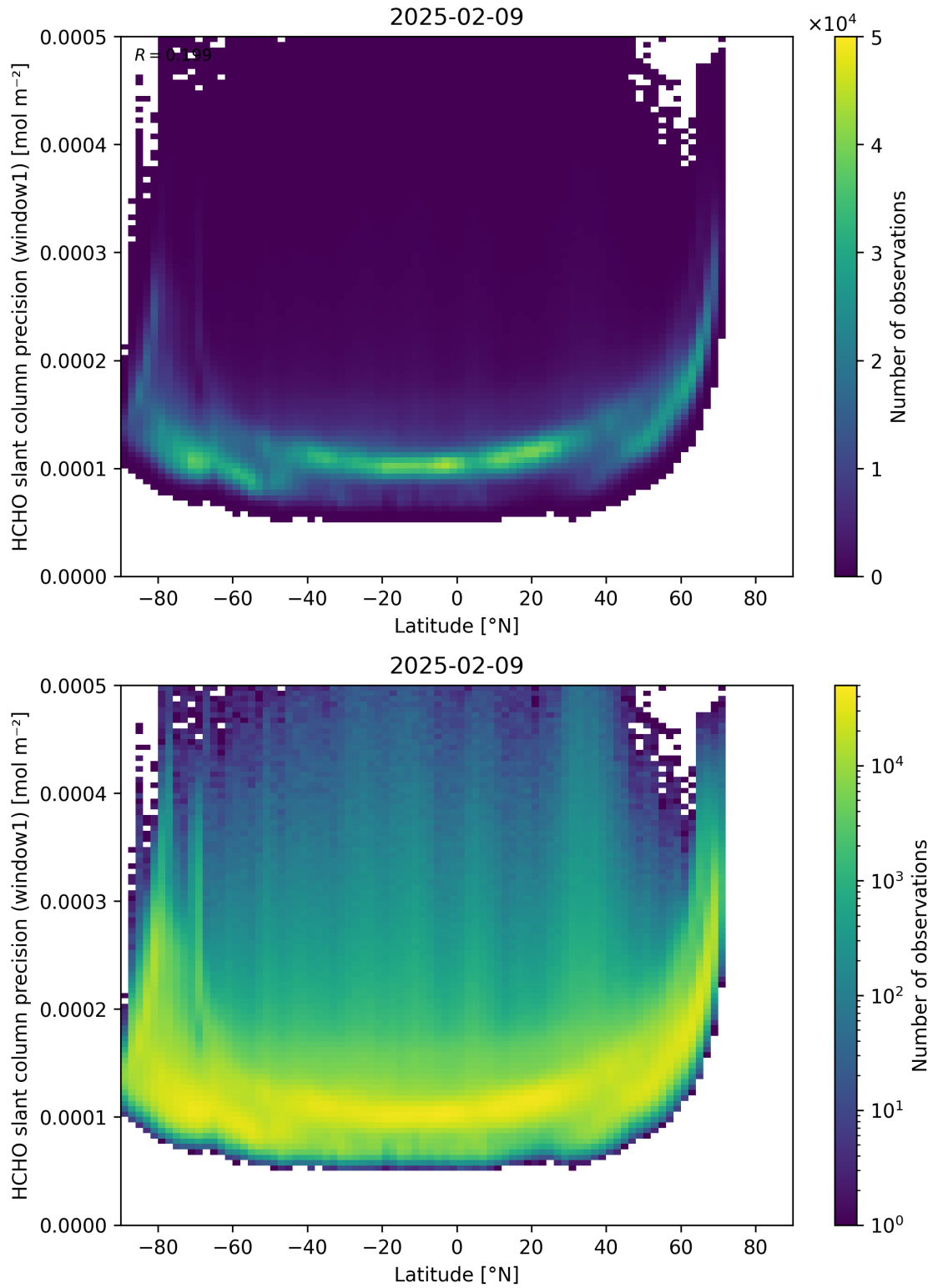
Figure 160: Scatter density plot of “Latitude” against “HCHO slant column precision (window1)” for 2025-02-08 to 2025-02-10.
