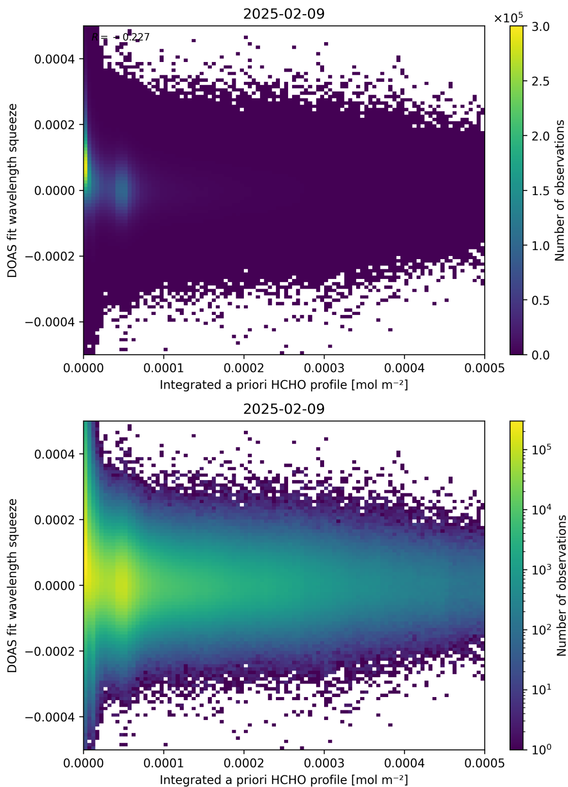
Figure 150: Scatter density plot of “Integrated a priori HCHO profile” against “DOAS fit wavelength squeeze” for 2025-02-08 to 2025-02-10.
