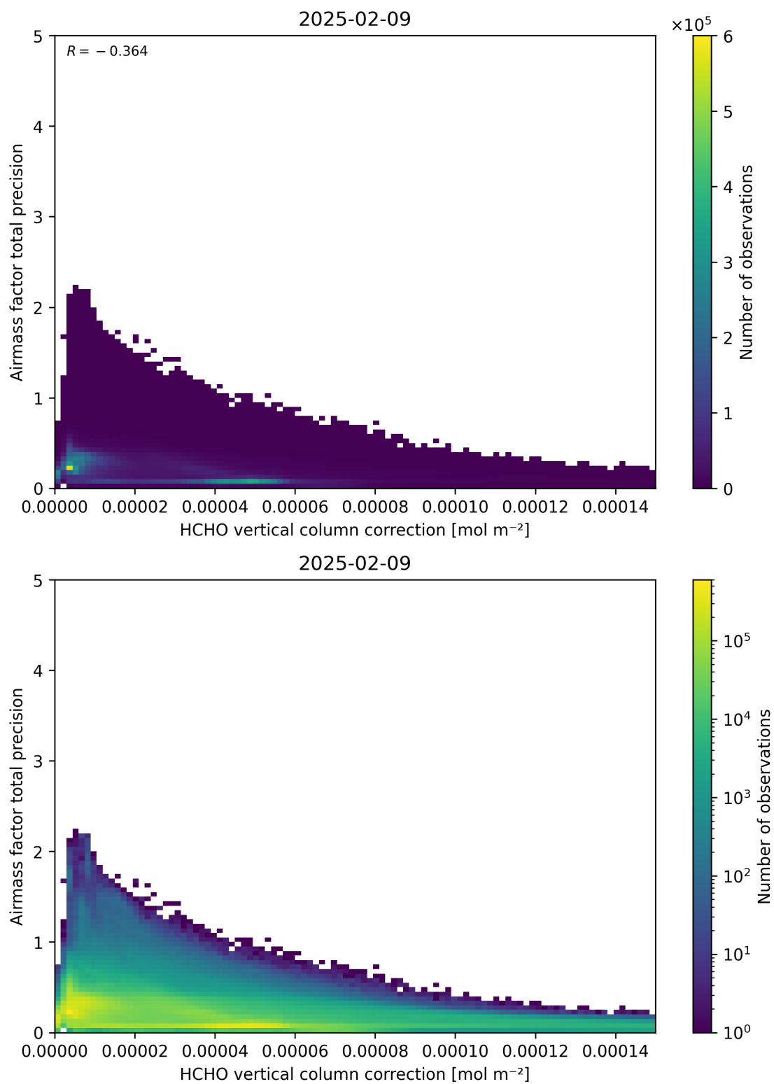
Figure 121: Scatter density plot of “HCHO vertical column correction” against “Airmass factor total precision” for 2025-02-08 to 2025-02-10.
