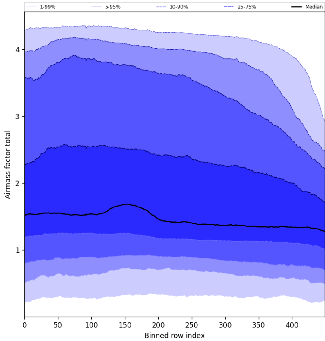
Figure 54: Along track statistics of “Airmass factor total” for 2025-02-08 to 2025-02-10
