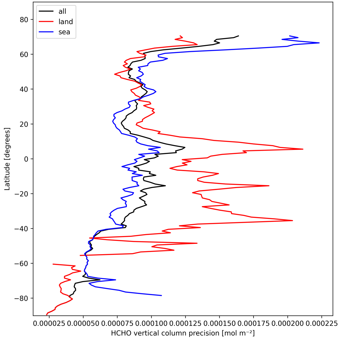
Figure 22: Zonal average of “HCHO vertical column precision” for 2025-02-08 to 2025-02-10.
