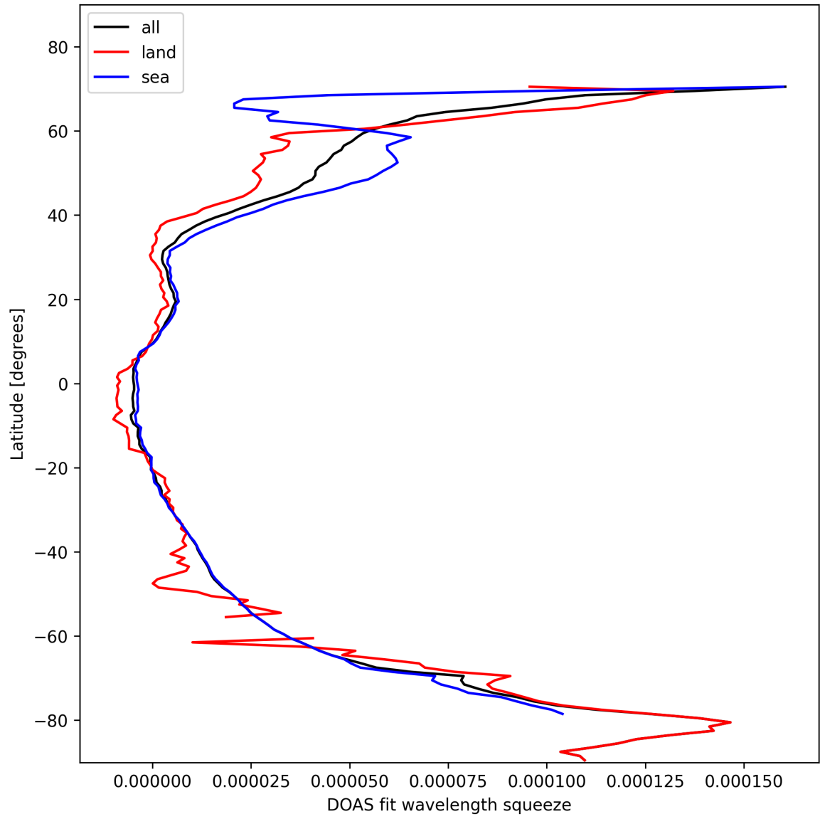
Figure 31: Zonal average of “DOAS fit wavelength squeeze” for 2025-02-08 to 2025-02-10.
