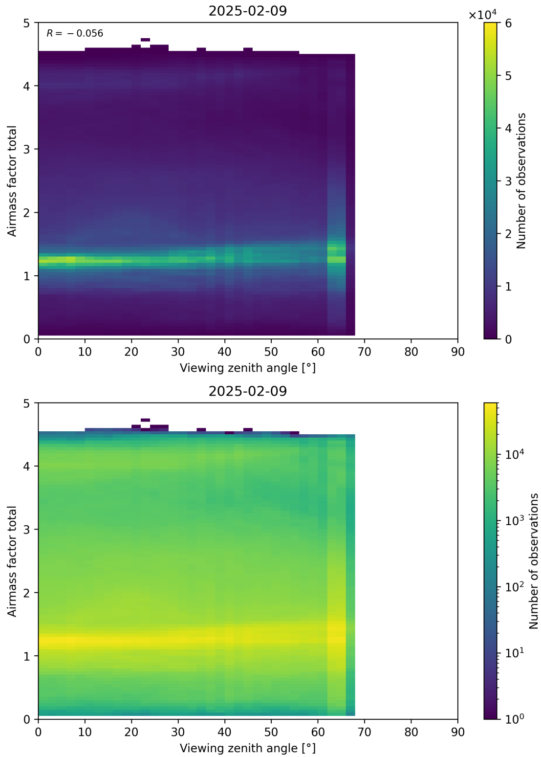
Figure 190: Scatter density plot of “Viewing zenith angle” against “Airmass factor total” for 2025-02-08 to 2025-02-10.
