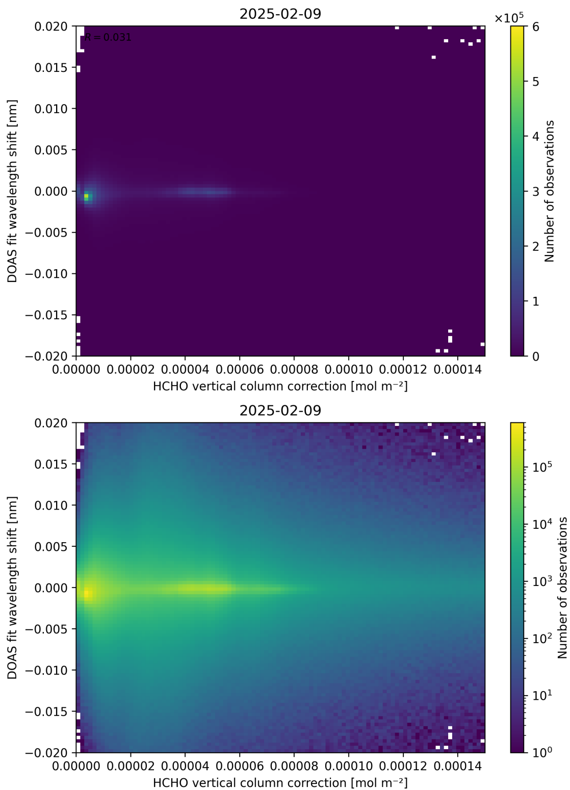
Figure 113: Scatter density plot of “HCHO vertical column correction” against “DOAS fit wavelength shift” for 2025-02-08 to 2025-02-10.
