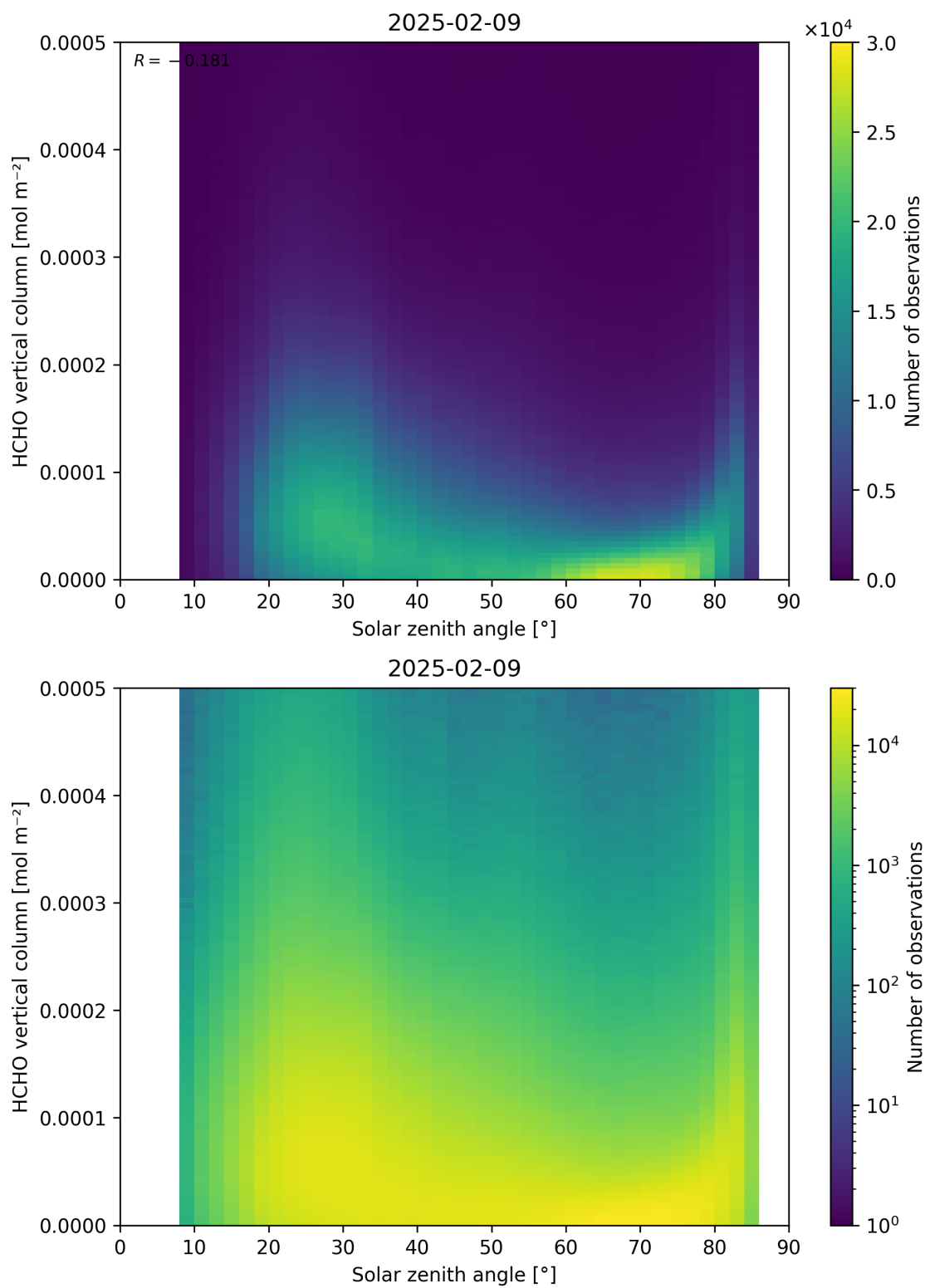
Figure 177: Scatter density plot of “Solar zenith angle” against “HCHO vertical column” for 2025-02-08 to 2025-02-10.
