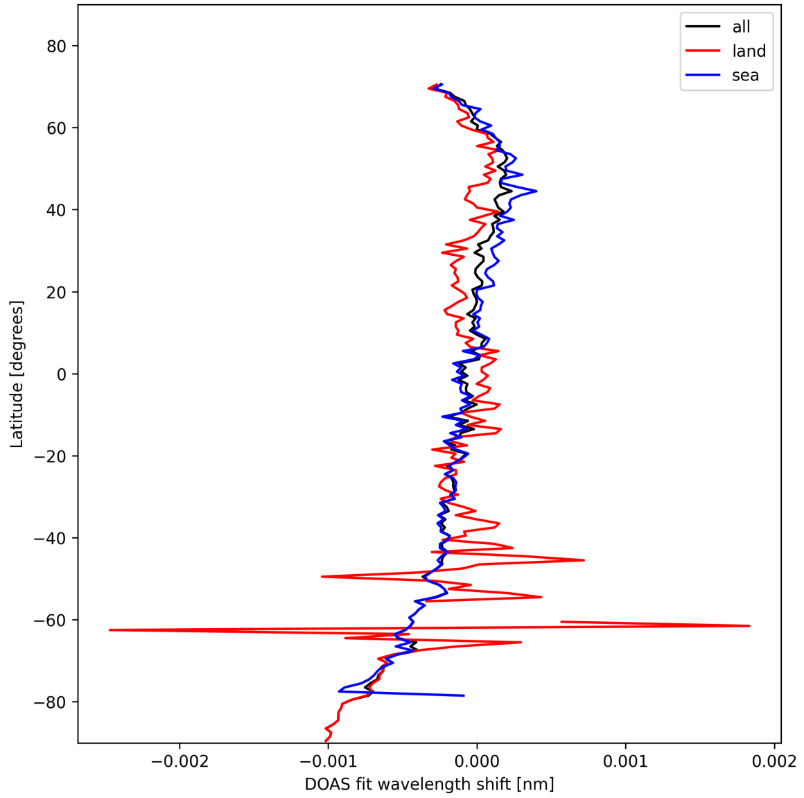
Figure 30: Zonal average of “DOAS fit wavelength shift” for 2025-02-08 to 2025-02-10.
