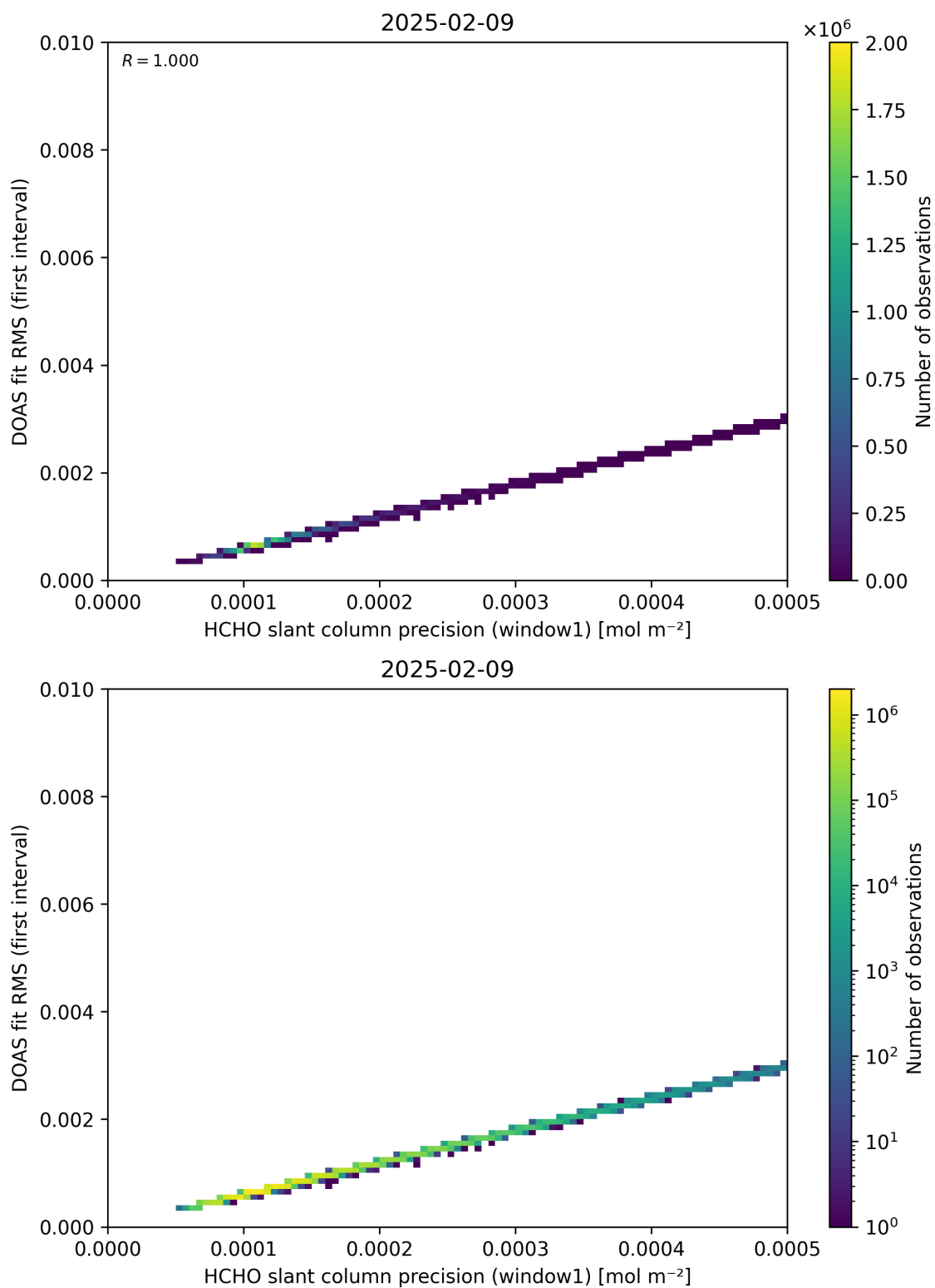
Figure 88: Scatter density plot of “HCHO slant column precision (window1)” against “DOAS fit RMS (first interval)” for 2025-02-08 to 2025-02-10.
