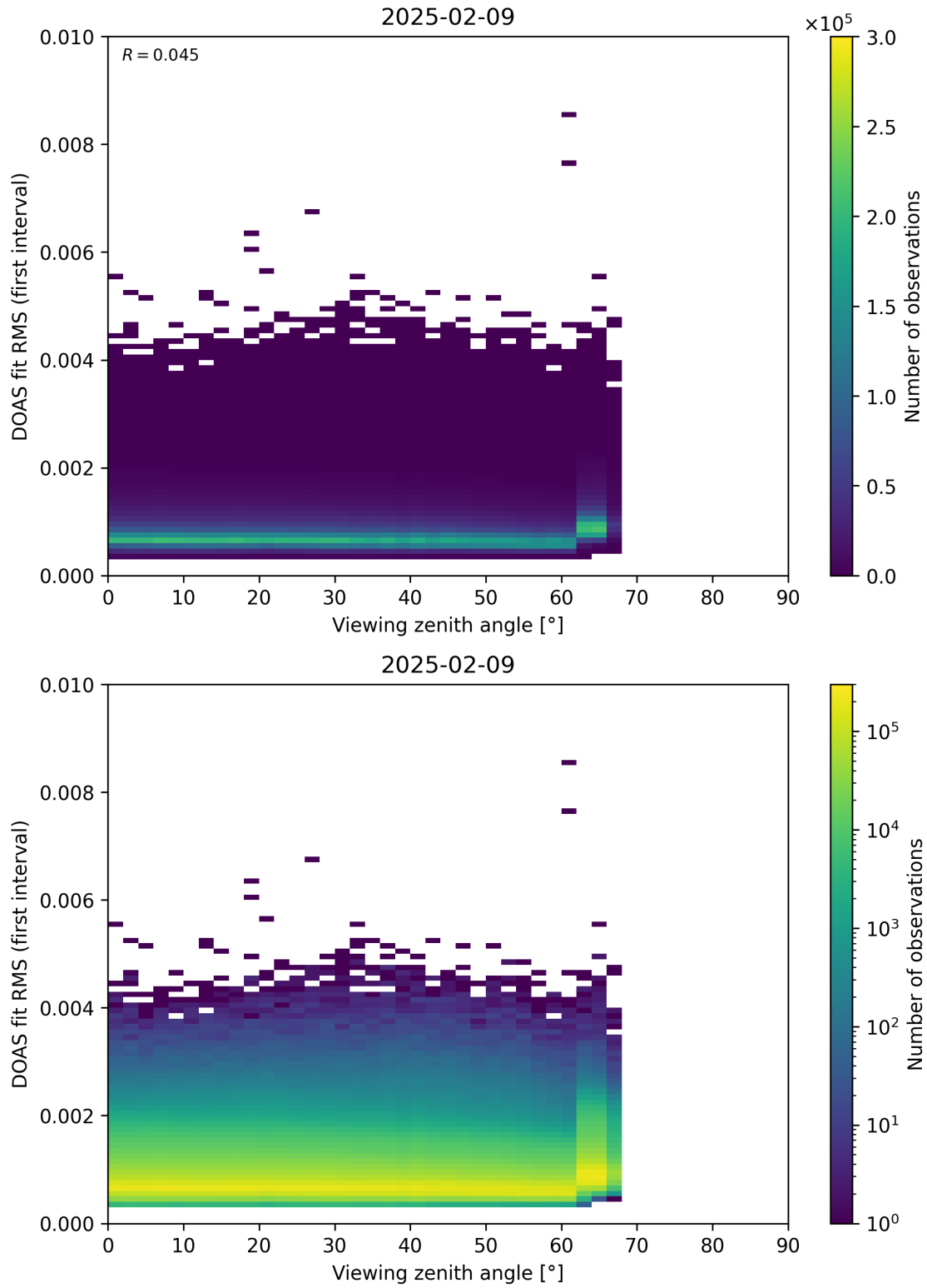
Figure 182: Scatter density plot of “Viewing zenith angle” against “DOAS fit RMS (first interval)” for 2025-02-08 to 2025-02-10.
