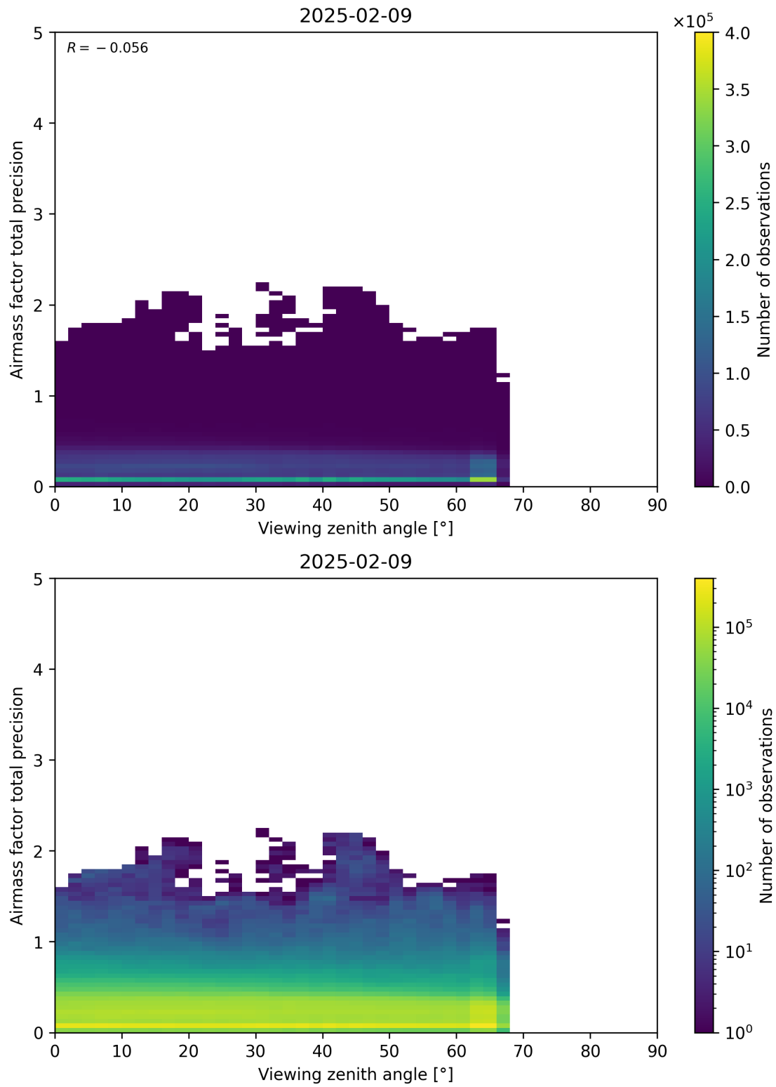
Figure 191: Scatter density plot of “Viewing zenith angle” against “Airmass factor total precision” for 2025-02-08 to 2025-02-10.
