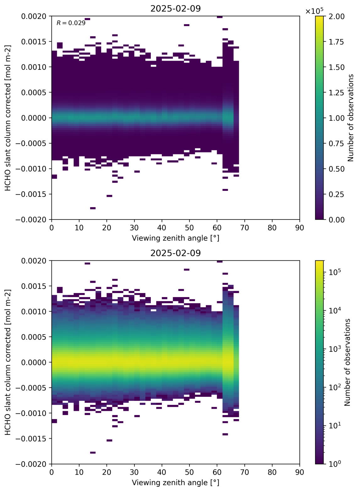
Figure 186: Scatter density plot of “Viewing zenith angle” against “HCHO slant column corrected” for 2025-02-08 to 2025-02-10.
