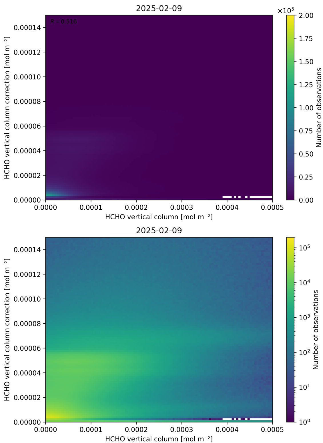
Figure 133: Scatter density plot of “HCHO vertical column” against “HCHO vertical column correction” for 2025-02-08 to 2025-02-10.
