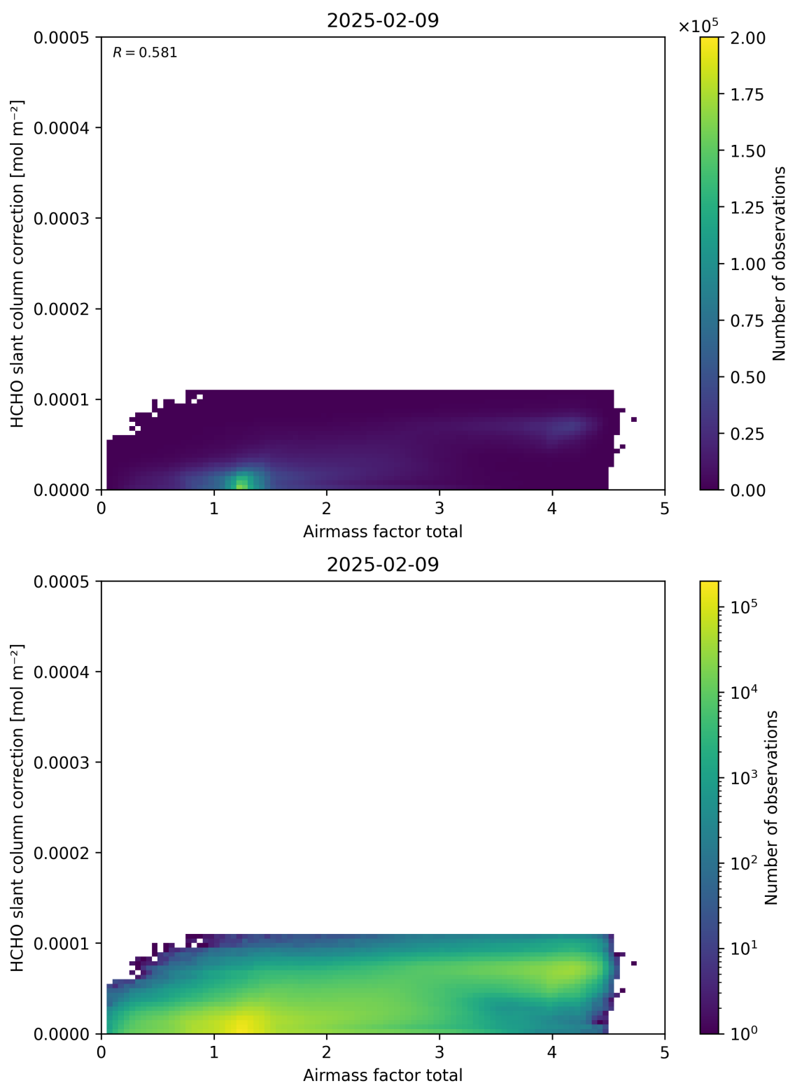
Figure 102: Scatter density plot of “Airmass factor total” against “HCHO slant column correction” for 2025-02-08 to 2025-02-10.
