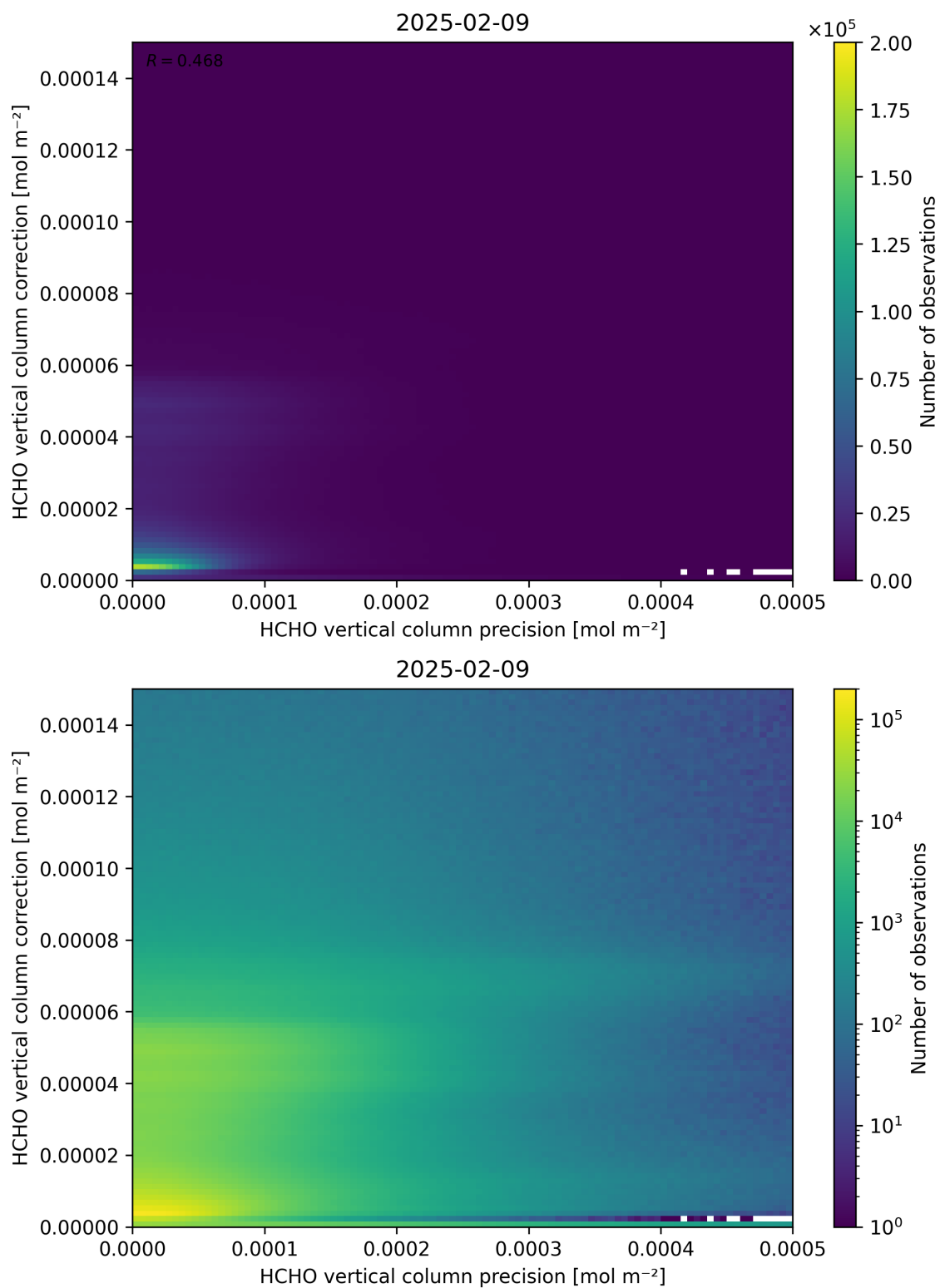
Figure 146: Scatter density plot of “HCHO vertical column precision” against “HCHO vertical column correction” for 2025-02-08 to 2025-02-10.
