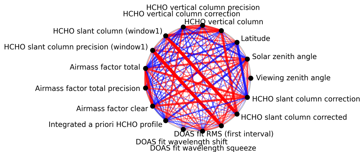
Figure 1: Map of correlation graph for 2025-02-08 to 2025-02-10.
