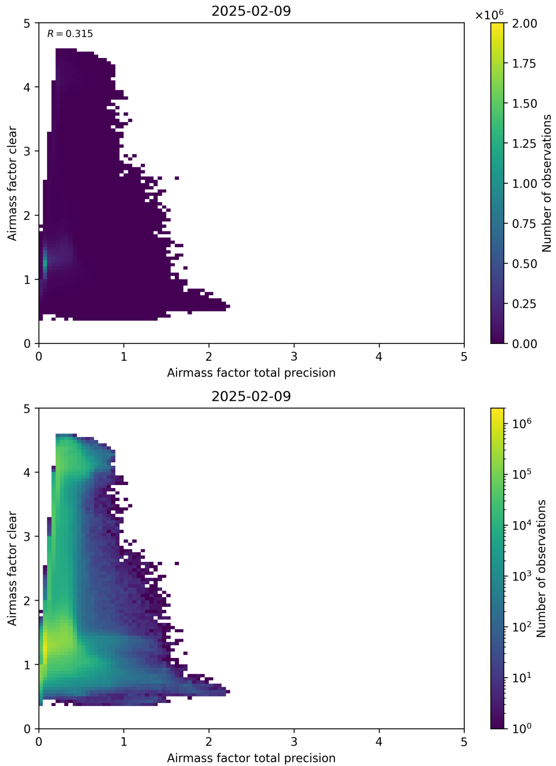
Figure 108: Scatter density plot of “Airmass factor total precision” against “Airmass factor clear” for 2025-02-08 to 2025-02-10.
