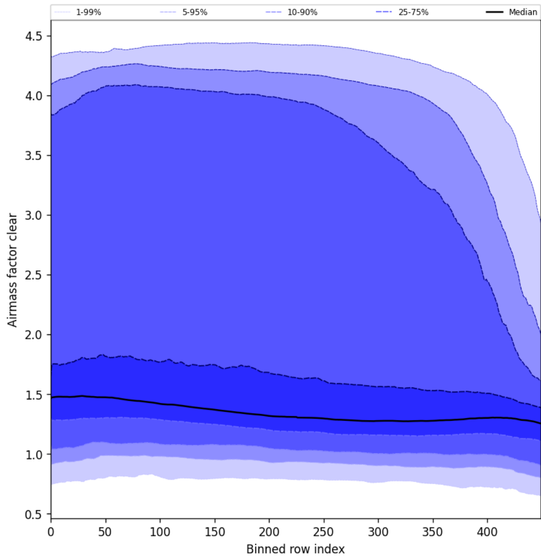
Figure 56: Along track statistics of “Airmass factor clear” for 2025-02-08 to 2025-02-10
