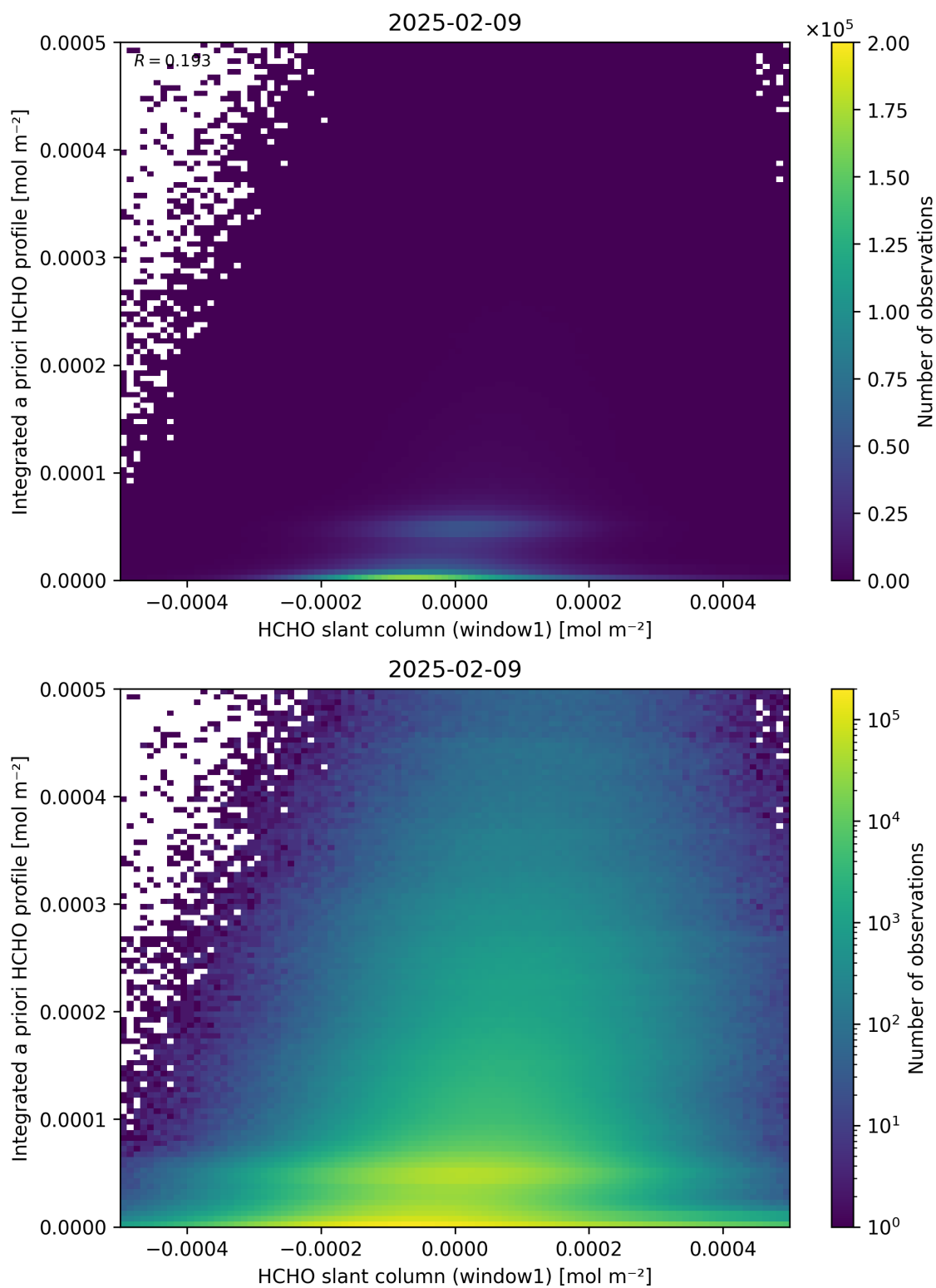
Figure 87: Scatter density plot of “HCHO slant column (window1)” against “Integrated a priori HCHO profile” for 2025-02-08 to 2025-02-10.
