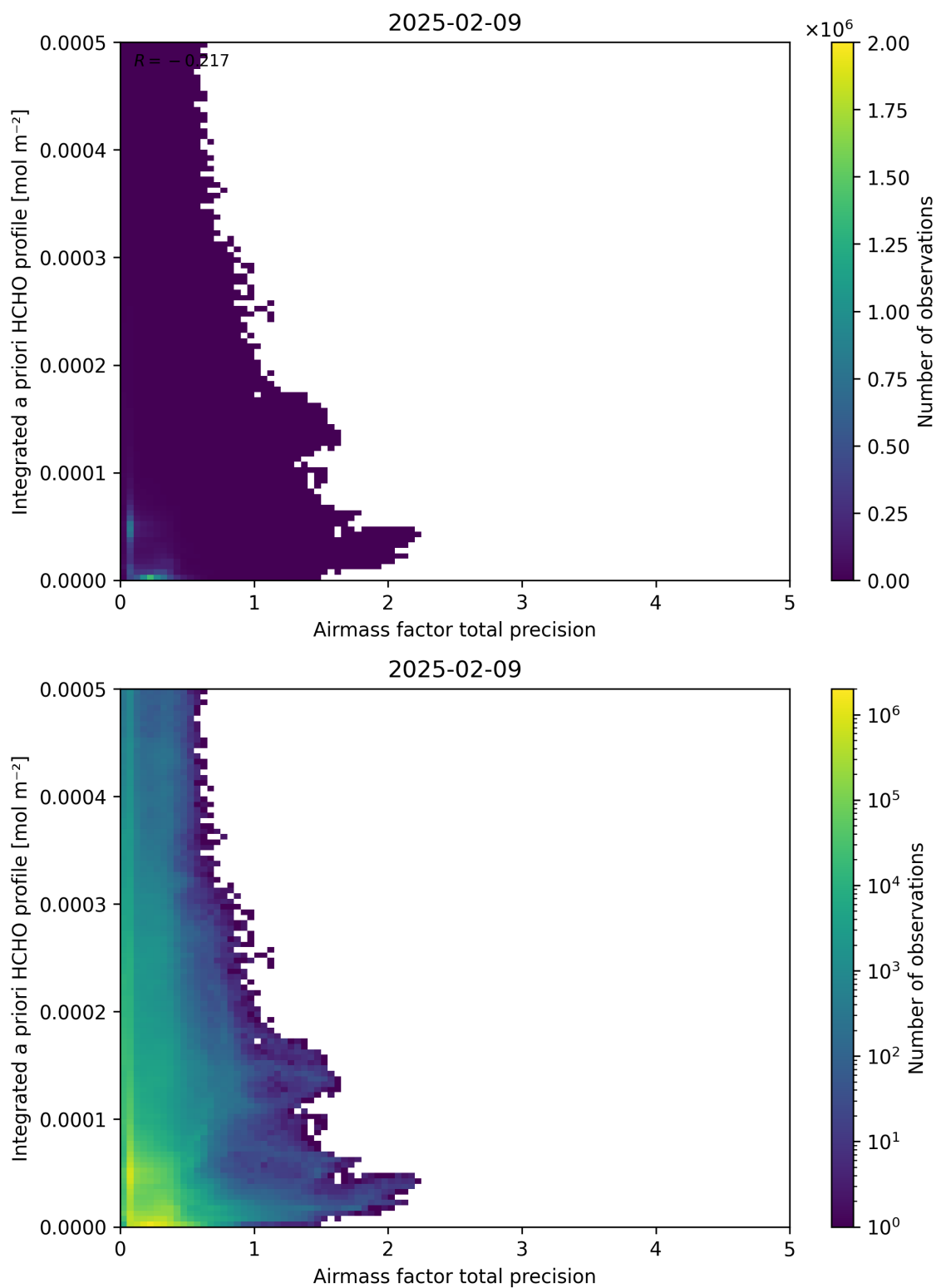
Figure 111: Scatter density plot of “Airmass factor total precision” against “Integrated a priori HCHO profile” for 2025-02-08 to 2025-02-10.
