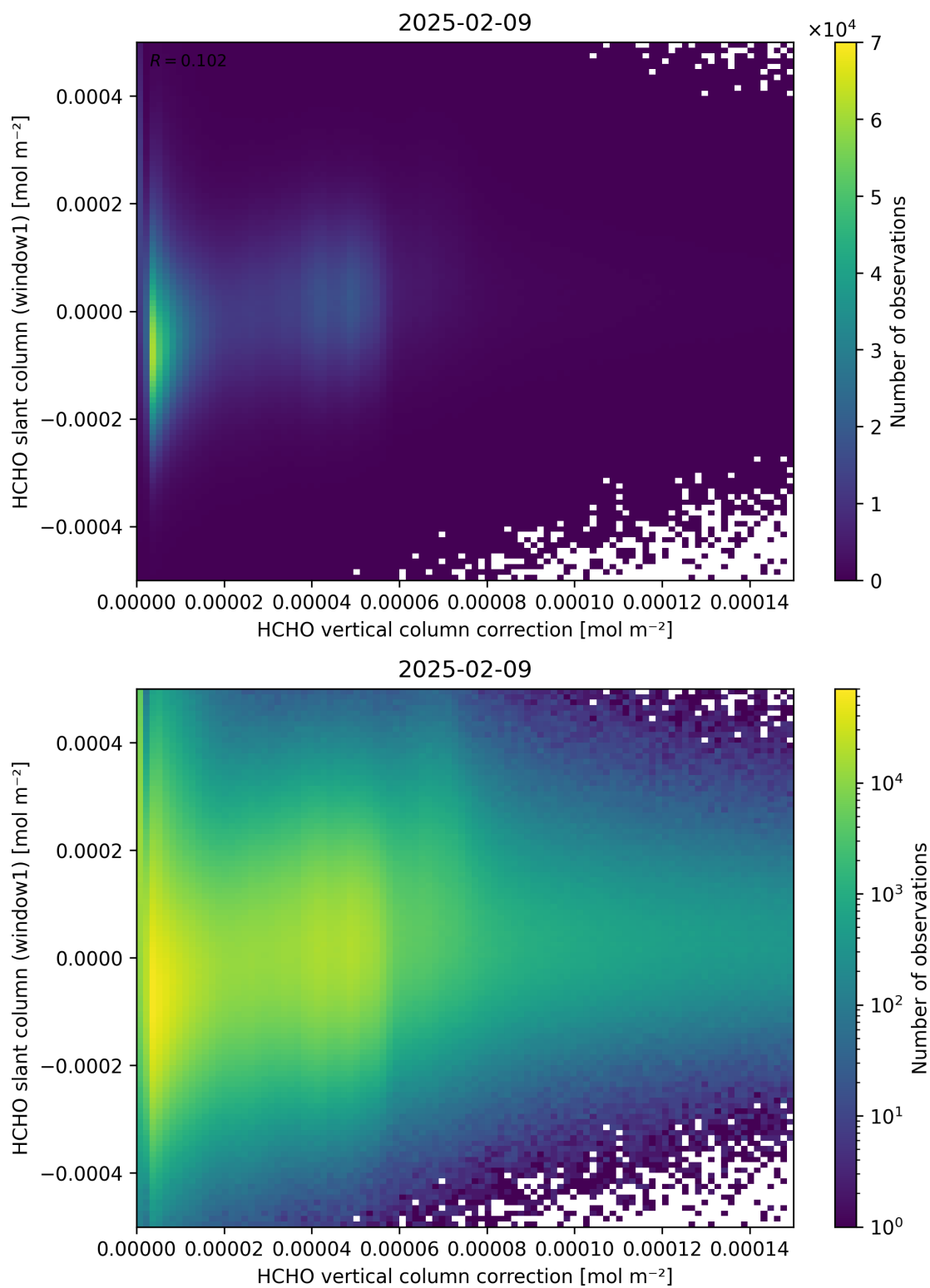
Figure 118: Scatter density plot of “HCHO vertical column correction” against “HCHO slant column (window1)” for 2025-02-08 to 2025-02-10.
