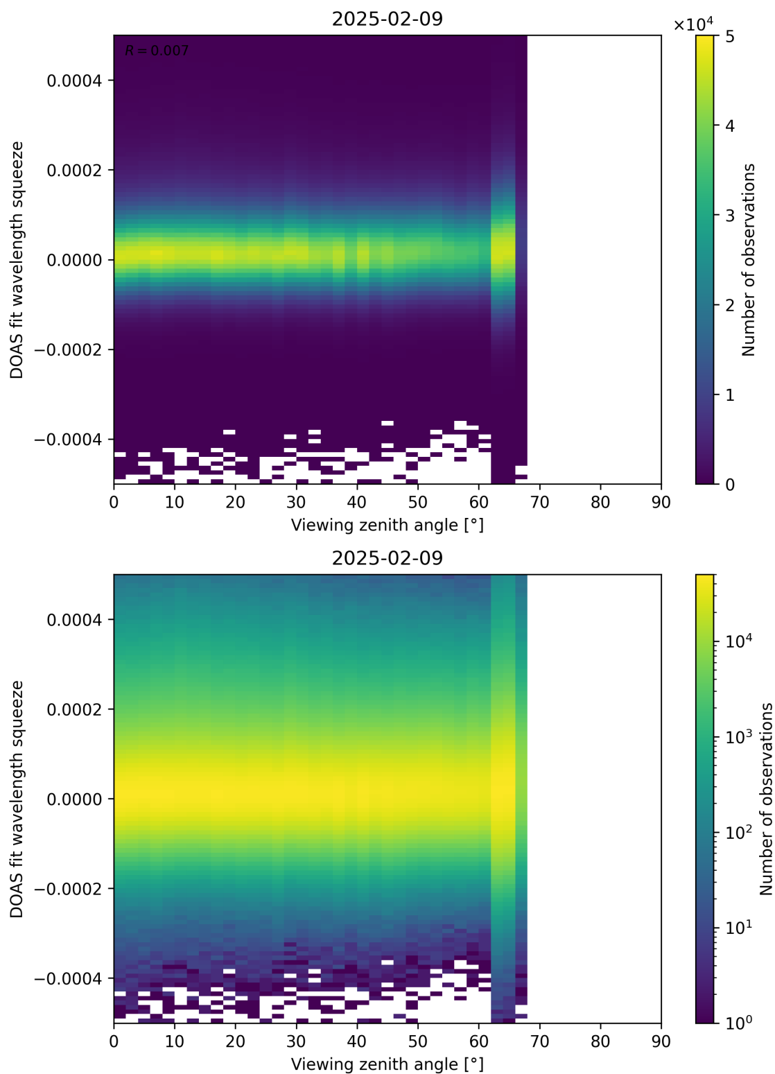
Figure 184: Scatter density plot of “Viewing zenith angle” against “DOAS fit wavelength squeeze” for 2025-02-08 to 2025-02-10.
