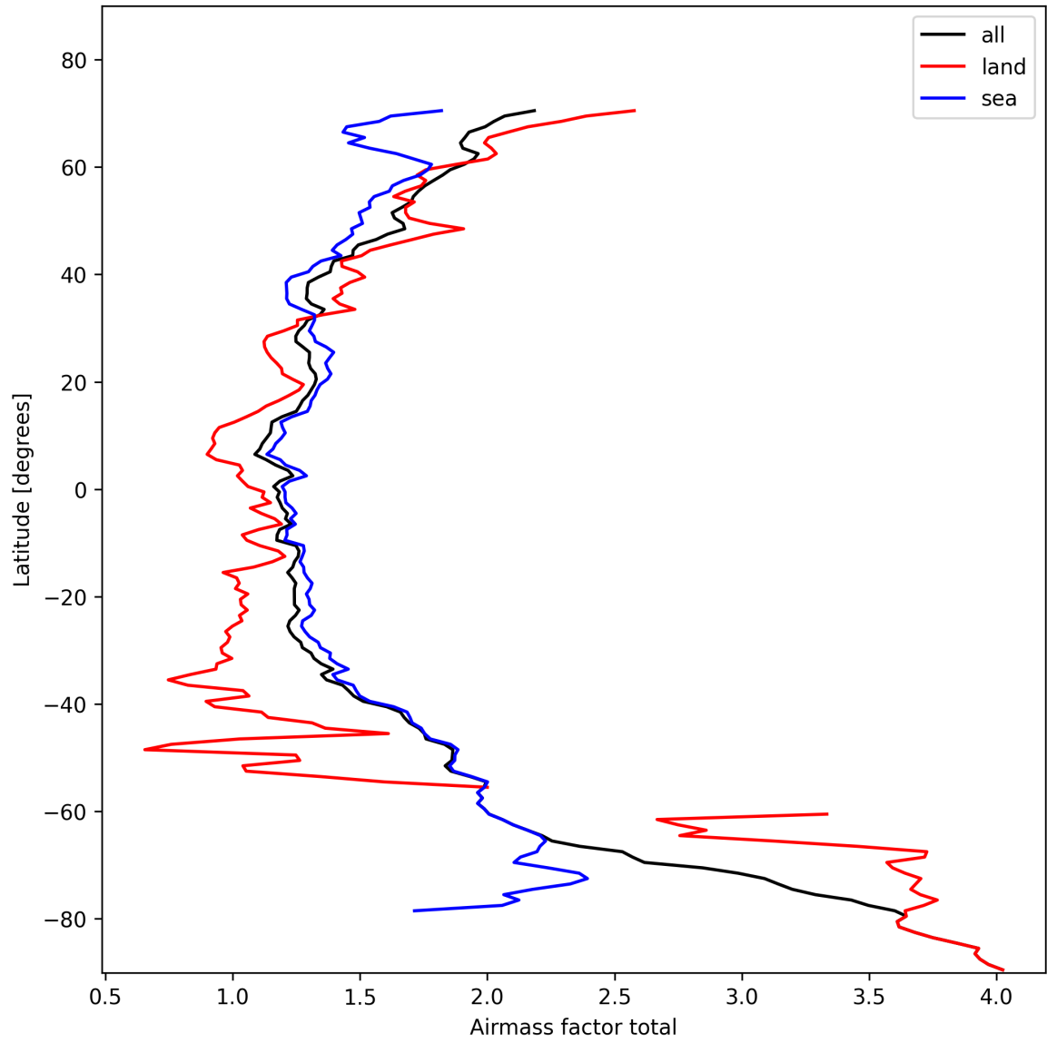
Figure 26: Zonal average of “Airmass factor total” for 2025-02-08 to 2025-02-10.
