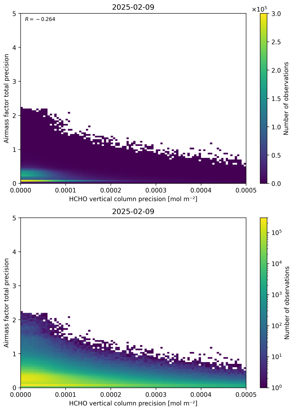
Figure 145: Scatter density plot of “HCHO vertical column precision” against “Airmass factor total precision” for 2025-02-08 to 2025-02-10.
