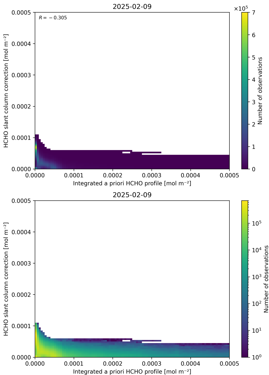
Figure 152: Scatter density plot of “Integrated a priori HCHO profile” against “HCHO slant column correction” for 2025-02-08 to 2025-02-10.
