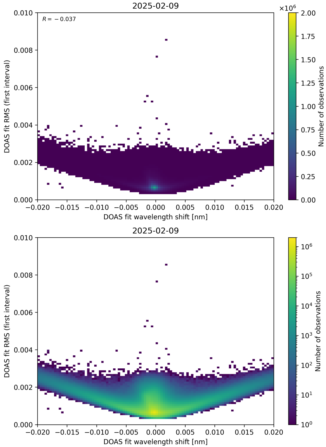
Figure 64: Scatter density plot of “DOAS fit wavelength shift” against “DOAS fit RMS (first interval)” for 2025-02-08 to 2025-02-10.
