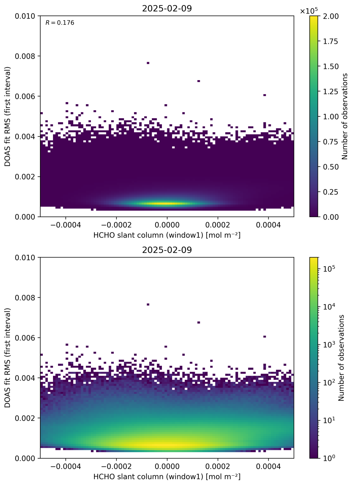
Figure 78: Scatter density plot of “HCHO slant column (window1)” against “DOAS fit RMS (first interval)” for 2025-02-08 to 2025-02-10.
