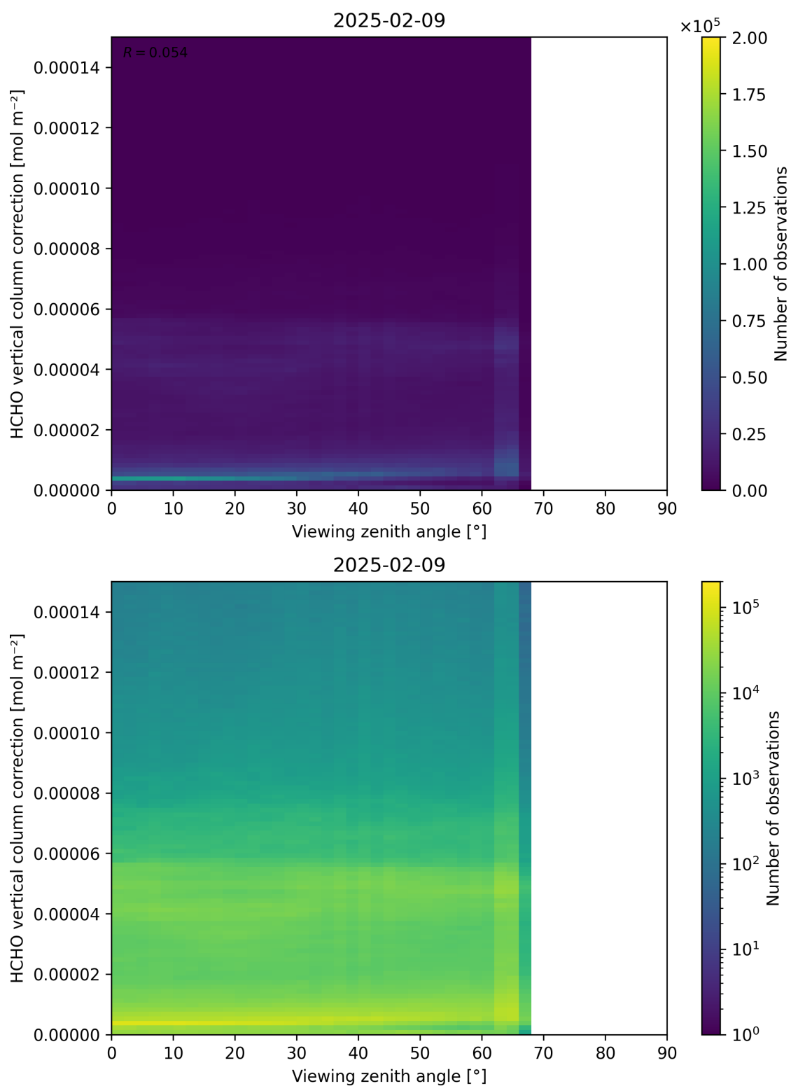
Figure 193: Scatter density plot of “Viewing zenith angle” against “HCHO vertical column correction” for 2025-02-08 to 2025-02-10.
