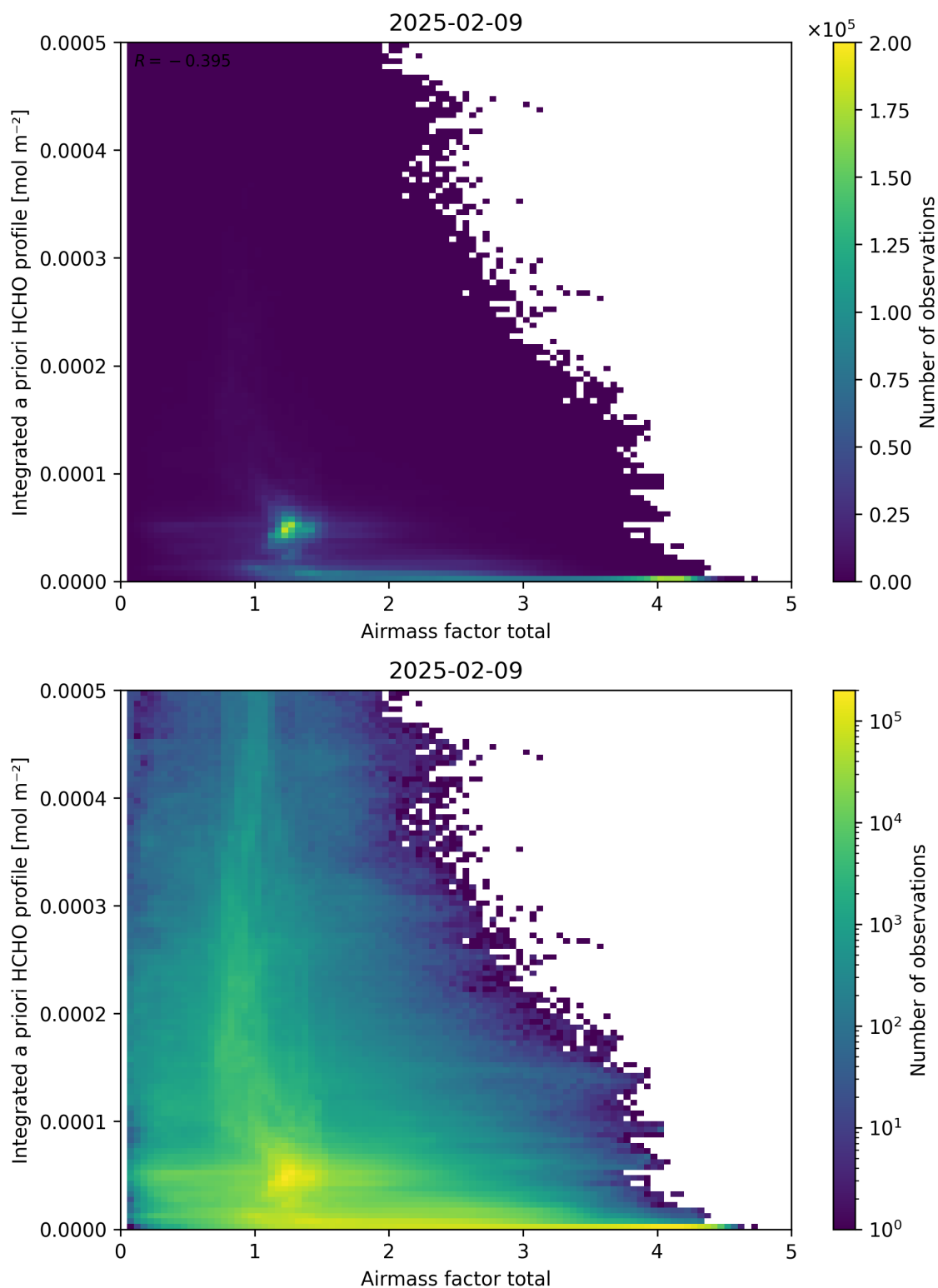
Figure 104: Scatter density plot of “Airmass factor total” against “Integrated a priori HCHO profile” for 2025-02-08 to 2025-02-10.
