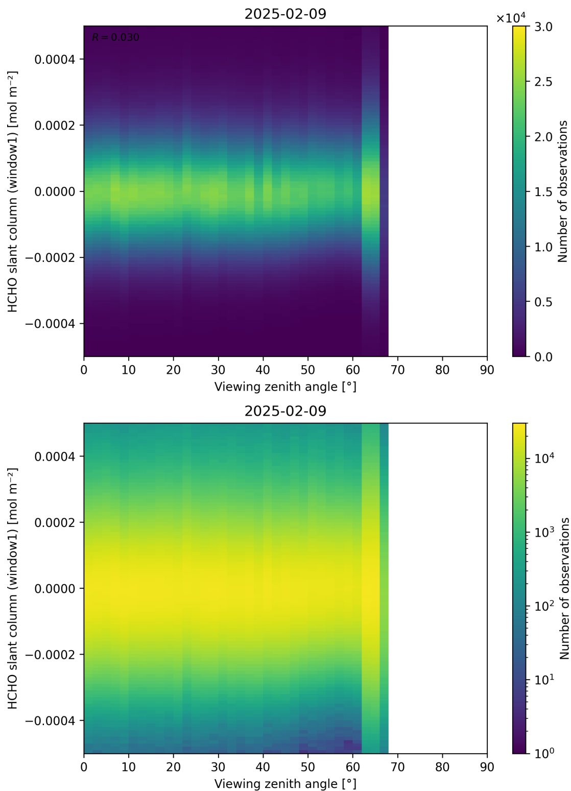
Figure 188: Scatter density plot of “Viewing zenith angle” against “HCHO slant column (window1)” for 2025-02-08 to 2025-02-10.
