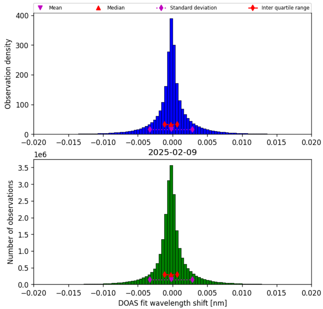
Figure 44: Histogram of “DOAS fit wavelength shift” for 2025-02-08 to 2025-02-10
