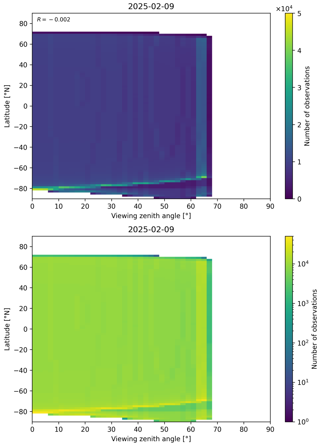
Figure 196: Scatter density plot of “Viewing zenith angle” against “Latitude” for 2025-02-08 to 2025-02-10.
