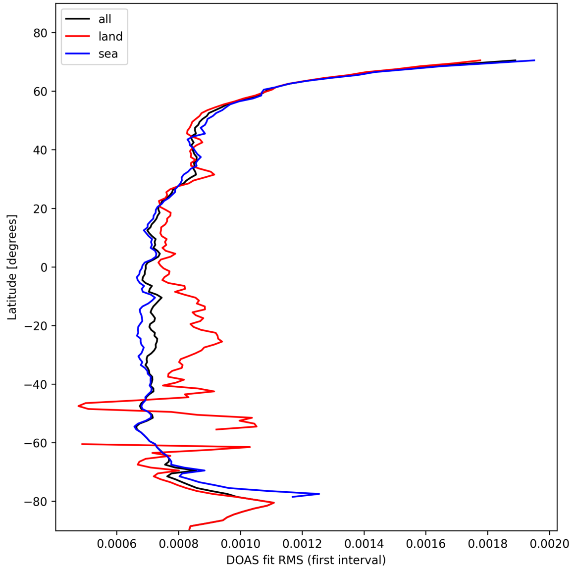
Figure 32: Zonal average of "DOAS fit RMS (first interval)" for 2025-02-08 to 2025-02-10.
