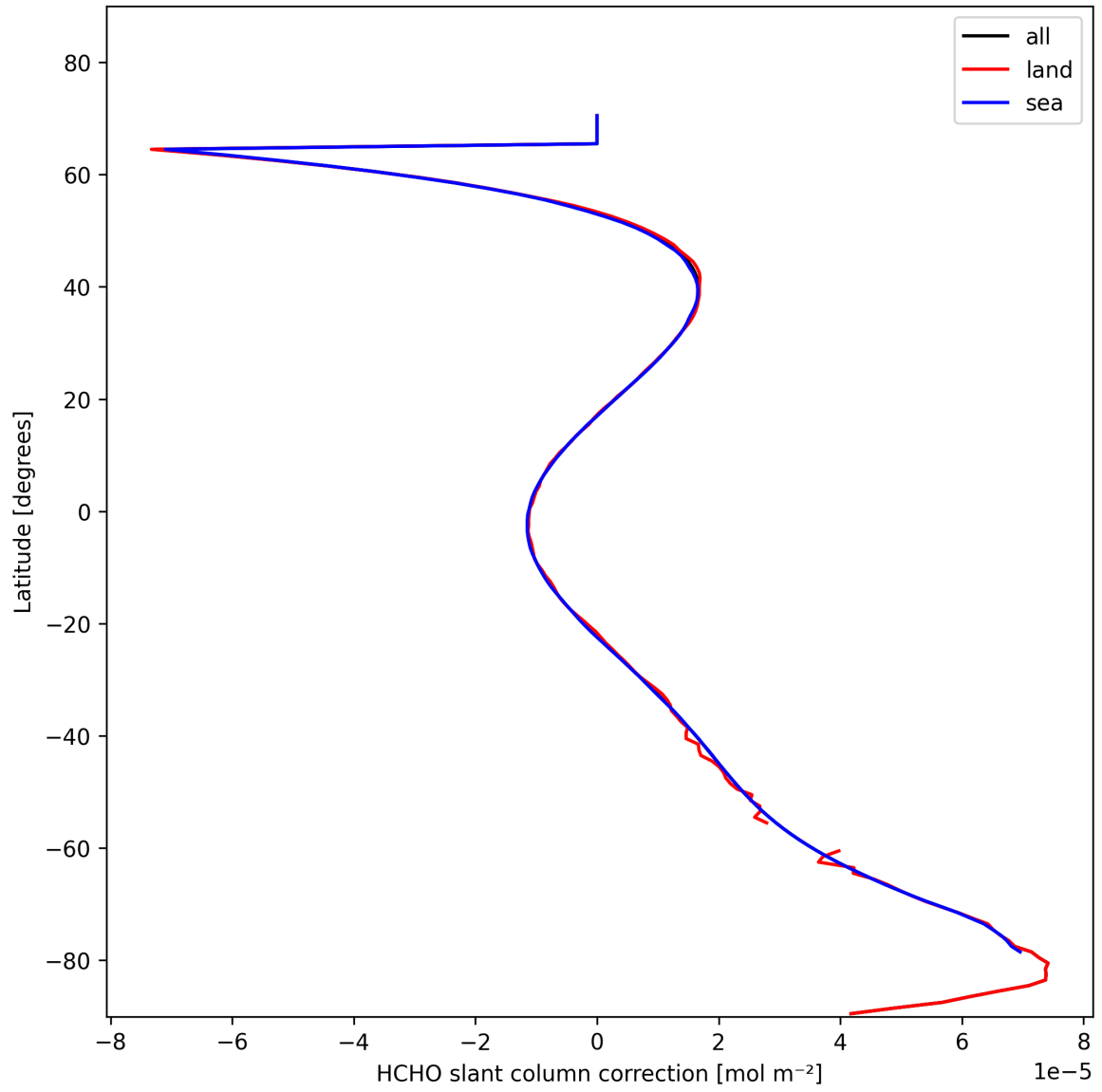
Figure 33: Zonal average of “HCHO slant column correction” for 2025-02-08 to 2025-02-10.
