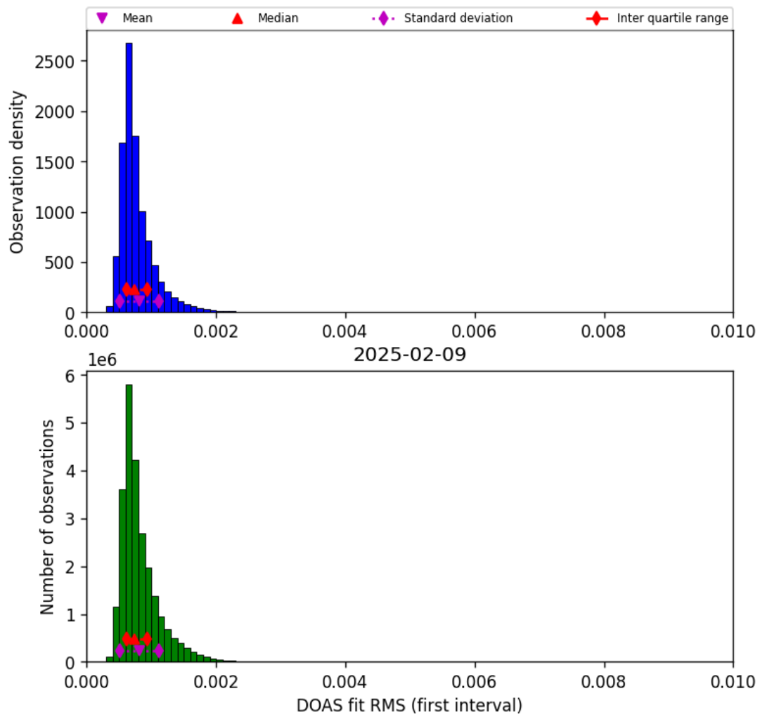
Figure 46: Histogram of “DOAS fit RMS (first interval)” for 2025-02-08 to 2025-02-10
