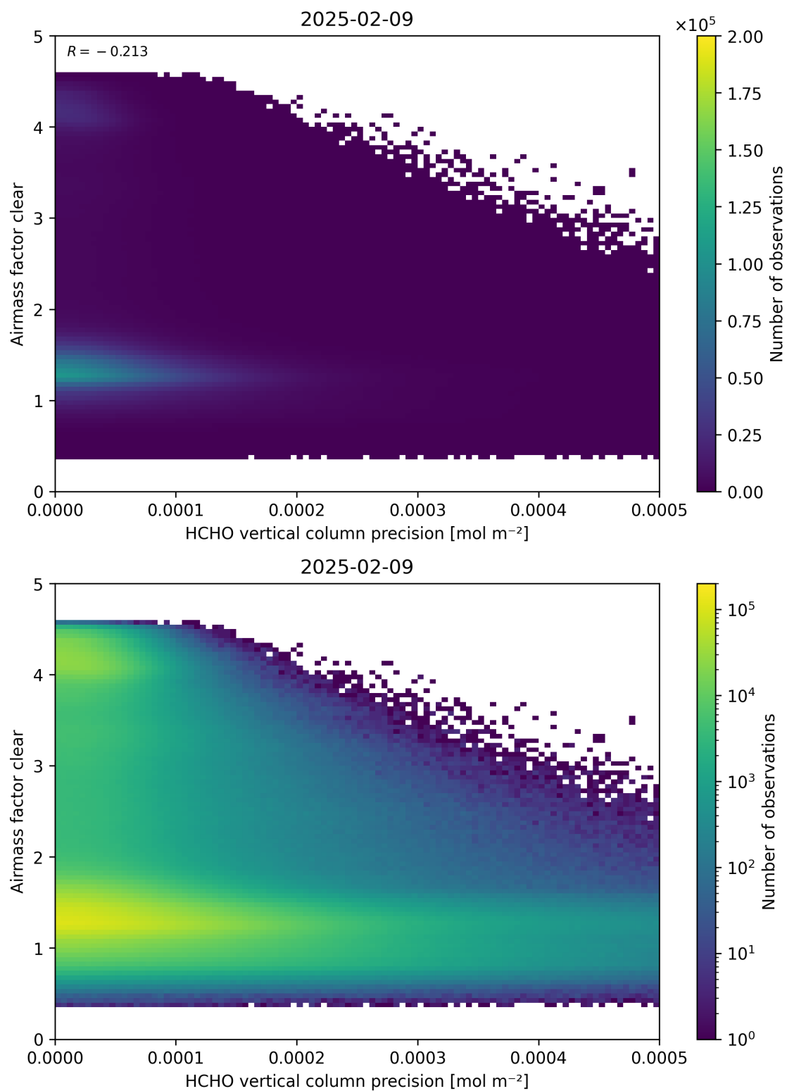
Figure 139: Scatter density plot of “HCHO vertical column precision” against “Airmass factor clear” for 2025-02-08 to 2025-02-10.
