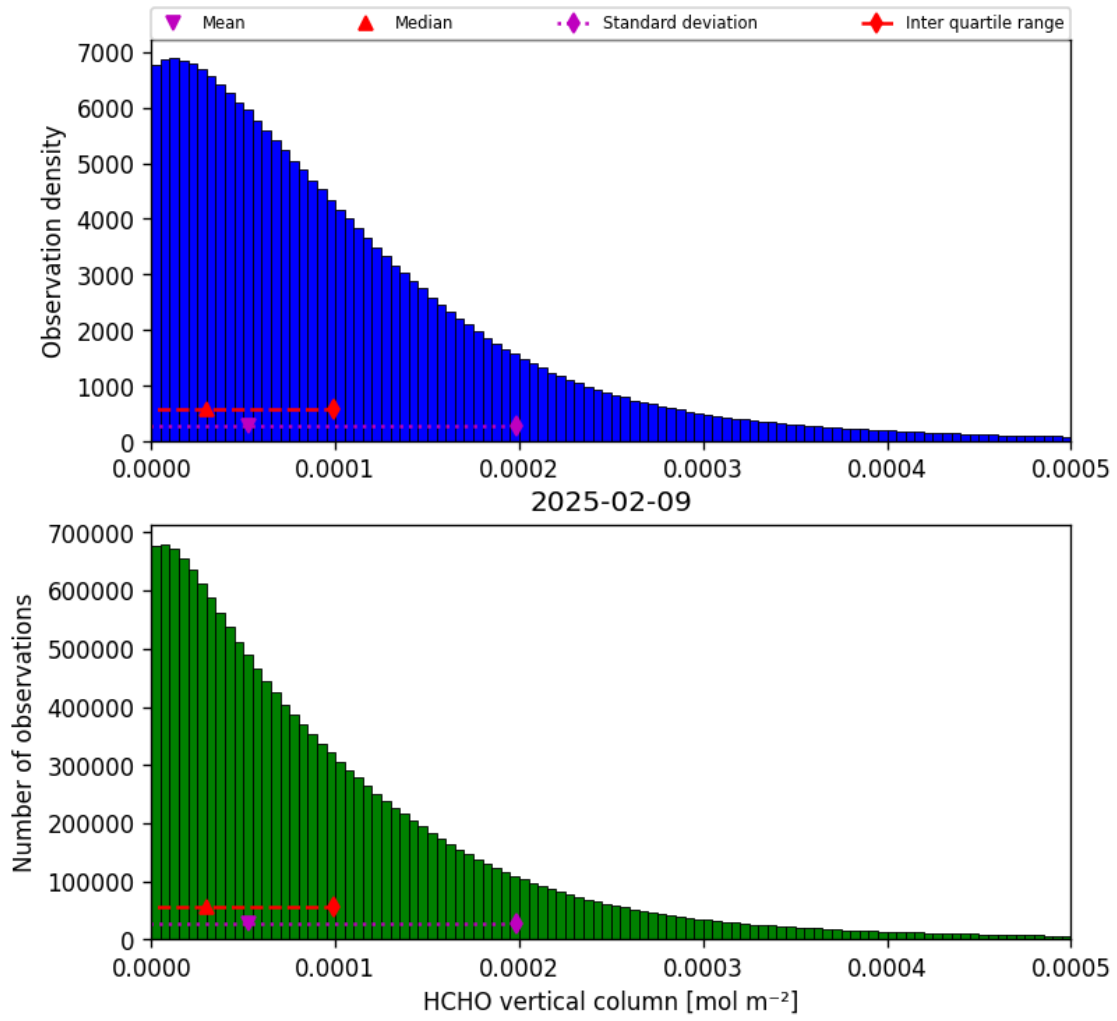
Figure 35: Histogram of “HCHO vertical column” for 2025-02-08 to 2025-02-10
