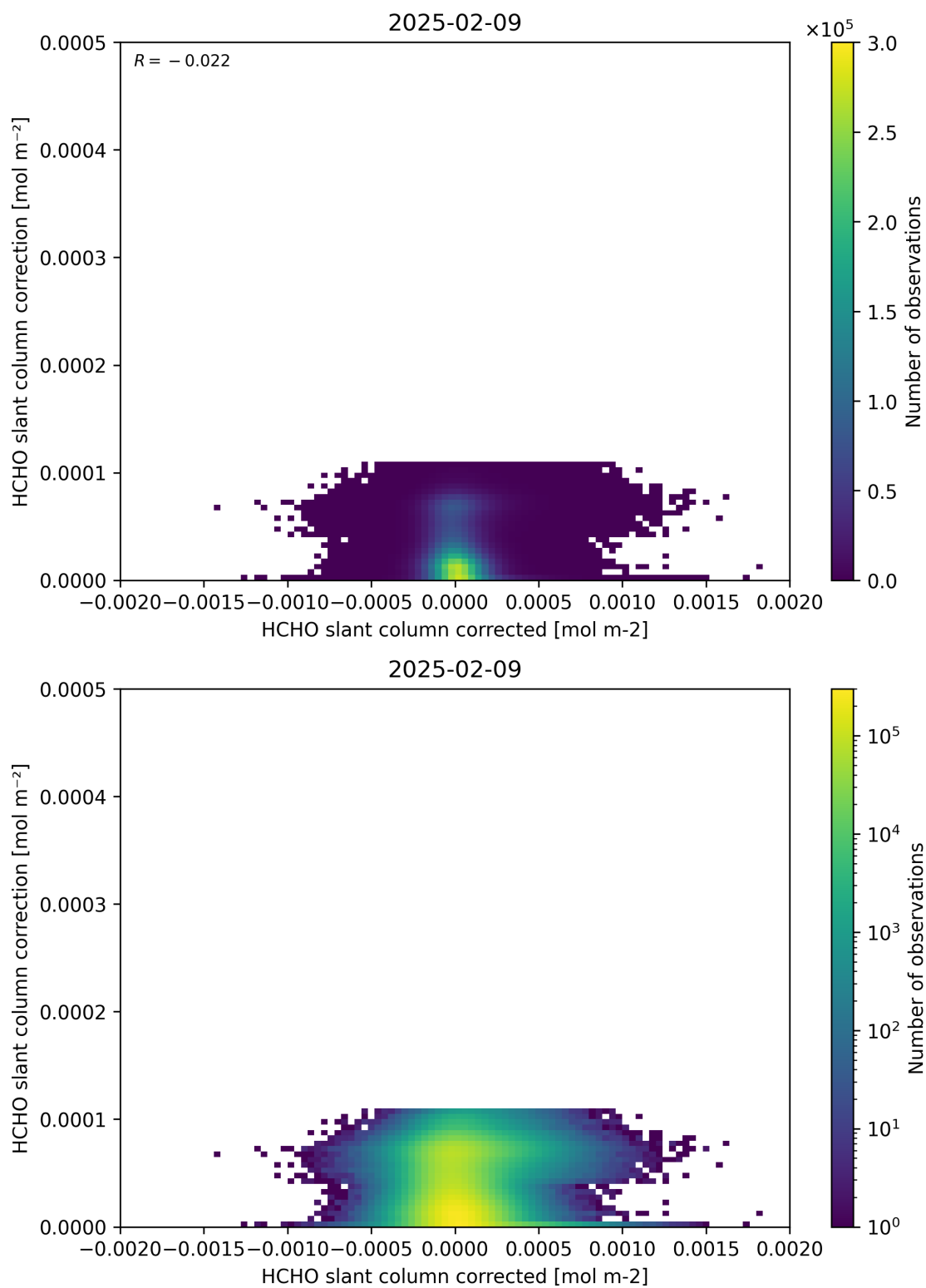
Figure 77: Scatter density plot of “HCHO slant column corrected” against “HCHO slant column correction” for 2025-02-08 to 2025-02-10.
