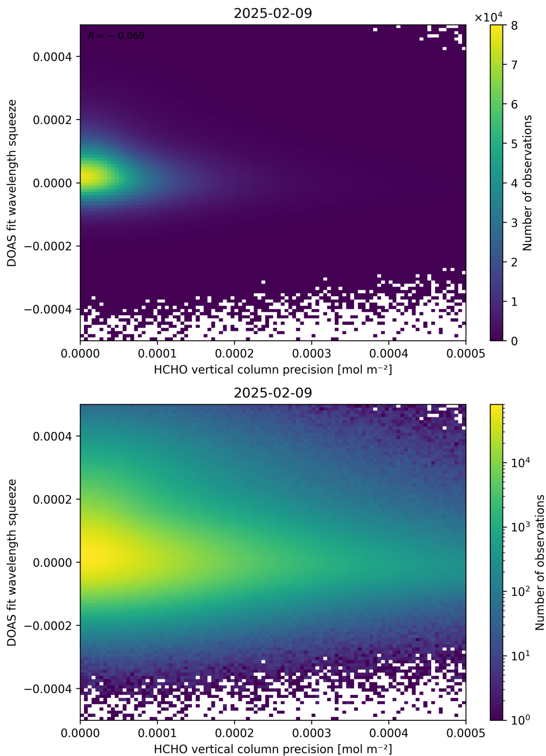
Figure 138: Scatter density plot of “HCHO vertical column precision” against “DOAS fit wavelength squeeze” for 2025-02-08 to 2025-02-10.
