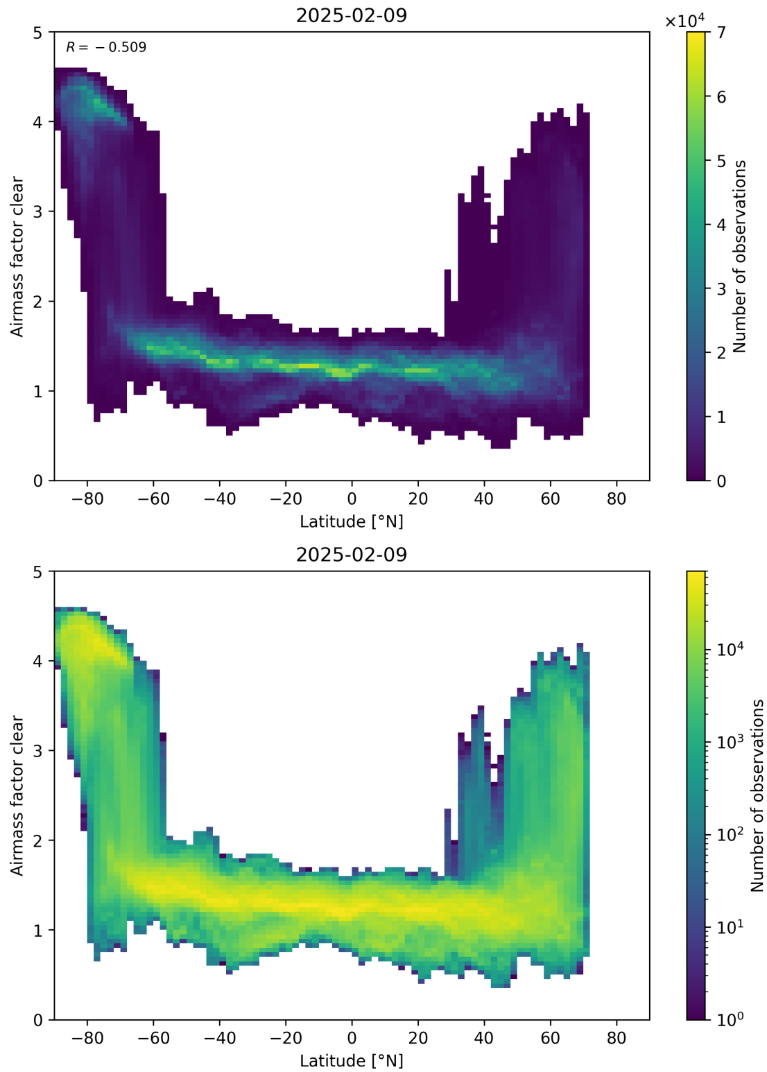
Figure 156: Scatter density plot of “Latitude” against “Airmass factor clear” for 2025-02-08 to 2025-02-10.
