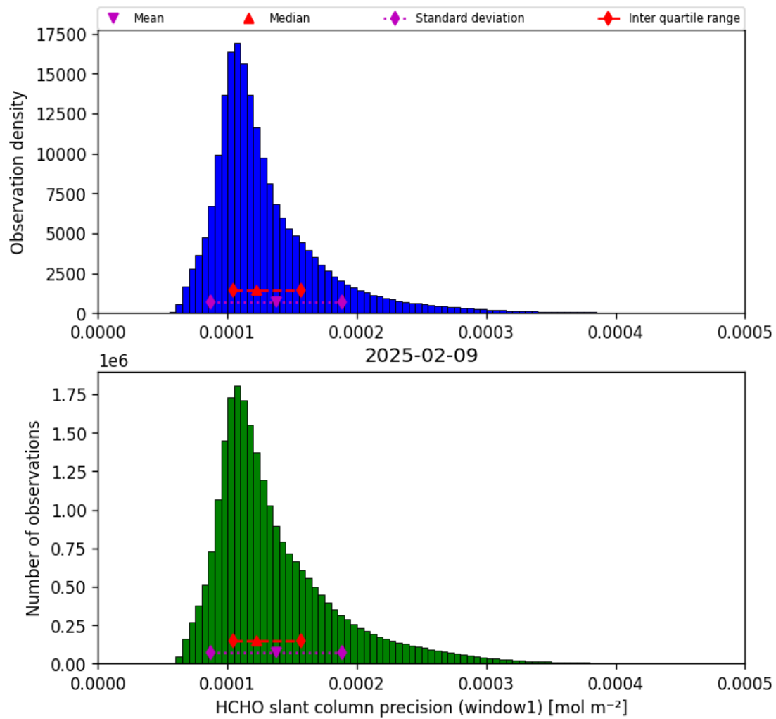
Figure 39: Histogram of “HCHO slant column precision (window1)” for 2025-02-08 to 2025-02-10
