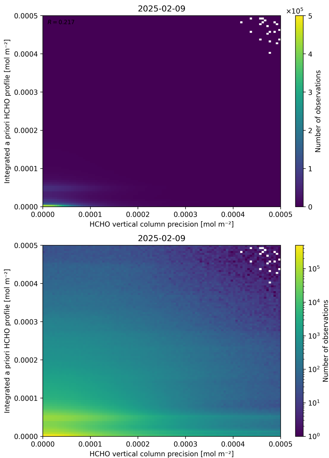
Figure 147: Scatter density plot of “HCHO vertical column precision” against “Integrated a priori HCHO profile” for 2025-02-08 to 2025-02-10.
