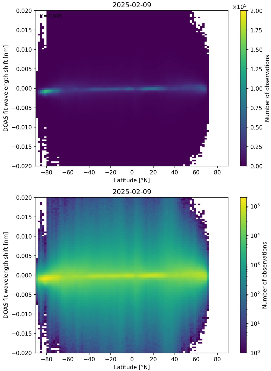
Figure 154: Scatter density plot of “Latitude” against “DOAS fit wavelength shift” for 2025-02-08 to 2025-02-10.
