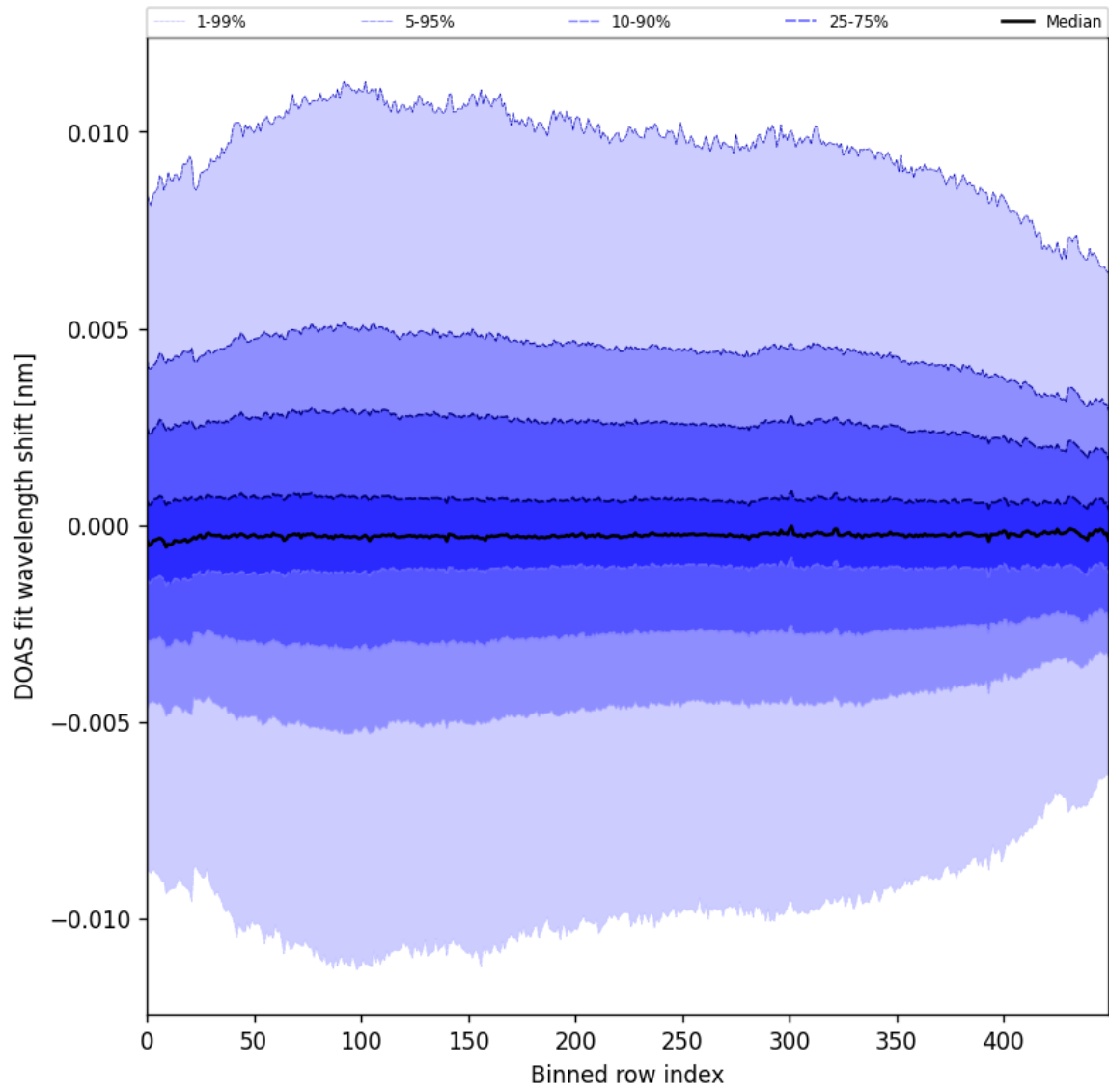
Figure 58: Along track statistics of “DOAS fit wavelength shift” for 2025-02-08 to 2025-02-10
