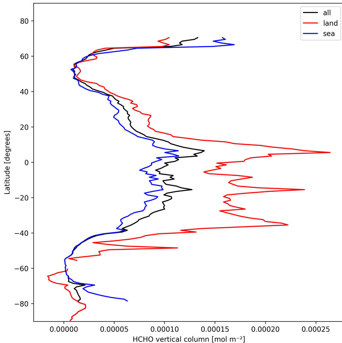
Figure 21: Zonal average of “HCHO vertical column” for 2025-02-08 to 2025-02-10.
