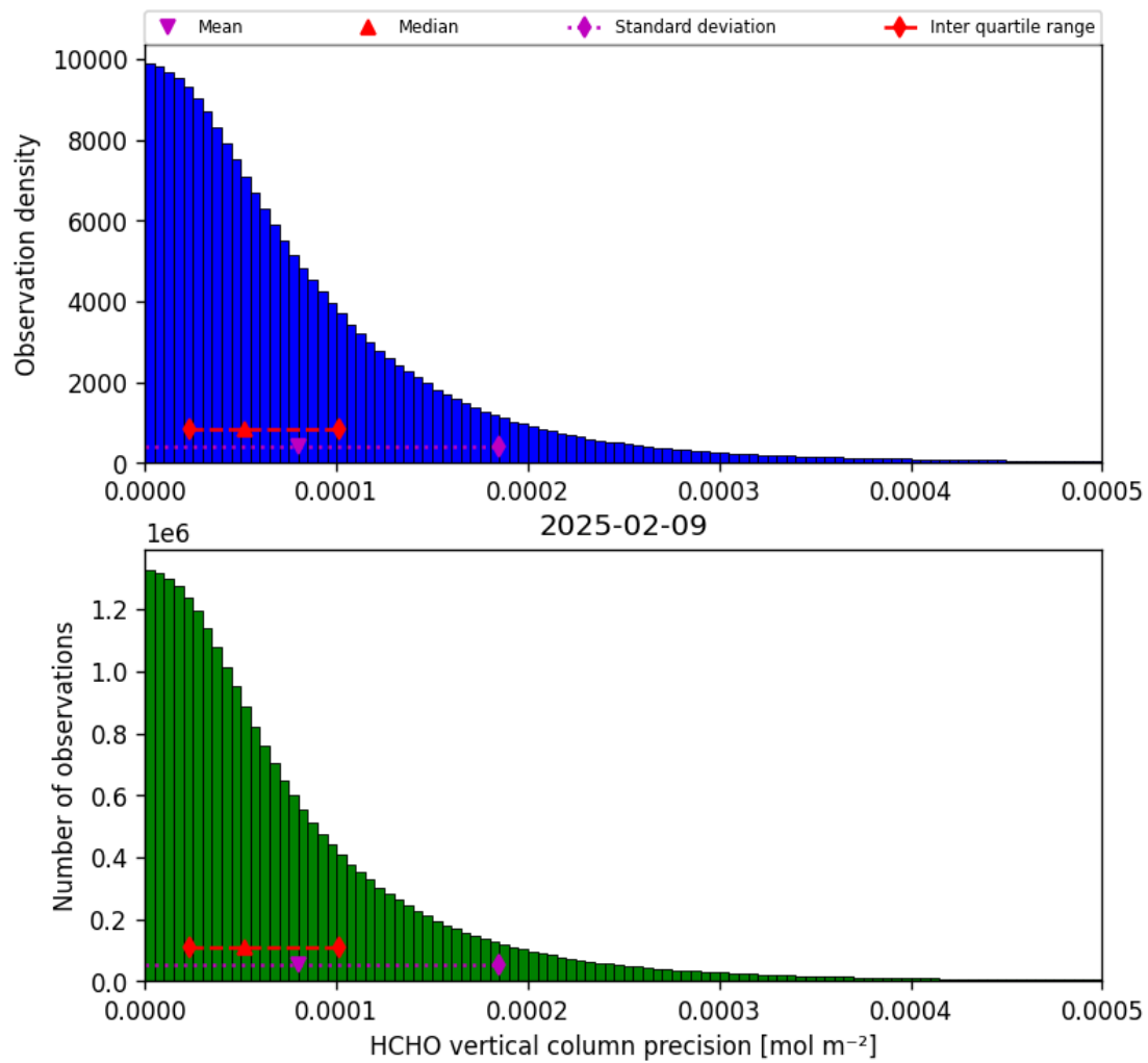
Figure 36: Histogram of “HCHO vertical column precision” for 2025-02-08 to 2025-02-10
