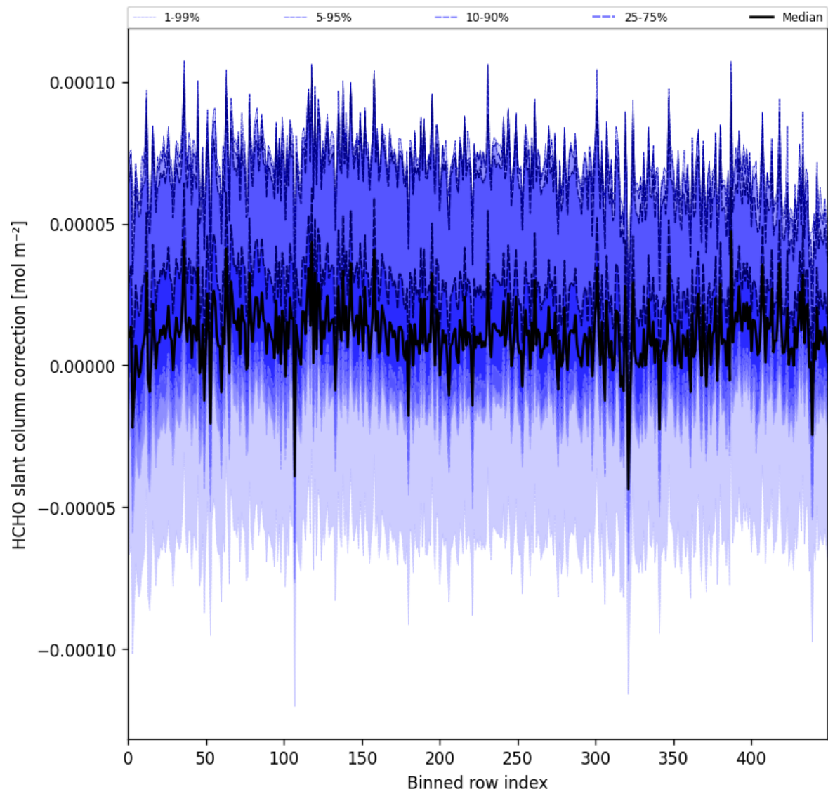
Figure 61: Along track statistics of “HCHO slant column correction” for 2025-02-08 to 2025-02-10
