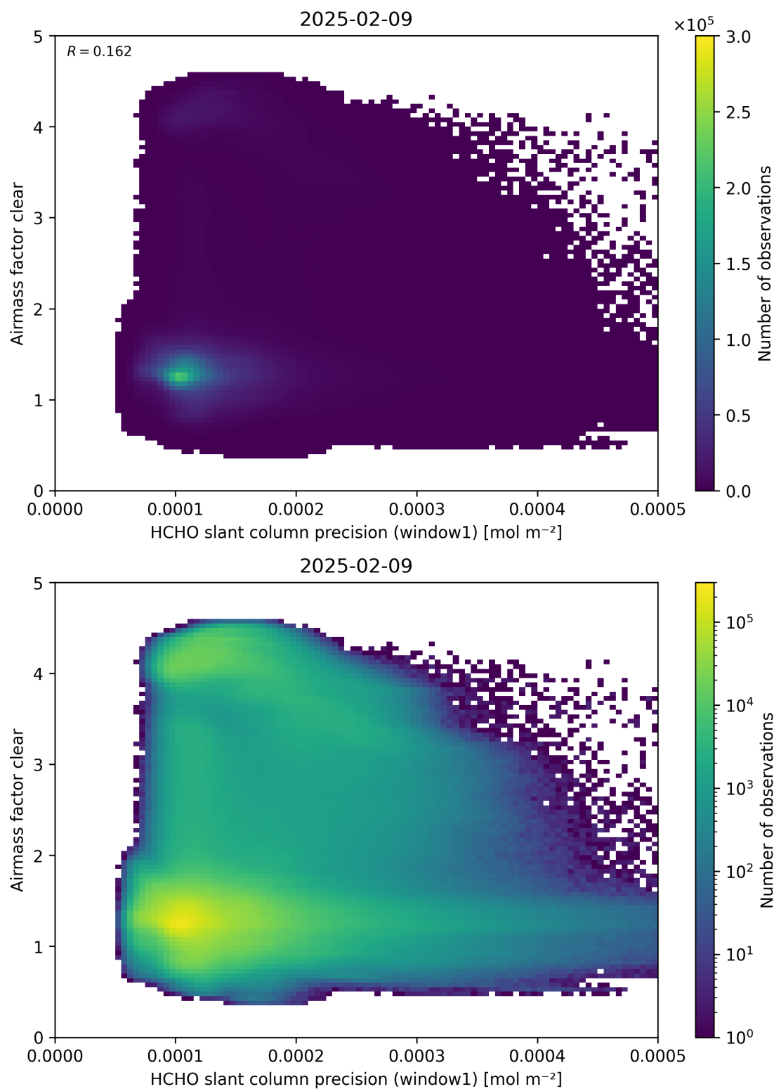
Figure 91: Scatter density plot of “HCHO slant column precision (window1)” against “Airmass factor clear” for 2025-02-08 to 2025-02-10.
