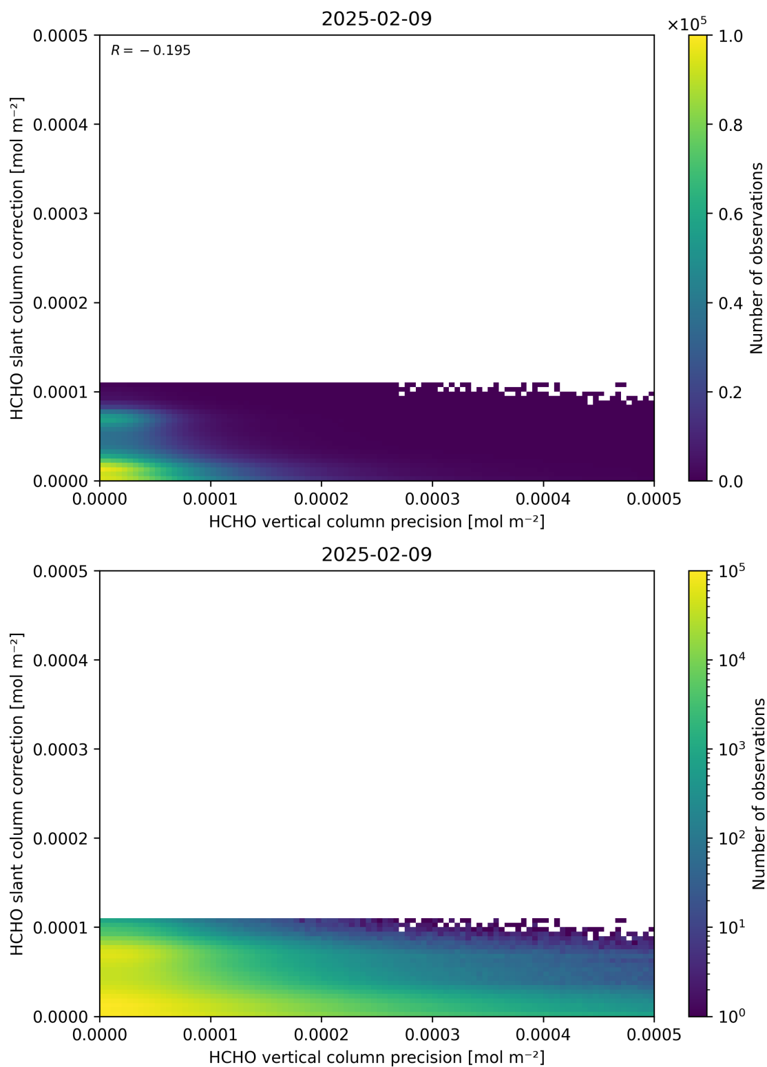
Figure 141: Scatter density plot of “HCHO vertical column precision” against “HCHO slant column correction” for 2025-02-08 to 2025-02-10.
