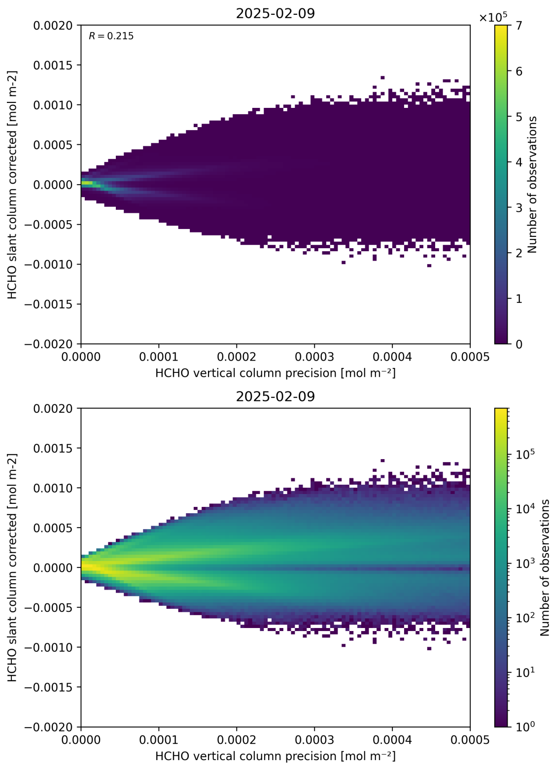
Figure 140: Scatter density plot of “HCHO vertical column precision” against “HCHO slant column corrected” for 2025-02-08 to 2025-02-10.
