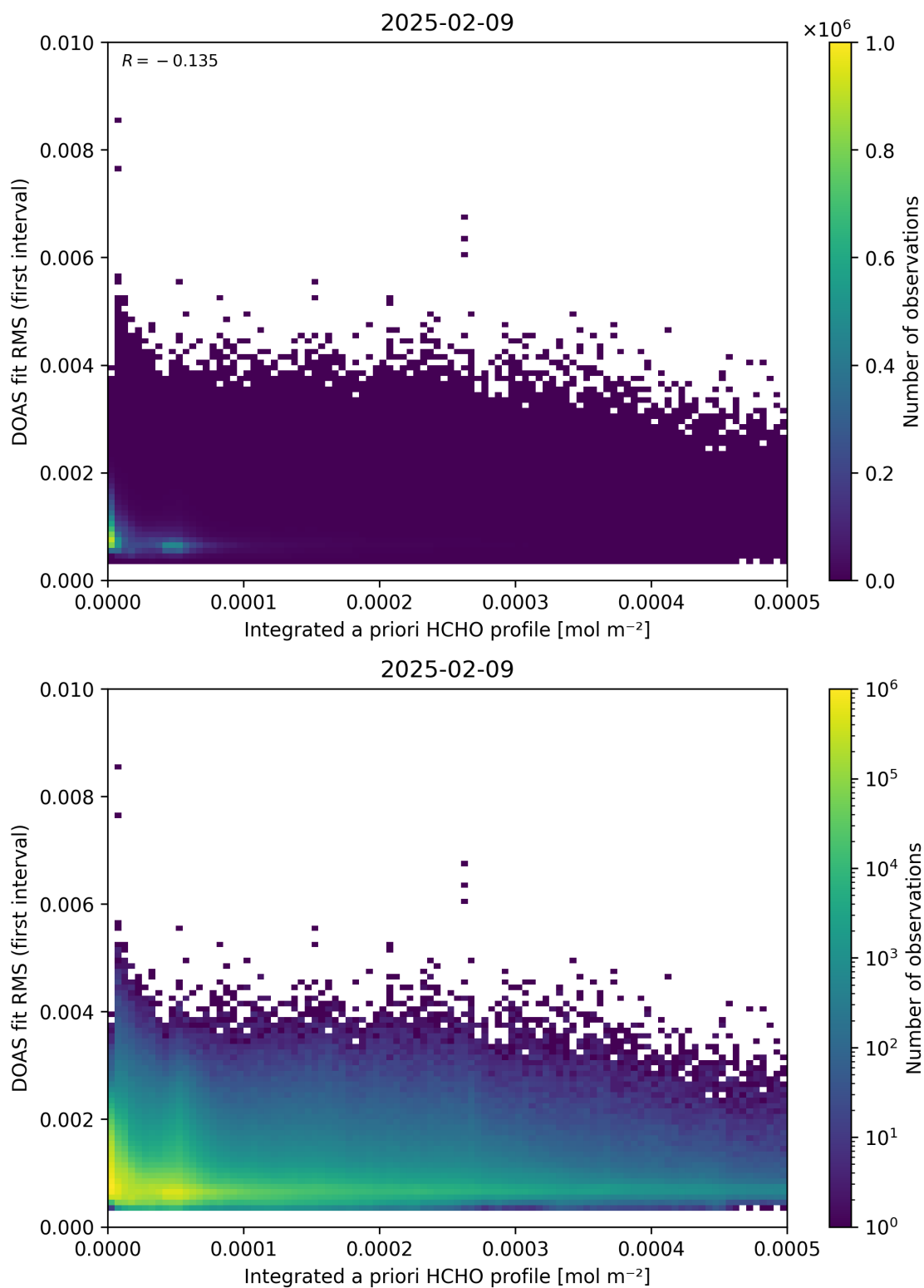
Figure 148: Scatter density plot of “Integrated a priori HCHO profile” against “DOAS fit RMS (first interval)” for 2025-02-08 to 2025-02-10.
