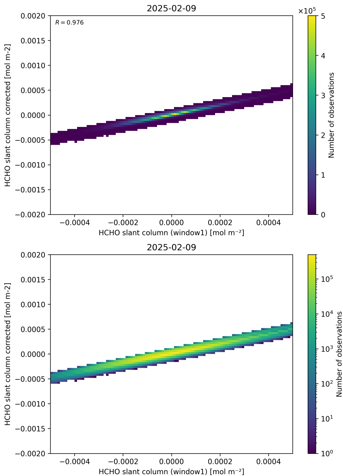
Figure 82: Scatter density plot of “HCHO slant column (window1)” against “HCHO slant column corrected” for 2025-02-08 to 2025-02-10.
