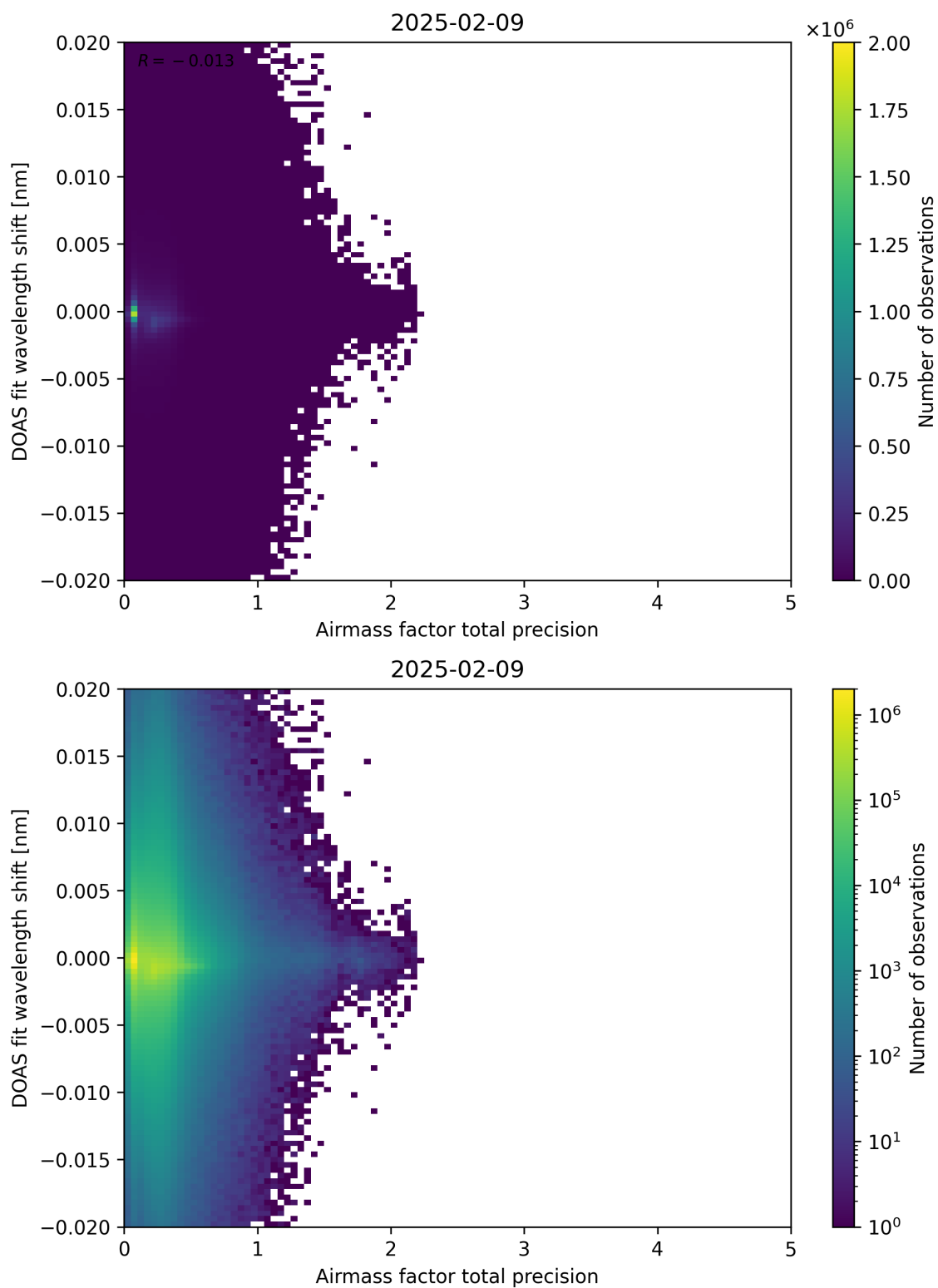
Figure 106: Scatter density plot of “Airmass factor total precision” against “DOAS fit wavelength shift” for 2025-02-08 to 2025-02-10.
