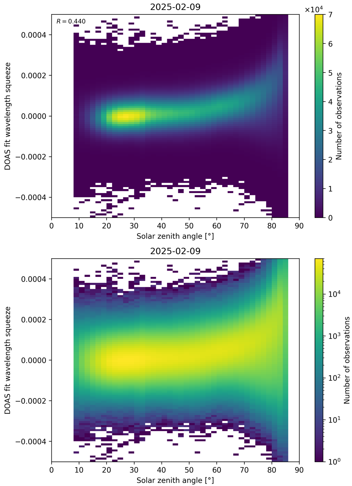
Figure 169: Scatter density plot of “Solar zenith angle” against “DOAS fit wavelength squeeze” for 2025-02-08 to 2025-02-10.
