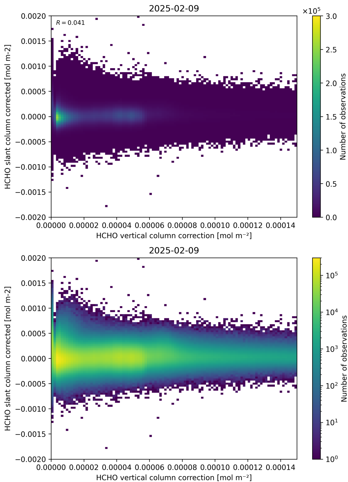
Figure 116: Scatter density plot of “HCHO vertical column correction” against “HCHO slant column corrected” for 2025-02-08 to 2025-02-10.
