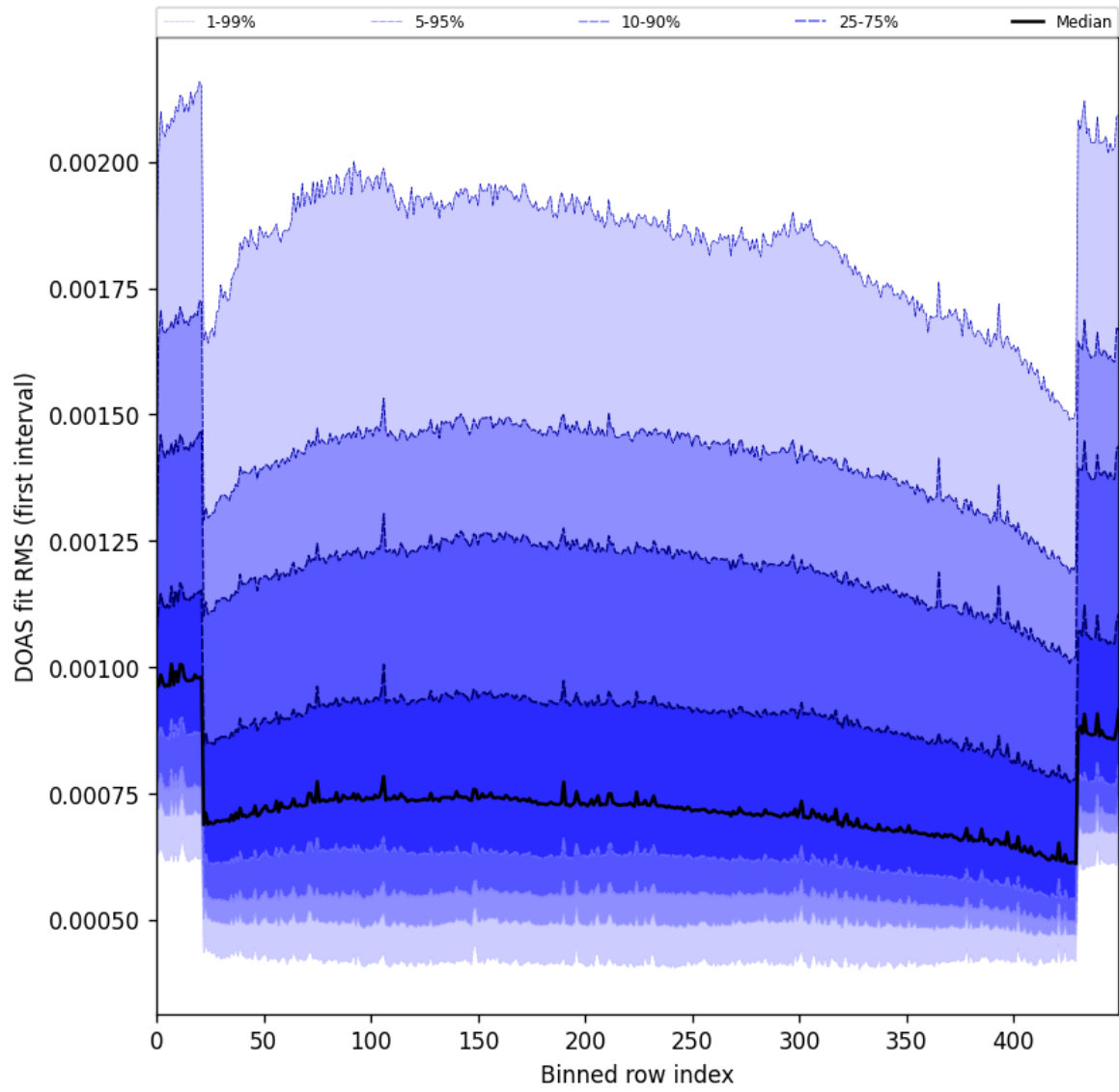
Figure 60: Along track statistics of “DOAS fit RMS (first interval)” for 2025-02-08 to 2025-02-10
