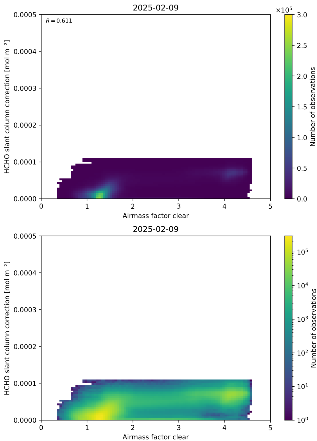
Figure 75: Scatter density plot of “Airmass factor clear” against “HCHO slant column correction” for 2025-02-08 to 2025-02-10.
