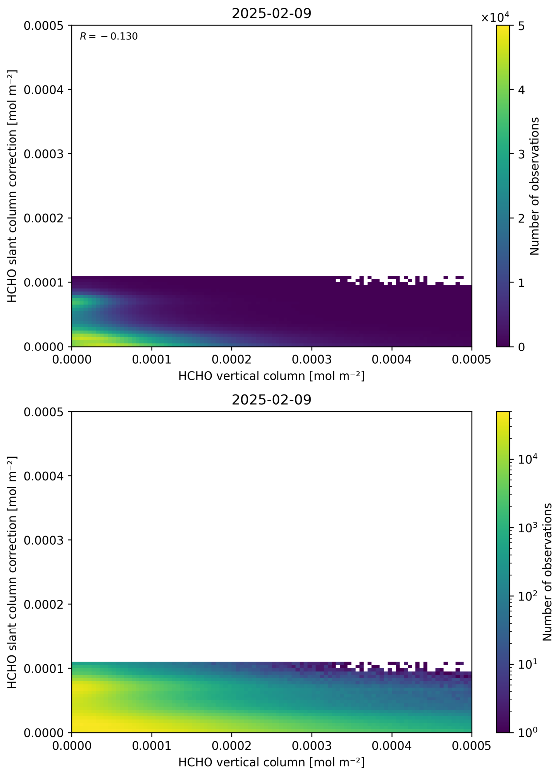
Figure 128: Scatter density plot of “HCHO vertical column” against “HCHO slant column correction” for 2025-02-08 to 2025-02-10.
