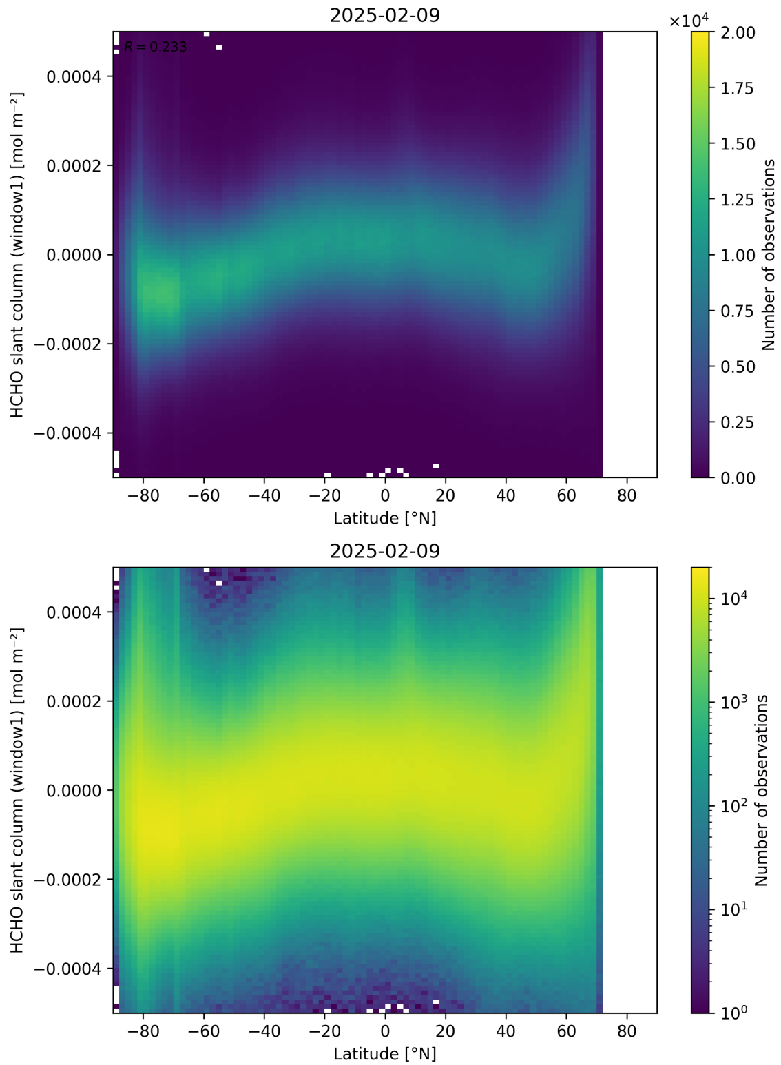
Figure 159: Scatter density plot of “Latitude” against “HCHO slant column (window1)” for 2025-02-08 to 2025-02-10.
