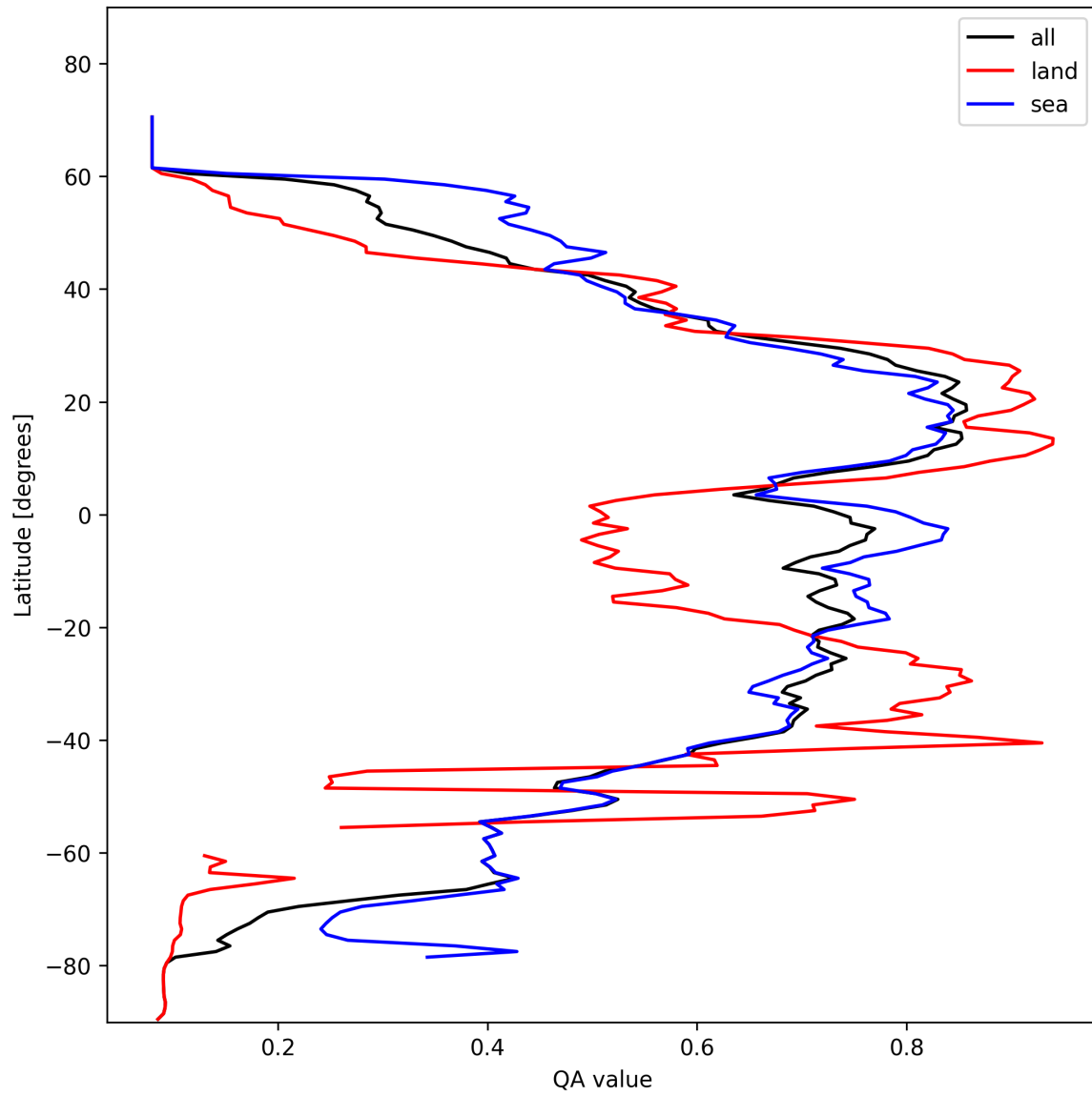
Figure 20: Zonal average of “QA value” for 2025-02-08 to 2025-02-10.
