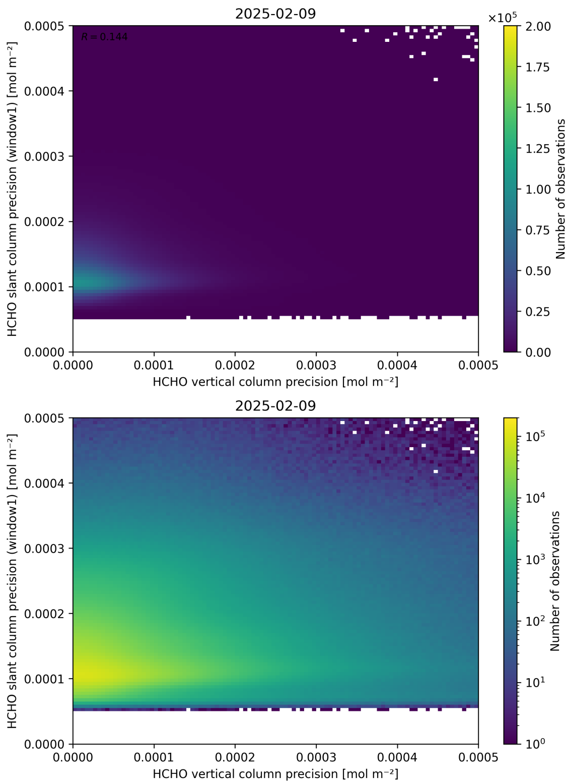
Figure 143: Scatter density plot of “HCHO vertical column precision” against “HCHO slant column precision (window1)” for 2025-02-08 to 2025-02-10.
