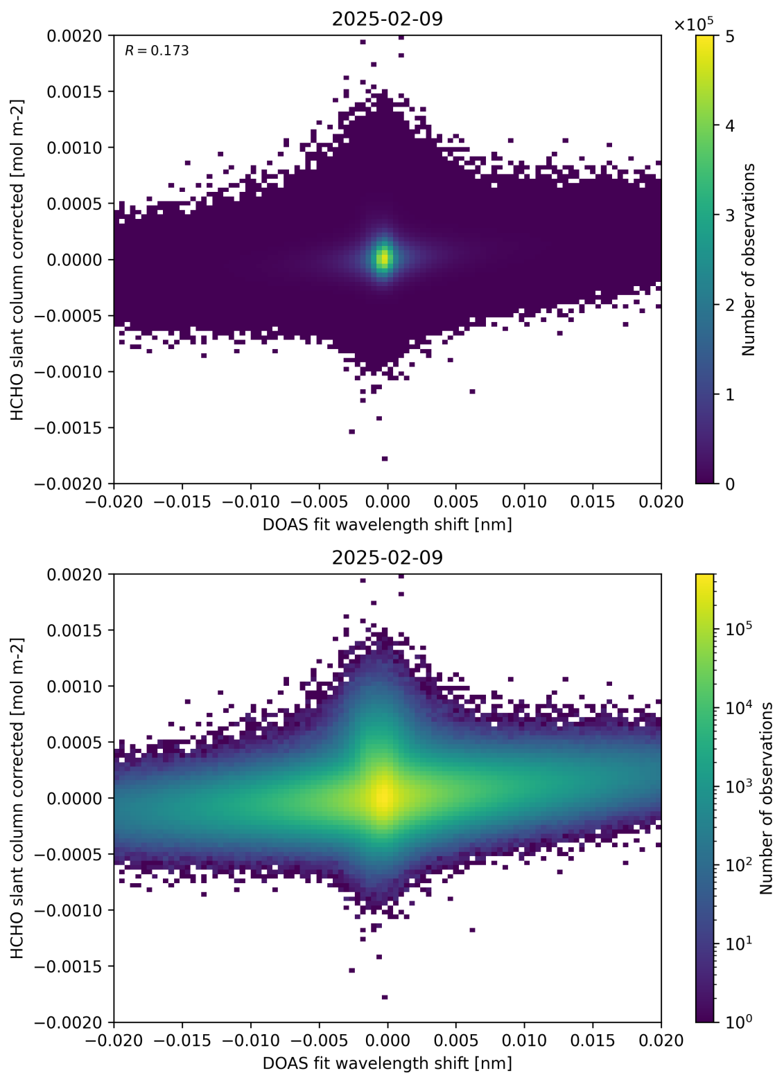
Figure 66: Scatter density plot of “DOAS fit wavelength shift” against “HCHO slant column corrected” for 2025-02-08 to 2025-02-10.
