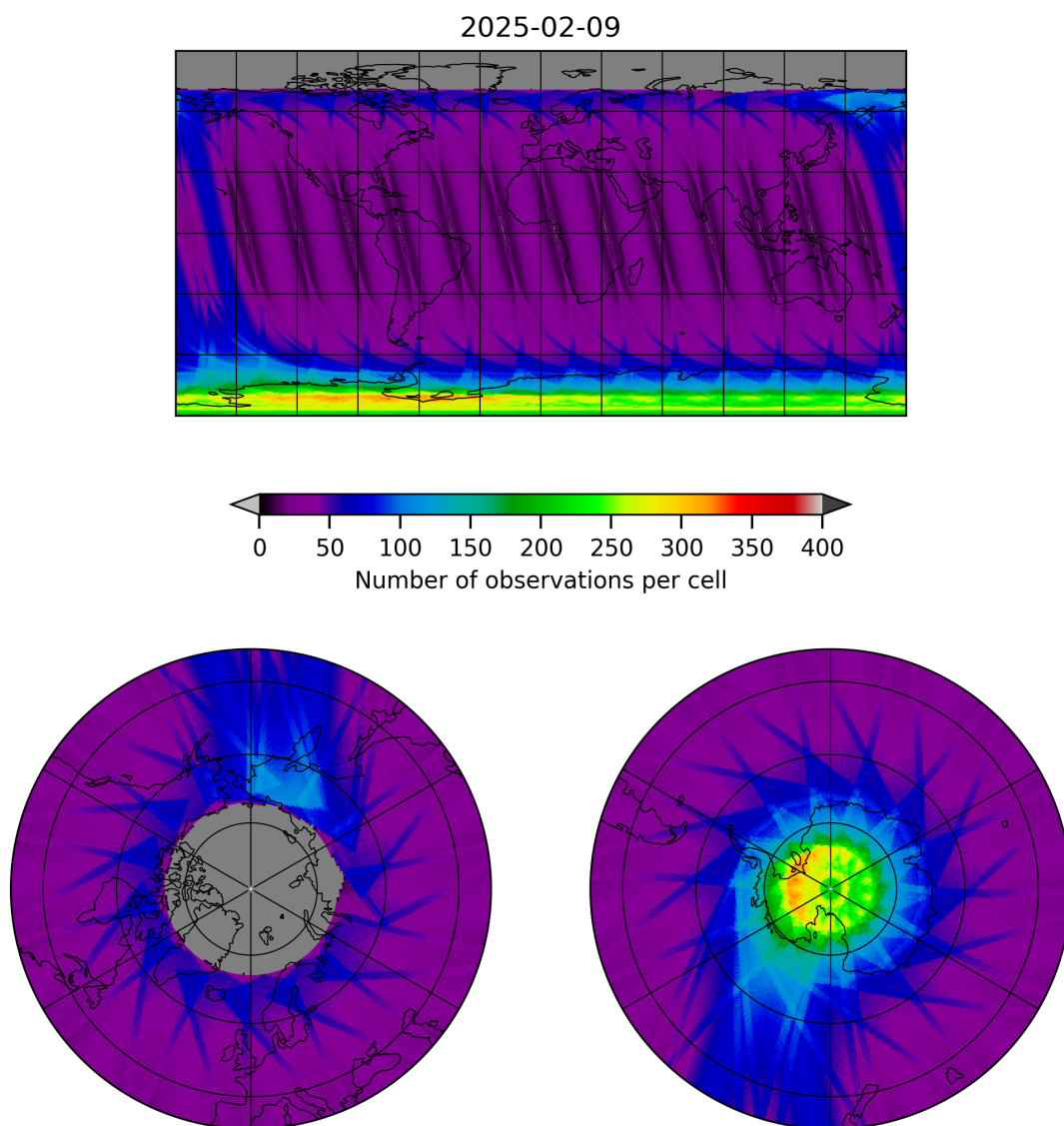
Figure 19: Map of the number of observations for 2025-02-08 to 2025-02-10
