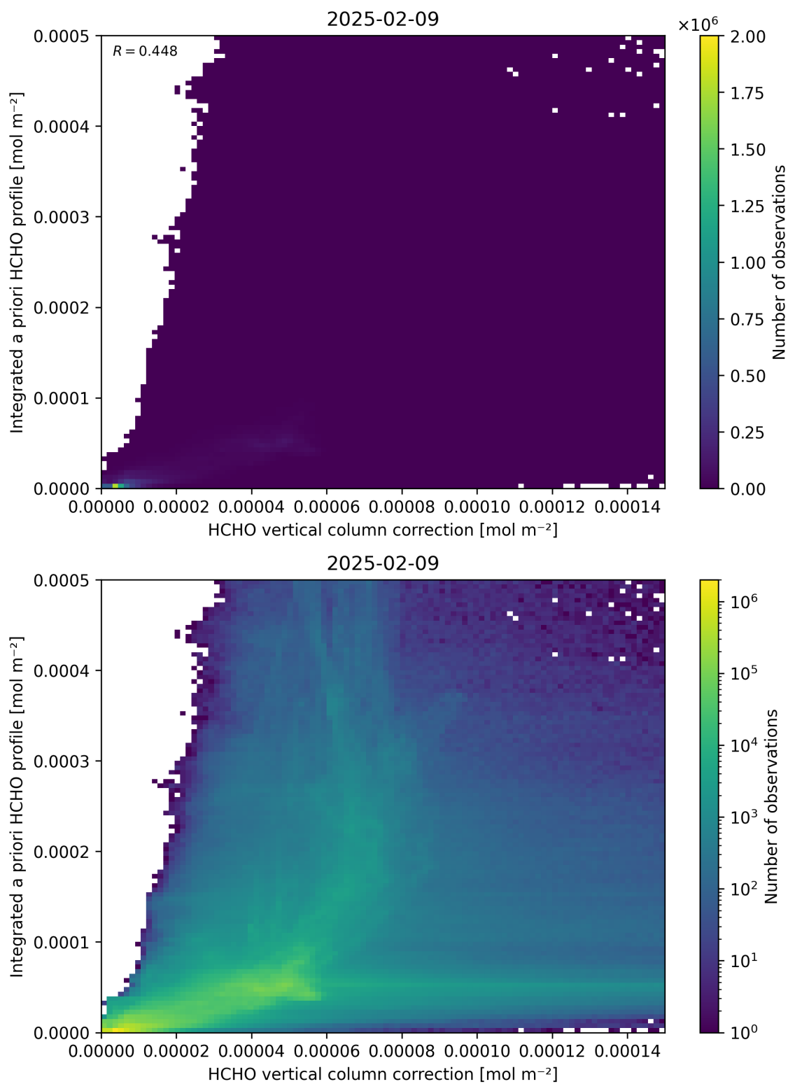
Figure 122: Scatter density plot of “HCHO vertical column correction” against “Integrated a priori HCHO profile” for 2025-02-08 to 2025-02-10.
