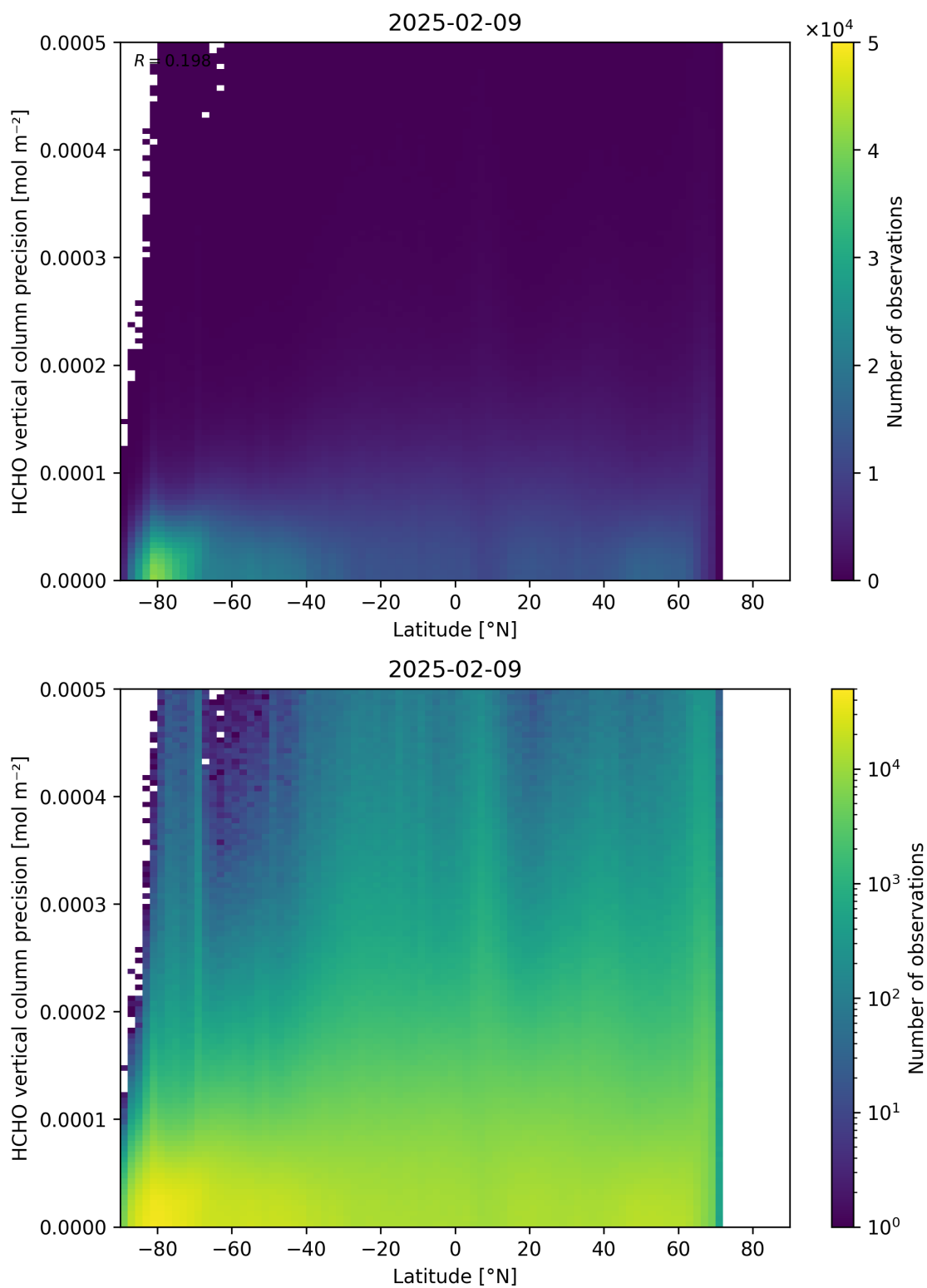
Figure 165: Scatter density plot of “Latitude” against “HCHO vertical column precision” for 2025-02-08 to 2025-02-10.
