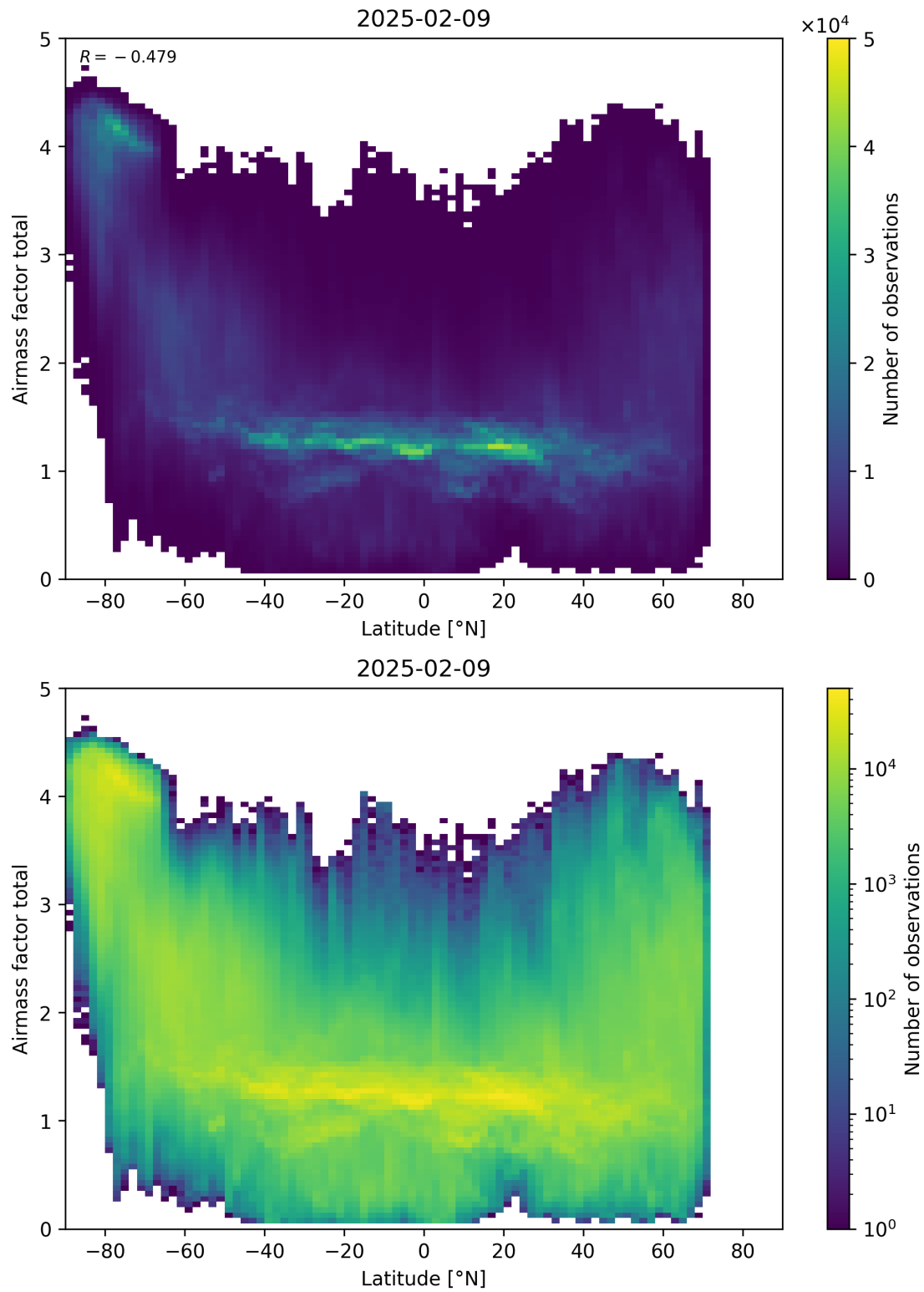
Figure 161: Scatter density plot of “Latitude” against “Airmass factor total” for 2025-02-08 to 2025-02-10.
