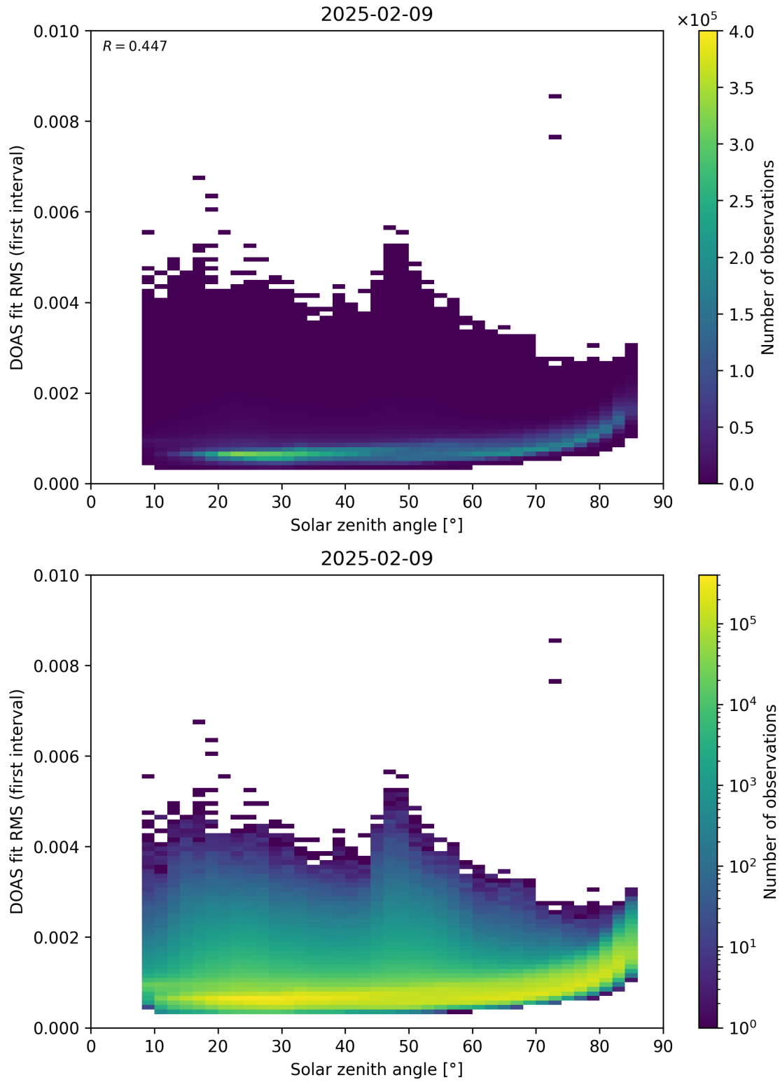
Figure 167: Scatter density plot of “Solar zenith angle” against “DOAS fit RMS (first interval)” for 2025-02-08 to 2025-02-10.
