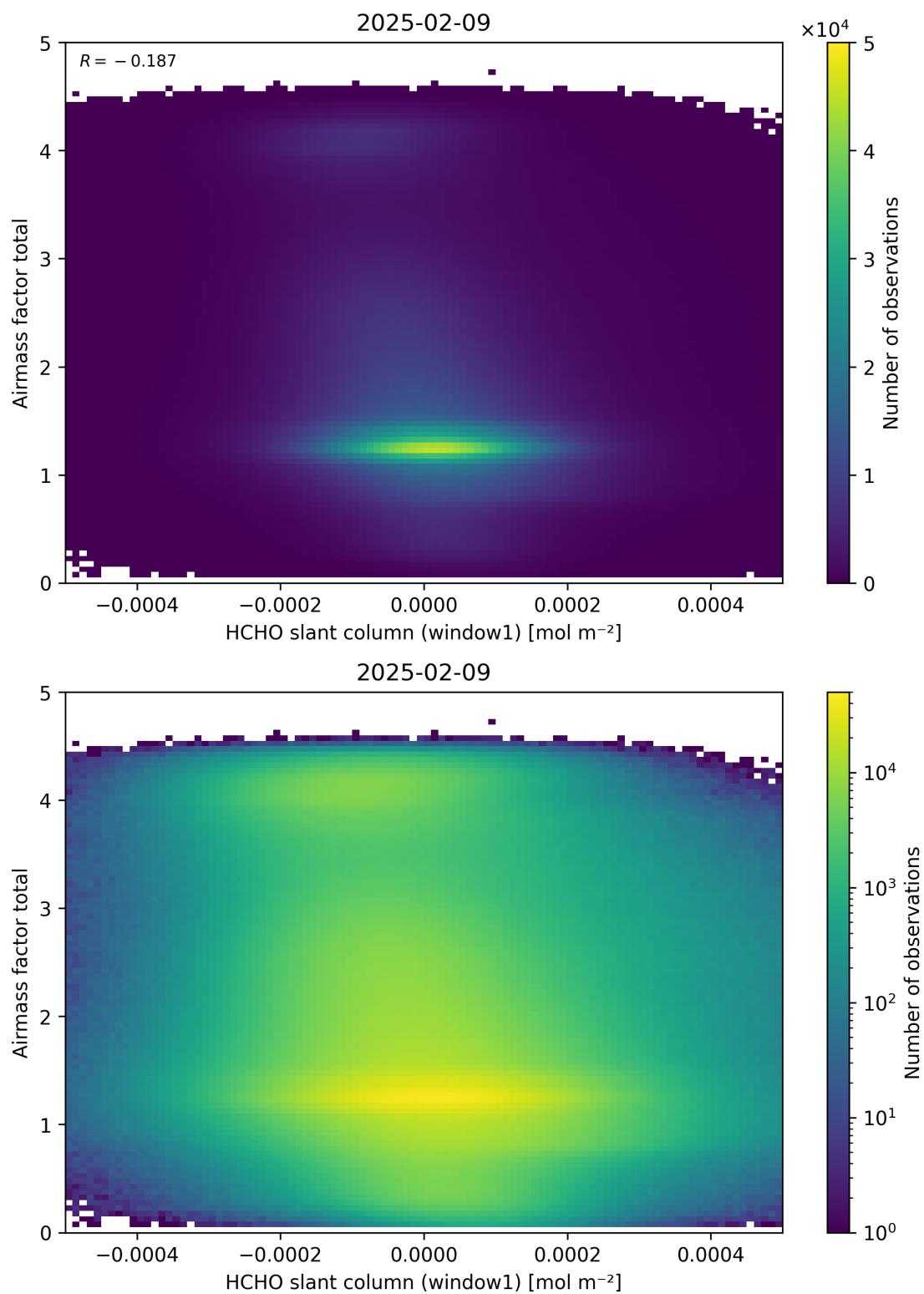
Figure 85: Scatter density plot of “HCHO slant column (window1)” against “Airmass factor total” for 2025-02-08 to 2025-02-10.
