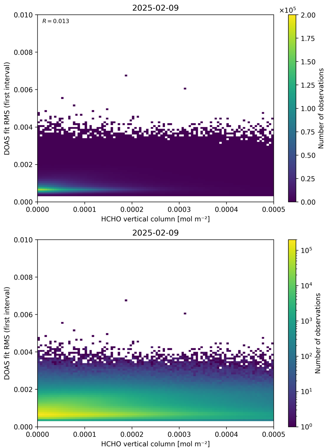
Figure 123: Scatter density plot of “HCHO vertical column” against “DOAS fit RMS (first interval)” for 2025-02-08 to 2025-02-10.
