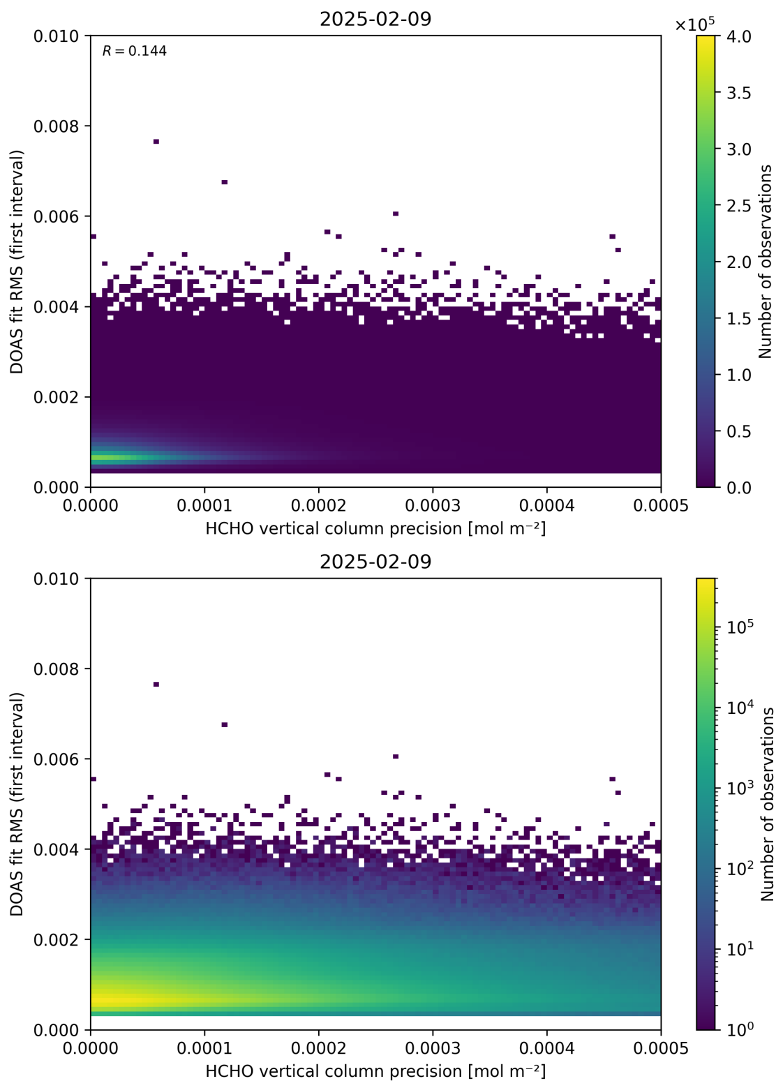
Figure 136: Scatter density plot of “HCHO vertical column precision” against “DOAS fit RMS (first interval)” for 2025-02-08 to 2025-02-10.
