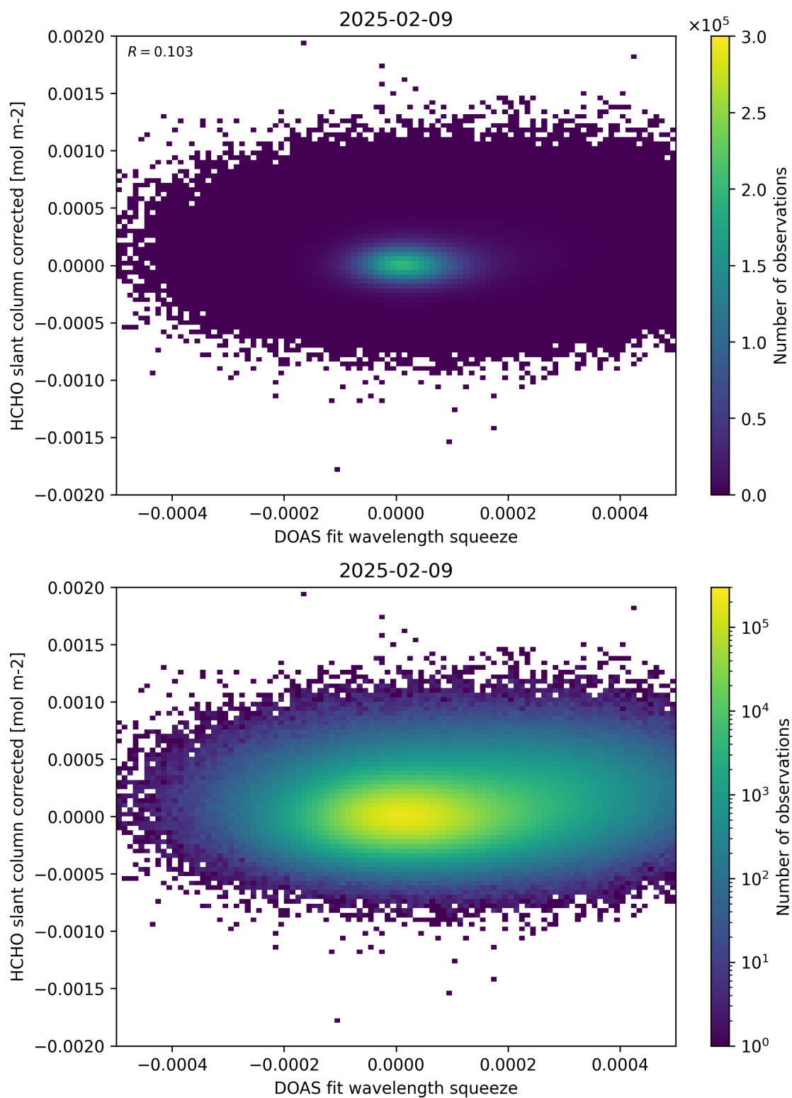
Figure 69: Scatter density plot of “DOAS fit wavelength squeeze” against “HCHO slant column corrected” for 2025-02-08 to 2025-02-10.
