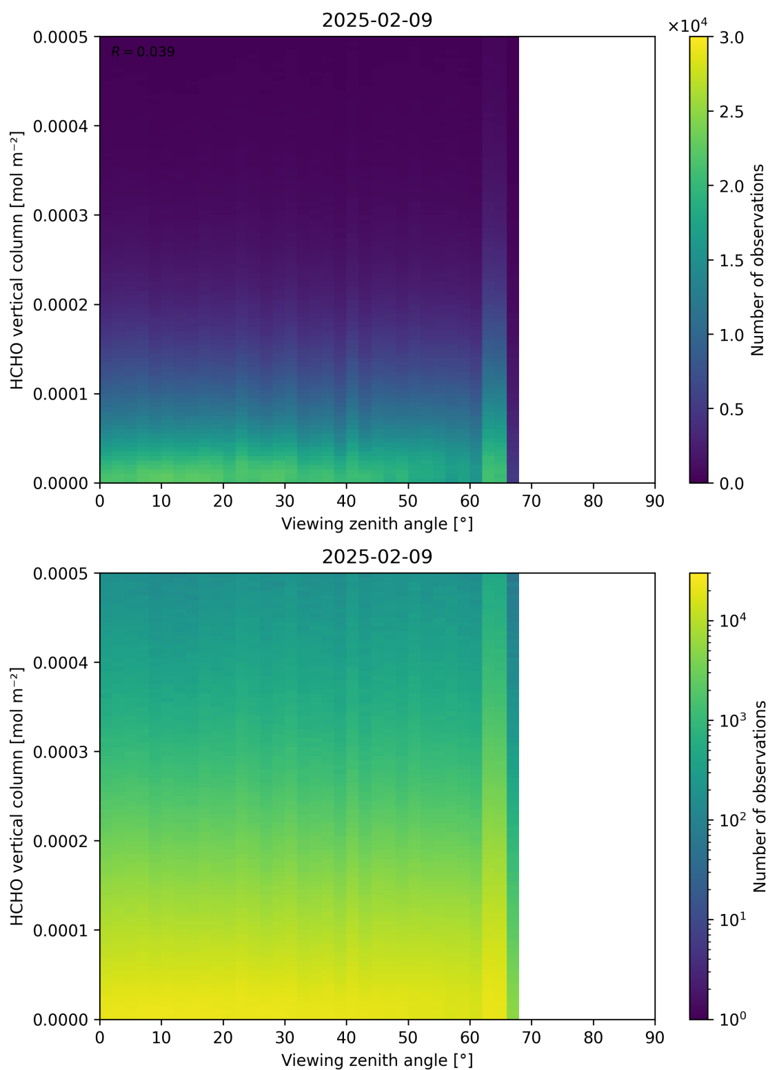
Figure 192: Scatter density plot of “Viewing zenith angle” against “HCHO vertical column” for 2025-02-08 to 2025-02-10.
