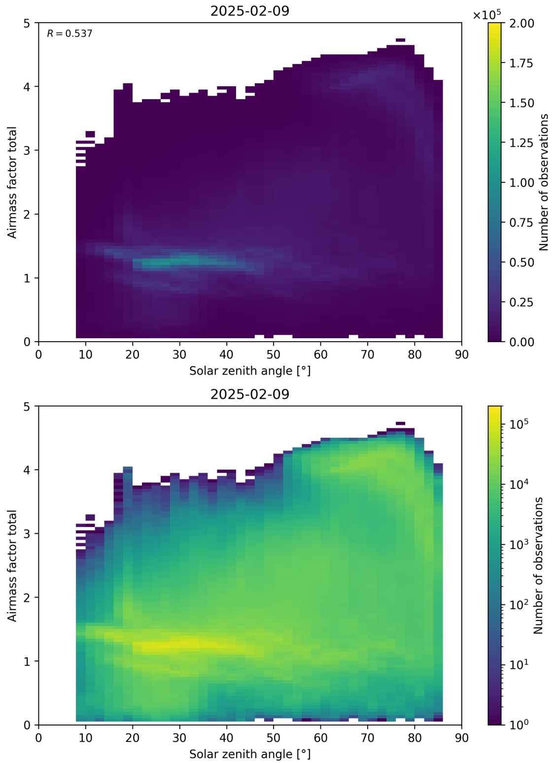
Figure 175: Scatter density plot of “Solar zenith angle” against “Airmass factor total” for 2025-02-08 to 2025-02-10.
