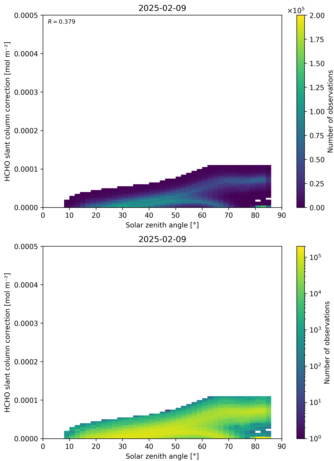
Figure 172: Scatter density plot of “Solar zenith angle” against “HCHO slant column correction” for 2025-02-08 to 2025-02-10.
