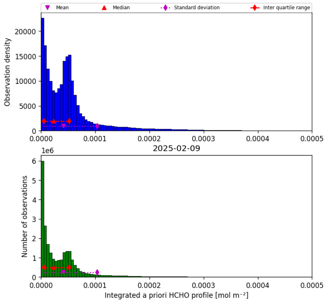
Figure 43: Histogram of “Integrated a priori HCHO profile” for 2025-02-08 to 2025-02-10
