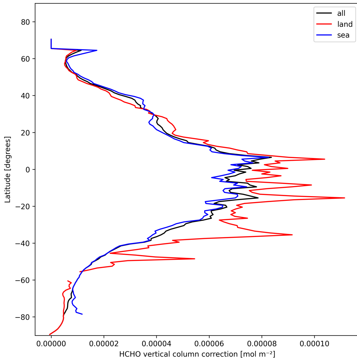
Figure 23: Zonal average of “HCHO vertical column correction” for 2025-02-08 to 2025-02-10.
