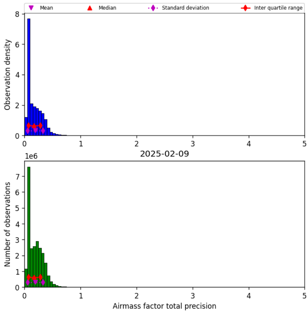
Figure 41: Histogram of “Airmass factor total precision” for 2025-02-08 to 2025-02-10
