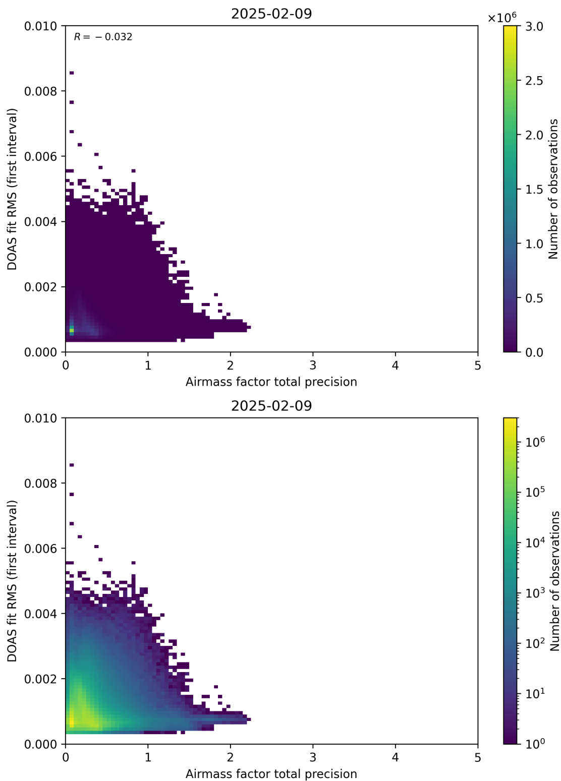
Figure 105: Scatter density plot of “Airmass factor total precision” against “DOAS fit RMS (first interval)” for 2025-02-08 to 2025-02-10.
