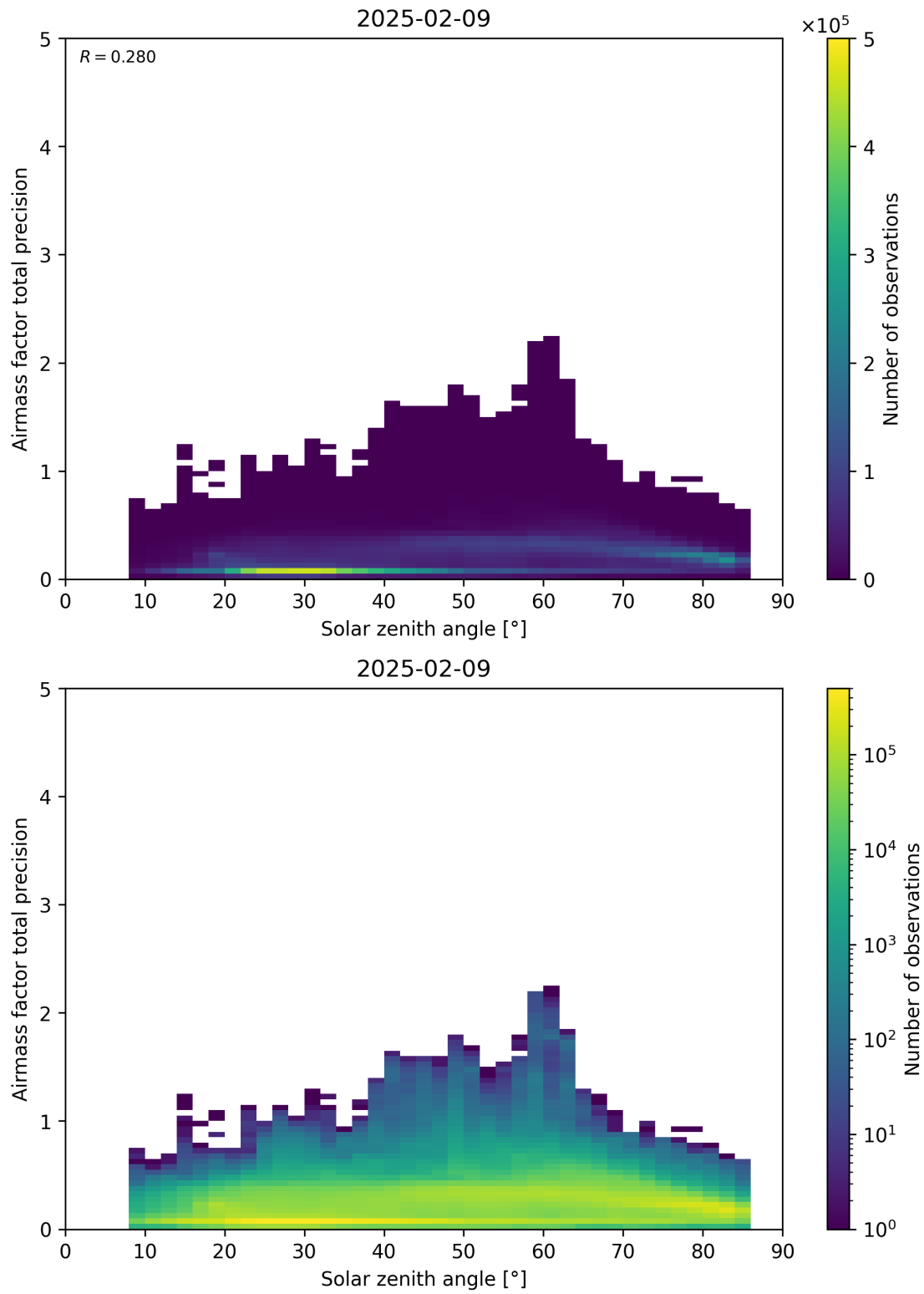
Figure 176: Scatter density plot of “Solar zenith angle” against “Airmass factor total precision” for 2025-02-08 to 2025-02-10.
