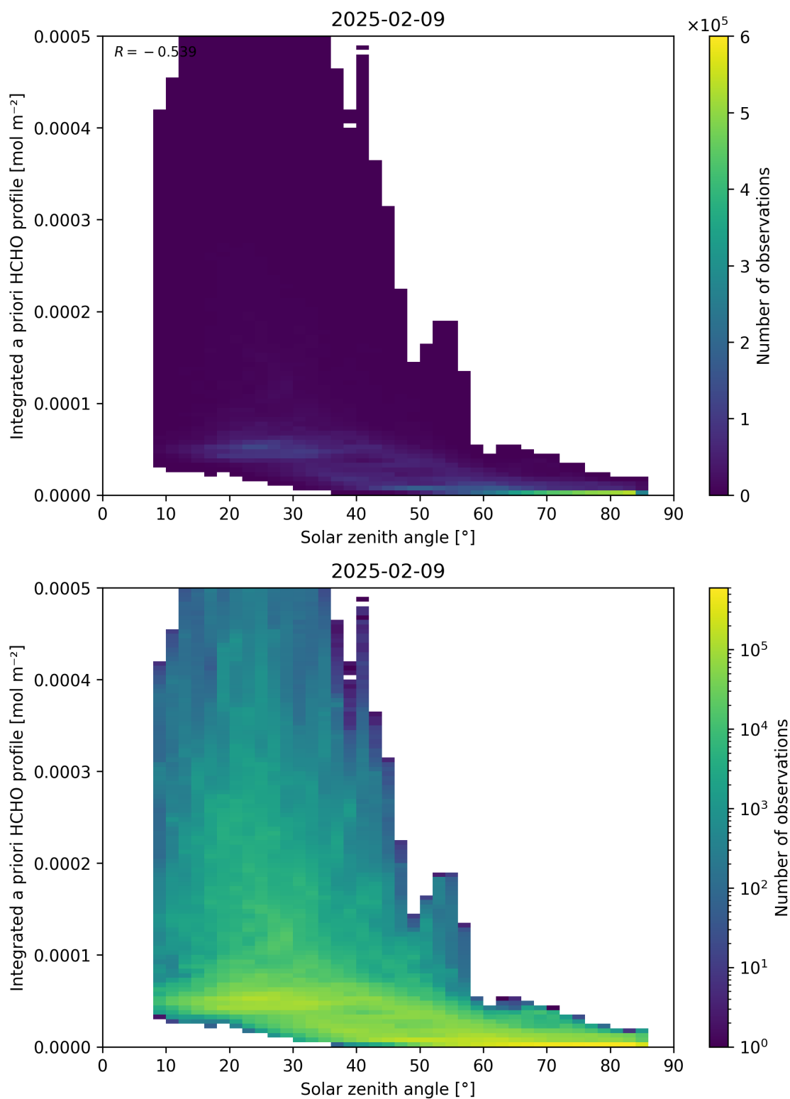
Figure 180: Scatter density plot of “Solar zenith angle” against “Integrated a priori HCHO profile” for 2025-02-08 to 2025-02-10.
