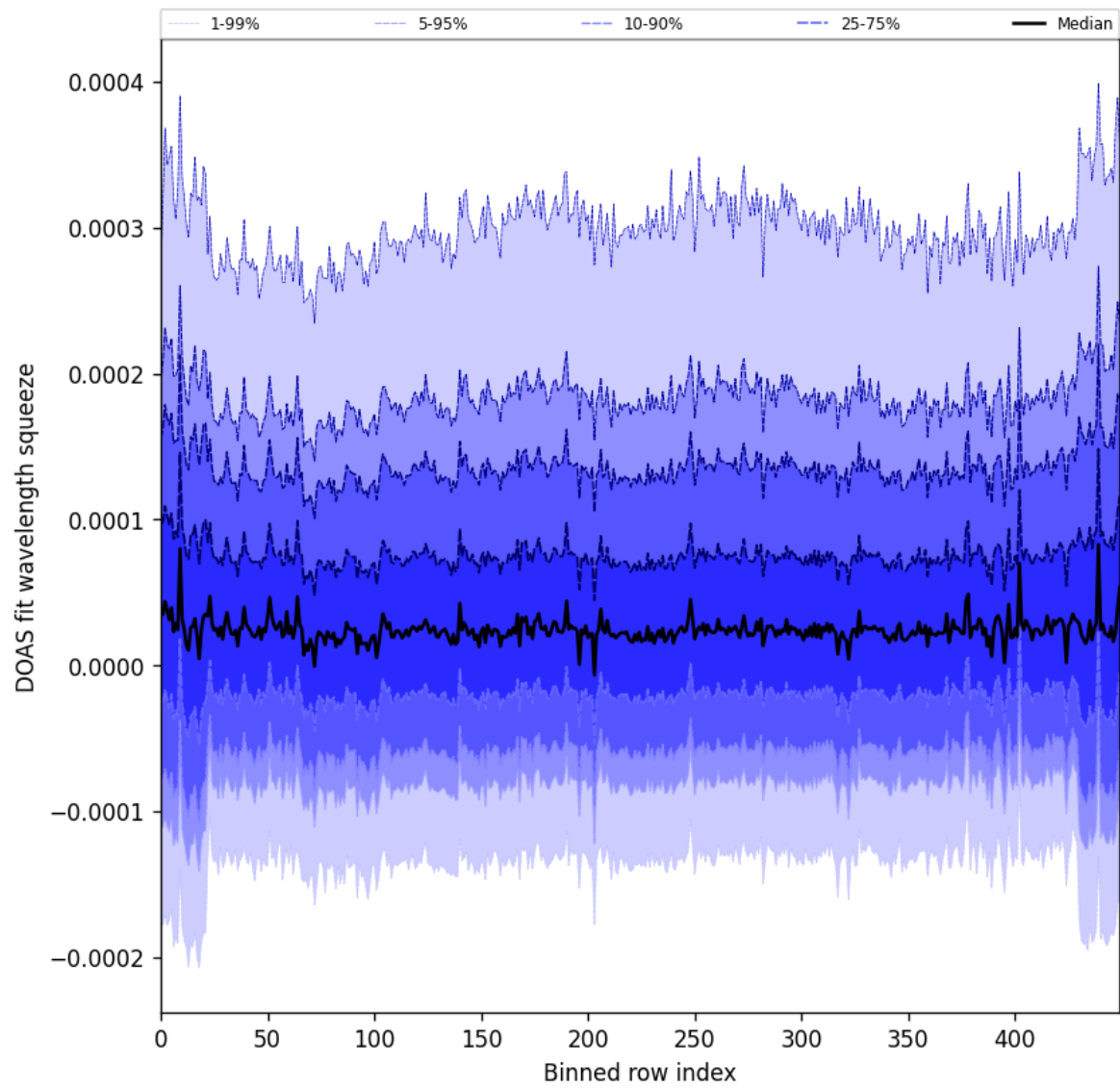
Figure 59: Along track statistics of “DOAS fit wavelength squeeze” for 2025-02-08 to 2025-02-10
