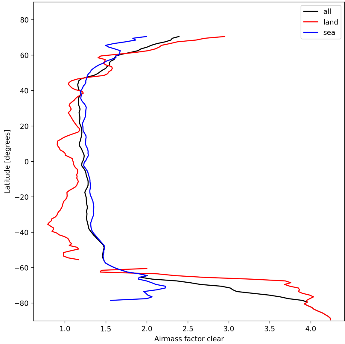
Figure 28: Zonal average of “Airmass factor clear” for 2025-02-08 to 2025-02-10.
