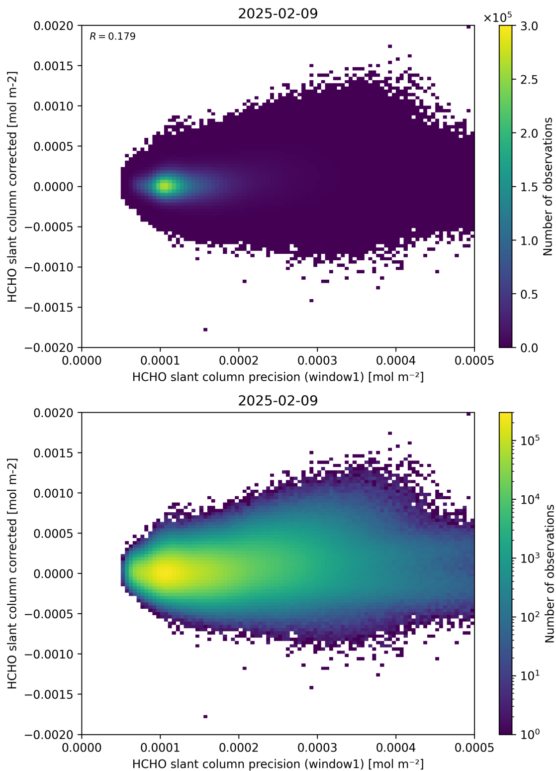
Figure 92: Scatter density plot of “HCHO slant column precision (window1)” against “HCHO slant column corrected” for 2025-02-08 to 2025-02-10.
