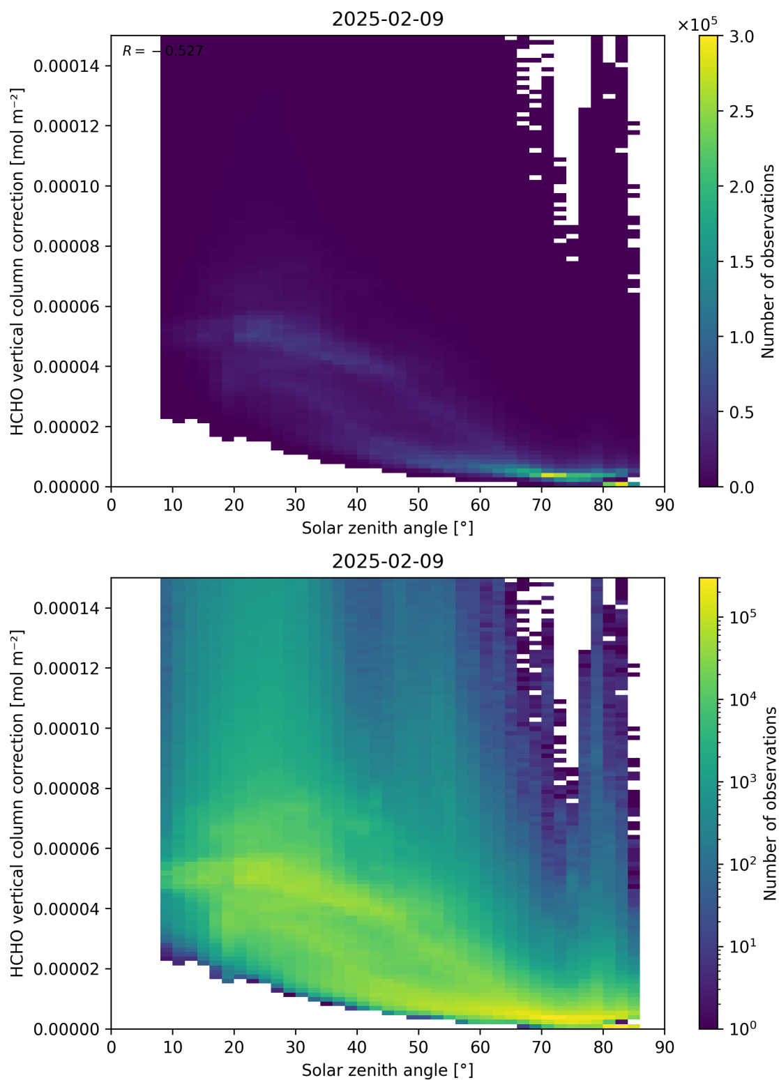
Figure 178: Scatter density plot of “Solar zenith angle” against “HCHO vertical column correction” for 2025-02-08 to 2025-02-10.
