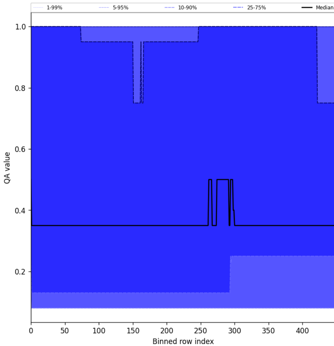
Figure 48: Along track statistics of “QA value” for 2025-02-08 to 2025-02-10
