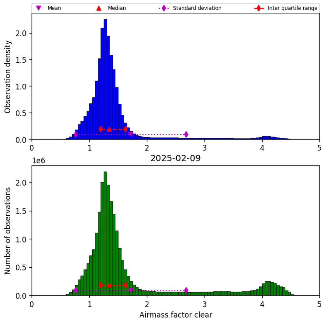
Figure 42: Histogram of “Airmass factor clear” for 2025-02-08 to 2025-02-10
