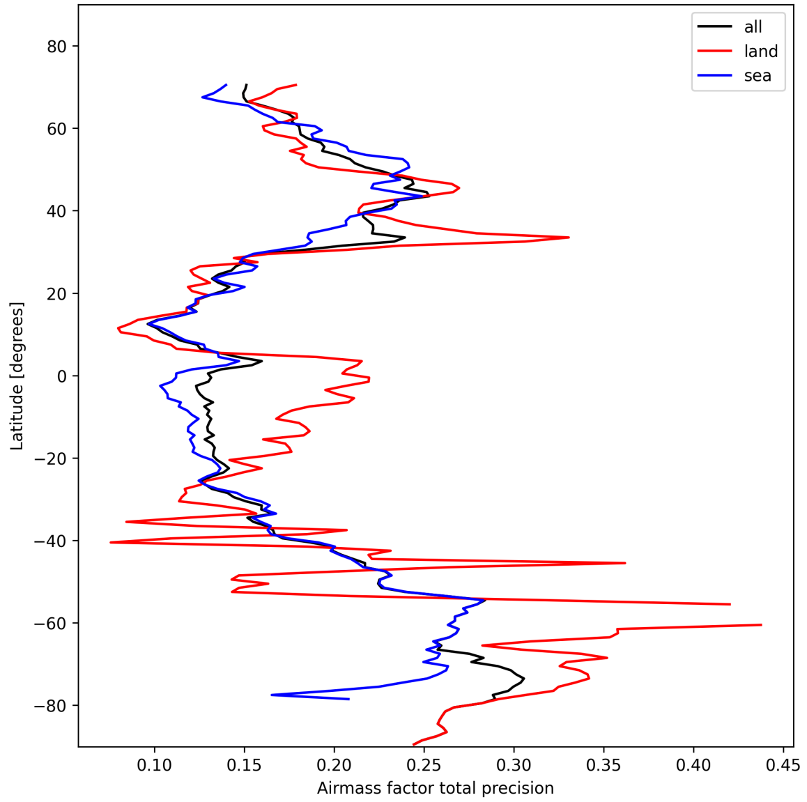
Figure 27: Zonal average of “Airmass factor total precision” for 2025-02-08 to 2025-02-10.
