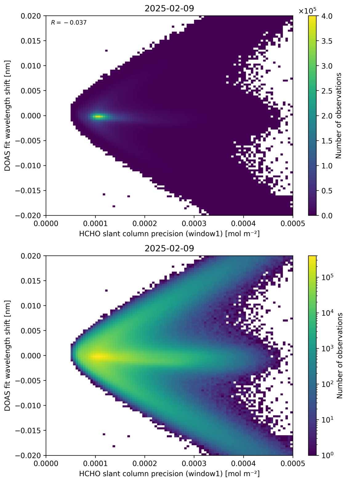
Figure 89: Scatter density plot of “HCHO slant column precision (window1)” against “DOAS fit wavelength shift” for 2025-02-08 to 2025-02-10.
