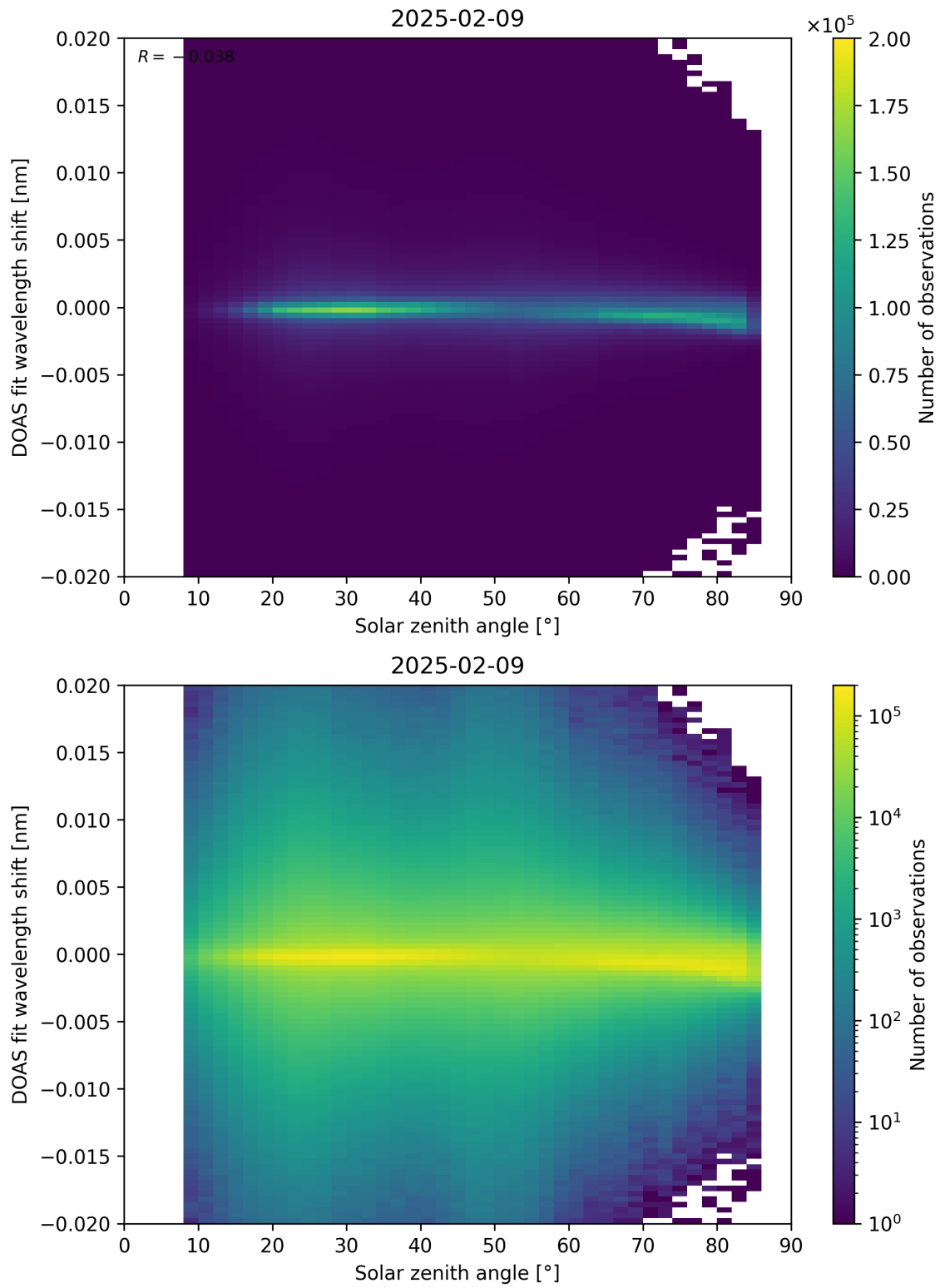
Figure 168: Scatter density plot of “Solar zenith angle” against “DOAS fit wavelength shift” for 2025-02-08 to 2025-02-10.
