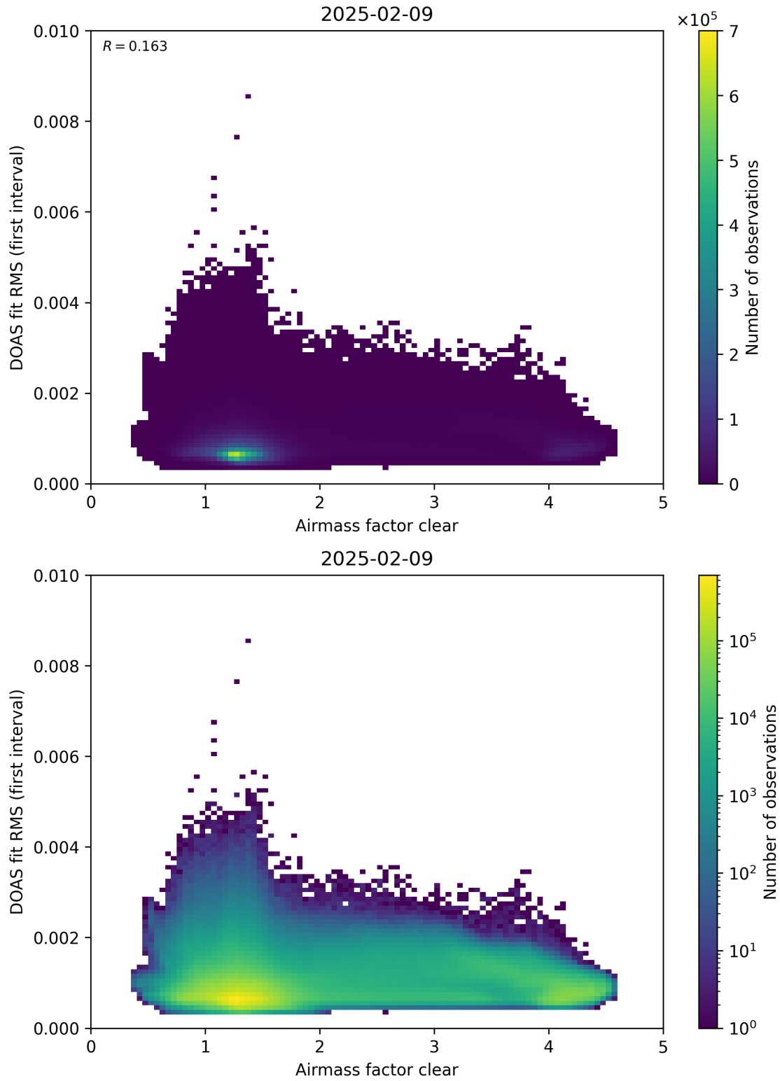
Figure 71: Scatter density plot of “Airmass factor clear” against “DOAS fit RMS (first interval)” for 2025-02-08 to 2025-02-10.
