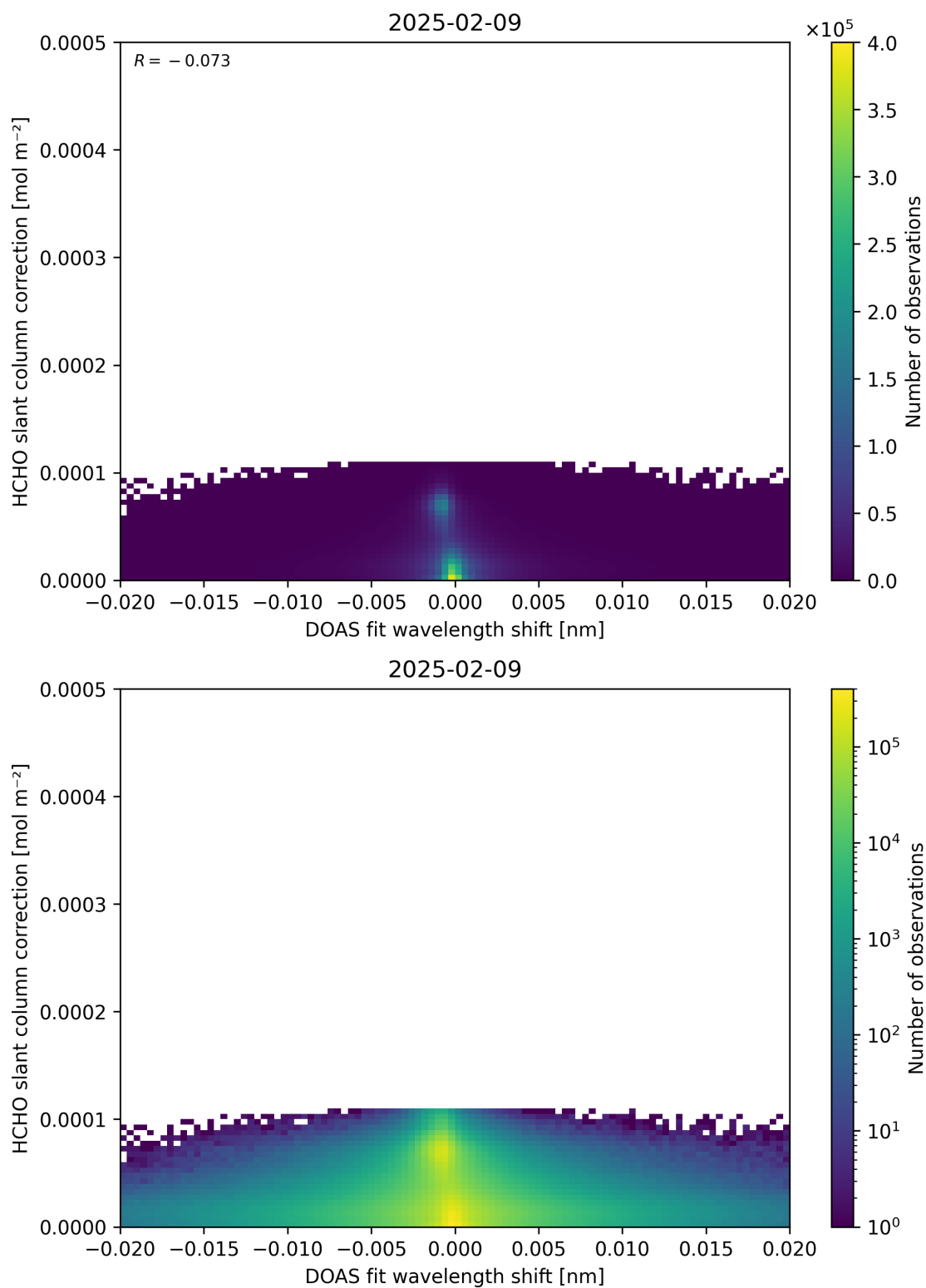
Figure 67: Scatter density plot of “DOAS fit wavelength shift” against “HCHO slant column correction” for 2025-02-08 to 2025-02-10.
