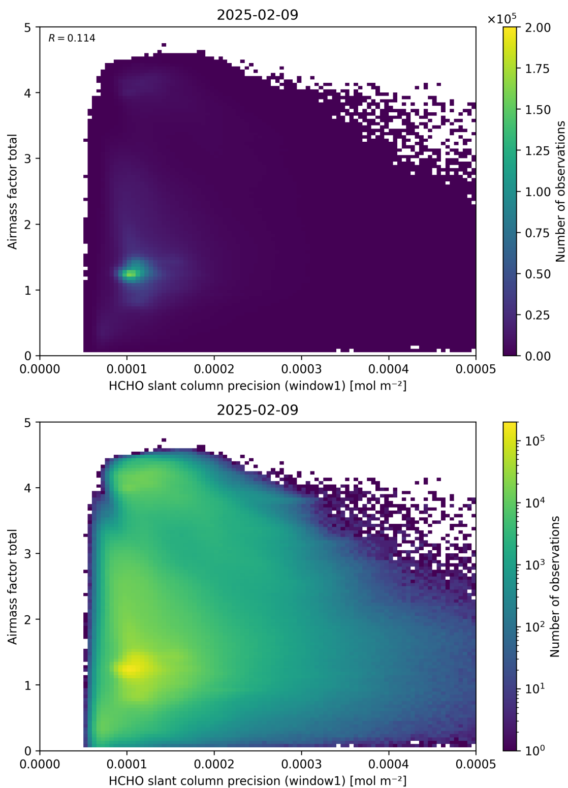
Figure 94: Scatter density plot of “HCHO slant column precision (window1)” against “Airmass factor total” for 2025-02-08 to 2025-02-10.
