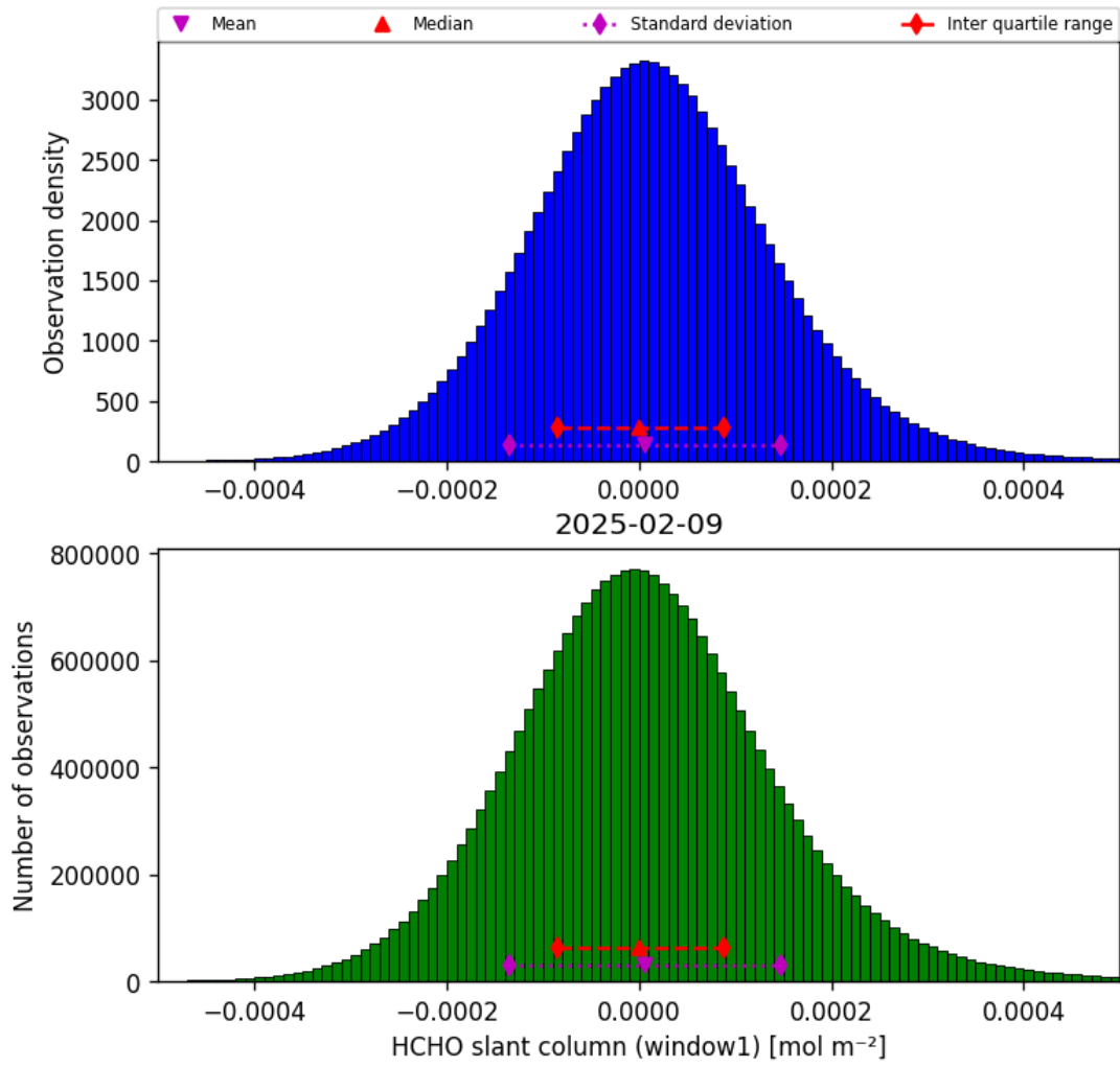
Figure 38: Histogram of “HCHO slant column (window1)” for 2025-02-08 to 2025-02-10
