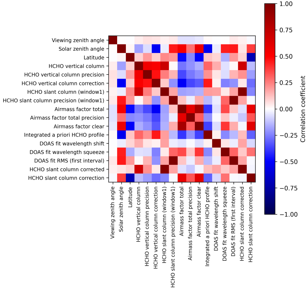
Figure 2: Map of correlation matrix for 2025-02-08 to 2025-02-10.
