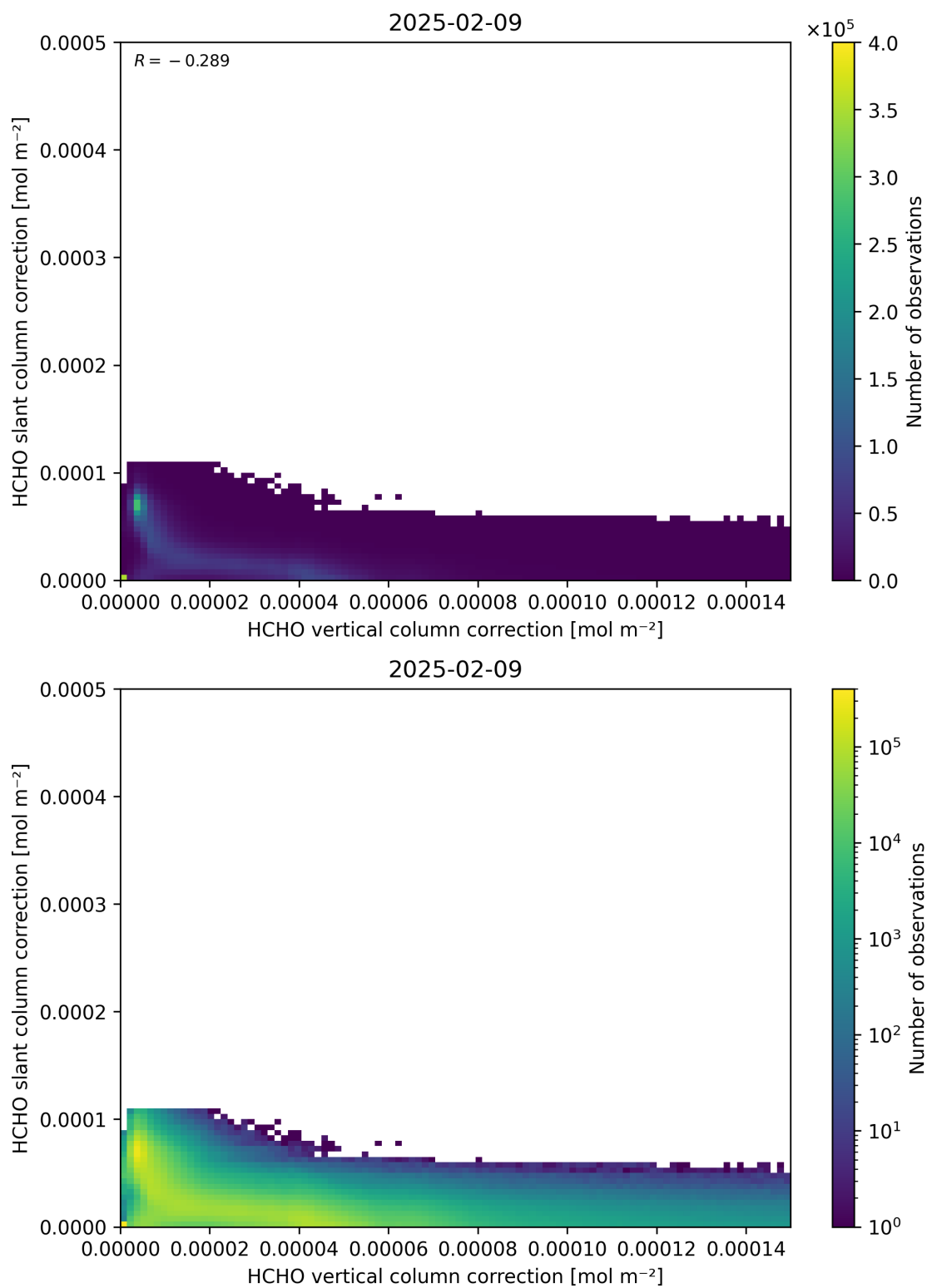
Figure 117: Scatter density plot of “HCHO vertical column correction” against “HCHO slant column correction” for 2025-02-08 to 2025-02-10.
