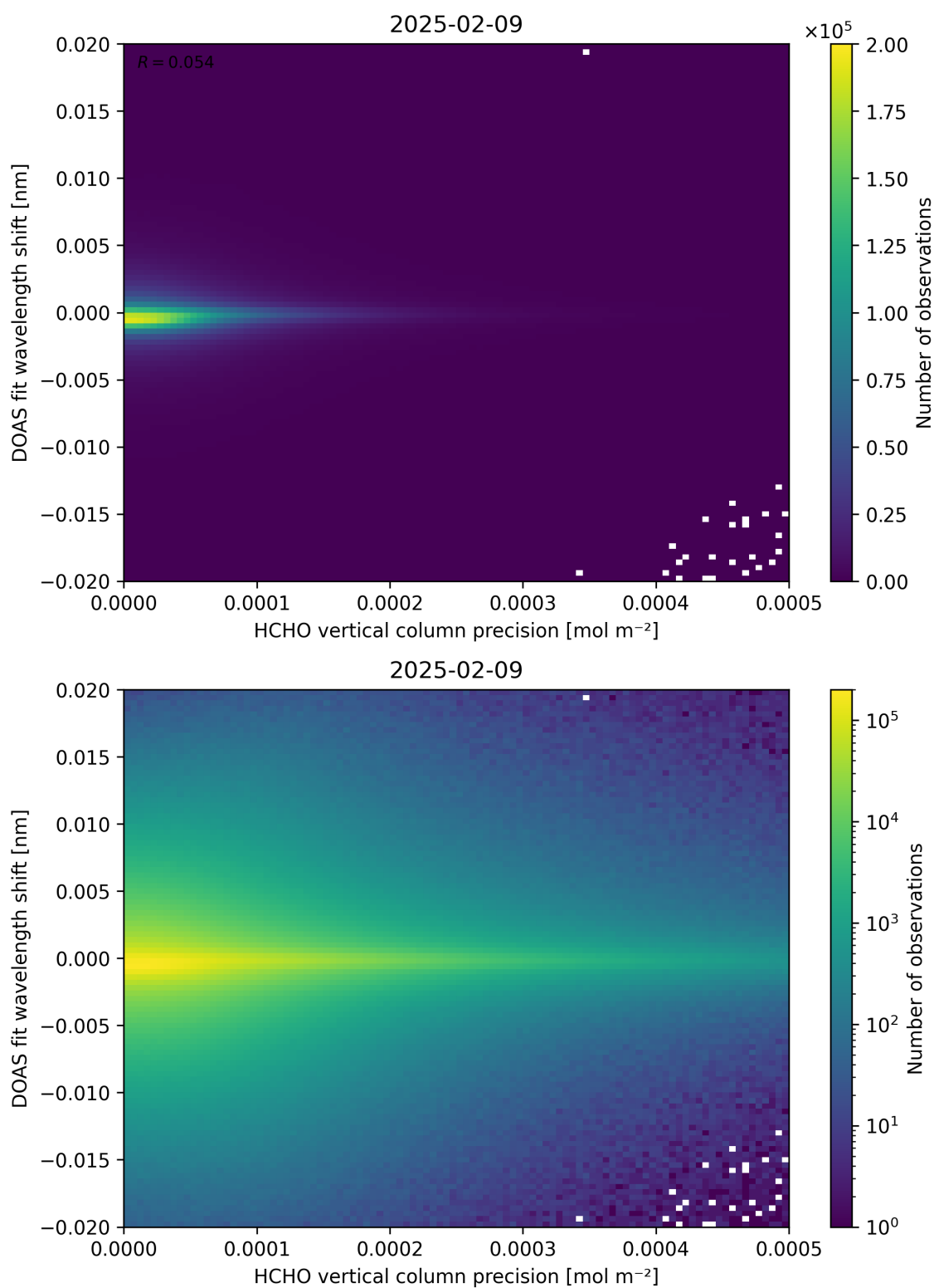
Figure 137: Scatter density plot of “HCHO vertical column precision” against “DOAS fit wavelength shift” for 2025-02-08 to 2025-02-10.
