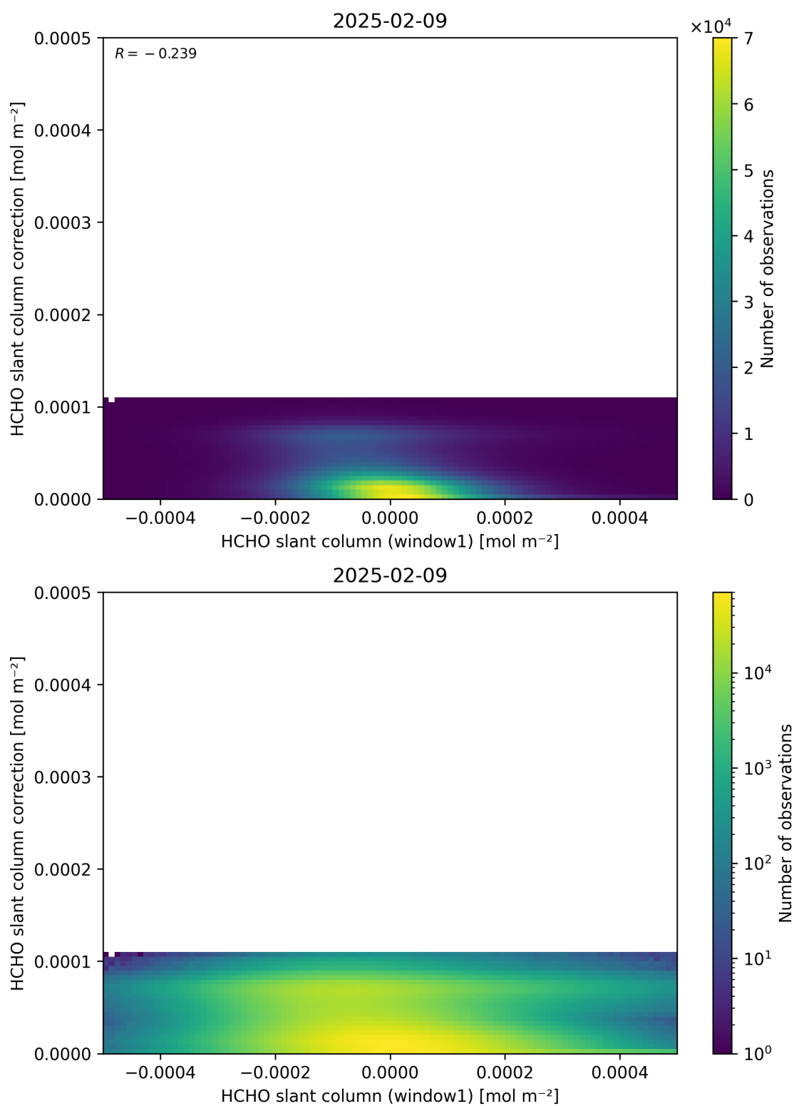
Figure 83: Scatter density plot of “HCHO slant column (window1)” against “HCHO slant column correction” for 2025-02-08 to 2025-02-10.
