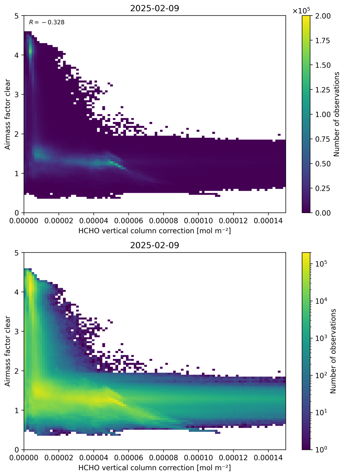
Figure 115: Scatter density plot of “HCHO vertical column correction” against “Airmass factor clear” for 2025-02-08 to 2025-02-10.
