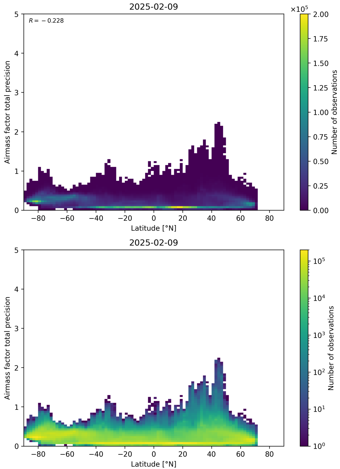
Figure 162: Scatter density plot of “Latitude” against “Airmass factor total precision” for 2025-02-08 to 2025-02-10.
