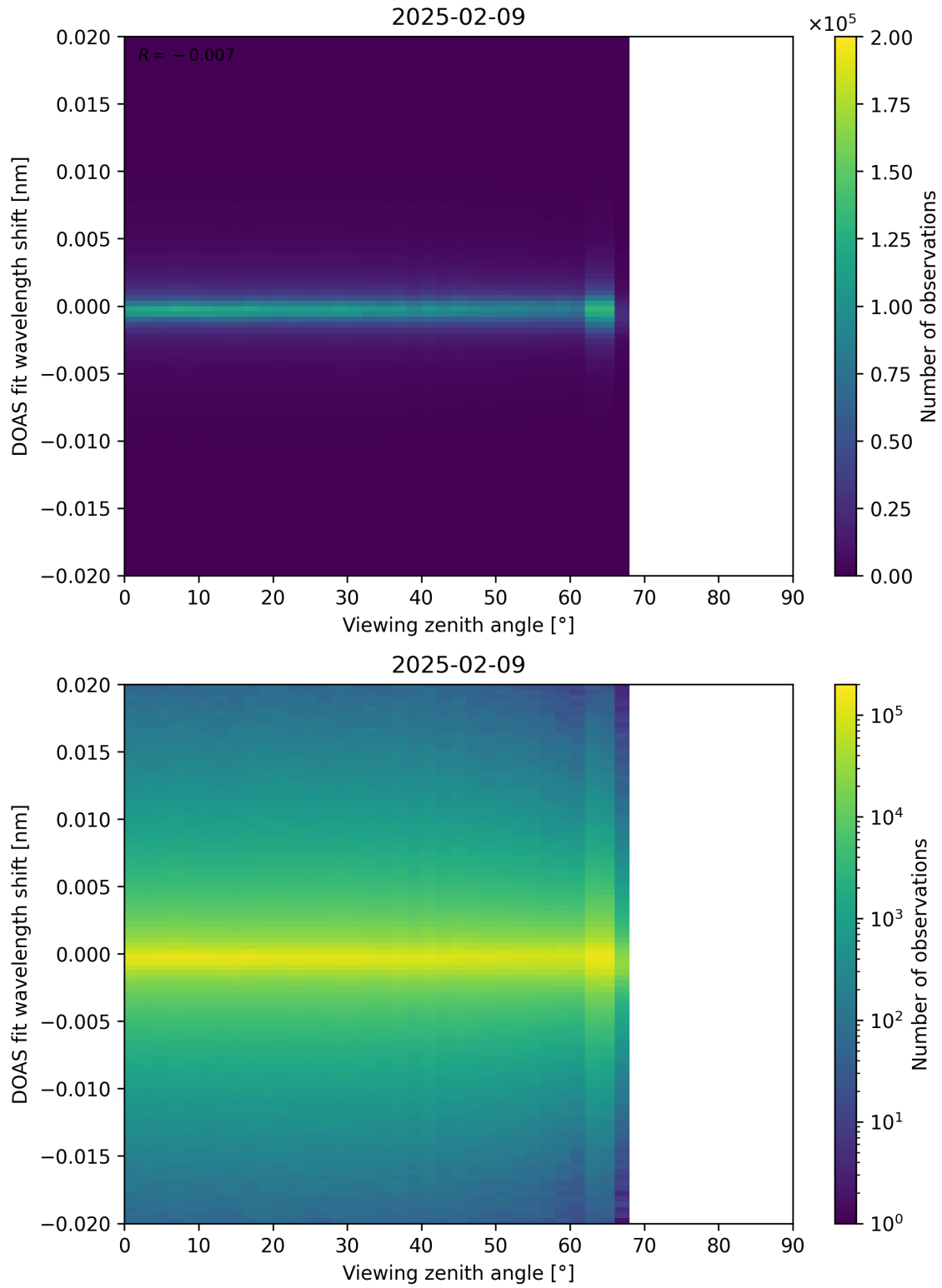
Figure 183: Scatter density plot of “Viewing zenith angle” against “DOAS fit wavelength shift” for 2025-02-08 to 2025-02-10.
