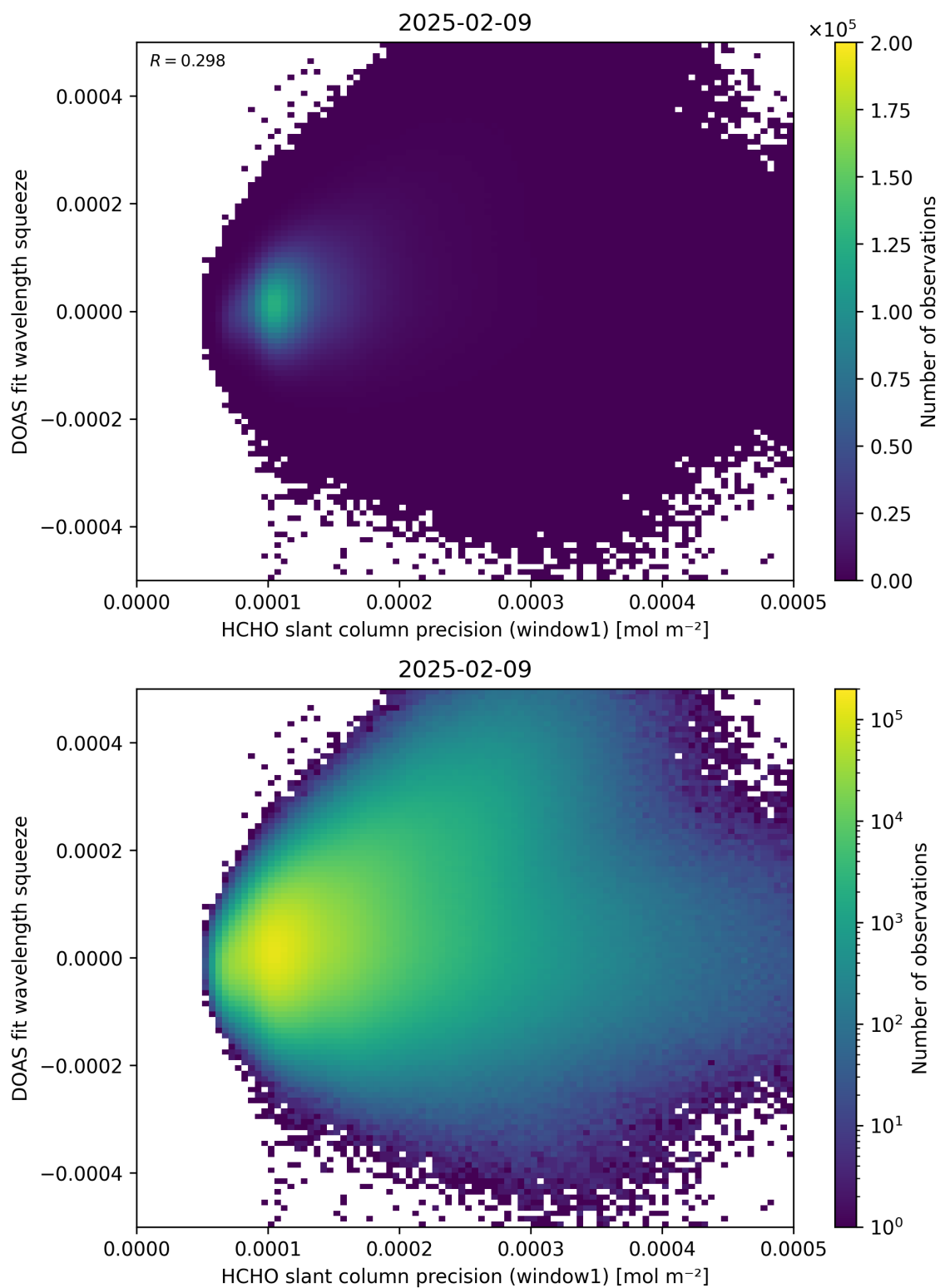
Figure 90: Scatter density plot of “HCHO slant column precision (window1)” against “DOAS fit wavelength squeeze” for 2025-02-08 to 2025-02-10.
