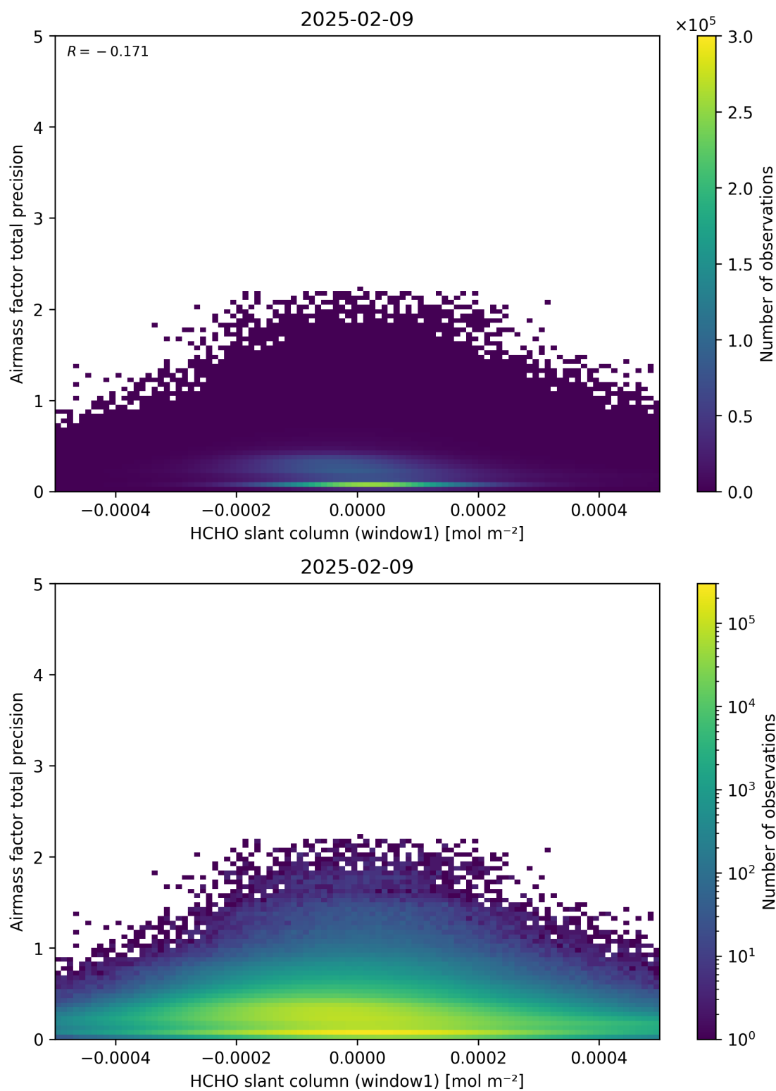
Figure 86: Scatter density plot of “HCHO slant column (window1)” against “Airmass factor total precision” for 2025-02-08 to 2025-02-10.
