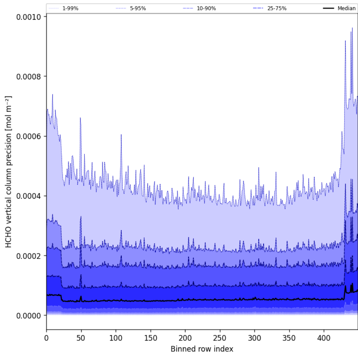
Figure 50: Along track statistics of “HCHO vertical column precision” for 2025-02-08 to 2025-02-10
