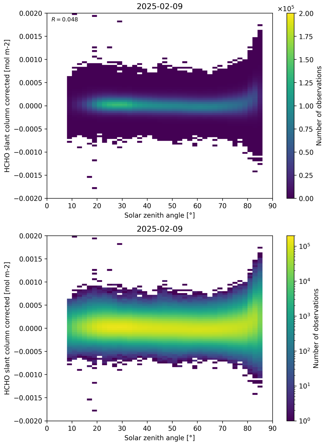
Figure 171: Scatter density plot of “Solar zenith angle” against “HCHO slant column corrected” for 2025-02-08 to 2025-02-10.
