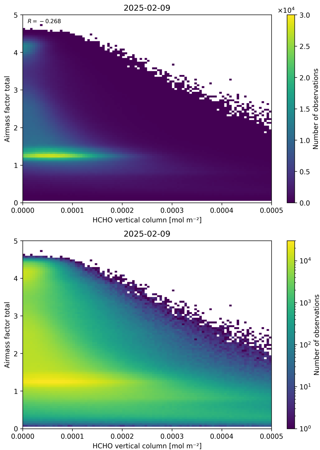
Figure 131: Scatter density plot of “HCHO vertical column” against “Airmass factor total” for 2025-02-08 to 2025-02-10.
