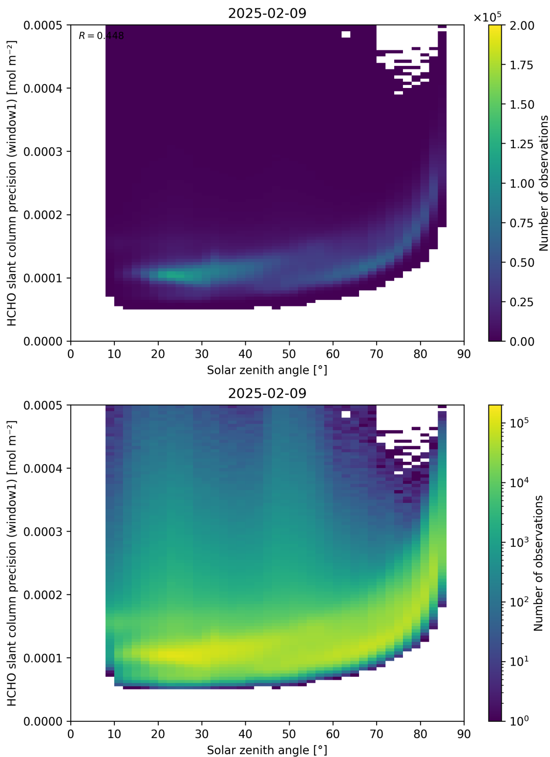
Figure 174: Scatter density plot of “Solar zenith angle” against “HCHO slant column precision (window1)” for 2025-02-08 to 2025-02-10.
