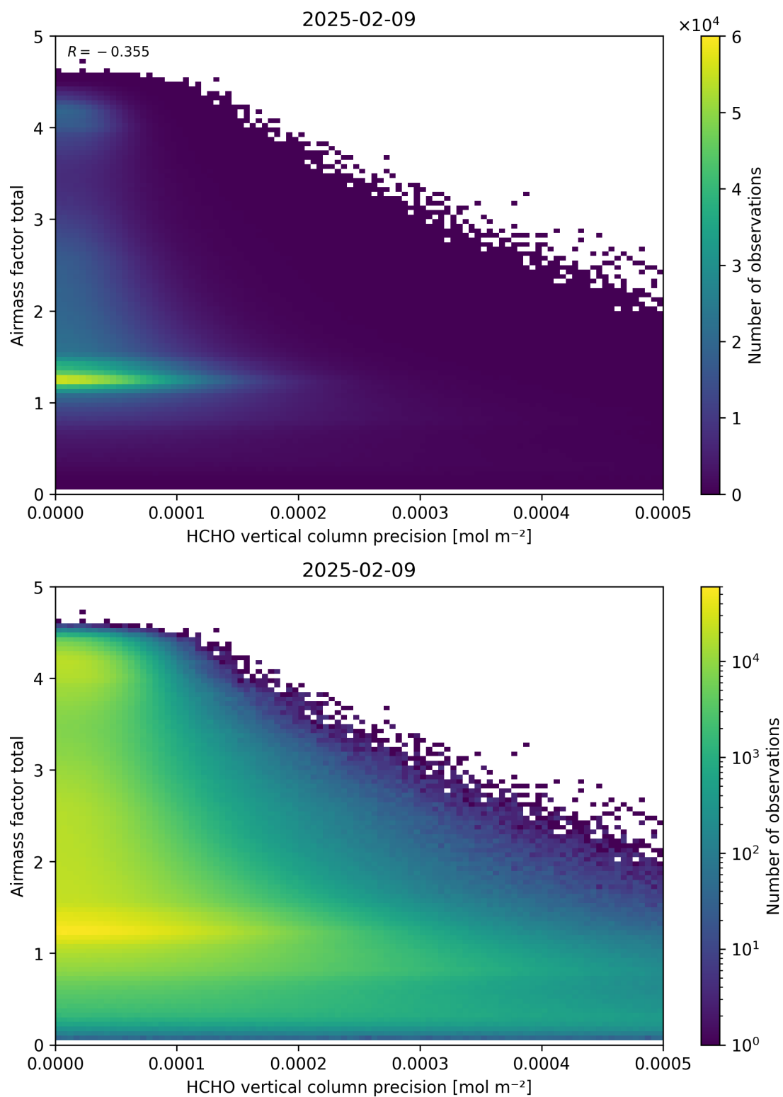
Figure 144: Scatter density plot of “HCHO vertical column precision” against “Airmass factor total” for 2025-02-08 to 2025-02-10.
