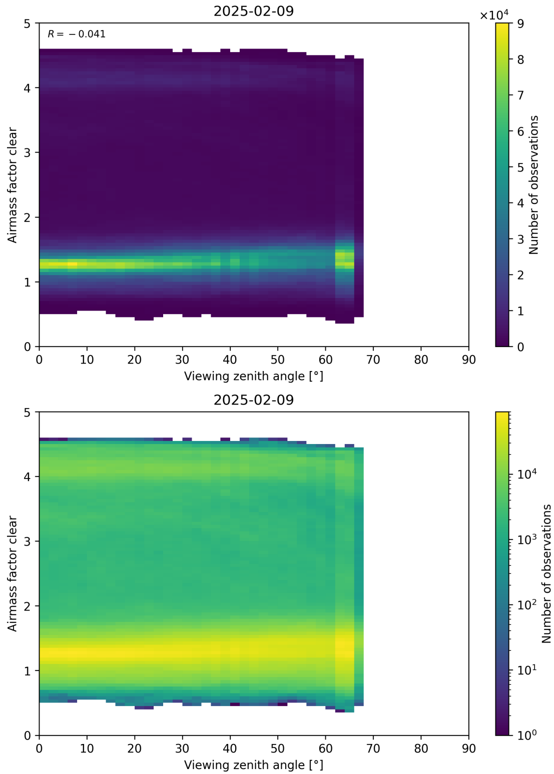
Figure 185: Scatter density plot of “Viewing zenith angle” against “Airmass factor clear” for 2025-02-08 to 2025-02-10.
