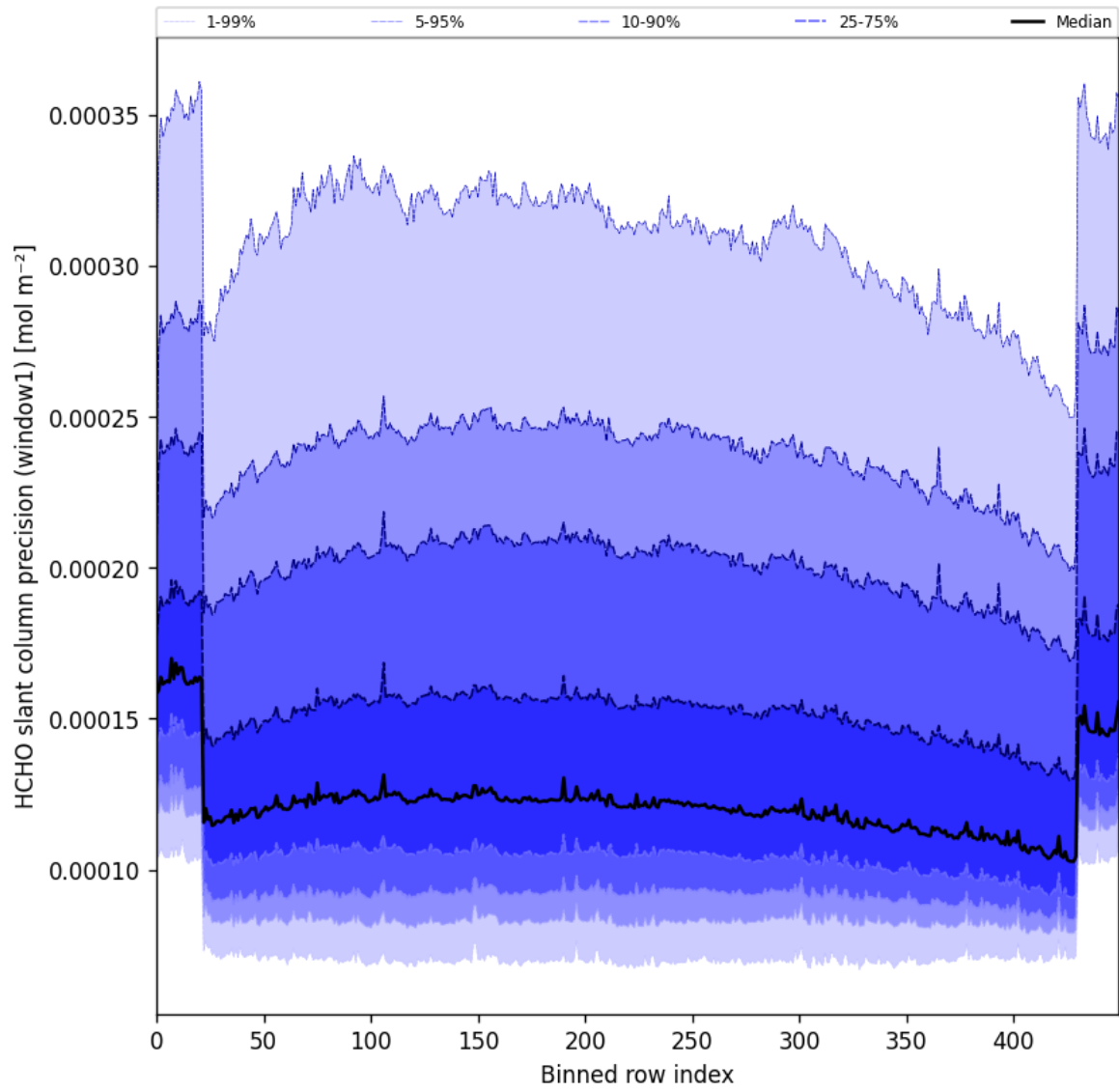
Figure 53: Along track statistics of “HCHO slant column precision (window1)” for 2025-02-08 to 2025-02-10
