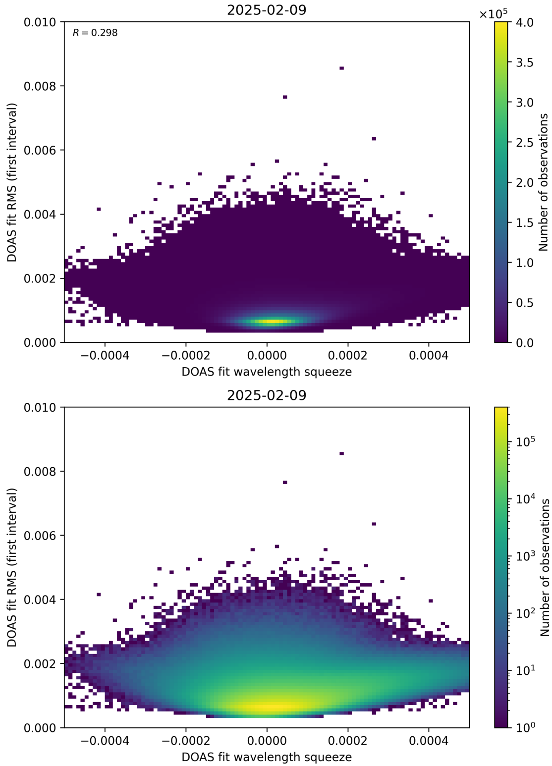
Figure 68: Scatter density plot of “DOAS fit wavelength squeeze” against “DOAS fit RMS (first interval)” for 2025-02-08 to 2025-02-10.
