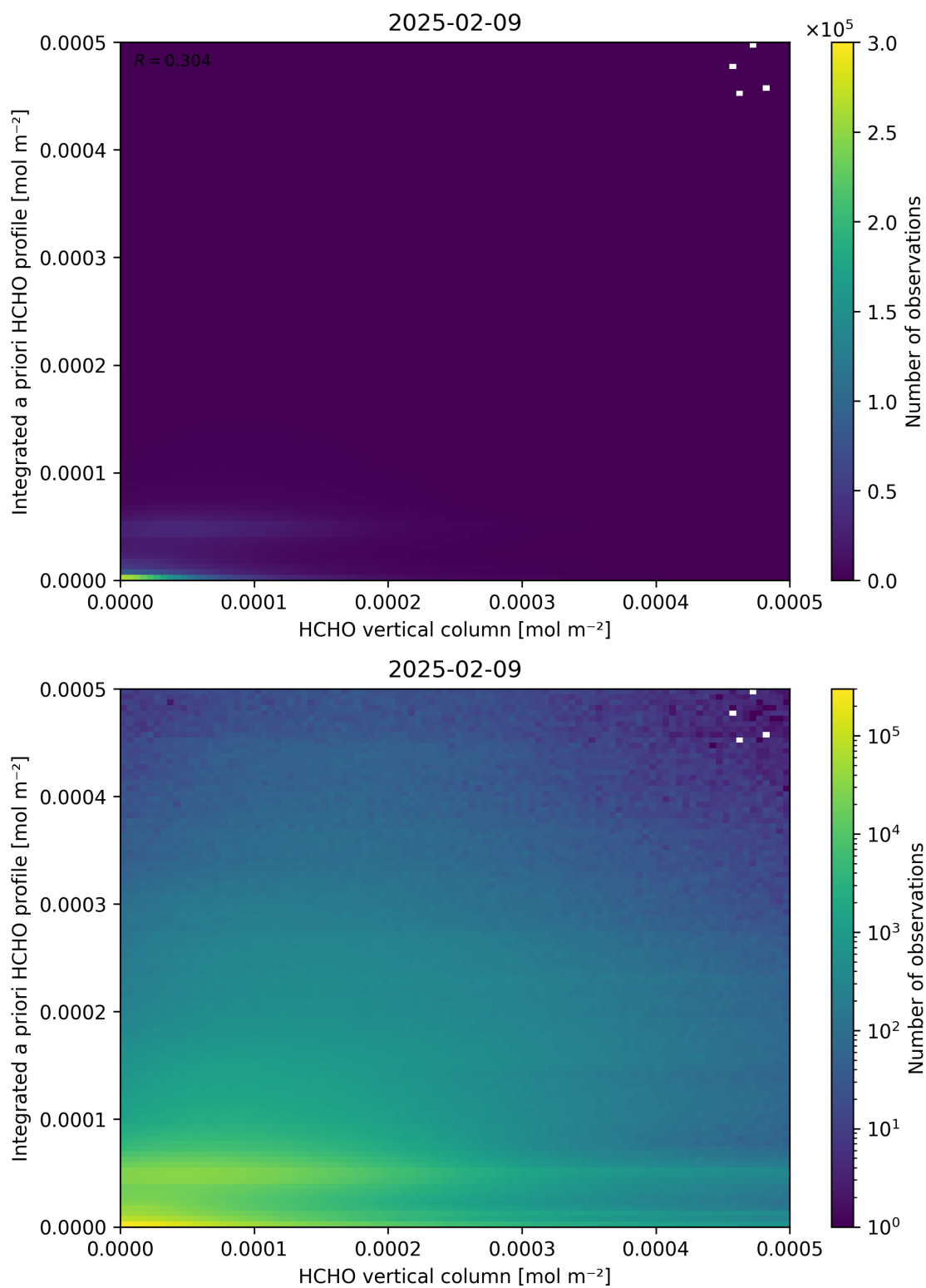
Figure 135: Scatter density plot of “HCHO vertical column” against “Integrated a priori HCHO profile” for 2025-02-08 to 2025-02-10.
