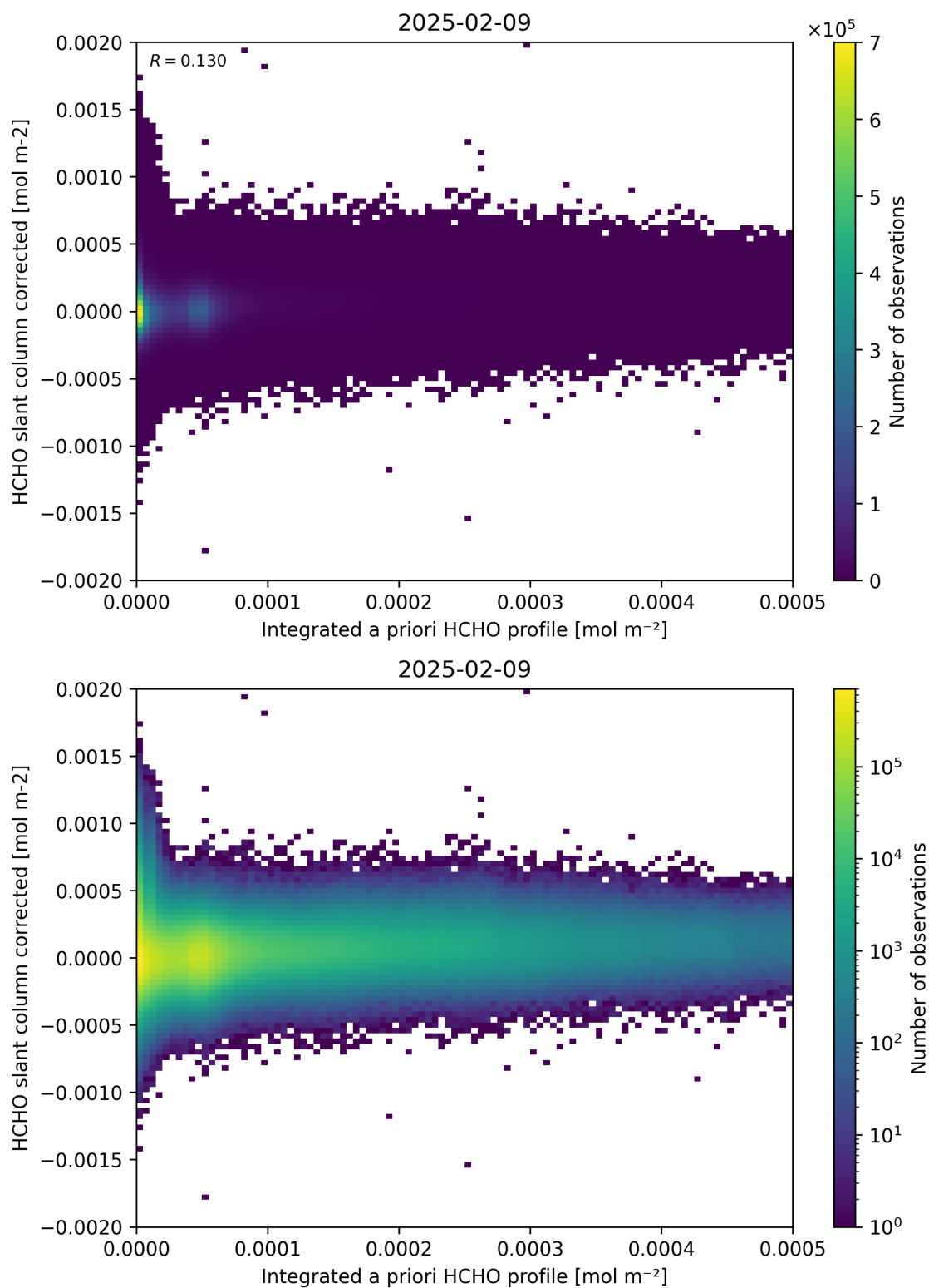
Figure 151: Scatter density plot of “Integrated a priori HCHO profile” against “HCHO slant column corrected” for 2025-02-08 to 2025-02-10.
