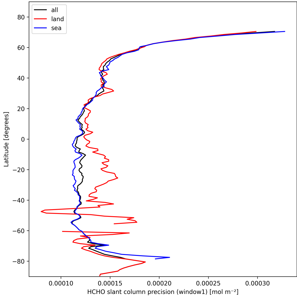
Figure 25: Zonal average of “HCHO slant column precision (window1)” for 2025-02-08 to 2025-02-10.
