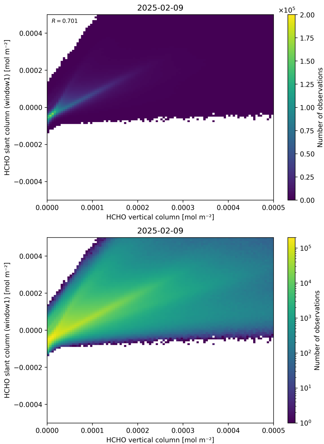
Figure 129: Scatter density plot of “HCHO vertical column” against “HCHO slant column (window1)” for 2025-02-08 to 2025-02-10.
