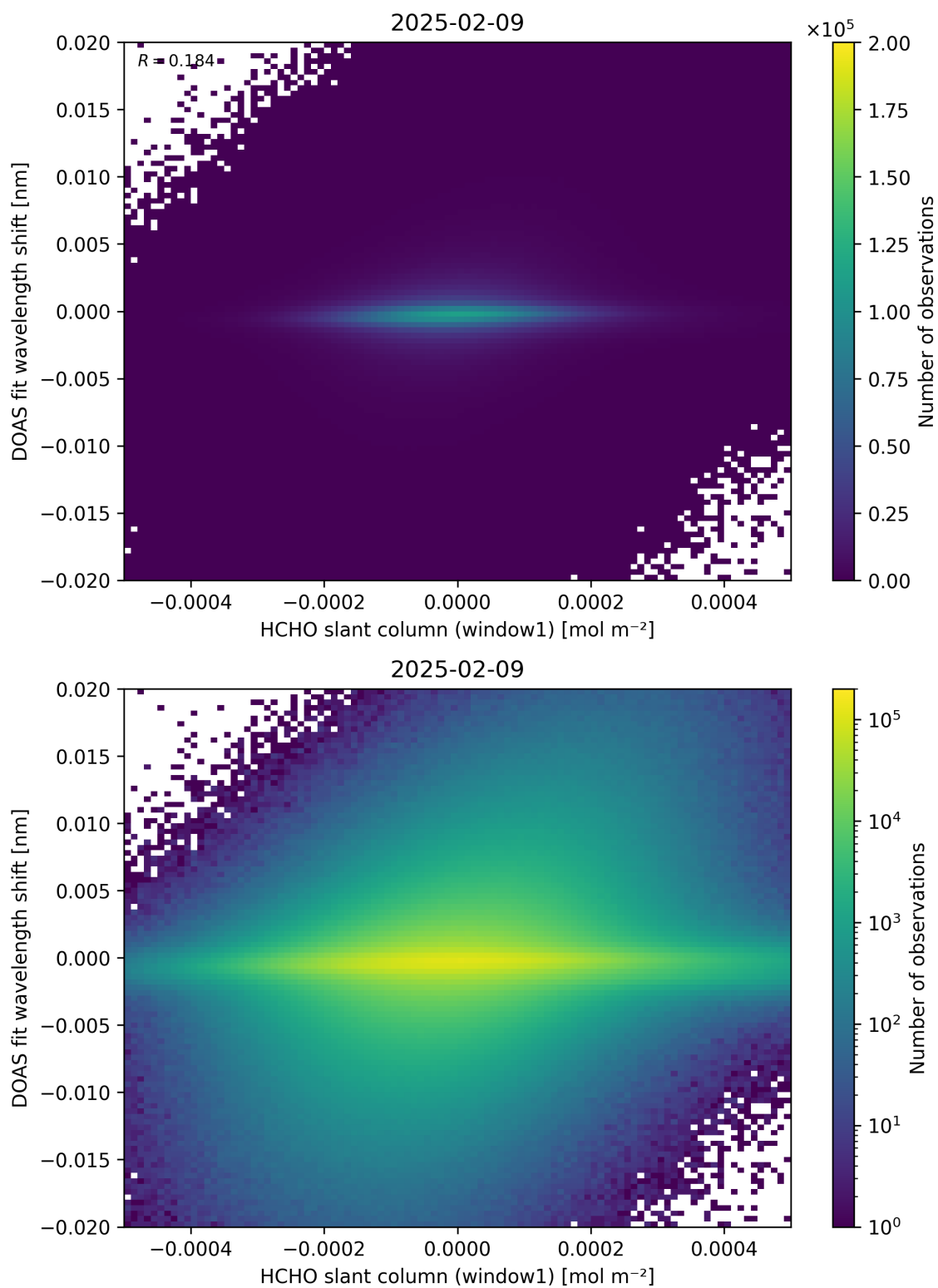
Figure 79: Scatter density plot of “HCHO slant column (window1)” against “DOAS fit wavelength shift” for 2025-02-08 to 2025-02-10.
