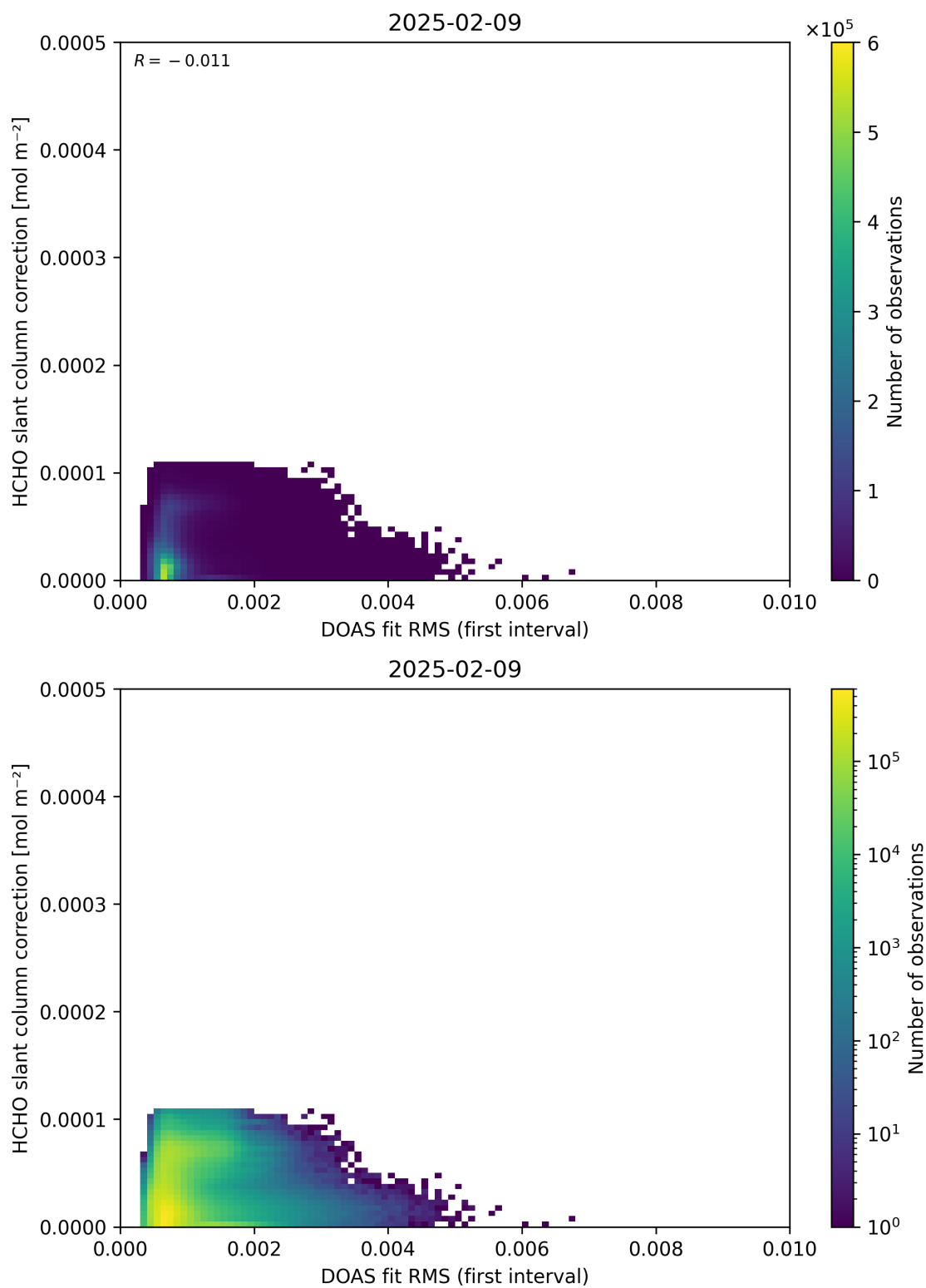
Figure 63: Scatter density plot of “DOAS fit RMS (first interval)” against “HCHO slant column correction” for 2025-02-08 to 2025-02-10.
