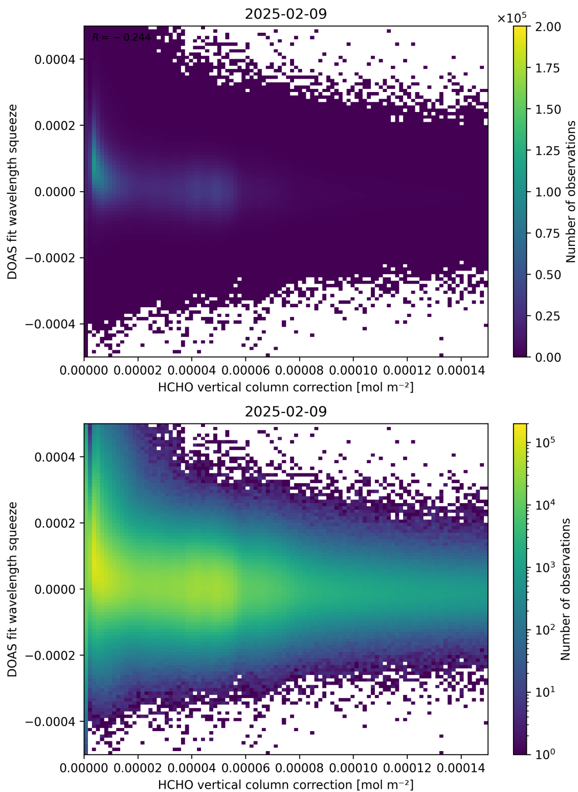
Figure 114: Scatter density plot of “HCHO vertical column correction” against “DOAS fit wavelength squeeze” for 2025-02-08 to 2025-02-10.
