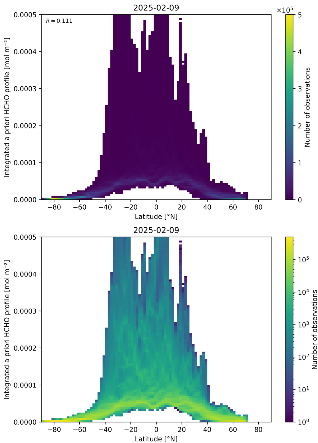
Figure 166: Scatter density plot of “Latitude” against “Integrated a priori HCHO profile” for 2025-02-08 to 2025-02-10.
