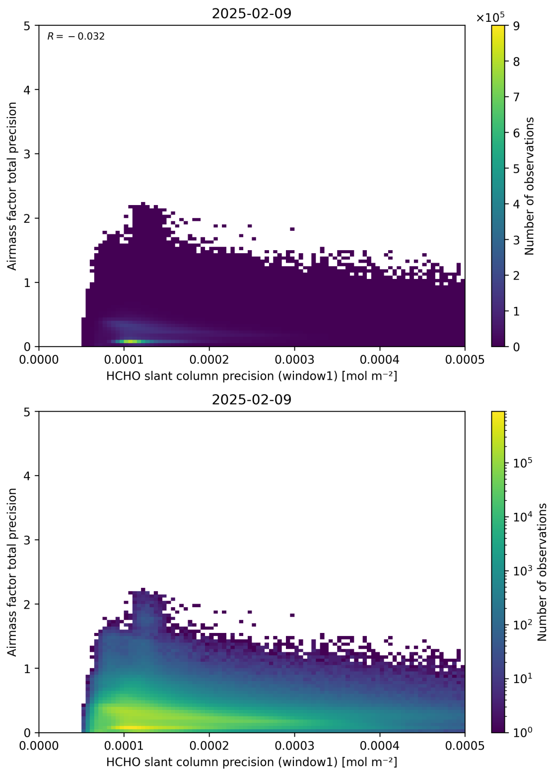
Figure 95: Scatter density plot of “HCHO slant column precision (window1)” against “Airmass factor total precision” for 2025-02-08 to 2025-02-10.
