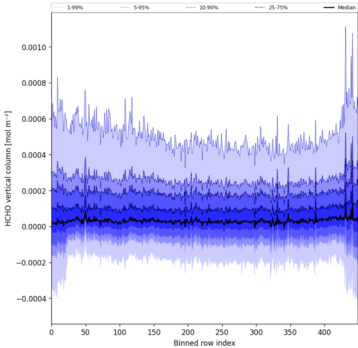
Figure 49: Along track statistics of “HCHO vertical column” for 2025-02-08 to 2025-02-10
