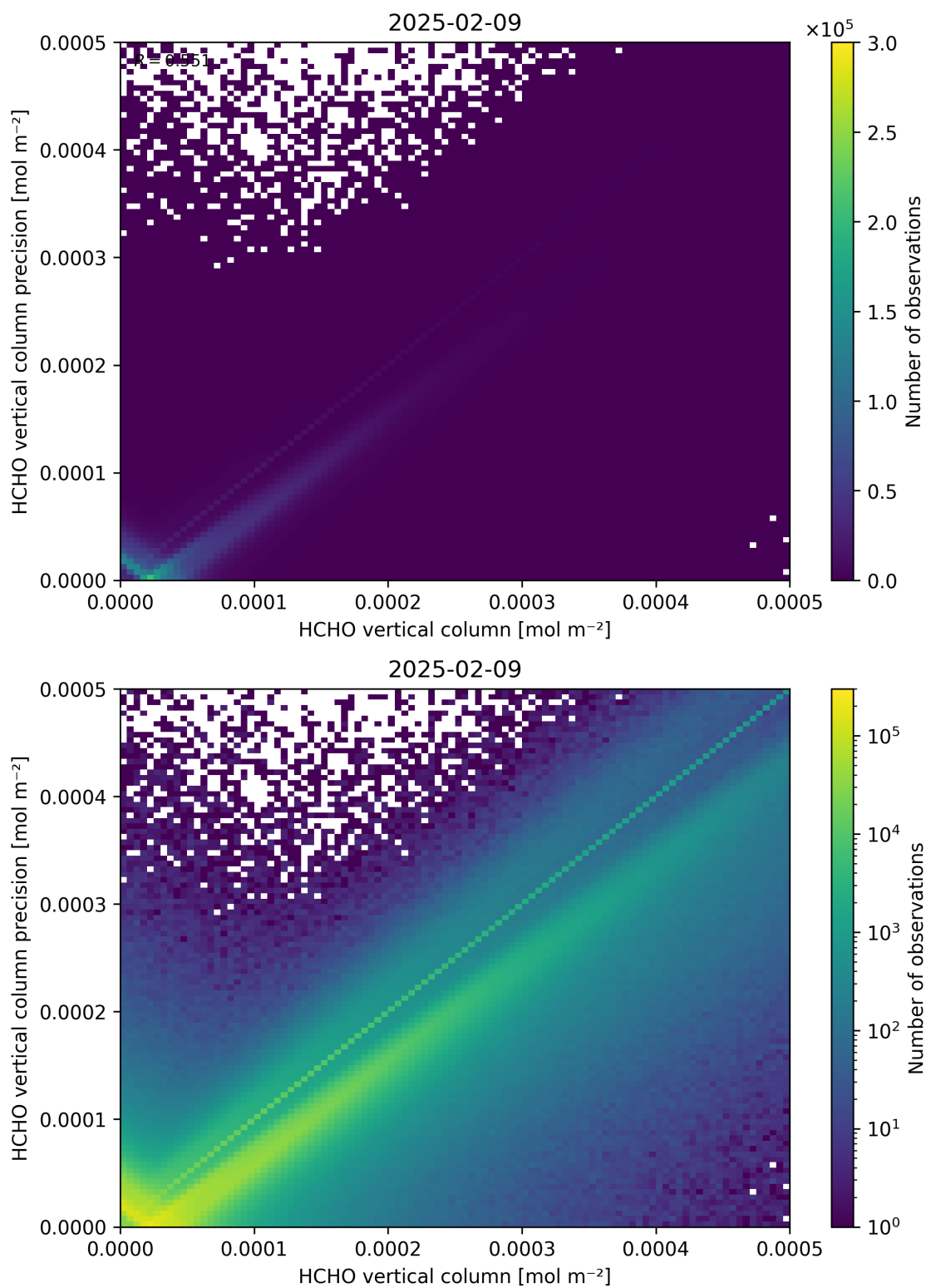
Figure 134: Scatter density plot of “HCHO vertical column” against “HCHO vertical column precision” for 2025-02-08 to 2025-02-10.
