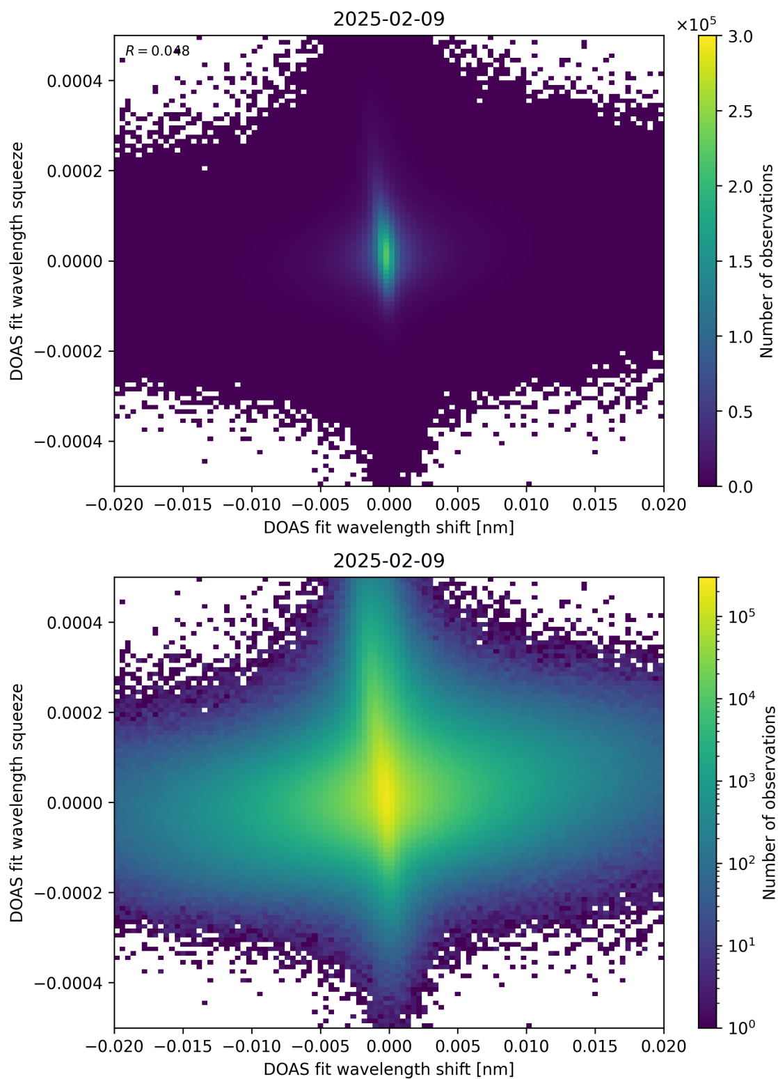
Figure 65: Scatter density plot of “DOAS fit wavelength shift” against “DOAS fit wavelength squeeze” for 2025-02-08 to 2025-02-10.
