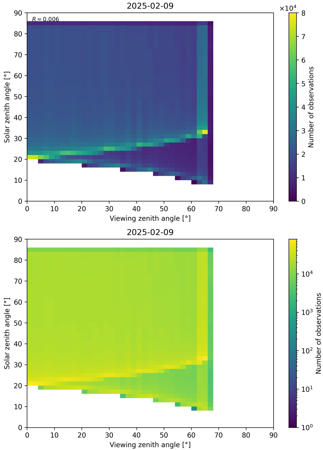
Figure 197: Scatter density plot of “Viewing zenith angle” against “Solar zenith angle” for 2025-02-08 to 2025-02-10.
