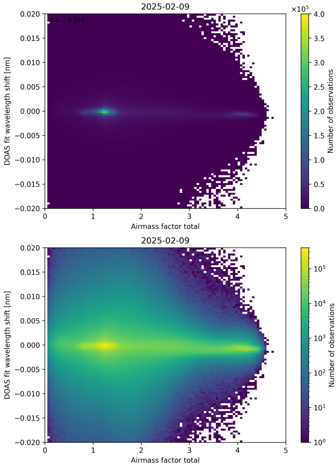
Figure 98: Scatter density plot of “Airmass factor total” against “DOAS fit wavelength shift” for 2025-02-08 to 2025-02-10.
