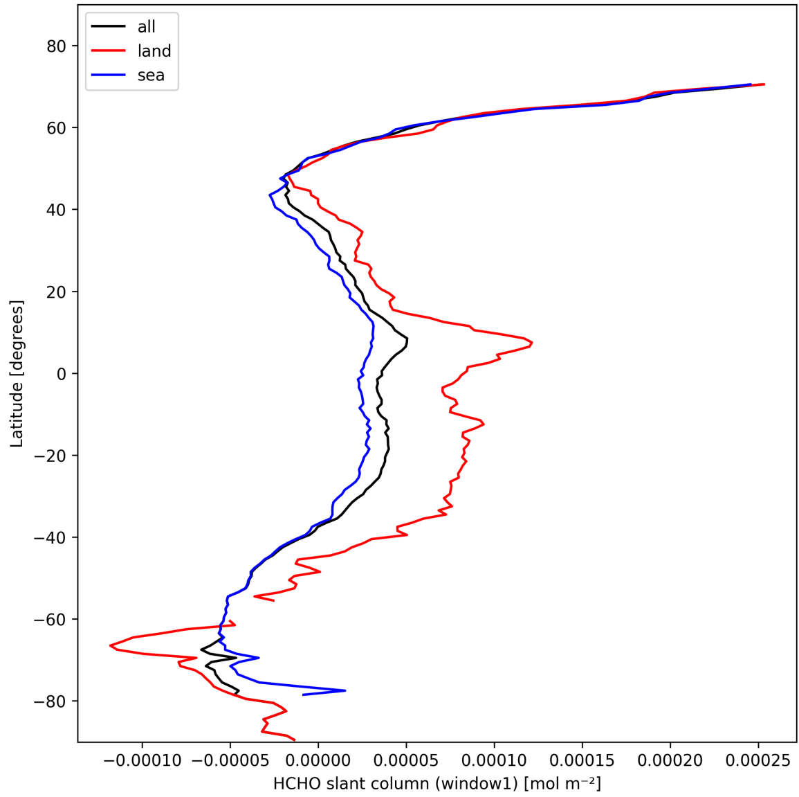
Figure 24: Zonal average of “HCHO slant column (window1)” for 2025-02-08 to 2025-02-10.
