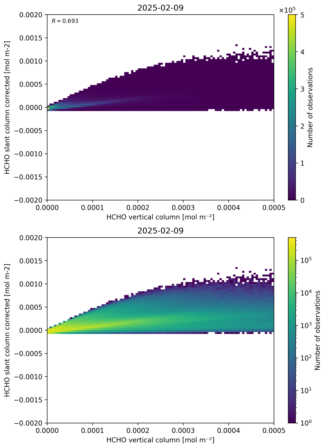
Figure 127: Scatter density plot of “HCHO vertical column” against “HCHO slant column corrected” for 2025-02-08 to 2025-02-10.
