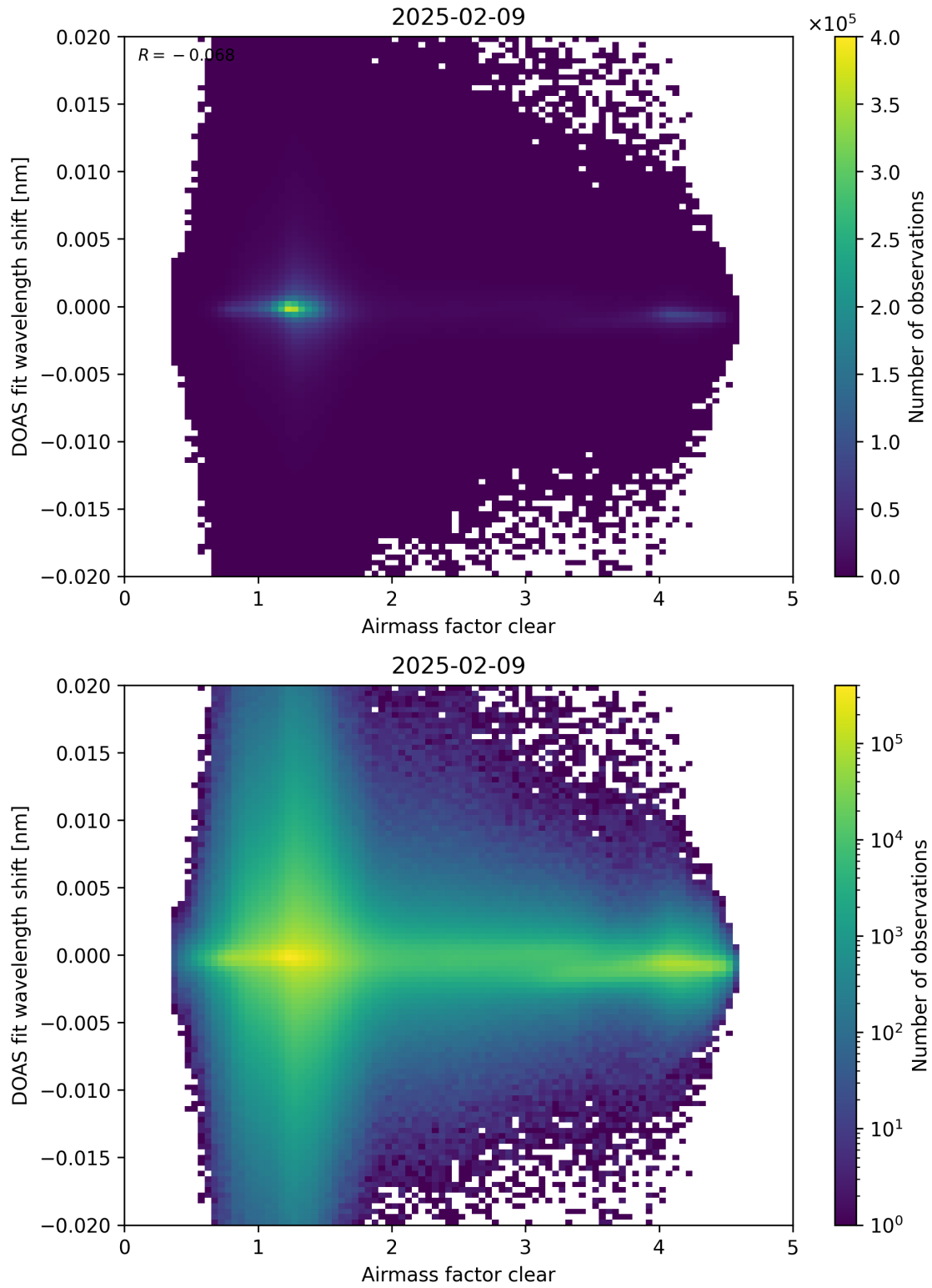
Figure 72: Scatter density plot of “Airmass factor clear” against “DOAS fit wavelength shift” for 2025-02-08 to 2025-02-10.
