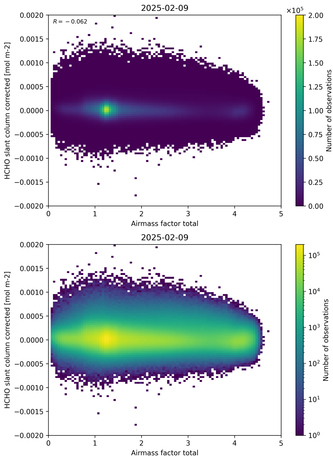
Figure 101: Scatter density plot of “Airmass factor total” against “HCHO slant column corrected” for 2025-02-08 to 2025-02-10.
