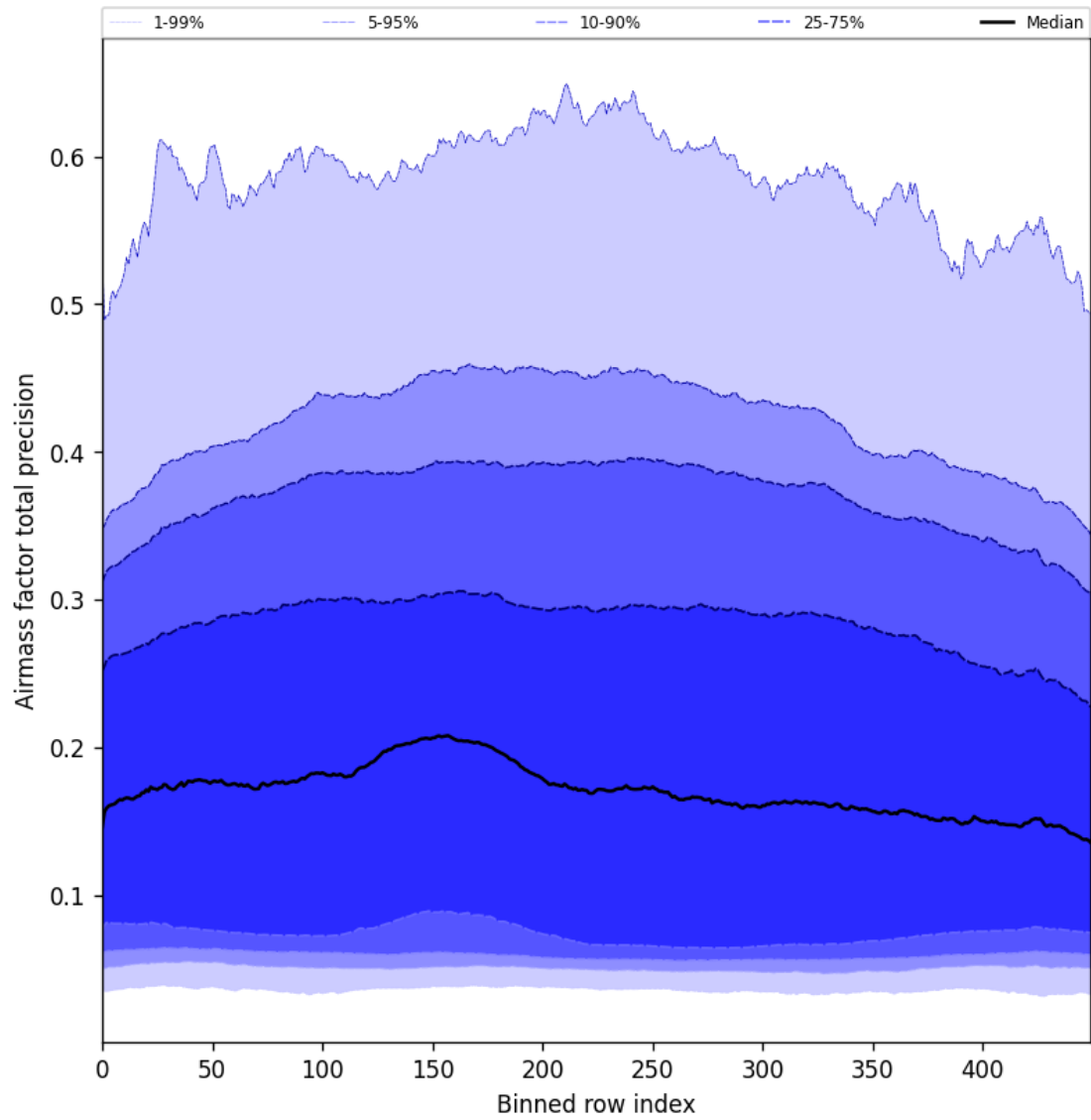
Figure 55: Along track statistics of “Airmass factor total precision” for 2025-02-08 to 2025-02-10
