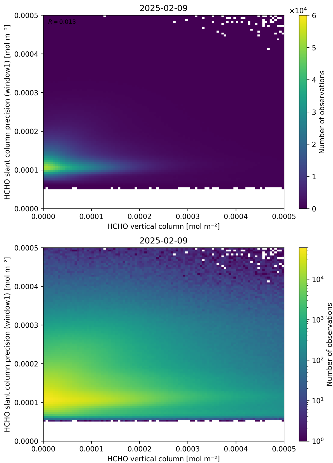
Figure 130: Scatter density plot of “HCHO vertical column” against “HCHO slant column precision (window1)” for 2025-02-08 to 2025-02-10.
