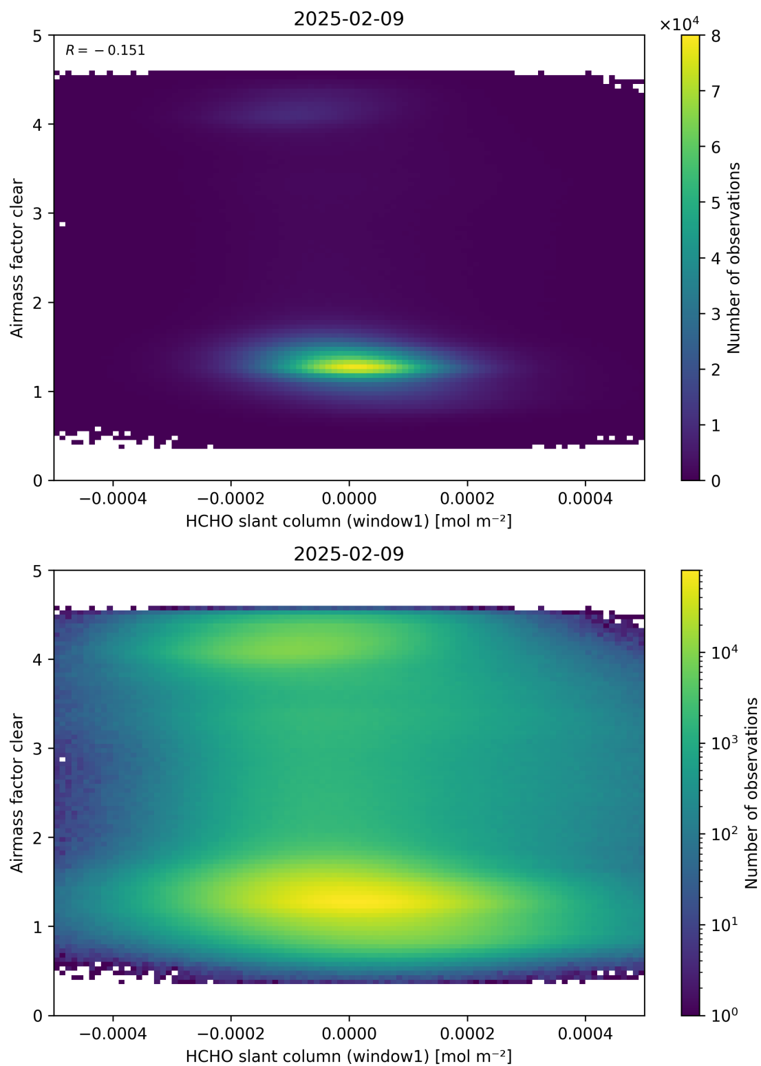
Figure 81: Scatter density plot of “HCHO slant column (window1)” against “Airmass factor clear” for 2025-02-08 to 2025-02-10.
