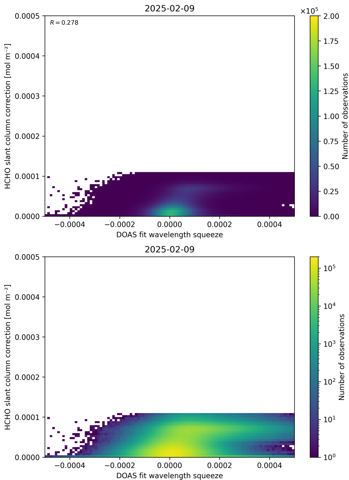
Figure 70: Scatter density plot of “DOAS fit wavelength squeeze” against “HCHO slant column correction” for 2025-02-08 to 2025-02-10.
