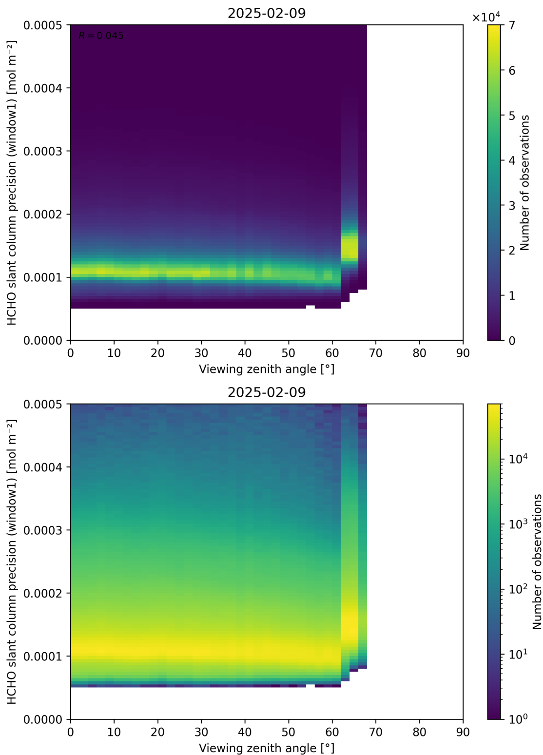
Figure 189: Scatter density plot of “Viewing zenith angle” against “HCHO slant column precision (window1)” for 2025-02-08 to 2025-02-10.
