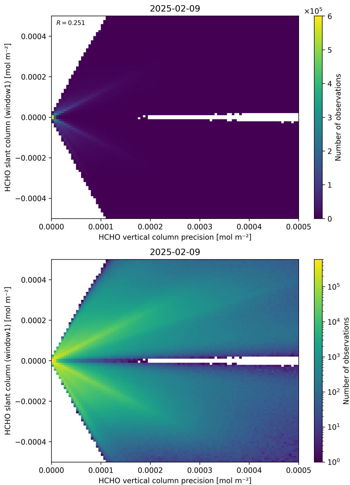
Figure 142: Scatter density plot of “HCHO vertical column precision” against “HCHO slant column (window1)” for 2025-02-08 to 2025-02-10.
