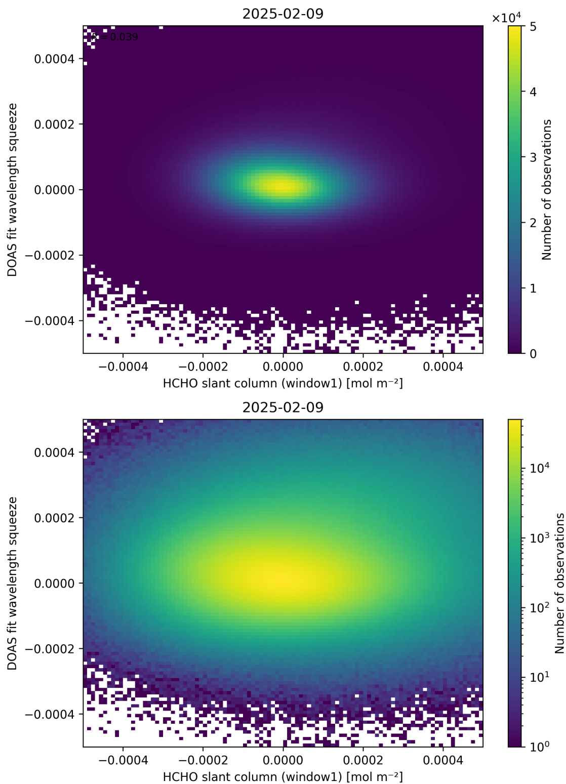
Figure 80: Scatter density plot of “HCHO slant column (window1)” against “DOAS fit wavelength squeeze” for 2025-02-08 to 2025-02-10.
