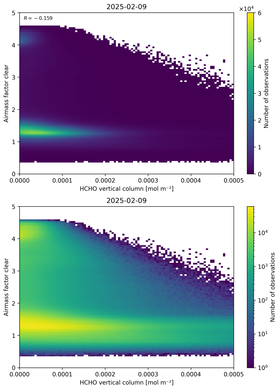
Figure 126: Scatter density plot of “HCHO vertical column” against “Airmass factor clear” for 2025-02-08 to 2025-02-10.
