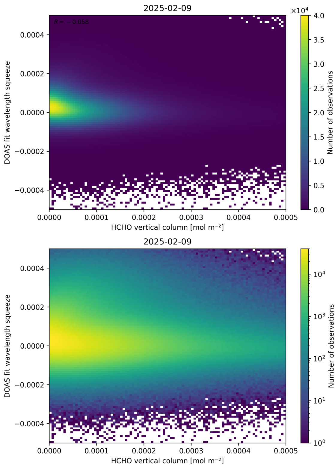
Figure 125: Scatter density plot of “HCHO vertical column” against “DOAS fit wavelength squeeze” for 2025-02-08 to 2025-02-10.
