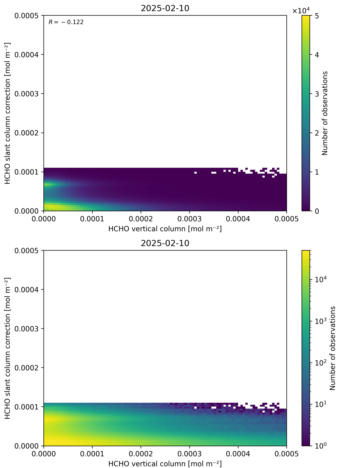
Figure 128: Scatter density plot of “HCHO vertical column” against “HCHO slant column correction” for 2025-02-09 to 2025-02-11.
