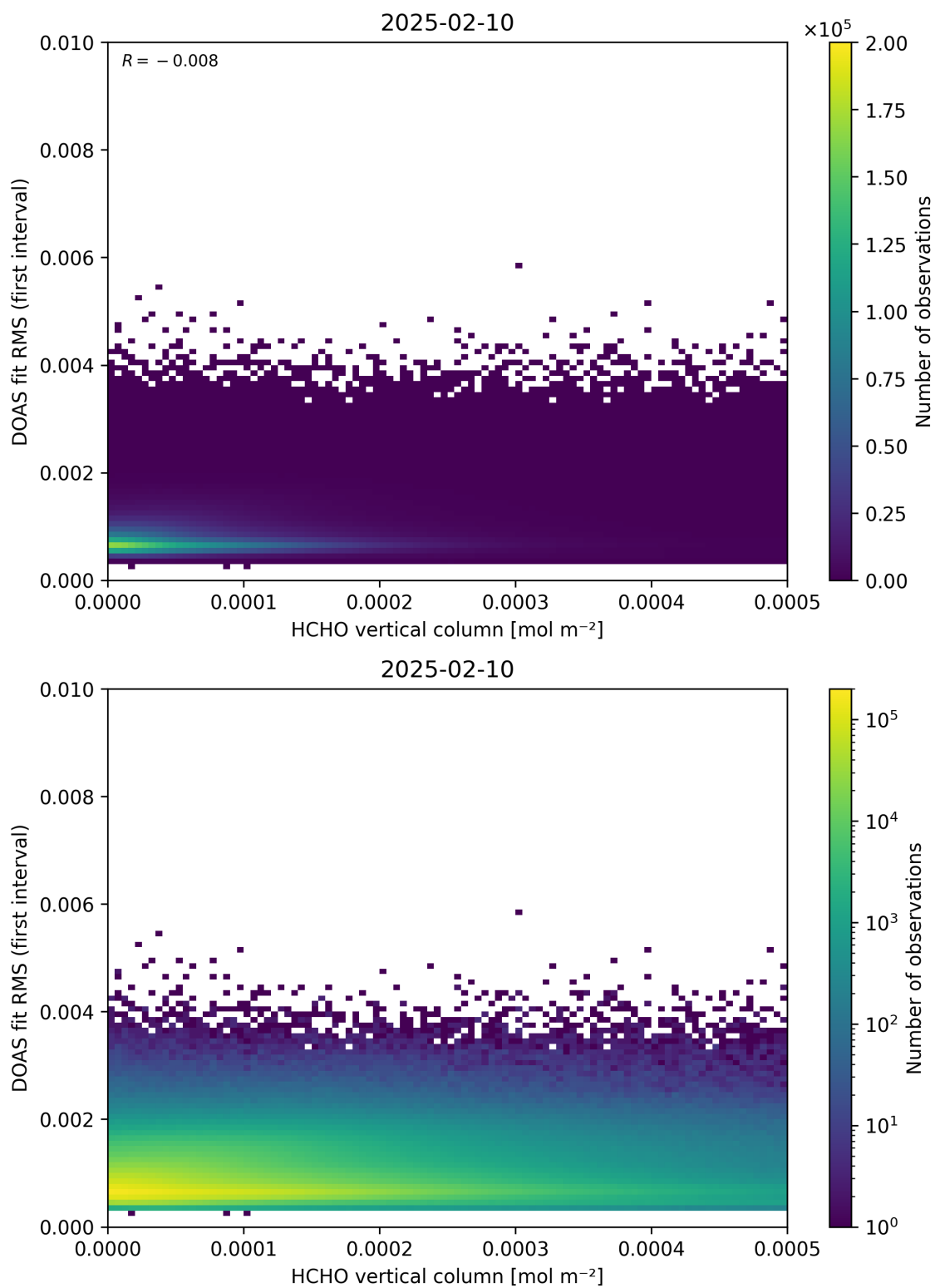
Figure 123: Scatter density plot of “HCHO vertical column” against “DOAS fit RMS (first interval)” for 2025-02-09 to 2025-02-11.
