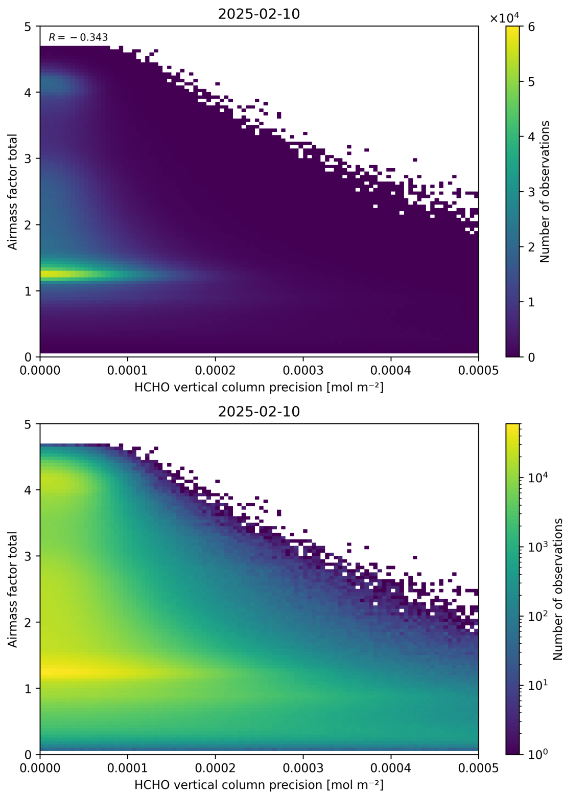
Figure 144: Scatter density plot of “HCHO vertical column precision” against “Airmass factor total” for 2025-02-09 to 2025-02-11.
