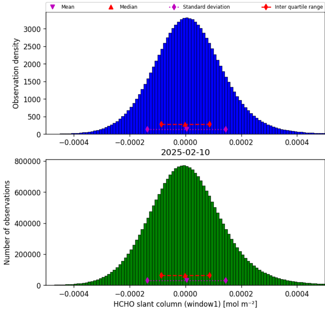
Figure 38: Histogram of “HCHO slant column (window1)” for 2025-02-09 to 2025-02-11
