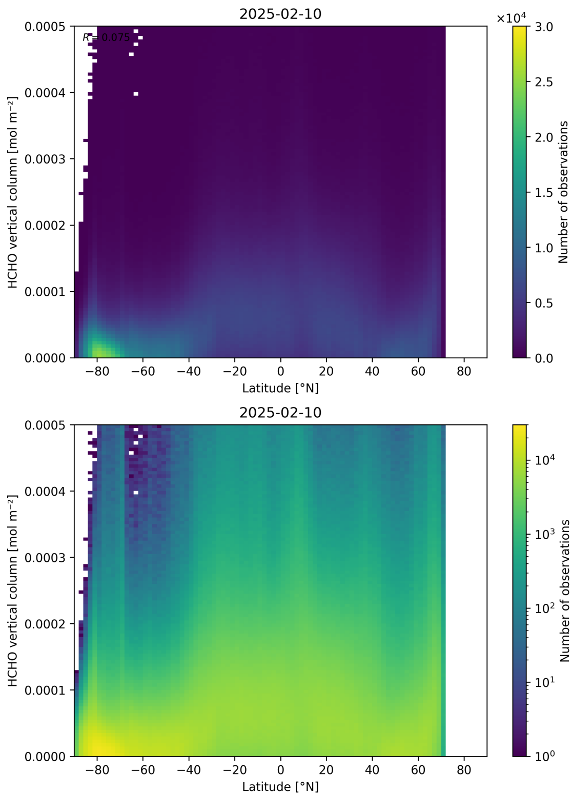
Figure 163: Scatter density plot of “Latitude” against “HCHO vertical column” for 2025-02-09 to 2025-02-11.
