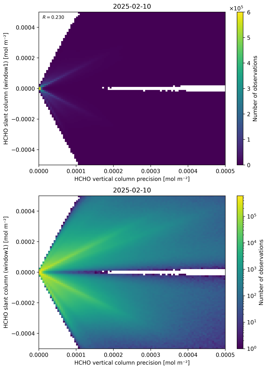
Figure 142: Scatter density plot of “HCHO vertical column precision” against “HCHO slant column (window1)” for 2025-02-09 to 2025-02-11.
