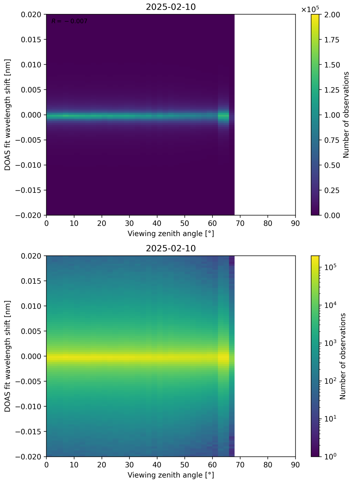
Figure 183: Scatter density plot of “Viewing zenith angle” against “DOAS fit wavelength shift” for 2025-02-09 to 2025-02-11.
