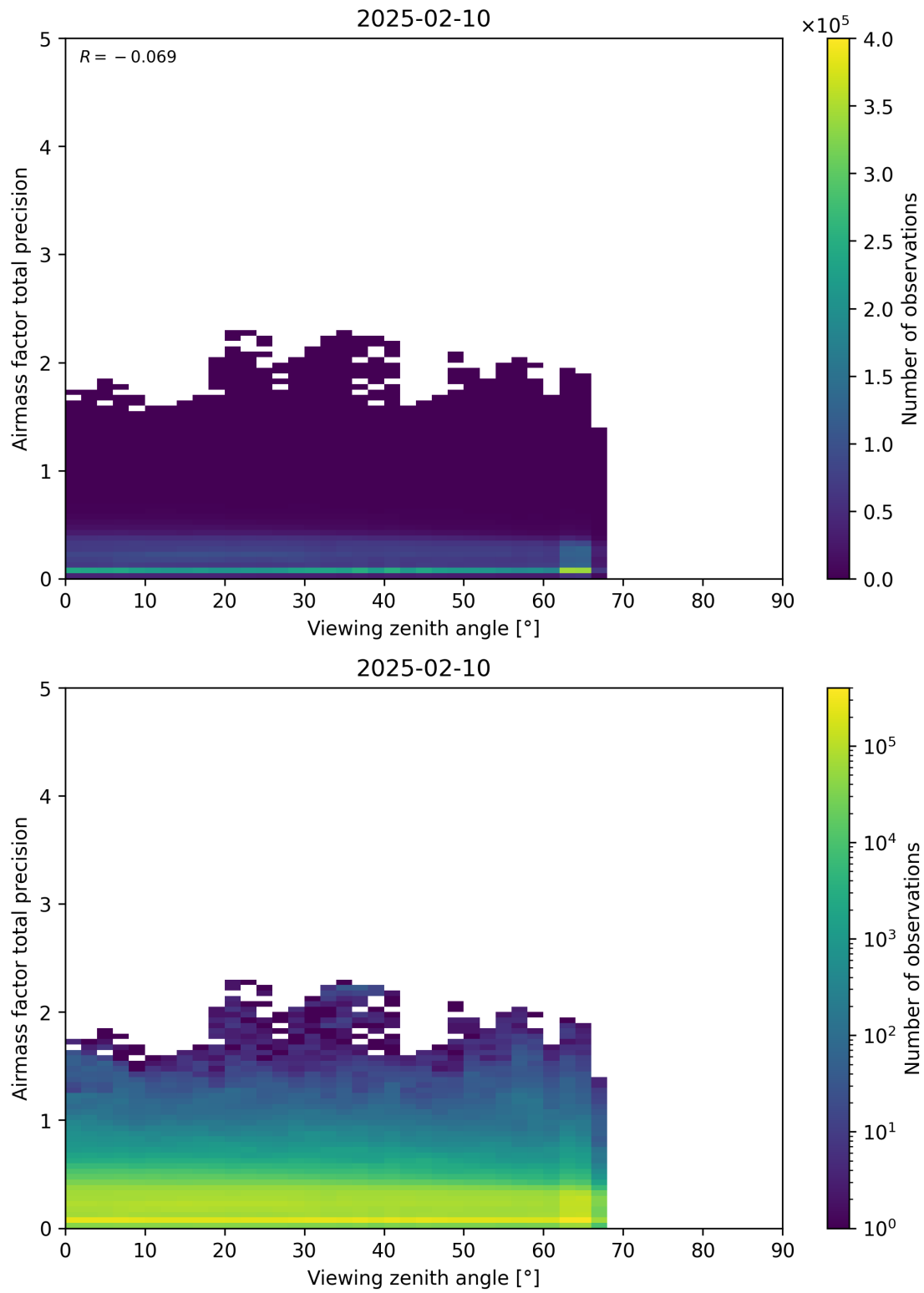
Figure 191: Scatter density plot of “Viewing zenith angle” against “Airmass factor total precision” for 2025-02-09 to 2025-02-11.
