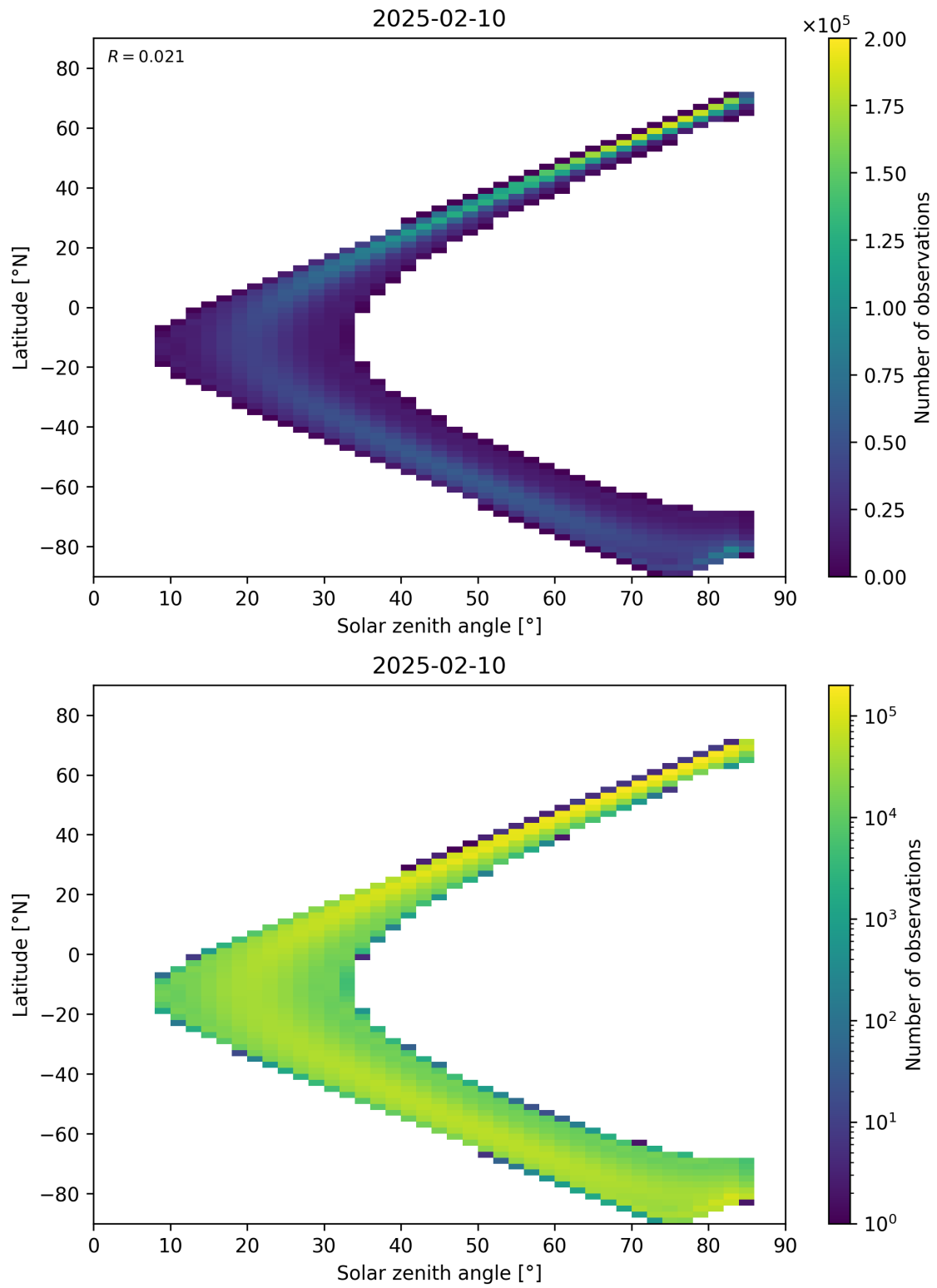
Figure 181: Scatter density plot of “Solar zenith angle” against “Latitude” for 2025-02-09 to 2025-02-11.
