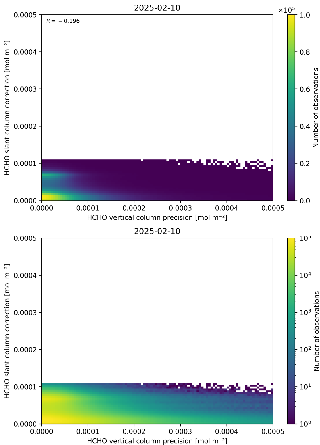
Figure 141: Scatter density plot of “HCHO vertical column precision” against “HCHO slant column correction” for 2025-02-09 to 2025-02-11.
