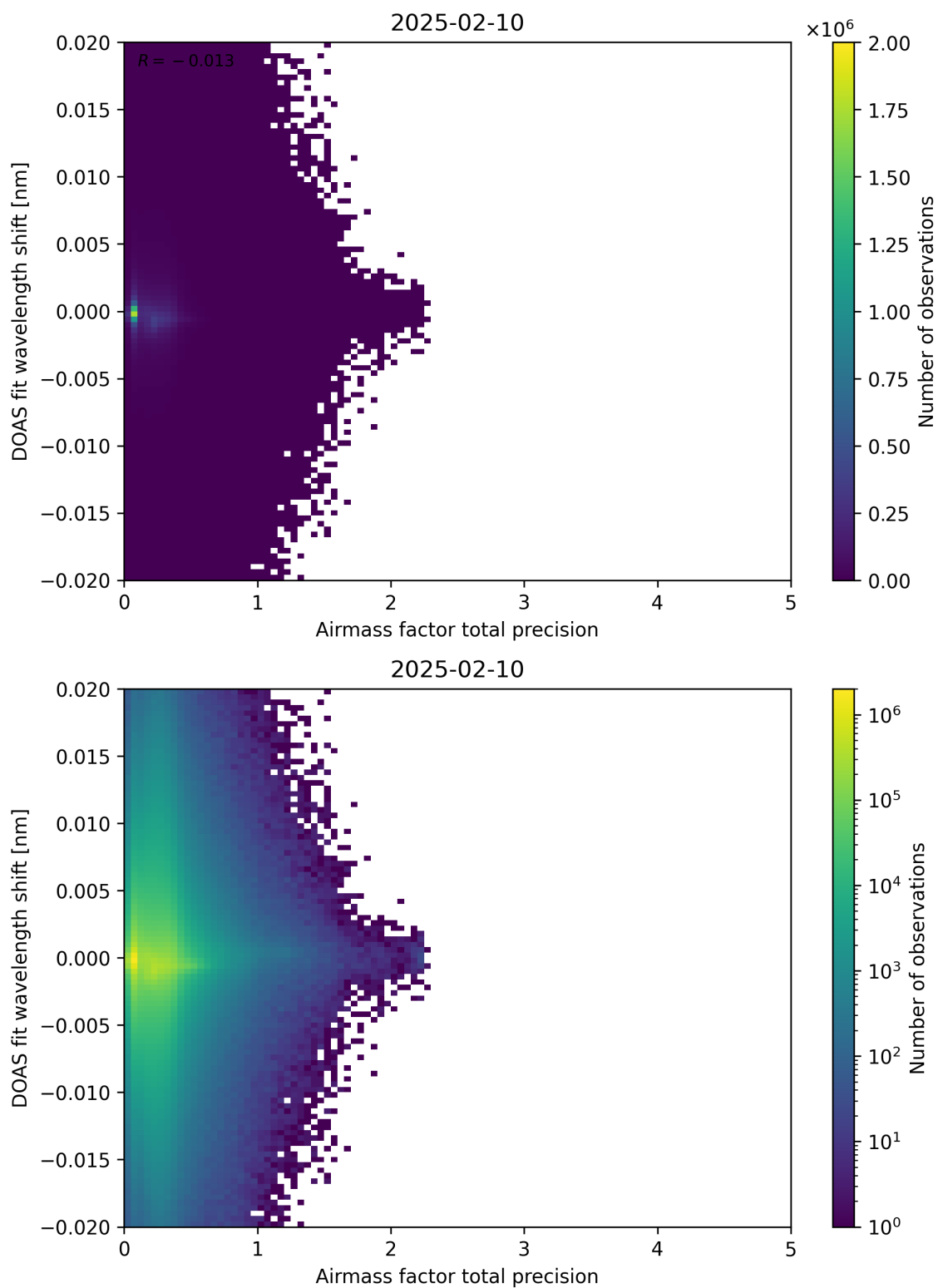
Figure 106: Scatter density plot of “Airmass factor total precision” against “DOAS fit wavelength shift” for 2025-02-09 to 2025-02-11.
