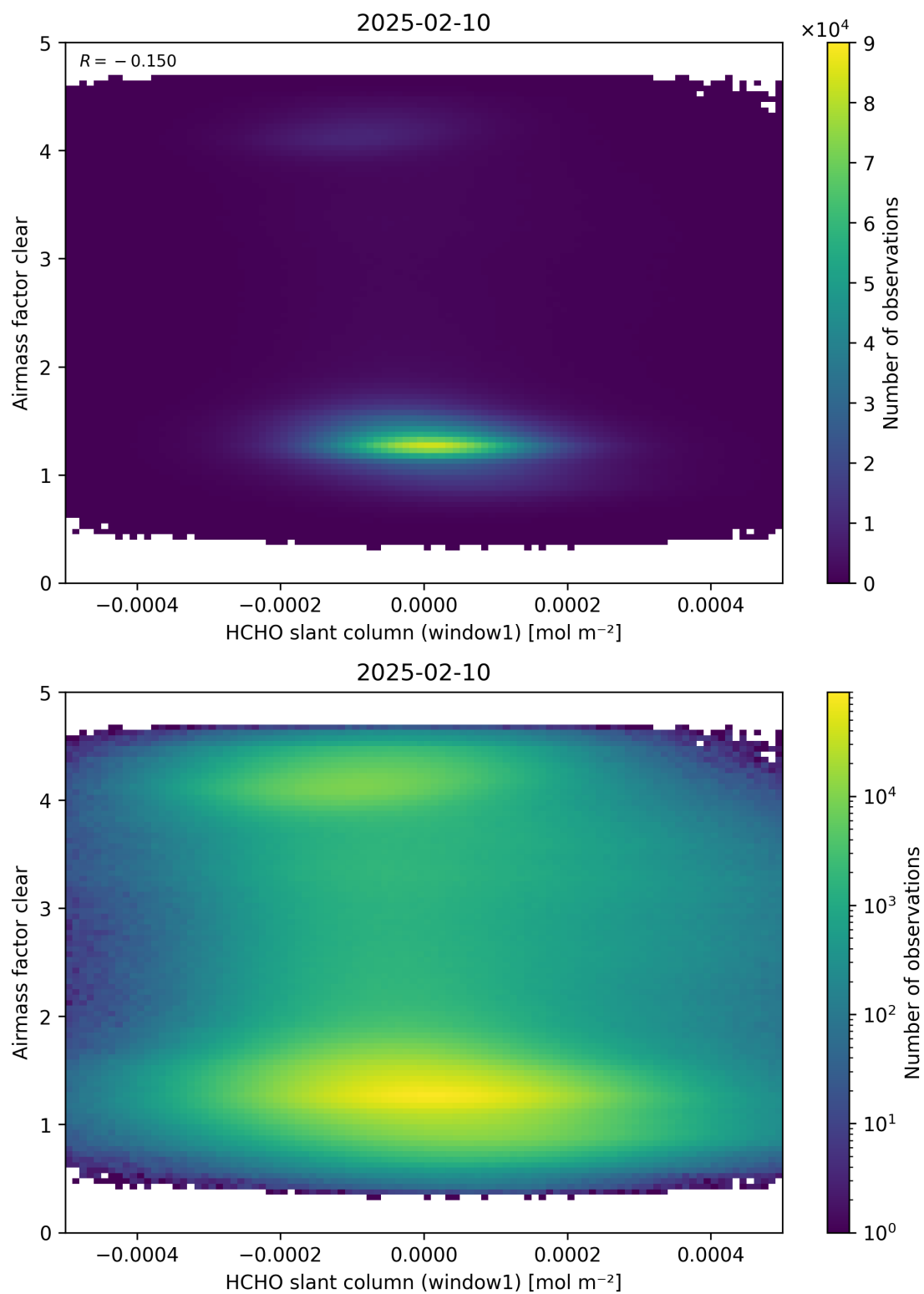
Figure 81: Scatter density plot of “HCHO slant column (window1)” against “Airmass factor clear” for 2025-02-09 to 2025-02-11.
