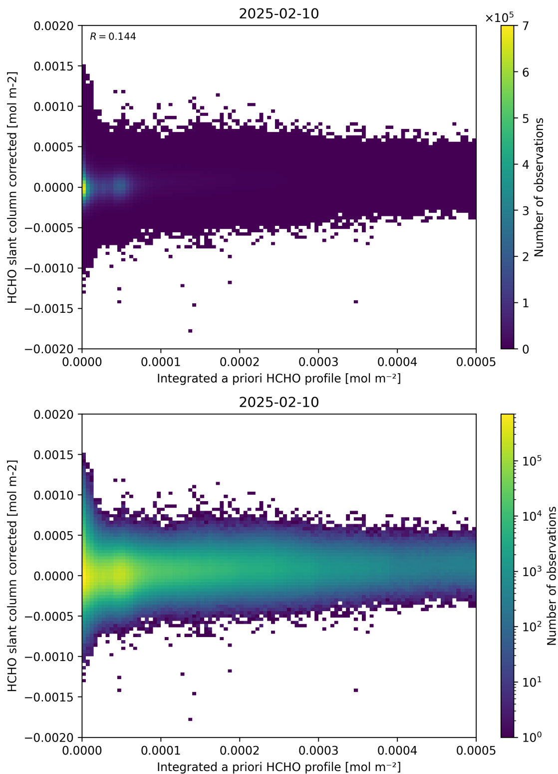
Figure 151: Scatter density plot of “Integrated a priori HCHO profile” against “HCHO slant column corrected” for 2025-02-09 to 2025-02-11.
