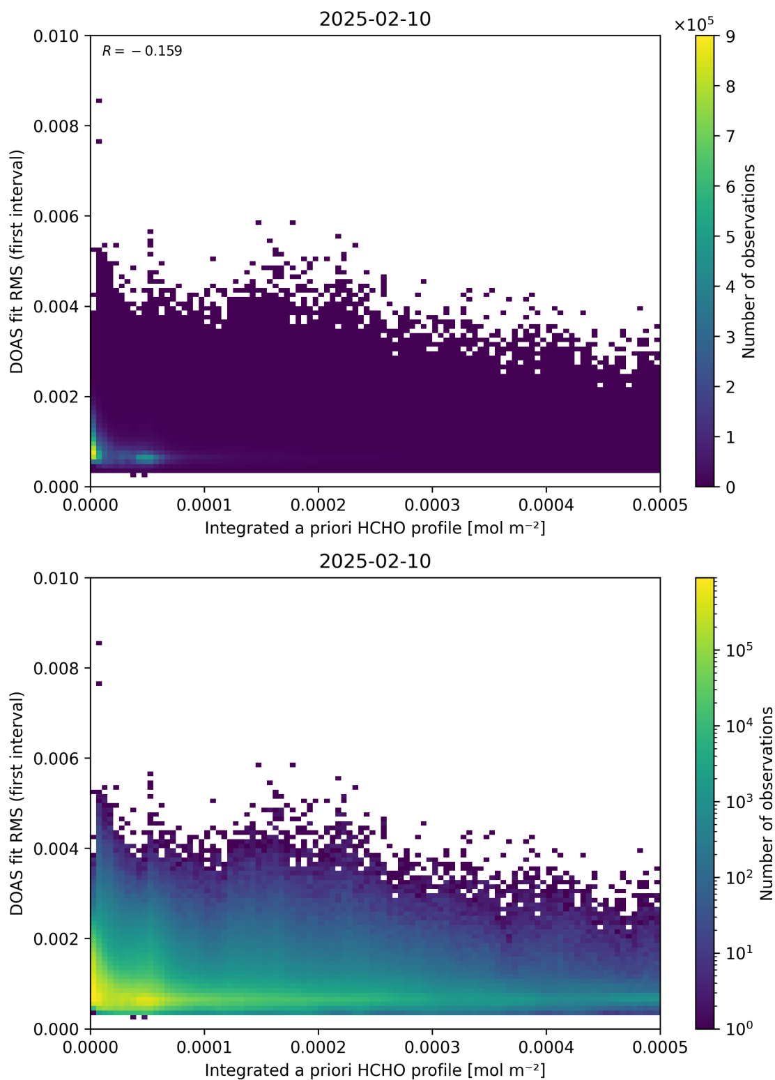
Figure 148: Scatter density plot of “Integrated a priori HCHO profile” against “DOAS fit RMS (first interval)” for 2025-02-09 to 2025-02-11.
