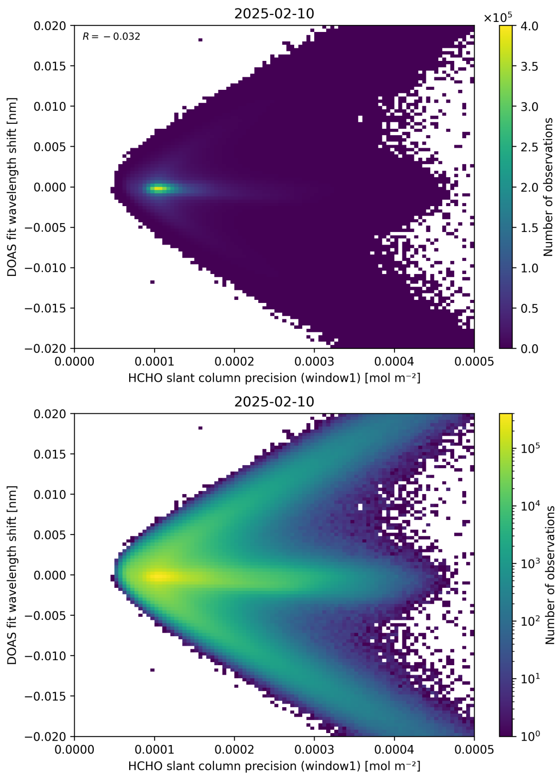
Figure 89: Scatter density plot of “HCHO slant column precision (window1)” against “DOAS fit wavelength shift” for 2025-02-09 to 2025-02-11.
