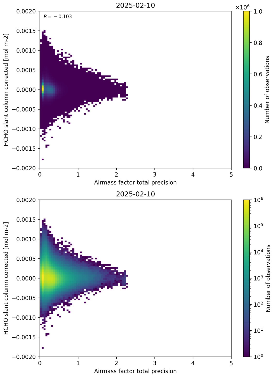
Figure 109: Scatter density plot of “Airmass factor total precision” against “HCHO slant column corrected” for 2025-02-09 to 2025-02-11.
