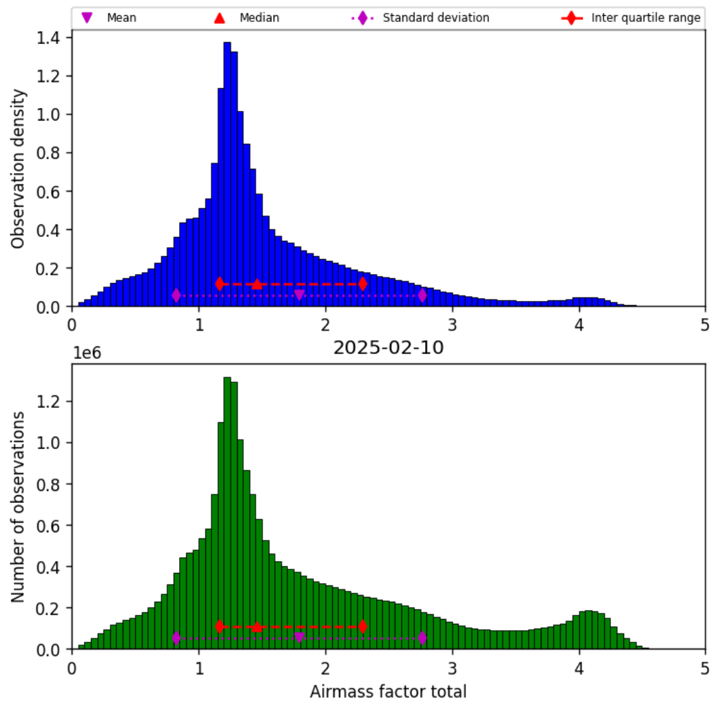
Figure 40: Histogram of “Airmass factor total” for 2025-02-09 to 2025-02-11
