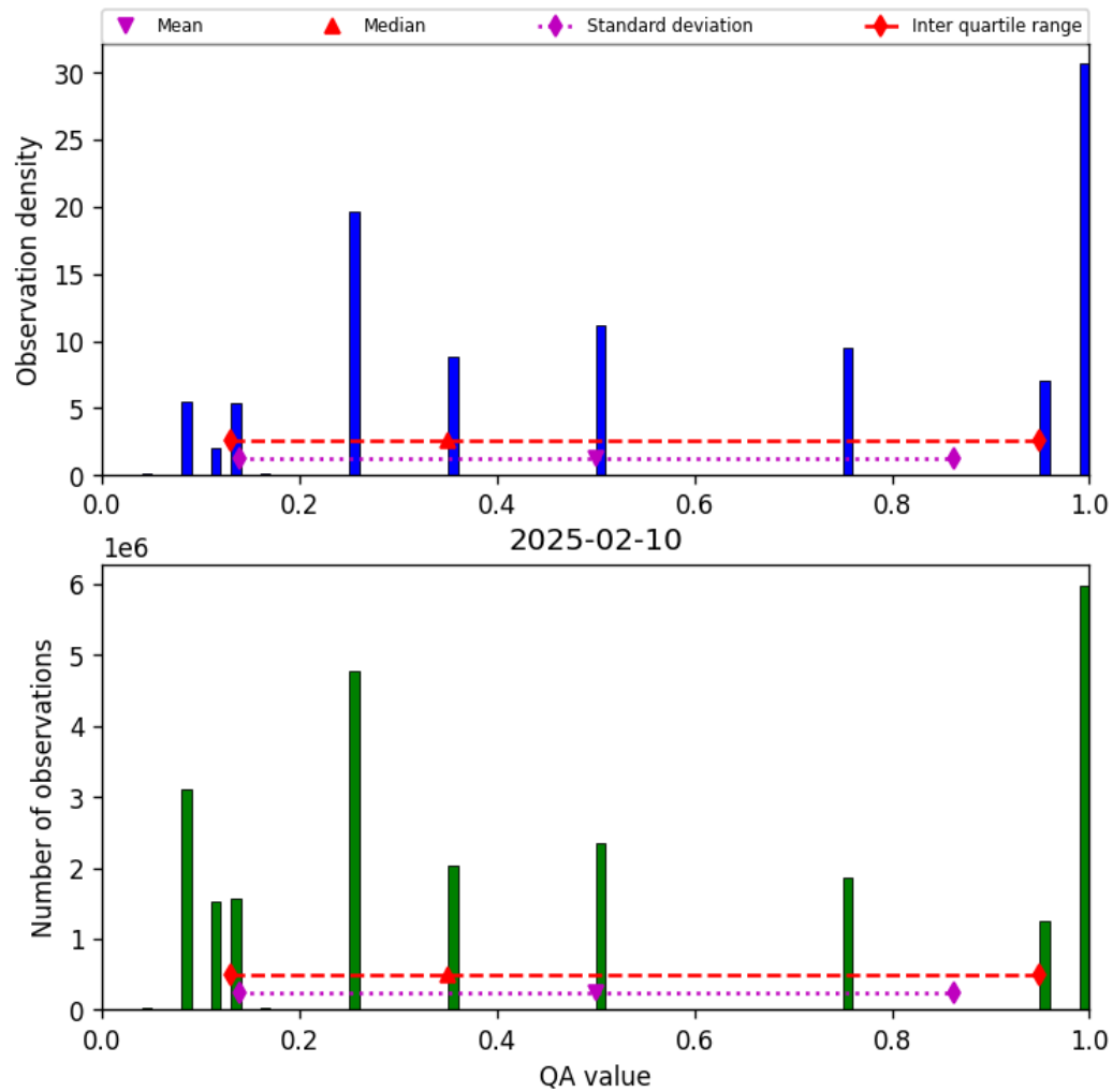
Figure 34: Histogram of “QA value” for 2025-02-09 to 2025-02-11
