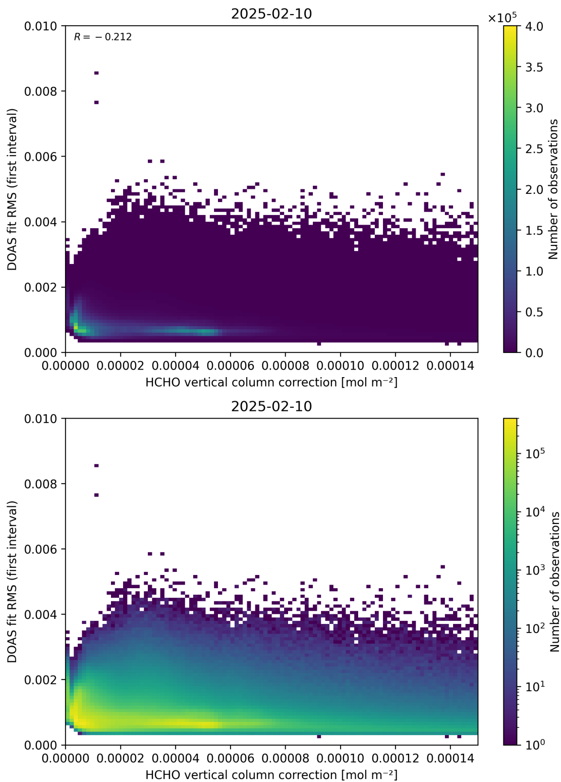
Figure 112: Scatter density plot of “HCHO vertical column correction” against “DOAS fit RMS (first interval)” for 2025-02-09 to 2025-02-11.
