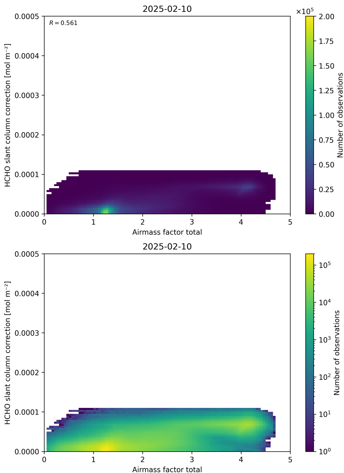
Figure 102: Scatter density plot of “Airmass factor total” against “HCHO slant column correction” for 2025-02-09 to 2025-02-11.
