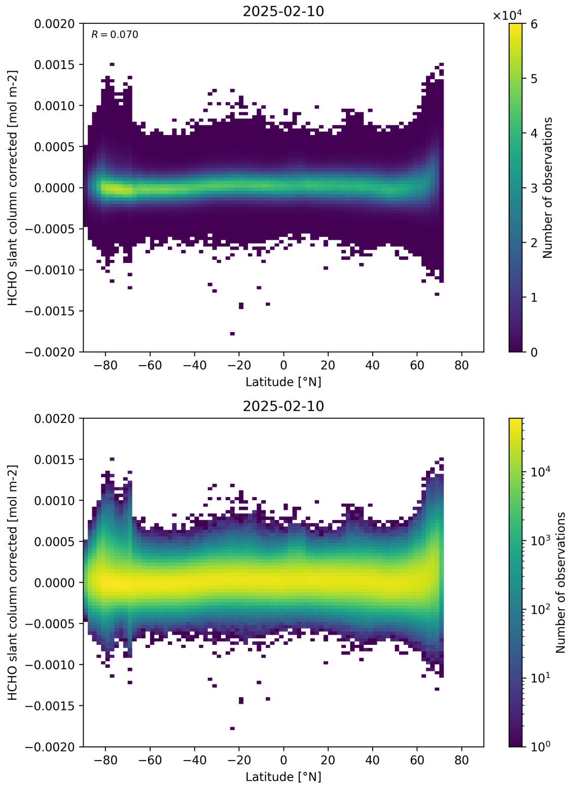
Figure 157: Scatter density plot of “Latitude” against “HCHO slant column corrected” for 2025-02-09 to 2025-02-11.
