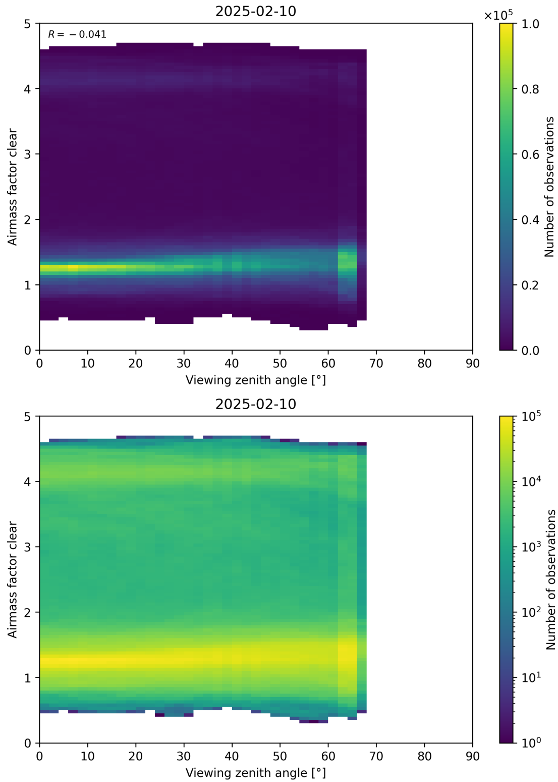
Figure 185: Scatter density plot of “Viewing zenith angle” against “Airmass factor clear” for 2025-02-09 to 2025-02-11.
