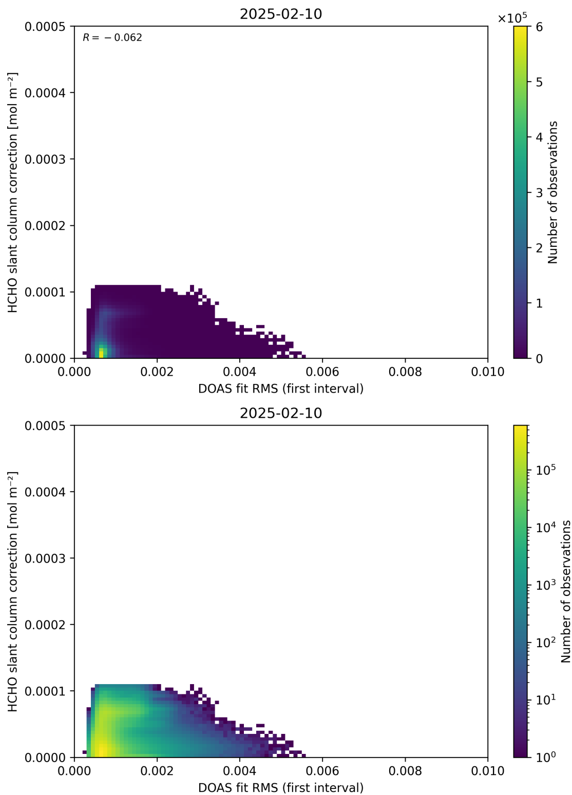
Figure 63: Scatter density plot of “DOAS fit RMS (first interval)” against “HCHO slant column correction” for 2025-02-09 to 2025-02-11.
