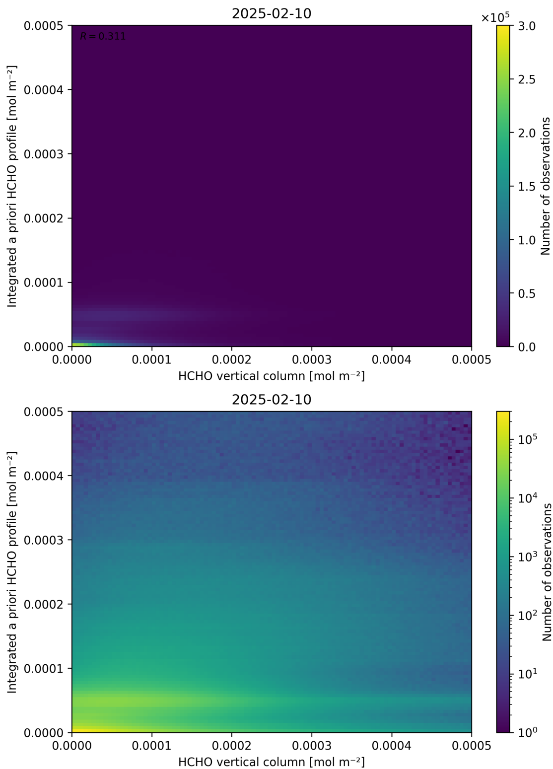
Figure 135: Scatter density plot of “HCHO vertical column” against “Integrated a priori HCHO profile” for 2025-02-09 to 2025-02-11.
