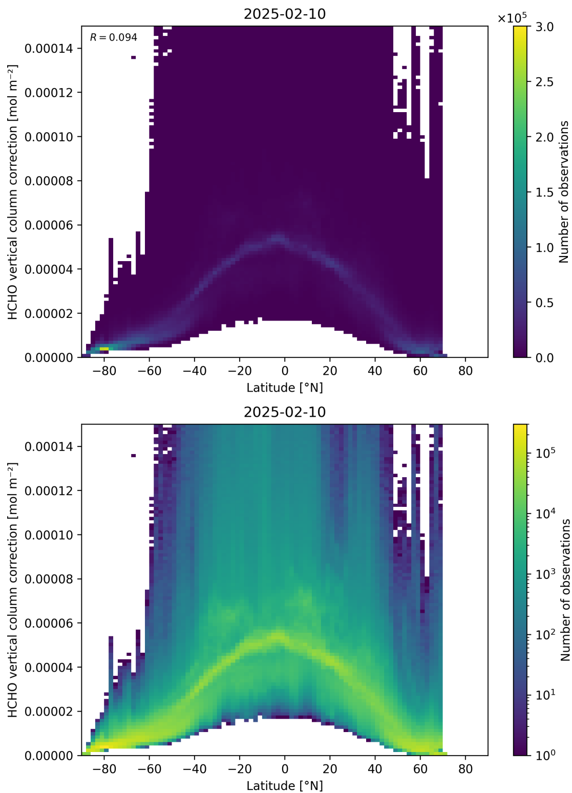
Figure 164: Scatter density plot of “Latitude” against “HCHO vertical column correction” for 2025-02-09 to 2025-02-11.
