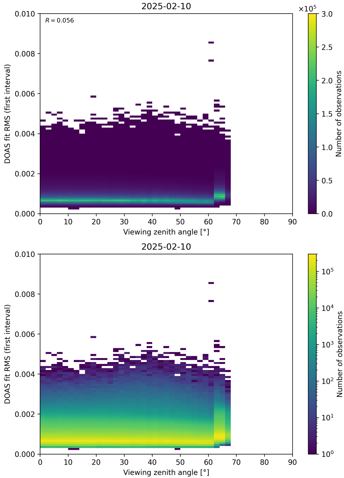
Figure 182: Scatter density plot of “Viewing zenith angle” against “DOAS fit RMS (first interval)” for 2025-02-09 to 2025-02-11.
