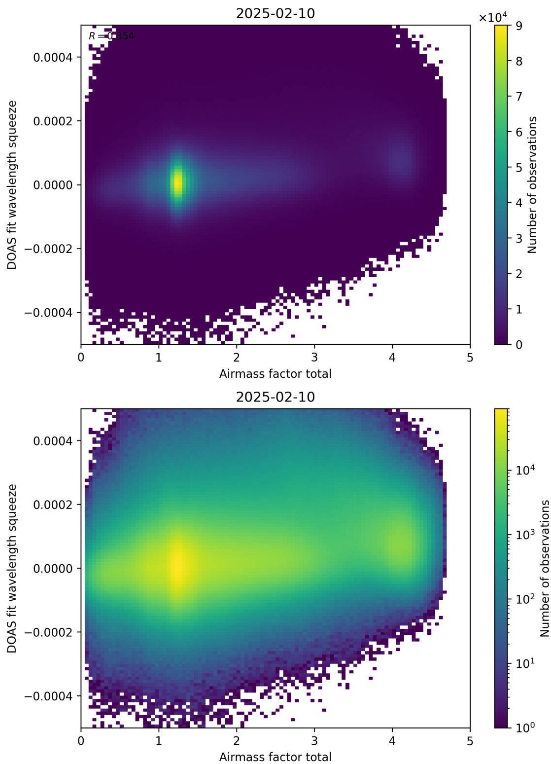
Figure 99: Scatter density plot of “Airmass factor total” against “DOAS fit wavelength squeeze” for 2025-02-09 to 2025-02-11.
