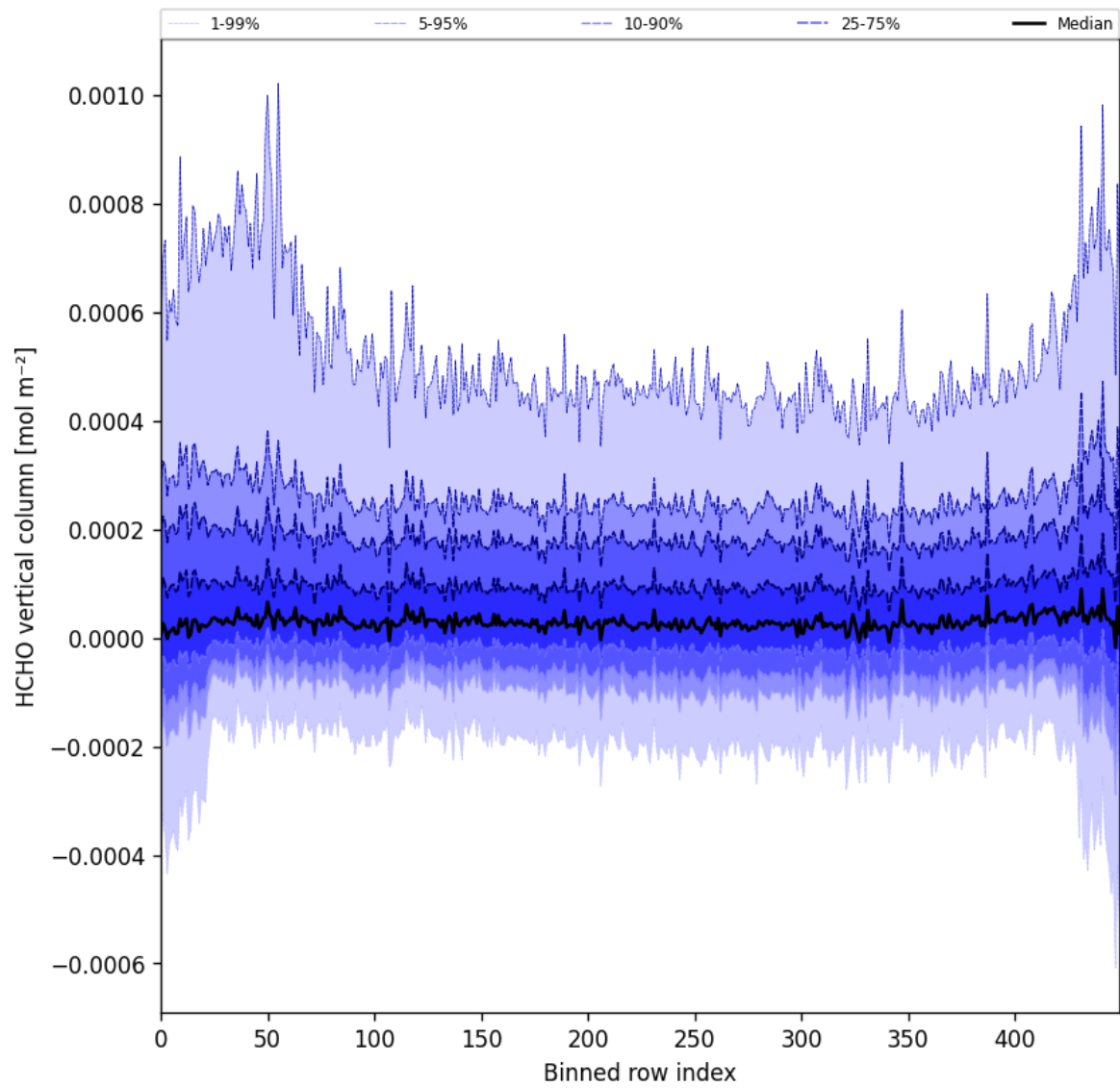
Figure 49: Along track statistics of “HCHO vertical column” for 2025-02-09 to 2025-02-11
