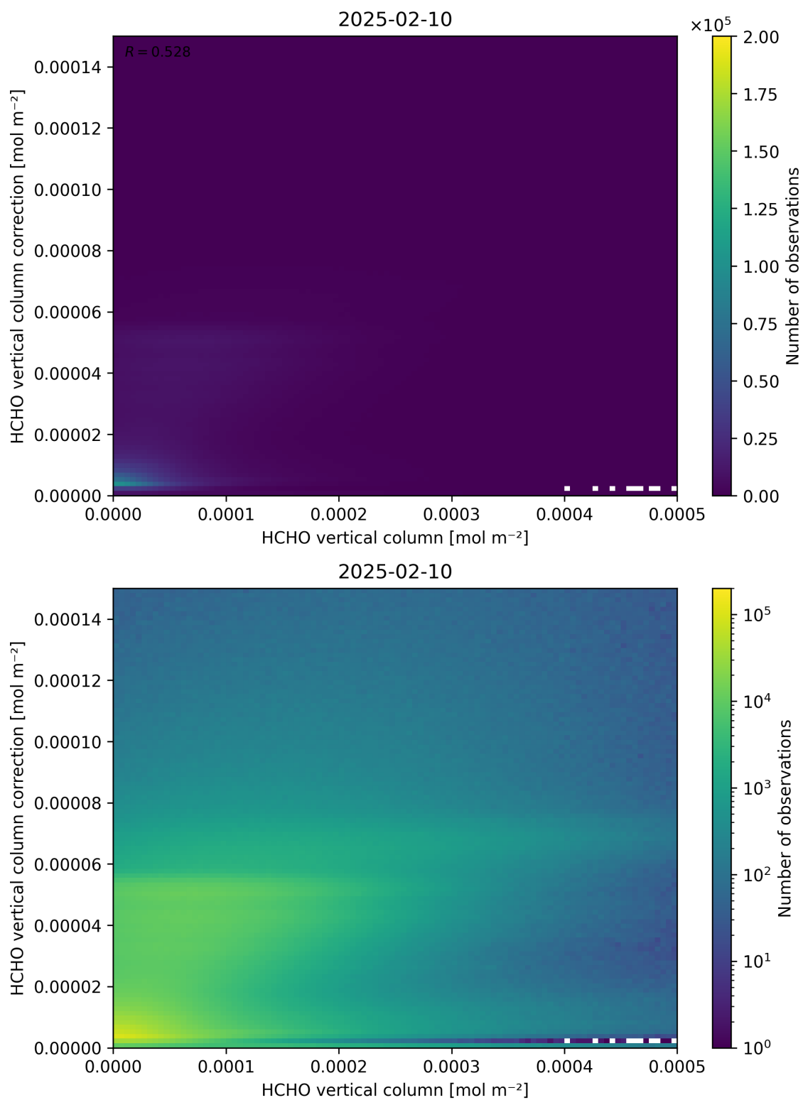
Figure 133: Scatter density plot of “HCHO vertical column” against “HCHO vertical column correction” for 2025-02-09 to 2025-02-11.
