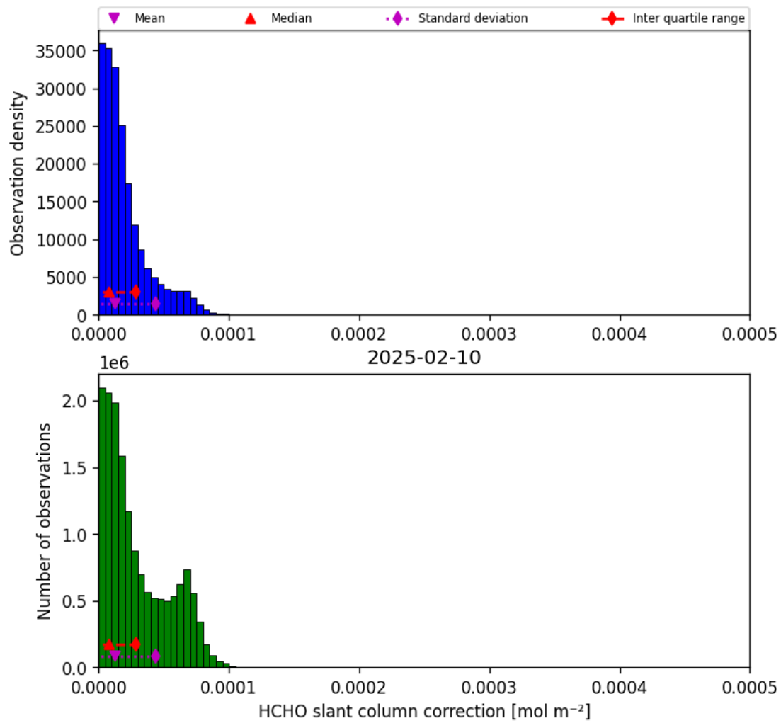
Figure 47: Histogram of “HCHO slant column correction” for 2025-02-09 to 2025-02-11
