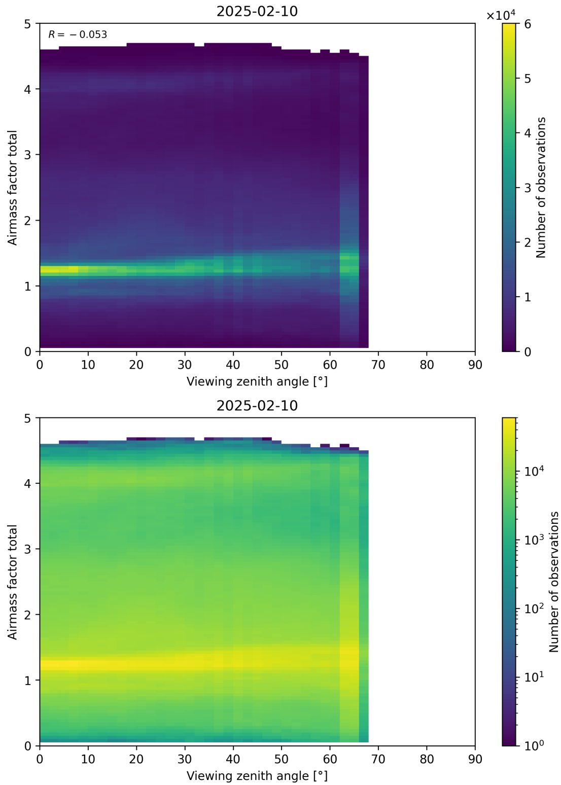
Figure 190: Scatter density plot of “Viewing zenith angle” against “Airmass factor total” for 2025-02-09 to 2025-02-11.
