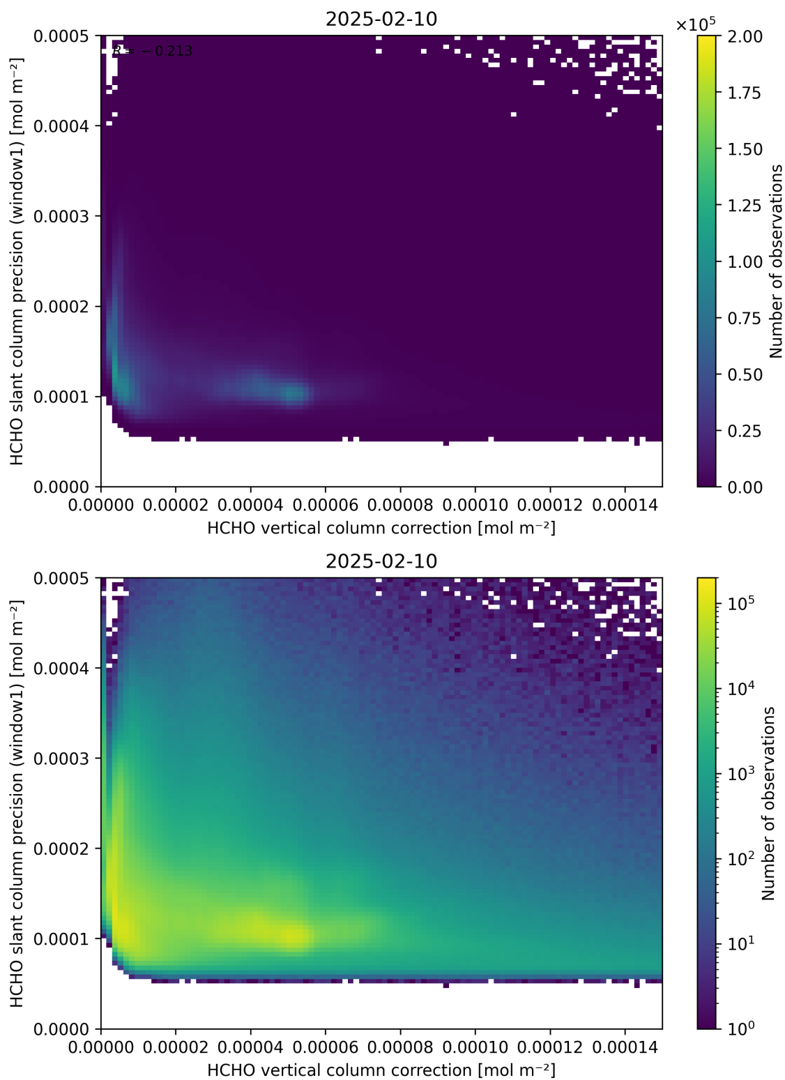
Figure 119: Scatter density plot of “HCHO vertical column correction” against “HCHO slant column precision (window1)” for 2025-02-09 to 2025-02-11.
