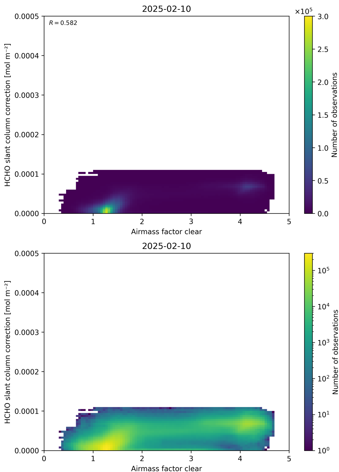
Figure 75: Scatter density plot of “Airmass factor clear” against “HCHO slant column correction” for 2025-02-09 to 2025-02-11.
