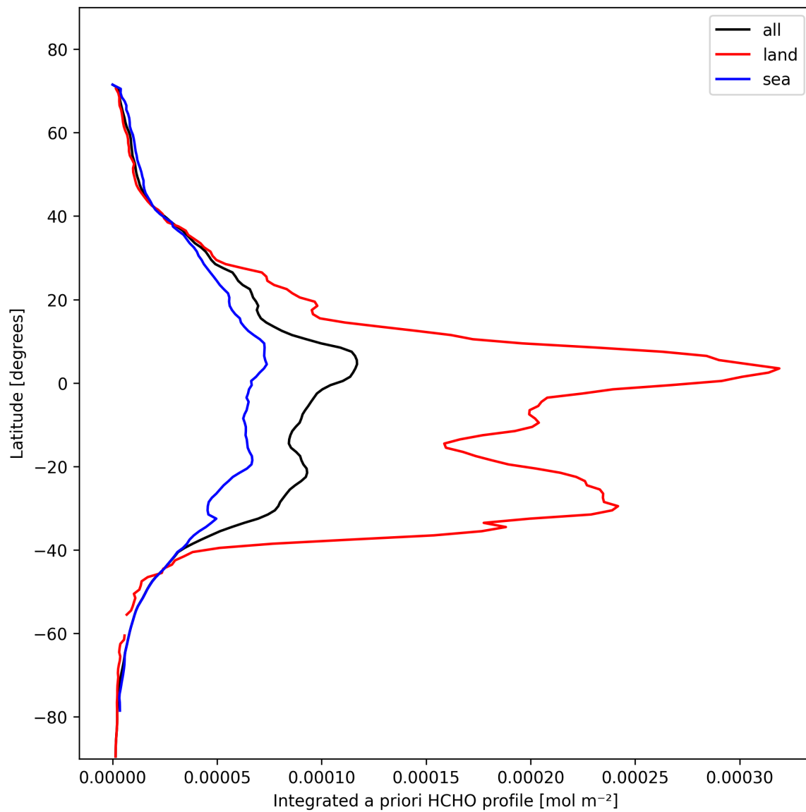
Figure 29: Zonal average of “Integrated a priori HCHO profile” for 2025-02-09 to 2025-02-11.
