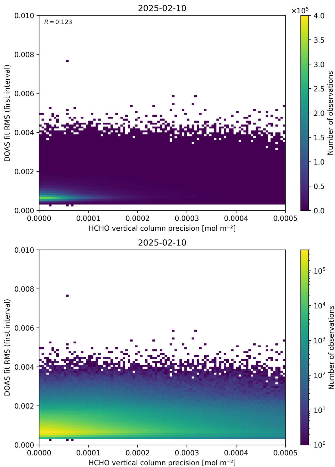
Figure 136: Scatter density plot of “HCHO vertical column precision” against “DOAS fit RMS (first interval)” for 2025-02-09 to 2025-02-11.
