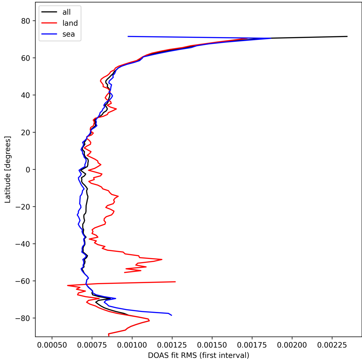
Figure 32: Zonal average of "DOAS fit RMS (first interval)" for 2025-02-09 to 2025-02-11.
