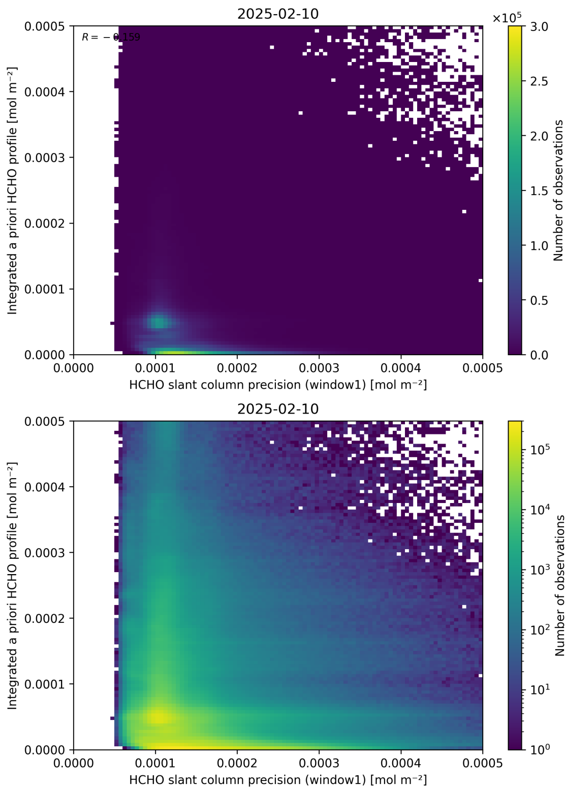
Figure 96: Scatter density plot of “HCHO slant column precision (window1)” against “Integrated a priori HCHO profile” for 2025-02-09 to 2025-02-11.
