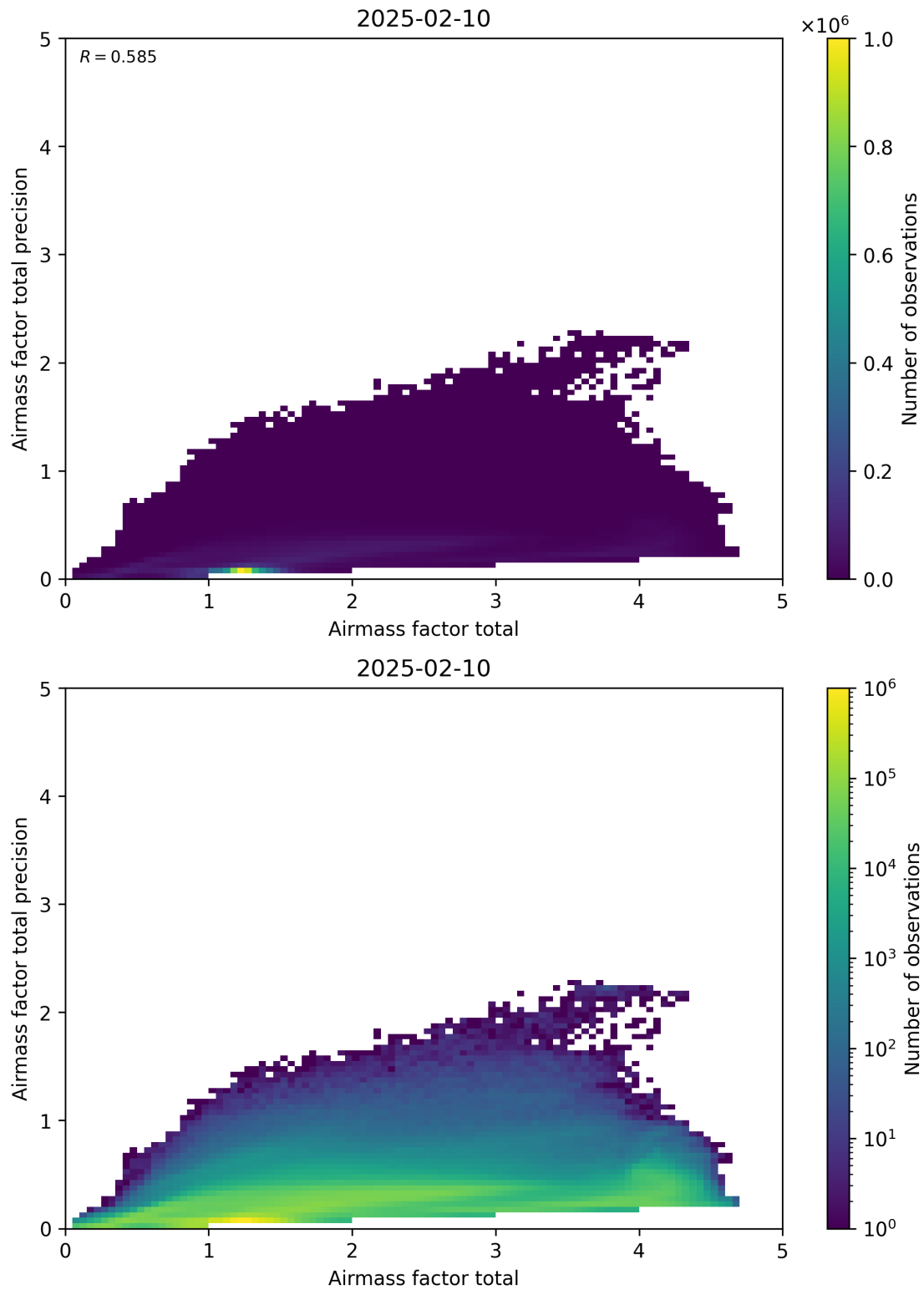
Figure 103: Scatter density plot of “Airmass factor total” against “Airmass factor total precision” for 2025-02-09 to 2025-02-11.
