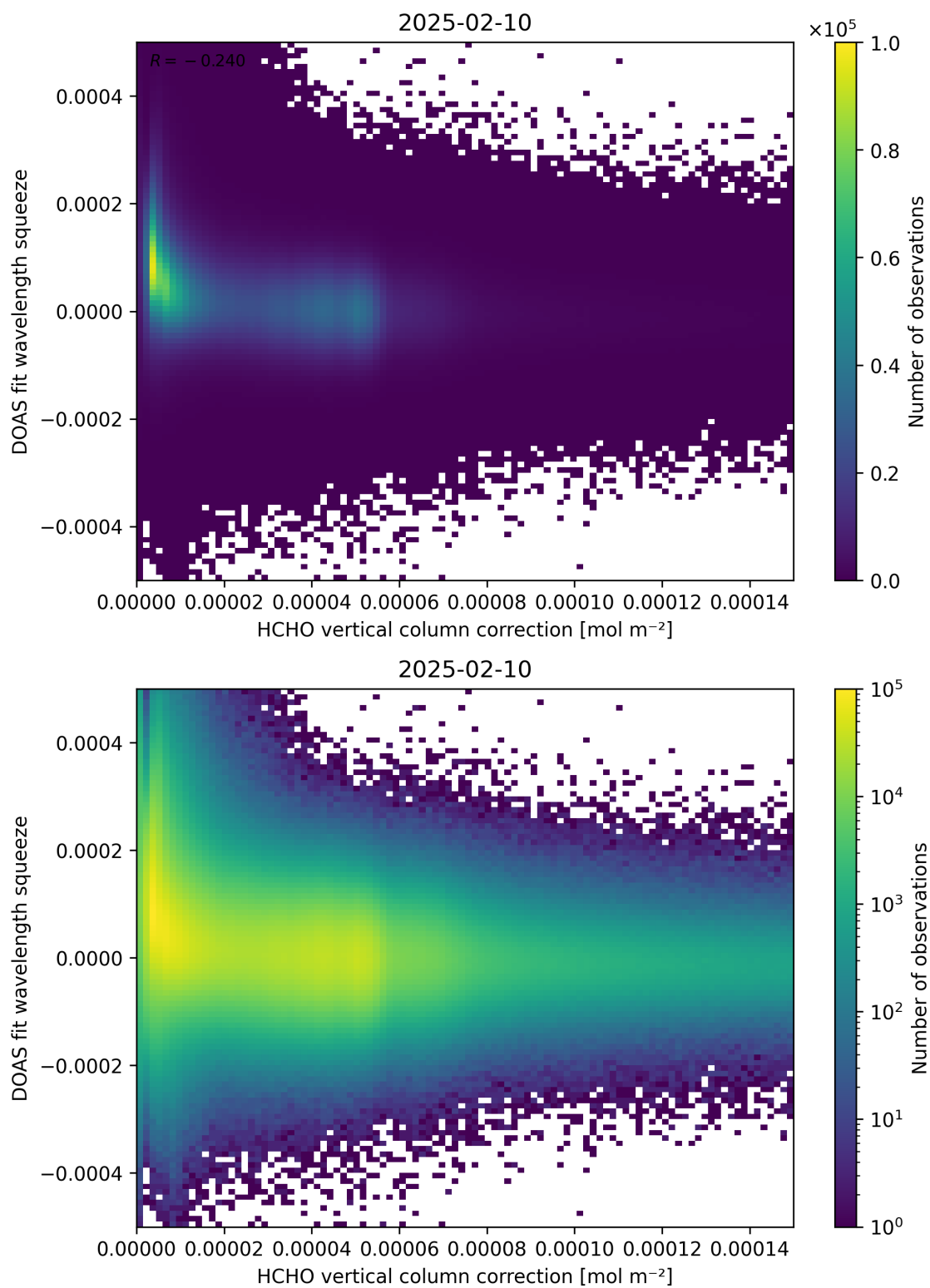
Figure 114: Scatter density plot of “HCHO vertical column correction” against “DOAS fit wavelength squeeze” for 2025-02-09 to 2025-02-11.
