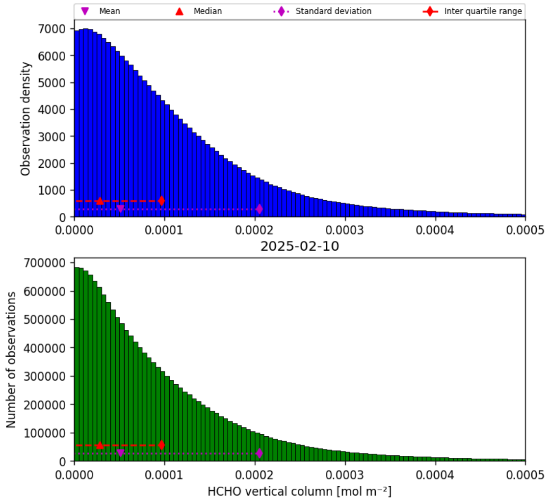
Figure 35: Histogram of “HCHO vertical column” for 2025-02-09 to 2025-02-11
