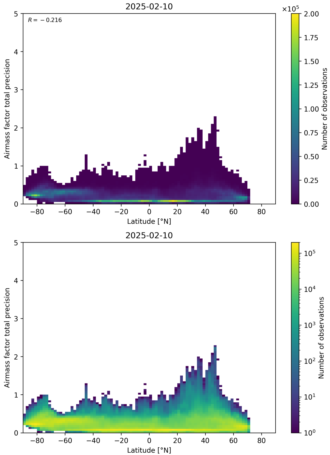
Figure 162: Scatter density plot of “Latitude” against “Airmass factor total precision” for 2025-02-09 to 2025-02-11.
