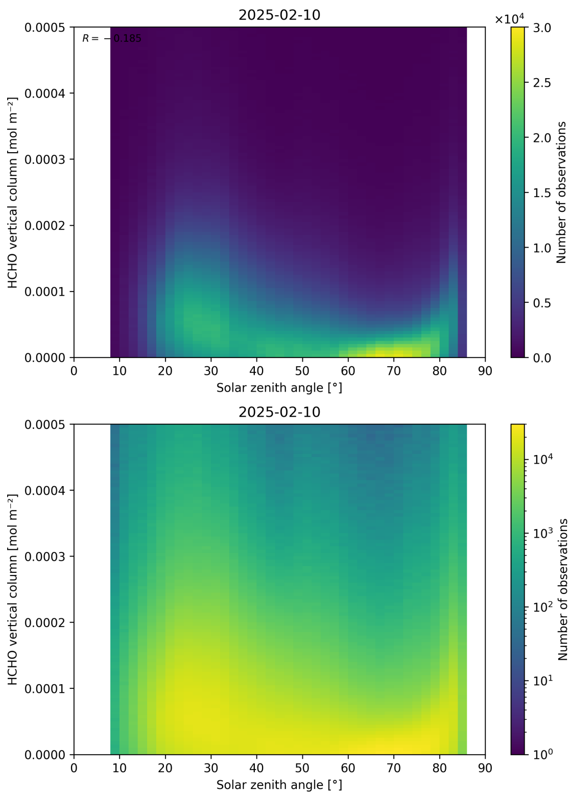
Figure 177: Scatter density plot of “Solar zenith angle” against “HCHO vertical column” for 2025-02-09 to 2025-02-11.
