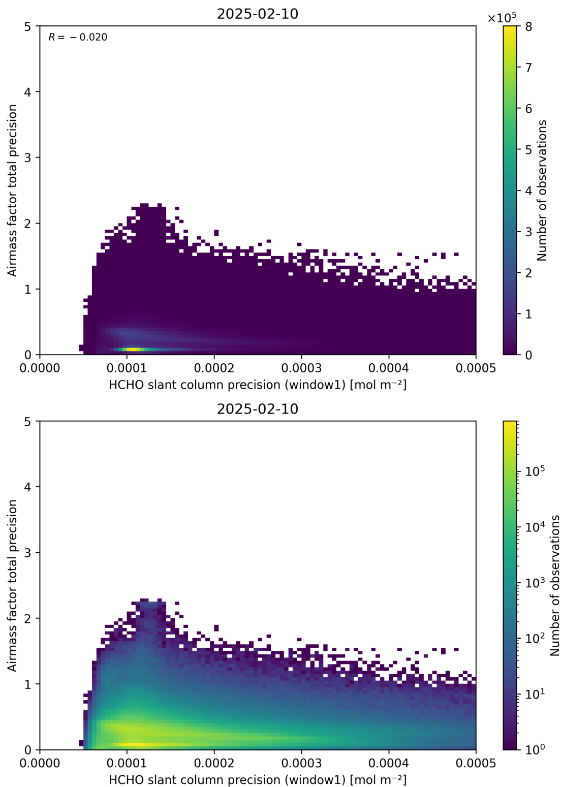
Figure 95: Scatter density plot of “HCHO slant column precision (window1)” against “Airmass factor total precision” for 2025-02-09 to 2025-02-11.
