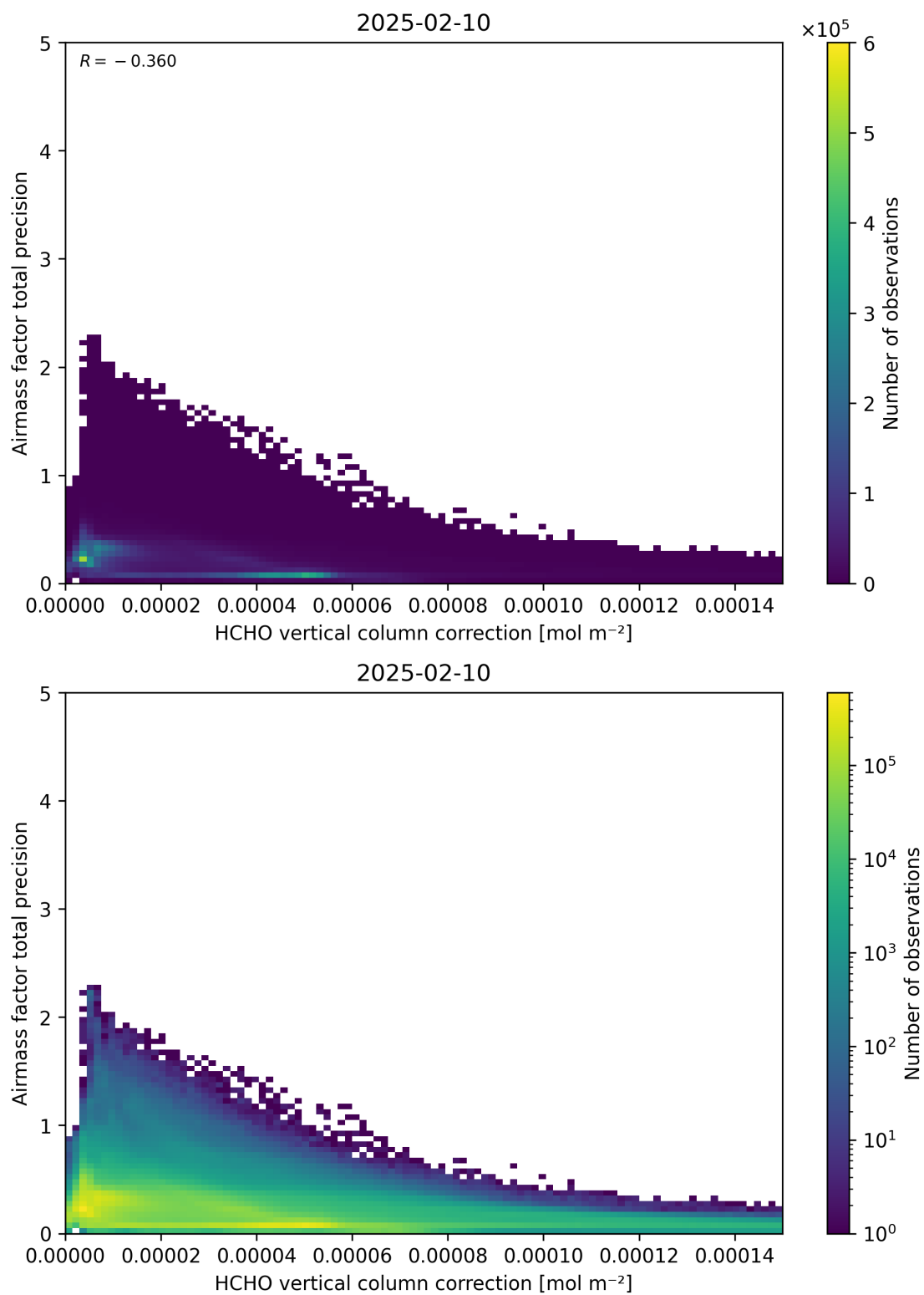
Figure 121: Scatter density plot of “HCHO vertical column correction” against “Airmass factor total precision” for 2025-02-09 to 2025-02-11.
