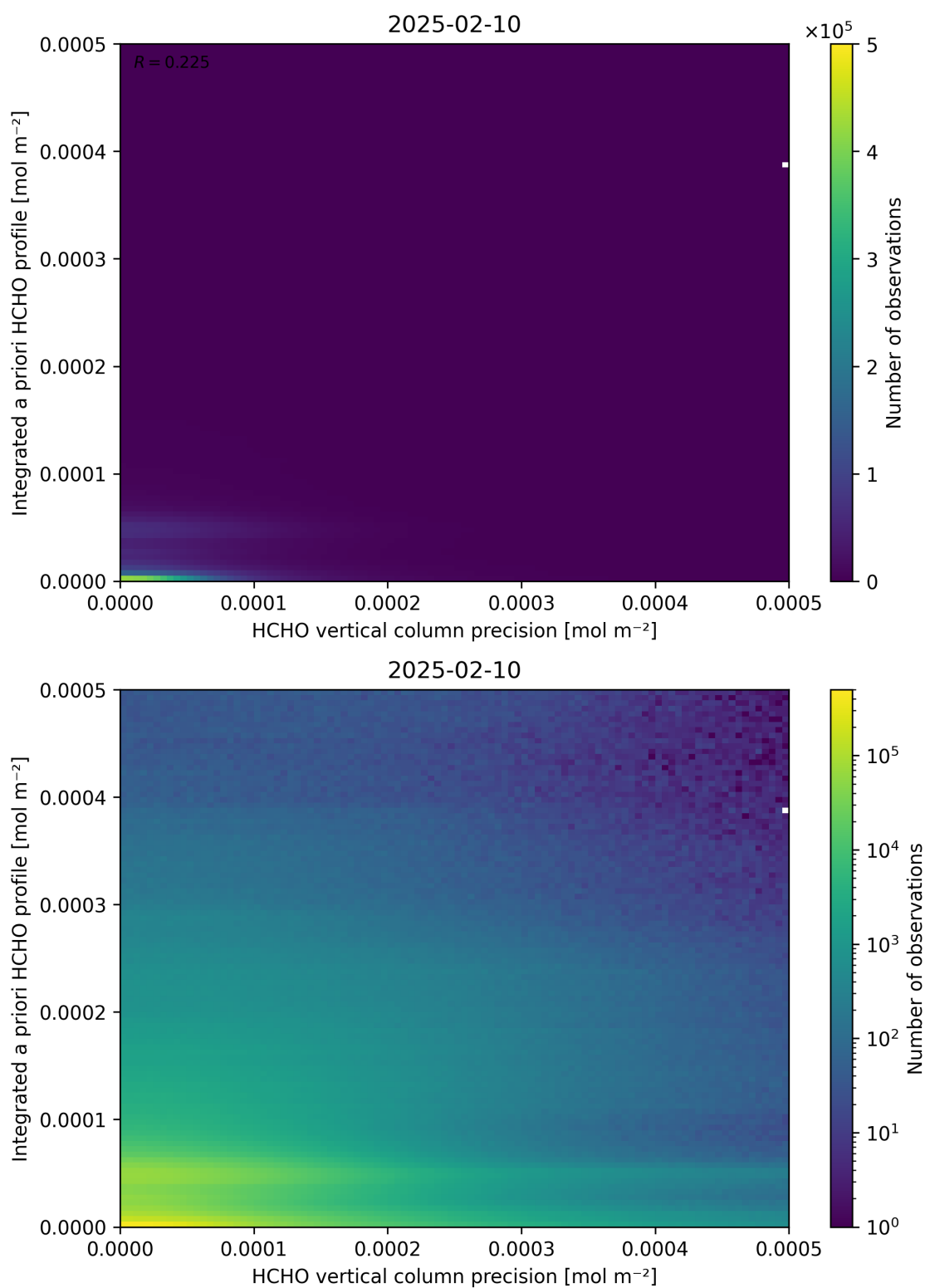
Figure 147: Scatter density plot of “HCHO vertical column precision” against “Integrated a priori HCHO profile” for 2025-02-09 to 2025-02-11.
