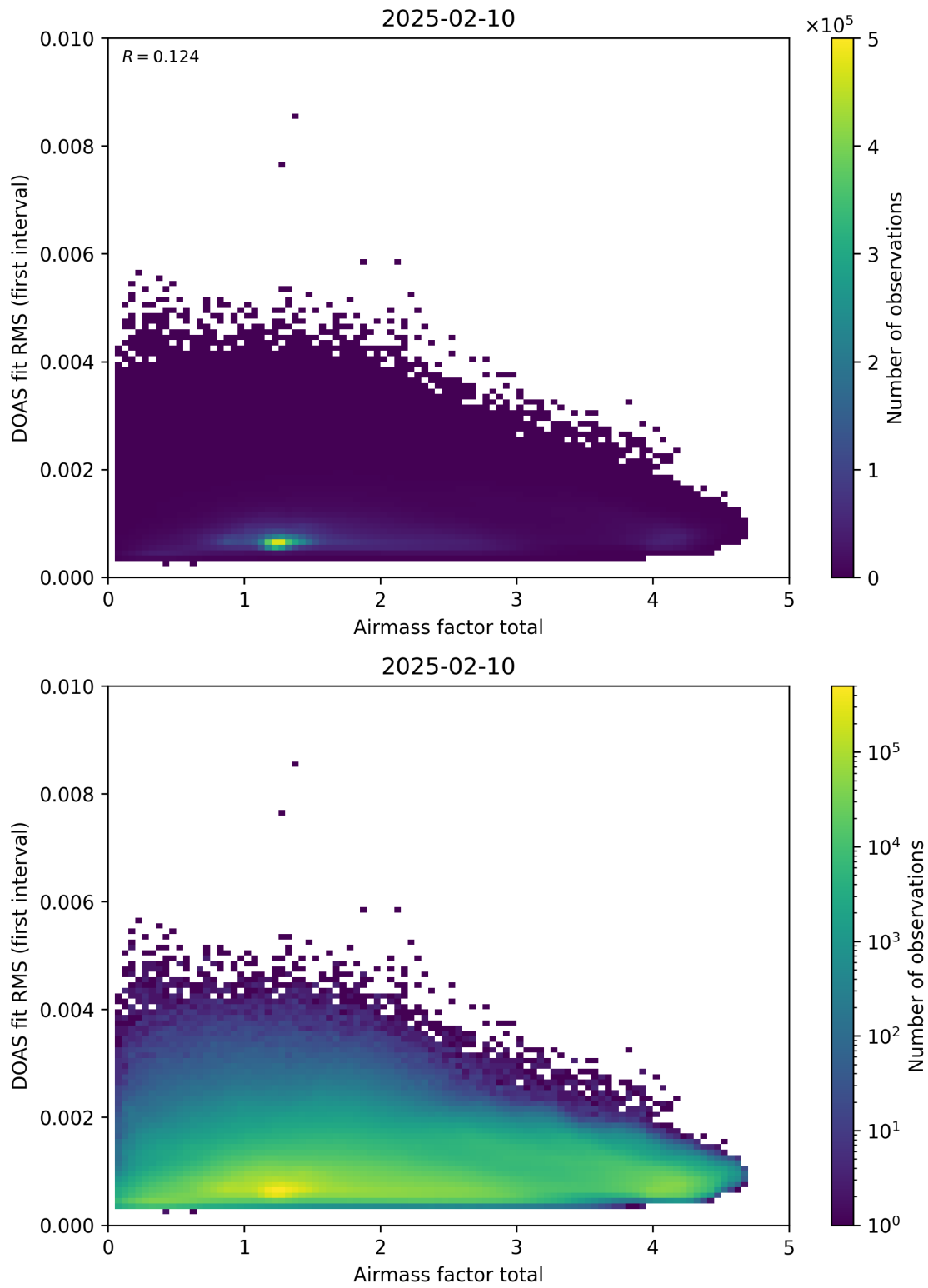
Figure 97: Scatter density plot of “Airmass factor total” against “DOAS fit RMS (first interval)” for 2025-02-09 to 2025-02-11.
