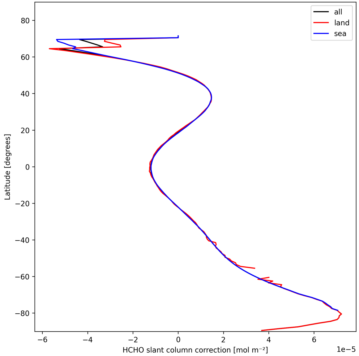
Figure 33: Zonal average of "HCHO slant column correction" for 2025-02-09 to 2025-02-11.
