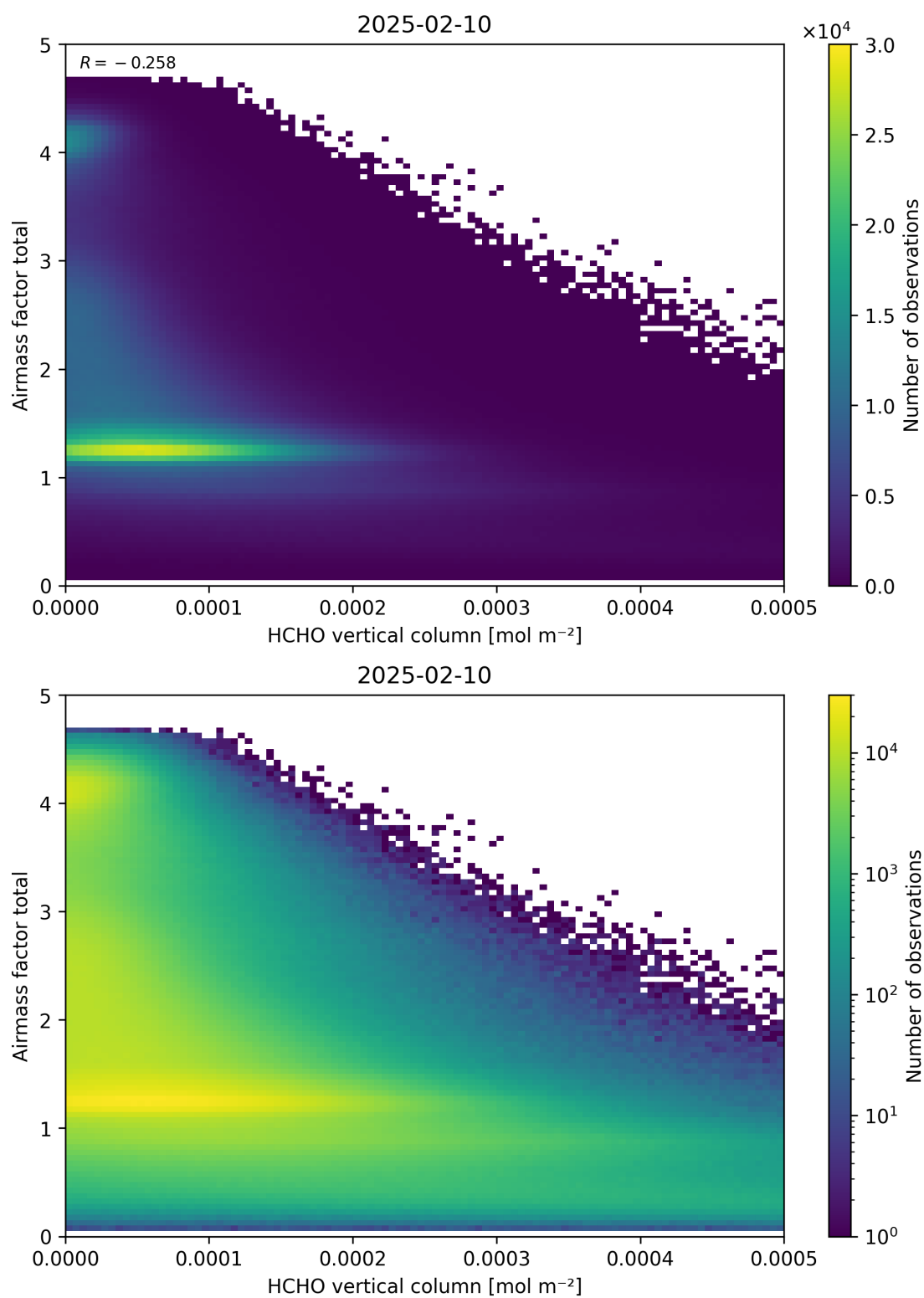
Figure 131: Scatter density plot of “HCHO vertical column” against “Airmass factor total” for 2025-02-09 to 2025-02-11.
