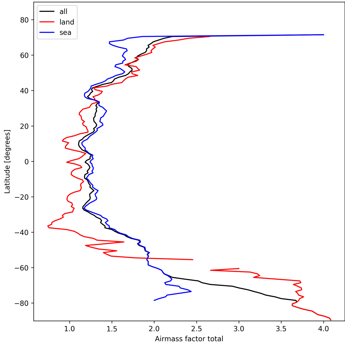
Figure 26: Zonal average of “Airmass factor total” for 2025-02-09 to 2025-02-11.
