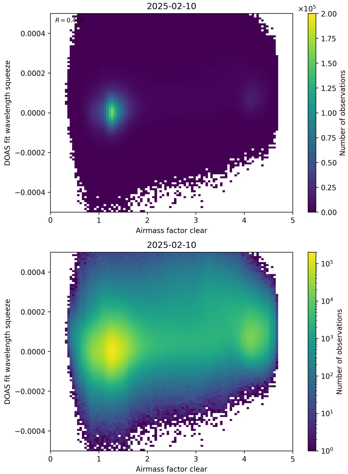
Figure 73: Scatter density plot of “Airmass factor clear” against “DOAS fit wavelength squeeze” for 2025-02-09 to 2025-02-11.
