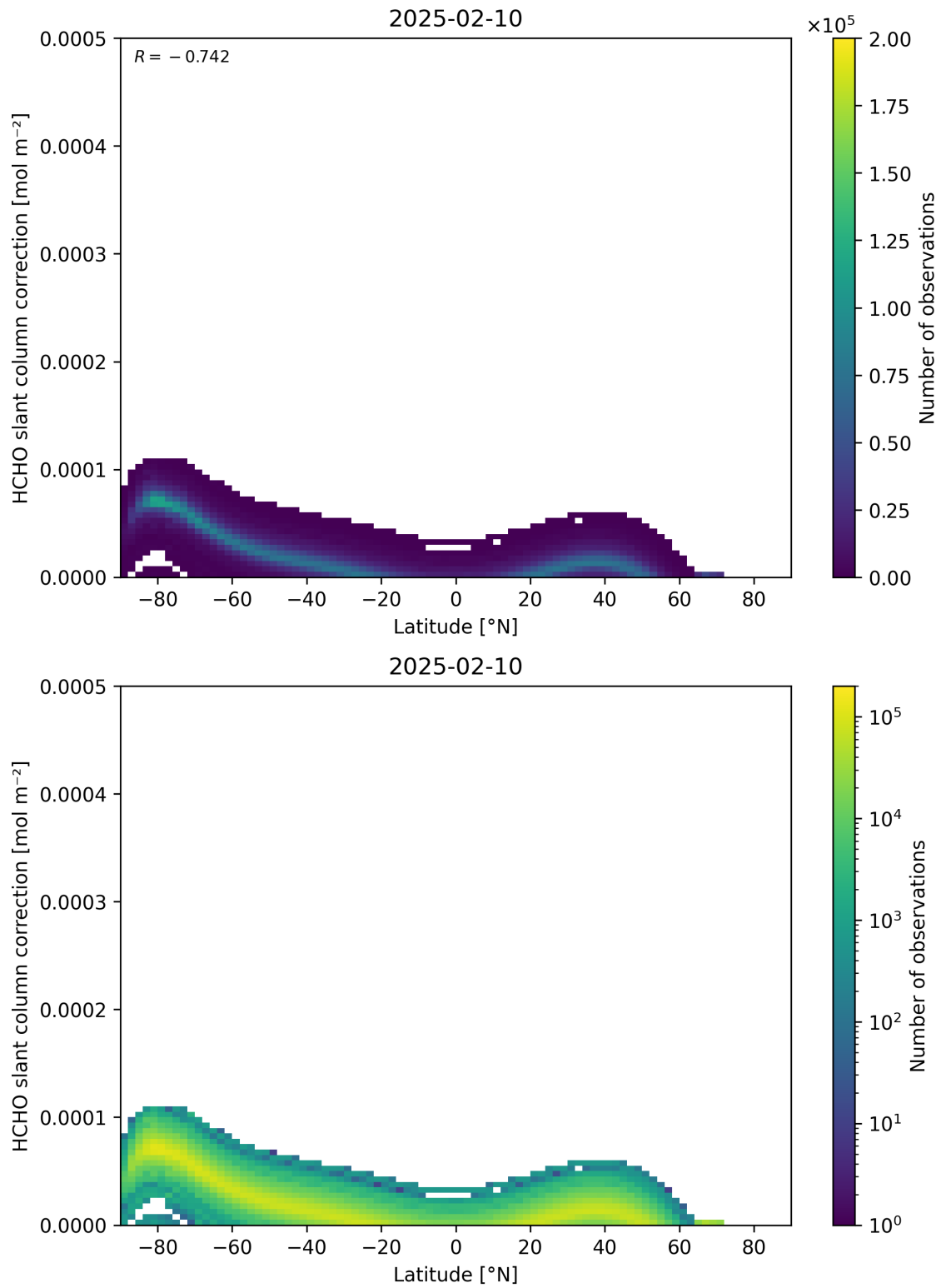
Figure 158: Scatter density plot of “Latitude” against “HCHO slant column correction” for 2025-02-09 to 2025-02-11.
