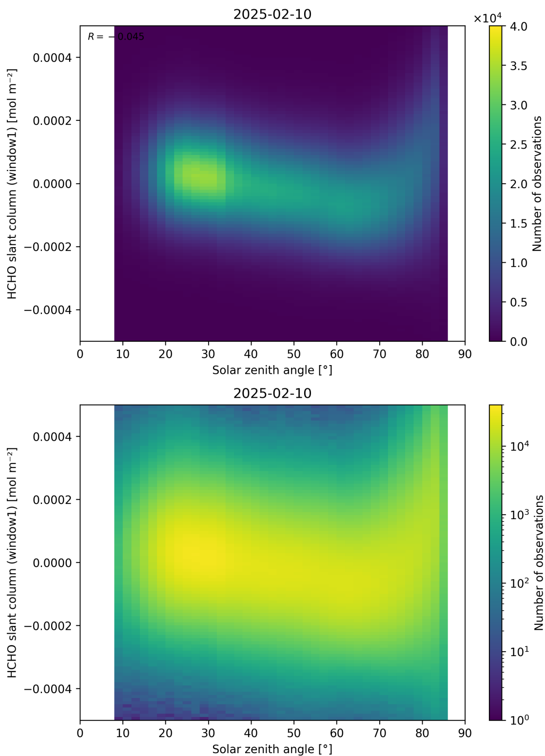
Figure 173: Scatter density plot of “Solar zenith angle” against “HCHO slant column (window1)” for 2025-02-09 to 2025-02-11.
