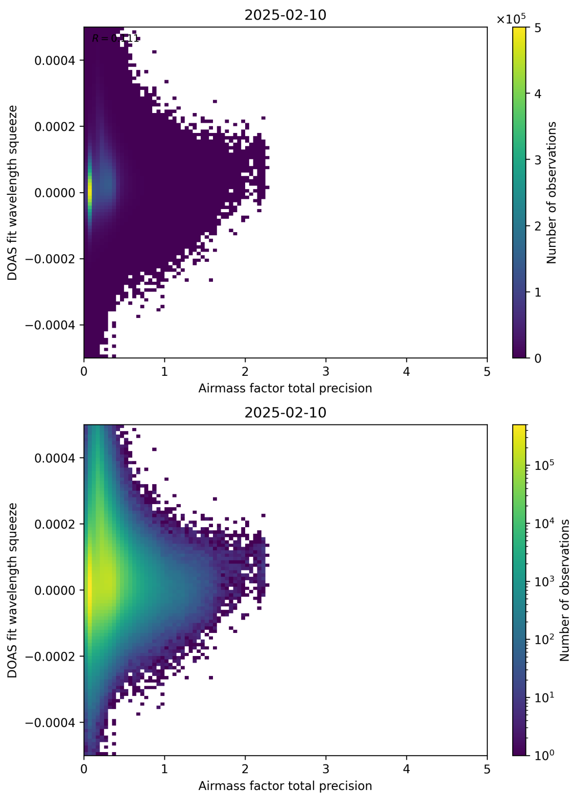
Figure 107: Scatter density plot of “Airmass factor total precision” against “DOAS fit wavelength squeeze” for 2025-02-09 to 2025-02-11.
