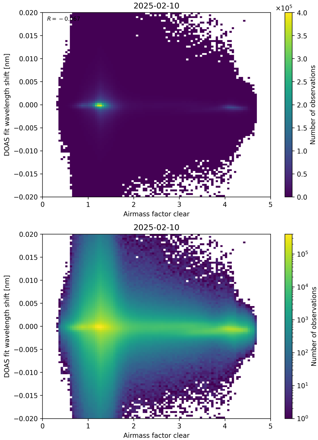
Figure 72: Scatter density plot of “Airmass factor clear” against “DOAS fit wavelength shift” for 2025-02-09 to 2025-02-11.
