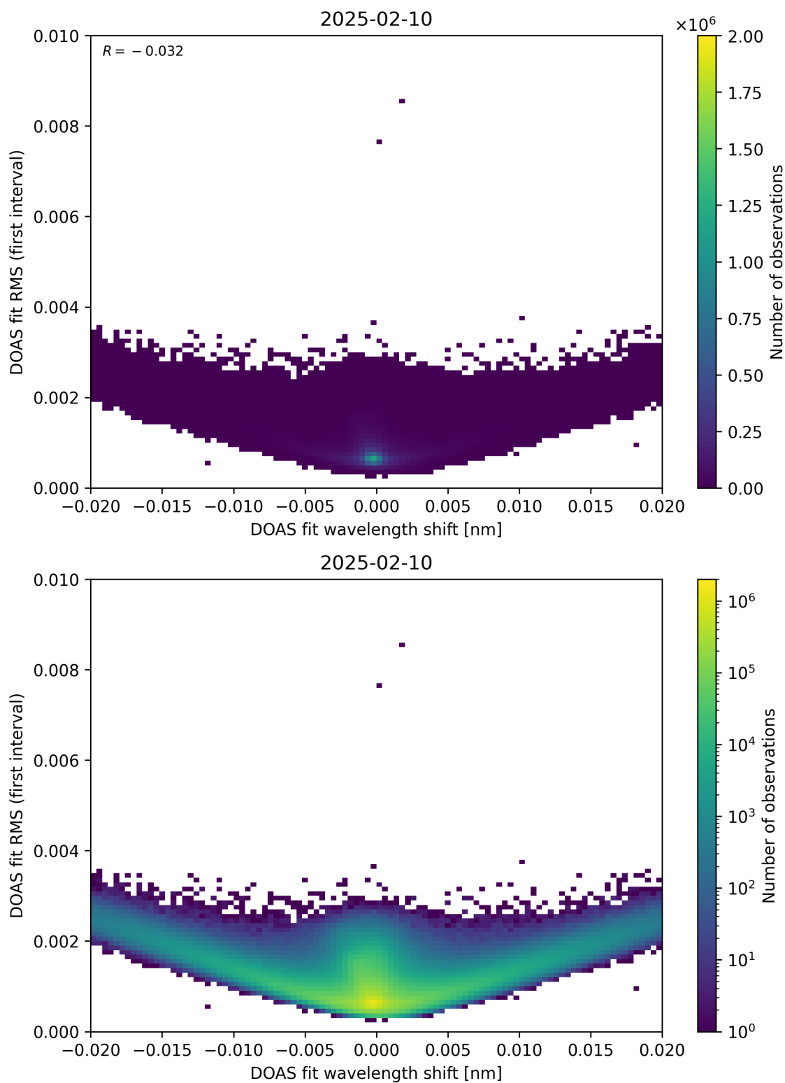
Figure 64: Scatter density plot of “DOAS fit wavelength shift” against “DOAS fit RMS (first interval)” for 2025-02-09 to 2025-02-11.
