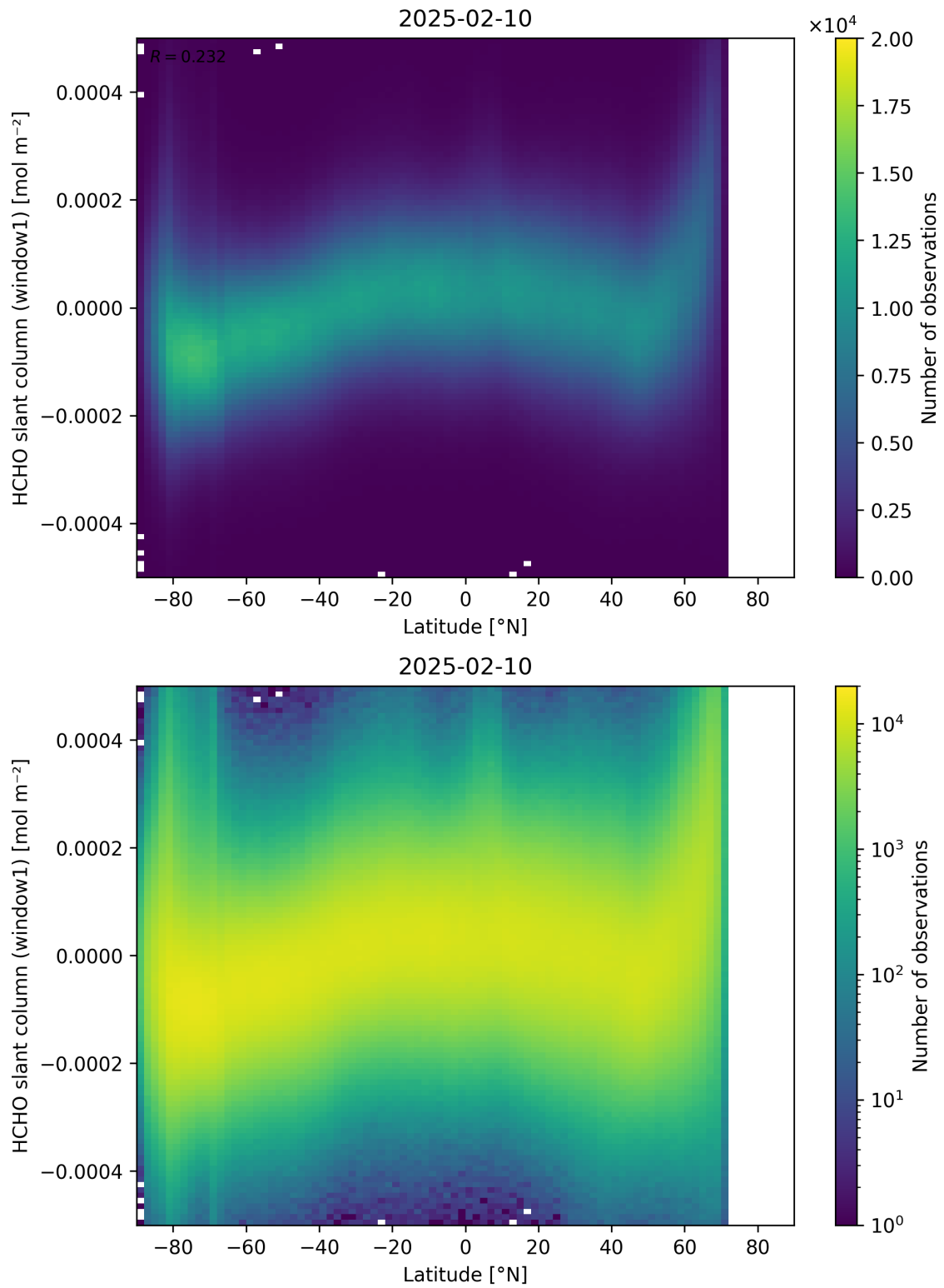
Figure 159: Scatter density plot of “Latitude” against “HCHO slant column (window1)” for 2025-02-09 to 2025-02-11.
