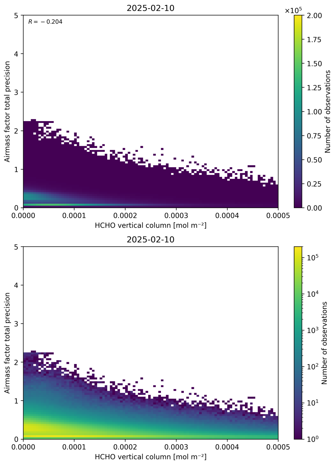
Figure 132: Scatter density plot of “HCHO vertical column” against “Airmass factor total precision” for 2025-02-09 to 2025-02-11.
