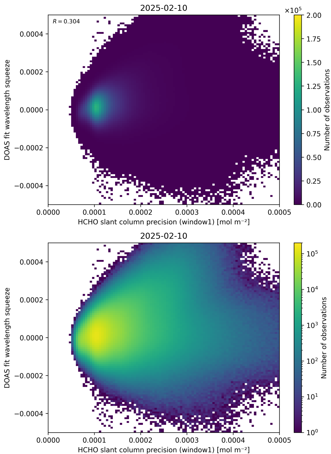
Figure 90: Scatter density plot of “HCHO slant column precision (window1)” against “DOAS fit wavelength squeeze” for 2025-02-09 to 2025-02-11.
