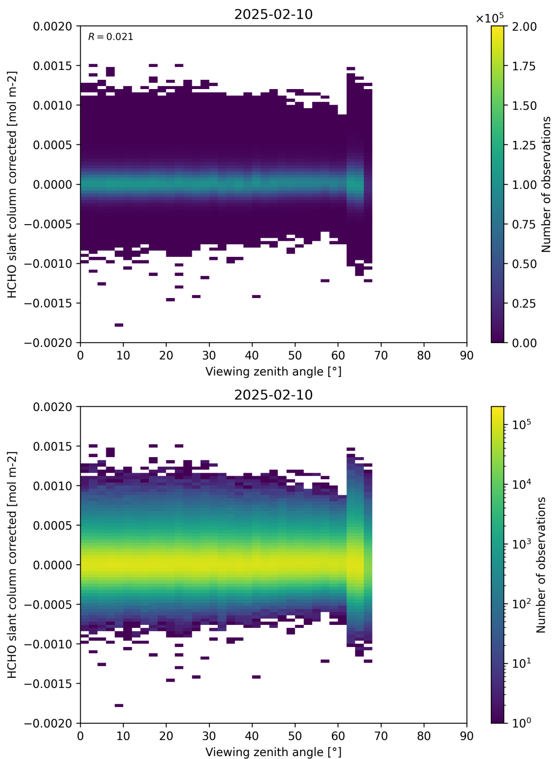
Figure 186: Scatter density plot of “Viewing zenith angle” against “HCHO slant column corrected” for 2025-02-09 to 2025-02-11.
