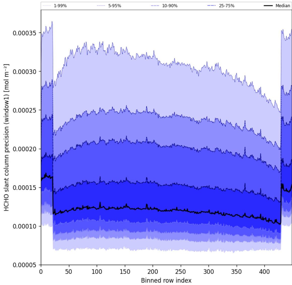
Figure 53: Along track statistics of “HCHO slant column precision (window1)” for 2025-02-09 to 2025-02-11
