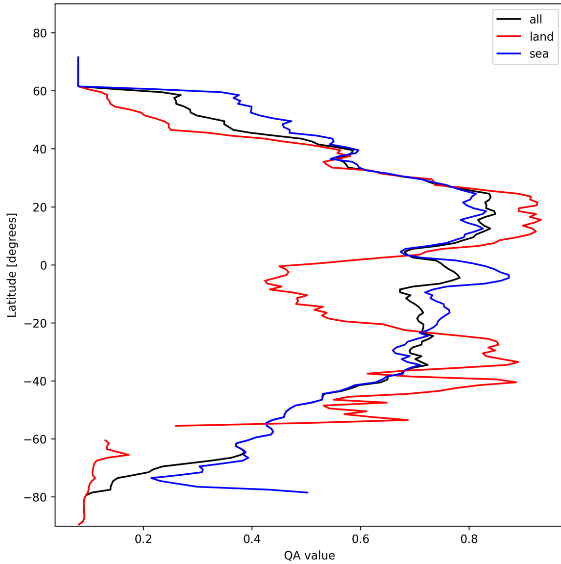
Figure 20: Zonal average of “QA value” for 2025-02-09 to 2025-02-11.
