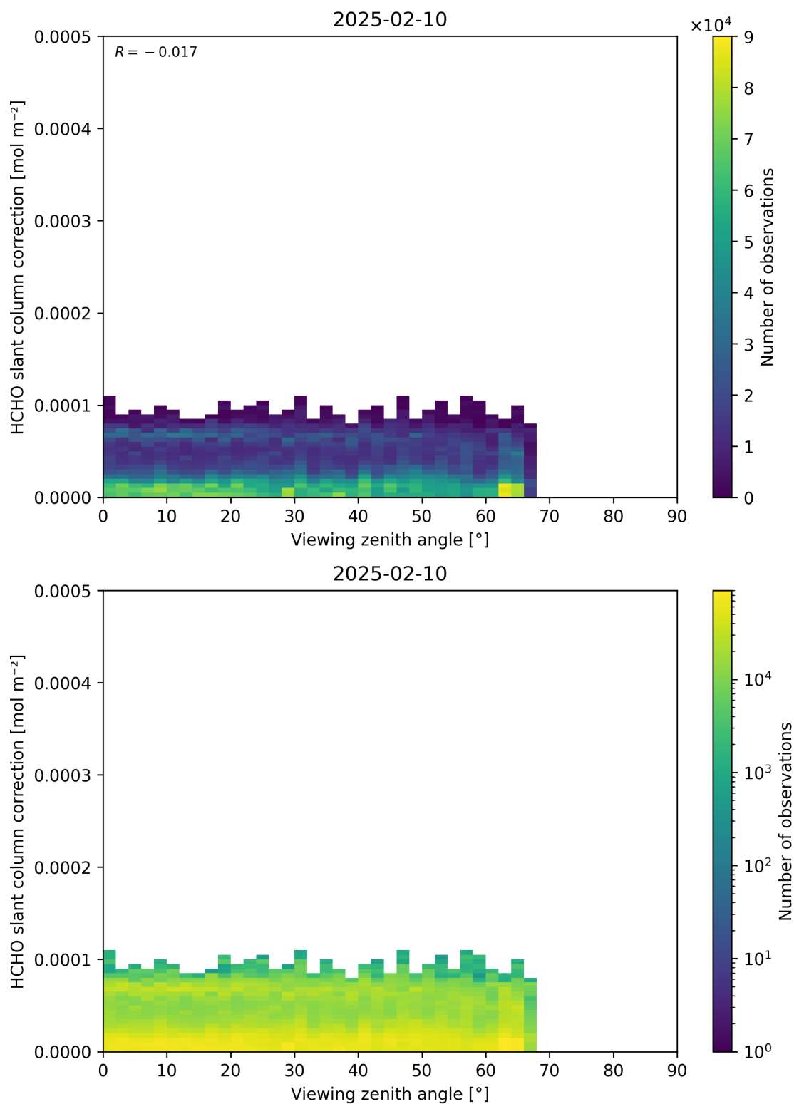
Figure 187: Scatter density plot of “Viewing zenith angle” against “HCHO slant column correction” for 2025-02-09 to 2025-02-11.
