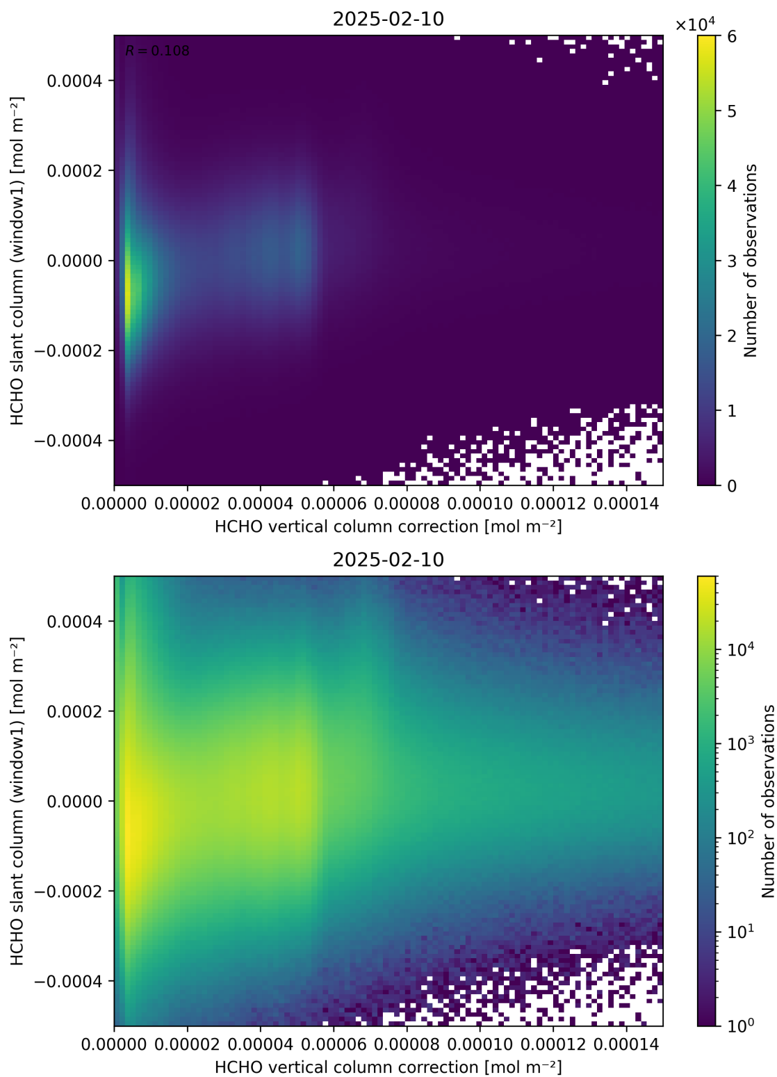
Figure 118: Scatter density plot of “HCHO vertical column correction” against “HCHO slant column (window1)” for 2025-02-09 to 2025-02-11.
