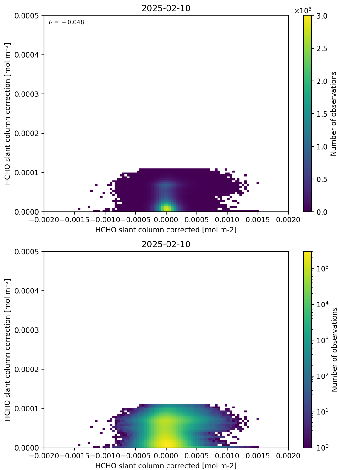
Figure 77: Scatter density plot of “HCHO slant column corrected” against “HCHO slant column correction” for 2025-02-09 to 2025-02-11.
