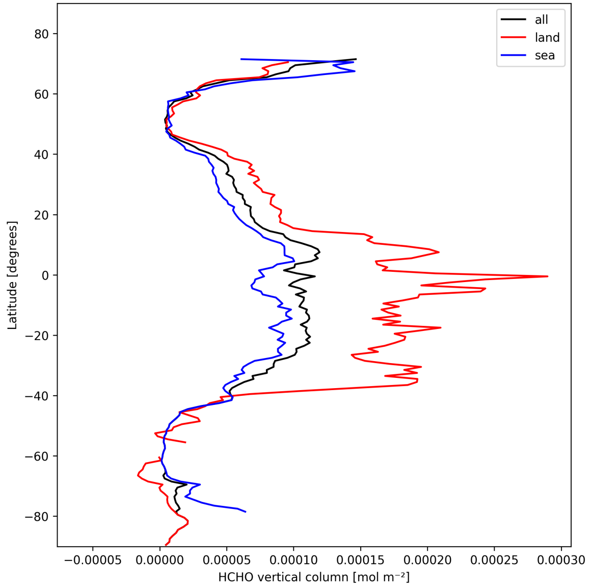
Figure 21: Zonal average of “HCHO vertical column” for 2025-02-09 to 2025-02-11.
