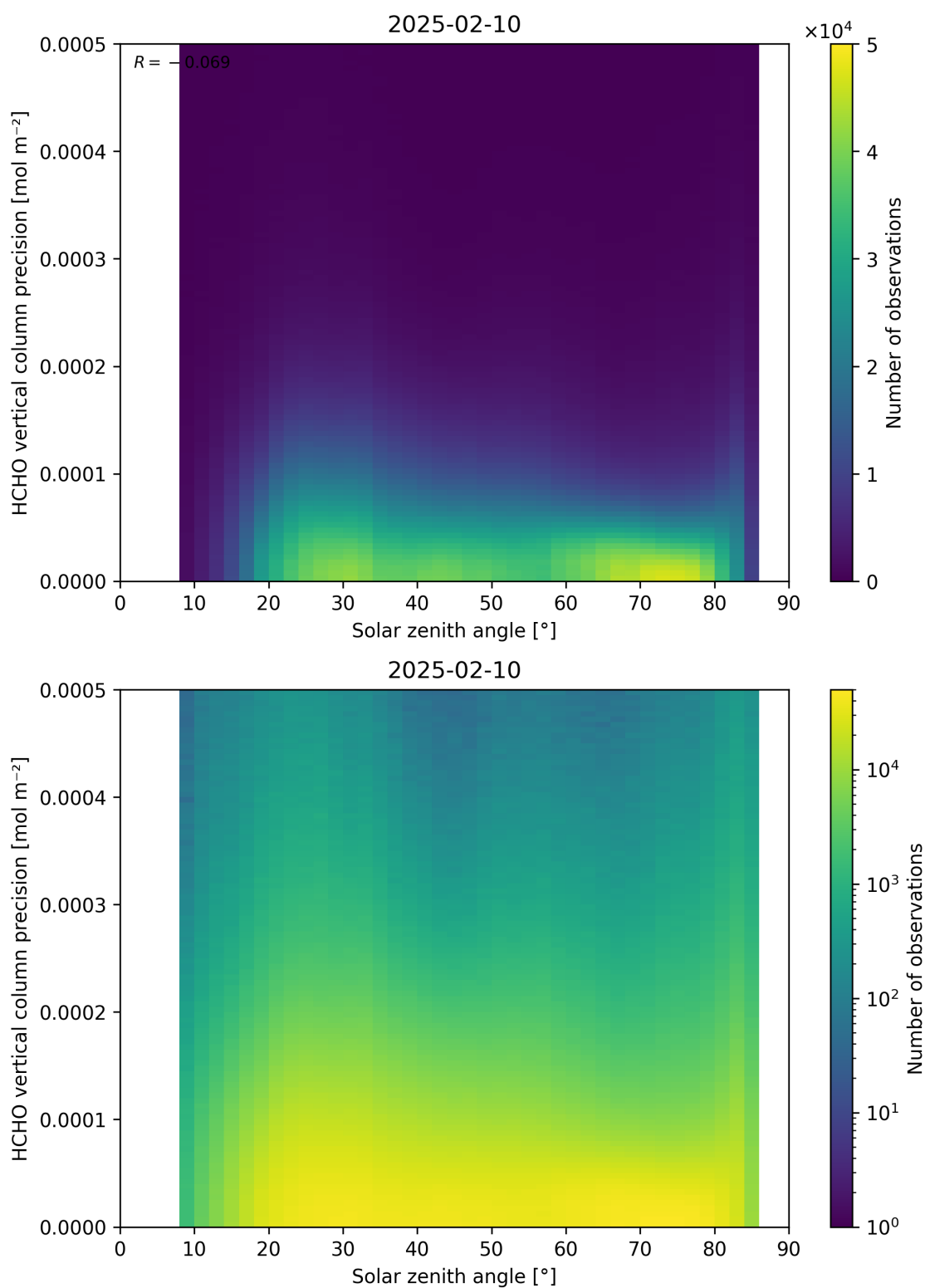
Figure 179: Scatter density plot of “Solar zenith angle” against “HCHO vertical column precision” for 2025-02-09 to 2025-02-11.
