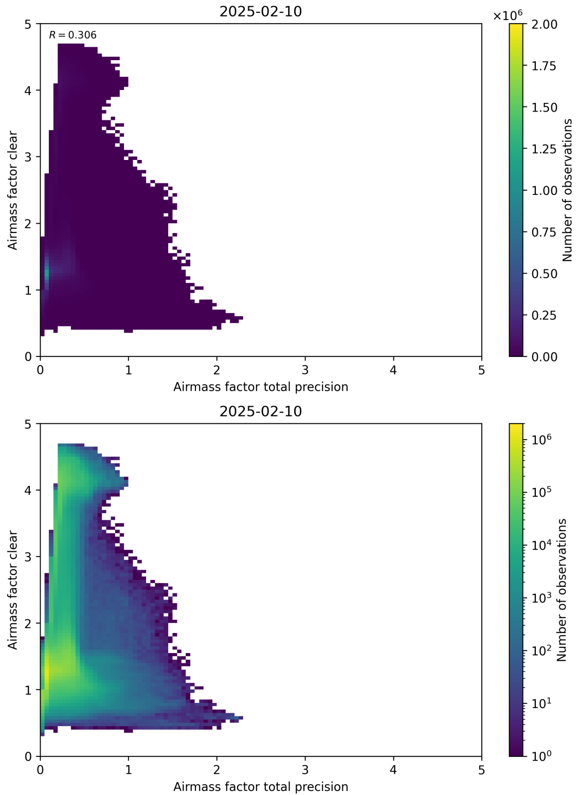
Figure 108: Scatter density plot of “Airmass factor total precision” against “Airmass factor clear” for 2025-02-09 to 2025-02-11.
