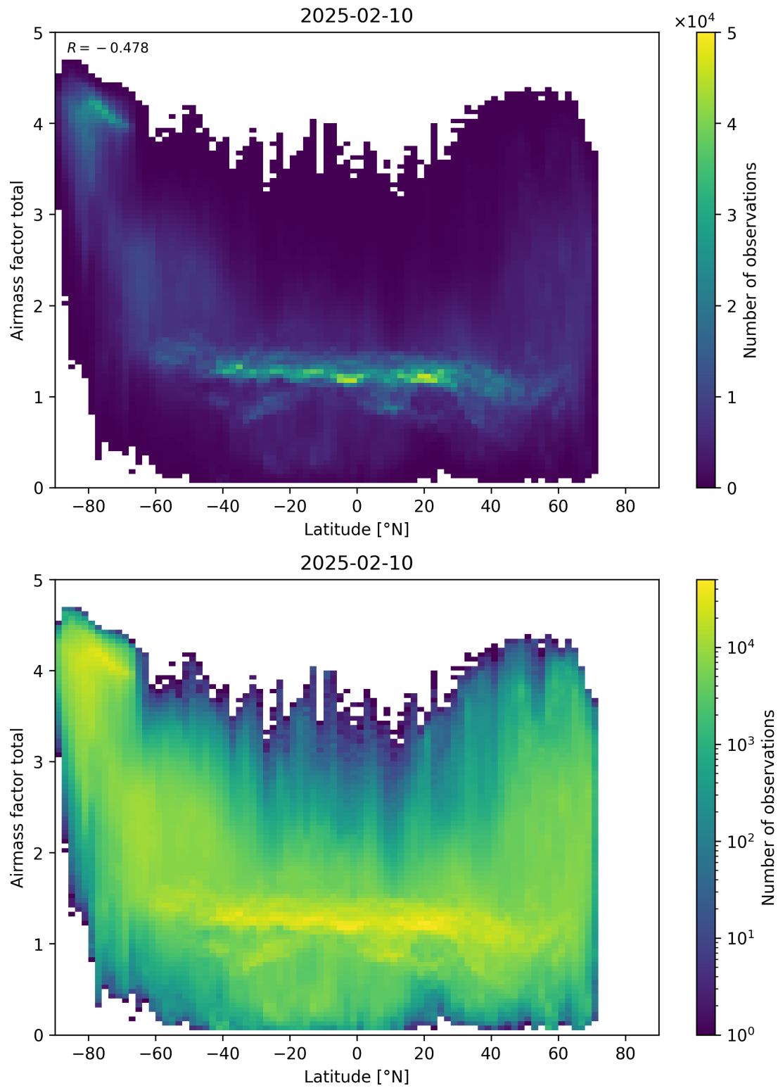
Figure 161: Scatter density plot of “Latitude” against “Airmass factor total” for 2025-02-09 to 2025-02-11.
