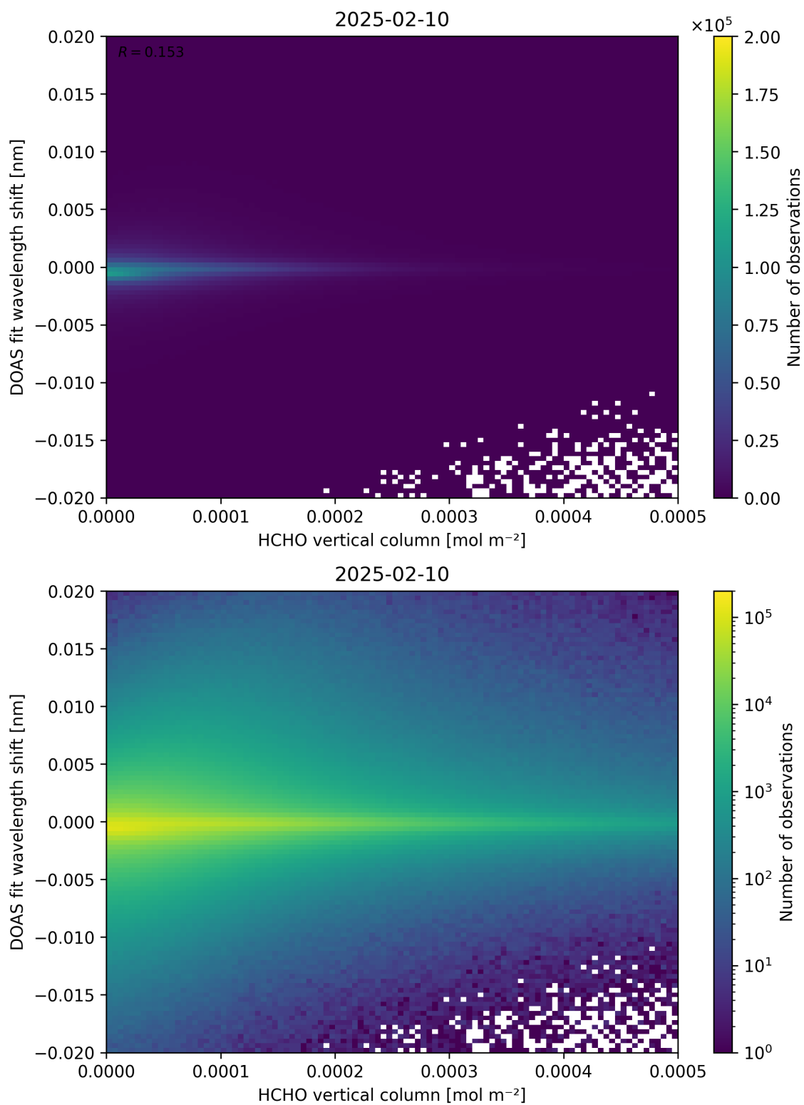
Figure 124: Scatter density plot of “HCHO vertical column” against “DOAS fit wavelength shift” for 2025-02-09 to 2025-02-11.
