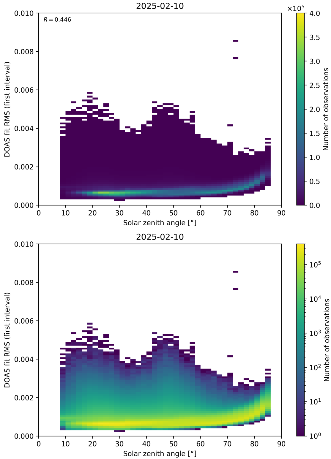
Figure 167: Scatter density plot of “Solar zenith angle” against “DOAS fit RMS (first interval)” for 2025-02-09 to 2025-02-11.
