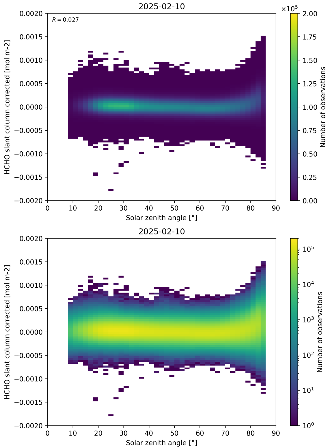
Figure 171: Scatter density plot of “Solar zenith angle” against “HCHO slant column corrected” for 2025-02-09 to 2025-02-11.
