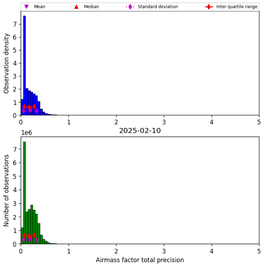
Figure 41: Histogram of “Airmass factor total precision” for 2025-02-09 to 2025-02-11
