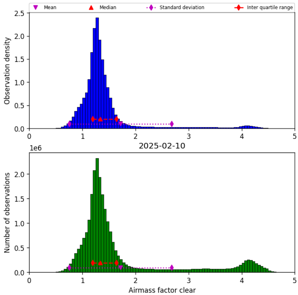
Figure 42: Histogram of “Airmass factor clear” for 2025-02-09 to 2025-02-11
