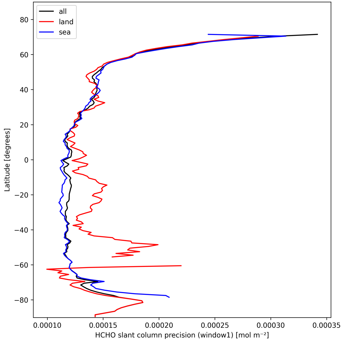
Figure 25: Zonal average of “HCHO slant column precision (window1)” for 2025-02-09 to 2025-02-11.
