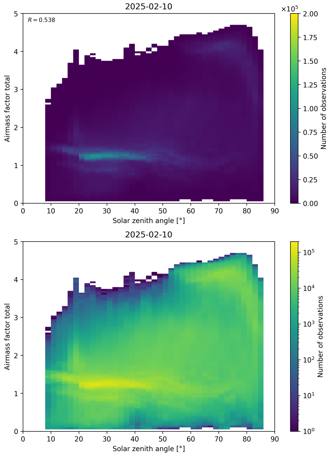
Figure 175: Scatter density plot of “Solar zenith angle” against “Airmass factor total” for 2025-02-09 to 2025-02-11.
