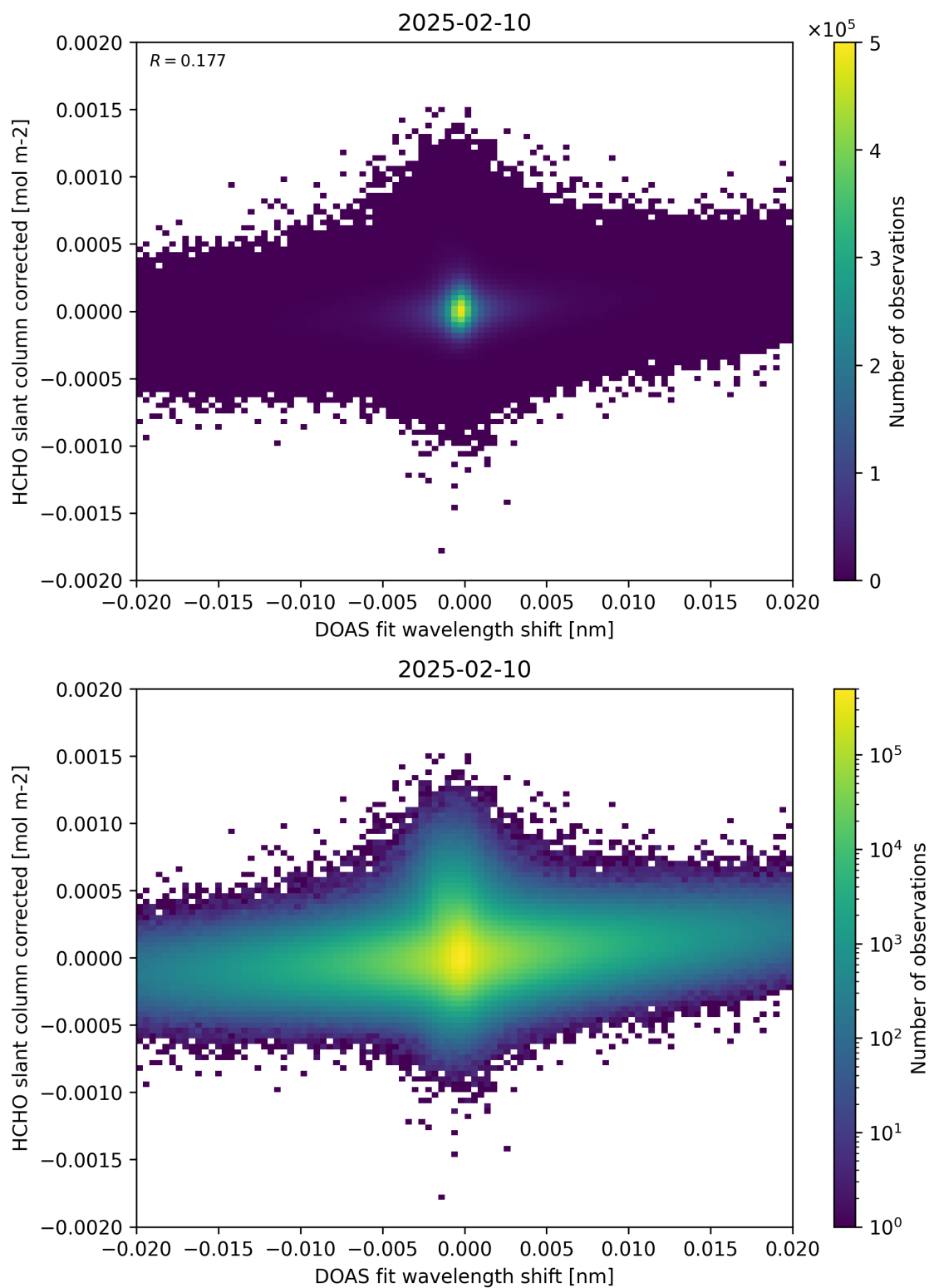
Figure 66: Scatter density plot of “DOAS fit wavelength shift” against “HCHO slant column corrected” for 2025-02-09 to 2025-02-11.
