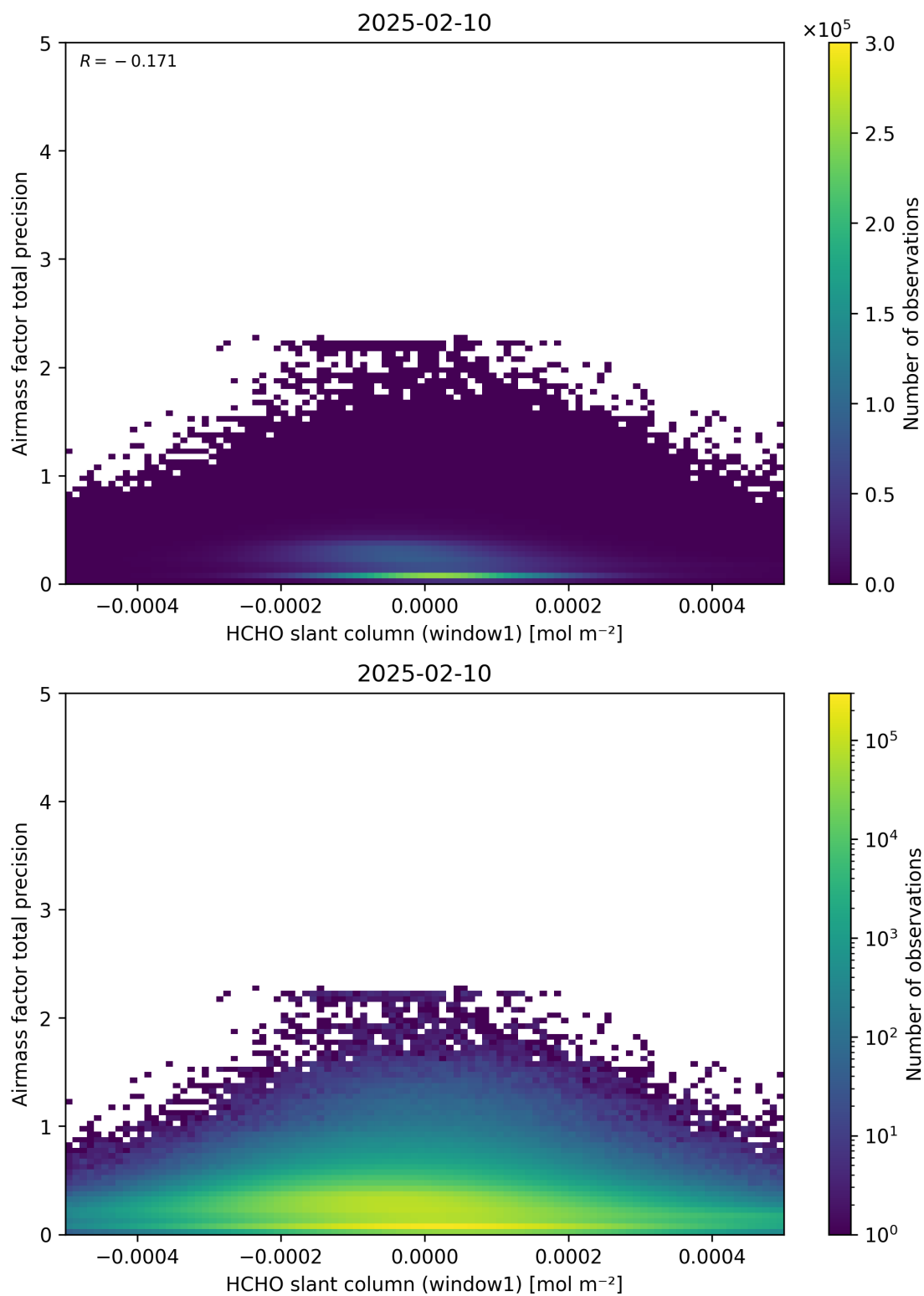
Figure 86: Scatter density plot of “HCHO slant column (window1)” against “Airmass factor total precision” for 2025-02-09 to 2025-02-11.
