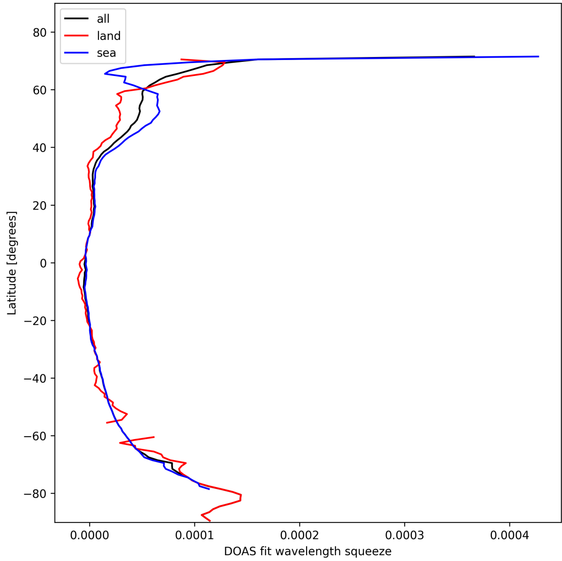
Figure 31: Zonal average of “DOAS fit wavelength squeeze” for 2025-02-09 to 2025-02-11.
