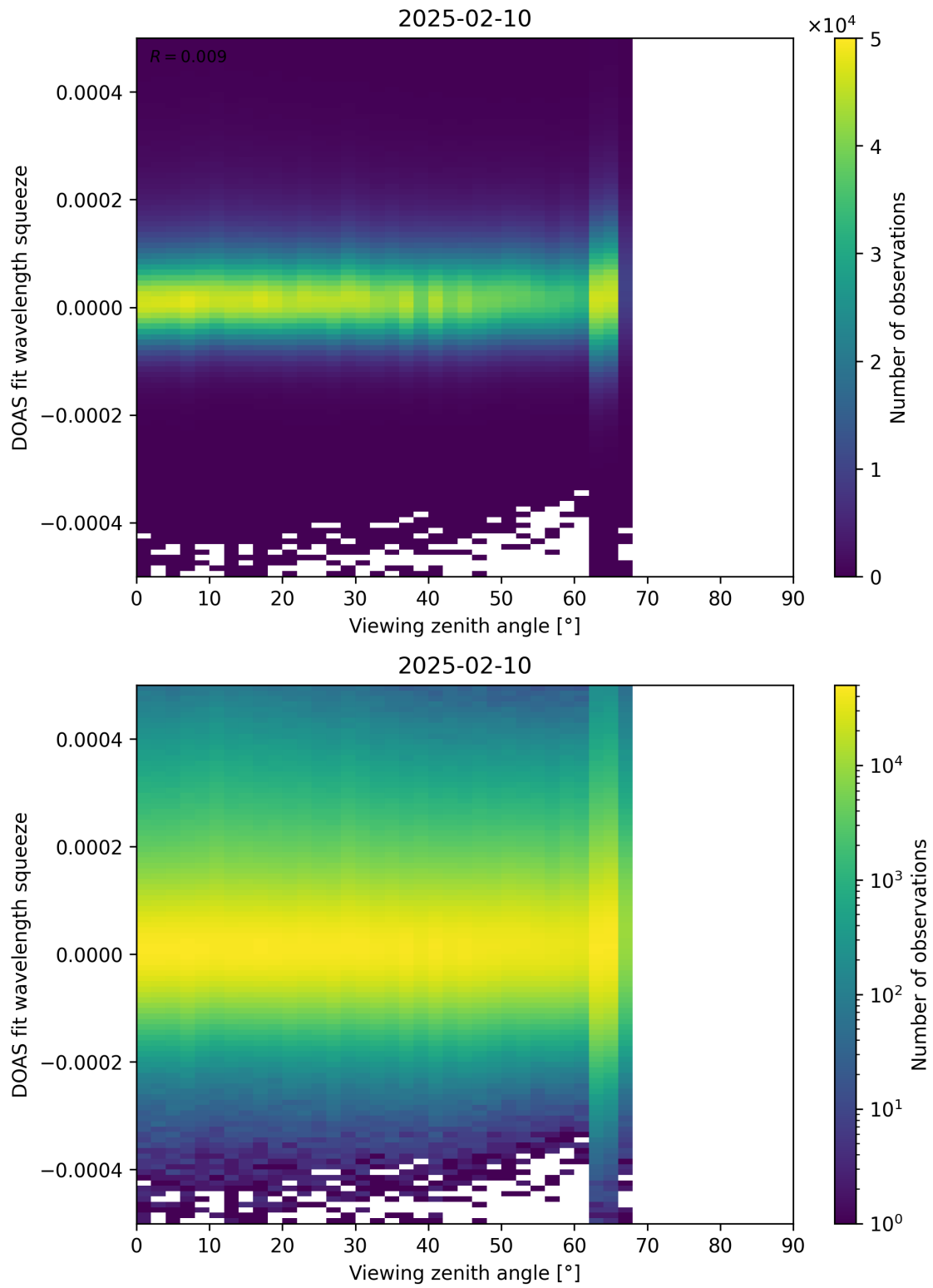
Figure 184: Scatter density plot of “Viewing zenith angle” against “DOAS fit wavelength squeeze” for 2025-02-09 to 2025-02-11.
