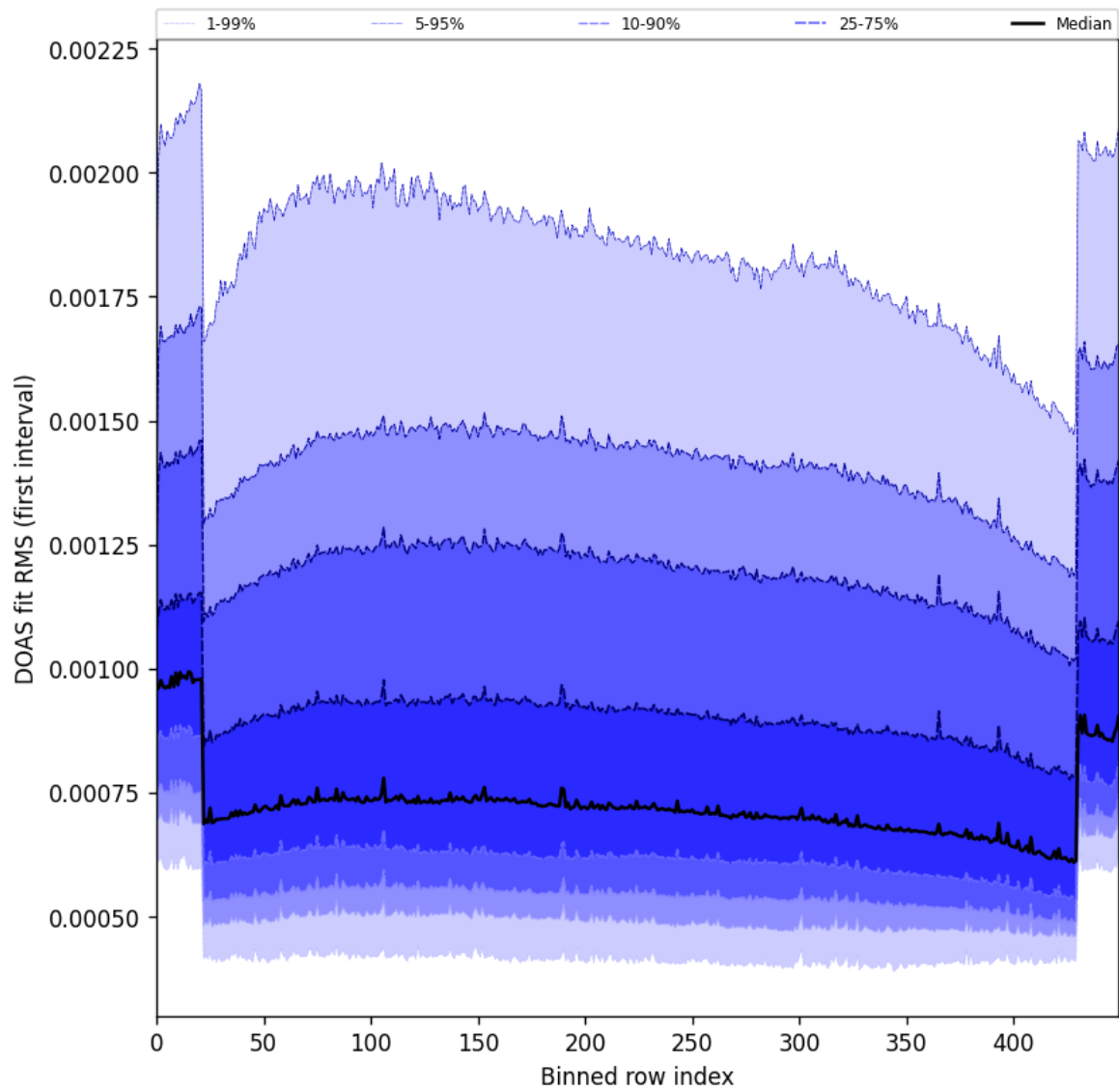
Figure 60: Along track statistics of “DOAS fit RMS (first interval)” for 2025-02-09 to 2025-02-11
