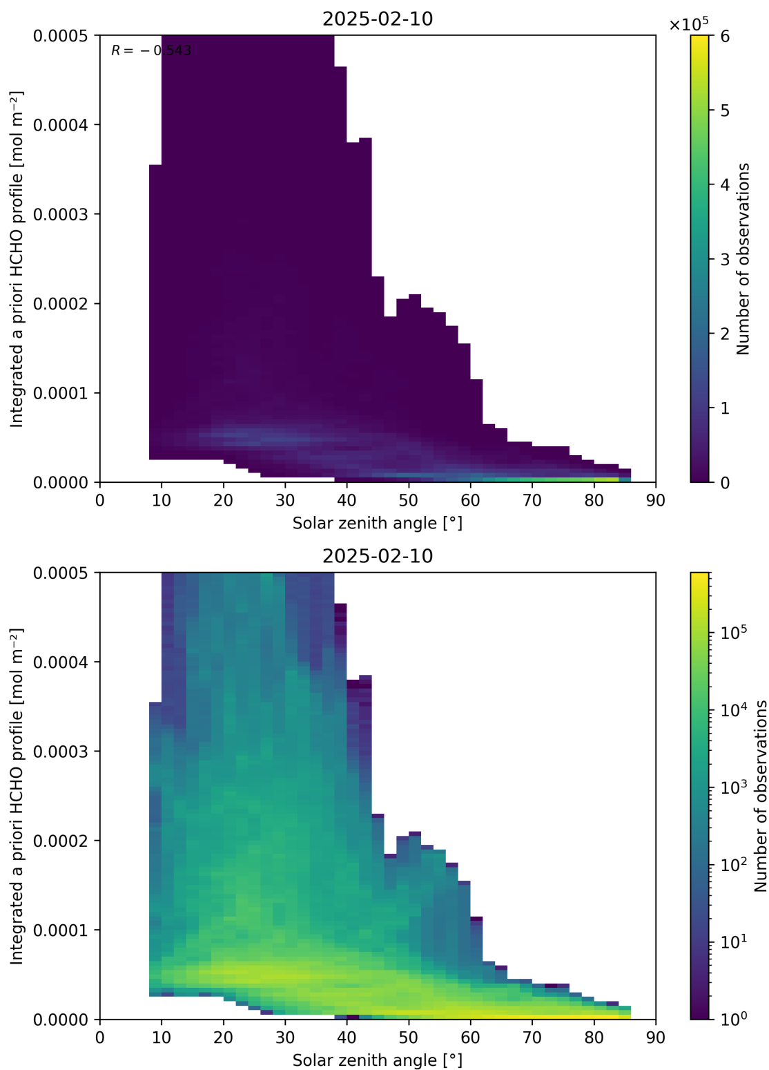
Figure 180: Scatter density plot of “Solar zenith angle” against “Integrated a priori HCHO profile” for 2025-02-09 to 2025-02-11.
