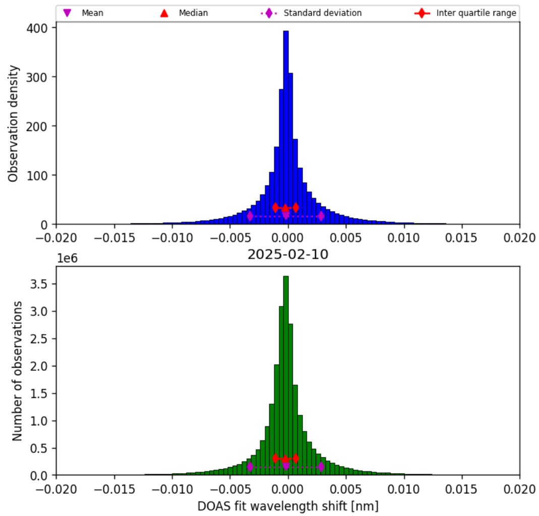
Figure 44: Histogram of “DOAS fit wavelength shift” for 2025-02-09 to 2025-02-11
