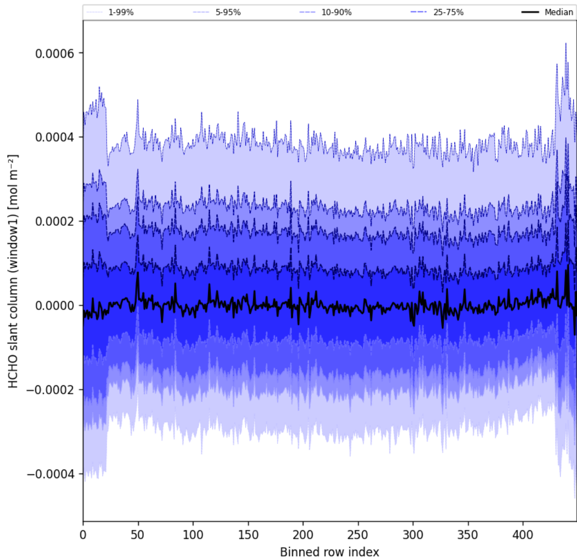
Figure 52: Along track statistics of “HCHO slant column (window1)” for 2025-02-09 to 2025-02-11
