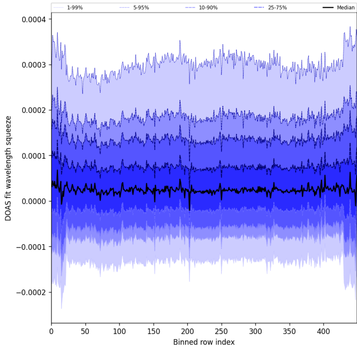
Figure 59: Along track statistics of “DOAS fit wavelength squeeze” for 2025-02-09 to 2025-02-11
