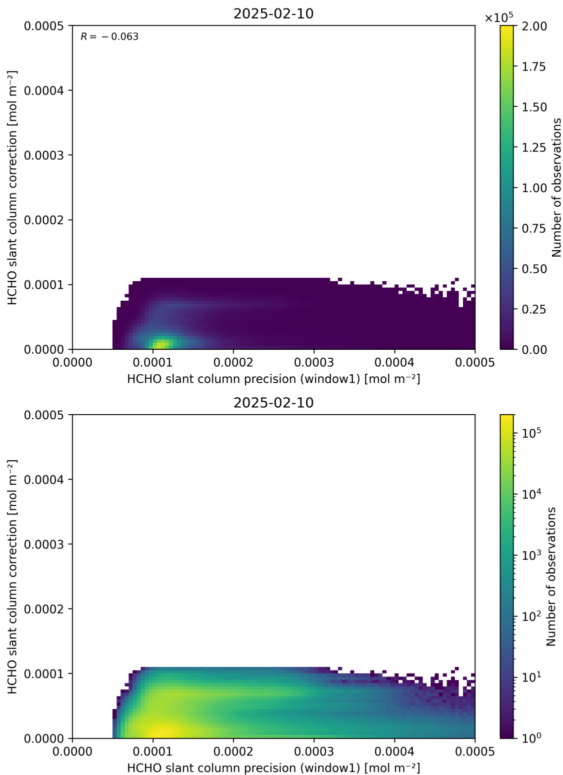
Figure 93: Scatter density plot of “HCHO slant column precision (window1)” against “HCHO slant column correction” for 2025-02-09 to 2025-02-11.
