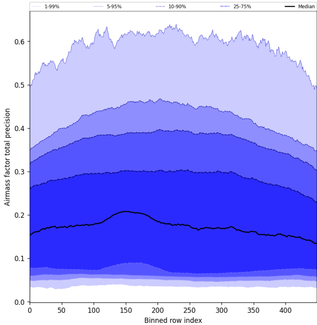
Figure 55: Along track statistics of “Airmass factor total precision” for 2025-02-09 to 2025-02-11
