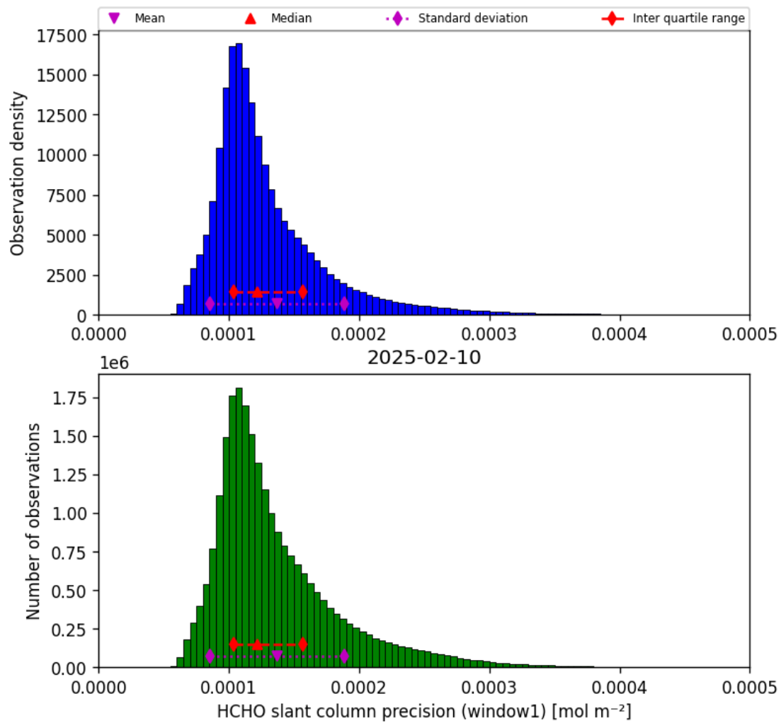
Figure 39: Histogram of “HCHO slant column precision (window1)” for 2025-02-09 to 2025-02-11
