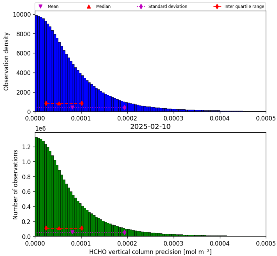
Figure 36: Histogram of “HCHO vertical column precision” for 2025-02-09 to 2025-02-11
