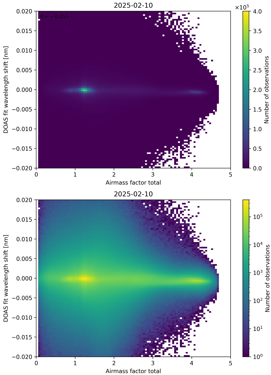
Figure 98: Scatter density plot of “Airmass factor total” against “DOAS fit wavelength shift” for 2025-02-09 to 2025-02-11.
