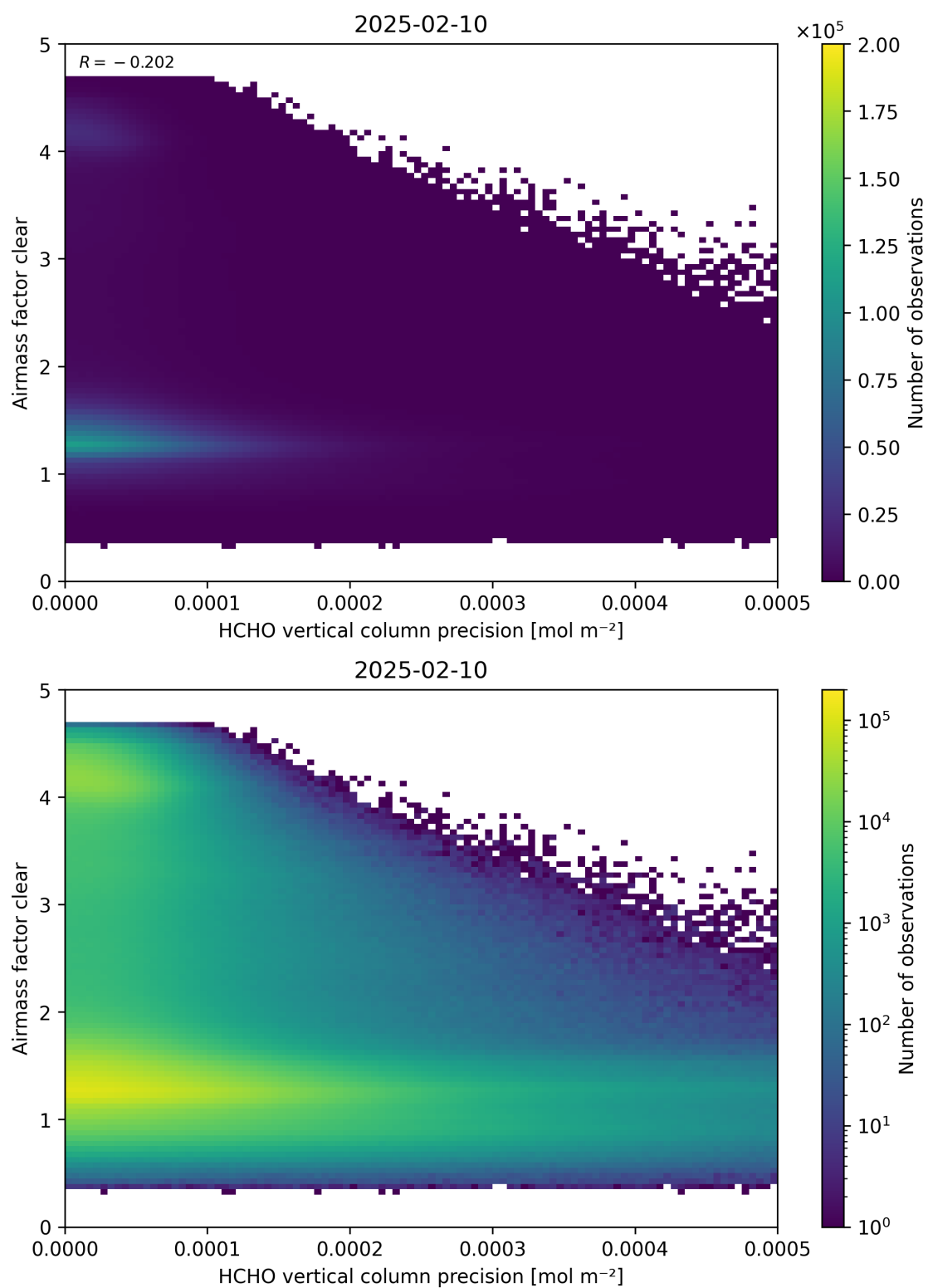
Figure 139: Scatter density plot of “HCHO vertical column precision” against “Airmass factor clear” for 2025-02-09 to 2025-02-11.
