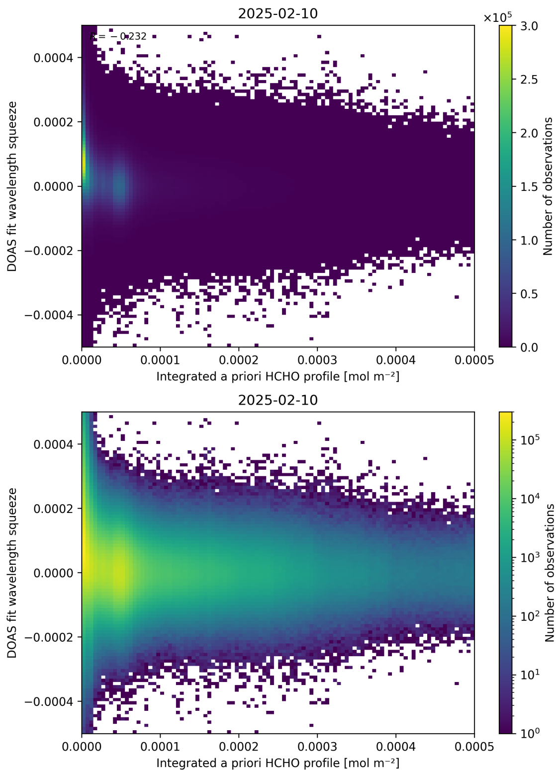
Figure 150: Scatter density plot of “Integrated a priori HCHO profile” against “DOAS fit wavelength squeeze” for 2025-02-09 to 2025-02-11.
