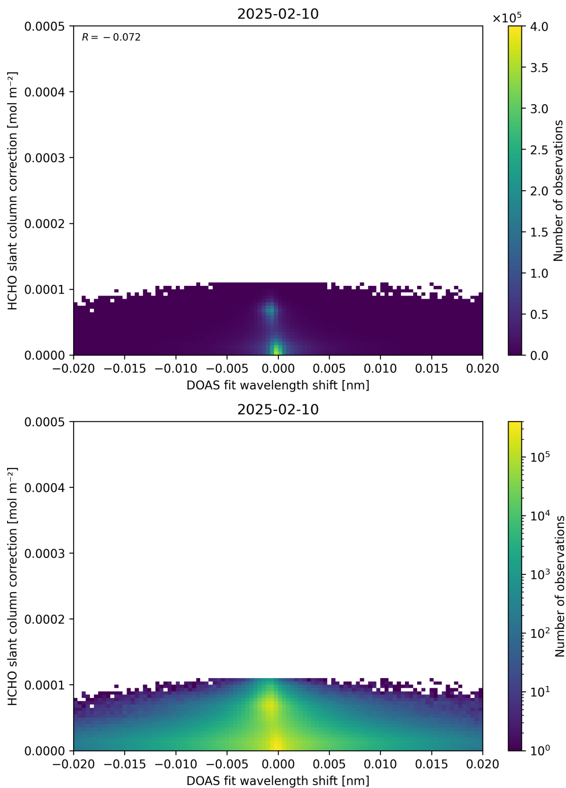
Figure 67: Scatter density plot of “DOAS fit wavelength shift” against “HCHO slant column correction” for 2025-02-09 to 2025-02-11.
