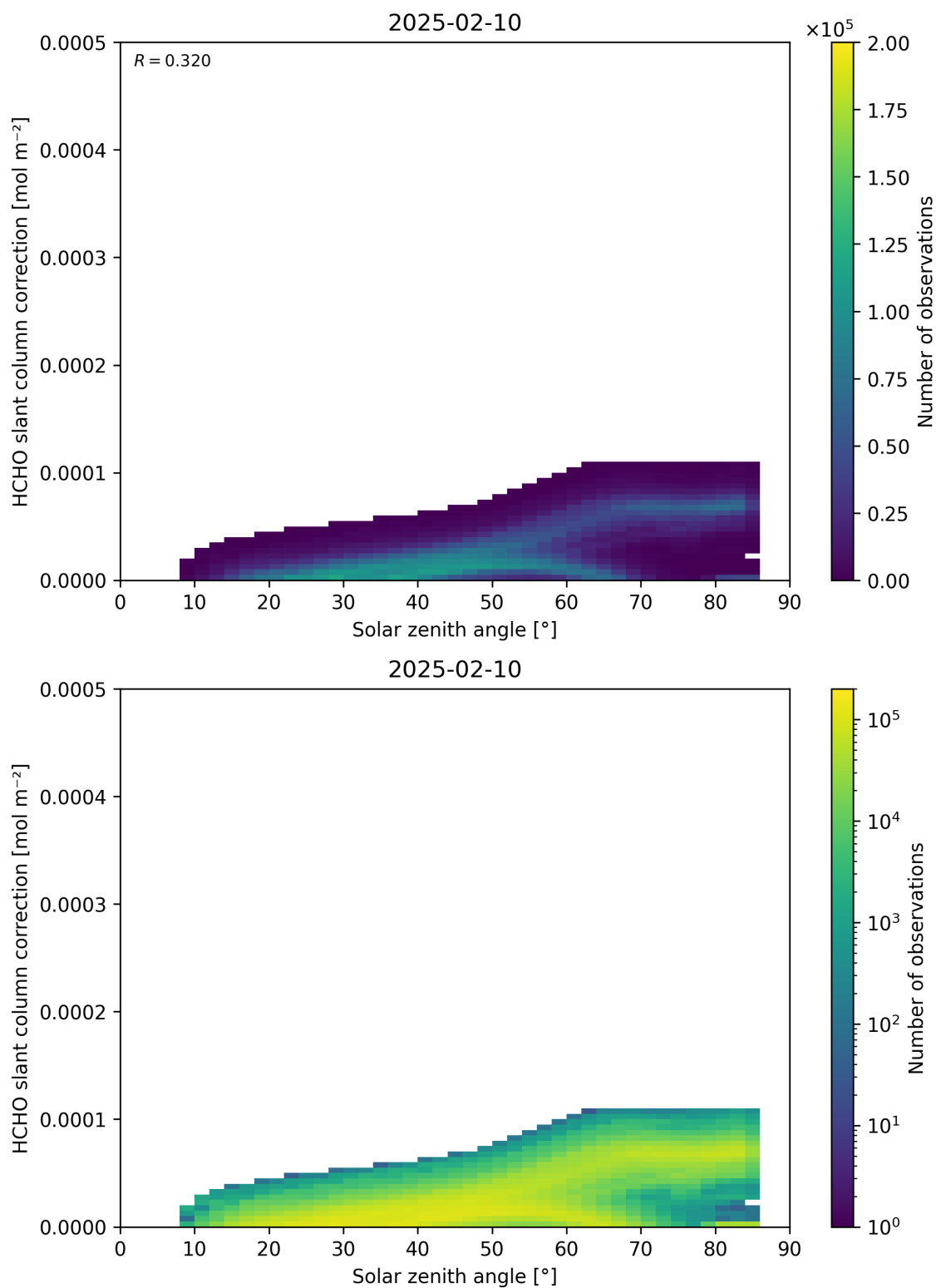
Figure 172: Scatter density plot of “Solar zenith angle” against “HCHO slant column correction” for 2025-02-09 to 2025-02-11.
