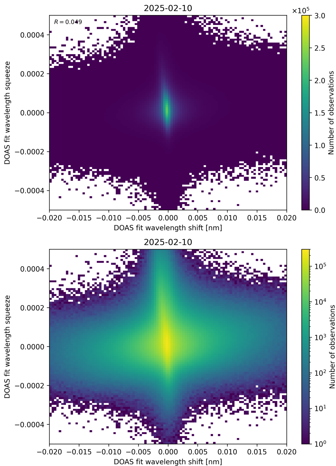
Figure 65: Scatter density plot of “DOAS fit wavelength shift” against “DOAS fit wavelength squeeze” for 2025-02-09 to 2025-02-11.
