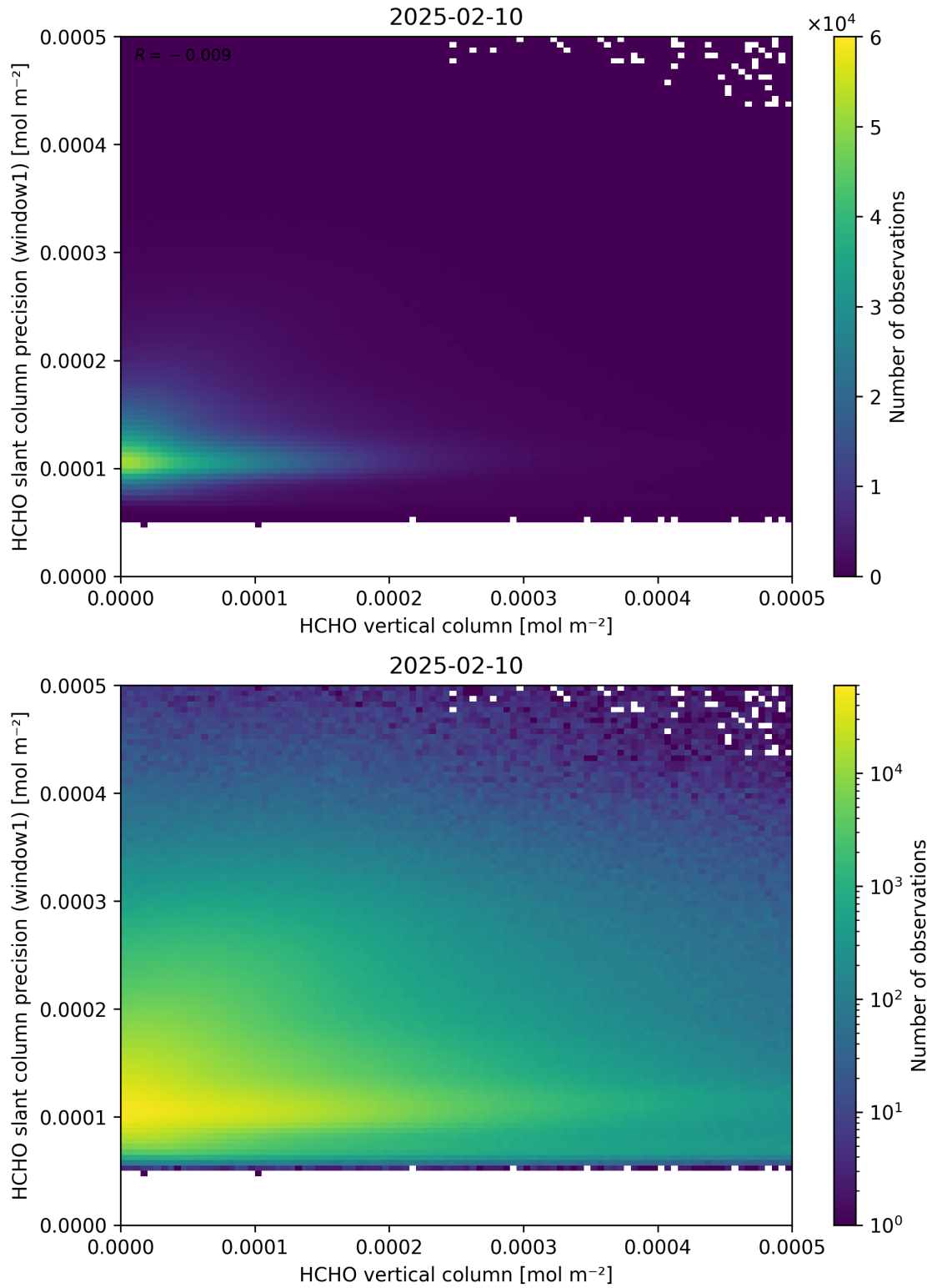
Figure 130: Scatter density plot of “HCHO vertical column” against “HCHO slant column precision (window1)” for 2025-02-09 to 2025-02-11.
