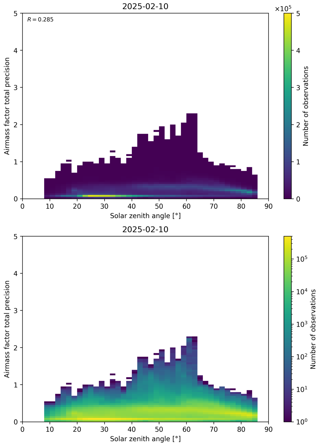
Figure 176: Scatter density plot of “Solar zenith angle” against “Airmass factor total precision” for 2025-02-09 to 2025-02-11.
