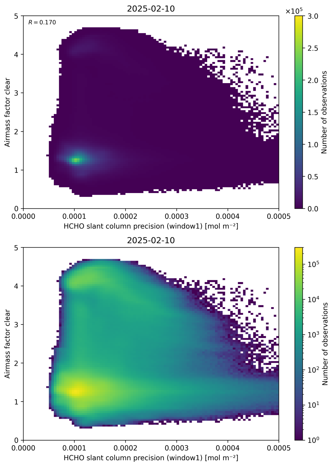
Figure 91: Scatter density plot of “HCHO slant column precision (window1)” against “Airmass factor clear” for 2025-02-09 to 2025-02-11.
