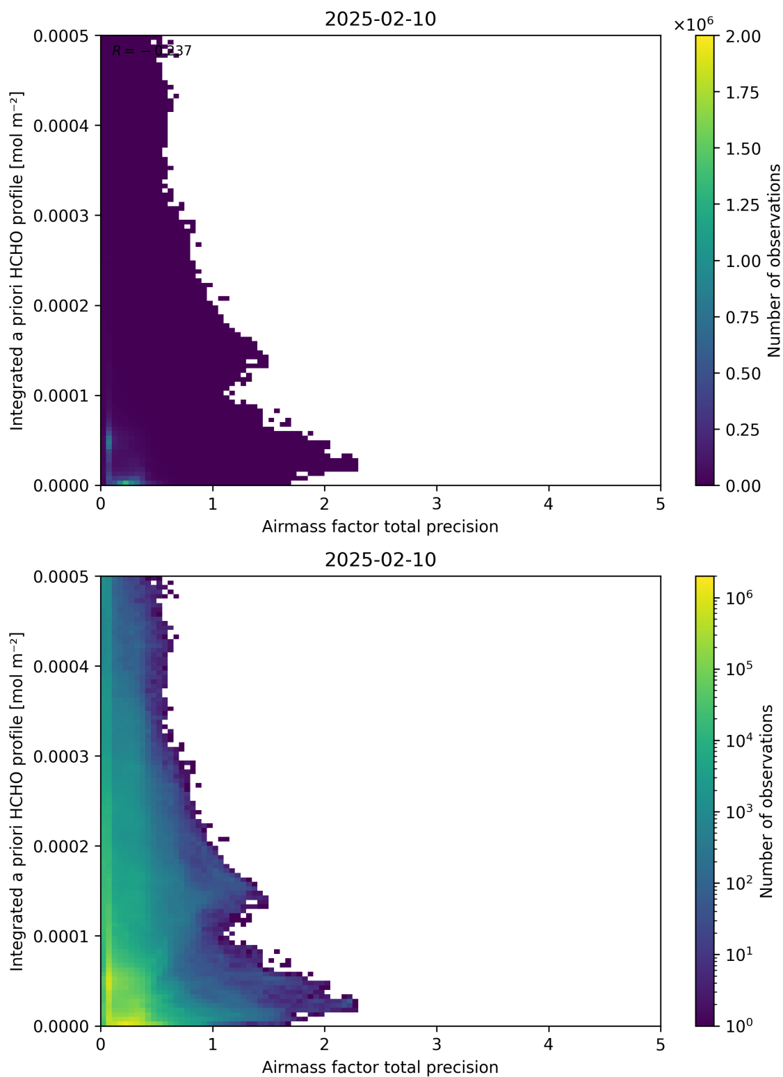
Figure 111: Scatter density plot of “Airmass factor total precision” against “Integrated a priori HCHO profile” for 2025-02-09 to 2025-02-11.
