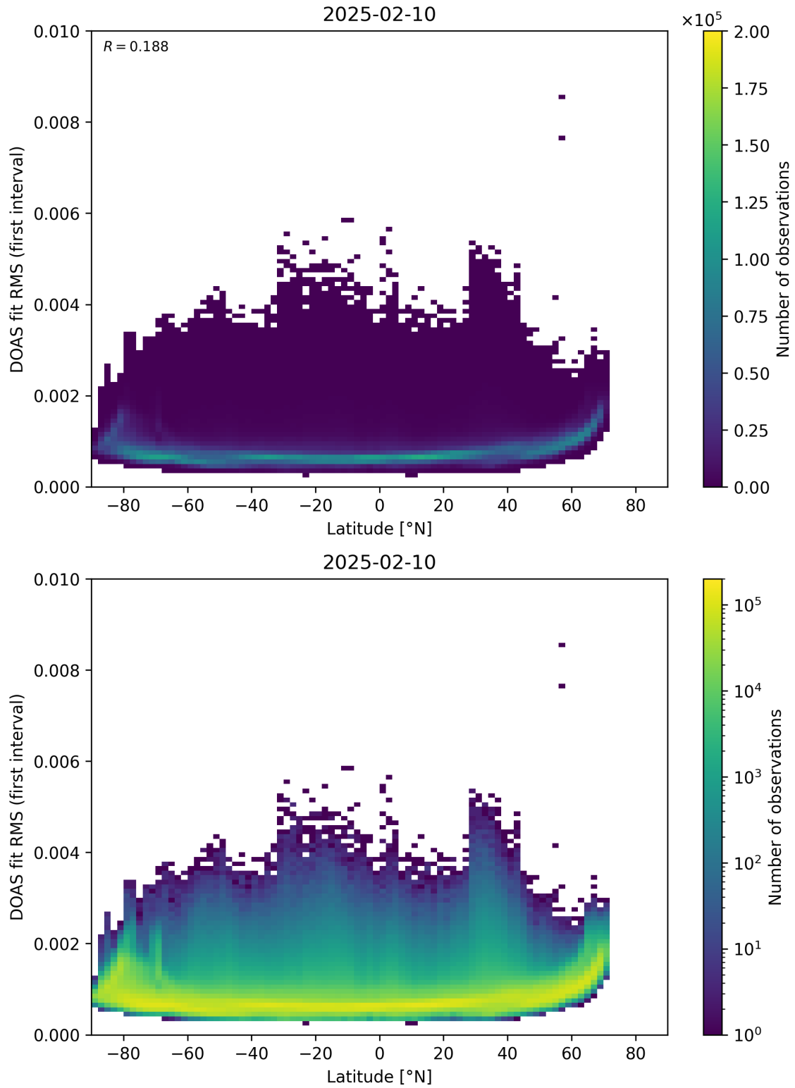
Figure 153: Scatter density plot of “Latitude” against “DOAS fit RMS (first interval)” for 2025-02-09 to 2025-02-11.
