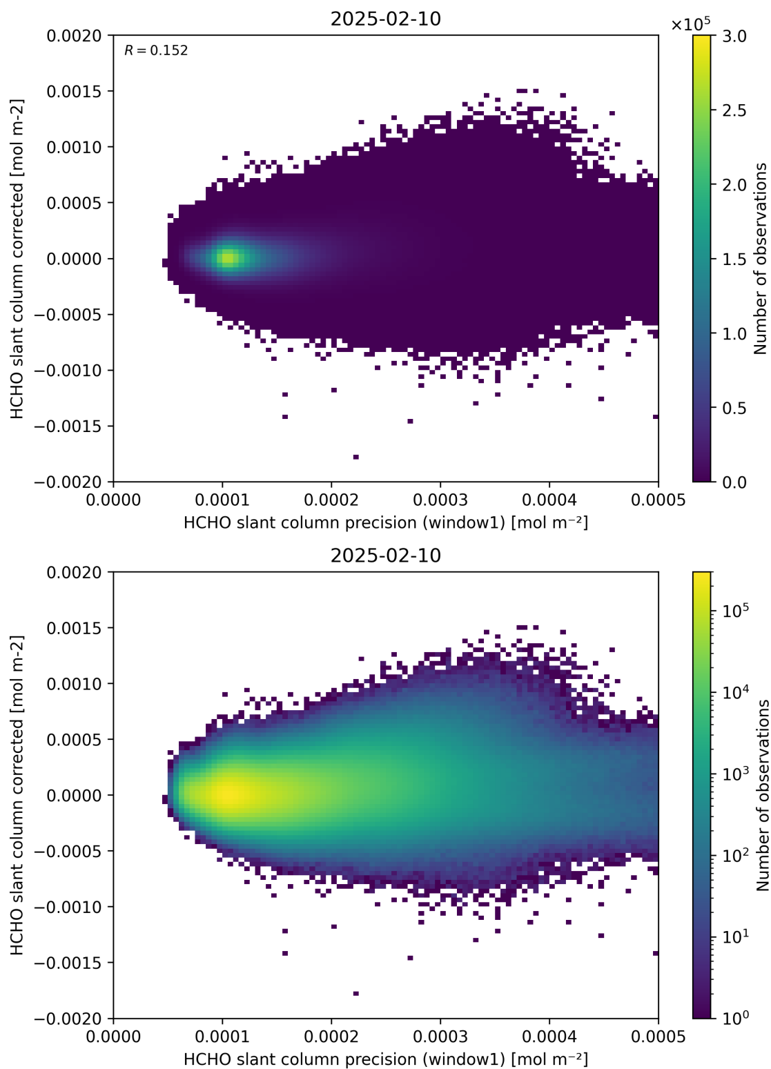
Figure 92: Scatter density plot of “HCHO slant column precision (window1)” against “HCHO slant column corrected” for 2025-02-09 to 2025-02-11.
