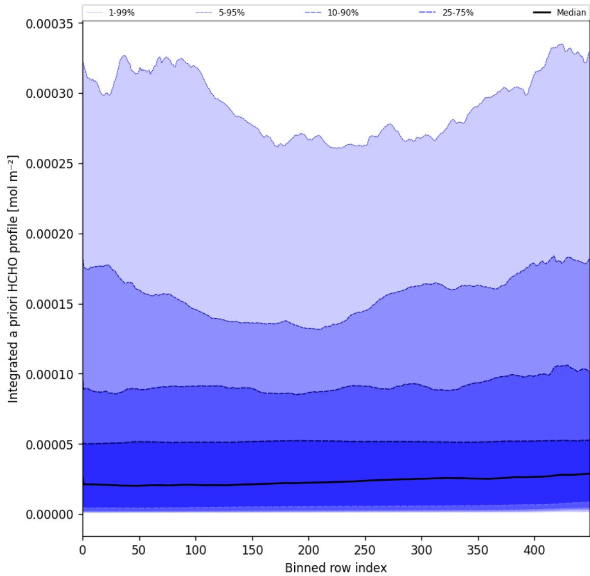
Figure 57: Along track statistics of “Integrated a priori HCHO profile” for 2025-02-09 to 2025-02-11
