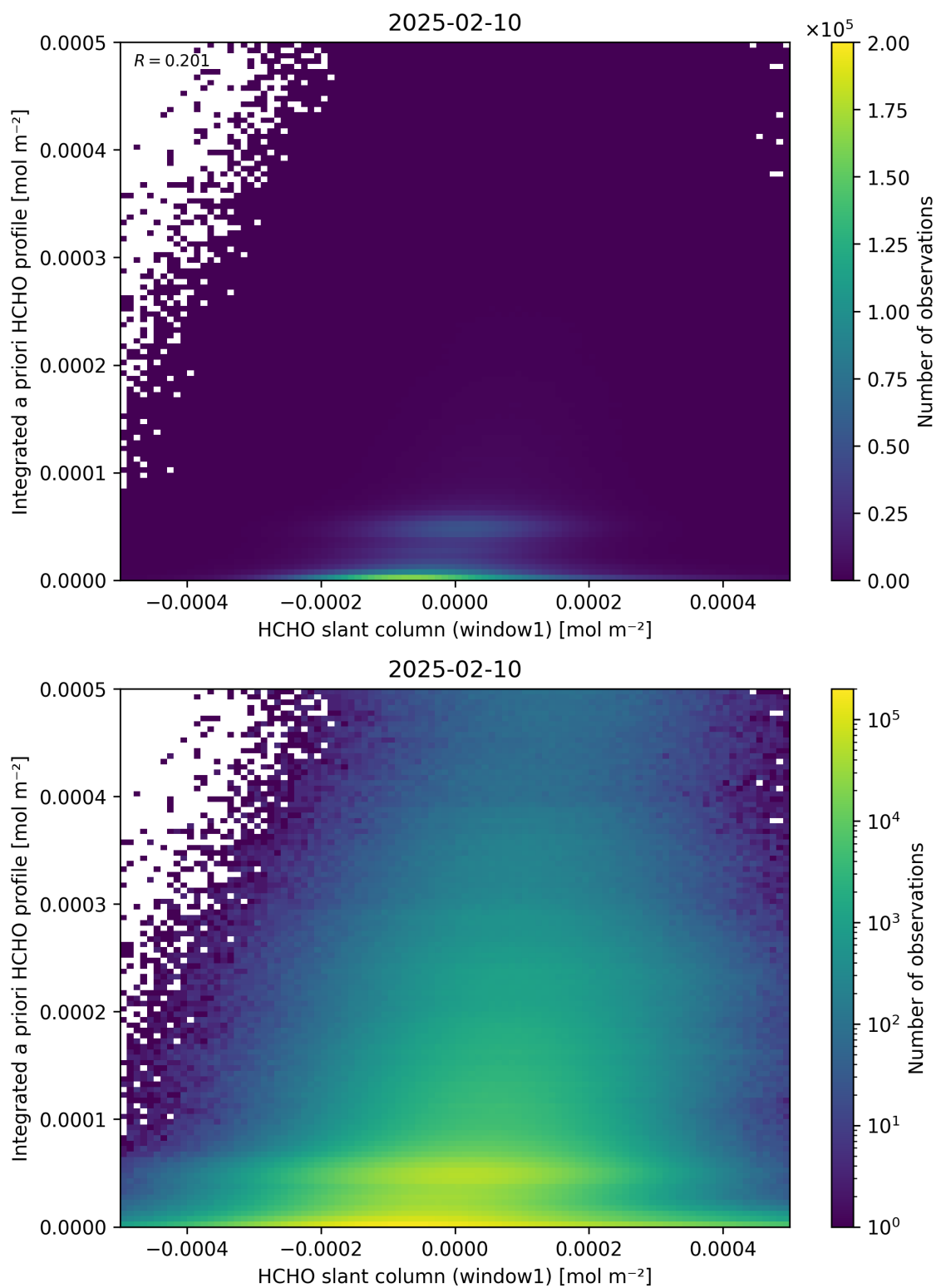
Figure 87: Scatter density plot of “HCHO slant column (window1)” against “Integrated a priori HCHO profile” for 2025-02-09 to 2025-02-11.
