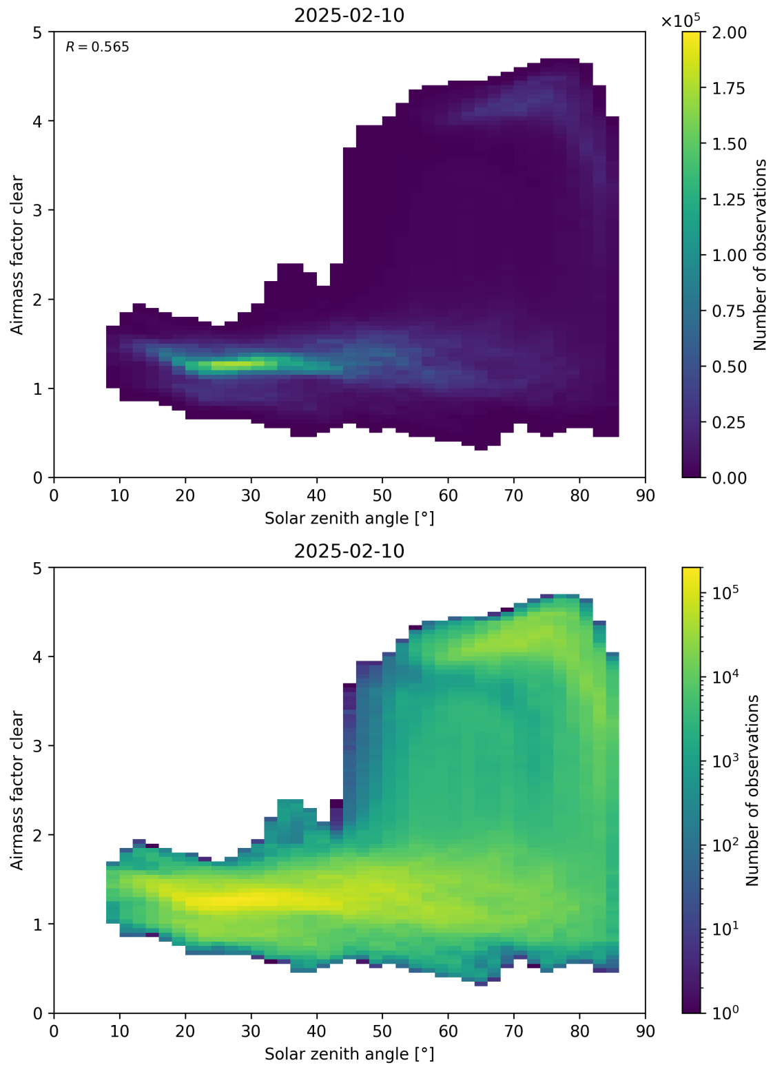
Figure 170: Scatter density plot of “Solar zenith angle” against “Airmass factor clear” for 2025-02-09 to 2025-02-11.
