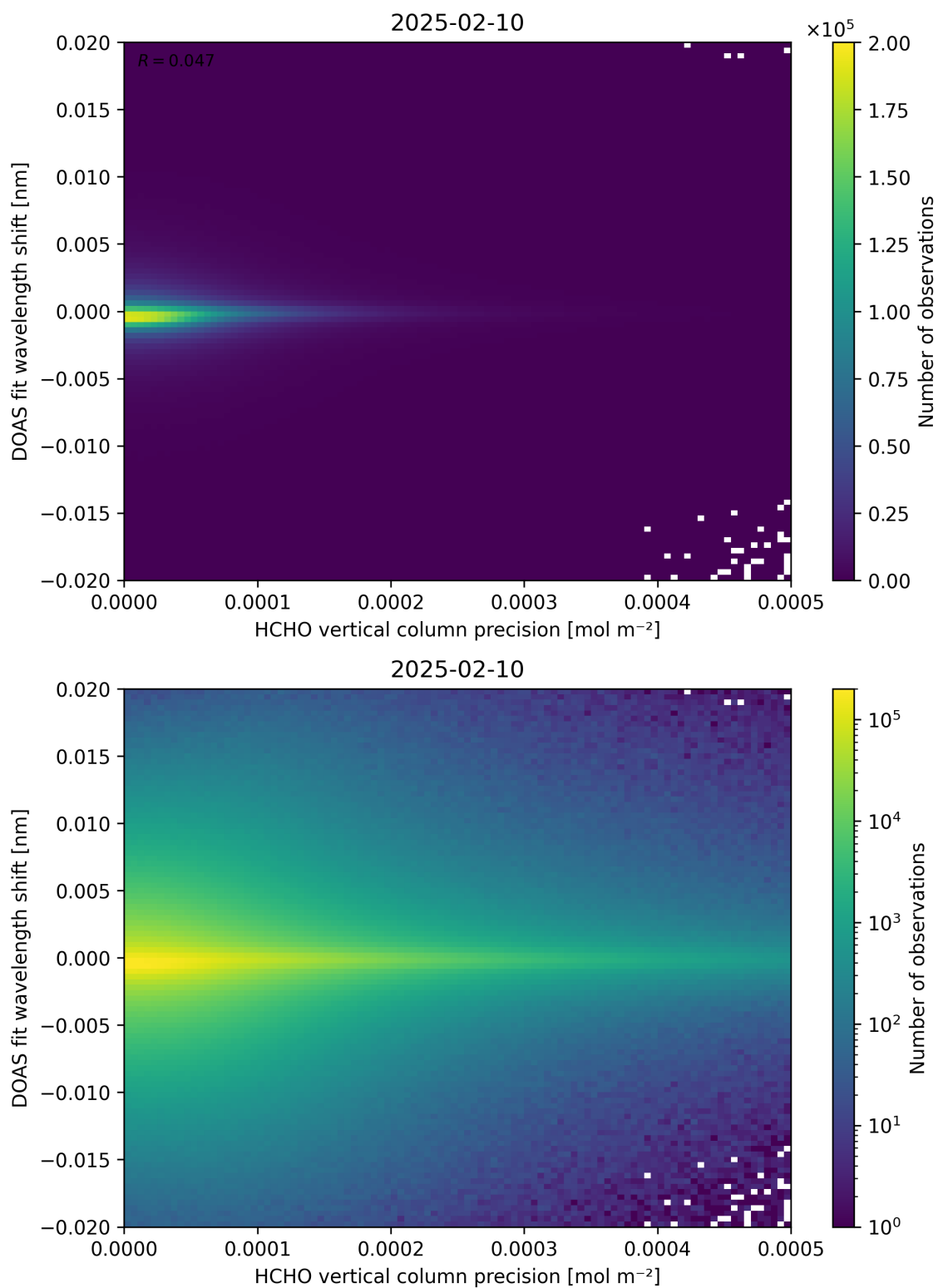
Figure 137: Scatter density plot of “HCHO vertical column precision” against “DOAS fit wavelength shift” for 2025-02-09 to 2025-02-11.
