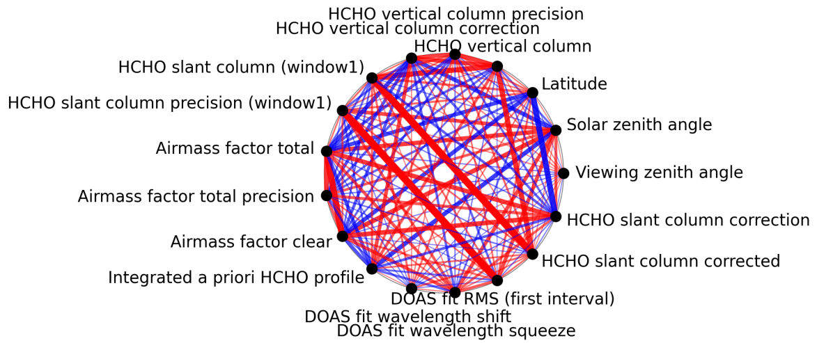
Figure 1: Map of correlation graph for 2025-02-09 to 2025-02-11.
