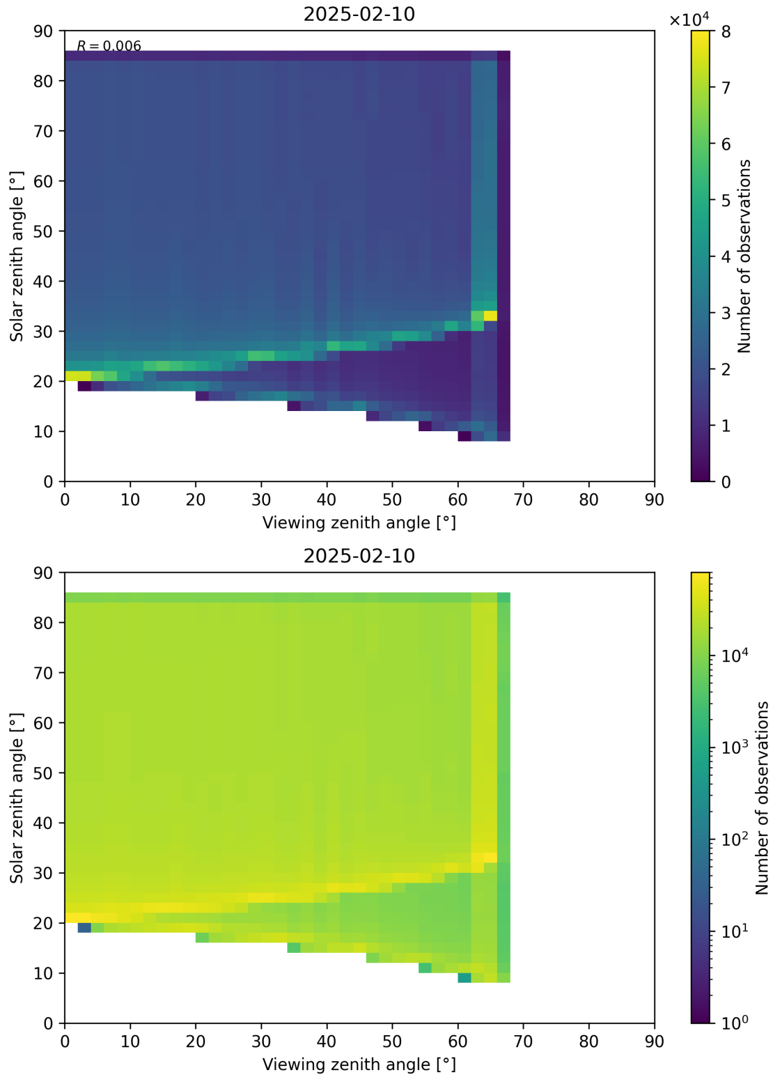
Figure 197: Scatter density plot of “Viewing zenith angle” against “Solar zenith angle” for 2025-02-09 to 2025-02-11.
