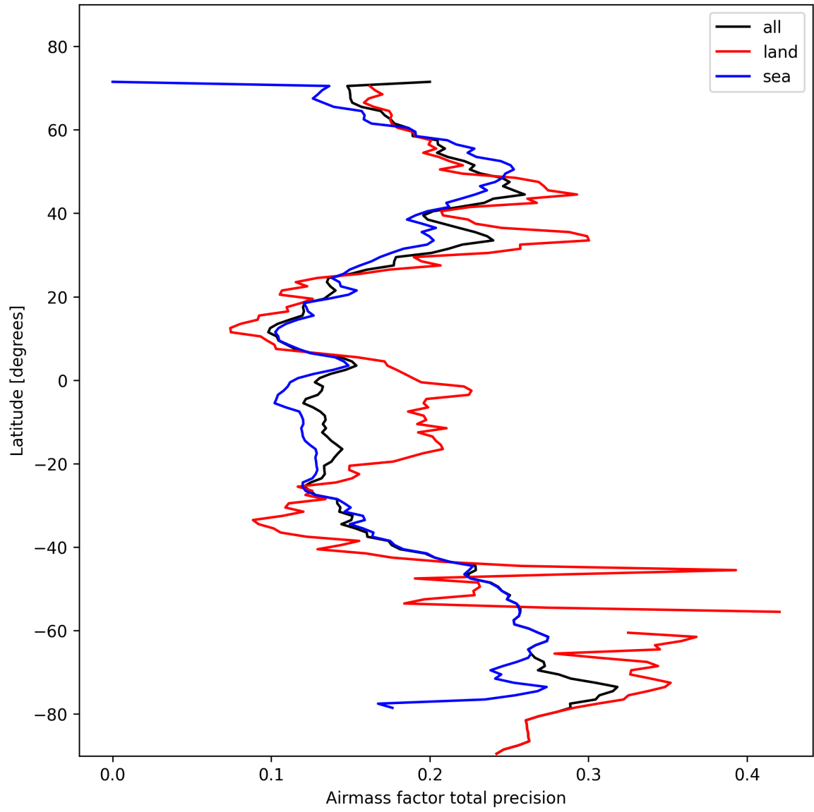
Figure 27: Zonal average of “Airmass factor total precision” for 2025-02-09 to 2025-02-11.
