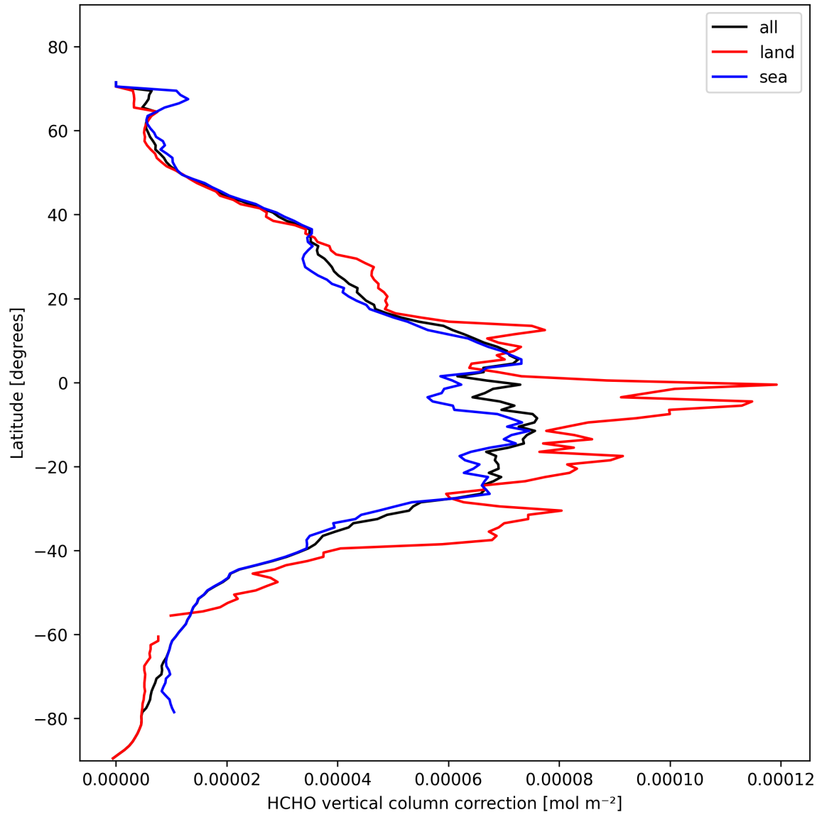
Figure 23: Zonal average of “HCHO vertical column correction” for 2025-02-09 to 2025-02-11.
