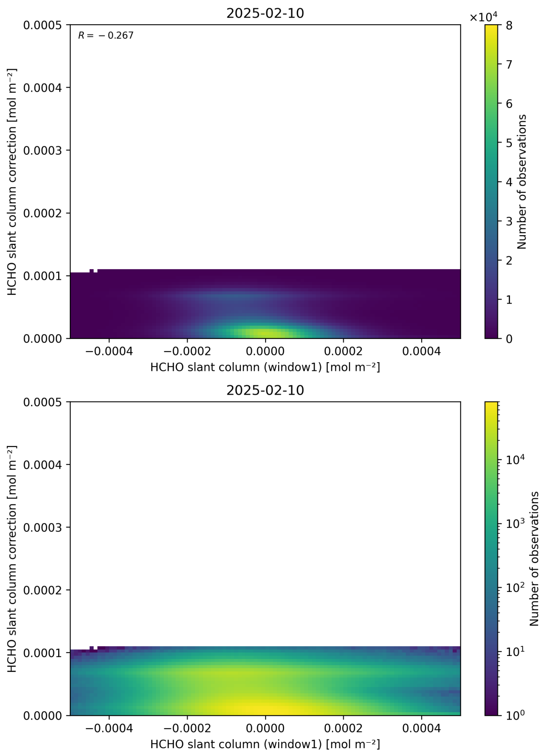
Figure 83: Scatter density plot of “HCHO slant column (window1)” against “HCHO slant column correction” for 2025-02-09 to 2025-02-11.
