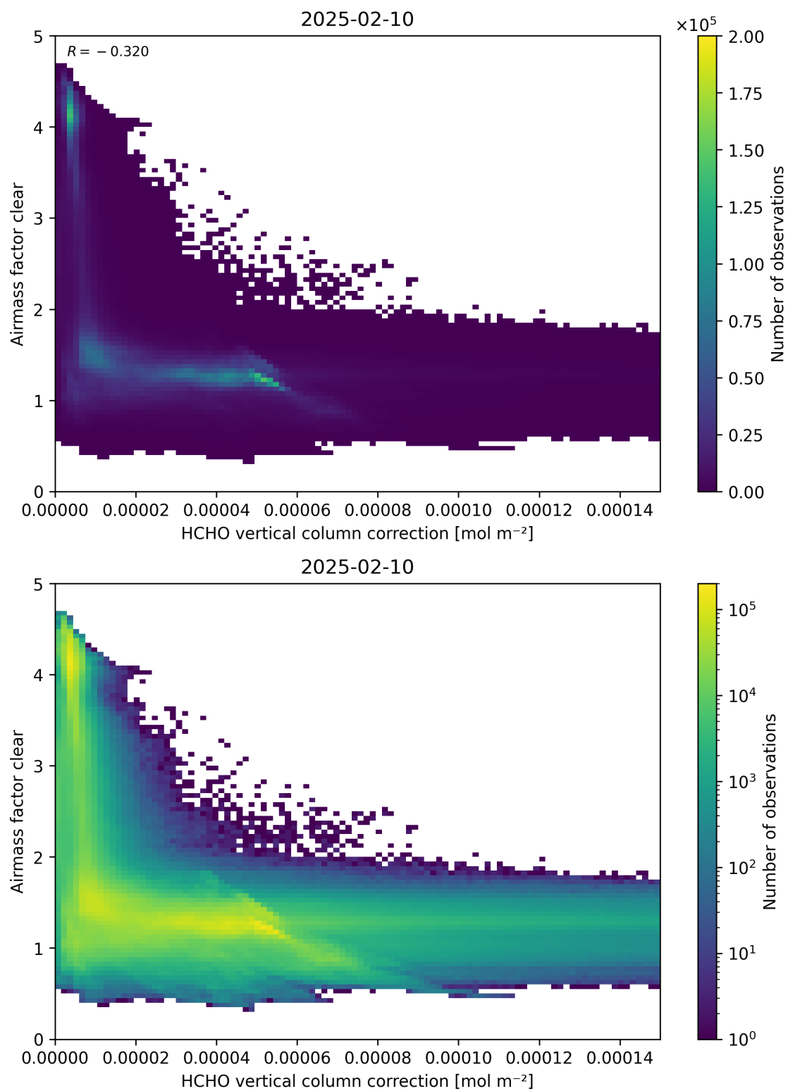
Figure 115: Scatter density plot of “HCHO vertical column correction” against “Airmass factor clear” for 2025-02-09 to 2025-02-11.
