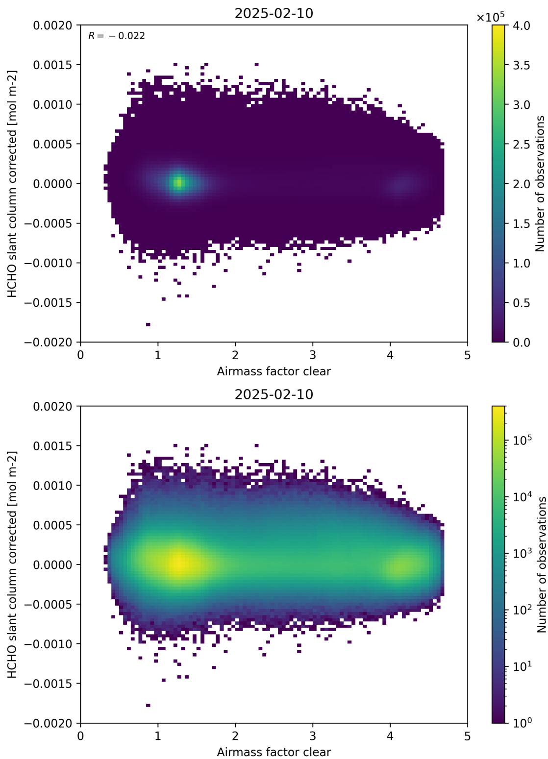
Figure 74: Scatter density plot of “Airmass factor clear” against “HCHO slant column corrected” for 2025-02-09 to 2025-02-11.
