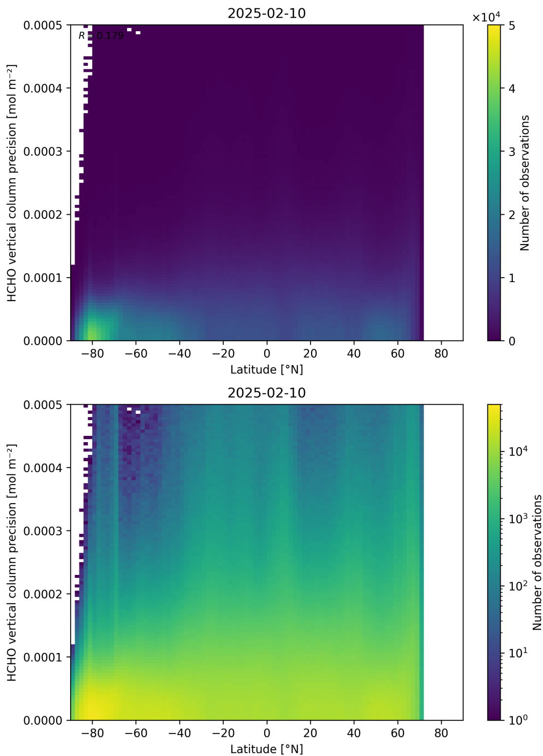
Figure 165: Scatter density plot of “Latitude” against “HCHO vertical column precision” for 2025-02-09 to 2025-02-11.
