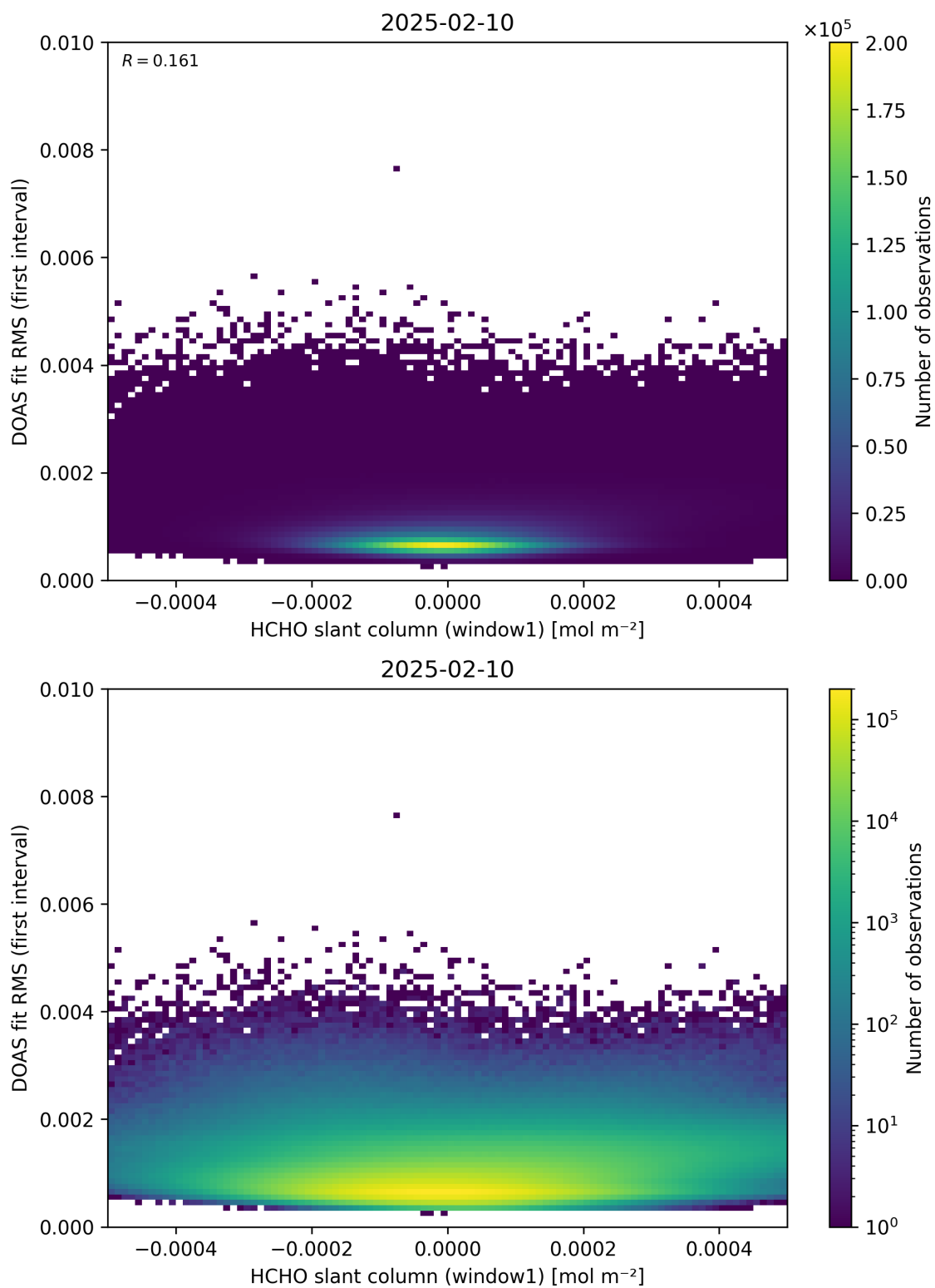
Figure 78: Scatter density plot of “HCHO slant column (window1)” against “DOAS fit RMS (first interval)” for 2025-02-09 to 2025-02-11.
