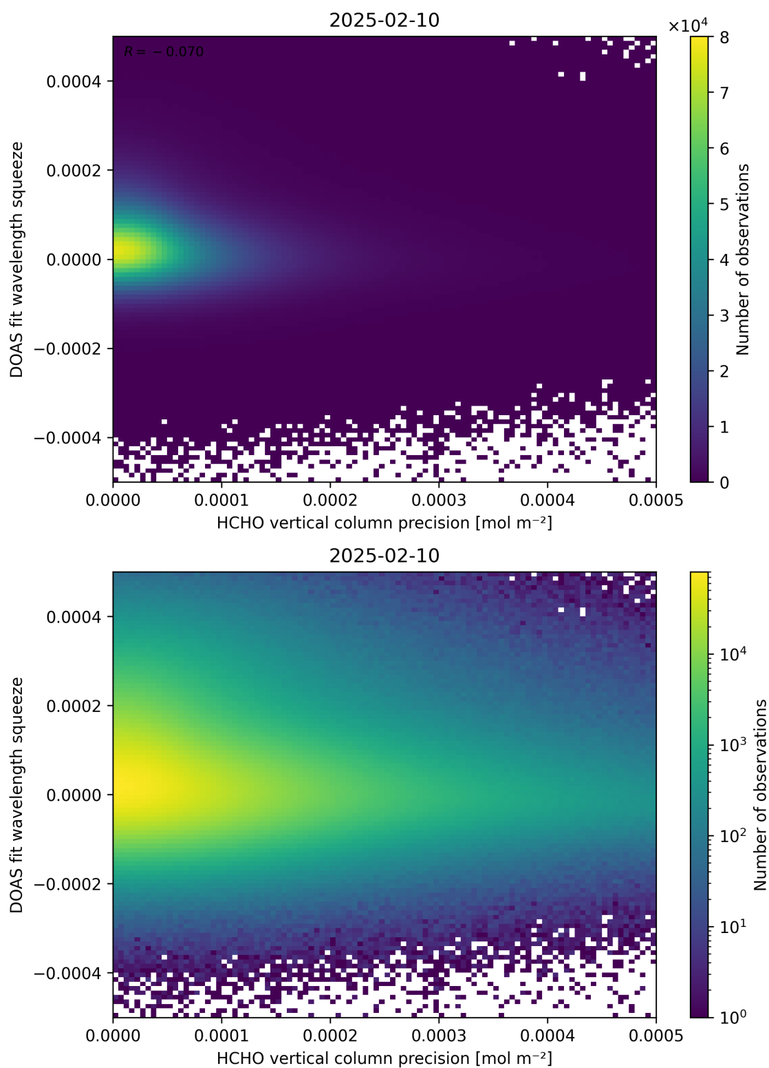
Figure 138: Scatter density plot of “HCHO vertical column precision” against “DOAS fit wavelength squeeze” for 2025-02-09 to 2025-02-11.
