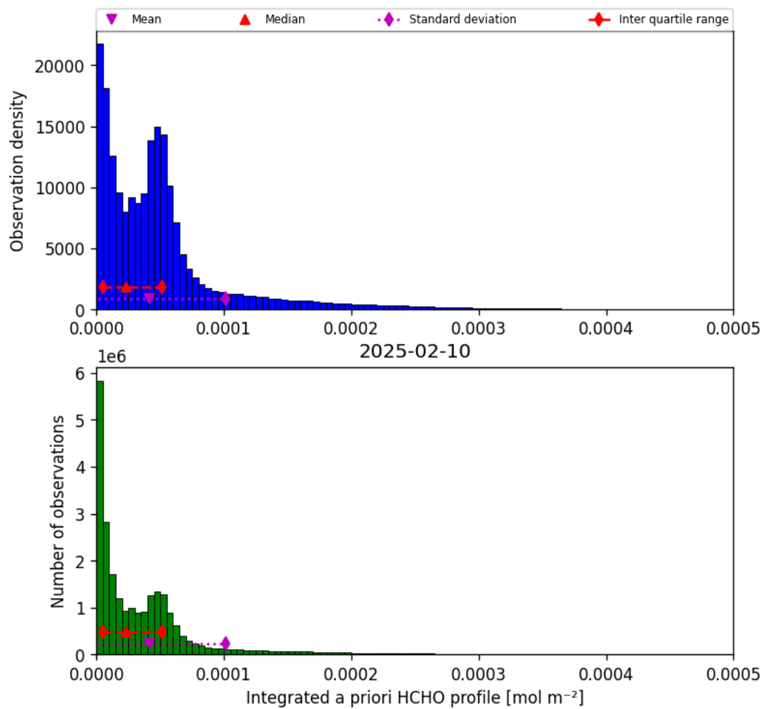
Figure 43: Histogram of “Integrated a priori HCHO profile” for 2025-02-09 to 2025-02-11
