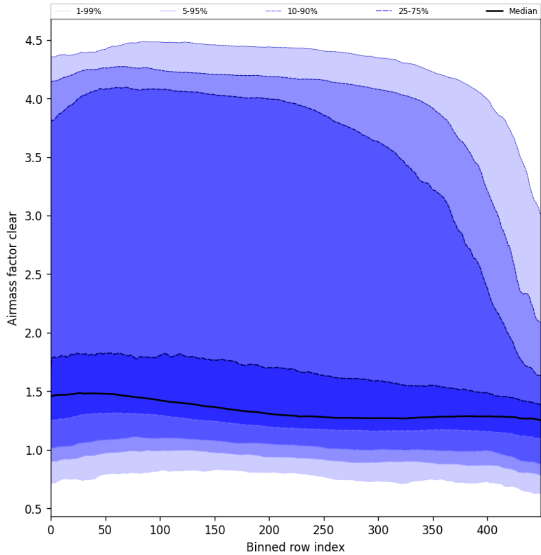
Figure 56: Along track statistics of “Air mass factor clear” for 2025-02-09 to 2025-02-11
