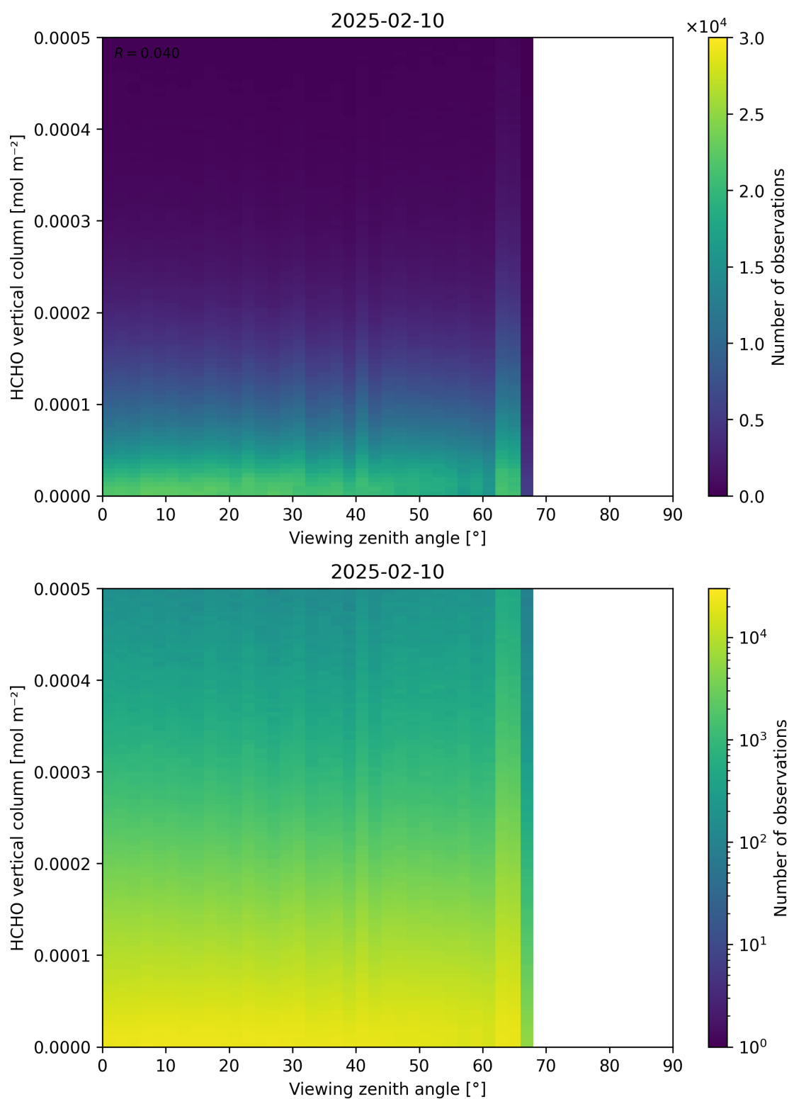
Figure 192: Scatter density plot of “Viewing zenith angle” against “HCHO vertical column” for 2025-02-09 to 2025-02-11.
