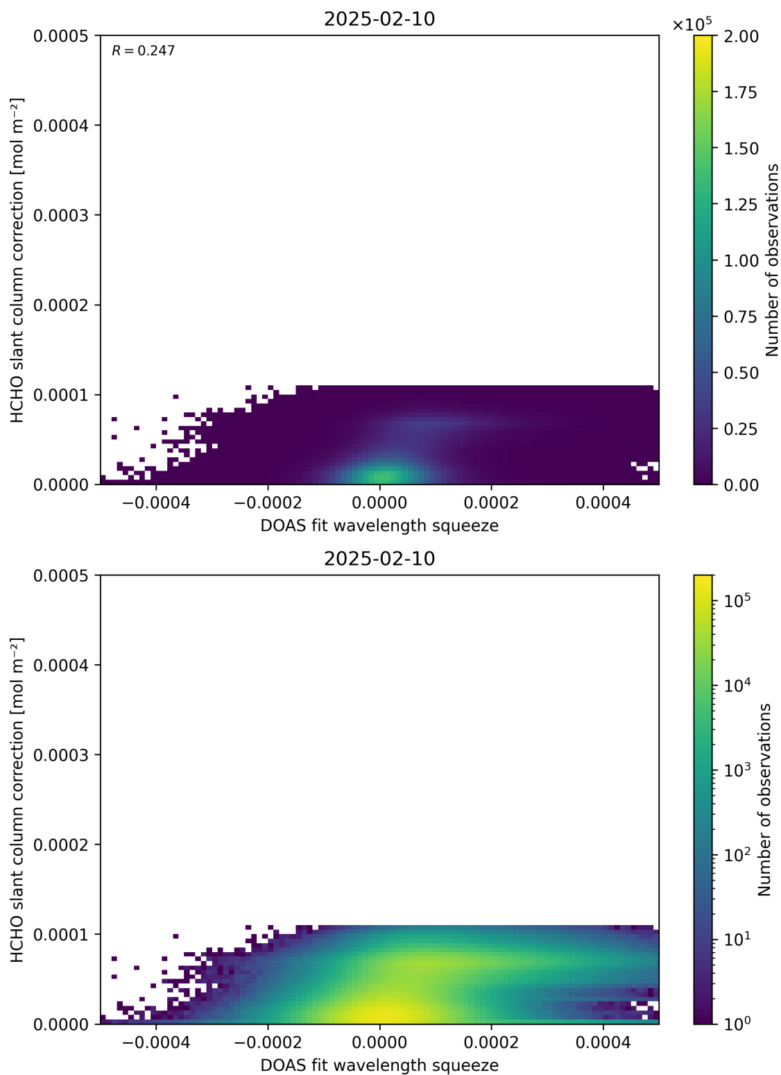
Figure 70: Scatter density plot of “DOAS fit wavelength squeeze” against “HCHO slant column correction” for 2025-02-09 to 2025-02-11.
