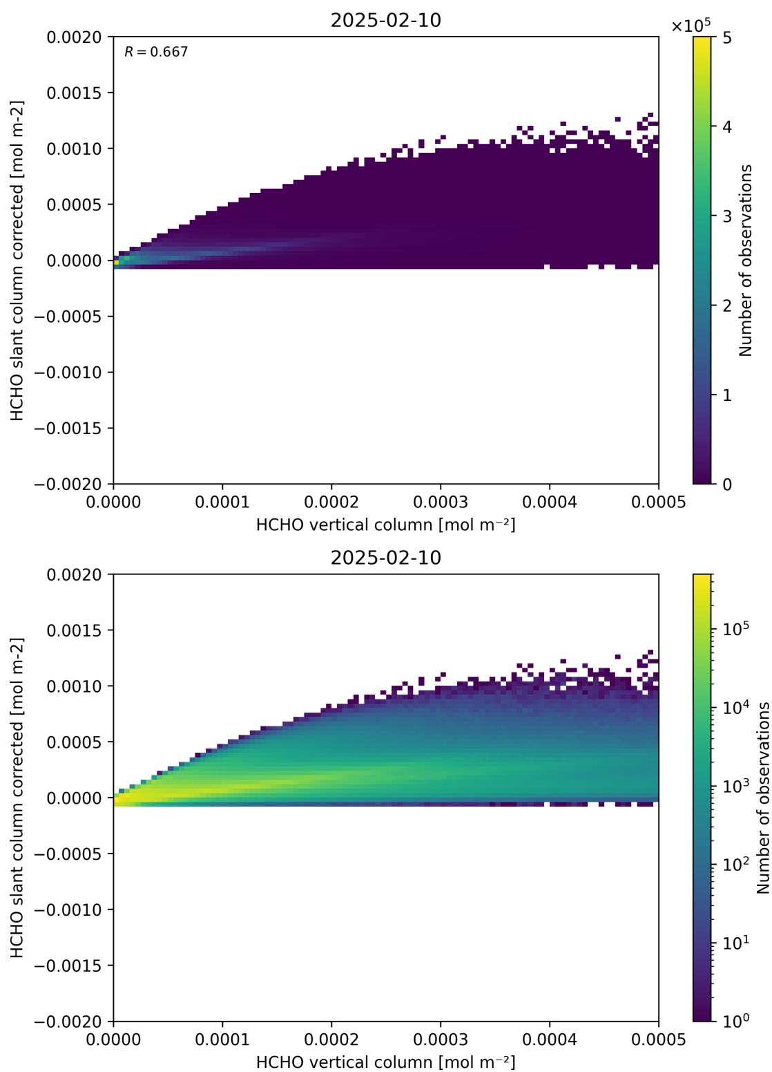
Figure 127: Scatter density plot of “HCHO vertical column” against “HCHO slant column corrected” for 2025-02-09 to 2025-02-11.
