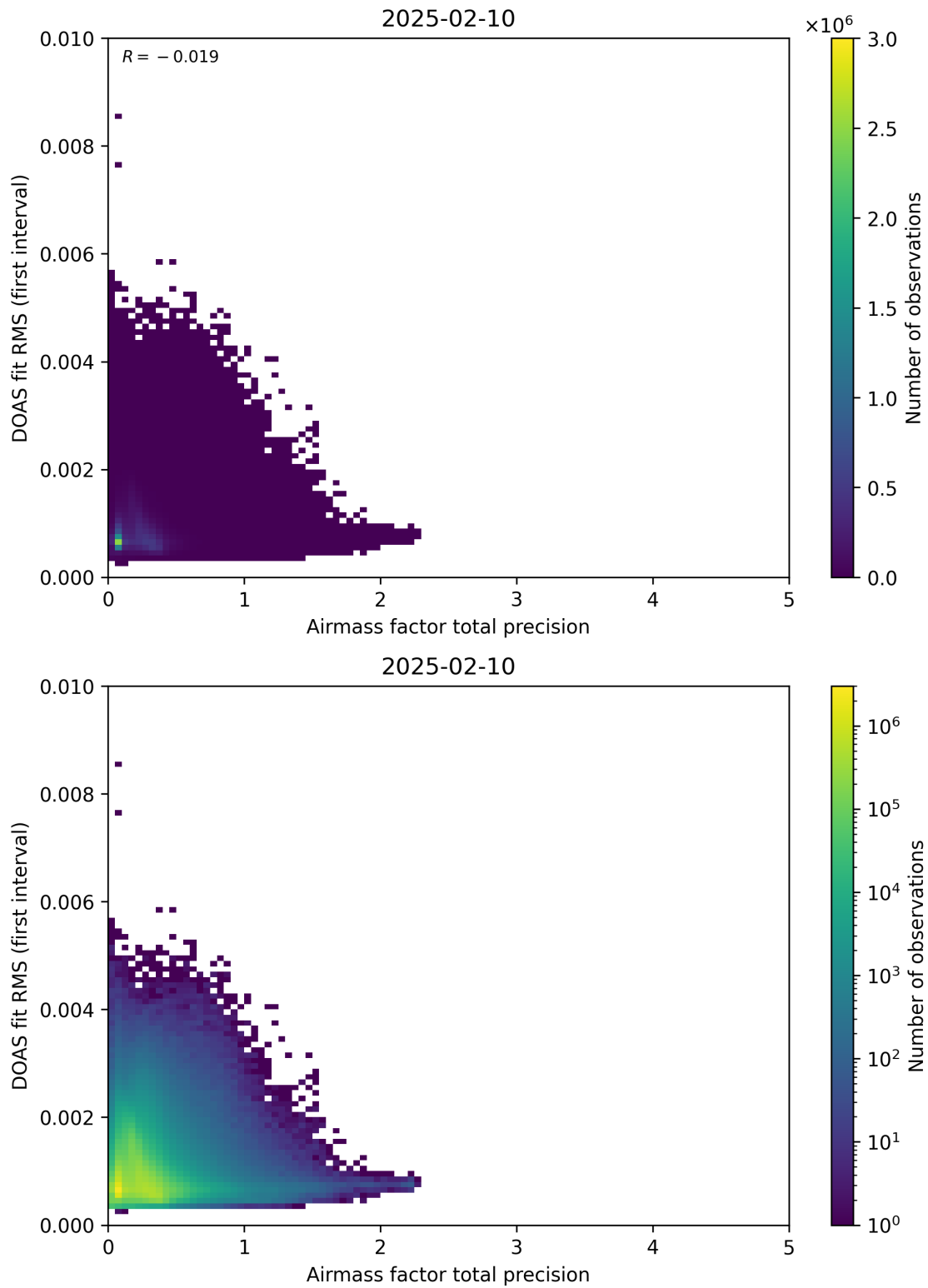
Figure 105: Scatter density plot of “Airmass factor total precision” against “DOAS fit RMS (first interval)” for 2025-02-09 to 2025-02-11.
