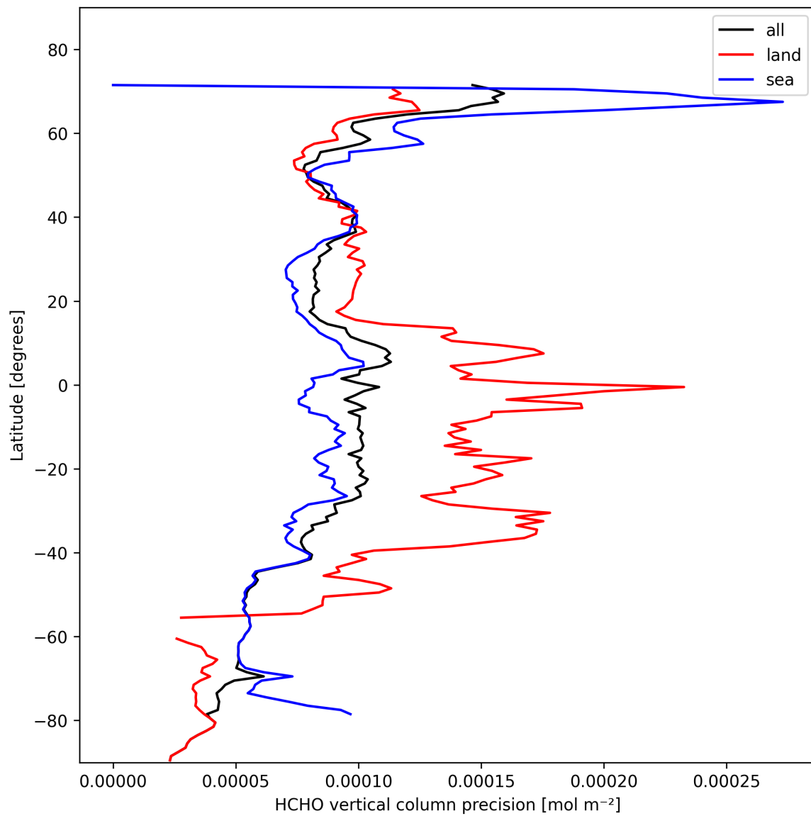
Figure 22: Zonal average of “HCHO vertical column precision” for 2025-02-09 to 2025-02-11.
