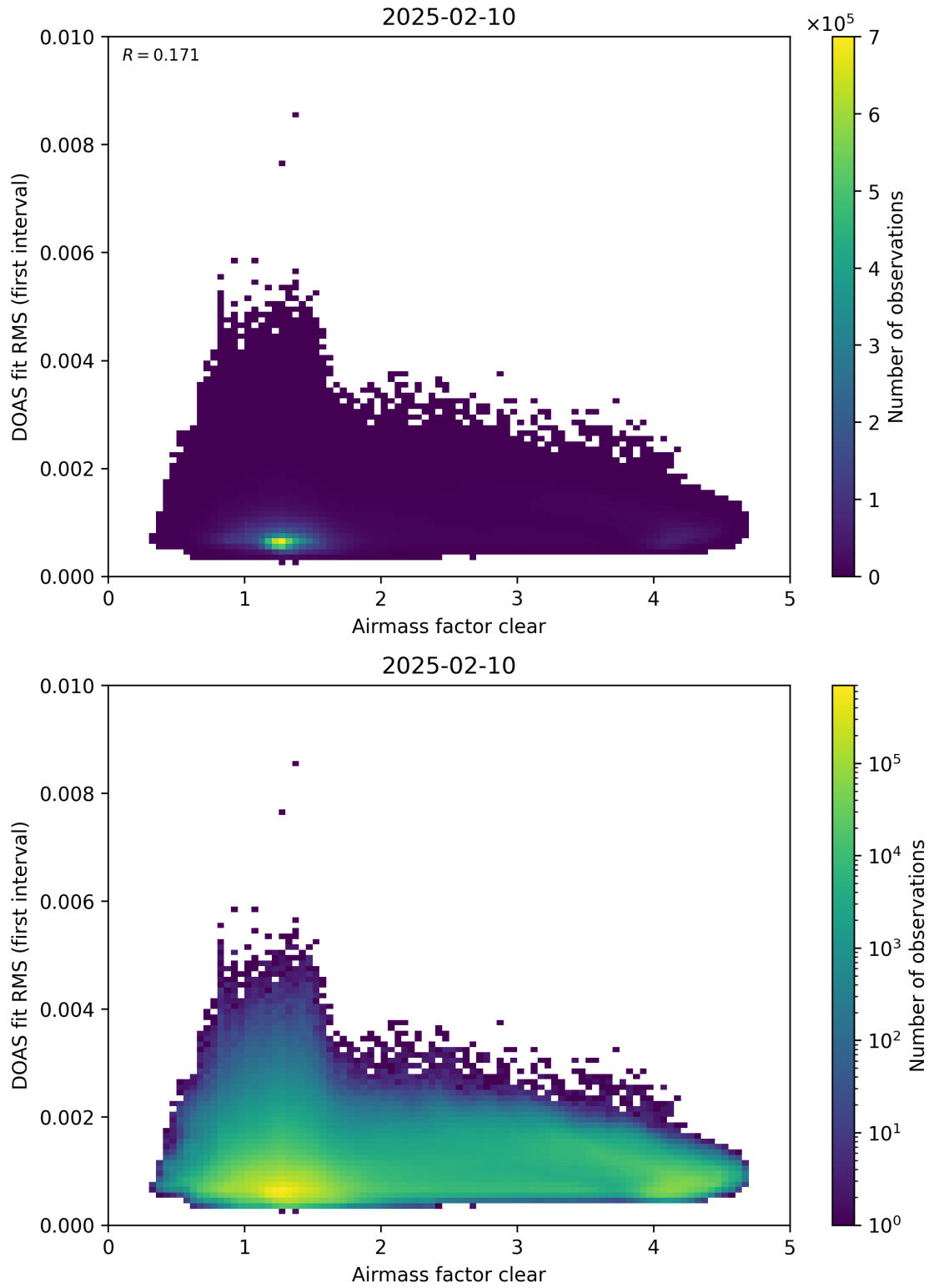
Figure 71: Scatter density plot of “Airmass factor clear” against “DOAS fit RMS (first interval)” for 2025-02-09 to 2025-02-11.
