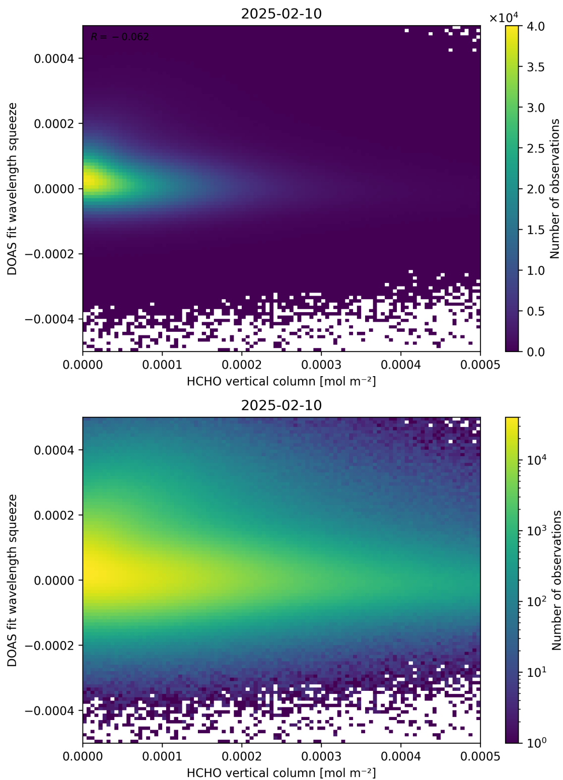
Figure 125: Scatter density plot of “HCHO vertical column” against “DOAS fit wavelength squeeze” for 2025-02-09 to 2025-02-11.
