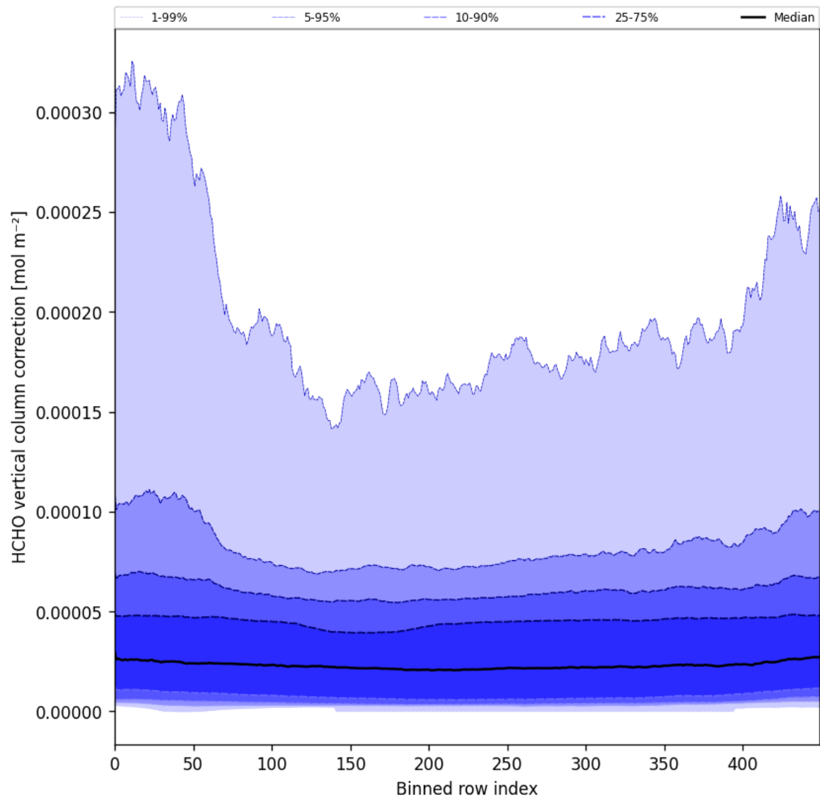
Figure 51: Along track statistics of “HCHO vertical column correction” for 2025-02-09 to 2025-02-11
