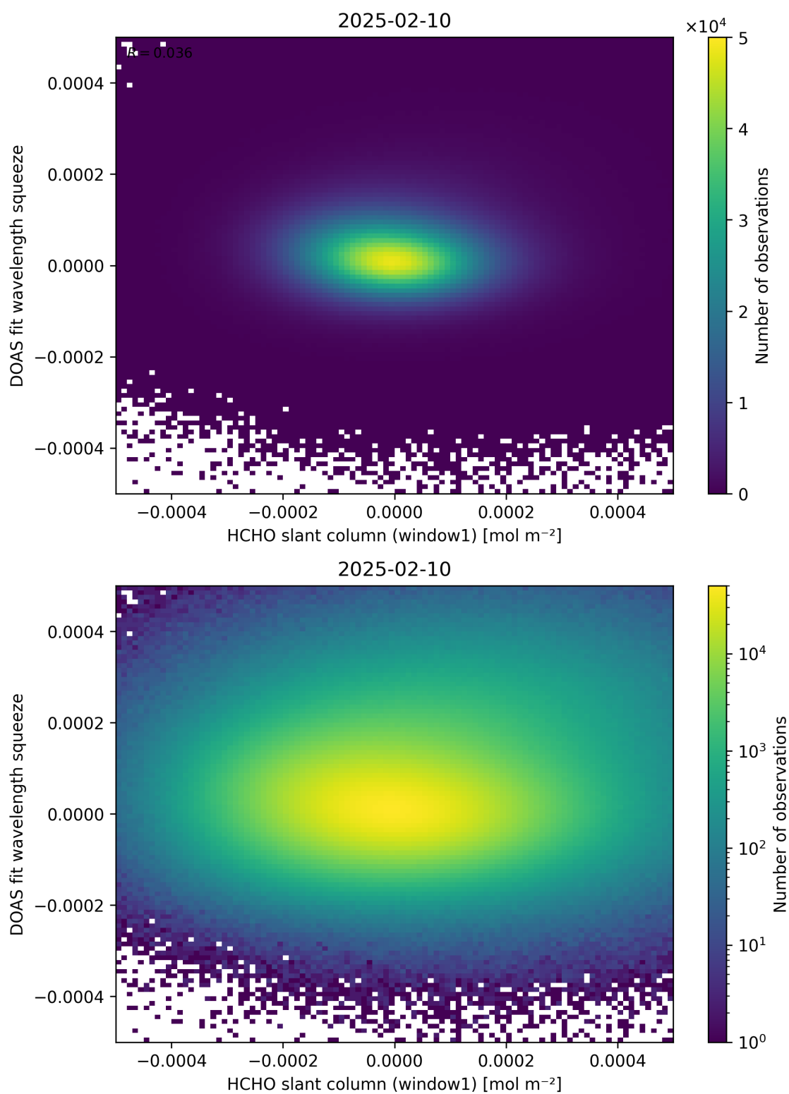
Figure 80: Scatter density plot of “HCHO slant column (window1)” against “DOAS fit wavelength squeeze” for 2025-02-09 to 2025-02-11.
