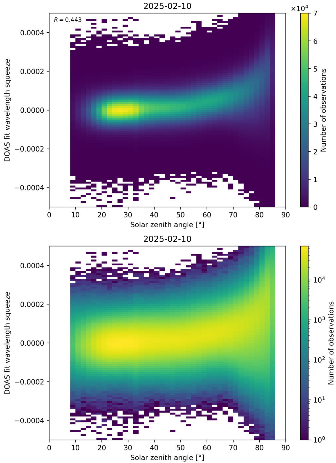
Figure 169: Scatter density plot of “Solar zenith angle” against “DOAS fit wavelength squeeze” for 2025-02-09 to 2025-02-11.
