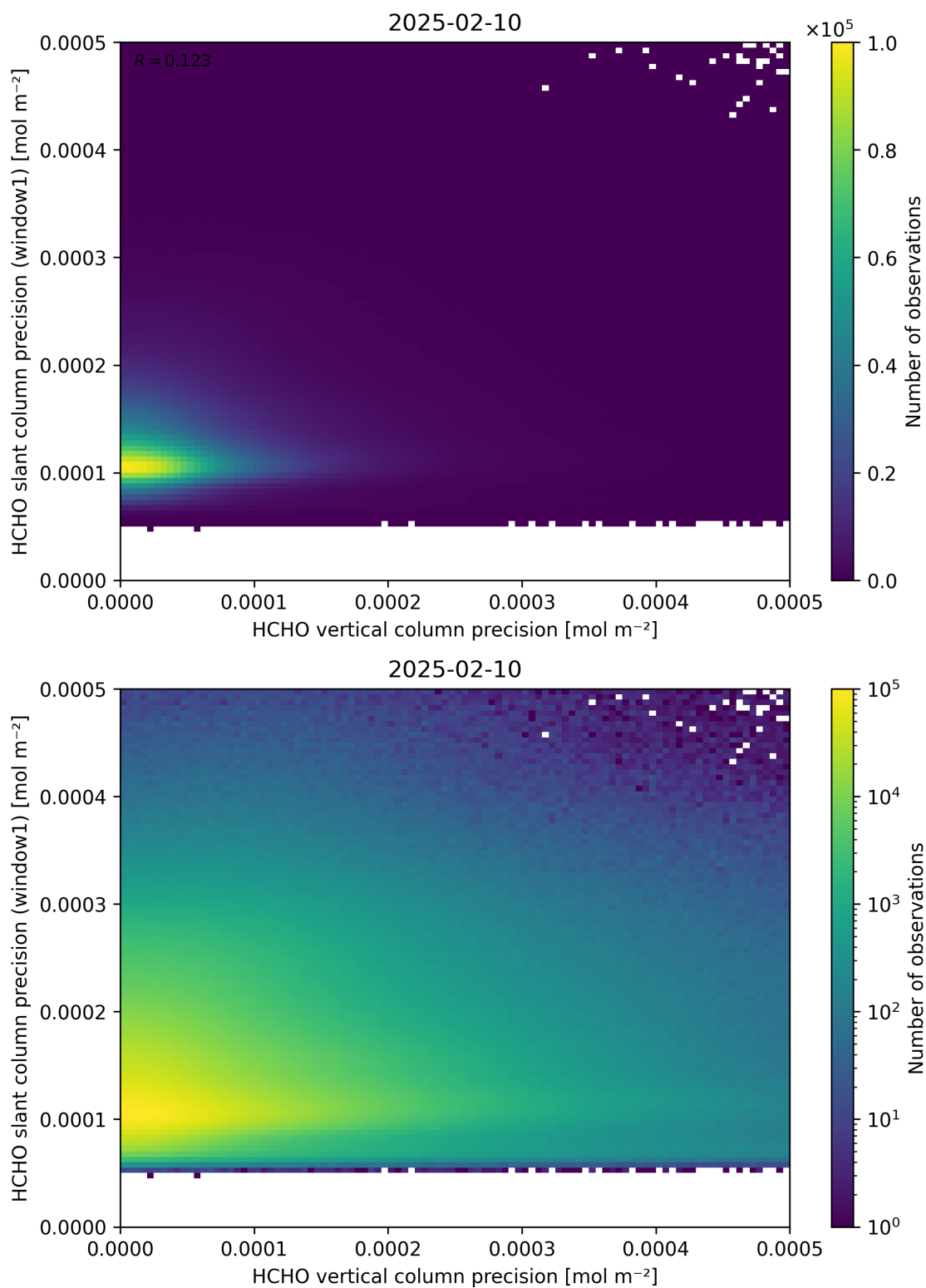
Figure 143: Scatter density plot of “HCHO vertical column precision” against “HCHO slant column precision (window1)” for 2025-02-09 to 2025-02-11.
