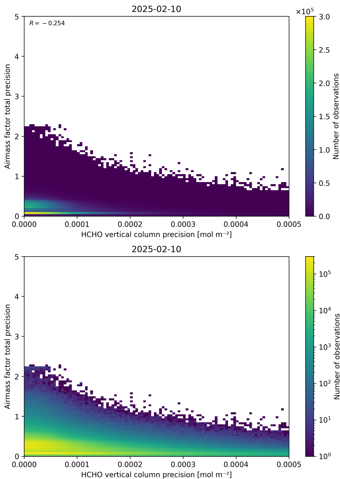
Figure 145: Scatter density plot of “HCHO vertical column precision” against “Airmass factor total precision” for 2025-02-09 to 2025-02-11.
