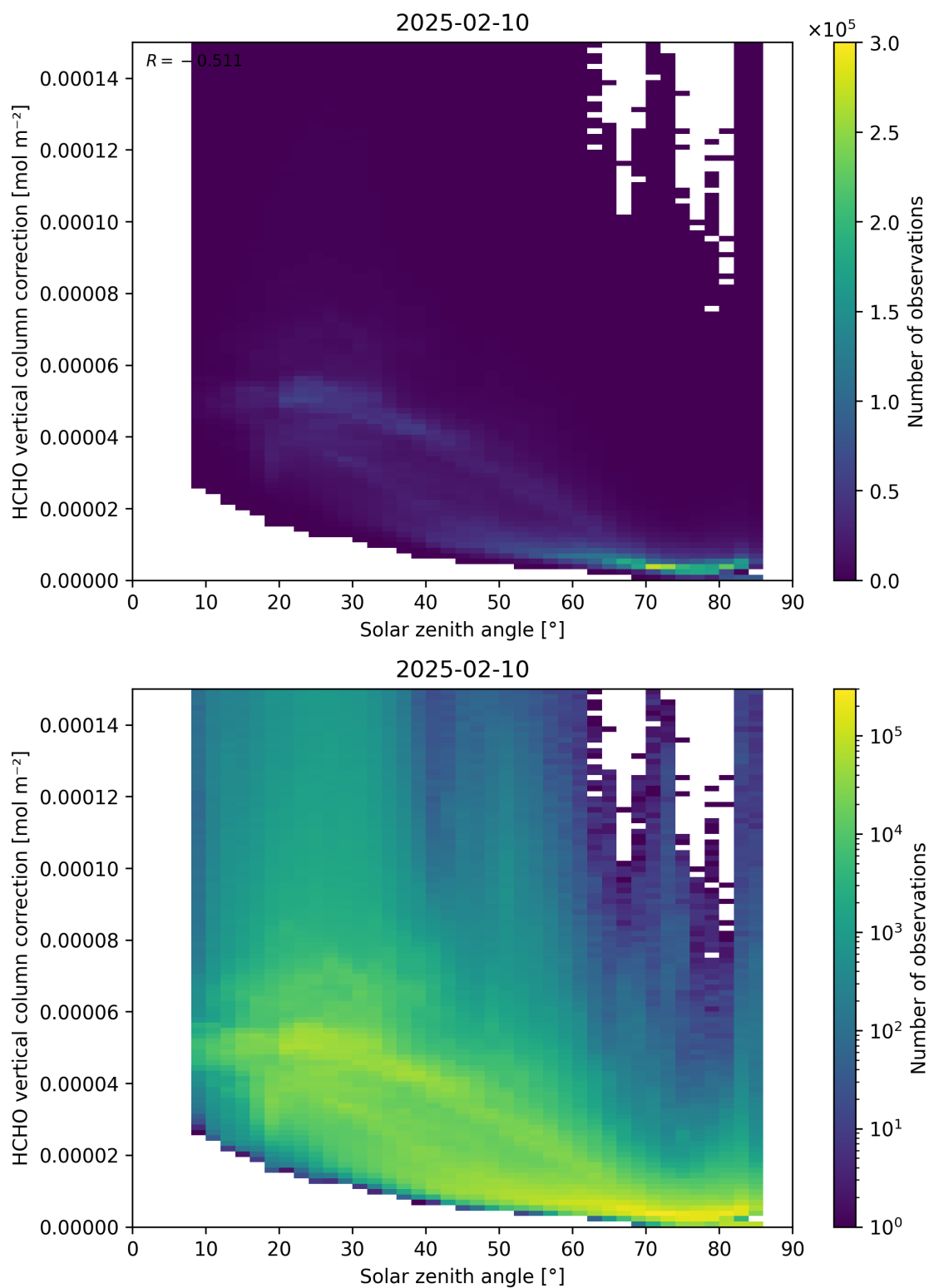
Figure 178: Scatter density plot of “Solar zenith angle” against “HCHO vertical column correction” for 2025-02-09 to 2025-02-11.
