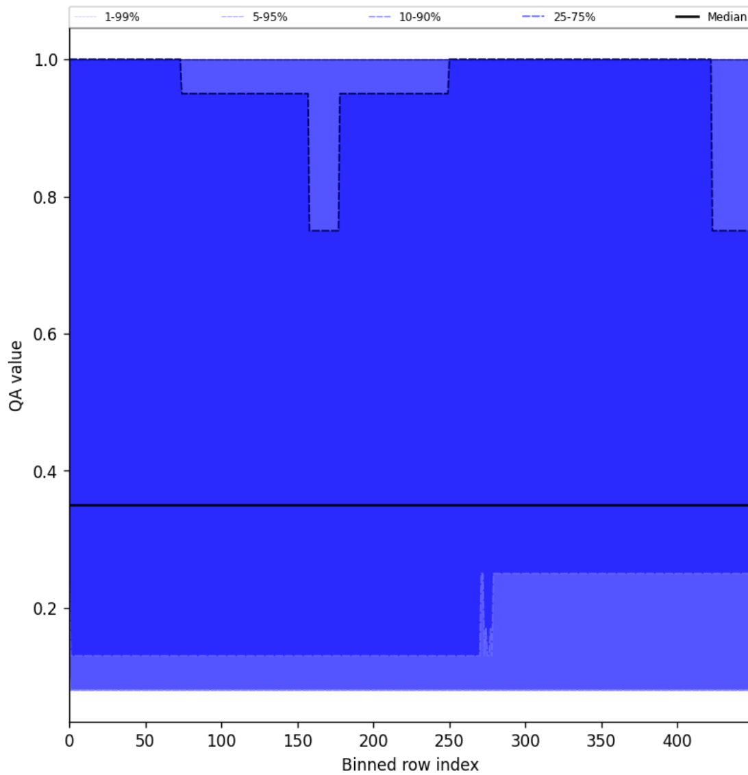
Figure 48: Along track statistics of “QA value” for 2025-02-09 to 2025-02-11
