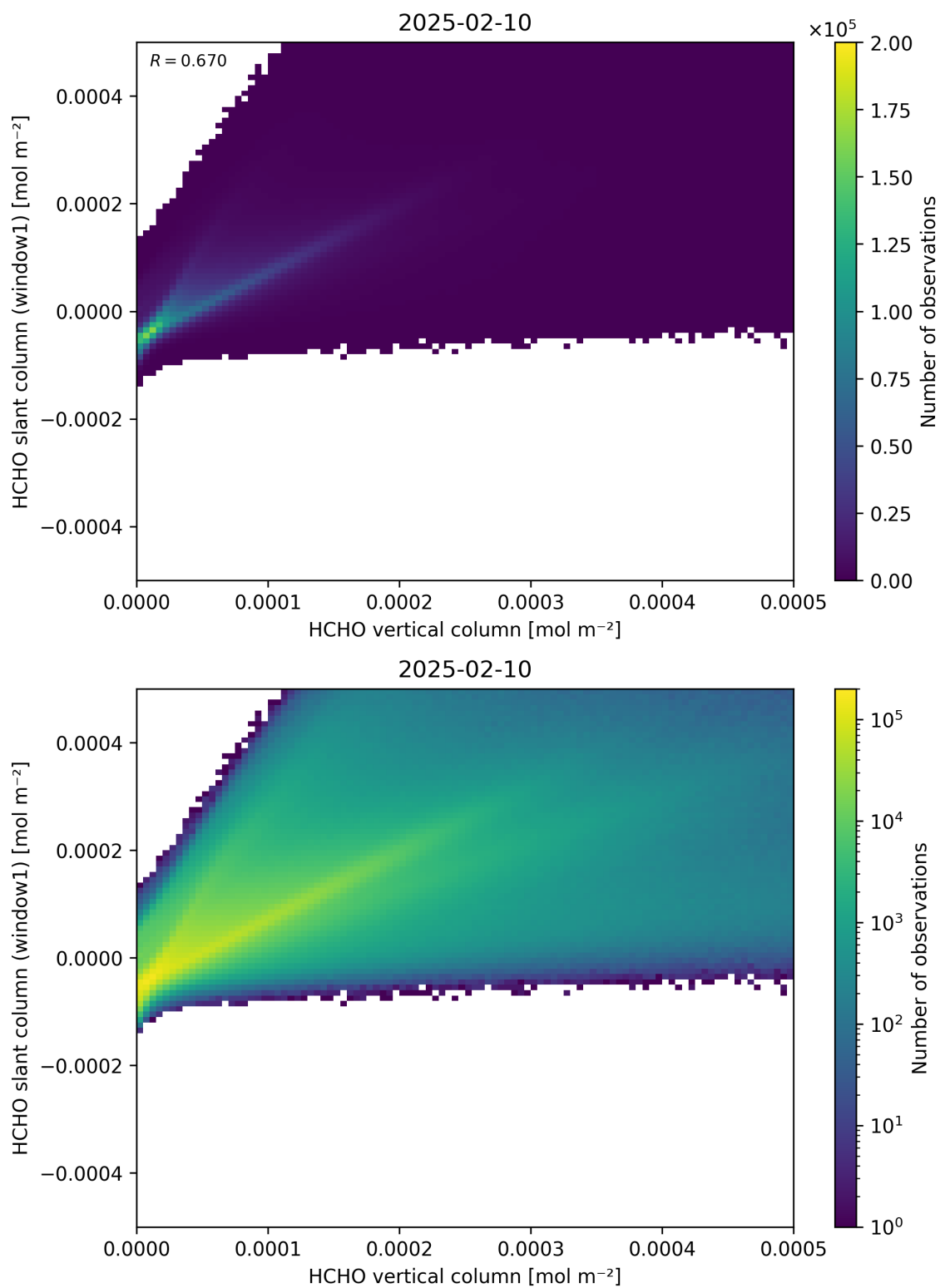
Figure 129: Scatter density plot of “HCHO vertical column” against “HCHO slant column (window1)” for 2025-02-09 to 2025-02-11.
