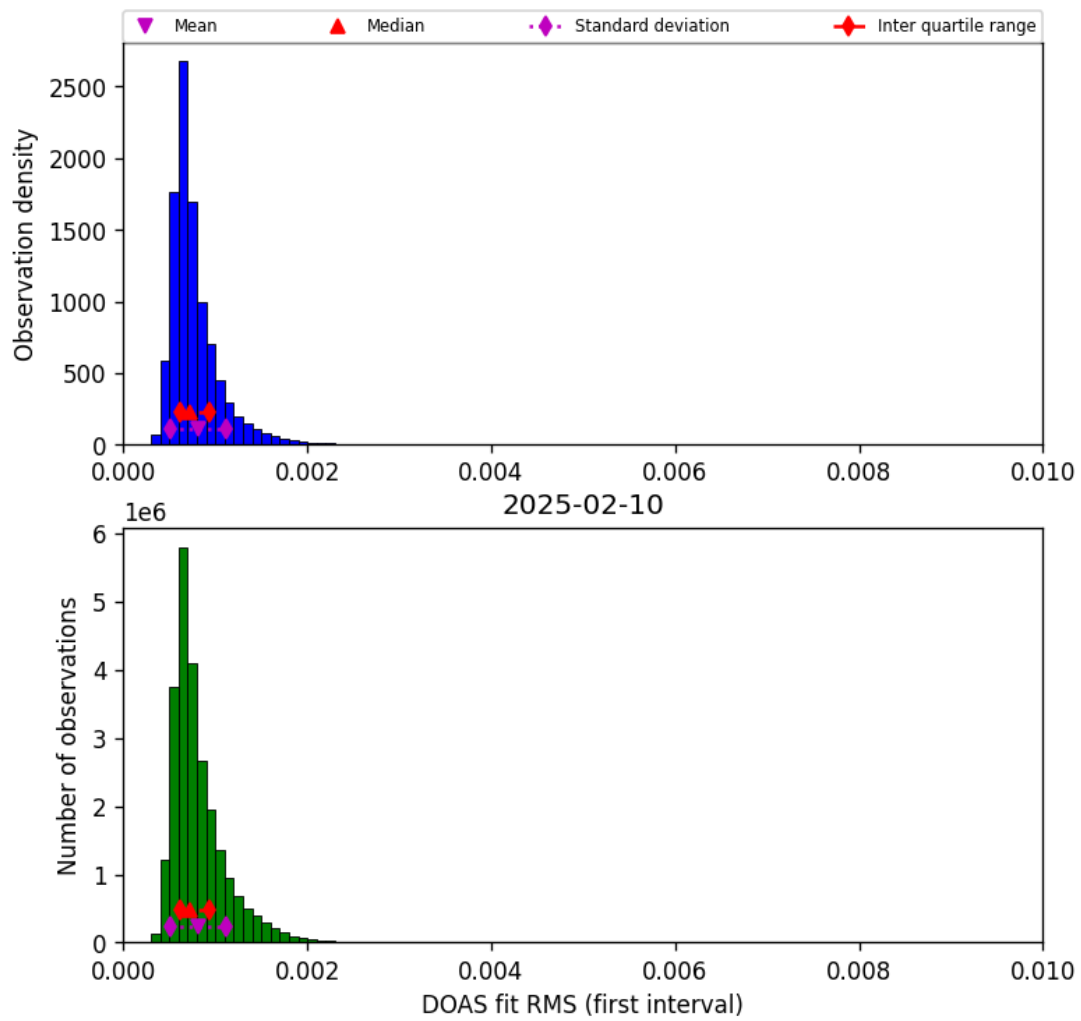
Figure 46: Histogram of “DOAS fit RMS (first interval)” for 2025-02-09 to 2025-02-11
