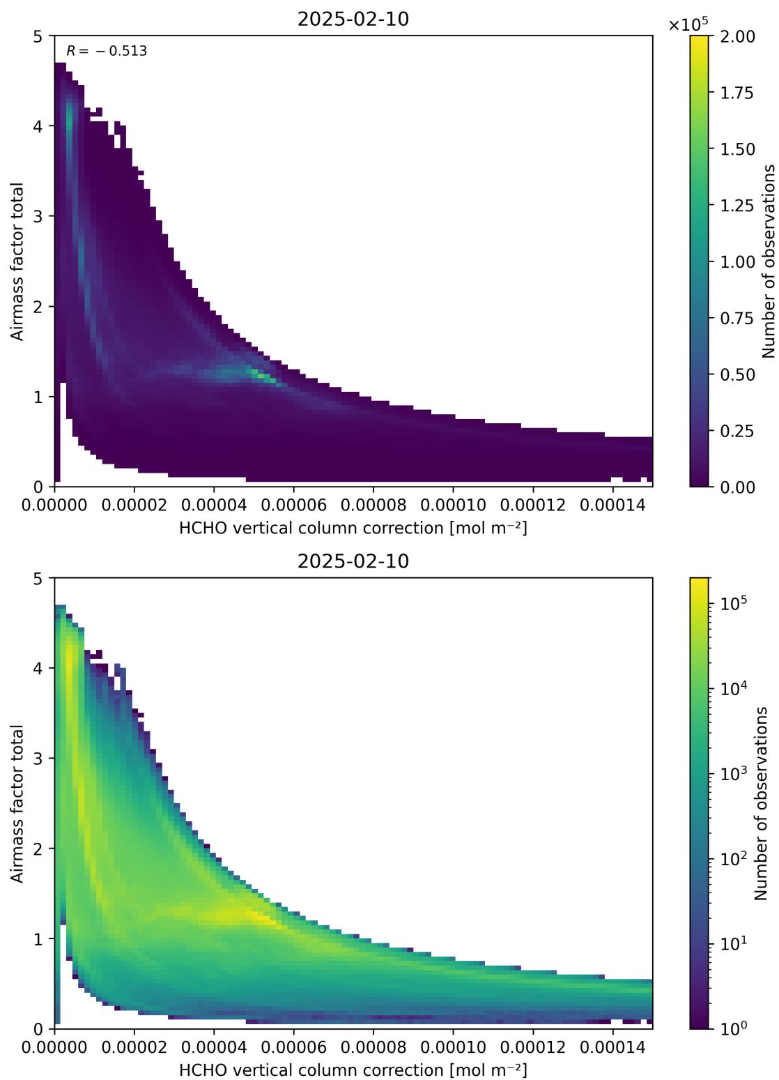
Figure 120: Scatter density plot of “HCHO vertical column correction” against “Airmass factor total” for 2025-02-09 to 2025-02-11.
