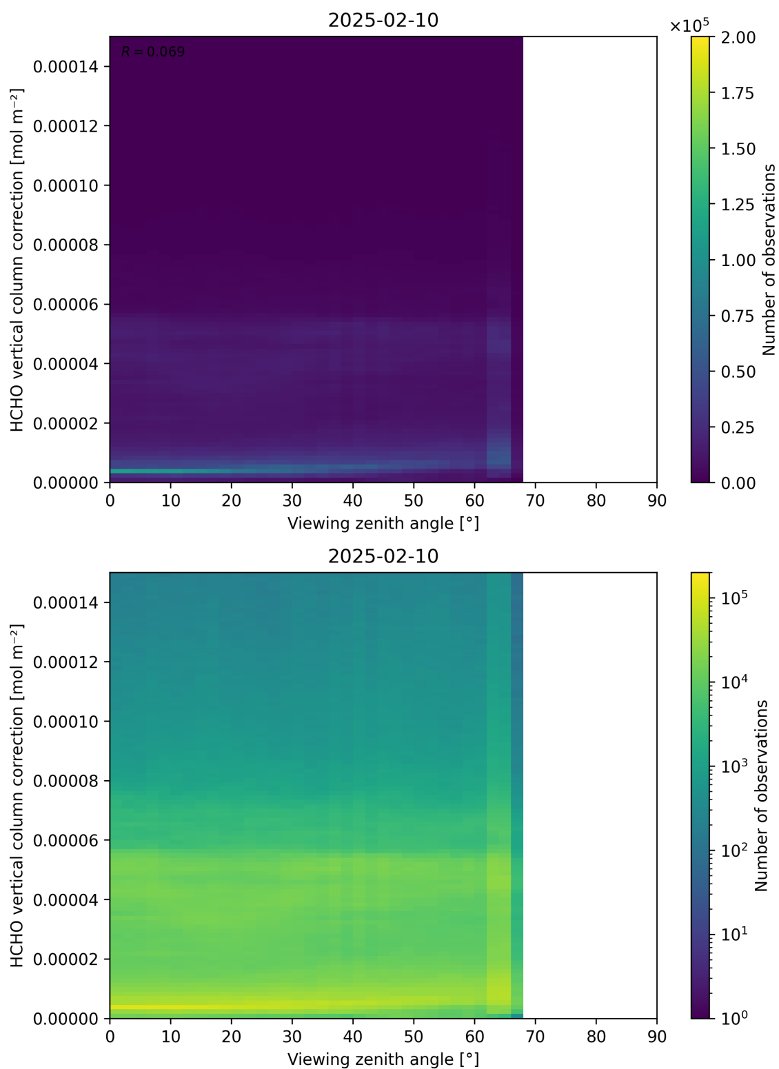
Figure 193: Scatter density plot of “Viewing zenith angle” against “HCHO vertical column correction” for 2025-02-09 to 2025-02-11.
