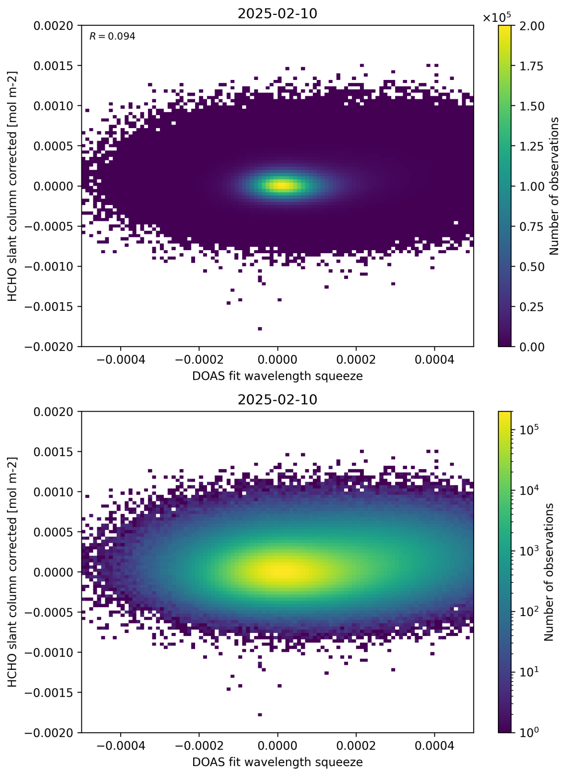
Figure 69: Scatter density plot of “DOAS fit wavelength squeeze” against “HCHO slant column corrected” for 2025-02-09 to 2025-02-11.
