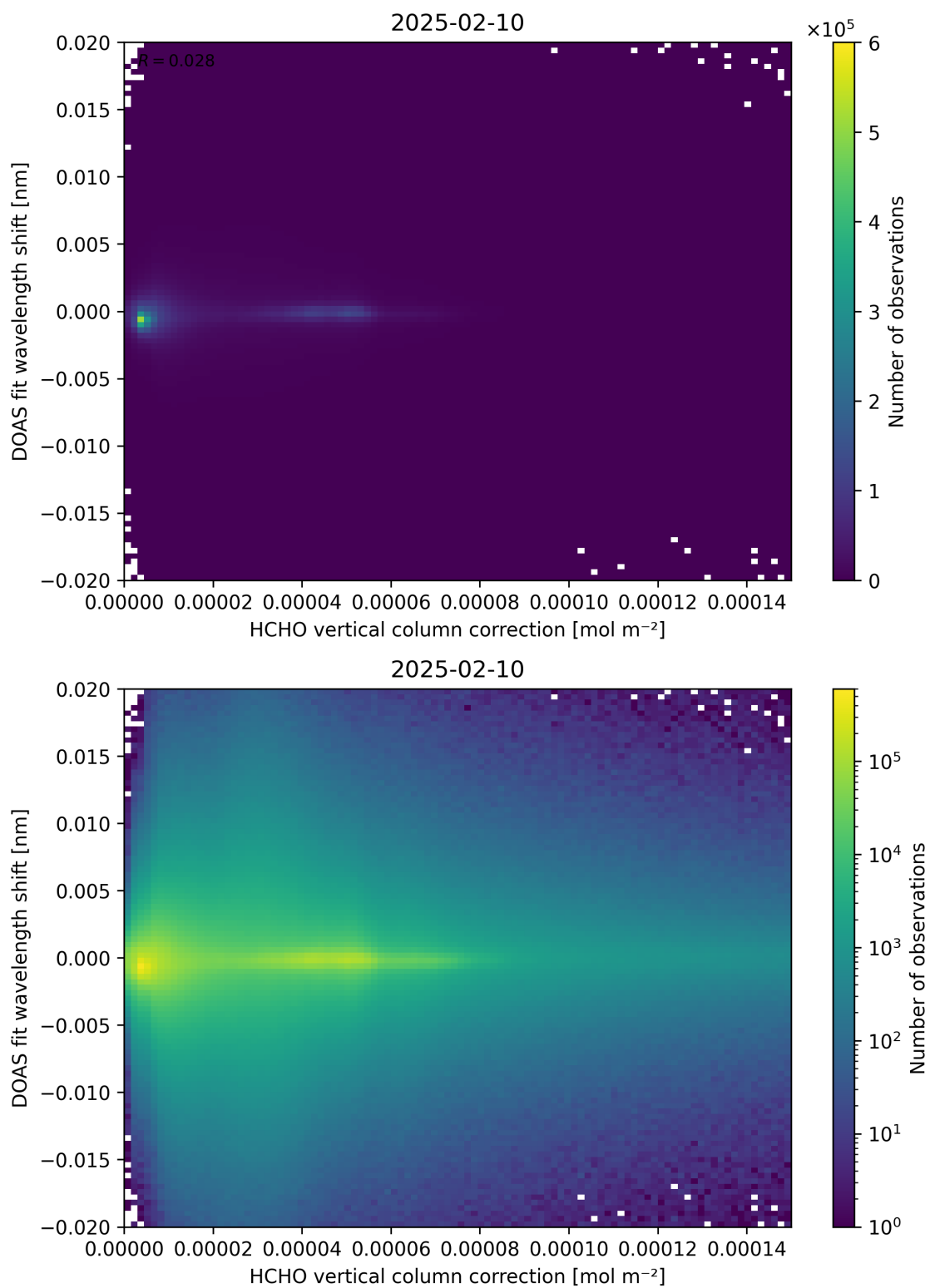
Figure 113: Scatter density plot of “HCHO vertical column correction” against “DOAS fit wavelength shift” for 2025-02-09 to 2025-02-11.
