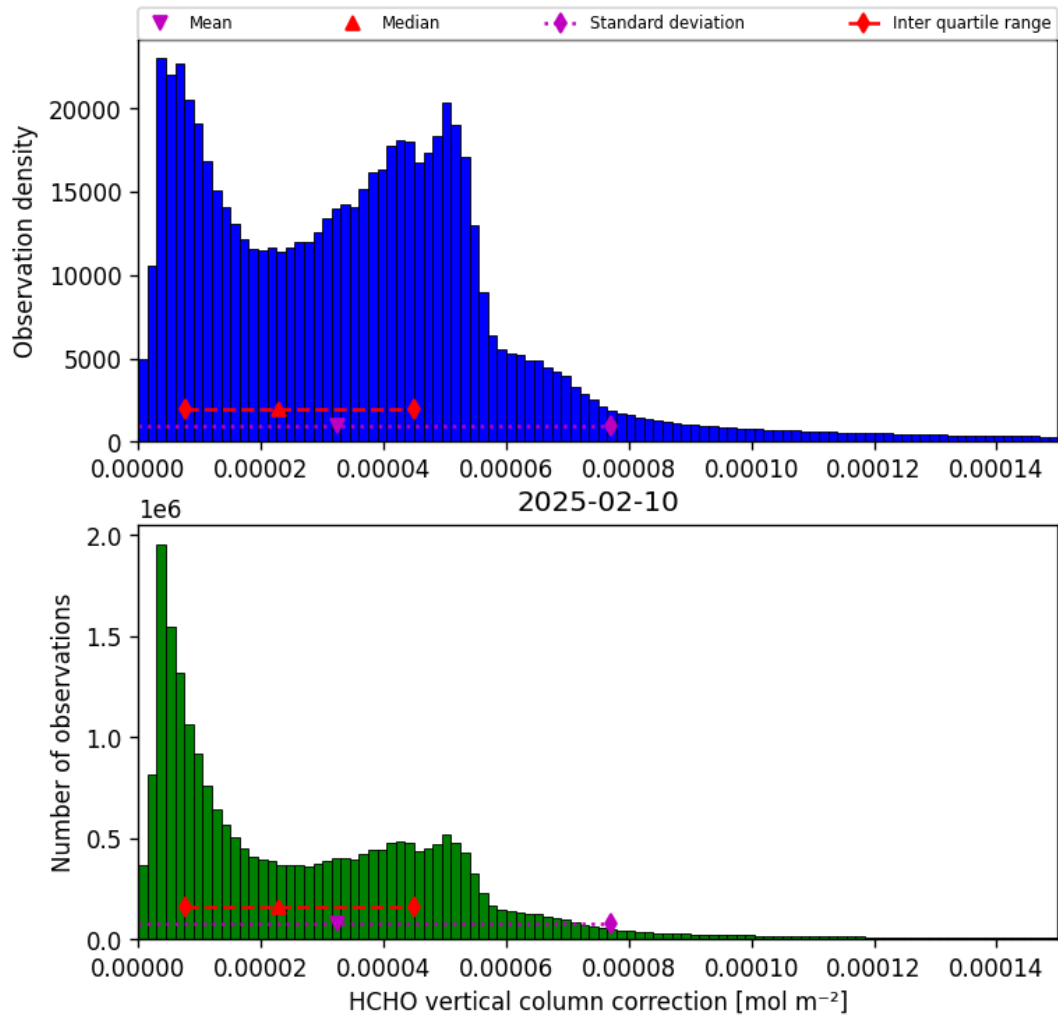
Figure 37: Histogram of “HCHO vertical column correction” for 2025-02-09 to 2025-02-11
