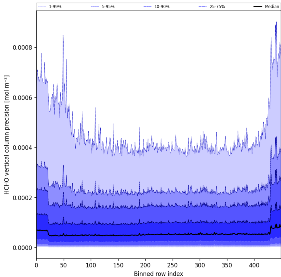
Figure 50: Along track statistics of “HCHO vertical column precision” for 2025-02-09 to 2025-02-11
