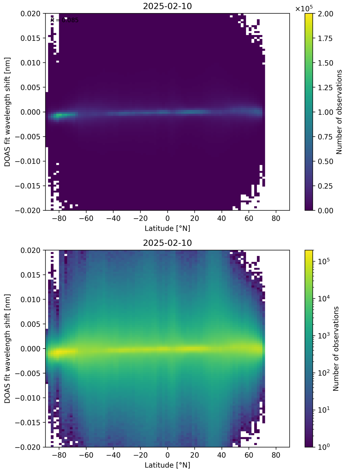
Figure 154: Scatter density plot of “Latitude” against “DOAS fit wavelength shift” for 2025-02-09 to 2025-02-11.
