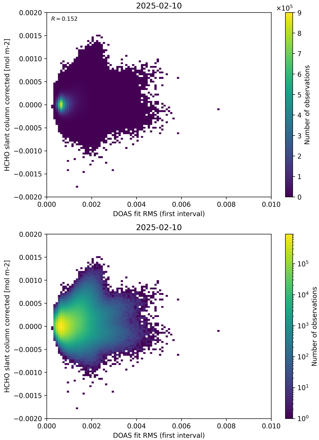
Figure 62: Scatter density plot of “DOAS fit RMS (first interval)” against “HCHO slant column corrected” for 2025-02-09 to 2025-02-11.
