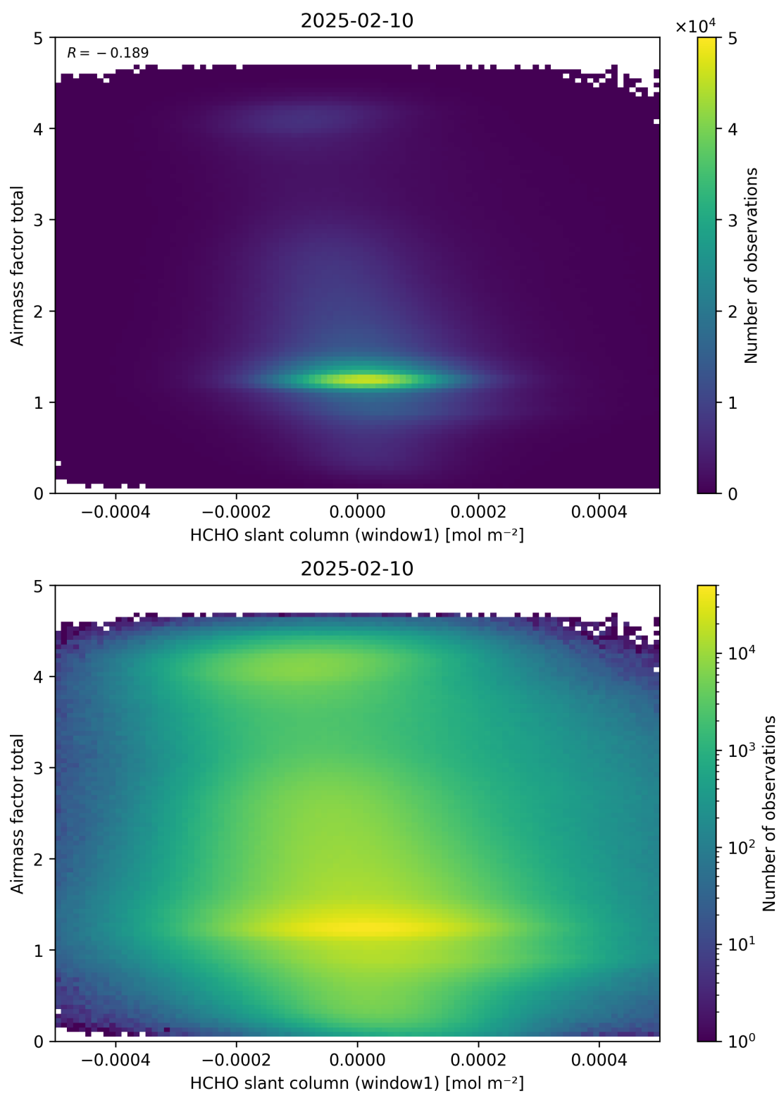
Figure 85: Scatter density plot of “HCHO slant column (window1)” against “Airmass factor total” for 2025-02-09 to 2025-02-11.
