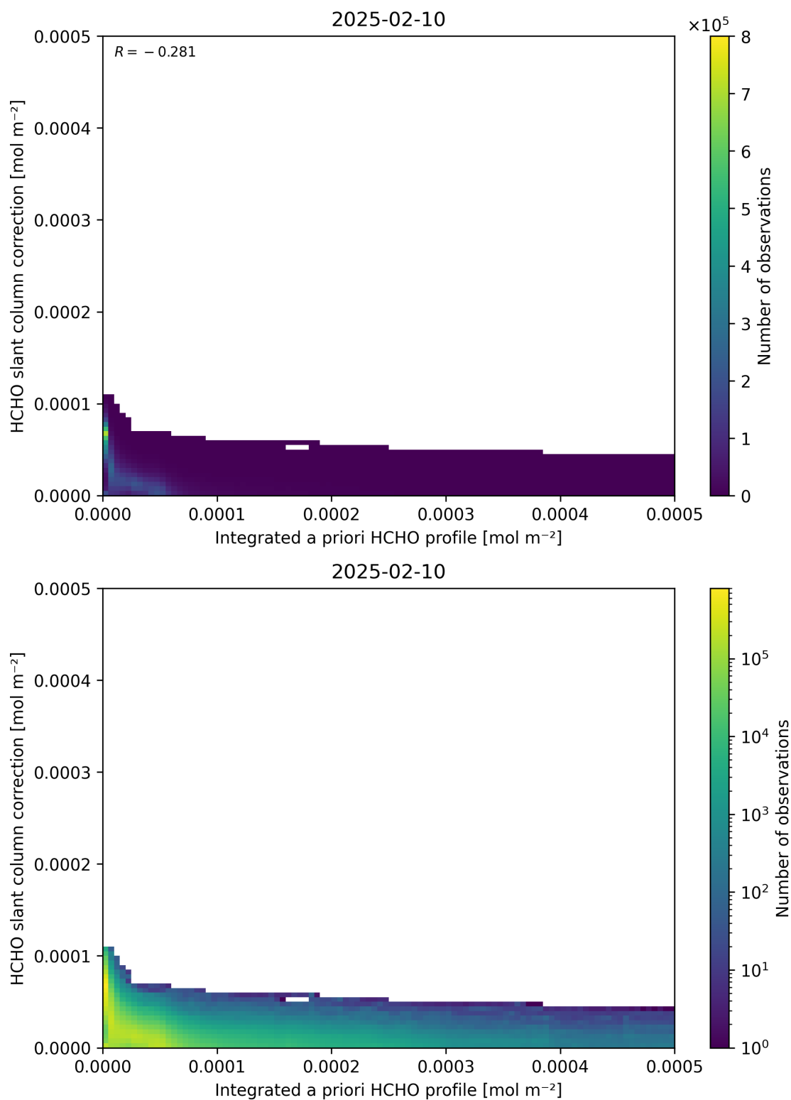
Figure 152: Scatter density plot of “Integrated a priori HCHO profile” against “HCHO slant column correction” for 2025-02-09 to 2025-02-11.
