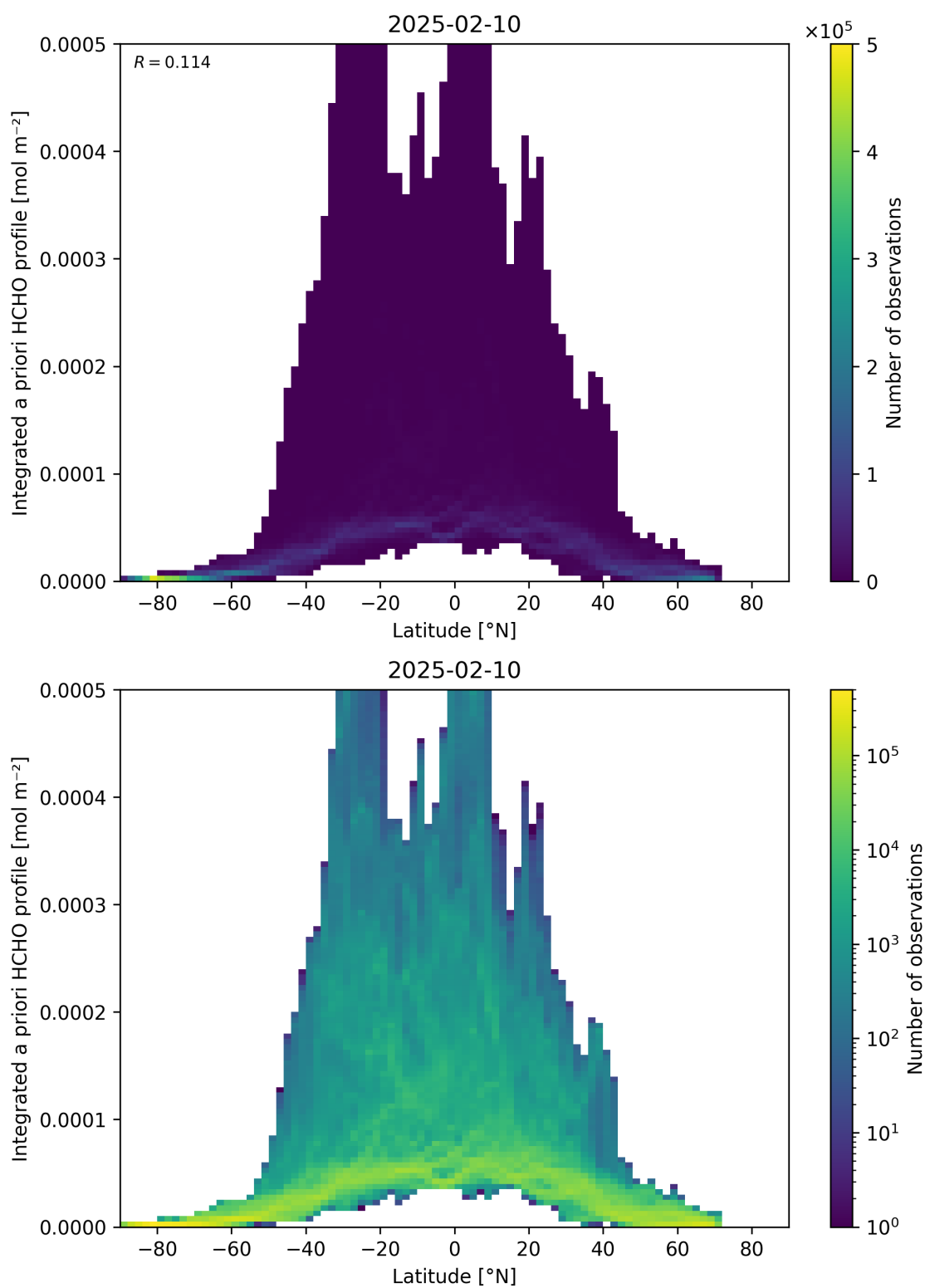
Figure 166: Scatter density plot of “Latitude” against “Integrated a priori HCHO profile” for 2025-02-09 to 2025-02-11.
