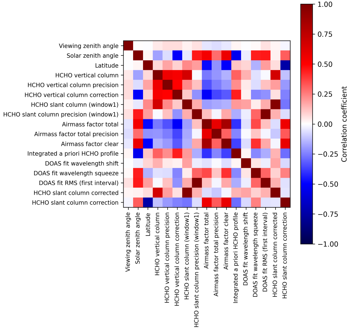
Figure 2: Map of correlation matrix for 2025-02-09 to 2025-02-11.
