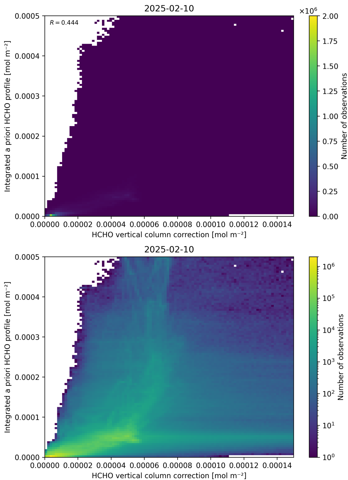
Figure 122: Scatter density plot of “HCHO vertical column correction” against “Integrated a priori HCHO profile” for 2025-02-09 to 2025-02-11.
