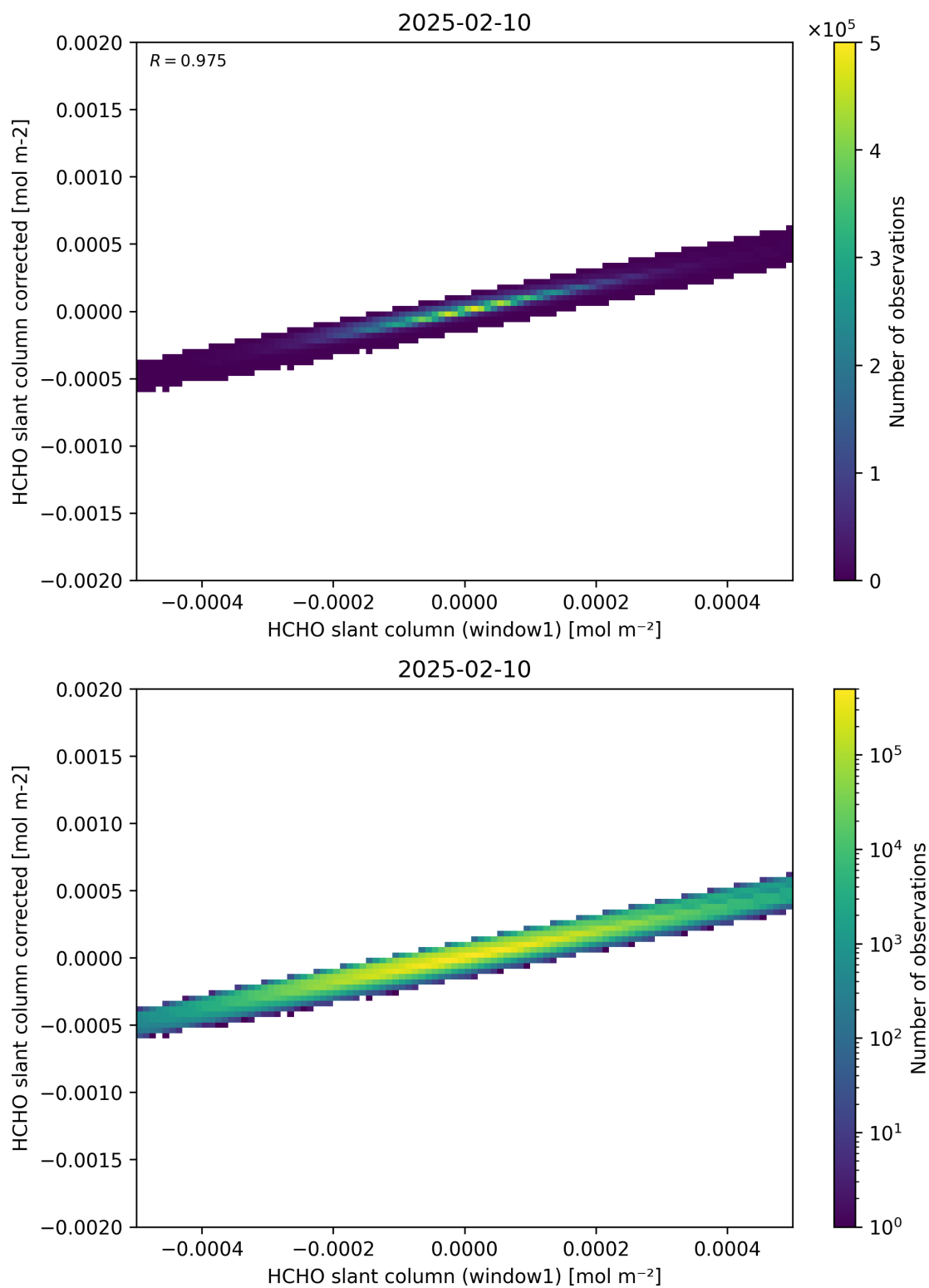
Figure 82: Scatter density plot of “HCHO slant column (window1)” against “HCHO slant column corrected” for 2025-02-09 to 2025-02-11.
