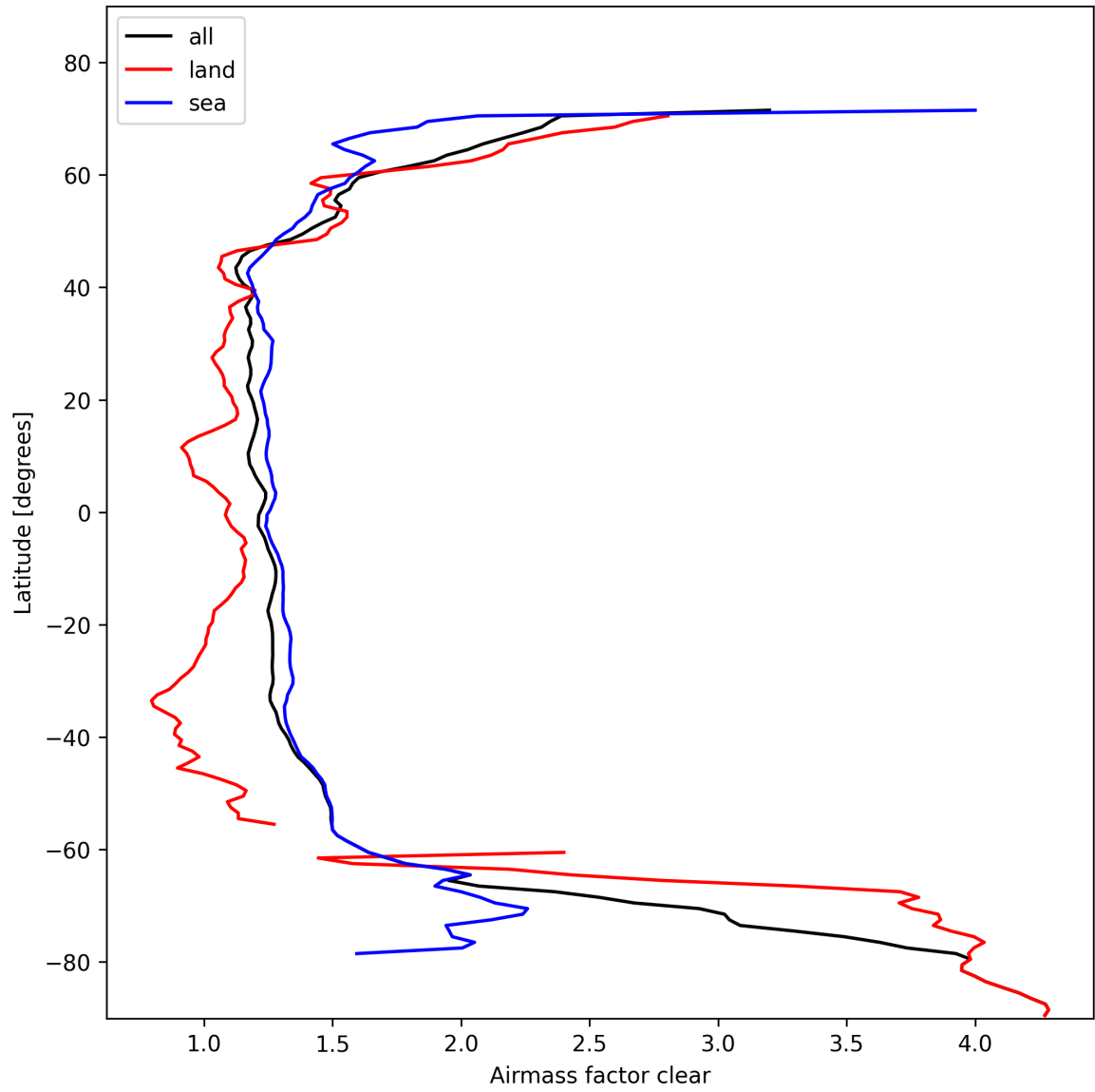
Figure 28: Zonal average of “Airmass factor clear” for 2025-02-09 to 2025-02-11.
