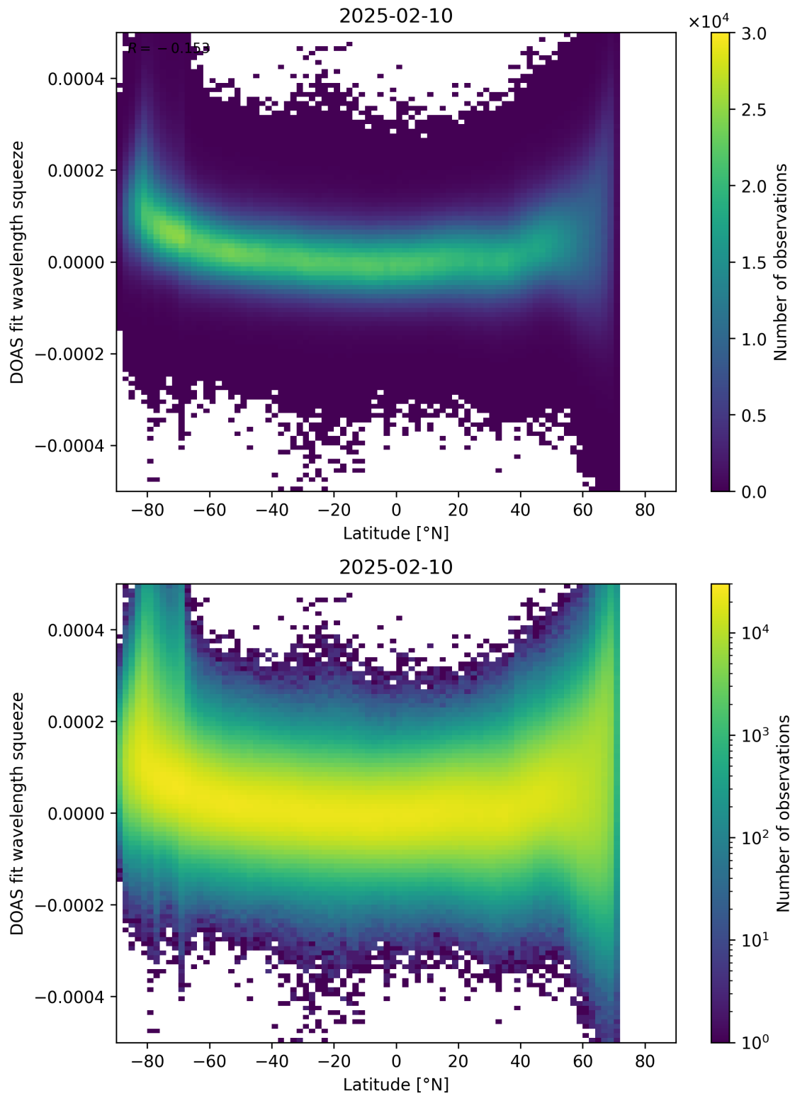
Figure 155: Scatter density plot of “Latitude” against “DOAS fit wavelength squeeze” for 2025-02-09 to 2025-02-11.
