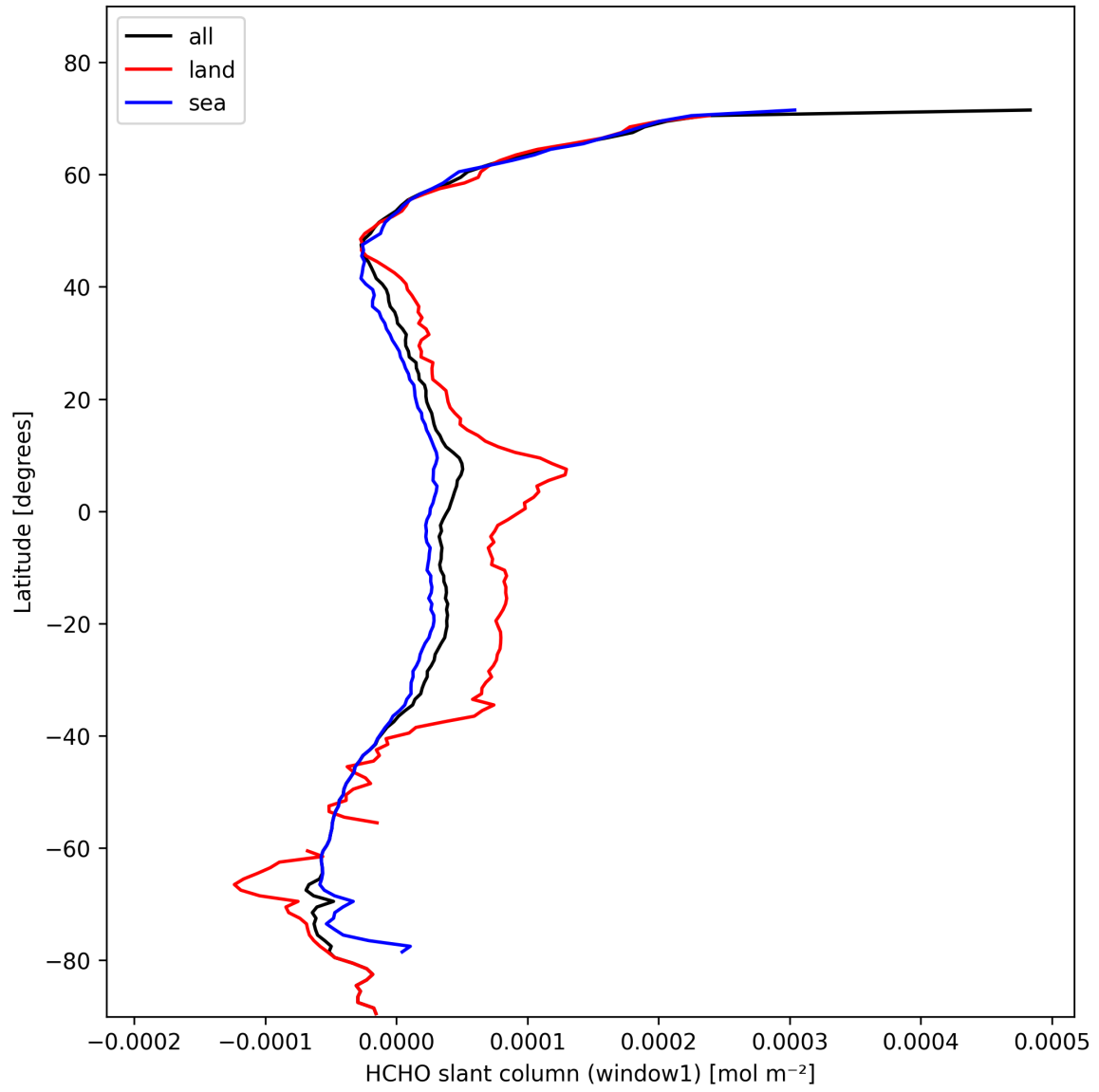
Figure 24: Zonal average of “HCHO slant column (window1)” for 2025-02-09 to 2025-02-11.
