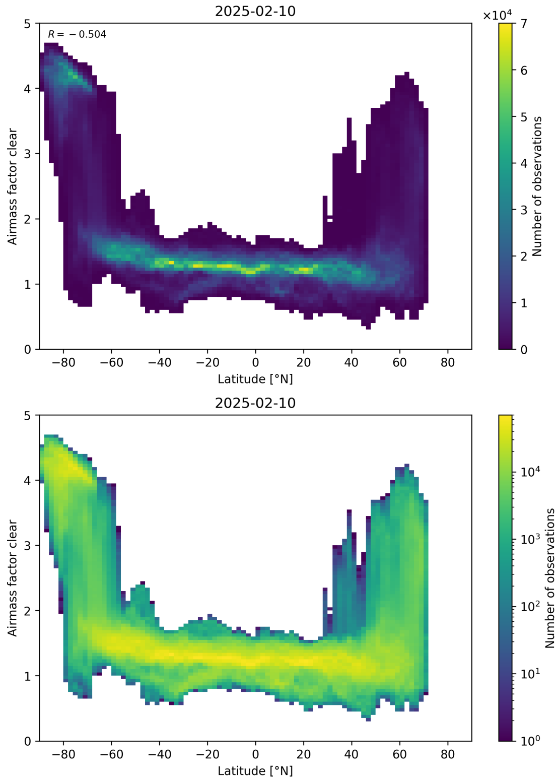
Figure 156: Scatter density plot of “Latitude” against “Airmass factor clear” for 2025-02-09 to 2025-02-11.
