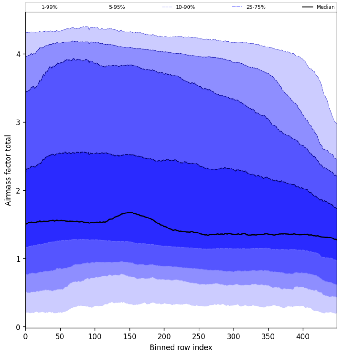
Figure 54: Along track statistics of “Airmass factor total” for 2025-02-09 to 2025-02-11
