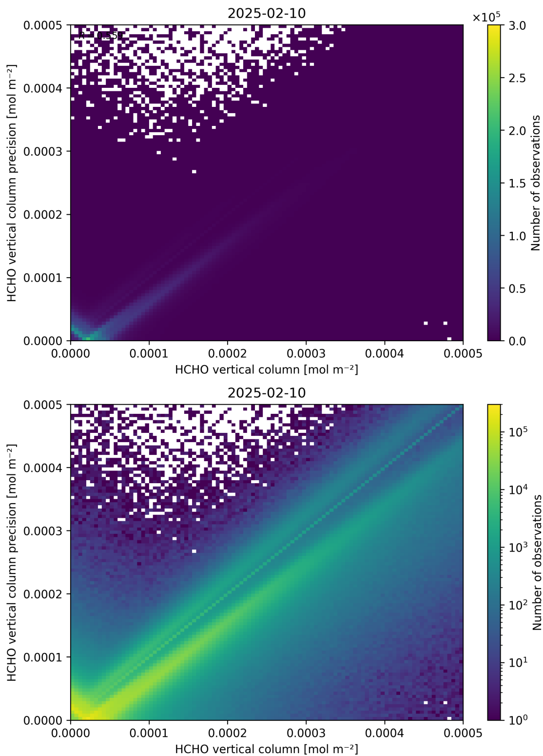
Figure 134: Scatter density plot of “HCHO vertical column” against “HCHO vertical column precision” for 2025-02-09 to 2025-02-11.
