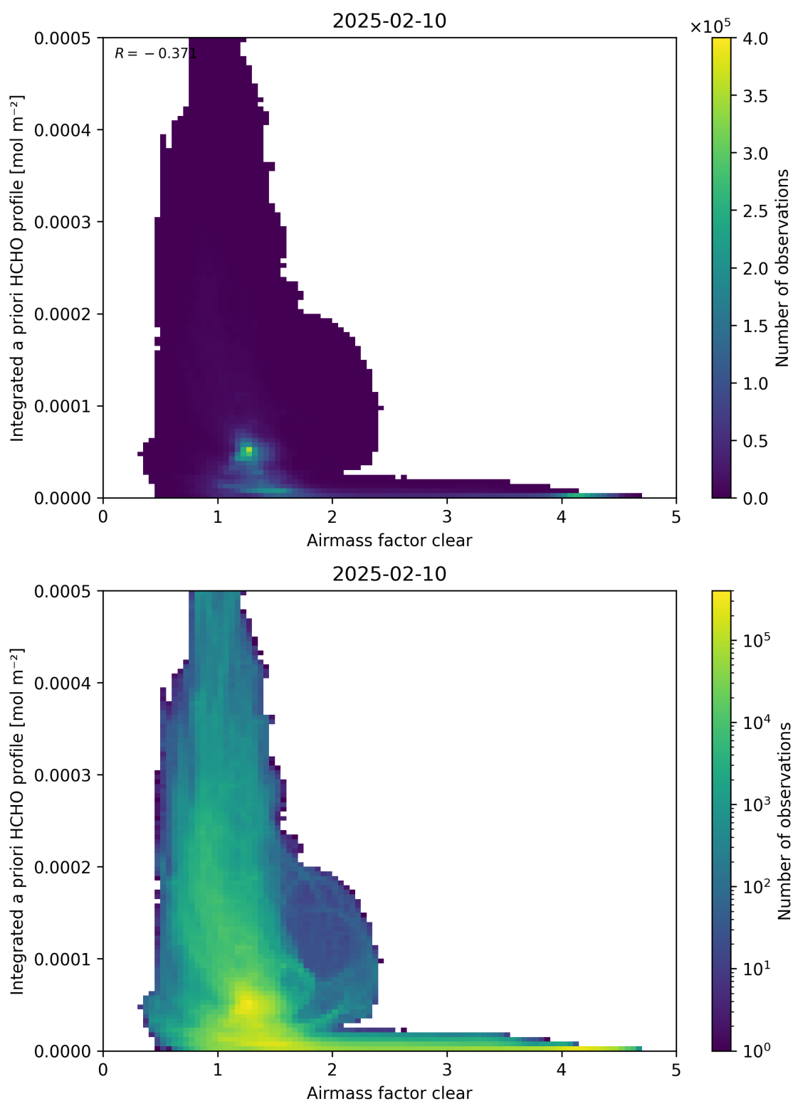
Figure 76: Scatter density plot of “Airmass factor clear” against “Integrated a priori HCHO profile” for 2025-02-09 to 2025-02-11.
