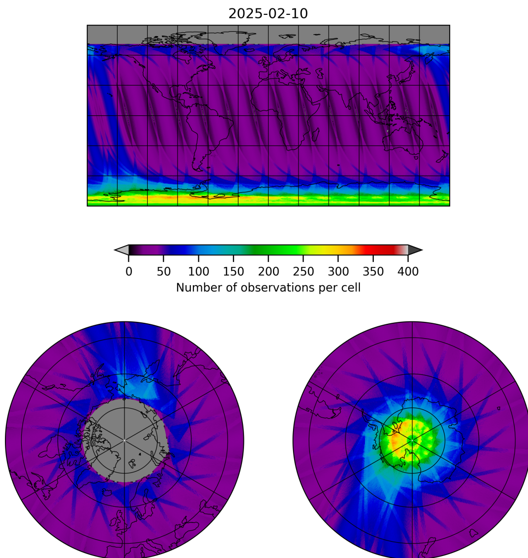
Figure 19: Map of the number of observations for 2025-02-09 to 2025-02-11
