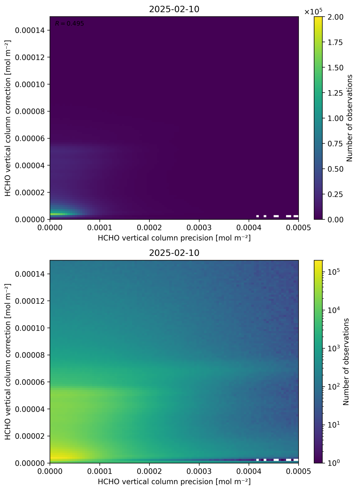
Figure 146: Scatter density plot of “HCHO vertical column precision” against “HCHO vertical column correction” for 2025-02-09 to 2025-02-11.
