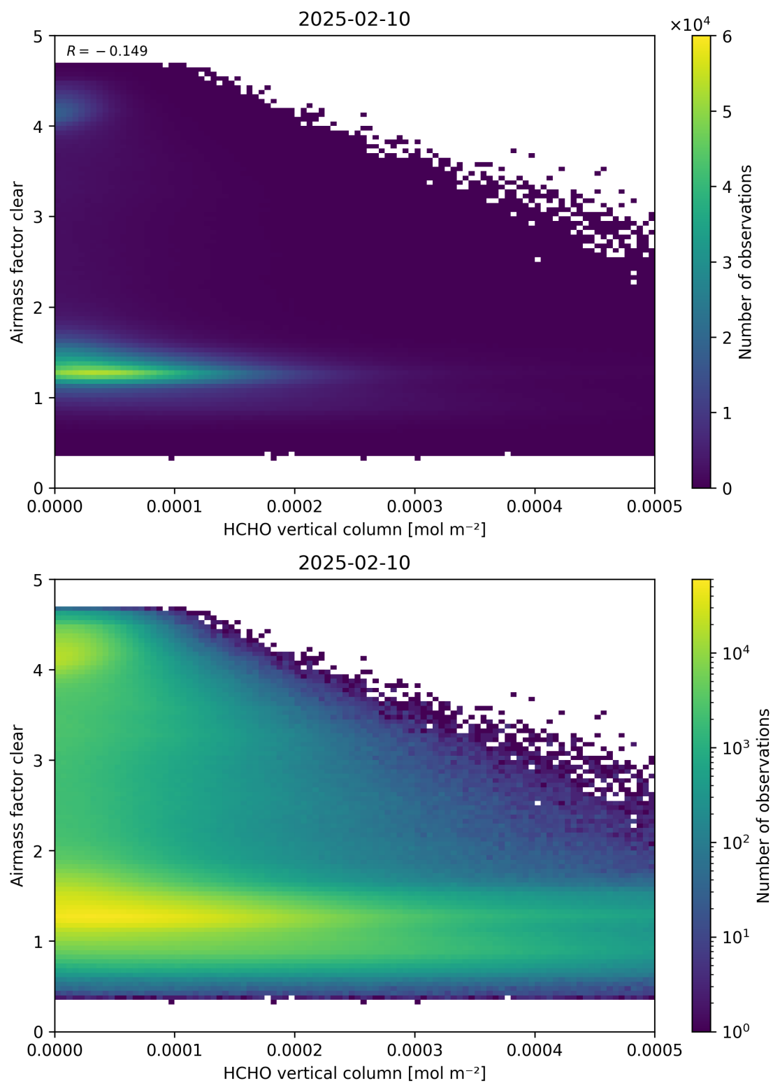
Figure 126: Scatter density plot of “HCHO vertical column” against “Airmass factor clear” for 2025-02-09 to 2025-02-11.
