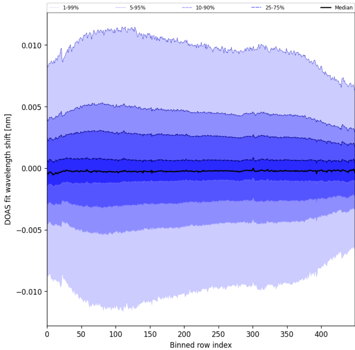
Figure 58: Along track statistics of “DOAS fit wavelength shift” for 2025-02-09 to 2025-02-11
