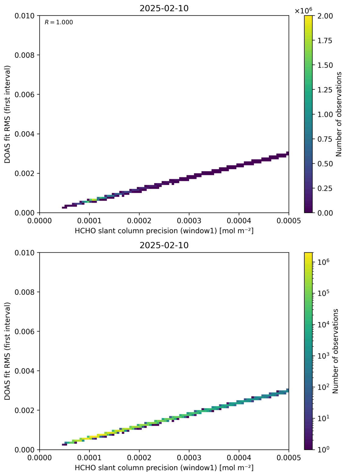
Figure 88: Scatter density plot of “HCHO slant column precision (window1)” against “DOAS fit RMS (first interval)” for 2025-02-09 to 2025-02-11.
