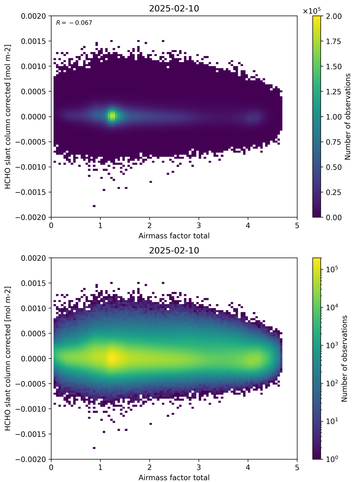
Figure 101: Scatter density plot of “Airmass factor total” against “HCHO slant column corrected” for 2025-02-09 to 2025-02-11.
