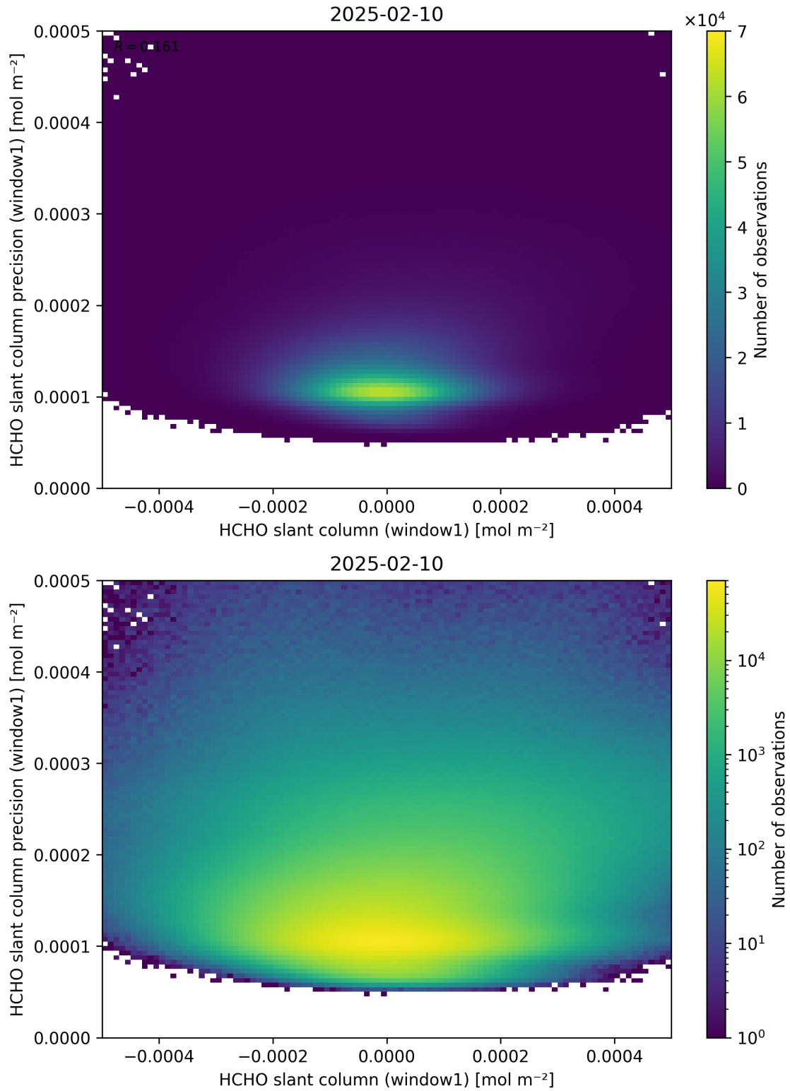
Figure 84: Scatter density plot of “HCHO slant column (window1)” against “HCHO slant column precision (window1)” for 2025-02-09 to 2025-02-11.
