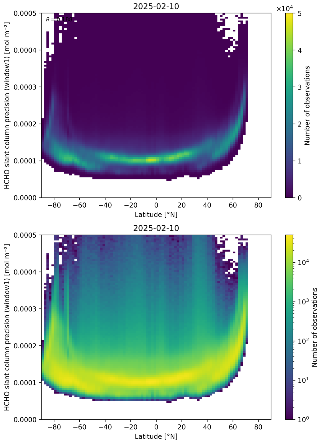
Figure 160: Scatter density plot of “Latitude” against “HCHO slant column precision (window1)” for 2025-02-09 to 2025-02-11.
