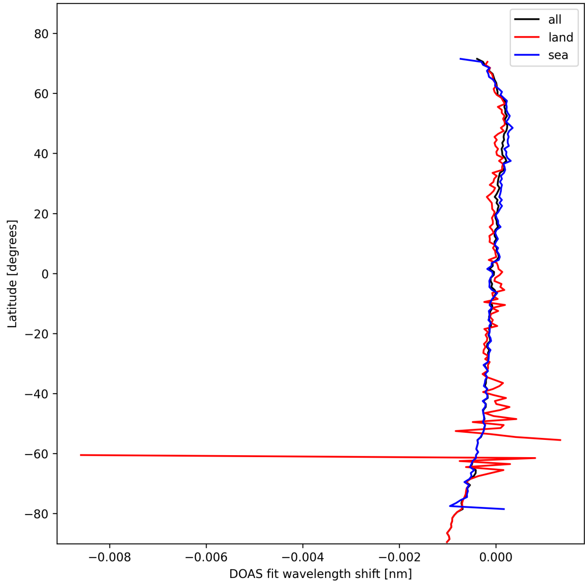
Figure 30: Zonal average of "DOAS fit wavelength shift" for 2025-02-09 to 2025-02-11.
