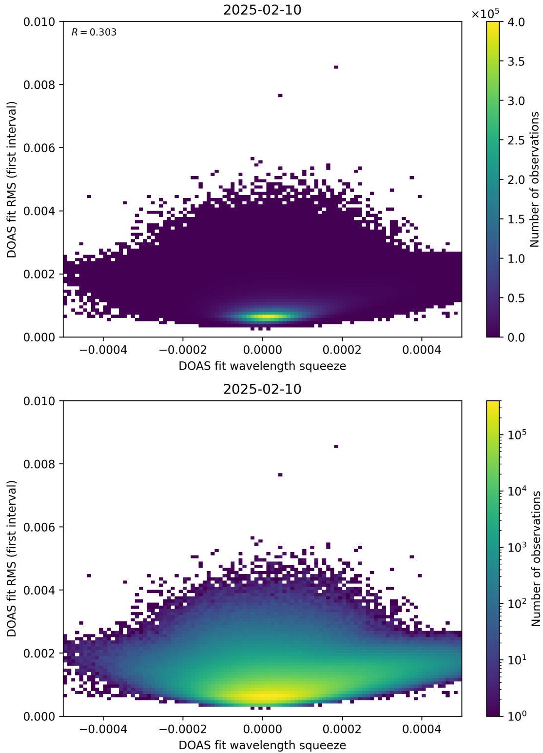
Figure 68: Scatter density plot of “DOAS fit wavelength squeeze” against “DOAS fit RMS (first interval)” for 2025-02-09 to 2025-02-11.
