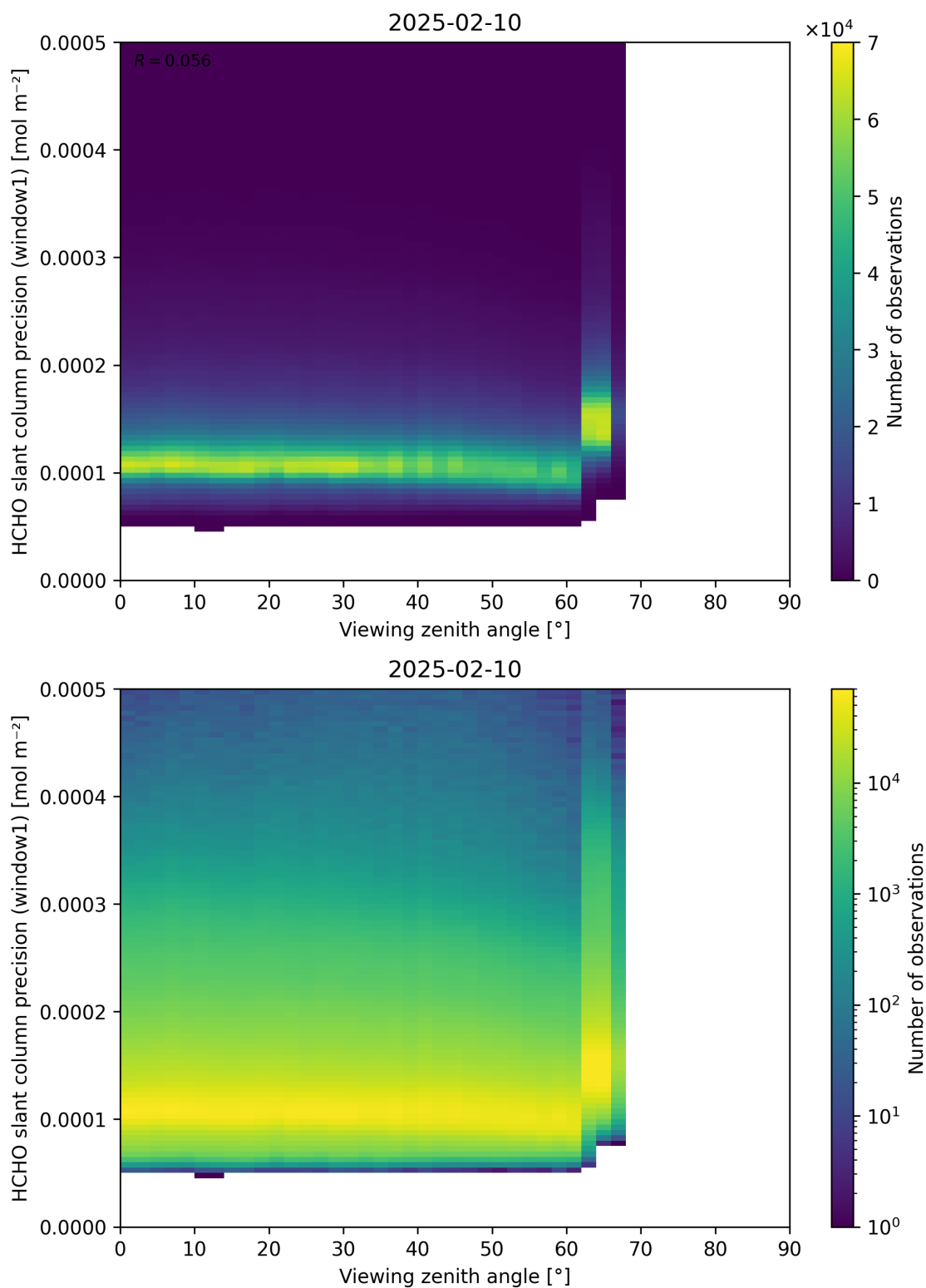
Figure 189: Scatter density plot of “Viewing zenith angle” against “HCHO slant column precision (window1)” for 2025-02-09 to 2025-02-11.
