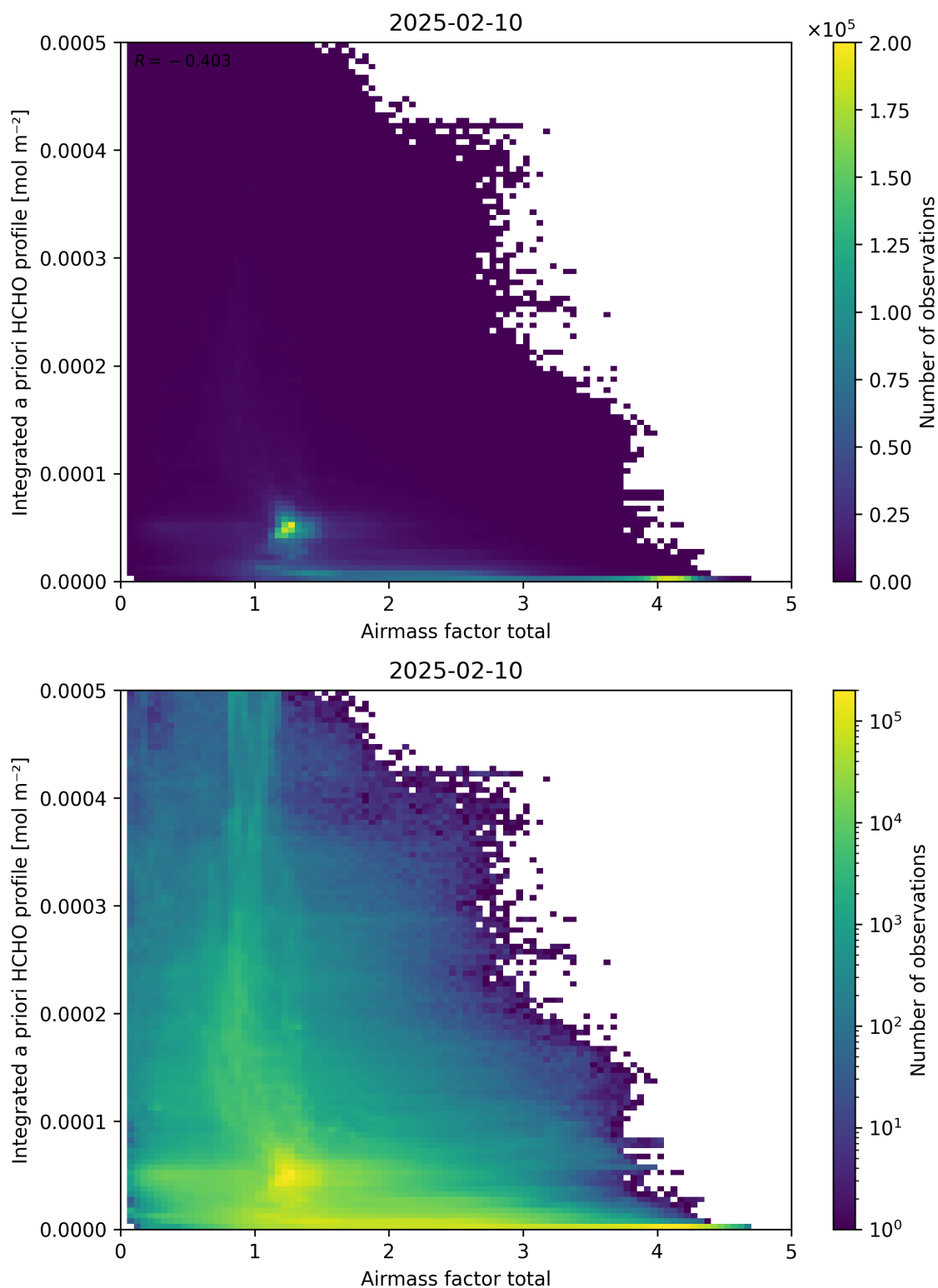
Figure 104: Scatter density plot of “Airmass factor total” against “Integrated a priori HCHO profile” for 2025-02-09 to 2025-02-11.
