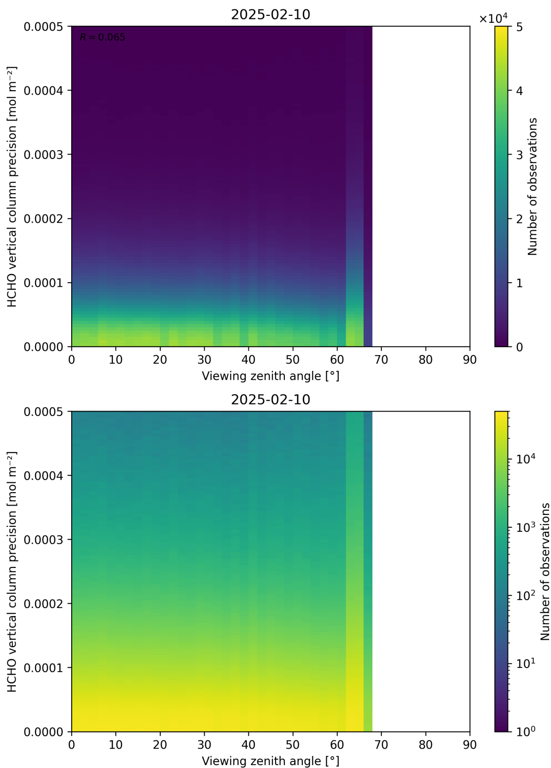
Figure 194: Scatter density plot of “Viewing zenith angle” against “HCHO vertical column precision” for 2025-02-09 to 2025-02-11.
