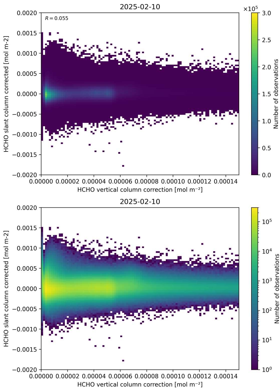
Figure 116: Scatter density plot of “HCHO vertical column correction” against “HCHO slant column corrected” for 2025-02-09 to 2025-02-11.
