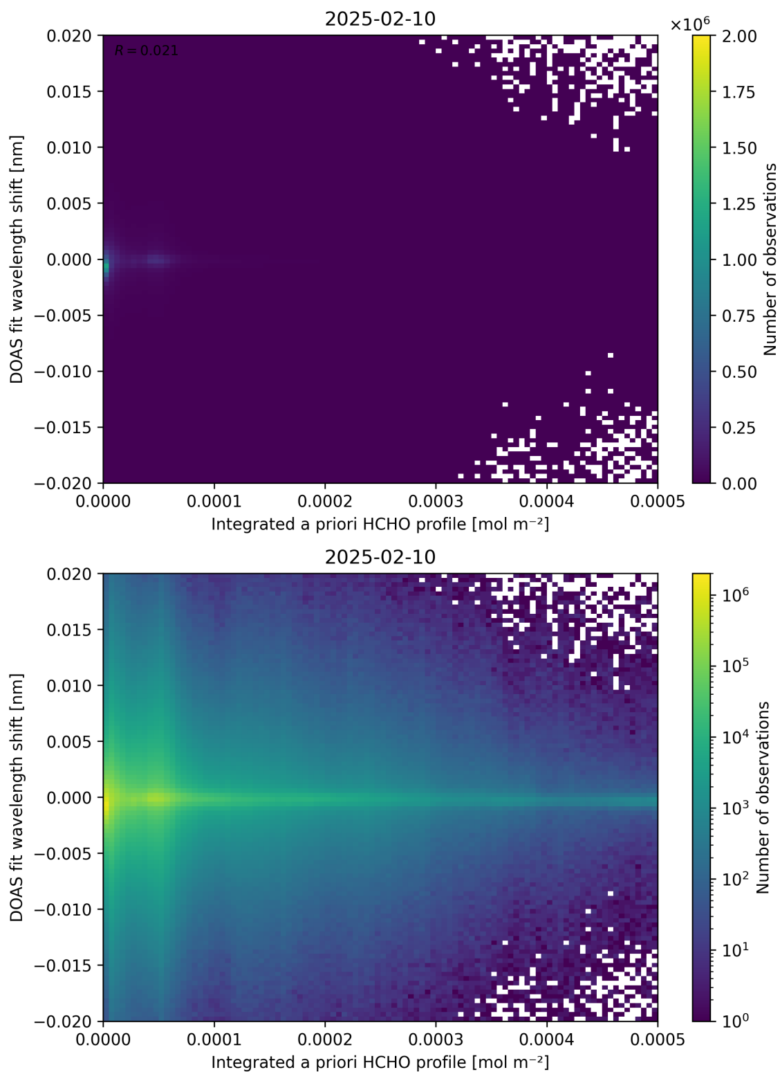
Figure 149: Scatter density plot of “Integrated a priori HCHO profile” against “DOAS fit wavelength shift” for 2025-02-09 to 2025-02-11.
