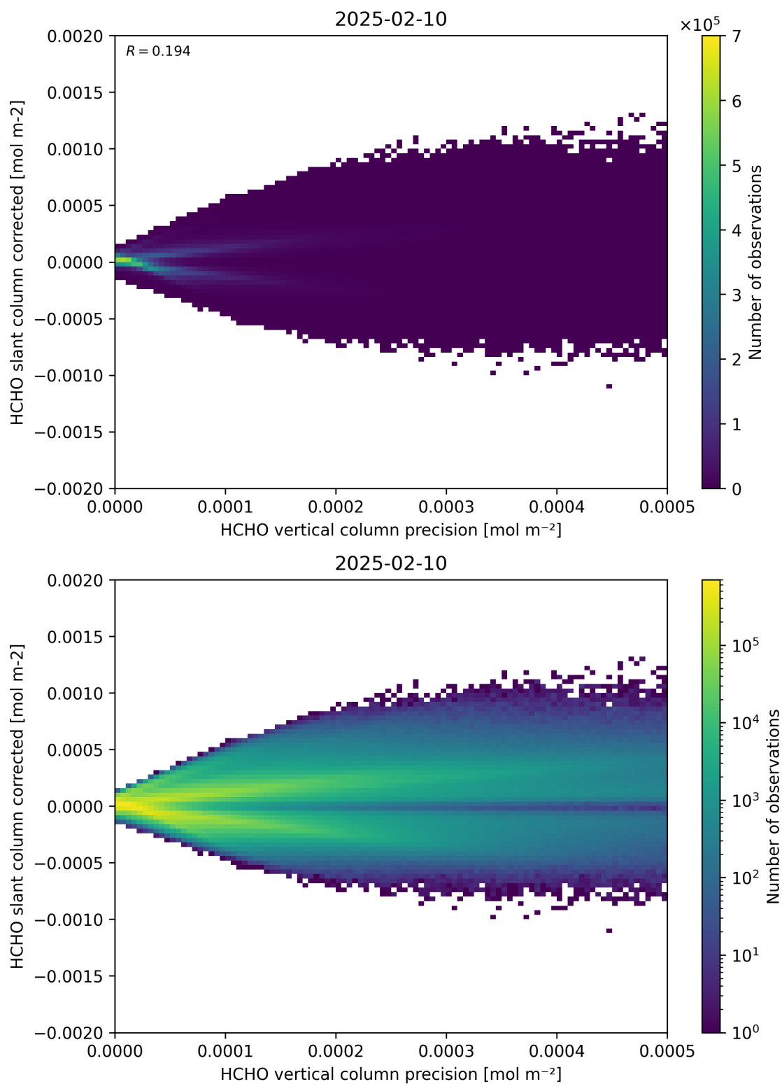
Figure 140: Scatter density plot of “HCHO vertical column precision” against “HCHO slant column corrected” for 2025-02-09 to 2025-02-11.
