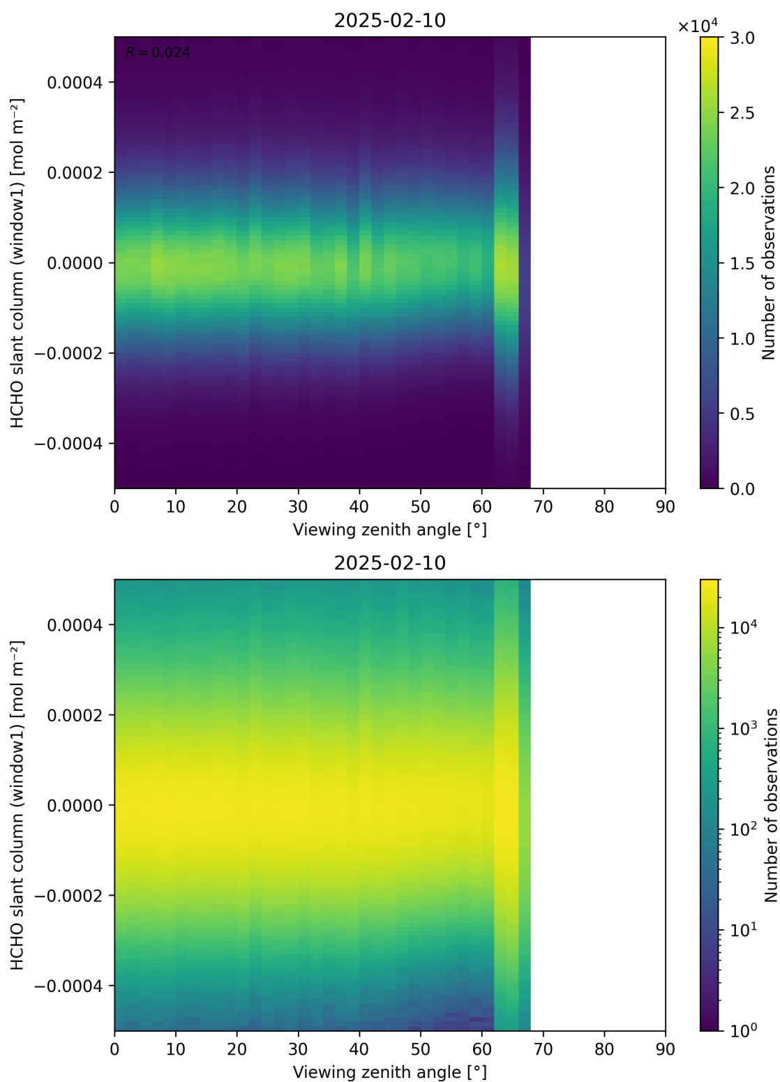
Figure 188: Scatter density plot of “Viewing zenith angle” against “HCHO slant column (window1)” for 2025-02-09 to 2025-02-11.
