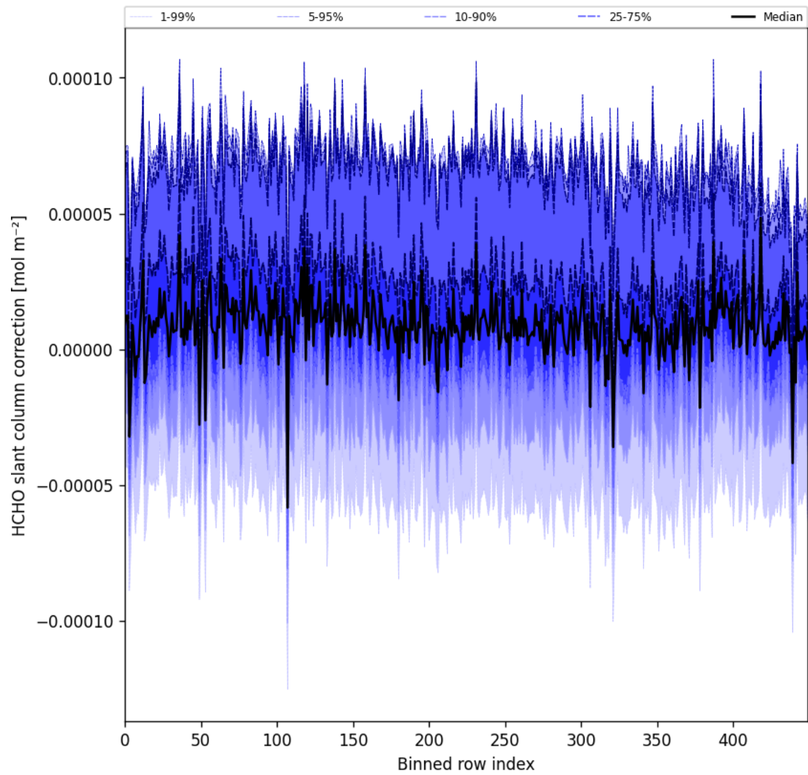
Figure 61: Along track statistics of “HCHO slant column correction” for 2025-02-09 to 2025-02-11
