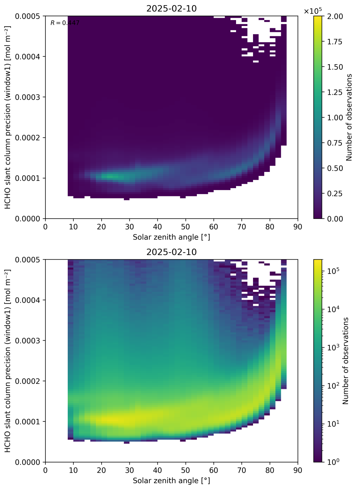
Figure 174: Scatter density plot of “Solar zenith angle” against “HCHO slant column precision (window1)” for 2025-02-09 to 2025-02-11.
