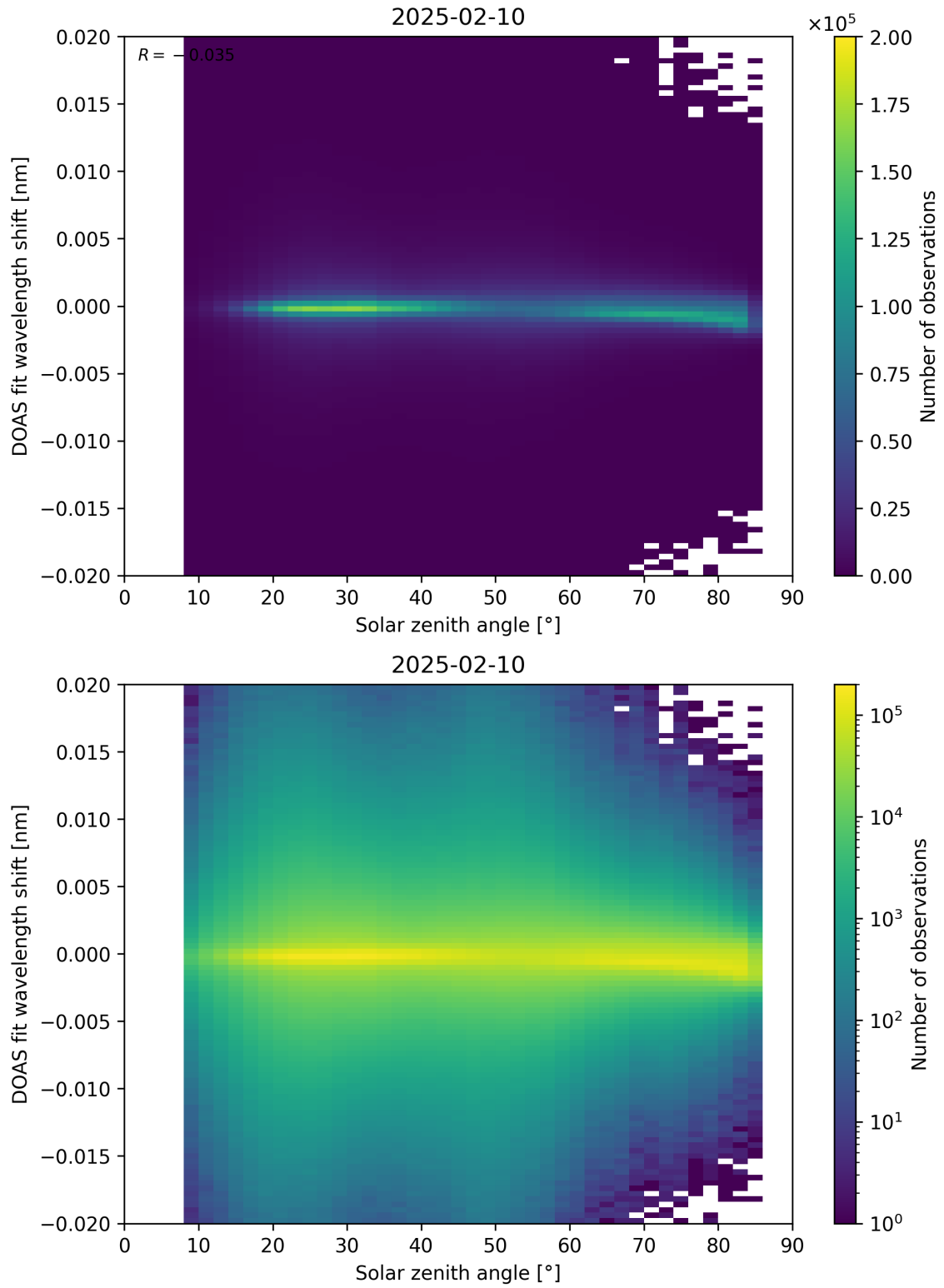
Figure 168: Scatter density plot of “Solar zenith angle” against “DOAS fit wavelength shift” for 2025-02-09 to 2025-02-11.
