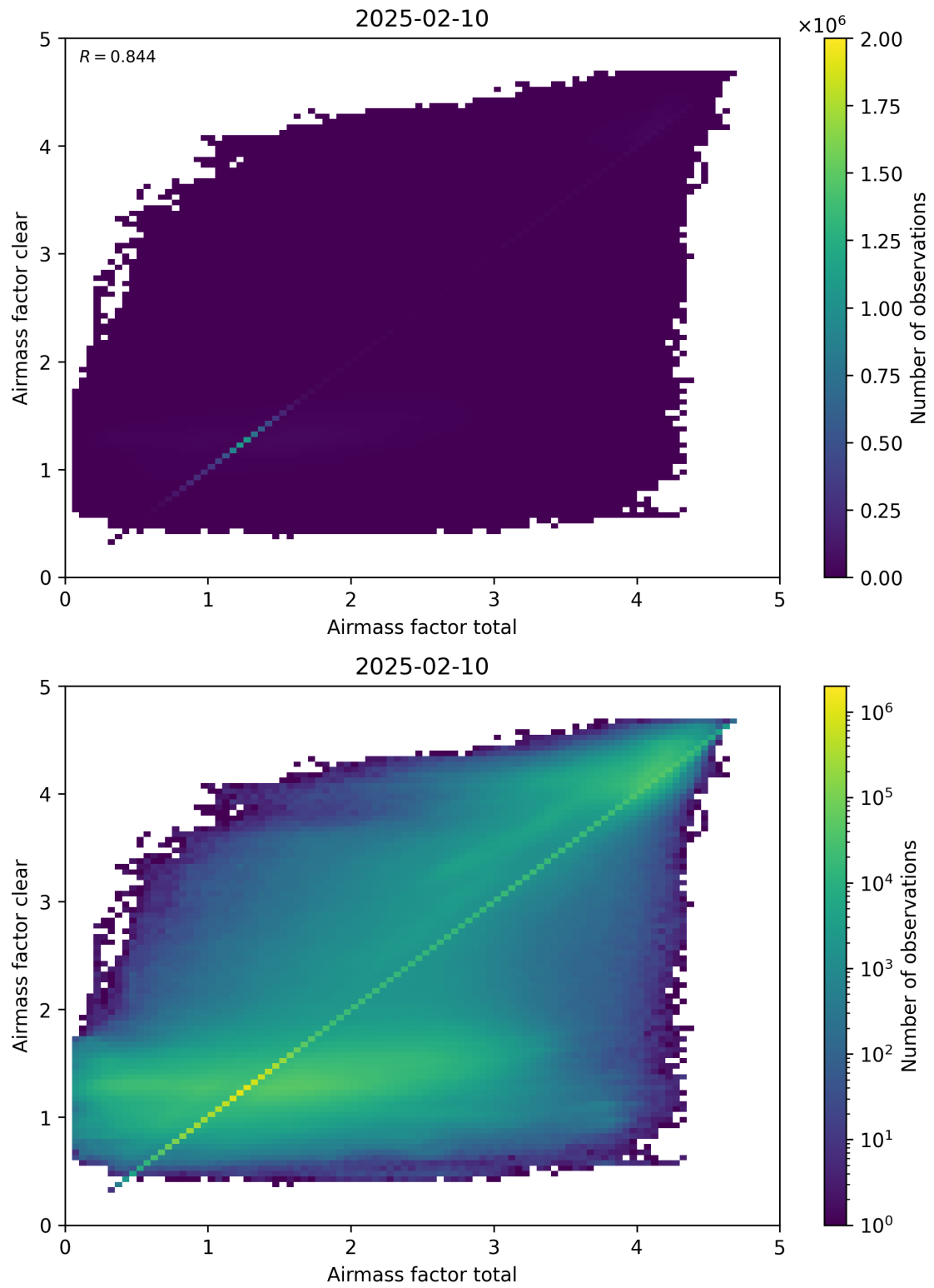
Figure 100: Scatter density plot of “Airmass factor total” against “Airmass factor clear” for 2025-02-09 to 2025-02-11.
