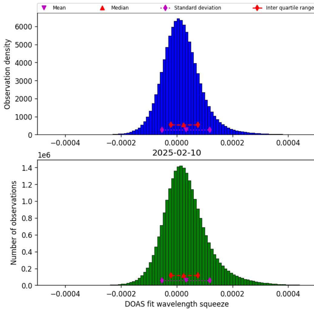
Figure 45: Histogram of “DOAS fit wavelength squeeze” for 2025-02-09 to 2025-02-11
