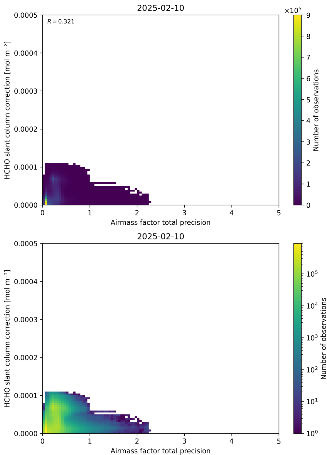
Figure 110: Scatter density plot of “Airmass factor total precision” against “HCHO slant column correction” for 2025-02-09 to 2025-02-11.
