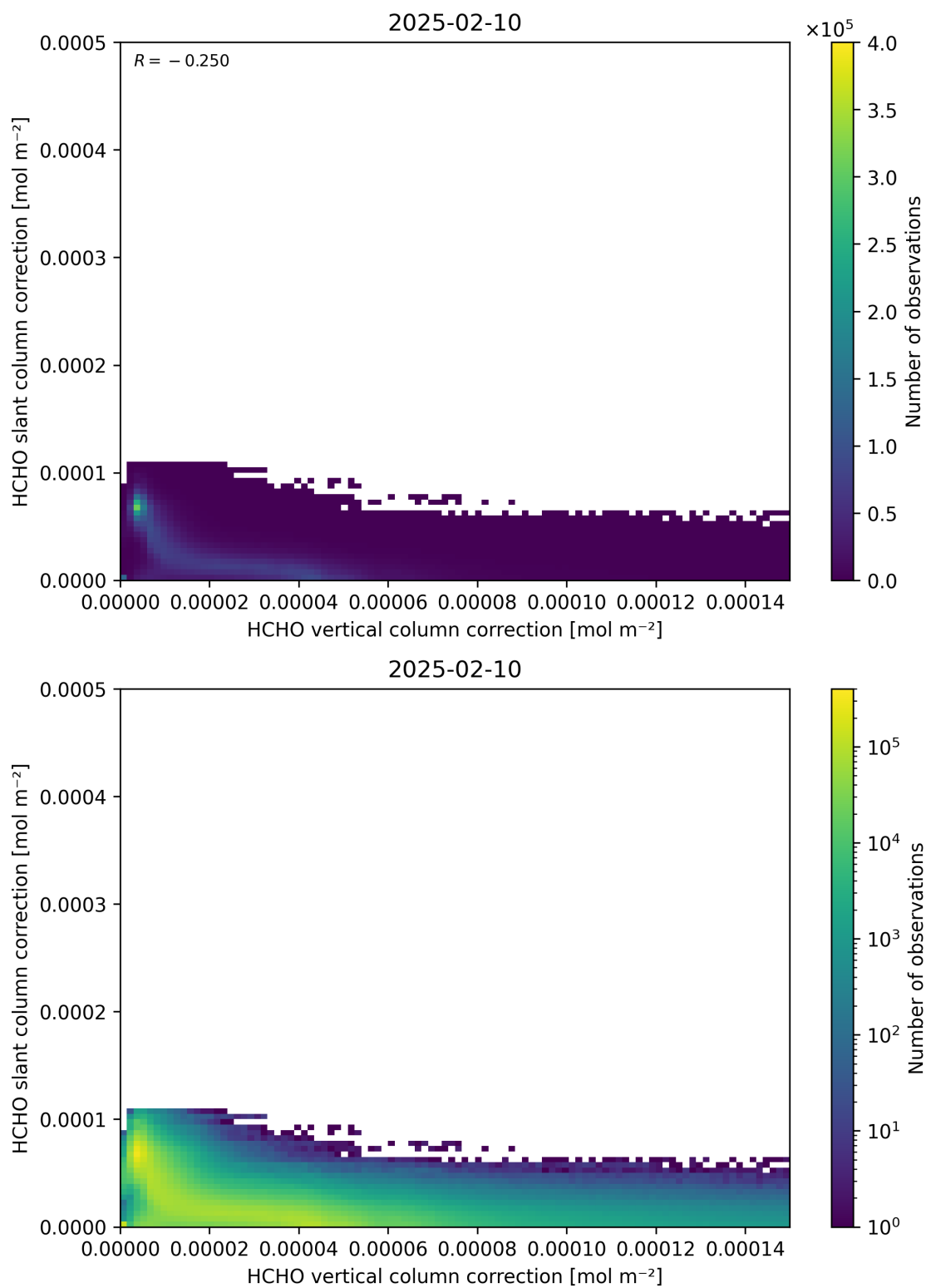
Figure 117: Scatter density plot of “HCHO vertical column correction” against “HCHO slant column correction” for 2025-02-09 to 2025-02-11.
