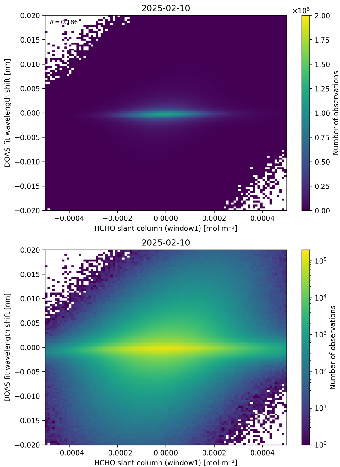
Figure 79: Scatter density plot of “HCHO slant column (window1)” against “DOAS fit wavelength shift” for 2025-02-09 to 2025-02-11.
