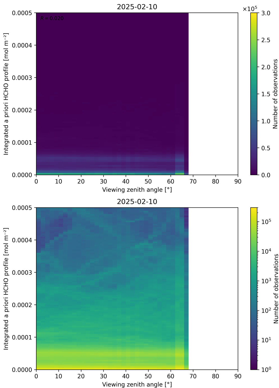
Figure 195: Scatter density plot of “Viewing zenith angle” against “Integrated a priori HCHO profile” for 2025-02-09 to 2025-02-11.
