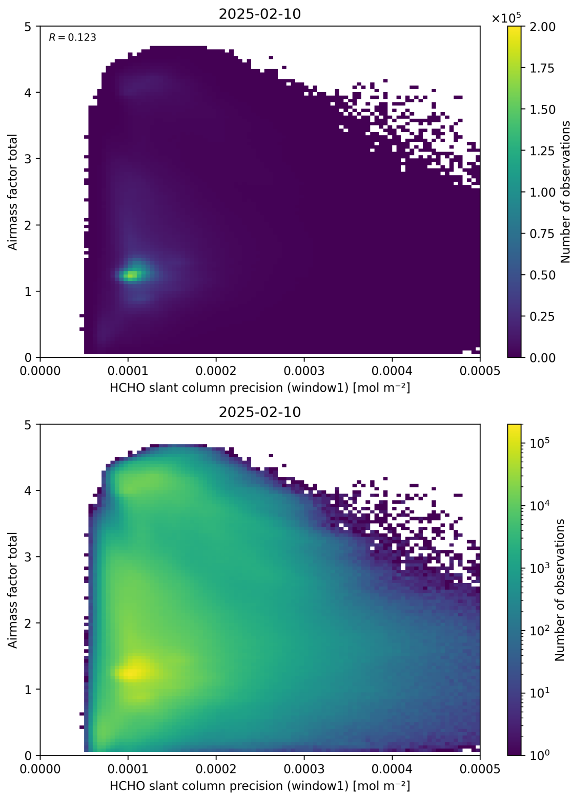
Figure 94: Scatter density plot of “HCHO slant column precision (window1)” against “Airmass factor total” for 2025-02-09 to 2025-02-11.
