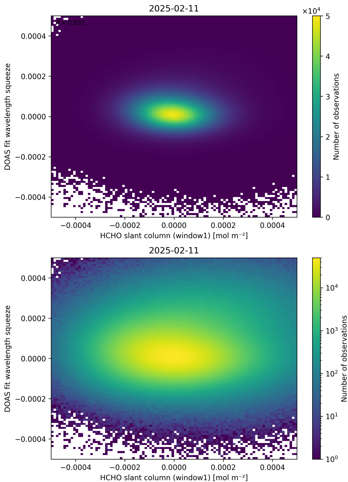
Figure 80: Scatter density plot of “HCHO slant column (window1)” against “DOAS fit wavelength squeeze” for 2025-02-10 to 2025-02-12.
