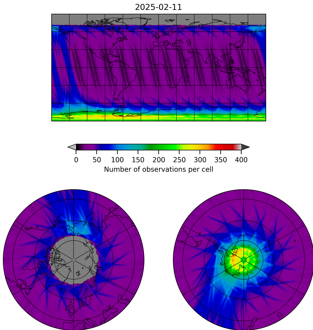
Figure 19: Map of the number of observations for 2025-02-10 to 2025-02-12
