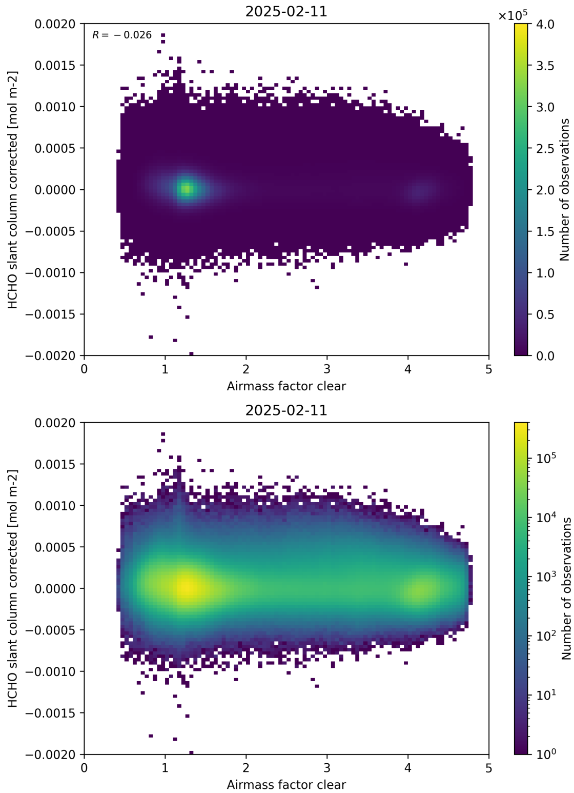
Figure 74: Scatter density plot of “Airmass factor clear” against “HCHO slant column corrected” for 2025-02-10 to 2025-02-12.
