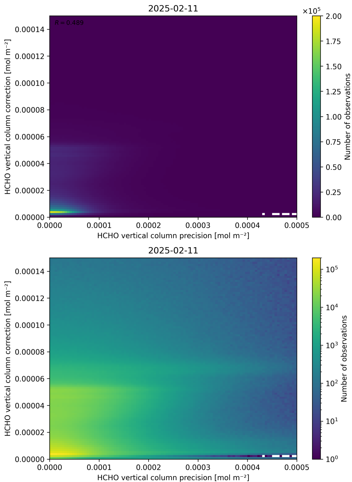
Figure 146: Scatter density plot of “HCHO vertical column precision” against “HCHO vertical column correction” for 2025-02-10 to 2025-02-12.
