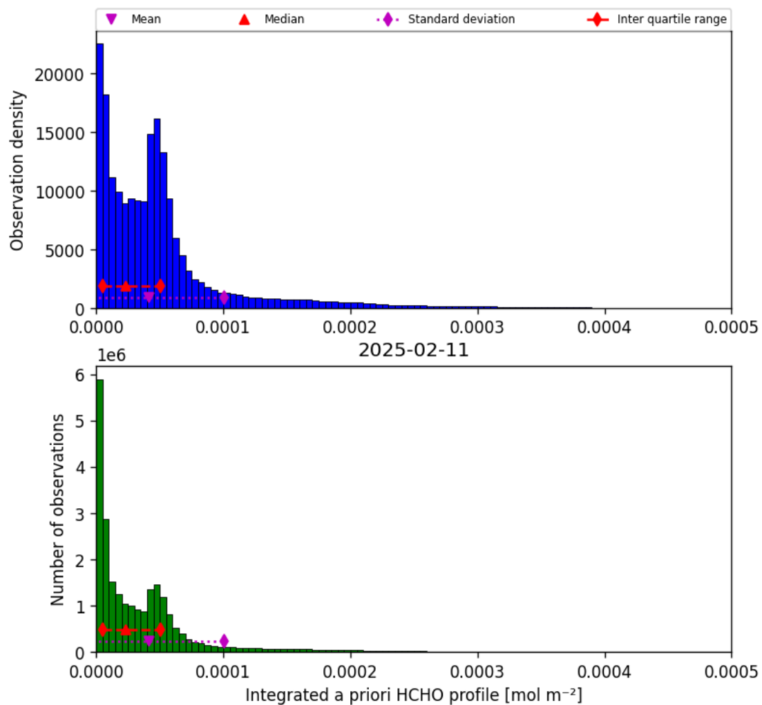
Figure 43: Histogram of “Integrated a priori HCHO profile” for 2025-02-10 to 2025-02-12
