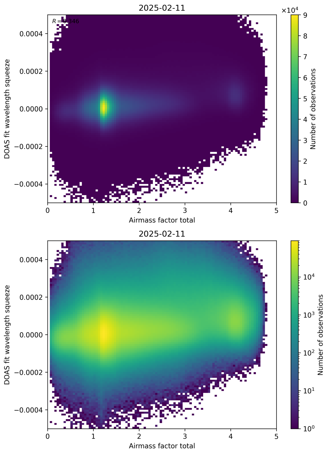
Figure 99: Scatter density plot of “Airmass factor total” against “DOAS fit wavelength squeeze” for 2025-02-10 to 2025-02-12.
