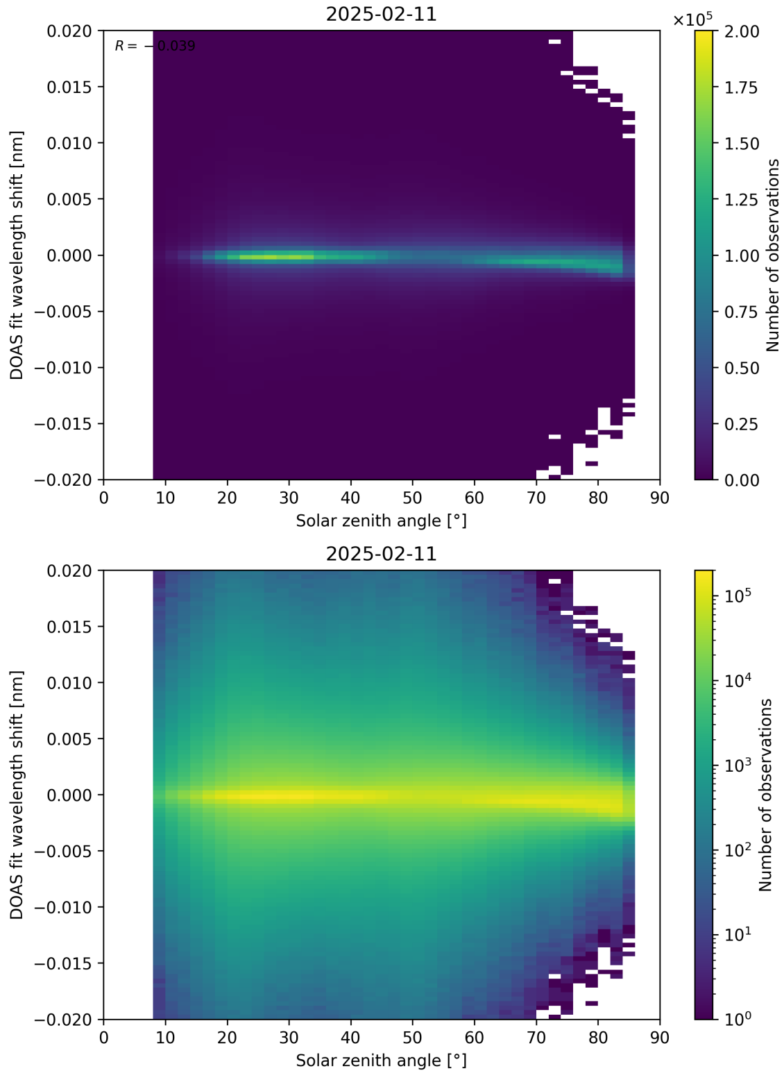
Figure 168: Scatter density plot of “Solar zenith angle” against “DOAS fit wavelength shift” for 2025-02-10 to 2025-02-12.
