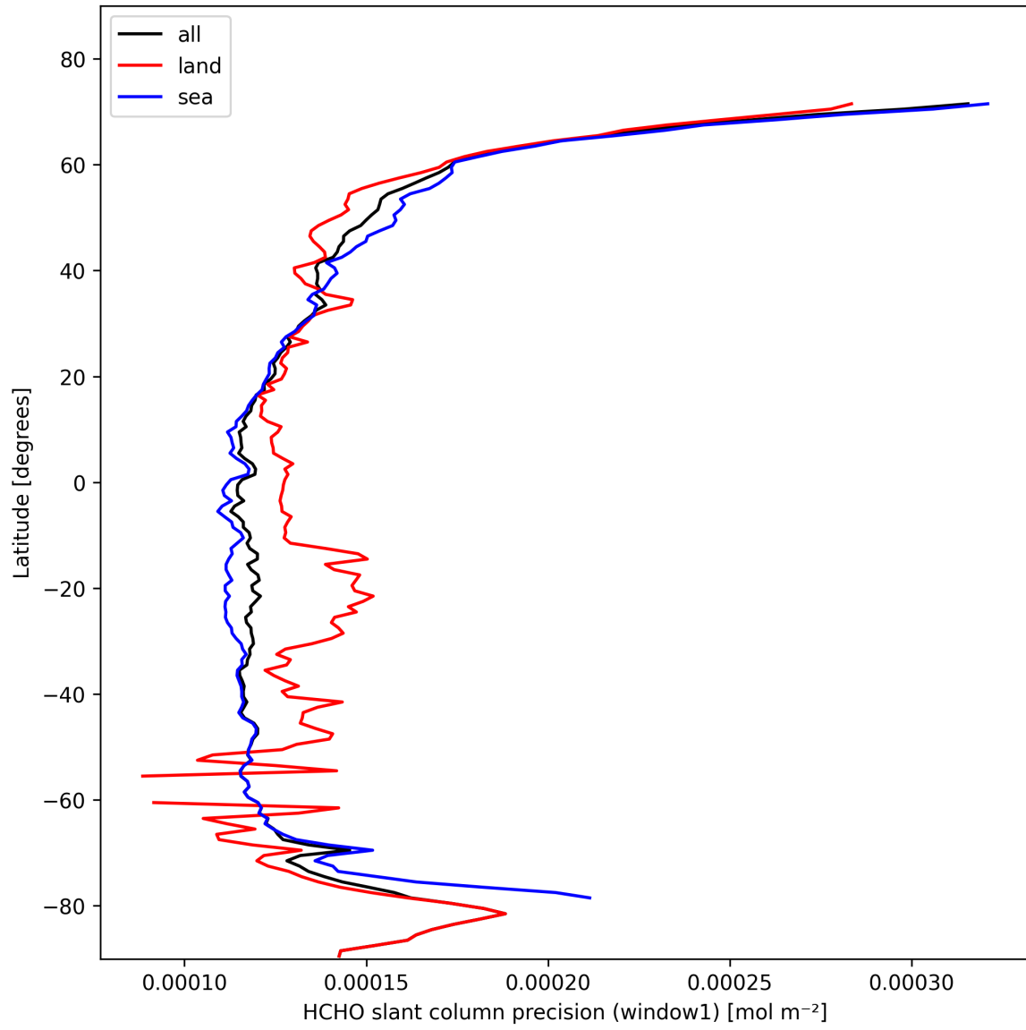
Figure 25: Zonal average of "HCHO slant column precision (window1)" for 2025-02-10 to 2025-02-12.
