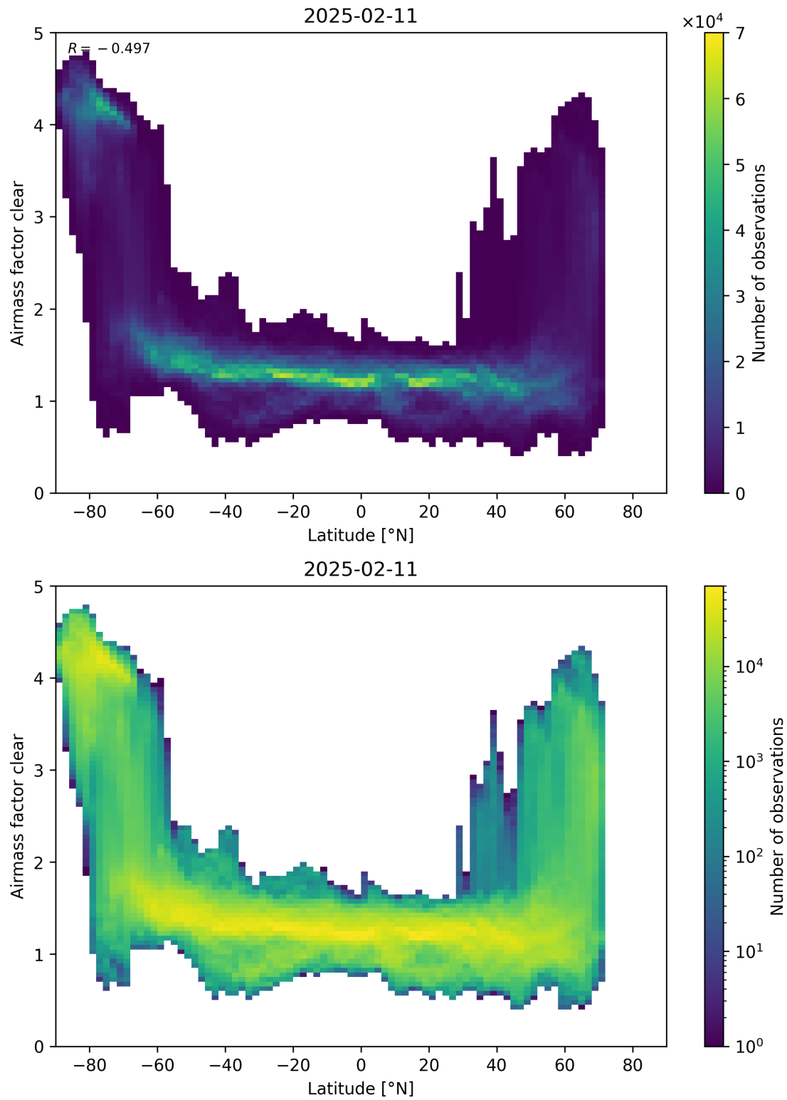
Figure 156: Scatter density plot of “Latitude” against “Airmass factor clear” for 2025-02-10 to 2025-02-12.
