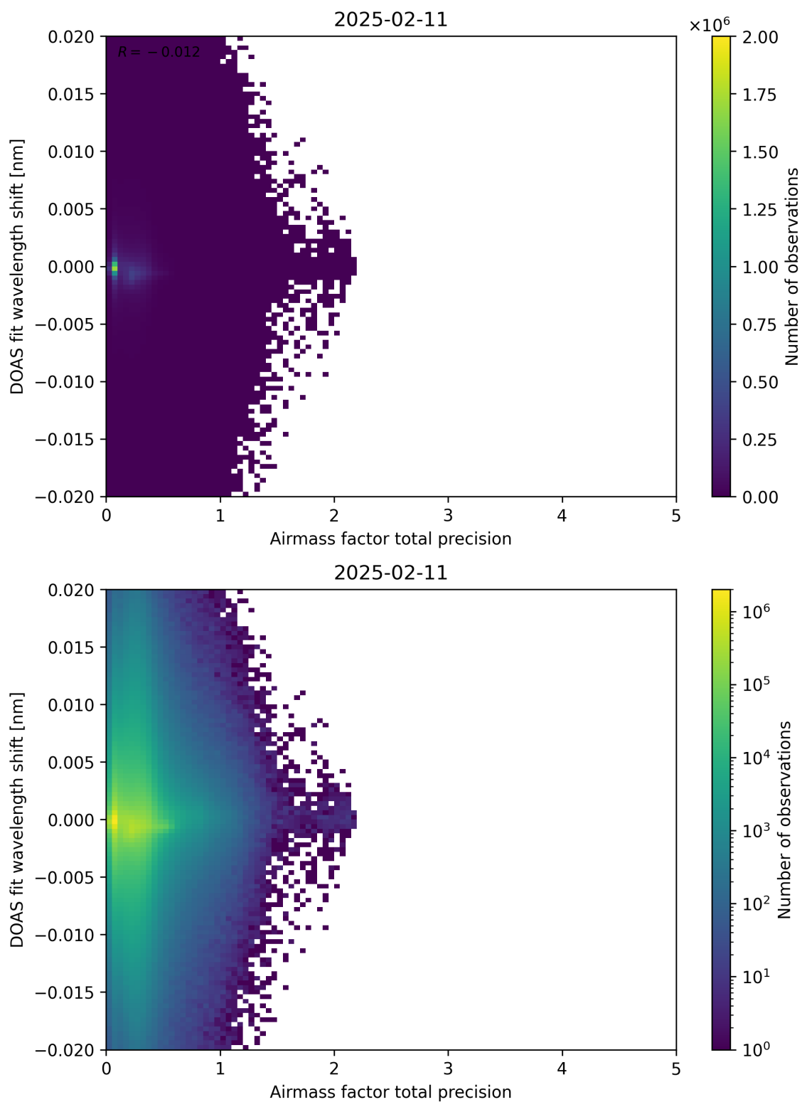
Figure 106: Scatter density plot of “Airmass factor total precision” against “DOAS fit wavelength shift” for 2025-02-10 to 2025-02-12.
