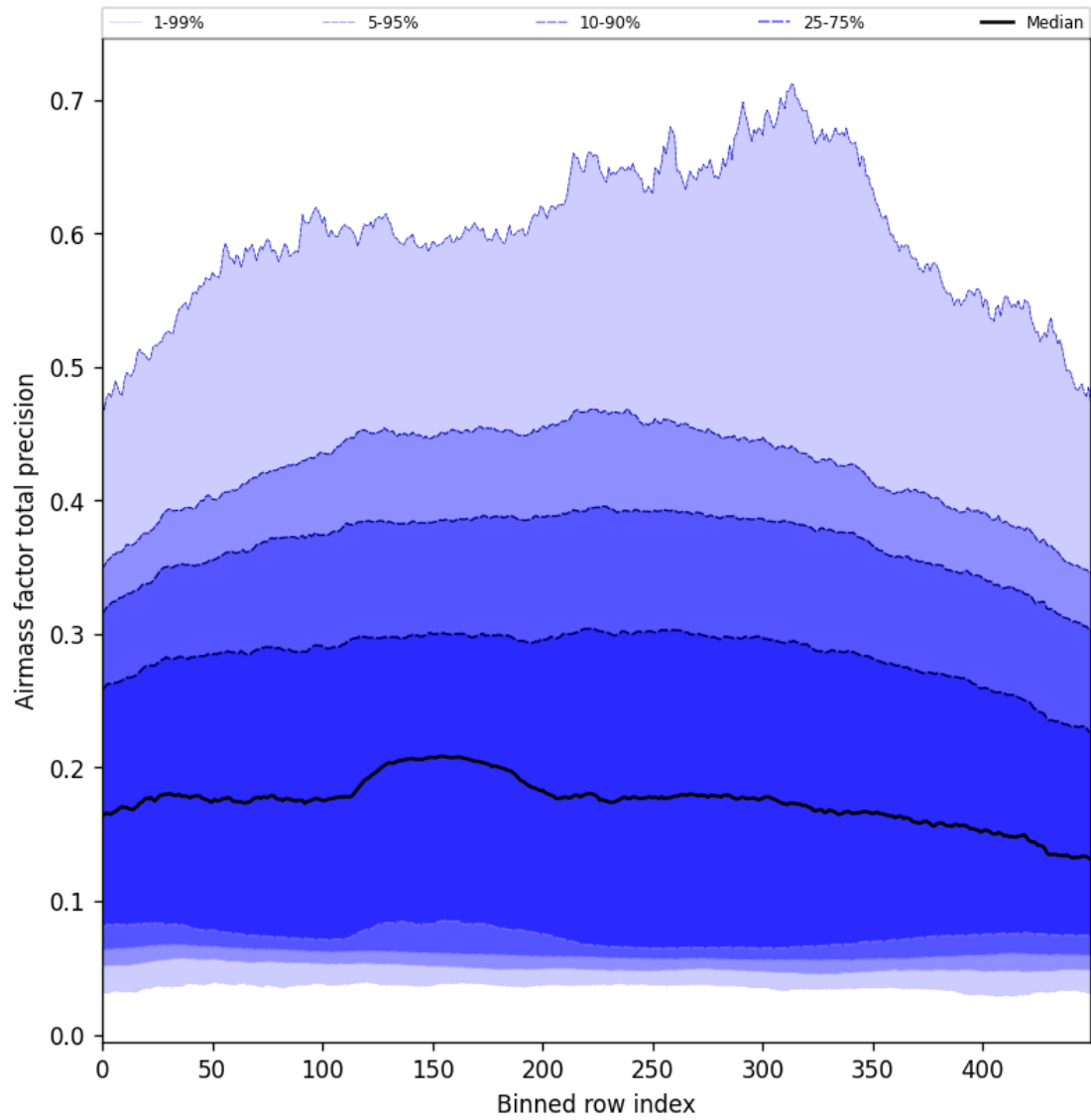
Figure 55: Along track statistics of “Airmass factor total precision” for 2025-02-10 to 2025-02-12
