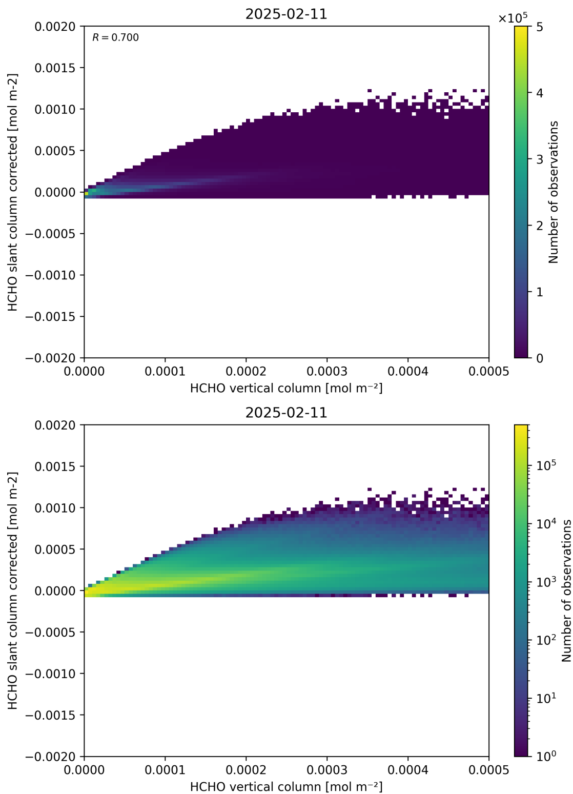
Figure 127: Scatter density plot of “HCHO vertical column” against “HCHO slant column corrected” for 2025-02-10 to 2025-02-12.
