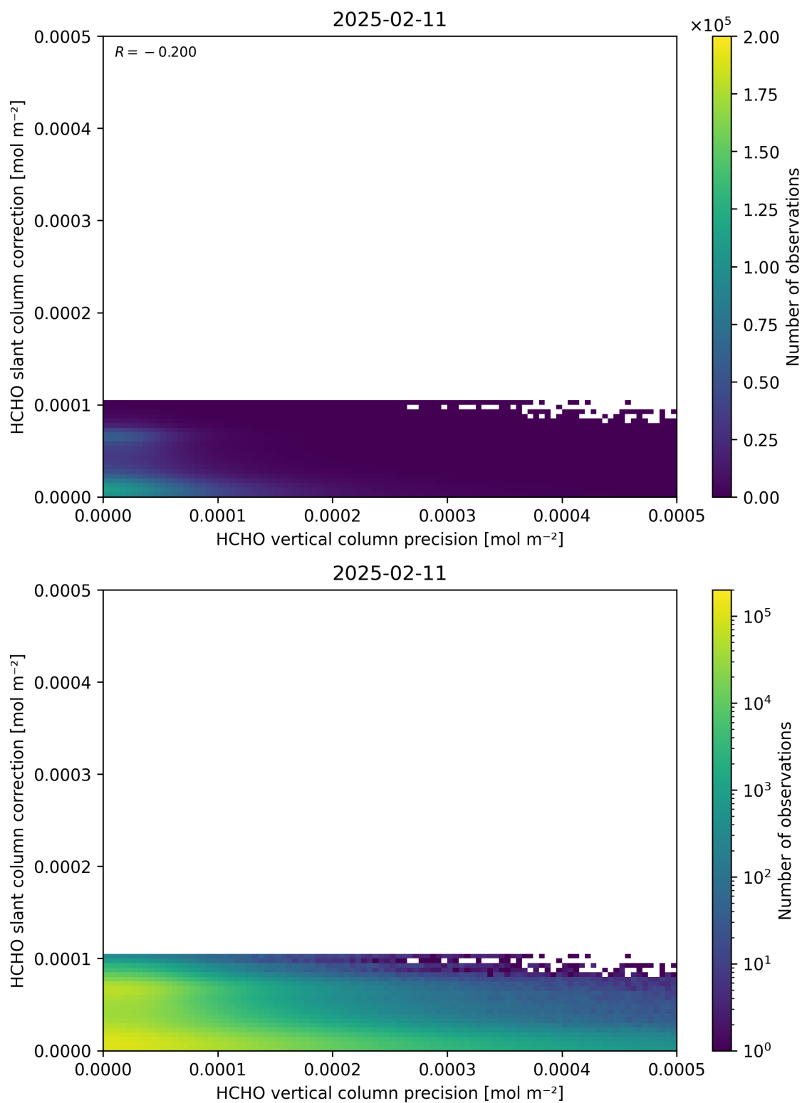
Figure 141: Scatter density plot of “HCHO vertical column precision” against “HCHO slant column correction” for 2025-02-10 to 2025-02-12.
