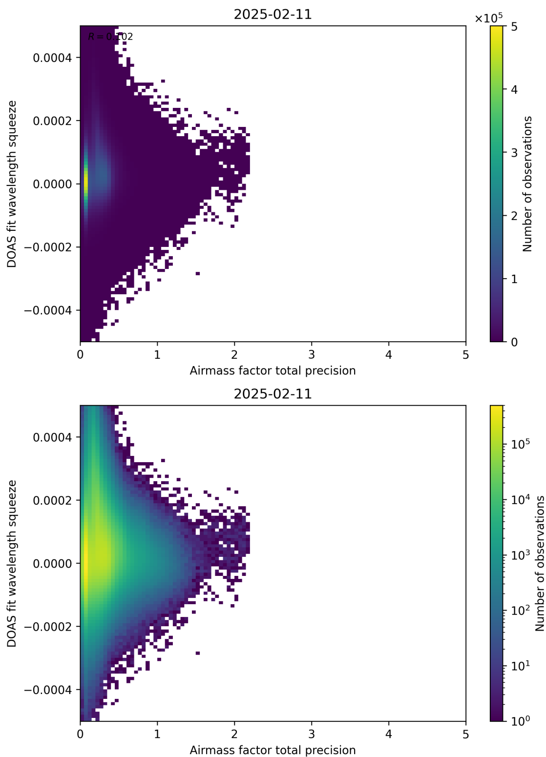
Figure 107: Scatter density plot of “Airmass factor total precision” against “DOAS fit wavelength squeeze” for 2025-02-10 to 2025-02-12.
