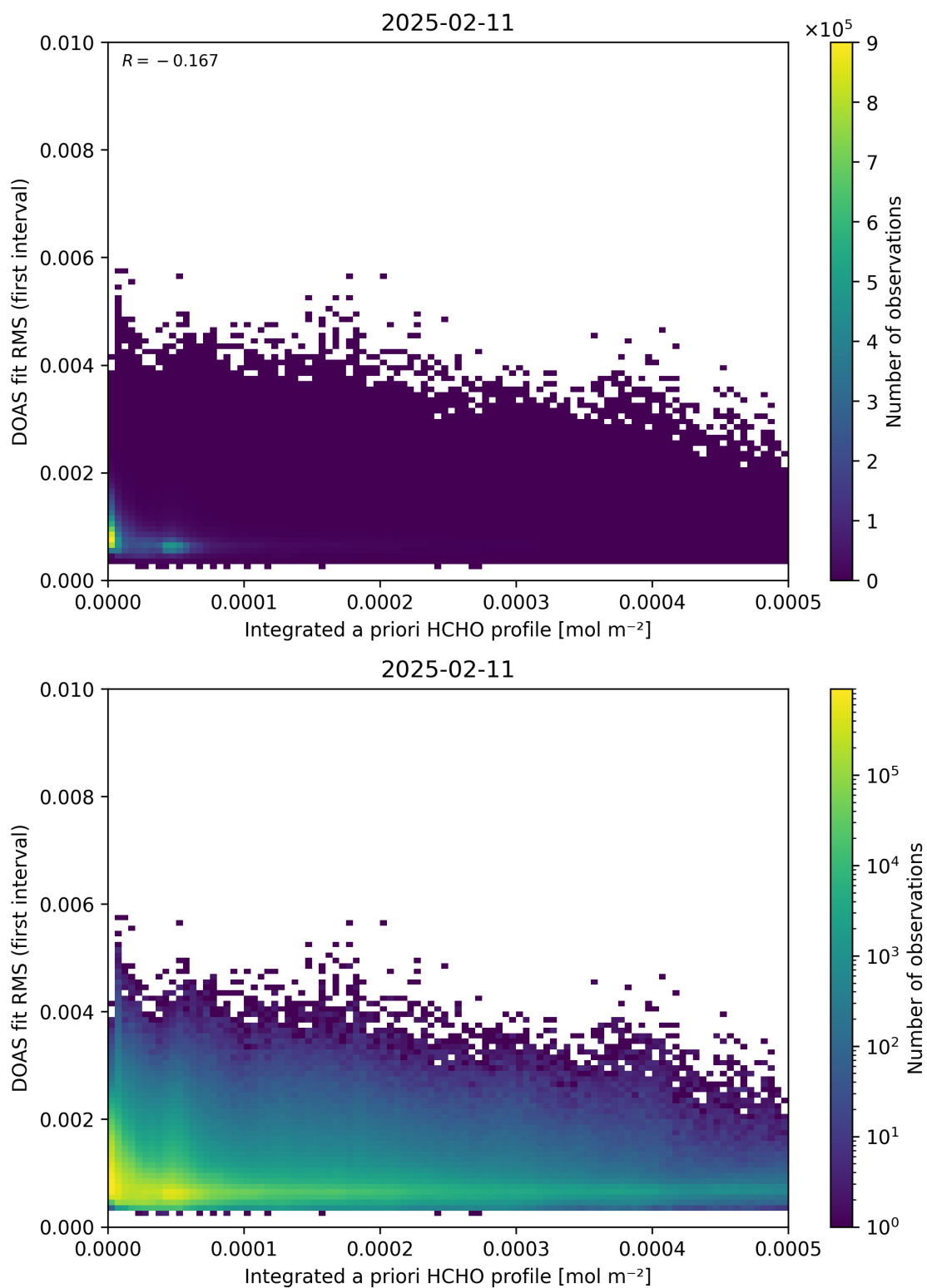
Figure 148: Scatter density plot of “Integrated a priori HCHO profile” against “DOAS fit RMS (first interval)” for 2025-02-10 to 2025-02-12.
