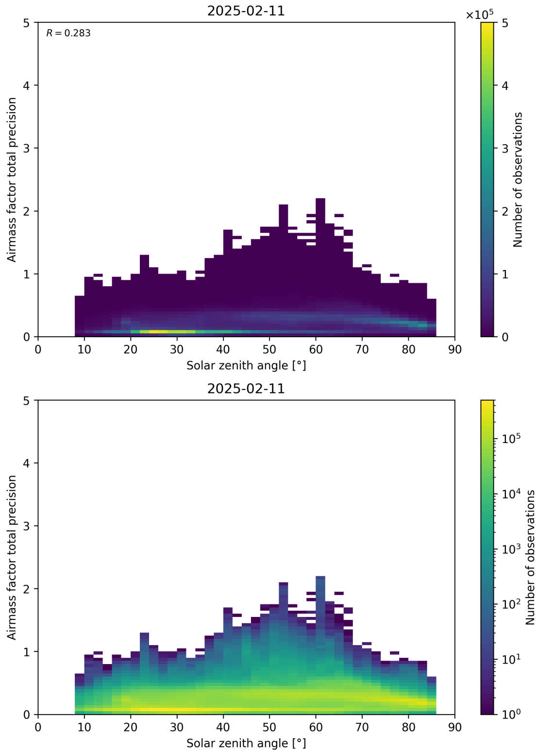
Figure 176: Scatter density plot of “Solar zenith angle” against “Airmass factor total precision” for 2025-02-10 to 2025-02-12.
