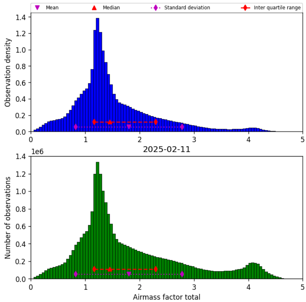
Figure 40: Histogram of “Airmass factor total” for 2025-02-10 to 2025-02-12
