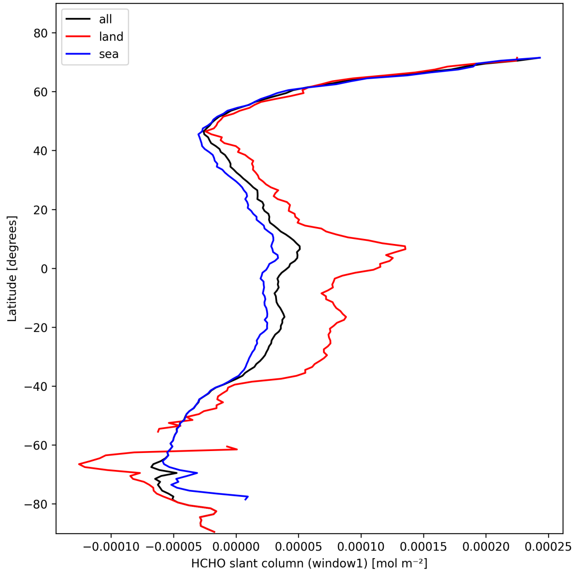
Figure 24: Zonal average of “HCHO slant column (window1)” for 2025-02-10 to 2025-02-12.
