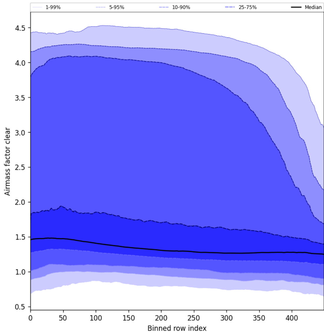
Figure 56: Along track statistics of “Air mass factor clear” for 2025-02-10 to 2025-02-12
