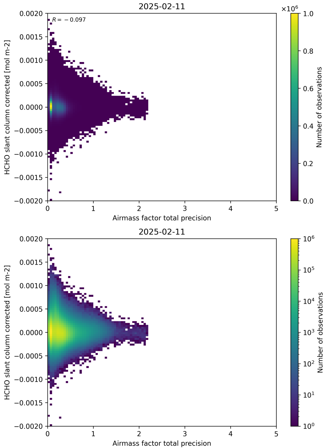
Figure 109: Scatter density plot of “Airmass factor total precision” against “HCHO slant column corrected” for 2025-02-10 to 2025-02-12.
