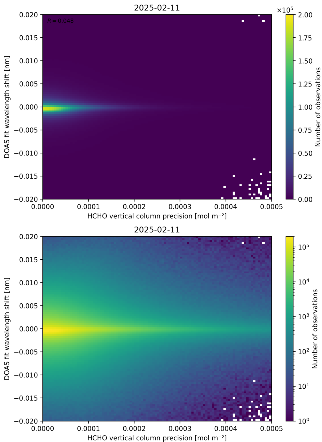
Figure 137: Scatter density plot of “HCHO vertical column precision” against “DOAS fit wavelength shift” for 2025-02-10 to 2025-02-12.
