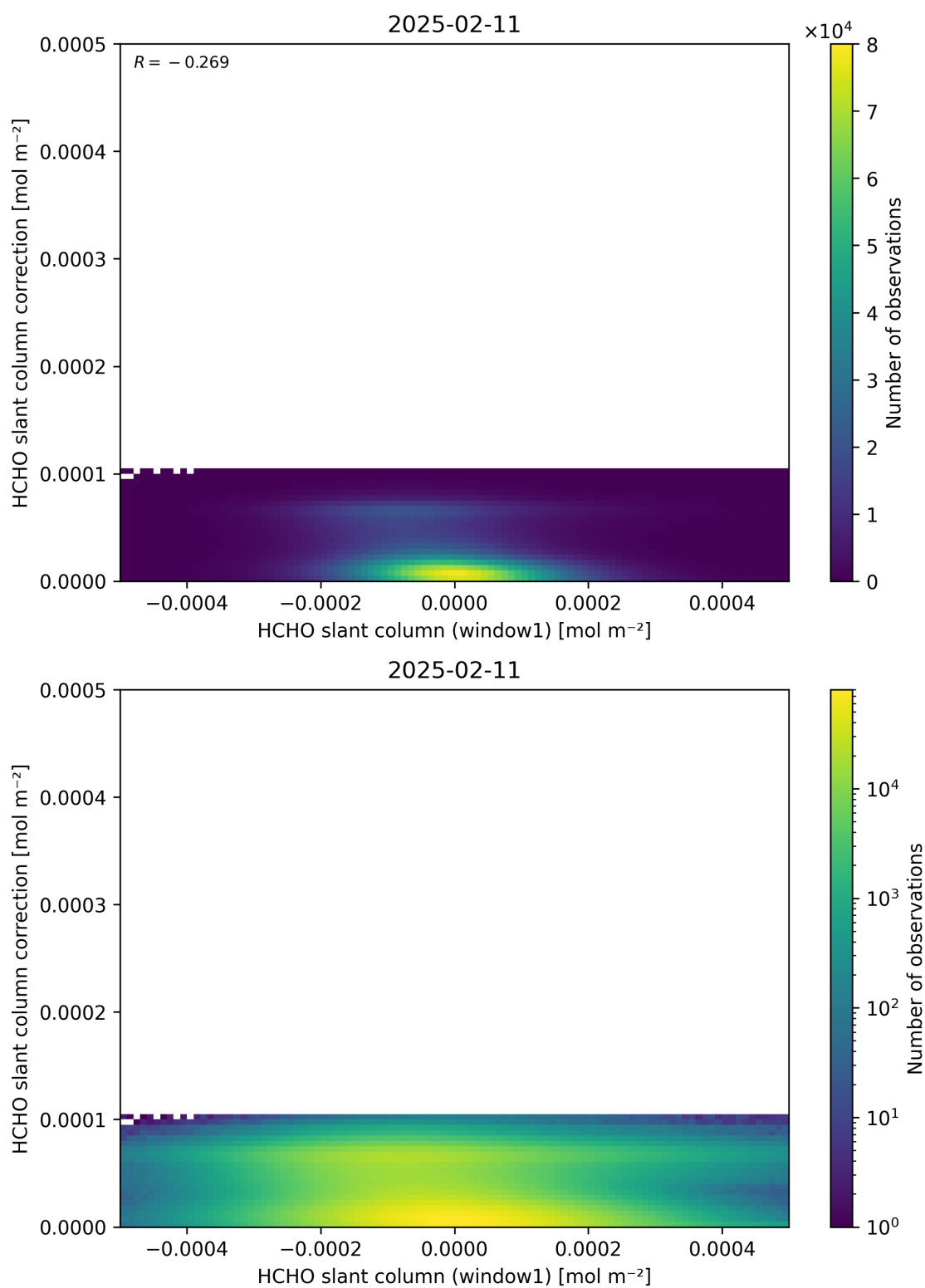
Figure 83: Scatter density plot of “HCHO slant column (window1)” against “HCHO slant column correction” for 2025-02-10 to 2025-02-12.
