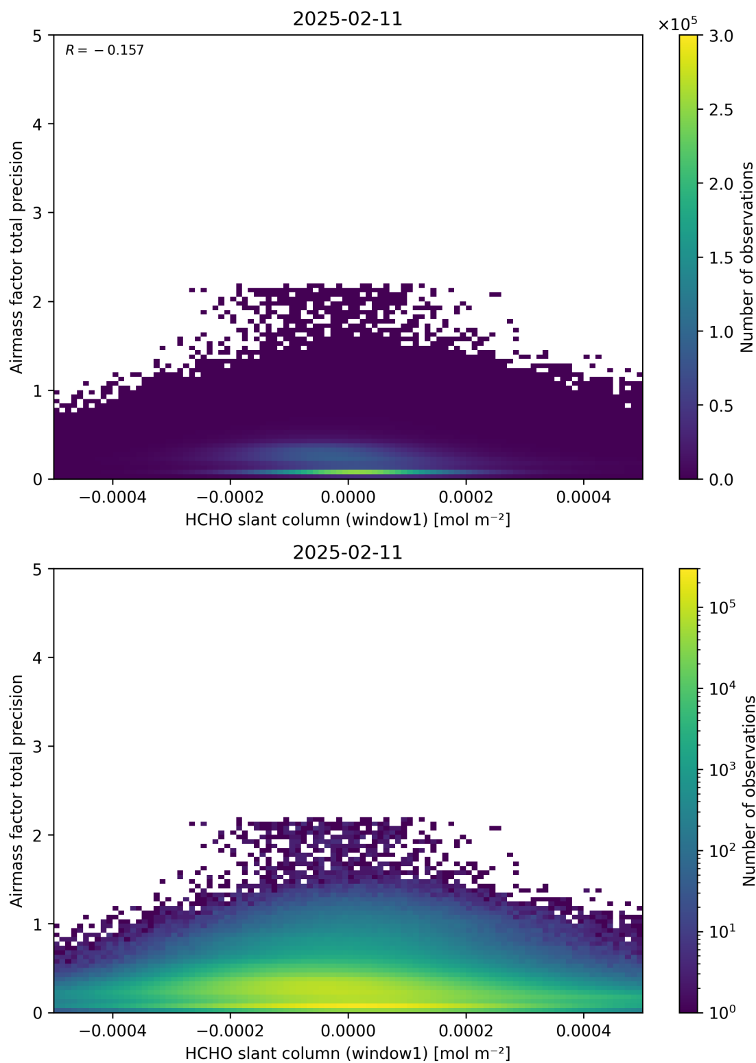
Figure 86: Scatter density plot of “HCHO slant column (window1)” against “Airmass factor total precision” for 2025-02-10 to 2025-02-12.
