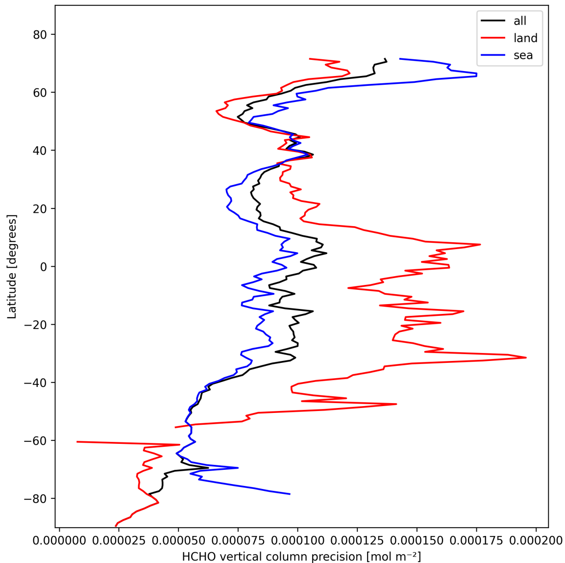
Figure 22: Zonal average of “HCHO vertical column precision” for 2025-02-10 to 2025-02-12.
