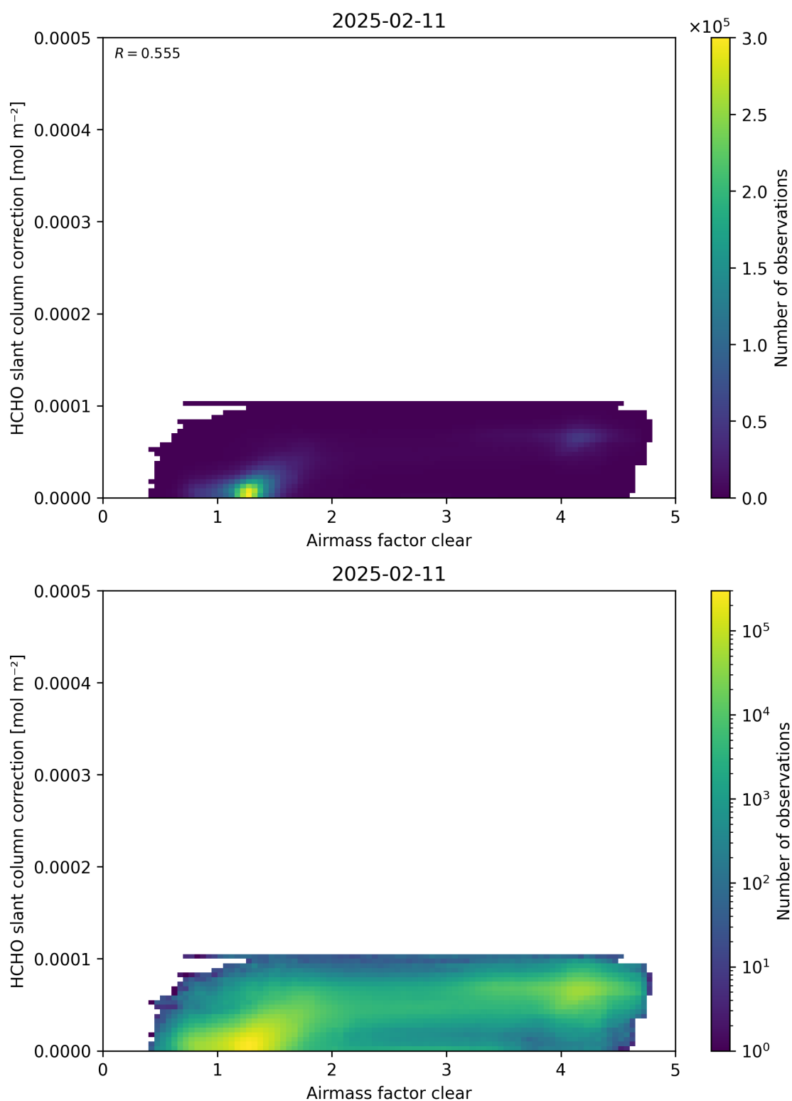
Figure 75: Scatter density plot of “Airmass factor clear” against “HCHO slant column correction” for 2025-02-10 to 2025-02-12.
