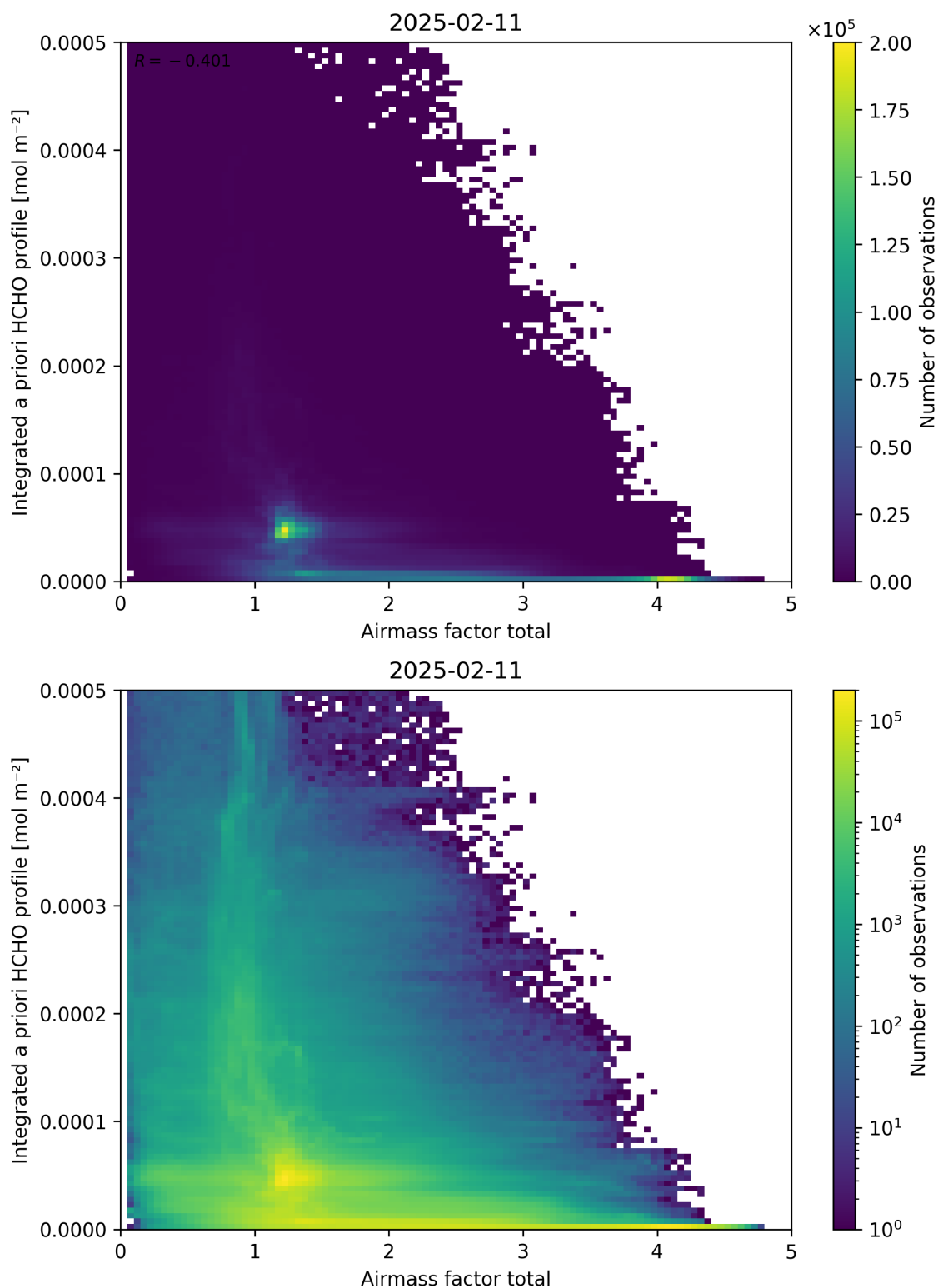
Figure 104: Scatter density plot of “Airmass factor total” against “Integrated a priori HCHO profile” for 2025-02-10 to 2025-02-12.
