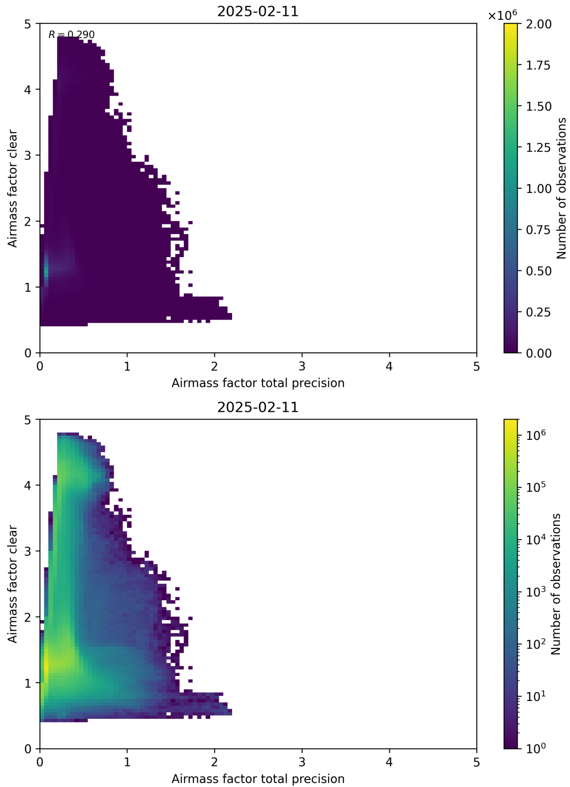
Figure 108: Scatter density plot of “Airmass factor total precision” against “Airmass factor clear” for 2025-02-10 to 2025-02-12.
