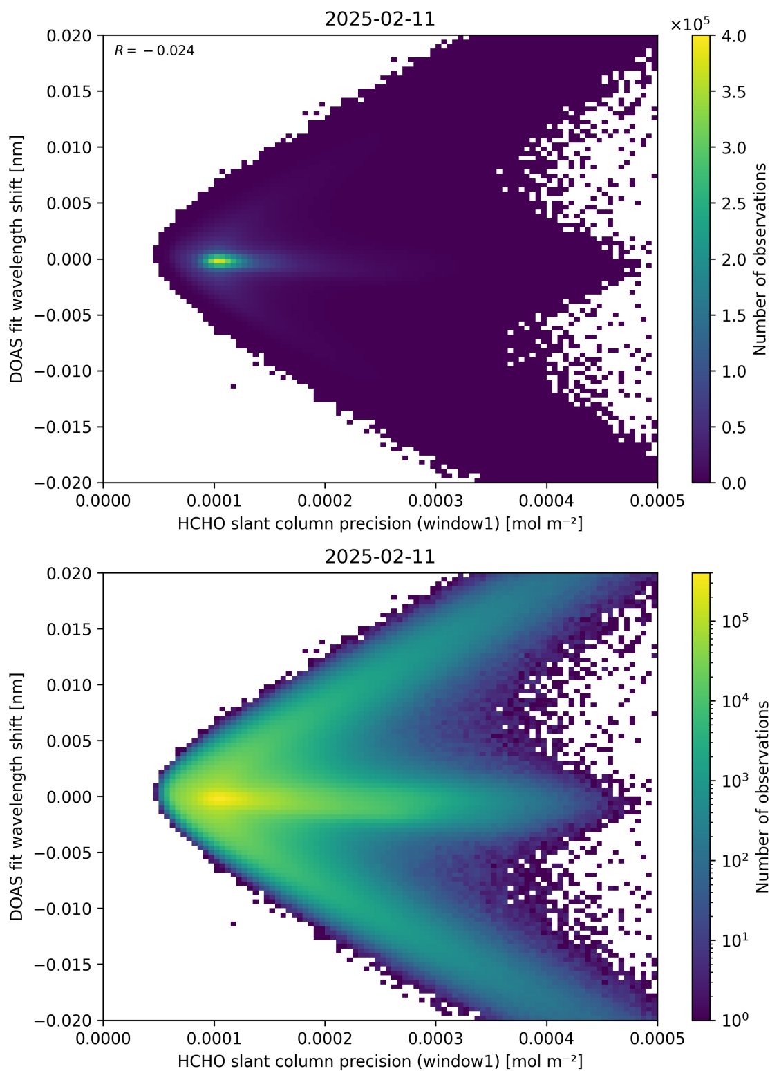
Figure 89: Scatter density plot of “HCHO slant column precision (window1)” against “DOAS fit wavelength shift” for 2025-02-10 to 2025-02-12.
