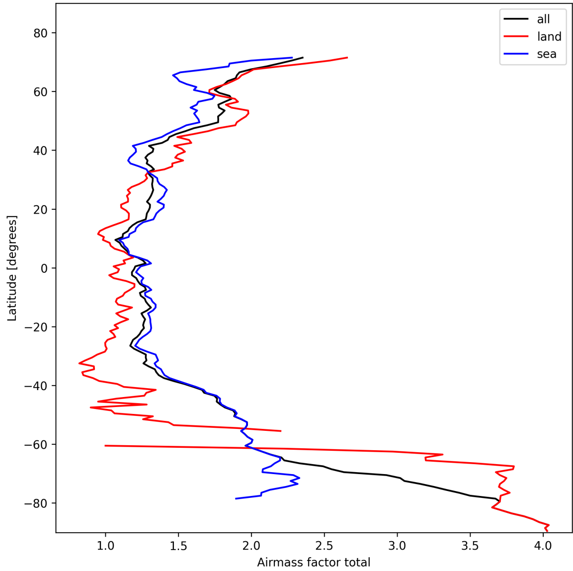
Figure 26: Zonal average of “Airmass factor total” for 2025-02-10 to 2025-02-12.
