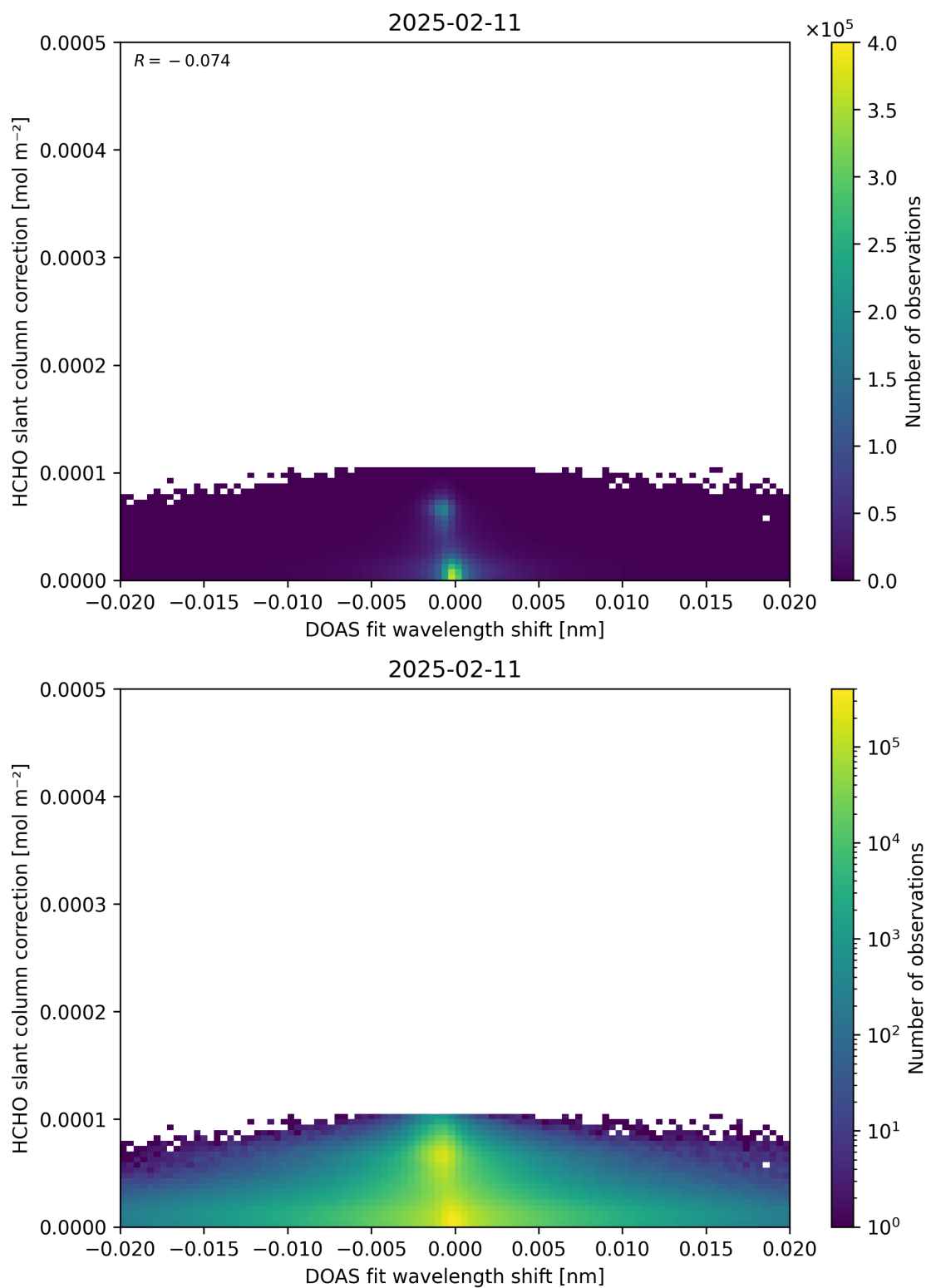
Figure 67: Scatter density plot of “DOAS fit wavelength shift” against “HCHO slant column correction” for 2025-02-10 to 2025-02-12.
