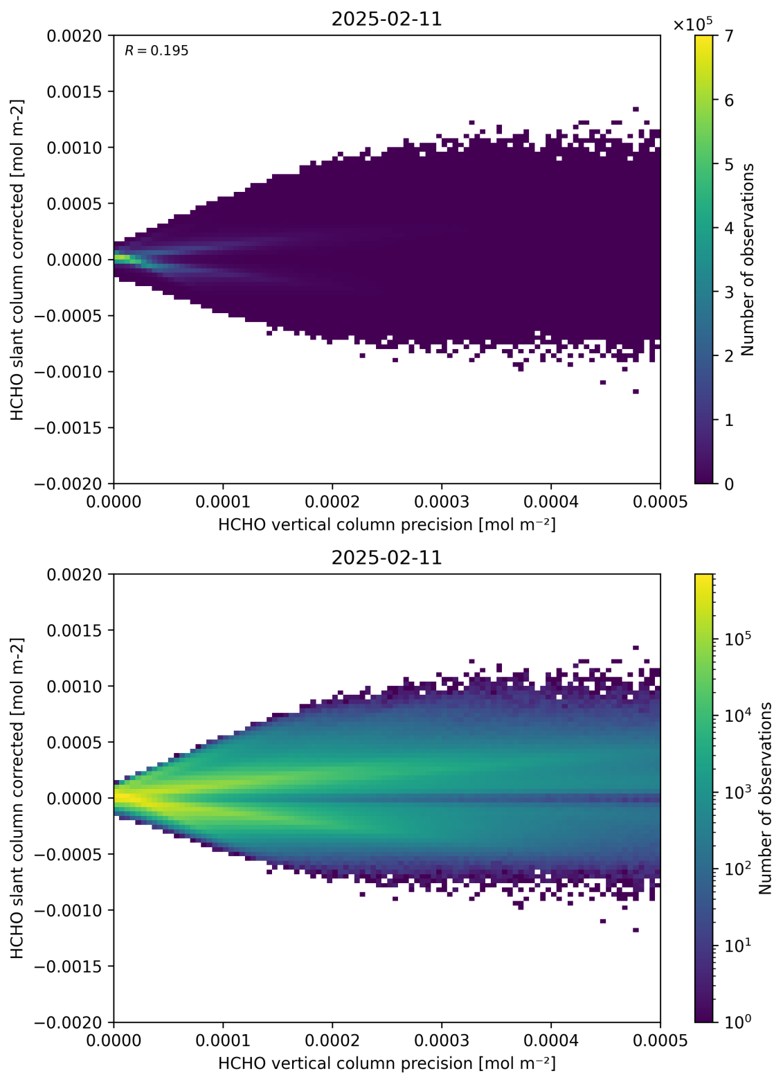
Figure 140: Scatter density plot of “HCHO vertical column precision” against “HCHO slant column corrected” for 2025-02-10 to 2025-02-12.
