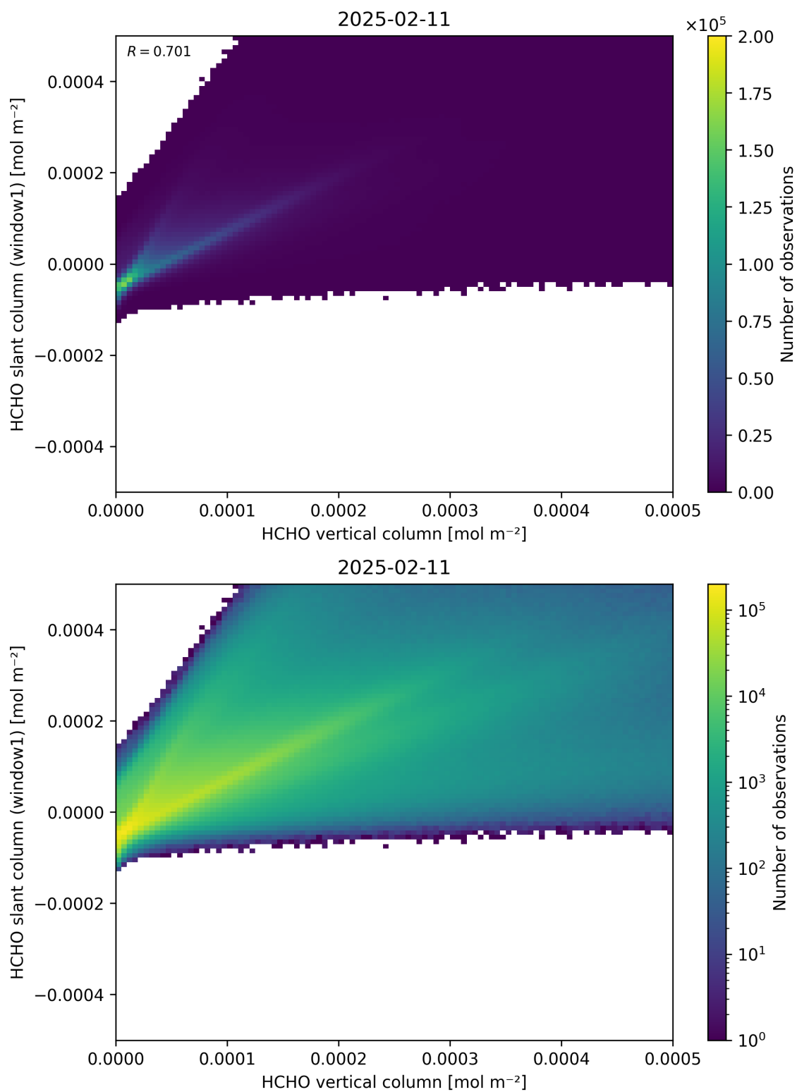
Figure 129: Scatter density plot of “HCHO vertical column” against “HCHO slant column (window1)” for 2025-02-10 to 2025-02-12.
