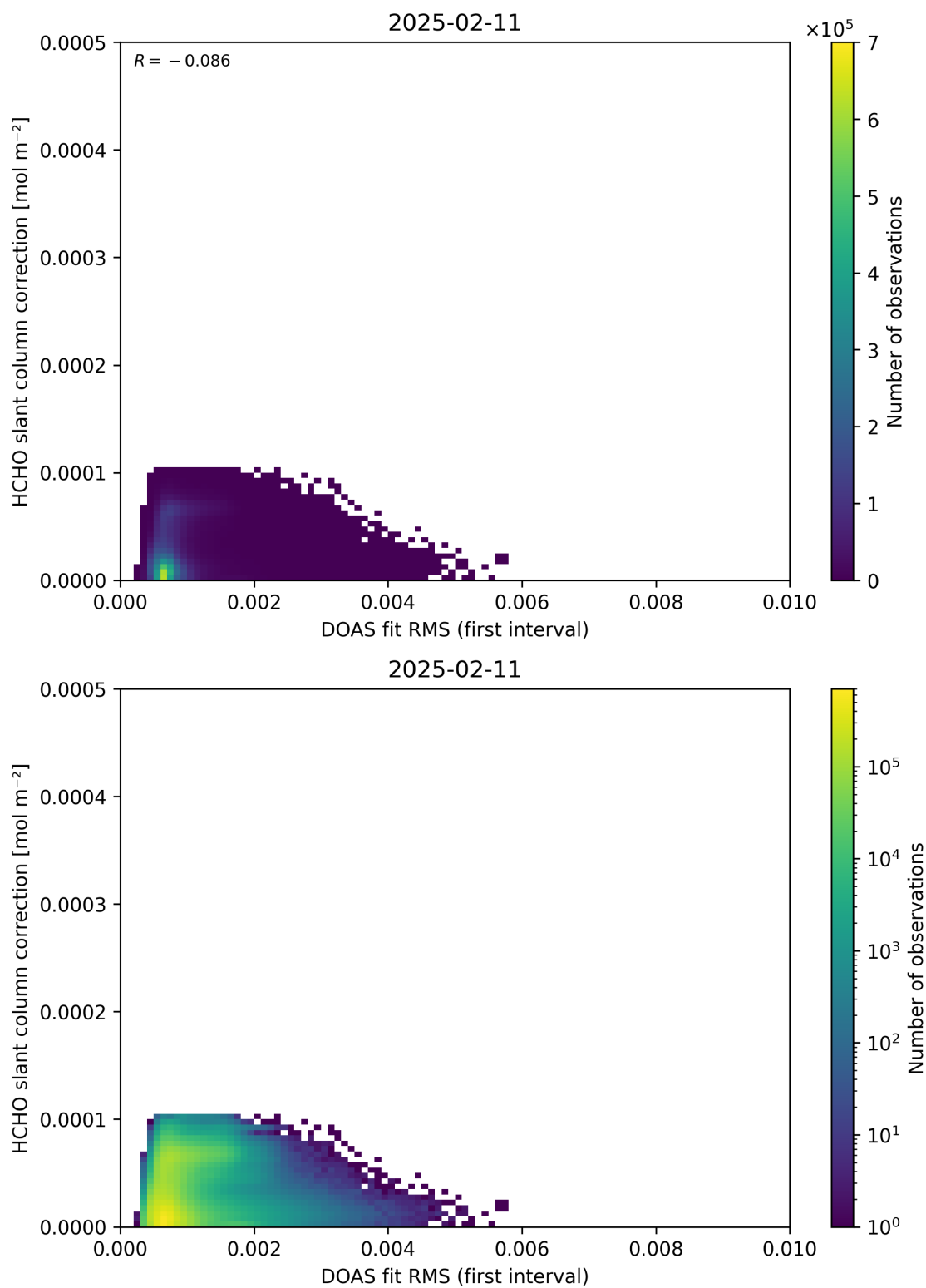
Figure 63: Scatter density plot of “DOAS fit RMS (first interval)” against “HCHO slant column correction” for 2025-02-10 to 2025-02-12.
