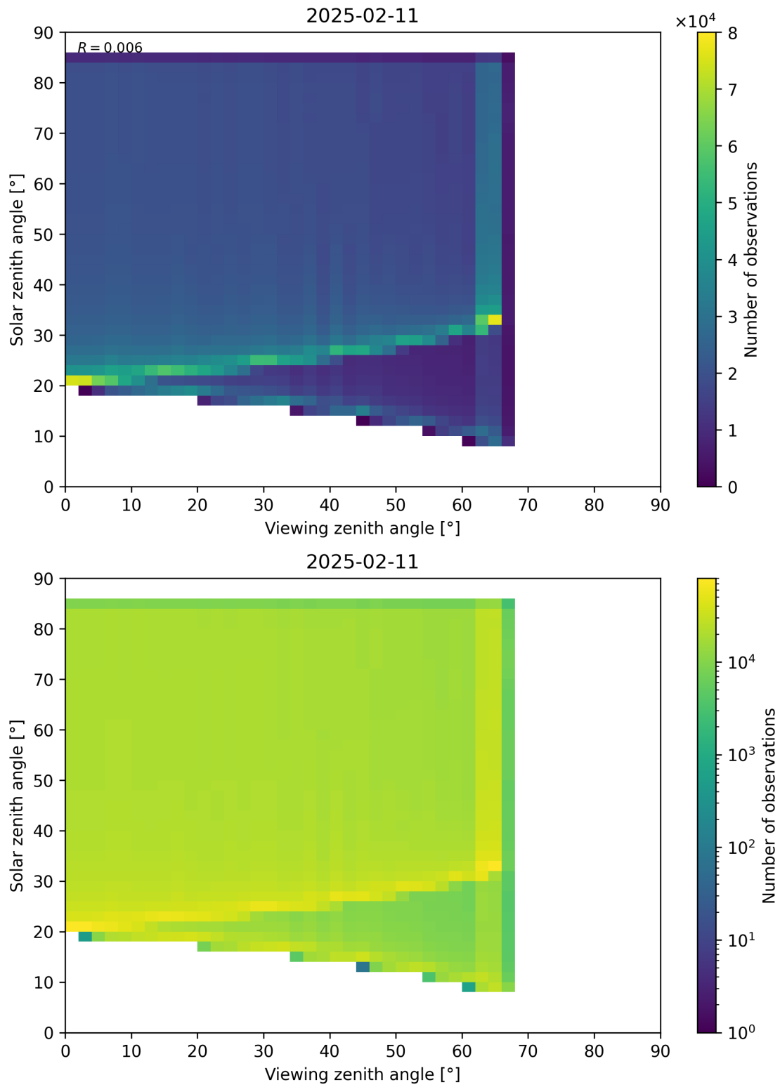
Figure 197: Scatter density plot of “Viewing zenith angle” against “Solar zenith angle” for 2025-02-10 to 2025-02-12.
