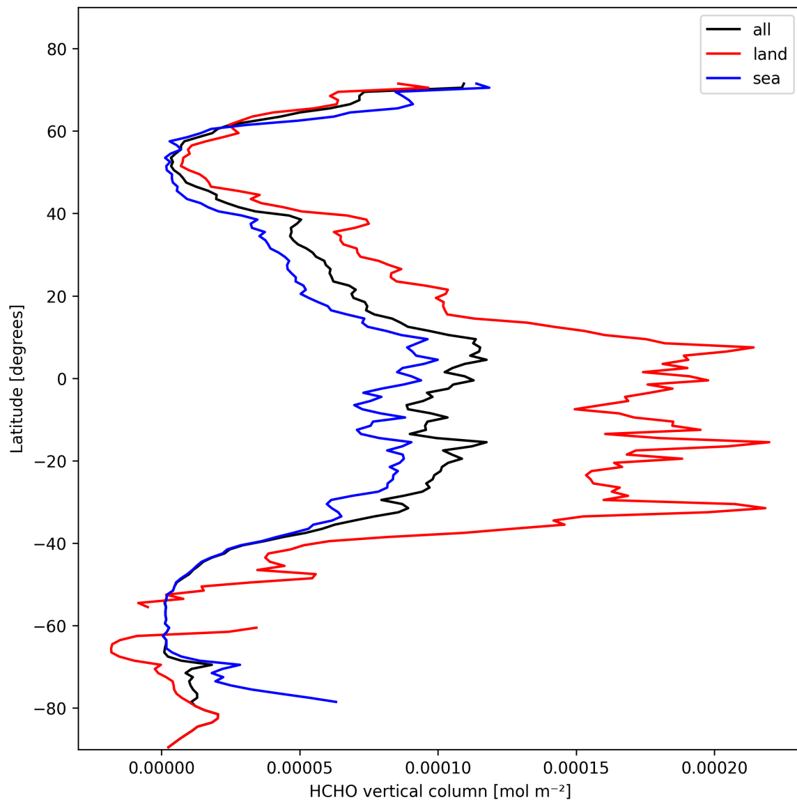
Figure 21: Zonal average of “HCHO vertical column” for 2025-02-10 to 2025-02-12.
