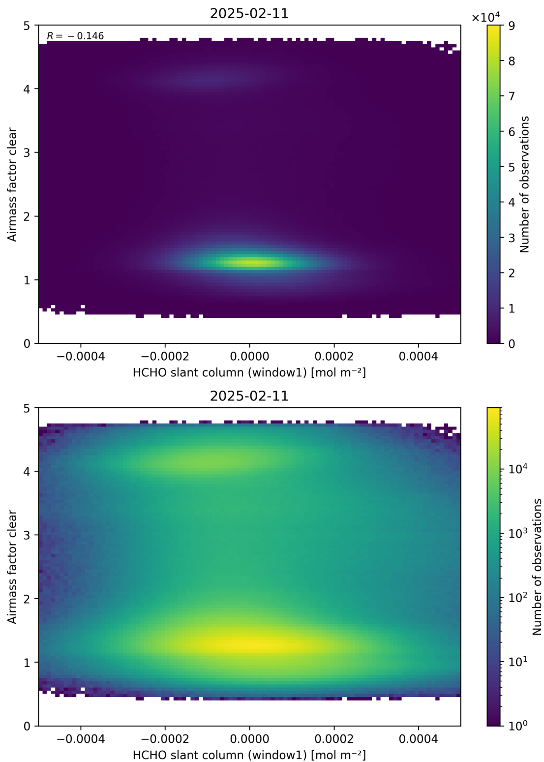
Figure 81: Scatter density plot of “HCHO slant column (window1)” against “Airmass factor clear” for 2025-02-10 to 2025-02-12.
