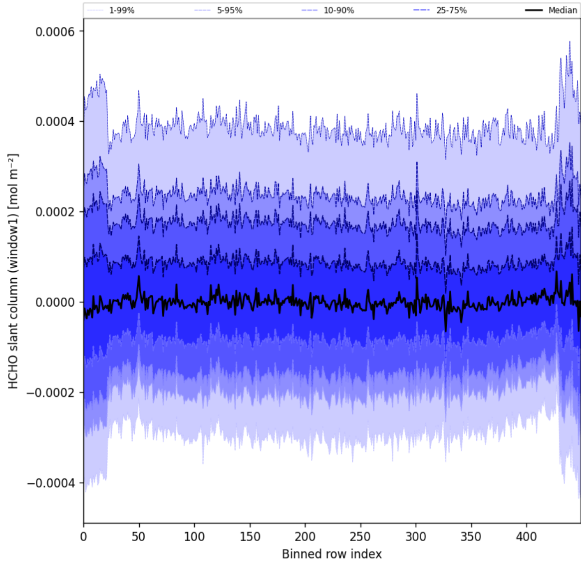
Figure 52: Along track statistics of “HCHO slant column (window1)” for 2025-02-10 to 2025-02-12
