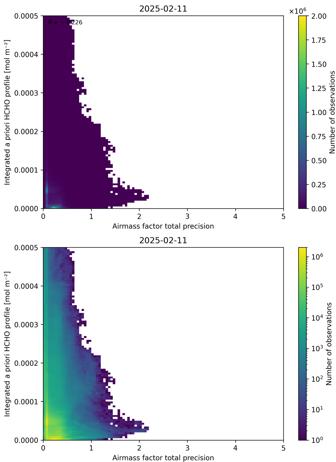
Figure 111: Scatter density plot of “Airmass factor total precision” against “Integrated a priori HCHO profile” for 2025-02-10 to 2025-02-12.
