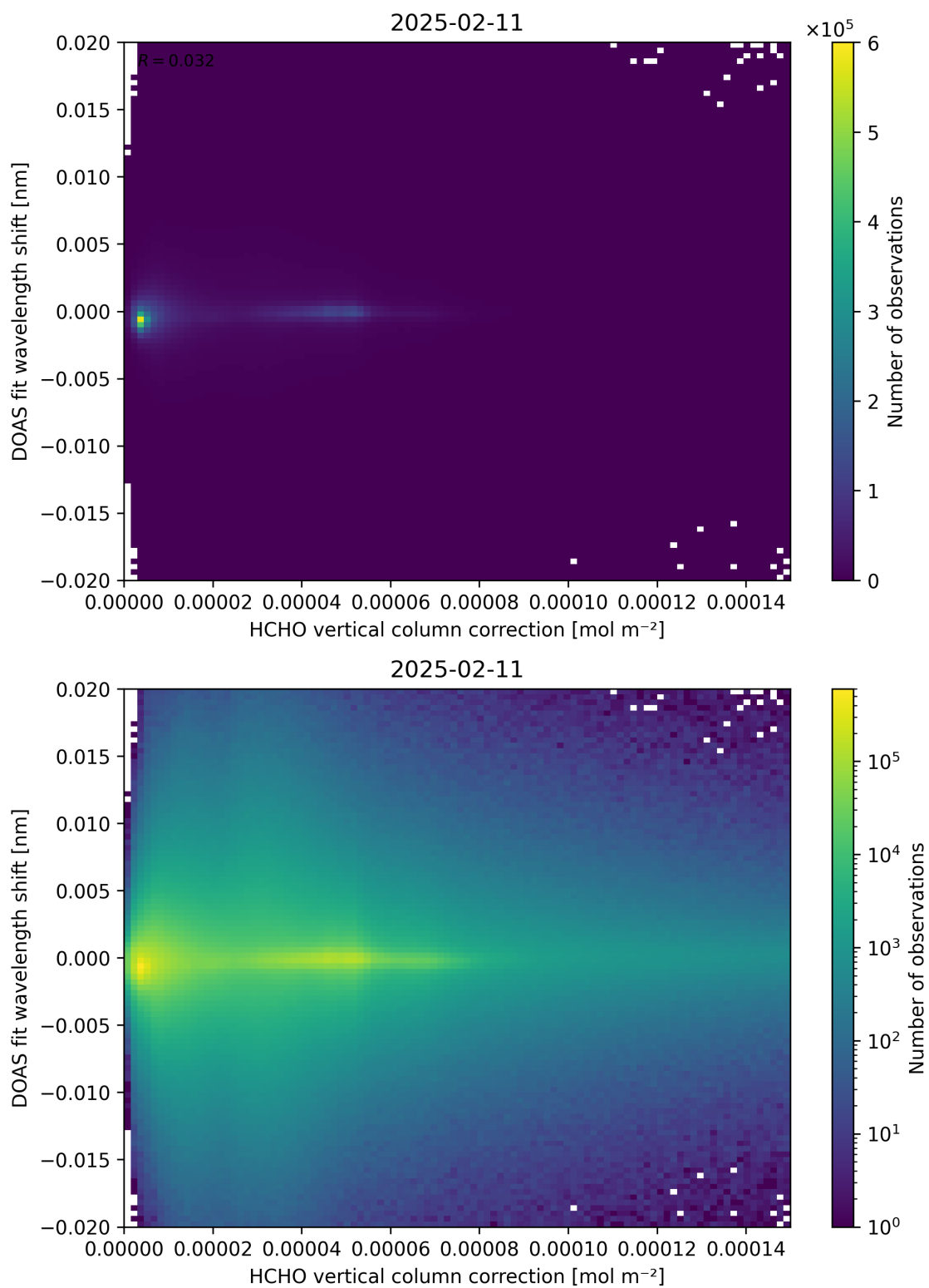
Figure 113: Scatter density plot of “HCHO vertical column correction” against “DOAS fit wavelength shift” for 2025-02-10 to 2025-02-12.
