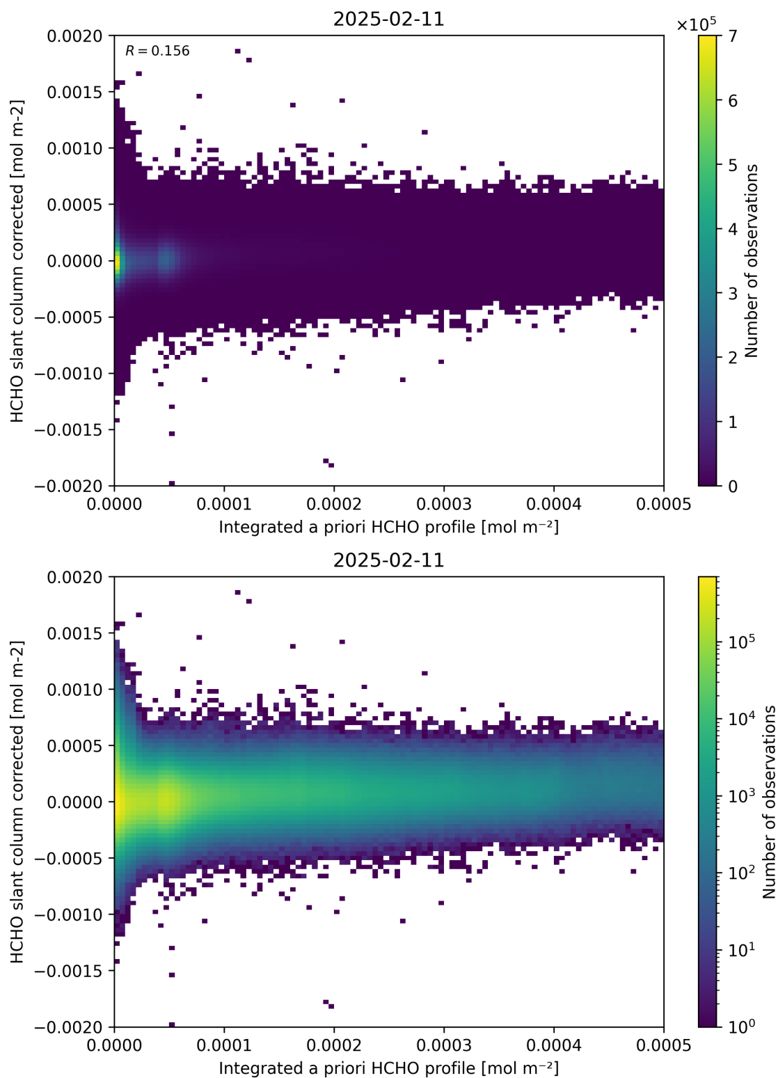
Figure 151: Scatter density plot of “Integrated a priori HCHO profile” against “HCHO slant column corrected” for 2025-02-10 to 2025-02-12.
