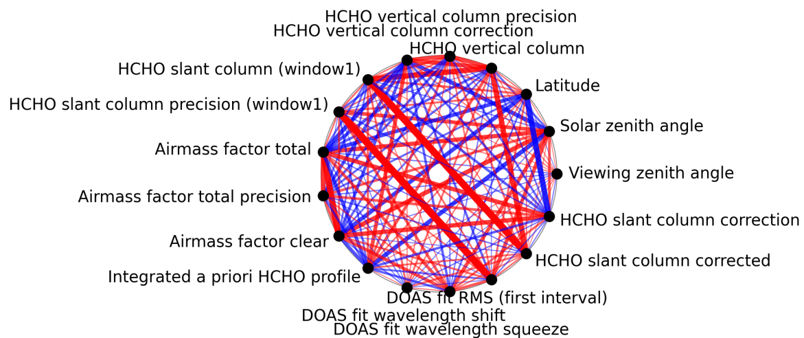
Figure 1: Map of correlation graph for 2025-02-10 to 2025-02-12.
