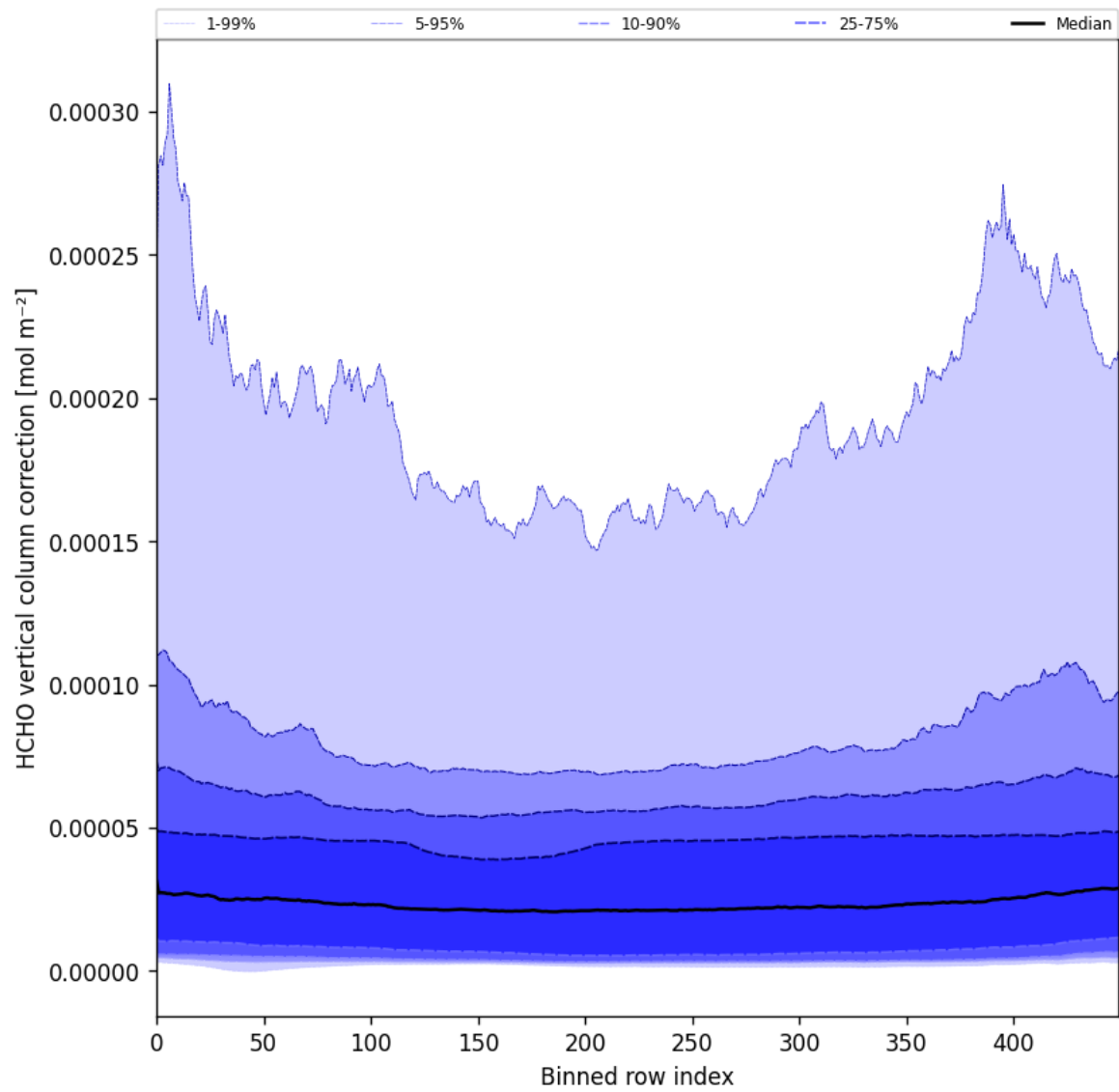
Figure 51: Along track statistics of “HCHO vertical column correction” for 2025-02-10 to 2025-02-12
