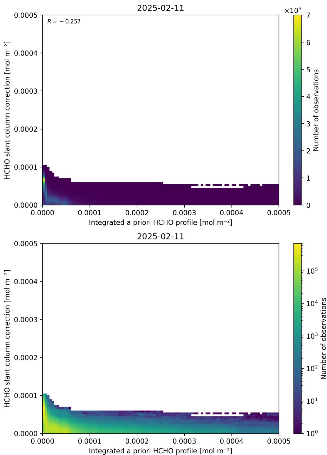
Figure 152: Scatter density plot of “Integrated a priori HCHO profile” against “HCHO slant column correction” for 2025-02-10 to 2025-02-12.
