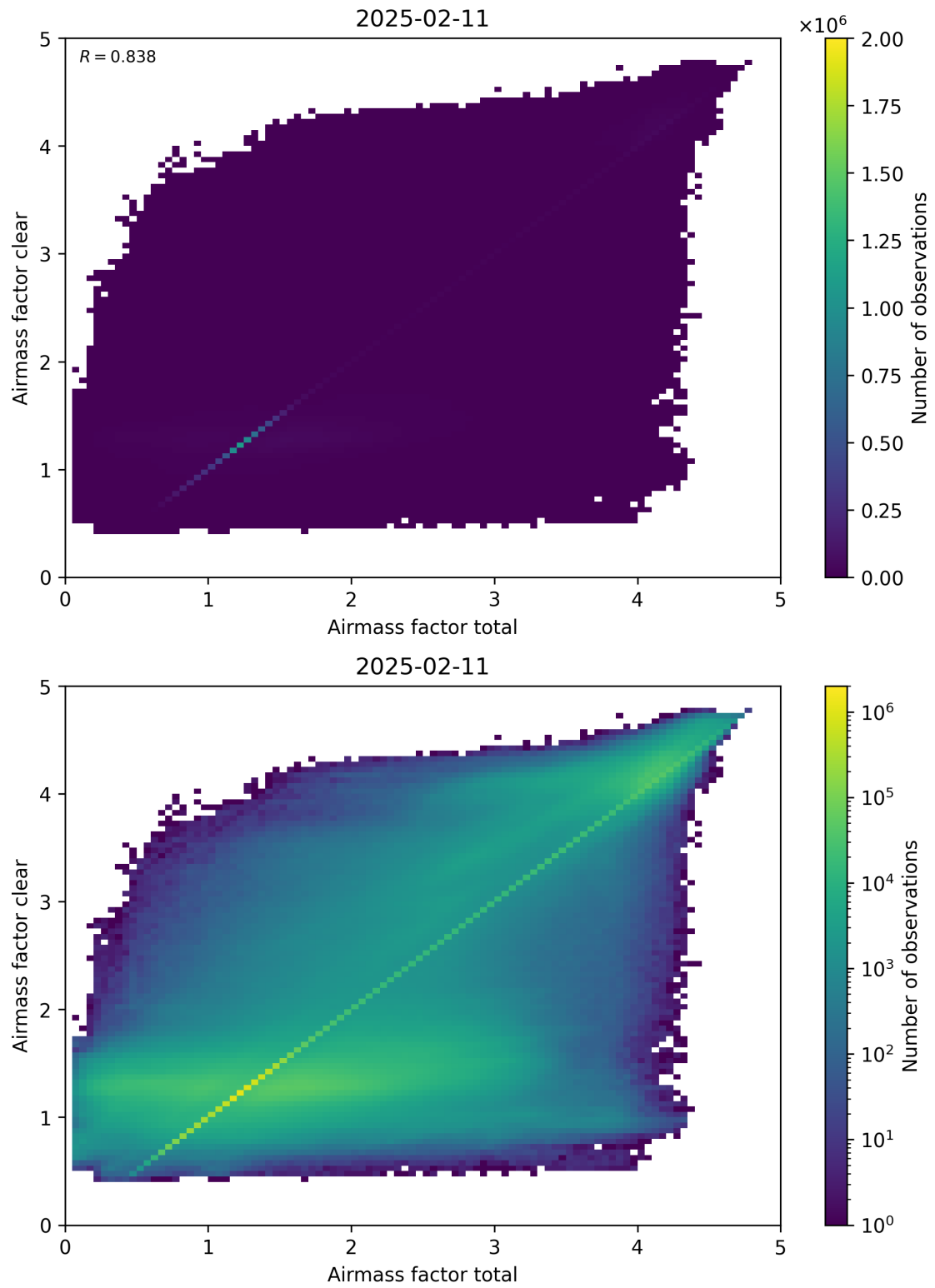
Figure 100: Scatter density plot of “Airmass factor total” against “Airmass factor clear” for 2025-02-10 to 2025-02-12.
