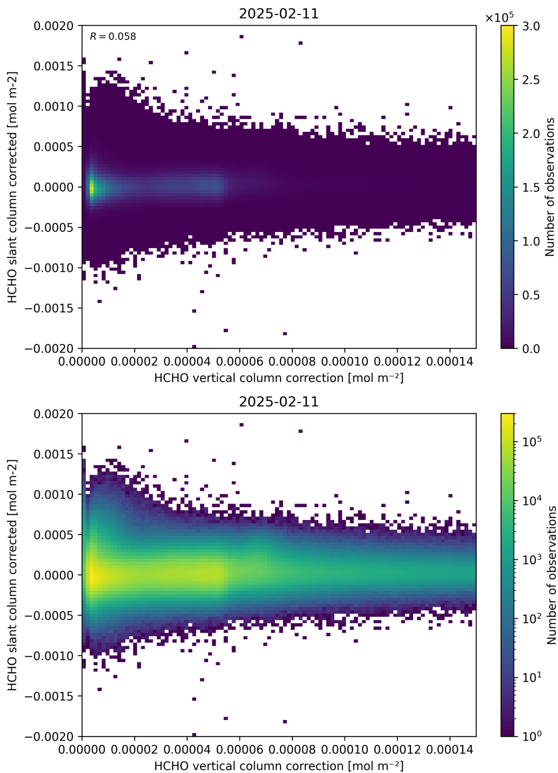
Figure 116: Scatter density plot of “HCHO vertical column correction” against “HCHO slant column corrected” for 2025-02-10 to 2025-02-12.
