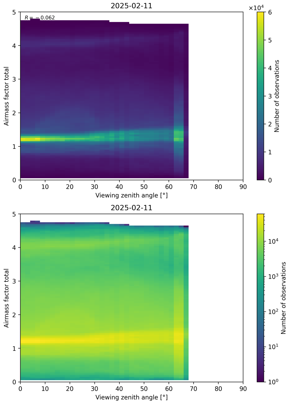
Figure 190: Scatter density plot of “Viewing zenith angle” against “Airmass factor total” for 2025-02-10 to 2025-02-12.
