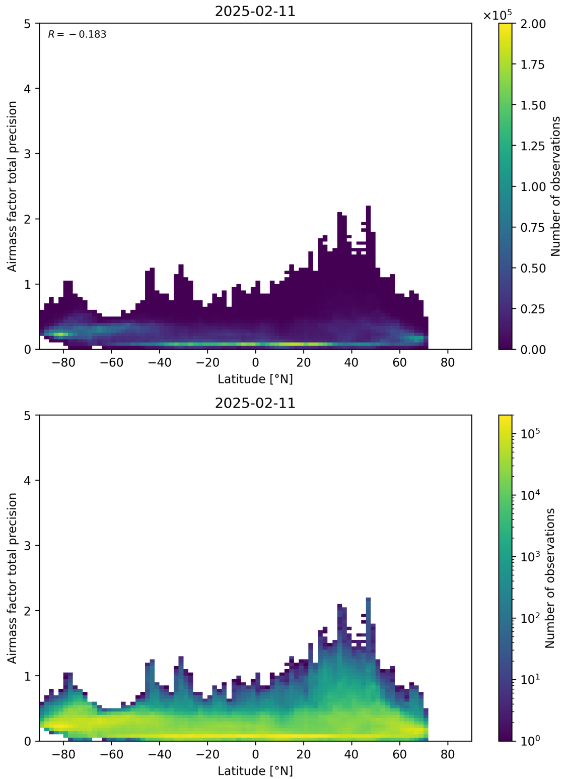
Figure 162: Scatter density plot of “Latitude” against “Airmass factor total precision” for 2025-02-10 to 2025-02-12.
