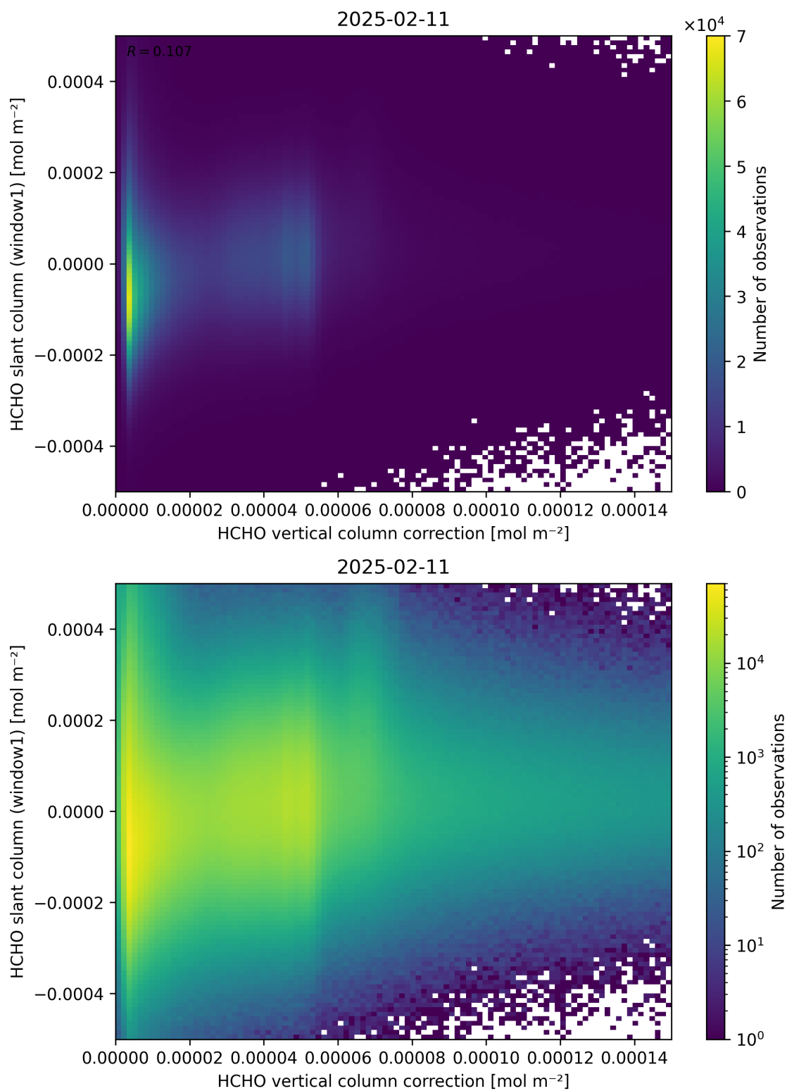
Figure 118: Scatter density plot of “HCHO vertical column correction” against “HCHO slant column (window1)” for 2025-02-10 to 2025-02-12.
