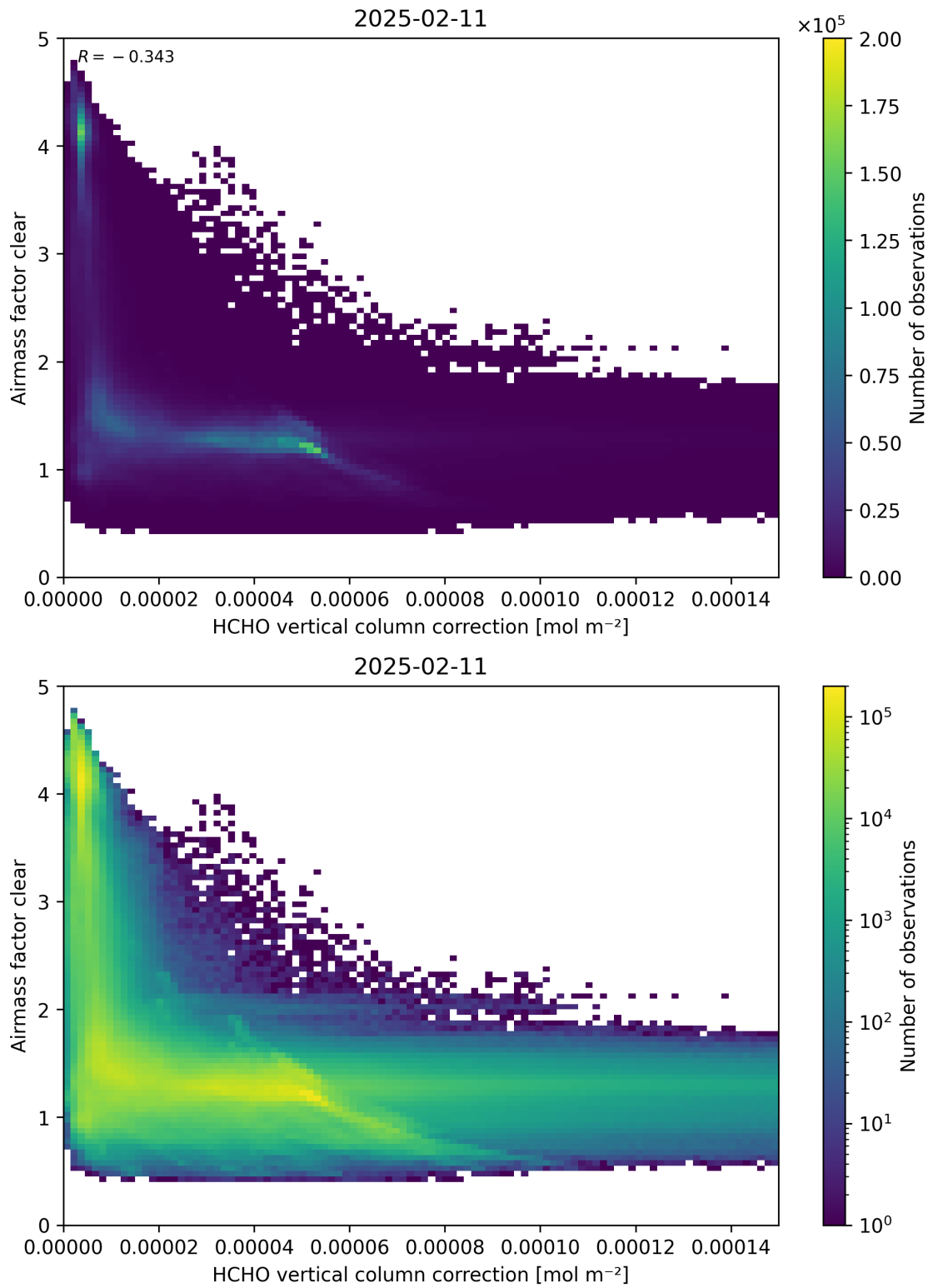
Figure 115: Scatter density plot of “HCHO vertical column correction” against “Airmass factor clear” for 2025-02-10 to 2025-02-12.
