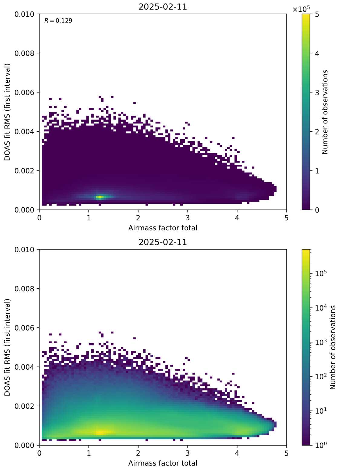
Figure 97: Scatter density plot of “Airmass factor total” against “DOAS fit RMS (first interval)” for 2025-02-10 to 2025-02-12.
