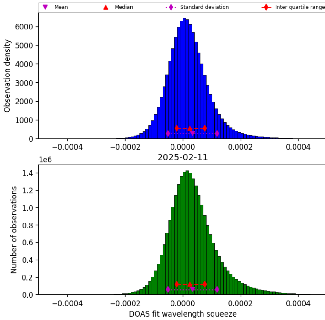
Figure 45: Histogram of “DOAS fit wavelength squeeze” for 2025-02-10 to 2025-02-12
