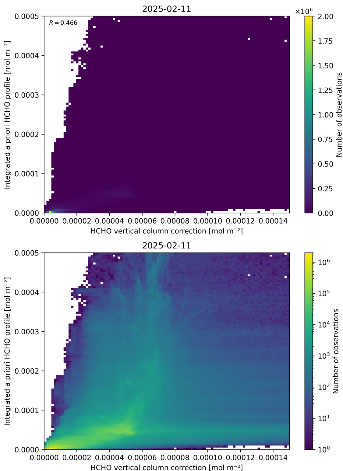
Figure 122: Scatter density plot of “HCHO vertical column correction” against “Integrated a priori HCHO profile” for 2025-02-10 to 2025-02-12.
