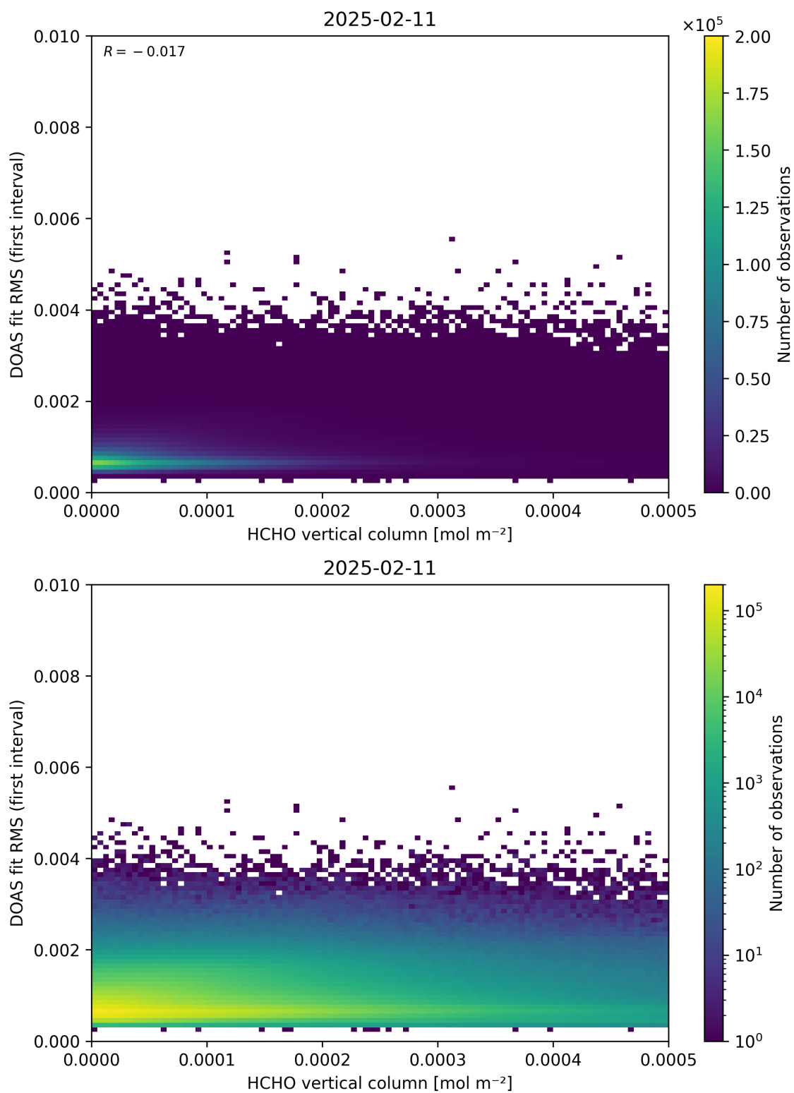
Figure 123: Scatter density plot of “HCHO vertical column” against “DOAS fit RMS (first interval)” for 2025-02-10 to 2025-02-12.
