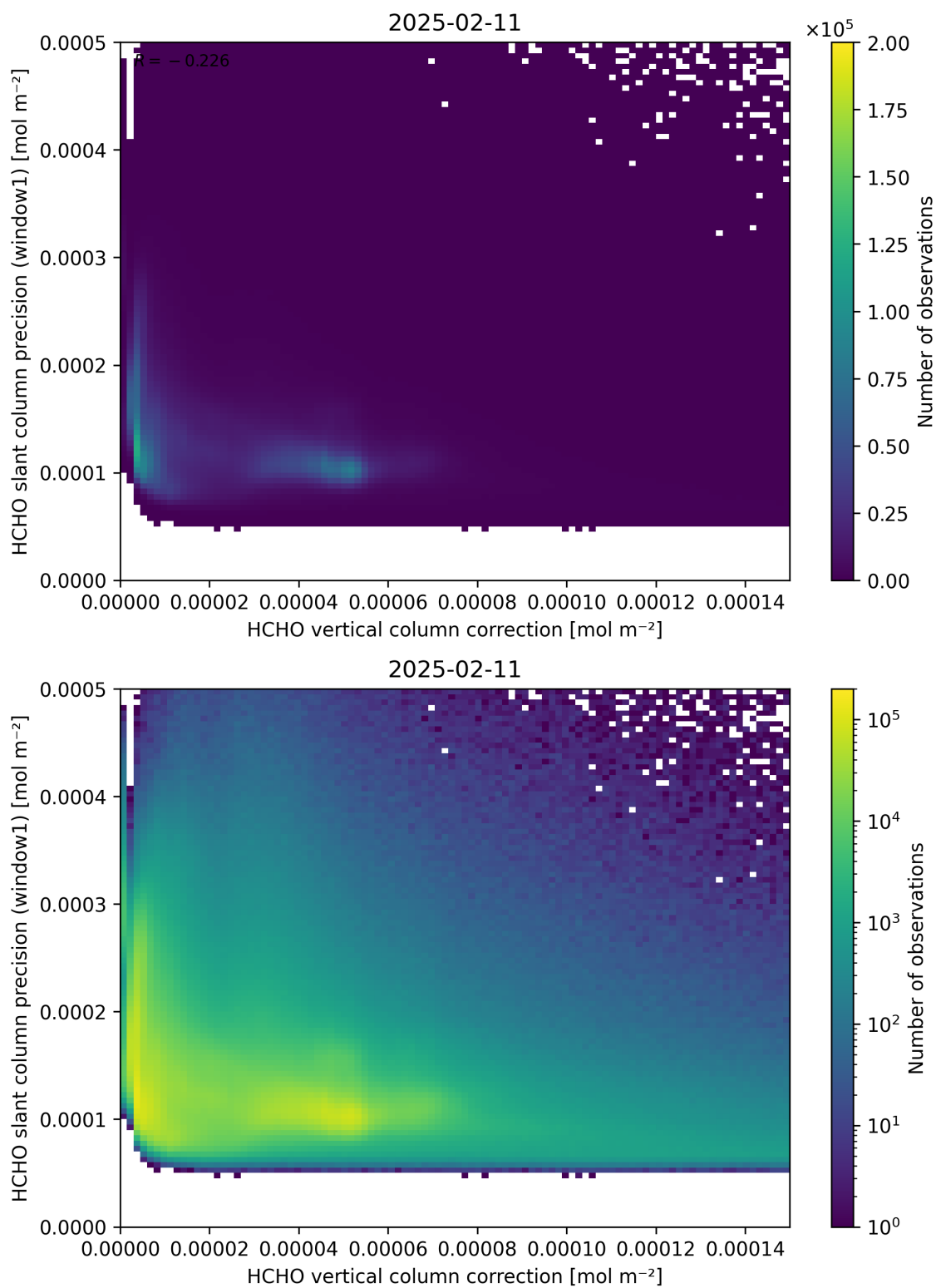
Figure 119: Scatter density plot of “HCHO vertical column correction” against “HCHO slant column precision (window1)” for 2025-02-10 to 2025-02-12.
