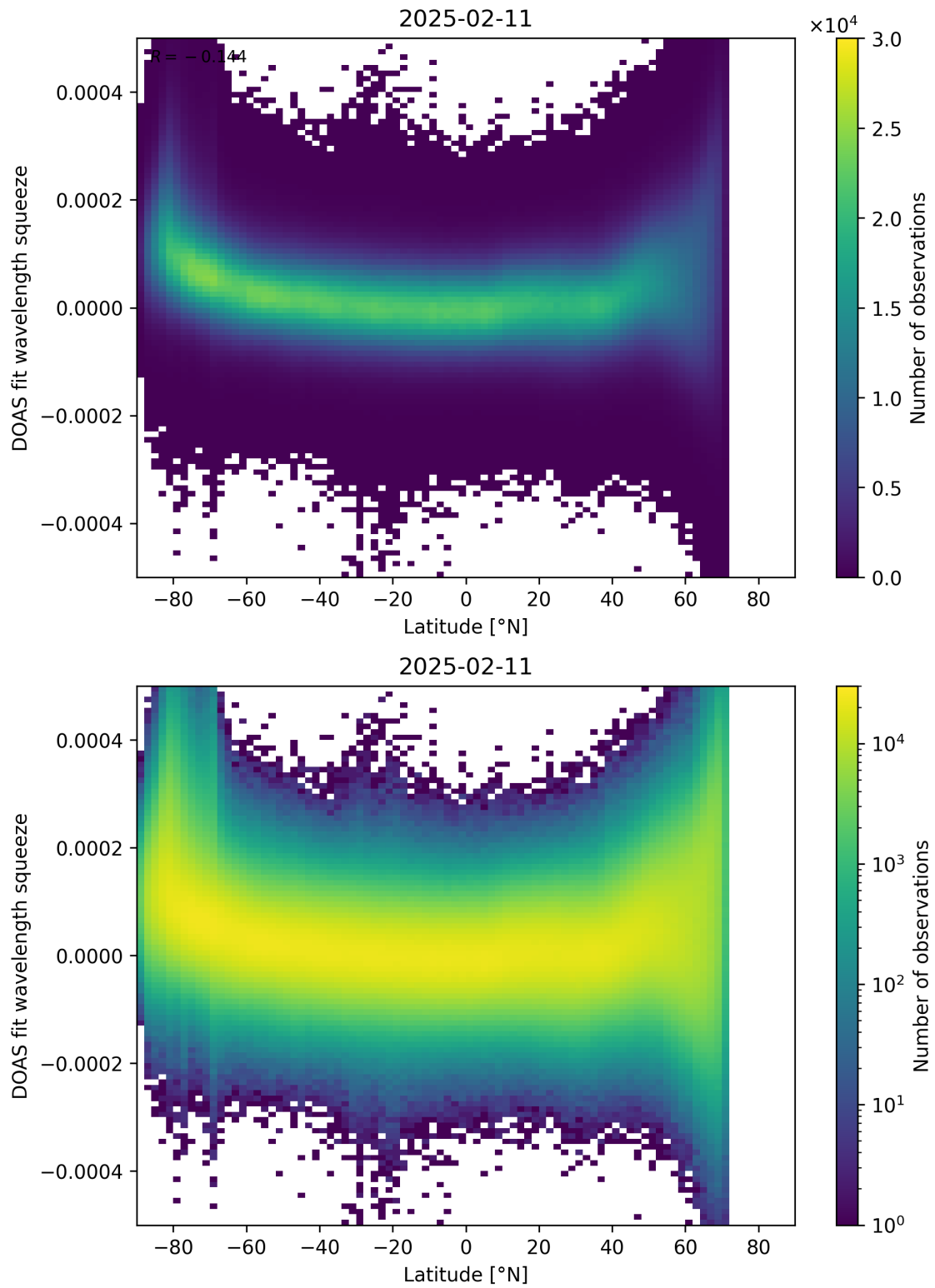
Figure 155: Scatter density plot of “Latitude” against “DOAS fit wavelength squeeze” for 2025-02-10 to 2025-02-12.
