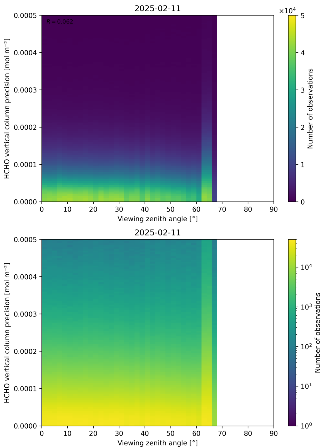
Figure 194: Scatter density plot of “Viewing zenith angle” against “HCHO vertical column precision” for 2025-02-10 to 2025-02-12.
