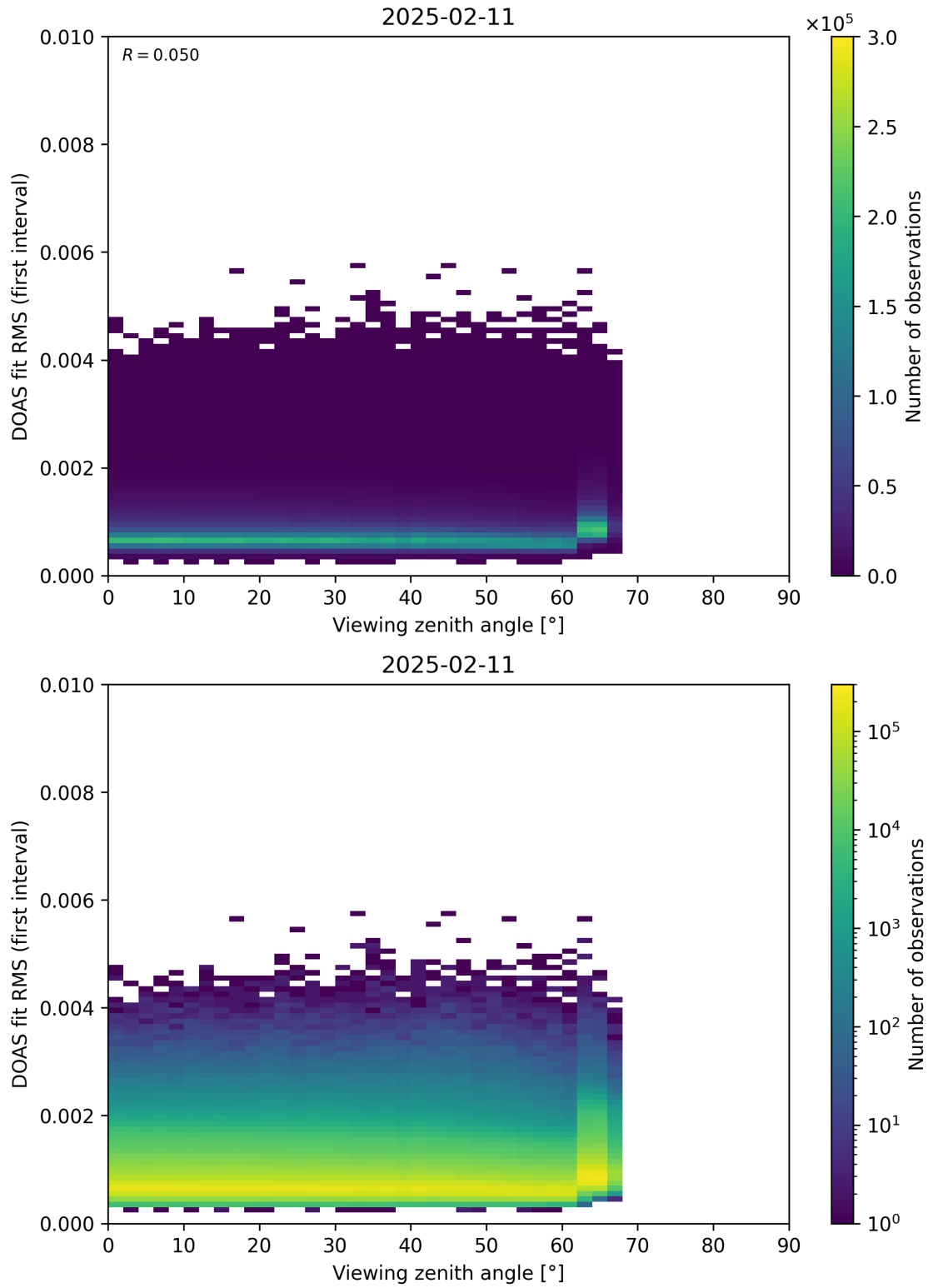
Figure 182: Scatter density plot of “Viewing zenith angle” against “DOAS fit RMS (first interval)” for 2025-02-10 to 2025-02-12.
