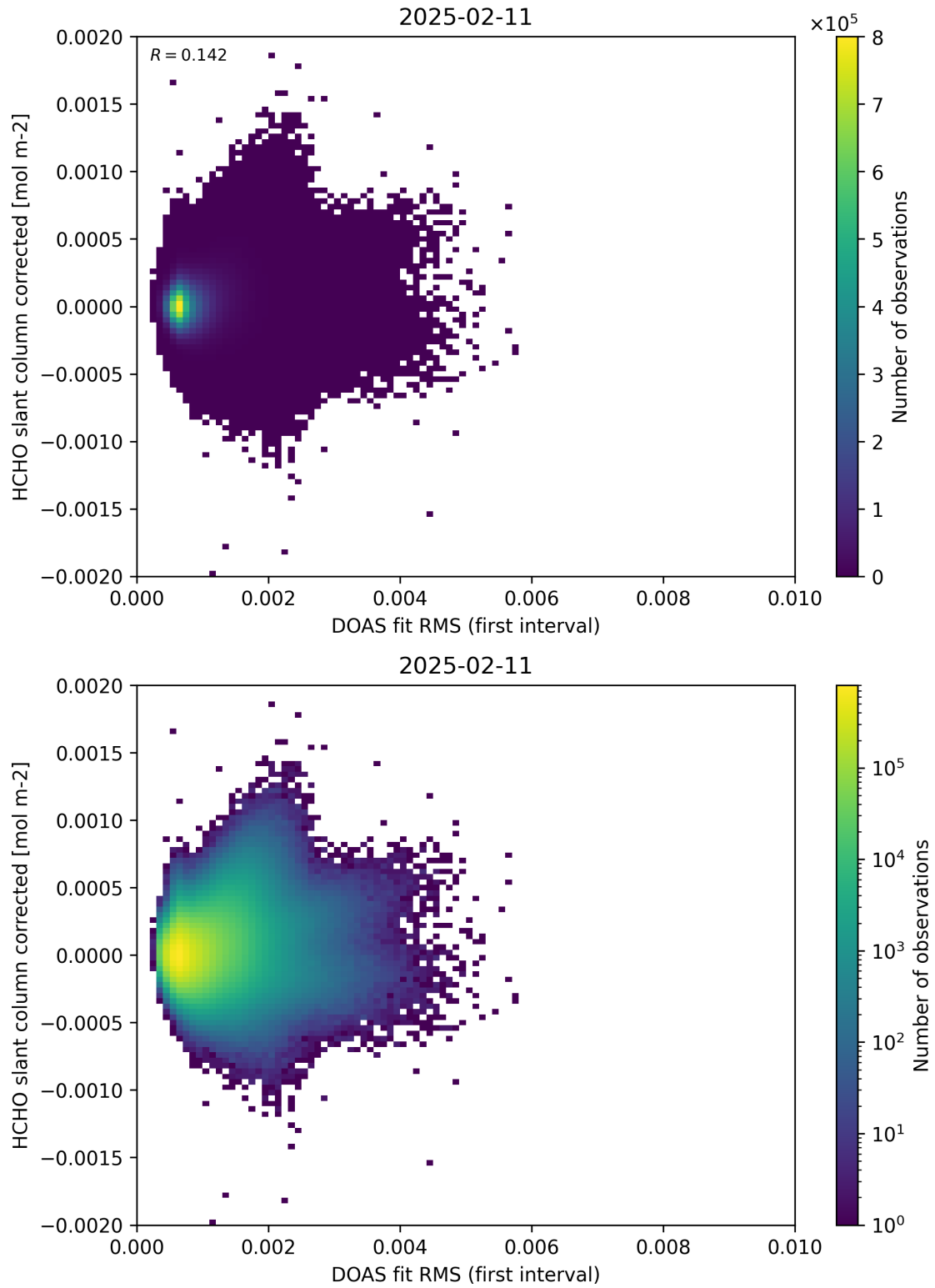
Figure 62: Scatter density plot of “DOAS fit RMS (first interval)” against “HCHO slant column corrected” for 2025-02-10 to 2025-02-12.
