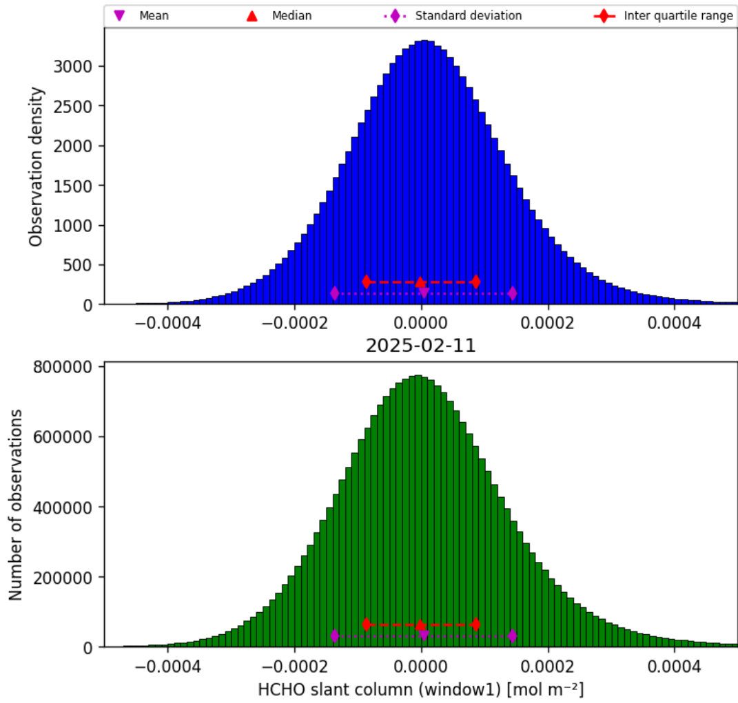
Figure 38: Histogram of “HCHO slant column (window1)” for 2025-02-10 to 2025-02-12
