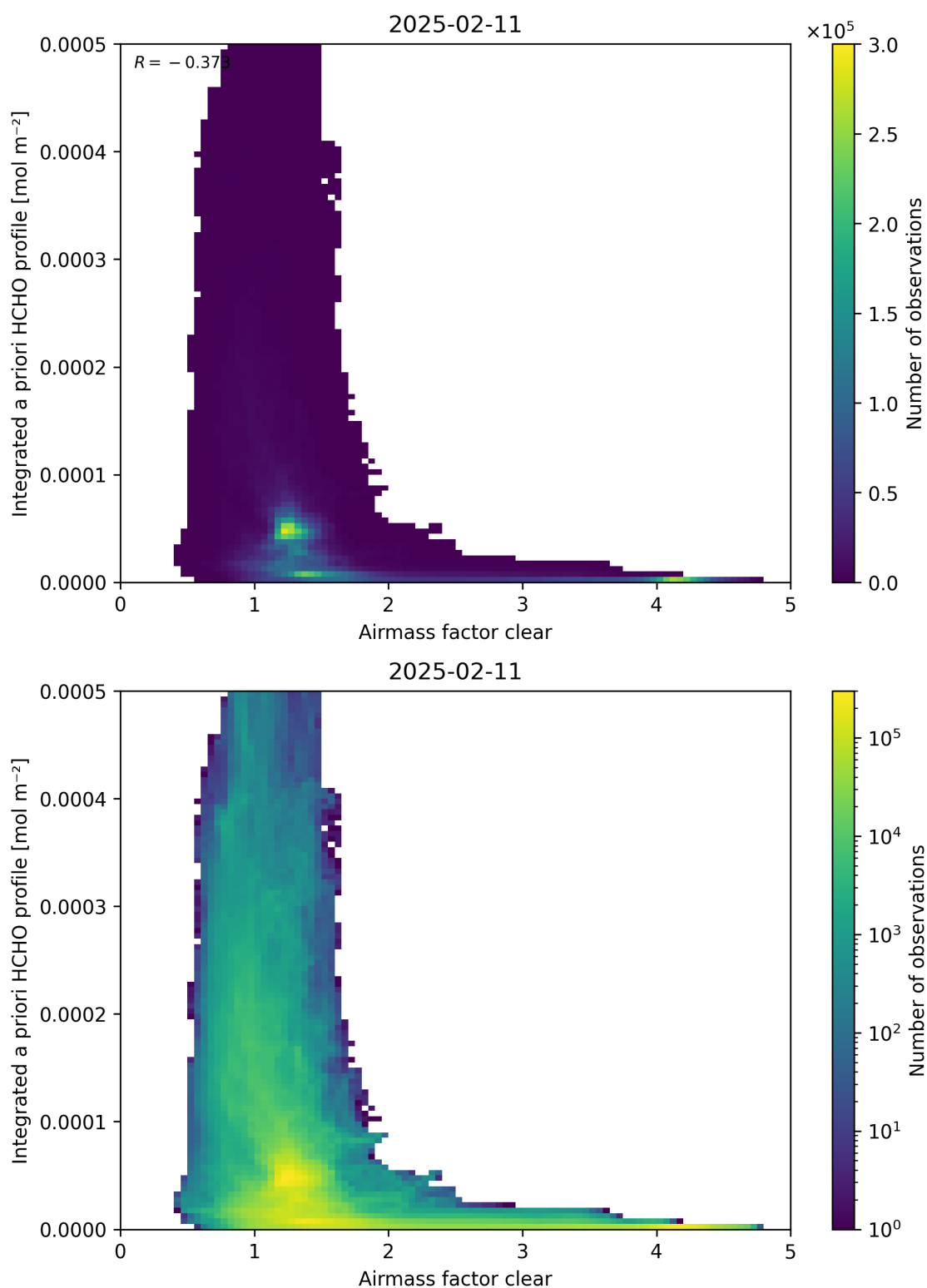
Figure 76: Scatter density plot of “Airmass factor clear” against “Integrated a priori HCHO profile” for 2025-02-10 to 2025-02-12.
