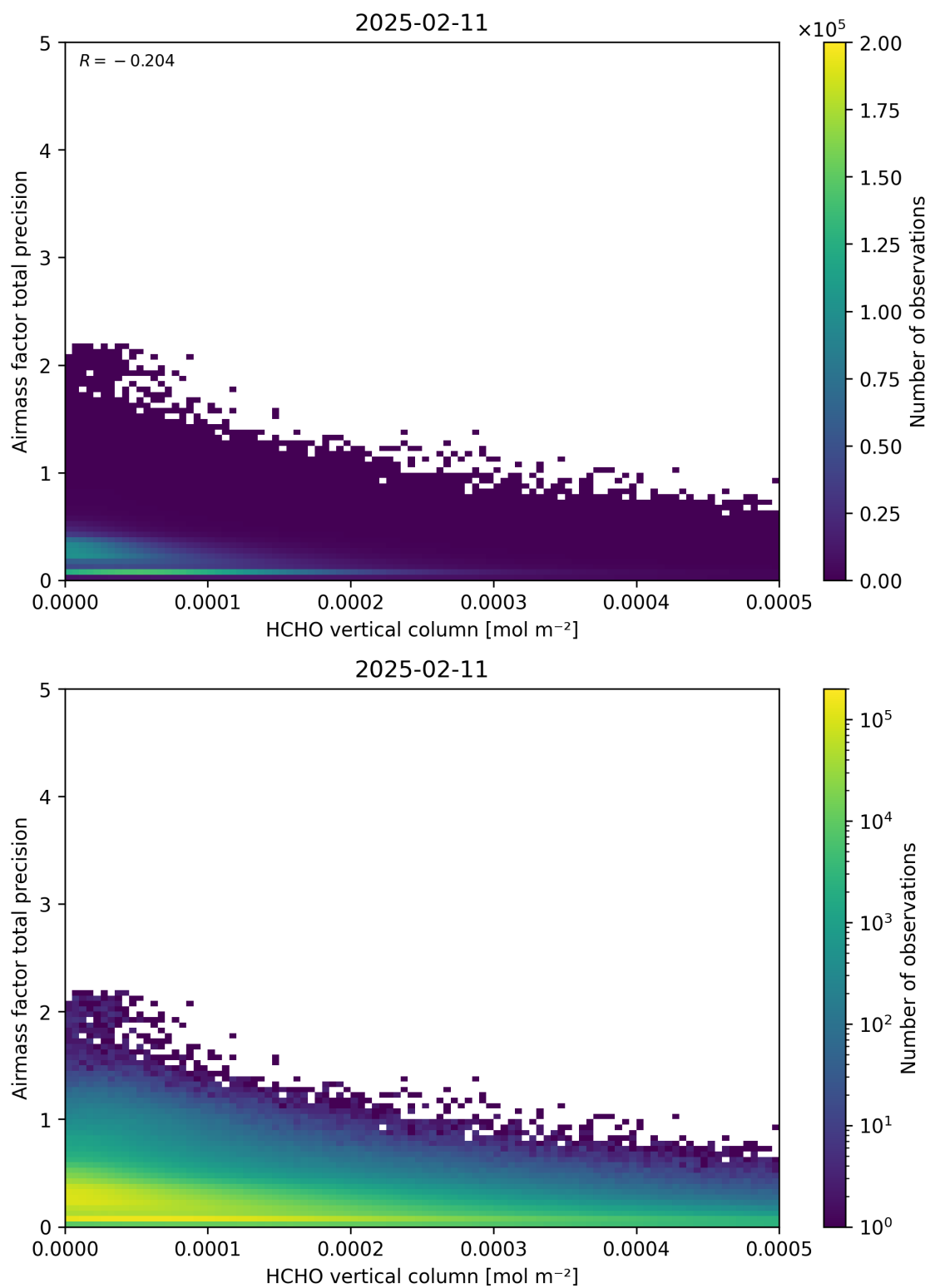
Figure 132: Scatter density plot of “HCHO vertical column” against “Airmass factor total precision” for 2025-02-10 to 2025-02-12.
