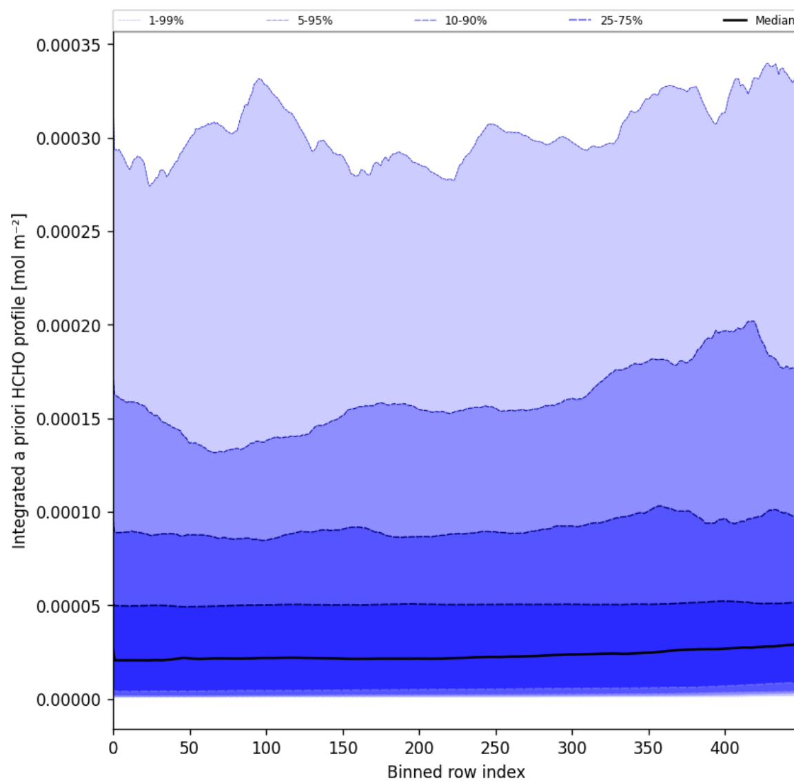
Figure 57: Along track statistics of "Integrated a priori HCHO profile" for 2025-02-10 to 2025-02-12
