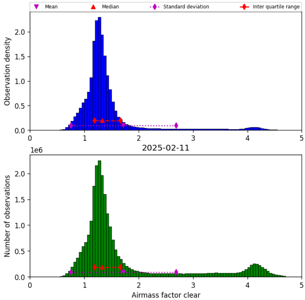
Figure 42: Histogram of “Airmass factor clear” for 2025-02-10 to 2025-02-12
