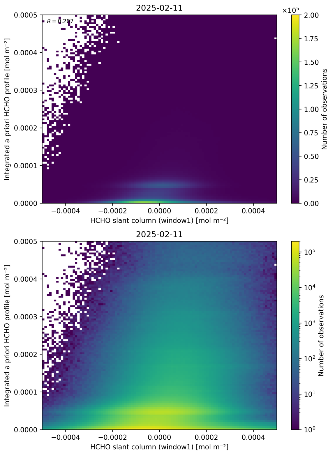
Figure 87: Scatter density plot of “HCHO slant column (window1)” against “Integrated a priori HCHO profile” for 2025-02-10 to 2025-02-12.
