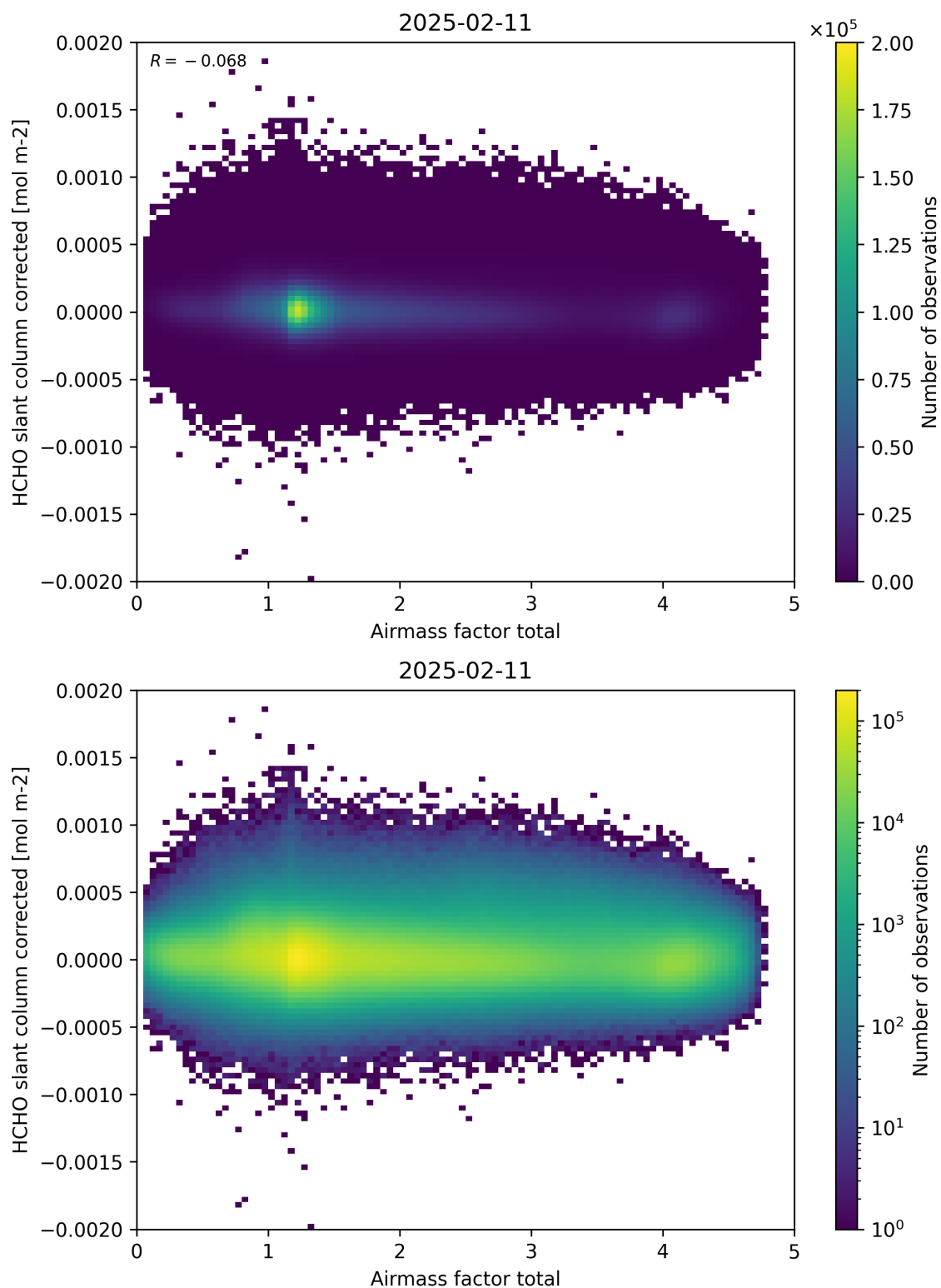
Figure 101: Scatter density plot of “Airmass factor total” against “HCHO slant column corrected” for 2025-02-10 to 2025-02-12.
