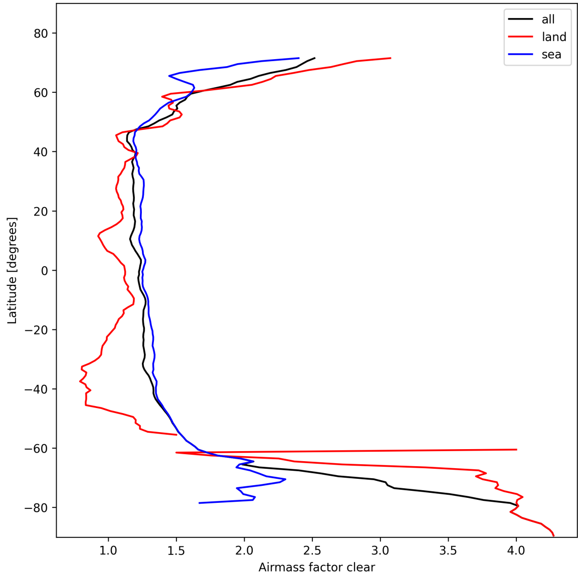
Figure 28: Zonal average of “Airmass factor clear” for 2025-02-10 to 2025-02-12.
