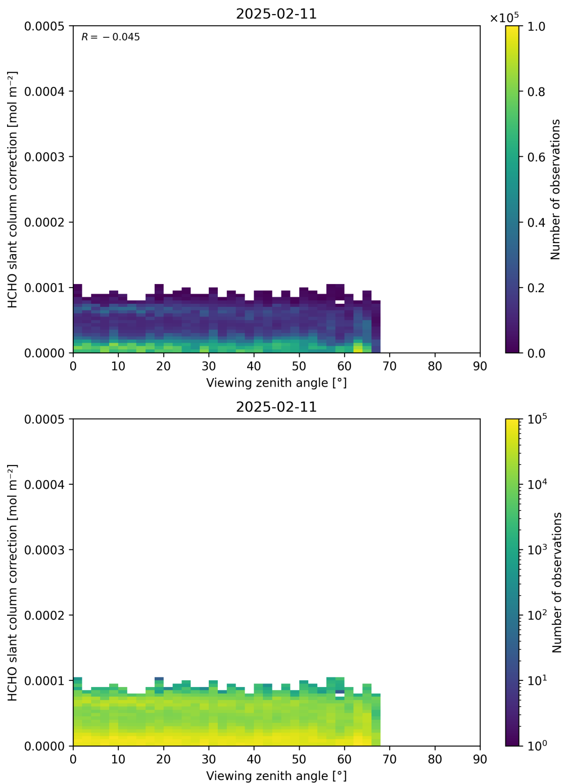
Figure 187: Scatter density plot of “Viewing zenith angle” against “HCHO slant column correction” for 2025-02-10 to 2025-02-12.
