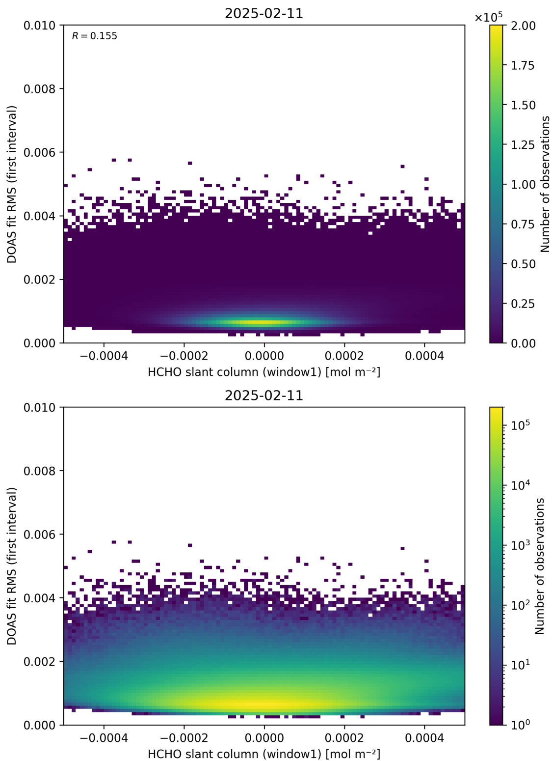
Figure 78: Scatter density plot of “HCHO slant column (window1)” against “DOAS fit RMS (first interval)” for 2025-02-10 to 2025-02-12.
