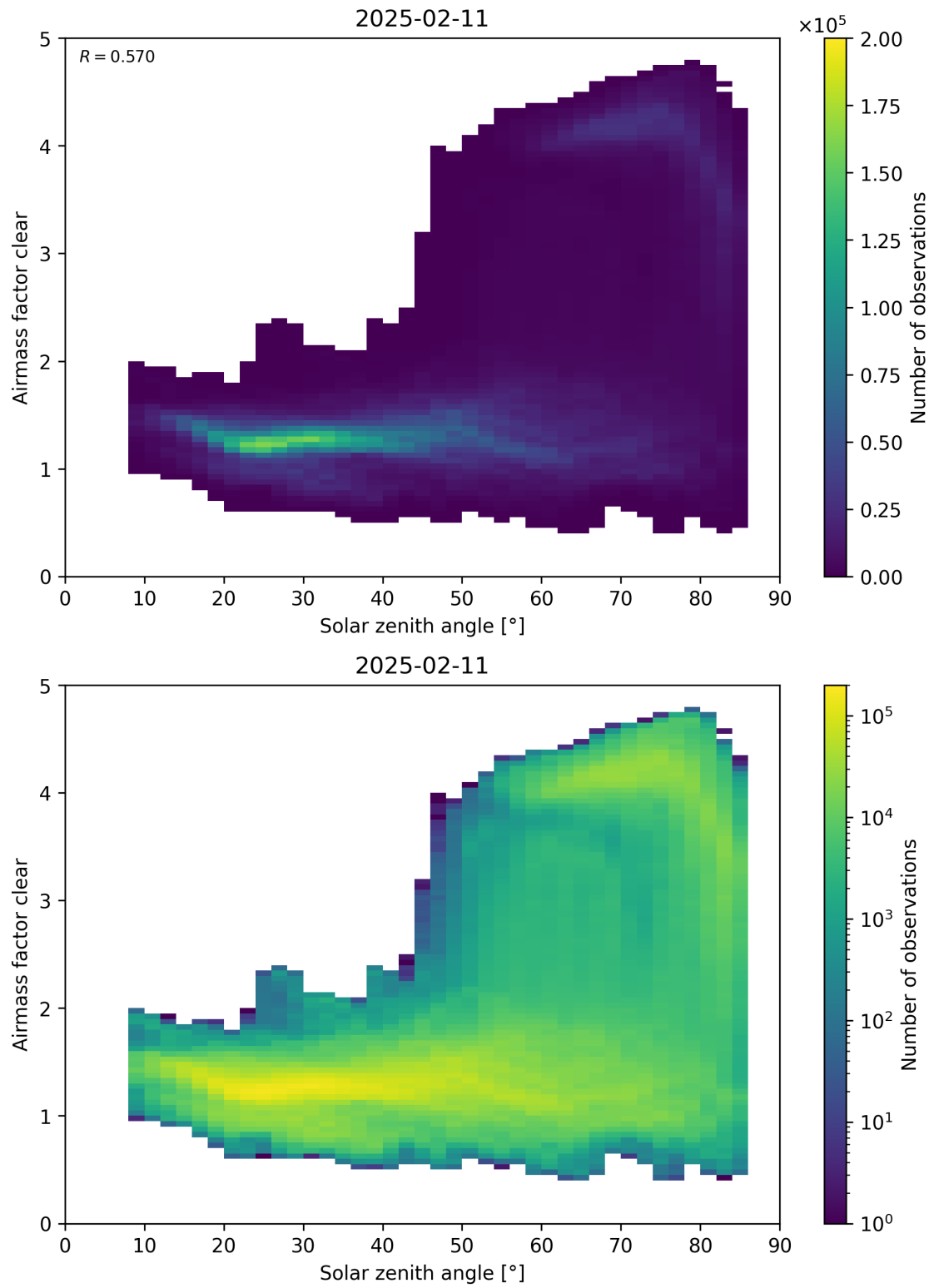
Figure 170: Scatter density plot of “Solar zenith angle” against “Airmass factor clear” for 2025-02-10 to 2025-02-12.
