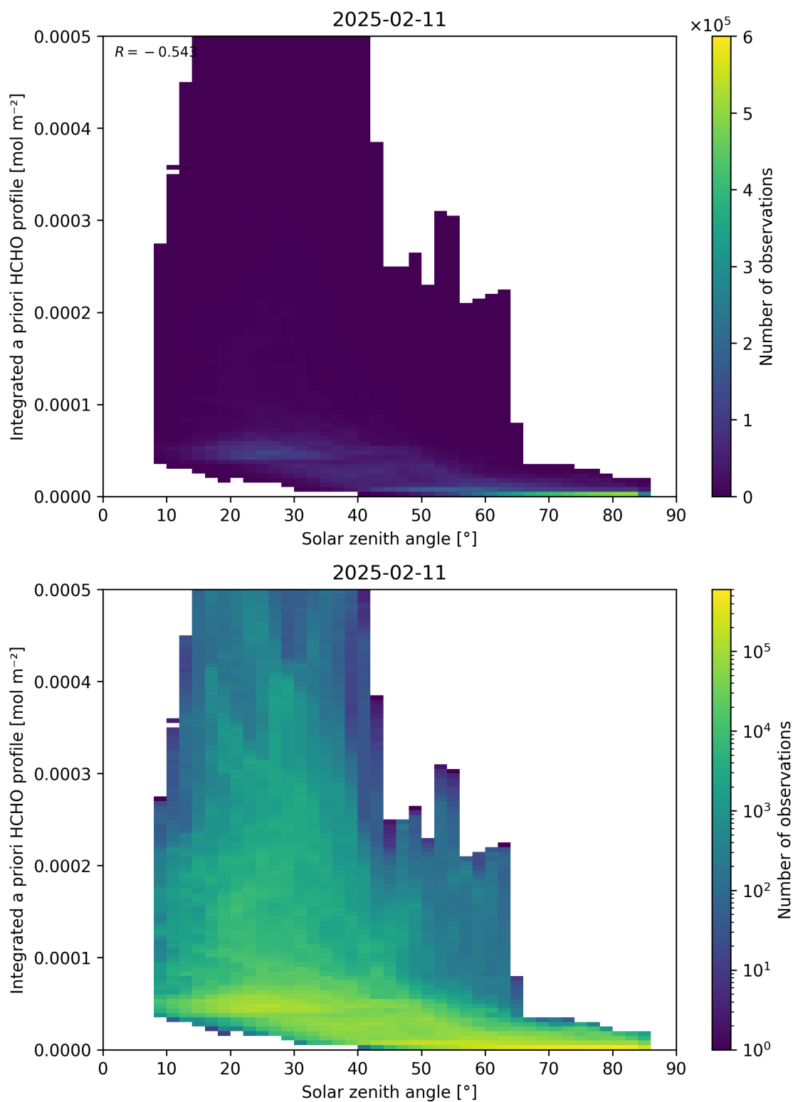
Figure 180: Scatter density plot of “Solar zenith angle” against “Integrated a priori HCHO profile” for 2025-02-10 to 2025-02-12.
