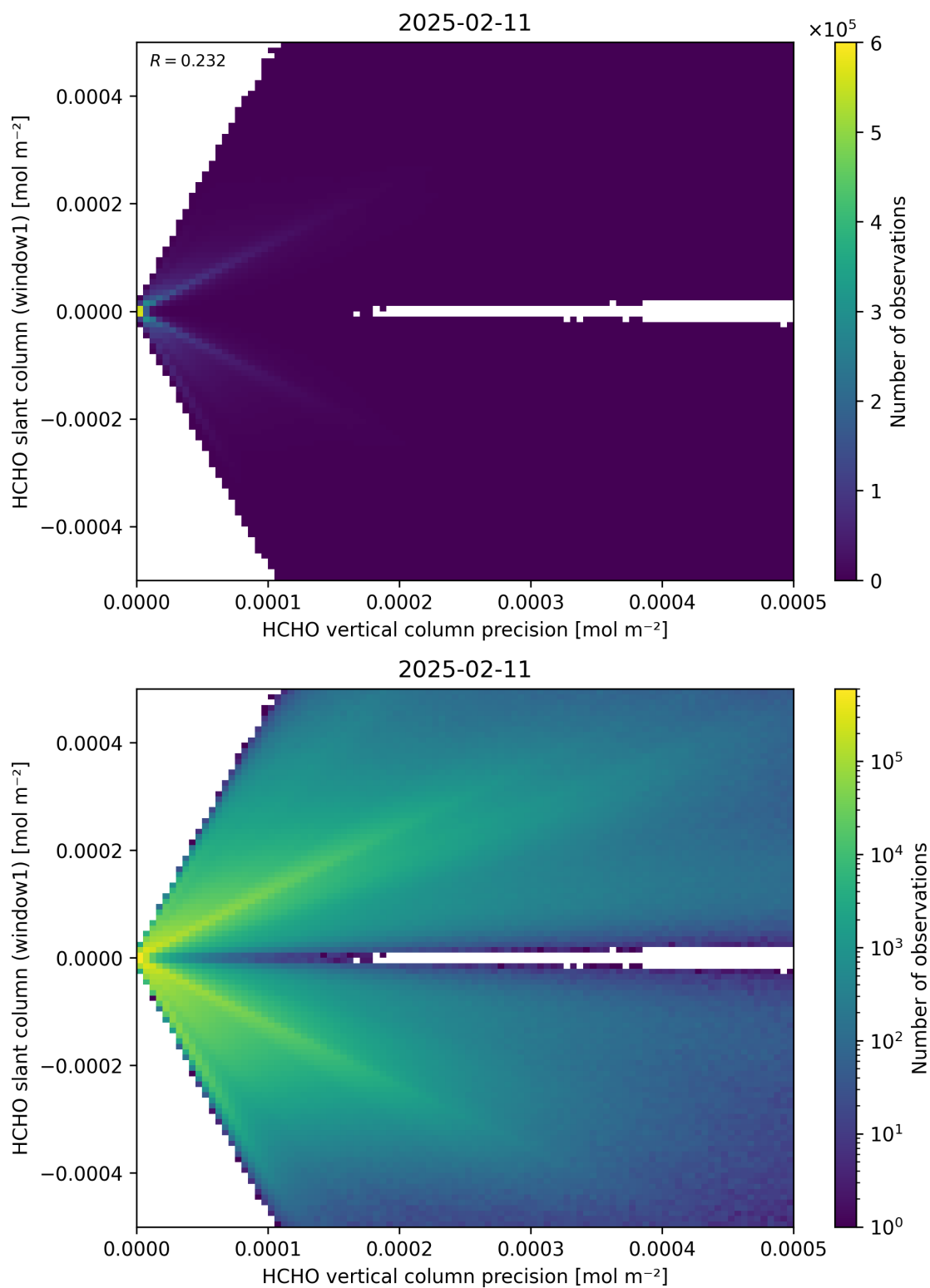
Figure 142: Scatter density plot of “HCHO vertical column precision” against “HCHO slant column (window1)” for 2025-02-10 to 2025-02-12.
