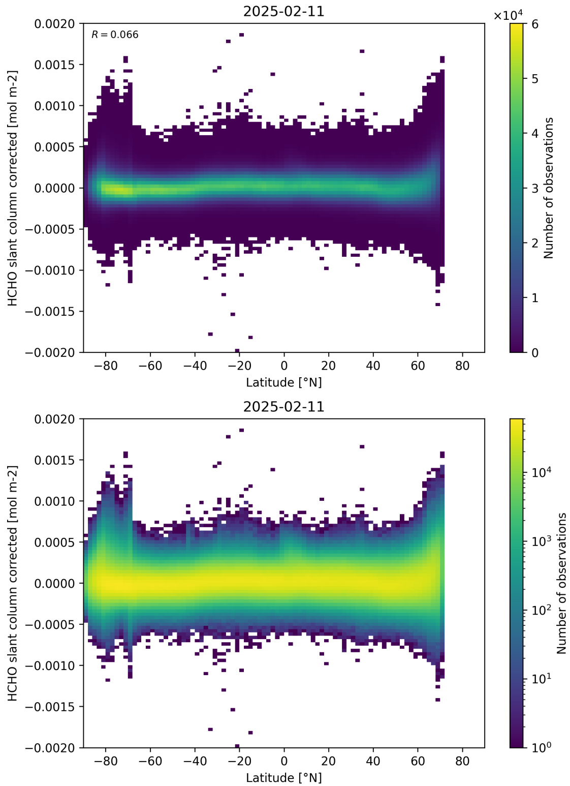
Figure 157: Scatter density plot of “Latitude” against “HCHO slant column corrected” for 2025-02-10 to 2025-02-12.
