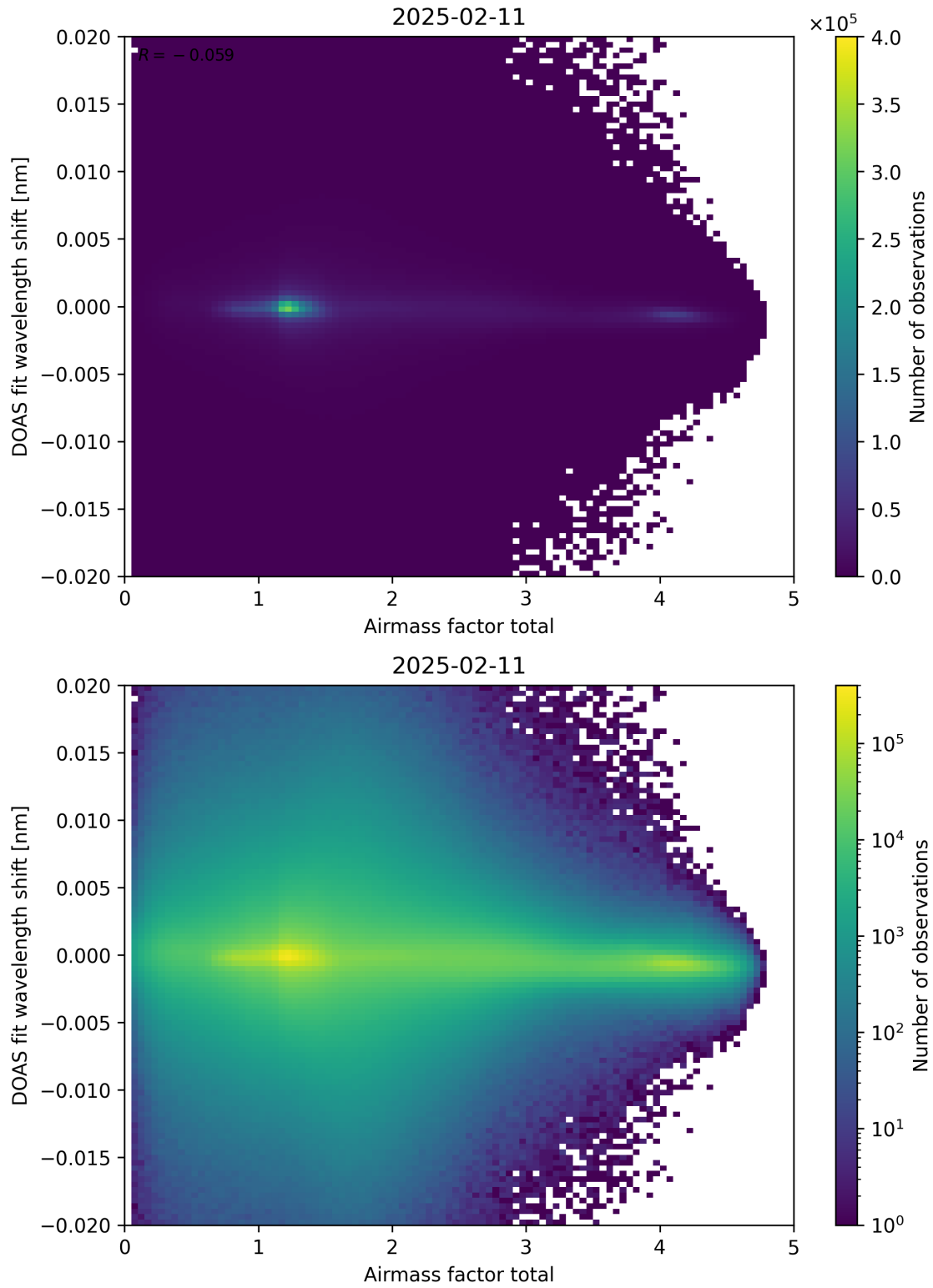
Figure 98: Scatter density plot of “Airmass factor total” against “DOAS fit wavelength shift” for 2025-02-10 to 2025-02-12.
