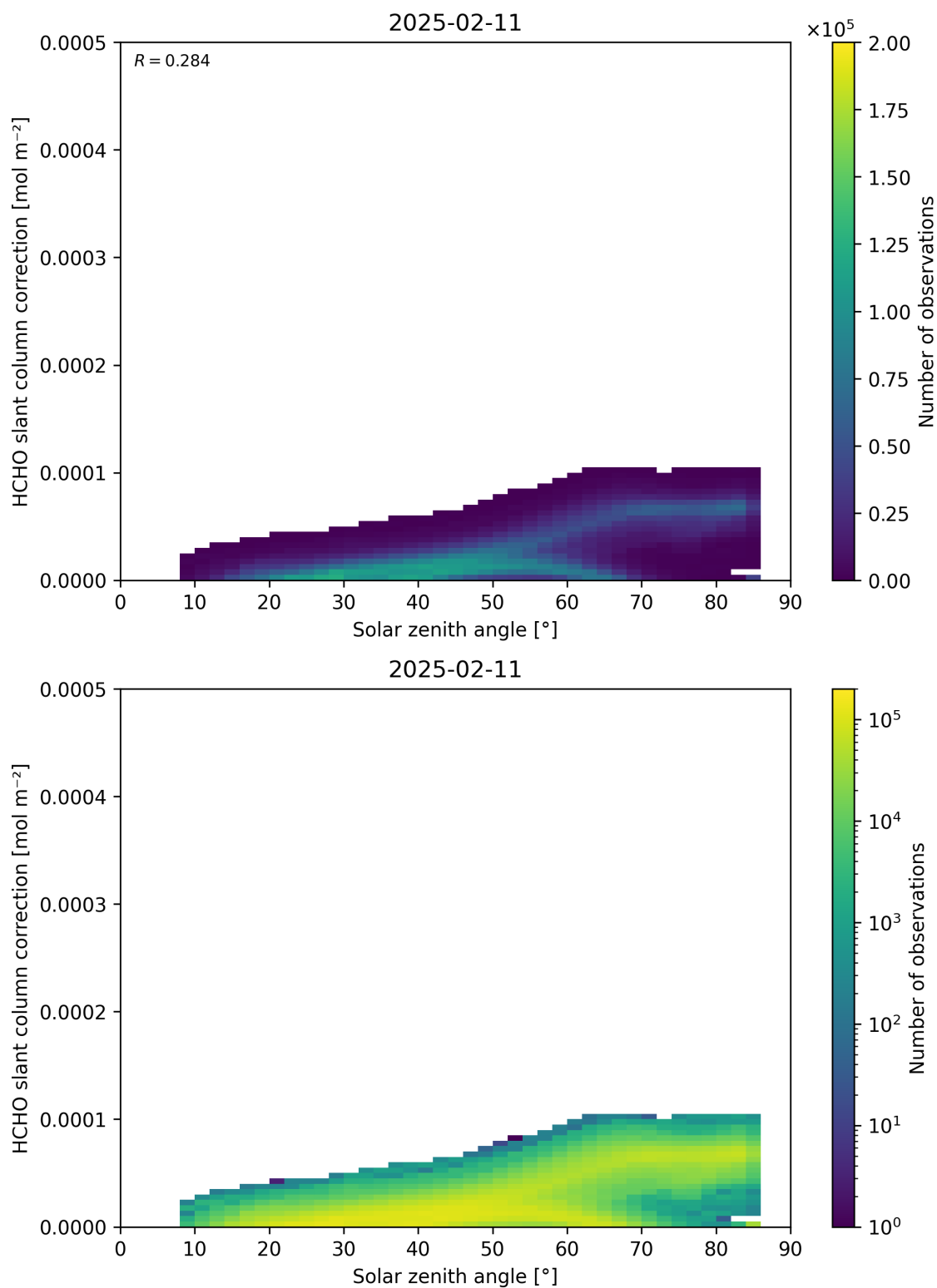
Figure 172: Scatter density plot of “Solar zenith angle” against “HCHO slant column correction” for 2025-02-10 to 2025-02-12.
