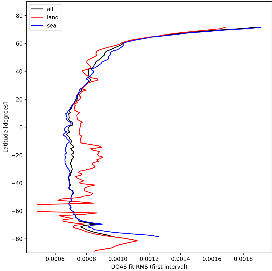
Figure 32: Zonal average of "DOAS fit RMS (first interval)" for 2025-02-10 to 2025-02-12.
