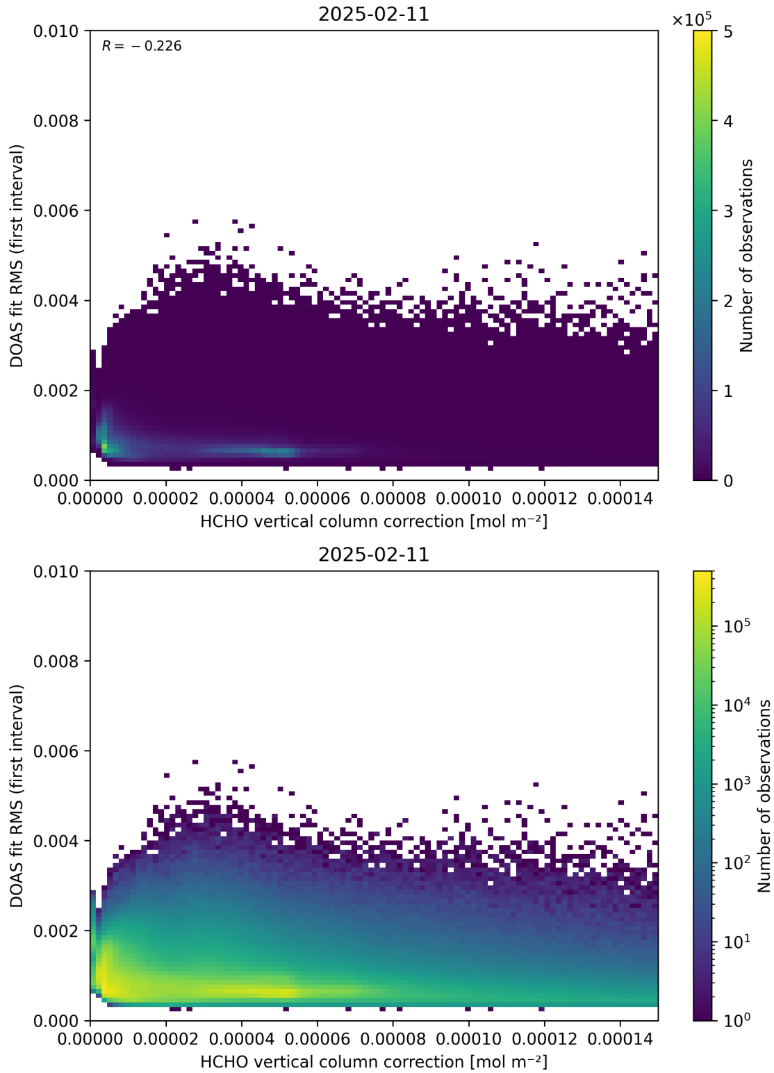
Figure 112: Scatter density plot of “HCHO vertical column correction” against “DOAS fit RMS (first interval)” for 2025-02-10 to 2025-02-12.
