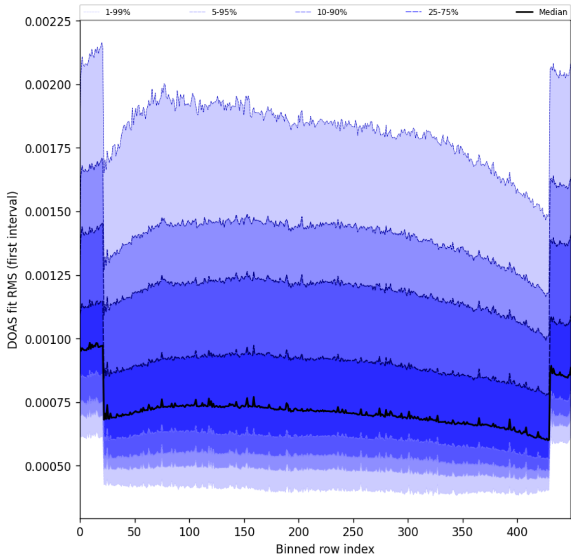
Figure 60: Along track statistics of “DOAS fit RMS (first interval)” for 2025-02-10 to 2025-02-12
