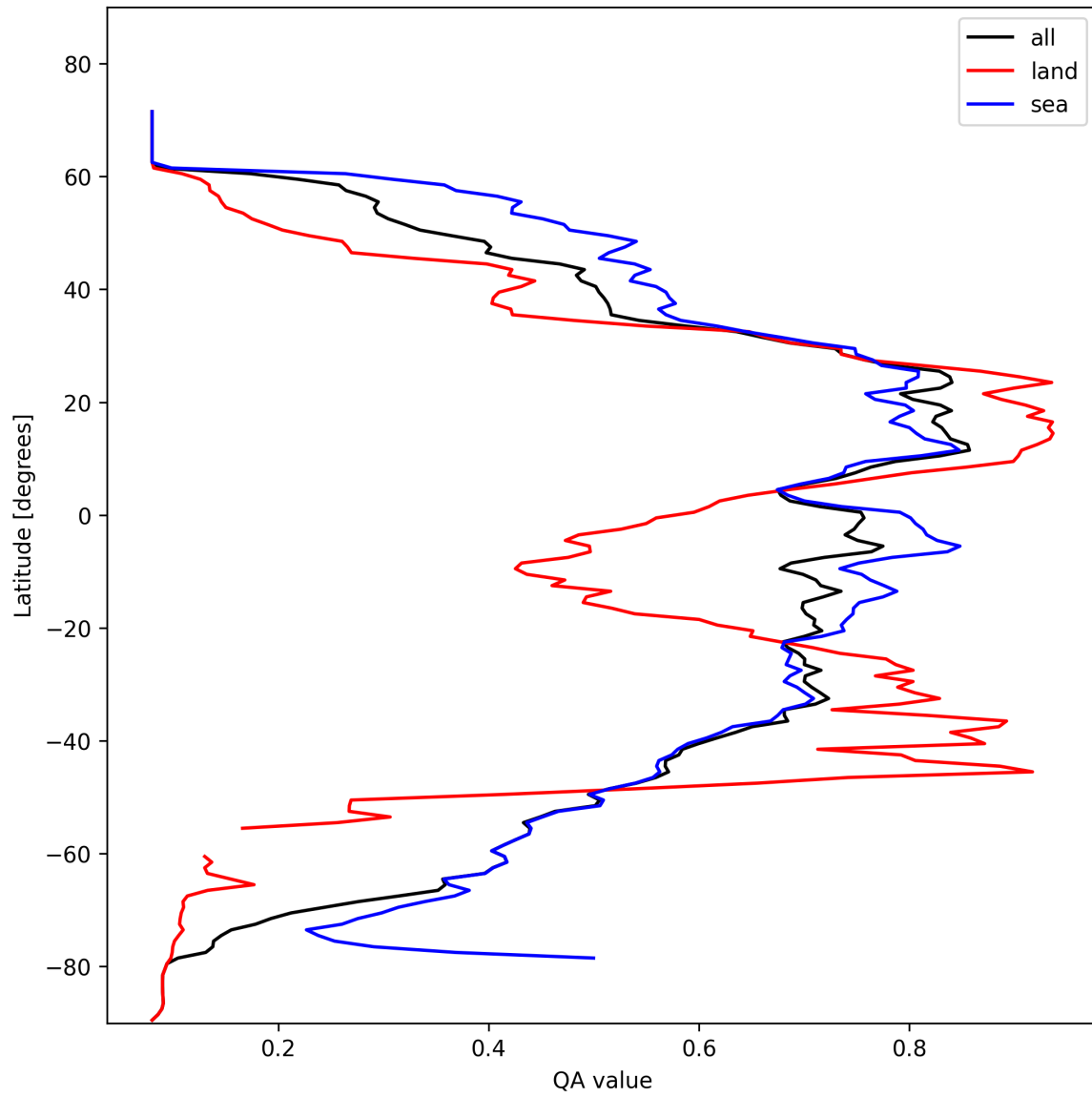
Figure 20: Zonal average of “QA value” for 2025-02-10 to 2025-02-12.
