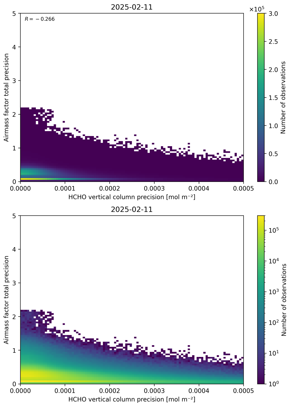
Figure 145: Scatter density plot of “HCHO vertical column precision” against “Airmass factor total precision” for 2025-02-10 to 2025-02-12.
