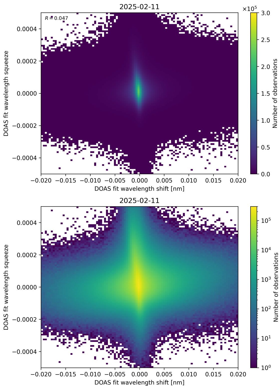
Figure 65: Scatter density plot of “DOAS fit wavelength shift” against “DOAS fit wavelength squeeze” for 2025-02-10 to 2025-02-12.
