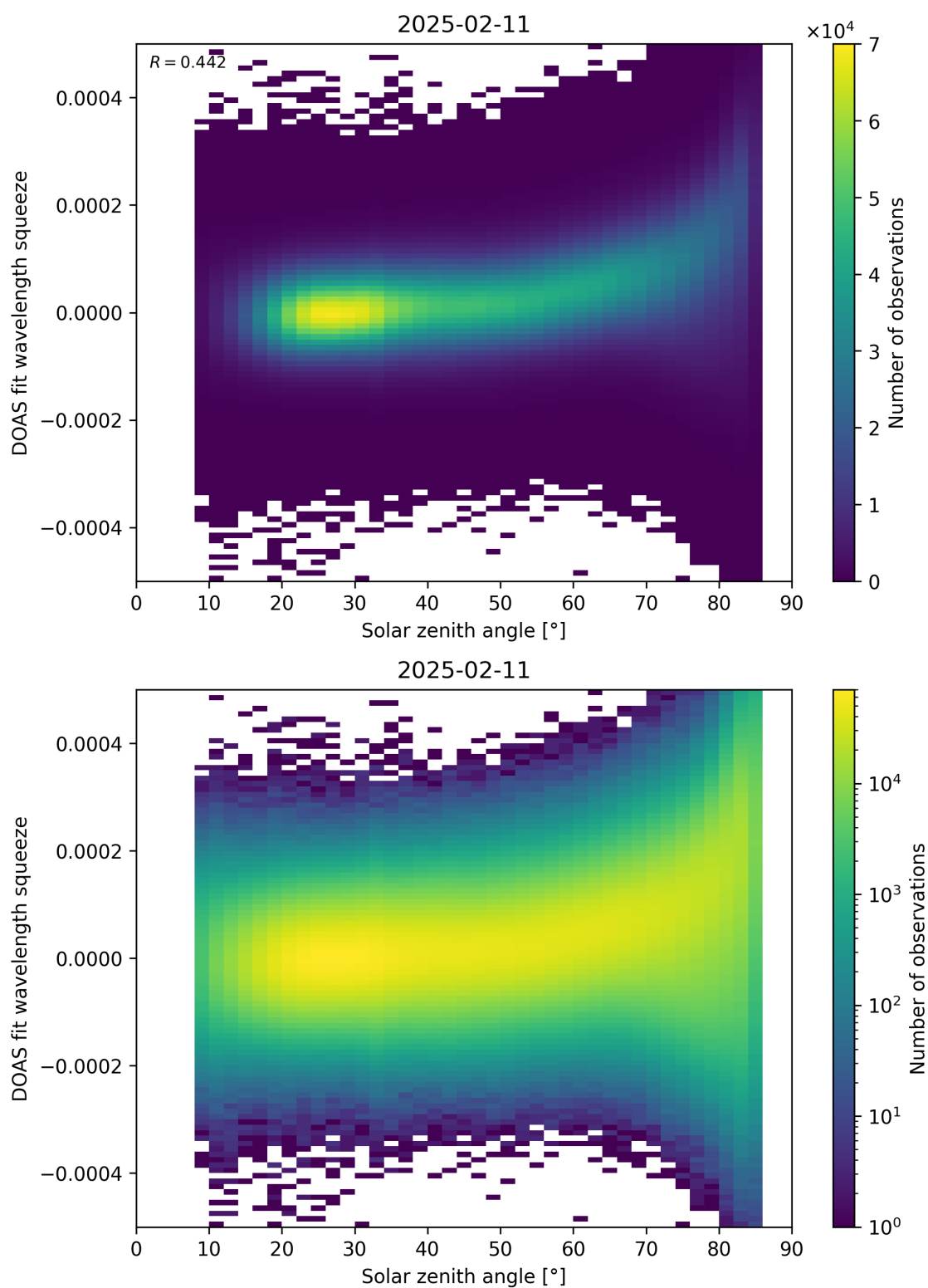
Figure 169: Scatter density plot of “Solar zenith angle” against “DOAS fit wavelength squeeze” for 2025-02-10 to 2025-02-12.
