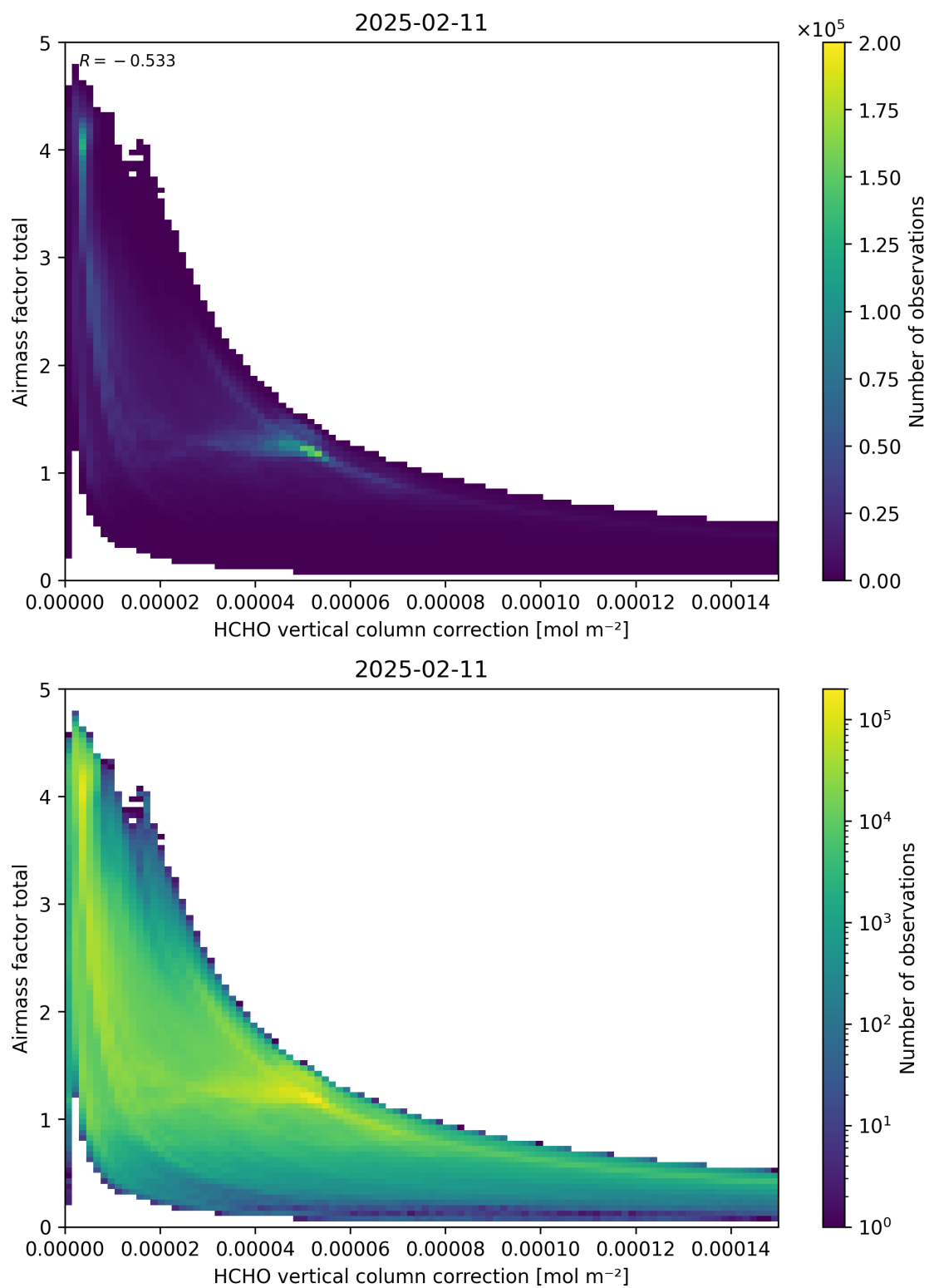
Figure 120: Scatter density plot of “HCHO vertical column correction” against “Airmass factor total” for 2025-02-10 to 2025-02-12.
