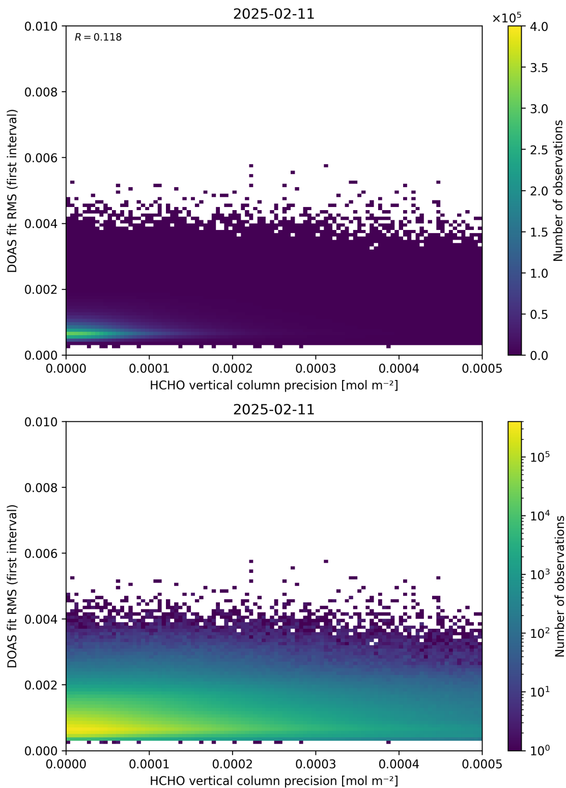
Figure 136: Scatter density plot of “HCHO vertical column precision” against “DOAS fit RMS (first interval)” for 2025-02-10 to 2025-02-12.
