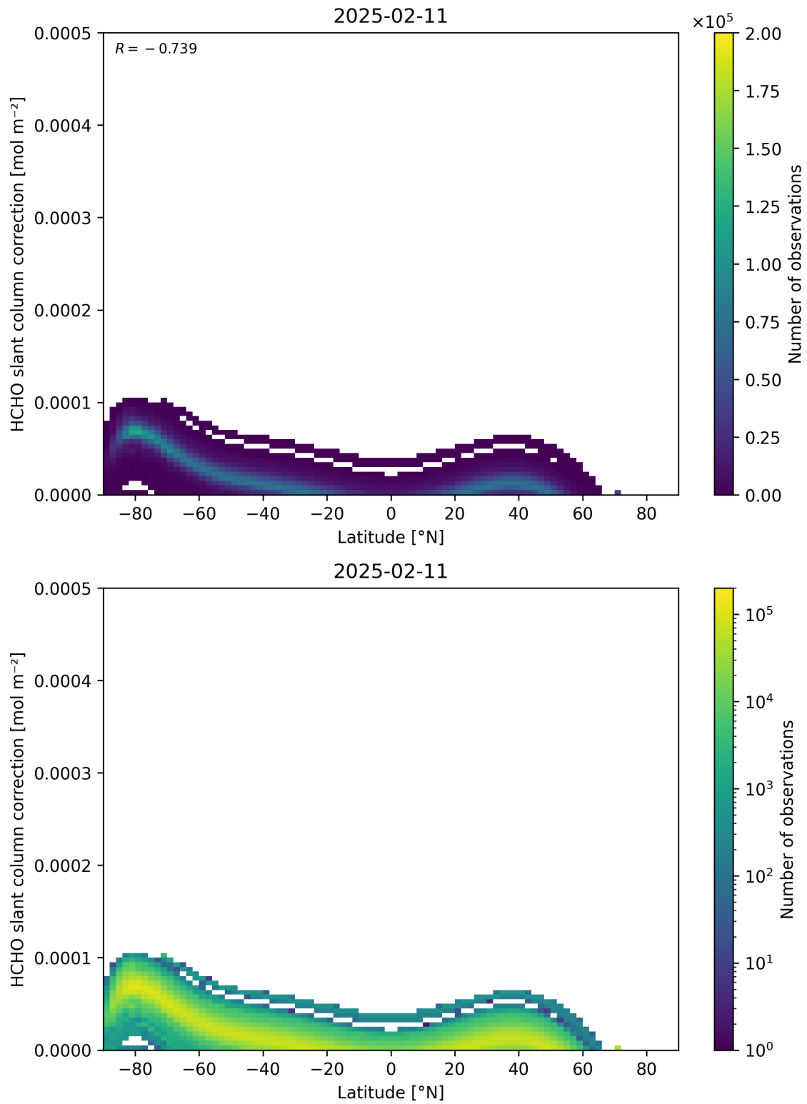
Figure 158: Scatter density plot of “Latitude” against “HCHO slant column correction” for 2025-02-10 to 2025-02-12.
