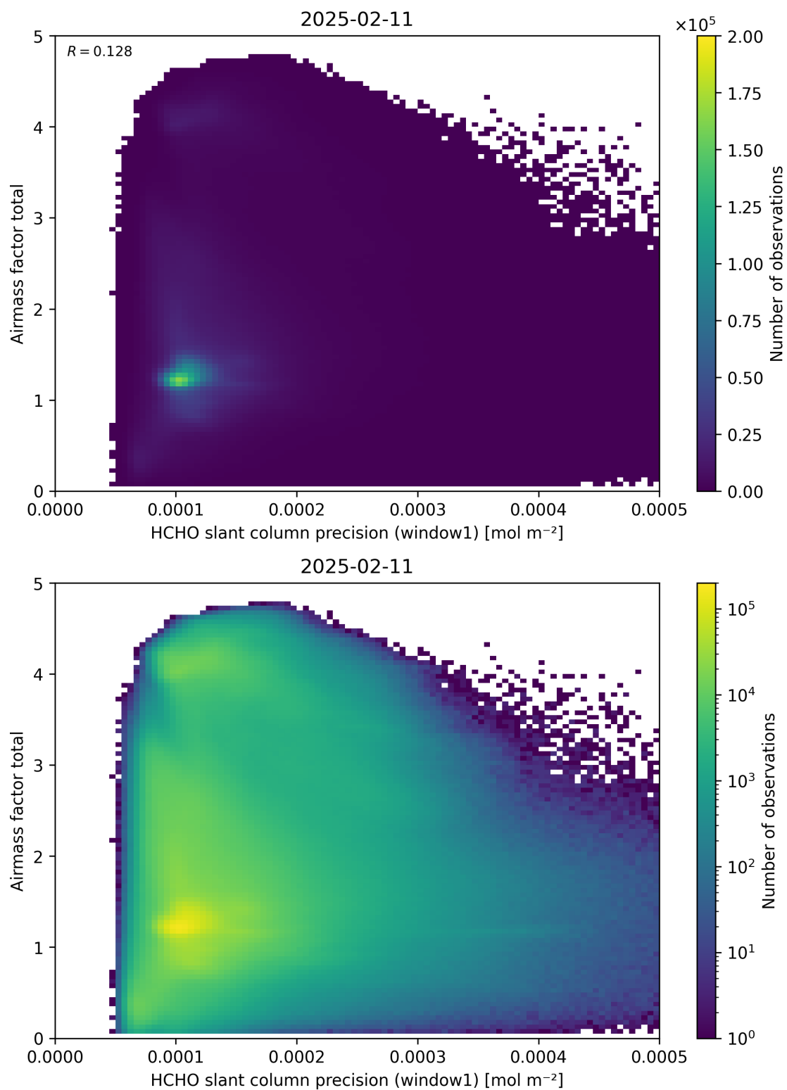
Figure 94: Scatter density plot of “HCHO slant column precision (window1)” against “Airmass factor total” for 2025-02-10 to 2025-02-12.
