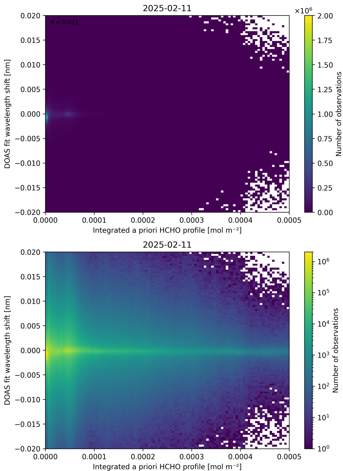
Figure 149: Scatter density plot of “Integrated a priori HCHO profile” against “DOAS fit wavelength shift” for 2025-02-10 to 2025-02-12.
