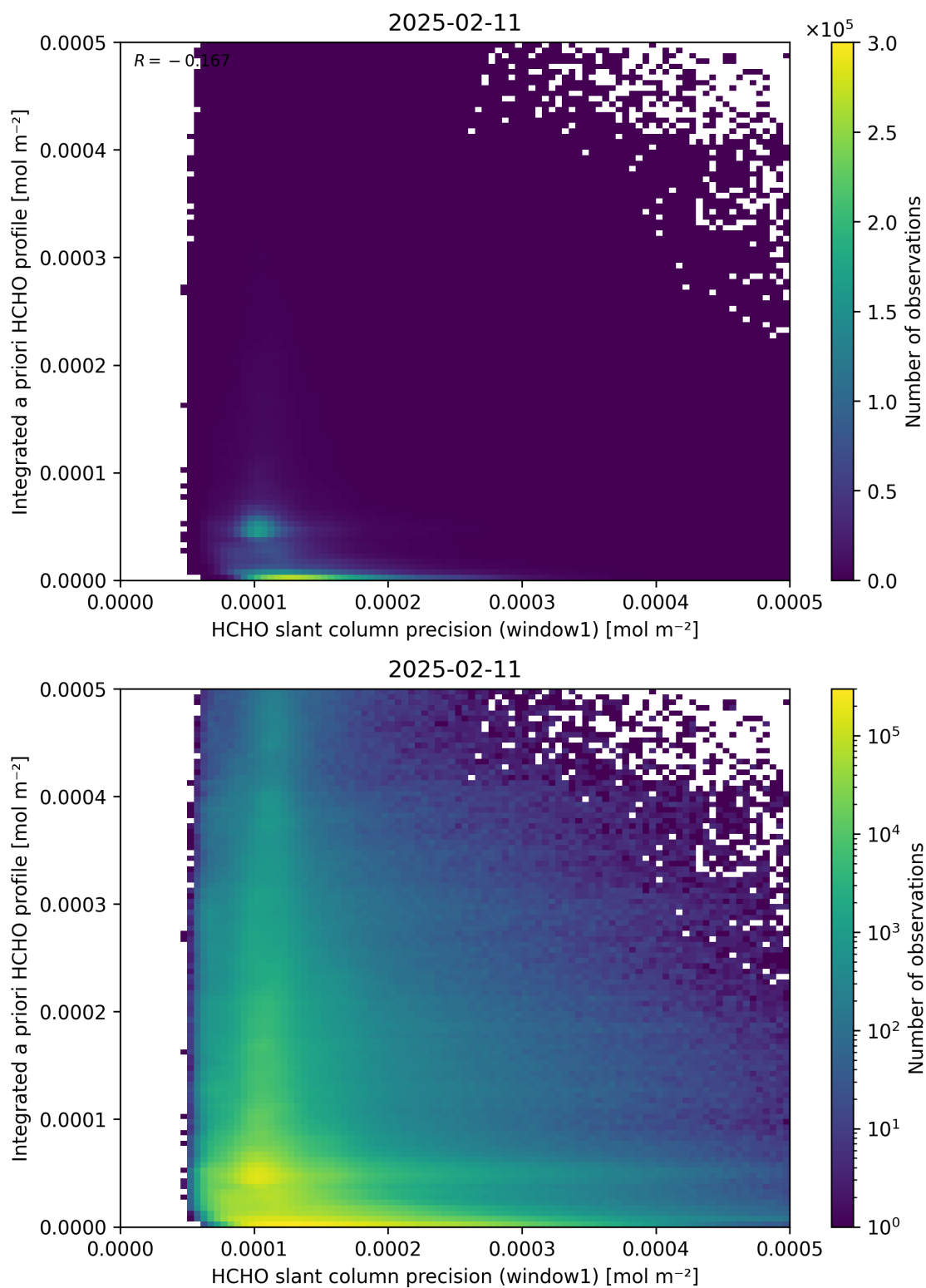
Figure 96: Scatter density plot of “HCHO slant column precision (window1)” against “Integrated a priori HCHO profile” for 2025-02-10 to 2025-02-12.
