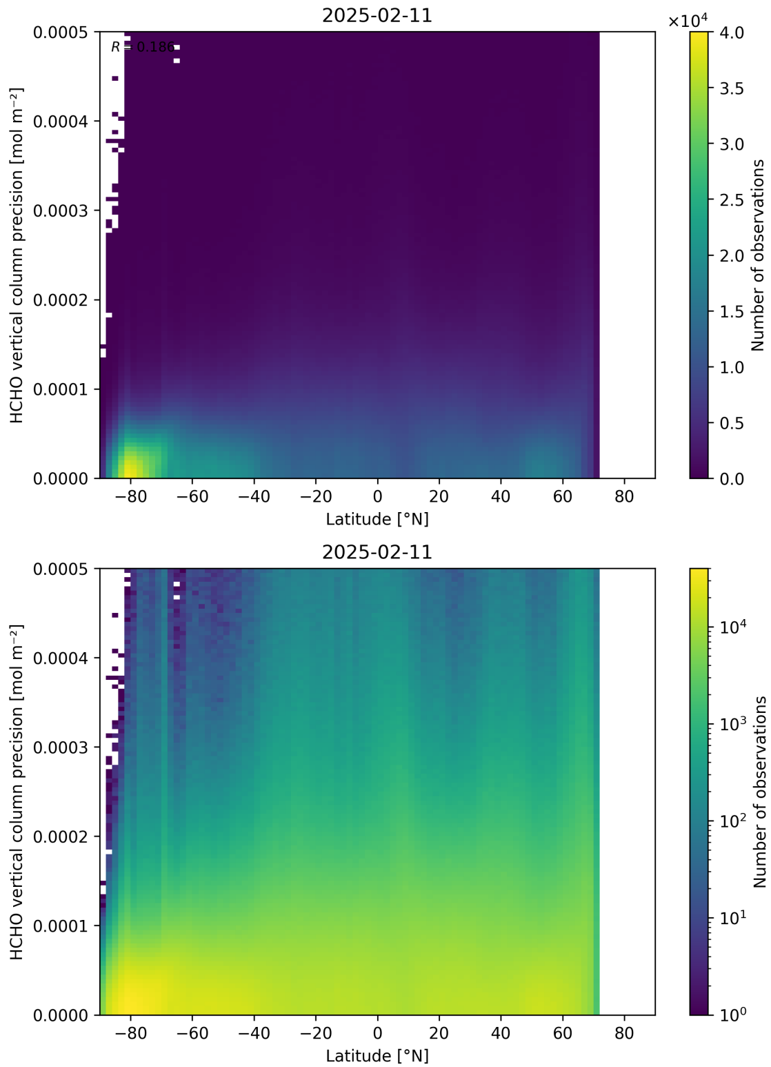
Figure 165: Scatter density plot of “Latitude” against “HCHO vertical column precision” for 2025-02-10 to 2025-02-12.
