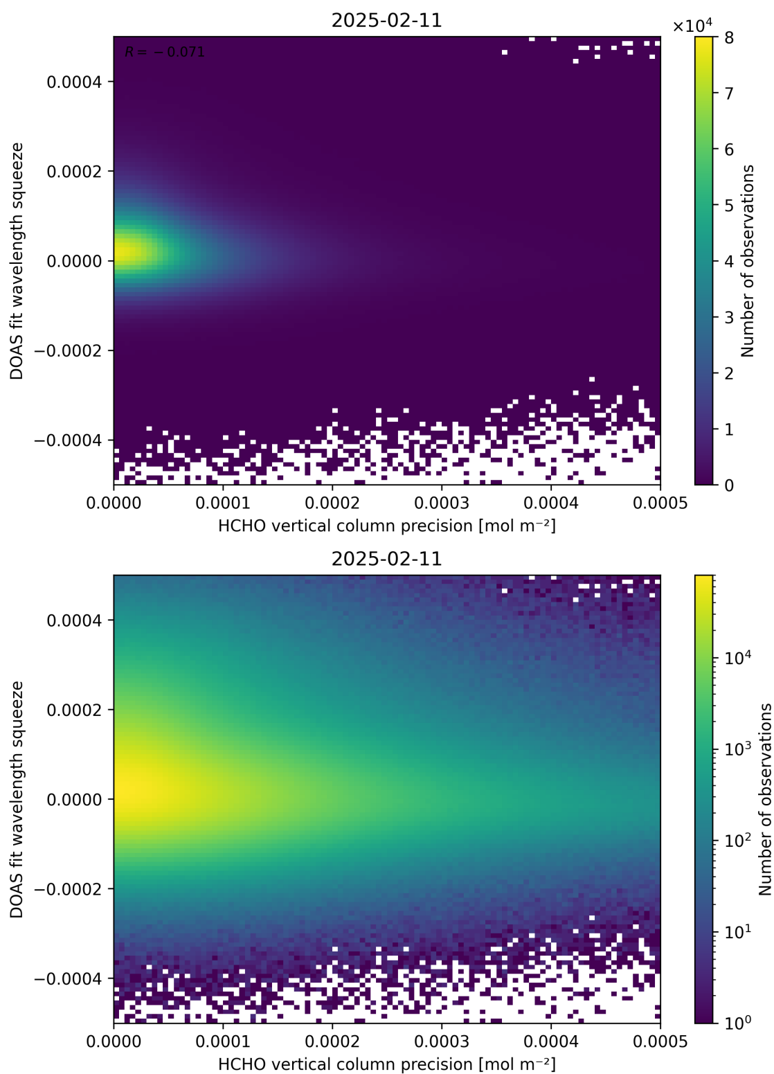
Figure 138: Scatter density plot of “HCHO vertical column precision” against “DOAS fit wavelength squeeze” for 2025-02-10 to 2025-02-12.
