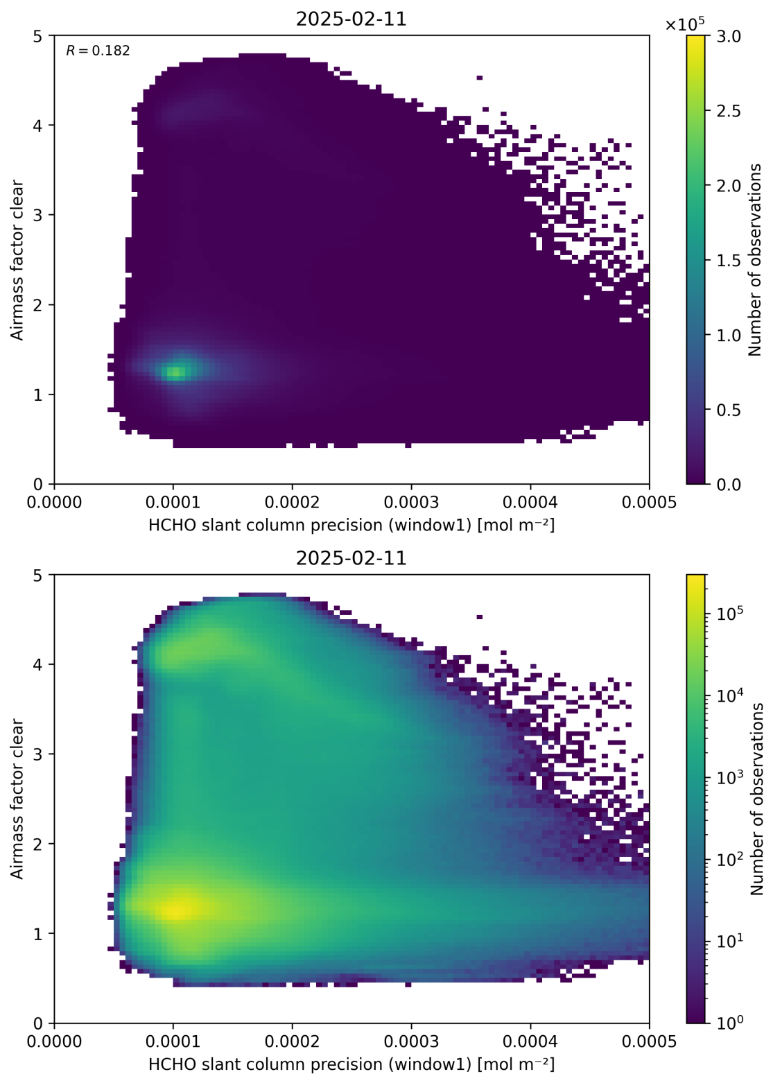
Figure 91: Scatter density plot of “HCHO slant column precision (window1)” against “Airmass factor clear” for 2025-02-10 to 2025-02-12.
