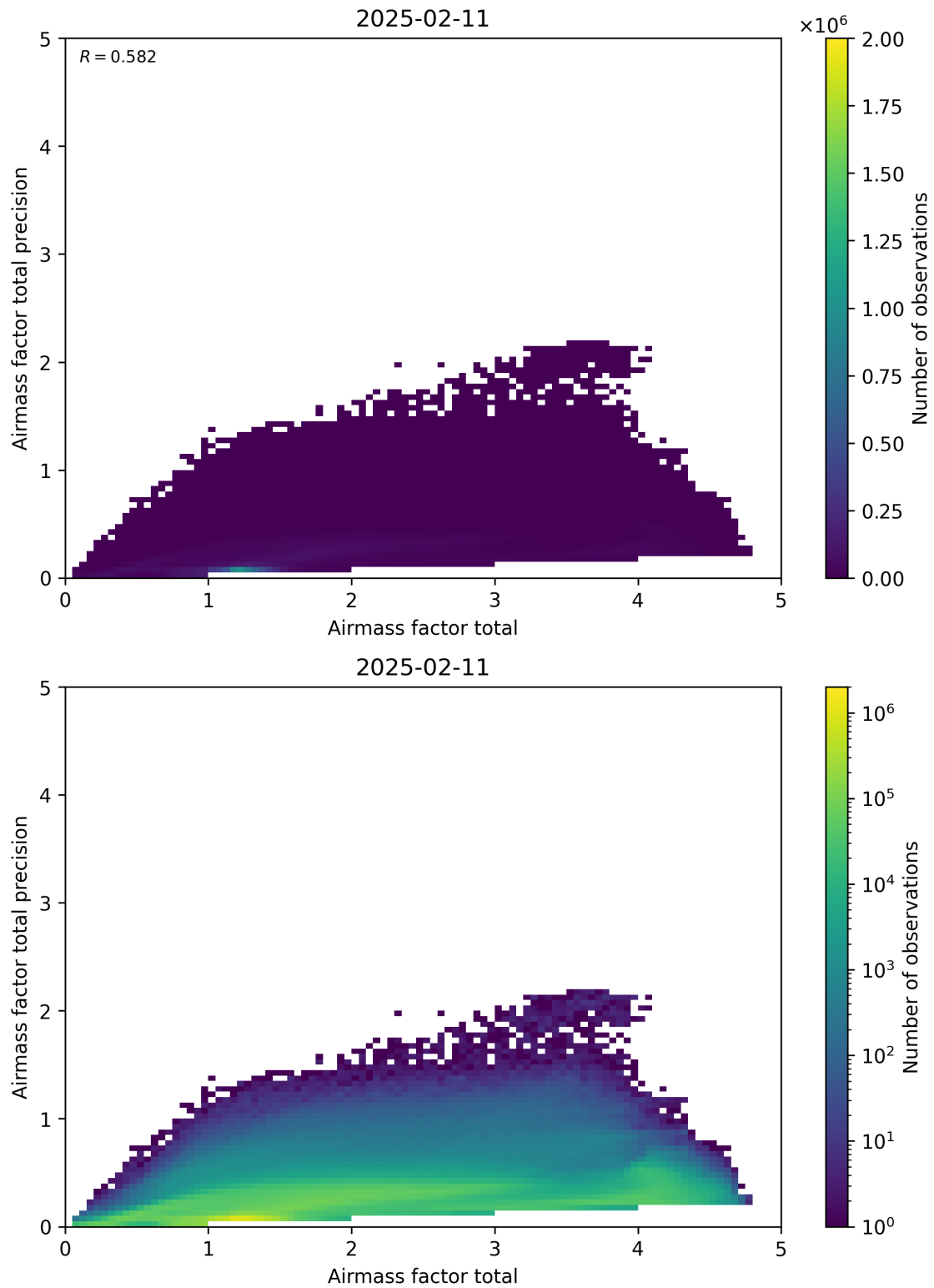
Figure 103: Scatter density plot of “Airmass factor total” against “Airmass factor total precision” for 2025-02-10 to 2025-02-12.
