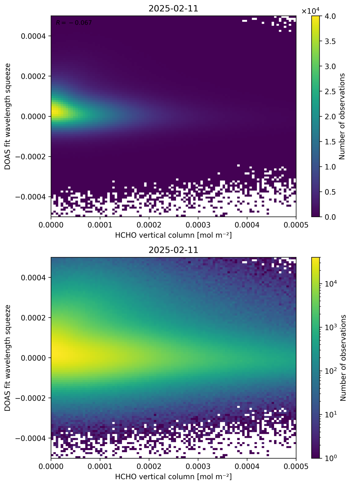
Figure 125: Scatter density plot of “HCHO vertical column” against “DOAS fit wavelength squeeze” for 2025-02-10 to 2025-02-12.
