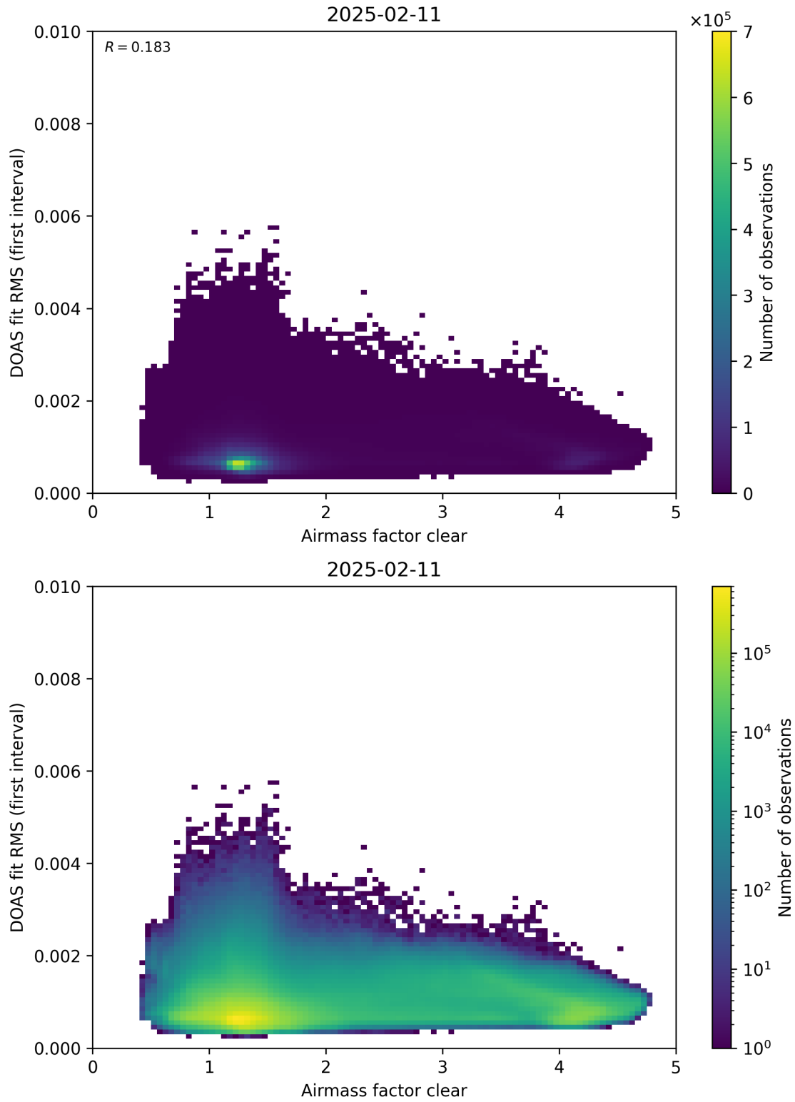
Figure 71: Scatter density plot of “Airmass factor clear” against “DOAS fit RMS (first interval)” for 2025-02-10 to 2025-02-12.
