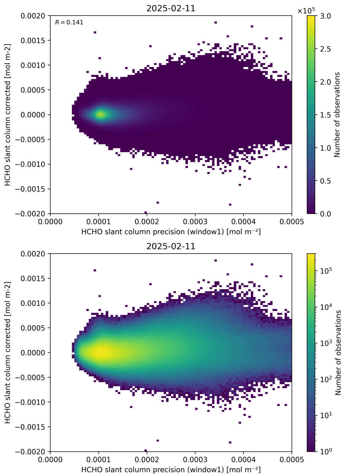
Figure 92: Scatter density plot of “HCHO slant column precision (window1)” against “HCHO slant column corrected” for 2025-02-10 to 2025-02-12.
