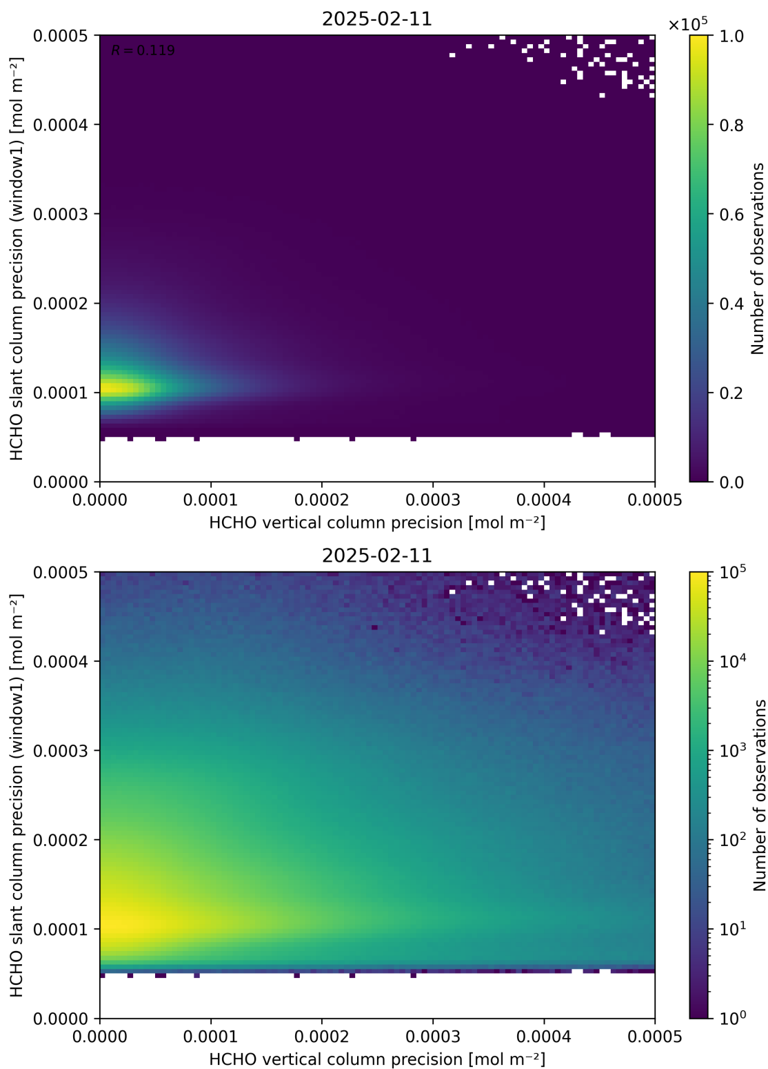
Figure 143: Scatter density plot of “HCHO vertical column precision” against “HCHO slant column precision (window1)” for 2025-02-10 to 2025-02-12.
