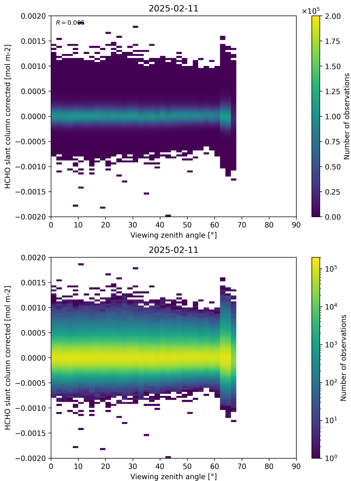
Figure 186: Scatter density plot of “Viewing zenith angle” against “HCHO slant column corrected” for 2025-02-10 to 2025-02-12.
