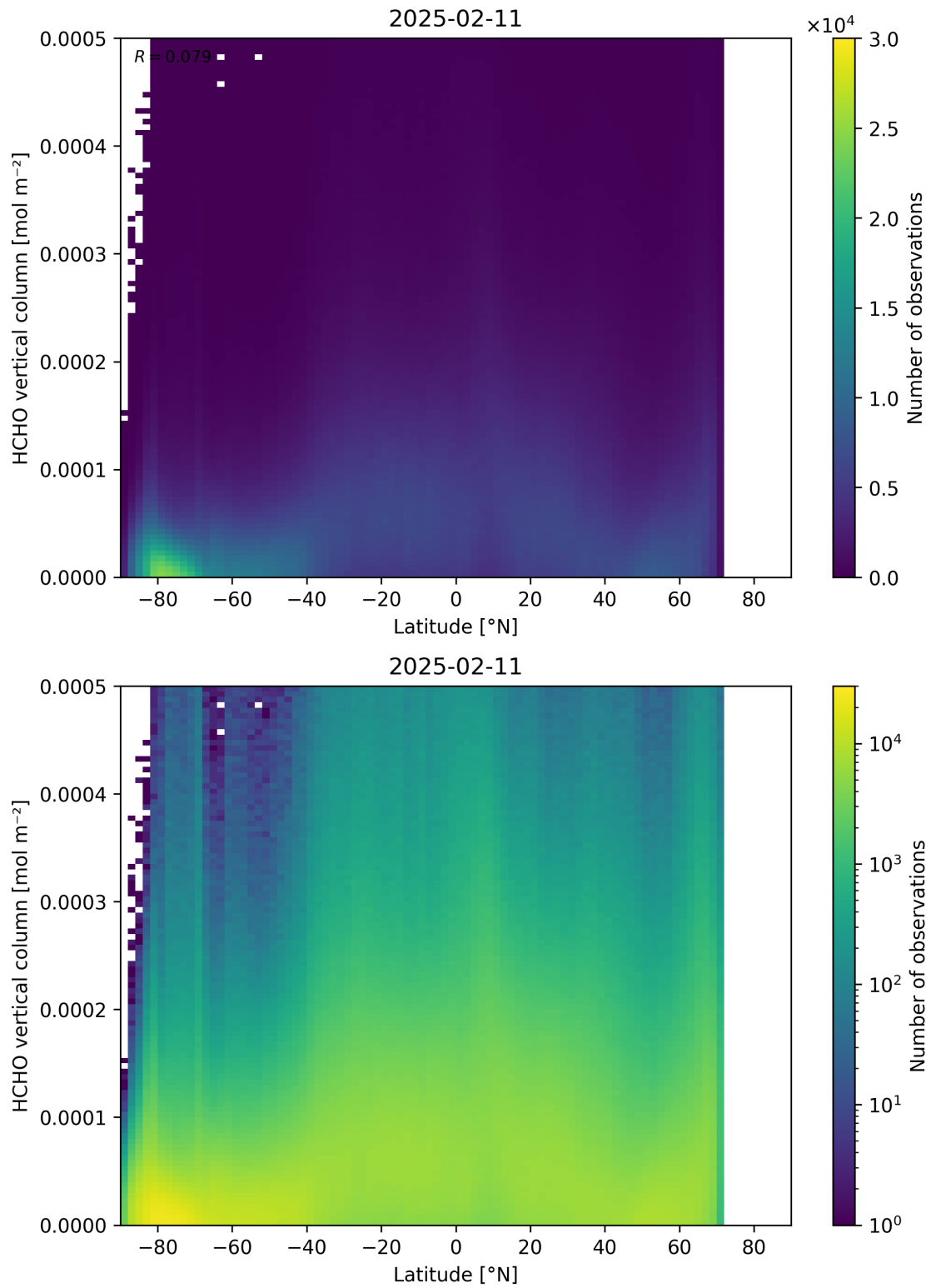
Figure 163: Scatter density plot of “Latitude” against “HCHO vertical column” for 2025-02-10 to 2025-02-12.
