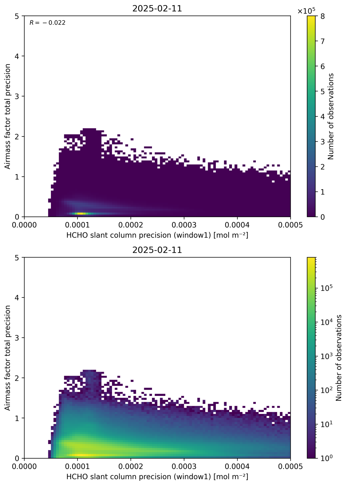
Figure 95: Scatter density plot of “HCHO slant column precision (window1)” against “Airmass factor total precision” for 2025-02-10 to 2025-02-12.
