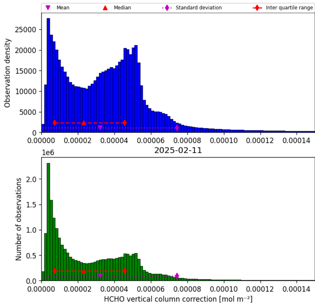
Figure 37: Histogram of “HCHO vertical column correction” for 2025-02-10 to 2025-02-12
