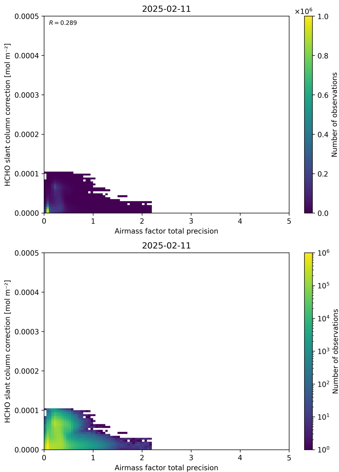
Figure 110: Scatter density plot of “Airmass factor total precision” against “HCHO slant column correction” for 2025-02-10 to 2025-02-12.
