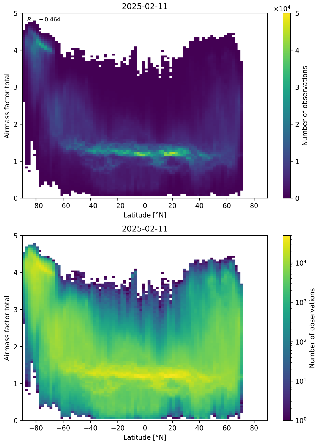
Figure 161: Scatter density plot of “Latitude” against “Airmass factor total” for 2025-02-10 to 2025-02-12.
