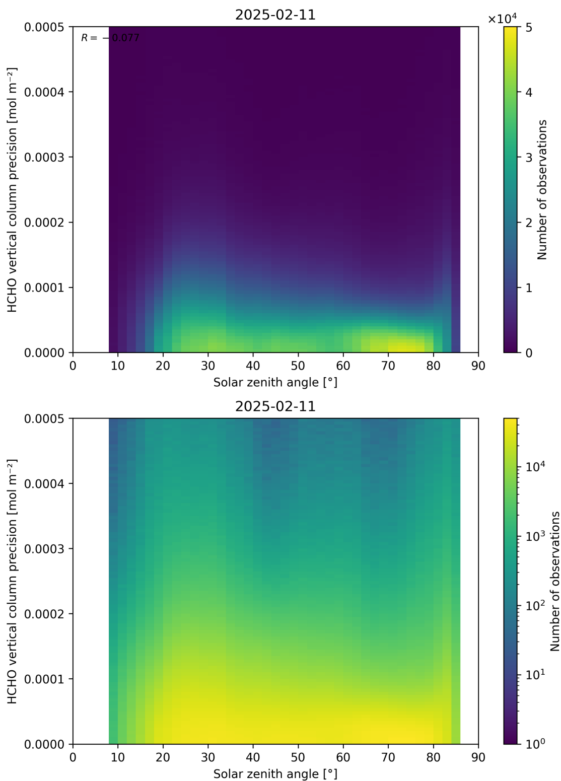
Figure 179: Scatter density plot of “Solar zenith angle” against “HCHO vertical column precision” for 2025-02-10 to 2025-02-12.
