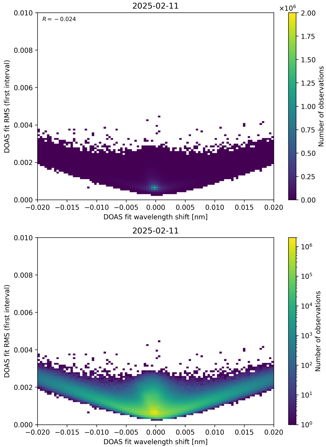
Figure 64: Scatter density plot of “DOAS fit wavelength shift” against “DOAS fit RMS (first interval)” for 2025-02-10 to 2025-02-12.
