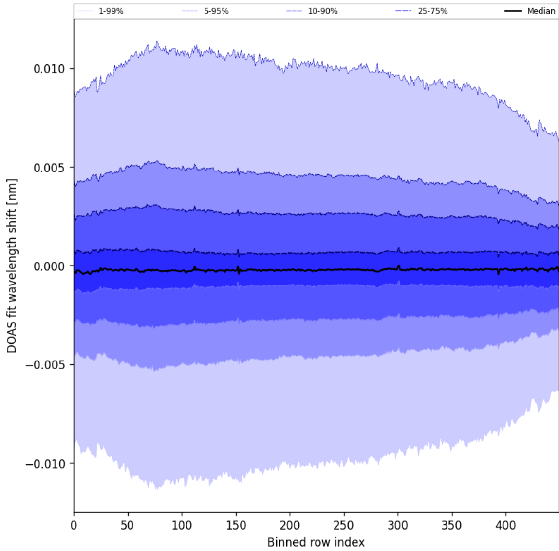
Figure 58: Along track statistics of “DOAS fit wavelength shift” for 2025-02-10 to 2025-02-12
