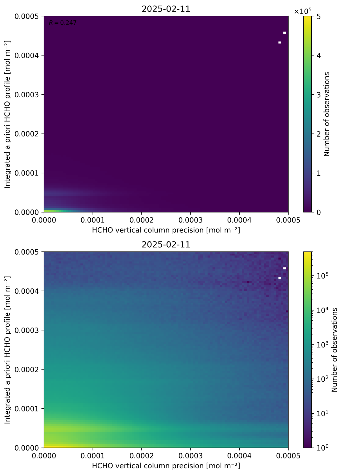
Figure 147: Scatter density plot of “HCHO vertical column precision” against “Integrated a priori HCHO profile” for 2025-02-10 to 2025-02-12.
