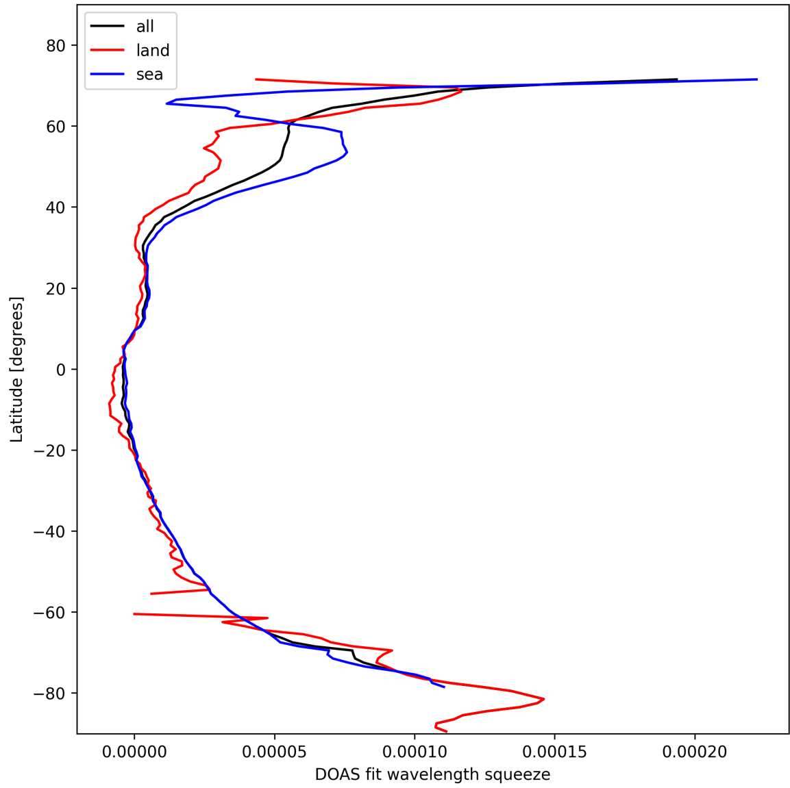
Figure 31: Zonal average of “DOAS fit wavelength squeeze” for 2025-02-10 to 2025-02-12.
