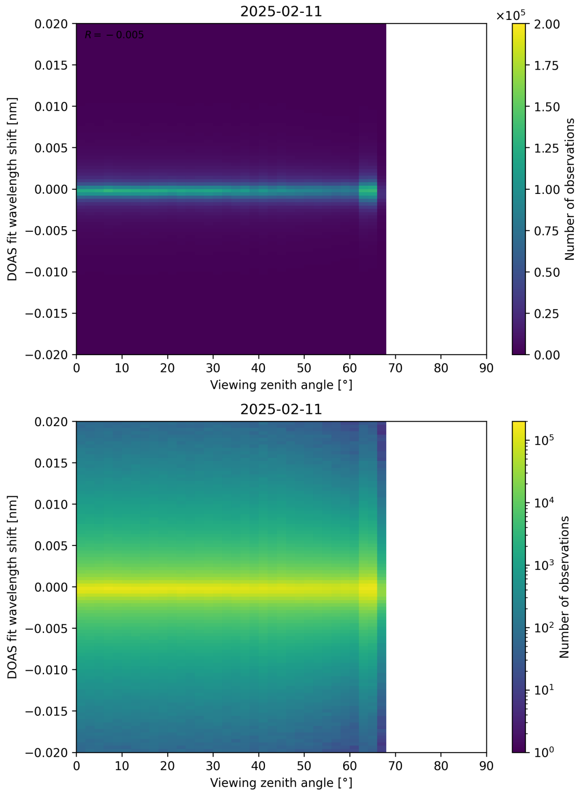
Figure 183: Scatter density plot of “Viewing zenith angle” against “DOAS fit wavelength shift” for 2025-02-10 to 2025-02-12.
