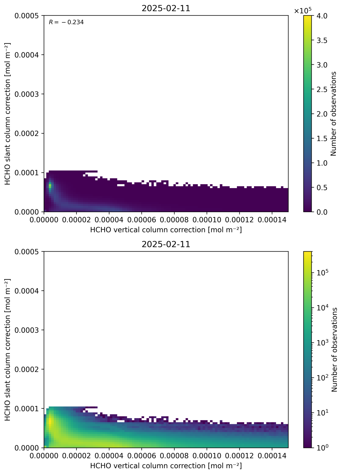
Figure 117: Scatter density plot of “HCHO vertical column correction” against “HCHO slant column correction” for 2025-02-10 to 2025-02-12.
