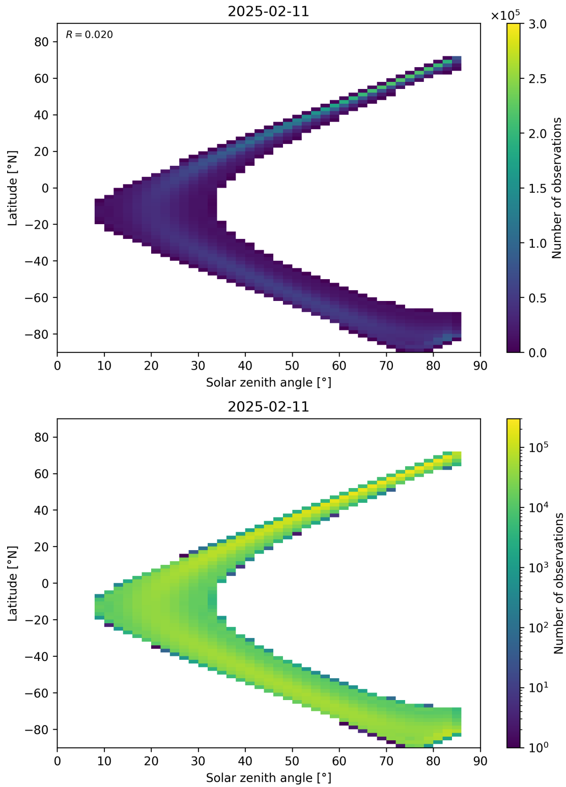
Figure 181: Scatter density plot of “Solar zenith angle” against “Latitude” for 2025-02-10 to 2025-02-12.
