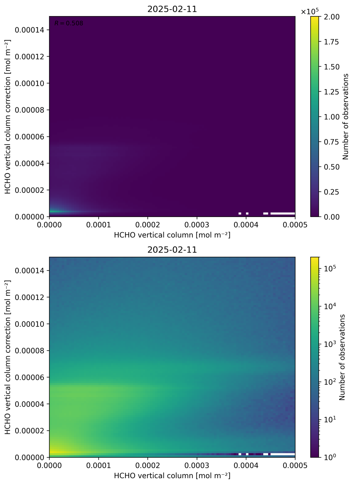
Figure 133: Scatter density plot of “HCHO vertical column” against “HCHO vertical column correction” for 2025-02-10 to 2025-02-12.
