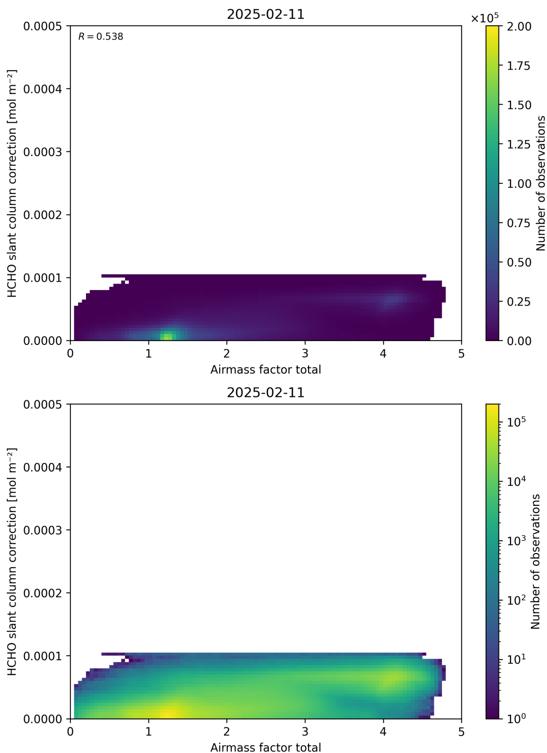
Figure 102: Scatter density plot of “Airmass factor total” against “HCHO slant column correction” for 2025-02-10 to 2025-02-12.
