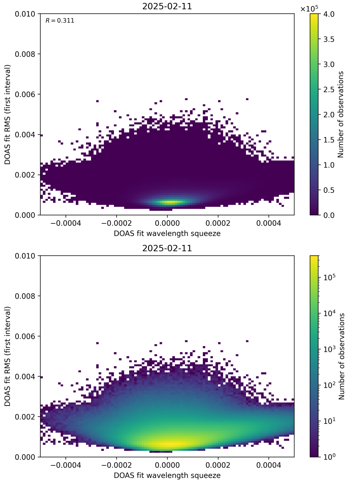
Figure 68: Scatter density plot of “DOAS fit wavelength squeeze” against “DOAS fit RMS (first interval)” for 2025-02-10 to 2025-02-12.
