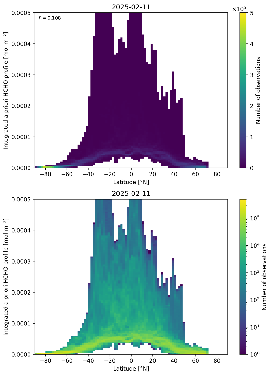
Figure 166: Scatter density plot of “Latitude” against “Integrated a priori HCHO profile” for 2025-02-10 to 2025-02-12.
