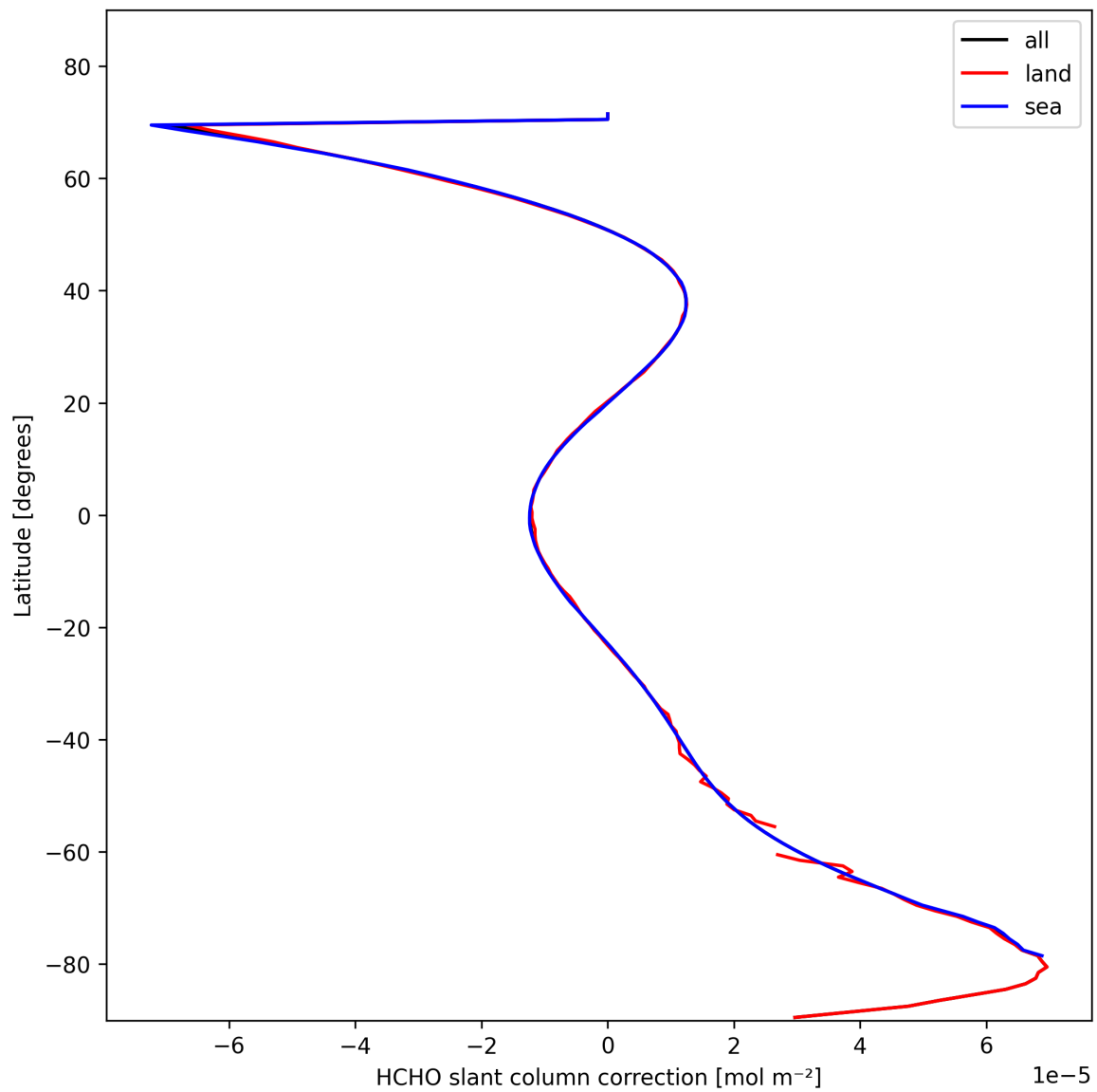
Figure 33: Zonal average of “HCHO slant column correction” for 2025-02-10 to 2025-02-12.
