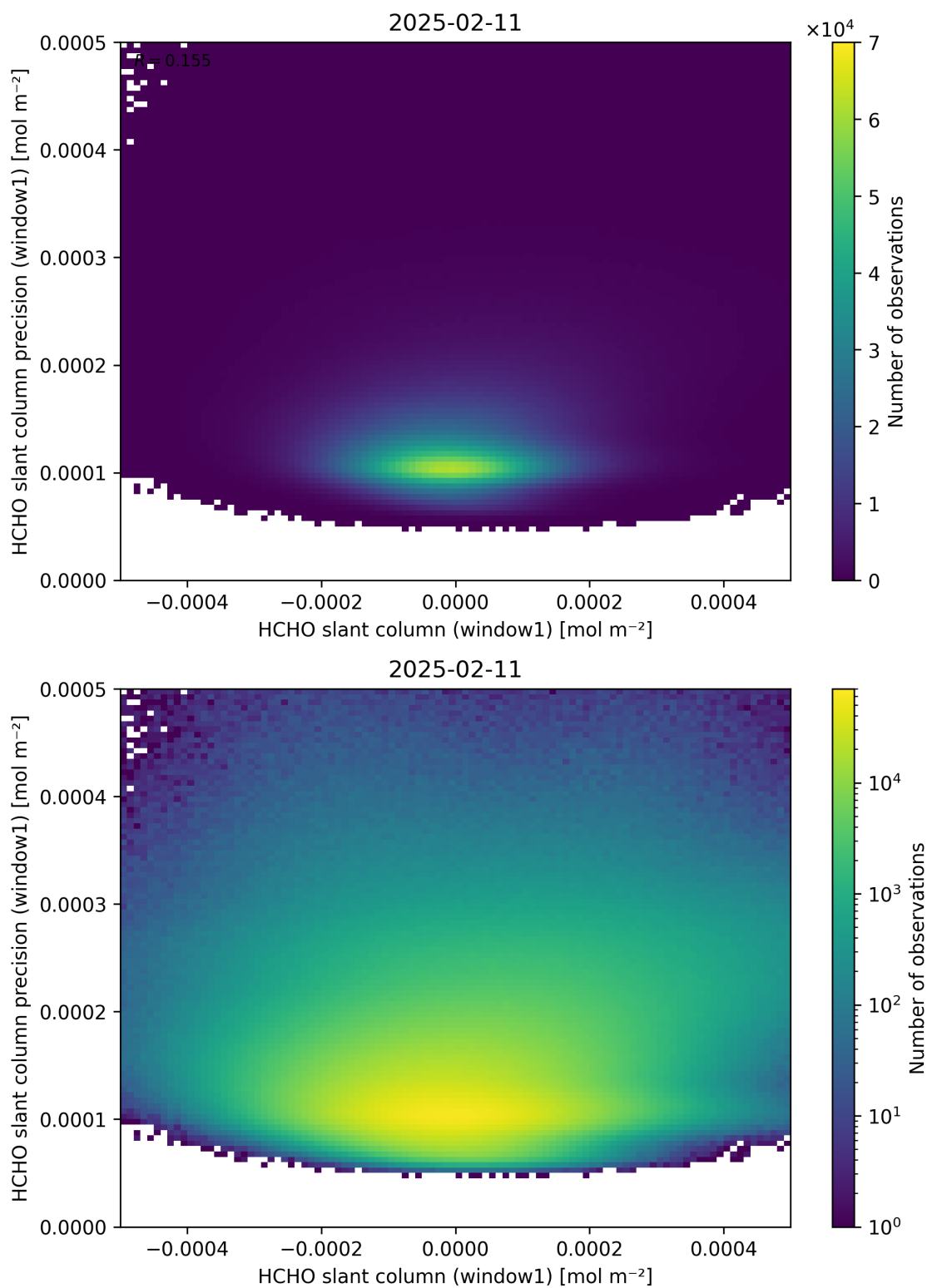
Figure 84: Scatter density plot of “HCHO slant column (window1)” against “HCHO slant column precision (window1)” for 2025-02-10 to 2025-02-12.
