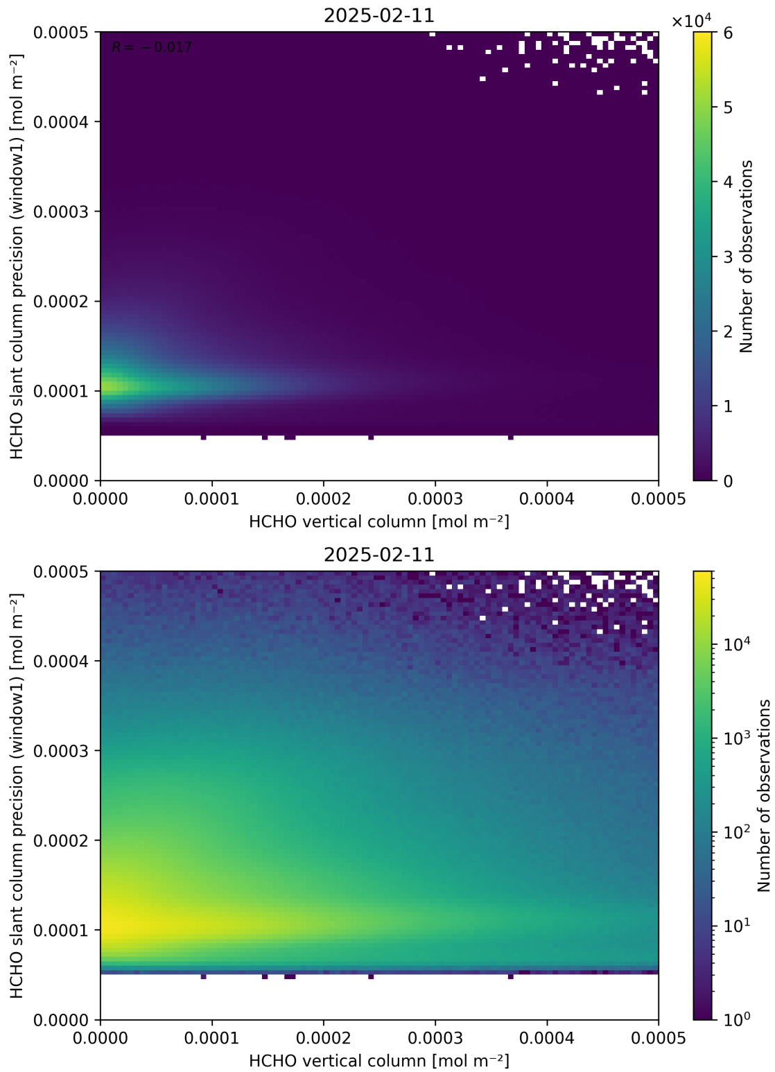
Figure 130: Scatter density plot of “HCHO vertical column” against “HCHO slant column precision (window1)” for 2025-02-10 to 2025-02-12.
