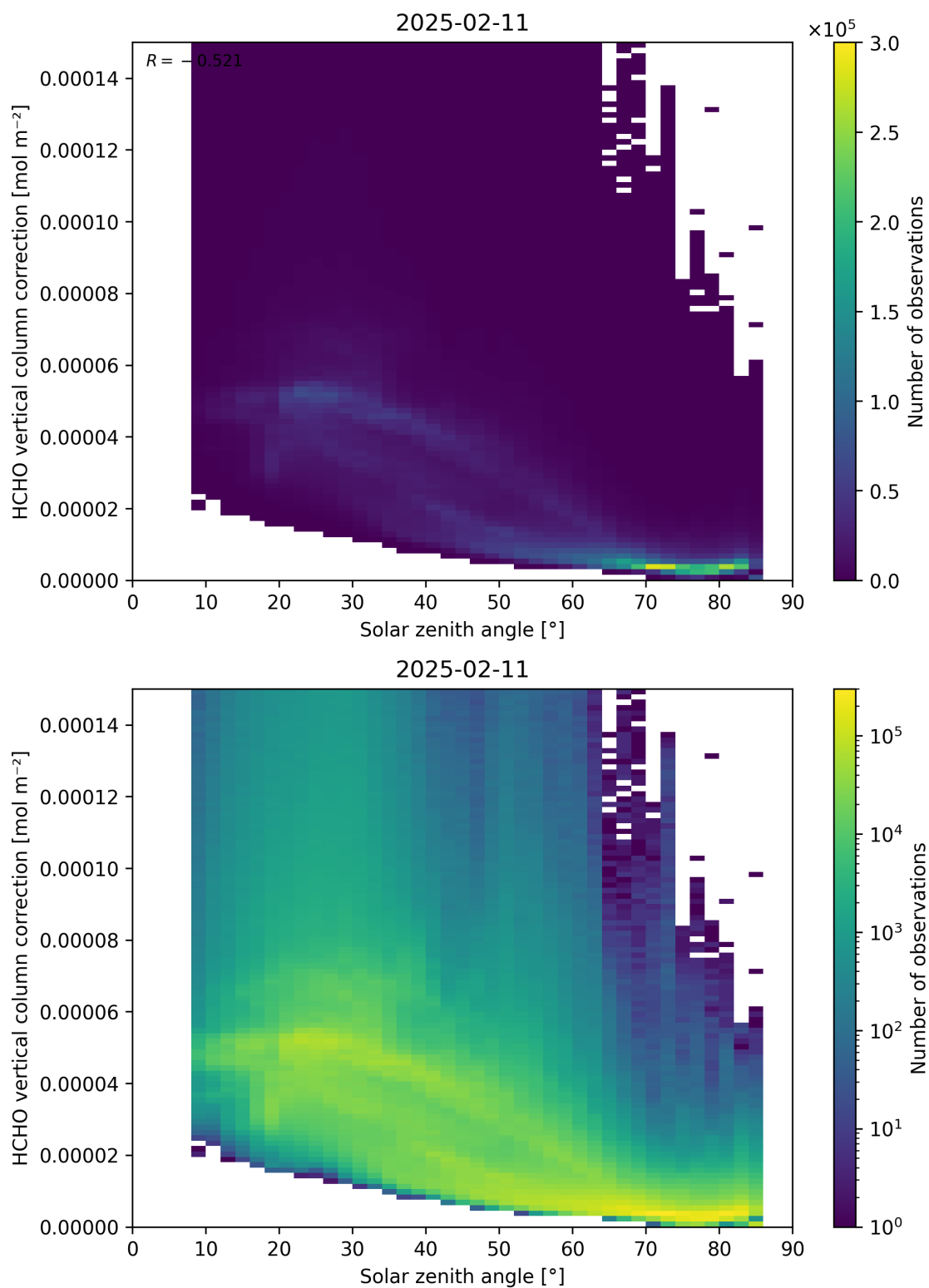
Figure 178: Scatter density plot of “Solar zenith angle” against “HCHO vertical column correction” for 2025-02-10 to 2025-02-12.
