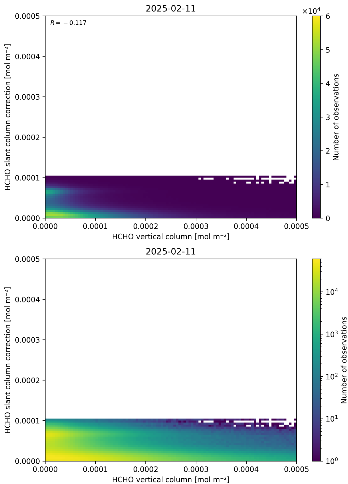
Figure 128: Scatter density plot of “HCHO vertical column” against “HCHO slant column correction” for 2025-02-10 to 2025-02-12.
