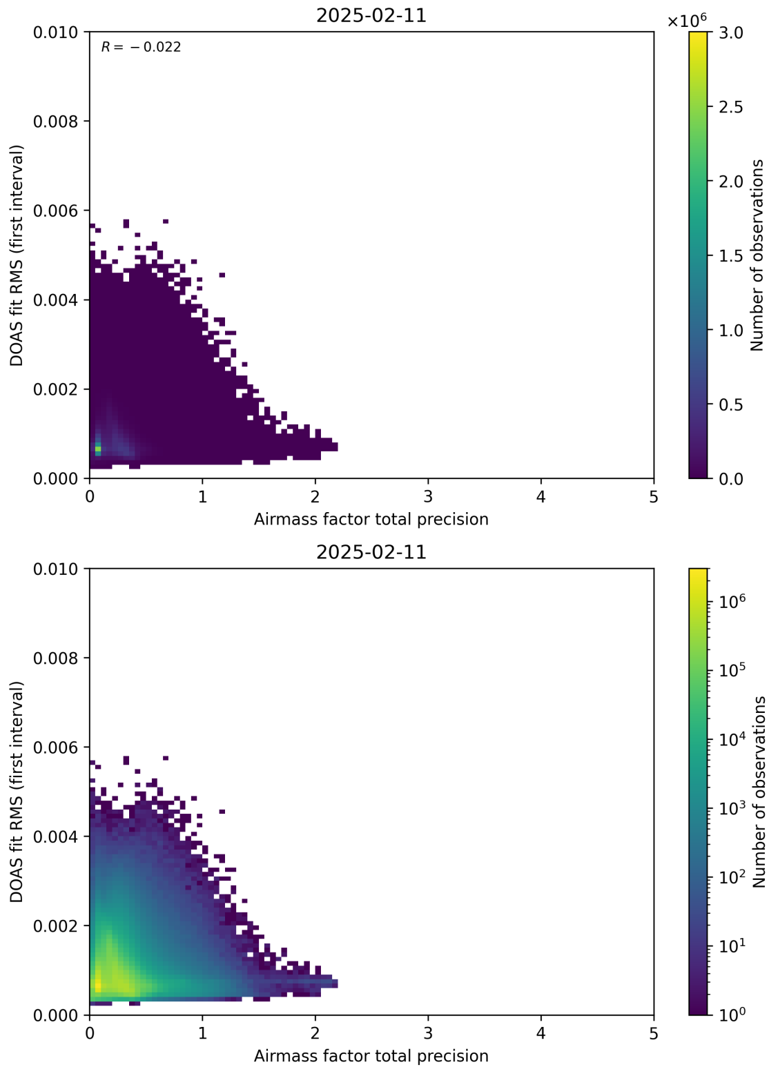
Figure 105: Scatter density plot of “Airmass factor total precision” against “DOAS fit RMS (first interval)” for 2025-02-10 to 2025-02-12.
