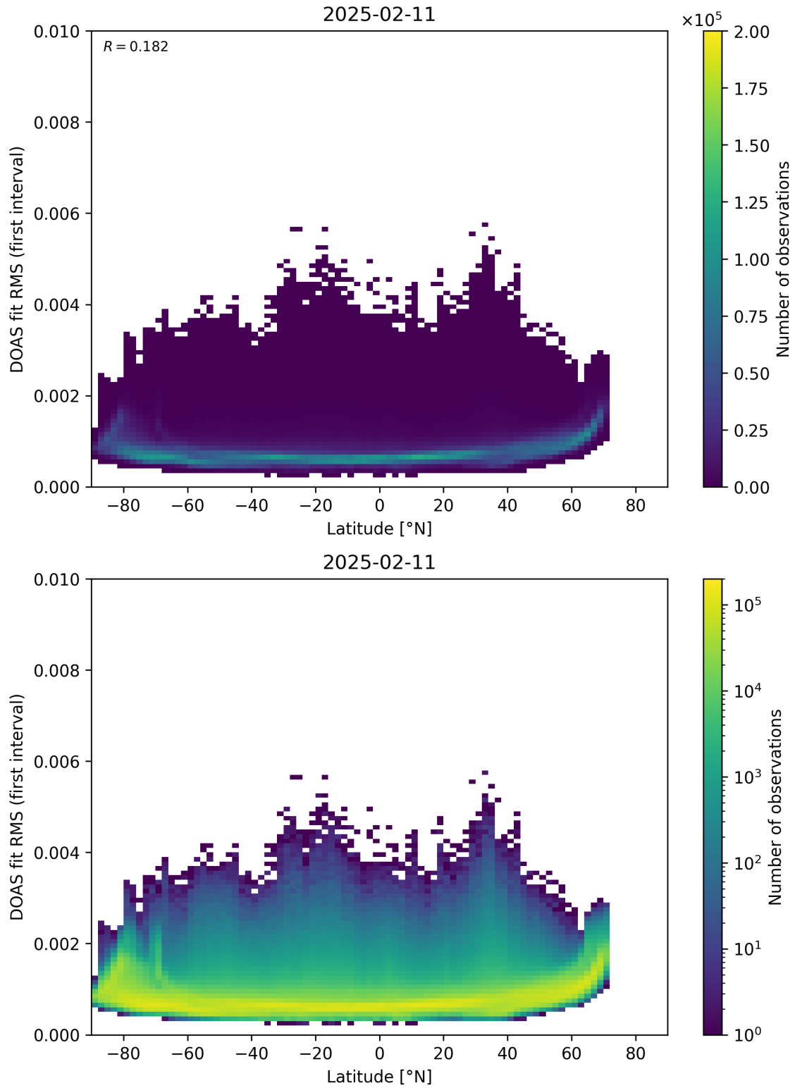
Figure 153: Scatter density plot of “Latitude” against “DOAS fit RMS (first interval)” for 2025-02-10 to 2025-02-12.
