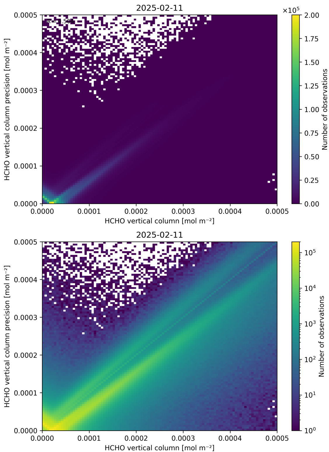
Figure 134: Scatter density plot of “HCHO vertical column” against “HCHO vertical column precision” for 2025-02-10 to 2025-02-12.
