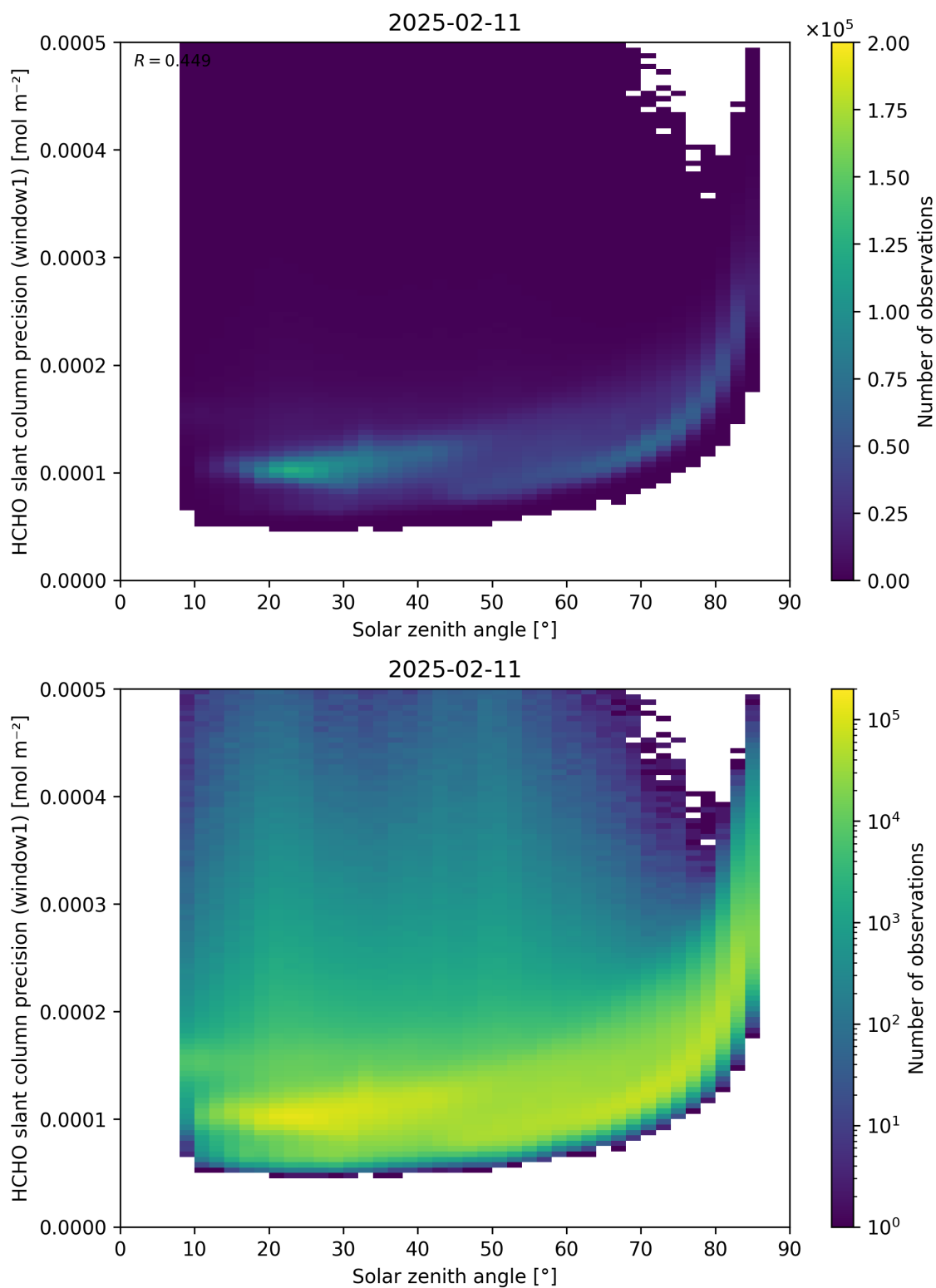
Figure 174: Scatter density plot of “Solar zenith angle” against “HCHO slant column precision (window1)” for 2025-02-10 to 2025-02-12.
