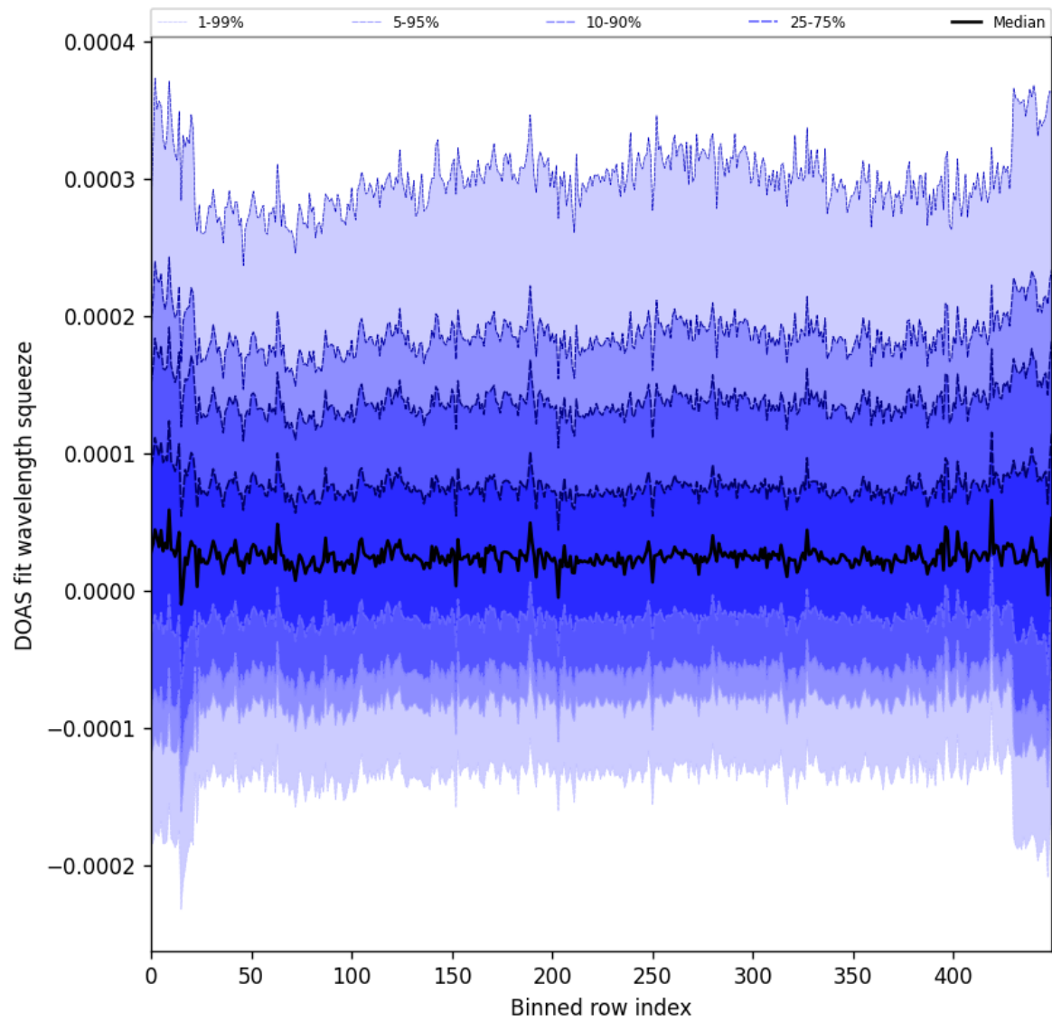
Figure 59: Along track statistics of “DOAS fit wavelength squeeze” for 2025-02-10 to 2025-02-12
