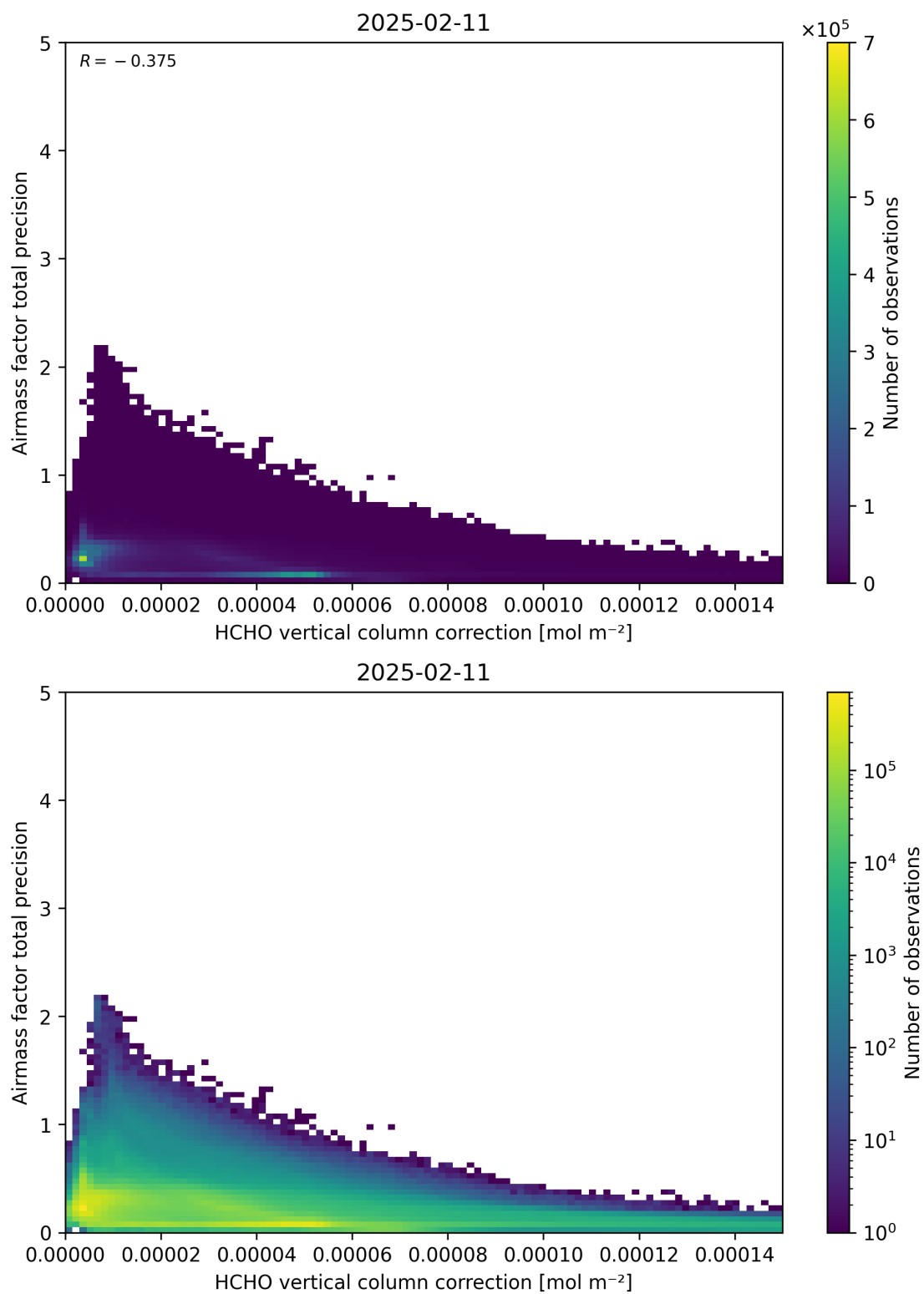
Figure 121: Scatter density plot of “HCHO vertical column correction” against “Airmass factor total precision” for 2025-02-10 to 2025-02-12.
