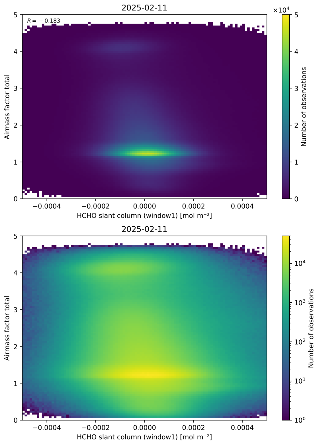
Figure 85: Scatter density plot of “HCHO slant column (window1)” against “Airmass factor total” for 2025-02-10 to 2025-02-12.
