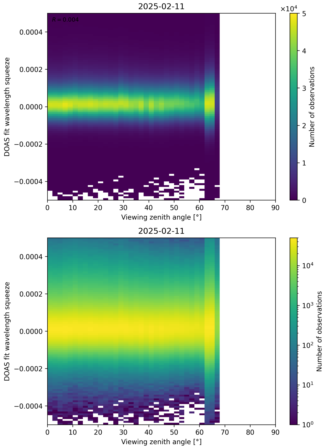
Figure 184: Scatter density plot of “Viewing zenith angle” against “DOAS fit wavelength squeeze” for 2025-02-10 to 2025-02-12.
