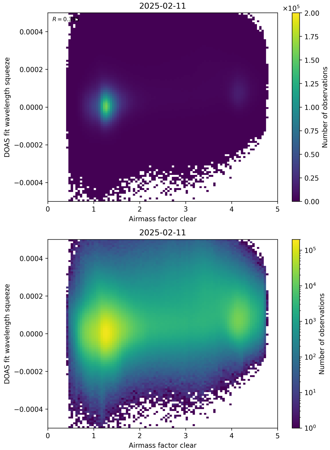
Figure 73: Scatter density plot of “Airmass factor clear” against “DOAS fit wavelength squeeze” for 2025-02-10 to 2025-02-12.
