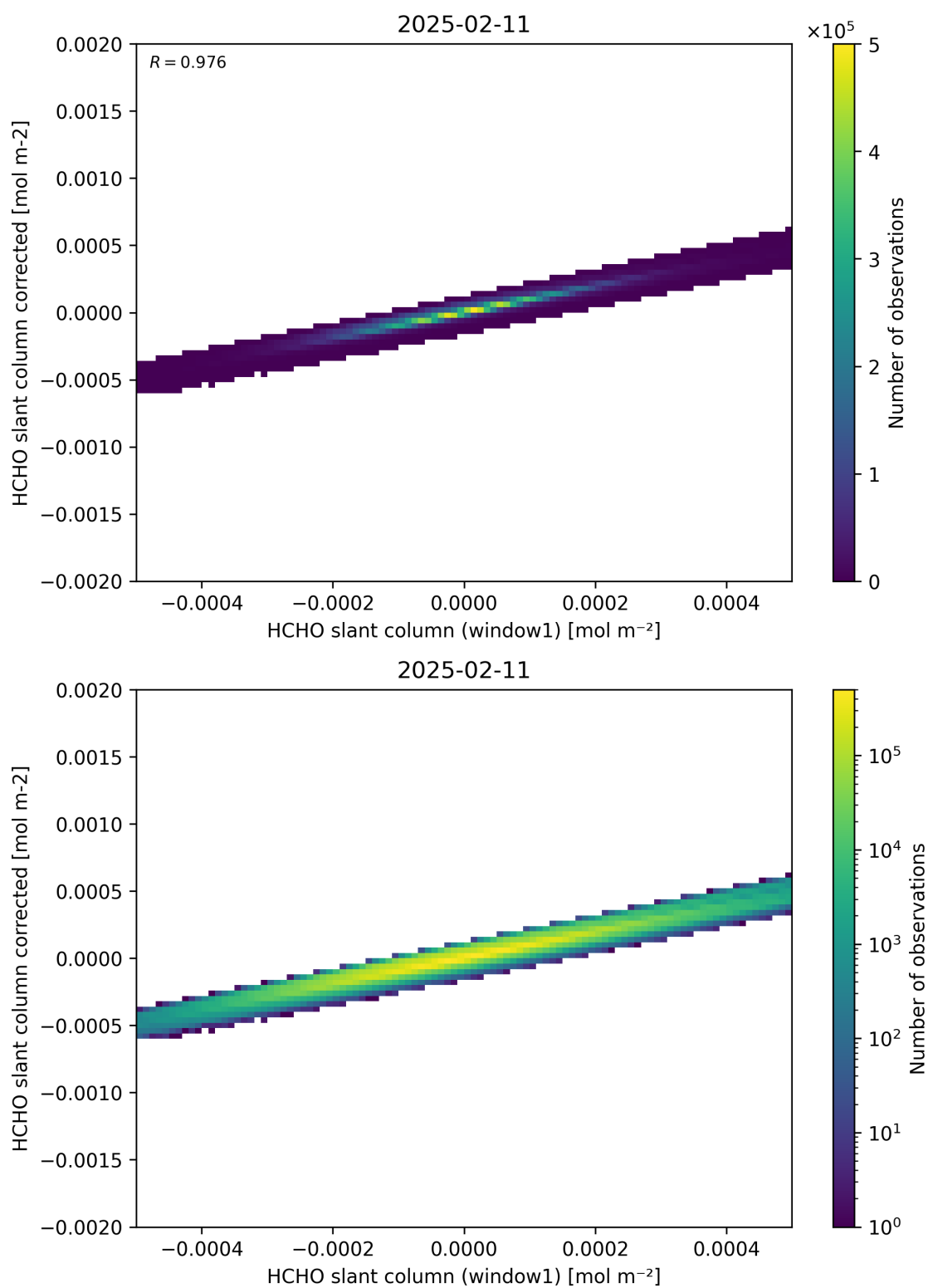
Figure 82: Scatter density plot of “HCHO slant column (window1)” against “HCHO slant column corrected” for 2025-02-10 to 2025-02-12.
