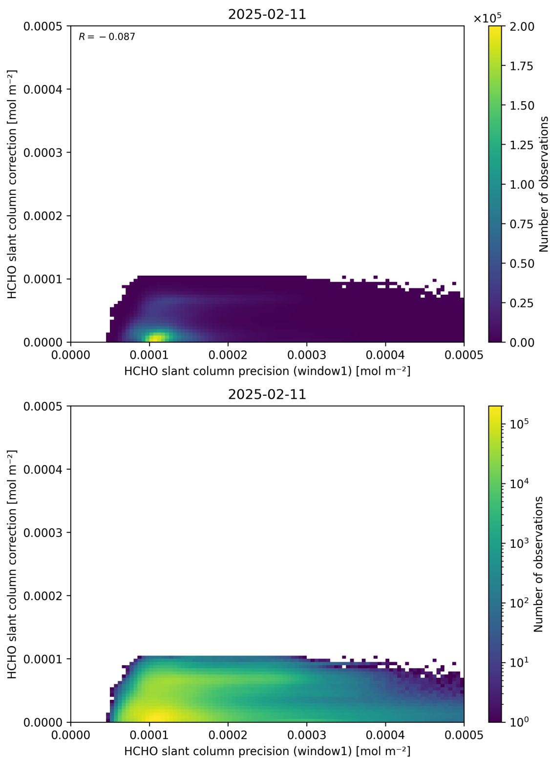
Figure 93: Scatter density plot of “HCHO slant column precision (window1)” against “HCHO slant column correction” for 2025-02-10 to 2025-02-12.
