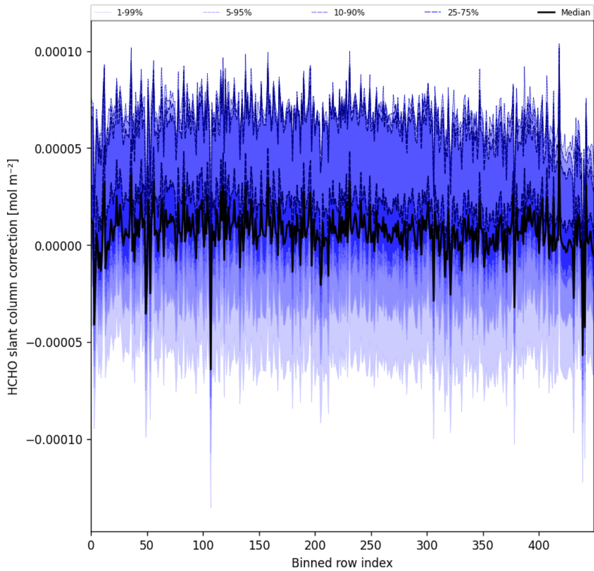
Figure 61: Along track statistics of “HCHO slant column correction” for 2025-02-10 to 2025-02-12
