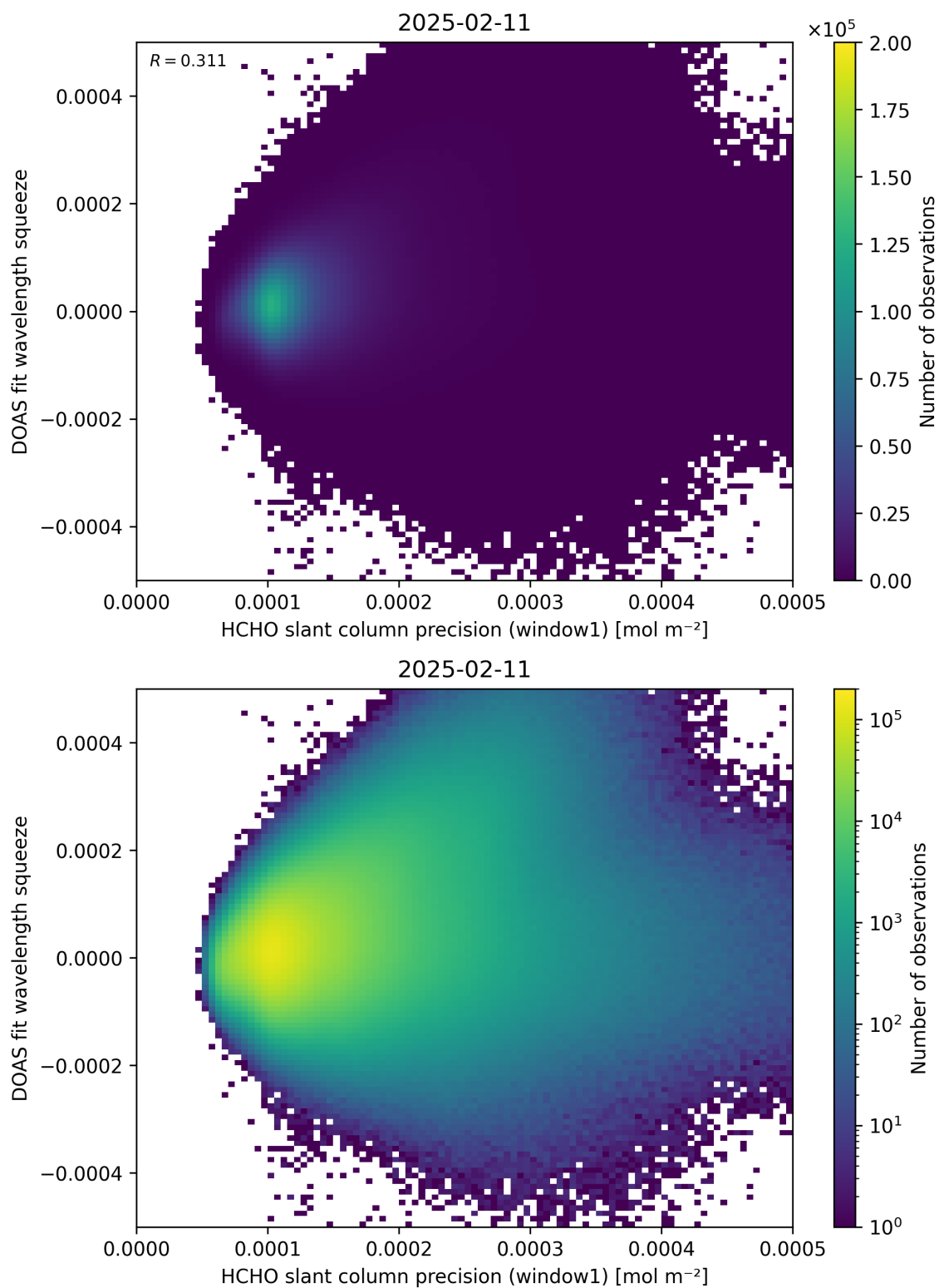
Figure 90: Scatter density plot of “HCHO slant column precision (window1)” against “DOAS fit wavelength squeeze” for 2025-02-10 to 2025-02-12.
