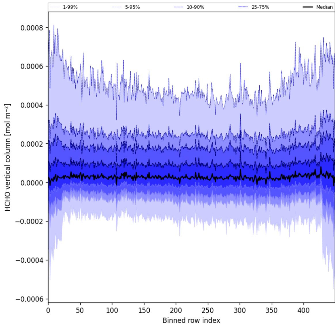
Figure 49: Along track statistics of “HCHO vertical column” for 2025-02-10 to 2025-02-12
