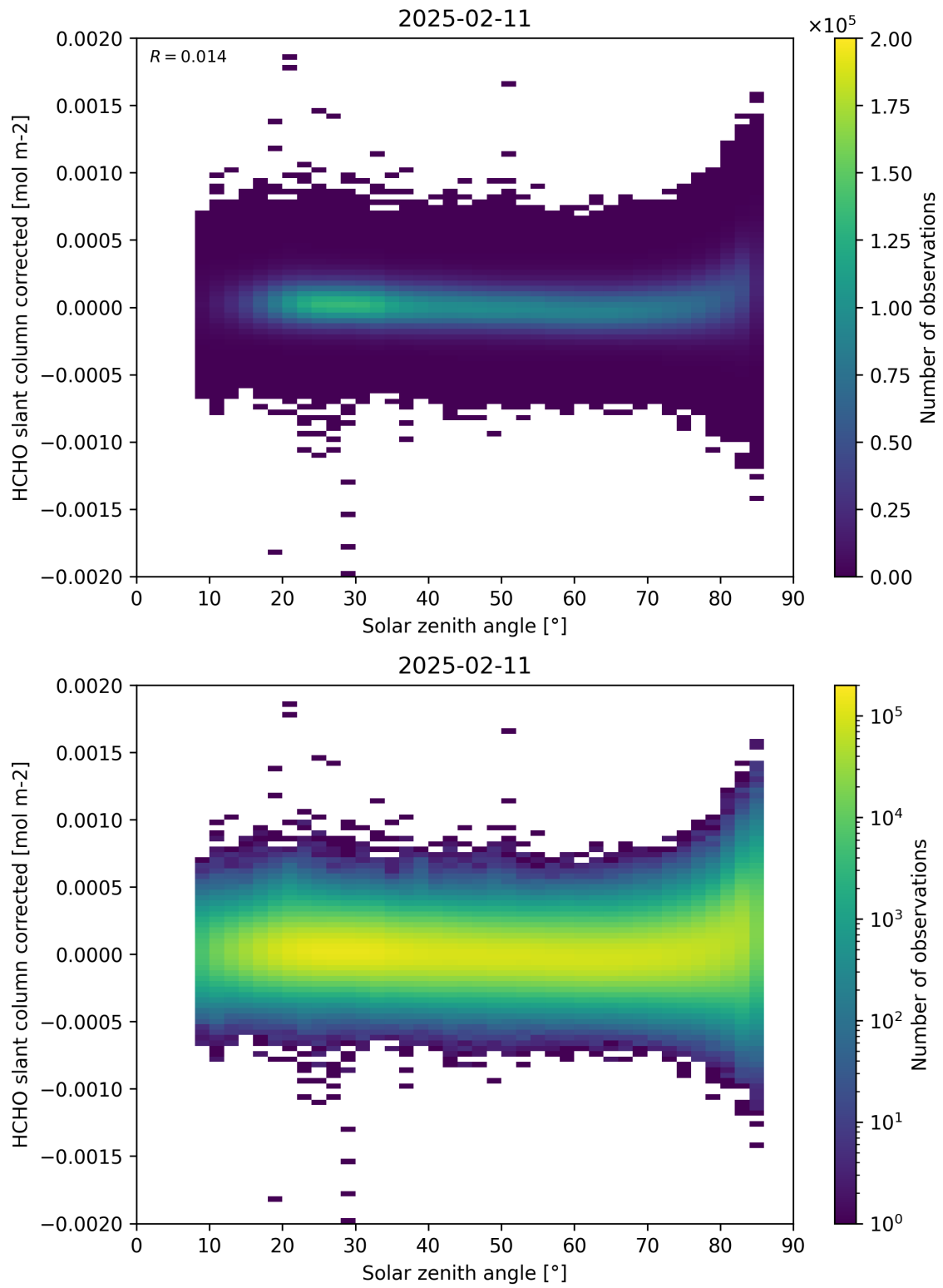
Figure 171: Scatter density plot of “Solar zenith angle” against “HCHO slant column corrected” for 2025-02-10 to 2025-02-12.
