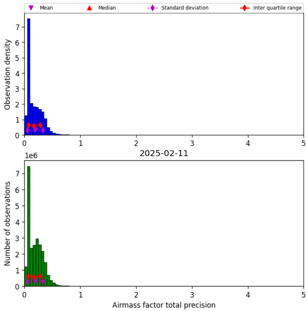
Figure 41: Histogram of “Airmass factor total precision” for 2025-02-10 to 2025-02-12
