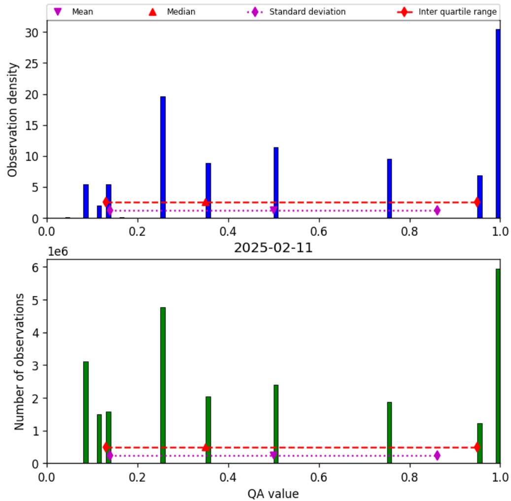
Figure 34: Histogram of “QA value” for 2025-02-10 to 2025-02-12
