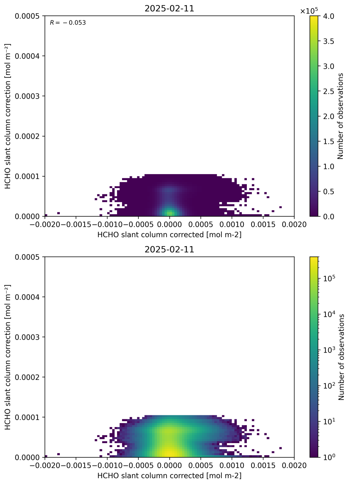
Figure 77: Scatter density plot of “HCHO slant column corrected” against “HCHO slant column correction” for 2025-02-10 to 2025-02-12.
