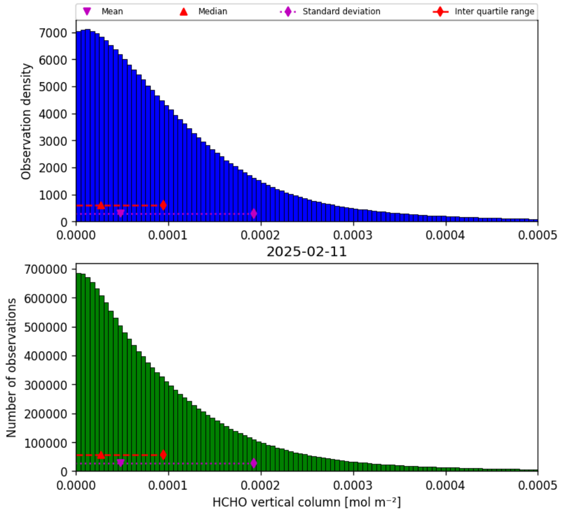
Figure 35: Histogram of “HCHO vertical column” for 2025-02-10 to 2025-02-12
