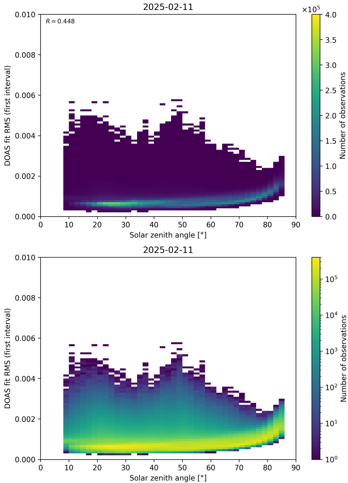
Figure 167: Scatter density plot of “Solar zenith angle” against “DOAS fit RMS (first interval)” for 2025-02-10 to 2025-02-12.
