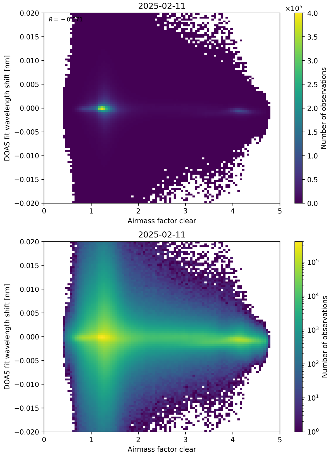
Figure 72: Scatter density plot of “Airmass factor clear” against “DOAS fit wavelength shift” for 2025-02-10 to 2025-02-12.
