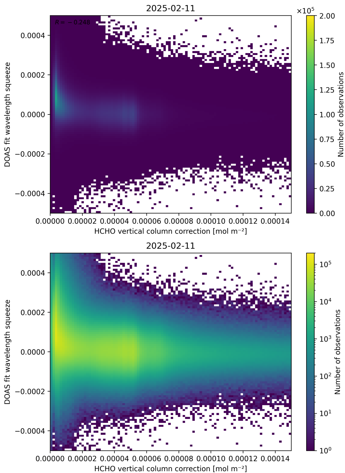
Figure 114: Scatter density plot of “HCHO vertical column correction” against “DOAS fit wavelength squeeze” for 2025-02-10 to 2025-02-12.
