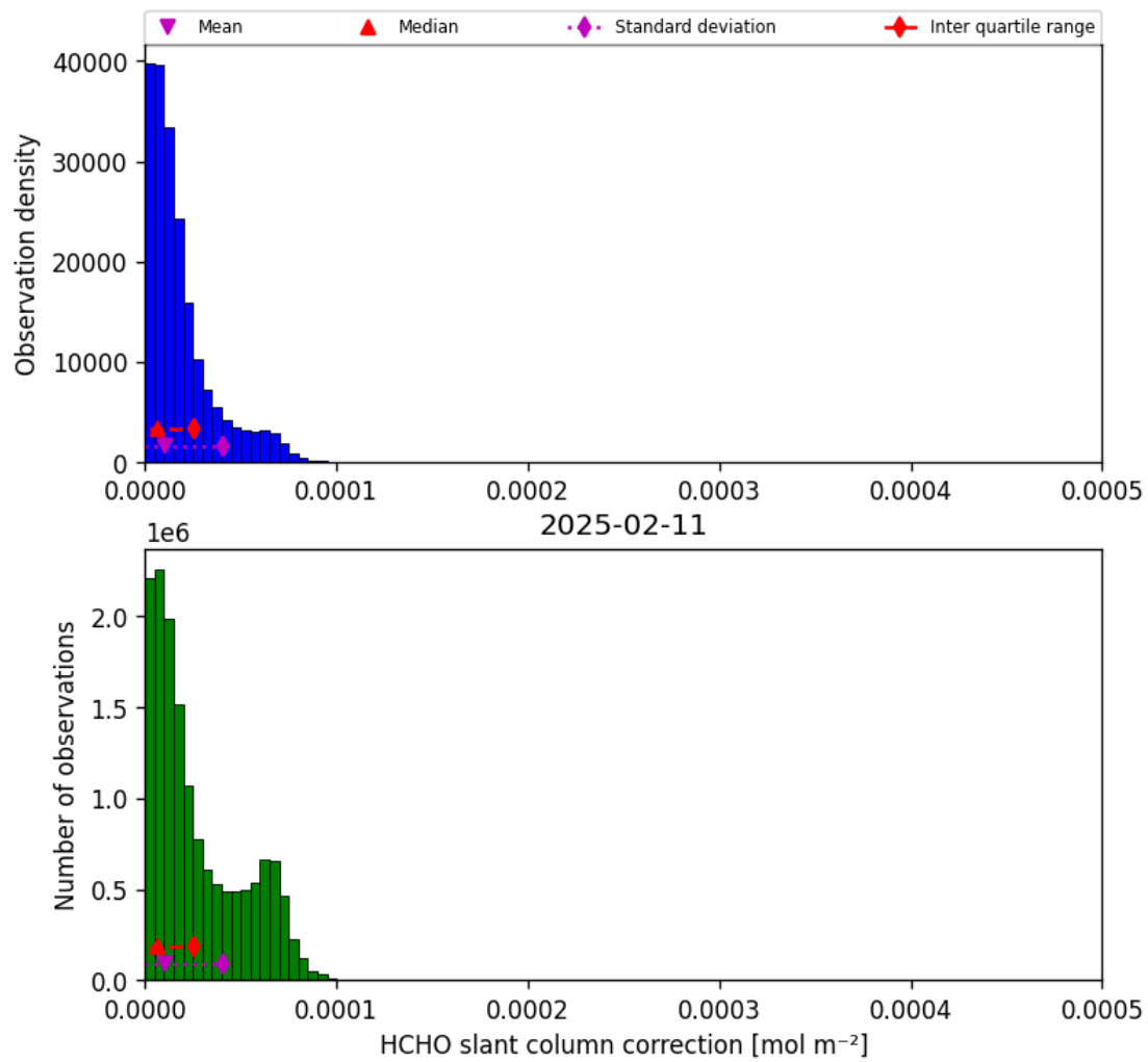
Figure 47: Histogram of “HCHO slant column correction” for 2025-02-10 to 2025-02-12
