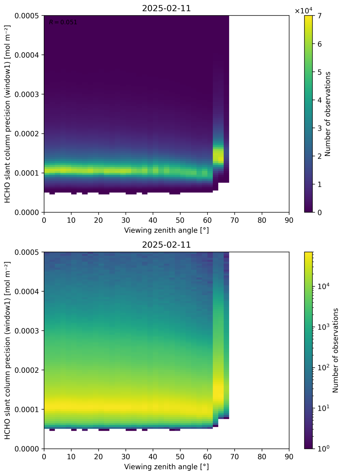
Figure 189: Scatter density plot of “Viewing zenith angle” against “HCHO slant column precision (window1)” for 2025-02-10 to 2025-02-12.
