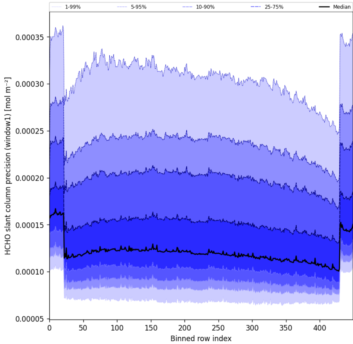
Figure 53: Along track statistics of “HCHO slant column precision (window1)” for 2025-02-10 to 2025-02-12
