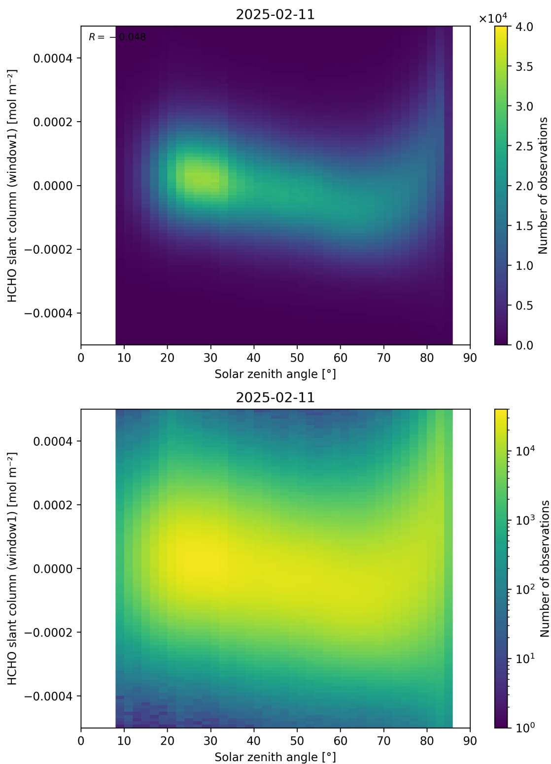
Figure 173: Scatter density plot of “Solar zenith angle” against “HCHO slant column (window1)” for 2025-02-10 to 2025-02-12.
