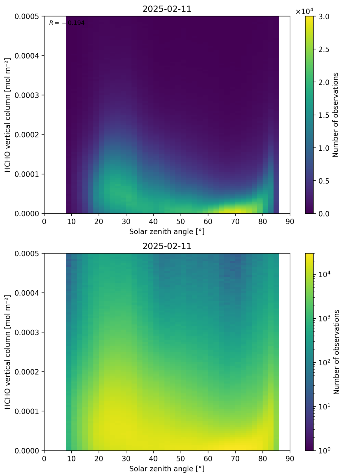
Figure 177: Scatter density plot of “Solar zenith angle” against “HCHO vertical column” for 2025-02-10 to 2025-02-12.
