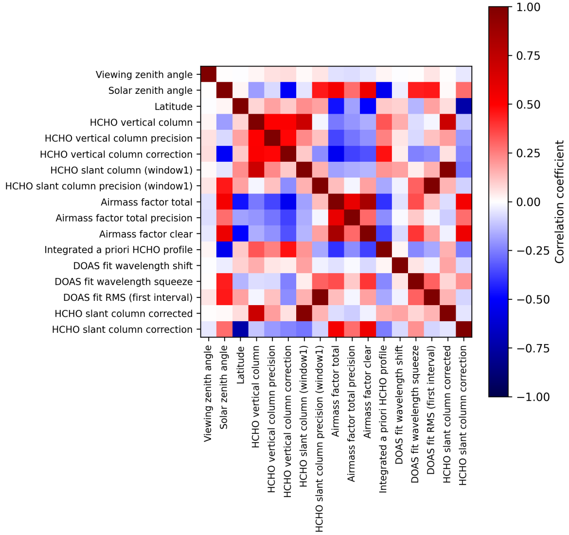
Figure 2: Map of correlation matrix for 2025-02-10 to 2025-02-12.
