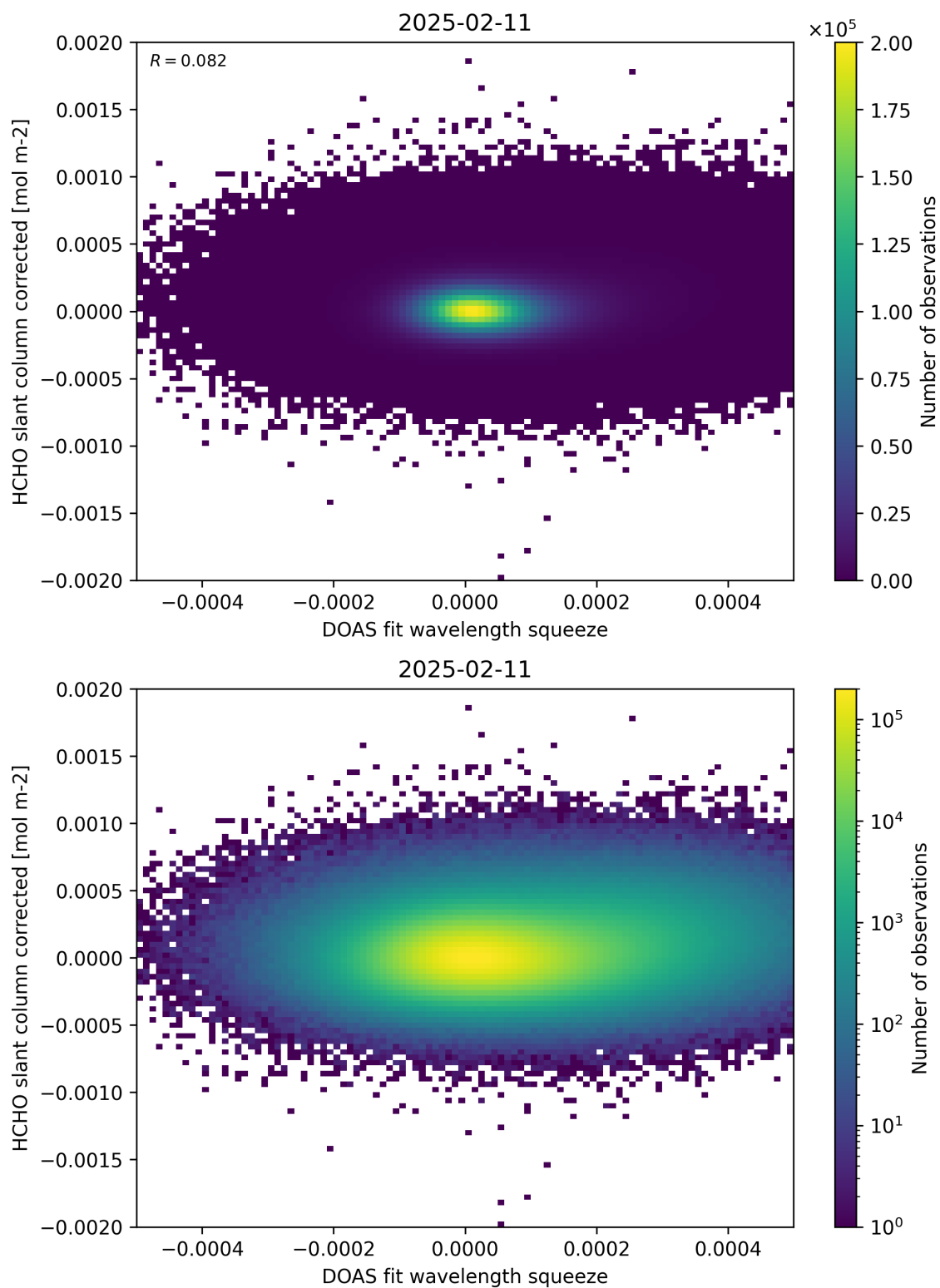
Figure 69: Scatter density plot of “DOAS fit wavelength squeeze” against “HCHO slant column corrected” for 2025-02-10 to 2025-02-12.
