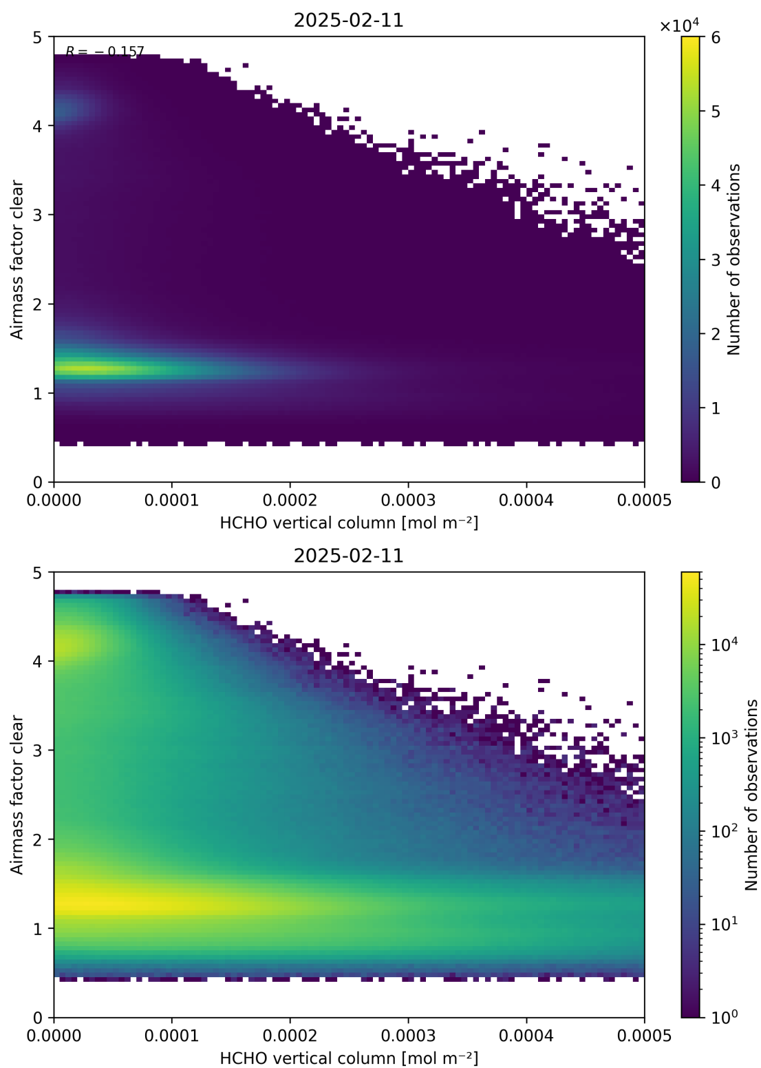
Figure 126: Scatter density plot of “HCHO vertical column” against “Airmass factor clear” for 2025-02-10 to 2025-02-12.
