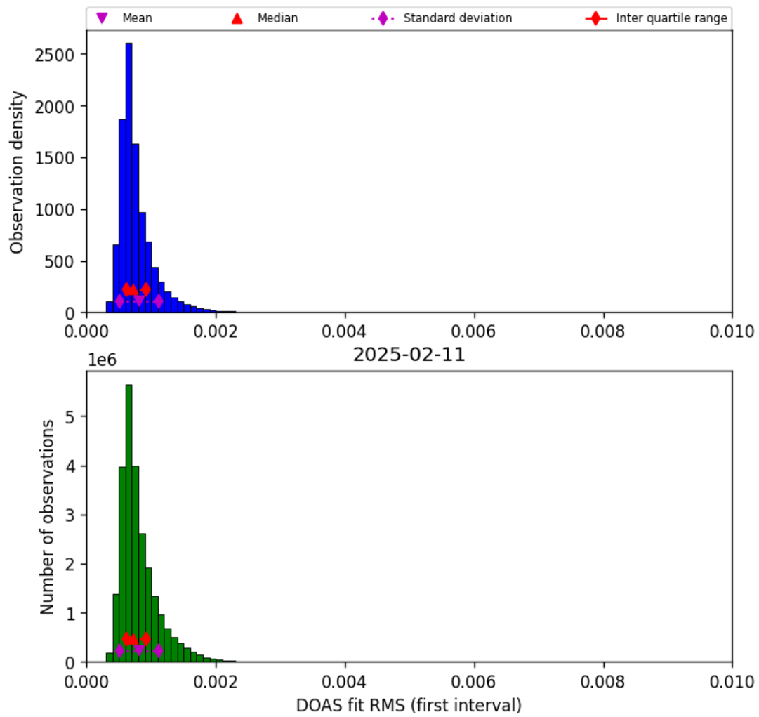
Figure 46: Histogram of “DOAS fit RMS (first interval)” for 2025-02-10 to 2025-02-12
