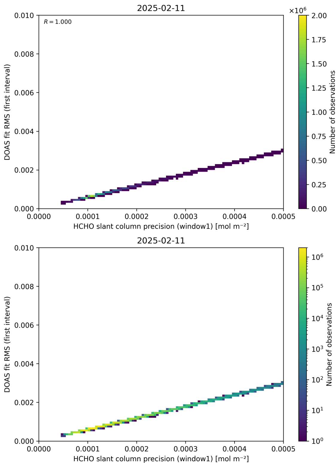
Figure 88: Scatter density plot of “HCHO slant column precision (window1)” against “DOAS fit RMS (first interval)” for 2025-02-10 to 2025-02-12.
