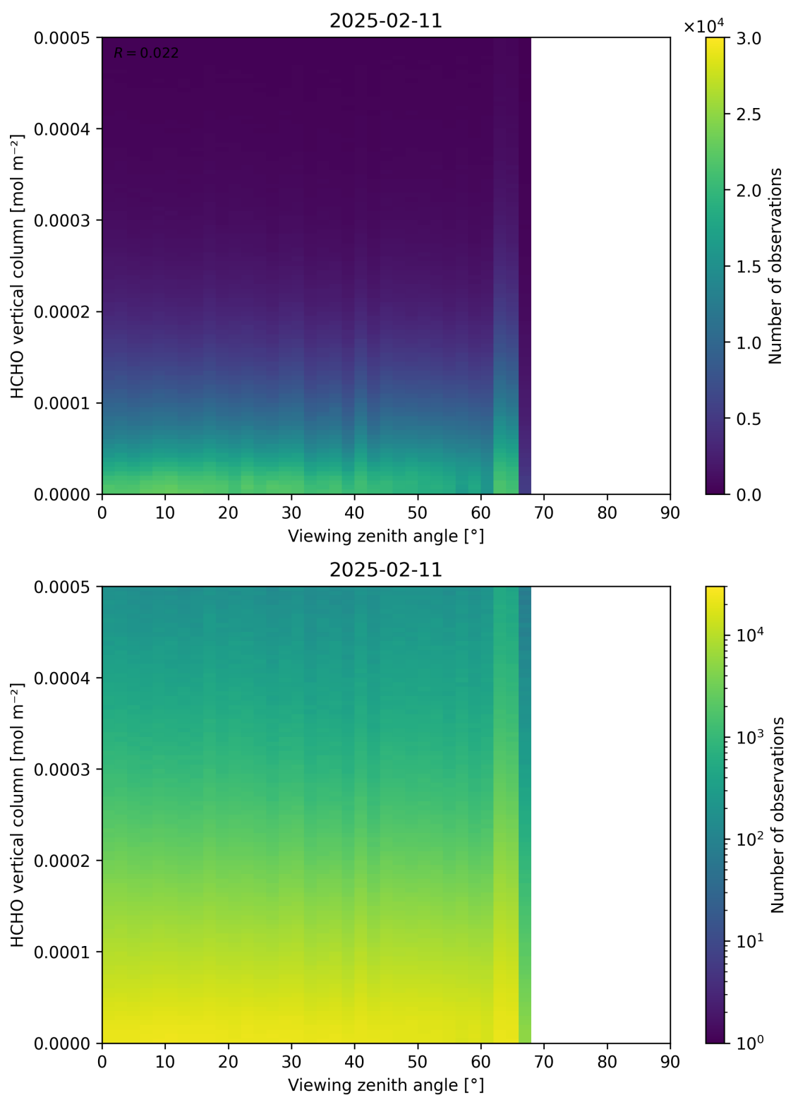
Figure 192: Scatter density plot of “Viewing zenith angle” against “HCHO vertical column” for 2025-02-10 to 2025-02-12.
