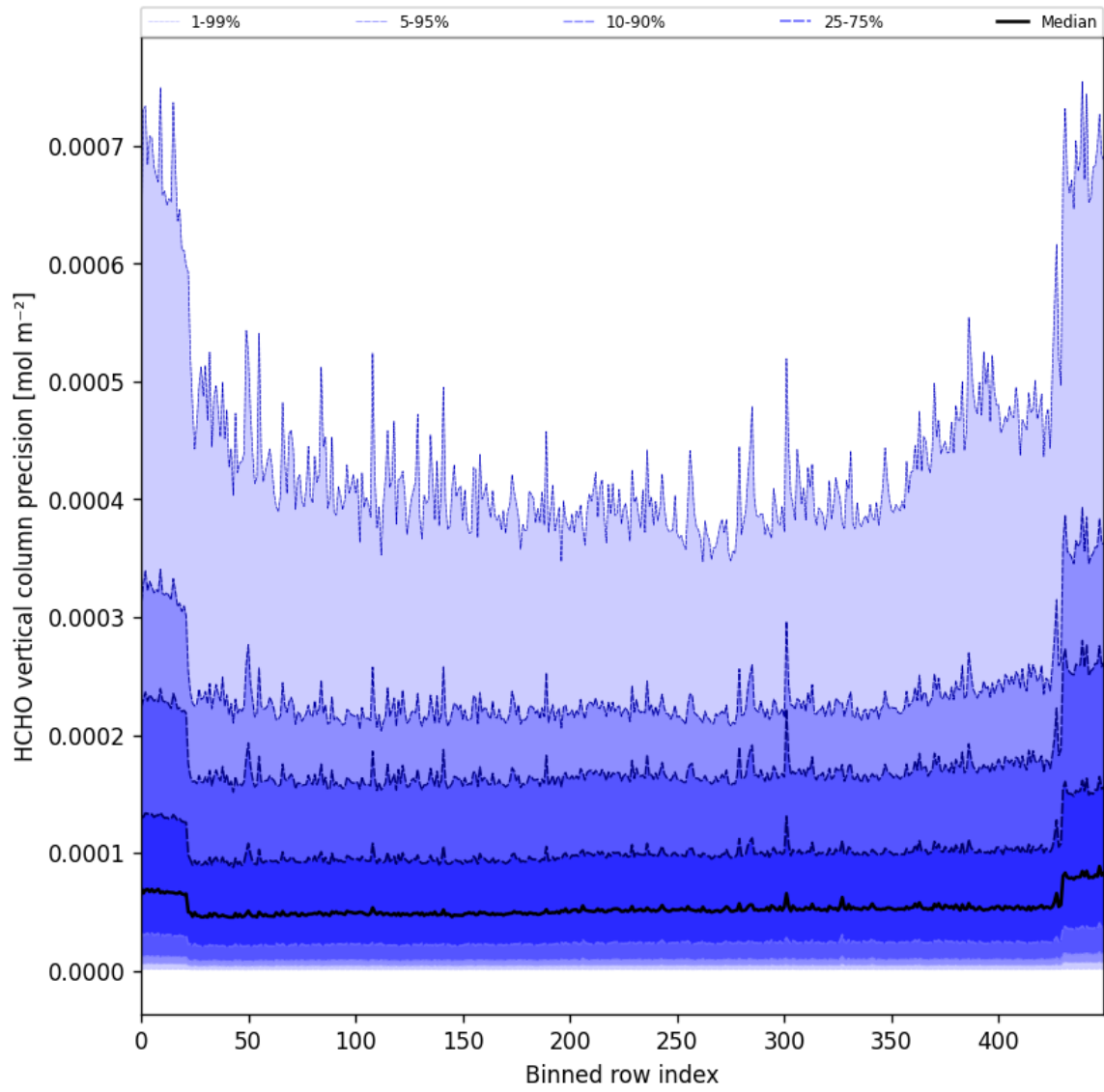
Figure 50: Along track statistics of “HCHO vertical column precision” for 2025-02-10 to 2025-02-12
