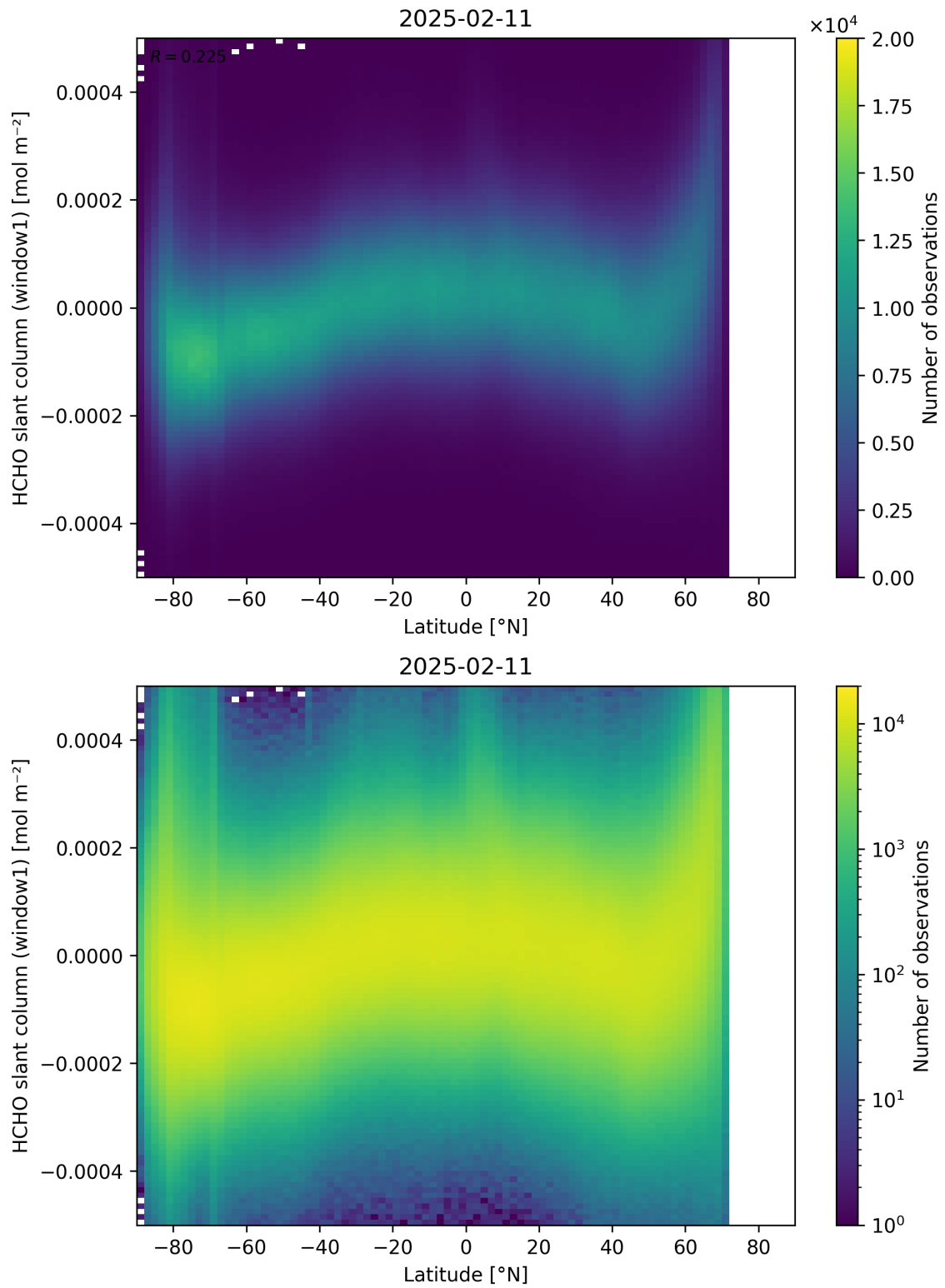
Figure 159: Scatter density plot of “Latitude” against “HCHO slant column (window1)” for 2025-02-10 to 2025-02-12.
