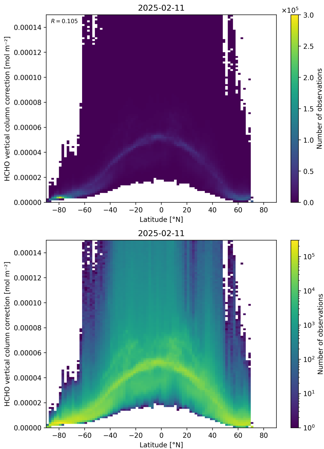
Figure 164: Scatter density plot of “Latitude” against “HCHO vertical column correction” for 2025-02-10 to 2025-02-12.
