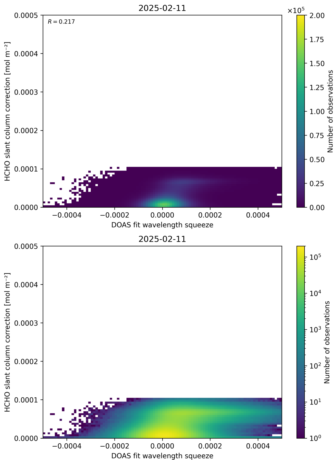
Figure 70: Scatter density plot of “DOAS fit wavelength squeeze” against “HCHO slant column correction” for 2025-02-10 to 2025-02-12.
