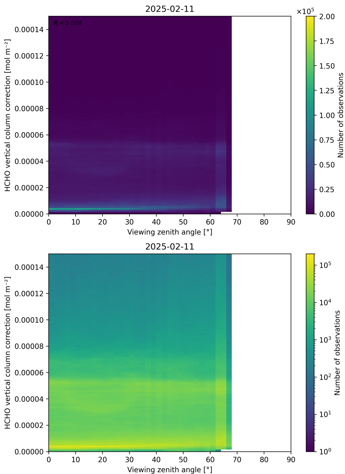
Figure 193: Scatter density plot of “Viewing zenith angle” against “HCHO vertical column correction” for 2025-02-10 to 2025-02-12.
