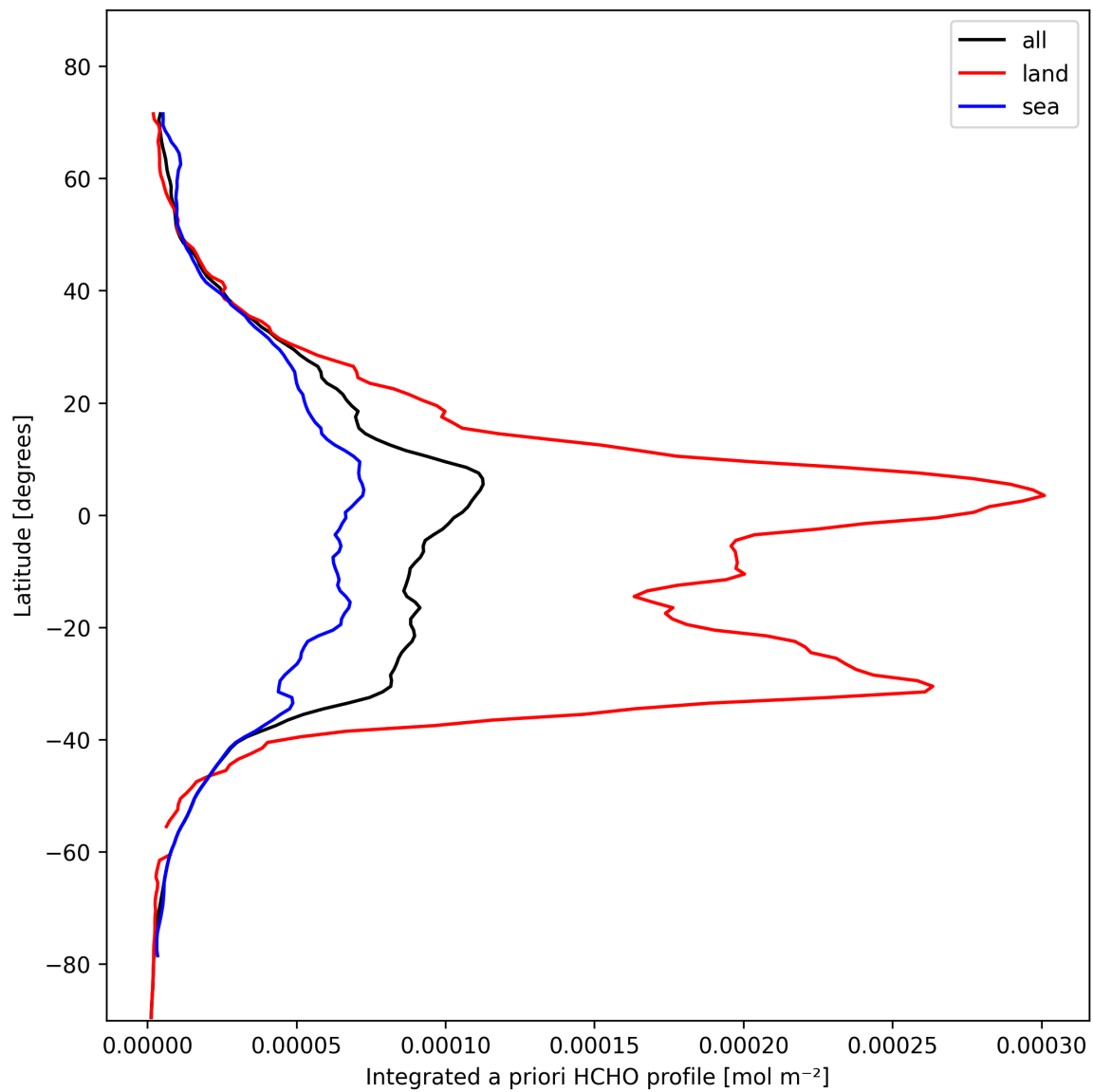
Figure 29: Zonal average of “Integrated a priori HCHO profile” for 2025-02-10 to 2025-02-12.
