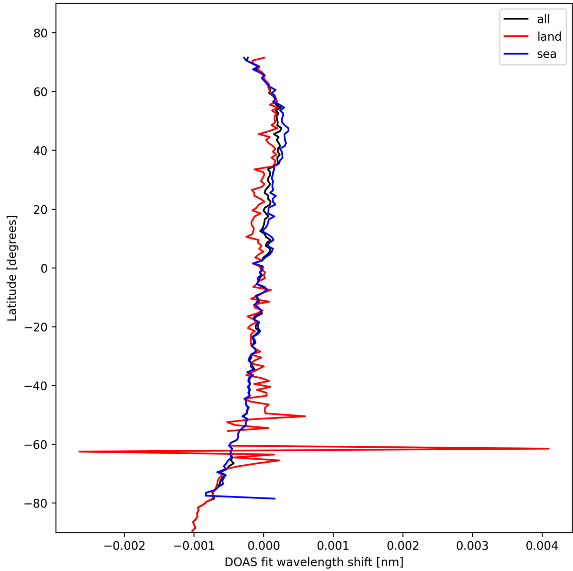
Figure 30: Zonal average of "DOAS fit wavelength shift" for 2025-02-10 to 2025-02-12.
