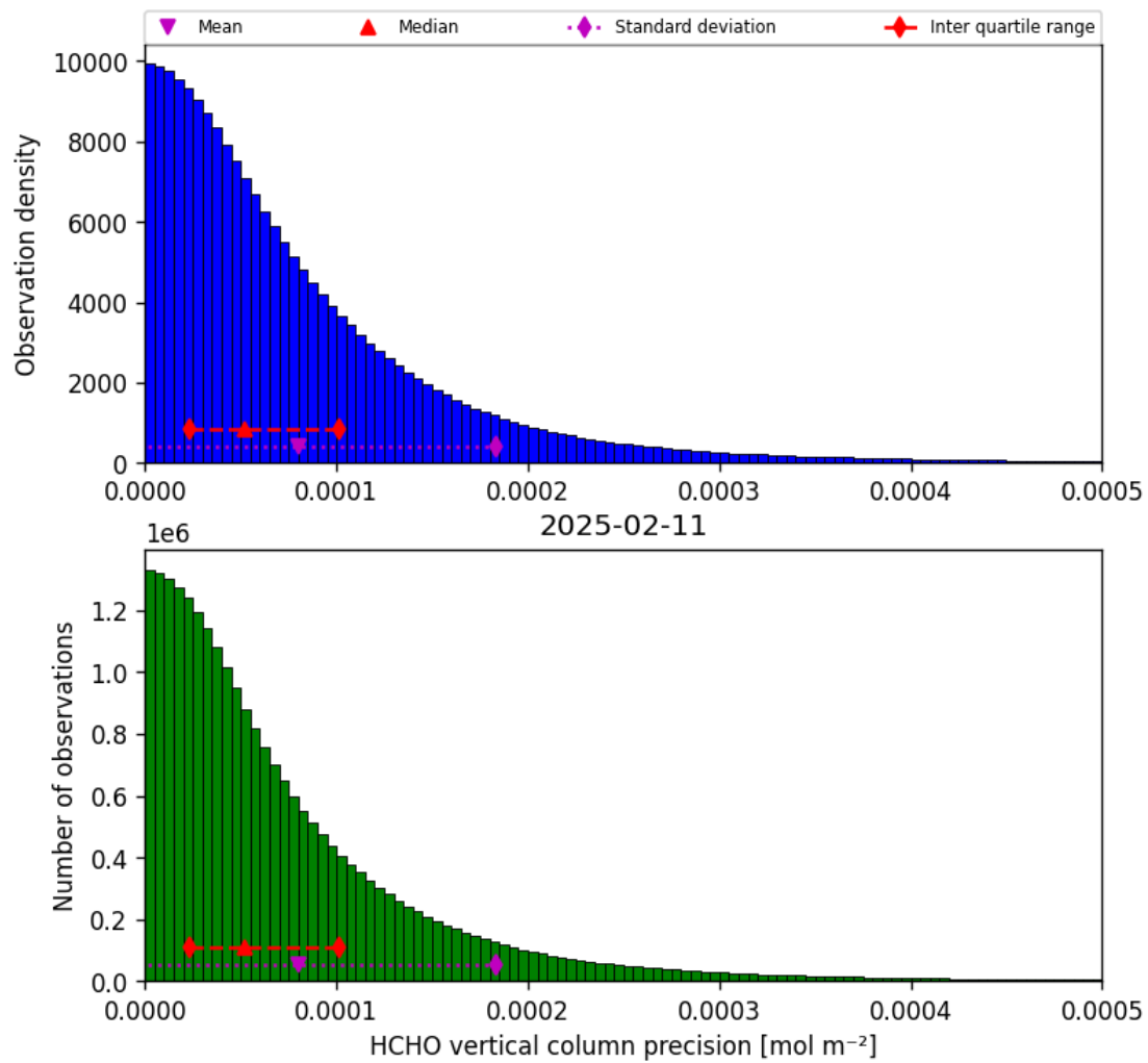
Figure 36: Histogram of “HCHO vertical column precision” for 2025-02-10 to 2025-02-12
