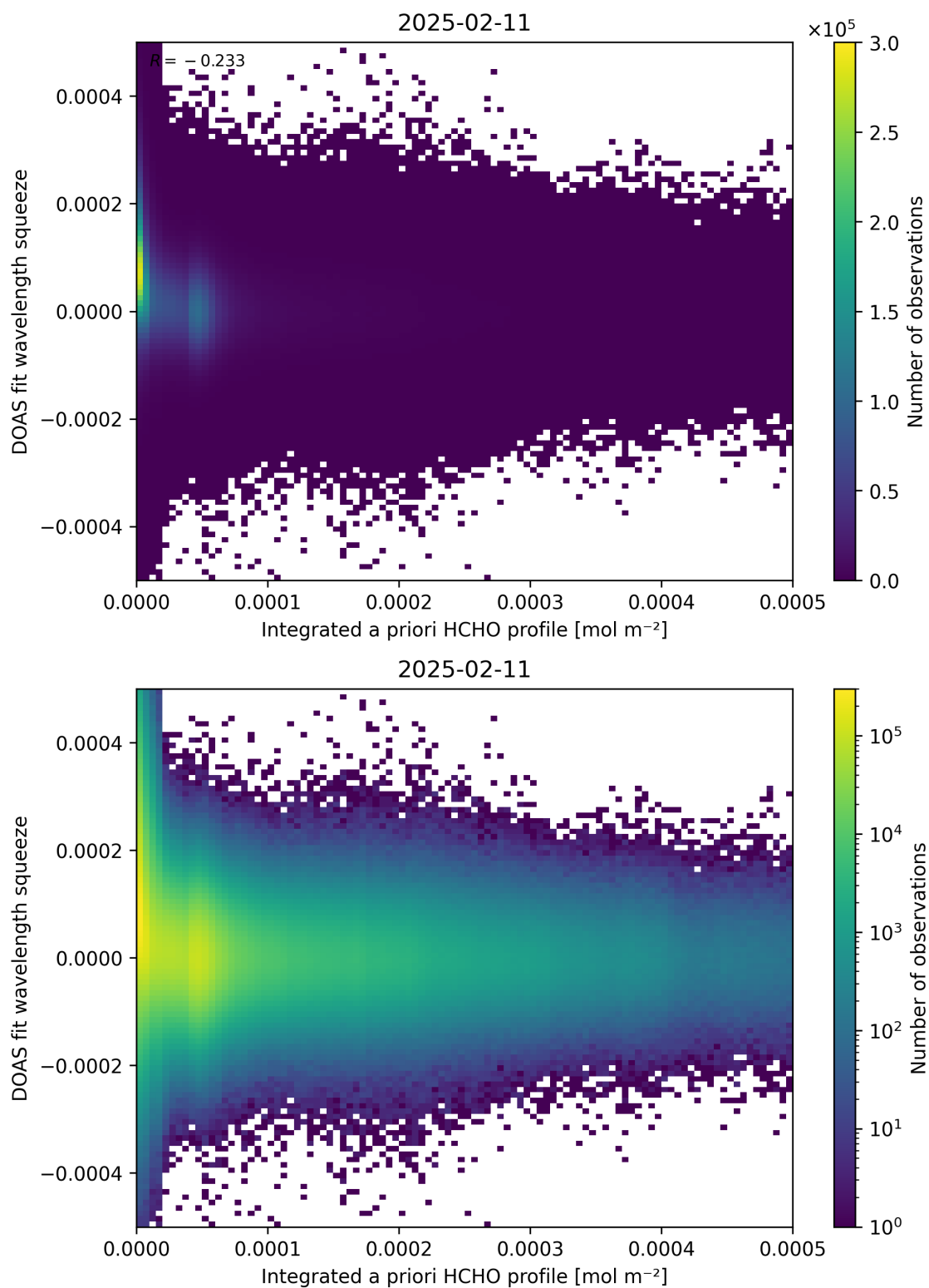
Figure 150: Scatter density plot of “Integrated a priori HCHO profile” against “DOAS fit wavelength squeeze” for 2025-02-10 to 2025-02-12.
