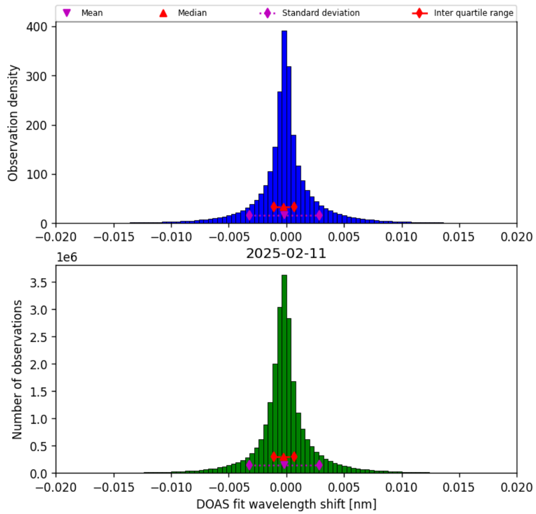
Figure 44: Histogram of “DOAS fit wavelength shift” for 2025-02-10 to 2025-02-12
