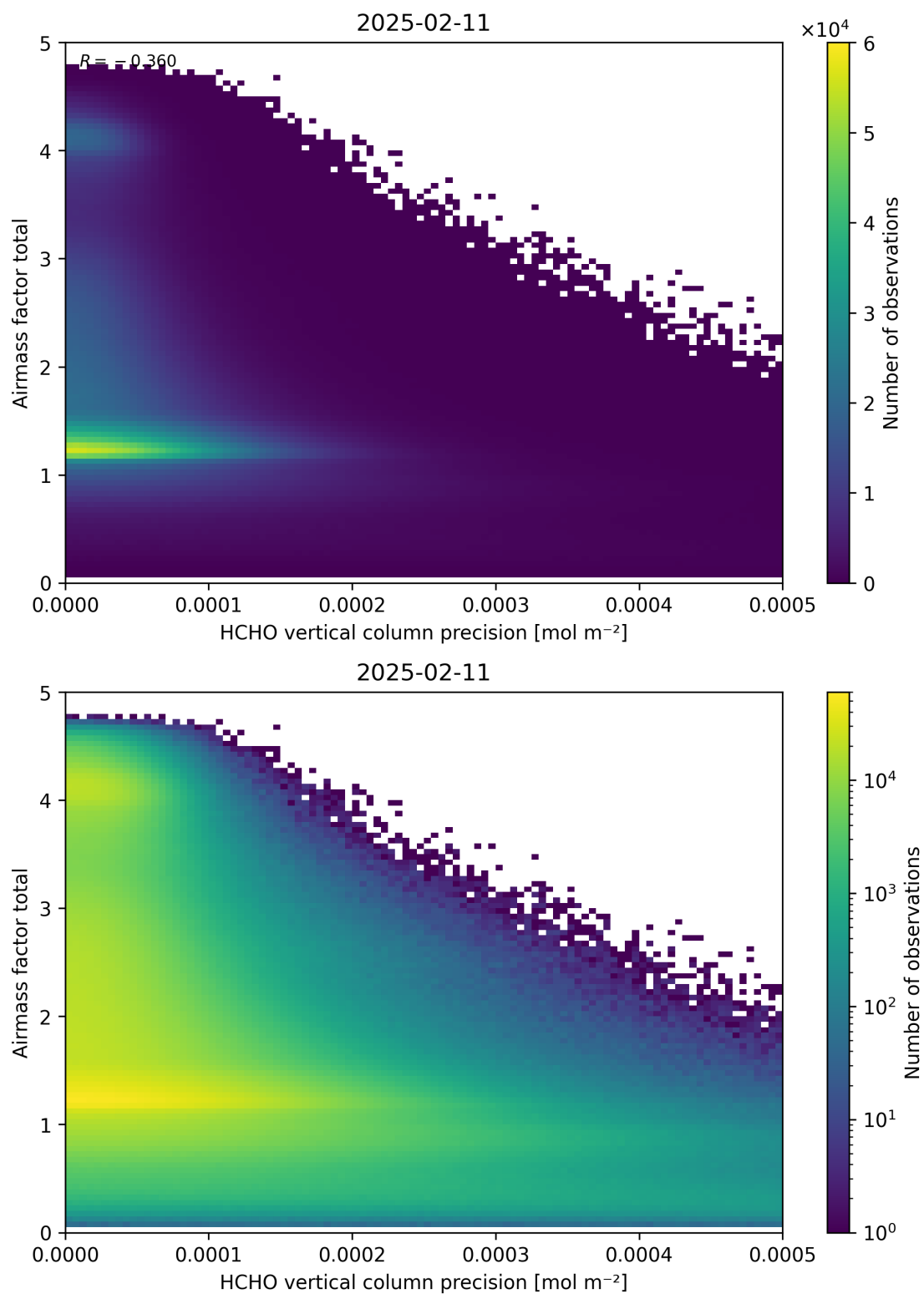
Figure 144: Scatter density plot of “HCHO vertical column precision” against “Airmass factor total” for 2025-02-10 to 2025-02-12.
