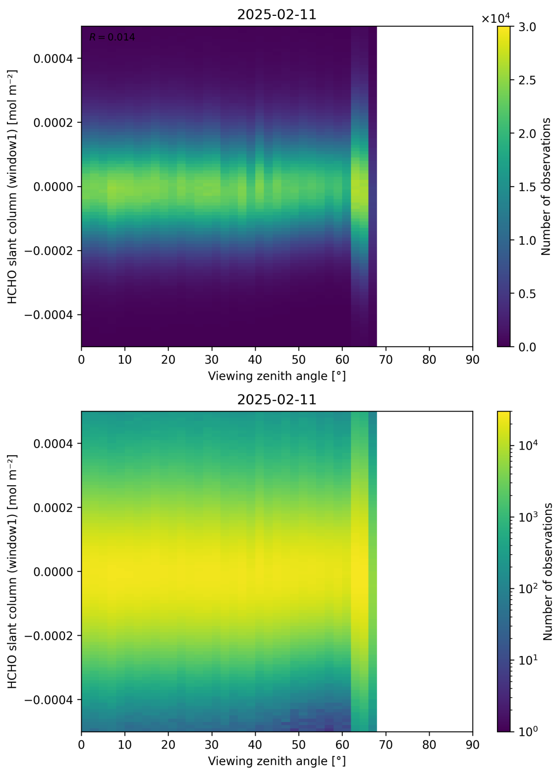
Figure 188: Scatter density plot of “Viewing zenith angle” against “HCHO slant column (window1)” for 2025-02-10 to 2025-02-12.
