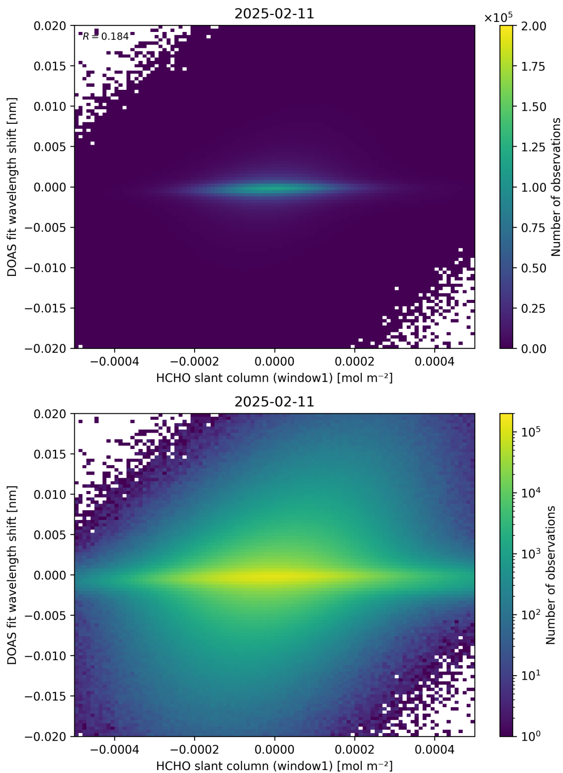
Figure 79: Scatter density plot of “HCHO slant column (window1)” against “DOAS fit wavelength shift” for 2025-02-10 to 2025-02-12.
