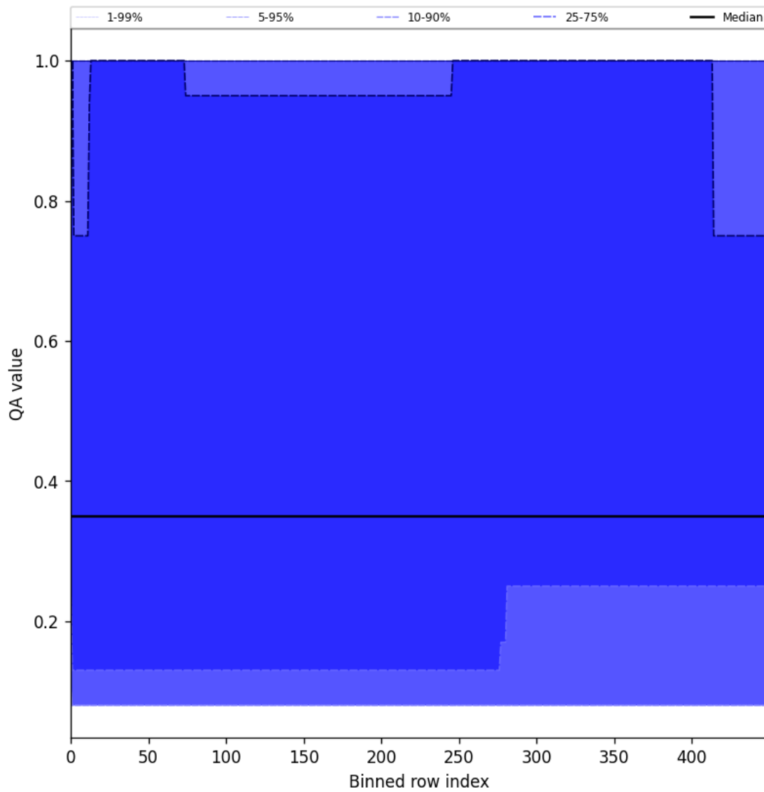
Figure 48: Along track statistics of “QA value” for 2025-02-10 to 2025-02-12
