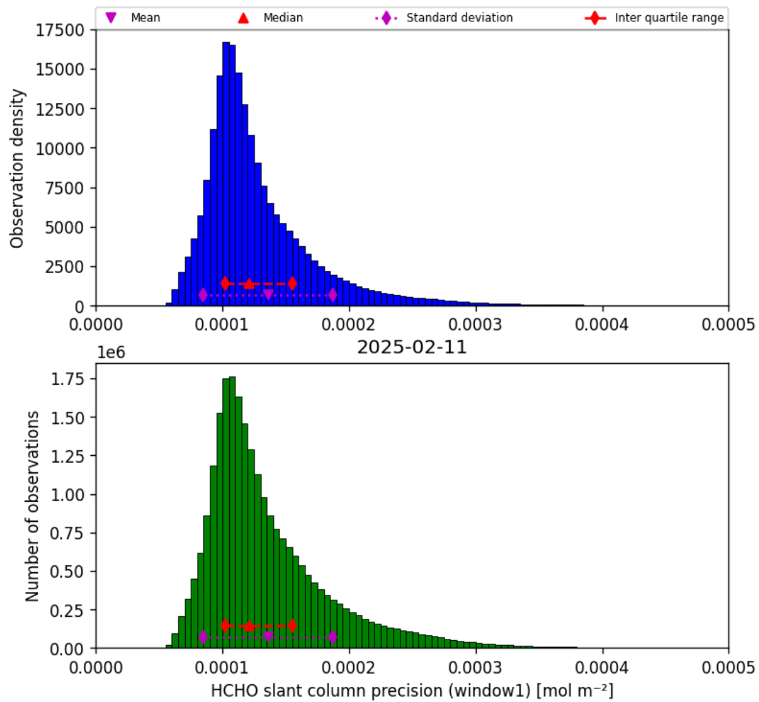
Figure 39: Histogram of “HCHO slant column precision (window1)” for 2025-02-10 to 2025-02-12
