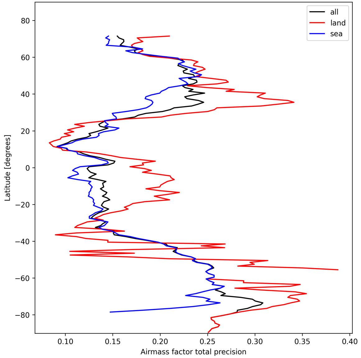
Figure 27: Zonal average of “Airmass factor total precision” for 2025-02-10 to 2025-02-12.
