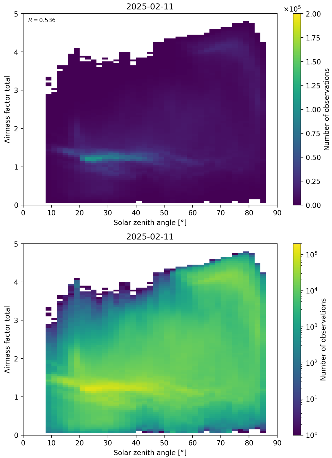
Figure 175: Scatter density plot of “Solar zenith angle” against “Airmass factor total” for 2025-02-10 to 2025-02-12.
