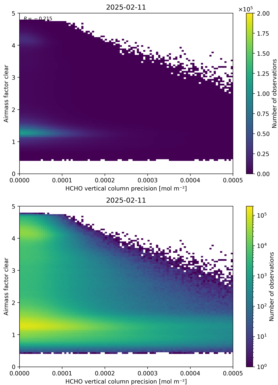
Figure 139: Scatter density plot of “HCHO vertical column precision” against “Airmass factor clear” for 2025-02-10 to 2025-02-12.
