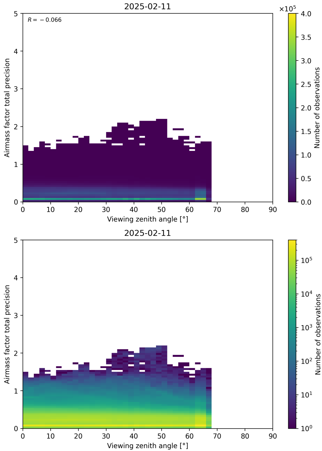
Figure 191: Scatter density plot of “Viewing zenith angle” against “Airmass factor total precision” for 2025-02-10 to 2025-02-12.
