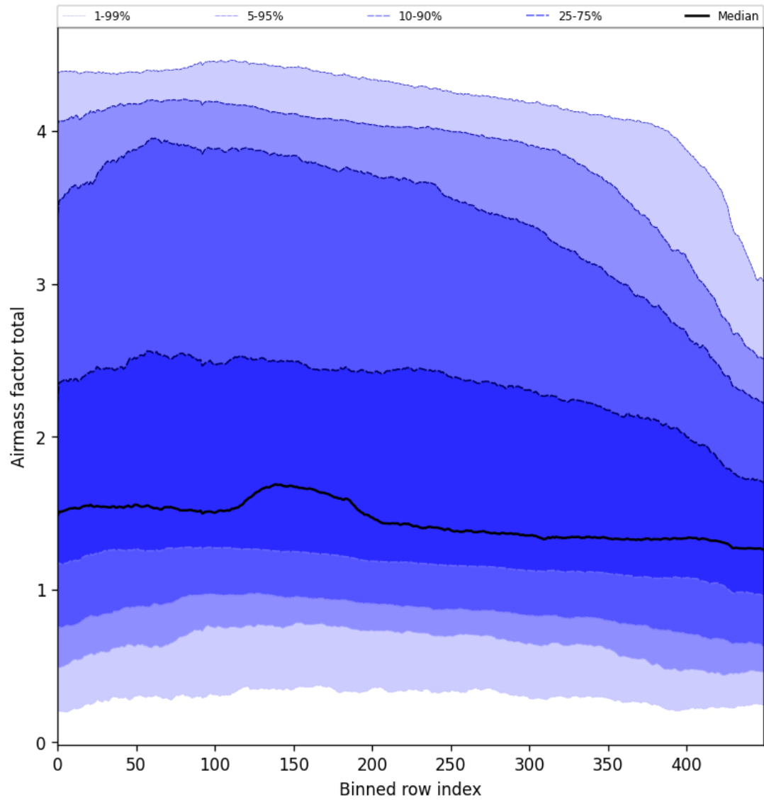
Figure 54: Along track statistics of “Airmass factor total” for 2025-02-10 to 2025-02-12
