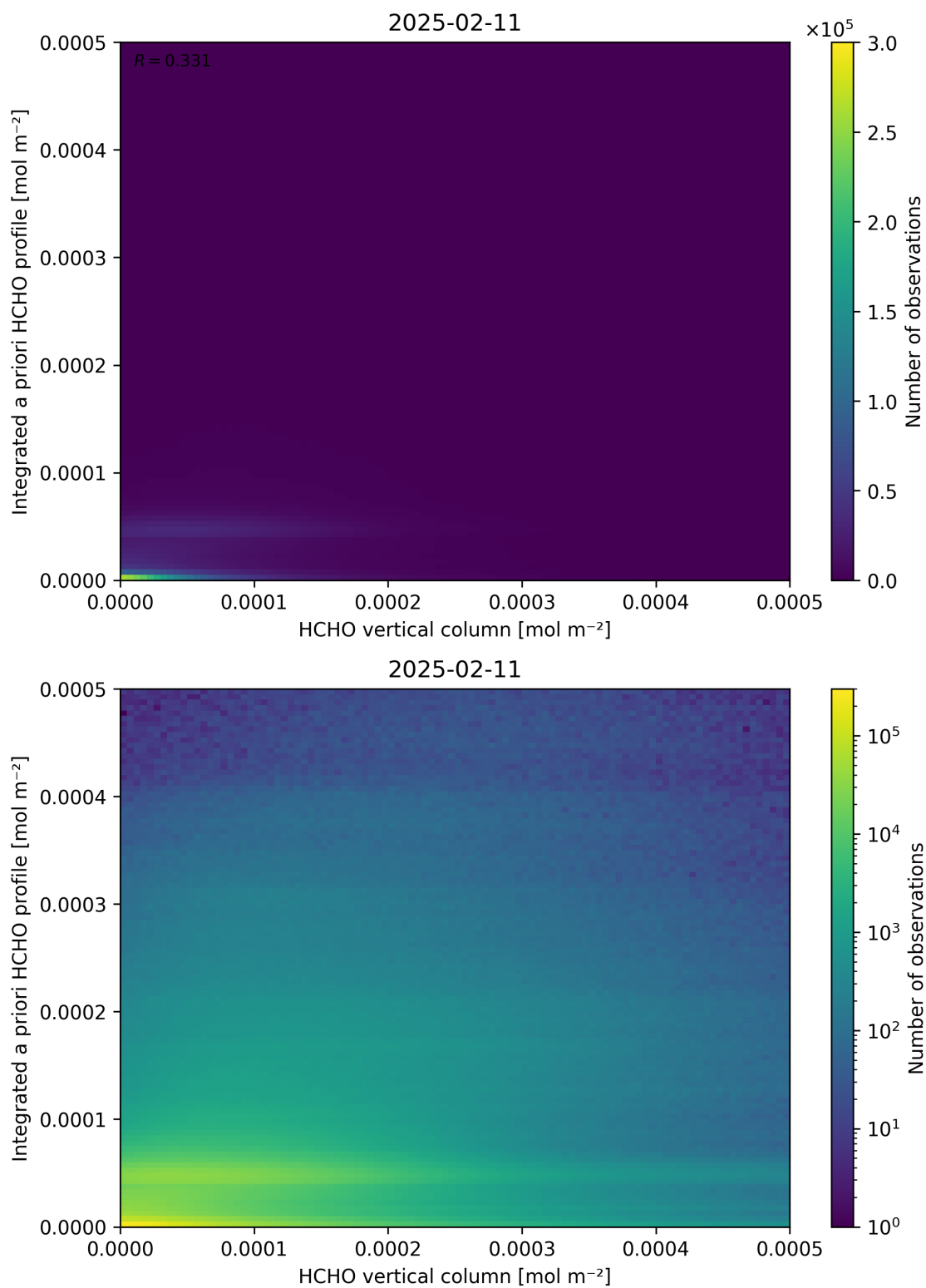
Figure 135: Scatter density plot of “HCHO vertical column” against “Integrated a priori HCHO profile” for 2025-02-10 to 2025-02-12.
