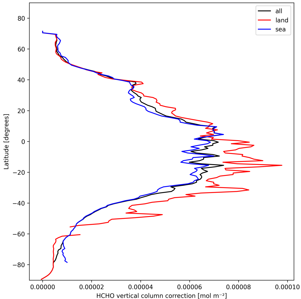
Figure 23: Zonal average of “HCHO vertical column correction” for 2025-02-10 to 2025-02-12.
