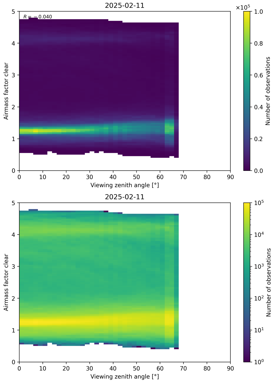
Figure 185: Scatter density plot of “Viewing zenith angle” against “Airmass factor clear” for 2025-02-10 to 2025-02-12.
