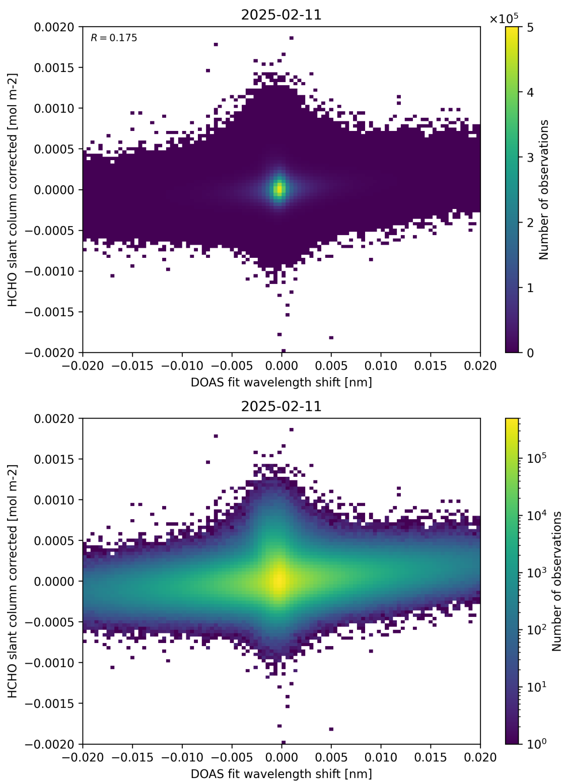
Figure 66: Scatter density plot of “DOAS fit wavelength shift” against “HCHO slant column corrected” for 2025-02-10 to 2025-02-12.
