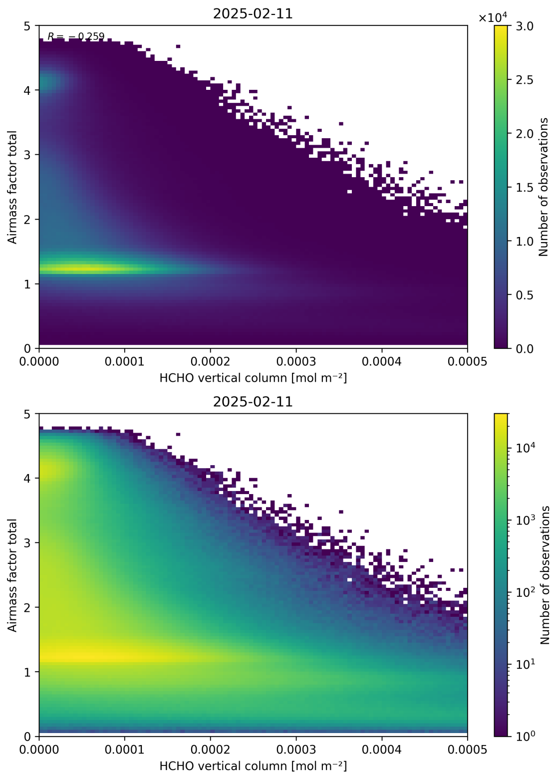
Figure 131: Scatter density plot of “HCHO vertical column” against “Airmass factor total” for 2025-02-10 to 2025-02-12.
