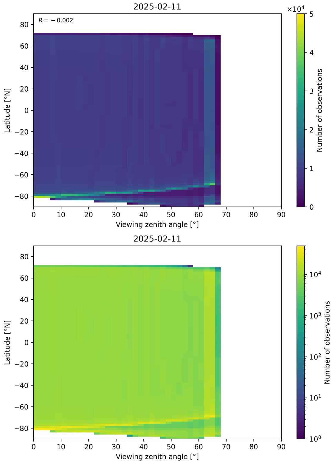
Figure 196: Scatter density plot of “Viewing zenith angle” against “Latitude” for 2025-02-10 to 2025-02-12.
