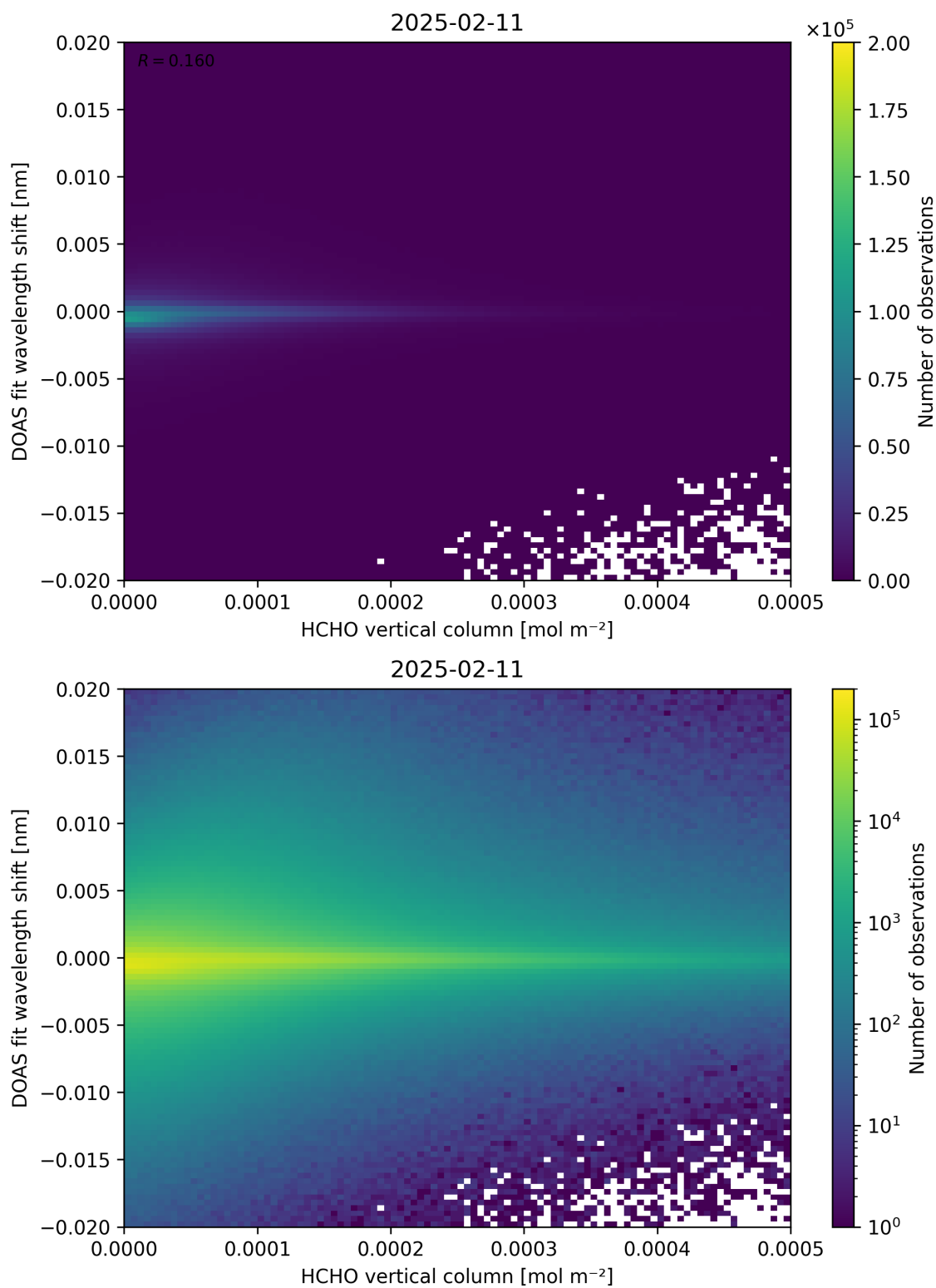
Figure 124: Scatter density plot of “HCHO vertical column” against “DOAS fit wavelength shift” for 2025-02-10 to 2025-02-12.
