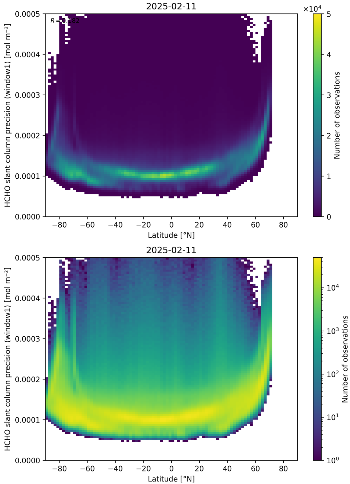
Figure 160: Scatter density plot of “Latitude” against “HCHO slant column precision (window1)” for 2025-02-10 to 2025-02-12.
