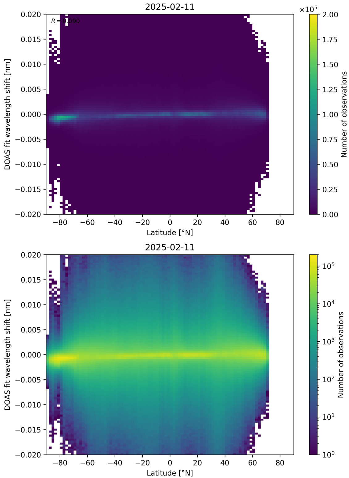
Figure 154: Scatter density plot of “Latitude” against “DOAS fit wavelength shift” for 2025-02-10 to 2025-02-12.
