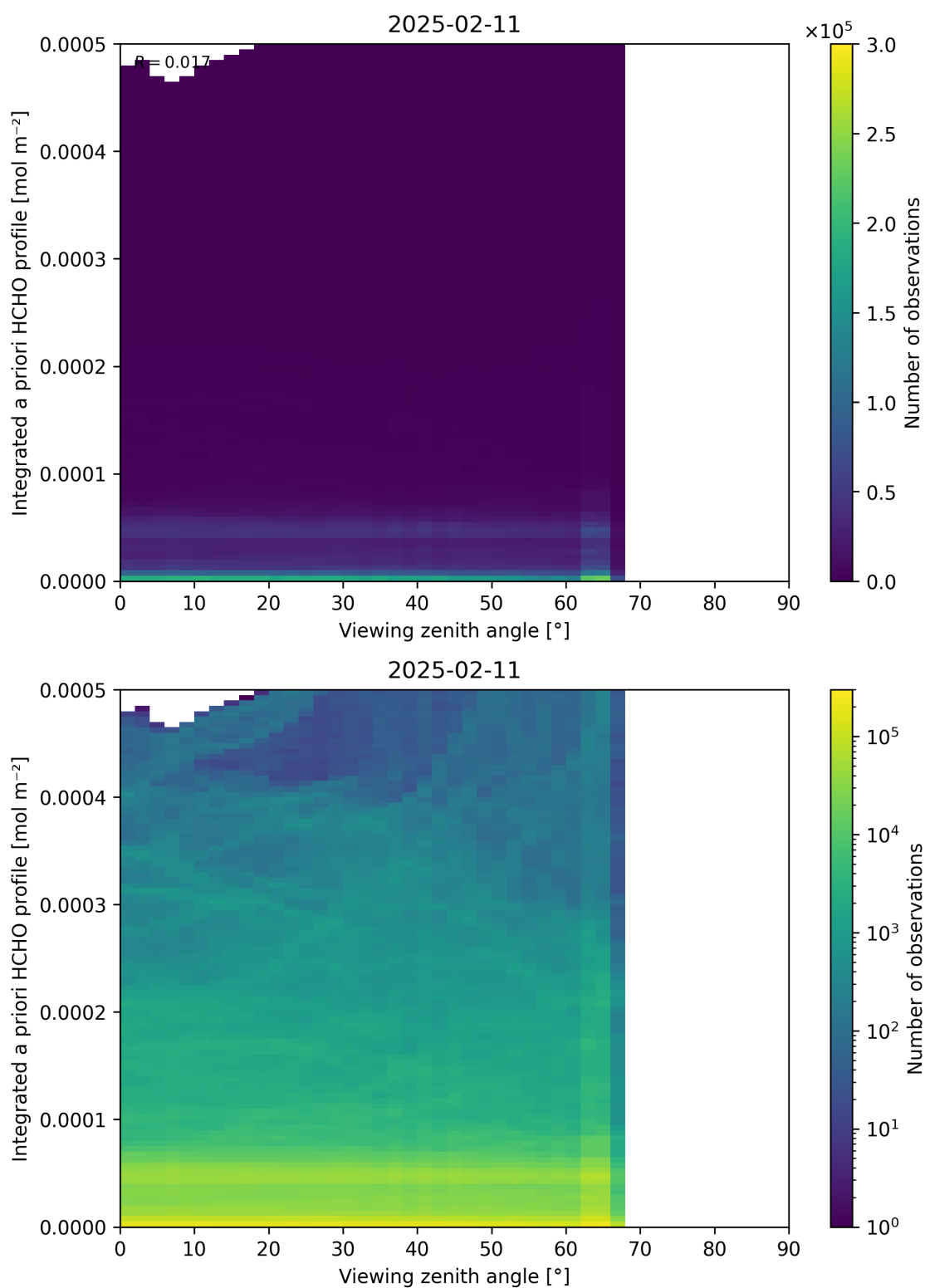
Figure 195: Scatter density plot of “Viewing zenith angle” against “Integrated a priori HCHO profile” for 2025-02-10 to 2025-02-12.
