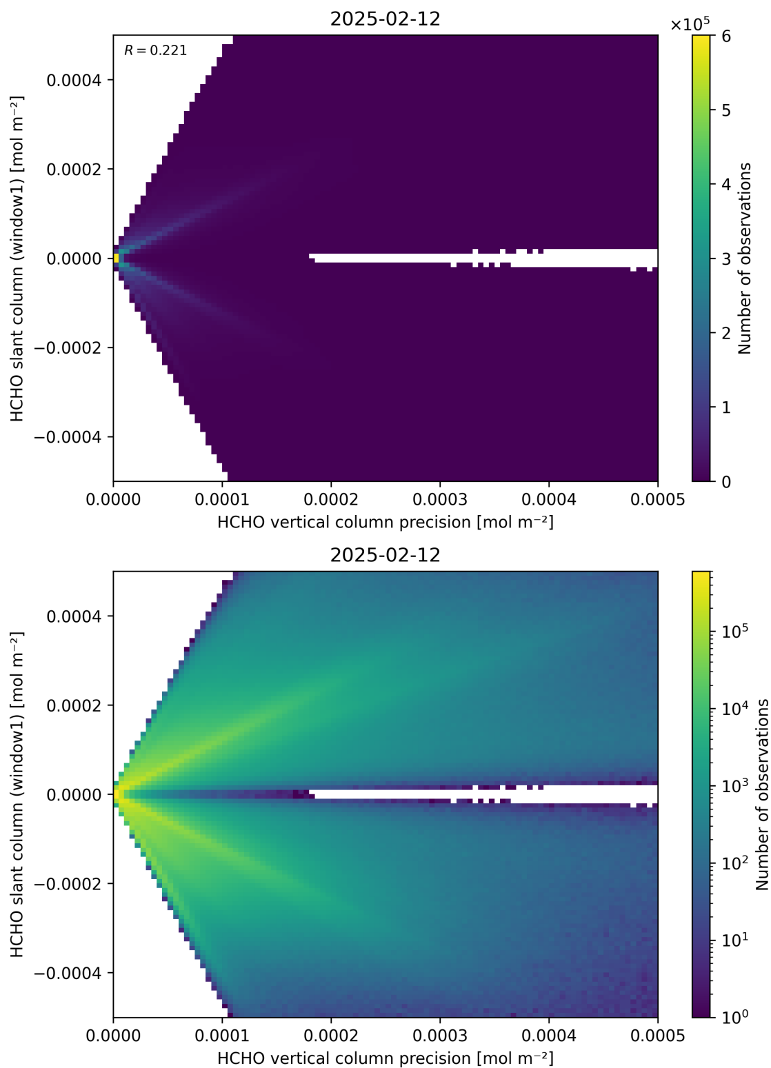
Figure 142: Scatter density plot of “HCHO vertical column precision” against “HCHO slant column (window1)” for 2025-02-11 to 2025-02-13.
