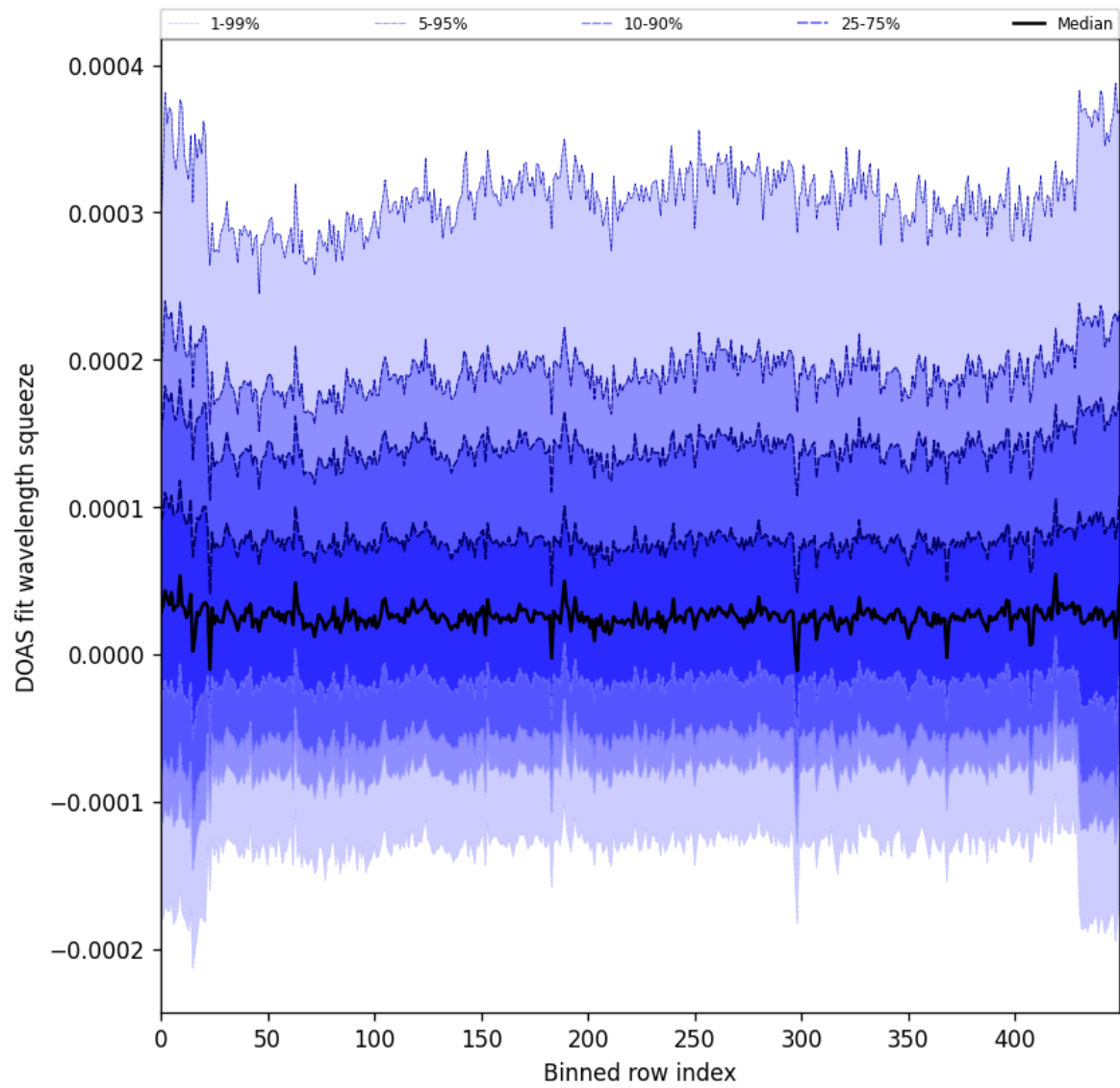
Figure 59: Along track statistics of “DOAS fit wavelength squeeze” for 2025-02-11 to 2025-02-13
