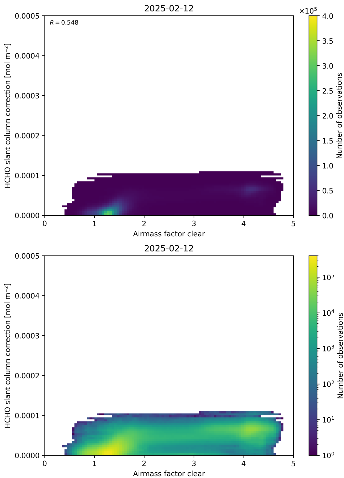
Figure 75: Scatter density plot of “Airmass factor clear” against “HCHO slant column correction” for 2025-02-11 to 2025-02-13.
