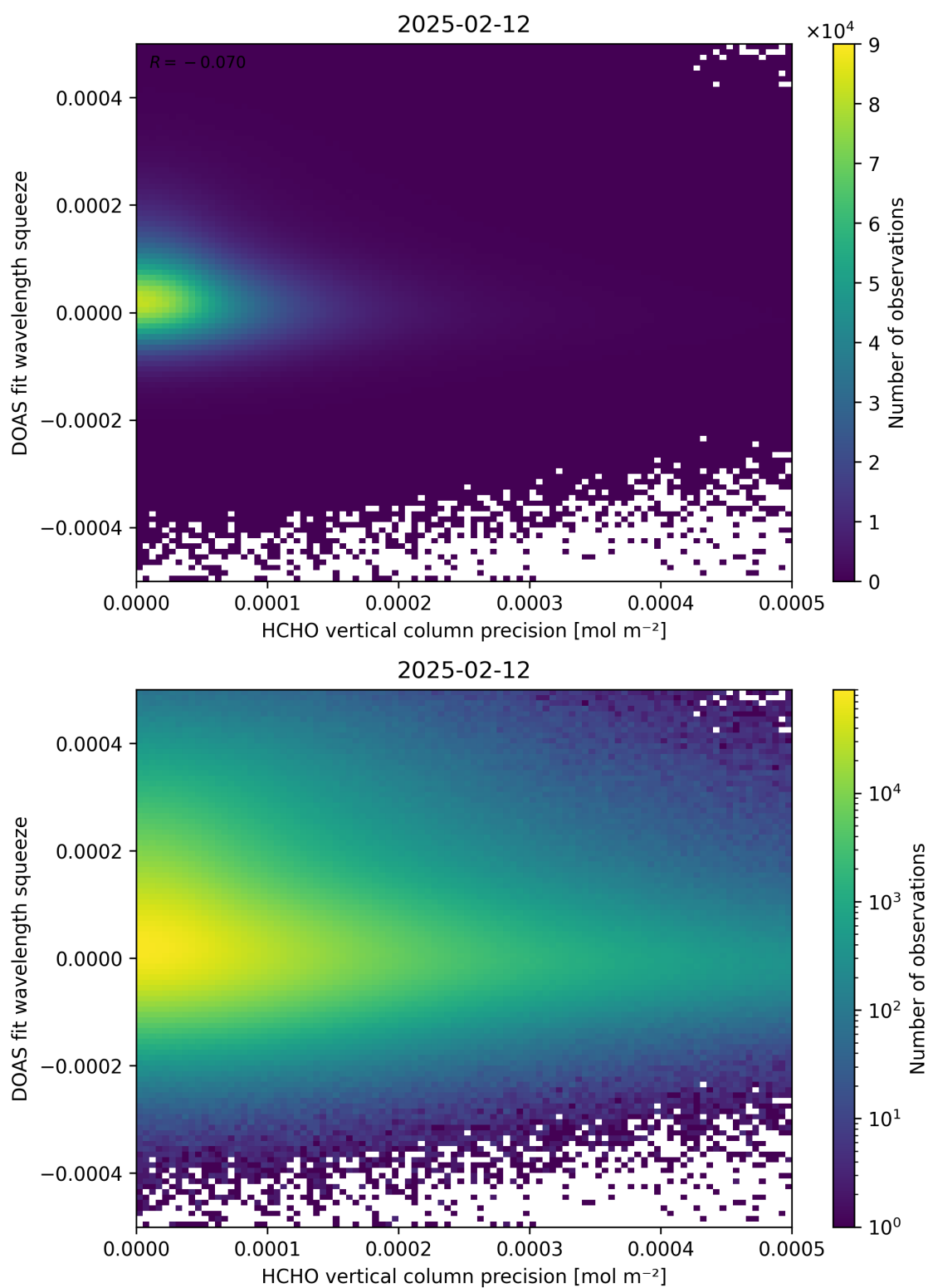
Figure 138: Scatter density plot of “HCHO vertical column precision” against “DOAS fit wavelength squeeze” for 2025-02-11 to 2025-02-13.
