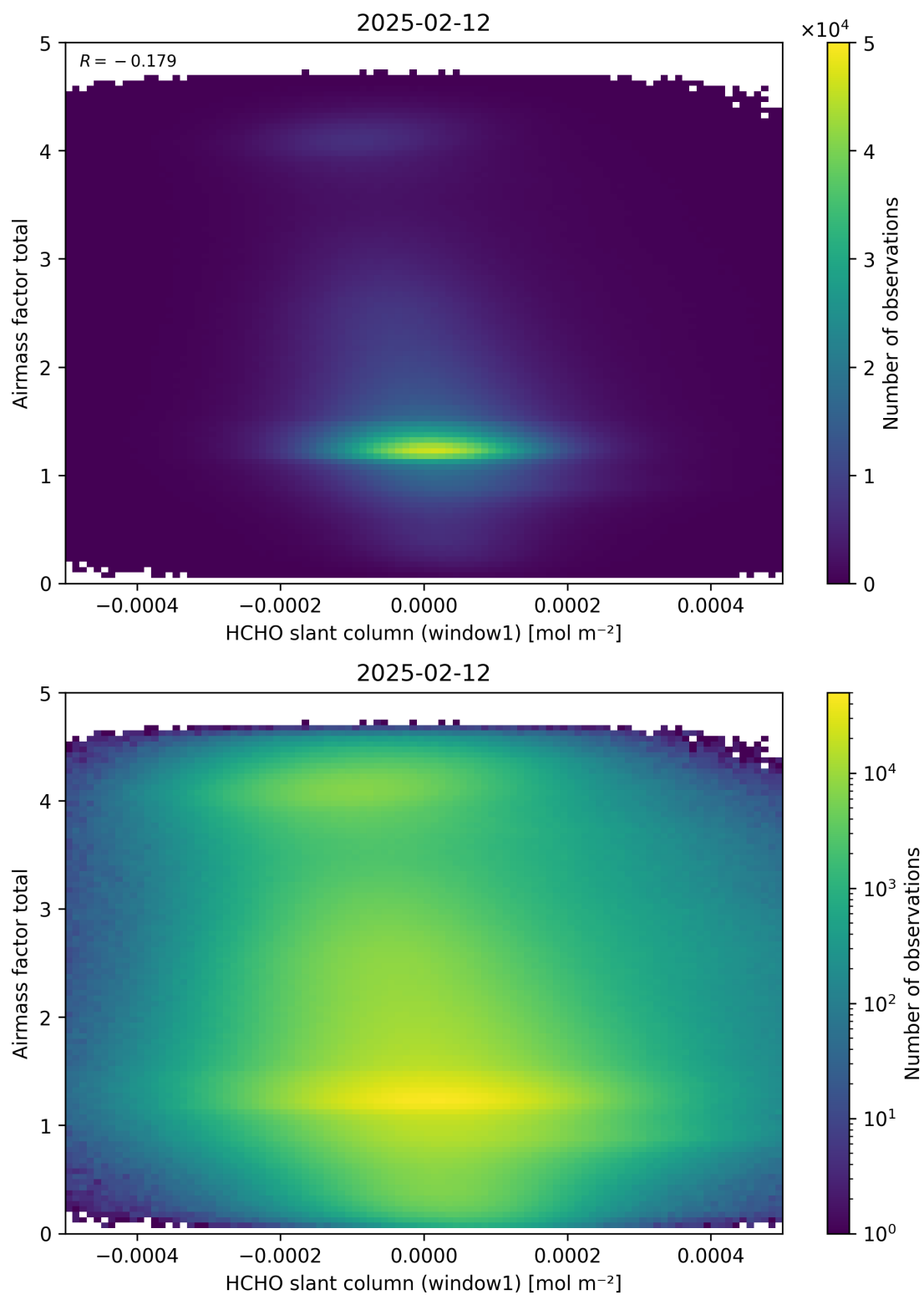
Figure 85: Scatter density plot of “HCHO slant column (window1)” against “Airmass factor total” for 2025-02-11 to 2025-02-13.
