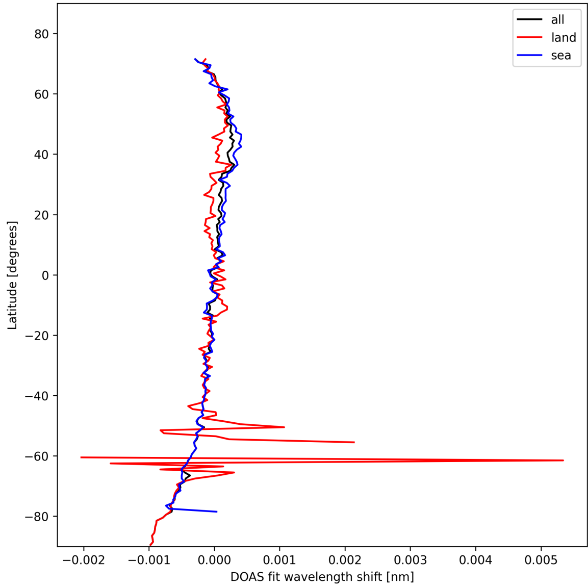
Figure 30: Zonal average of "DOAS fit wavelength shift" for 2025-02-11 to 2025-02-13.
