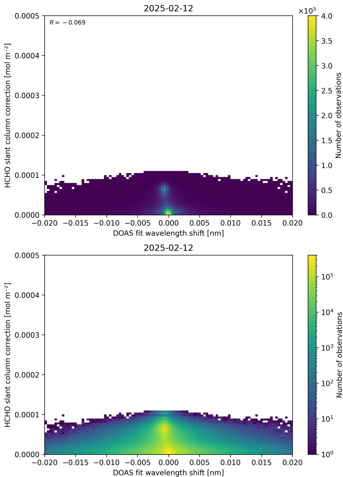
Figure 67: Scatter density plot of “DOAS fit wavelength shift” against “HCHO slant column correction” for 2025-02-11 to 2025-02-13.
