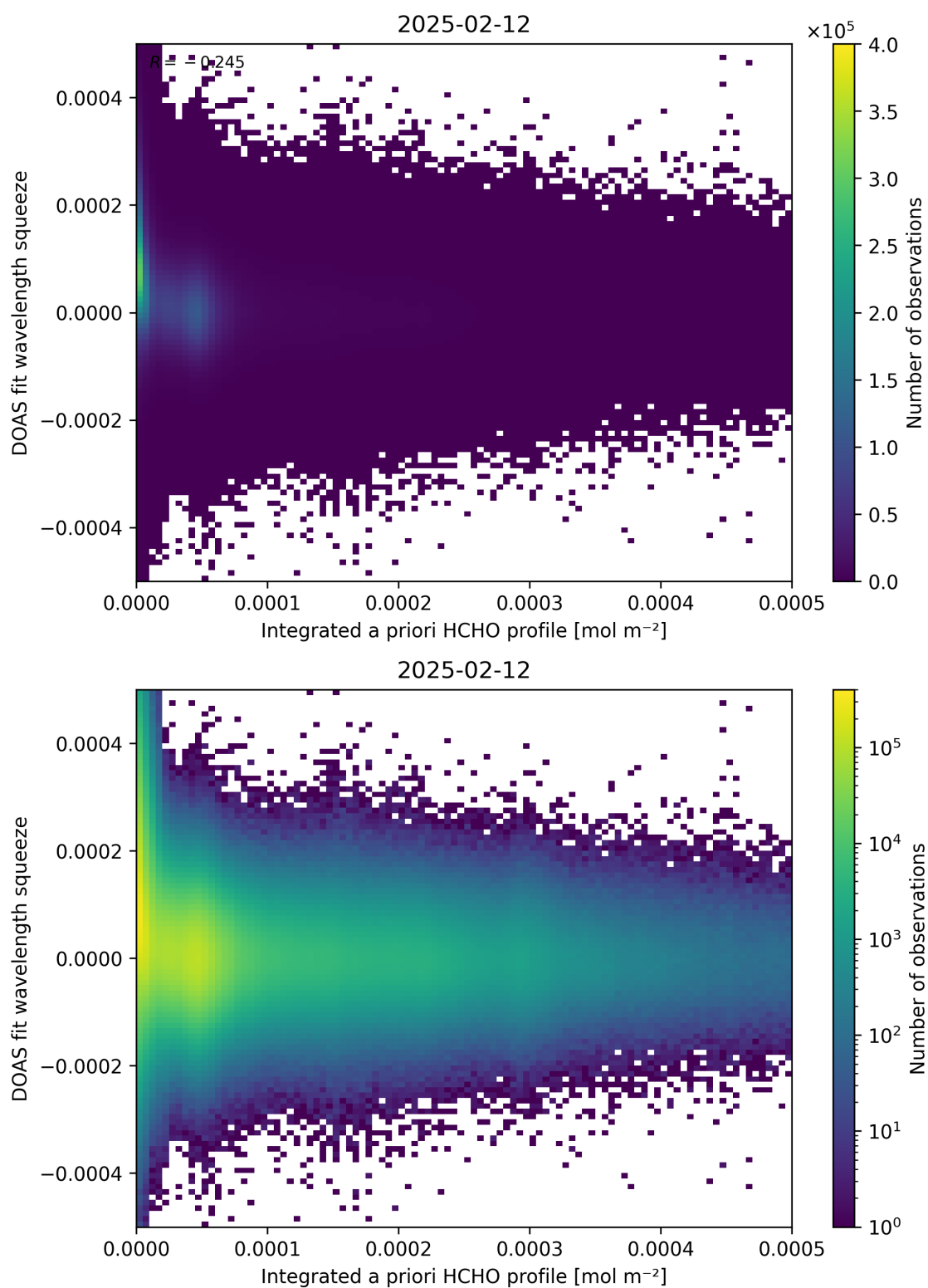
Figure 150: Scatter density plot of “Integrated a priori HCHO profile” against “DOAS fit wavelength squeeze” for 2025-02-11 to 2025-02-13.
