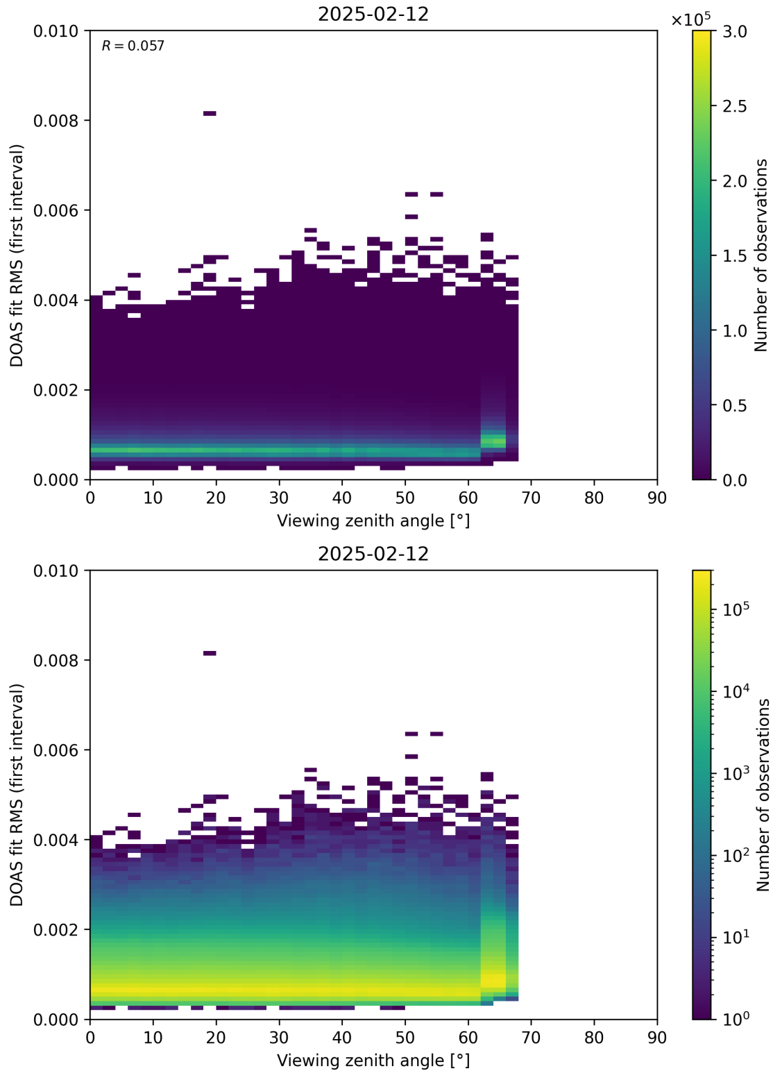
Figure 182: Scatter density plot of “Viewing zenith angle” against “DOAS fit RMS (first interval)” for 2025-02-11 to 2025-02-13.
