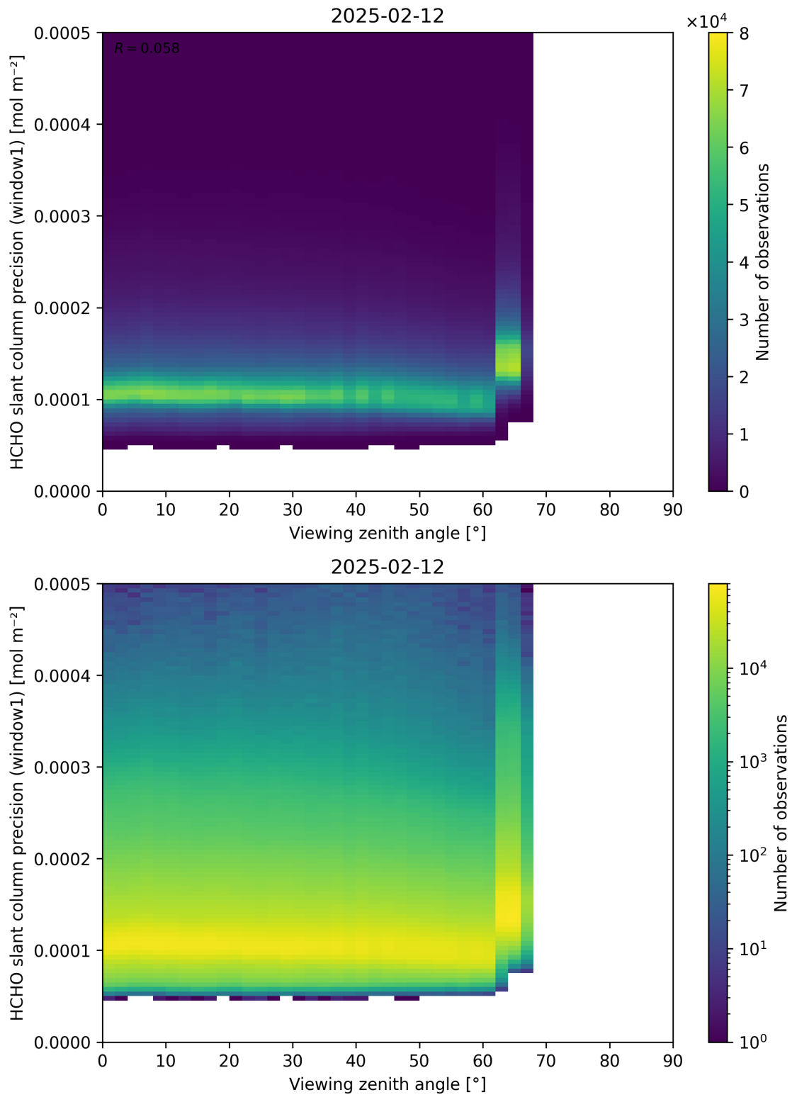
Figure 189: Scatter density plot of “Viewing zenith angle” against “HCHO slant column precision (window1)” for 2025-02-11 to 2025-02-13.
