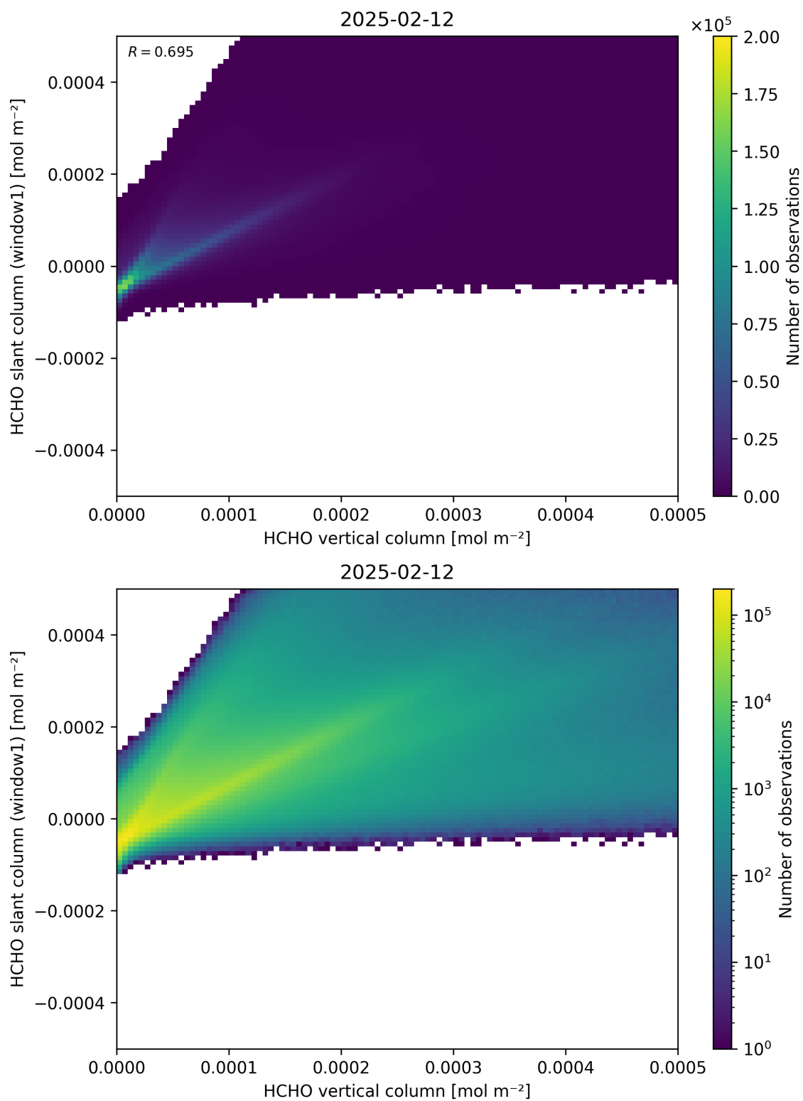
Figure 129: Scatter density plot of “HCHO vertical column” against “HCHO slant column (window1)” for 2025-02-11 to 2025-02-13.
