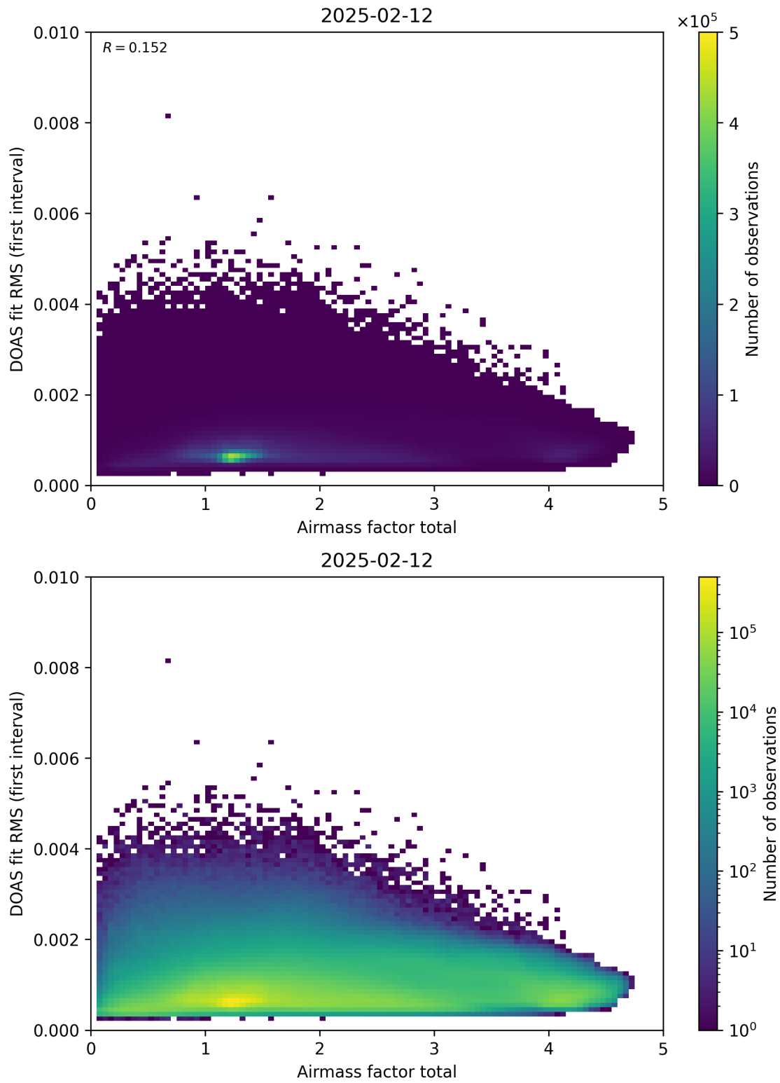
Figure 97: Scatter density plot of “Airmass factor total” against “DOAS fit RMS (first interval)” for 2025-02-11 to 2025-02-13.
