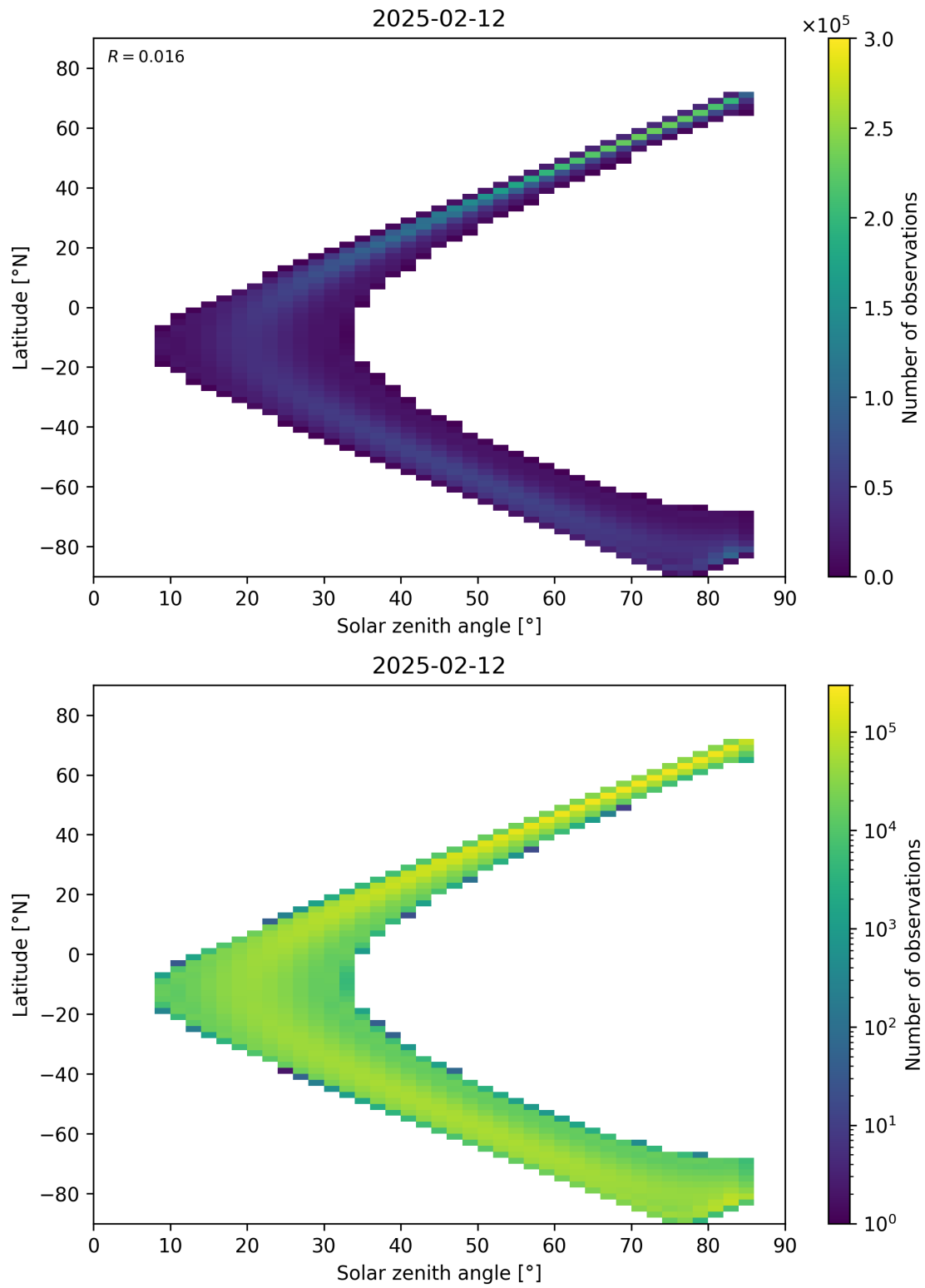
Figure 181: Scatter density plot of “Solar zenith angle” against “Latitude” for 2025-02-11 to 2025-02-13.
