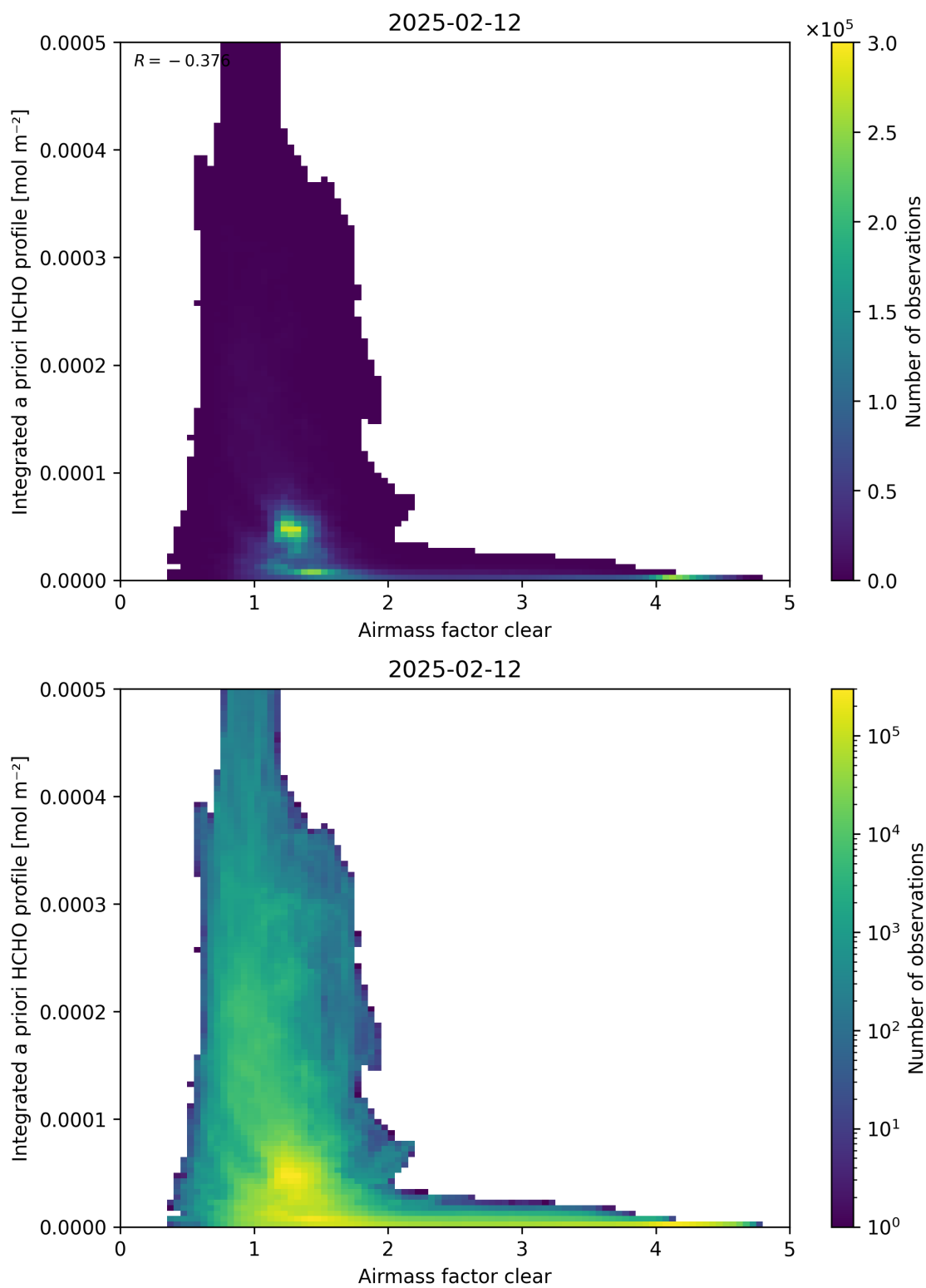
Figure 76: Scatter density plot of “Airmass factor clear” against “Integrated a priori HCHO profile” for 2025-02-11 to 2025-02-13.
