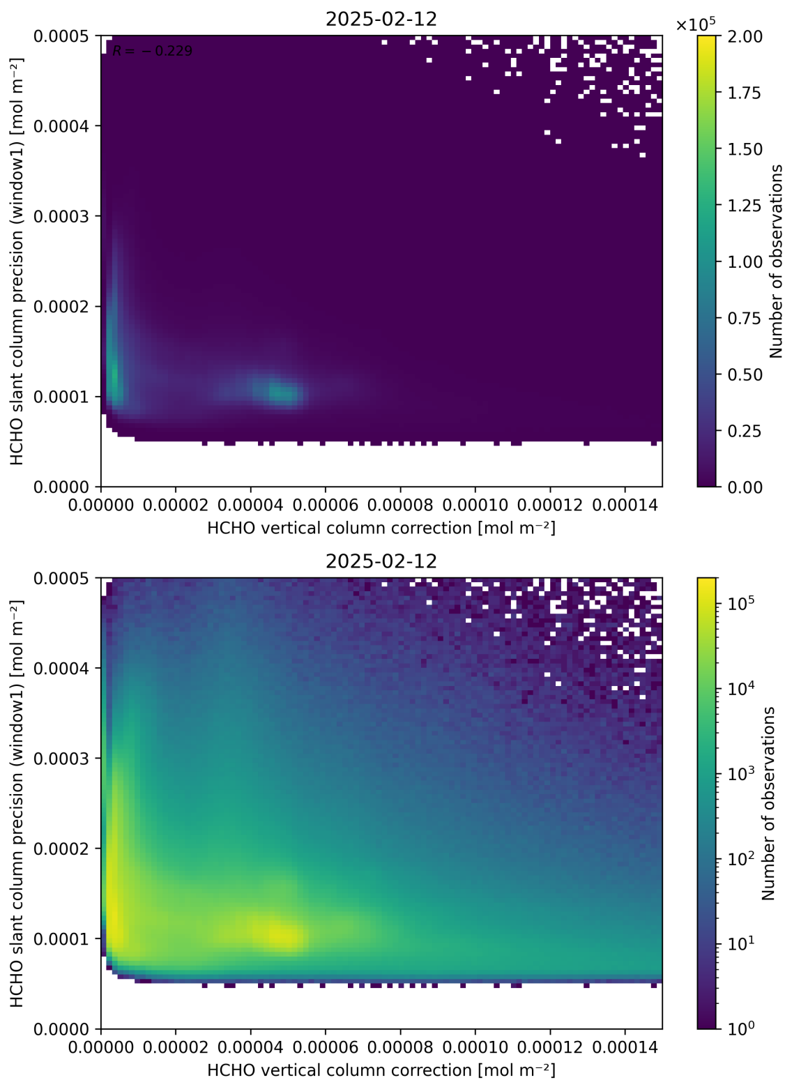
Figure 119: Scatter density plot of “HCHO vertical column correction” against “HCHO slant column precision (window1)” for 2025-02-11 to 2025-02-13.
