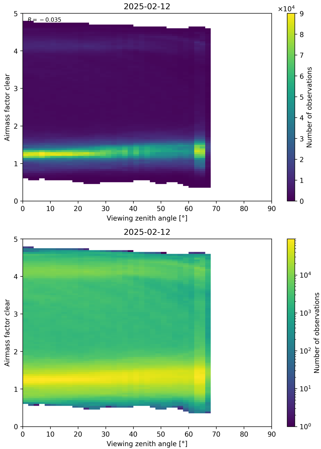
Figure 185: Scatter density plot of “Viewing zenith angle” against “Airmass factor clear” for 2025-02-11 to 2025-02-13.
