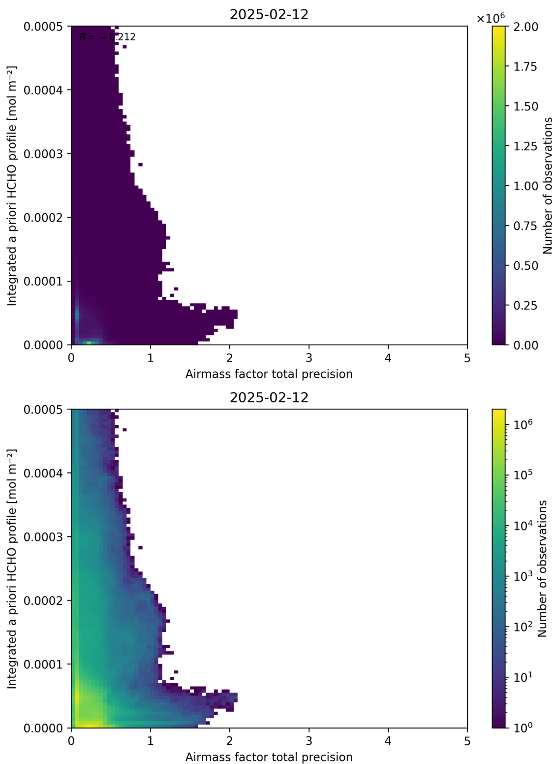
Figure 111: Scatter density plot of “Airmass factor total precision” against “Integrated a priori HCHO profile” for 2025-02-11 to 2025-02-13.
