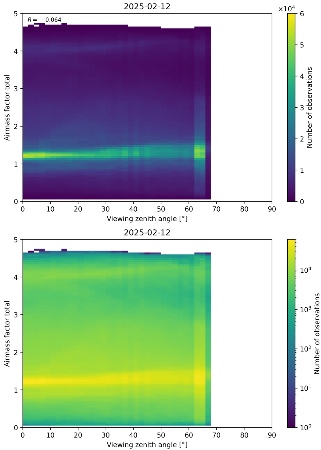
Figure 190: Scatter density plot of “Viewing zenith angle” against “Airmass factor total” for 2025-02-11 to 2025-02-13.
