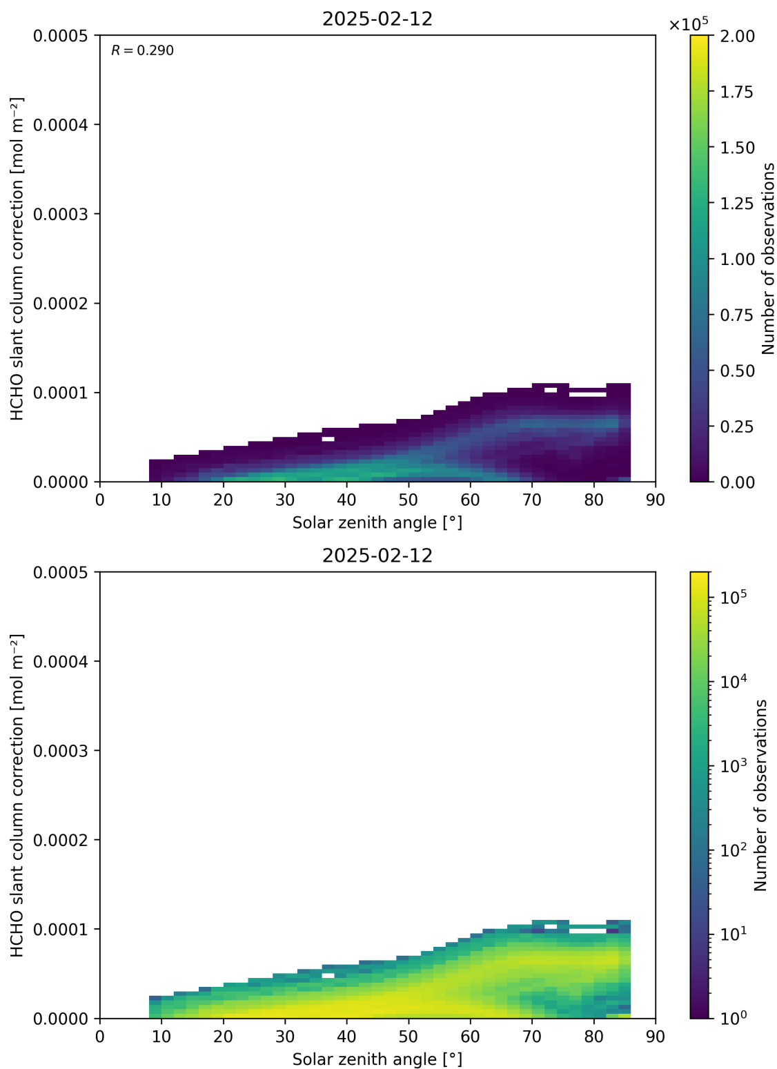
Figure 172: Scatter density plot of “Solar zenith angle” against “HCHO slant column correction” for 2025-02-11 to 2025-02-13.
