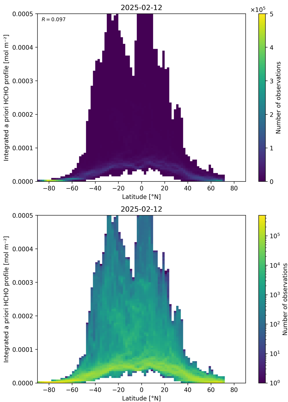
Figure 166: Scatter density plot of “Latitude” against “Integrated a priori HCHO profile” for 2025-02-11 to 2025-02-13.
