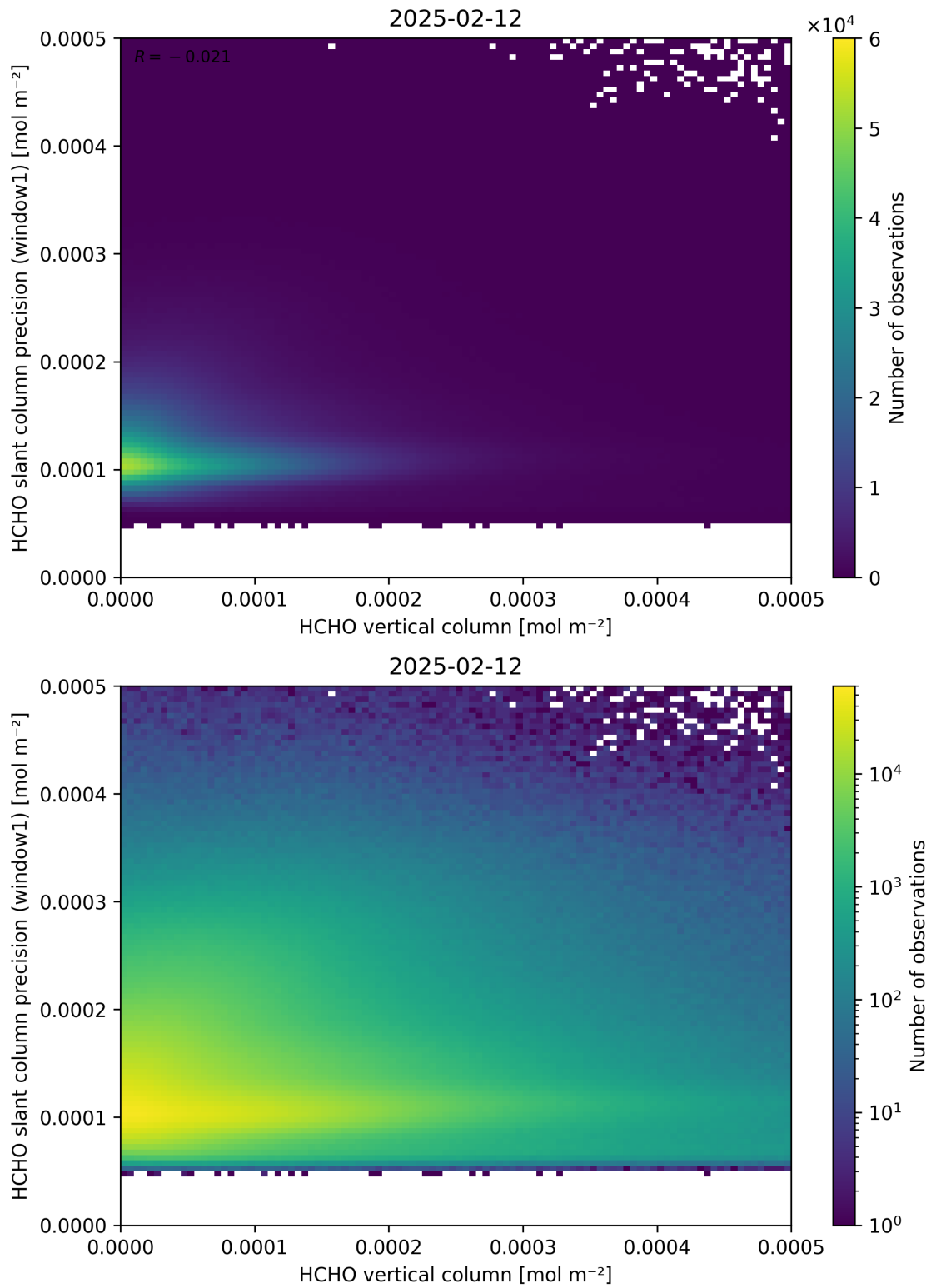
Figure 130: Scatter density plot of “HCHO vertical column” against “HCHO slant column precision (window1)” for 2025-02-11 to 2025-02-13.
