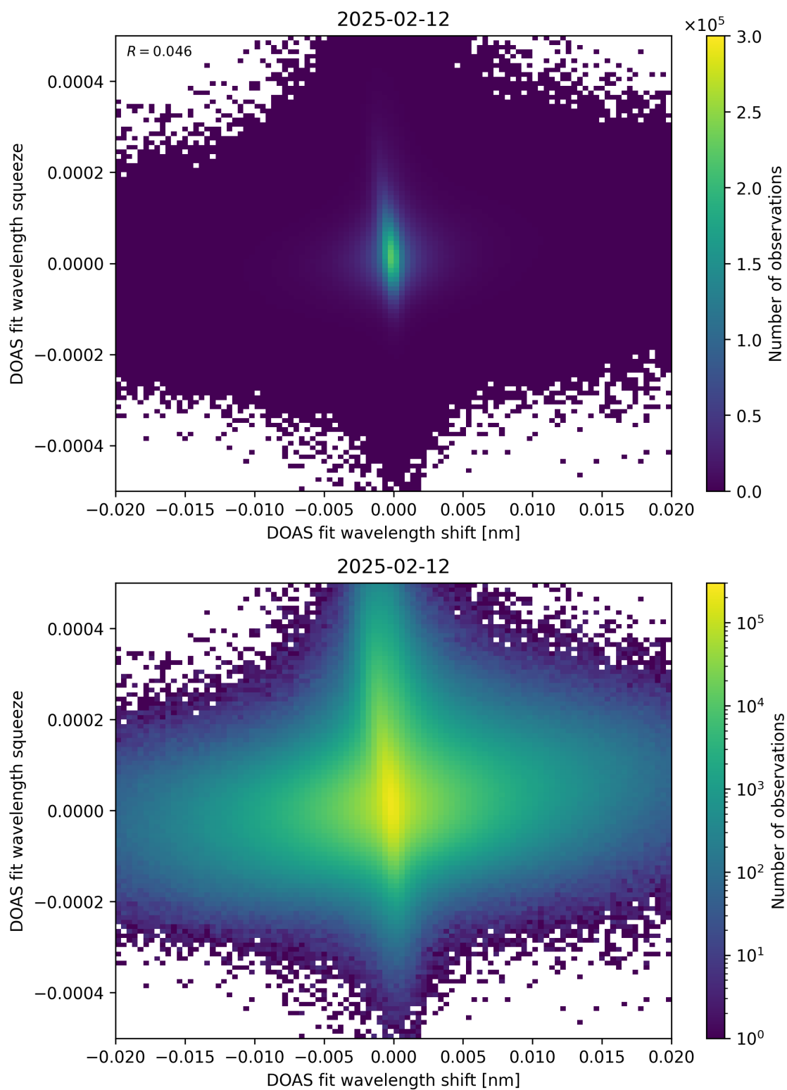
Figure 65: Scatter density plot of “DOAS fit wavelength shift” against “DOAS fit wavelength squeeze” for 2025-02-11 to 2025-02-13.
