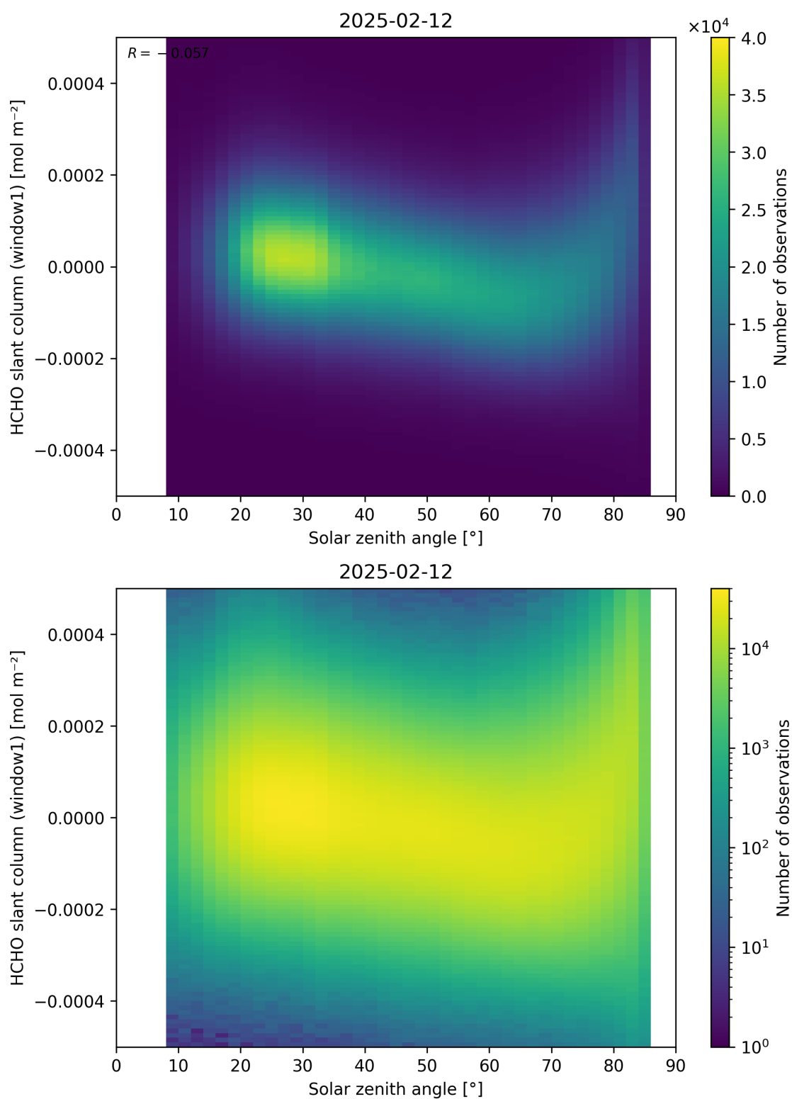
Figure 173: Scatter density plot of “Solar zenith angle” against “HCHO slant column (window1)” for 2025-02-11 to 2025-02-13.
