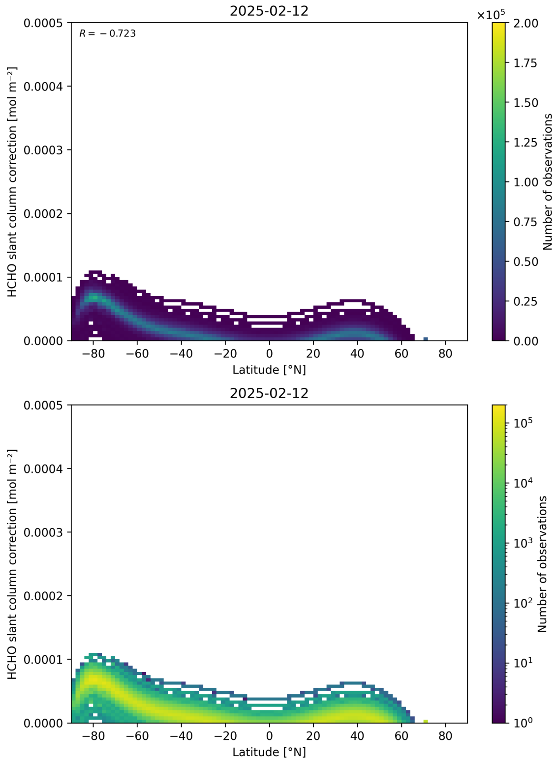
Figure 158: Scatter density plot of “Latitude” against “HCHO slant column correction” for 2025-02-11 to 2025-02-13.
