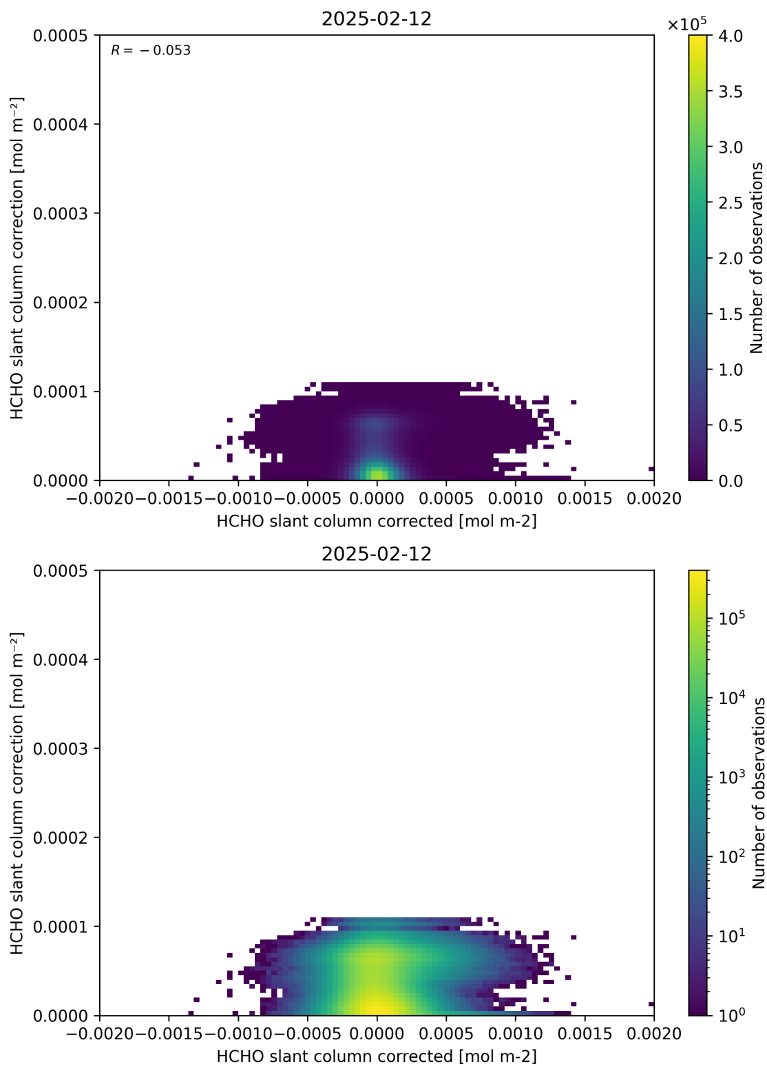
Figure 77: Scatter density plot of “HCHO slant column corrected” against “HCHO slant column correction” for 2025-02-11 to 2025-02-13.
