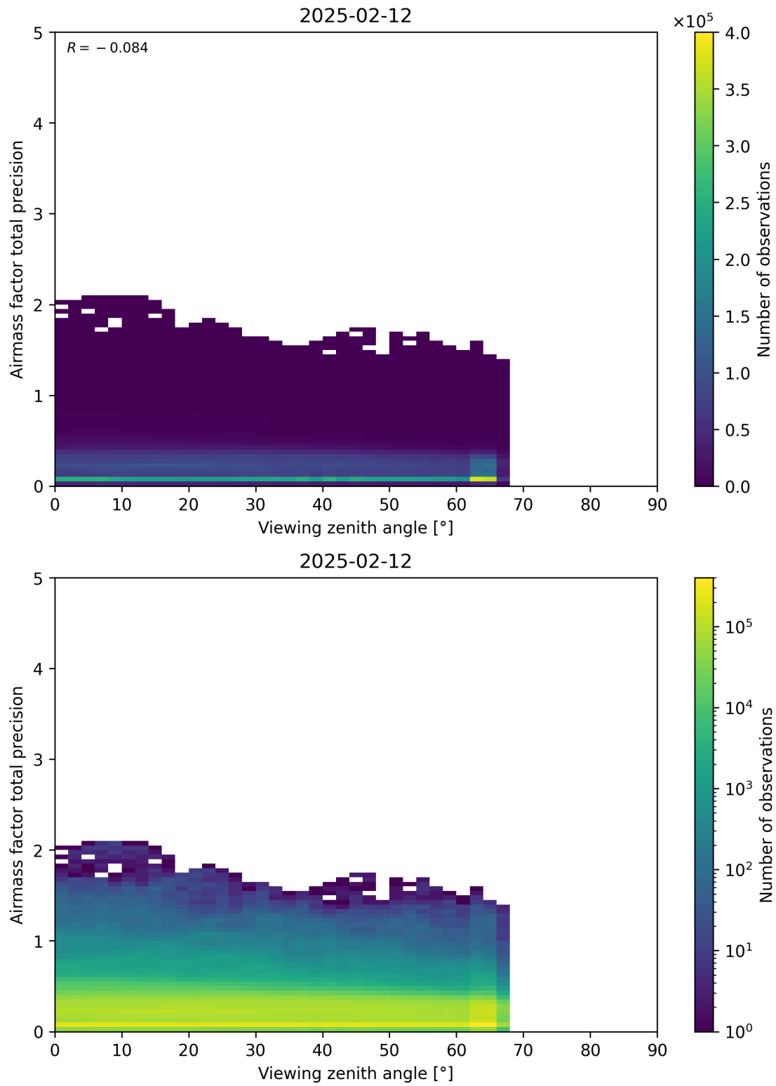
Figure 191: Scatter density plot of “Viewing zenith angle” against “Airmass factor total precision” for 2025-02-11 to 2025-02-13.
