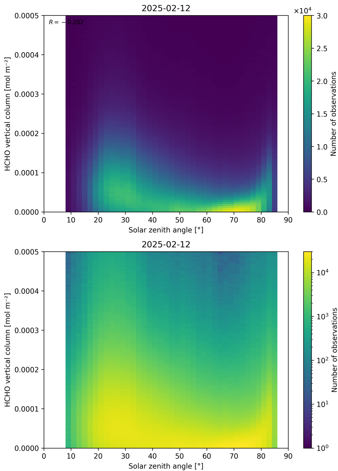
Figure 177: Scatter density plot of “Solar zenith angle” against “HCHO vertical column” for 2025-02-11 to 2025-02-13.
