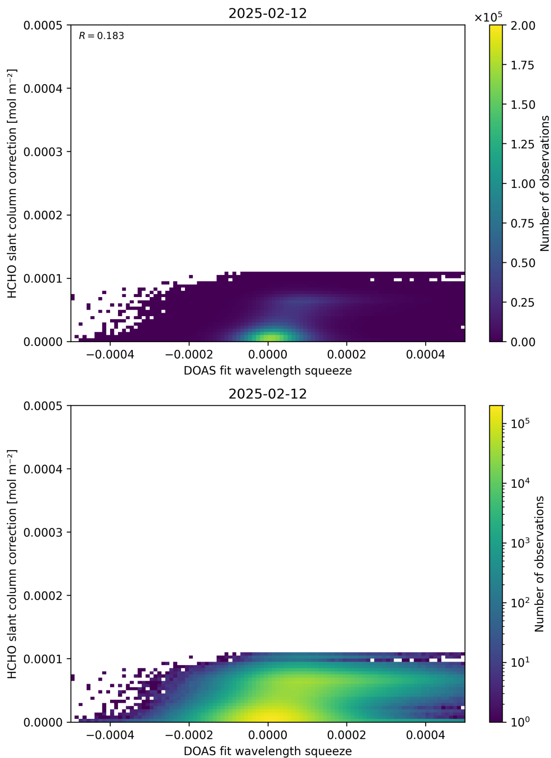
Figure 70: Scatter density plot of “DOAS fit wavelength squeeze” against “HCHO slant column correction” for 2025-02-11 to 2025-02-13.
