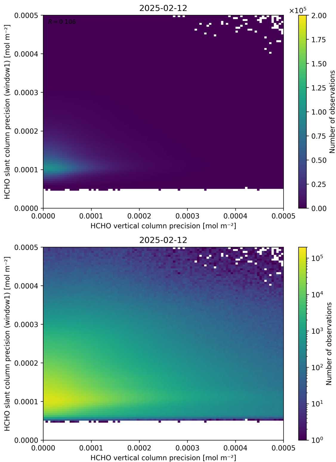
Figure 143: Scatter density plot of “HCHO vertical column precision” against “HCHO slant column precision (window1)” for 2025-02-11 to 2025-02-13.
