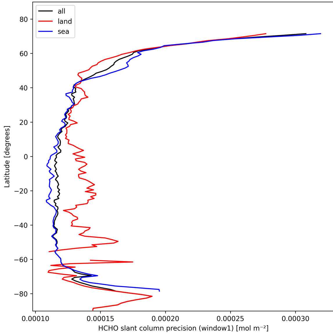
Figure 25: Zonal average of "HCHO slant column precision (window1)" for 2025-02-11 to 2025-02-13.
