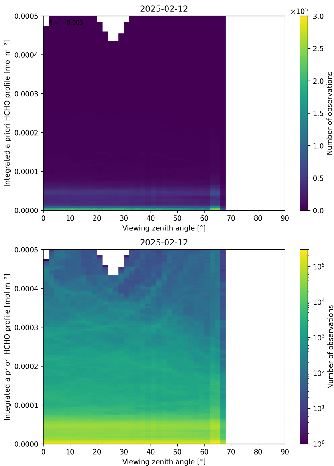
Figure 195: Scatter density plot of “Viewing zenith angle” against “Integrated a priori HCHO profile” for 2025-02-11 to 2025-02-13.
