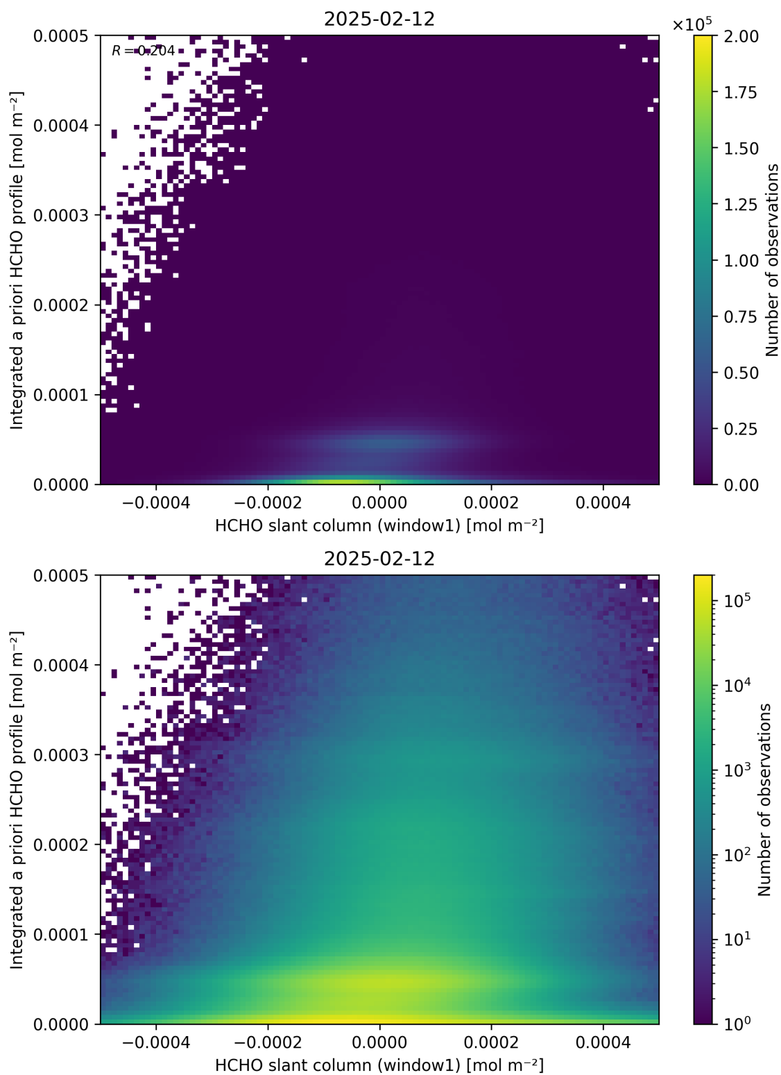
Figure 87: Scatter density plot of “HCHO slant column (window1)” against “Integrated a priori HCHO profile” for 2025-02-11 to 2025-02-13.
