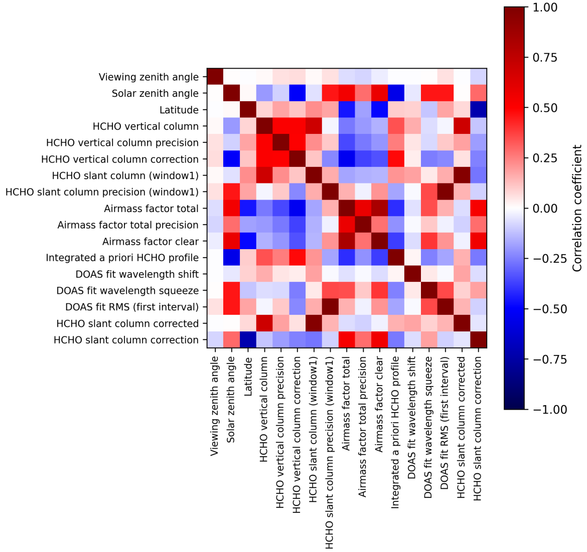
Figure 2: Map of correlation matrix for 2025-02-11 to 2025-02-13.
