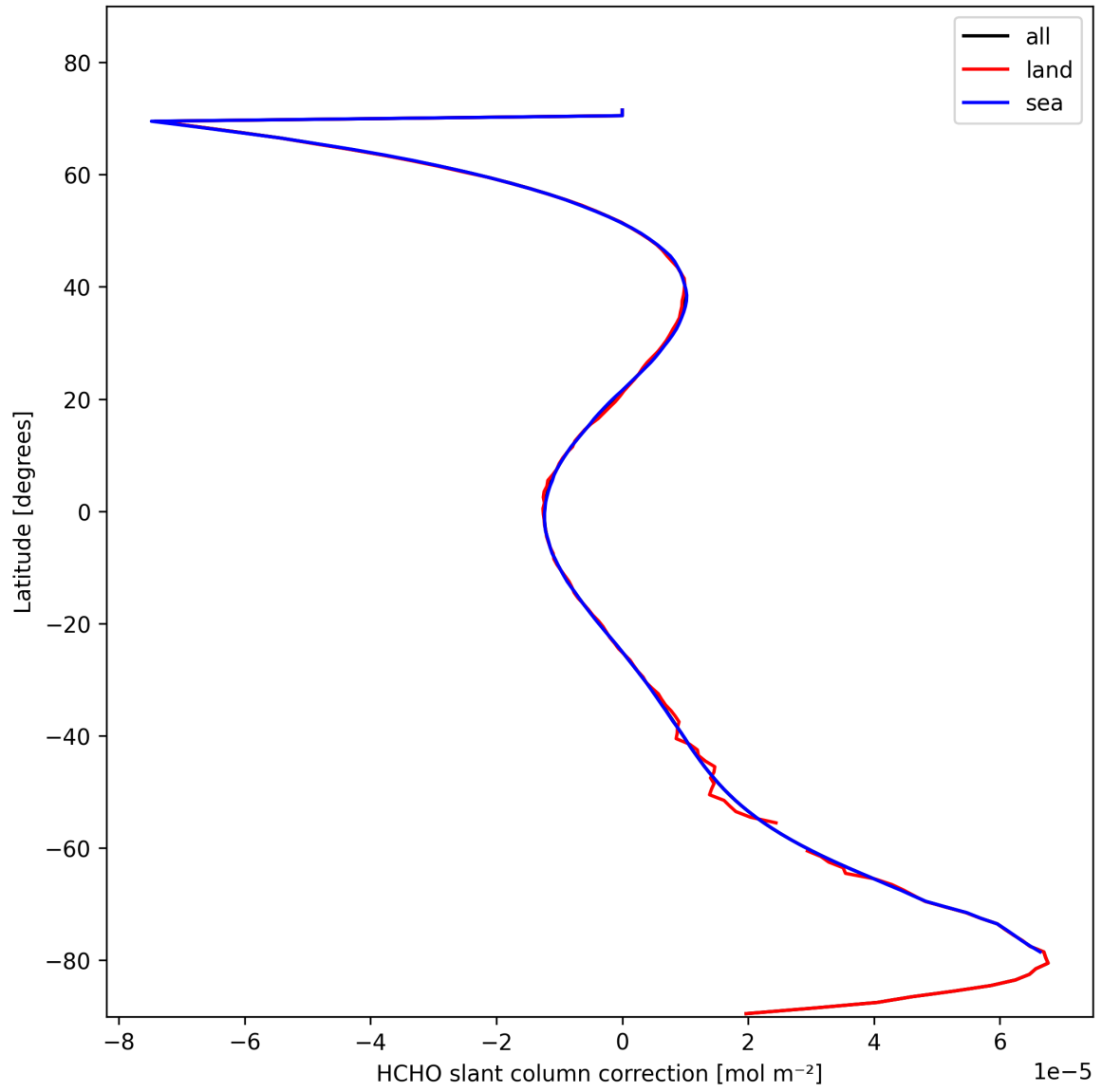
Figure 33: Zonal average of “HCHO slant column correction” for 2025-02-11 to 2025-02-13.
