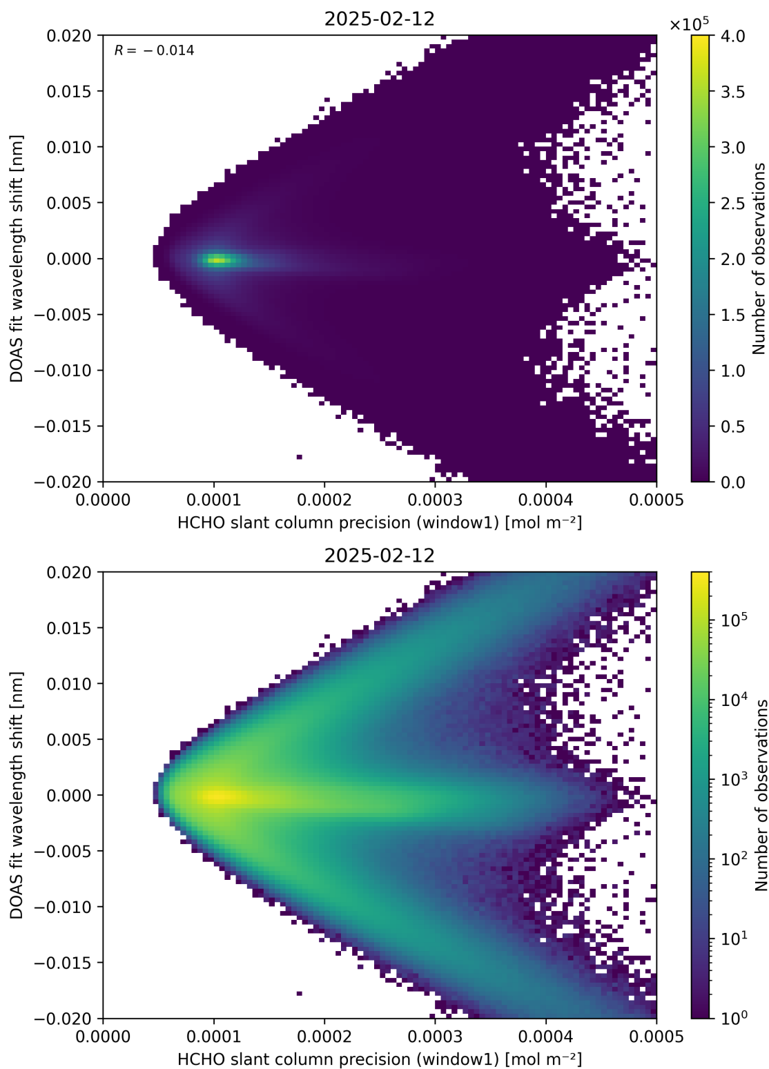
Figure 89: Scatter density plot of “HCHO slant column precision (window1)” against “DOAS fit wavelength shift” for 2025-02-11 to 2025-02-13.
