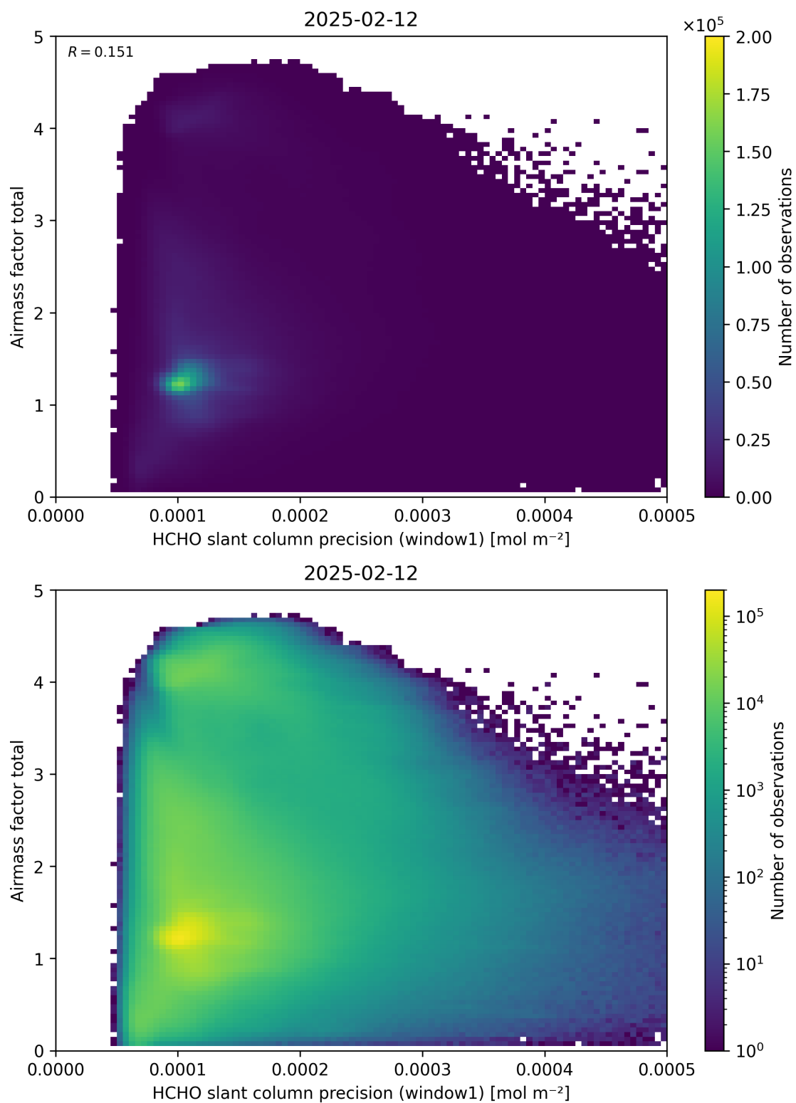
Figure 94: Scatter density plot of “HCHO slant column precision (window1)” against “Airmass factor total” for 2025-02-11 to 2025-02-13.
