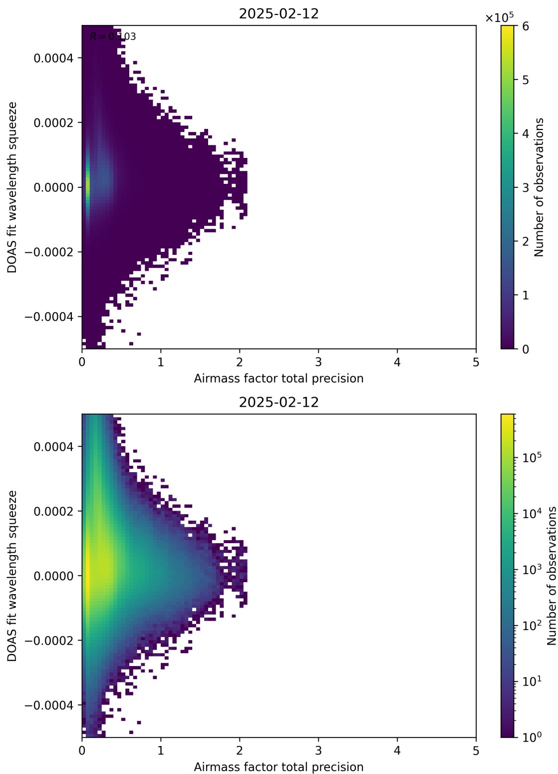
Figure 107: Scatter density plot of “Airmass factor total precision” against “DOAS fit wavelength squeeze” for 2025-02-11 to 2025-02-13.
