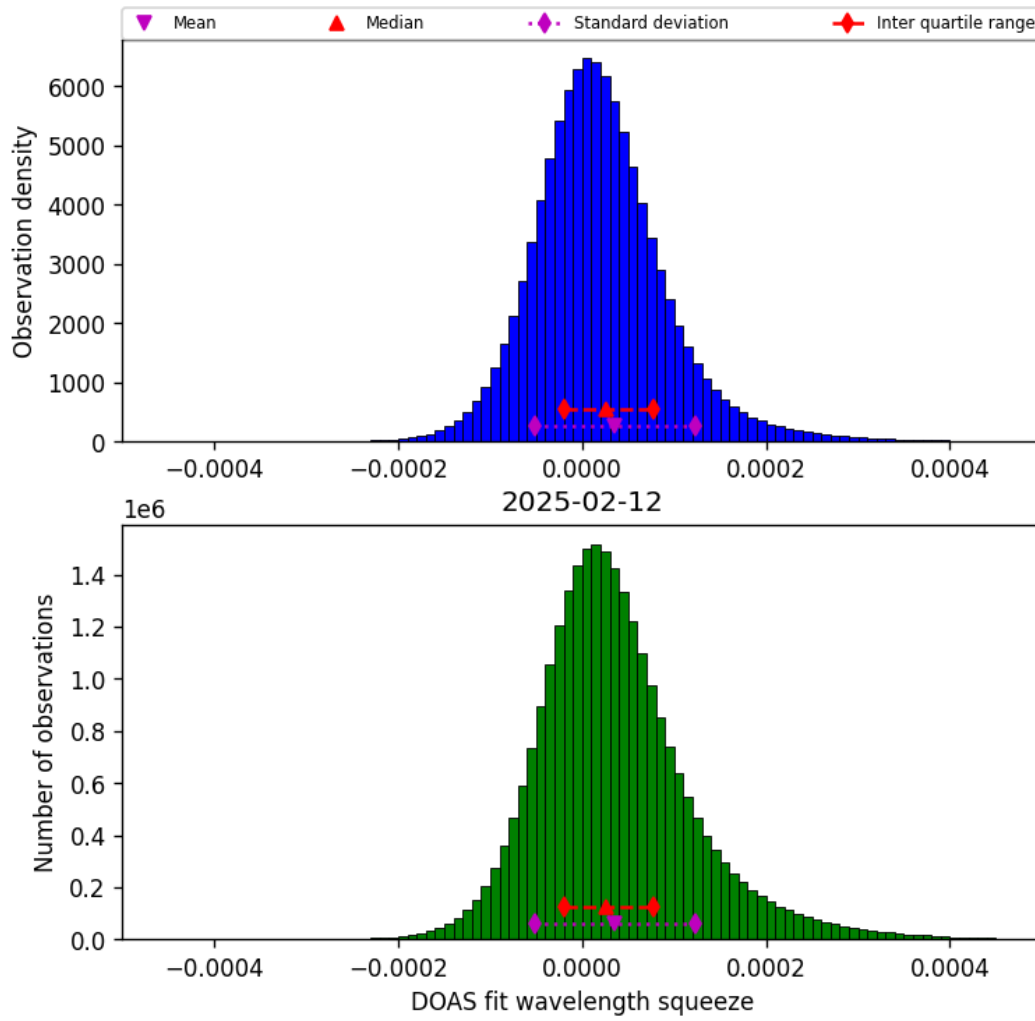
Figure 45: Histogram of “DOAS fit wavelength squeeze” for 2025-02-11 to 2025-02-13
