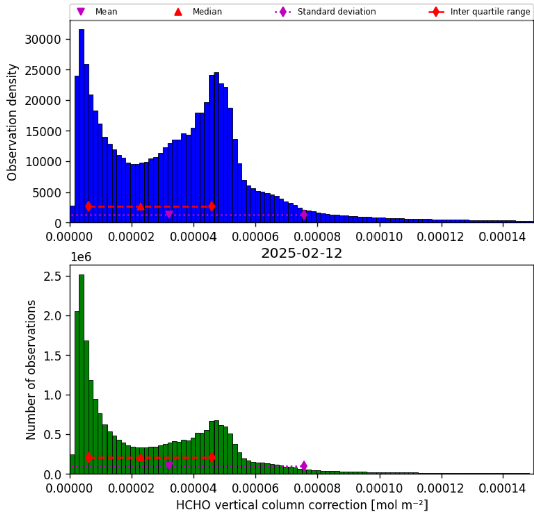
Figure 37: Histogram of “HCHO vertical column correction” for 2025-02-11 to 2025-02-13
