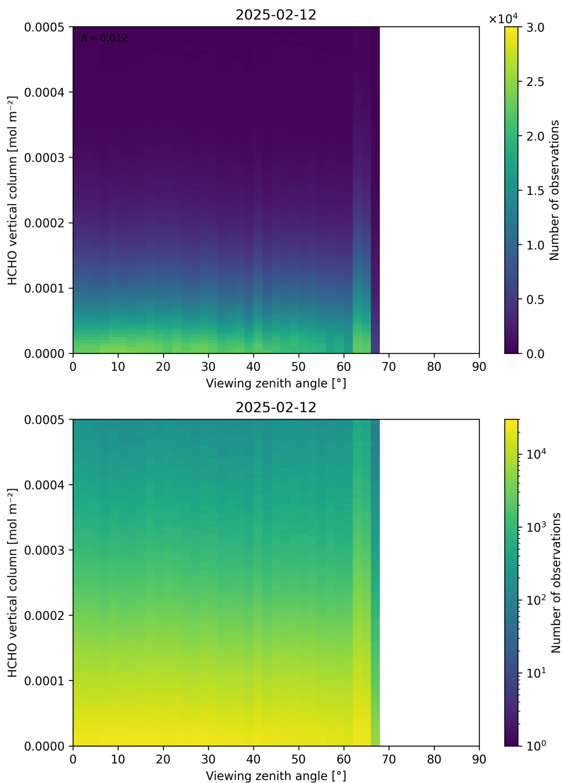
Figure 192: Scatter density plot of “Viewing zenith angle” against “HCHO vertical column” for 2025-02-11 to 2025-02-13.
