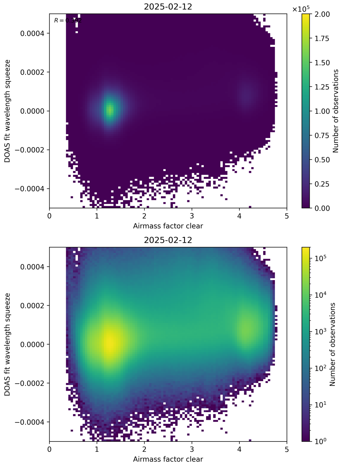
Figure 73: Scatter density plot of “Airmass factor clear” against “DOAS fit wavelength squeeze” for 2025-02-11 to 2025-02-13.
