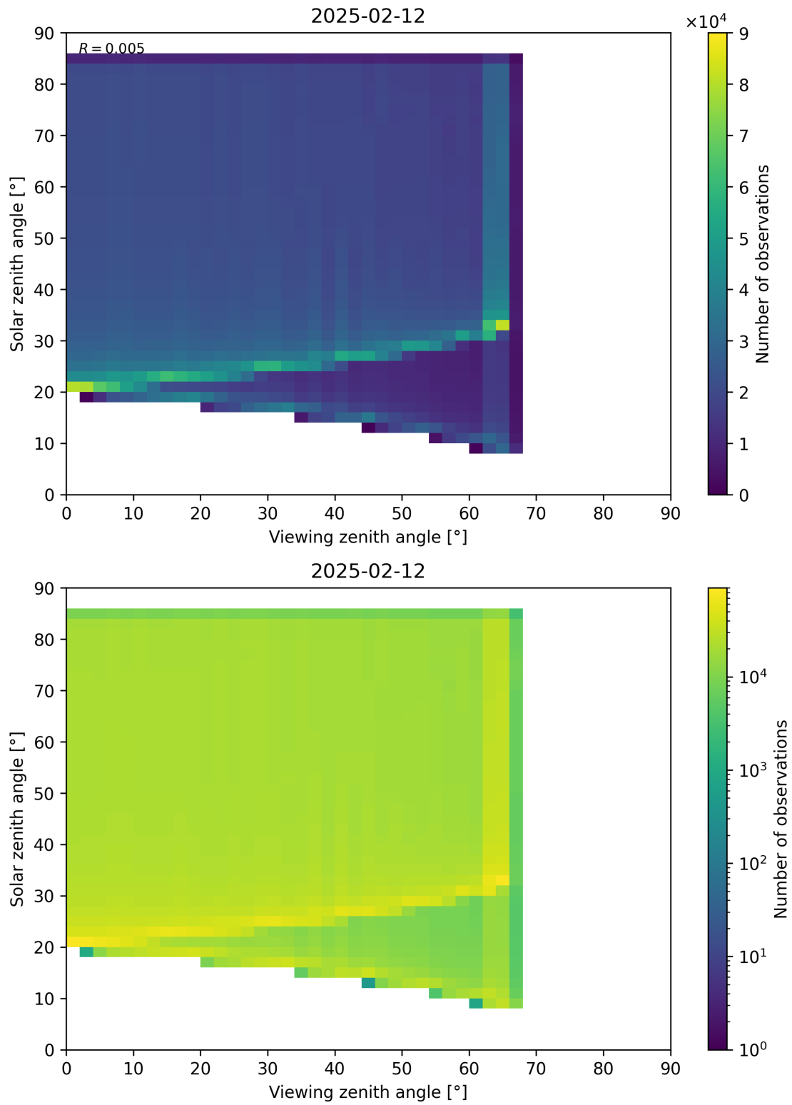
Figure 197: Scatter density plot of “Viewing zenith angle” against “Solar zenith angle” for 2025-02-11 to 2025-02-13.
