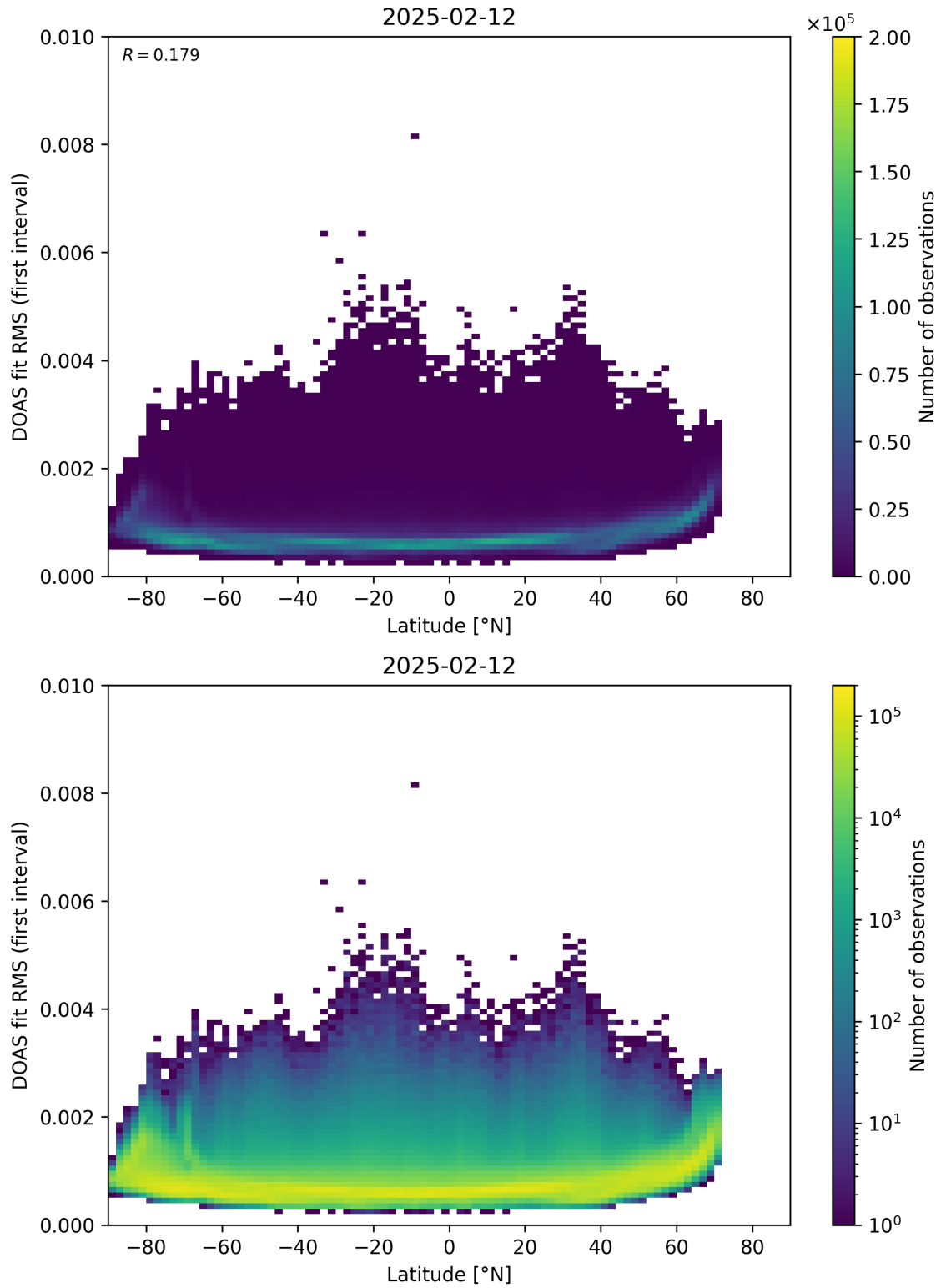
Figure 153: Scatter density plot of “Latitude” against “DOAS fit RMS (first interval)” for 2025-02-11 to 2025-02-13.
