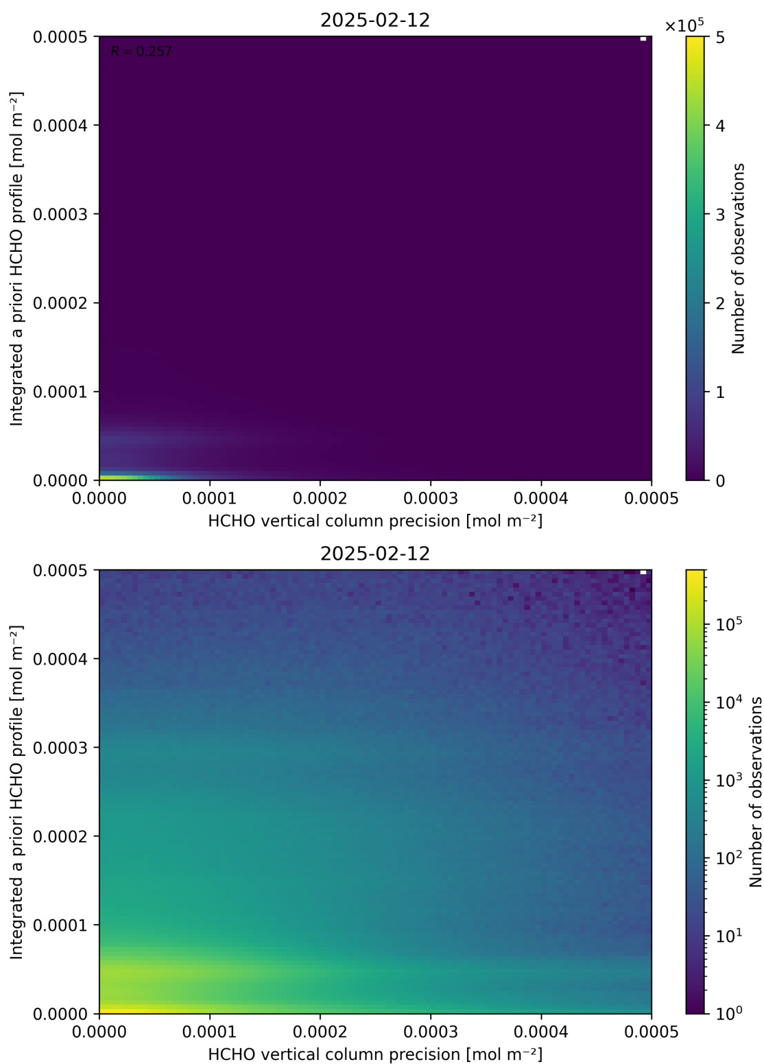
Figure 147: Scatter density plot of “HCHO vertical column precision” against “Integrated a priori HCHO profile” for 2025-02-11 to 2025-02-13.
