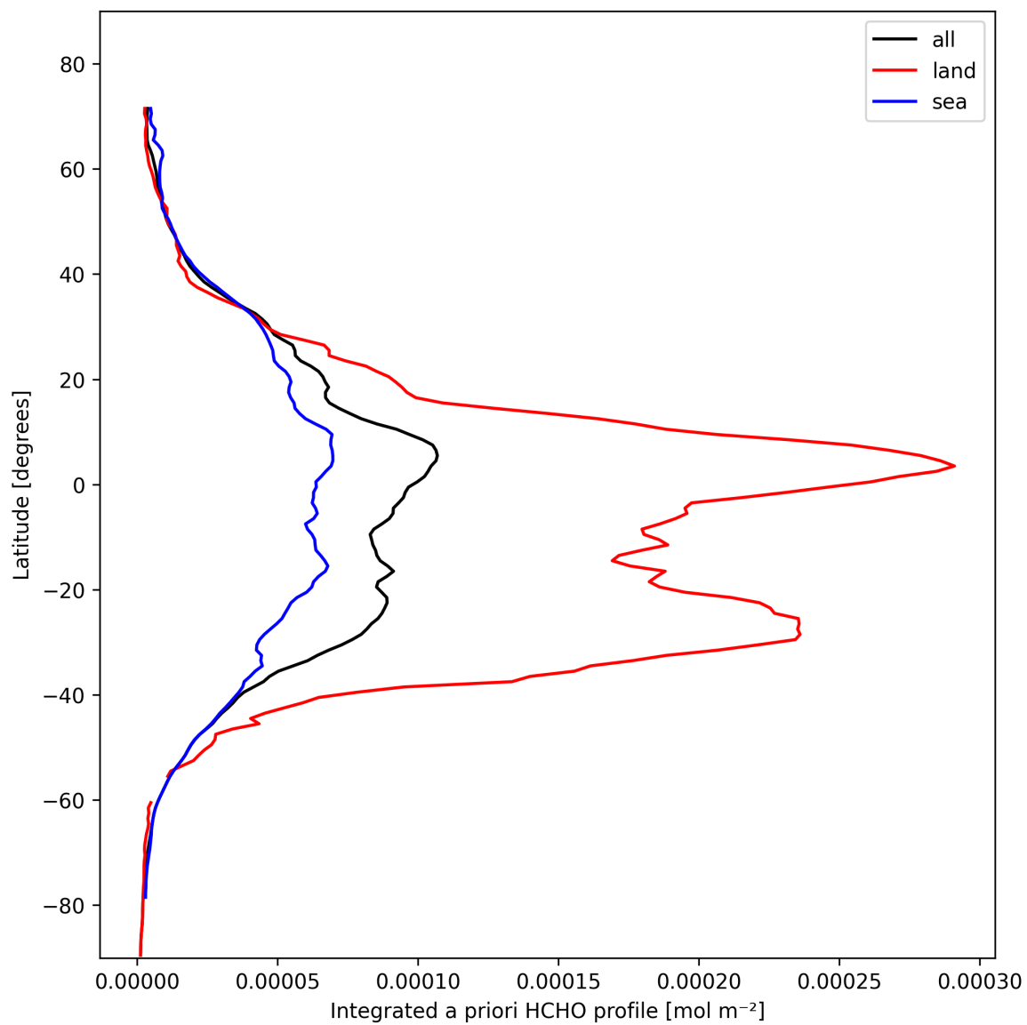
Figure 29: Zonal average of “Integrated a priori HCHO profile” for 2025-02-11 to 2025-02-13.
