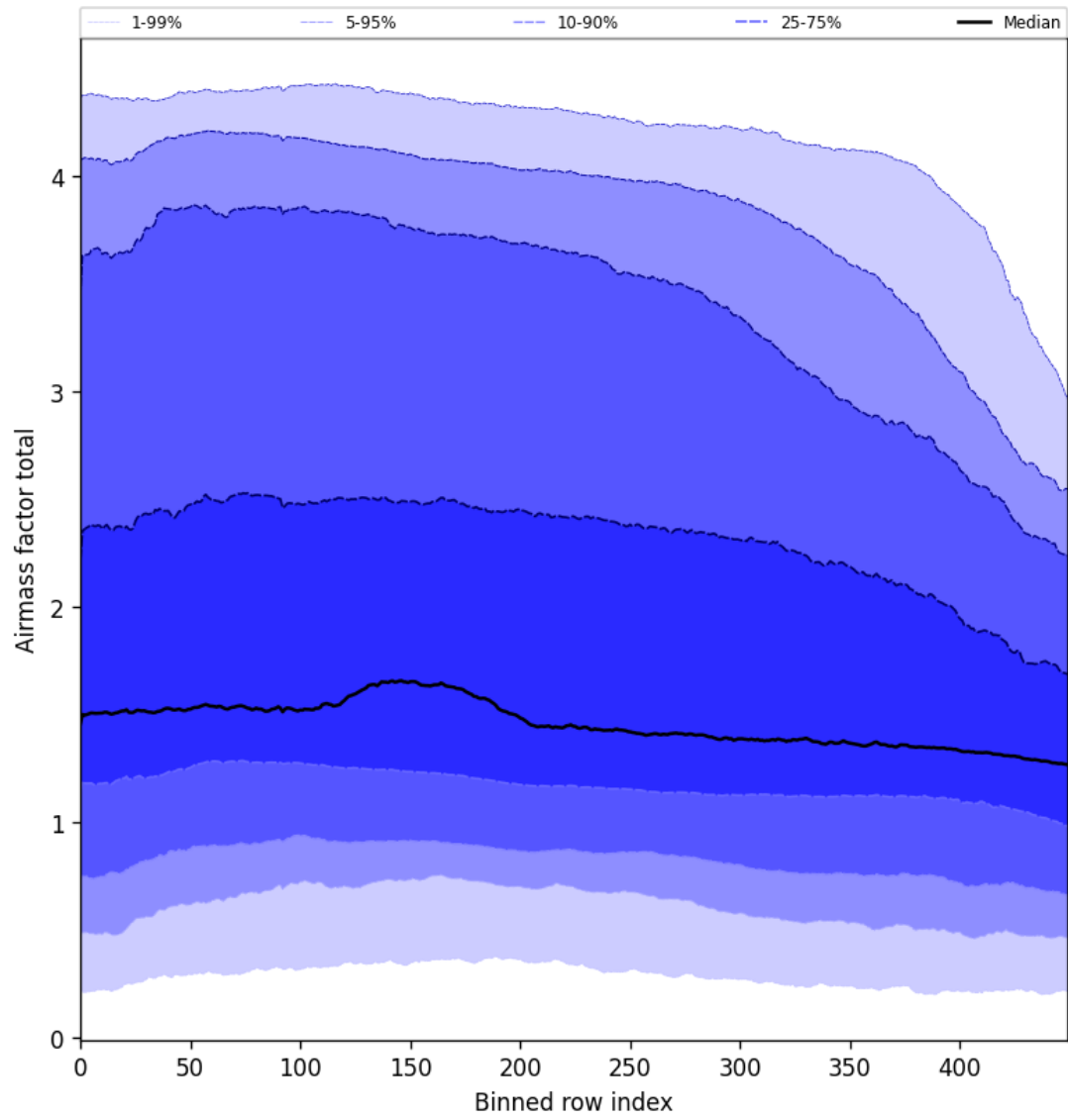
Figure 54: Along track statistics of “Airmass factor total” for 2025-02-11 to 2025-02-13
