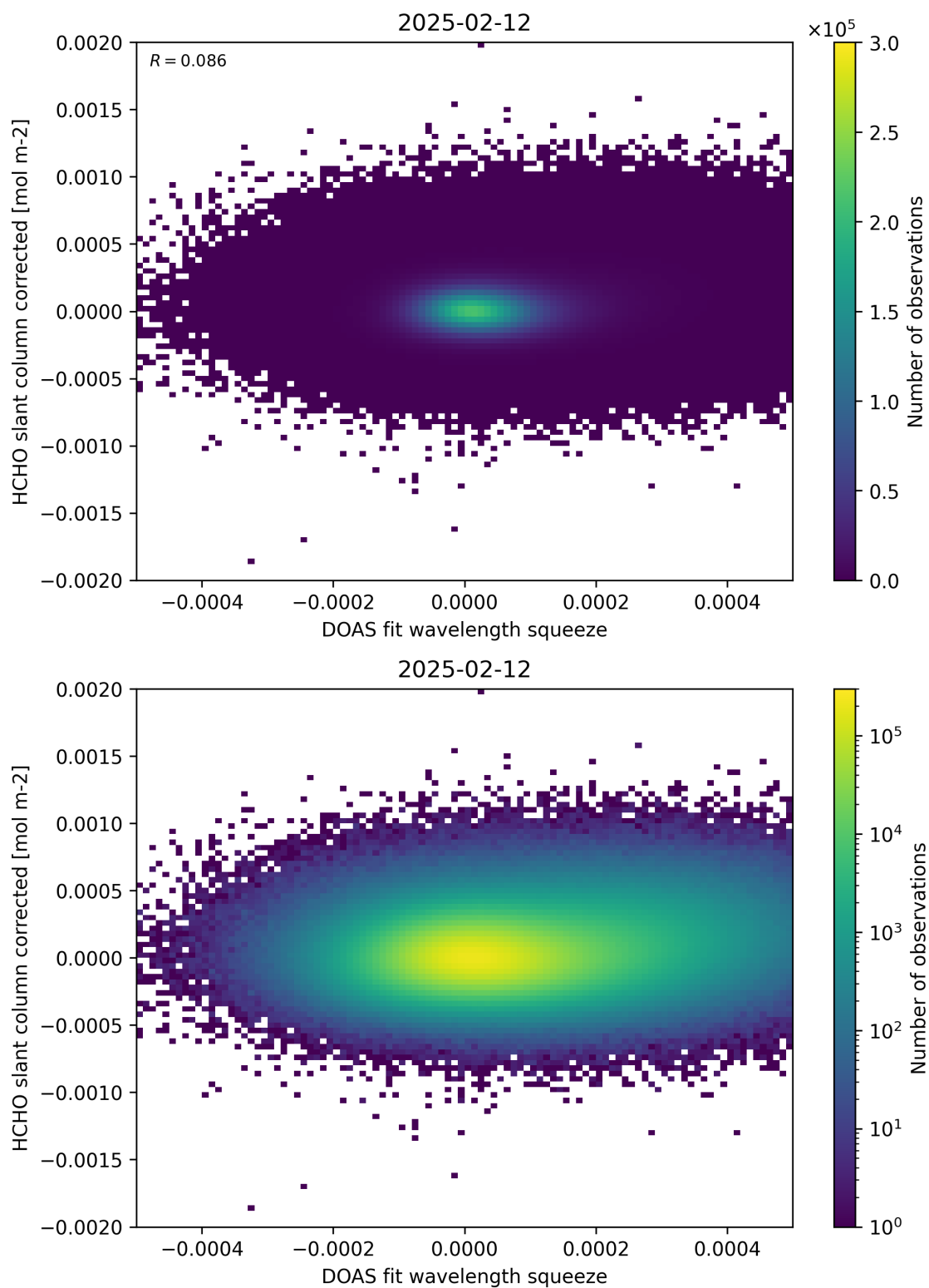
Figure 69: Scatter density plot of “DOAS fit wavelength squeeze” against “HCHO slant column corrected” for 2025-02-11 to 2025-02-13.
