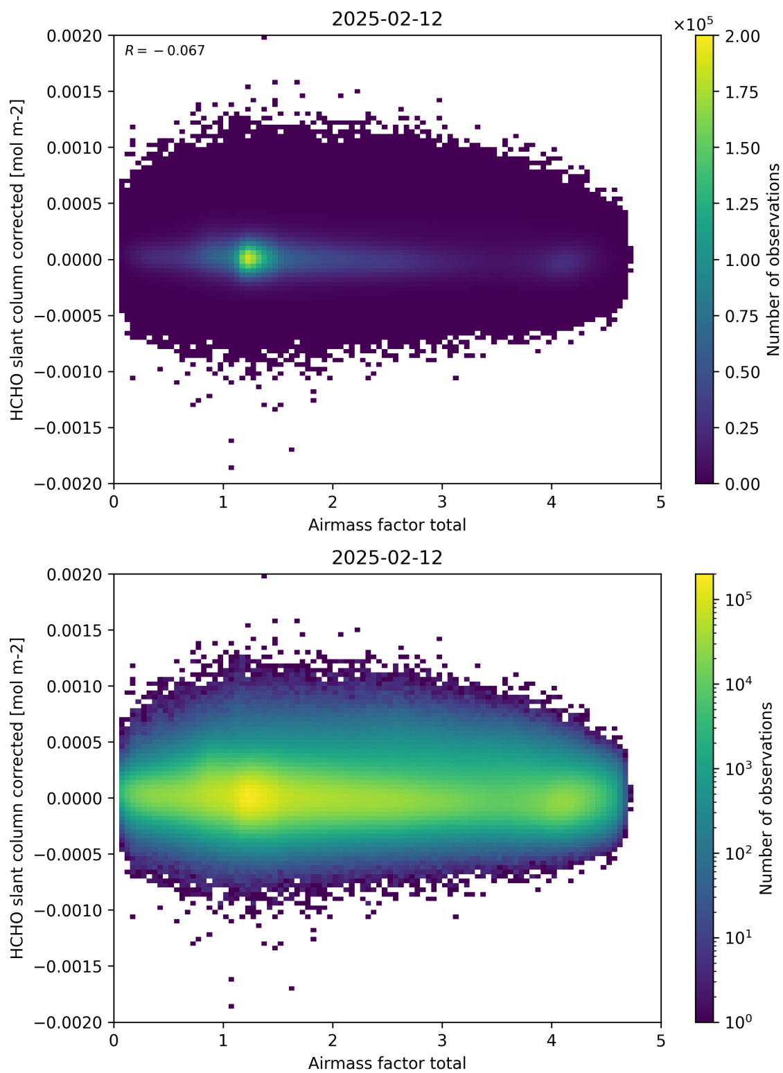
Figure 101: Scatter density plot of “Airmass factor total” against “HCHO slant column corrected” for 2025-02-11 to 2025-02-13.
