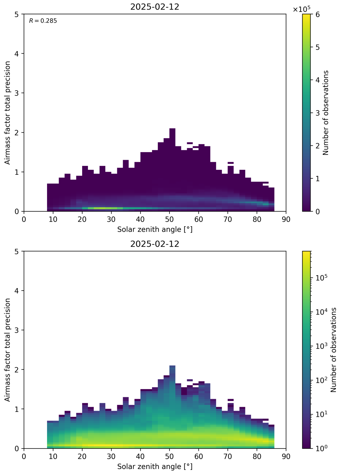
Figure 176: Scatter density plot of “Solar zenith angle” against “Airmass factor total precision” for 2025-02-11 to 2025-02-13.
