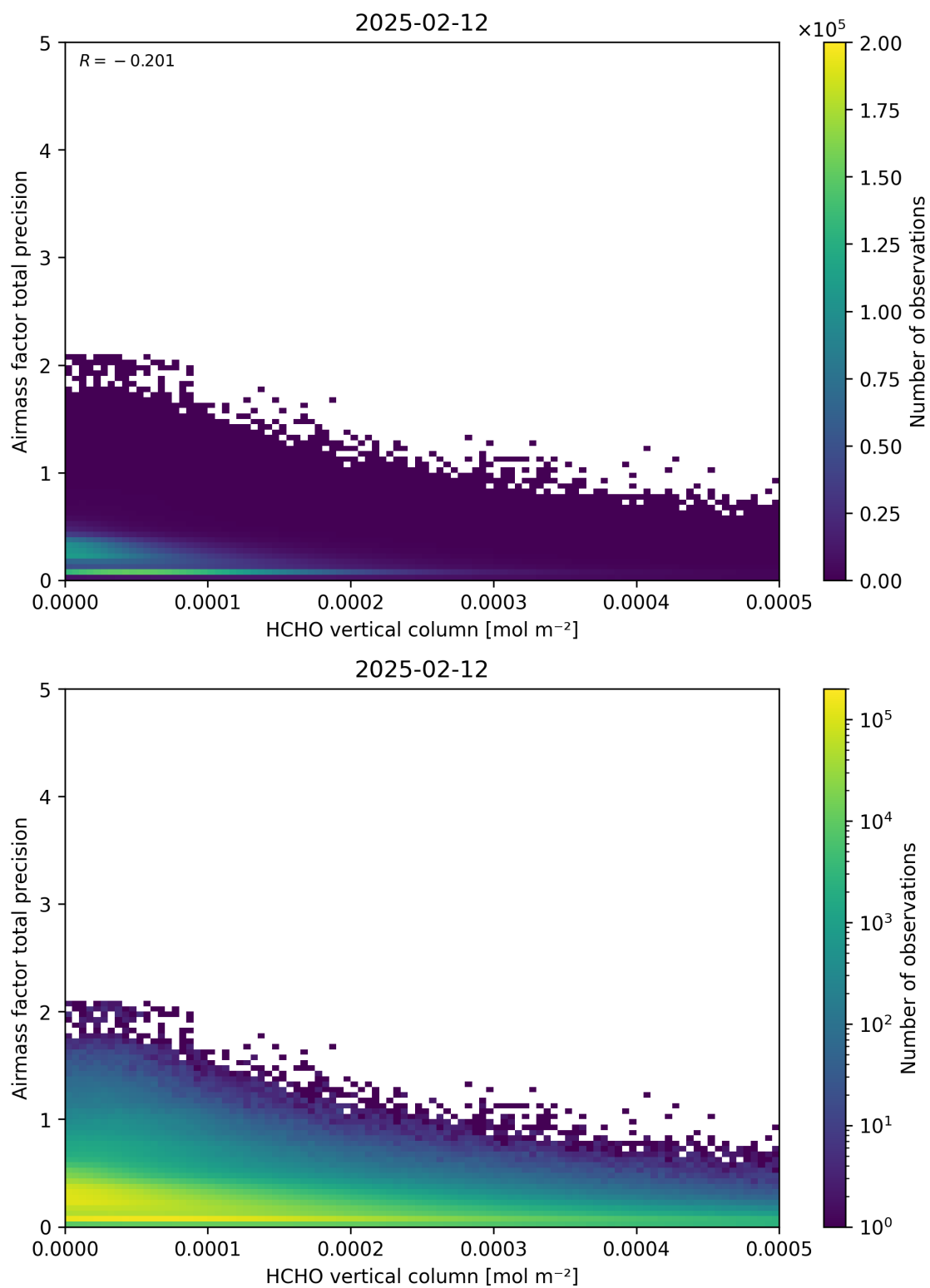
Figure 132: Scatter density plot of “HCHO vertical column” against “Airmass factor total precision” for 2025-02-11 to 2025-02-13.
