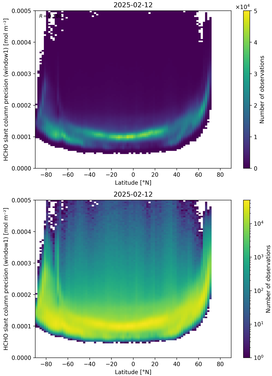
Figure 160: Scatter density plot of “Latitude” against “HCHO slant column precision (window1)” for 2025-02-11 to 2025-02-13.
