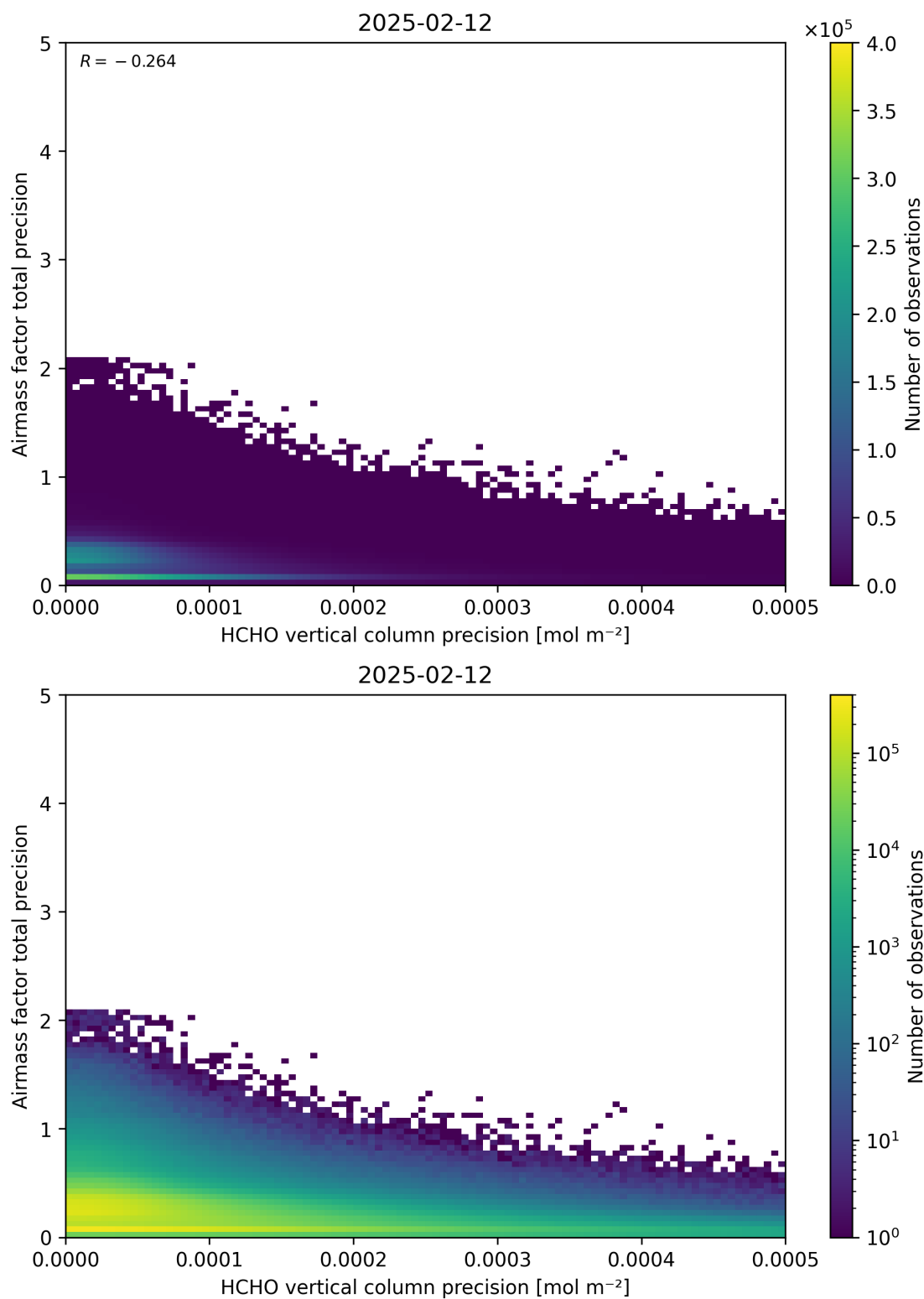
Figure 145: Scatter density plot of “HCHO vertical column precision” against “Airmass factor total precision” for 2025-02-11 to 2025-02-13.
