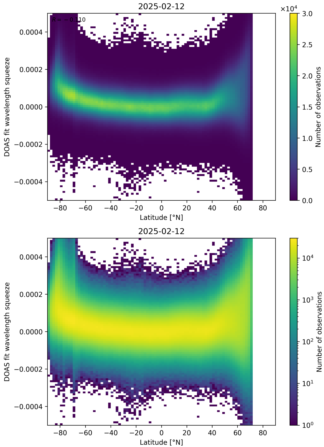
Figure 155: Scatter density plot of “Latitude” against “DOAS fit wavelength squeeze” for 2025-02-11 to 2025-02-13.
