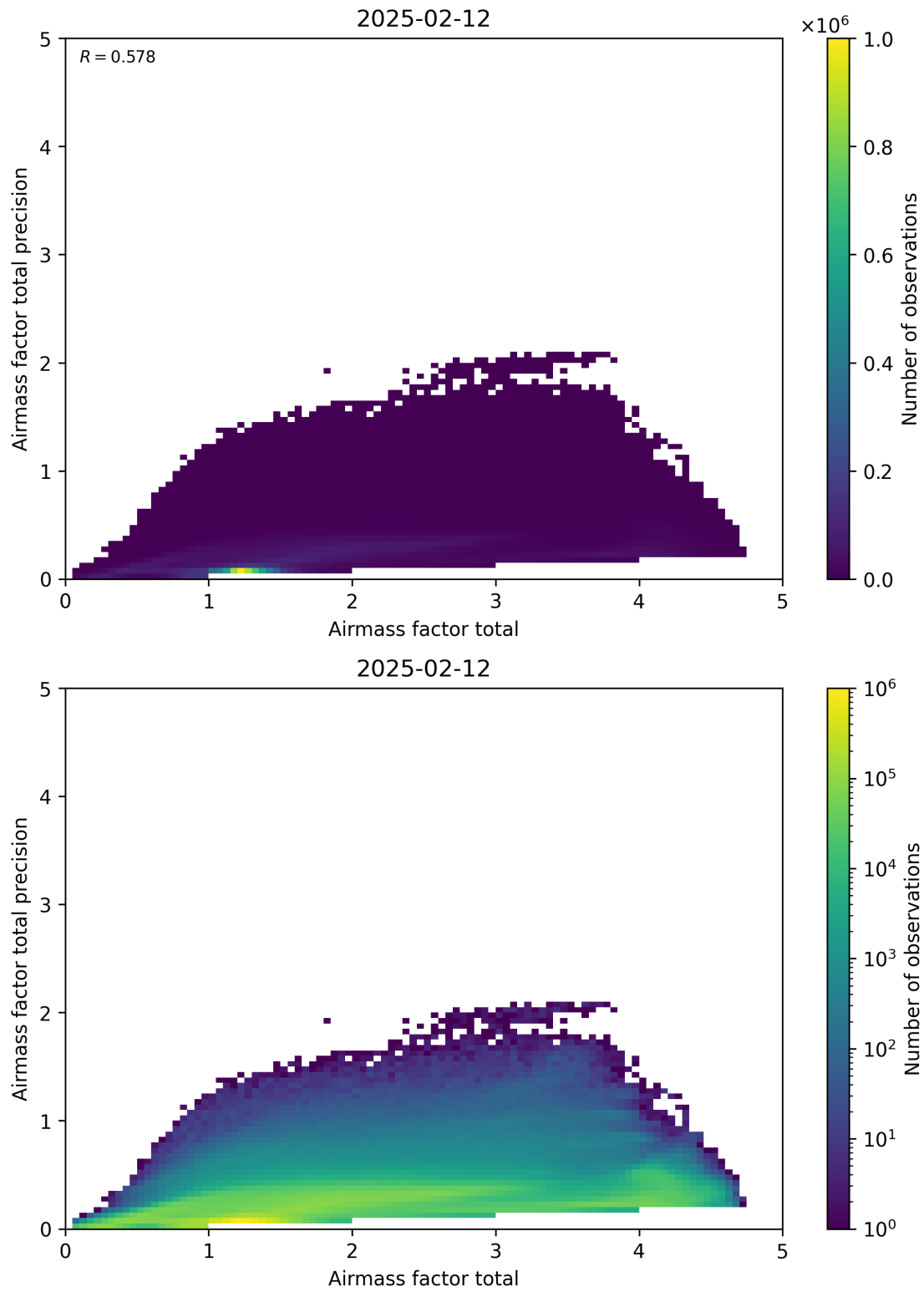
Figure 103: Scatter density plot of “Airmass factor total” against “Airmass factor total precision” for 2025-02-11 to 2025-02-13.
