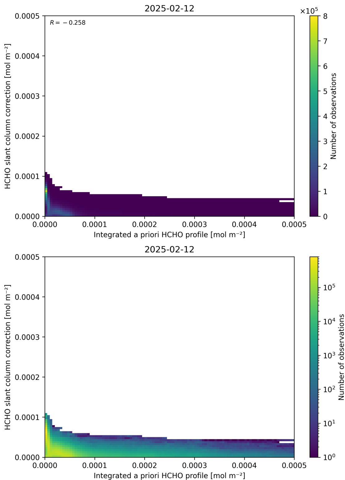
Figure 152: Scatter density plot of “Integrated a priori HCHO profile” against “HCHO slant column correction” for 2025-02-11 to 2025-02-13.
