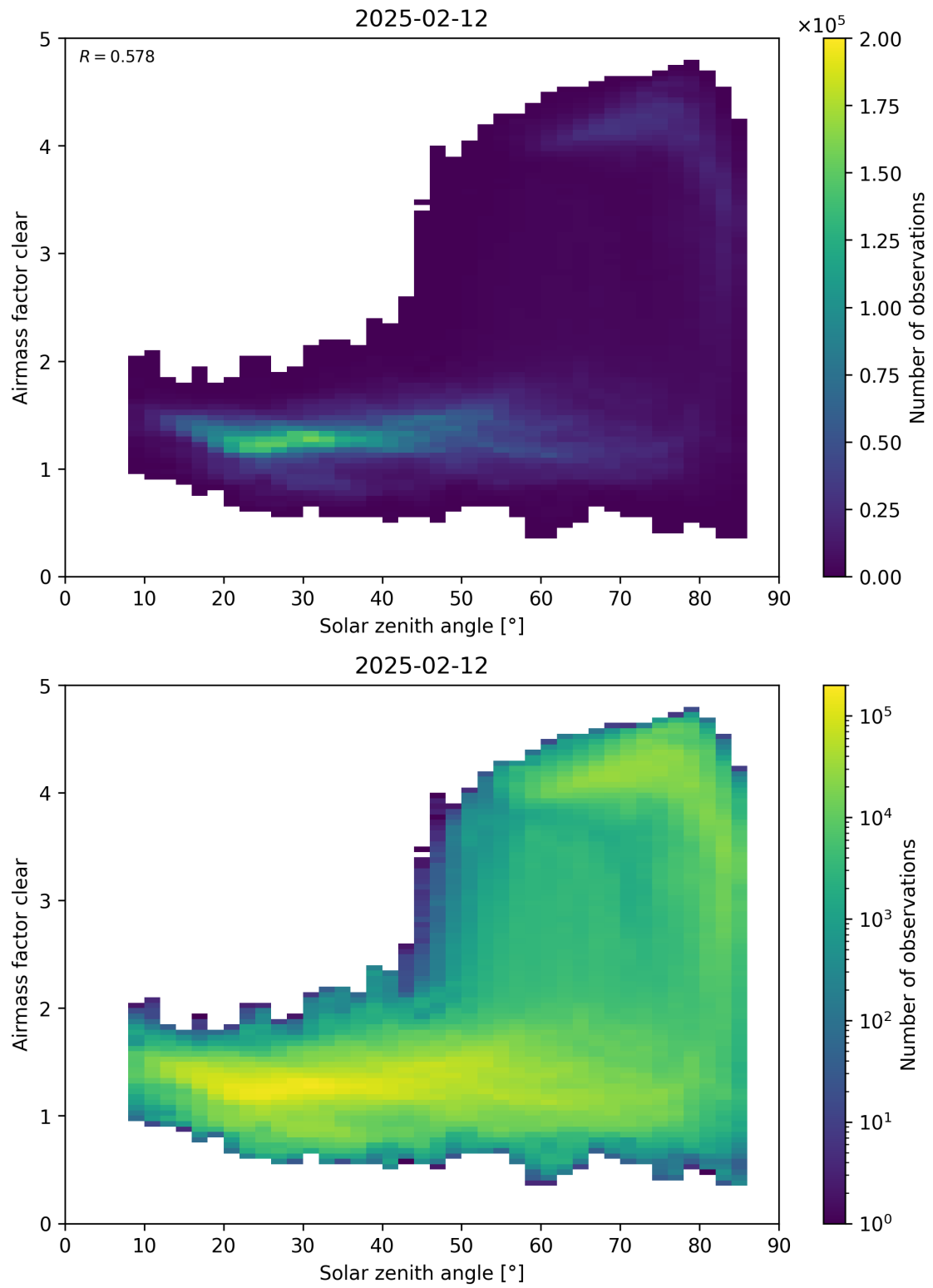
Figure 170: Scatter density plot of “Solar zenith angle” against “Airmass factor clear” for 2025-02-11 to 2025-02-13.
