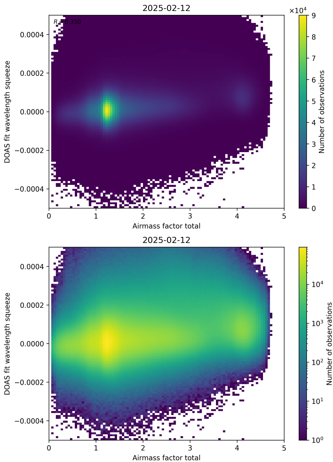
Figure 99: Scatter density plot of “Airmass factor total” against “DOAS fit wavelength squeeze” for 2025-02-11 to 2025-02-13.
