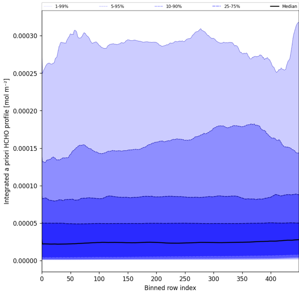
Figure 57: Along track statistics of “Integrated a priori HCHO profile” for 2025-02-11 to 2025-02-13
