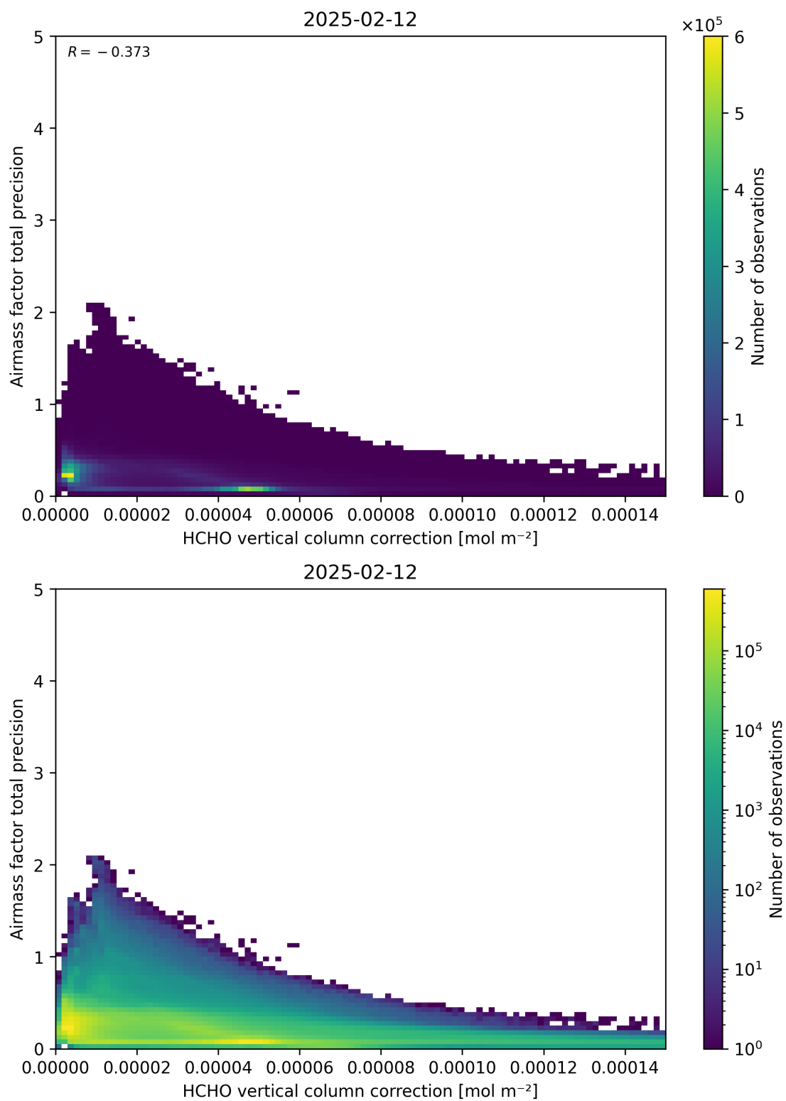
Figure 121: Scatter density plot of “HCHO vertical column correction” against “Airmass factor total precision” for 2025-02-11 to 2025-02-13.
