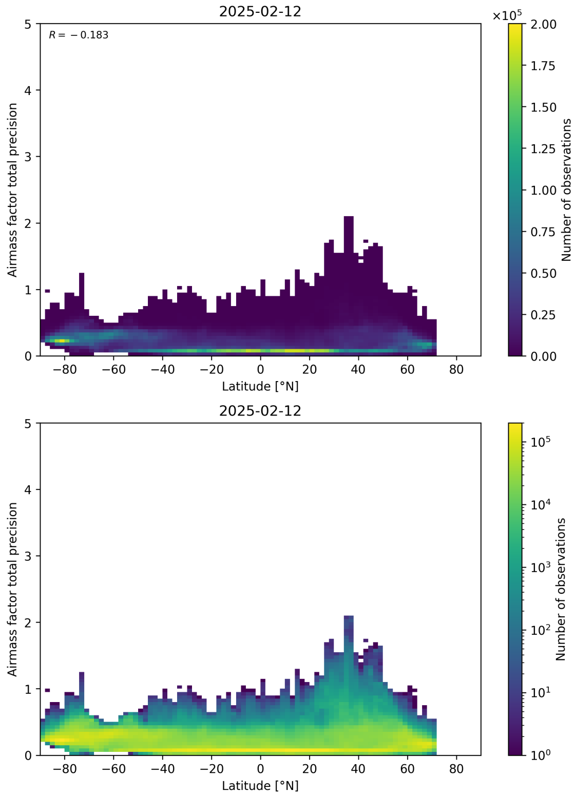
Figure 162: Scatter density plot of “Latitude” against “Airmass factor total precision” for 2025-02-11 to 2025-02-13.
