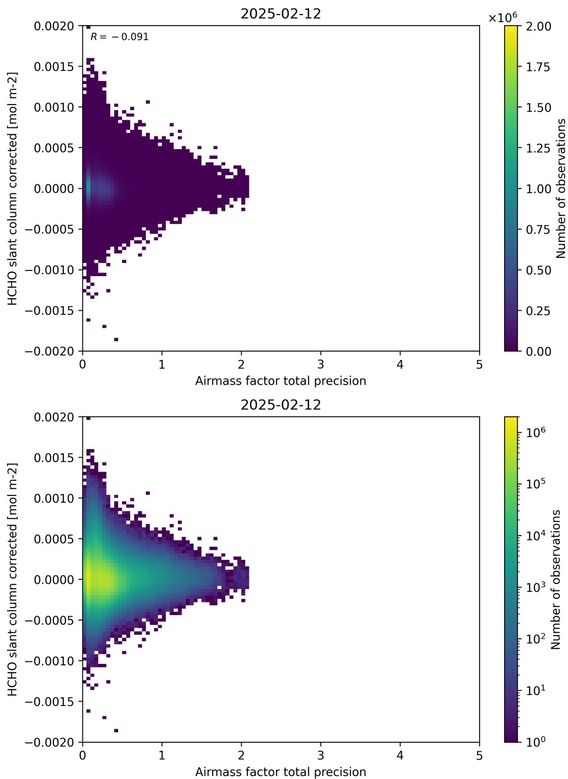
Figure 109: Scatter density plot of “Airmass factor total precision” against “HCHO slant column corrected” for 2025-02-11 to 2025-02-13.
