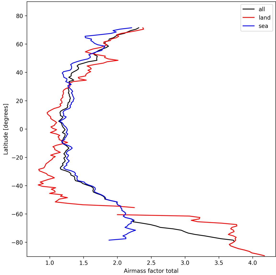
Figure 26: Zonal average of “Airmass factor total” for 2025-02-11 to 2025-02-13.
