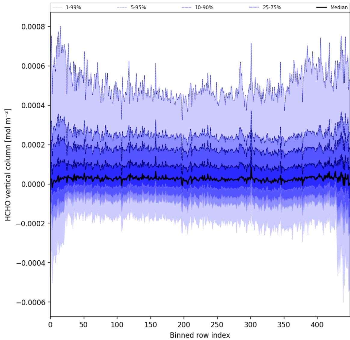
Figure 49: Along track statistics of “HCHO vertical column” for 2025-02-11 to 2025-02-13
