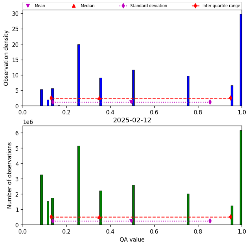
Figure 34: Histogram of “QA value” for 2025-02-11 to 2025-02-13
