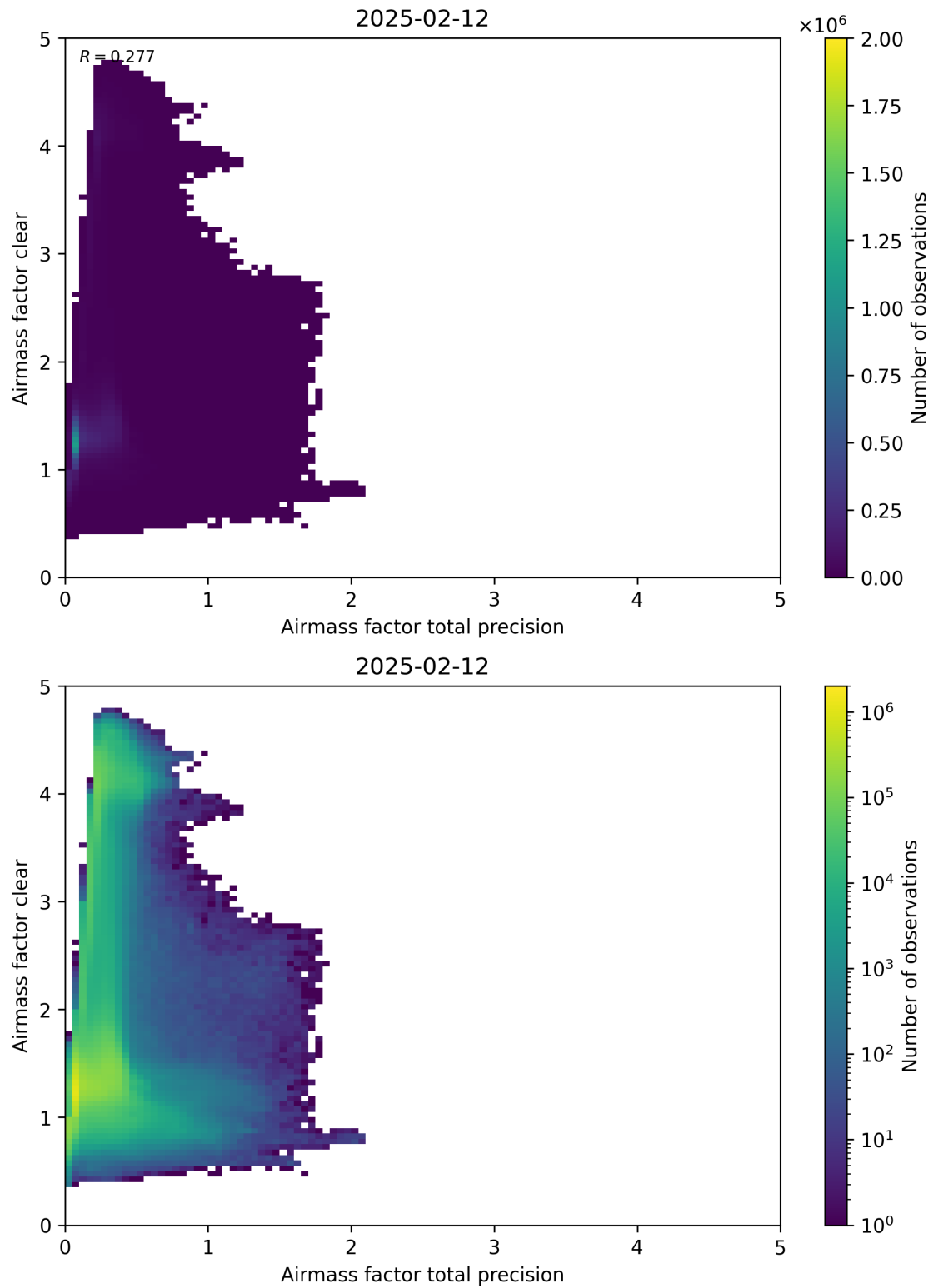
Figure 108: Scatter density plot of “Airmass factor total precision” against “Airmass factor clear” for 2025-02-11 to 2025-02-13.
