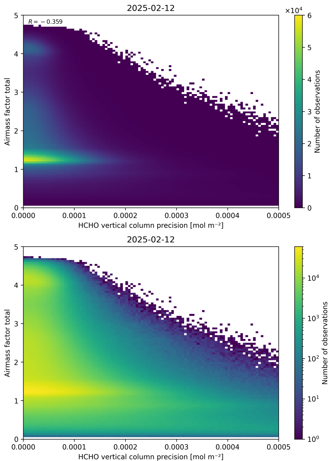
Figure 144: Scatter density plot of “HCHO vertical column precision” against “Airmass factor total” for 2025-02-11 to 2025-02-13.
