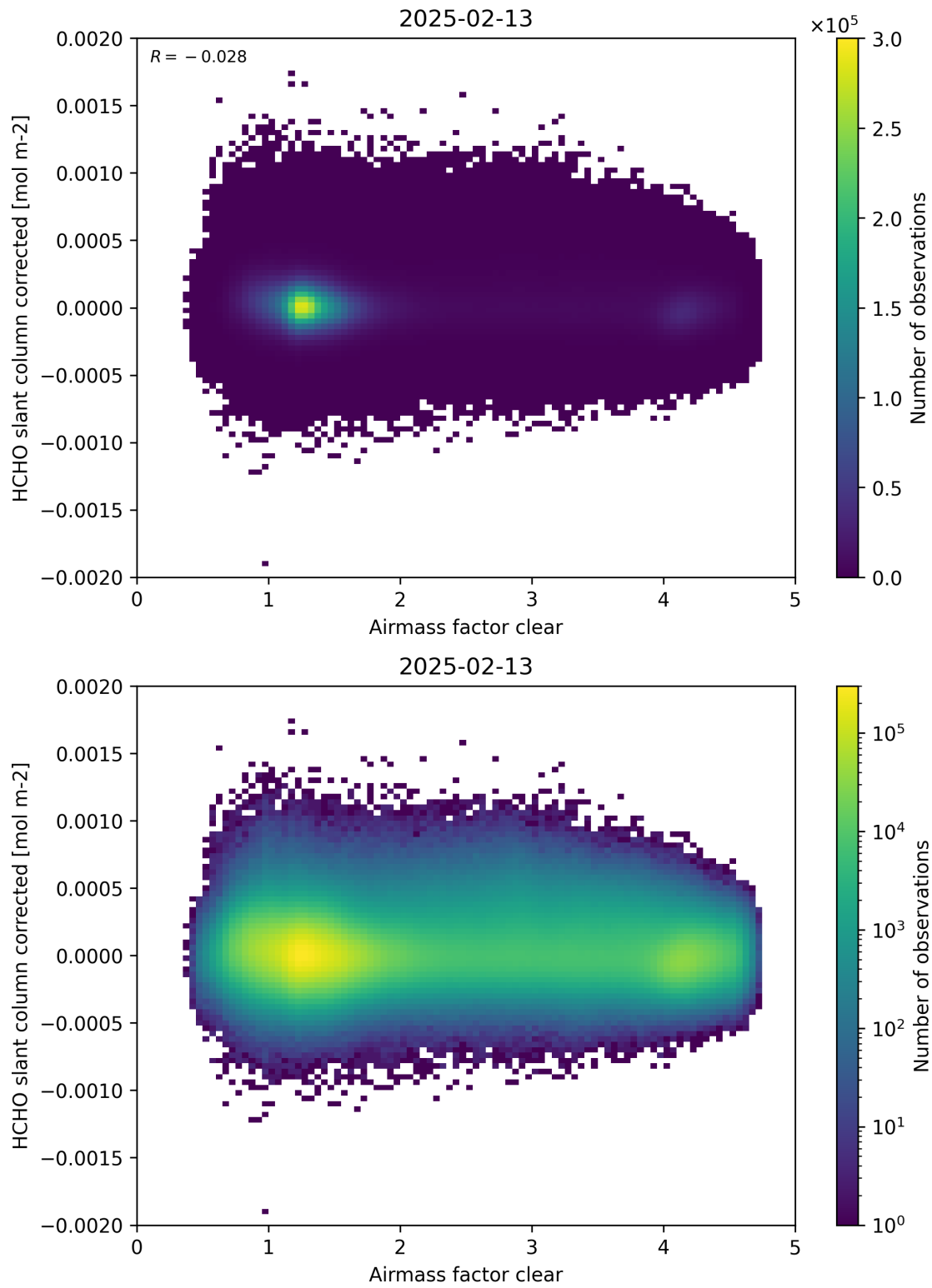
Figure 74: Scatter density plot of “Airmass factor clear” against “HCHO slant column corrected” for 2025-02-13 to 2025-02-14.
