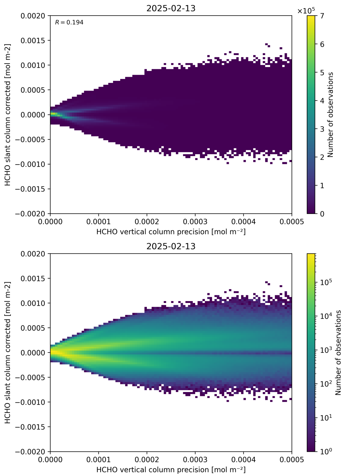
Figure 140: Scatter density plot of “HCHO vertical column precision” against “HCHO slant column corrected” for 2025-02-13 to 2025-02-14.
