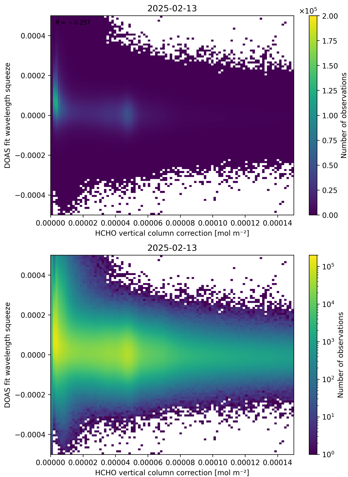
Figure 114: Scatter density plot of “HCHO vertical column correction” against “DOAS fit wavelength squeeze” for 2025-02-13 to 2025-02-14.
