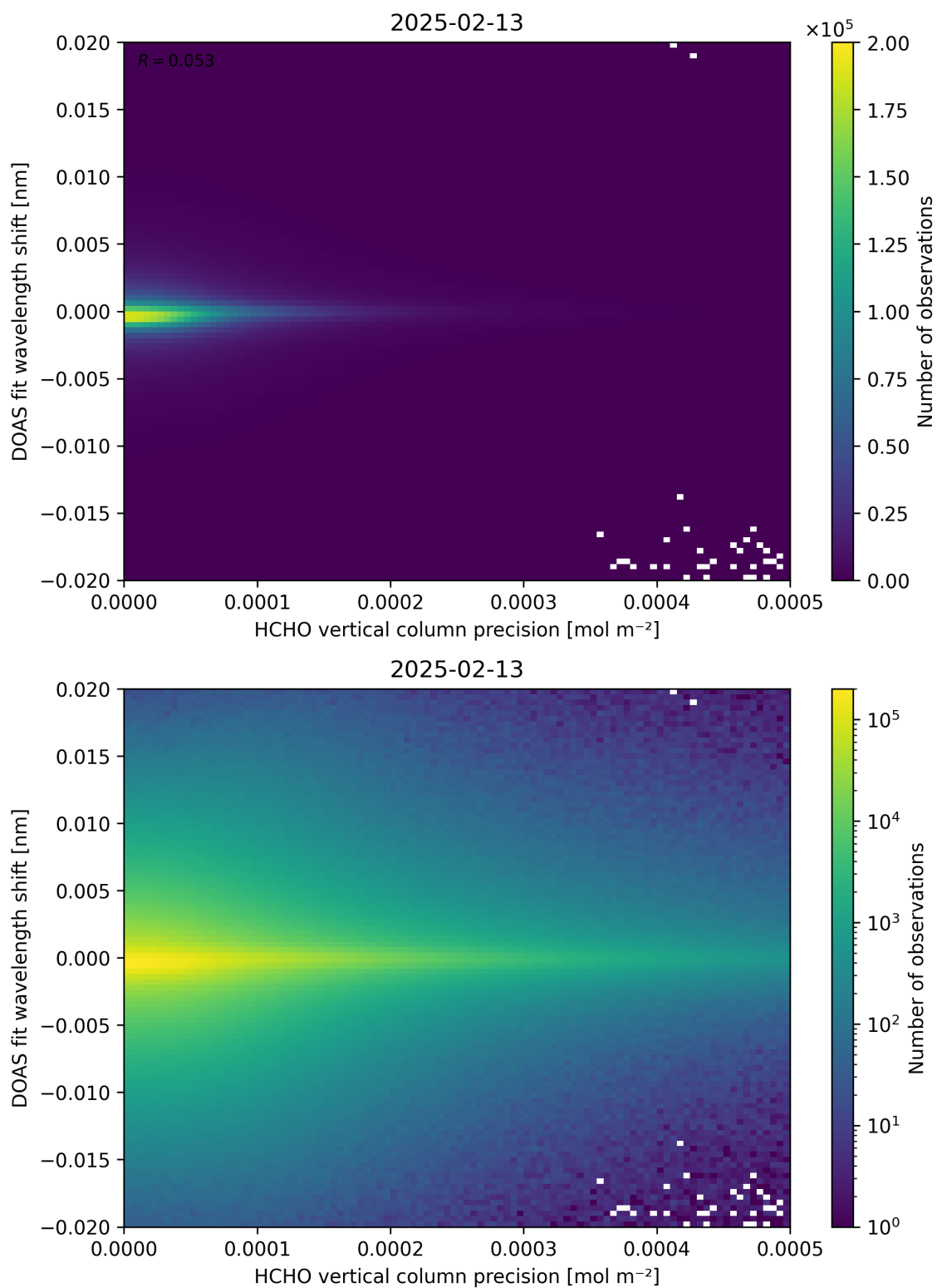
Figure 137: Scatter density plot of “HCHO vertical column precision” against “DOAS fit wavelength shift” for 2025-02-13 to 2025-02-14.
