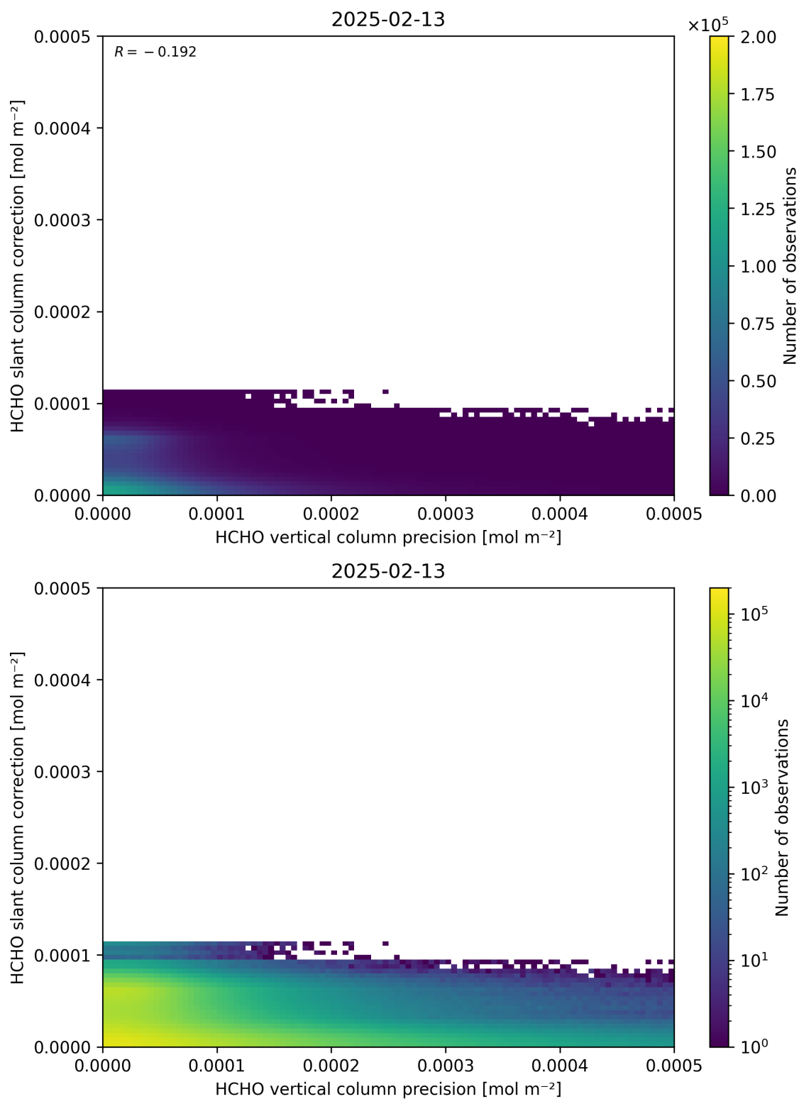
Figure 141: Scatter density plot of “HCHO vertical column precision” against “HCHO slant column correction” for 2025-02-13 to 2025-02-14.
