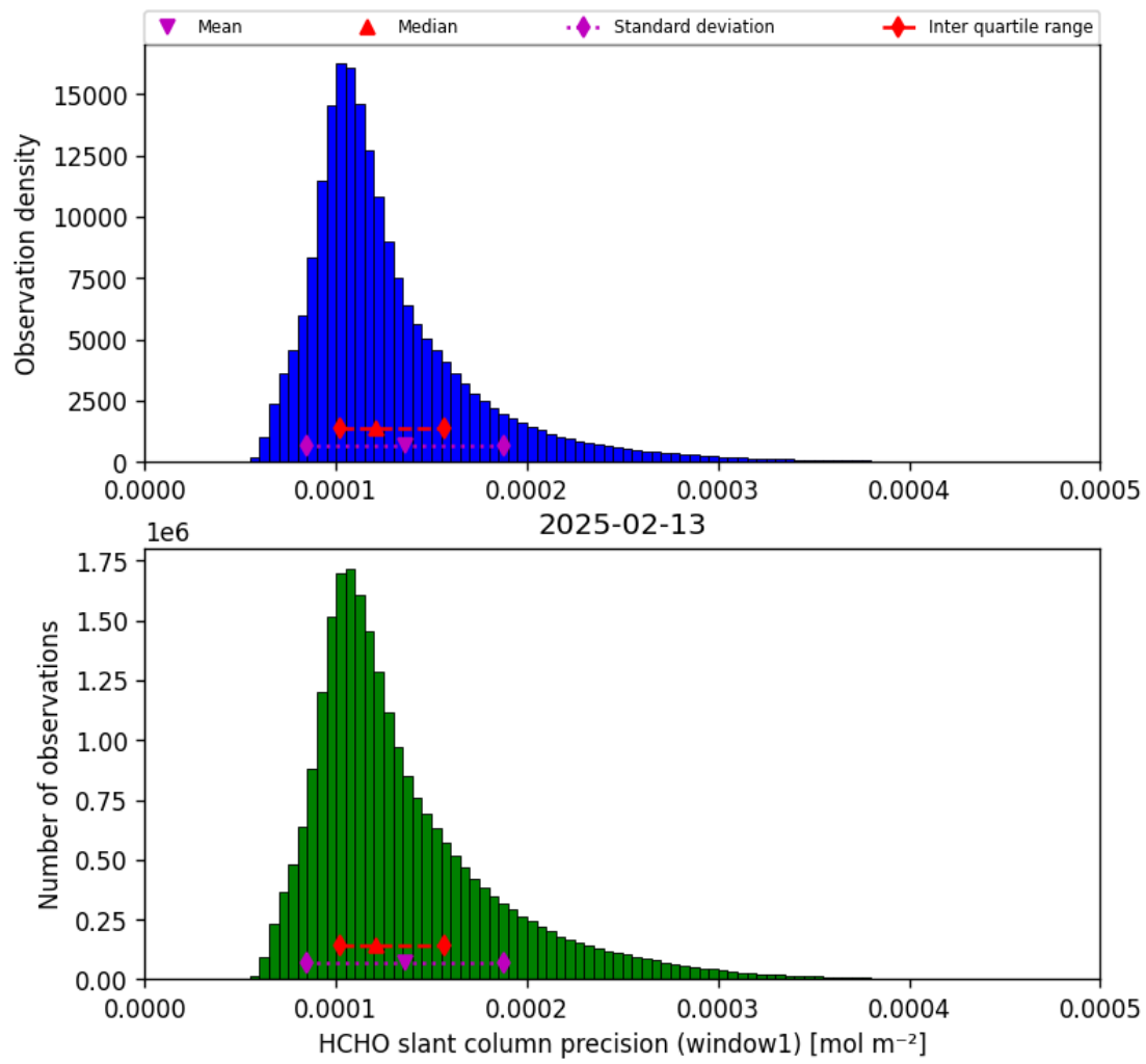
Figure 39: Histogram of “HCHO slant column precision (window1)” for 2025-02-13 to 2025-02-14
