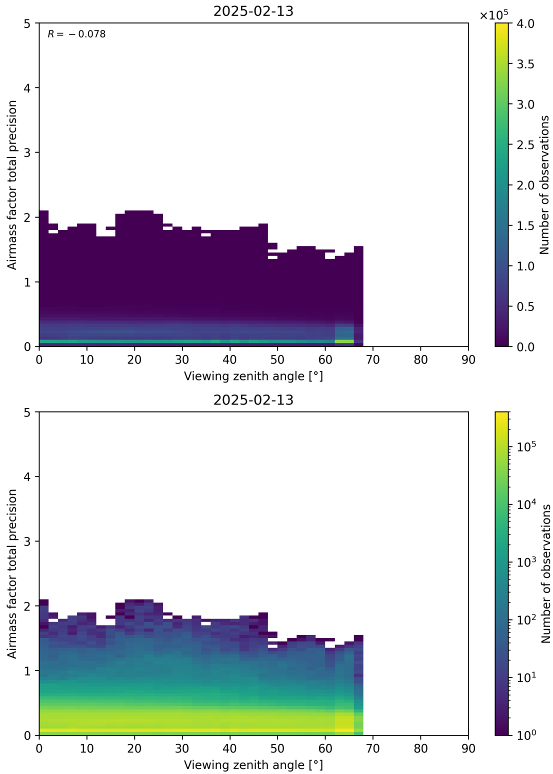
Figure 191: Scatter density plot of “Viewing zenith angle” against “Airmass factor total precision” for 2025-02-13 to 2025-02-14.
