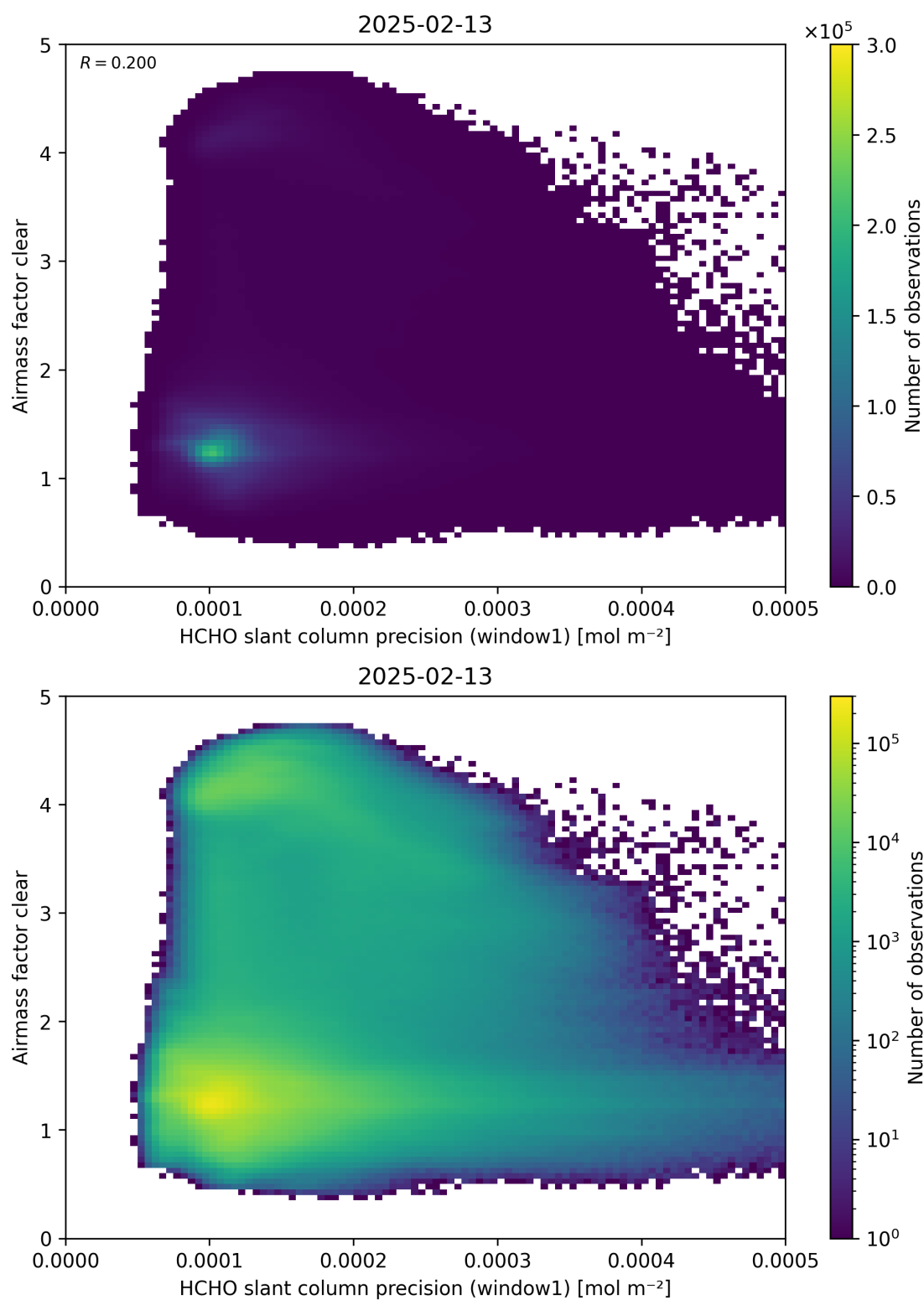
Figure 91: Scatter density plot of “HCHO slant column precision (window1)” against “Airmass factor clear” for 2025-02-13 to 2025-02-14.
