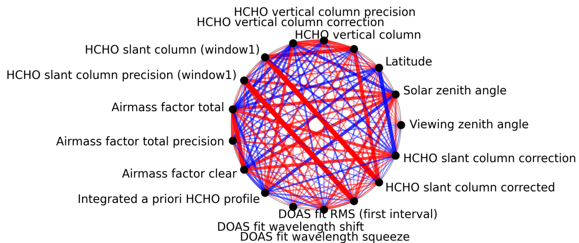
Figure 1: Map of correlation graph for 2025-02-13 to 2025-02-14.
