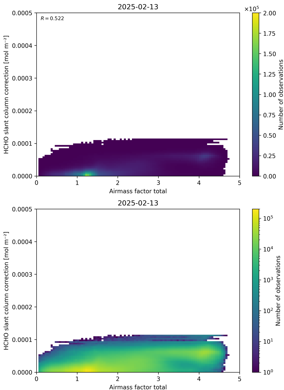
Figure 102: Scatter density plot of “Airmass factor total” against “HCHO slant column correction” for 2025-02-13 to 2025-02-14.
