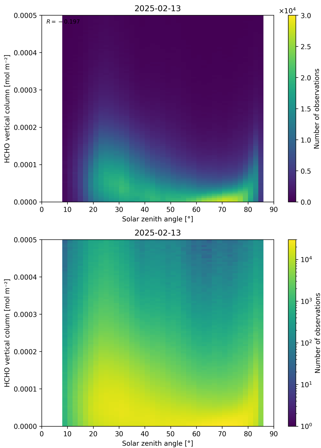
Figure 177: Scatter density plot of “Solar zenith angle” against “HCHO vertical column” for 2025-02-13 to 2025-02-14.
