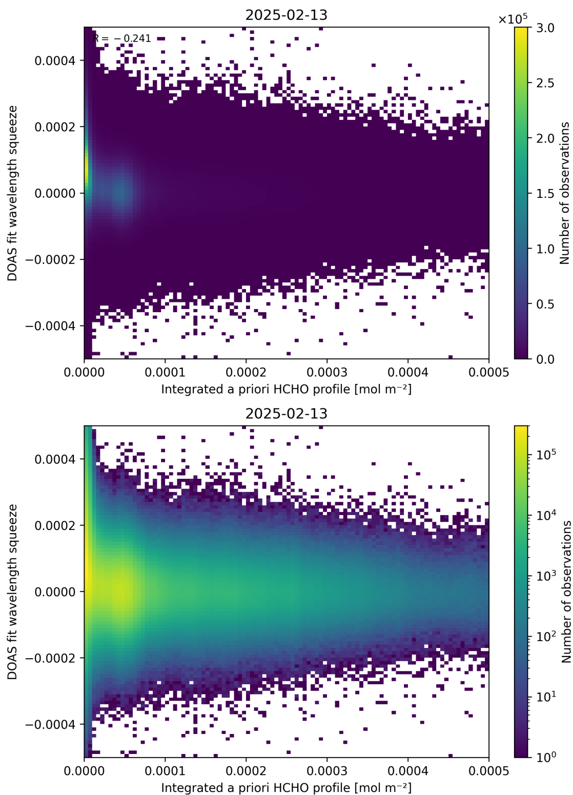
Figure 150: Scatter density plot of “Integrated a priori HCHO profile” against “DOAS fit wavelength squeeze” for 2025-02-13 to 2025-02-14.
