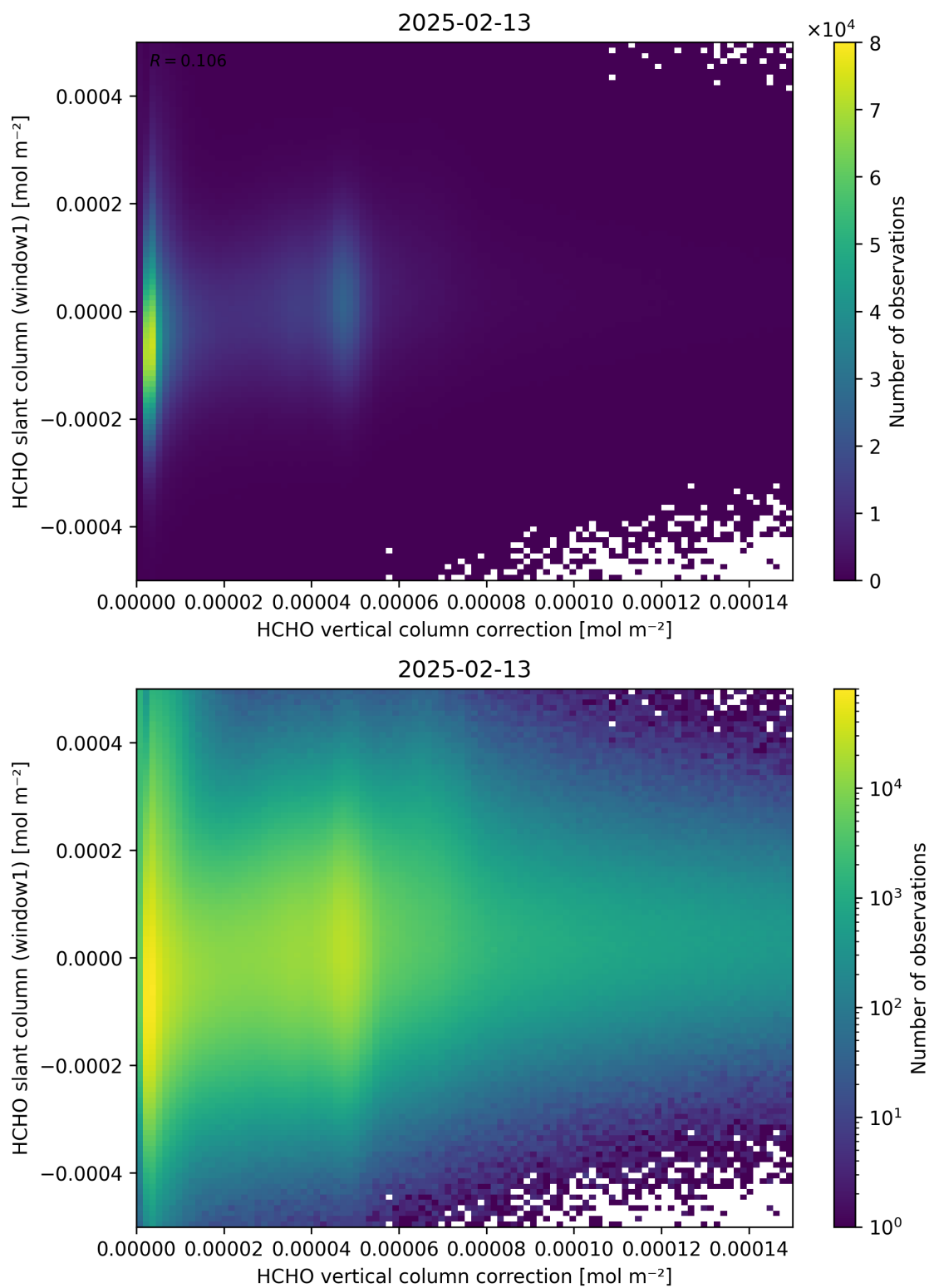
Figure 118: Scatter density plot of “HCHO vertical column correction” against “HCHO slant column (window1)” for 2025-02-13 to 2025-02-14.
