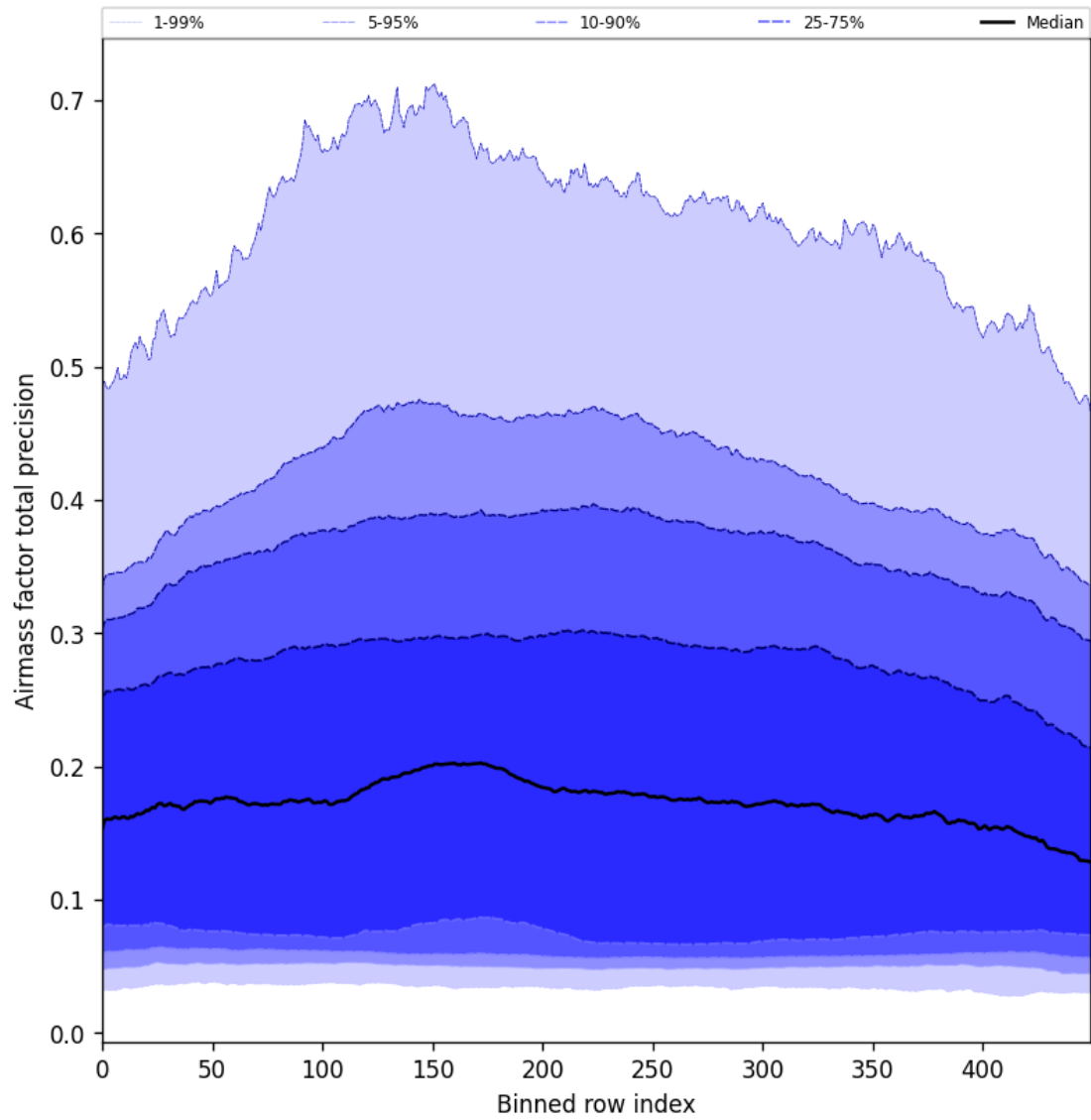
Figure 55: Along track statistics of “Airmass factor total precision” for 2025-02-13 to 2025-02-14
