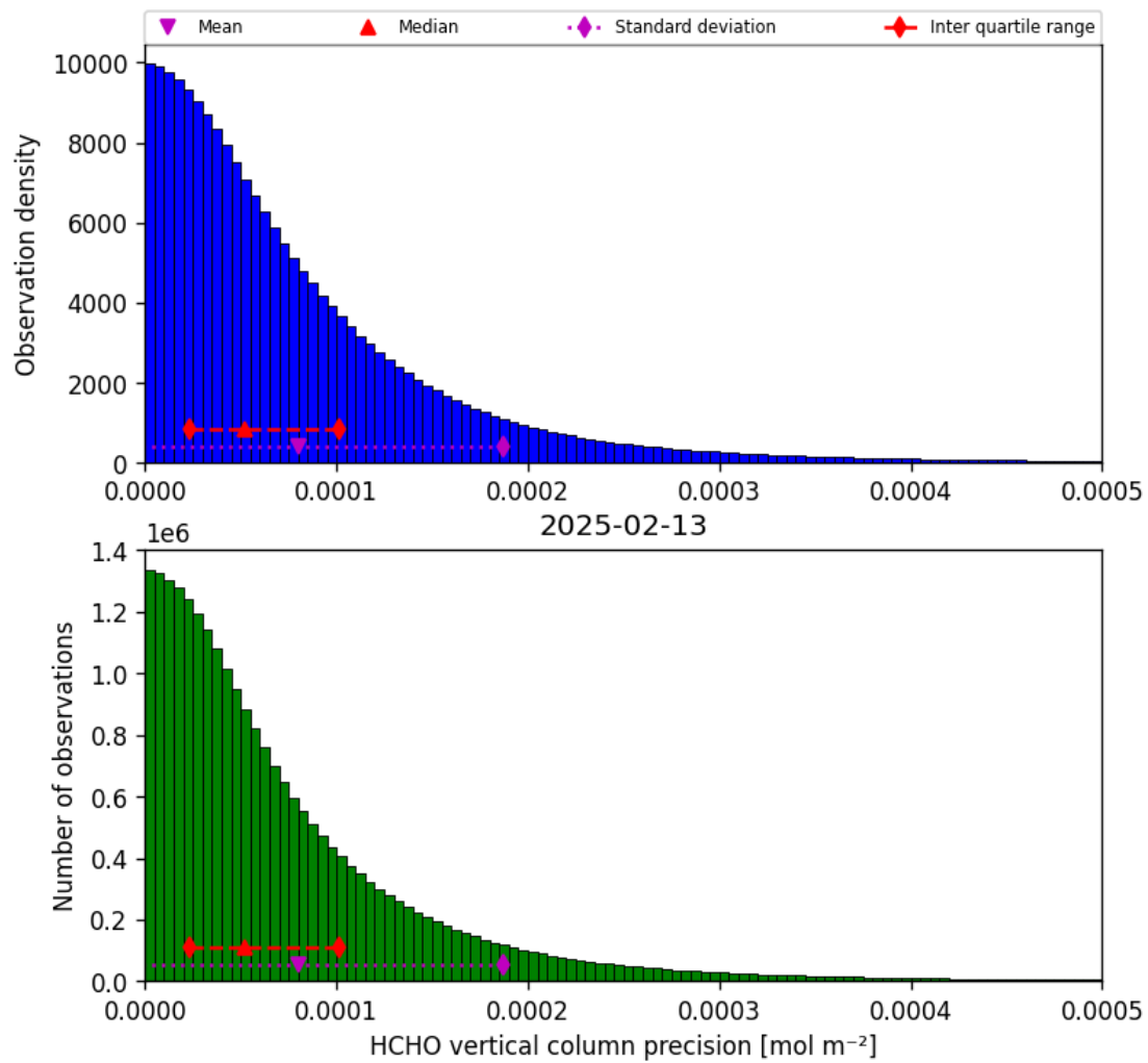
Figure 36: Histogram of “HCHO vertical column precision” for 2025-02-13 to 2025-02-14
