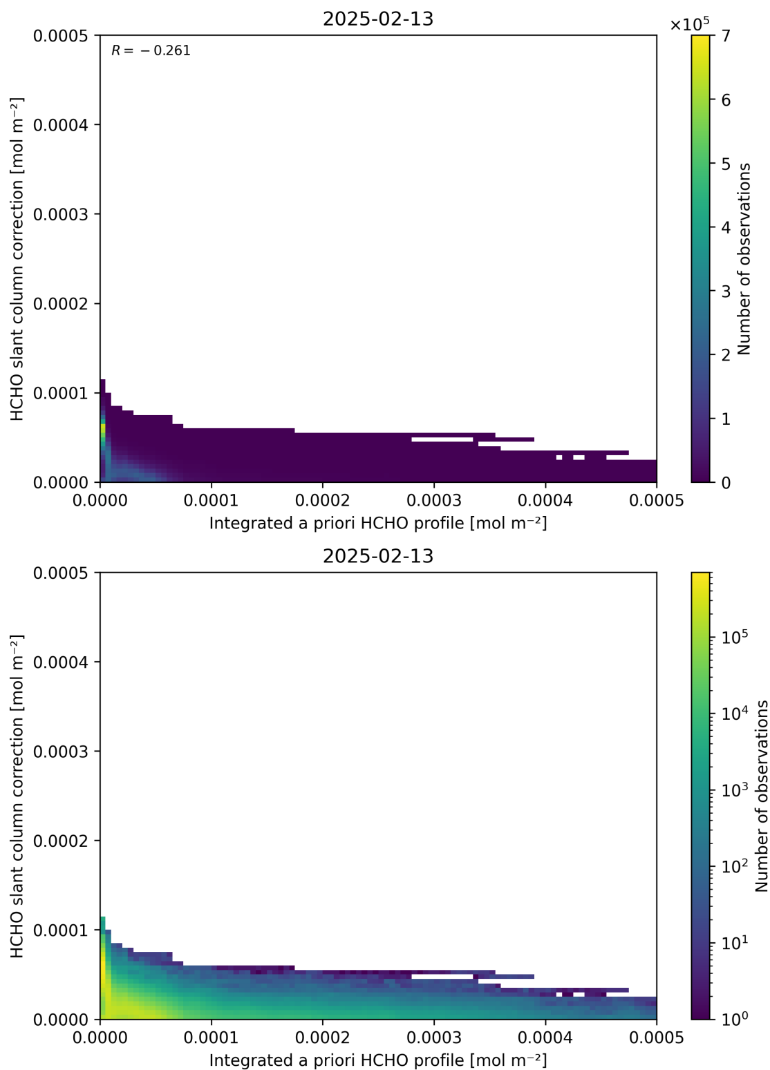
Figure 152: Scatter density plot of “Integrated a priori HCHO profile” against “HCHO slant column correction” for 2025-02-13 to 2025-02-14.
