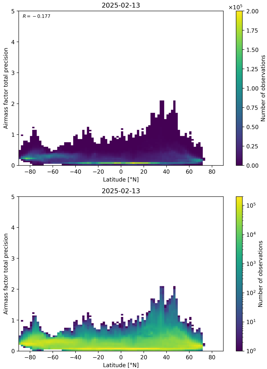
Figure 162: Scatter density plot of “Latitude” against “Airmass factor total precision” for 2025-02-13 to 2025-02-14.
