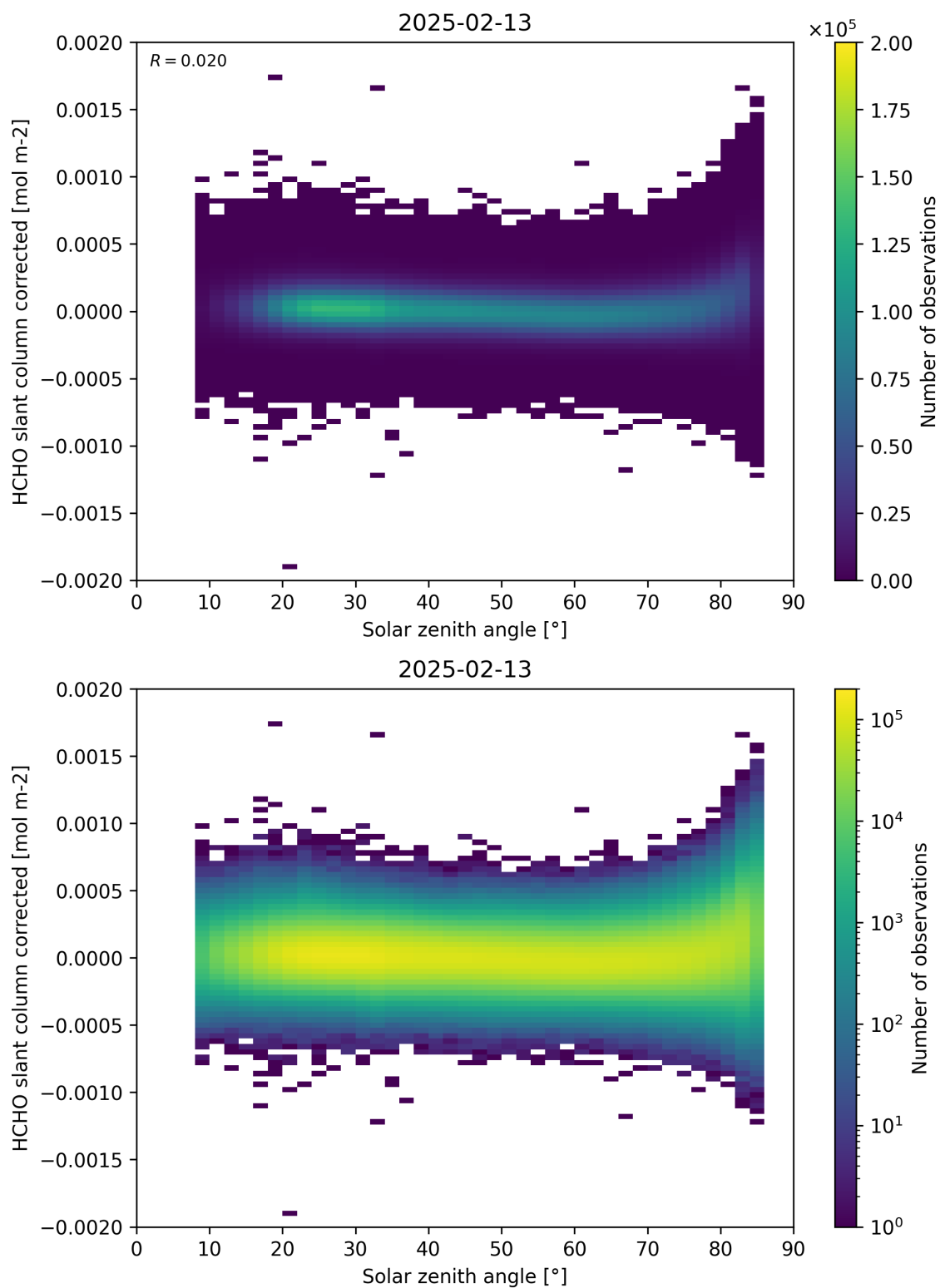
Figure 171: Scatter density plot of “Solar zenith angle” against “HCHO slant column corrected” for 2025-02-13 to 2025-02-14.
