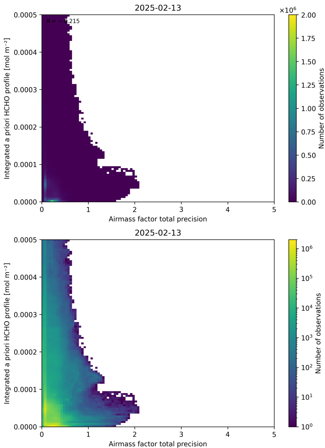
Figure 111: Scatter density plot of “Airmass factor total precision” against “Integrated a priori HCHO profile” for 2025-02-13 to 2025-02-14.
