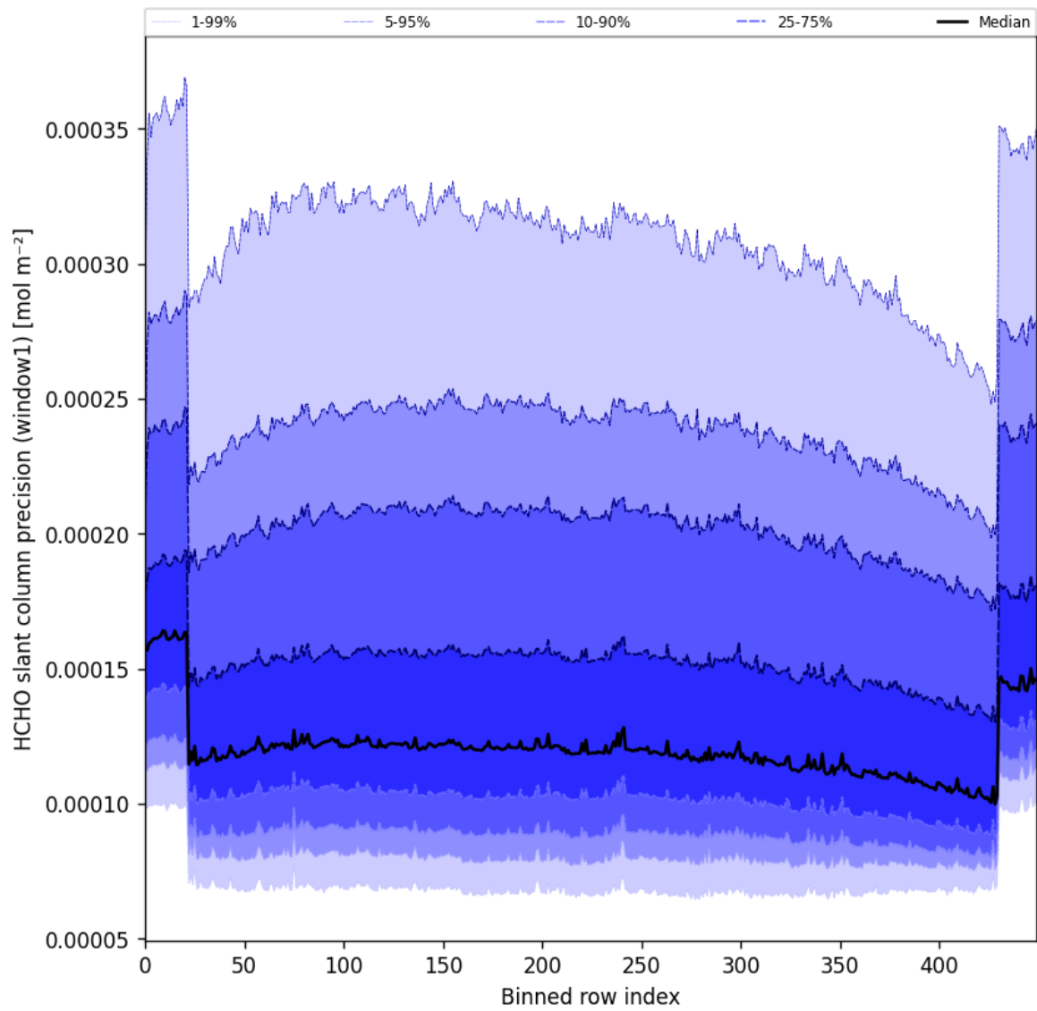
Figure 53: Along track statistics of "HCHO slant column precision (window1)" for 2025-02-13 to 2025-02-14
