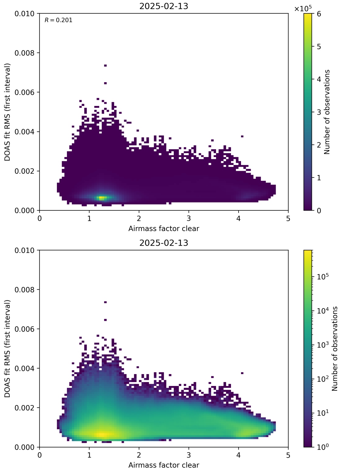
Figure 71: Scatter density plot of “Airmass factor clear” against “DOAS fit RMS (first interval)” for 2025-02-13 to 2025-02-14.
