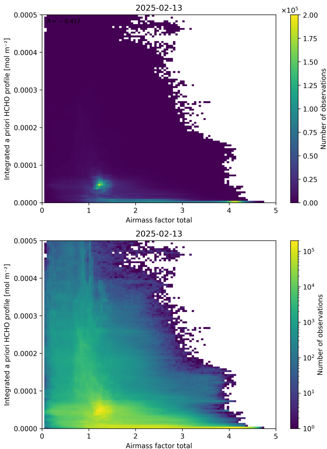
Figure 104: Scatter density plot of “Airmass factor total” against “Integrated a priori HCHO profile” for 2025-02-13 to 2025-02-14.
