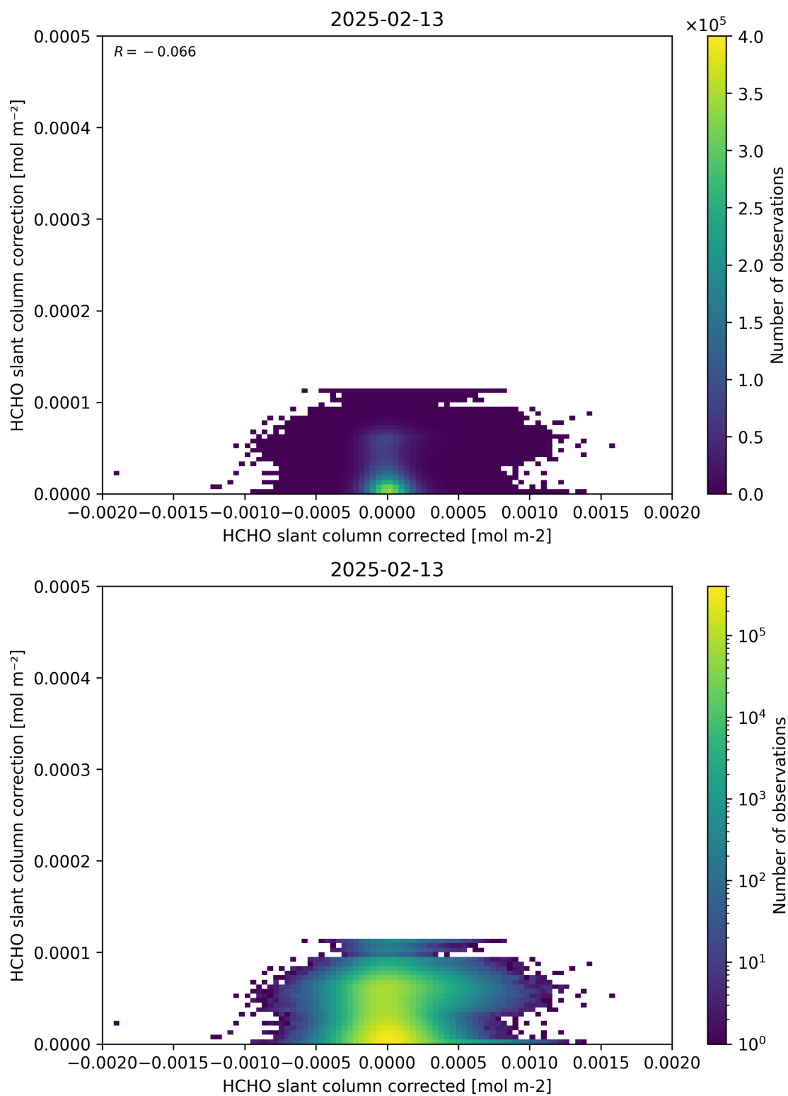
Figure 77: Scatter density plot of “HCHO slant column corrected” against “HCHO slant column correction” for 2025-02-13 to 2025-02-14.
