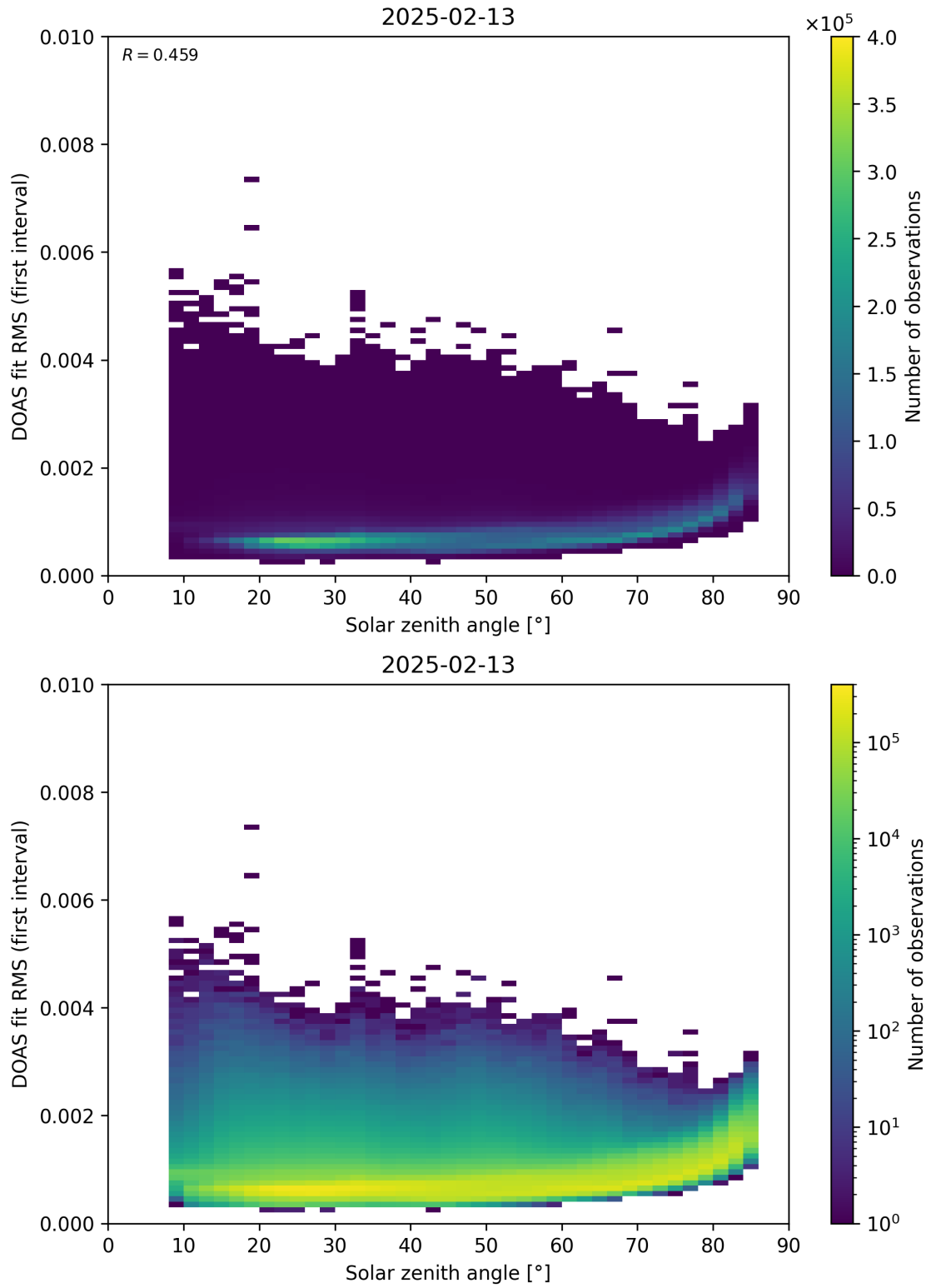
Figure 167: Scatter density plot of “Solar zenith angle” against “DOAS fit RMS (first interval)” for 2025-02-13 to 2025-02-14.
