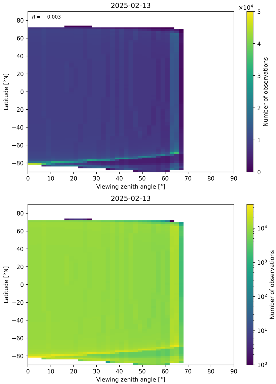
Figure 196: Scatter density plot of “Viewing zenith angle” against “Latitude” for 2025-02-13 to 2025-02-14.
