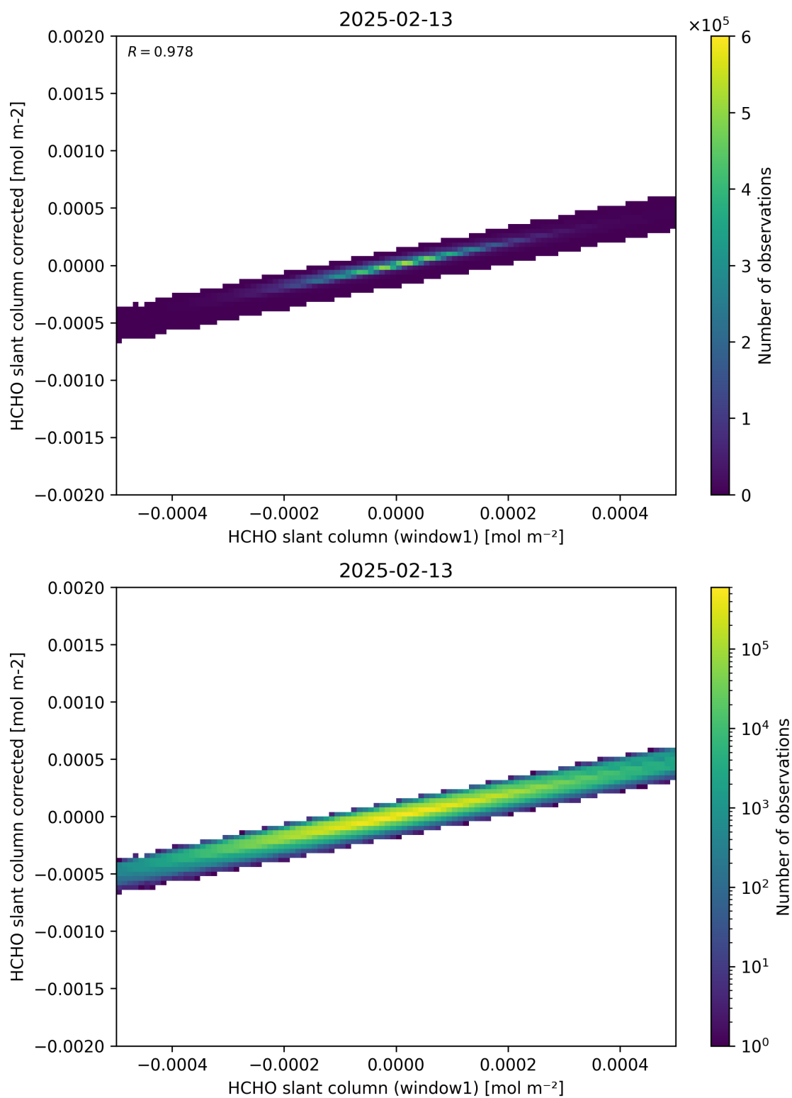
Figure 82: Scatter density plot of “HCHO slant column (window1)” against “HCHO slant column corrected” for 2025-02-13 to 2025-02-14.
