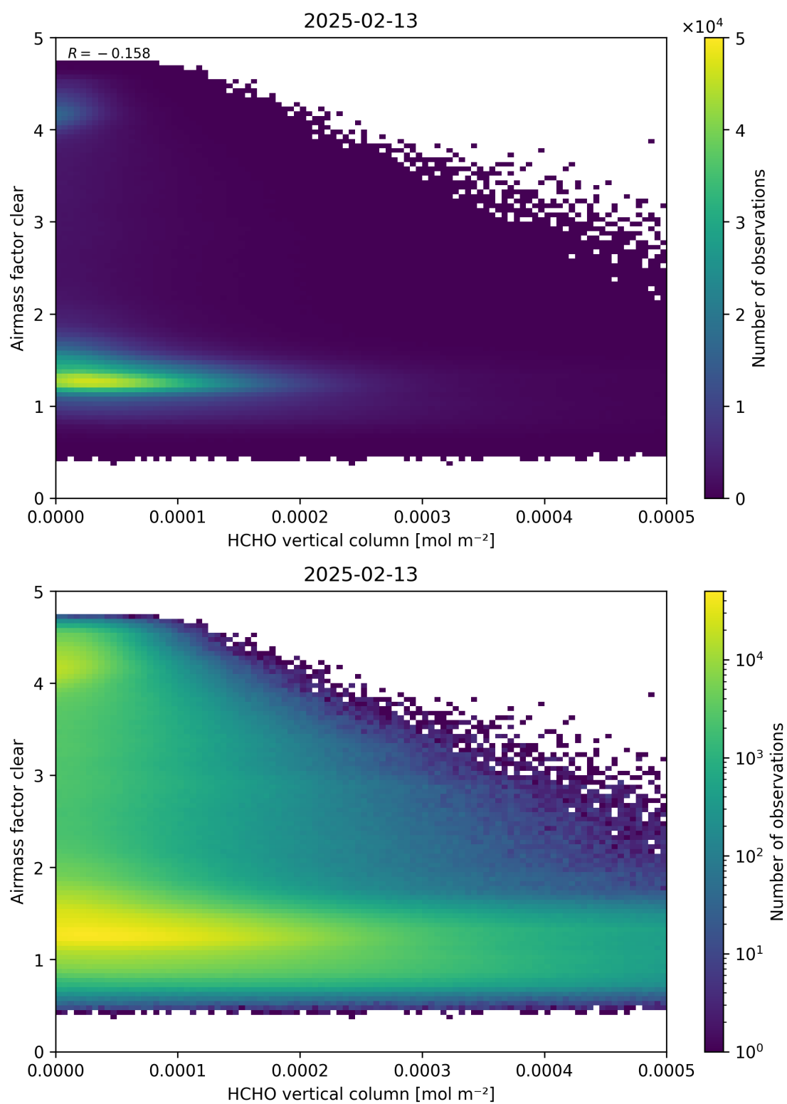
Figure 126: Scatter density plot of “HCHO vertical column” against “Airmass factor clear” for 2025-02-13 to 2025-02-14.
