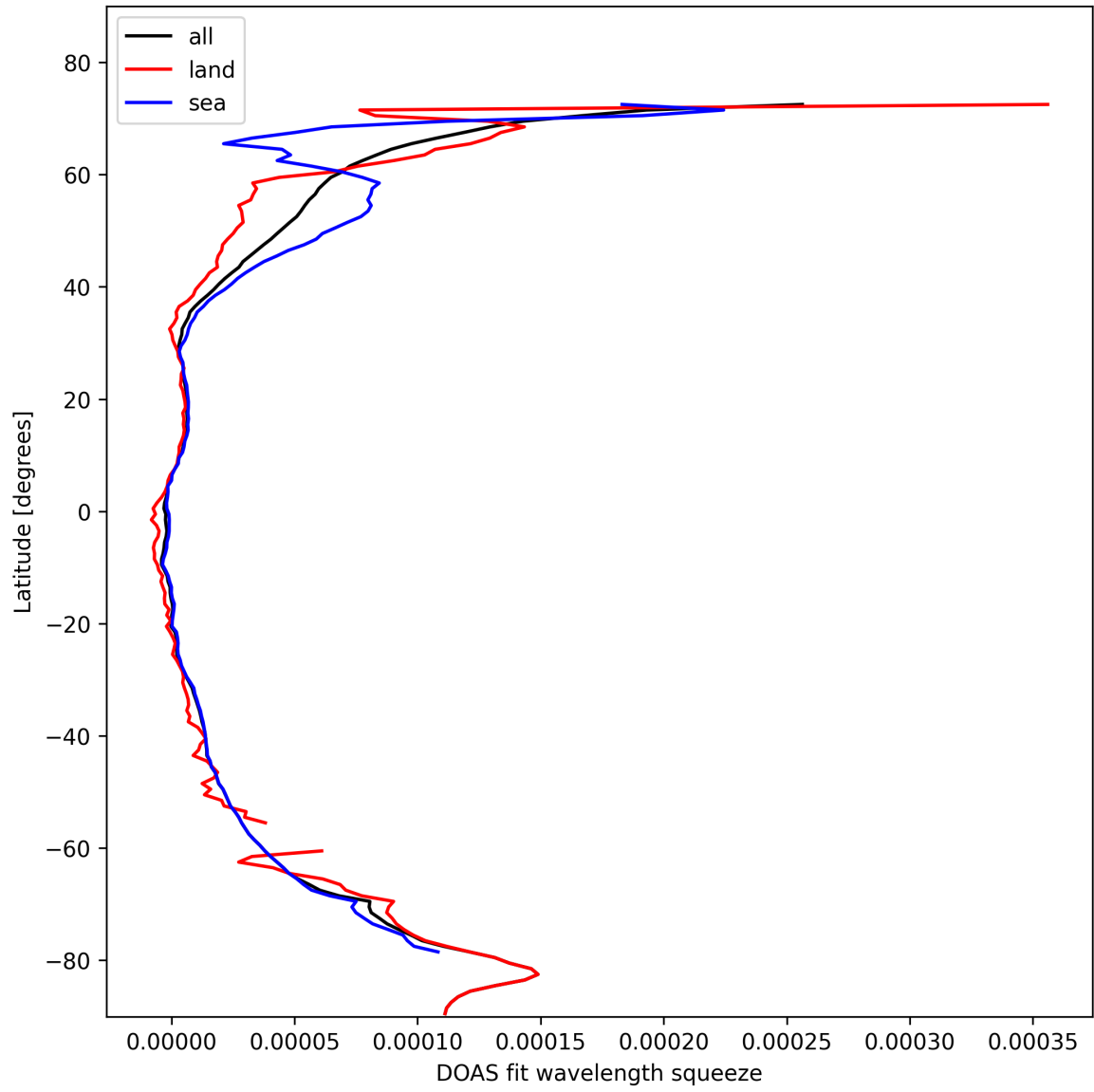
Figure 31: Zonal average of “DOAS fit wavelength squeeze” for 2025-02-13 to 2025-02-14.
