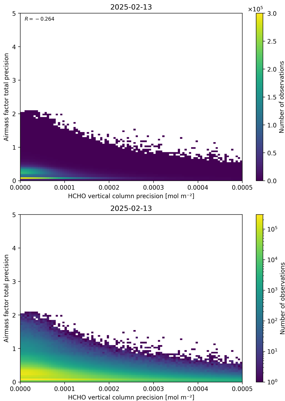
Figure 145: Scatter density plot of “HCHO vertical column precision” against “Airmass factor total precision” for 2025-02-13 to 2025-02-14.
