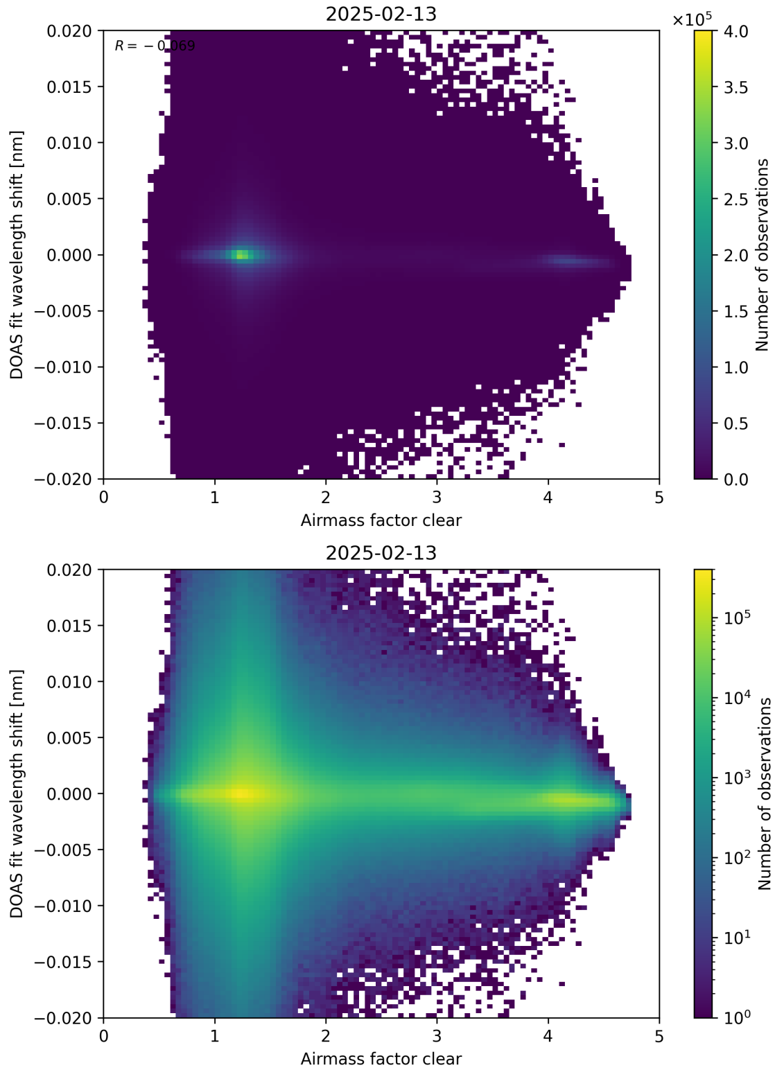
Figure 72: Scatter density plot of “Airmass factor clear” against “DOAS fit wavelength shift” for 2025-02-13 to 2025-02-14.
