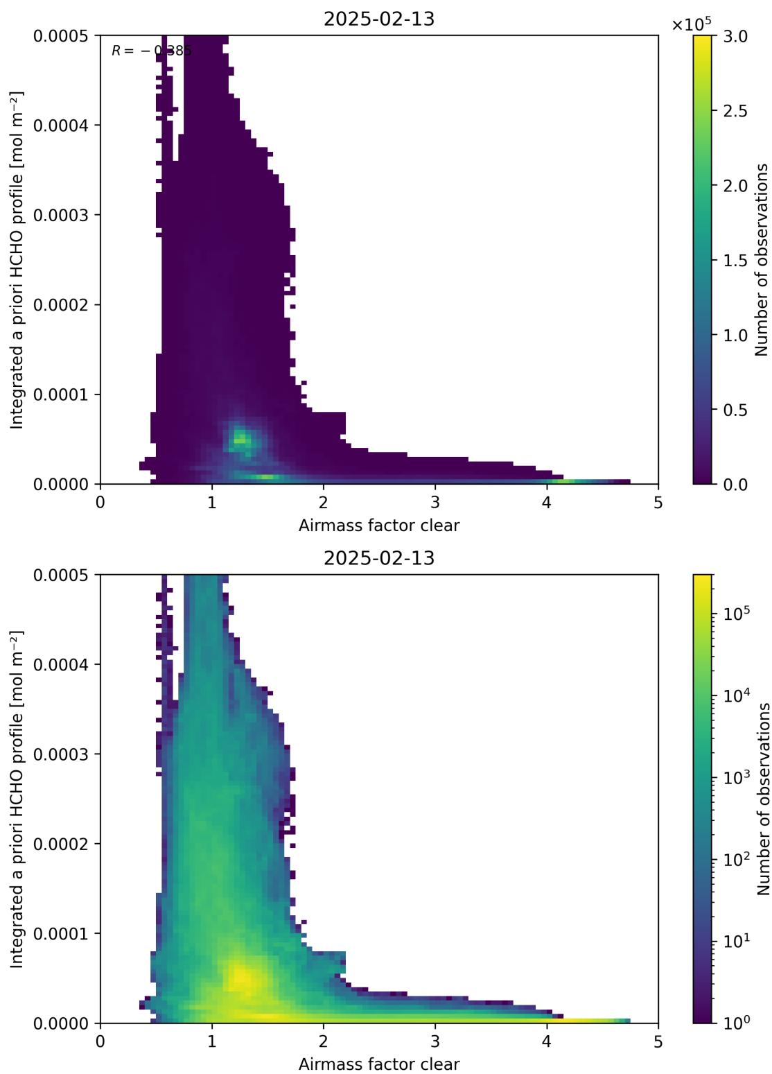
Figure 76: Scatter density plot of “Airmass factor clear” against “Integrated a priori HCHO profile” for 2025-02-13 to 2025-02-14.
