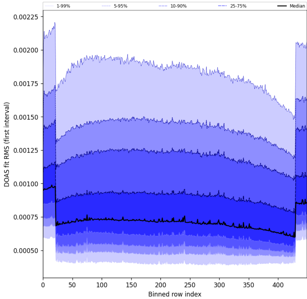
Figure 60: Along track statistics of “DOAS fit RMS (first interval)” for 2025-02-13 to 2025-02-14
