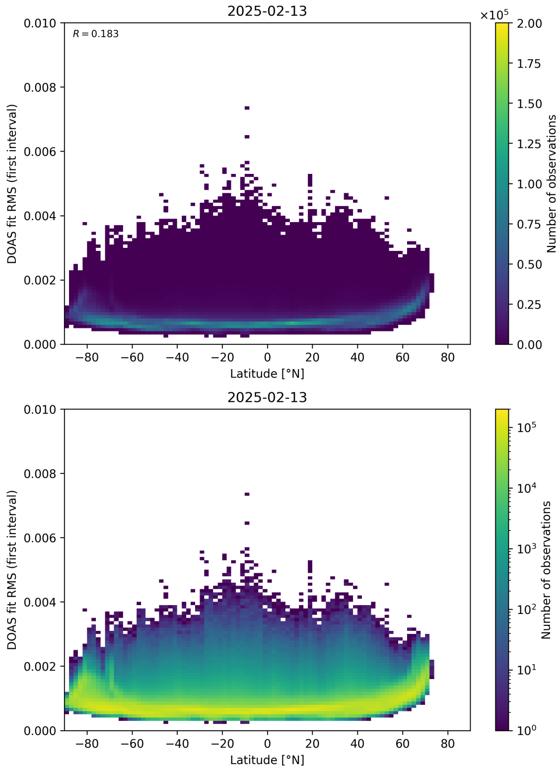
Figure 153: Scatter density plot of “Latitude” against “DOAS fit RMS (first interval)” for 2025-02-13 to 2025-02-14.
