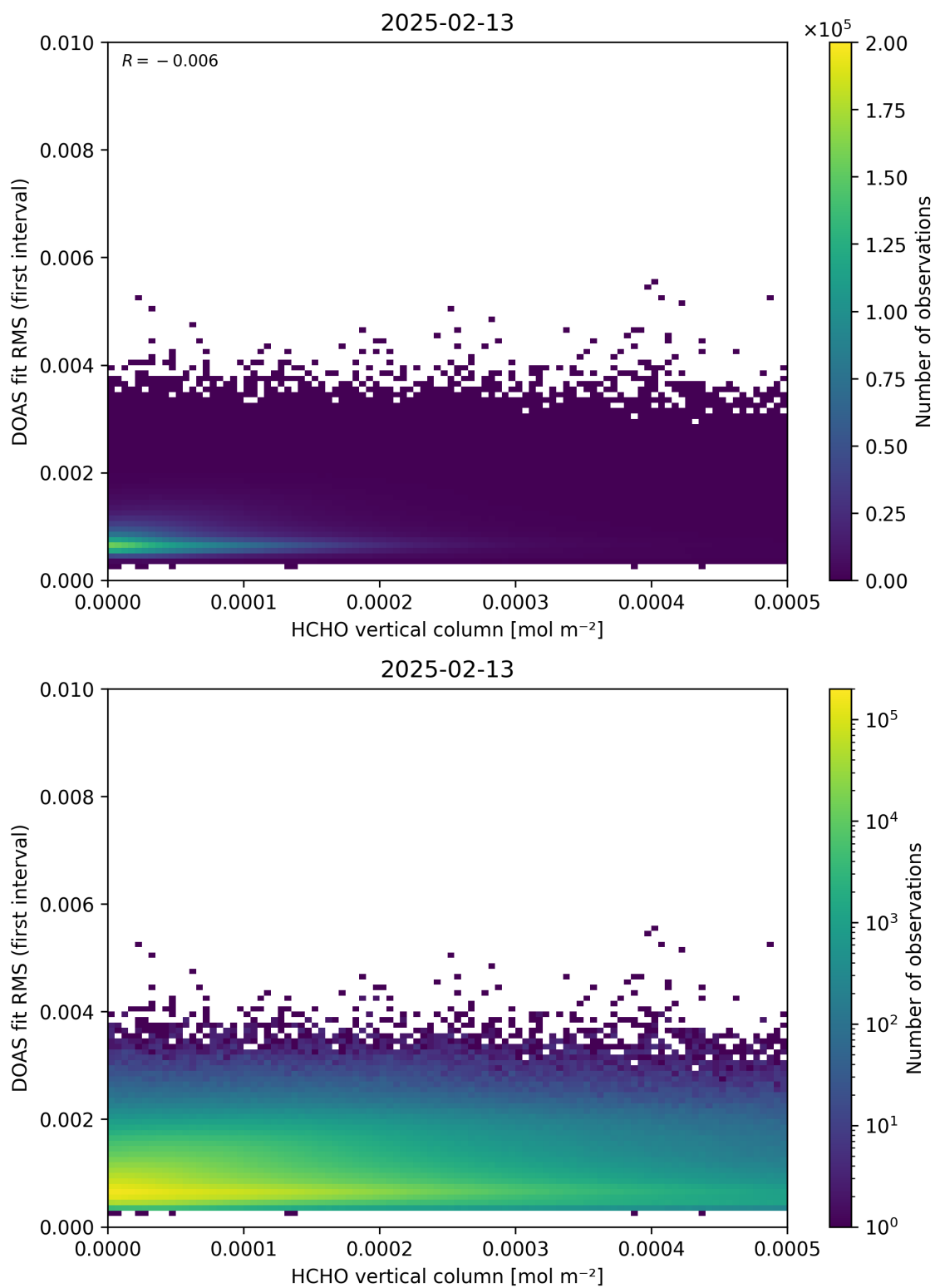
Figure 123: Scatter density plot of “HCHO vertical column” against “DOAS fit RMS (first interval)” for 2025-02-13 to 2025-02-14.
