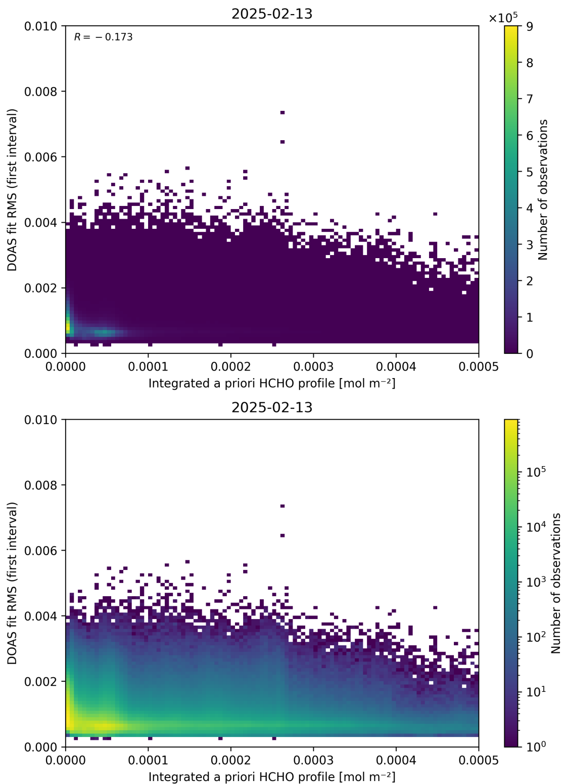
Figure 148: Scatter density plot of “Integrated a priori HCHO profile” against “DOAS fit RMS (first interval)” for 2025-02-13 to 2025-02-14.
