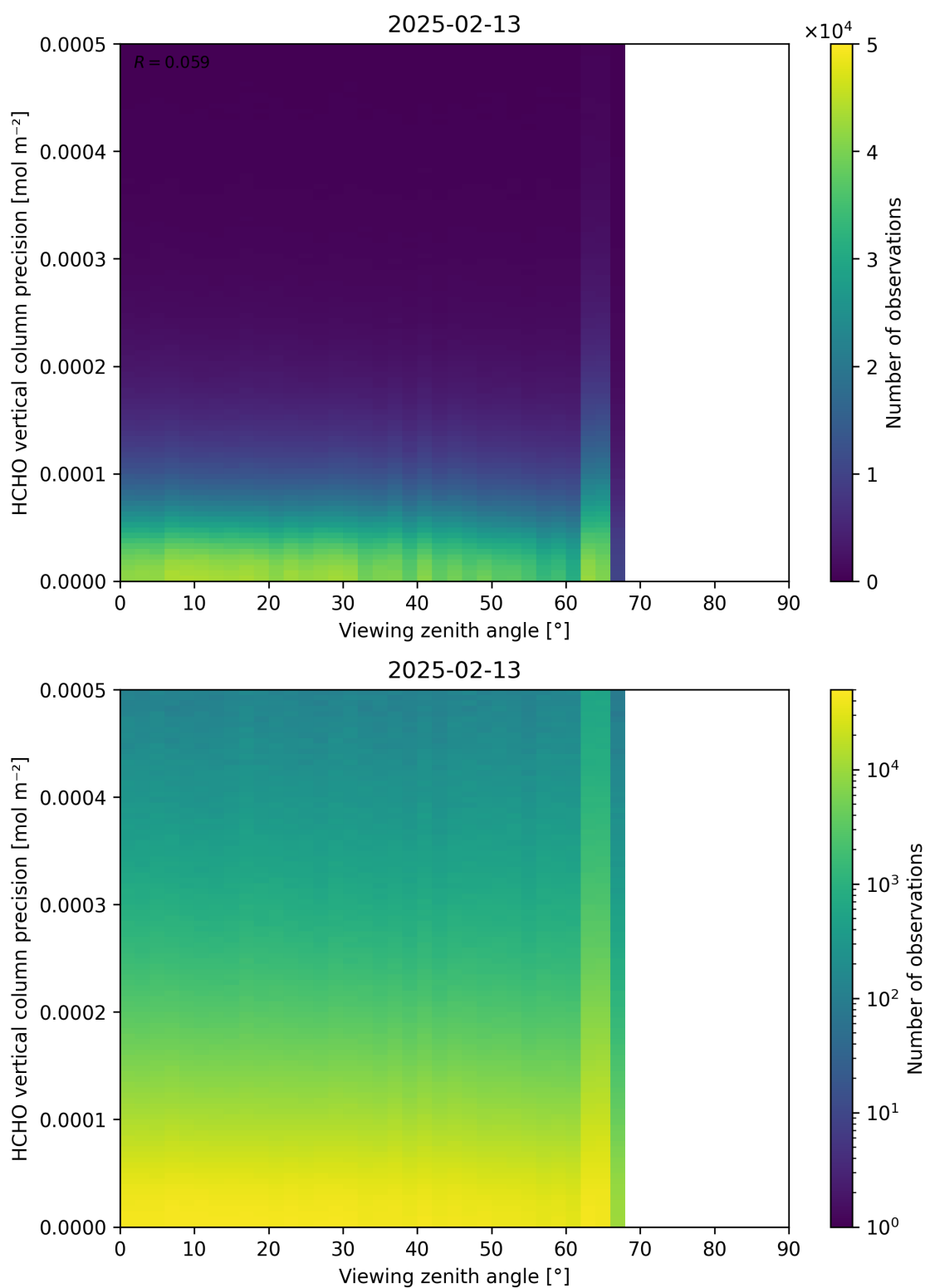
Figure 194: Scatter density plot of “Viewing zenith angle” against “HCHO vertical column precision” for 2025-02-13 to 2025-02-14.
