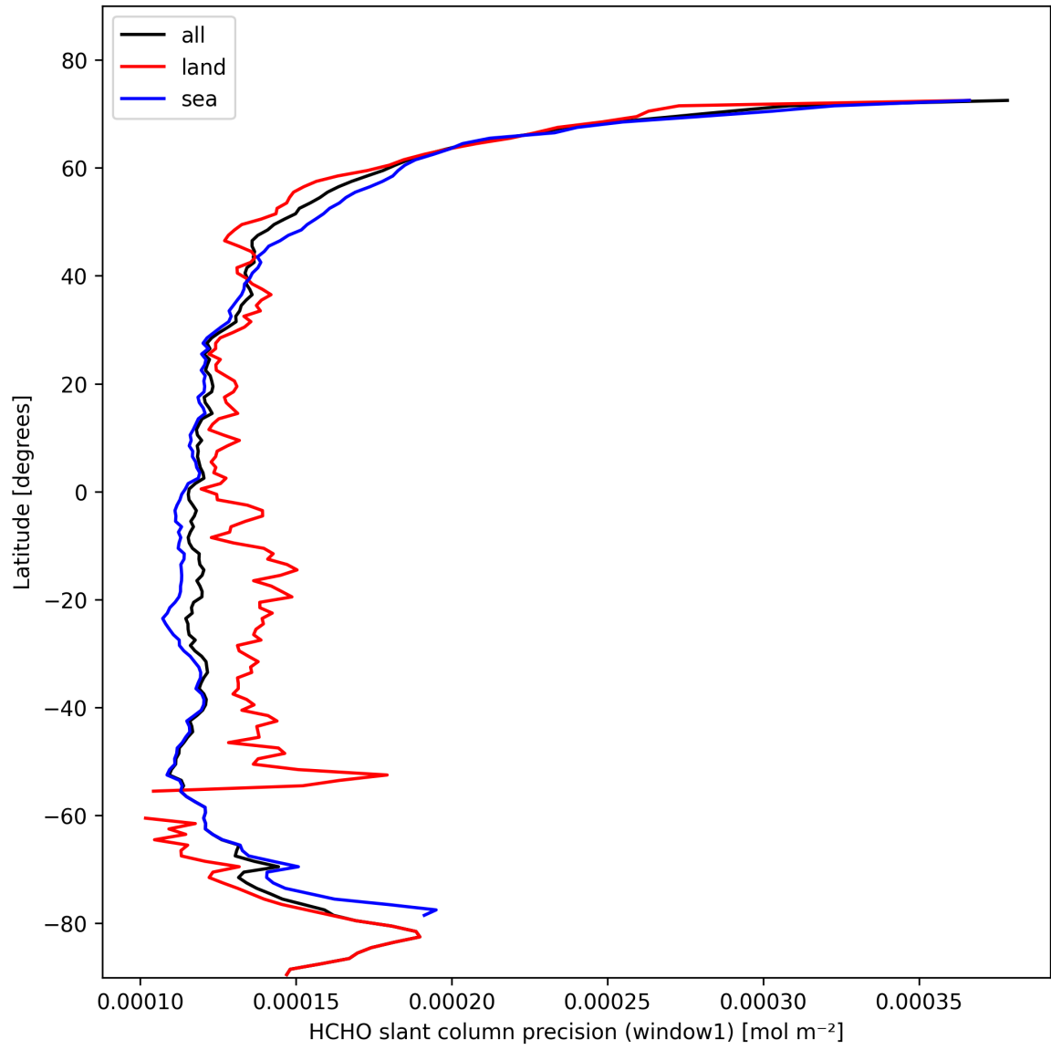
Figure 25: Zonal average of "HCHO slant column precision (window1)" for 2025-02-13 to 2025-02-14.
