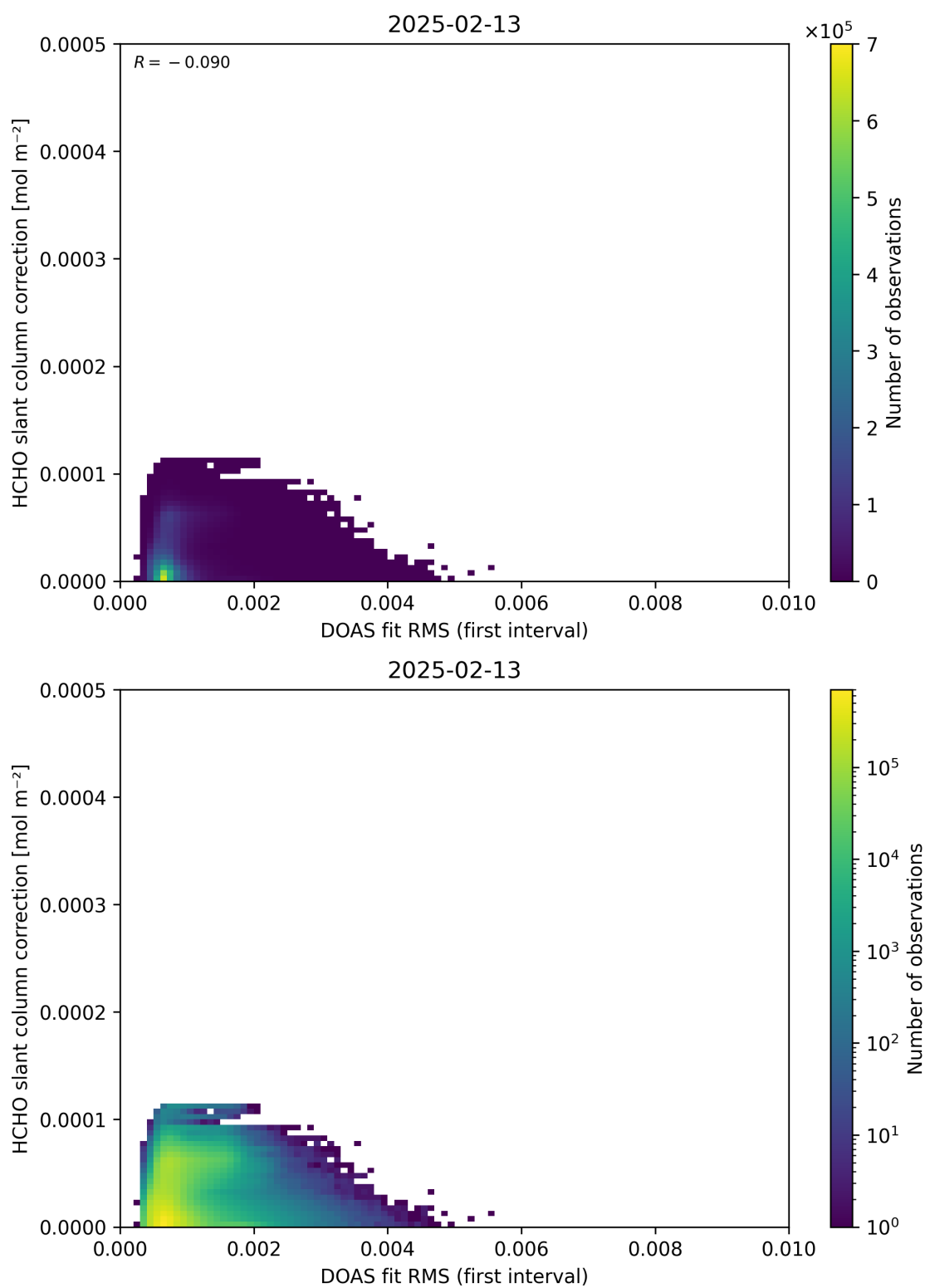
Figure 63: Scatter density plot of “DOAS fit RMS (first interval)” against “HCHO slant column correction” for 2025-02-13 to 2025-02-14.
