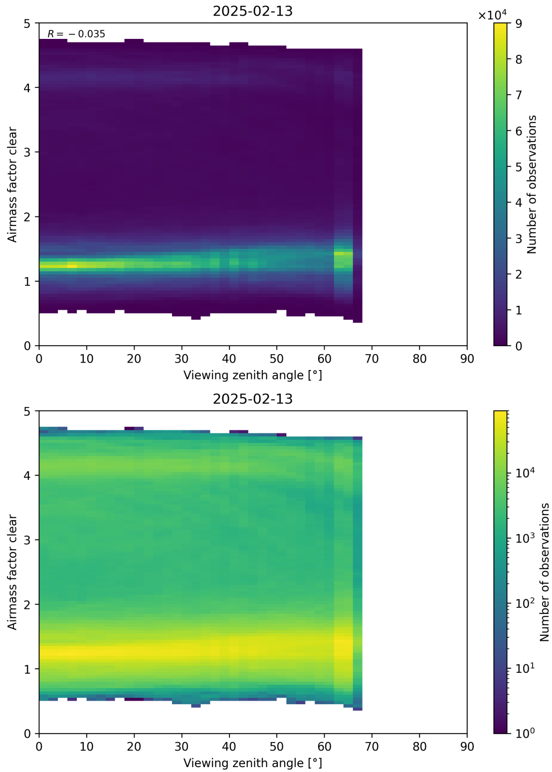
Figure 185: Scatter density plot of “Viewing zenith angle” against “Airmass factor clear” for 2025-02-13 to 2025-02-14.
