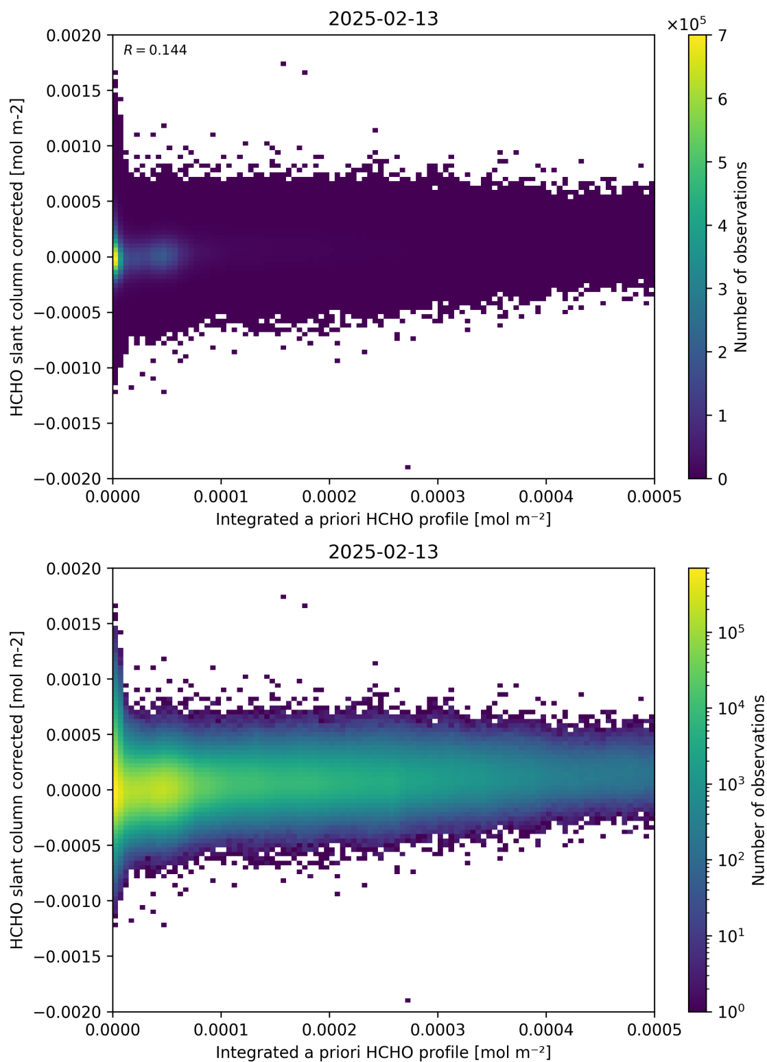
Figure 151: Scatter density plot of “Integrated a priori HCHO profile” against “HCHO slant column corrected” for 2025-02-13 to 2025-02-14.
