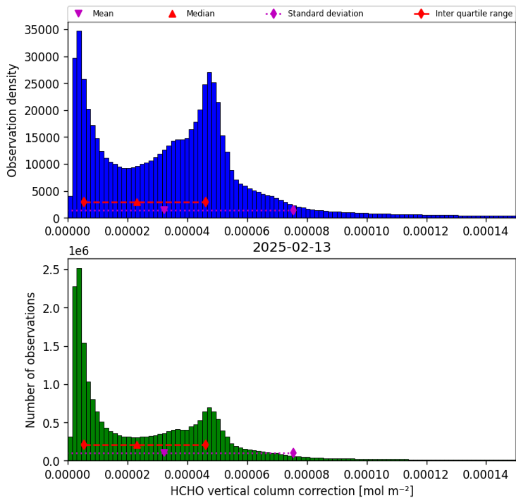
Figure 37: Histogram of “HCHO vertical column correction” for 2025-02-13 to 2025-02-14
