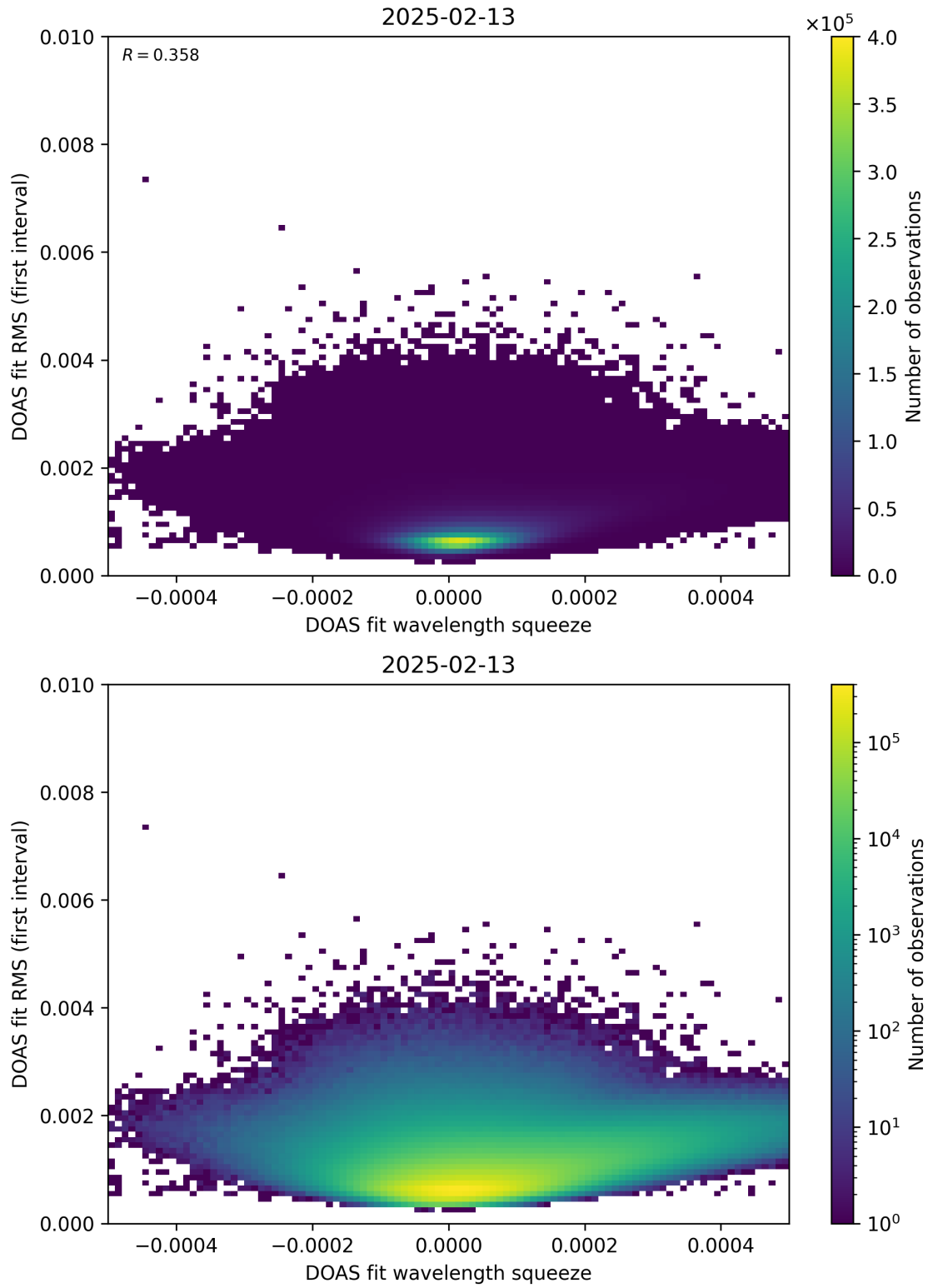
Figure 68: Scatter density plot of “DOAS fit wavelength squeeze” against “DOAS fit RMS (first interval)” for 2025-02-13 to 2025-02-14.
