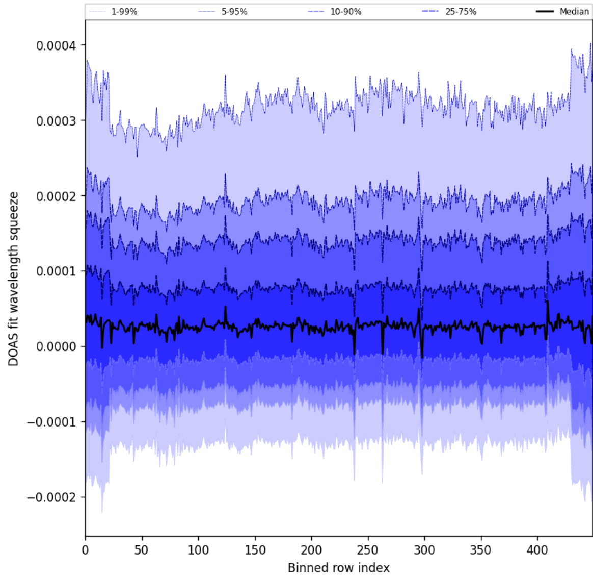
Figure 59: Along track statistics of “DOAS fit wavelength squeeze” for 2025-02-13 to 2025-02-14
