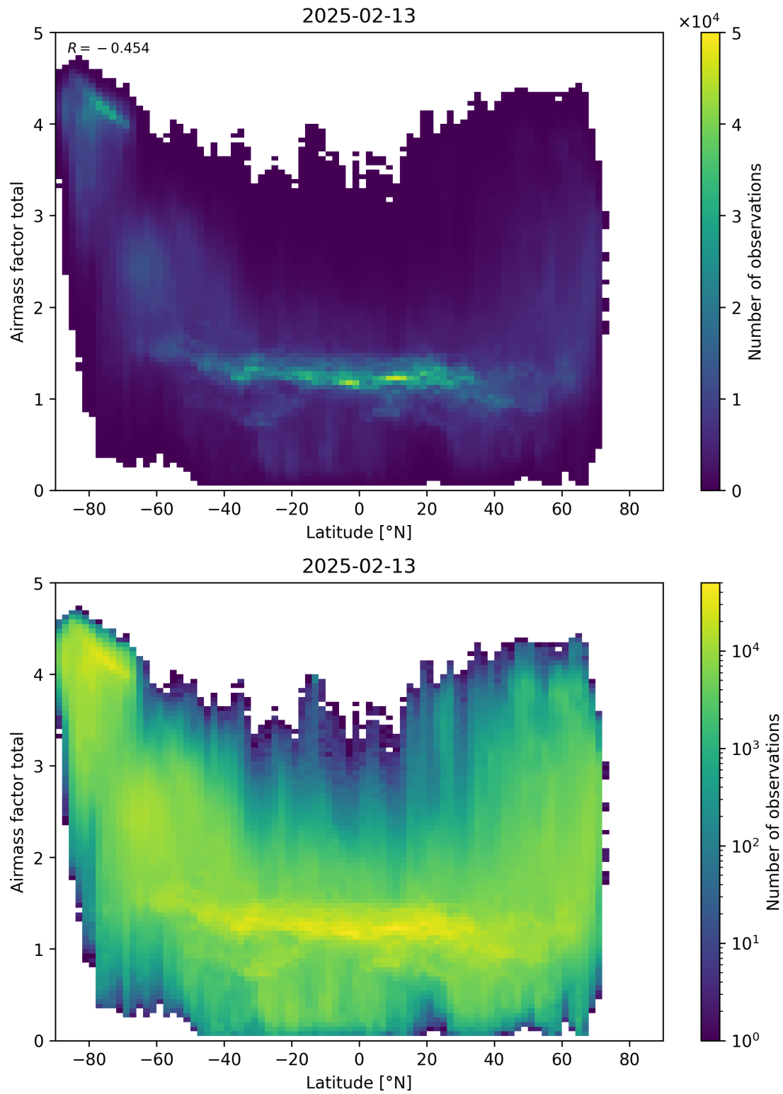
Figure 161: Scatter density plot of “Latitude” against “Airmass factor total” for 2025-02-13 to 2025-02-14.
