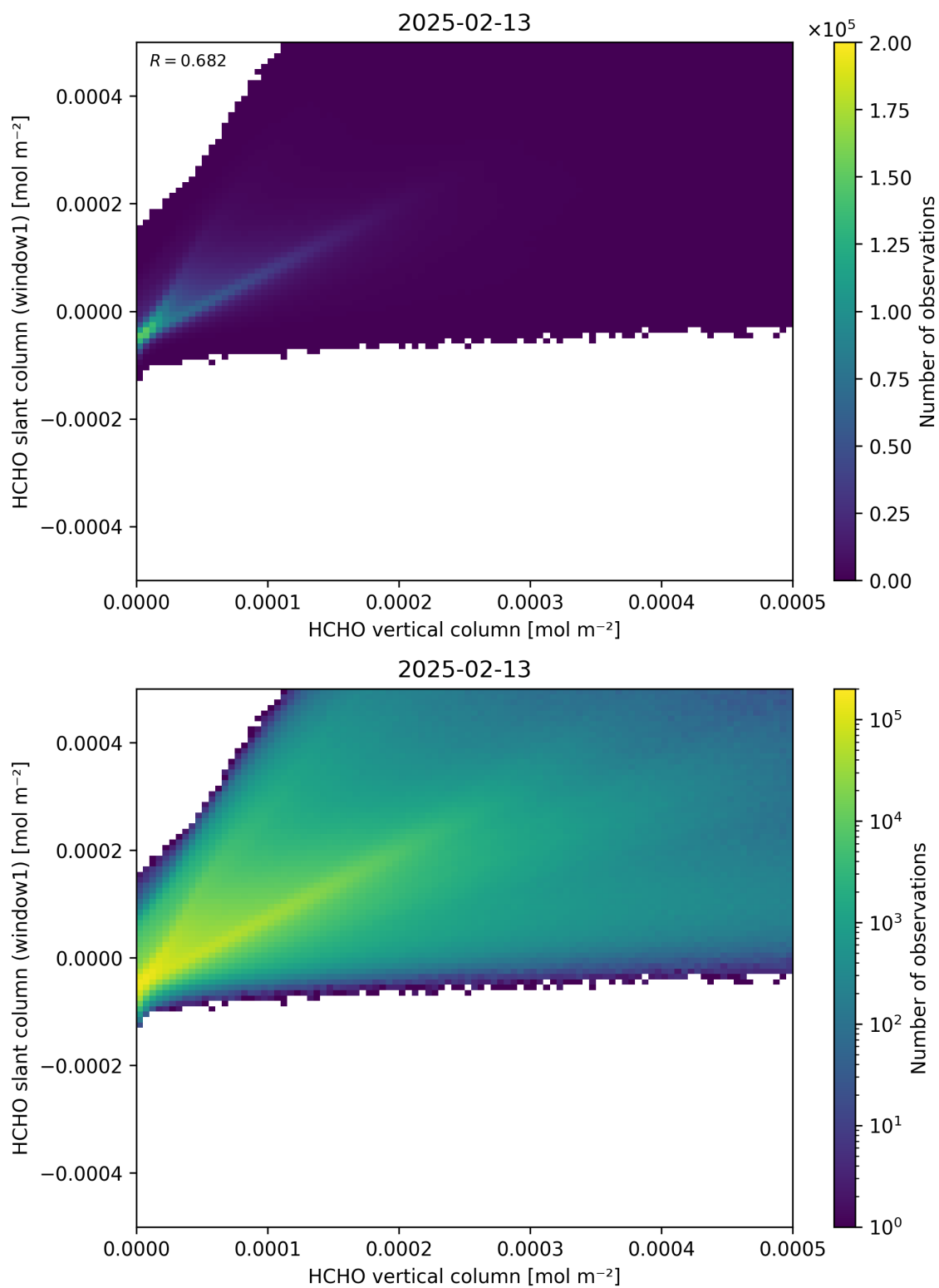
Figure 129: Scatter density plot of “HCHO vertical column” against “HCHO slant column (window1)” for 2025-02-13 to 2025-02-14.
