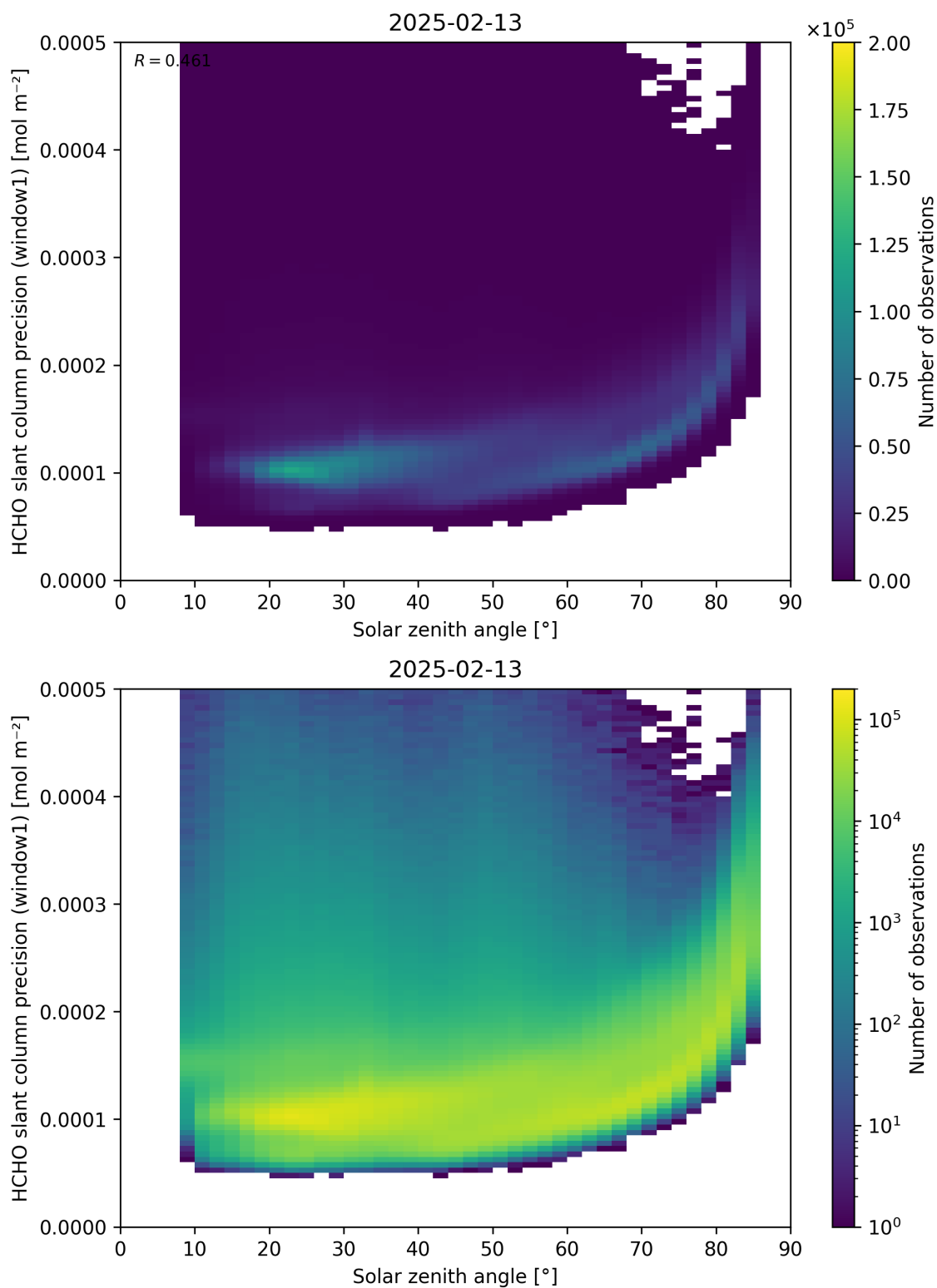
Figure 174: Scatter density plot of “Solar zenith angle” against “HCHO slant column precision (window1)” for 2025-02-13 to 2025-02-14.
