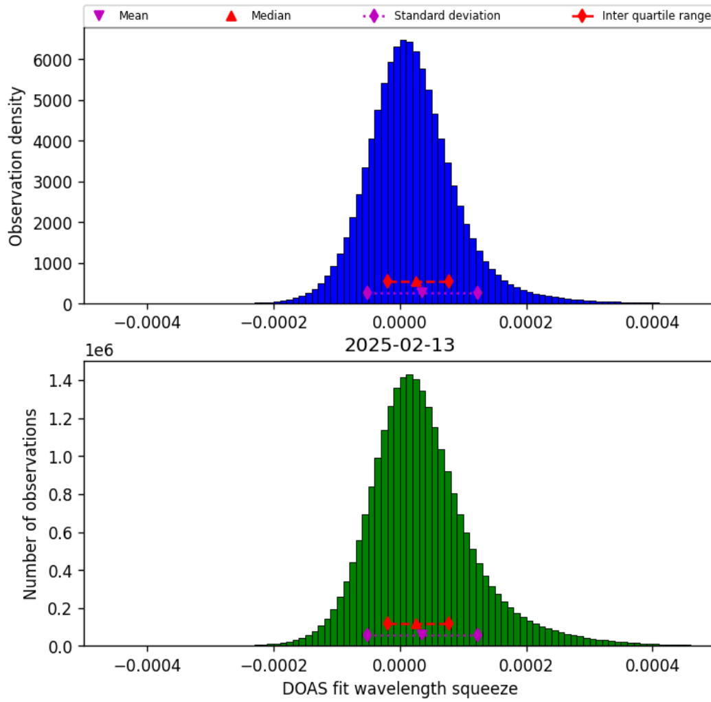
Figure 45: Histogram of “DOAS fit wavelength squeeze” for 2025-02-13 to 2025-02-14
