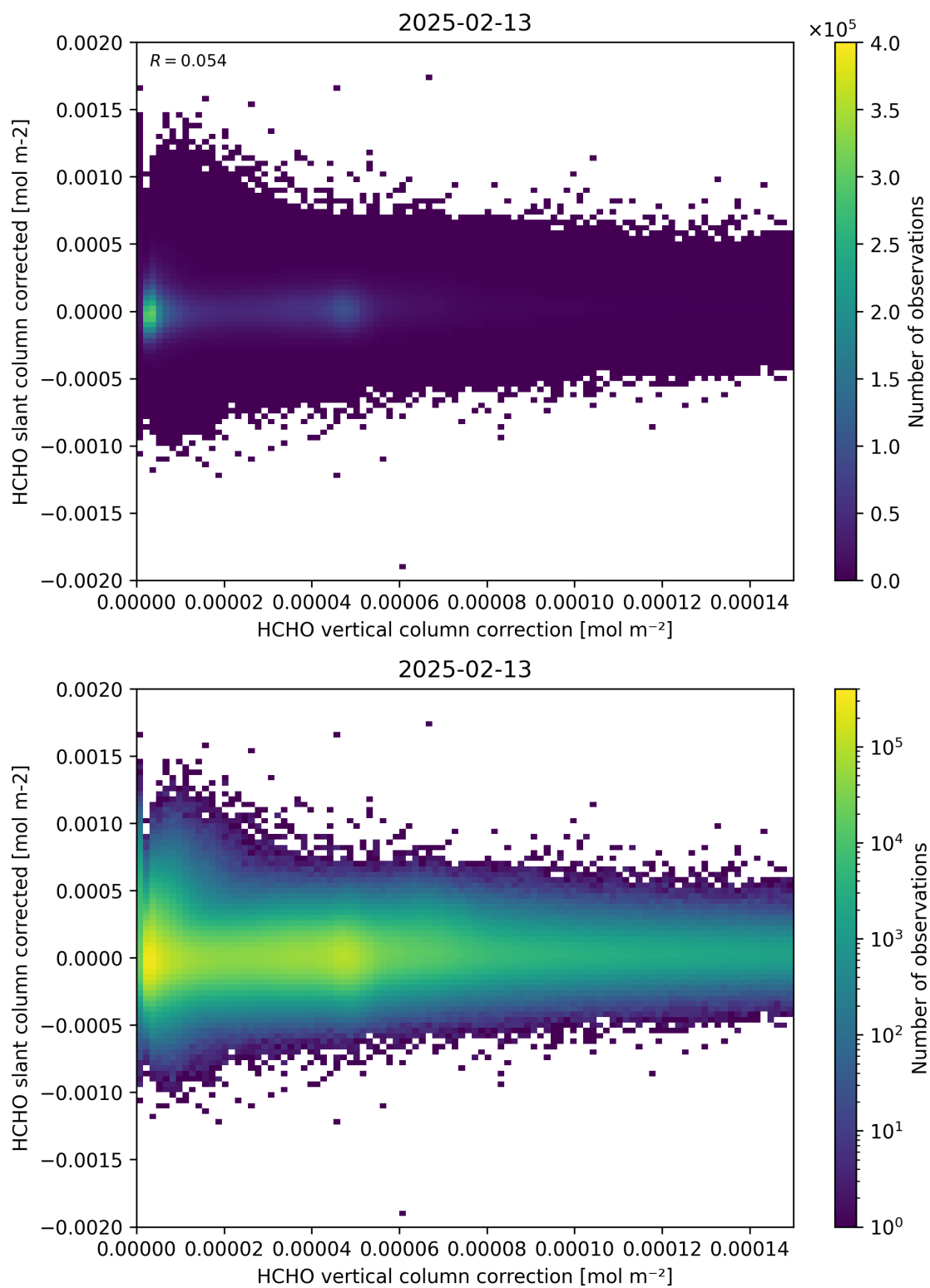
Figure 116: Scatter density plot of “HCHO vertical column correction” against “HCHO slant column corrected” for 2025-02-13 to 2025-02-14.
