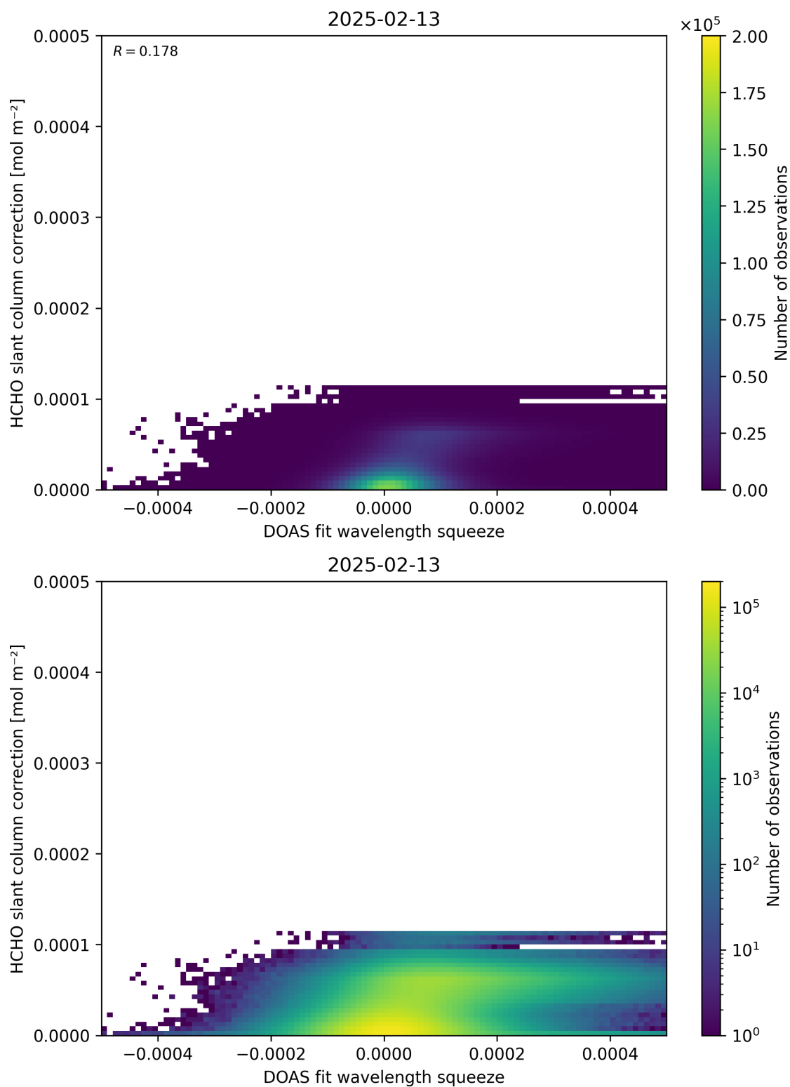
Figure 70: Scatter density plot of “DOAS fit wavelength squeeze” against “HCHO slant column correction” for 2025-02-13 to 2025-02-14.
