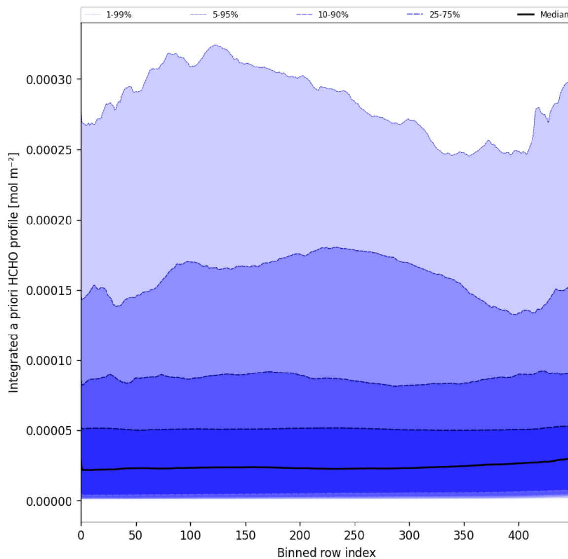
Figure 57: Along track statistics of "Integrated a priori HCHO profile" for 2025-02-13 to 2025-02-14
