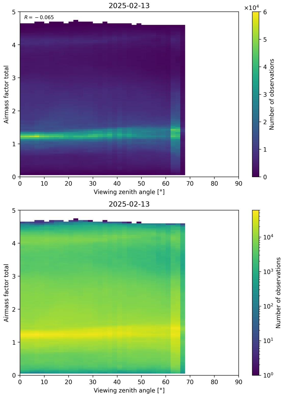
Figure 190: Scatter density plot of “Viewing zenith angle” against “Airmass factor total” for 2025-02-13 to 2025-02-14.
