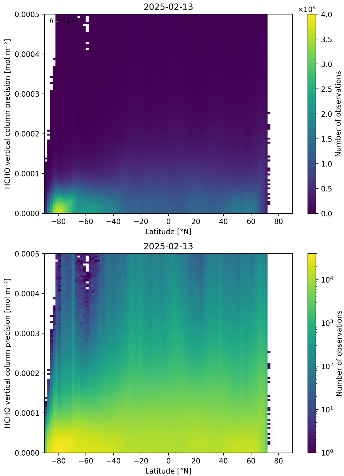
Figure 165: Scatter density plot of “Latitude” against “HCHO vertical column precision” for 2025-02-13 to 2025-02-14.
