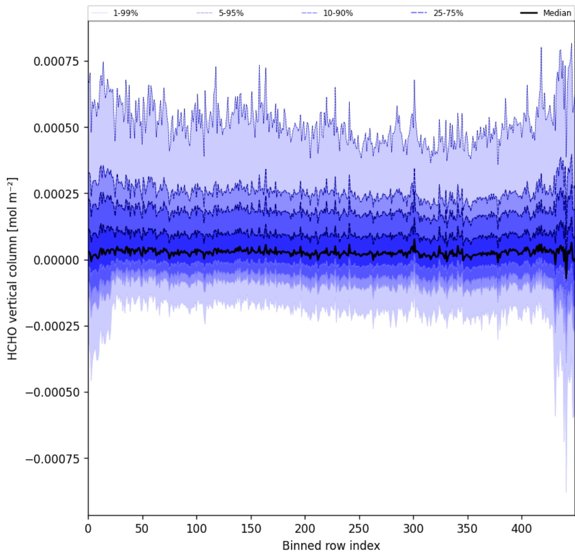
Figure 49: Along track statistics of “HCHO vertical column” for 2025-02-13 to 2025-02-14
