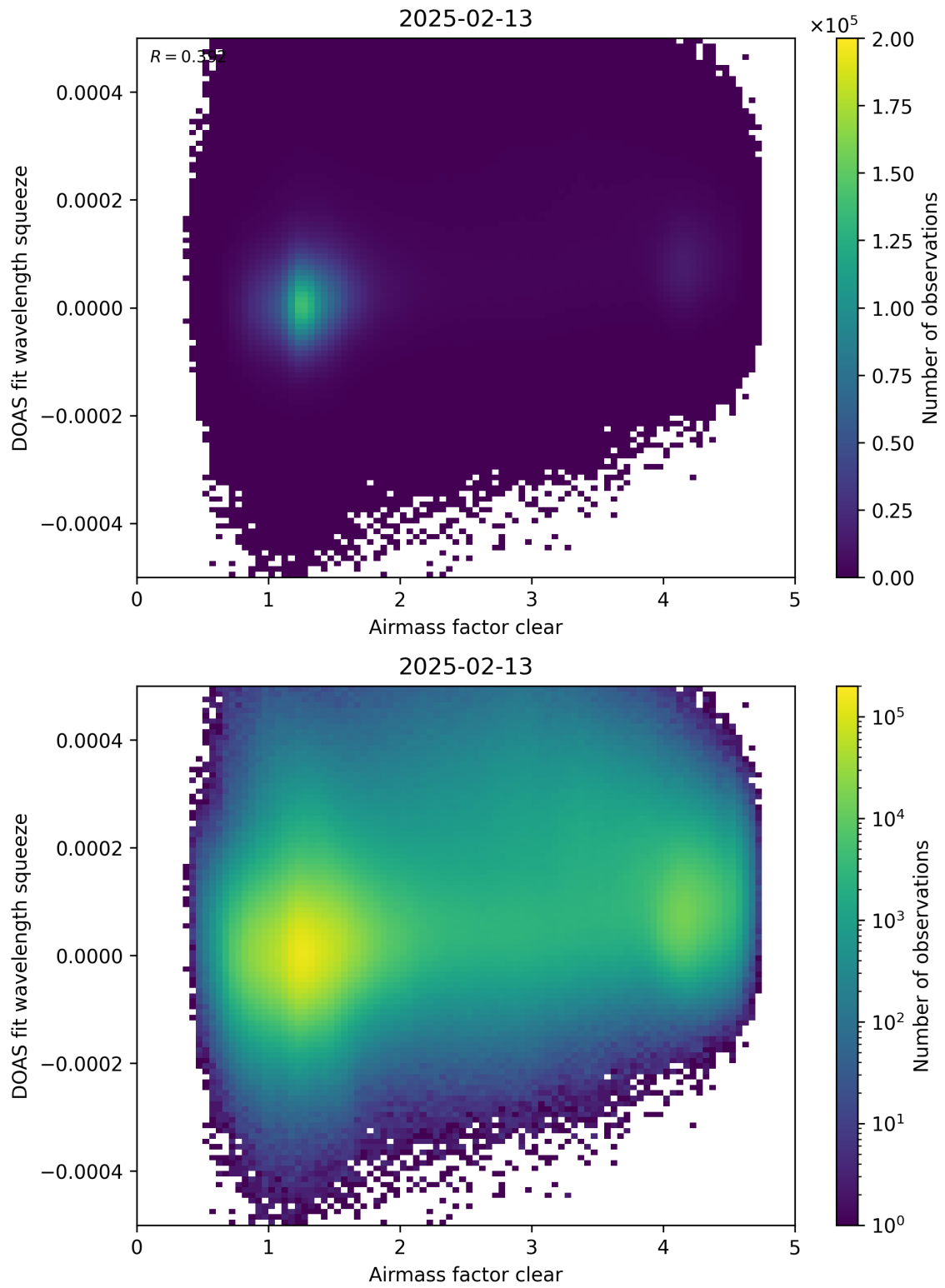
Figure 73: Scatter density plot of “Airmass factor clear” against “DOAS fit wavelength squeeze” for 2025-02-13 to 2025-02-14.
