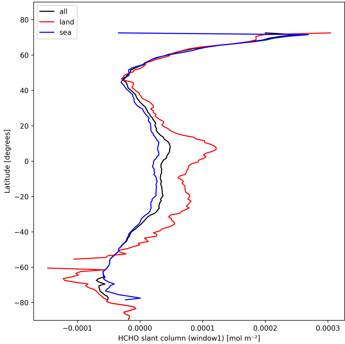
Figure 24: Zonal average of “HCHO slant column (window1)” for 2025-02-13 to 2025-02-14.
