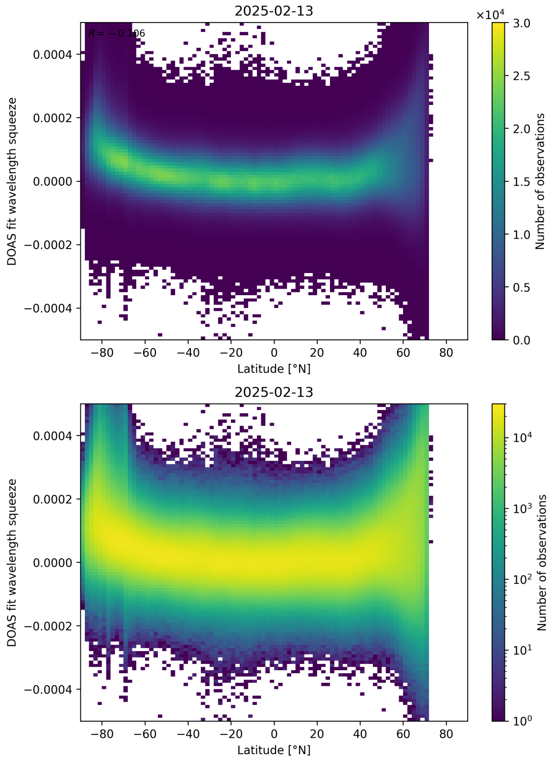
Figure 155: Scatter density plot of “Latitude” against “DOAS fit wavelength squeeze” for 2025-02-13 to 2025-02-14.
