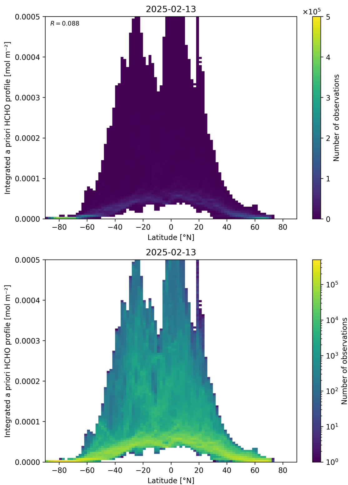
Figure 166: Scatter density plot of “Latitude” against “Integrated a priori HCHO profile” for 2025-02-13 to 2025-02-14.
