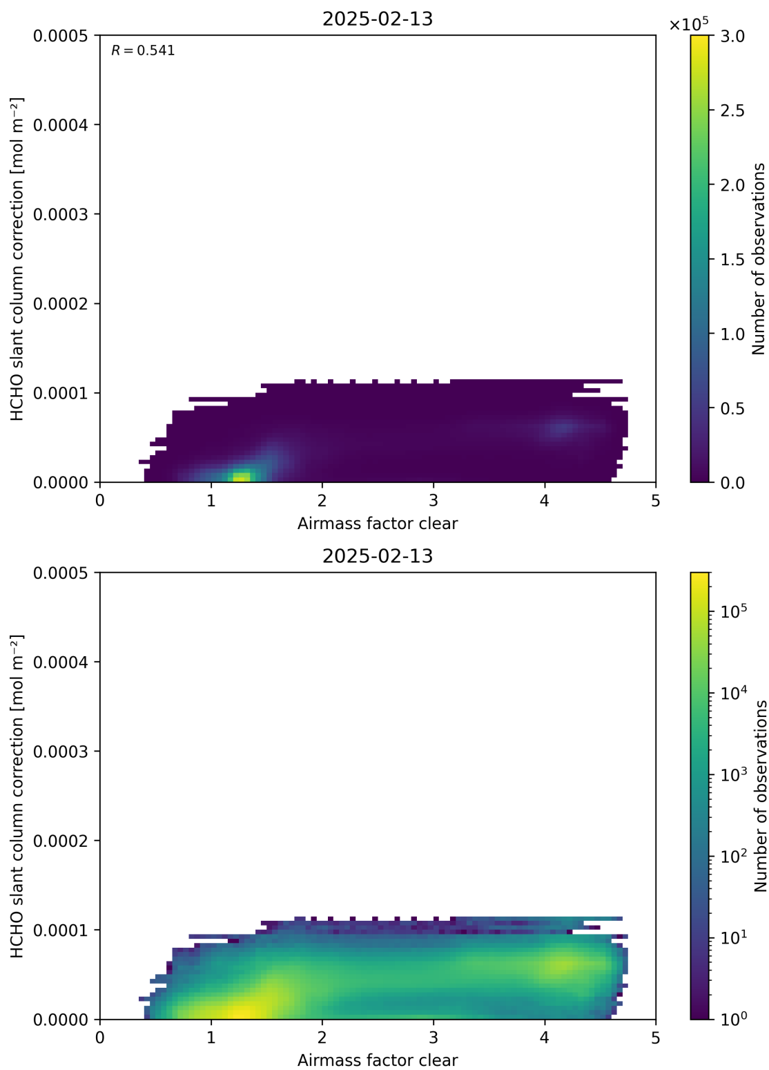
Figure 75: Scatter density plot of “Airmass factor clear” against “HCHO slant column correction” for 2025-02-13 to 2025-02-14.
