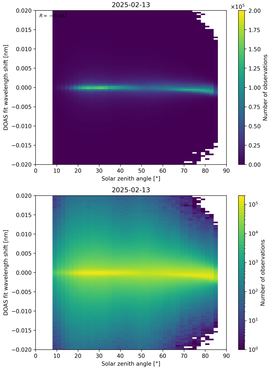
Figure 168: Scatter density plot of “Solar zenith angle” against “DOAS fit wavelength shift” for 2025-02-13 to 2025-02-14.
