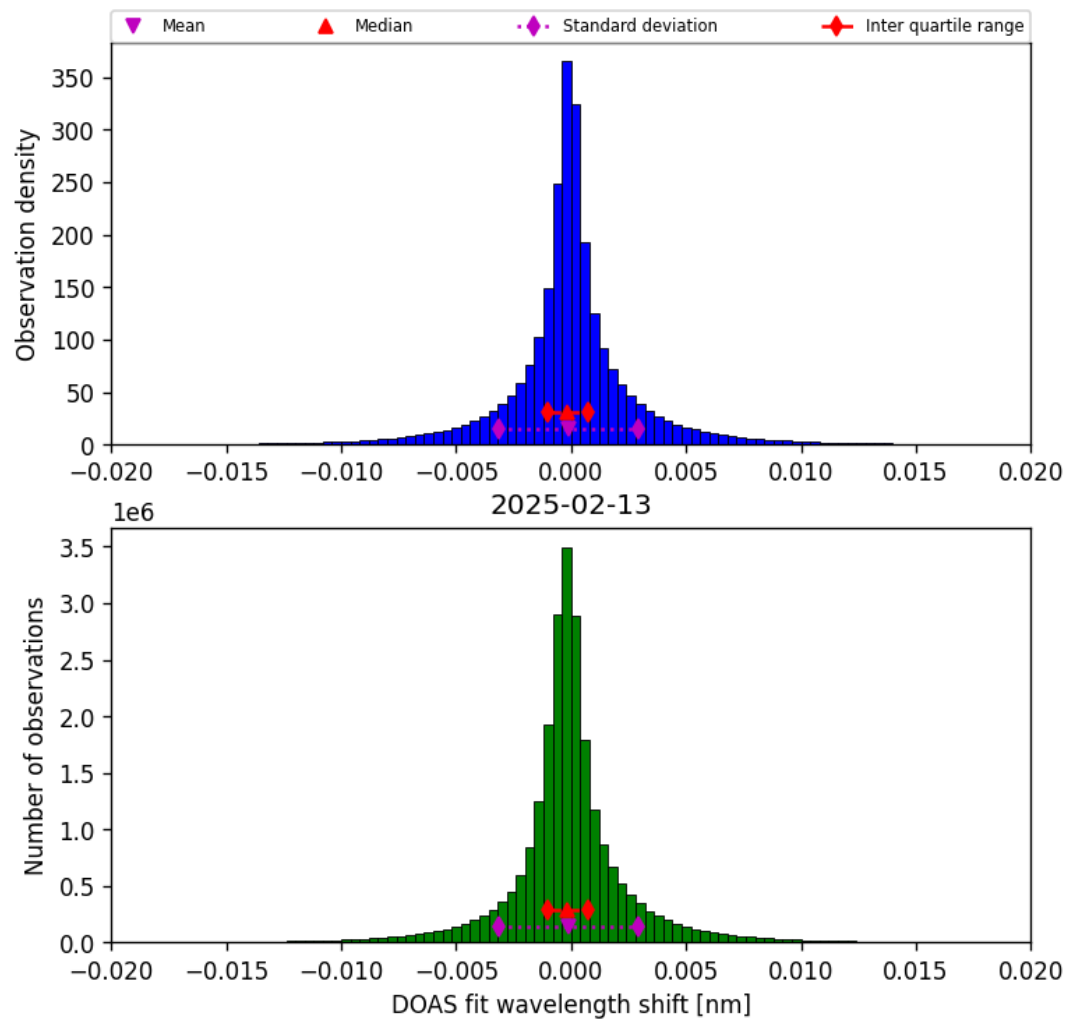
Figure 44: Histogram of “DOAS fit wavelength shift” for 2025-02-13 to 2025-02-14
