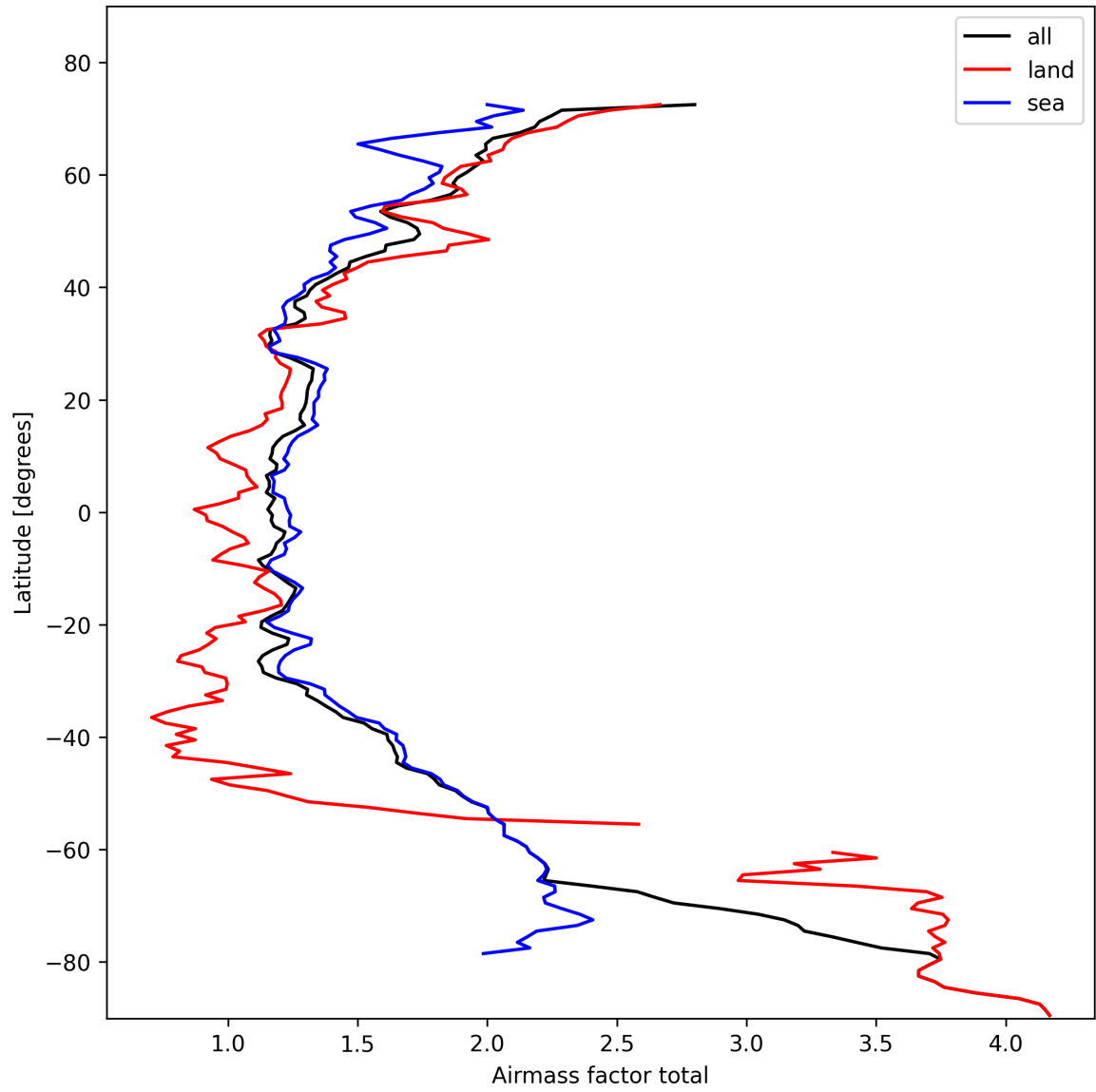
Figure 26: Zonal average of “Airmass factor total” for 2025-02-13 to 2025-02-14.
