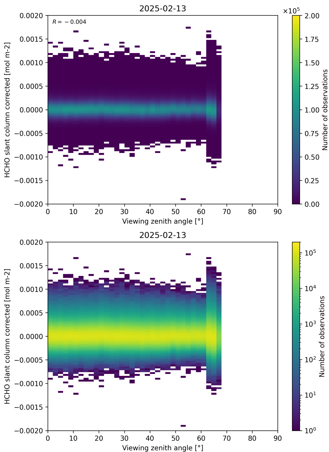
Figure 186: Scatter density plot of “Viewing zenith angle” against “HCHO slant column corrected” for 2025-02-13 to 2025-02-14.
