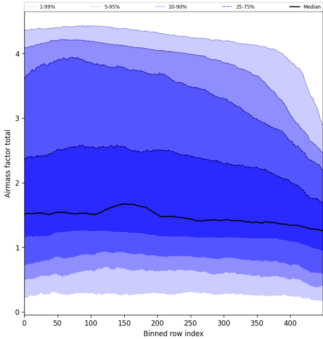
Figure 54: Along track statistics of “Airmass factor total” for 2025-02-13 to 2025-02-14
