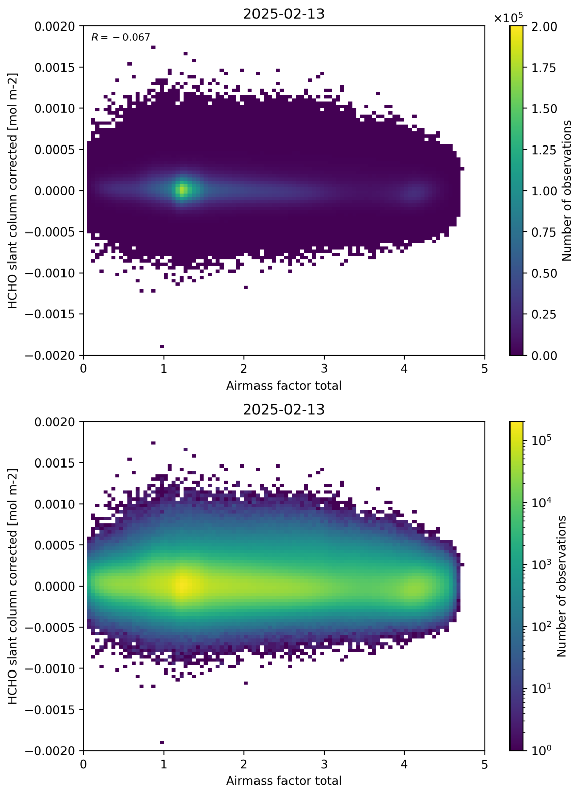
Figure 101: Scatter density plot of “Airmass factor total” against “HCHO slant column corrected” for 2025-02-13 to 2025-02-14.
