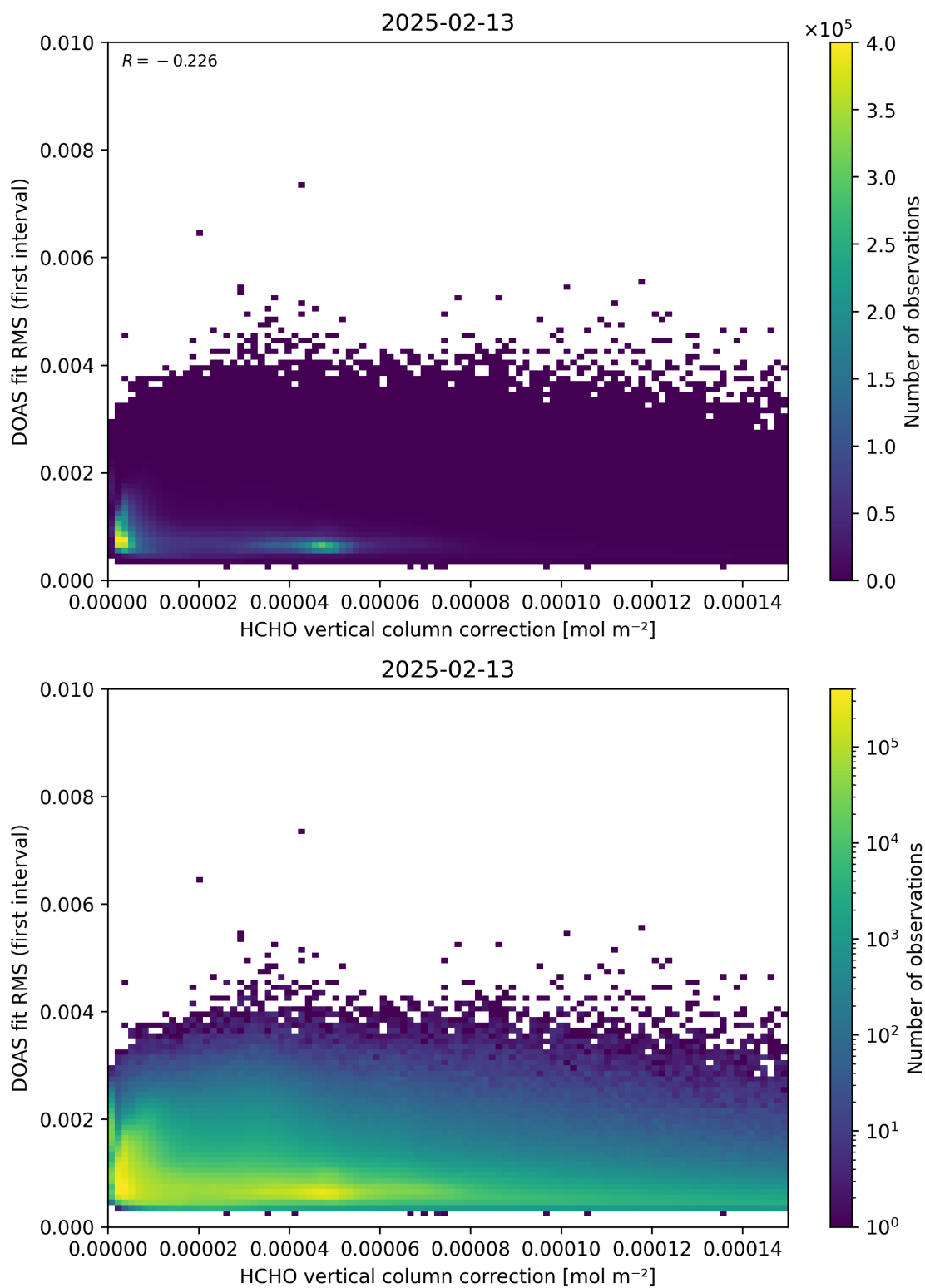
Figure 112: Scatter density plot of “HCHO vertical column correction” against “DOAS fit RMS (first interval)” for 2025-02-13 to 2025-02-14.
