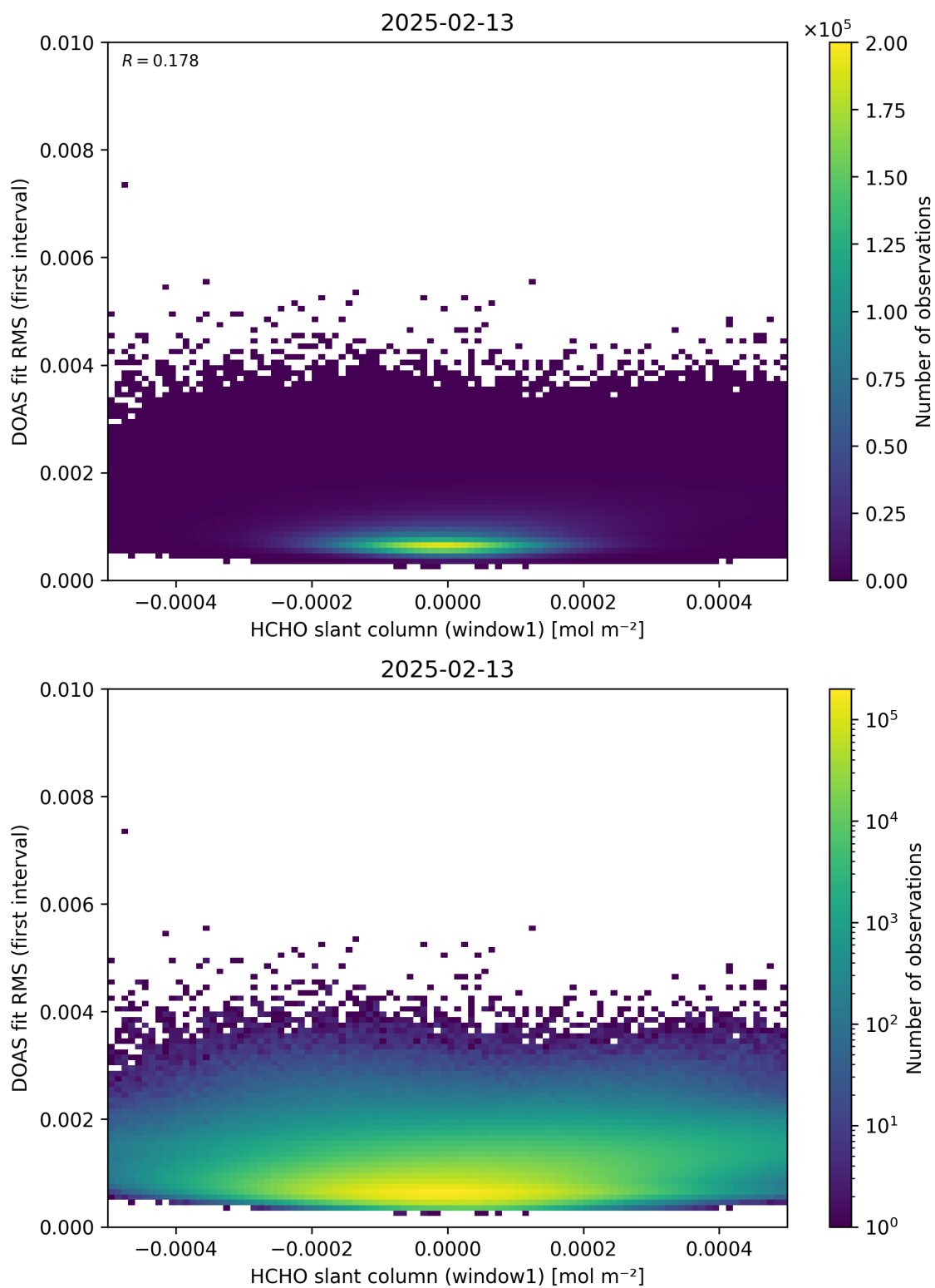
Figure 78: Scatter density plot of “HCHO slant column (window1)” against “DOAS fit RMS (first interval)” for 2025-02-13 to 2025-02-14.
