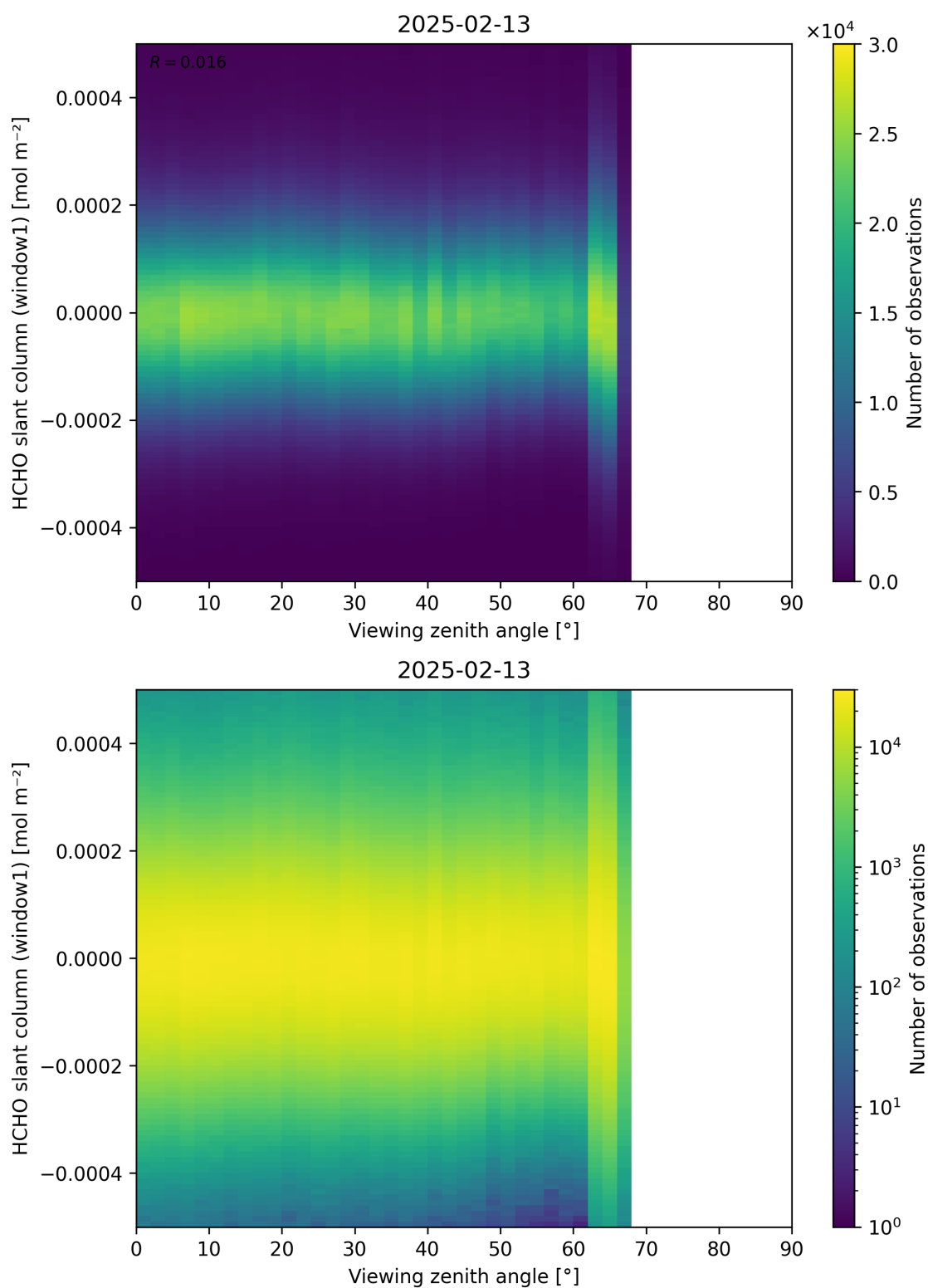
Figure 188: Scatter density plot of “Viewing zenith angle” against “HCHO slant column (window1)” for 2025-02-13 to 2025-02-14.
