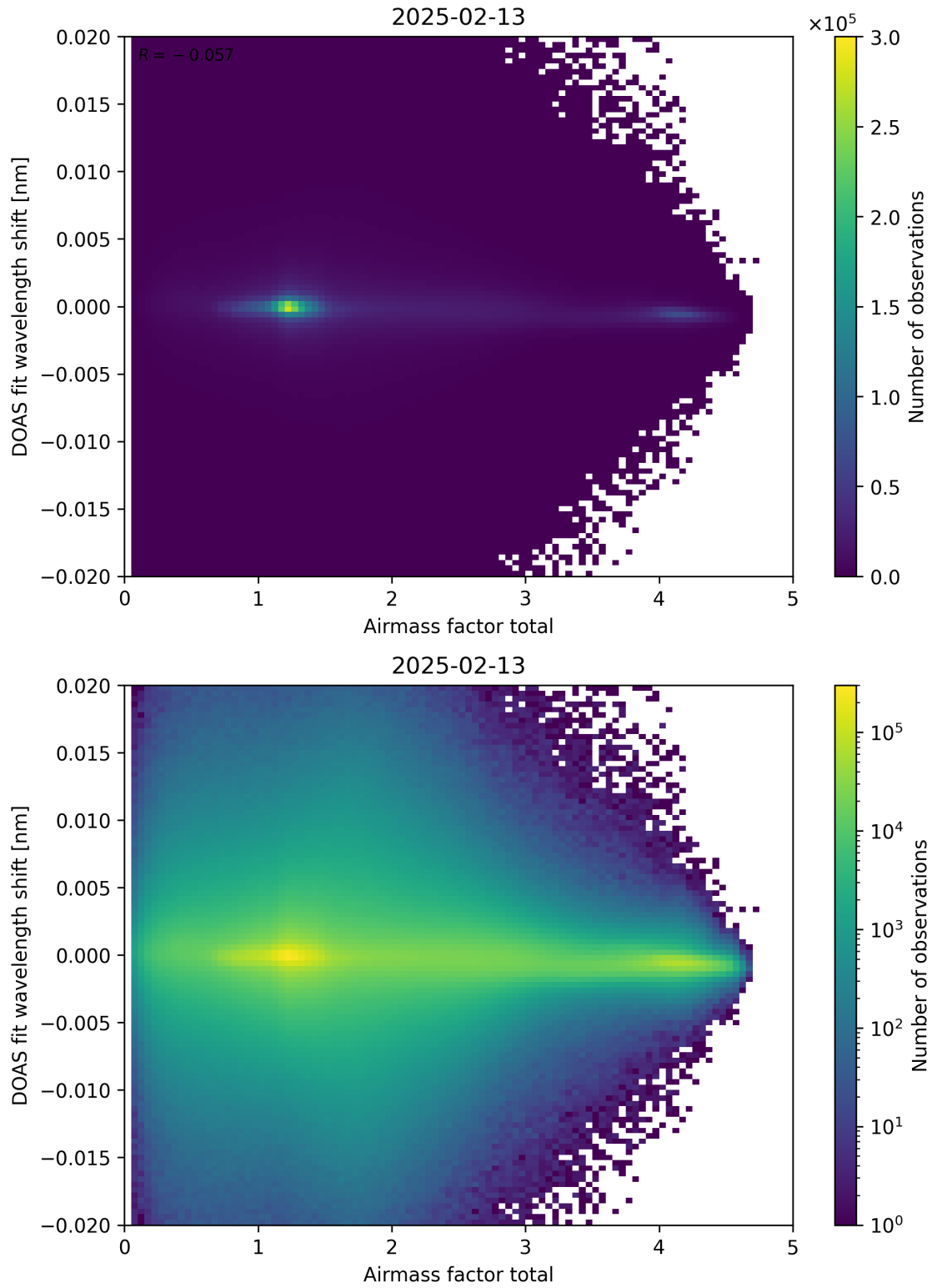
Figure 98: Scatter density plot of “Airmass factor total” against “DOAS fit wavelength shift” for 2025-02-13 to 2025-02-14.
