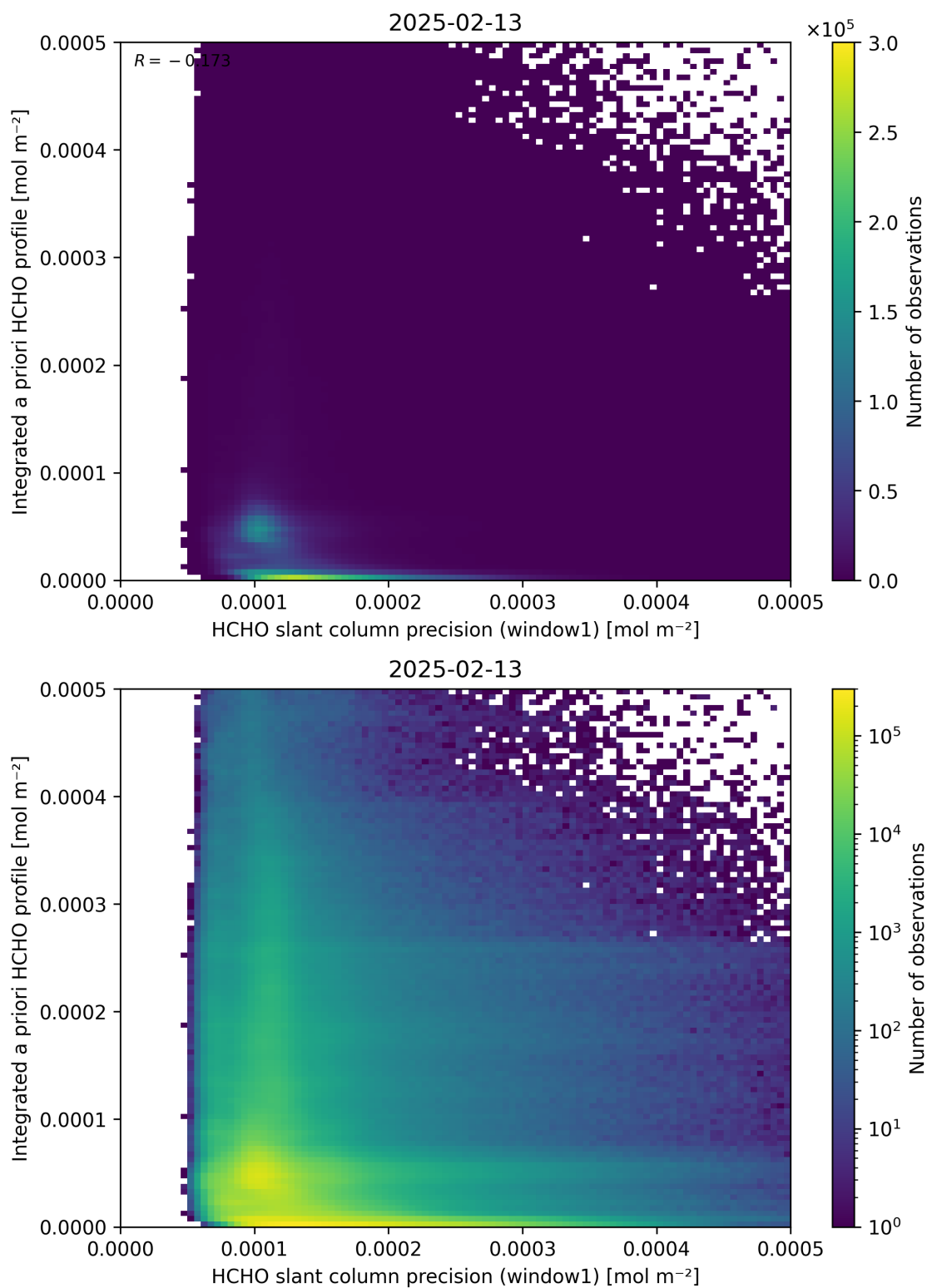
Figure 96: Scatter density plot of “HCHO slant column precision (window1)” against “Integrated a priori HCHO profile” for 2025-02-13 to 2025-02-14.
