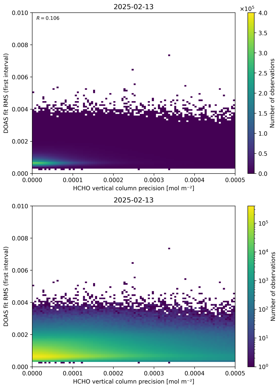
Figure 136: Scatter density plot of “HCHO vertical column precision” against “DOAS fit RMS (first interval)” for 2025-02-13 to 2025-02-14.
