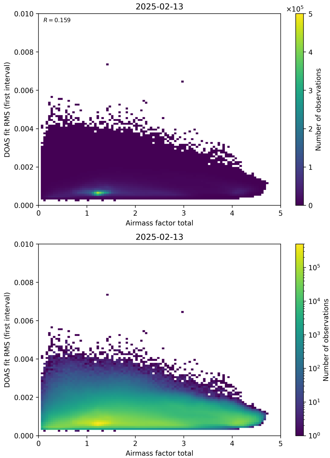
Figure 97: Scatter density plot of “Airmass factor total” against “DOAS fit RMS (first interval)” for 2025-02-13 to 2025-02-14.
