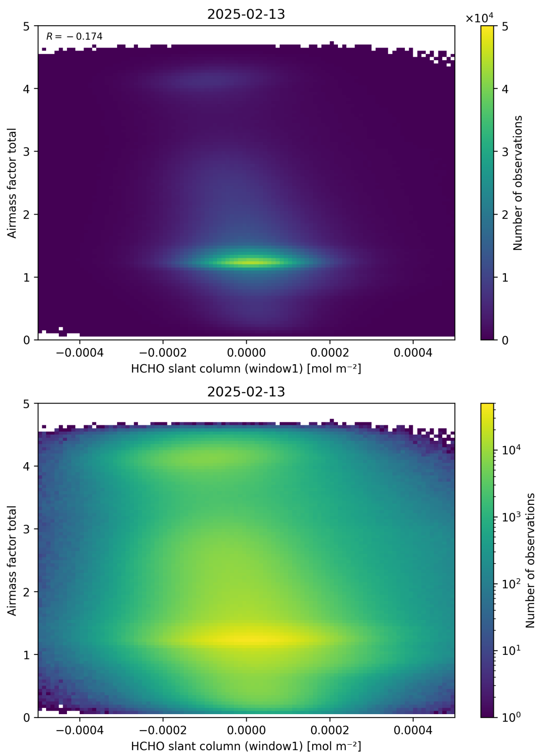
Figure 85: Scatter density plot of “HCHO slant column (window1)” against “Airmass factor total” for 2025-02-13 to 2025-02-14.
