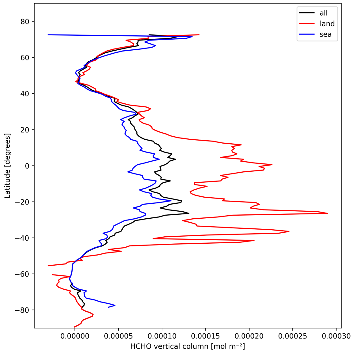
Figure 21: Zonal average of “HCHO vertical column” for 2025-02-13 to 2025-02-14.
