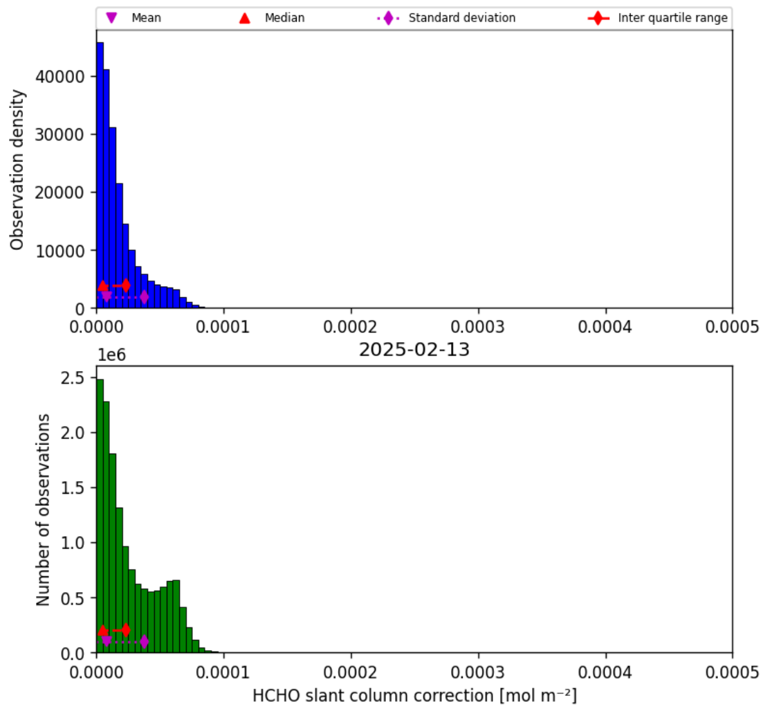
Figure 47: Histogram of “HCHO slant column correction” for 2025-02-13 to 2025-02-14
