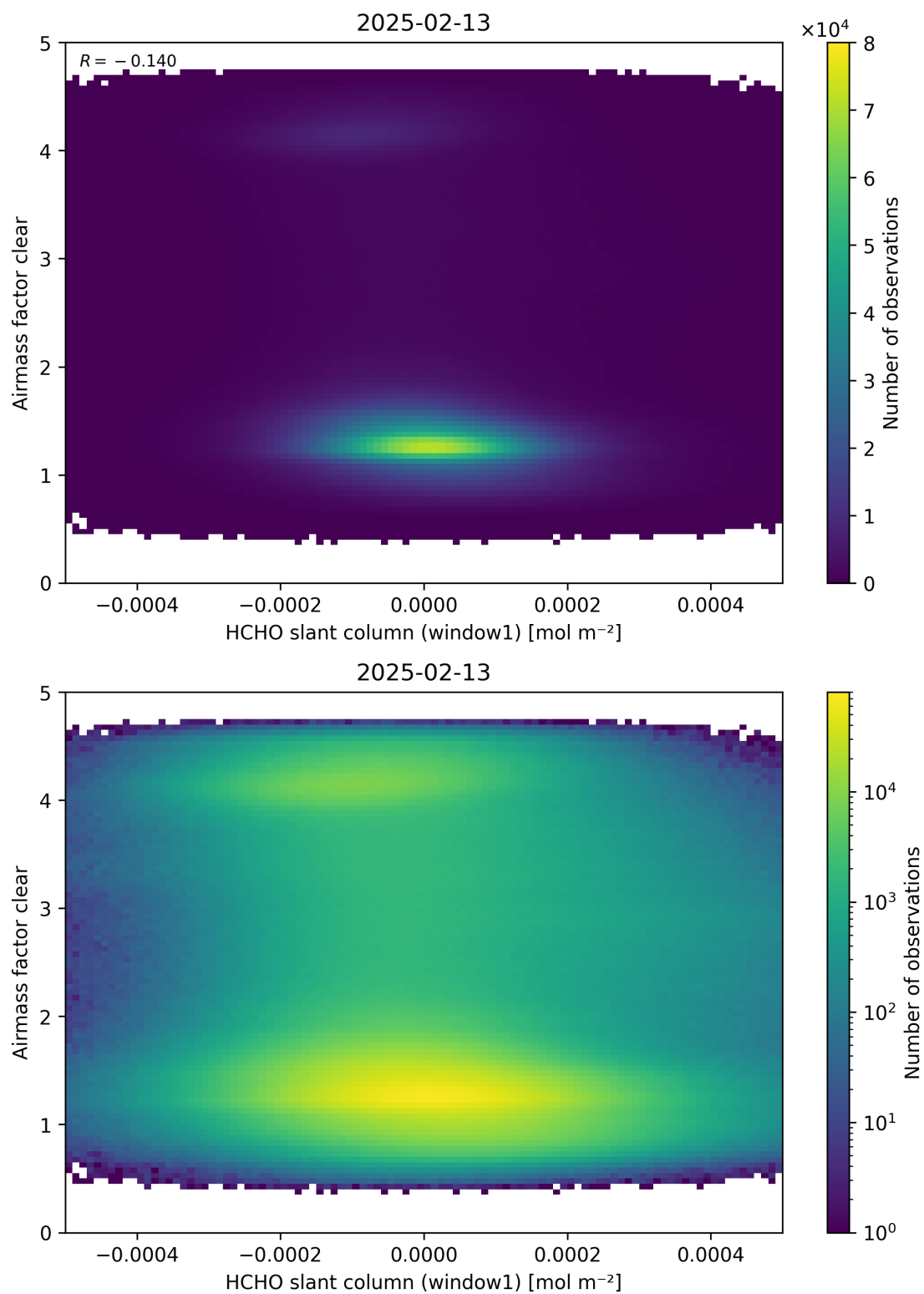
Figure 81: Scatter density plot of “HCHO slant column (window1)” against “Airmass factor clear” for 2025-02-13 to 2025-02-14.
