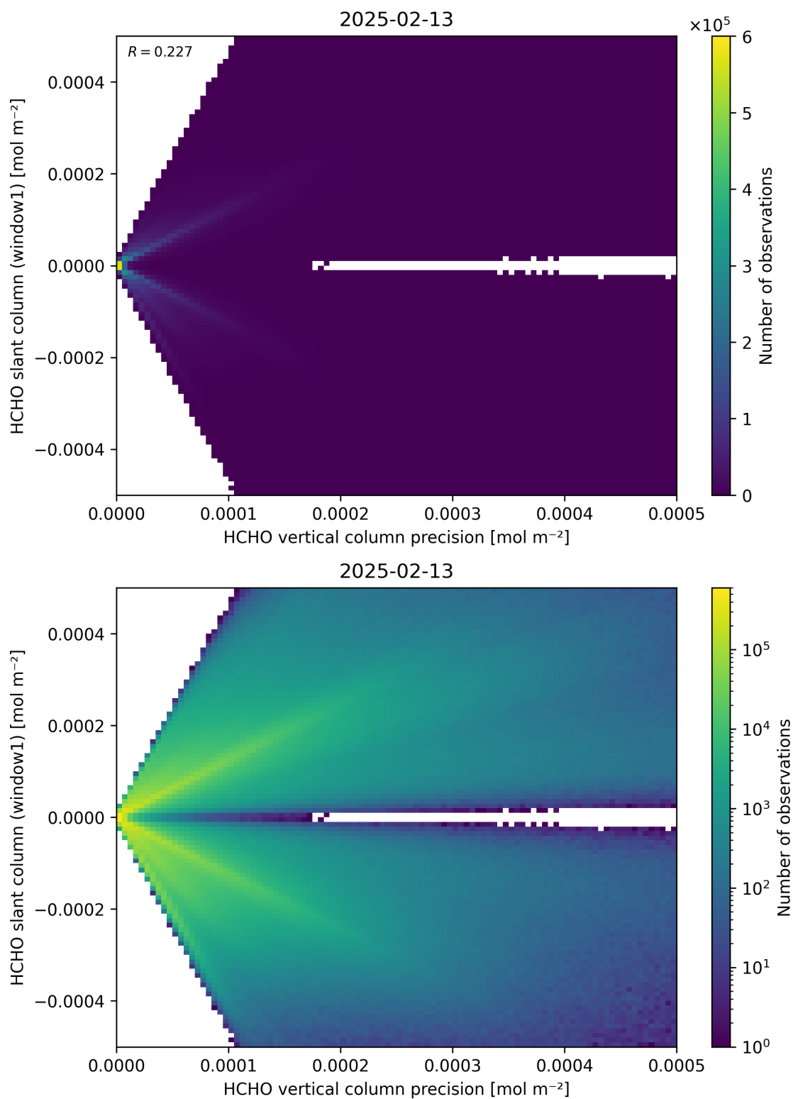
Figure 142: Scatter density plot of “HCHO vertical column precision” against “HCHO slant column (window1)” for 2025-02-13 to 2025-02-14.
