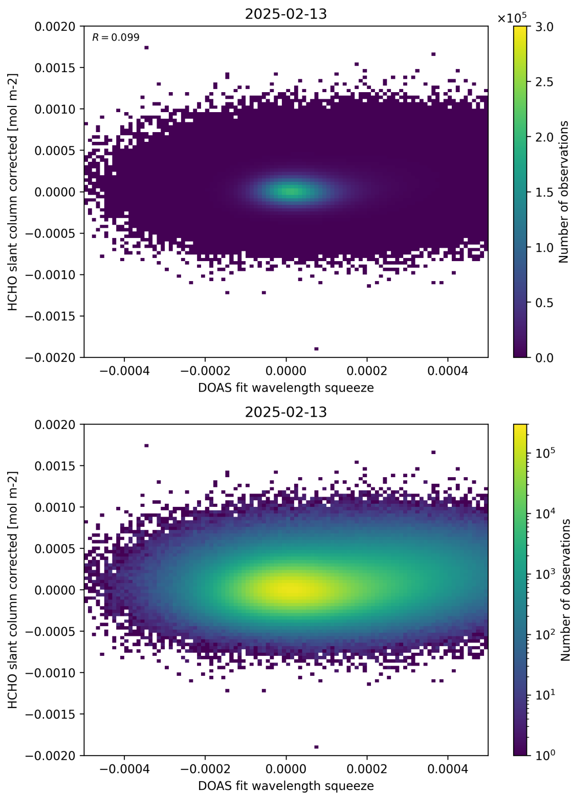
Figure 69: Scatter density plot of “DOAS fit wavelength squeeze” against “HCHO slant column corrected” for 2025-02-13 to 2025-02-14.
