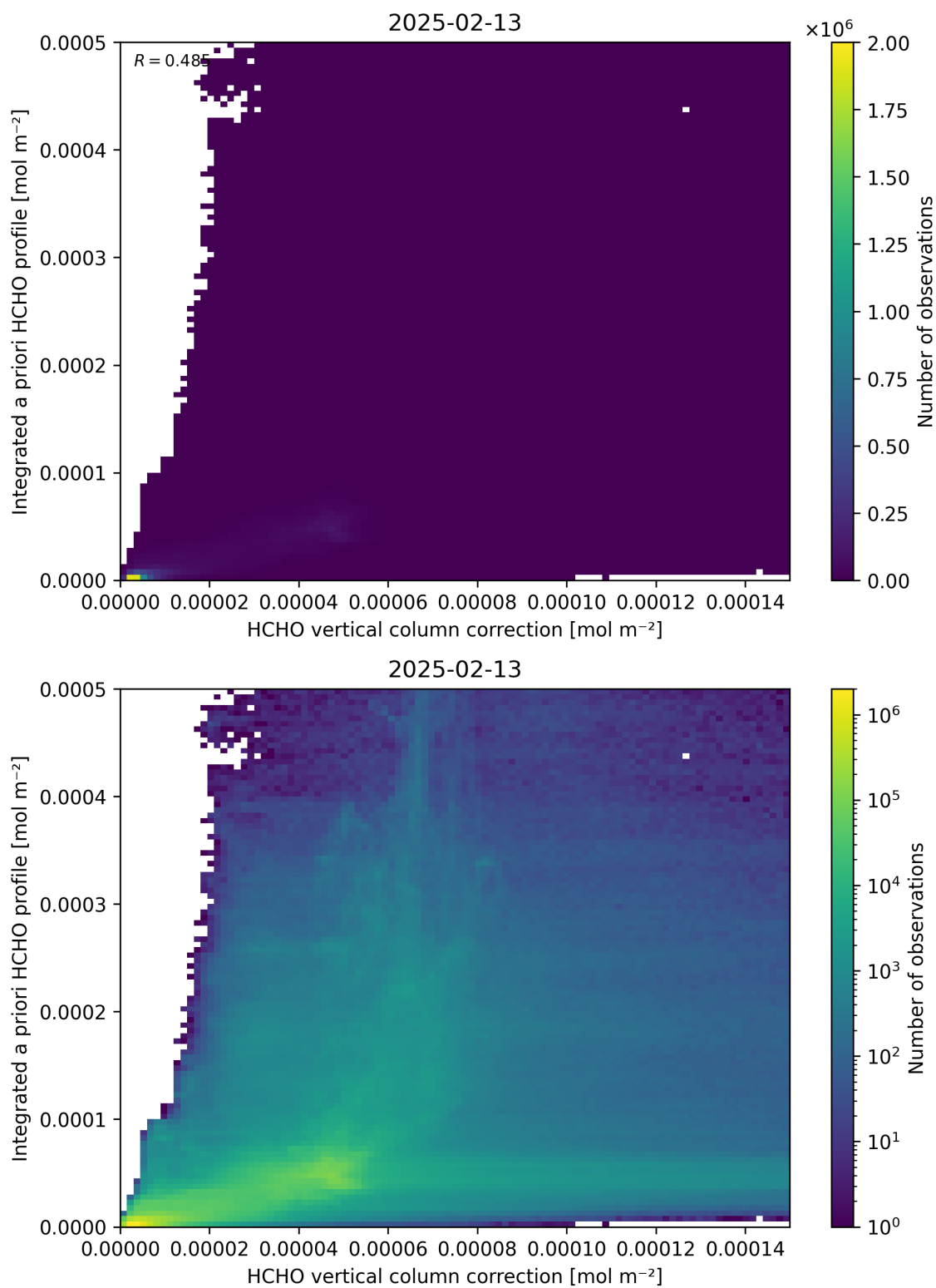
Figure 122: Scatter density plot of “HCHO vertical column correction” against “Integrated a priori HCHO profile” for 2025-02-13 to 2025-02-14.
