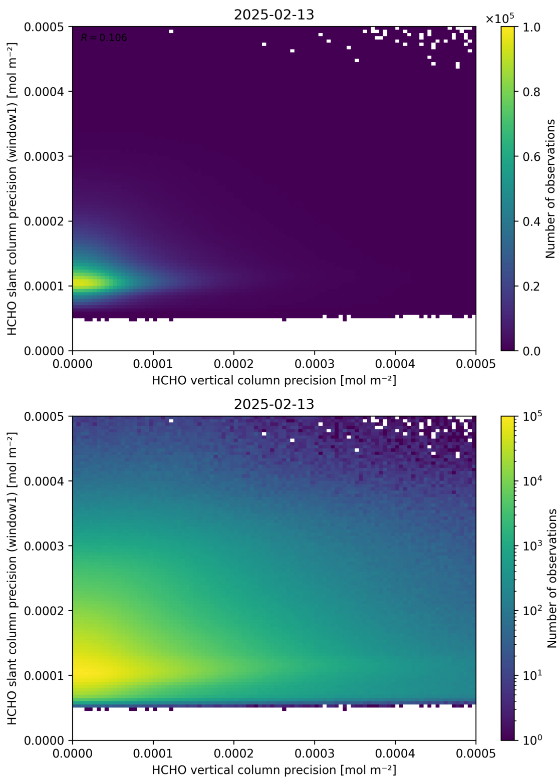
Figure 143: Scatter density plot of “HCHO vertical column precision” against “HCHO slant column precision (window1)” for 2025-02-13 to 2025-02-14.
