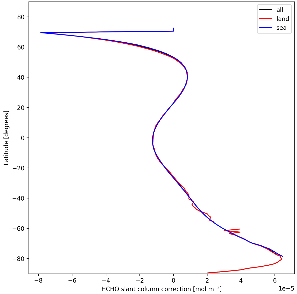
Figure 33: Zonal average of "HCHO slant column correction" for 2025-02-13 to 2025-02-14.
