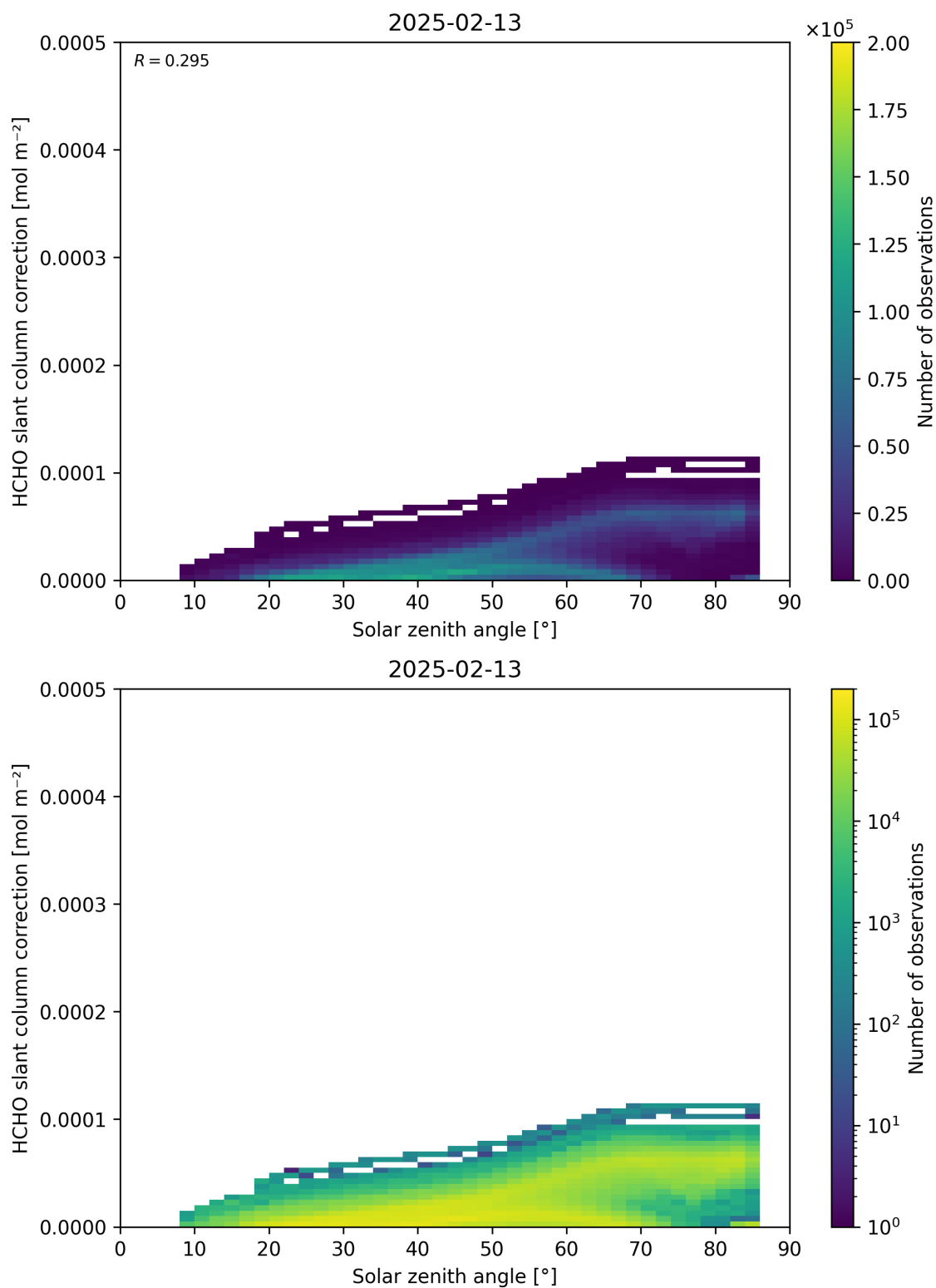
Figure 172: Scatter density plot of “Solar zenith angle” against “HCHO slant column correction” for 2025-02-13 to 2025-02-14.
