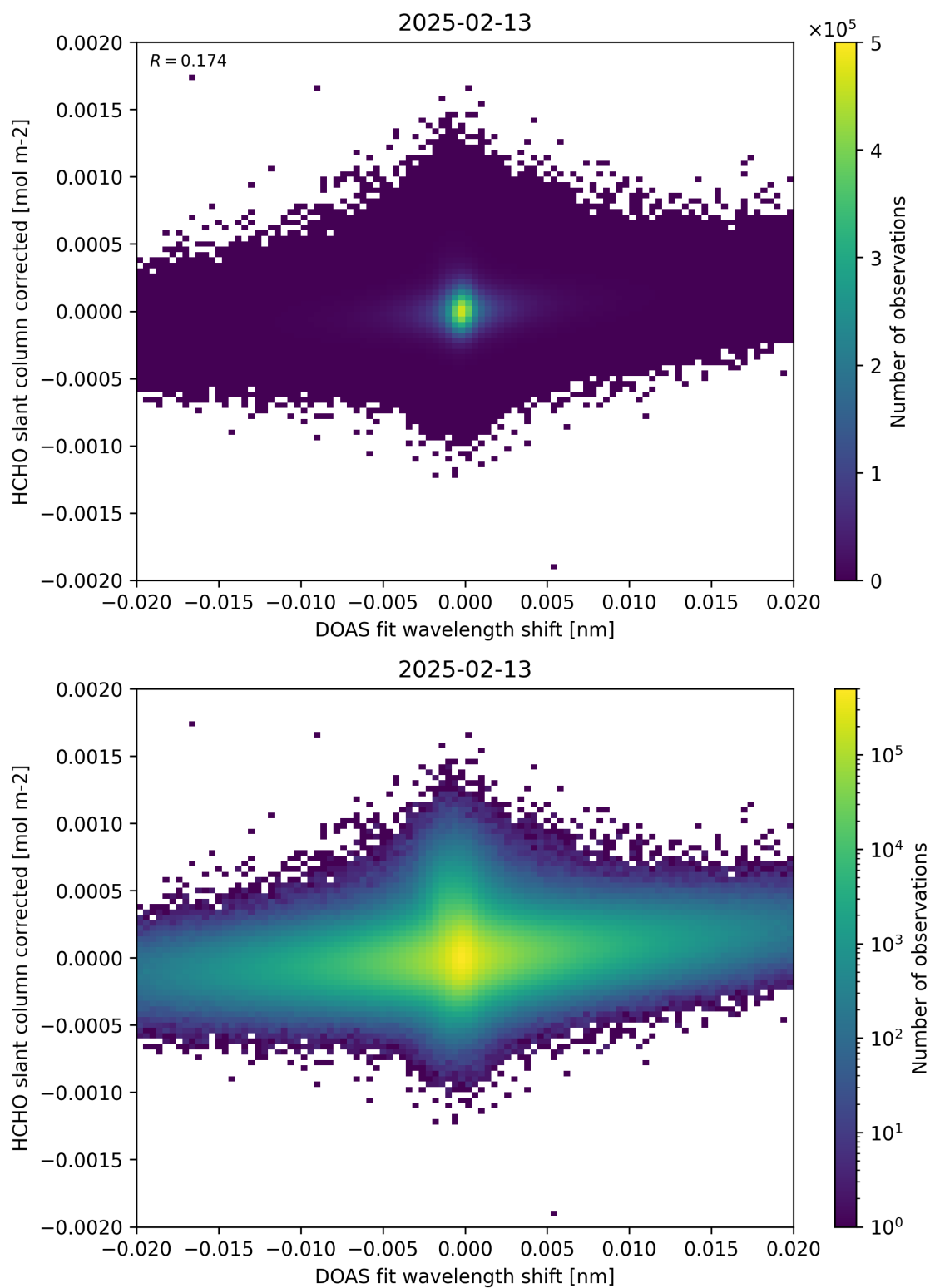
Figure 66: Scatter density plot of “DOAS fit wavelength shift” against “HCHO slant column corrected” for 2025-02-13 to 2025-02-14.
