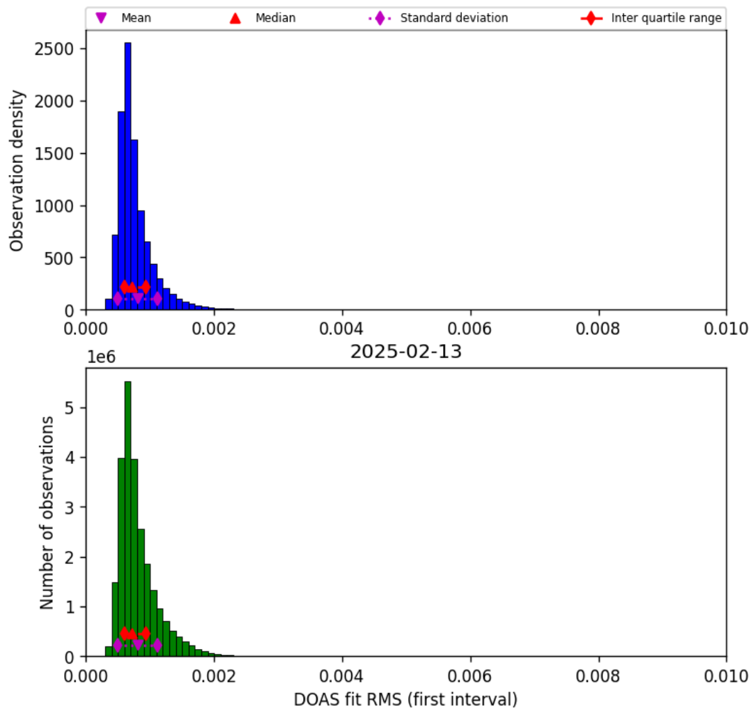
Figure 46: Histogram of “DOAS fit RMS (first interval)” for 2025-02-13 to 2025-02-14
