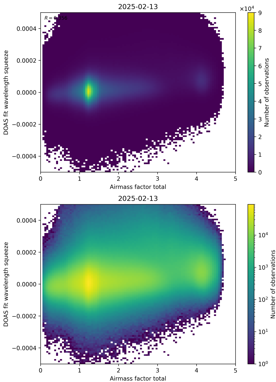
Figure 99: Scatter density plot of “Airmass factor total” against “DOAS fit wavelength squeeze” for 2025-02-13 to 2025-02-14.
