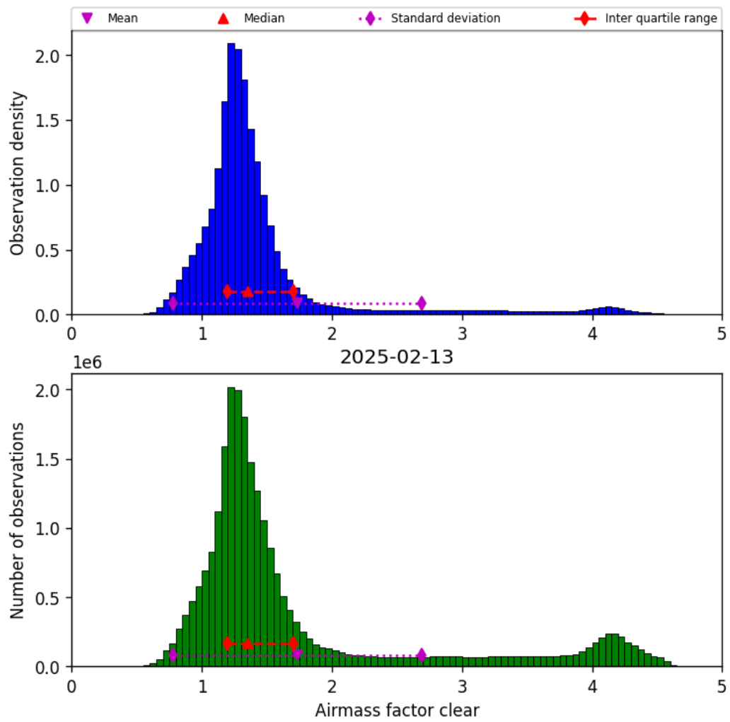
Figure 42: Histogram of “Airmass factor clear” for 2025-02-13 to 2025-02-14
