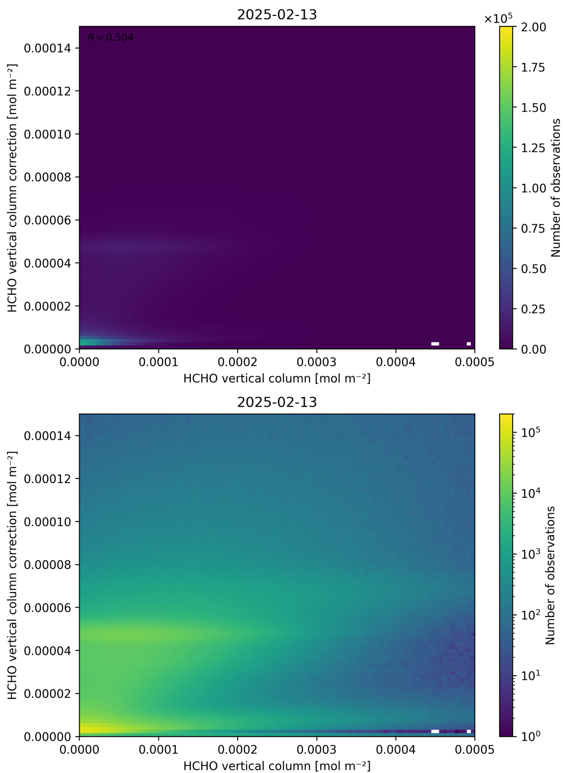
Figure 133: Scatter density plot of “HCHO vertical column” against “HCHO vertical column correction” for 2025-02-13 to 2025-02-14.
