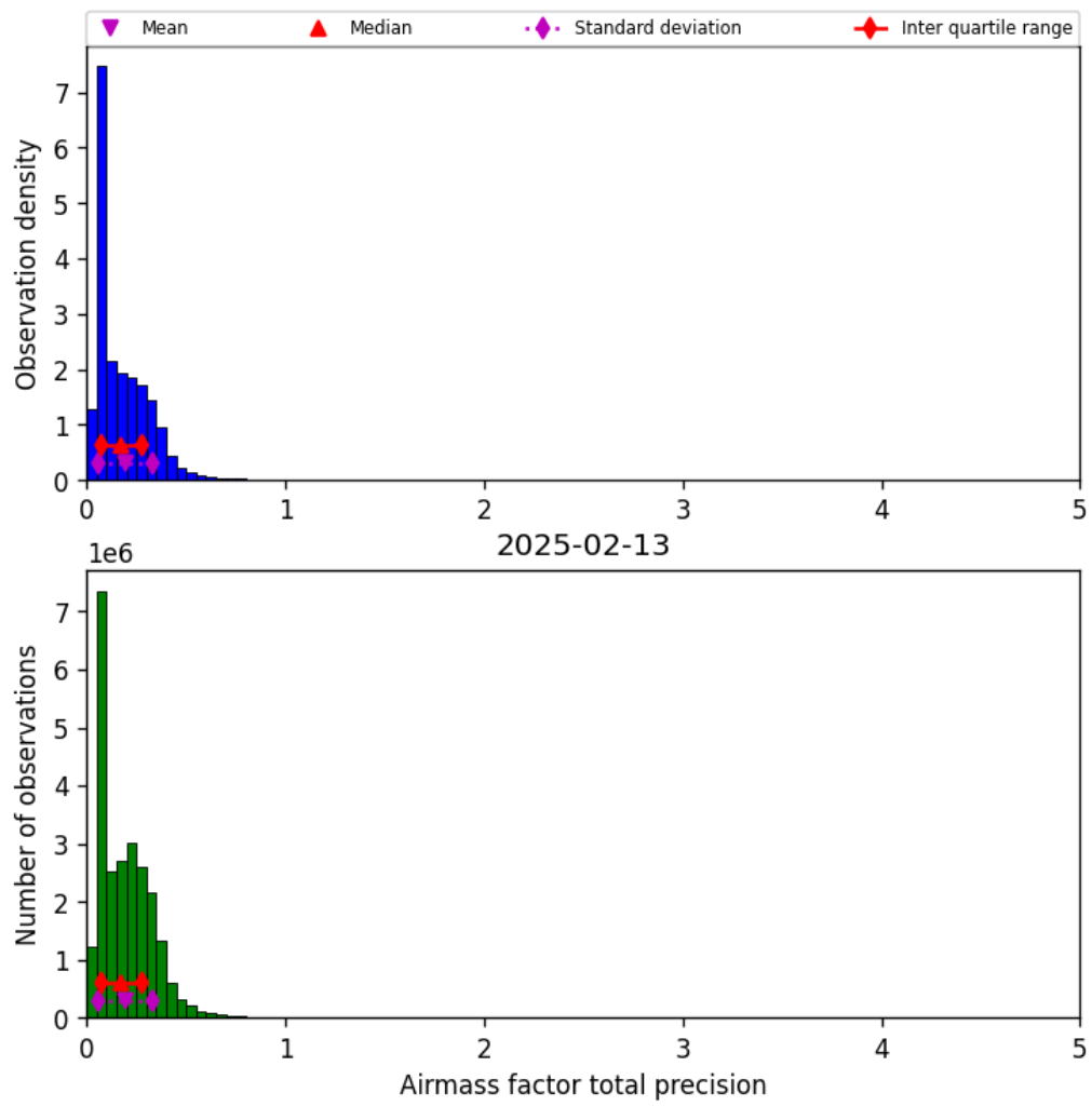
Figure 41: Histogram of “Airmass factor total precision” for 2025-02-13 to 2025-02-14
