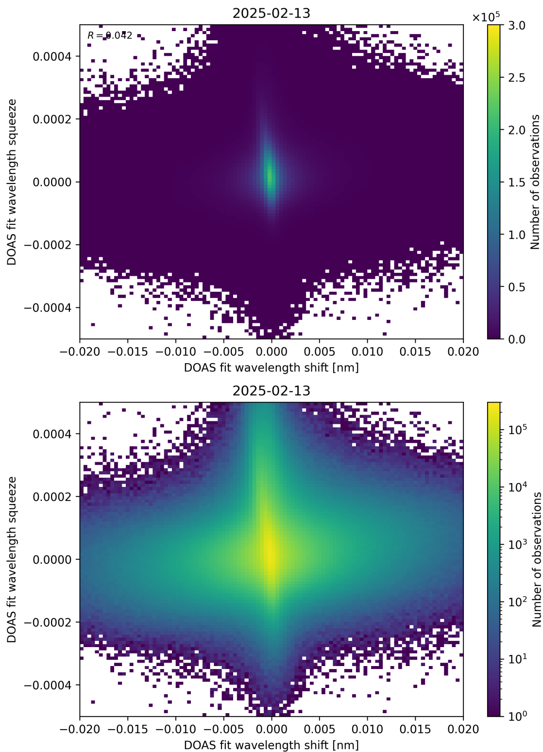
Figure 65: Scatter density plot of “DOAS fit wavelength shift” against “DOAS fit wavelength squeeze” for 2025-02-13 to 2025-02-14.
