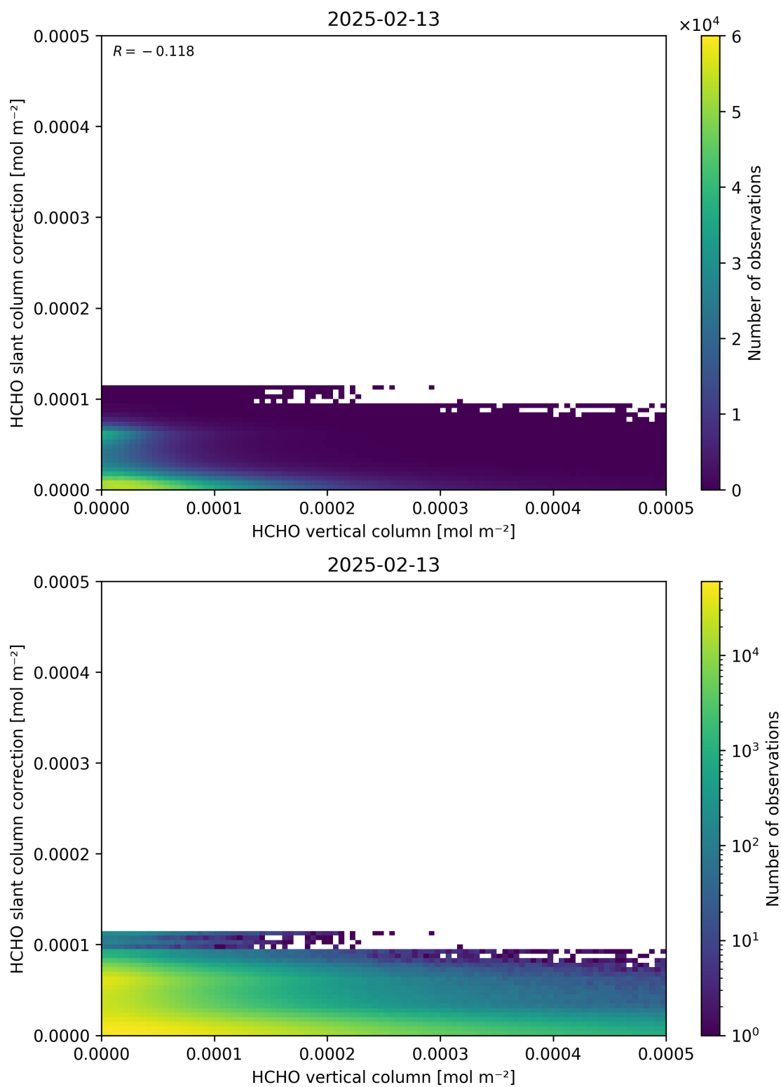
Figure 128: Scatter density plot of “HCHO vertical column” against “HCHO slant column correction” for 2025-02-13 to 2025-02-14.
