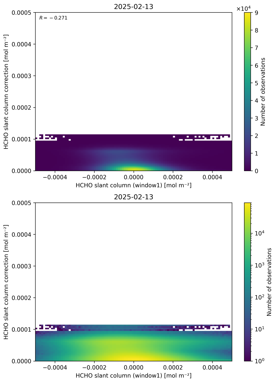
Figure 83: Scatter density plot of “HCHO slant column (window1)” against “HCHO slant column correction” for 2025-02-13 to 2025-02-14.
