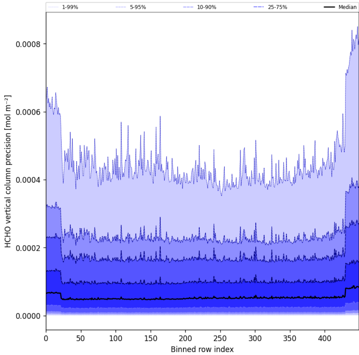
Figure 50: Along track statistics of “HCHO vertical column precision” for 2025-02-13 to 2025-02-14
