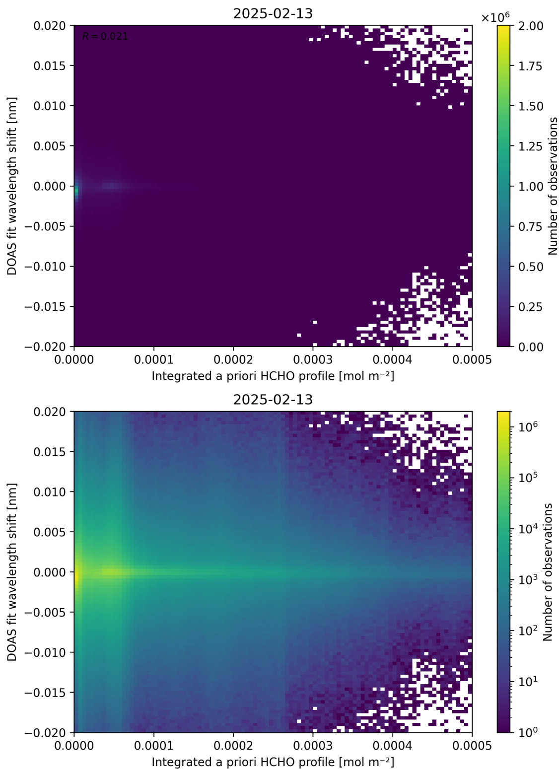
Figure 149: Scatter density plot of “Integrated a priori HCHO profile” against “DOAS fit wavelength shift” for 2025-02-13 to 2025-02-14.
