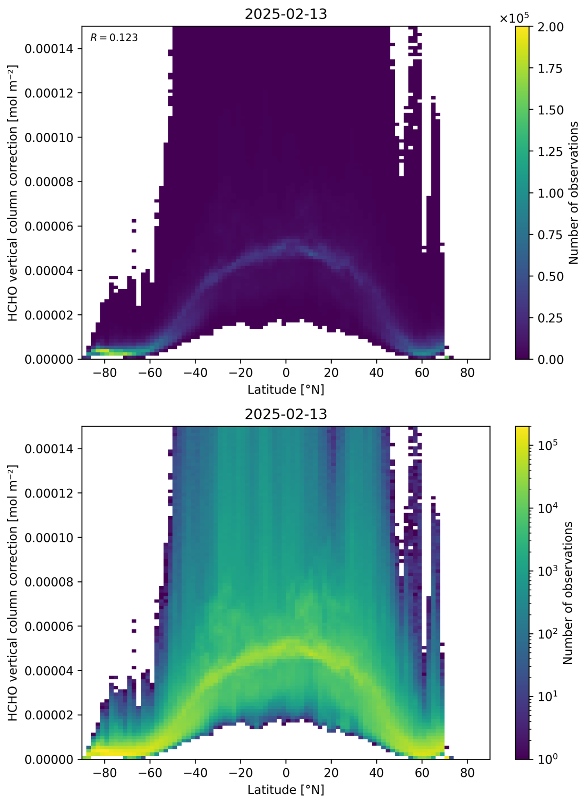
Figure 164: Scatter density plot of “Latitude” against “HCHO vertical column correction” for 2025-02-13 to 2025-02-14.
