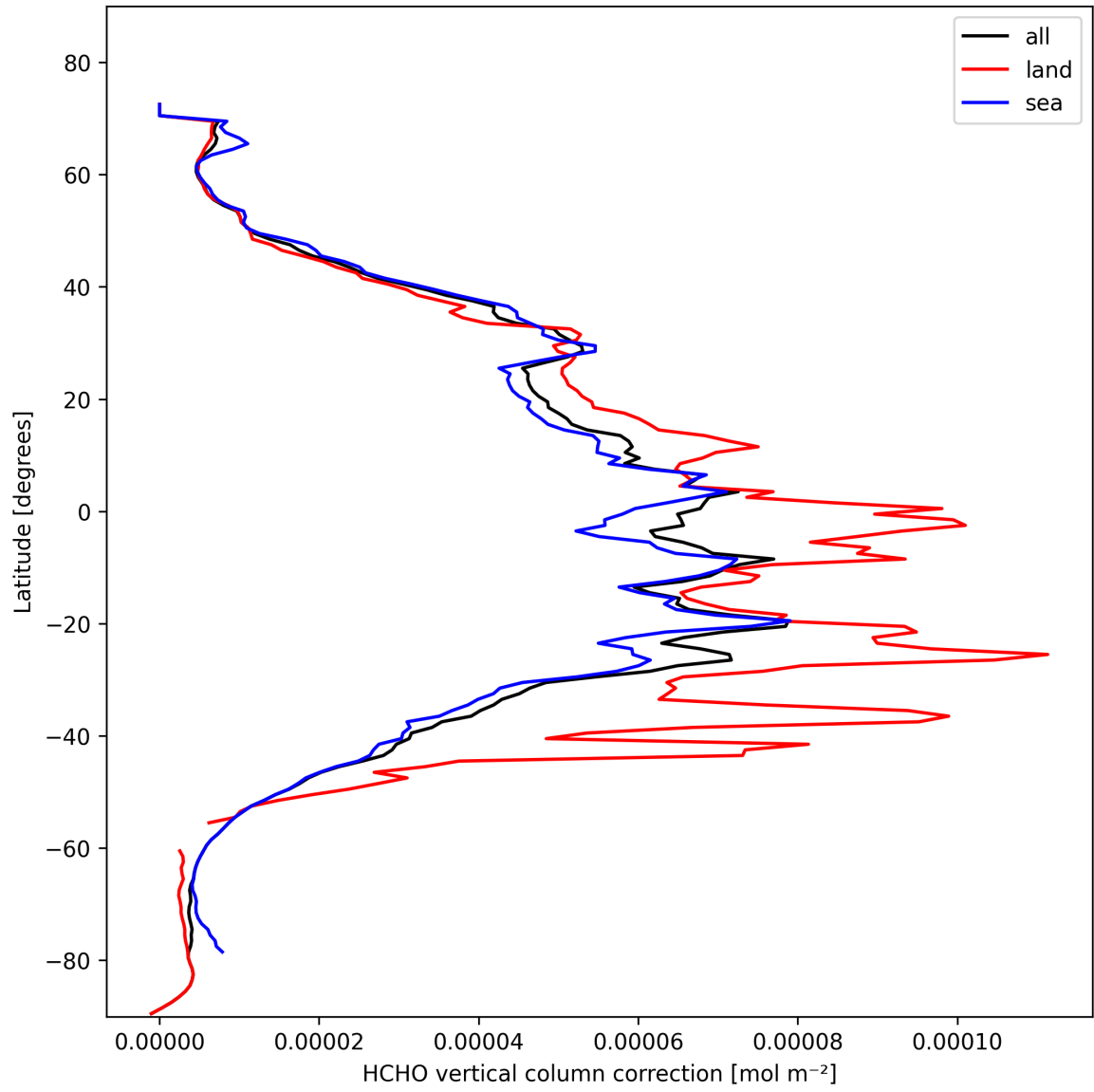
Figure 23: Zonal average of “HCHO vertical column correction” for 2025-02-13 to 2025-02-14.
