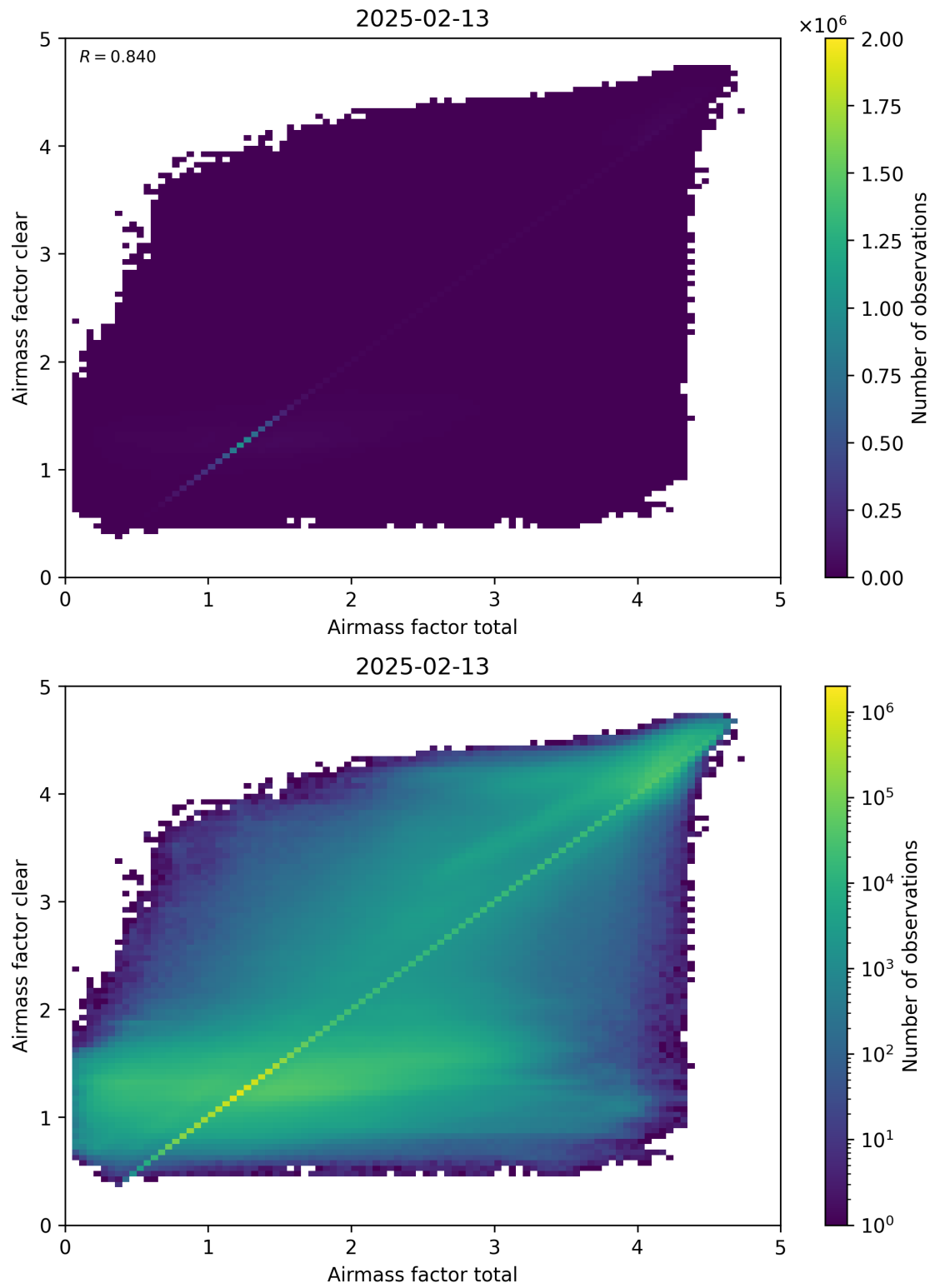
Figure 100: Scatter density plot of “Airmass factor total” against “Airmass factor clear” for 2025-02-13 to 2025-02-14.
