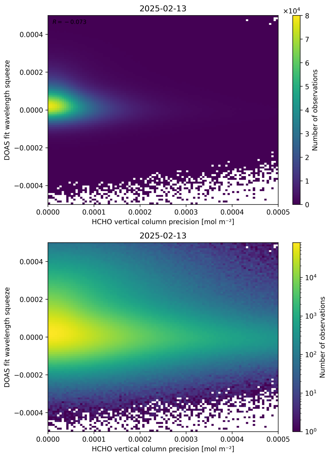
Figure 138: Scatter density plot of “HCHO vertical column precision” against “DOAS fit wavelength squeeze” for 2025-02-13 to 2025-02-14.
