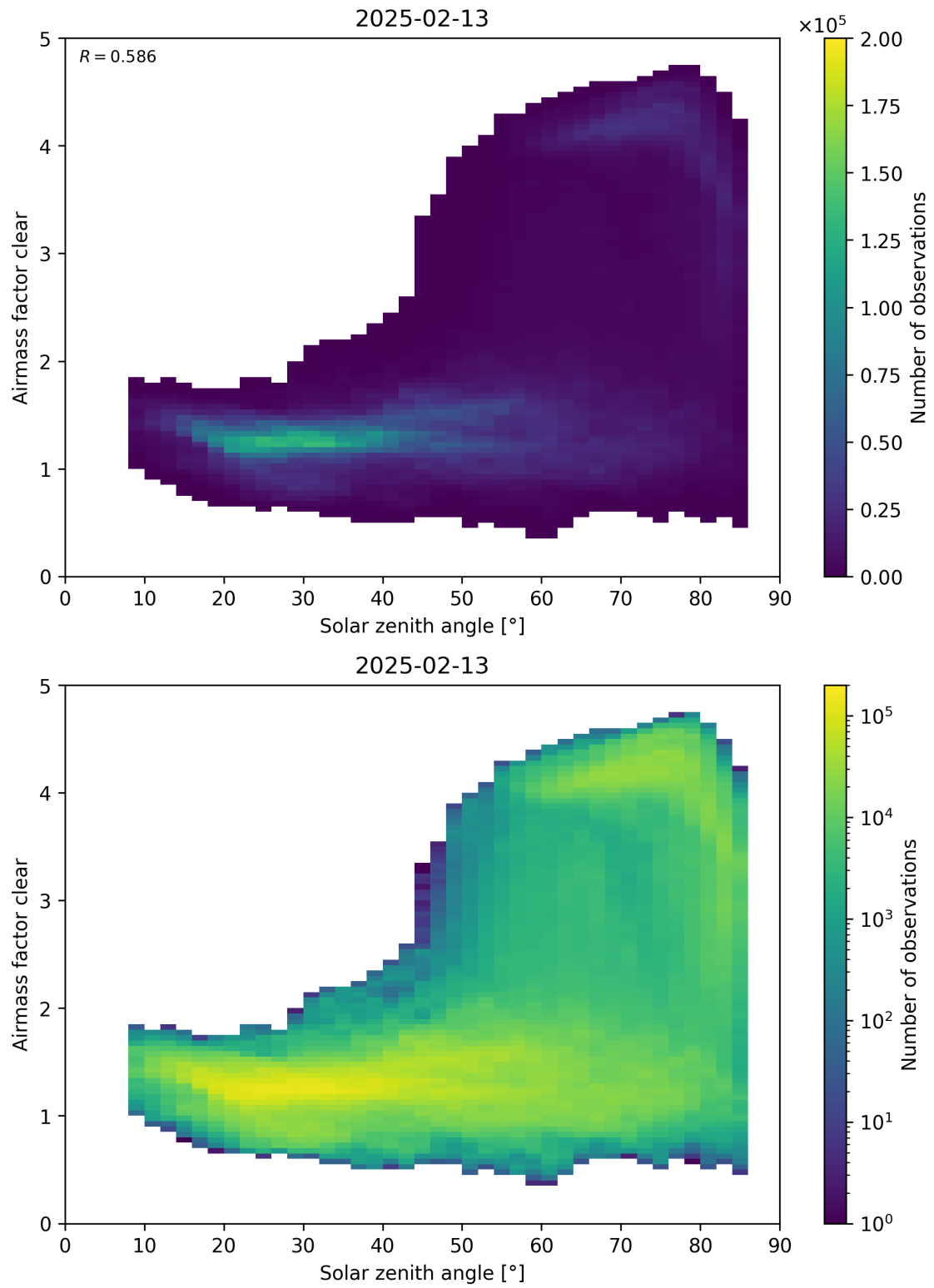
Figure 170: Scatter density plot of “Solar zenith angle” against “Airmass factor clear” for 2025-02-13 to 2025-02-14.
