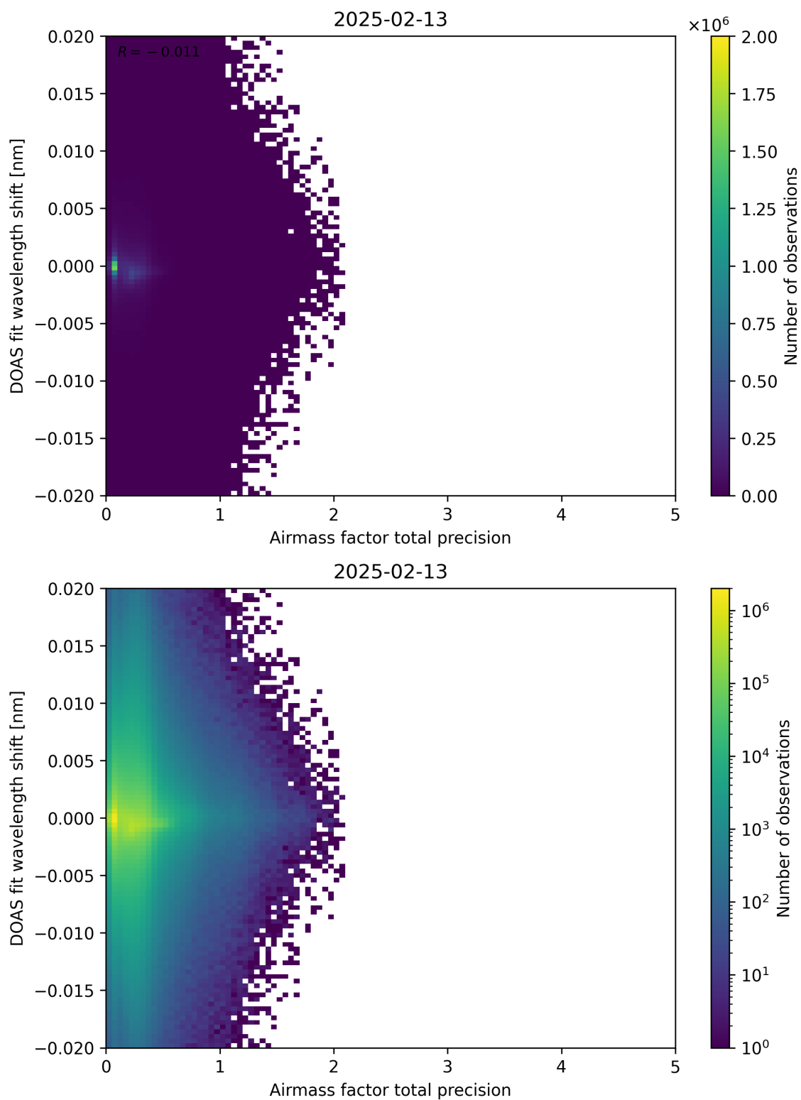
Figure 106: Scatter density plot of “Airmass factor total precision” against “DOAS fit wavelength shift” for 2025-02-13 to 2025-02-14.
