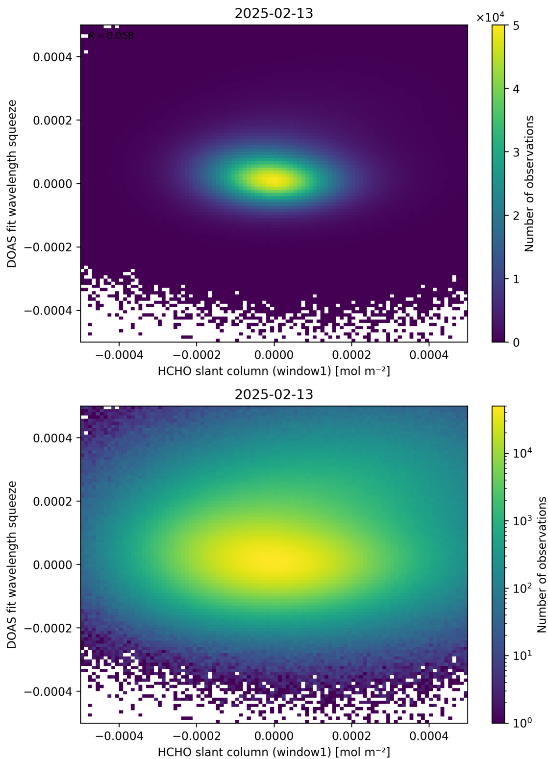
Figure 80: Scatter density plot of “HCHO slant column (window1)” against “DOAS fit wavelength squeeze” for 2025-02-13 to 2025-02-14.
