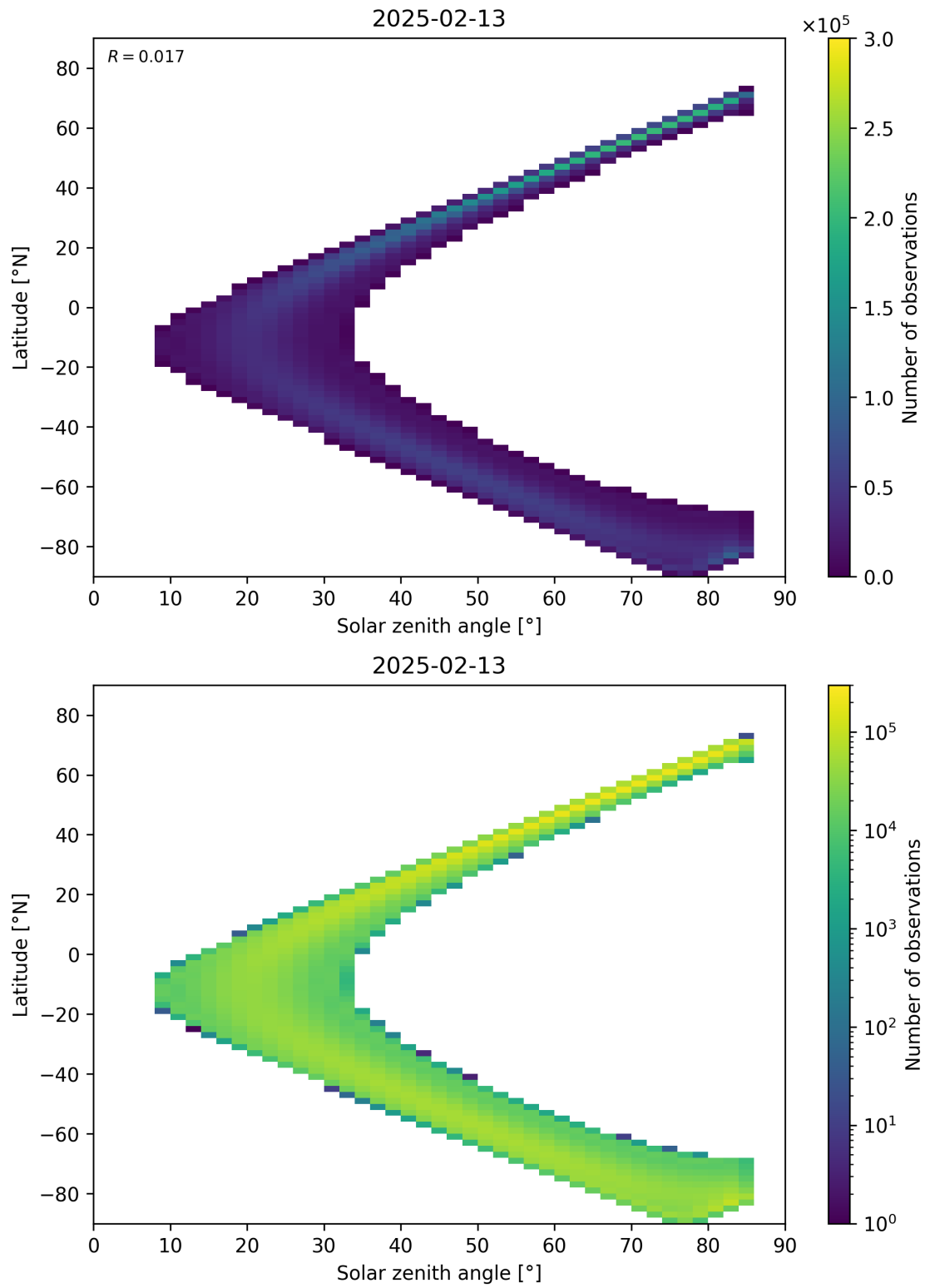
Figure 181: Scatter density plot of “Solar zenith angle” against “Latitude” for 2025-02-13 to 2025-02-14.
