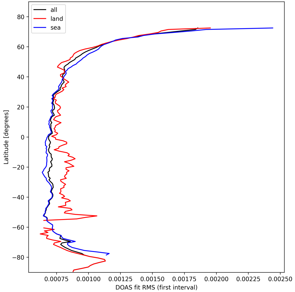
Figure 32: Zonal average of “DOAS fit RMS (first interval)” for 2025-02-13 to 2025-02-14.
