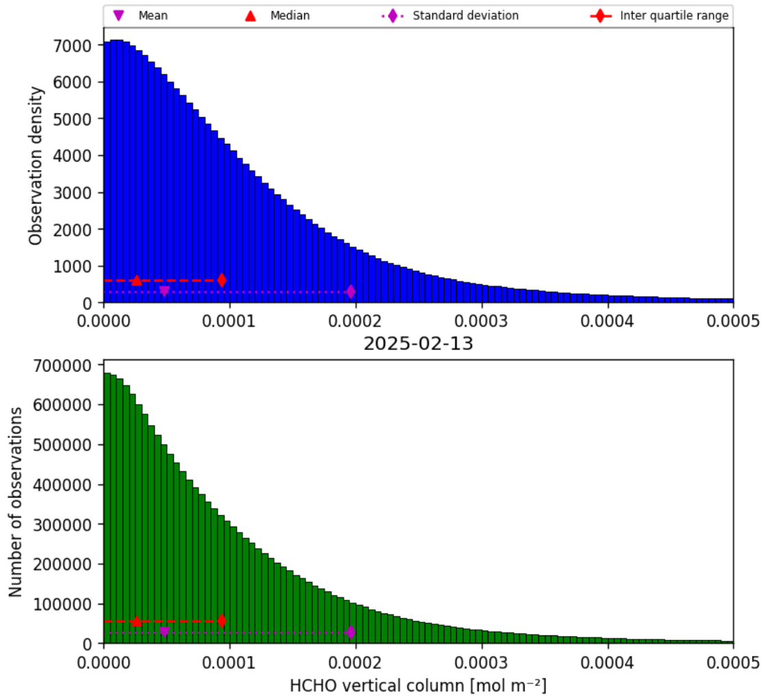
Figure 35: Histogram of “HCHO vertical column” for 2025-02-13 to 2025-02-14
