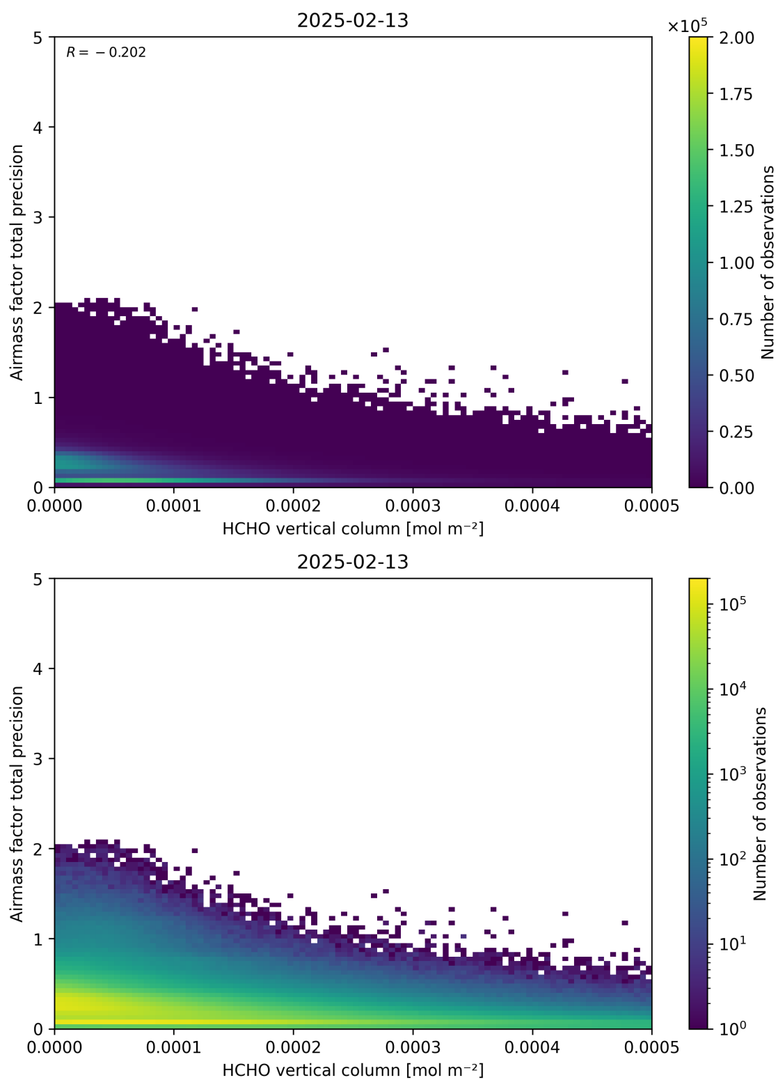
Figure 132: Scatter density plot of “HCHO vertical column” against “Airmass factor total precision” for 2025-02-13 to 2025-02-14.
