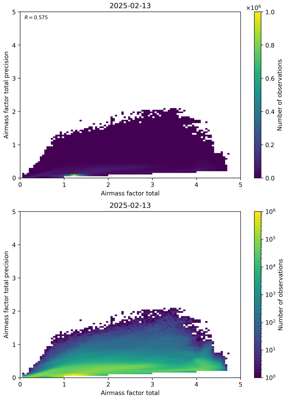
Figure 103: Scatter density plot of “Airmass factor total” against “Airmass factor total precision” for 2025-02-13 to 2025-02-14.
