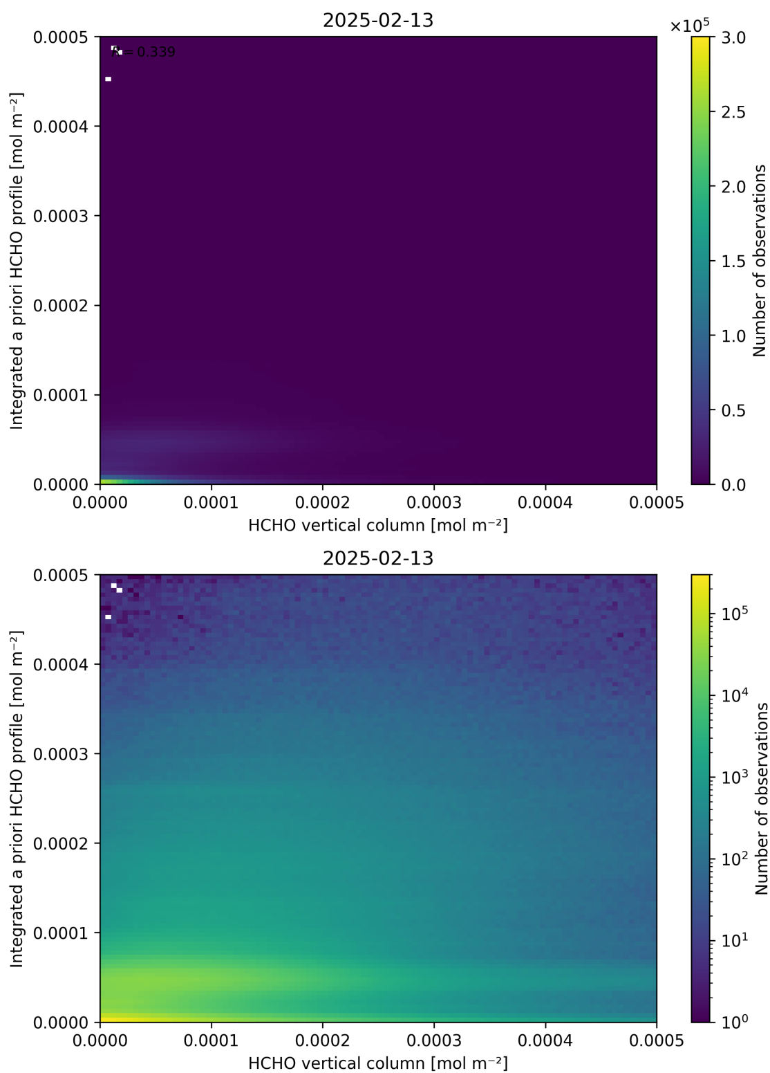
Figure 135: Scatter density plot of “HCHO vertical column” against “Integrated a priori HCHO profile” for 2025-02-13 to 2025-02-14.
