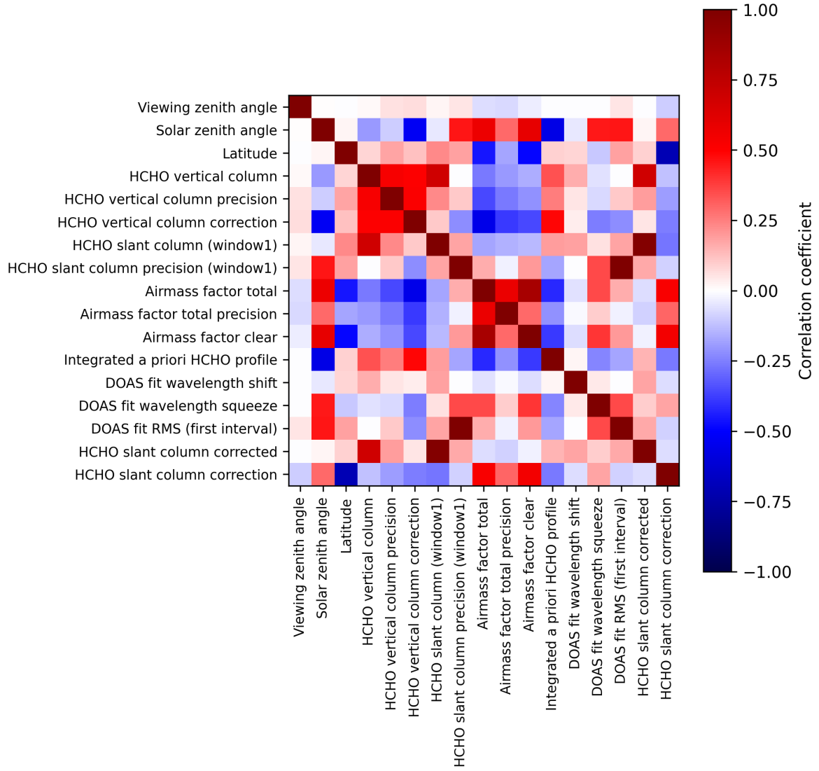
Figure 2: Map of correlation matrix for 2025-02-13 to 2025-02-14.
