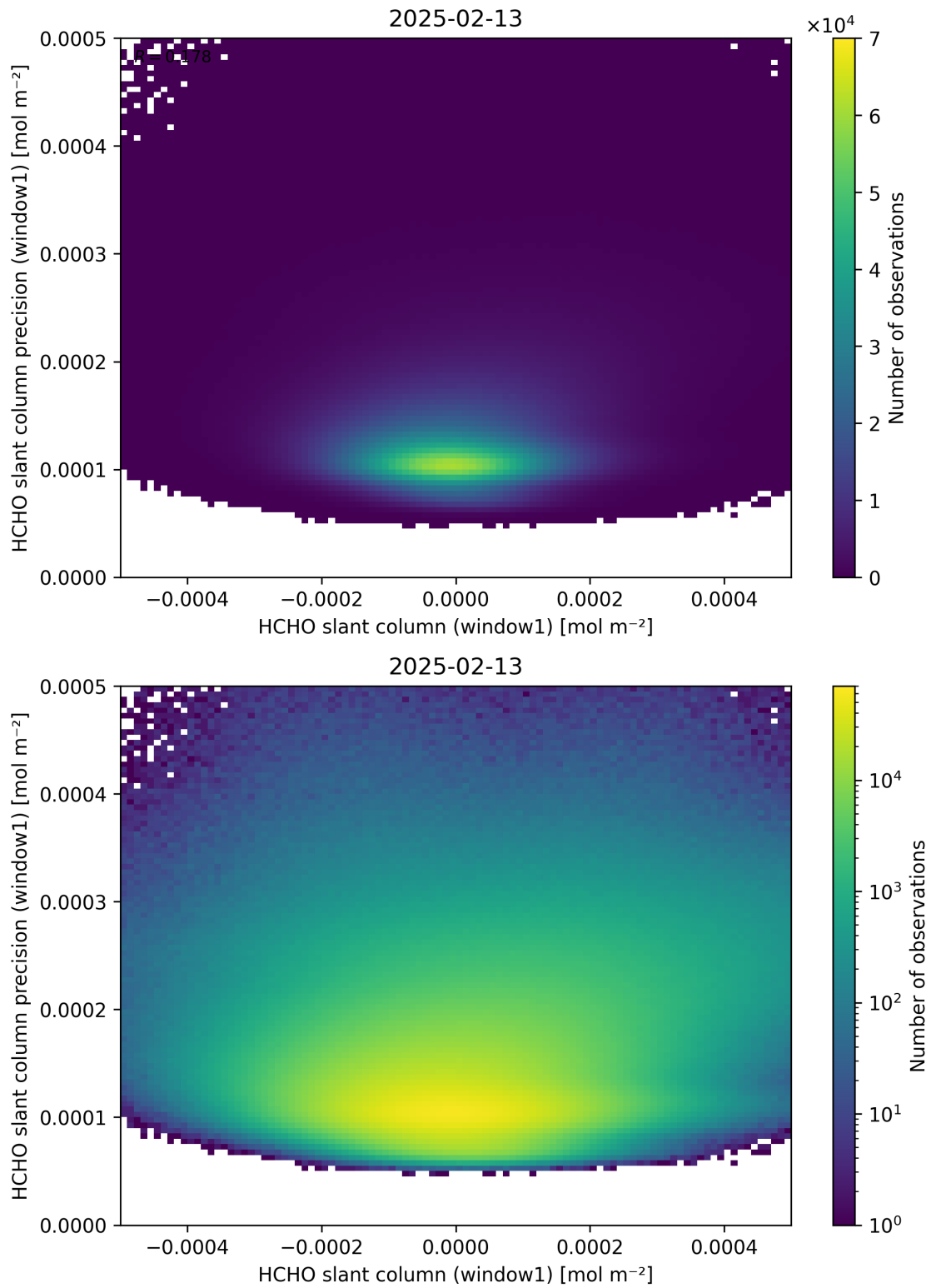
Figure 84: Scatter density plot of “HCHO slant column (window1)” against “HCHO slant column precision (window1)” for 2025-02-13 to 2025-02-14.
