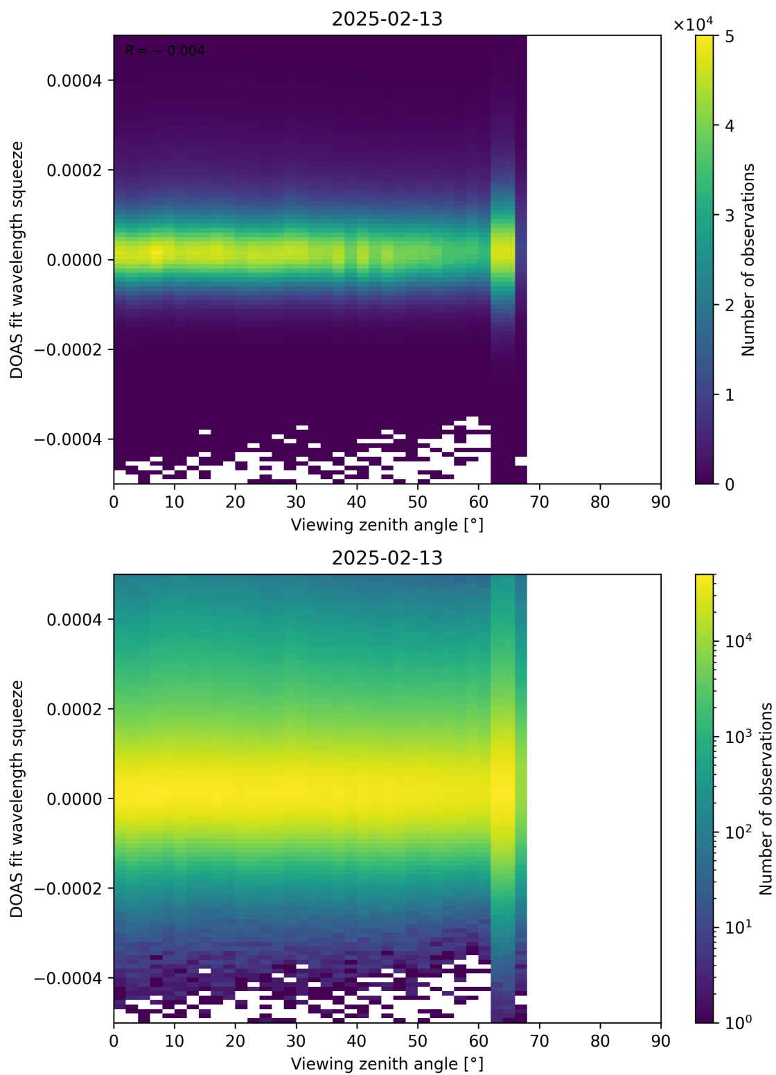
Figure 184: Scatter density plot of “Viewing zenith angle” against “DOAS fit wavelength squeeze” for 2025-02-13 to 2025-02-14.
