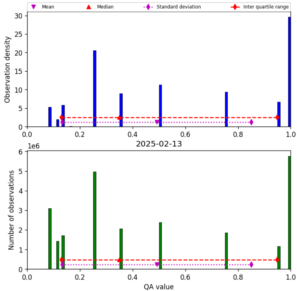
Figure 34: Histogram of “QA value” for 2025-02-13 to 2025-02-14
