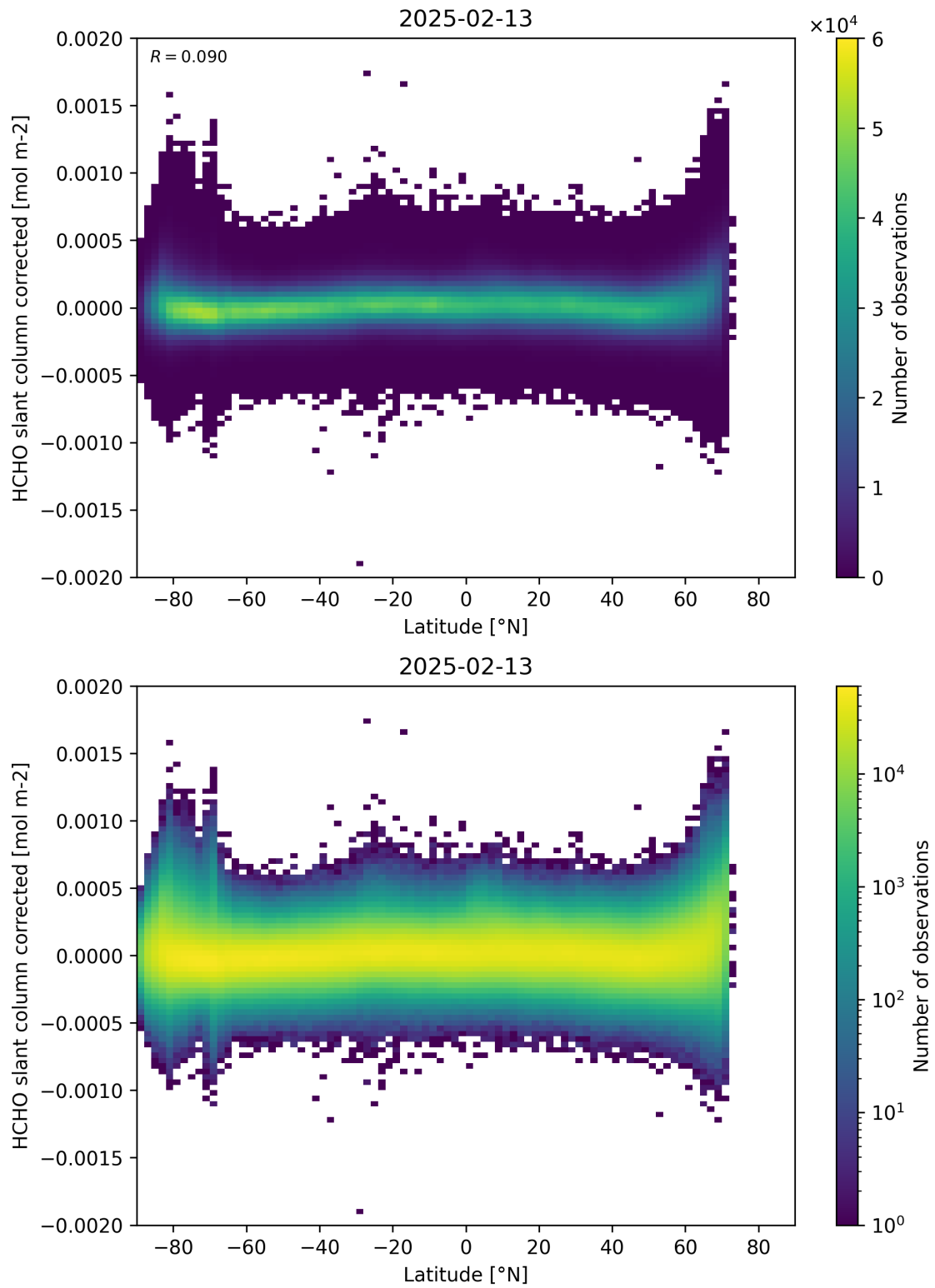
Figure 157: Scatter density plot of “Latitude” against “HCHO slant column corrected” for 2025-02-13 to 2025-02-14.
