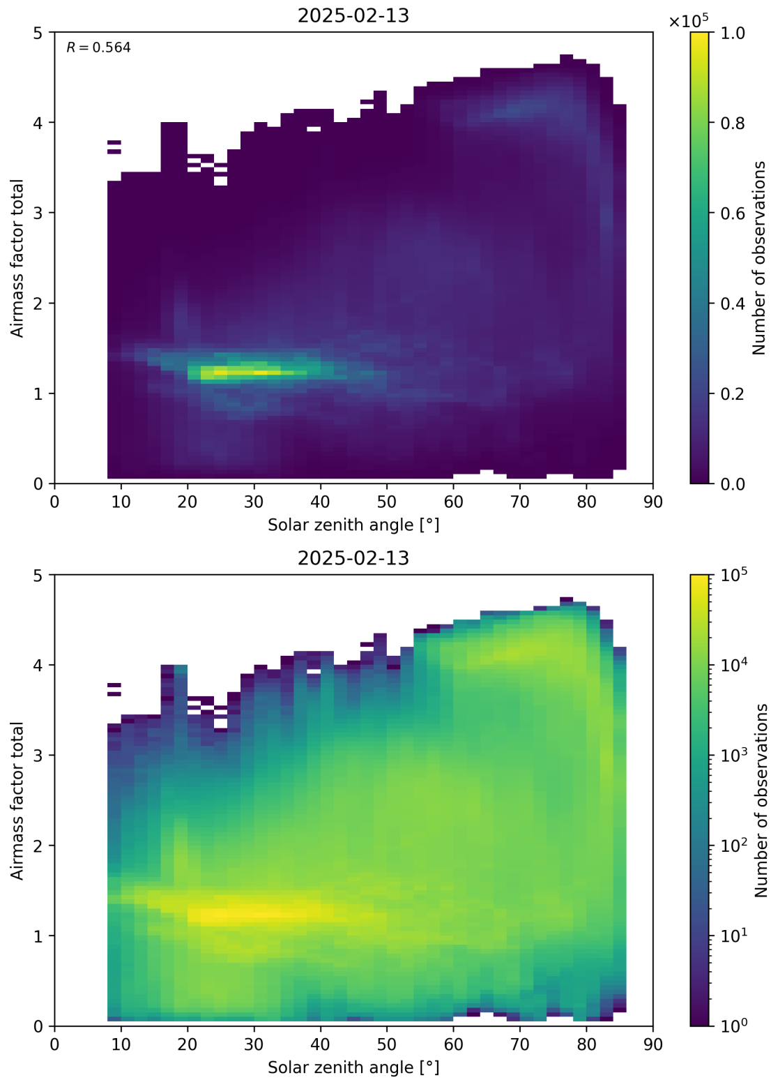
Figure 175: Scatter density plot of “Solar zenith angle” against “Airmass factor total” for 2025-02-13 to 2025-02-14.
