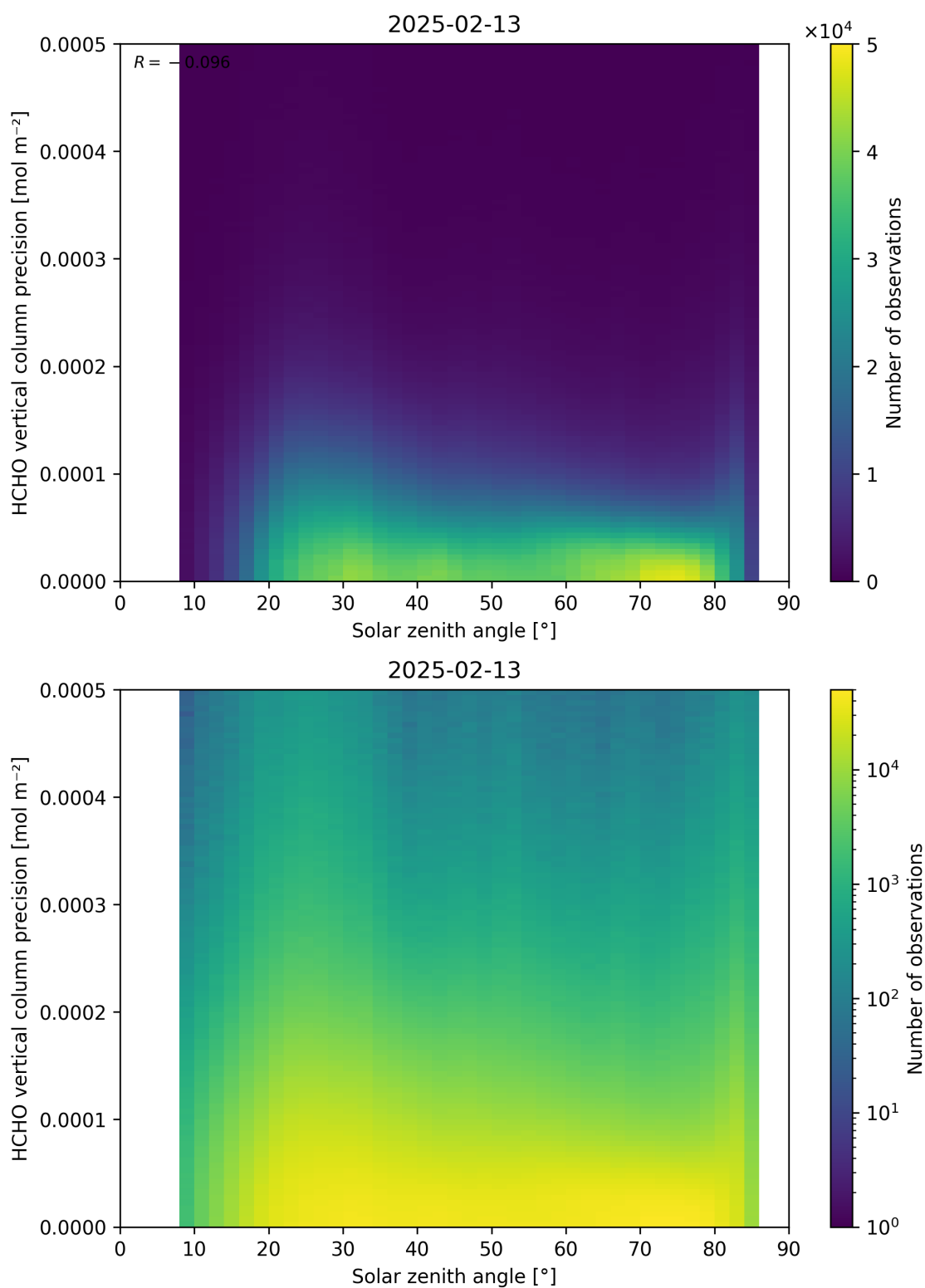
Figure 179: Scatter density plot of “Solar zenith angle” against “HCHO vertical column precision” for 2025-02-13 to 2025-02-14.
