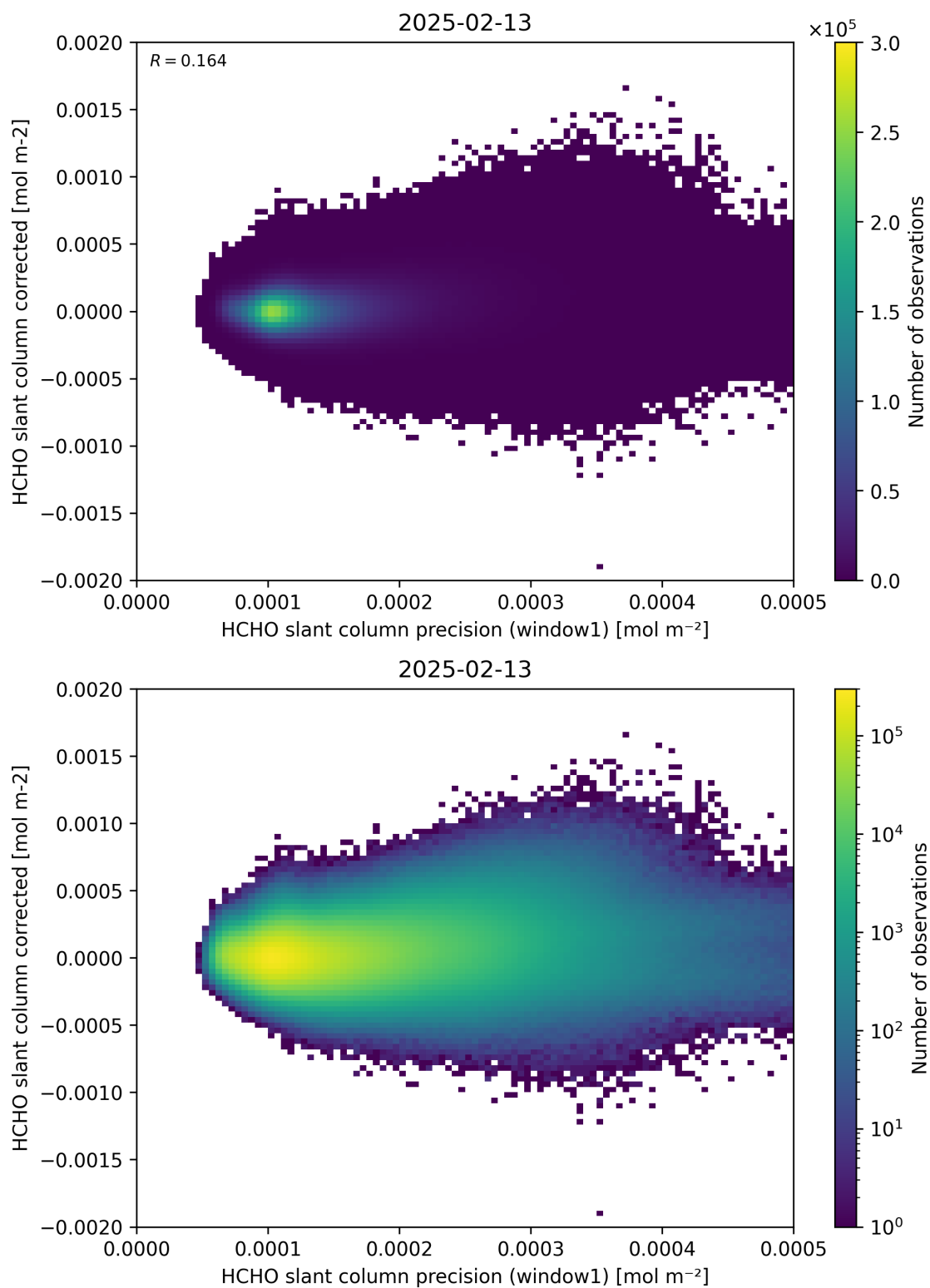
Figure 92: Scatter density plot of “HCHO slant column precision (window1)” against “HCHO slant column corrected” for 2025-02-13 to 2025-02-14.
