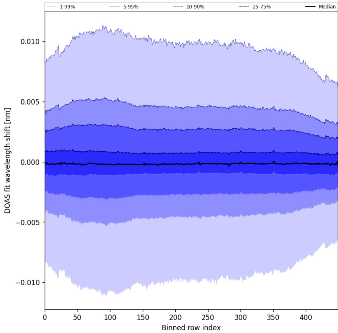
Figure 58: Along track statistics of “DOAS fit wavelength shift” for 2025-02-13 to 2025-02-14
