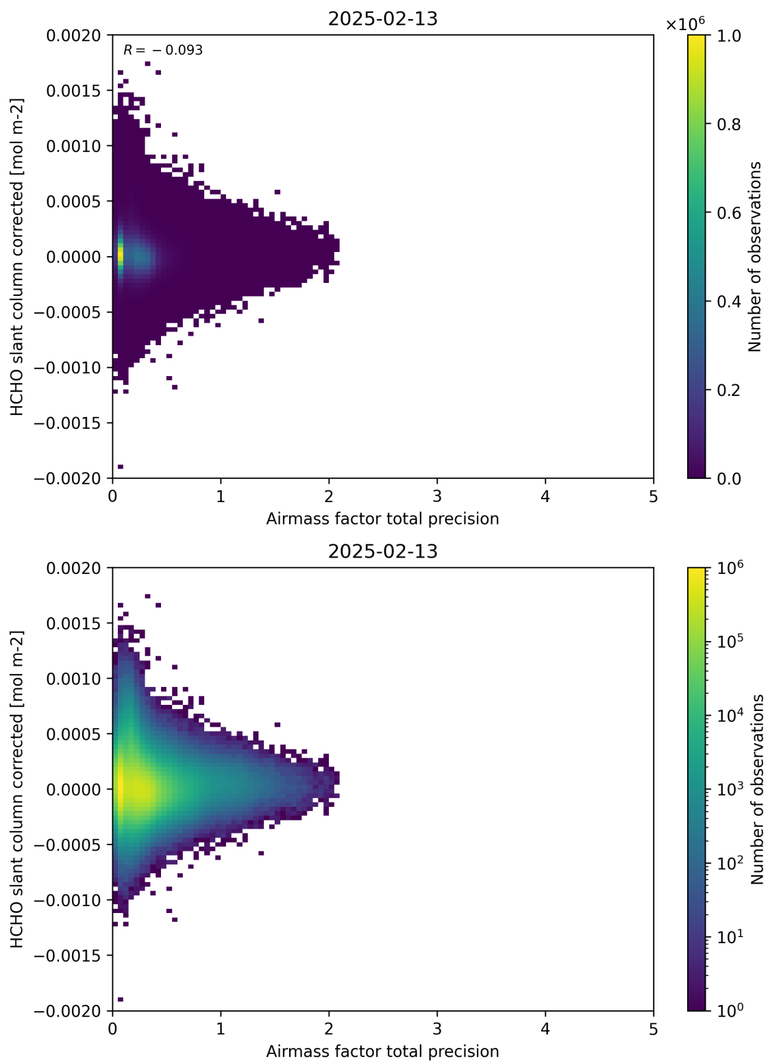
Figure 109: Scatter density plot of “Airmass factor total precision” against “HCHO slant column corrected” for 2025-02-13 to 2025-02-14.
