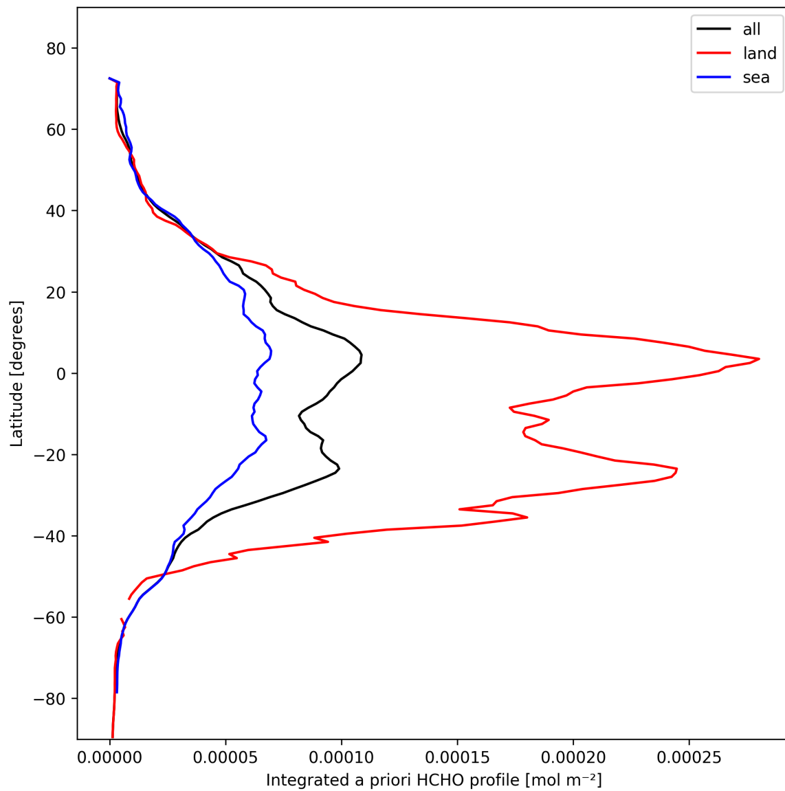
Figure 29: Zonal average of “Integrated a priori HCHO profile” for 2025-02-13 to 2025-02-14.
