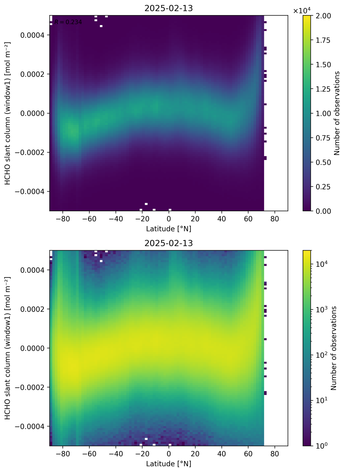
Figure 159: Scatter density plot of “Latitude” against “HCHO slant column (window1)” for 2025-02-13 to 2025-02-14.
