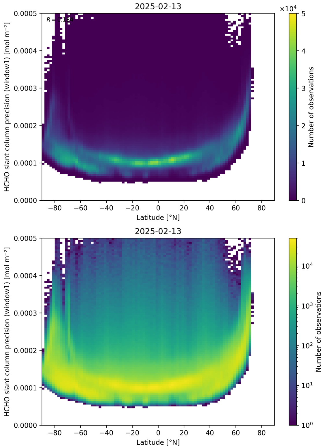
Figure 160: Scatter density plot of “Latitude” against “HCHO slant column precision (window1)” for 2025-02-13 to 2025-02-14.
