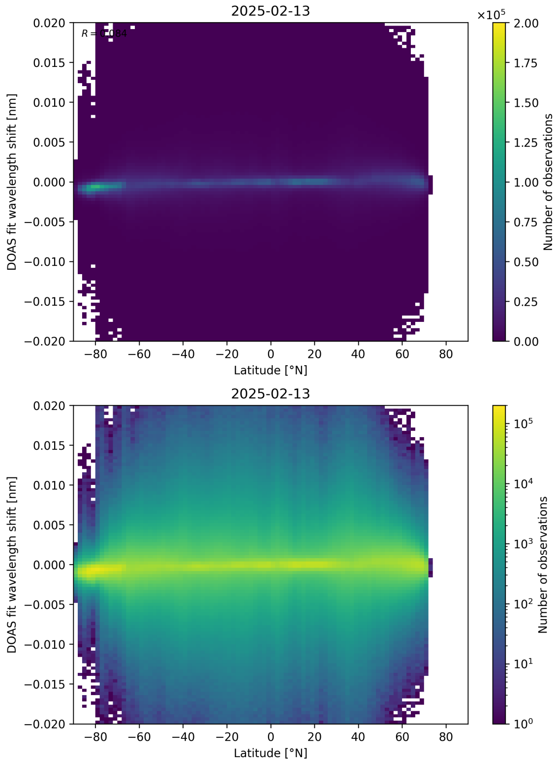
Figure 154: Scatter density plot of “Latitude” against “DOAS fit wavelength shift” for 2025-02-13 to 2025-02-14.
