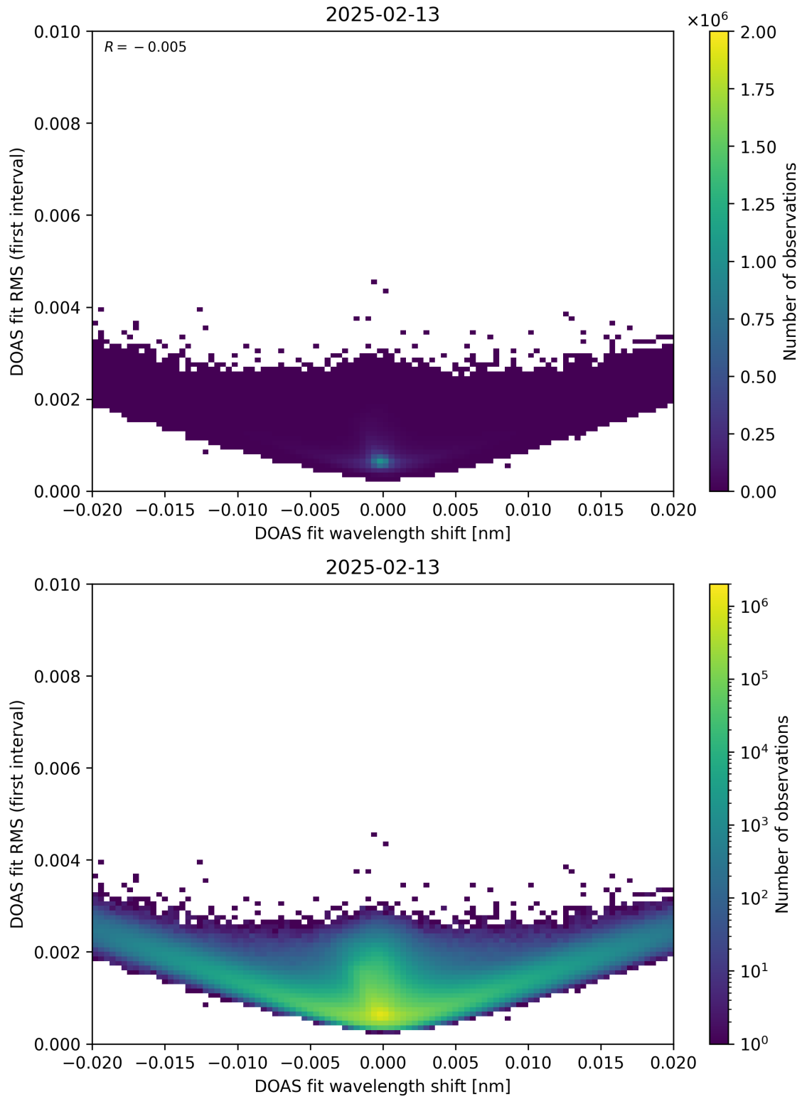
Figure 64: Scatter density plot of “DOAS fit wavelength shift” against “DOAS fit RMS (first interval)” for 2025-02-13 to 2025-02-14.
