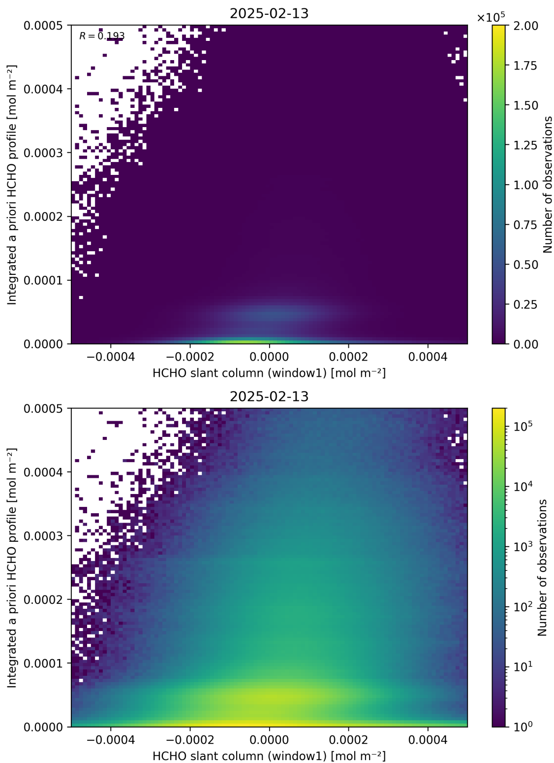
Figure 87: Scatter density plot of “HCHO slant column (window1)” against “Integrated a priori HCHO profile” for 2025-02-13 to 2025-02-14.
