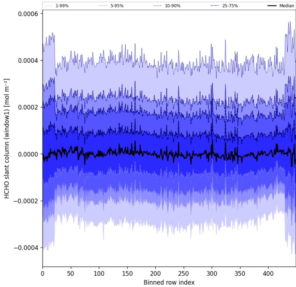
Figure 52: Along track statistics of “HCHO slant column (window1)” for 2025-02-13 to 2025-02-14
