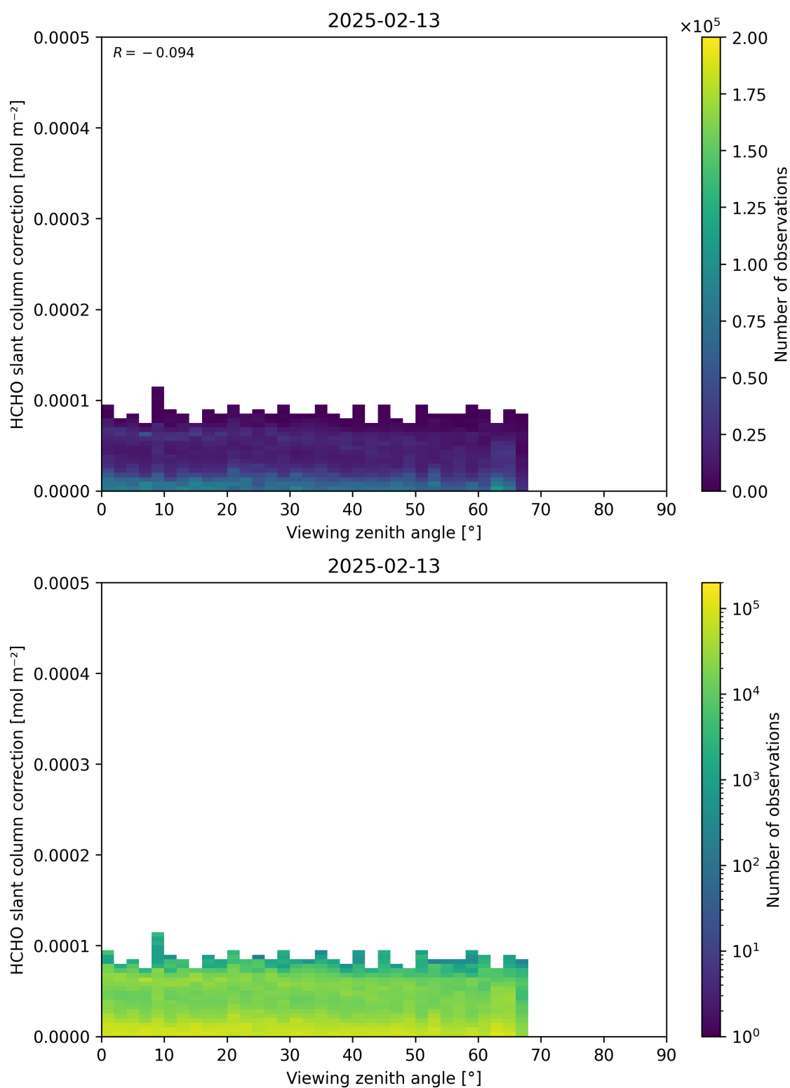
Figure 187: Scatter density plot of “Viewing zenith angle” against “HCHO slant column correction” for 2025-02-13 to 2025-02-14.
