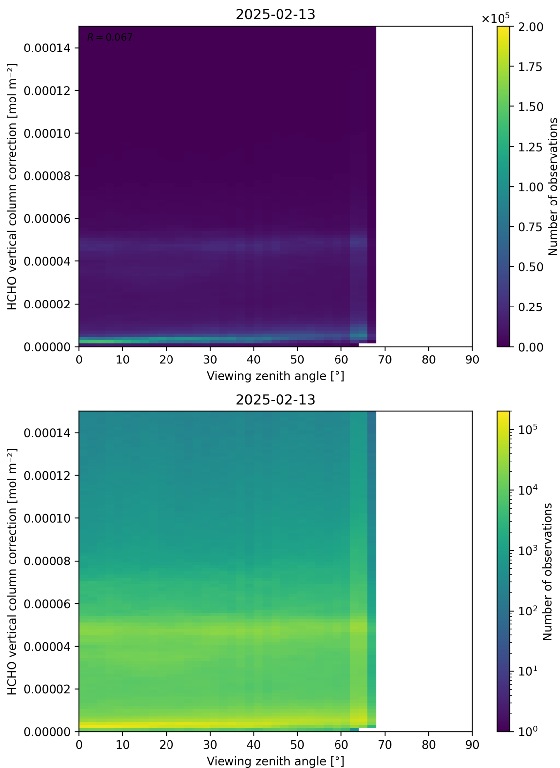
Figure 193: Scatter density plot of “Viewing zenith angle” against “HCHO vertical column correction” for 2025-02-13 to 2025-02-14.
