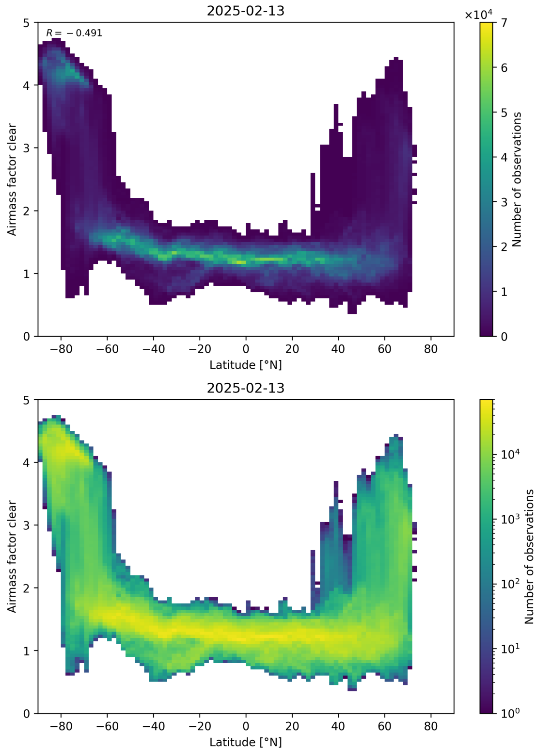
Figure 156: Scatter density plot of “Latitude” against “Airmass factor clear” for 2025-02-13 to 2025-02-14.
