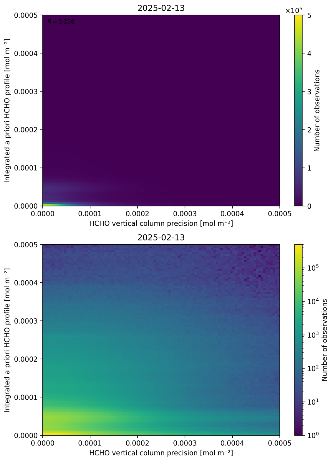
Figure 147: Scatter density plot of “HCHO vertical column precision” against “Integrated a priori HCHO profile” for 2025-02-13 to 2025-02-14.
