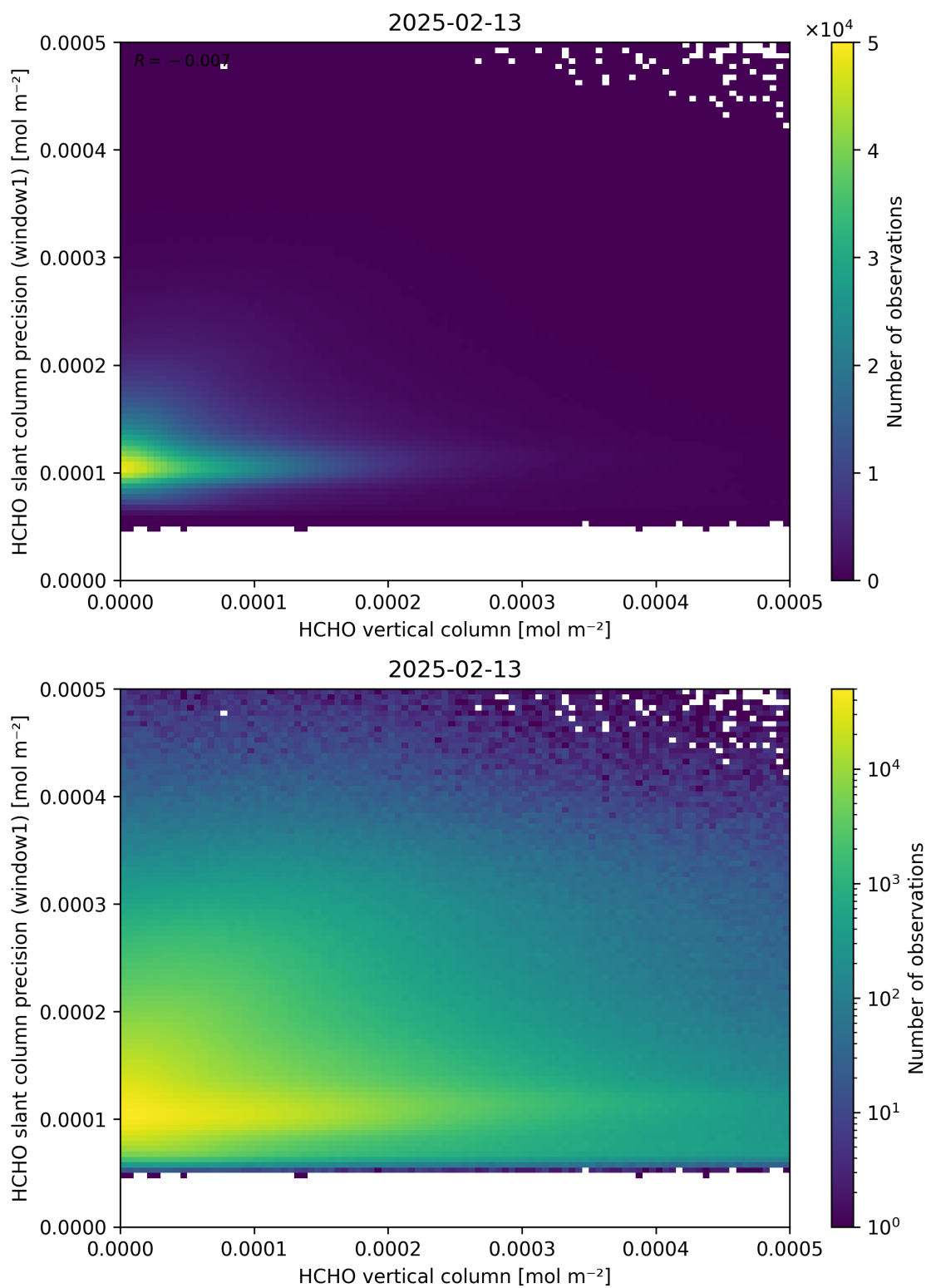
Figure 130: Scatter density plot of “HCHO vertical column” against “HCHO slant column precision (window1)” for 2025-02-13 to 2025-02-14.
