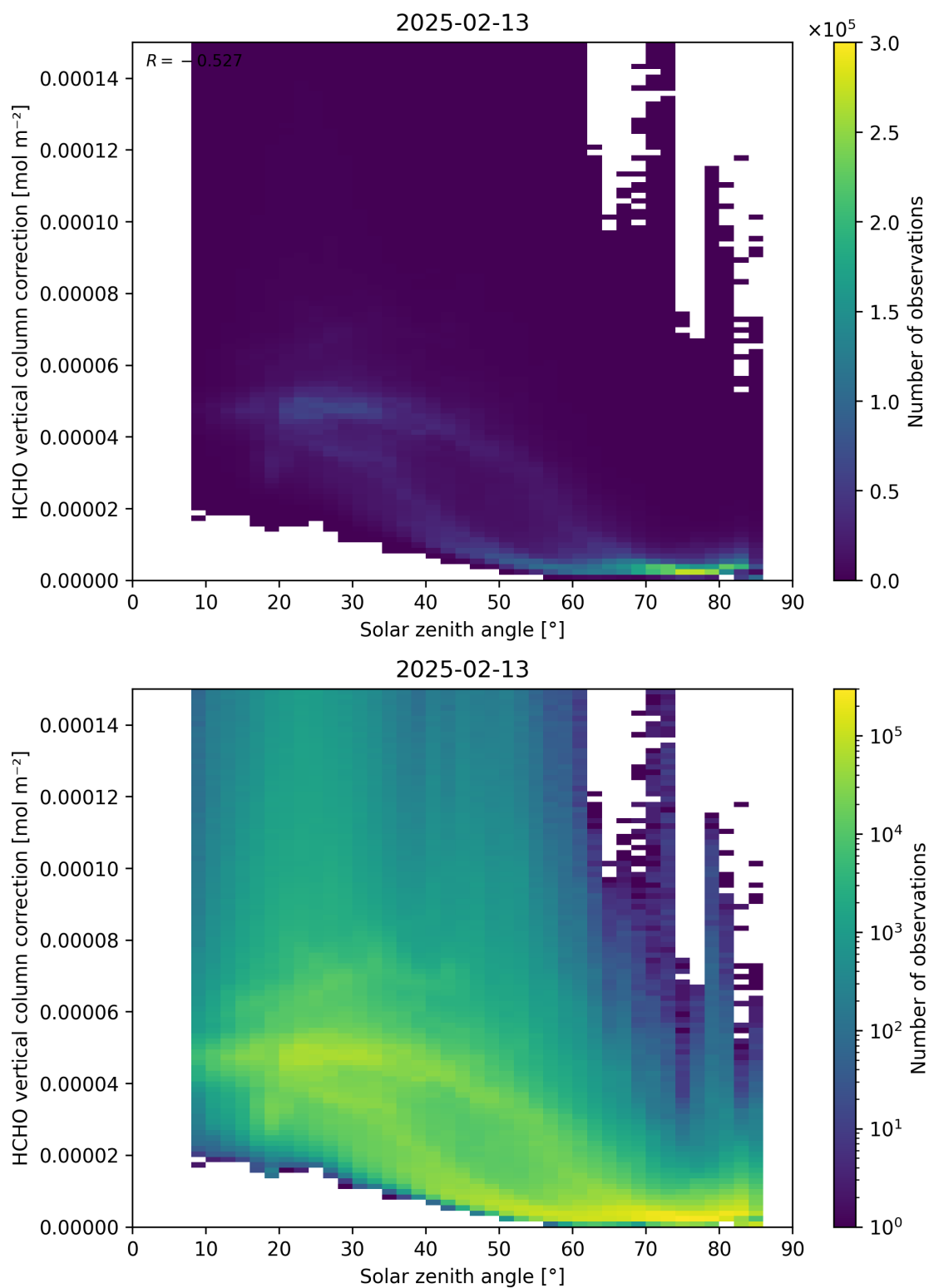
Figure 178: Scatter density plot of “Solar zenith angle” against “HCHO vertical column correction” for 2025-02-13 to 2025-02-14.
