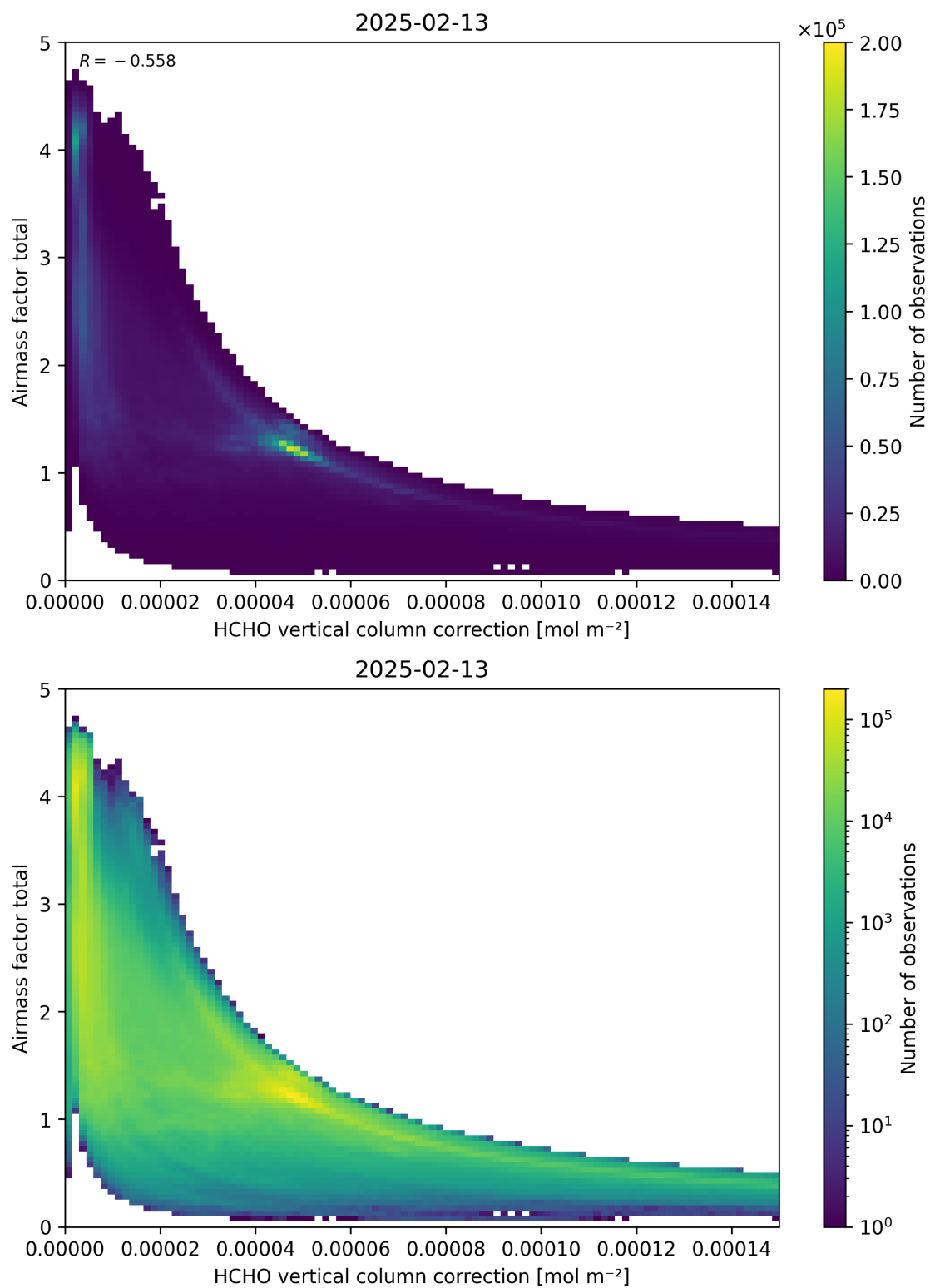
Figure 120: Scatter density plot of “HCHO vertical column correction” against “Airmass factor total” for 2025-02-13 to 2025-02-14.
