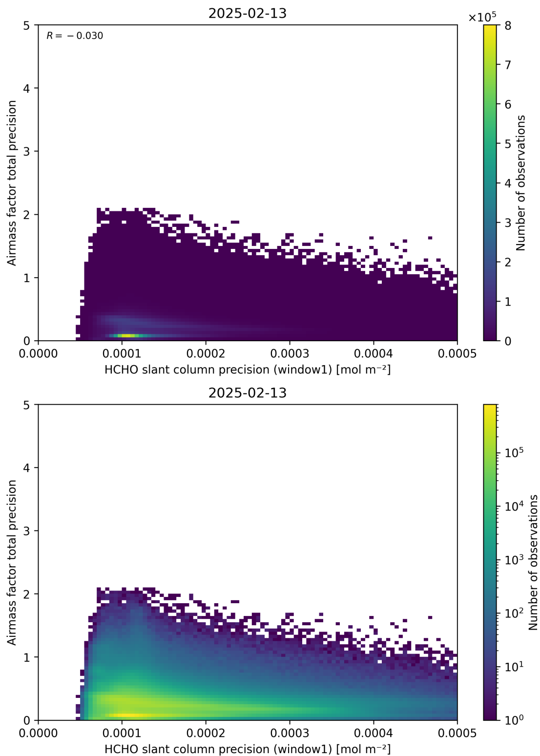
Figure 95: Scatter density plot of “HCHO slant column precision (window1)” against “Airmass factor total precision” for 2025-02-13 to 2025-02-14.
