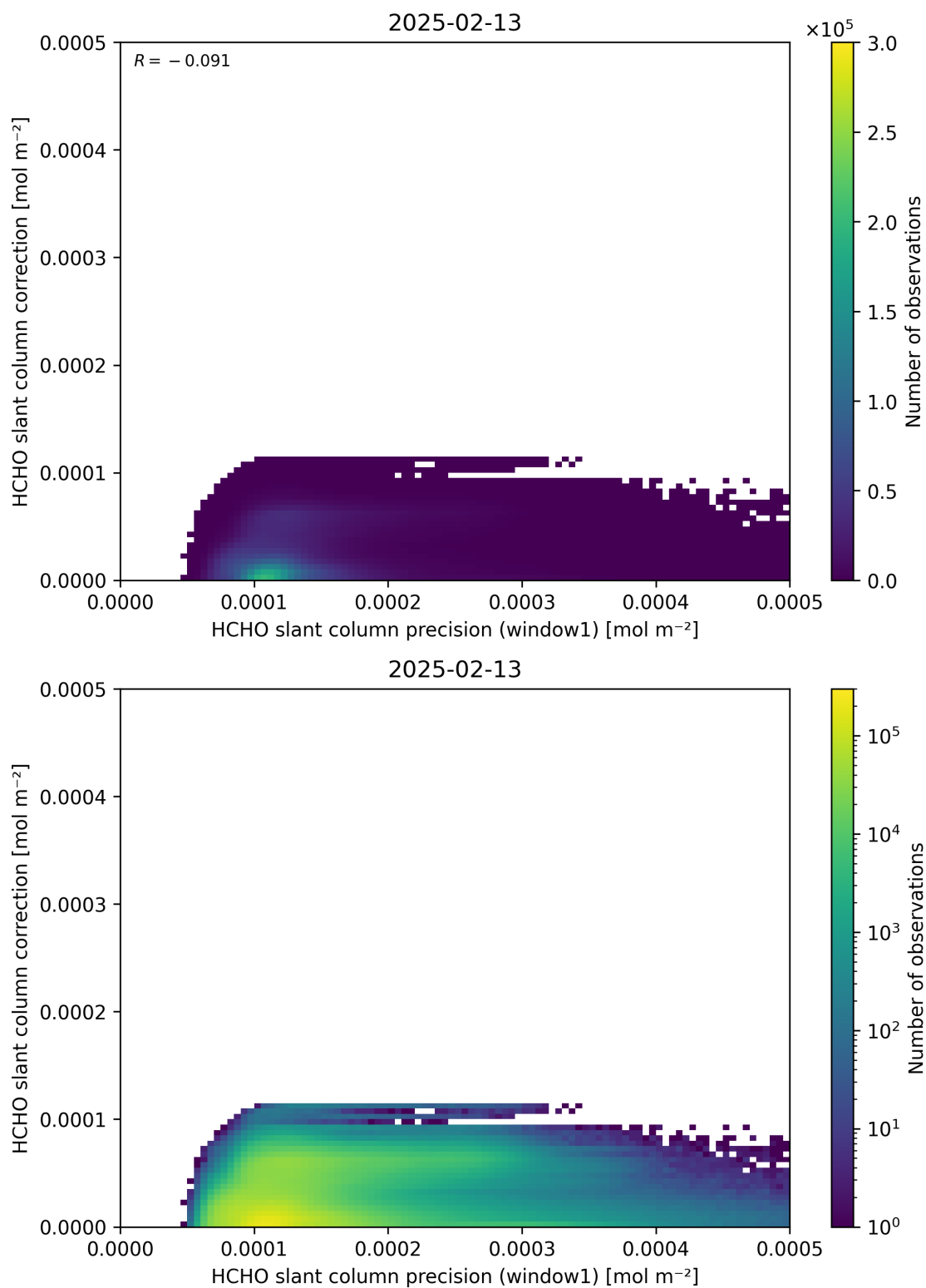
Figure 93: Scatter density plot of “HCHO slant column precision (window1)” against “HCHO slant column correction” for 2025-02-13 to 2025-02-14.
