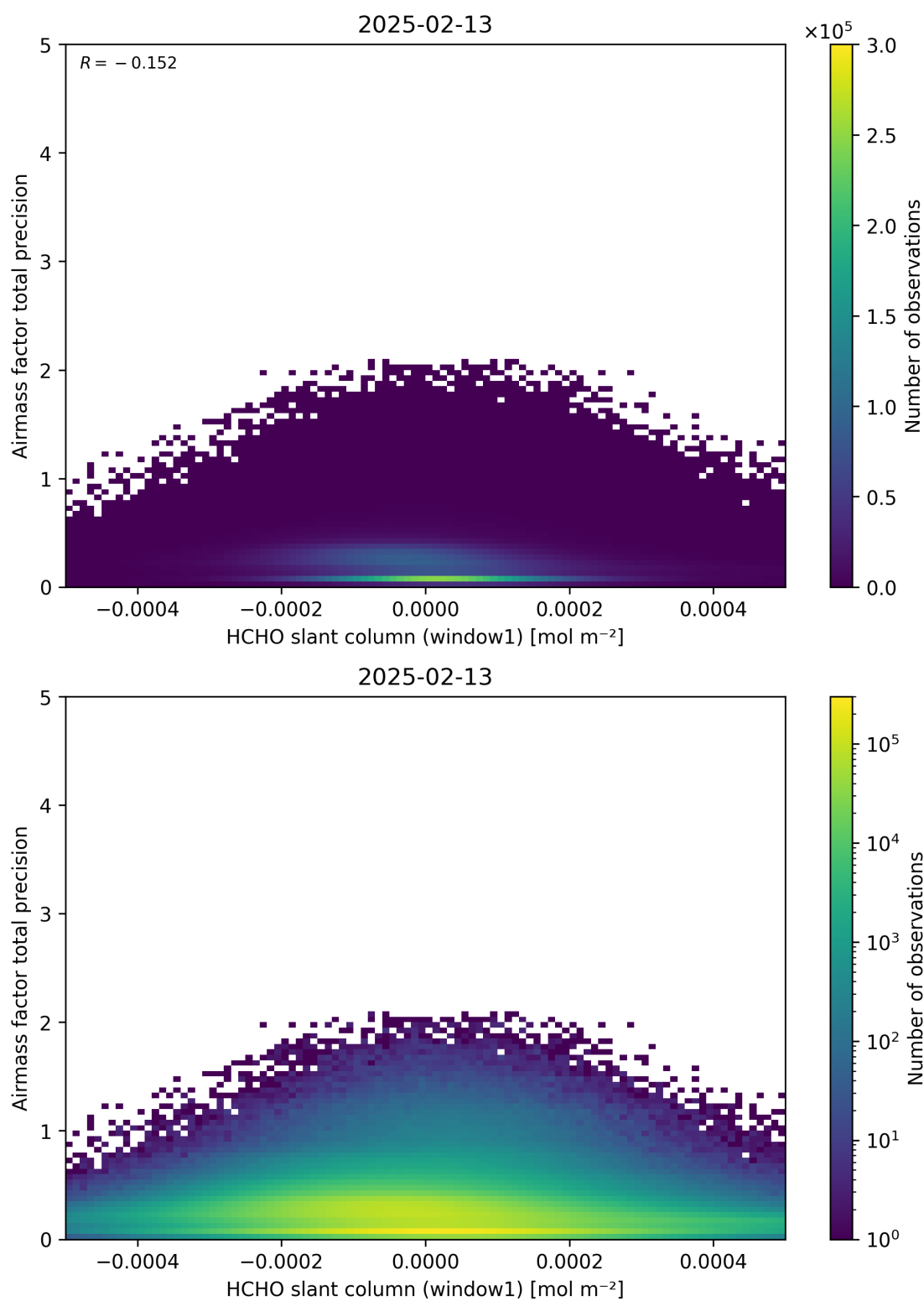
Figure 86: Scatter density plot of “HCHO slant column (window1)” against “Airmass factor total precision” for 2025-02-13 to 2025-02-14.
