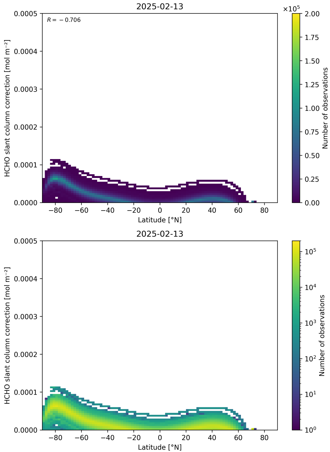
Figure 158: Scatter density plot of “Latitude” against “HCHO slant column correction” for 2025-02-13 to 2025-02-14.
