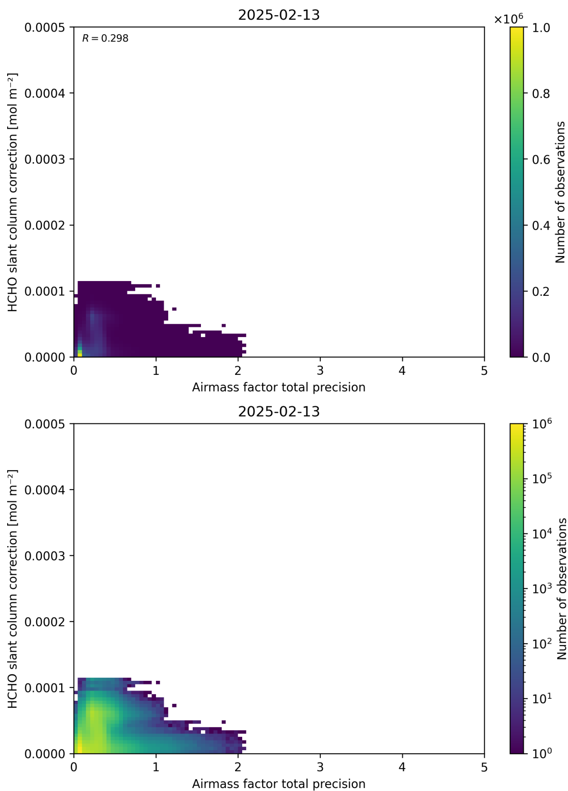
Figure 110: Scatter density plot of “Airmass factor total precision” against “HCHO slant column correction” for 2025-02-13 to 2025-02-14.
