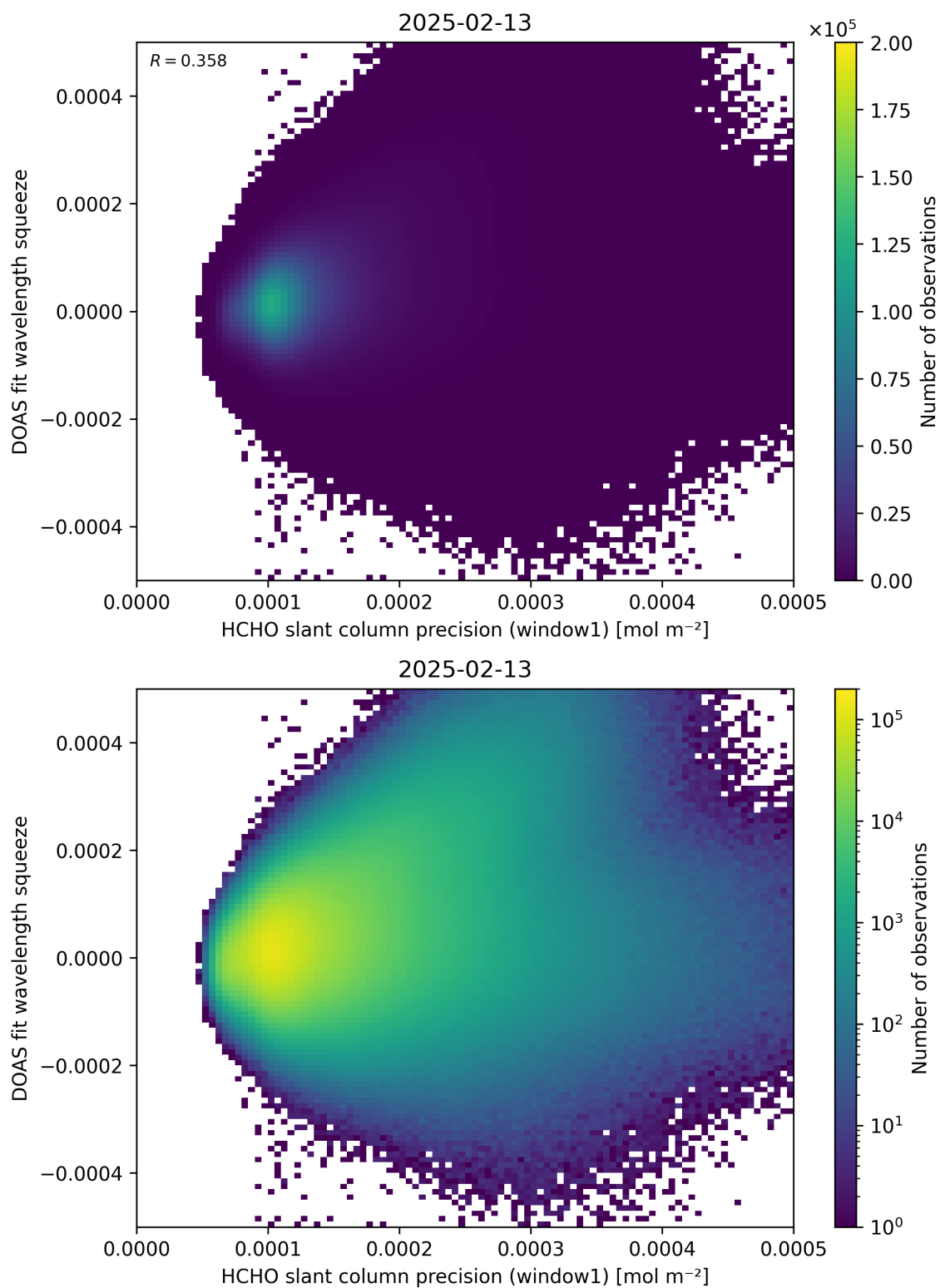
Figure 90: Scatter density plot of “HCHO slant column precision (window1)” against “DOAS fit wavelength squeeze” for 2025-02-13 to 2025-02-14.
