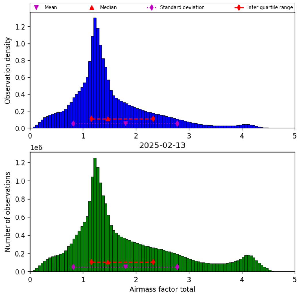
Figure 40: Histogram of “Airmass factor total” for 2025-02-13 to 2025-02-14
