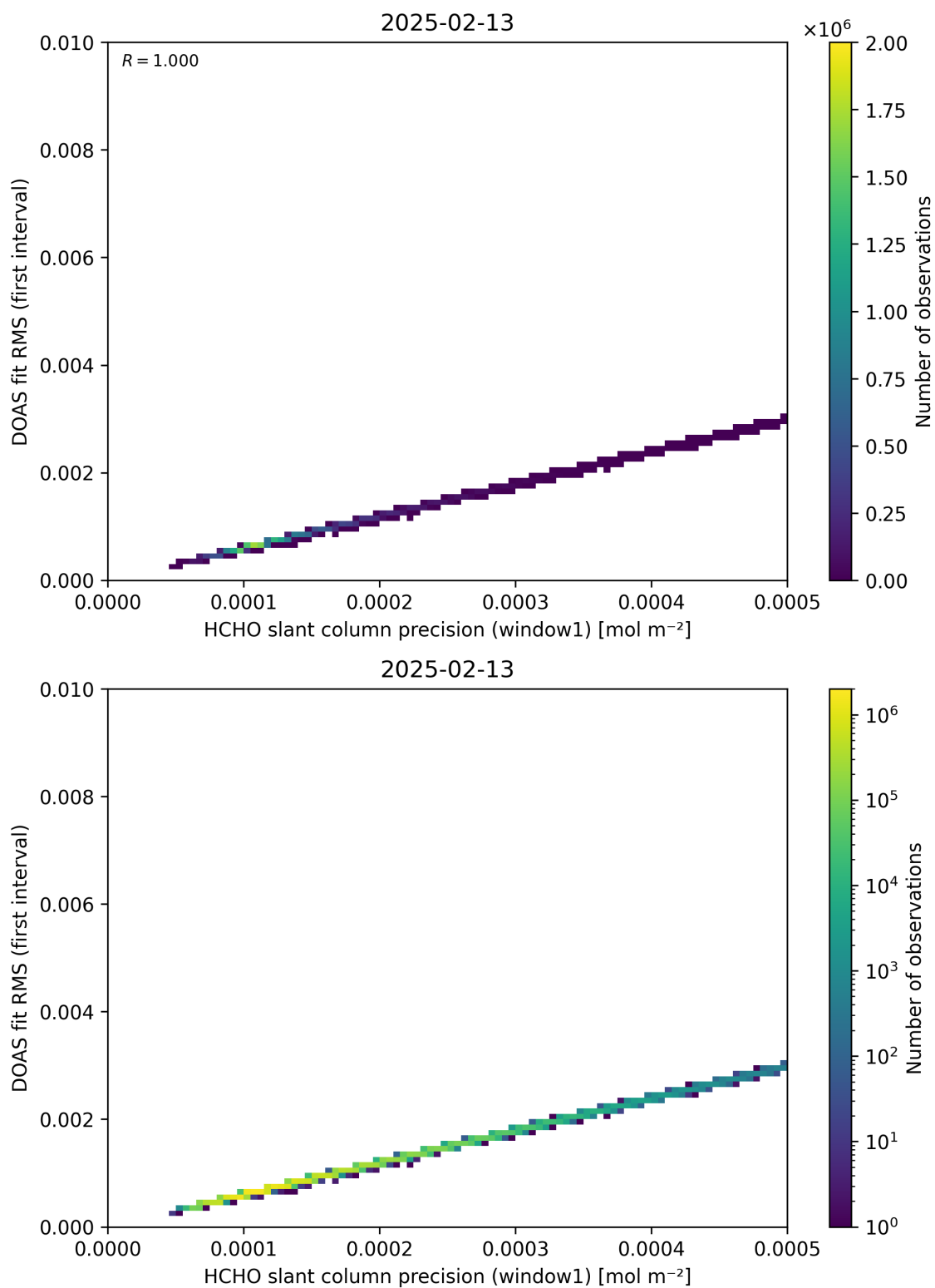
Figure 88: Scatter density plot of “HCHO slant column precision (window1)” against “DOAS fit RMS (first interval)” for 2025-02-13 to 2025-02-14.
