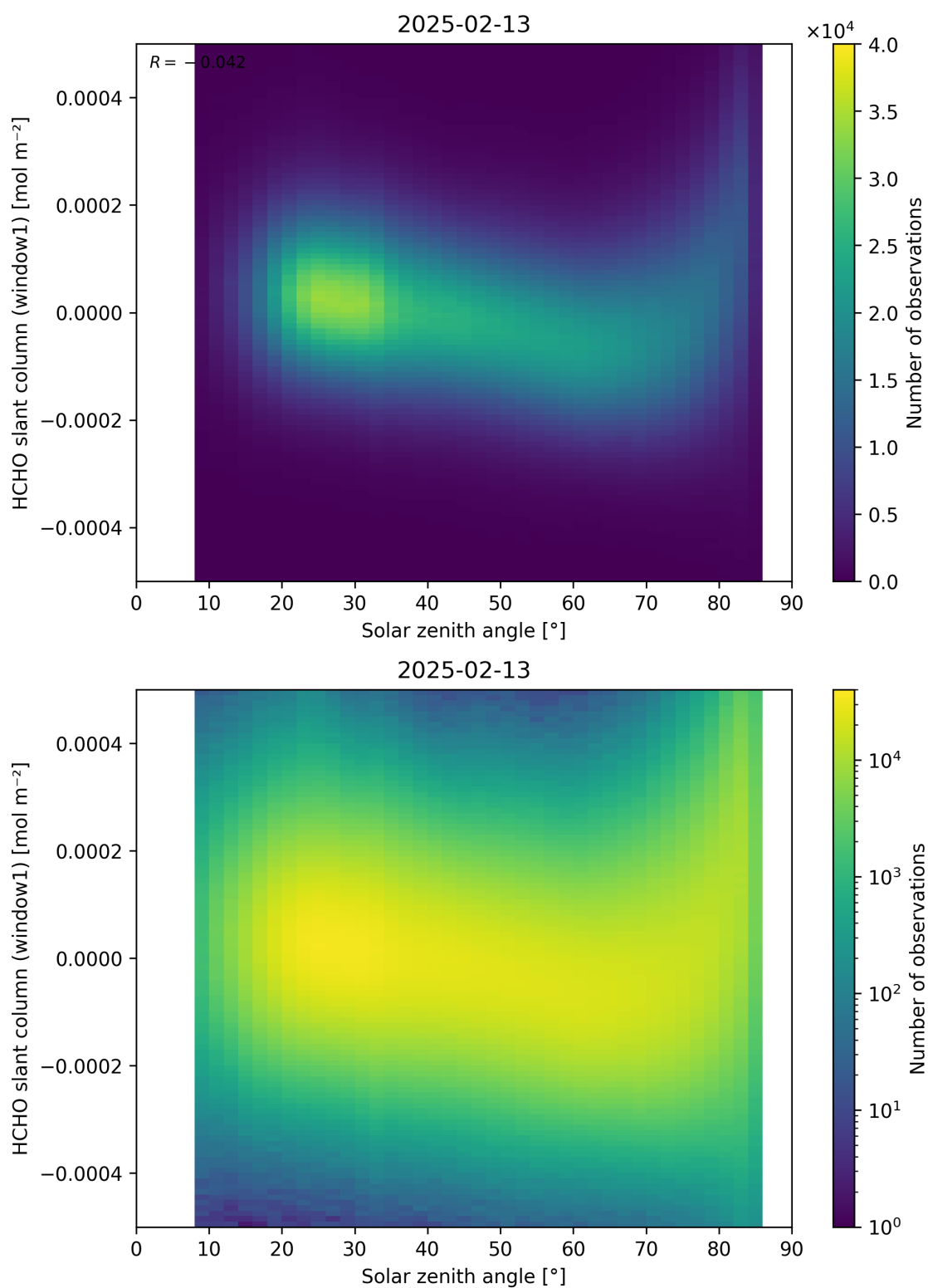
Figure 173: Scatter density plot of “Solar zenith angle” against “HCHO slant column (window1)” for 2025-02-13 to 2025-02-14.
