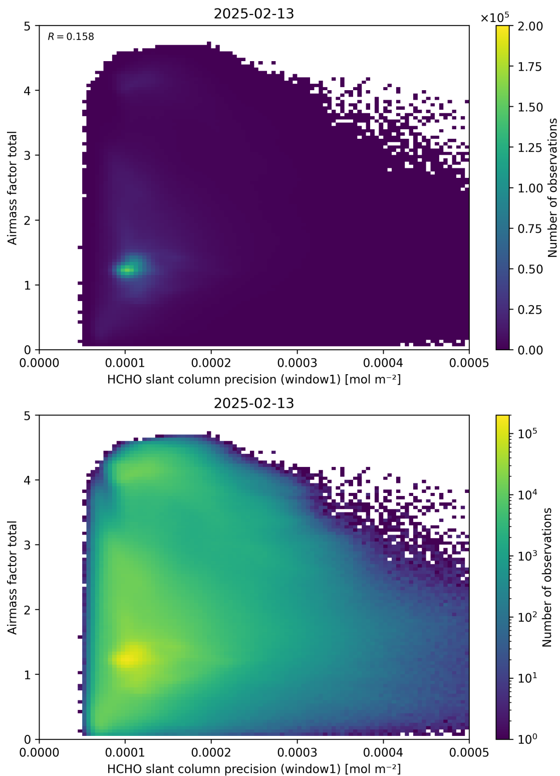
Figure 94: Scatter density plot of “HCHO slant column precision (window1)” against “Airmass factor total” for 2025-02-13 to 2025-02-14.
