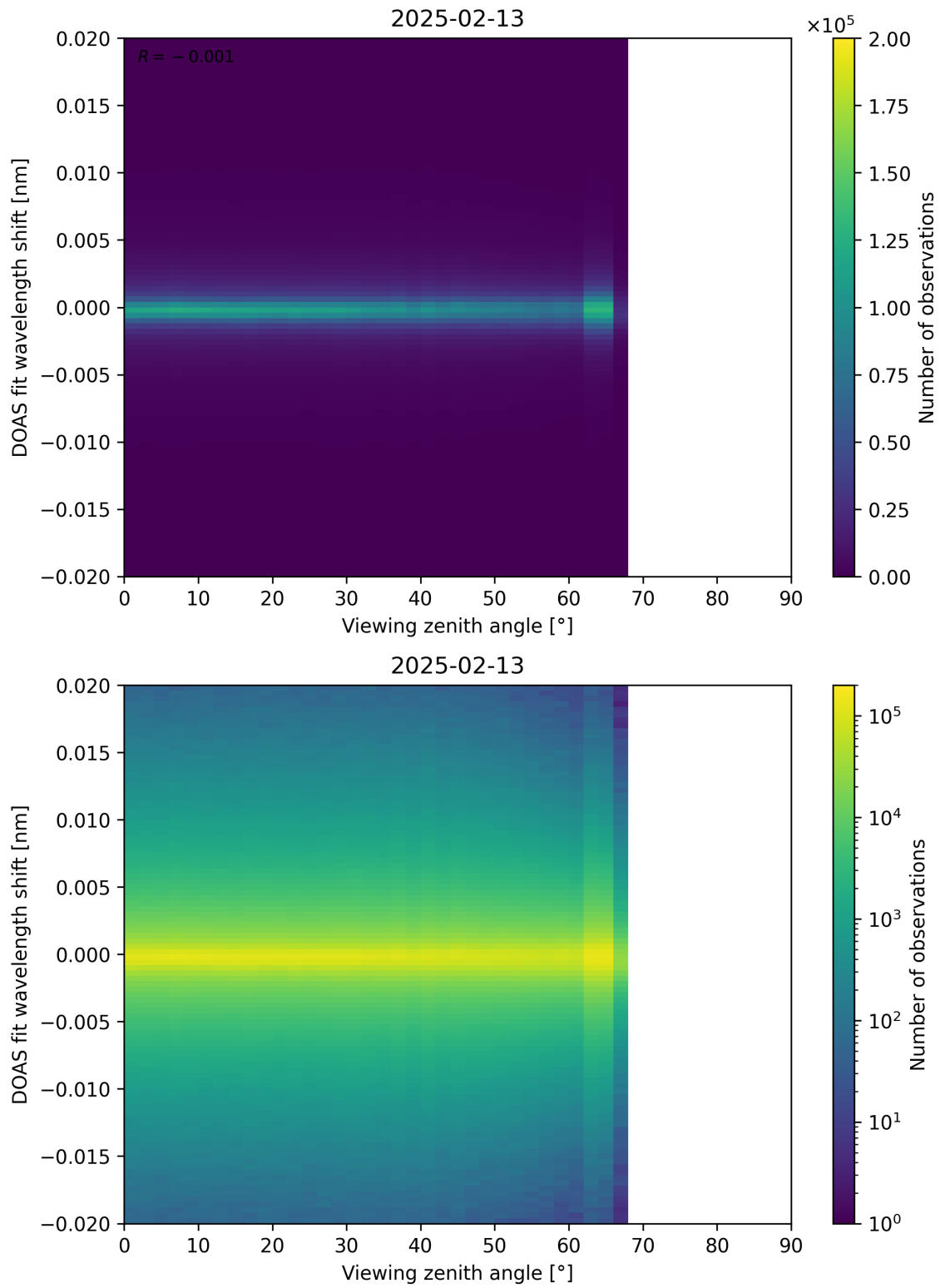
Figure 183: Scatter density plot of “Viewing zenith angle” against “DOAS fit wavelength shift” for 2025-02-13 to 2025-02-14.
