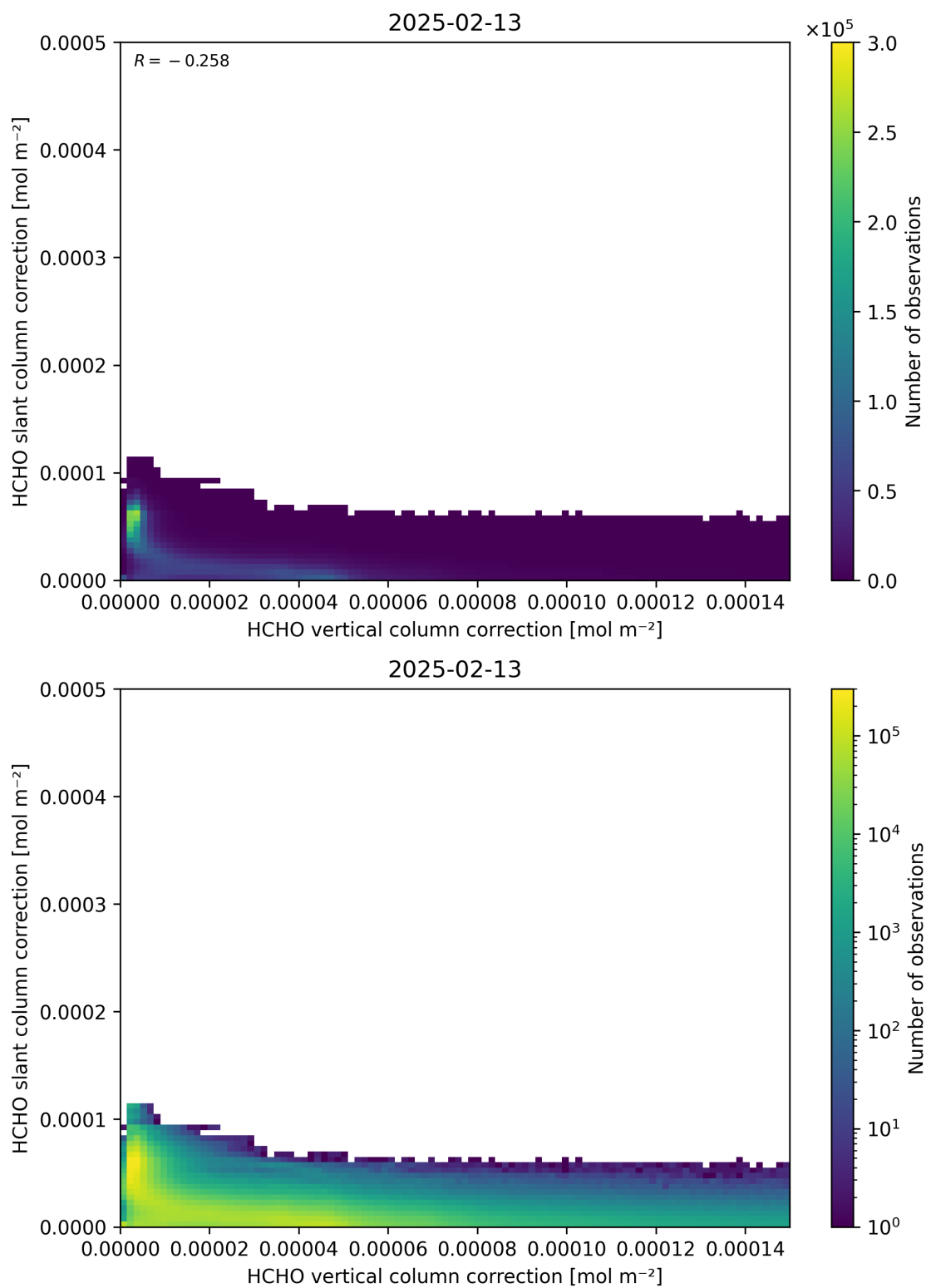
Figure 117: Scatter density plot of “HCHO vertical column correction” against “HCHO slant column correction” for 2025-02-13 to 2025-02-14.
