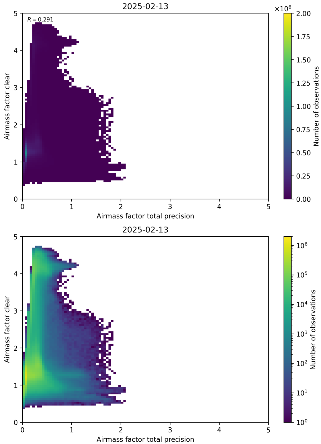
Figure 108: Scatter density plot of “Airmass factor total precision” against “Airmass factor clear” for 2025-02-13 to 2025-02-14.
