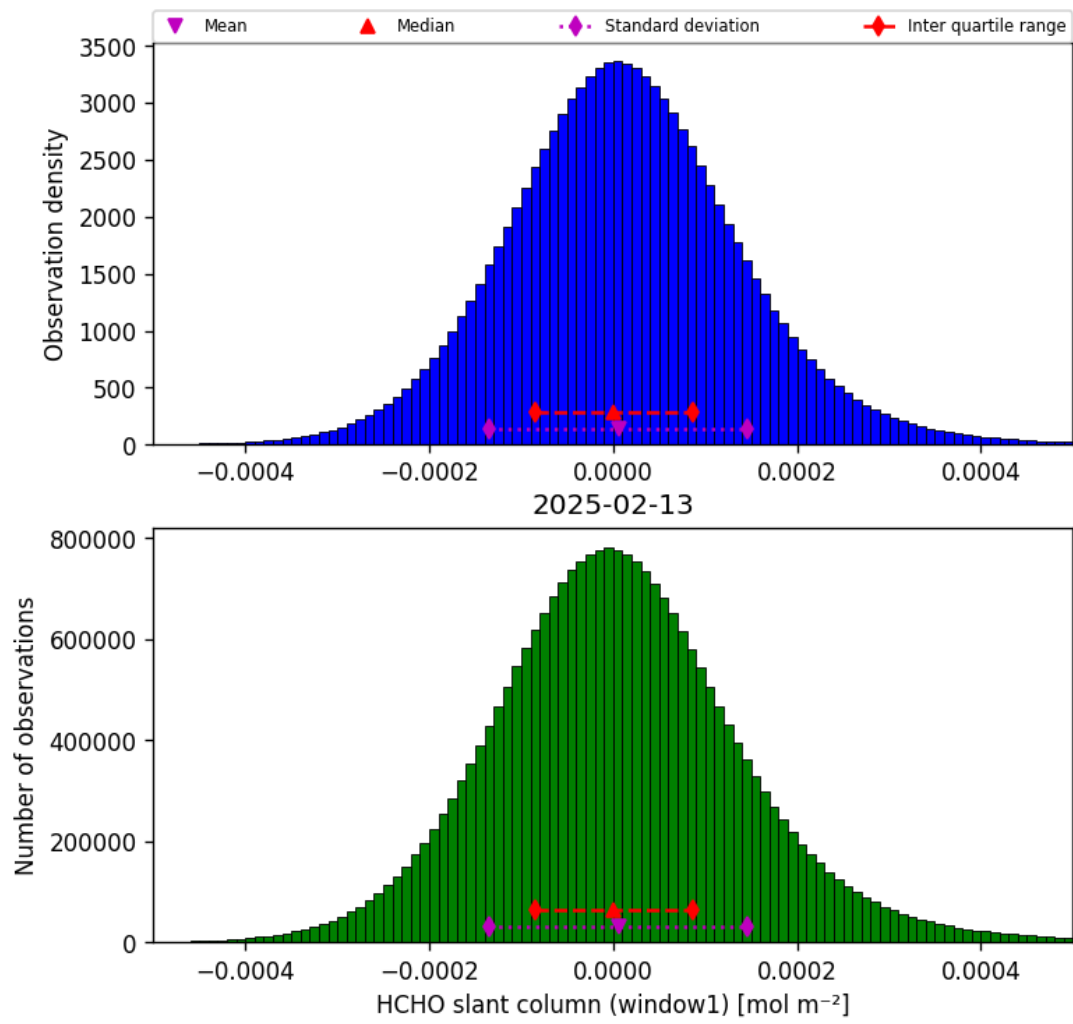
Figure 38: Histogram of “HCHO slant column (window1)” for 2025-02-13 to 2025-02-14
