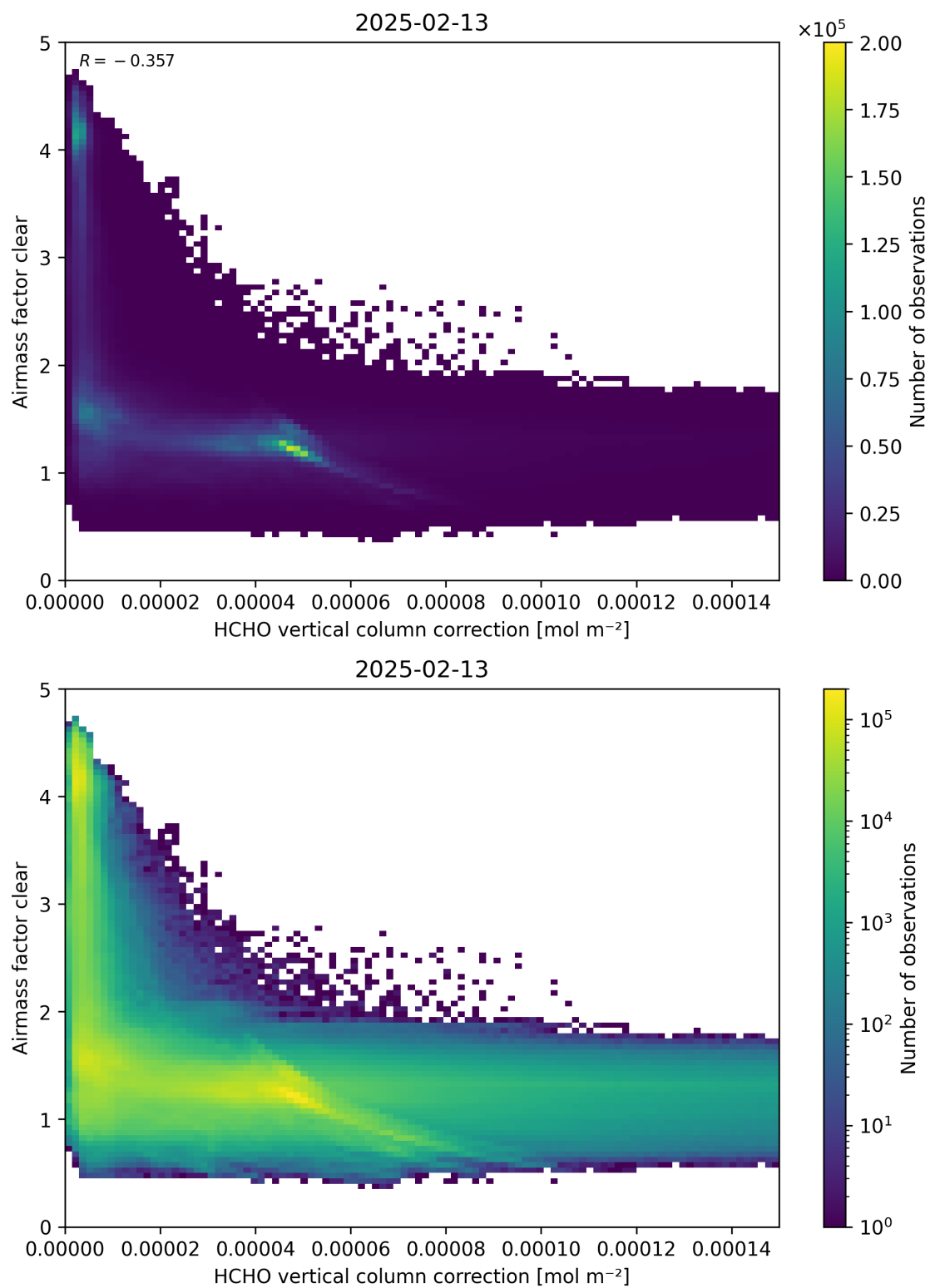
Figure 115: Scatter density plot of “HCHO vertical column correction” against “Airmass factor clear” for 2025-02-13 to 2025-02-14.
