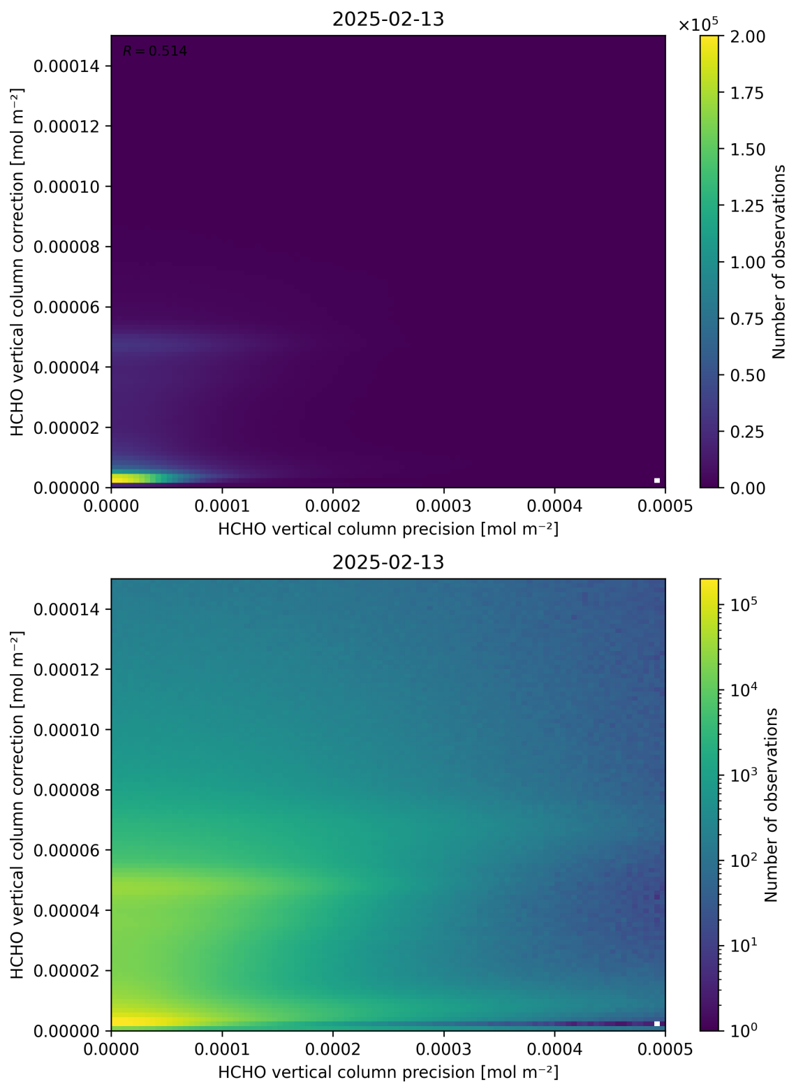
Figure 146: Scatter density plot of “HCHO vertical column precision” against “HCHO vertical column correction” for 2025-02-13 to 2025-02-14.
