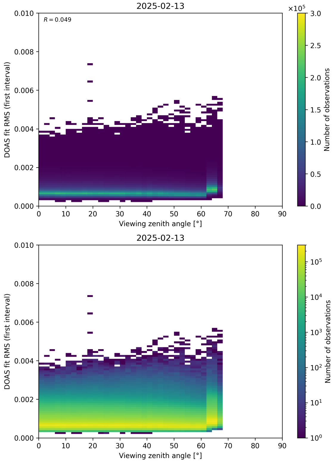
Figure 182: Scatter density plot of “Viewing zenith angle” against “DOAS fit RMS (first interval)” for 2025-02-13 to 2025-02-14.
