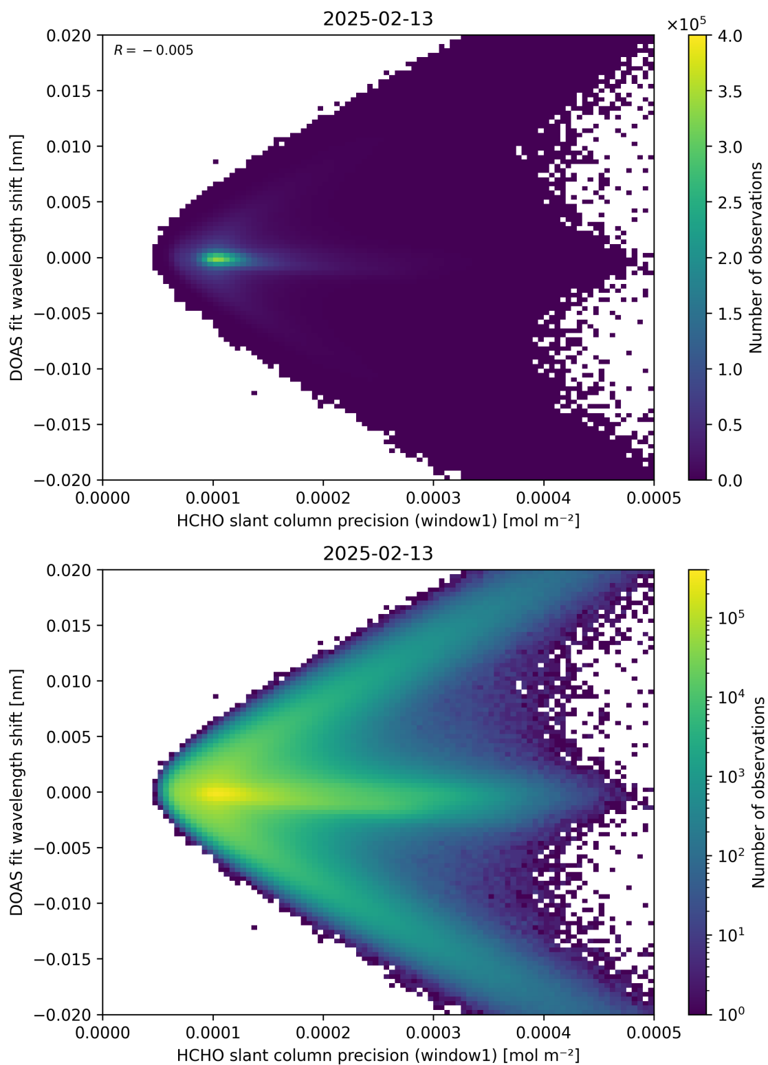
Figure 89: Scatter density plot of “HCHO slant column precision (window1)” against “DOAS fit wavelength shift” for 2025-02-13 to 2025-02-14.
