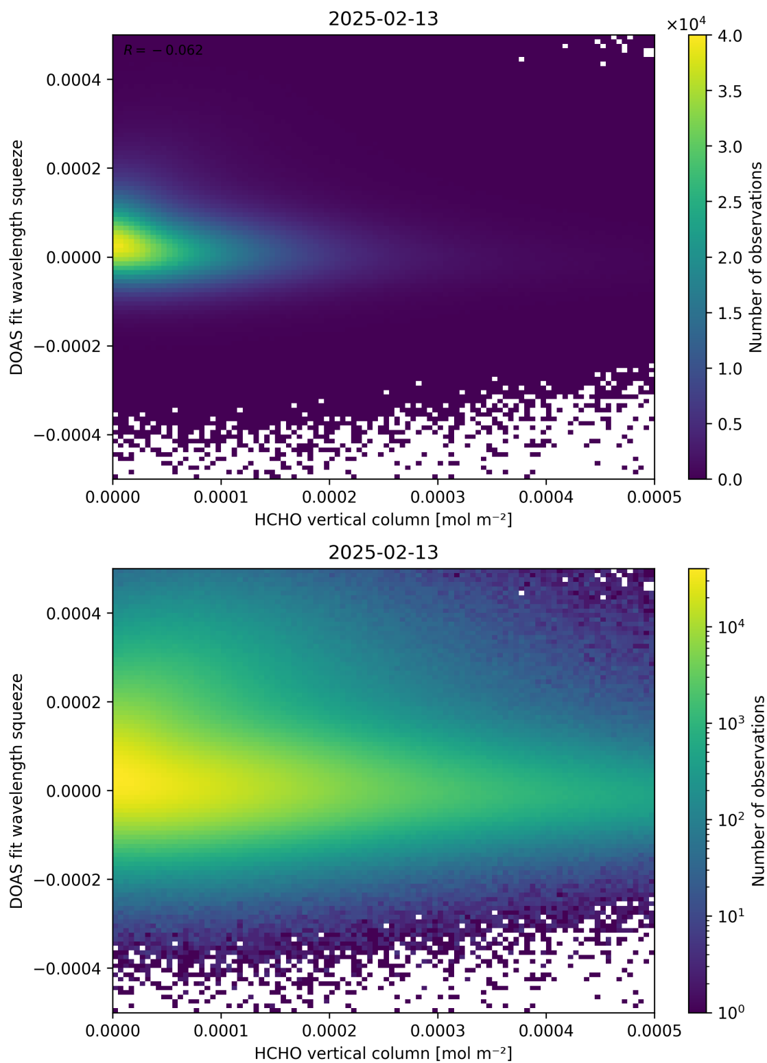
Figure 125: Scatter density plot of “HCHO vertical column” against “DOAS fit wavelength squeeze” for 2025-02-13 to 2025-02-14.
