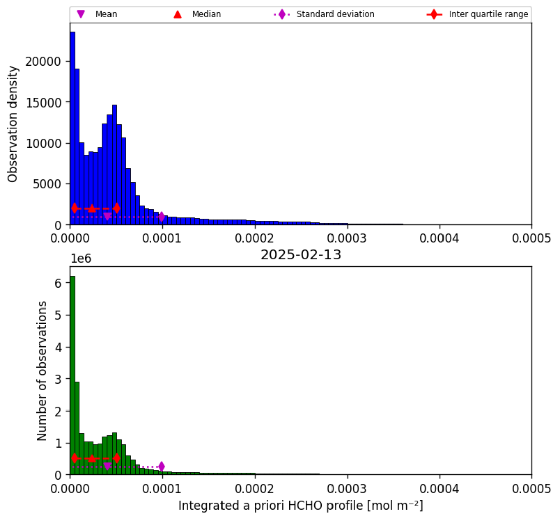
Figure 43: Histogram of “Integrated a priori HCHO profile” for 2025-02-13 to 2025-02-14
