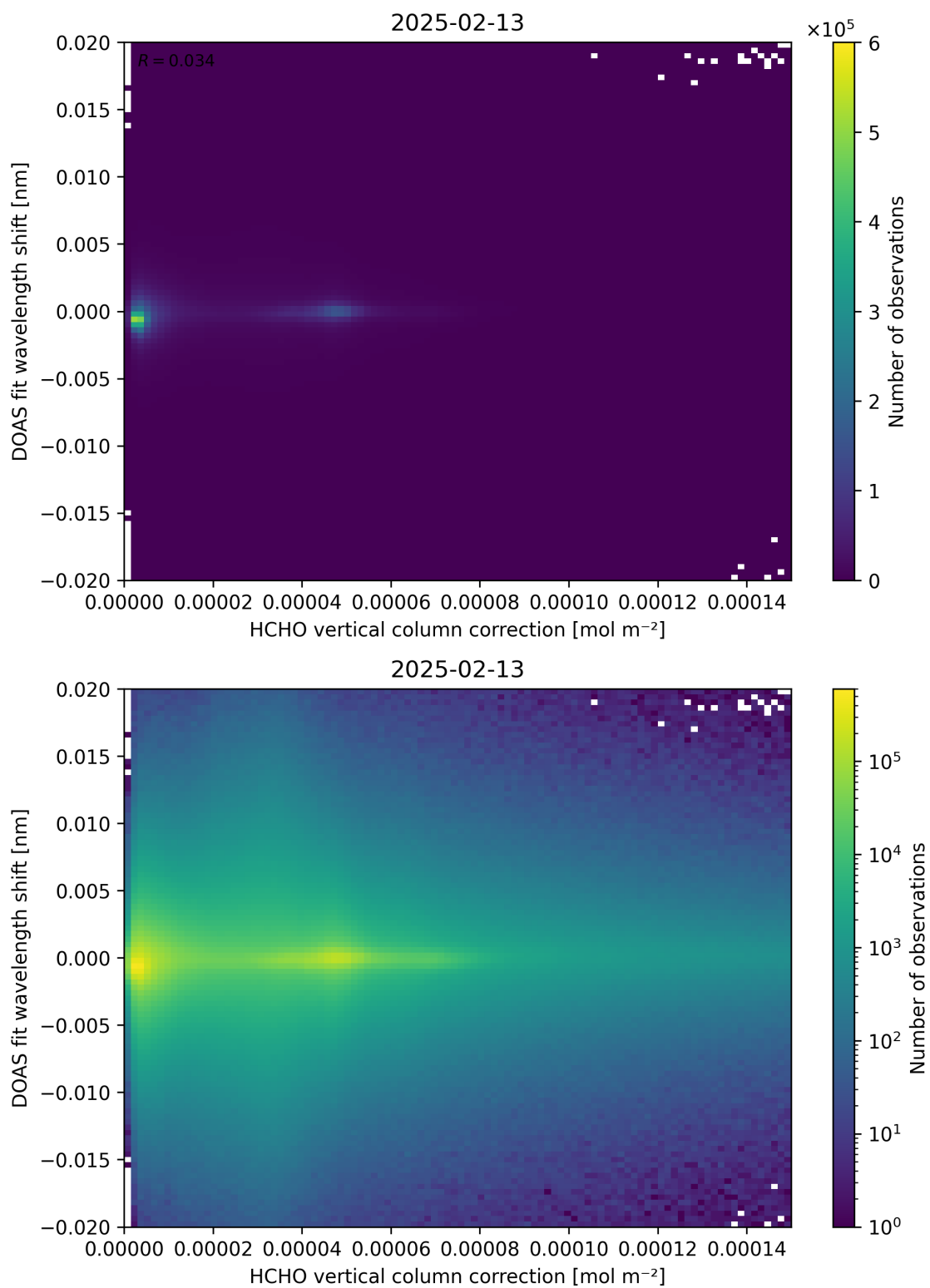
Figure 113: Scatter density plot of “HCHO vertical column correction” against “DOAS fit wavelength shift” for 2025-02-13 to 2025-02-14.
