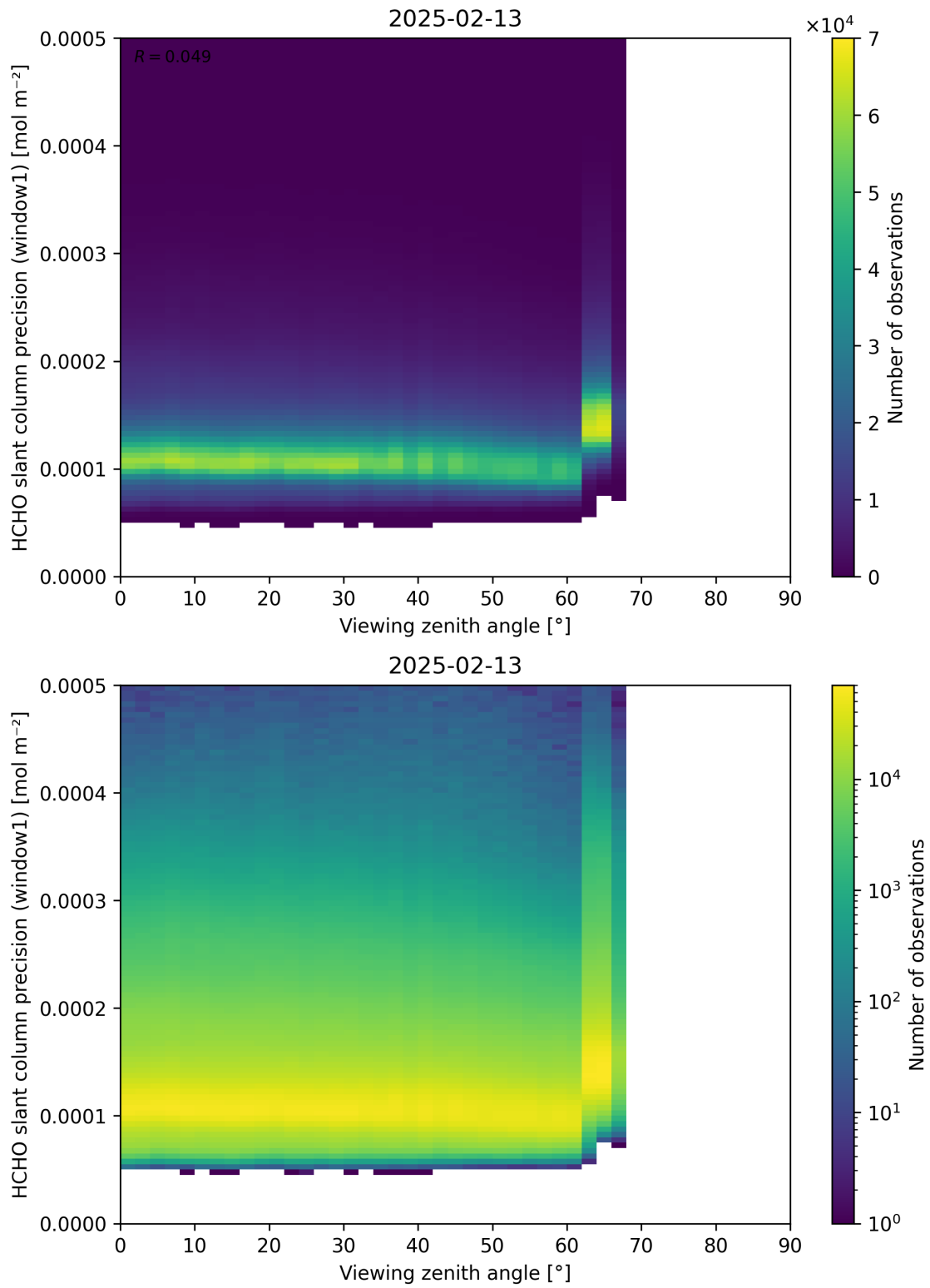
Figure 189: Scatter density plot of “Viewing zenith angle” against “HCHO slant column precision (window1)” for 2025-02-13 to 2025-02-14.
