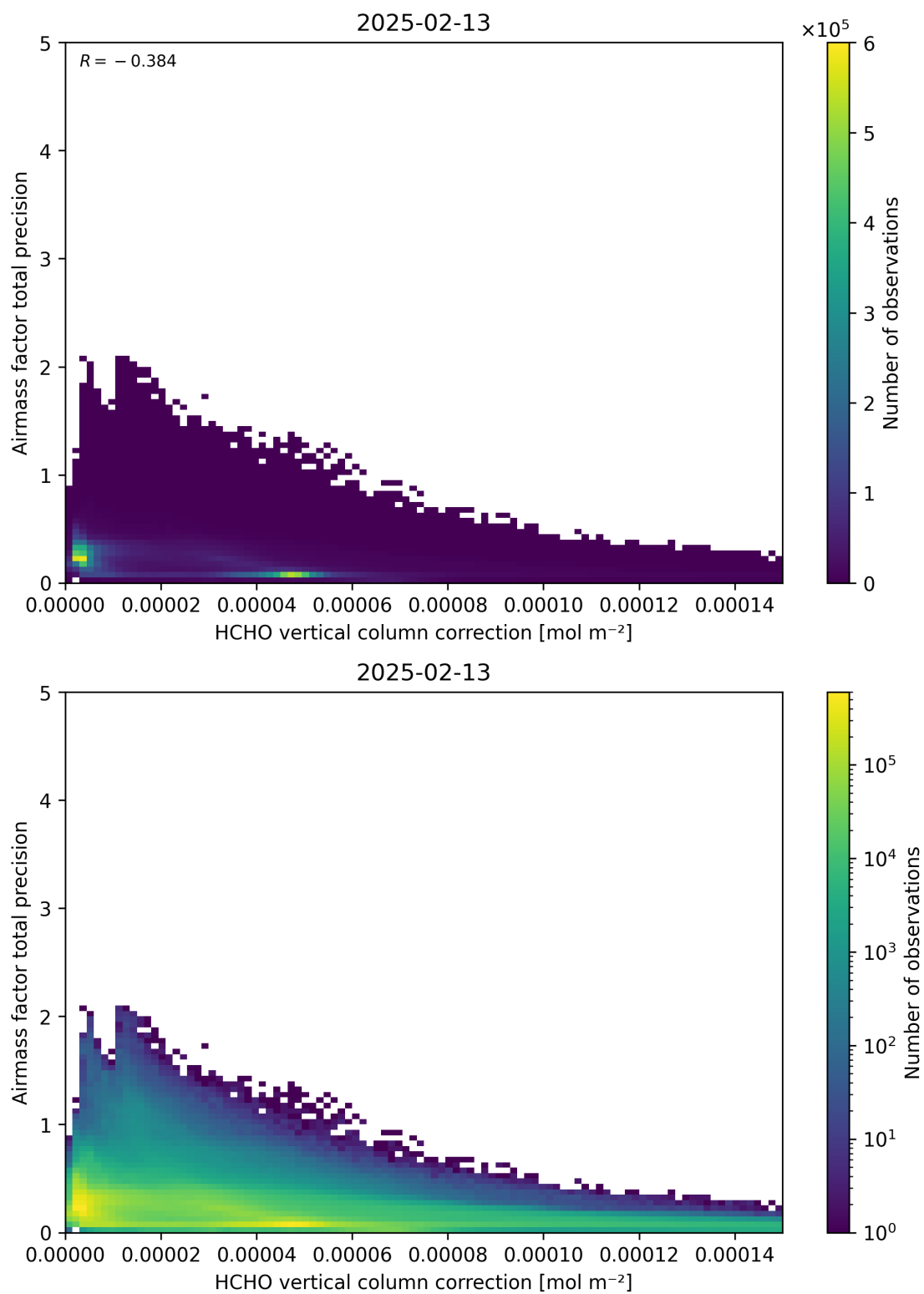
Figure 121: Scatter density plot of “HCHO vertical column correction” against “Airmass factor total precision” for 2025-02-13 to 2025-02-14.
