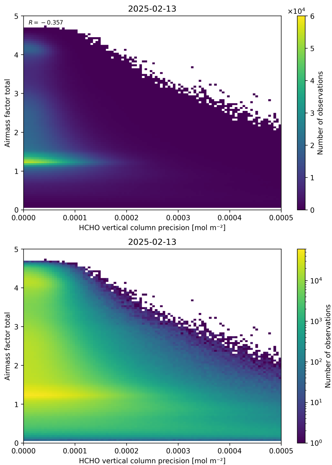
Figure 144: Scatter density plot of “HCHO vertical column precision” against “Airmass factor total” for 2025-02-13 to 2025-02-14.
