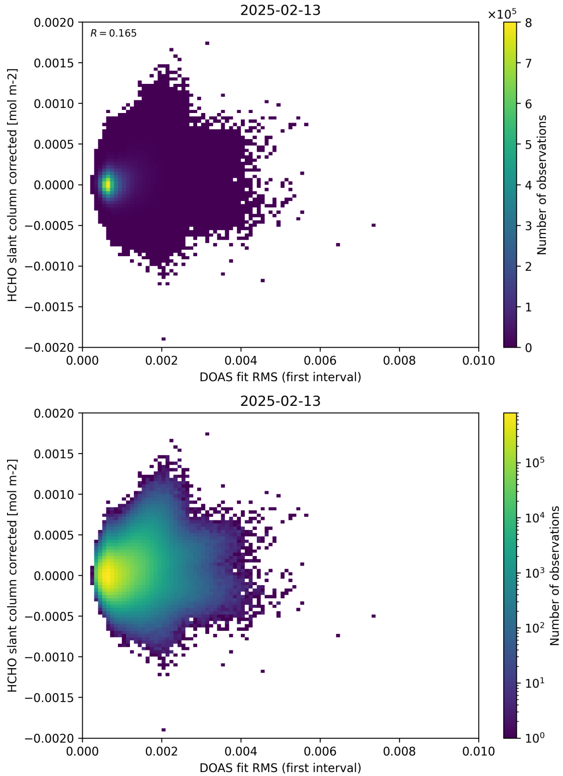
Figure 62: Scatter density plot of “DOAS fit RMS (first interval)” against “HCHO slant column corrected” for 2025-02-13 to 2025-02-14.
