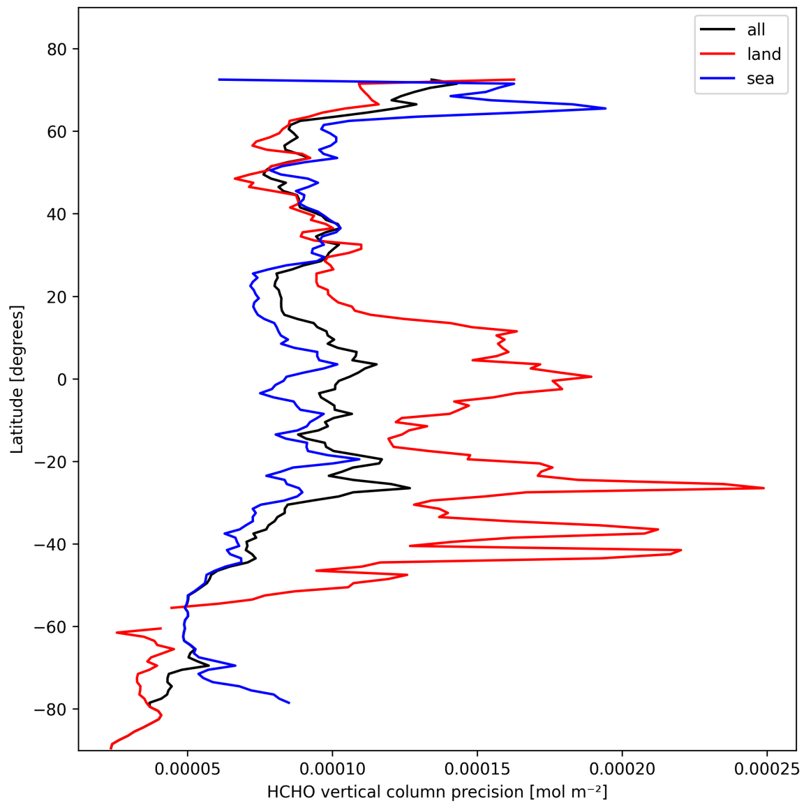
Figure 22: Zonal average of “HCHO vertical column precision” for 2025-02-13 to 2025-02-14.
