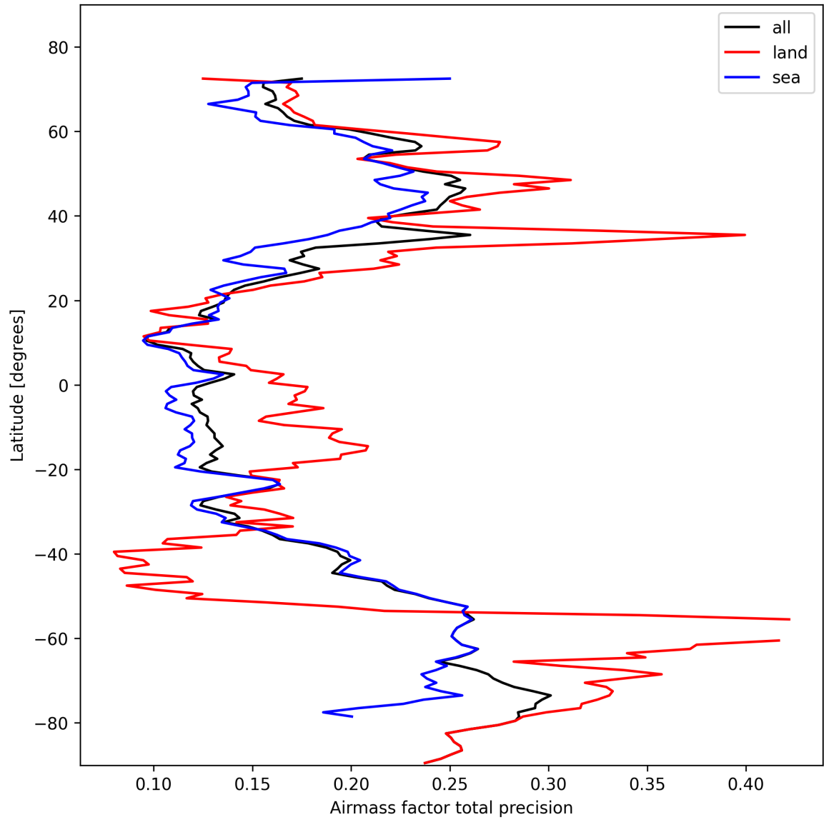
Figure 27: Zonal average of “Airmass factor total precision” for 2025-02-13 to 2025-02-14.
