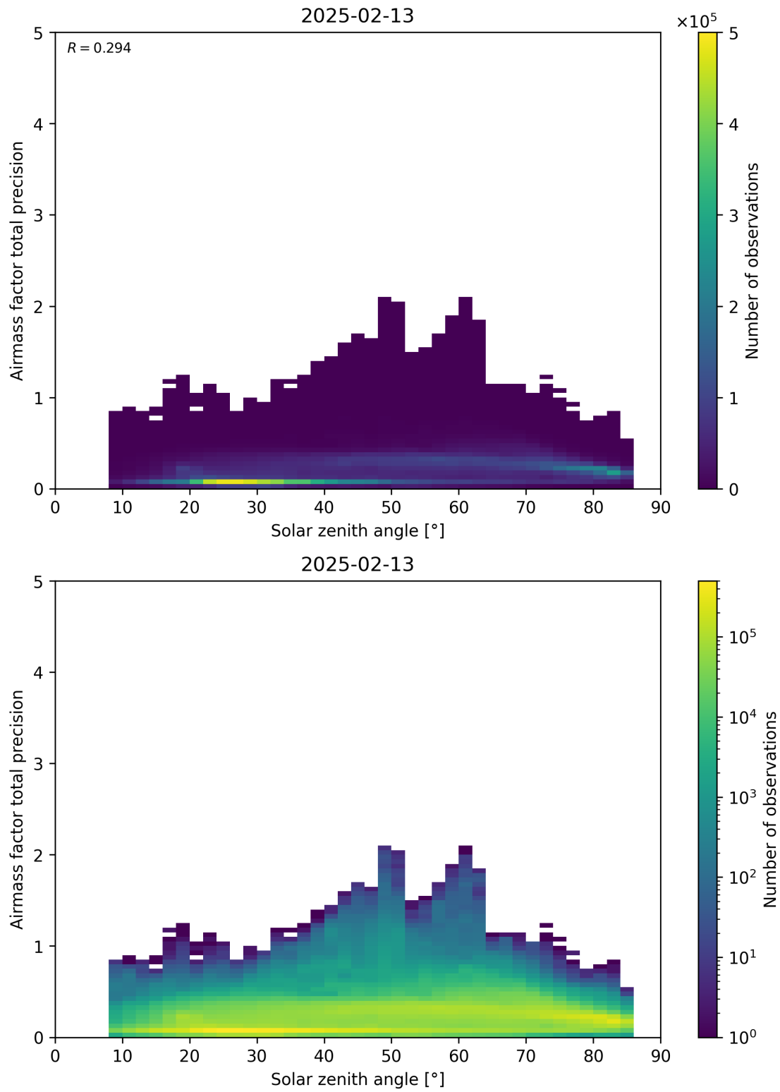
Figure 176: Scatter density plot of “Solar zenith angle” against “Airmass factor total precision” for 2025-02-13 to 2025-02-14.
