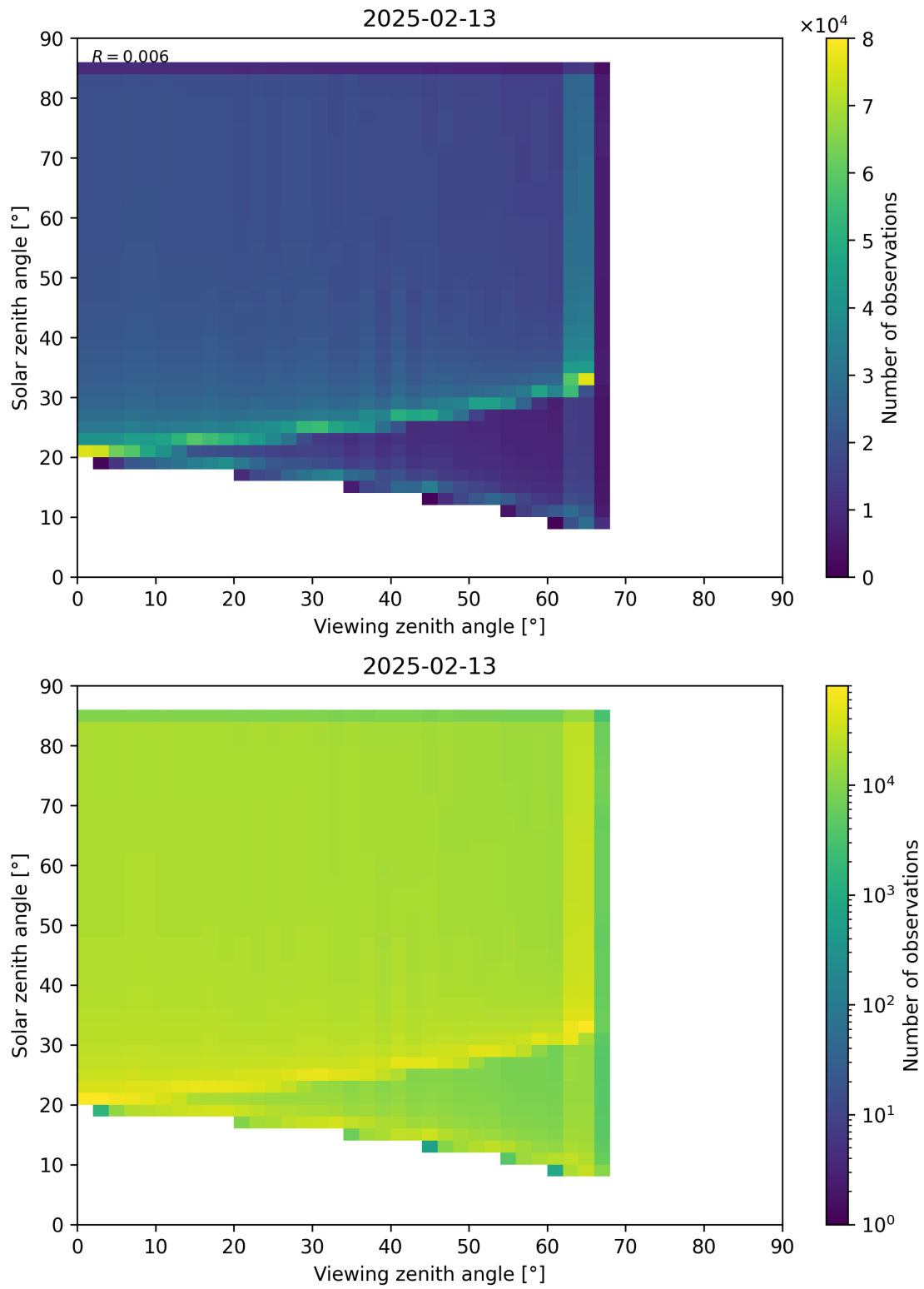
Figure 197: Scatter density plot of “Viewing zenith angle” against “Solar zenith angle” for 2025-02-13 to 2025-02-14.
