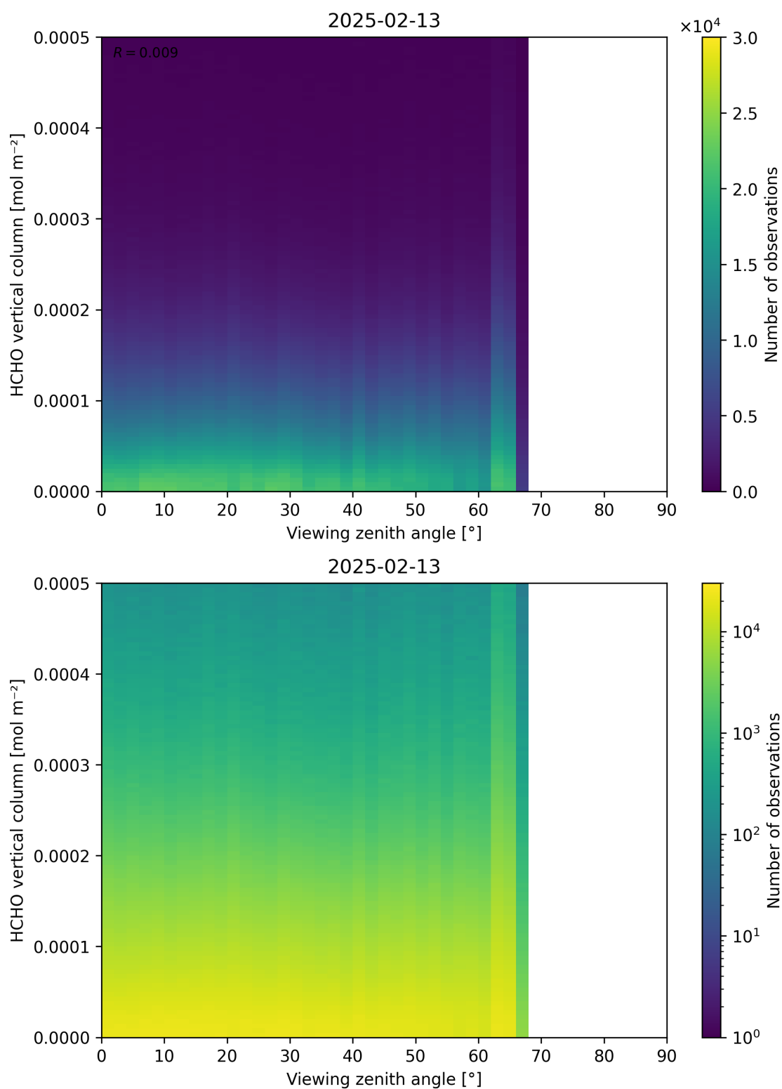
Figure 192: Scatter density plot of “Viewing zenith angle” against “HCHO vertical column” for 2025-02-13 to 2025-02-14.
