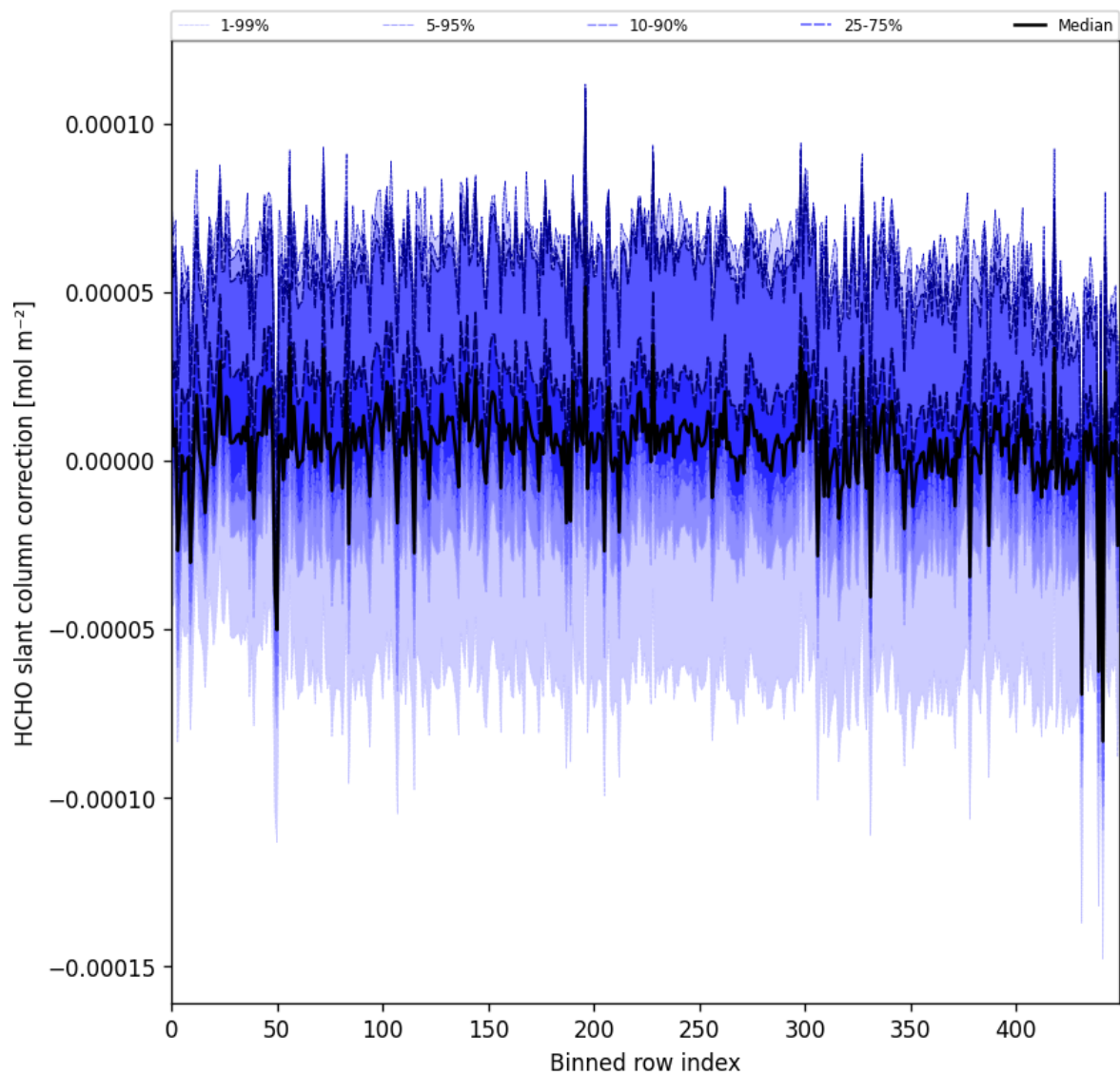
Figure 61: Along track statistics of “HCHO slant column correction” for 2025-02-13 to 2025-02-14
