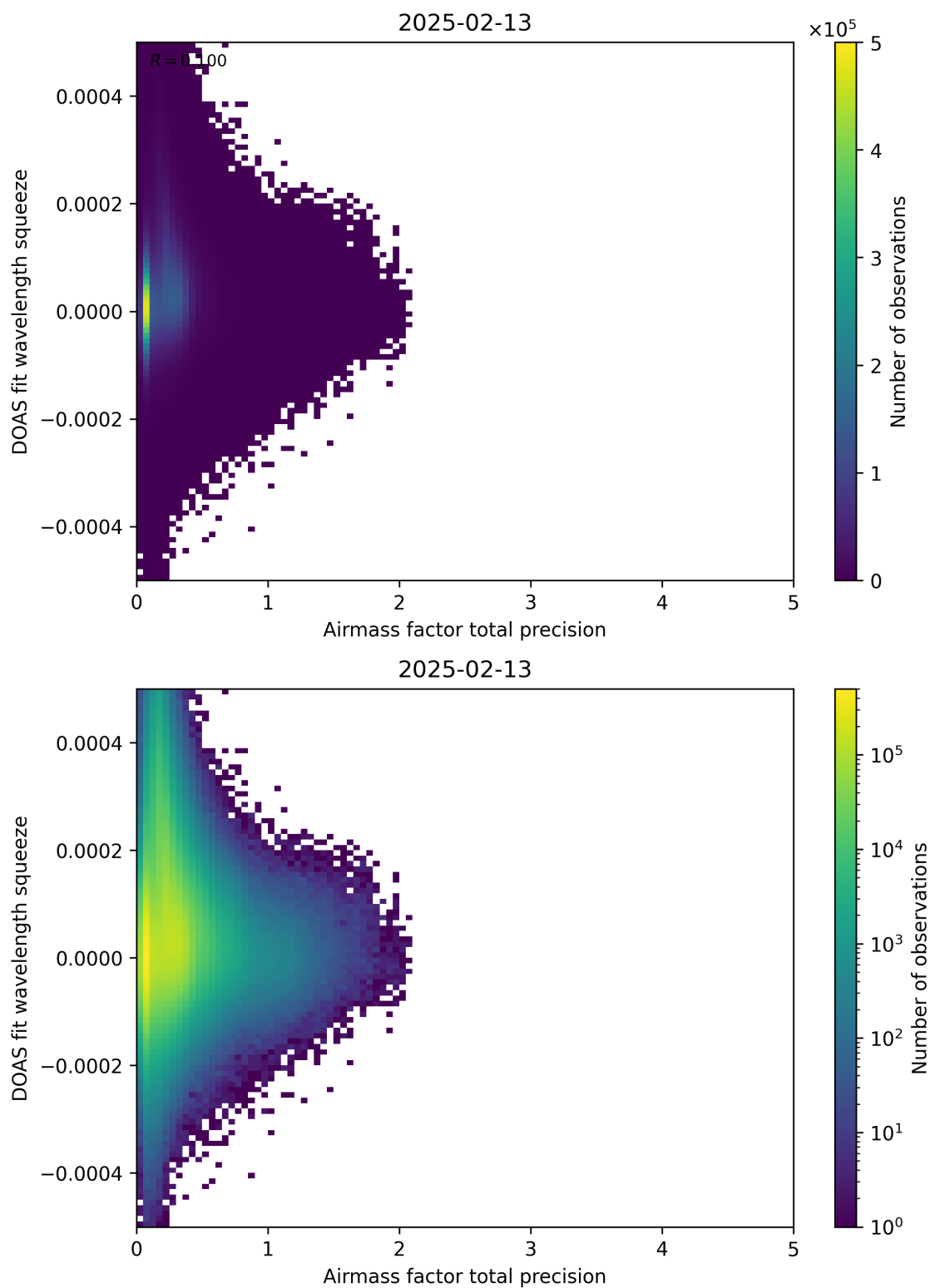
Figure 107: Scatter density plot of “Airmass factor total precision” against “DOAS fit wavelength squeeze” for 2025-02-13 to 2025-02-14.
