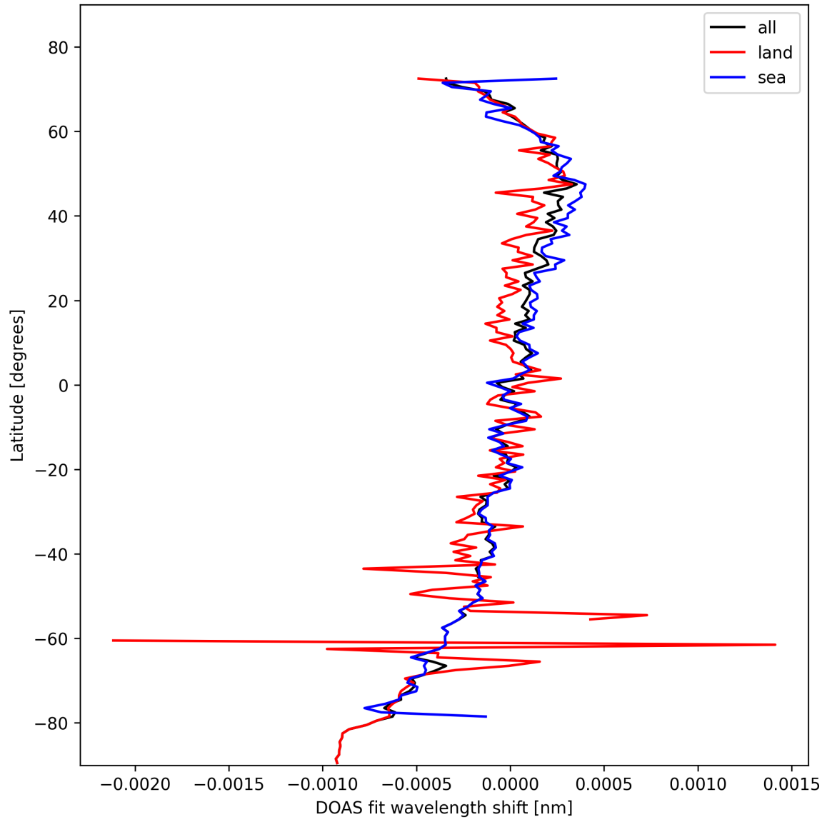
Figure 30: Zonal average of “DOAS fit wavelength shift” for 2025-02-13 to 2025-02-14.
