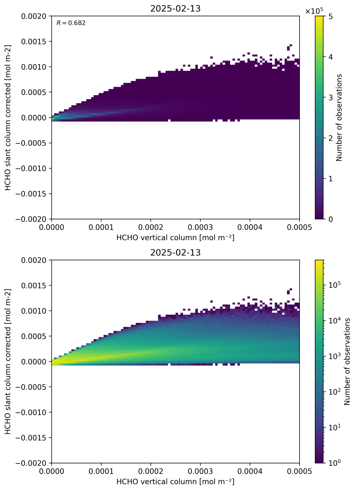
Figure 127: Scatter density plot of “HCHO vertical column” against “HCHO slant column corrected” for 2025-02-13 to 2025-02-14.
