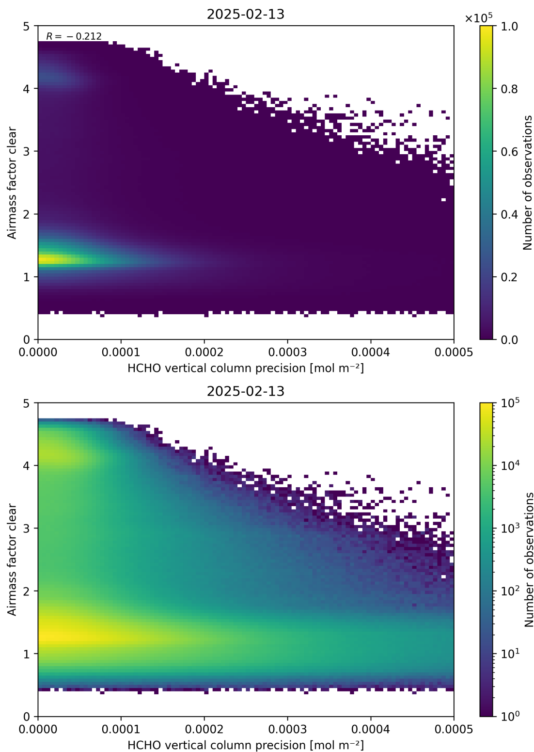
Figure 139: Scatter density plot of “HCHO vertical column precision” against “Airmass factor clear” for 2025-02-13 to 2025-02-14.
