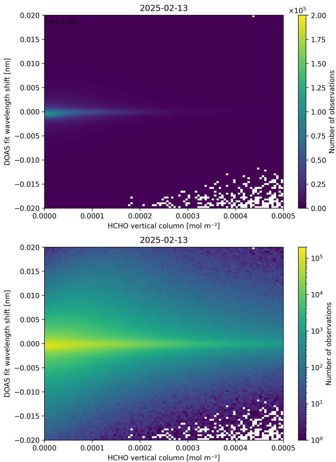
Figure 124: Scatter density plot of “HCHO vertical column” against “DOAS fit wavelength shift” for 2025-02-13 to 2025-02-14.
