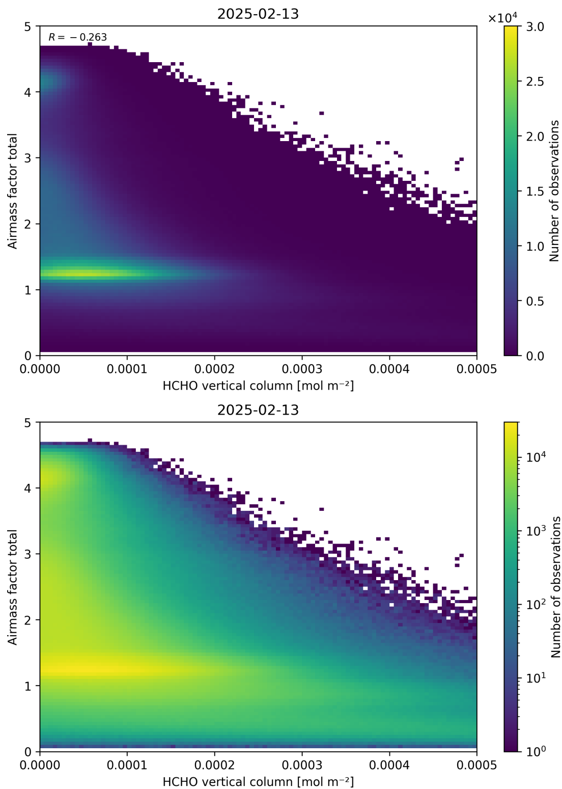
Figure 131: Scatter density plot of “HCHO vertical column” against “Airmass factor total” for 2025-02-13 to 2025-02-14.
