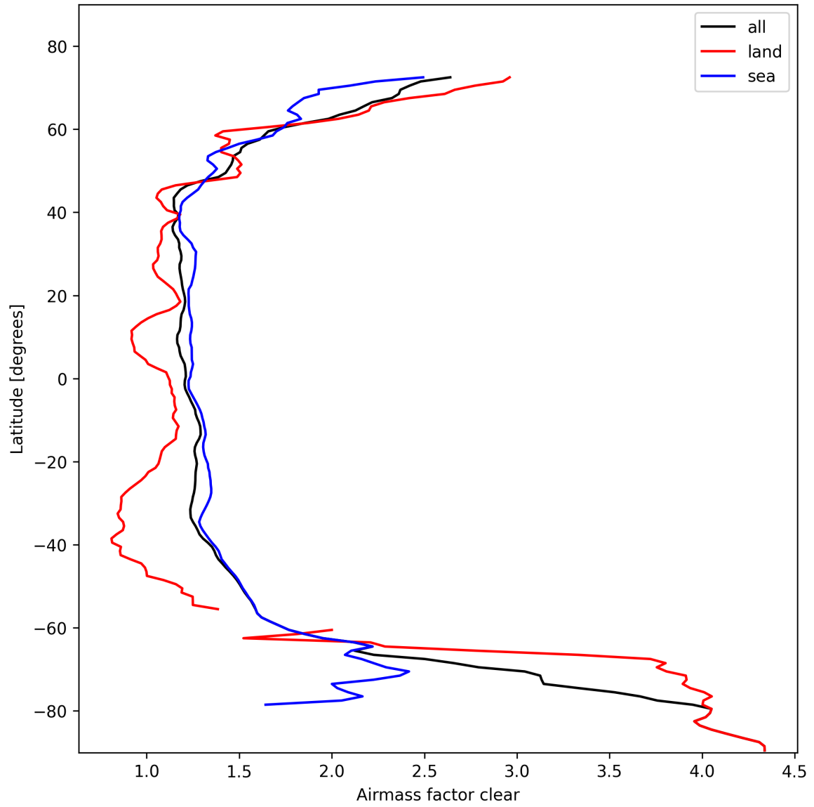
Figure 28: Zonal average of “Airmass factor clear” for 2025-02-13 to 2025-02-15.
