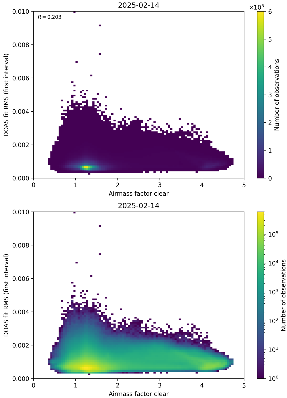
Figure 71: Scatter density plot of “Airmass factor clear” against “DOAS fit RMS (first interval)” for 2025-02-13 to 2025-02-15.
