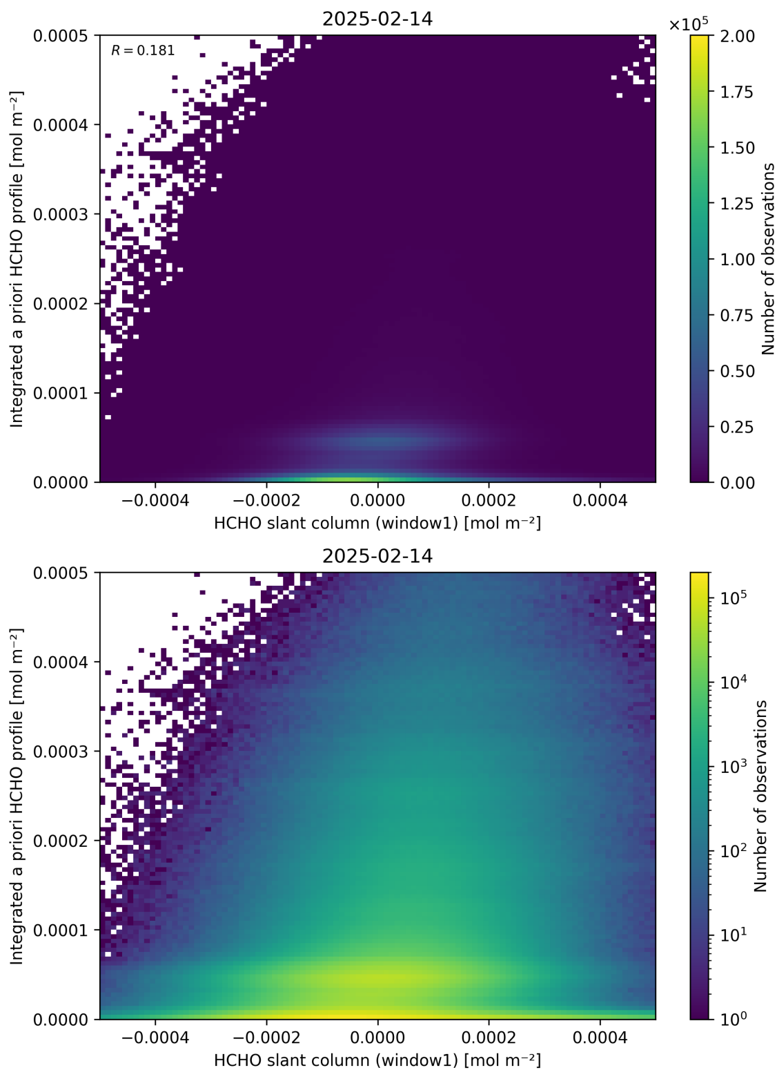
Figure 87: Scatter density plot of “HCHO slant column (window1)” against “Integrated a priori HCHO profile” for 2025-02-13 to 2025-02-15.
