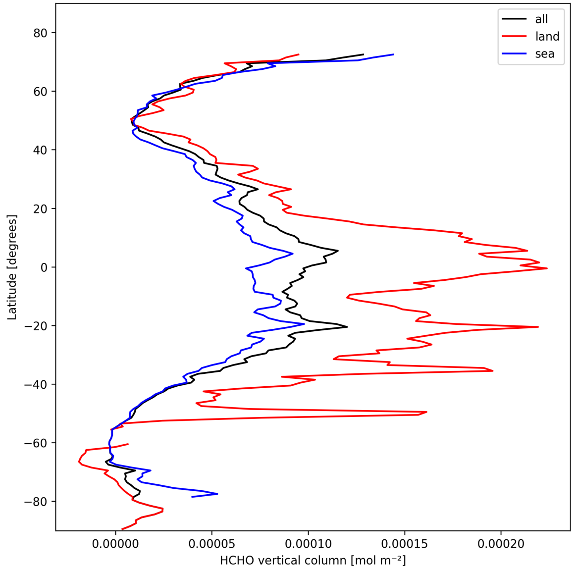
Figure 21: Zonal average of “HCHO vertical column” for 2025-02-13 to 2025-02-15.
