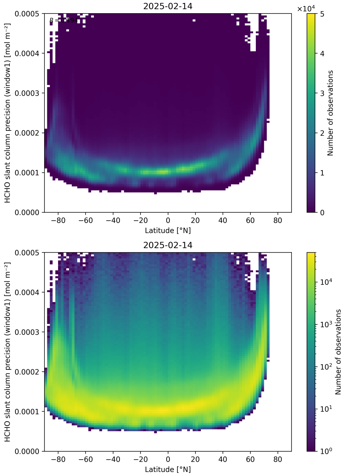
Figure 160: Scatter density plot of “Latitude” against “HCHO slant column precision (window1)” for 2025-02-13 to 2025-02-15.
