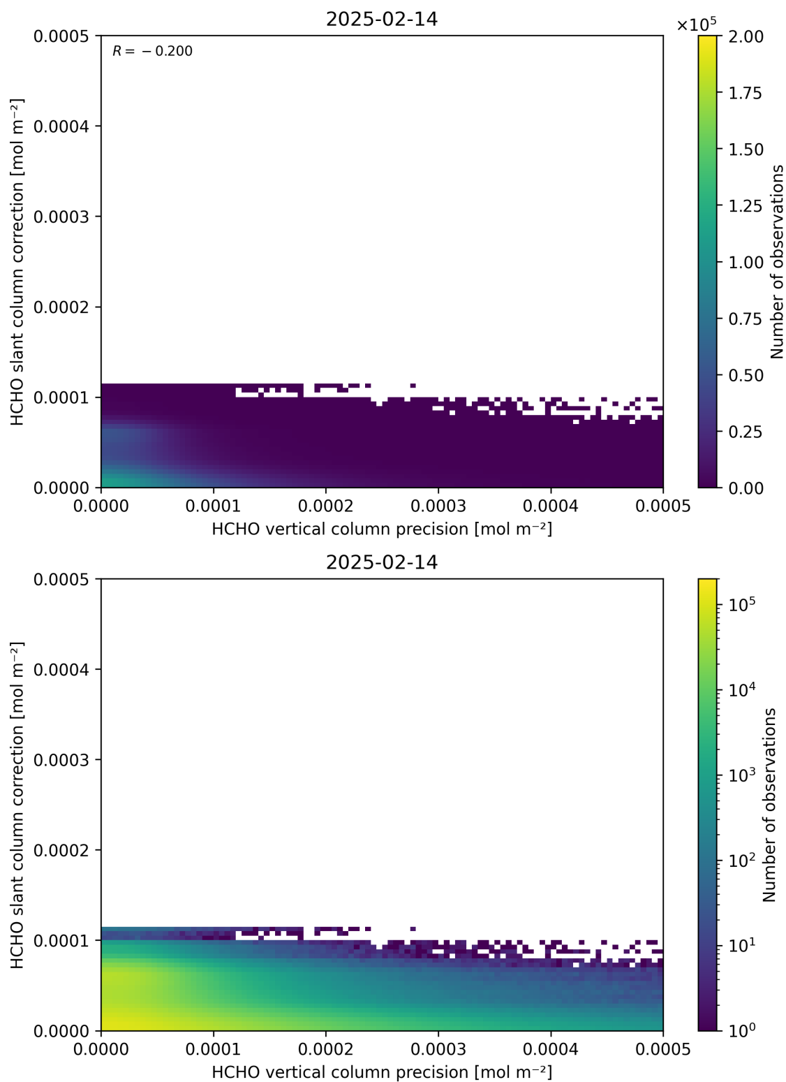
Figure 141: Scatter density plot of “HCHO vertical column precision” against “HCHO slant column correction” for 2025-02-13 to 2025-02-15.
