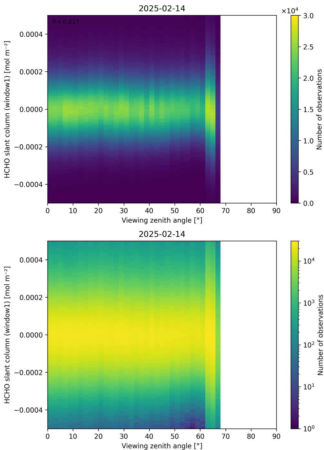
Figure 188: Scatter density plot of “Viewing zenith angle” against “HCHO slant column (window1)” for 2025-02-13 to 2025-02-15.
