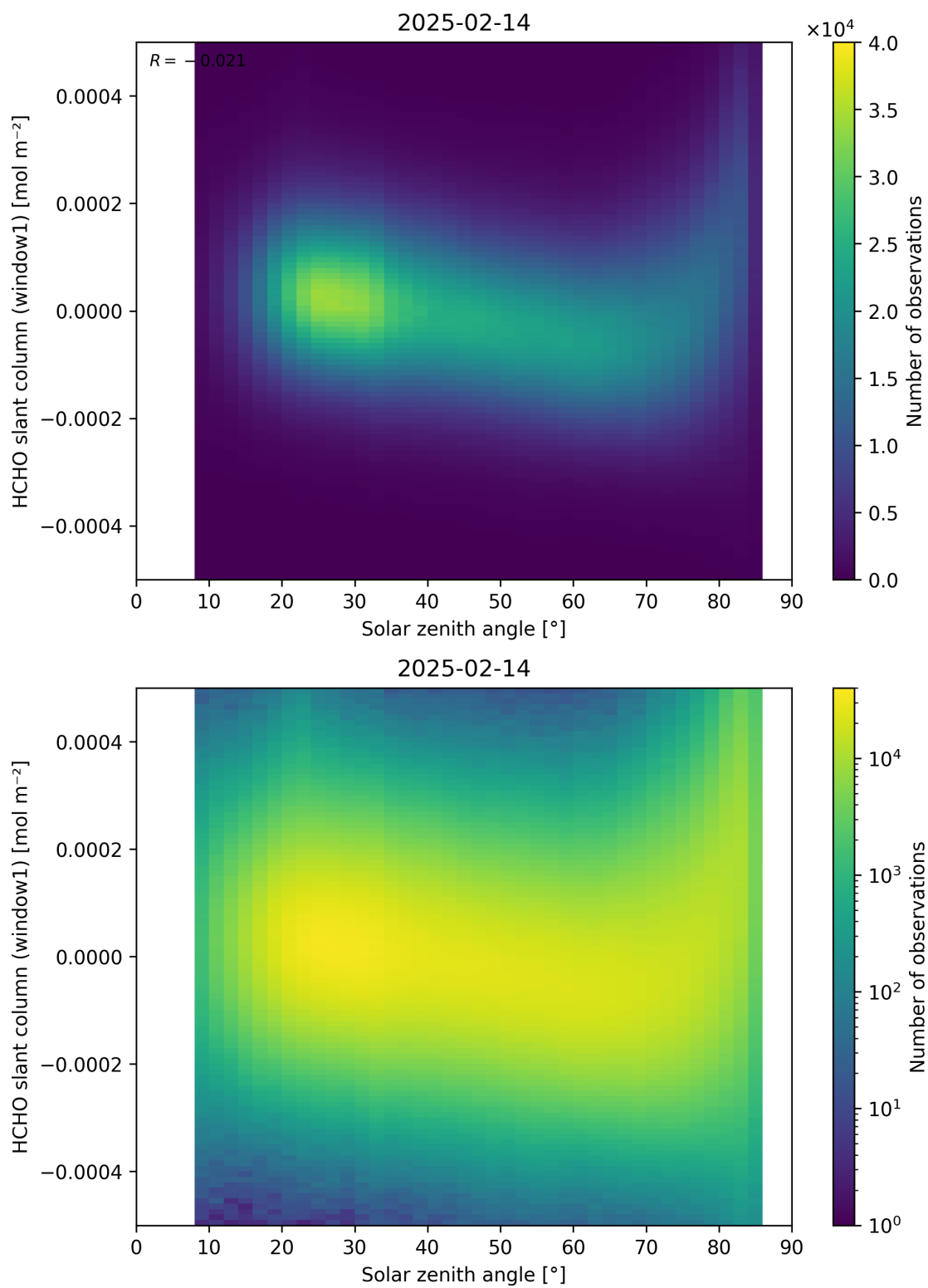
Figure 173: Scatter density plot of “Solar zenith angle” against “HCHO slant column (window1)” for 2025-02-13 to 2025-02-15.
