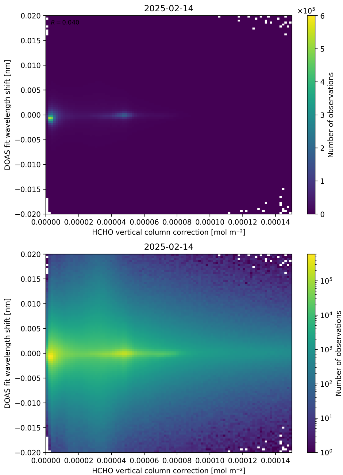
Figure 113: Scatter density plot of “HCHO vertical column correction” against “DOAS fit wavelength shift” for 2025-02-13 to 2025-02-15.
