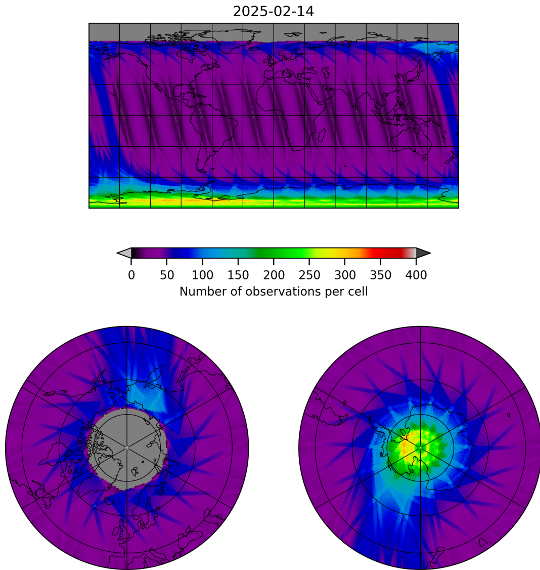
Figure 19: Map of the number of observations for 2025-02-13 to 2025-02-15
