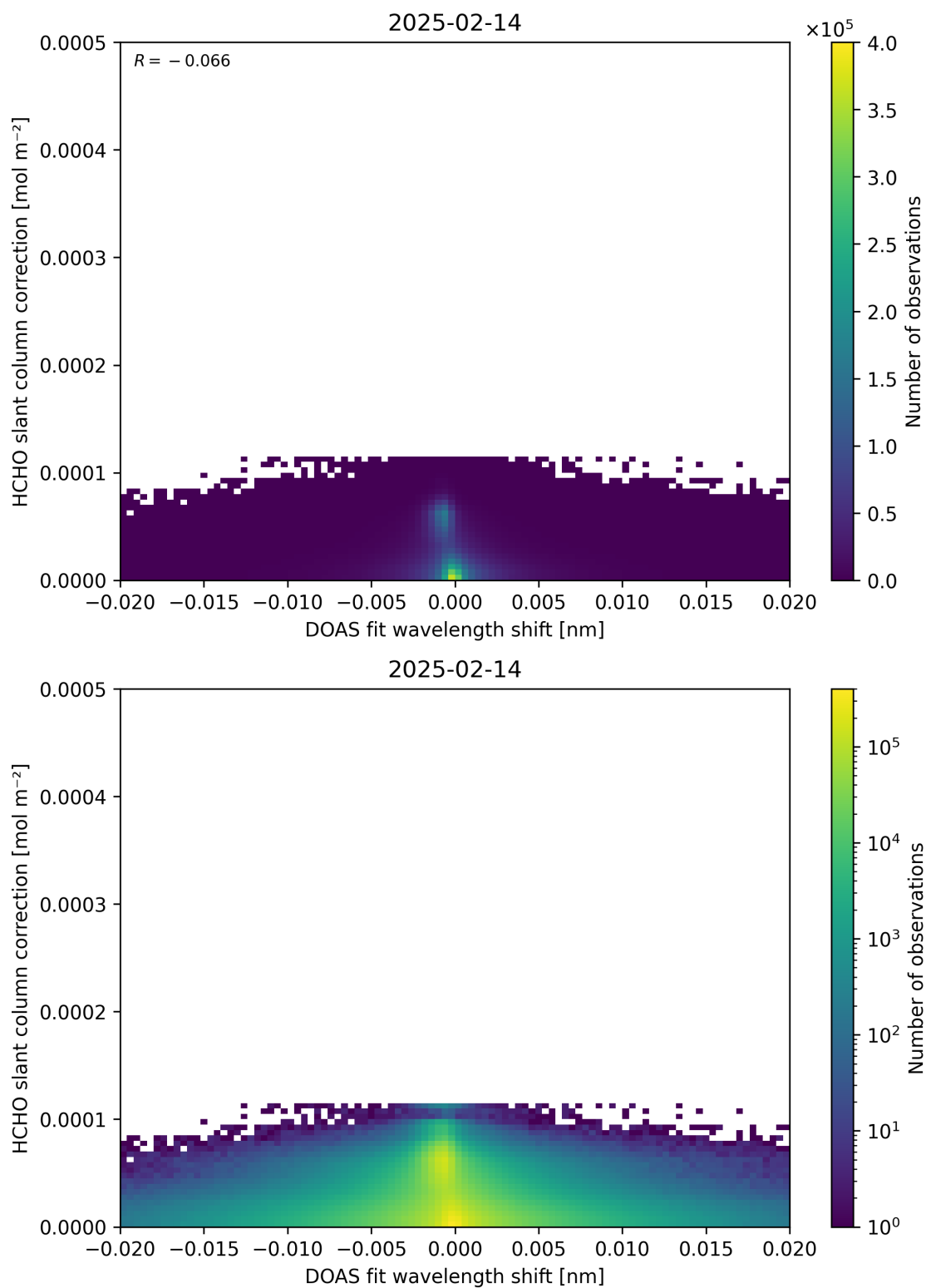
Figure 67: Scatter density plot of “DOAS fit wavelength shift” against “HCHO slant column correction” for 2025-02-13 to 2025-02-15.
