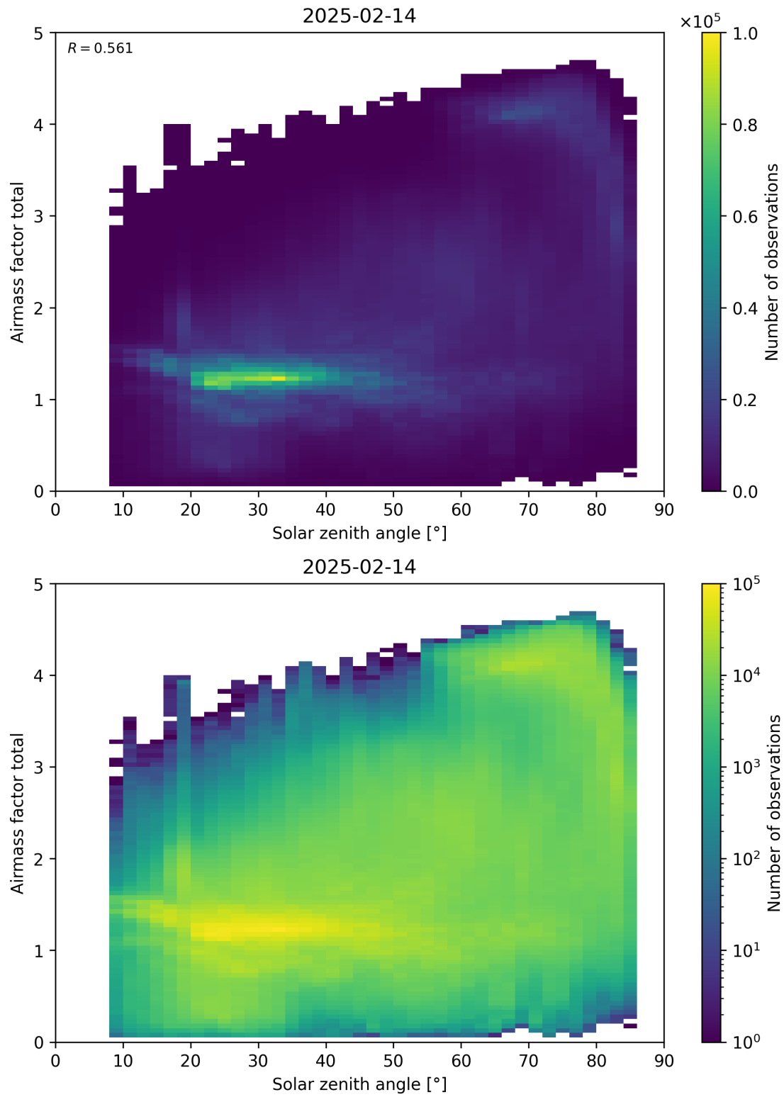
Figure 175: Scatter density plot of “Solar zenith angle” against “Airmass factor total” for 2025-02-13 to 2025-02-15.
