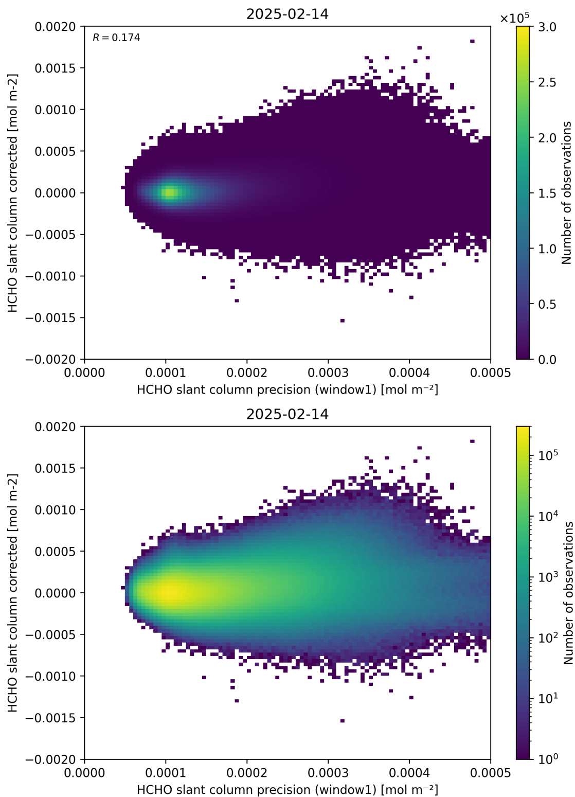
Figure 92: Scatter density plot of “HCHO slant column precision (window1)” against “HCHO slant column corrected” for 2025-02-13 to 2025-02-15.
