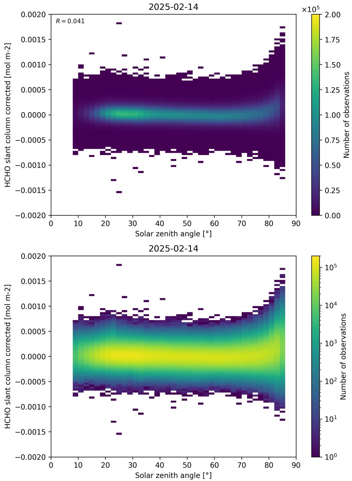
Figure 171: Scatter density plot of “Solar zenith angle” against “HCHO slant column corrected” for 2025-02-13 to 2025-02-15.
