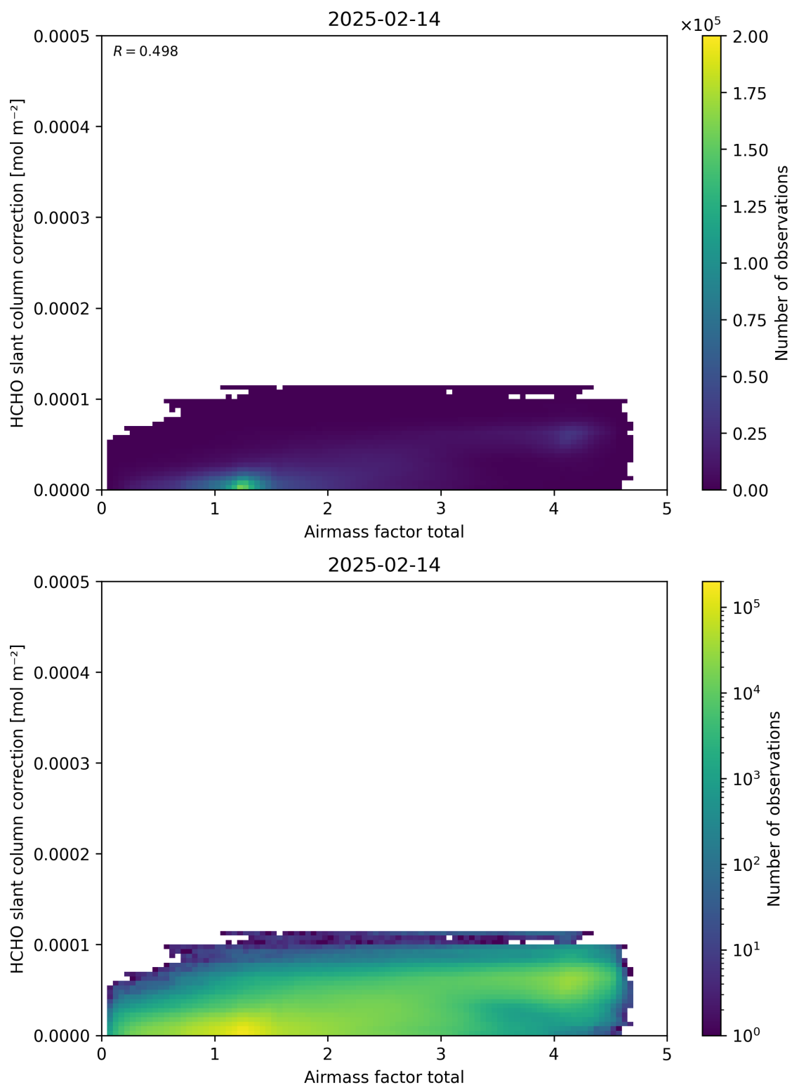
Figure 102: Scatter density plot of “Airmass factor total” against “HCHO slant column correction” for 2025-02-13 to 2025-02-15.
