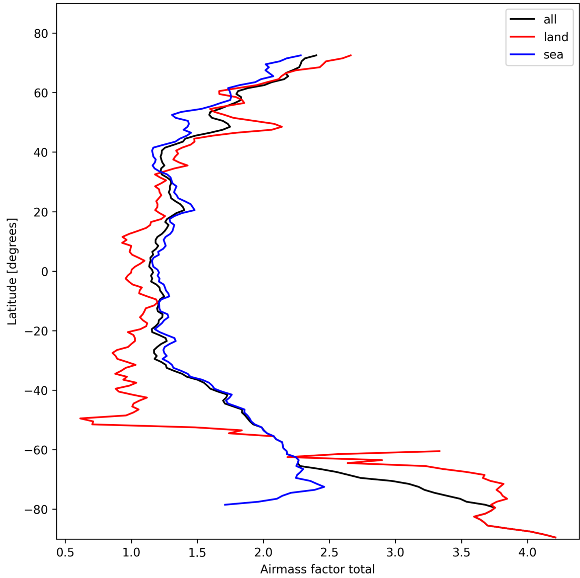
Figure 26: Zonal average of “Airmass factor total” for 2025-02-13 to 2025-02-15.
