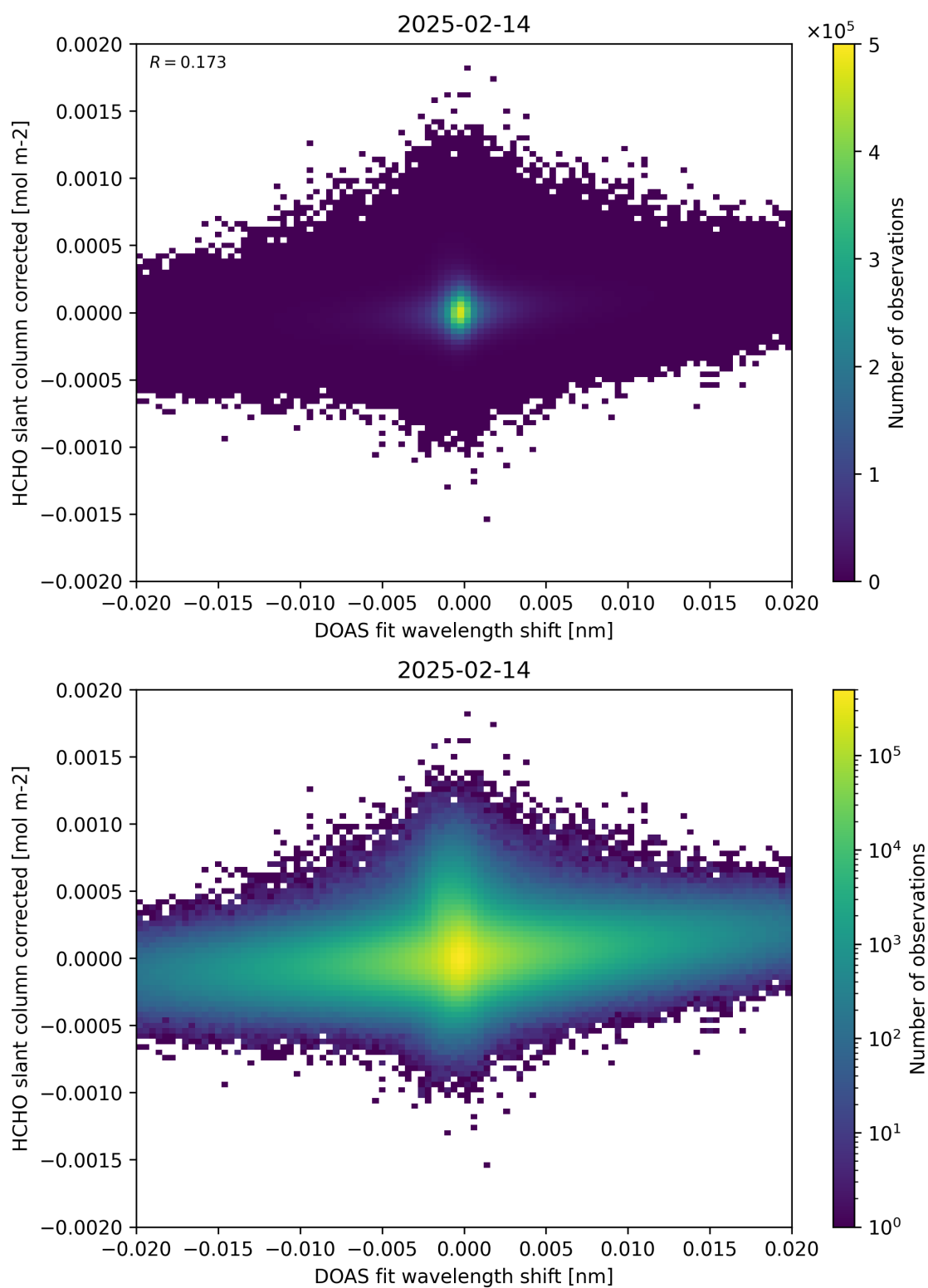
Figure 66: Scatter density plot of “DOAS fit wavelength shift” against “HCHO slant column corrected” for 2025-02-13 to 2025-02-15.
