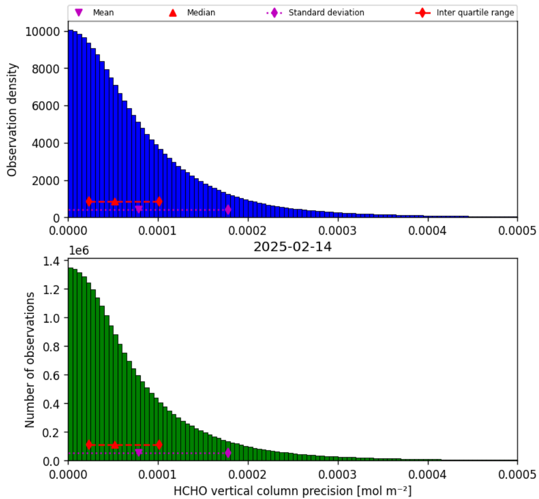
Figure 36: Histogram of “HCHO vertical column precision” for 2025-02-13 to 2025-02-15
