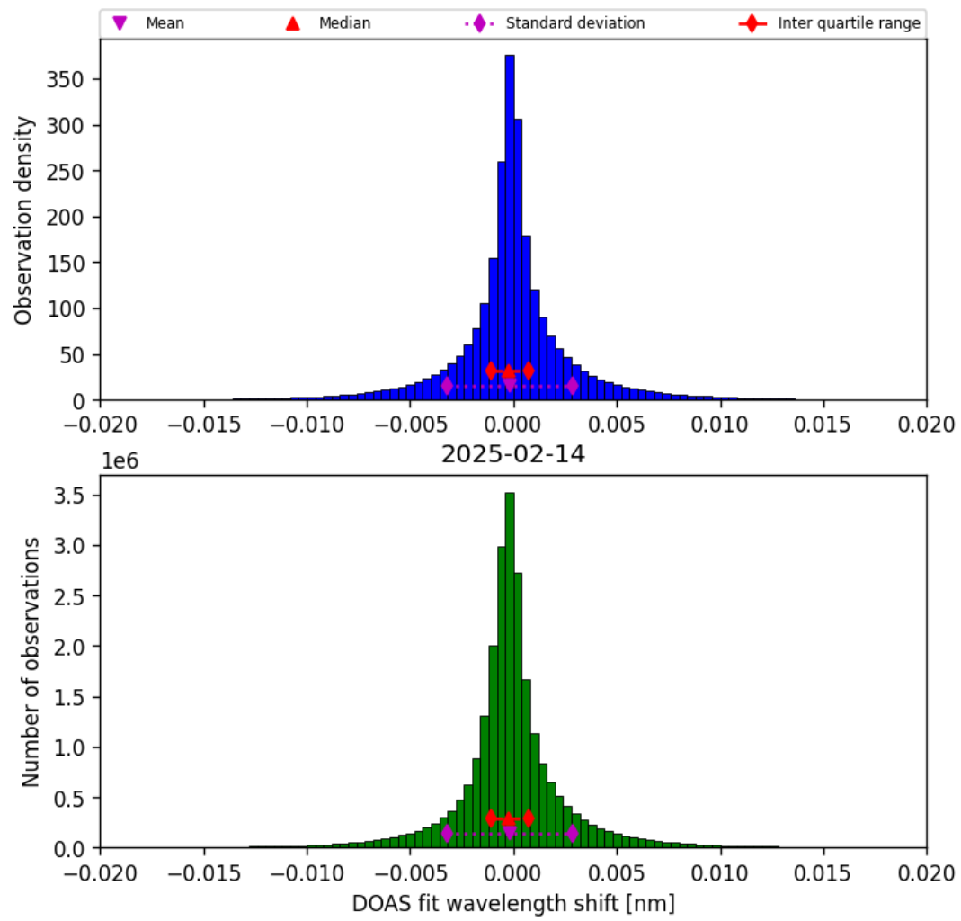
Figure 44: Histogram of “DOAS fit wavelength shift” for 2025-02-13 to 2025-02-15
