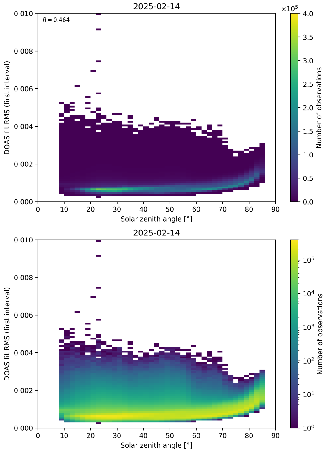
Figure 167: Scatter density plot of “Solar zenith angle” against “DOAS fit RMS (first interval)” for 2025-02-13 to 2025-02-15.
