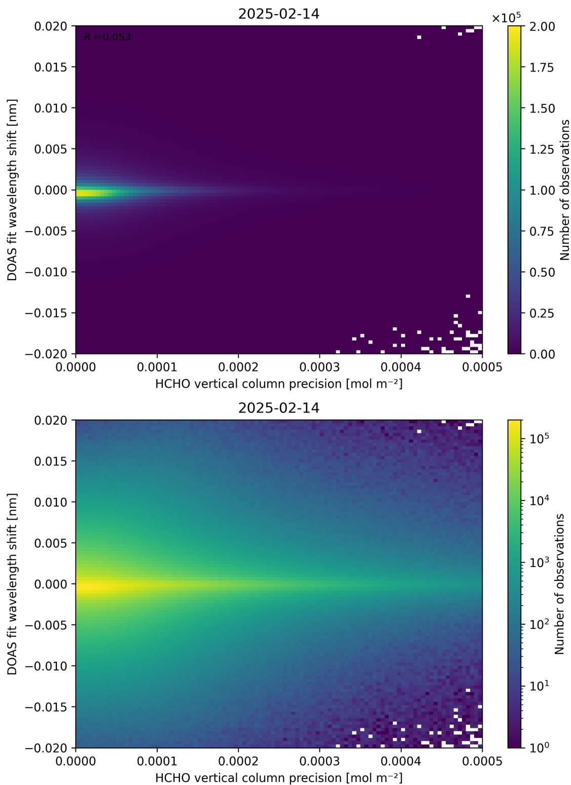
Figure 137: Scatter density plot of “HCHO vertical column precision” against “DOAS fit wavelength shift” for 2025-02-13 to 2025-02-15.
