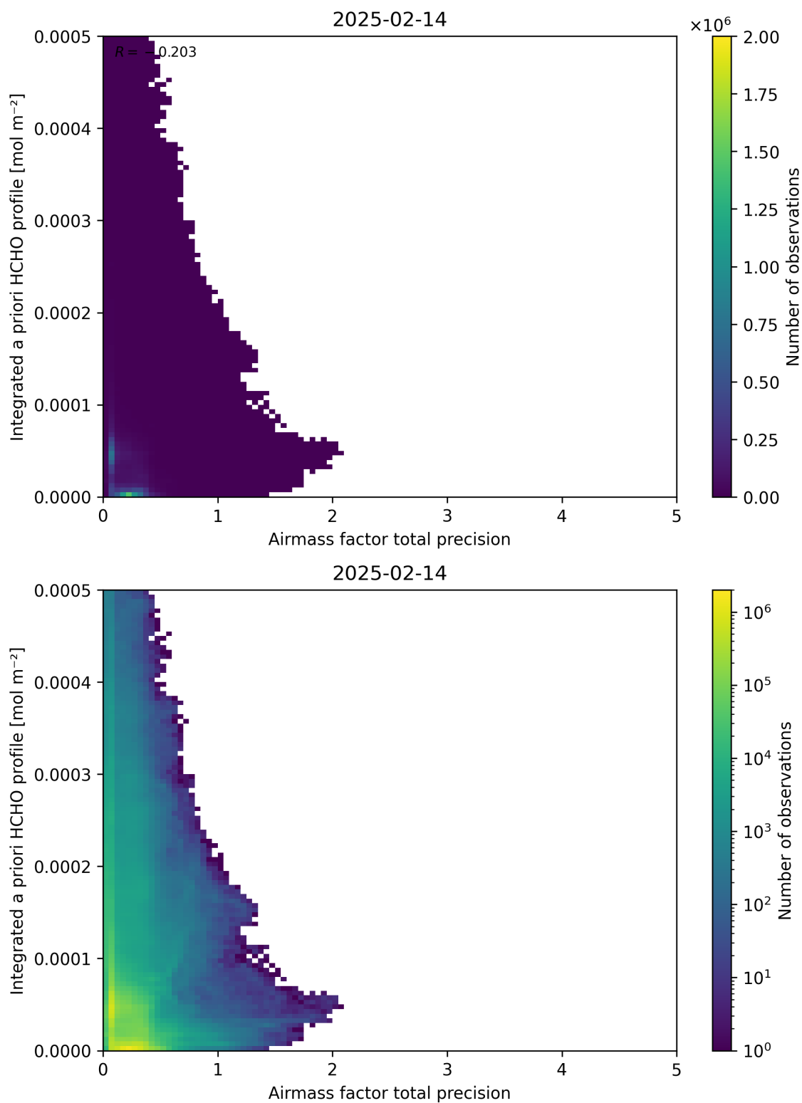
Figure 111: Scatter density plot of “Airmass factor total precision” against “Integrated a priori HCHO profile” for 2025-02-13 to 2025-02-15.
