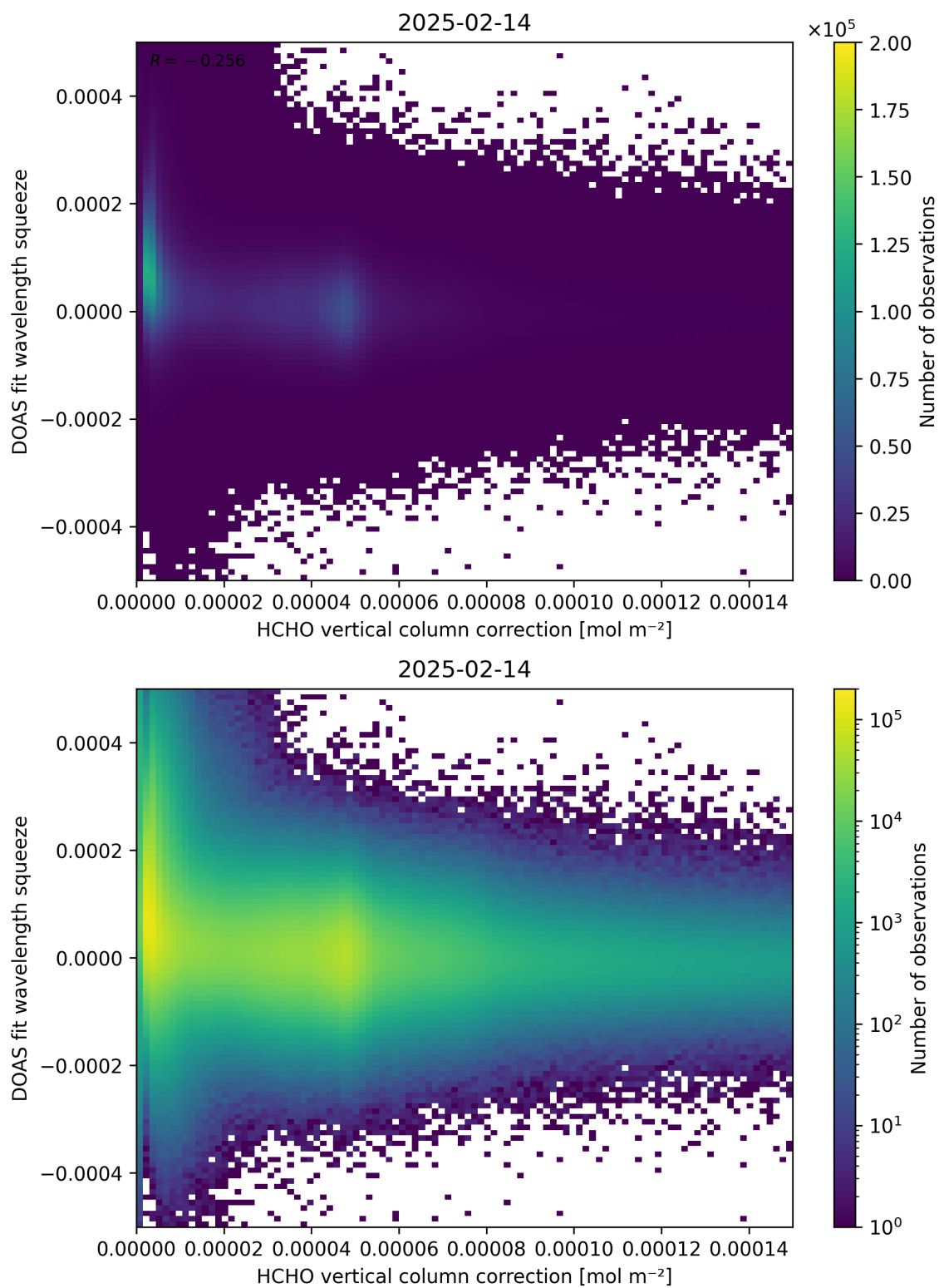
Figure 114: Scatter density plot of “HCHO vertical column correction” against “DOAS fit wavelength squeeze” for 2025-02-13 to 2025-02-15.
