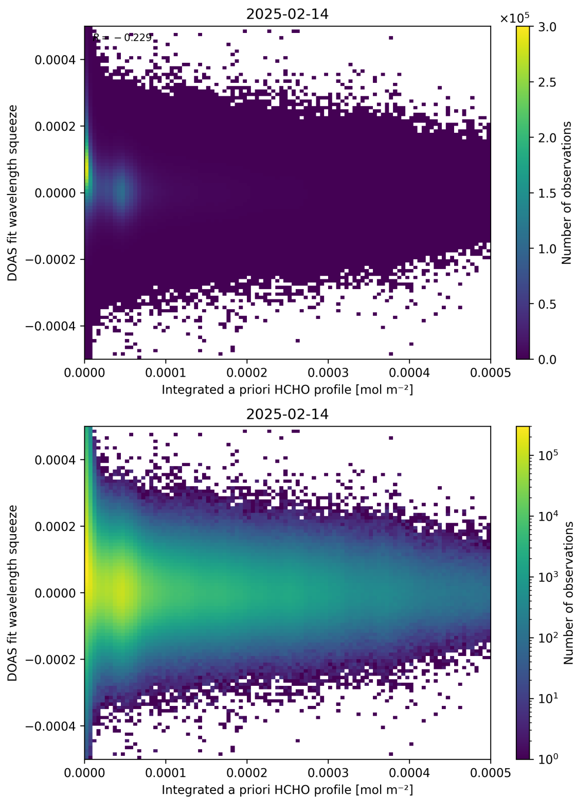
Figure 150: Scatter density plot of “Integrated a priori HCHO profile” against “DOAS fit wavelength squeeze” for 2025-02-13 to 2025-02-15.
