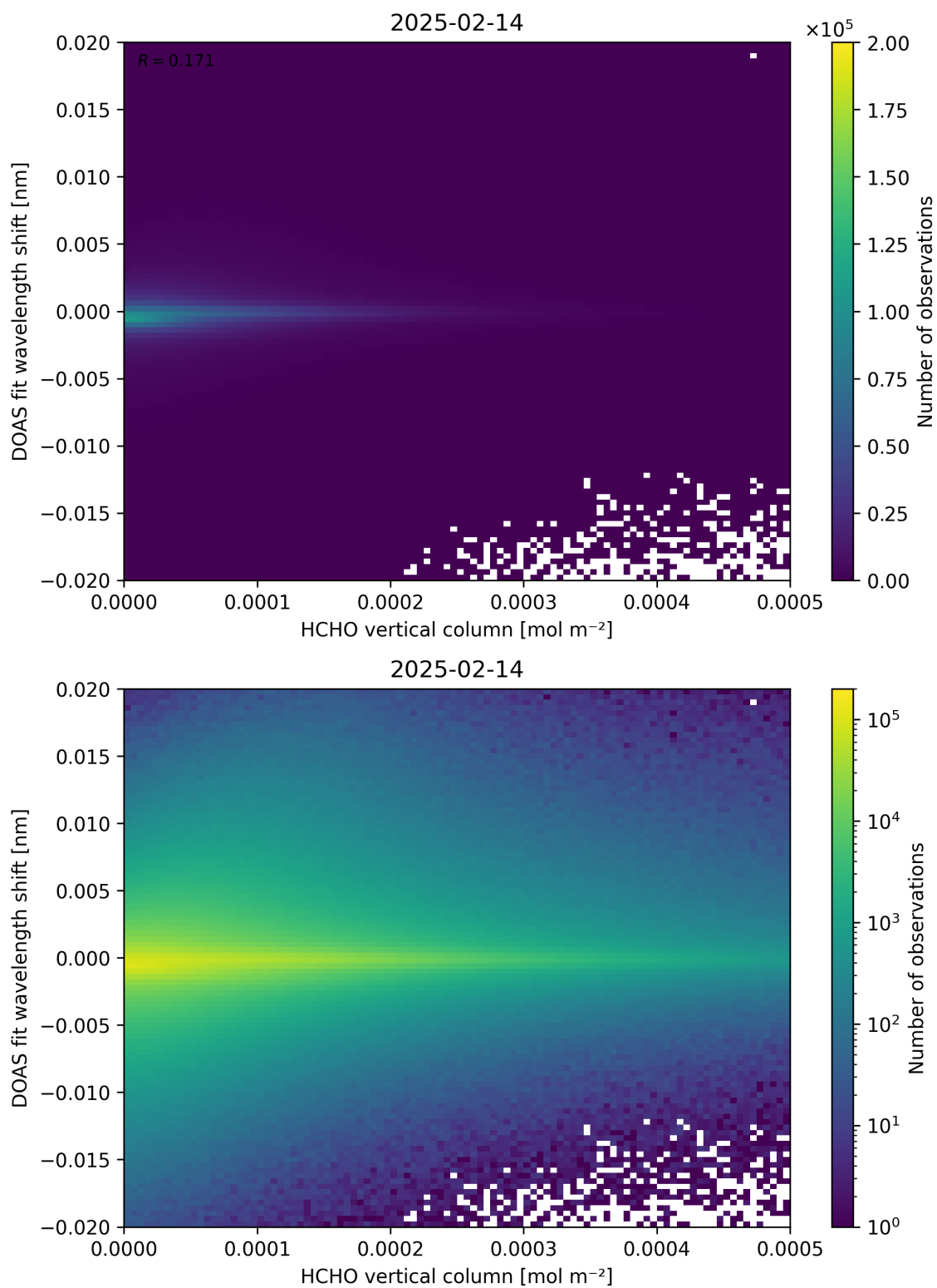
Figure 124: Scatter density plot of “HCHO vertical column” against “DOAS fit wavelength shift” for 2025-02-13 to 2025-02-15.
