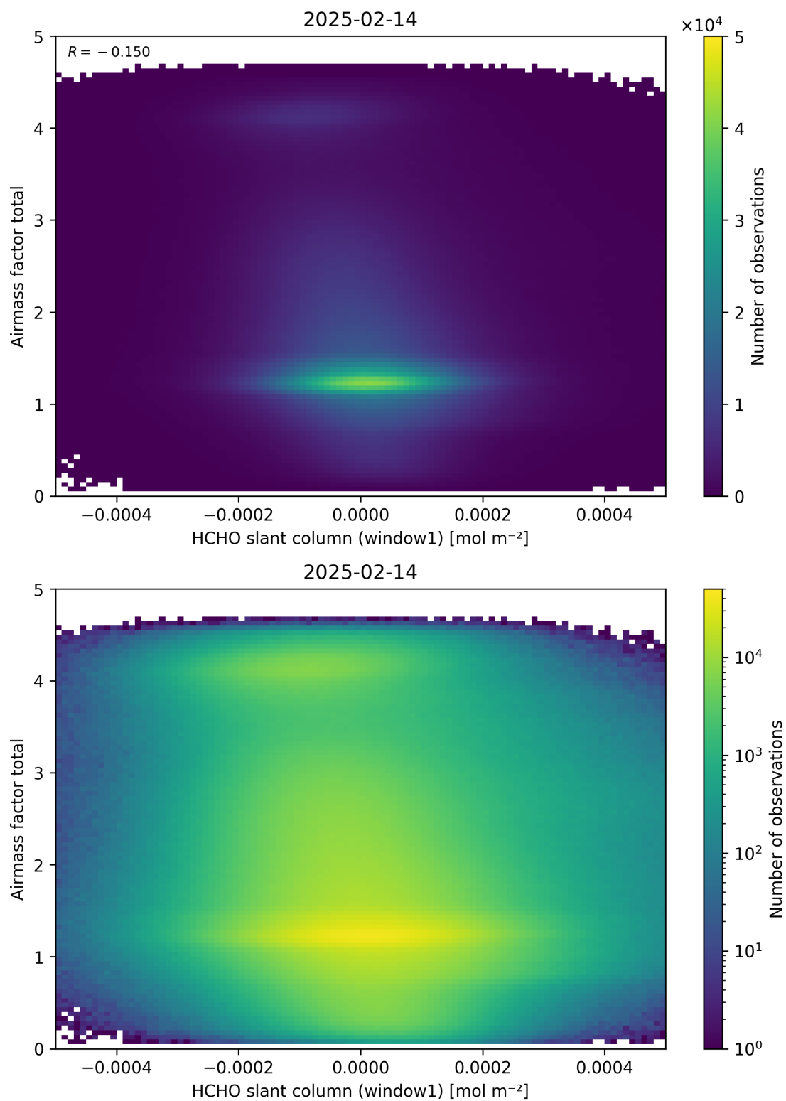
Figure 85: Scatter density plot of “HCHO slant column (window1)” against “Airmass factor total” for 2025-02-13 to 2025-02-15.
