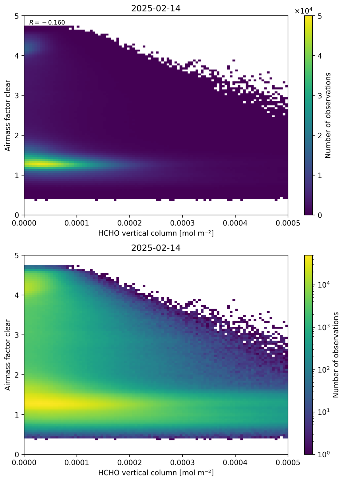
Figure 126: Scatter density plot of “HCHO vertical column” against “Airmass factor clear” for 2025-02-13 to 2025-02-15.
