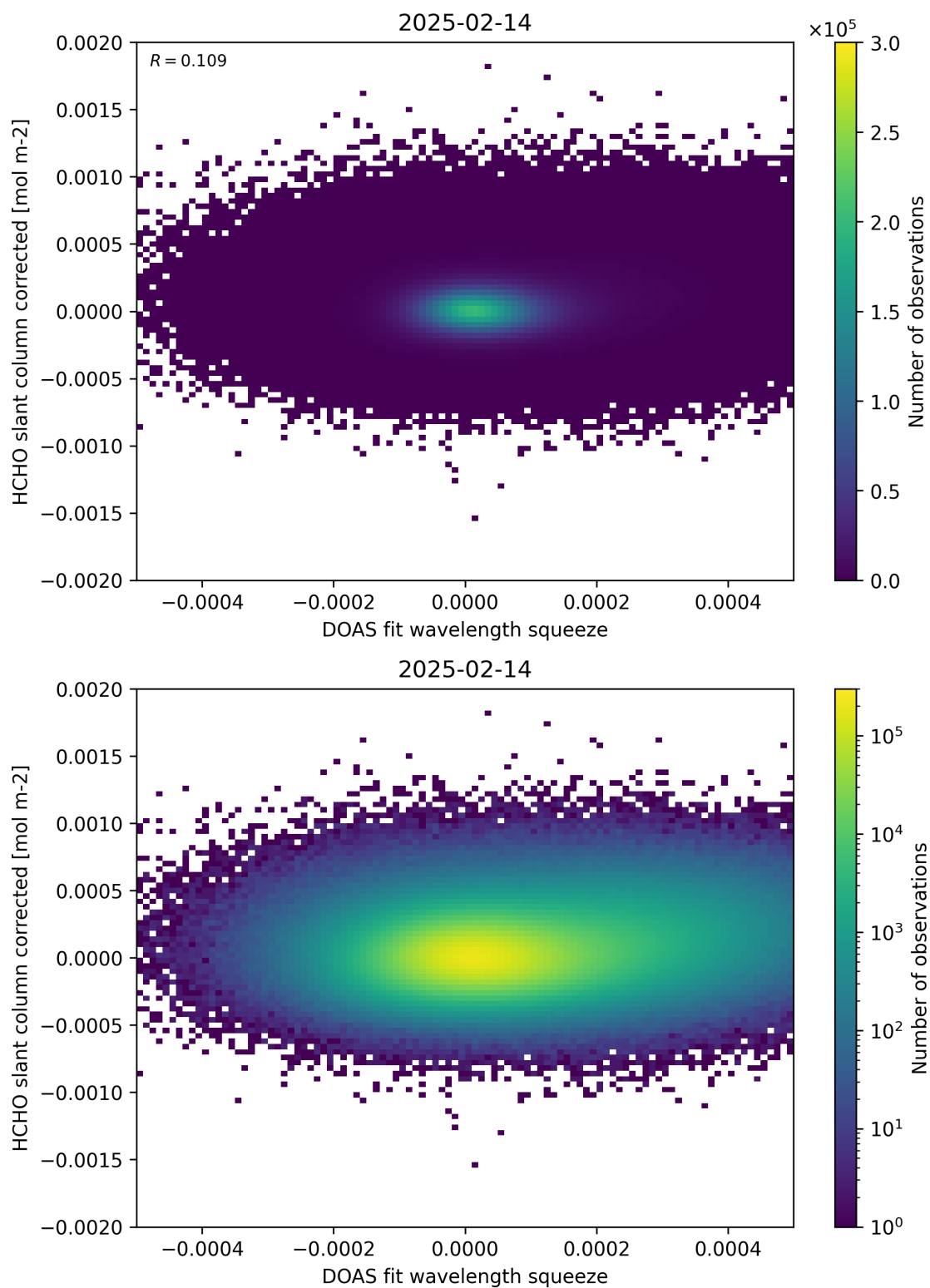
Figure 69: Scatter density plot of “DOAS fit wavelength squeeze” against “HCHO slant column corrected” for 2025-02-13 to 2025-02-15.
