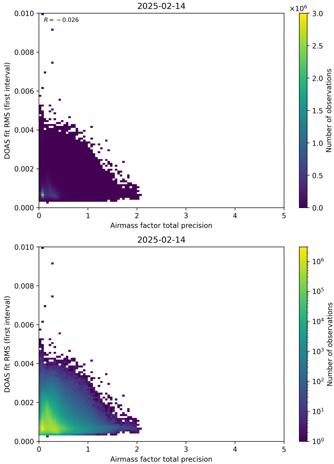
Figure 105: Scatter density plot of “Airmass factor total precision” against “DOAS fit RMS (first interval)” for 2025-02-13 to 2025-02-15.
