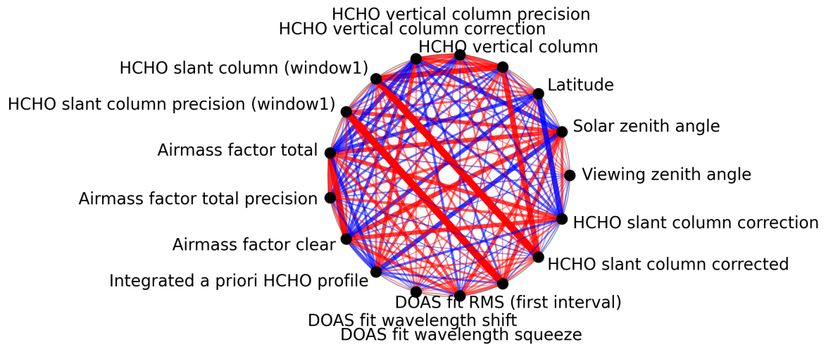
Figure 1: Map of correlation graph for 2025-02-13 to 2025-02-15.
