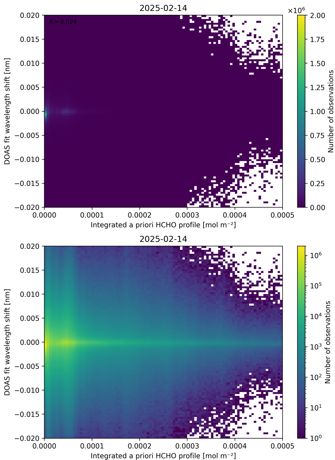
Figure 149: Scatter density plot of “Integrated a priori HCHO profile” against “DOAS fit wavelength shift” for 2025-02-13 to 2025-02-15.
