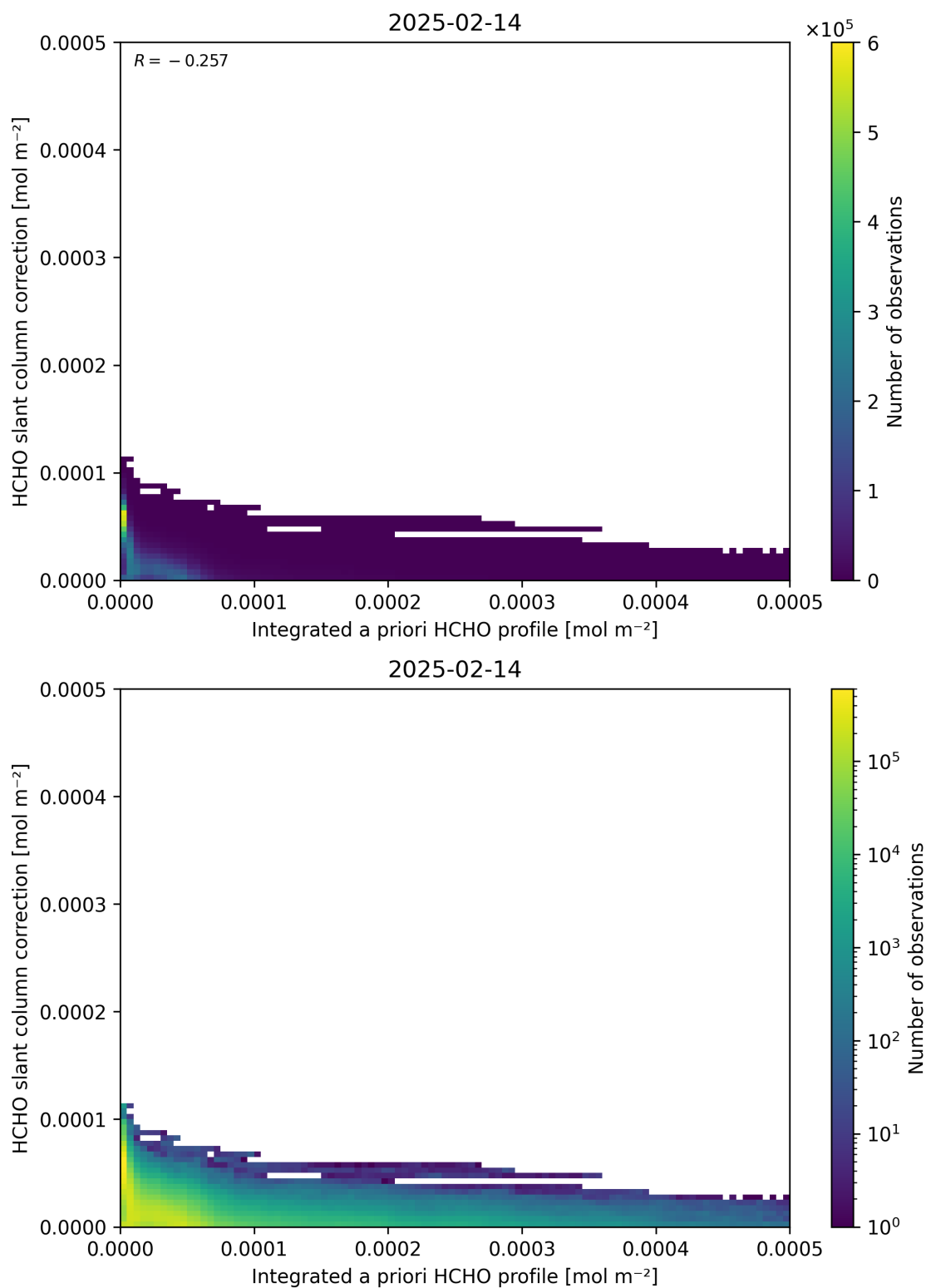
Figure 152: Scatter density plot of “Integrated a priori HCHO profile” against “HCHO slant column correction” for 2025-02-13 to 2025-02-15.
