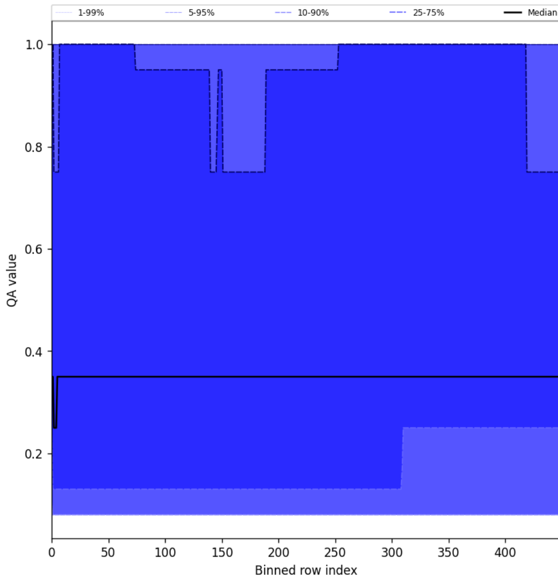
Figure 48: Along track statistics of “QA value” for 2025-02-13 to 2025-02-15
