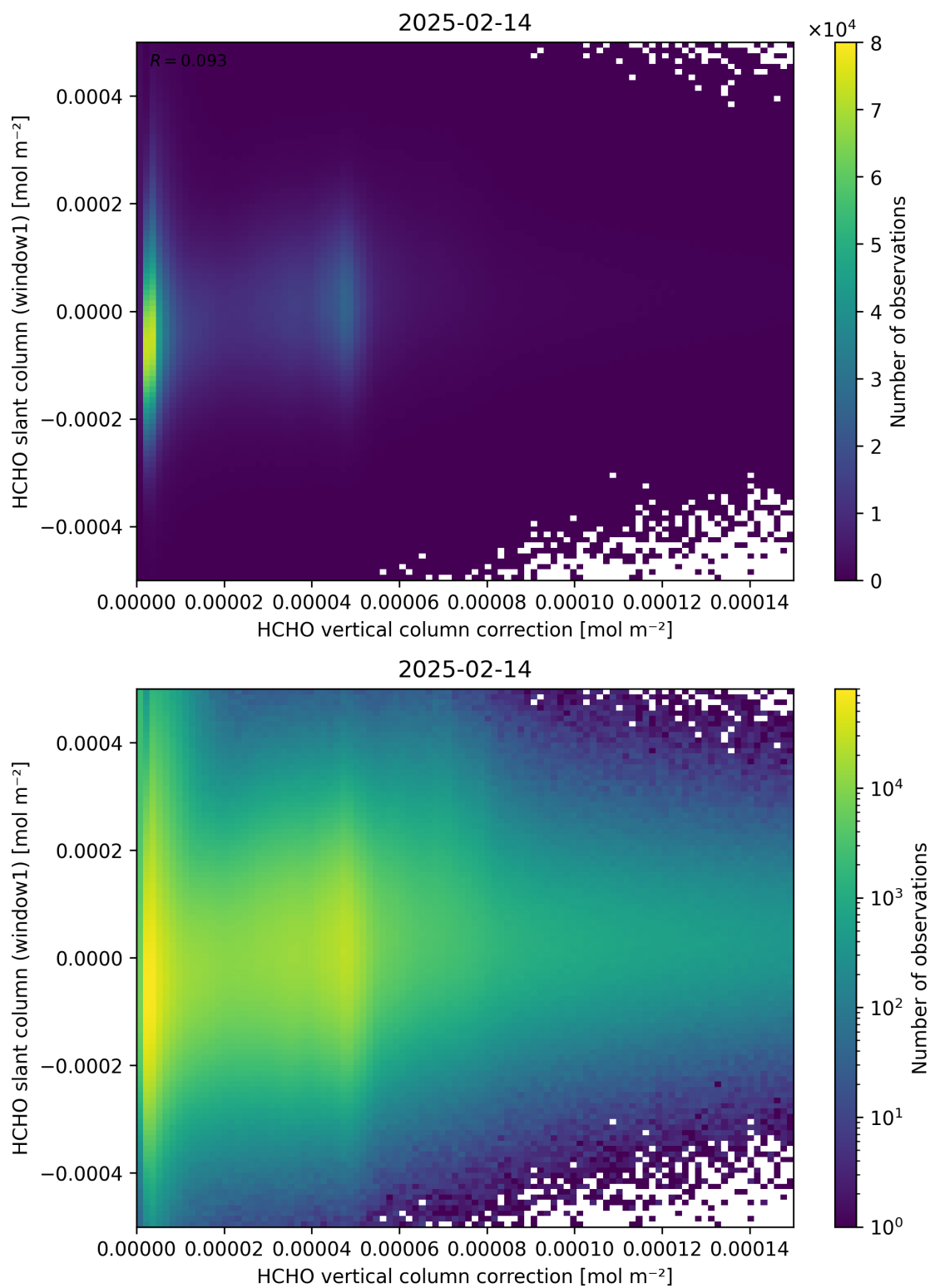
Figure 118: Scatter density plot of “HCHO vertical column correction” against “HCHO slant column (window1)” for 2025-02-13 to 2025-02-15.
