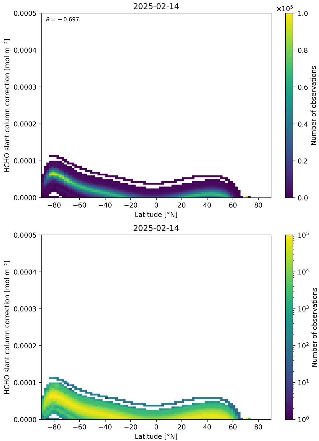
Figure 158: Scatter density plot of “Latitude” against “HCHO slant column correction” for 2025-02-13 to 2025-02-15.
