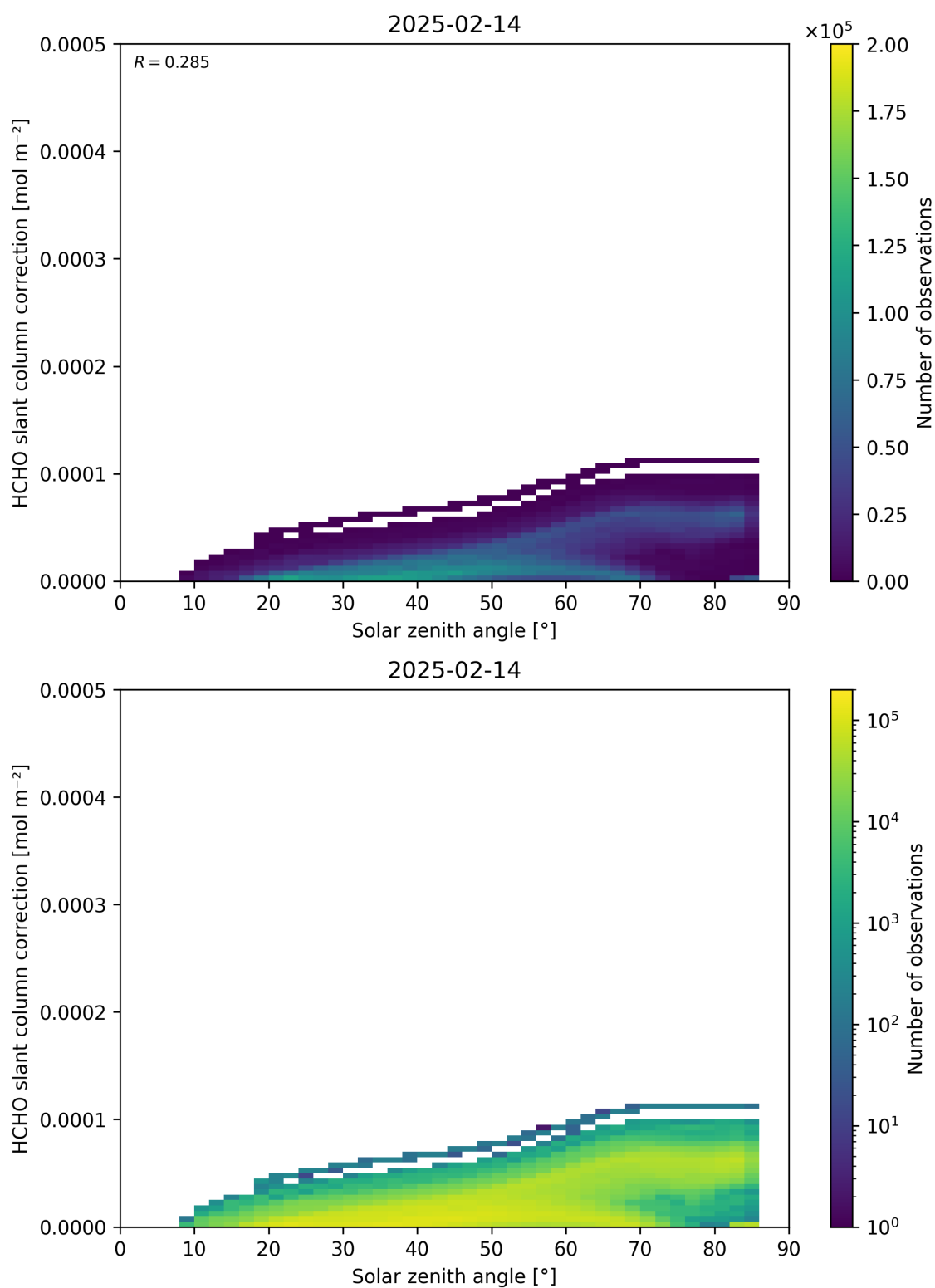
Figure 172: Scatter density plot of “Solar zenith angle” against “HCHO slant column correction” for 2025-02-13 to 2025-02-15.
