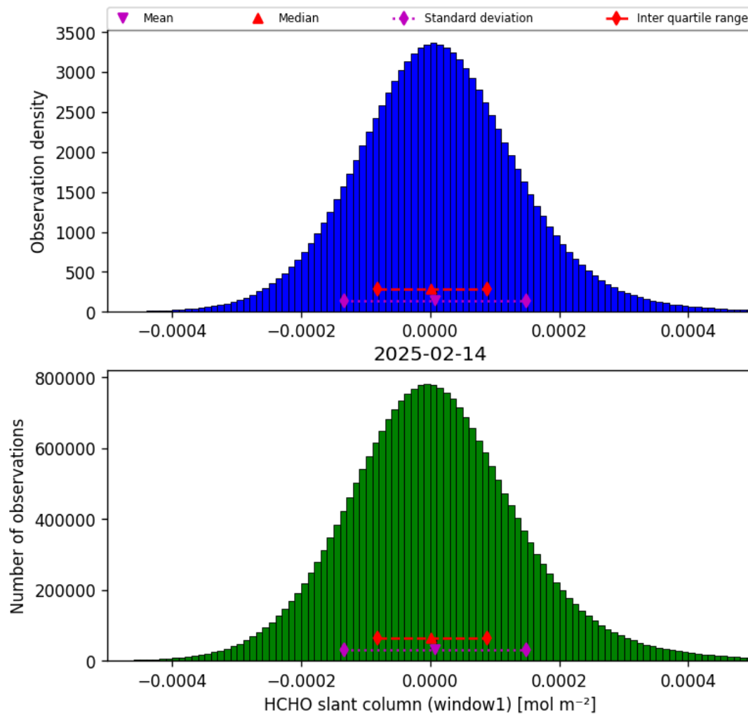
Figure 38: Histogram of “HCHO slant column (window1)” for 2025-02-13 to 2025-02-15
