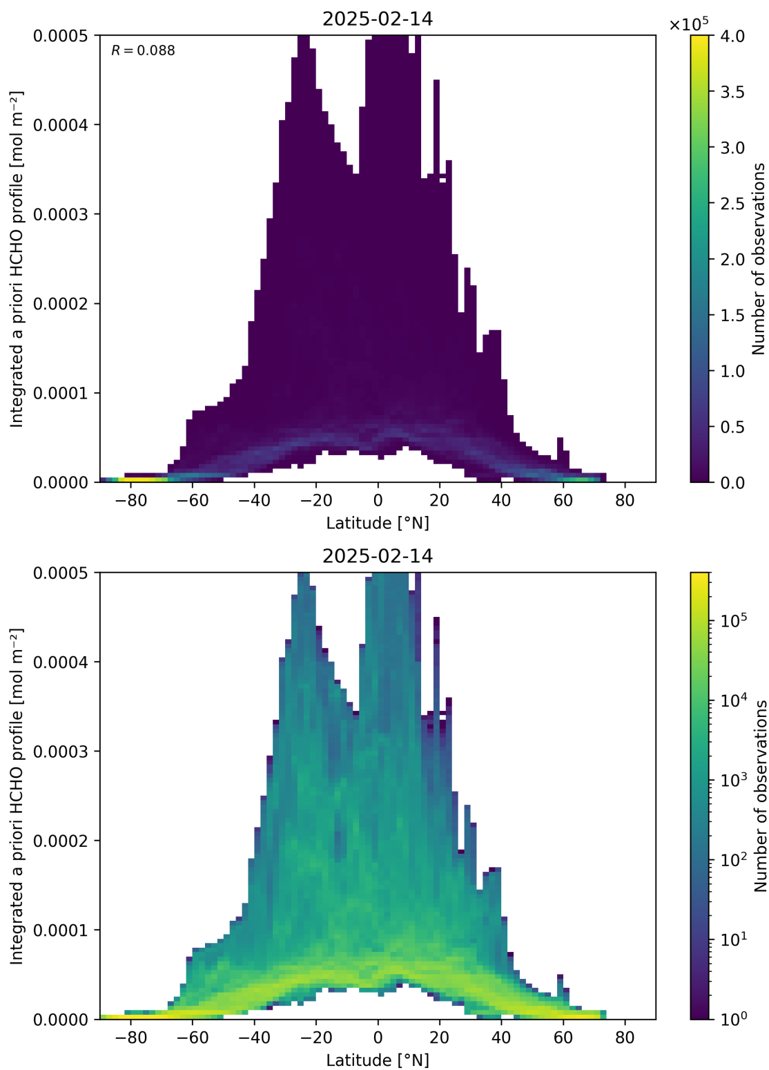
Figure 166: Scatter density plot of “Latitude” against “Integrated a priori HCHO profile” for 2025-02-13 to 2025-02-15.
