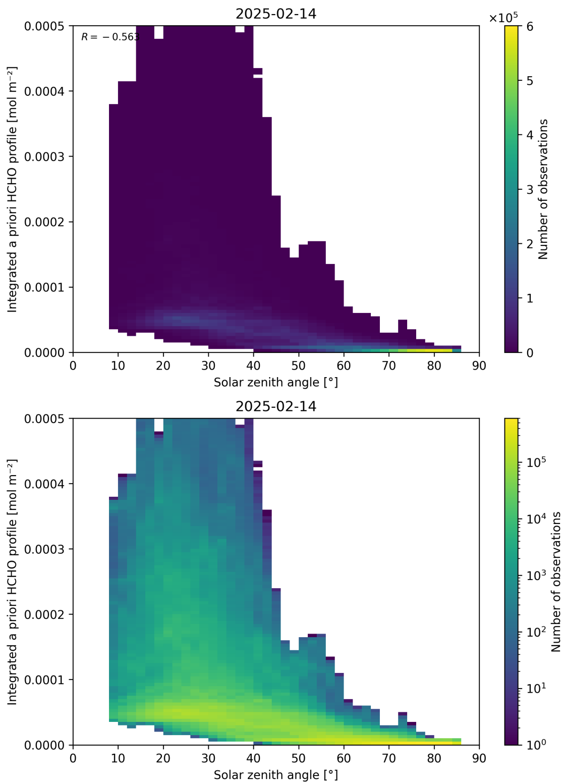
Figure 180: Scatter density plot of “Solar zenith angle” against “Integrated a priori HCHO profile” for 2025-02-13 to 2025-02-15.
