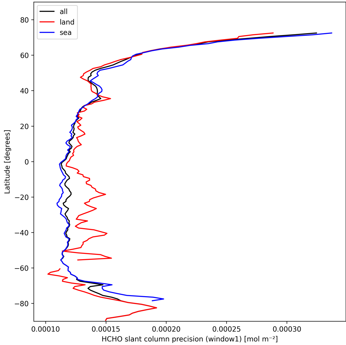
Figure 25: Zonal average of “HCHO slant column precision (window1)” for 2025-02-13 to 2025-02-15.
