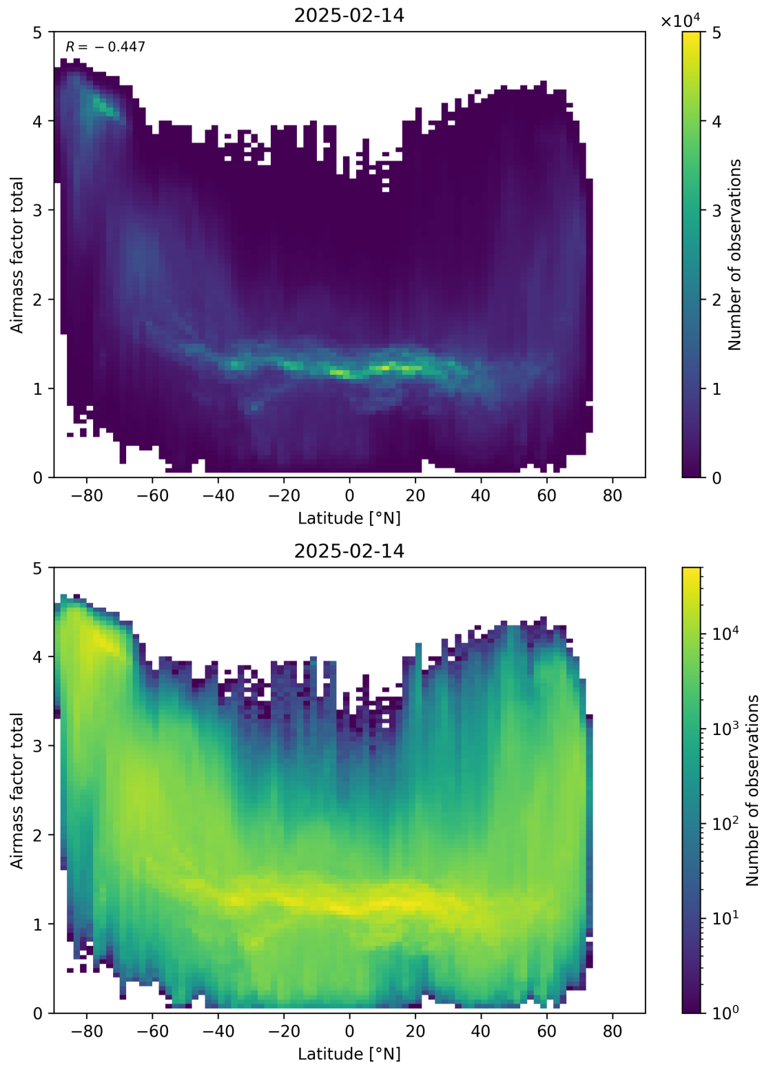
Figure 161: Scatter density plot of “Latitude” against “Airmass factor total” for 2025-02-13 to 2025-02-15.
