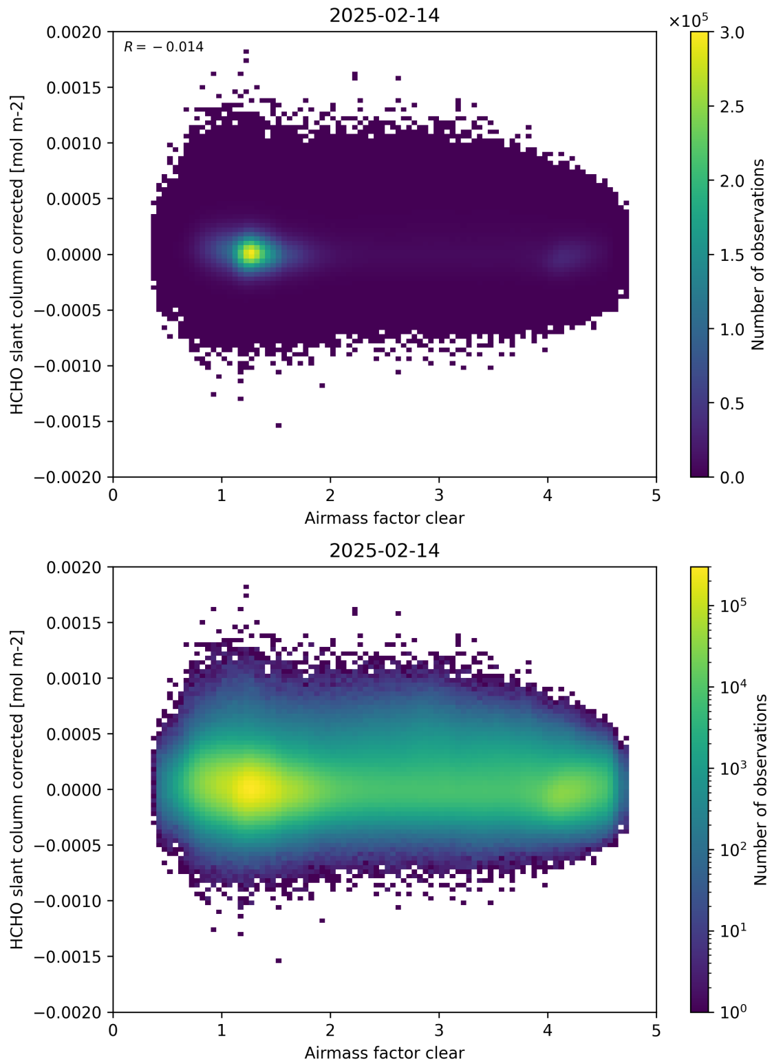
Figure 74: Scatter density plot of “Airmass factor clear” against “HCHO slant column corrected” for 2025-02-13 to 2025-02-15.
