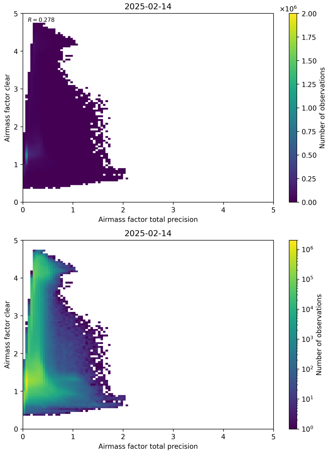
Figure 108: Scatter density plot of “Airmass factor total precision” against “Airmass factor clear” for 2025-02-13 to 2025-02-15.
