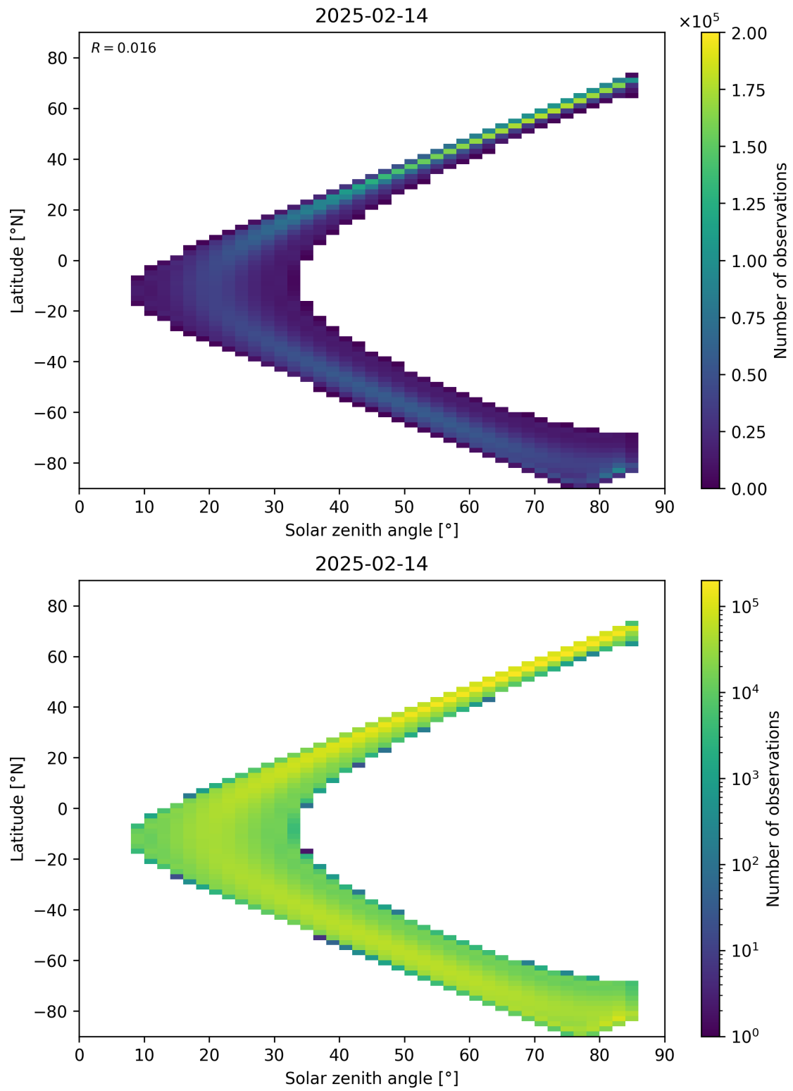
Figure 181: Scatter density plot of “Solar zenith angle” against “Latitude” for 2025-02-13 to 2025-02-15.
