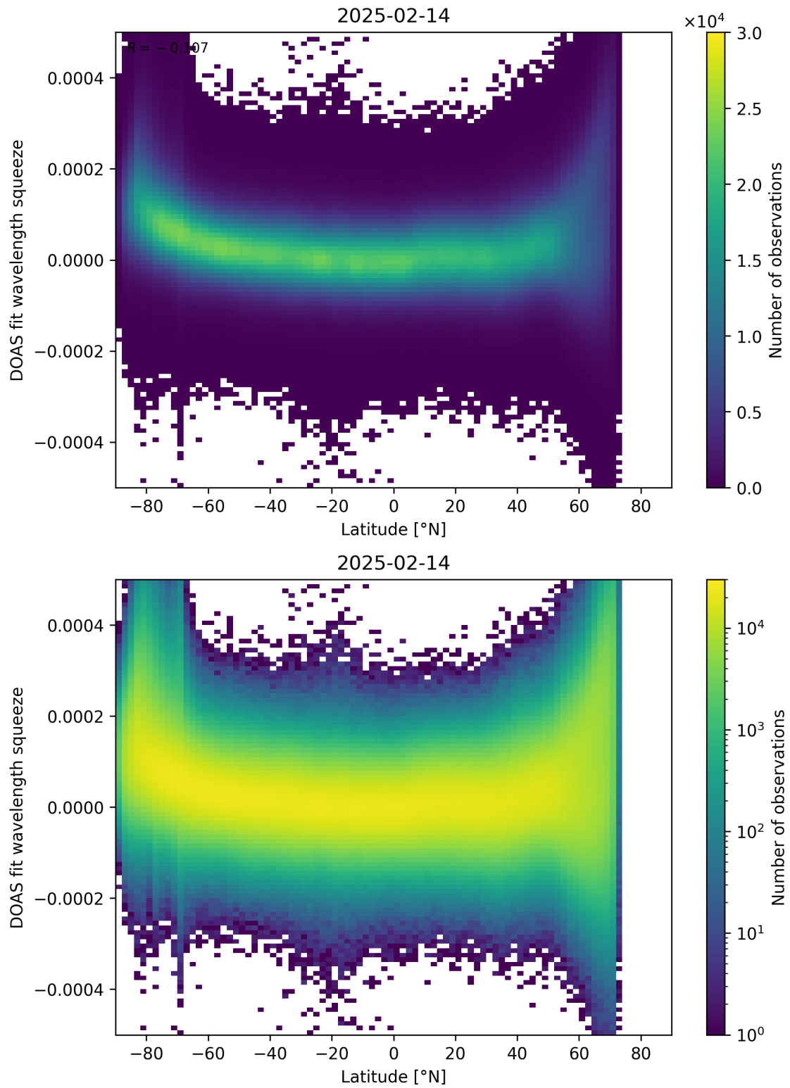
Figure 155: Scatter density plot of “Latitude” against “DOAS fit wavelength squeeze” for 2025-02-13 to 2025-02-15.
