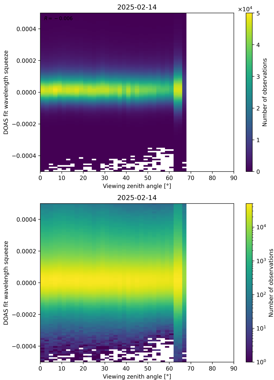
Figure 184: Scatter density plot of “Viewing zenith angle” against “DOAS fit wavelength squeeze” for 2025-02-13 to 2025-02-15.
