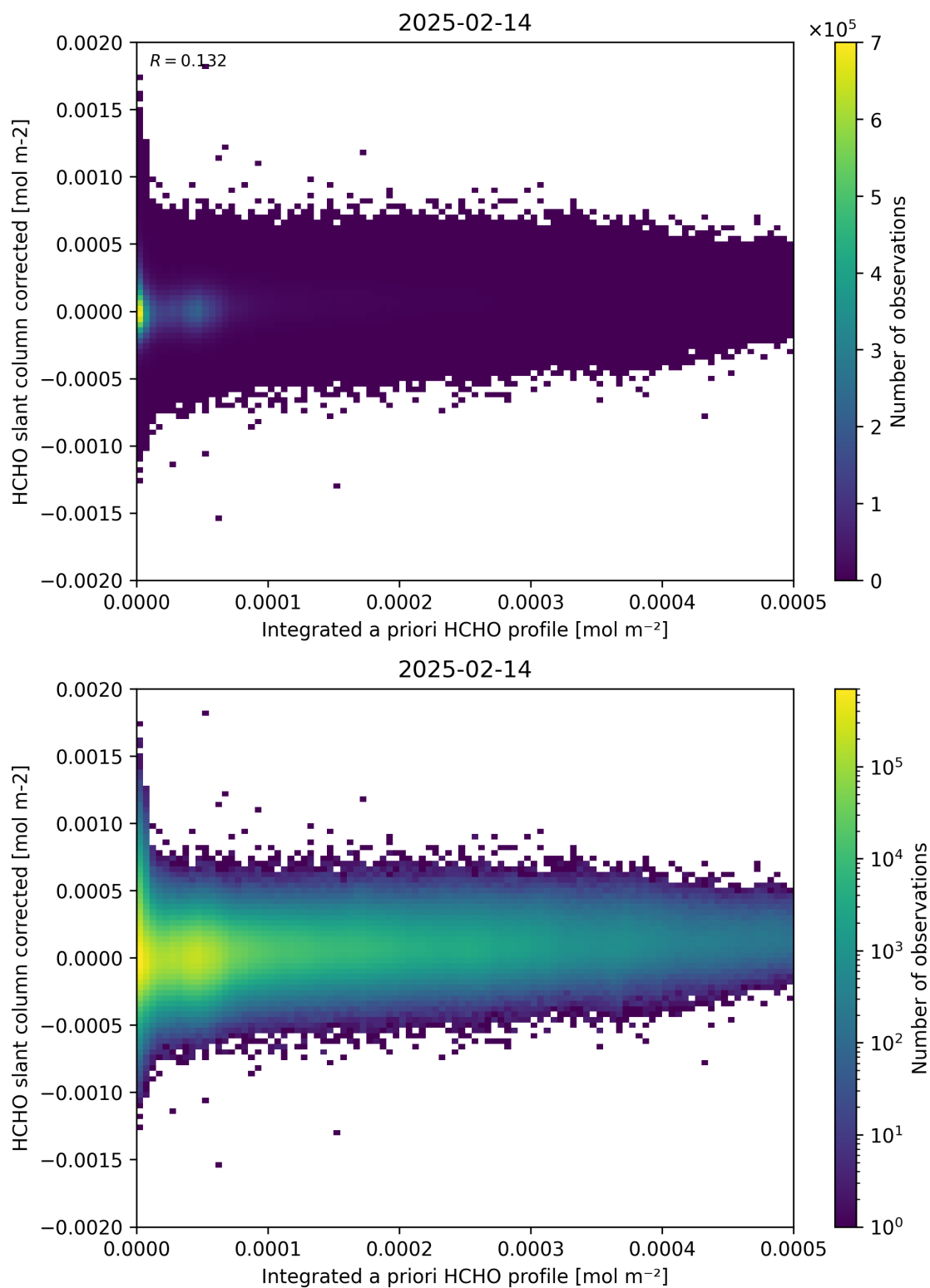
Figure 151: Scatter density plot of “Integrated a priori HCHO profile” against “HCHO slant column corrected” for 2025-02-13 to 2025-02-15.
