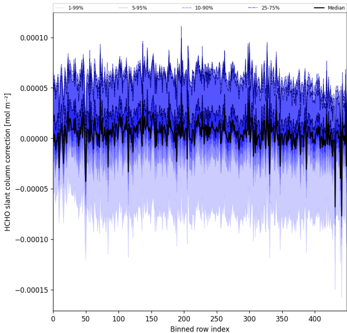
Figure 61: Along track statistics of “HCHO slant column correction” for 2025-02-13 to 2025-02-15
