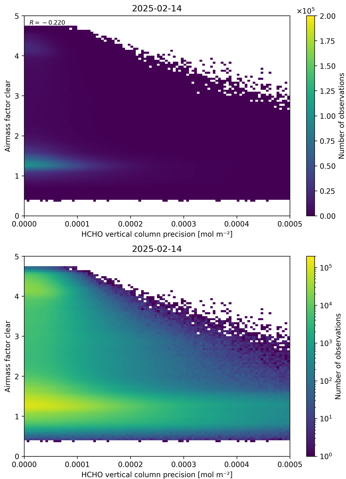
Figure 139: Scatter density plot of “HCHO vertical column precision” against “Airmass factor clear” for 2025-02-13 to 2025-02-15.
