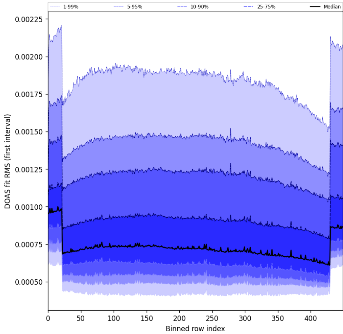
Figure 60: Along track statistics of “DOAS fit RMS (first interval)” for 2025-02-13 to 2025-02-15
