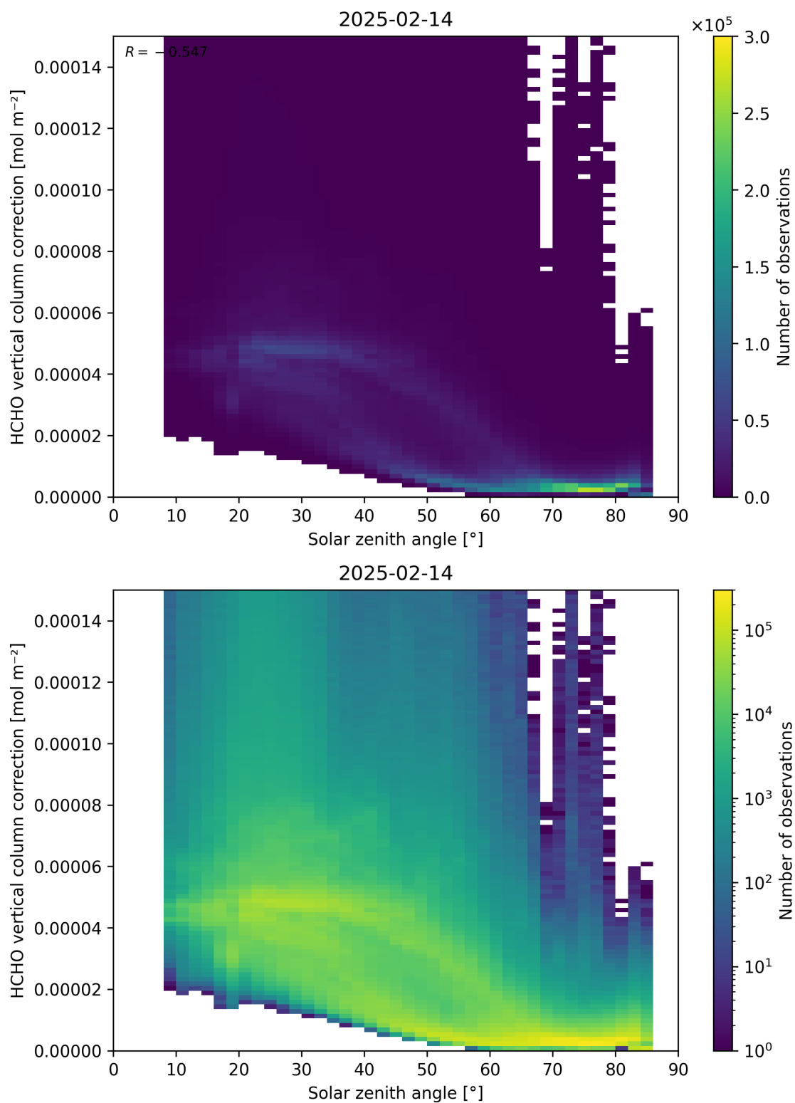
Figure 178: Scatter density plot of “Solar zenith angle” against “HCHO vertical column correction” for 2025-02-13 to 2025-02-15.
