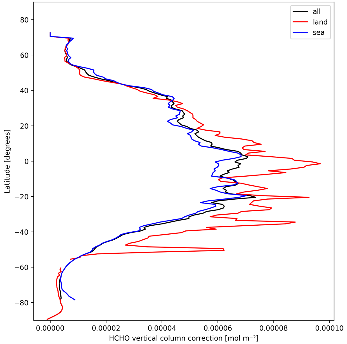
Figure 23: Zonal average of “HCHO vertical column correction” for 2025-02-13 to 2025-02-15.
