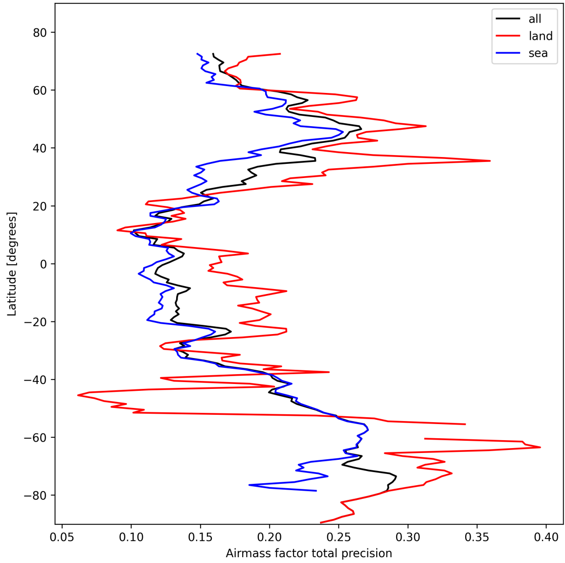
Figure 27: Zonal average of “Airmass factor total precision” for 2025-02-13 to 2025-02-15.
