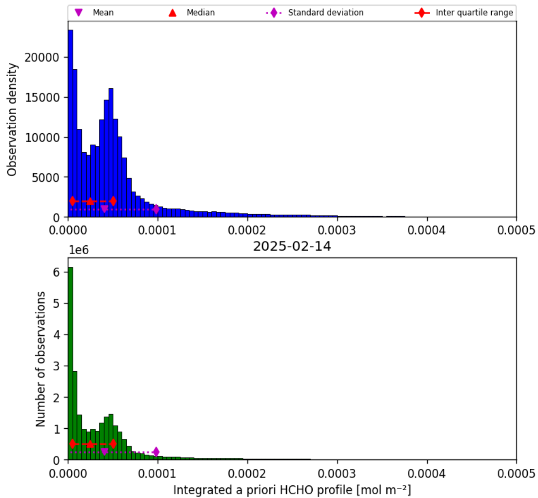
Figure 43: Histogram of “Integrated a priori HCHO profile” for 2025-02-13 to 2025-02-15
