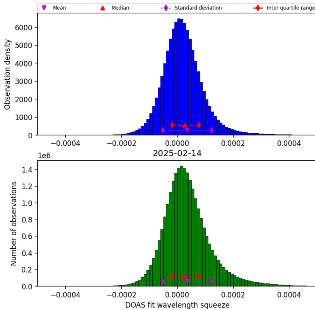
Figure 45: Histogram of “DOAS fit wavelength squeeze” for 2025-02-13 to 2025-02-15
