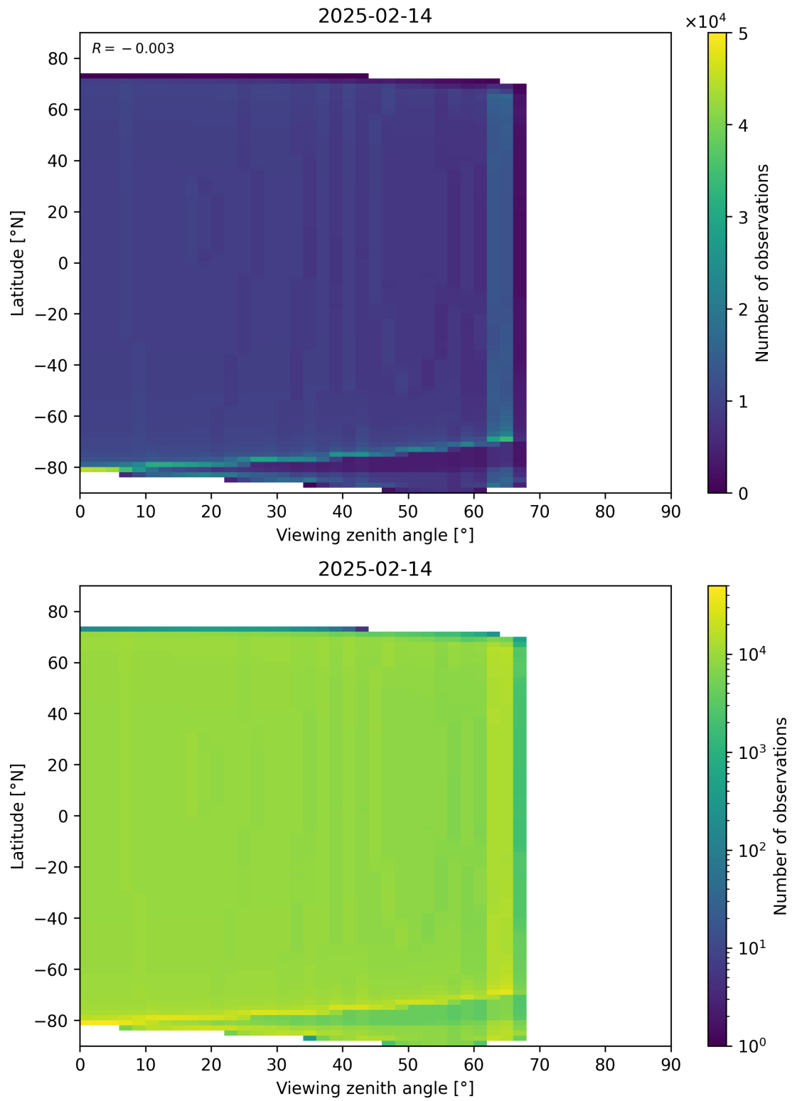
Figure 196: Scatter density plot of “Viewing zenith angle” against “Latitude” for 2025-02-13 to 2025-02-15.
