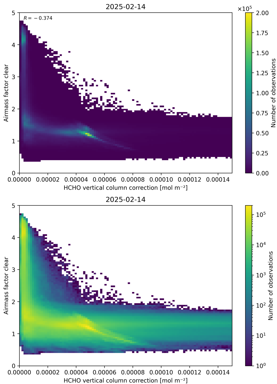
Figure 115: Scatter density plot of “HCHO vertical column correction” against “Airmass factor clear” for 2025-02-13 to 2025-02-15.
