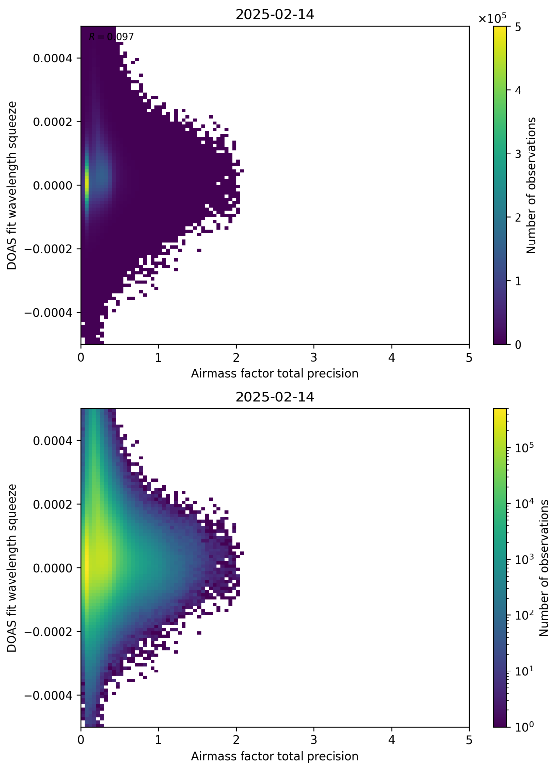
Figure 107: Scatter density plot of “Airmass factor total precision” against “DOAS fit wavelength squeeze” for 2025-02-13 to 2025-02-15.
