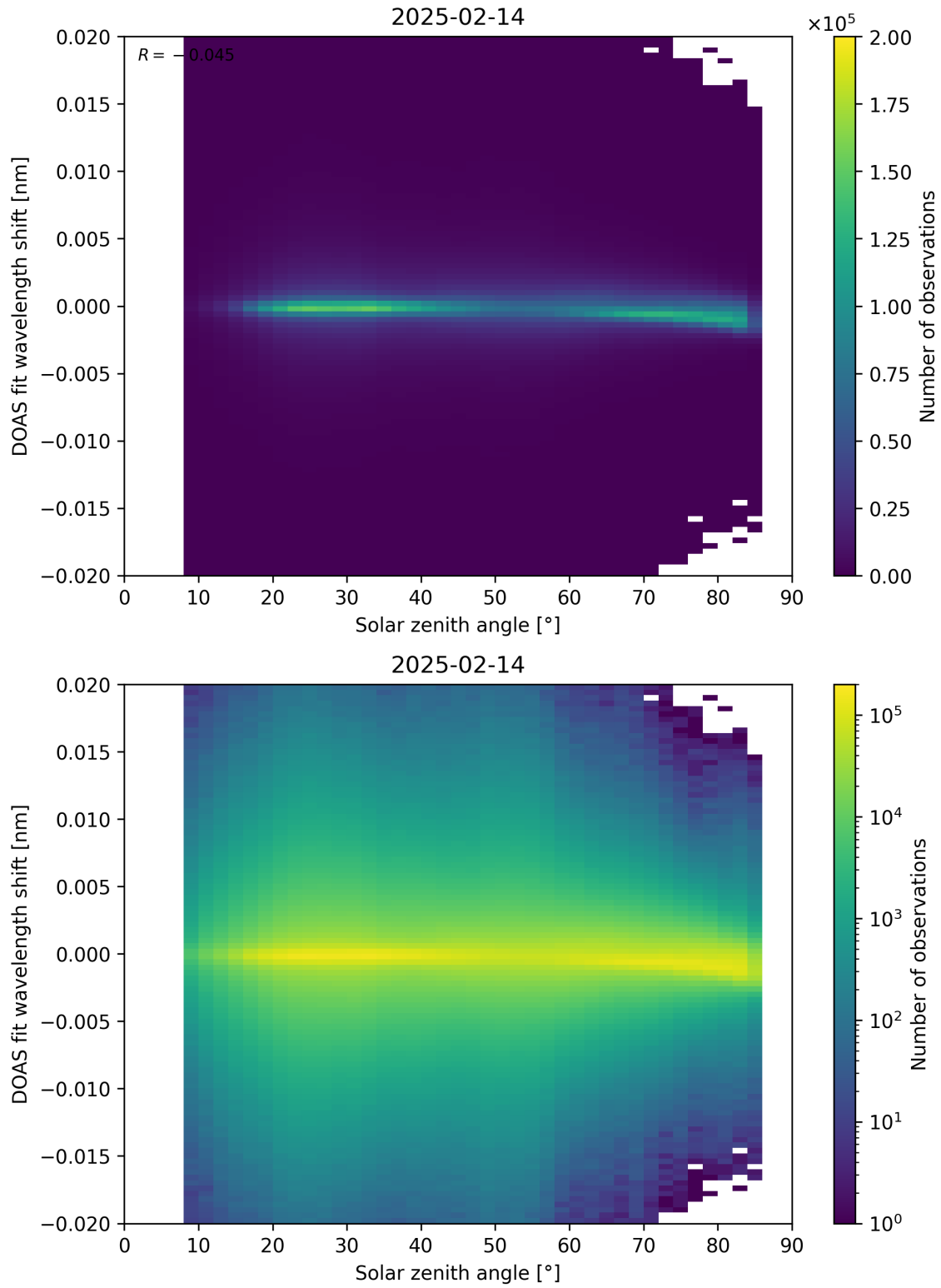
Figure 168: Scatter density plot of “Solar zenith angle” against “DOAS fit wavelength shift” for 2025-02-13 to 2025-02-15.
