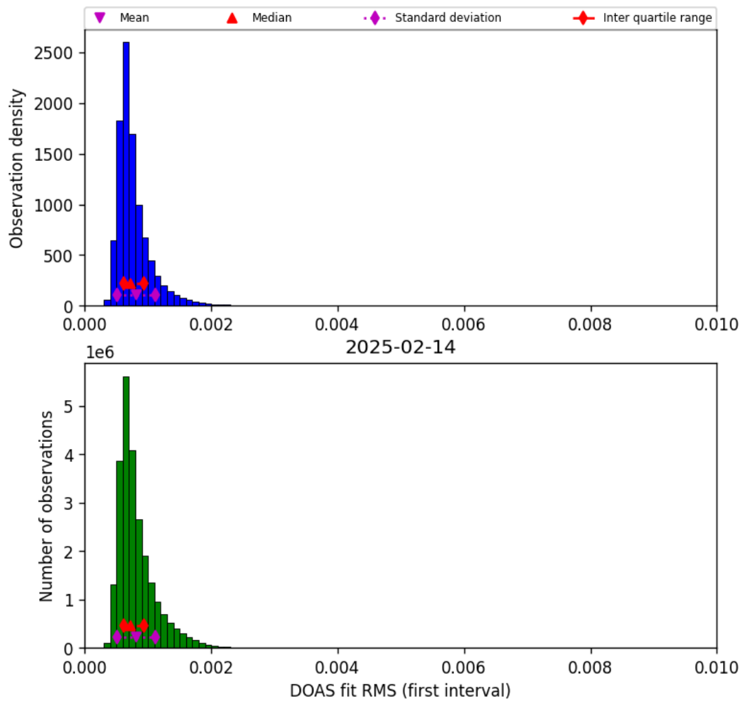
Figure 46: Histogram of “DOAS fit RMS (first interval)” for 2025-02-13 to 2025-02-15
