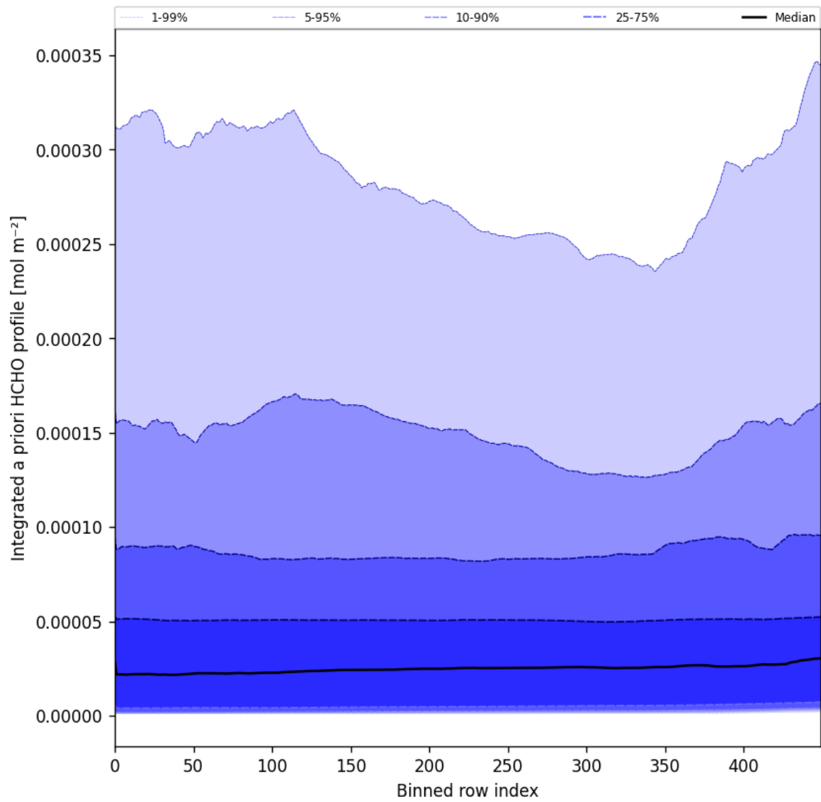
Figure 57: Along track statistics of "Integrated a priori HCHO profile" for 2025-02-13 to 2025-02-15
