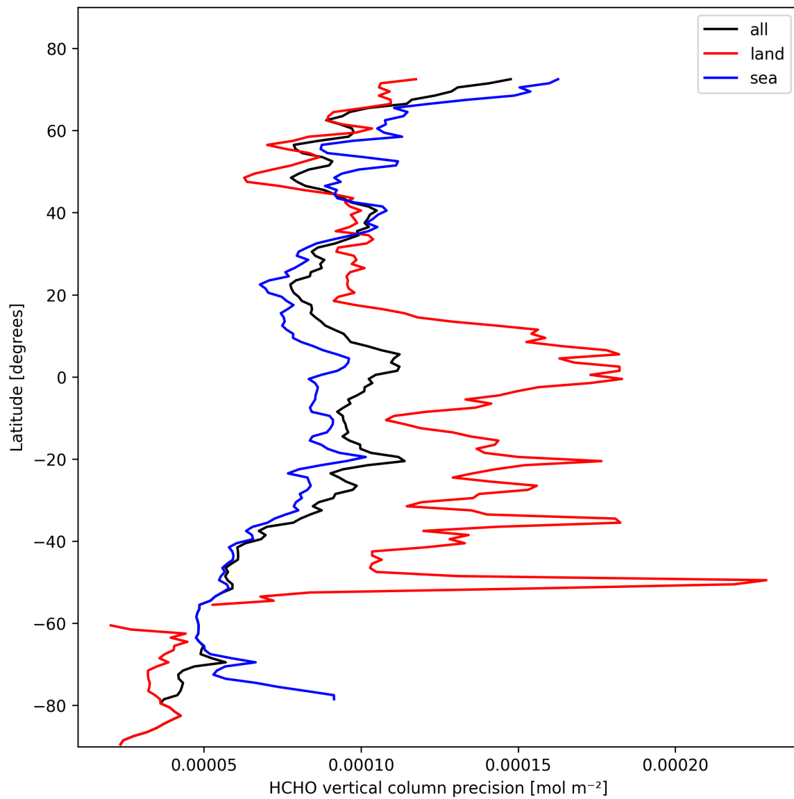
Figure 22: Zonal average of “HCHO vertical column precision” for 2025-02-13 to 2025-02-15.
