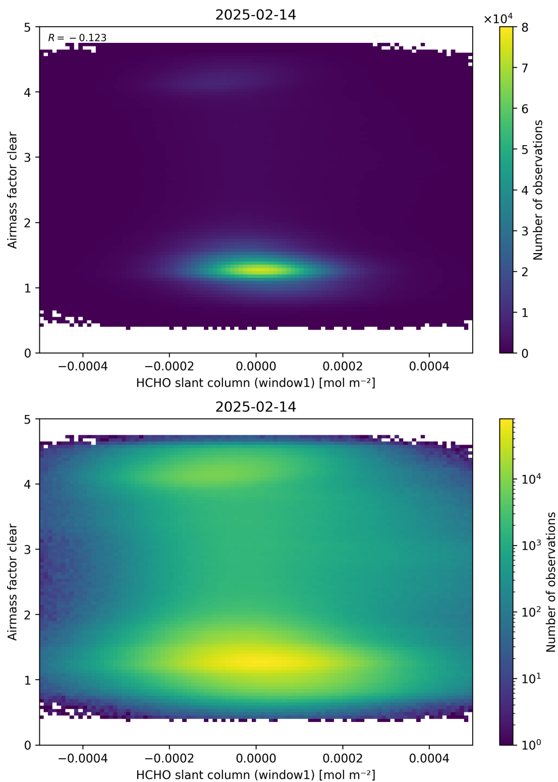
Figure 81: Scatter density plot of “HCHO slant column (window1)” against “Airmass factor clear” for 2025-02-13 to 2025-02-15.
