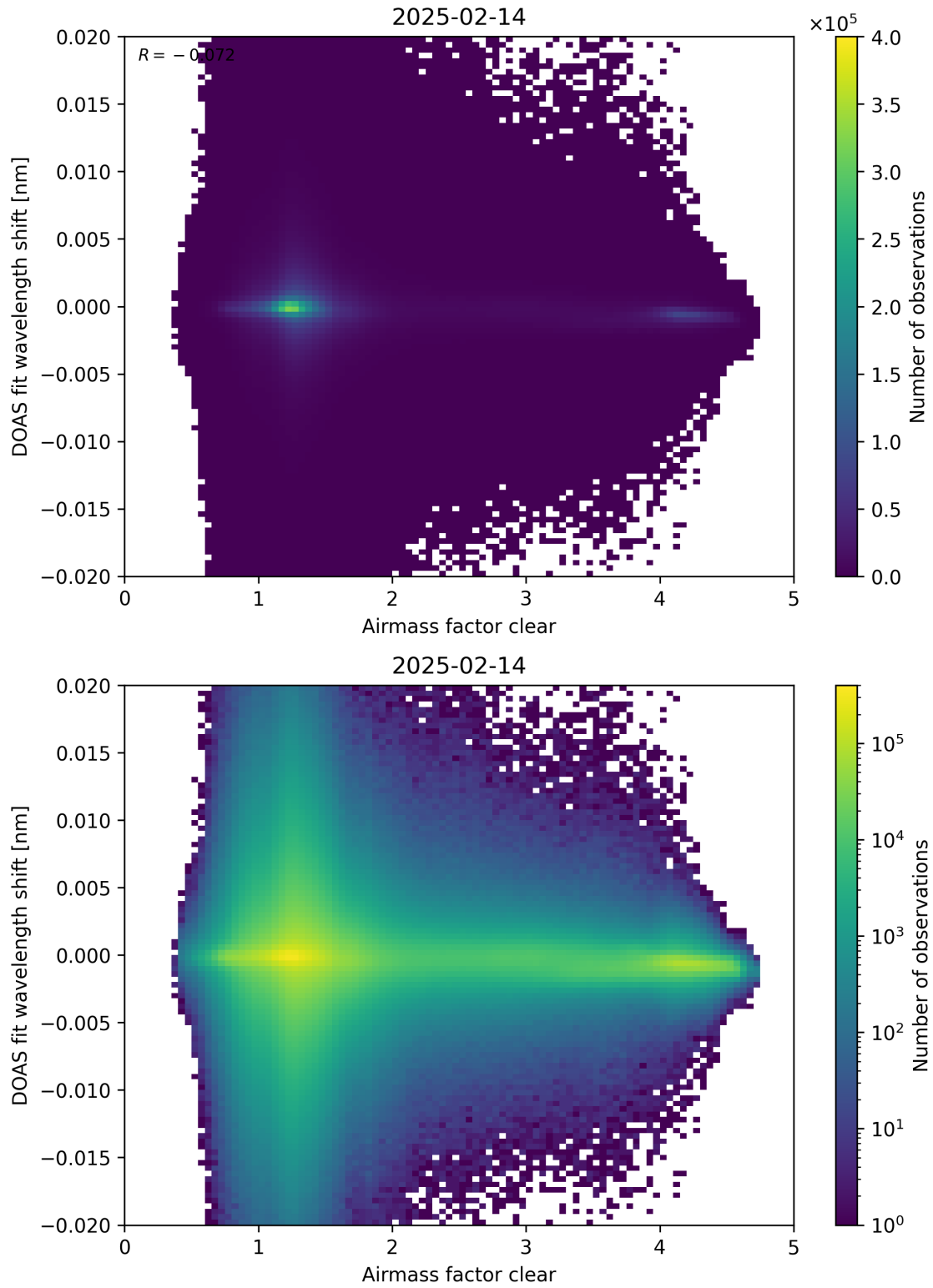
Figure 72: Scatter density plot of “Airmass factor clear” against “DOAS fit wavelength shift” for 2025-02-13 to 2025-02-15.
