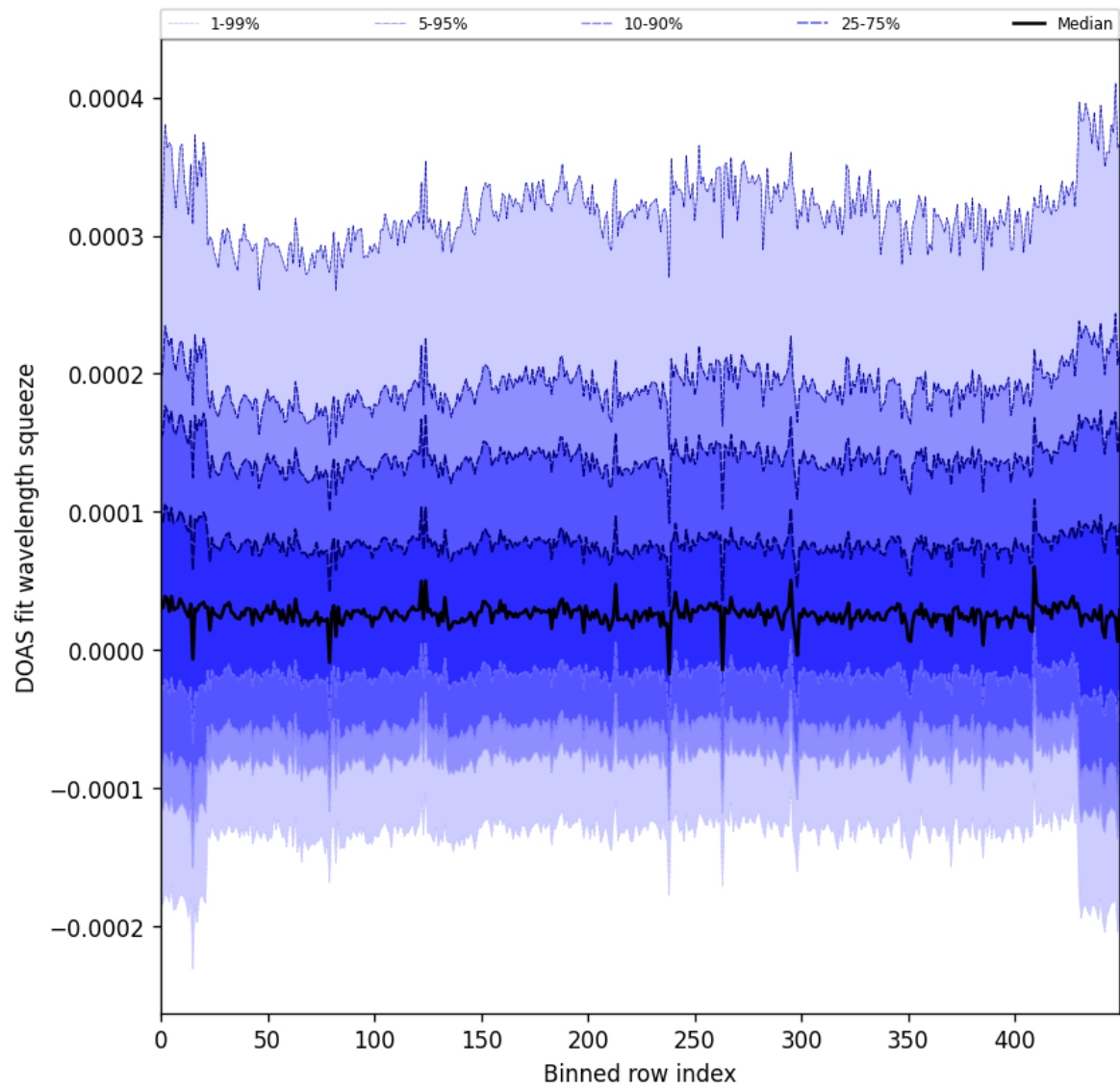
Figure 59: Along track statistics of “DOAS fit wavelength squeeze” for 2025-02-13 to 2025-02-15
