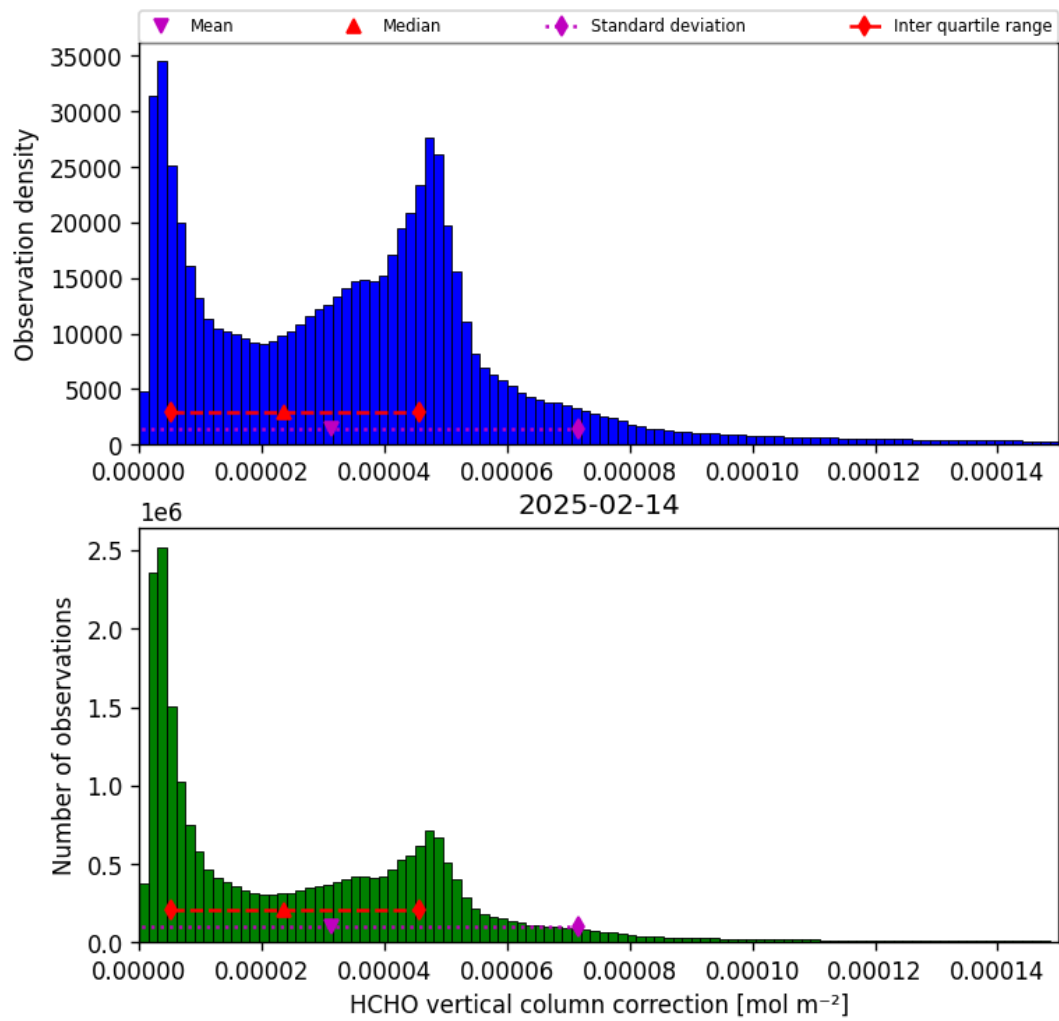
Figure 37: Histogram of “HCHO vertical column correction” for 2025-02-13 to 2025-02-15
