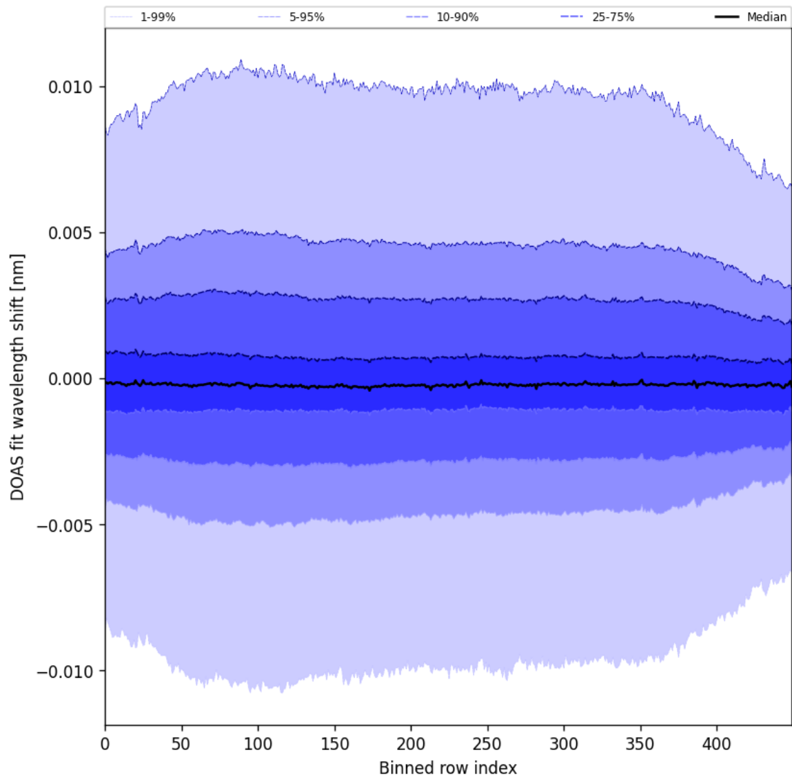
Figure 58: Along track statistics of “DOAS fit wavelength shift” for 2025-02-13 to 2025-02-15
