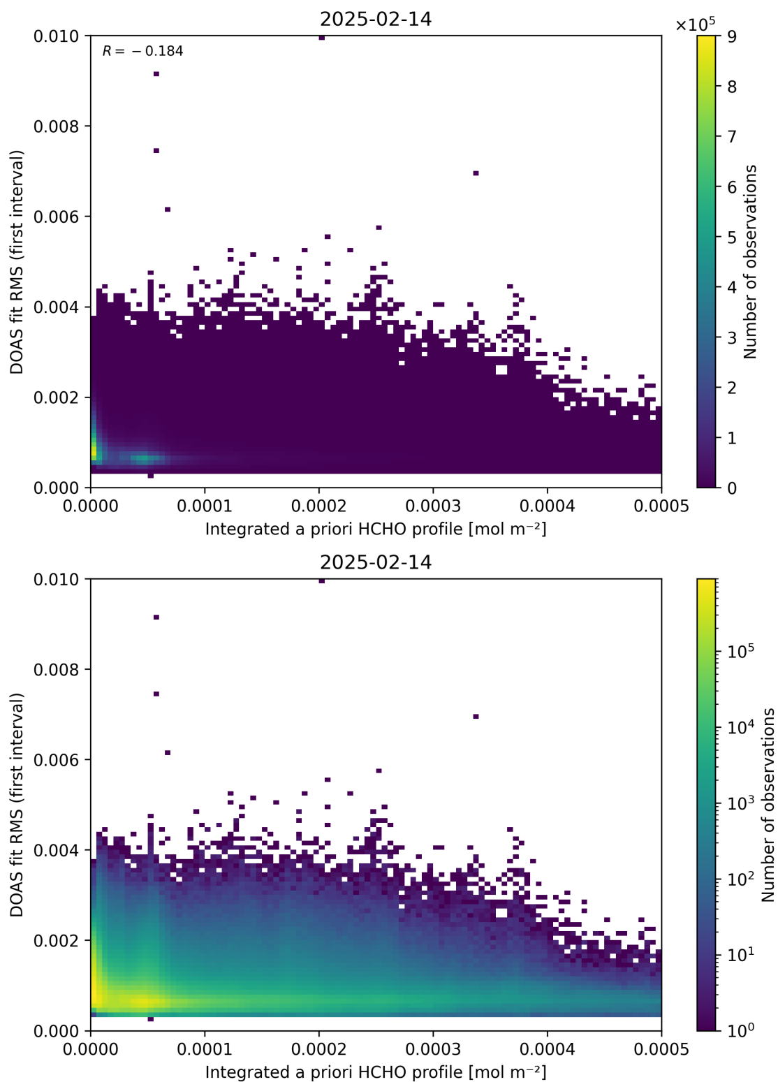
Figure 148: Scatter density plot of “Integrated a priori HCHO profile” against “DOAS fit RMS (first interval)” for 2025-02-13 to 2025-02-15.
