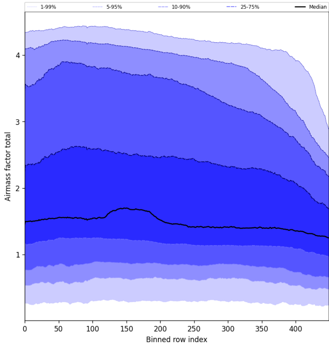
Figure 54: Along track statistics of “Airmass factor total” for 2025-02-13 to 2025-02-15
