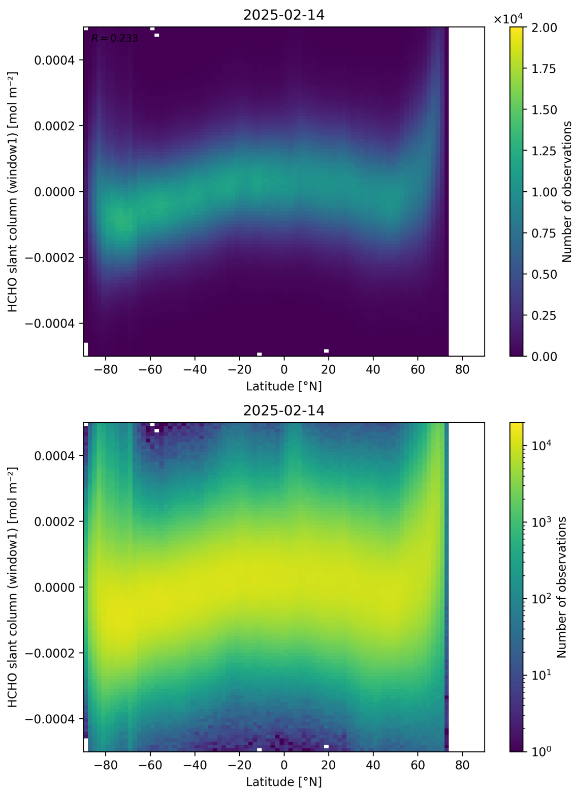
Figure 159: Scatter density plot of “Latitude” against “HCHO slant column (window1)” for 2025-02-13 to 2025-02-15.
