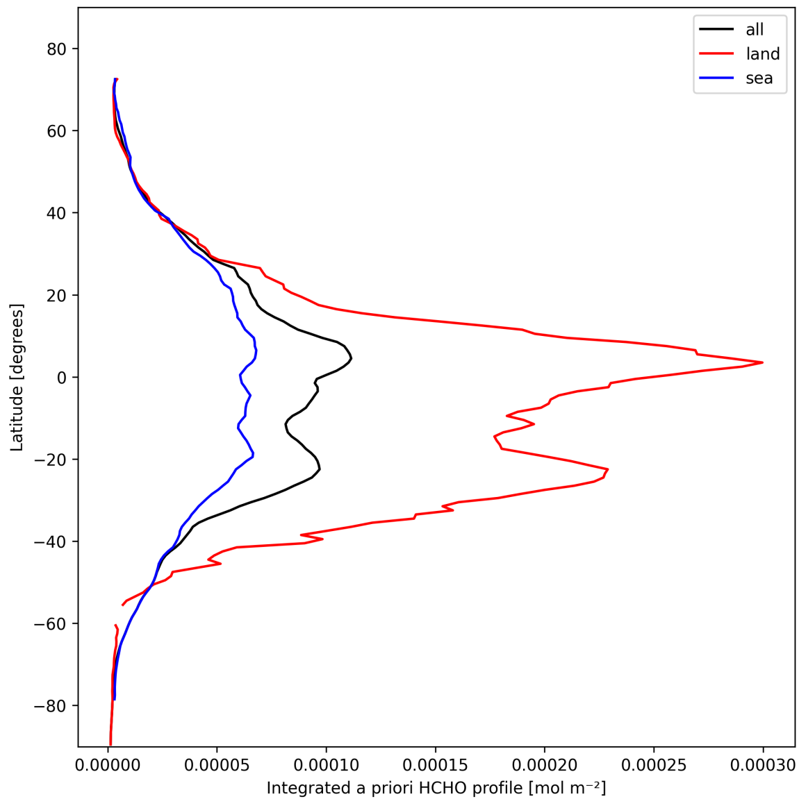
Figure 29: Zonal average of “Integrated a priori HCHO profile” for 2025-02-13 to 2025-02-15.
