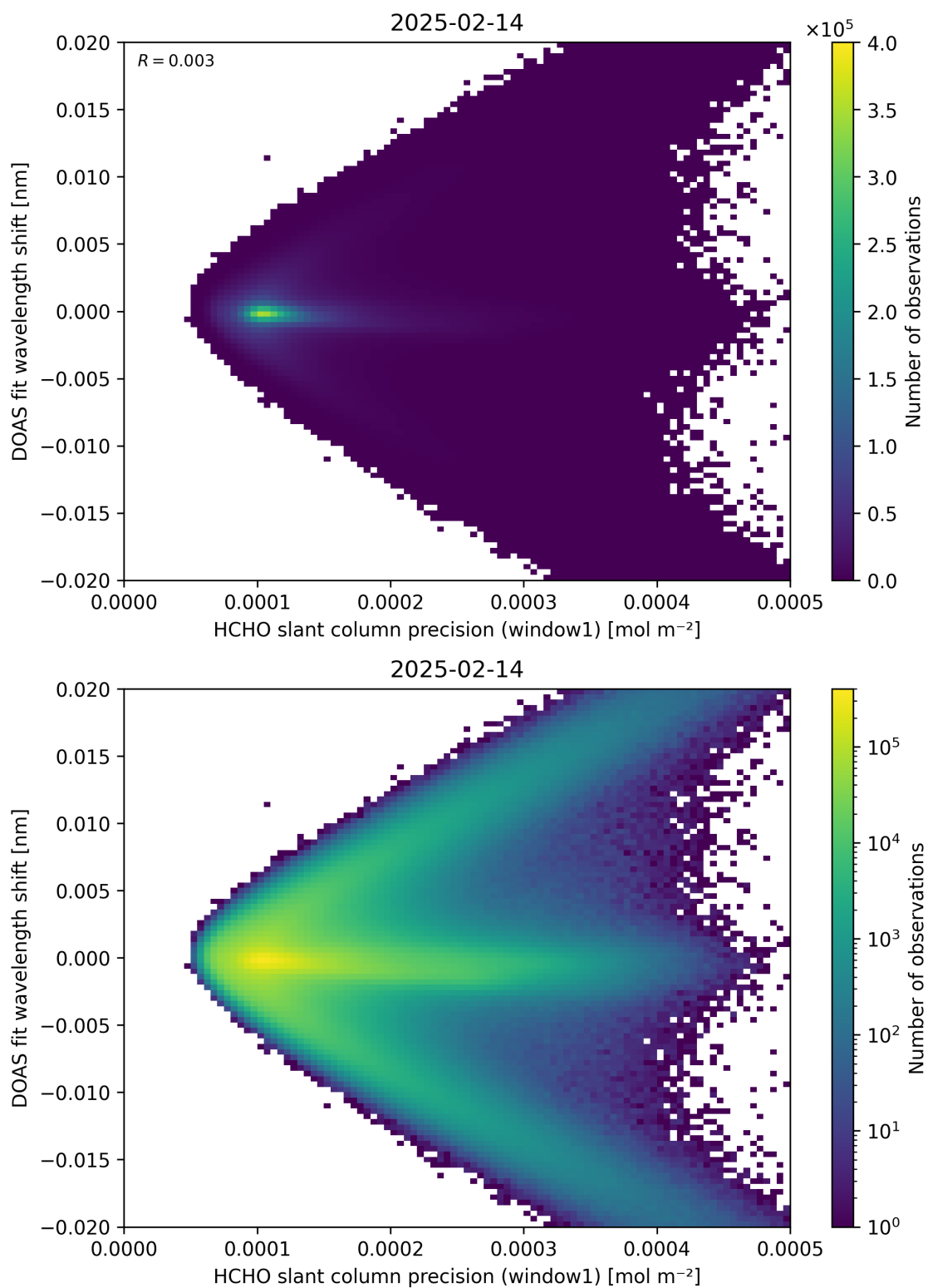
Figure 89: Scatter density plot of “HCHO slant column precision (window1)” against “DOAS fit wavelength shift” for 2025-02-13 to 2025-02-15.
