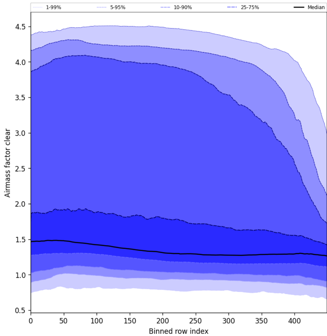
Figure 56: Along track statistics of “Air mass factor clear” for 2025-02-13 to 2025-02-15
