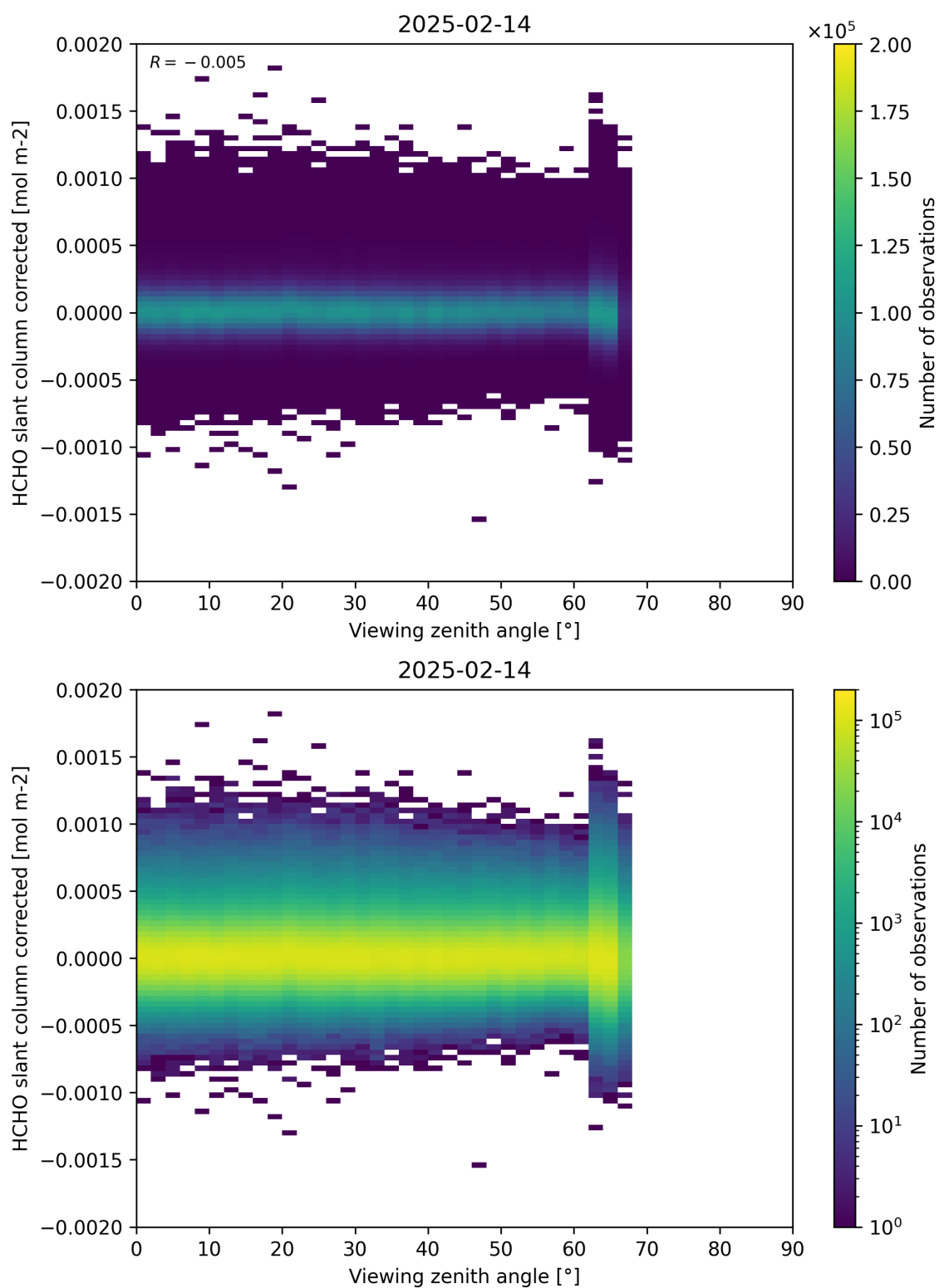
Figure 186: Scatter density plot of “Viewing zenith angle” against “HCHO slant column corrected” for 2025-02-13 to 2025-02-15.
