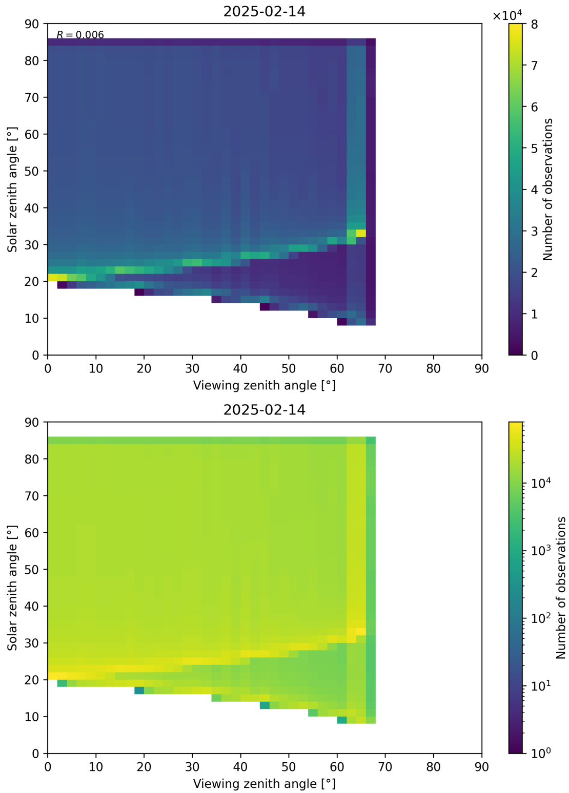
Figure 197: Scatter density plot of “Viewing zenith angle” against “Solar zenith angle” for 2025-02-13 to 2025-02-15.
