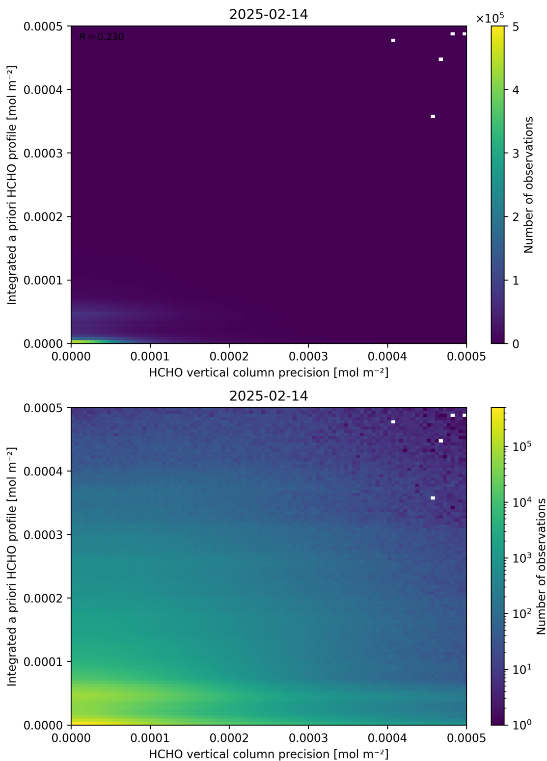
Figure 147: Scatter density plot of “HCHO vertical column precision” against “Integrated a priori HCHO profile” for 2025-02-13 to 2025-02-15.
