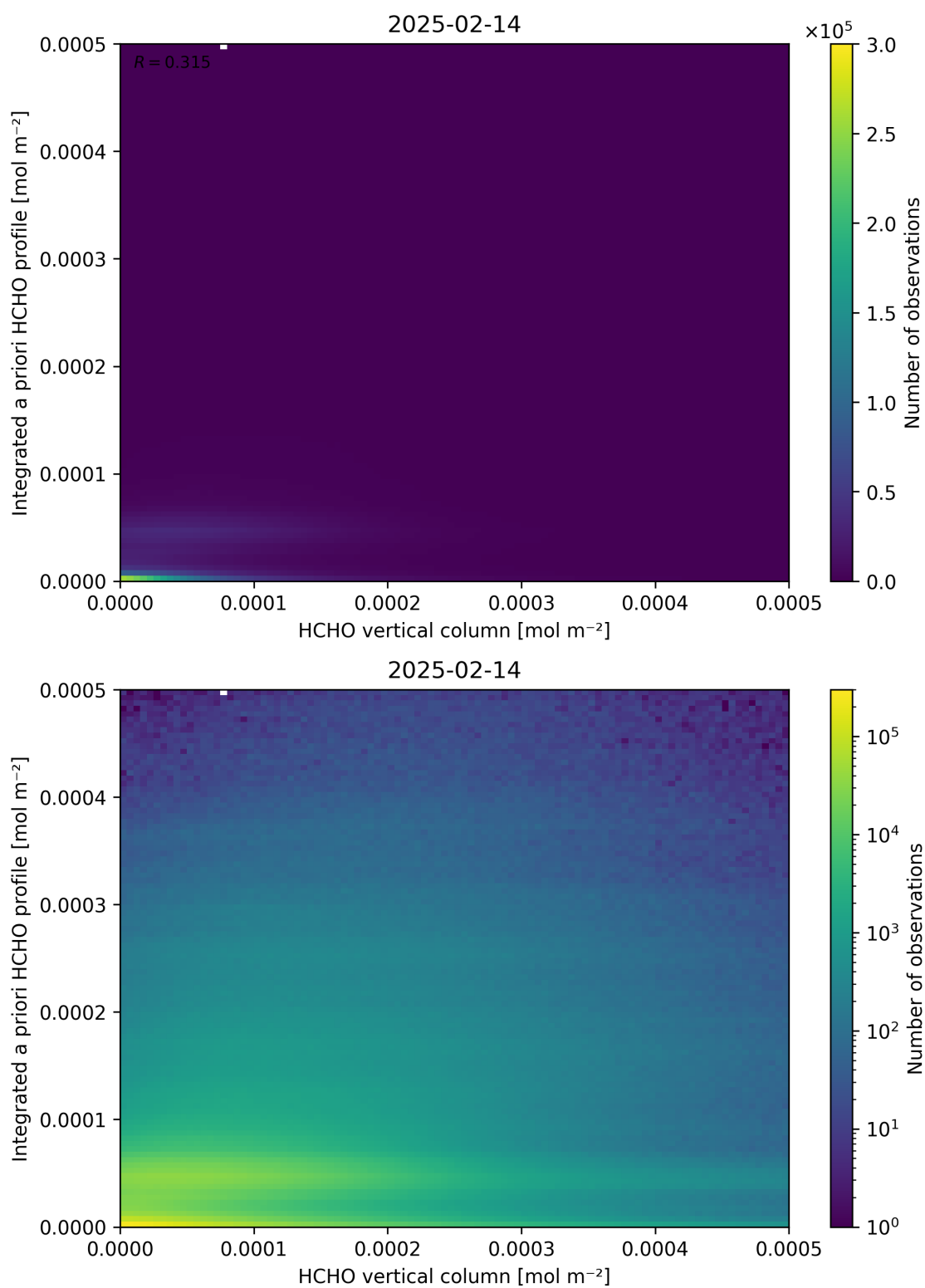
Figure 135: Scatter density plot of “HCHO vertical column” against “Integrated a priori HCHO profile” for 2025-02-13 to 2025-02-15.
