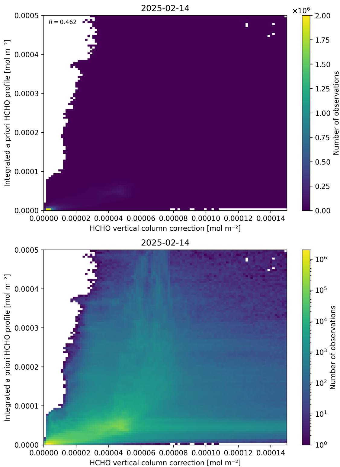
Figure 122: Scatter density plot of “HCHO vertical column correction” against “Integrated a priori HCHO profile” for 2025-02-13 to 2025-02-15.
