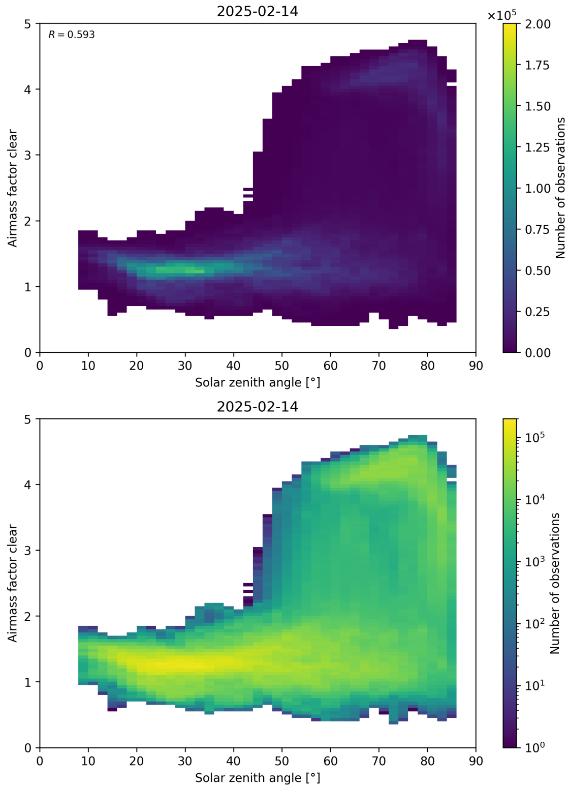
Figure 170: Scatter density plot of “Solar zenith angle” against “Airmass factor clear” for 2025-02-13 to 2025-02-15.
