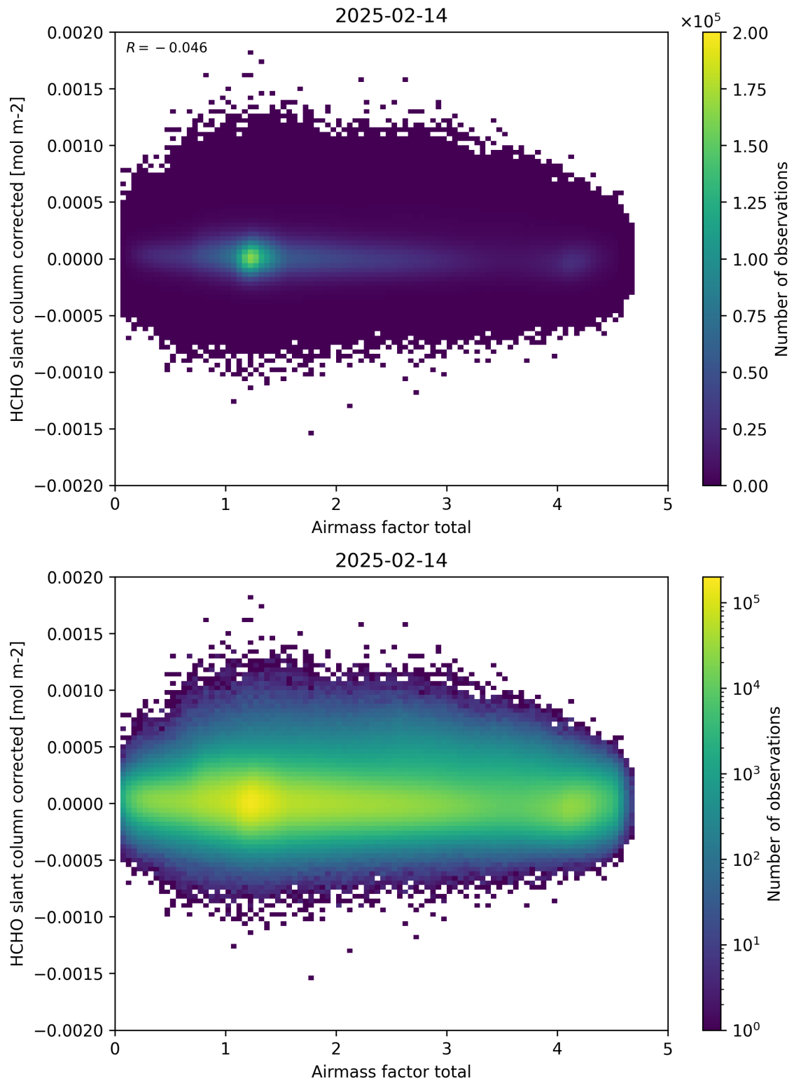
Figure 101: Scatter density plot of “Airmass factor total” against “HCHO slant column corrected” for 2025-02-13 to 2025-02-15.
