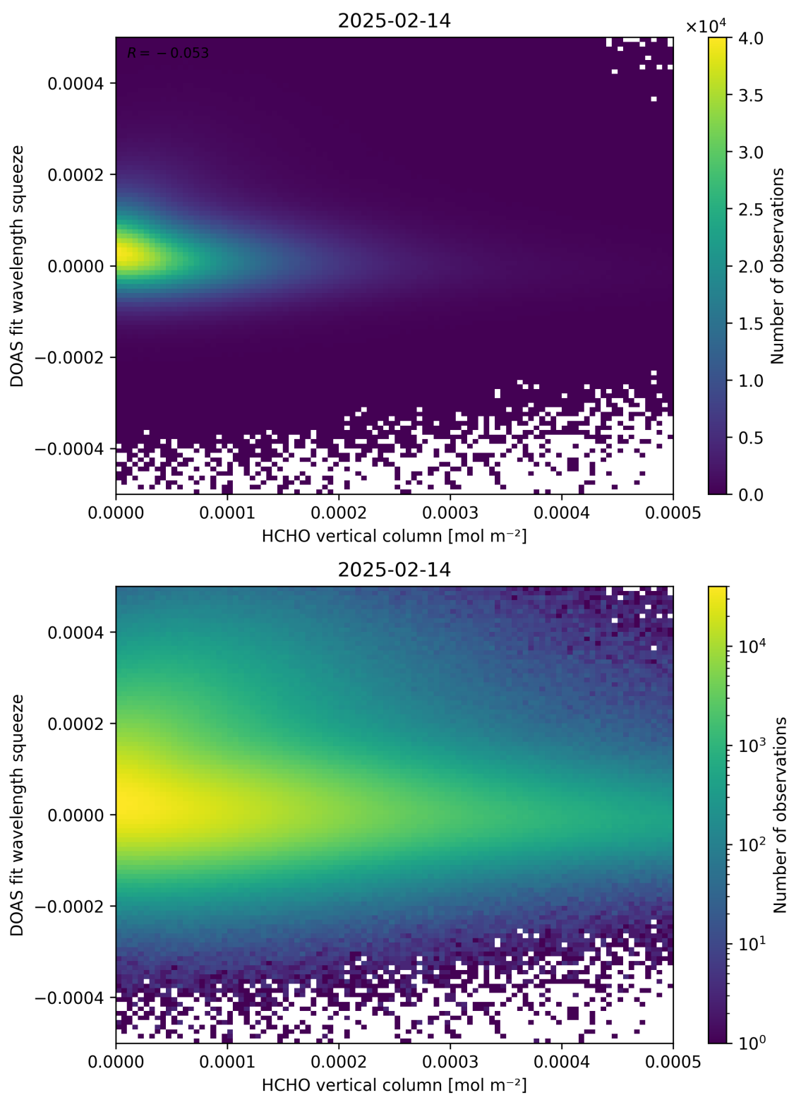
Figure 125: Scatter density plot of “HCHO vertical column” against “DOAS fit wavelength squeeze” for 2025-02-13 to 2025-02-15.
