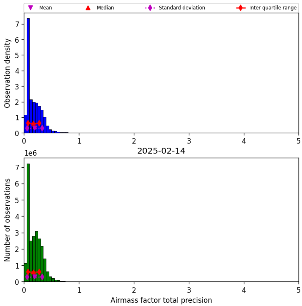
Figure 41: Histogram of “Airmass factor total precision” for 2025-02-13 to 2025-02-15
