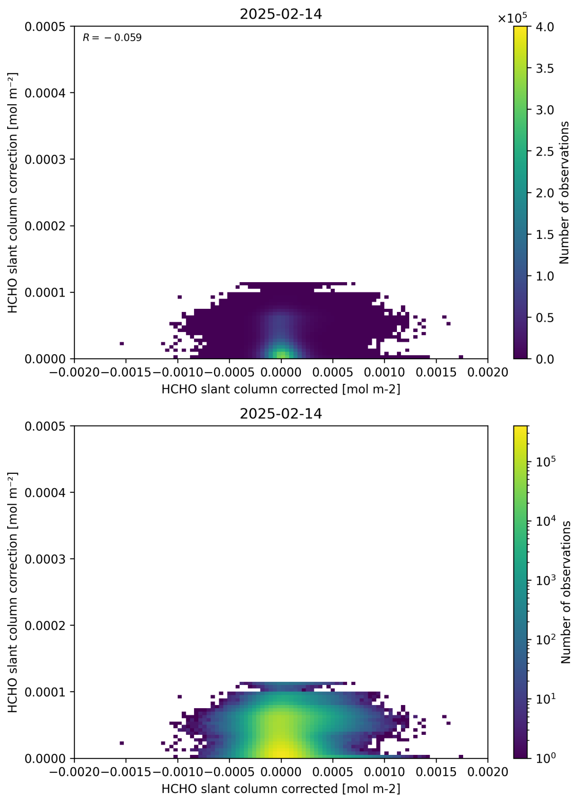
Figure 77: Scatter density plot of “HCHO slant column corrected” against “HCHO slant column correction” for 2025-02-13 to 2025-02-15.
