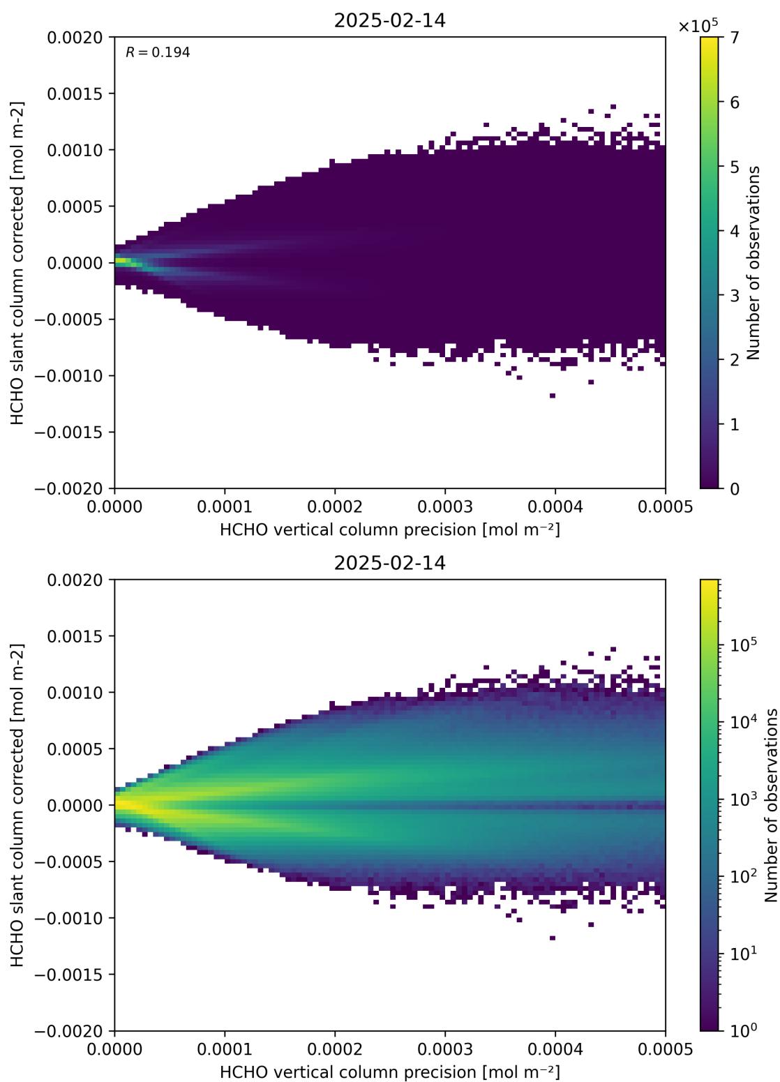
Figure 140: Scatter density plot of “HCHO vertical column precision” against “HCHO slant column corrected” for 2025-02-13 to 2025-02-15.
