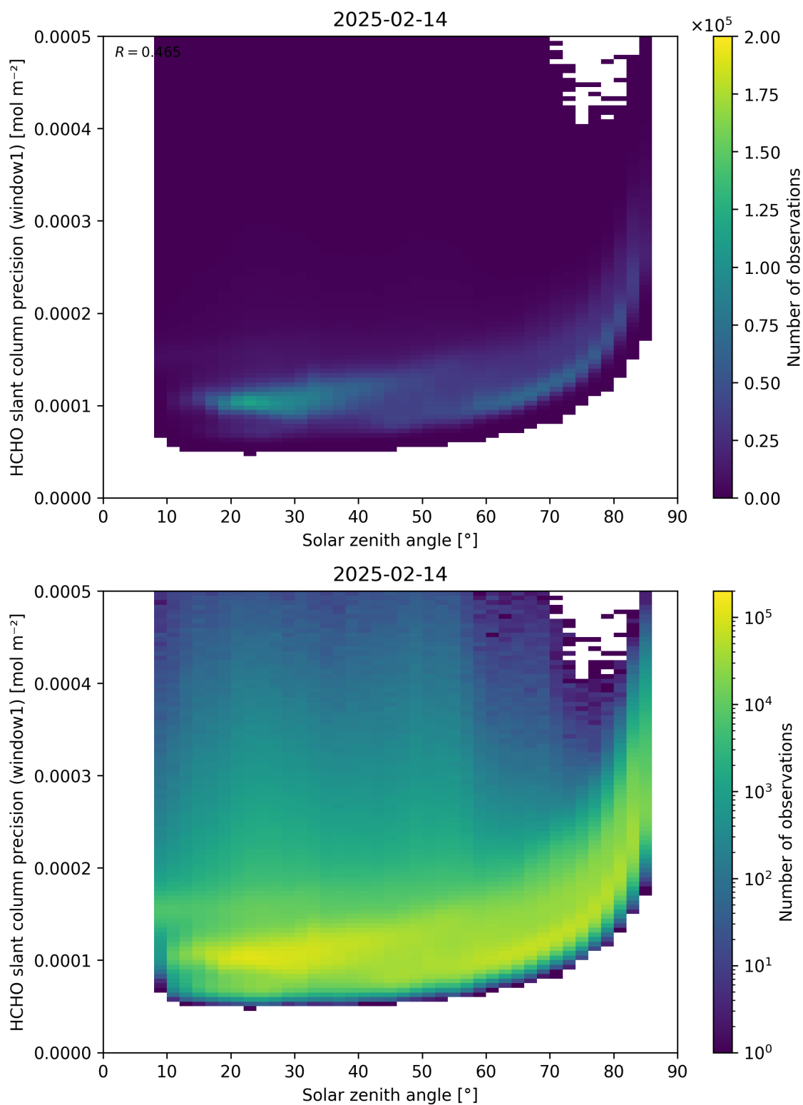
Figure 174: Scatter density plot of “Solar zenith angle” against “HCHO slant column precision (window1)” for 2025-02-13 to 2025-02-15.
