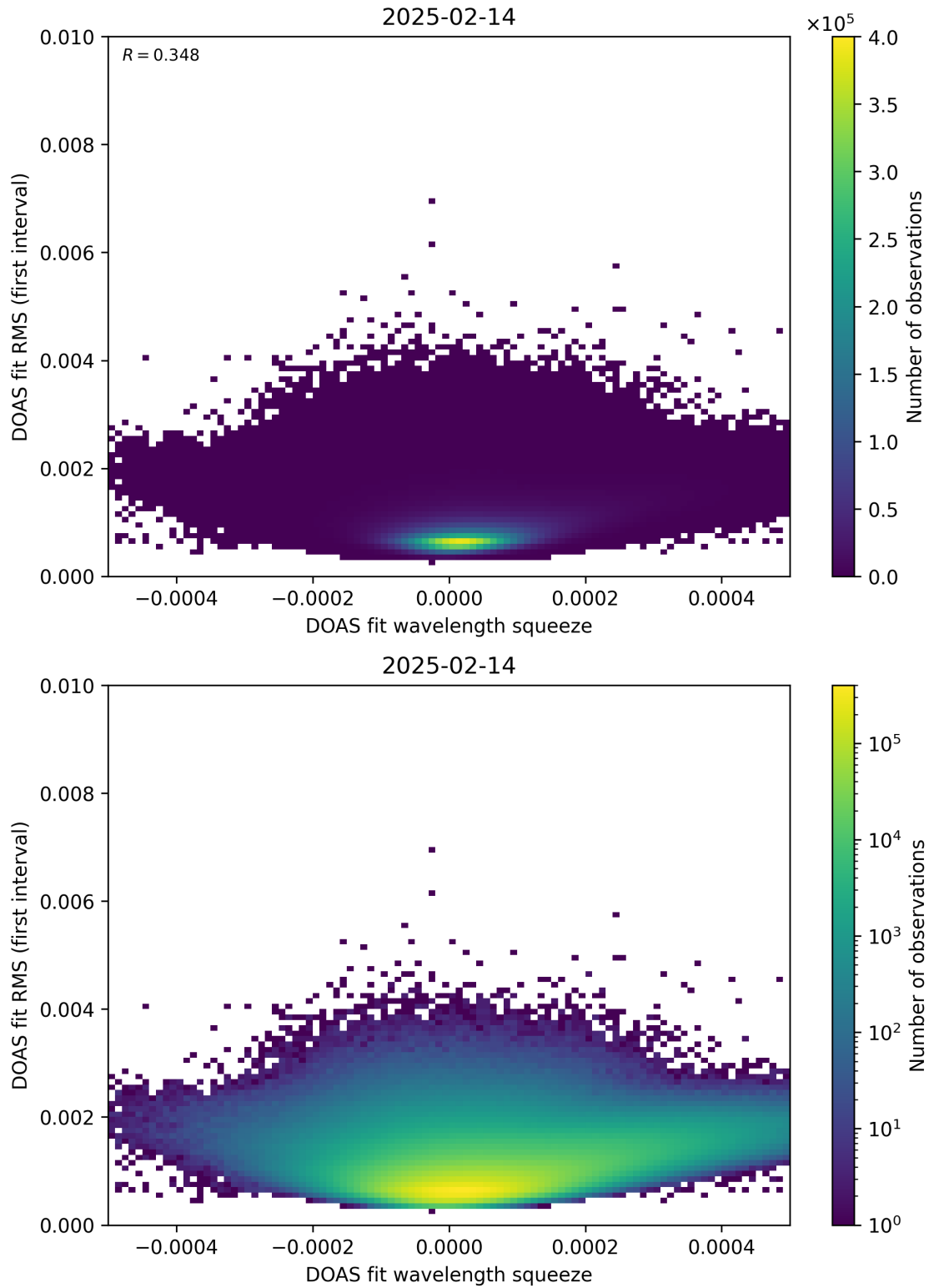
Figure 68: Scatter density plot of “DOAS fit wavelength squeeze” against “DOAS fit RMS (first interval)” for 2025-02-13 to 2025-02-15.
