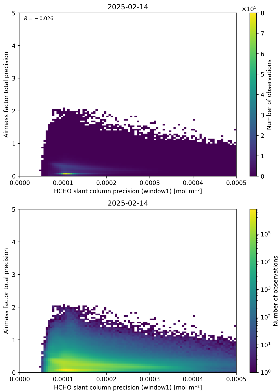
Figure 95: Scatter density plot of “HCHO slant column precision (window1)” against “Airmass factor total precision” for 2025-02-13 to 2025-02-15.
