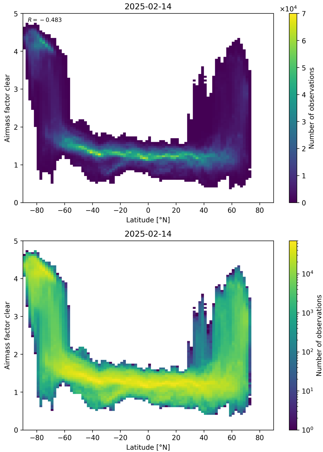
Figure 156: Scatter density plot of “Latitude” against “Airmass factor clear” for 2025-02-13 to 2025-02-15.
