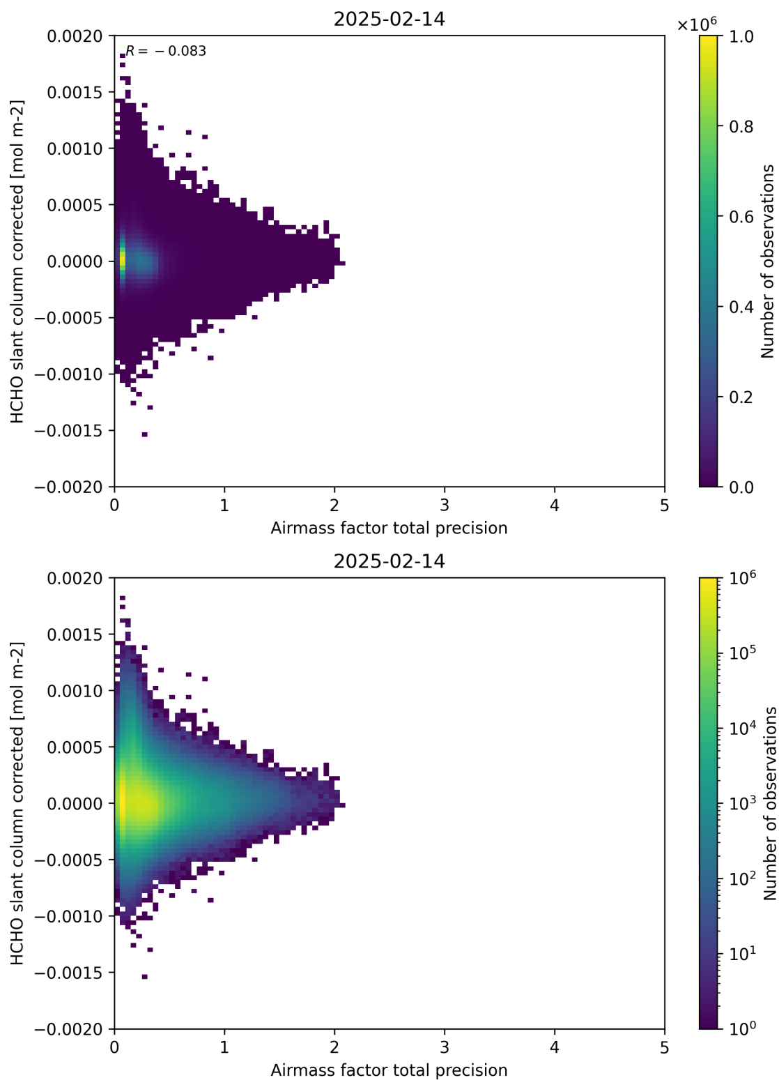
Figure 109: Scatter density plot of “Airmass factor total precision” against “HCHO slant column corrected” for 2025-02-13 to 2025-02-15.
