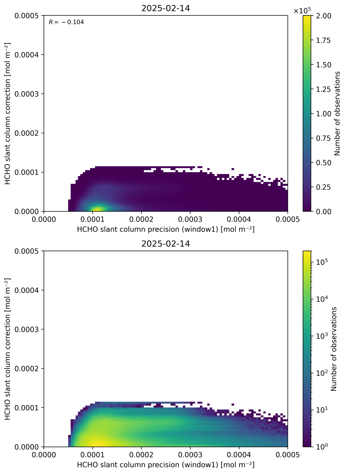
Figure 93: Scatter density plot of “HCHO slant column precision (window1)” against “HCHO slant column correction” for 2025-02-13 to 2025-02-15.
