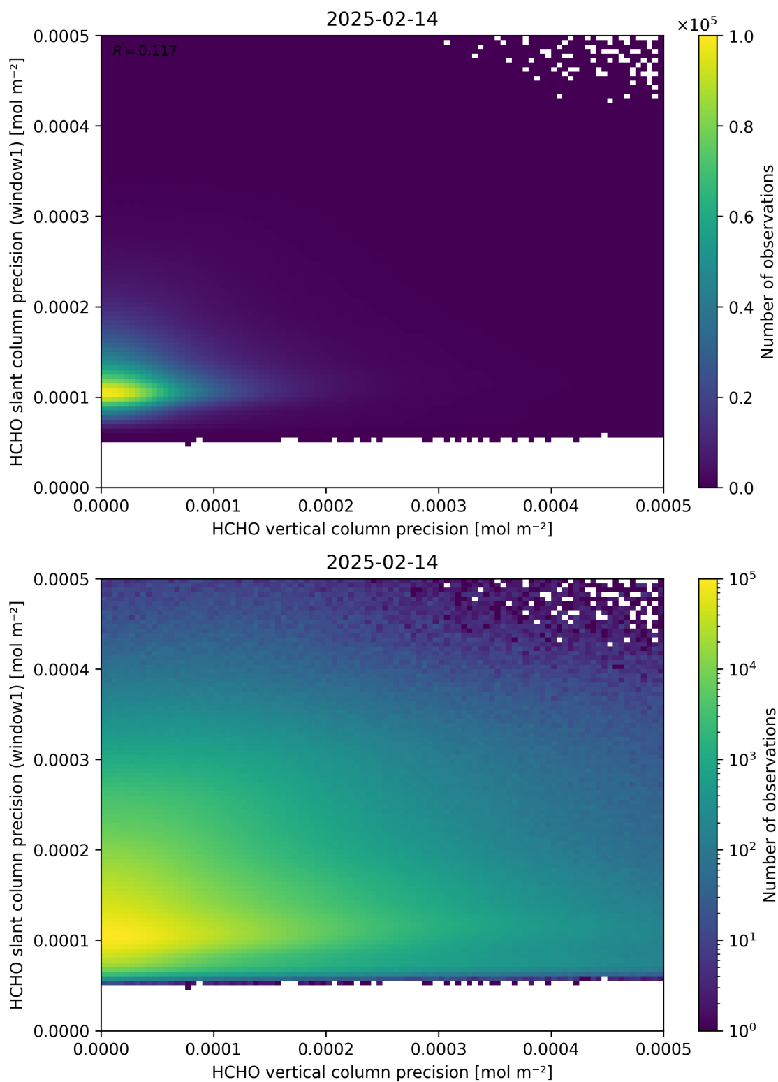
Figure 143: Scatter density plot of “HCHO vertical column precision” against “HCHO slant column precision (window1)” for 2025-02-13 to 2025-02-15.
