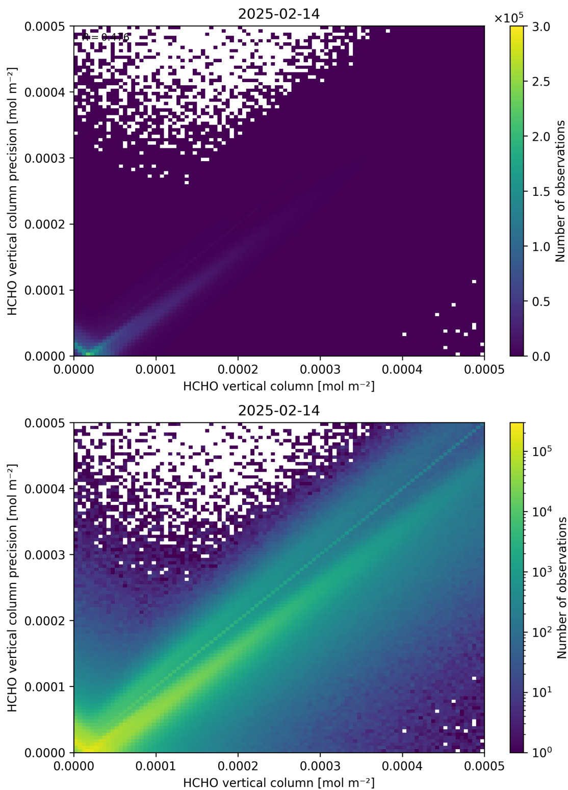
Figure 134: Scatter density plot of “HCHO vertical column” against “HCHO vertical column precision” for 2025-02-13 to 2025-02-15.
