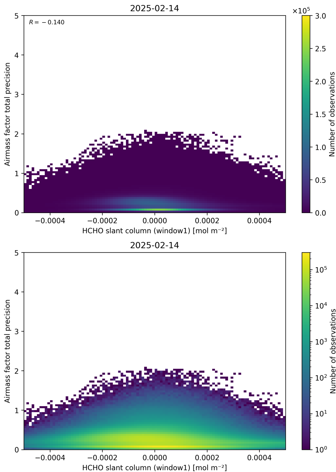
Figure 86: Scatter density plot of “HCHO slant column (window1)” against “Airmass factor total precision” for 2025-02-13 to 2025-02-15.
