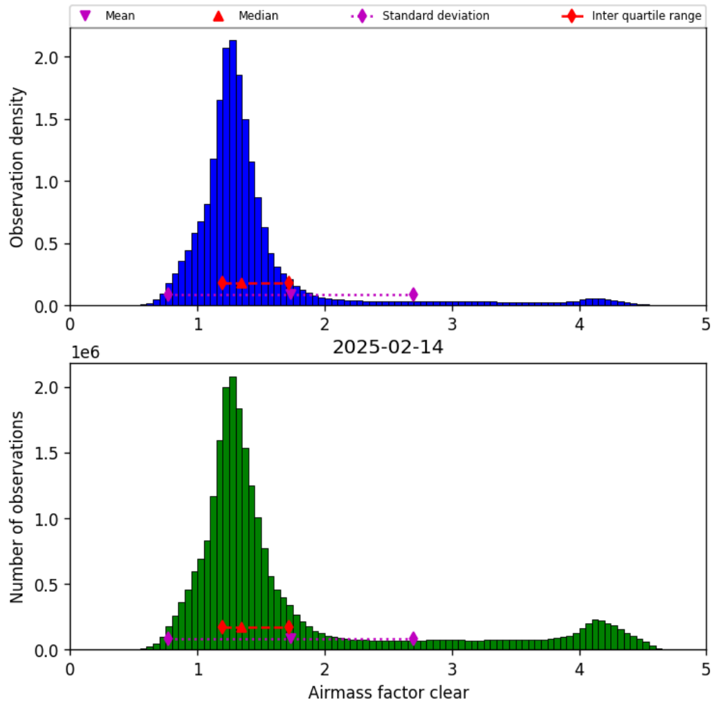
Figure 42: Histogram of “Airmass factor clear” for 2025-02-13 to 2025-02-15
