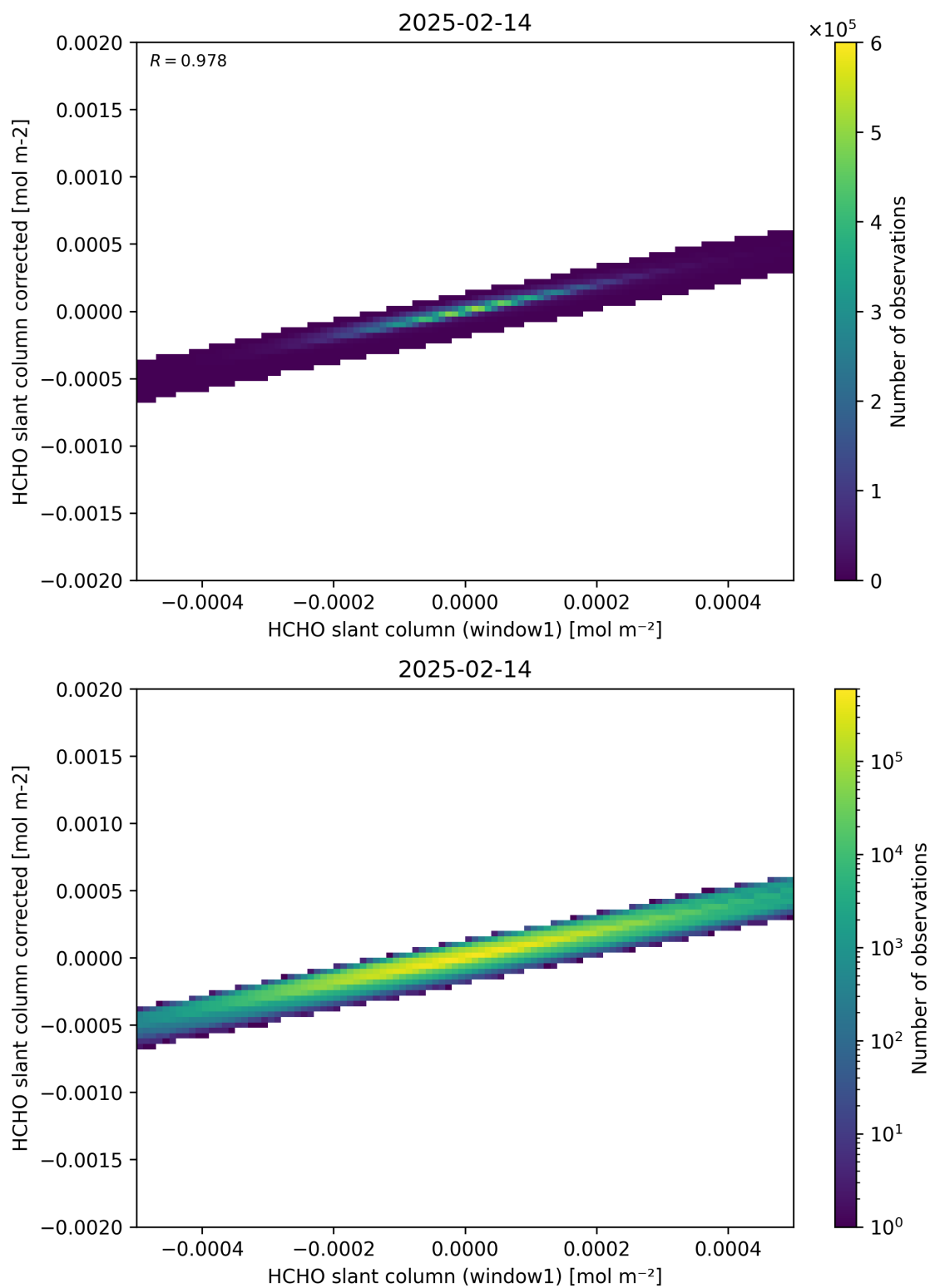
Figure 82: Scatter density plot of “HCHO slant column (window1)” against “HCHO slant column corrected” for 2025-02-13 to 2025-02-15.
