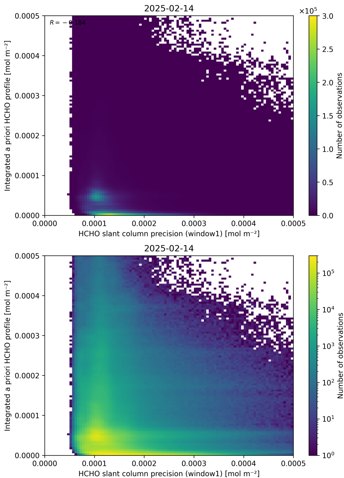
Figure 96: Scatter density plot of “HCHO slant column precision (window1)” against “Integrated a priori HCHO profile” for 2025-02-13 to 2025-02-15.
