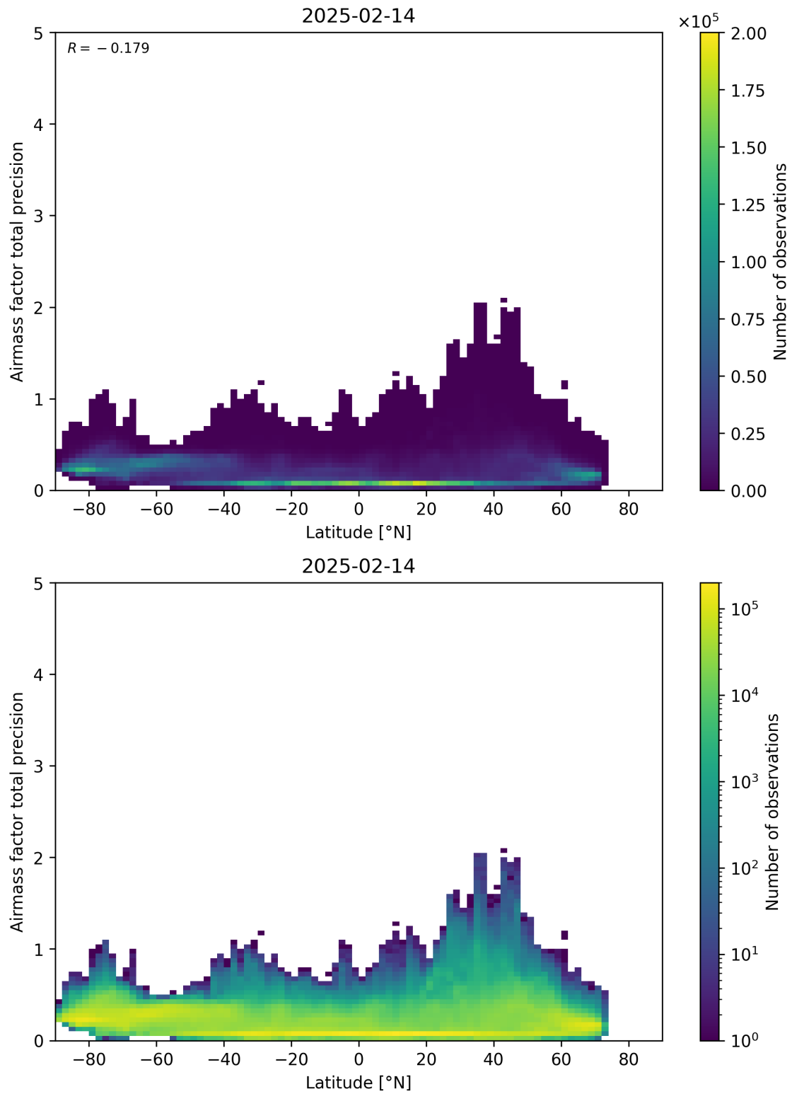
Figure 162: Scatter density plot of “Latitude” against “Airmass factor total precision” for 2025-02-13 to 2025-02-15.
