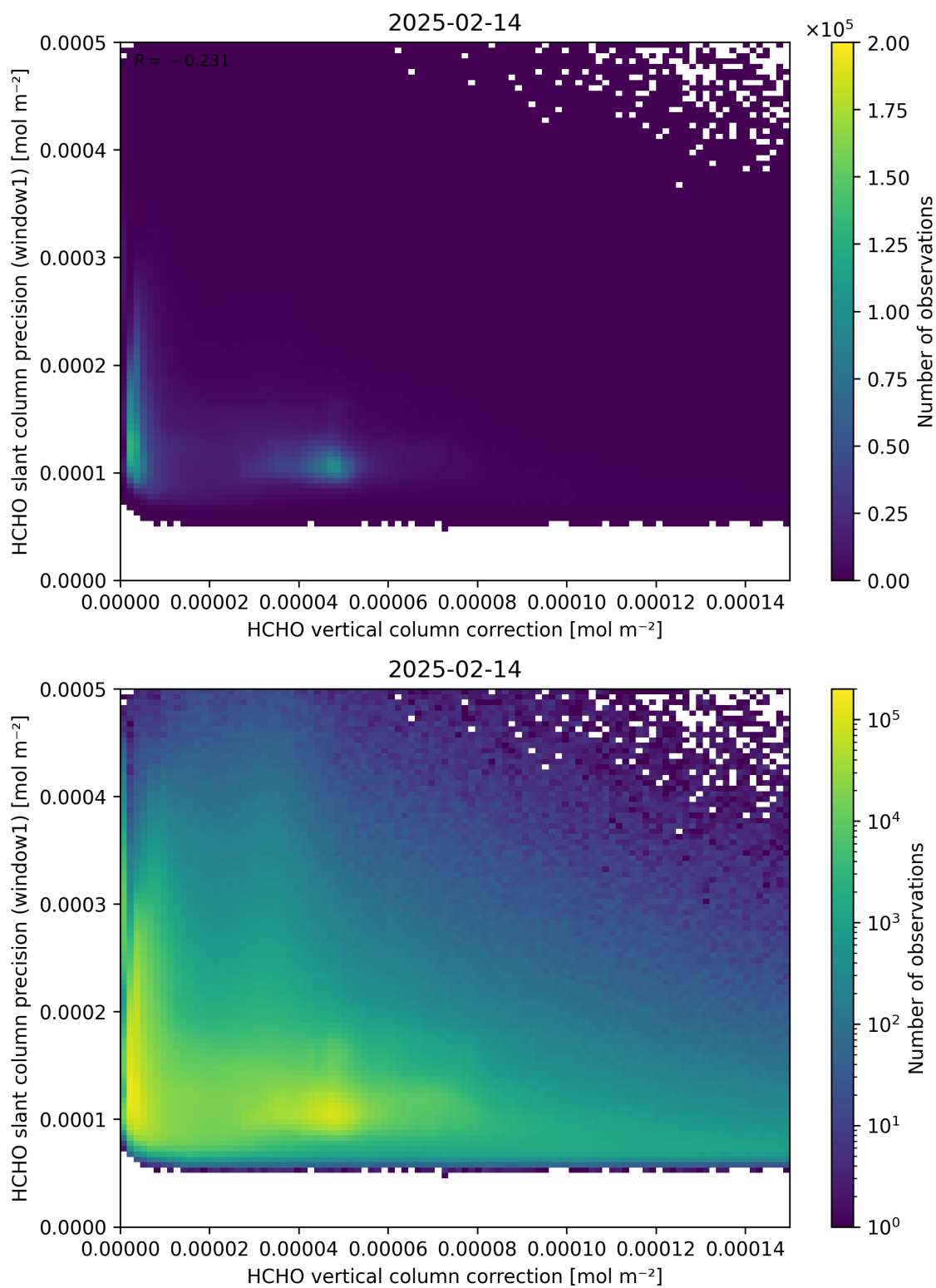
Figure 119: Scatter density plot of “HCHO vertical column correction” against “HCHO slant column precision (window1)” for 2025-02-13 to 2025-02-15.
