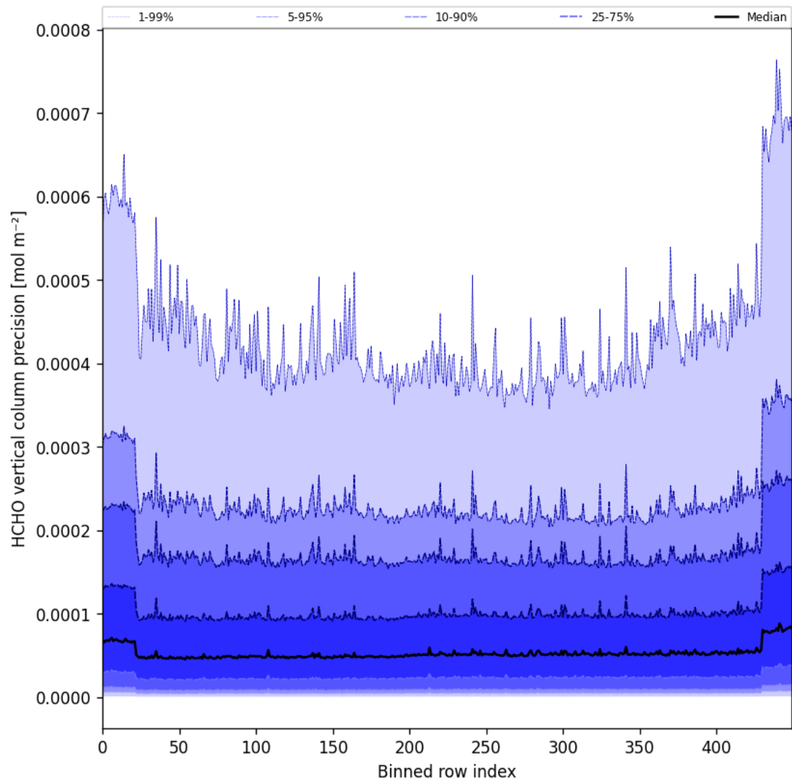
Figure 50: Along track statistics of “HCHO vertical column precision” for 2025-02-13 to 2025-02-15
