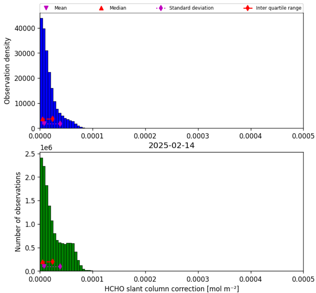
Figure 47: Histogram of “HCHO slant column correction” for 2025-02-13 to 2025-02-15
