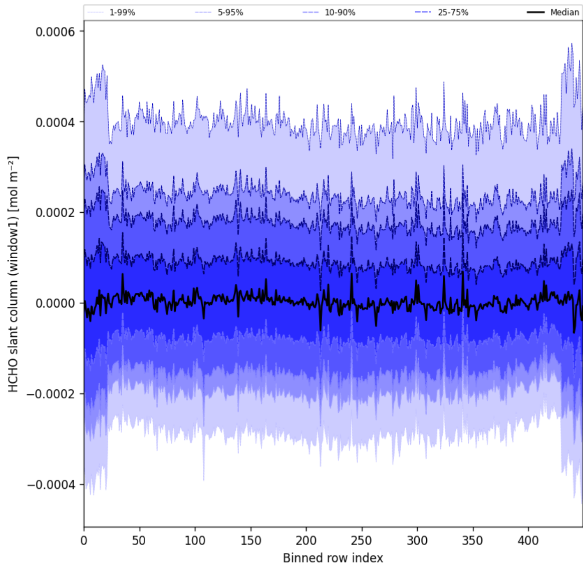
Figure 52: Along track statistics of “HCHO slant column (window1)” for 2025-02-13 to 2025-02-15
