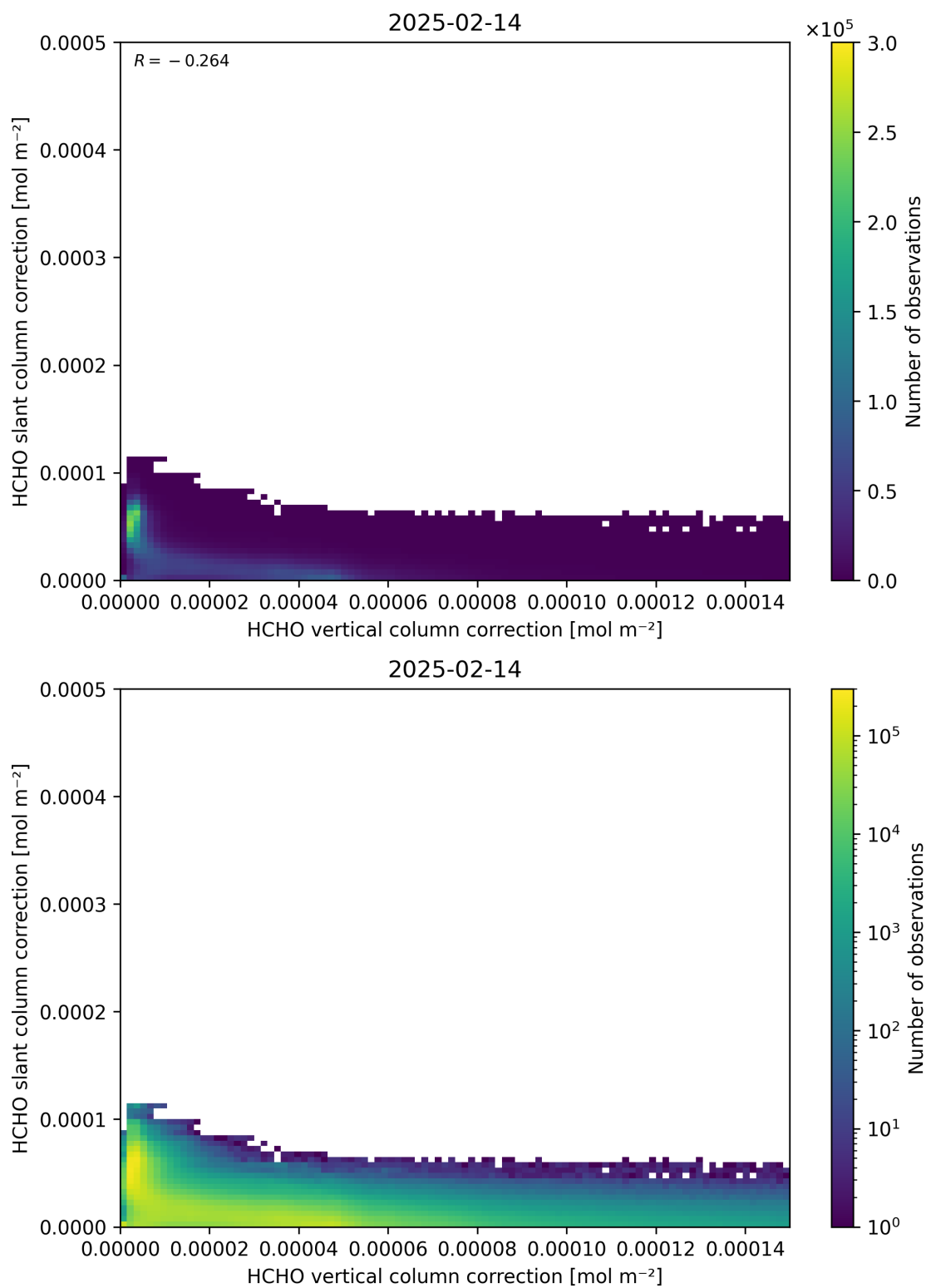
Figure 117: Scatter density plot of “HCHO vertical column correction” against “HCHO slant column correction” for 2025-02-13 to 2025-02-15.
