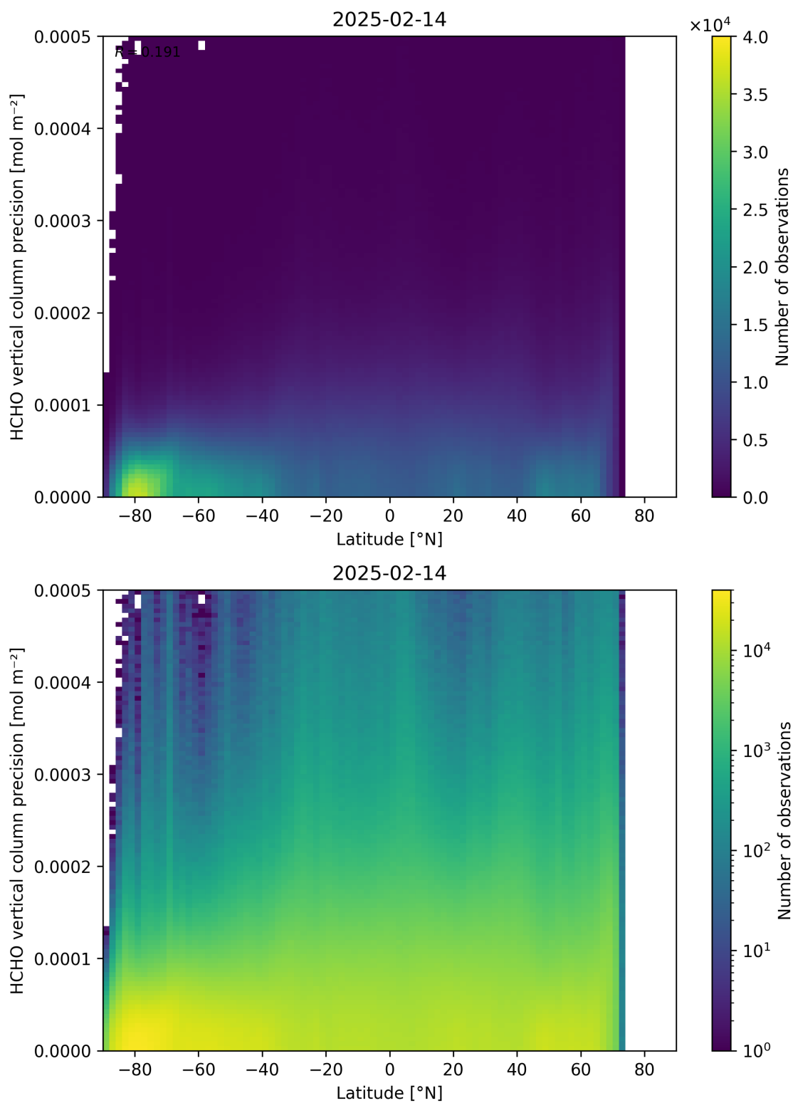
Figure 165: Scatter density plot of “Latitude” against “HCHO vertical column precision” for 2025-02-13 to 2025-02-15.
