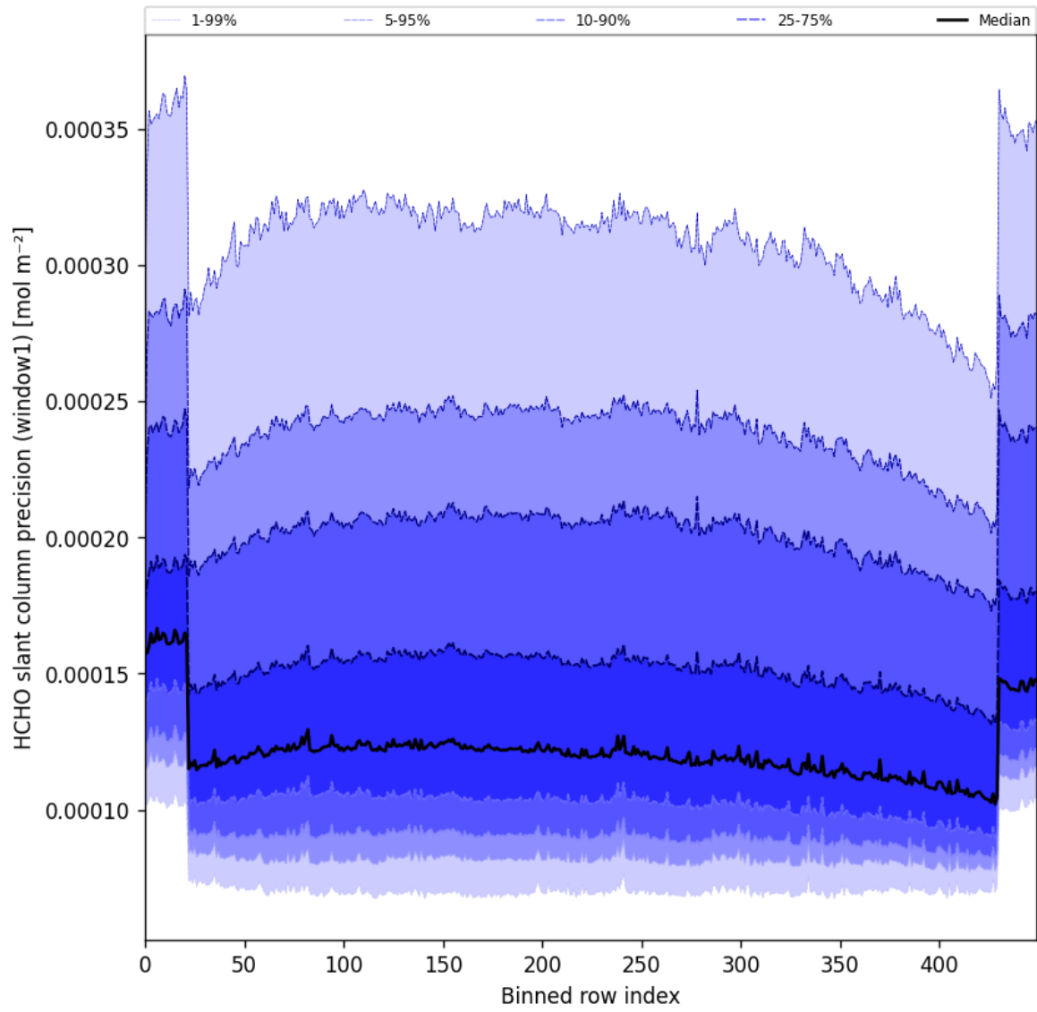
Figure 53: Along track statistics of "HCHO slant column precision (window1)" for 2025-02-13 to 2025-02-15
