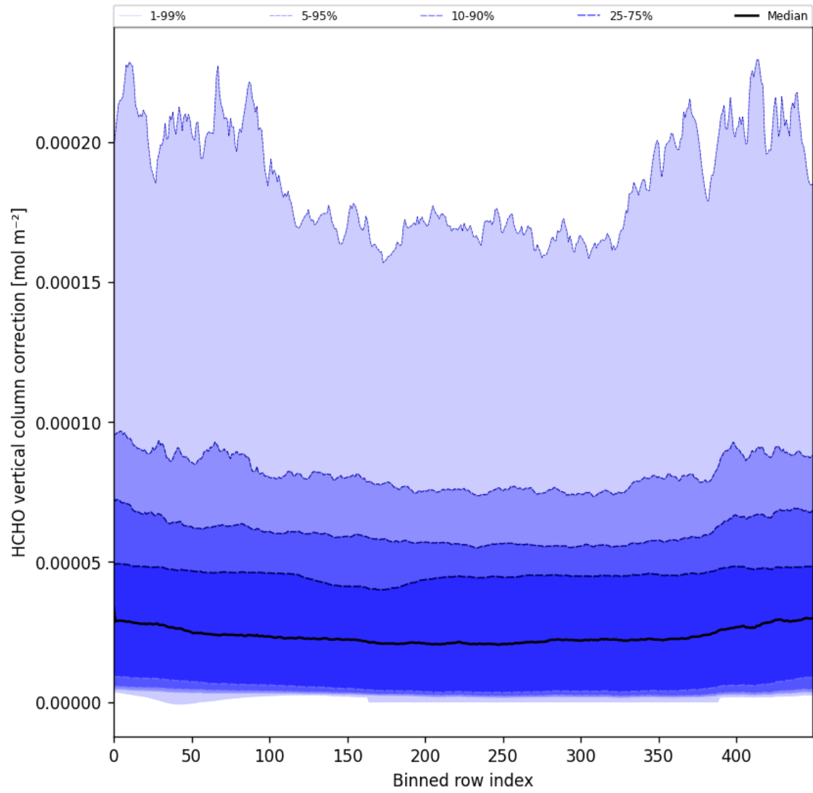
Figure 51: Along track statistics of “HCHO vertical column correction” for 2025-02-13 to 2025-02-15
