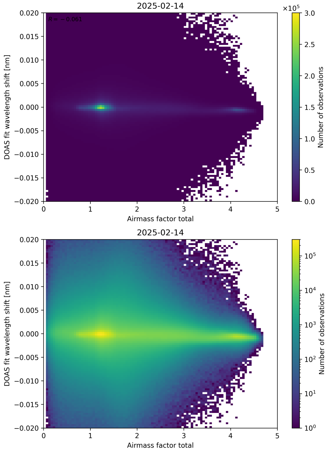
Figure 98: Scatter density plot of “Airmass factor total” against “DOAS fit wavelength shift” for 2025-02-13 to 2025-02-15.
