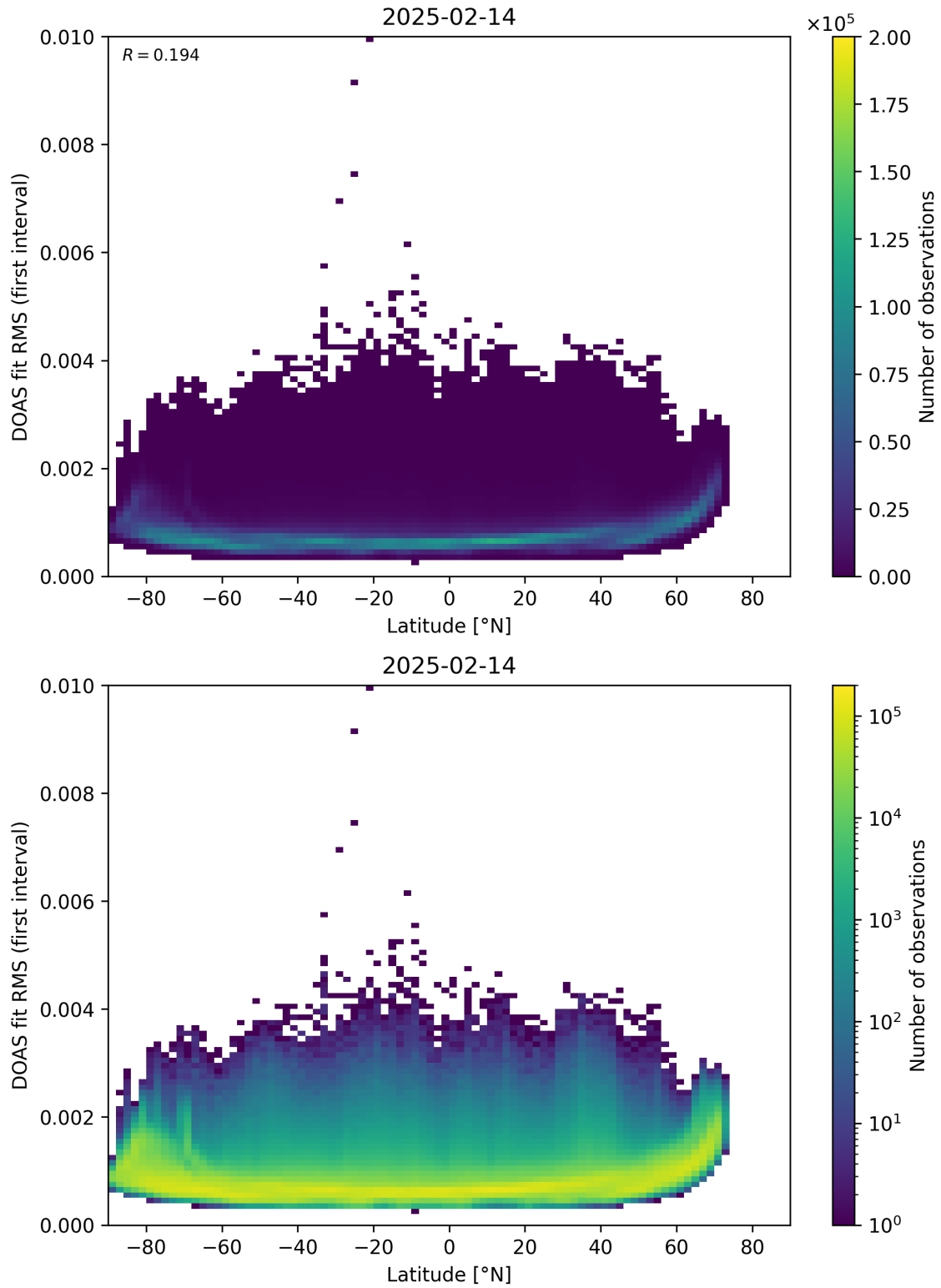
Figure 153: Scatter density plot of “Latitude” against “DOAS fit RMS (first interval)” for 2025-02-13 to 2025-02-15.
