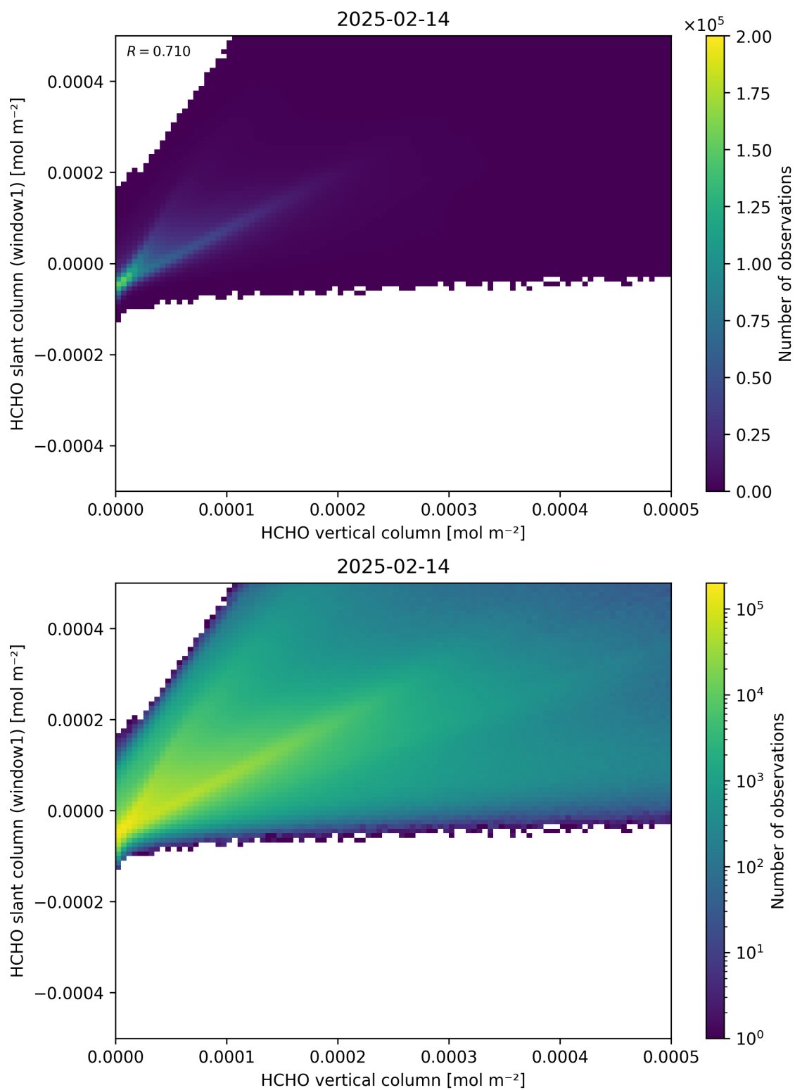
Figure 129: Scatter density plot of “HCHO vertical column” against “HCHO slant column (window1)” for 2025-02-13 to 2025-02-15.
