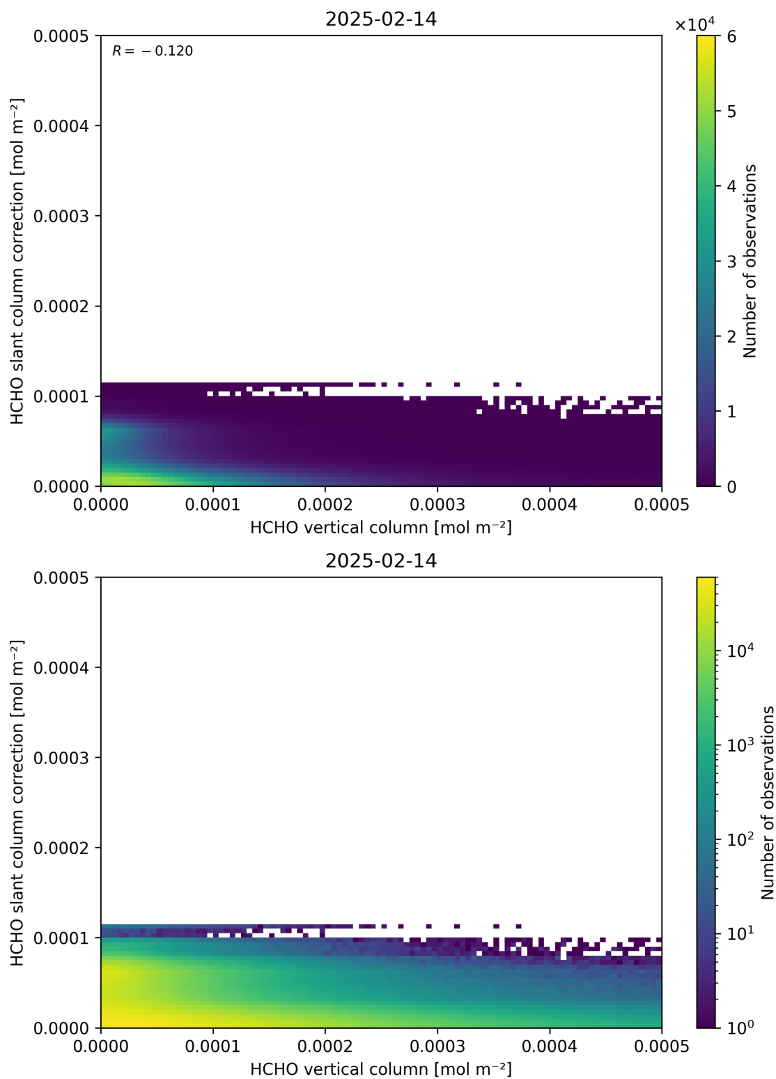
Figure 128: Scatter density plot of “HCHO vertical column” against “HCHO slant column correction” for 2025-02-13 to 2025-02-15.
