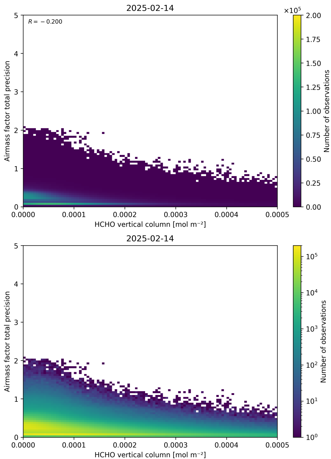
Figure 132: Scatter density plot of “HCHO vertical column” against “Airmass factor total precision” for 2025-02-13 to 2025-02-15.
