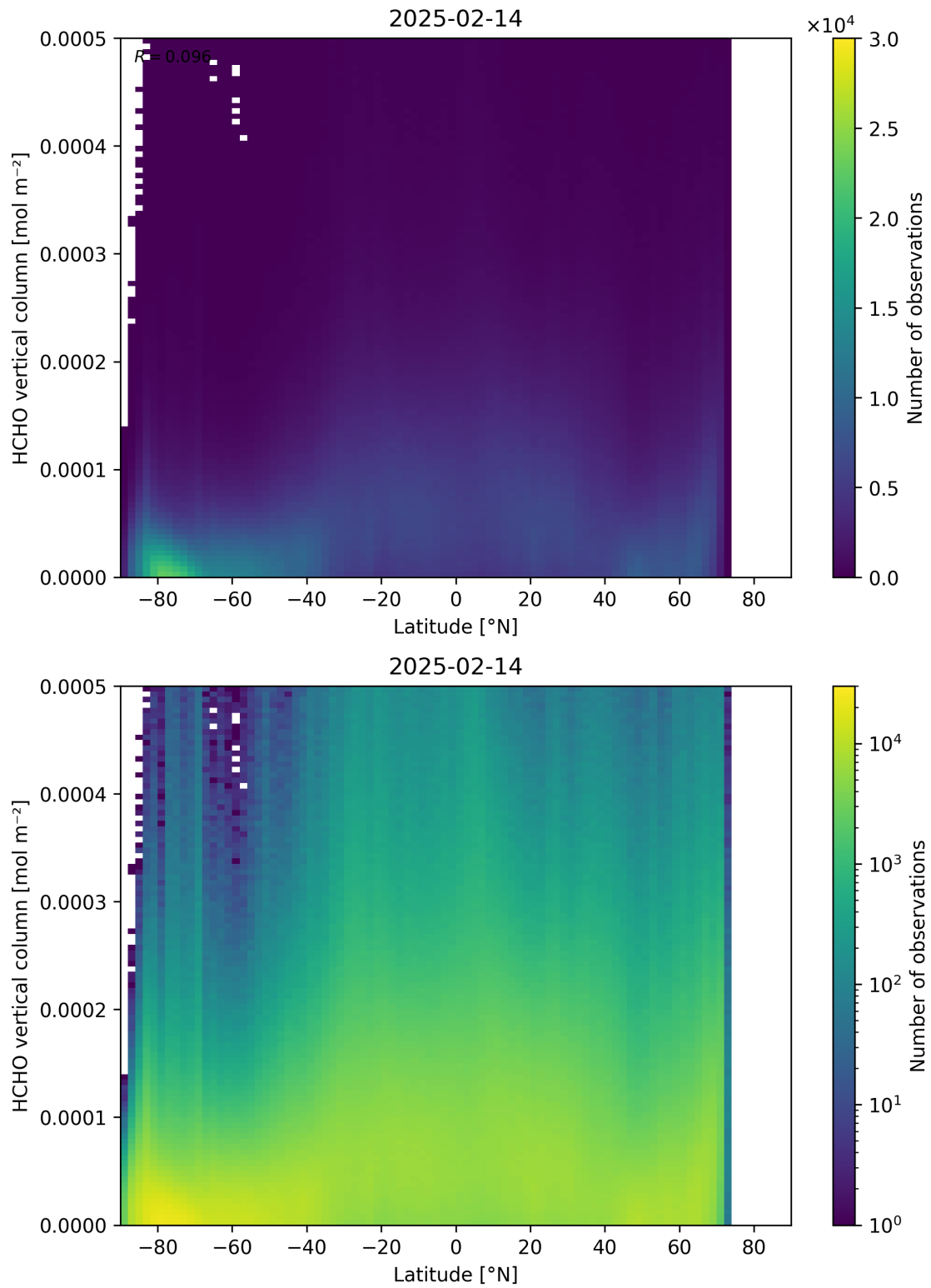
Figure 163: Scatter density plot of “Latitude” against “HCHO vertical column” for 2025-02-13 to 2025-02-15.
