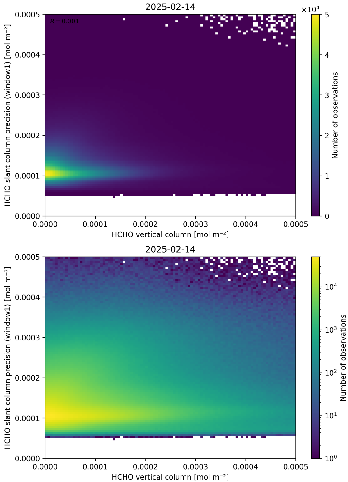
Figure 130: Scatter density plot of “HCHO vertical column” against “HCHO slant column precision (window1)” for 2025-02-13 to 2025-02-15.
