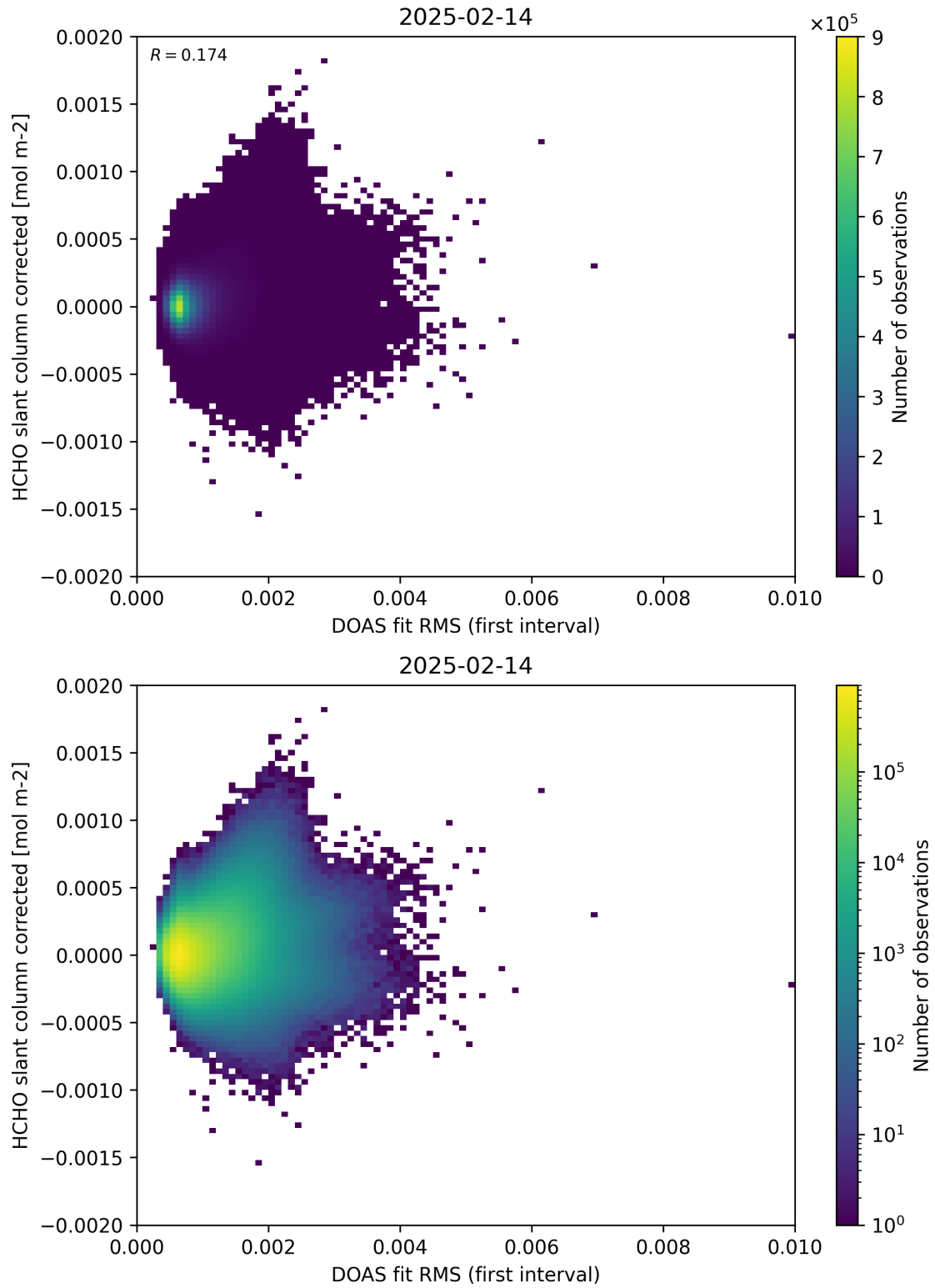
Figure 62: Scatter density plot of “DOAS fit RMS (first interval)” against “HCHO slant column corrected” for 2025-02-13 to 2025-02-15.
