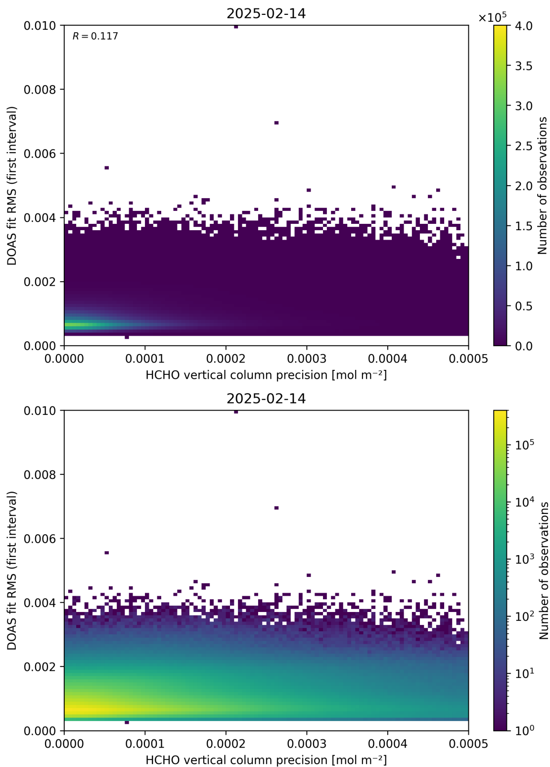
Figure 136: Scatter density plot of “HCHO vertical column precision” against “DOAS fit RMS (first interval)” for 2025-02-13 to 2025-02-15.
