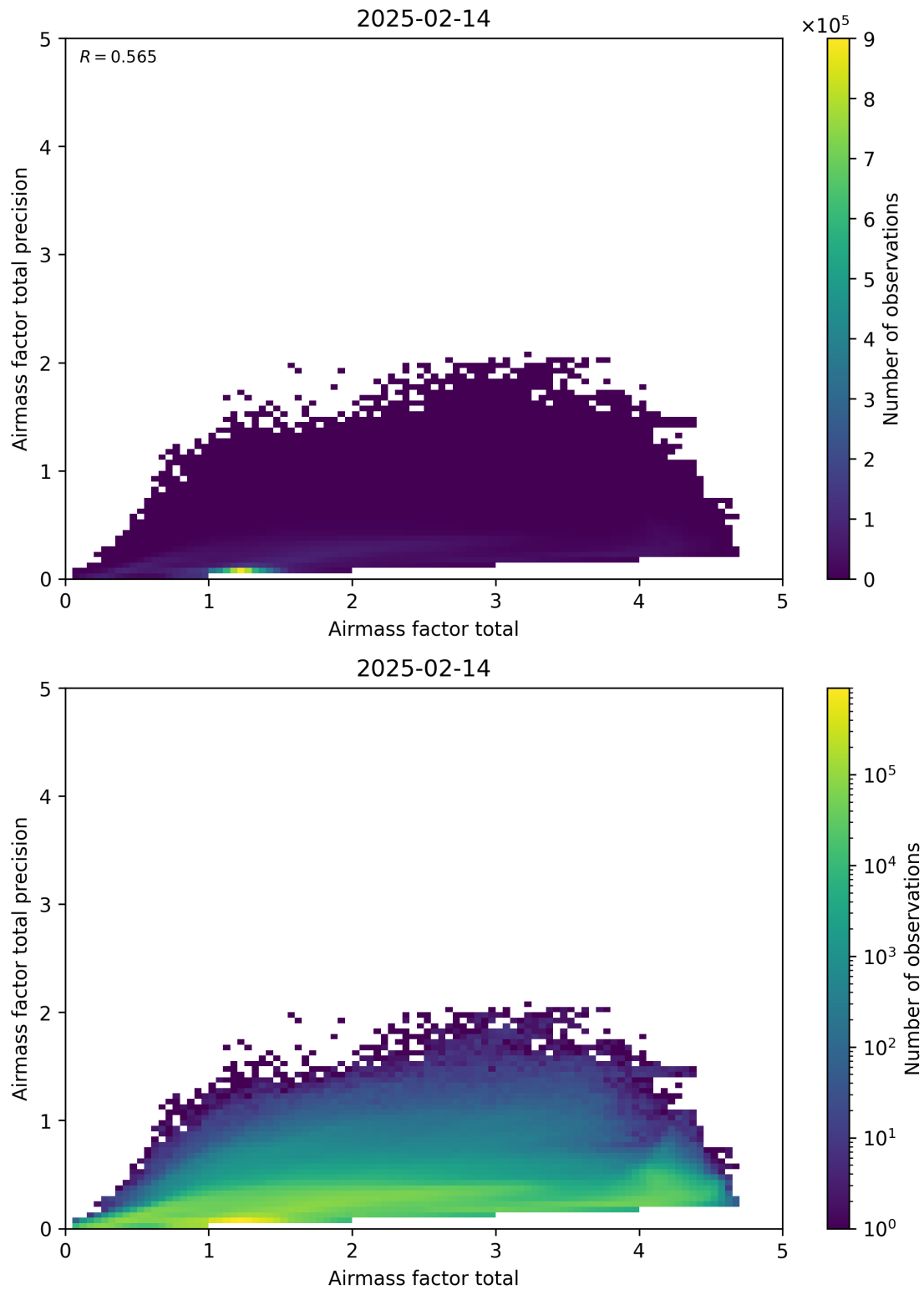
Figure 103: Scatter density plot of “Airmass factor total” against “Airmass factor total precision” for 2025-02-13 to 2025-02-15.
