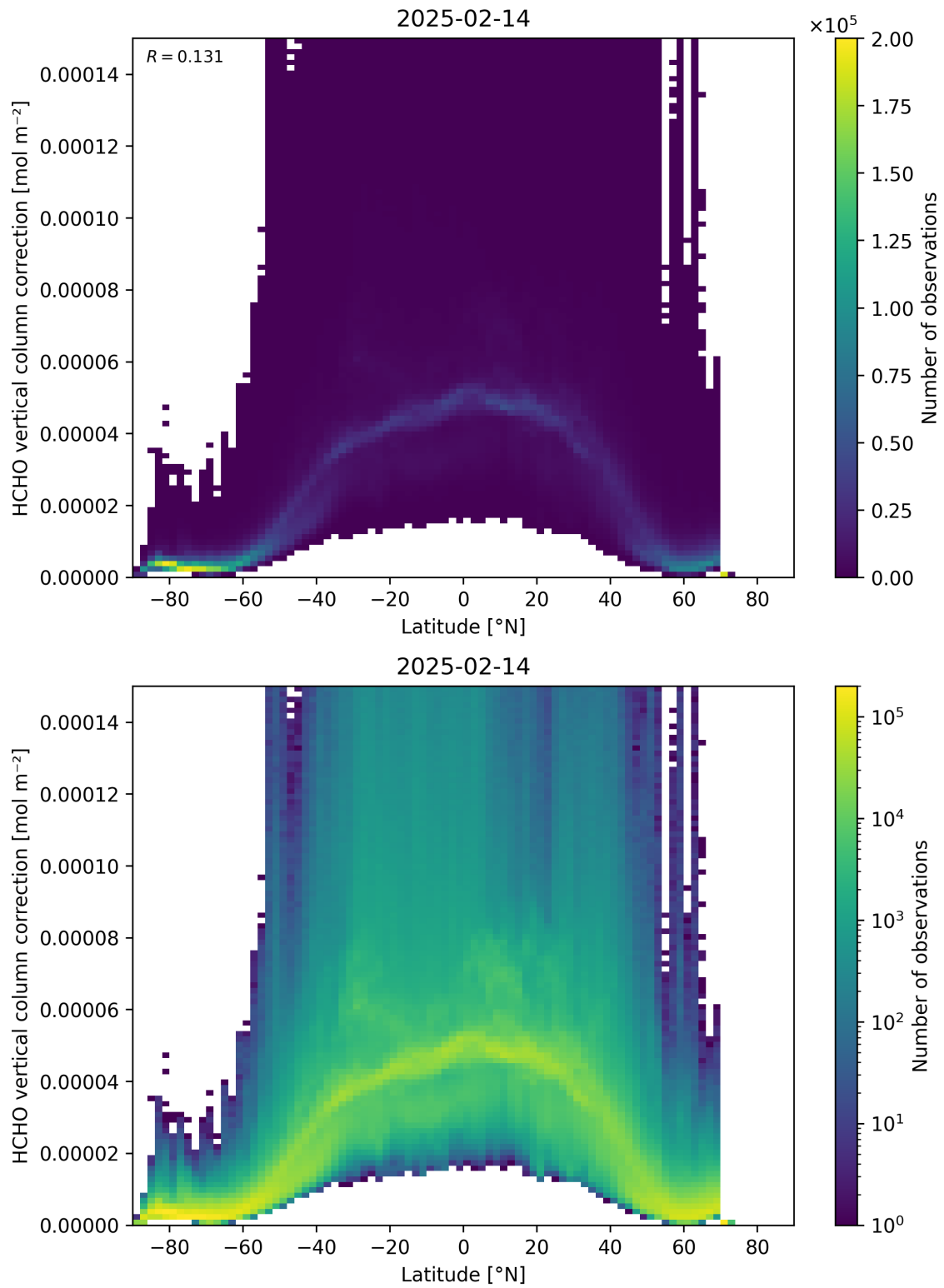
Figure 164: Scatter density plot of “Latitude” against “HCHO vertical column correction” for 2025-02-13 to 2025-02-15.
