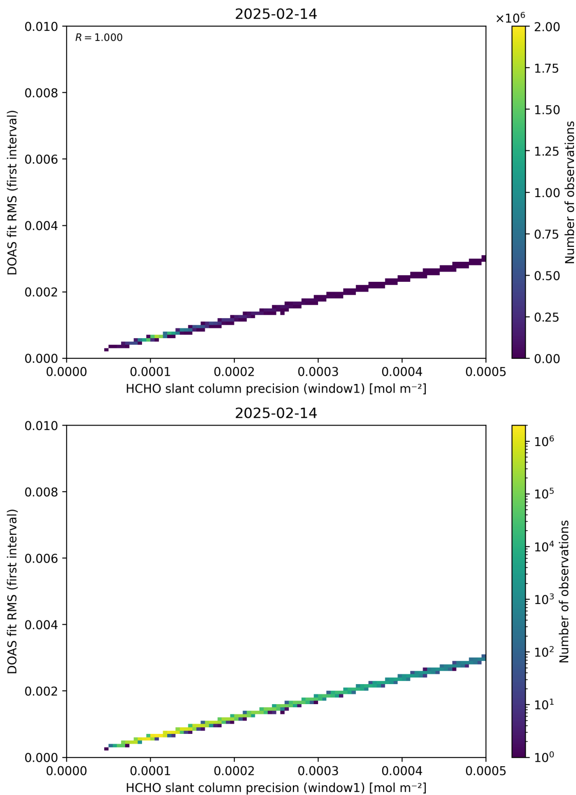
Figure 88: Scatter density plot of “HCHO slant column precision (window1)” against “DOAS fit RMS (first interval)” for 2025-02-13 to 2025-02-15.
