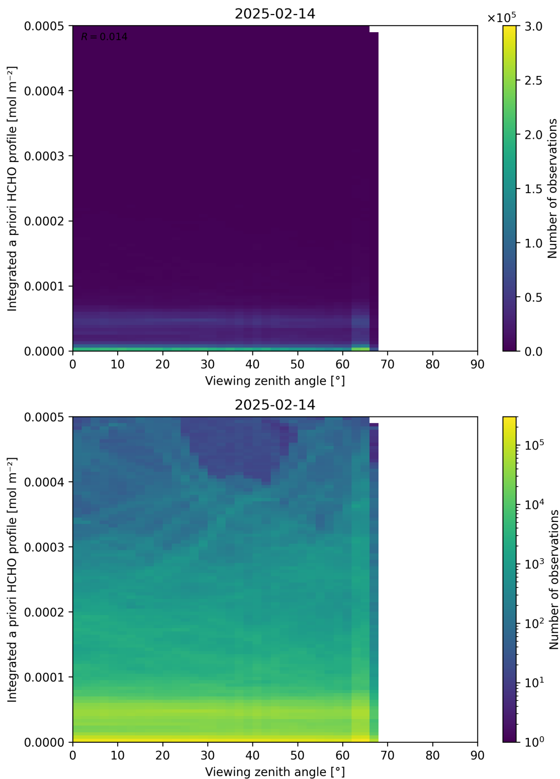
Figure 195: Scatter density plot of “Viewing zenith angle” against “Integrated a priori HCHO profile” for 2025-02-13 to 2025-02-15.
