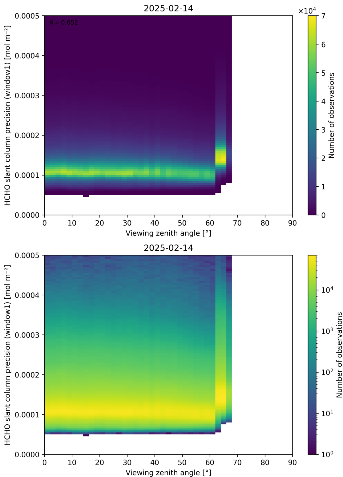
Figure 189: Scatter density plot of “Viewing zenith angle” against “HCHO slant column precision (window1)” for 2025-02-13 to 2025-02-15.
