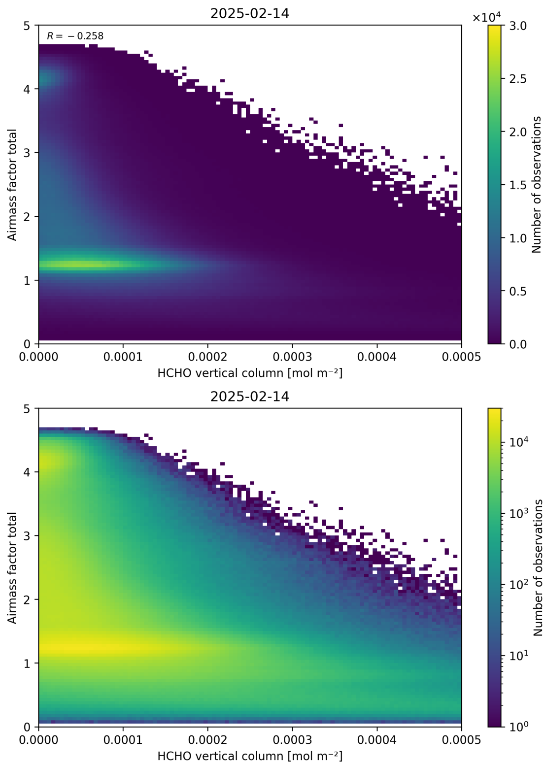
Figure 131: Scatter density plot of “HCHO vertical column” against “Airmass factor total” for 2025-02-13 to 2025-02-15.
