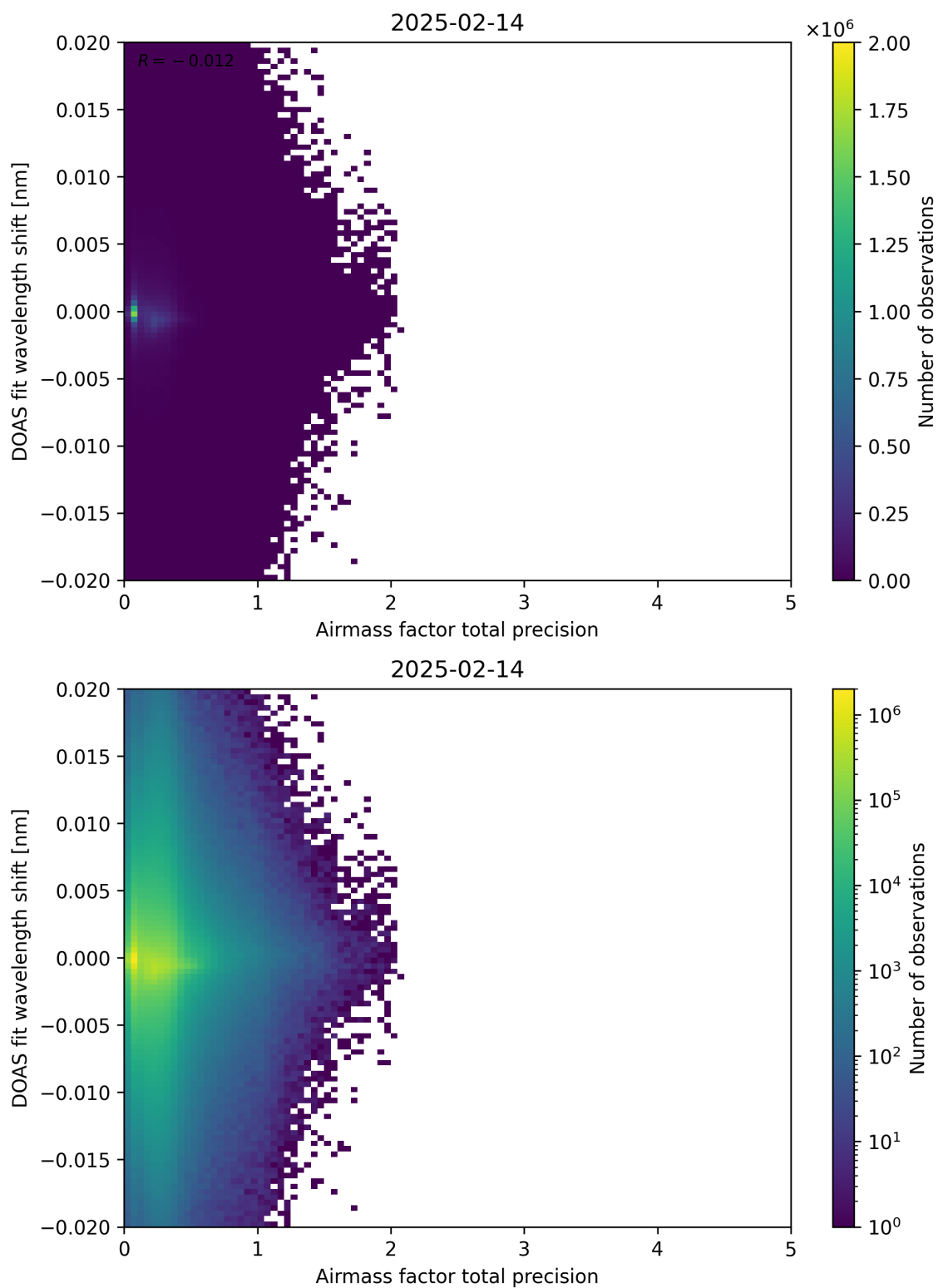
Figure 106: Scatter density plot of “Airmass factor total precision” against “DOAS fit wavelength shift” for 2025-02-13 to 2025-02-15.
