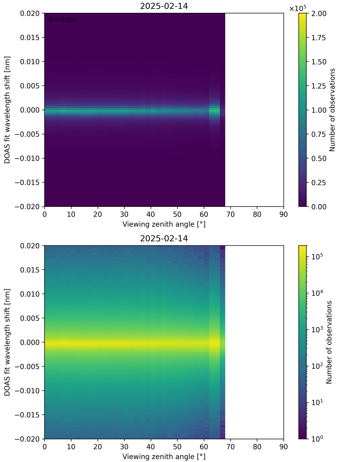
Figure 183: Scatter density plot of “Viewing zenith angle” against “DOAS fit wavelength shift” for 2025-02-13 to 2025-02-15.
