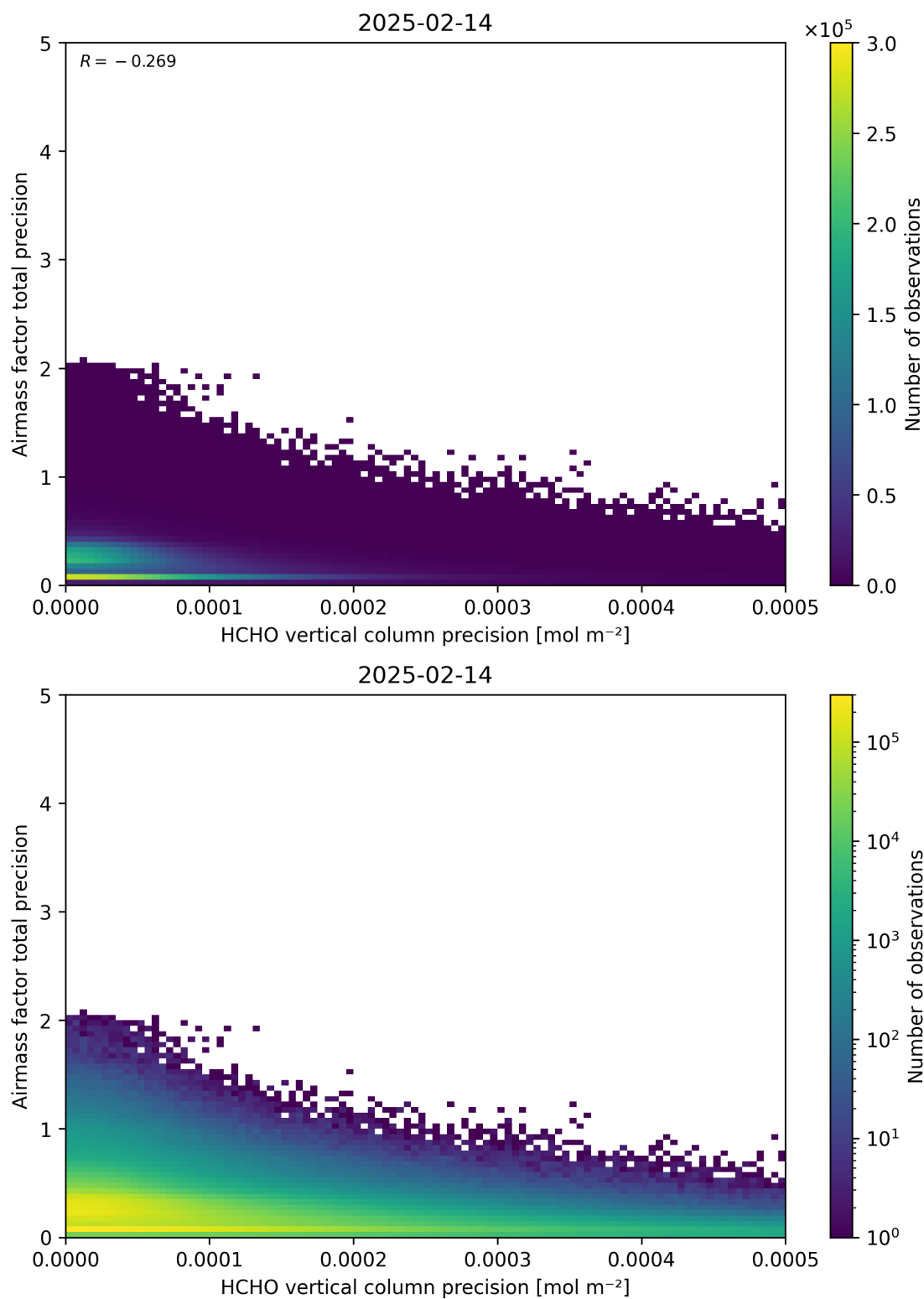
Figure 145: Scatter density plot of “HCHO vertical column precision” against “Airmass factor total precision” for 2025-02-13 to 2025-02-15.
