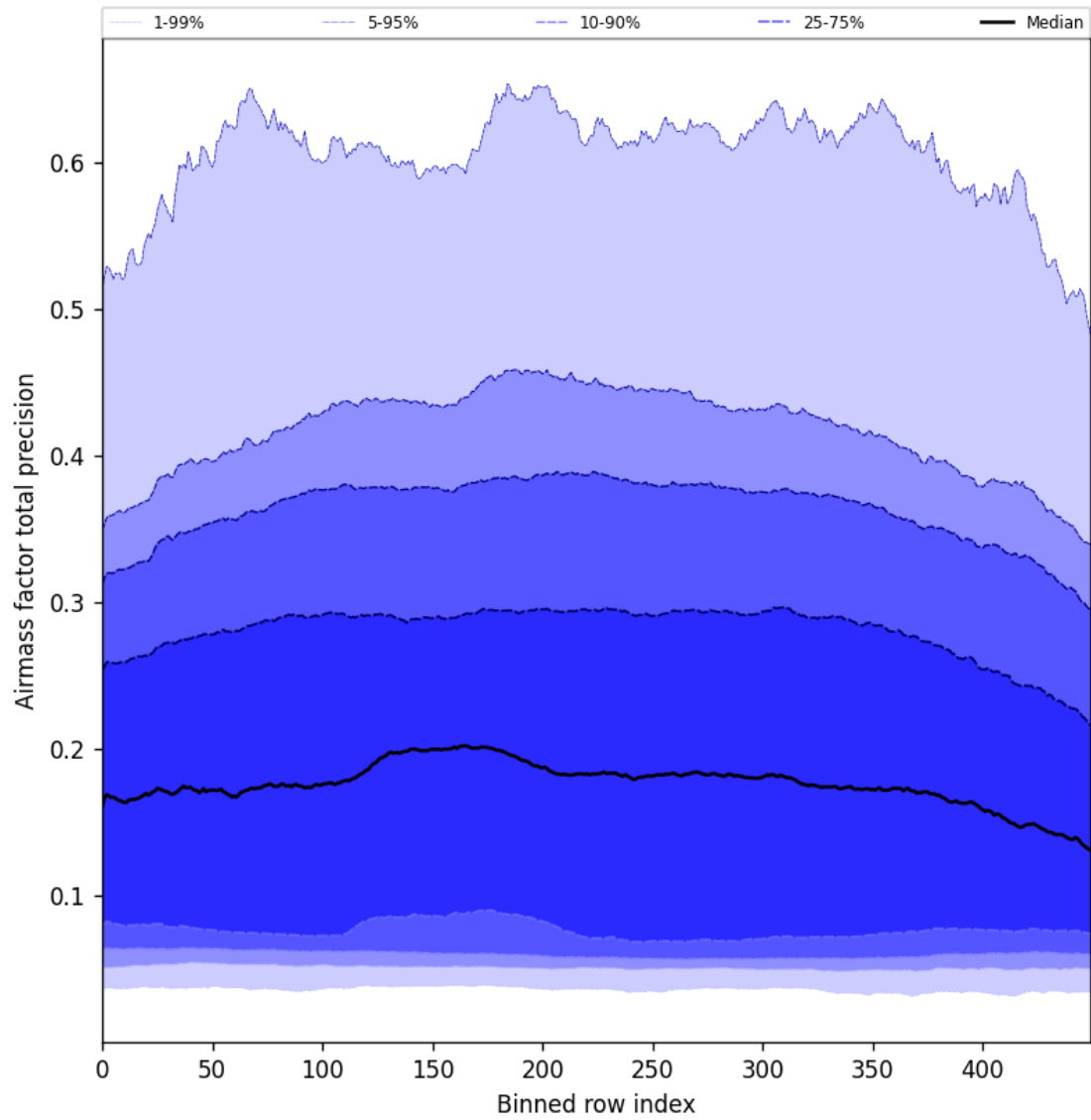
Figure 55: Along track statistics of “Airmass factor total precision” for 2025-02-13 to 2025-02-15
