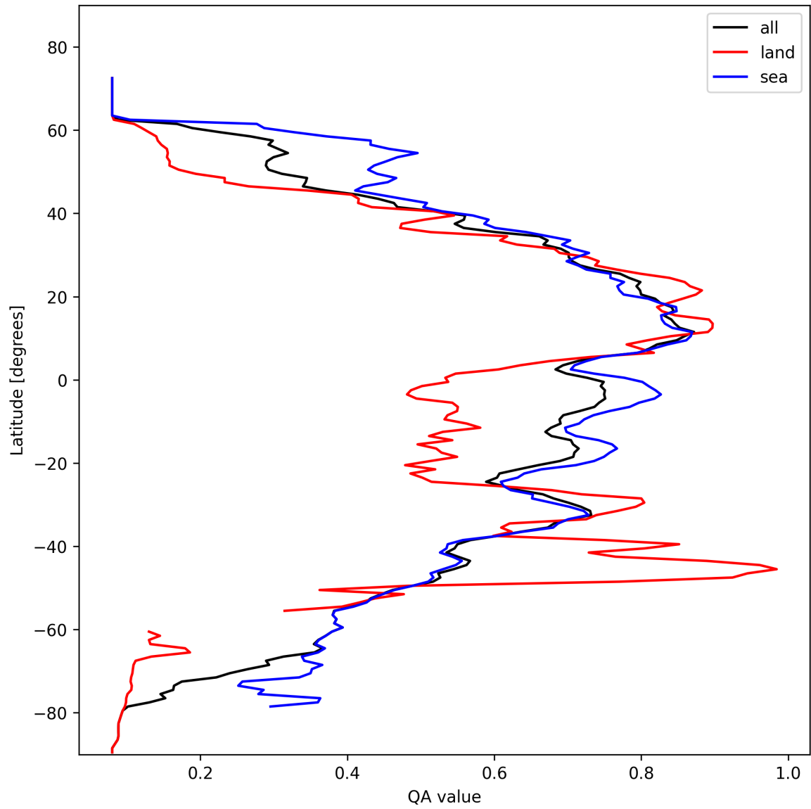
Figure 20: Zonal average of “QA value” for 2025-02-13 to 2025-02-15.
