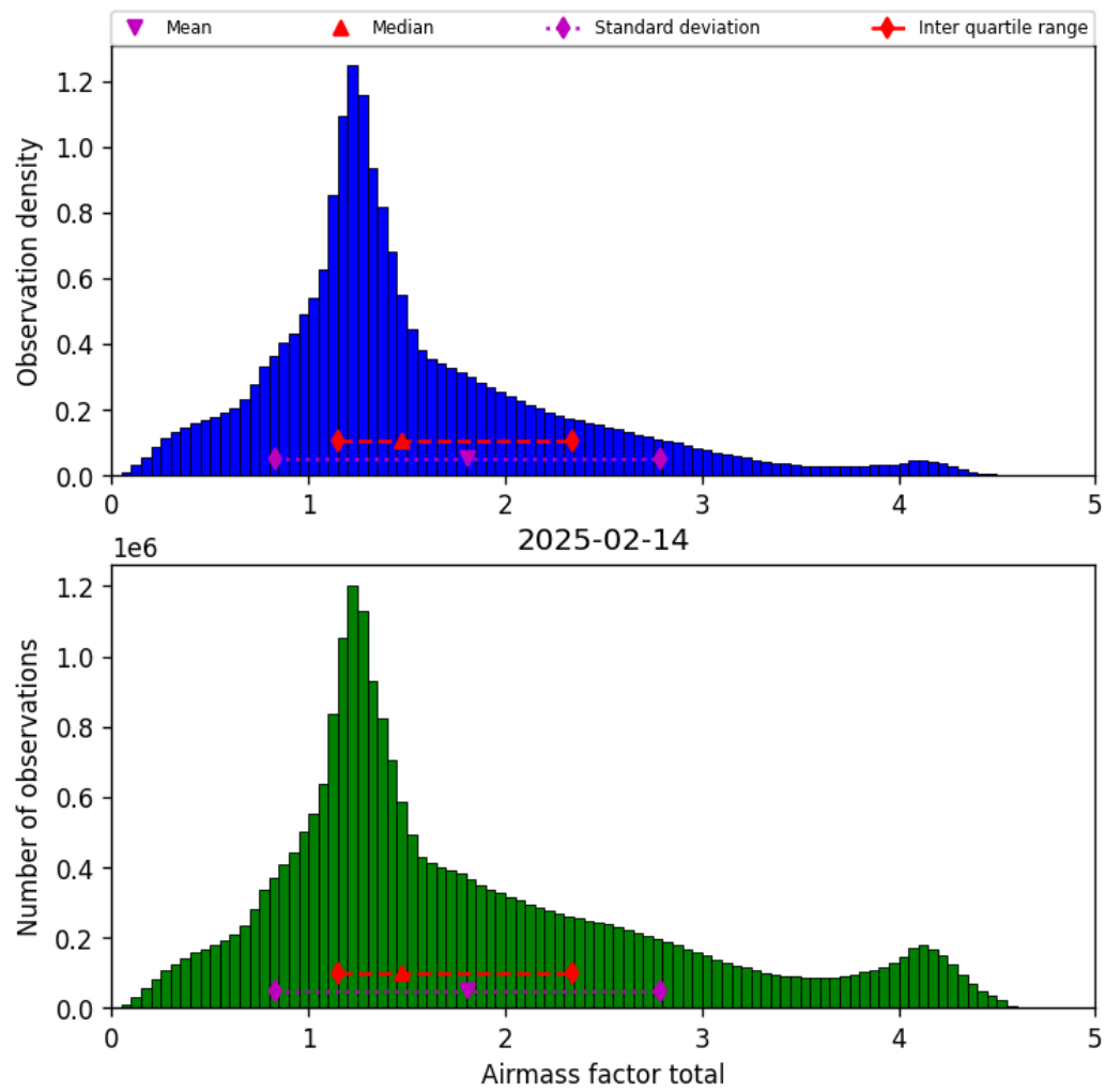
Figure 40: Histogram of “Airmass factor total” for 2025-02-13 to 2025-02-15
