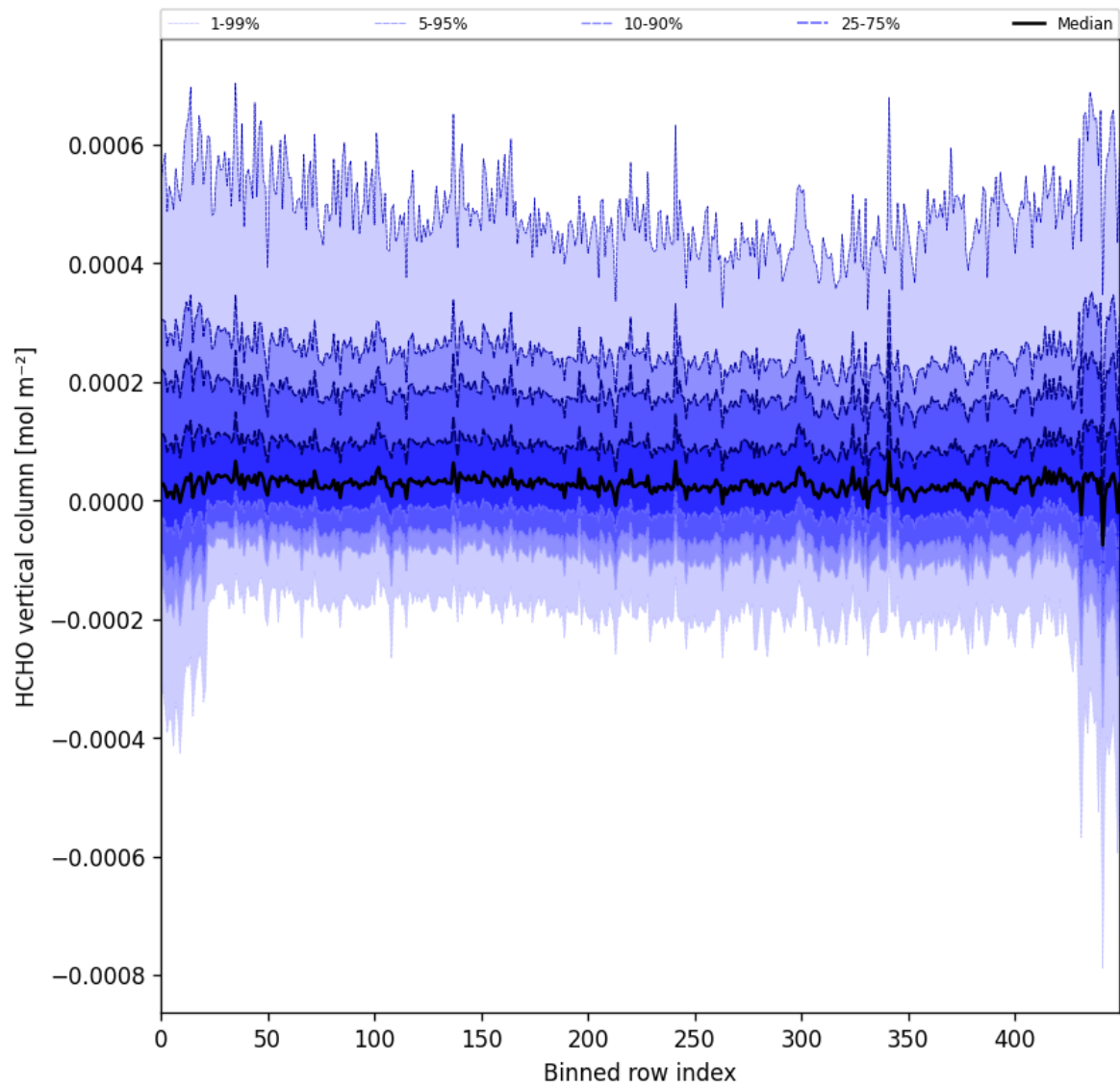
Figure 49: Along track statistics of “HCHO vertical column” for 2025-02-13 to 2025-02-15
