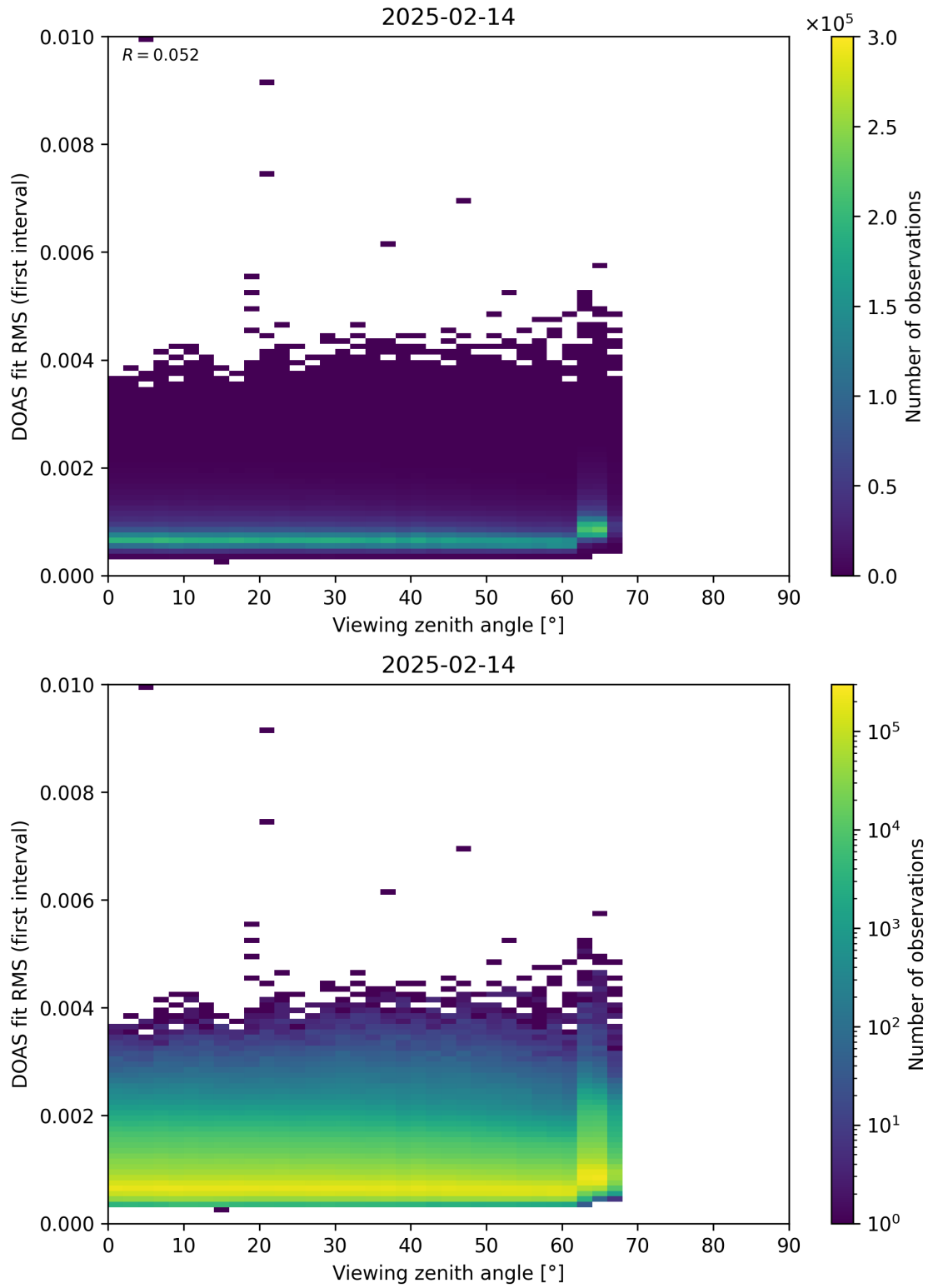
Figure 182: Scatter density plot of “Viewing zenith angle” against “DOAS fit RMS (first interval)” for 2025-02-13 to 2025-02-15.
