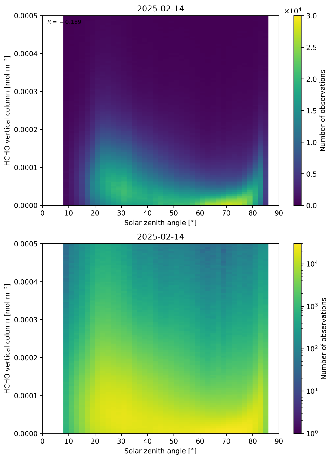
Figure 177: Scatter density plot of “Solar zenith angle” against “HCHO vertical column” for 2025-02-13 to 2025-02-15.
