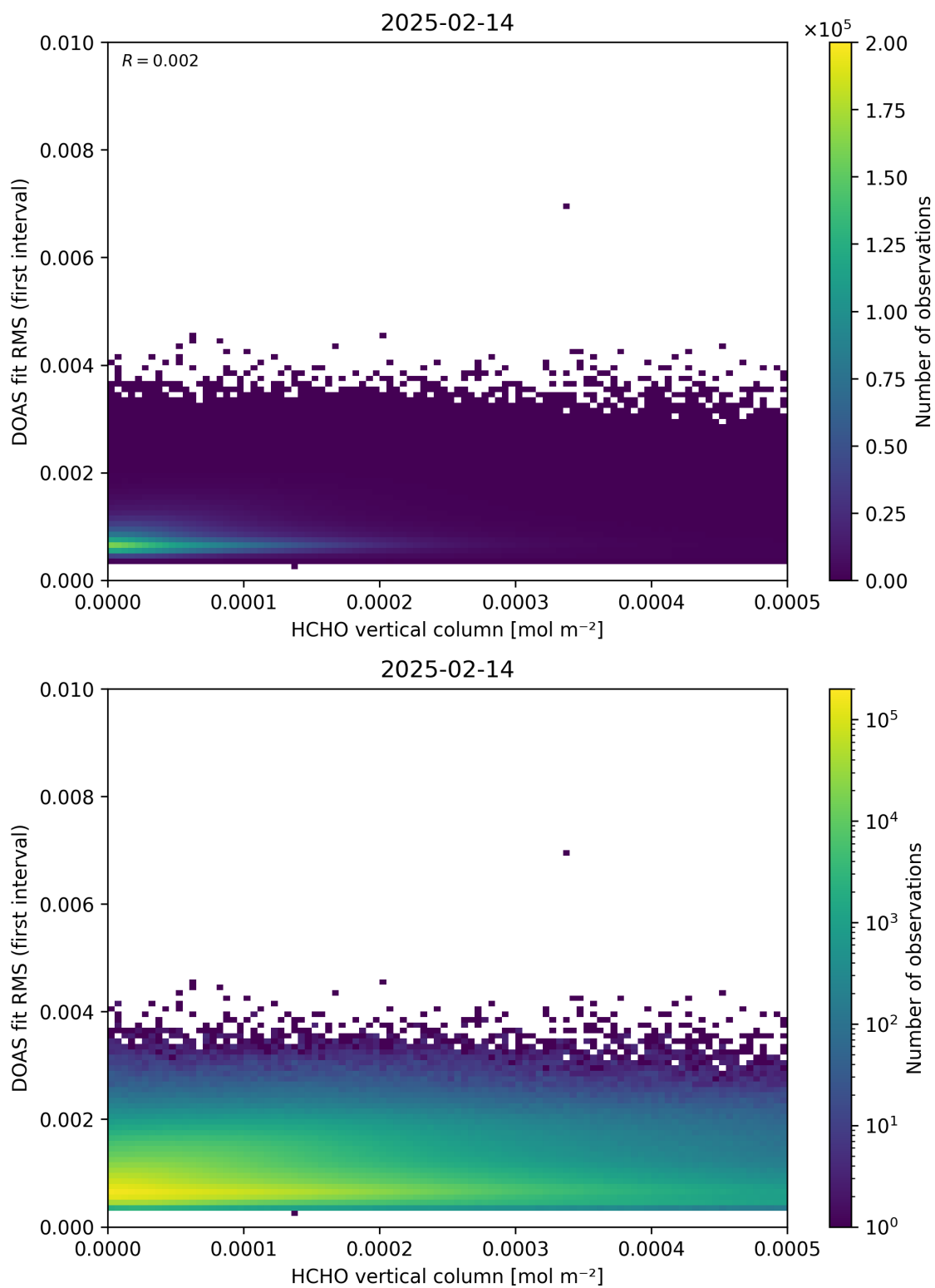
Figure 123: Scatter density plot of “HCHO vertical column” against “DOAS fit RMS (first interval)” for 2025-02-13 to 2025-02-15.
