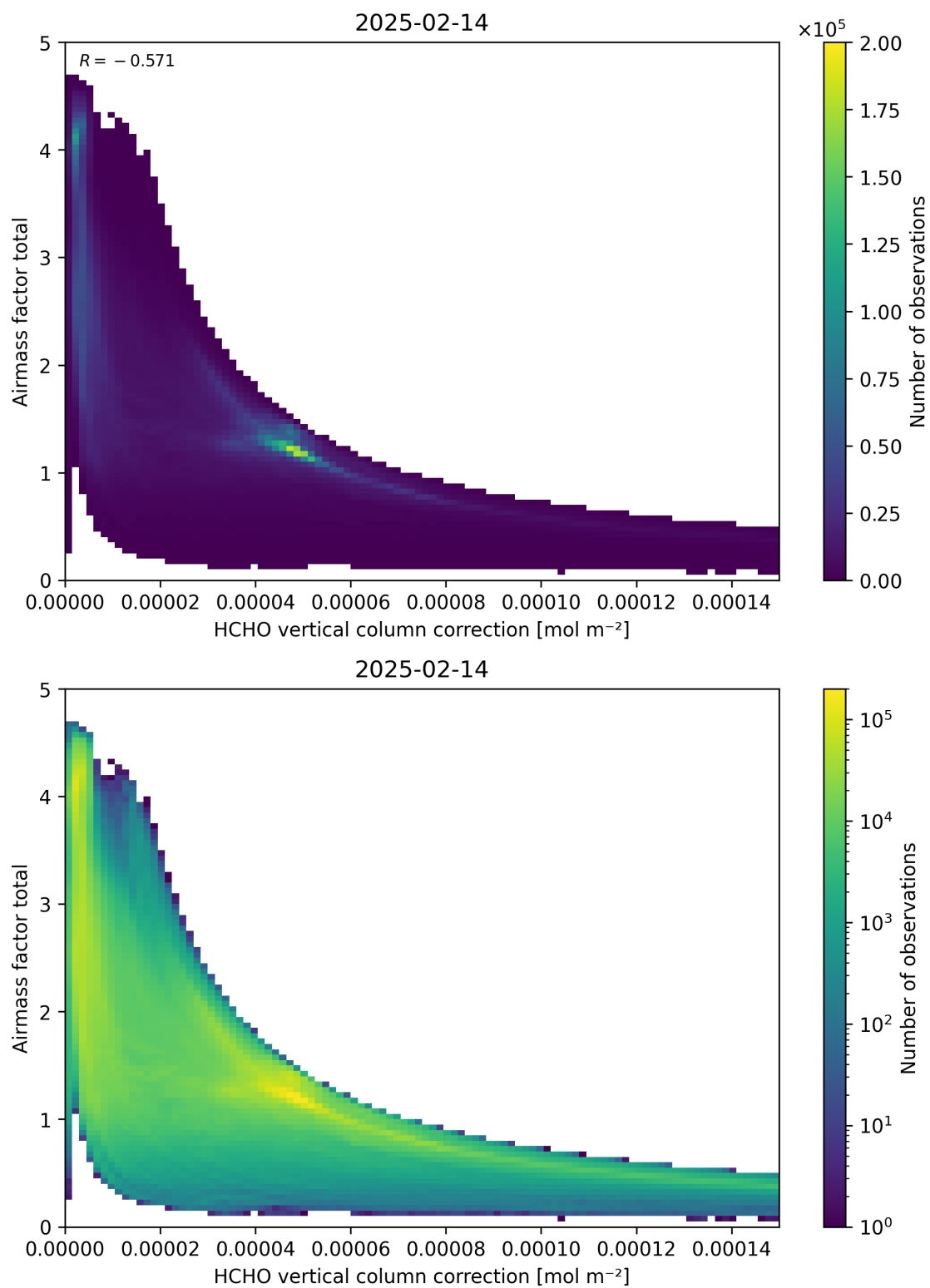
Figure 120: Scatter density plot of “HCHO vertical column correction” against “Airmass factor total” for 2025-02-13 to 2025-02-15.
