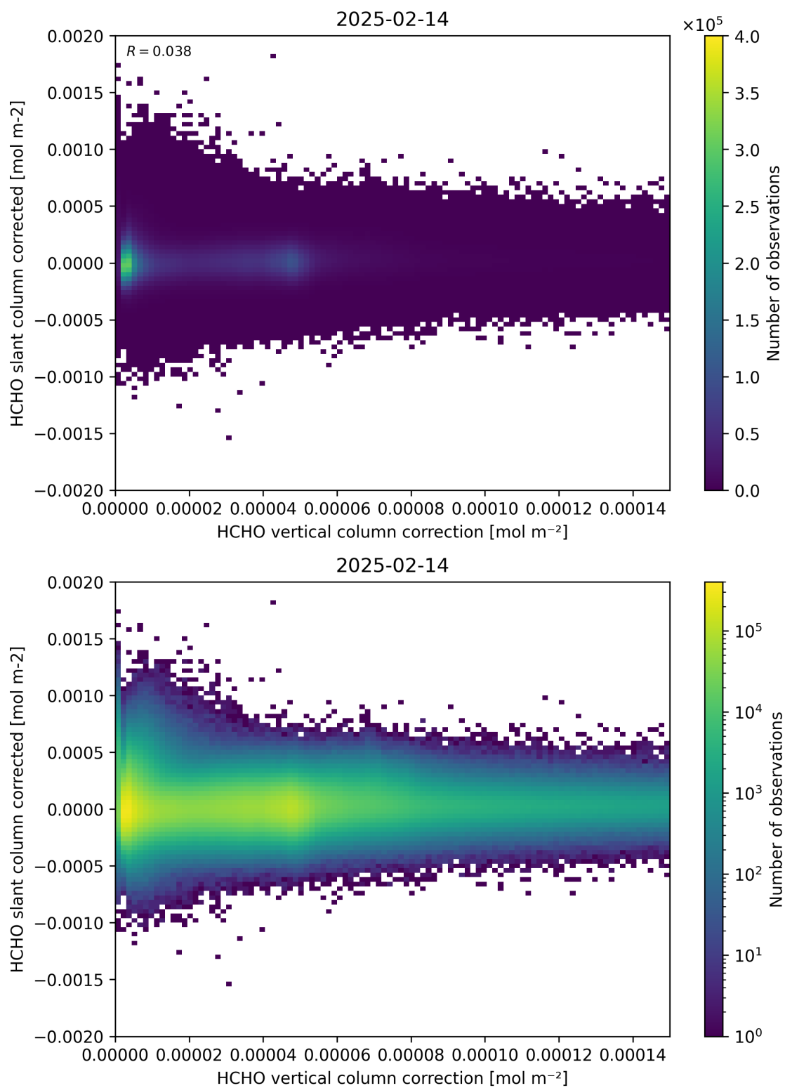
Figure 116: Scatter density plot of “HCHO vertical column correction” against “HCHO slant column corrected” for 2025-02-13 to 2025-02-15.
