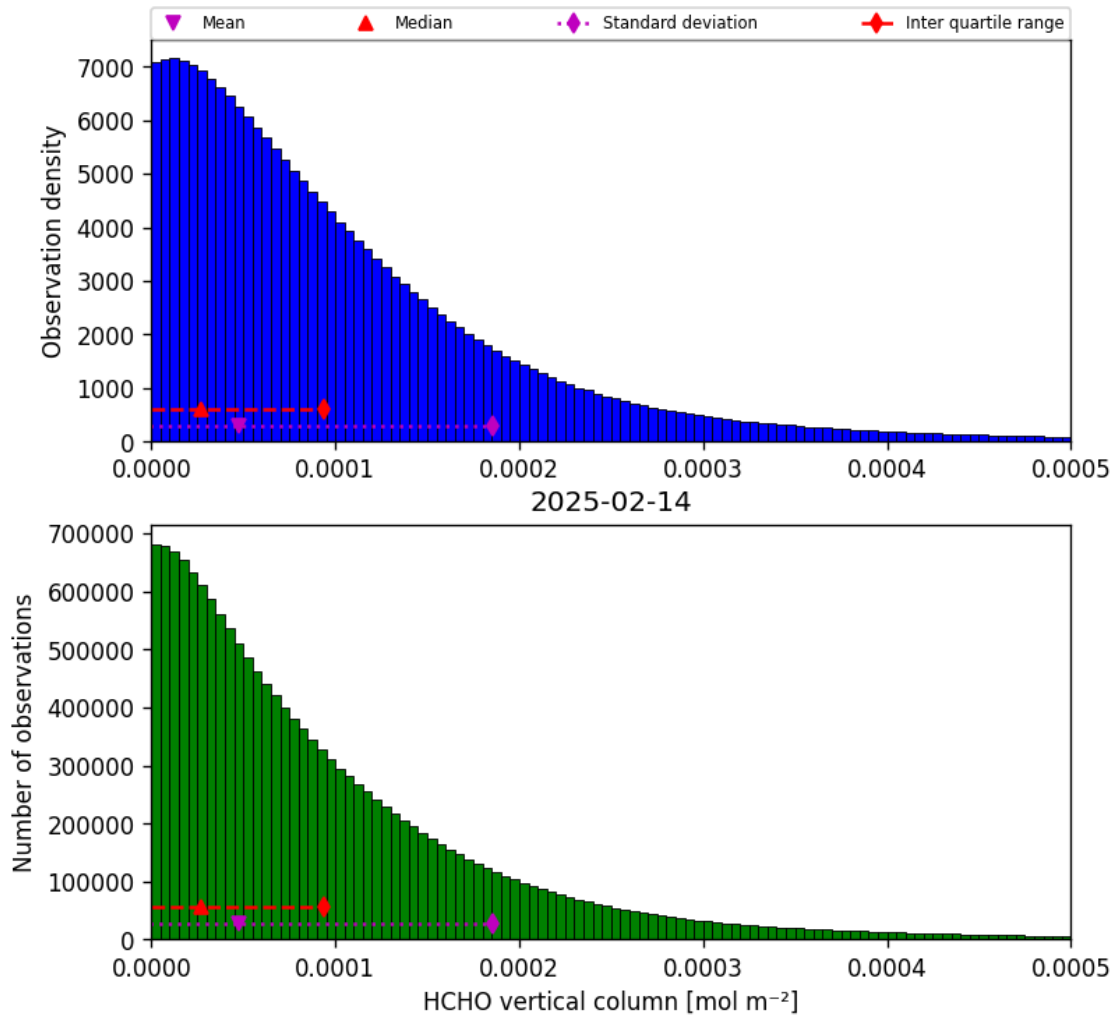
Figure 35: Histogram of “HCHO vertical column” for 2025-02-13 to 2025-02-15
