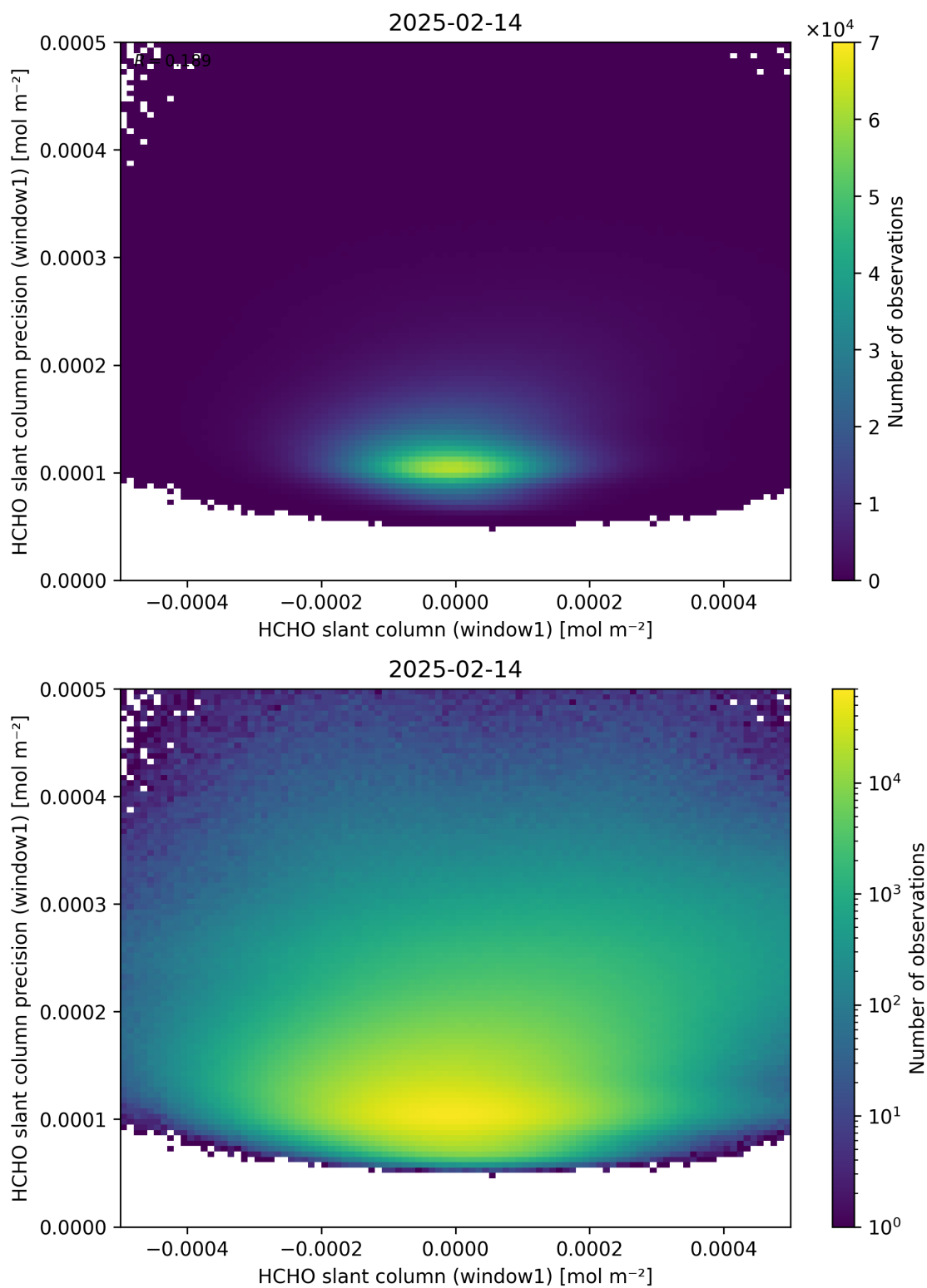
Figure 84: Scatter density plot of “HCHO slant column (window1)” against “HCHO slant column precision (window1)” for 2025-02-13 to 2025-02-15.
