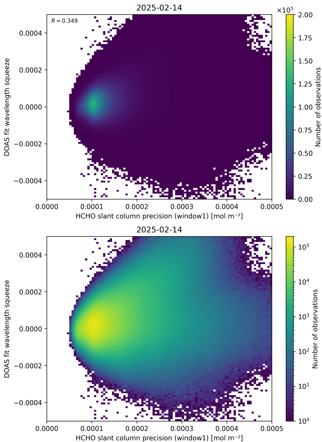
Figure 90: Scatter density plot of “HCHO slant column precision (window1)” against “DOAS fit wavelength squeeze” for 2025-02-13 to 2025-02-15.
