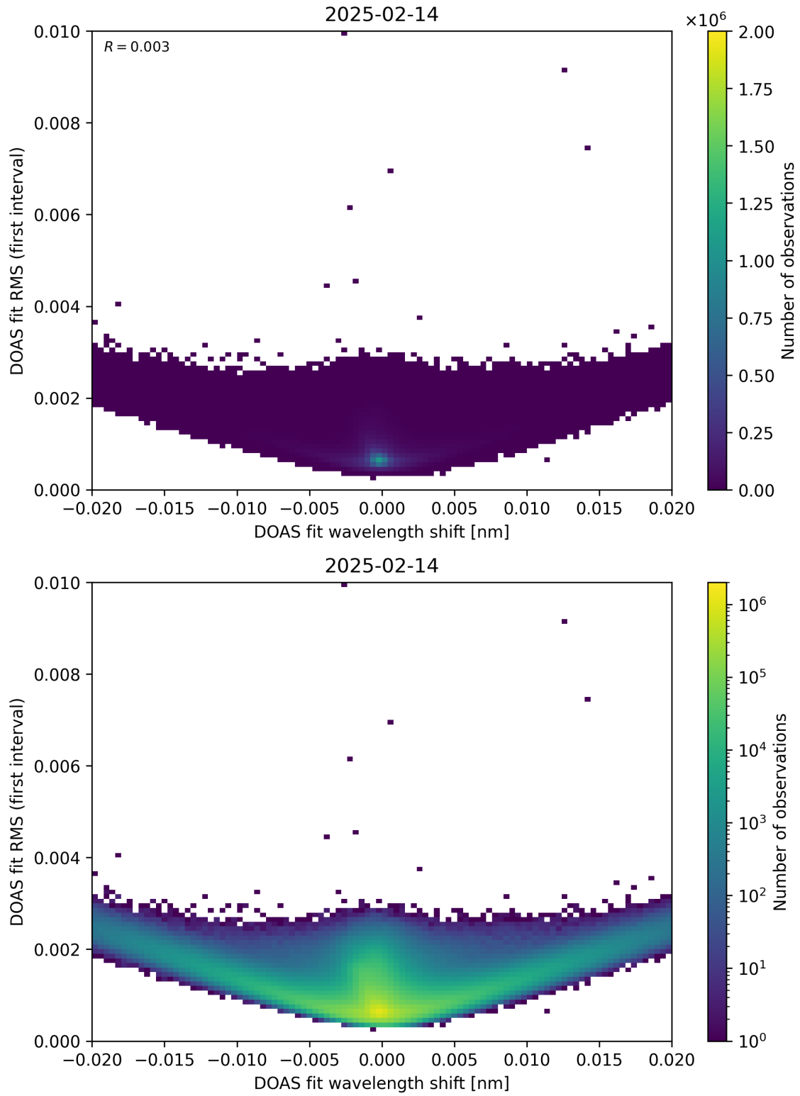
Figure 64: Scatter density plot of “DOAS fit wavelength shift” against “DOAS fit RMS (first interval)” for 2025-02-13 to 2025-02-15.
