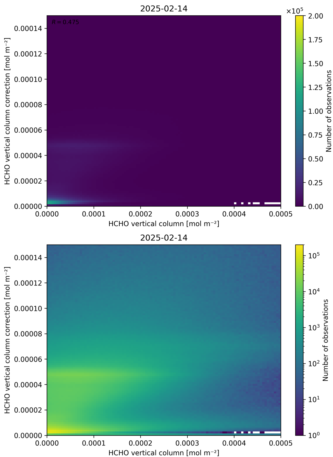
Figure 133: Scatter density plot of “HCHO vertical column” against “HCHO vertical column correction” for 2025-02-13 to 2025-02-15.
