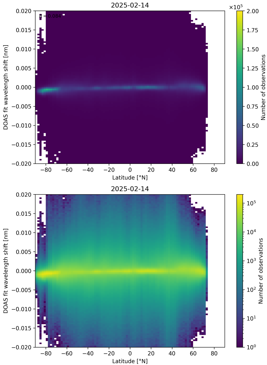
Figure 154: Scatter density plot of “Latitude” against “DOAS fit wavelength shift” for 2025-02-13 to 2025-02-15.
