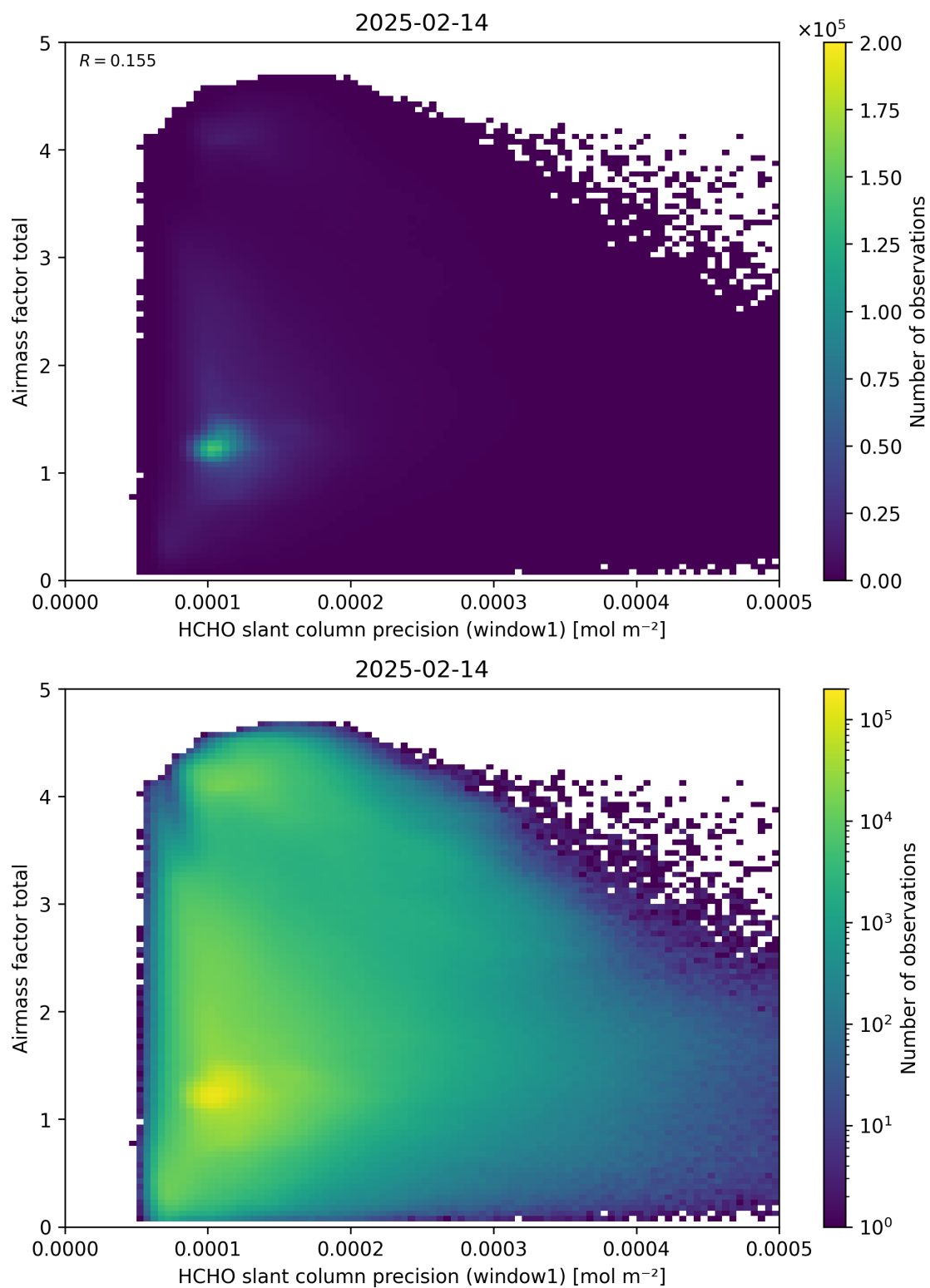
Figure 94: Scatter density plot of “HCHO slant column precision (window1)” against “Airmass factor total” for 2025-02-13 to 2025-02-15.
