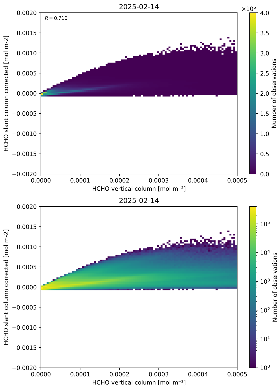
Figure 127: Scatter density plot of “HCHO vertical column” against “HCHO slant column corrected” for 2025-02-13 to 2025-02-15.
