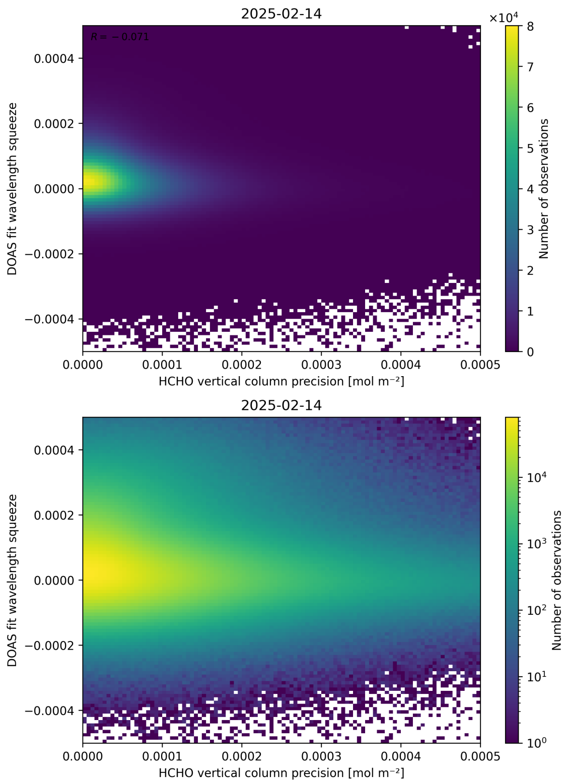
Figure 138: Scatter density plot of “HCHO vertical column precision” against “DOAS fit wavelength squeeze” for 2025-02-13 to 2025-02-15.
