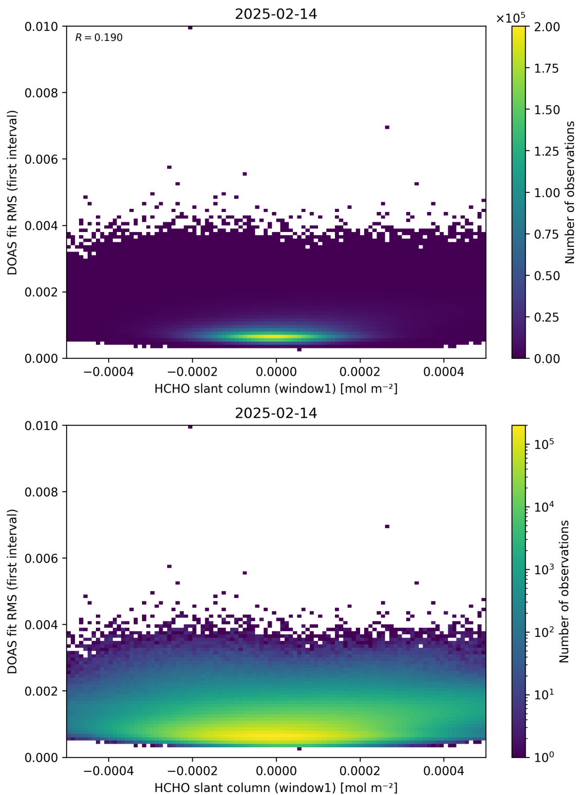
Figure 78: Scatter density plot of “HCHO slant column (window1)” against “DOAS fit RMS (first interval)” for 2025-02-13 to 2025-02-15.
