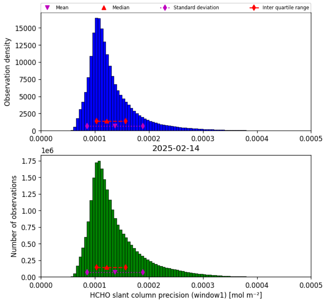
Figure 39: Histogram of “HCHO slant column precision (window1)” for 2025-02-13 to 2025-02-15
