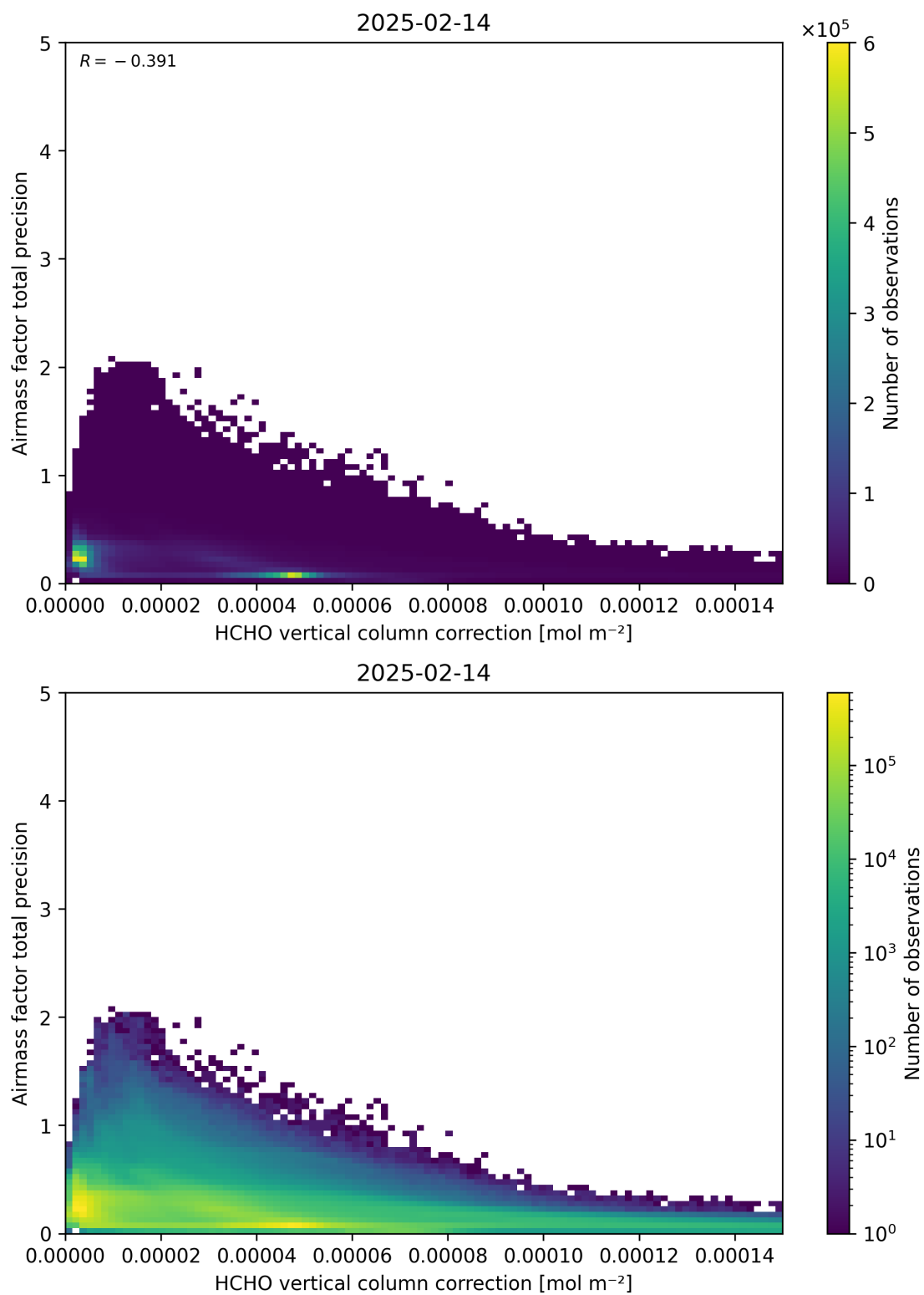
Figure 121: Scatter density plot of “HCHO vertical column correction” against “Airmass factor total precision” for 2025-02-13 to 2025-02-15.
