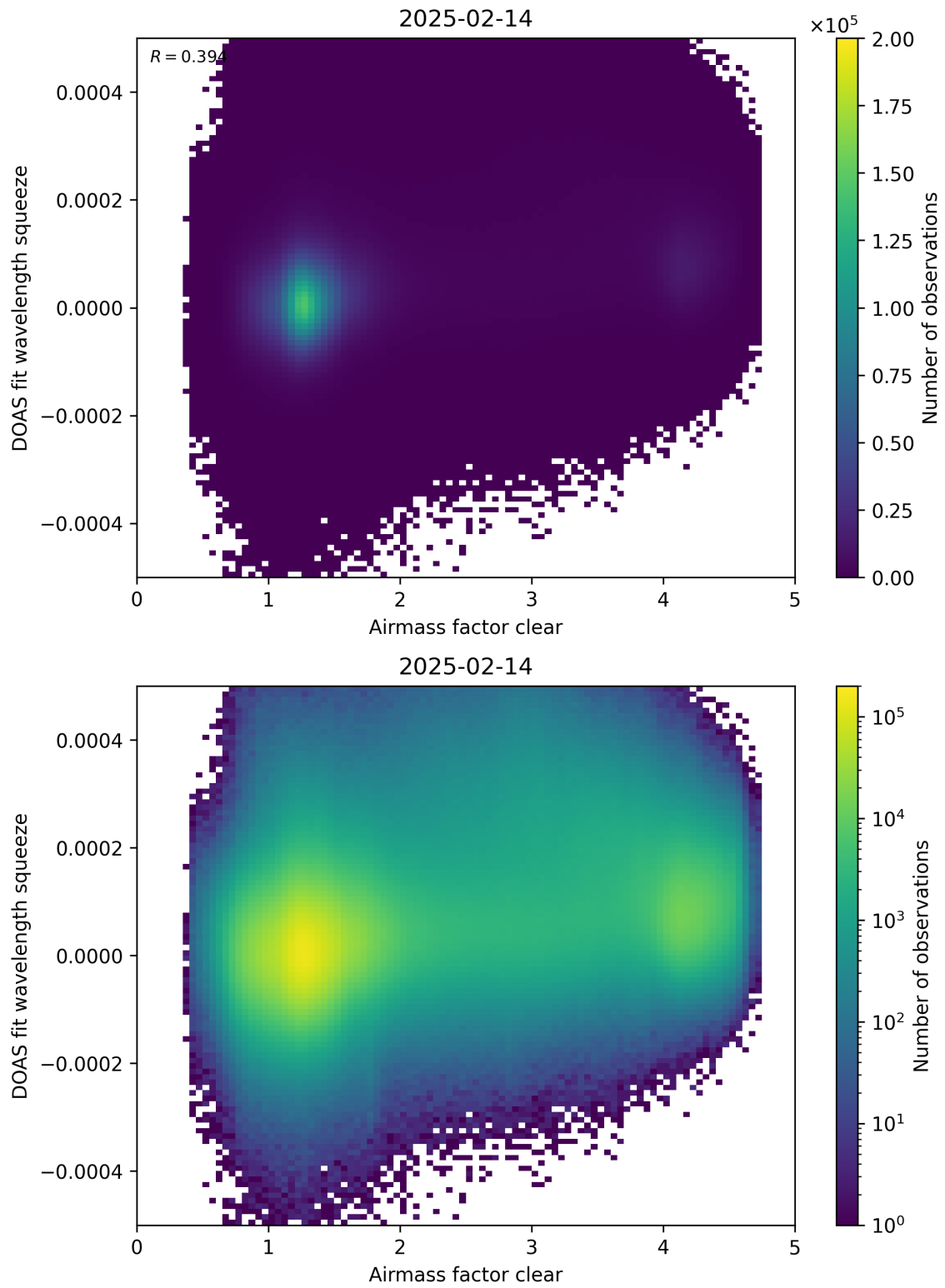
Figure 73: Scatter density plot of “Airmass factor clear” against “DOAS fit wavelength squeeze” for 2025-02-13 to 2025-02-15.
