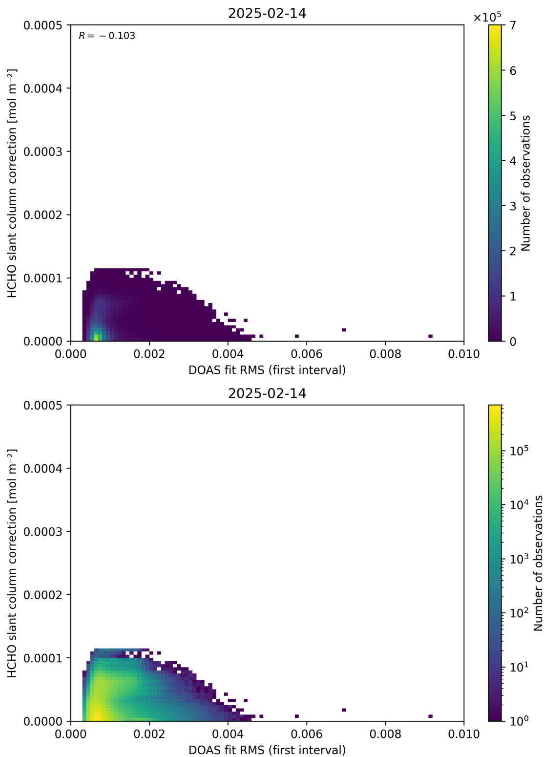
Figure 63: Scatter density plot of “DOAS fit RMS (first interval)” against “HCHO slant column correction” for 2025-02-13 to 2025-02-15.
