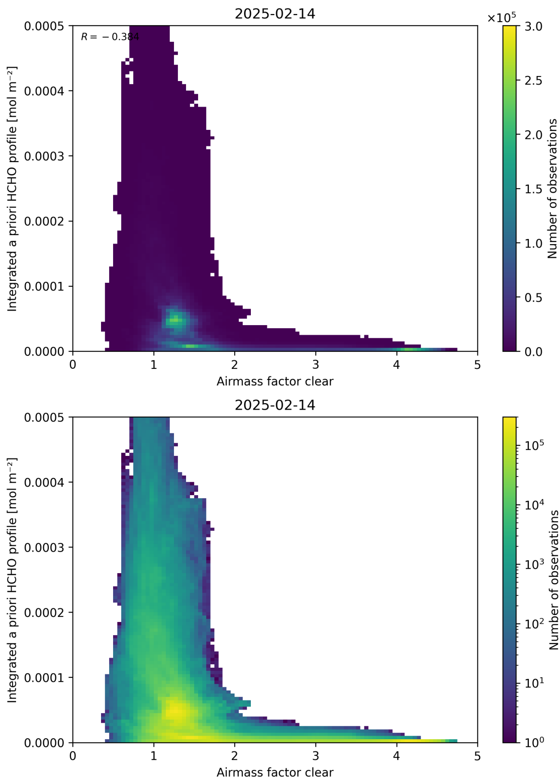
Figure 76: Scatter density plot of “Airmass factor clear” against “Integrated a priori HCHO profile” for 2025-02-13 to 2025-02-15.
