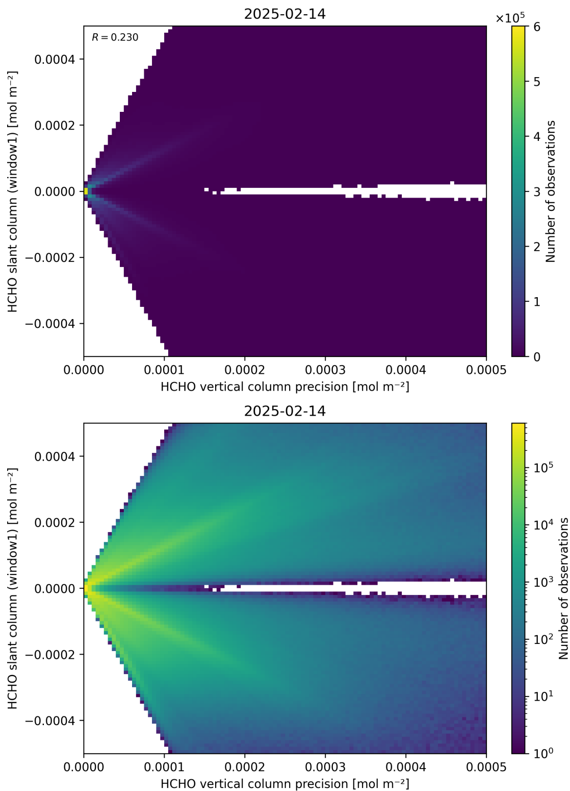
Figure 142: Scatter density plot of “HCHO vertical column precision” against “HCHO slant column (window1)” for 2025-02-13 to 2025-02-15.
