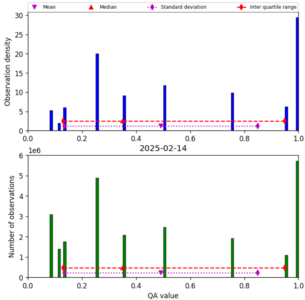
Figure 34: Histogram of “QA value” for 2025-02-13 to 2025-02-15
