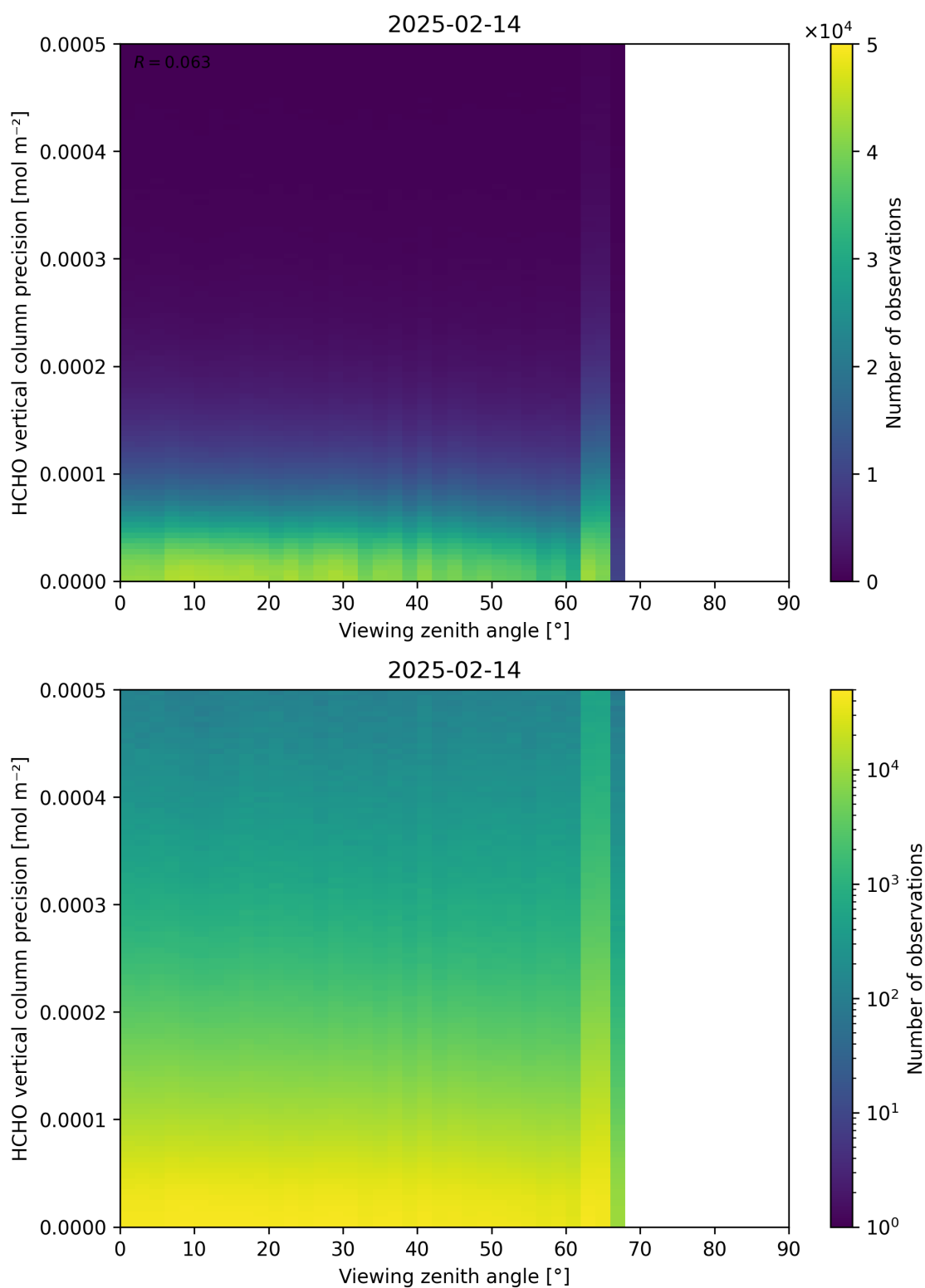
Figure 194: Scatter density plot of “Viewing zenith angle” against “HCHO vertical column precision” for 2025-02-13 to 2025-02-15.
