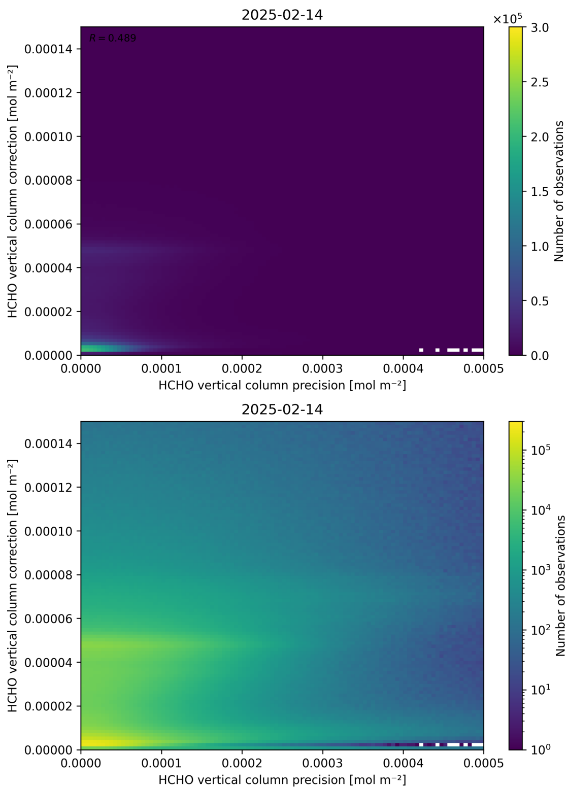
Figure 146: Scatter density plot of “HCHO vertical column precision” against “HCHO vertical column correction” for 2025-02-13 to 2025-02-15.
