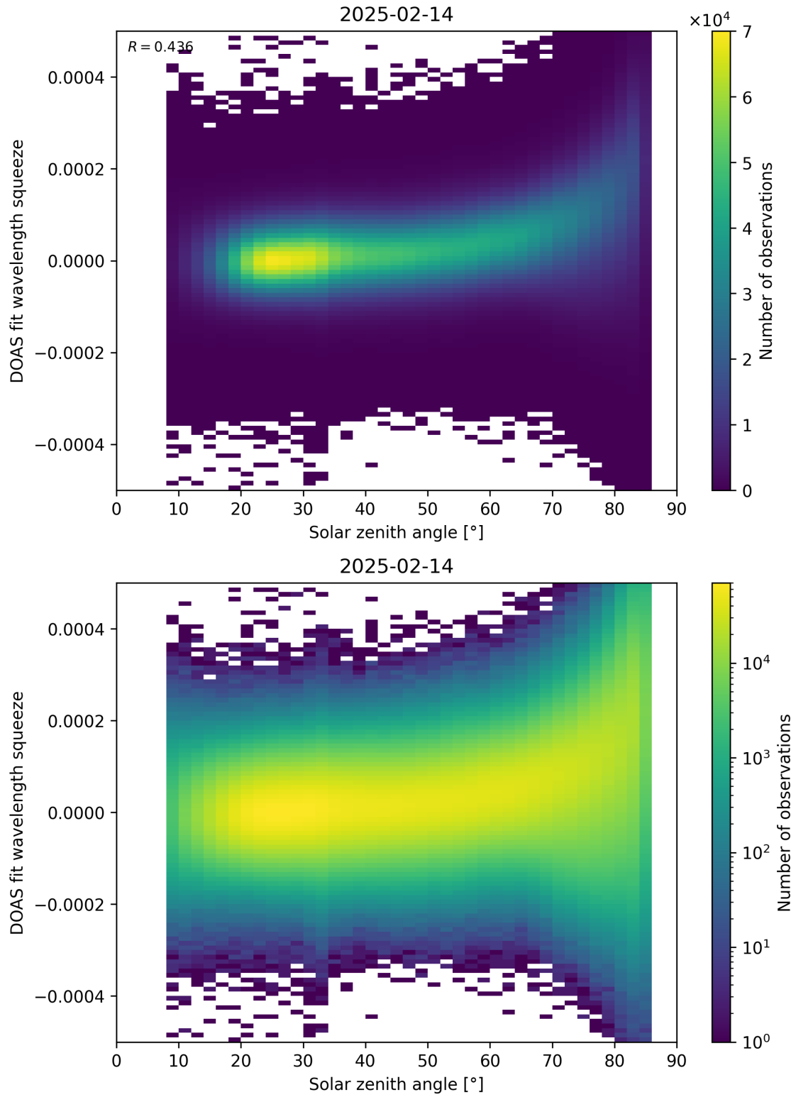
Figure 169: Scatter density plot of “Solar zenith angle” against “DOAS fit wavelength squeeze” for 2025-02-13 to 2025-02-15.
