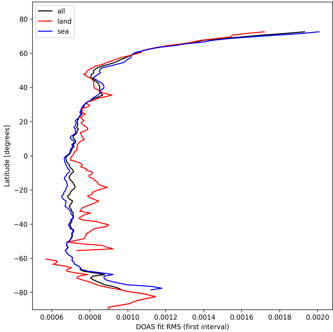
Figure 32: Zonal average of “DOAS fit RMS (first interval)” for 2025-02-13 to 2025-02-15.
