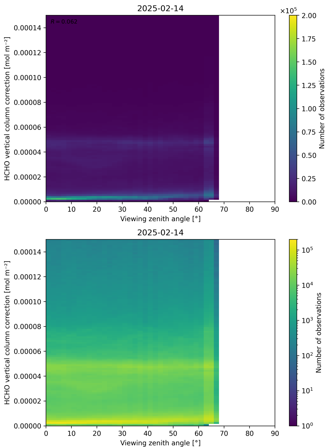
Figure 193: Scatter density plot of “Viewing zenith angle” against “HCHO vertical column correction” for 2025-02-13 to 2025-02-15.
