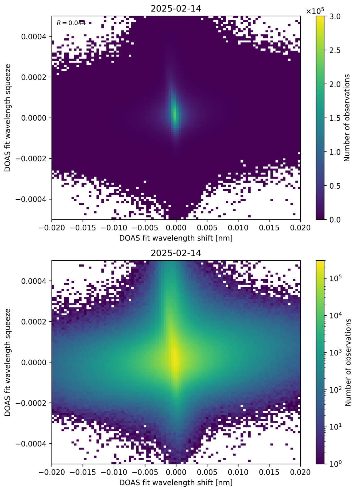
Figure 65: Scatter density plot of “DOAS fit wavelength shift” against “DOAS fit wavelength squeeze” for 2025-02-13 to 2025-02-15.
