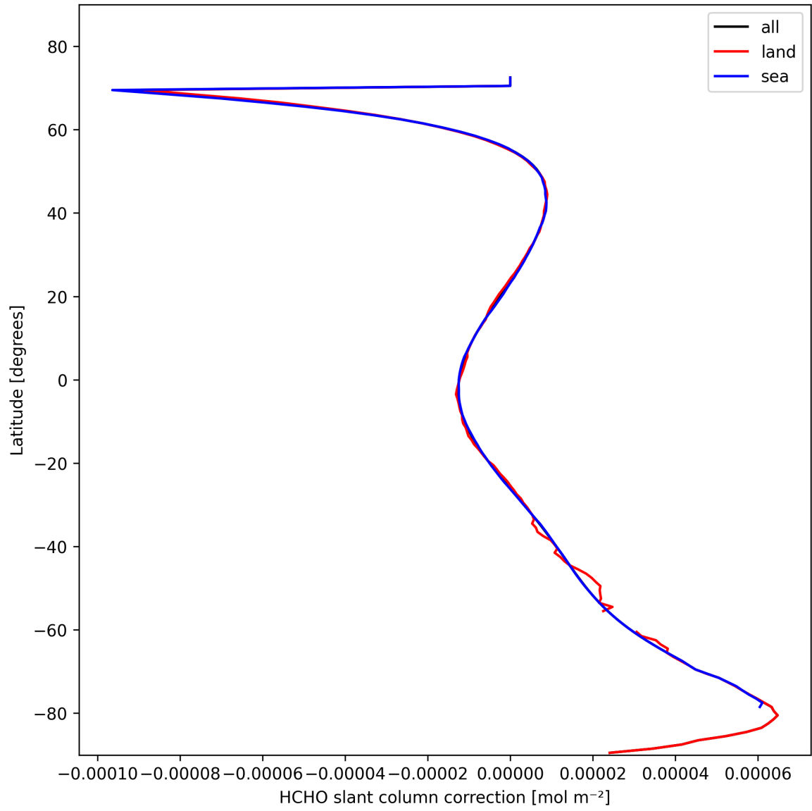
Figure 33: Zonal average of “HCHO slant column correction” for 2025-02-13 to 2025-02-15.
