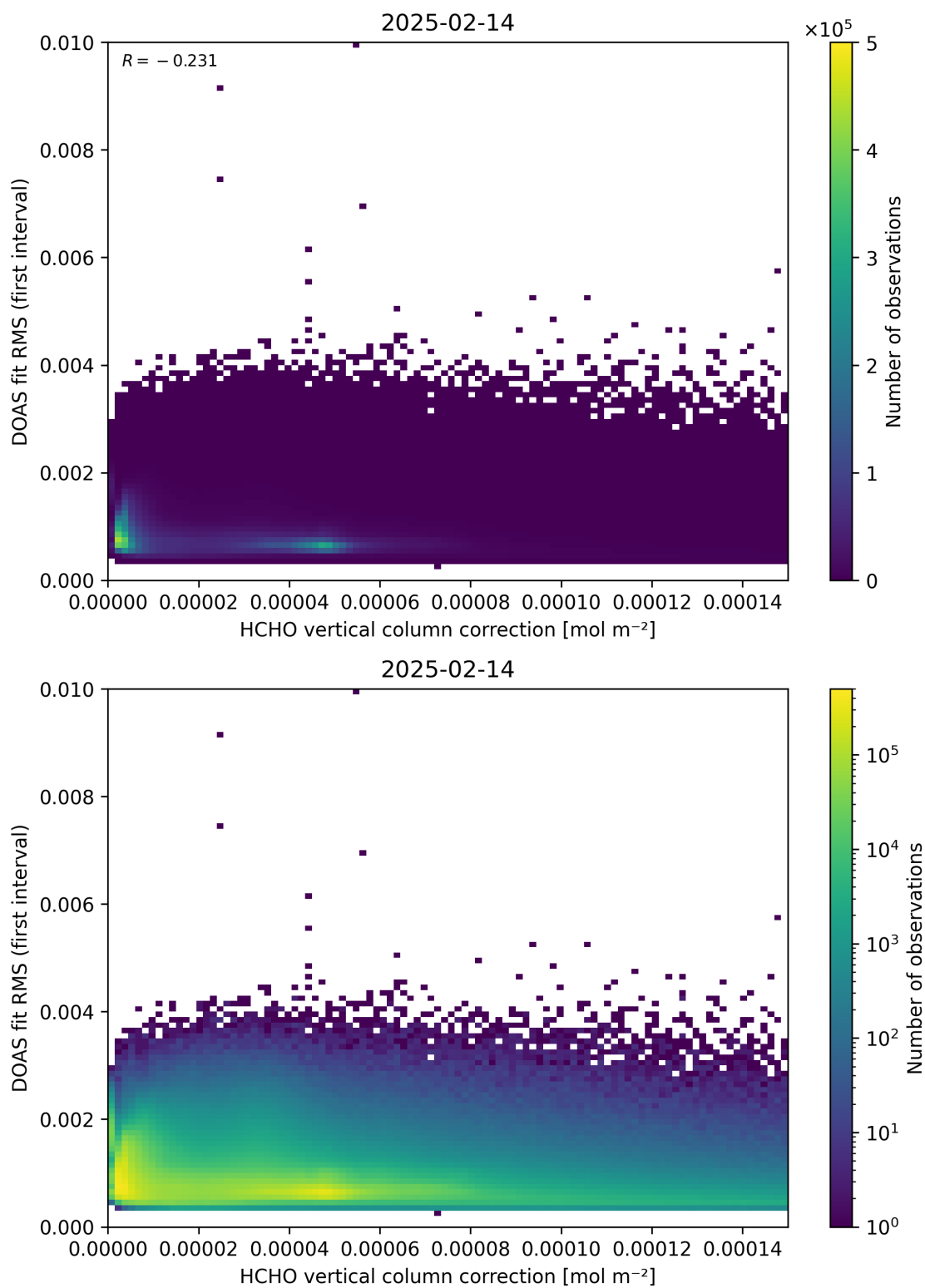
Figure 112: Scatter density plot of “HCHO vertical column correction” against “DOAS fit RMS (first interval)” for 2025-02-13 to 2025-02-15.
