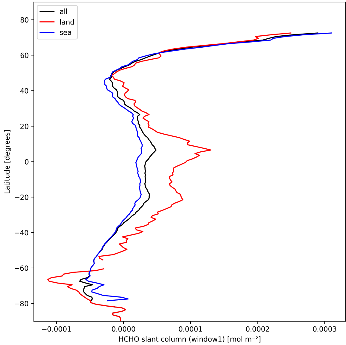
Figure 24: Zonal average of “HCHO slant column (window1)” for 2025-02-13 to 2025-02-15.
