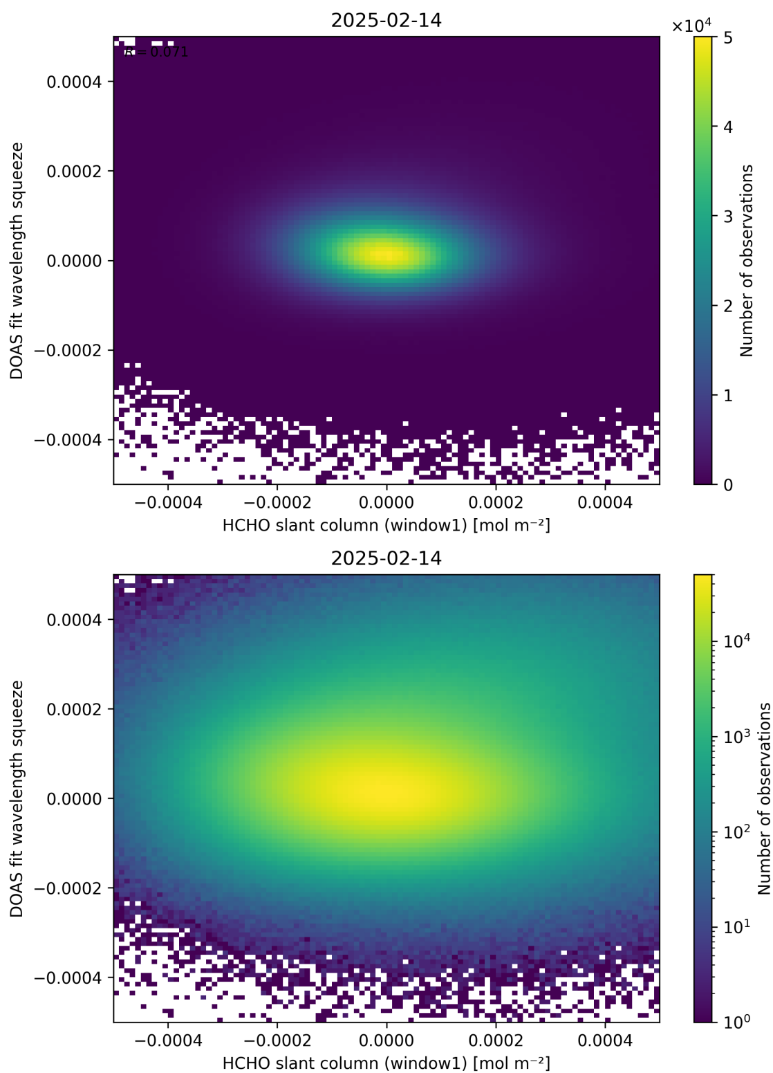
Figure 80: Scatter density plot of “HCHO slant column (window1)” against “DOAS fit wavelength squeeze” for 2025-02-13 to 2025-02-15.
