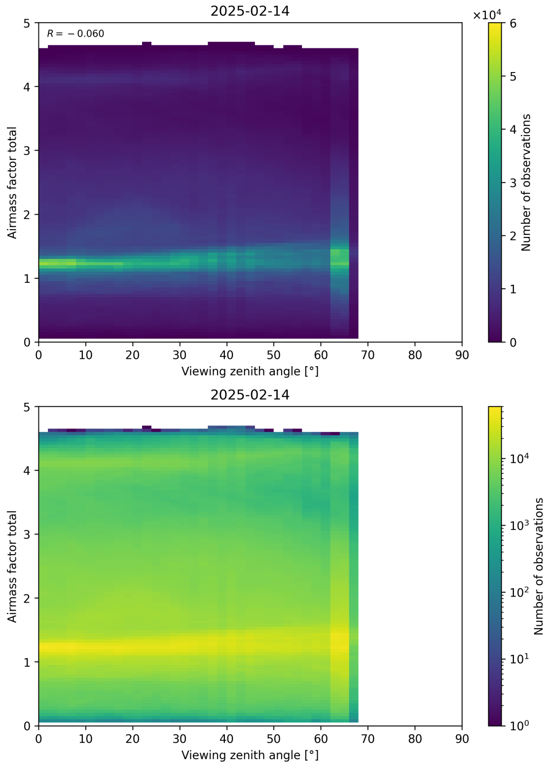
Figure 190: Scatter density plot of “Viewing zenith angle” against “Airmass factor total” for 2025-02-13 to 2025-02-15.
