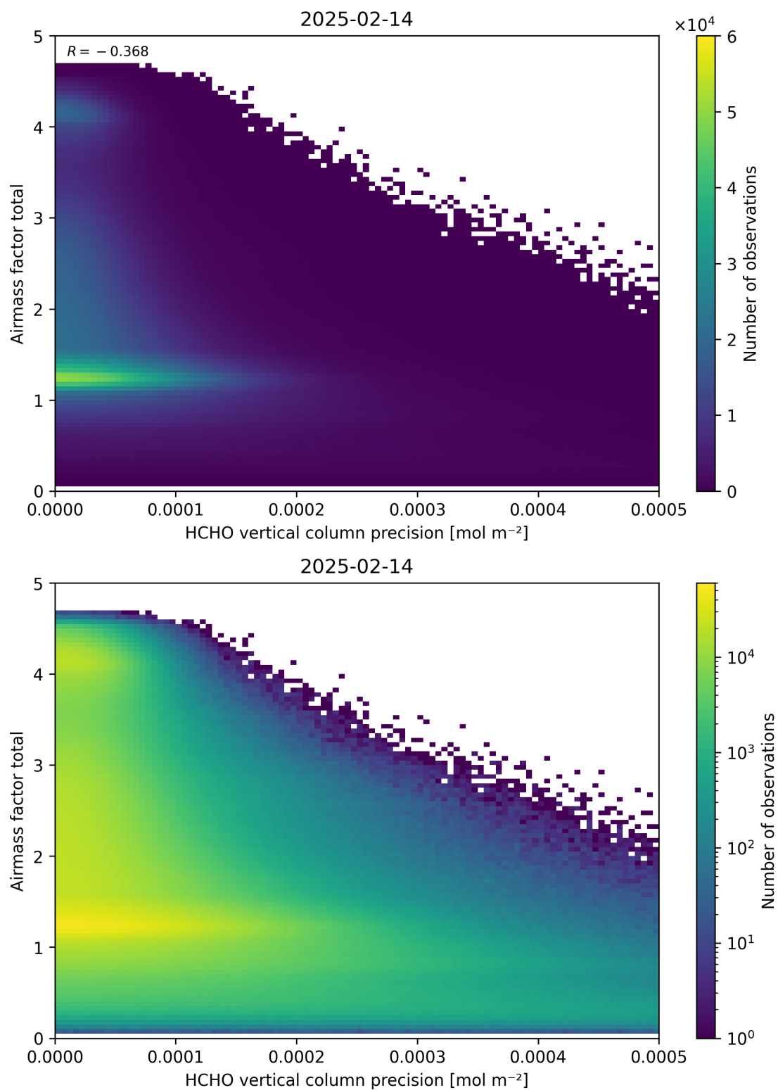
Figure 144: Scatter density plot of “HCHO vertical column precision” against “Airmass factor total” for 2025-02-13 to 2025-02-15.
