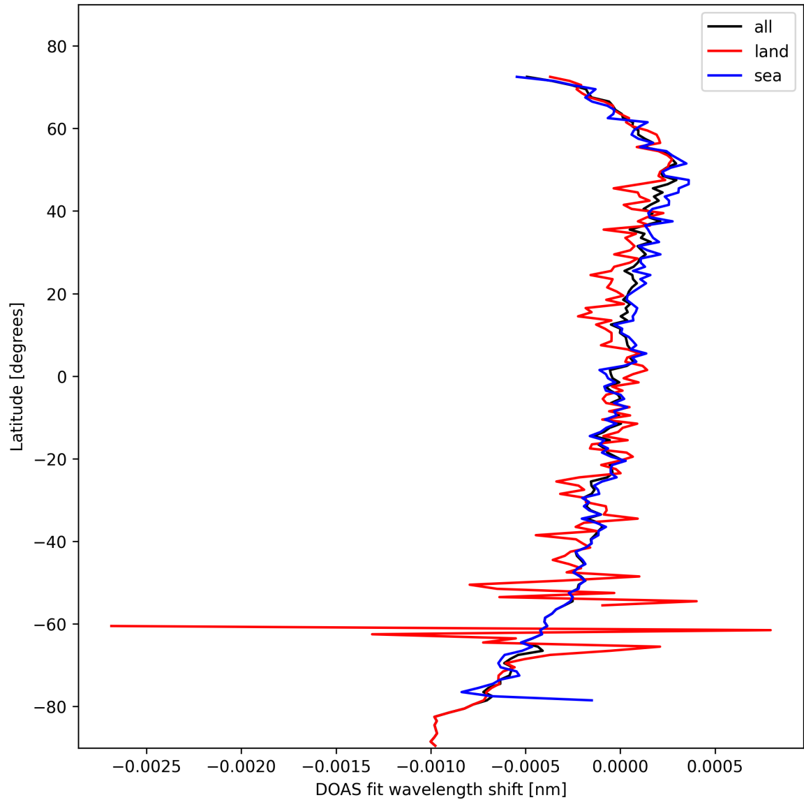
Figure 30: Zonal average of “DOAS fit wavelength shift” for 2025-02-13 to 2025-02-15.
