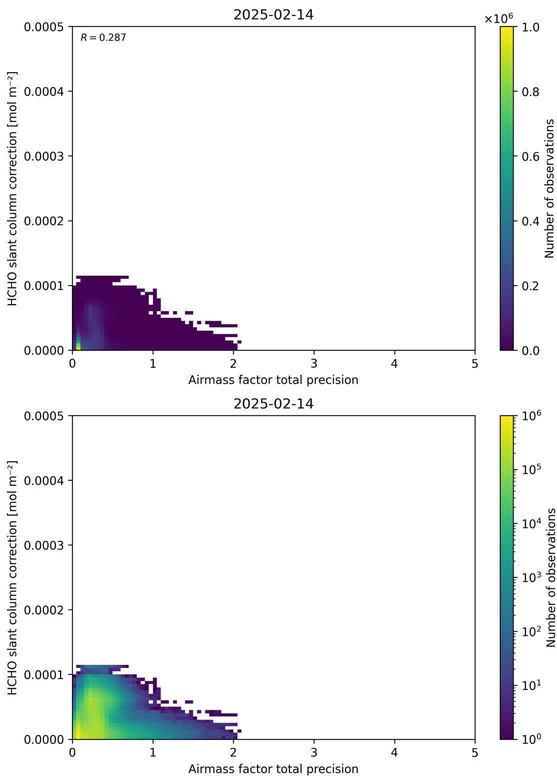
Figure 110: Scatter density plot of “Airmass factor total precision” against “HCHO slant column correction” for 2025-02-13 to 2025-02-15.
