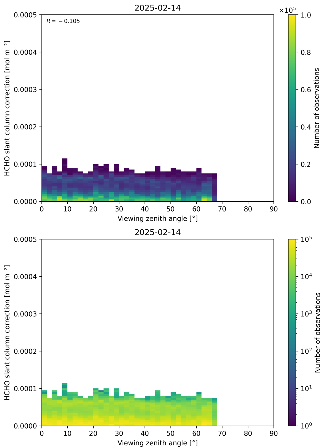
Figure 187: Scatter density plot of “Viewing zenith angle” against “HCHO slant column correction” for 2025-02-13 to 2025-02-15.
