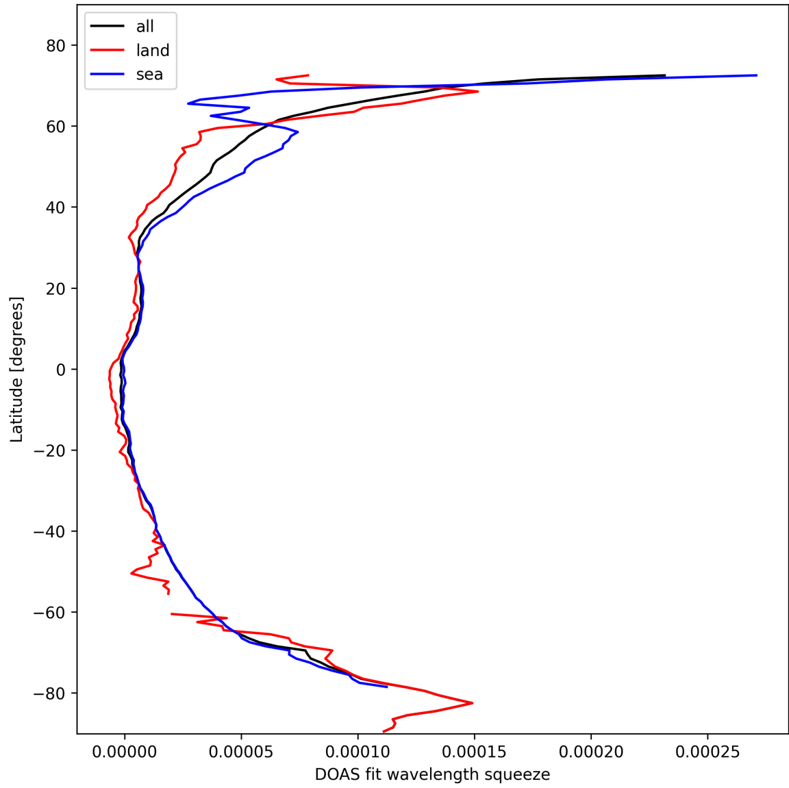
Figure 31: Zonal average of “DOAS fit wavelength squeeze” for 2025-02-13 to 2025-02-15.
