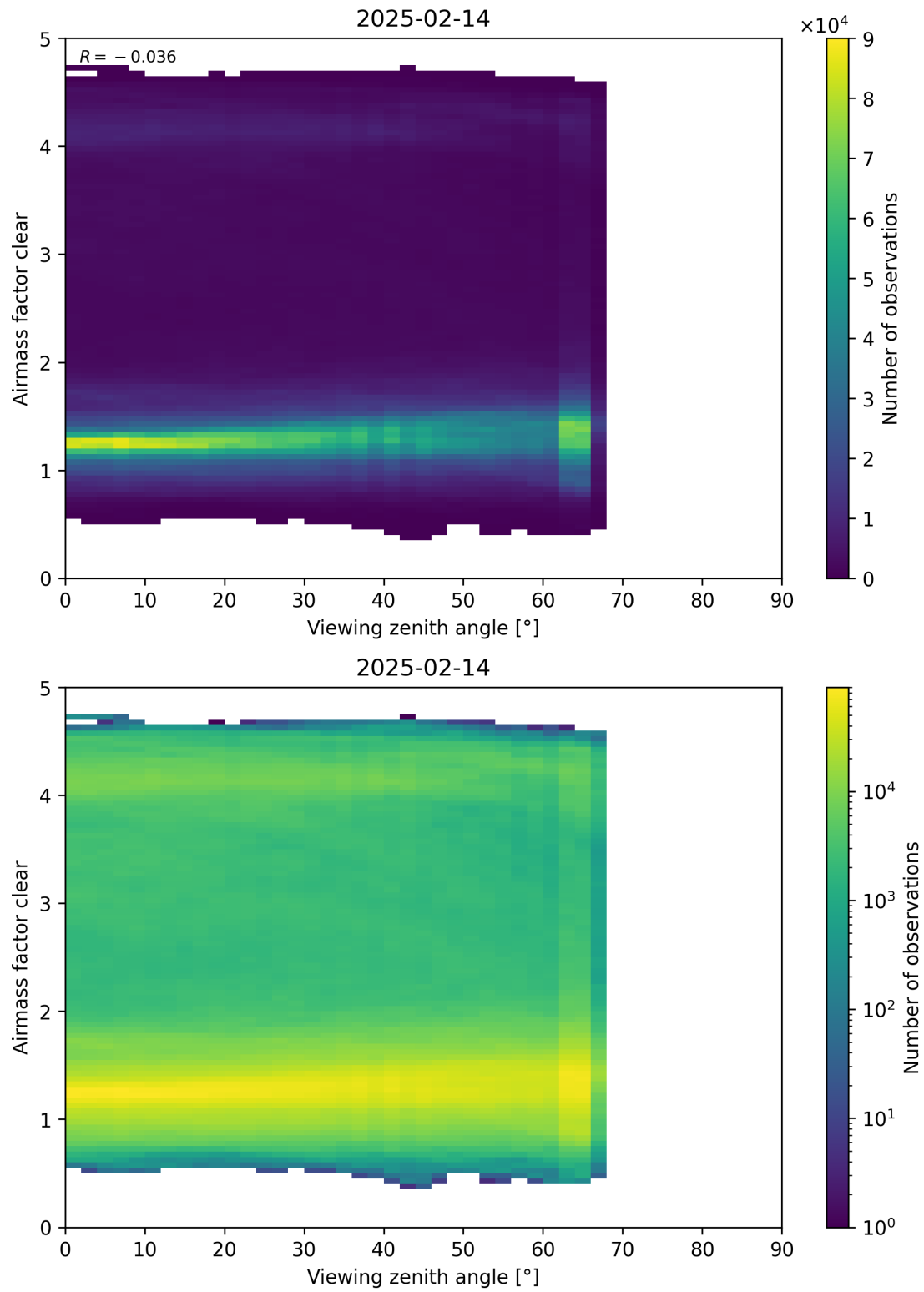
Figure 185: Scatter density plot of “Viewing zenith angle” against “Airmass factor clear” for 2025-02-13 to 2025-02-15.
