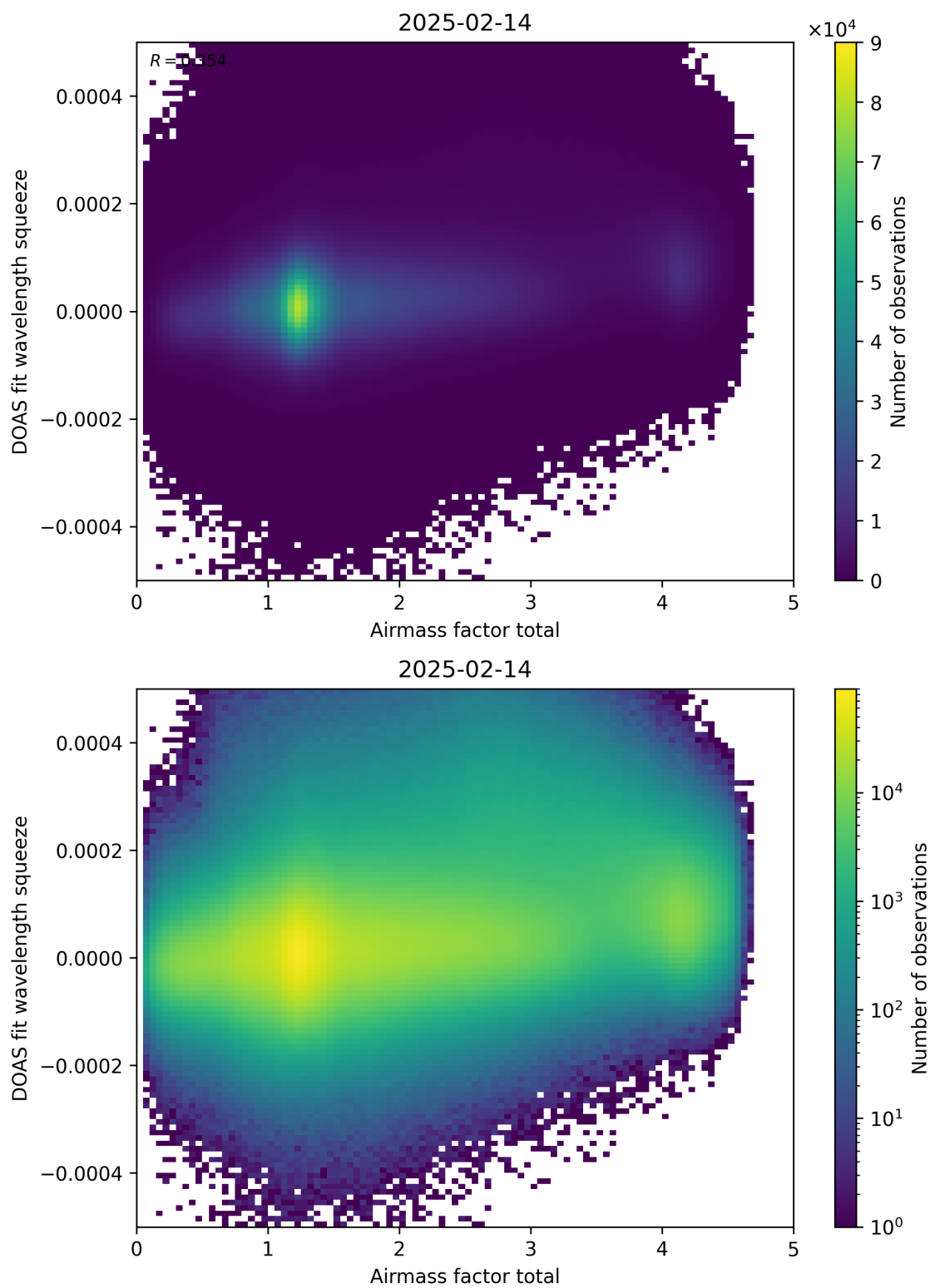
Figure 99: Scatter density plot of “Airmass factor total” against “DOAS fit wavelength squeeze” for 2025-02-13 to 2025-02-15.
