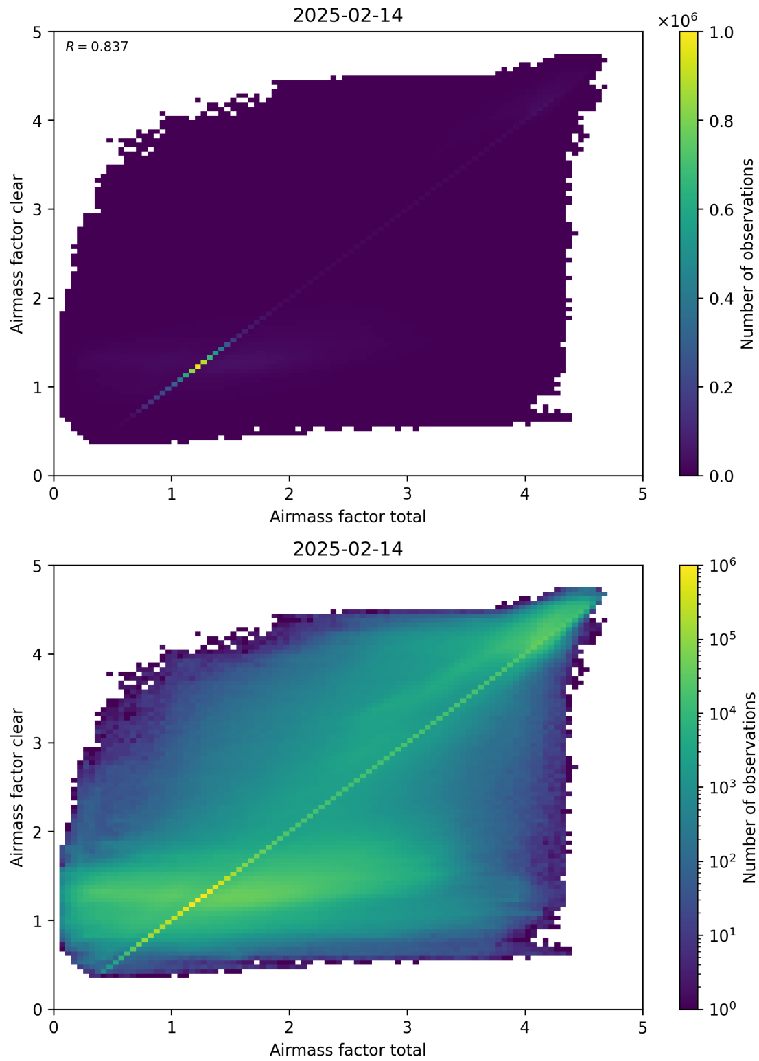
Figure 100: Scatter density plot of “Airmass factor total” against “Airmass factor clear” for 2025-02-13 to 2025-02-15.
