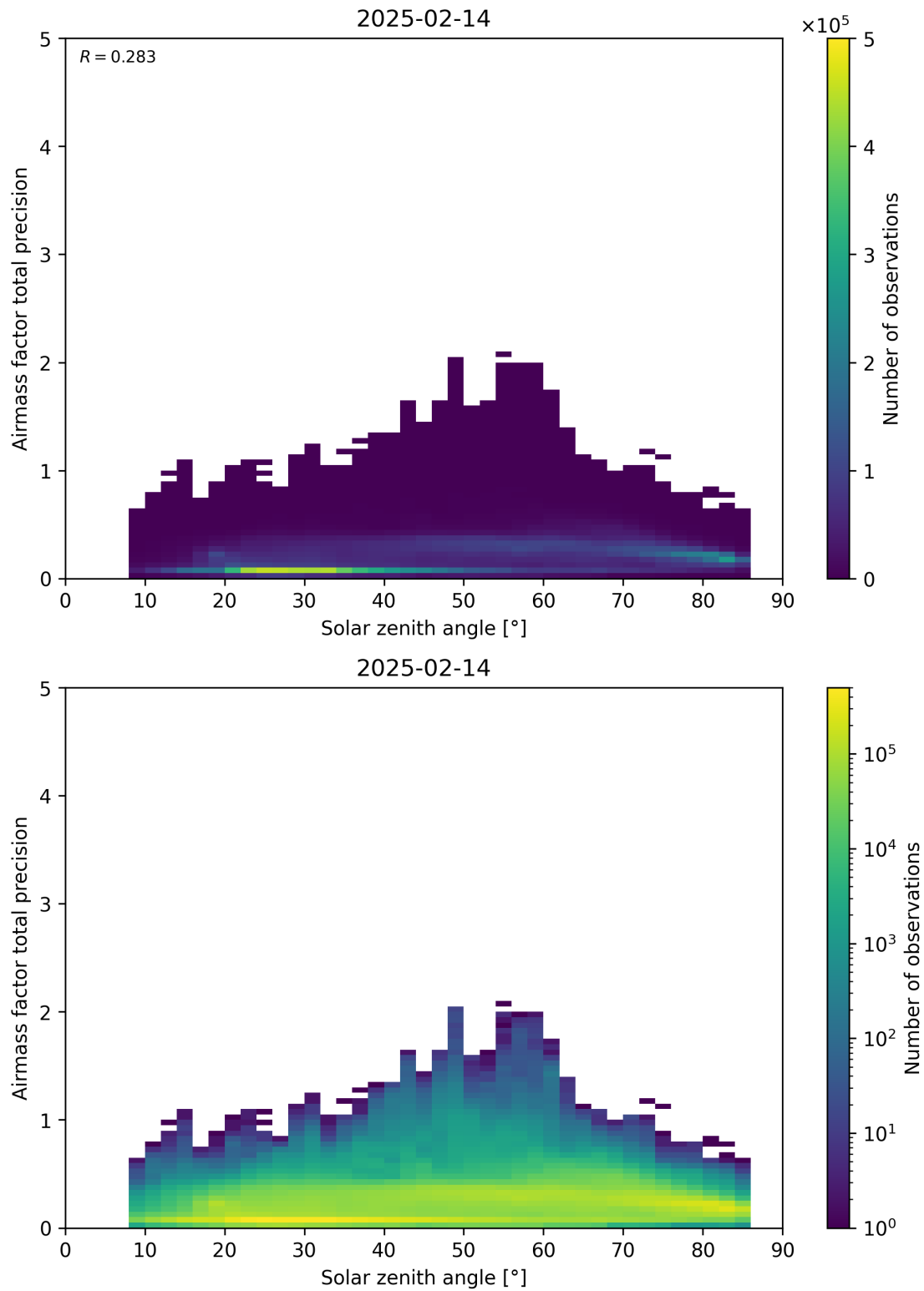
Figure 176: Scatter density plot of “Solar zenith angle” against “Airmass factor total precision” for 2025-02-13 to 2025-02-15.
