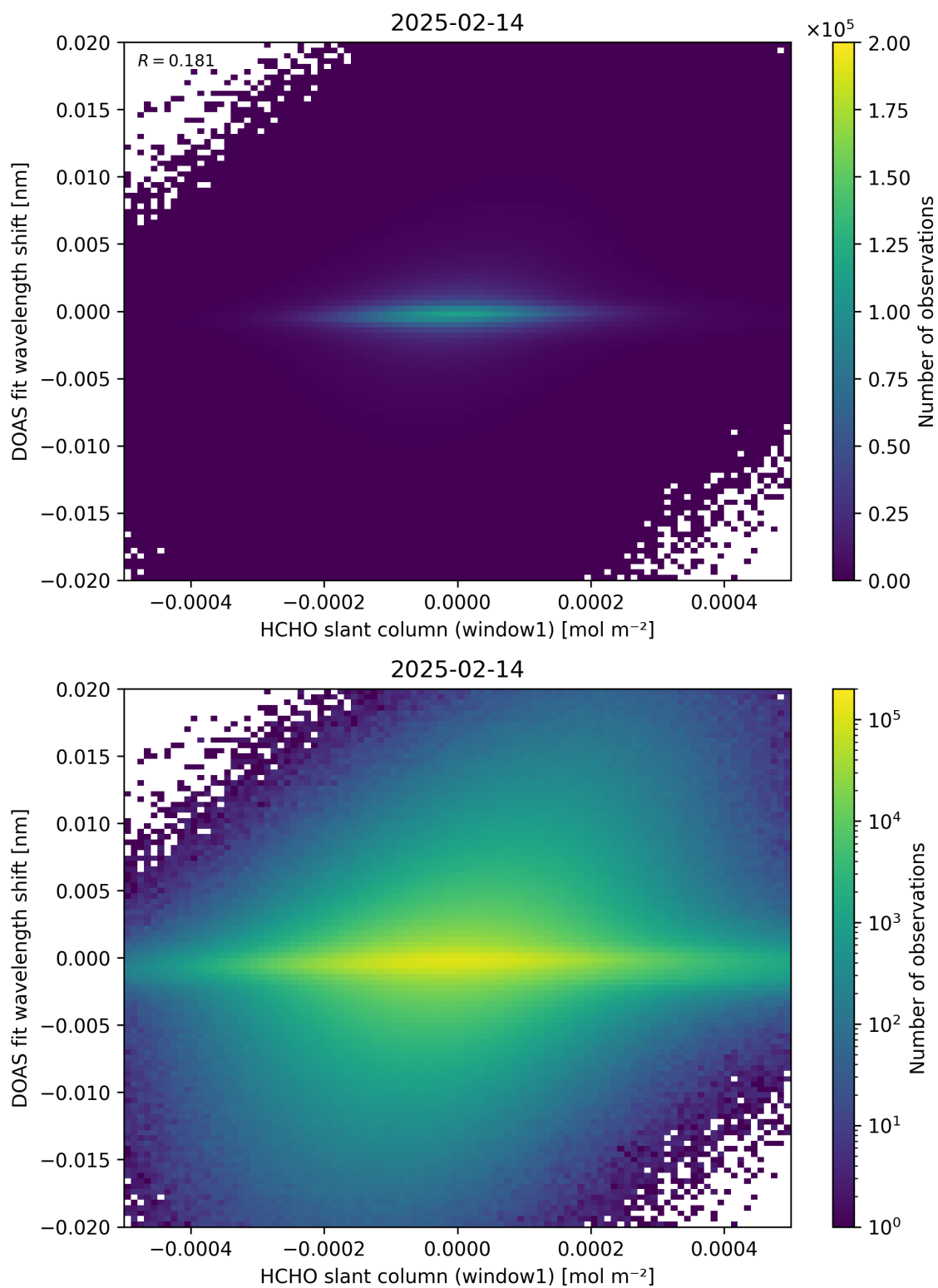
Figure 79: Scatter density plot of “HCHO slant column (window1)” against “DOAS fit wavelength shift” for 2025-02-13 to 2025-02-15.
