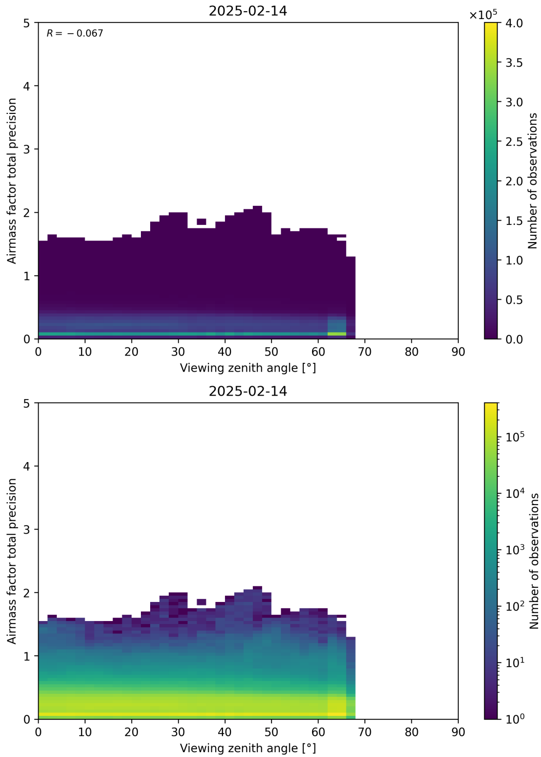
Figure 191: Scatter density plot of “Viewing zenith angle” against “Airmass factor total precision” for 2025-02-13 to 2025-02-15.
