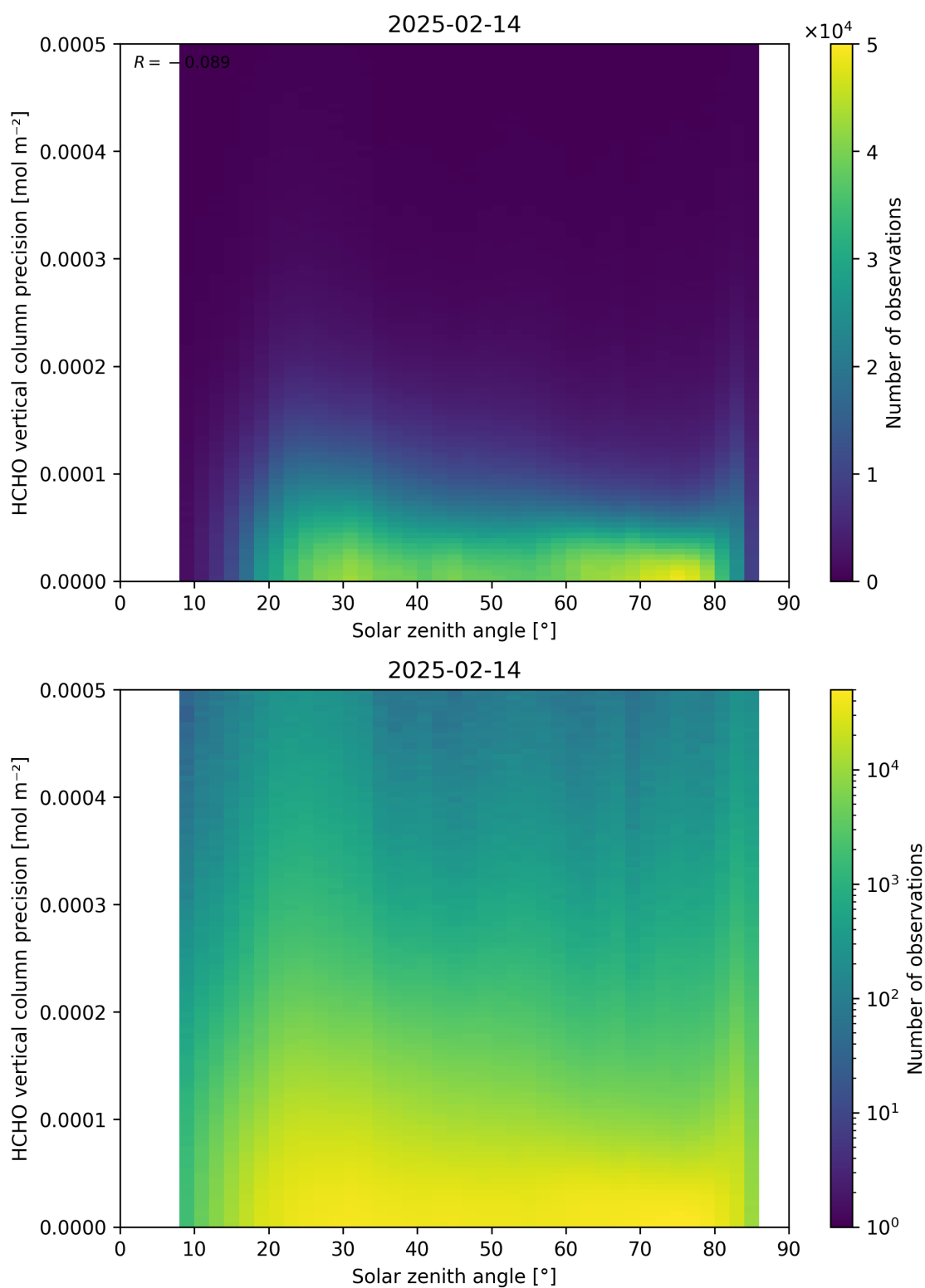
Figure 179: Scatter density plot of “Solar zenith angle” against “HCHO vertical column precision” for 2025-02-13 to 2025-02-15.
