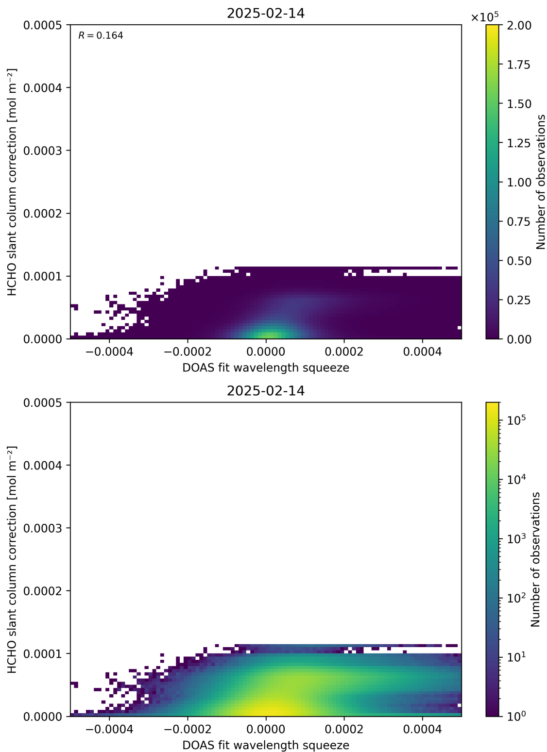
Figure 70: Scatter density plot of “DOAS fit wavelength squeeze” against “HCHO slant column correction” for 2025-02-13 to 2025-02-15.
