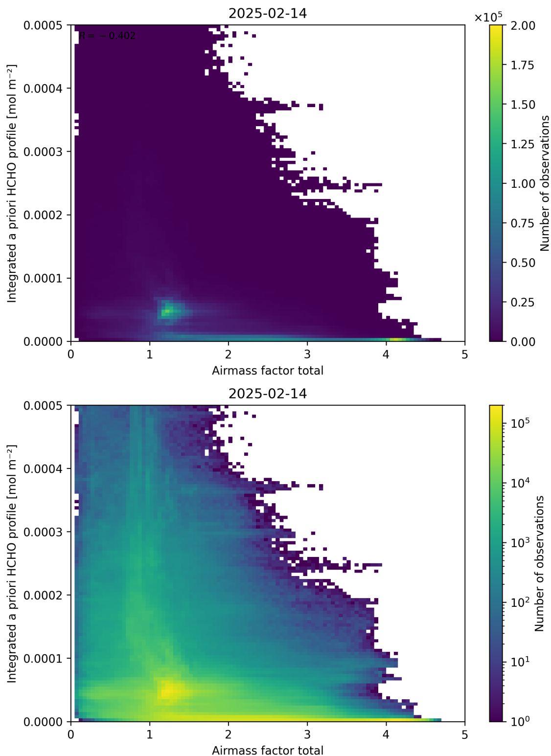
Figure 104: Scatter density plot of “Airmass factor total” against “Integrated a priori HCHO profile” for 2025-02-13 to 2025-02-15.
