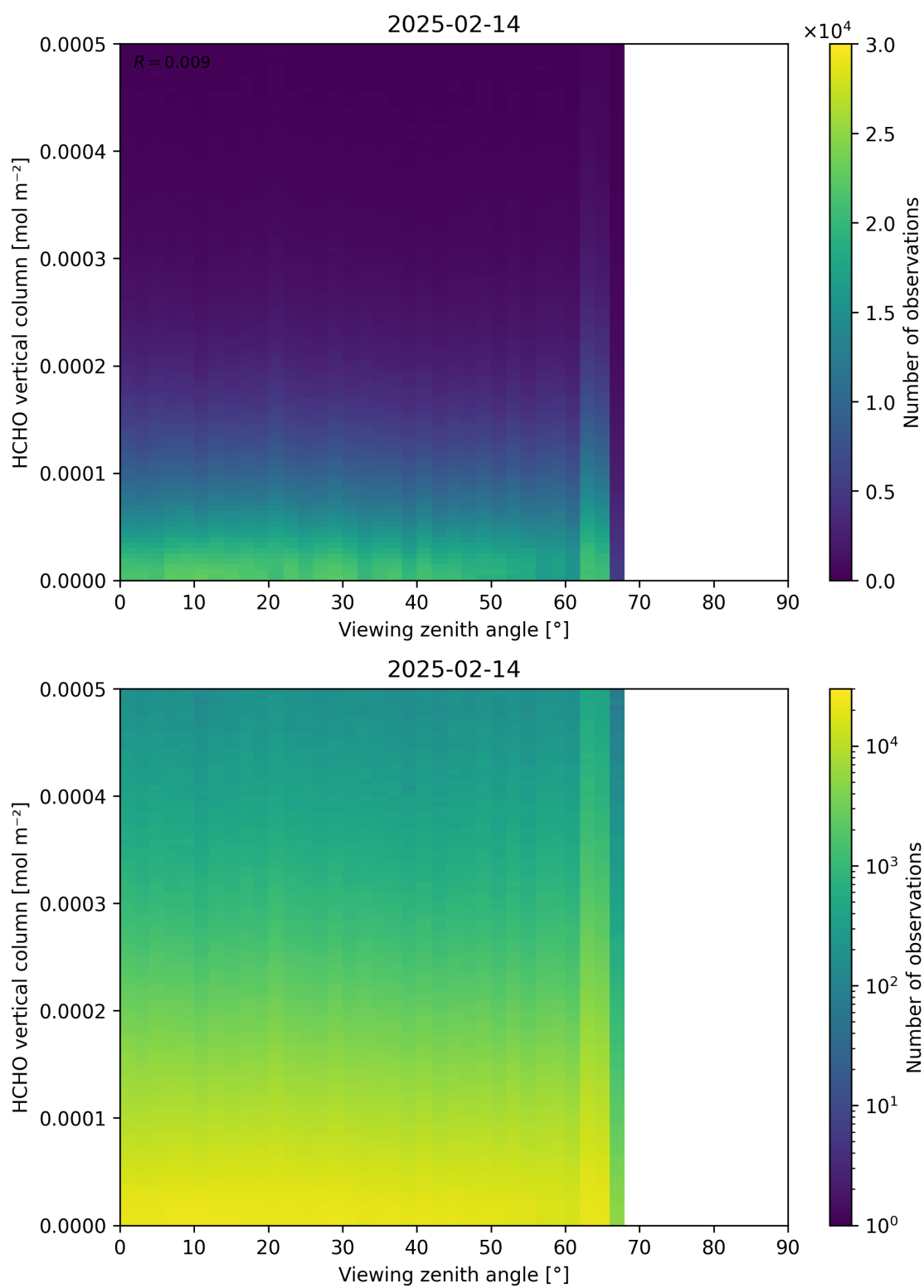
Figure 192: Scatter density plot of “Viewing zenith angle” against “HCHO vertical column” for 2025-02-13 to 2025-02-15.
