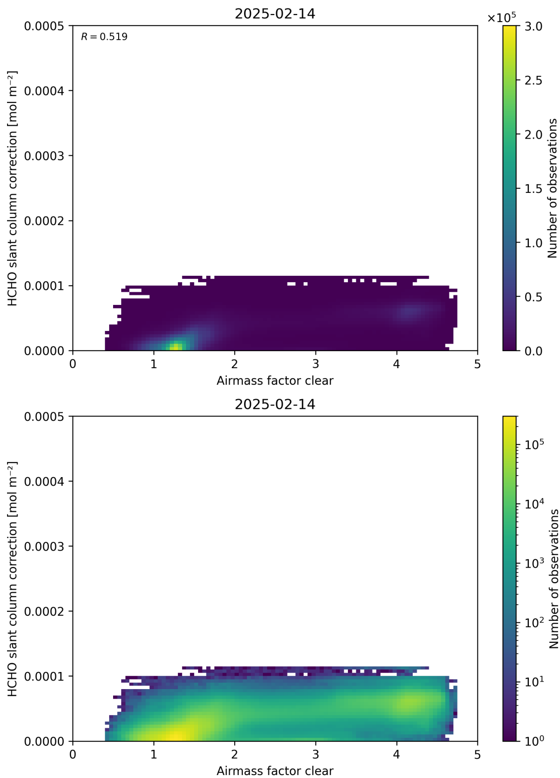
Figure 75: Scatter density plot of “Airmass factor clear” against “HCHO slant column correction” for 2025-02-13 to 2025-02-15.
