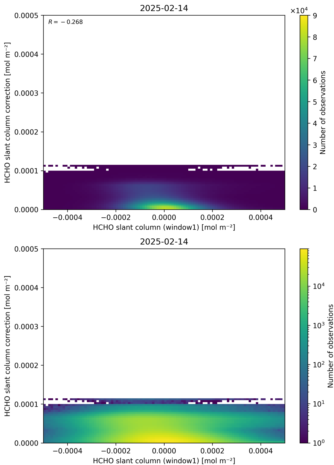
Figure 83: Scatter density plot of “HCHO slant column (window1)” against “HCHO slant column correction” for 2025-02-13 to 2025-02-15.
