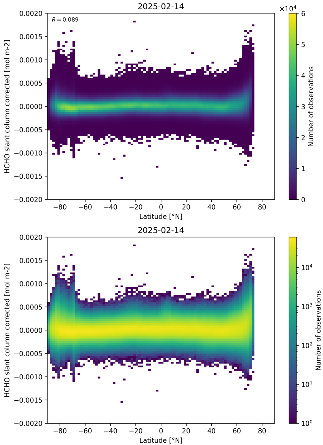
Figure 157: Scatter density plot of “Latitude” against “HCHO slant column corrected” for 2025-02-13 to 2025-02-15.
