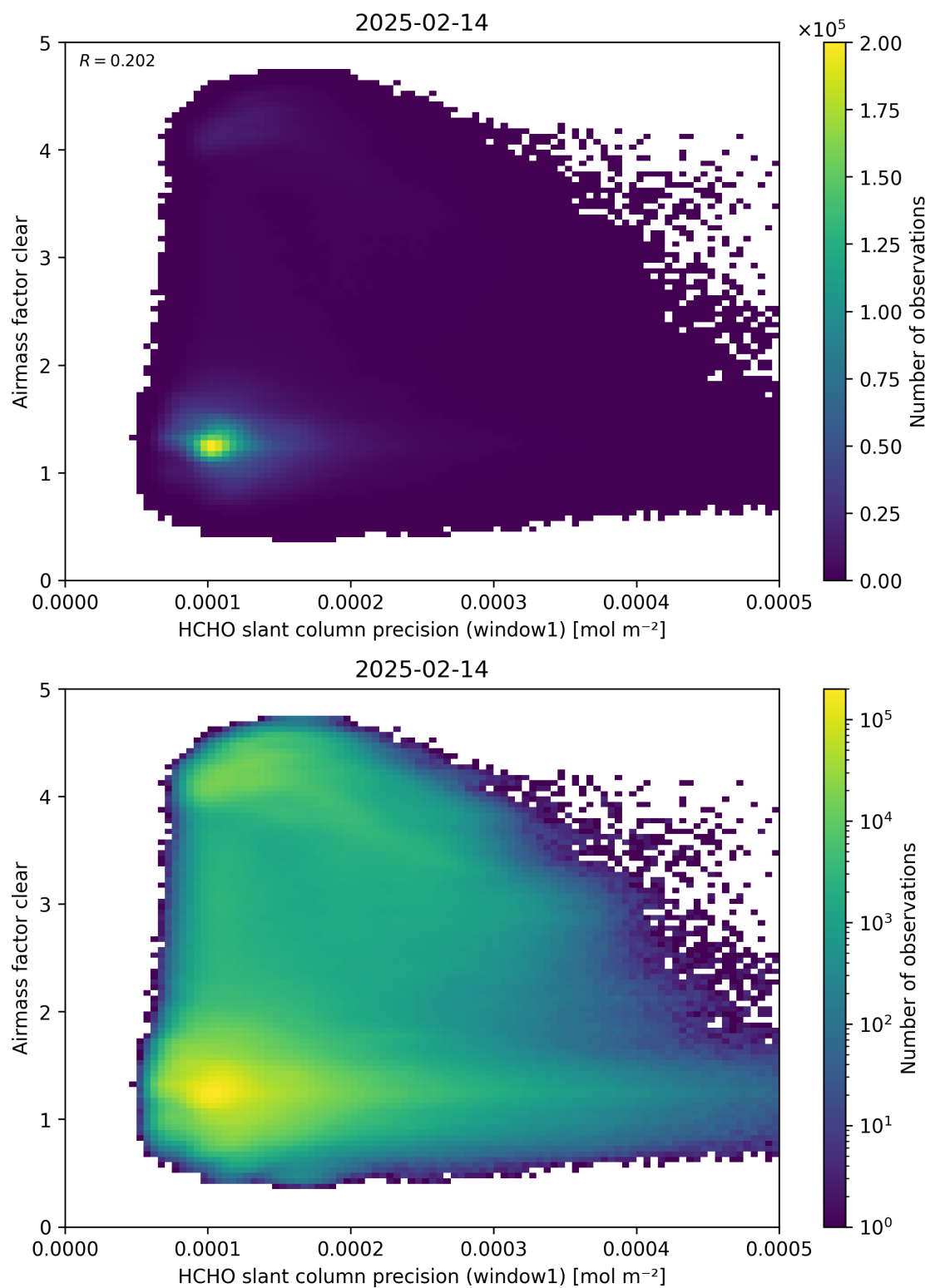
Figure 91: Scatter density plot of “HCHO slant column precision (window1)” against “Airmass factor clear” for 2025-02-13 to 2025-02-15.
