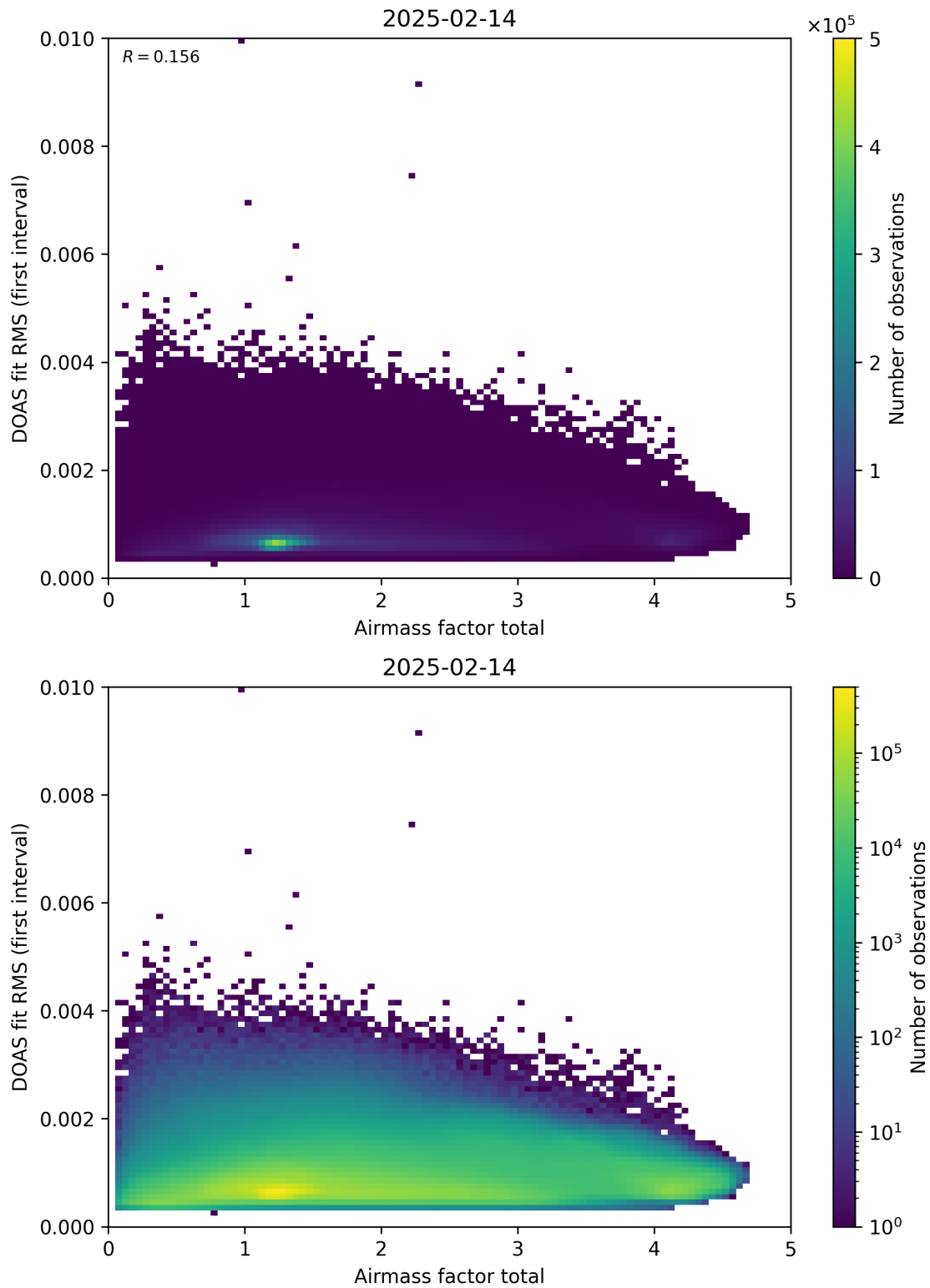
Figure 97: Scatter density plot of “Airmass factor total” against “DOAS fit RMS (first interval)” for 2025-02-13 to 2025-02-15.
