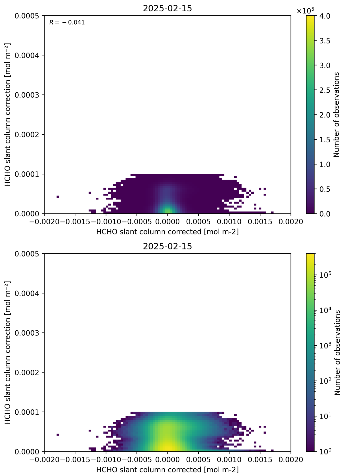
Figure 77: Scatter density plot of “HCHO slant column corrected” against “HCHO slant column correction” for 2025-02-14 to 2025-02-16.
