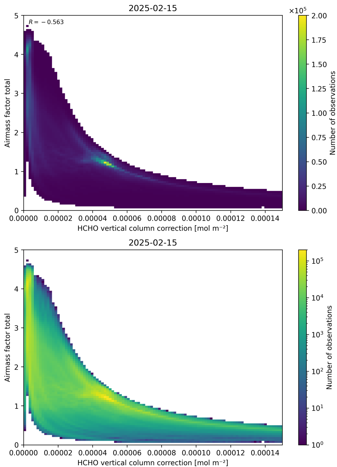
Figure 120: Scatter density plot of “HCHO vertical column correction” against “Airmass factor total” for 2025-02-14 to 2025-02-16.
