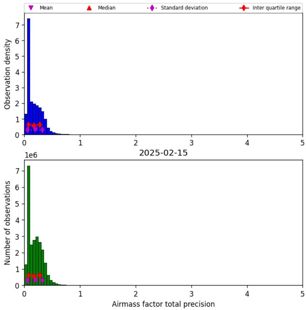
Figure 41: Histogram of “Airmass factor total precision” for 2025-02-14 to 2025-02-16
