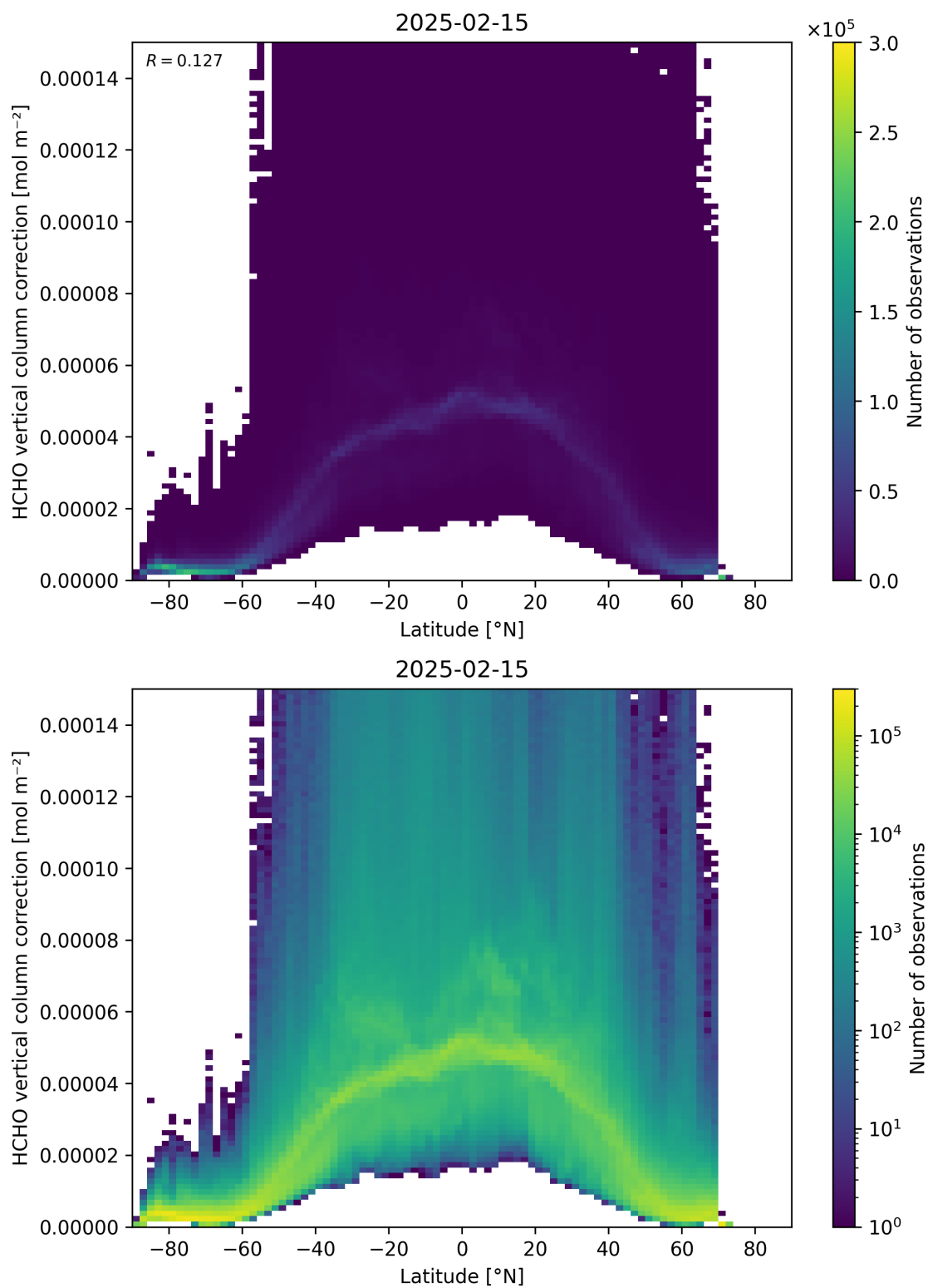
Figure 164: Scatter density plot of “Latitude” against “HCHO vertical column correction” for 2025-02-14 to 2025-02-16.
