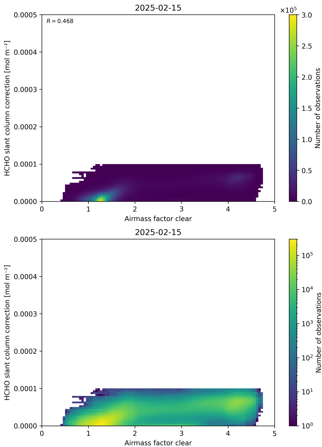
Figure 75: Scatter density plot of “Airmass factor clear” against “HCHO slant column correction” for 2025-02-14 to 2025-02-16.
