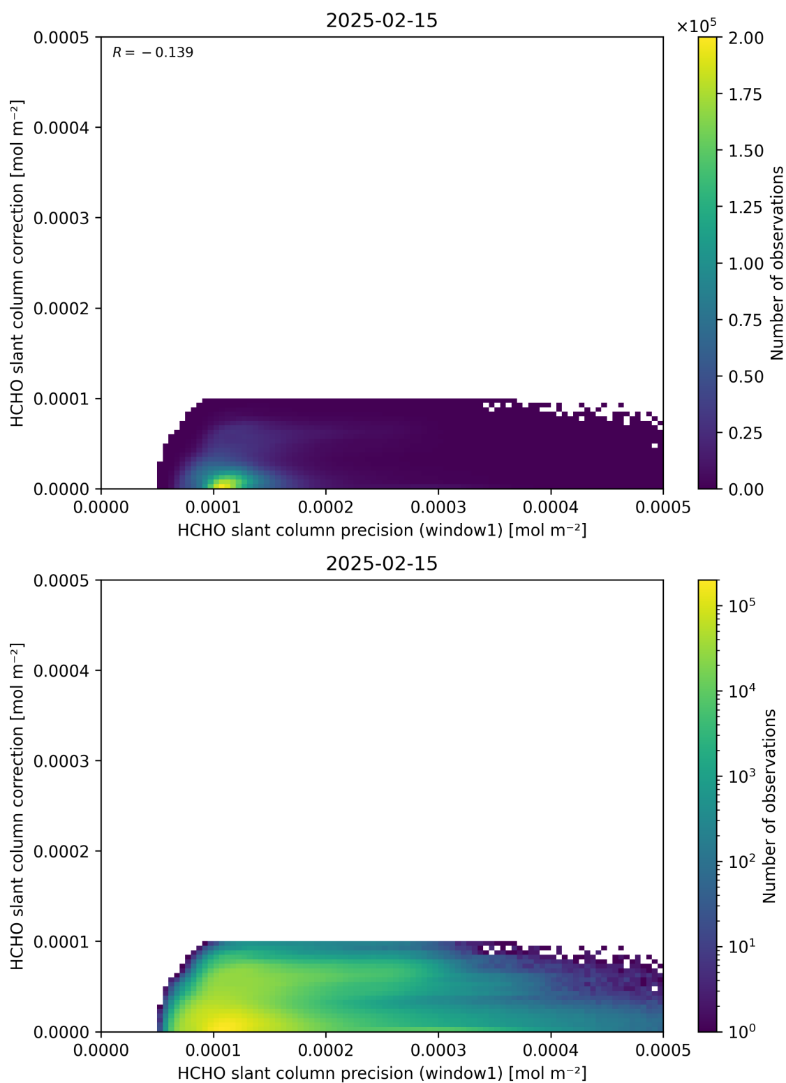
Figure 93: Scatter density plot of “HCHO slant column precision (window1)” against “HCHO slant column correction” for 2025-02-14 to 2025-02-16.
