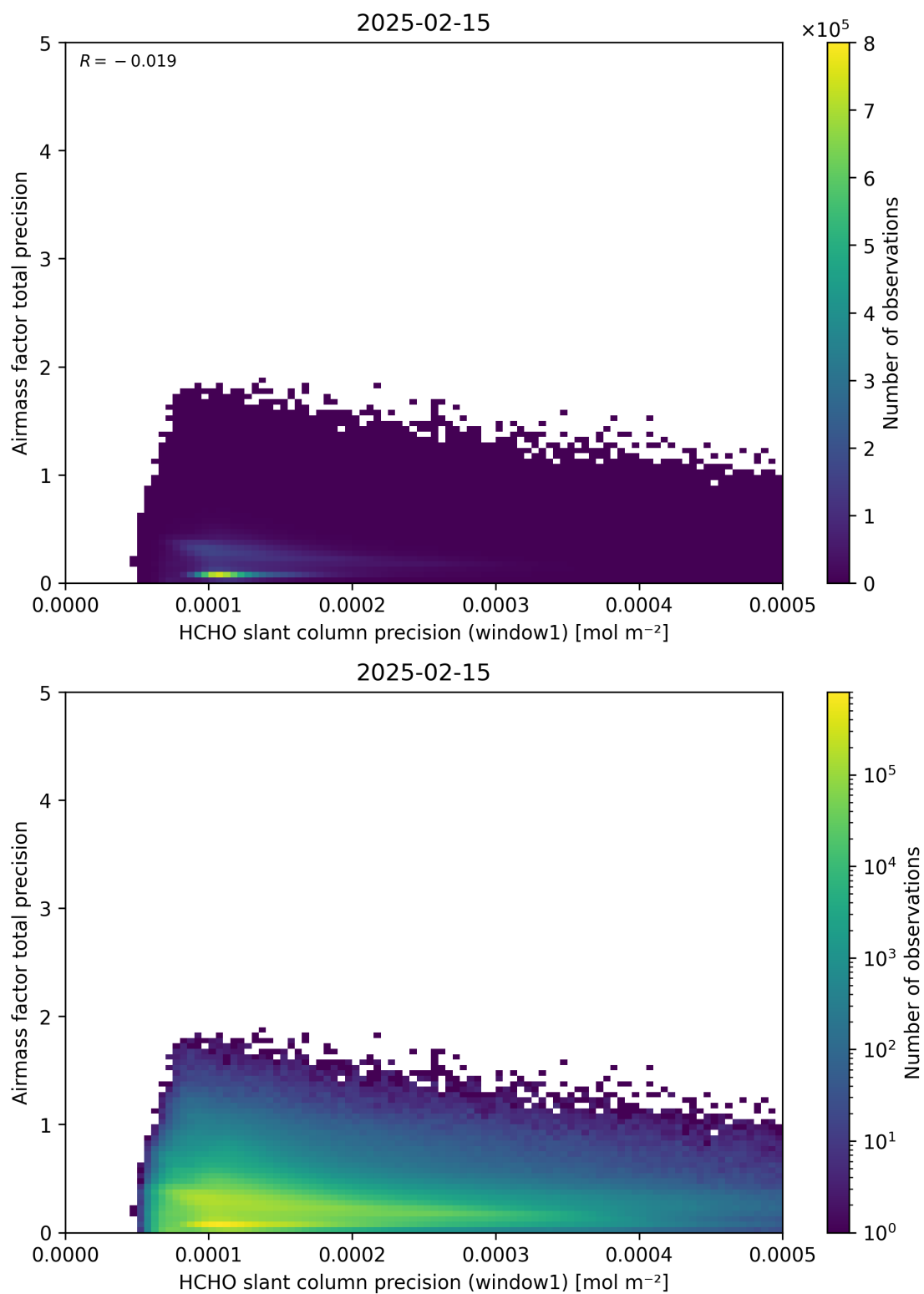
Figure 95: Scatter density plot of “HCHO slant column precision (window1)” against “Airmass factor total precision” for 2025-02-14 to 2025-02-16.
