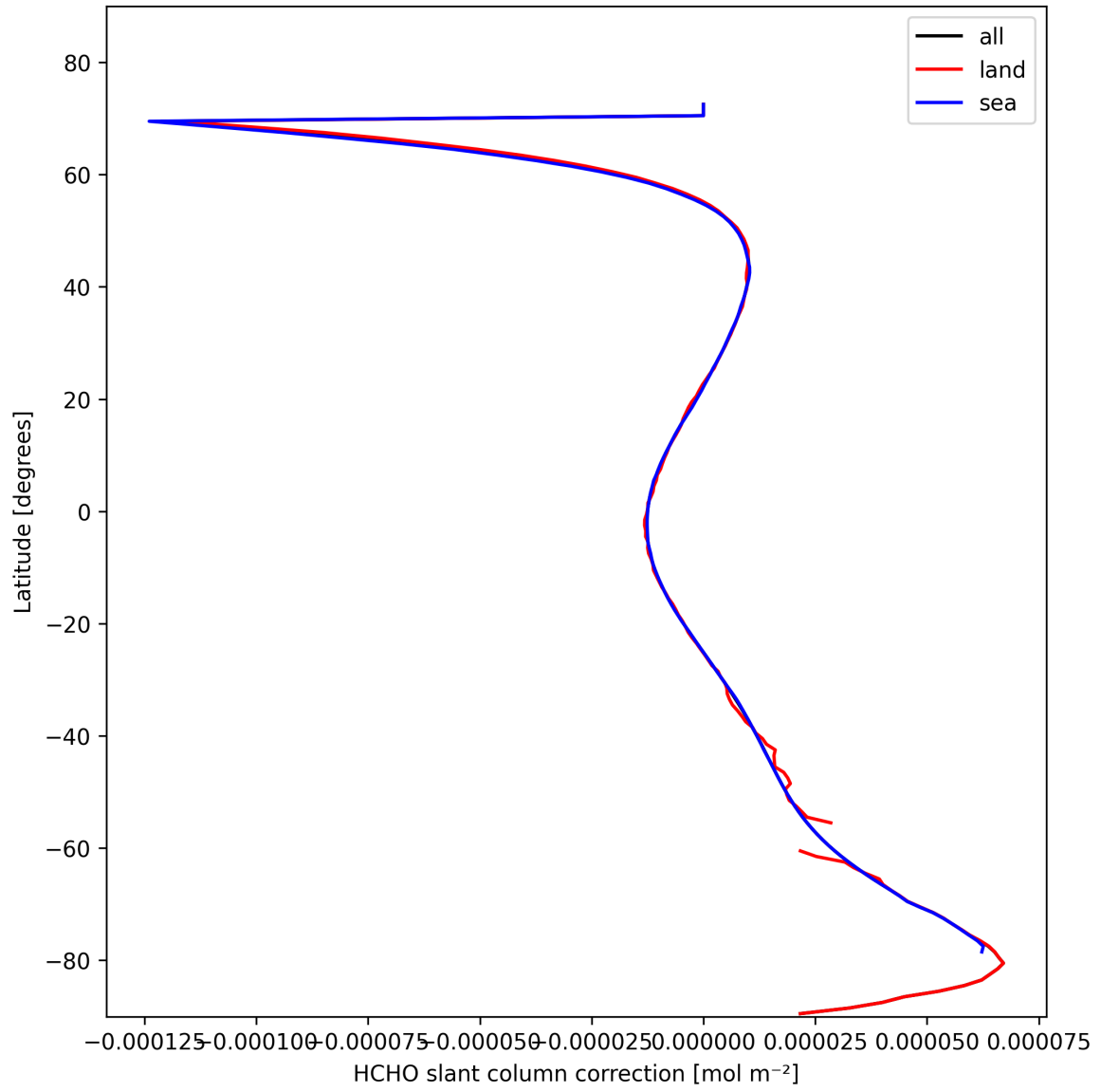
Figure 33: Zonal average of “HCHO slant column correction” for 2025-02-14 to 2025-02-16.
