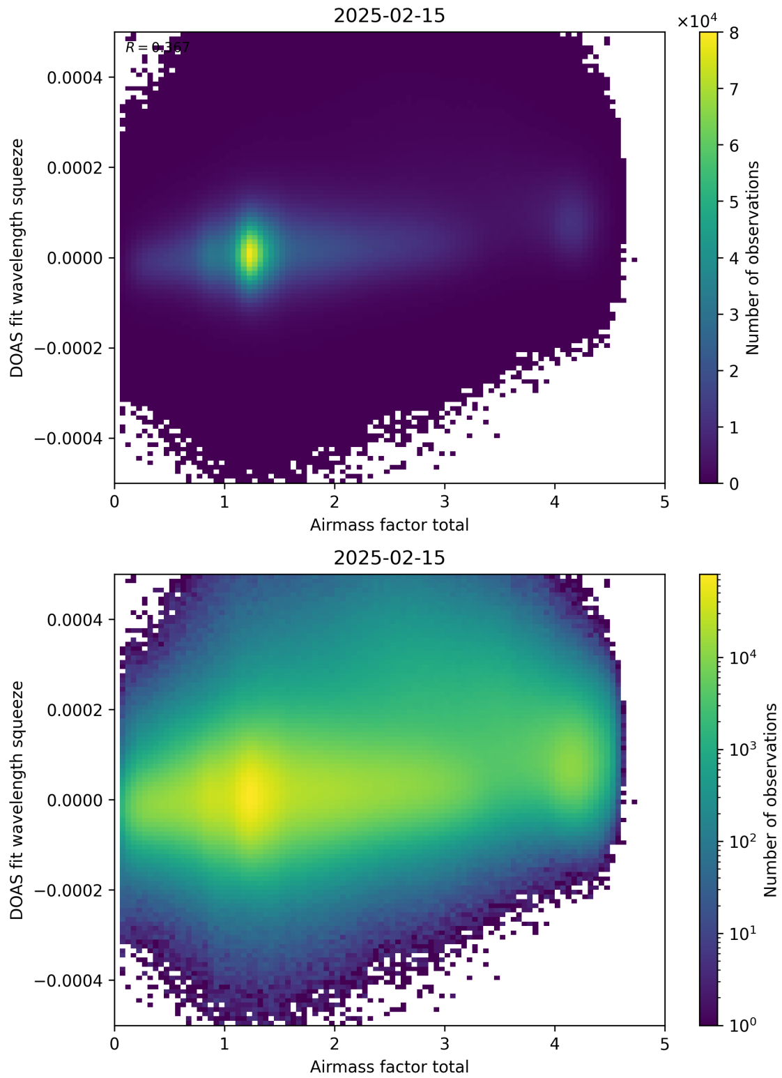
Figure 99: Scatter density plot of “Airmass factor total” against “DOAS fit wavelength squeeze” for 2025-02-14 to 2025-02-16.
