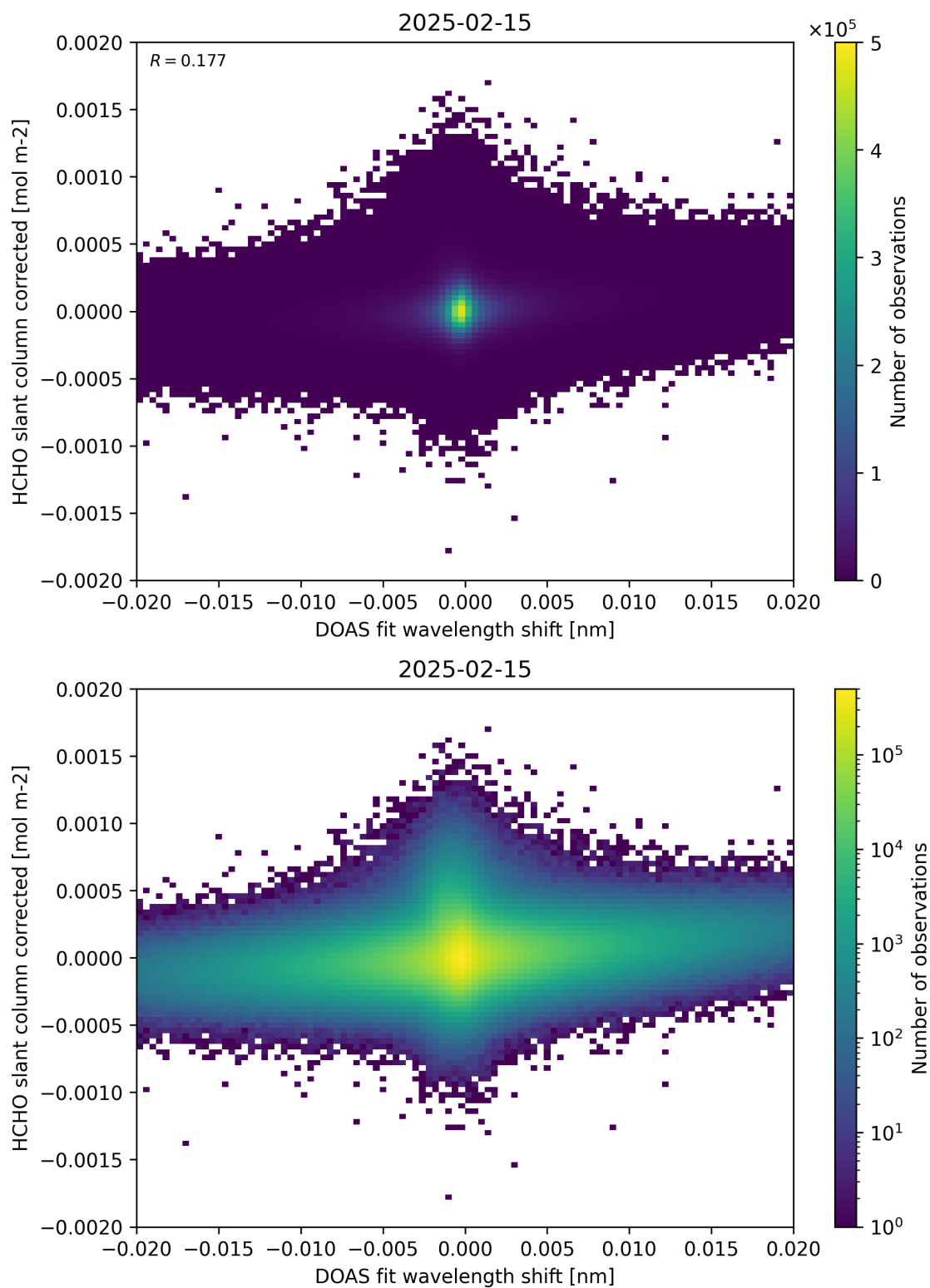
Figure 66: Scatter density plot of “DOAS fit wavelength shift” against “HCHO slant column corrected” for 2025-02-14 to 2025-02-16.
