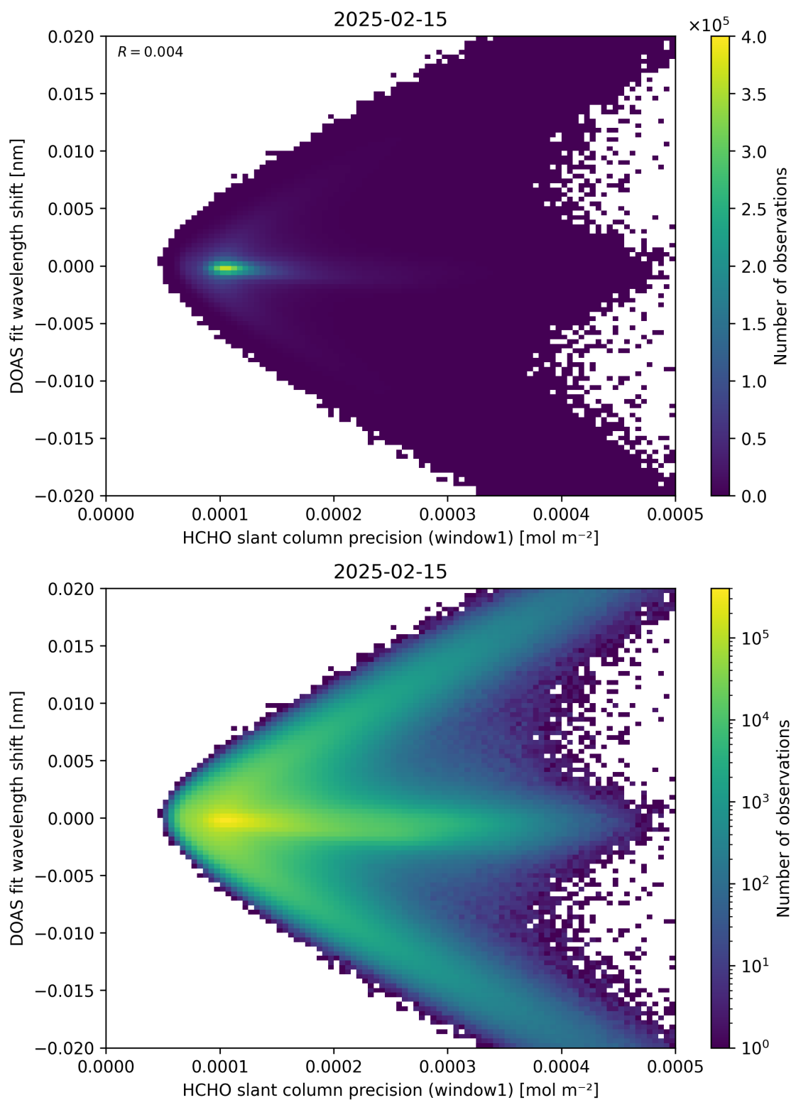
Figure 89: Scatter density plot of “HCHO slant column precision (window1)” against “DOAS fit wavelength shift” for 2025-02-14 to 2025-02-16.
