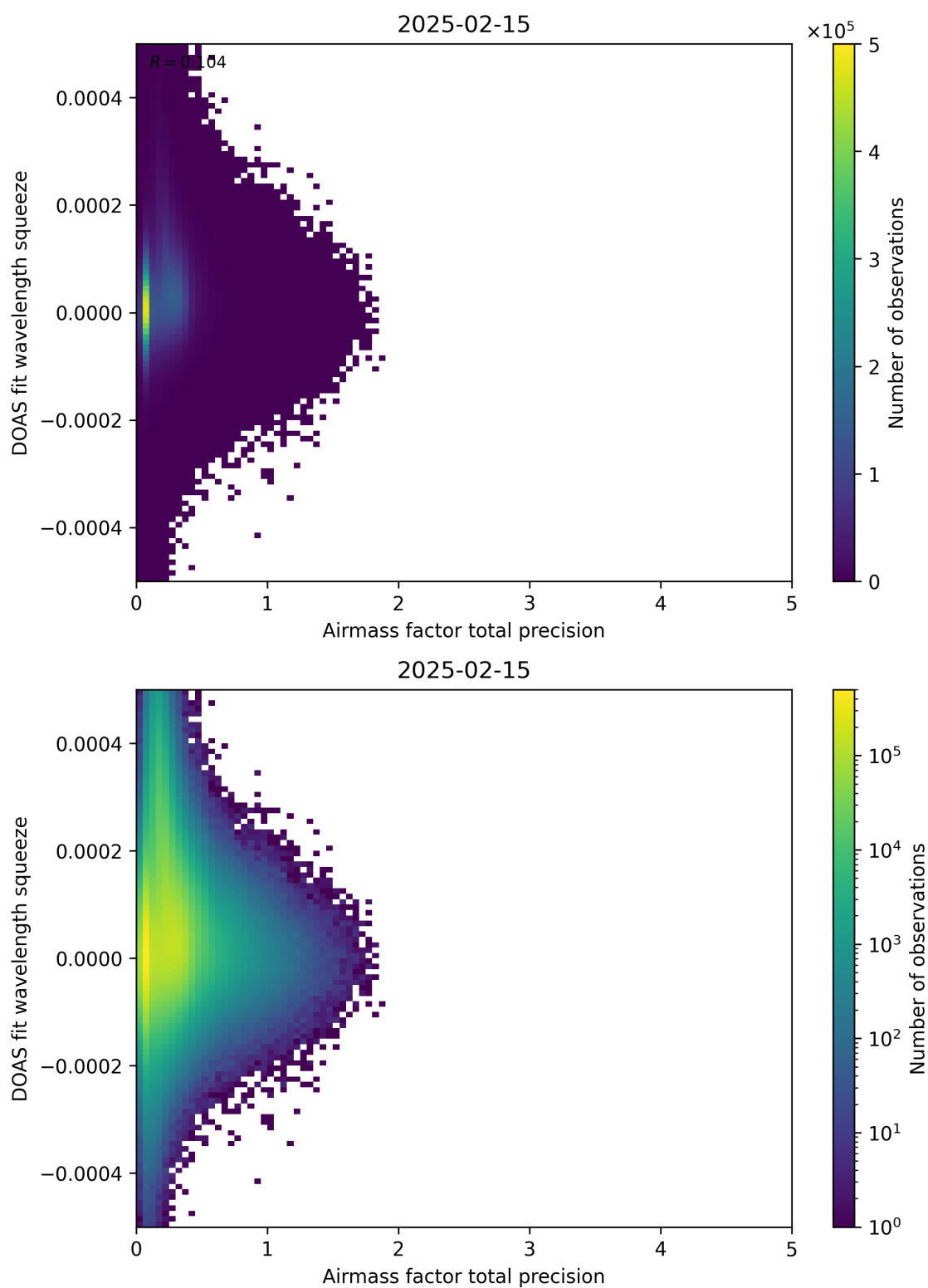
Figure 107: Scatter density plot of “Airmass factor total precision” against “DOAS fit wavelength squeeze” for 2025-02-14 to 2025-02-16.
