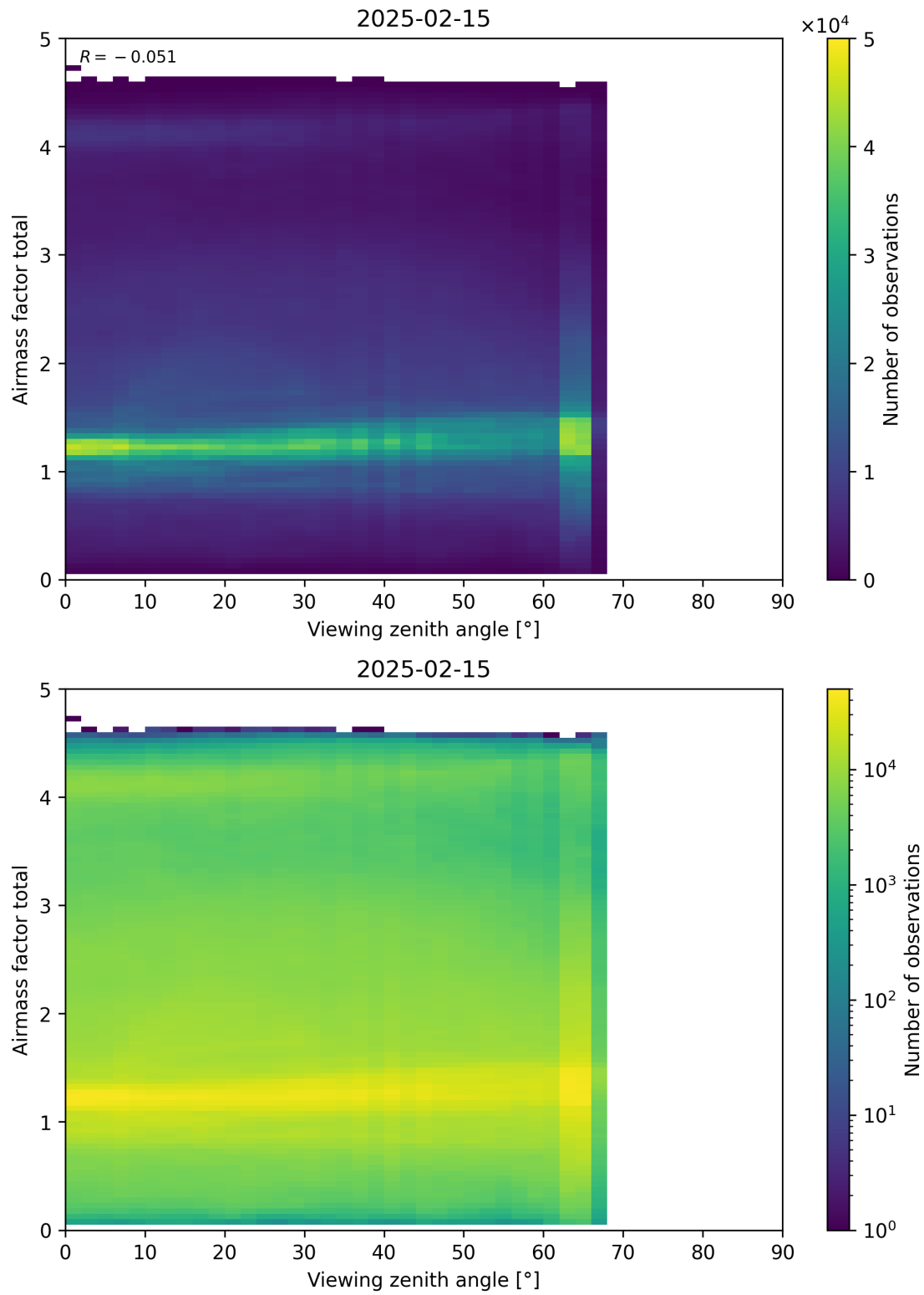
Figure 190: Scatter density plot of “Viewing zenith angle” against “Airmass factor total” for 2025-02-14 to 2025-02-16.
