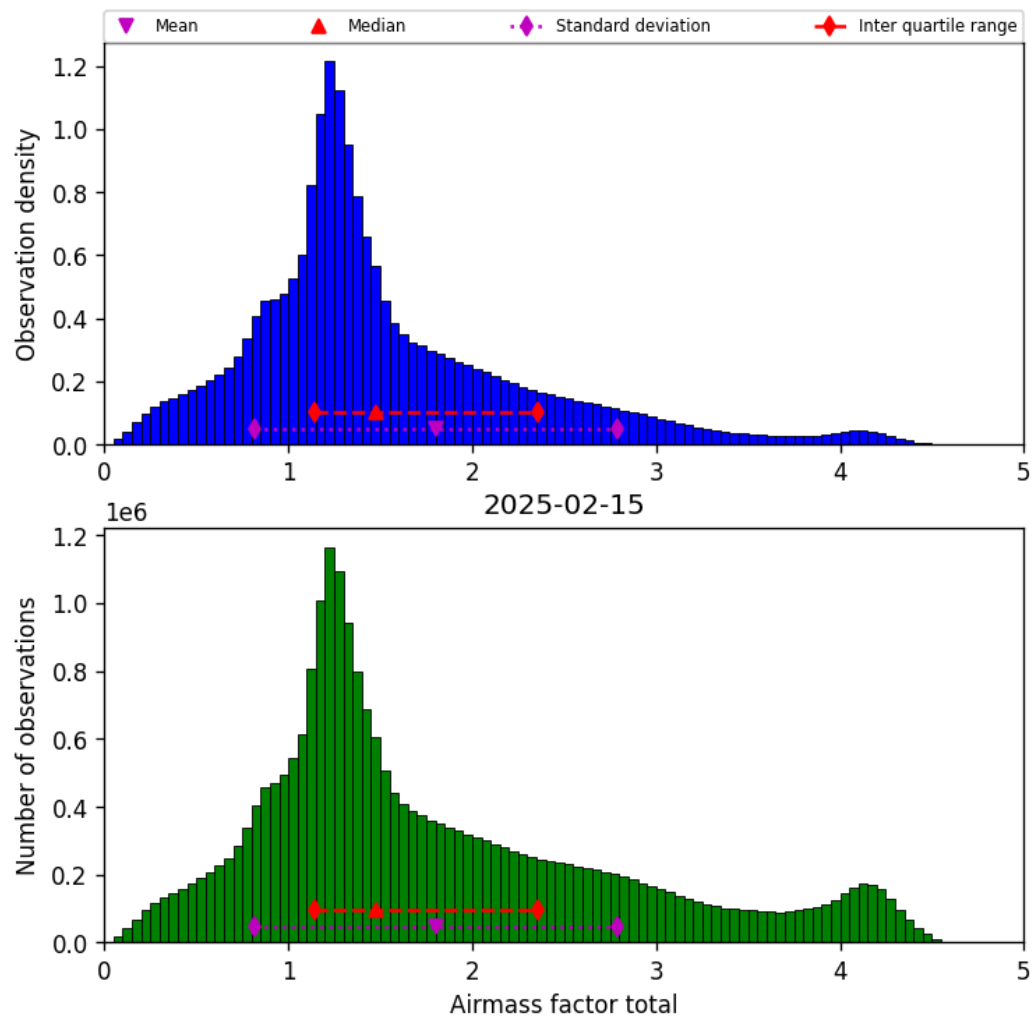
Figure 40: Histogram of “Airmass factor total” for 2025-02-14 to 2025-02-16
