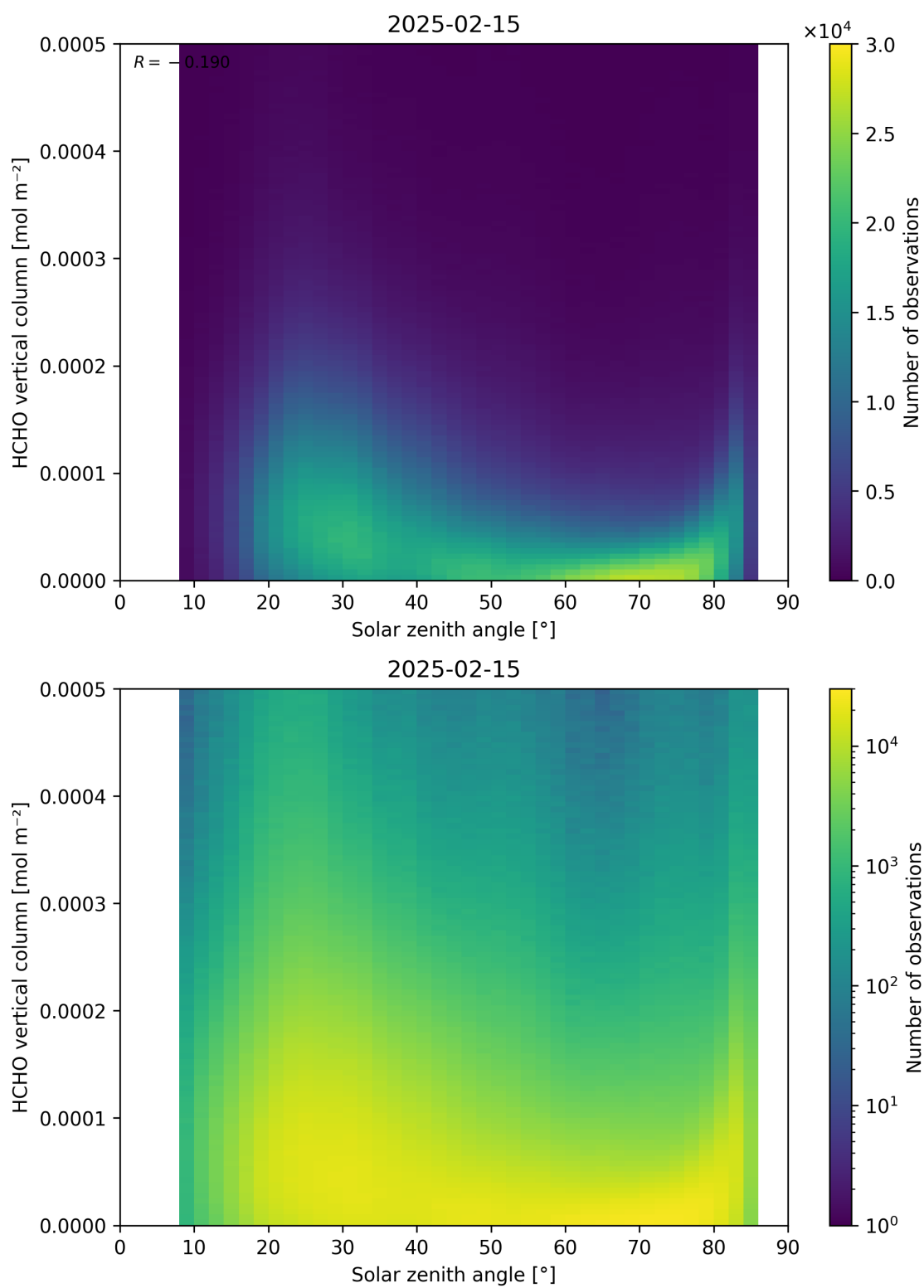
Figure 177: Scatter density plot of “Solar zenith angle” against “HCHO vertical column” for 2025-02-14 to 2025-02-16.
