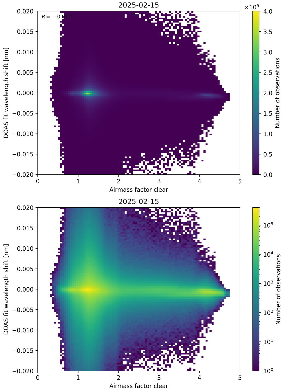
Figure 72: Scatter density plot of “Airmass factor clear” against “DOAS fit wavelength shift” for 2025-02-14 to 2025-02-16.
