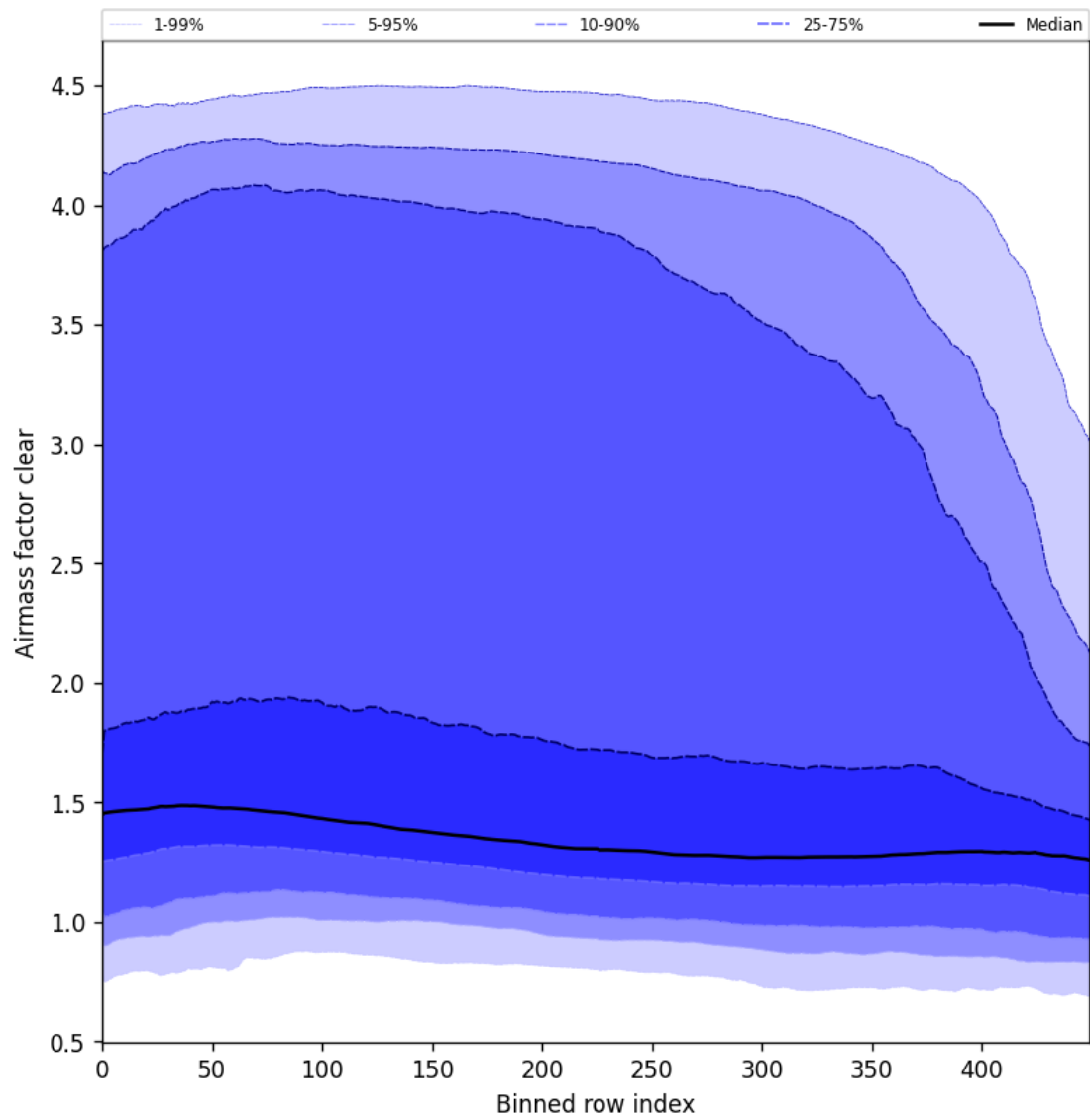
Figure 56: Along track statistics of “Airmass factor clear” for 2025-02-14 to 2025-02-16
