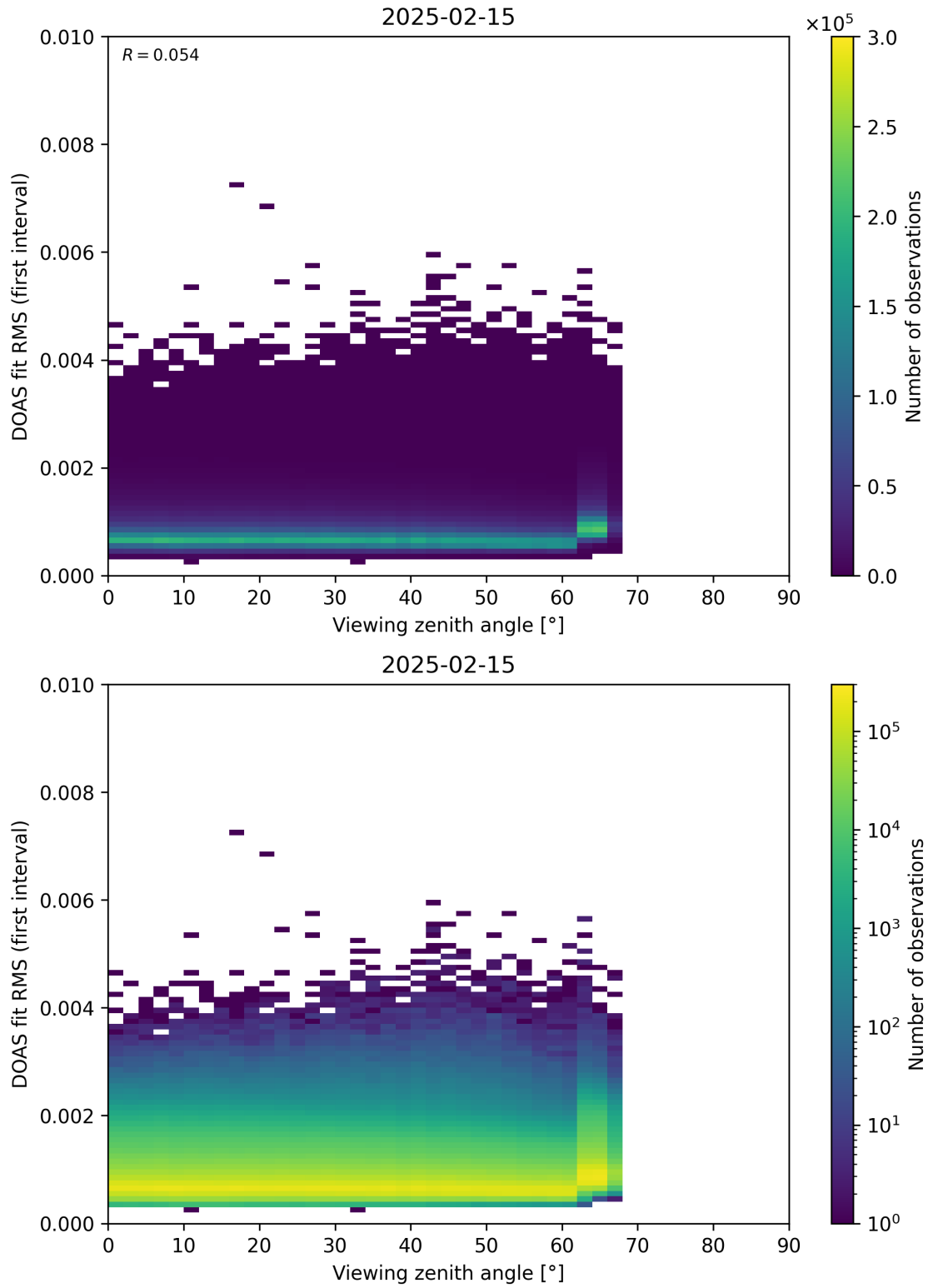
Figure 182: Scatter density plot of “Viewing zenith angle” against “DOAS fit RMS (first interval)” for 2025-02-14 to 2025-02-16.
