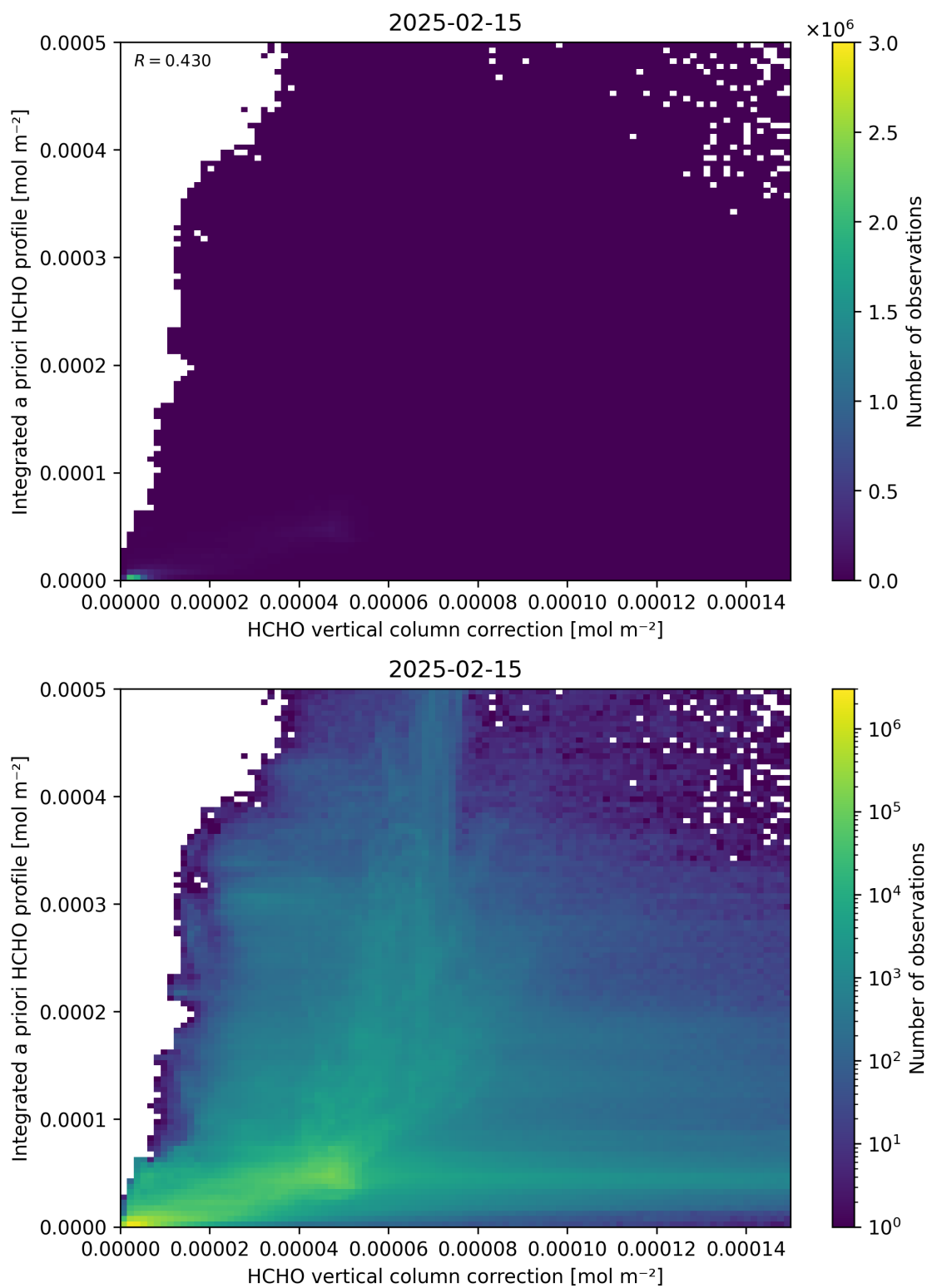
Figure 122: Scatter density plot of “HCHO vertical column correction” against “Integrated a priori HCHO profile” for 2025-02-14 to 2025-02-16.
