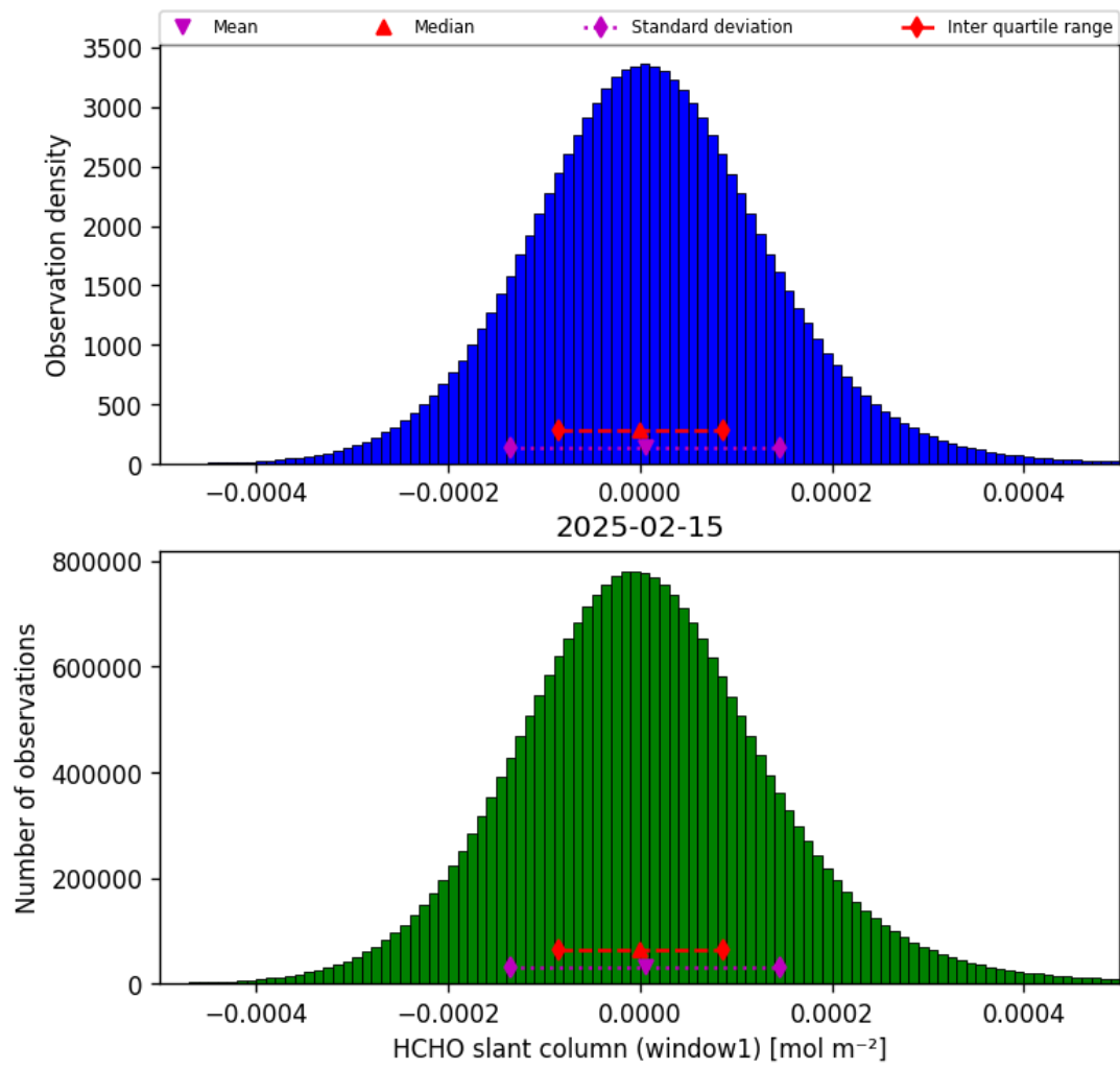
Figure 38: Histogram of “HCHO slant column (window1)” for 2025-02-14 to 2025-02-16
