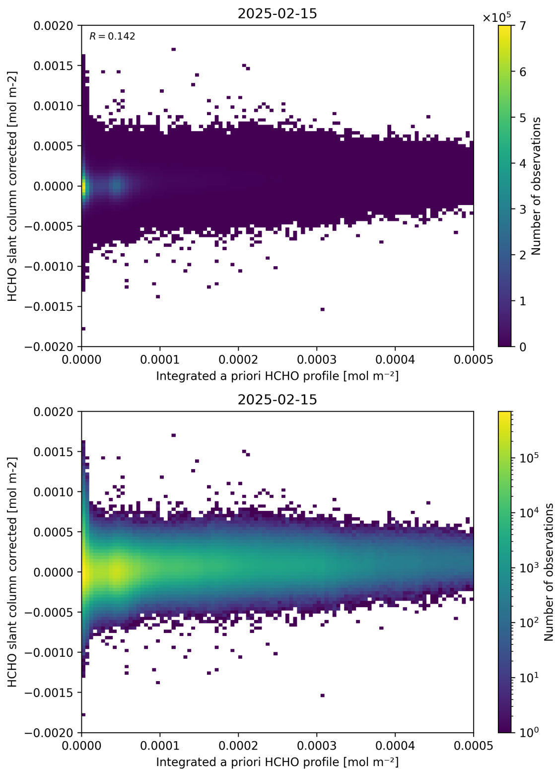
Figure 151: Scatter density plot of “Integrated a priori HCHO profile” against “HCHO slant column corrected” for 2025-02-14 to 2025-02-16.
