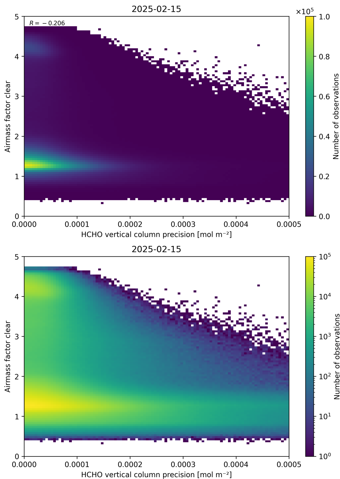
Figure 139: Scatter density plot of “HCHO vertical column precision” against “Airmass factor clear” for 2025-02-14 to 2025-02-16.
