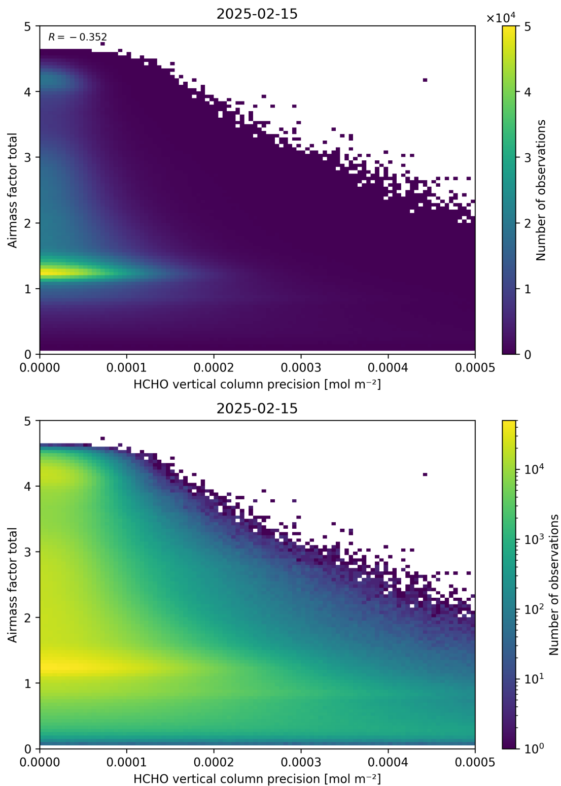
Figure 144: Scatter density plot of “HCHO vertical column precision” against “Airmass factor total” for 2025-02-14 to 2025-02-16.
