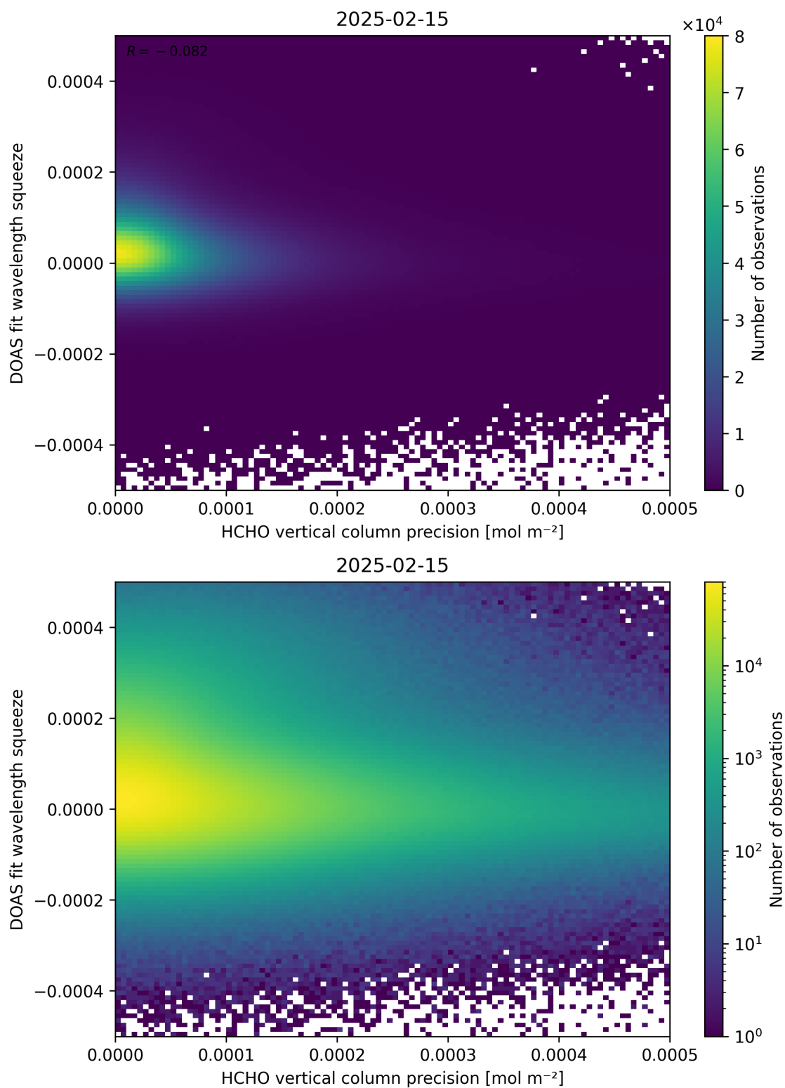
Figure 138: Scatter density plot of “HCHO vertical column precision” against “DOAS fit wavelength squeeze” for 2025-02-14 to 2025-02-16.
