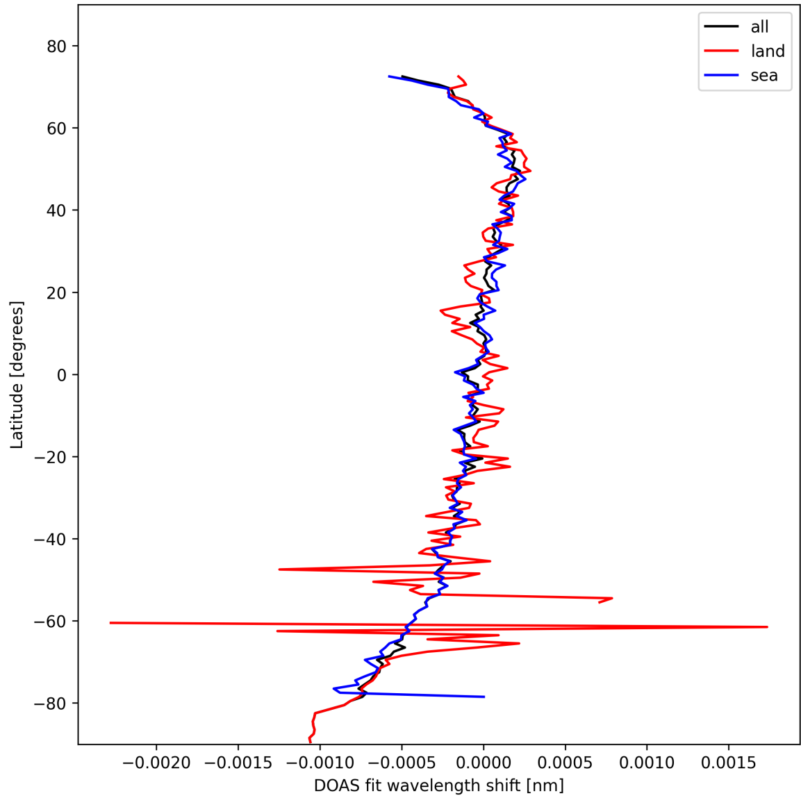
Figure 30: Zonal average of "DOAS fit wavelength shift" for 2025-02-14 to 2025-02-16.
