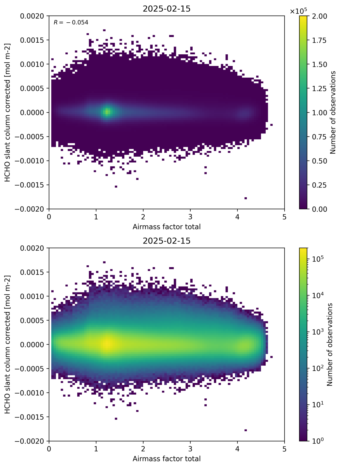
Figure 101: Scatter density plot of “Airmass factor total” against “HCHO slant column corrected” for 2025-02-14 to 2025-02-16.
