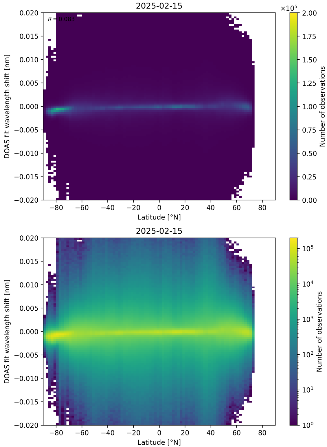
Figure 154: Scatter density plot of “Latitude” against “DOAS fit wavelength shift” for 2025-02-14 to 2025-02-16.
