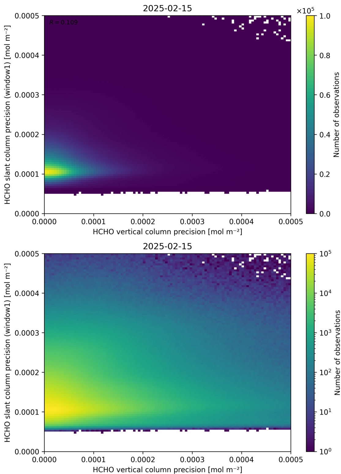
Figure 143: Scatter density plot of “HCHO vertical column precision” against “HCHO slant column precision (window1)” for 2025-02-14 to 2025-02-16.
