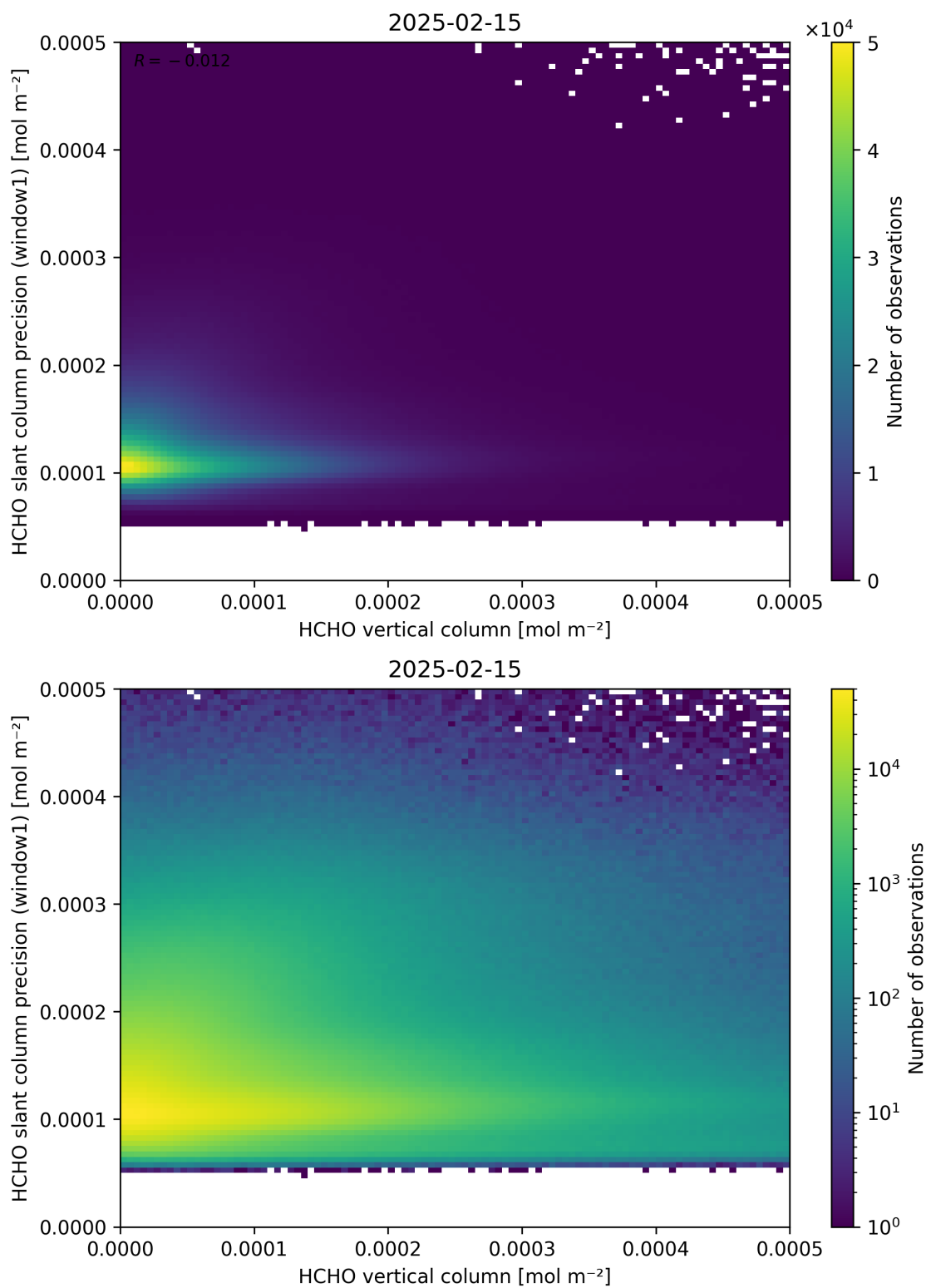
Figure 130: Scatter density plot of “HCHO vertical column” against “HCHO slant column precision (window1)” for 2025-02-14 to 2025-02-16.
