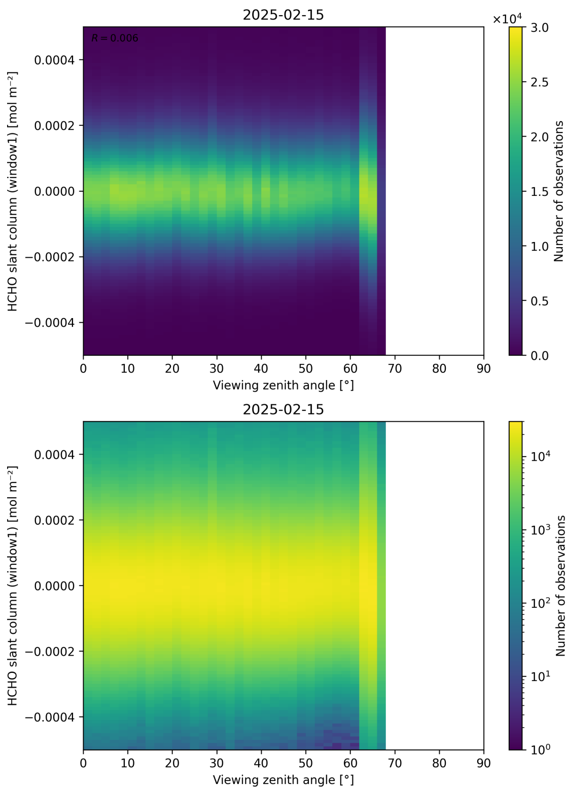
Figure 188: Scatter density plot of “Viewing zenith angle” against “HCHO slant column (window1)” for 2025-02-14 to 2025-02-16.
