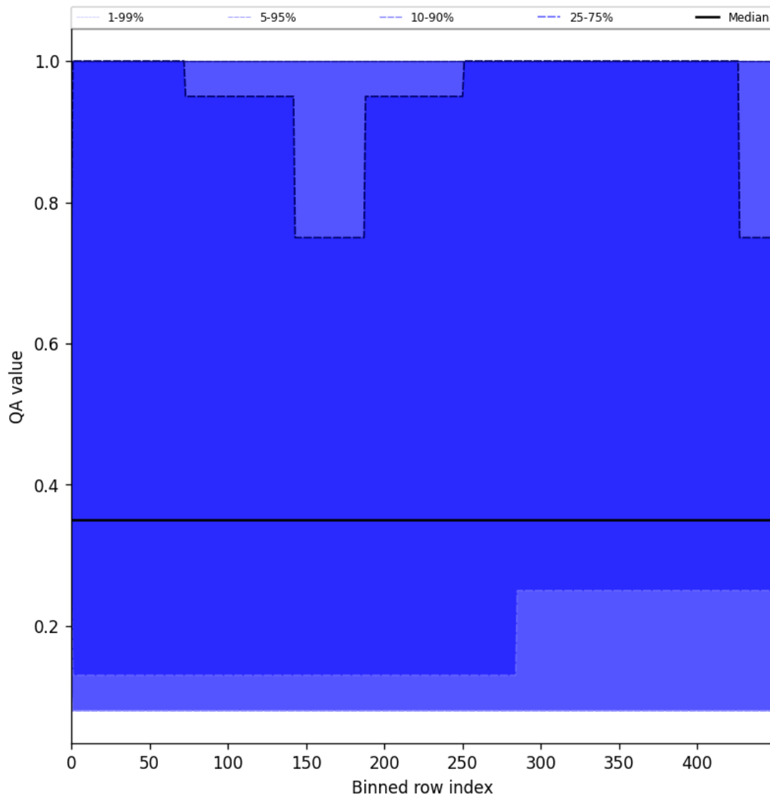
Figure 48: Along track statistics of “QA value” for 2025-02-14 to 2025-02-16
