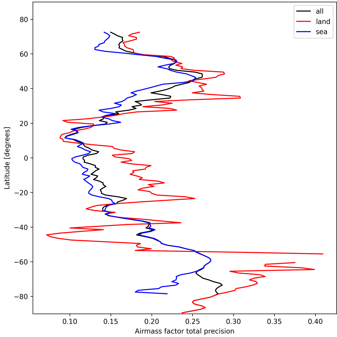
Figure 27: Zonal average of “Airmass factor total precision” for 2025-02-14 to 2025-02-16.
