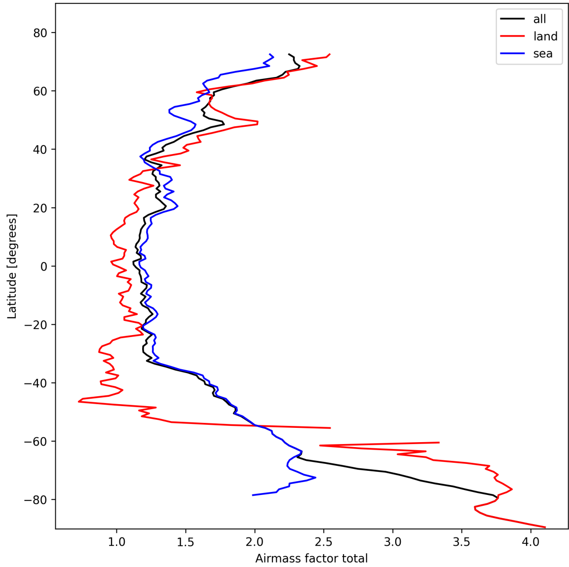
Figure 26: Zonal average of “Airmass factor total” for 2025-02-14 to 2025-02-16.
