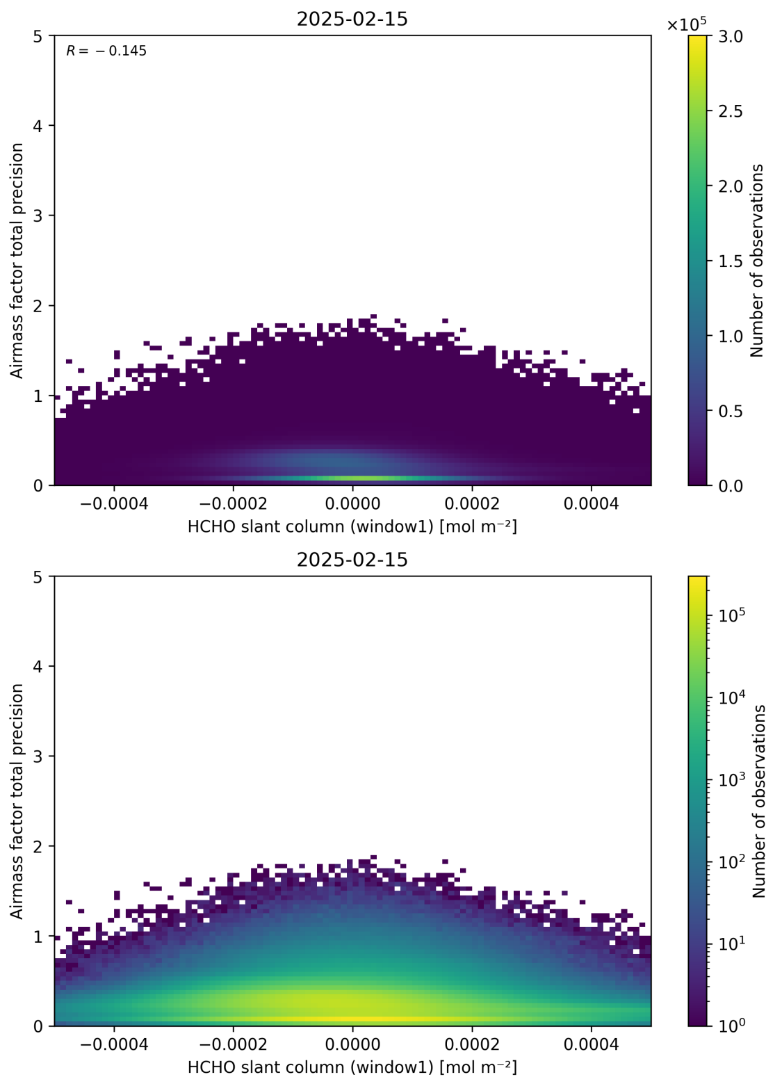
Figure 86: Scatter density plot of “HCHO slant column (window1)” against “Airmass factor total precision” for 2025-02-14 to 2025-02-16.
