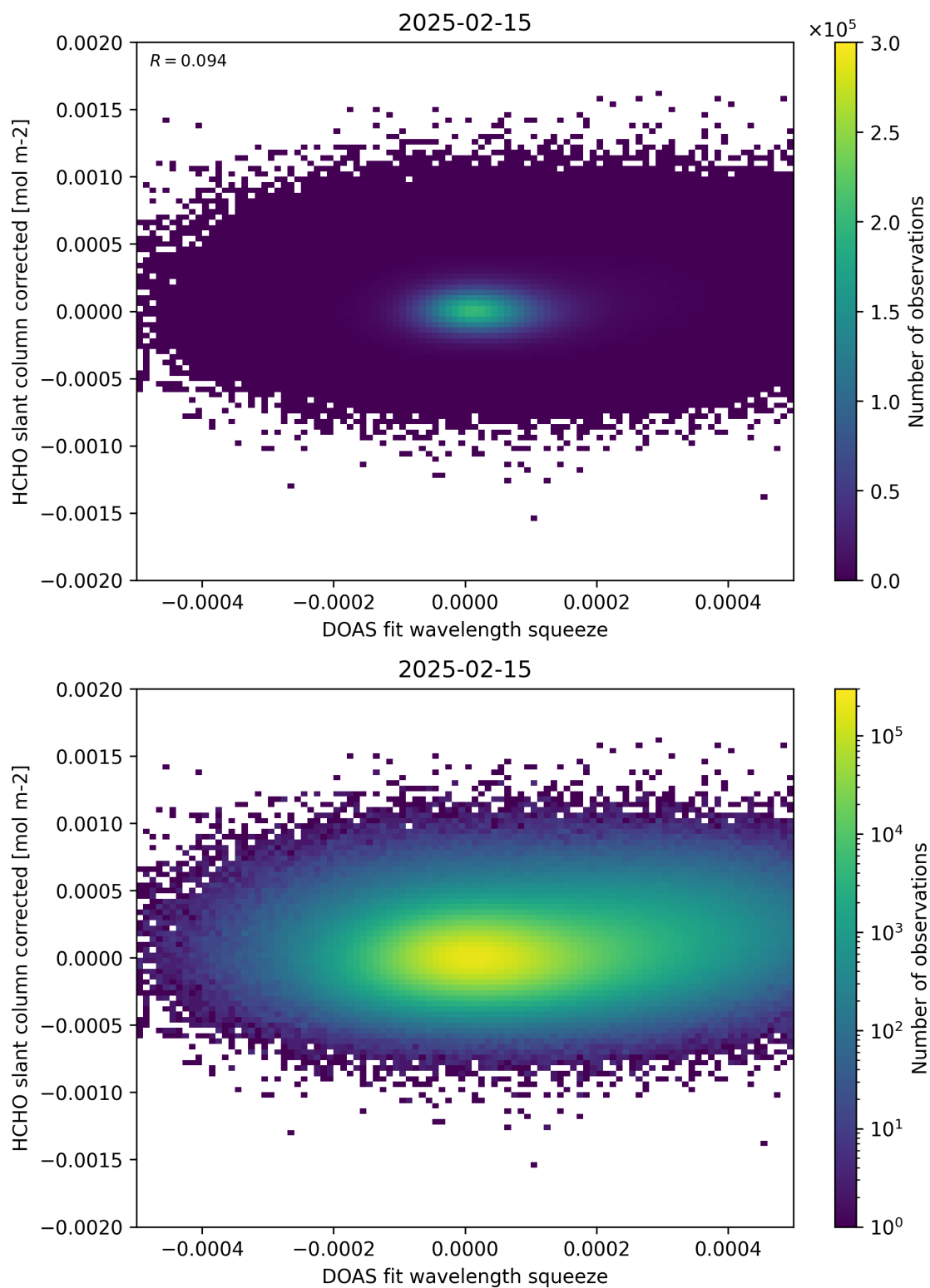
Figure 69: Scatter density plot of “DOAS fit wavelength squeeze” against “HCHO slant column corrected” for 2025-02-14 to 2025-02-16.
