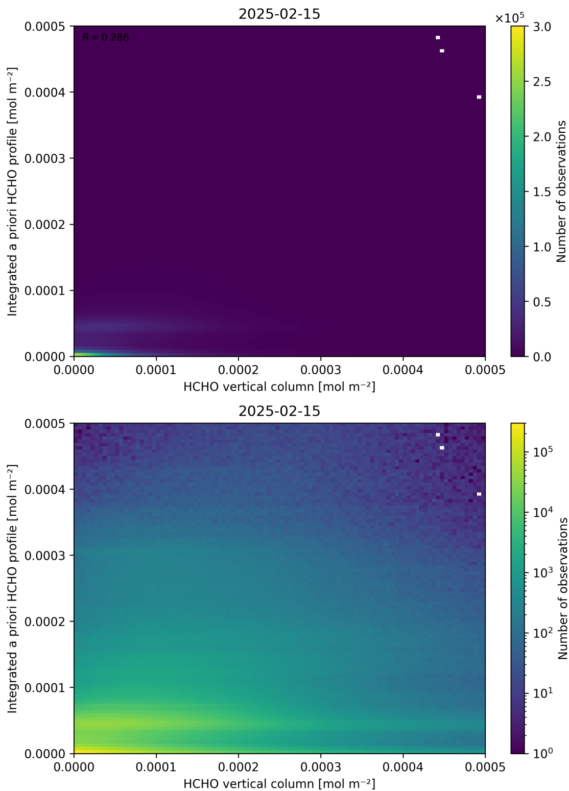
Figure 135: Scatter density plot of “HCHO vertical column” against “Integrated a priori HCHO profile” for 2025-02-14 to 2025-02-16.
