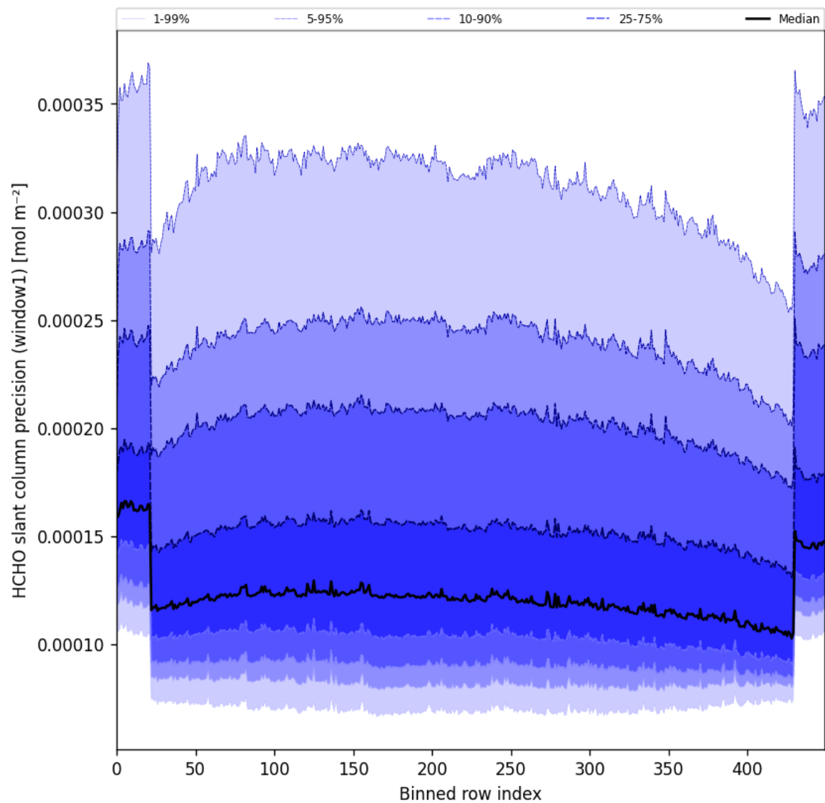
Figure 53: Along track statistics of “HCHO slant column precision (window1)” for 2025-02-14 to 2025-02-16
