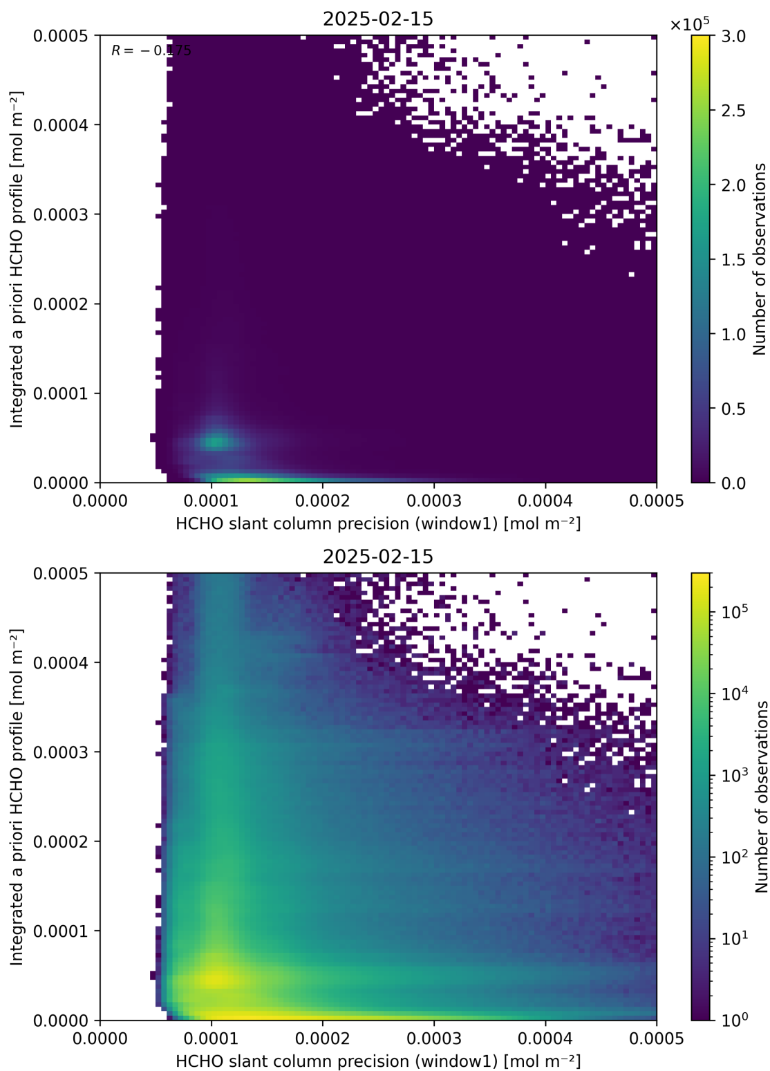
Figure 96: Scatter density plot of “HCHO slant column precision (window1)” against “Integrated a priori HCHO profile” for 2025-02-14 to 2025-02-16.
