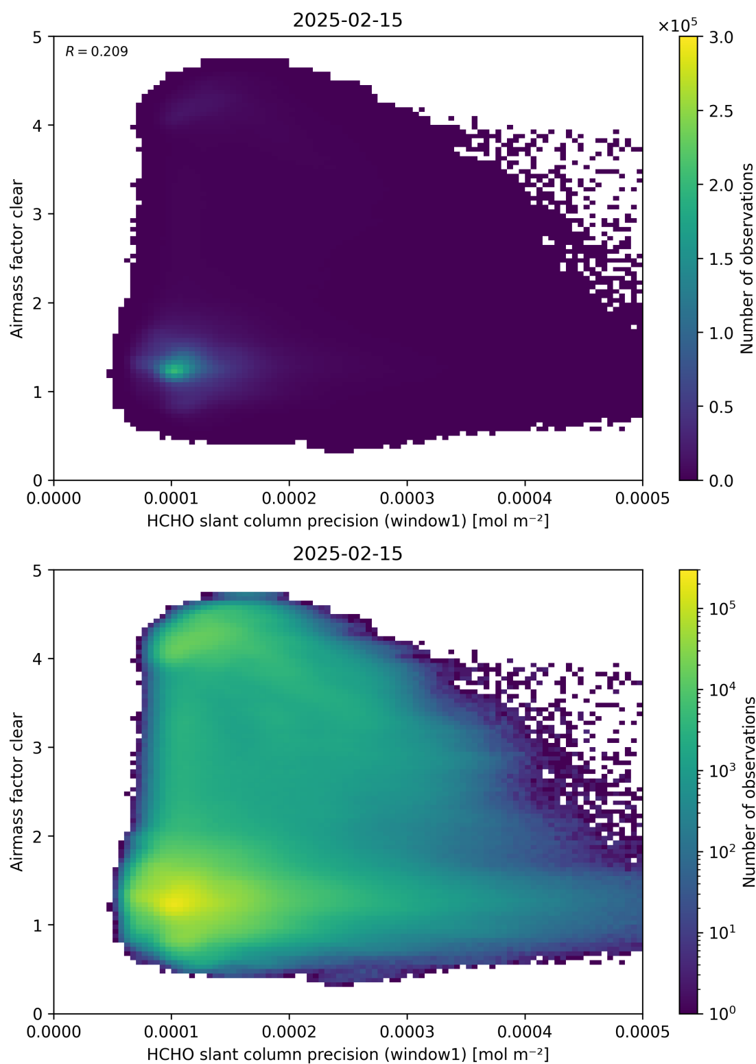
Figure 91: Scatter density plot of “HCHO slant column precision (window1)” against “Airmass factor clear” for 2025-02-14 to 2025-02-16.
