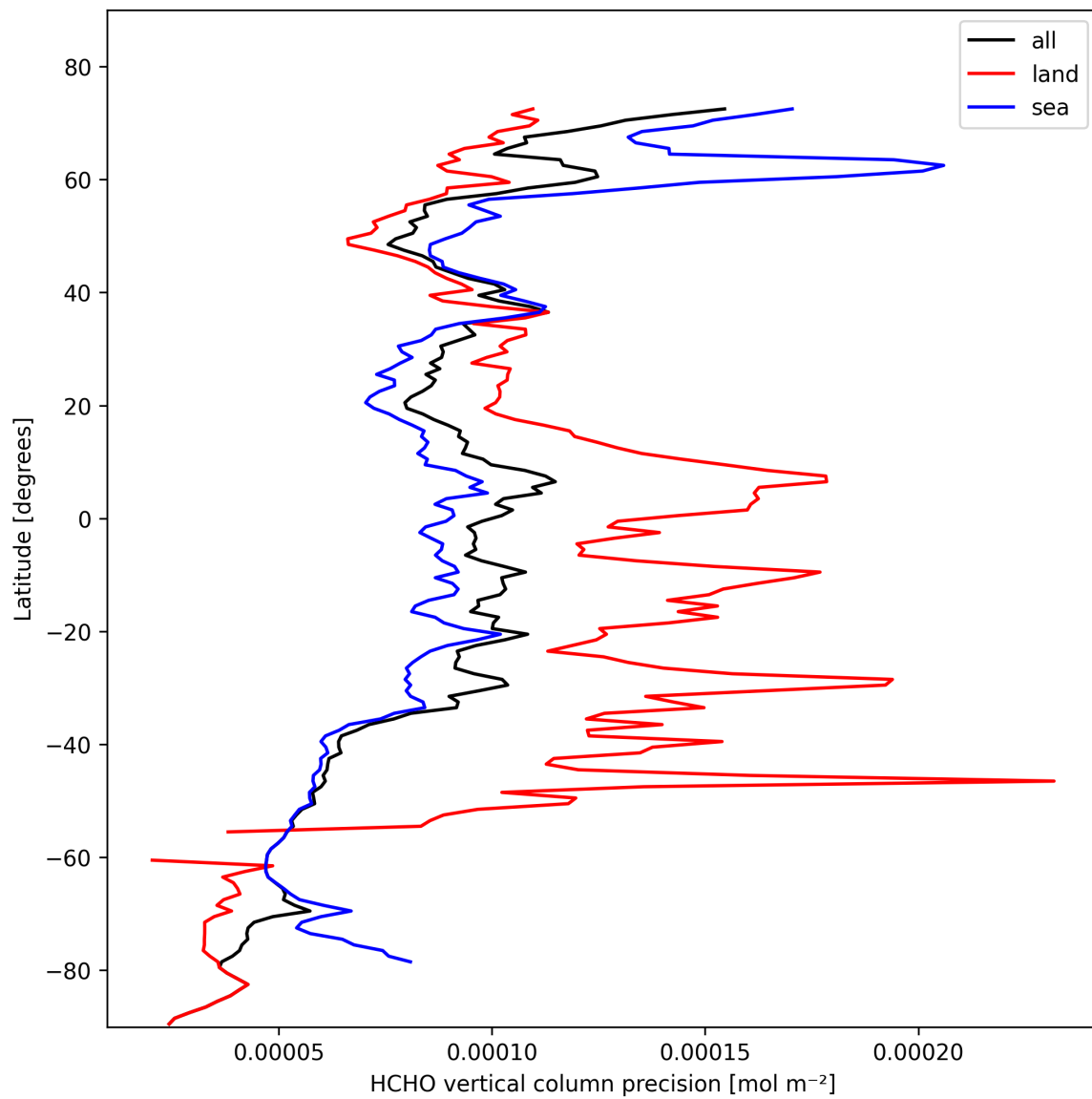
Figure 22: Zonal average of “HCHO vertical column precision” for 2025-02-14 to 2025-02-16.
