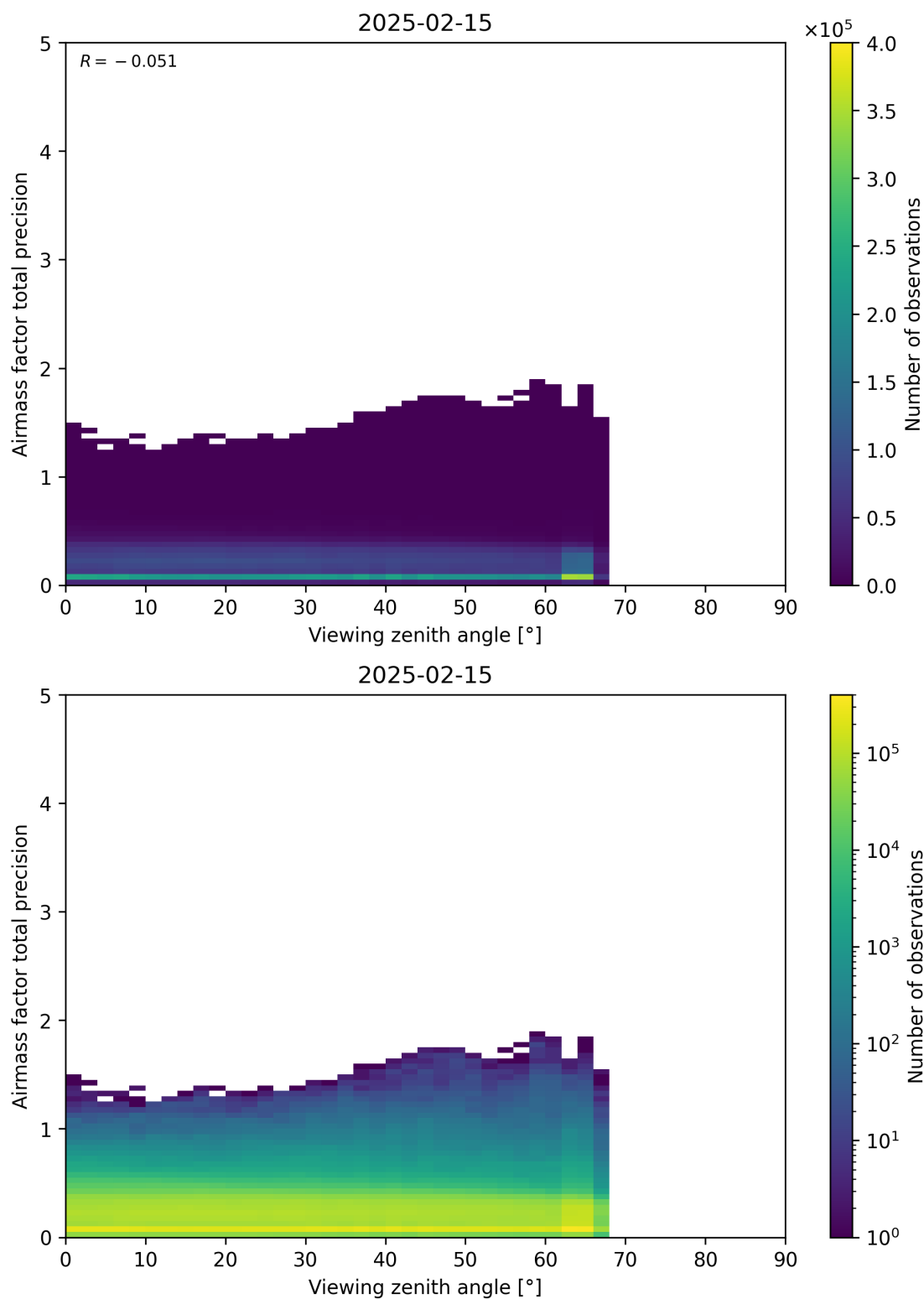
Figure 191: Scatter density plot of “Viewing zenith angle” against “Airmass factor total precision” for 2025-02-14 to 2025-02-16.
