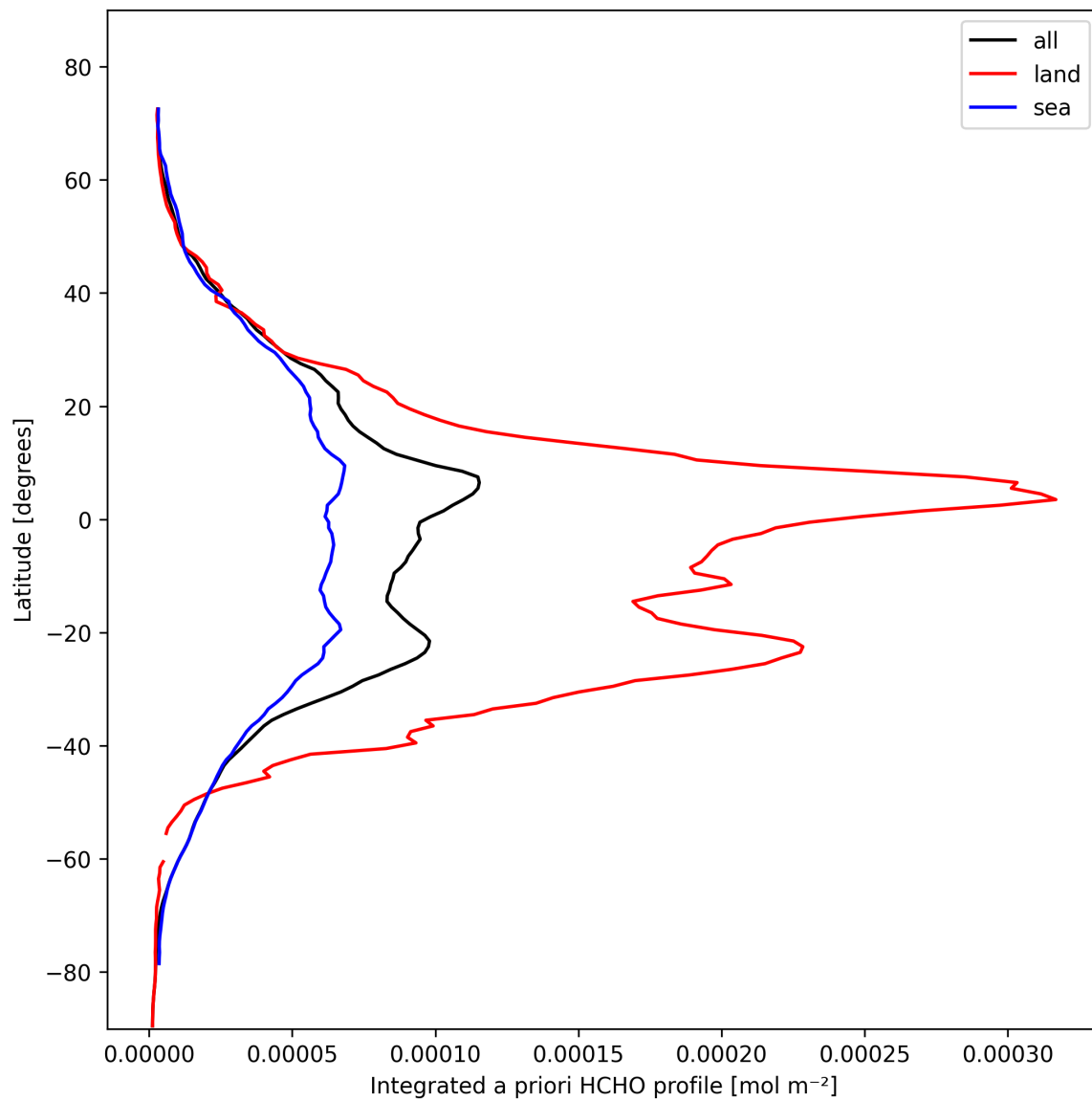
Figure 29: Zonal average of “Integrated a priori HCHO profile” for 2025-02-14 to 2025-02-16.
