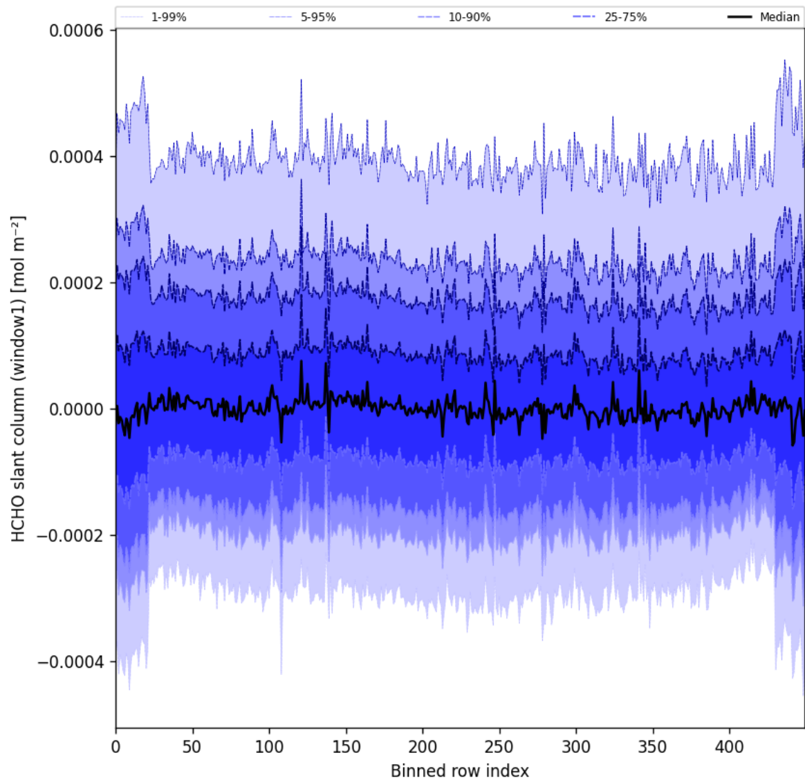
Figure 52: Along track statistics of “HCHO slant column (window1)” for 2025-02-14 to 2025-02-16
