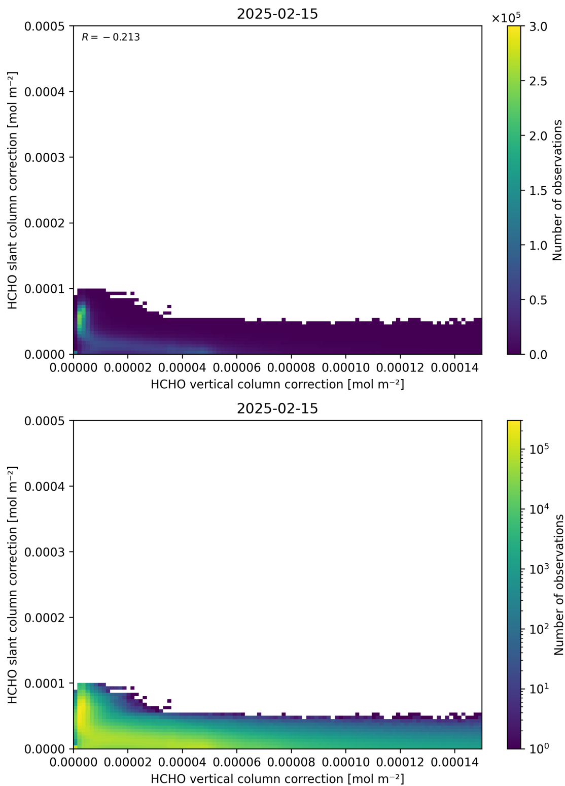
Figure 117: Scatter density plot of “HCHO vertical column correction” against “HCHO slant column correction” for 2025-02-14 to 2025-02-16.
