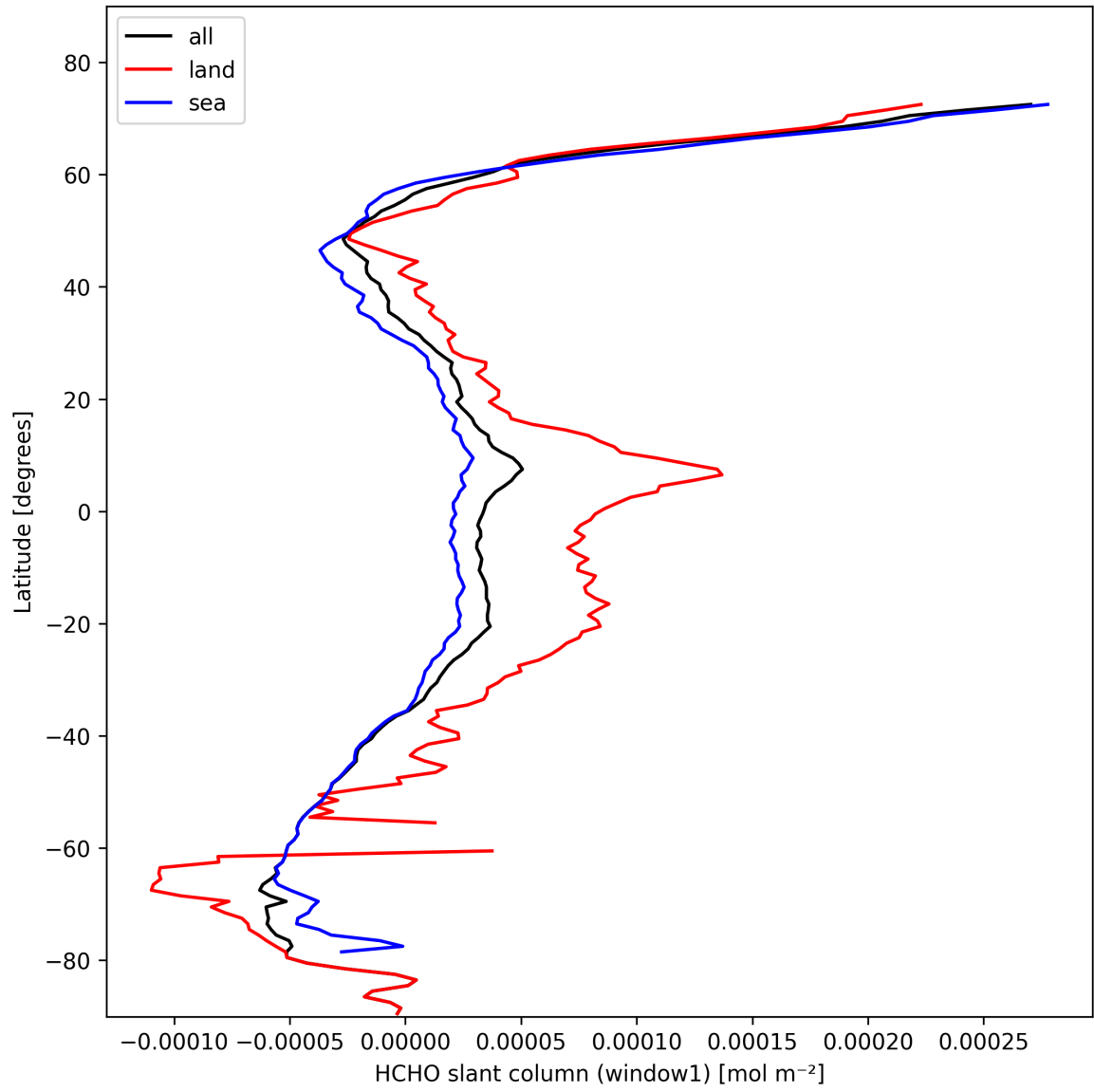
Figure 24: Zonal average of “HCHO slant column (window1)” for 2025-02-14 to 2025-02-16.
