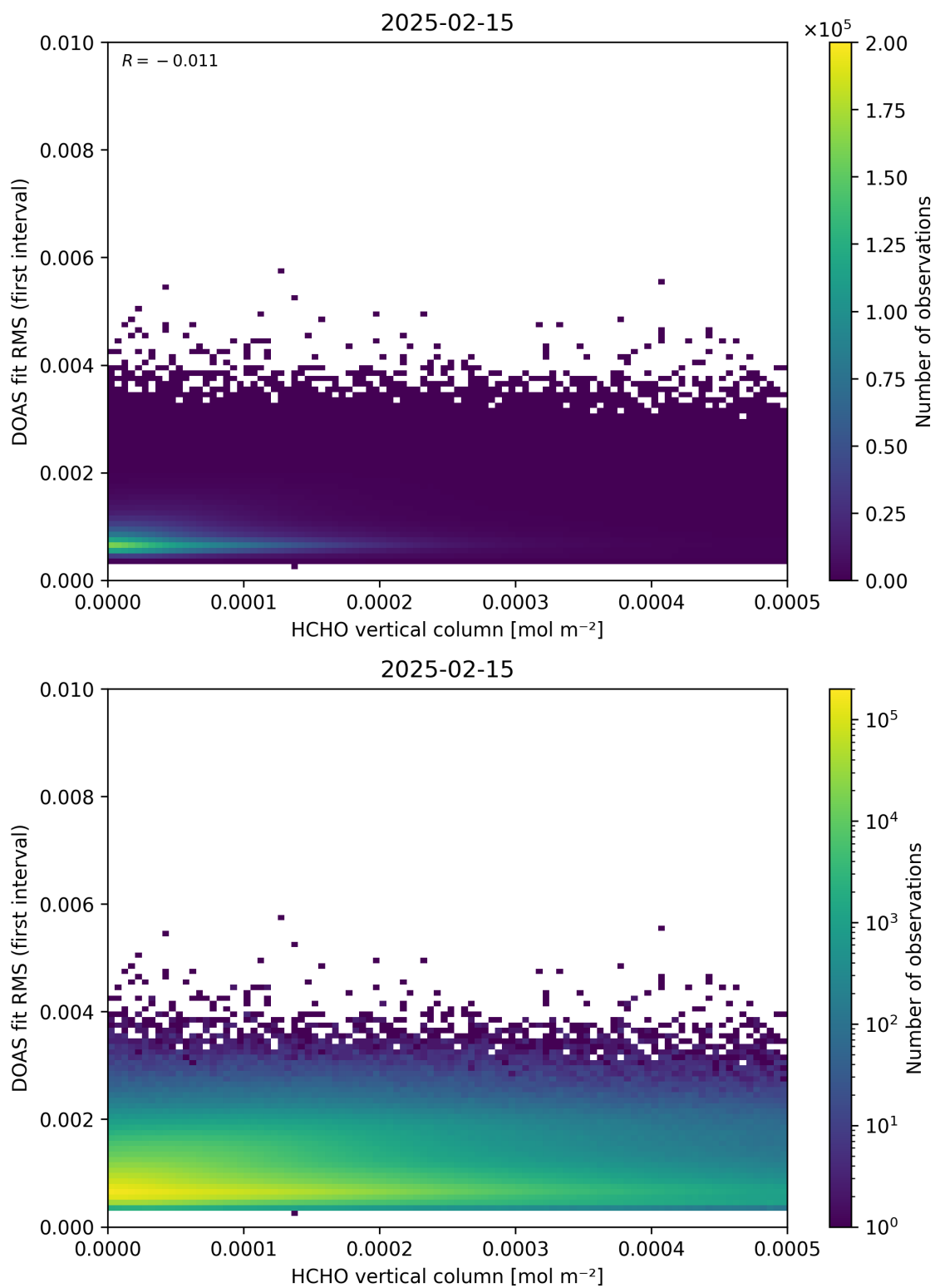
Figure 123: Scatter density plot of “HCHO vertical column” against “DOAS fit RMS (first interval)” for 2025-02-14 to 2025-02-16.
