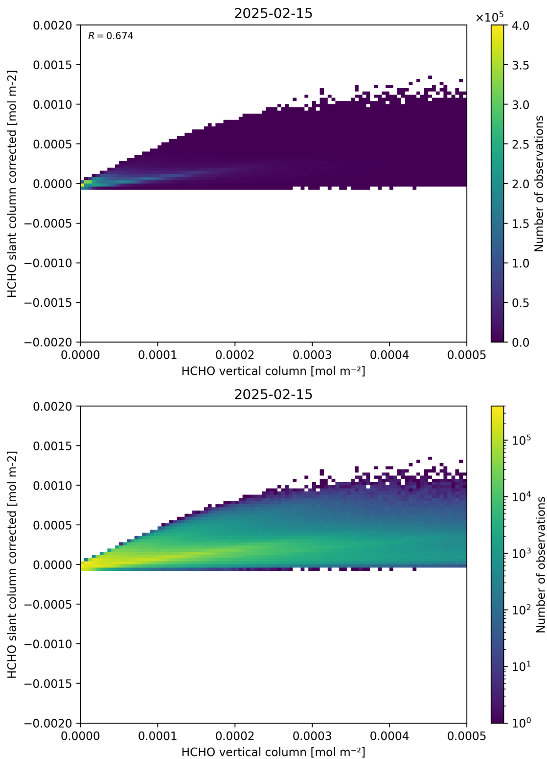
Figure 127: Scatter density plot of “HCHO vertical column” against “HCHO slant column corrected” for 2025-02-14 to 2025-02-16.
