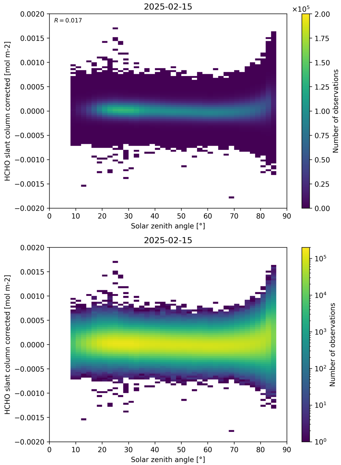
Figure 171: Scatter density plot of “Solar zenith angle” against “HCHO slant column corrected” for 2025-02-14 to 2025-02-16.
