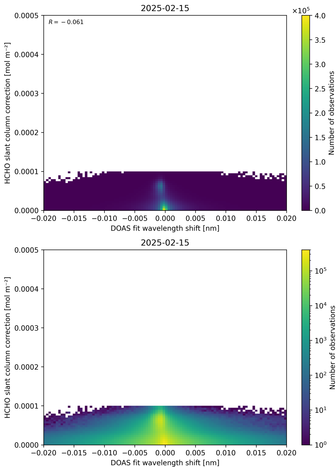
Figure 67: Scatter density plot of “DOAS fit wavelength shift” against “HCHO slant column correction” for 2025-02-14 to 2025-02-16.
