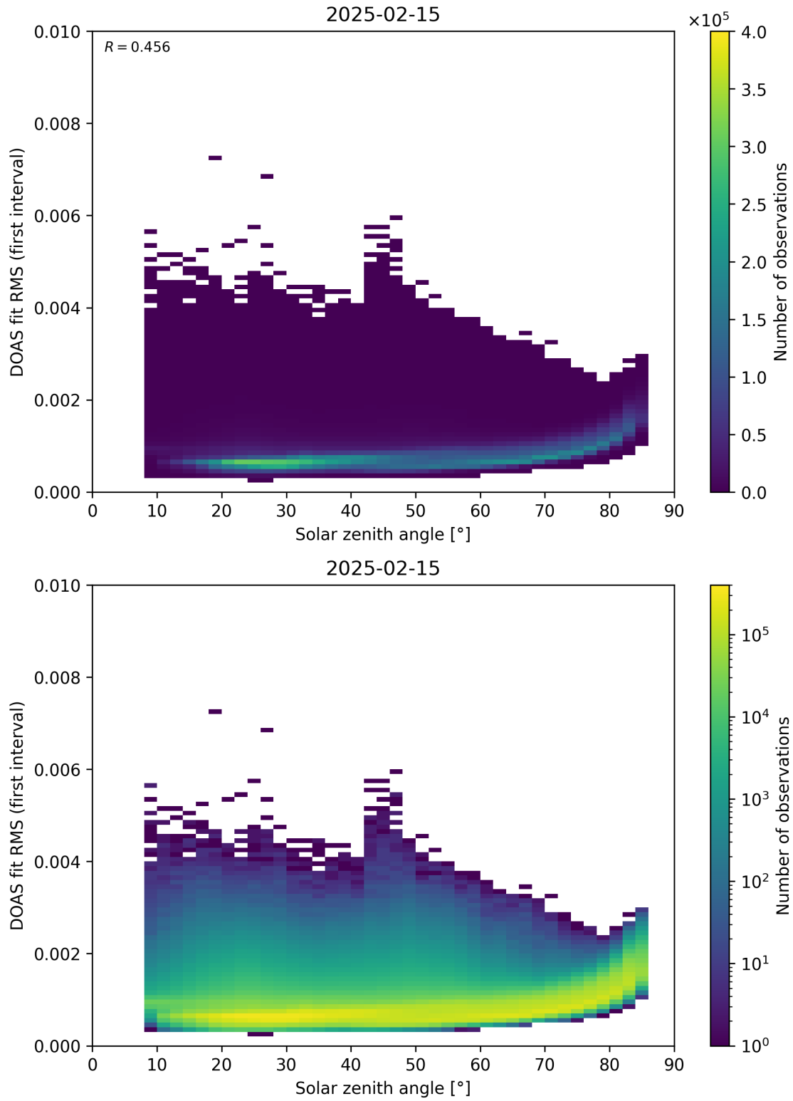
Figure 167: Scatter density plot of “Solar zenith angle” against “DOAS fit RMS (first interval)” for 2025-02-14 to 2025-02-16.
