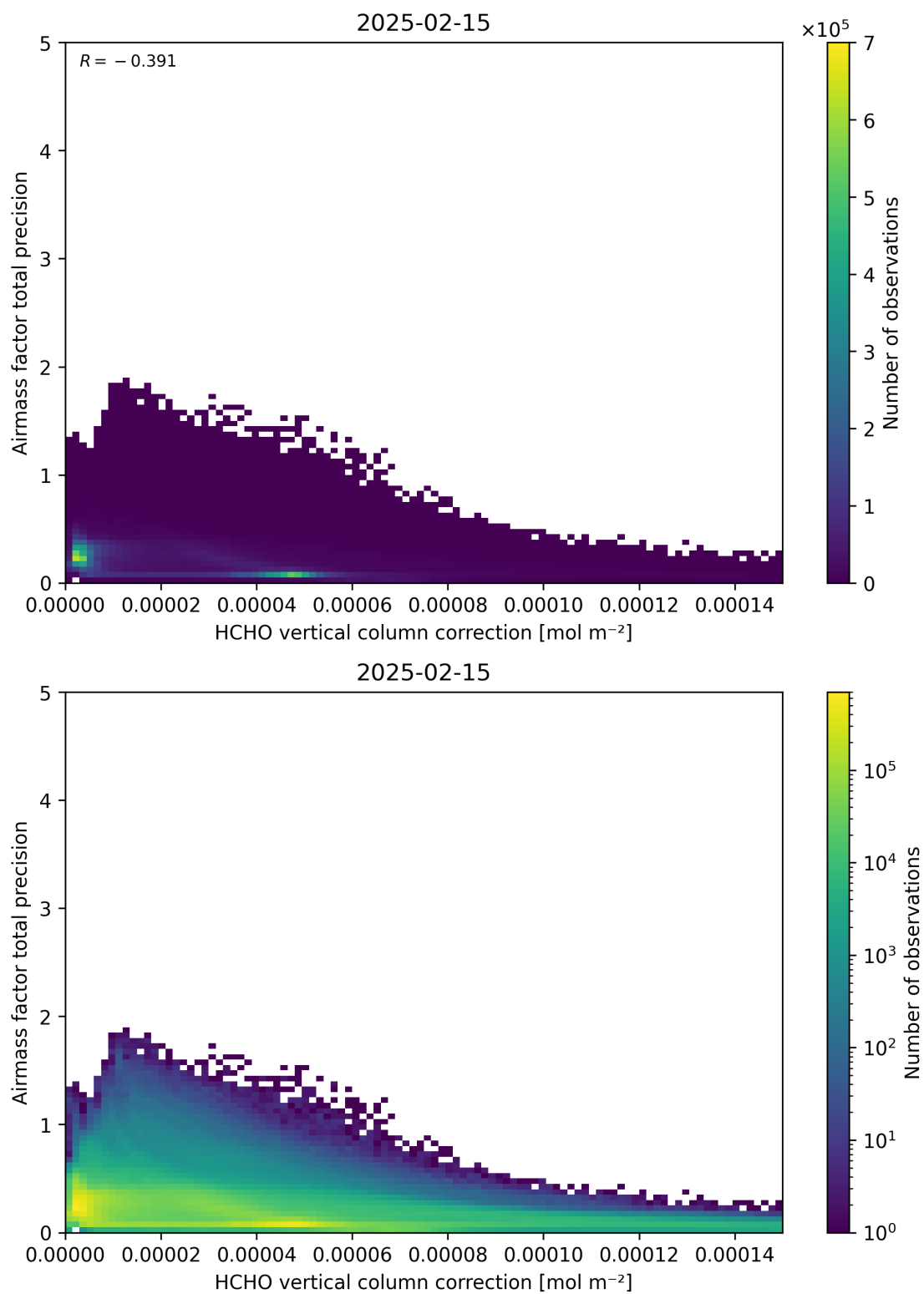
Figure 121: Scatter density plot of “HCHO vertical column correction” against “Airmass factor total precision” for 2025-02-14 to 2025-02-16.
