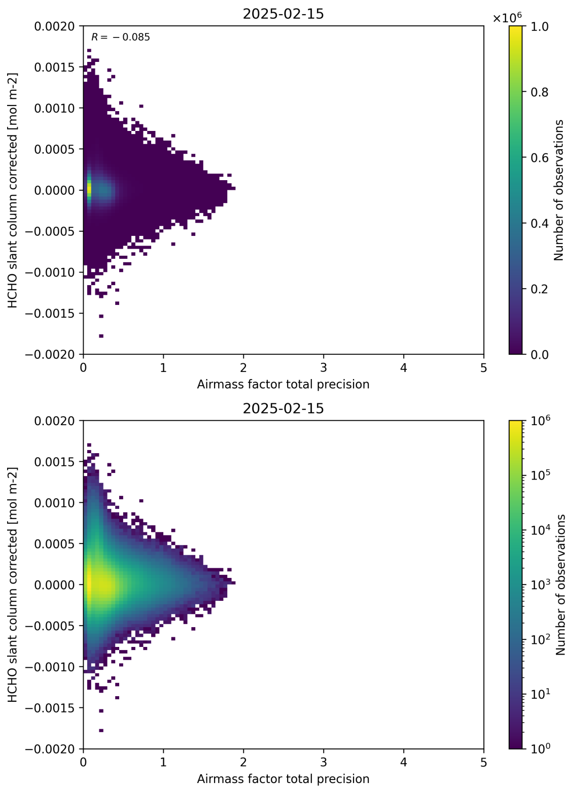
Figure 109: Scatter density plot of “Airmass factor total precision” against “HCHO slant column corrected” for 2025-02-14 to 2025-02-16.
