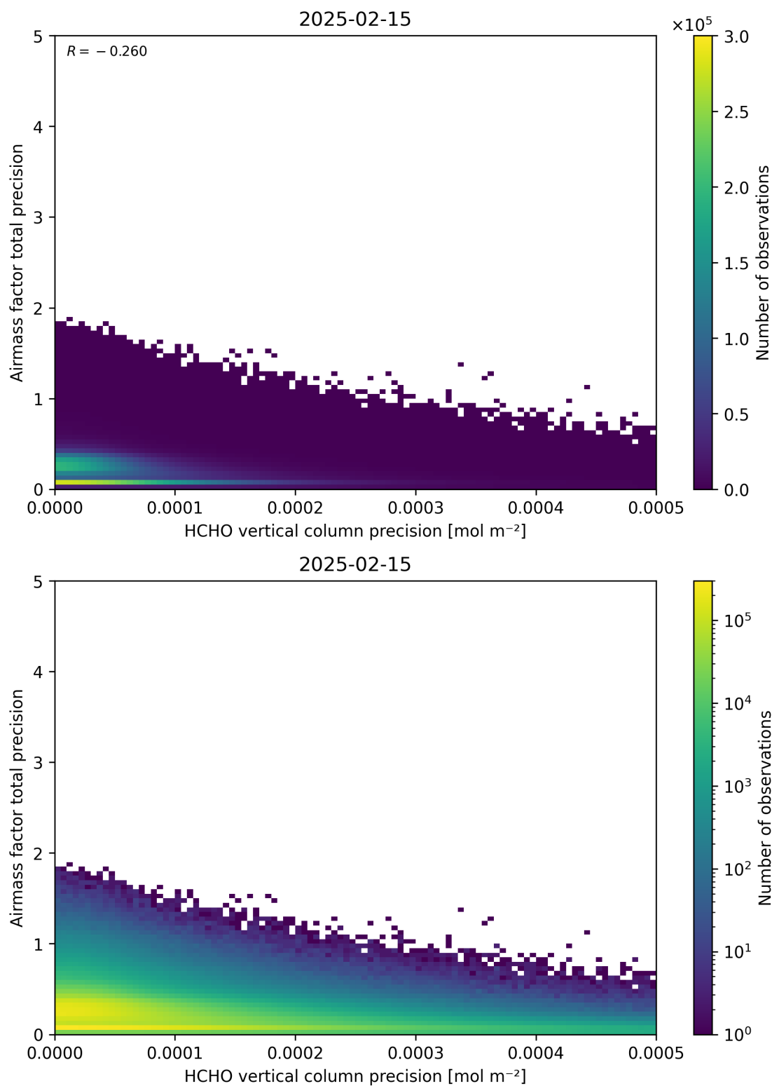
Figure 145: Scatter density plot of “HCHO vertical column precision” against “Airmass factor total precision” for 2025-02-14 to 2025-02-16.
