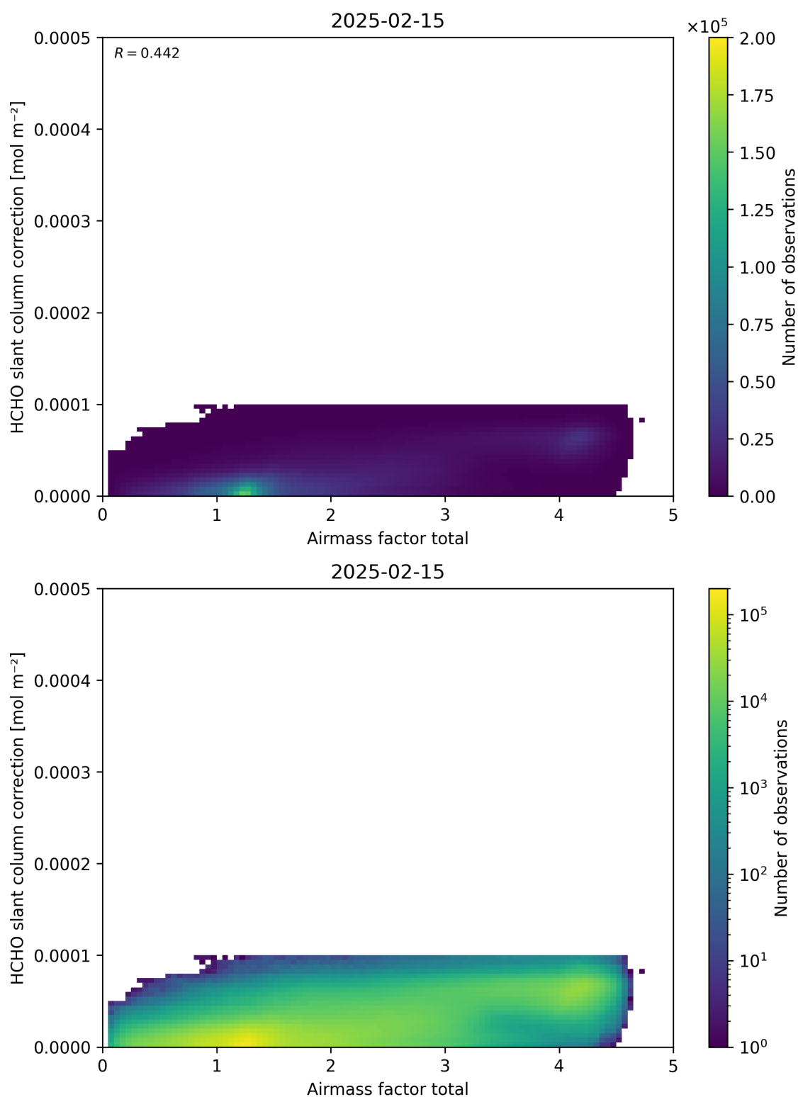
Figure 102: Scatter density plot of “Airmass factor total” against “HCHO slant column correction” for 2025-02-14 to 2025-02-16.
