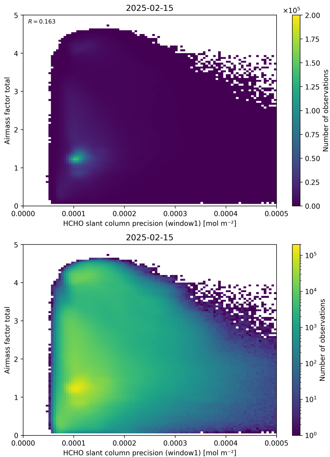
Figure 94: Scatter density plot of “HCHO slant column precision (window1)” against “Airmass factor total” for 2025-02-14 to 2025-02-16.
