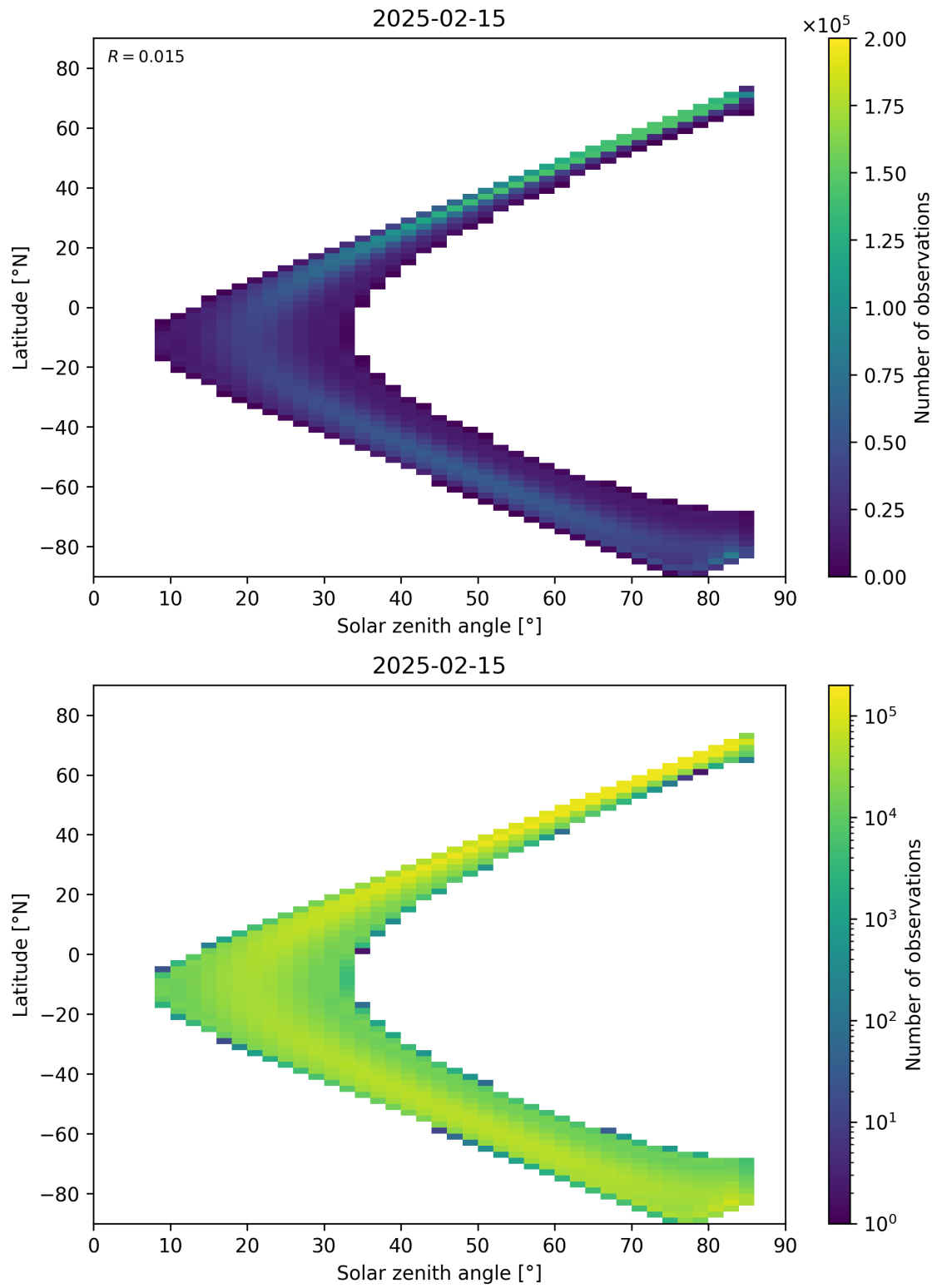
Figure 181: Scatter density plot of “Solar zenith angle” against “Latitude” for 2025-02-14 to 2025-02-16.
