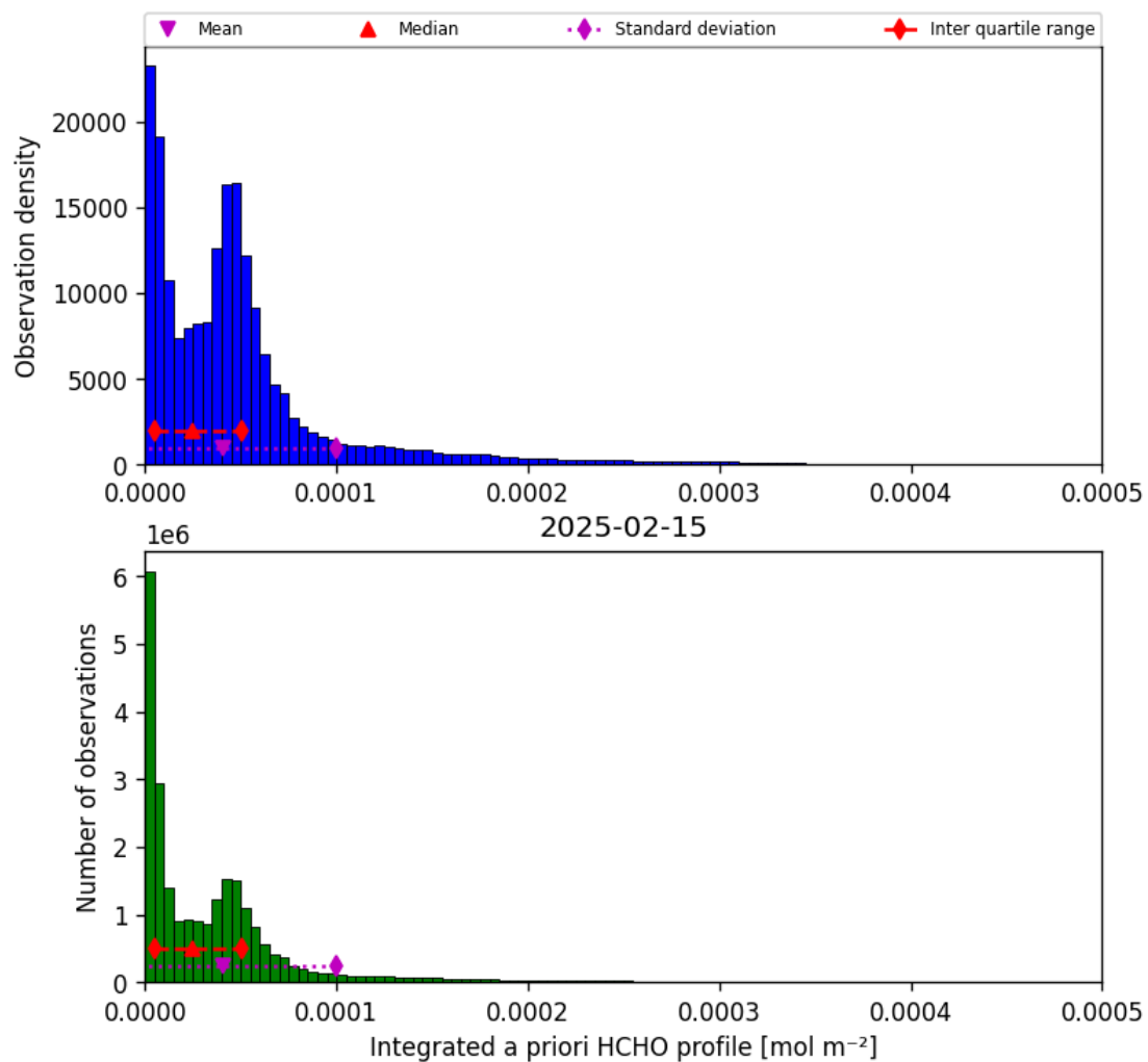
Figure 43: Histogram of “Integrated a priori HCHO profile” for 2025-02-14 to 2025-02-16
