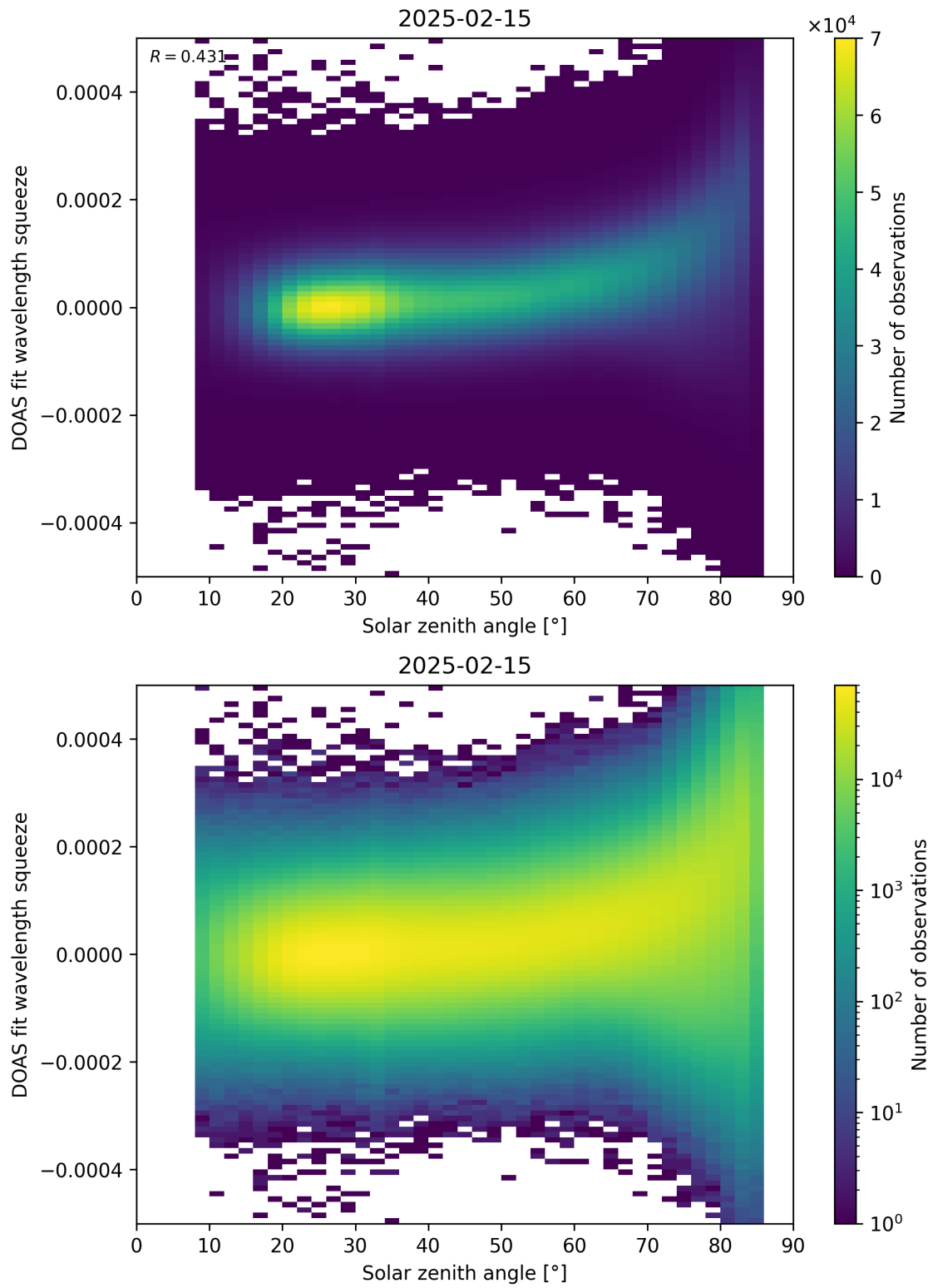
Figure 169: Scatter density plot of “Solar zenith angle” against “DOAS fit wavelength squeeze” for 2025-02-14 to 2025-02-16.
