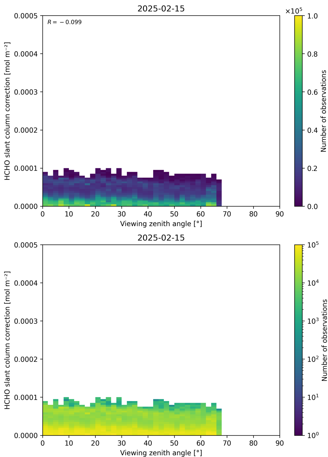
Figure 187: Scatter density plot of “Viewing zenith angle” against “HCHO slant column correction” for 2025-02-14 to 2025-02-16.
