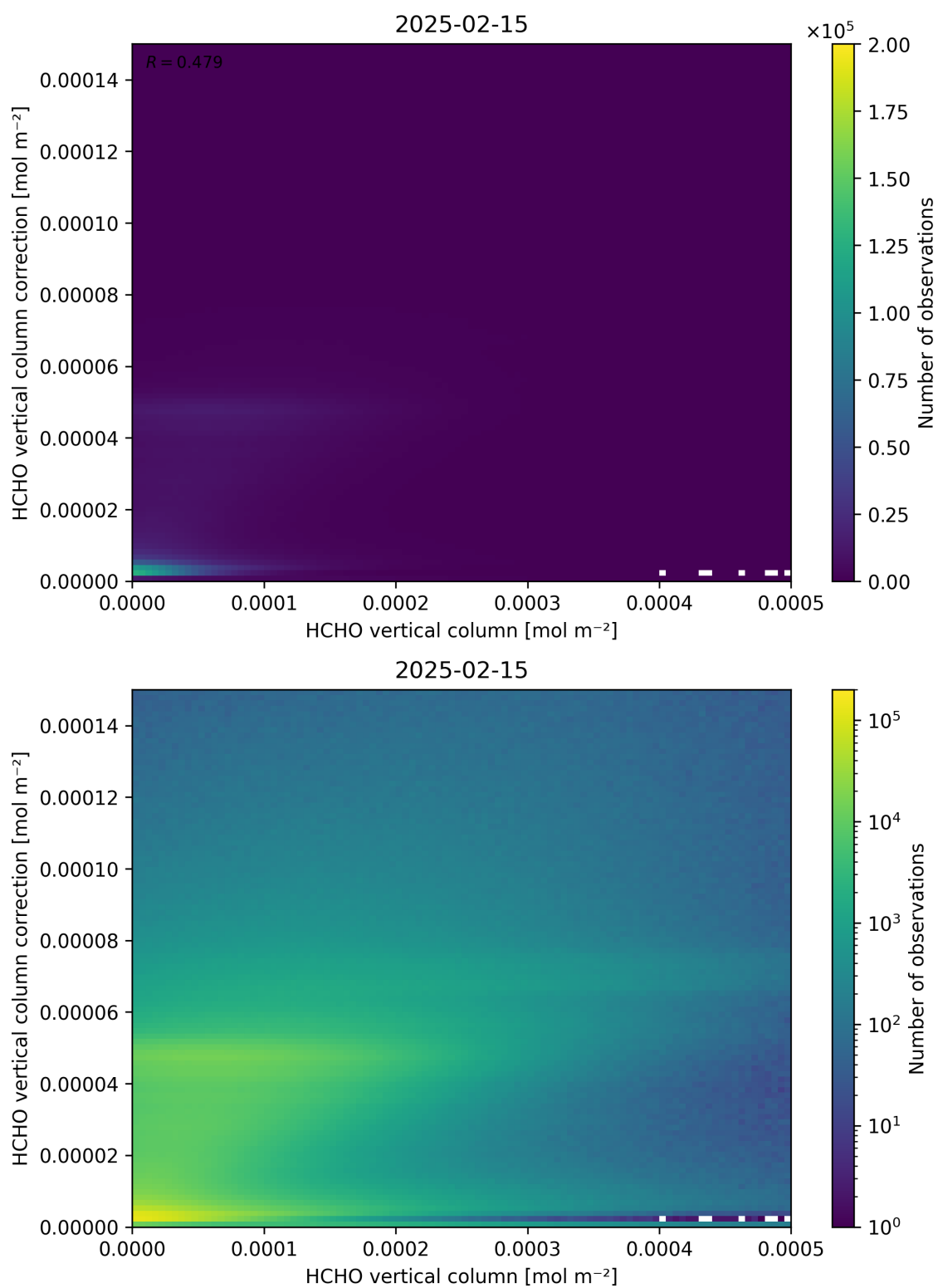
Figure 133: Scatter density plot of “HCHO vertical column” against “HCHO vertical column correction” for 2025-02-14 to 2025-02-16.
