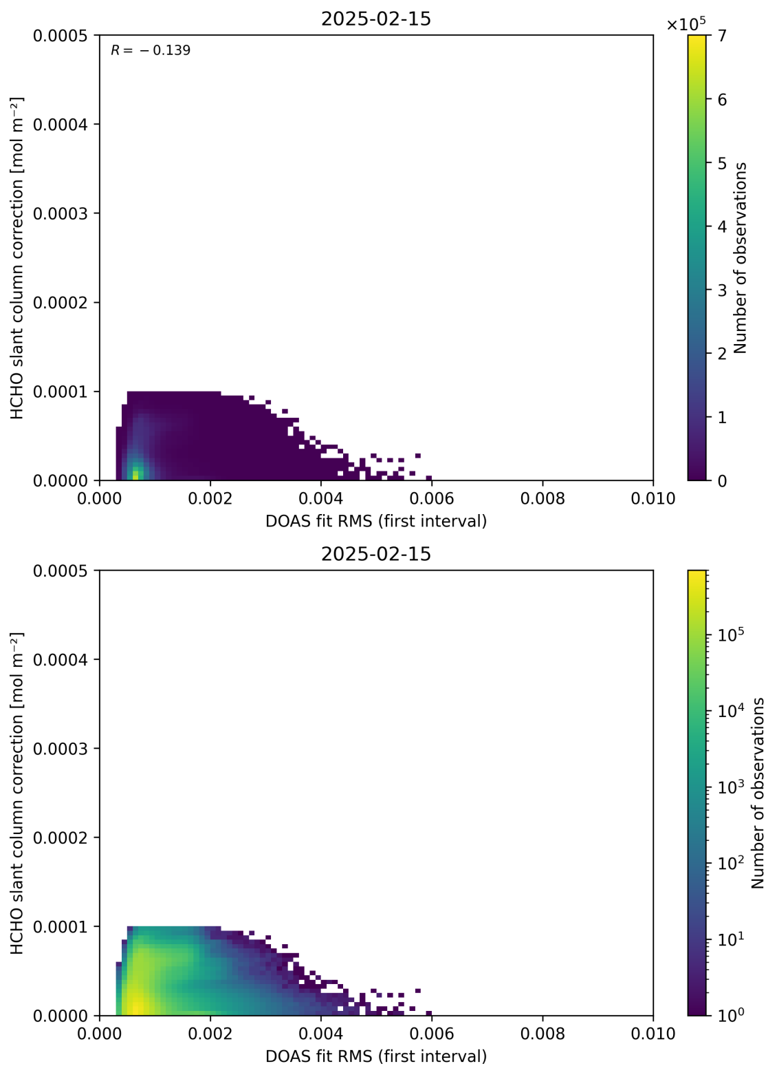
Figure 63: Scatter density plot of “DOAS fit RMS (first interval)” against “HCHO slant column correction” for 2025-02-14 to 2025-02-16.
