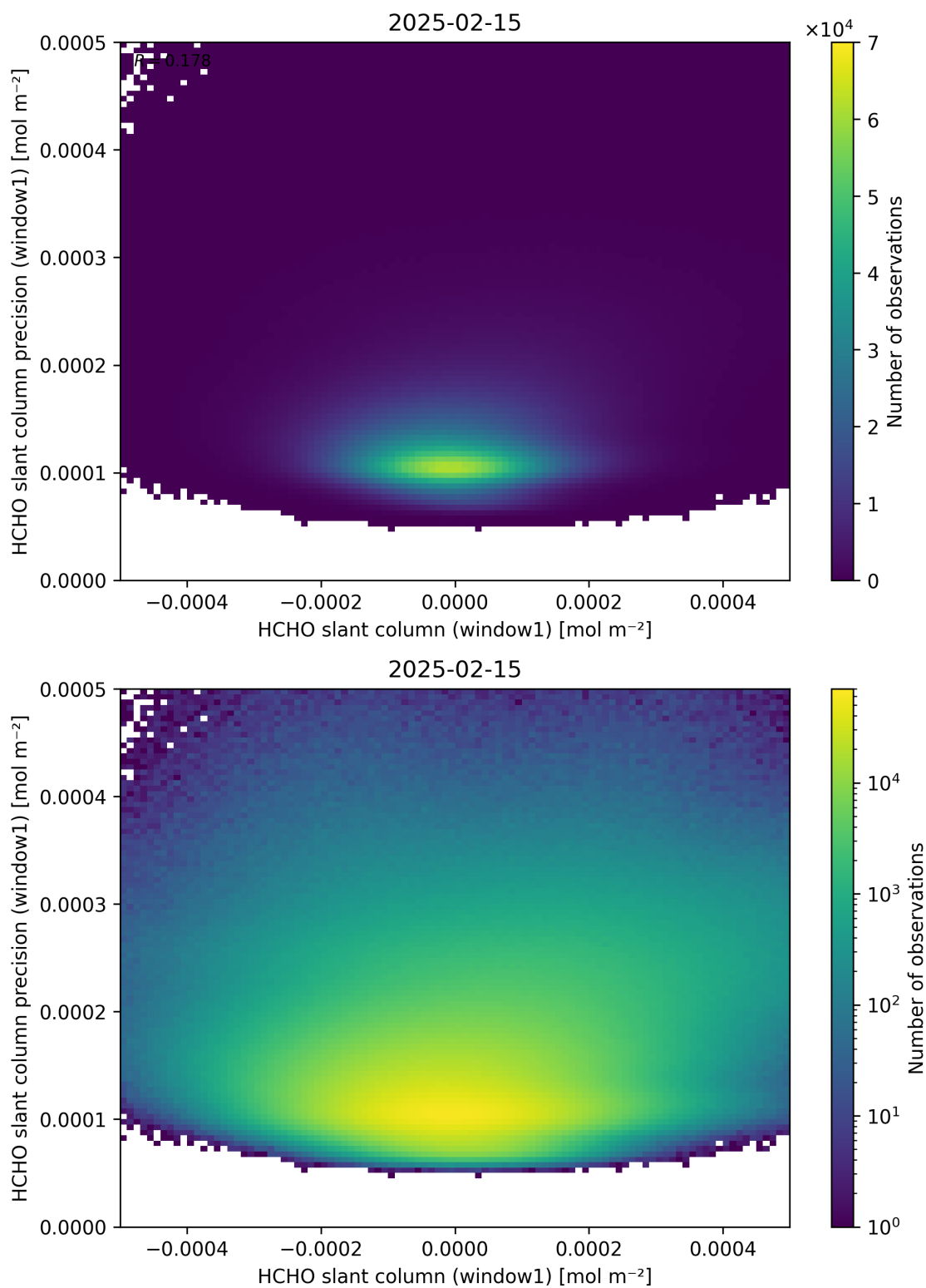
Figure 84: Scatter density plot of “HCHO slant column (window1)” against “HCHO slant column precision (window1)” for 2025-02-14 to 2025-02-16.
