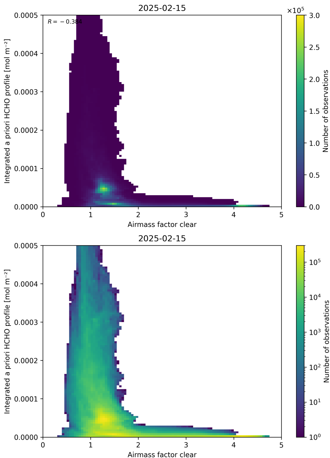
Figure 76: Scatter density plot of “Airmass factor clear” against “Integrated a priori HCHO profile” for 2025-02-14 to 2025-02-16.
