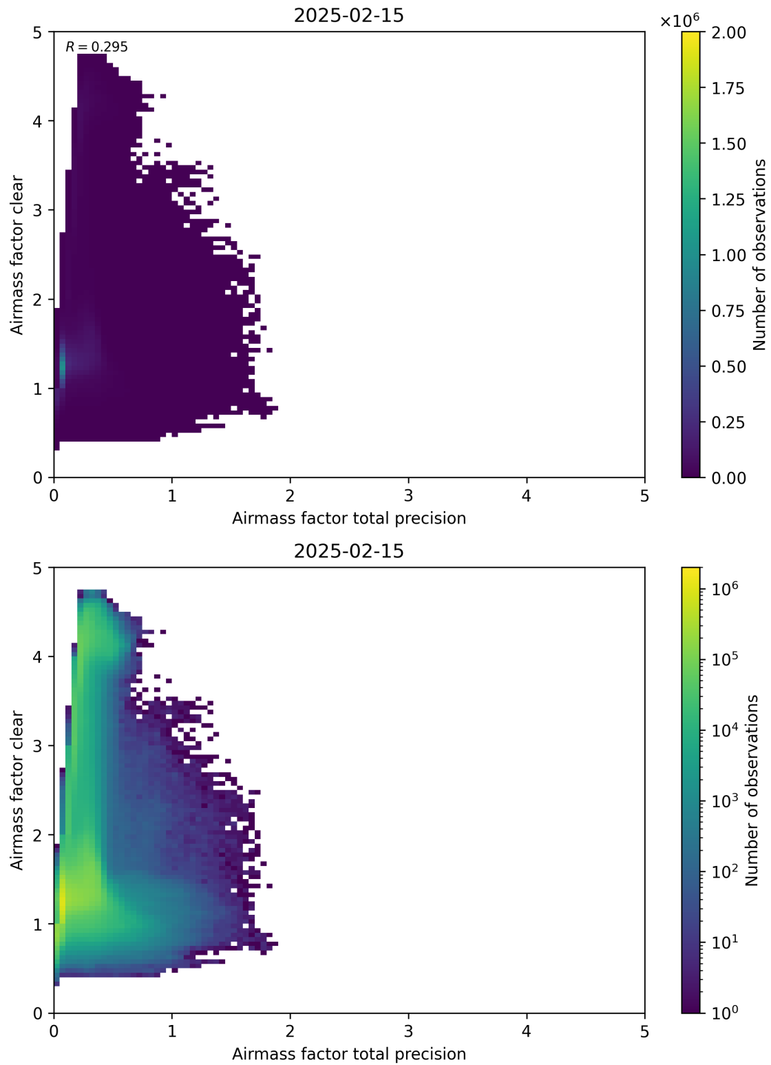
Figure 108: Scatter density plot of “Airmass factor total precision” against “Airmass factor clear” for 2025-02-14 to 2025-02-16.
