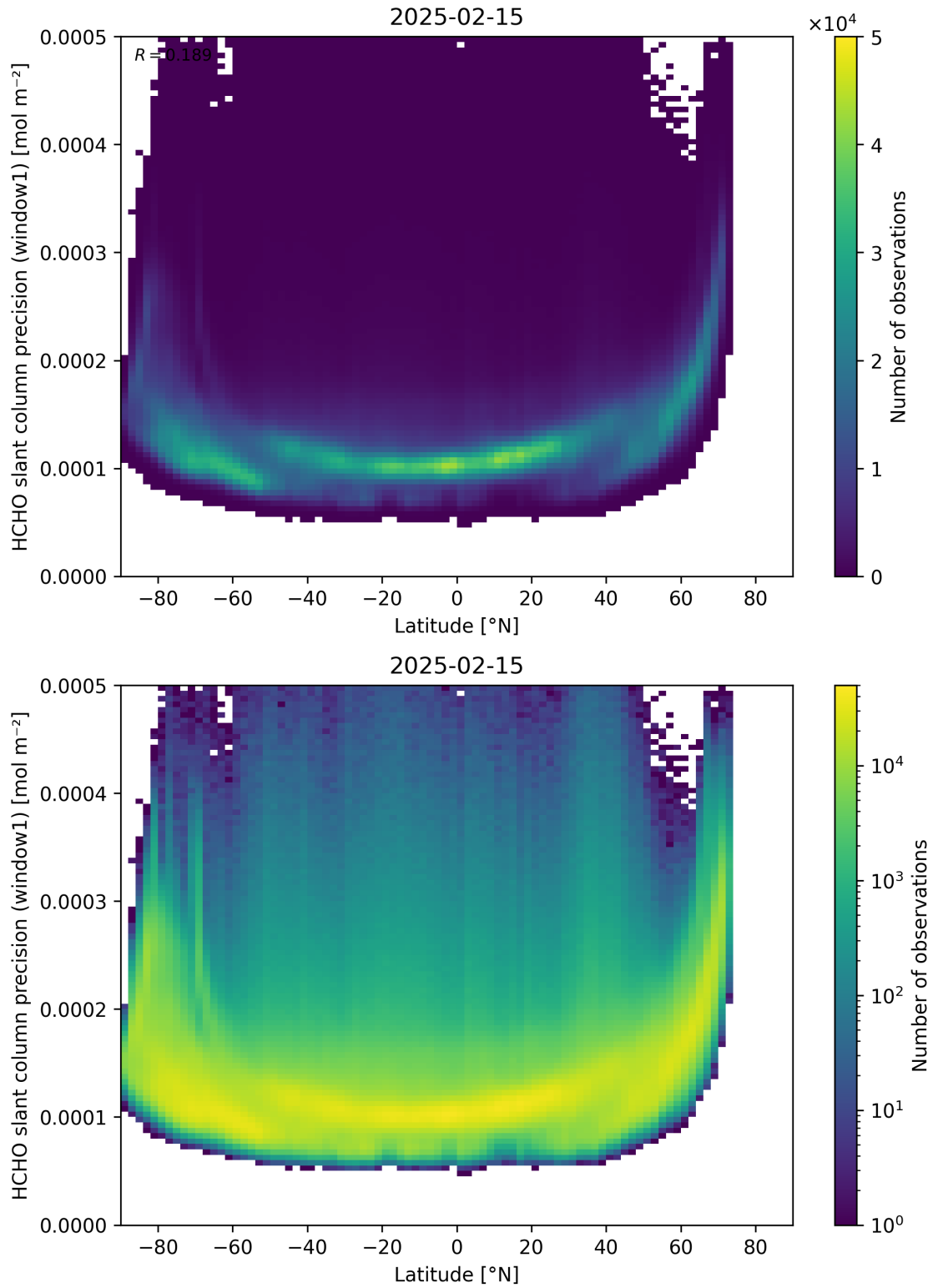
Figure 160: Scatter density plot of “Latitude” against “HCHO slant column precision (window1)” for 2025-02-14 to 2025-02-16.
