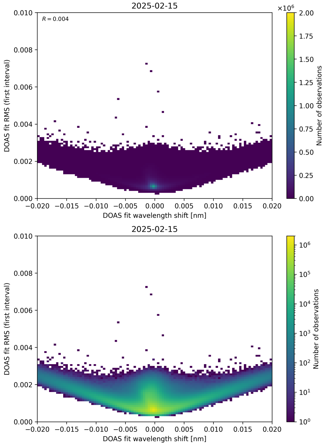
Figure 64: Scatter density plot of “DOAS fit wavelength shift” against “DOAS fit RMS (first interval)” for 2025-02-14 to 2025-02-16.
