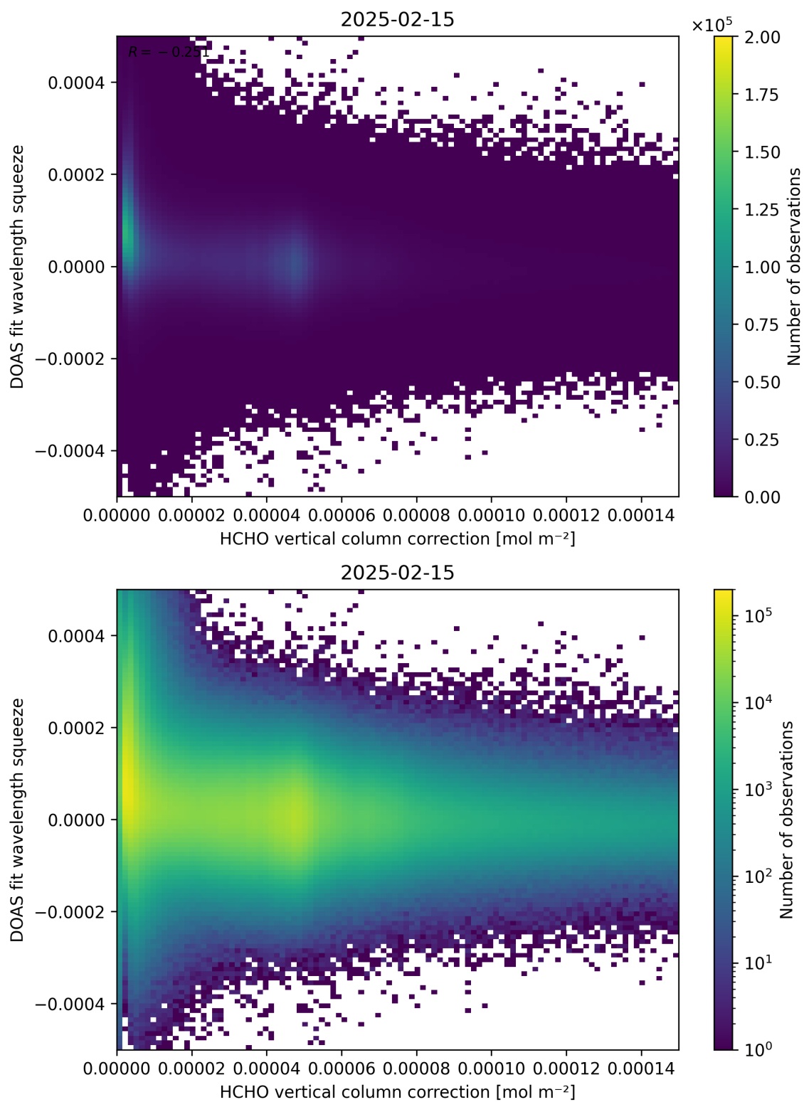
Figure 114: Scatter density plot of “HCHO vertical column correction” against “DOAS fit wavelength squeeze” for 2025-02-14 to 2025-02-16.
