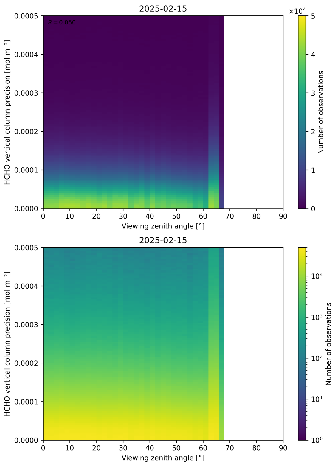
Figure 194: Scatter density plot of “Viewing zenith angle” against “HCHO vertical column precision” for 2025-02-14 to 2025-02-16.
