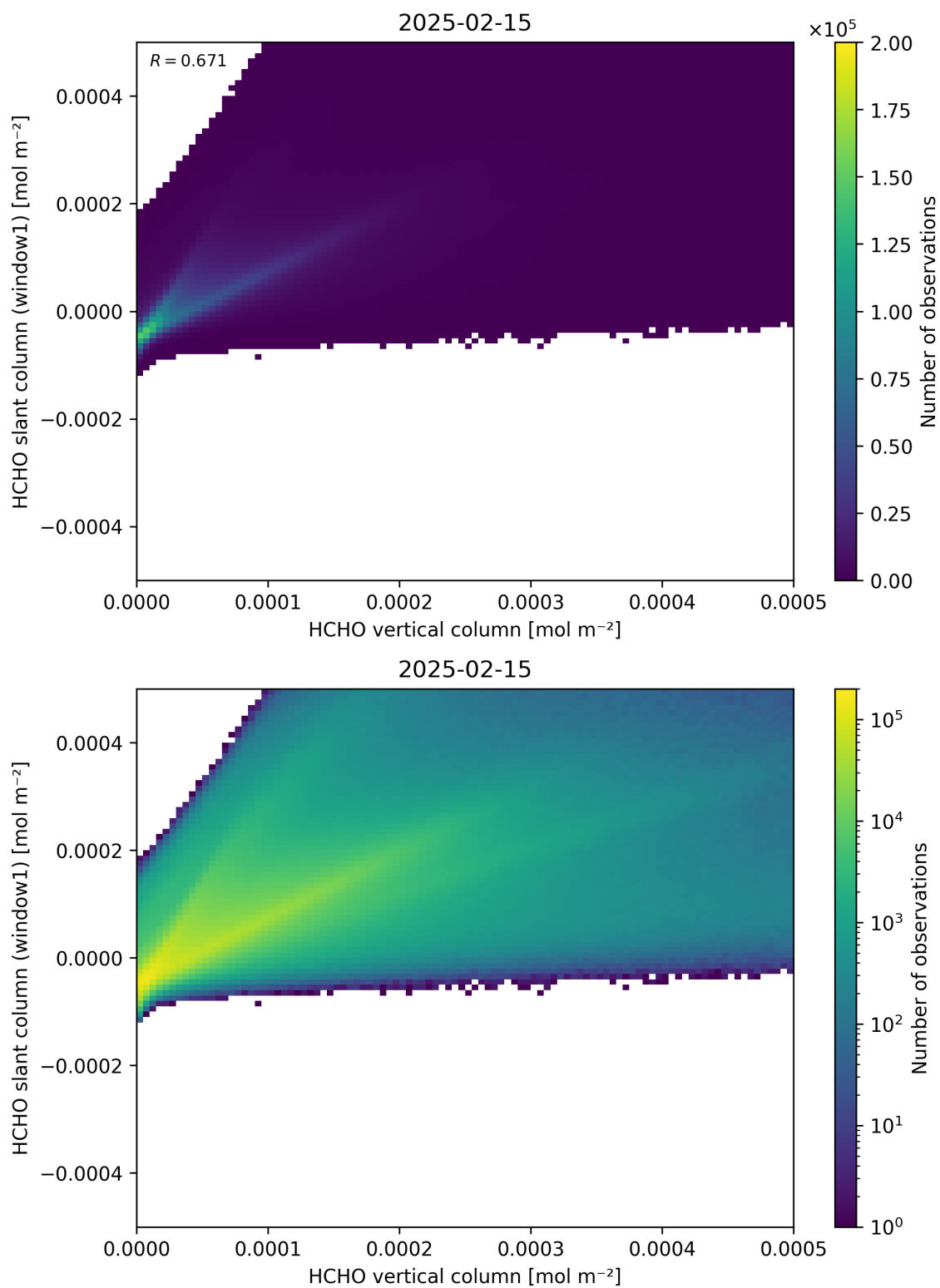
Figure 129: Scatter density plot of “HCHO vertical column” against “HCHO slant column (window1)” for 2025-02-14 to 2025-02-16.
