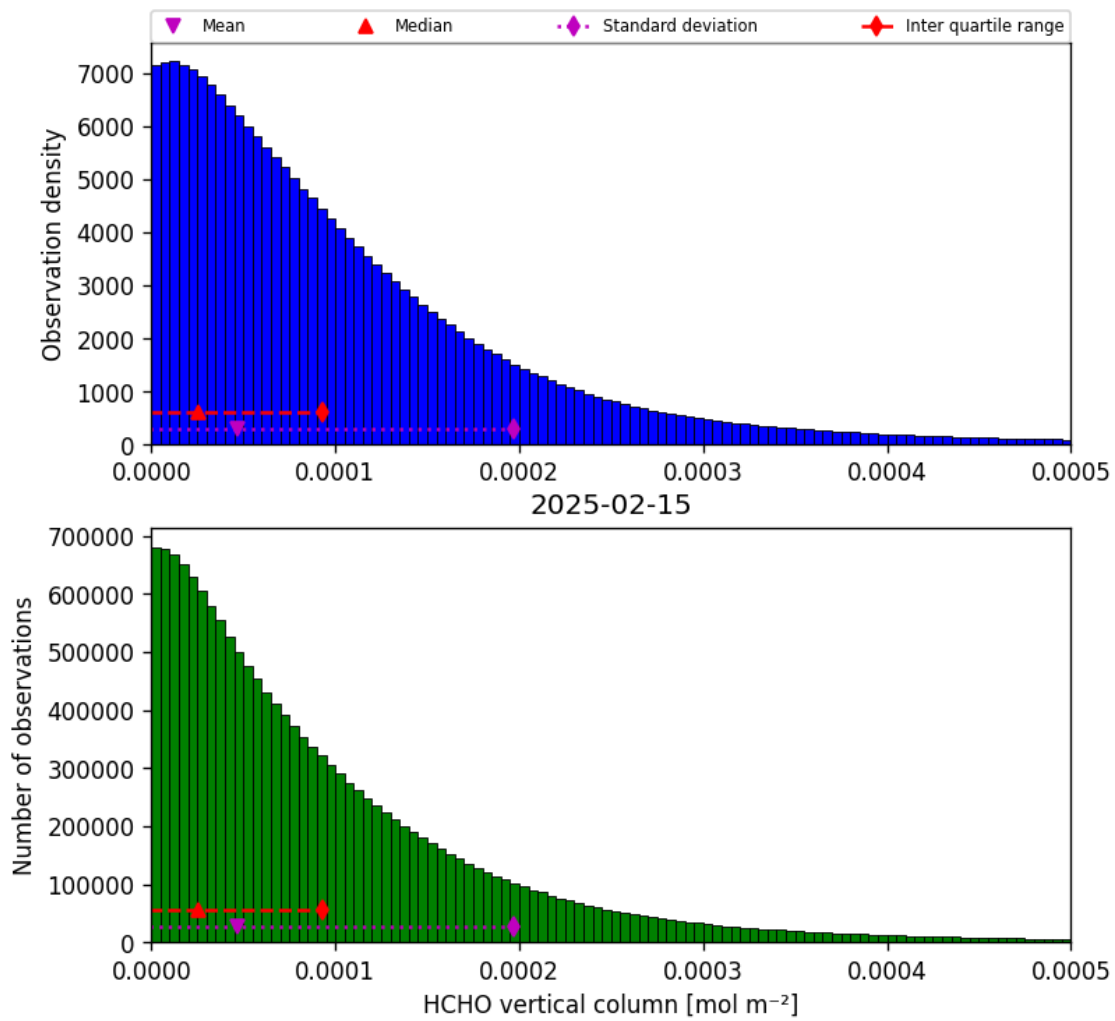
Figure 35: Histogram of “HCHO vertical column” for 2025-02-14 to 2025-02-16
