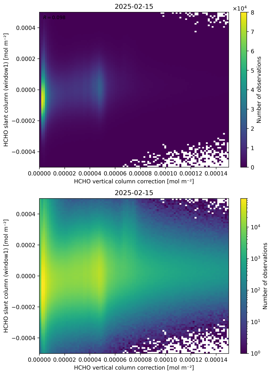
Figure 118: Scatter density plot of “HCHO vertical column correction” against “HCHO slant column (window1)” for 2025-02-14 to 2025-02-16.
