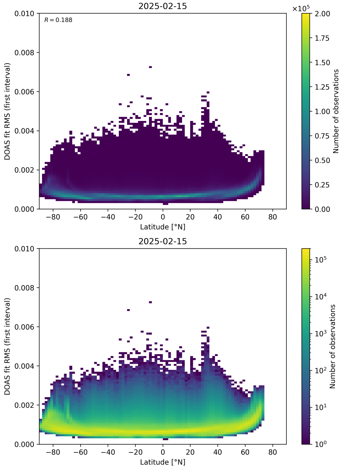
Figure 153: Scatter density plot of “Latitude” against “DOAS fit RMS (first interval)” for 2025-02-14 to 2025-02-16.
