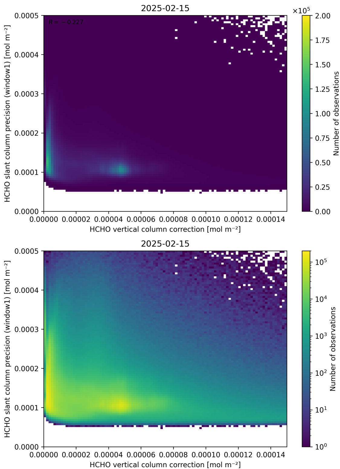
Figure 119: Scatter density plot of “HCHO vertical column correction” against “HCHO slant column precision (window1)” for 2025-02-14 to 2025-02-16.
