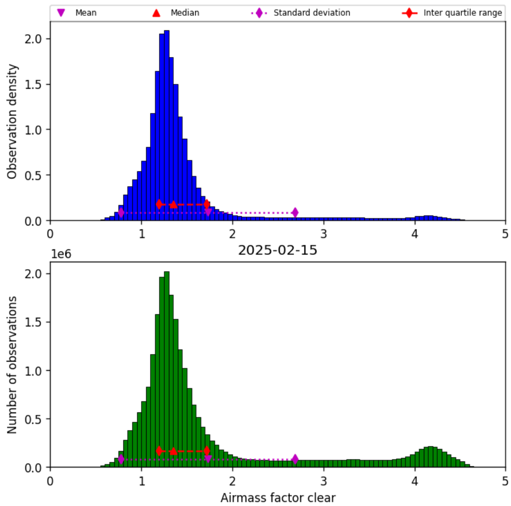
Figure 42: Histogram of “Airmass factor clear” for 2025-02-14 to 2025-02-16
