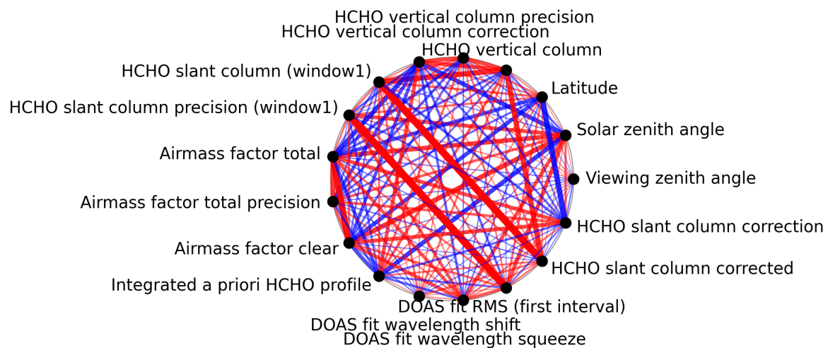
Figure 1: Map of correlation graph for 2025-02-14 to 2025-02-16.
