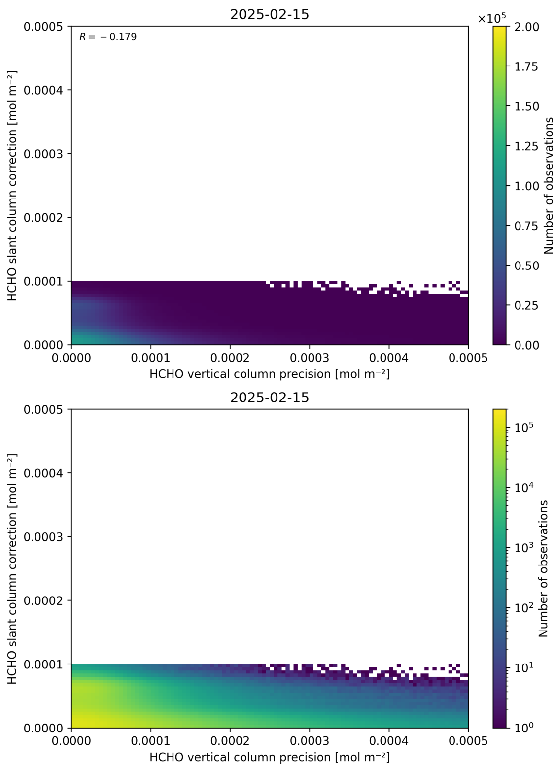
Figure 141: Scatter density plot of “HCHO vertical column precision” against “HCHO slant column correction” for 2025-02-14 to 2025-02-16.
