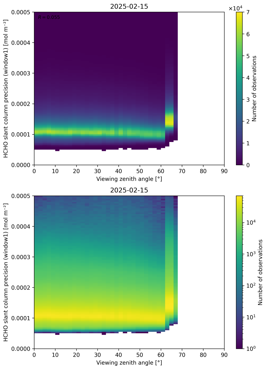
Figure 189: Scatter density plot of “Viewing zenith angle” against “HCHO slant column precision (window1)” for 2025-02-14 to 2025-02-16.
