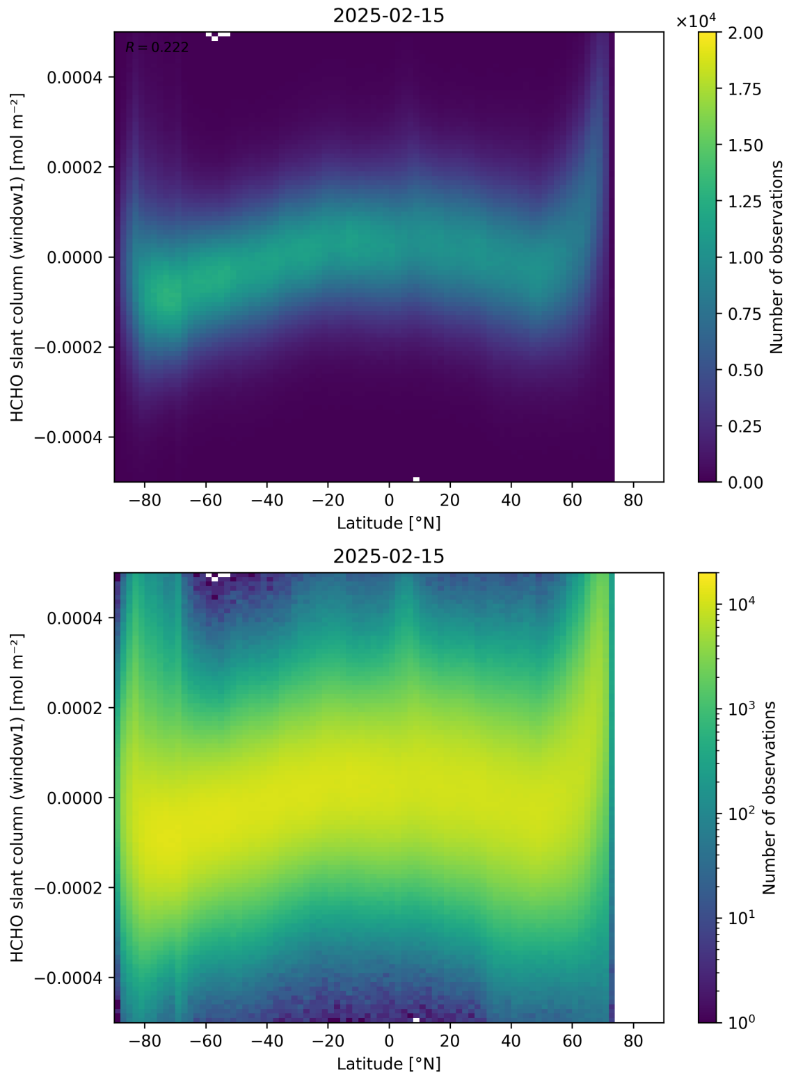
Figure 159: Scatter density plot of “Latitude” against “HCHO slant column (window1)” for 2025-02-14 to 2025-02-16.
