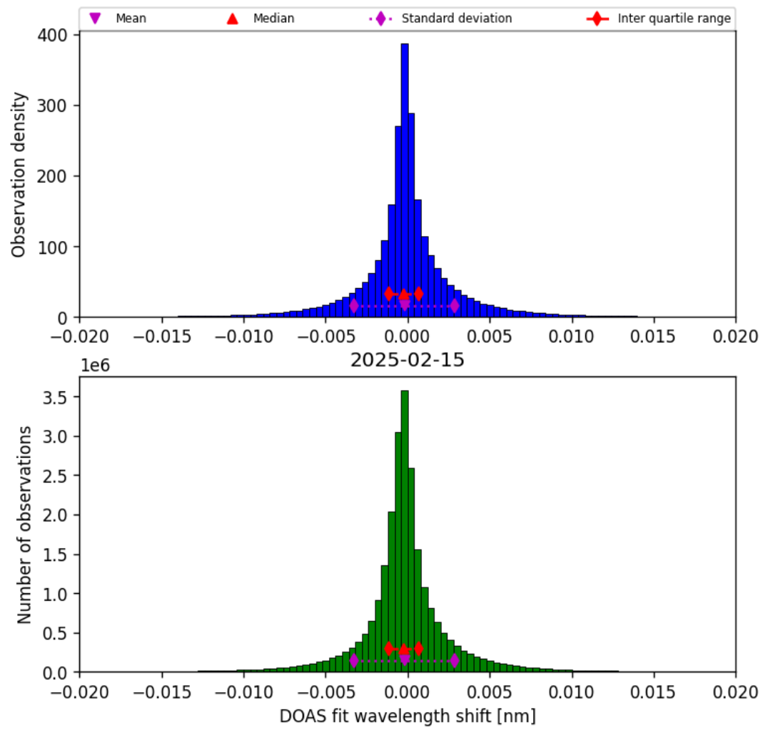
Figure 44: Histogram of “DOAS fit wavelength shift” for 2025-02-14 to 2025-02-16
