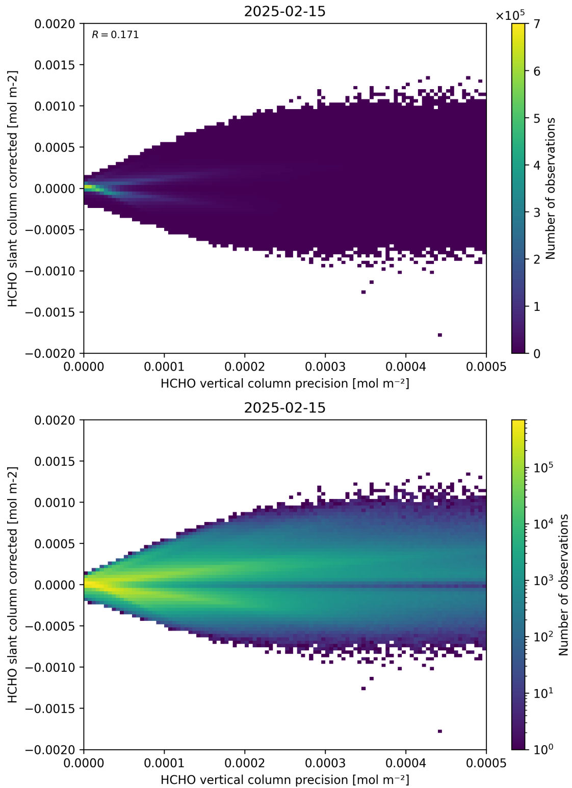
Figure 140: Scatter density plot of “HCHO vertical column precision” against “HCHO slant column corrected” for 2025-02-14 to 2025-02-16.
