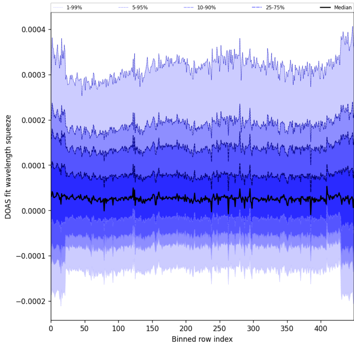
Figure 59: Along track statistics of “DOAS fit wavelength squeeze” for 2025-02-14 to 2025-02-16
