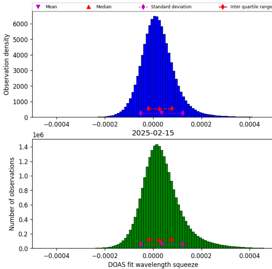
Figure 45: Histogram of “DOAS fit wavelength squeeze” for 2025-02-14 to 2025-02-16
