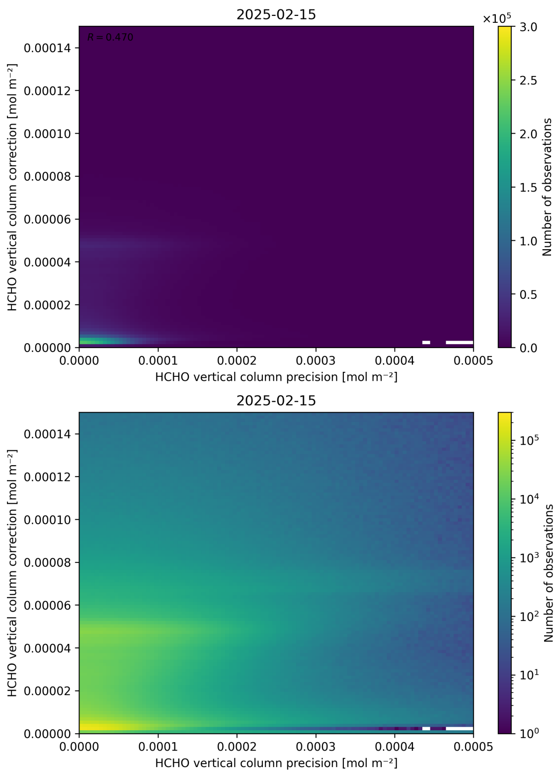
Figure 146: Scatter density plot of “HCHO vertical column precision” against “HCHO vertical column correction” for 2025-02-14 to 2025-02-16.
