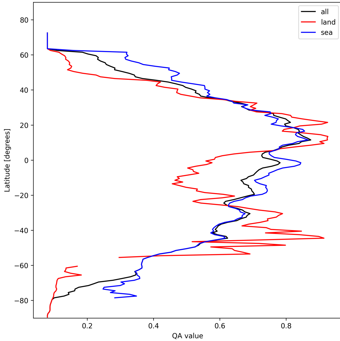
Figure 20: Zonal average of “QA value” for 2025-02-14 to 2025-02-16.
