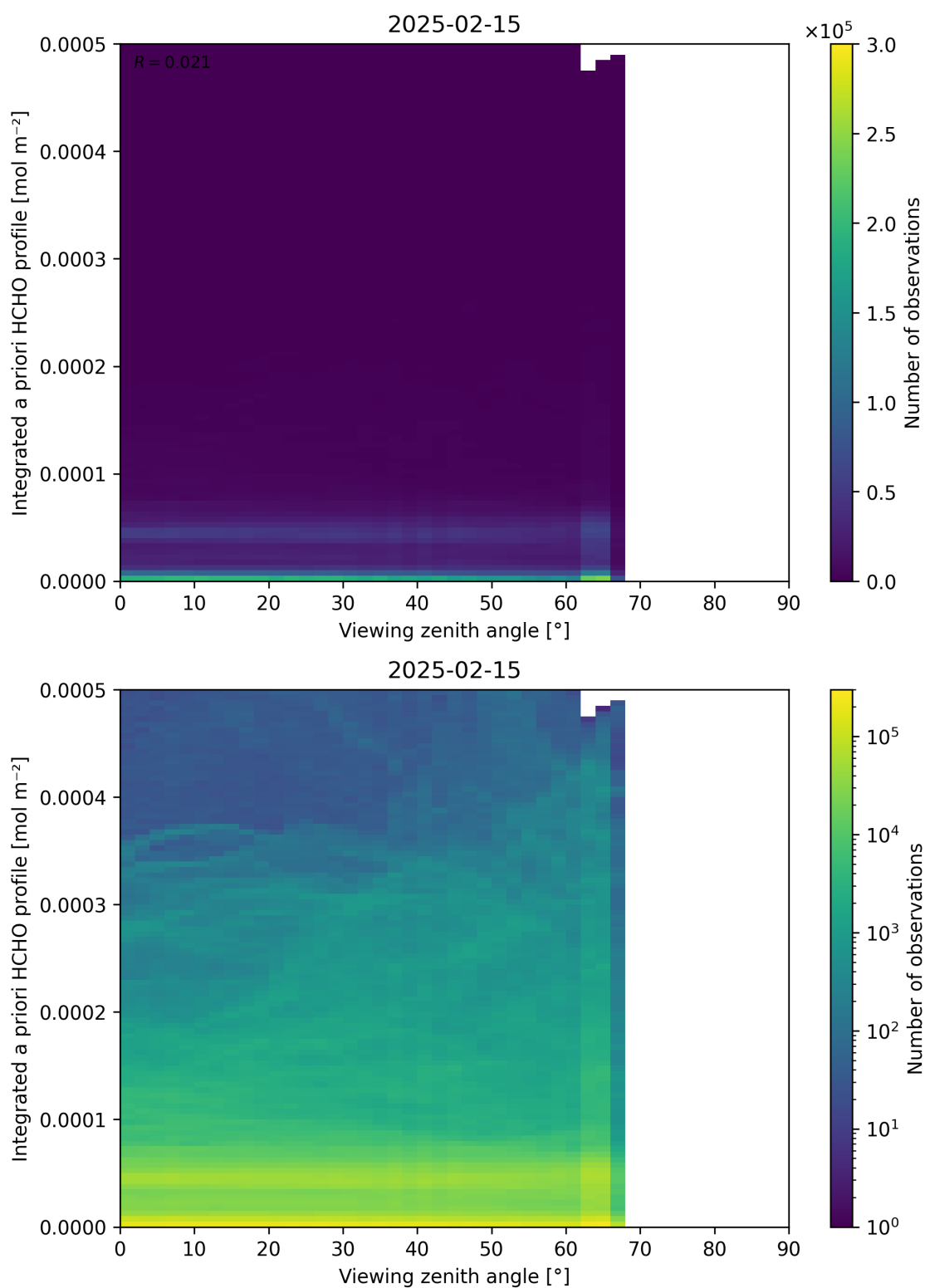
Figure 195: Scatter density plot of “Viewing zenith angle” against “Integrated a priori HCHO profile” for 2025-02-14 to 2025-02-16.
