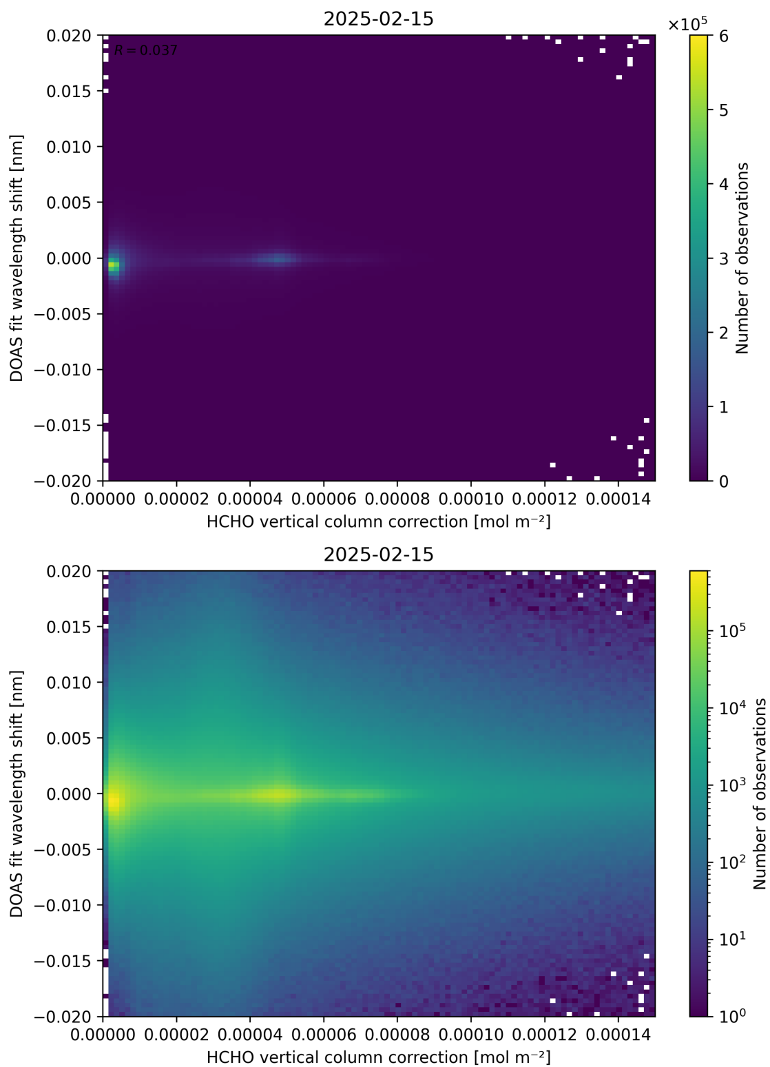
Figure 113: Scatter density plot of “HCHO vertical column correction” against “DOAS fit wavelength shift” for 2025-02-14 to 2025-02-16.
