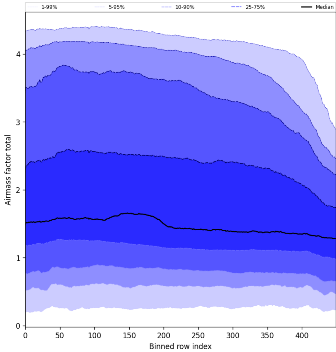
Figure 54: Along track statistics of “Airmass factor total” for 2025-02-14 to 2025-02-16
