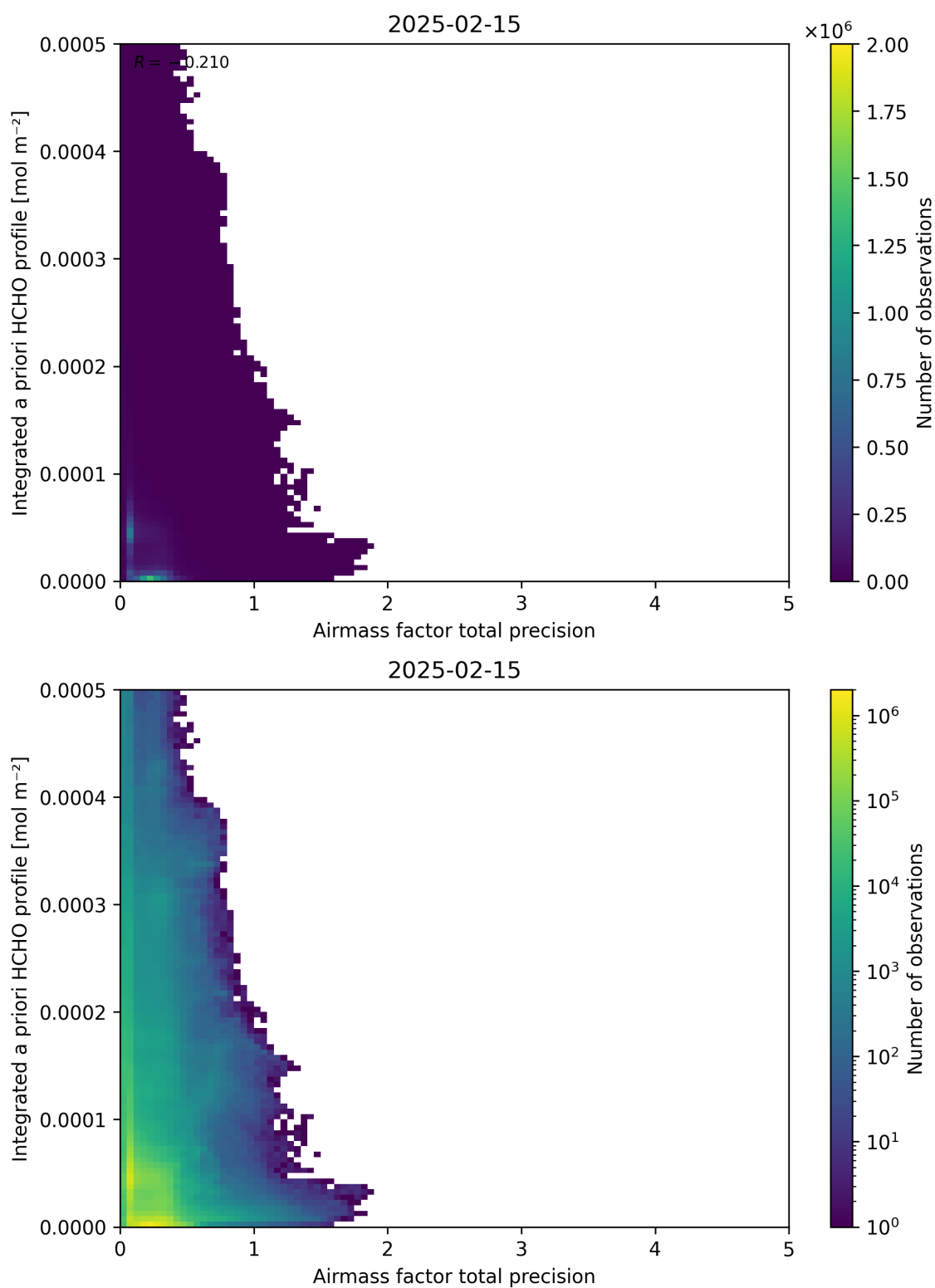
Figure 111: Scatter density plot of “Airmass factor total precision” against “Integrated a priori HCHO profile” for 2025-02-14 to 2025-02-16.
