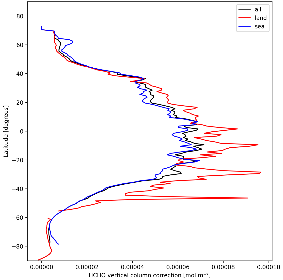
Figure 23: Zonal average of “HCHO vertical column correction” for 2025-02-14 to 2025-02-16.
