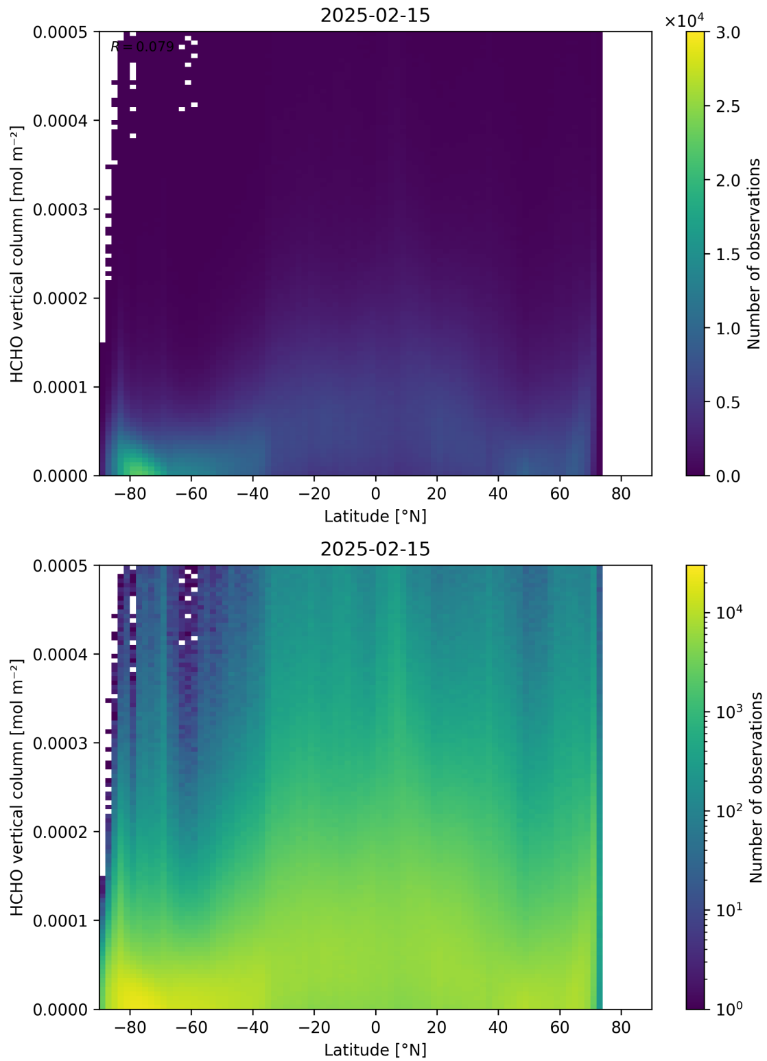
Figure 163: Scatter density plot of “Latitude” against “HCHO vertical column” for 2025-02-14 to 2025-02-16.
