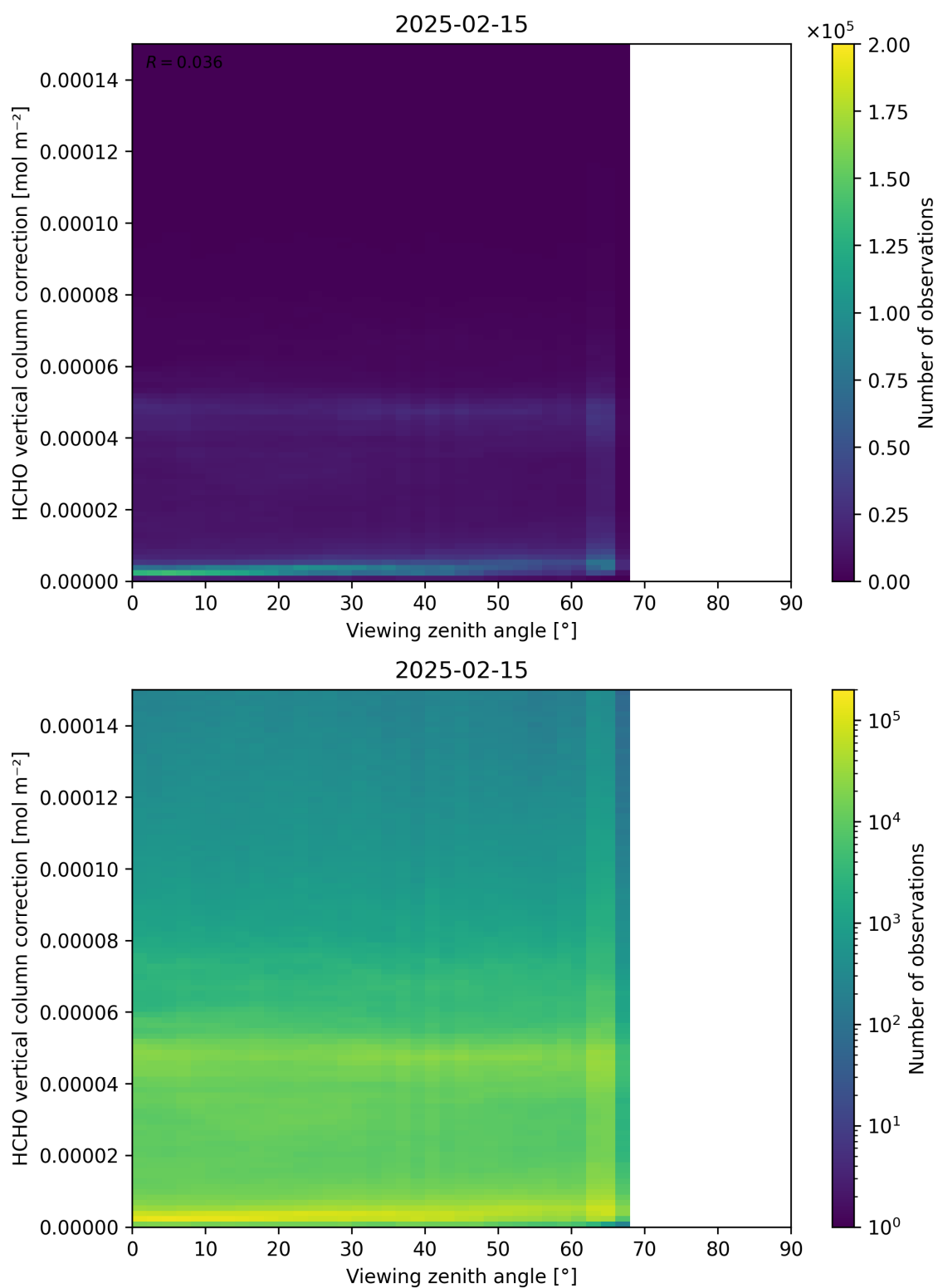
Figure 193: Scatter density plot of “Viewing zenith angle” against “HCHO vertical column correction” for 2025-02-14 to 2025-02-16.
