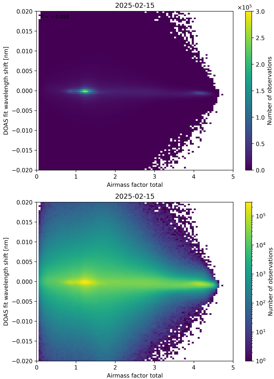
Figure 98: Scatter density plot of “Airmass factor total” against “DOAS fit wavelength shift” for 2025-02-14 to 2025-02-16.
