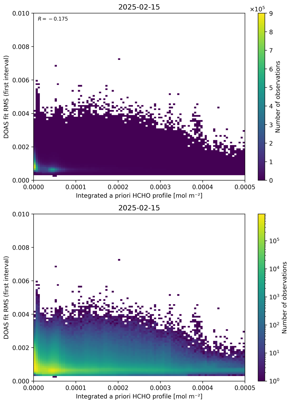
Figure 148: Scatter density plot of “Integrated a priori HCHO profile” against “DOAS fit RMS (first interval)” for 2025-02-14 to 2025-02-16.
