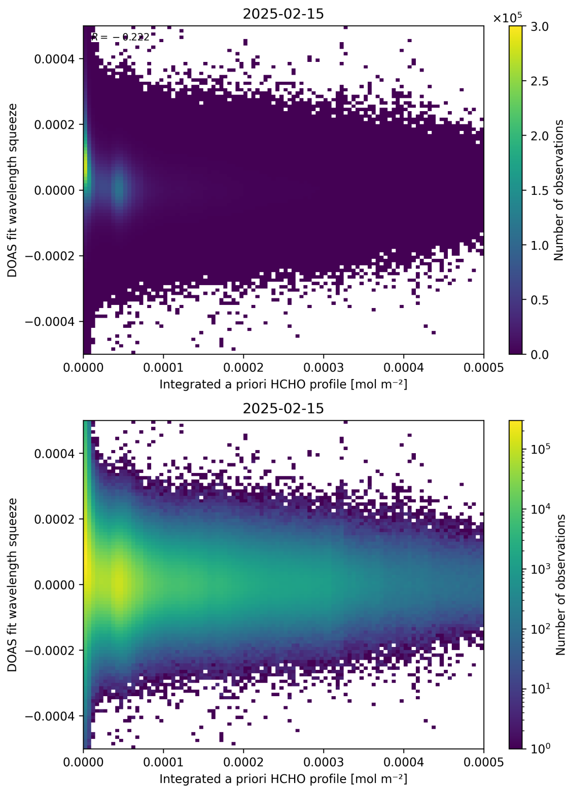
Figure 150: Scatter density plot of “Integrated a priori HCHO profile” against “DOAS fit wavelength squeeze” for 2025-02-14 to 2025-02-16.
