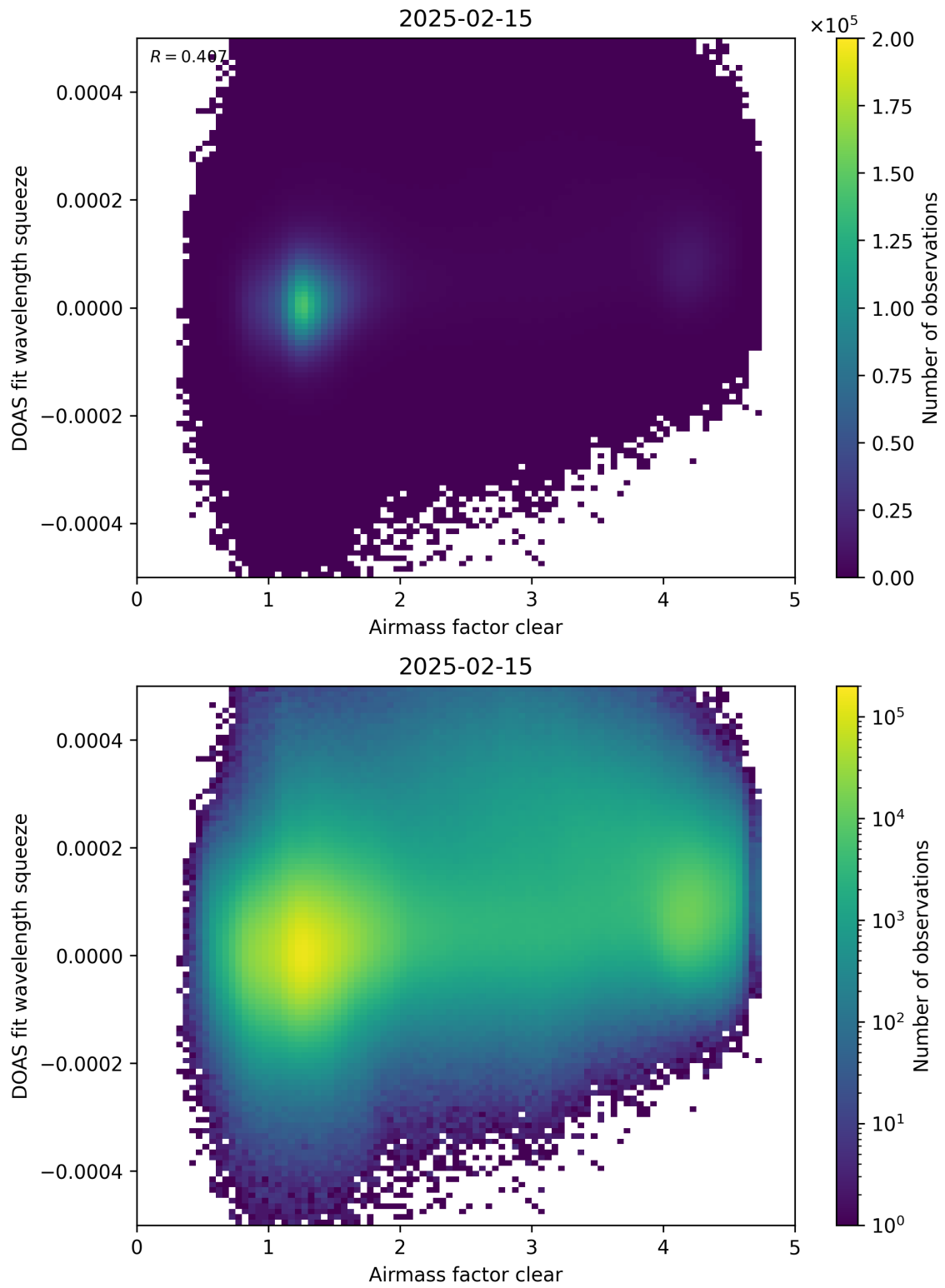
Figure 73: Scatter density plot of “Airmass factor clear” against “DOAS fit wavelength squeeze” for 2025-02-14 to 2025-02-16.
