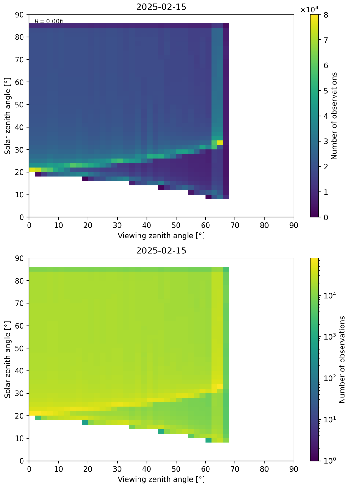
Figure 197: Scatter density plot of “Viewing zenith angle” against “Solar zenith angle” for 2025-02-14 to 2025-02-16.
