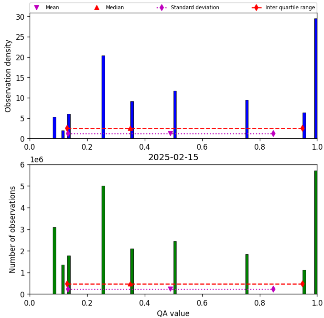
Figure 34: Histogram of “QA value” for 2025-02-14 to 2025-02-16
