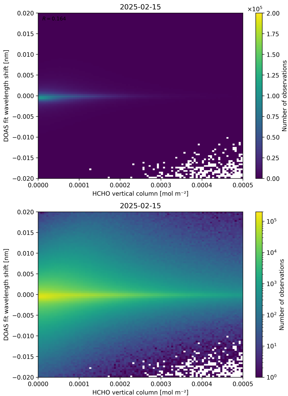
Figure 124: Scatter density plot of “HCHO vertical column” against “DOAS fit wavelength shift” for 2025-02-14 to 2025-02-16.
