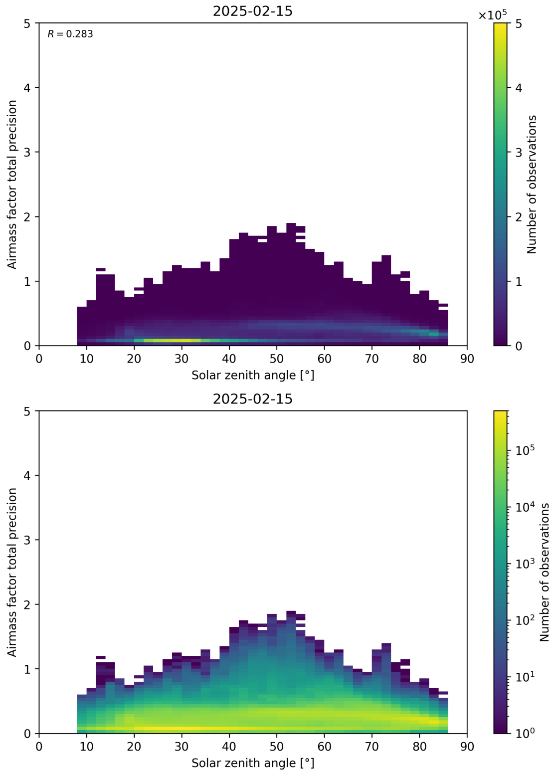
Figure 176: Scatter density plot of “Solar zenith angle” against “Airmass factor total precision” for 2025-02-14 to 2025-02-16.
