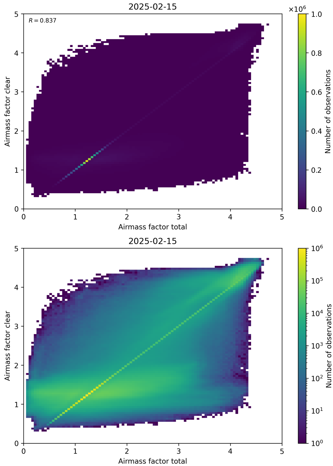
Figure 100: Scatter density plot of “Airmass factor total” against “Airmass factor clear” for 2025-02-14 to 2025-02-16.
