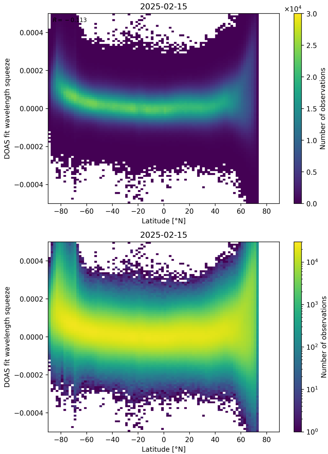
Figure 155: Scatter density plot of “Latitude” against “DOAS fit wavelength squeeze” for 2025-02-14 to 2025-02-16.
