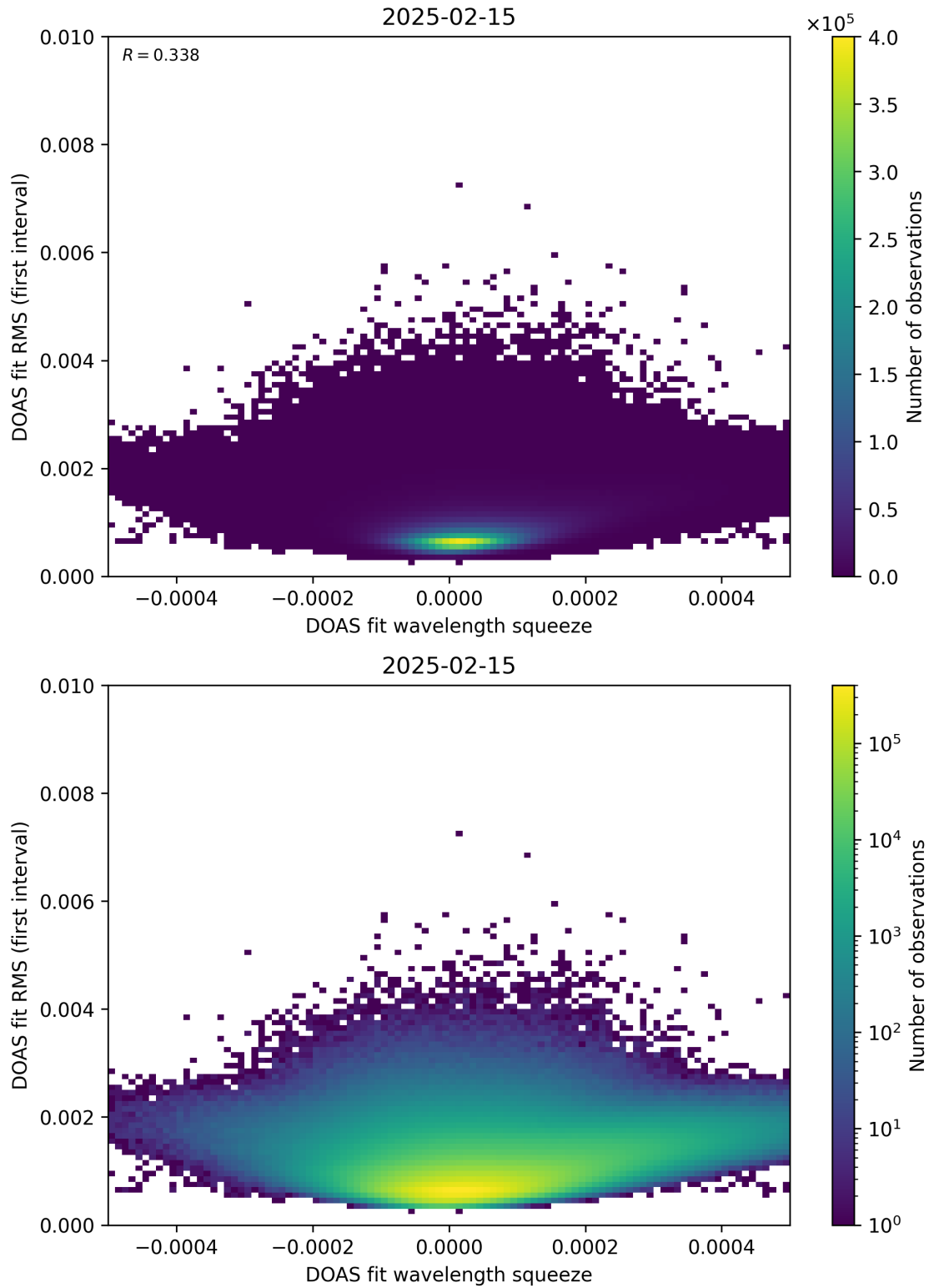
Figure 68: Scatter density plot of “DOAS fit wavelength squeeze” against “DOAS fit RMS (first interval)” for 2025-02-14 to 2025-02-16.
