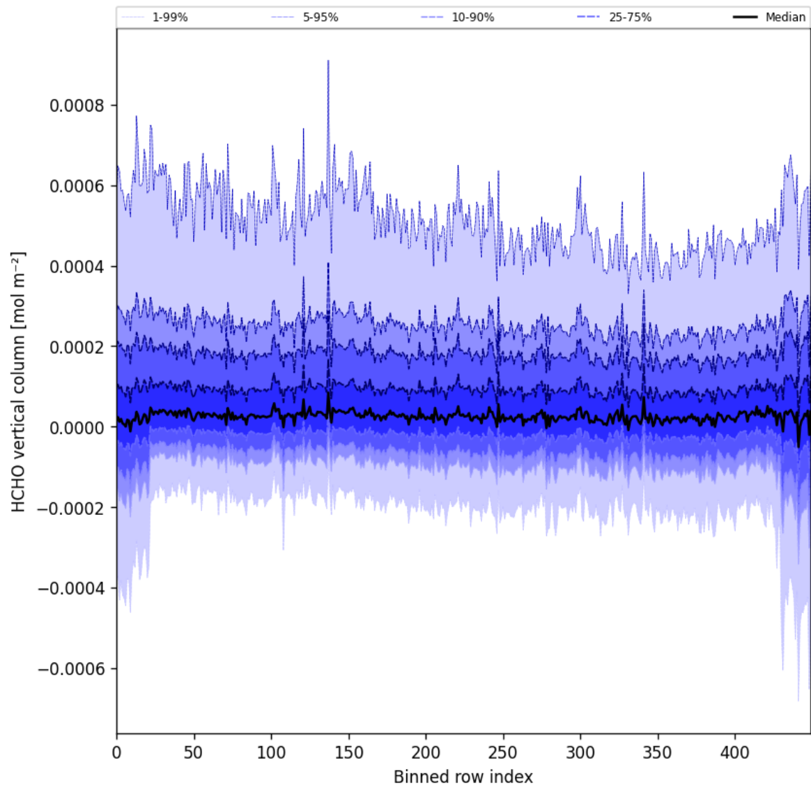
Figure 49: Along track statistics of “HCHO vertical column” for 2025-02-14 to 2025-02-16
