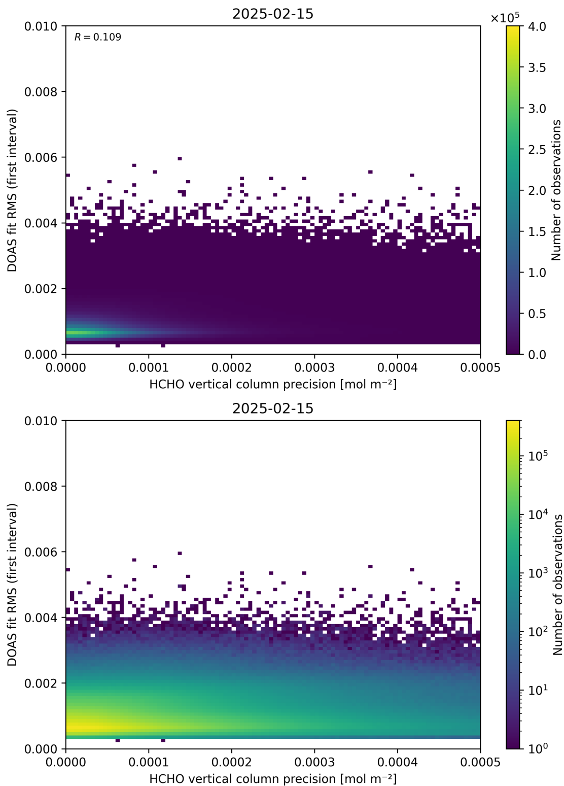
Figure 136: Scatter density plot of “HCHO vertical column precision” against “DOAS fit RMS (first interval)” for 2025-02-14 to 2025-02-16.
