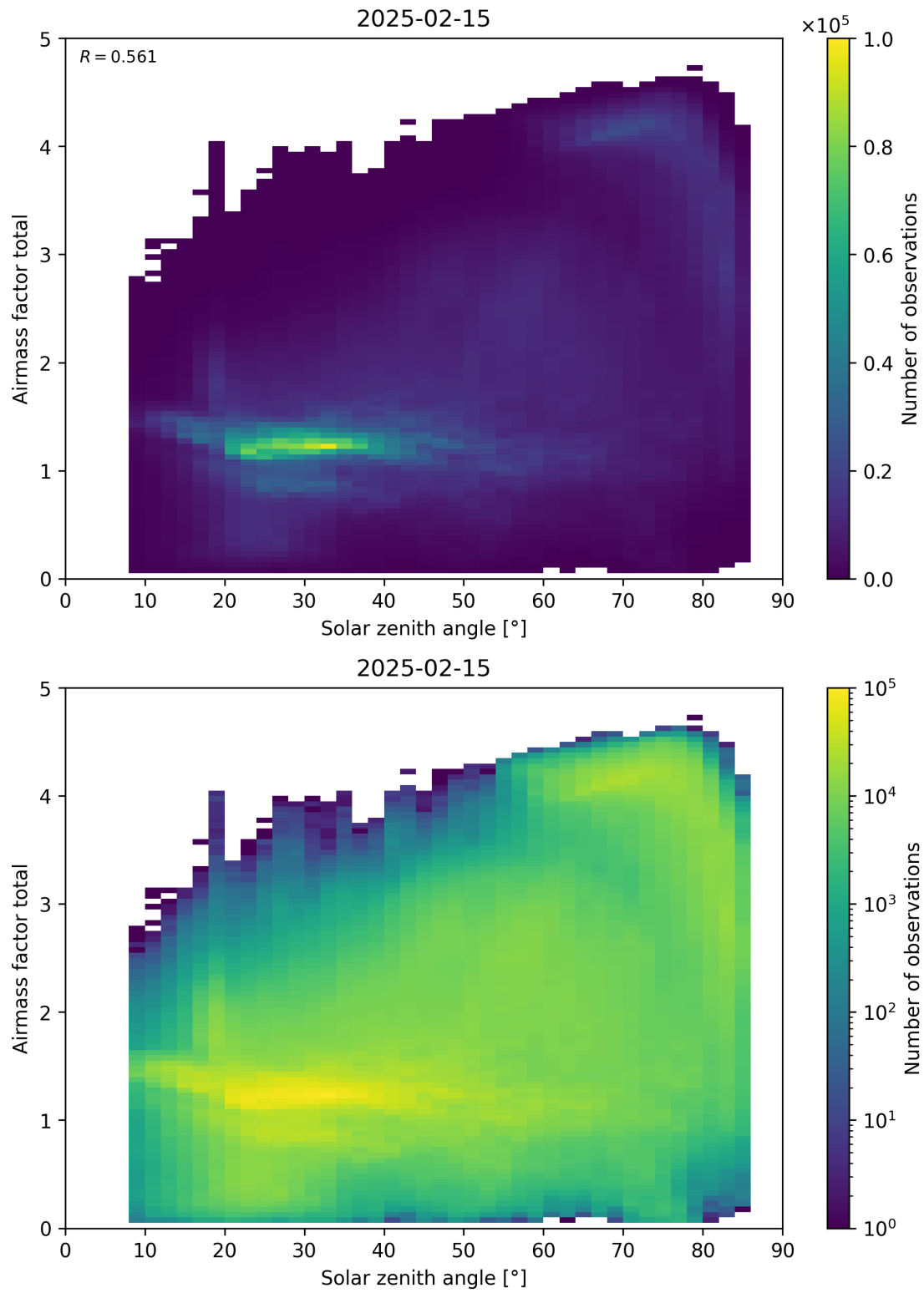
Figure 175: Scatter density plot of “Solar zenith angle” against “Airmass factor total” for 2025-02-14 to 2025-02-16.
