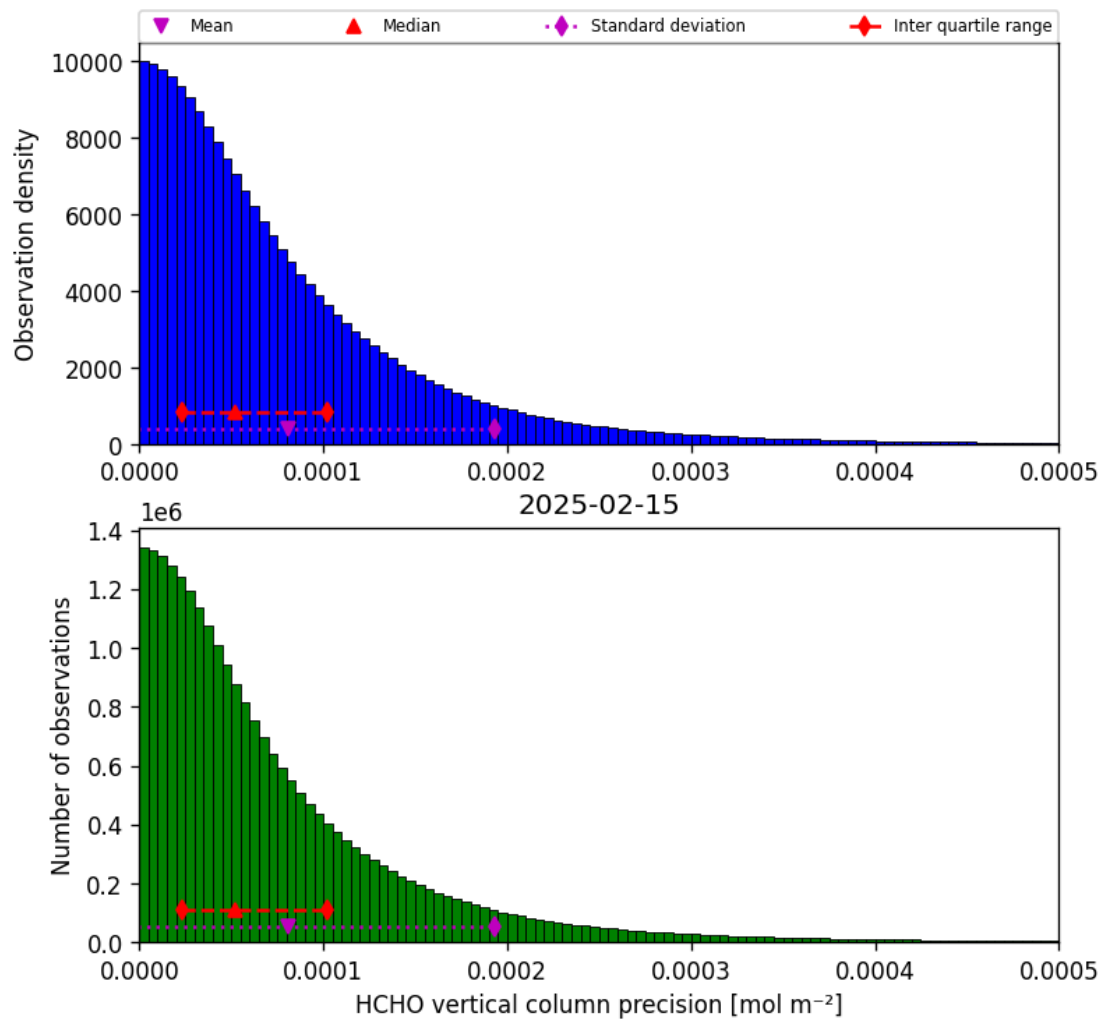
Figure 36: Histogram of "HCHO vertical column precision" for 2025-02-14 to 2025-02-16
