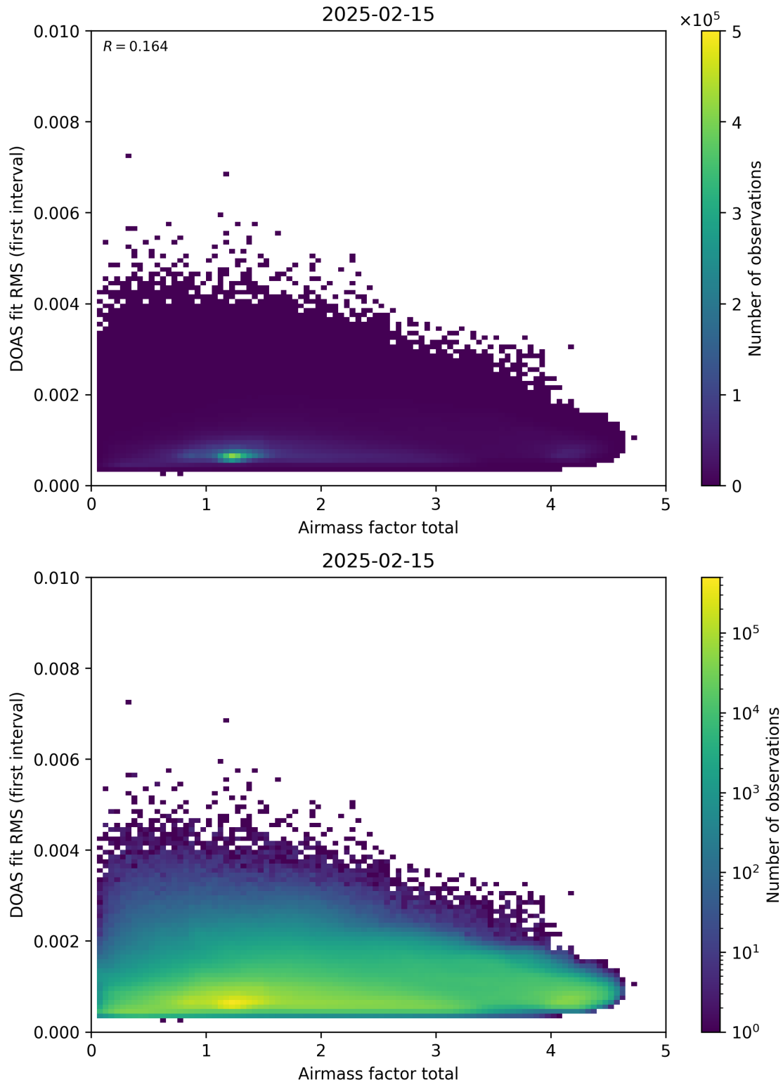
Figure 97: Scatter density plot of “Airmass factor total” against “DOAS fit RMS (first interval)” for 2025-02-14 to 2025-02-16.
