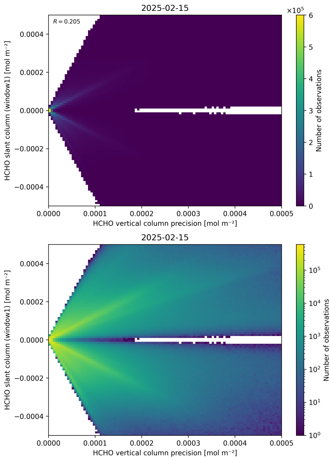
Figure 142: Scatter density plot of “HCHO vertical column precision” against “HCHO slant column (window1)” for 2025-02-14 to 2025-02-16.
