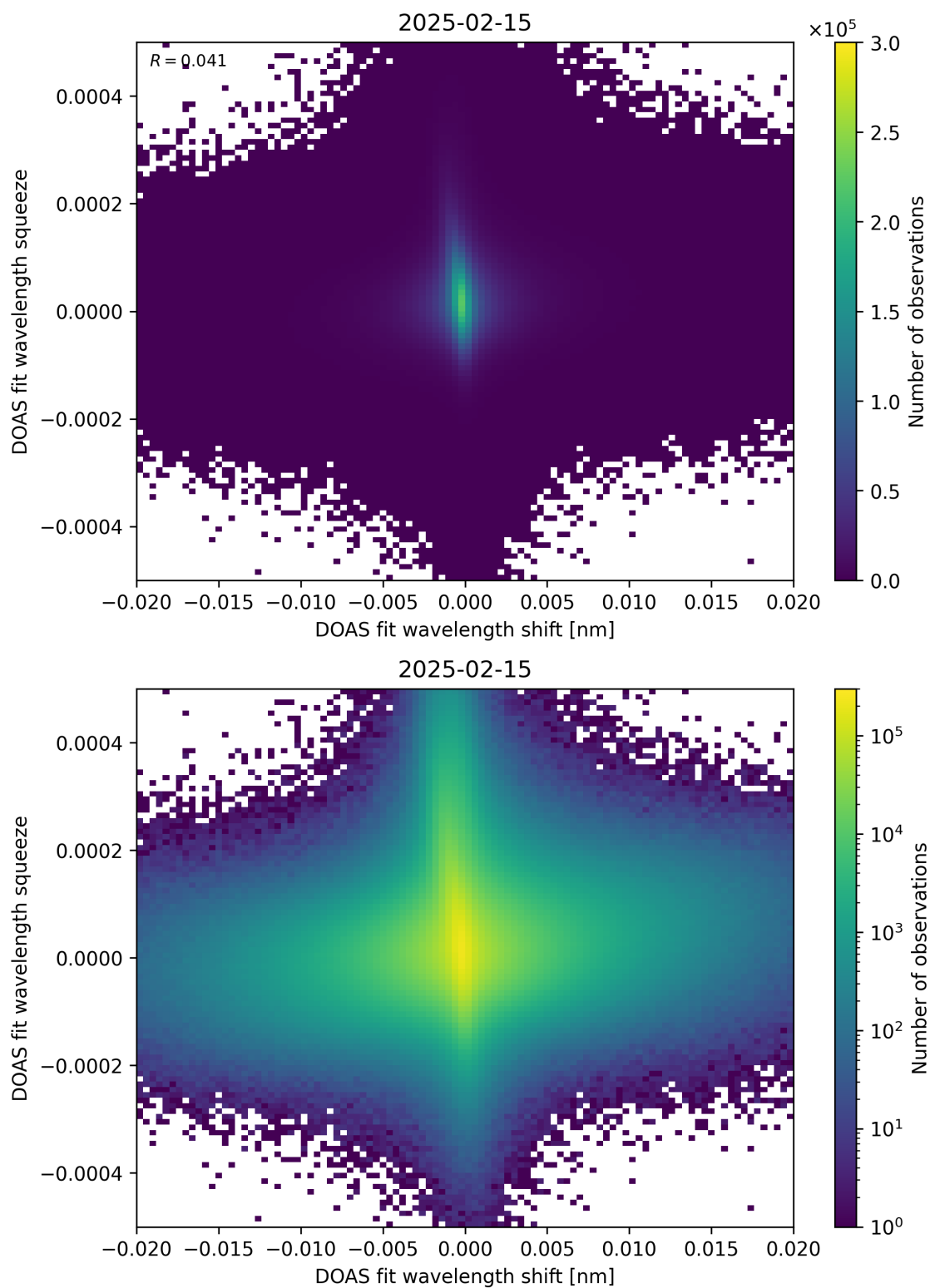
Figure 65: Scatter density plot of “DOAS fit wavelength shift” against “DOAS fit wavelength squeeze” for 2025-02-14 to 2025-02-16.
