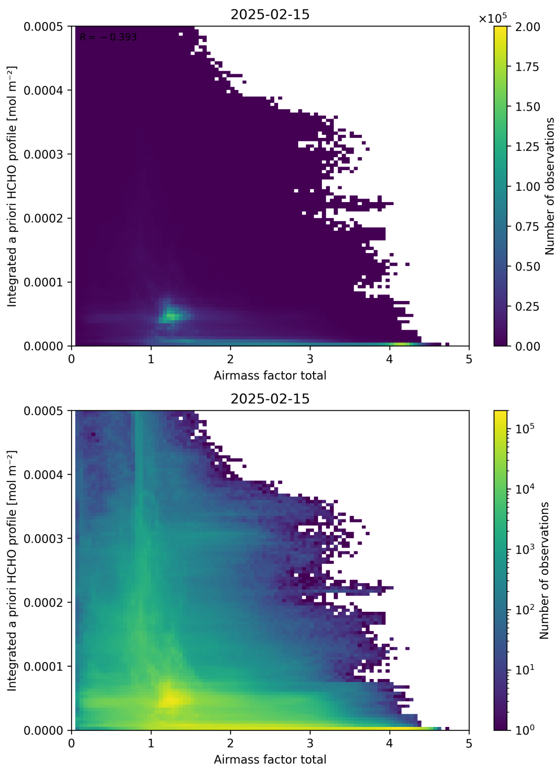
Figure 104: Scatter density plot of “Airmass factor total” against “Integrated a priori HCHO profile” for 2025-02-14 to 2025-02-16.
