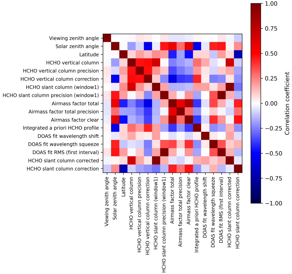
Figure 2: Map of correlation matrix for 2025-02-14 to 2025-02-16.
