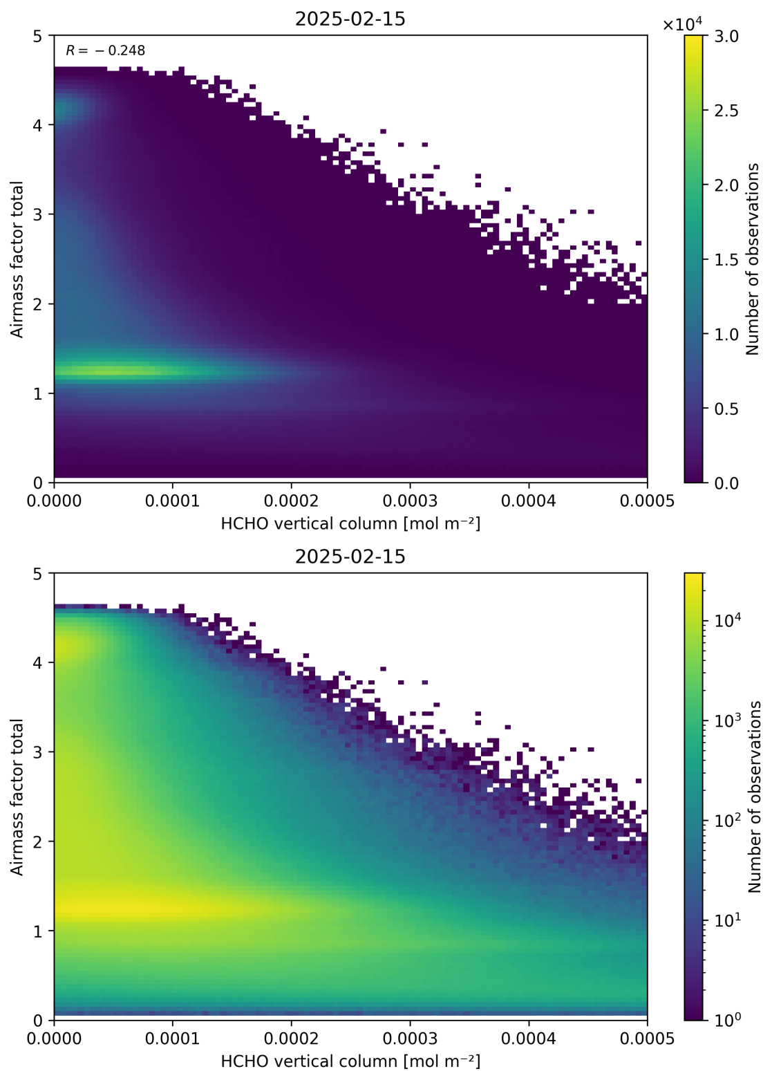
Figure 131: Scatter density plot of “HCHO vertical column” against “Airmass factor total” for 2025-02-14 to 2025-02-16.
