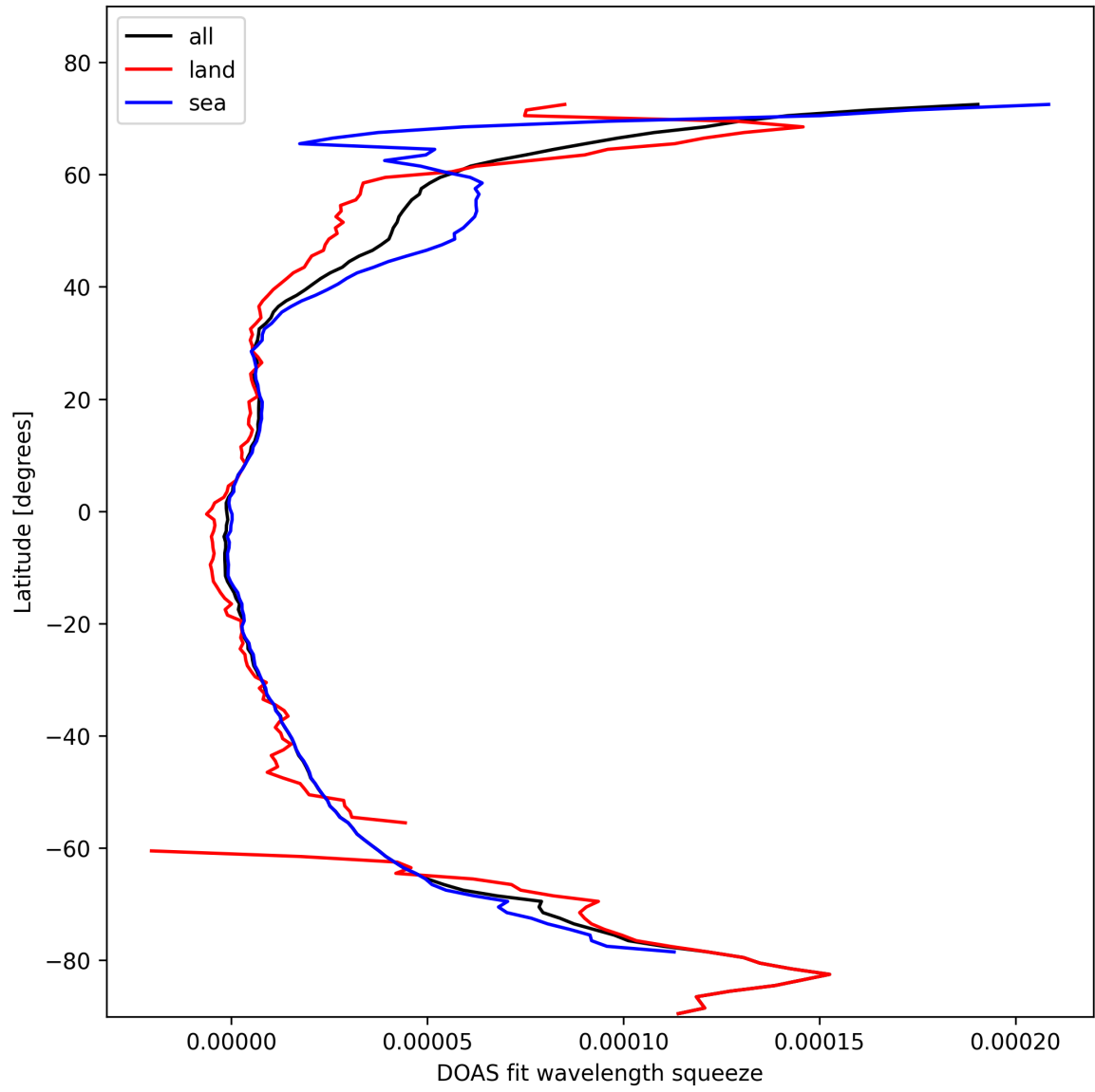
Figure 31: Zonal average of “DOAS fit wavelength squeeze” for 2025-02-14 to 2025-02-16.
