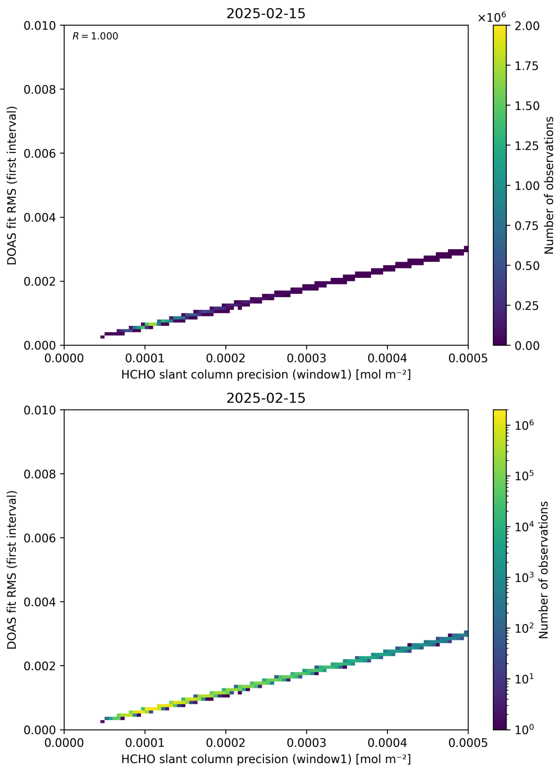
Figure 88: Scatter density plot of “HCHO slant column precision (window1)” against “DOAS fit RMS (first interval)” for 2025-02-14 to 2025-02-16.
