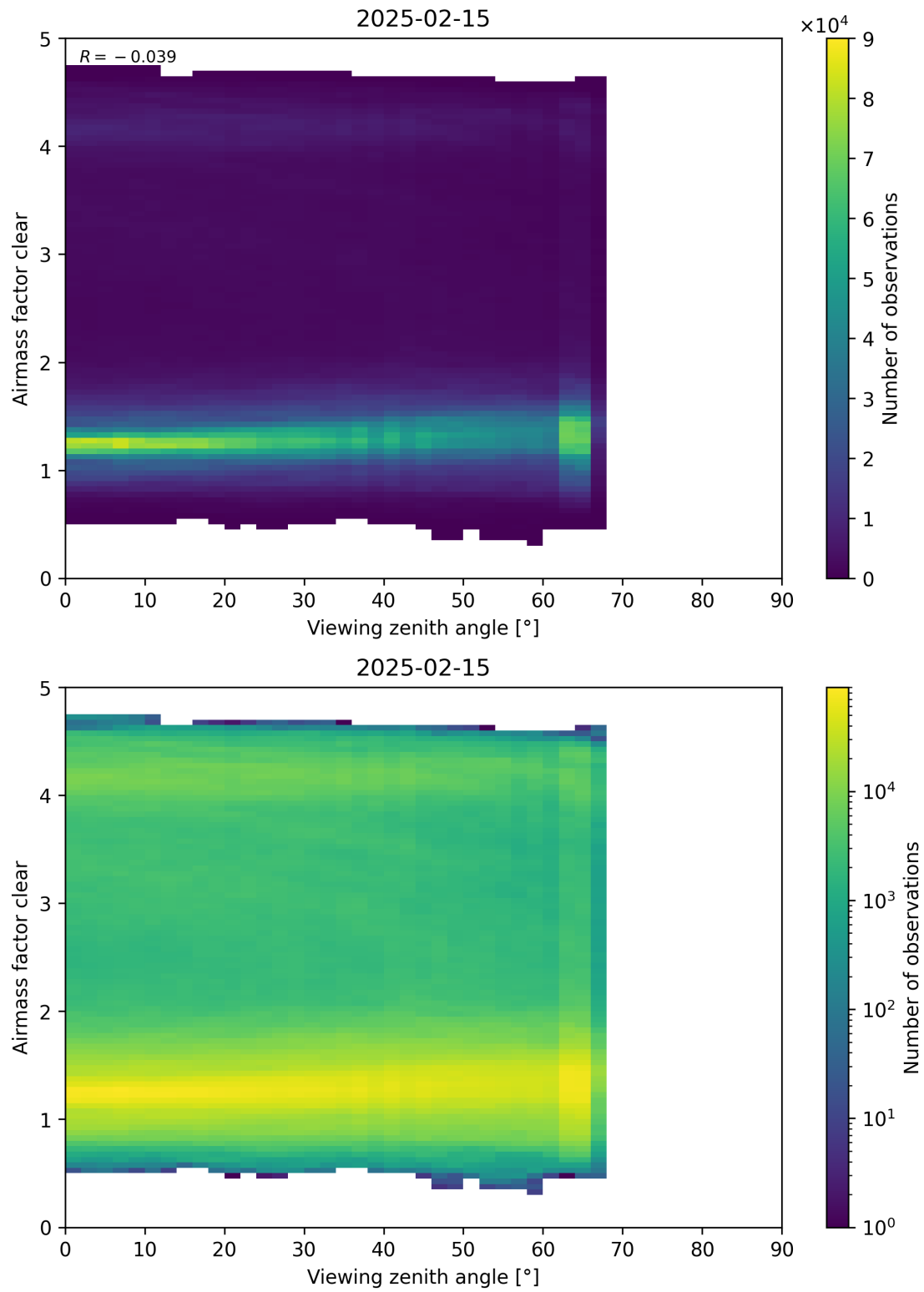
Figure 185: Scatter density plot of “Viewing zenith angle” against “Airmass factor clear” for 2025-02-14 to 2025-02-16.
