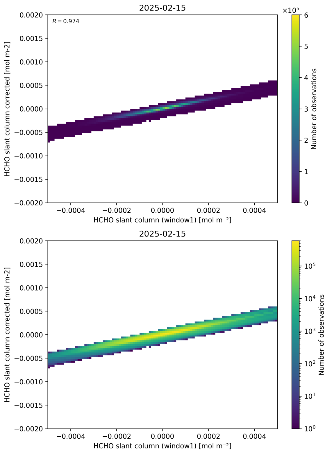
Figure 82: Scatter density plot of “HCHO slant column (window1)” against “HCHO slant column corrected” for 2025-02-14 to 2025-02-16.
