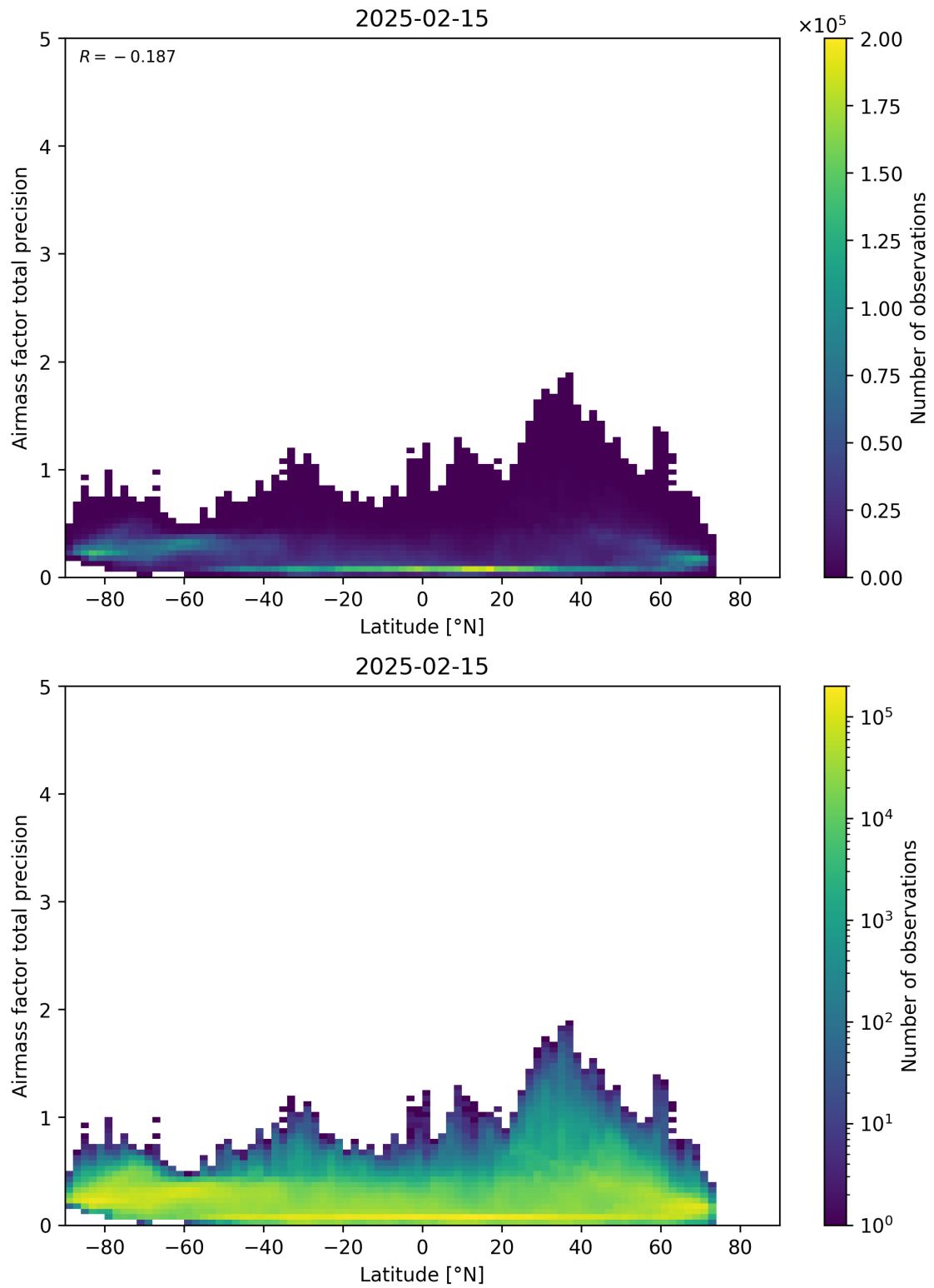
Figure 162: Scatter density plot of “Latitude” against “Airmass factor total precision” for 2025-02-14 to 2025-02-16.
