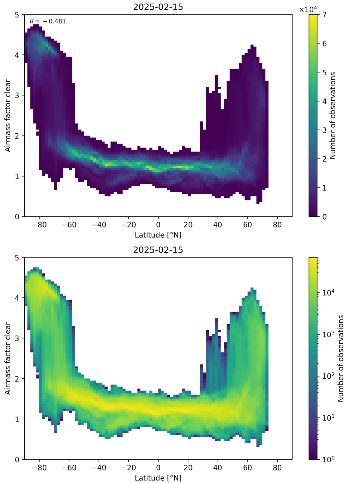
Figure 156: Scatter density plot of “Latitude” against “Airmass factor clear” for 2025-02-14 to 2025-02-16.
