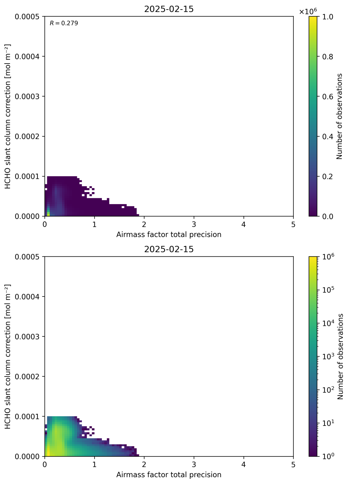
Figure 110: Scatter density plot of “Airmass factor total precision” against “HCHO slant column correction” for 2025-02-14 to 2025-02-16.
