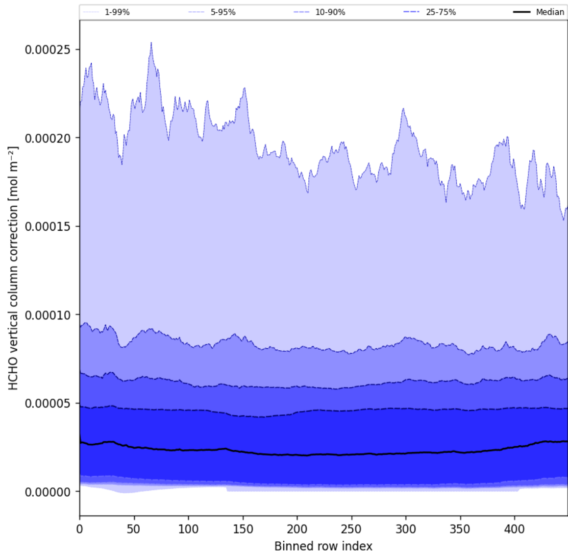
Figure 51: Along track statistics of “HCHO vertical column correction” for 2025-02-14 to 2025-02-16
