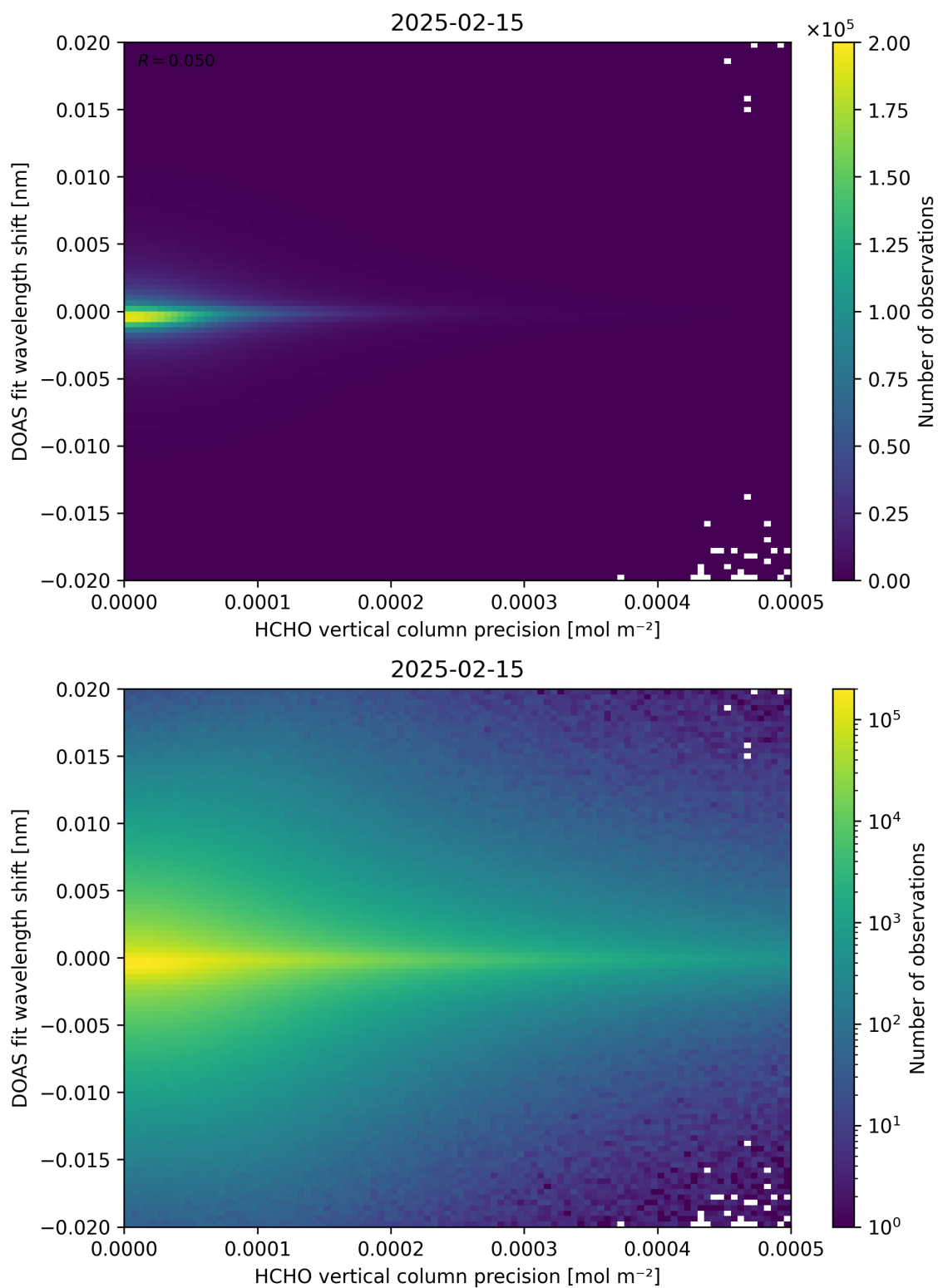
Figure 137: Scatter density plot of “HCHO vertical column precision” against “DOAS fit wavelength shift” for 2025-02-14 to 2025-02-16.
