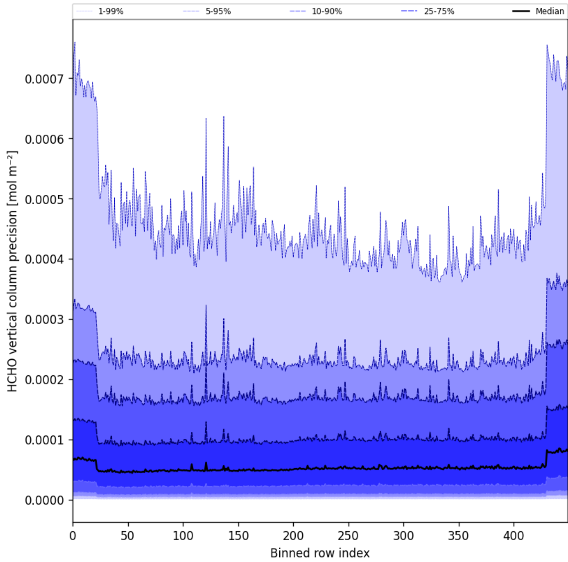
Figure 50: Along track statistics of “HCHO vertical column precision” for 2025-02-14 to 2025-02-16
