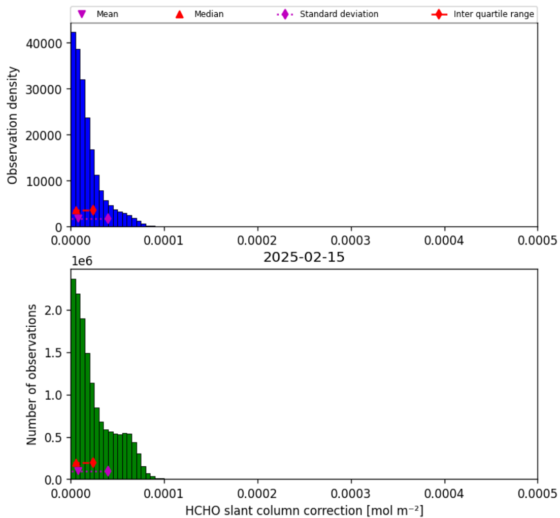
Figure 47: Histogram of “HCHO slant column correction” for 2025-02-14 to 2025-02-16
