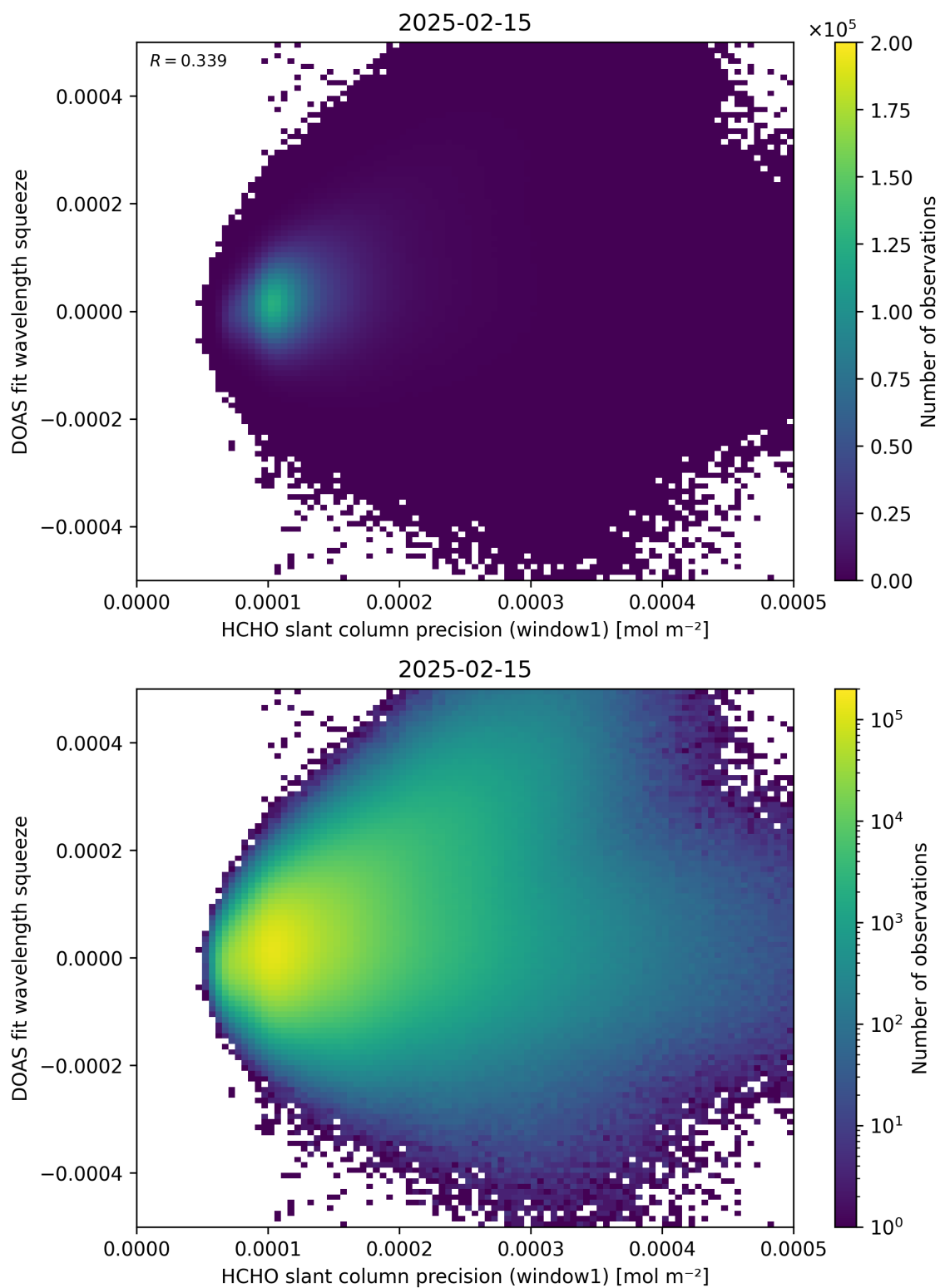
Figure 90: Scatter density plot of “HCHO slant column precision (window1)” against “DOAS fit wavelength squeeze” for 2025-02-14 to 2025-02-16.
