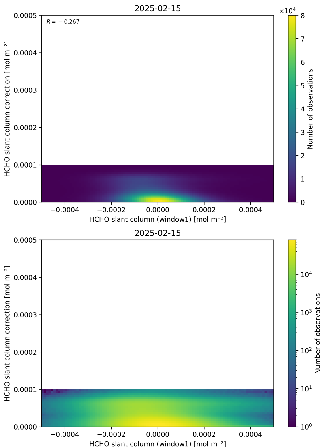
Figure 83: Scatter density plot of “HCHO slant column (window1)” against “HCHO slant column correction” for 2025-02-14 to 2025-02-16.
