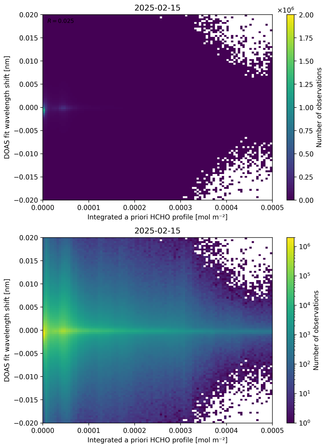
Figure 149: Scatter density plot of “Integrated a priori HCHO profile” against “DOAS fit wavelength shift” for 2025-02-14 to 2025-02-16.
