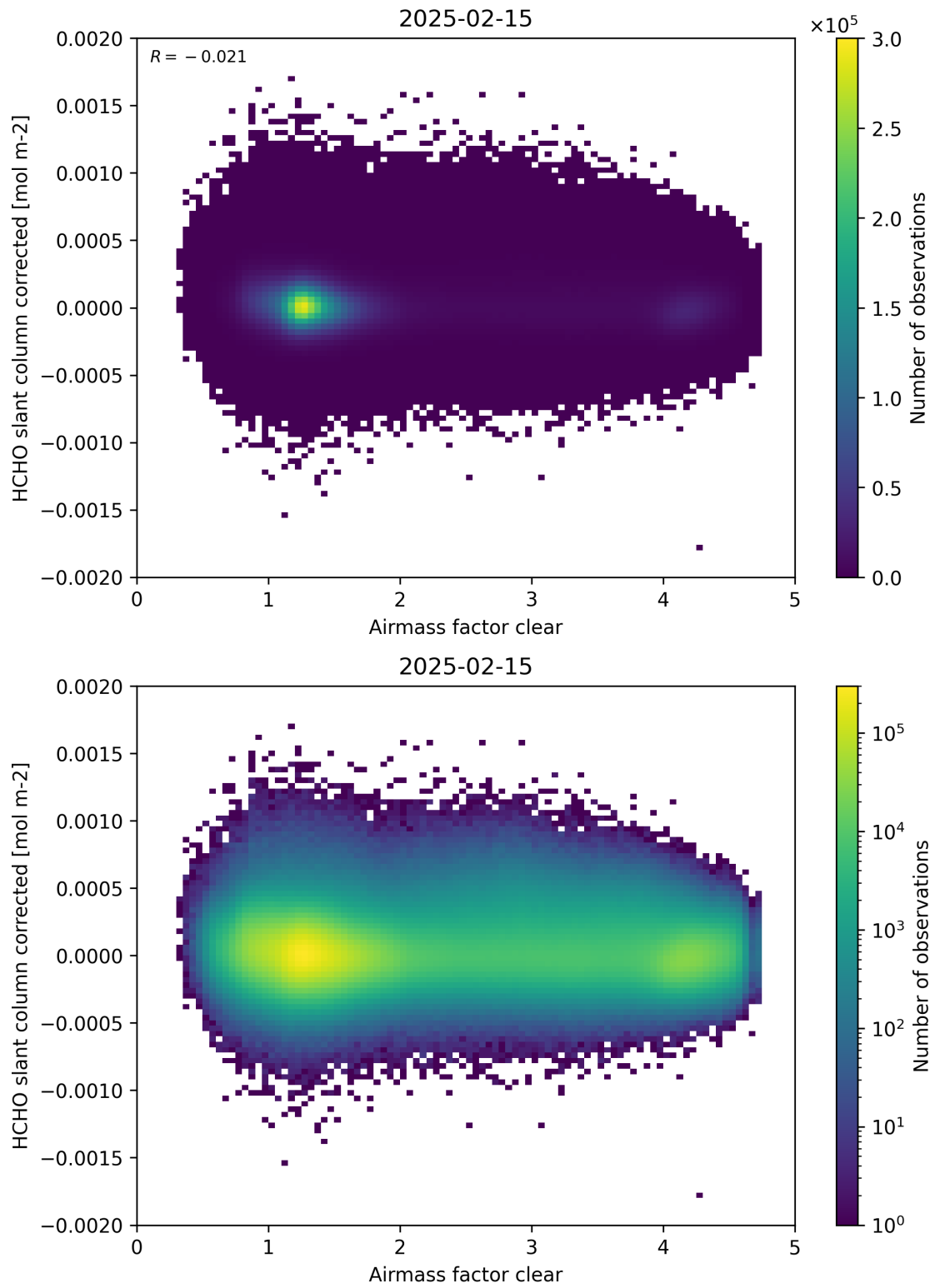
Figure 74: Scatter density plot of “Airmass factor clear” against “HCHO slant column corrected” for 2025-02-14 to 2025-02-16.
