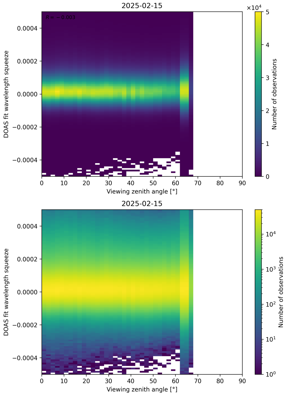
Figure 184: Scatter density plot of “Viewing zenith angle” against “DOAS fit wavelength squeeze” for 2025-02-14 to 2025-02-16.
