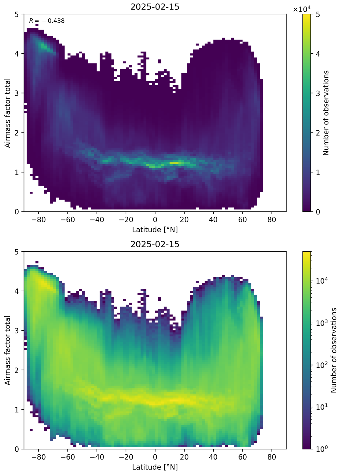
Figure 161: Scatter density plot of “Latitude” against “Airmass factor total” for 2025-02-14 to 2025-02-16.
