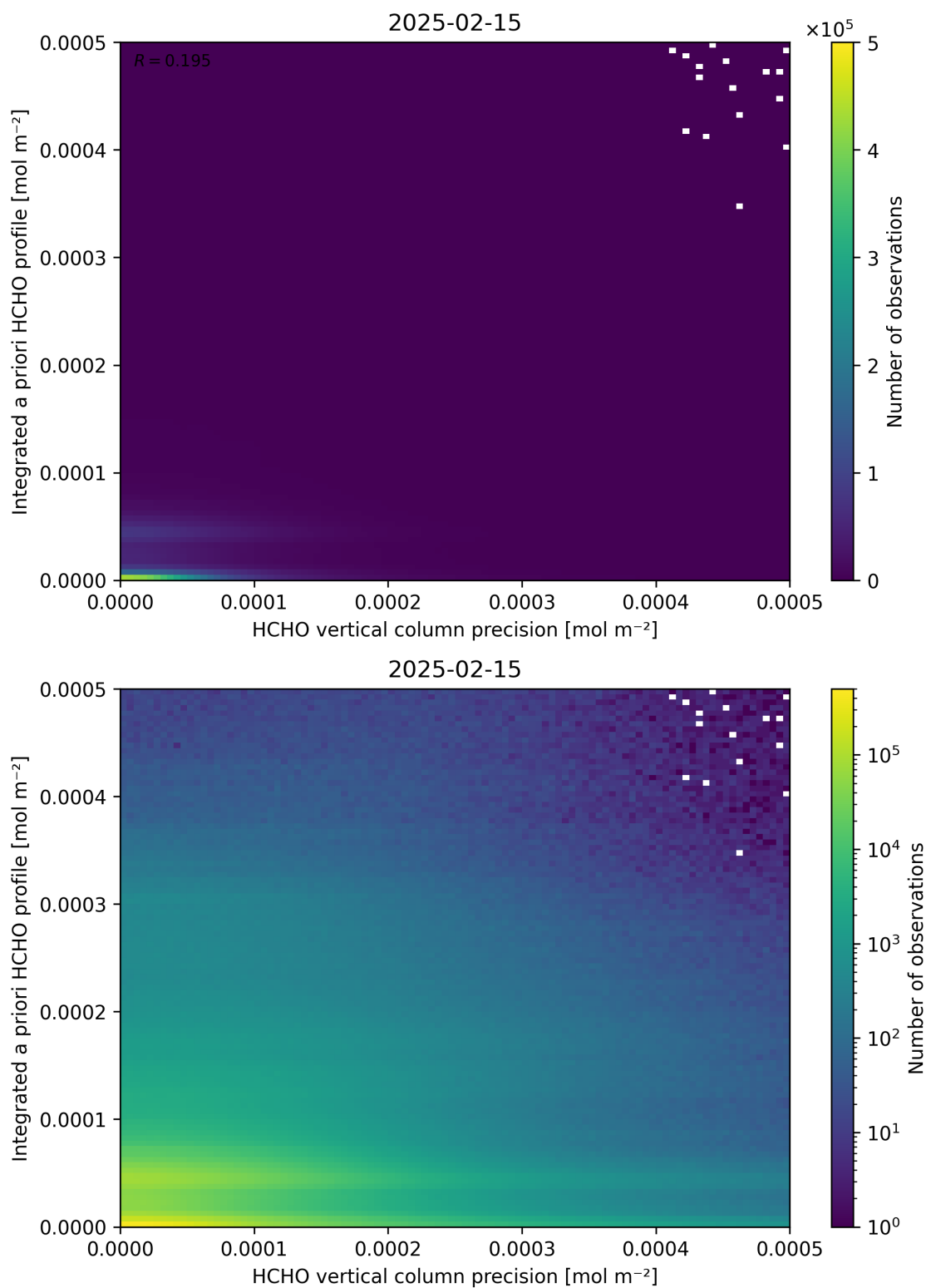
Figure 147: Scatter density plot of “HCHO vertical column precision” against “Integrated a priori HCHO profile” for 2025-02-14 to 2025-02-16.
