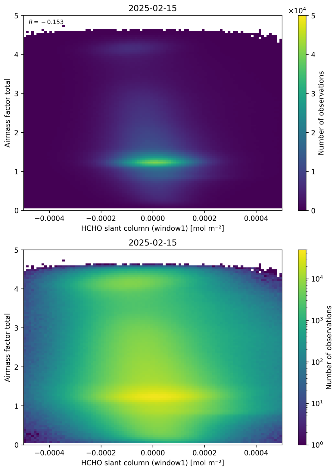
Figure 85: Scatter density plot of “HCHO slant column (window1)” against “Airmass factor total” for 2025-02-14 to 2025-02-16.
