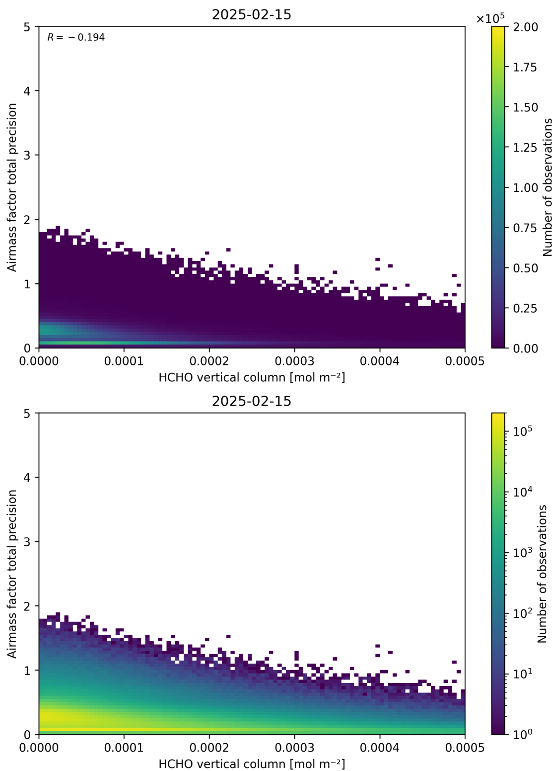
Figure 132: Scatter density plot of “HCHO vertical column” against “Airmass factor total precision” for 2025-02-14 to 2025-02-16.
