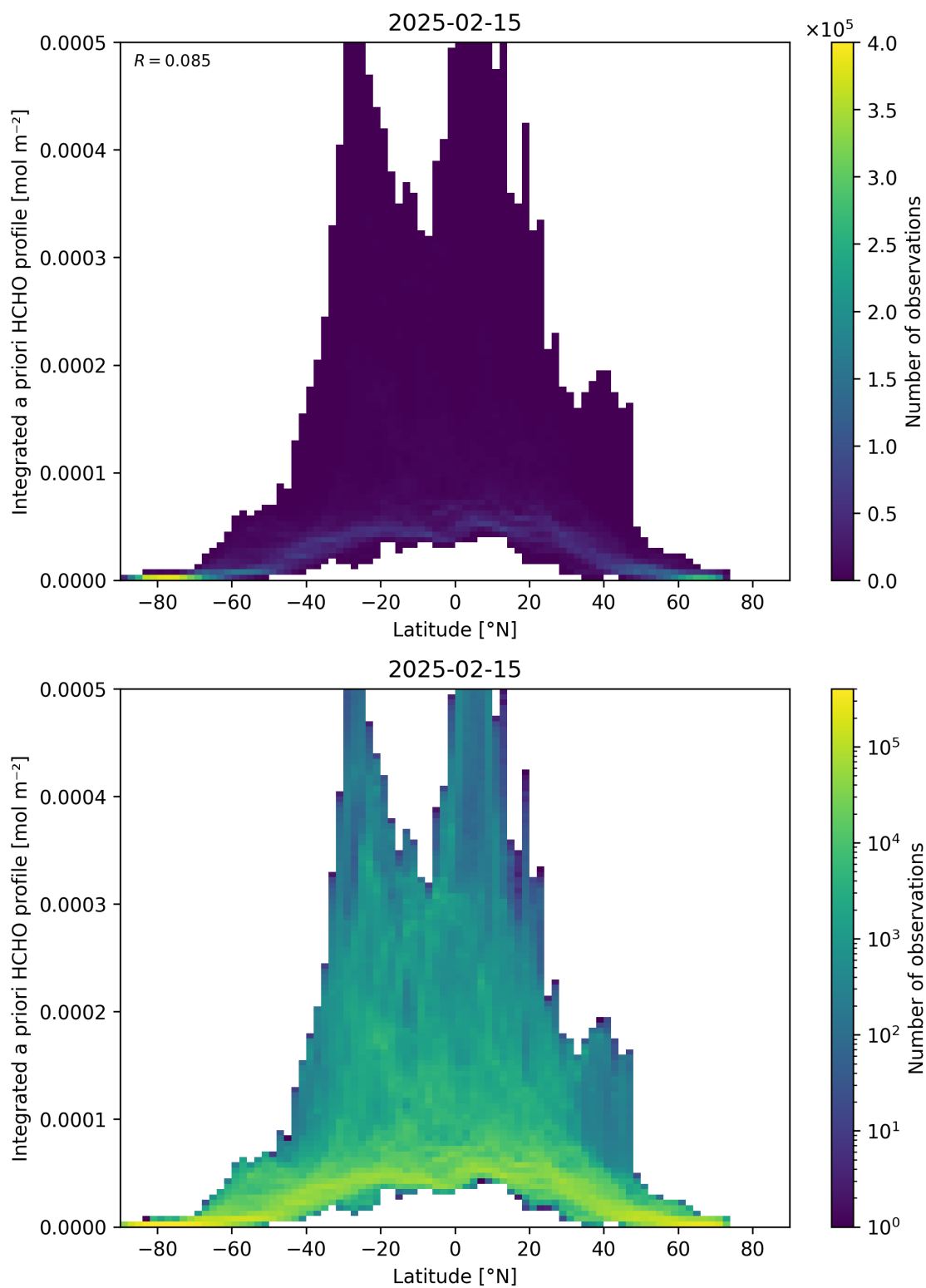
Figure 166: Scatter density plot of “Latitude” against “Integrated a priori HCHO profile” for 2025-02-14 to 2025-02-16.
