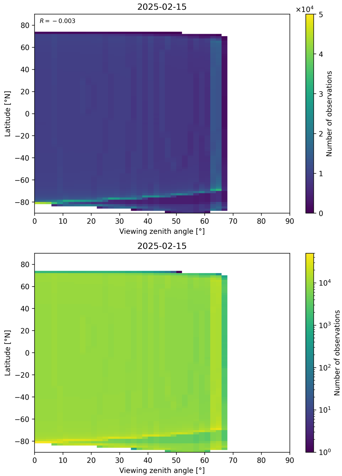
Figure 196: Scatter density plot of “Viewing zenith angle” against “Latitude” for 2025-02-14 to 2025-02-16.
