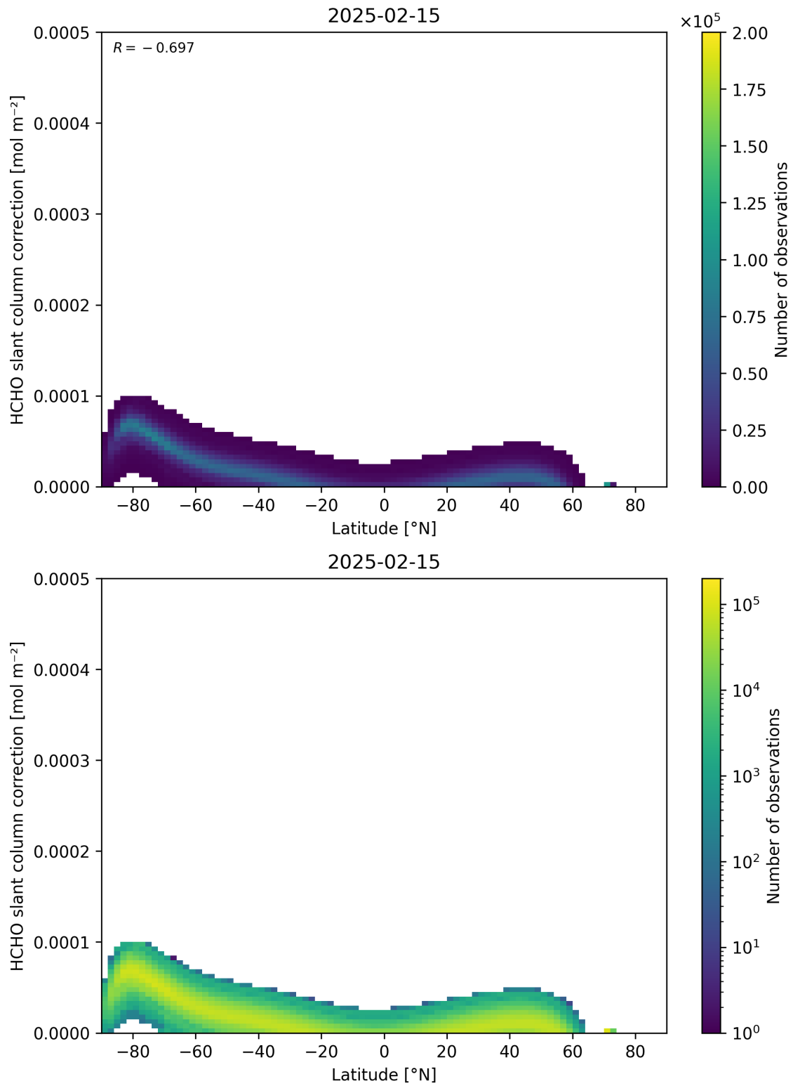
Figure 158: Scatter density plot of “Latitude” against “HCHO slant column correction” for 2025-02-14 to 2025-02-16.
