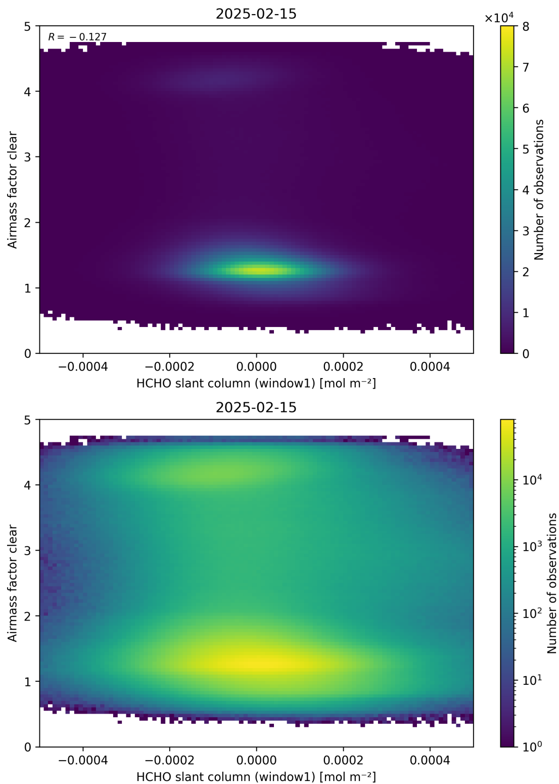
Figure 81: Scatter density plot of “HCHO slant column (window1)” against “Airmass factor clear” for 2025-02-14 to 2025-02-16.
