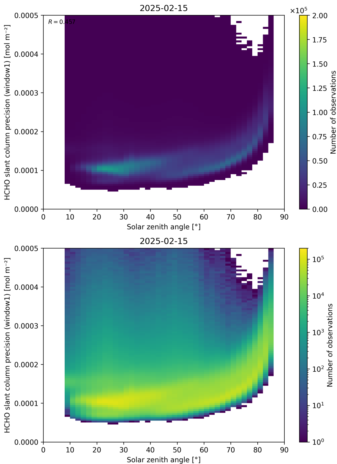
Figure 174: Scatter density plot of “Solar zenith angle” against “HCHO slant column precision (window1)” for 2025-02-14 to 2025-02-16.
