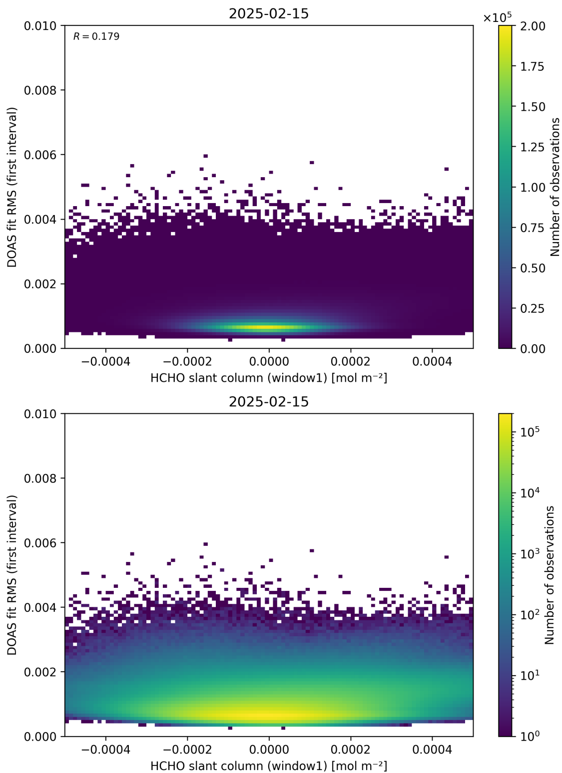
Figure 78: Scatter density plot of “HCHO slant column (window1)” against “DOAS fit RMS (first interval)” for 2025-02-14 to 2025-02-16.
