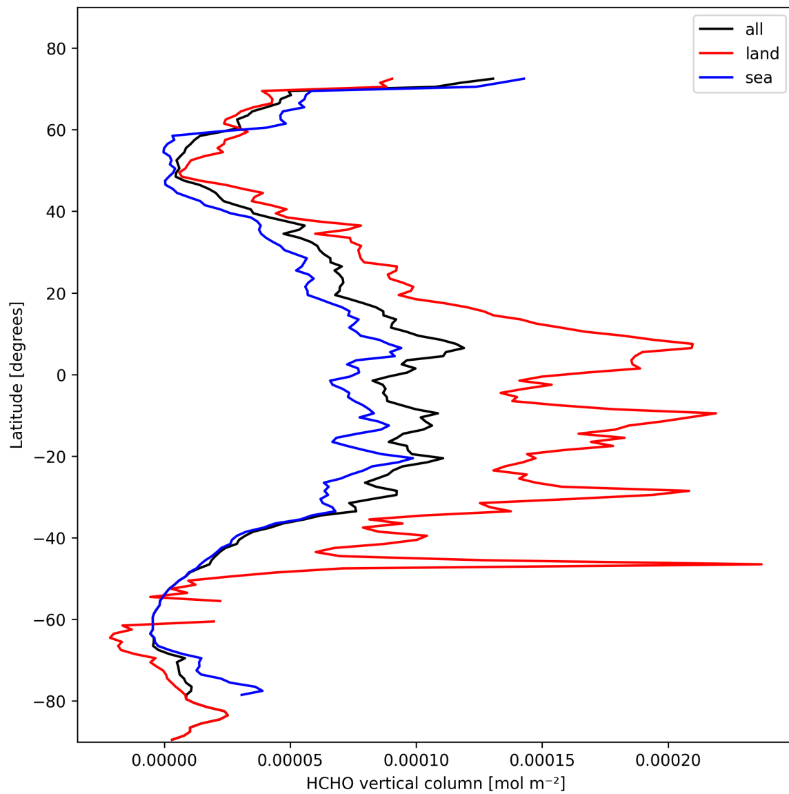
Figure 21: Zonal average of “HCHO vertical column” for 2025-02-14 to 2025-02-16.
