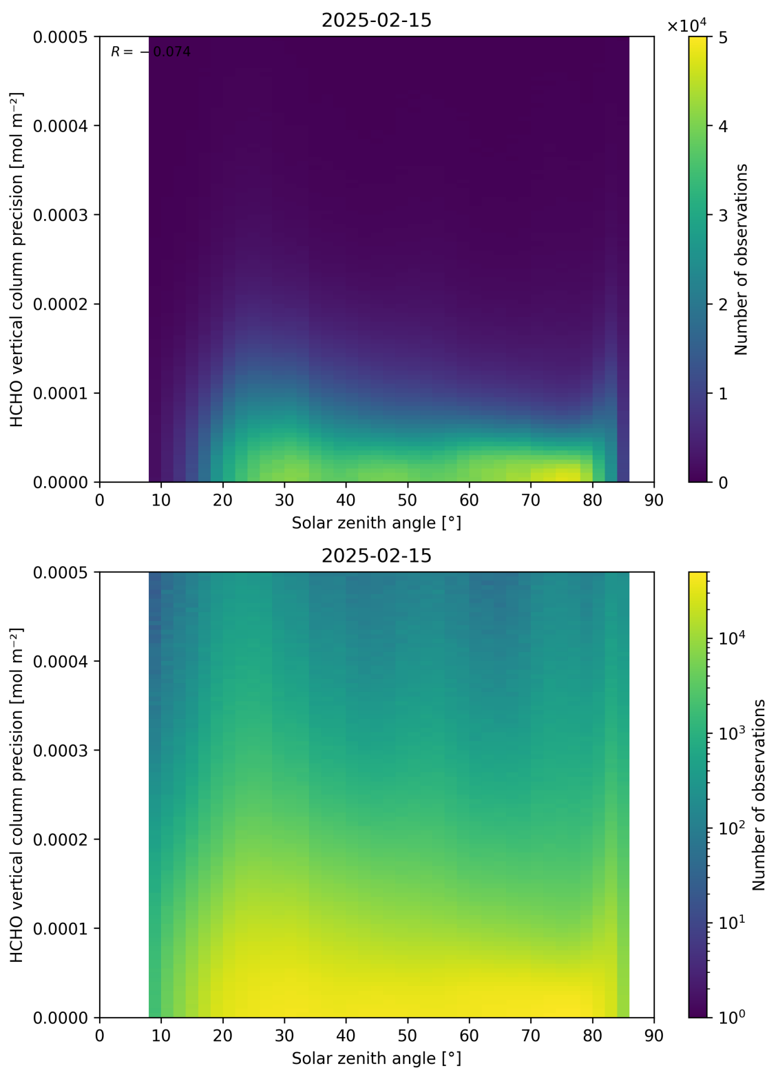
Figure 179: Scatter density plot of “Solar zenith angle” against “HCHO vertical column precision” for 2025-02-14 to 2025-02-16.
