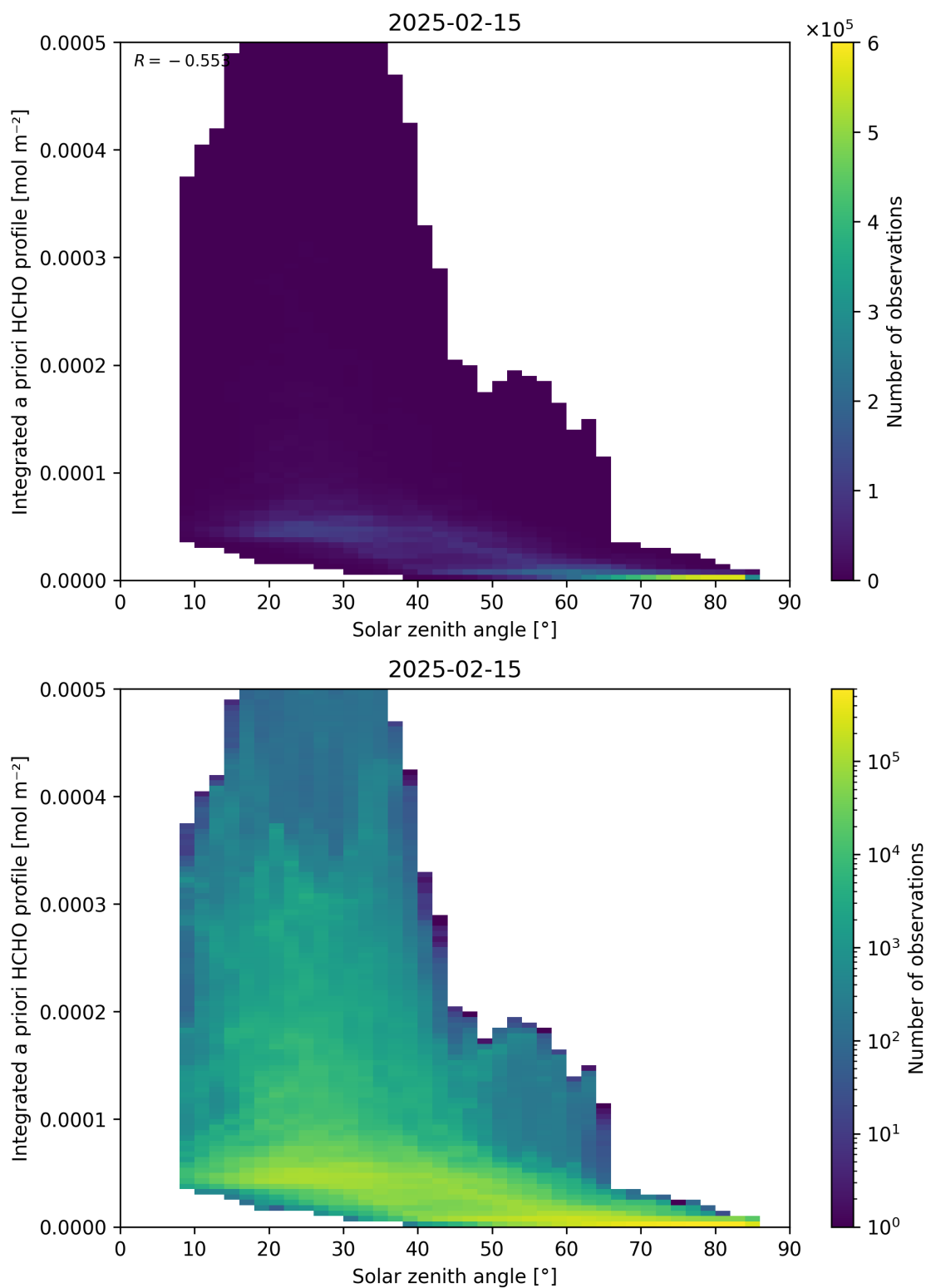
Figure 180: Scatter density plot of “Solar zenith angle” against “Integrated a priori HCHO profile” for 2025-02-14 to 2025-02-16.
