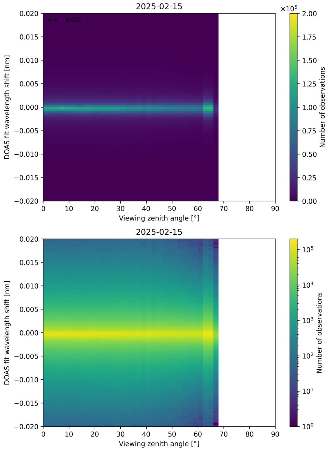
Figure 183: Scatter density plot of “Viewing zenith angle” against “DOAS fit wavelength shift” for 2025-02-14 to 2025-02-16.
