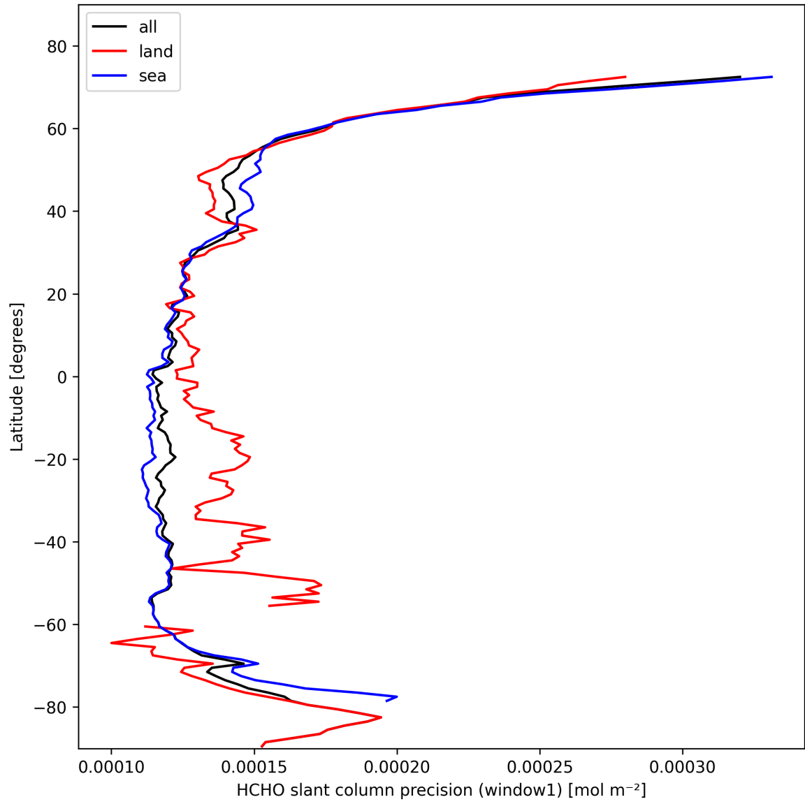
Figure 25: Zonal average of "HCHO slant column precision (window1)" for 2025-02-14 to 2025-02-16.
