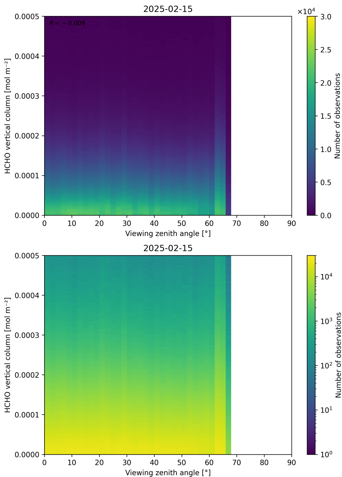
Figure 192: Scatter density plot of “Viewing zenith angle” against “HCHO vertical column” for 2025-02-14 to 2025-02-16.
