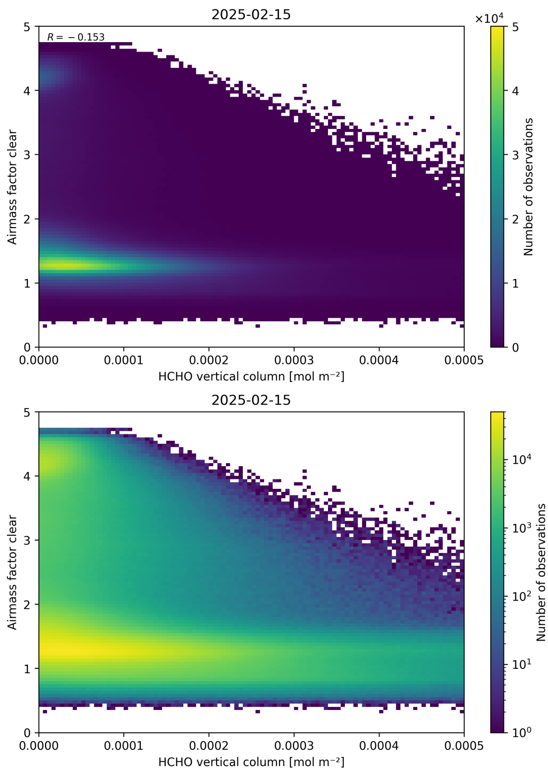
Figure 126: Scatter density plot of “HCHO vertical column” against “Airmass factor clear” for 2025-02-14 to 2025-02-16.
