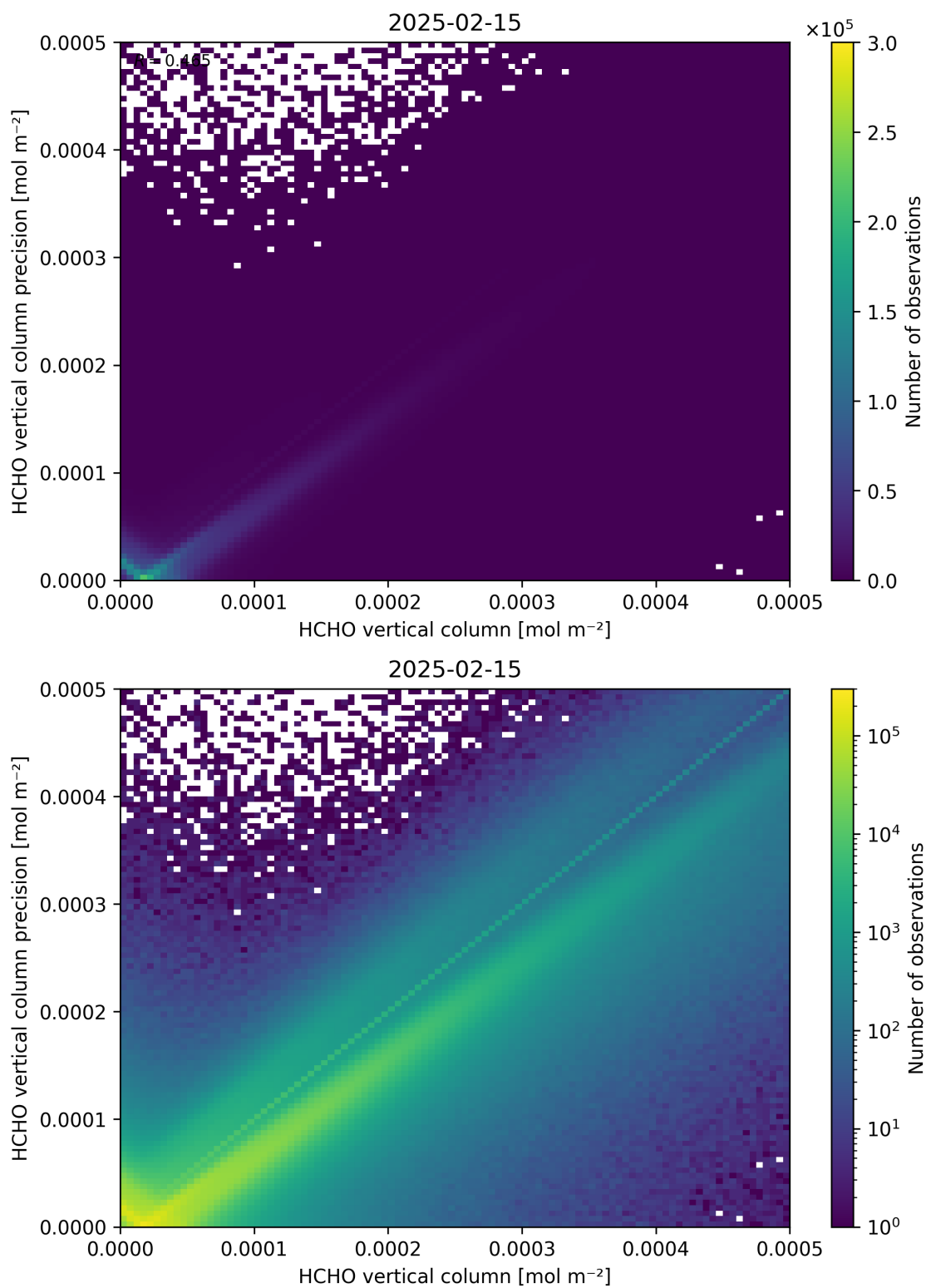
Figure 134: Scatter density plot of “HCHO vertical column” against “HCHO vertical column precision” for 2025-02-14 to 2025-02-16.
