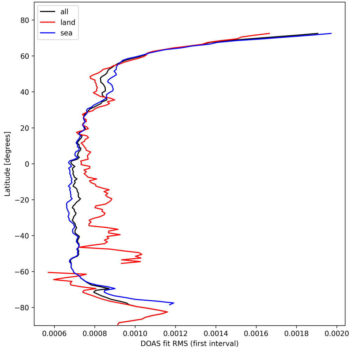
Figure 32: Zonal average of “DOAS fit RMS (first interval)” for 2025-02-14 to 2025-02-16.
