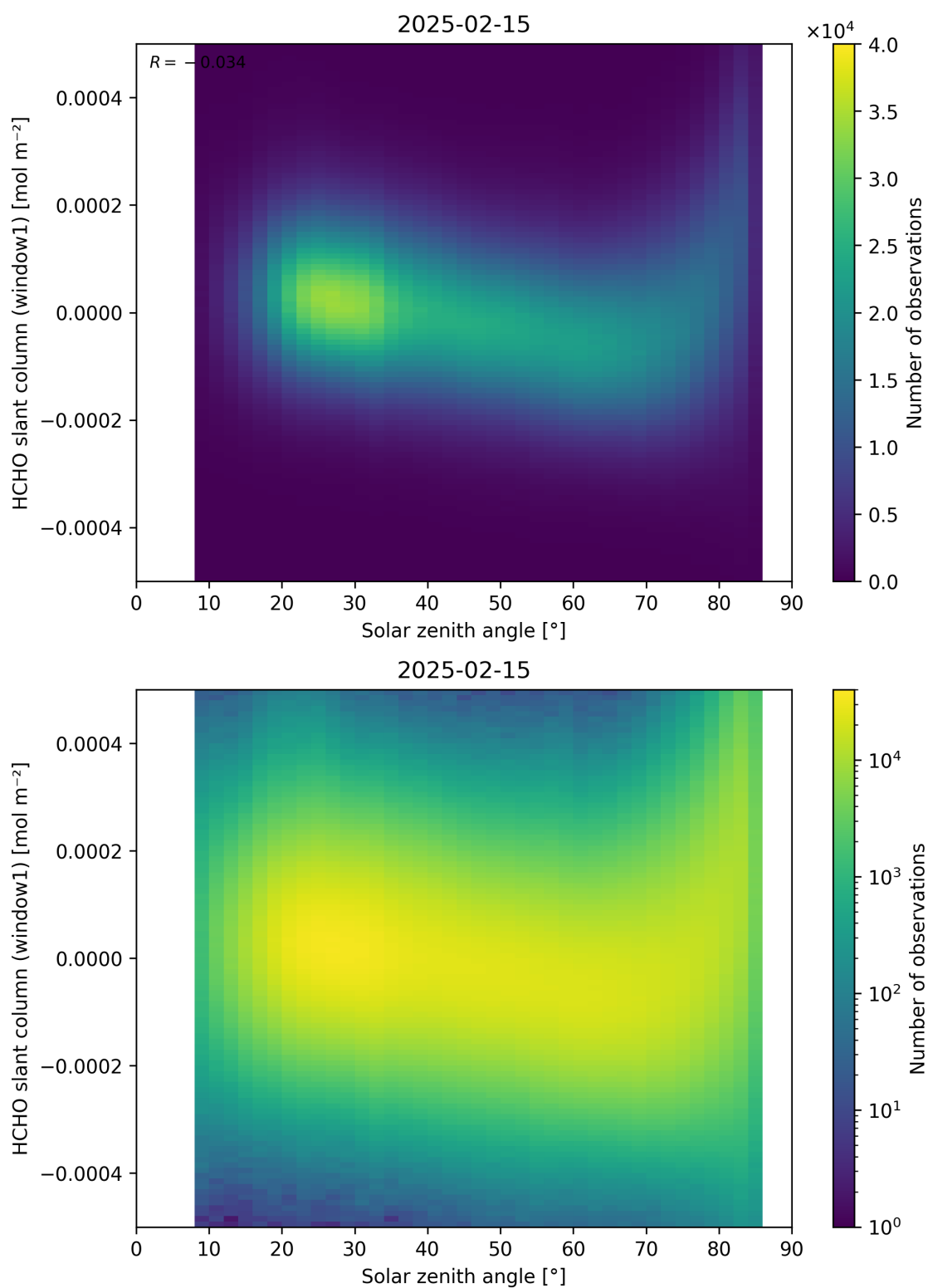
Figure 173: Scatter density plot of “Solar zenith angle” against “HCHO slant column (window1)” for 2025-02-14 to 2025-02-16.
