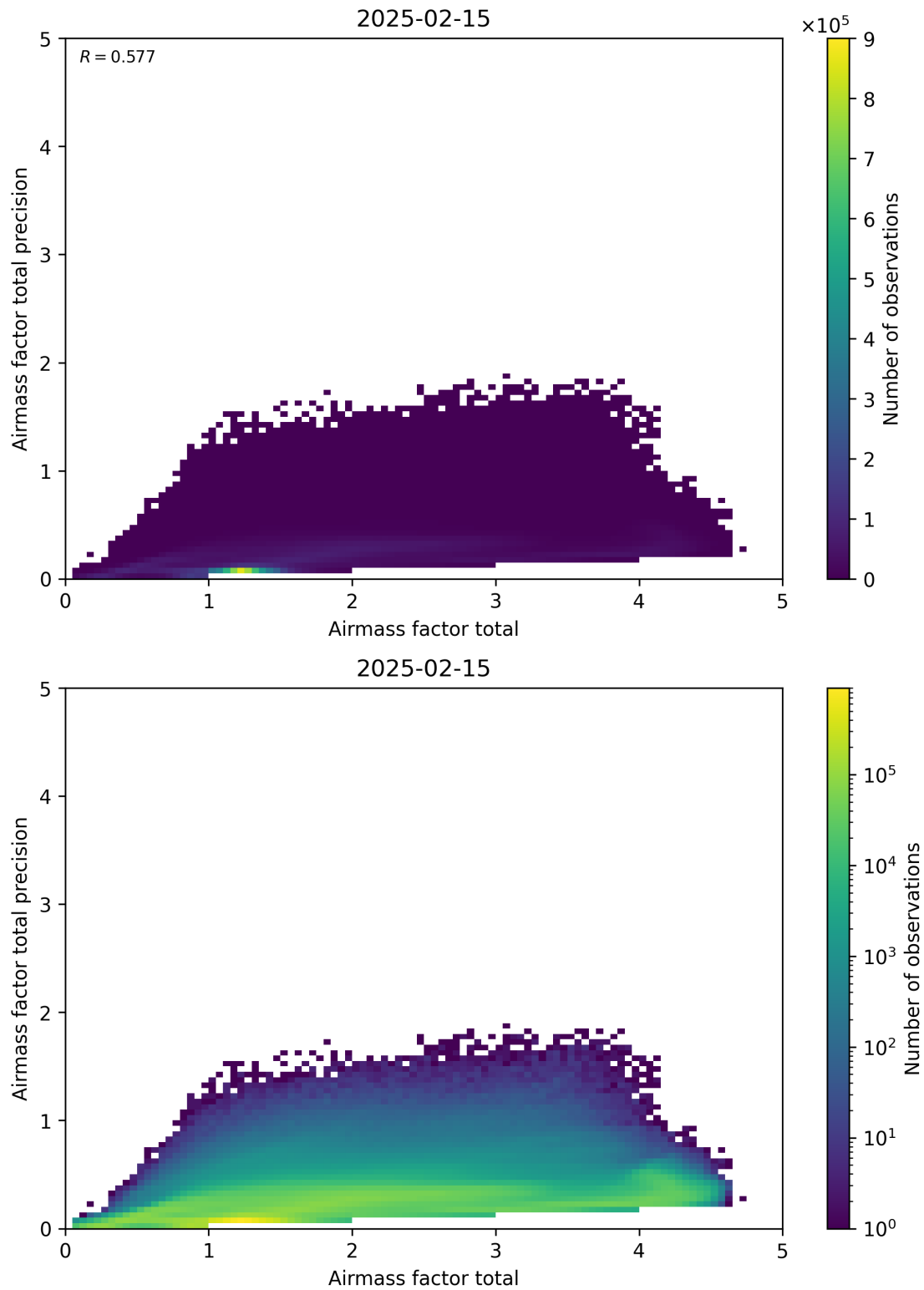
Figure 103: Scatter density plot of “Airmass factor total” against “Airmass factor total precision” for 2025-02-14 to 2025-02-16.
