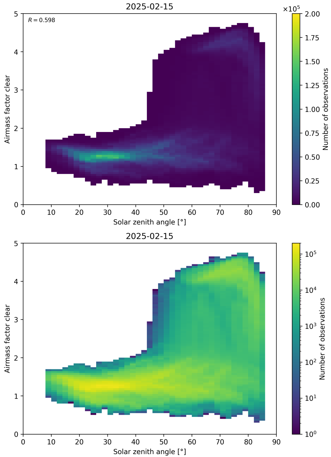
Figure 170: Scatter density plot of “Solar zenith angle” against “Airmass factor clear” for 2025-02-14 to 2025-02-16.
