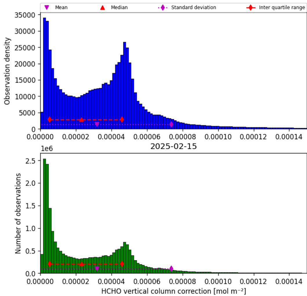
Figure 37: Histogram of “HCHO vertical column correction” for 2025-02-14 to 2025-02-16
