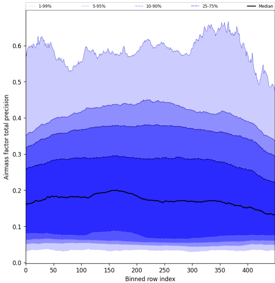
Figure 55: Along track statistics of “Airmass factor total precision” for 2025-02-14 to 2025-02-16
