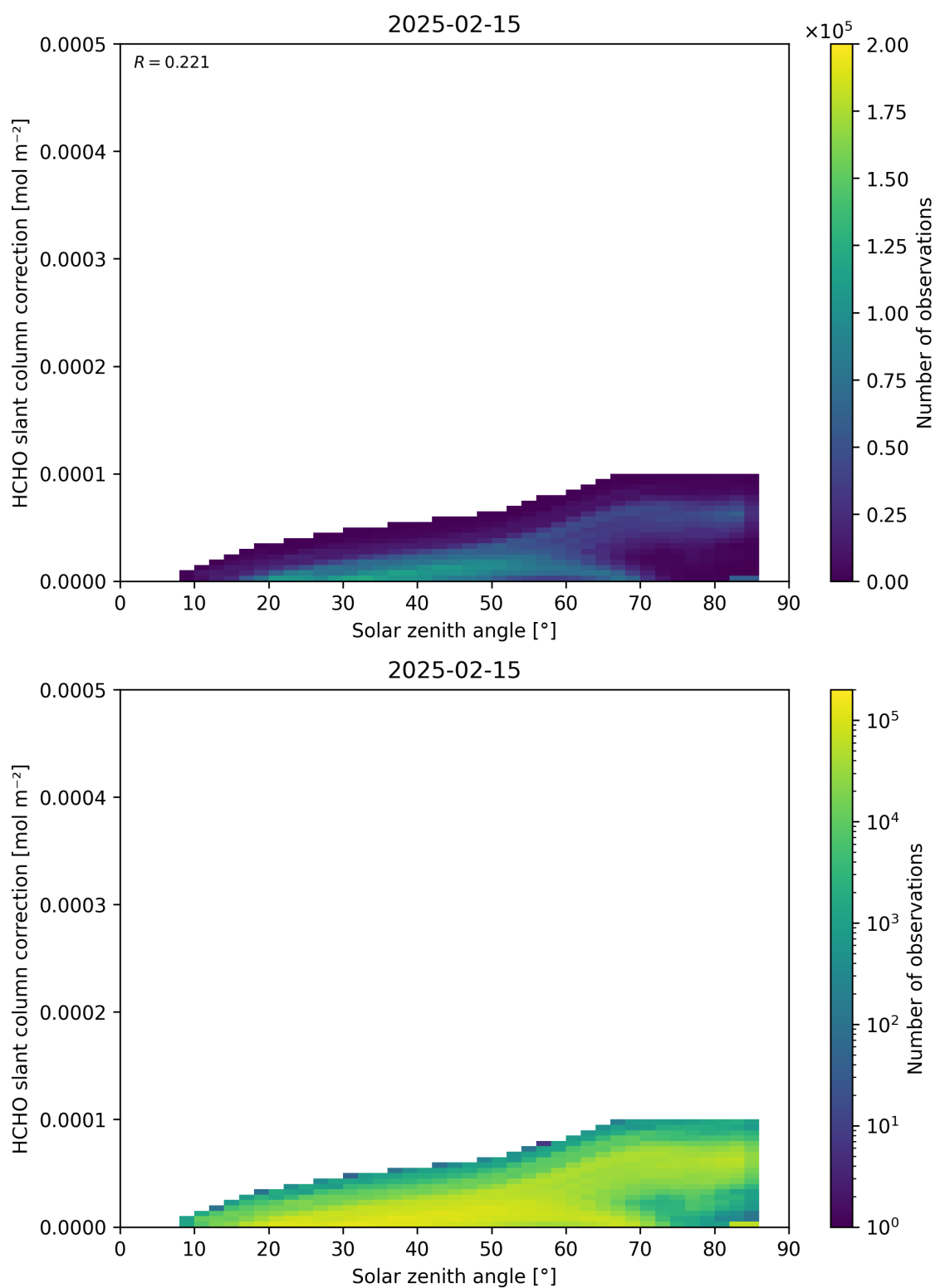
Figure 172: Scatter density plot of “Solar zenith angle” against “HCHO slant column correction” for 2025-02-14 to 2025-02-16.
