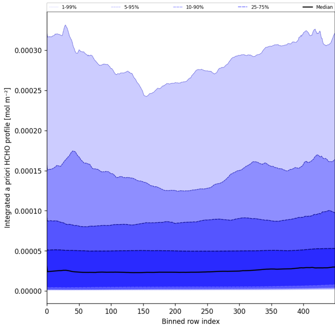
Figure 57: Along track statistics of “Integrated a priori HCHO profile” for 2025-02-14 to 2025-02-16
