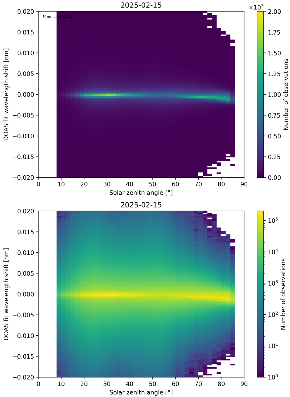
Figure 168: Scatter density plot of “Solar zenith angle” against “DOAS fit wavelength shift” for 2025-02-14 to 2025-02-16.
