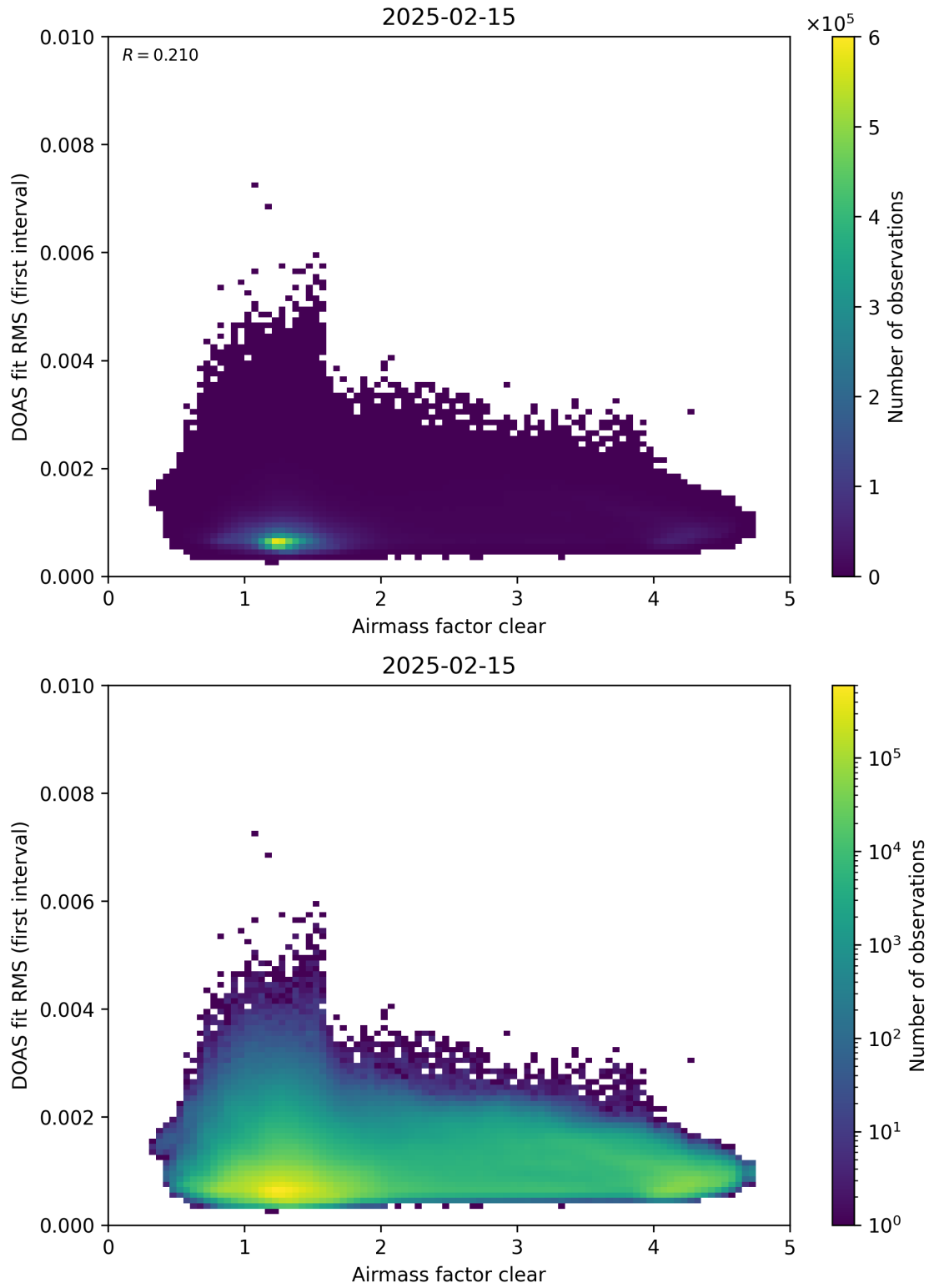
Figure 71: Scatter density plot of “Airmass factor clear” against “DOAS fit RMS (first interval)” for 2025-02-14 to 2025-02-16.
