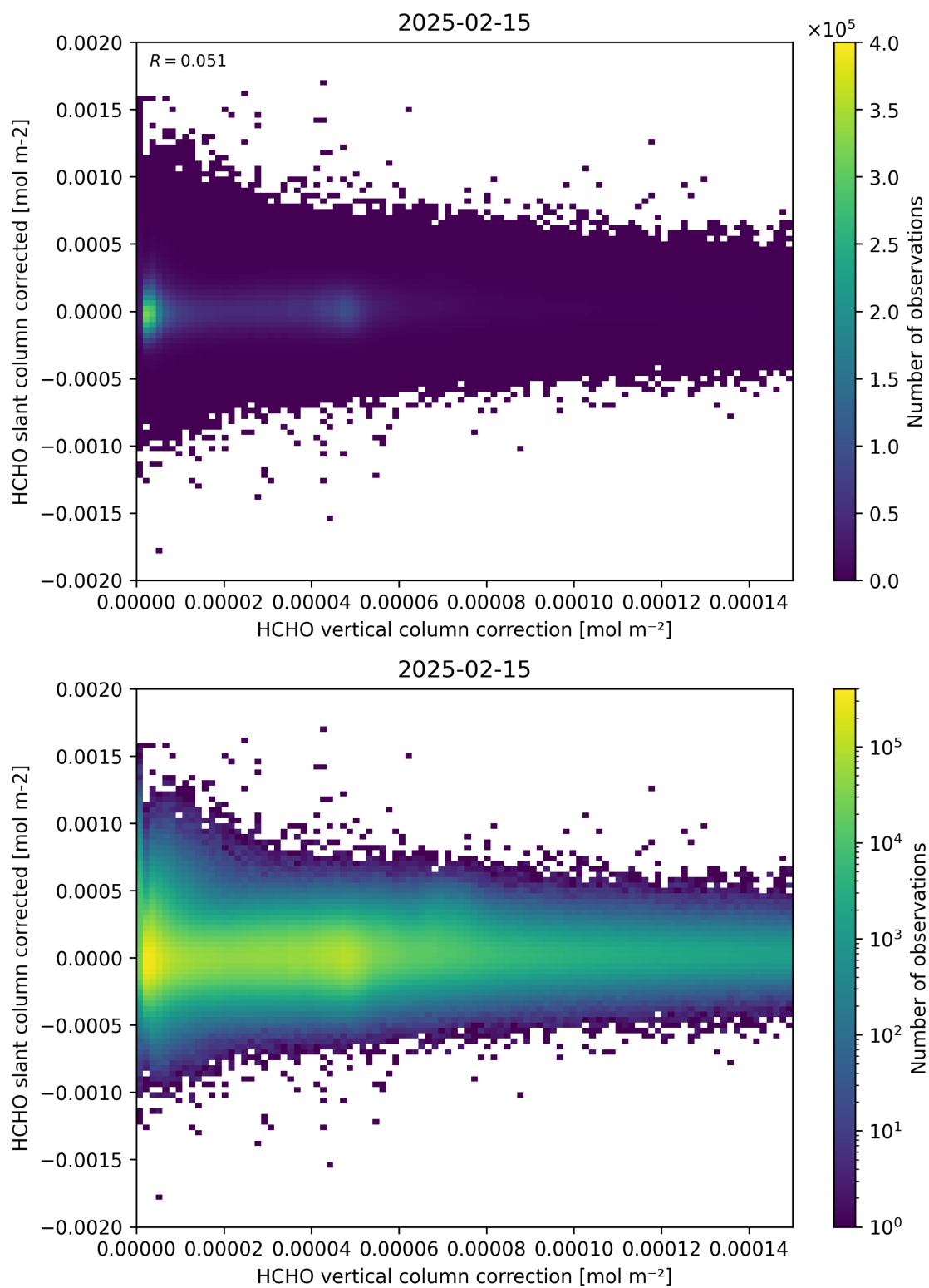
Figure 116: Scatter density plot of “HCHO vertical column correction” against “HCHO slant column corrected” for 2025-02-14 to 2025-02-16.
