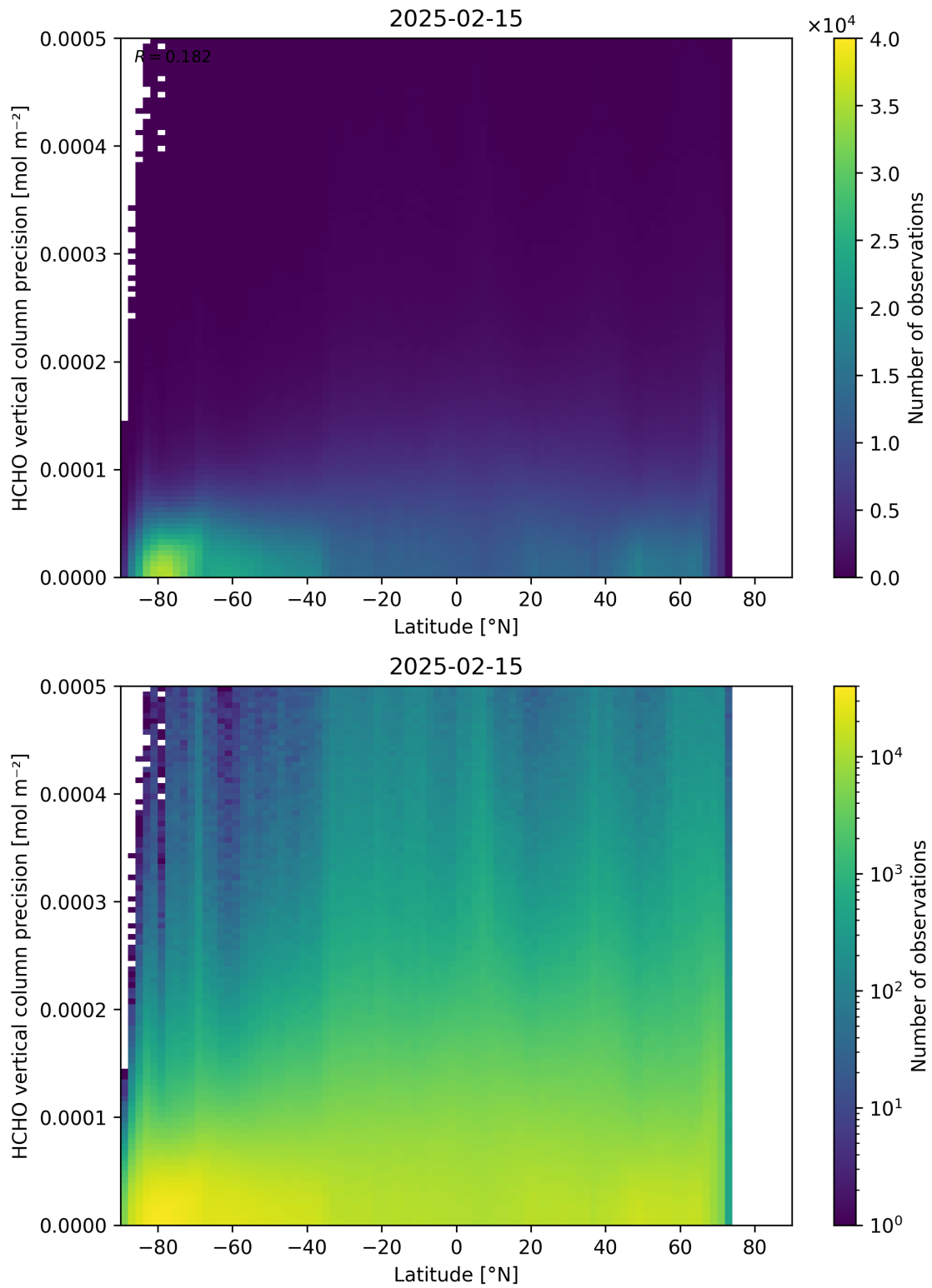
Figure 165: Scatter density plot of “Latitude” against “HCHO vertical column precision” for 2025-02-14 to 2025-02-16.
