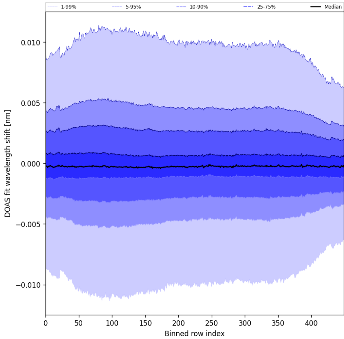
Figure 58: Along track statistics of “DOAS fit wavelength shift” for 2025-02-14 to 2025-02-16
