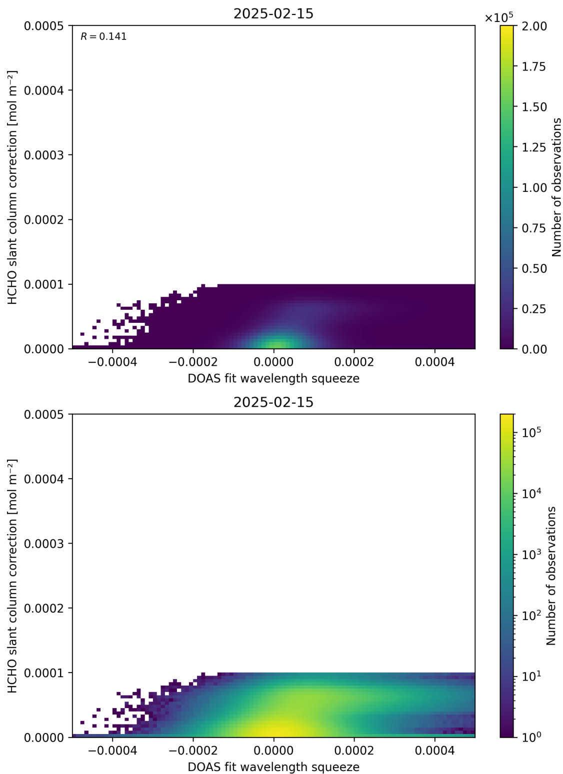
Figure 70: Scatter density plot of “DOAS fit wavelength squeeze” against “HCHO slant column correction” for 2025-02-14 to 2025-02-16.
