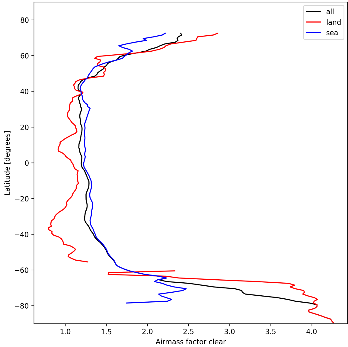
Figure 28: Zonal average of “Airmass factor clear” for 2025-02-14 to 2025-02-16.
