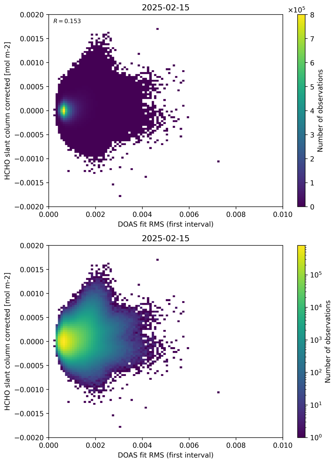
Figure 62: Scatter density plot of “DOAS fit RMS (first interval)” against “HCHO slant column corrected” for 2025-02-14 to 2025-02-16.
