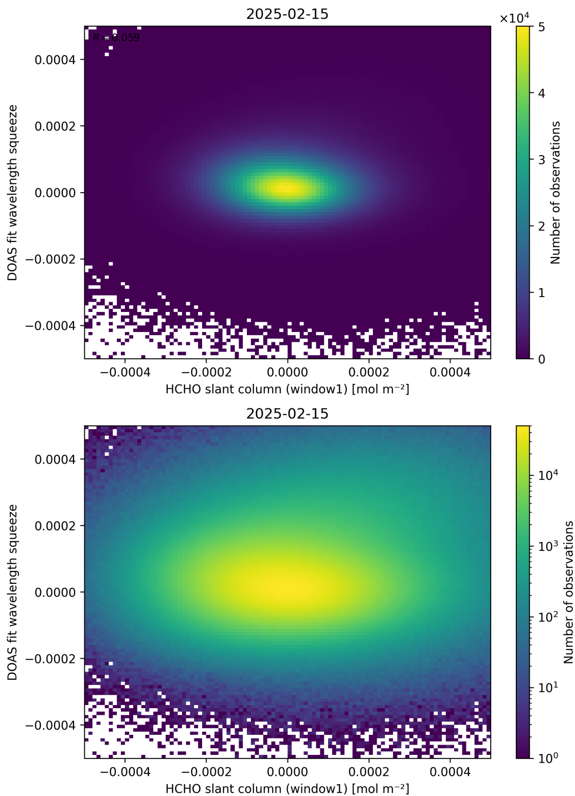
Figure 80: Scatter density plot of “HCHO slant column (window1)” against “DOAS fit wavelength squeeze” for 2025-02-14 to 2025-02-16.
