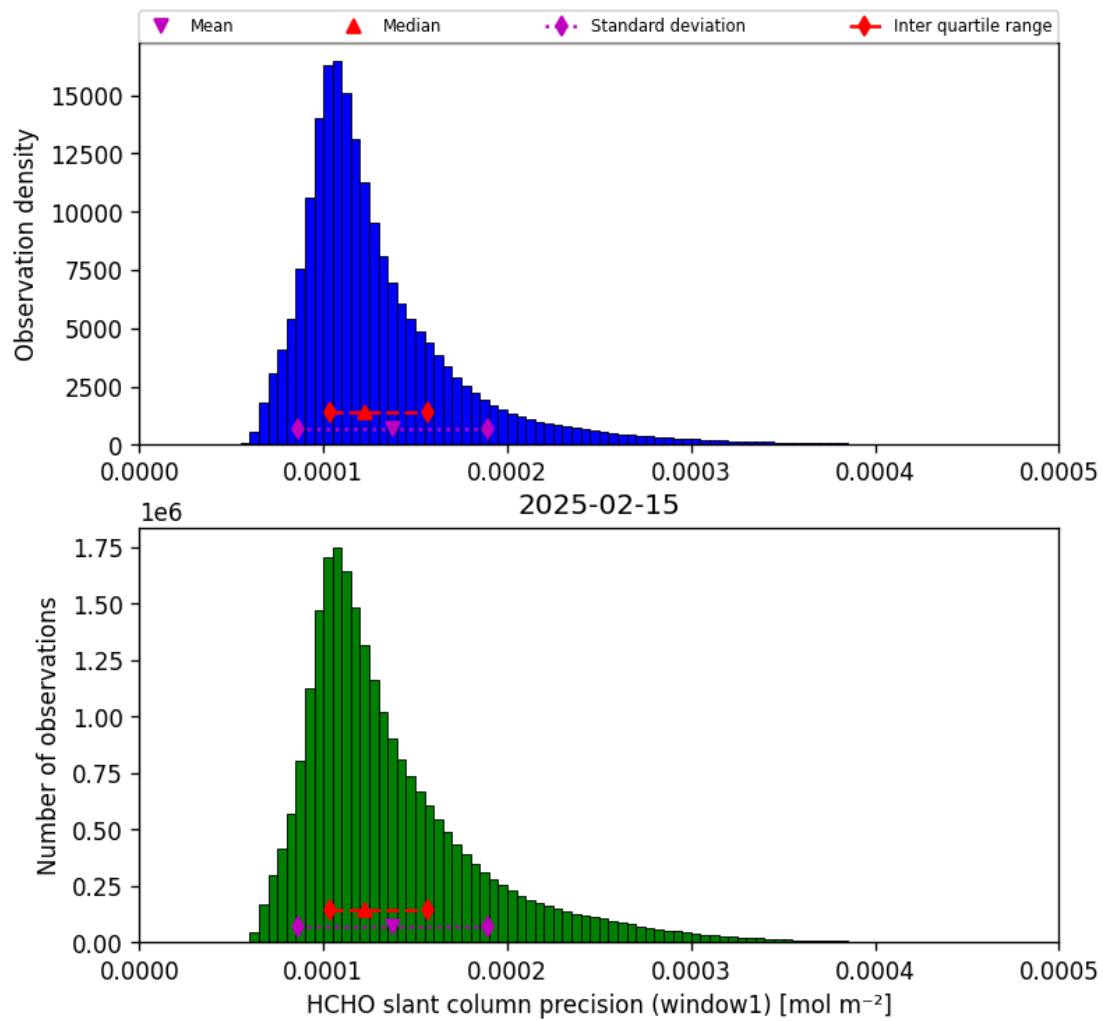
Figure 39: Histogram of “HCHO slant column precision (window1)” for 2025-02-14 to 2025-02-16
