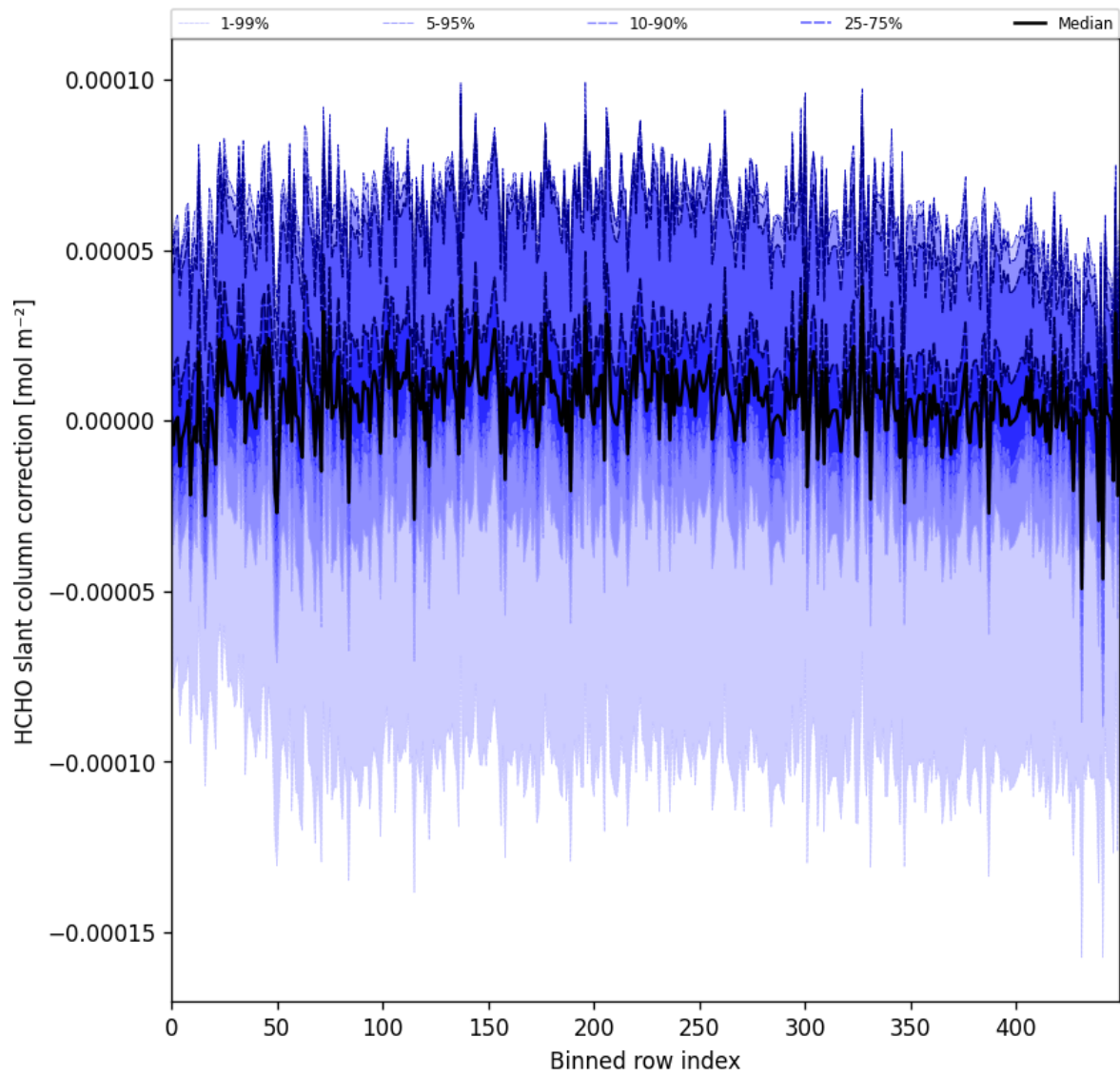
Figure 61: Along track statistics of “HCHO slant column correction” for 2025-02-14 to 2025-02-16
