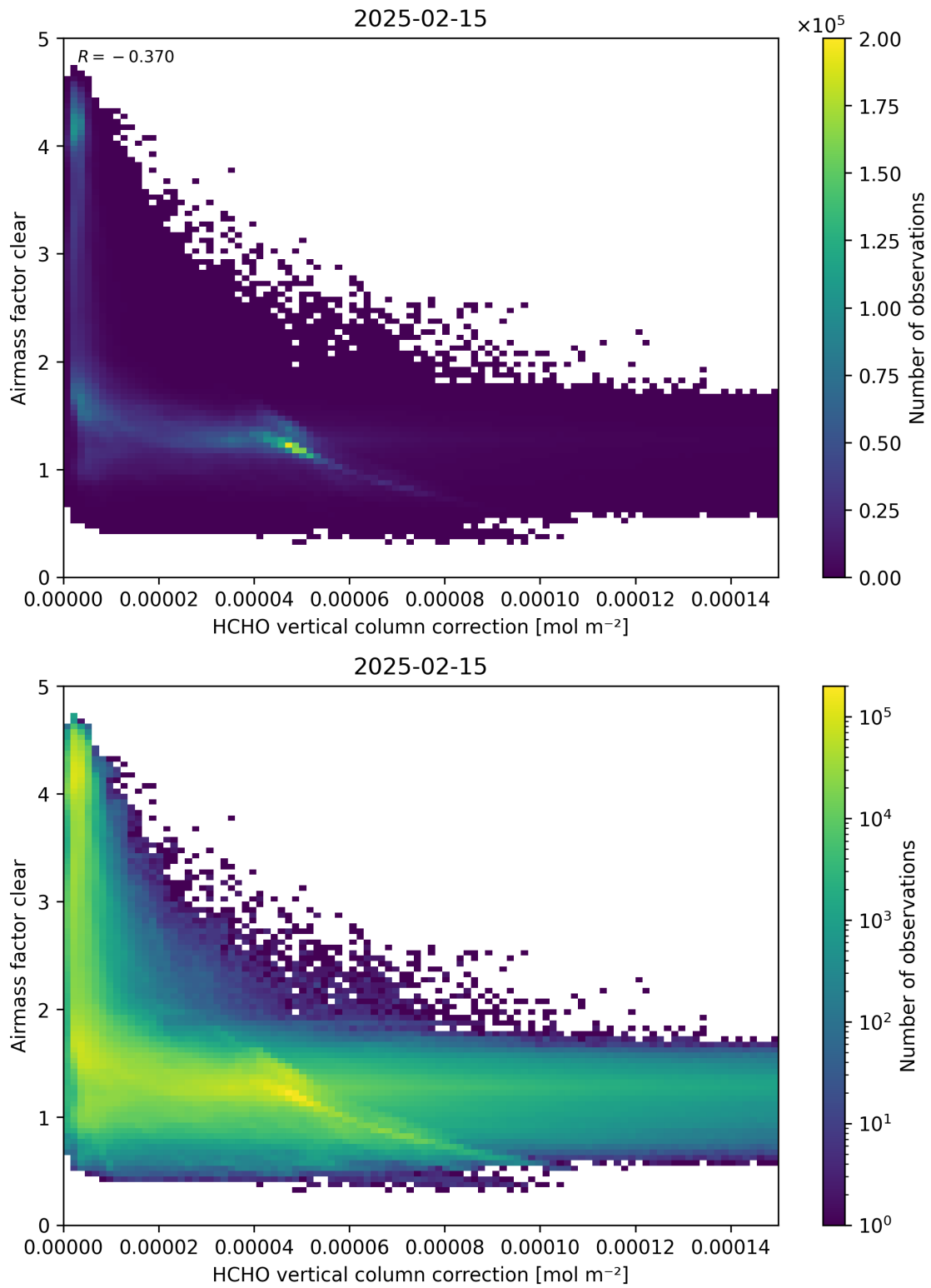
Figure 115: Scatter density plot of “HCHO vertical column correction” against “Airmass factor clear” for 2025-02-14 to 2025-02-16.
