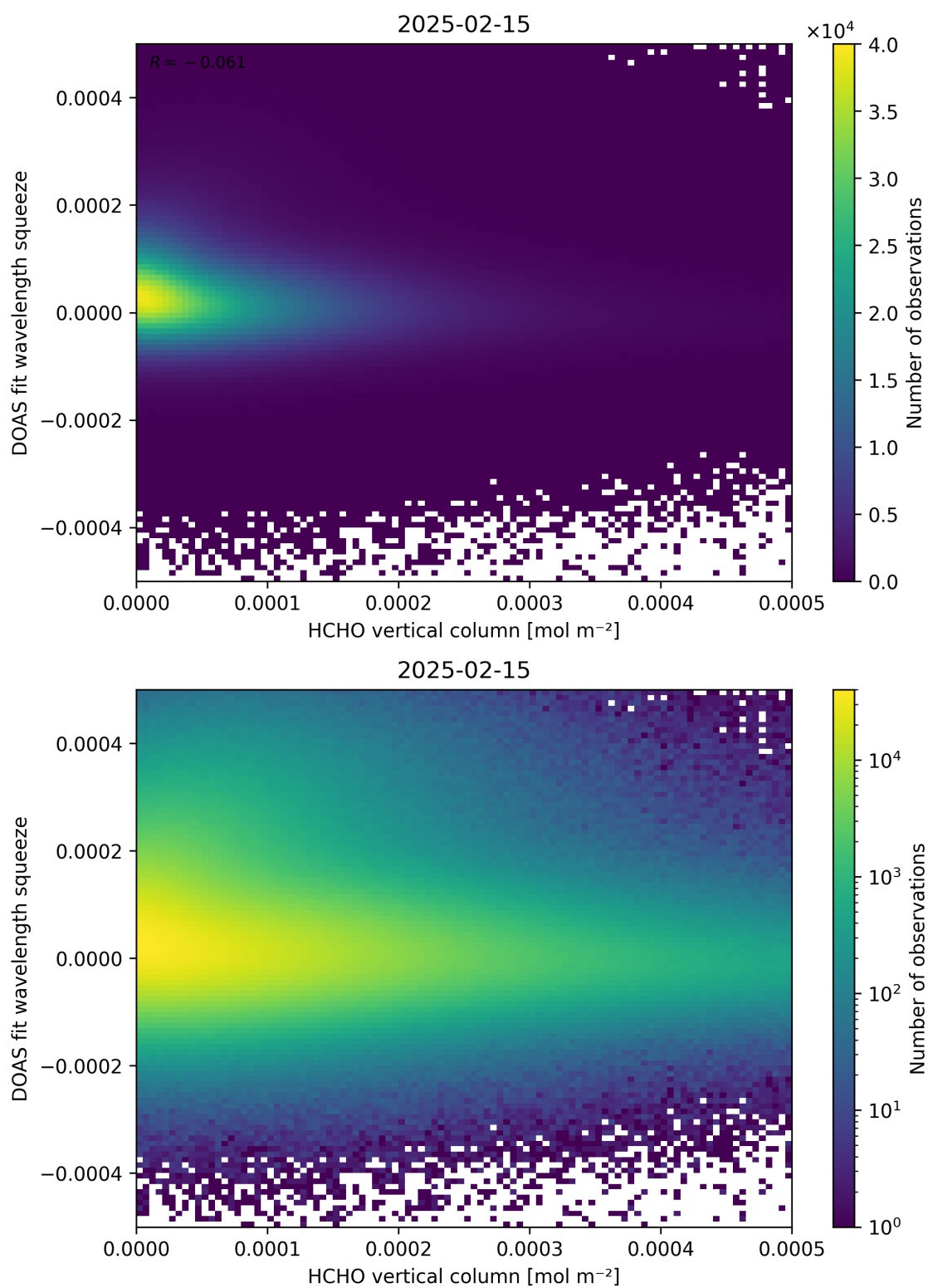
Figure 125: Scatter density plot of “HCHO vertical column” against “DOAS fit wavelength squeeze” for 2025-02-14 to 2025-02-16.
