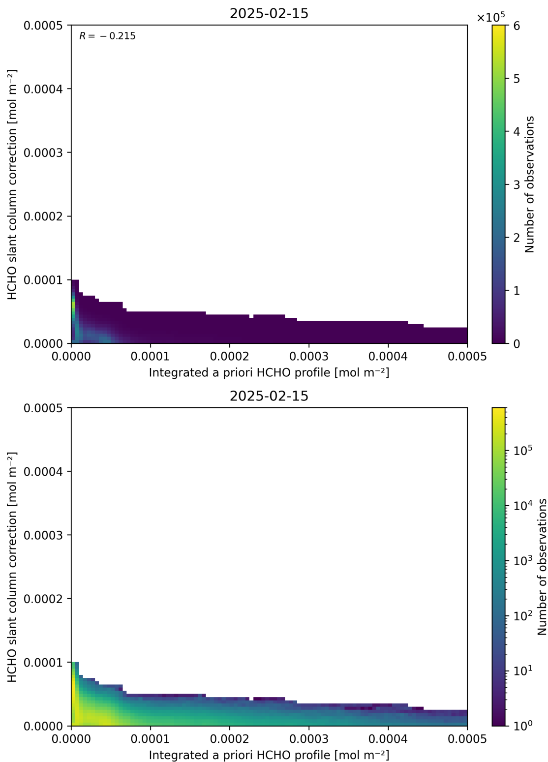
Figure 152: Scatter density plot of “Integrated a priori HCHO profile” against “HCHO slant column correction” for 2025-02-14 to 2025-02-16.
