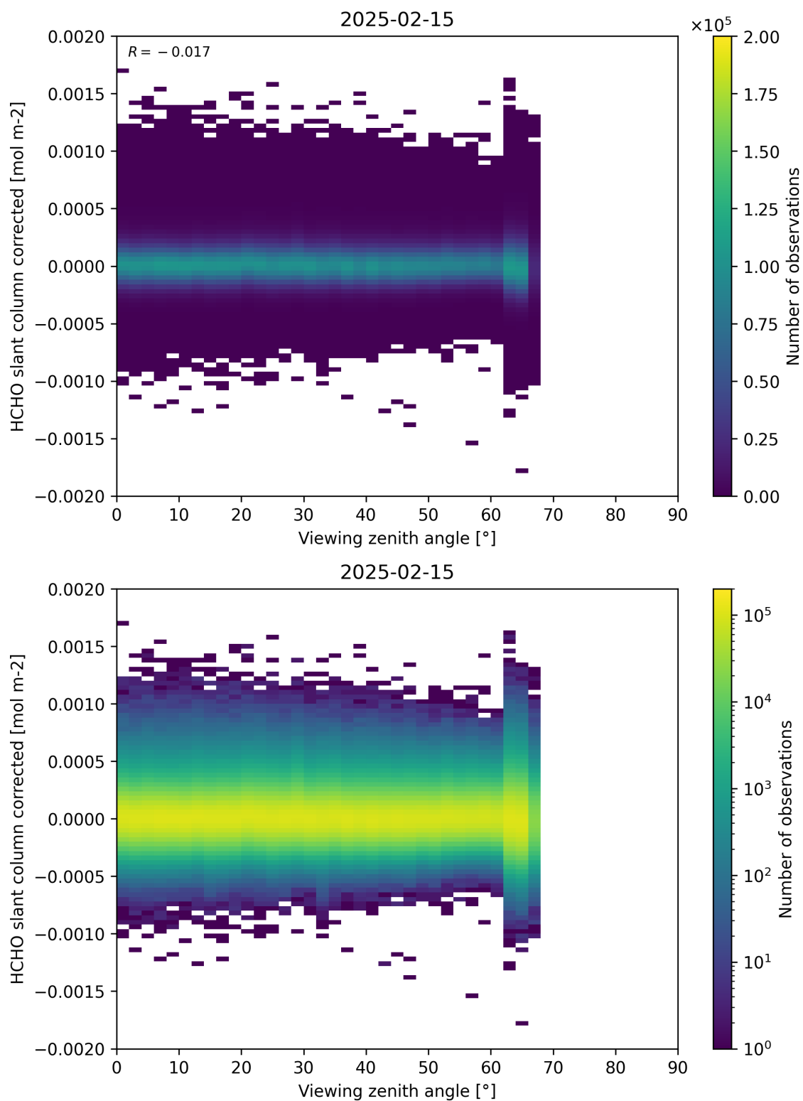
Figure 186: Scatter density plot of “Viewing zenith angle” against “HCHO slant column corrected” for 2025-02-14 to 2025-02-16.
