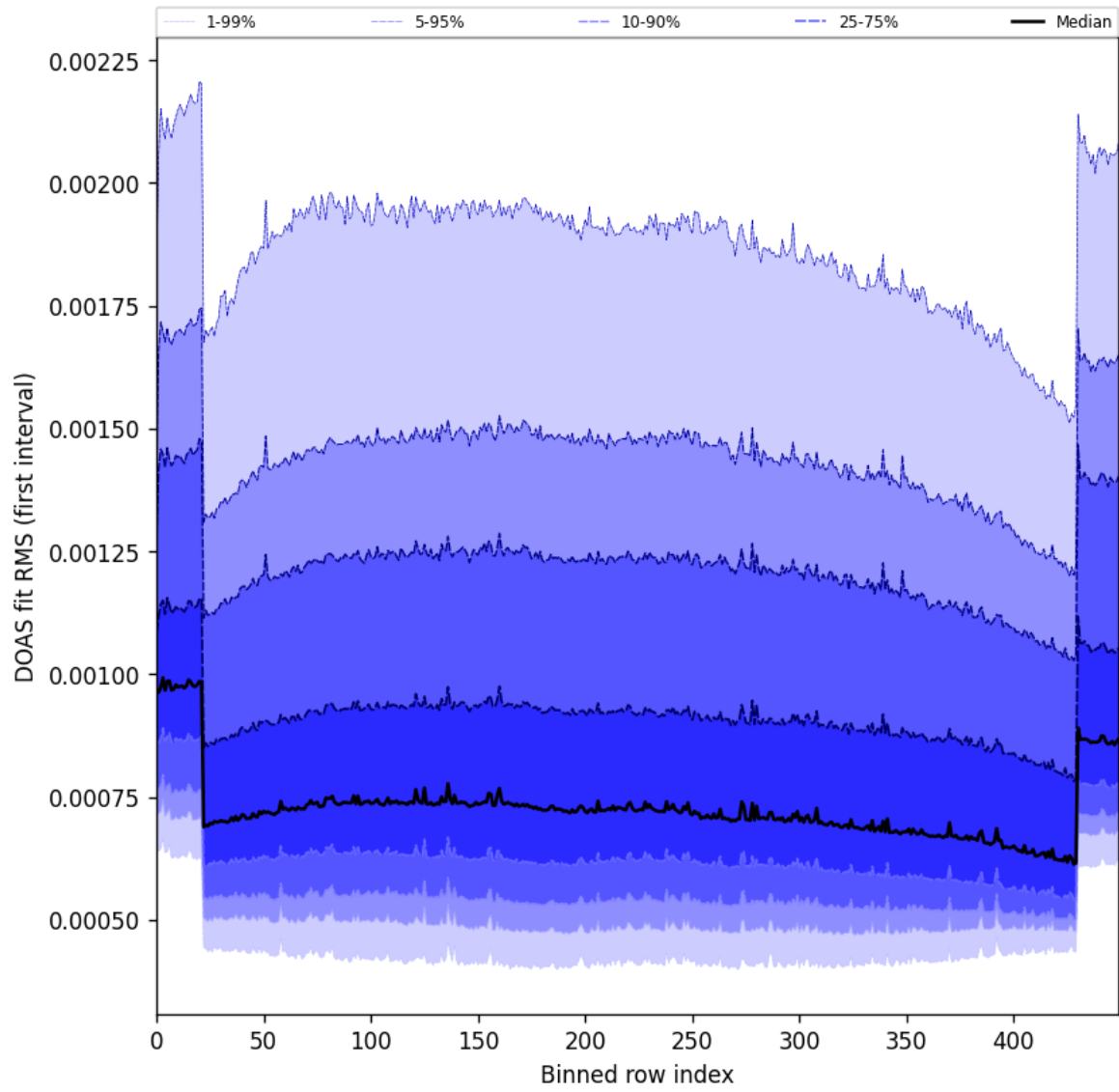
Figure 60: Along track statistics of “DOAS fit RMS (first interval)” for 2025-02-14 to 2025-02-16
