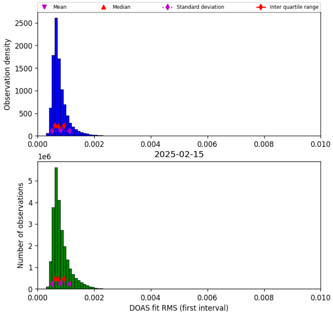
Figure 46: Histogram of “DOAS fit RMS (first interval)” for 2025-02-14 to 2025-02-16
