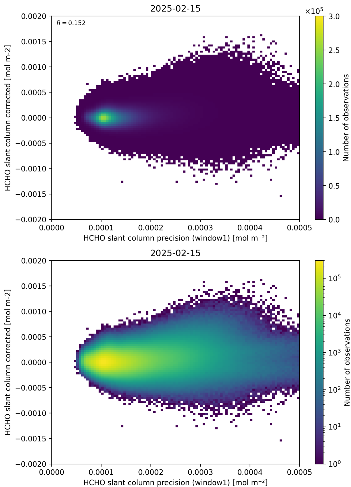
Figure 92: Scatter density plot of “HCHO slant column precision (window1)” against “HCHO slant column corrected” for 2025-02-14 to 2025-02-16.
