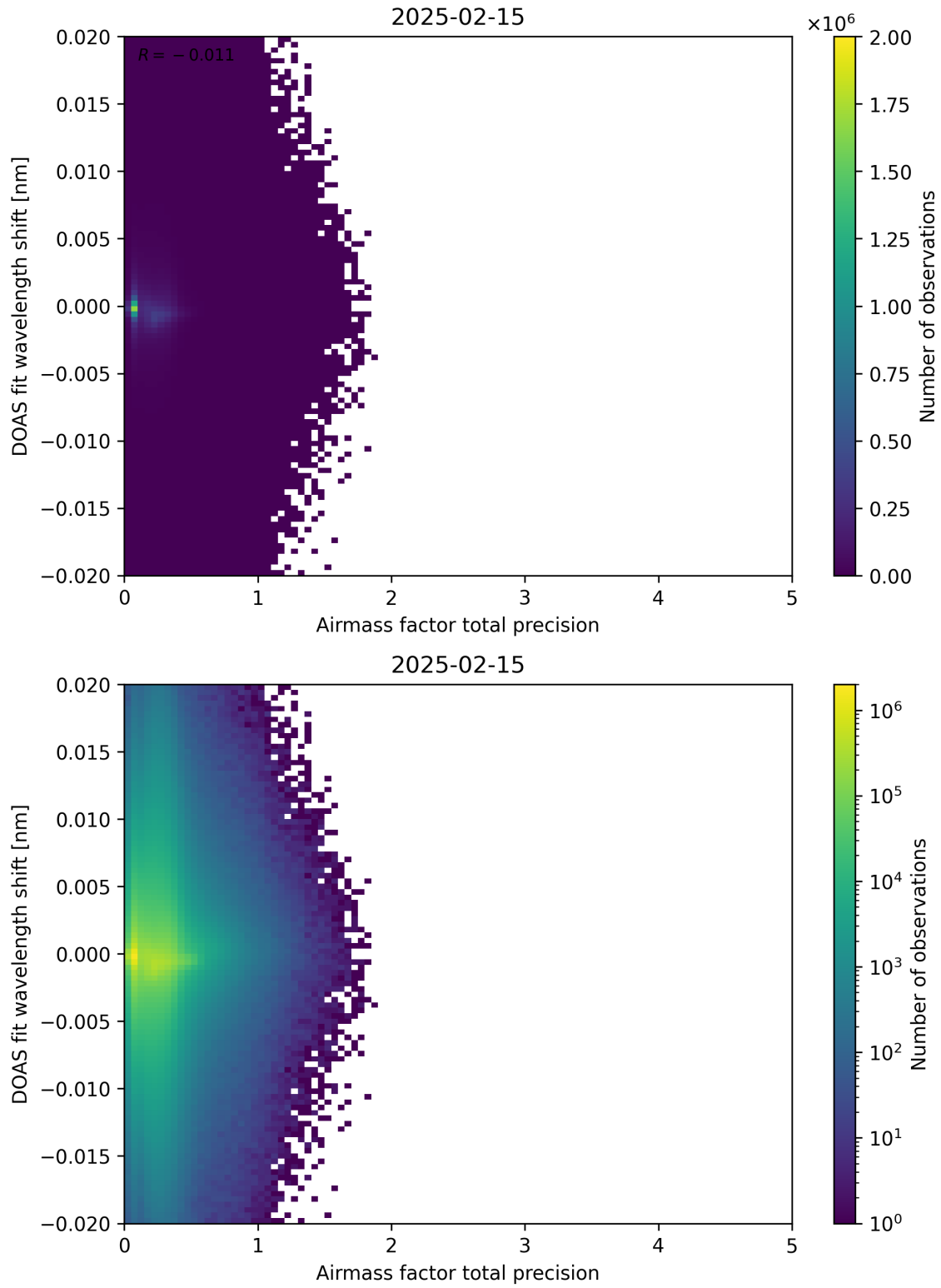
Figure 106: Scatter density plot of “Airmass factor total precision” against “DOAS fit wavelength shift” for 2025-02-14 to 2025-02-16.
