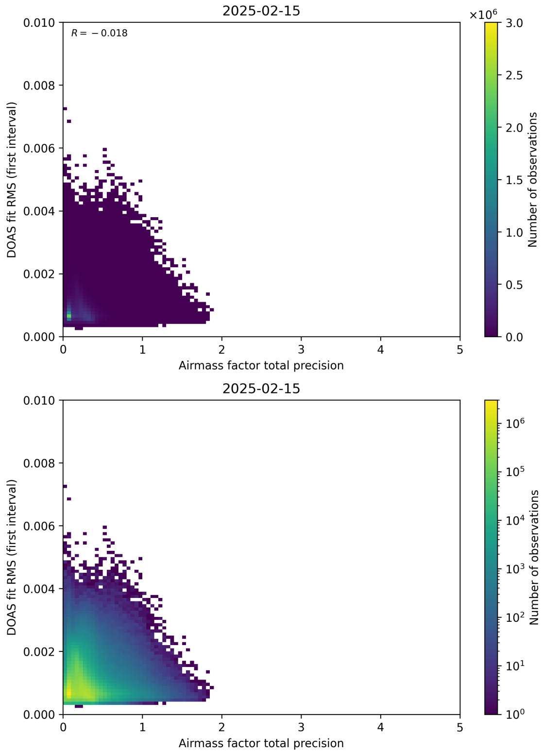
Figure 105: Scatter density plot of “Airmass factor total precision” against “DOAS fit RMS (first interval)” for 2025-02-14 to 2025-02-16.
