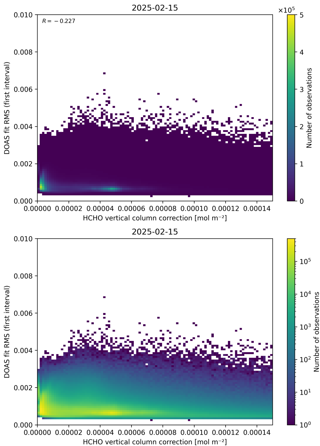
Figure 112: Scatter density plot of “HCHO vertical column correction” against “DOAS fit RMS (first interval)” for 2025-02-14 to 2025-02-16.
