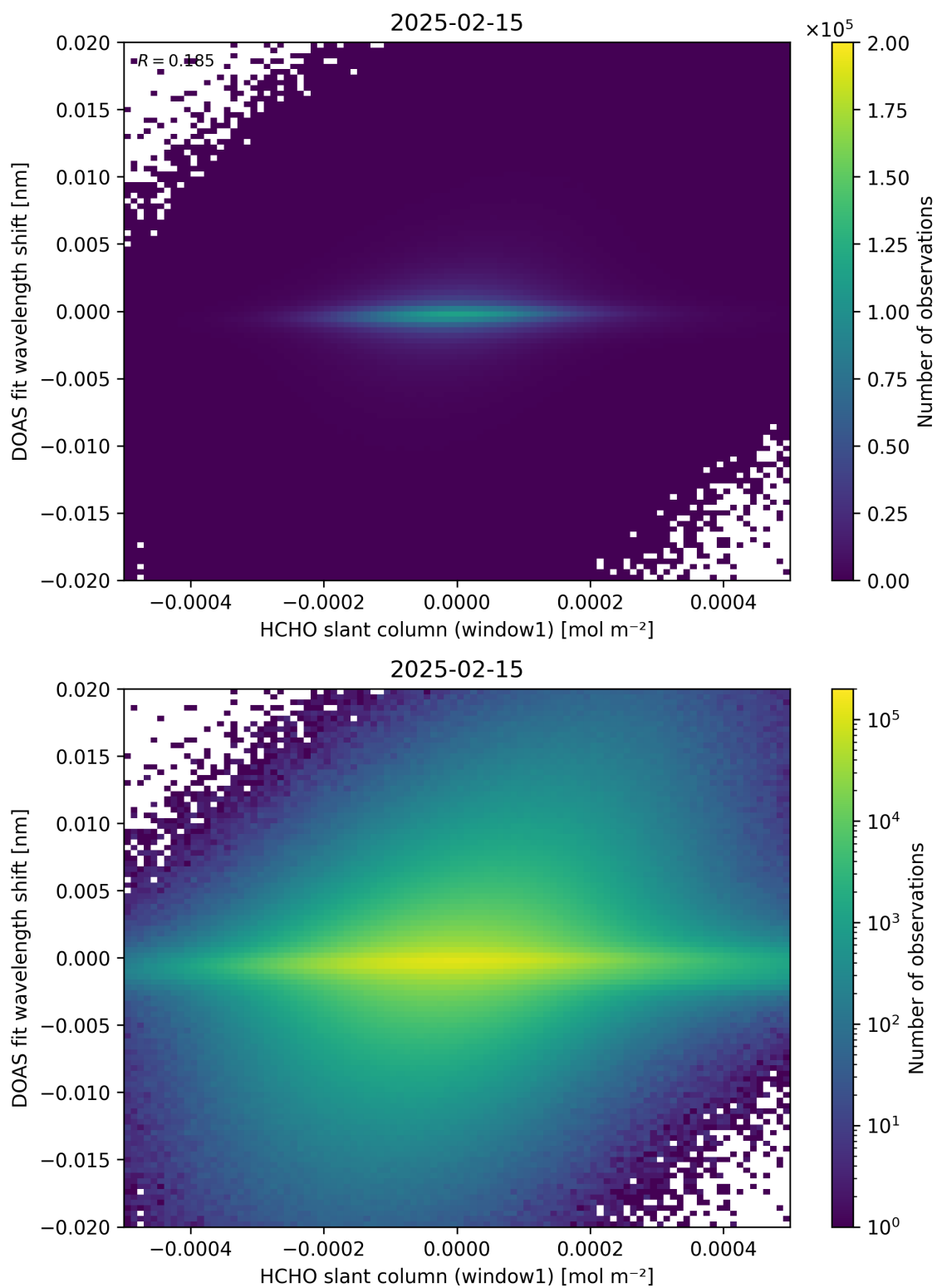
Figure 79: Scatter density plot of “HCHO slant column (window1)” against “DOAS fit wavelength shift” for 2025-02-14 to 2025-02-16.
