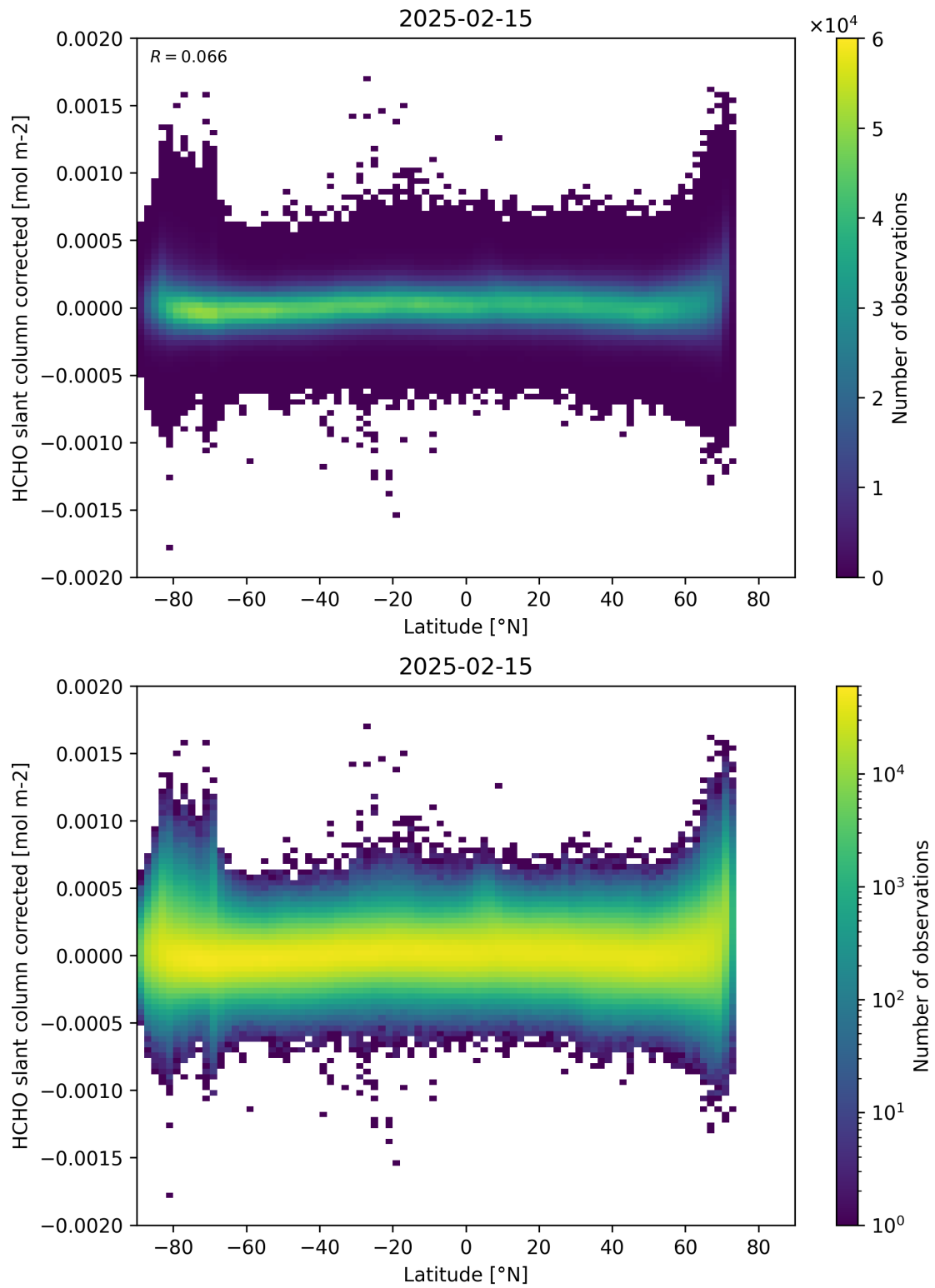
Figure 157: Scatter density plot of “Latitude” against “HCHO slant column corrected” for 2025-02-14 to 2025-02-16.
