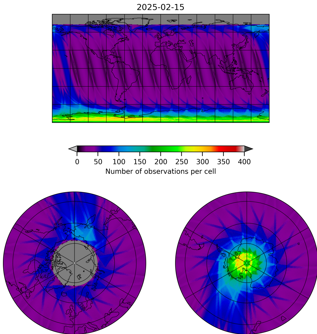
Figure 19: Map of the number of observations for 2025-02-14 to 2025-02-16
