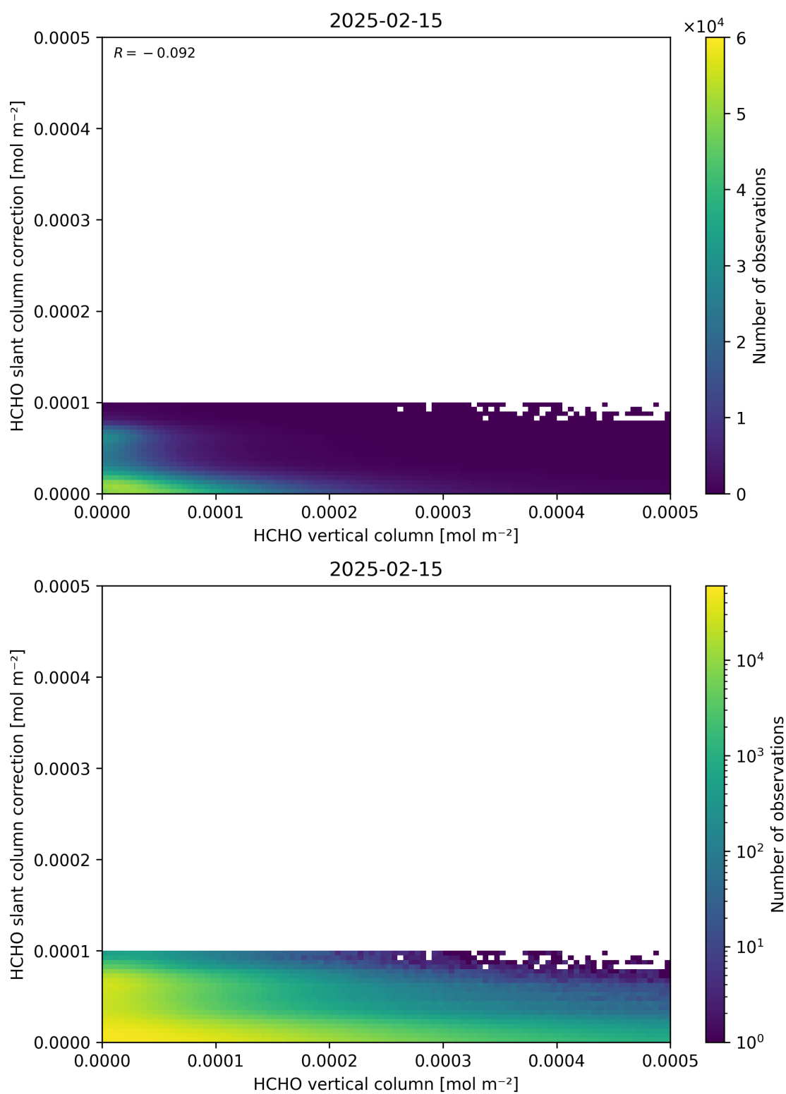
Figure 128: Scatter density plot of “HCHO vertical column” against “HCHO slant column correction” for 2025-02-14 to 2025-02-16.
