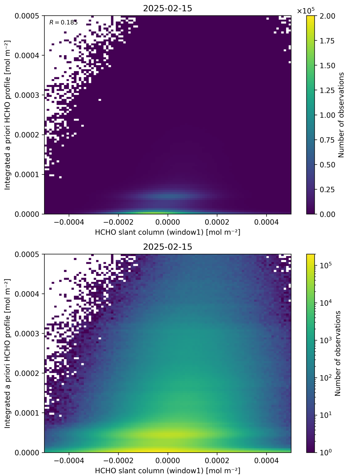
Figure 87: Scatter density plot of “HCHO slant column (window1)” against “Integrated a priori HCHO profile” for 2025-02-14 to 2025-02-16.
