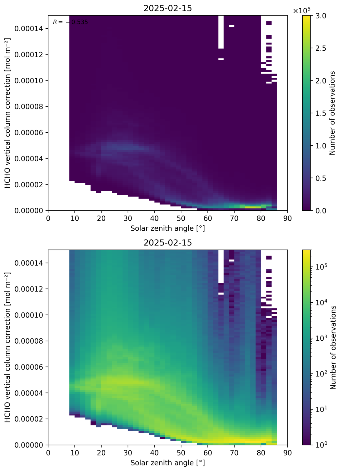
Figure 178: Scatter density plot of “Solar zenith angle” against “HCHO vertical column correction” for 2025-02-14 to 2025-02-16.
