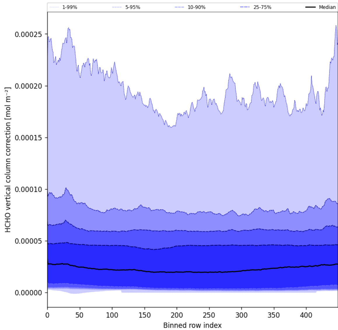
Figure 51: Along track statistics of “HCHO vertical column correction” for 2025-02-15 to 2025-02-17
