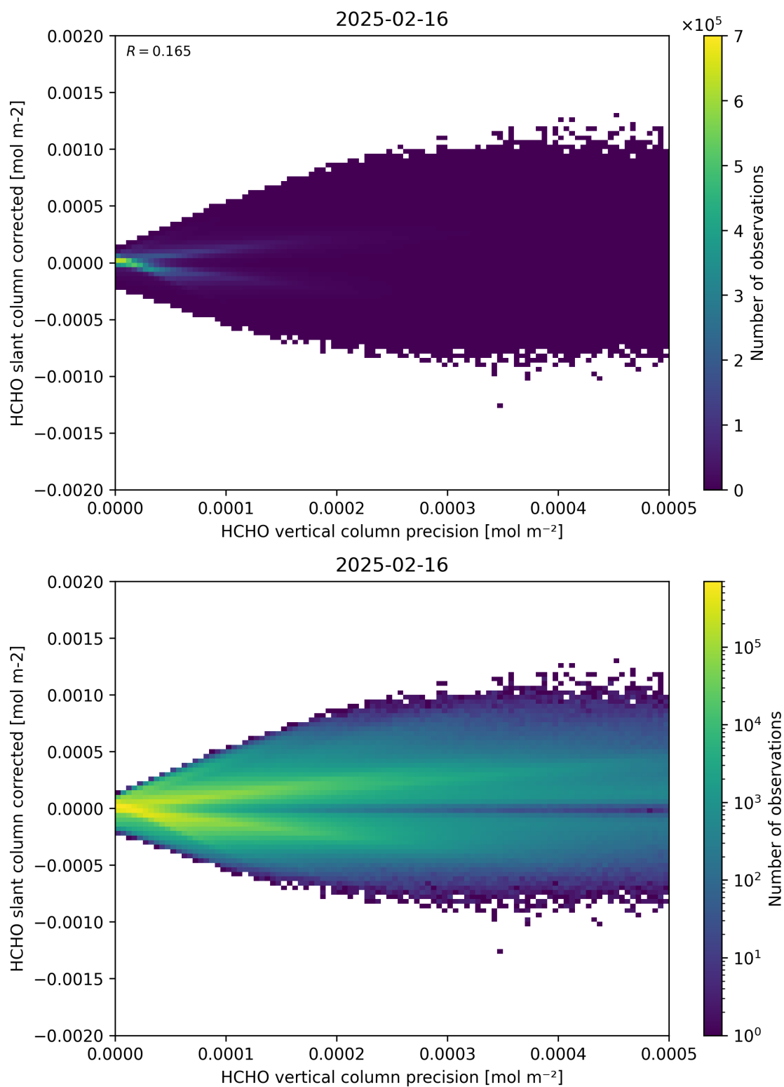
Figure 140: Scatter density plot of “HCHO vertical column precision” against “HCHO slant column corrected” for 2025-02-15 to 2025-02-17.
