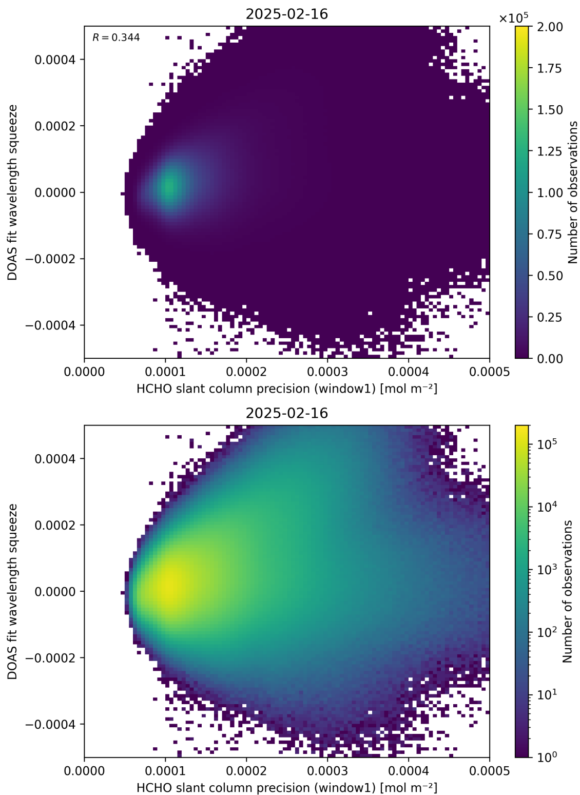
Figure 90: Scatter density plot of “HCHO slant column precision (window1)” against “DOAS fit wavelength squeeze” for 2025-02-15 to 2025-02-17.
