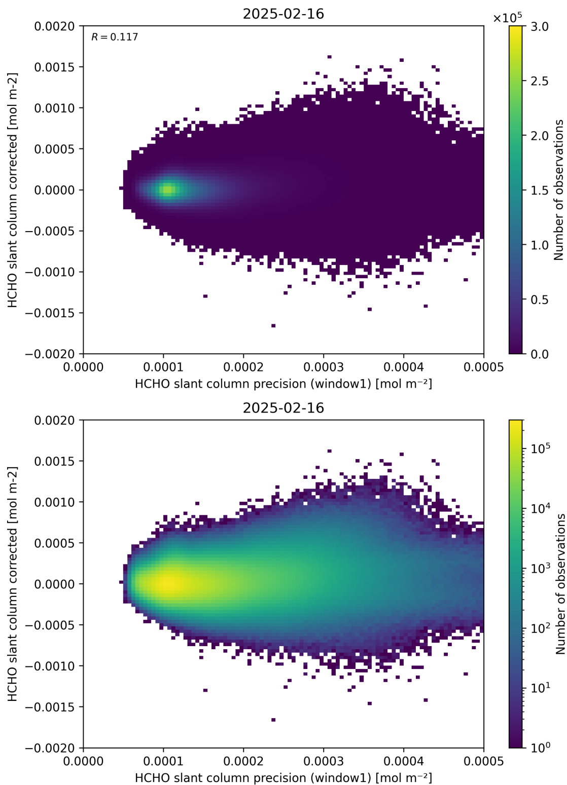
Figure 92: Scatter density plot of “HCHO slant column precision (window1)” against “HCHO slant column corrected” for 2025-02-15 to 2025-02-17.
