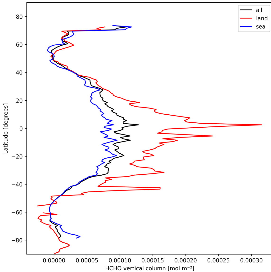
Figure 21: Zonal average of “HCHO vertical column” for 2025-02-15 to 2025-02-17.
