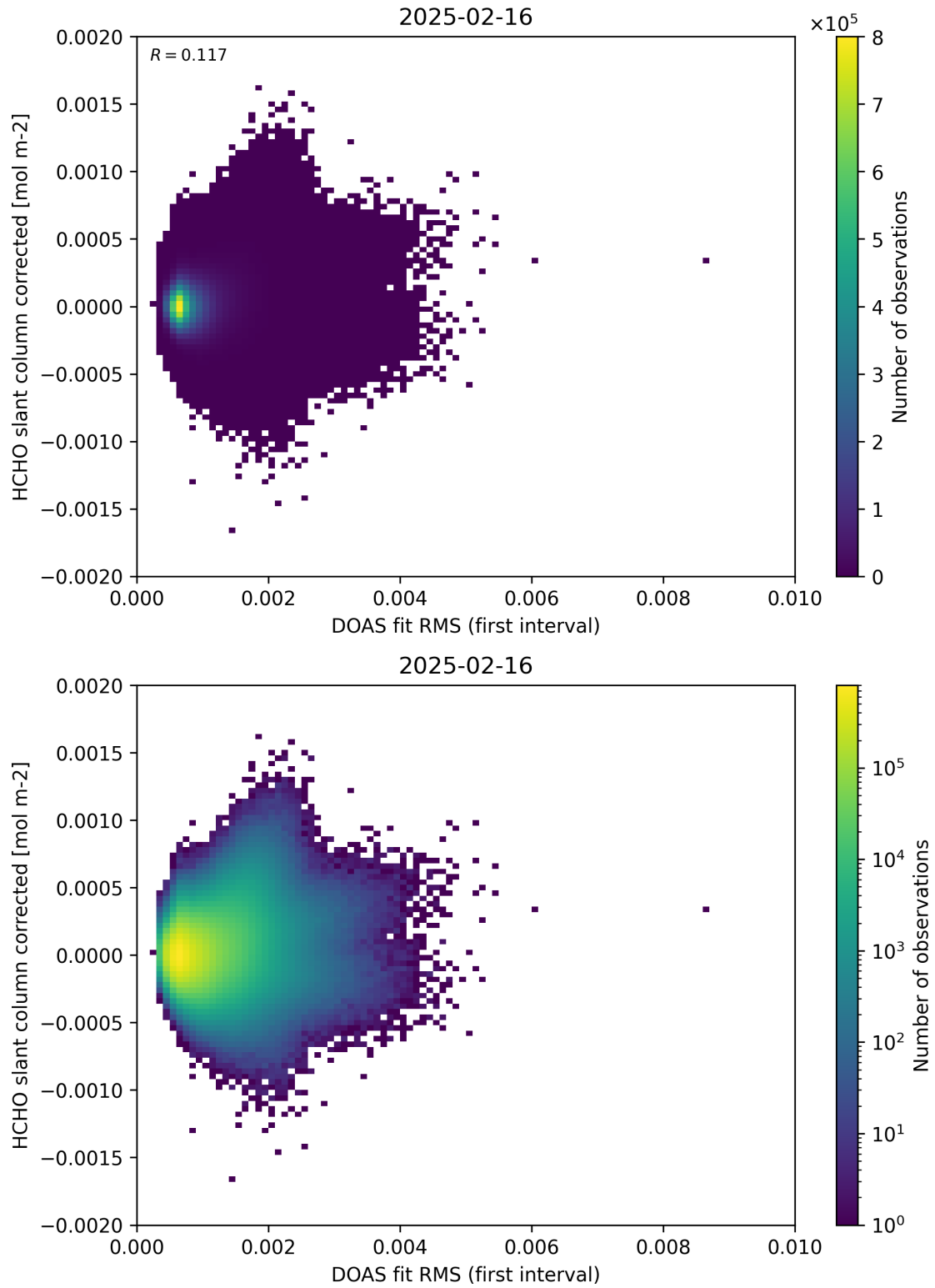
Figure 62: Scatter density plot of “DOAS fit RMS (first interval)” against “HCHO slant column corrected” for 2025-02-15 to 2025-02-17.
