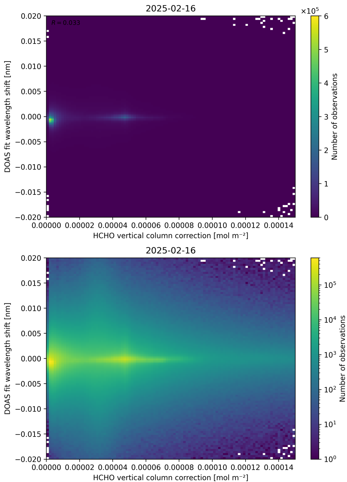
Figure 113: Scatter density plot of “HCHO vertical column correction” against “DOAS fit wavelength shift” for 2025-02-15 to 2025-02-17.
