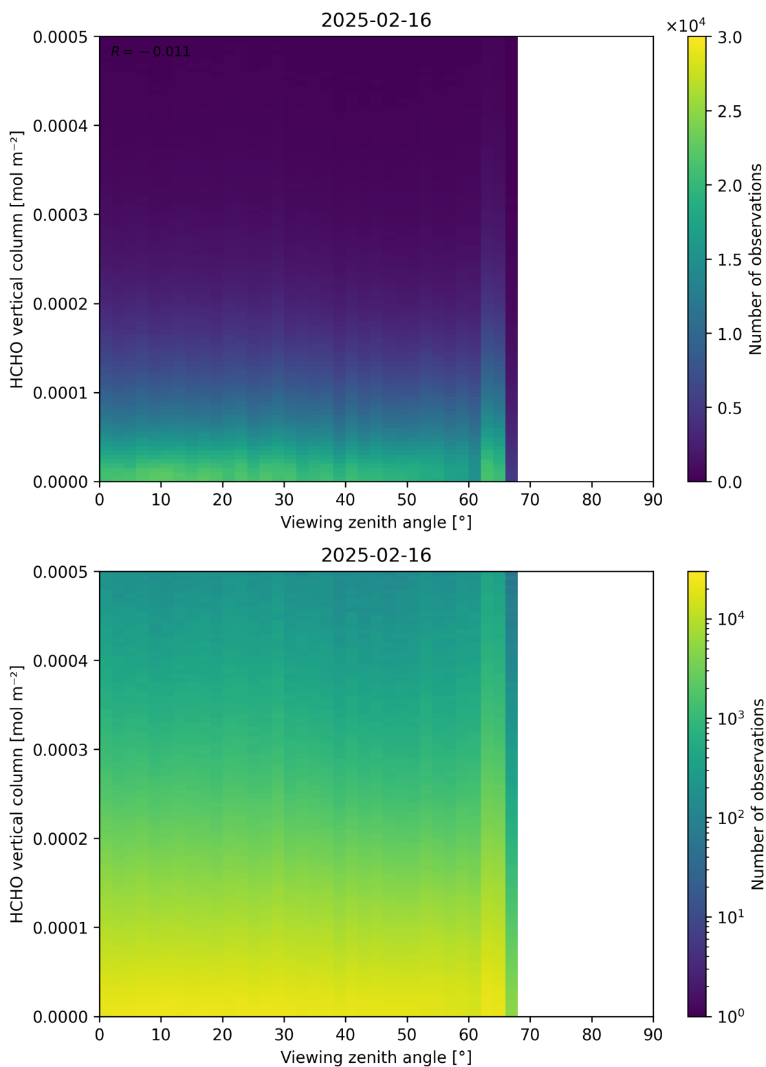
Figure 192: Scatter density plot of “Viewing zenith angle” against “HCHO vertical column” for 2025-02-15 to 2025-02-17.
