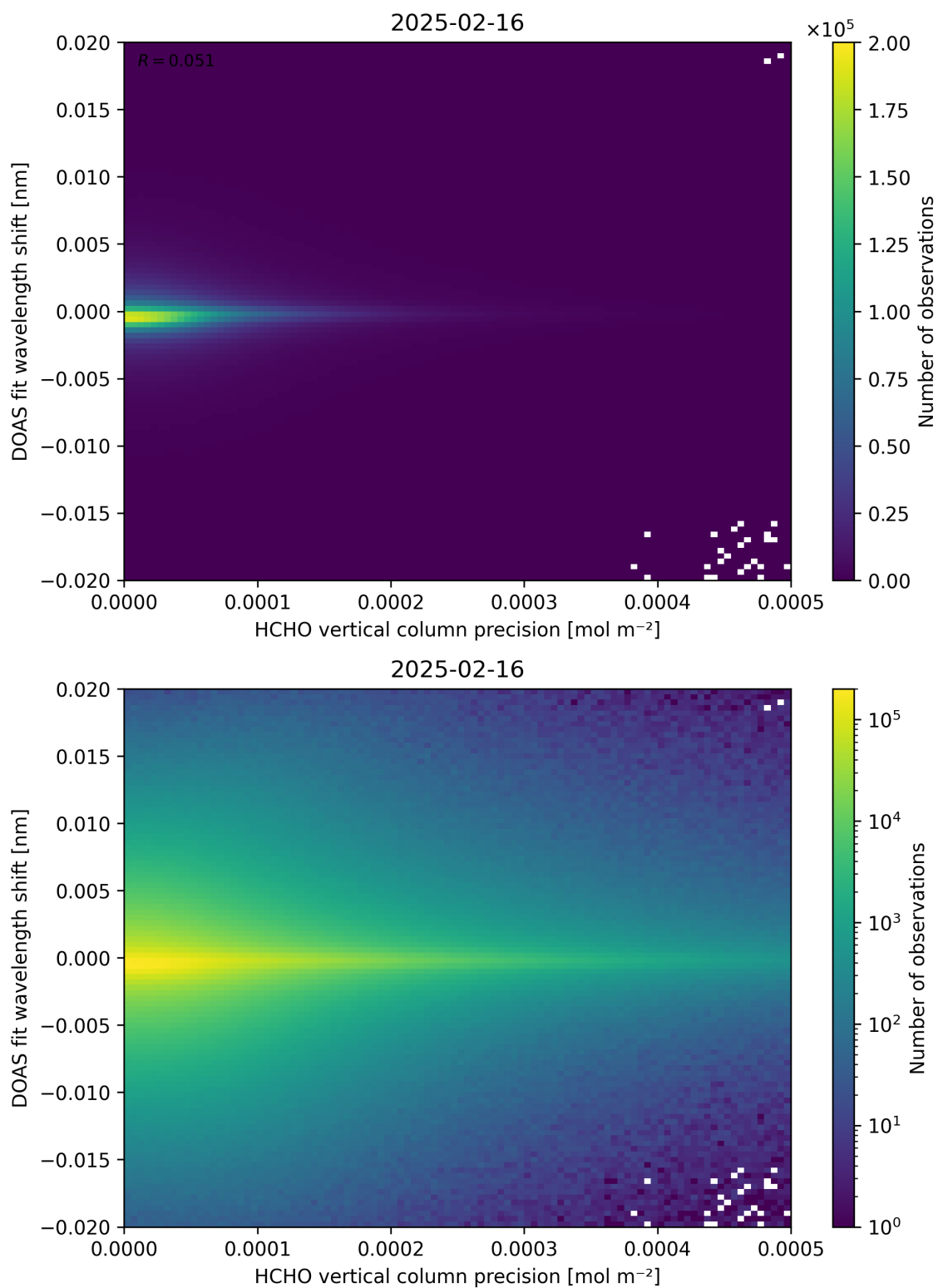
Figure 137: Scatter density plot of “HCHO vertical column precision” against “DOAS fit wavelength shift” for 2025-02-15 to 2025-02-17.
