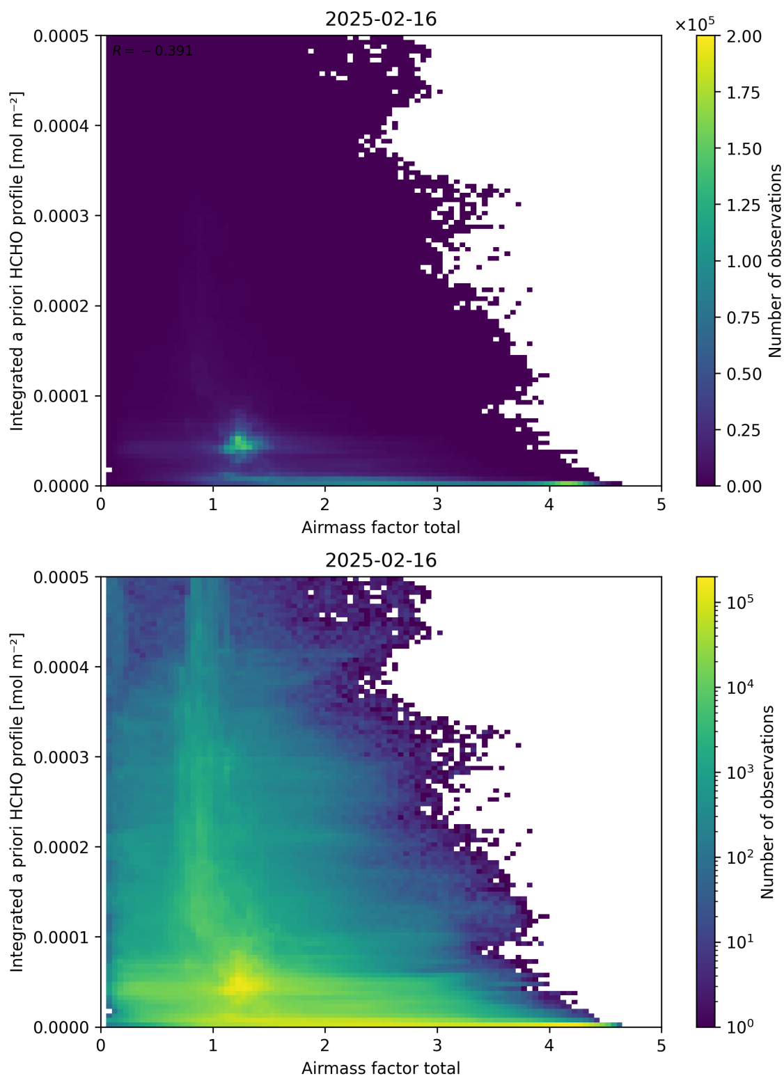
Figure 104: Scatter density plot of “Airmass factor total” against “Integrated a priori HCHO profile” for 2025-02-15 to 2025-02-17.
