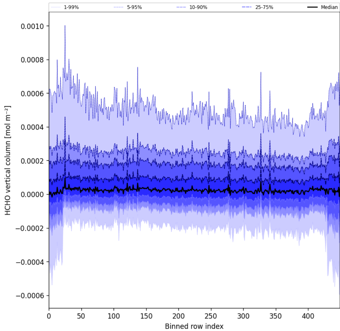
Figure 49: Along track statistics of “HCHO vertical column” for 2025-02-15 to 2025-02-17
