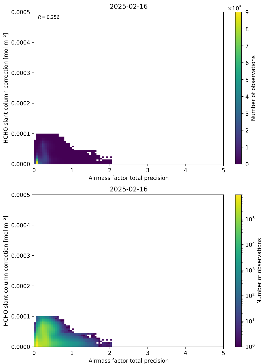
Figure 110: Scatter density plot of “Airmass factor total precision” against “HCHO slant column correction” for 2025-02-15 to 2025-02-17.
