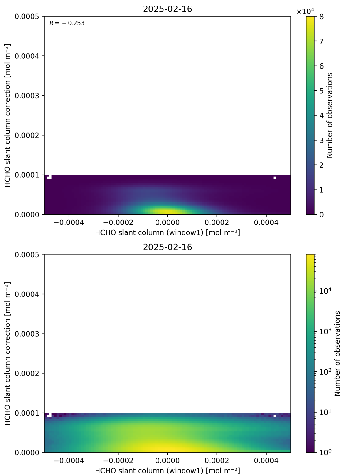
Figure 83: Scatter density plot of “HCHO slant column (window1)” against “HCHO slant column correction” for 2025-02-15 to 2025-02-17.
