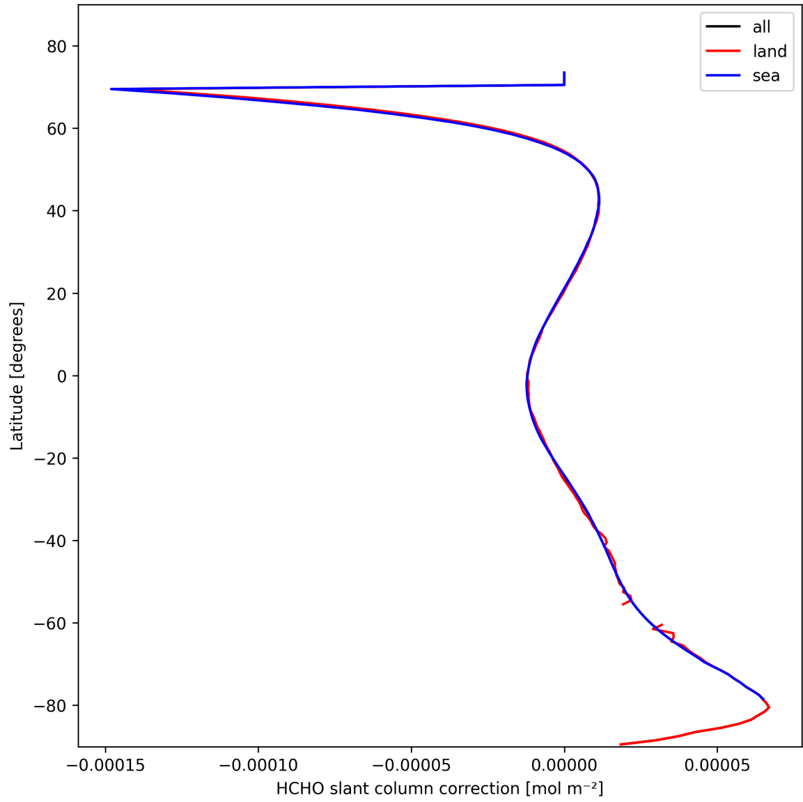
Figure 33: Zonal average of “HCHO slant column correction” for 2025-02-15 to 2025-02-17.
