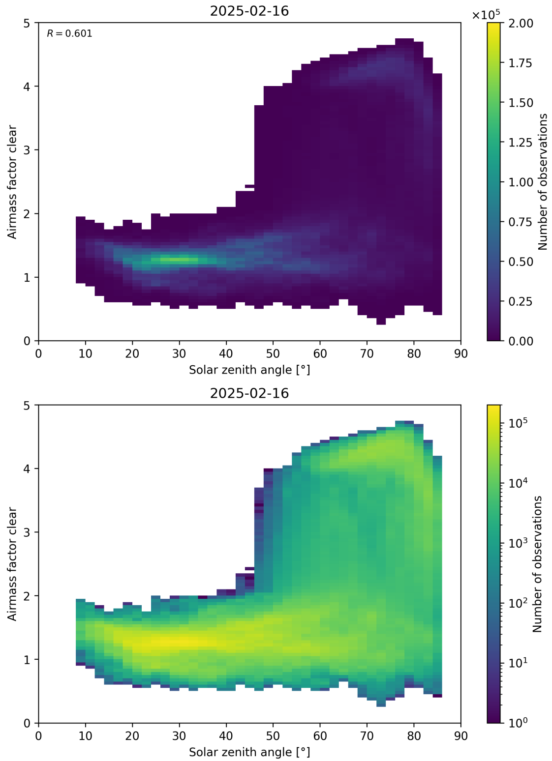
Figure 170: Scatter density plot of “Solar zenith angle” against “Airmass factor clear” for 2025-02-15 to 2025-02-17.
