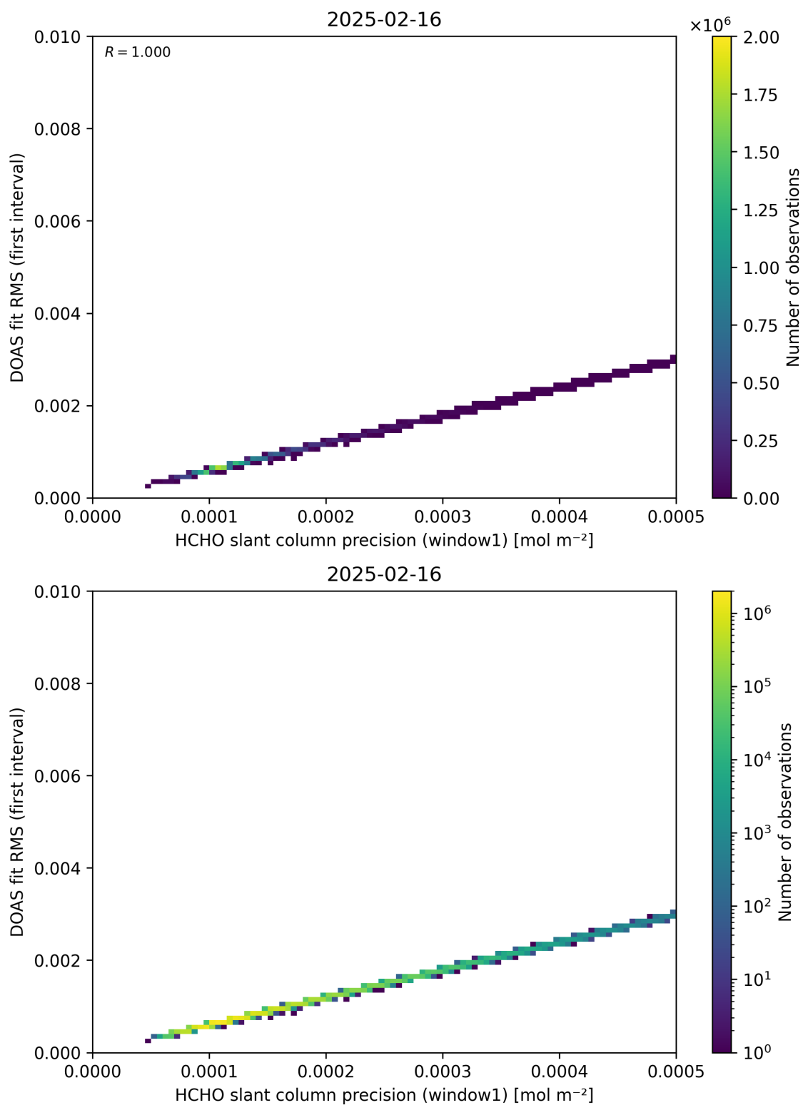
Figure 88: Scatter density plot of “HCHO slant column precision (window1)” against “DOAS fit RMS (first interval)” for 2025-02-15 to 2025-02-17.
