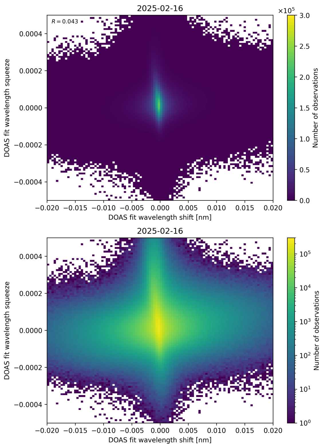
Figure 65: Scatter density plot of “DOAS fit wavelength shift” against “DOAS fit wavelength squeeze” for 2025-02-15 to 2025-02-17.
