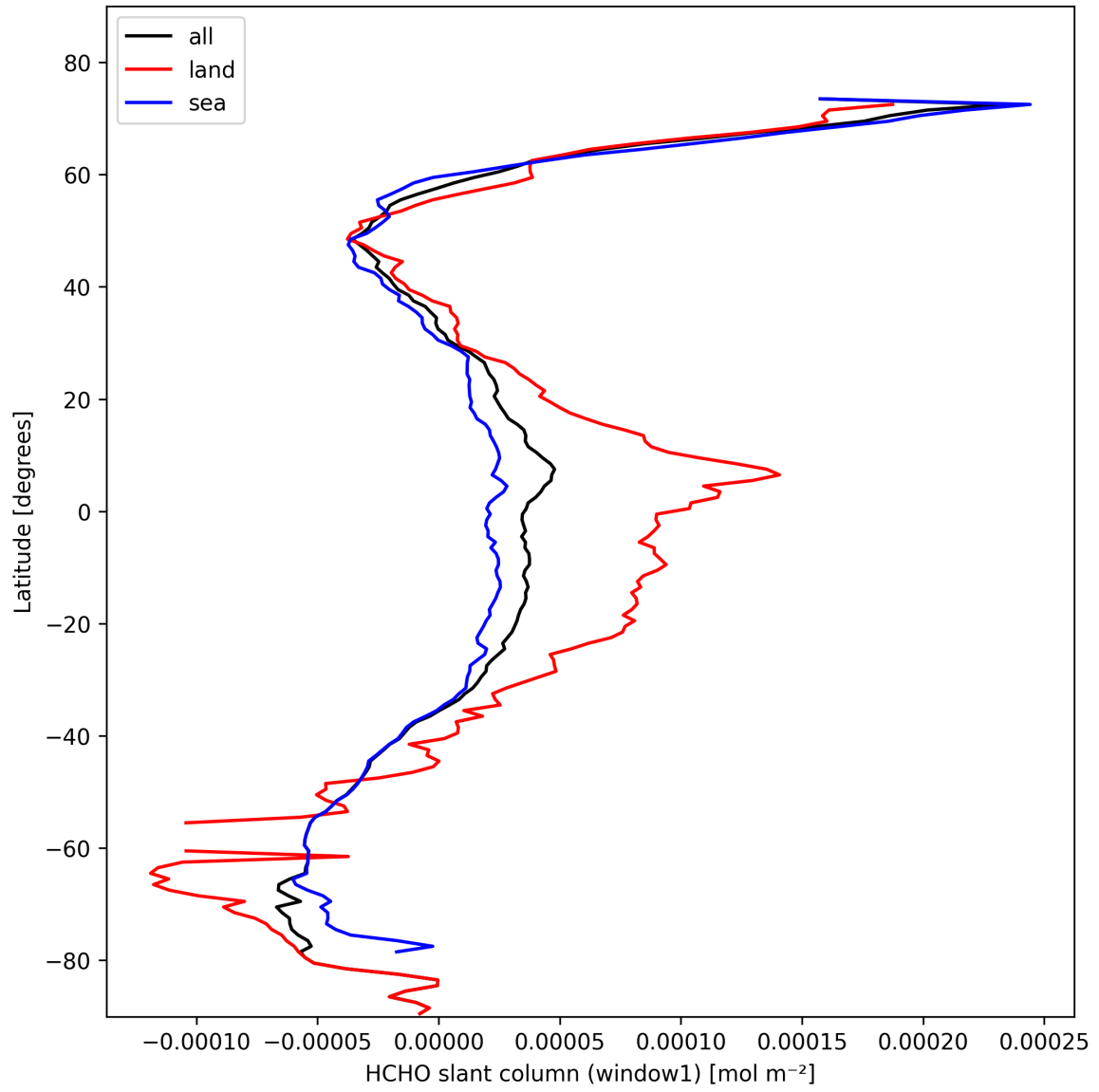
Figure 24: Zonal average of “HCHO slant column (window1)” for 2025-02-15 to 2025-02-17.
