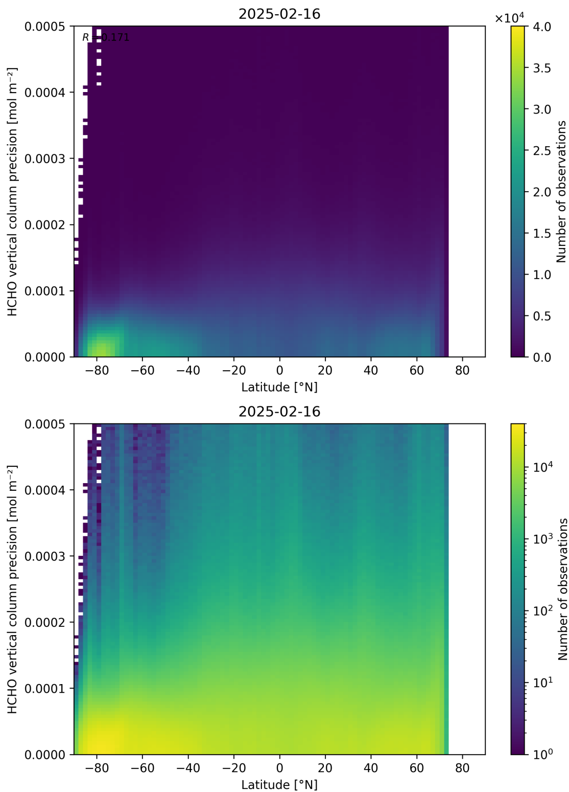
Figure 165: Scatter density plot of “Latitude” against “HCHO vertical column precision” for 2025-02-15 to 2025-02-17.
