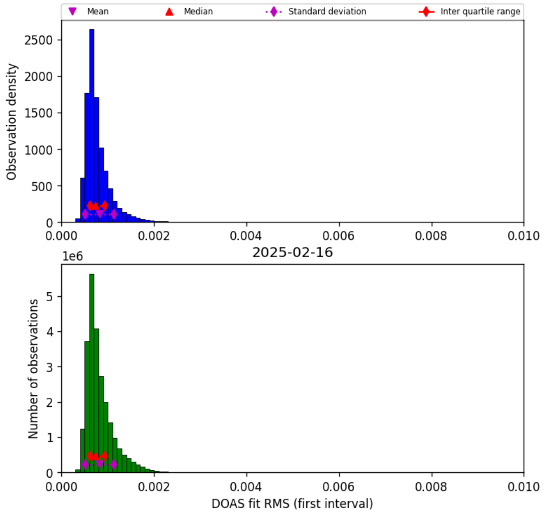
Figure 46: Histogram of “DOAS fit RMS (first interval)” for 2025-02-15 to 2025-02-17
