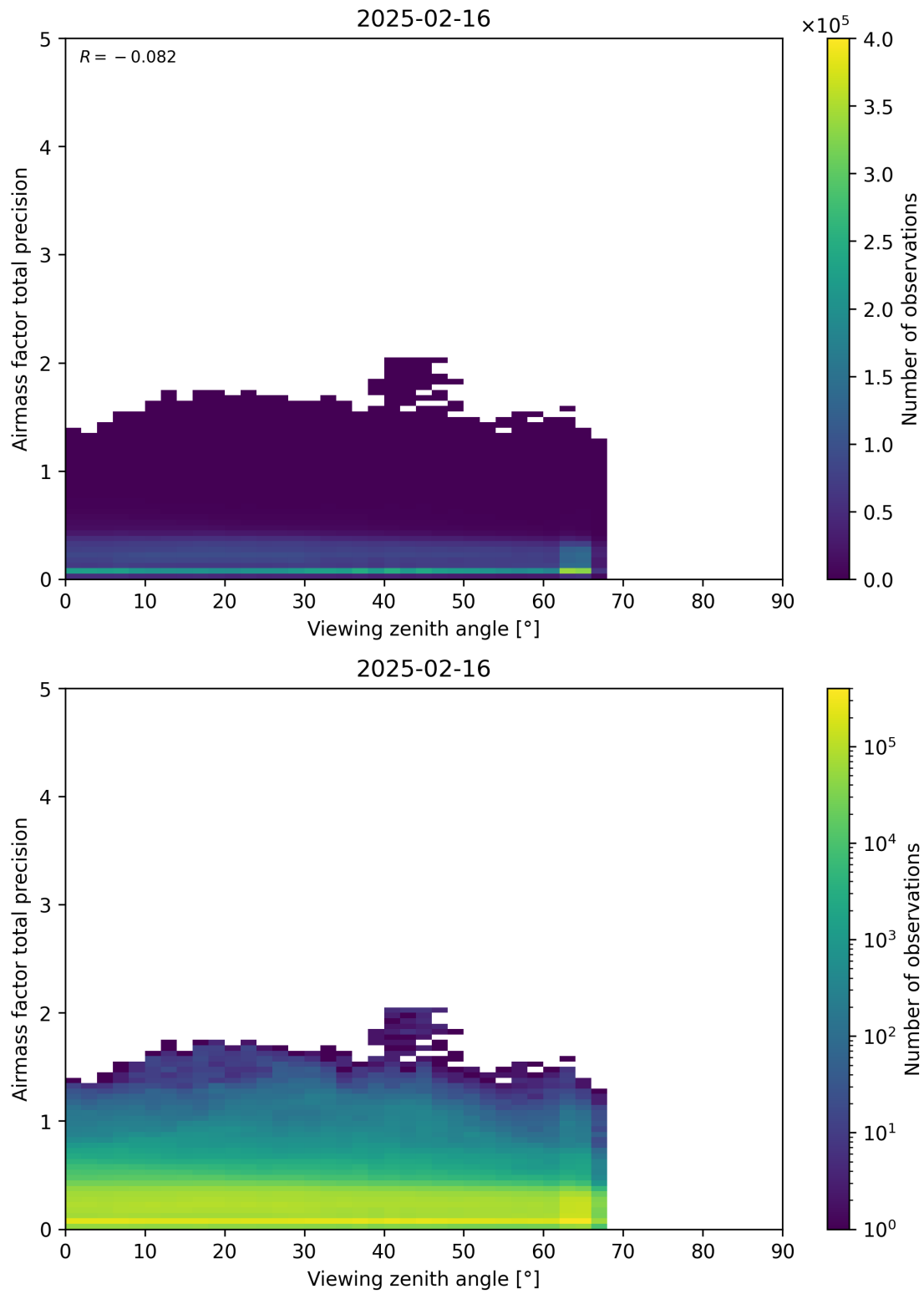
Figure 191: Scatter density plot of “Viewing zenith angle” against “Airmass factor total precision” for 2025-02-15 to 2025-02-17.
