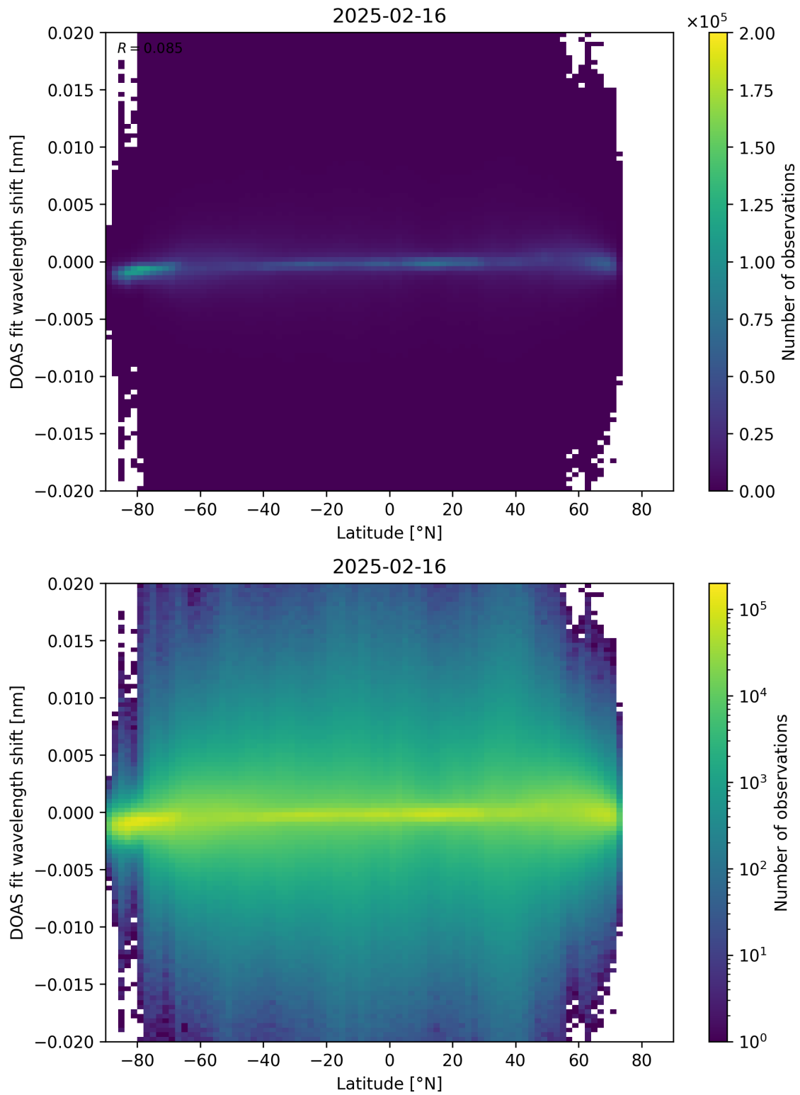
Figure 154: Scatter density plot of “Latitude” against “DOAS fit wavelength shift” for 2025-02-15 to 2025-02-17.
