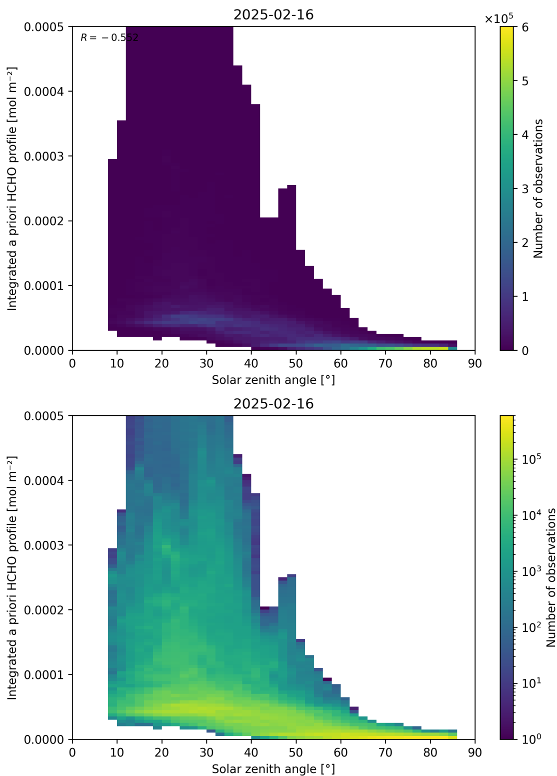
Figure 180: Scatter density plot of “Solar zenith angle” against “Integrated a priori HCHO profile” for 2025-02-15 to 2025-02-17.
