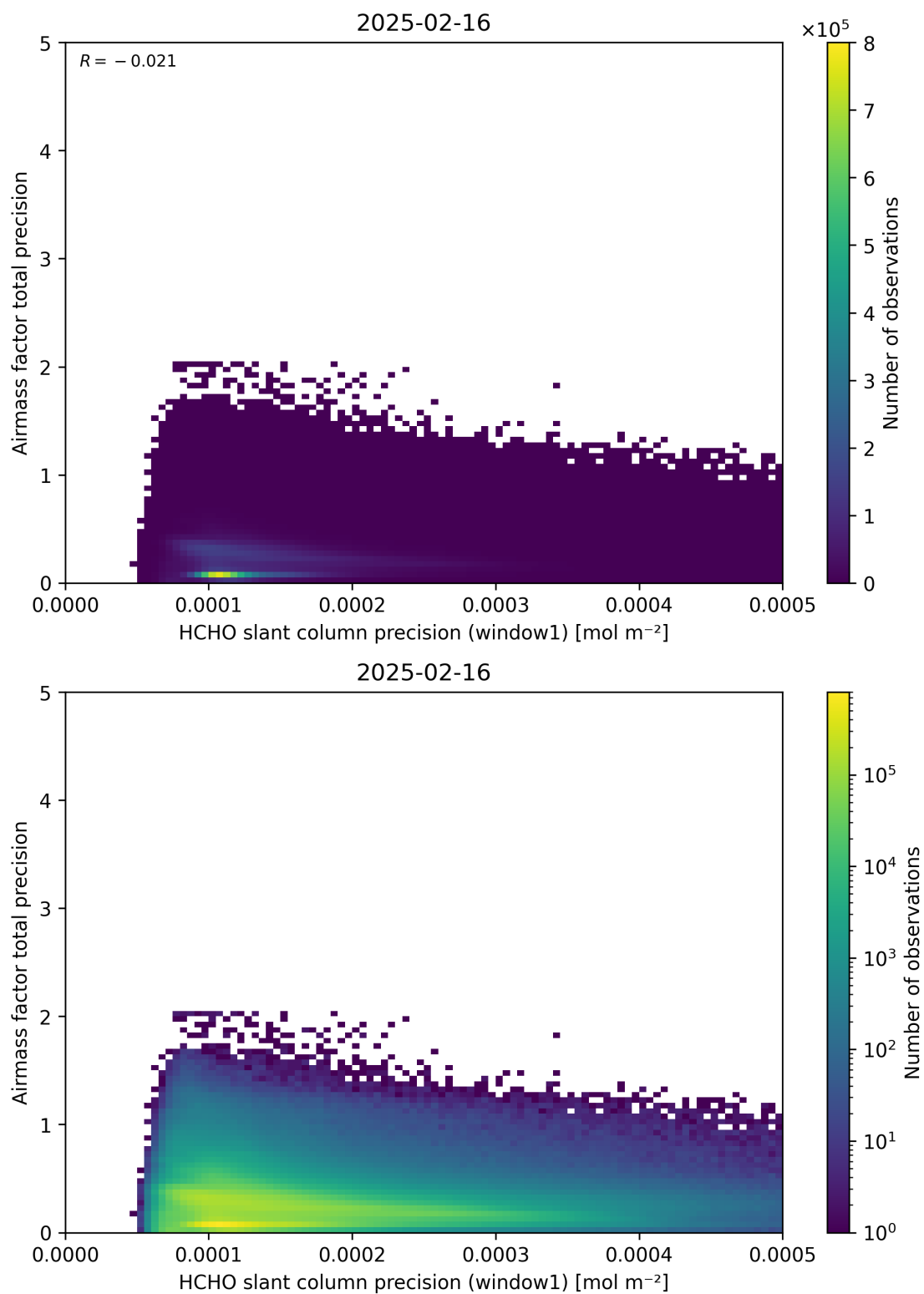
Figure 95: Scatter density plot of “HCHO slant column precision (window1)” against “Airmass factor total precision” for 2025-02-15 to 2025-02-17.
