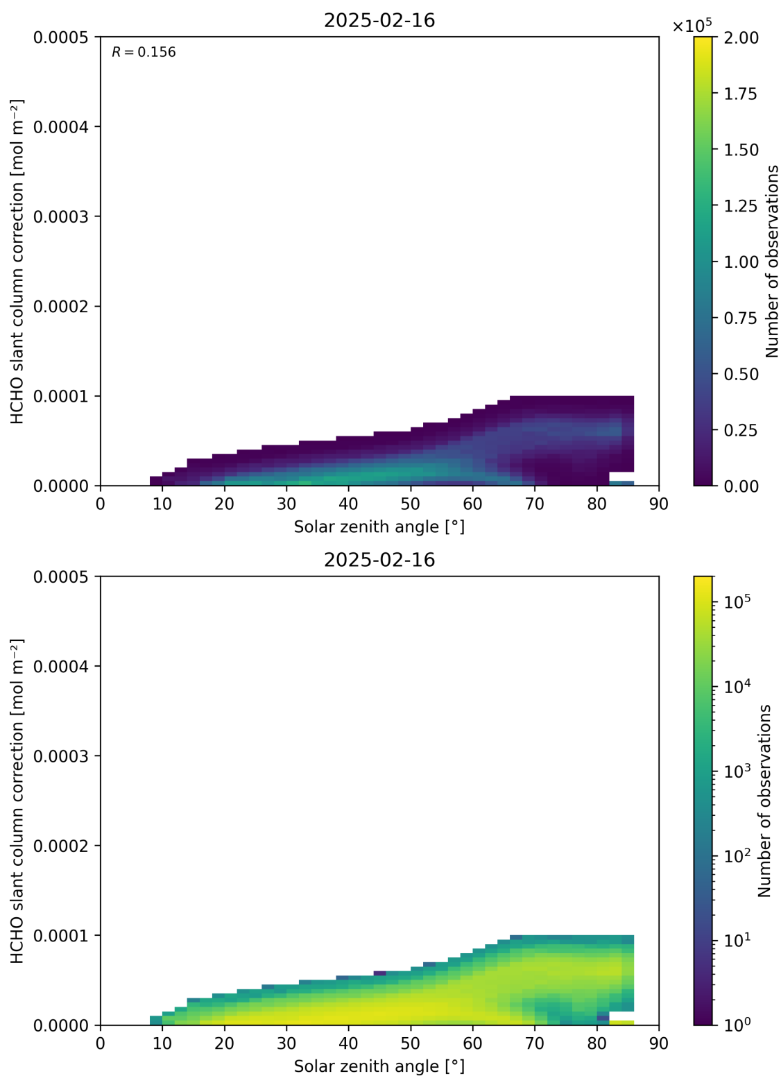
Figure 172: Scatter density plot of “Solar zenith angle” against “HCHO slant column correction” for 2025-02-15 to 2025-02-17.
