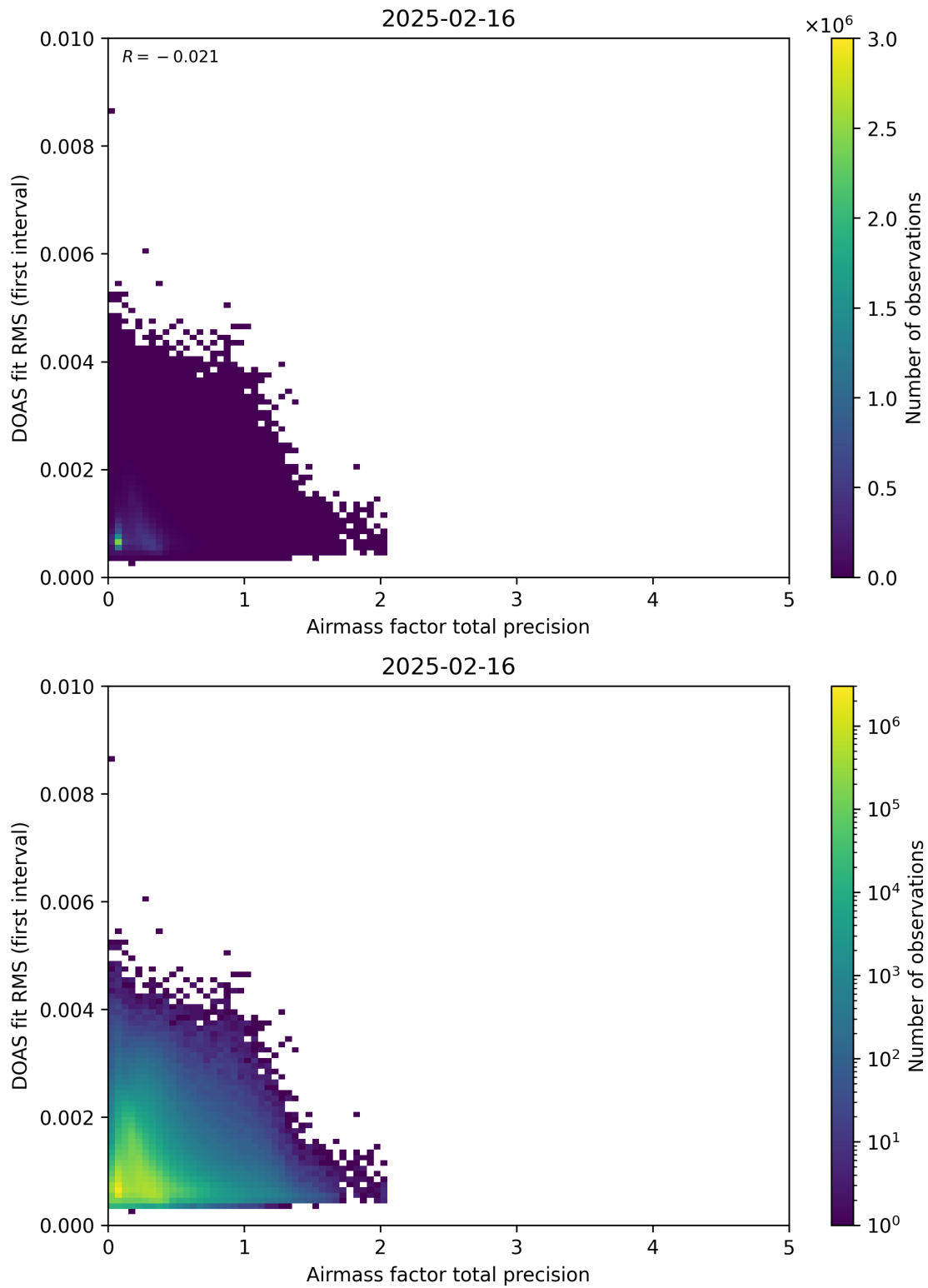
Figure 105: Scatter density plot of “Airmass factor total precision” against “DOAS fit RMS (first interval)” for 2025-02-15 to 2025-02-17.
