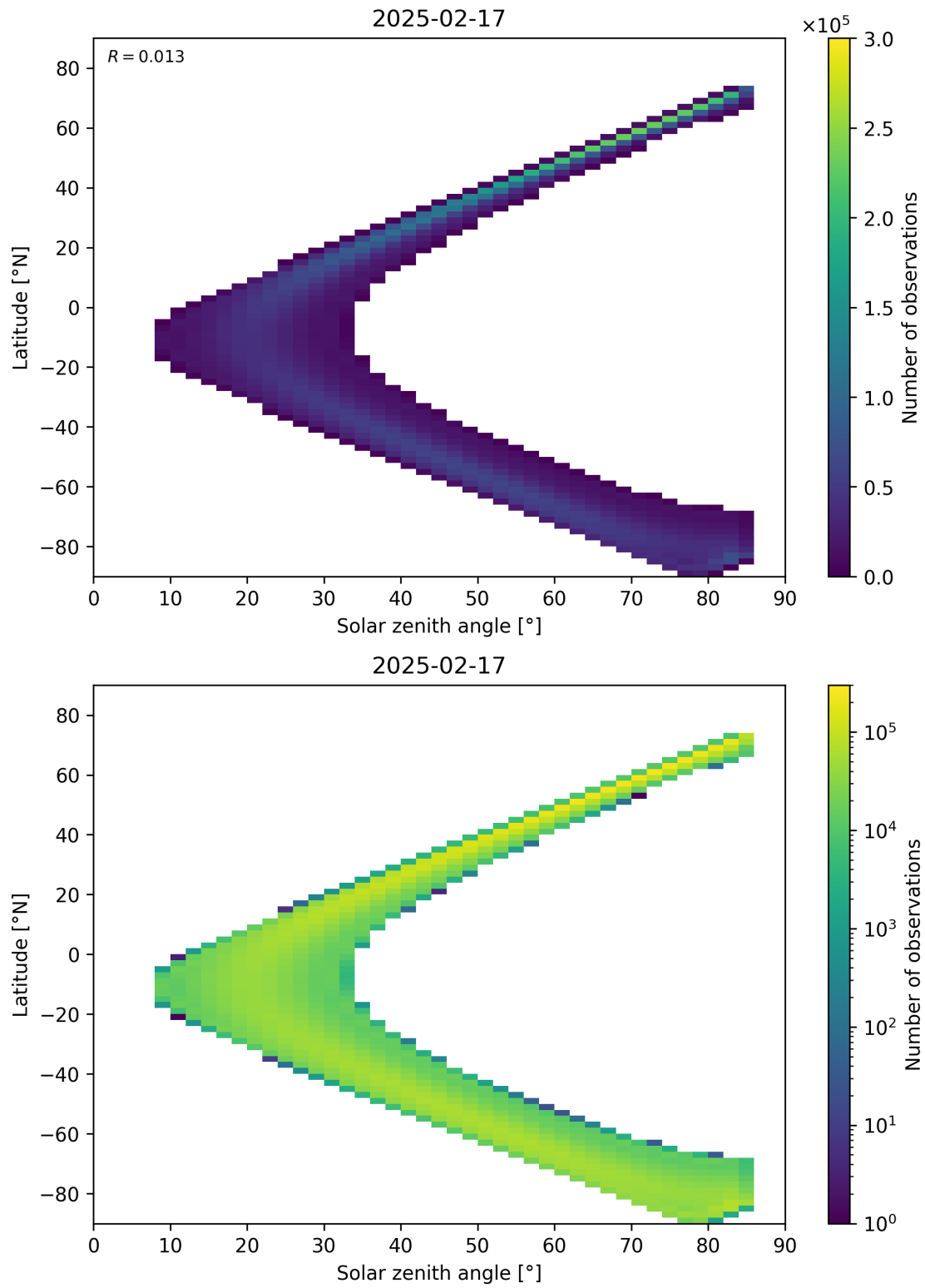
Figure 181: Scatter density plot of “Solar zenith angle” against “Latitude” for 2025-02-16 to 2025-02-18.
