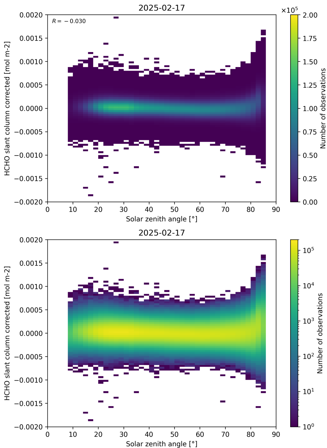
Figure 171: Scatter density plot of “Solar zenith angle” against “HCHO slant column corrected” for 2025-02-16 to 2025-02-18.
