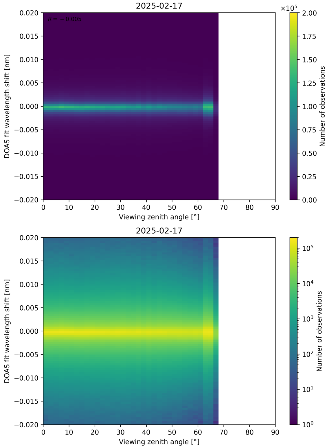
Figure 183: Scatter density plot of “Viewing zenith angle” against “DOAS fit wavelength shift” for 2025-02-16 to 2025-02-18.
