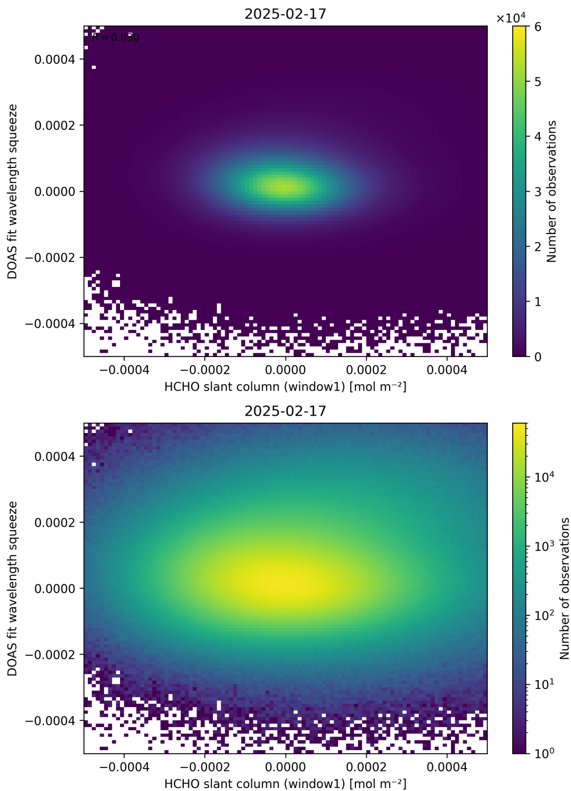
Figure 80: Scatter density plot of “HCHO slant column (window1)” against “DOAS fit wavelength squeeze” for 2025-02-16 to 2025-02-18.
