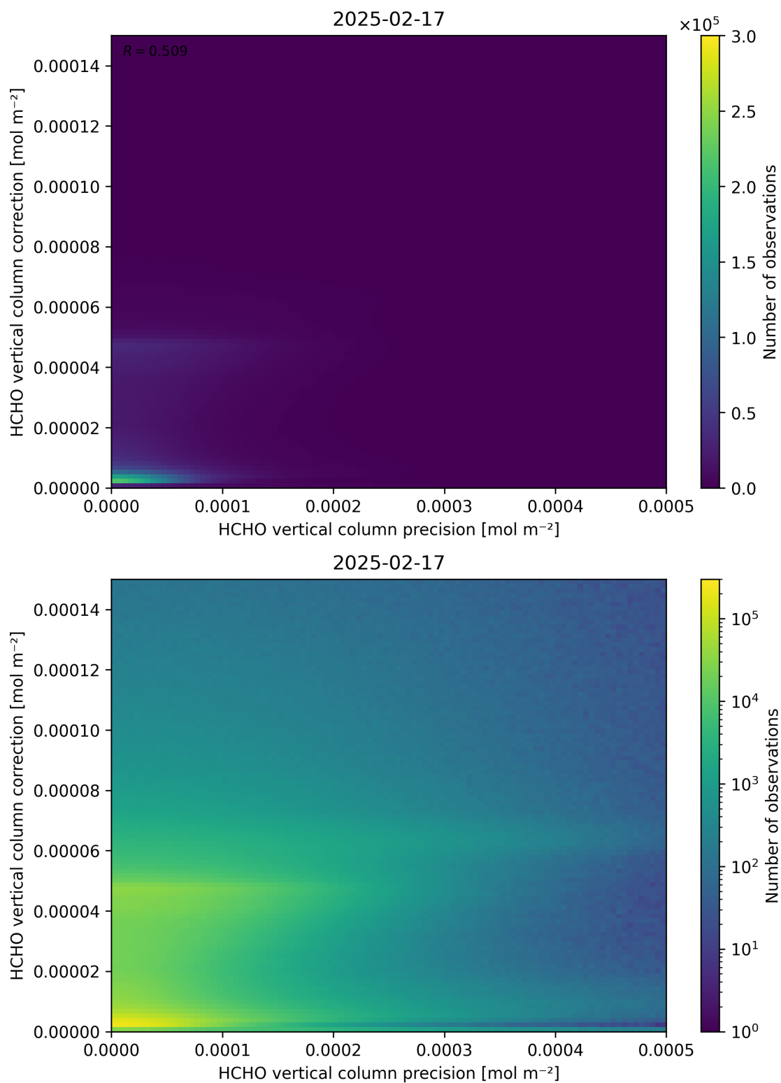
Figure 146: Scatter density plot of “HCHO vertical column precision” against “HCHO vertical column correction” for 2025-02-16 to 2025-02-18.
