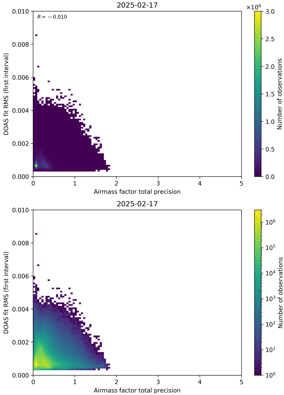
Figure 105: Scatter density plot of “Airmass factor total precision” against “DOAS fit RMS (first interval)” for 2025-02-16 to 2025-02-18.
