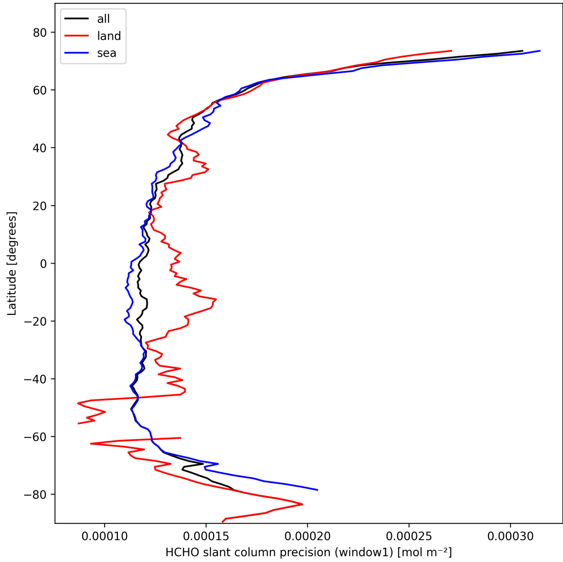
Figure 25: Zonal average of “HCHO slant column precision (window1)” for 2025-02-16 to 2025-02-18.
