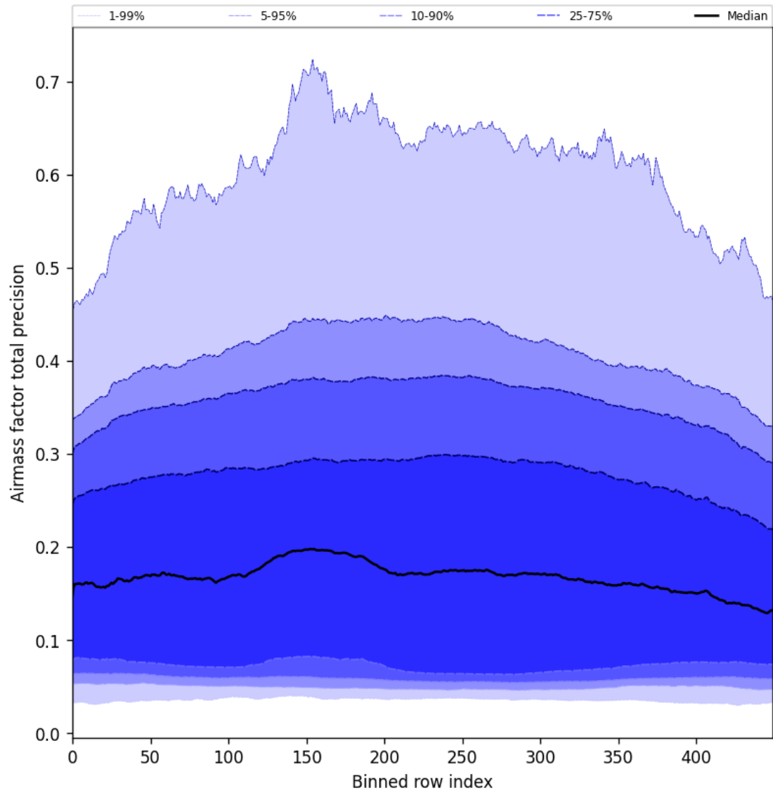
Figure 55: Along track statistics of “Airmass factor total precision” for 2025-02-16 to 2025-02-18
