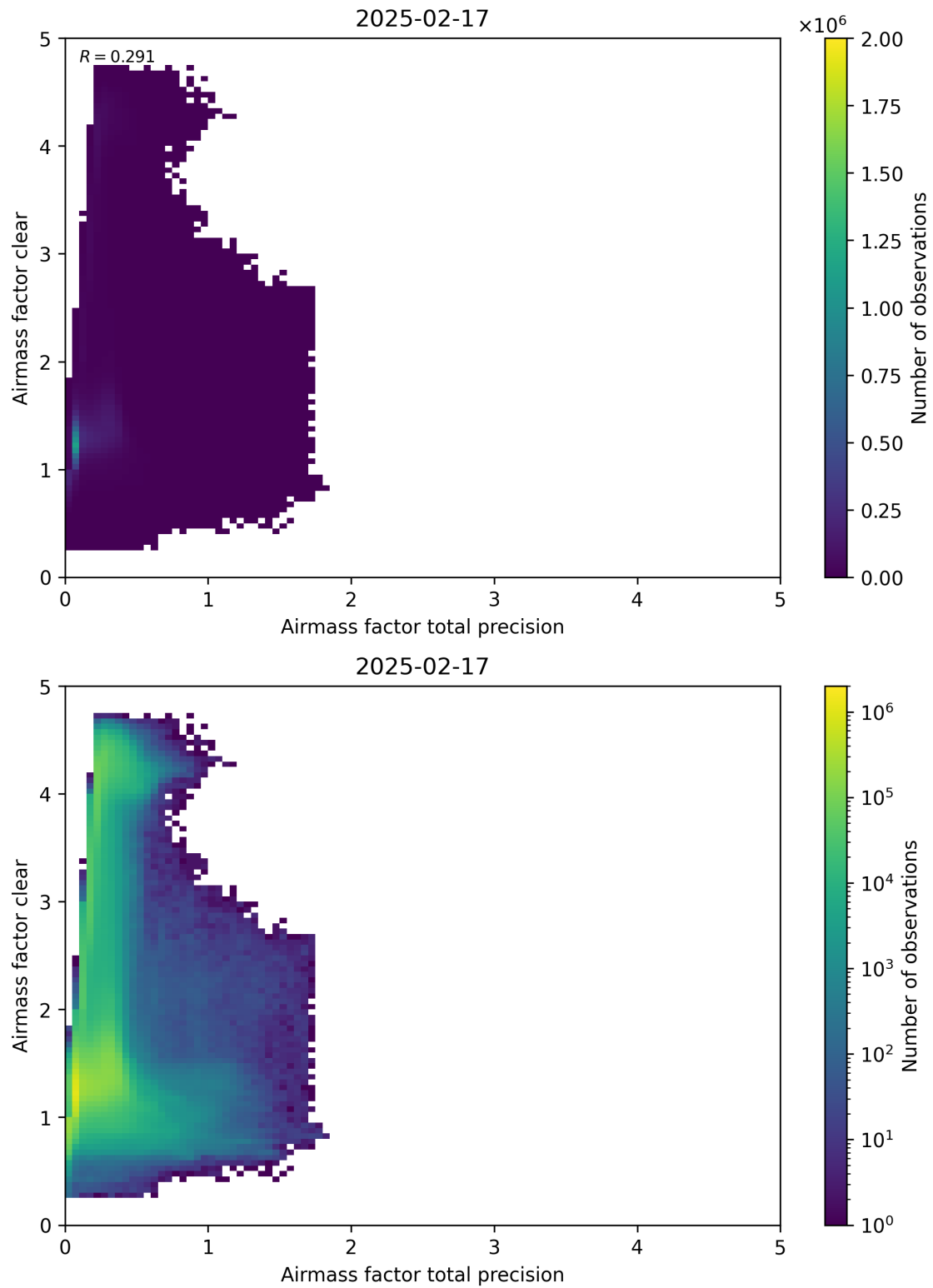
Figure 108: Scatter density plot of “Airmass factor total precision” against “Airmass factor clear” for 2025-02-16 to 2025-02-18.
