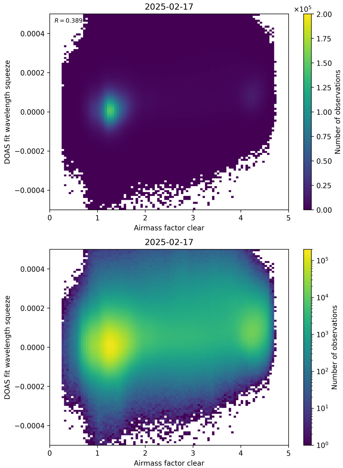
Figure 73: Scatter density plot of “Airmass factor clear” against “DOAS fit wavelength squeeze” for 2025-02-16 to 2025-02-18.
