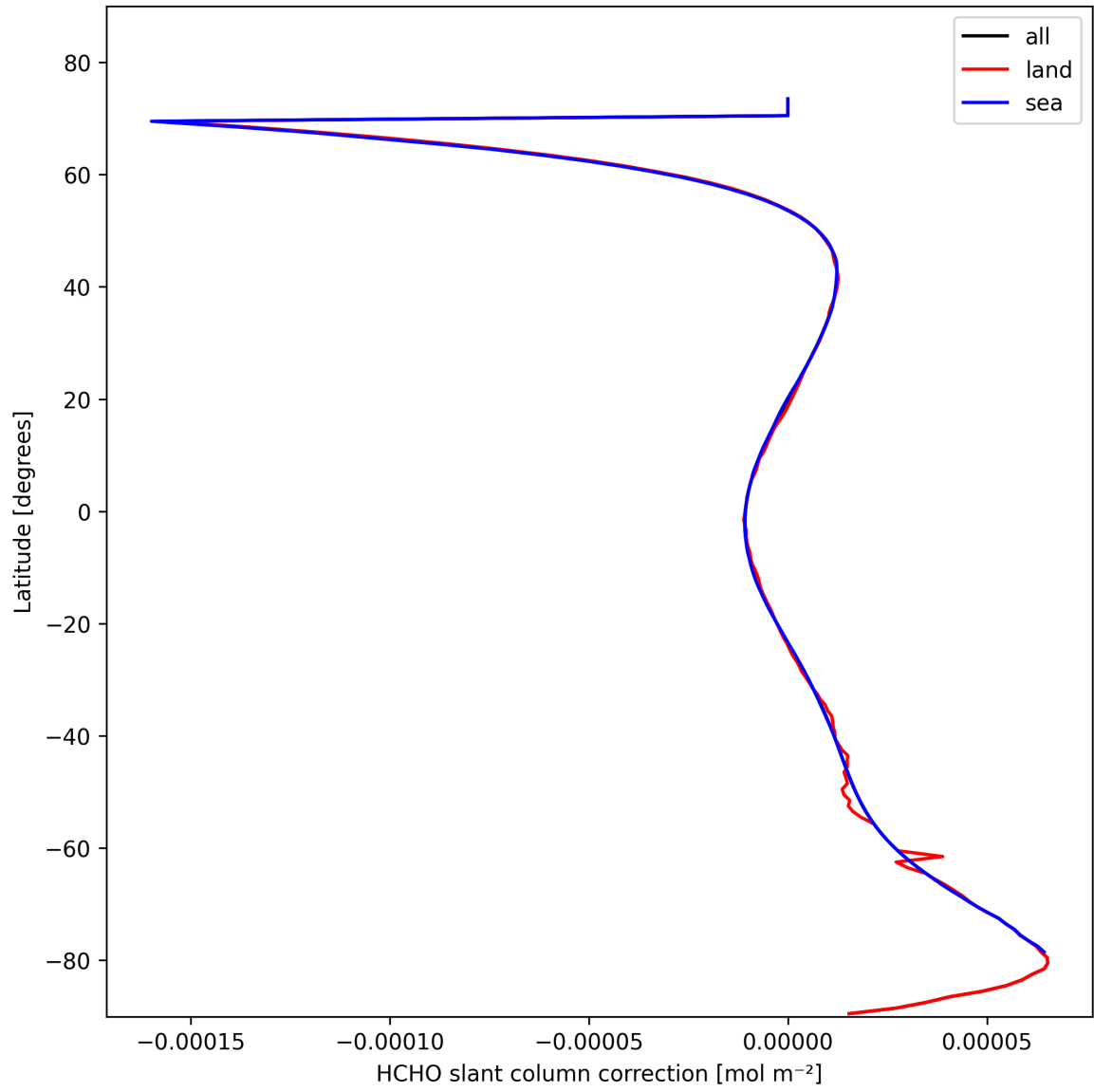
Figure 33: Zonal average of “HCHO slant column correction” for 2025-02-16 to 2025-02-18.
