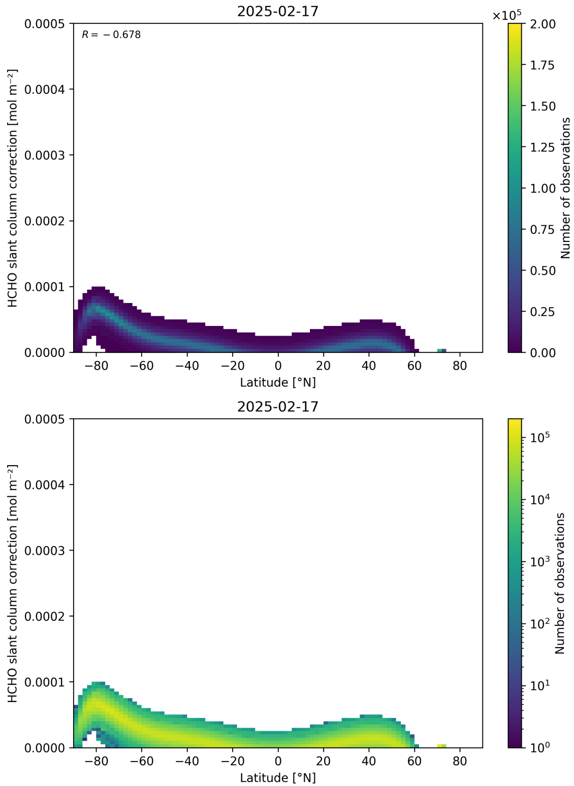
Figure 158: Scatter density plot of “Latitude” against “HCHO slant column correction” for 2025-02-16 to 2025-02-18.
