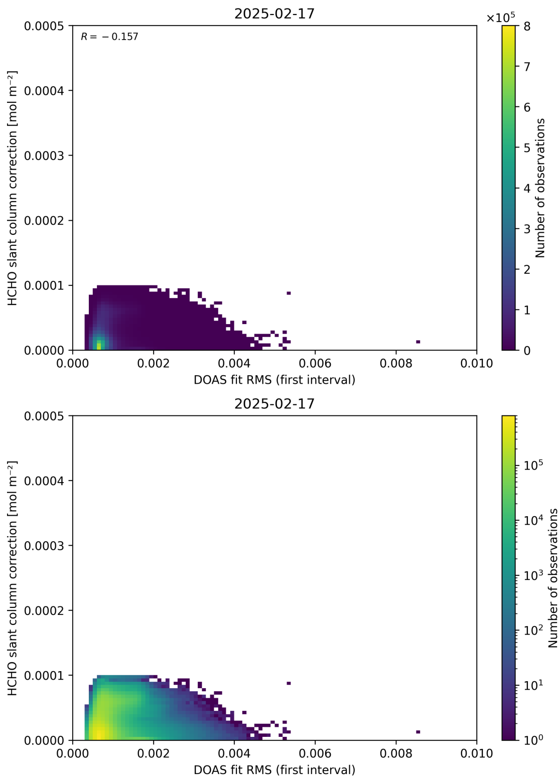
Figure 63: Scatter density plot of “DOAS fit RMS (first interval)” against “HCHO slant column correction” for 2025-02-16 to 2025-02-18.
