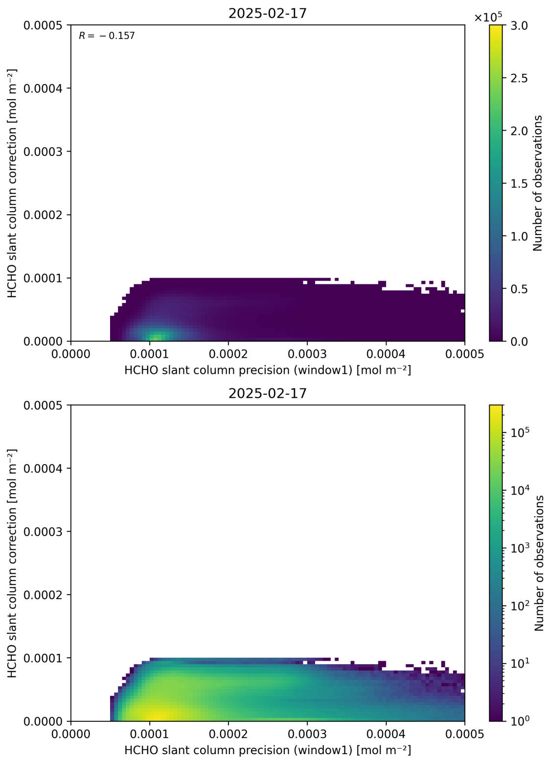
Figure 93: Scatter density plot of “HCHO slant column precision (window1)” against “HCHO slant column correction” for 2025-02-16 to 2025-02-18.
