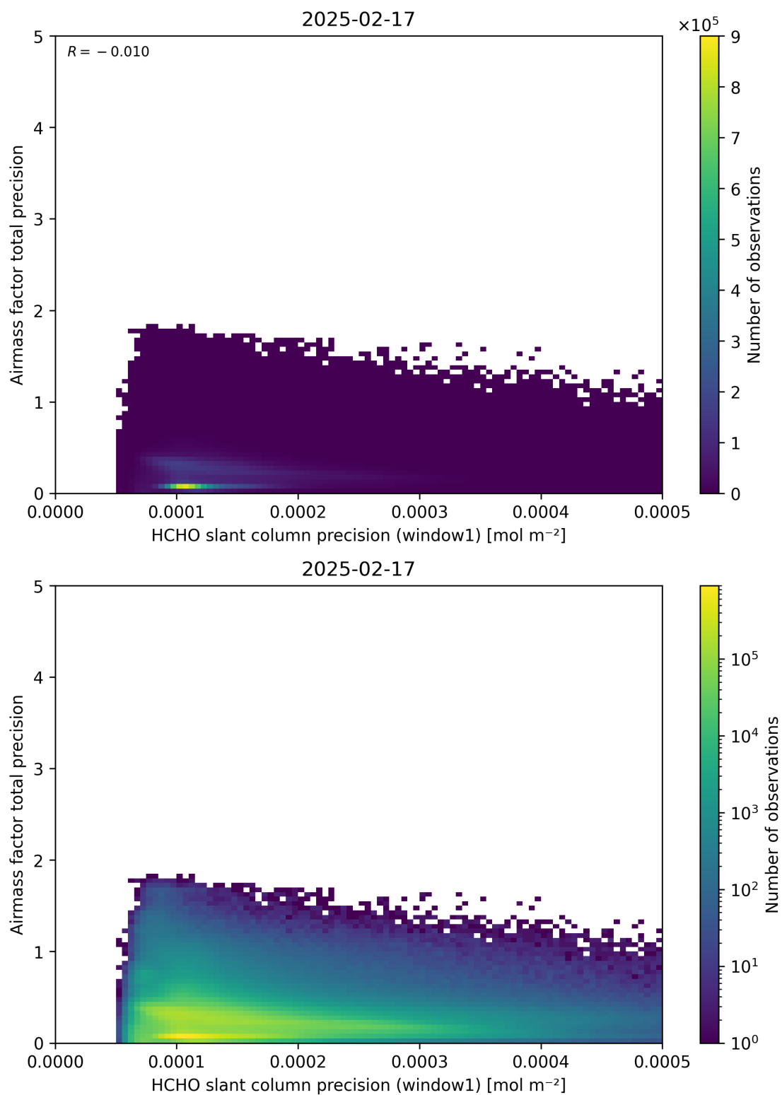
Figure 95: Scatter density plot of “HCHO slant column precision (window1)” against “Airmass factor total precision” for 2025-02-16 to 2025-02-18.
