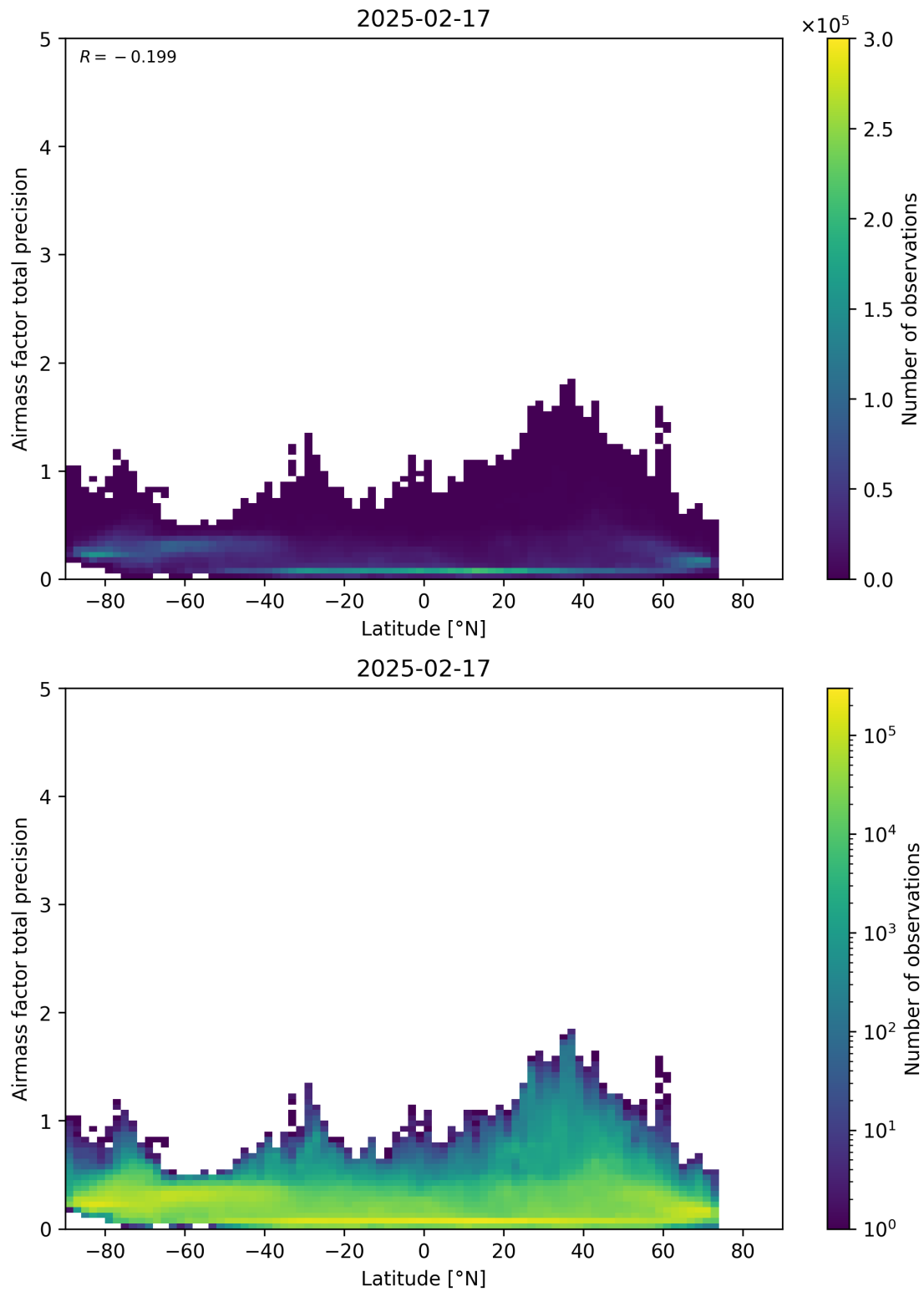
Figure 162: Scatter density plot of “Latitude” against “Airmass factor total precision” for 2025-02-16 to 2025-02-18.
