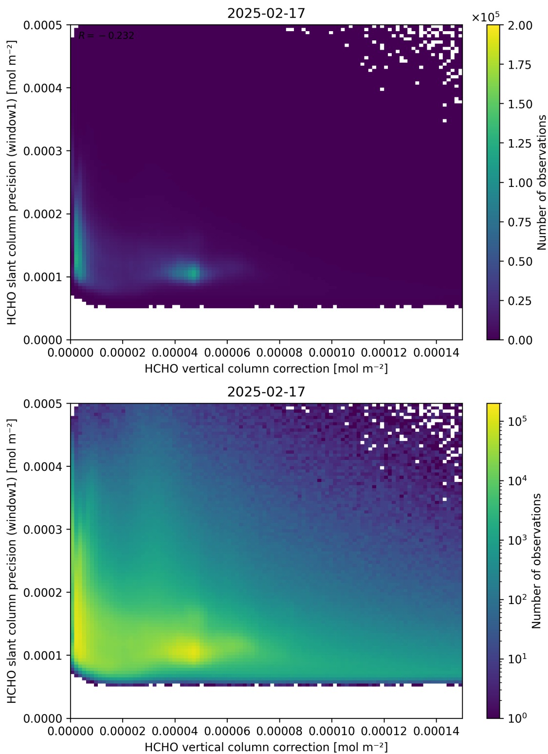
Figure 119: Scatter density plot of “HCHO vertical column correction” against “HCHO slant column precision (window1)” for 2025-02-16 to 2025-02-18.
