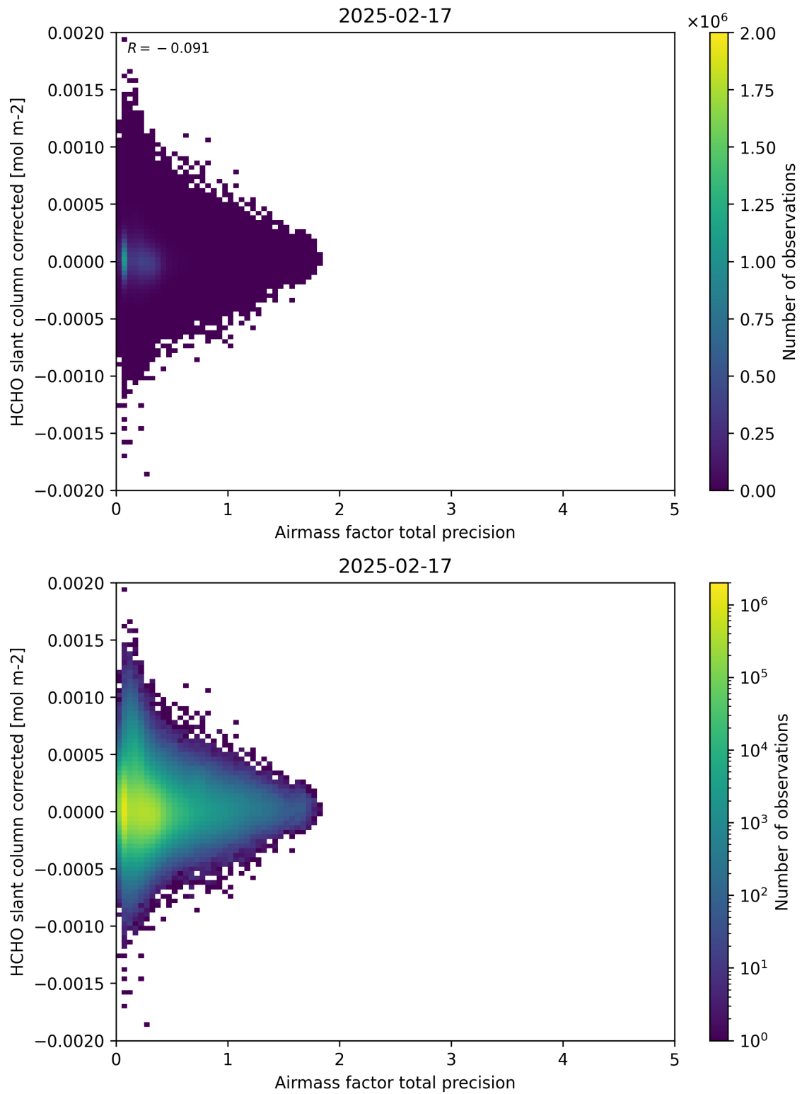
Figure 109: Scatter density plot of “Airmass factor total precision” against “HCHO slant column corrected” for 2025-02-16 to 2025-02-18.
