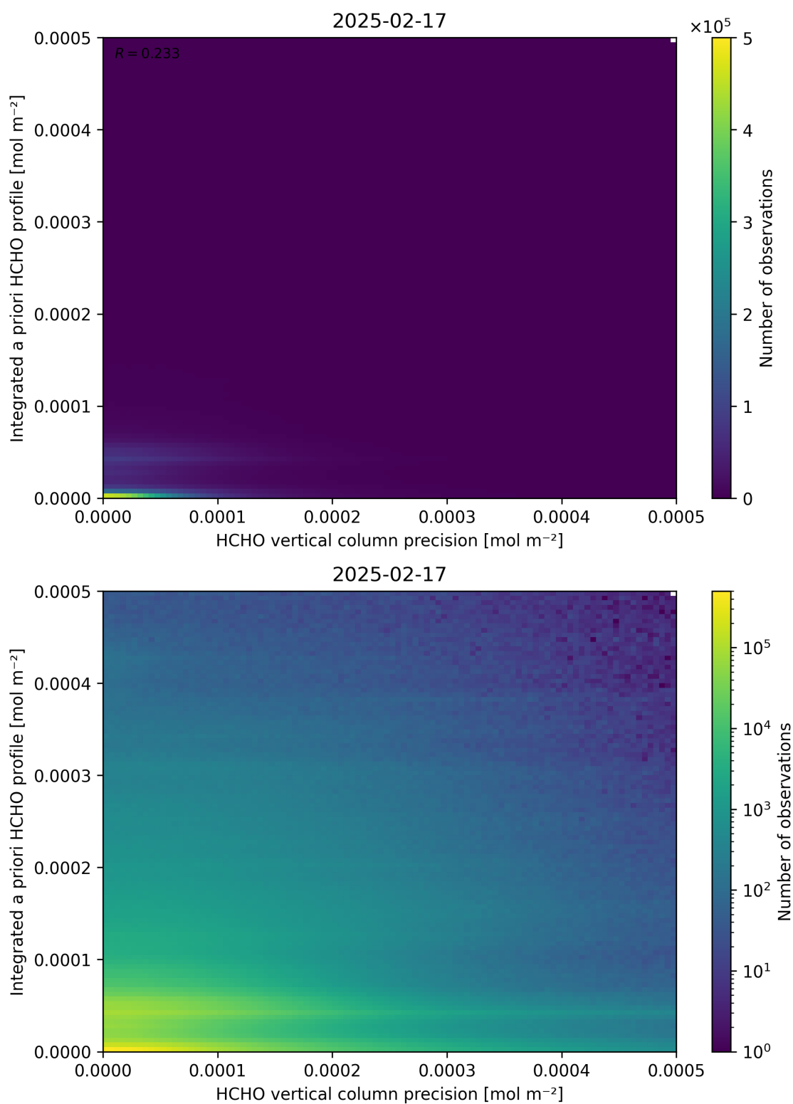
Figure 147: Scatter density plot of “HCHO vertical column precision” against “Integrated a priori HCHO profile” for 2025-02-16 to 2025-02-18.
