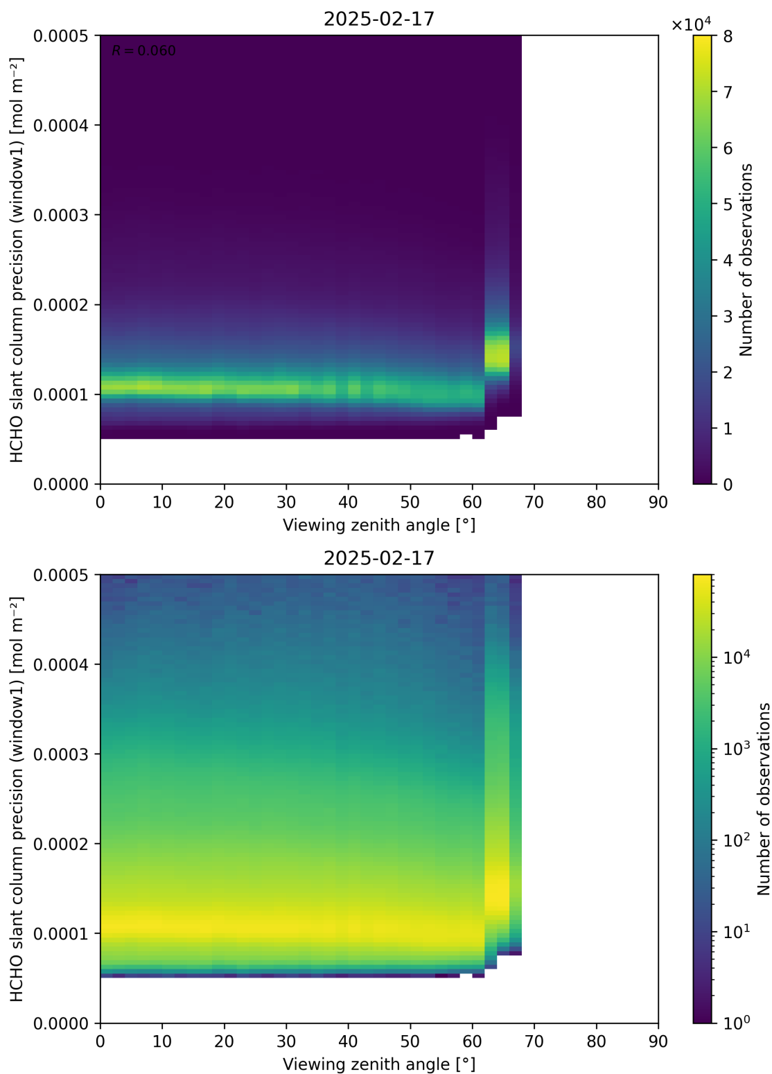
Figure 189: Scatter density plot of “Viewing zenith angle” against “HCHO slant column precision (window1)” for 2025-02-16 to 2025-02-18.
