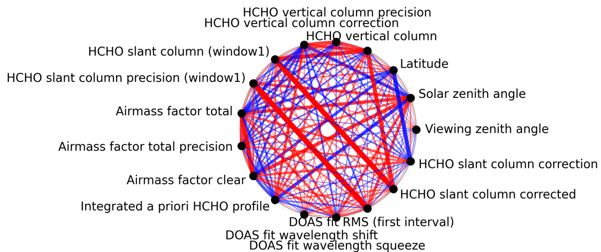
Figure 1: Map of correlation graph for 2025-02-16 to 2025-02-18.
