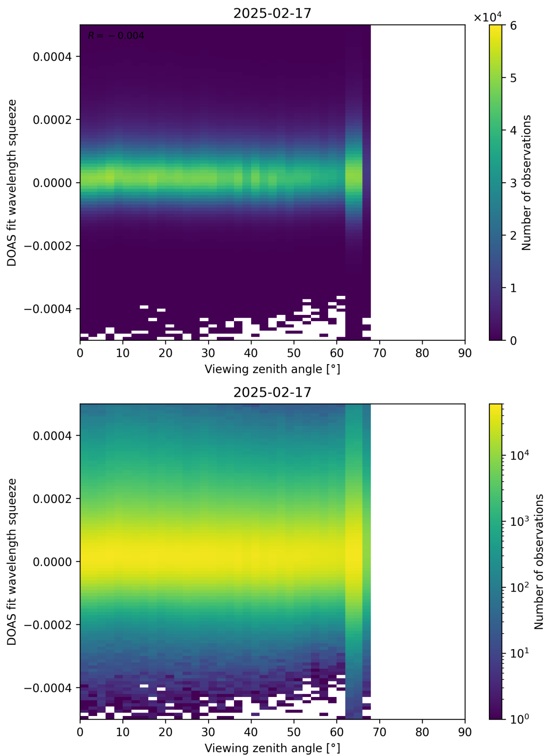
Figure 184: Scatter density plot of “Viewing zenith angle” against “DOAS fit wavelength squeeze” for 2025-02-16 to 2025-02-18.
