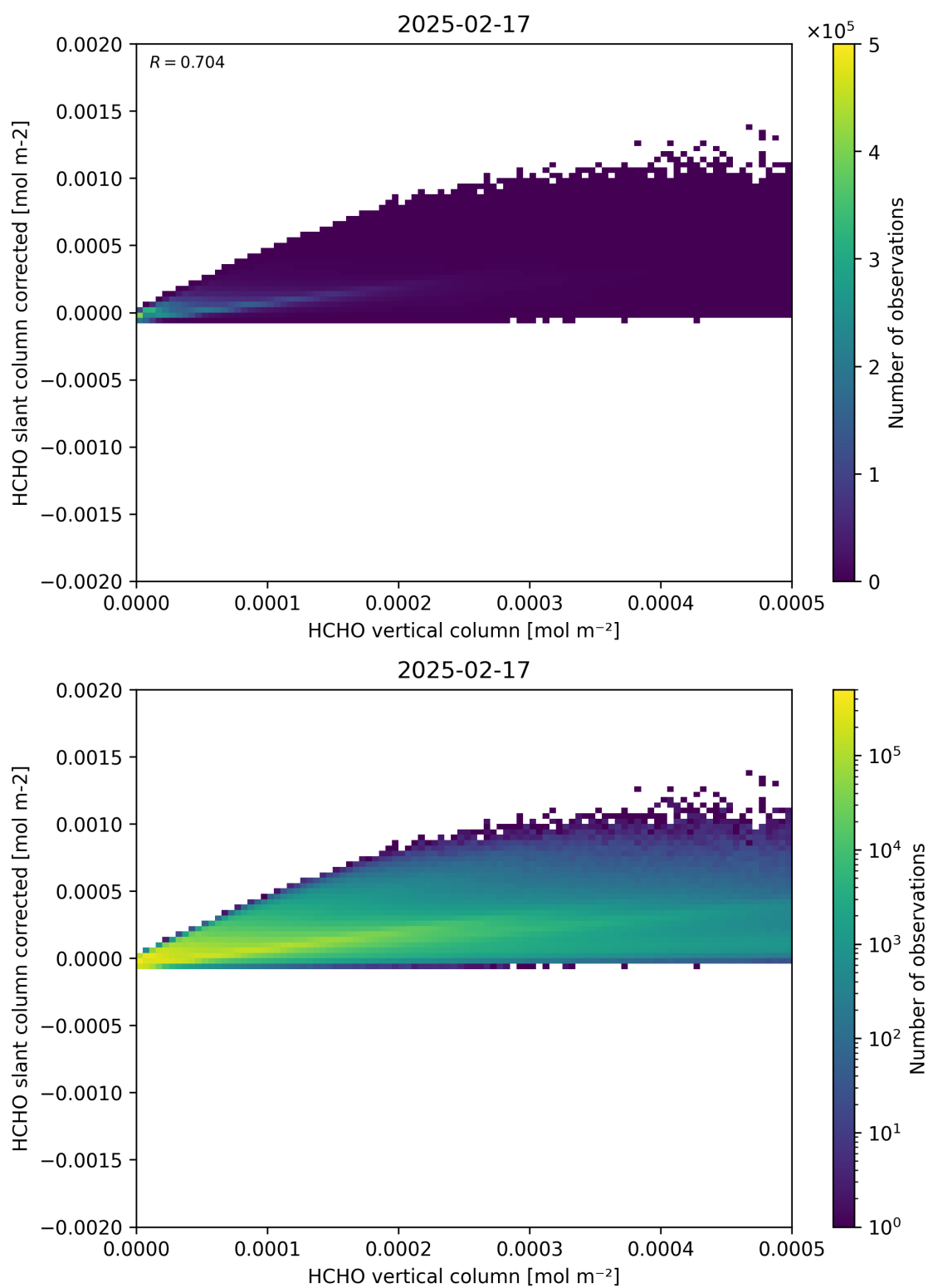
Figure 127: Scatter density plot of “HCHO vertical column” against “HCHO slant column corrected” for 2025-02-16 to 2025-02-18.
