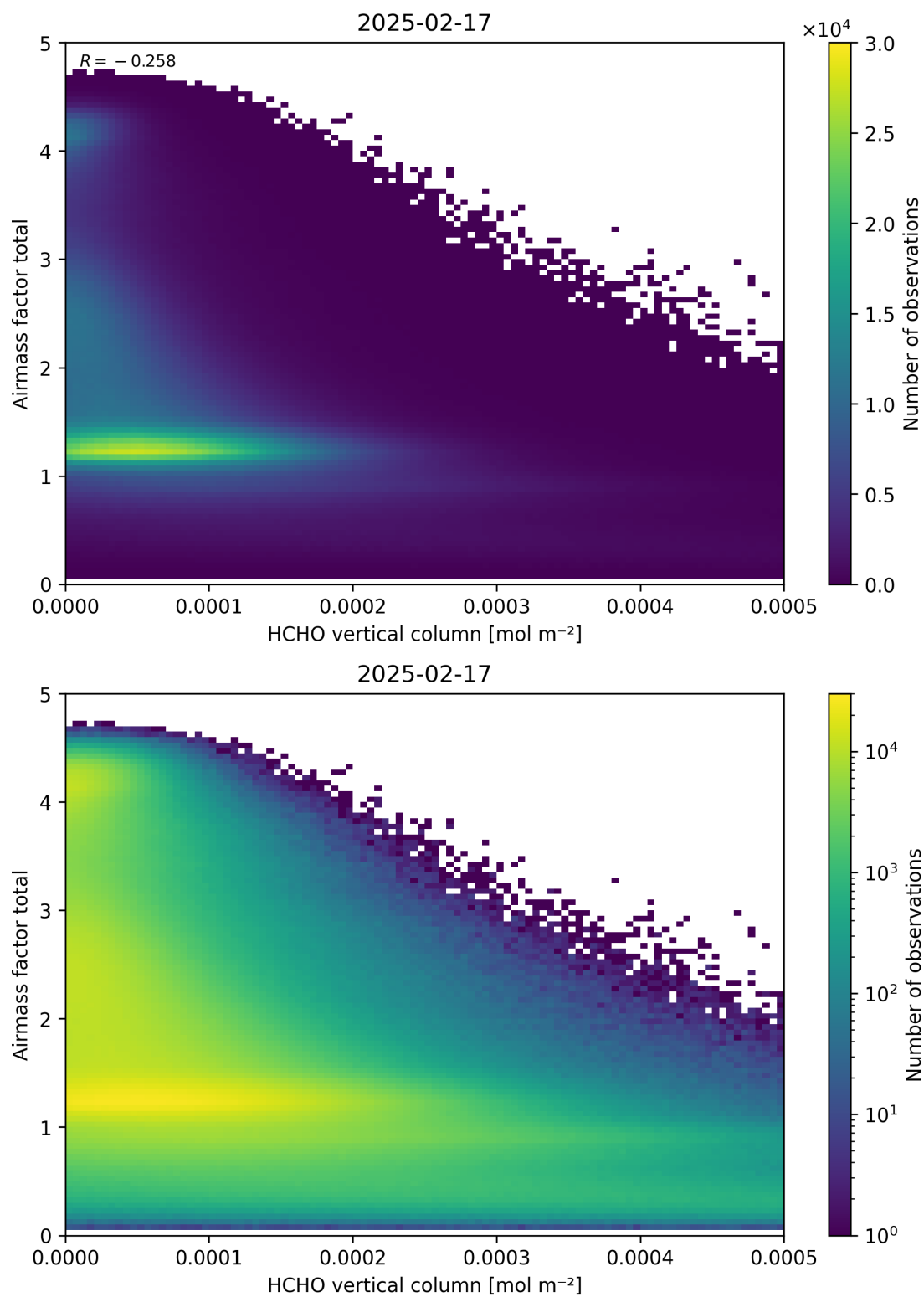
Figure 131: Scatter density plot of “HCHO vertical column” against “Airmass factor total” for 2025-02-16 to 2025-02-18.
