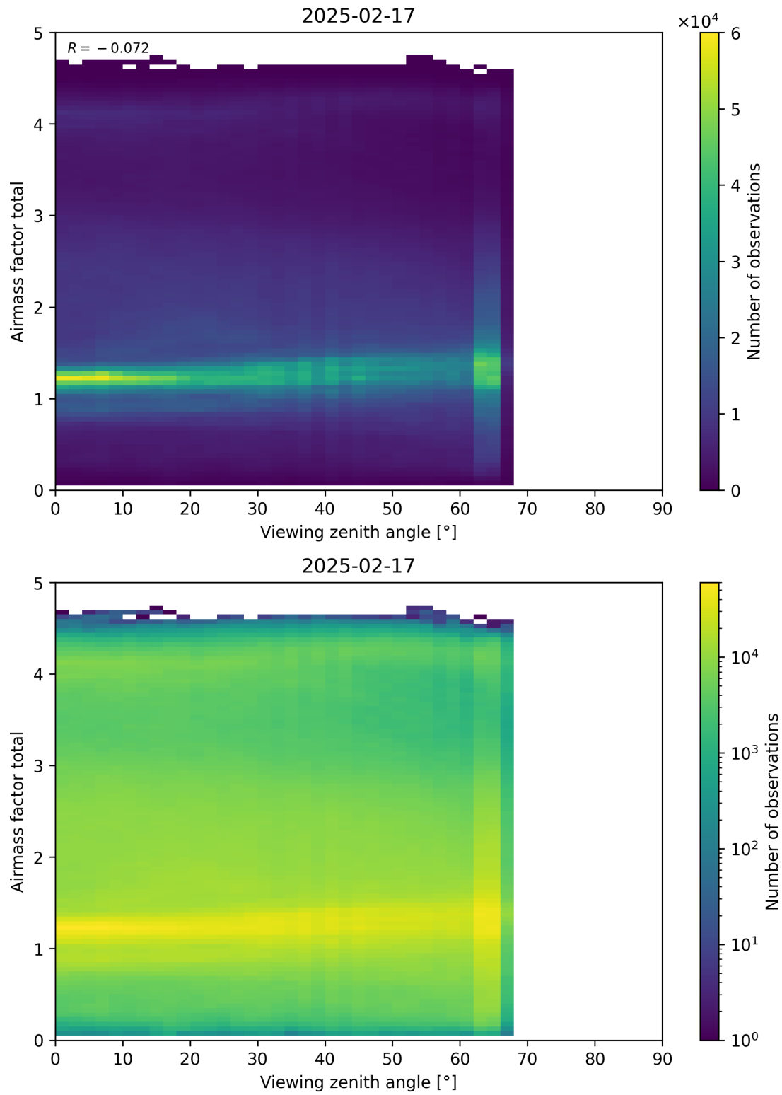
Figure 190: Scatter density plot of “Viewing zenith angle” against “Airmass factor total” for 2025-02-16 to 2025-02-18.
