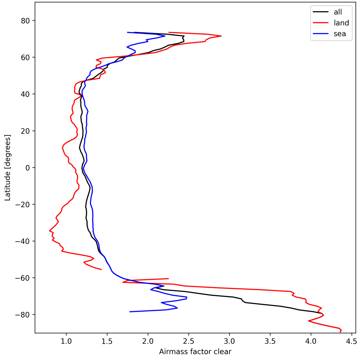
Figure 28: Zonal average of “Airmass factor clear” for 2025-02-16 to 2025-02-18.
