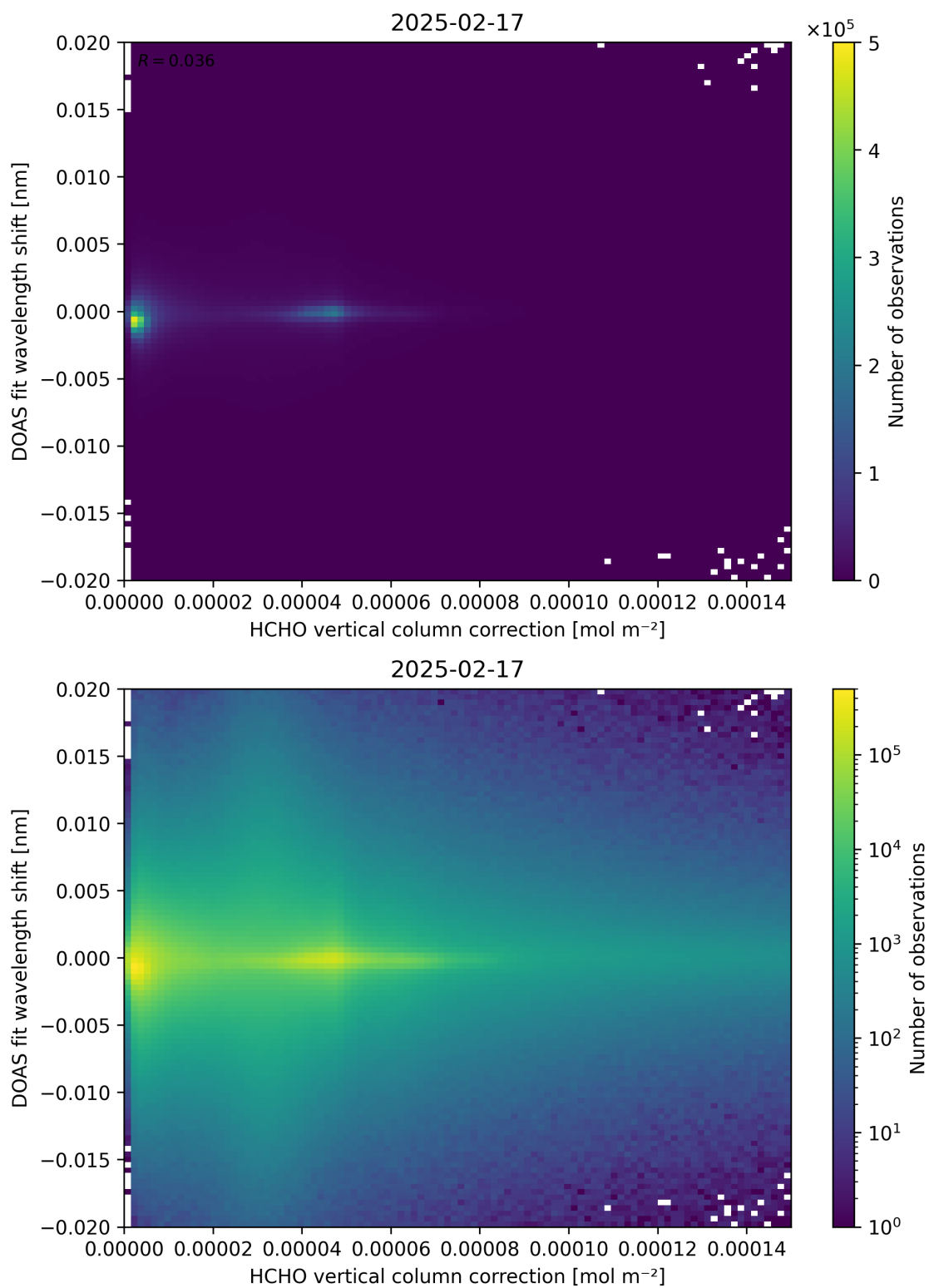
Figure 113: Scatter density plot of “HCHO vertical column correction” against “DOAS fit wavelength shift” for 2025-02-16 to 2025-02-18.
