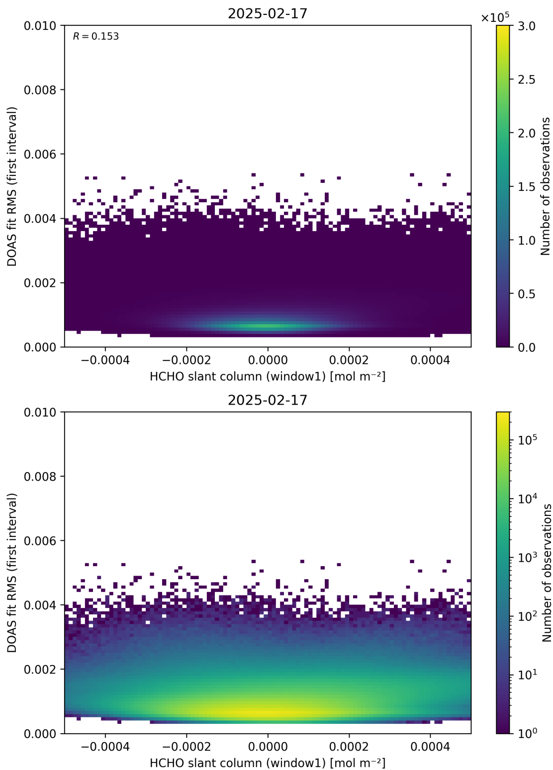
Figure 78: Scatter density plot of “HCHO slant column (window1)” against “DOAS fit RMS (first interval)” for 2025-02-16 to 2025-02-18.
