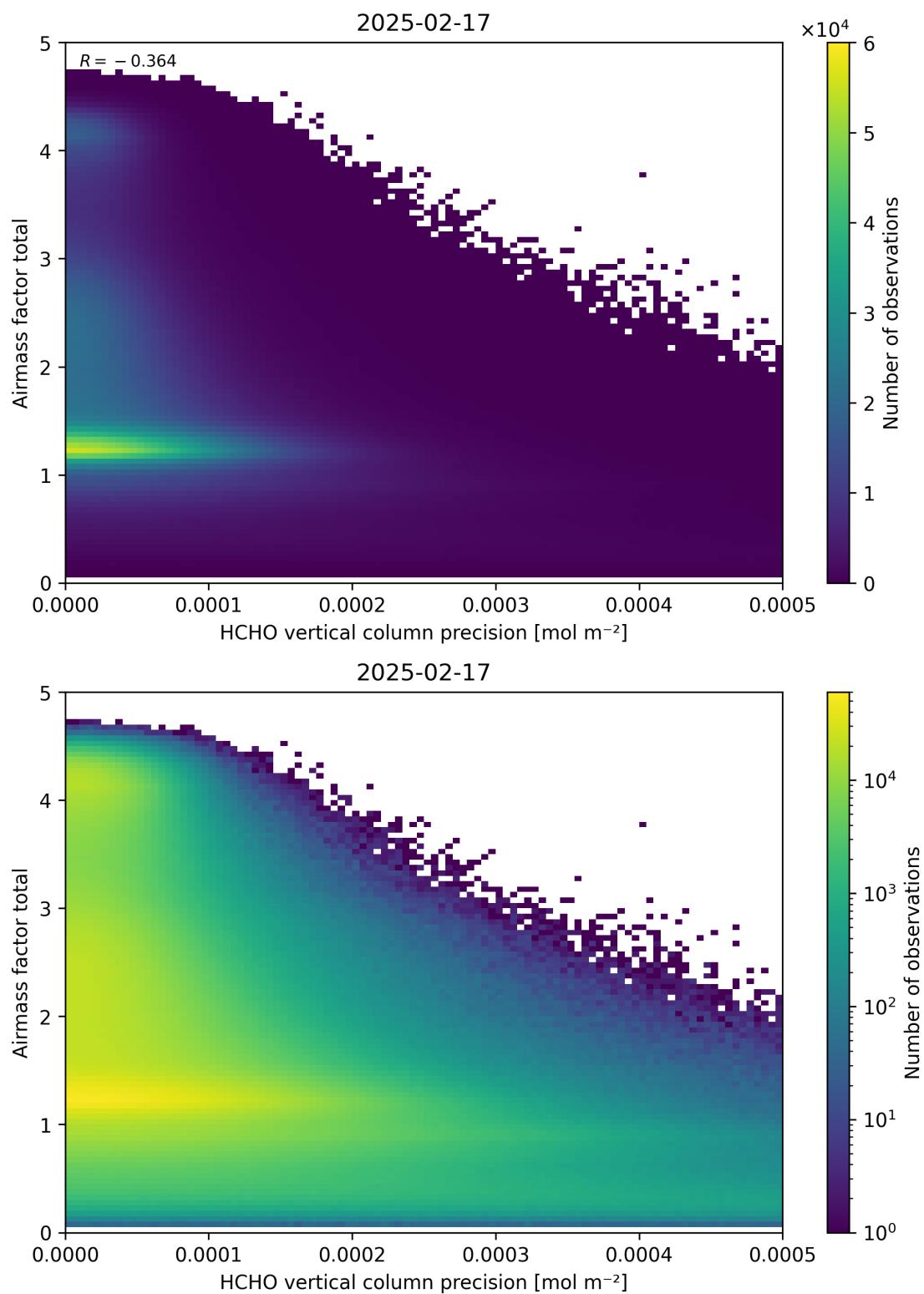
Figure 144: Scatter density plot of “HCHO vertical column precision” against “Airmass factor total” for 2025-02-16 to 2025-02-18.
