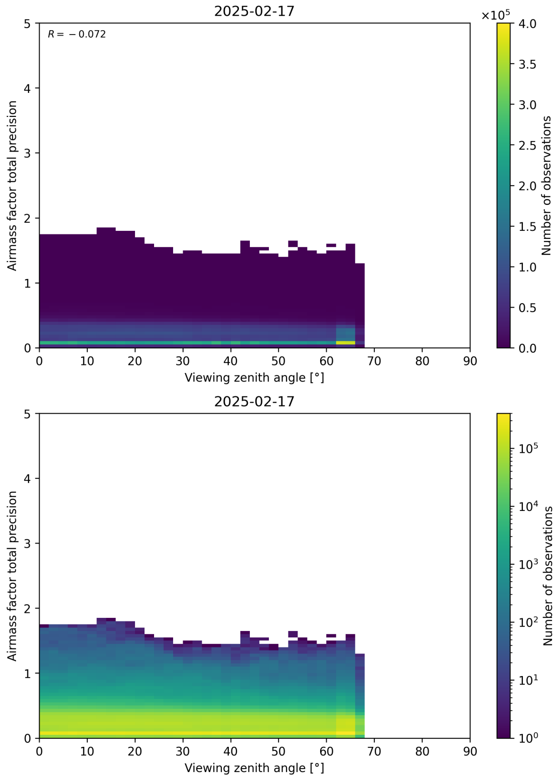
Figure 191: Scatter density plot of “Viewing zenith angle” against “Airmass factor total precision” for 2025-02-16 to 2025-02-18.
