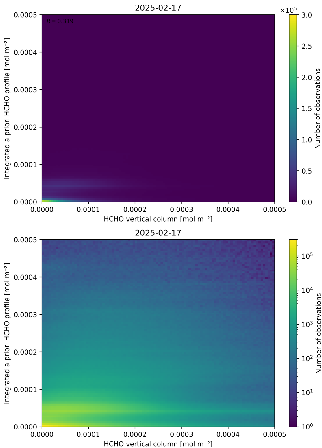
Figure 135: Scatter density plot of “HCHO vertical column” against “Integrated a priori HCHO profile” for 2025-02-16 to 2025-02-18.
