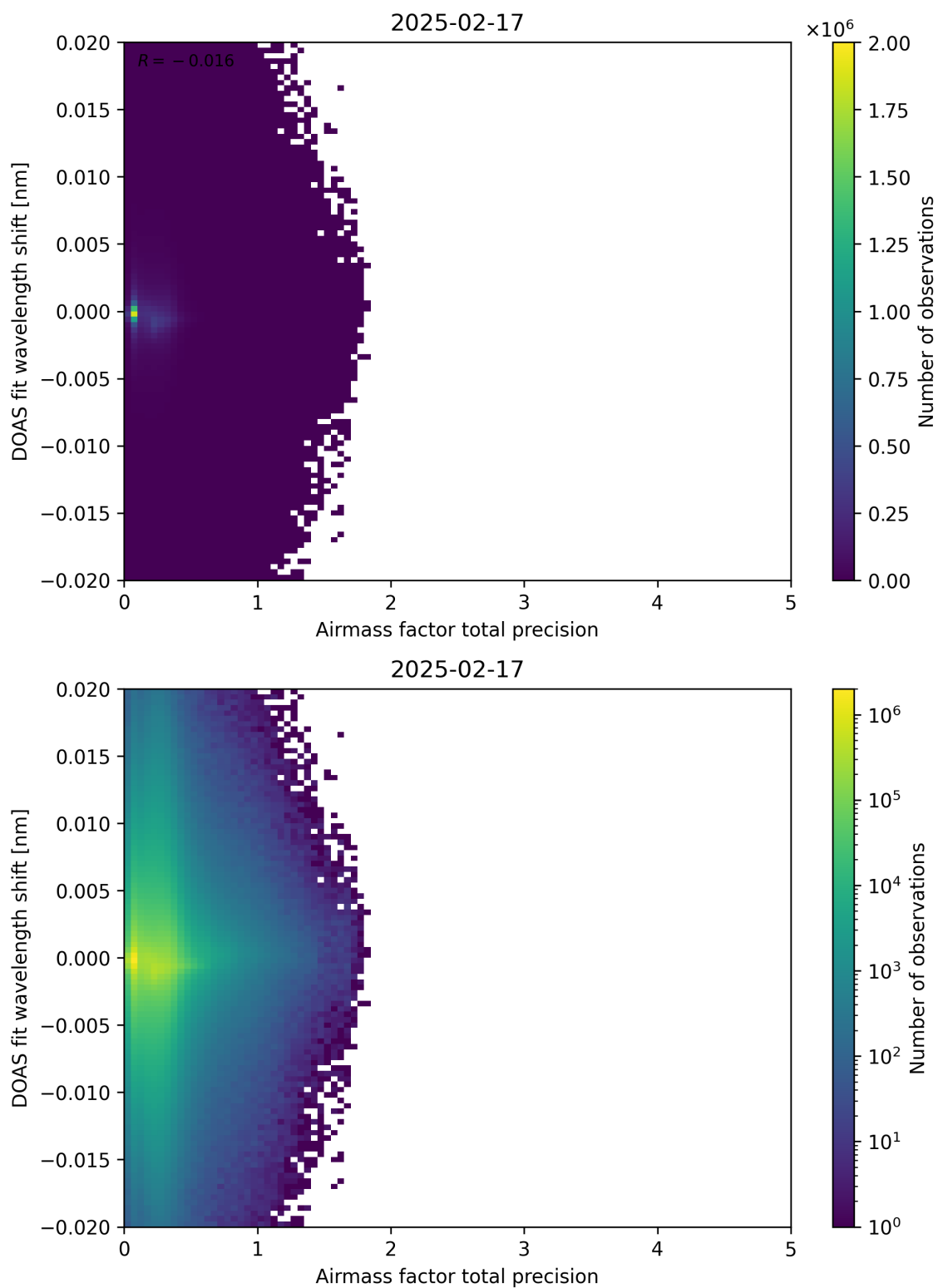
Figure 106: Scatter density plot of “Airmass factor total precision” against “DOAS fit wavelength shift” for 2025-02-16 to 2025-02-18.
