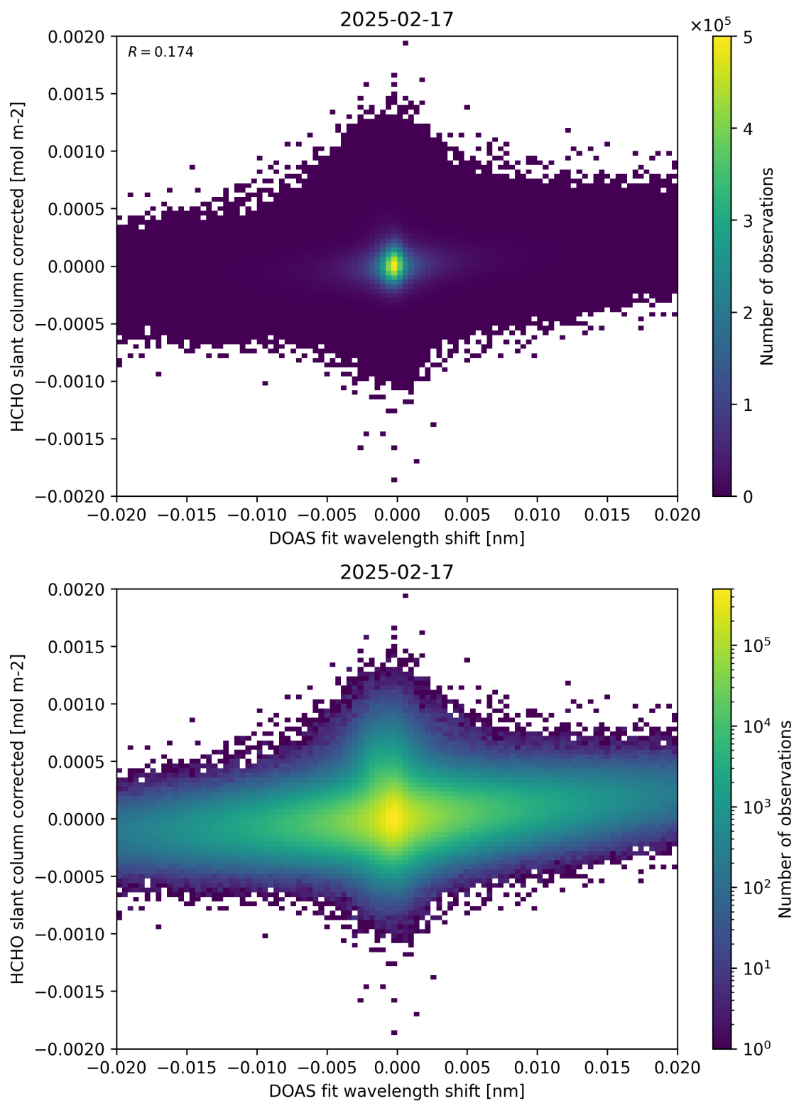
Figure 66: Scatter density plot of “DOAS fit wavelength shift” against “HCHO slant column corrected” for 2025-02-16 to 2025-02-18.
