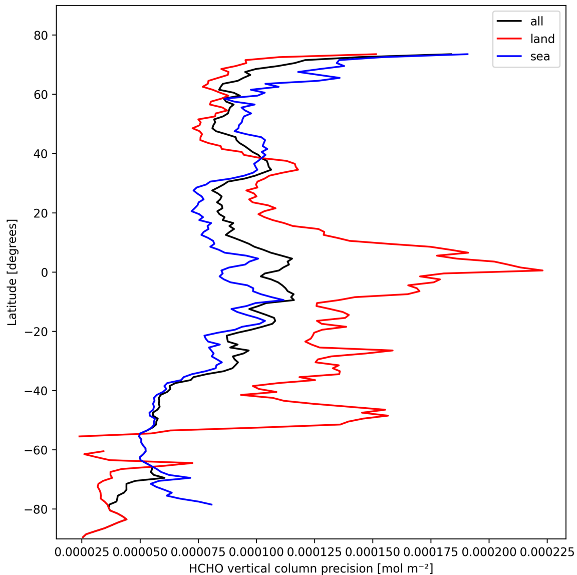
Figure 22: Zonal average of “HCHO vertical column precision” for 2025-02-16 to 2025-02-18.
