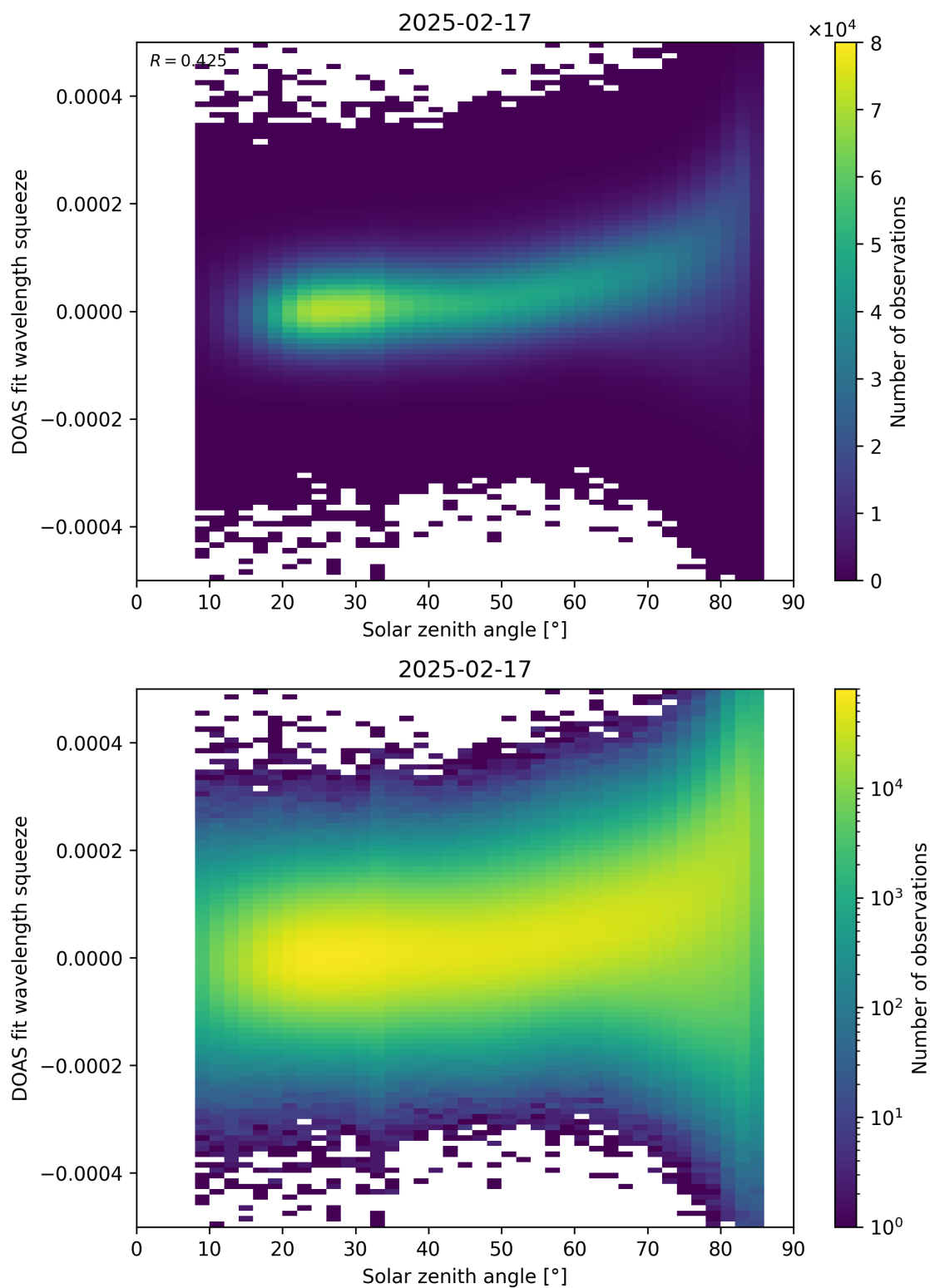
Figure 169: Scatter density plot of “Solar zenith angle” against “DOAS fit wavelength squeeze” for 2025-02-16 to 2025-02-18.
