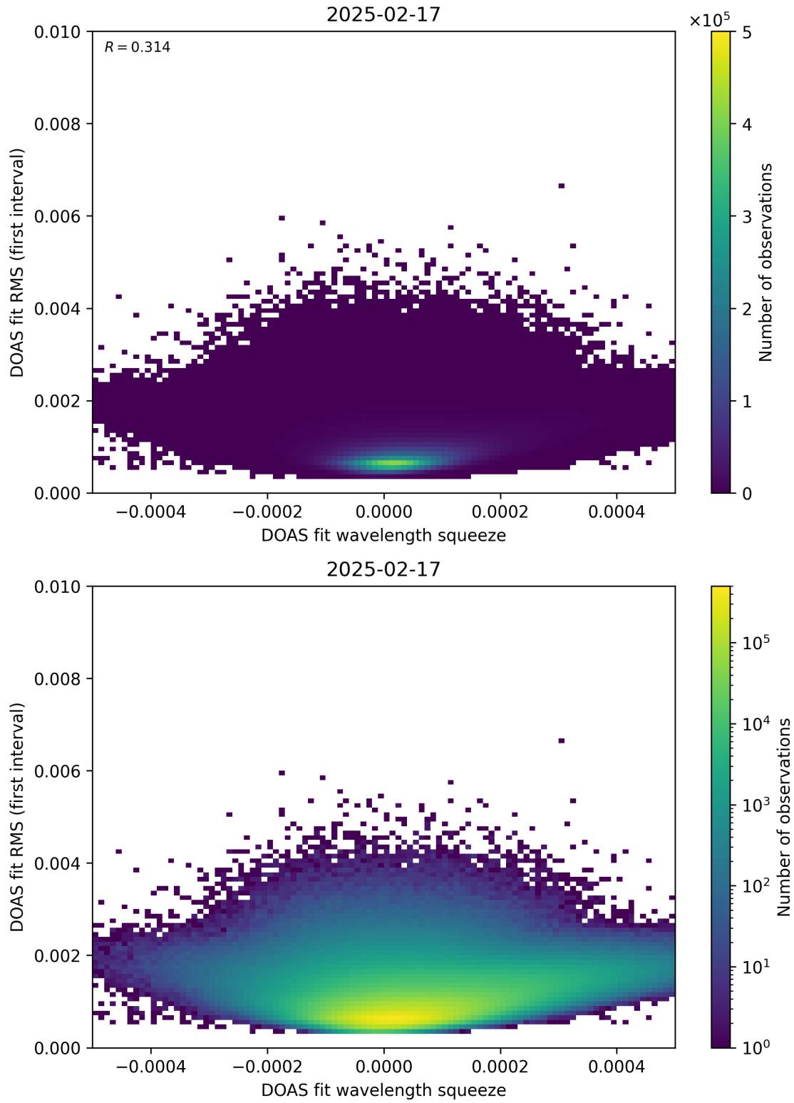
Figure 68: Scatter density plot of “DOAS fit wavelength squeeze” against “DOAS fit RMS (first interval)” for 2025-02-16 to 2025-02-18.
