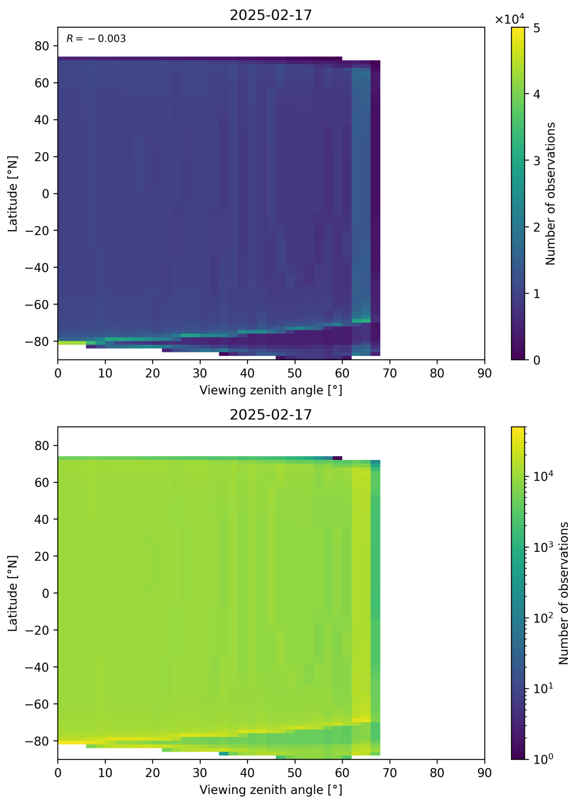
Figure 196: Scatter density plot of “Viewing zenith angle” against “Latitude” for 2025-02-16 to 2025-02-18.
