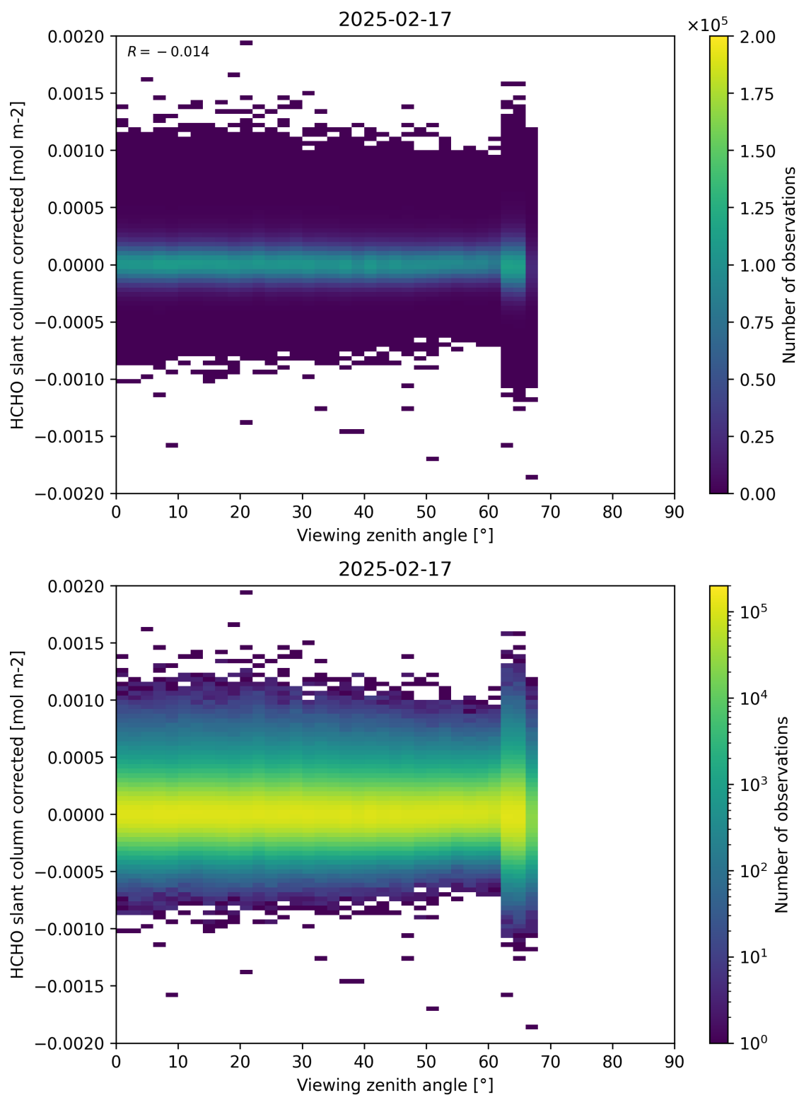
Figure 186: Scatter density plot of “Viewing zenith angle” against “HCHO slant column corrected” for 2025-02-16 to 2025-02-18.
