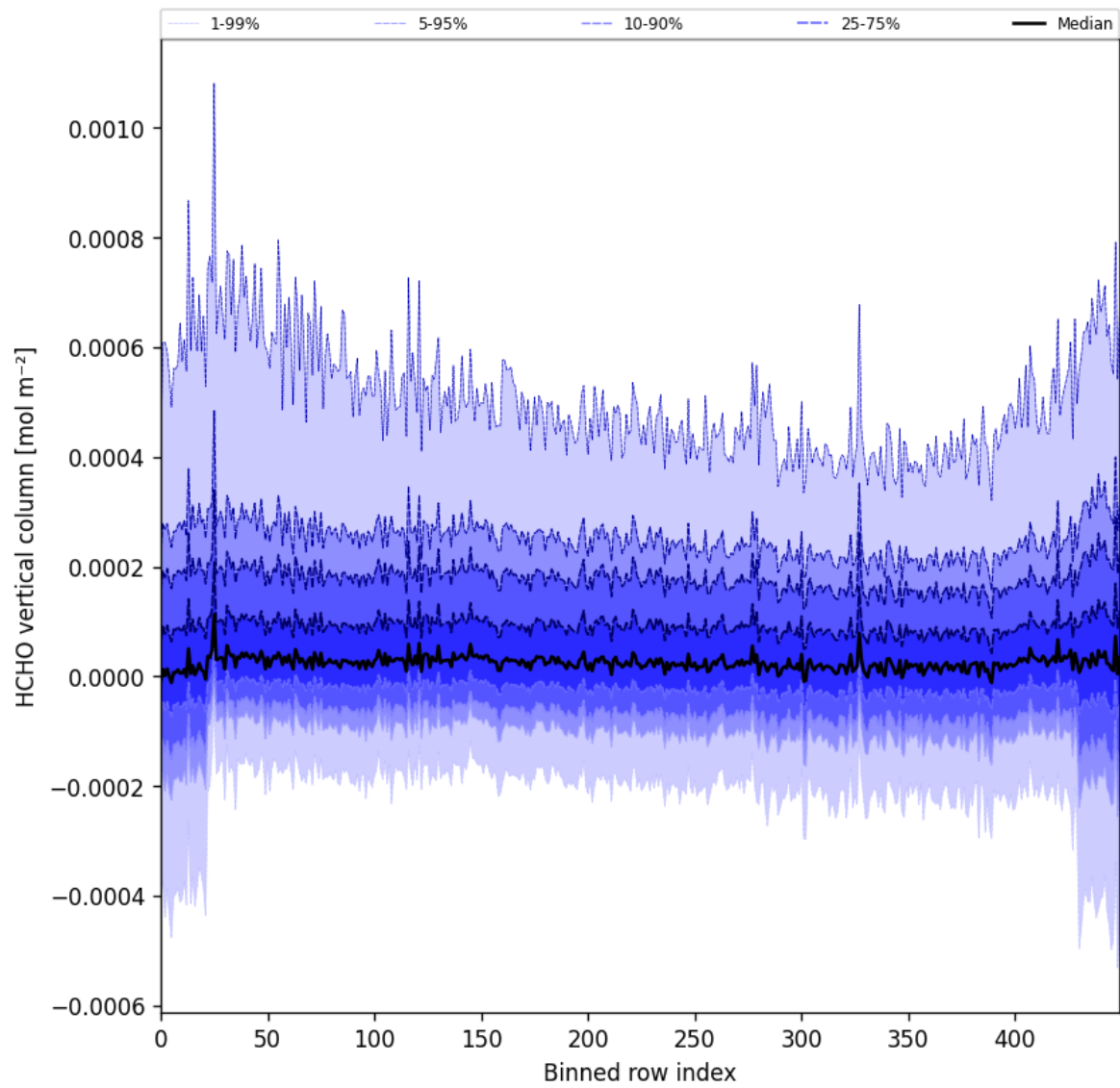
Figure 49: Along track statistics of “HCHO vertical column” for 2025-02-16 to 2025-02-18
