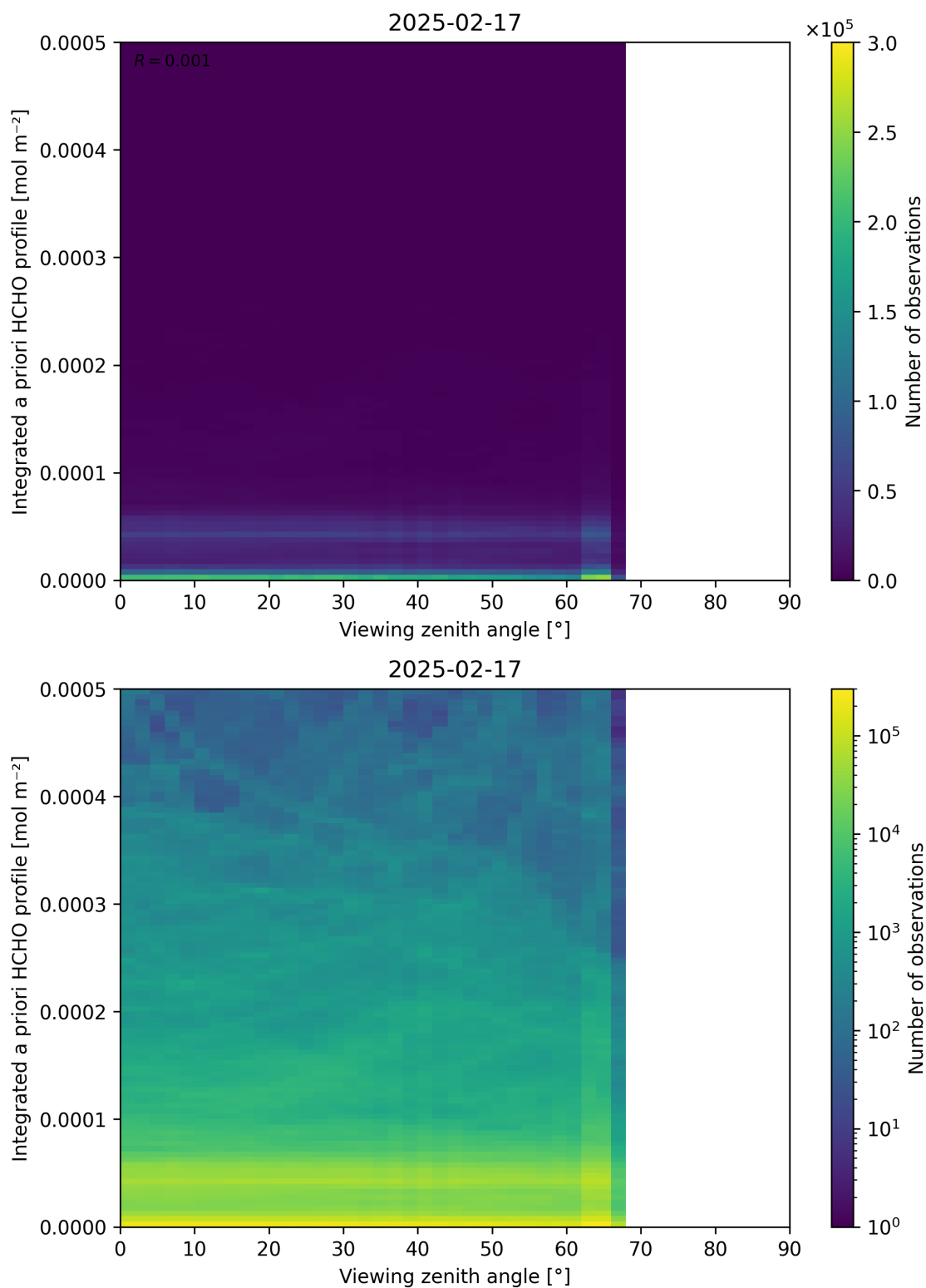
Figure 195: Scatter density plot of “Viewing zenith angle” against “Integrated a priori HCHO profile” for 2025-02-16 to 2025-02-18.
