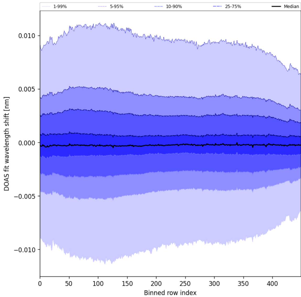
Figure 58: Along track statistics of “DOAS fit wavelength shift” for 2025-02-16 to 2025-02-18
