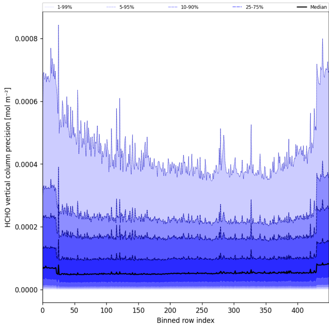
Figure 50: Along track statistics of “HCHO vertical column precision” for 2025-02-16 to 2025-02-18
