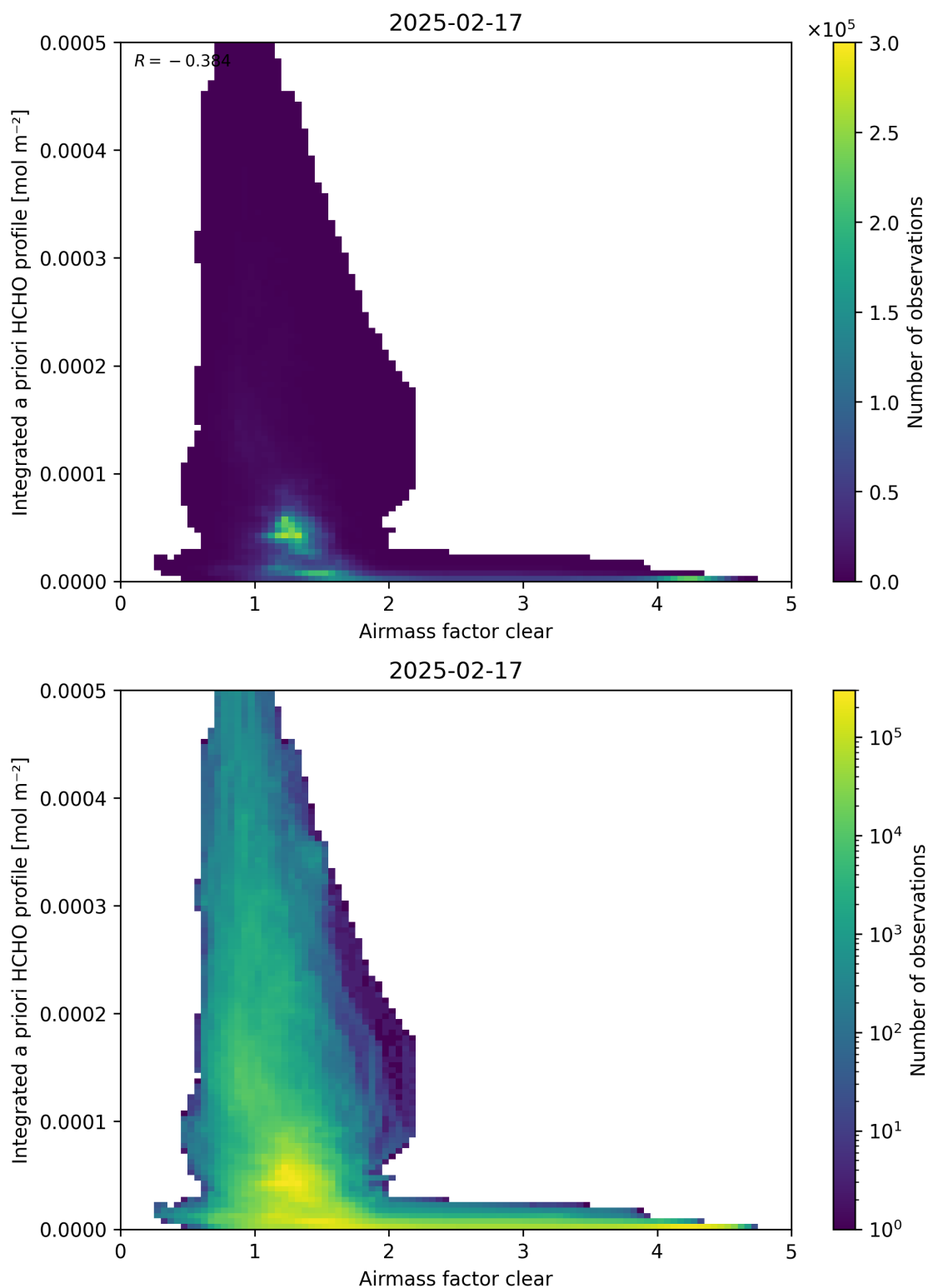
Figure 76: Scatter density plot of “Airmass factor clear” against “Integrated a priori HCHO profile” for 2025-02-16 to 2025-02-18.
