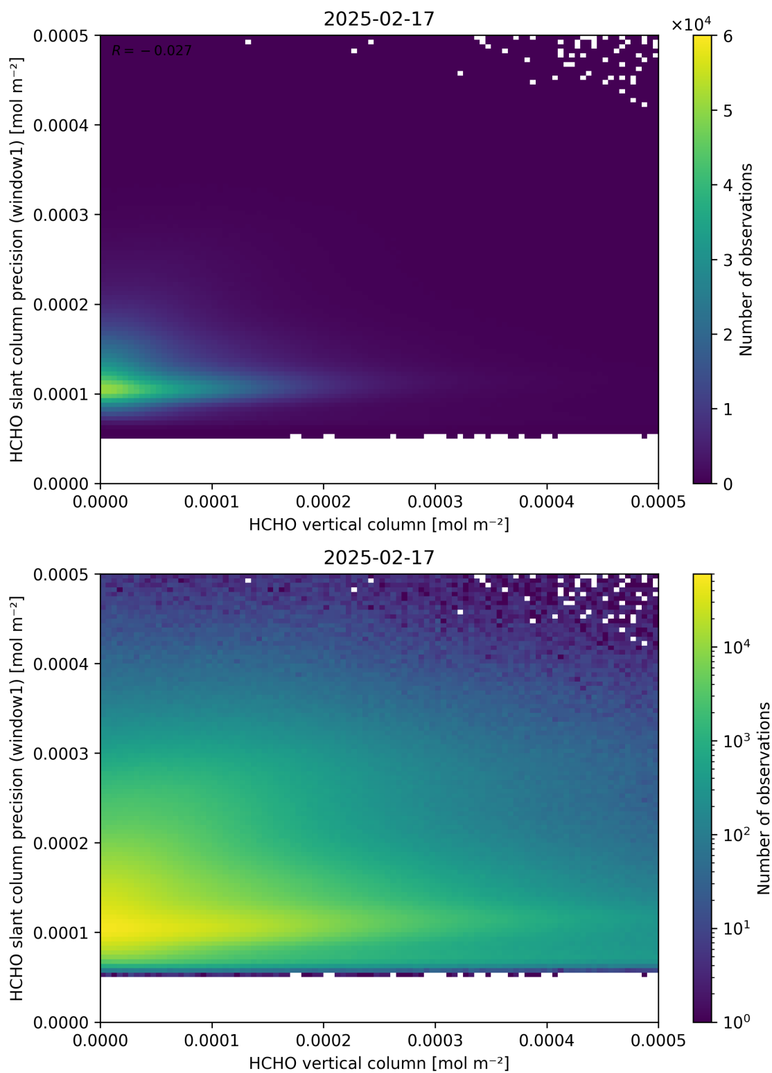
Figure 130: Scatter density plot of “HCHO vertical column” against “HCHO slant column precision (window1)” for 2025-02-16 to 2025-02-18.
