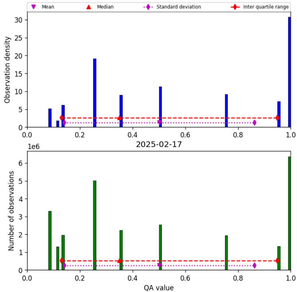
Figure 34: Histogram of “QA value” for 2025-02-16 to 2025-02-18
