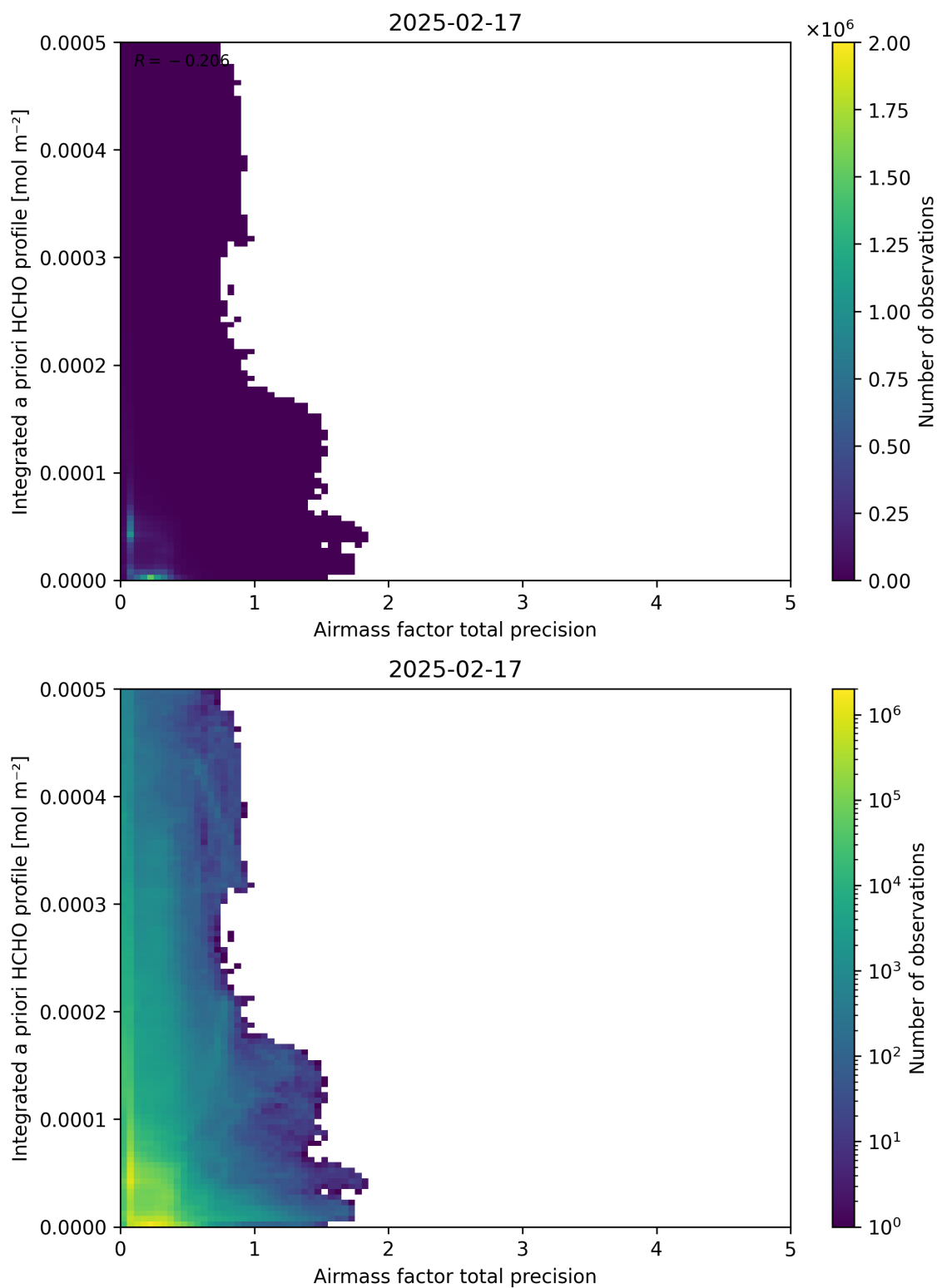
Figure 111: Scatter density plot of “Airmass factor total precision” against “Integrated a priori HCHO profile” for 2025-02-16 to 2025-02-18.
