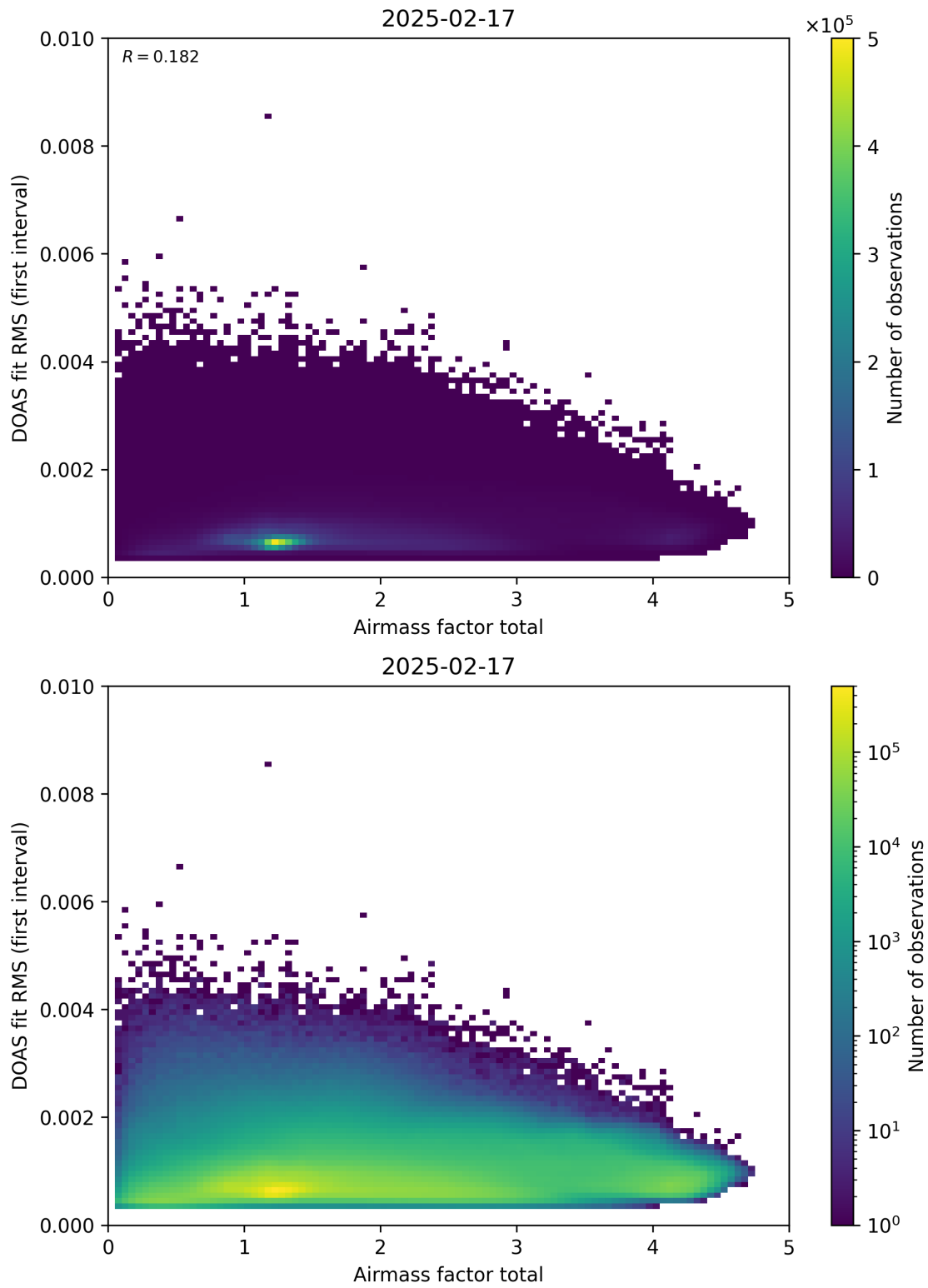
Figure 97: Scatter density plot of “Airmass factor total” against “DOAS fit RMS (first interval)” for 2025-02-16 to 2025-02-18.
