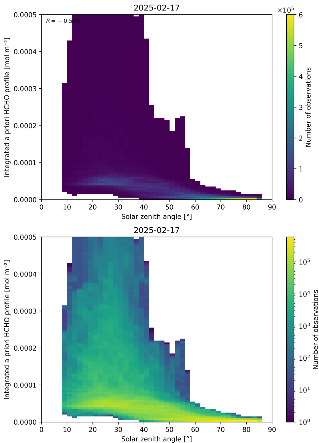
Figure 180: Scatter density plot of “Solar zenith angle” against “Integrated a priori HCHO profile” for 2025-02-16 to 2025-02-18.
