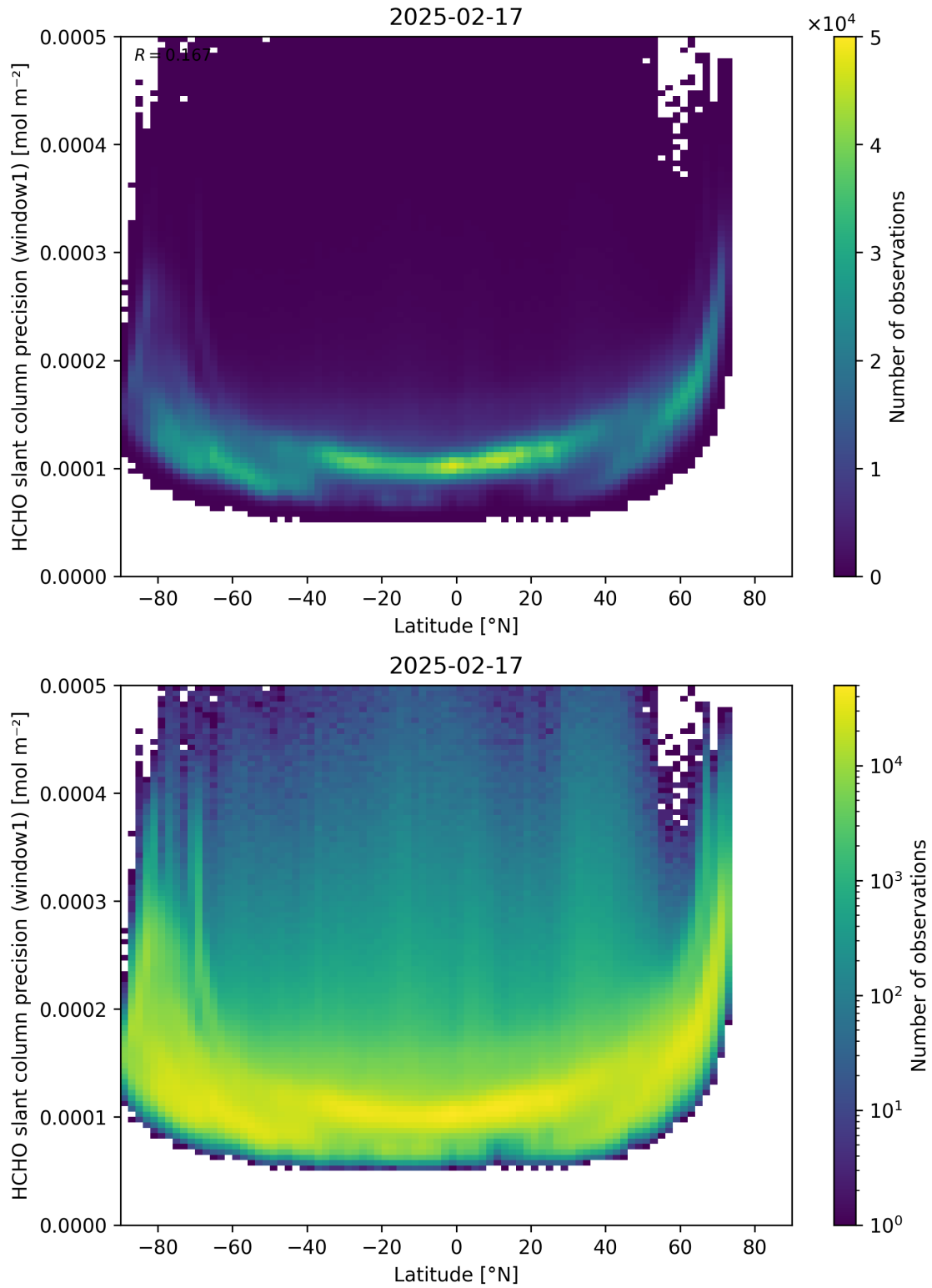
Figure 160: Scatter density plot of “Latitude” against “HCHO slant column precision (window1)” for 2025-02-16 to 2025-02-18.
