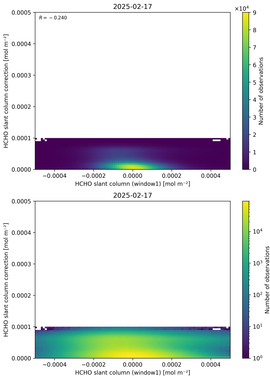
Figure 83: Scatter density plot of “HCHO slant column (window1)” against “HCHO slant column correction” for 2025-02-16 to 2025-02-18.
