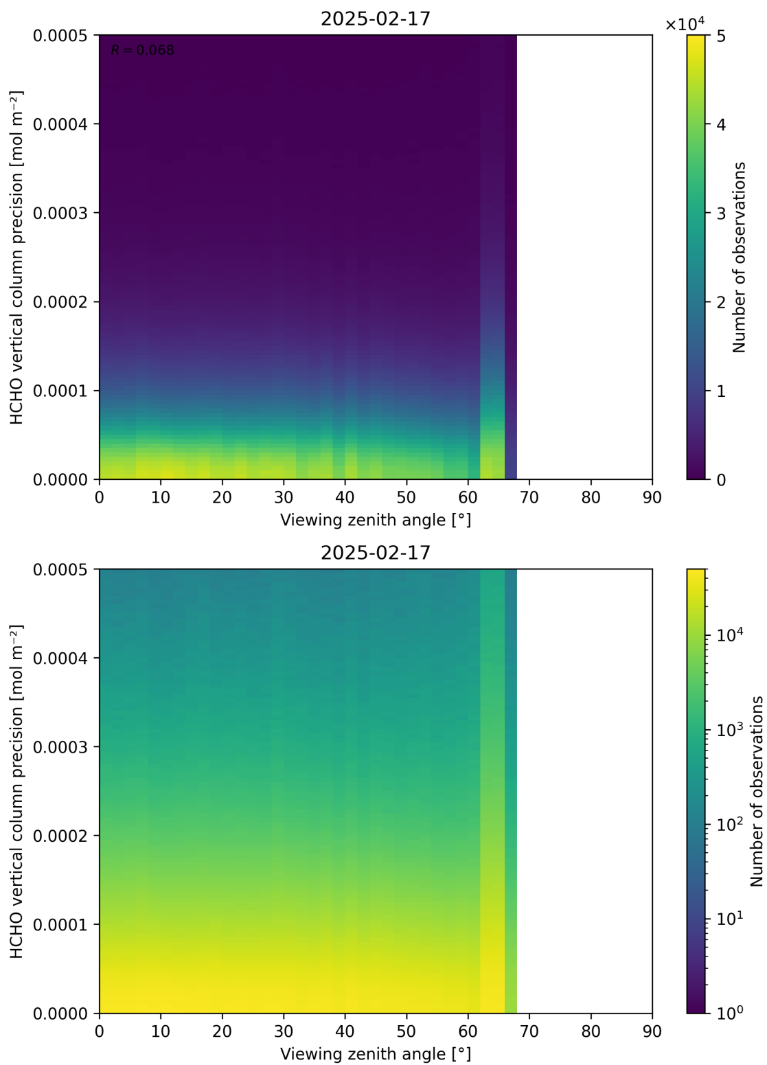
Figure 194: Scatter density plot of “Viewing zenith angle” against “HCHO vertical column precision” for 2025-02-16 to 2025-02-18.
