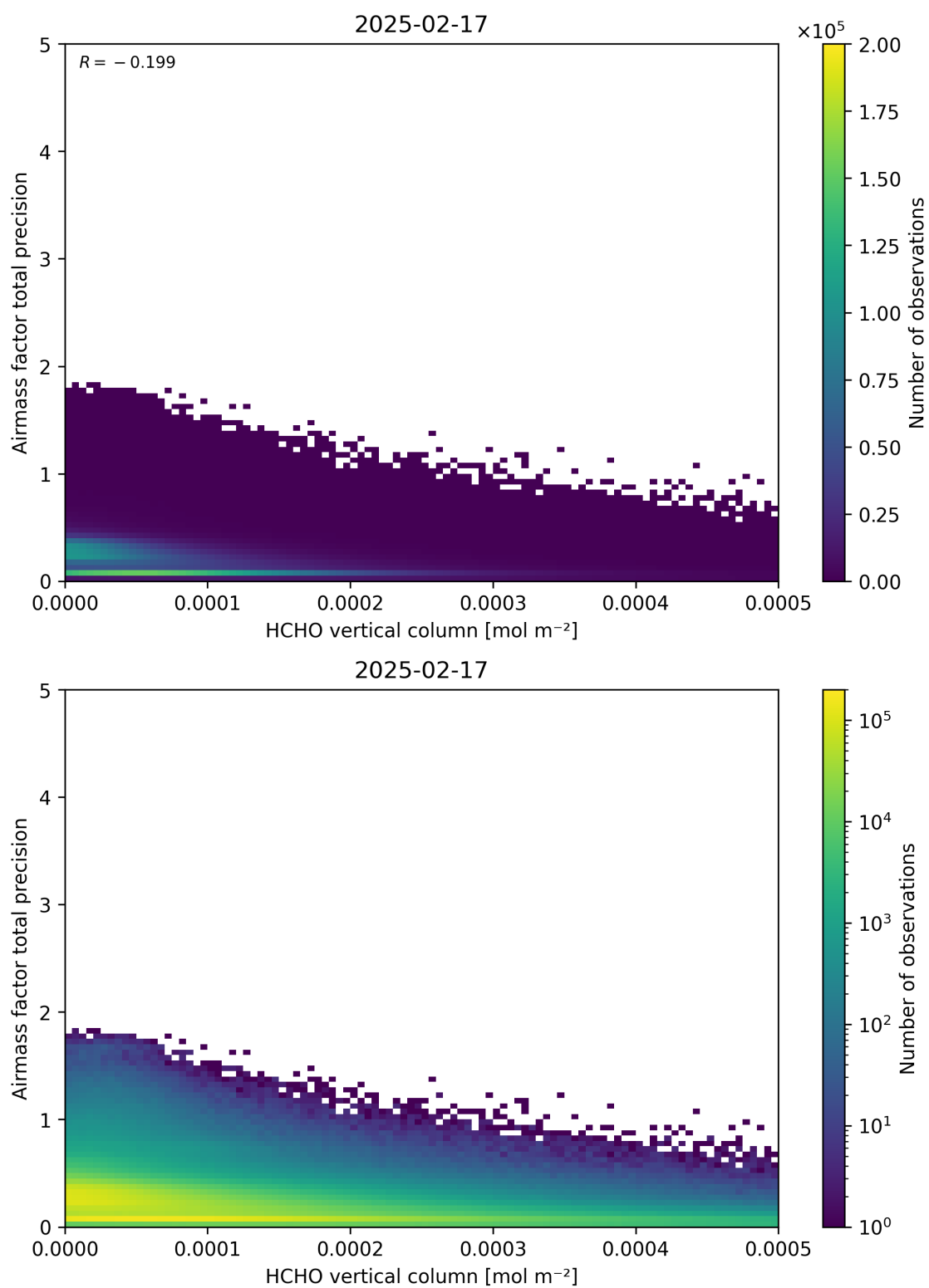
Figure 132: Scatter density plot of “HCHO vertical column” against “Airmass factor total precision” for 2025-02-16 to 2025-02-18.
