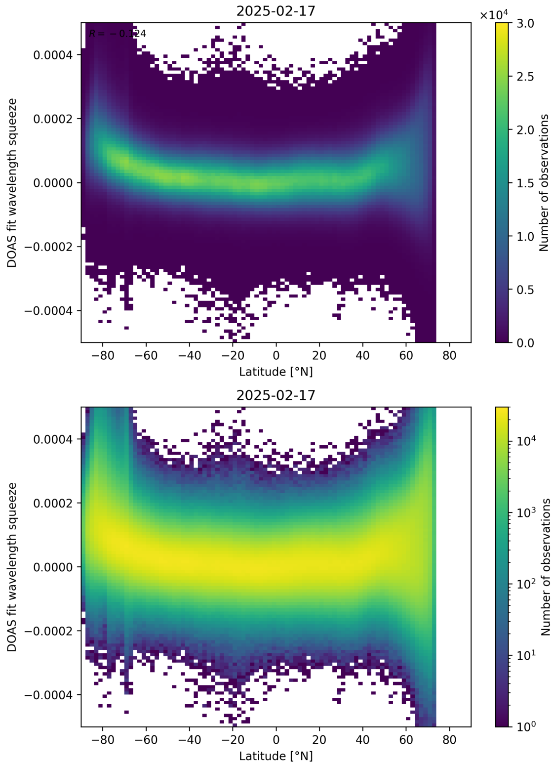
Figure 155: Scatter density plot of “Latitude” against “DOAS fit wavelength squeeze” for 2025-02-16 to 2025-02-18.
