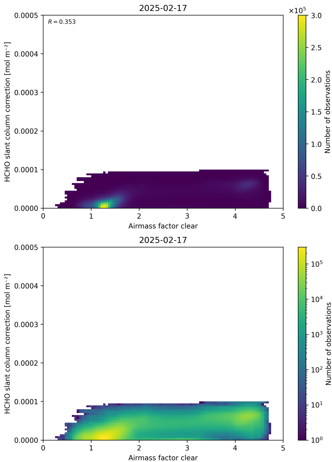
Figure 75: Scatter density plot of “Airmass factor clear” against “HCHO slant column correction” for 2025-02-16 to 2025-02-18.
