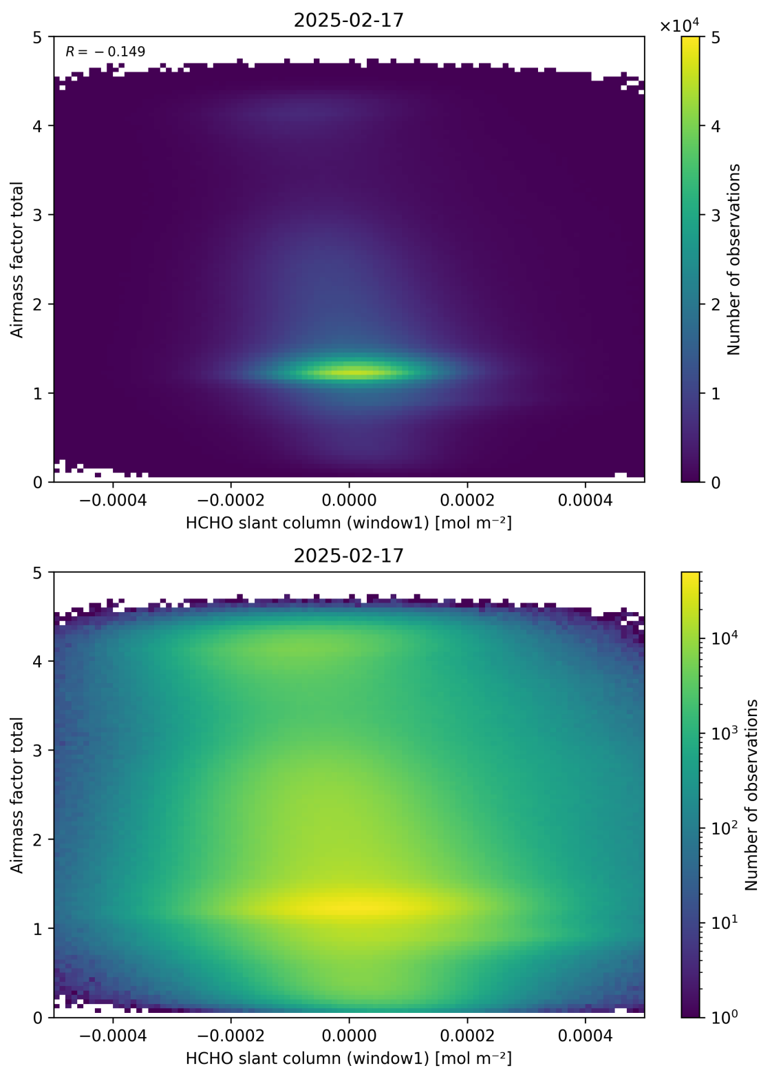
Figure 85: Scatter density plot of “HCHO slant column (window1)” against “Airmass factor total” for 2025-02-16 to 2025-02-18.
