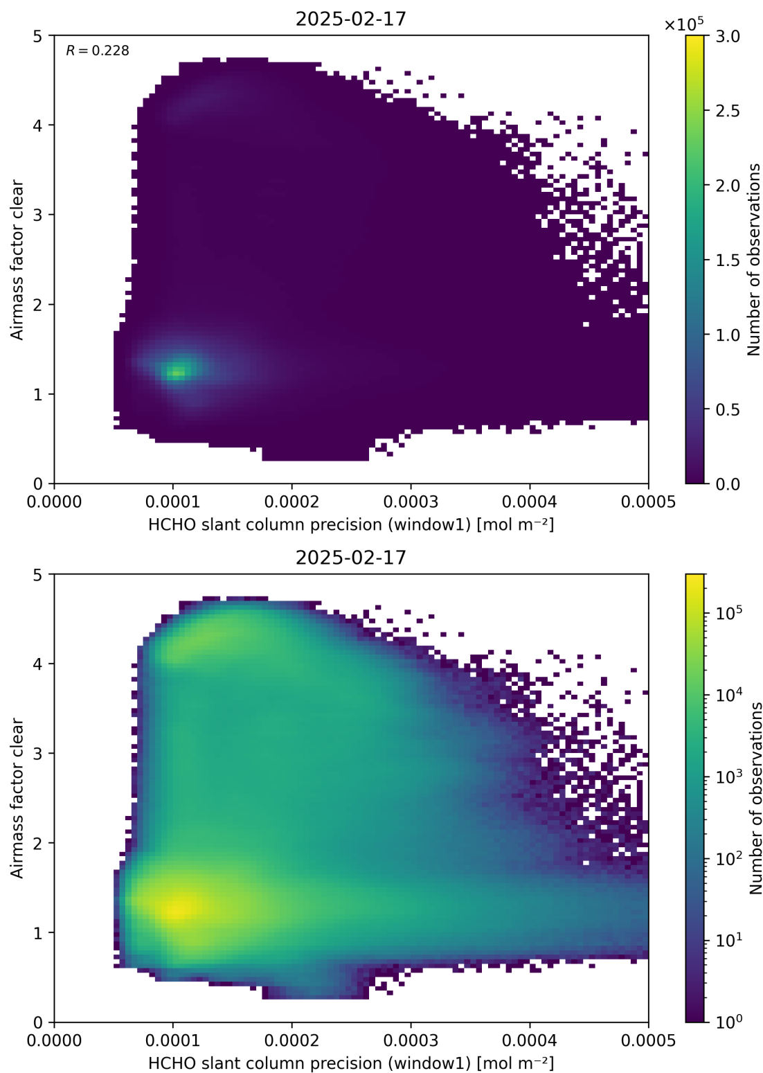
Figure 91: Scatter density plot of “HCHO slant column precision (window1)” against “Airmass factor clear” for 2025-02-16 to 2025-02-18.
