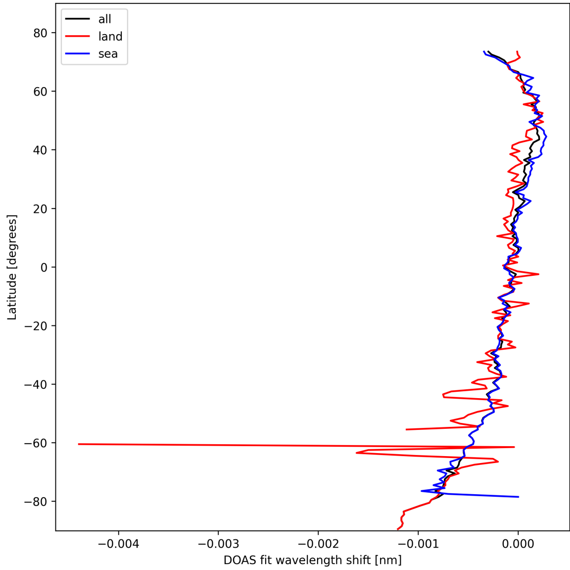
Figure 30: Zonal average of "DOAS fit wavelength shift" for 2025-02-16 to 2025-02-18.
