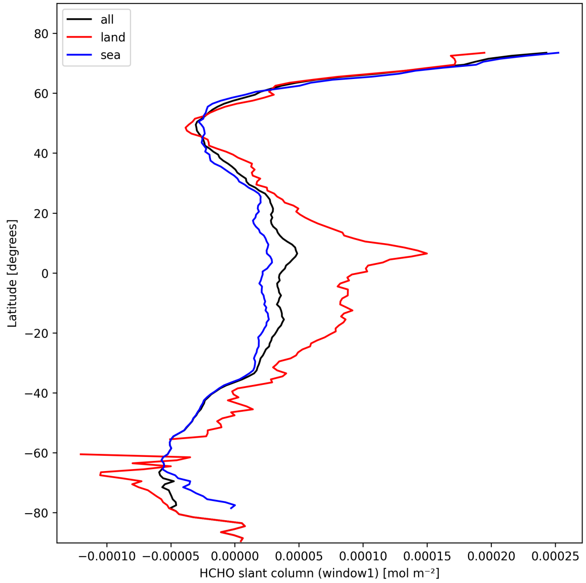
Figure 24: Zonal average of “HCHO slant column (window1)” for 2025-02-16 to 2025-02-18.
