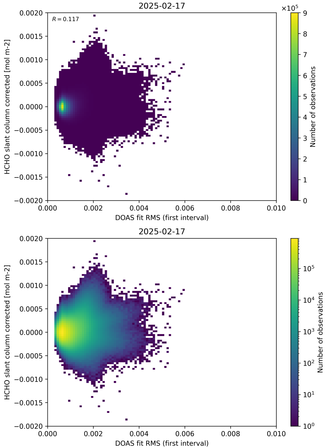
Figure 62: Scatter density plot of “DOAS fit RMS (first interval)” against “HCHO slant column corrected” for 2025-02-16 to 2025-02-18.
