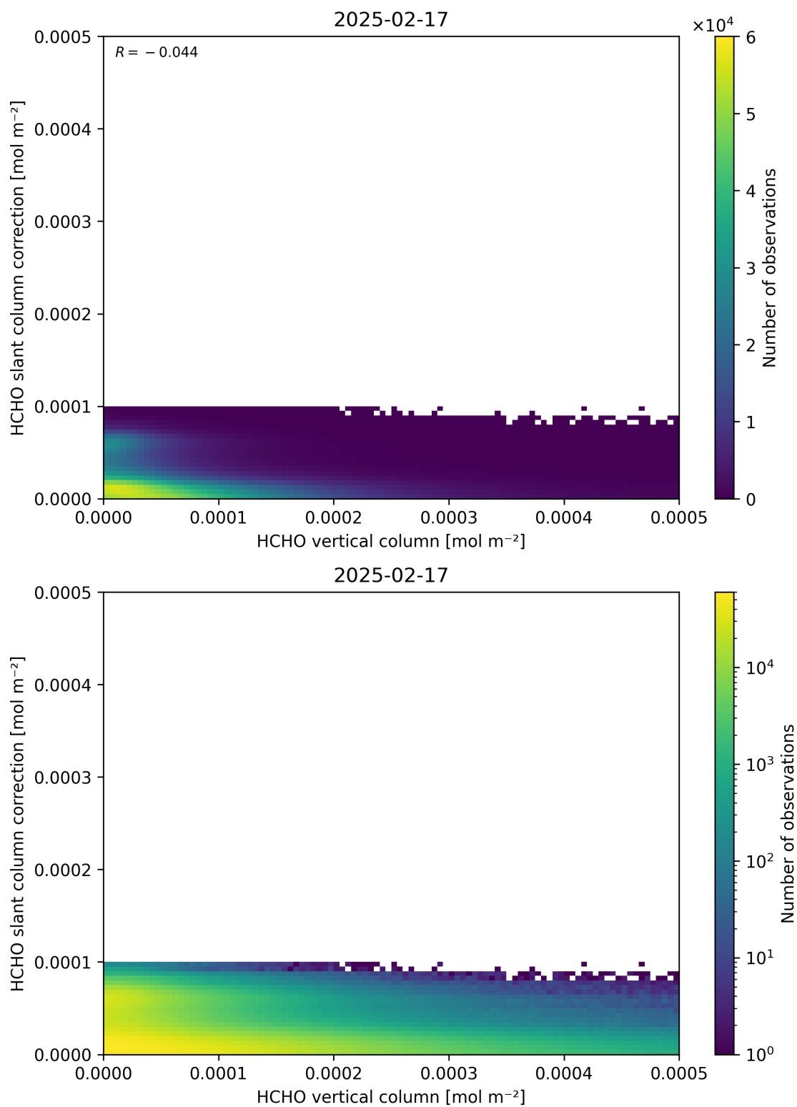
Figure 128: Scatter density plot of “HCHO vertical column” against “HCHO slant column correction” for 2025-02-16 to 2025-02-18.
