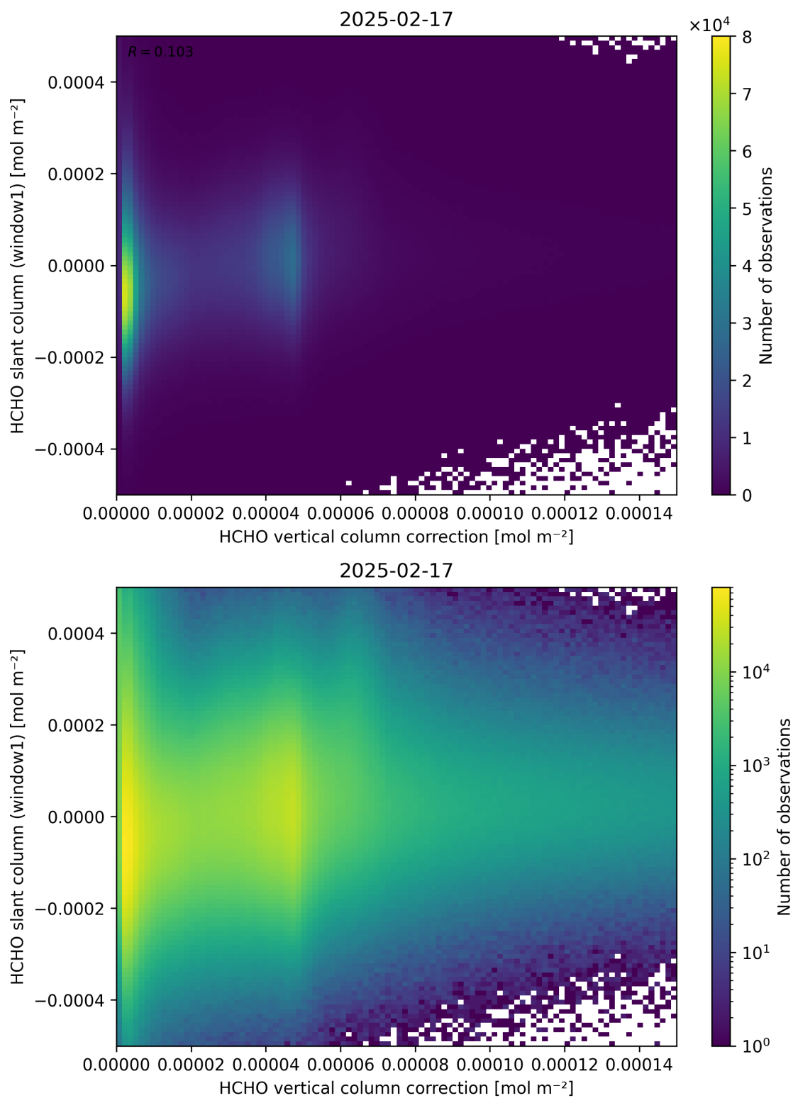
Figure 118: Scatter density plot of “HCHO vertical column correction” against “HCHO slant column (window1)” for 2025-02-16 to 2025-02-18.
