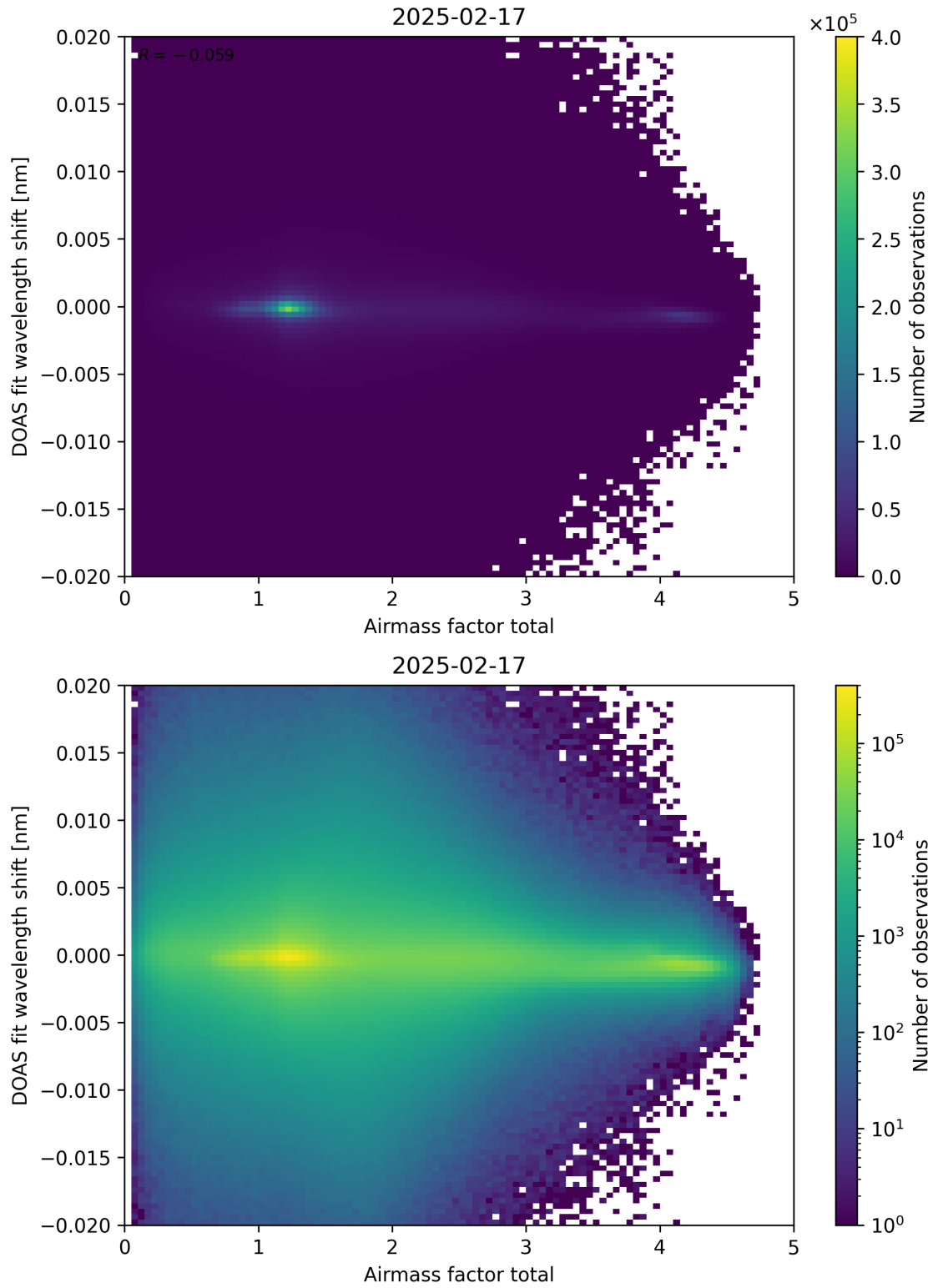
Figure 98: Scatter density plot of “Airmass factor total” against “DOAS fit wavelength shift” for 2025-02-16 to 2025-02-18.
