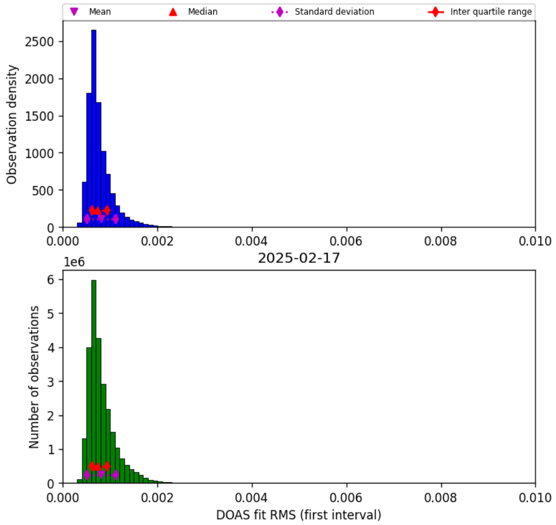
Figure 46: Histogram of “DOAS fit RMS (first interval)” for 2025-02-16 to 2025-02-18
