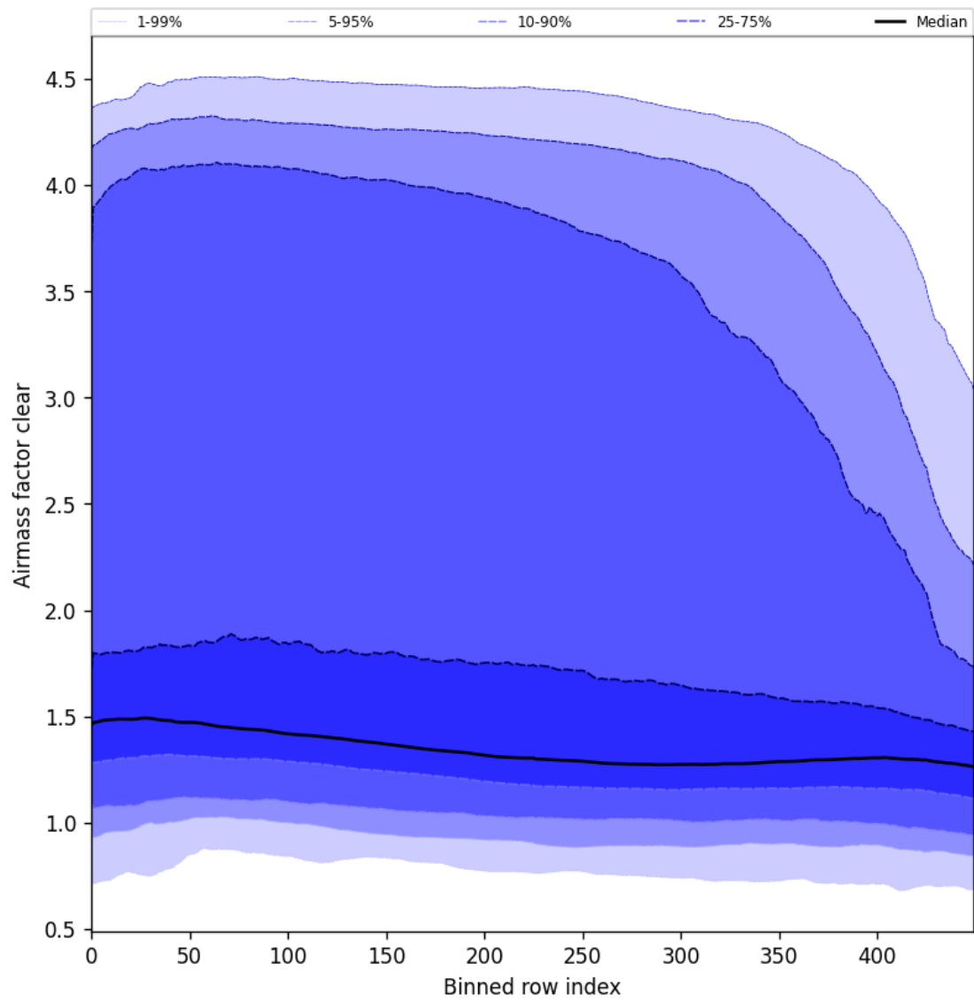
Figure 56: Along track statistics of “Airmass factor clear” for 2025-02-16 to 2025-02-18
