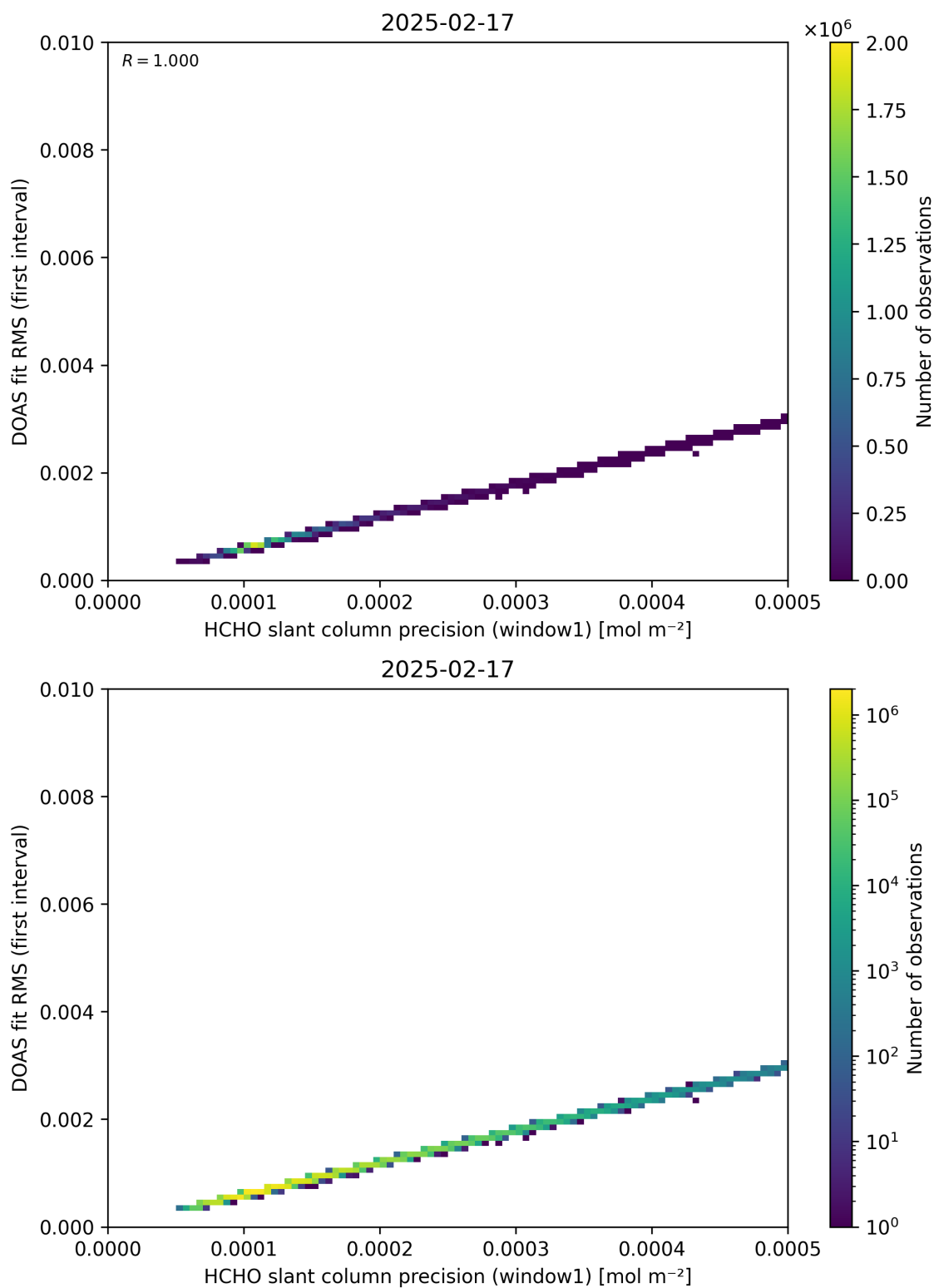
Figure 88: Scatter density plot of “HCHO slant column precision (window1)” against “DOAS fit RMS (first interval)” for 2025-02-16 to 2025-02-18.
