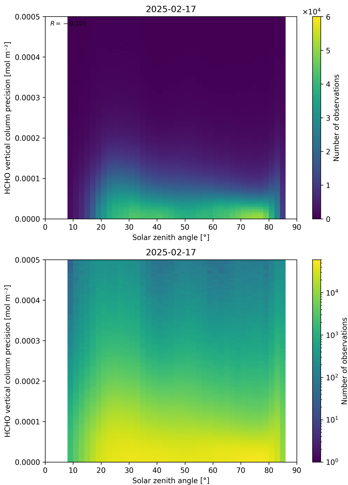
Figure 179: Scatter density plot of “Solar zenith angle” against “HCHO vertical column precision” for 2025-02-16 to 2025-02-18.
