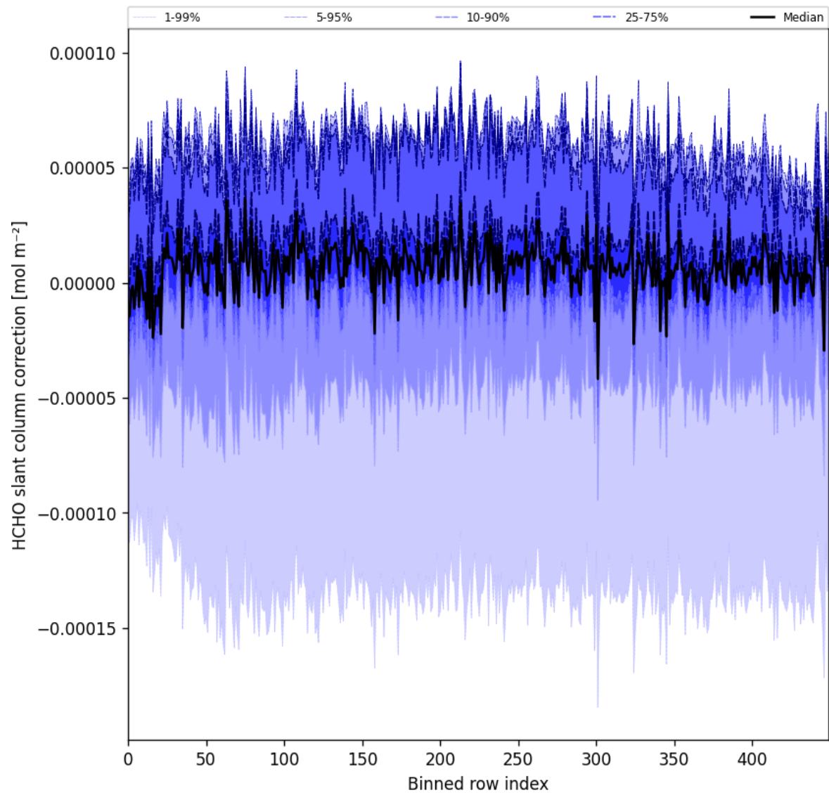
Figure 61: Along track statistics of “HCHO slant column correction” for 2025-02-16 to 2025-02-18
