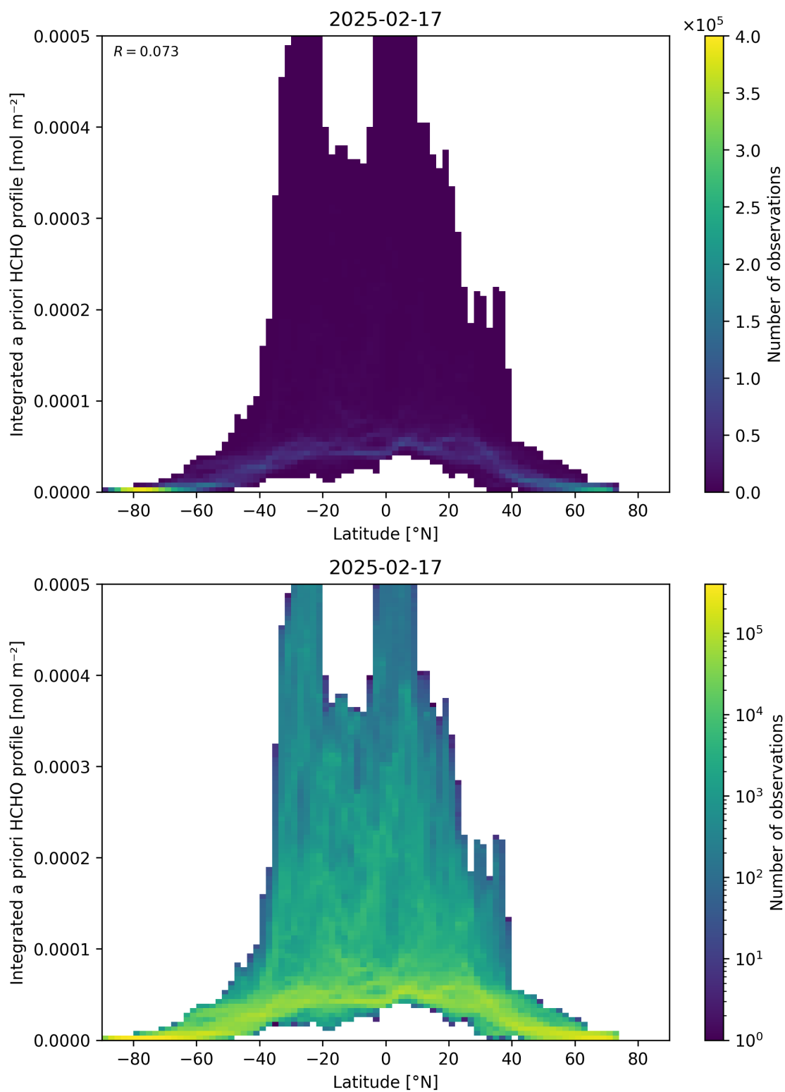
Figure 166: Scatter density plot of “Latitude” against “Integrated a priori HCHO profile” for 2025-02-16 to 2025-02-18.
