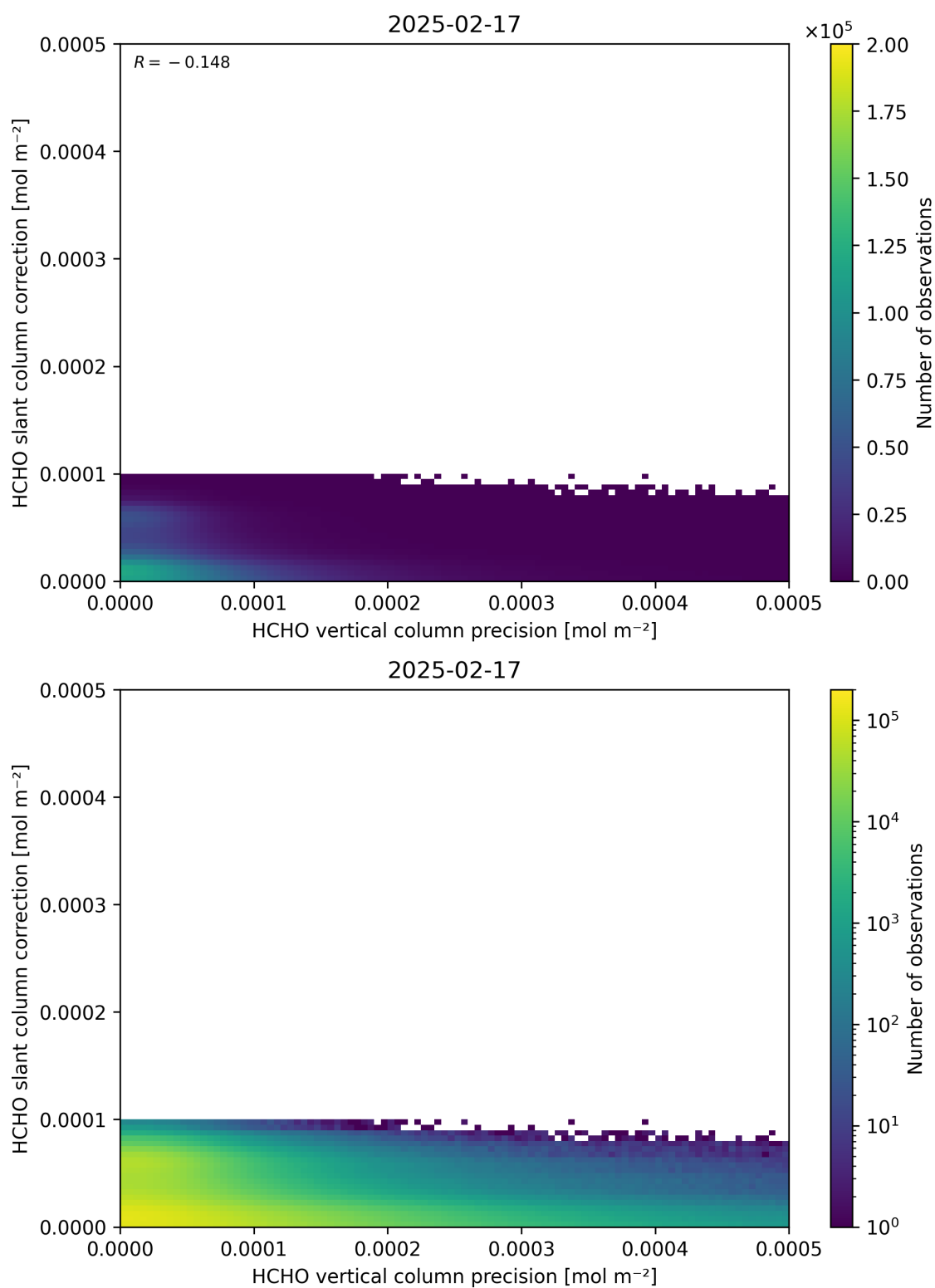
Figure 141: Scatter density plot of “HCHO vertical column precision” against “HCHO slant column correction” for 2025-02-16 to 2025-02-18.
