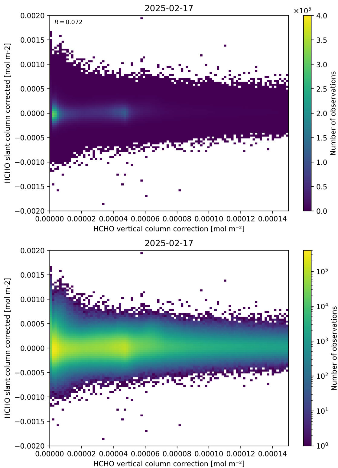
Figure 116: Scatter density plot of “HCHO vertical column correction” against “HCHO slant column corrected” for 2025-02-16 to 2025-02-18.
