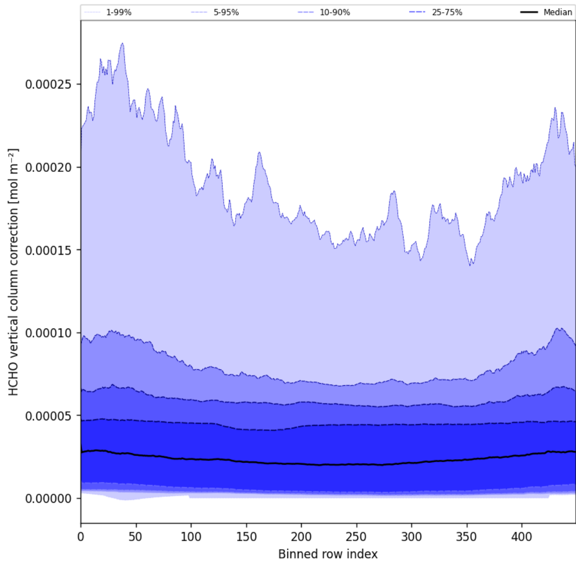
Figure 51: Along track statistics of “HCHO vertical column correction” for 2025-02-16 to 2025-02-18
