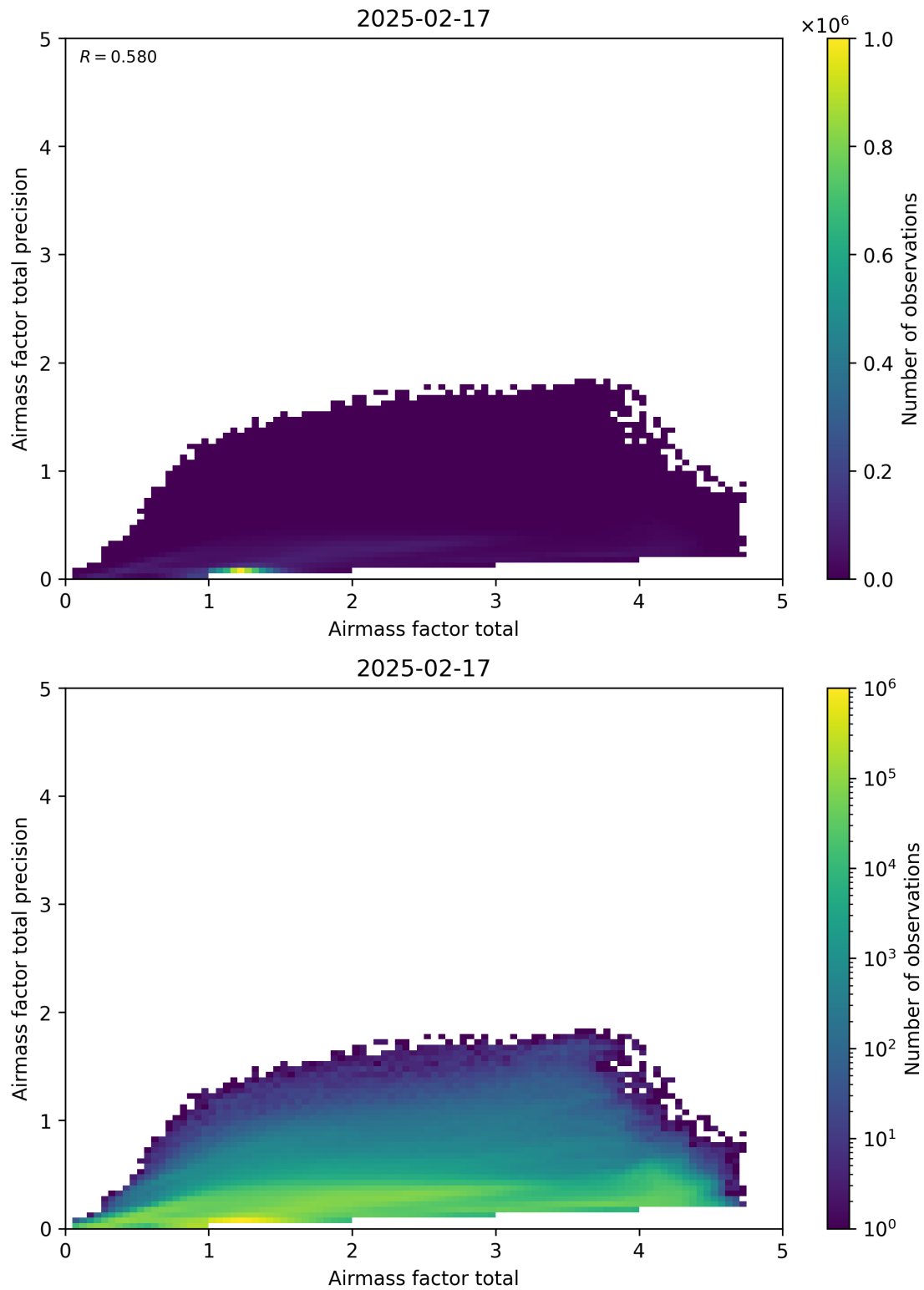
Figure 103: Scatter density plot of “Airmass factor total” against “Airmass factor total precision” for 2025-02-16 to 2025-02-18.
