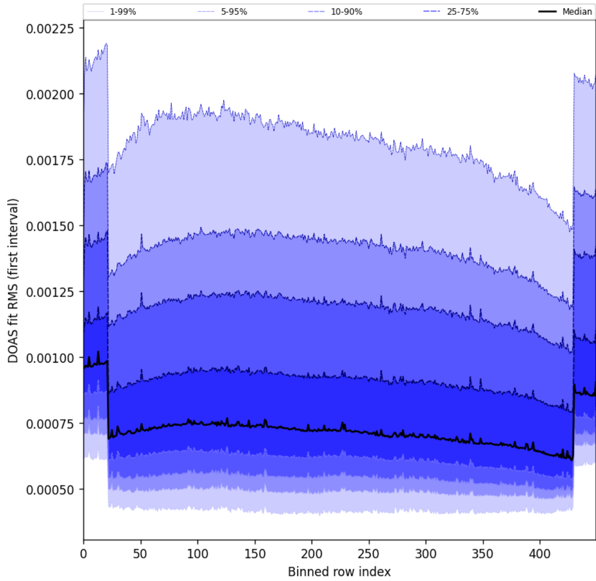
Figure 60: Along track statistics of “DOAS fit RMS (first interval)” for 2025-02-16 to 2025-02-18
