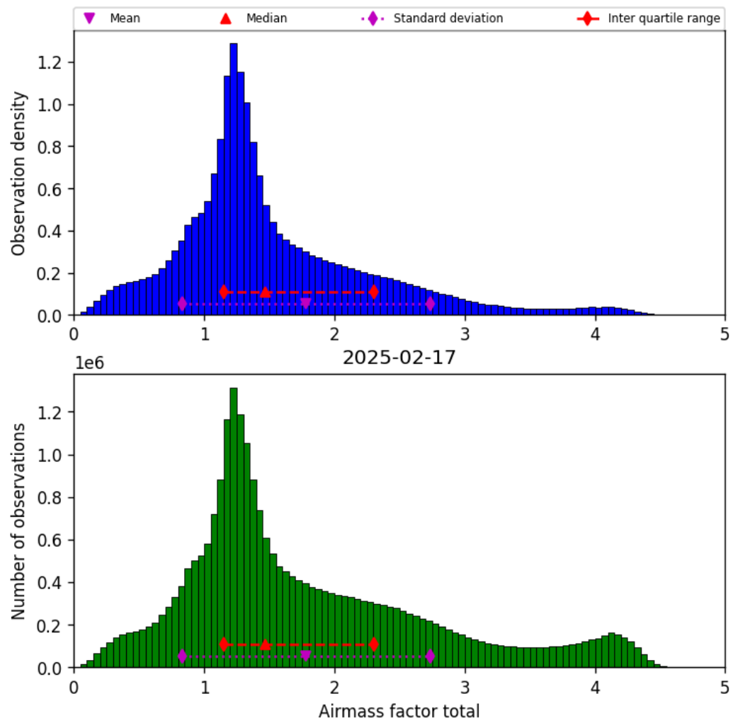
Figure 40: Histogram of “Airmass factor total” for 2025-02-16 to 2025-02-18
