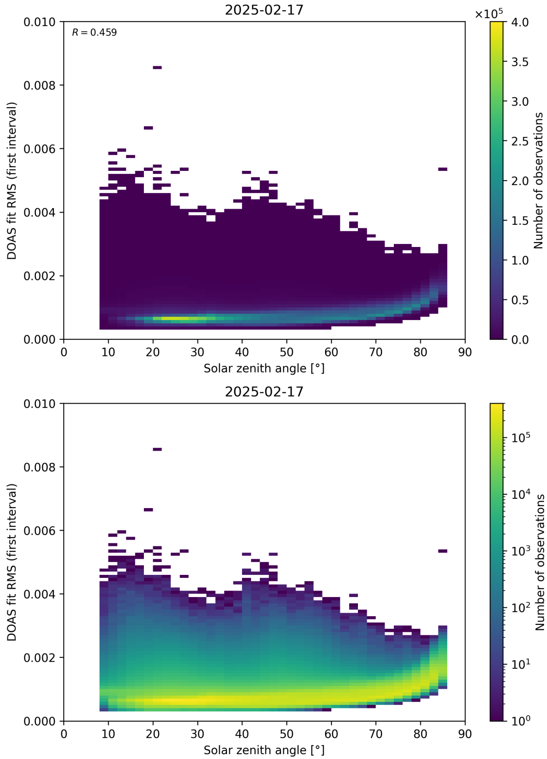
Figure 167: Scatter density plot of “Solar zenith angle” against “DOAS fit RMS (first interval)” for 2025-02-16 to 2025-02-18.
