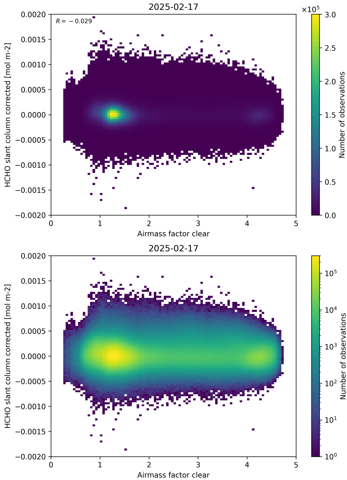
Figure 74: Scatter density plot of “Airmass factor clear” against “HCHO slant column corrected” for 2025-02-16 to 2025-02-18.
