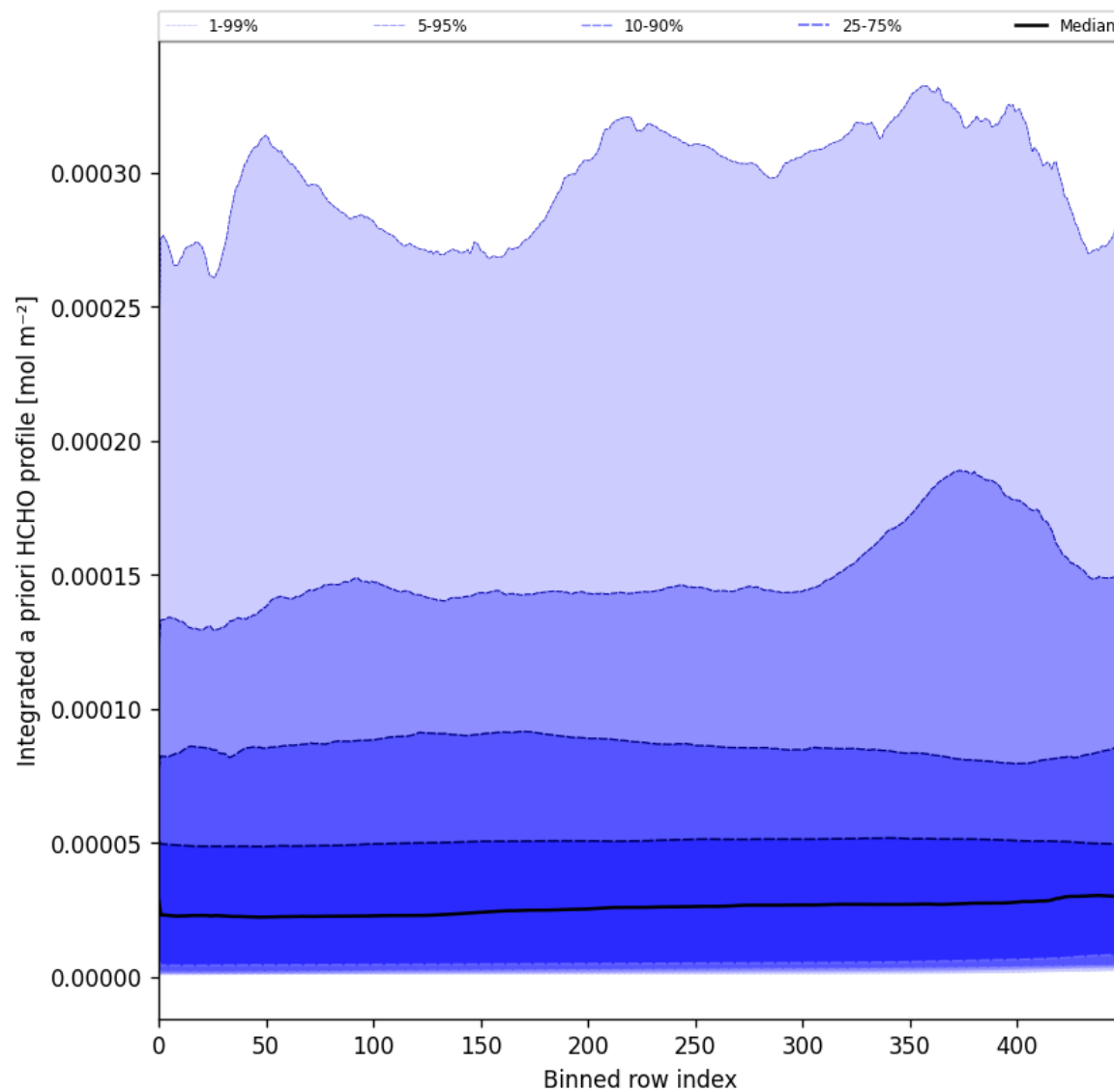
Figure 57: Along track statistics of “Integrated a priori HCHO profile” for 2025-02-16 to 2025-02-18
