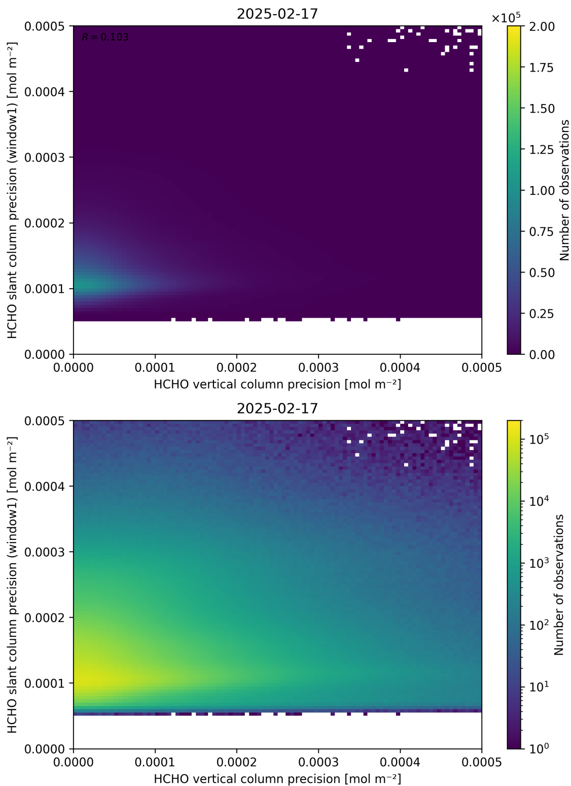
Figure 143: Scatter density plot of “HCHO vertical column precision” against “HCHO slant column precision (window1)” for 2025-02-16 to 2025-02-18.
