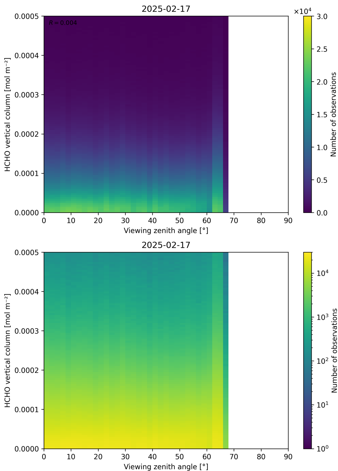
Figure 192: Scatter density plot of “Viewing zenith angle” against “HCHO vertical column” for 2025-02-16 to 2025-02-18.
