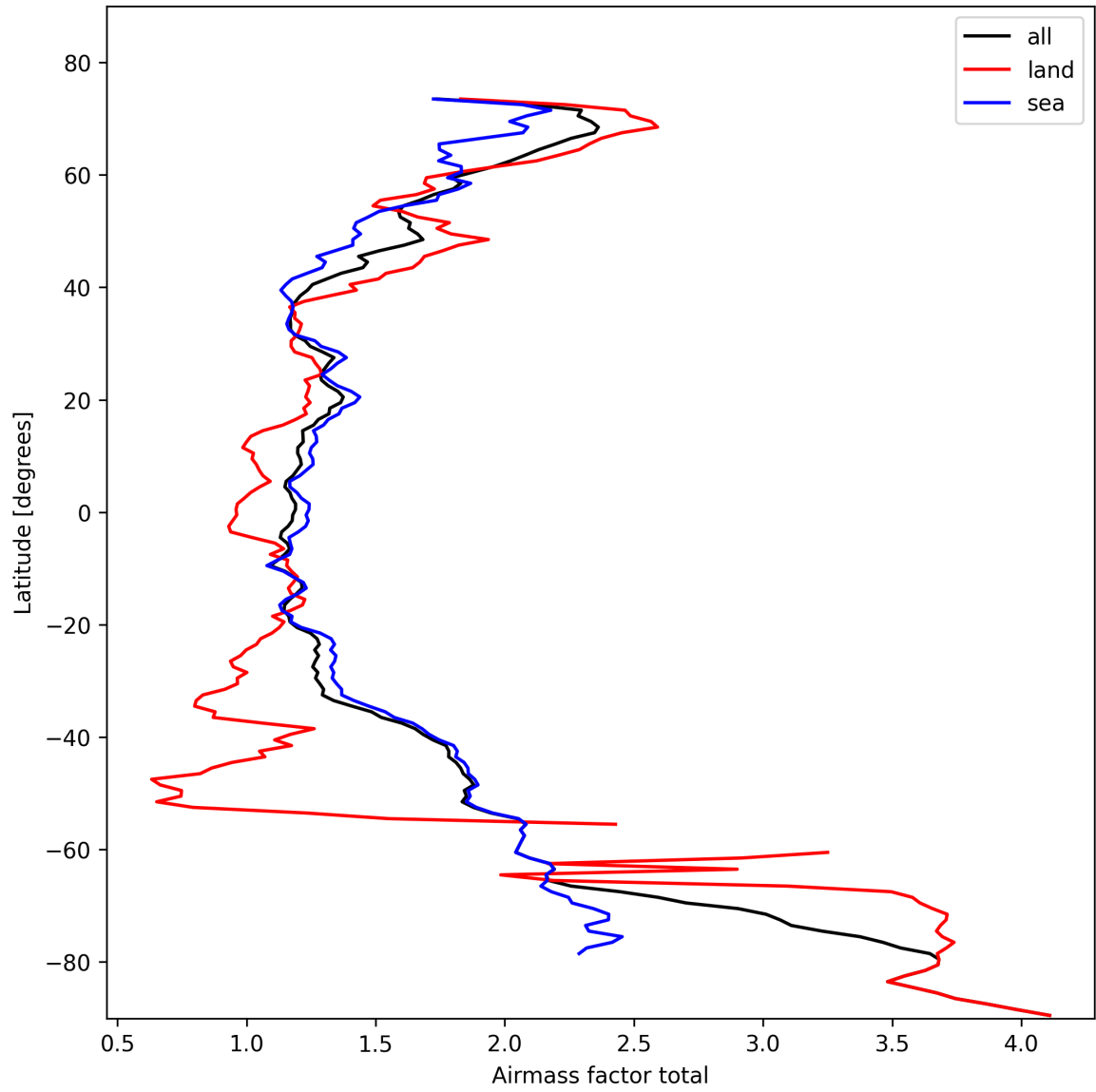
Figure 26: Zonal average of “Airmass factor total” for 2025-02-16 to 2025-02-18.
