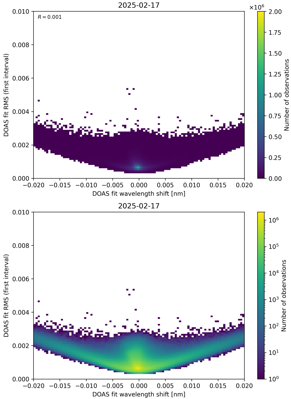
Figure 64: Scatter density plot of “DOAS fit wavelength shift” against “DOAS fit RMS (first interval)” for 2025-02-16 to 2025-02-18.
