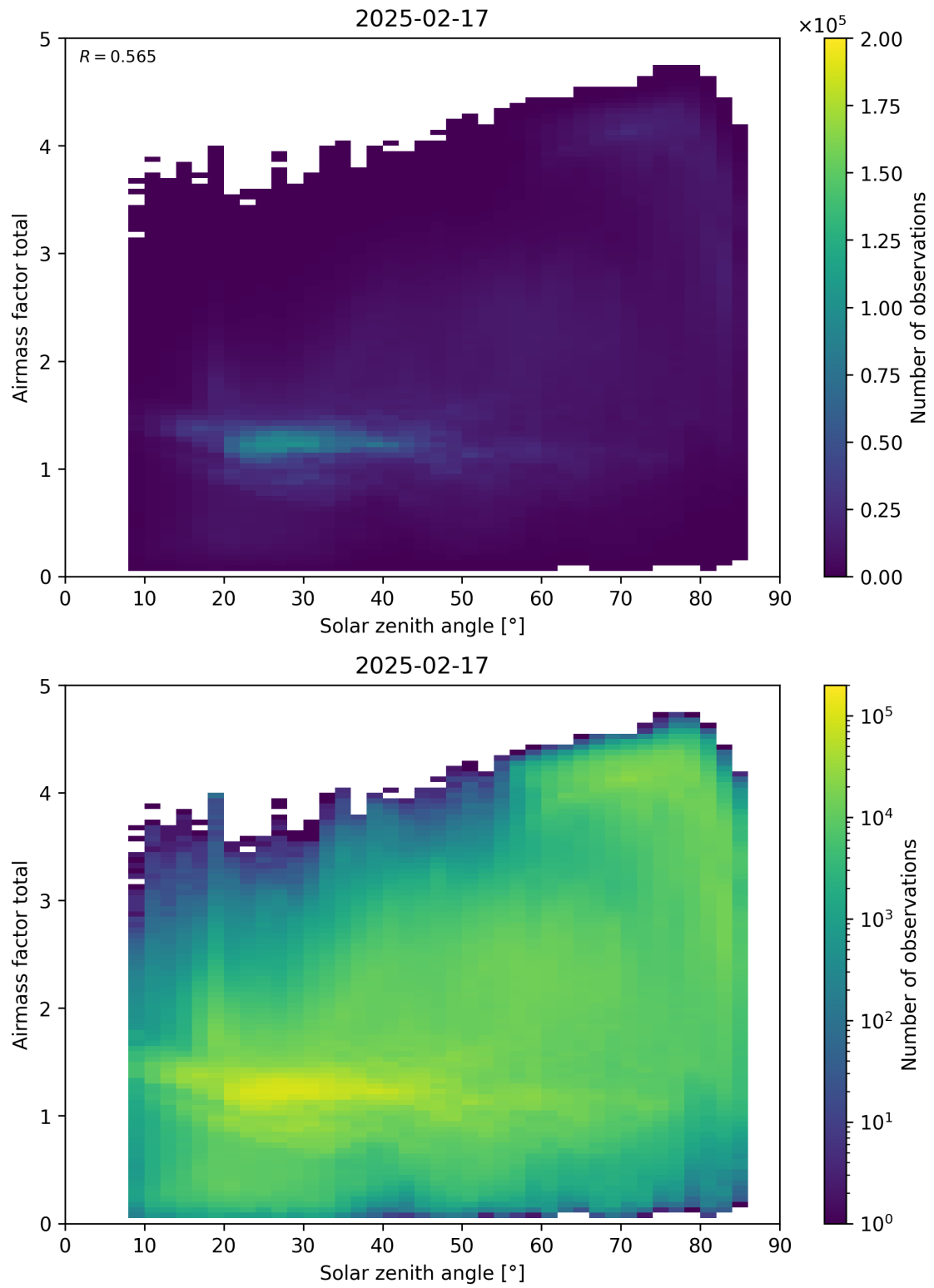
Figure 175: Scatter density plot of “Solar zenith angle” against “Airmass factor total” for 2025-02-16 to 2025-02-18.
