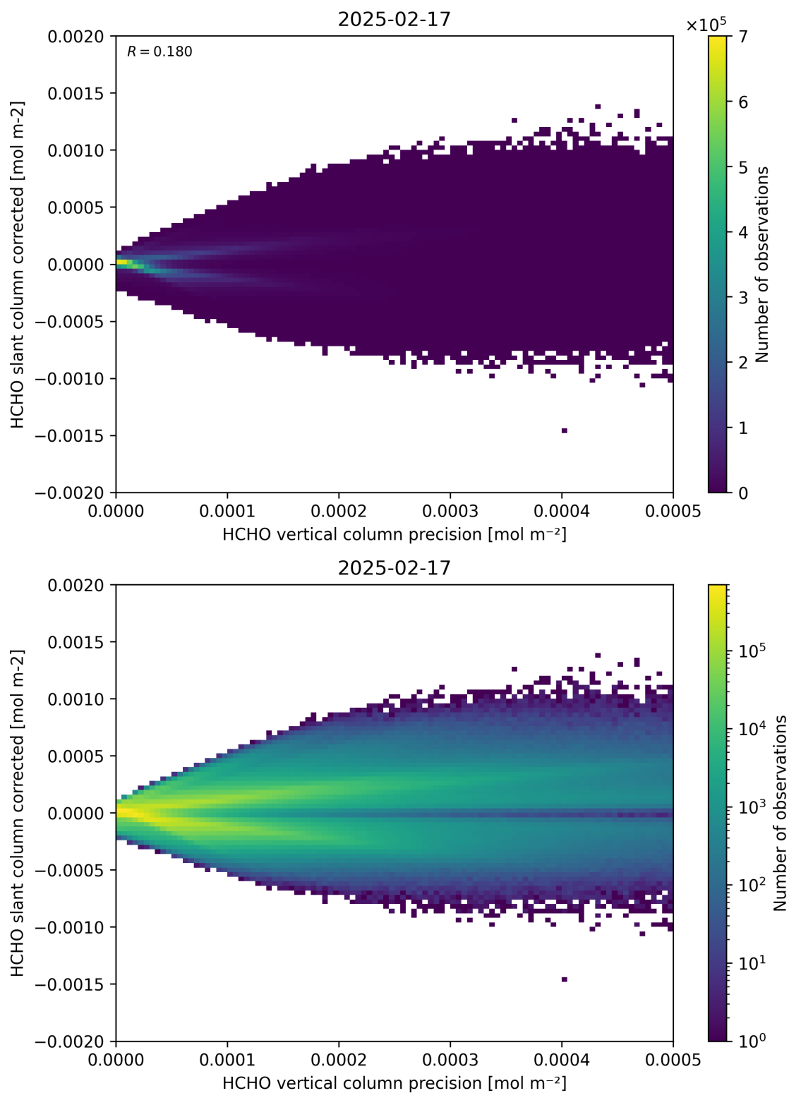
Figure 140: Scatter density plot of “HCHO vertical column precision” against “HCHO slant column corrected” for 2025-02-16 to 2025-02-18.
