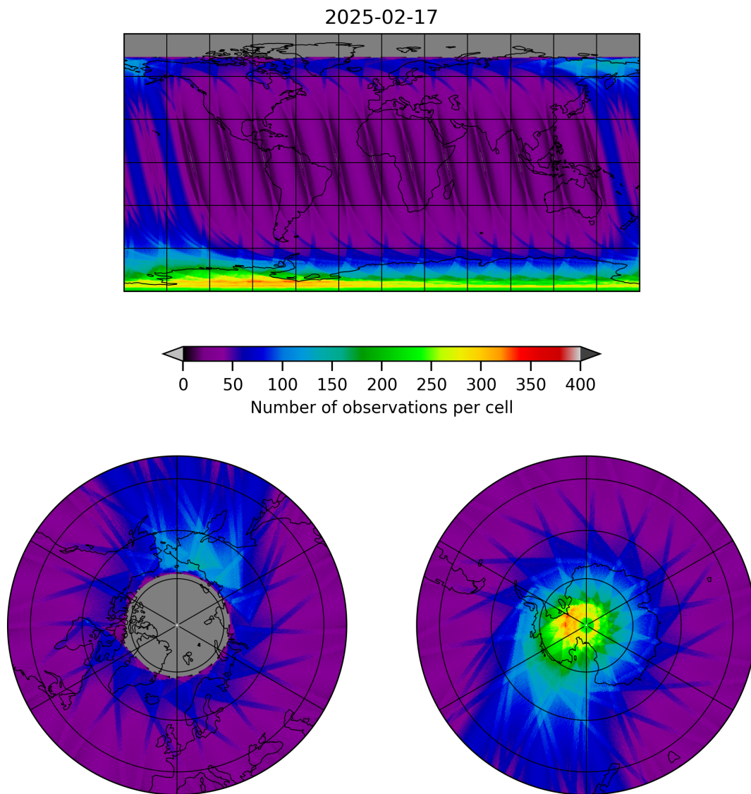
Figure 19: Map of the number of observations for 2025-02-16 to 2025-02-18
