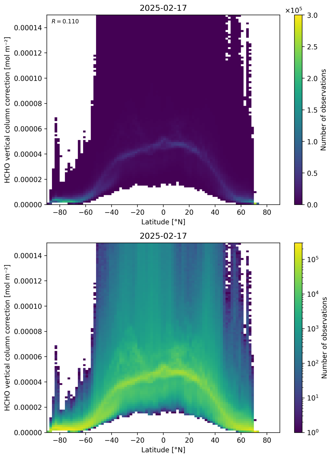
Figure 164: Scatter density plot of “Latitude” against “HCHO vertical column correction” for 2025-02-16 to 2025-02-18.
