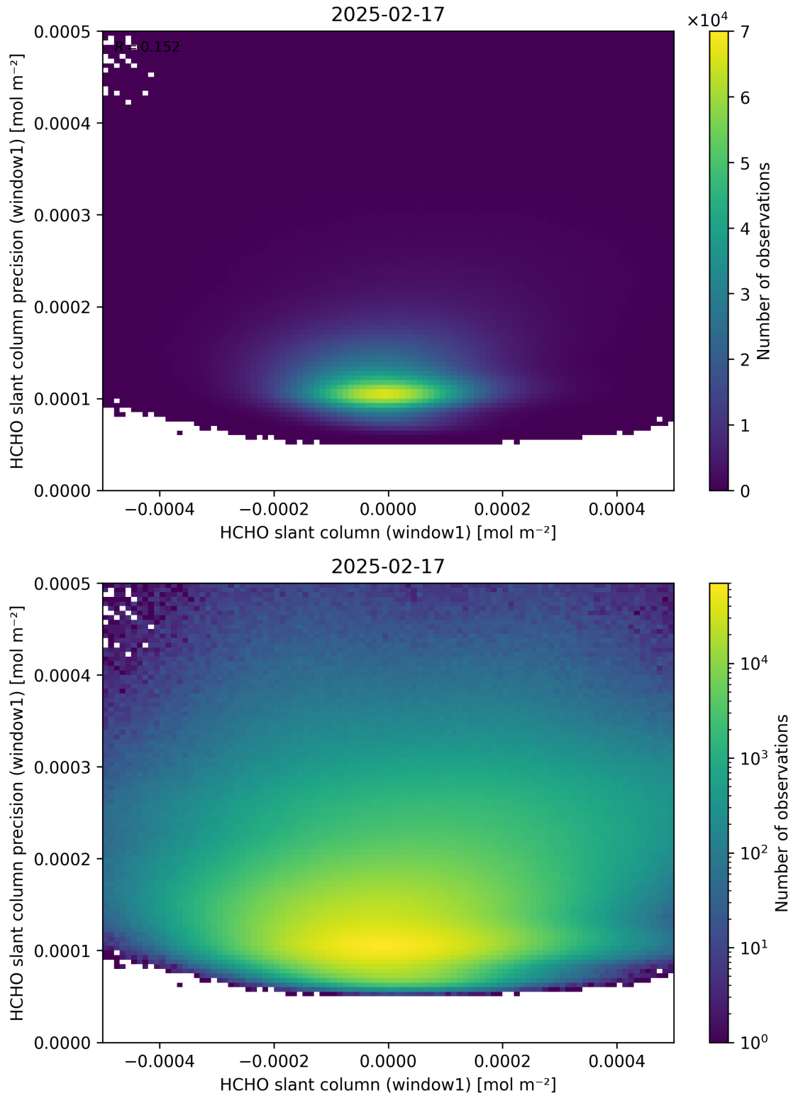
Figure 84: Scatter density plot of “HCHO slant column (window1)” against “HCHO slant column precision (window1)” for 2025-02-16 to 2025-02-18.
