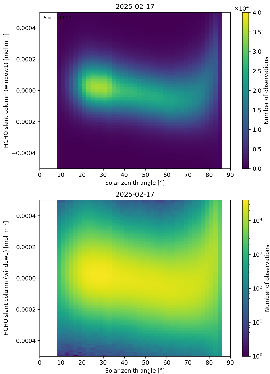
Figure 173: Scatter density plot of “Solar zenith angle” against “HCHO slant column (window1)” for 2025-02-16 to 2025-02-18.
