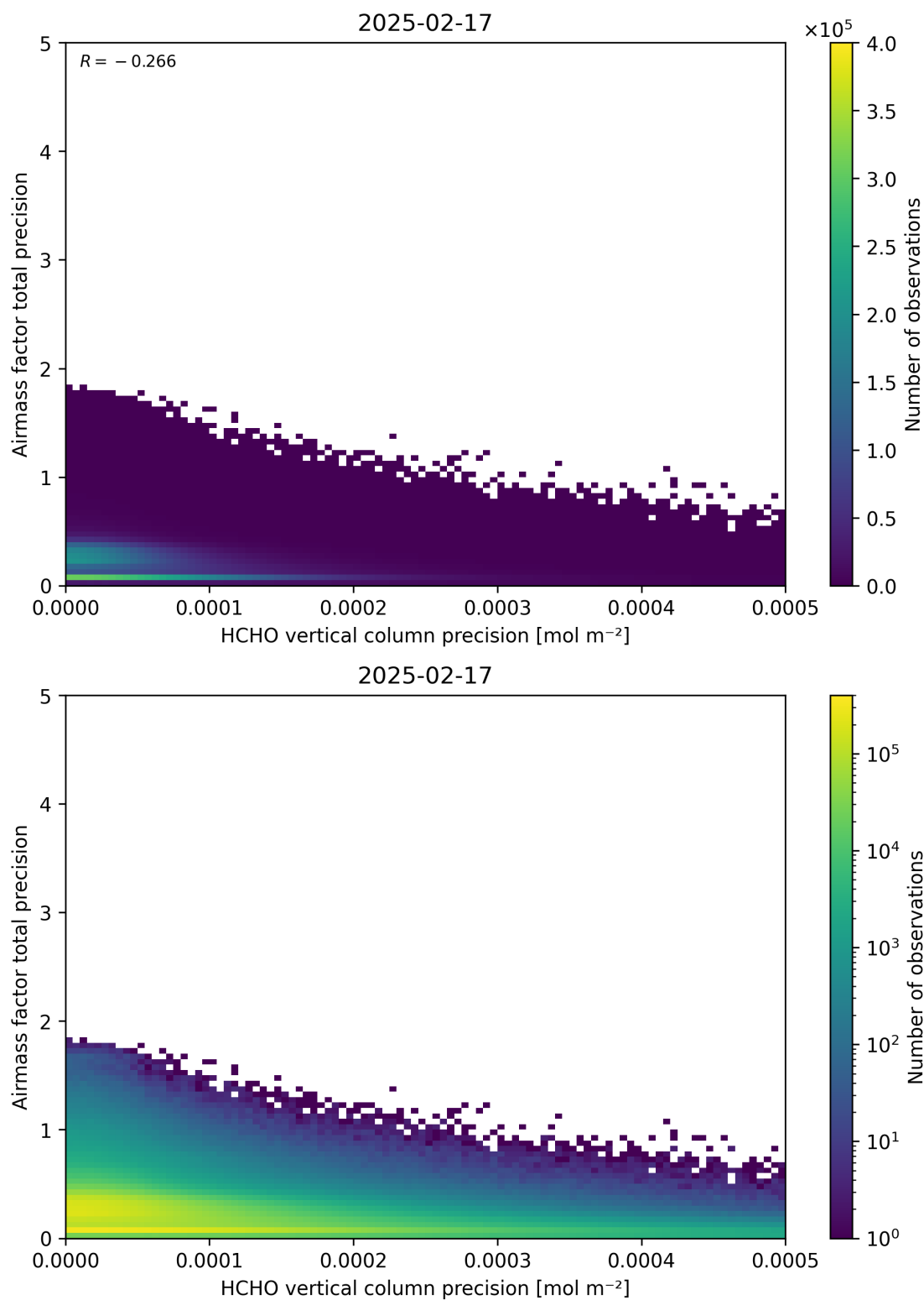
Figure 145: Scatter density plot of “HCHO vertical column precision” against “Airmass factor total precision” for 2025-02-16 to 2025-02-18.
