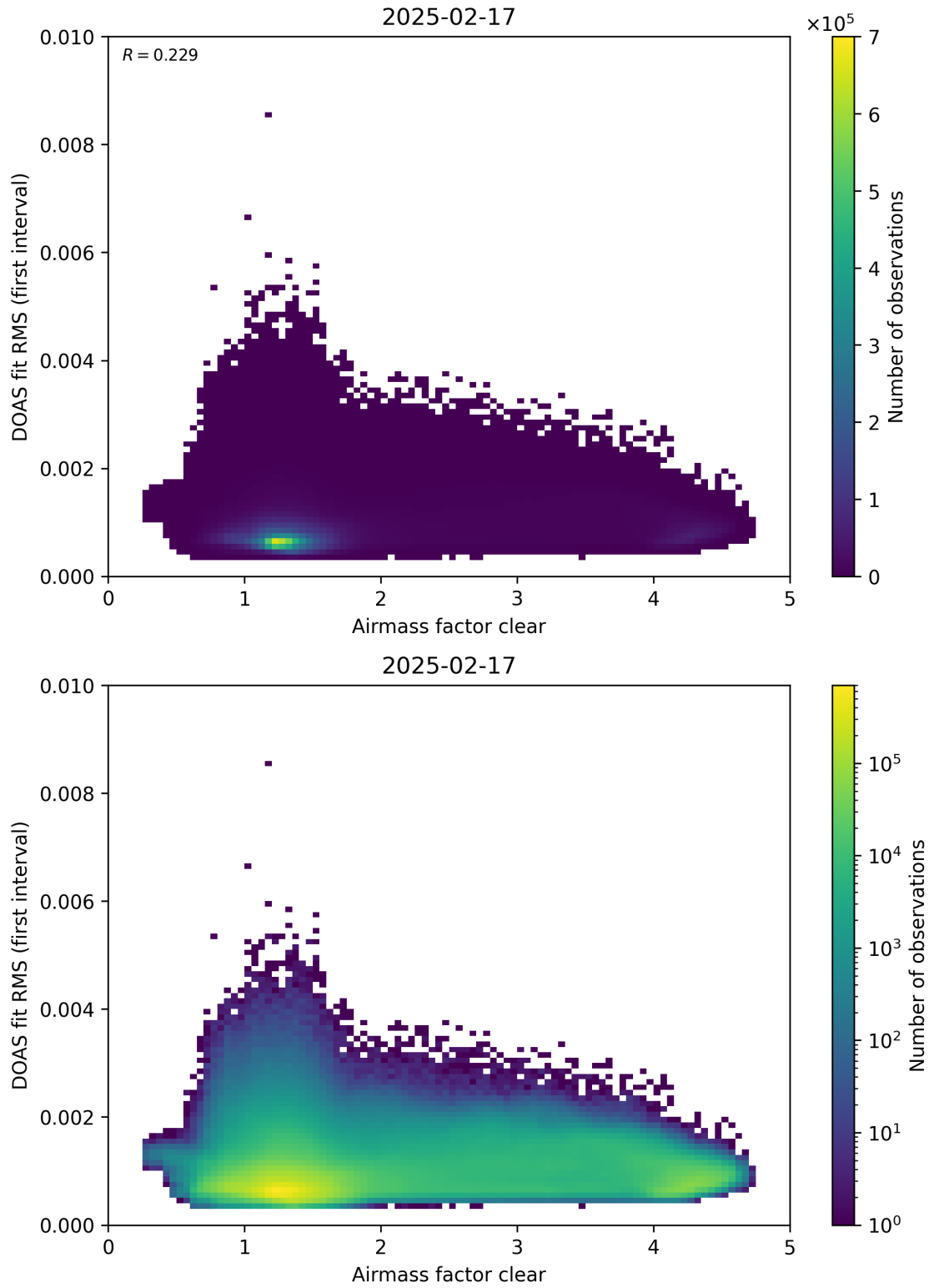
Figure 71: Scatter density plot of “Airmass factor clear” against “DOAS fit RMS (first interval)” for 2025-02-16 to 2025-02-18.
