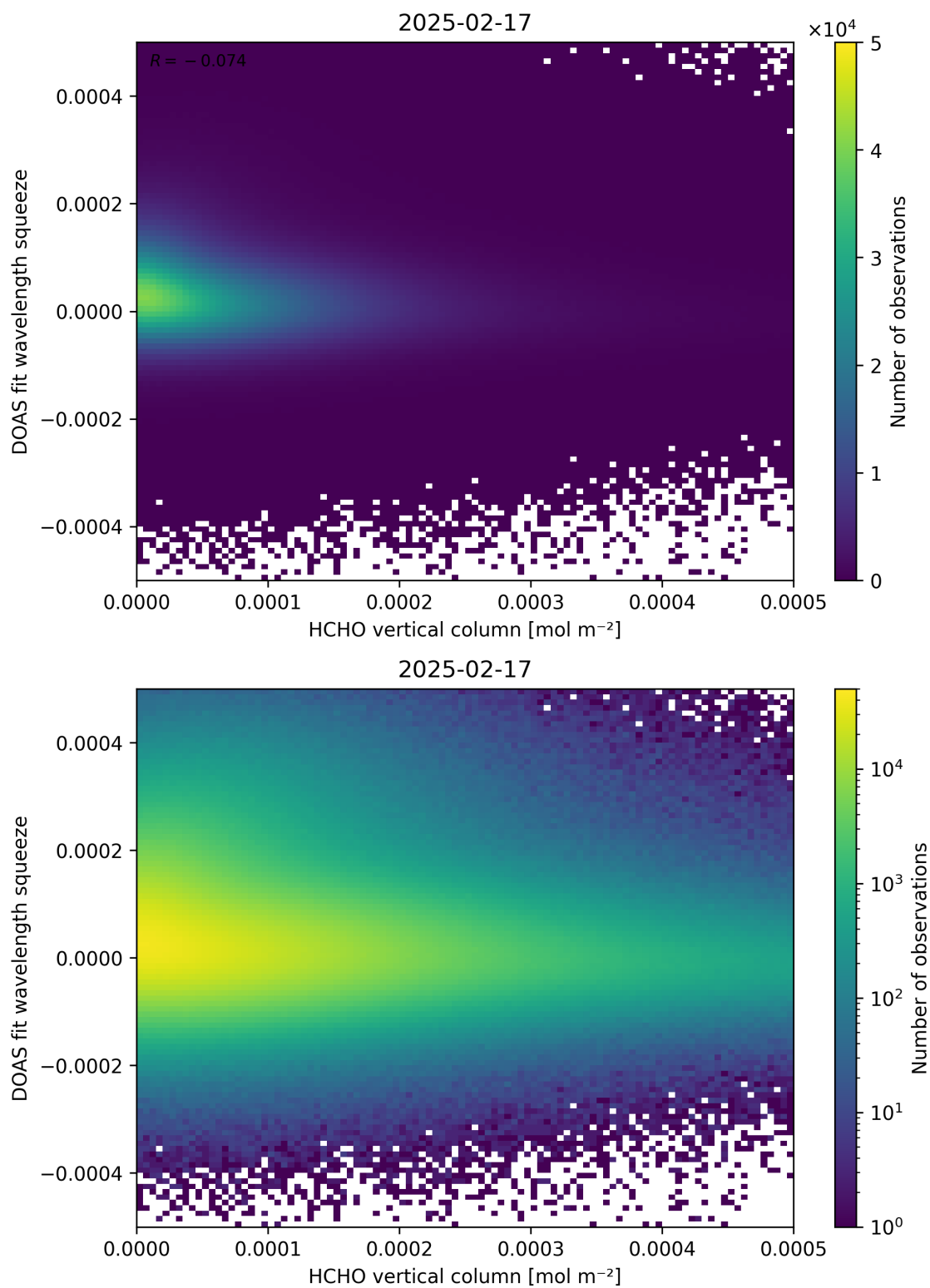
Figure 125: Scatter density plot of “HCHO vertical column” against “DOAS fit wavelength squeeze” for 2025-02-16 to 2025-02-18.
