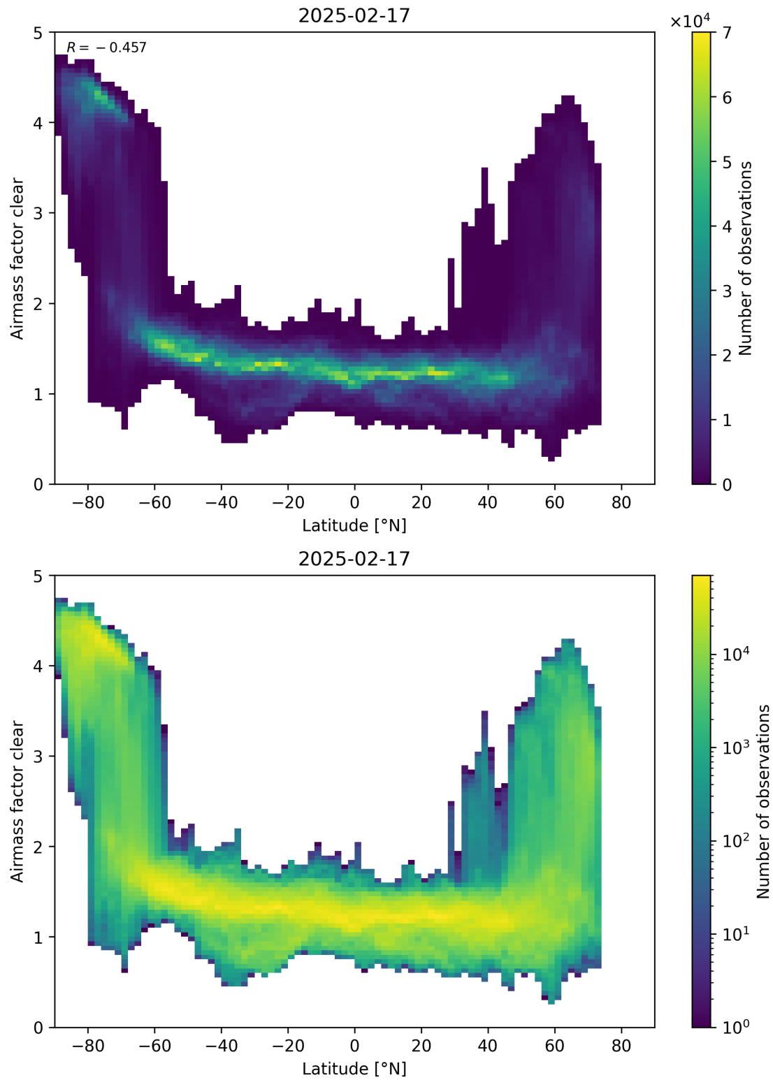
Figure 156: Scatter density plot of “Latitude” against “Airmass factor clear” for 2025-02-16 to 2025-02-18.
