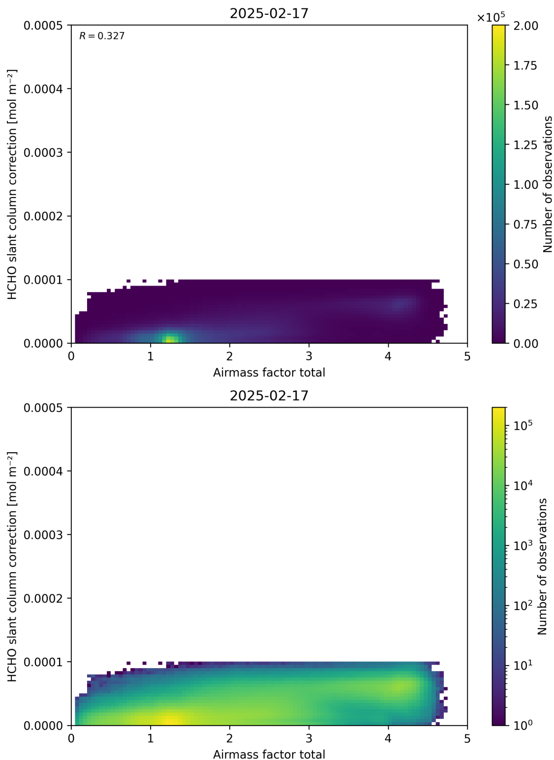
Figure 102: Scatter density plot of “Airmass factor total” against “HCHO slant column correction” for 2025-02-16 to 2025-02-18.
