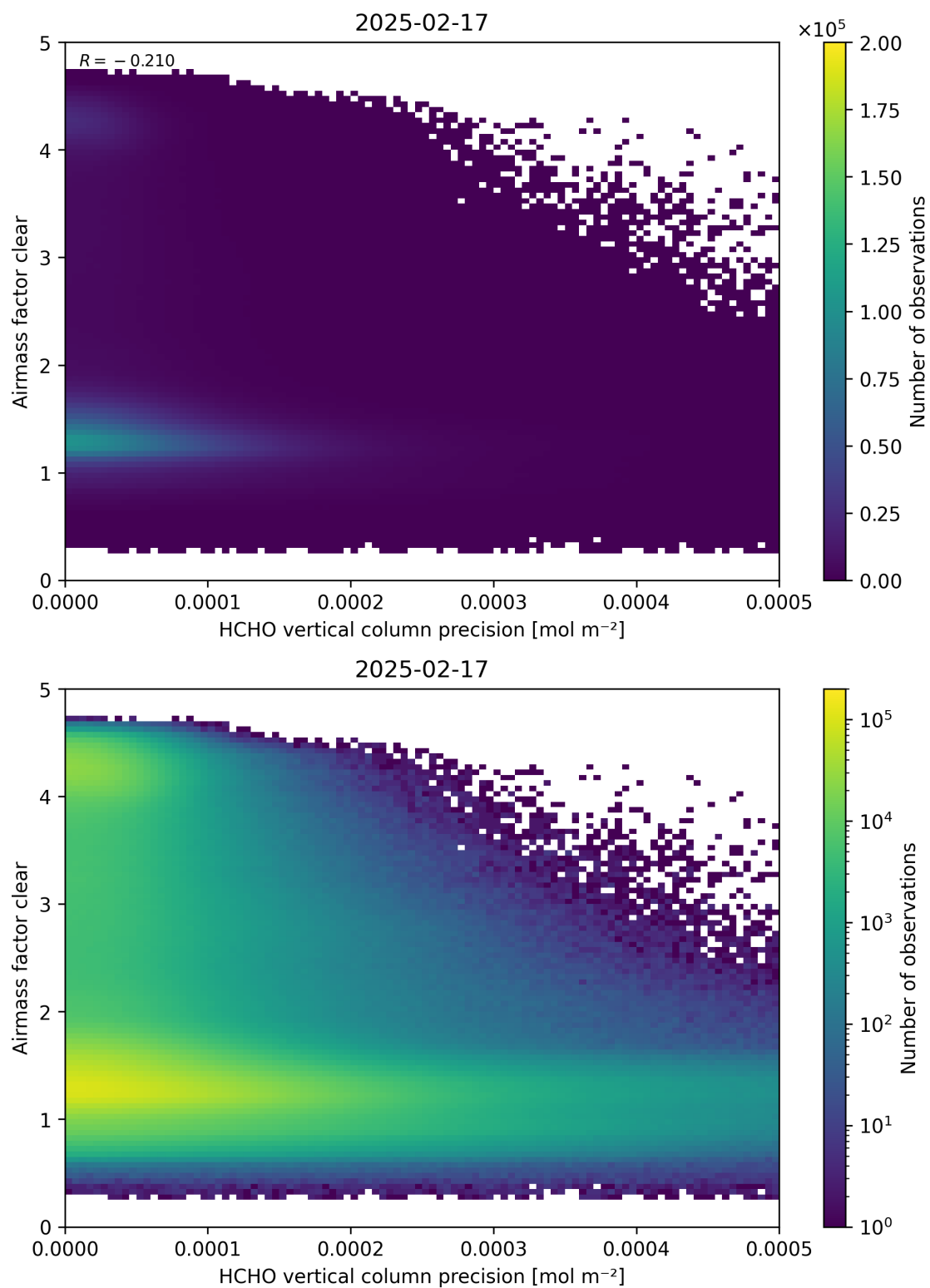
Figure 139: Scatter density plot of “HCHO vertical column precision” against “Airmass factor clear” for 2025-02-16 to 2025-02-18.
