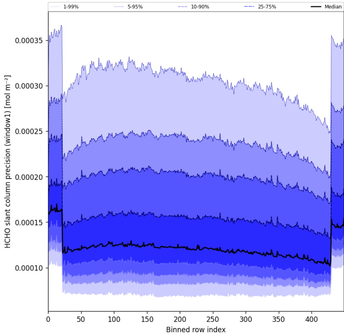
Figure 53: Along track statistics of “HCHO slant column precision (window1)” for 2025-02-16 to 2025-02-18
