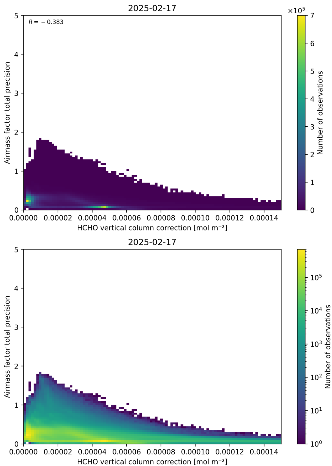
Figure 121: Scatter density plot of “HCHO vertical column correction” against “Airmass factor total precision” for 2025-02-16 to 2025-02-18.
