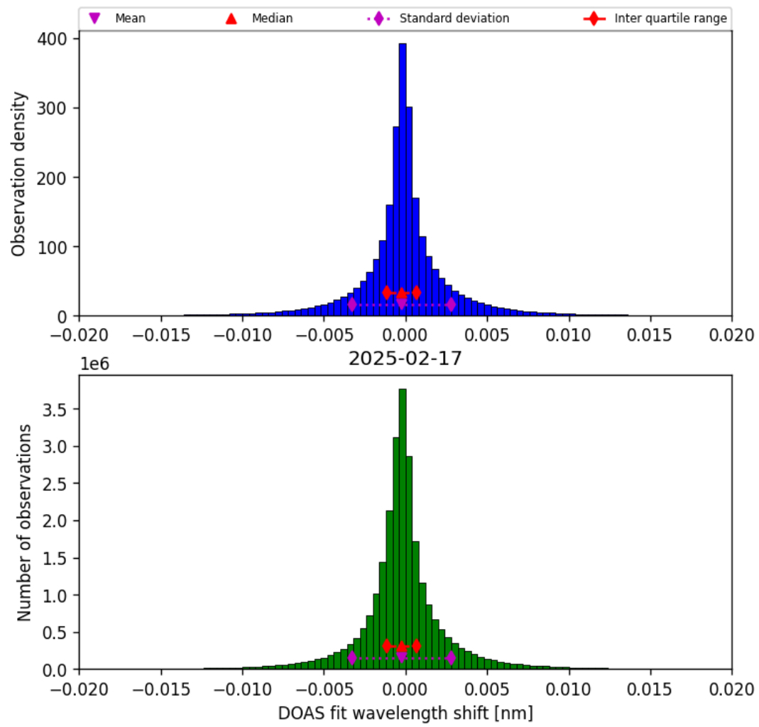
Figure 44: Histogram of “DOAS fit wavelength shift” for 2025-02-16 to 2025-02-18
