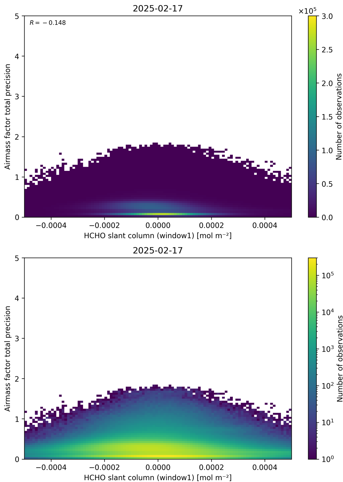
Figure 86: Scatter density plot of “HCHO slant column (window1)” against “Airmass factor total precision” for 2025-02-16 to 2025-02-18.
