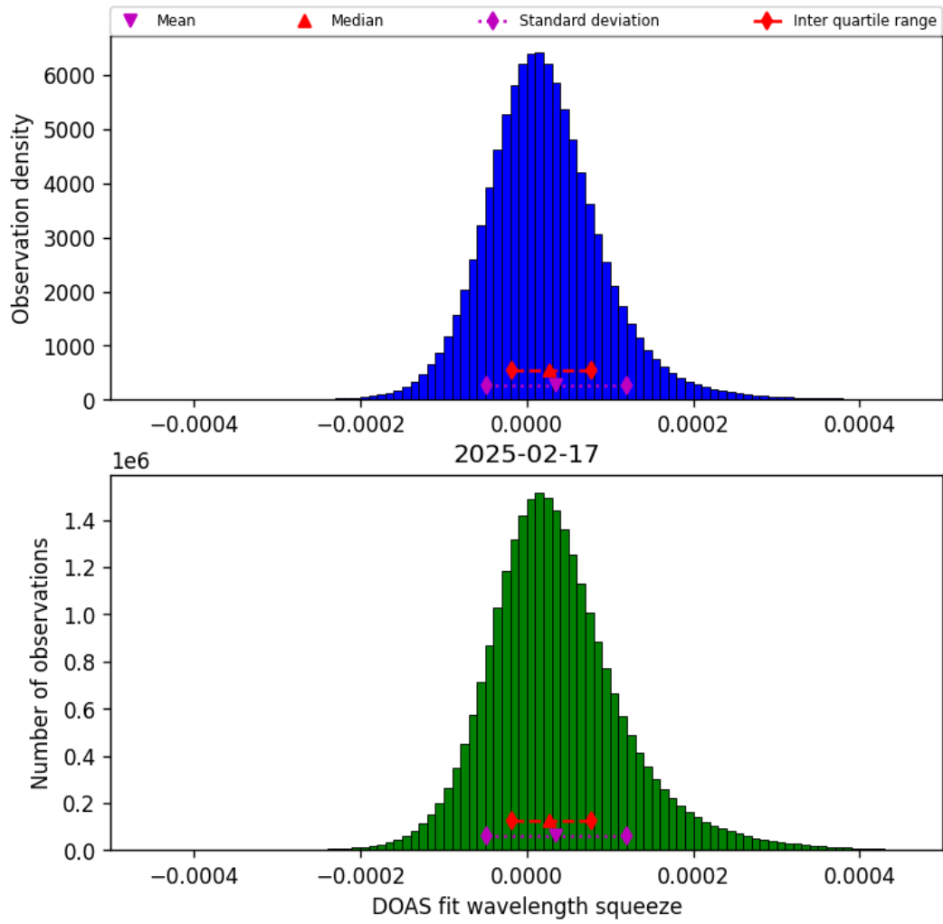
Figure 45: Histogram of “DOAS fit wavelength squeeze” for 2025-02-16 to 2025-02-18
