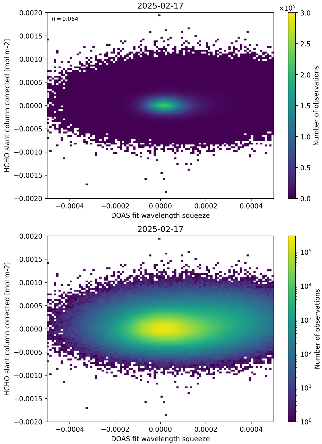
Figure 69: Scatter density plot of “DOAS fit wavelength squeeze” against “HCHO slant column corrected” for 2025-02-16 to 2025-02-18.
