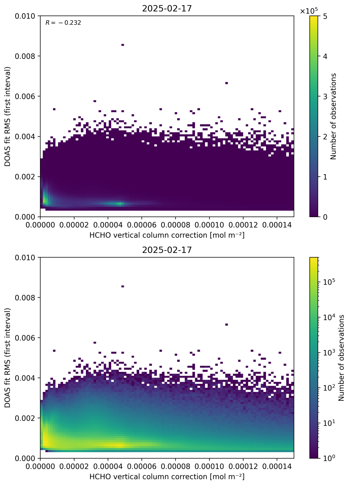
Figure 112: Scatter density plot of “HCHO vertical column correction” against “DOAS fit RMS (first interval)” for 2025-02-16 to 2025-02-18.
