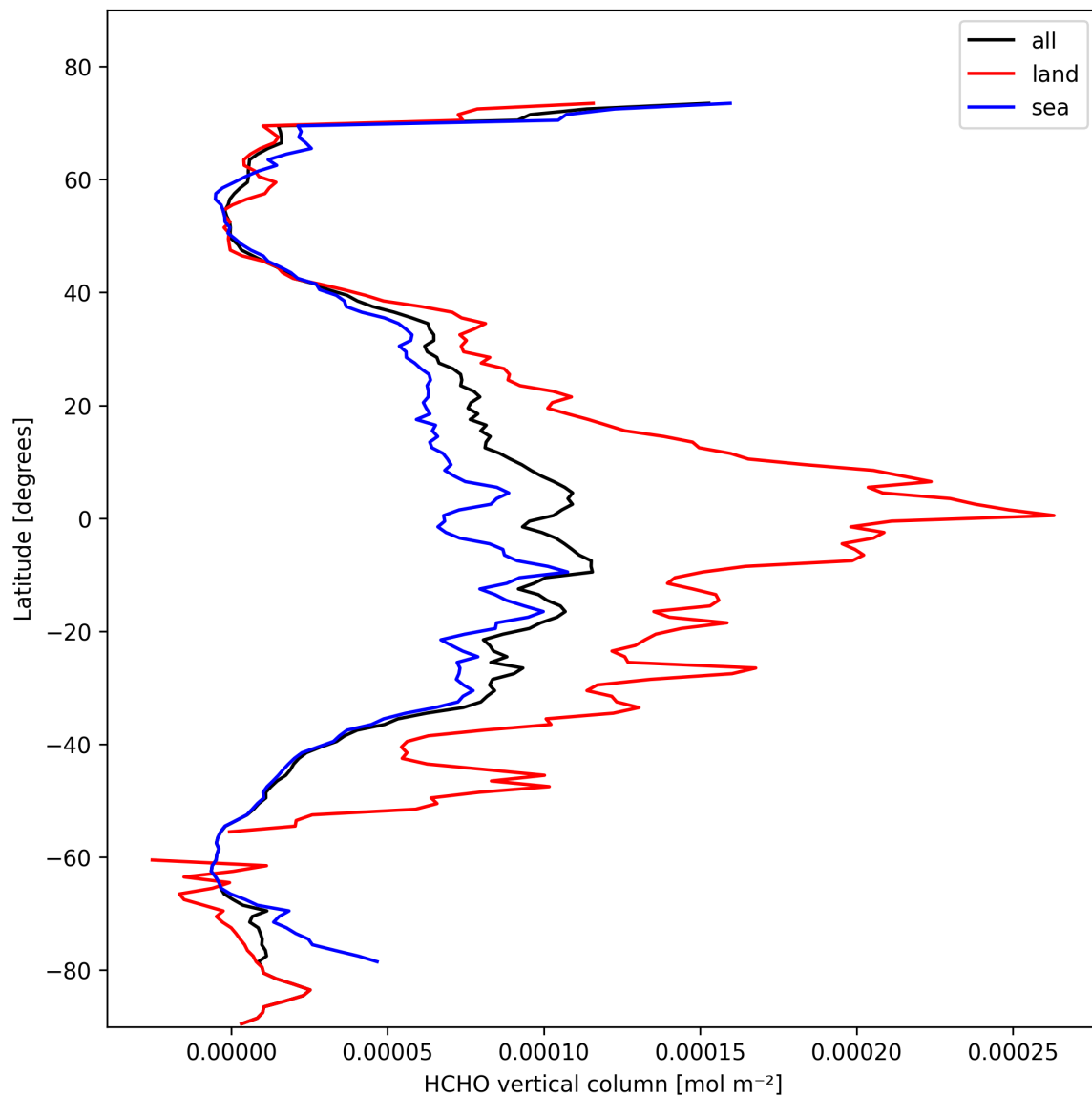
Figure 21: Zonal average of “HCHO vertical column” for 2025-02-16 to 2025-02-18.
