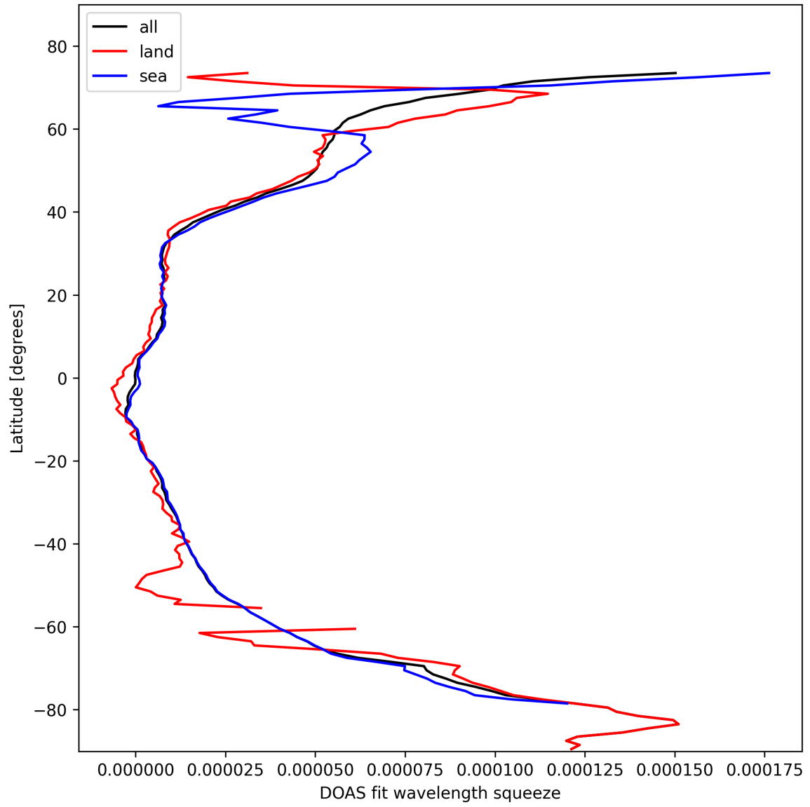
Figure 31: Zonal average of “DOAS fit wavelength squeeze” for 2025-02-16 to 2025-02-18.
