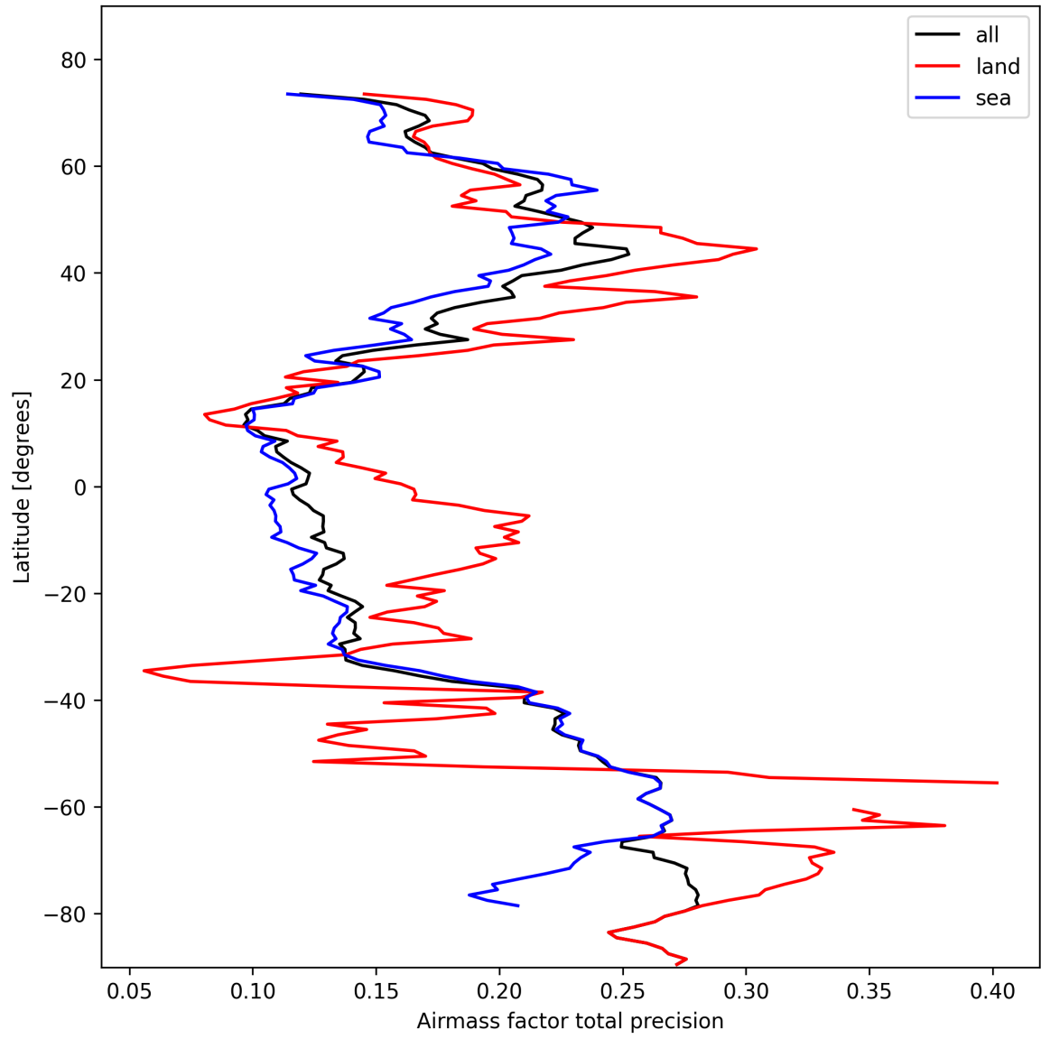
Figure 27: Zonal average of “Airmass factor total precision” for 2025-02-16 to 2025-02-18.
