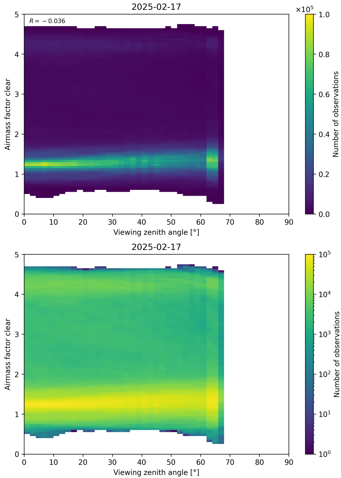
Figure 185: Scatter density plot of “Viewing zenith angle” against “Airmass factor clear” for 2025-02-16 to 2025-02-18.
