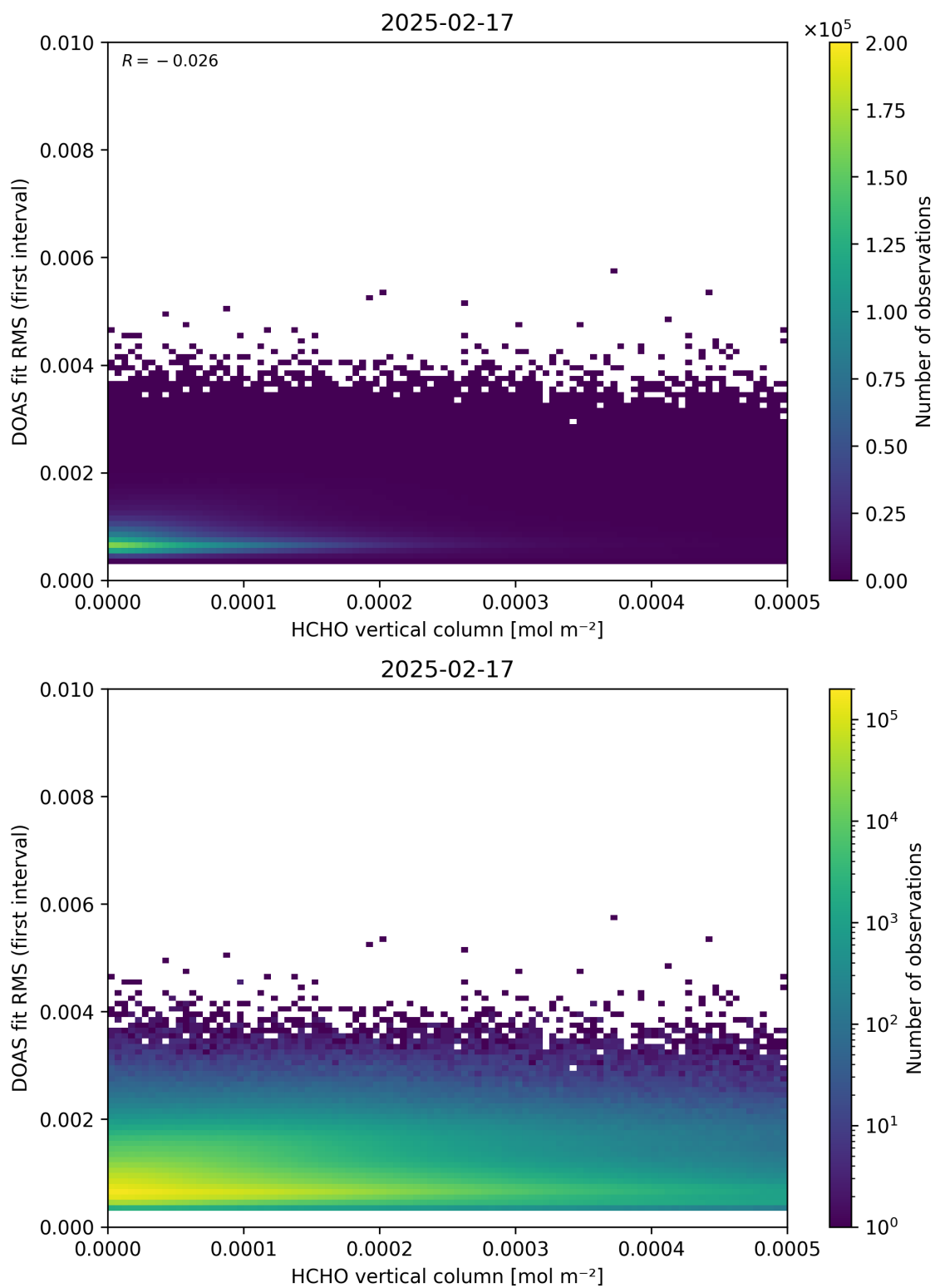
Figure 123: Scatter density plot of “HCHO vertical column” against “DOAS fit RMS (first interval)” for 2025-02-16 to 2025-02-18.
