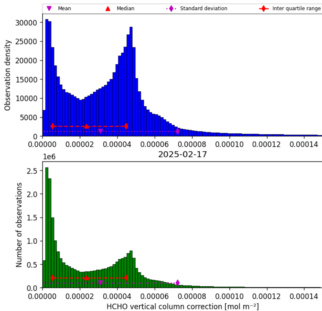
Figure 37: Histogram of “HCHO vertical column correction” for 2025-02-16 to 2025-02-18
