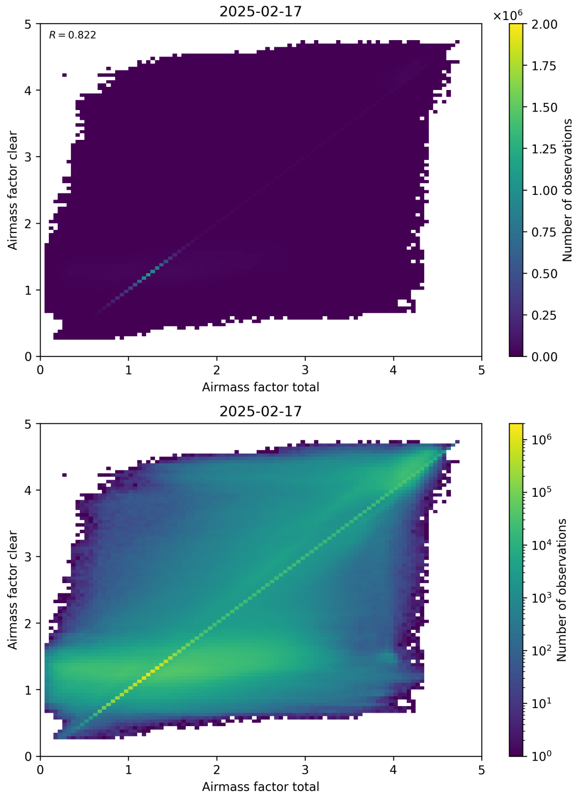
Figure 100: Scatter density plot of “Airmass factor total” against “Airmass factor clear” for 2025-02-16 to 2025-02-18.
