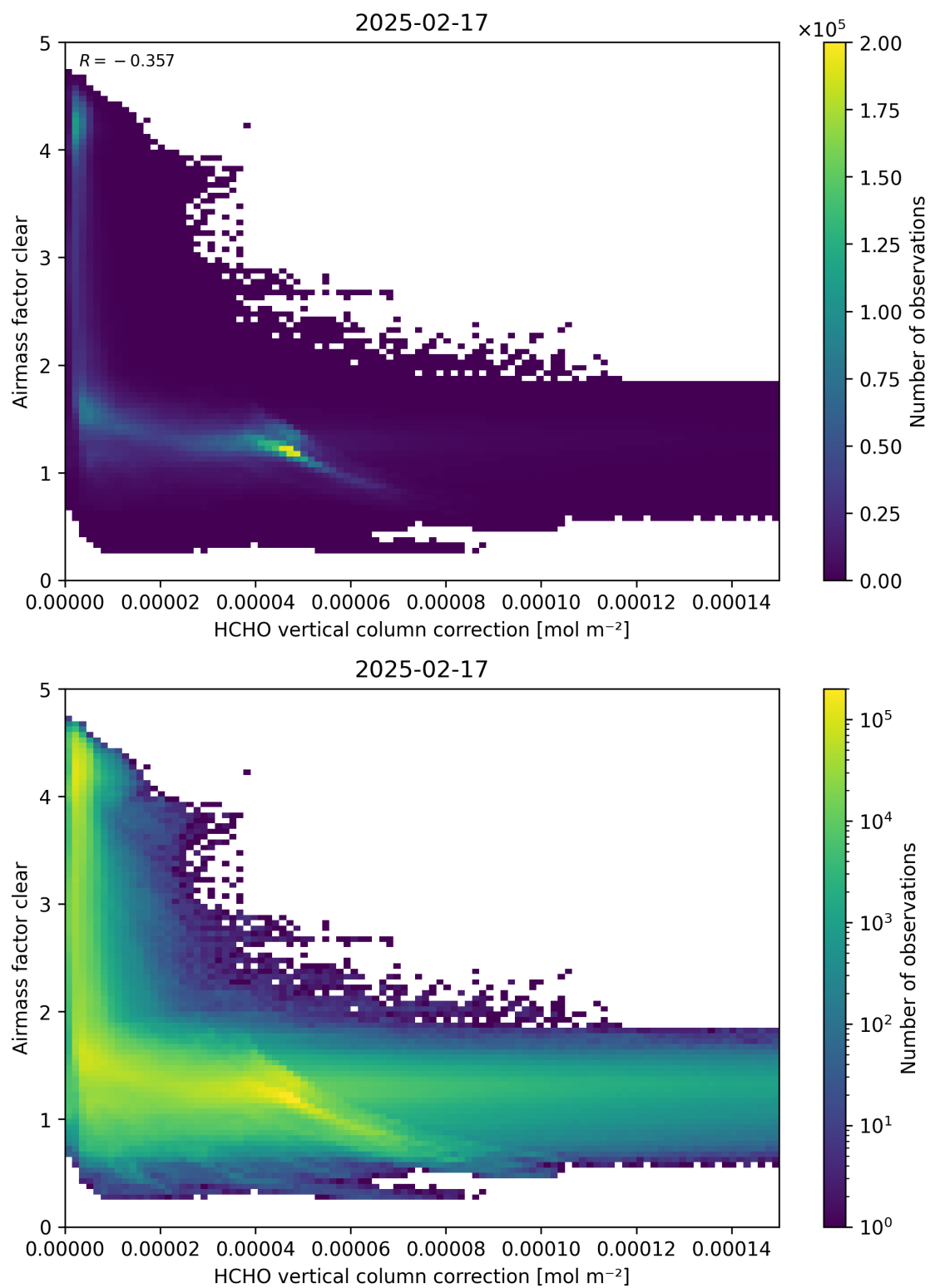
Figure 115: Scatter density plot of “HCHO vertical column correction” against “Airmass factor clear” for 2025-02-16 to 2025-02-18.
