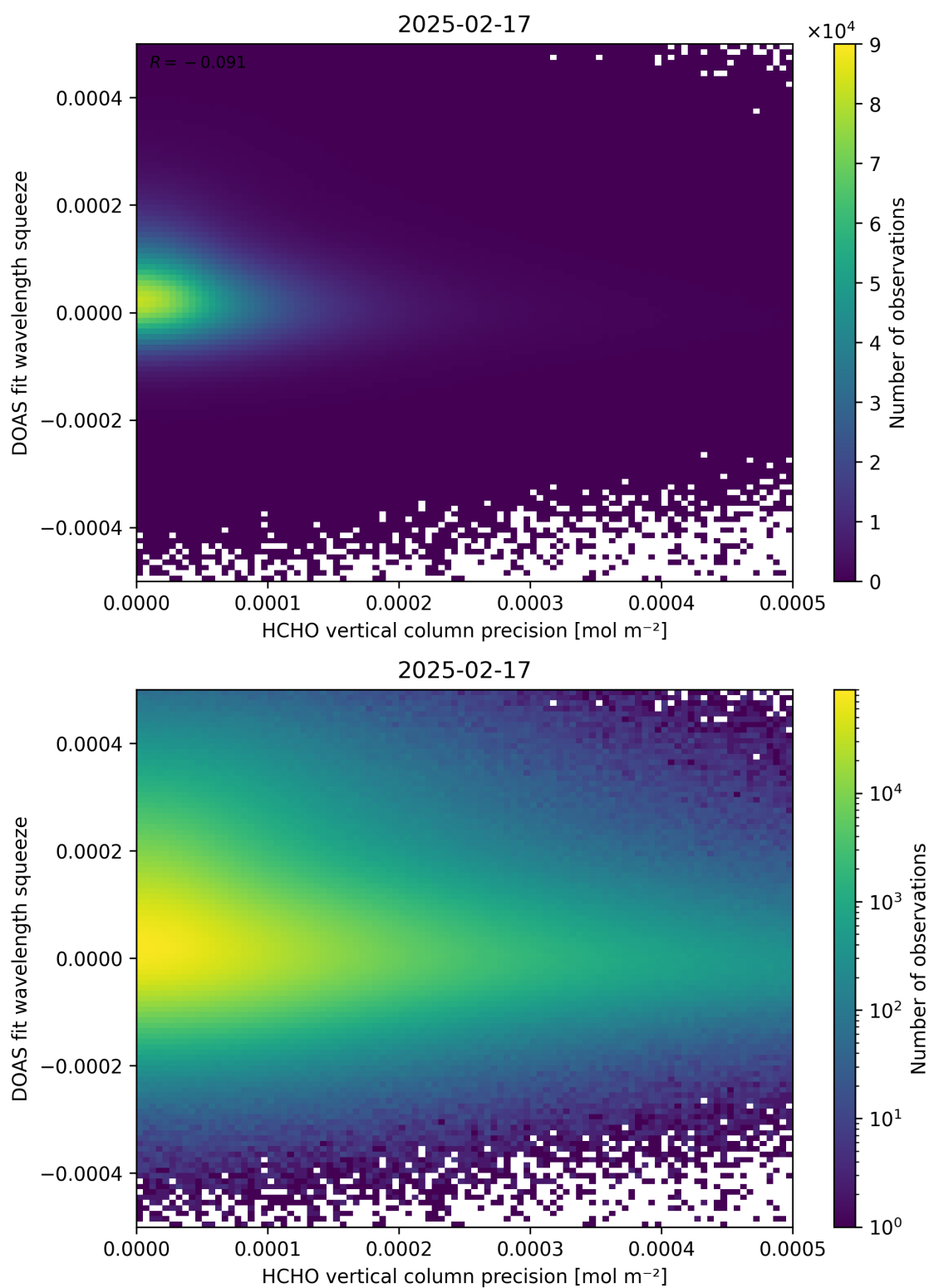
Figure 138: Scatter density plot of “HCHO vertical column precision” against “DOAS fit wavelength squeeze” for 2025-02-16 to 2025-02-18.
