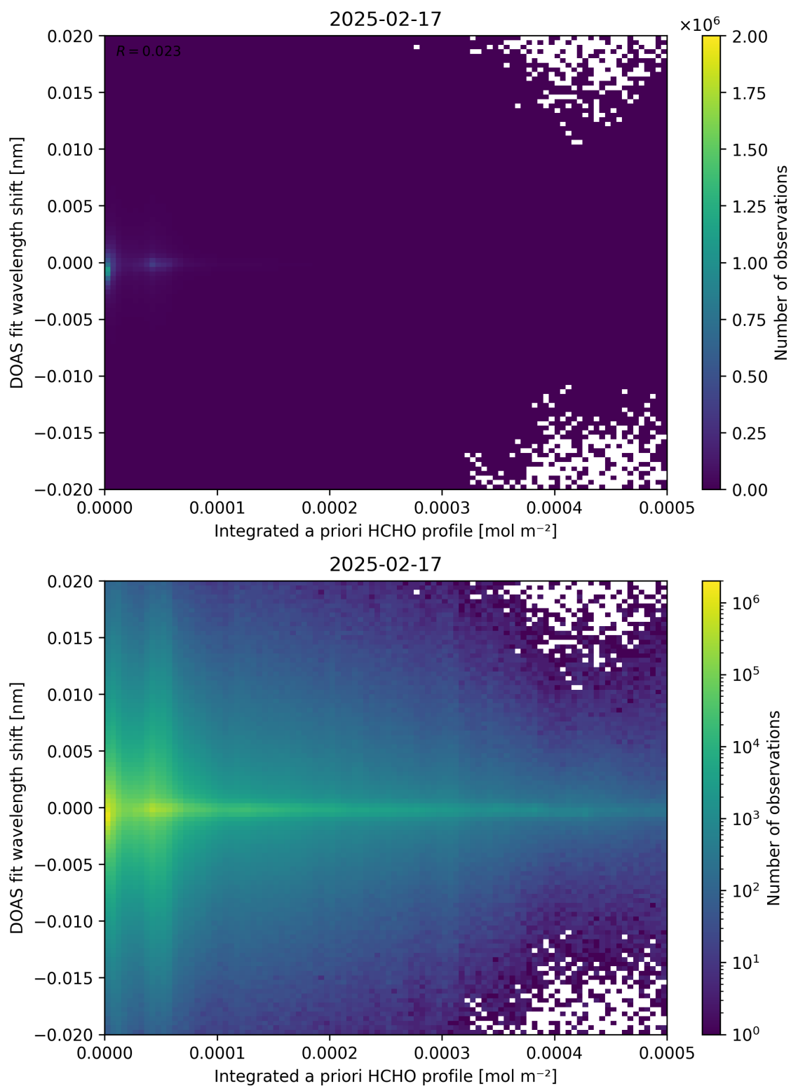
Figure 149: Scatter density plot of “Integrated a priori HCHO profile” against “DOAS fit wavelength shift” for 2025-02-16 to 2025-02-18.
