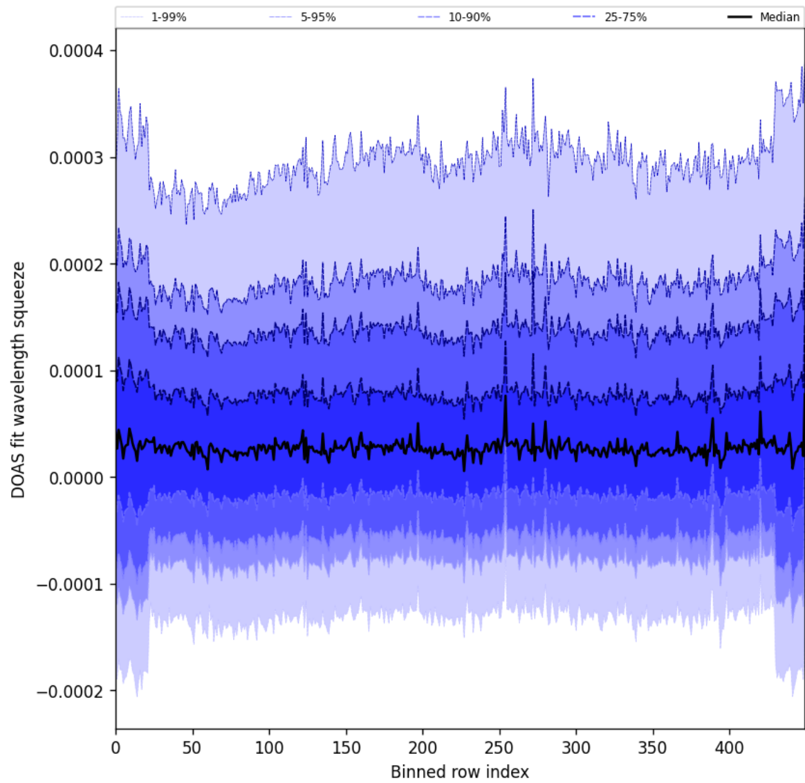
Figure 59: Along track statistics of “DOAS fit wavelength squeeze” for 2025-02-16 to 2025-02-18
