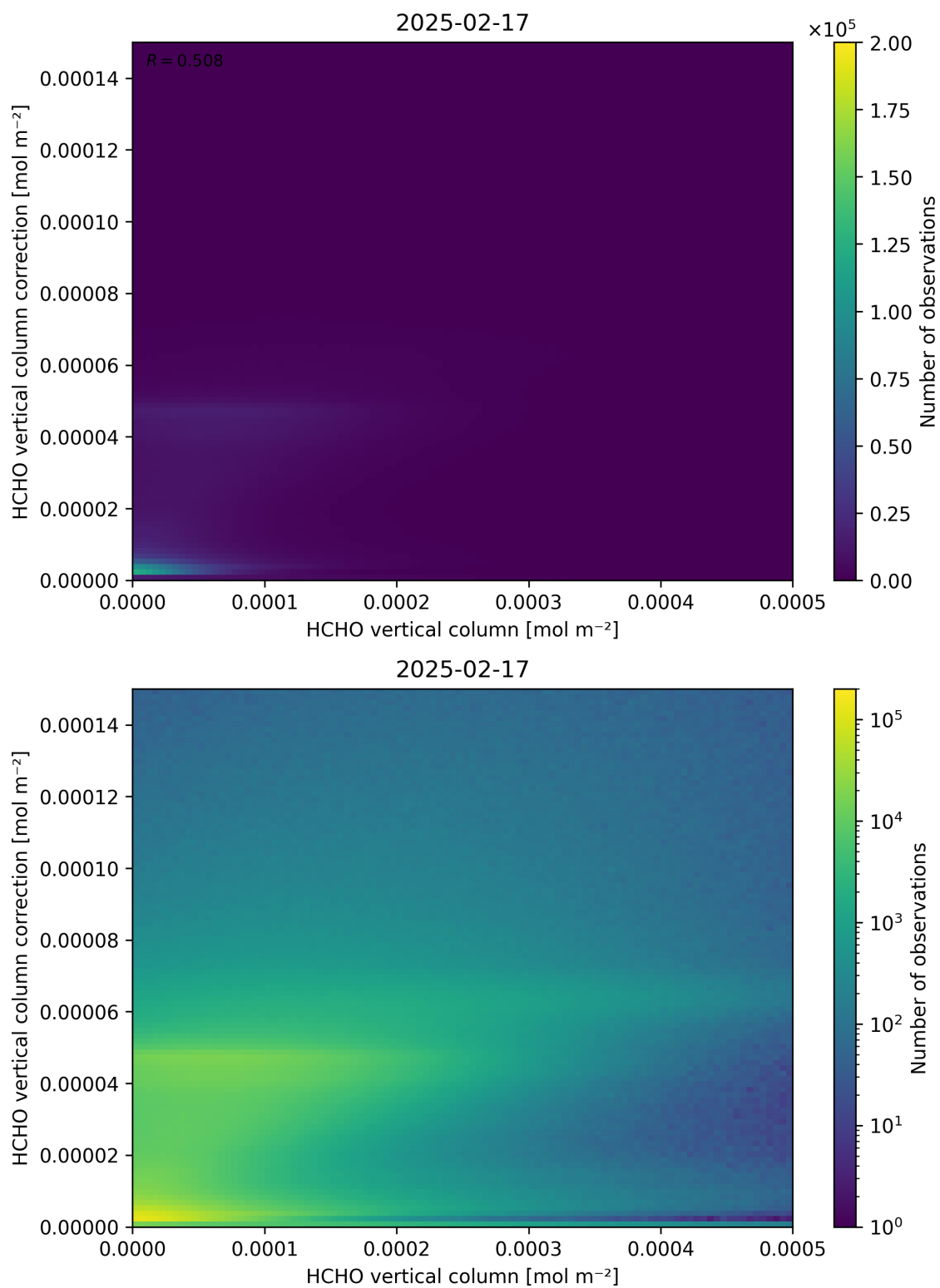
Figure 133: Scatter density plot of “HCHO vertical column” against “HCHO vertical column correction” for 2025-02-16 to 2025-02-18.
