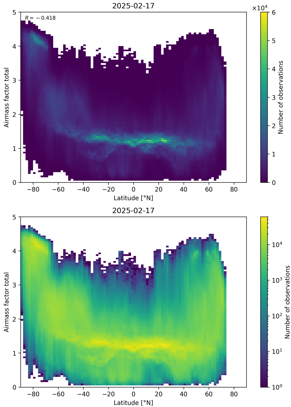
Figure 161: Scatter density plot of “Latitude” against “Airmass factor total” for 2025-02-16 to 2025-02-18.
