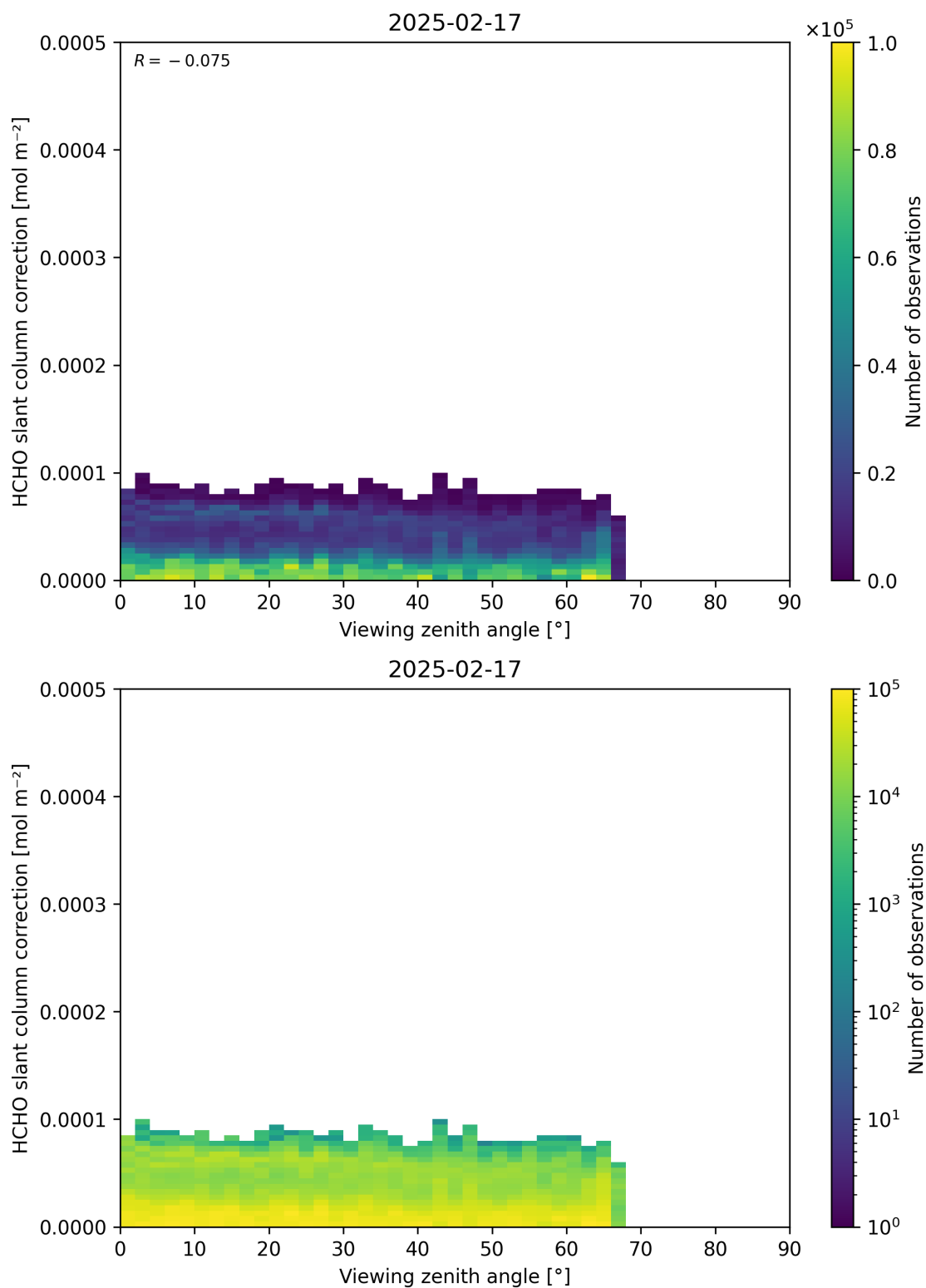
Figure 187: Scatter density plot of “Viewing zenith angle” against “HCHO slant column correction” for 2025-02-16 to 2025-02-18.
