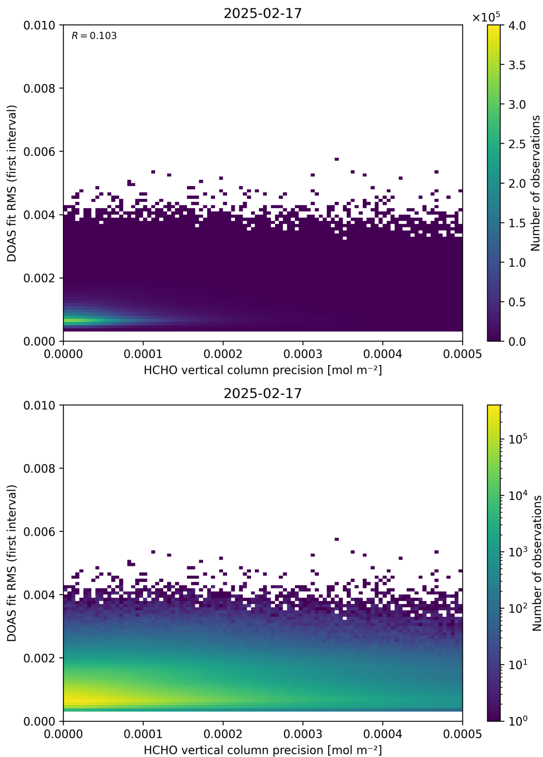
Figure 136: Scatter density plot of “HCHO vertical column precision” against “DOAS fit RMS (first interval)” for 2025-02-16 to 2025-02-18.
