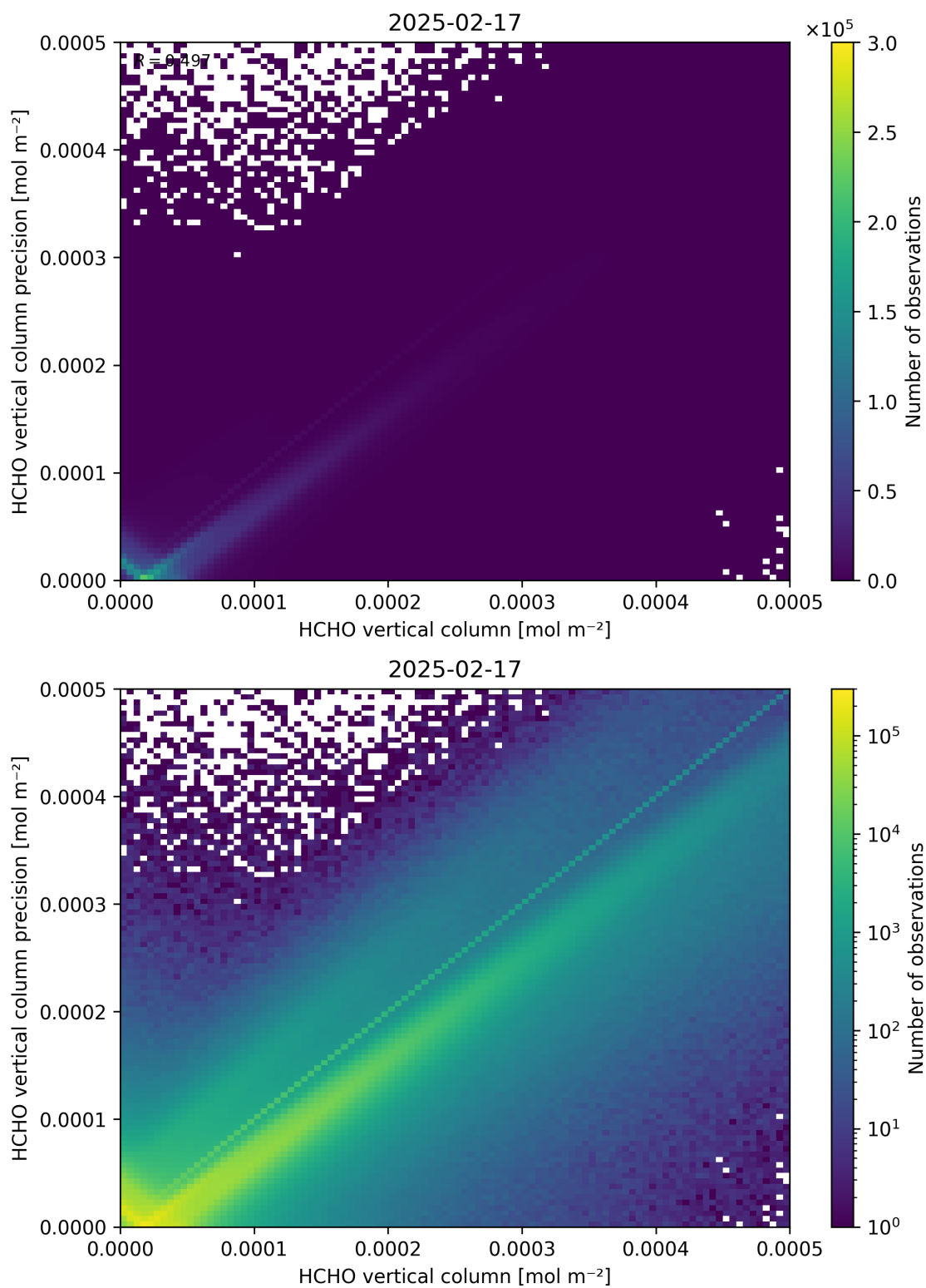
Figure 134: Scatter density plot of “HCHO vertical column” against “HCHO vertical column precision” for 2025-02-16 to 2025-02-18.
