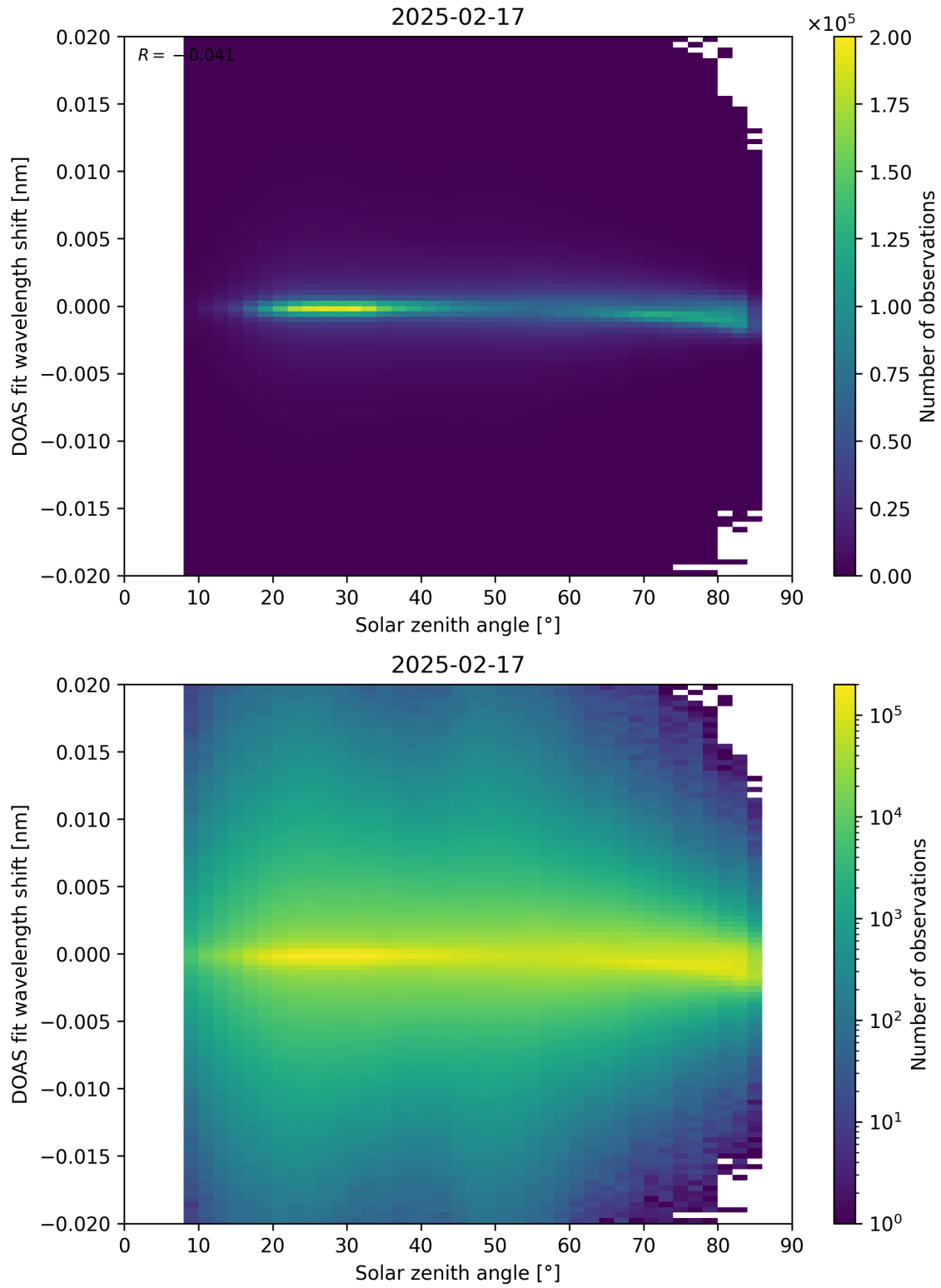
Figure 168: Scatter density plot of “Solar zenith angle” against “DOAS fit wavelength shift” for 2025-02-16 to 2025-02-18.
