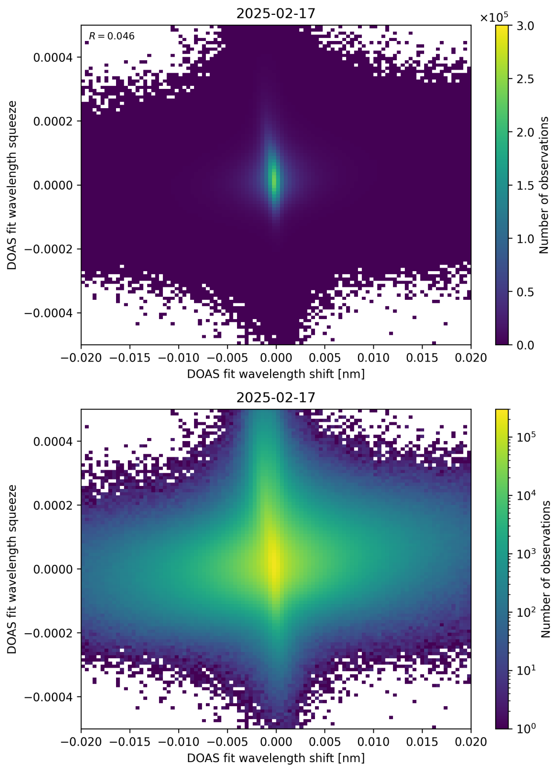
Figure 65: Scatter density plot of “DOAS fit wavelength shift” against “DOAS fit wavelength squeeze” for 2025-02-16 to 2025-02-18.
