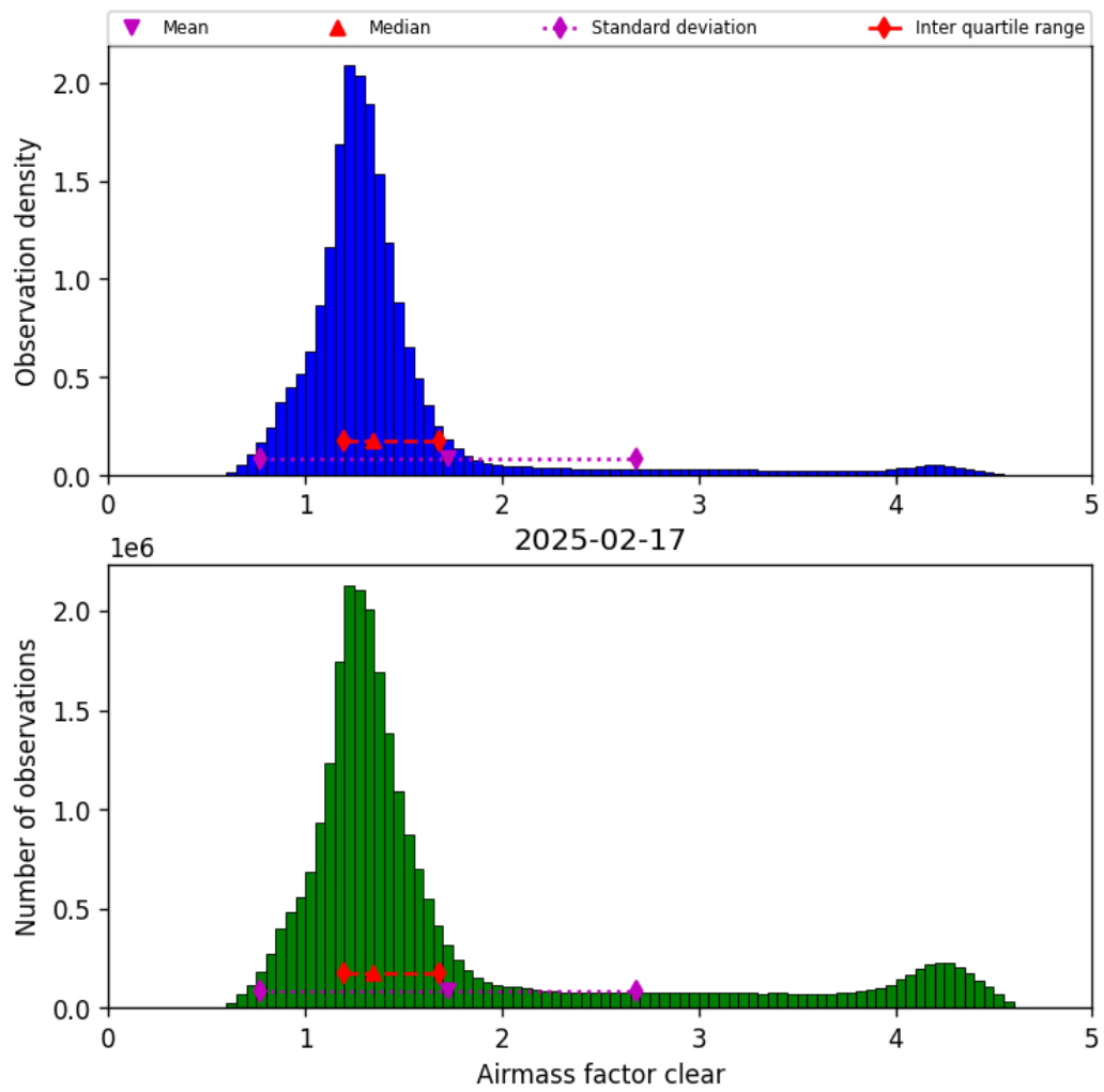
Figure 42: Histogram of “Airmass factor clear” for 2025-02-16 to 2025-02-18
