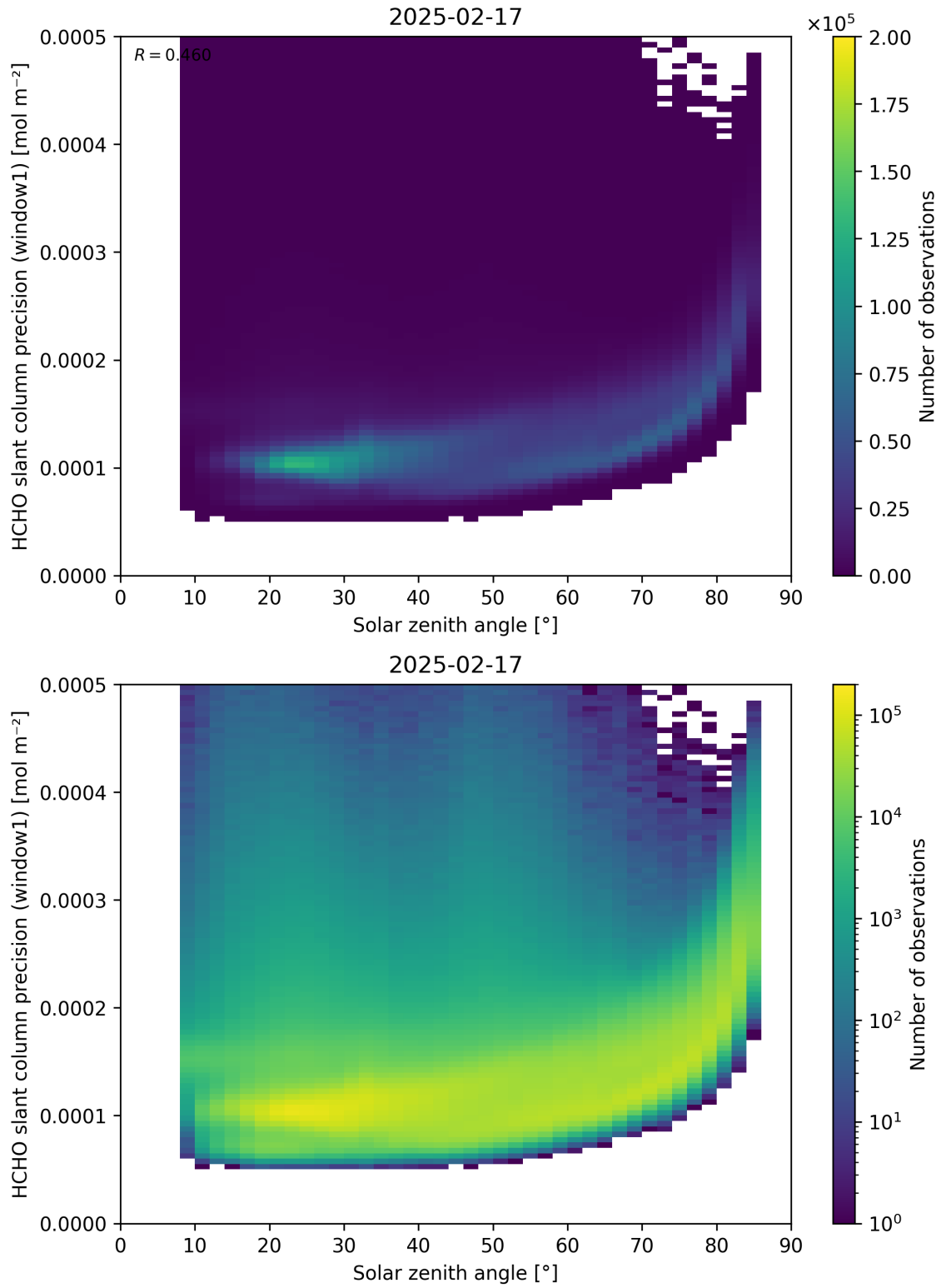
Figure 174: Scatter density plot of “Solar zenith angle” against “HCHO slant column precision (window1)” for 2025-02-16 to 2025-02-18.
