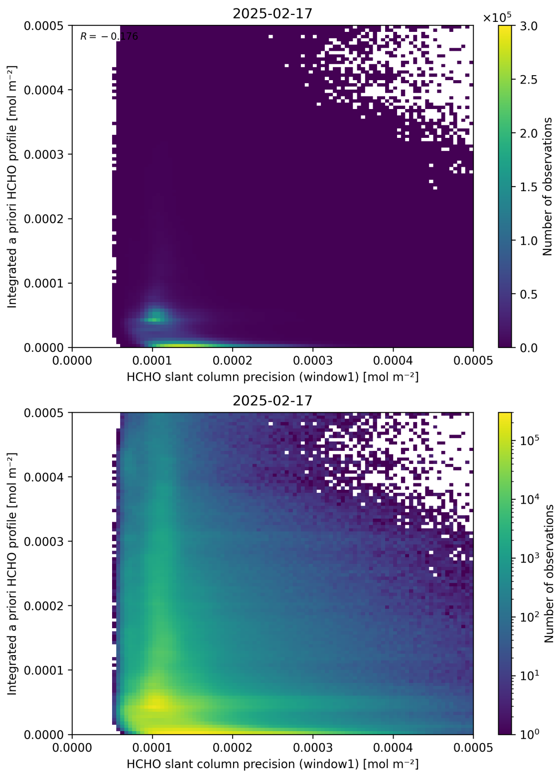
Figure 96: Scatter density plot of “HCHO slant column precision (window1)” against “Integrated a priori HCHO profile” for 2025-02-16 to 2025-02-18.
