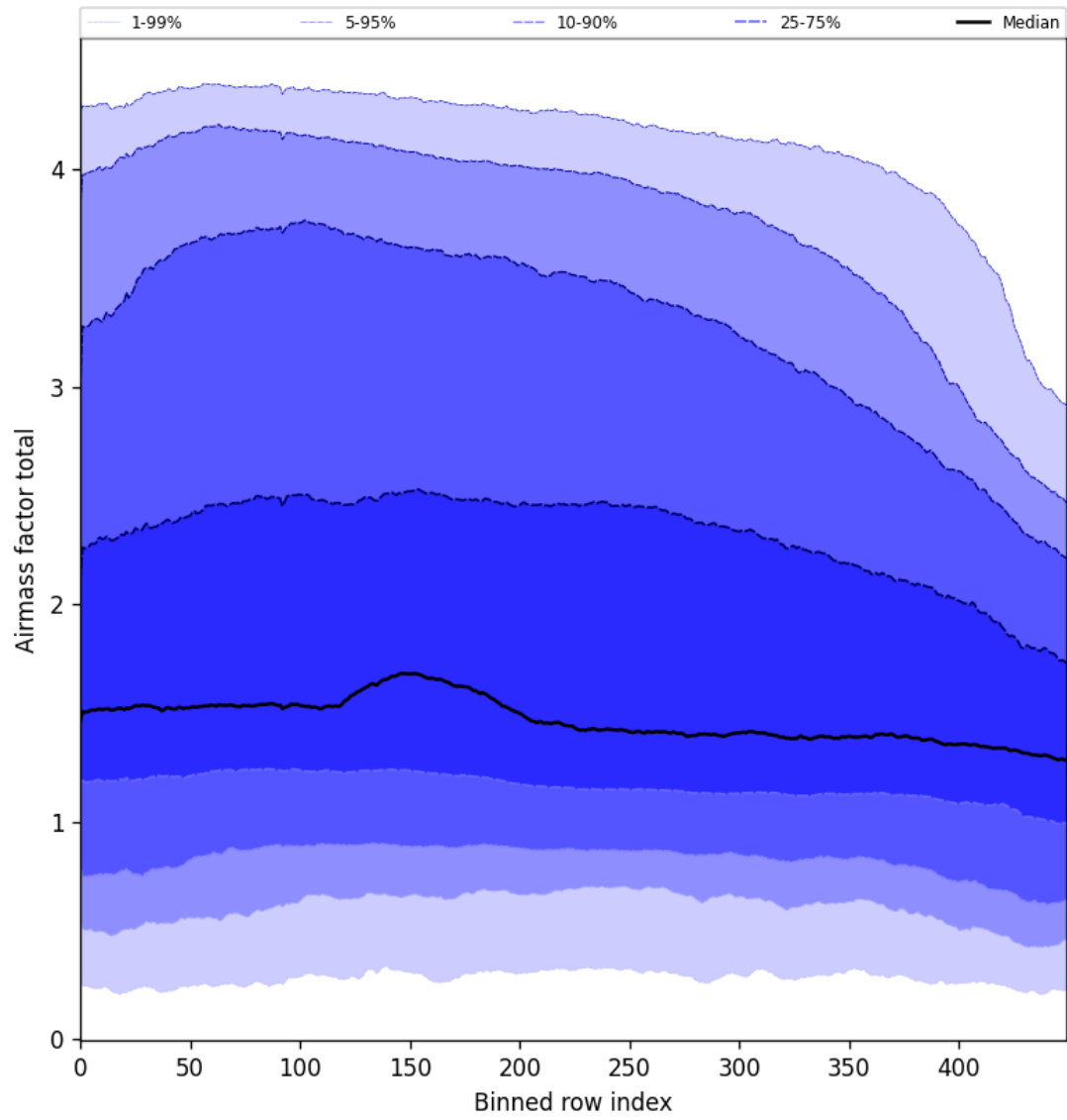
Figure 54: Along track statistics of “Airmass factor total” for 2025-02-16 to 2025-02-18
