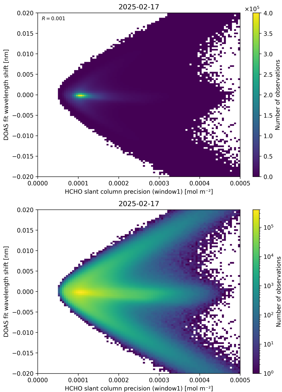
Figure 89: Scatter density plot of “HCHO slant column precision (window1)” against “DOAS fit wavelength shift” for 2025-02-16 to 2025-02-18.
