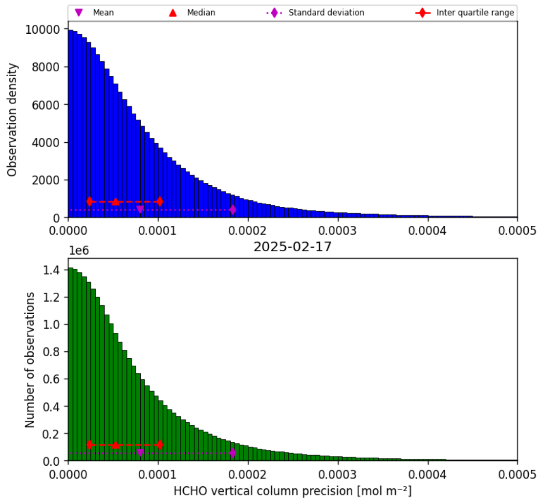
Figure 36: Histogram of “HCHO vertical column precision” for 2025-02-16 to 2025-02-18
