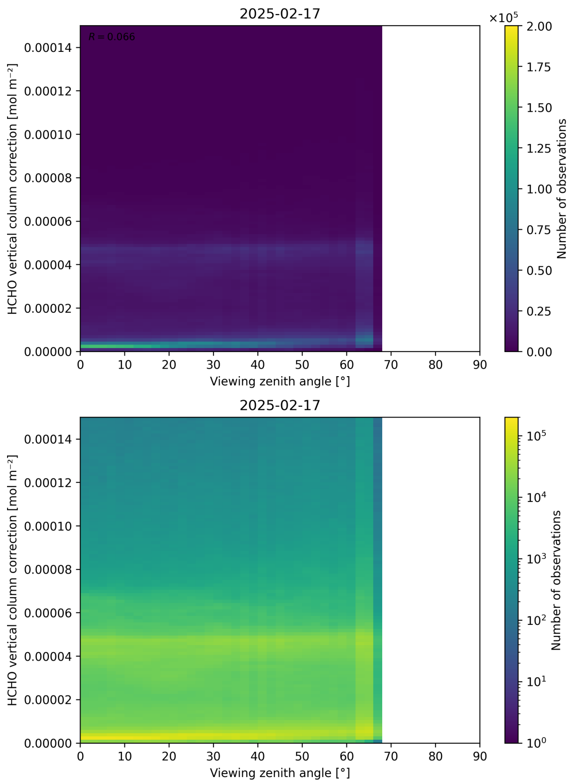
Figure 193: Scatter density plot of “Viewing zenith angle” against “HCHO vertical column correction” for 2025-02-16 to 2025-02-18.
