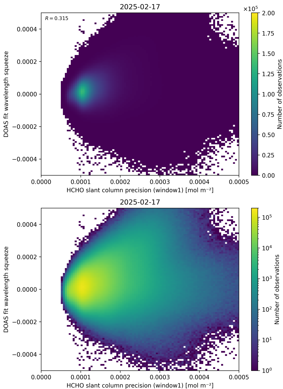
Figure 90: Scatter density plot of “HCHO slant column precision (window1)” against “DOAS fit wavelength squeeze” for 2025-02-16 to 2025-02-18.
