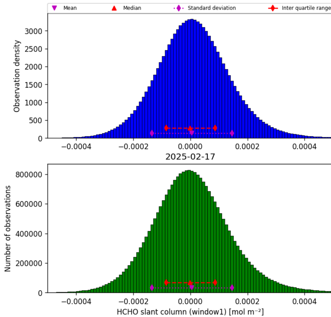
Figure 38: Histogram of “HCHO slant column (window1)” for 2025-02-16 to 2025-02-18
