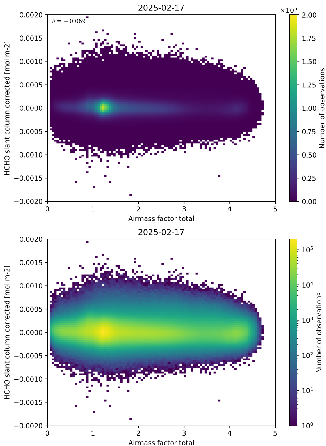
Figure 101: Scatter density plot of “Airmass factor total” against “HCHO slant column corrected” for 2025-02-16 to 2025-02-18.
