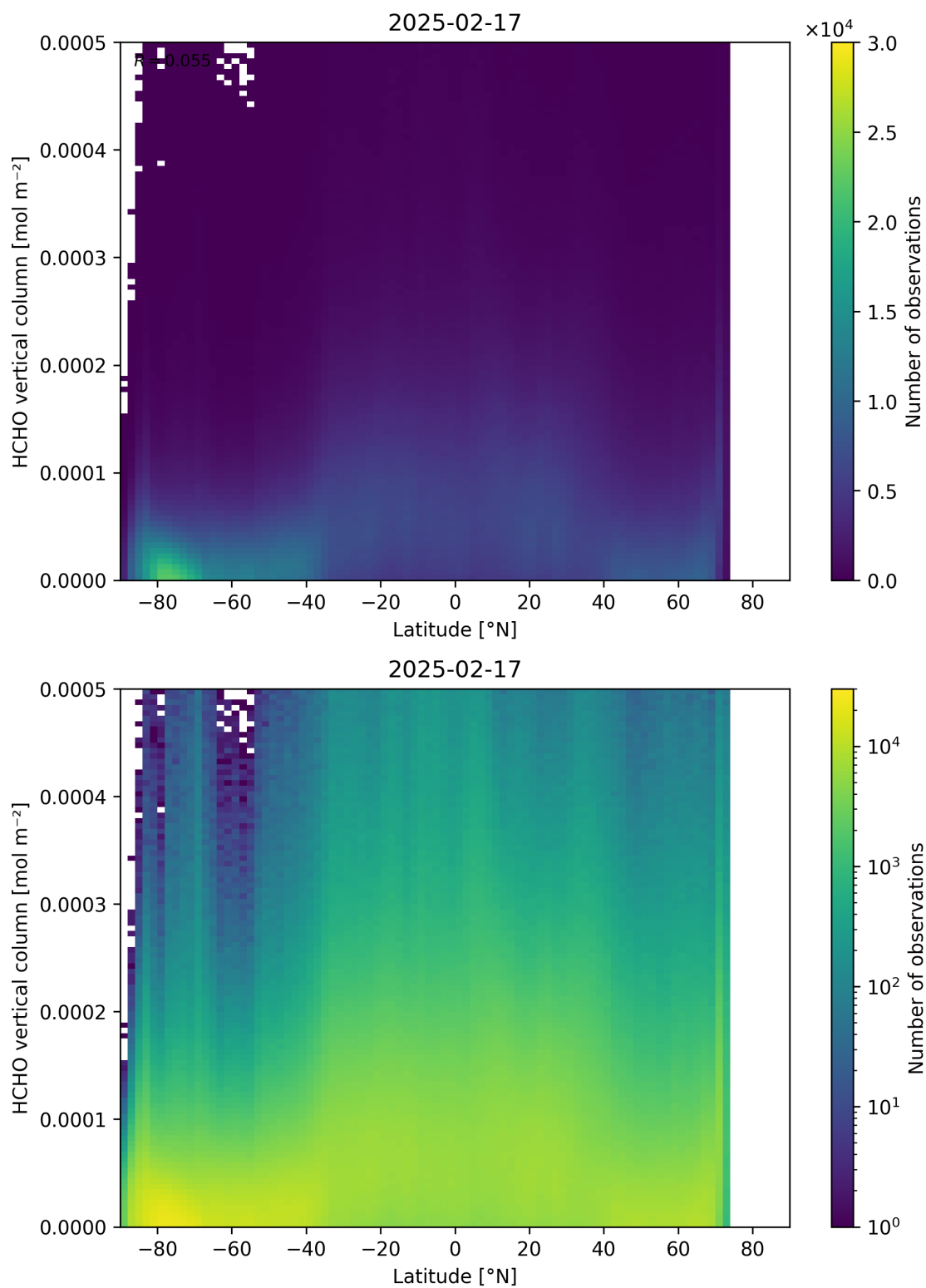
Figure 163: Scatter density plot of “Latitude” against “HCHO vertical column” for 2025-02-16 to 2025-02-18.
