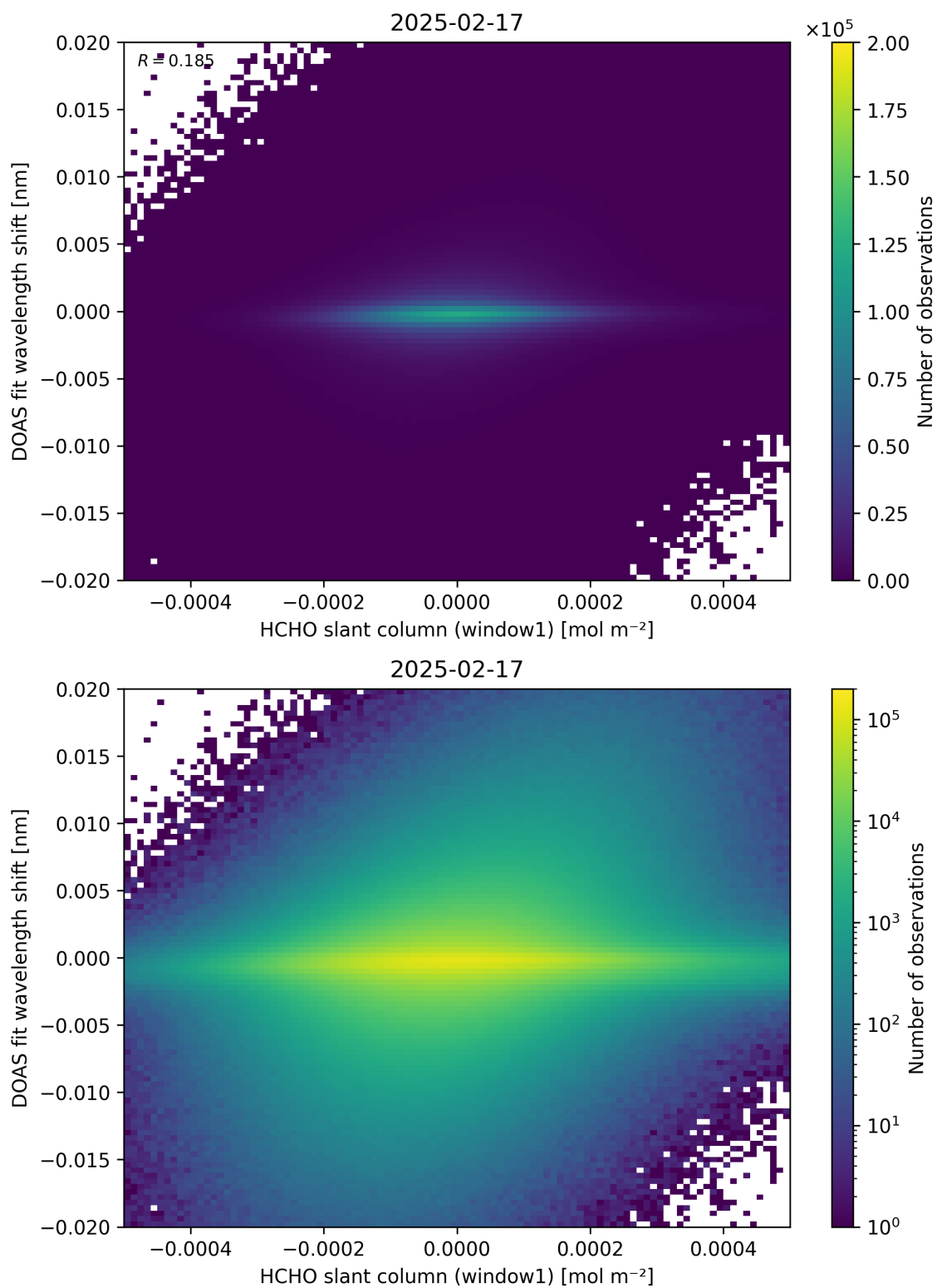
Figure 79: Scatter density plot of “HCHO slant column (window1)” against “DOAS fit wavelength shift” for 2025-02-16 to 2025-02-18.
