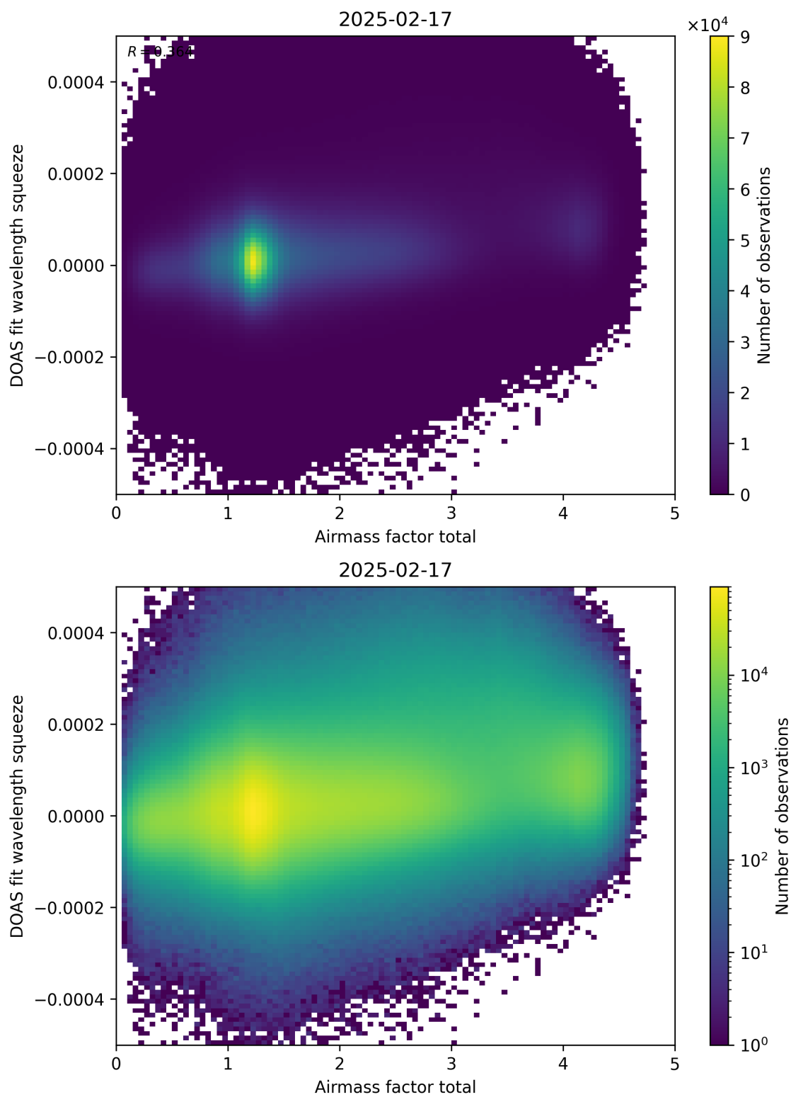
Figure 99: Scatter density plot of “Airmass factor total” against “DOAS fit wavelength squeeze” for 2025-02-16 to 2025-02-18.
