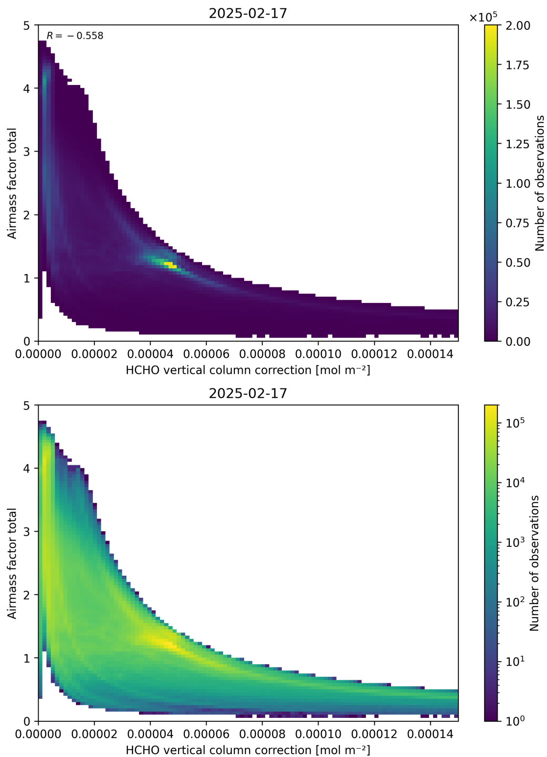
Figure 120: Scatter density plot of “HCHO vertical column correction” against “Airmass factor total” for 2025-02-16 to 2025-02-18.
