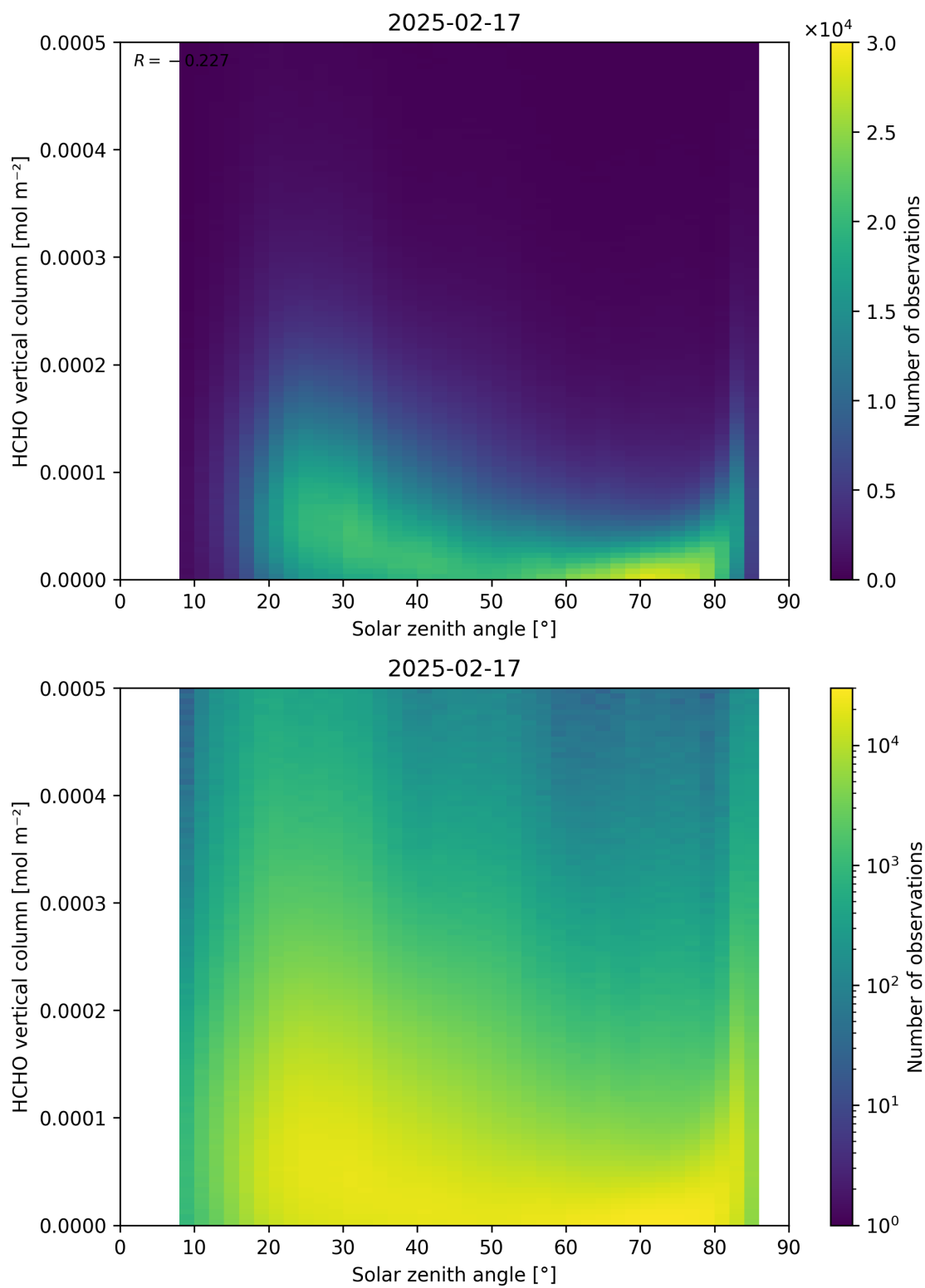
Figure 177: Scatter density plot of “Solar zenith angle” against “HCHO vertical column” for 2025-02-16 to 2025-02-18.
