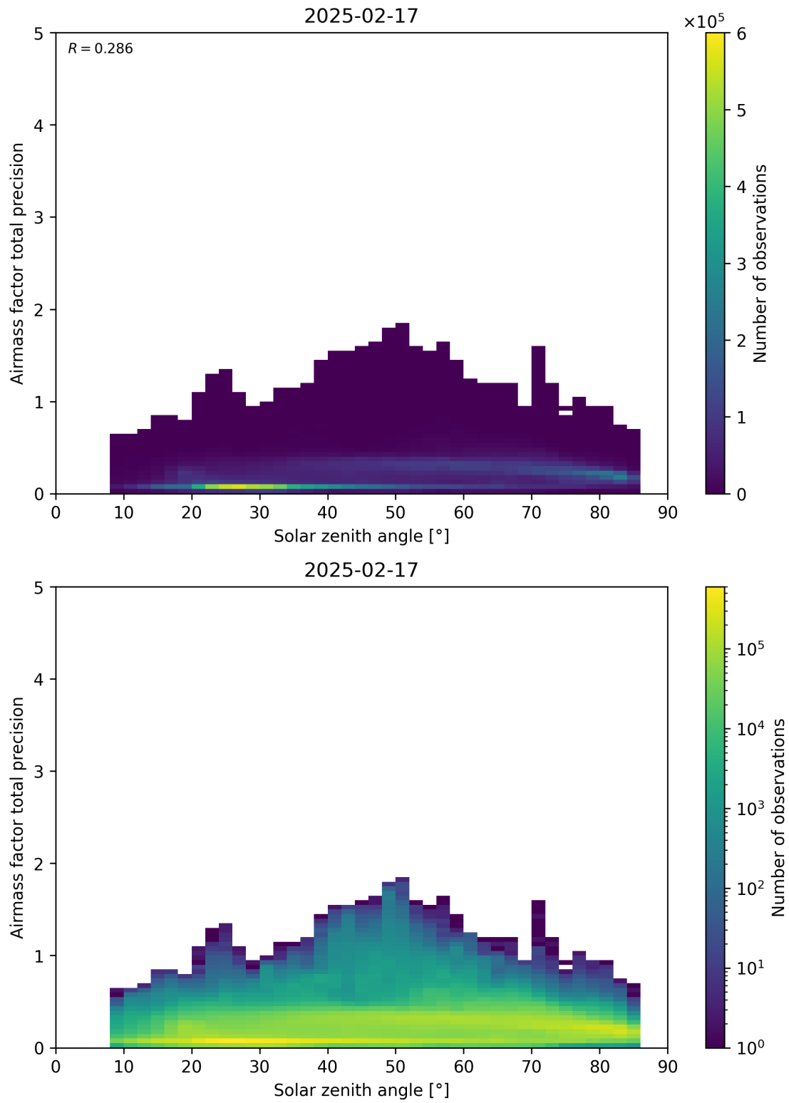
Figure 176: Scatter density plot of “Solar zenith angle” against “Airmass factor total precision” for 2025-02-16 to 2025-02-18.
