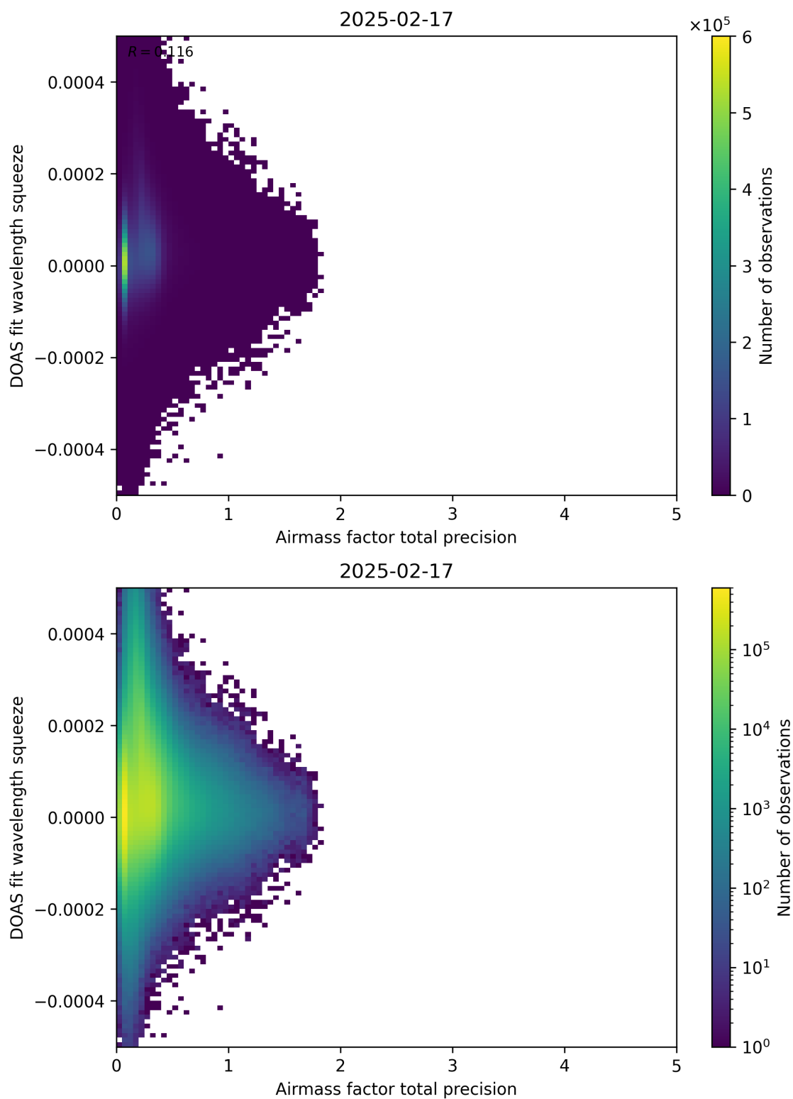
Figure 107: Scatter density plot of “Airmass factor total precision” against “DOAS fit wavelength squeeze” for 2025-02-16 to 2025-02-18.
