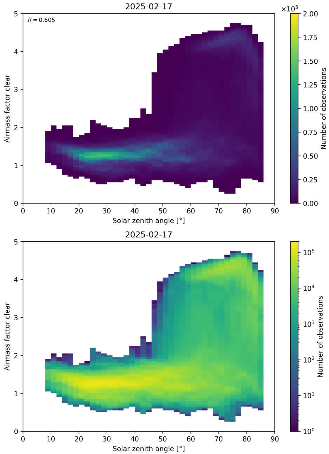
Figure 170: Scatter density plot of “Solar zenith angle” against “Airmass factor clear” for 2025-02-16 to 2025-02-18.
