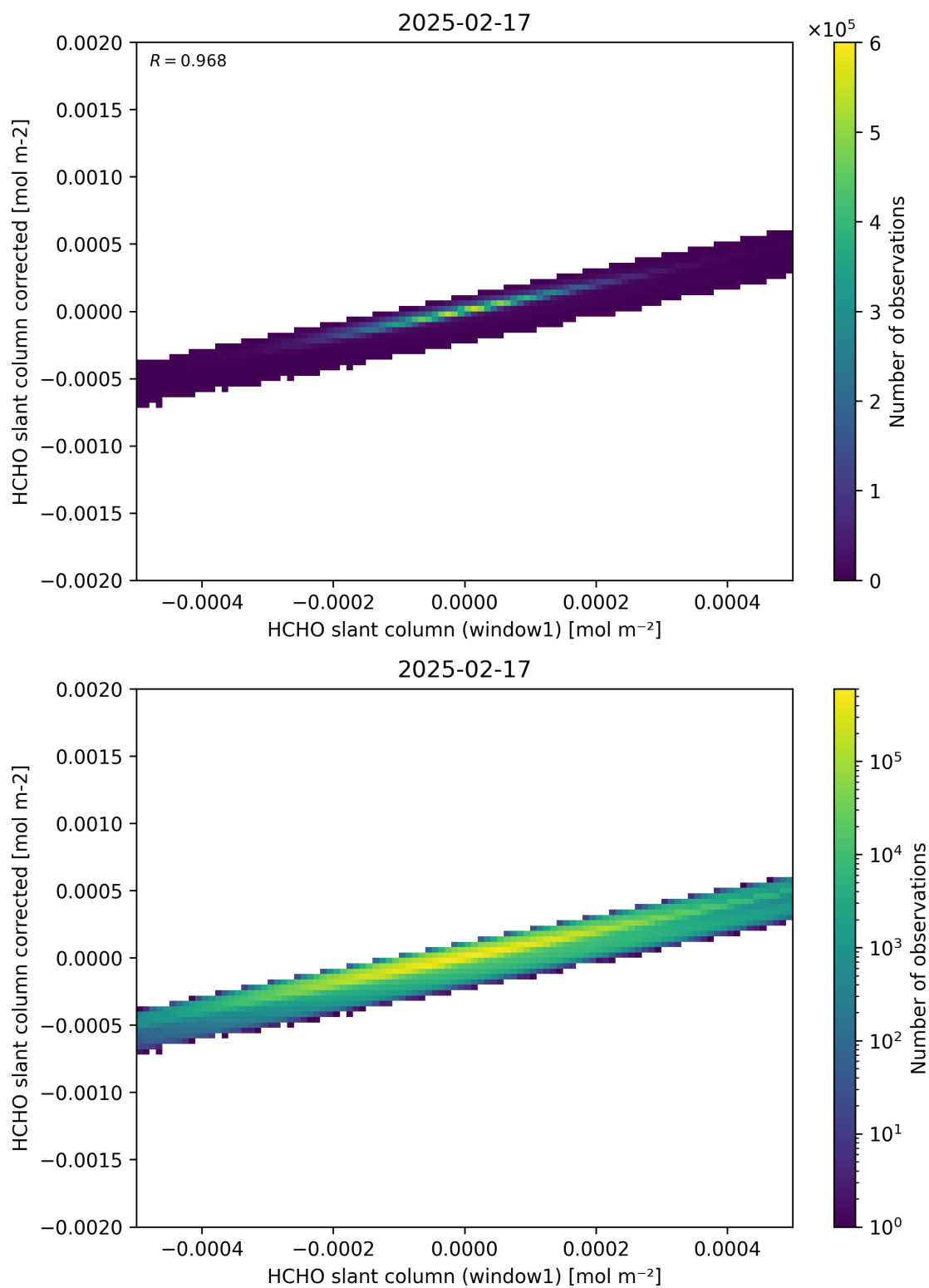
Figure 82: Scatter density plot of “HCHO slant column (window1)” against “HCHO slant column corrected” for 2025-02-16 to 2025-02-18.
