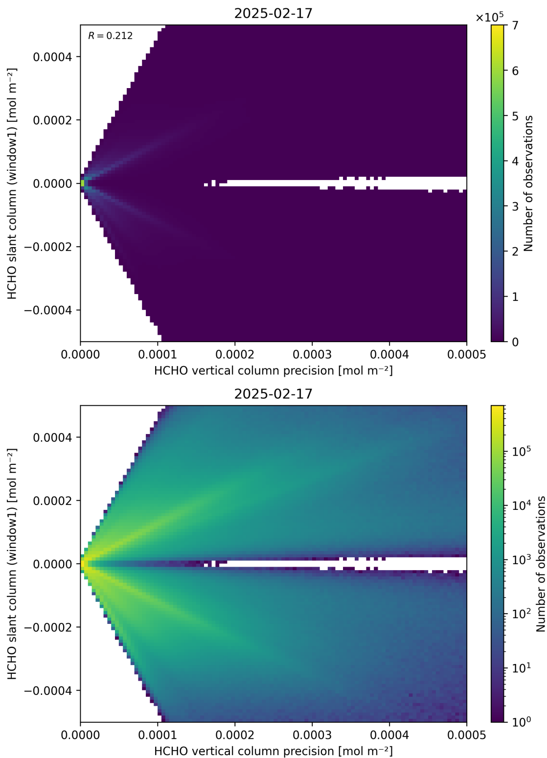
Figure 142: Scatter density plot of “HCHO vertical column precision” against “HCHO slant column (window1)” for 2025-02-16 to 2025-02-18.
