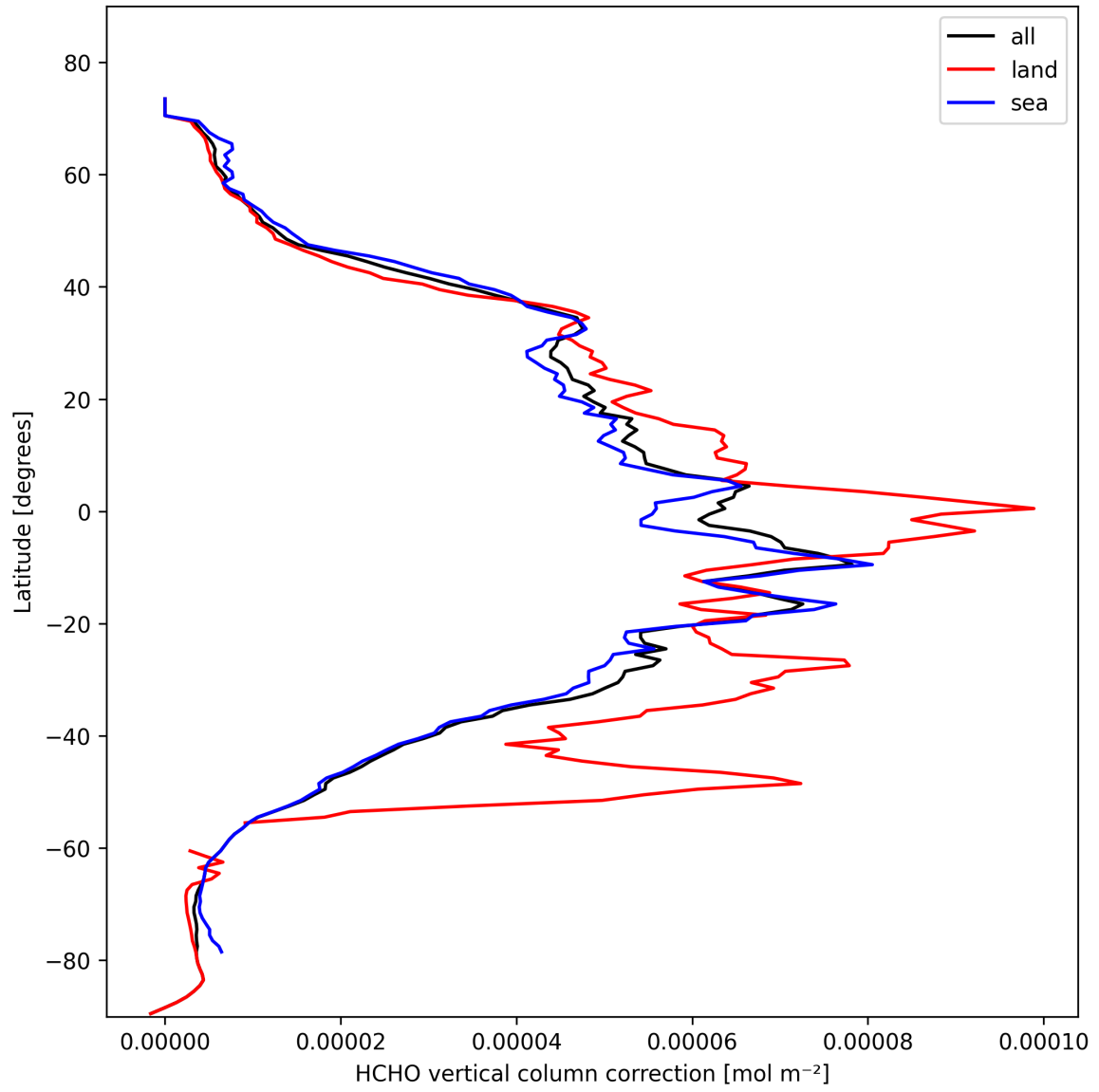
Figure 23: Zonal average of “HCHO vertical column correction” for 2025-02-16 to 2025-02-18.
