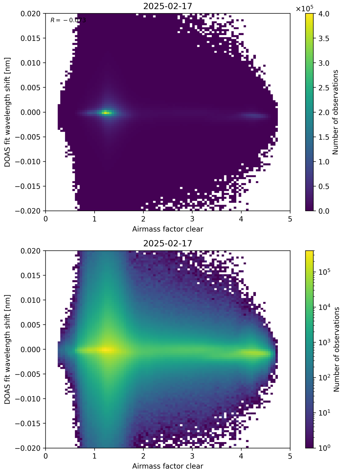
Figure 72: Scatter density plot of “Airmass factor clear” against “DOAS fit wavelength shift” for 2025-02-16 to 2025-02-18.
