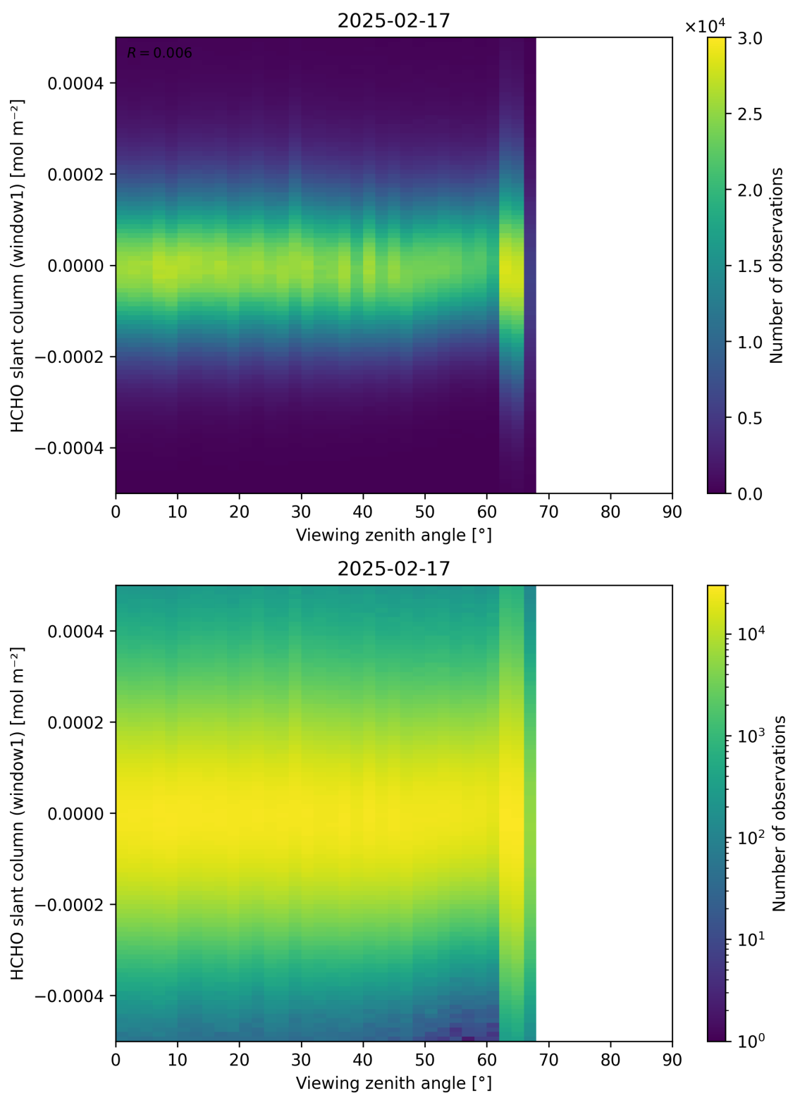
Figure 188: Scatter density plot of “Viewing zenith angle” against “HCHO slant column (window1)” for 2025-02-16 to 2025-02-18.
