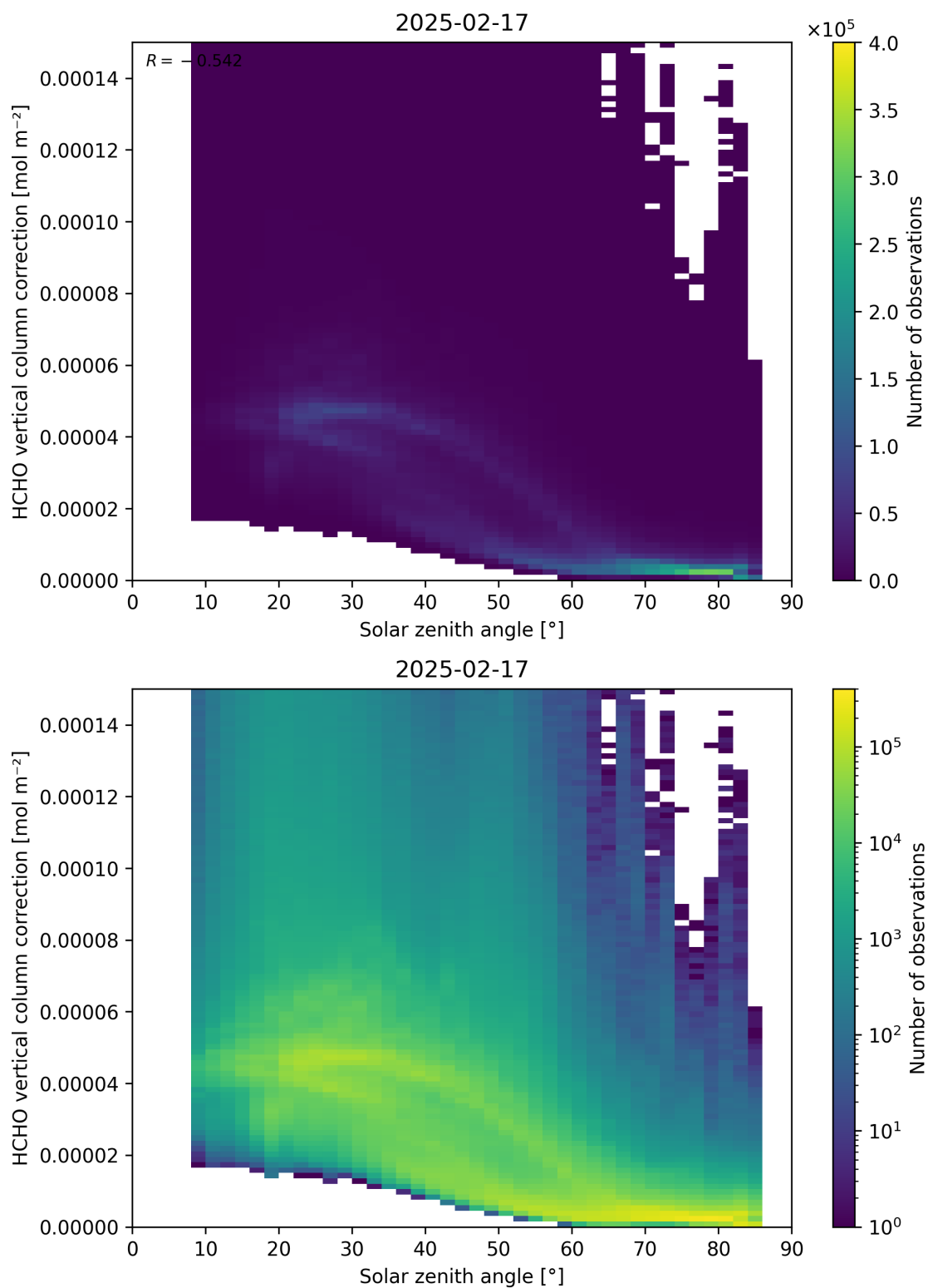
Figure 178: Scatter density plot of “Solar zenith angle” against “HCHO vertical column correction” for 2025-02-16 to 2025-02-18.
