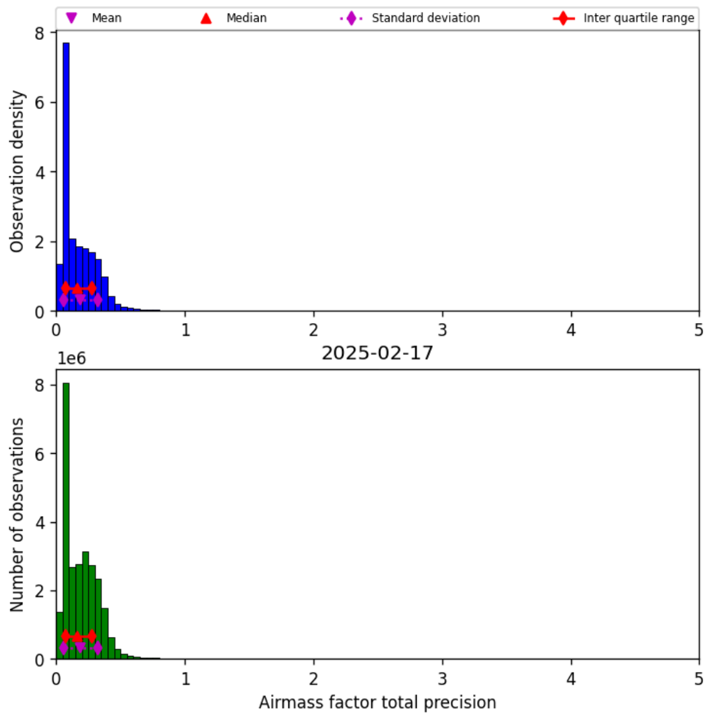
Figure 41: Histogram of “Airmass factor total precision” for 2025-02-16 to 2025-02-18
