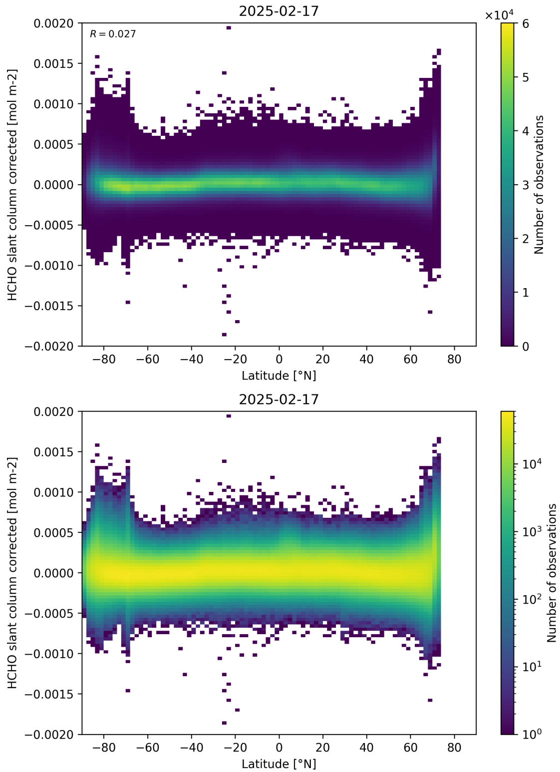
Figure 157: Scatter density plot of “Latitude” against “HCHO slant column corrected” for 2025-02-16 to 2025-02-18.
