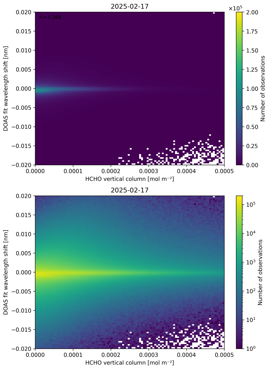
Figure 124: Scatter density plot of “HCHO vertical column” against “DOAS fit wavelength shift” for 2025-02-16 to 2025-02-18.
