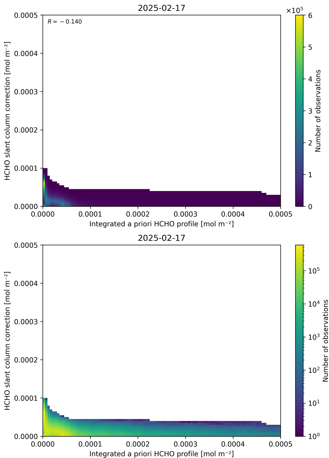
Figure 152: Scatter density plot of “Integrated a priori HCHO profile” against “HCHO slant column correction” for 2025-02-16 to 2025-02-18.
