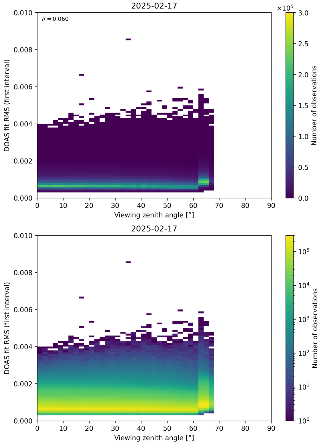
Figure 182: Scatter density plot of “Viewing zenith angle” against “DOAS fit RMS (first interval)” for 2025-02-16 to 2025-02-18.
