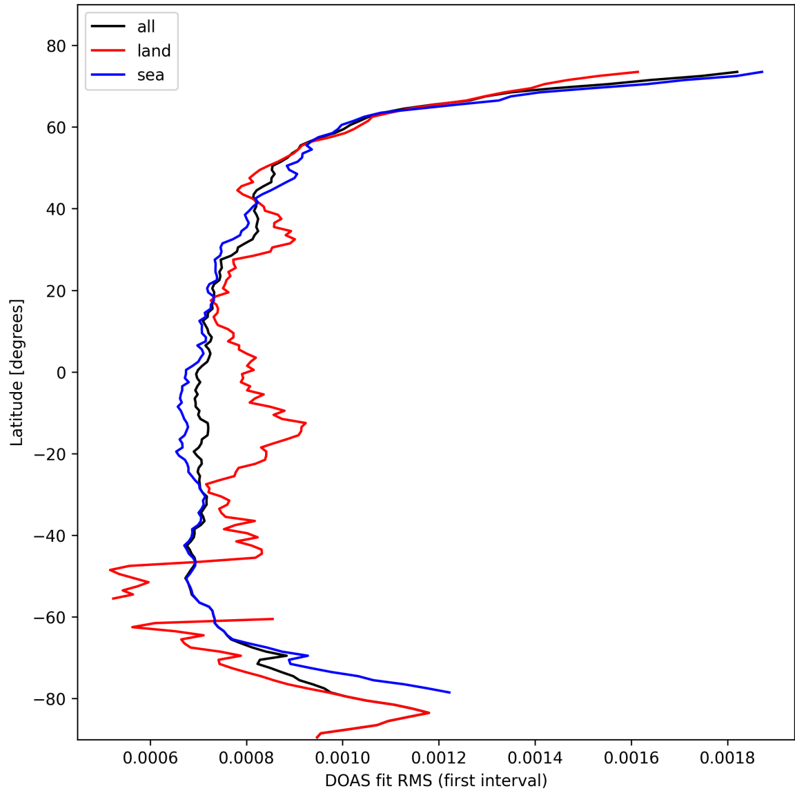
Figure 32: Zonal average of “DOAS fit RMS (first interval)” for 2025-02-16 to 2025-02-18.
