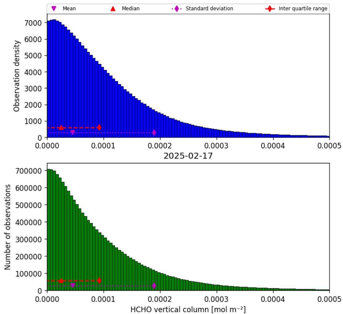
Figure 35: Histogram of “HCHO vertical column” for 2025-02-16 to 2025-02-18
