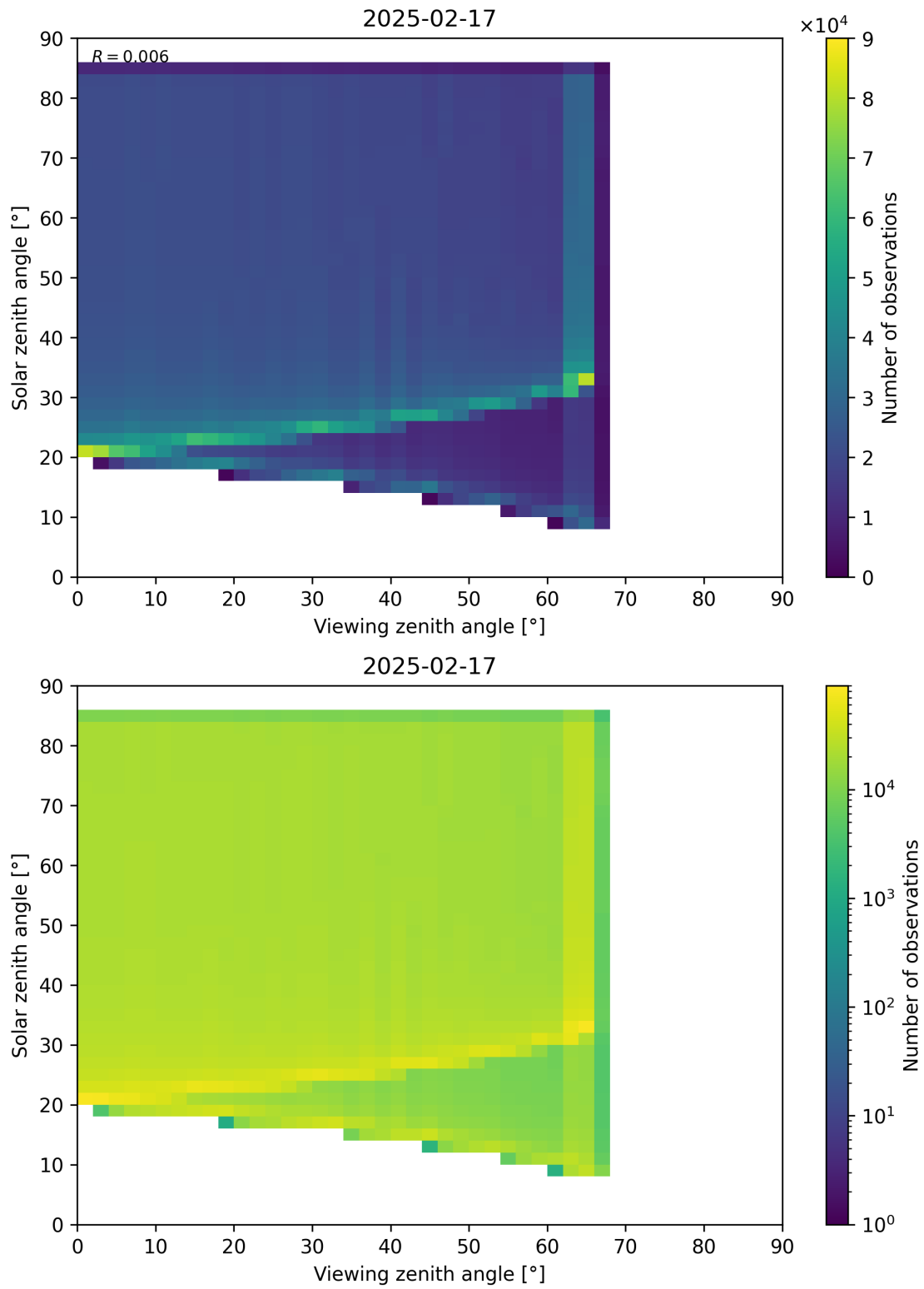
Figure 197: Scatter density plot of “Viewing zenith angle” against “Solar zenith angle” for 2025-02-16 to 2025-02-18.
