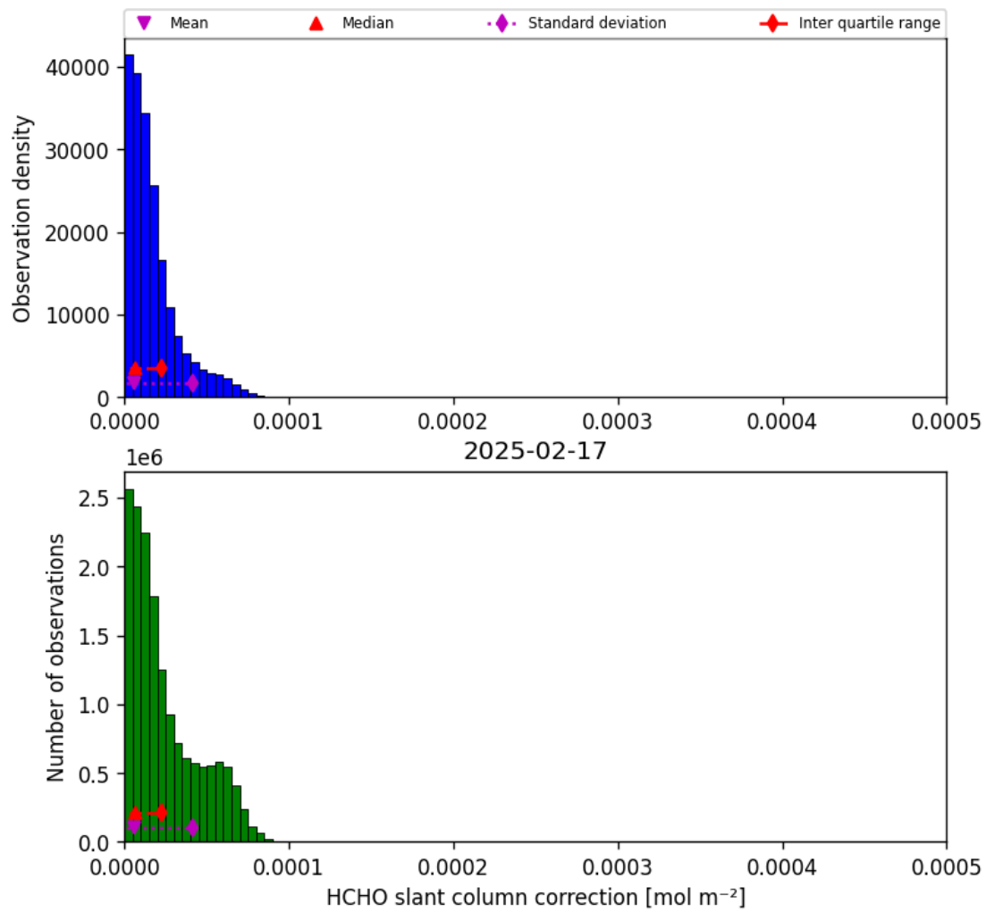
Figure 47: Histogram of “HCHO slant column correction” for 2025-02-16 to 2025-02-18
