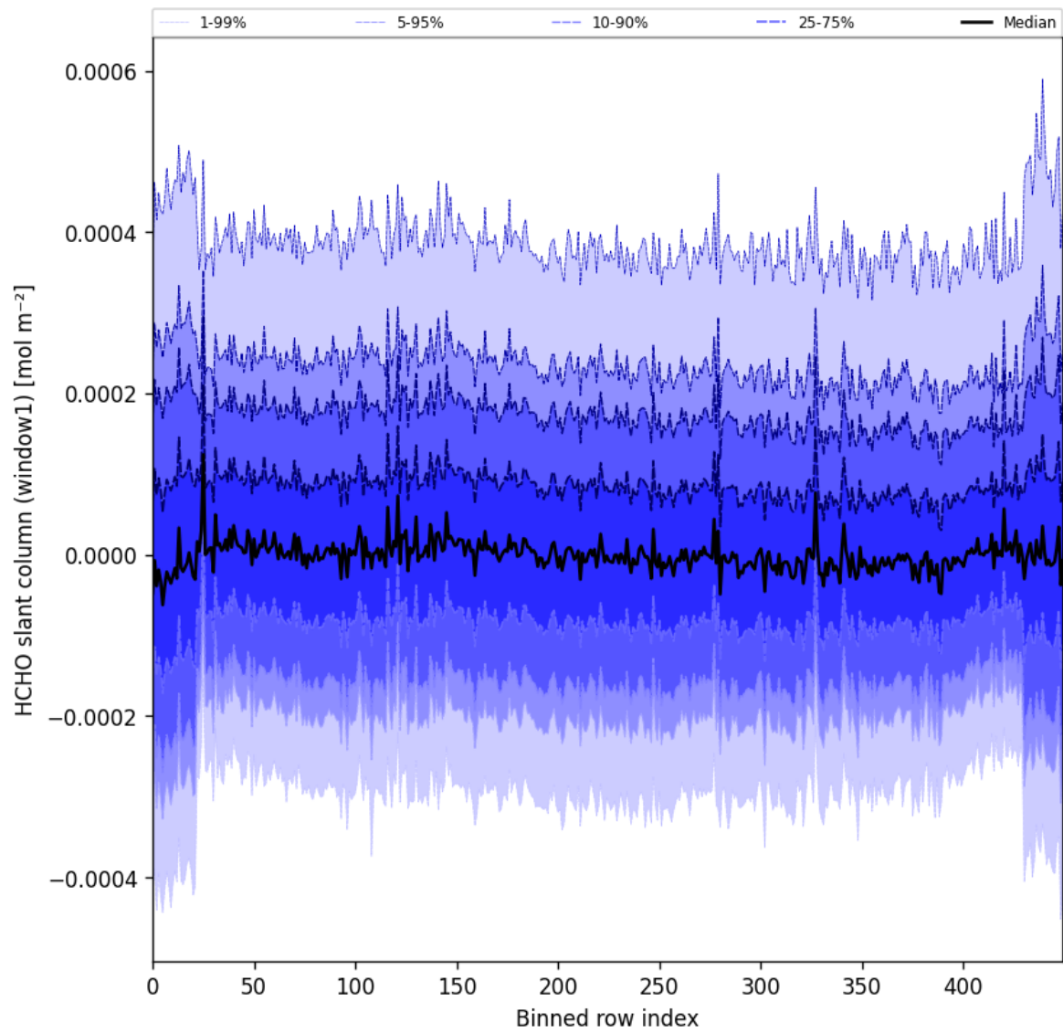
Figure 52: Along track statistics of “HCHO slant column (window1)” for 2025-02-16 to 2025-02-18
