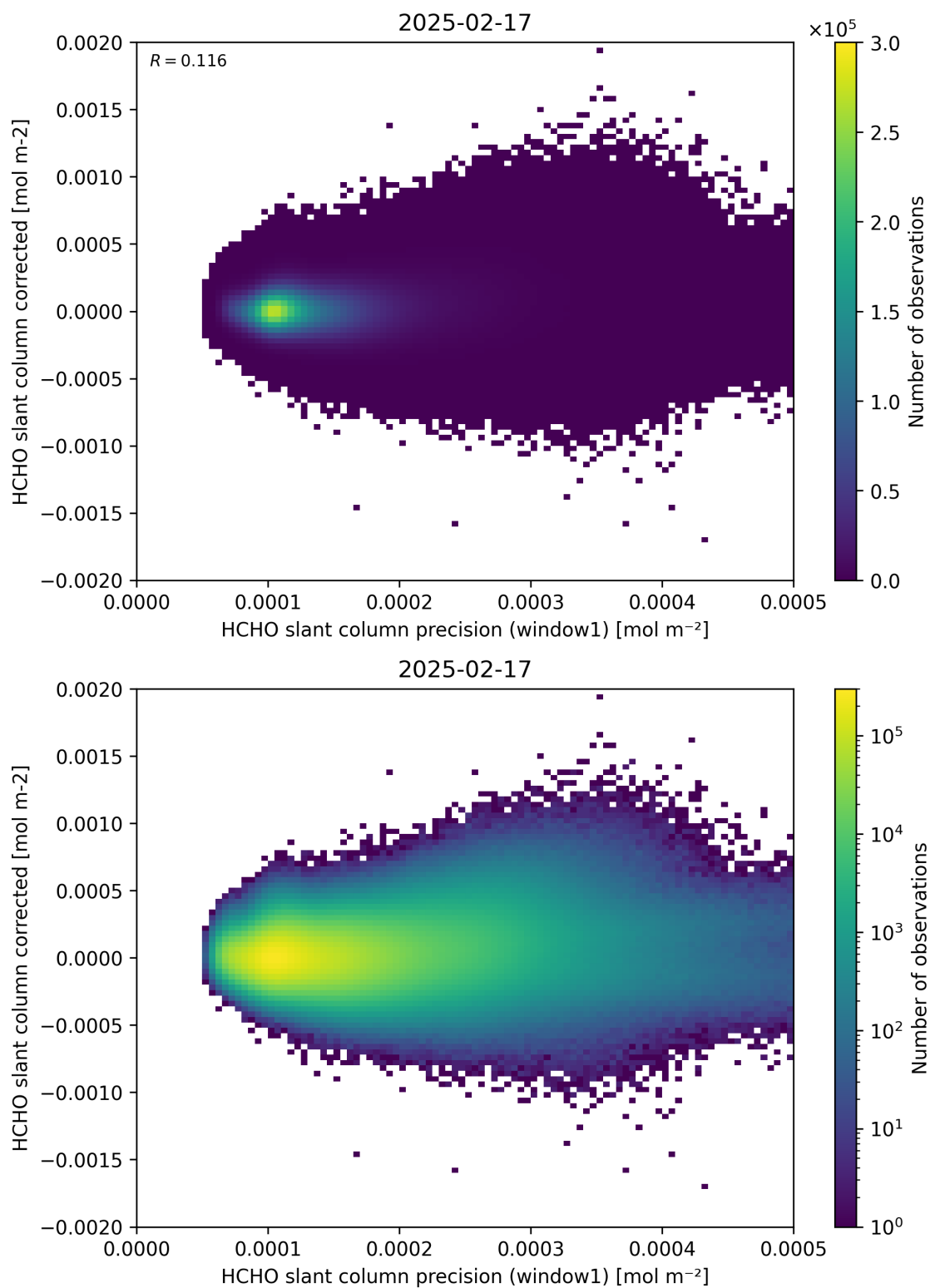
Figure 92: Scatter density plot of “HCHO slant column precision (window1)” against “HCHO slant column corrected” for 2025-02-16 to 2025-02-18.
