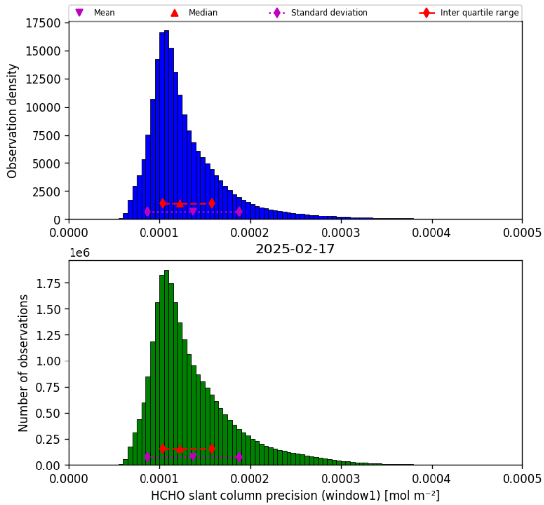
Figure 39: Histogram of “HCHO slant column precision (window1)” for 2025-02-16 to 2025-02-18
