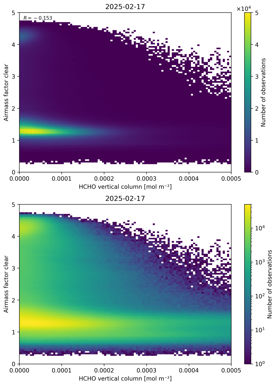
Figure 126: Scatter density plot of “HCHO vertical column” against “Airmass factor clear” for 2025-02-16 to 2025-02-18.
