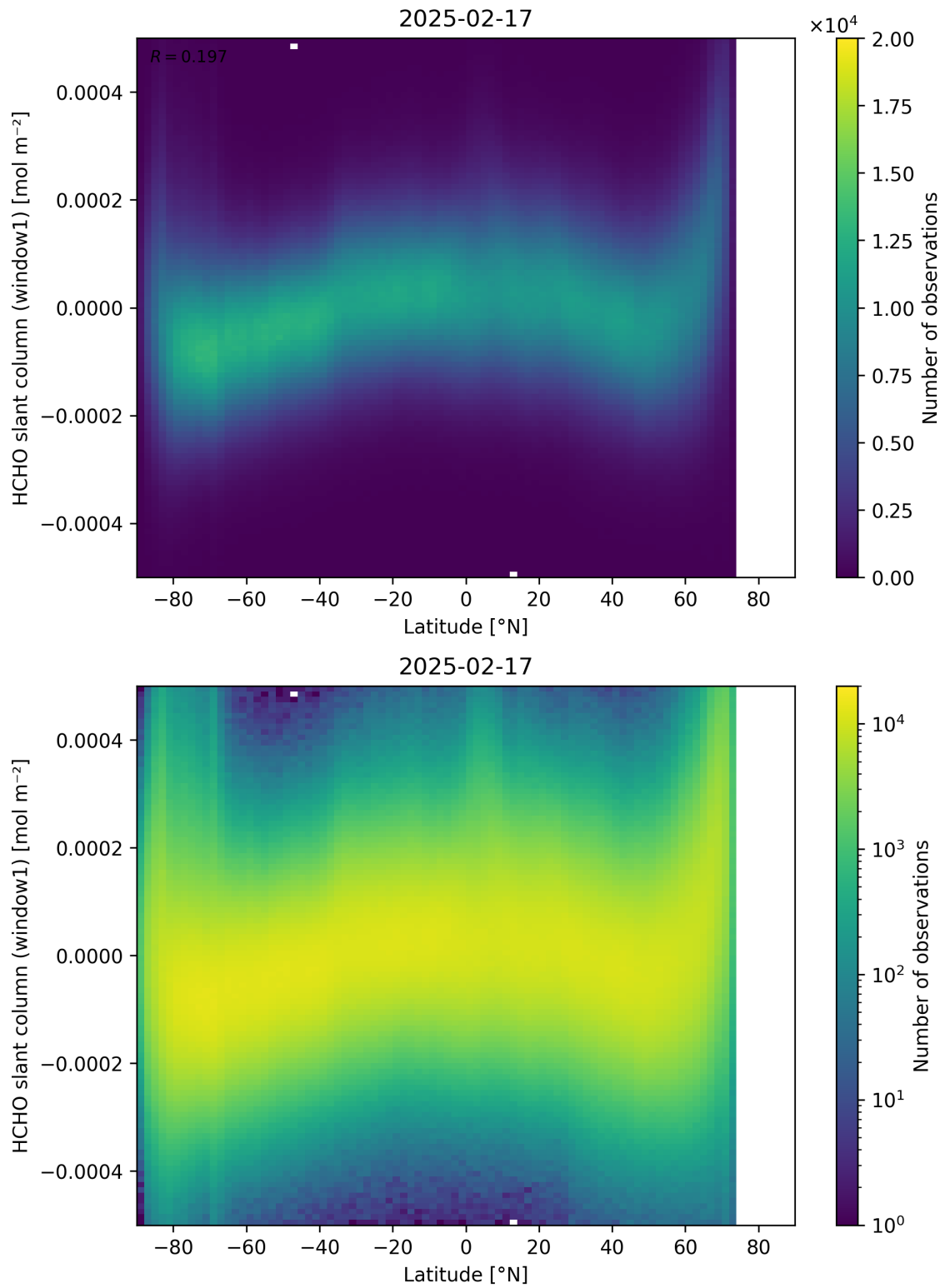
Figure 159: Scatter density plot of “Latitude” against “HCHO slant column (window1)” for 2025-02-16 to 2025-02-18.
