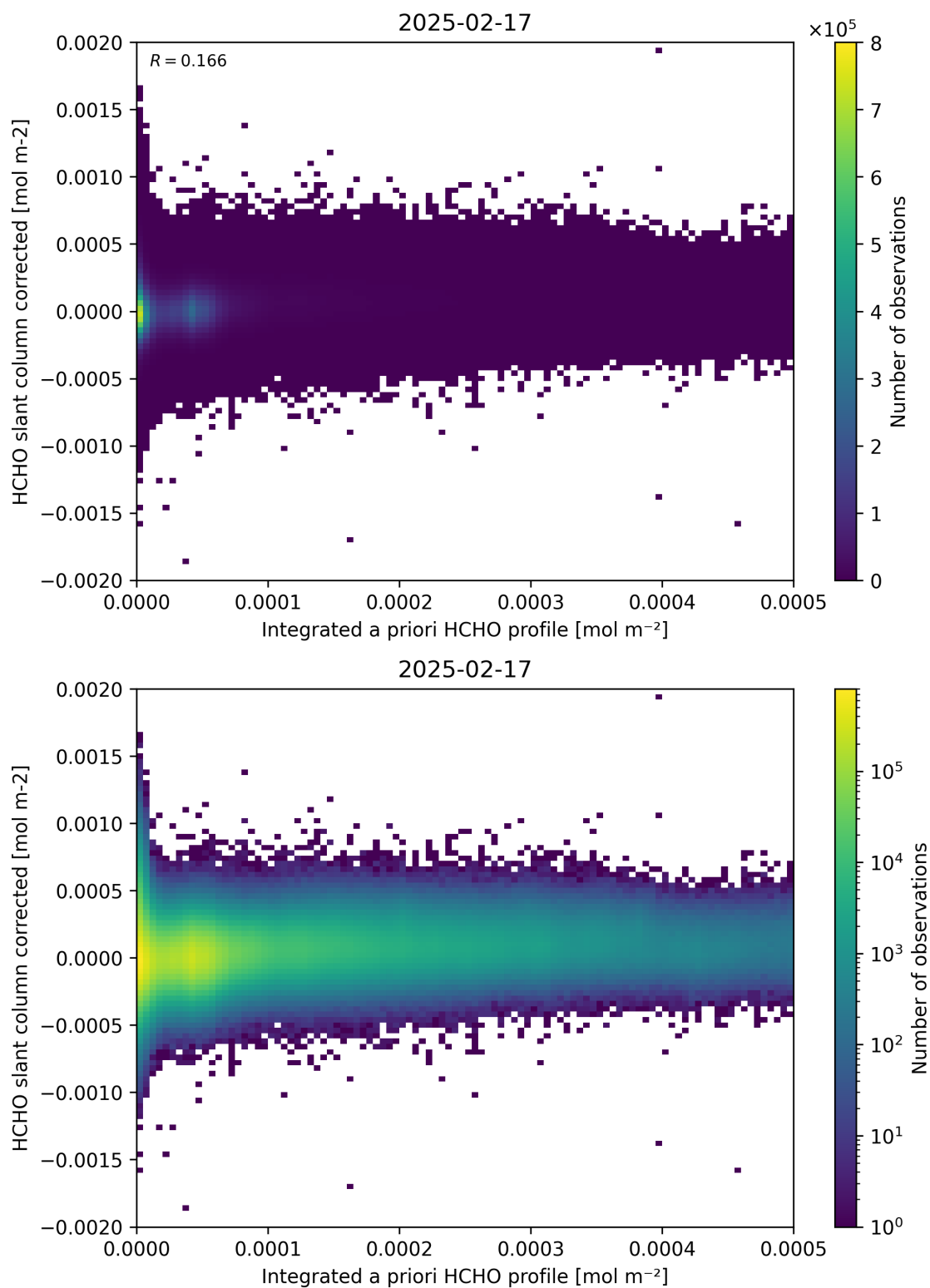
Figure 151: Scatter density plot of “Integrated a priori HCHO profile” against “HCHO slant column corrected” for 2025-02-16 to 2025-02-18.
