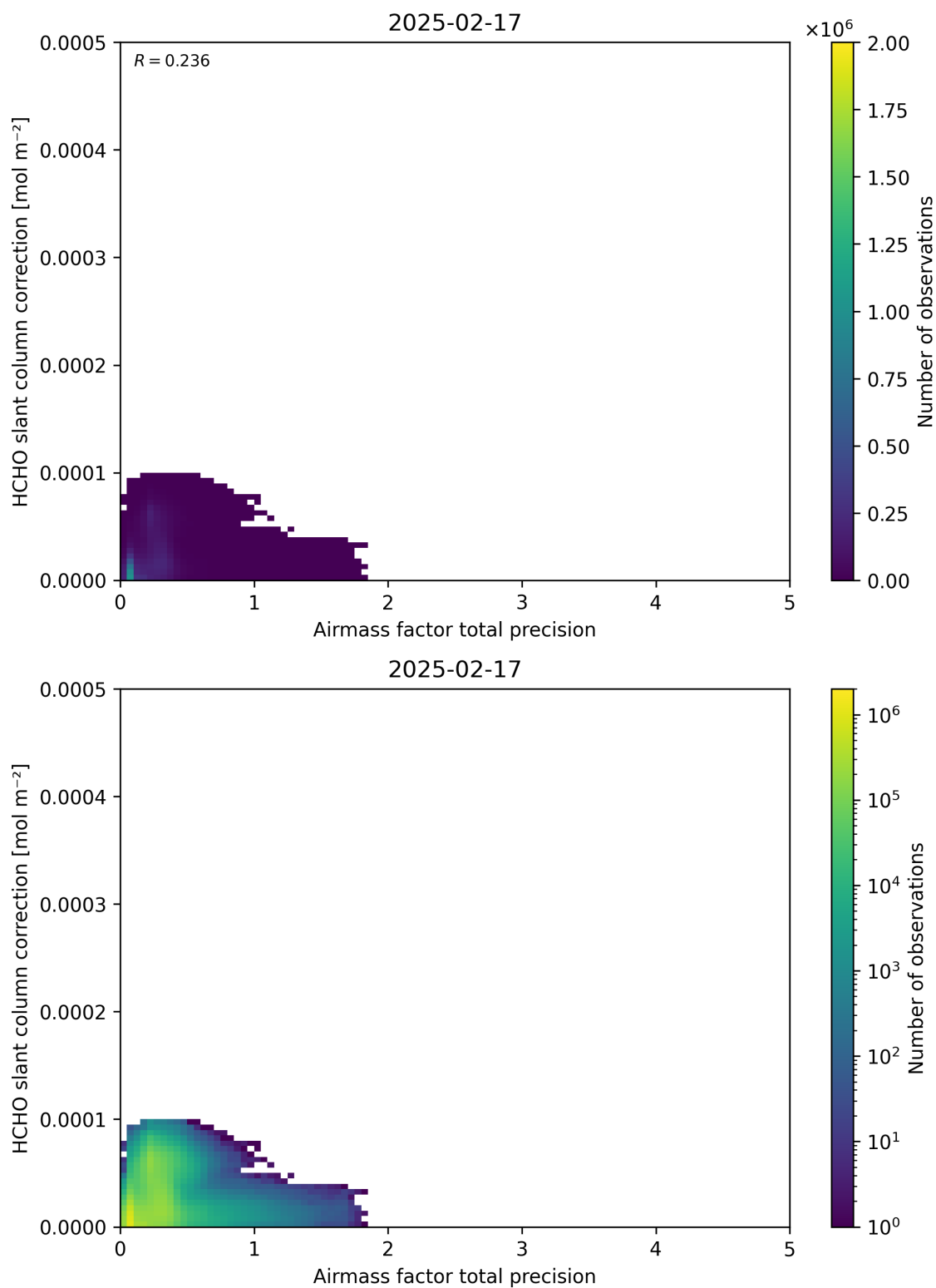
Figure 110: Scatter density plot of “Airmass factor total precision” against “HCHO slant column correction” for 2025-02-16 to 2025-02-18.
