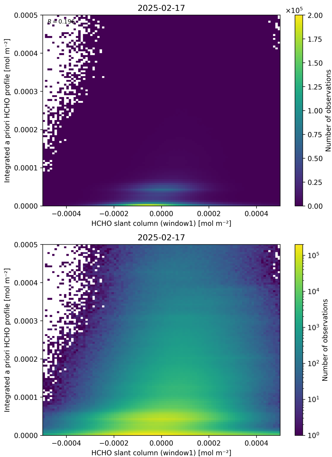
Figure 87: Scatter density plot of “HCHO slant column (window1)” against “Integrated a priori HCHO profile” for 2025-02-16 to 2025-02-18.
