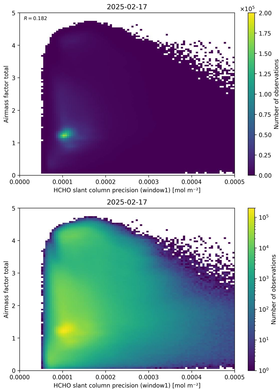
Figure 94: Scatter density plot of “HCHO slant column precision (window1)” against “Airmass factor total” for 2025-02-16 to 2025-02-18.
