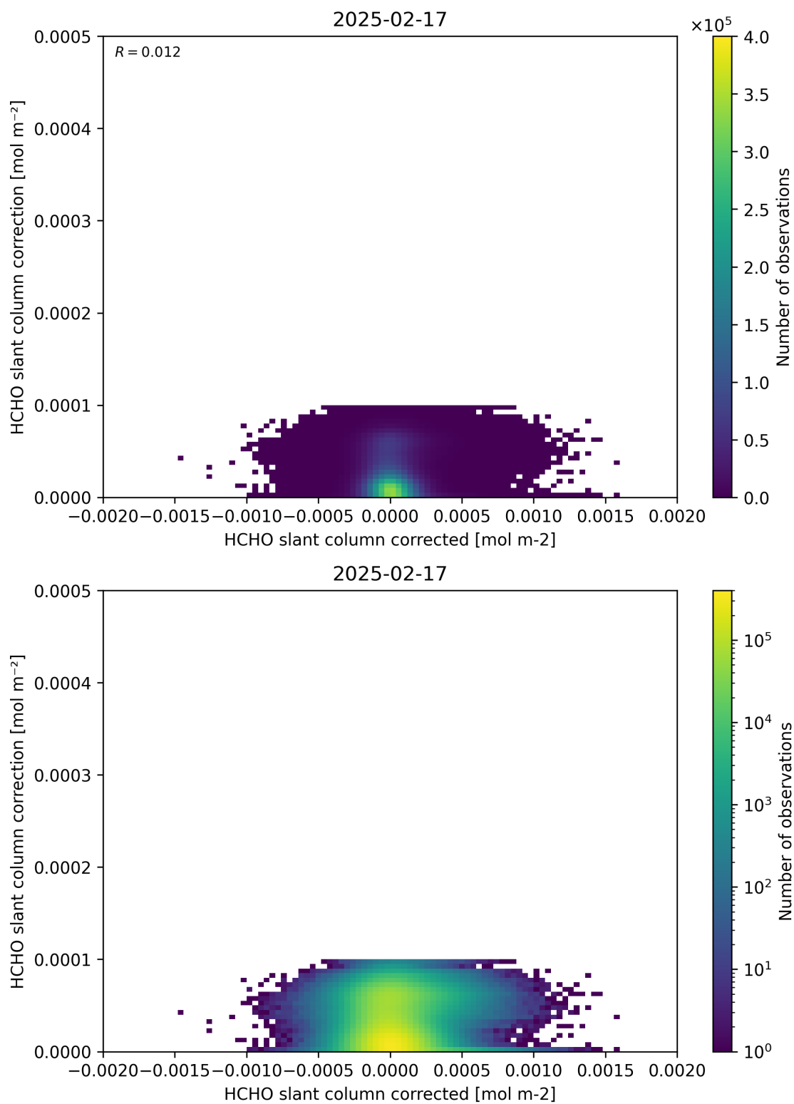
Figure 77: Scatter density plot of “HCHO slant column corrected” against “HCHO slant column correction” for 2025-02-16 to 2025-02-18.
