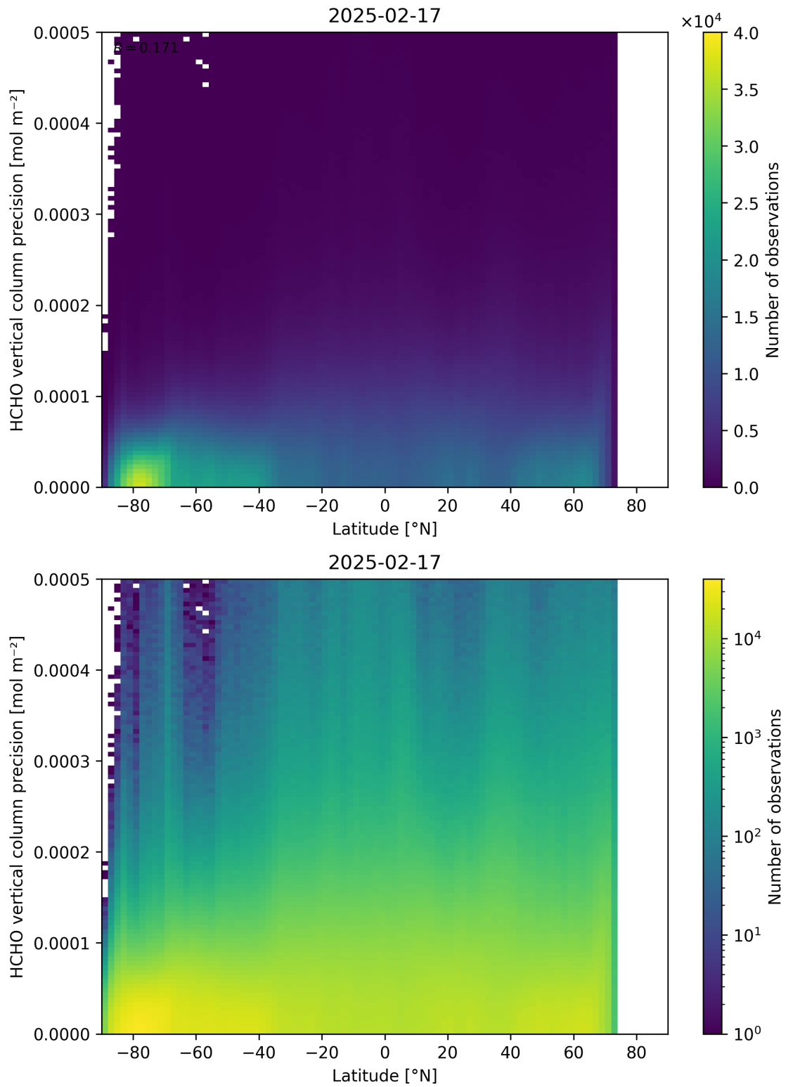
Figure 165: Scatter density plot of “Latitude” against “HCHO vertical column precision” for 2025-02-16 to 2025-02-18.
