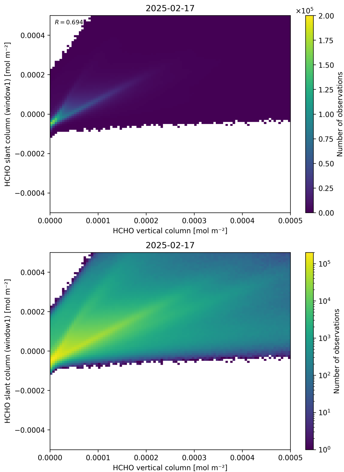
Figure 129: Scatter density plot of “HCHO vertical column” against “HCHO slant column (window1)” for 2025-02-16 to 2025-02-18.
