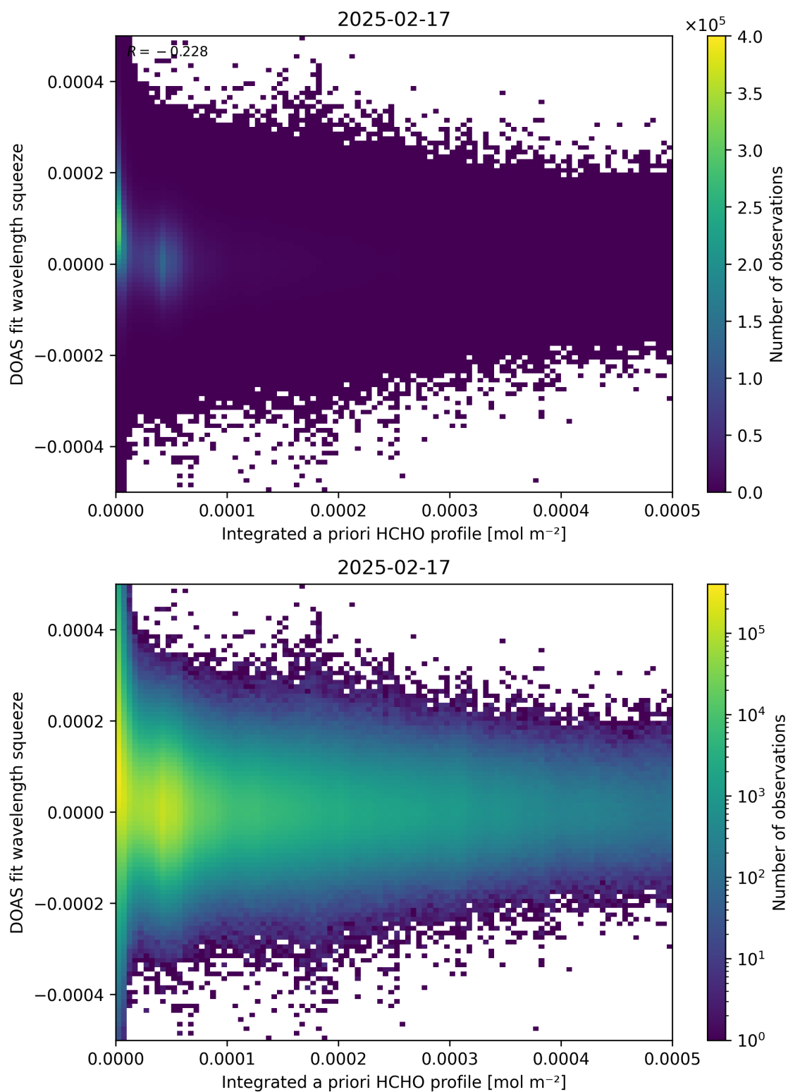
Figure 150: Scatter density plot of “Integrated a priori HCHO profile” against “DOAS fit wavelength squeeze” for 2025-02-16 to 2025-02-18.
