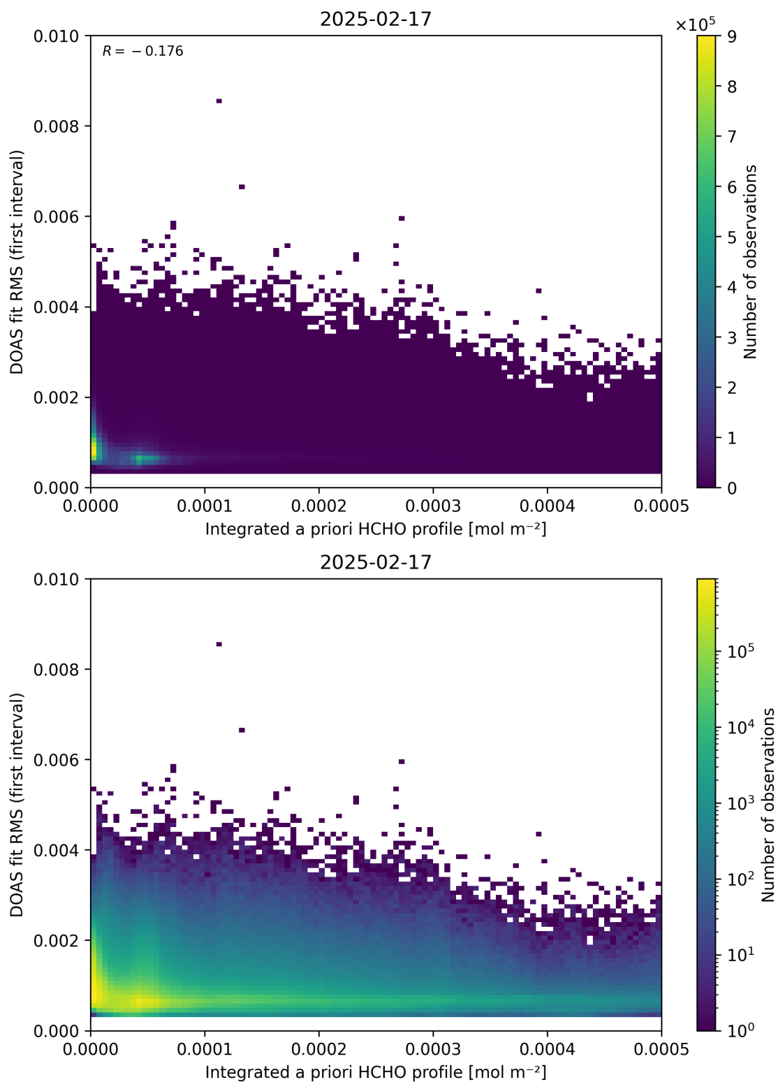
Figure 148: Scatter density plot of “Integrated a priori HCHO profile” against “DOAS fit RMS (first interval)” for 2025-02-16 to 2025-02-18.
