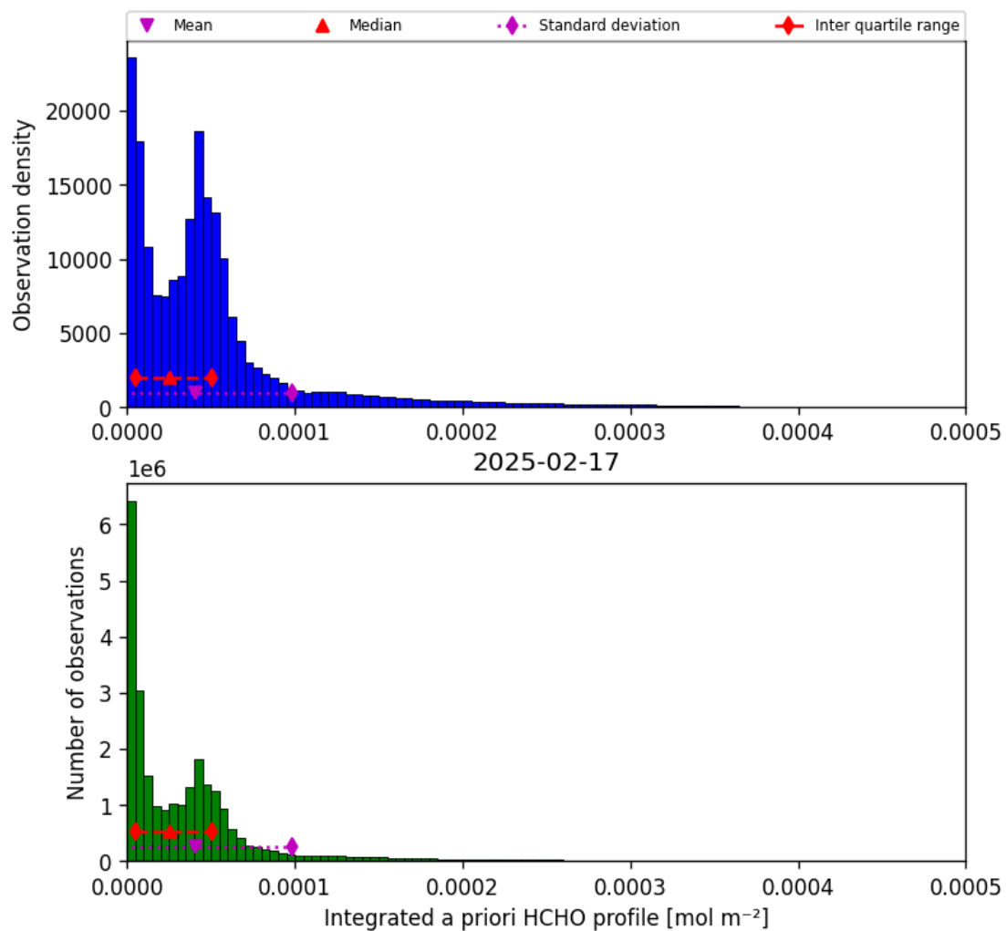
Figure 43: Histogram of “Integrated a priori HCHO profile” for 2025-02-16 to 2025-02-18
