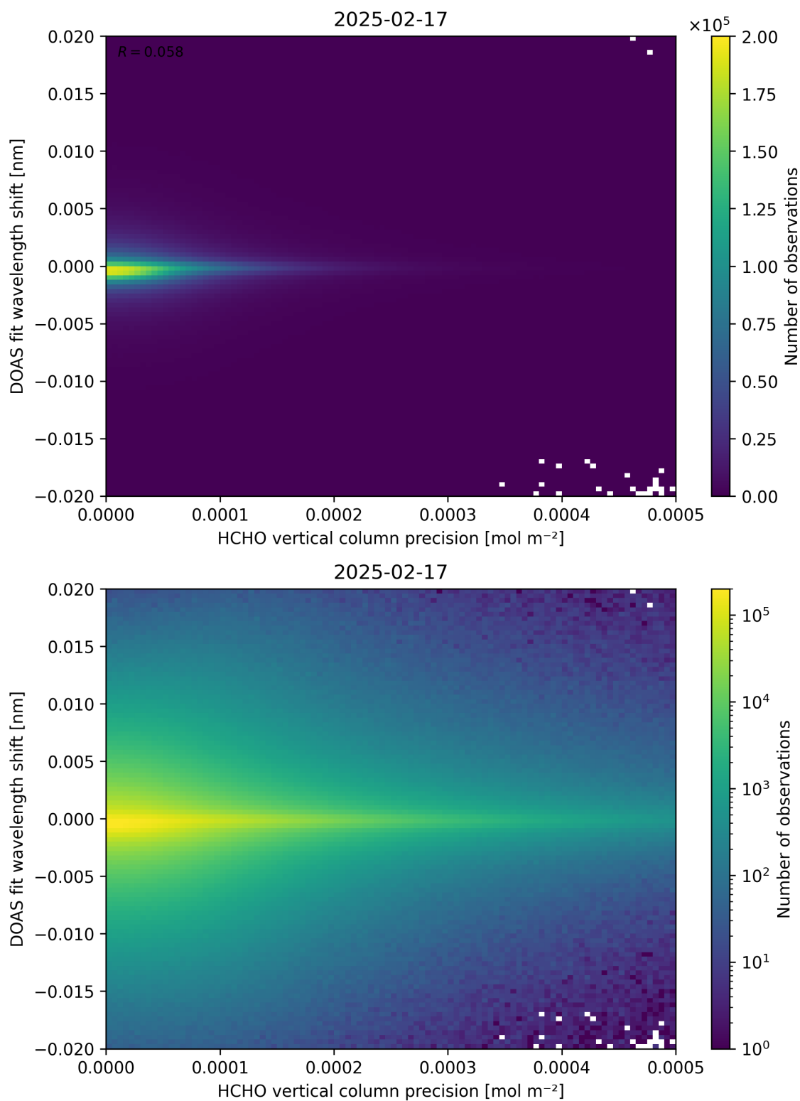
Figure 137: Scatter density plot of “HCHO vertical column precision” against “DOAS fit wavelength shift” for 2025-02-16 to 2025-02-18.
