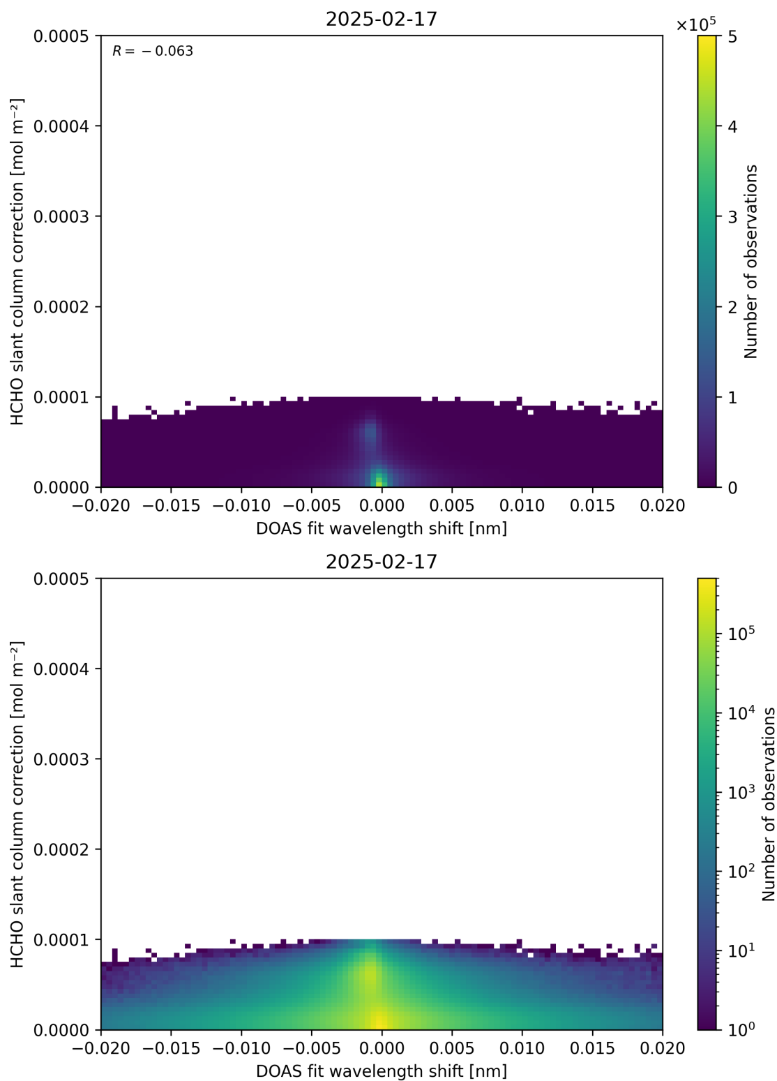
Figure 67: Scatter density plot of “DOAS fit wavelength shift” against “HCHO slant column correction” for 2025-02-16 to 2025-02-18.
