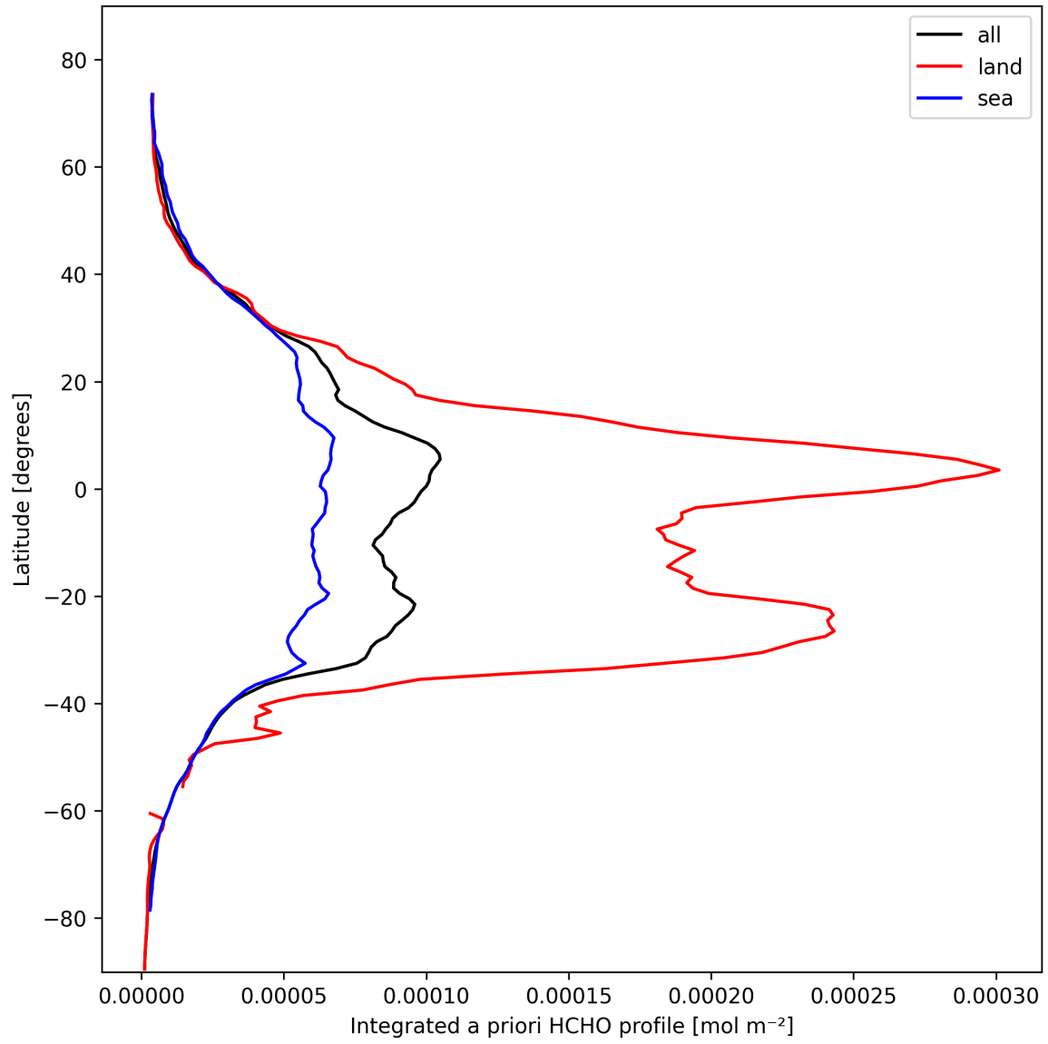
Figure 29: Zonal average of “Integrated a priori HCHO profile” for 2025-02-16 to 2025-02-18.
