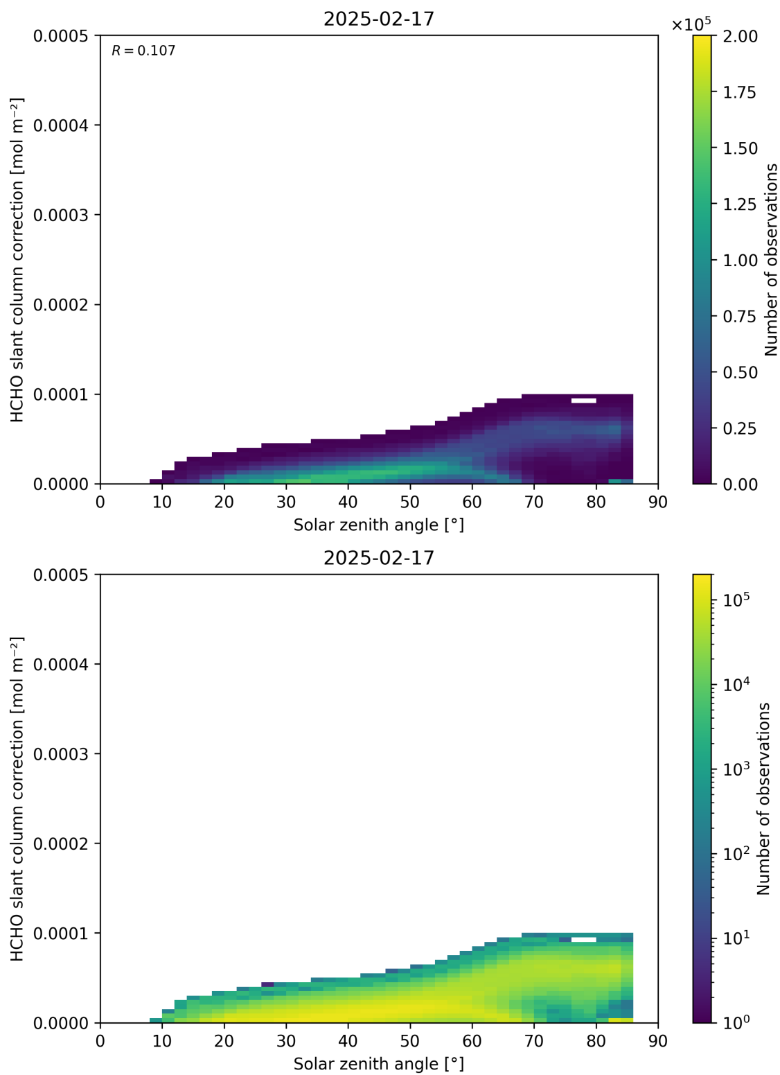
Figure 172: Scatter density plot of “Solar zenith angle” against “HCHO slant column correction” for 2025-02-16 to 2025-02-18.
