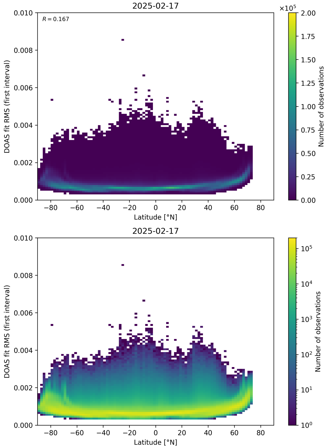
Figure 153: Scatter density plot of “Latitude” against “DOAS fit RMS (first interval)” for 2025-02-16 to 2025-02-18.
