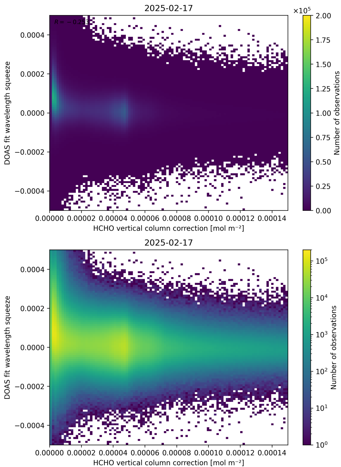
Figure 114: Scatter density plot of “HCHO vertical column correction” against “DOAS fit wavelength squeeze” for 2025-02-16 to 2025-02-18.
