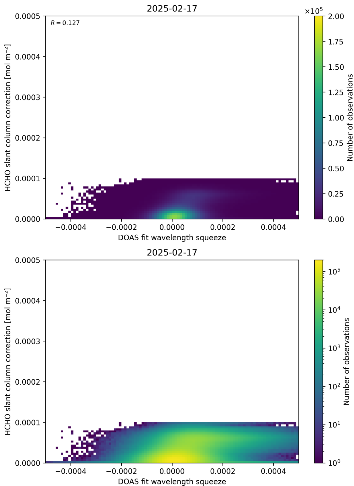
Figure 70: Scatter density plot of “DOAS fit wavelength squeeze” against “HCHO slant column correction” for 2025-02-16 to 2025-02-18.
