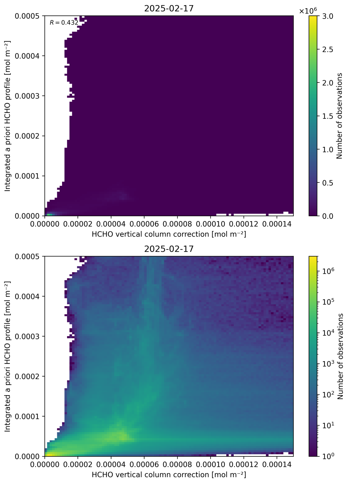
Figure 122: Scatter density plot of “HCHO vertical column correction” against “Integrated a priori HCHO profile” for 2025-02-16 to 2025-02-18.
