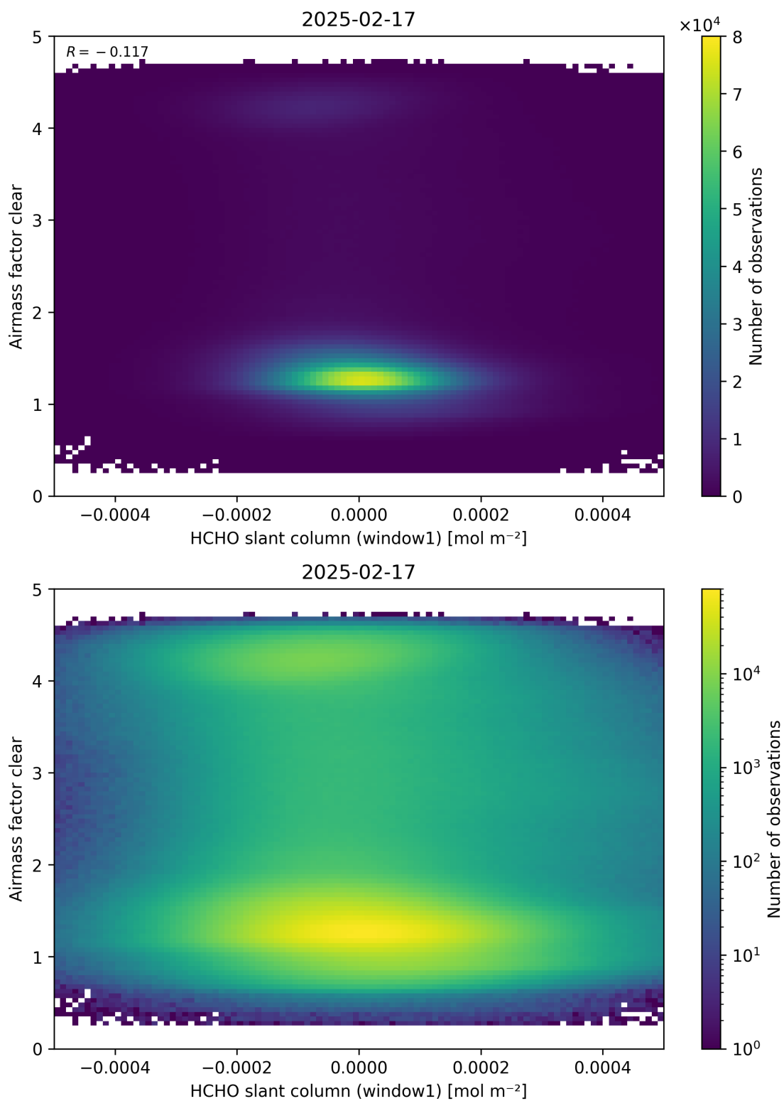
Figure 81: Scatter density plot of “HCHO slant column (window1)” against “Airmass factor clear” for 2025-02-16 to 2025-02-18.
