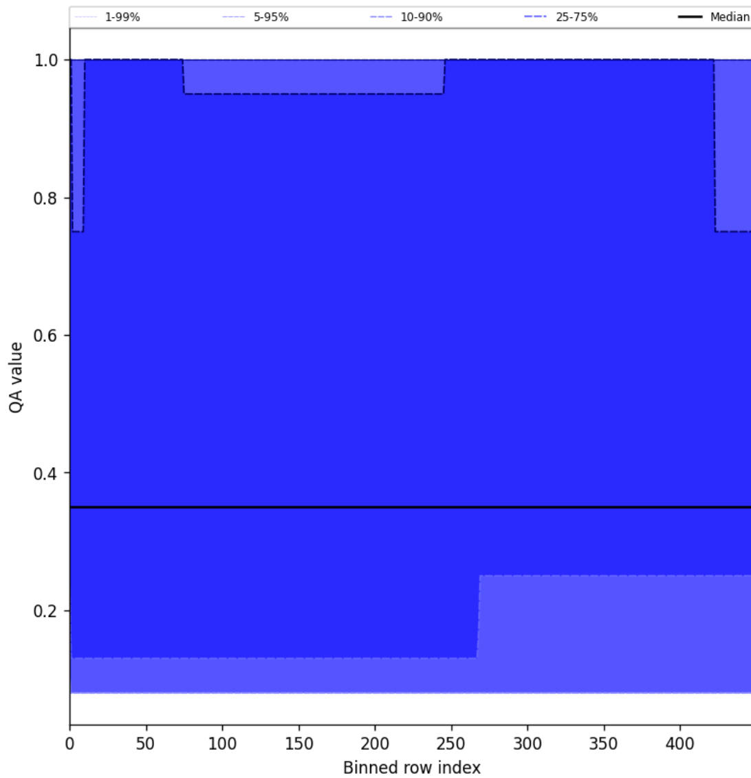
Figure 48: Along track statistics of "QA value" for 2025-02-16 to 2025-02-18
