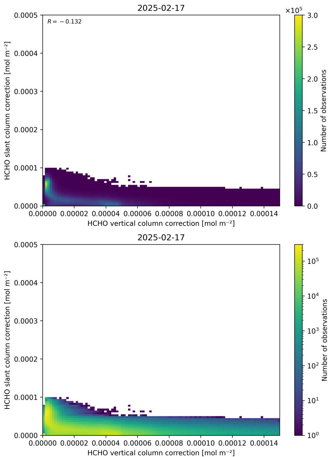
Figure 117: Scatter density plot of “HCHO vertical column correction” against “HCHO slant column correction” for 2025-02-16 to 2025-02-18.
