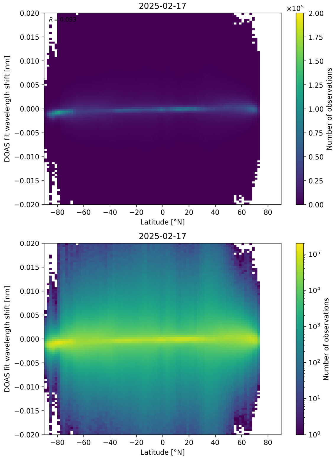
Figure 154: Scatter density plot of “Latitude” against “DOAS fit wavelength shift” for 2025-02-16 to 2025-02-18.
