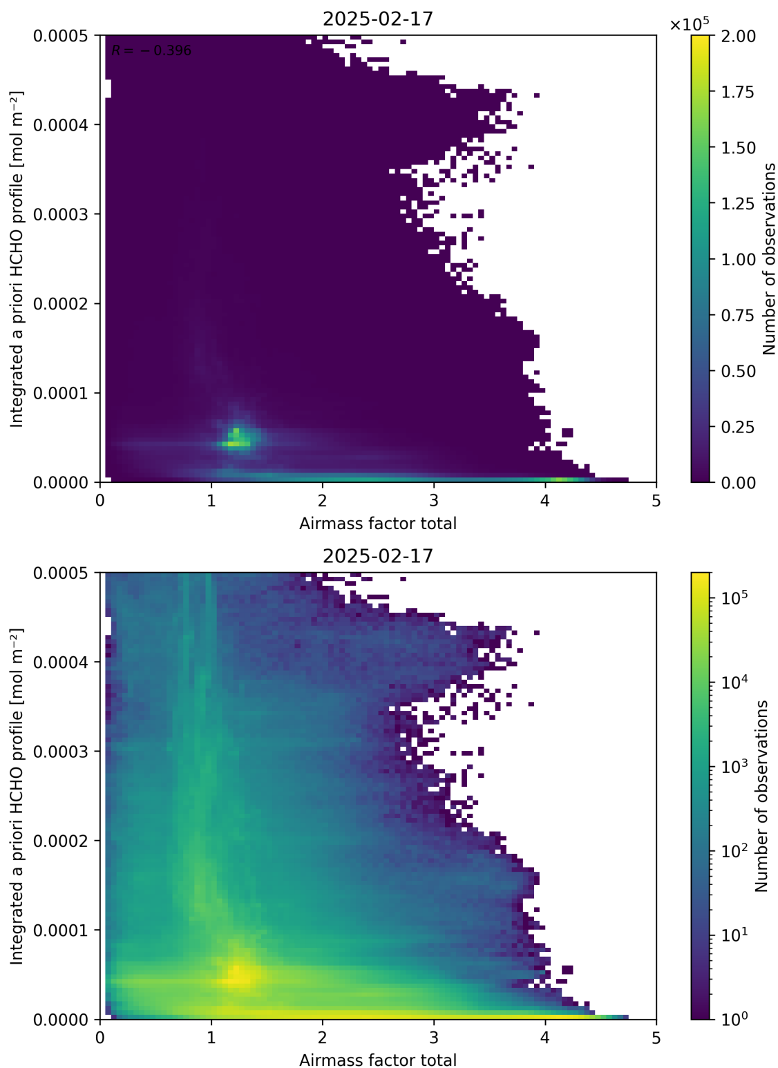
Figure 104: Scatter density plot of “Airmass factor total” against “Integrated a priori HCHO profile” for 2025-02-16 to 2025-02-18.
