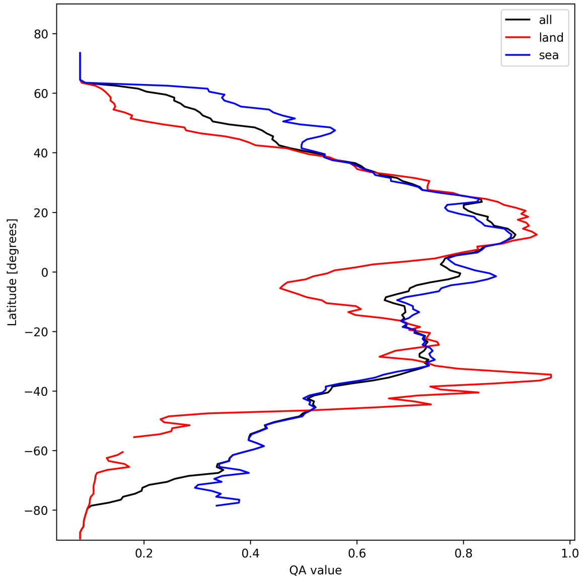
Figure 20: Zonal average of “QA value” for 2025-02-16 to 2025-02-18.
