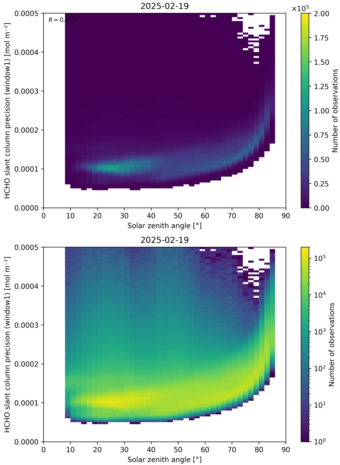
Figure 174: Scatter density plot of “Solar zenith angle” against “HCHO slant column precision (window1)” for 2025-02-19 to 2025-02-20.
