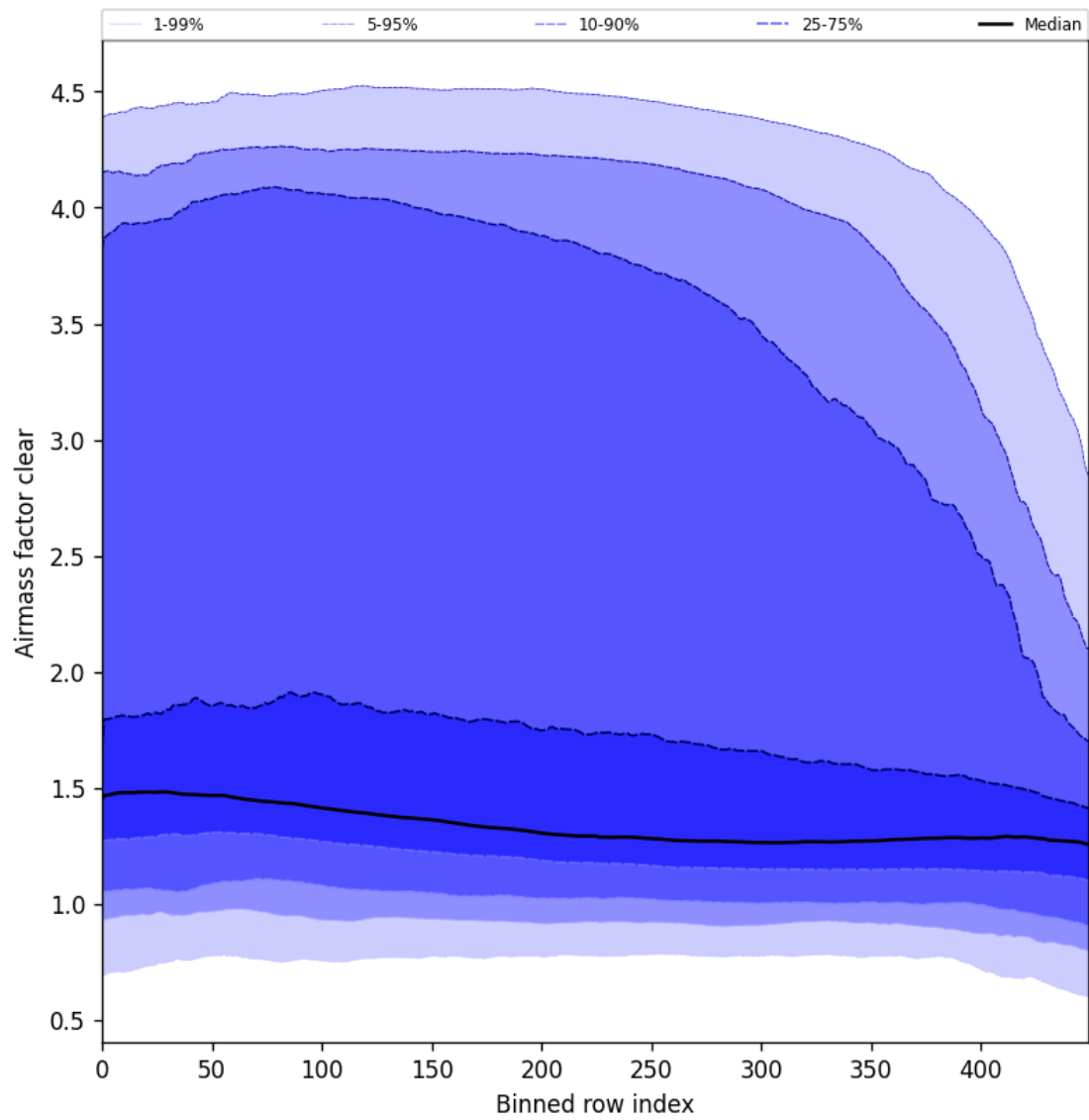
Figure 56: Along track statistics of “Airmass factor clear” for 2025-02-19 to 2025-02-20
