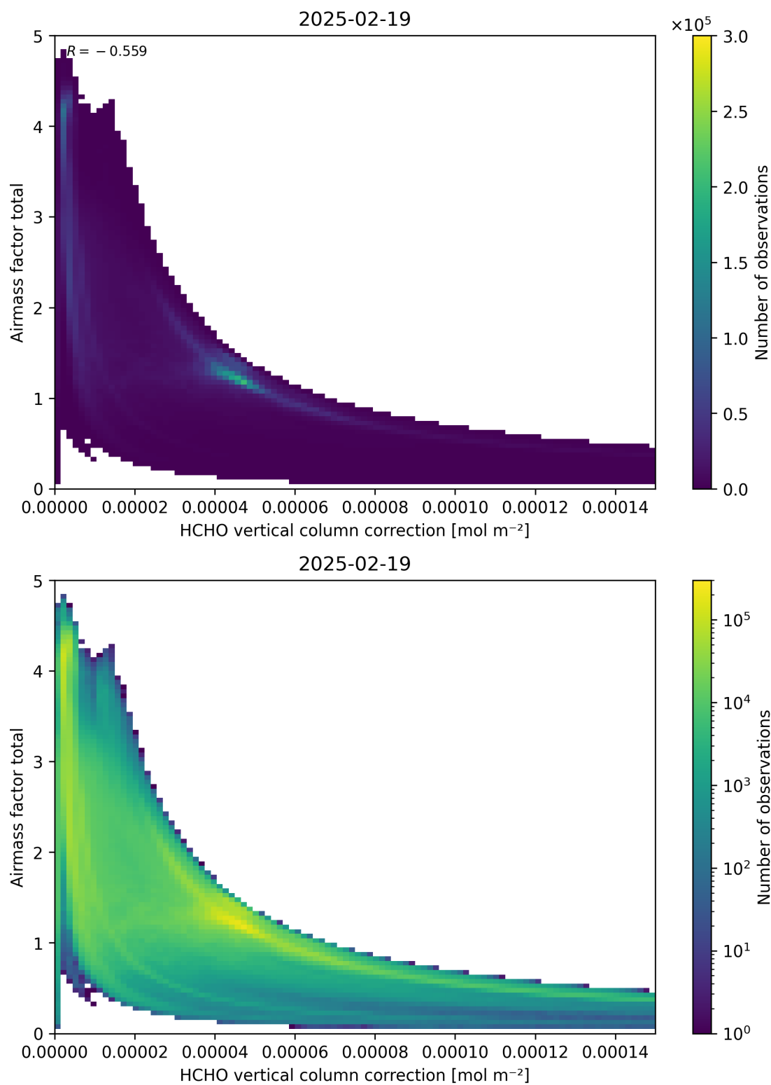
Figure 120: Scatter density plot of “HCHO vertical column correction” against “Airmass factor total” for 2025-02-19 to 2025-02-20.
