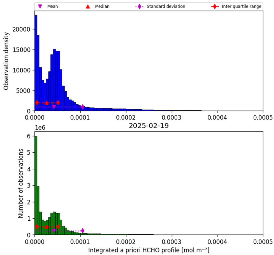
Figure 43: Histogram of “Integrated a priori HCHO profile” for 2025-02-19 to 2025-02-20
