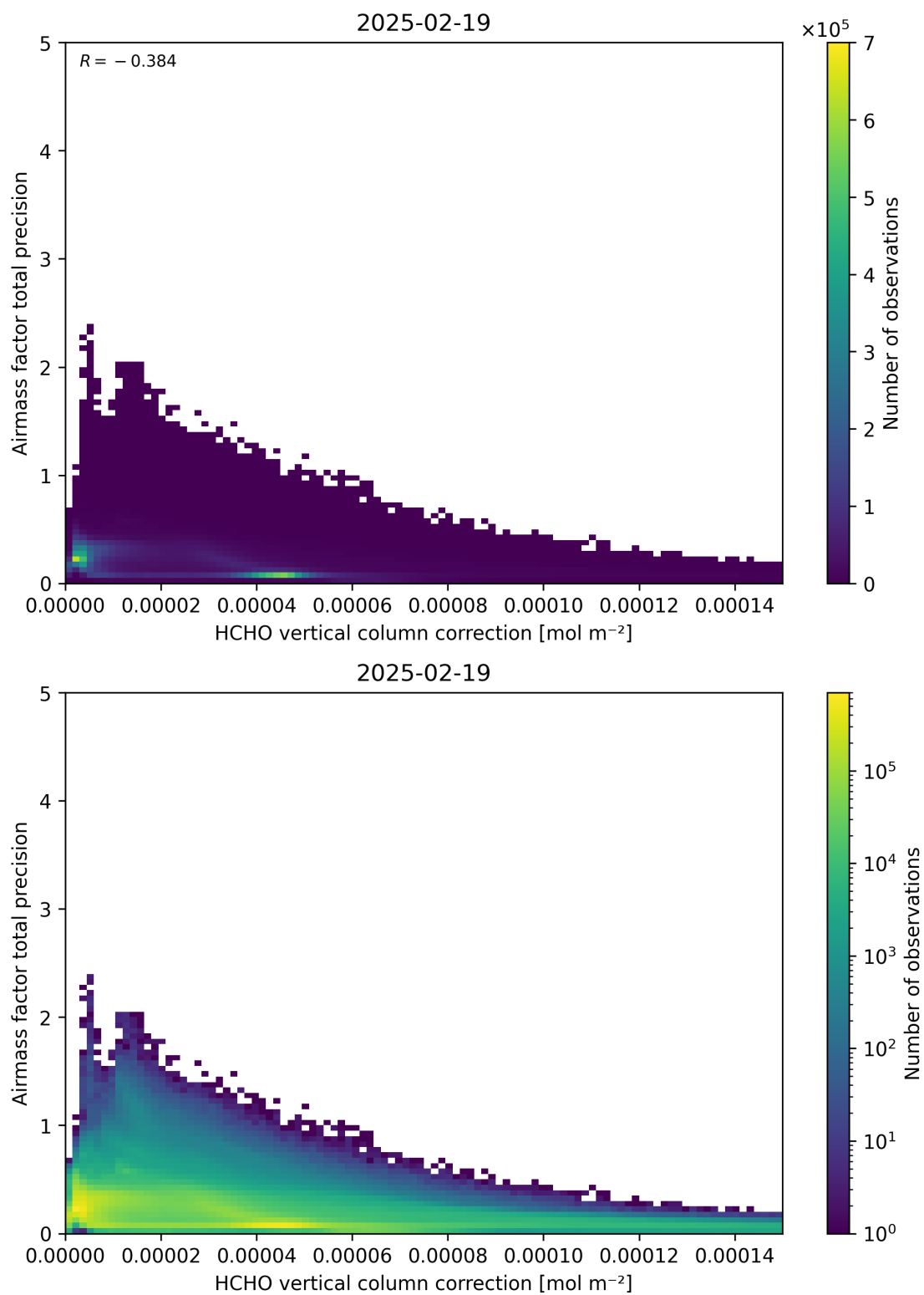
Figure 121: Scatter density plot of “HCHO vertical column correction” against “Airmass factor total precision” for 2025-02-19 to 2025-02-20.
