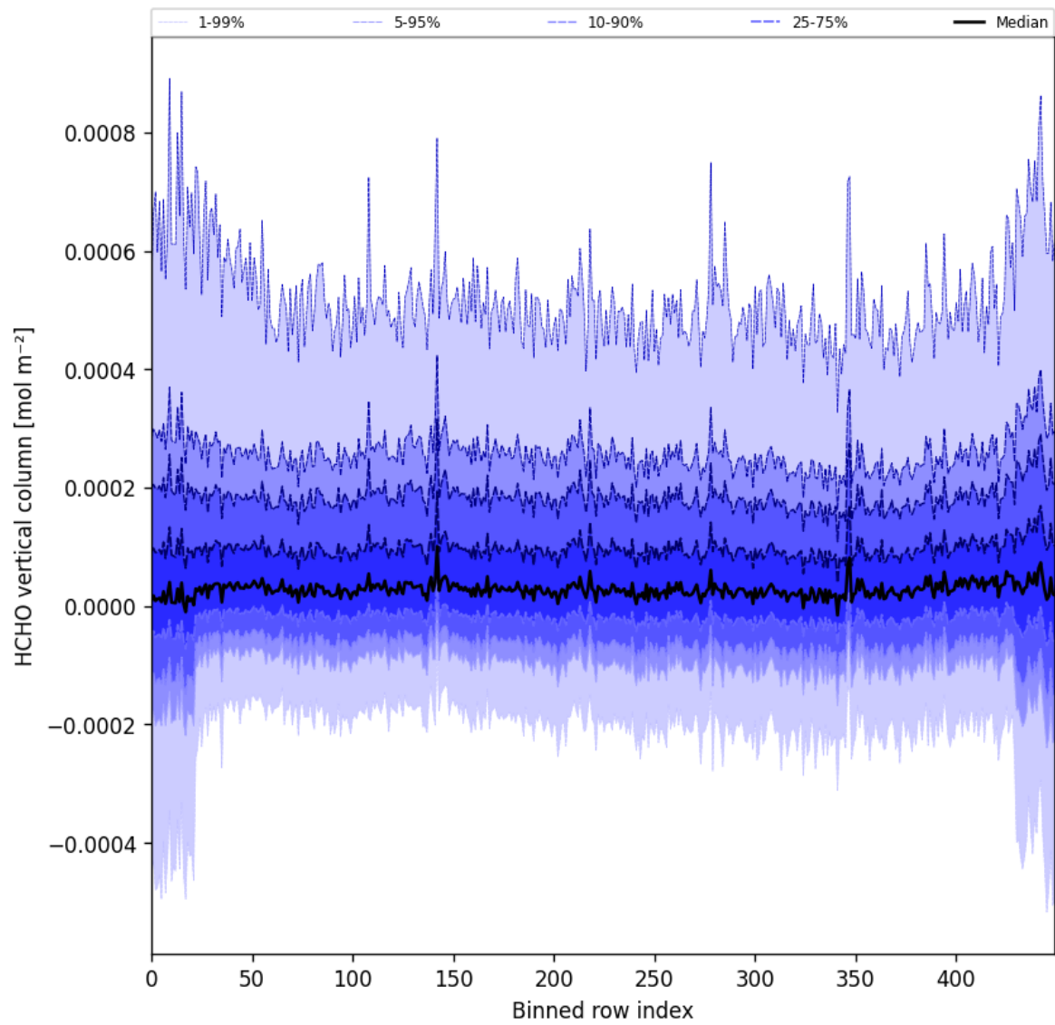
Figure 49: Along track statistics of “HCHO vertical column” for 2025-02-19 to 2025-02-20
