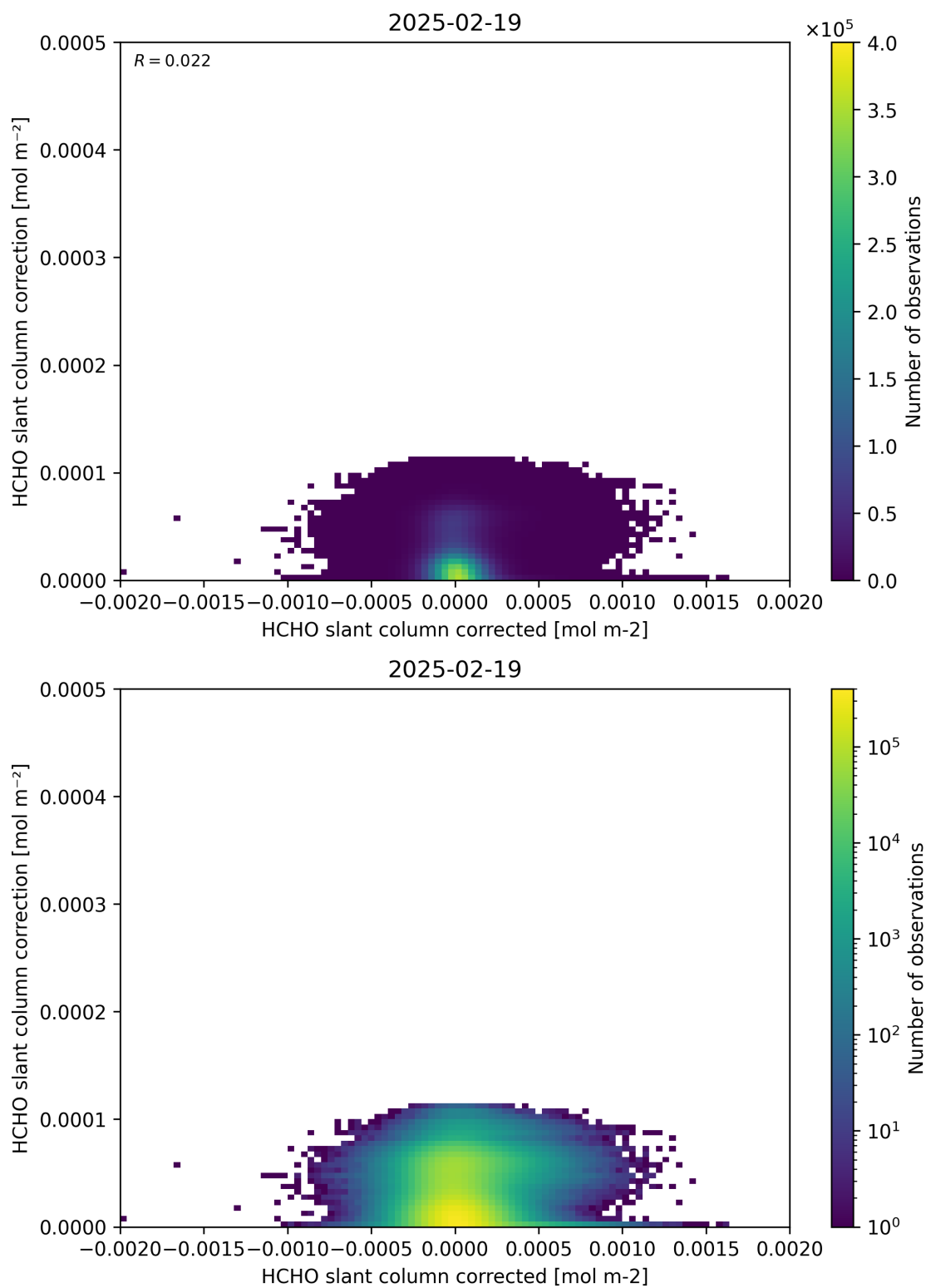
Figure 77: Scatter density plot of “HCHO slant column corrected” against “HCHO slant column correction” for 2025-02-19 to 2025-02-20.
