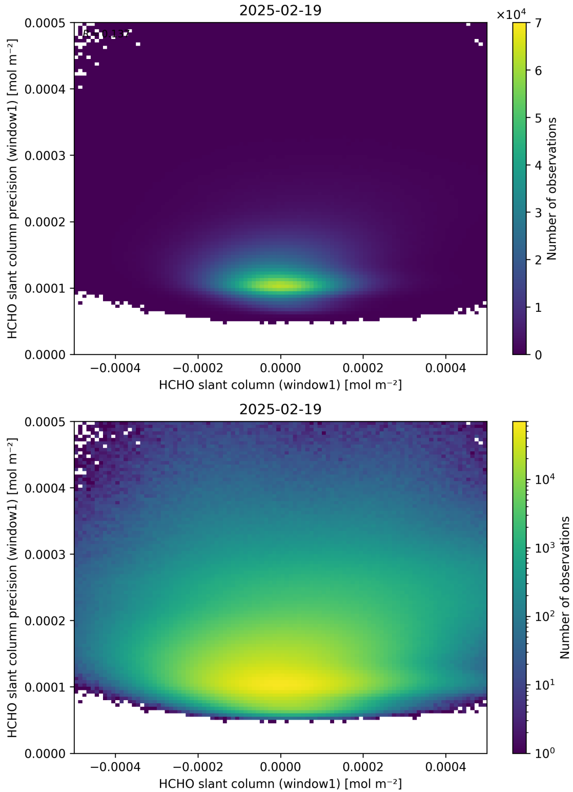
Figure 84: Scatter density plot of “HCHO slant column (window1)” against “HCHO slant column precision (window1)” for 2025-02-19 to 2025-02-20.
