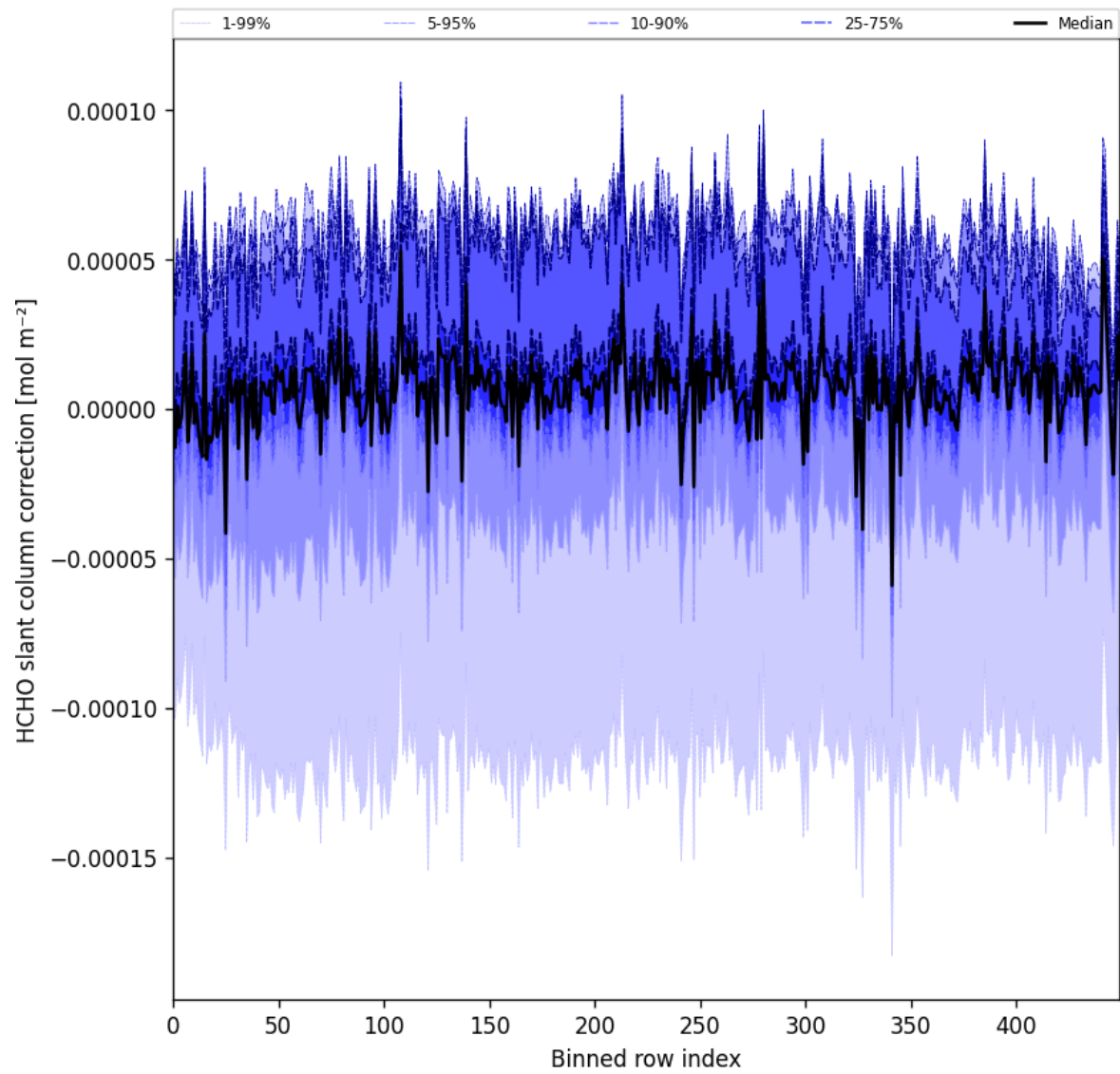
Figure 61: Along track statistics of “HCHO slant column correction” for 2025-02-19 to 2025-02-20
