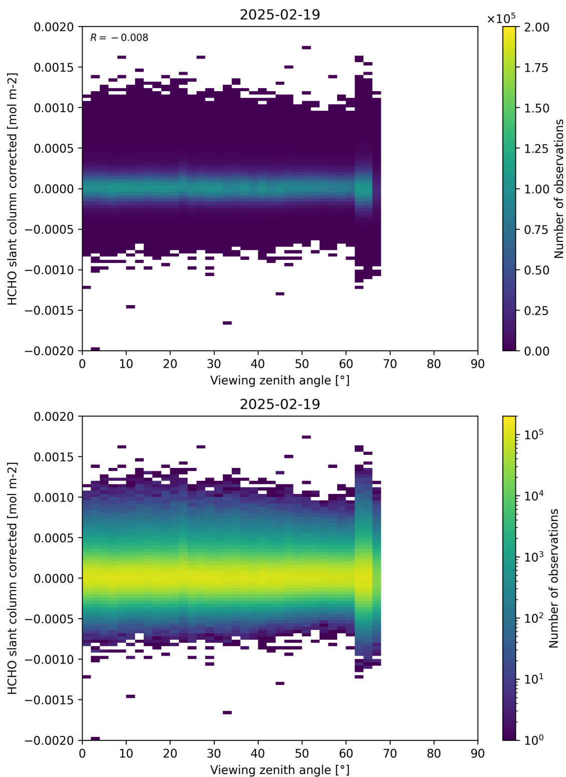
Figure 186: Scatter density plot of “Viewing zenith angle” against “HCHO slant column corrected” for 2025-02-19 to 2025-02-20.
