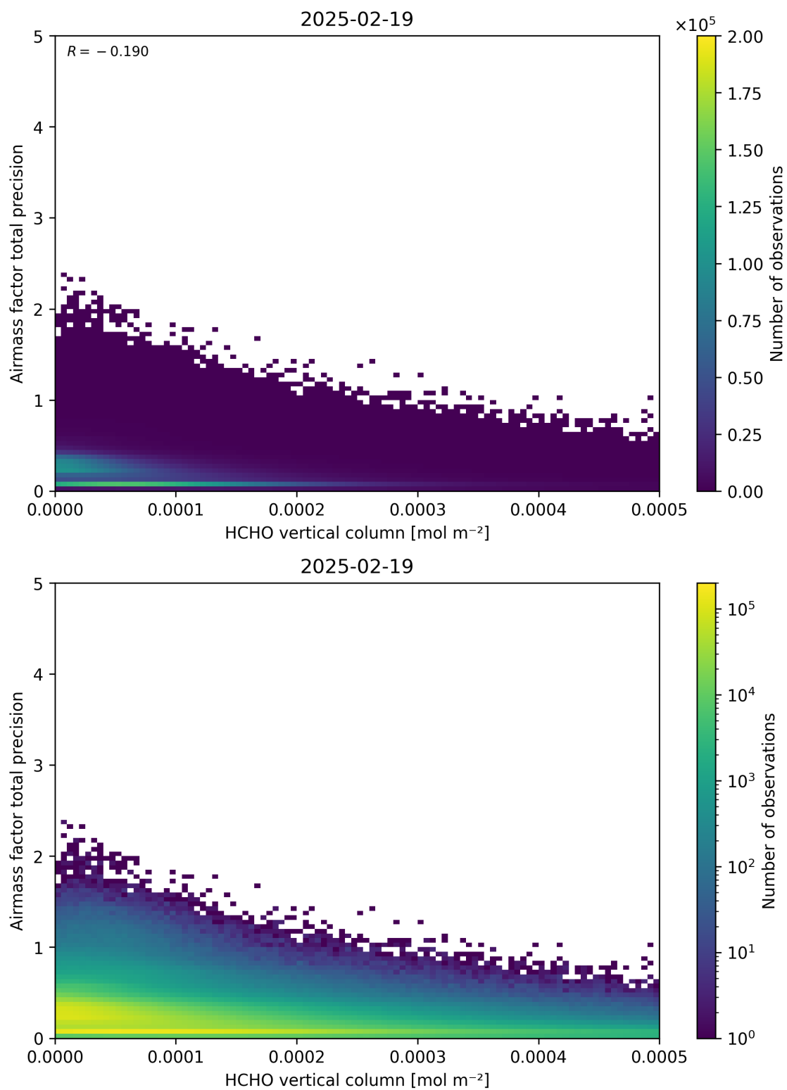
Figure 132: Scatter density plot of “HCHO vertical column” against “Airmass factor total precision” for 2025-02-19 to 2025-02-20.
