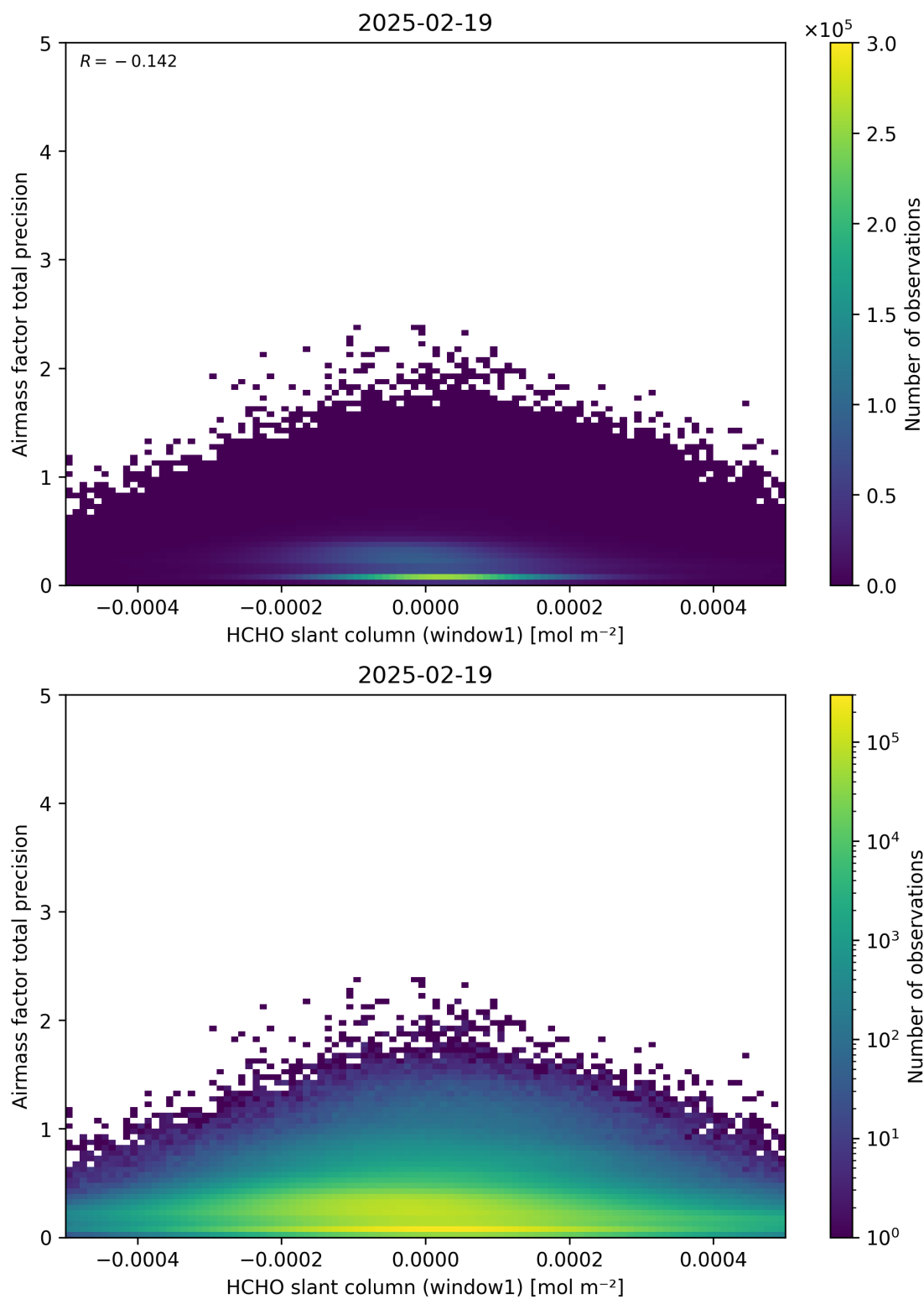
Figure 86: Scatter density plot of “HCHO slant column (window1)” against “Airmass factor total precision” for 2025-02-19 to 2025-02-20.
