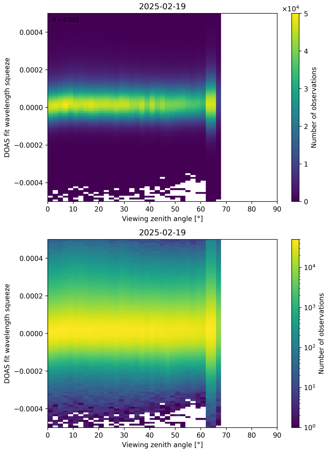
Figure 184: Scatter density plot of “Viewing zenith angle” against “DOAS fit wavelength squeeze” for 2025-02-19 to 2025-02-20.
