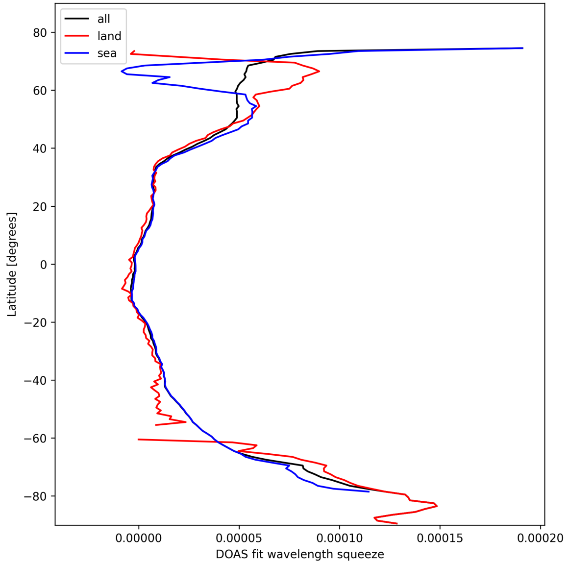
Figure 31: Zonal average of “DOAS fit wavelength squeeze” for 2025-02-19 to 2025-02-20.
