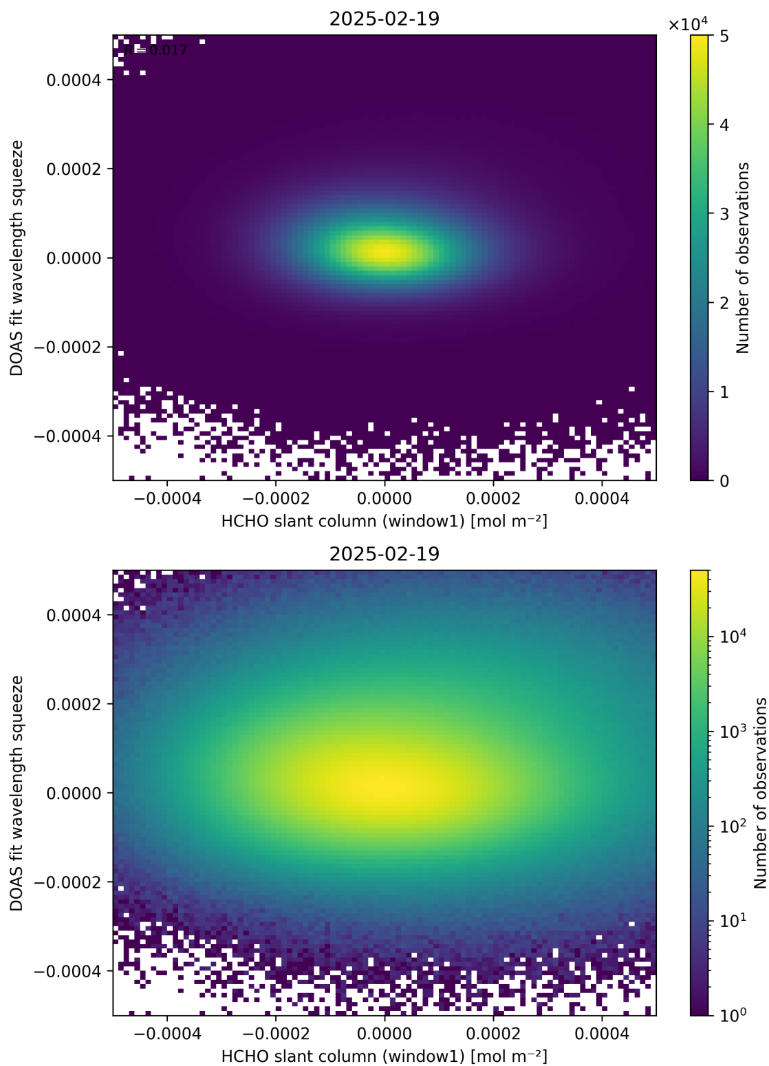
Figure 80: Scatter density plot of “HCHO slant column (window1)” against “DOAS fit wavelength squeeze” for 2025-02-19 to 2025-02-20.
