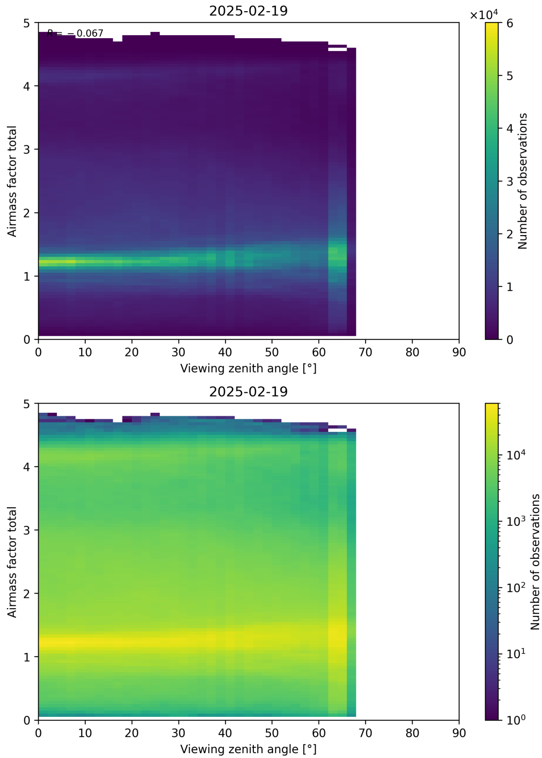
Figure 190: Scatter density plot of “Viewing zenith angle” against “Airmass factor total” for 2025-02-19 to 2025-02-20.
