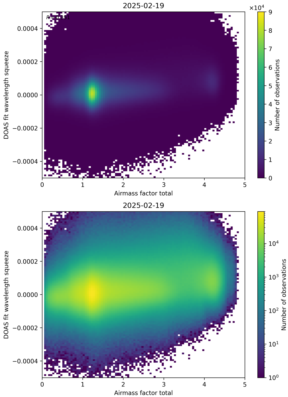
Figure 99: Scatter density plot of “Airmass factor total” against “DOAS fit wavelength squeeze” for 2025-02-19 to 2025-02-20.
