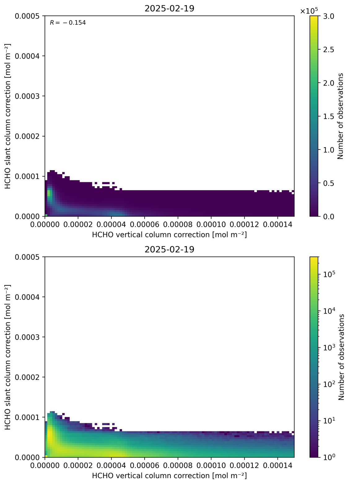
Figure 117: Scatter density plot of “HCHO vertical column correction” against “HCHO slant column correction” for 2025-02-19 to 2025-02-20.
