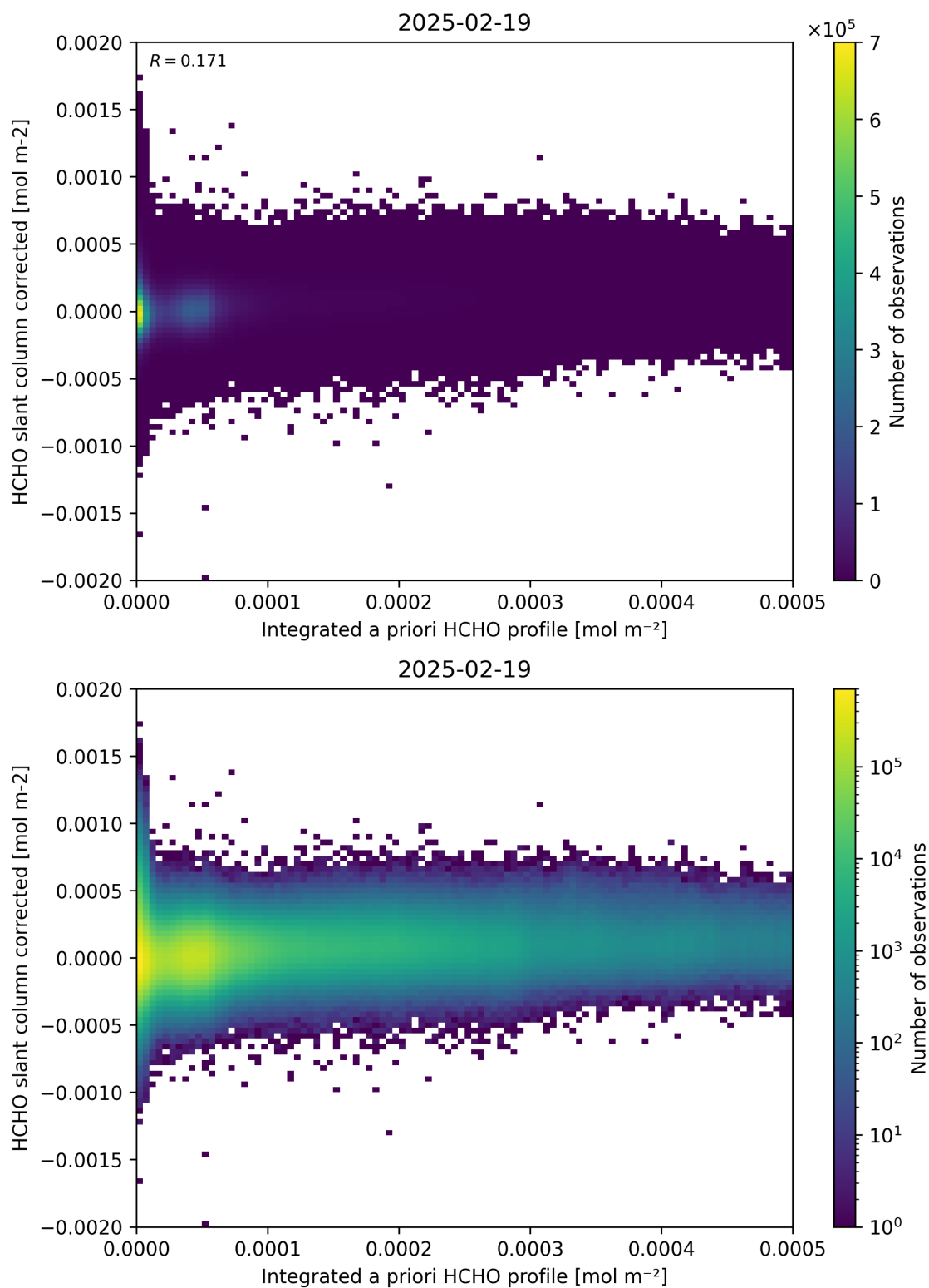
Figure 151: Scatter density plot of “Integrated a priori HCHO profile” against “HCHO slant column corrected” for 2025-02-19 to 2025-02-20.
