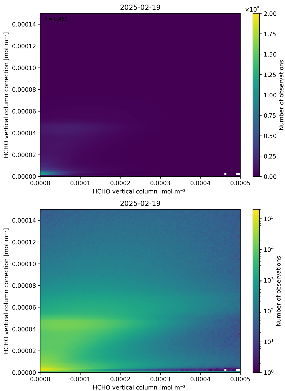
Figure 133: Scatter density plot of “HCHO vertical column” against “HCHO vertical column correction” for 2025-02-19 to 2025-02-20.
