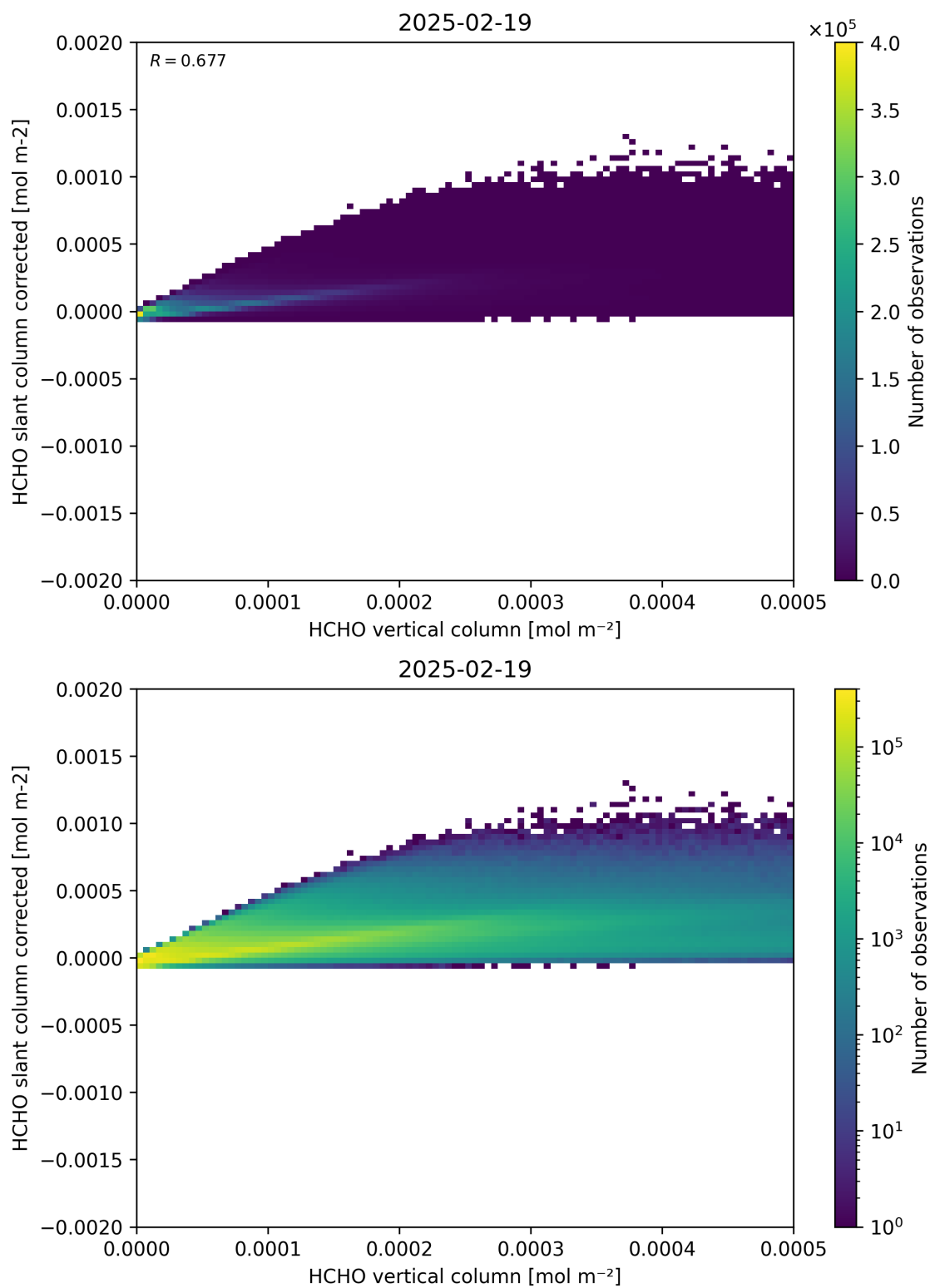
Figure 127: Scatter density plot of “HCHO vertical column” against “HCHO slant column corrected” for 2025-02-19 to 2025-02-20.
