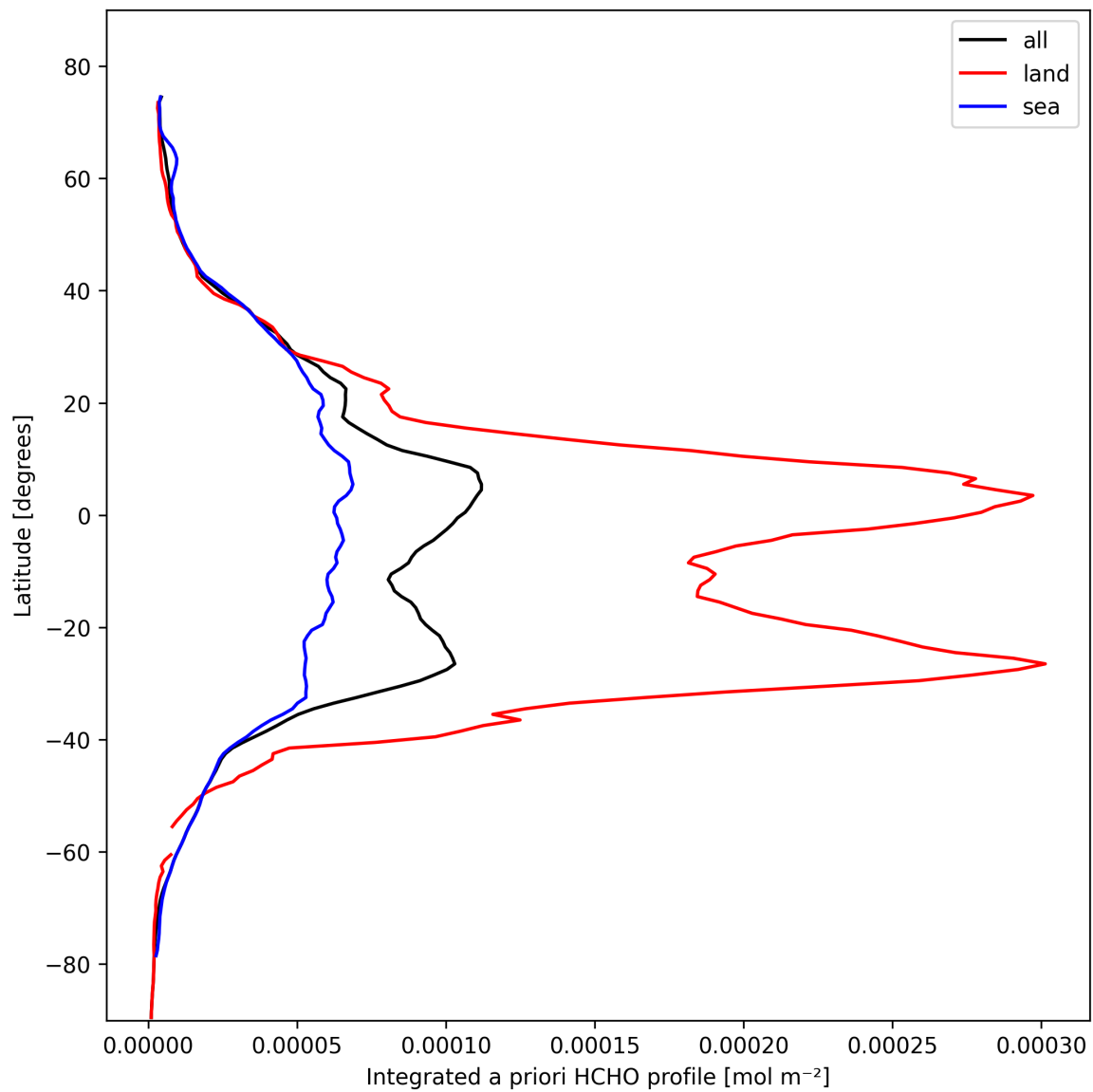
Figure 29: Zonal average of “Integrated a priori HCHO profile” for 2025-02-19 to 2025-02-20.
