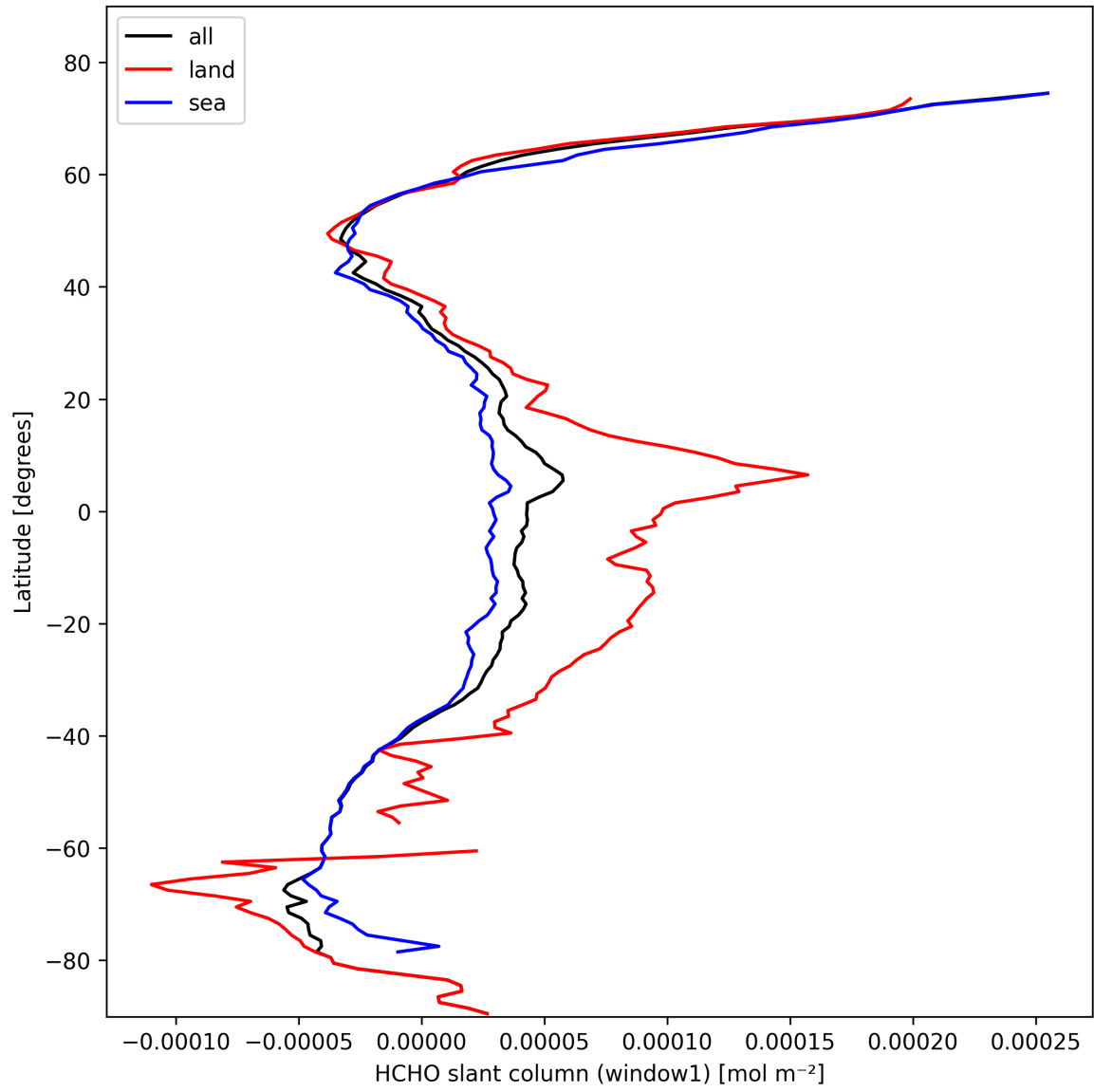
Figure 24: Zonal average of “HCHO slant column (window1)” for 2025-02-19 to 2025-02-20.
