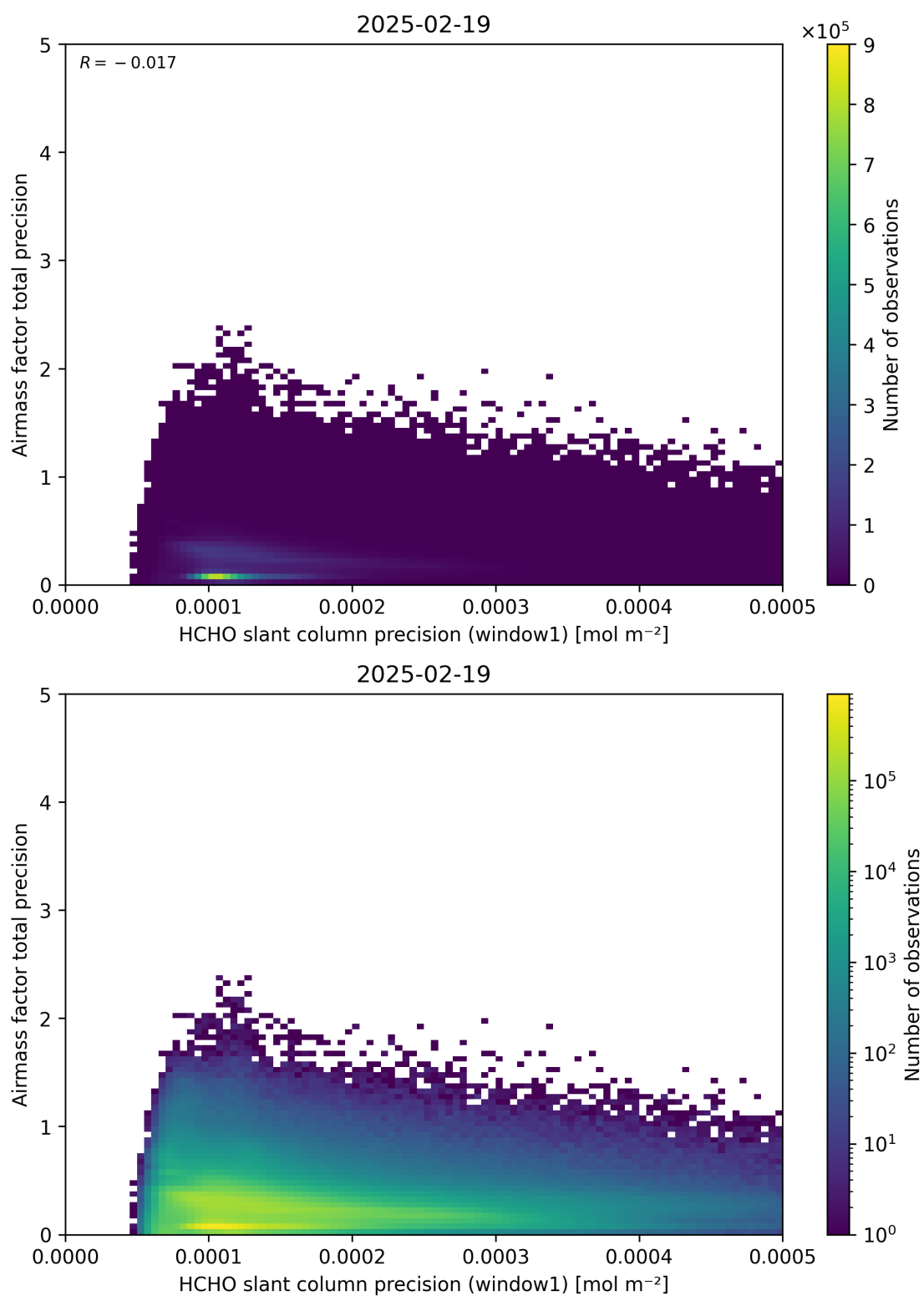
Figure 95: Scatter density plot of “HCHO slant column precision (window1)” against “Airmass factor total precision” for 2025-02-19 to 2025-02-20.
