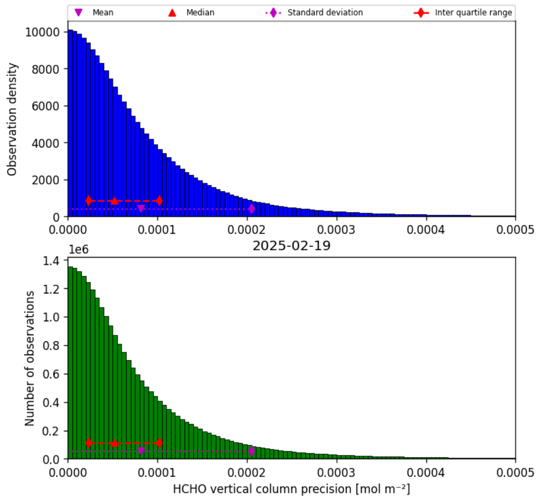
Figure 36: Histogram of “HCHO vertical column precision” for 2025-02-19 to 2025-02-20
