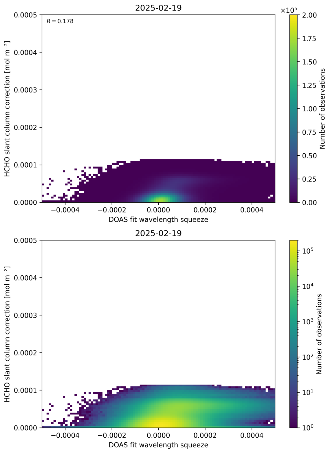
Figure 70: Scatter density plot of “DOAS fit wavelength squeeze” against “HCHO slant column correction” for 2025-02-19 to 2025-02-20.
