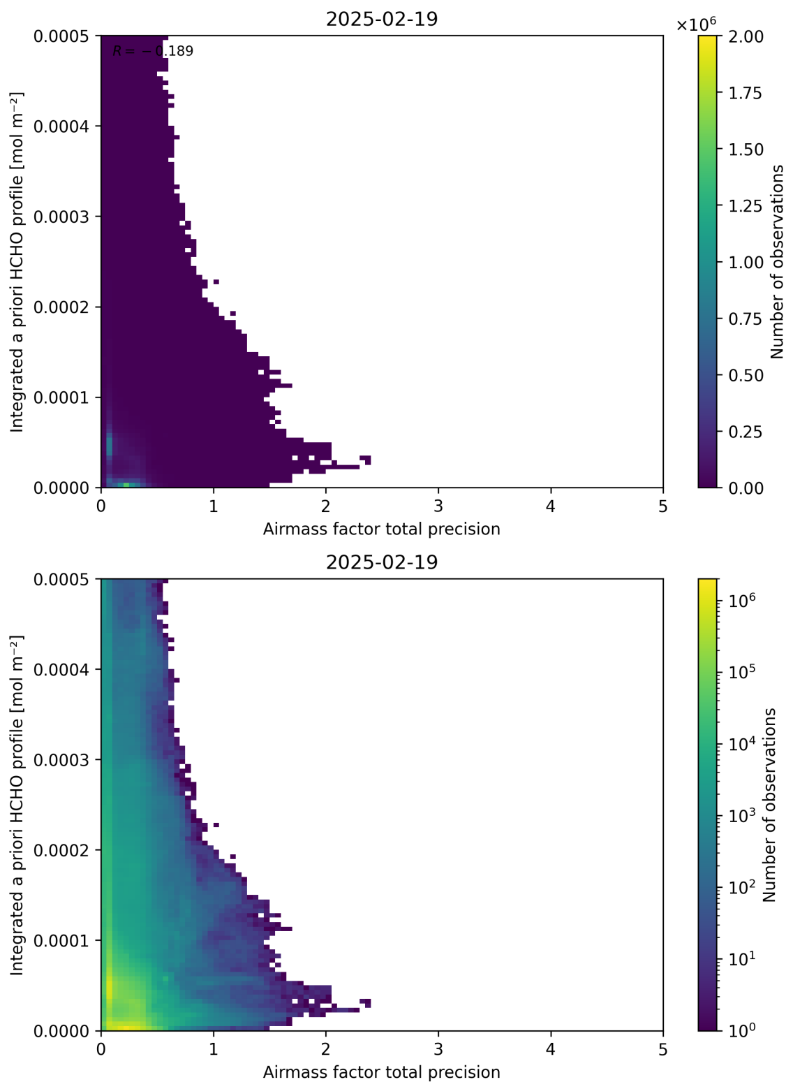
Figure 111: Scatter density plot of “Airmass factor total precision” against “Integrated a priori HCHO profile” for 2025-02-19 to 2025-02-20.
