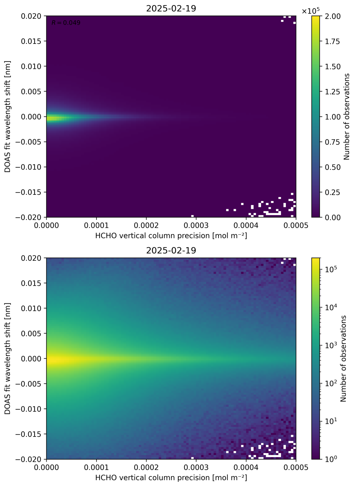
Figure 137: Scatter density plot of “HCHO vertical column precision” against “DOAS fit wavelength shift” for 2025-02-19 to 2025-02-20.
