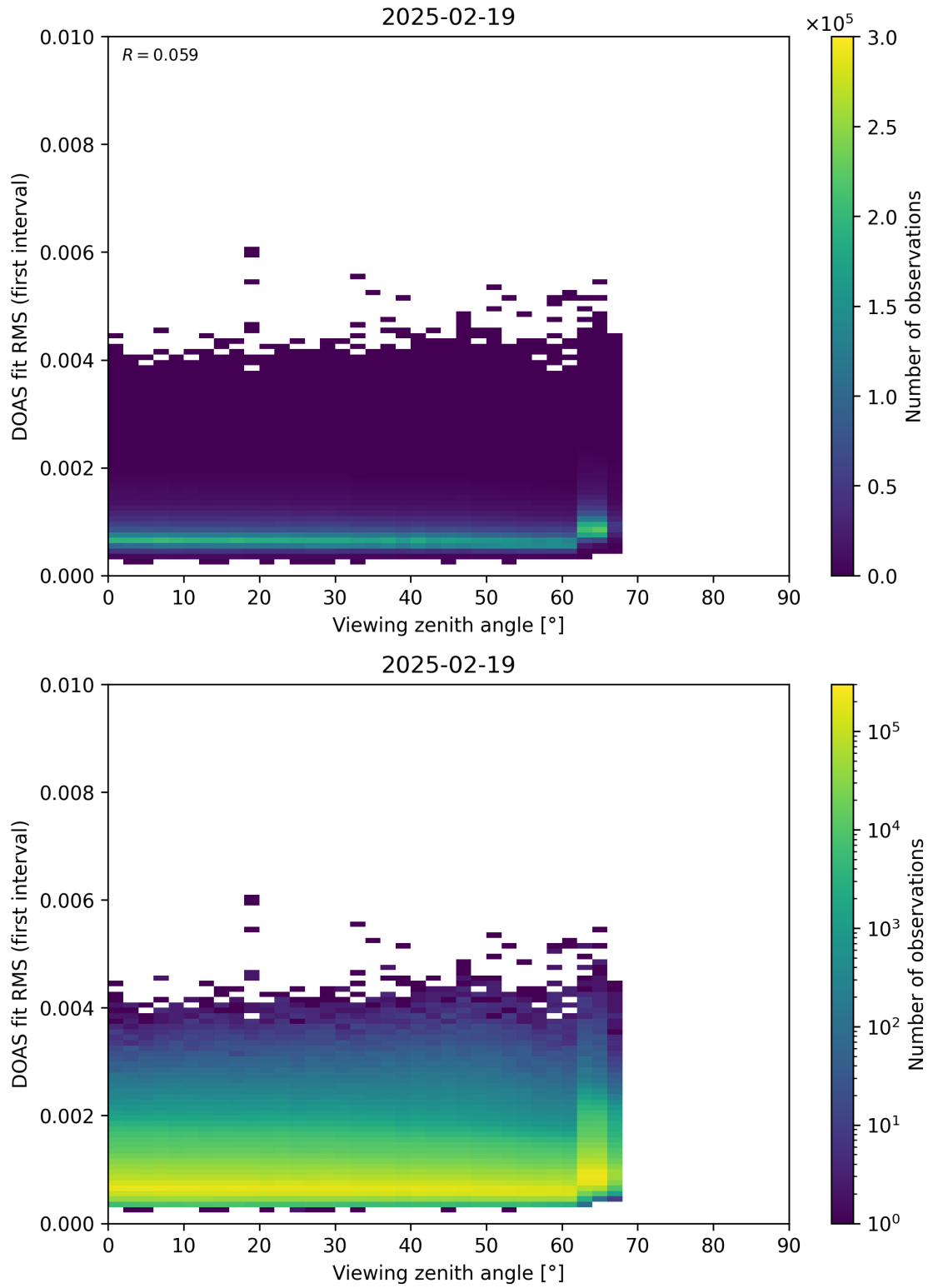
Figure 182: Scatter density plot of “Viewing zenith angle” against “DOAS fit RMS (first interval)” for 2025-02-19 to 2025-02-20.
