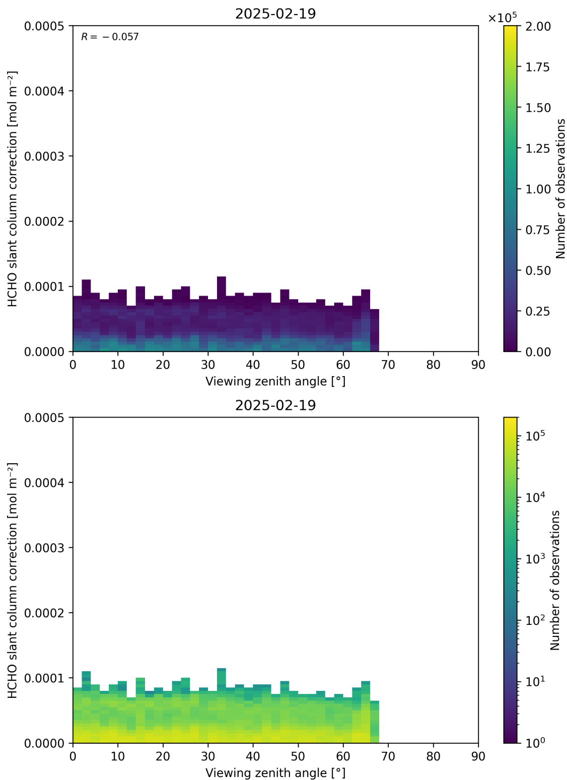
Figure 187: Scatter density plot of “Viewing zenith angle” against “HCHO slant column correction” for 2025-02-19 to 2025-02-20.
