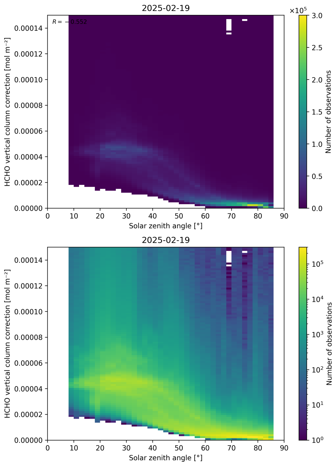
Figure 178: Scatter density plot of “Solar zenith angle” against “HCHO vertical column correction” for 2025-02-19 to 2025-02-20.
