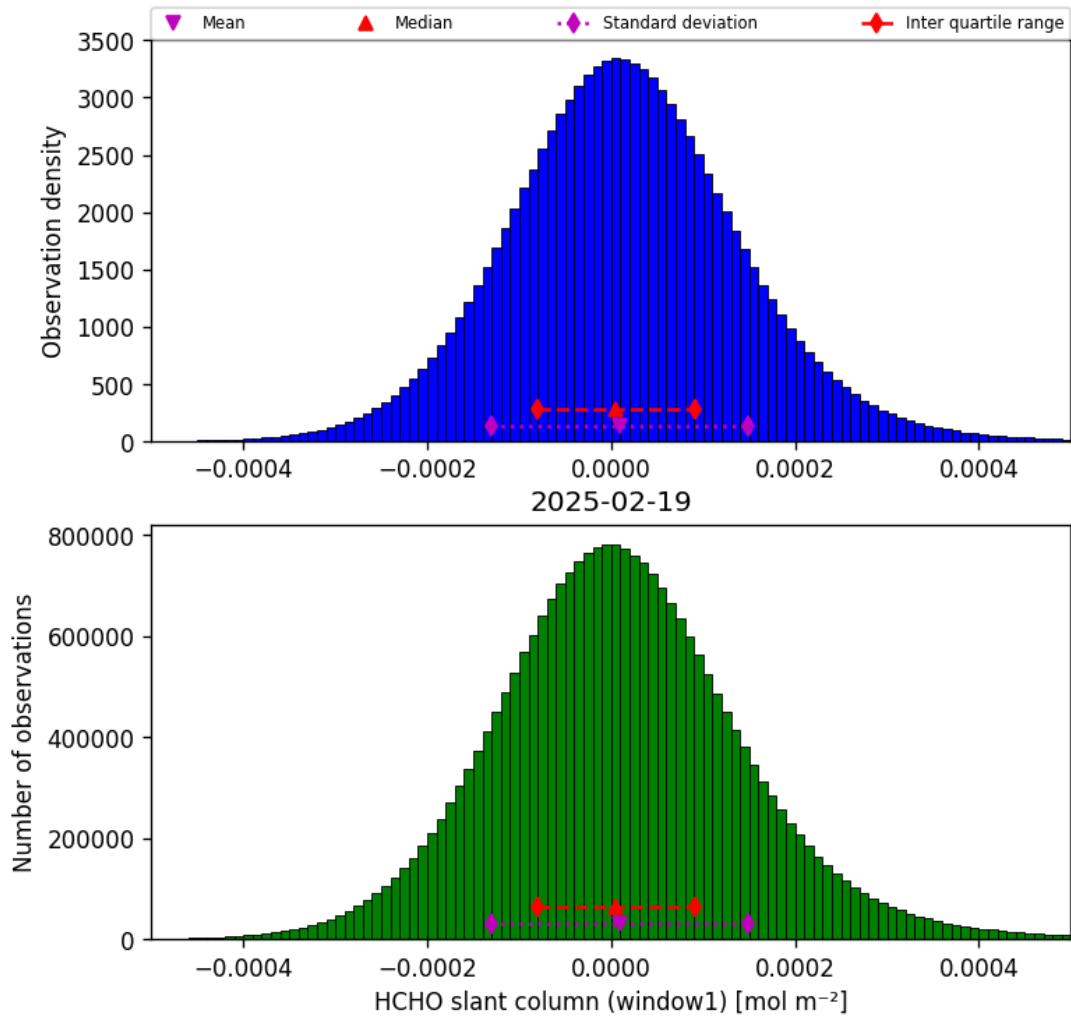
Figure 38: Histogram of “HCHO slant column (window1)” for 2025-02-19 to 2025-02-20
