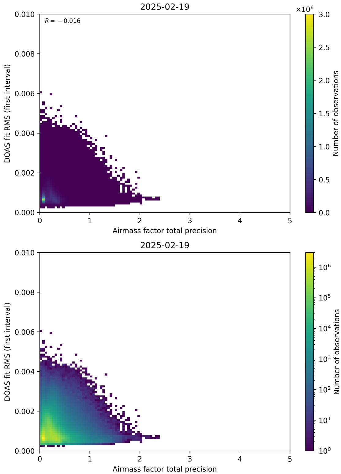
Figure 105: Scatter density plot of “Airmass factor total precision” against “DOAS fit RMS (first interval)” for 2025-02-19 to 2025-02-20.
