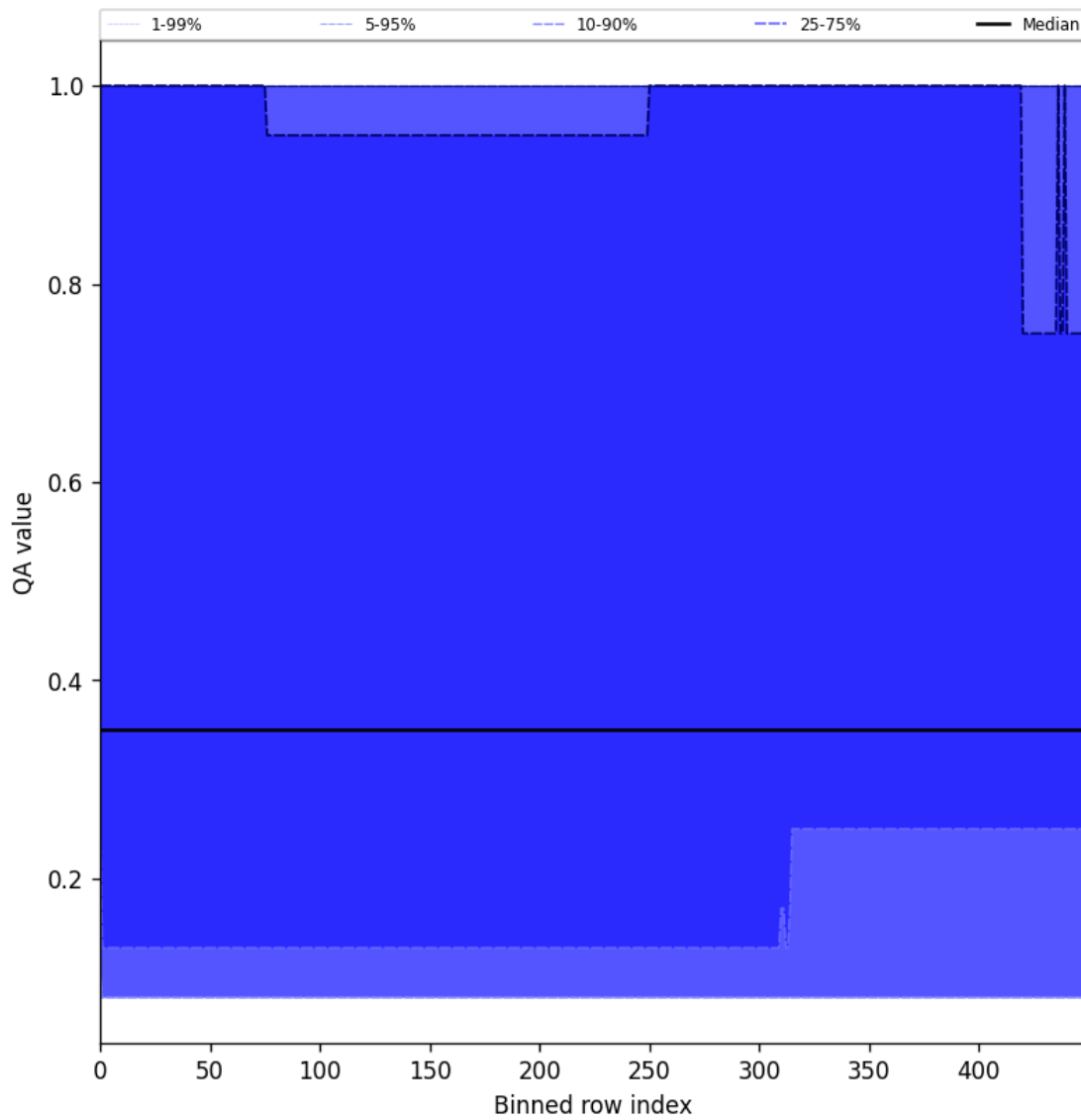
Figure 48: Along track statistics of “QA value” for 2025-02-19 to 2025-02-20
