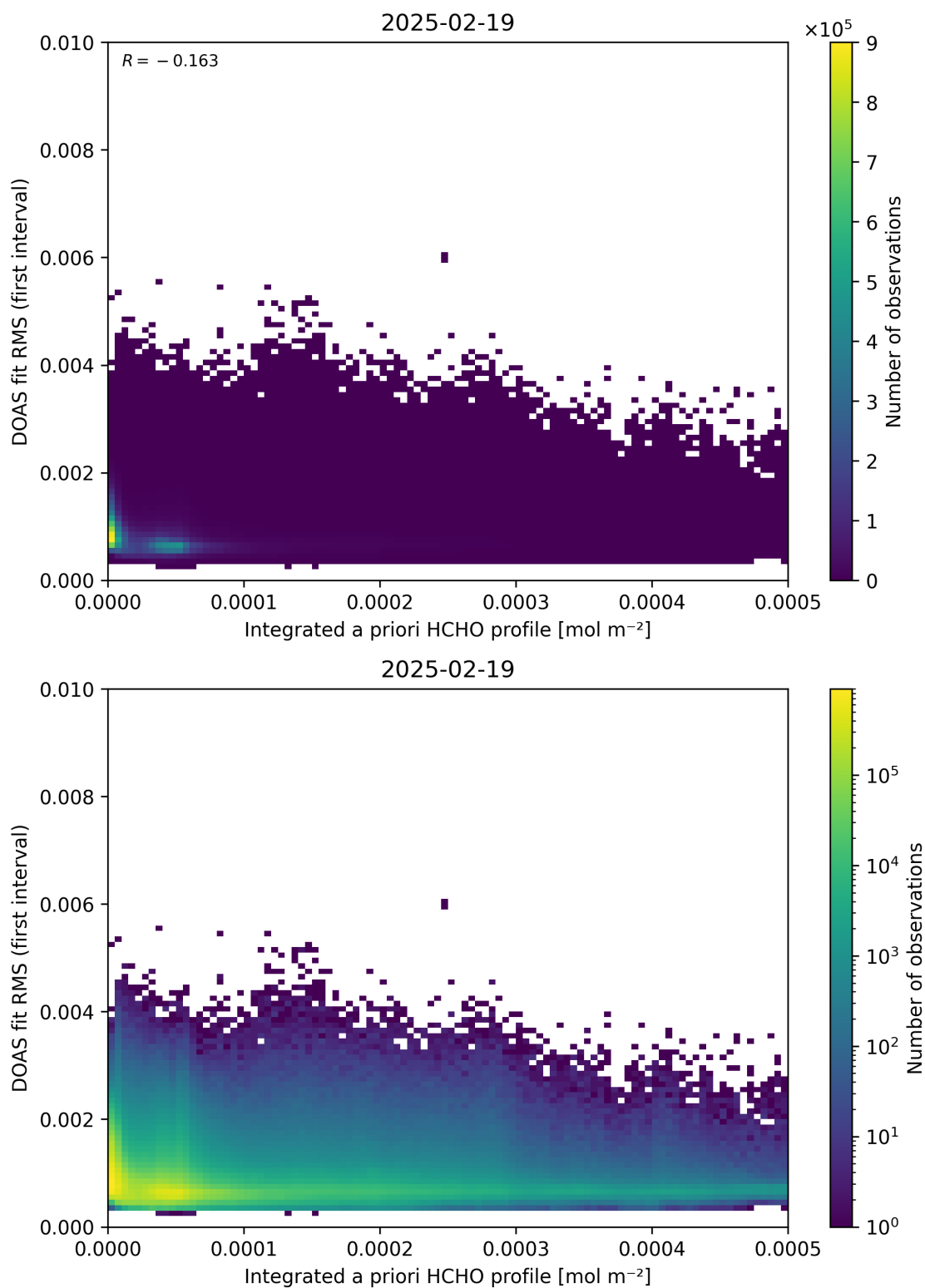
Figure 148: Scatter density plot of “Integrated a priori HCHO profile” against “DOAS fit RMS (first interval)” for 2025-02-19 to 2025-02-20.
