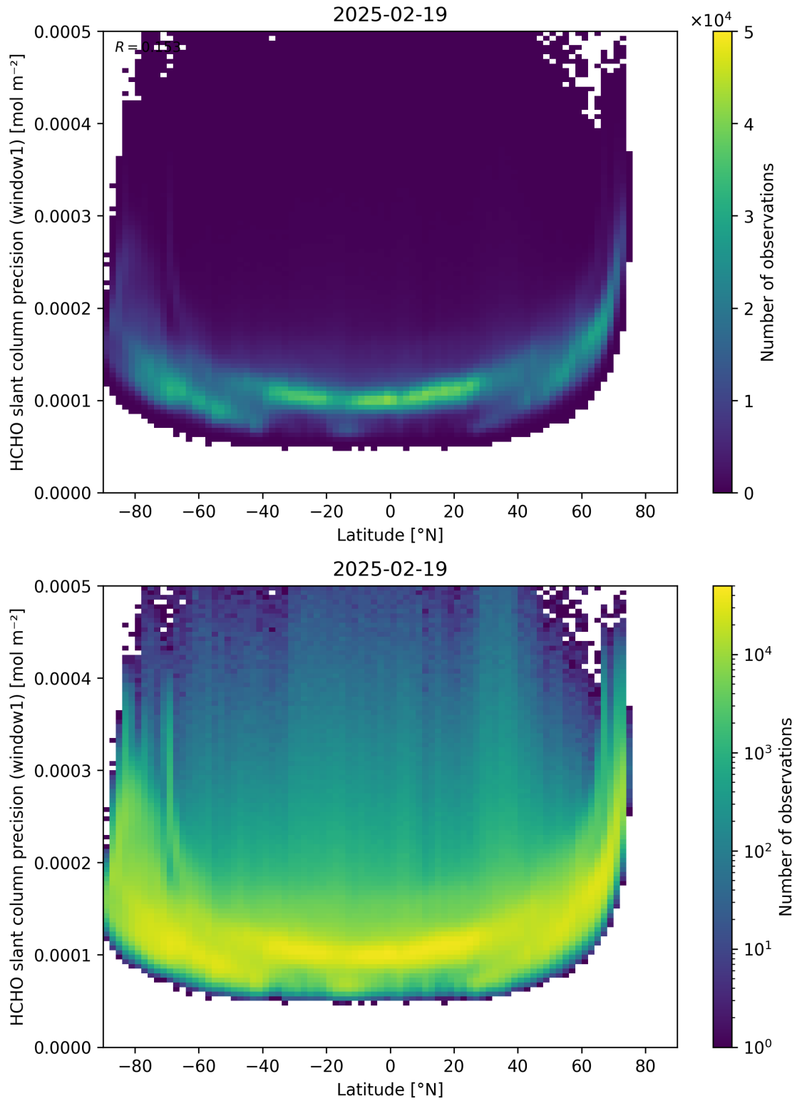
Figure 160: Scatter density plot of “Latitude” against “HCHO slant column precision (window1)” for 2025-02-19 to 2025-02-20.
