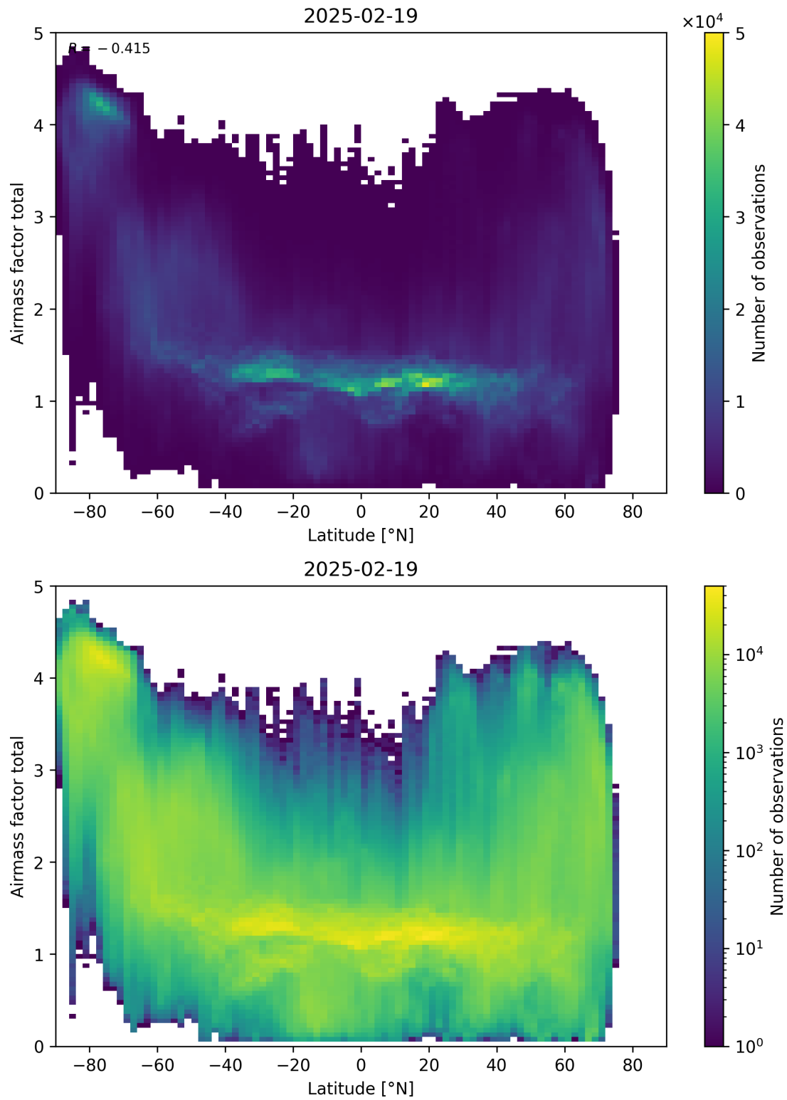
Figure 161: Scatter density plot of “Latitude” against “Airmass factor total” for 2025-02-19 to 2025-02-20.
