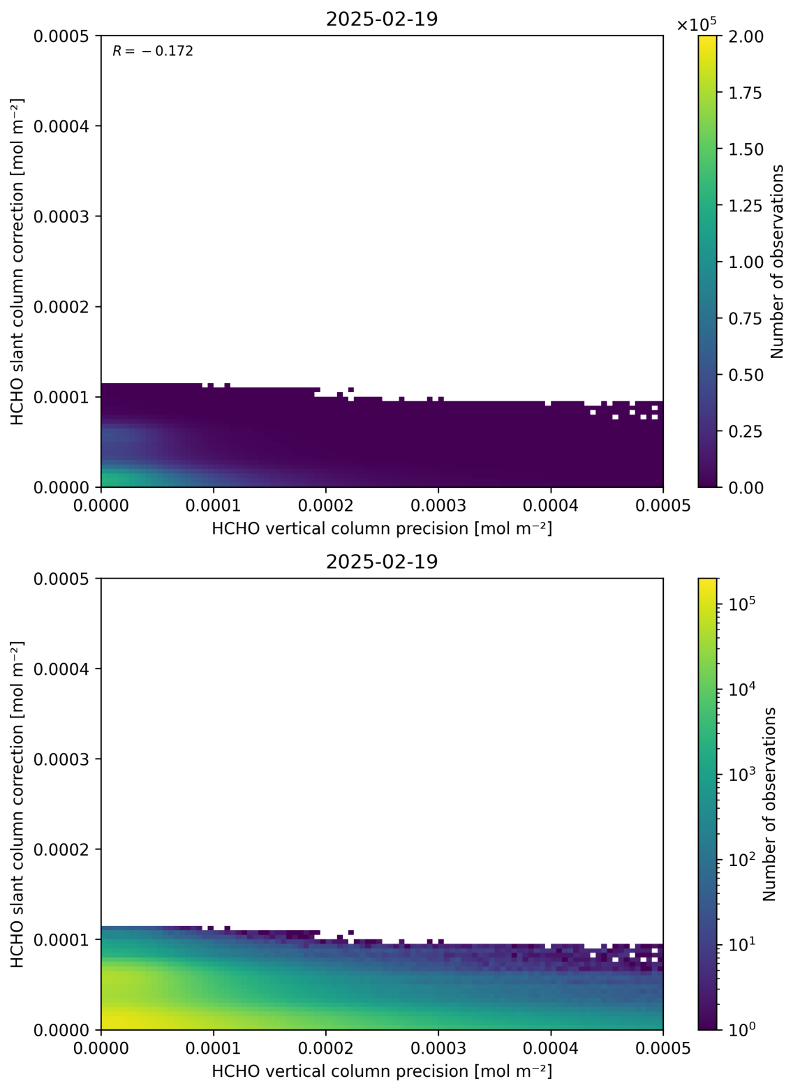
Figure 141: Scatter density plot of “HCHO vertical column precision” against “HCHO slant column correction” for 2025-02-19 to 2025-02-20.
