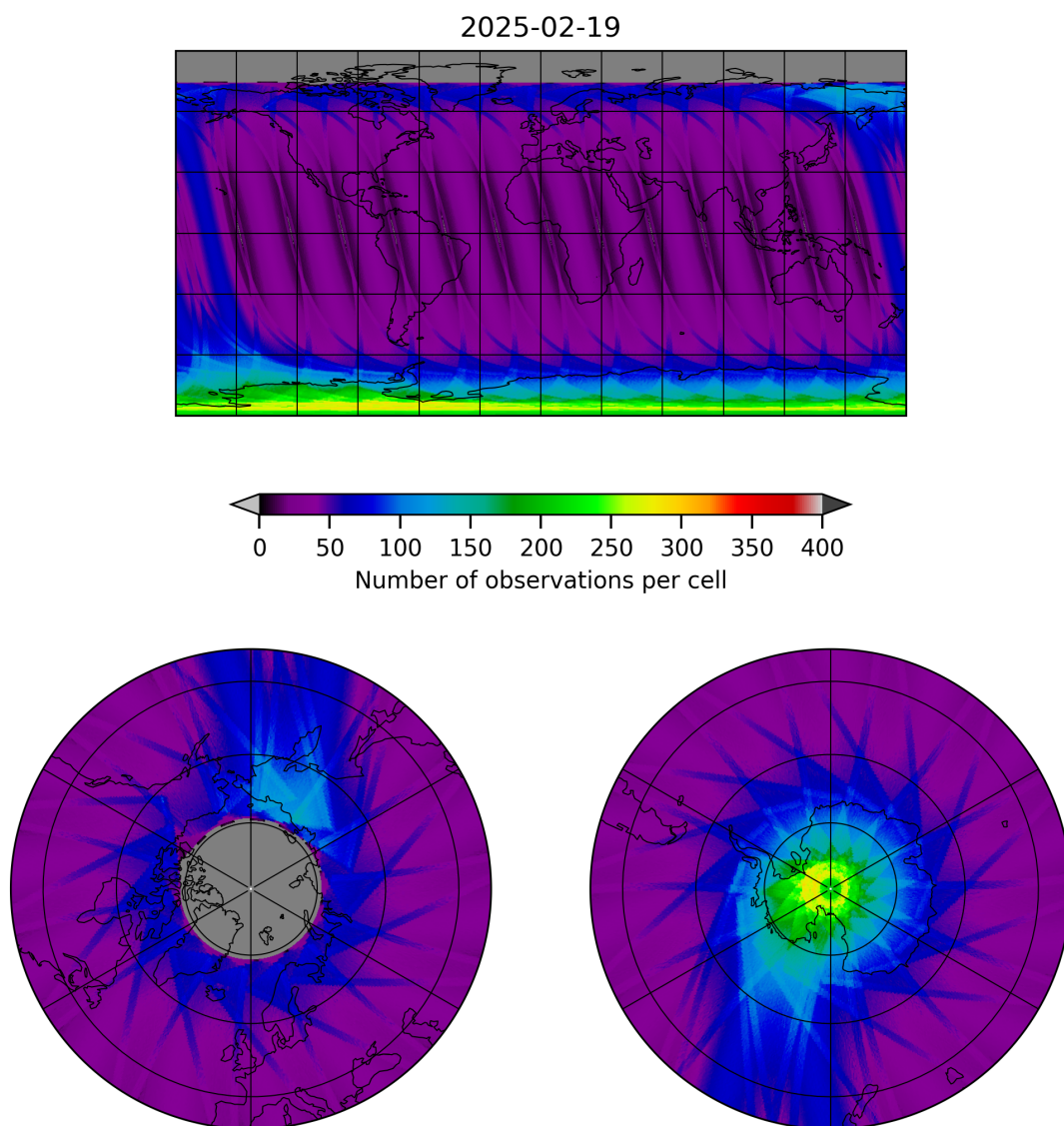
Figure 19: Map of the number of observations for 2025-02-19 to 2025-02-20
