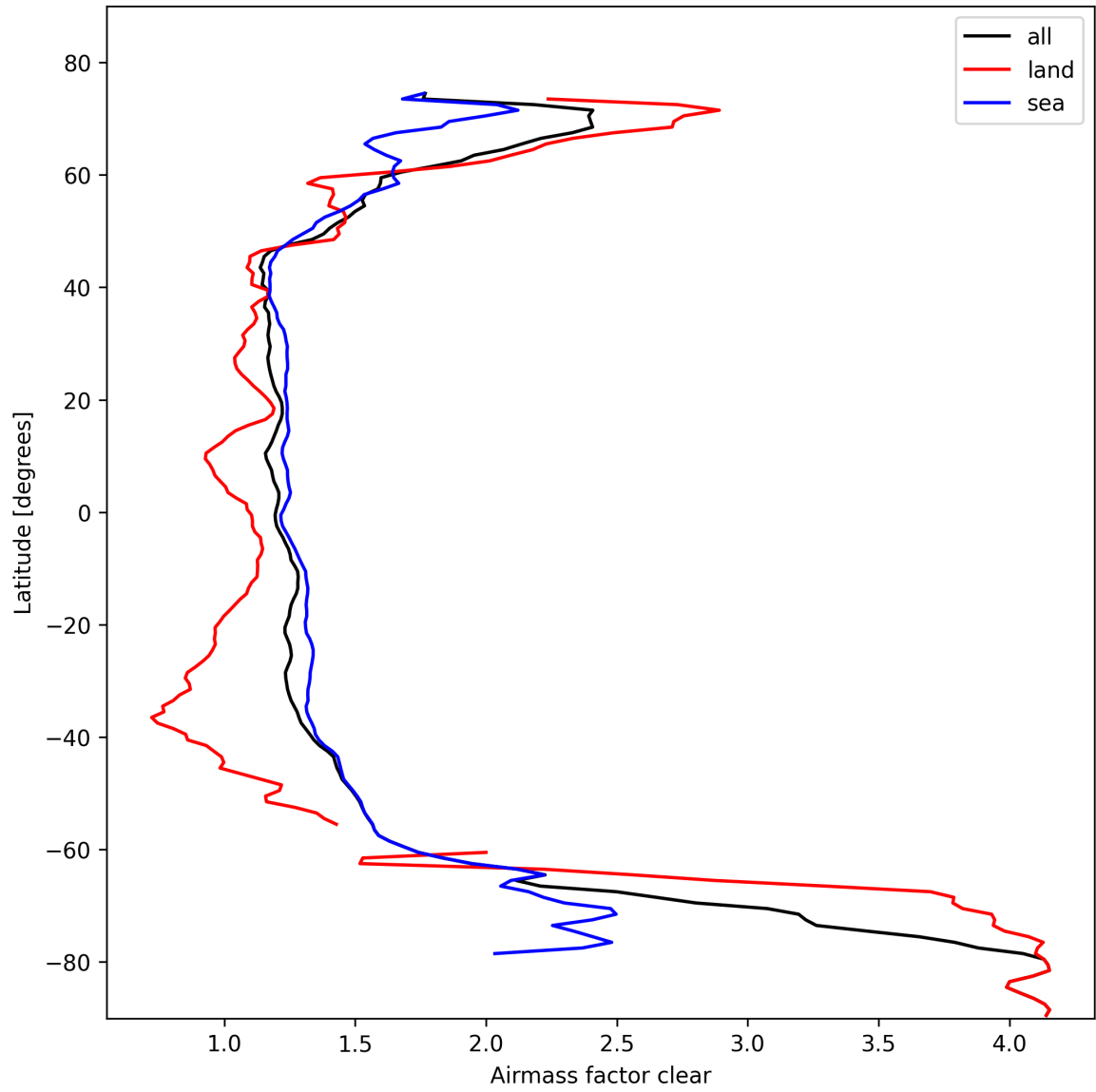
Figure 28: Zonal average of “Airmass factor clear” for 2025-02-19 to 2025-02-20.
