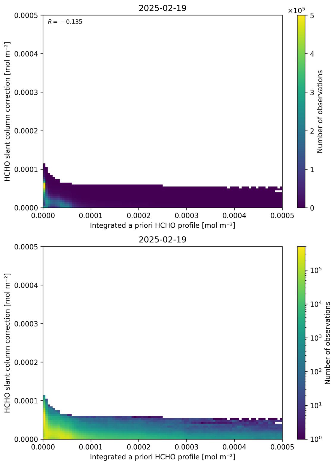
Figure 152: Scatter density plot of “Integrated a priori HCHO profile” against “HCHO slant column correction” for 2025-02-19 to 2025-02-20.
