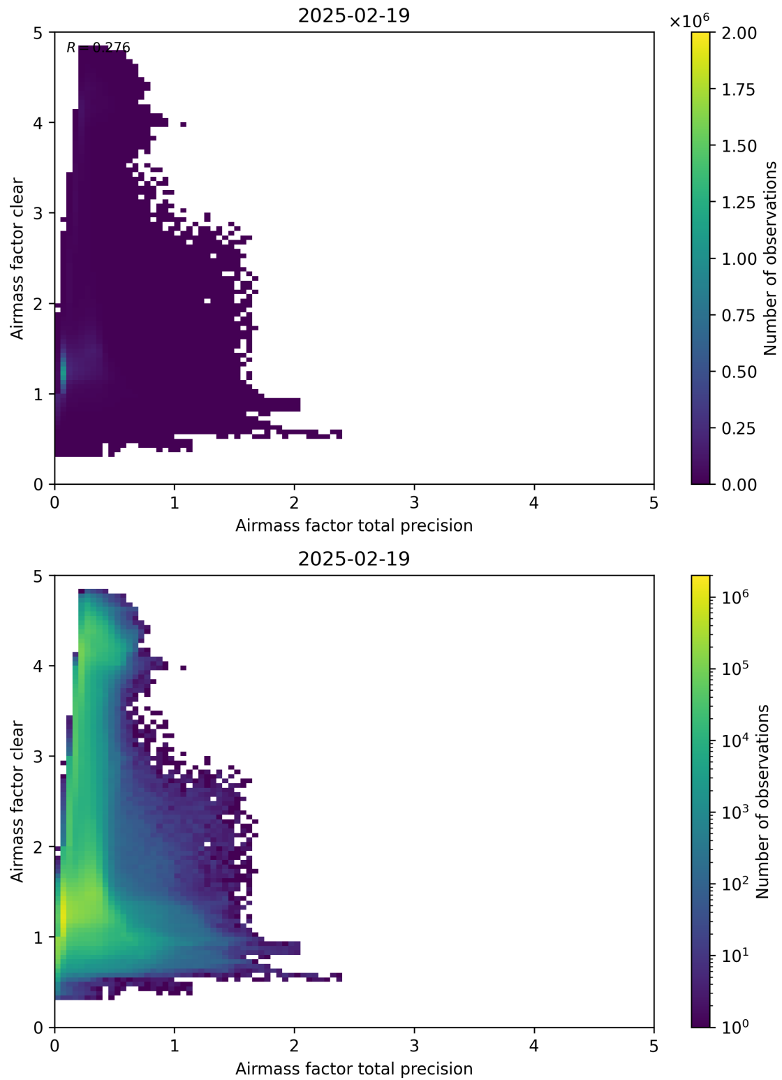
Figure 108: Scatter density plot of “Airmass factor total precision” against “Airmass factor clear” for 2025-02-19 to 2025-02-20.
