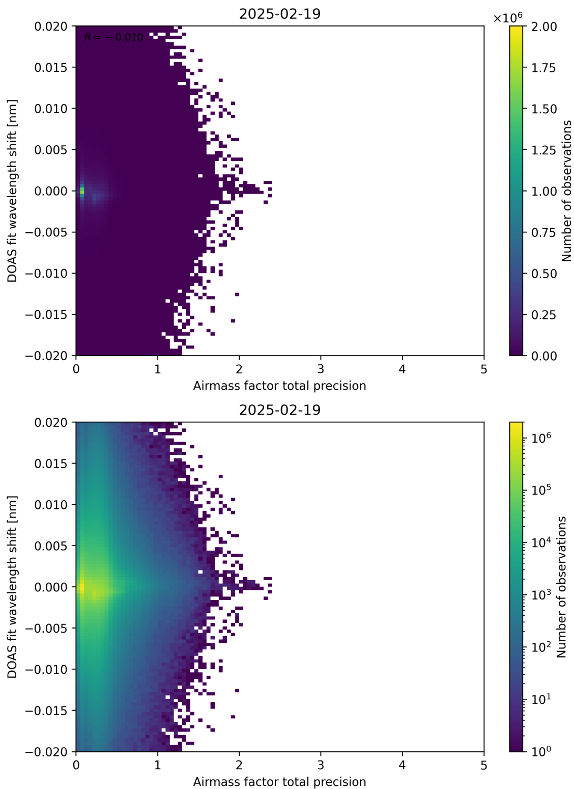
Figure 106: Scatter density plot of “Airmass factor total precision” against “DOAS fit wavelength shift” for 2025-02-19 to 2025-02-20.
