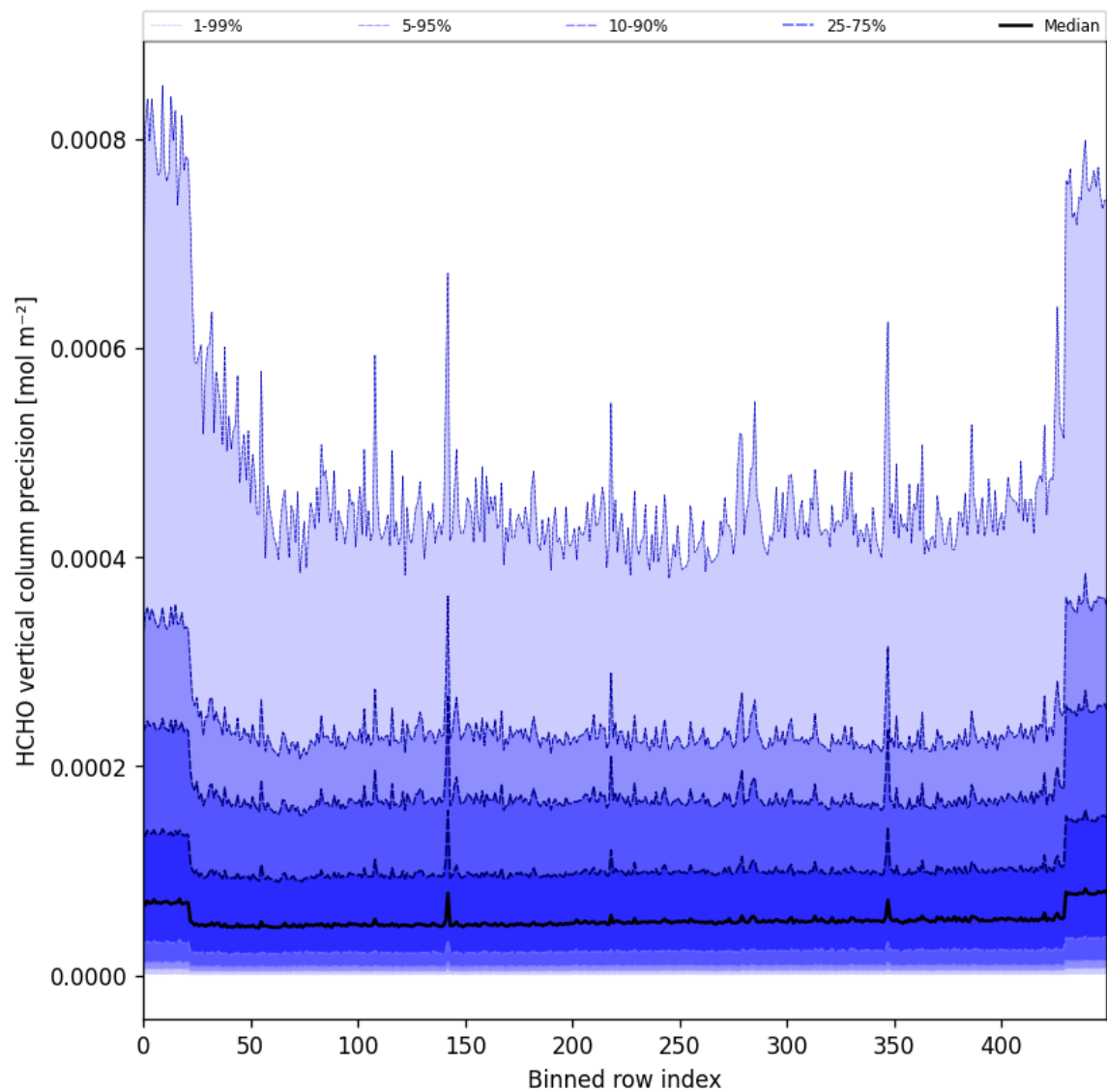
Figure 50: Along track statistics of “HCHO vertical column precision” for 2025-02-19 to 2025-02-20
