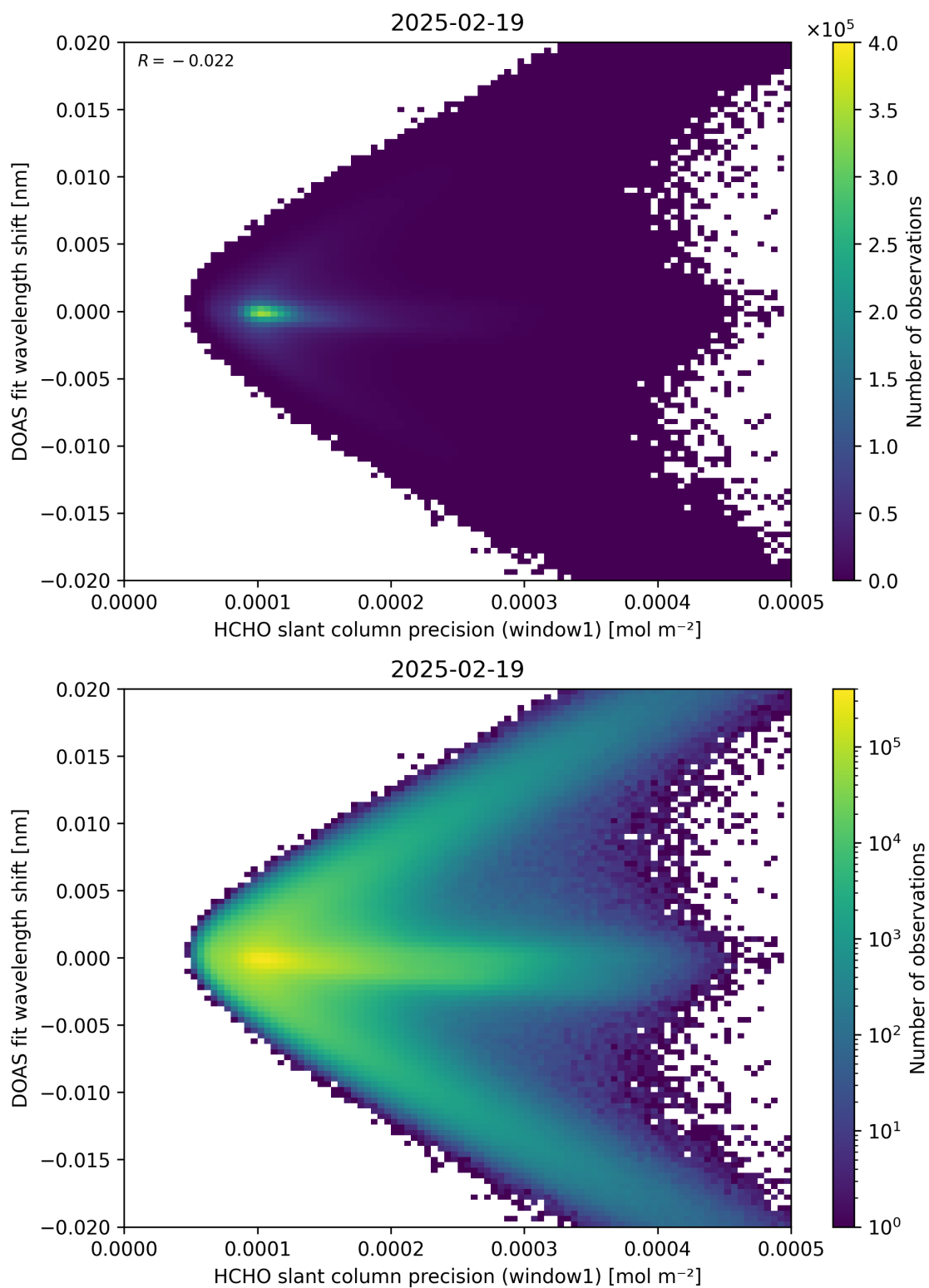
Figure 89: Scatter density plot of “HCHO slant column precision (window1)” against “DOAS fit wavelength shift” for 2025-02-19 to 2025-02-20.
