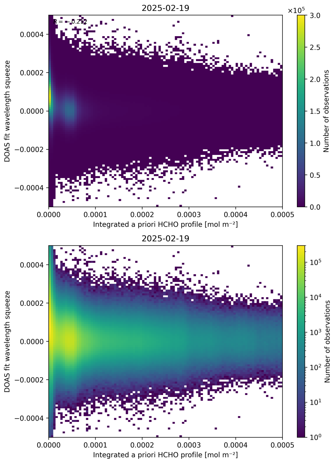
Figure 150: Scatter density plot of “Integrated a priori HCHO profile” against “DOAS fit wavelength squeeze” for 2025-02-19 to 2025-02-20.
