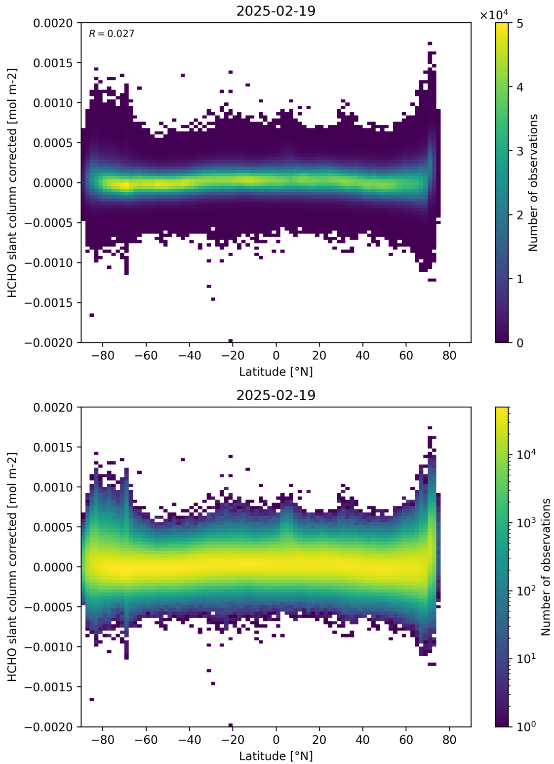
Figure 157: Scatter density plot of “Latitude” against “HCHO slant column corrected” for 2025-02-19 to 2025-02-20.
