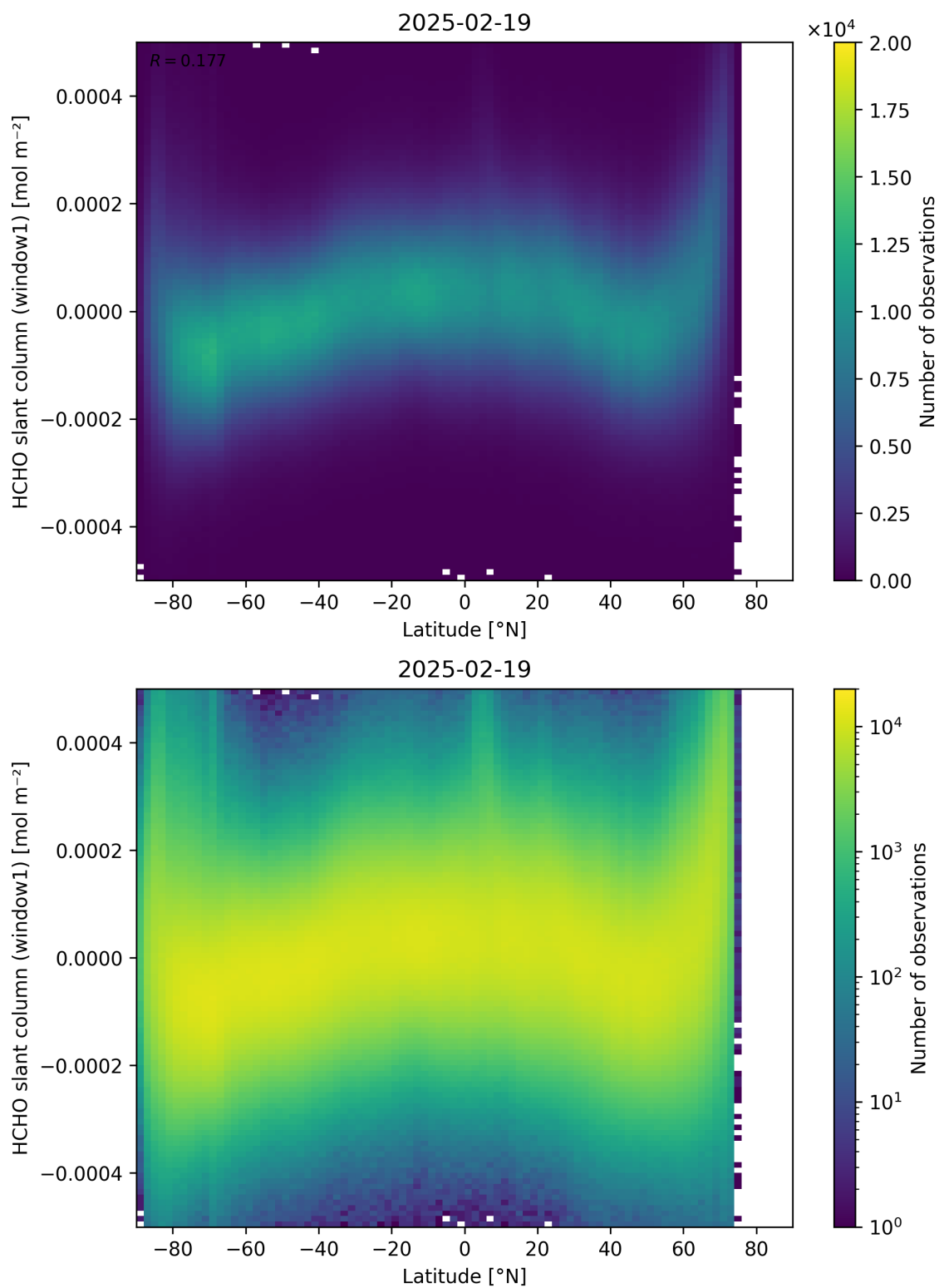
Figure 159: Scatter density plot of “Latitude” against “HCHO slant column (window1)” for 2025-02-19 to 2025-02-20.
