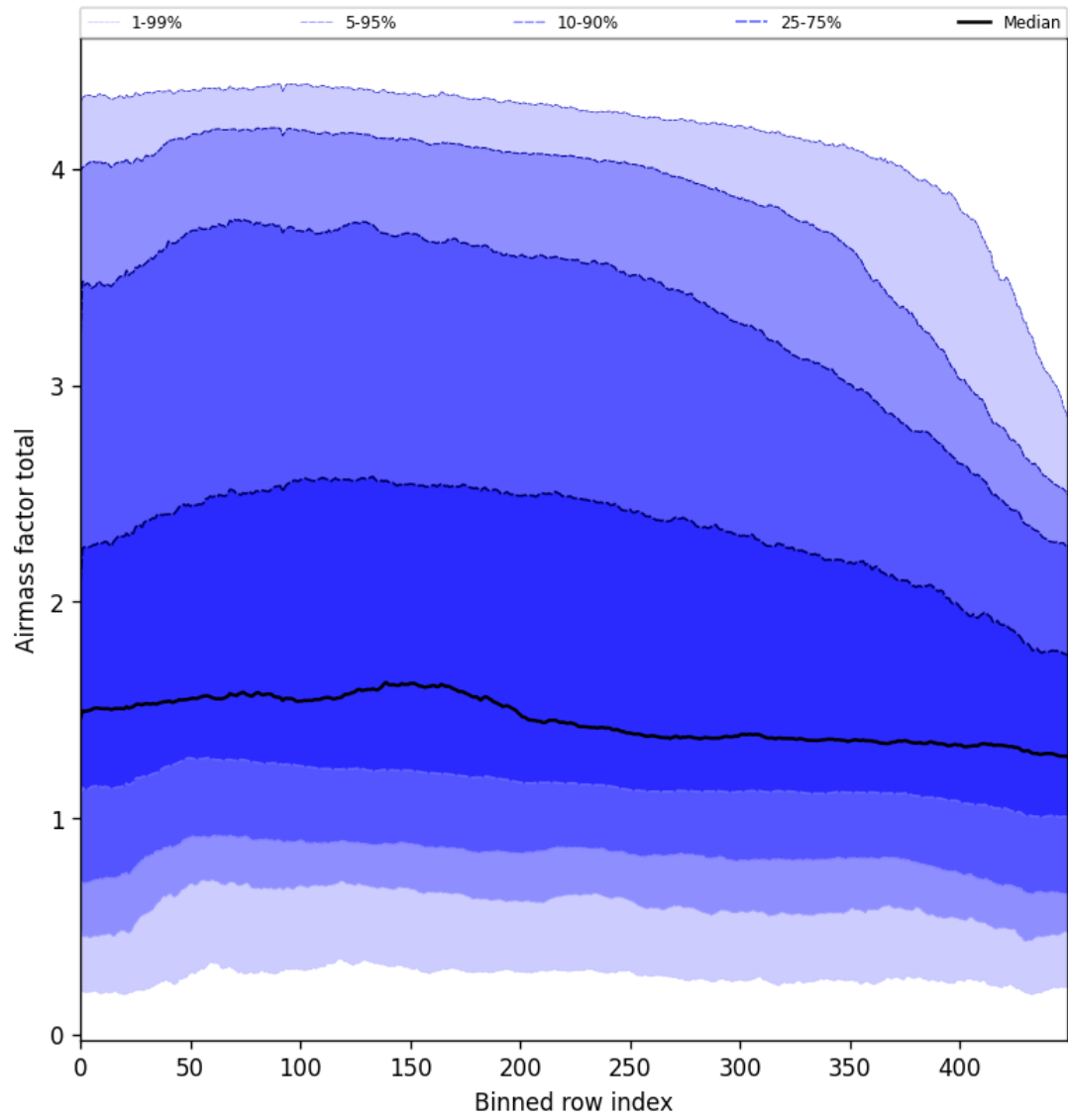
Figure 54: Along track statistics of “Airmass factor total” for 2025-02-19 to 2025-02-20
