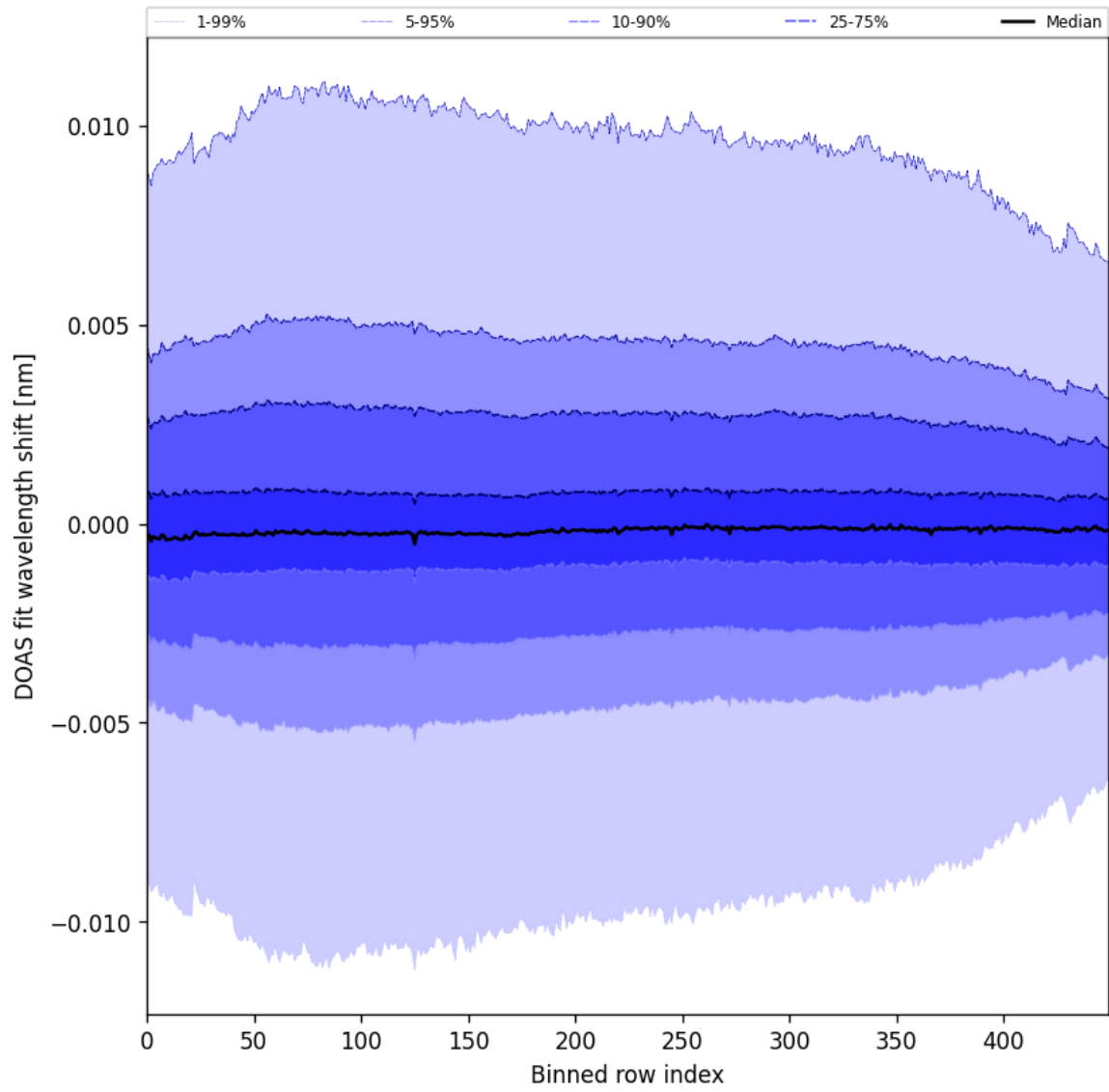
Figure 58: Along track statistics of “DOAS fit wavelength shift” for 2025-02-19 to 2025-02-20
