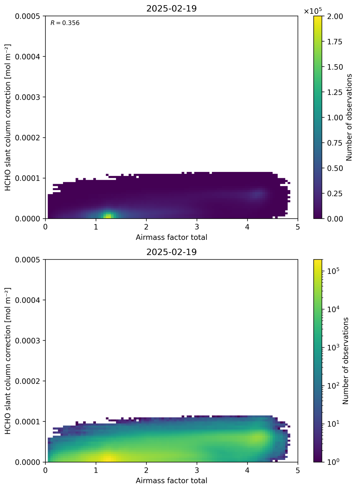
Figure 102: Scatter density plot of “Airmass factor total” against “HCHO slant column correction” for 2025-02-19 to 2025-02-20.
