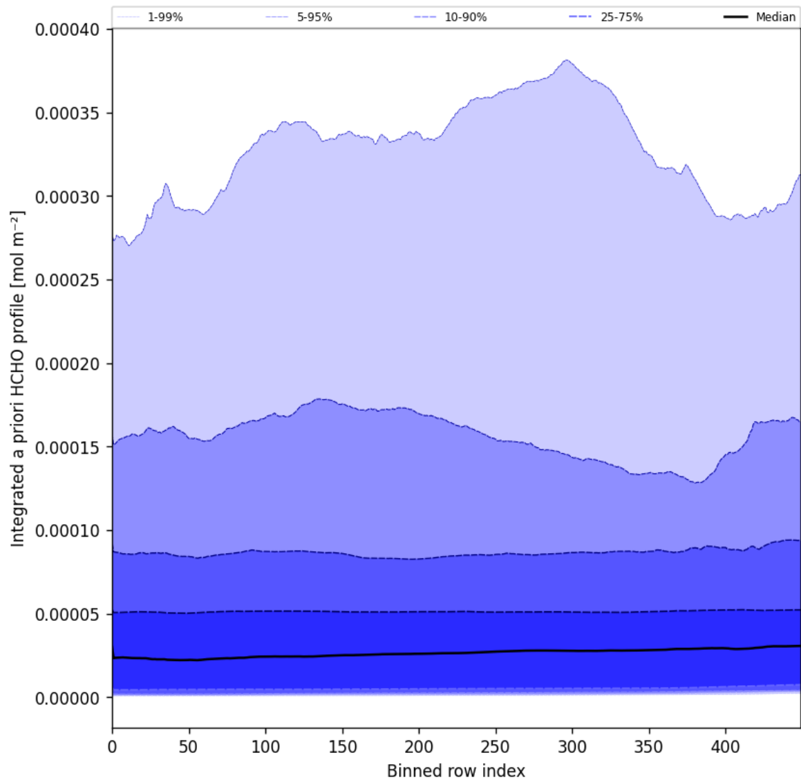
Figure 57: Along track statistics of “Integrated a priori HCHO profile” for 2025-02-19 to 2025-02-20
