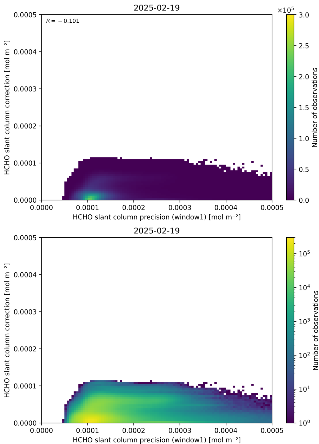
Figure 93: Scatter density plot of “HCHO slant column precision (window1)” against “HCHO slant column correction” for 2025-02-19 to 2025-02-20.
