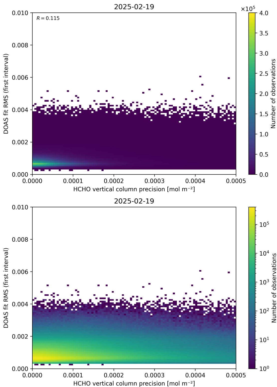
Figure 136: Scatter density plot of “HCHO vertical column precision” against “DOAS fit RMS (first interval)” for 2025-02-19 to 2025-02-20.
