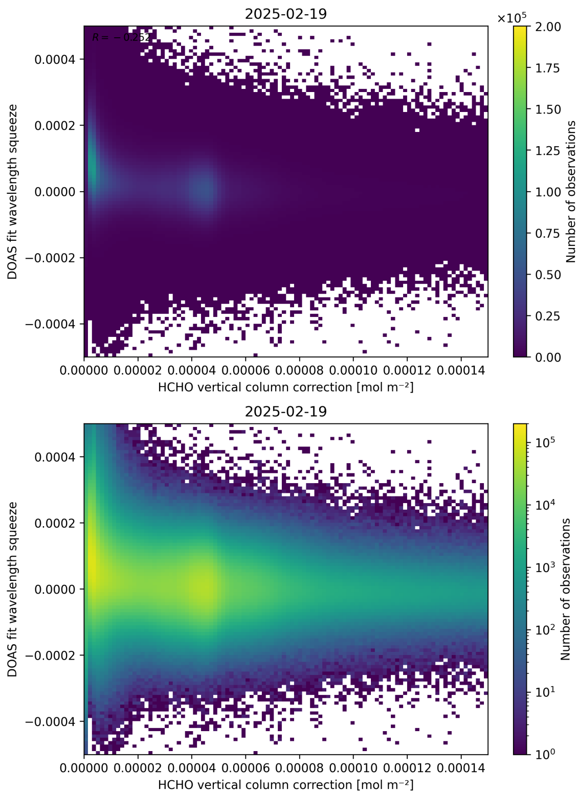
Figure 114: Scatter density plot of “HCHO vertical column correction” against “DOAS fit wavelength squeeze” for 2025-02-19 to 2025-02-20.
