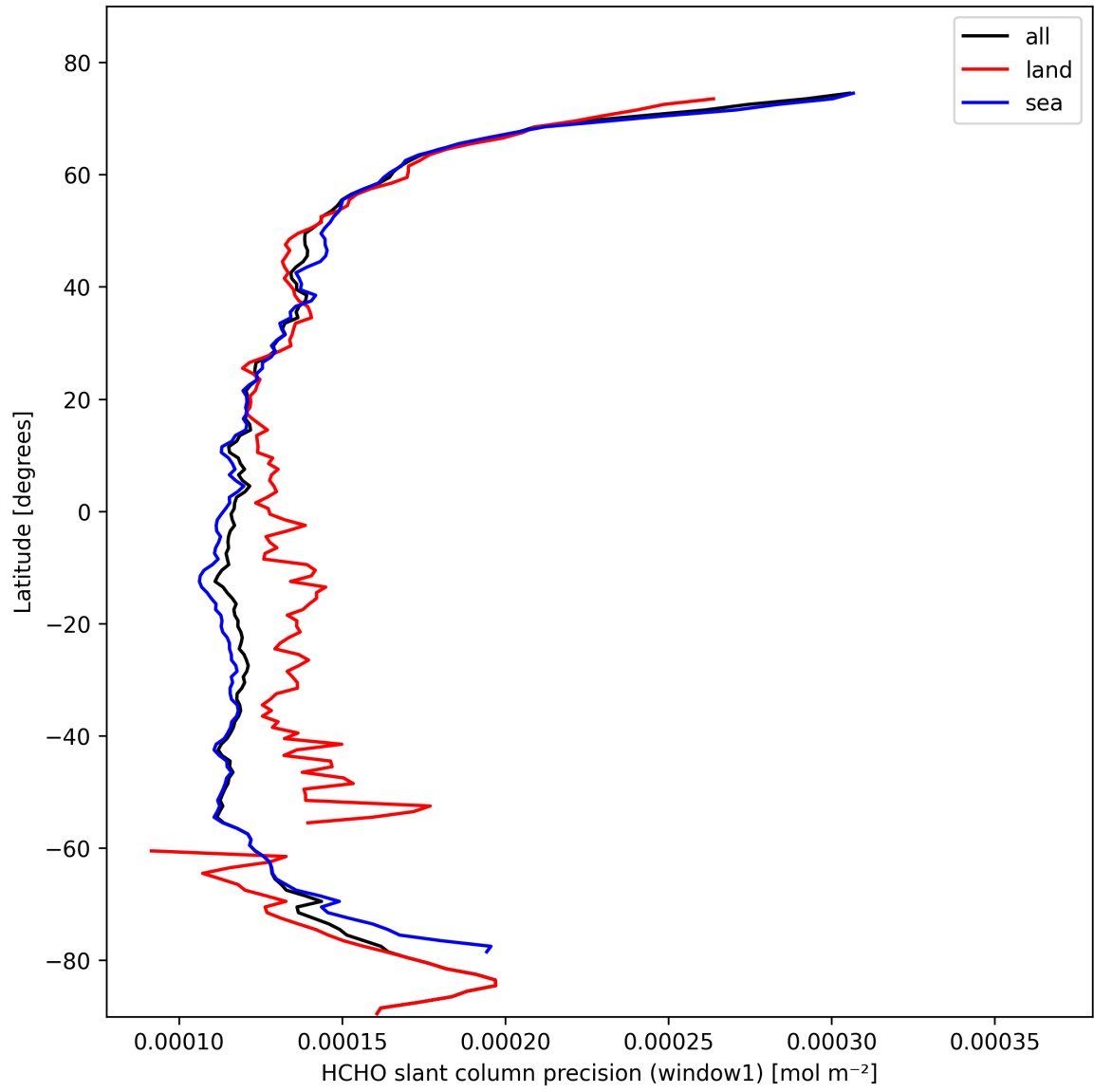
Figure 25: Zonal average of “HCHO slant column precision (window1)” for 2025-02-19 to 2025-02-20.
