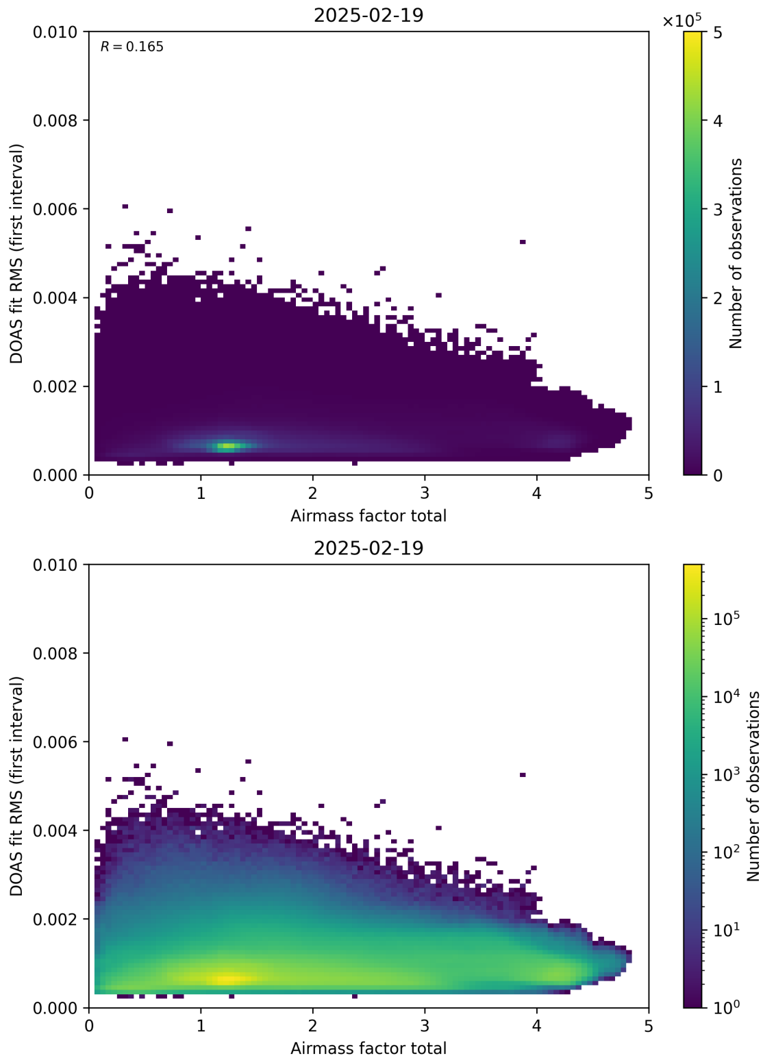
Figure 97: Scatter density plot of “Airmass factor total” against “DOAS fit RMS (first interval)” for 2025-02-19 to 2025-02-20.
