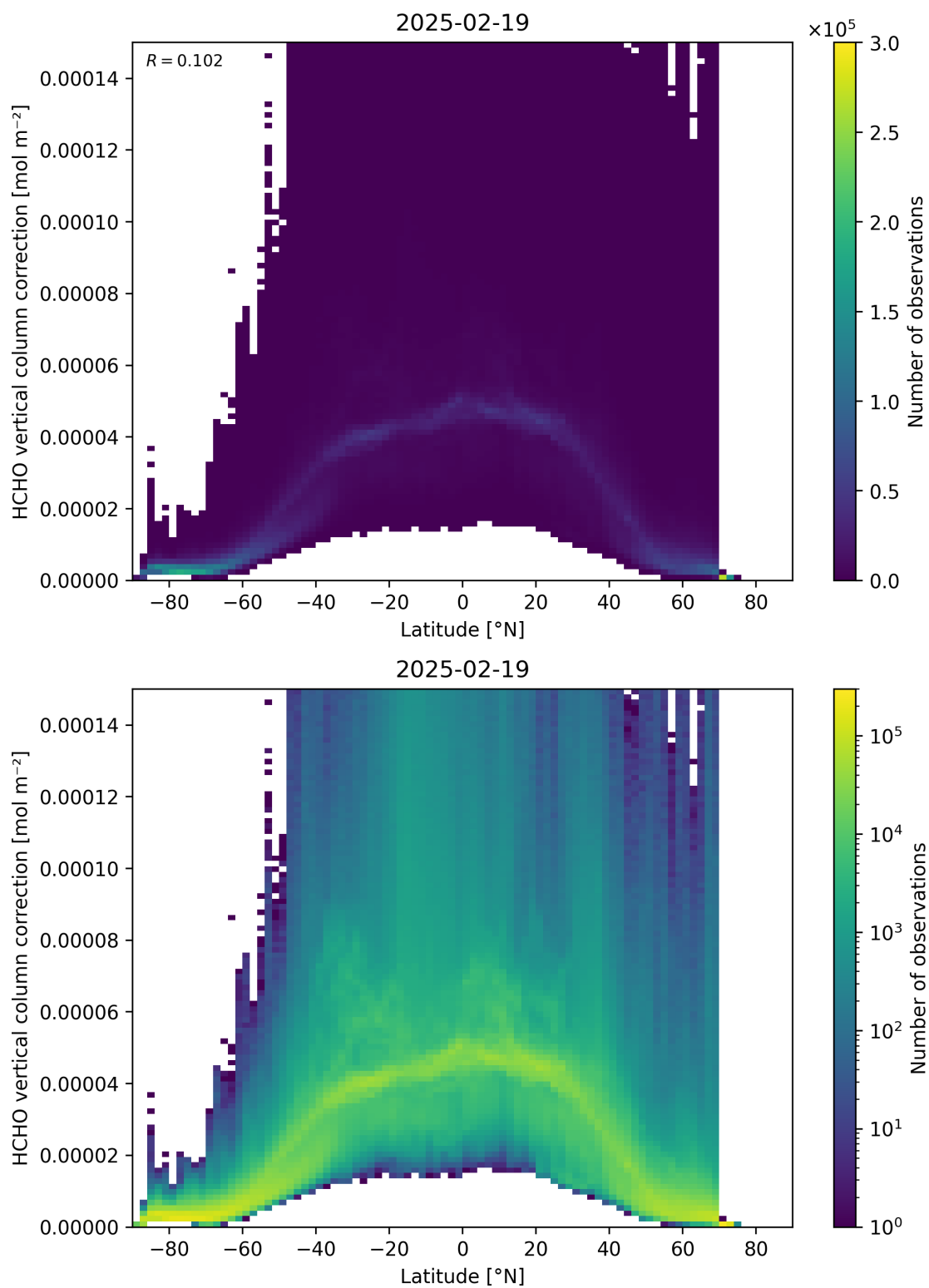
Figure 164: Scatter density plot of “Latitude” against “HCHO vertical column correction” for 2025-02-19 to 2025-02-20.
