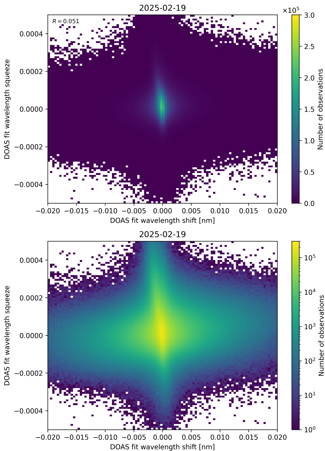
Figure 65: Scatter density plot of “DOAS fit wavelength shift” against “DOAS fit wavelength squeeze” for 2025-02-19 to 2025-02-20.
