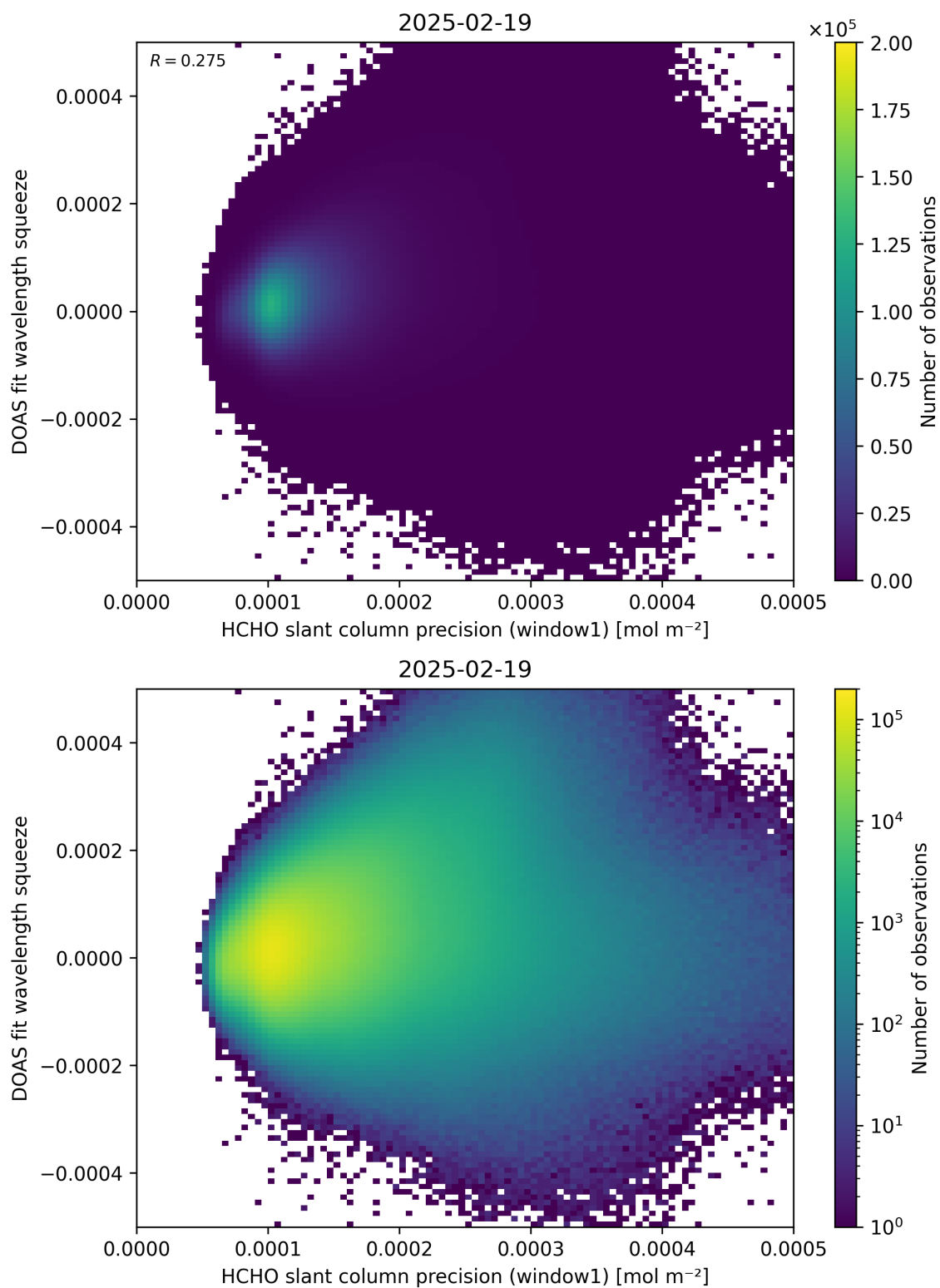
Figure 90: Scatter density plot of “HCHO slant column precision (window1)” against “DOAS fit wavelength squeeze” for 2025-02-19 to 2025-02-20.
