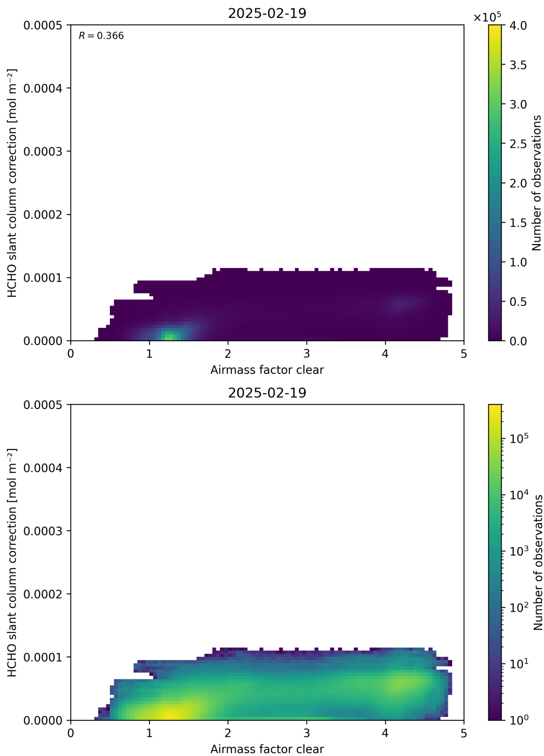
Figure 75: Scatter density plot of “Airmass factor clear” against “HCHO slant column correction” for 2025-02-19 to 2025-02-20.
