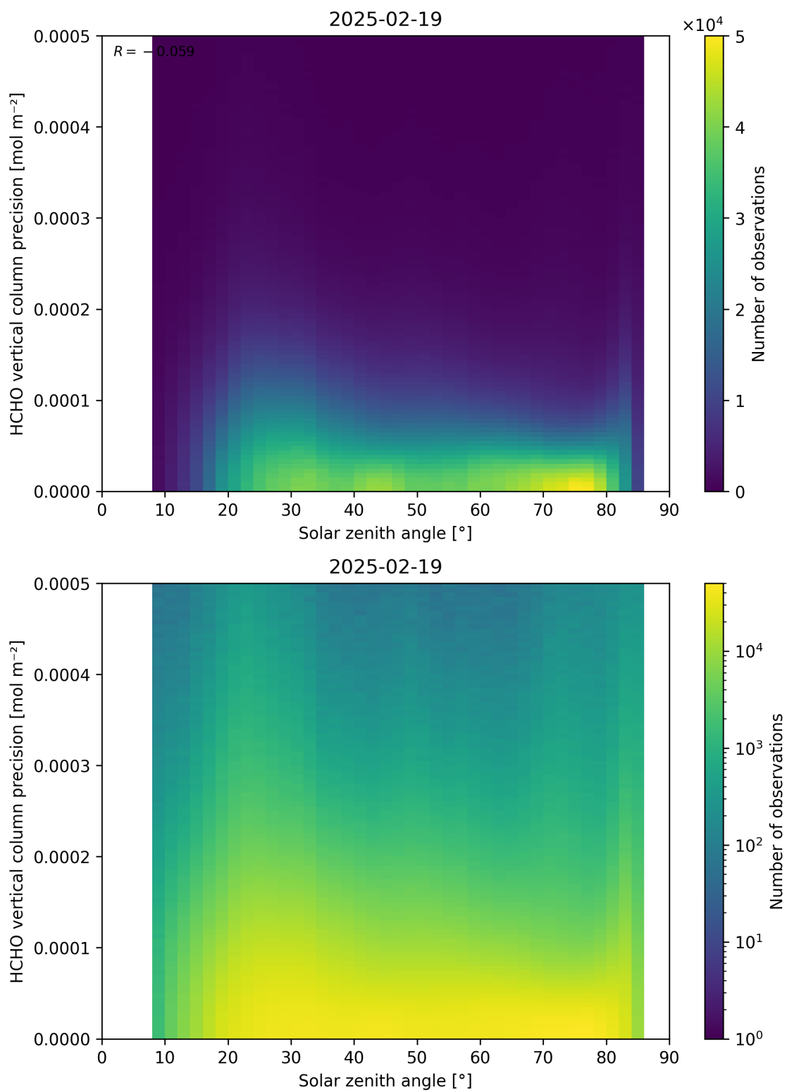
Figure 179: Scatter density plot of “Solar zenith angle” against “HCHO vertical column precision” for 2025-02-19 to 2025-02-20.
