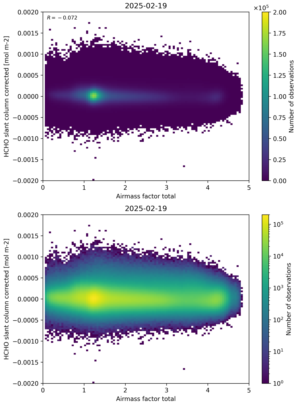
Figure 101: Scatter density plot of “Airmass factor total” against “HCHO slant column corrected” for 2025-02-19 to 2025-02-20.
