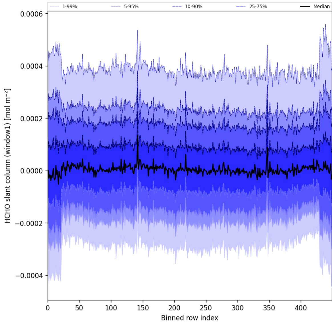
Figure 52: Along track statistics of “HCHO slant column (window1)” for 2025-02-19 to 2025-02-20
