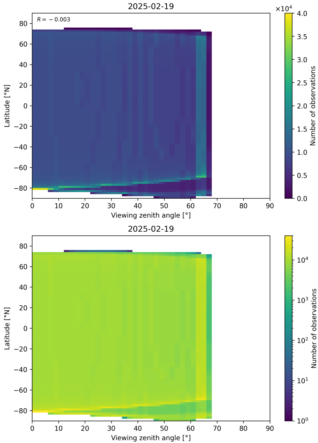
Figure 196: Scatter density plot of “Viewing zenith angle” against “Latitude” for 2025-02-19 to 2025-02-20.
