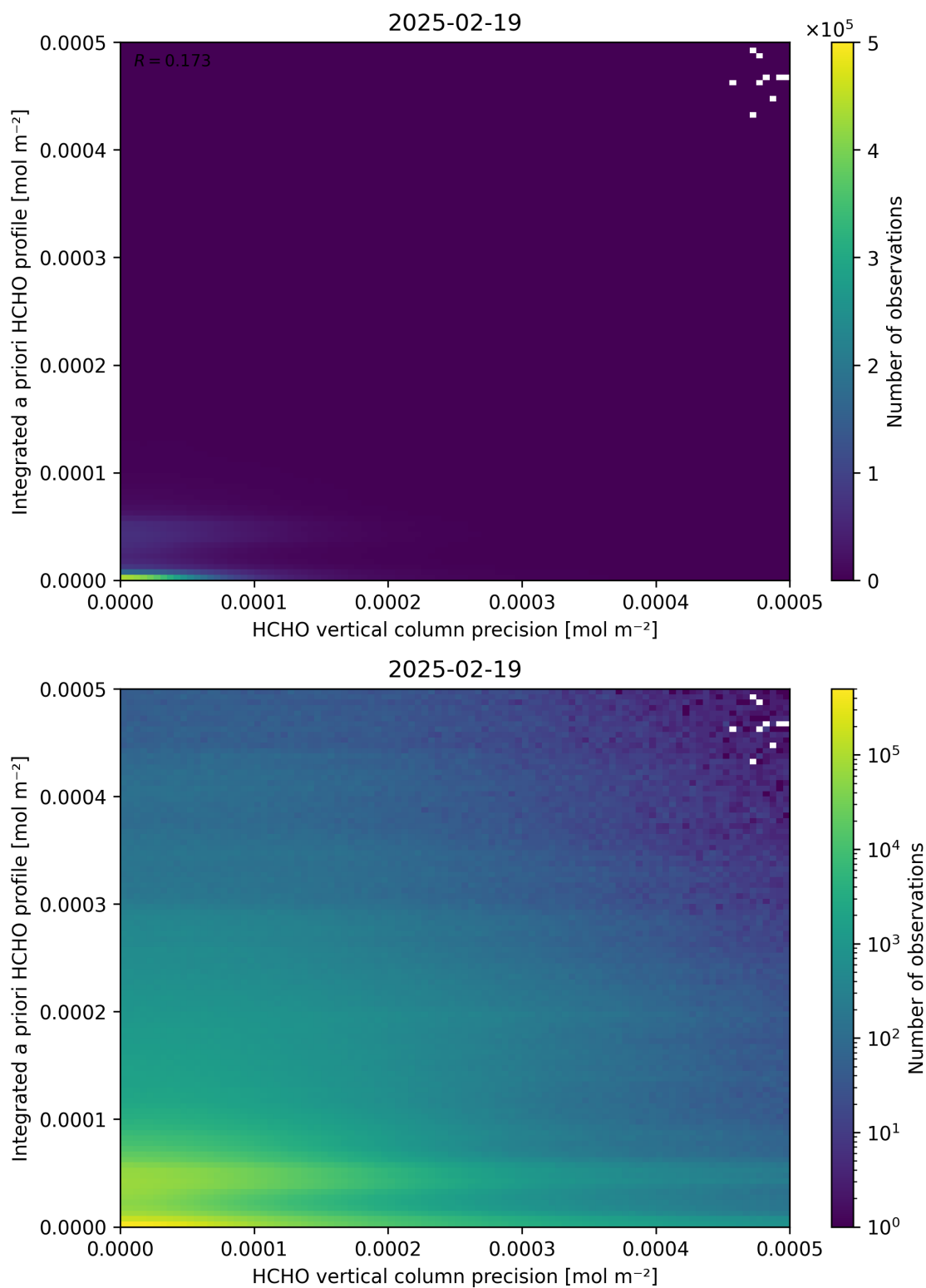
Figure 147: Scatter density plot of “HCHO vertical column precision” against “Integrated a priori HCHO profile” for 2025-02-19 to 2025-02-20.
