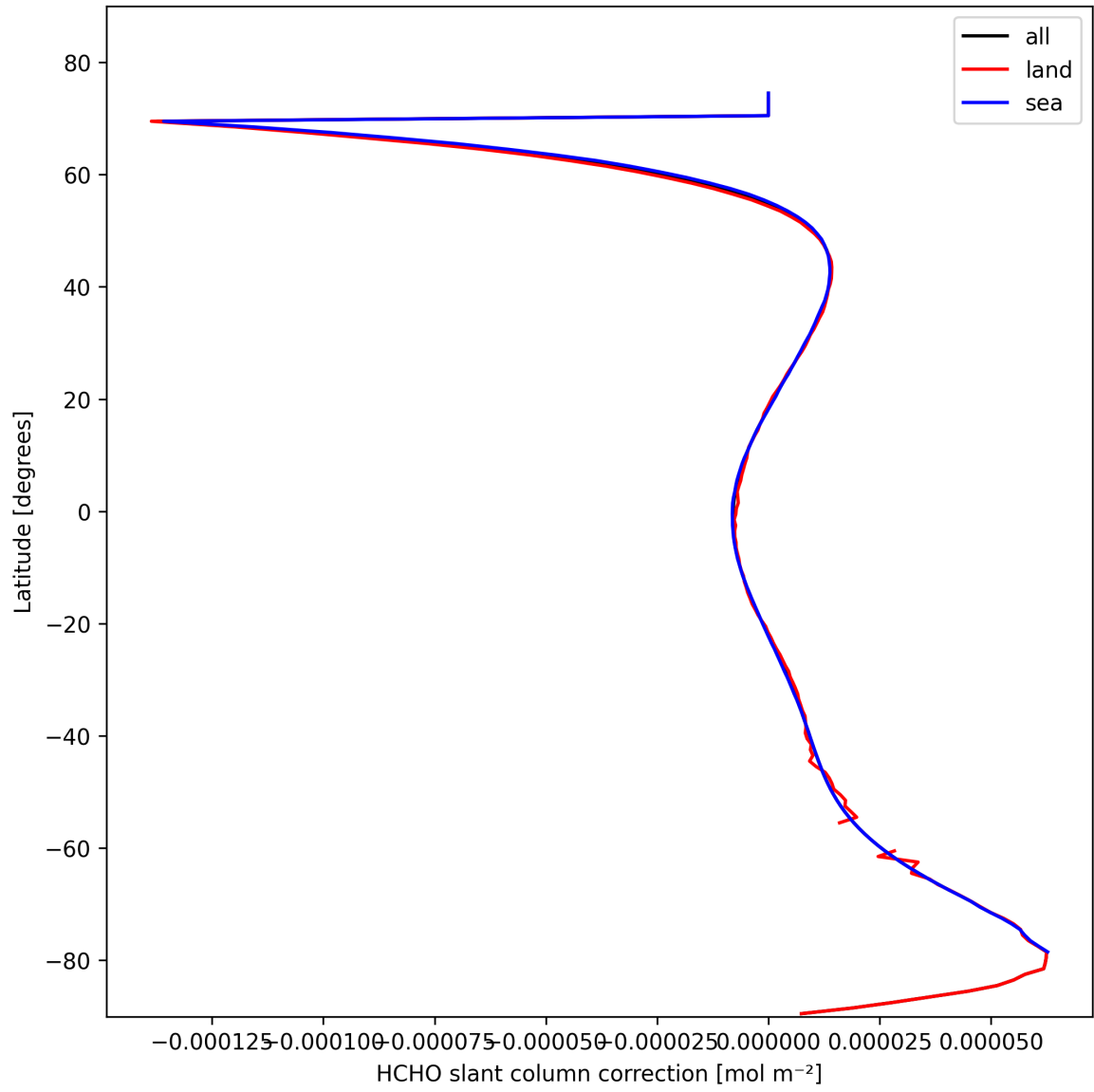
Figure 33: Zonal average of “HCHO slant column correction” for 2025-02-19 to 2025-02-20.
