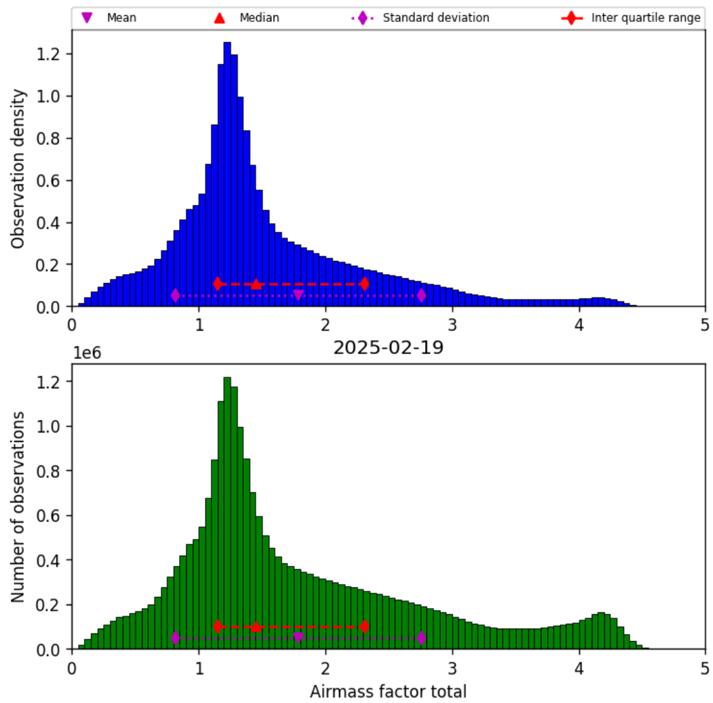
Figure 40: Histogram of “Airmass factor total” for 2025-02-19 to 2025-02-20
