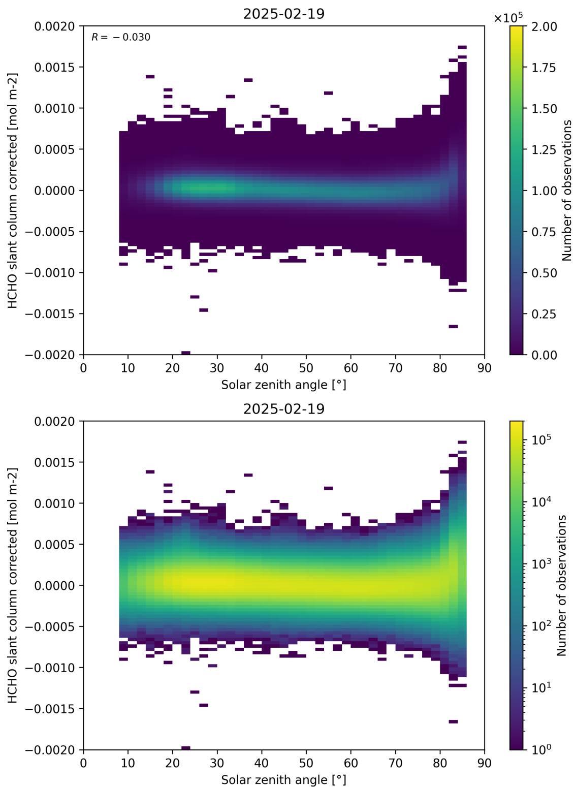
Figure 171: Scatter density plot of “Solar zenith angle” against “HCHO slant column corrected” for 2025-02-19 to 2025-02-20.
