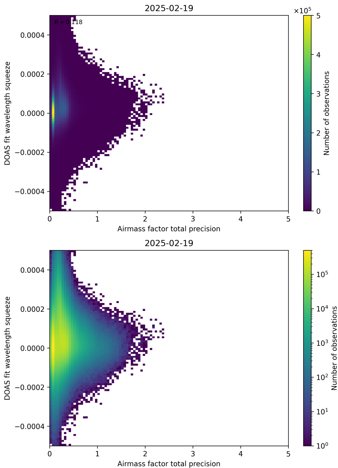
Figure 107: Scatter density plot of “Airmass factor total precision” against “DOAS fit wavelength squeeze” for 2025-02-19 to 2025-02-20.
