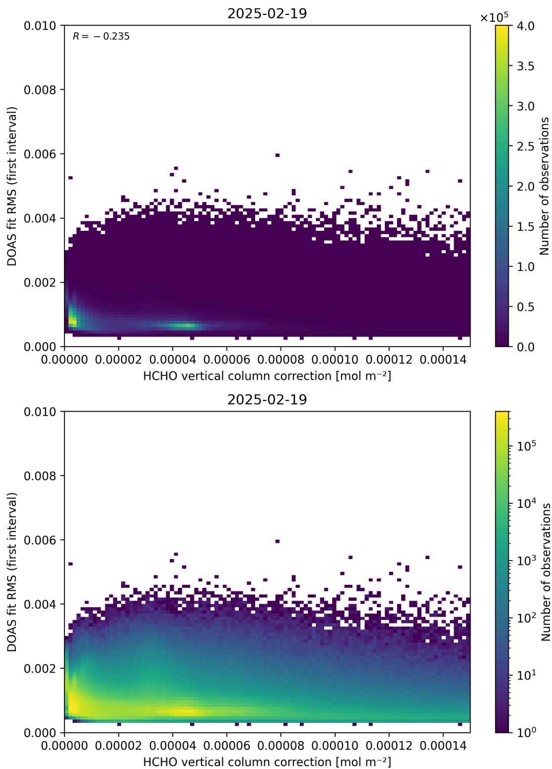
Figure 112: Scatter density plot of “HCHO vertical column correction” against “DOAS fit RMS (first interval)” for 2025-02-19 to 2025-02-20.
