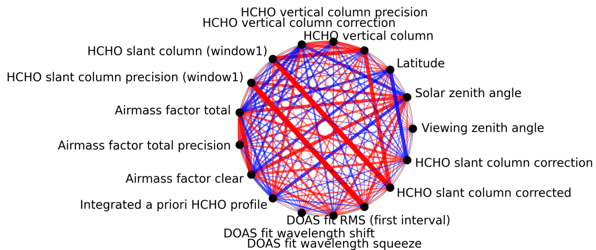
Figure 1: Map of correlation graph for 2025-02-19 to 2025-02-20.
