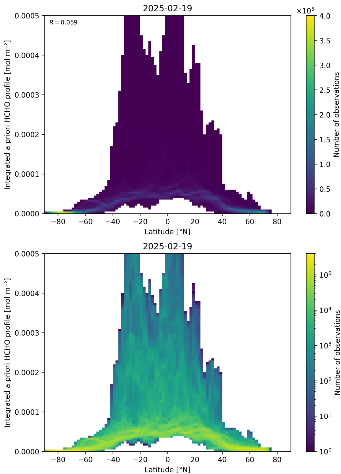
Figure 166: Scatter density plot of “Latitude” against “Integrated a priori HCHO profile” for 2025-02-19 to 2025-02-20.
