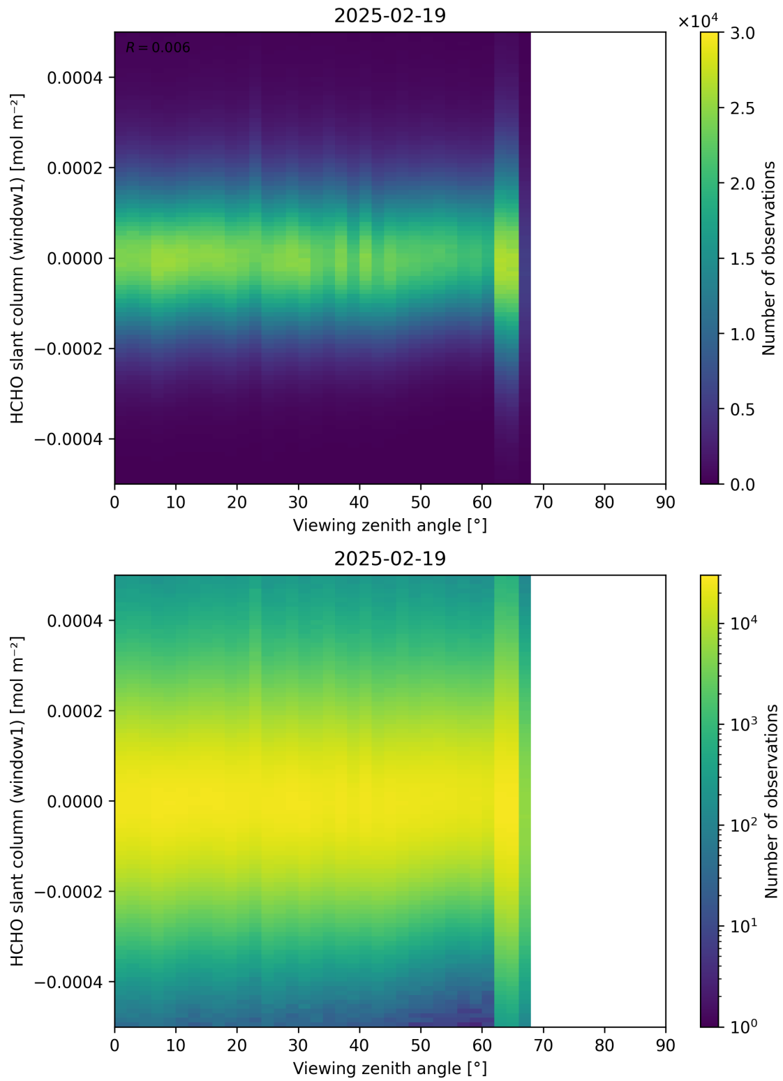
Figure 188: Scatter density plot of “Viewing zenith angle” against “HCHO slant column (window1)” for 2025-02-19 to 2025-02-20.
