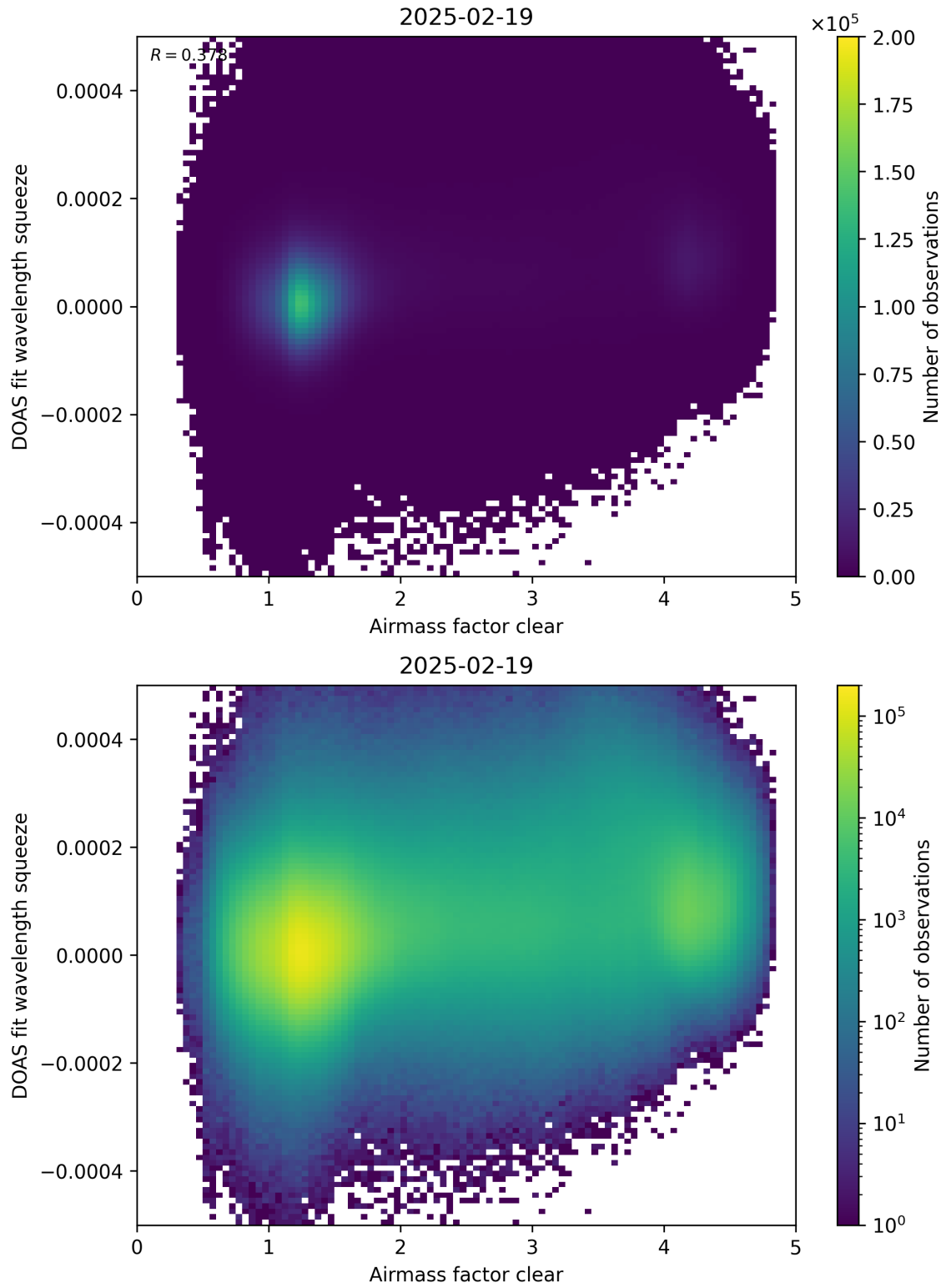
Figure 73: Scatter density plot of “Airmass factor clear” against “DOAS fit wavelength squeeze” for 2025-02-19 to 2025-02-20.
