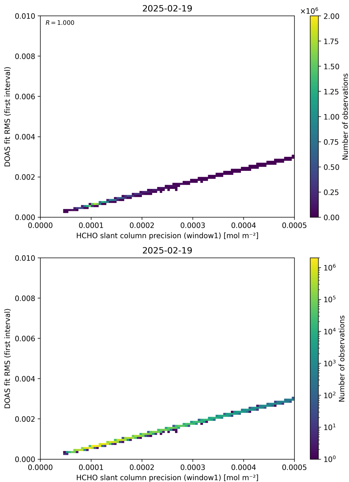
Figure 88: Scatter density plot of “HCHO slant column precision (window1)” against “DOAS fit RMS (first interval)” for 2025-02-19 to 2025-02-20.
