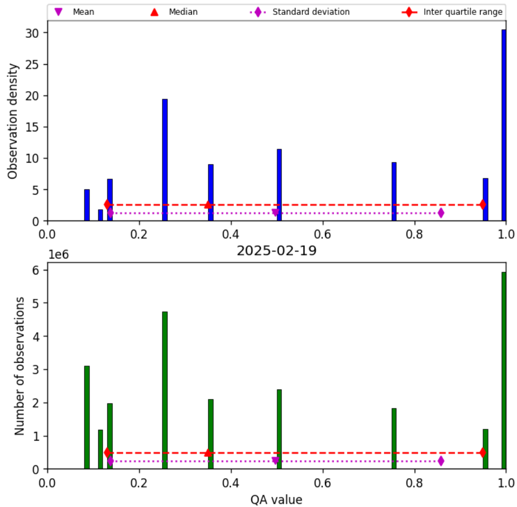
Figure 34: Histogram of “QA value” for 2025-02-19 to 2025-02-20
