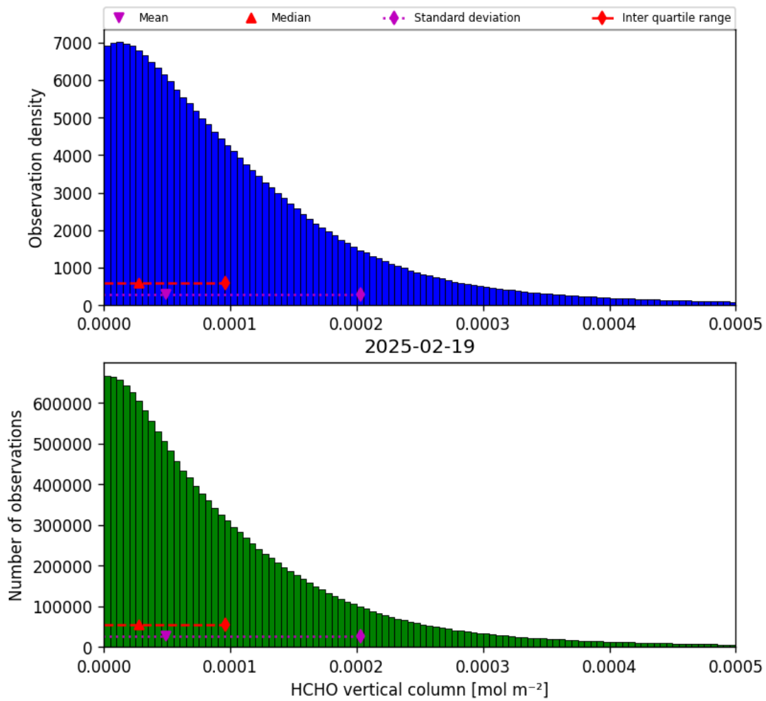
Figure 35: Histogram of “HCHO vertical column” for 2025-02-19 to 2025-02-20
