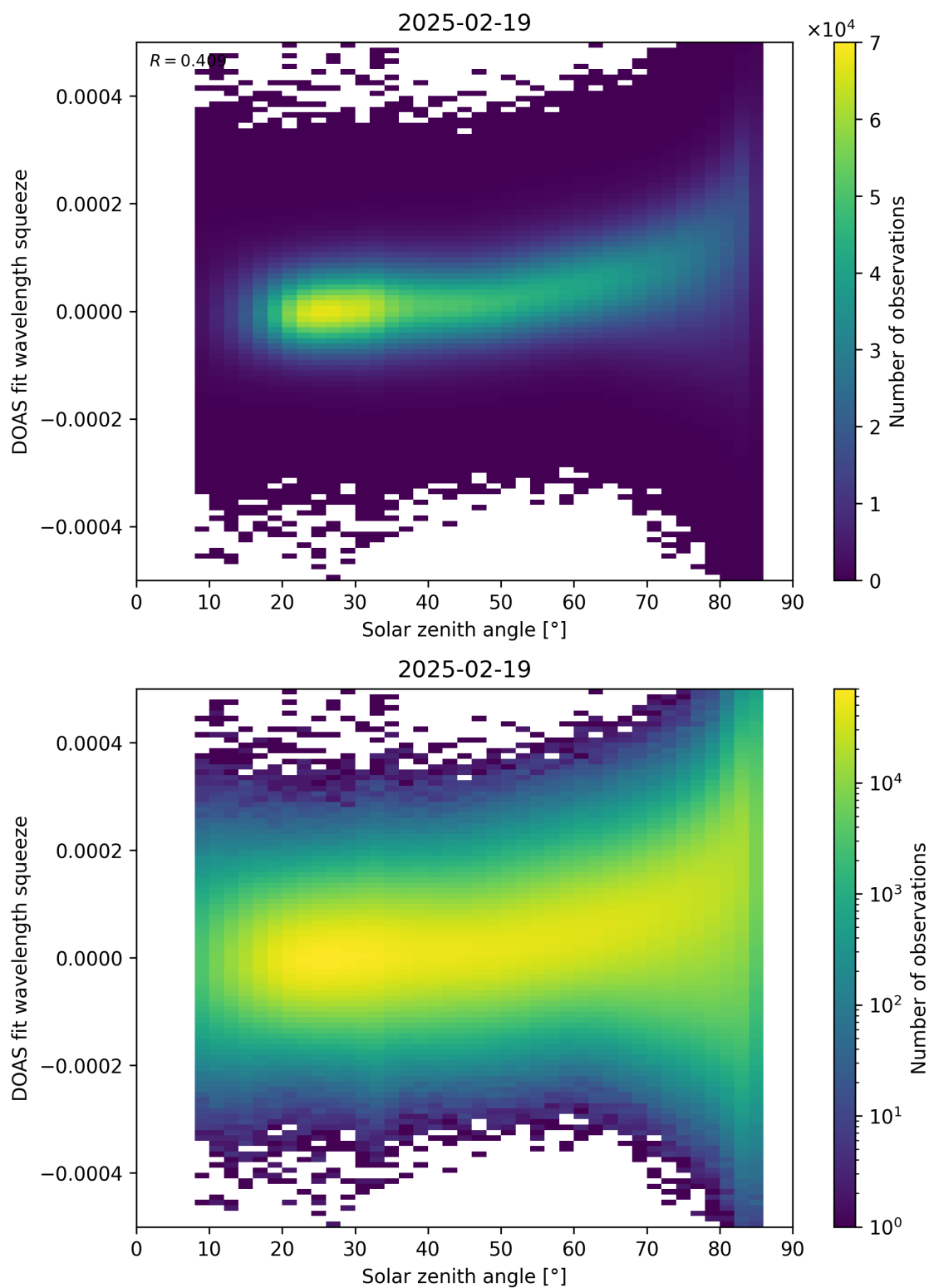
Figure 169: Scatter density plot of “Solar zenith angle” against “DOAS fit wavelength squeeze” for 2025-02-19 to 2025-02-20.
