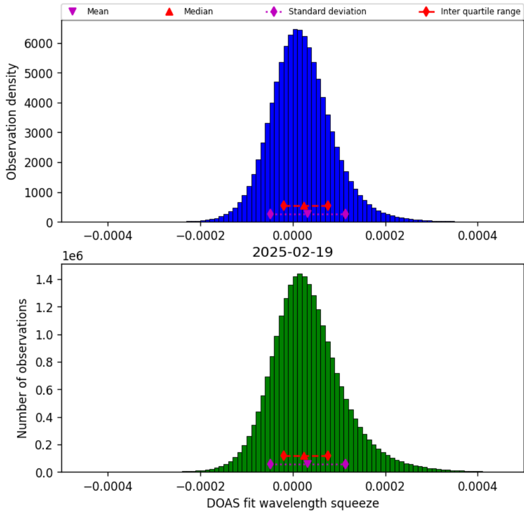
Figure 45: Histogram of “DOAS fit wavelength squeeze” for 2025-02-19 to 2025-02-20
