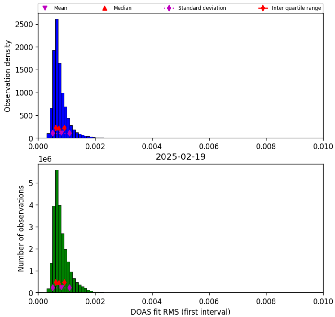
Figure 46: Histogram of “DOAS fit RMS (first interval)” for 2025-02-19 to 2025-02-20
