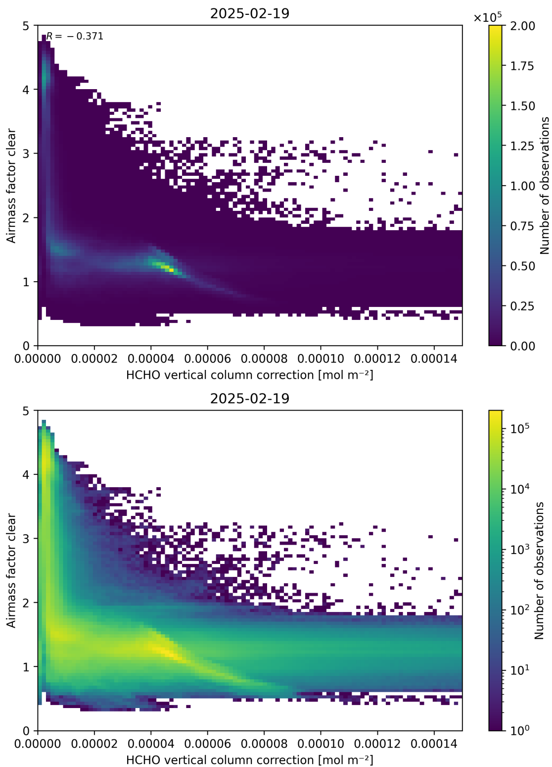
Figure 115: Scatter density plot of “HCHO vertical column correction” against “Air mass factor clear” for 2025-02-19 to 2025-02-20.
