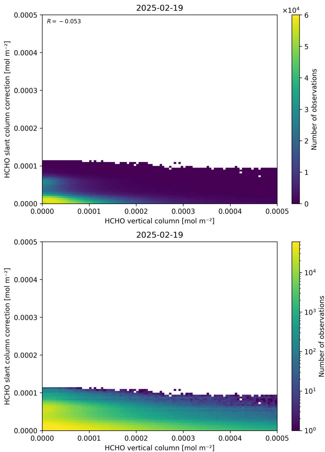
Figure 128: Scatter density plot of “HCHO vertical column” against “HCHO slant column correction” for 2025-02-19 to 2025-02-20.
