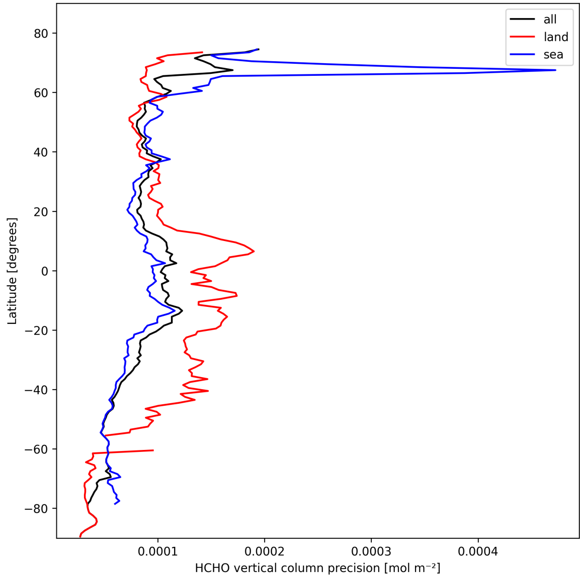
Figure 22: Zonal average of “HCHO vertical column precision” for 2025-02-19 to 2025-02-20.
