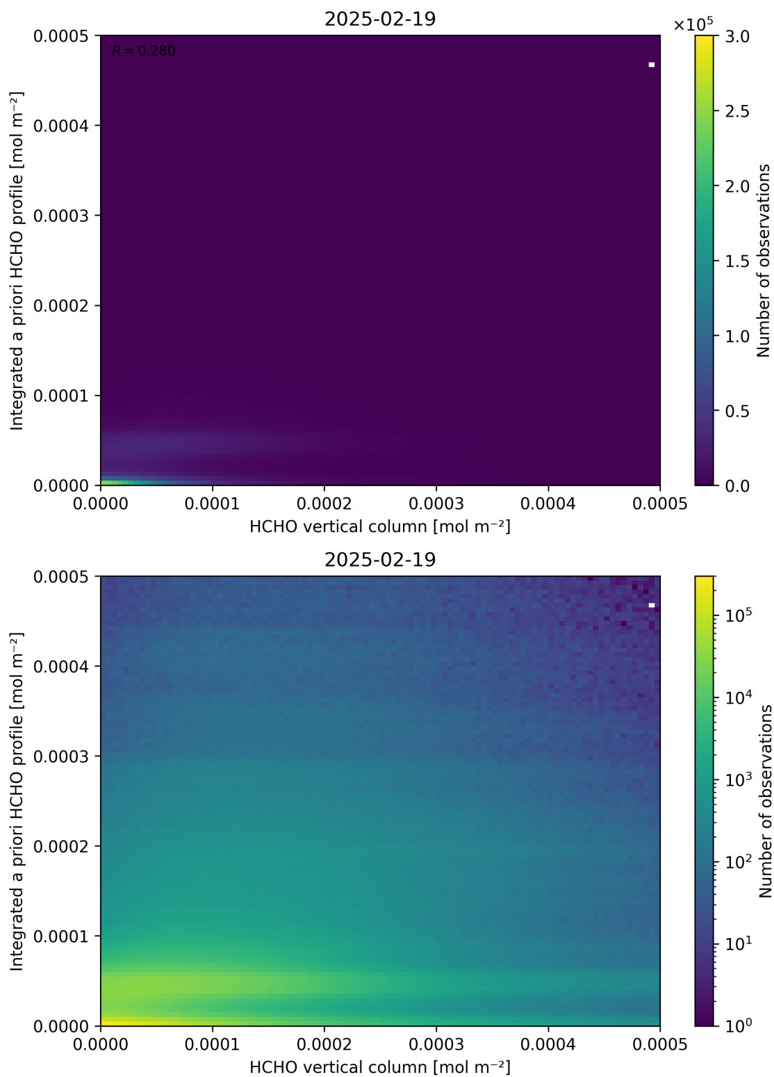
Figure 135: Scatter density plot of “HCHO vertical column” against “Integrated a priori HCHO profile” for 2025-02-19 to 2025-02-20.
