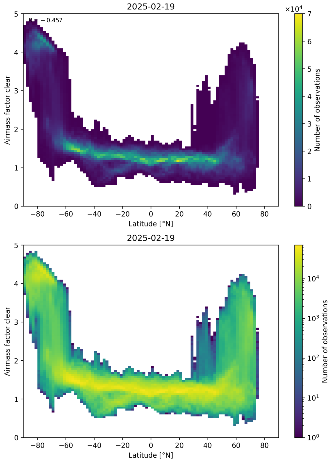
Figure 156: Scatter density plot of “Latitude” against “Airmass factor clear” for 2025-02-19 to 2025-02-20.
