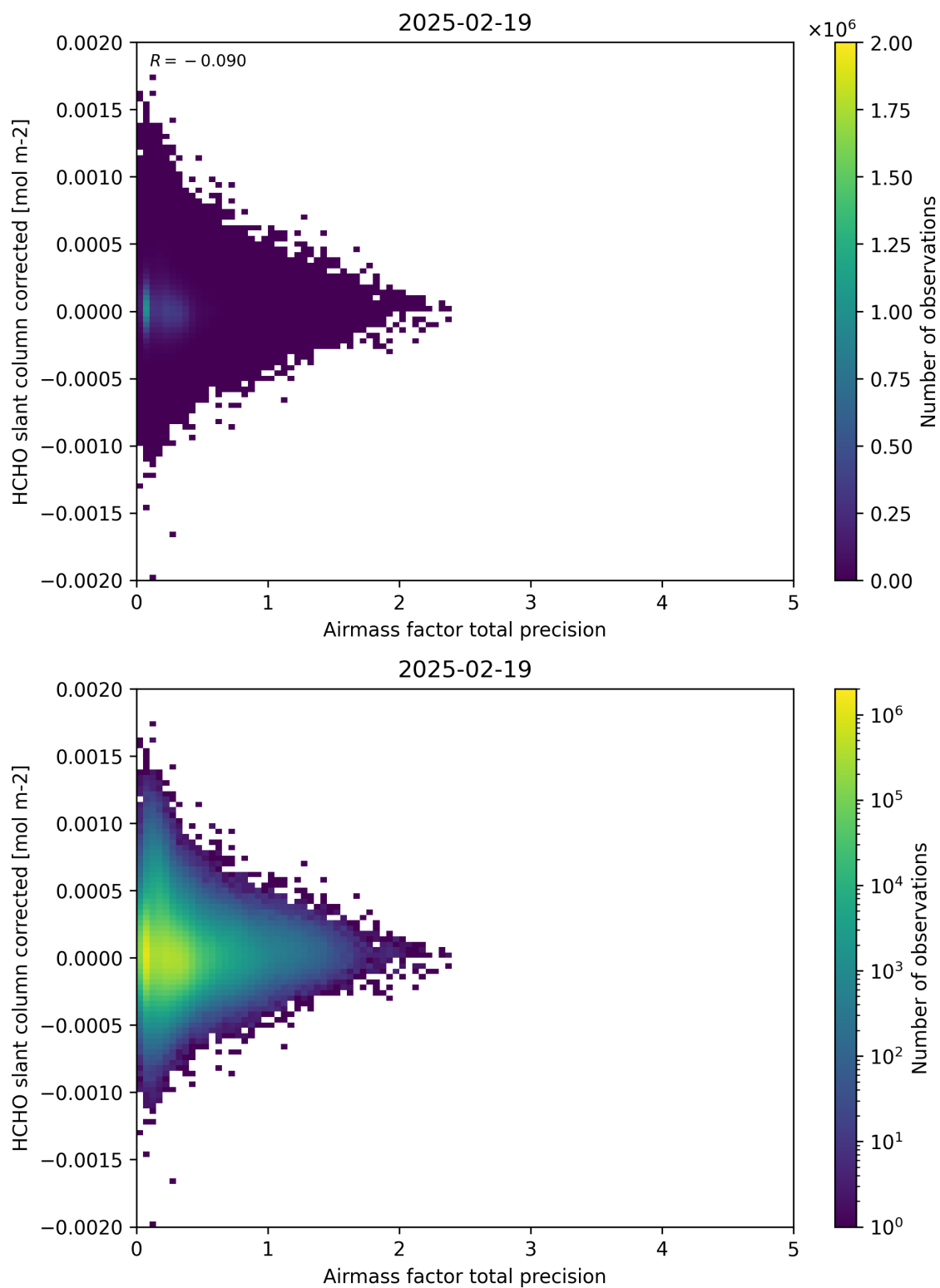
Figure 109: Scatter density plot of “Airmass factor total precision” against “HCHO slant column corrected” for 2025-02-19 to 2025-02-20.
