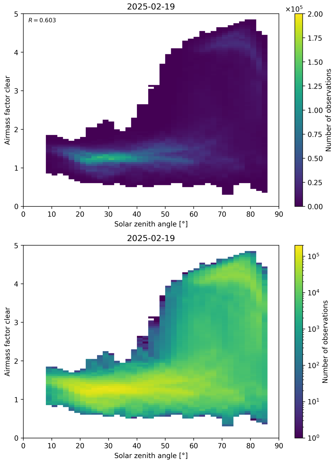
Figure 170: Scatter density plot of “Solar zenith angle” against “Airmass factor clear” for 2025-02-19 to 2025-02-20.
