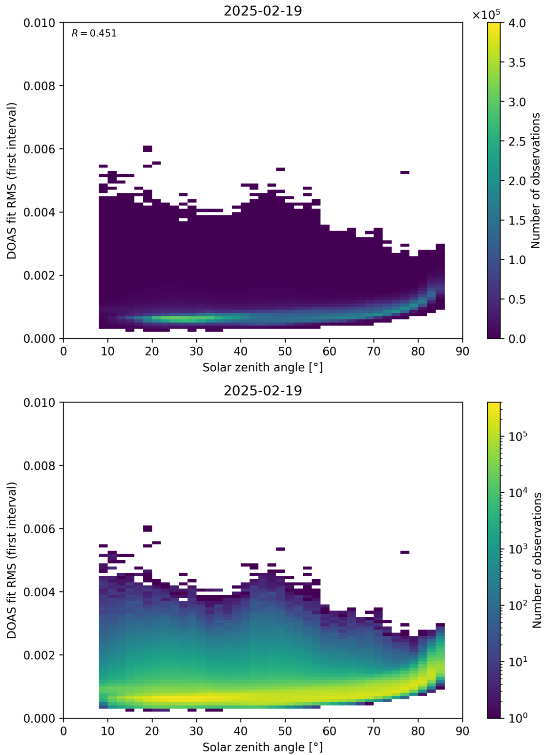
Figure 167: Scatter density plot of “Solar zenith angle” against “DOAS fit RMS (first interval)” for 2025-02-19 to 2025-02-20.
