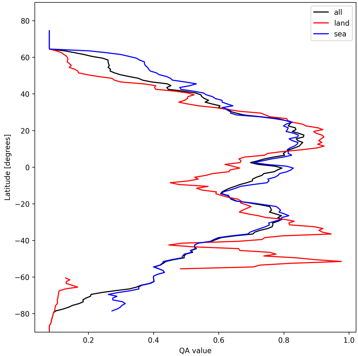
Figure 20: Zonal average of “QA value” for 2025-02-19 to 2025-02-20.
