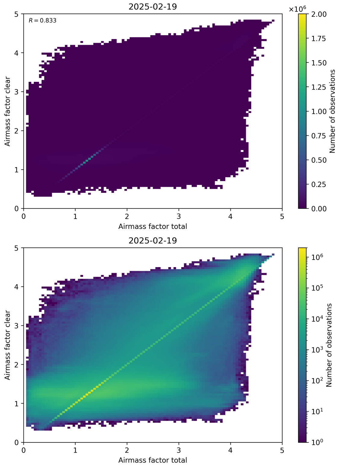
Figure 100: Scatter density plot of “Airmass factor total” against “Airmass factor clear” for 2025-02-19 to 2025-02-20.
