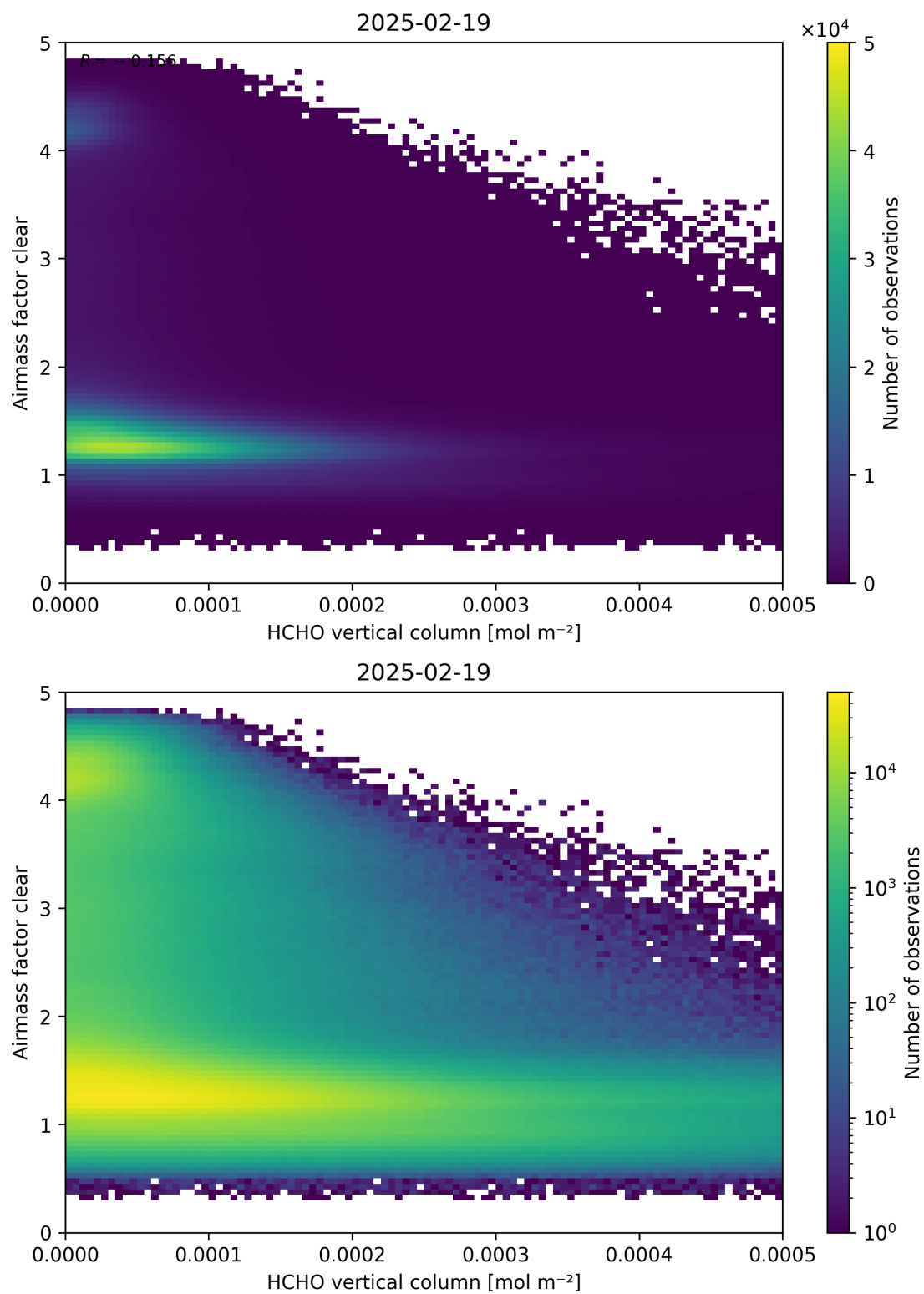
Figure 126: Scatter density plot of “HCHO vertical column” against “Airmass factor clear” for 2025-02-19 to 2025-02-20.
