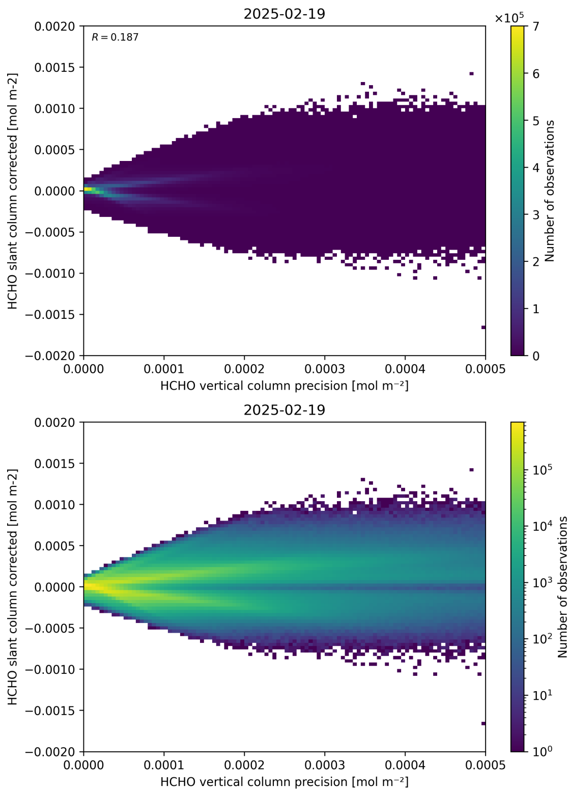
Figure 140: Scatter density plot of “HCHO vertical column precision” against “HCHO slant column corrected” for 2025-02-19 to 2025-02-20.
