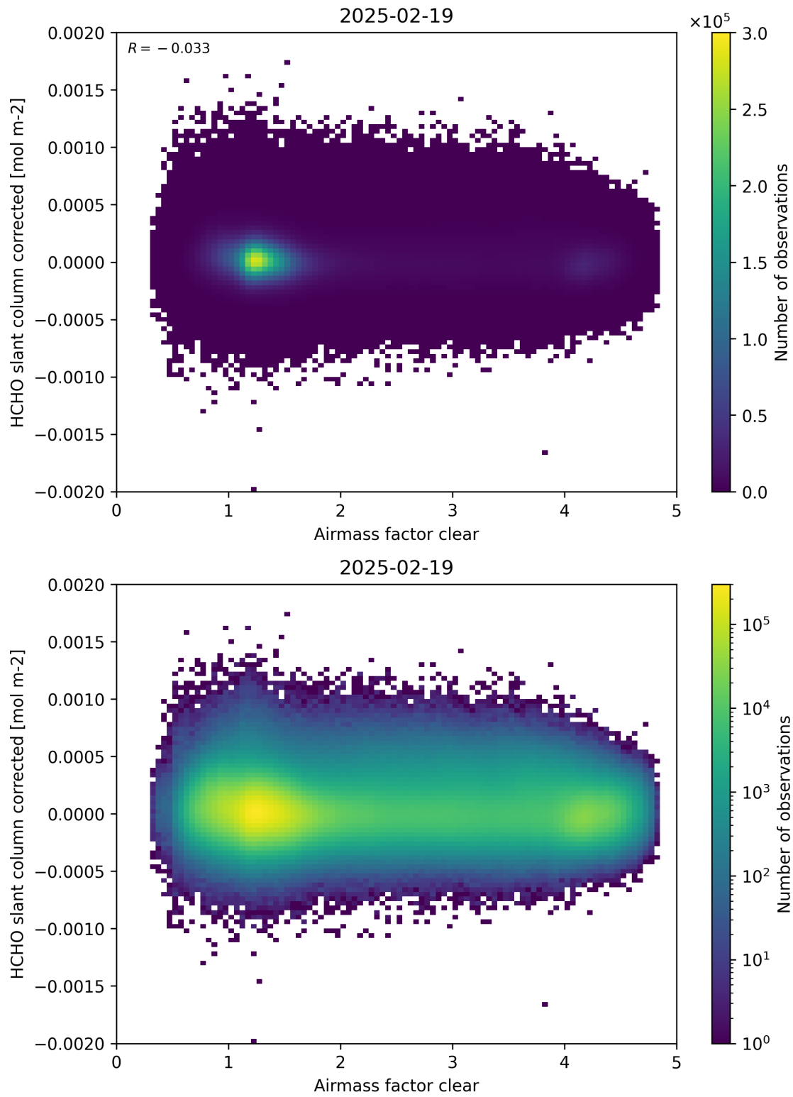
Figure 74: Scatter density plot of “Airmass factor clear” against “HCHO slant column corrected” for 2025-02-19 to 2025-02-20.
