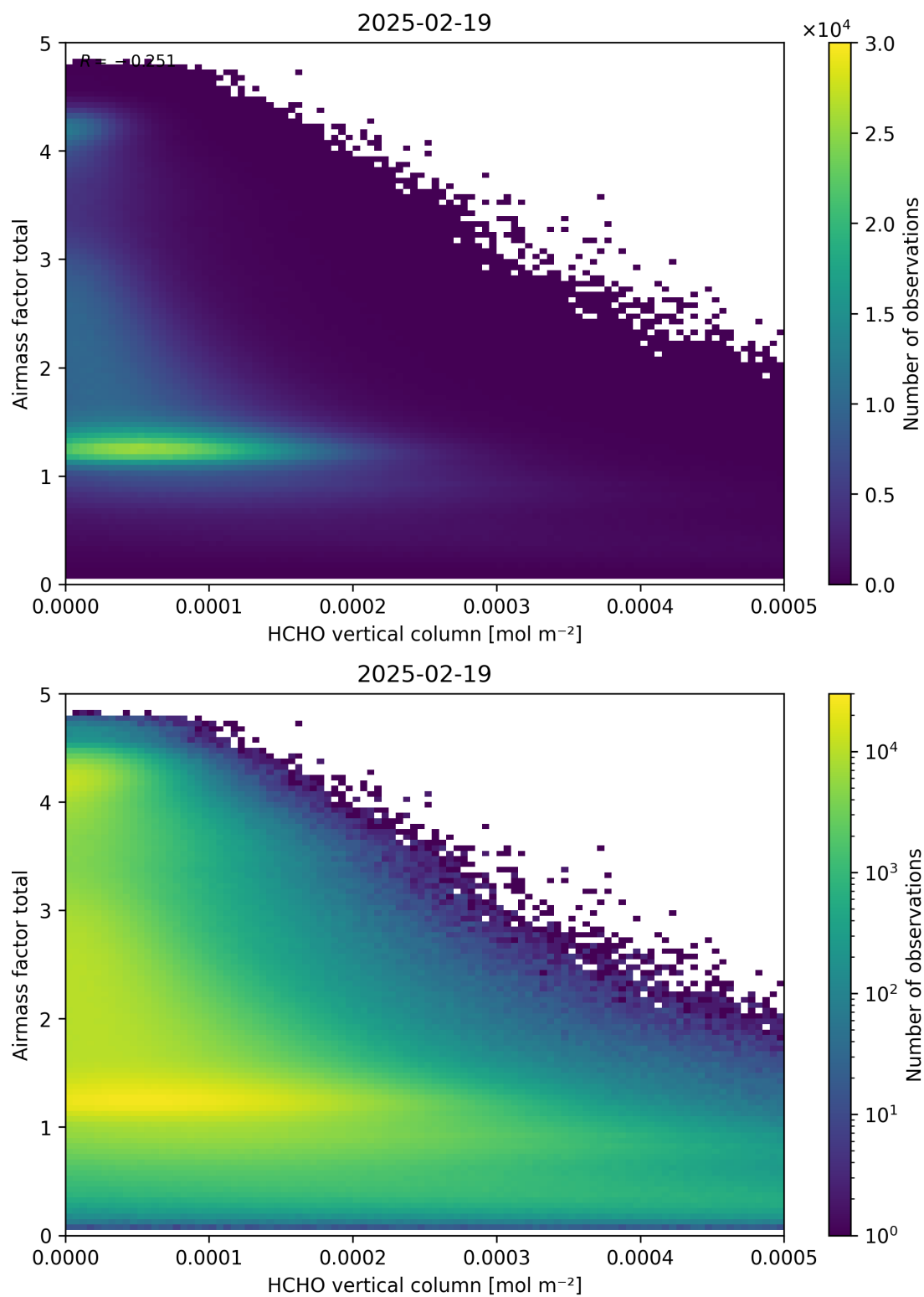
Figure 131: Scatter density plot of “HCHO vertical column” against “Airmass factor total” for 2025-02-19 to 2025-02-20.
