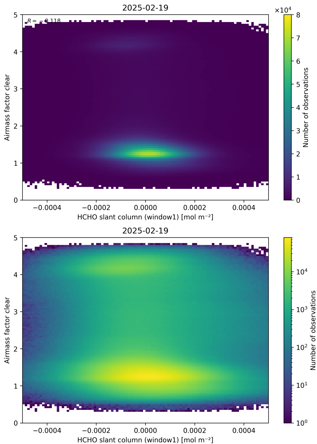
Figure 81: Scatter density plot of “HCHO slant column (window1)” against “Airmass factor clear” for 2025-02-19 to 2025-02-20.
