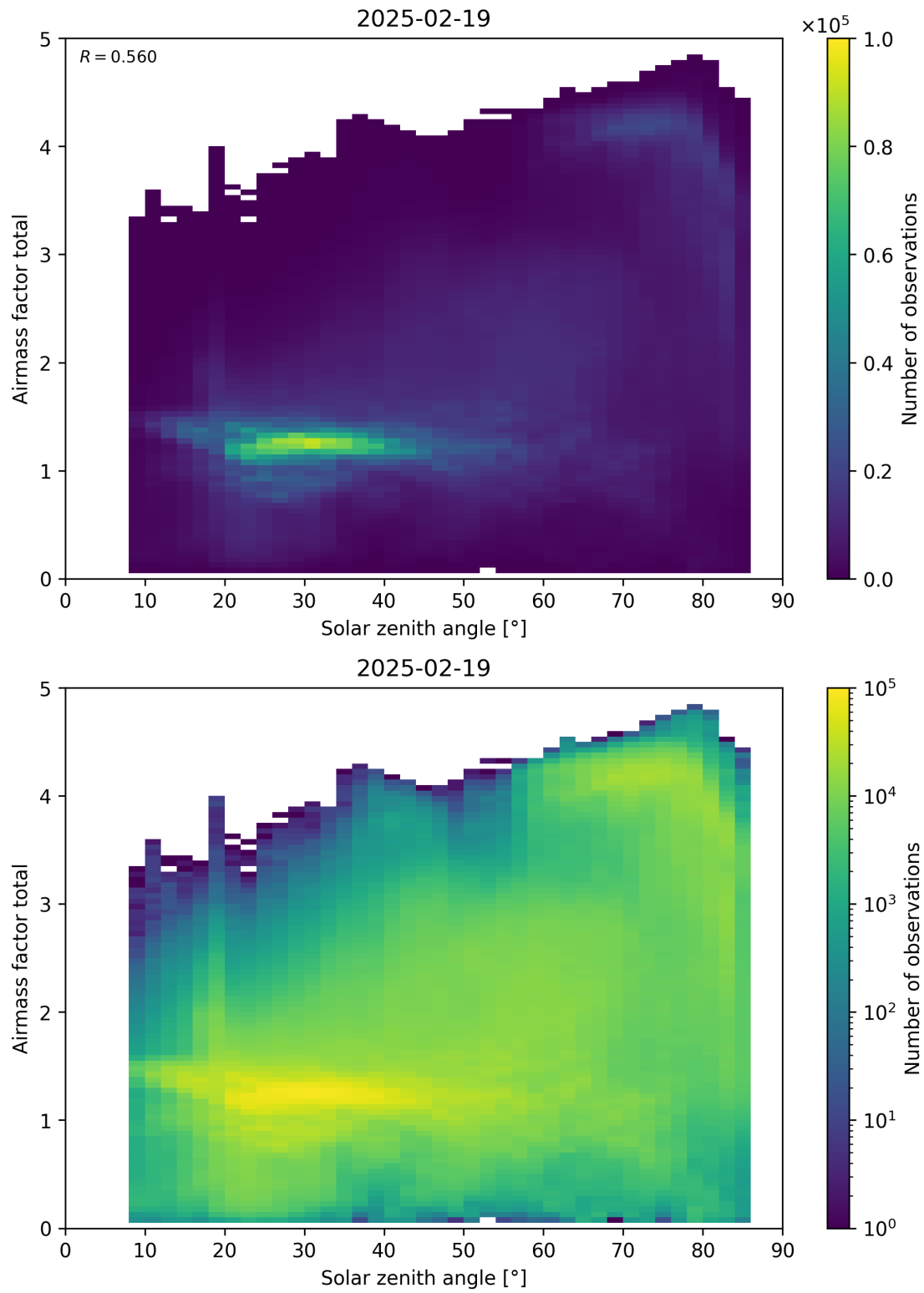
Figure 175: Scatter density plot of “Solar zenith angle” against “Airmass factor total” for 2025-02-19 to 2025-02-20.
