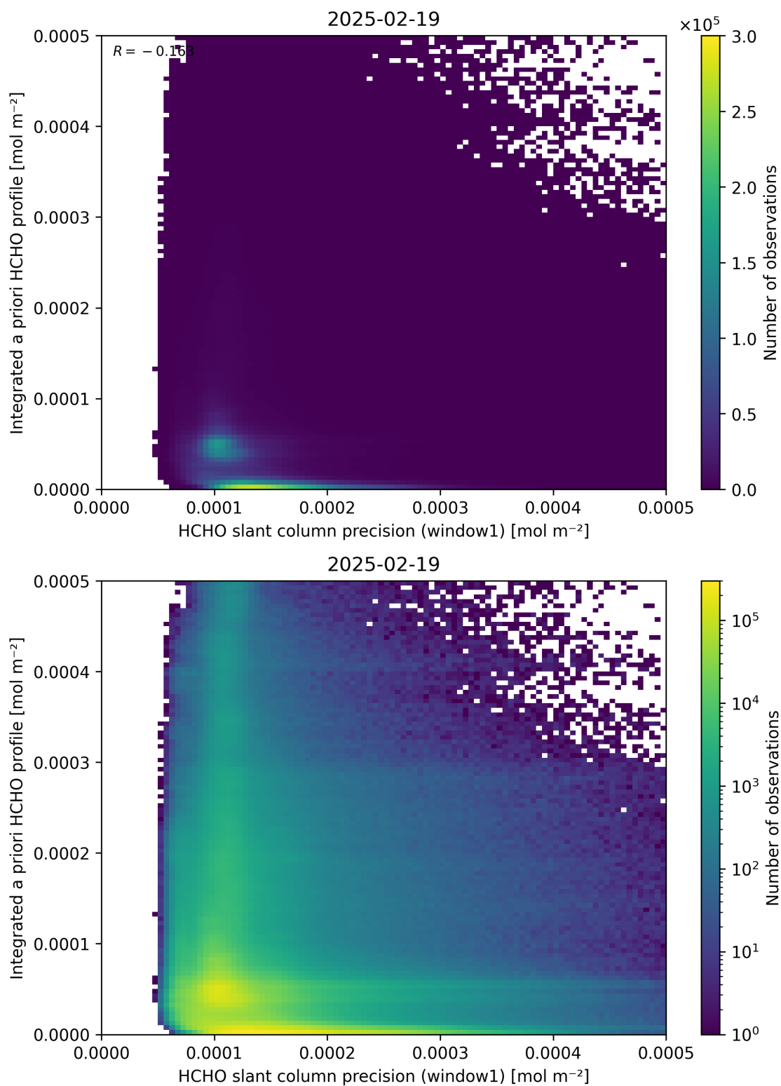
Figure 96: Scatter density plot of “HCHO slant column precision (window1)” against “Integrated a priori HCHO profile” for 2025-02-19 to 2025-02-20.
