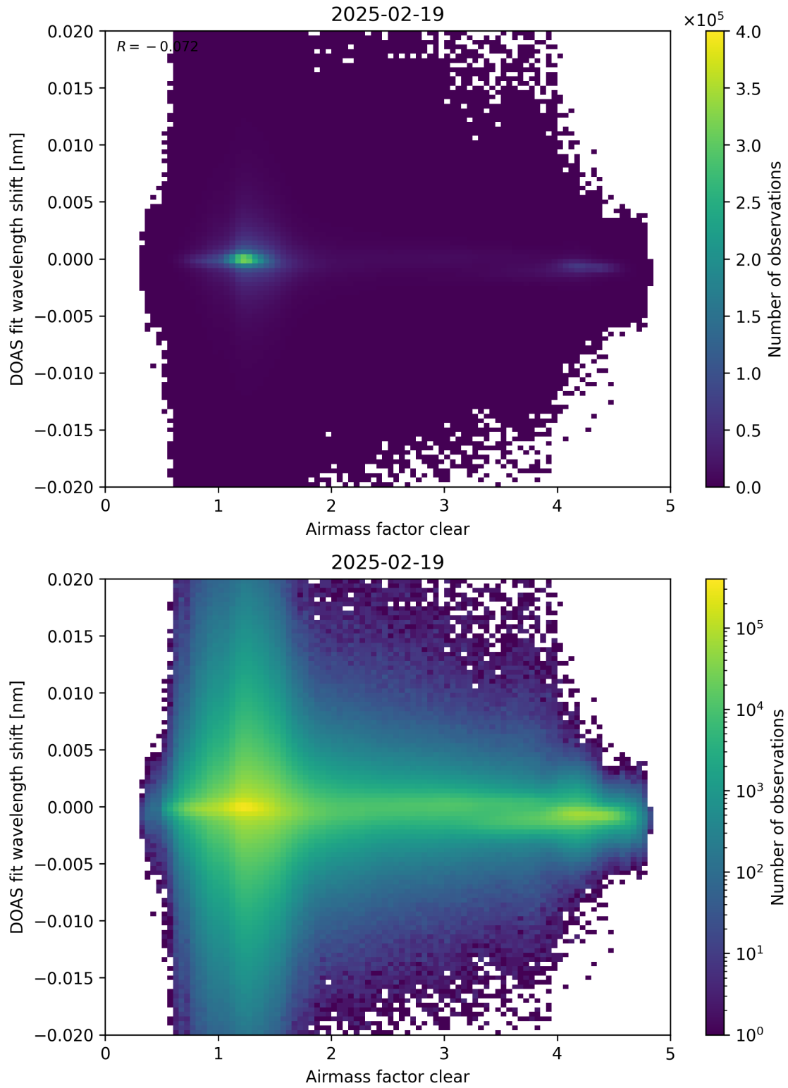
Figure 72: Scatter density plot of “Airmass factor clear” against “DOAS fit wavelength shift” for 2025-02-19 to 2025-02-20.
