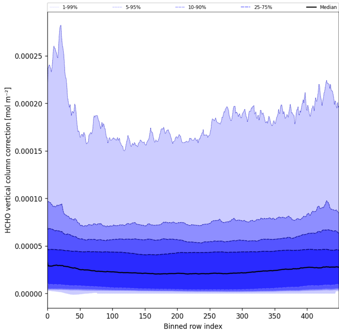
Figure 51: Along track statistics of "HCHO vertical column correction" for 2025-02-19 to 2025-02-20
