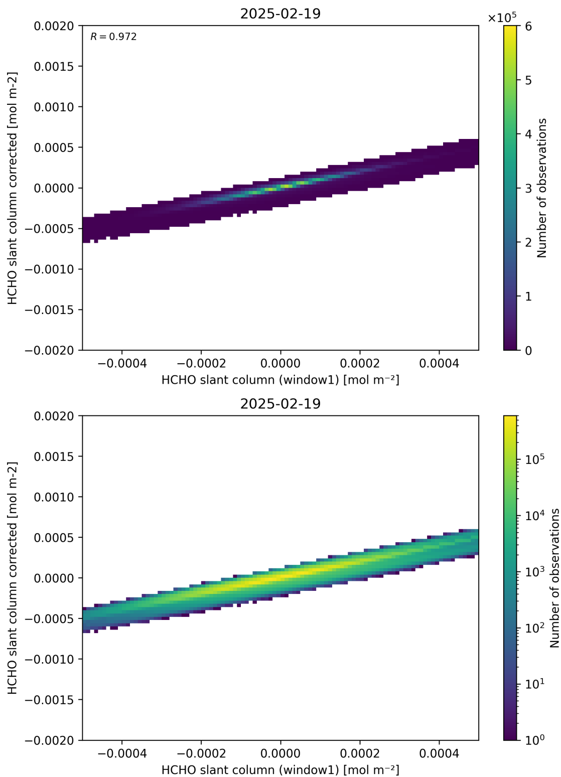
Figure 82: Scatter density plot of “HCHO slant column (window1)” against “HCHO slant column corrected” for 2025-02-19 to 2025-02-20.
