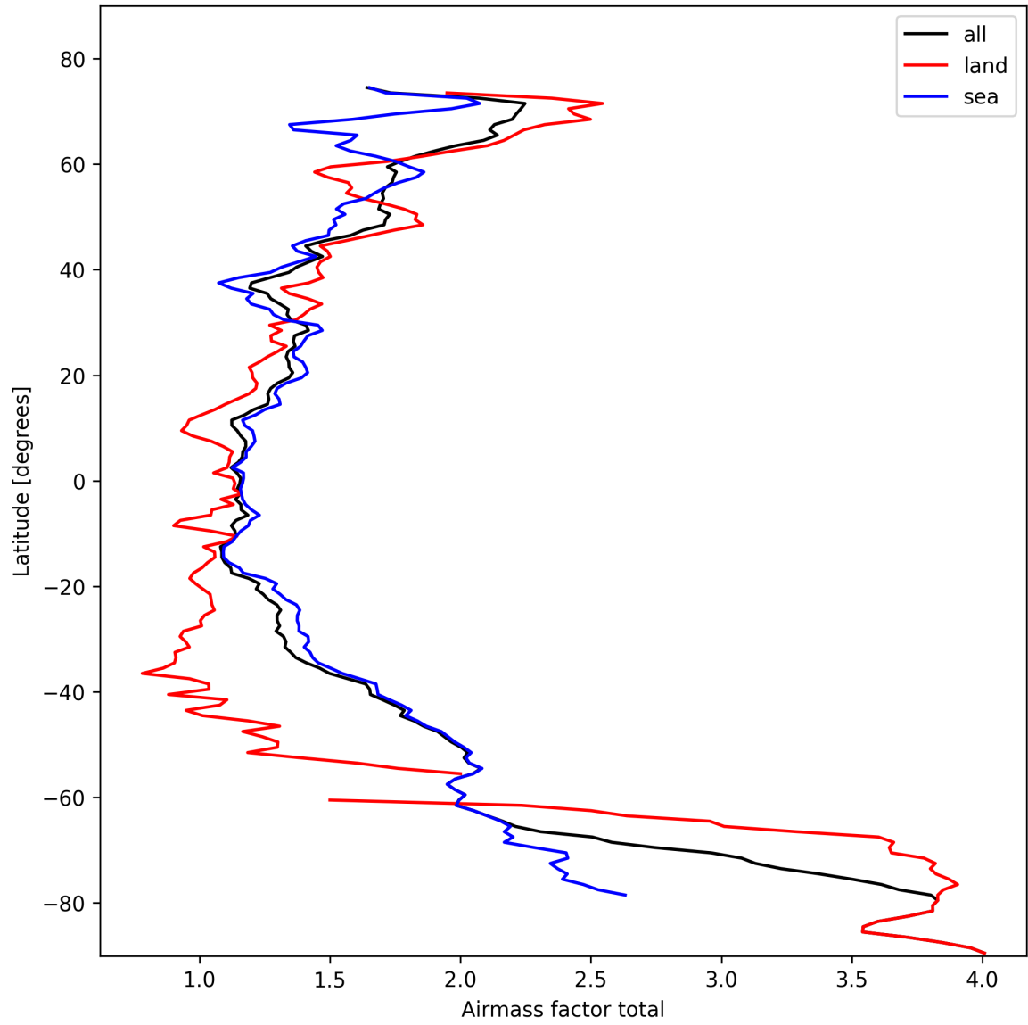
Figure 26: Zonal average of “Airmass factor total” for 2025-02-19 to 2025-02-20.
