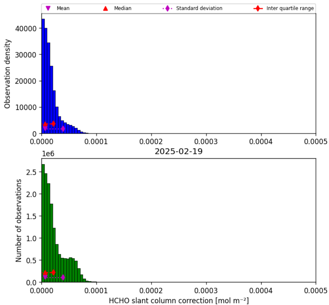
Figure 47: Histogram of “HCHO slant column correction” for 2025-02-19 to 2025-02-20
