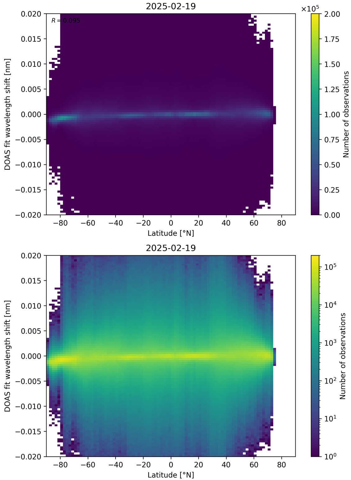
Figure 154: Scatter density plot of “Latitude” against “DOAS fit wavelength shift” for 2025-02-19 to 2025-02-20.
