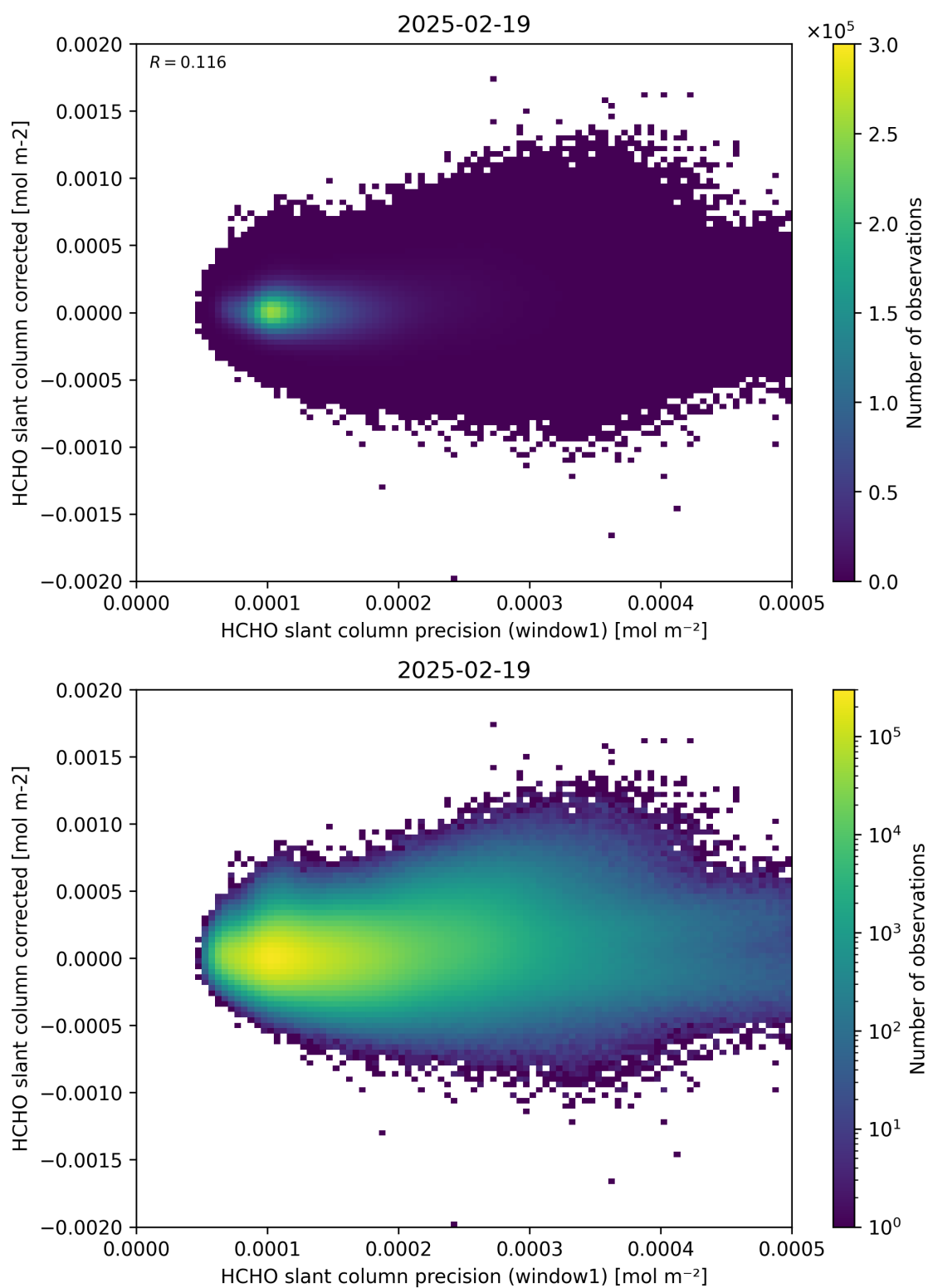
Figure 92: Scatter density plot of “HCHO slant column precision (window1)” against “HCHO slant column corrected” for 2025-02-19 to 2025-02-20.
