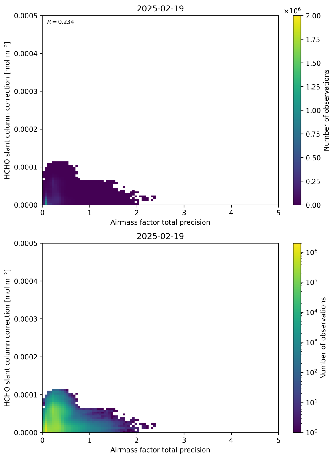
Figure 110: Scatter density plot of “Airmass factor total precision” against “HCHO slant column correction” for 2025-02-19 to 2025-02-20.
