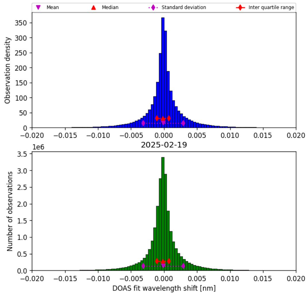
Figure 44: Histogram of “DOAS fit wavelength shift” for 2025-02-19 to 2025-02-20
