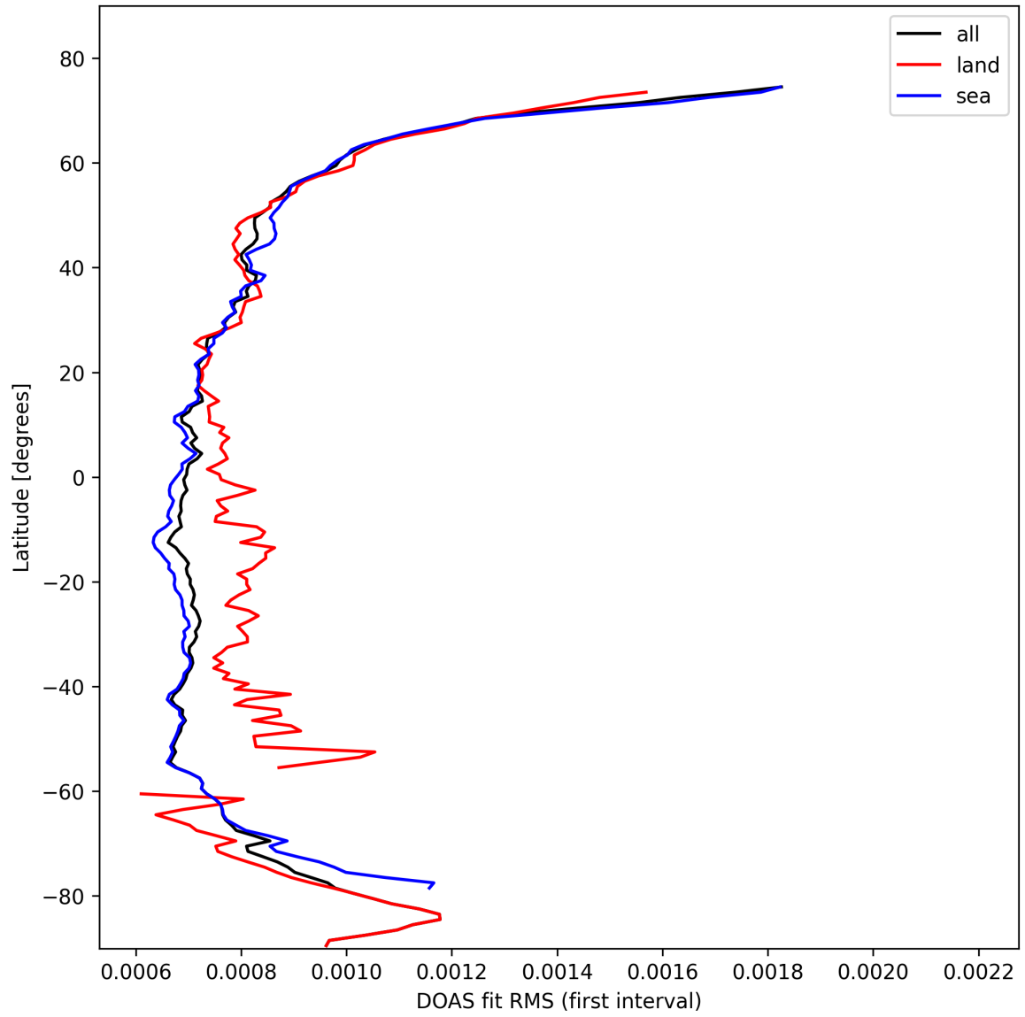
Figure 32: Zonal average of “DOAS fit RMS (first interval)” for 2025-02-19 to 2025-02-20.
