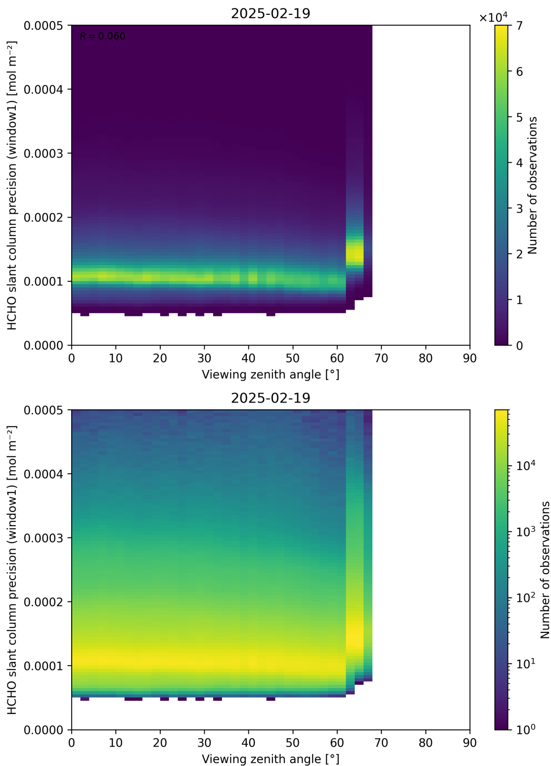
Figure 189: Scatter density plot of “Viewing zenith angle” against “HCHO slant column precision (window1)” for 2025-02-19 to 2025-02-20.
