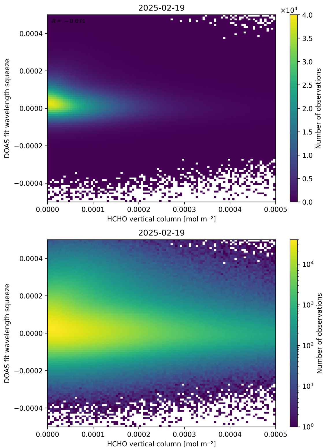
Figure 125: Scatter density plot of “HCHO vertical column” against “DOAS fit wavelength squeeze” for 2025-02-19 to 2025-02-20.
