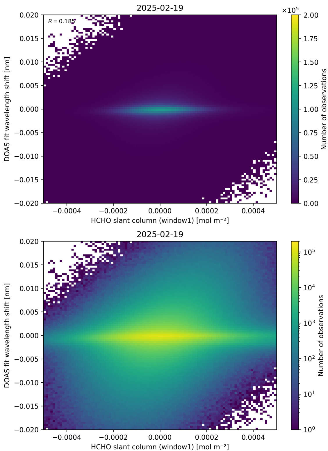
Figure 79: Scatter density plot of “HCHO slant column (window1)” against “DOAS fit wavelength shift” for 2025-02-19 to 2025-02-20.
