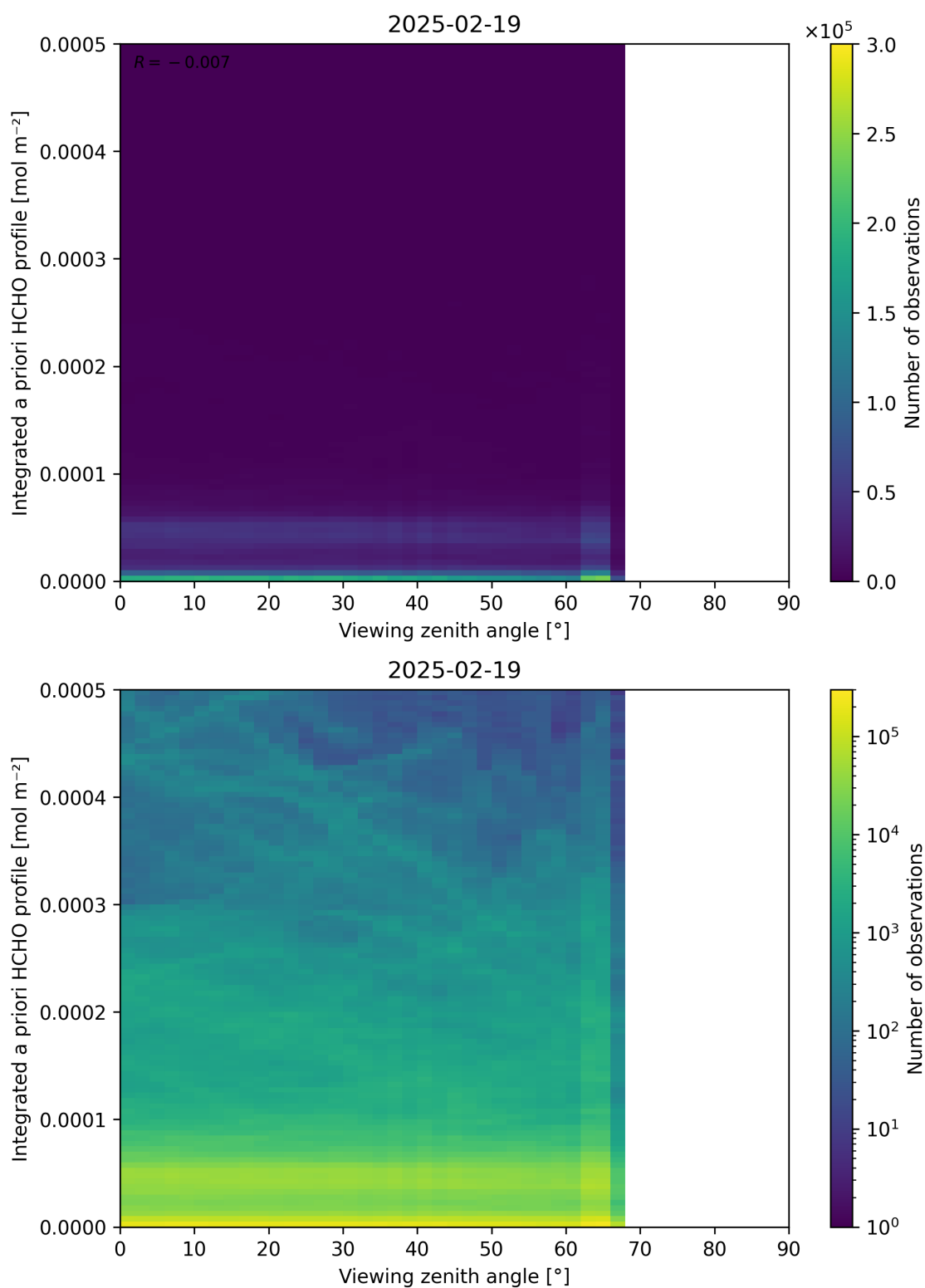
Figure 195: Scatter density plot of “Viewing zenith angle” against “Integrated a priori HCHO profile” for 2025-02-19 to 2025-02-20.
