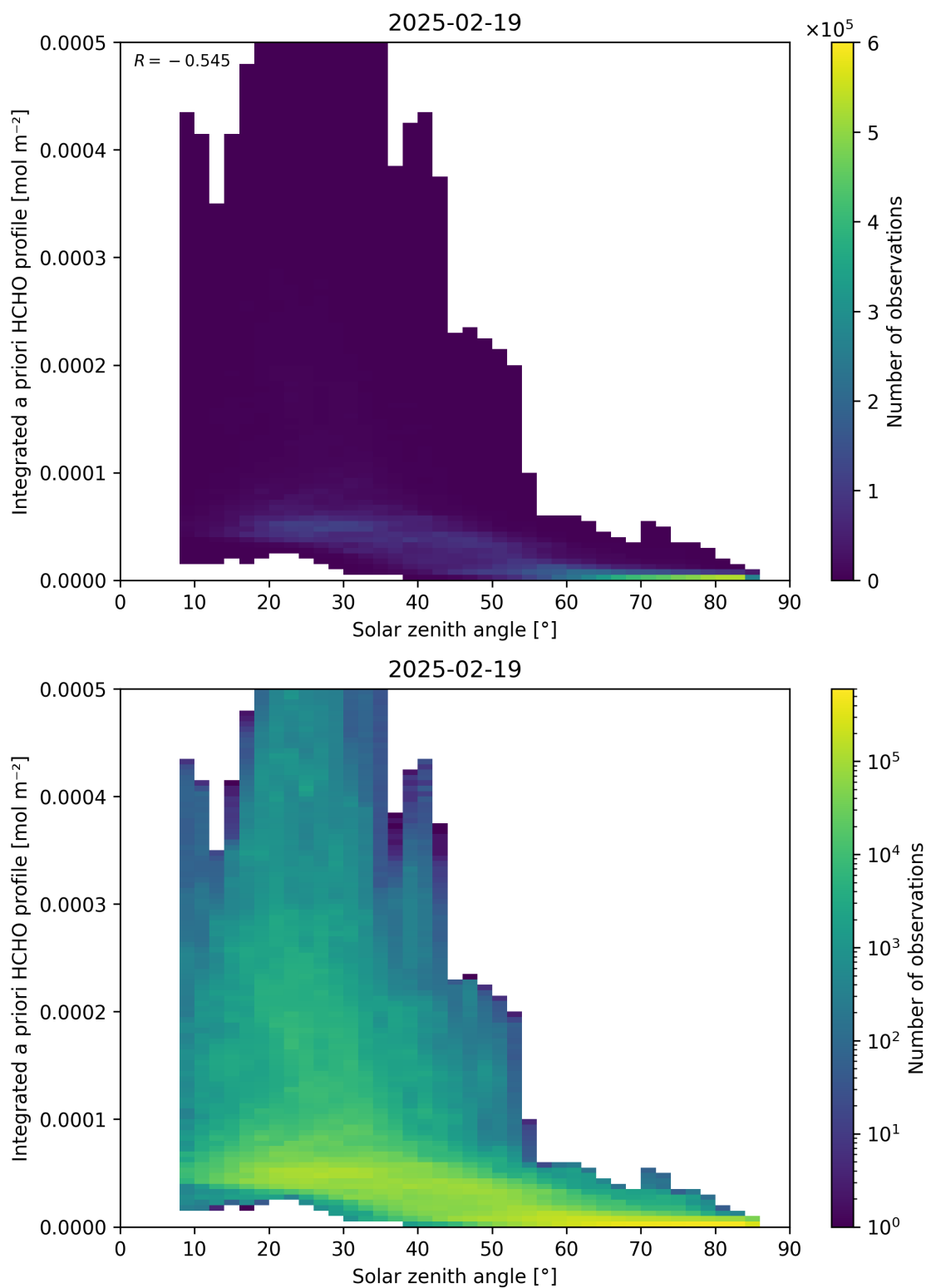
Figure 180: Scatter density plot of “Solar zenith angle” against “Integrated a priori HCHO profile” for 2025-02-19 to 2025-02-20.
