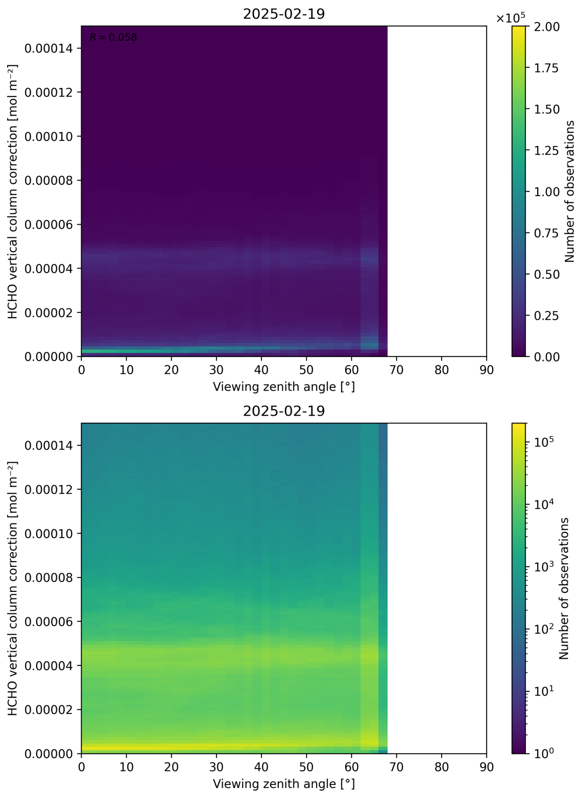
Figure 193: Scatter density plot of “Viewing zenith angle” against “HCHO vertical column correction” for 2025-02-19 to 2025-02-20.
