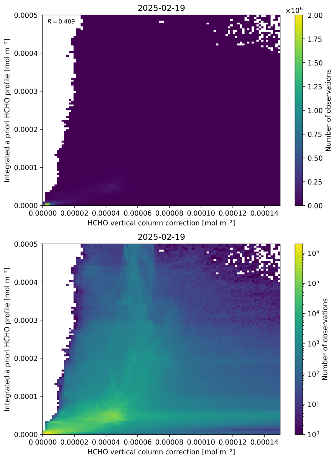
Figure 122: Scatter density plot of “HCHO vertical column correction” against “Integrated a priori HCHO profile” for 2025-02-19 to 2025-02-20.
