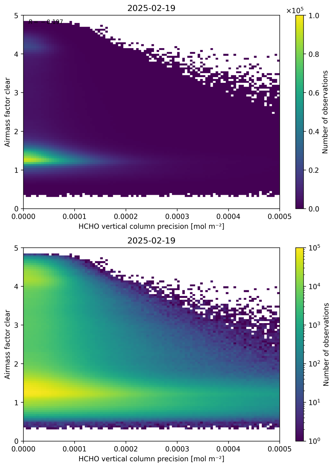
Figure 139: Scatter density plot of “HCHO vertical column precision” against “Airmass factor clear” for 2025-02-19 to 2025-02-20.
