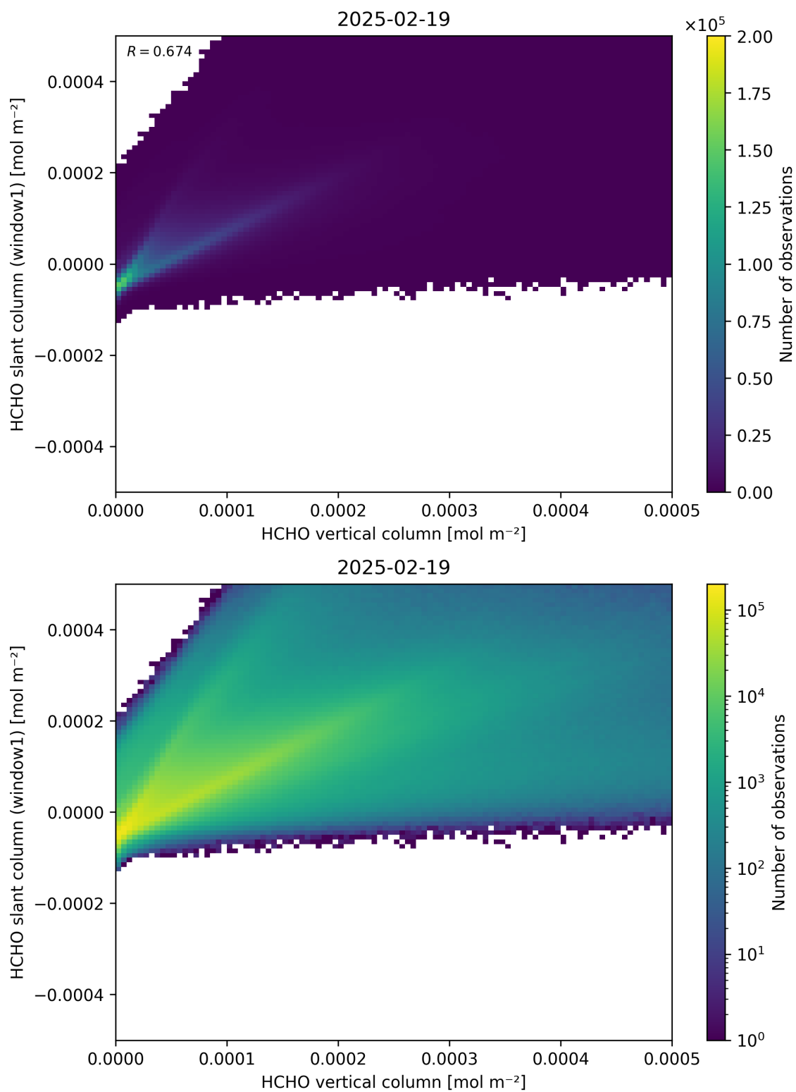
Figure 129: Scatter density plot of “HCHO vertical column” against “HCHO slant column (window1)” for 2025-02-19 to 2025-02-20.
