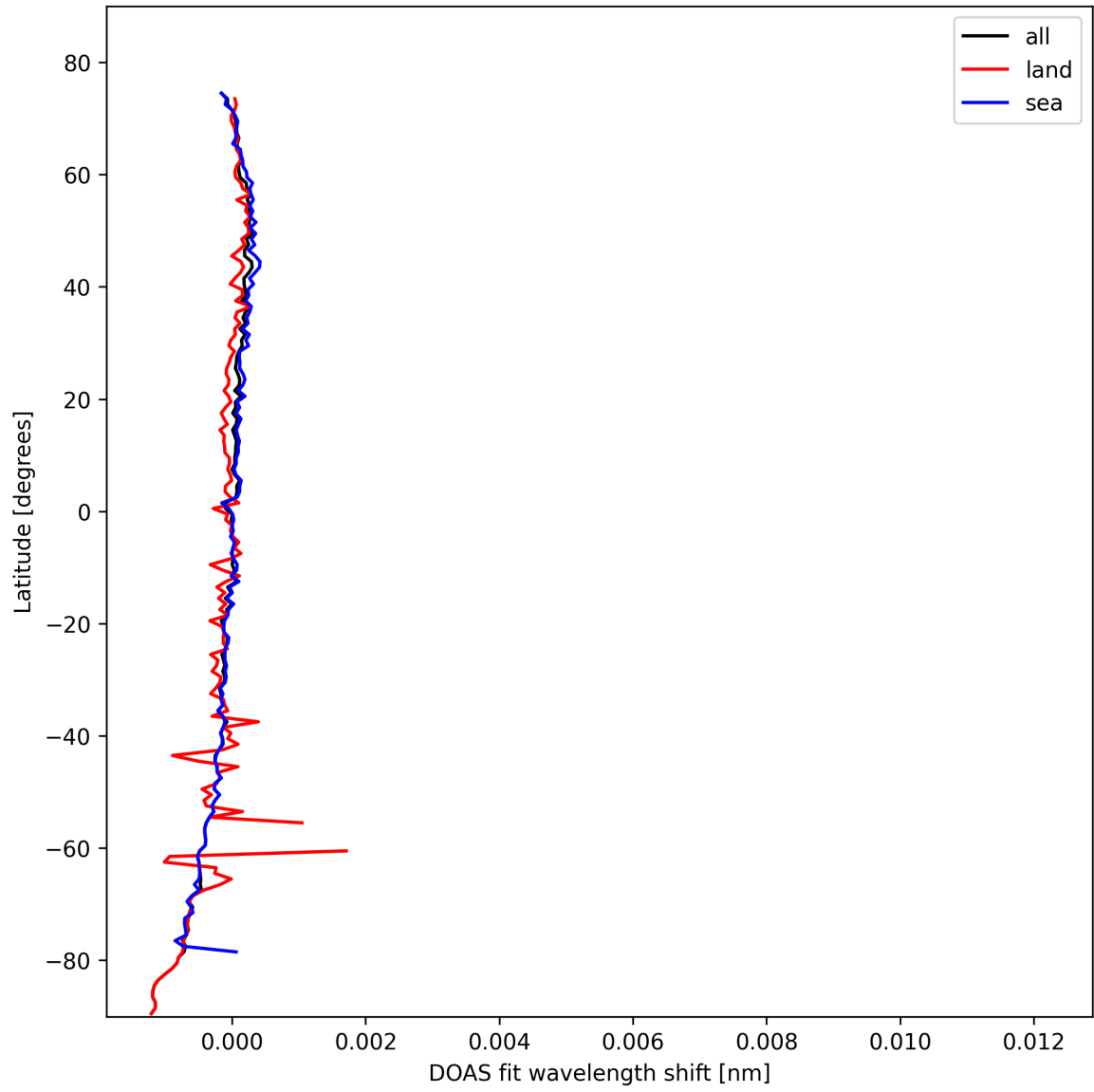
Figure 30: Zonal average of “DOAS fit wavelength shift” for 2025-02-19 to 2025-02-20.
