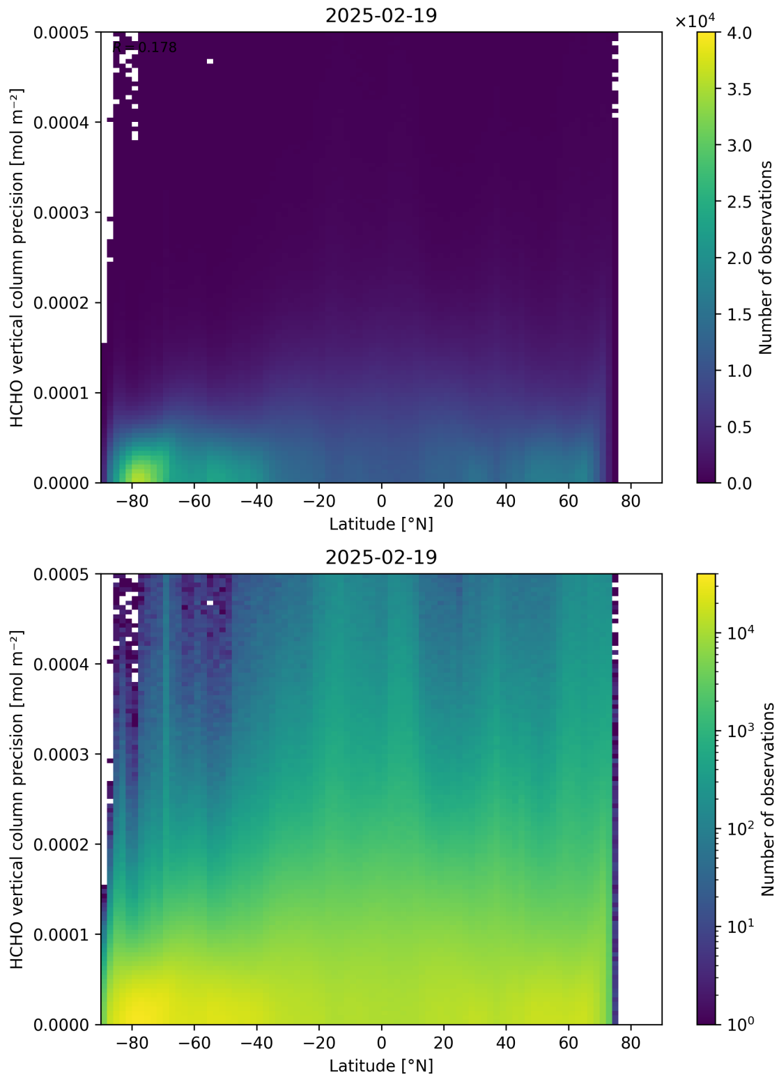
Figure 165: Scatter density plot of “Latitude” against “HCHO vertical column precision” for 2025-02-19 to 2025-02-20.
