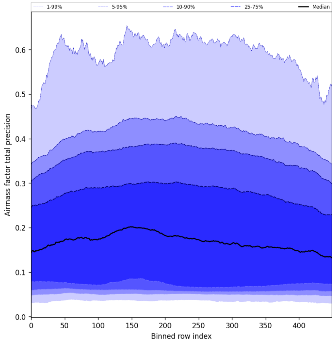
Figure 55: Along track statistics of “Airmass factor total precision” for 2025-02-19 to 2025-02-20
