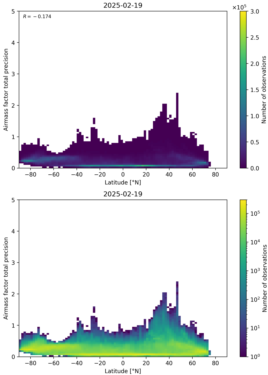
Figure 162: Scatter density plot of “Latitude” against “Airmass factor total precision” for 2025-02-19 to 2025-02-20.
