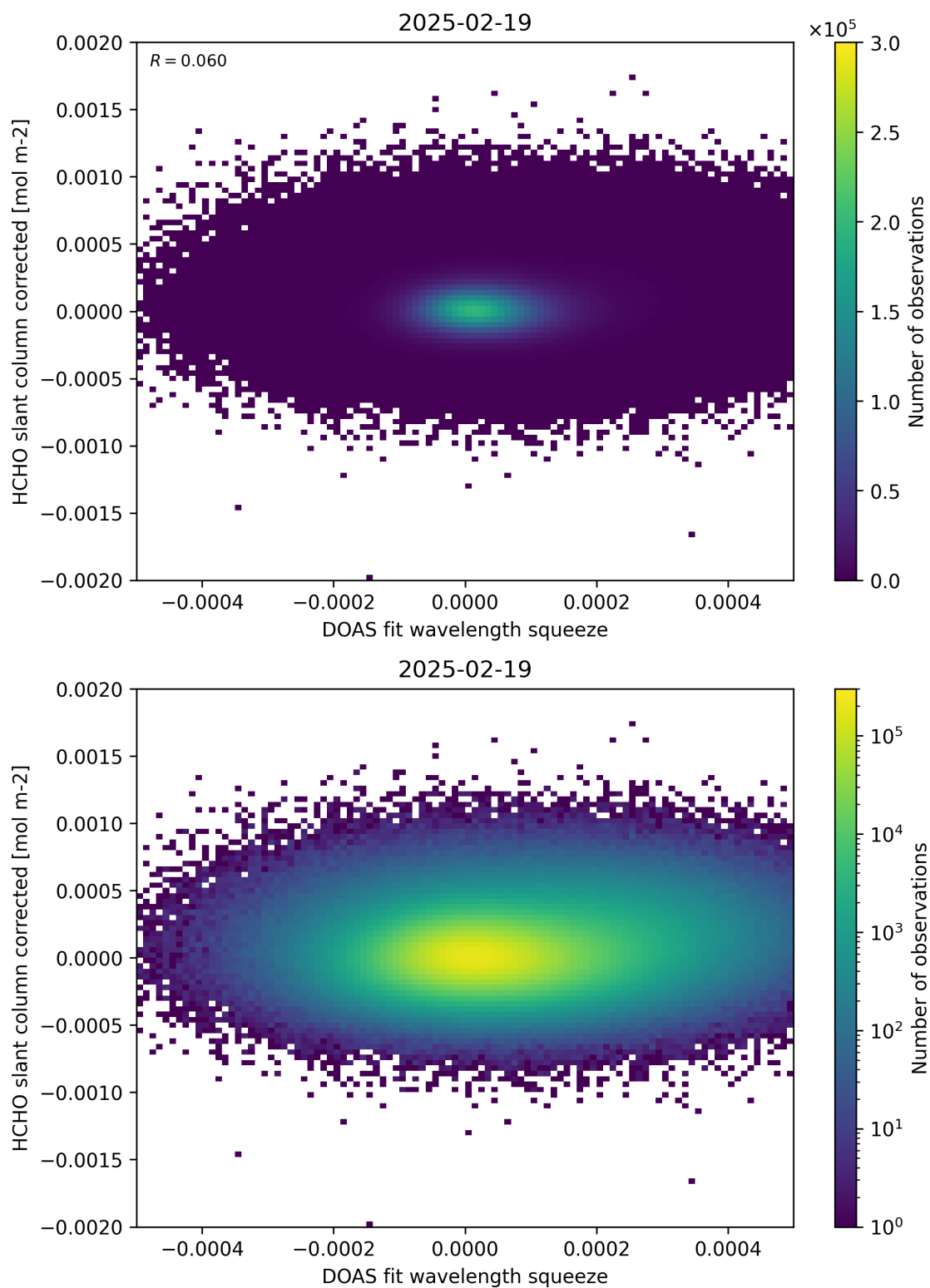
Figure 69: Scatter density plot of “DOAS fit wavelength squeeze” against “HCHO slant column corrected” for 2025-02-19 to 2025-02-20.
