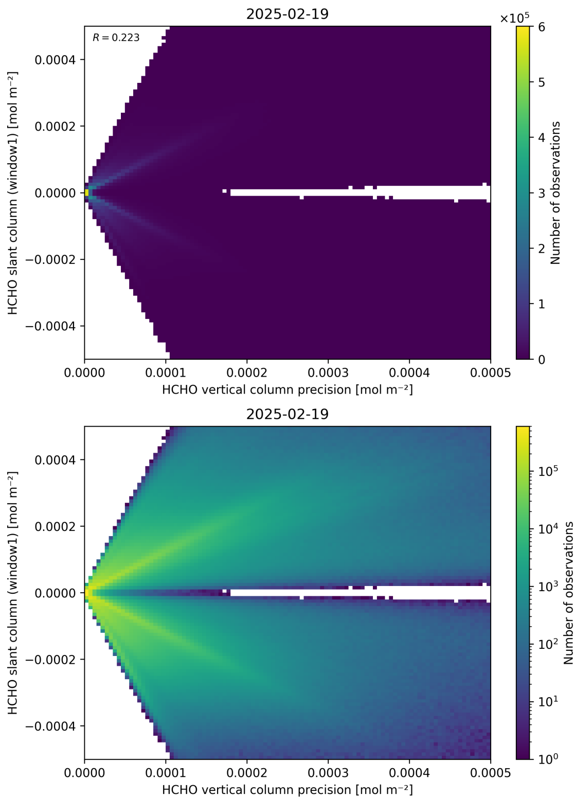
Figure 142: Scatter density plot of “HCHO vertical column precision” against “HCHO slant column (window1)” for 2025-02-19 to 2025-02-20.
