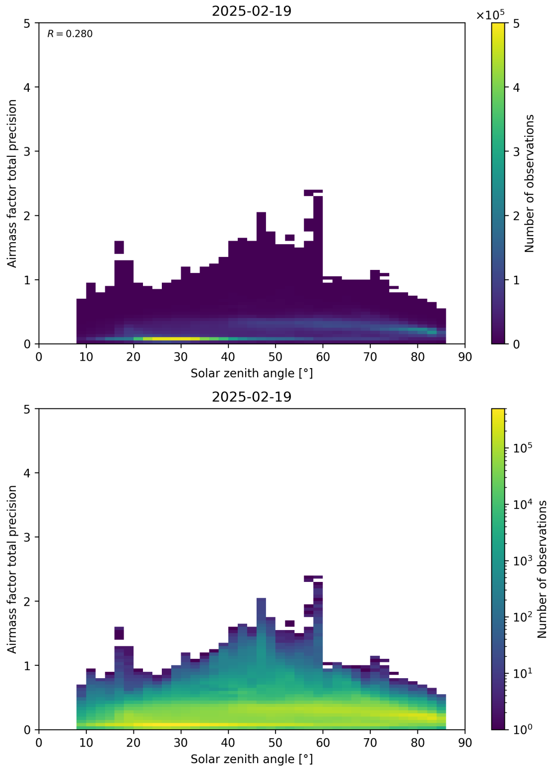
Figure 176: Scatter density plot of “Solar zenith angle” against “Airmass factor total precision” for 2025-02-19 to 2025-02-20.
