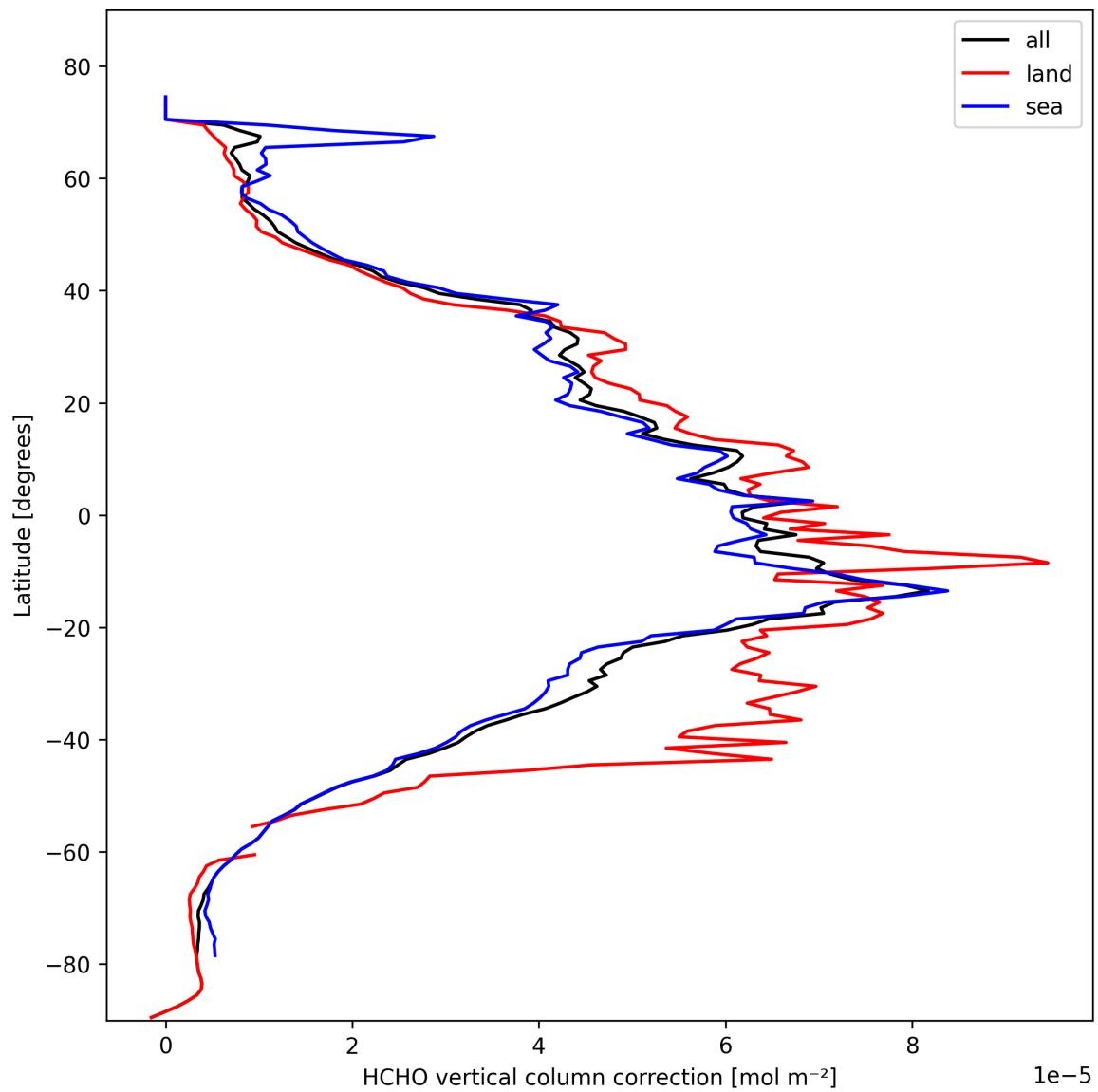
Figure 23: Zonal average of “HCHO vertical column correction” for 2025-02-19 to 2025-02-20.
