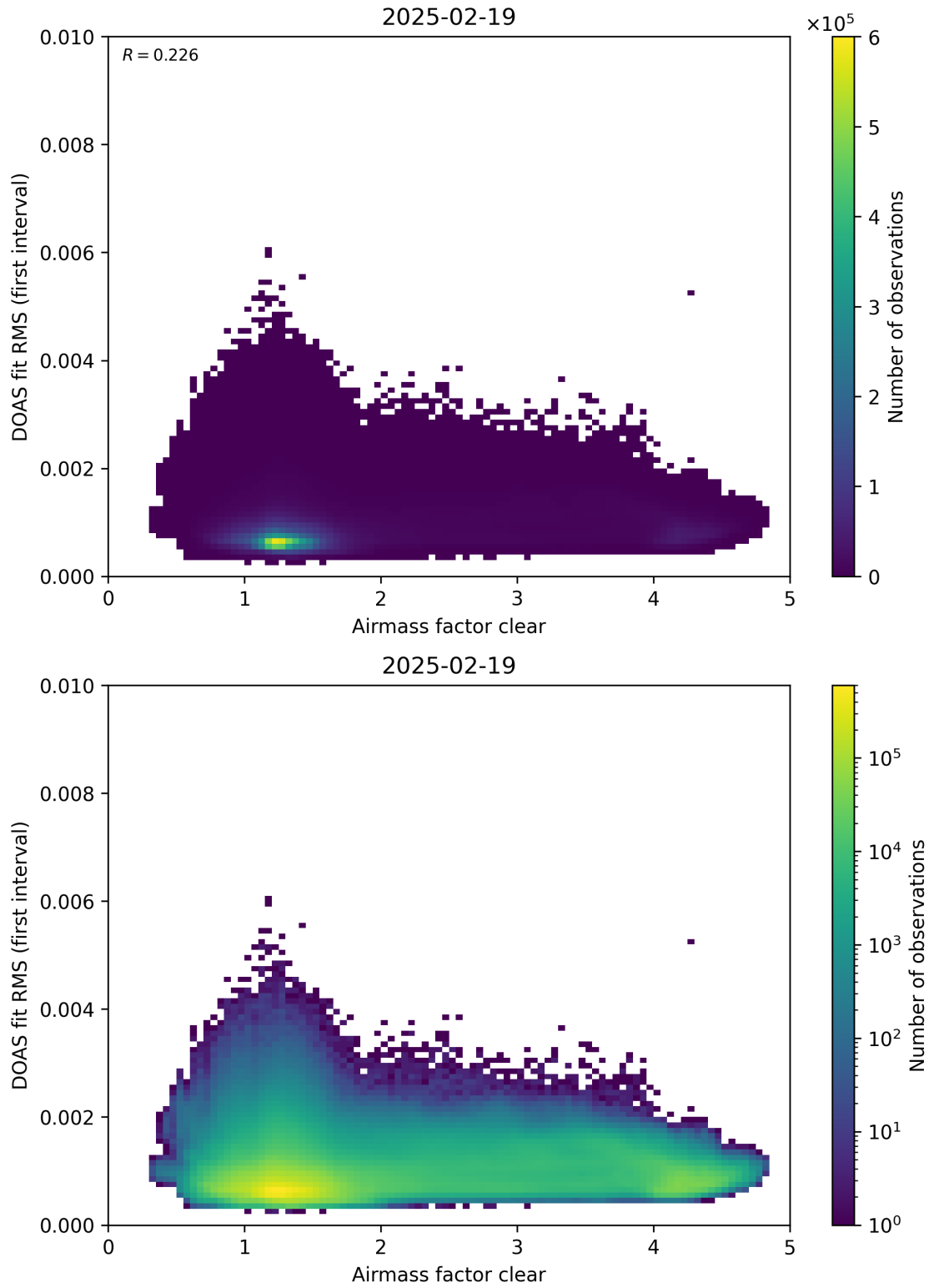
Figure 71: Scatter density plot of “Airmass factor clear” against “DOAS fit RMS (first interval)” for 2025-02-19 to 2025-02-20.
