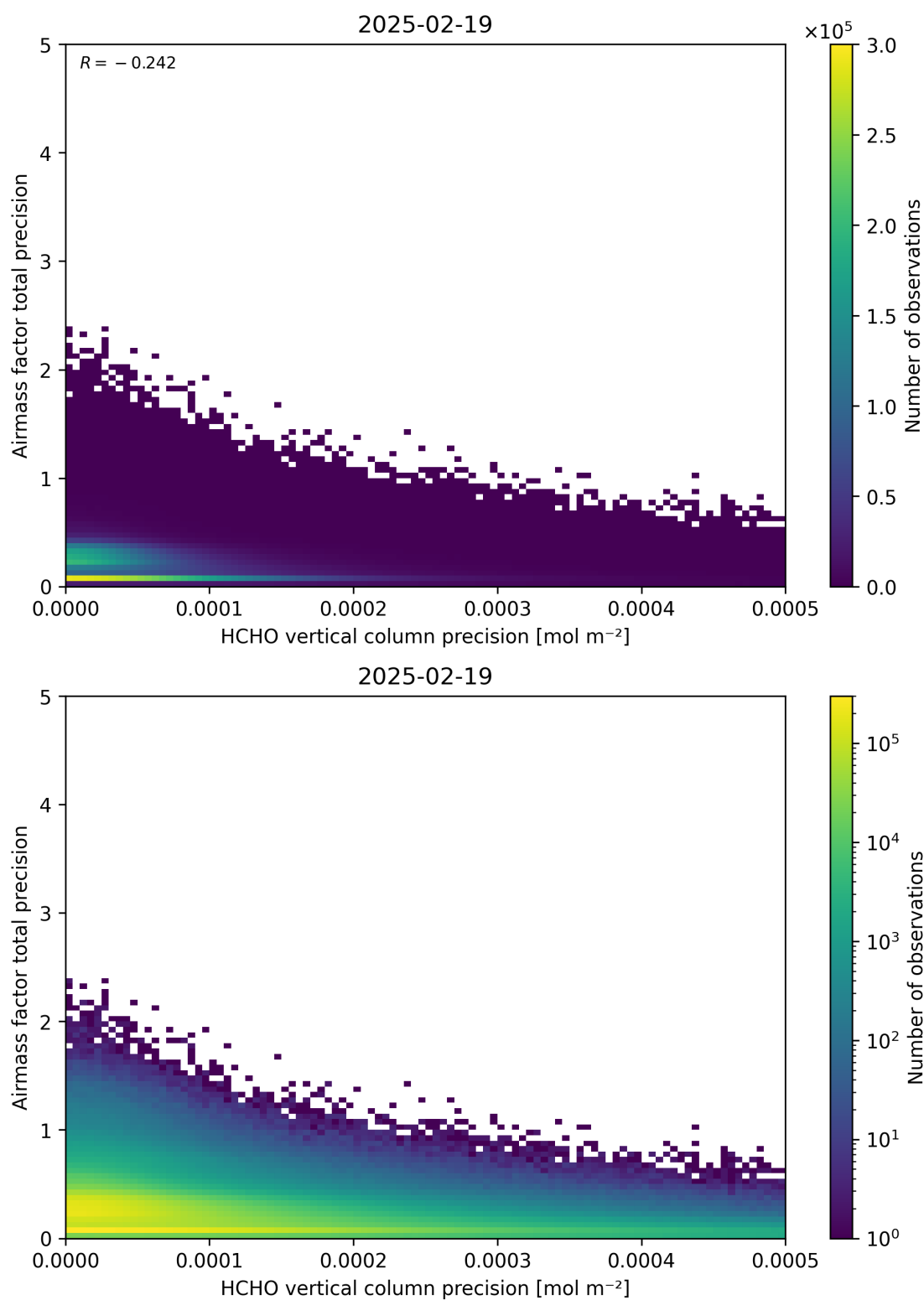
Figure 145: Scatter density plot of “HCHO vertical column precision” against “Airmass factor total precision” for 2025-02-19 to 2025-02-20.
