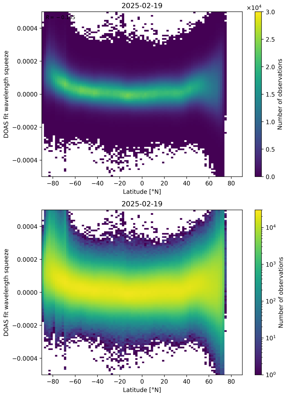
Figure 155: Scatter density plot of “Latitude” against “DOAS fit wavelength squeeze” for 2025-02-19 to 2025-02-20.
