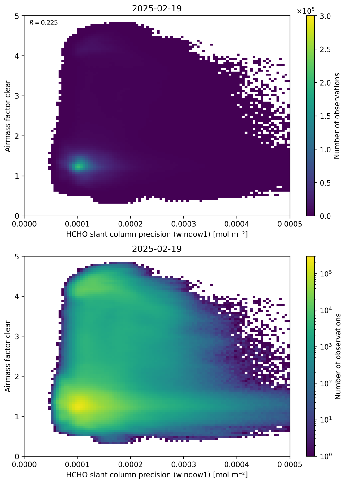
Figure 91: Scatter density plot of “HCHO slant column precision (window1)” against “Airmass factor clear” for 2025-02-19 to 2025-02-20.
