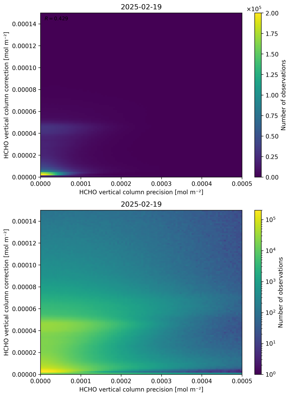
Figure 146: Scatter density plot of “HCHO vertical column precision” against “HCHO vertical column correction” for 2025-02-19 to 2025-02-20.
