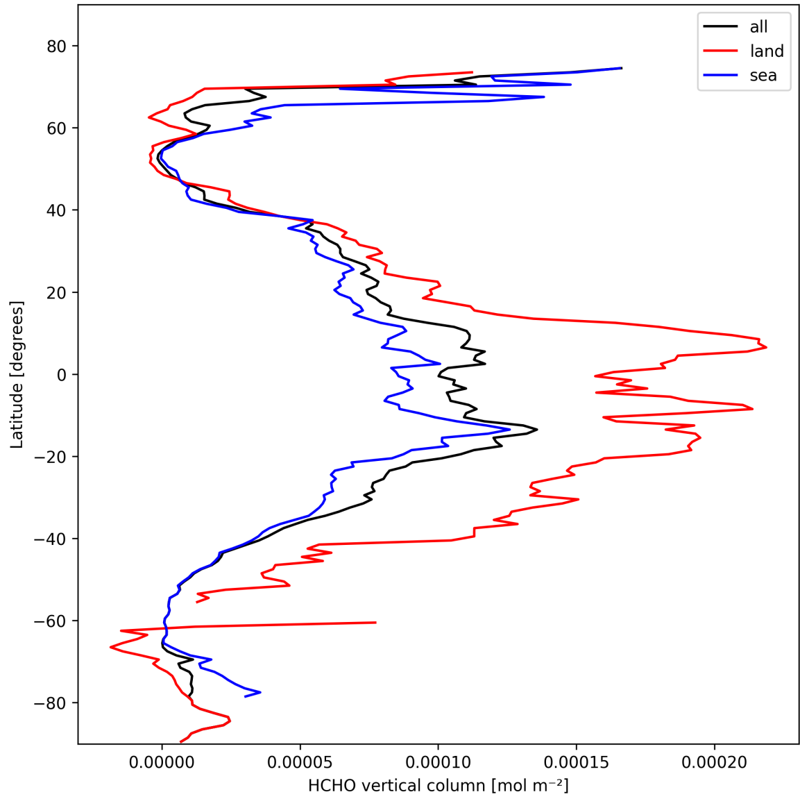
Figure 21: Zonal average of “HCHO vertical column” for 2025-02-19 to 2025-02-20.
