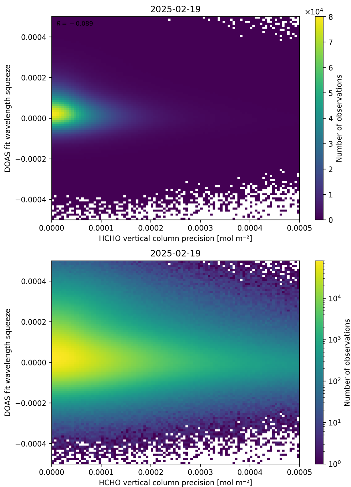
Figure 138: Scatter density plot of “HCHO vertical column precision” against “DOAS fit wavelength squeeze” for 2025-02-19 to 2025-02-20.
