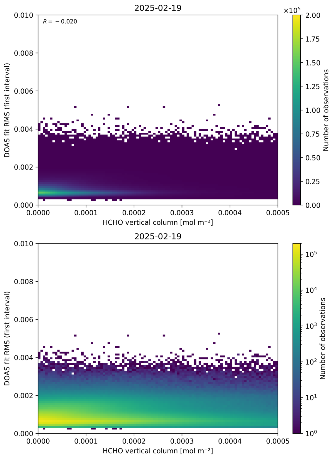
Figure 123: Scatter density plot of “HCHO vertical column” against “DOAS fit RMS (first interval)” for 2025-02-19 to 2025-02-20.
