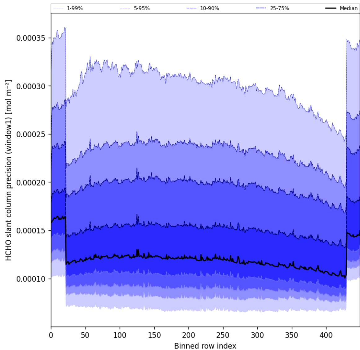
Figure 53: Along track statistics of “HCHO slant column precision (window1)” for 2025-02-19 to 2025-02-20
