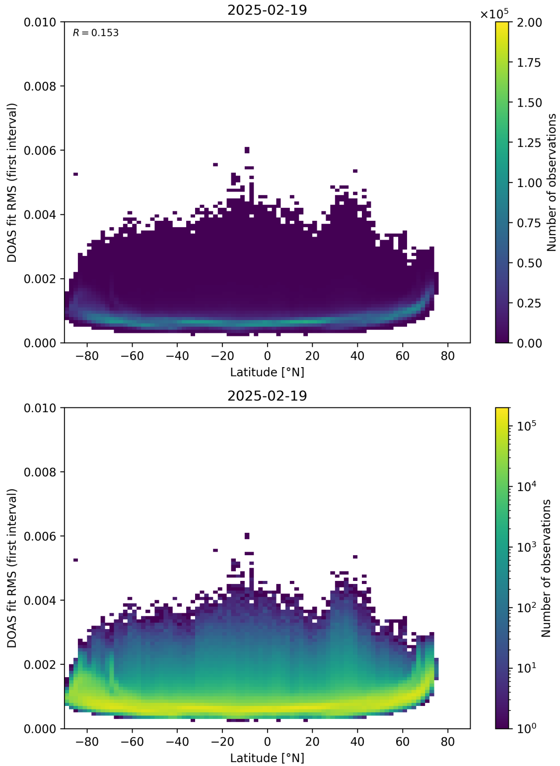
Figure 153: Scatter density plot of “Latitude” against “DOAS fit RMS (first interval)” for 2025-02-19 to 2025-02-20.
