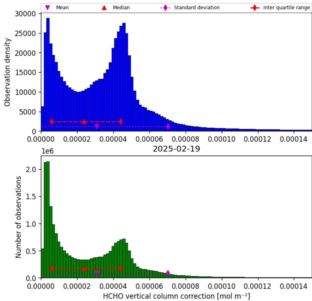
Figure 37: Histogram of “HCHO vertical column correction” for 2025-02-19 to 2025-02-20
