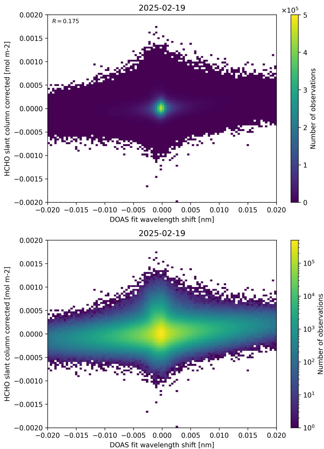
Figure 66: Scatter density plot of “DOAS fit wavelength shift” against “HCHO slant column corrected” for 2025-02-19 to 2025-02-20.
