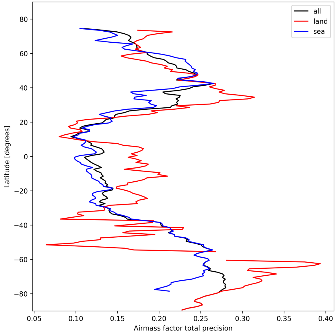
Figure 27: Zonal average of “Airmass factor total precision” for 2025-02-19 to 2025-02-20.
