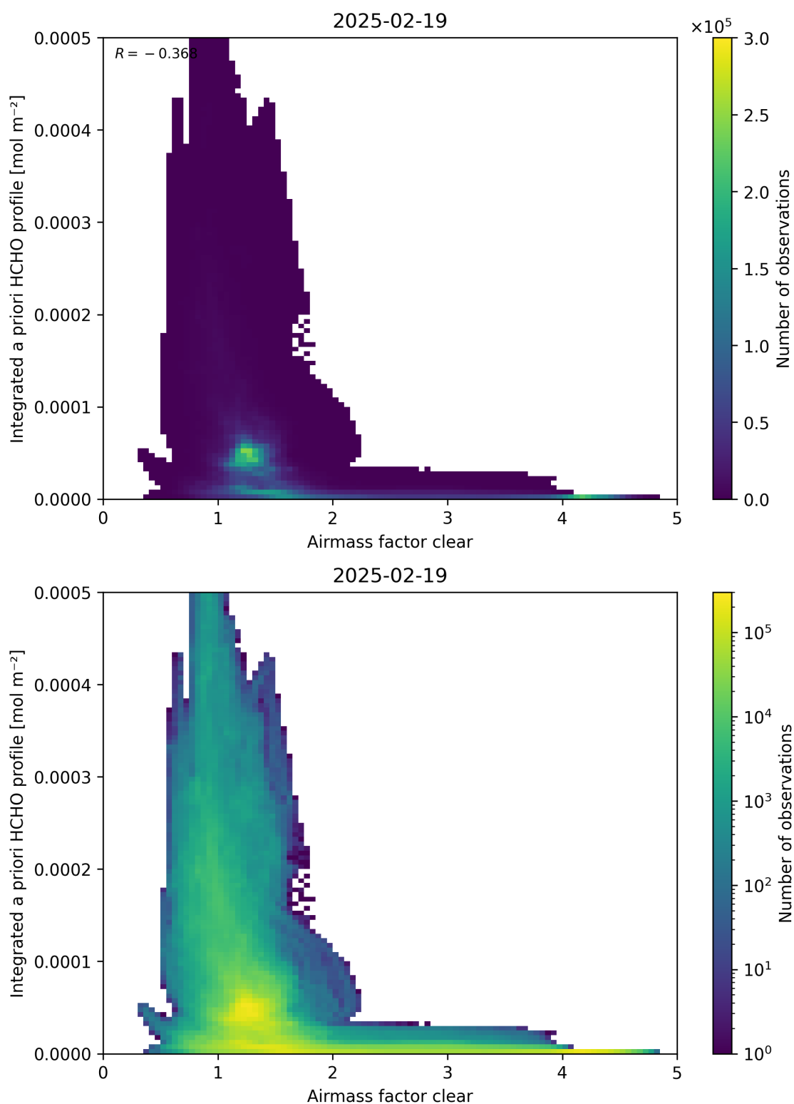
Figure 76: Scatter density plot of “Airmass factor clear” against “Integrated a priori HCHO profile” for 2025-02-19 to 2025-02-20.
