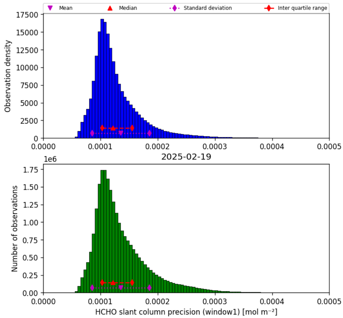
Figure 39: Histogram of “HCHO slant column precision (window1)” for 2025-02-19 to 2025-02-20
