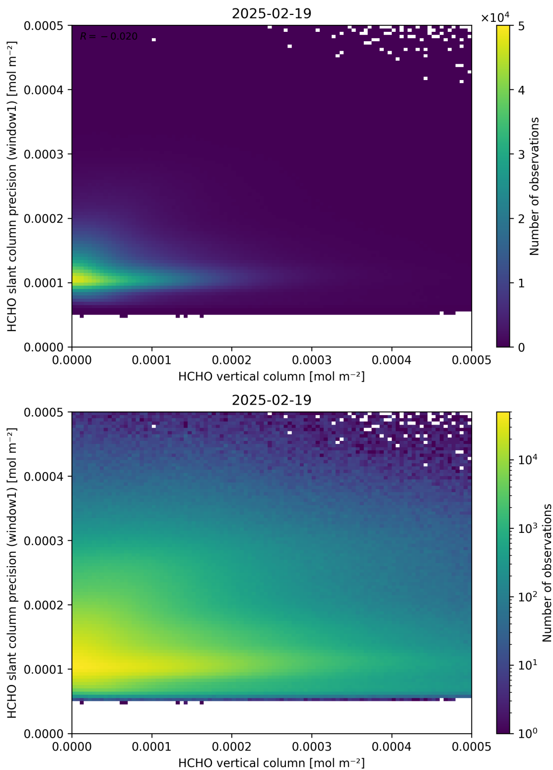
Figure 130: Scatter density plot of “HCHO vertical column” against “HCHO slant column precision (window1)” for 2025-02-19 to 2025-02-20.
