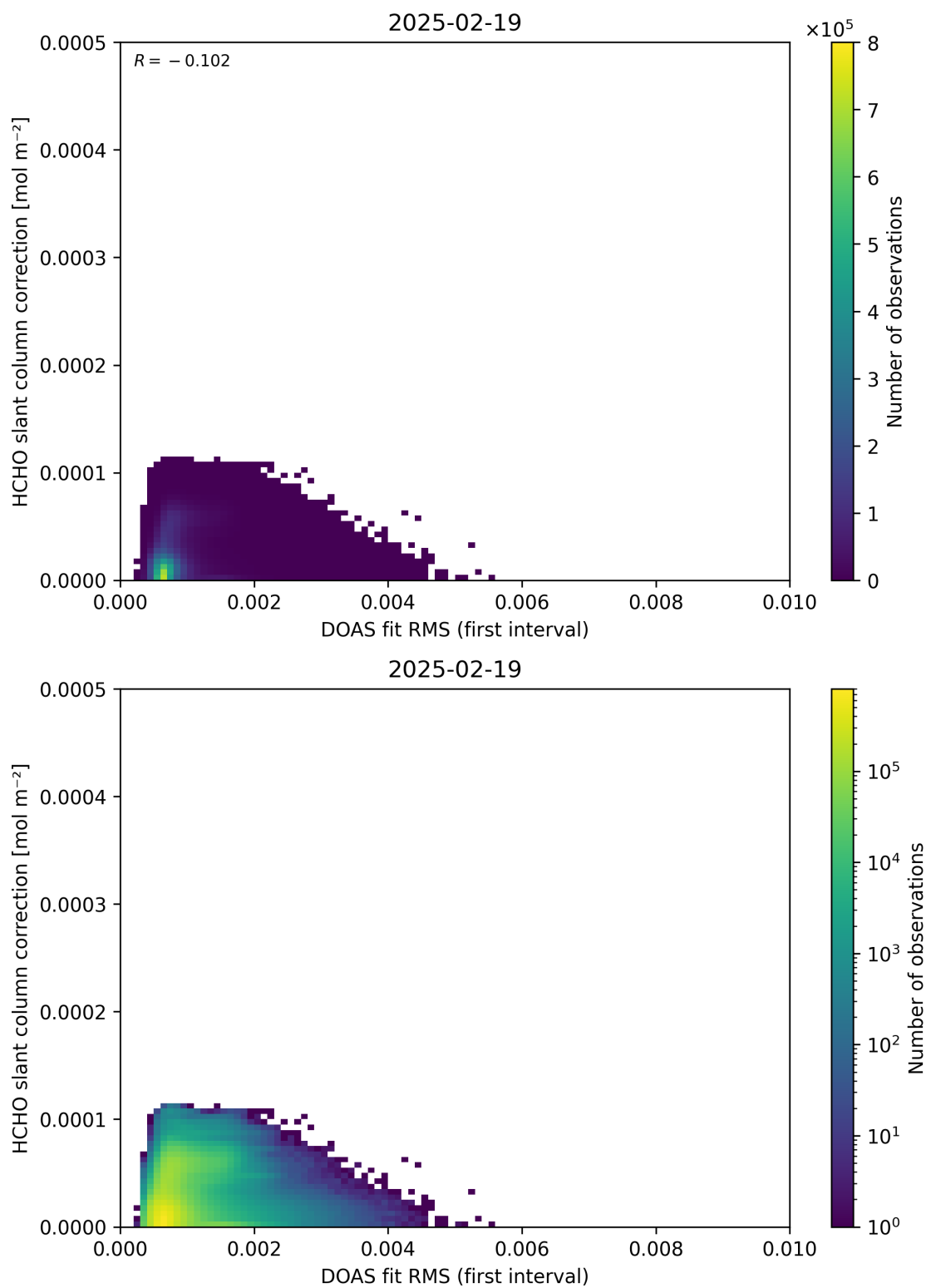
Figure 63: Scatter density plot of “DOAS fit RMS (first interval)” against “HCHO slant column correction” for 2025-02-19 to 2025-02-20.
