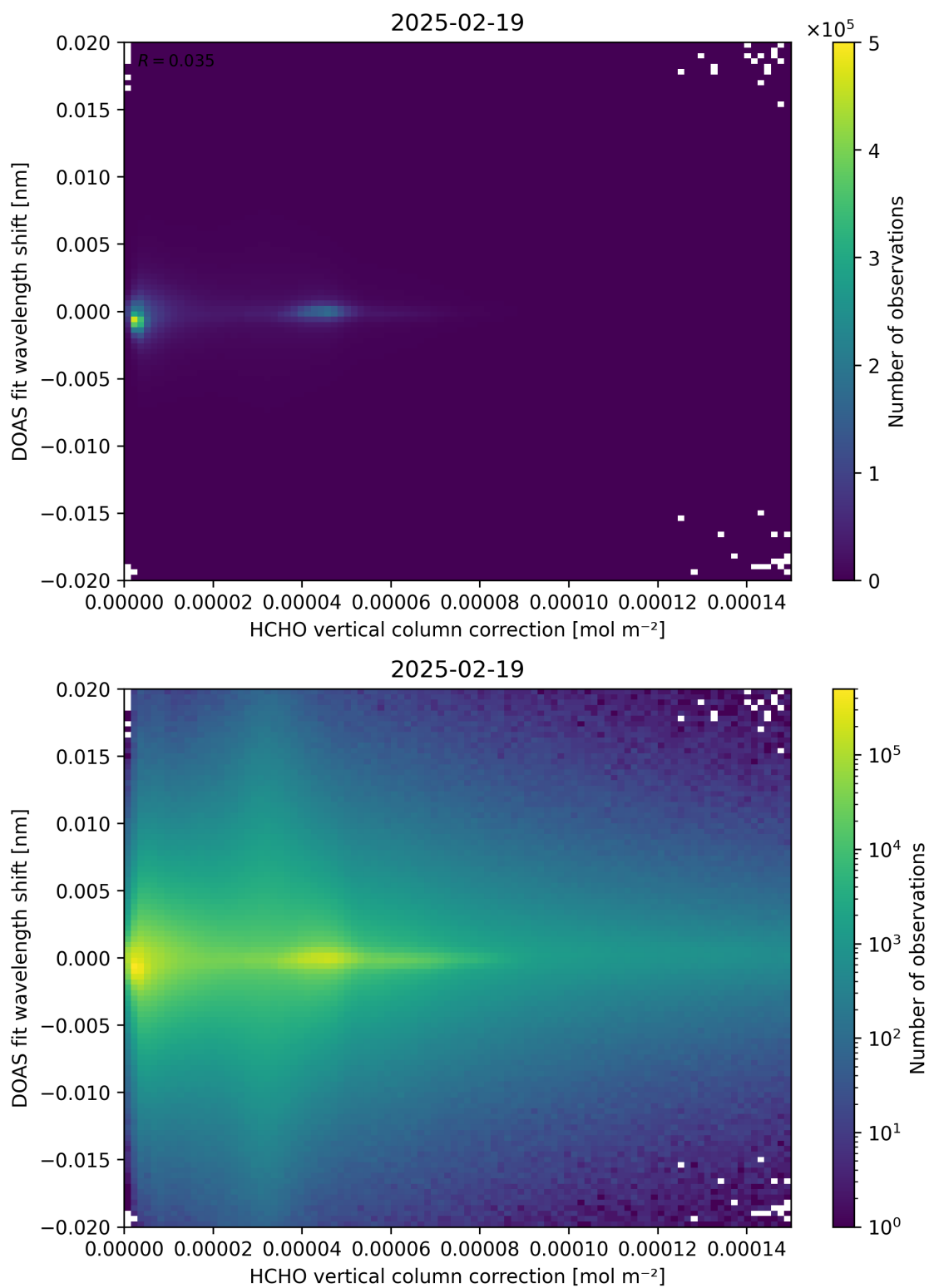
Figure 113: Scatter density plot of “HCHO vertical column correction” against “DOAS fit wavelength shift” for 2025-02-19 to 2025-02-20.
