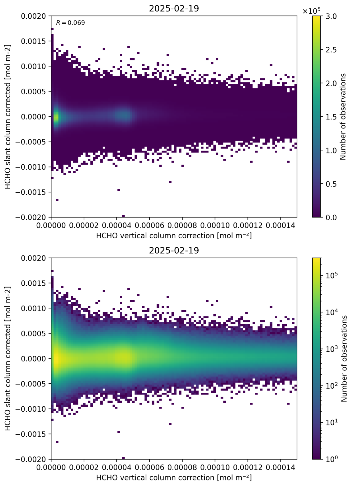
Figure 116: Scatter density plot of “HCHO vertical column correction” against “HCHO slant column corrected” for 2025-02-19 to 2025-02-20.
