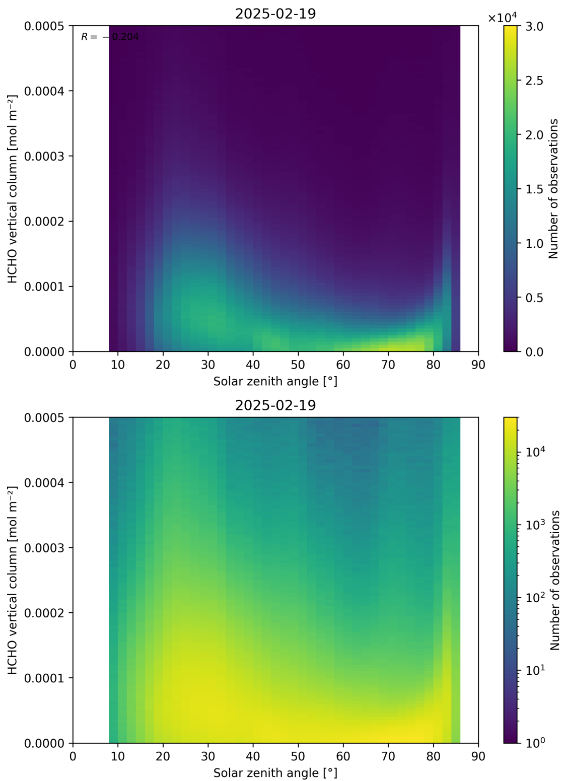
Figure 177: Scatter density plot of “Solar zenith angle” against “HCHO vertical column” for 2025-02-19 to 2025-02-20.
