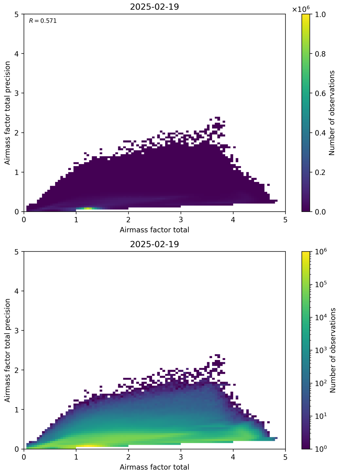
Figure 103: Scatter density plot of “Airmass factor total” against “Airmass factor total precision” for 2025-02-19 to 2025-02-20.
