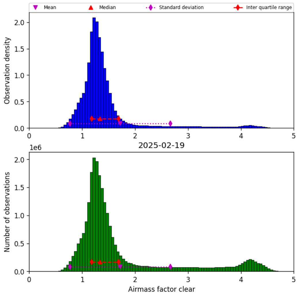
Figure 42: Histogram of “Airmass factor clear” for 2025-02-19 to 2025-02-20
