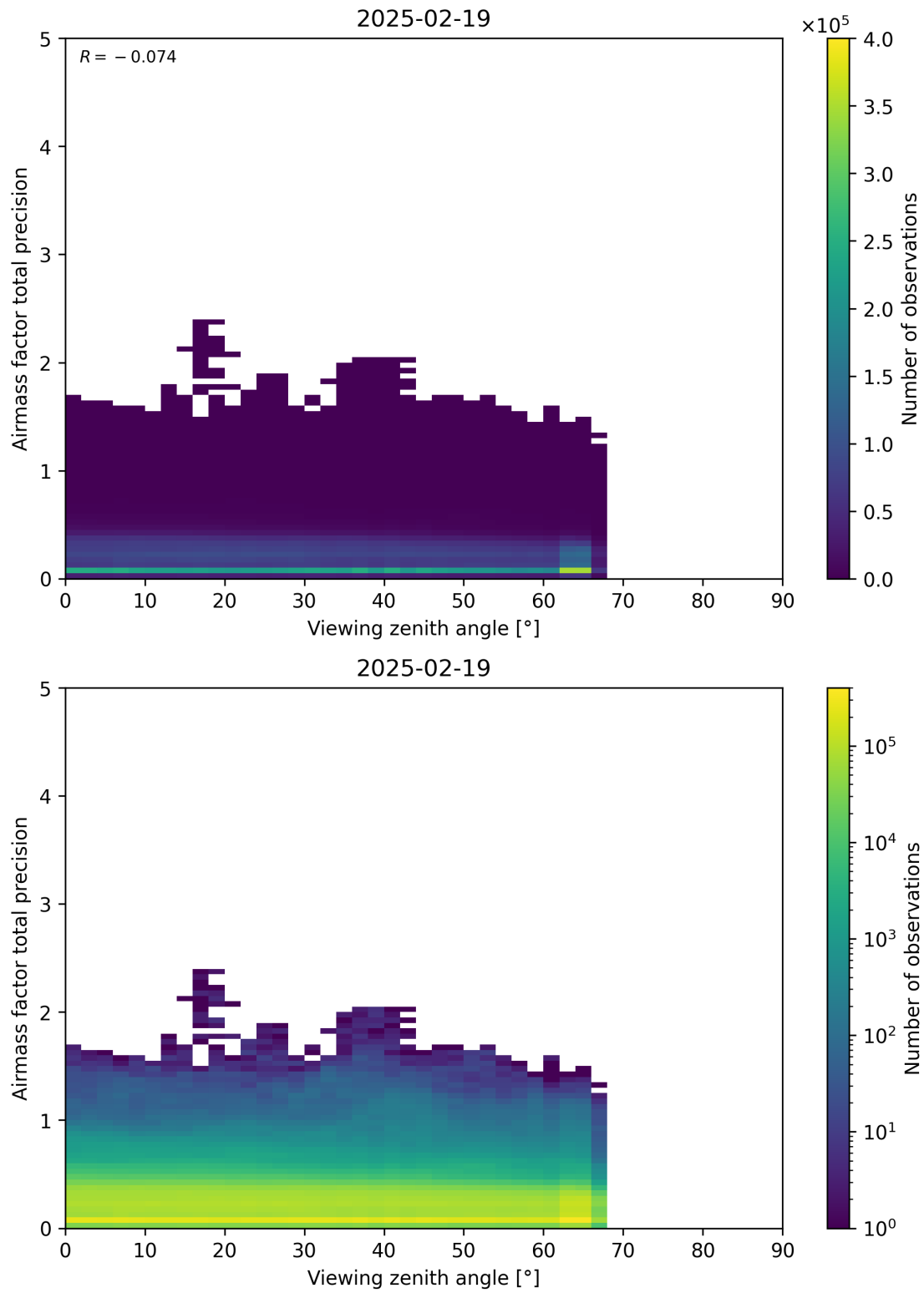
Figure 191: Scatter density plot of “Viewing zenith angle” against “Airmass factor total precision” for 2025-02-19 to 2025-02-20.
