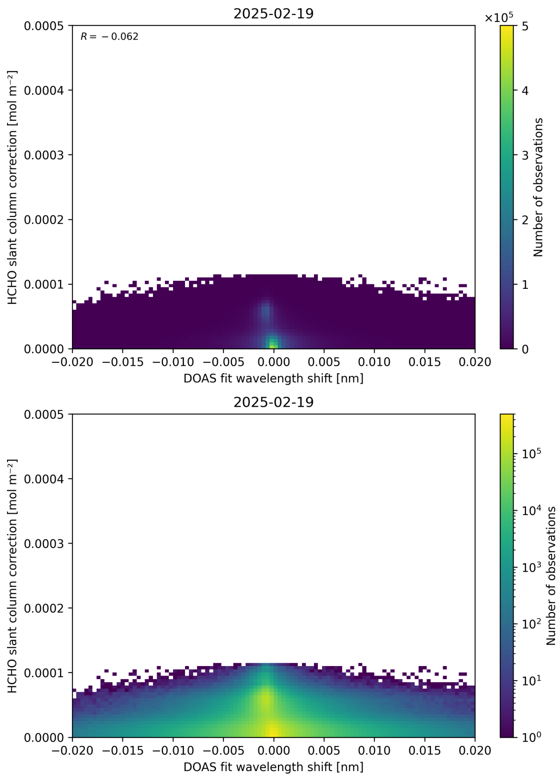
Figure 67: Scatter density plot of “DOAS fit wavelength shift” against “HCHO slant column correction” for 2025-02-19 to 2025-02-20.
