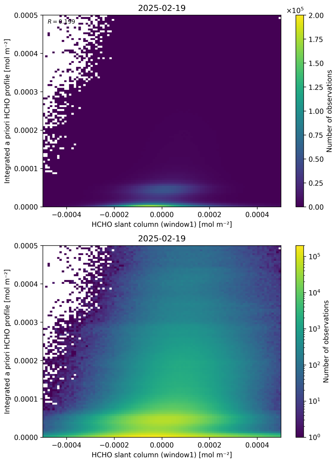
Figure 87: Scatter density plot of “HCHO slant column (window1)” against “Integrated a priori HCHO profile” for 2025-02-19 to 2025-02-20.
