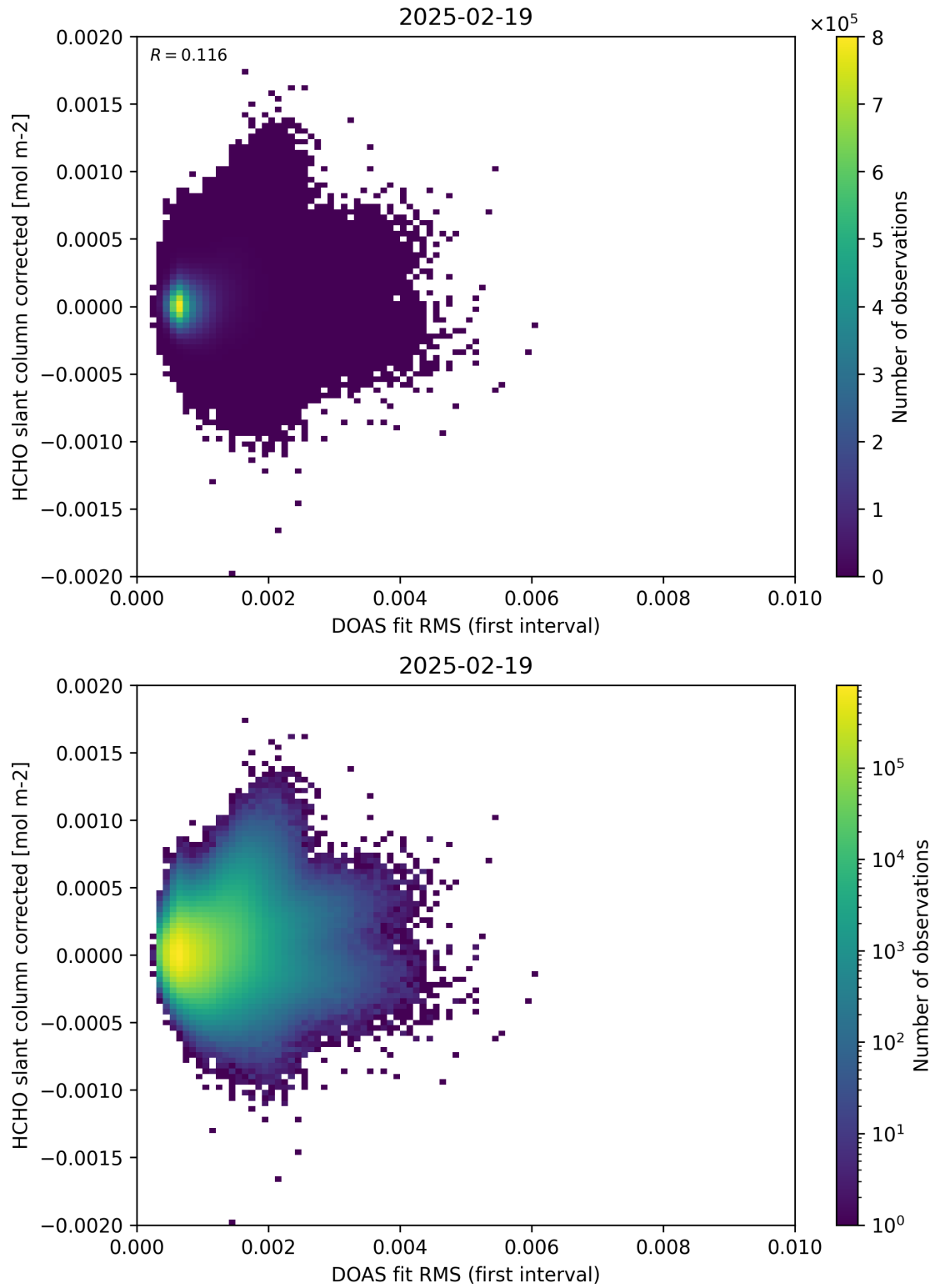
Figure 62: Scatter density plot of “DOAS fit RMS (first interval)” against “HCHO slant column corrected” for 2025-02-19 to 2025-02-20.
