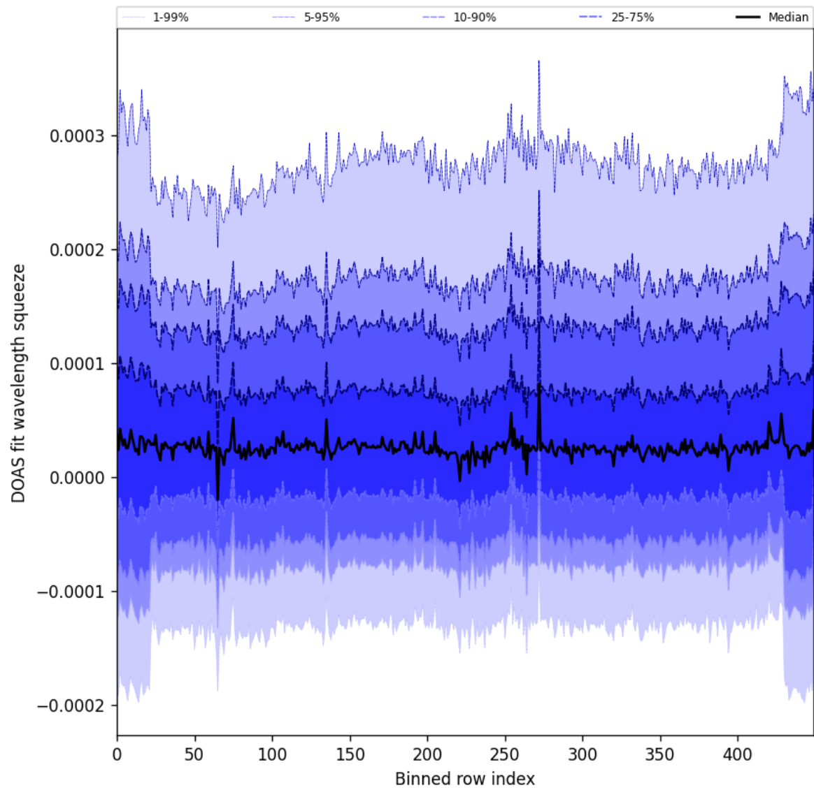
Figure 59: Along track statistics of “DOAS fit wavelength squeeze” for 2025-02-19 to 2025-02-20
