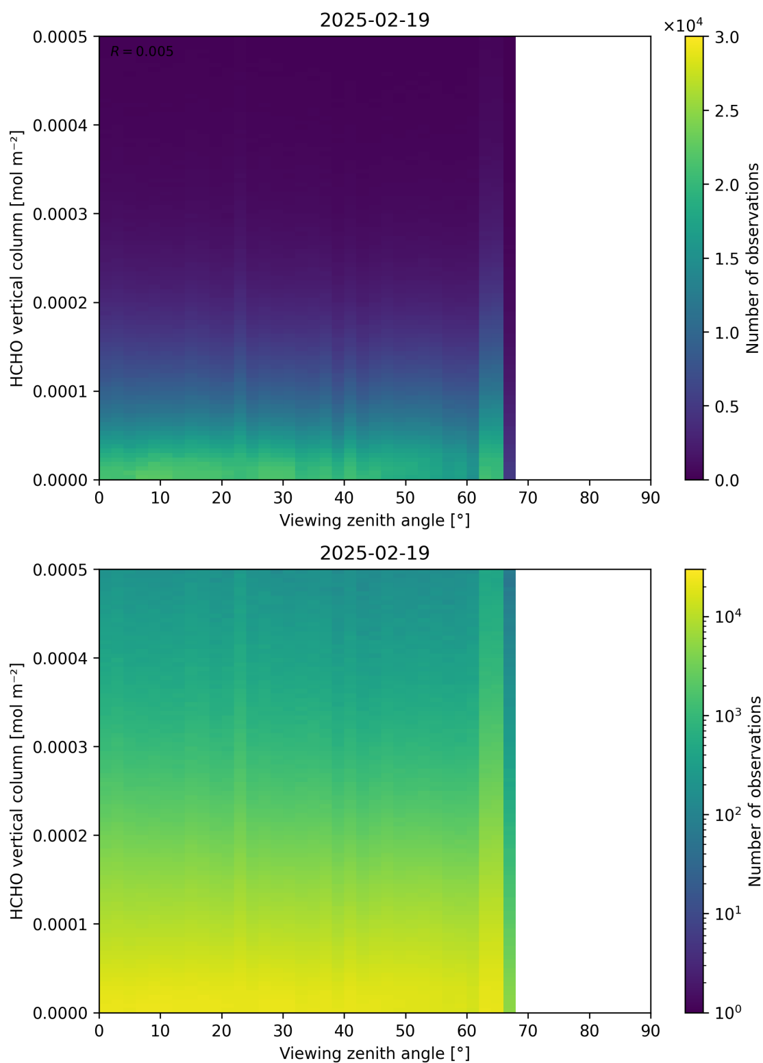
Figure 192: Scatter density plot of “Viewing zenith angle” against “HCHO vertical column” for 2025-02-19 to 2025-02-20.
