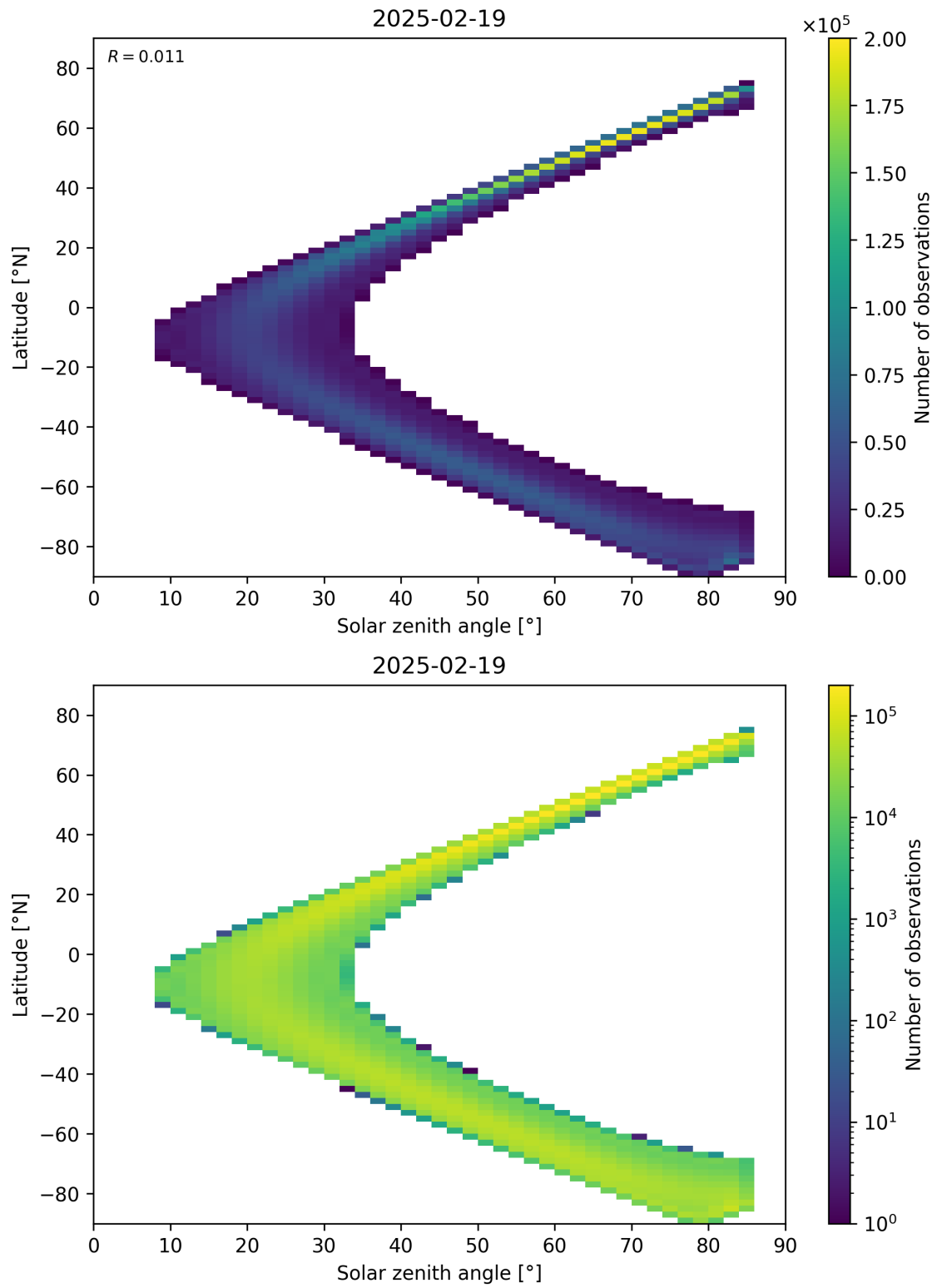
Figure 181: Scatter density plot of “Solar zenith angle” against “Latitude” for 2025-02-19 to 2025-02-20.
