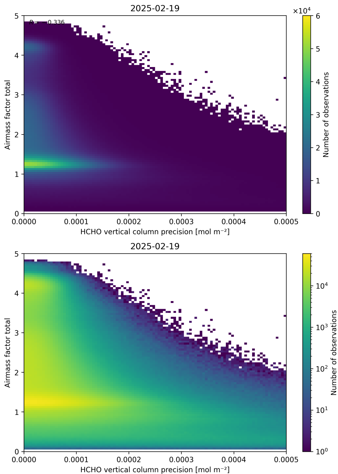
Figure 144: Scatter density plot of “HCHO vertical column precision” against “Airmass factor total” for 2025-02-19 to 2025-02-20.
