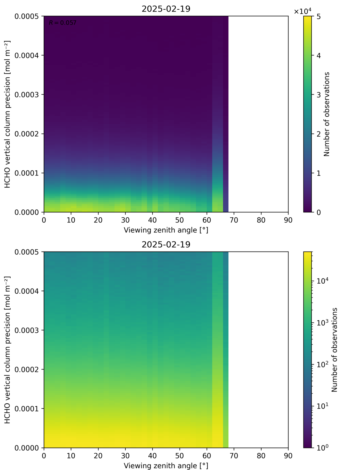
Figure 194: Scatter density plot of “Viewing zenith angle” against “HCHO vertical column precision” for 2025-02-19 to 2025-02-20.
