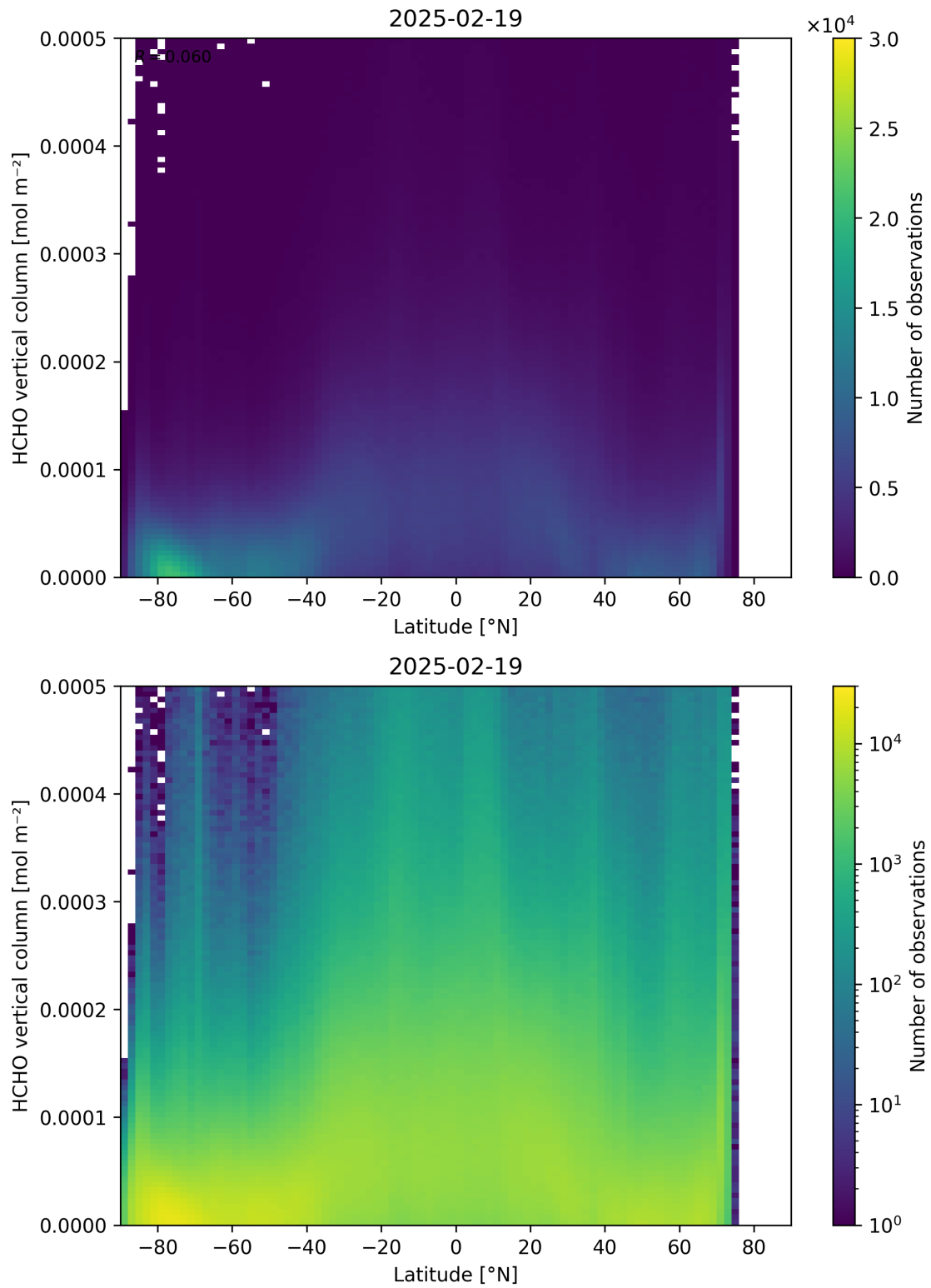
Figure 163: Scatter density plot of “Latitude” against “HCHO vertical column” for 2025-02-19 to 2025-02-20.
