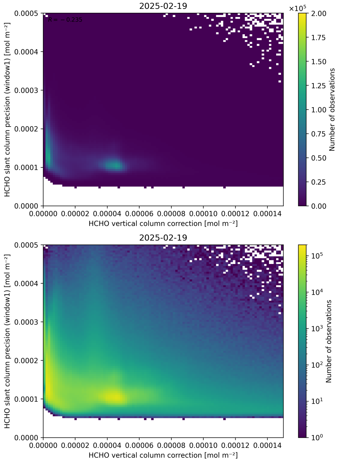
Figure 119: Scatter density plot of “HCHO vertical column correction” against “HCHO slant column precision (window1)” for 2025-02-19 to 2025-02-20.
