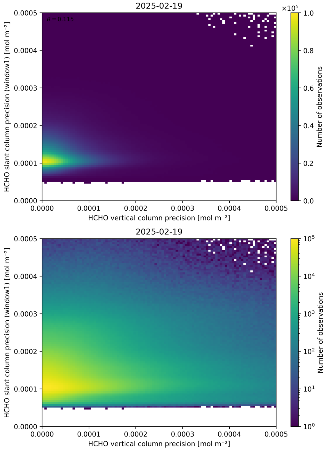
Figure 143: Scatter density plot of “HCHO vertical column precision” against “HCHO slant column precision (window1)” for 2025-02-19 to 2025-02-20.
