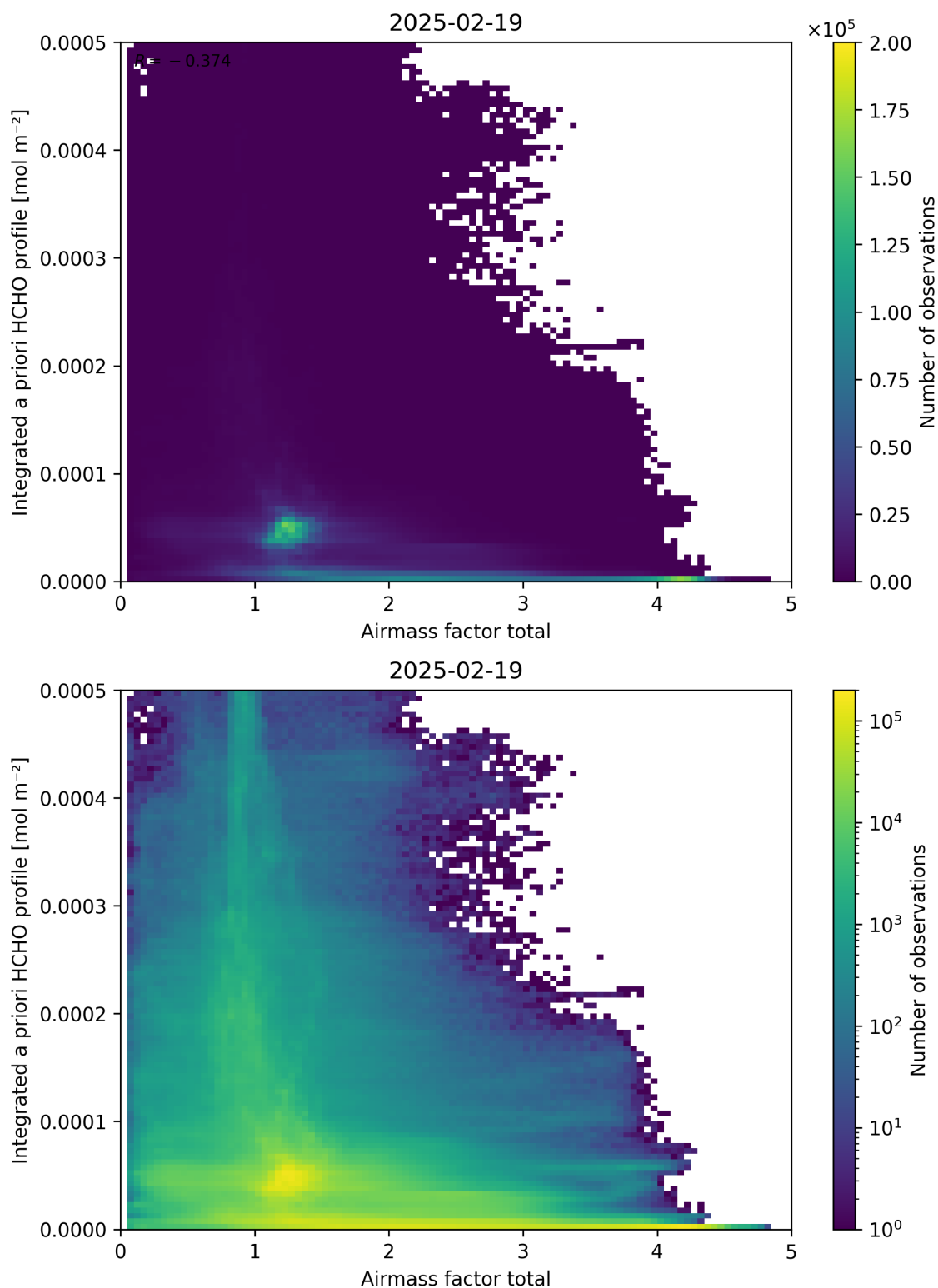
Figure 104: Scatter density plot of “Airmass factor total” against “Integrated a priori HCHO profile” for 2025-02-19 to 2025-02-20.
