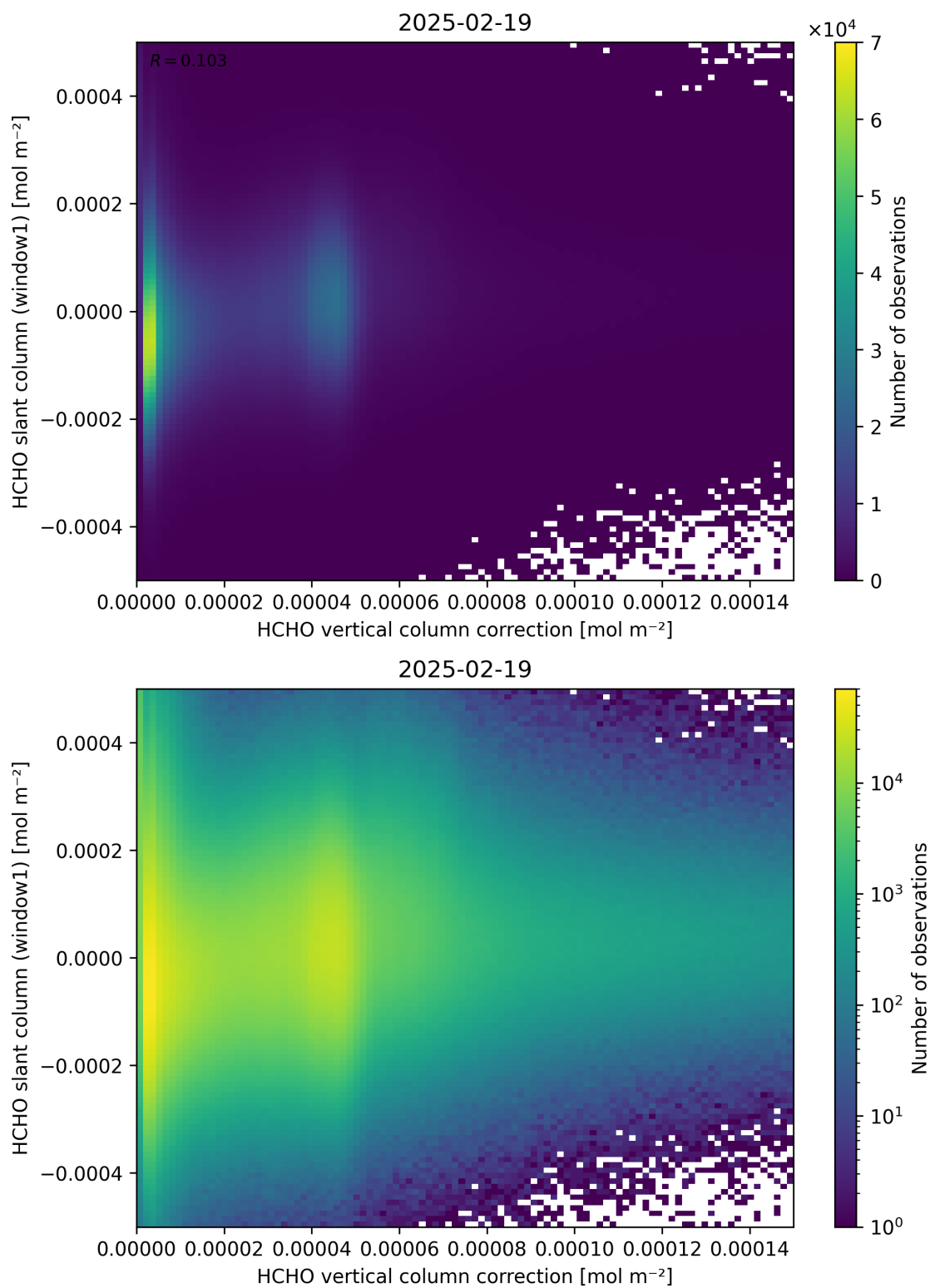
Figure 118: Scatter density plot of “HCHO vertical column correction” against “HCHO slant column (window1)” for 2025-02-19 to 2025-02-20.
