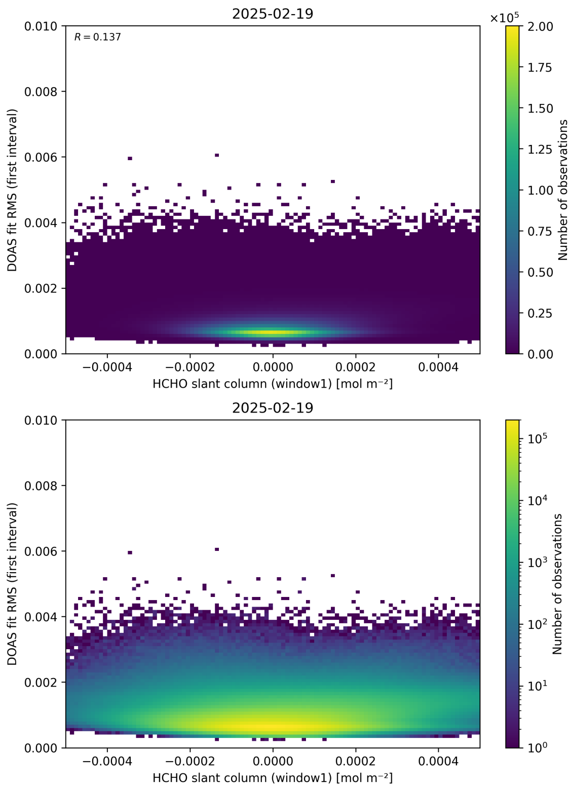
Figure 78: Scatter density plot of “HCHO slant column (window1)” against “DOAS fit RMS (first interval)” for 2025-02-19 to 2025-02-20.
