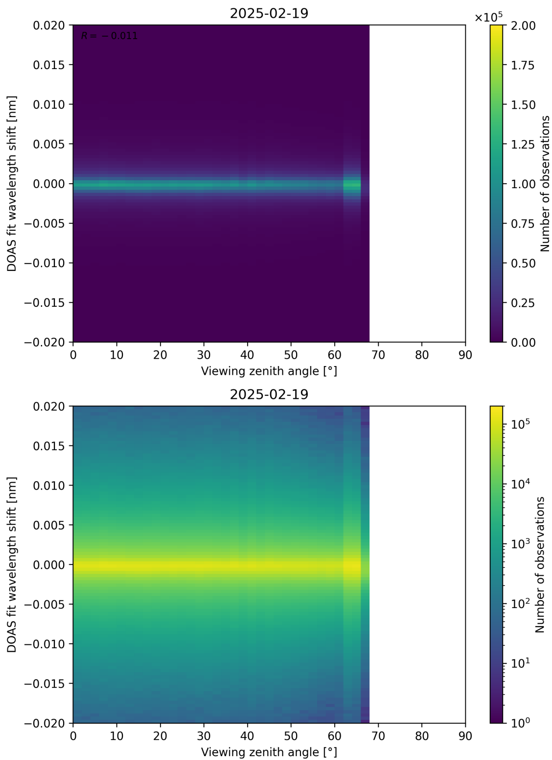
Figure 183: Scatter density plot of “Viewing zenith angle” against “DOAS fit wavelength shift” for 2025-02-19 to 2025-02-20.
