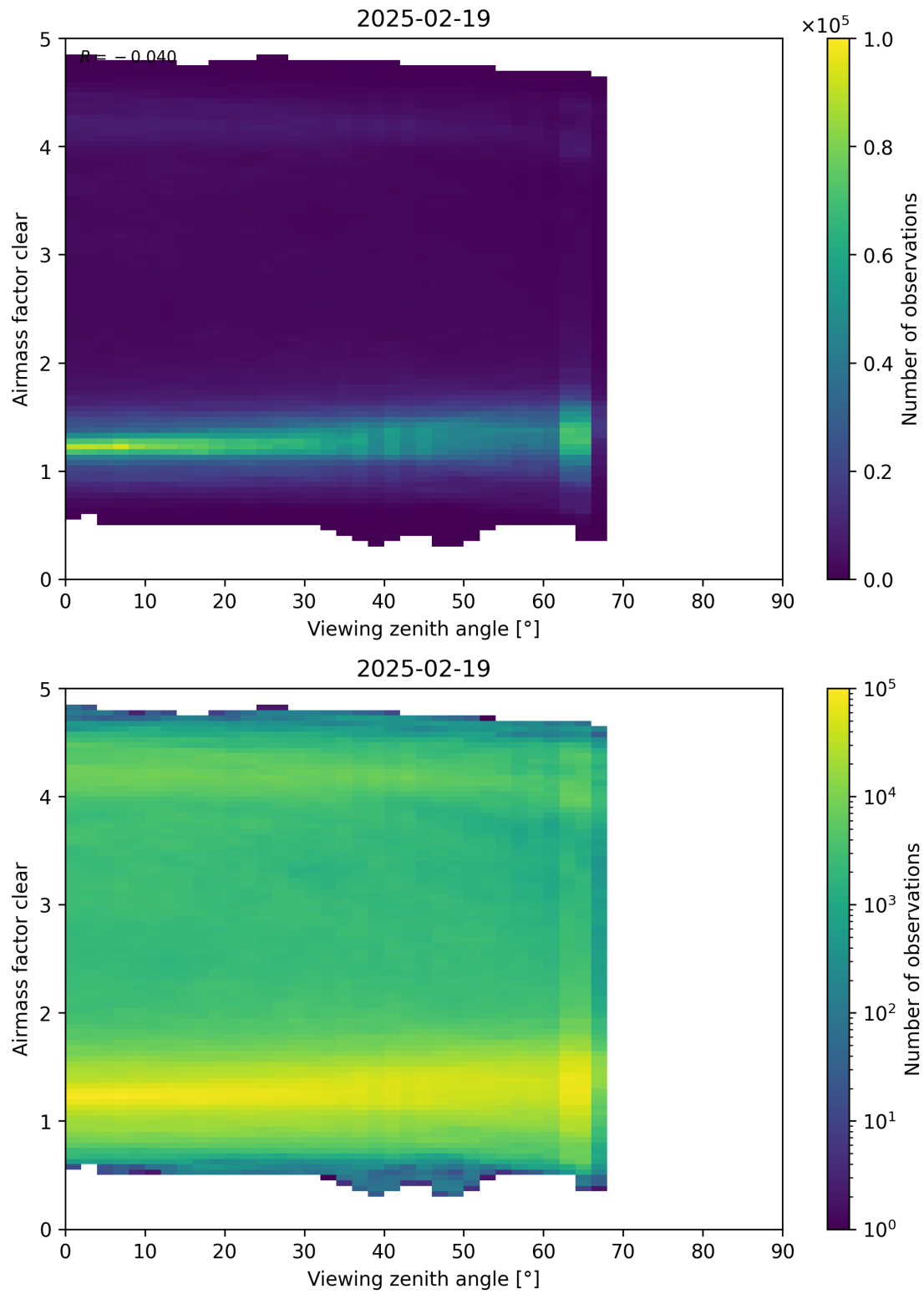
Figure 185: Scatter density plot of “Viewing zenith angle” against “Airmass factor clear” for 2025-02-19 to 2025-02-20.
