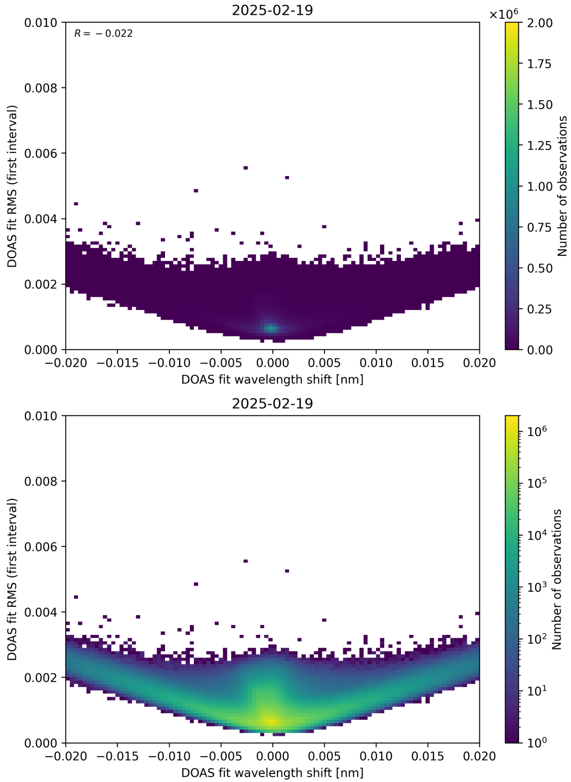
Figure 64: Scatter density plot of “DOAS fit wavelength shift” against “DOAS fit RMS (first interval)” for 2025-02-19 to 2025-02-20.
