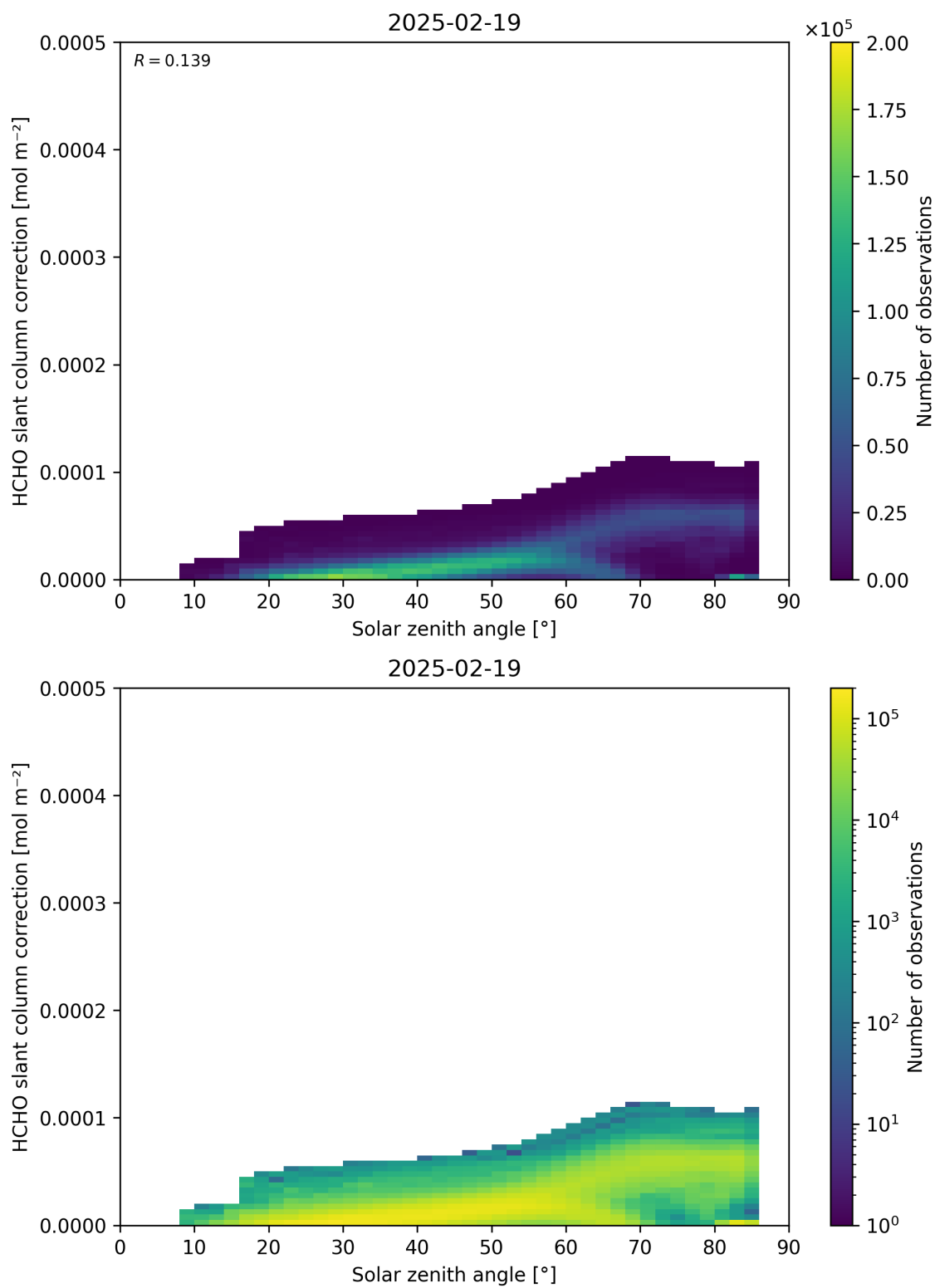
Figure 172: Scatter density plot of “Solar zenith angle” against “HCHO slant column correction” for 2025-02-19 to 2025-02-20.
