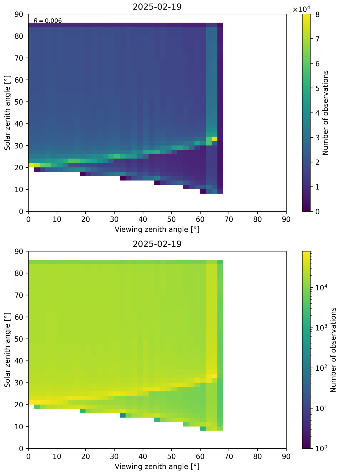
Figure 197: Scatter density plot of “Viewing zenith angle” against “Solar zenith angle” for 2025-02-19 to 2025-02-20.
