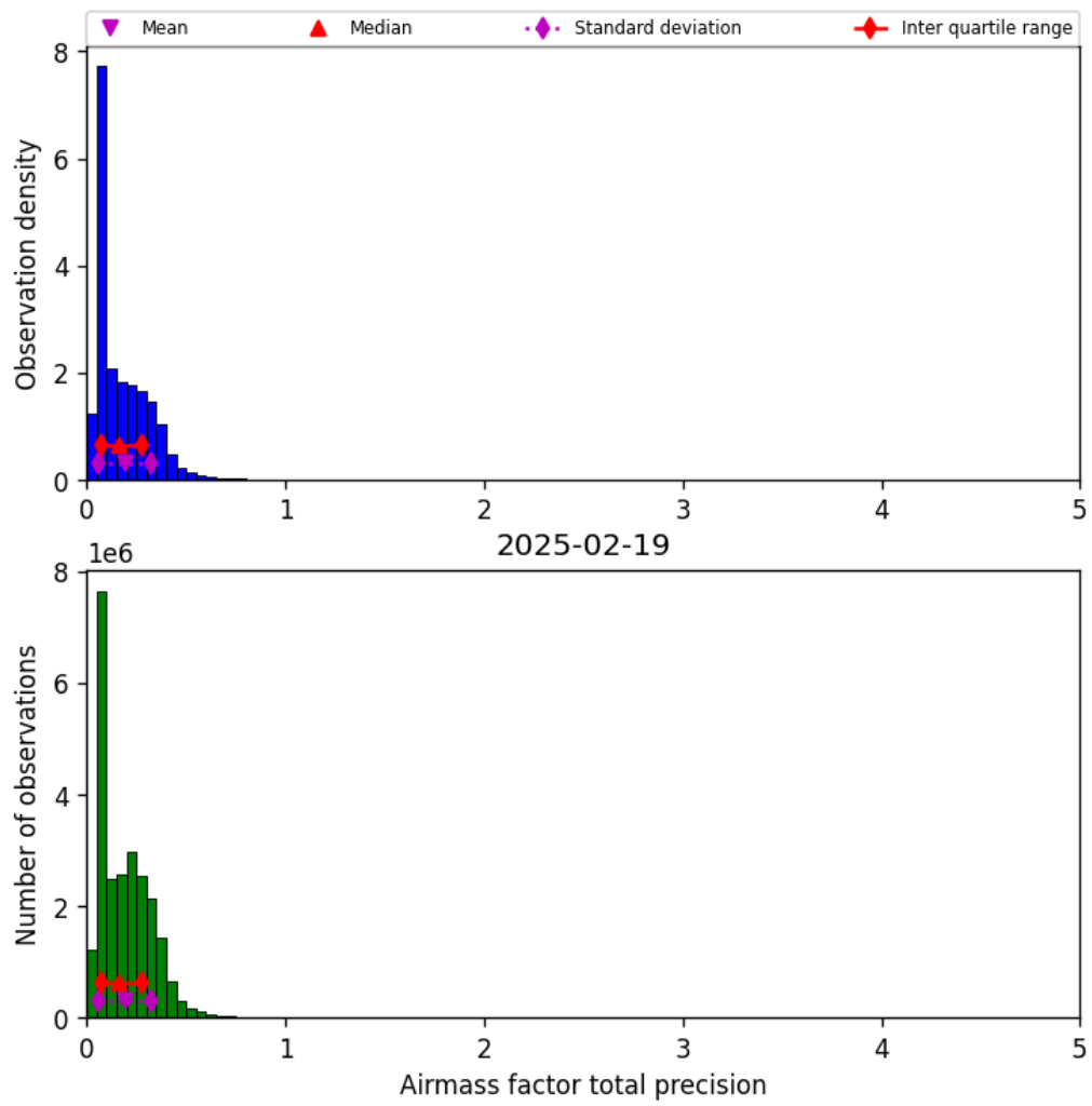
Figure 41: Histogram of “Airmass factor total precision” for 2025-02-19 to 2025-02-20
