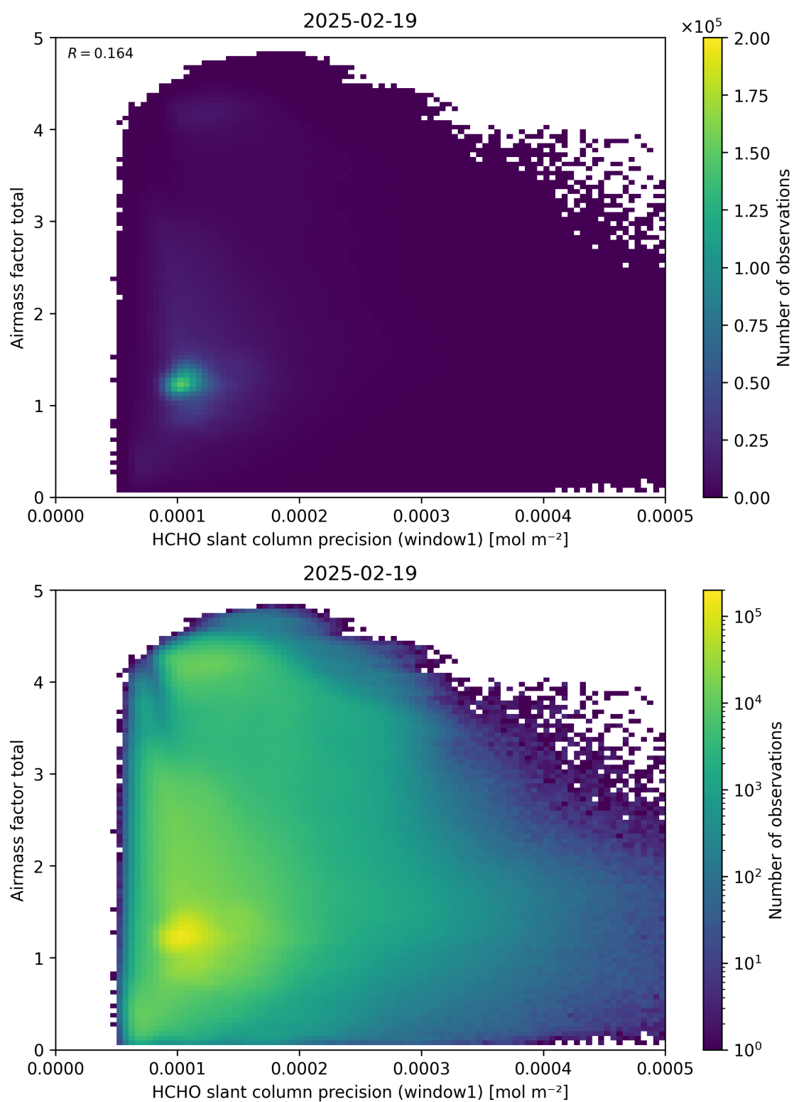
Figure 94: Scatter density plot of “HCHO slant column precision (window1)” against “Airmass factor total” for 2025-02-19 to 2025-02-20.
