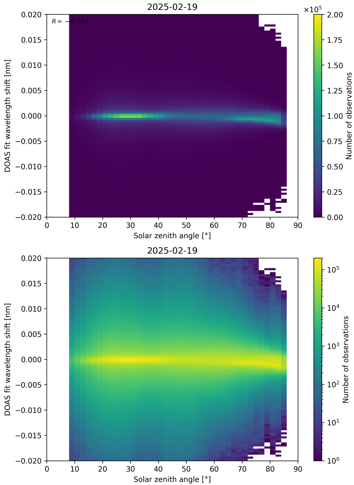
Figure 168: Scatter density plot of “Solar zenith angle” against “DOAS fit wavelength shift” for 2025-02-19 to 2025-02-20.
