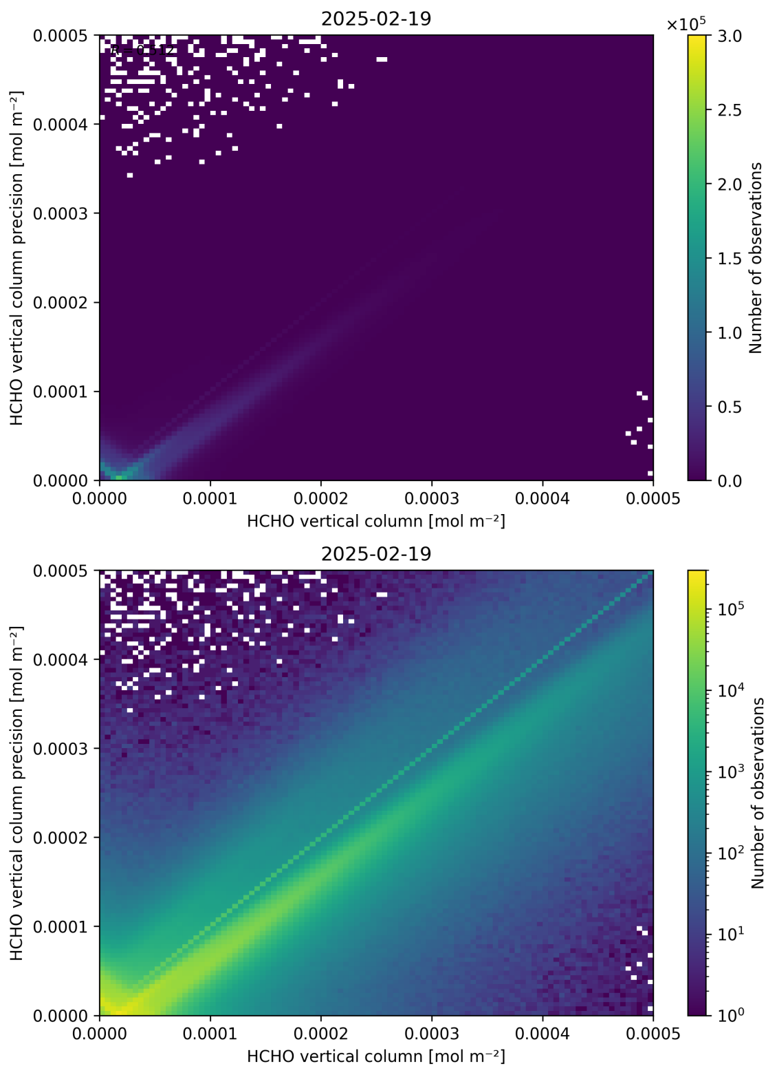
Figure 134: Scatter density plot of “HCHO vertical column” against “HCHO vertical column precision” for 2025-02-19 to 2025-02-20.
