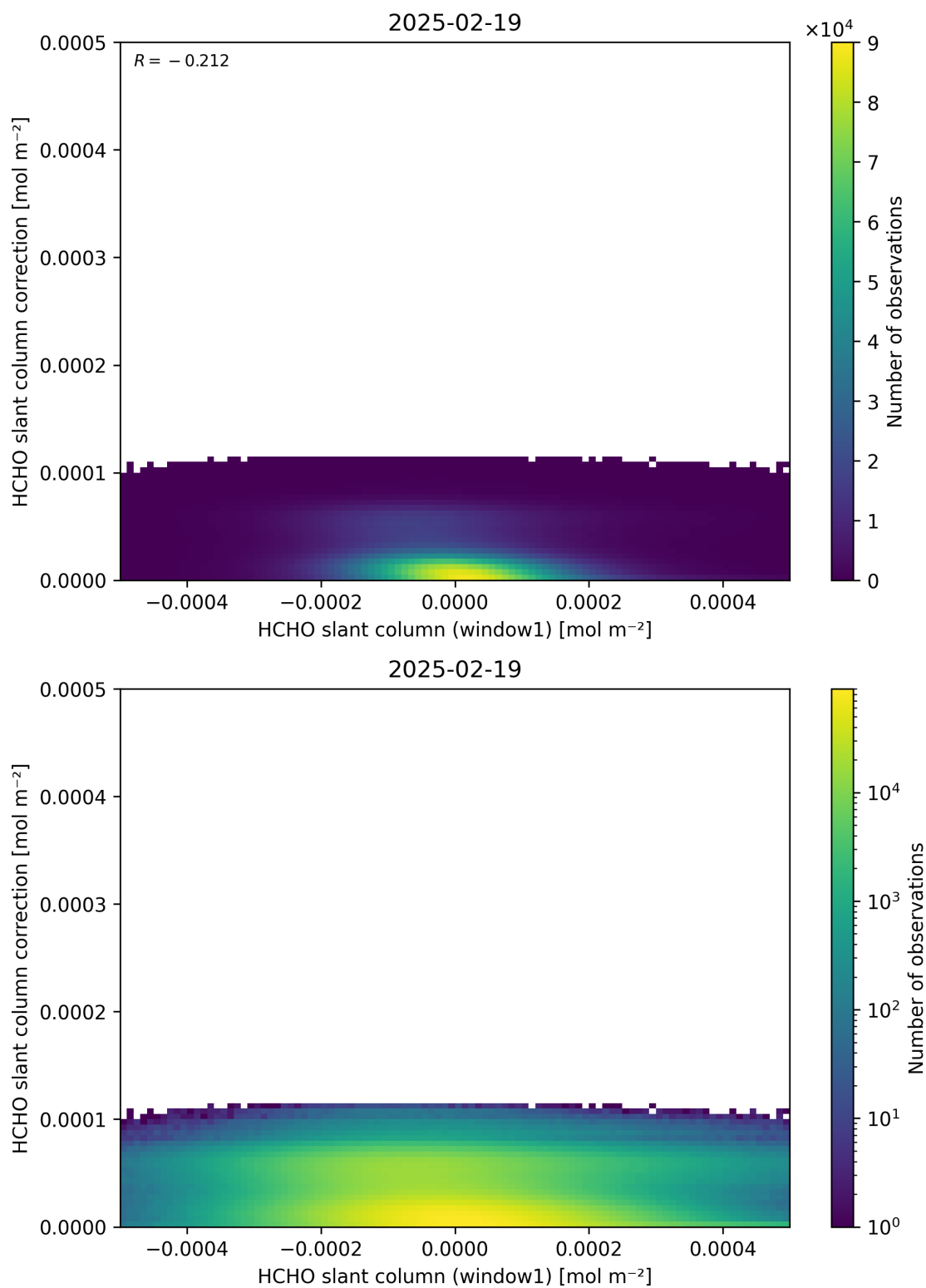
Figure 83: Scatter density plot of “HCHO slant column (window1)” against “HCHO slant column correction” for 2025-02-19 to 2025-02-20.
