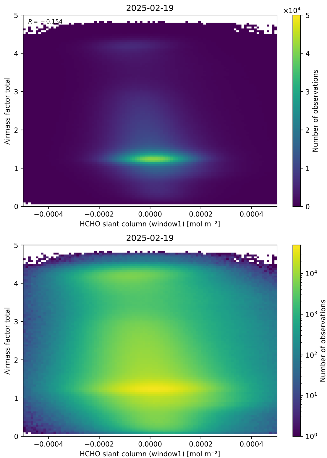
Figure 85: Scatter density plot of “HCHO slant column (window1)” against “Airmass factor total” for 2025-02-19 to 2025-02-20.
