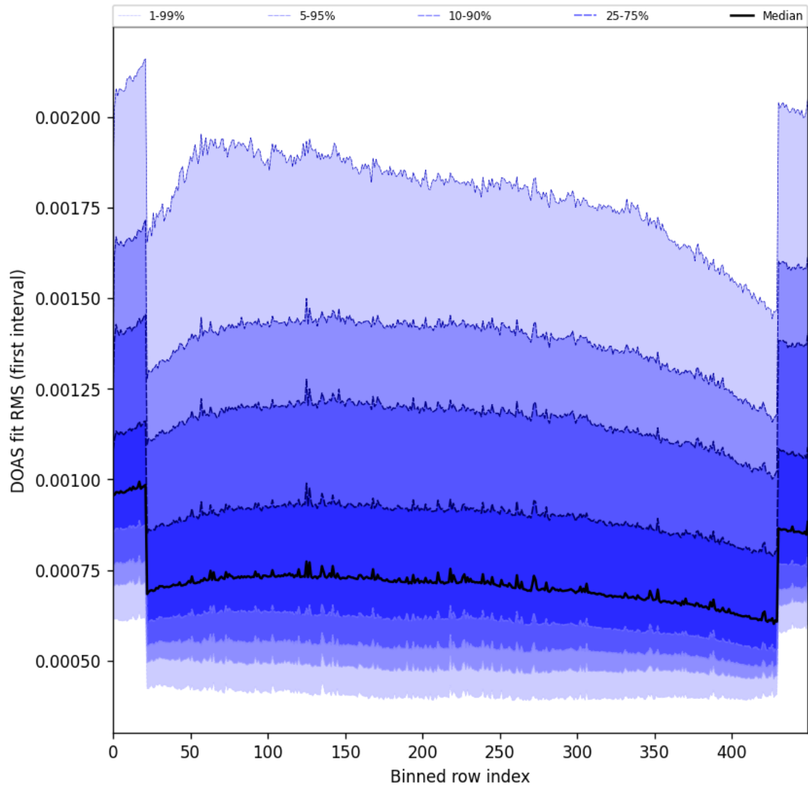
Figure 60: Along track statistics of “DOAS fit RMS (first interval)” for 2025-02-19 to 2025-02-20
