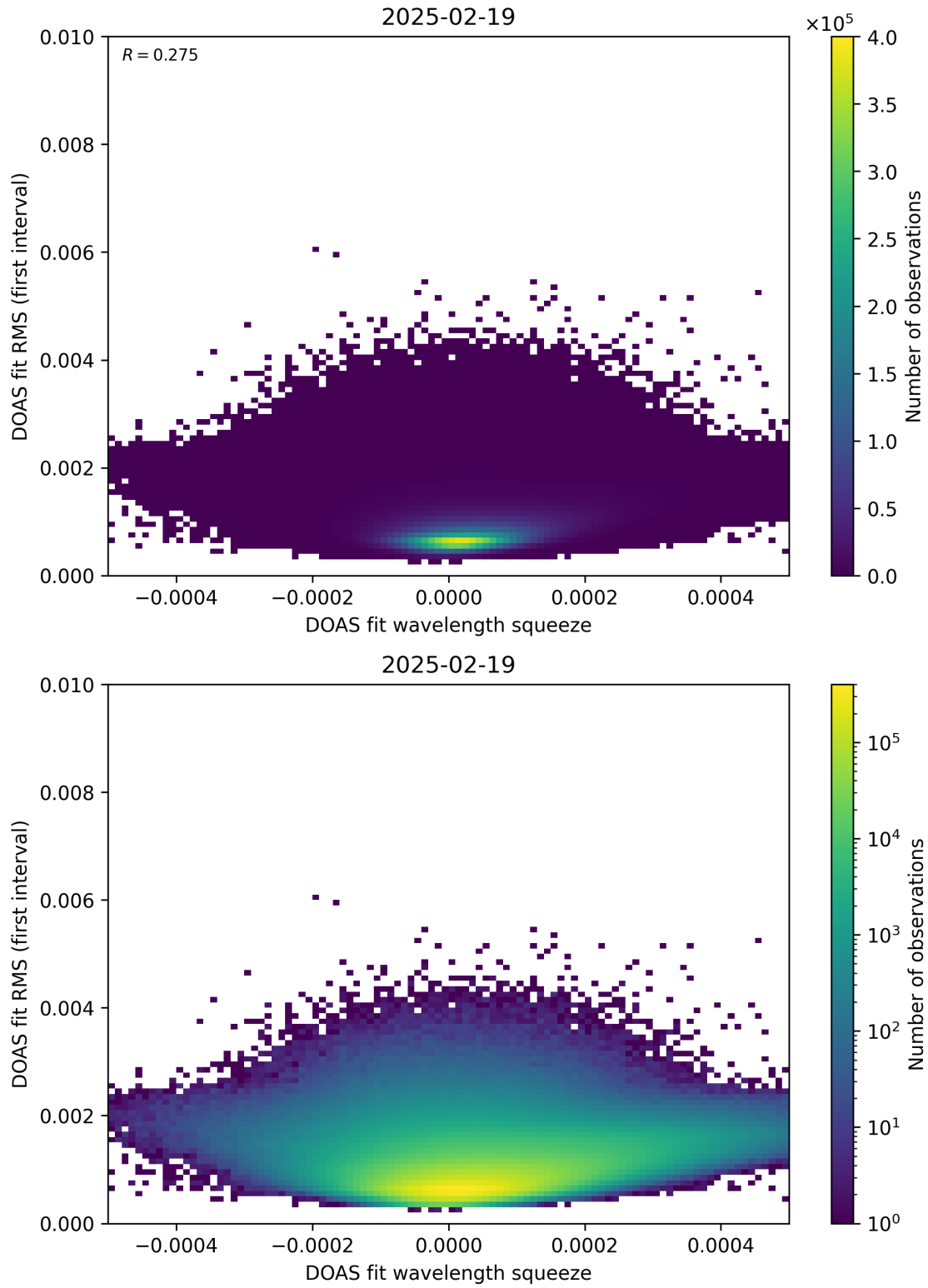
Figure 68: Scatter density plot of “DOAS fit wavelength squeeze” against “DOAS fit RMS (first interval)” for 2025-02-19 to 2025-02-20.
