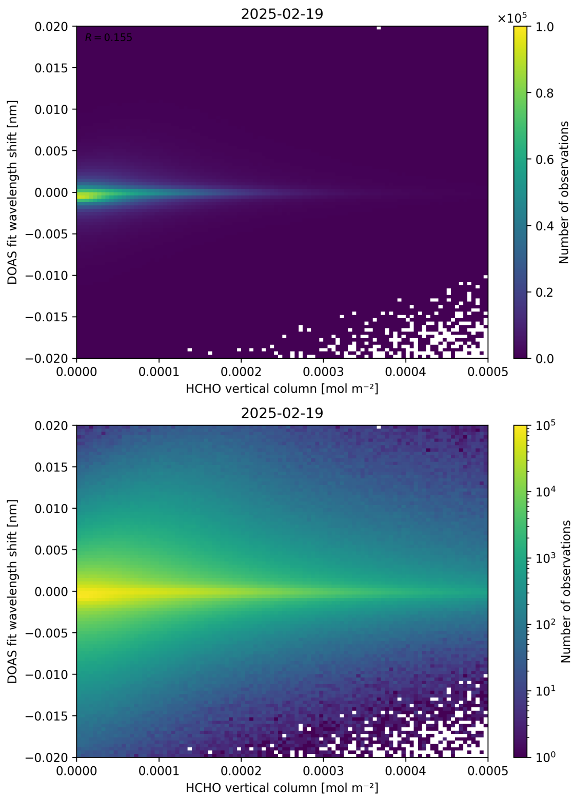
Figure 124: Scatter density plot of “HCHO vertical column” against “DOAS fit wavelength shift” for 2025-02-19 to 2025-02-20.
