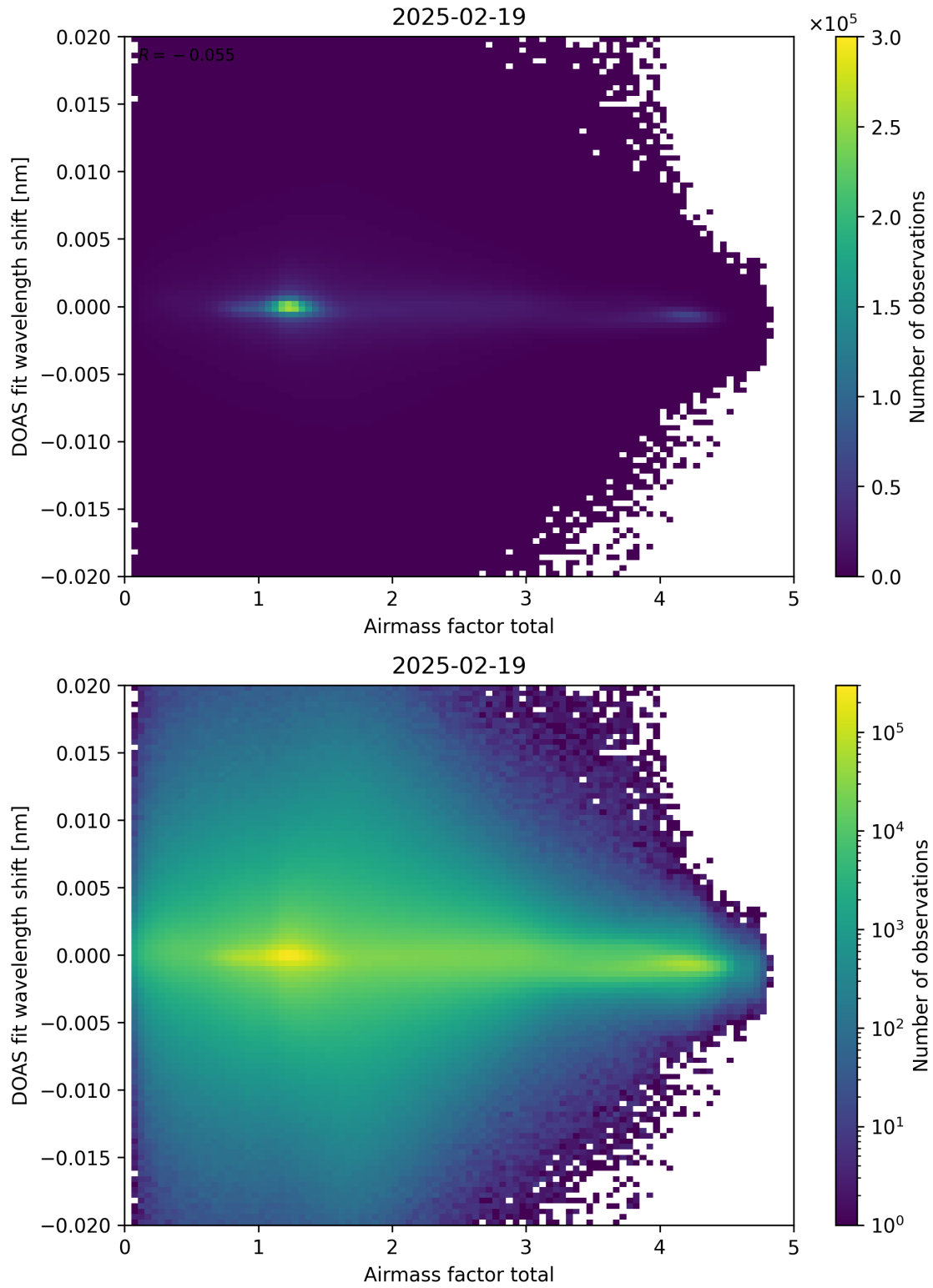
Figure 98: Scatter density plot of “Airmass factor total” against “DOAS fit wavelength shift” for 2025-02-19 to 2025-02-20.
