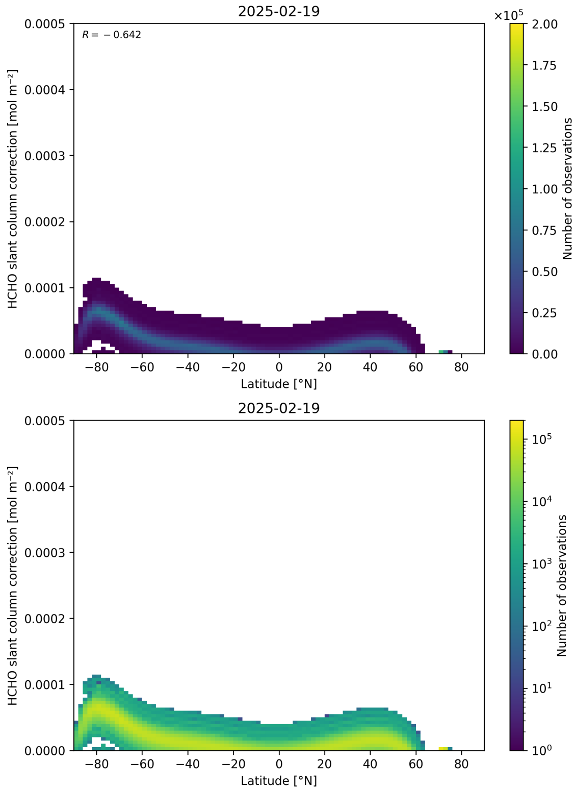
Figure 158: Scatter density plot of “Latitude” against “HCHO slant column correction” for 2025-02-19 to 2025-02-20.
