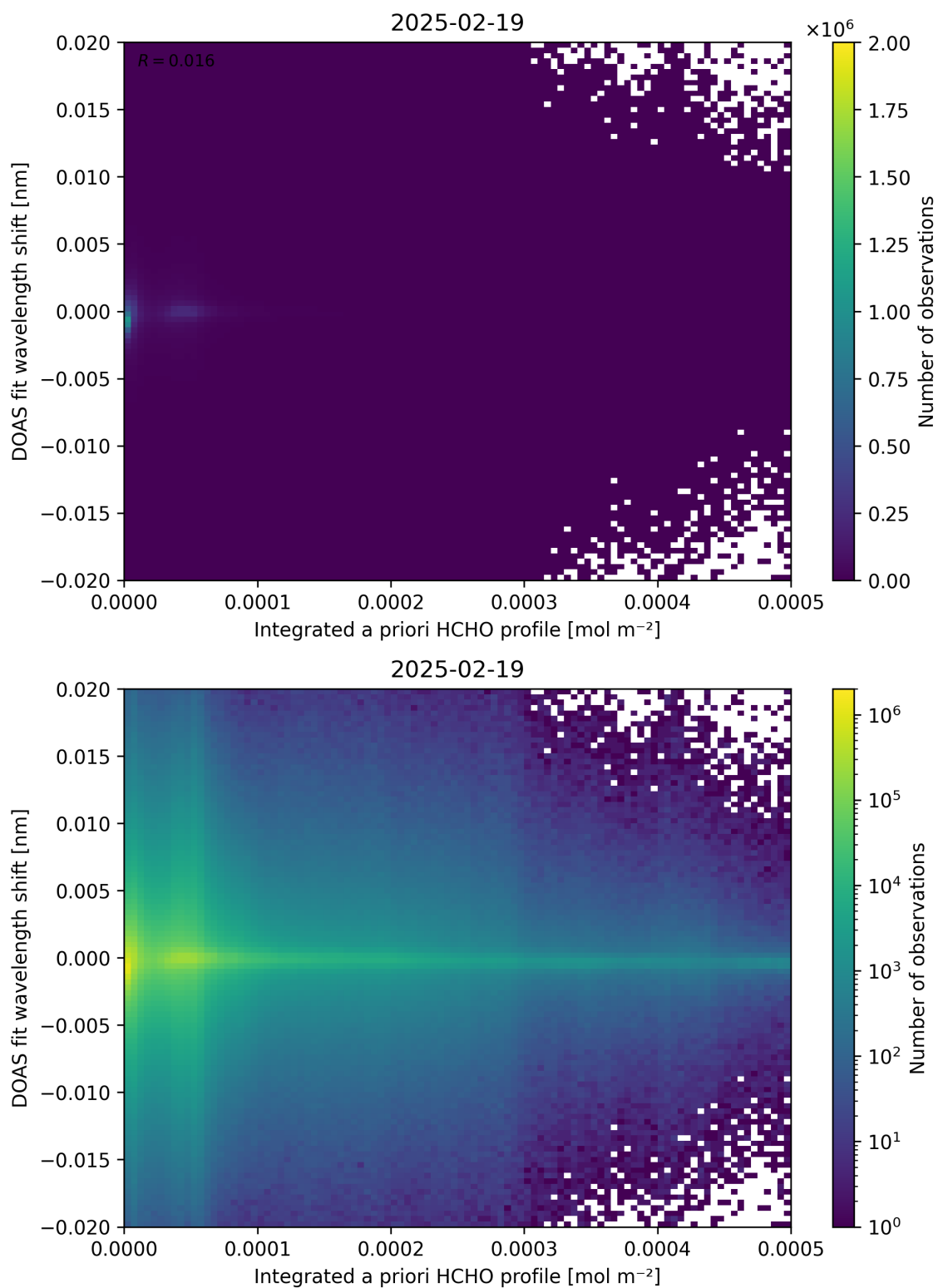
Figure 149: Scatter density plot of “Integrated a priori HCHO profile” against “DOAS fit wavelength shift” for 2025-02-19 to 2025-02-20.
