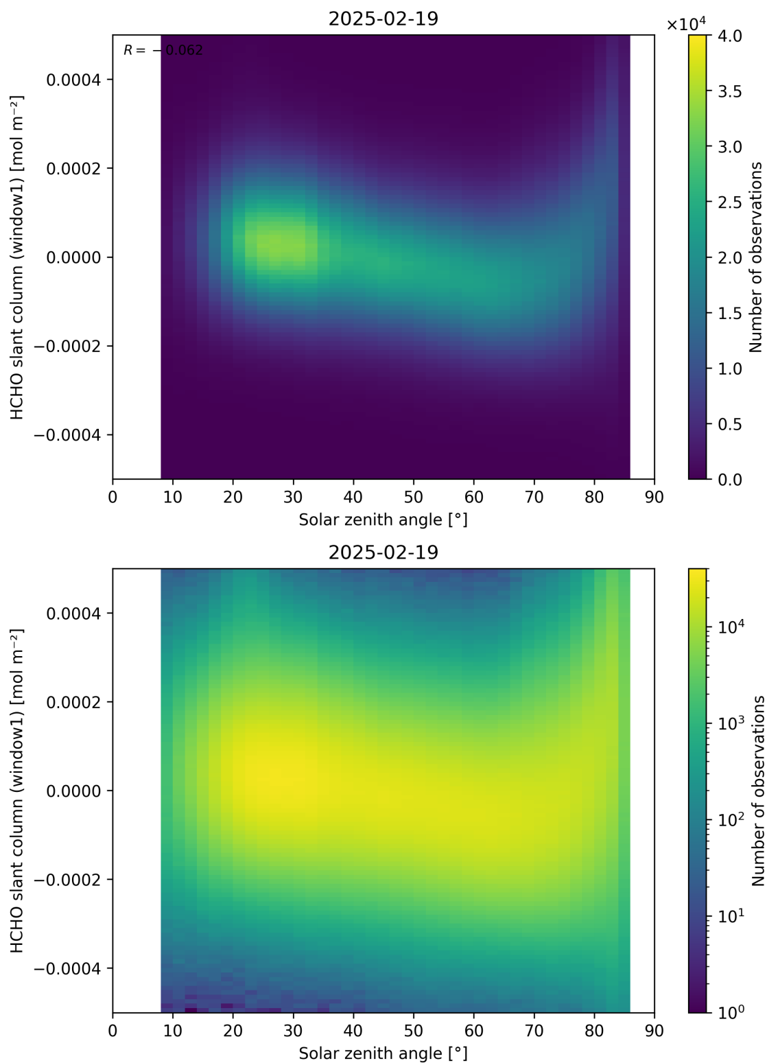
Figure 173: Scatter density plot of “Solar zenith angle” against “HCHO slant column (window1)” for 2025-02-19 to 2025-02-20.
