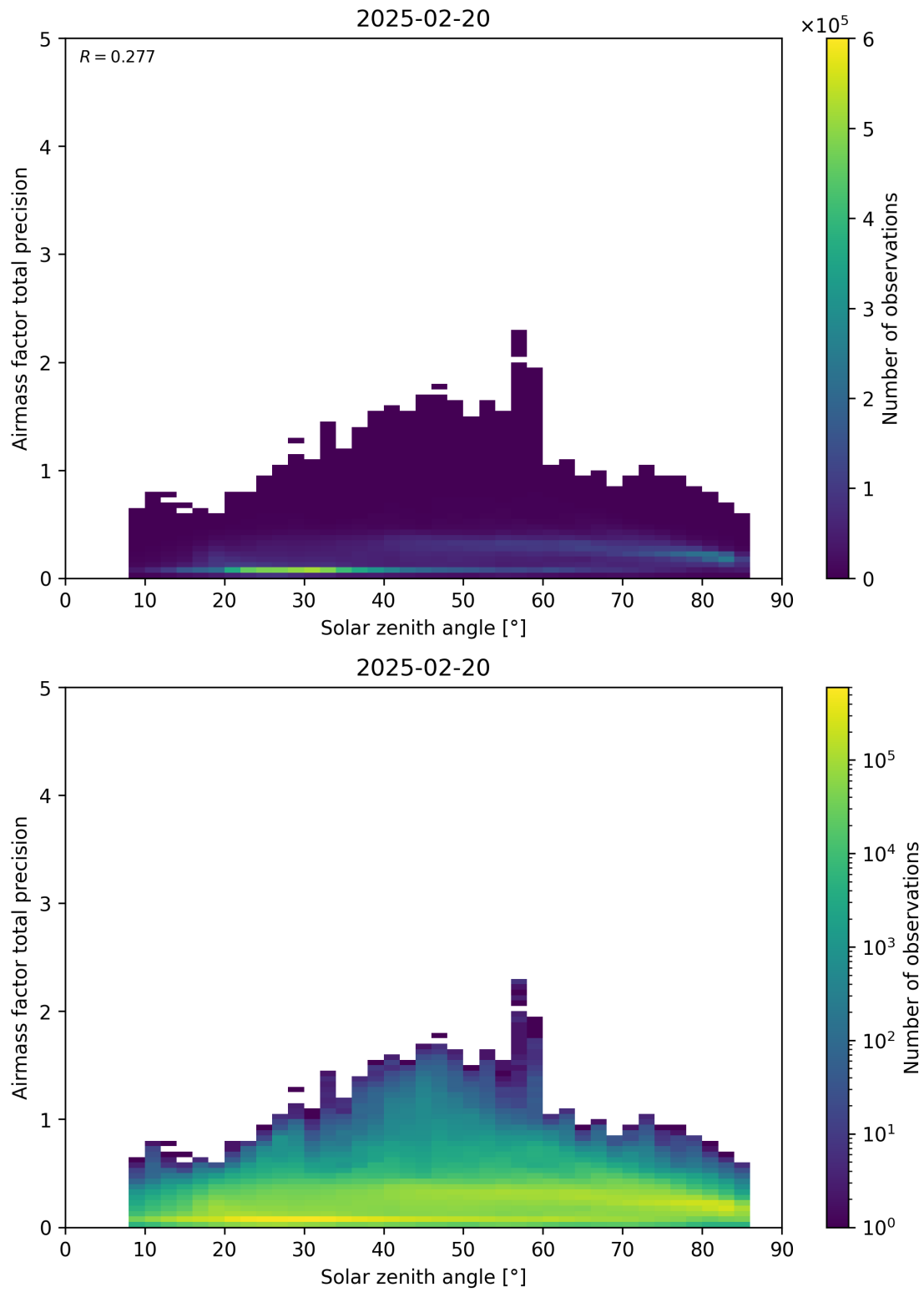
Figure 176: Scatter density plot of “Solar zenith angle” against “Airmass factor total precision” for 2025-02-19 to 2025-02-21.
