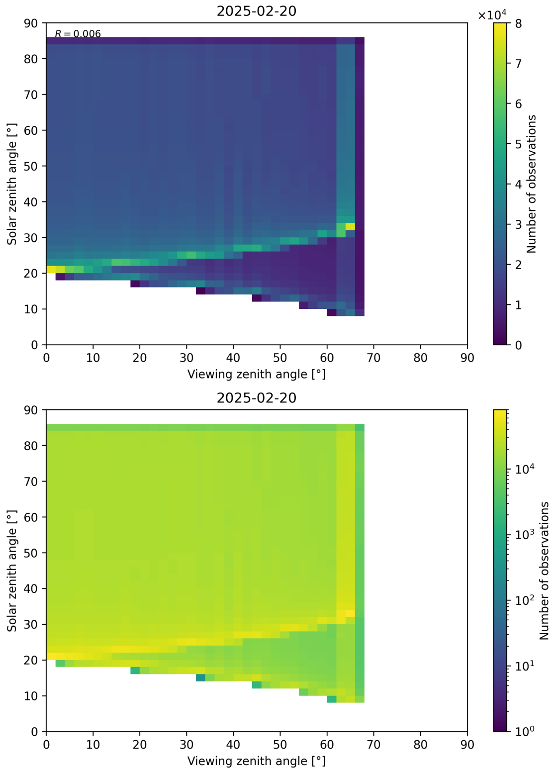
Figure 197: Scatter density plot of “Viewing zenith angle” against “Solar zenith angle” for 2025-02-19 to 2025-02-21.
