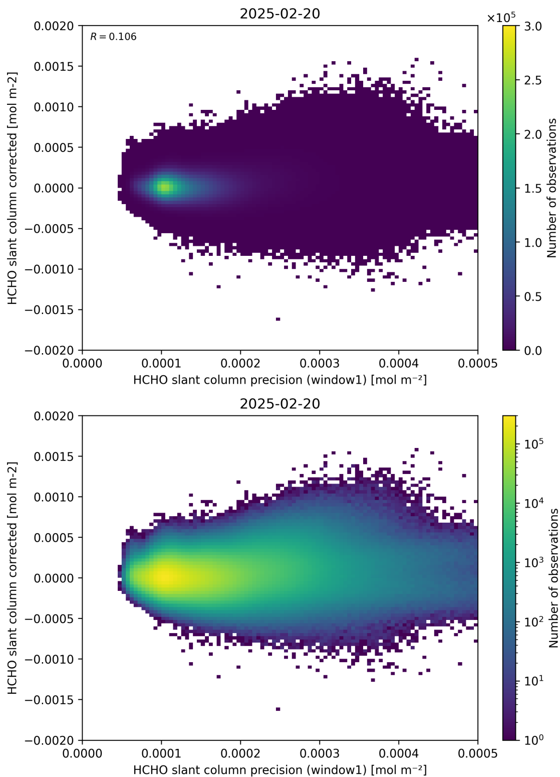
Figure 92: Scatter density plot of “HCHO slant column precision (window1)” against “HCHO slant column corrected” for 2025-02-19 to 2025-02-21.
