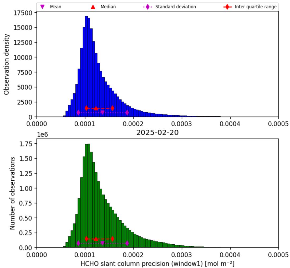
Figure 39: Histogram of “HCHO slant column precision (window1)” for 2025-02-19 to 2025-02-21
