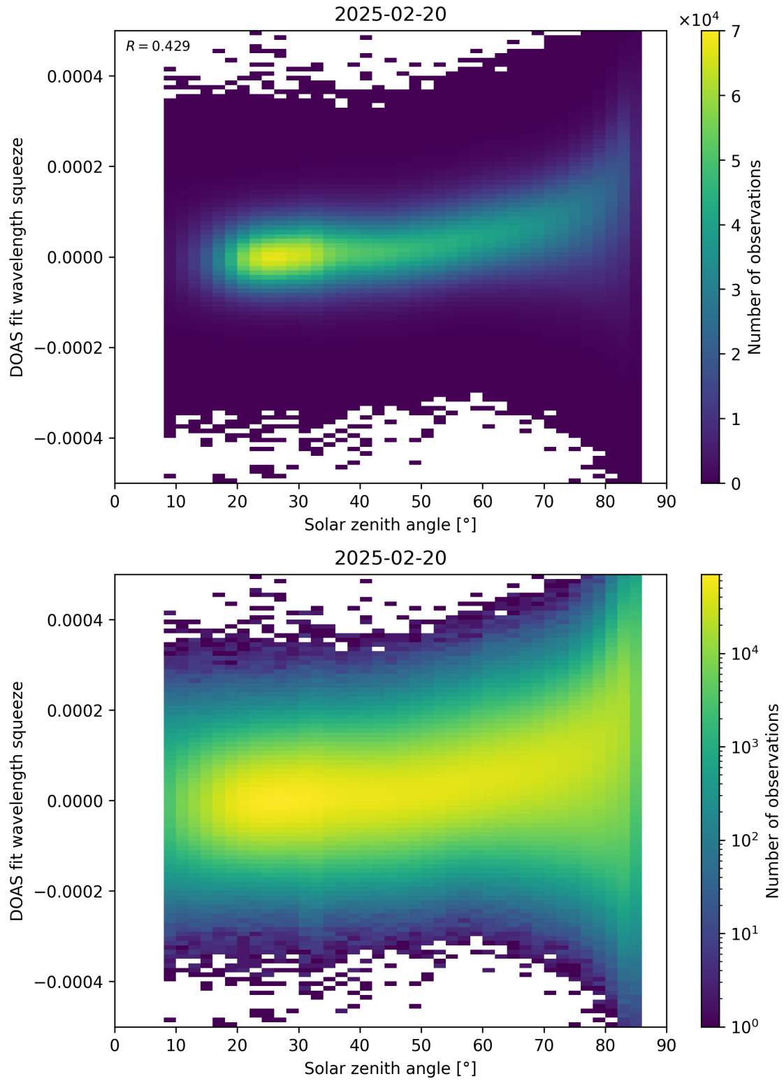
Figure 169: Scatter density plot of “Solar zenith angle” against “DOAS fit wavelength squeeze” for 2025-02-19 to 2025-02-21.
