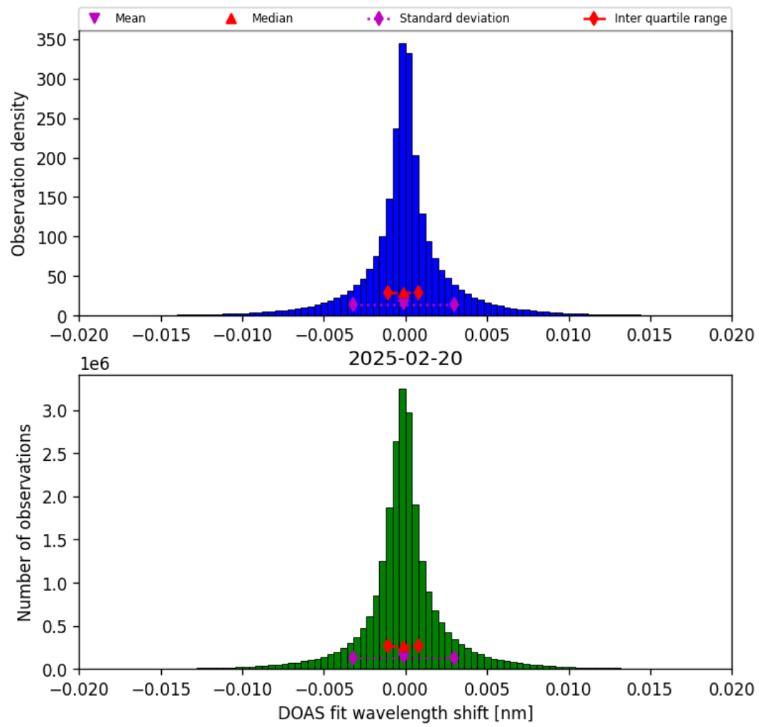
Figure 44: Histogram of “DOAS fit wavelength shift” for 2025-02-19 to 2025-02-21
