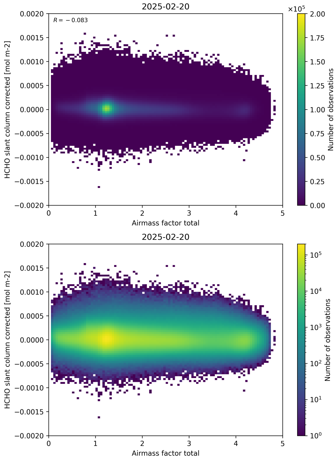
Figure 101: Scatter density plot of “Airmass factor total” against “HCHO slant column corrected” for 2025-02-19 to 2025-02-21.
