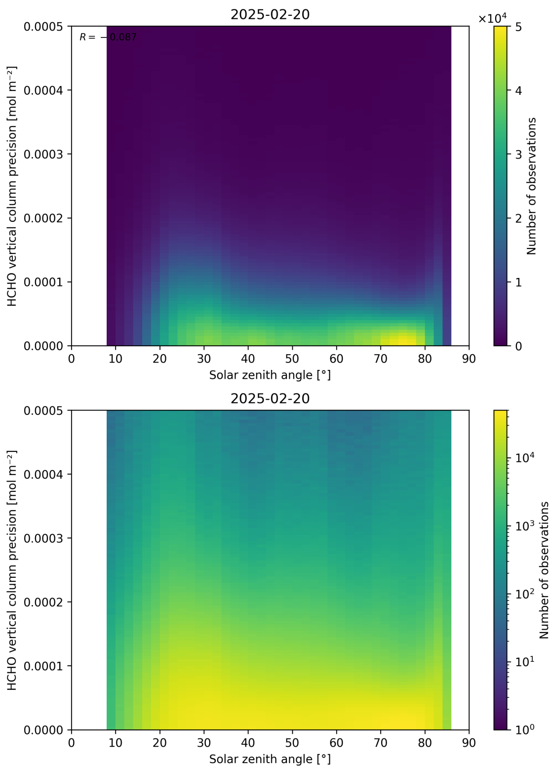
Figure 179: Scatter density plot of “Solar zenith angle” against “HCHO vertical column precision” for 2025-02-19 to 2025-02-21.
