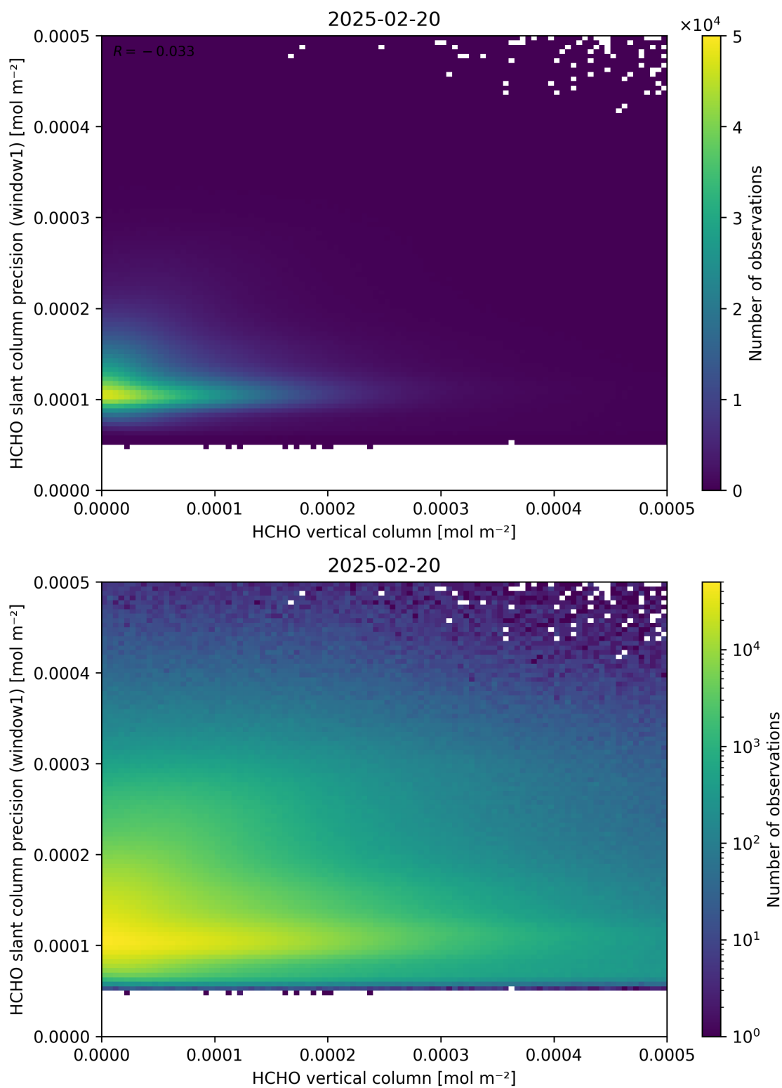
Figure 130: Scatter density plot of “HCHO vertical column” against “HCHO slant column precision (window1)” for 2025-02-19 to 2025-02-21.
