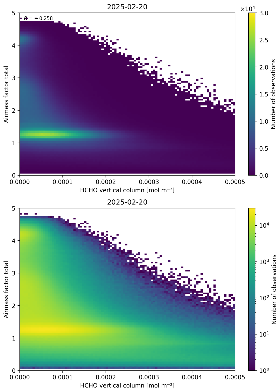
Figure 131: Scatter density plot of “HCHO vertical column” against “Airmass factor total” for 2025-02-19 to 2025-02-21.
