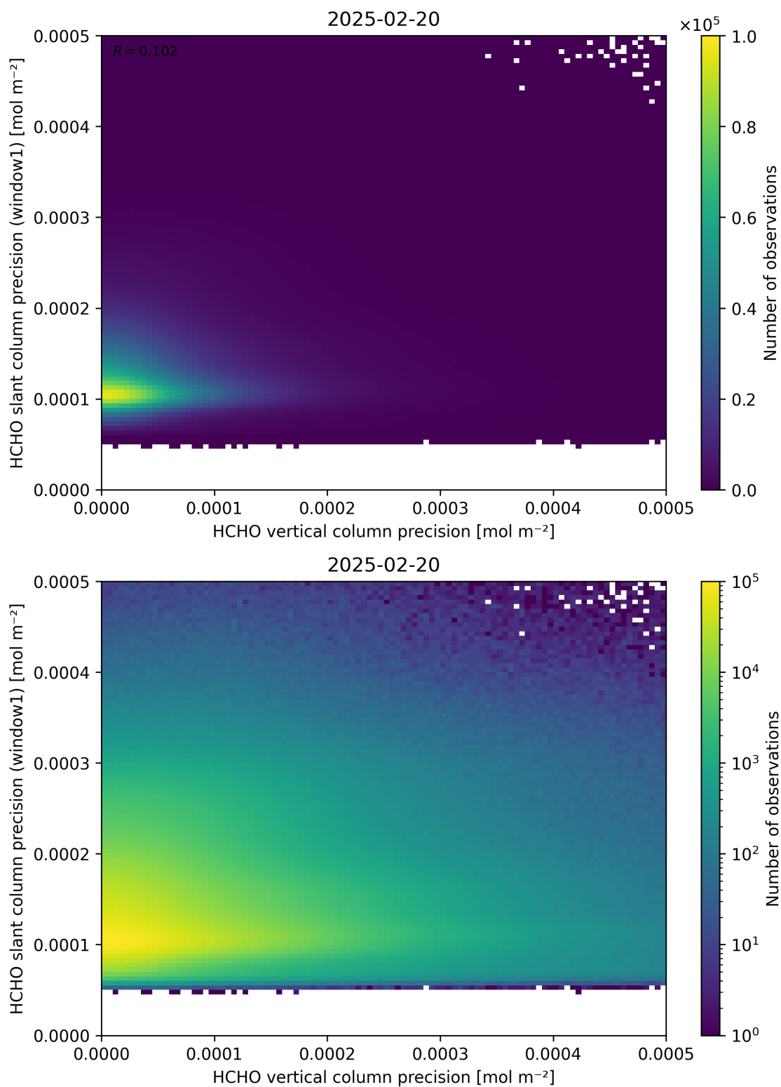
Figure 143: Scatter density plot of “HCHO vertical column precision” against “HCHO slant column precision (window1)” for 2025-02-19 to 2025-02-21.
