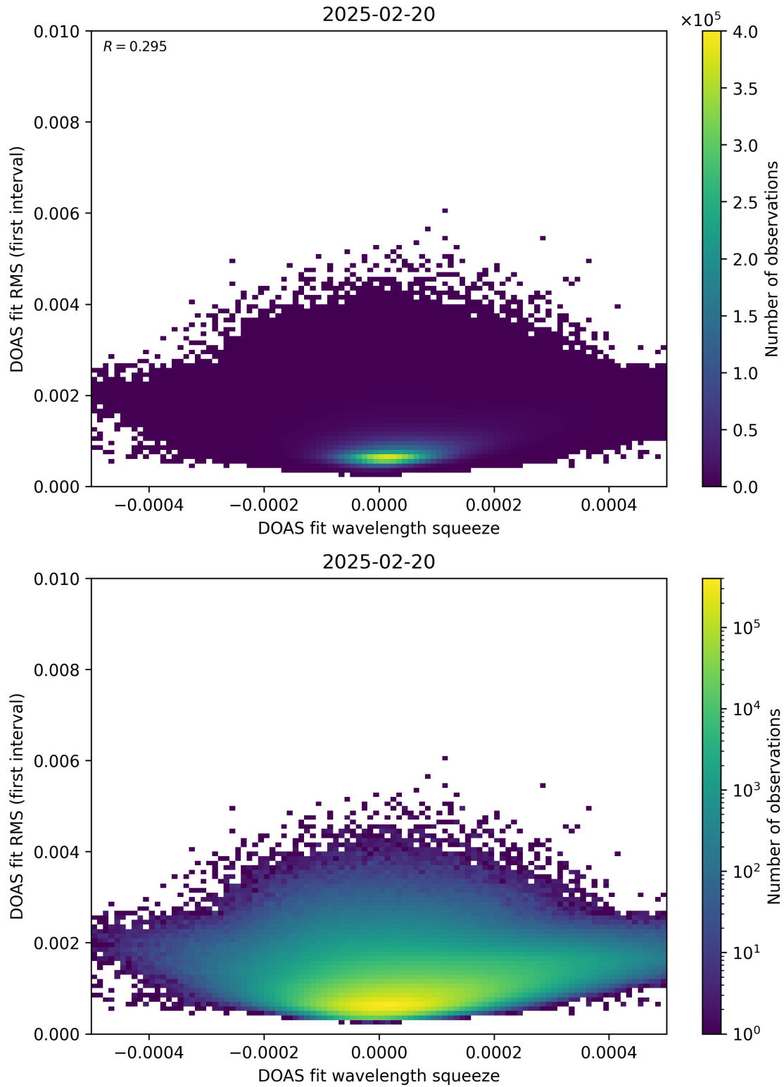
Figure 68: Scatter density plot of “DOAS fit wavelength squeeze” against “DOAS fit RMS (first interval)” for 2025-02-19 to 2025-02-21.
