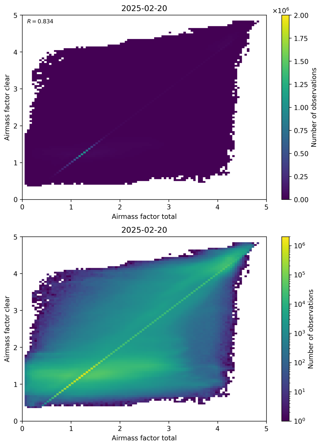
Figure 100: Scatter density plot of “Airmass factor total” against “Airmass factor clear” for 2025-02-19 to 2025-02-21.
