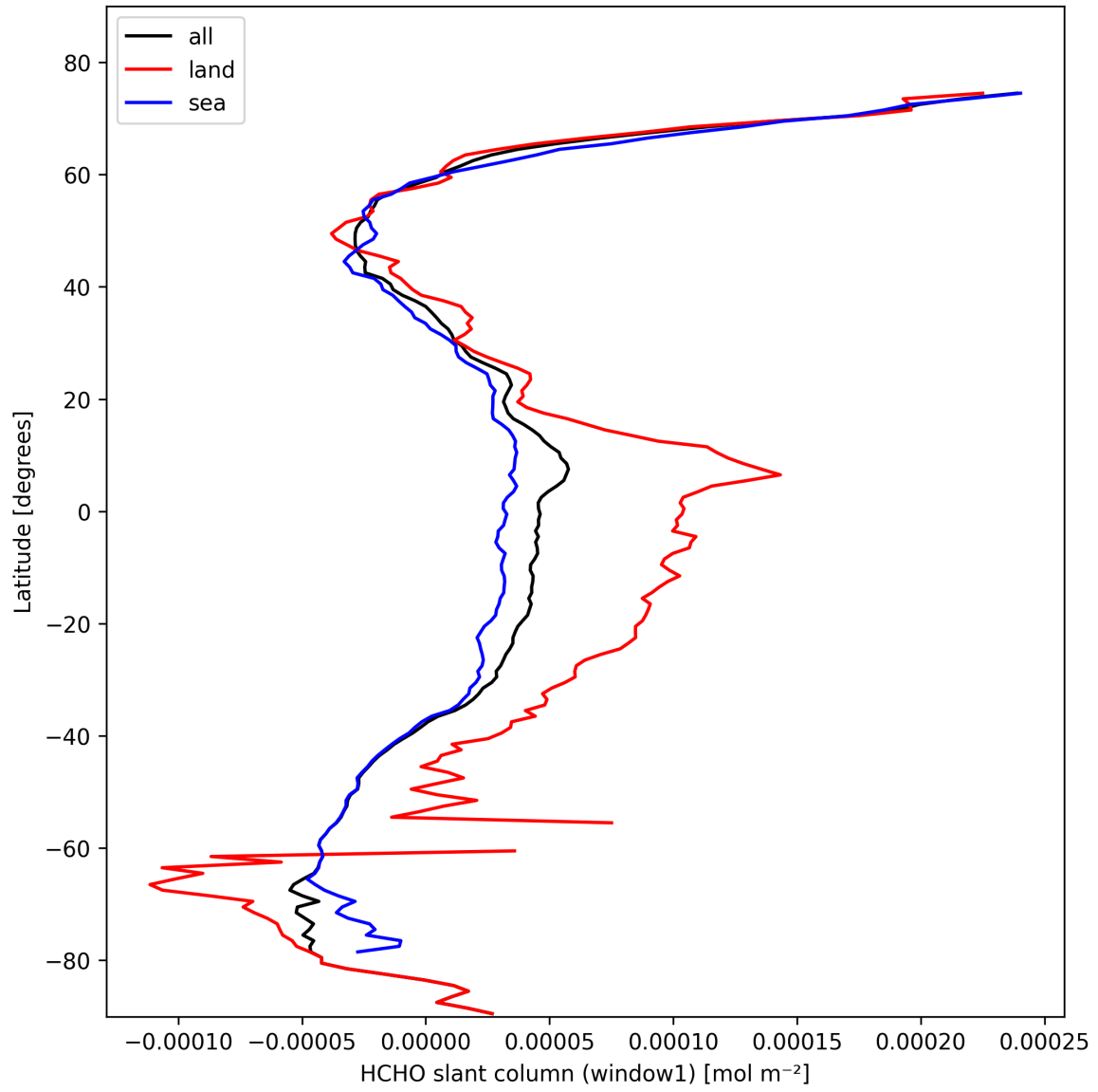
Figure 24: Zonal average of “HCHO slant column (window1)” for 2025-02-19 to 2025-02-21.
