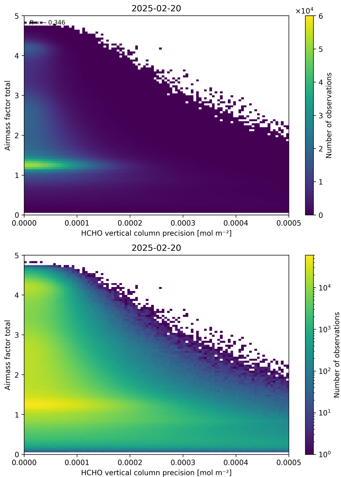
Figure 144: Scatter density plot of “HCHO vertical column precision” against “Airmass factor total” for 2025-02-19 to 2025-02-21.
