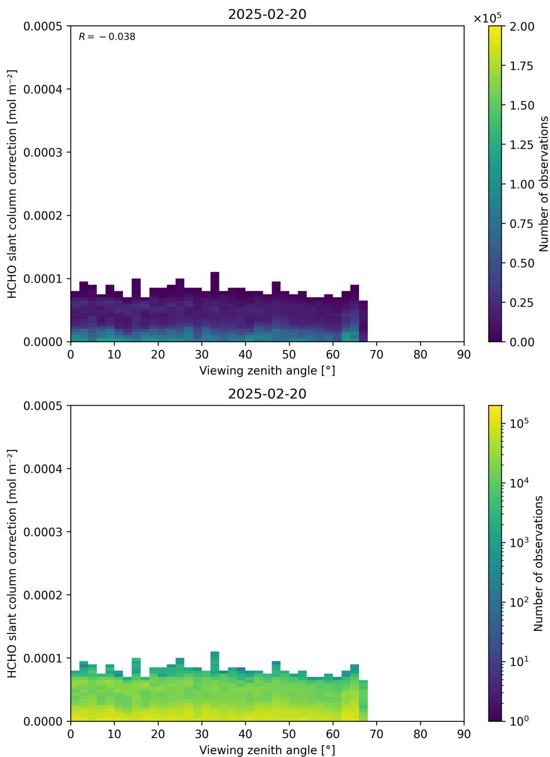
Figure 187: Scatter density plot of “Viewing zenith angle” against “HCHO slant column correction” for 2025-02-19 to 2025-02-21.
