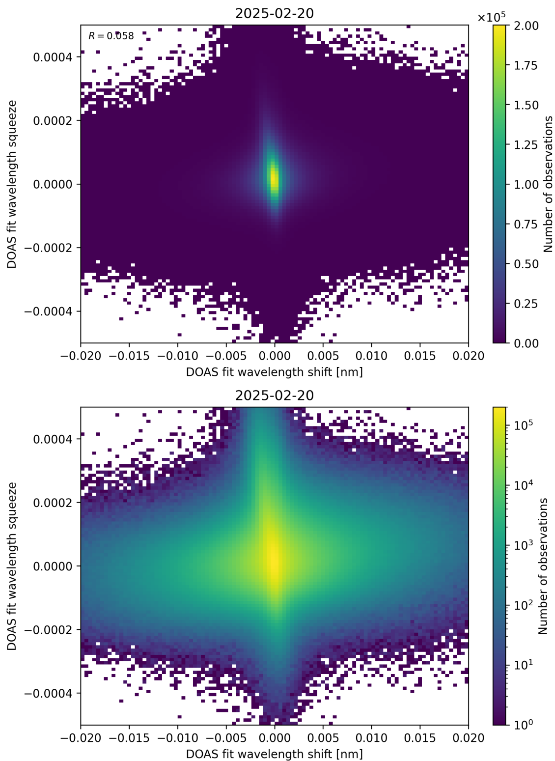
Figure 65: Scatter density plot of “DOAS fit wavelength shift” against “DOAS fit wavelength squeeze” for 2025-02-19 to 2025-02-21.
