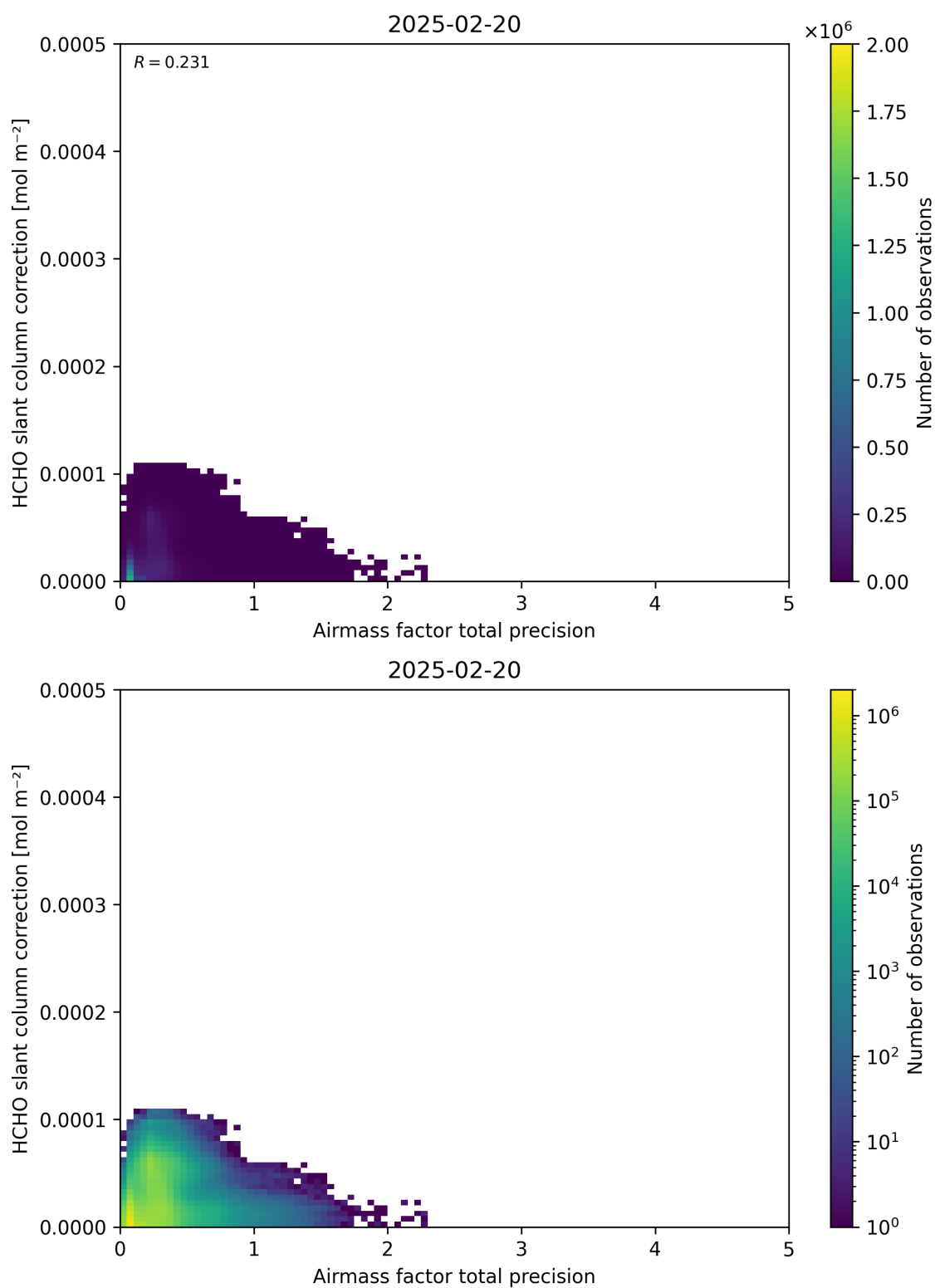
Figure 110: Scatter density plot of “Airmass factor total precision” against “HCHO slant column correction” for 2025-02-19 to 2025-02-21.
