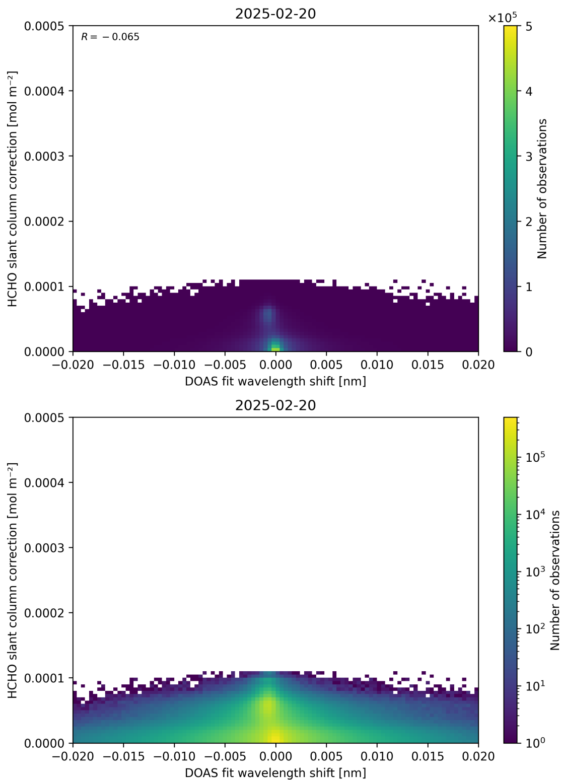
Figure 67: Scatter density plot of “DOAS fit wavelength shift” against “HCHO slant column correction” for 2025-02-19 to 2025-02-21.
