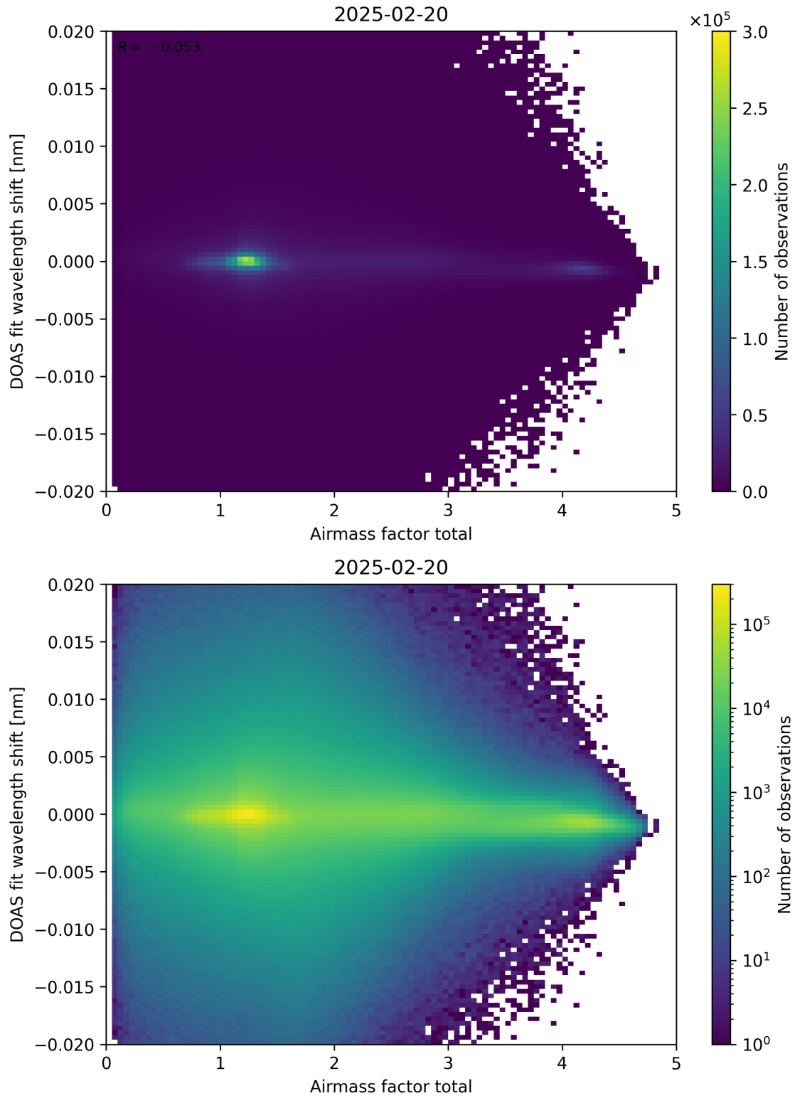
Figure 98: Scatter density plot of “Airmass factor total” against “DOAS fit wavelength shift” for 2025-02-19 to 2025-02-21.
