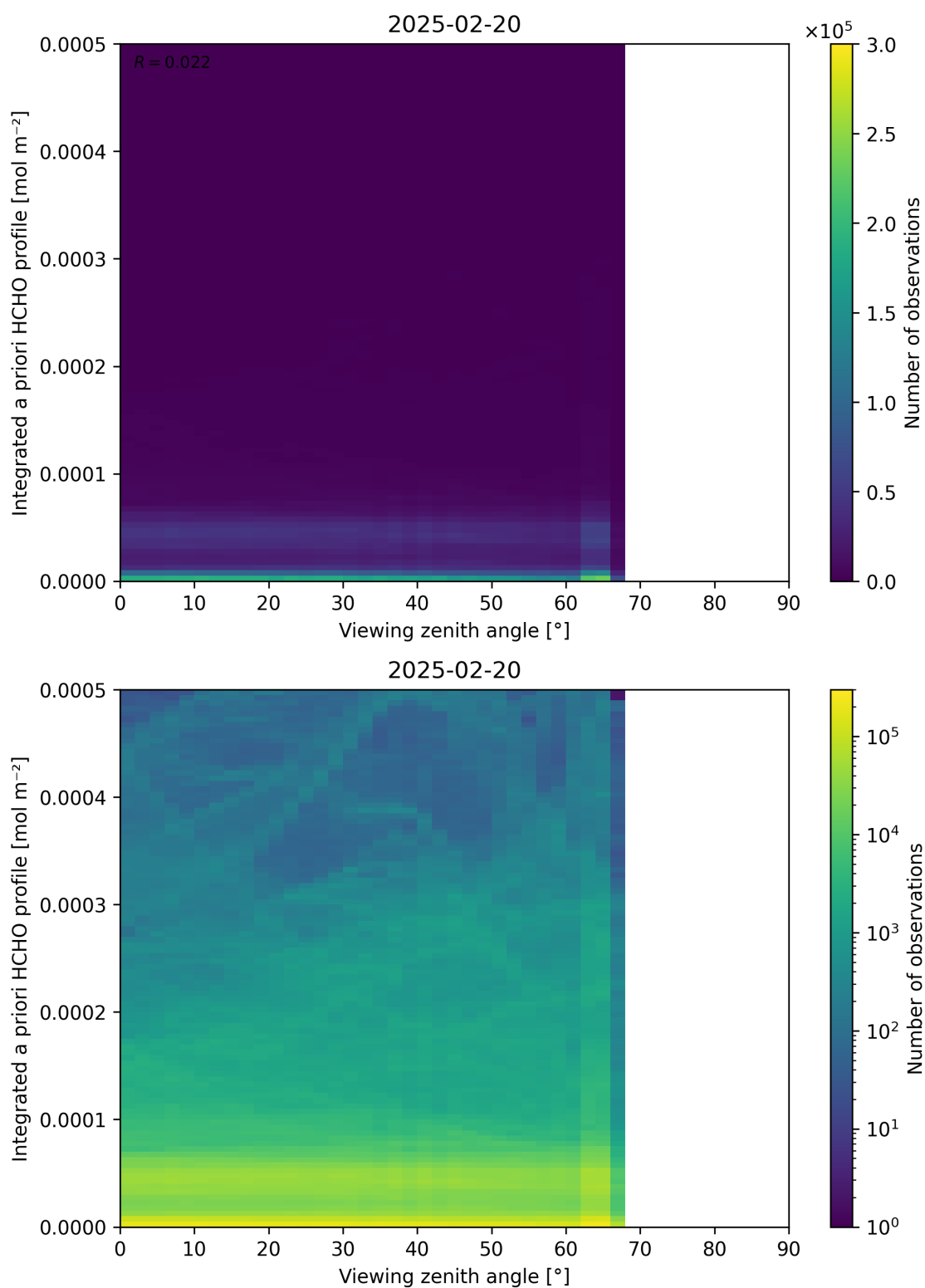
Figure 195: Scatter density plot of “Viewing zenith angle” against “Integrated a priori HCHO profile” for 2025-02-19 to 2025-02-21.
