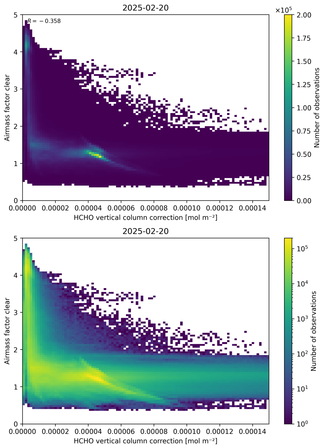
Figure 115: Scatter density plot of “HCHO vertical column correction” against “Airmass factor clear” for 2025-02-19 to 2025-02-21.
