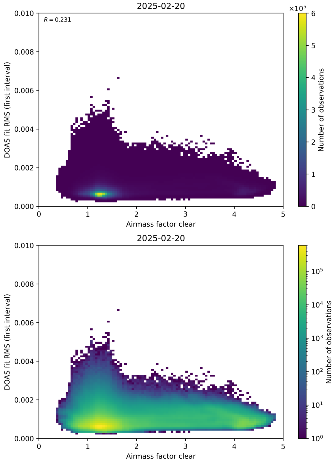
Figure 71: Scatter density plot of “Airmass factor clear” against “DOAS fit RMS (first interval)” for 2025-02-19 to 2025-02-21.
