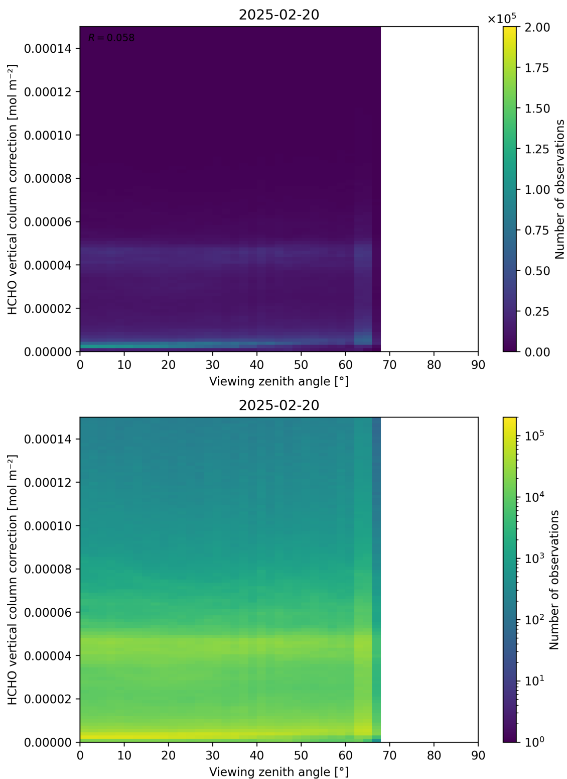
Figure 193: Scatter density plot of “Viewing zenith angle” against “HCHO vertical column correction” for 2025-02-19 to 2025-02-21.
