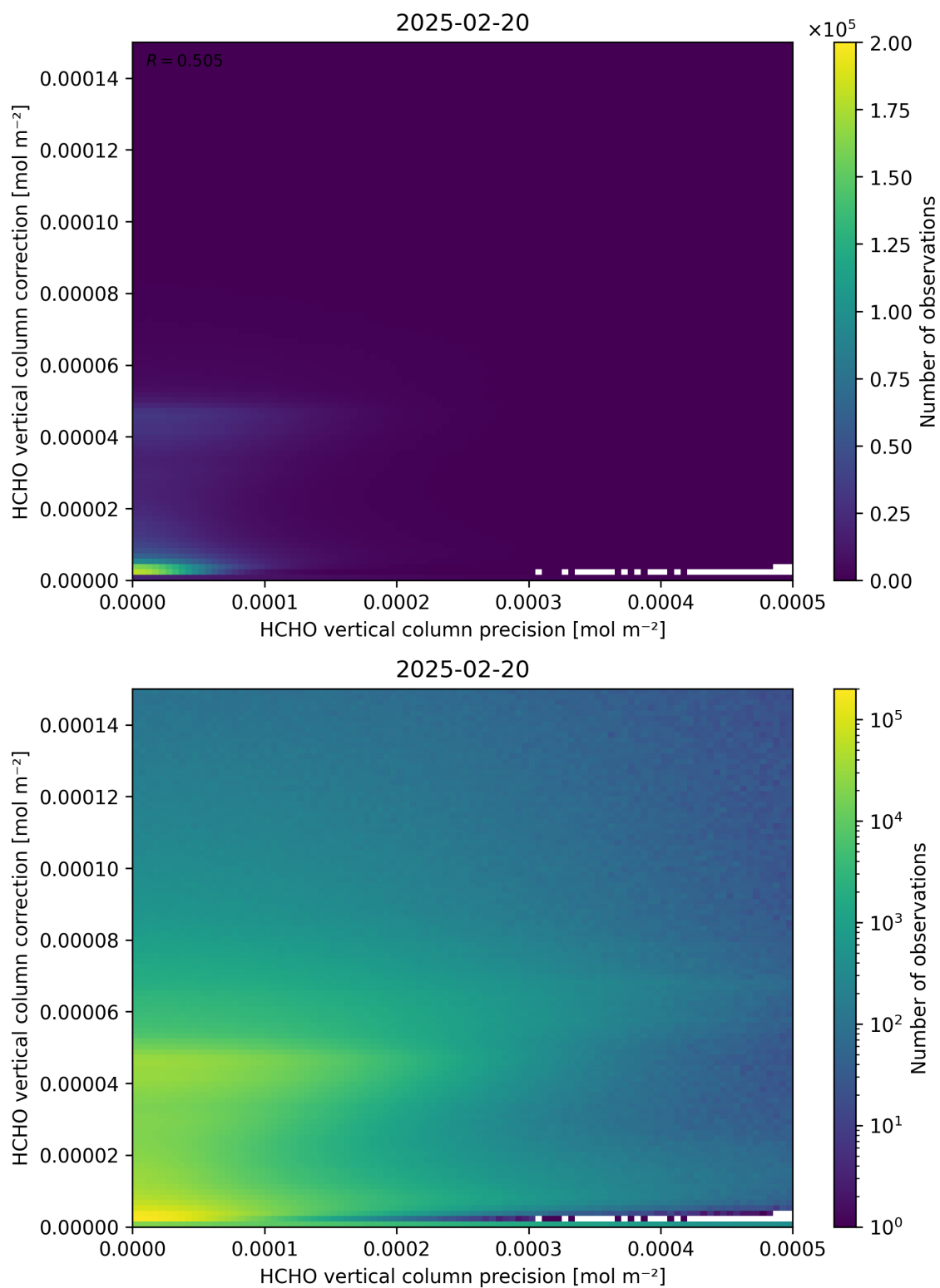
Figure 146: Scatter density plot of “HCHO vertical column precision” against “HCHO vertical column correction” for 2025-02-19 to 2025-02-21.
