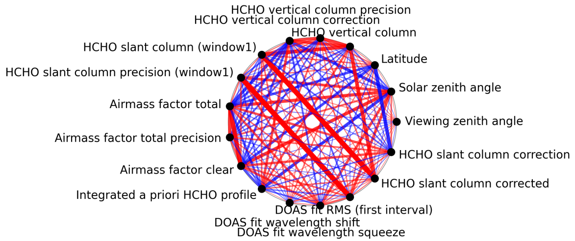
Figure 1: Map of correlation graph for 2025-02-19 to 2025-02-21.
