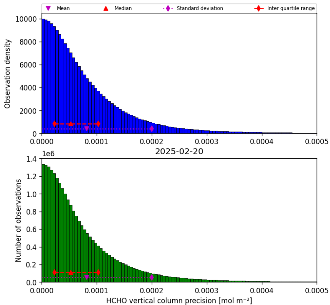
Figure 36: Histogram of “HCHO vertical column precision” for 2025-02-19 to 2025-02-21
