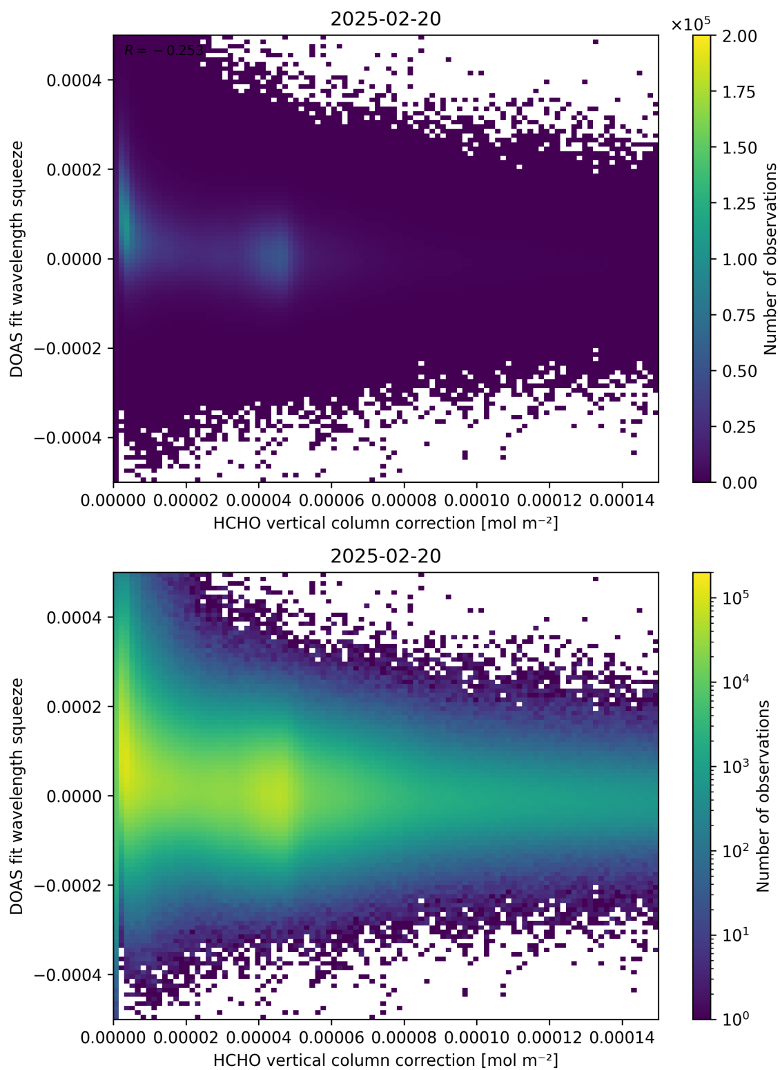
Figure 114: Scatter density plot of “HCHO vertical column correction” against “DOAS fit wavelength squeeze” for 2025-02-19 to 2025-02-21.
