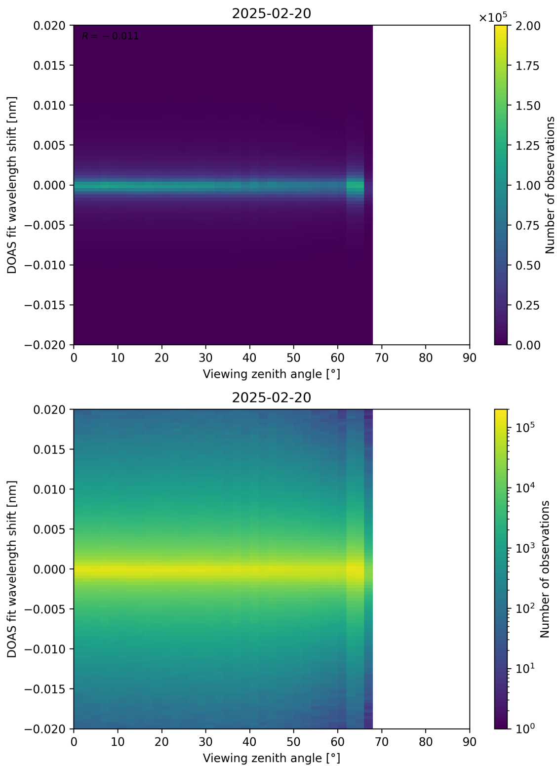
Figure 183: Scatter density plot of “Viewing zenith angle” against “DOAS fit wavelength shift” for 2025-02-19 to 2025-02-21.
