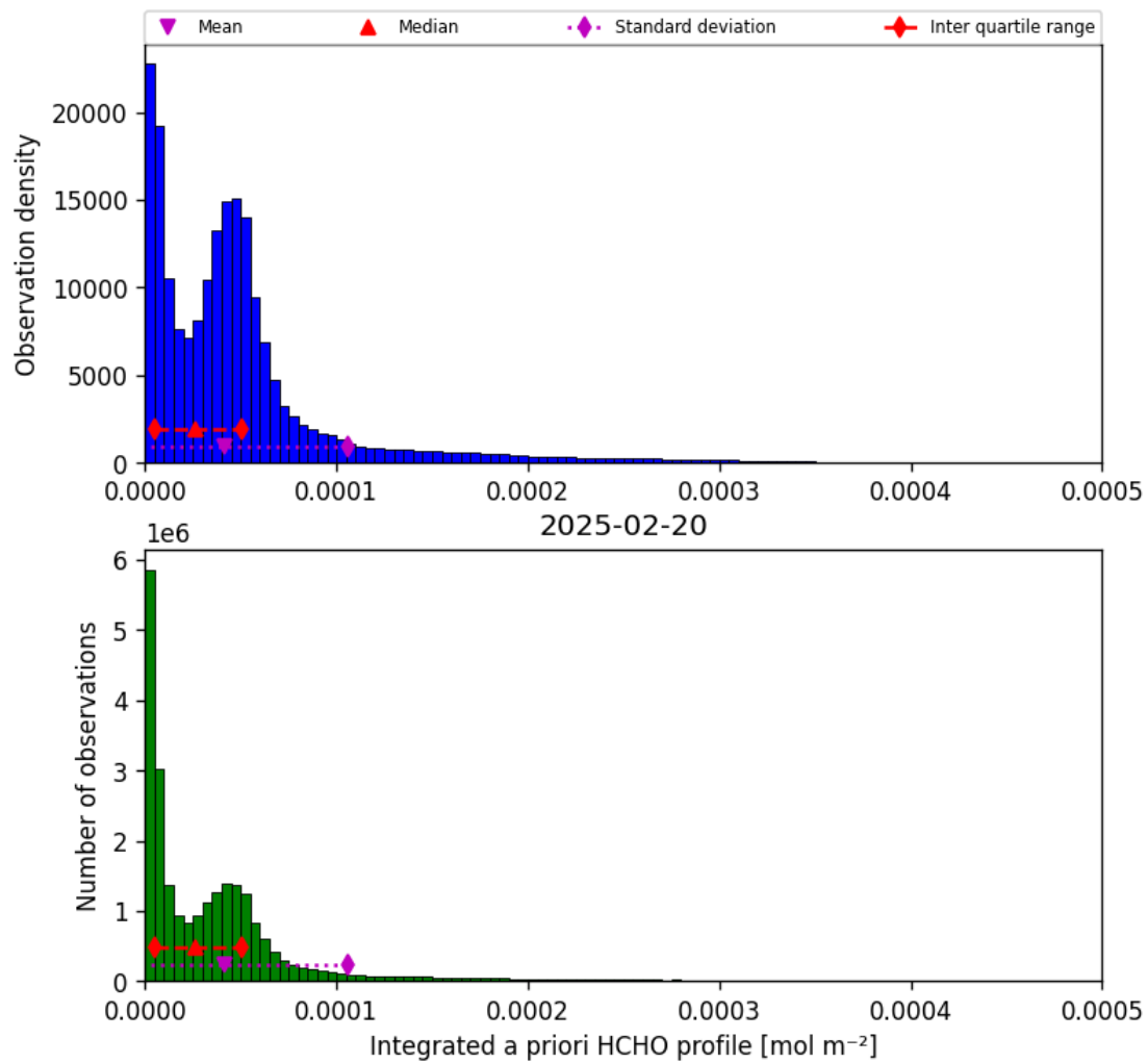
Figure 43: Histogram of “Integrated a priori HCHO profile” for 2025-02-19 to 2025-02-21
