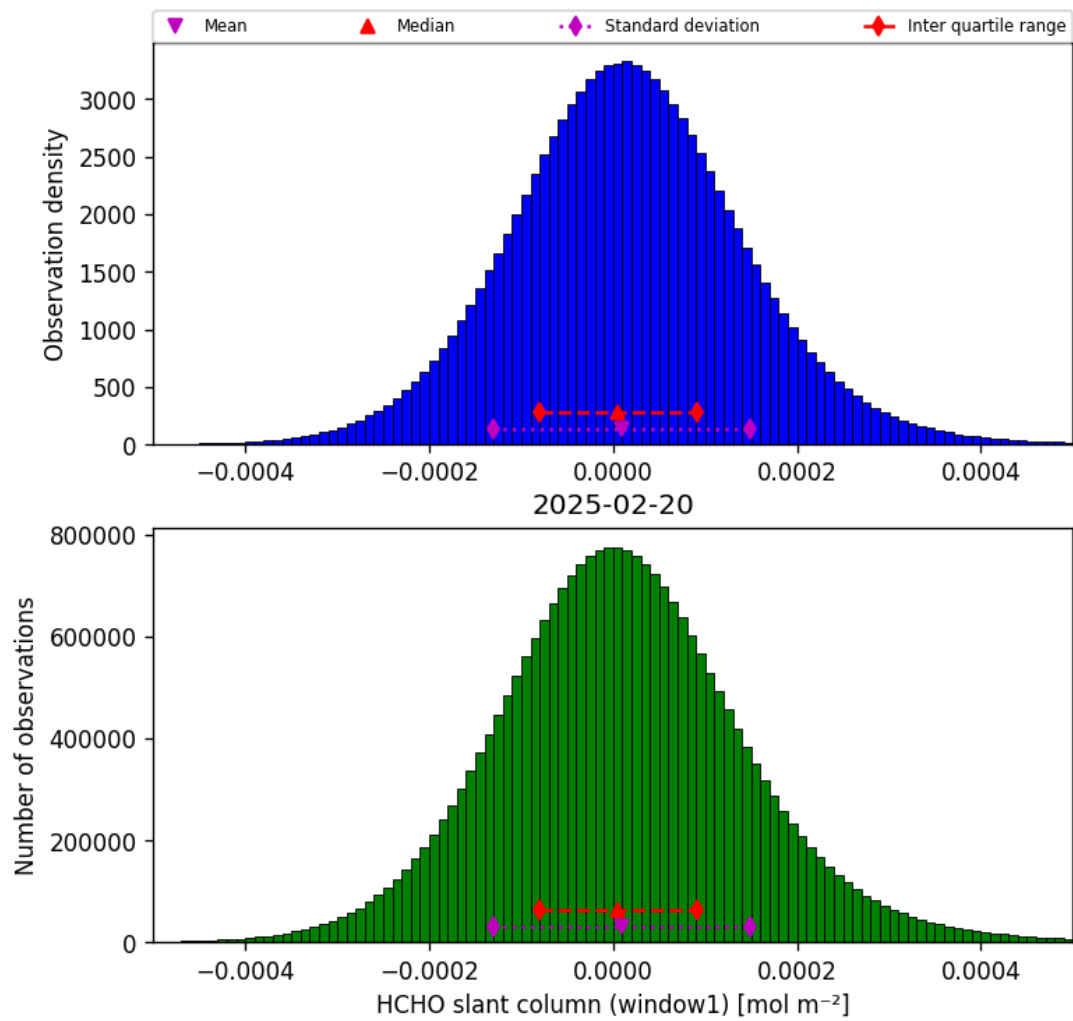
Figure 38: Histogram of “HCHO slant column (window1)” for 2025-02-19 to 2025-02-21
