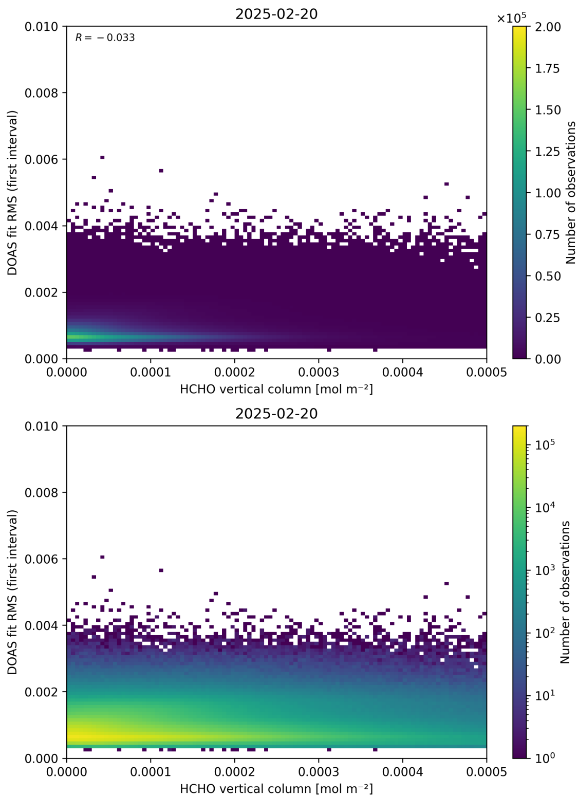
Figure 123: Scatter density plot of “HCHO vertical column” against “DOAS fit RMS (first interval)” for 2025-02-19 to 2025-02-21.
