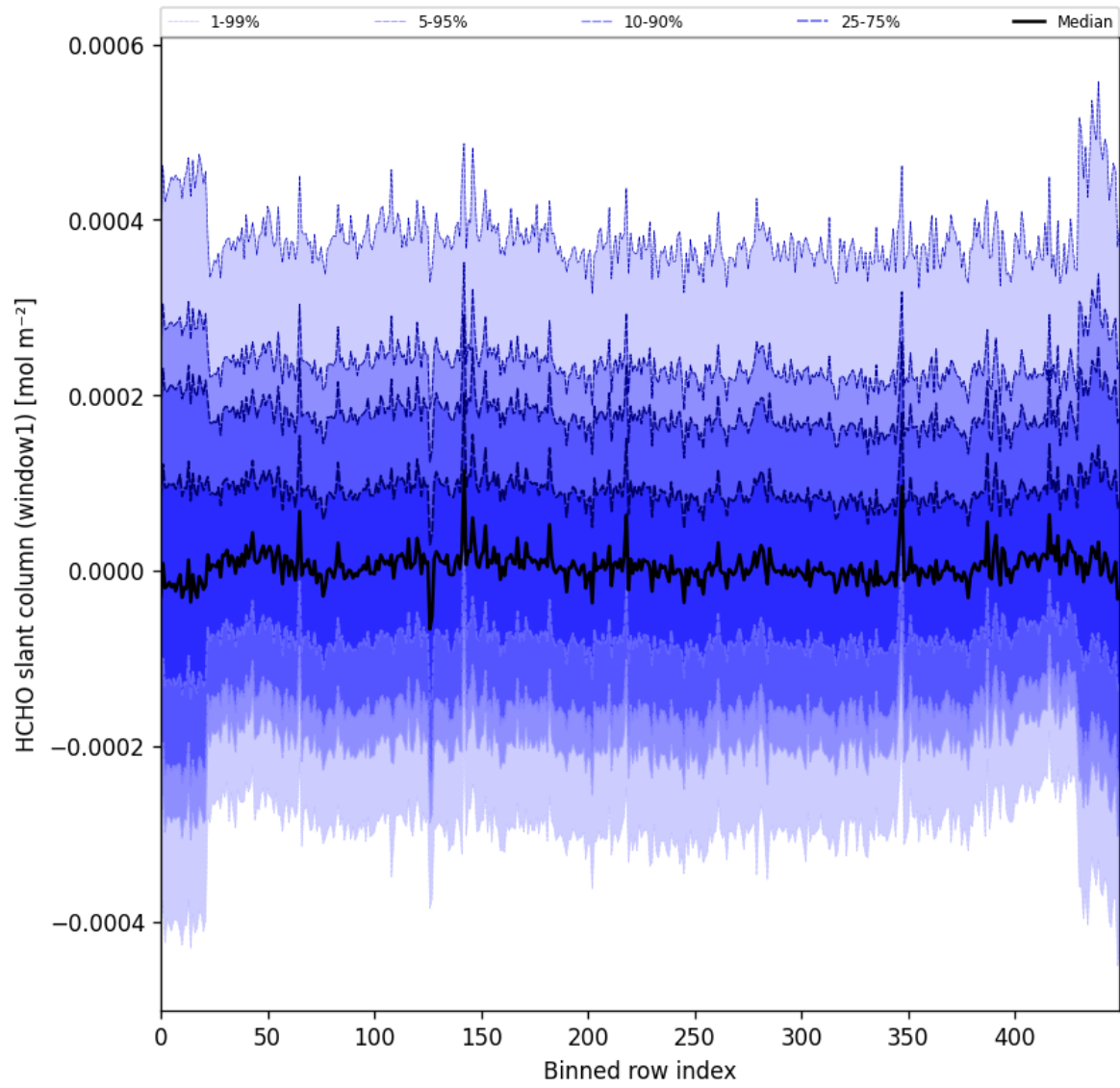
Figure 52: Along track statistics of “HCHO slant column (window1)” for 2025-02-19 to 2025-02-21
