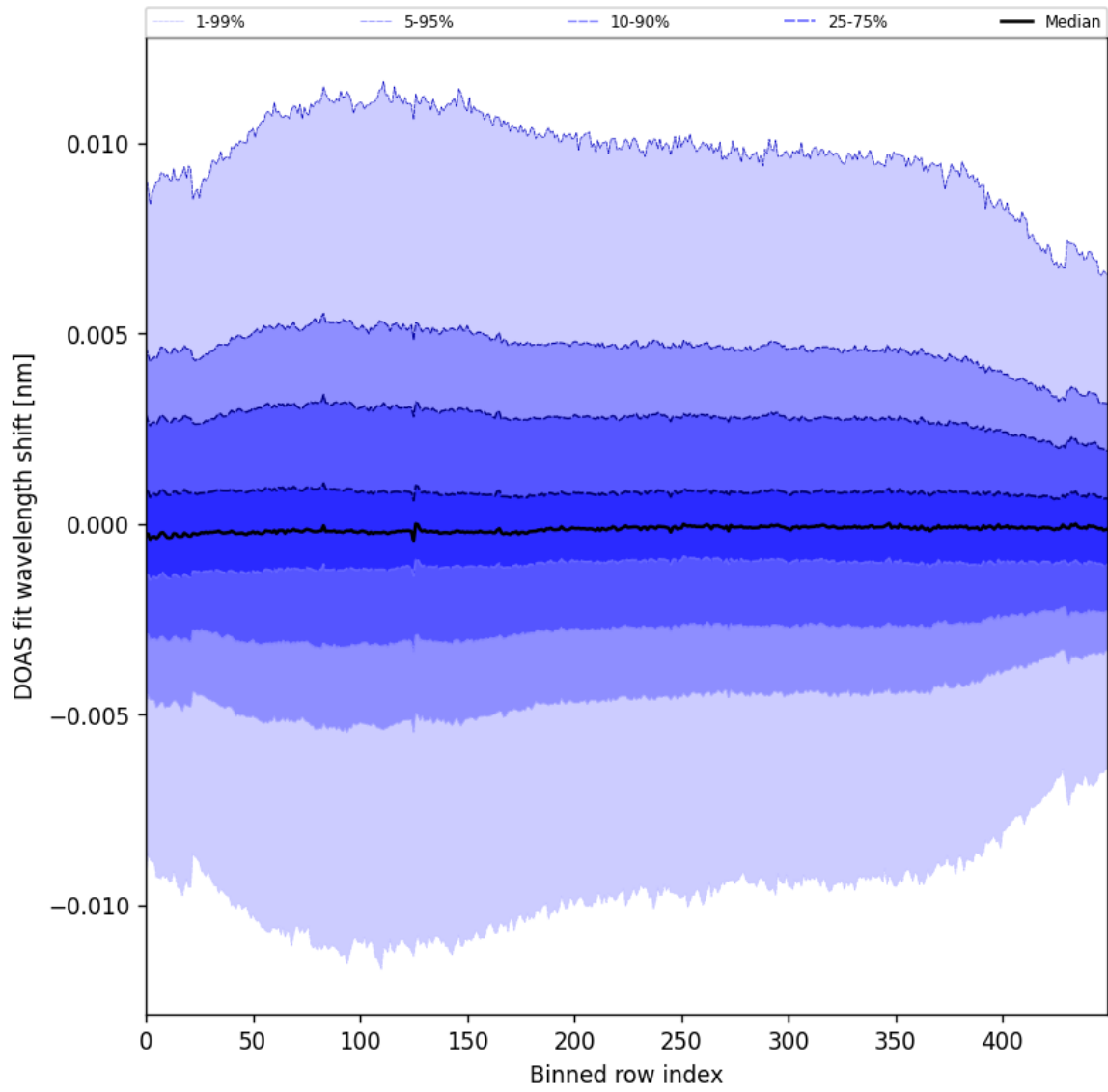
Figure 58: Along track statistics of “DOAS fit wavelength shift” for 2025-02-19 to 2025-02-21
