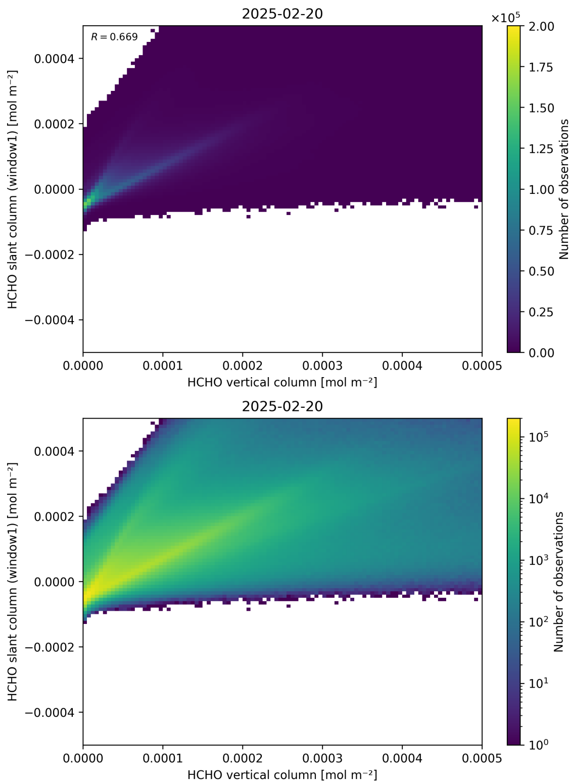
Figure 129: Scatter density plot of “HCHO vertical column” against “HCHO slant column (window1)” for 2025-02-19 to 2025-02-21.
