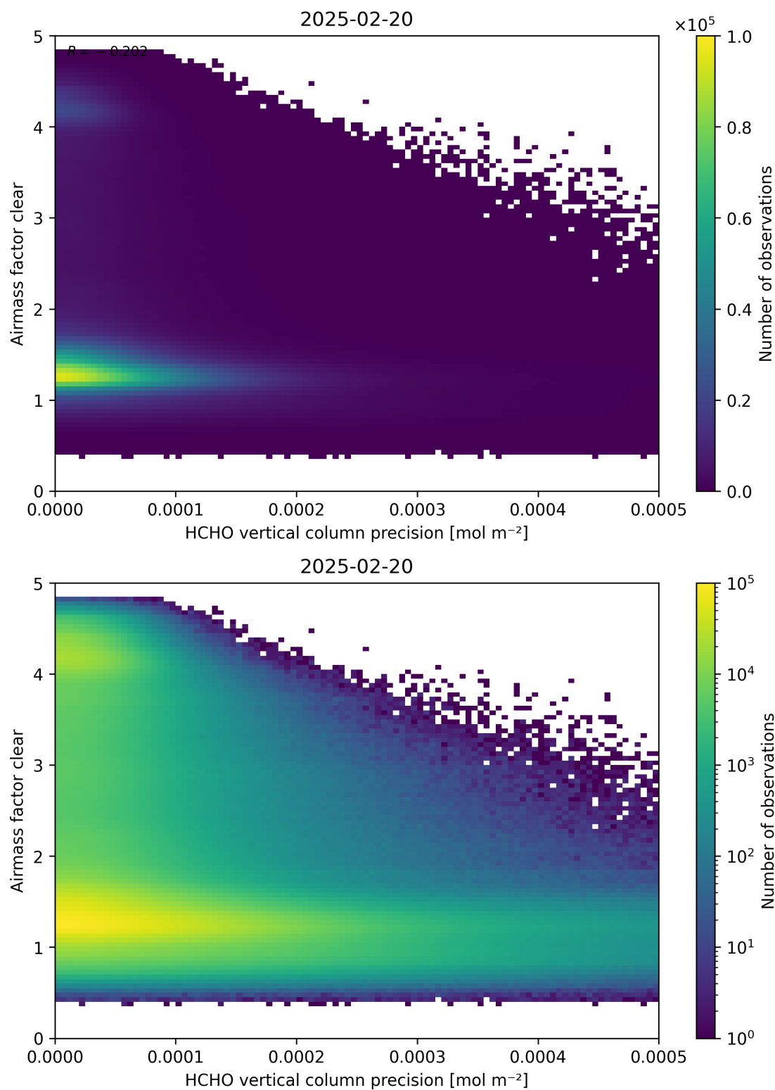
Figure 139: Scatter density plot of “HCHO vertical column precision” against “Airmass factor clear” for 2025-02-19 to 2025-02-21.
