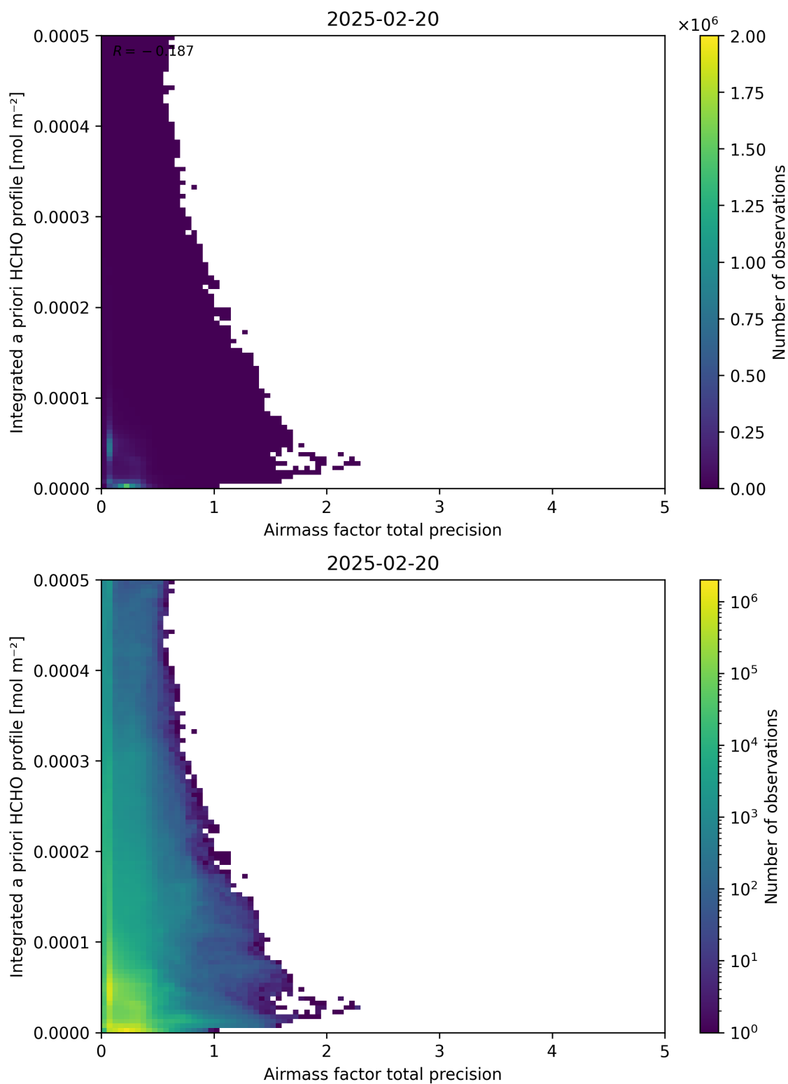
Figure 111: Scatter density plot of “Airmass factor total precision” against “Integrated a priori HCHO profile” for 2025-02-19 to 2025-02-21.
