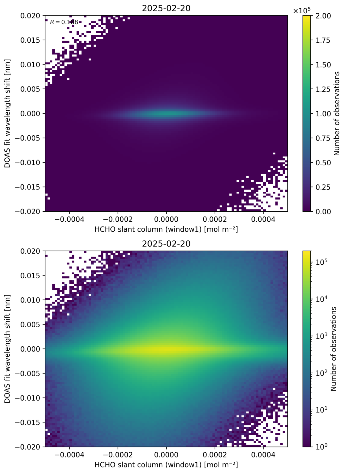
Figure 79: Scatter density plot of “HCHO slant column (window1)” against “DOAS fit wavelength shift” for 2025-02-19 to 2025-02-21.
