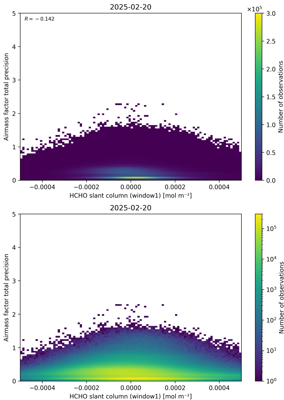
Figure 86: Scatter density plot of “HCHO slant column (window1)” against “Airmass factor total precision” for 2025-02-19 to 2025-02-21.
