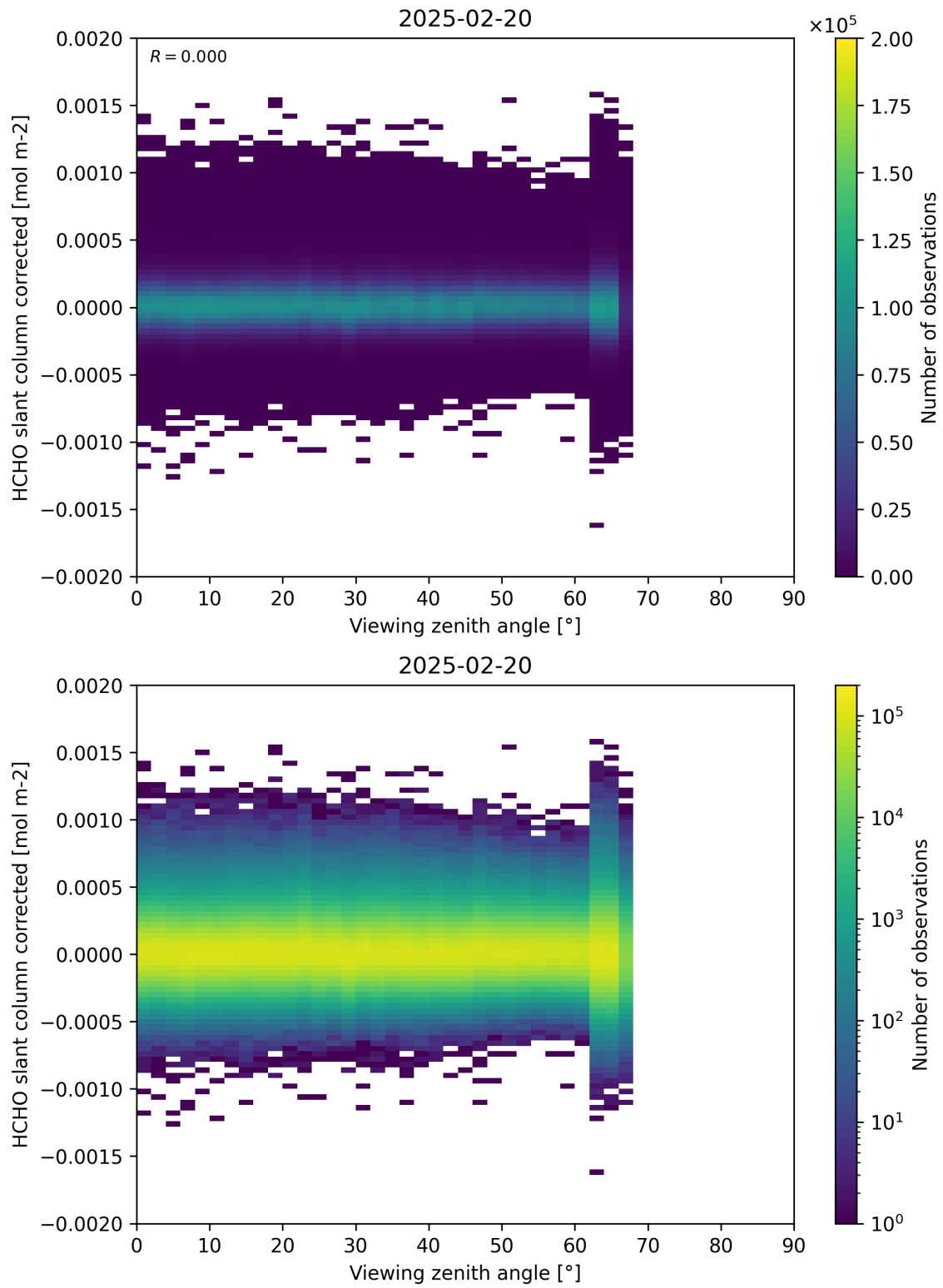
Figure 186: Scatter density plot of “Viewing zenith angle” against “HCHO slant column corrected” for 2025-02-19 to 2025-02-21.
