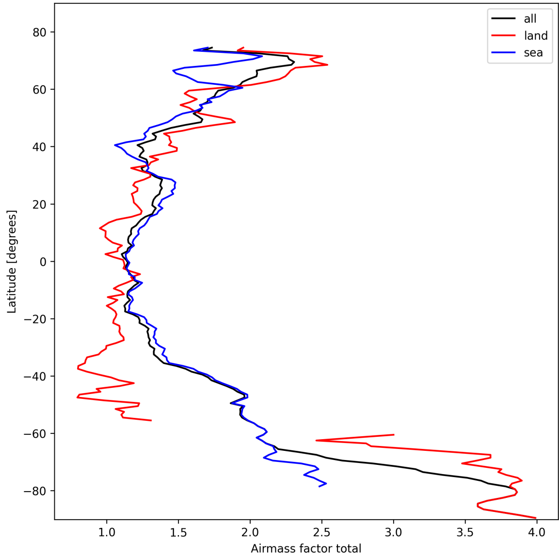
Figure 26: Zonal average of “Airmass factor total” for 2025-02-19 to 2025-02-21.
