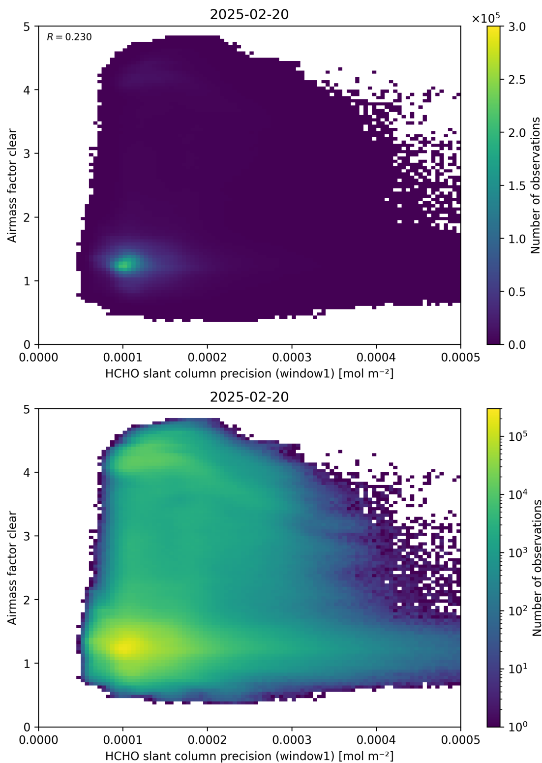
Figure 91: Scatter density plot of “HCHO slant column precision (window1)” against “Airmass factor clear” for 2025-02-19 to 2025-02-21.
