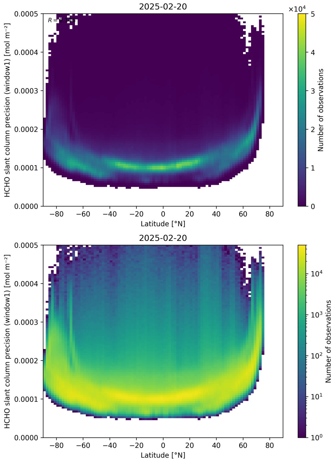
Figure 160: Scatter density plot of “Latitude” against “HCHO slant column precision (window1)” for 2025-02-19 to 2025-02-21.
