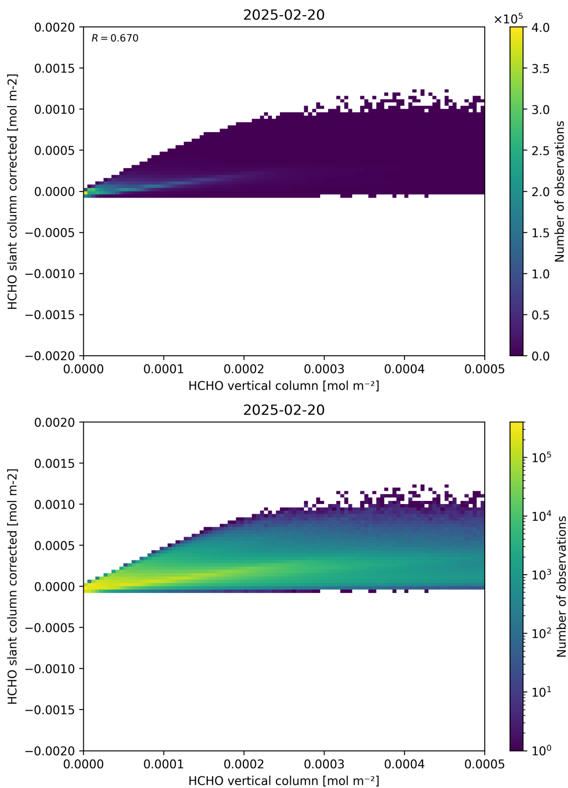
Figure 127: Scatter density plot of “HCHO vertical column” against “HCHO slant column corrected” for 2025-02-19 to 2025-02-21.
