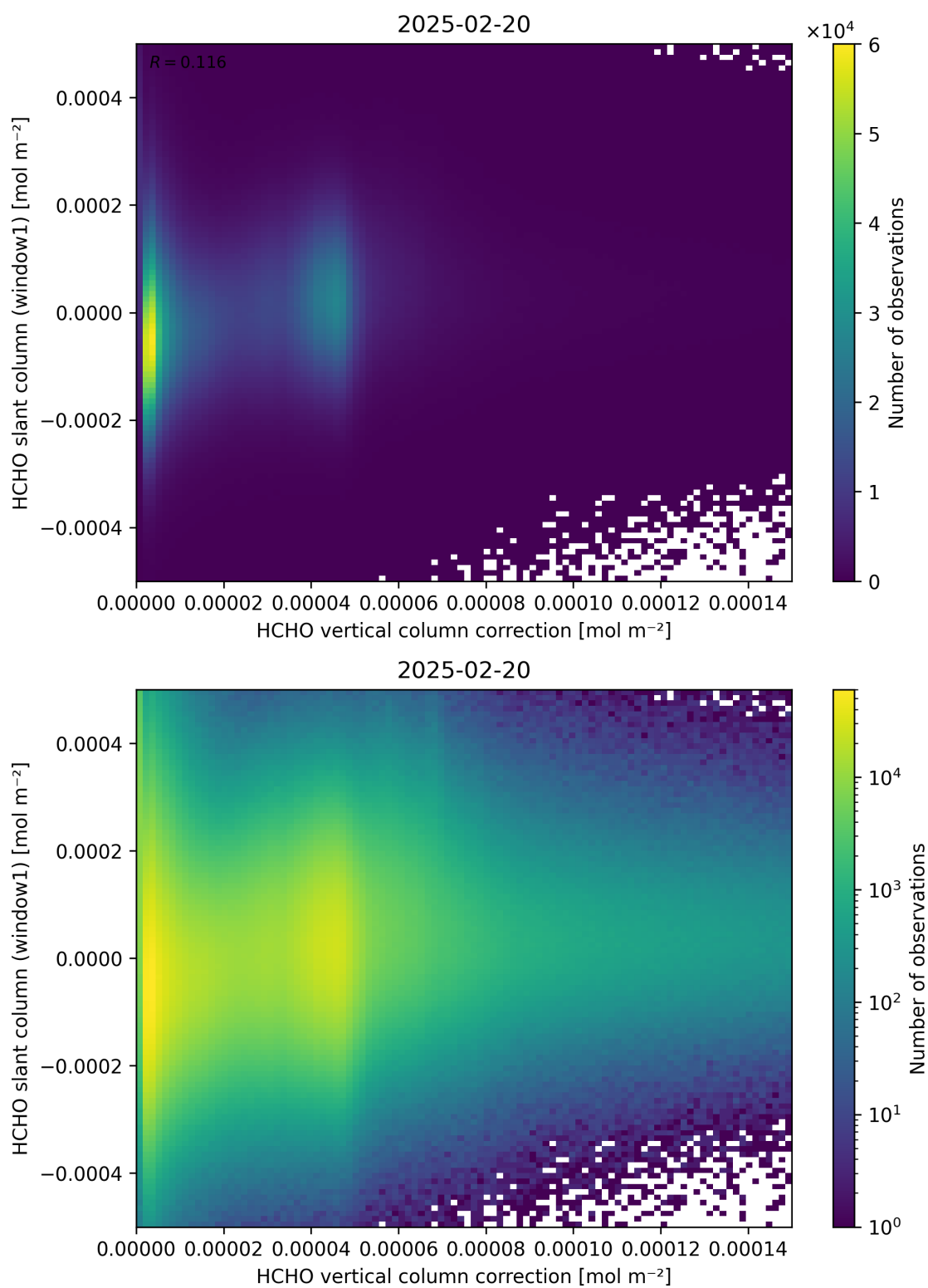
Figure 118: Scatter density plot of “HCHO vertical column correction” against “HCHO slant column (window1)” for 2025-02-19 to 2025-02-21.
