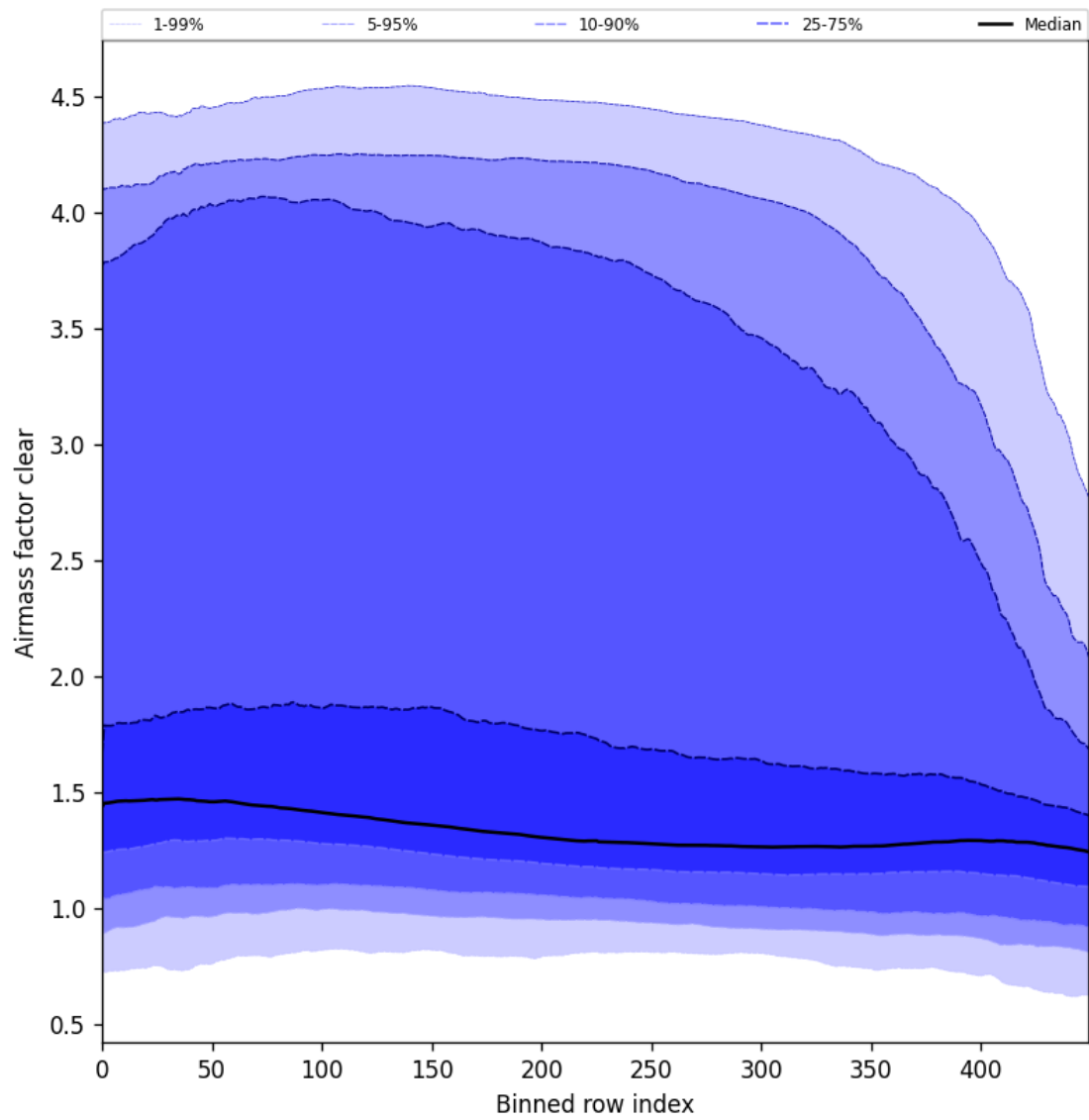
Figure 56: Along track statistics of “Air mass factor clear” for 2025-02-19 to 2025-02-21
