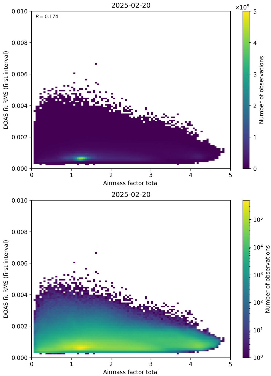
Figure 97: Scatter density plot of “Airmass factor total” against “DOAS fit RMS (first interval)” for 2025-02-19 to 2025-02-21.
