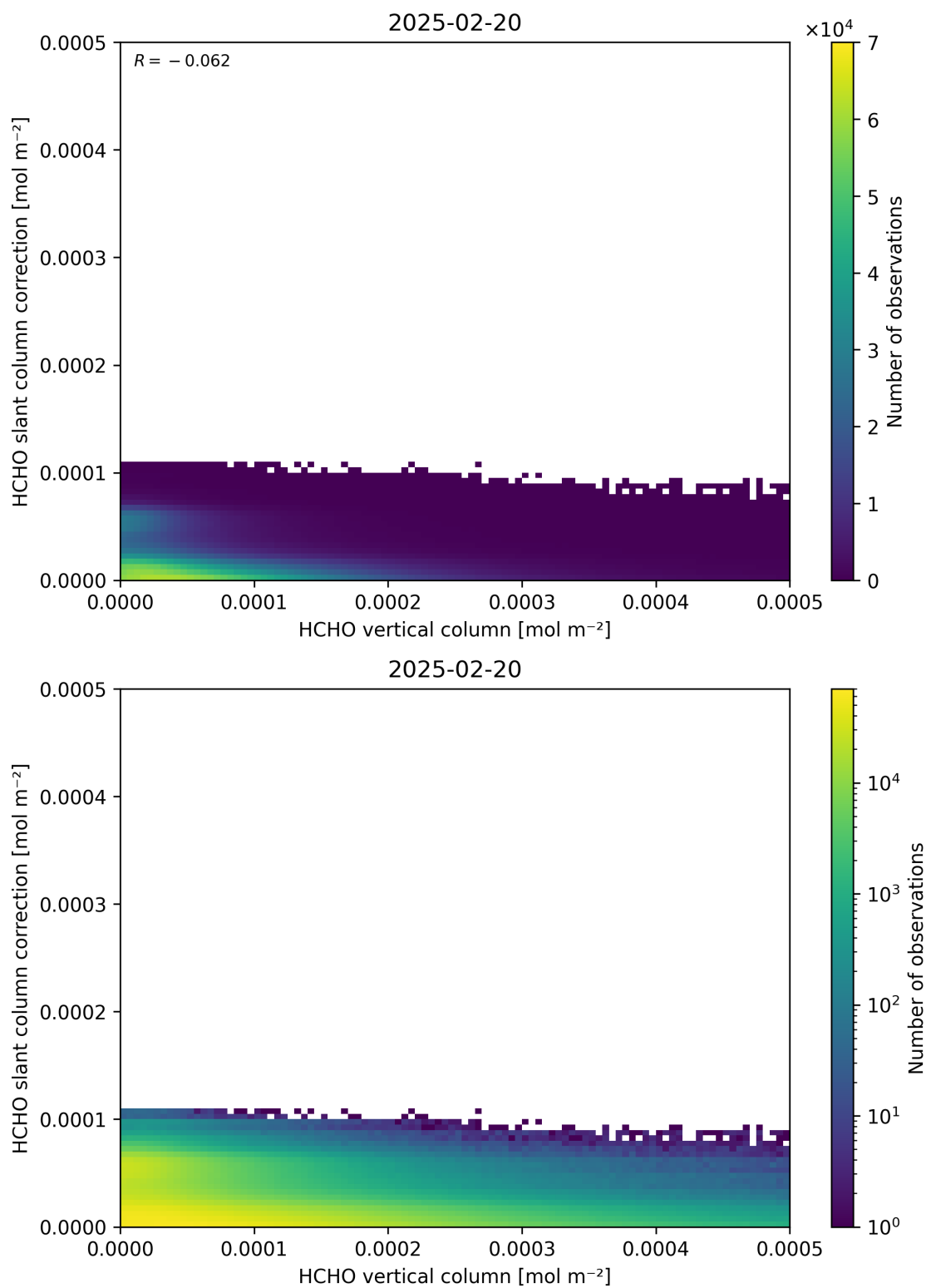
Figure 128: Scatter density plot of “HCHO vertical column” against “HCHO slant column correction” for 2025-02-19 to 2025-02-21.
