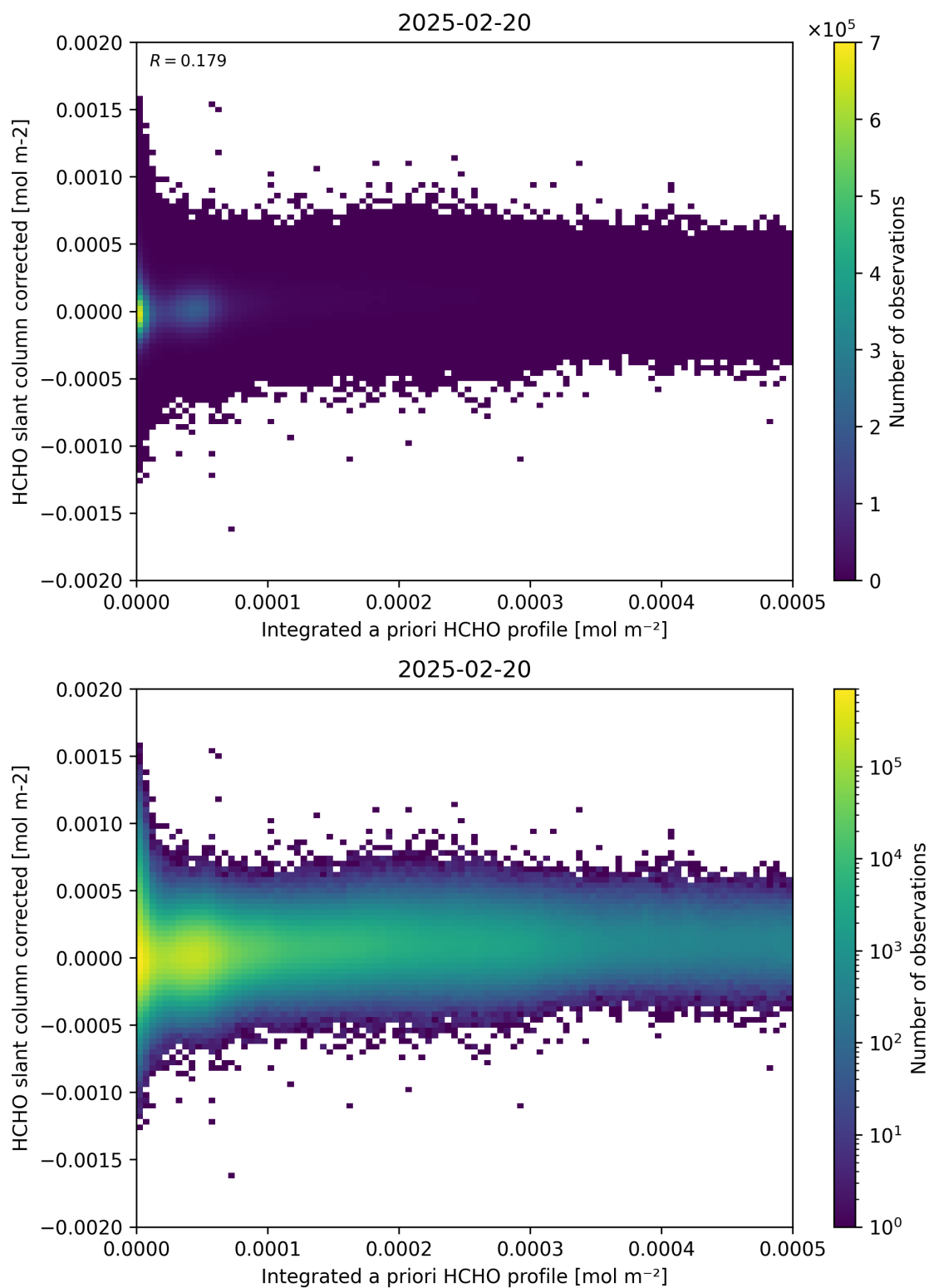
Figure 151: Scatter density plot of “Integrated a priori HCHO profile” against “HCHO slant column corrected” for 2025-02-19 to 2025-02-21.
