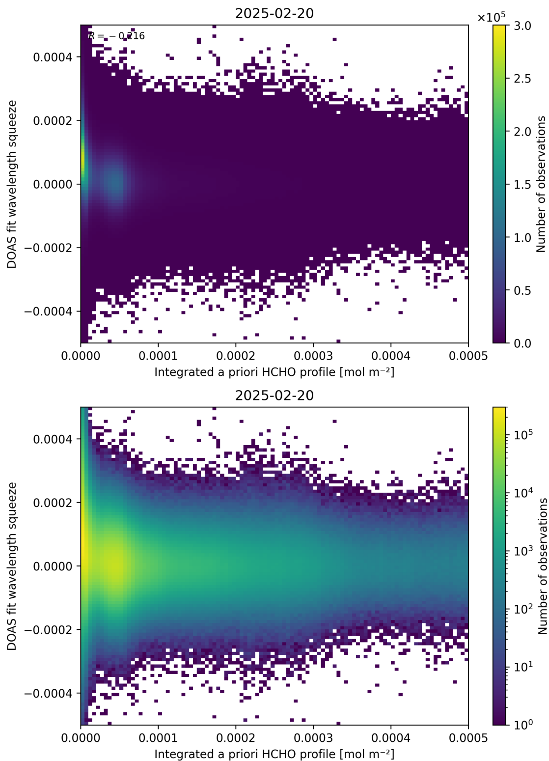
Figure 150: Scatter density plot of “Integrated a priori HCHO profile” against “DOAS fit wavelength squeeze” for 2025-02-19 to 2025-02-21.
