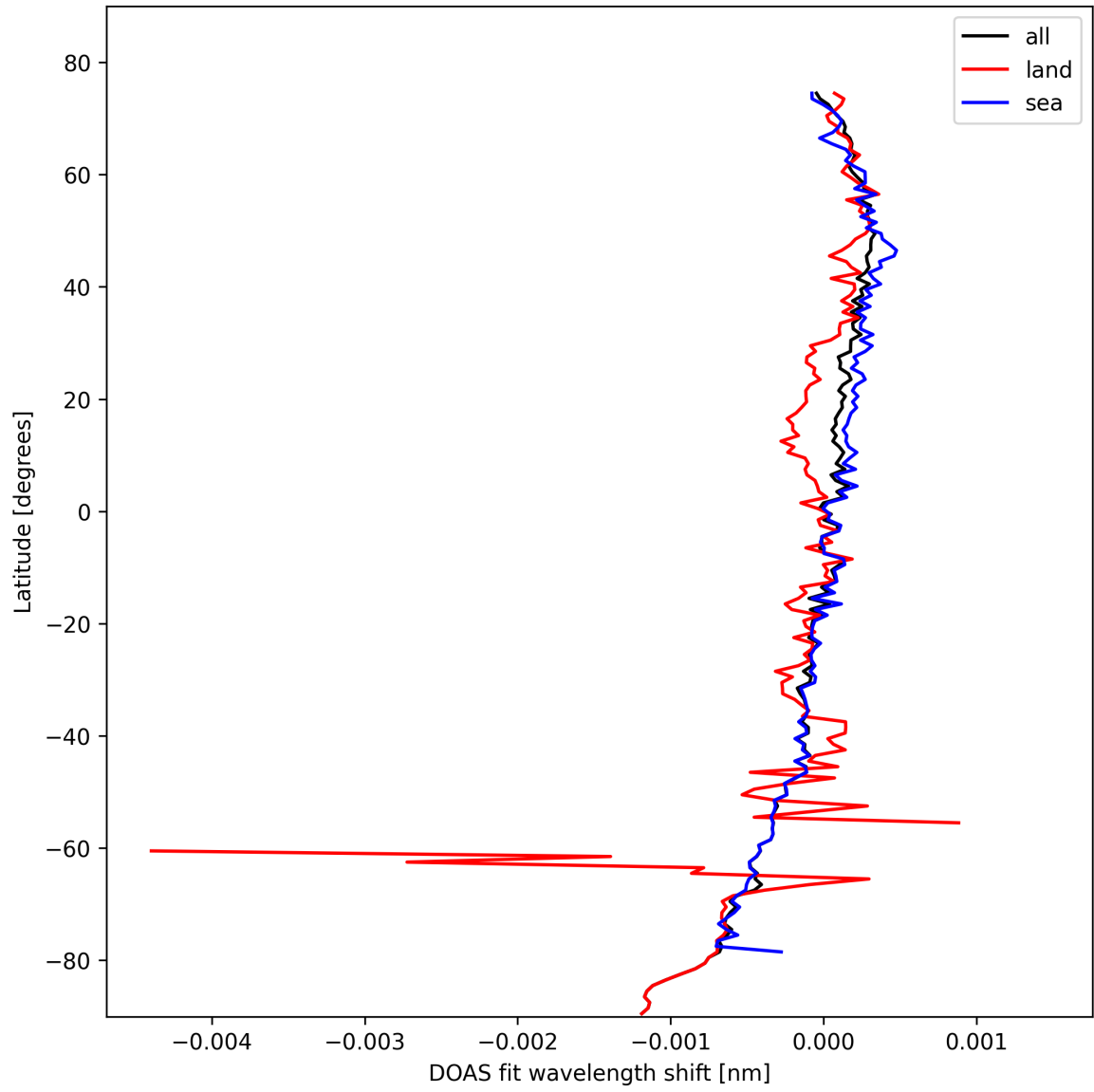
Figure 30: Zonal average of “DOAS fit wavelength shift” for 2025-02-19 to 2025-02-21.
