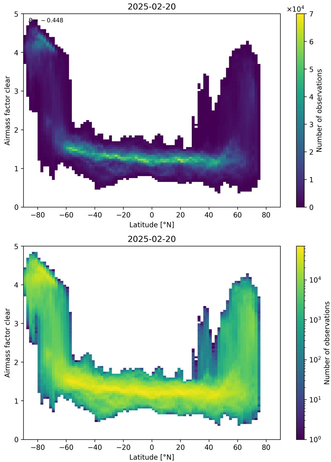
Figure 156: Scatter density plot of “Latitude” against “Airmass factor clear” for 2025-02-19 to 2025-02-21.
