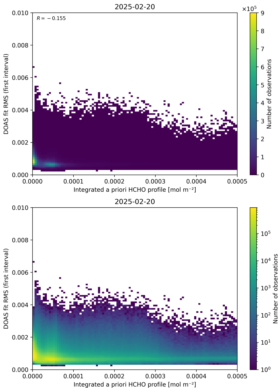
Figure 148: Scatter density plot of “Integrated a priori HCHO profile” against “DOAS fit RMS (first interval)” for 2025-02-19 to 2025-02-21.
