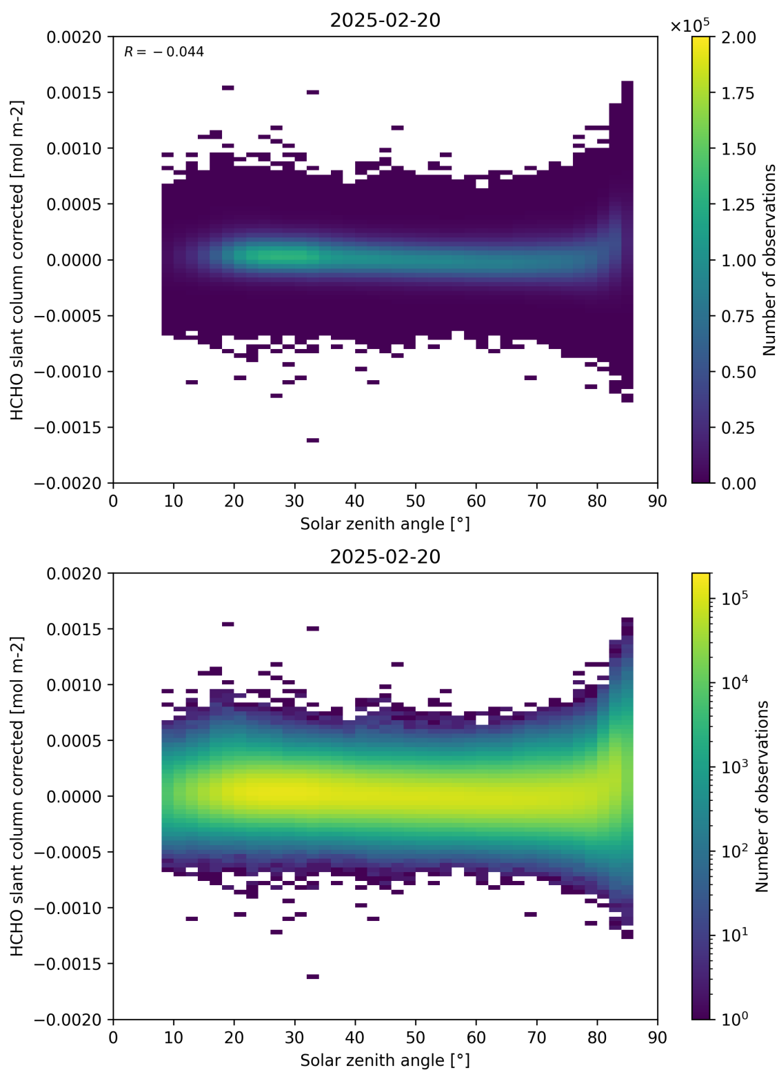
Figure 171: Scatter density plot of “Solar zenith angle” against “HCHO slant column corrected” for 2025-02-19 to 2025-02-21.
