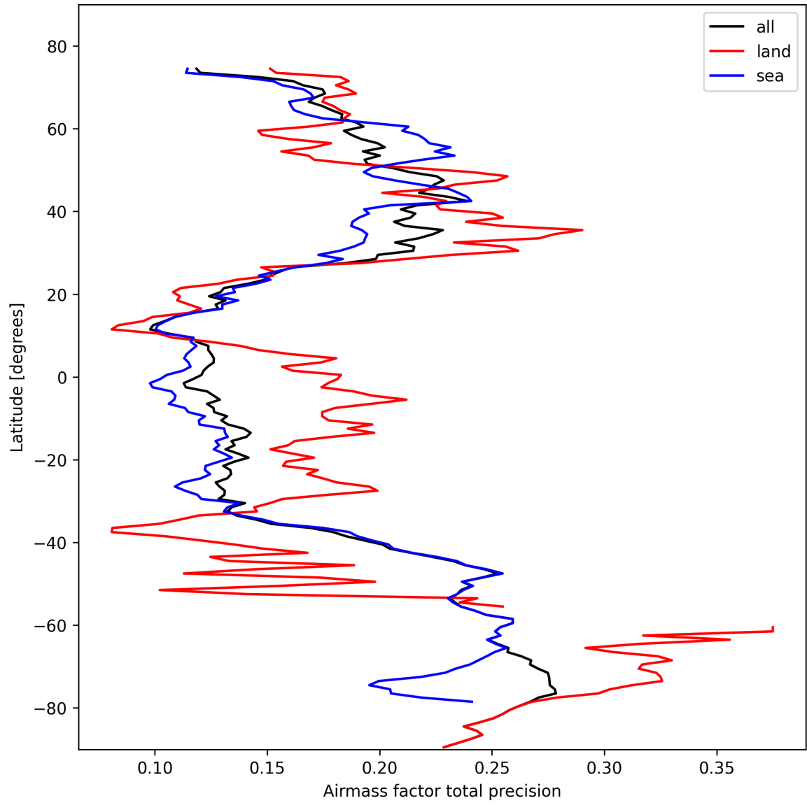
Figure 27: Zonal average of “Airmass factor total precision” for 2025-02-19 to 2025-02-21.
