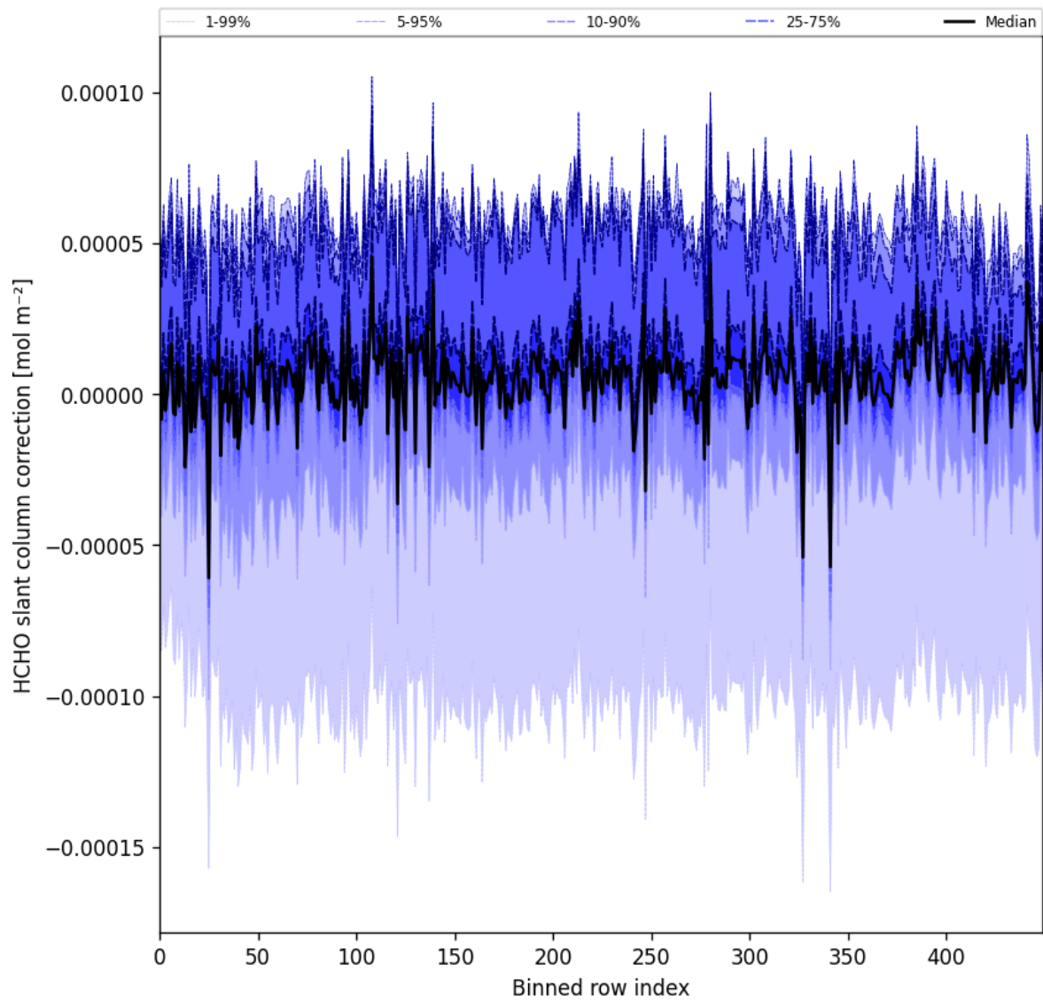
Figure 61: Along track statistics of “HCHO slant column correction” for 2025-02-19 to 2025-02-21
