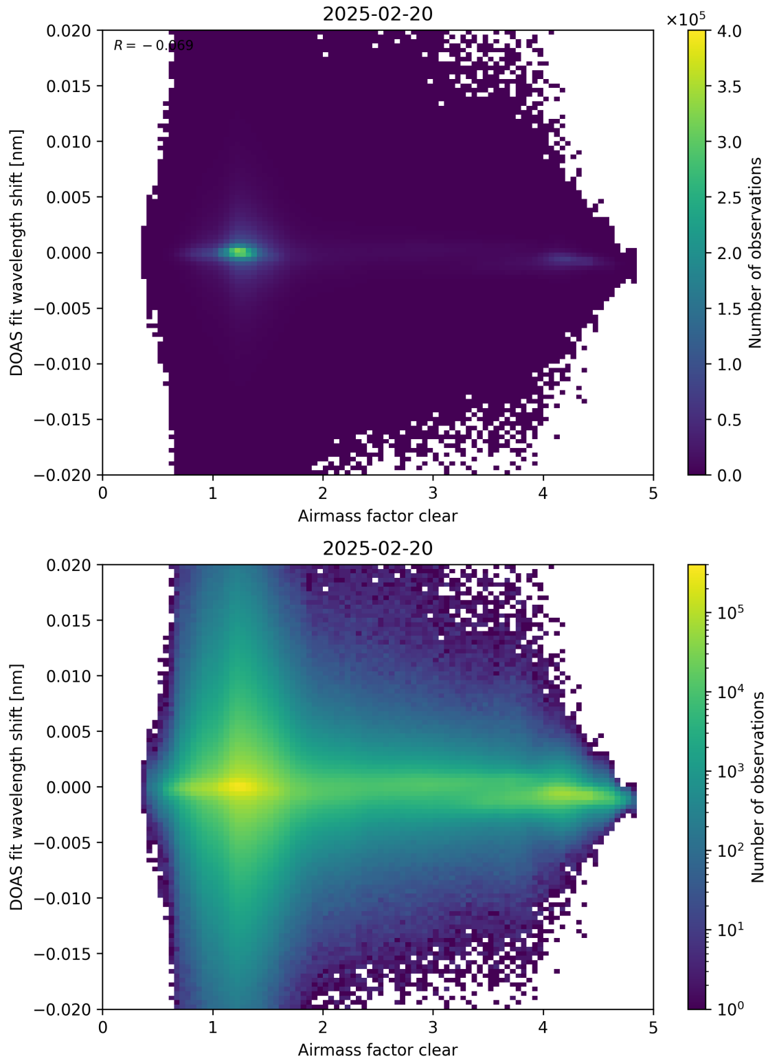
Figure 72: Scatter density plot of “Airmass factor clear” against “DOAS fit wavelength shift” for 2025-02-19 to 2025-02-21.
