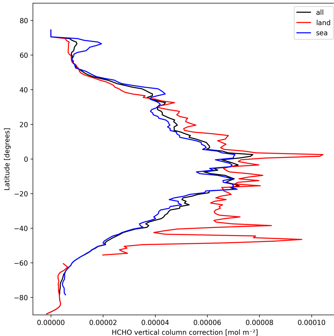
Figure 23: Zonal average of “HCHO vertical column correction” for 2025-02-19 to 2025-02-21.
