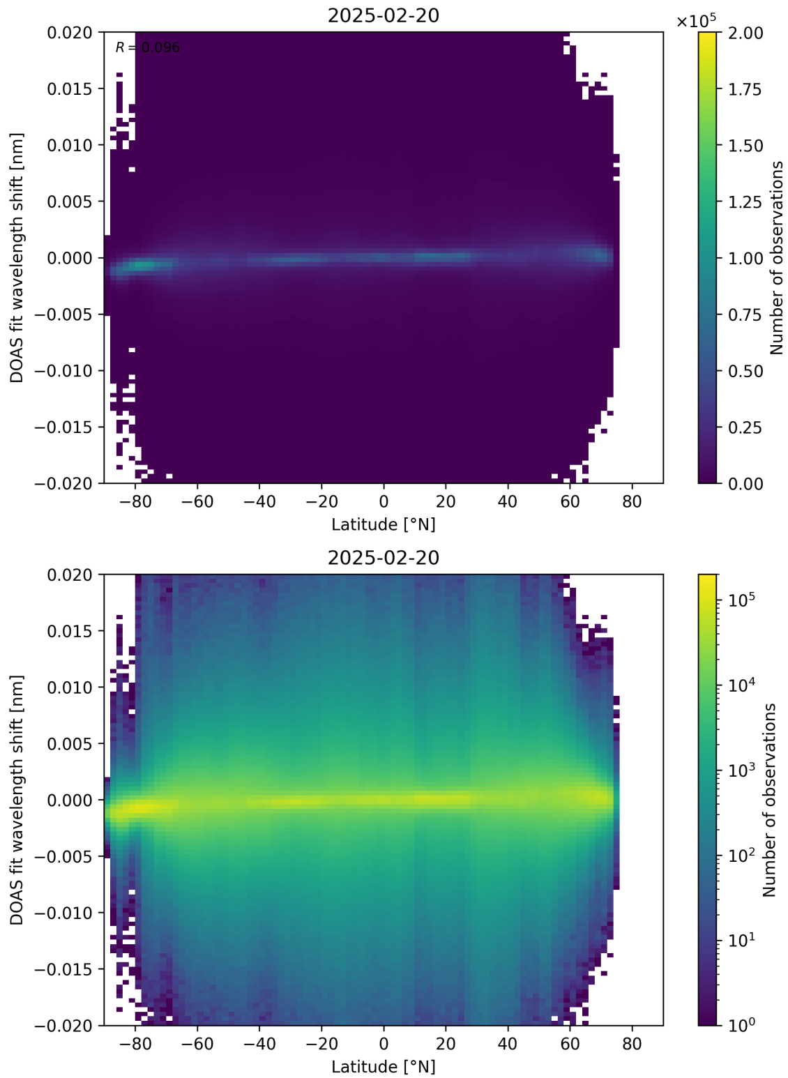
Figure 154: Scatter density plot of “Latitude” against “DOAS fit wavelength shift” for 2025-02-19 to 2025-02-21.
