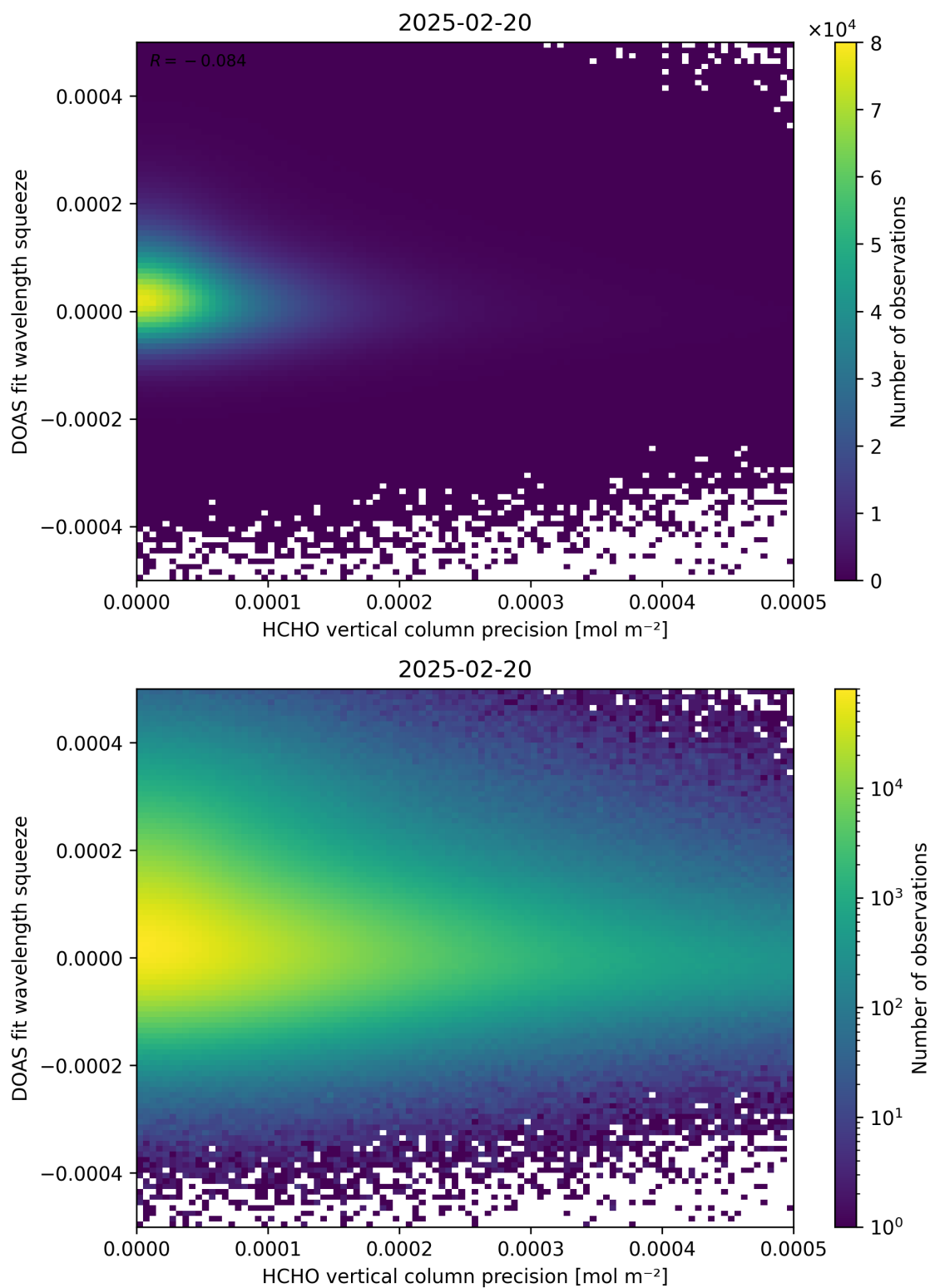
Figure 138: Scatter density plot of “HCHO vertical column precision” against “DOAS fit wavelength squeeze” for 2025-02-19 to 2025-02-21.
