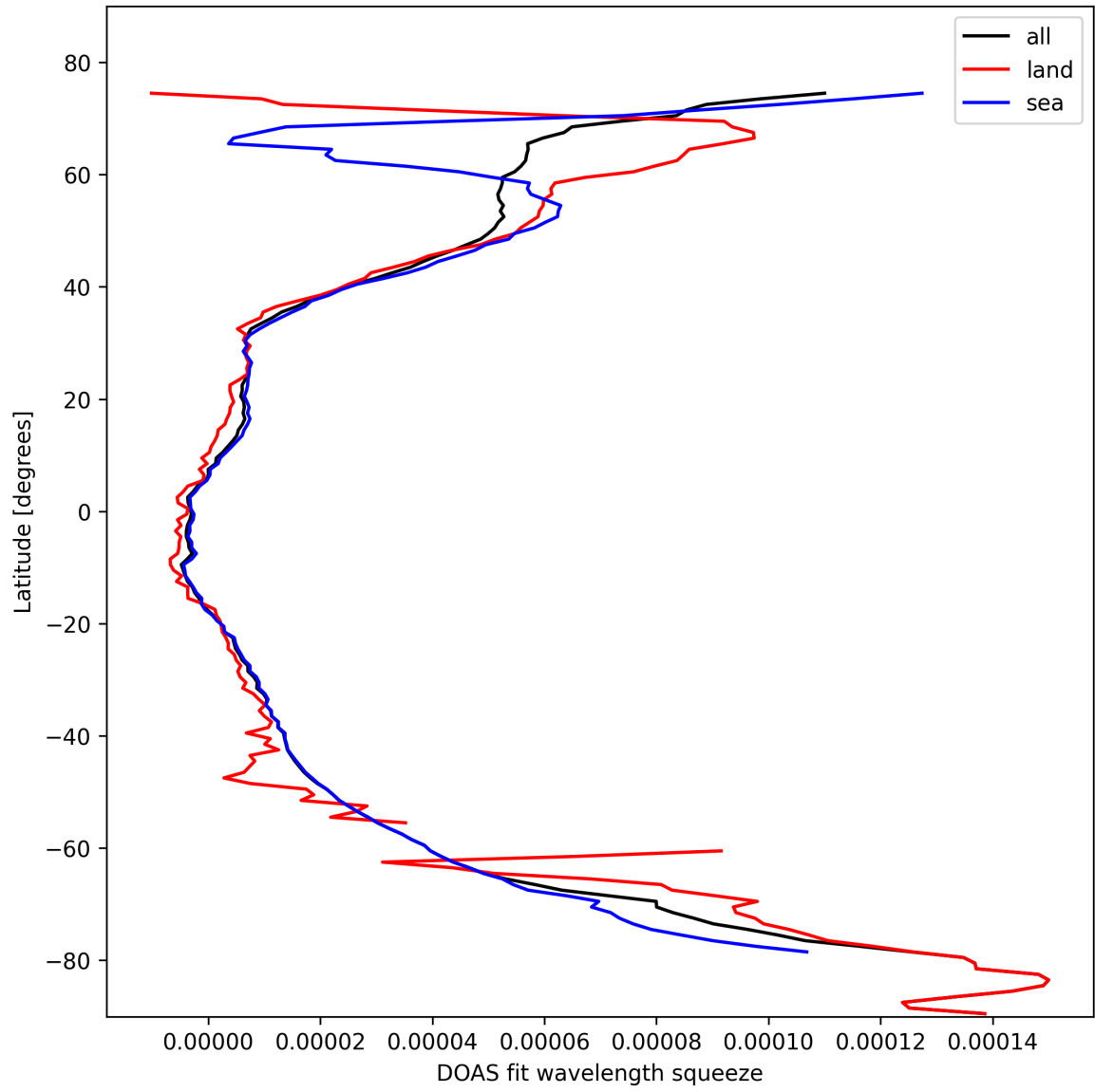
Figure 31: Zonal average of “DOAS fit wavelength squeeze” for 2025-02-19 to 2025-02-21.
