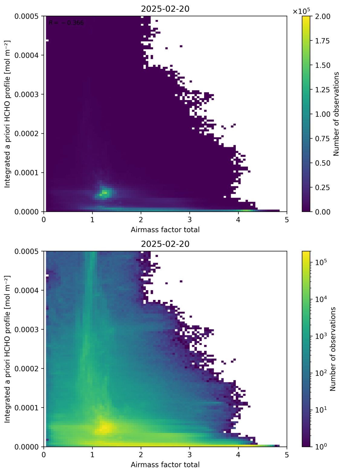
Figure 104: Scatter density plot of “Airmass factor total” against “Integrated a priori HCHO profile” for 2025-02-19 to 2025-02-21.
