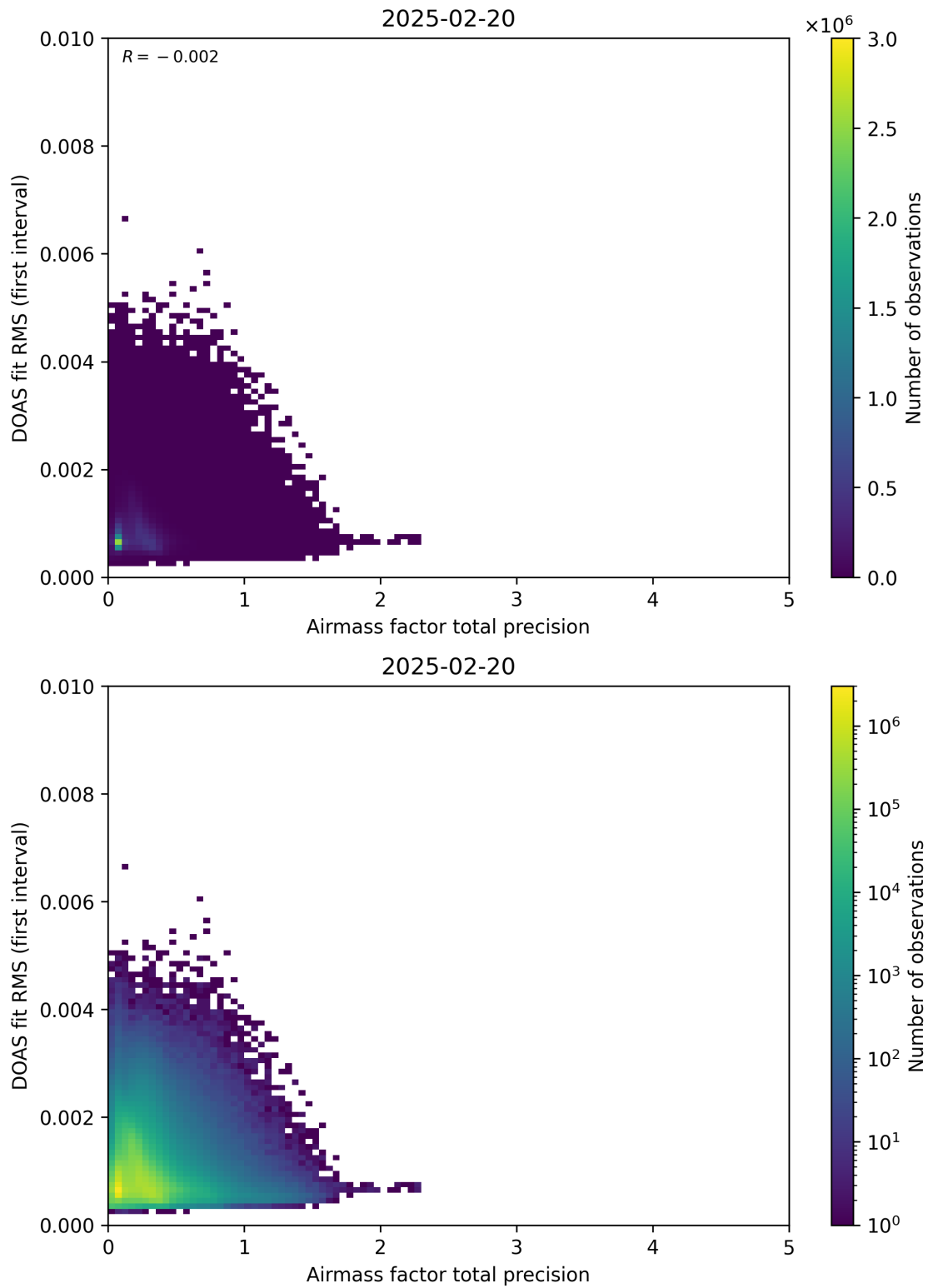
Figure 105: Scatter density plot of “Airmass factor total precision” against “DOAS fit RMS (first interval)” for 2025-02-19 to 2025-02-21.
