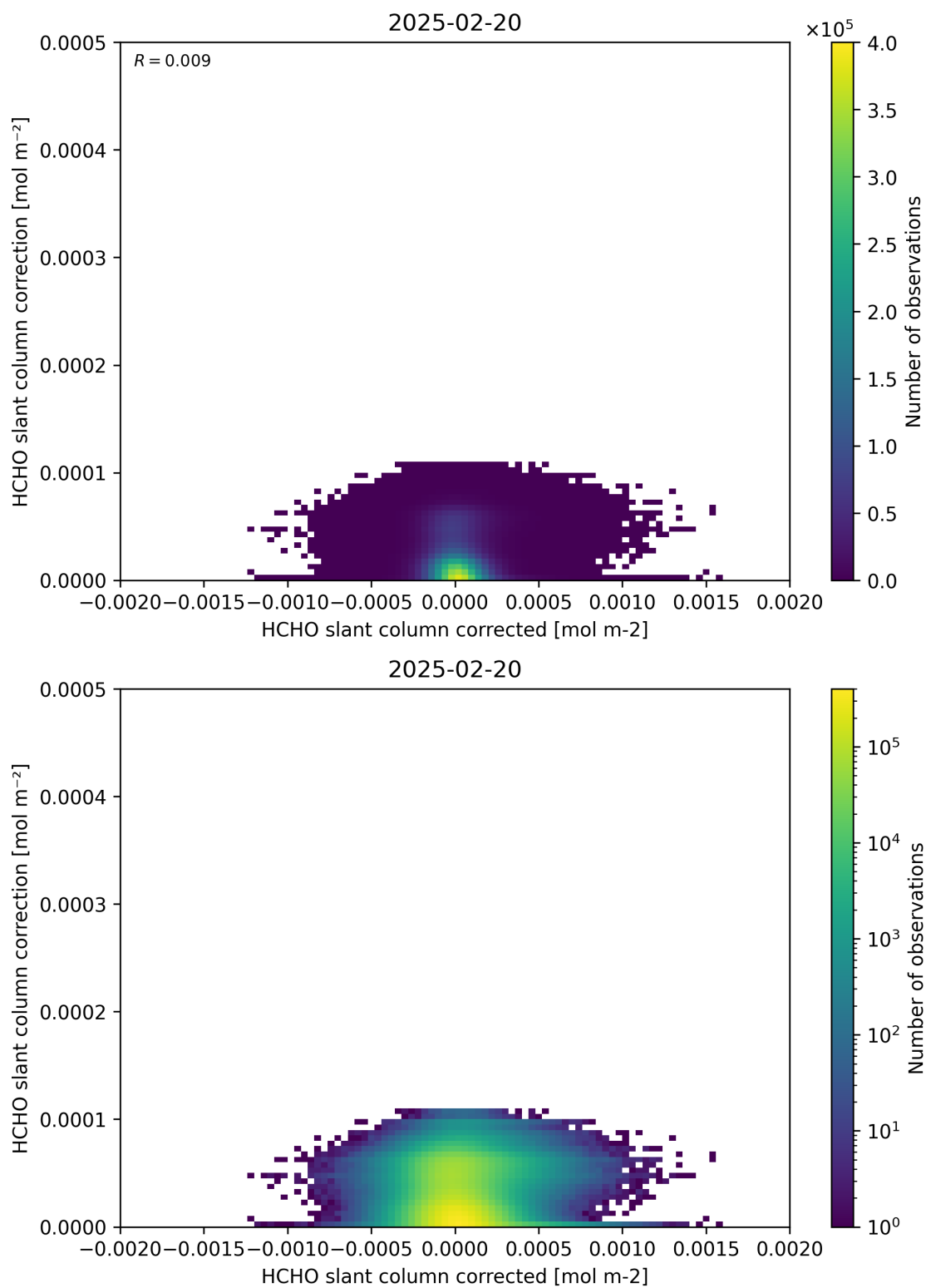
Figure 77: Scatter density plot of “HCHO slant column corrected” against “HCHO slant column correction” for 2025-02-19 to 2025-02-21.
