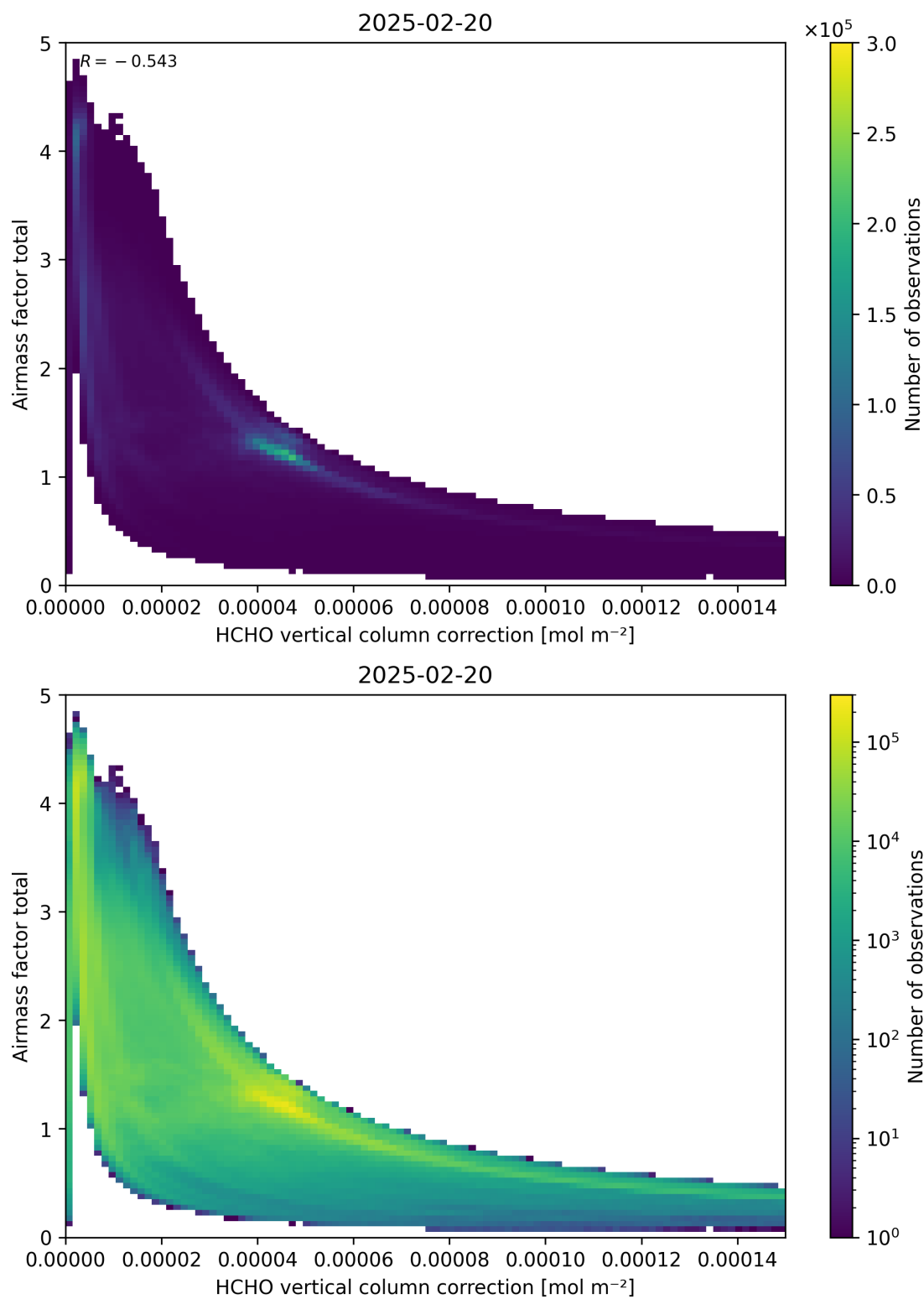
Figure 120: Scatter density plot of “HCHO vertical column correction” against “Airmass factor total” for 2025-02-19 to 2025-02-21.
