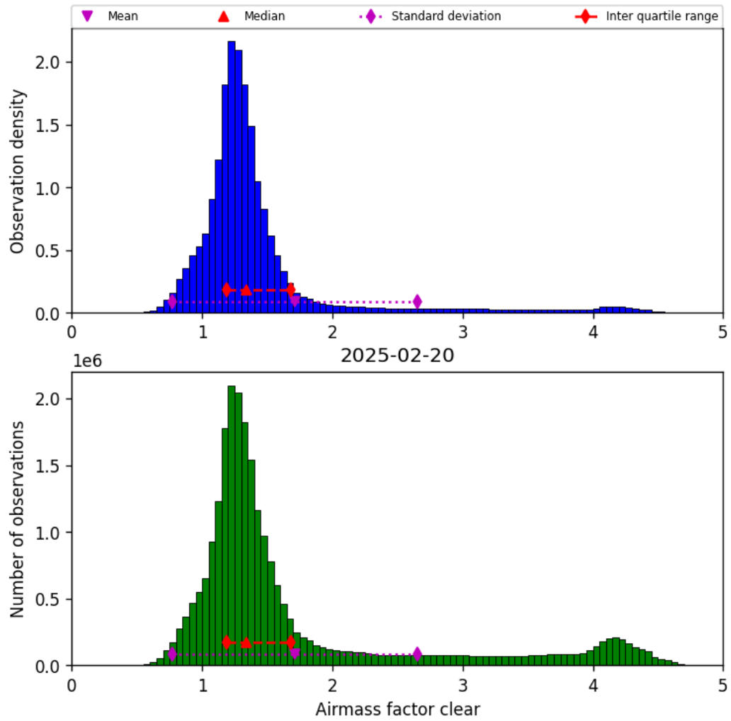
Figure 42: Histogram of “Airmass factor clear” for 2025-02-19 to 2025-02-21
