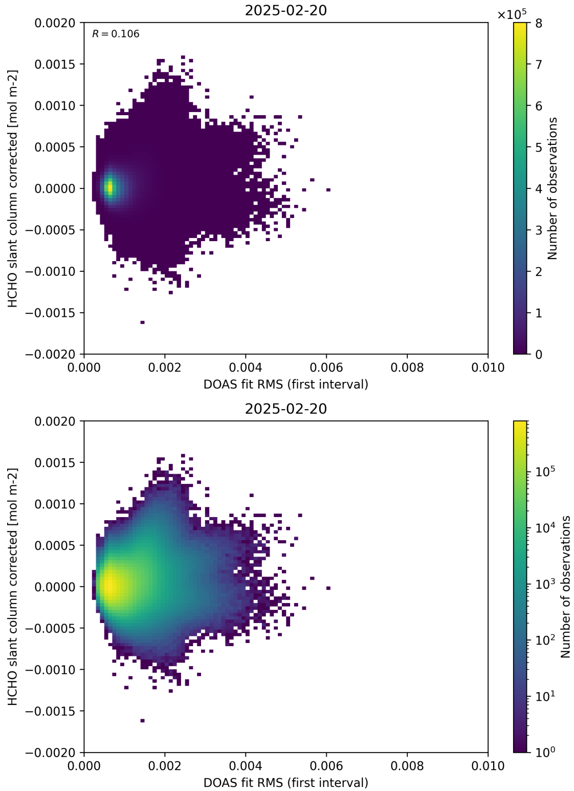
Figure 62: Scatter density plot of “DOAS fit RMS (first interval)” against “HCHO slant column corrected” for 2025-02-19 to 2025-02-21.
