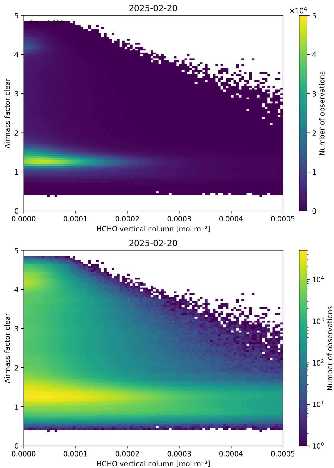
Figure 126: Scatter density plot of “HCHO vertical column” against “Airmass factor clear” for 2025-02-19 to 2025-02-21.
