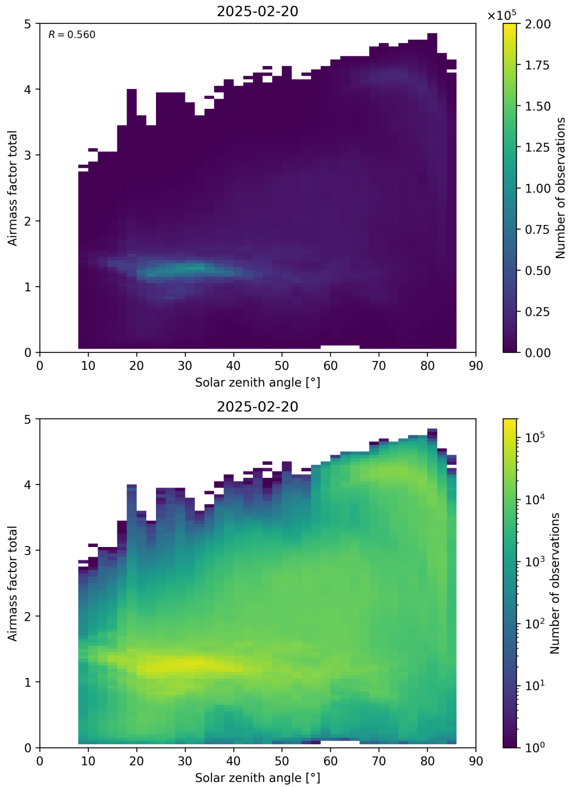
Figure 175: Scatter density plot of “Solar zenith angle” against “Airmass factor total” for 2025-02-19 to 2025-02-21.
