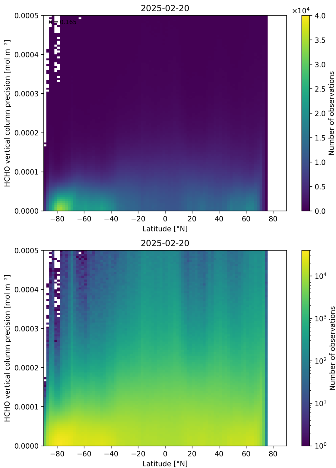
Figure 165: Scatter density plot of “Latitude” against “HCHO vertical column precision” for 2025-02-19 to 2025-02-21.
