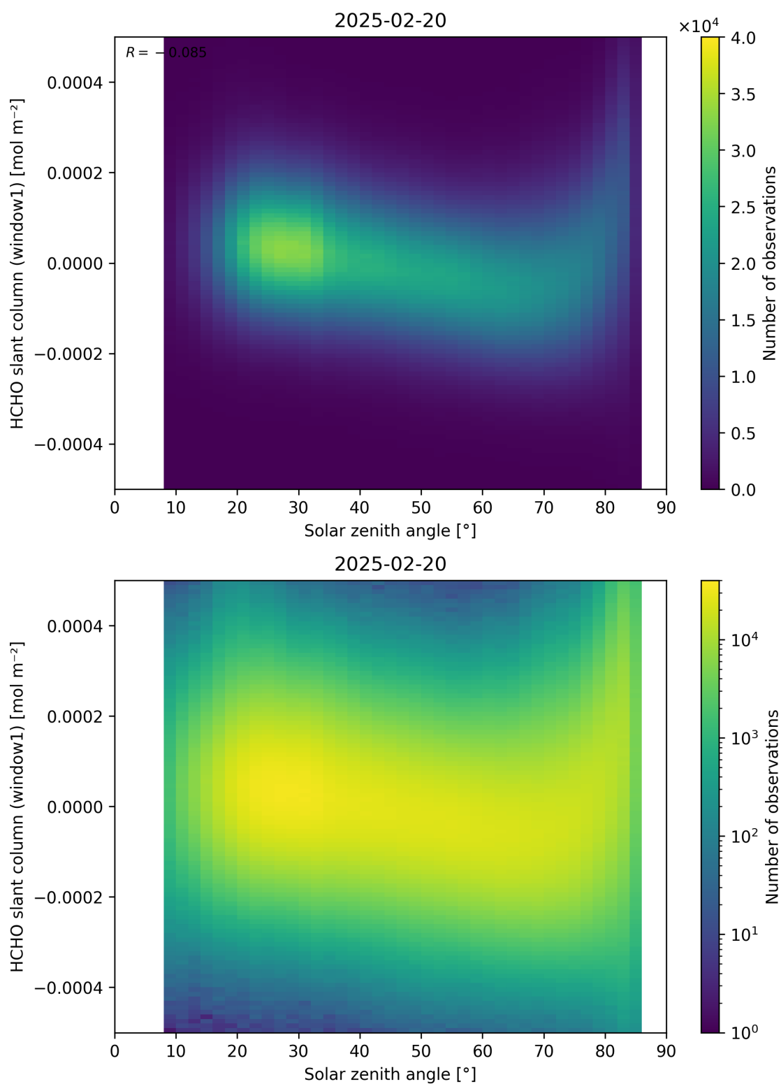
Figure 173: Scatter density plot of “Solar zenith angle” against “HCHO slant column (window1)” for 2025-02-19 to 2025-02-21.
