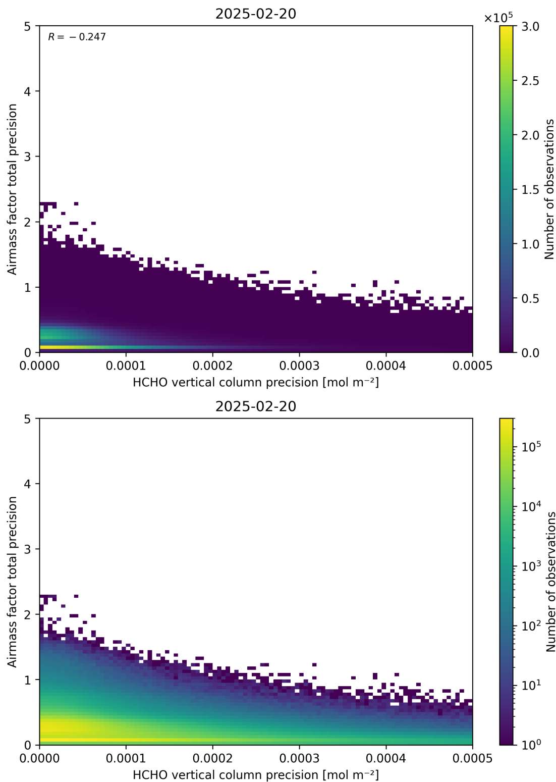
Figure 145: Scatter density plot of “HCHO vertical column precision” against “Airmass factor total precision” for 2025-02-19 to 2025-02-21.
