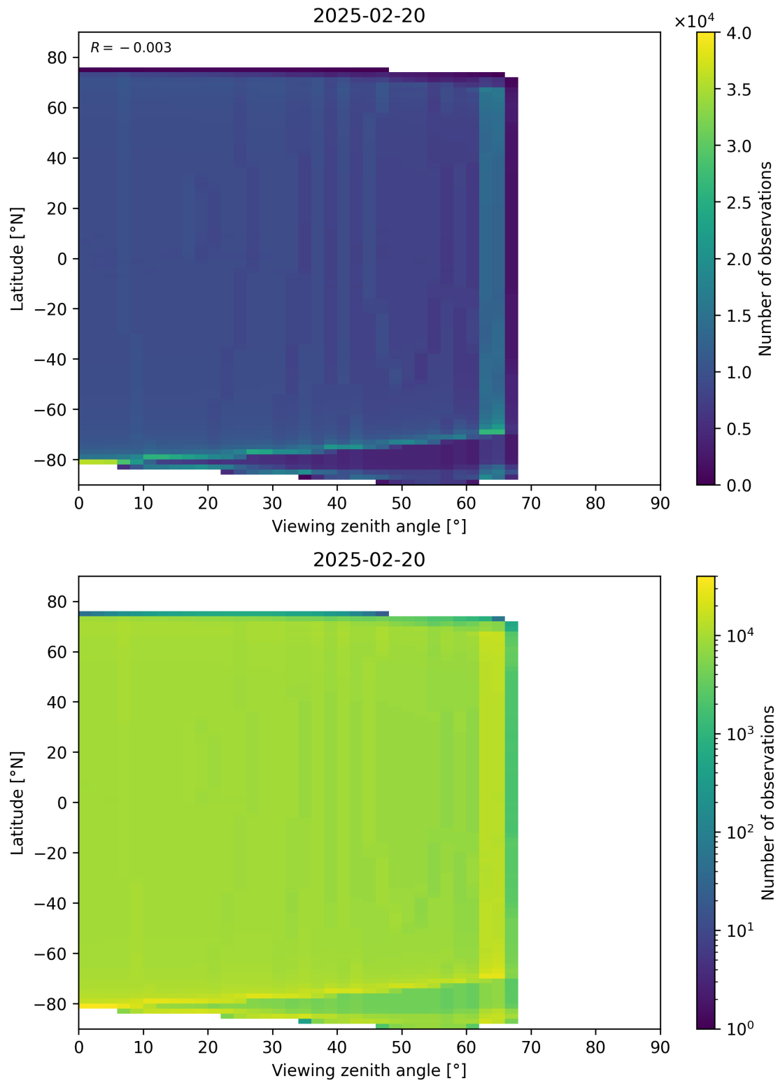
Figure 196: Scatter density plot of “Viewing zenith angle” against “Latitude” for 2025-02-19 to 2025-02-21.
