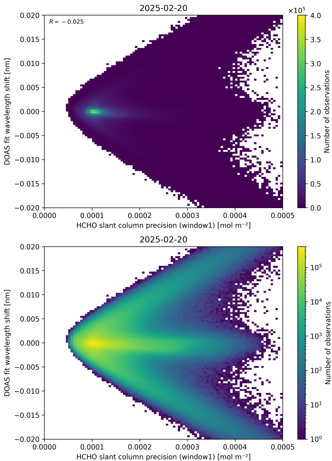
Figure 89: Scatter density plot of “HCHO slant column precision (window1)” against “DOAS fit wavelength shift” for 2025-02-19 to 2025-02-21.
