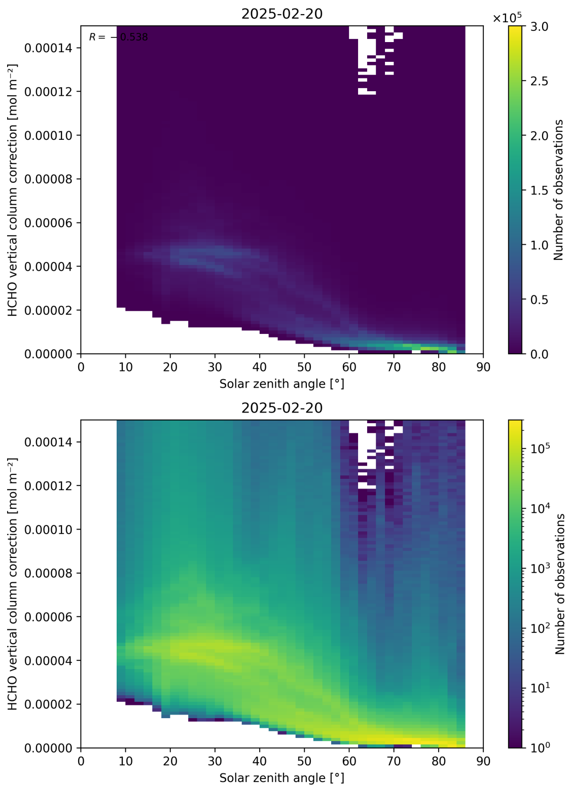
Figure 178: Scatter density plot of “Solar zenith angle” against “HCHO vertical column correction” for 2025-02-19 to 2025-02-21.
