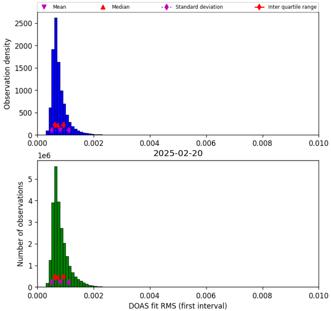
Figure 46: Histogram of “DOAS fit RMS (first interval)” for 2025-02-19 to 2025-02-21
