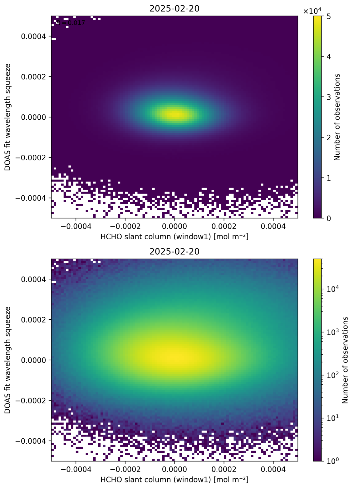
Figure 80: Scatter density plot of “HCHO slant column (window1)” against “DOAS fit wavelength squeeze” for 2025-02-19 to 2025-02-21.
