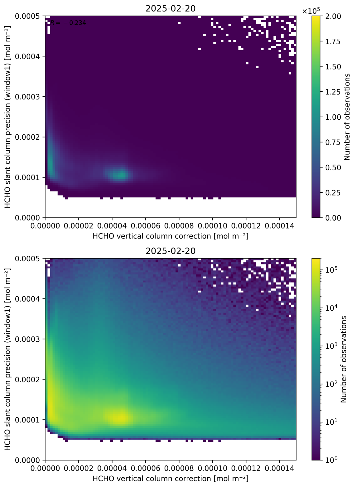
Figure 119: Scatter density plot of “HCHO vertical column correction” against “HCHO slant column precision (window1)” for 2025-02-19 to 2025-02-21.
