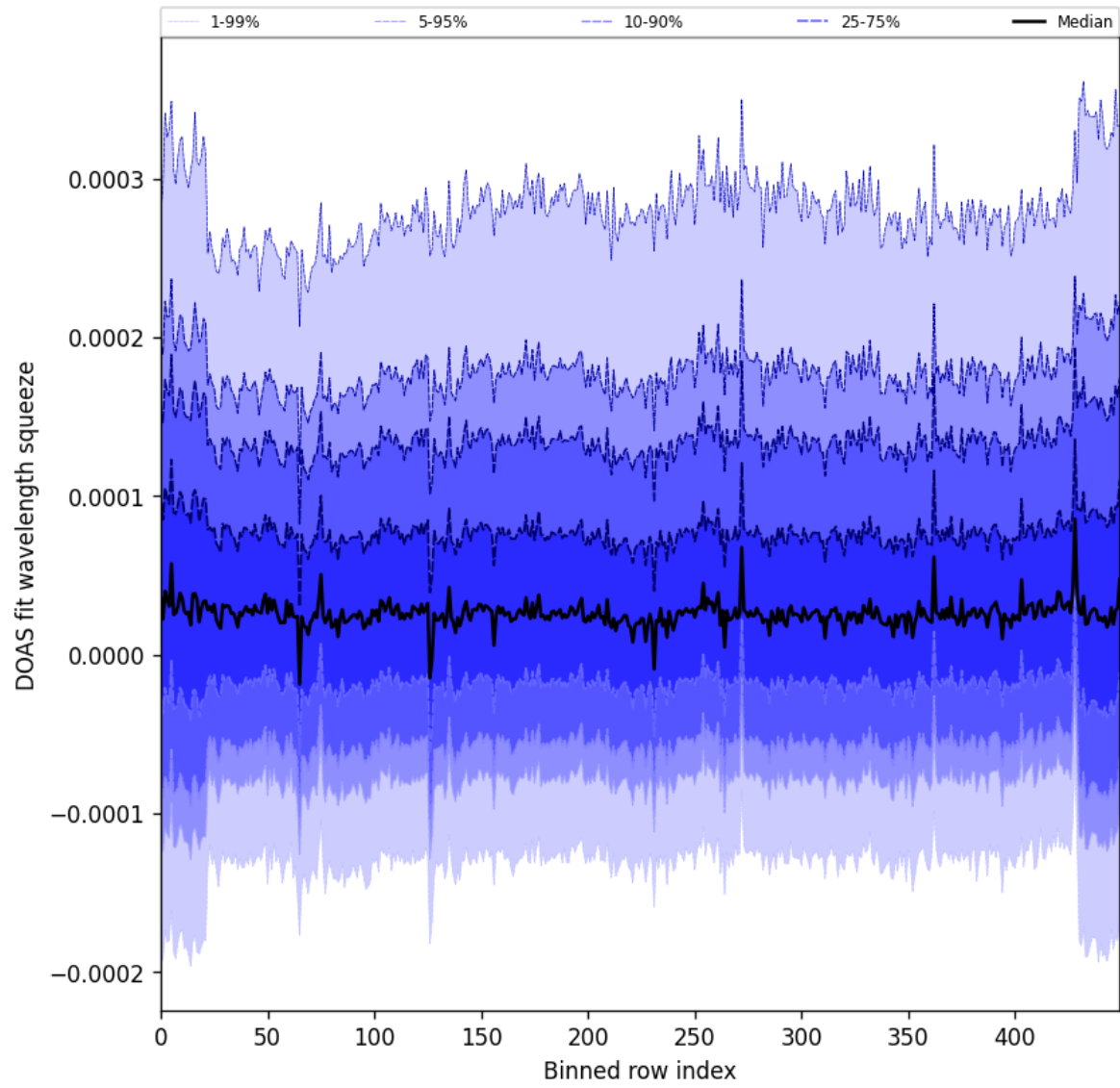
Figure 59: Along track statistics of “DOAS fit wavelength squeeze” for 2025-02-19 to 2025-02-21
