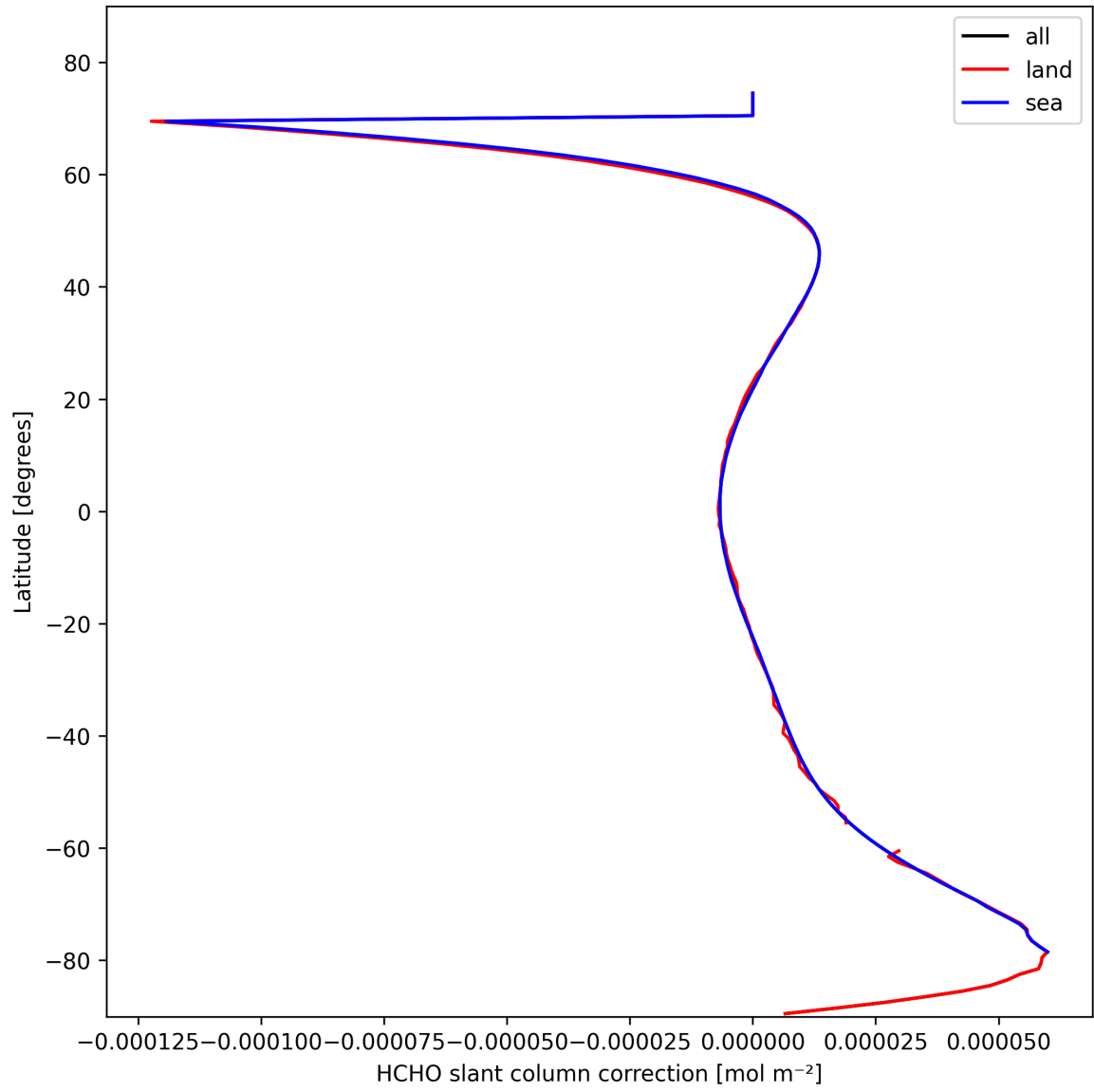
Figure 33: Zonal average of “HCHO slant column correction” for 2025-02-19 to 2025-02-21.
