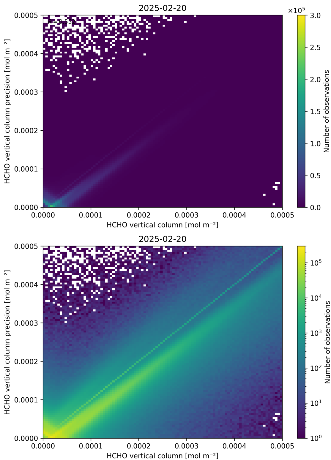
Figure 134: Scatter density plot of “HCHO vertical column” against “HCHO vertical column precision” for 2025-02-19 to 2025-02-21.
