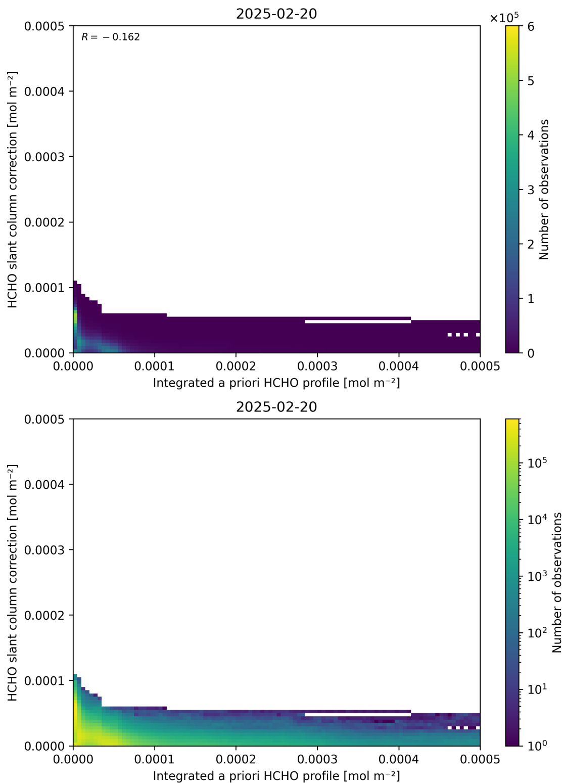
Figure 152: Scatter density plot of “Integrated a priori HCHO profile” against “HCHO slant column correction” for 2025-02-19 to 2025-02-21.
