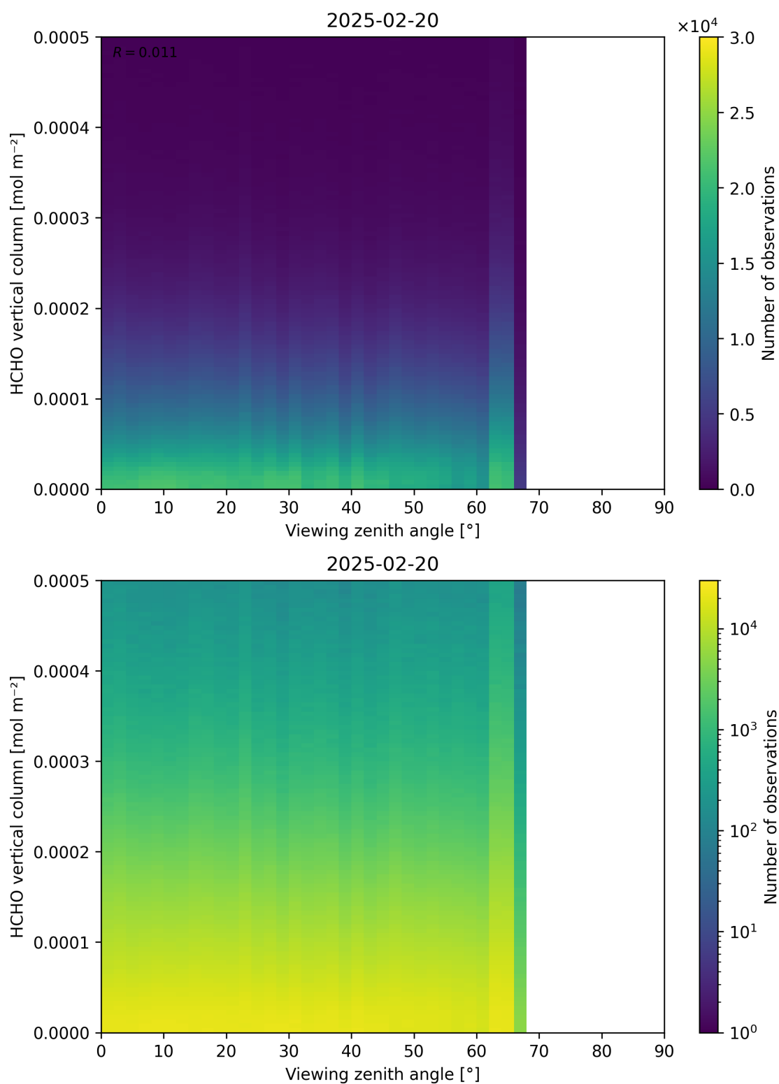
Figure 192: Scatter density plot of “Viewing zenith angle” against “HCHO vertical column” for 2025-02-19 to 2025-02-21.
