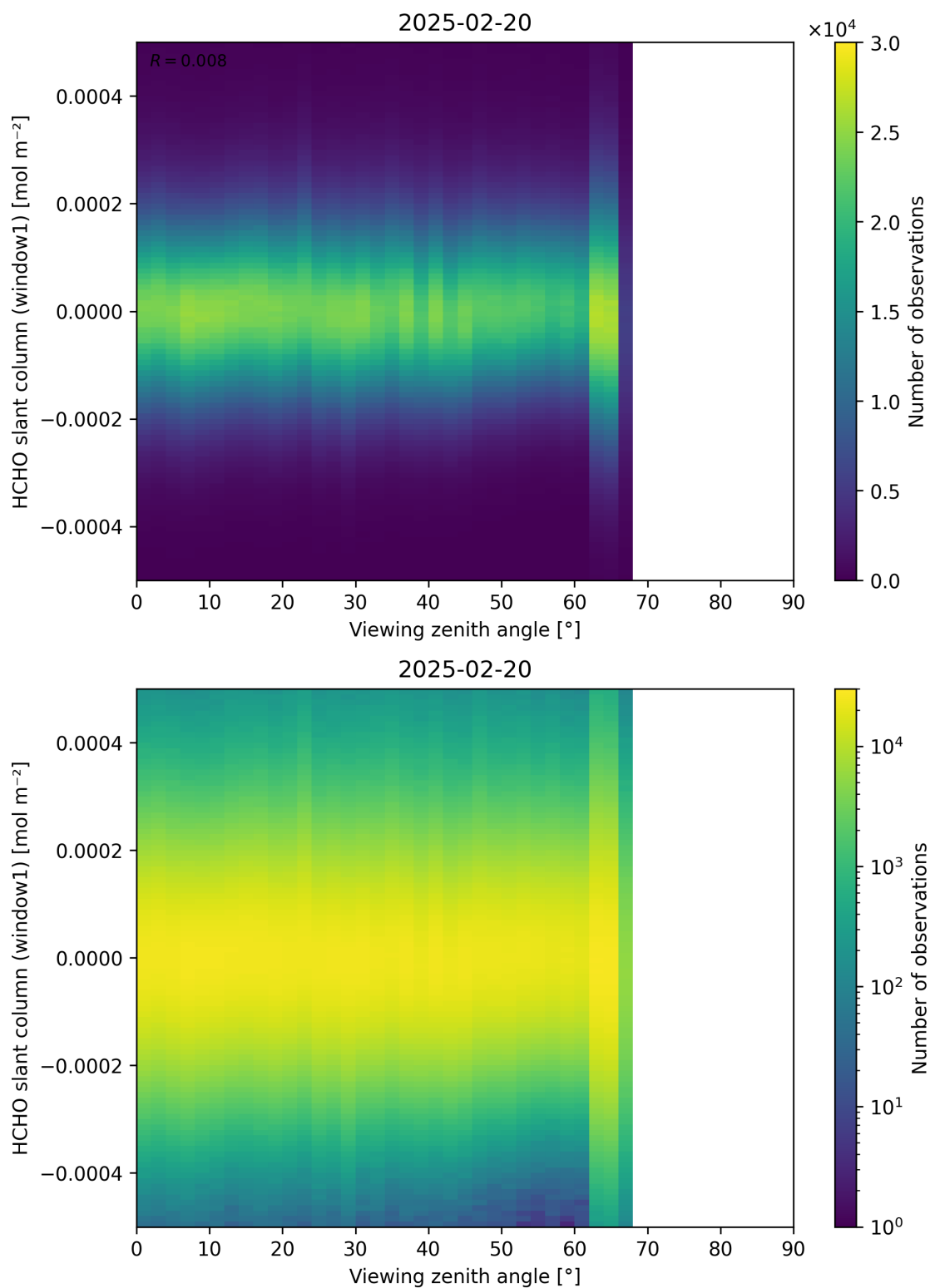
Figure 188: Scatter density plot of “Viewing zenith angle” against “HCHO slant column (window1)” for 2025-02-19 to 2025-02-21.
