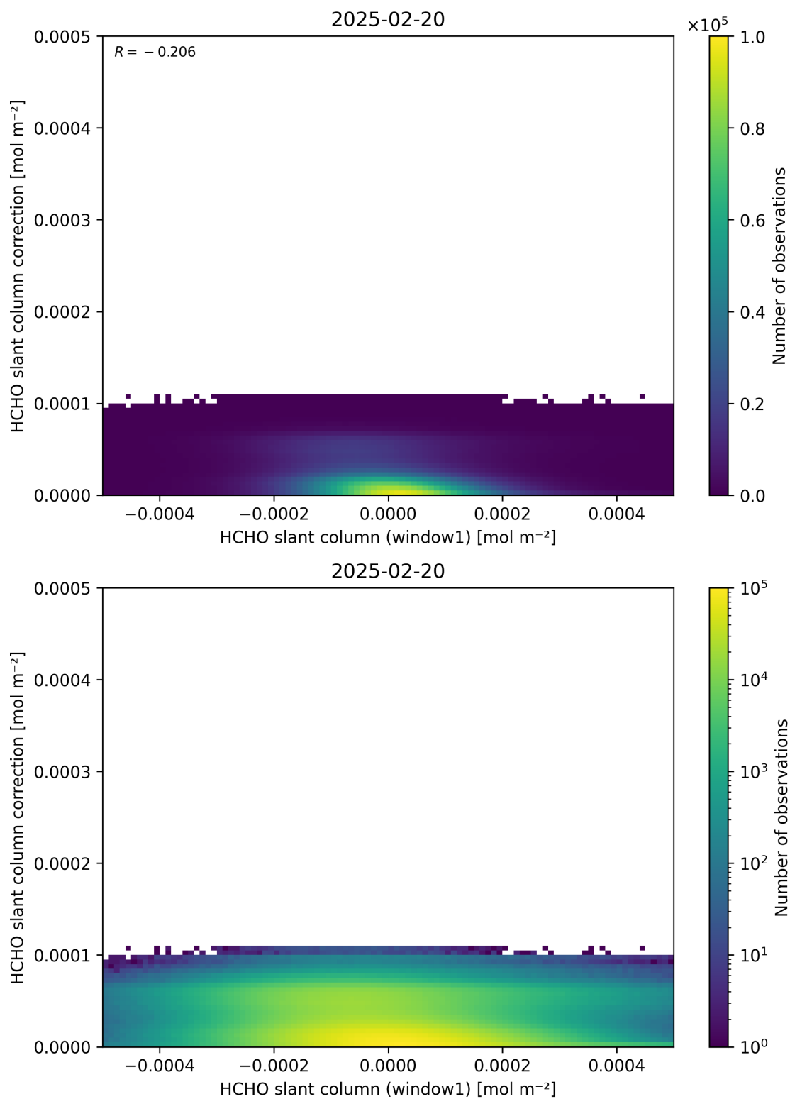
Figure 83: Scatter density plot of “HCHO slant column (window1)” against “HCHO slant column correction” for 2025-02-19 to 2025-02-21.
