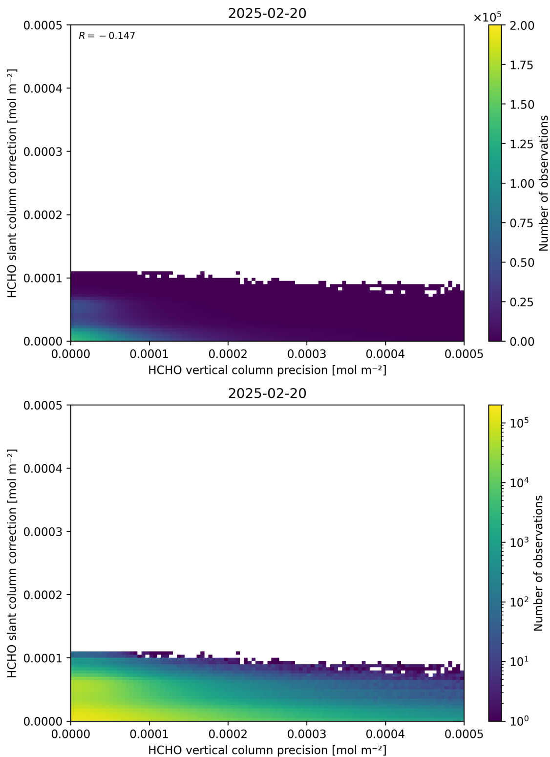
Figure 141: Scatter density plot of “HCHO vertical column precision” against “HCHO slant column correction” for 2025-02-19 to 2025-02-21.
