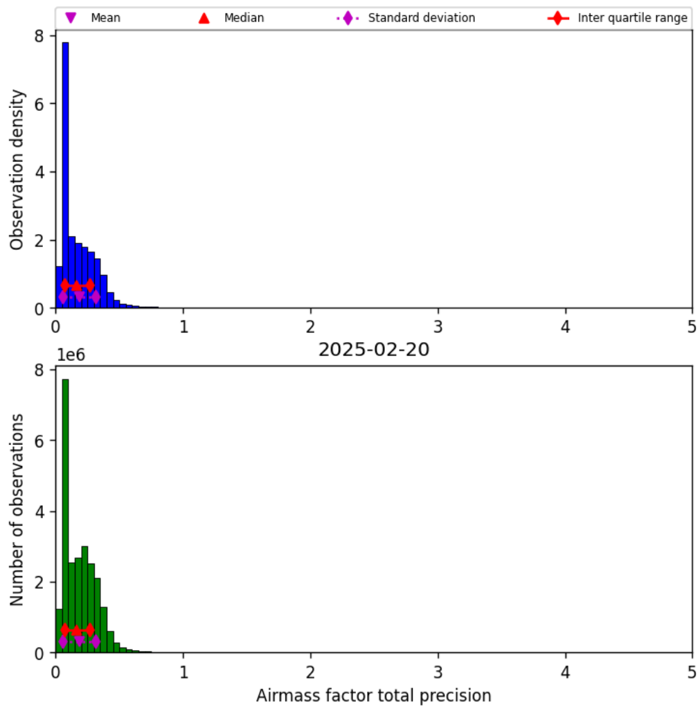
Figure 41: Histogram of “Airmass factor total precision” for 2025-02-19 to 2025-02-21
