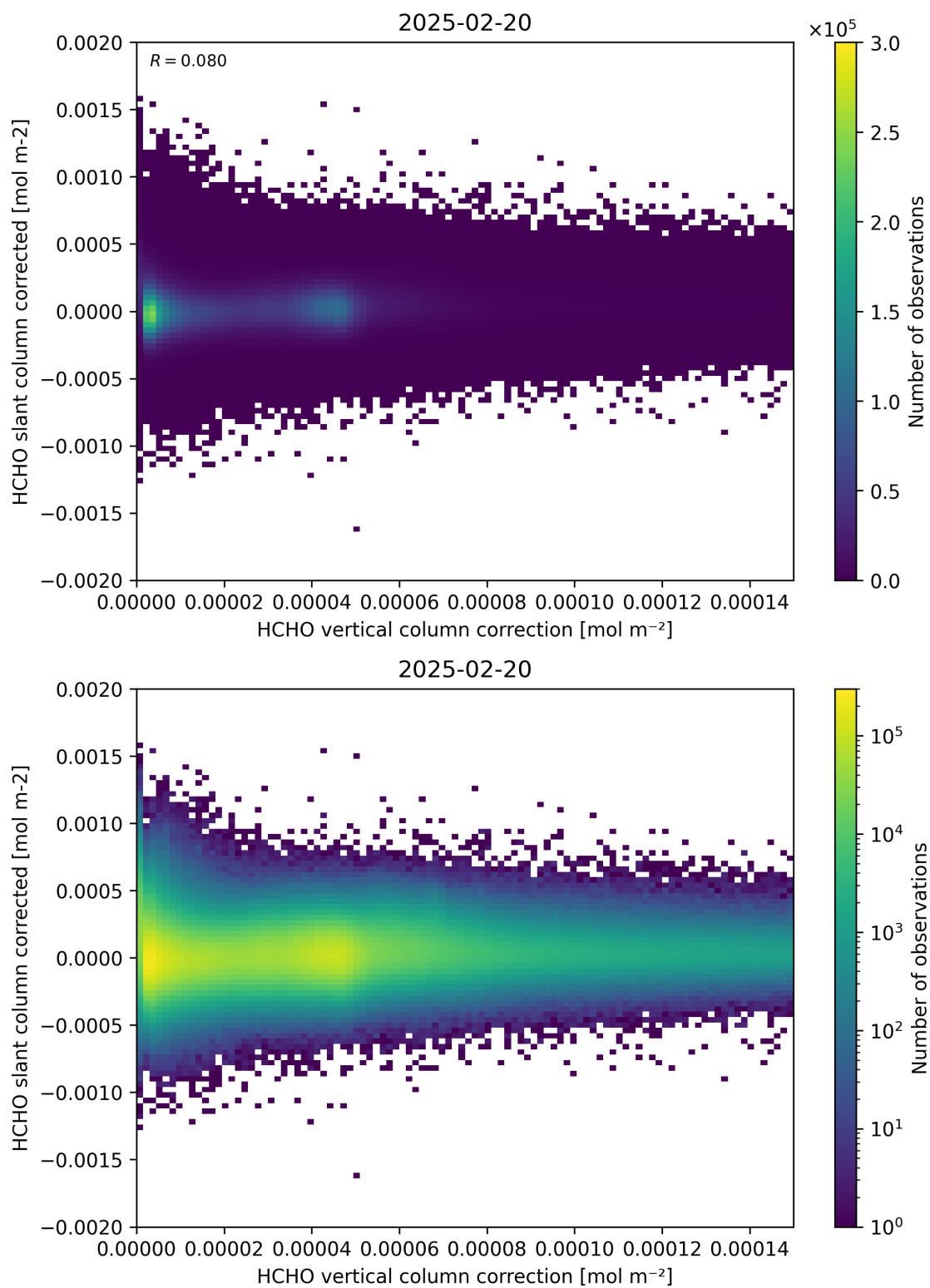
Figure 116: Scatter density plot of “HCHO vertical column correction” against “HCHO slant column corrected” for 2025-02-19 to 2025-02-21.
