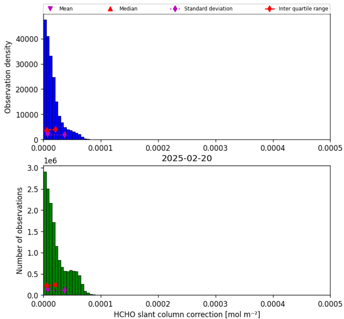
Figure 47: Histogram of “HCHO slant column correction” for 2025-02-19 to 2025-02-21
