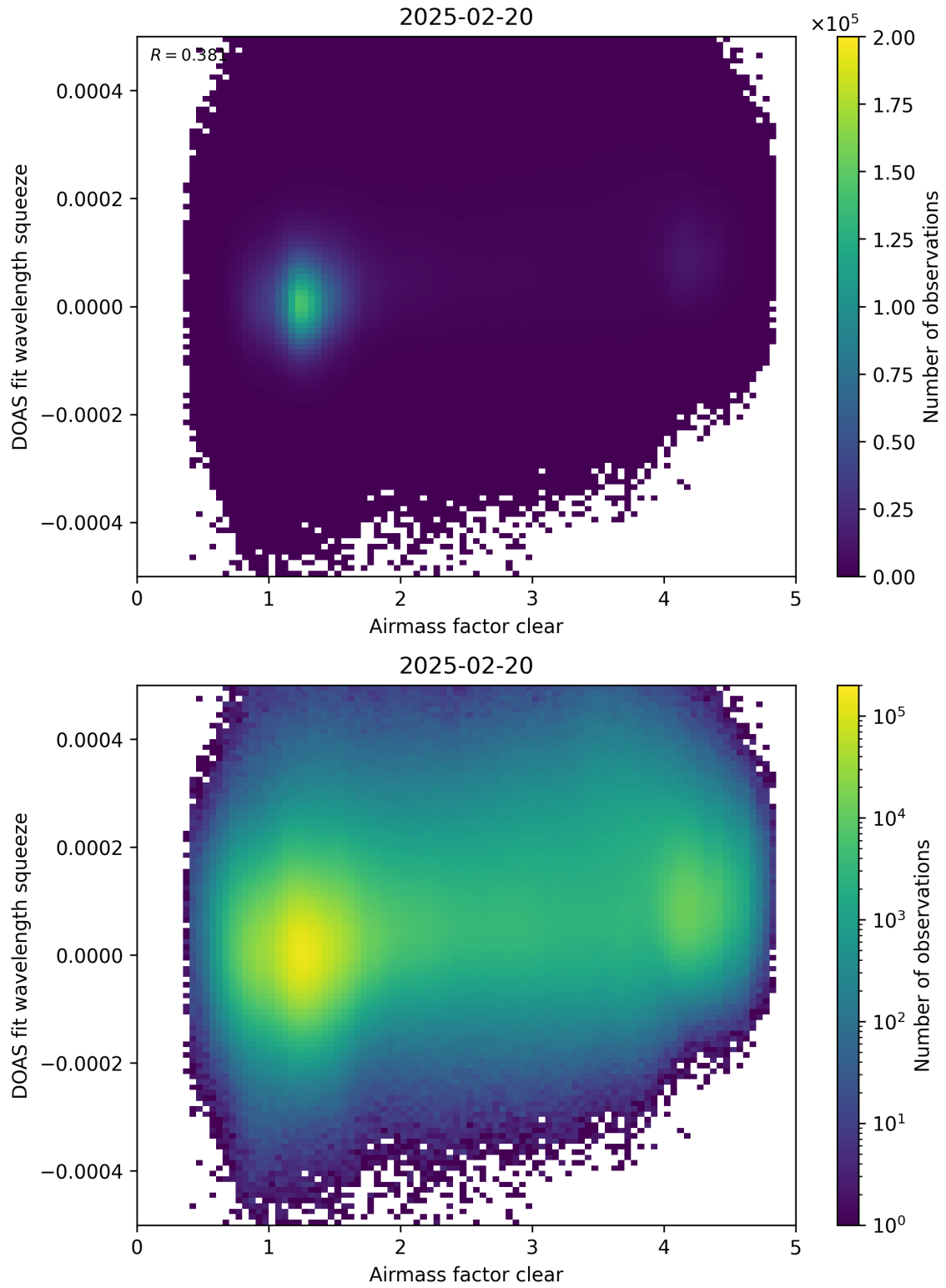
Figure 73: Scatter density plot of “Airmass factor clear” against “DOAS fit wavelength squeeze” for 2025-02-19 to 2025-02-21.
