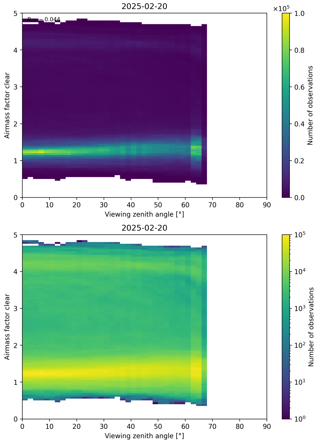
Figure 185: Scatter density plot of “Viewing zenith angle” against “Airmass factor clear” for 2025-02-19 to 2025-02-21.
