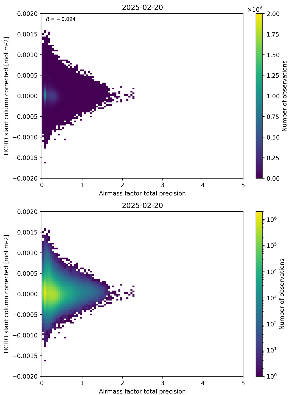
Figure 109: Scatter density plot of “Airmass factor total precision” against “HCHO slant column corrected” for 2025-02-19 to 2025-02-21.
