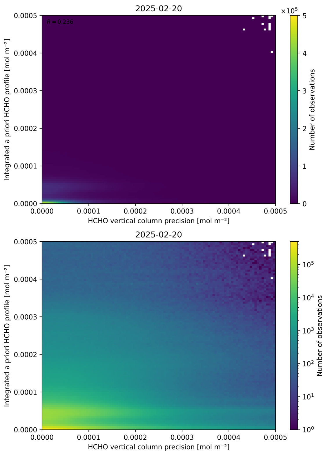
Figure 147: Scatter density plot of “HCHO vertical column precision” against “Integrated a priori HCHO profile” for 2025-02-19 to 2025-02-21.
