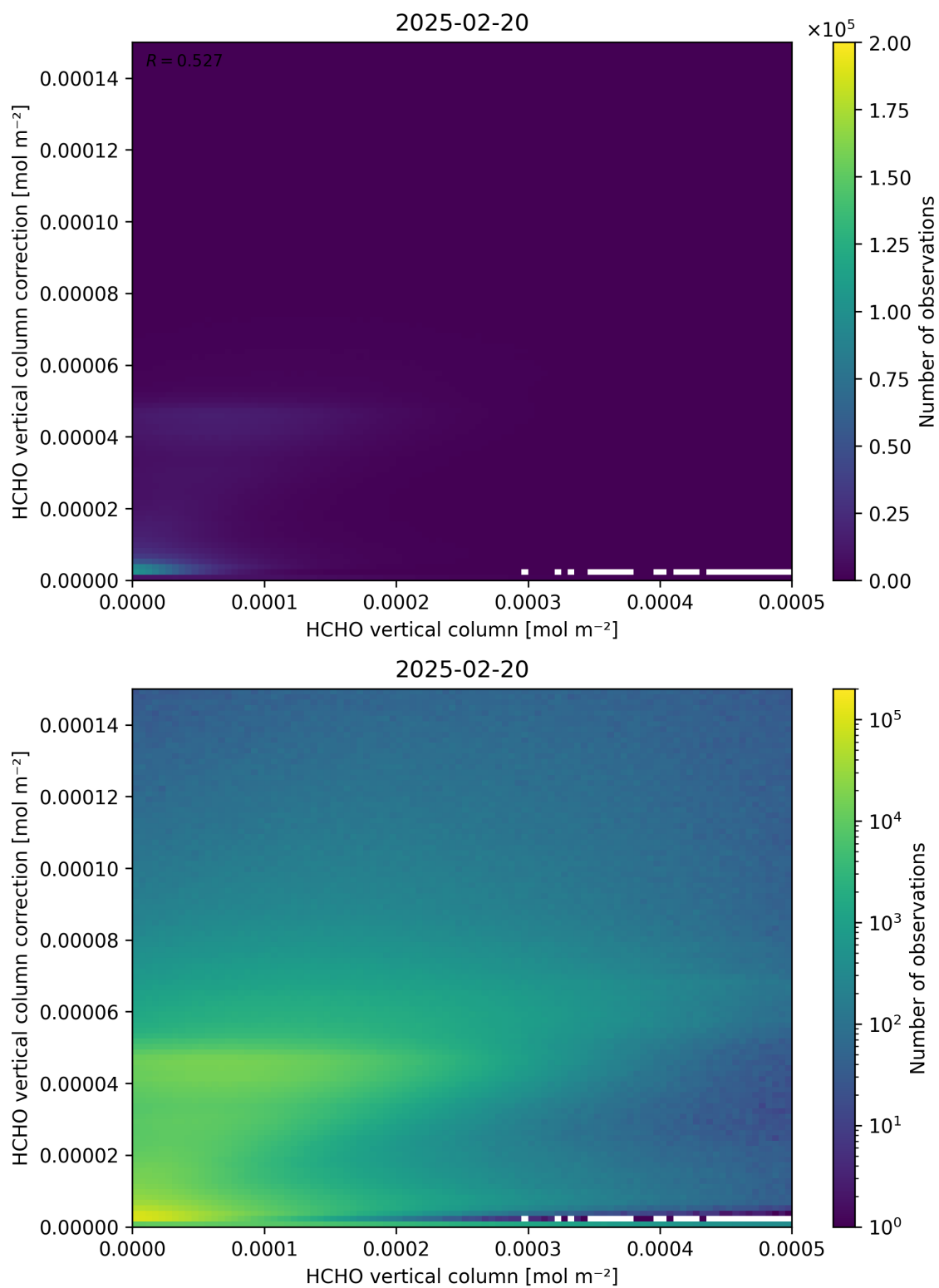
Figure 133: Scatter density plot of “HCHO vertical column” against “HCHO vertical column correction” for 2025-02-19 to 2025-02-21.
