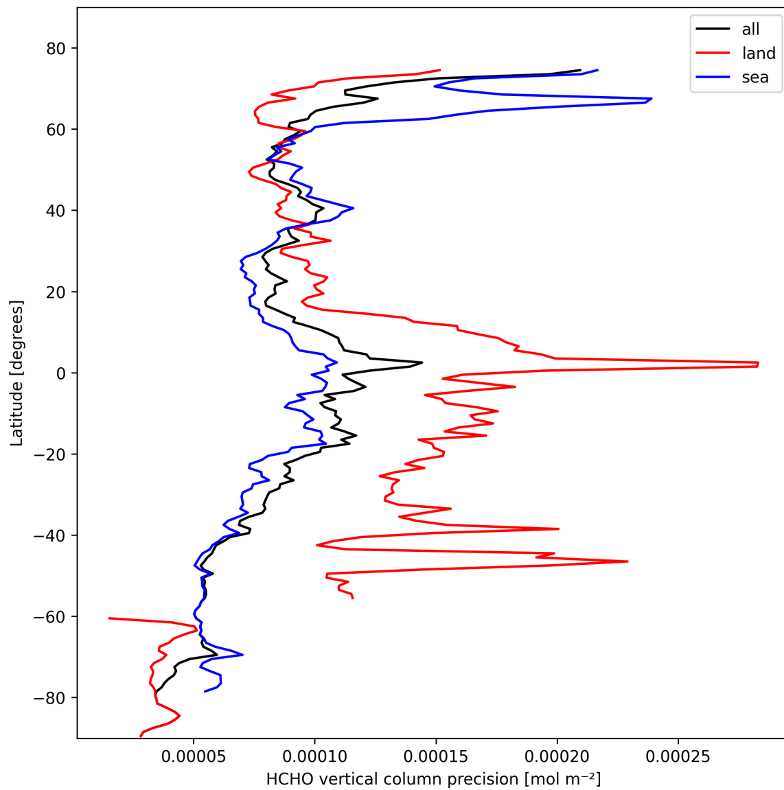
Figure 22: Zonal average of “HCHO vertical column precision” for 2025-02-19 to 2025-02-21.
