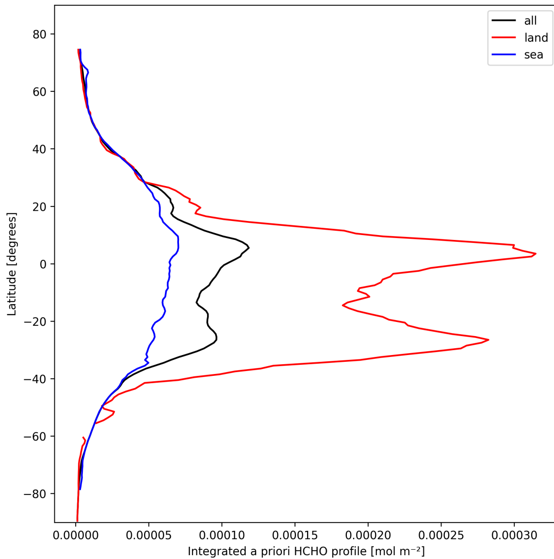
Figure 29: Zonal average of “Integrated a priori HCHO profile” for 2025-02-19 to 2025-02-21.
