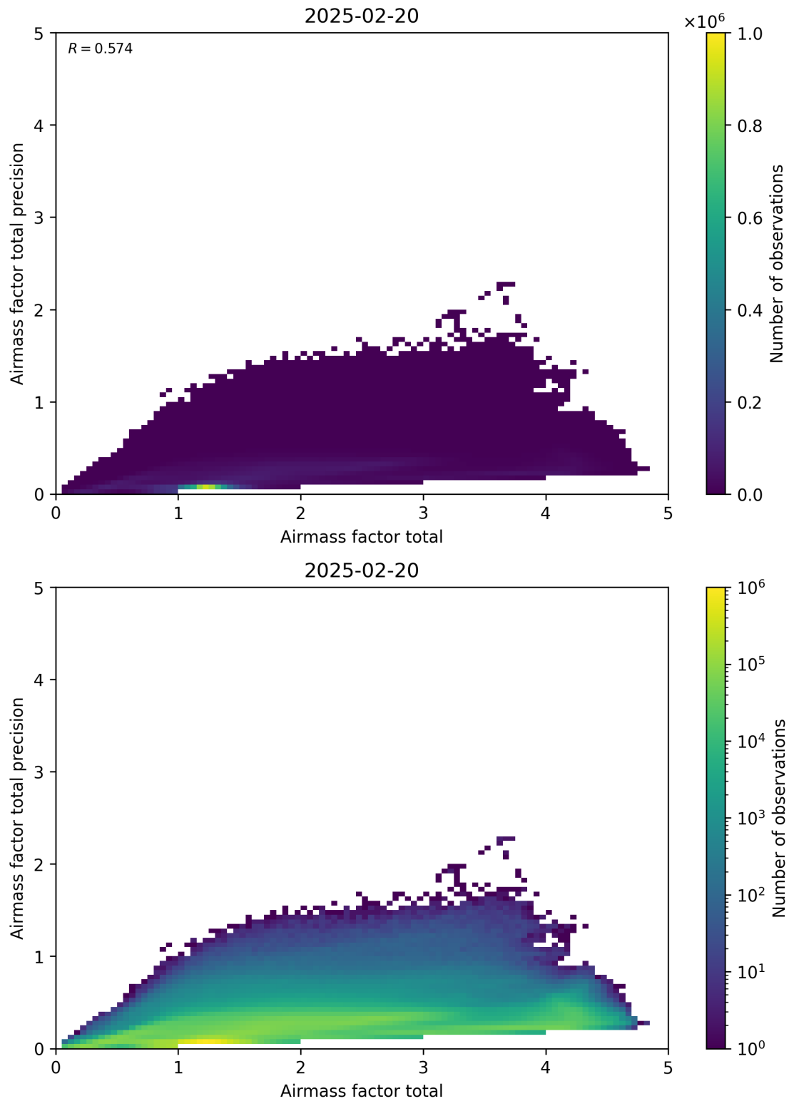
Figure 103: Scatter density plot of “Airmass factor total” against “Airmass factor total precision” for 2025-02-19 to 2025-02-21.
