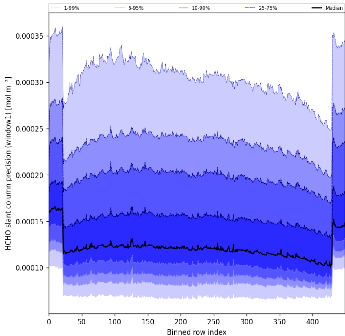
Figure 53: Along track statistics of “HCHO slant column precision (window1)” for 2025-02-19 to 2025-02-21
