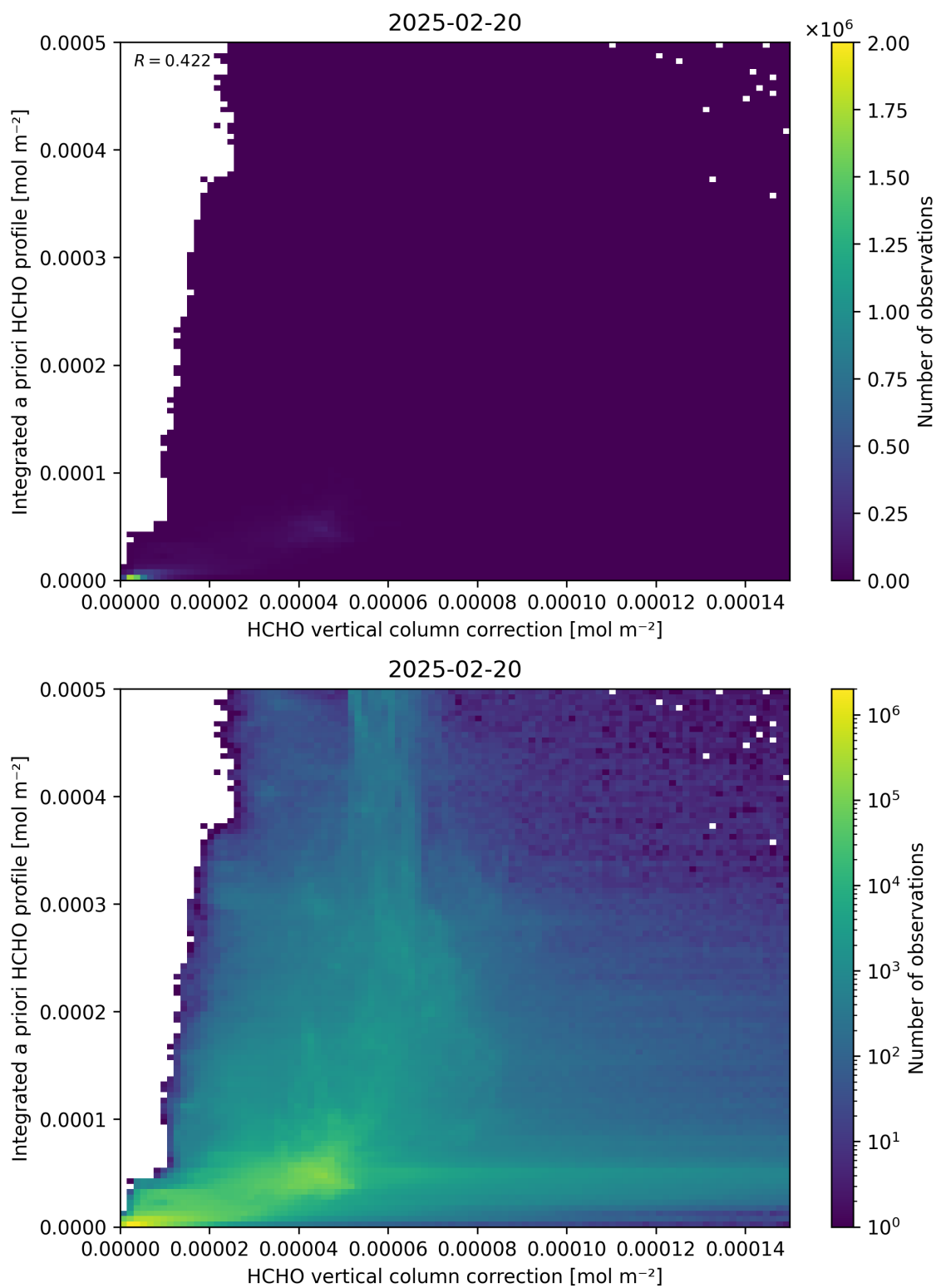
Figure 122: Scatter density plot of “HCHO vertical column correction” against “Integrated a priori HCHO profile” for 2025-02-19 to 2025-02-21.
