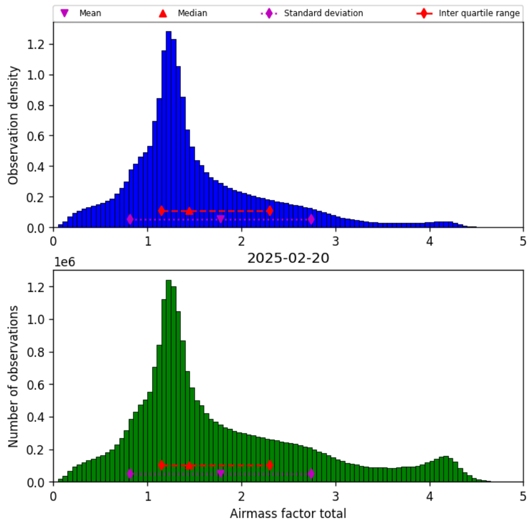
Figure 40: Histogram of “Airmass factor total” for 2025-02-19 to 2025-02-21
