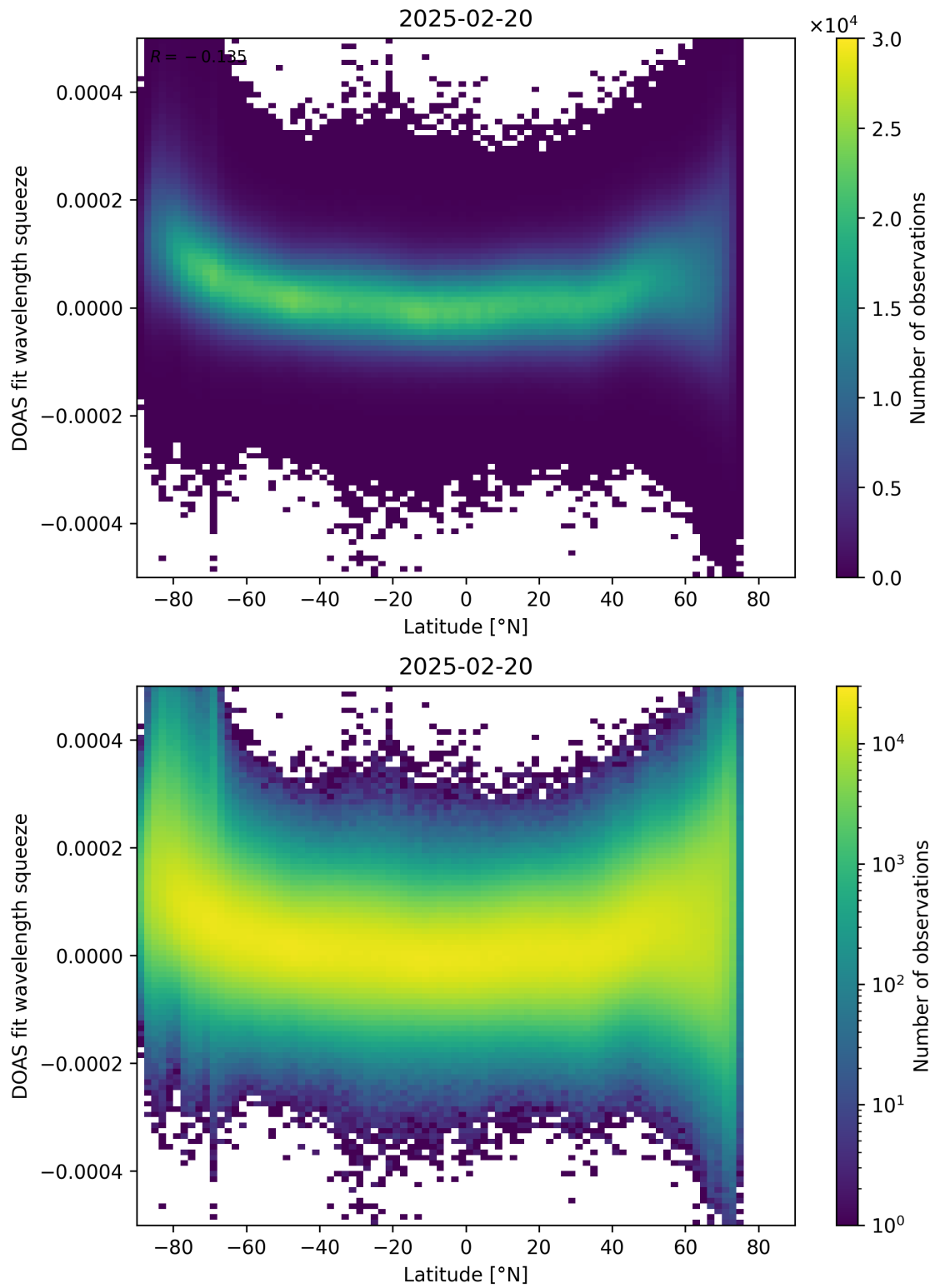
Figure 155: Scatter density plot of “Latitude” against “DOAS fit wavelength squeeze” for 2025-02-19 to 2025-02-21.
