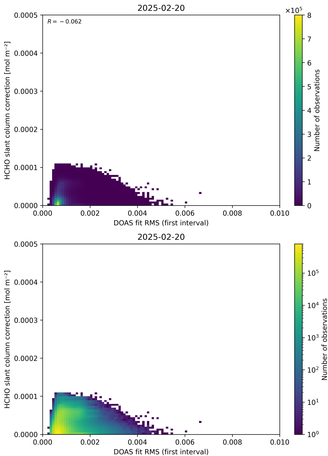
Figure 63: Scatter density plot of “DOAS fit RMS (first interval)” against “HCHO slant column correction” for 2025-02-19 to 2025-02-21.
