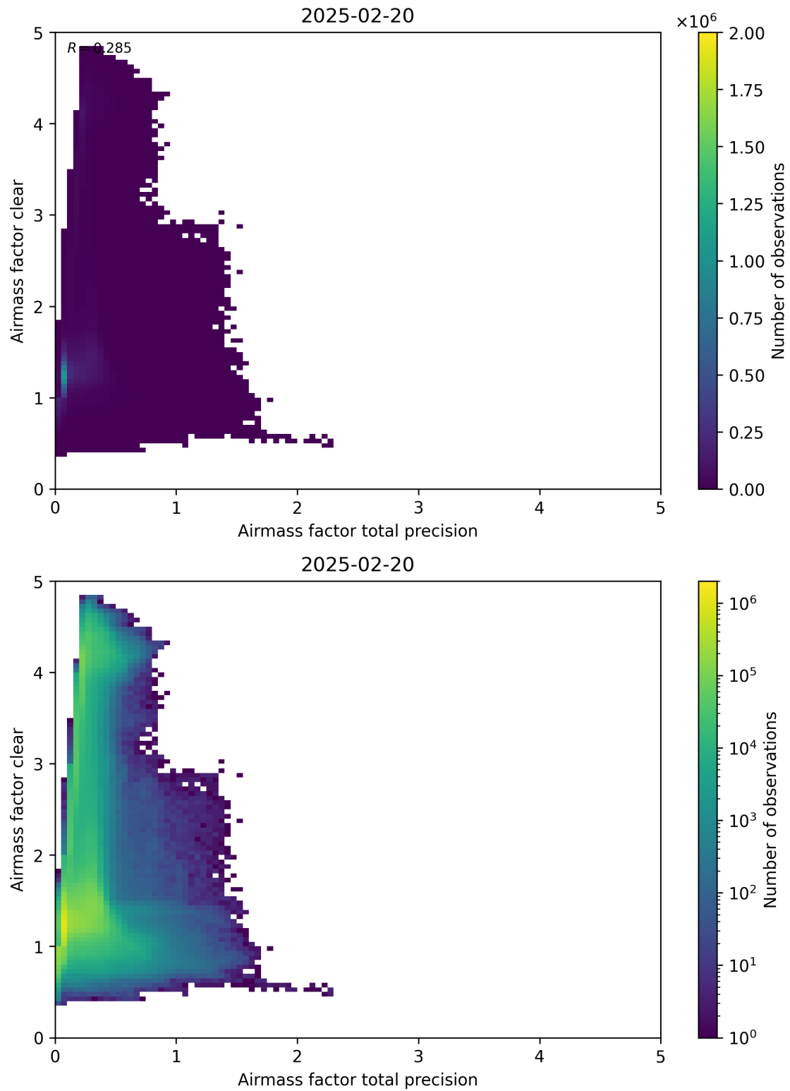
Figure 108: Scatter density plot of “Airmass factor total precision” against “Airmass factor clear” for 2025-02-19 to 2025-02-21.
