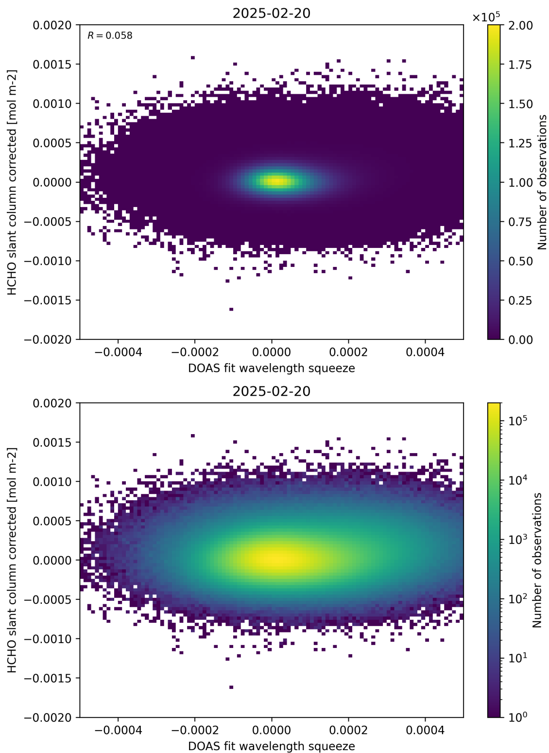
Figure 69: Scatter density plot of “DOAS fit wavelength squeeze” against “HCHO slant column corrected” for 2025-02-19 to 2025-02-21.
