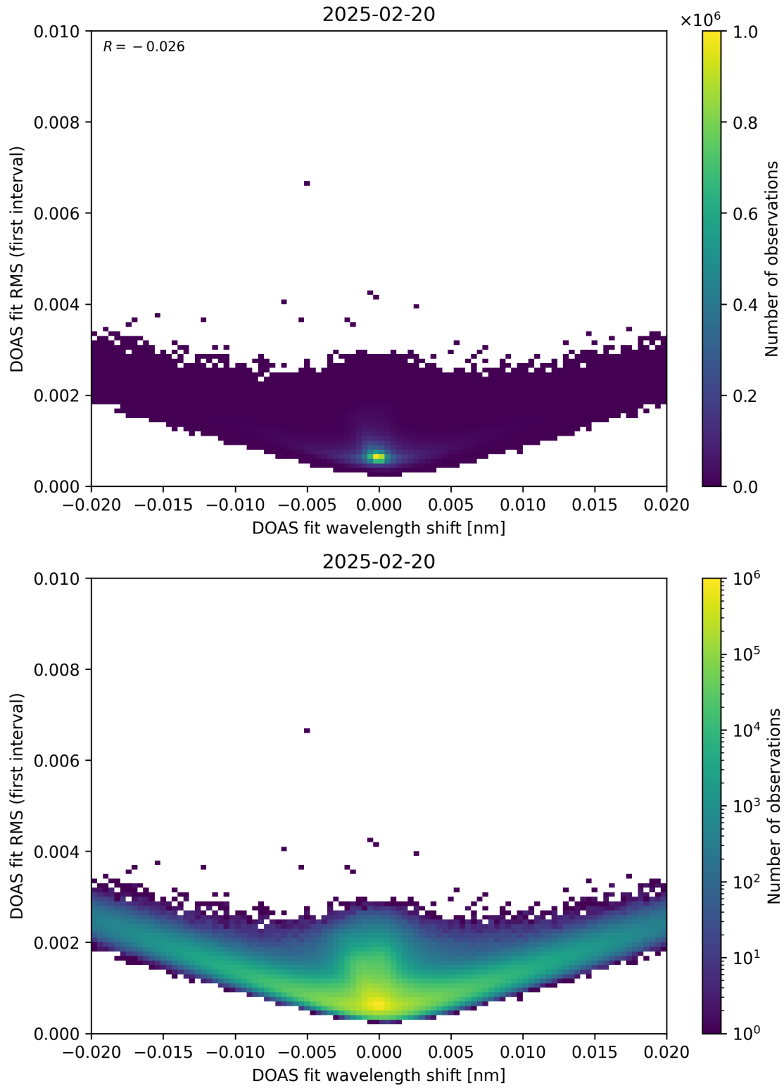
Figure 64: Scatter density plot of “DOAS fit wavelength shift” against “DOAS fit RMS (first interval)” for 2025-02-19 to 2025-02-21.
