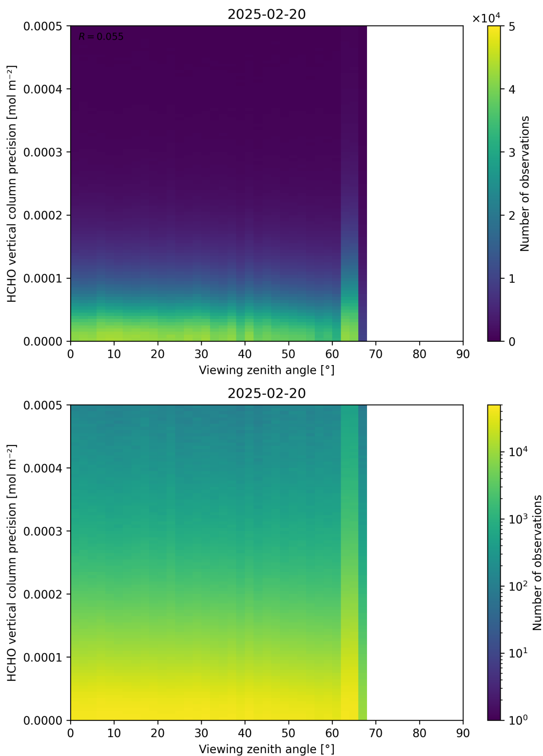
Figure 194: Scatter density plot of “Viewing zenith angle” against “HCHO vertical column precision” for 2025-02-19 to 2025-02-21.
