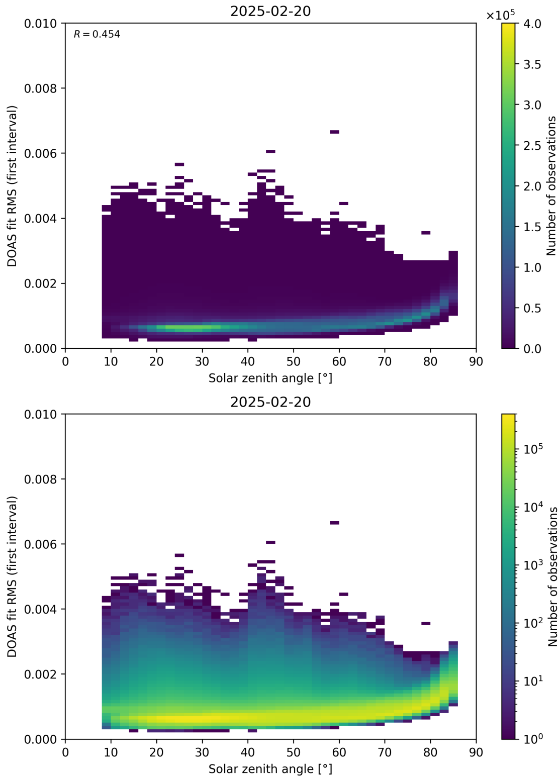
Figure 167: Scatter density plot of “Solar zenith angle” against “DOAS fit RMS (first interval)” for 2025-02-19 to 2025-02-21.
