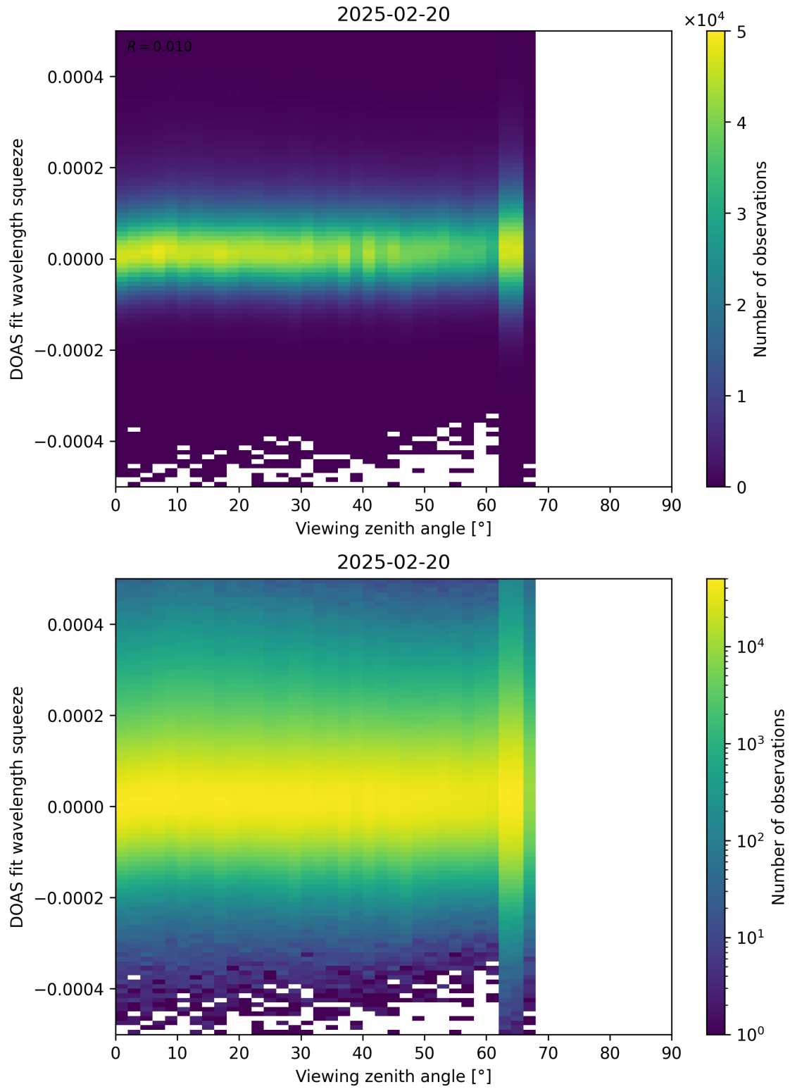
Figure 184: Scatter density plot of “Viewing zenith angle” against “DOAS fit wavelength squeeze” for 2025-02-19 to 2025-02-21.
