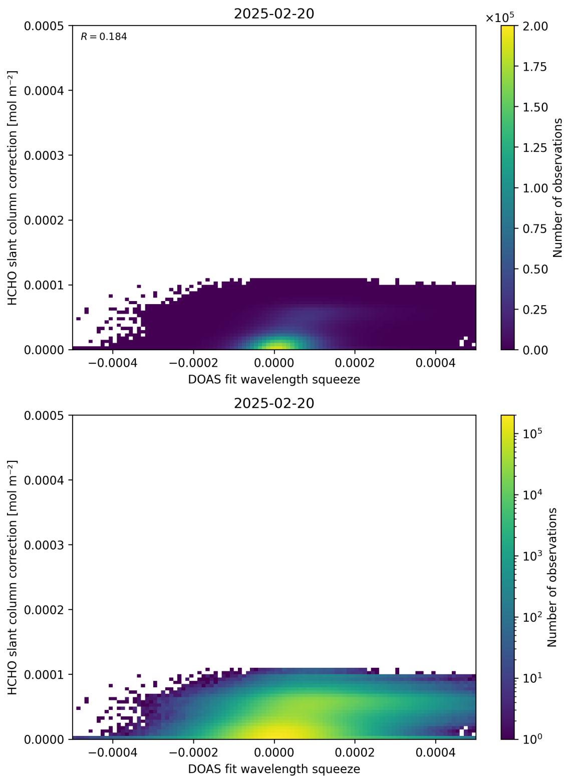
Figure 70: Scatter density plot of “DOAS fit wavelength squeeze” against “HCHO slant column correction” for 2025-02-19 to 2025-02-21.
