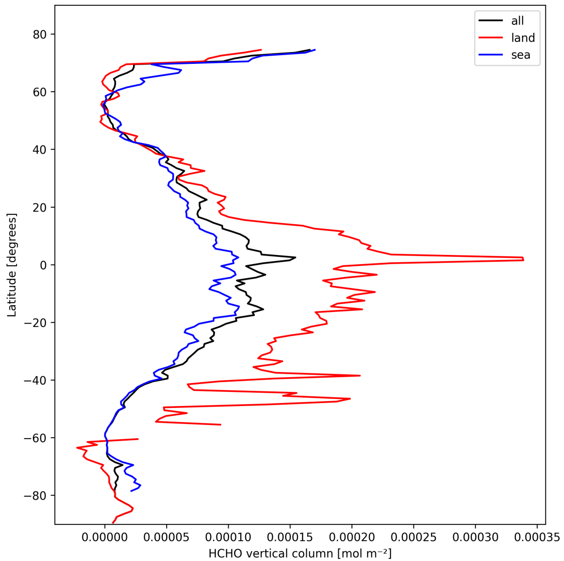
Figure 21: Zonal average of “HCHO vertical column” for 2025-02-19 to 2025-02-21.
