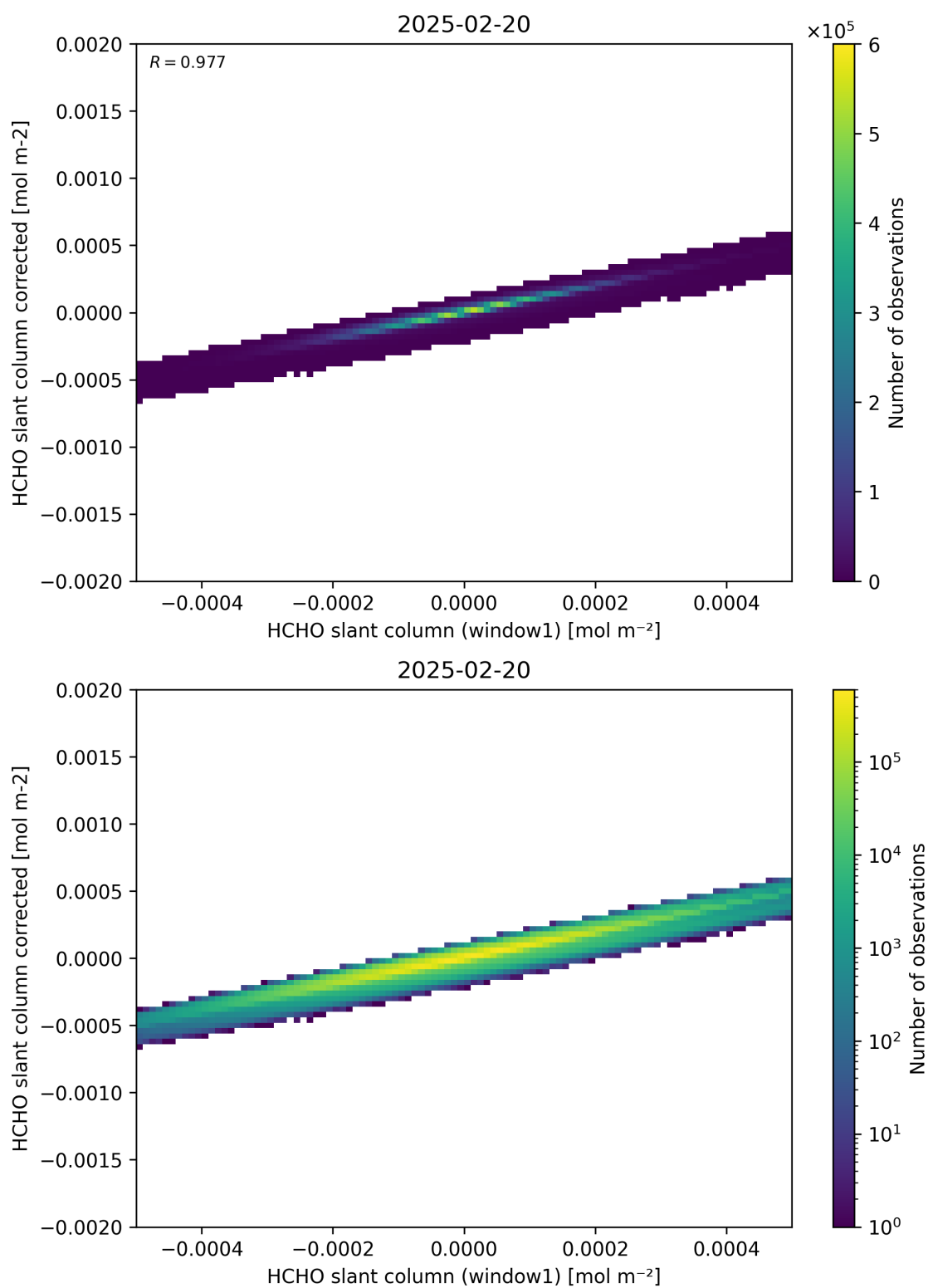
Figure 82: Scatter density plot of “HCHO slant column (window1)” against “HCHO slant column corrected” for 2025-02-19 to 2025-02-21.
