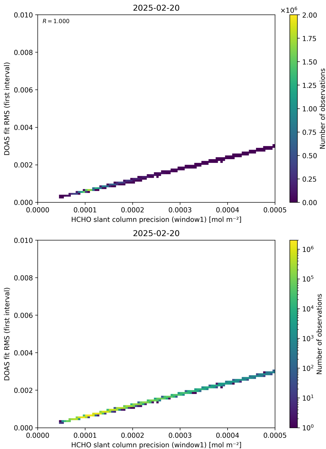
Figure 88: Scatter density plot of “HCHO slant column precision (window1)” against “DOAS fit RMS (first interval)” for 2025-02-19 to 2025-02-21.
