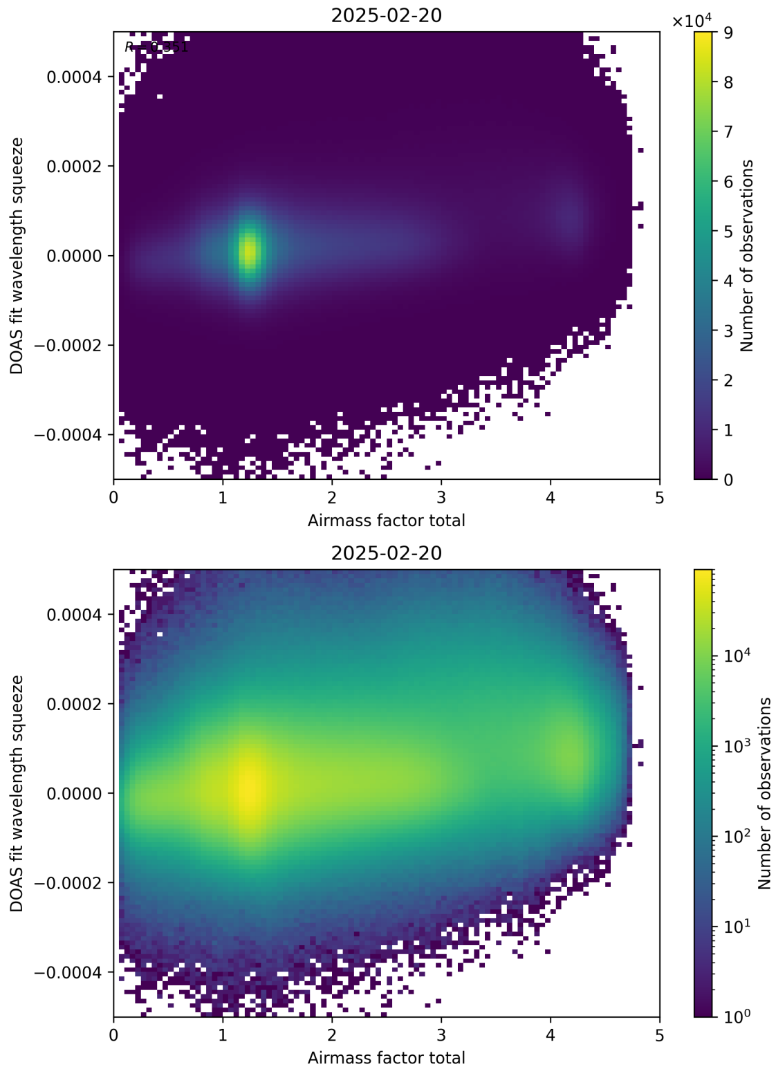
Figure 99: Scatter density plot of “Airmass factor total” against “DOAS fit wavelength squeeze” for 2025-02-19 to 2025-02-21.
