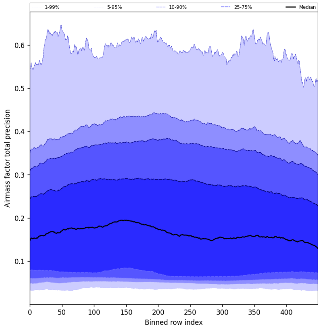
Figure 55: Along track statistics of “Airmass factor total precision” for 2025-02-19 to 2025-02-21
