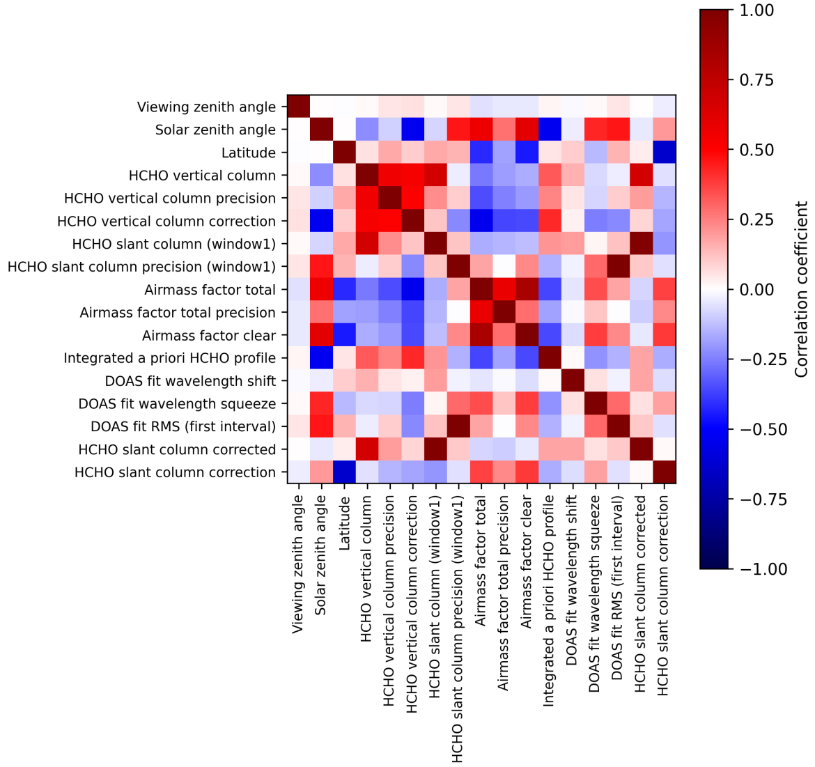
Figure 2: Map of correlation matrix for 2025-02-19 to 2025-02-21.
