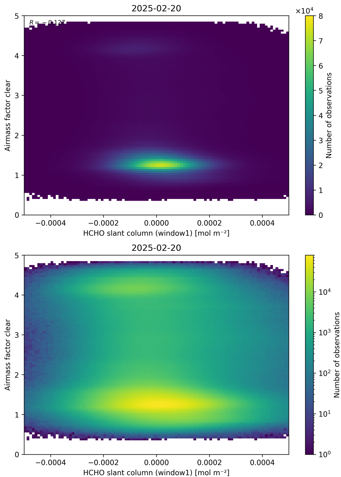
Figure 81: Scatter density plot of “HCHO slant column (window1)” against “Airmass factor clear” for 2025-02-19 to 2025-02-21.
