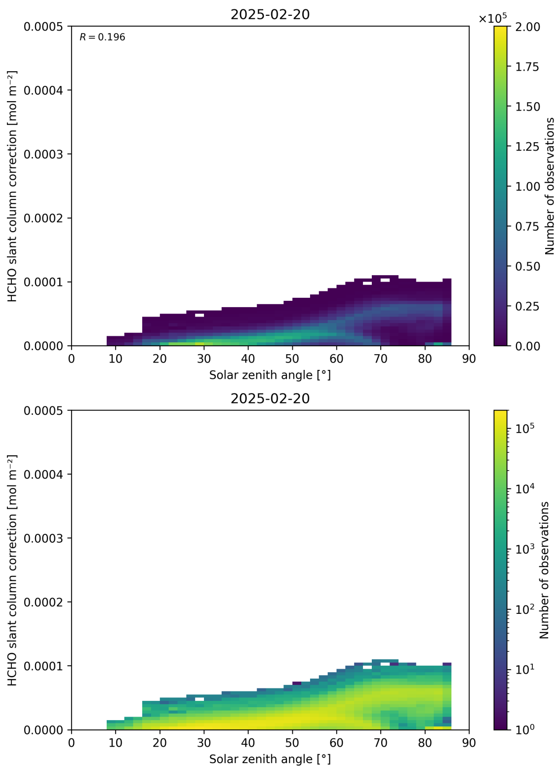
Figure 172: Scatter density plot of “Solar zenith angle” against “HCHO slant column correction” for 2025-02-19 to 2025-02-21.
