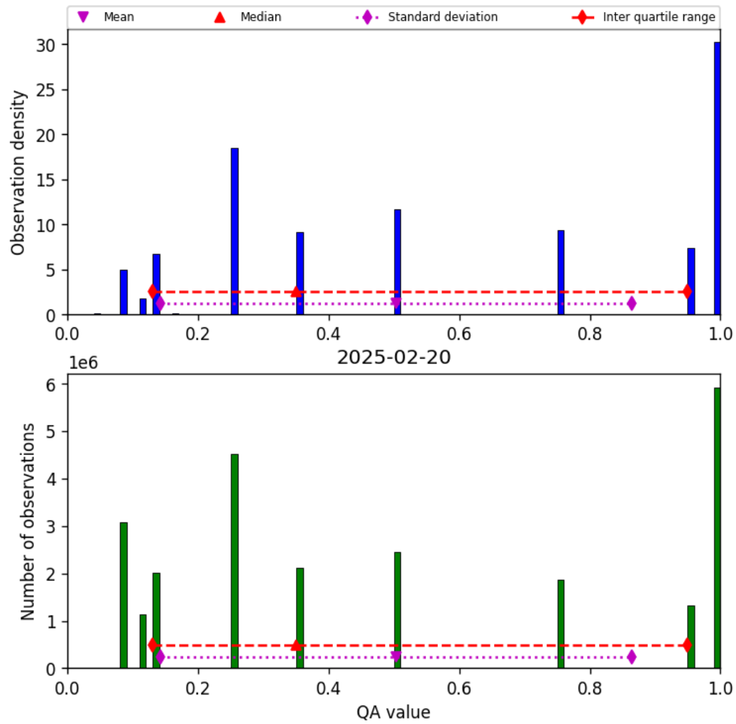
Figure 34: Histogram of “QA value” for 2025-02-19 to 2025-02-21
