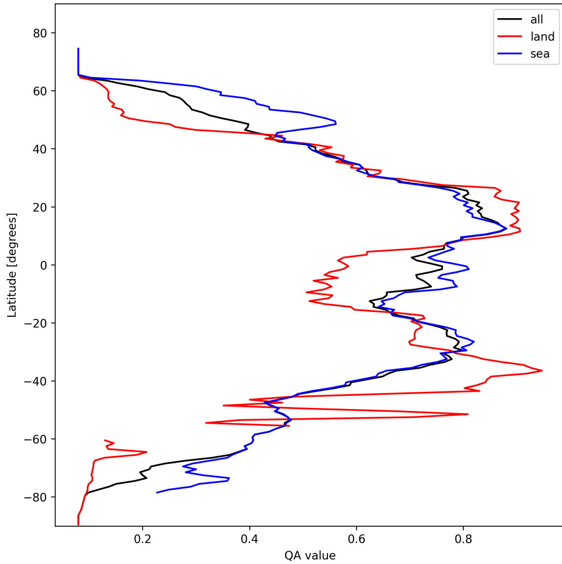
Figure 20: Zonal average of “QA value” for 2025-02-19 to 2025-02-21.
