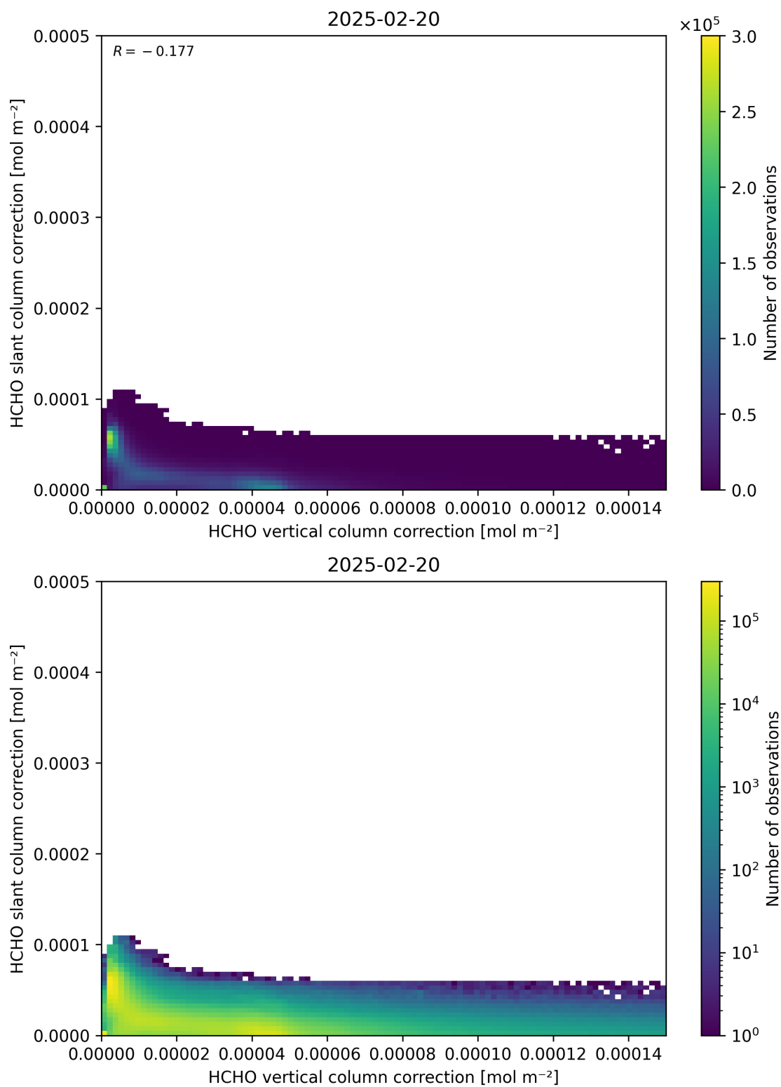
Figure 117: Scatter density plot of “HCHO vertical column correction” against “HCHO slant column correction” for 2025-02-19 to 2025-02-21.
