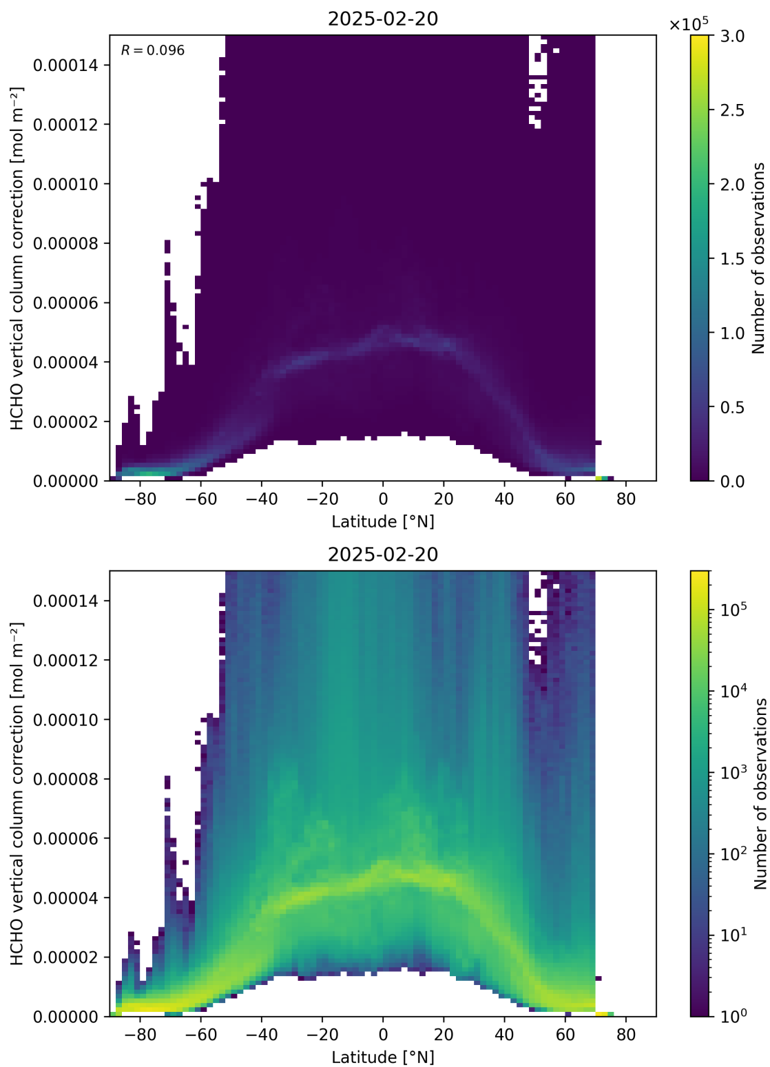
Figure 164: Scatter density plot of “Latitude” against “HCHO vertical column correction” for 2025-02-19 to 2025-02-21.
