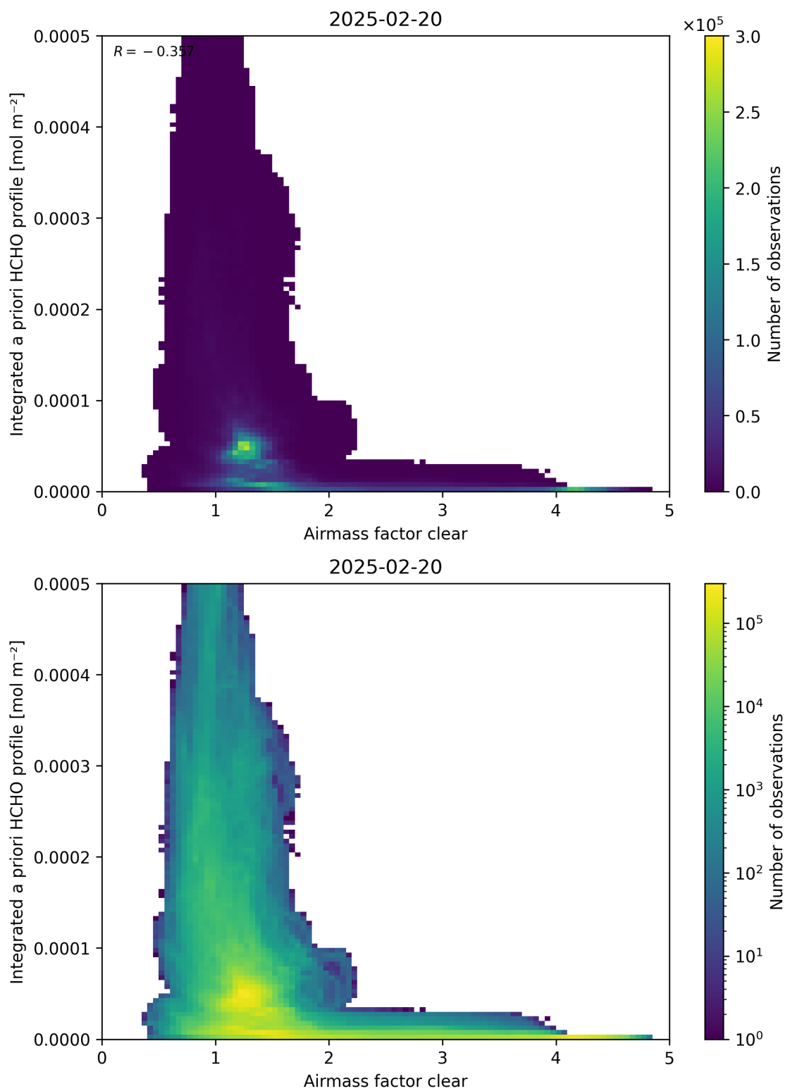
Figure 76: Scatter density plot of “Airmass factor clear” against “Integrated a priori HCHO profile” for 2025-02-19 to 2025-02-21.
