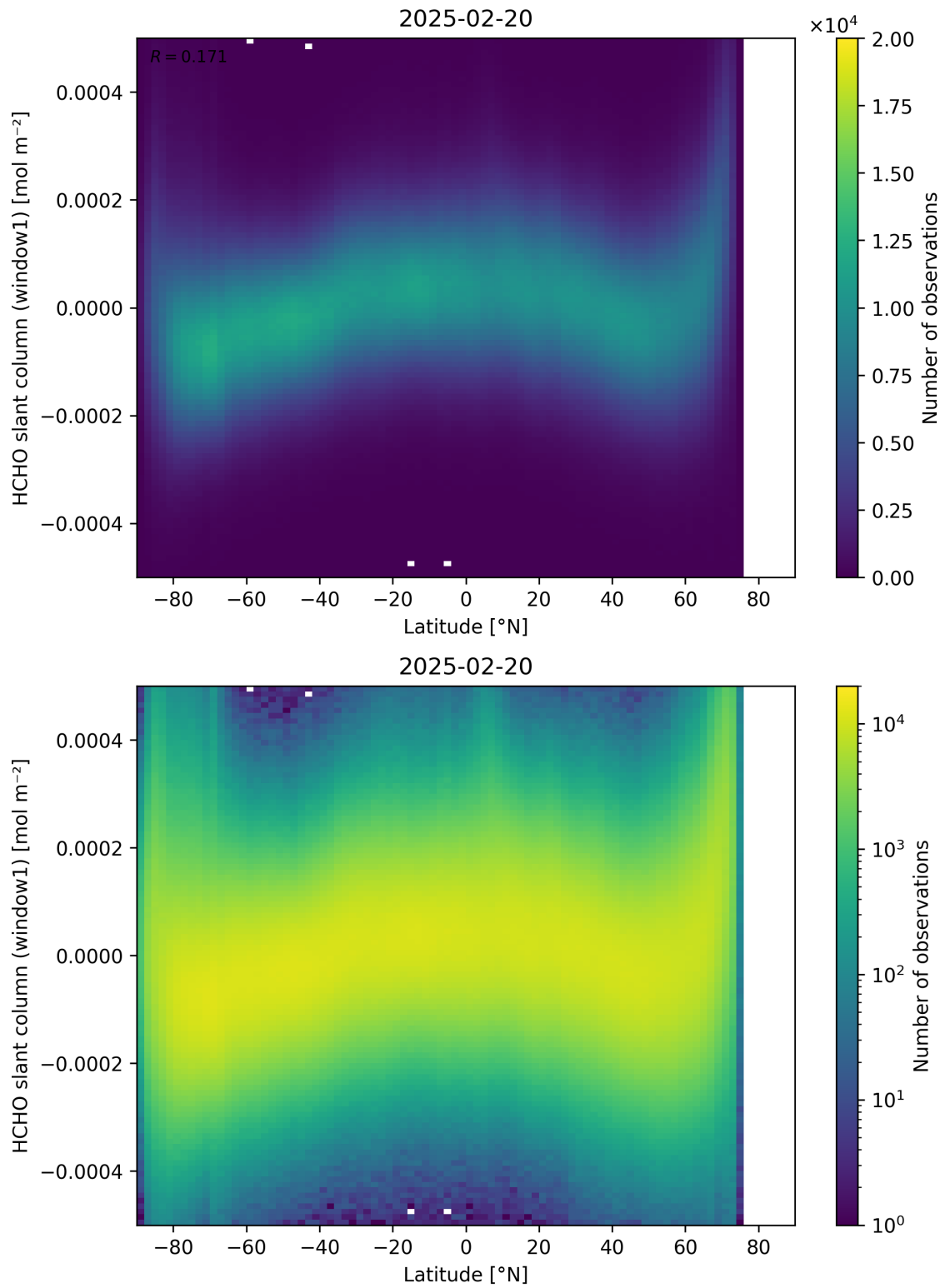
Figure 159: Scatter density plot of “Latitude” against “HCHO slant column (window1)” for 2025-02-19 to 2025-02-21.
