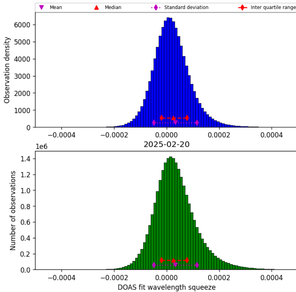
Figure 45: Histogram of “DOAS fit wavelength squeeze” for 2025-02-19 to 2025-02-21
