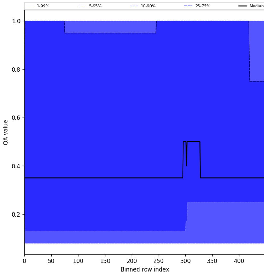
Figure 48: Along track statistics of “QA value” for 2025-02-19 to 2025-02-21
