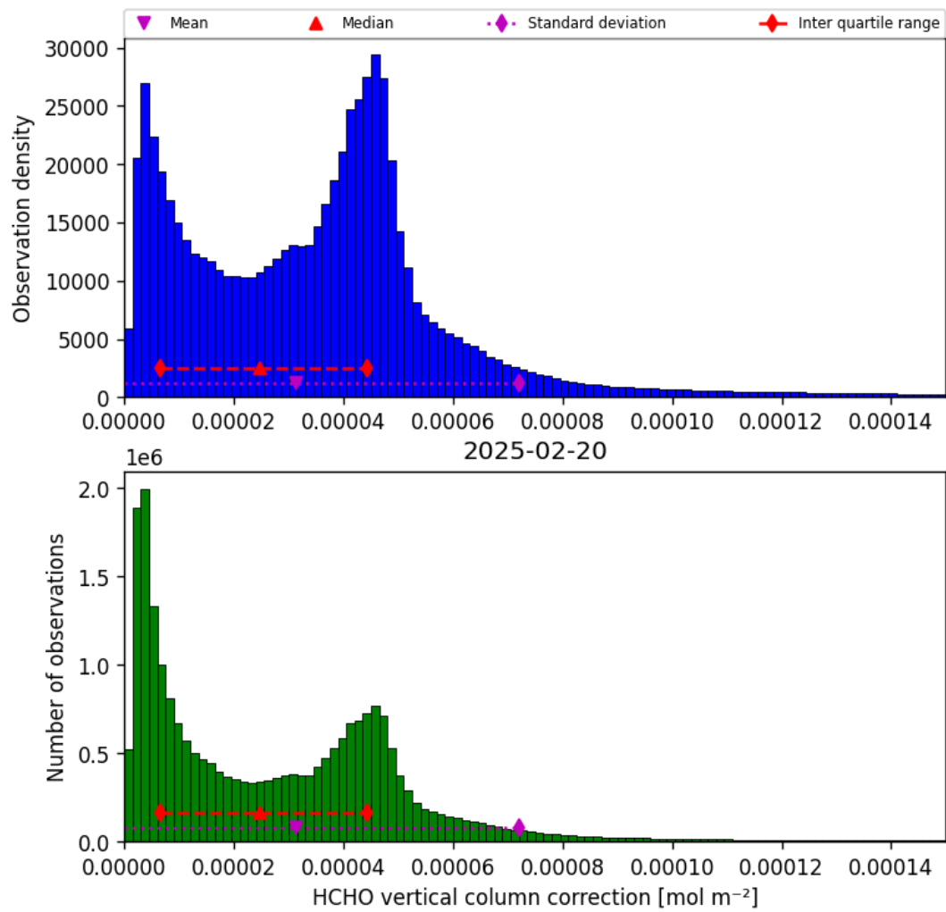
Figure 37: Histogram of “HCHO vertical column correction” for 2025-02-19 to 2025-02-21
