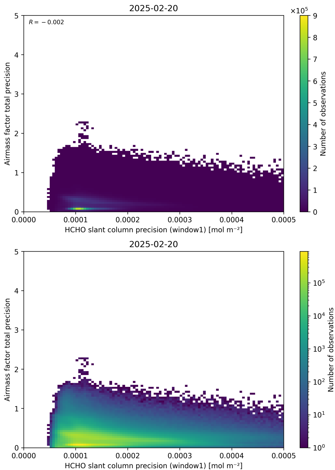
Figure 95: Scatter density plot of “HCHO slant column precision (window1)” against “Airmass factor total precision” for 2025-02-19 to 2025-02-21.
