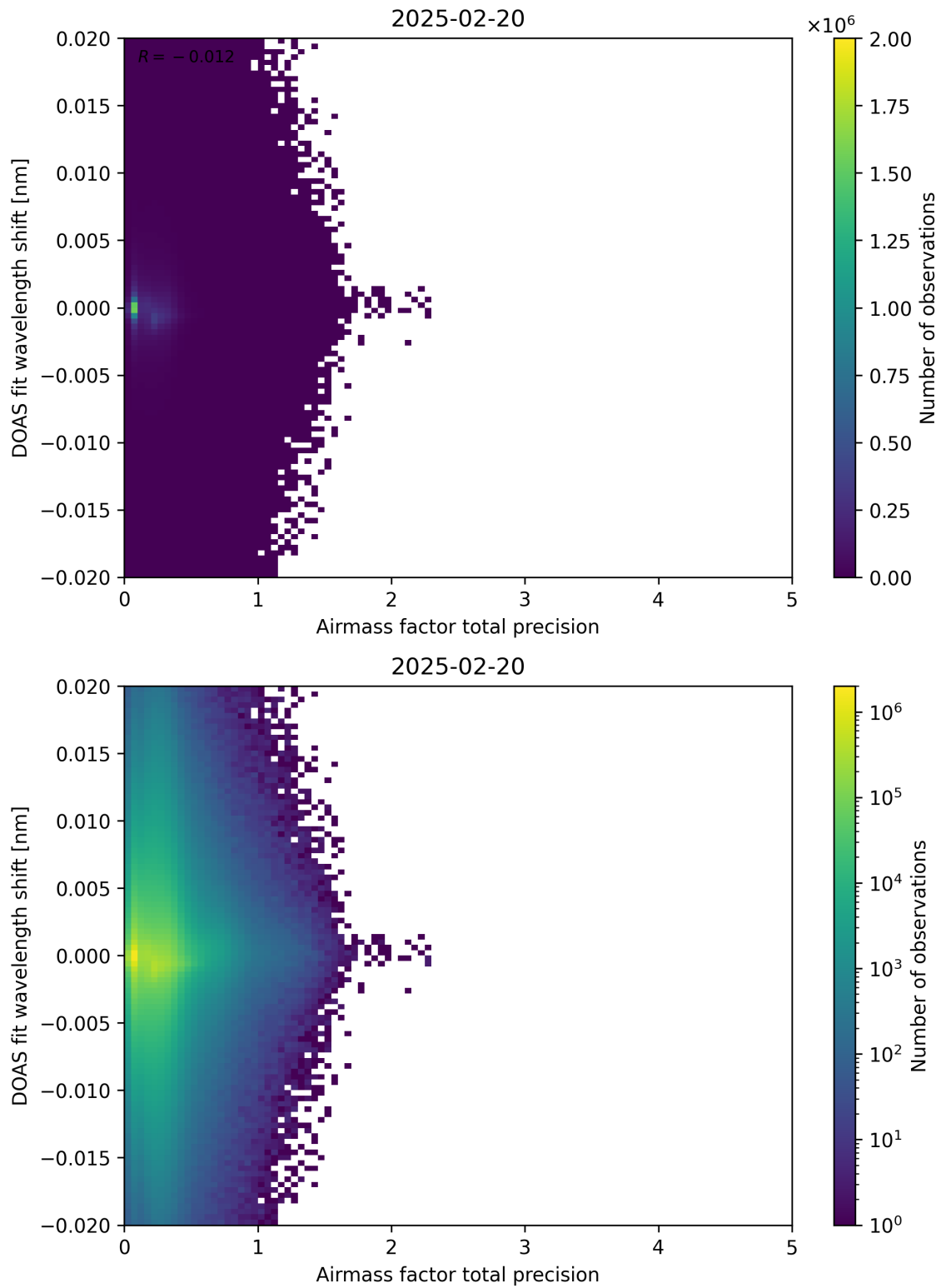
Figure 106: Scatter density plot of “Airmass factor total precision” against “DOAS fit wavelength shift” for 2025-02-19 to 2025-02-21.
