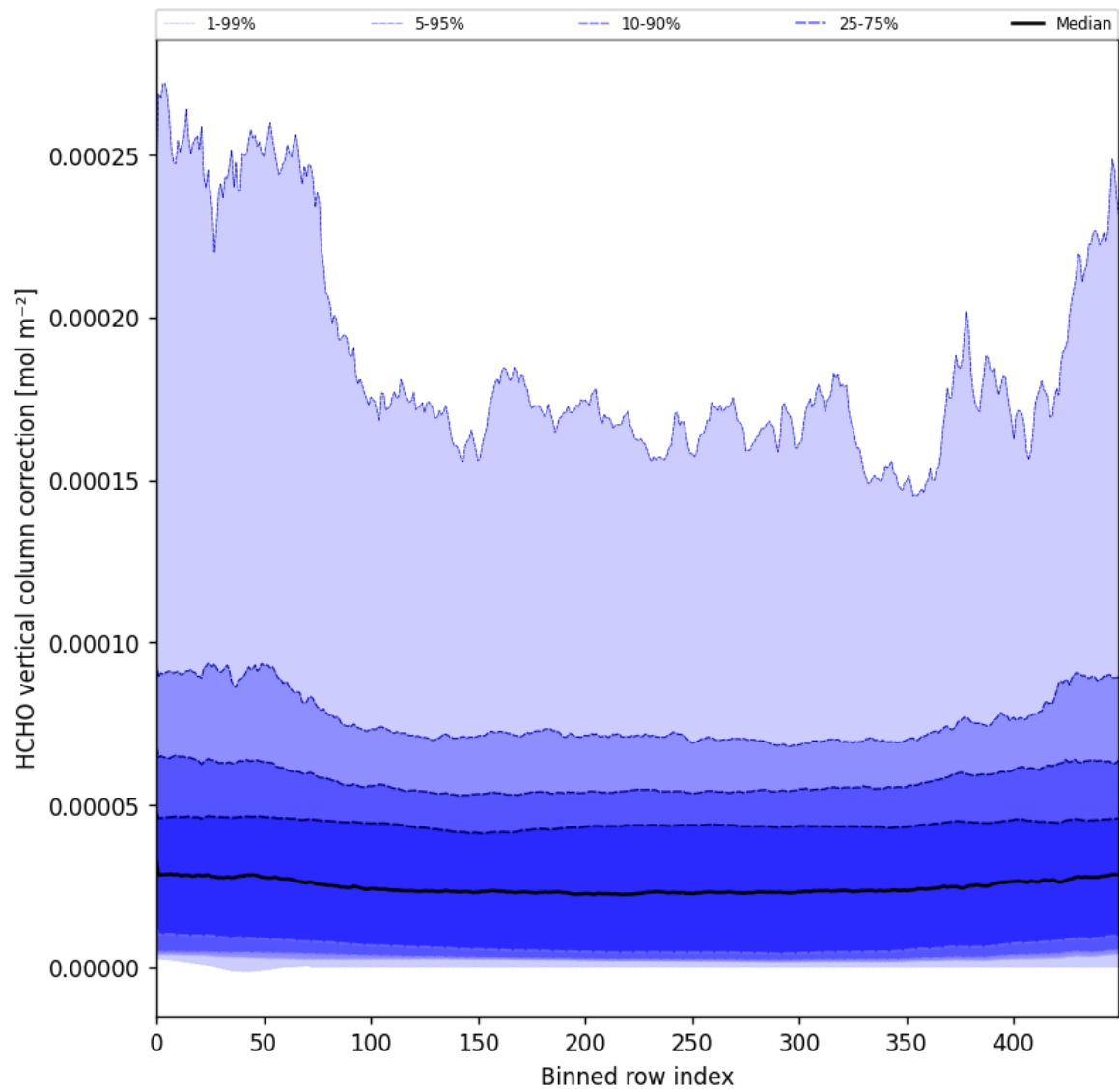
Figure 51: Along track statistics of “HCHO vertical column correction” for 2025-02-19 to 2025-02-21
