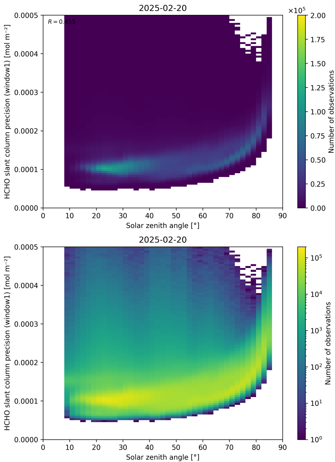
Figure 174: Scatter density plot of “Solar zenith angle” against “HCHO slant column precision (window1)” for 2025-02-19 to 2025-02-21.
