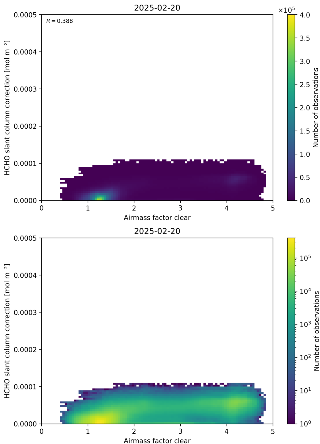
Figure 75: Scatter density plot of “Airmass factor clear” against “HCHO slant column correction” for 2025-02-19 to 2025-02-21.
