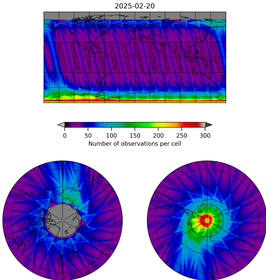
Figure 19: Map of the number of observations for 2025-02-19 to 2025-02-21
