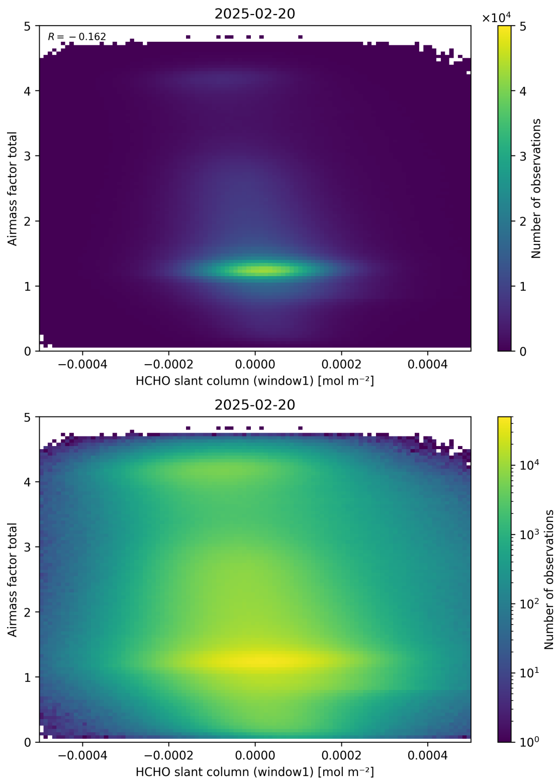
Figure 85: Scatter density plot of “HCHO slant column (window1)” against “Airmass factor total” for 2025-02-19 to 2025-02-21.
