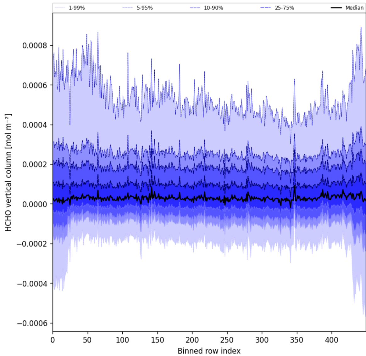
Figure 49: Along track statistics of “HCHO vertical column” for 2025-02-19 to 2025-02-21
