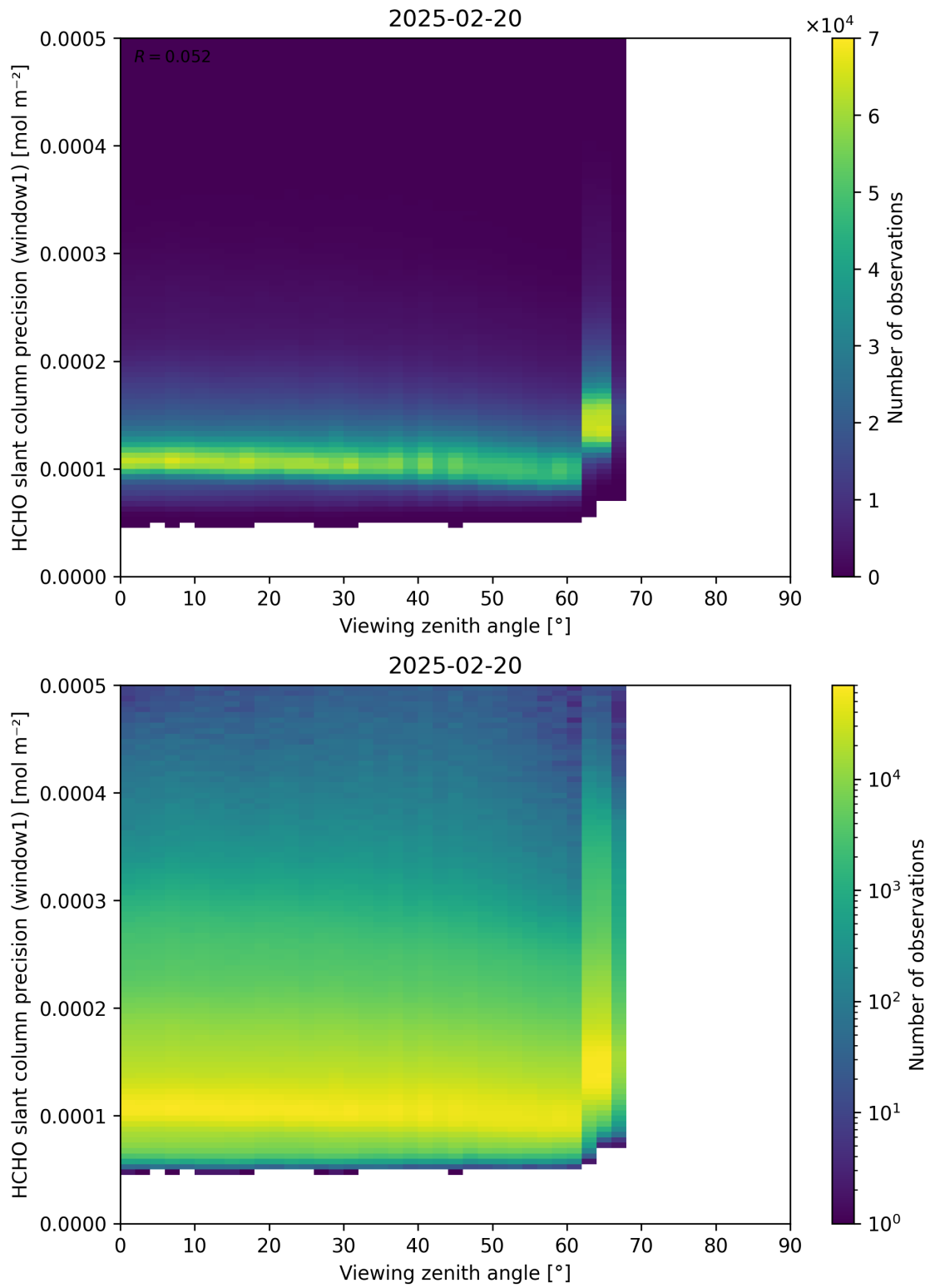
Figure 189: Scatter density plot of “Viewing zenith angle” against “HCHO slant column precision (window1)” for 2025-02-19 to 2025-02-21.
