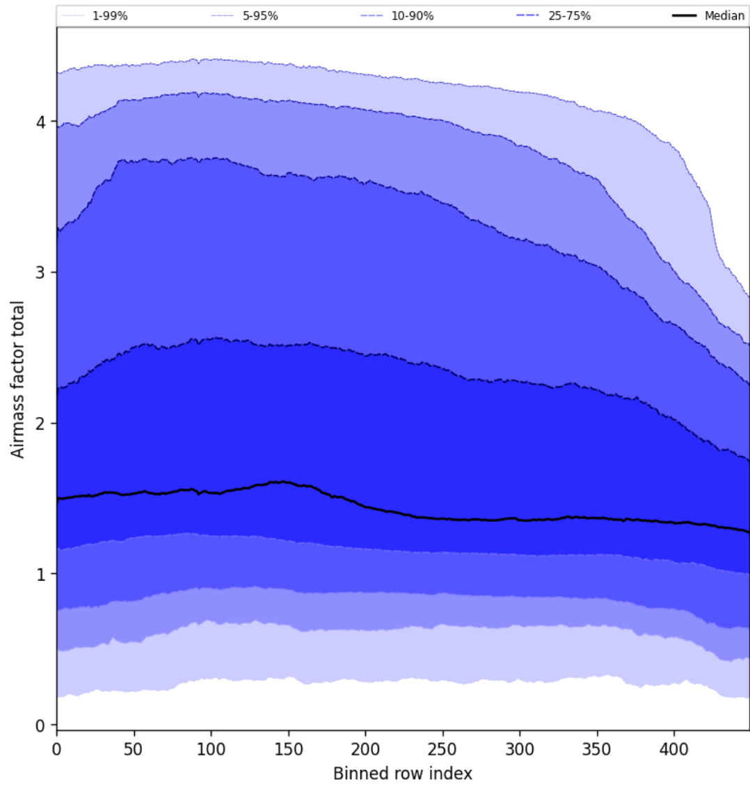
Figure 54: Along track statistics of “Airmass factor total” for 2025-02-19 to 2025-02-21
