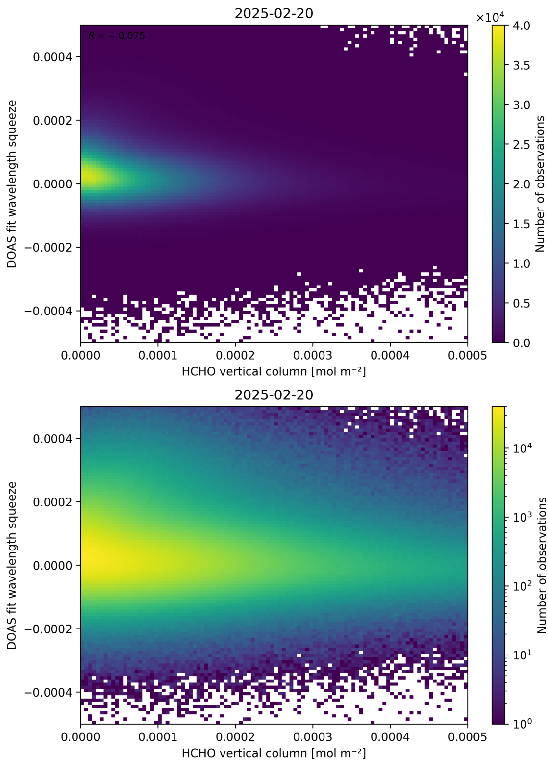
Figure 125: Scatter density plot of “HCHO vertical column” against “DOAS fit wavelength squeeze” for 2025-02-19 to 2025-02-21.
