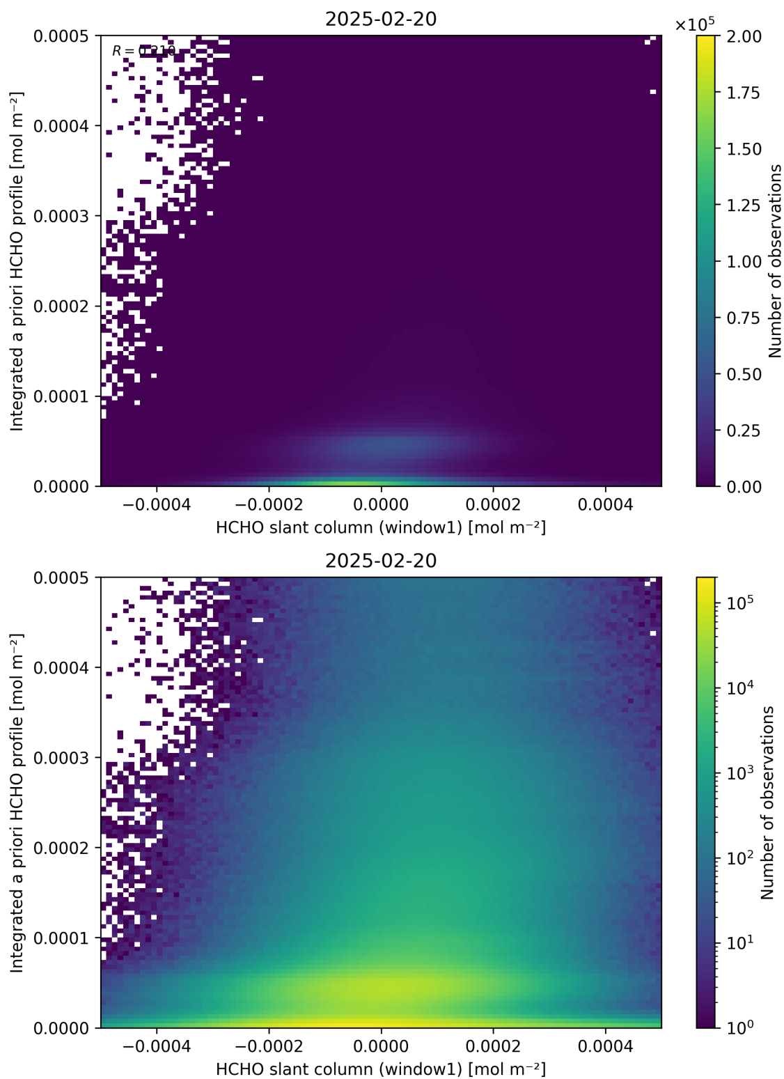
Figure 87: Scatter density plot of “HCHO slant column (window1)” against “Integrated a priori HCHO profile” for 2025-02-19 to 2025-02-21.
