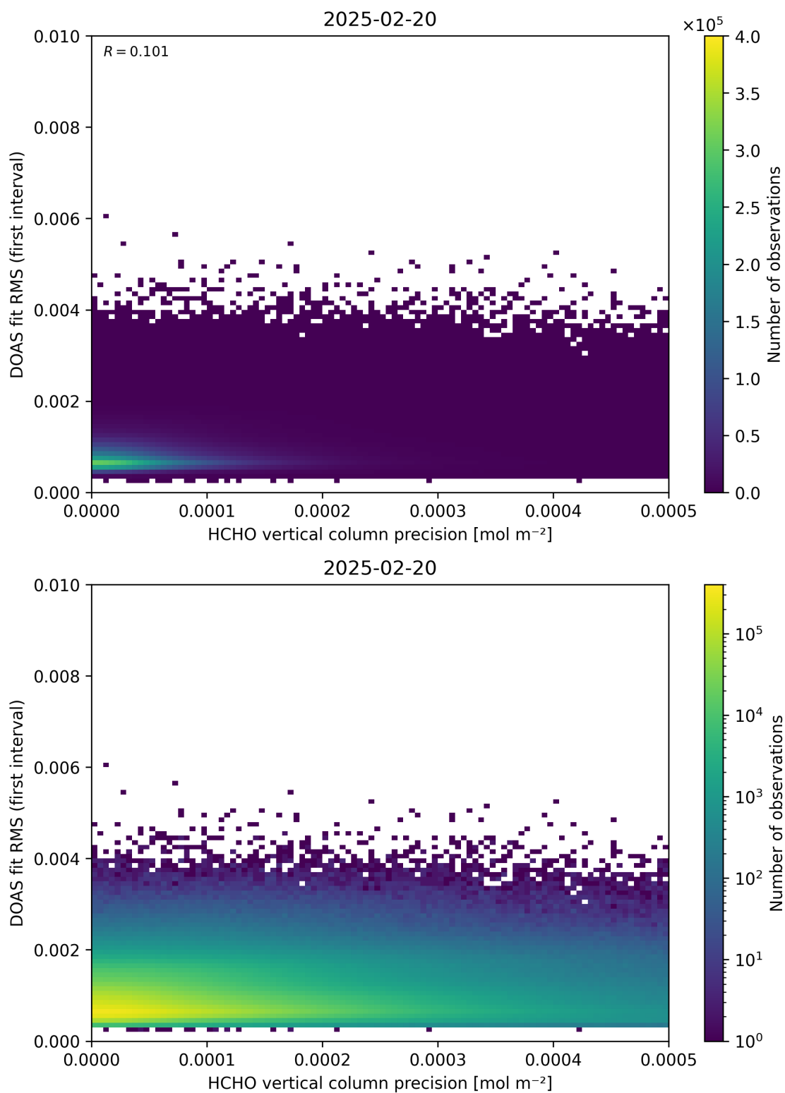
Figure 136: Scatter density plot of “HCHO vertical column precision” against “DOAS fit RMS (first interval)” for 2025-02-19 to 2025-02-21.
