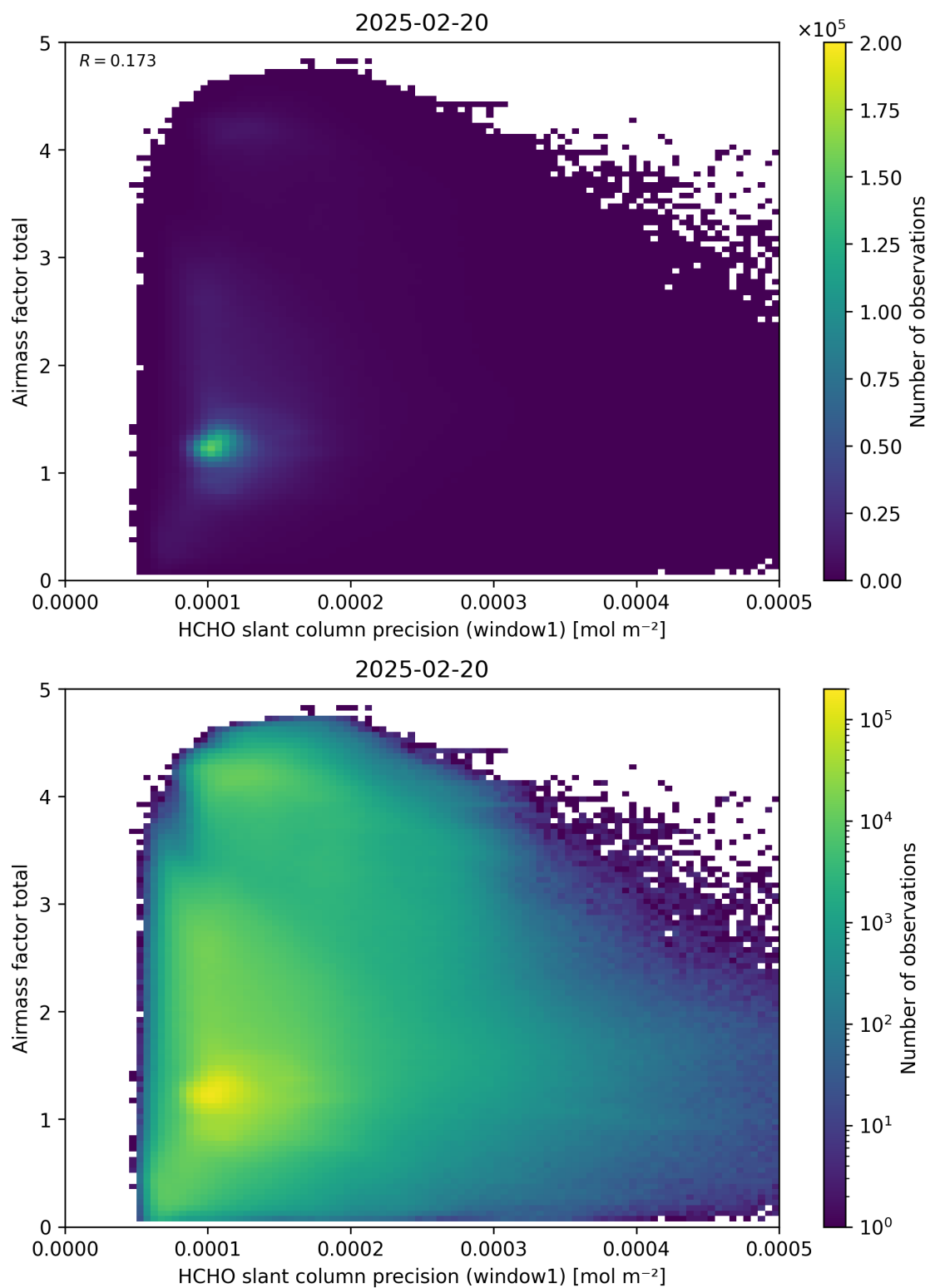
Figure 94: Scatter density plot of “HCHO slant column precision (window1)” against “Airmass factor total” for 2025-02-19 to 2025-02-21.
