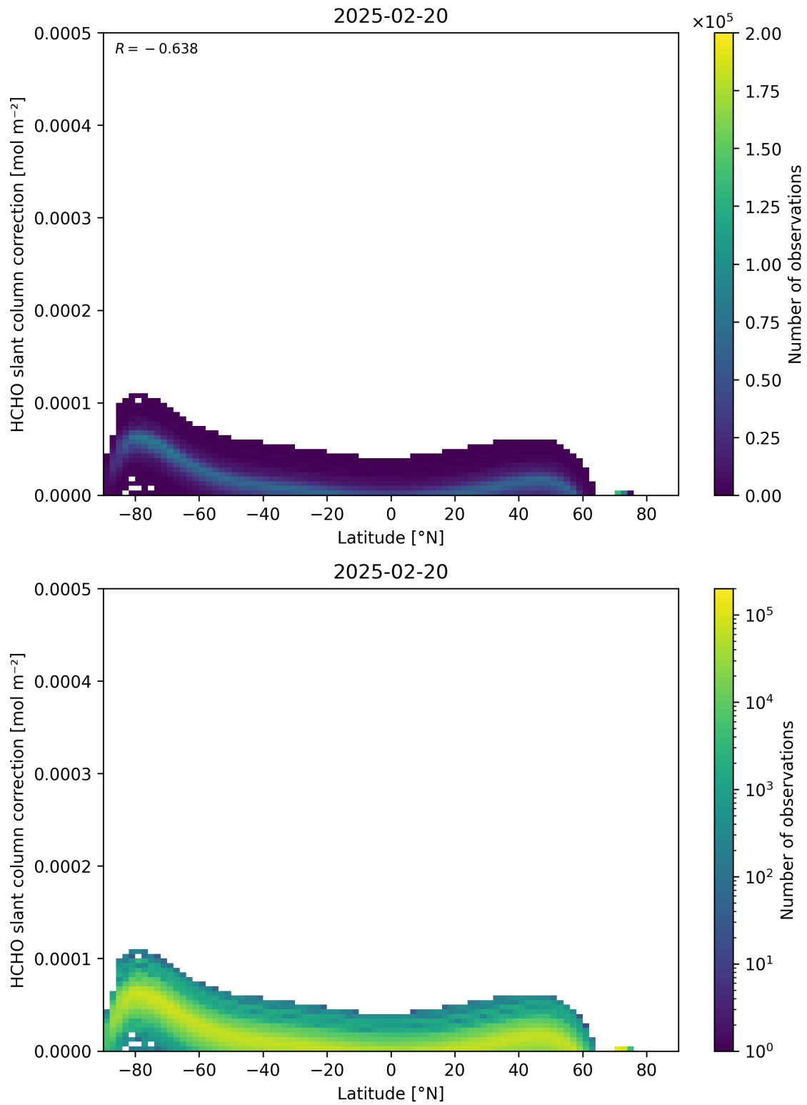
Figure 158: Scatter density plot of “Latitude” against “HCHO slant column correction” for 2025-02-19 to 2025-02-21.
