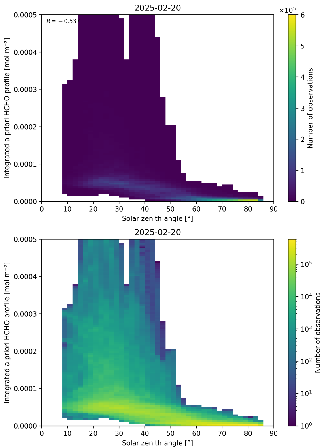
Figure 180: Scatter density plot of “Solar zenith angle” against “Integrated a priori HCHO profile” for 2025-02-19 to 2025-02-21.
