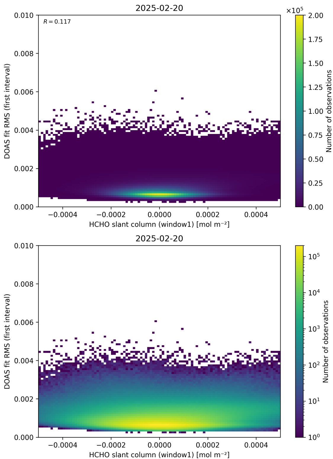
Figure 78: Scatter density plot of “HCHO slant column (window1)” against “DOAS fit RMS (first interval)” for 2025-02-19 to 2025-02-21.
