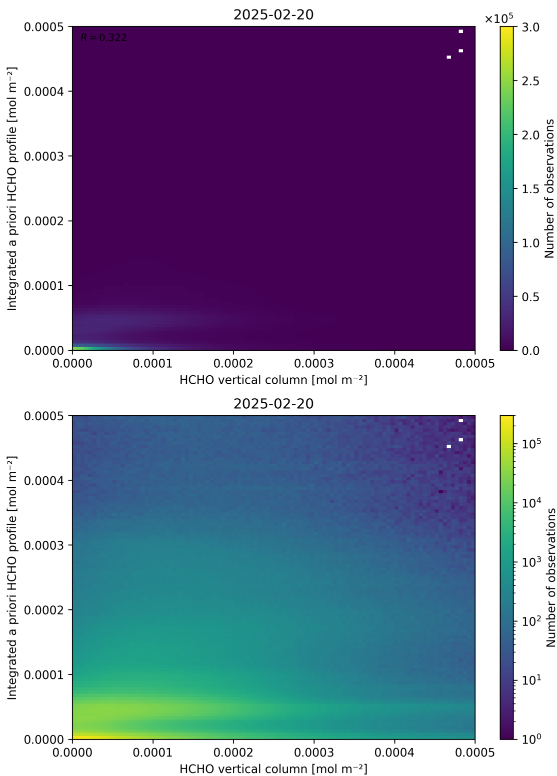
Figure 135: Scatter density plot of “HCHO vertical column” against “Integrated a priori HCHO profile” for 2025-02-19 to 2025-02-21.
