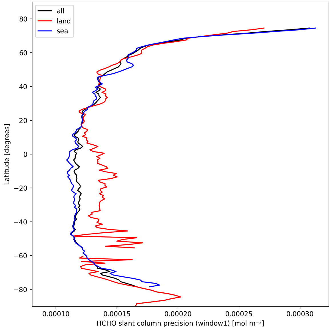
Figure 25: Zonal average of “HCHO slant column precision (window1)” for 2025-02-19 to 2025-02-21.
