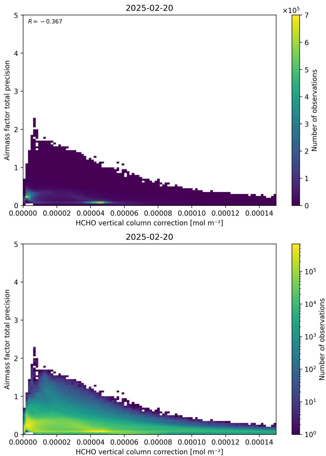
Figure 121: Scatter density plot of “HCHO vertical column correction” against “Airmass factor total precision” for 2025-02-19 to 2025-02-21.
