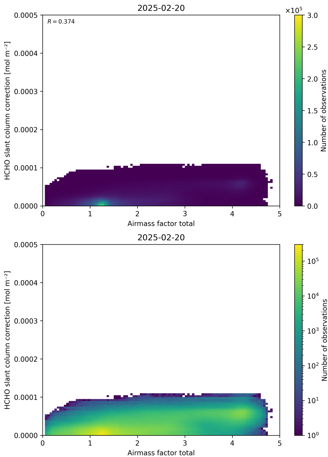
Figure 102: Scatter density plot of “Airmass factor total” against “HCHO slant column correction” for 2025-02-19 to 2025-02-21.
