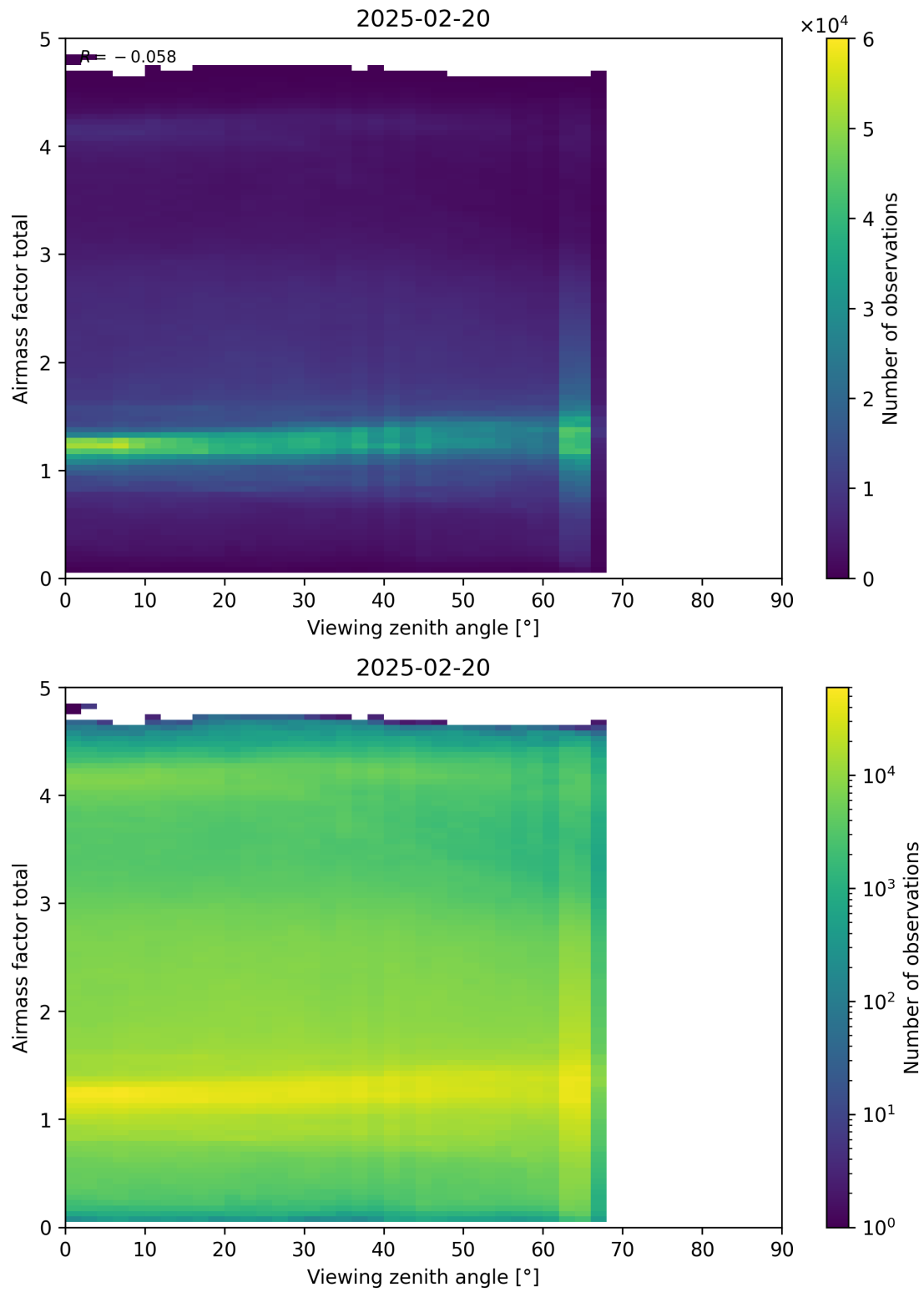
Figure 190: Scatter density plot of “Viewing zenith angle” against “Airmass factor total” for 2025-02-19 to 2025-02-21.
