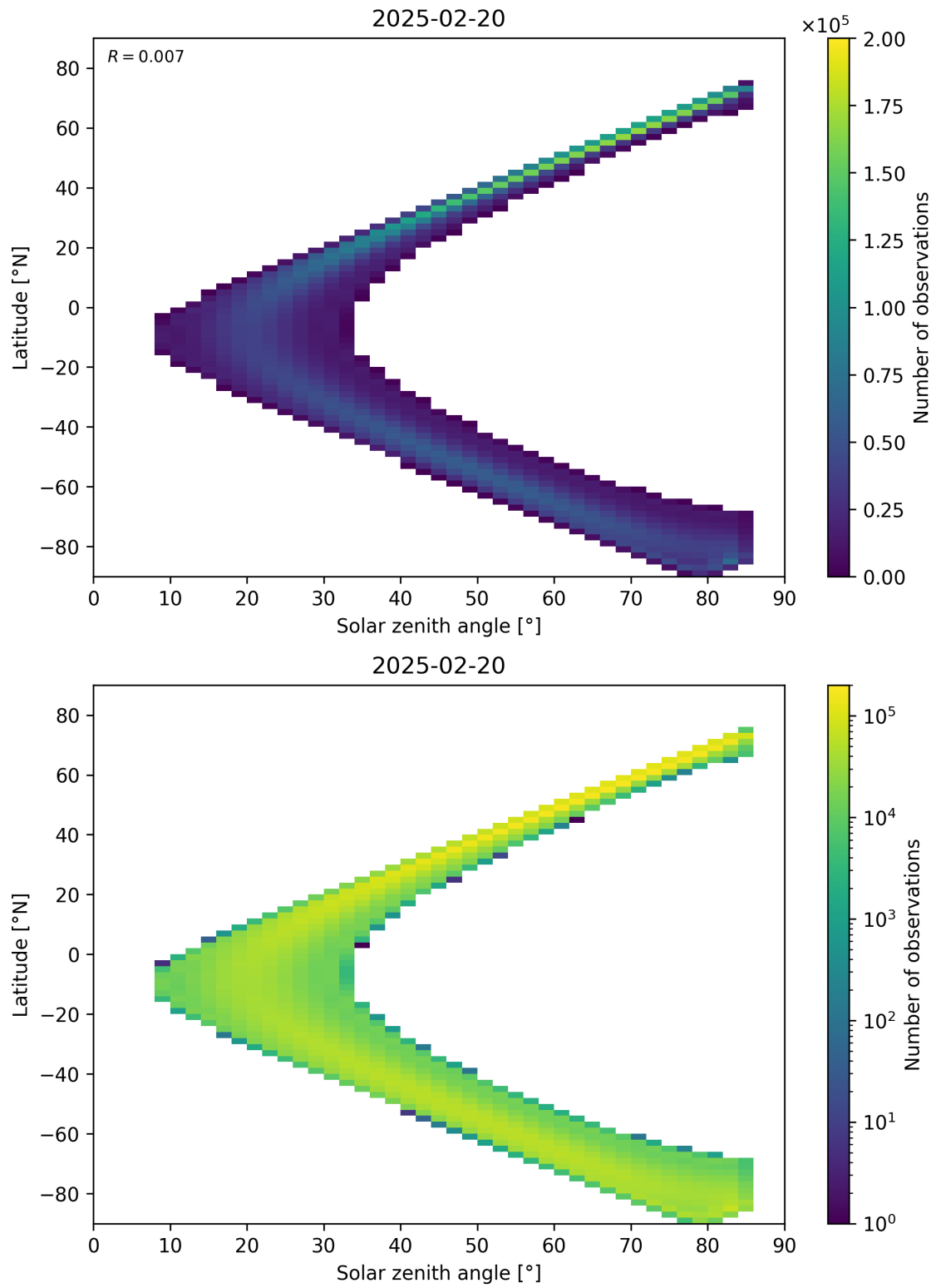
Figure 181: Scatter density plot of “Solar zenith angle” against “Latitude” for 2025-02-19 to 2025-02-21.
