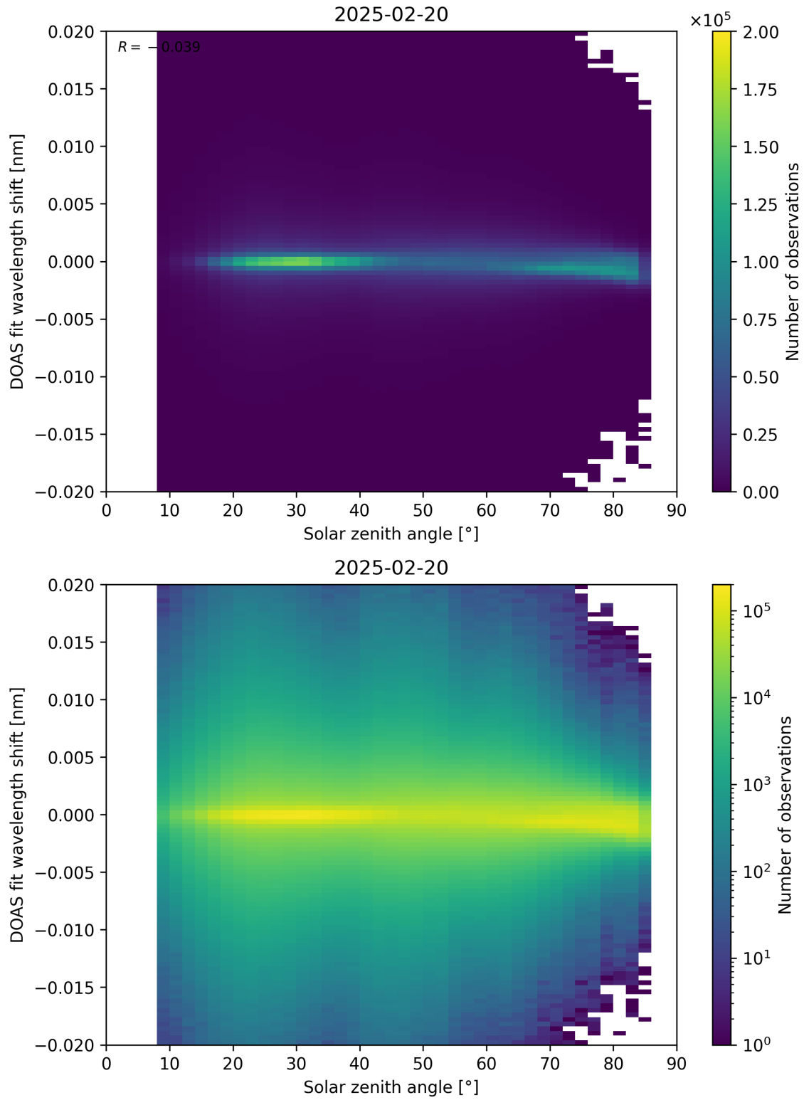
Figure 168: Scatter density plot of “Solar zenith angle” against “DOAS fit wavelength shift” for 2025-02-19 to 2025-02-21.
