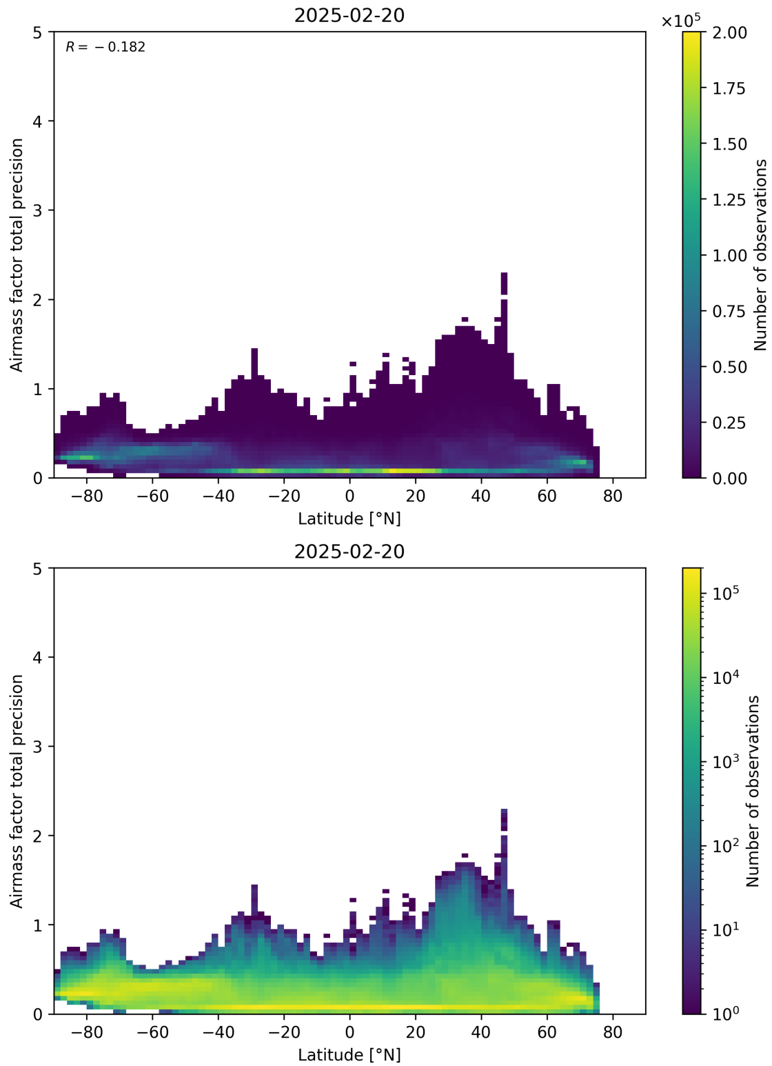
Figure 162: Scatter density plot of “Latitude” against “Airmass factor total precision” for 2025-02-19 to 2025-02-21.
