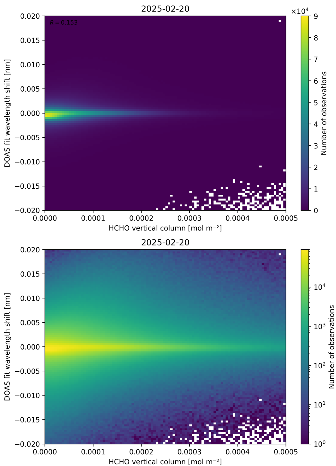
Figure 124: Scatter density plot of “HCHO vertical column” against “DOAS fit wavelength shift” for 2025-02-19 to 2025-02-21.
