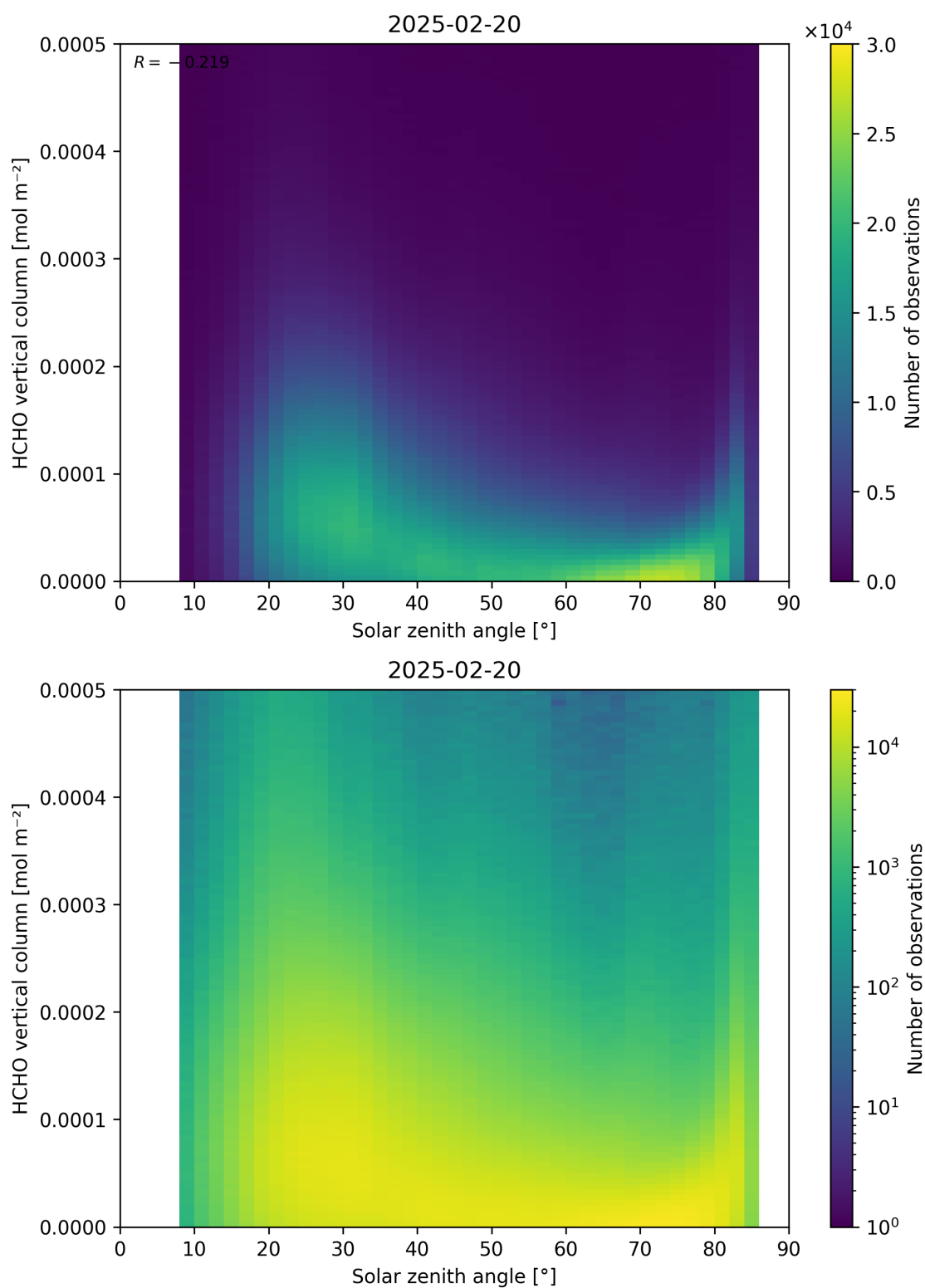
Figure 177: Scatter density plot of “Solar zenith angle” against “HCHO vertical column” for 2025-02-19 to 2025-02-21.
