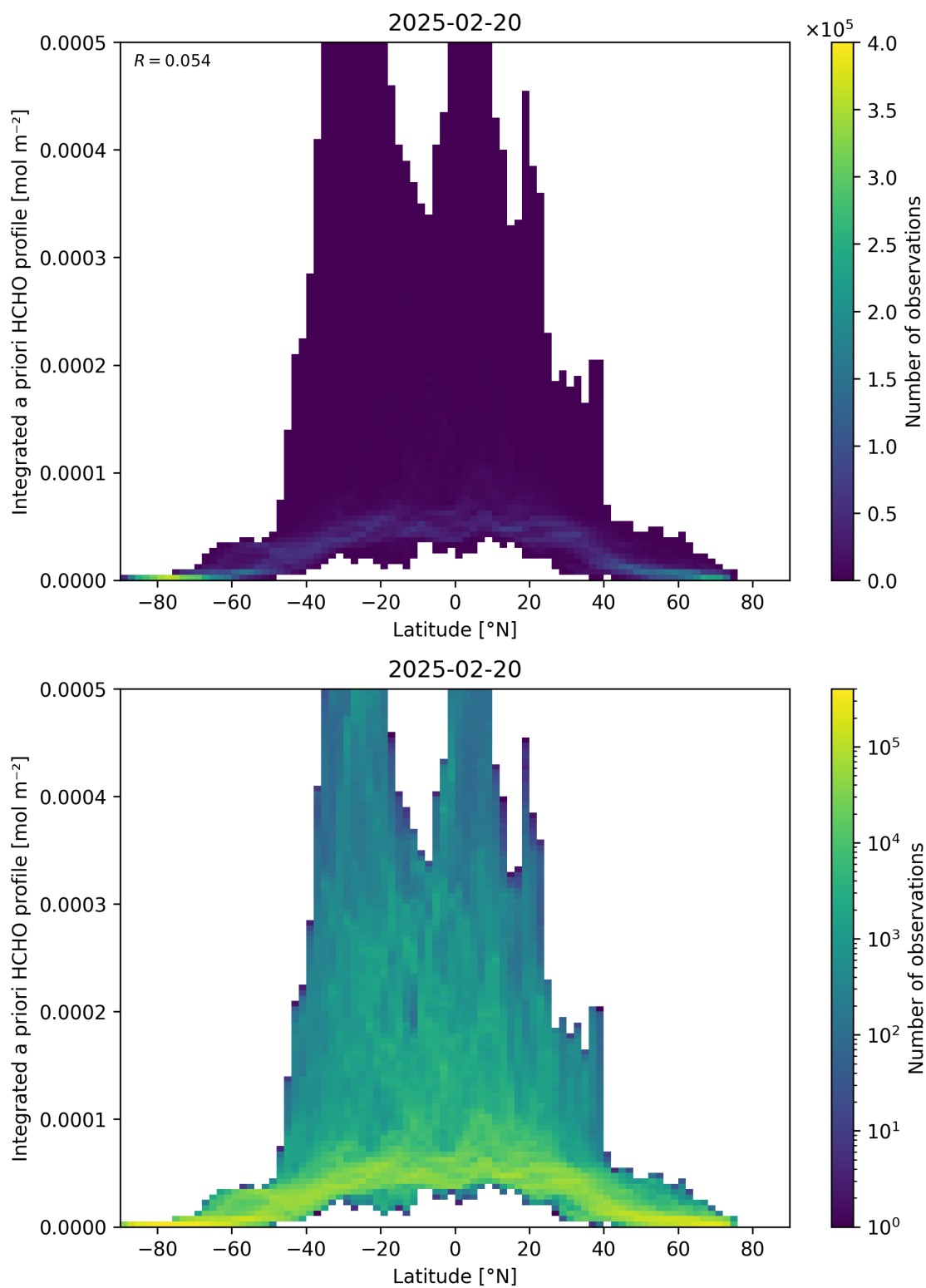
Figure 166: Scatter density plot of “Latitude” against “Integrated a priori HCHO profile” for 2025-02-19 to 2025-02-21.
