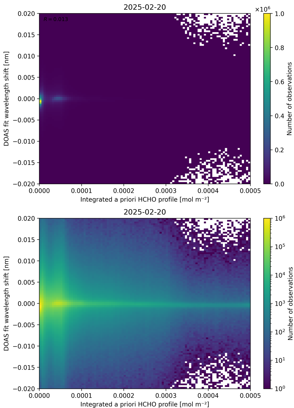
Figure 149: Scatter density plot of “Integrated a priori HCHO profile” against “DOAS fit wavelength shift” for 2025-02-19 to 2025-02-21.
