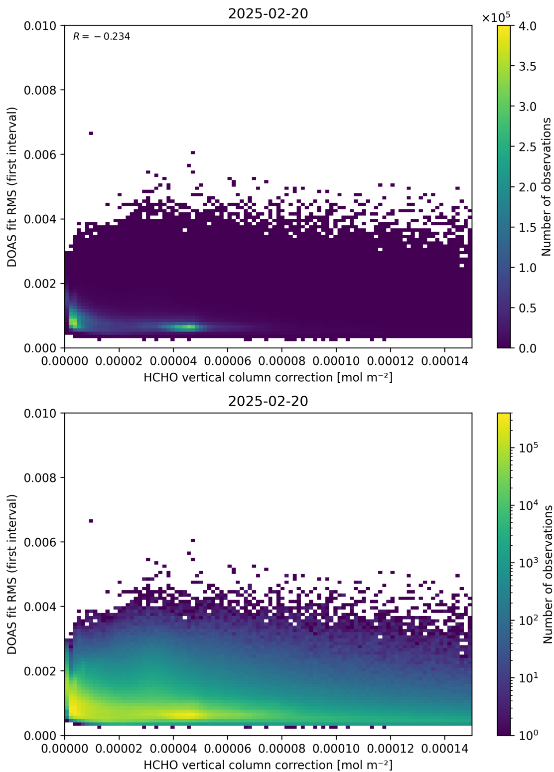
Figure 112: Scatter density plot of “HCHO vertical column correction” against “DOAS fit RMS (first interval)” for 2025-02-19 to 2025-02-21.
