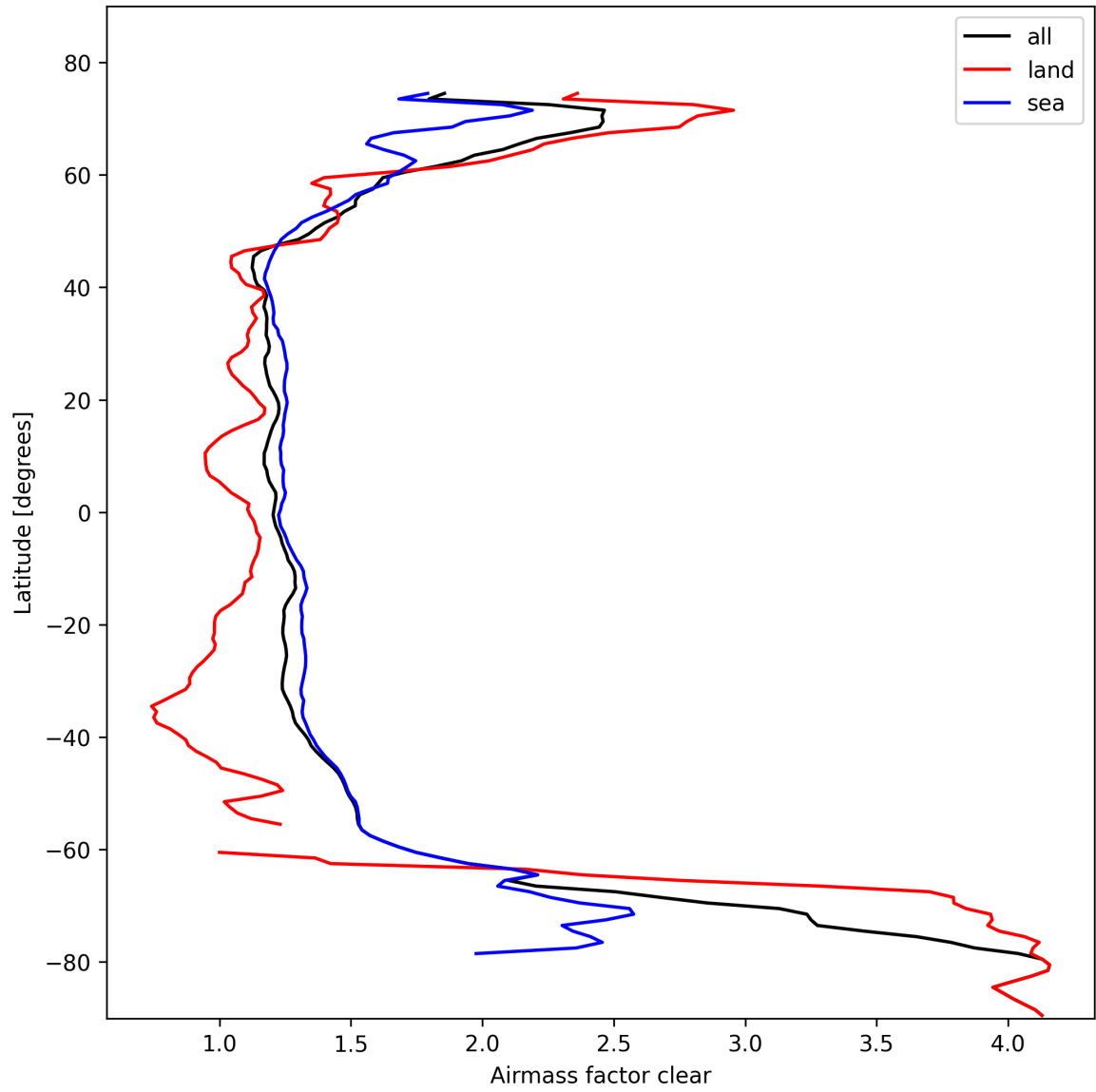
Figure 28: Zonal average of “Airmass factor clear” for 2025-02-19 to 2025-02-21.
