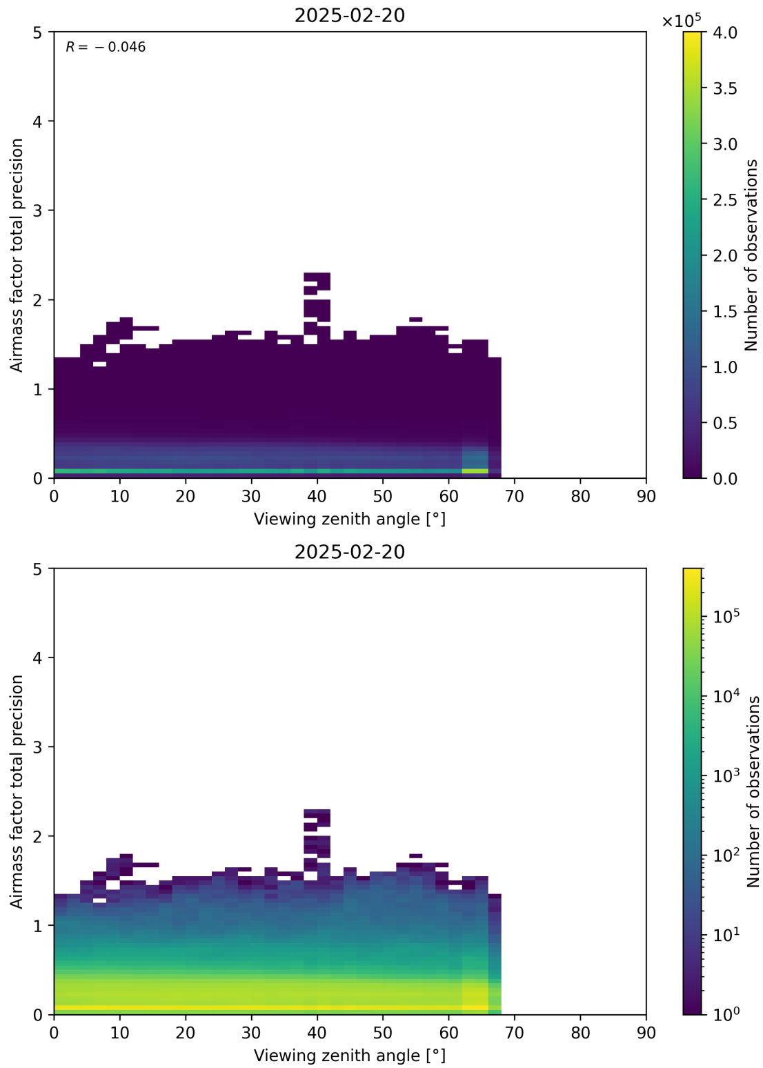
Figure 191: Scatter density plot of “Viewing zenith angle” against “Airmass factor total precision” for 2025-02-19 to 2025-02-21.
