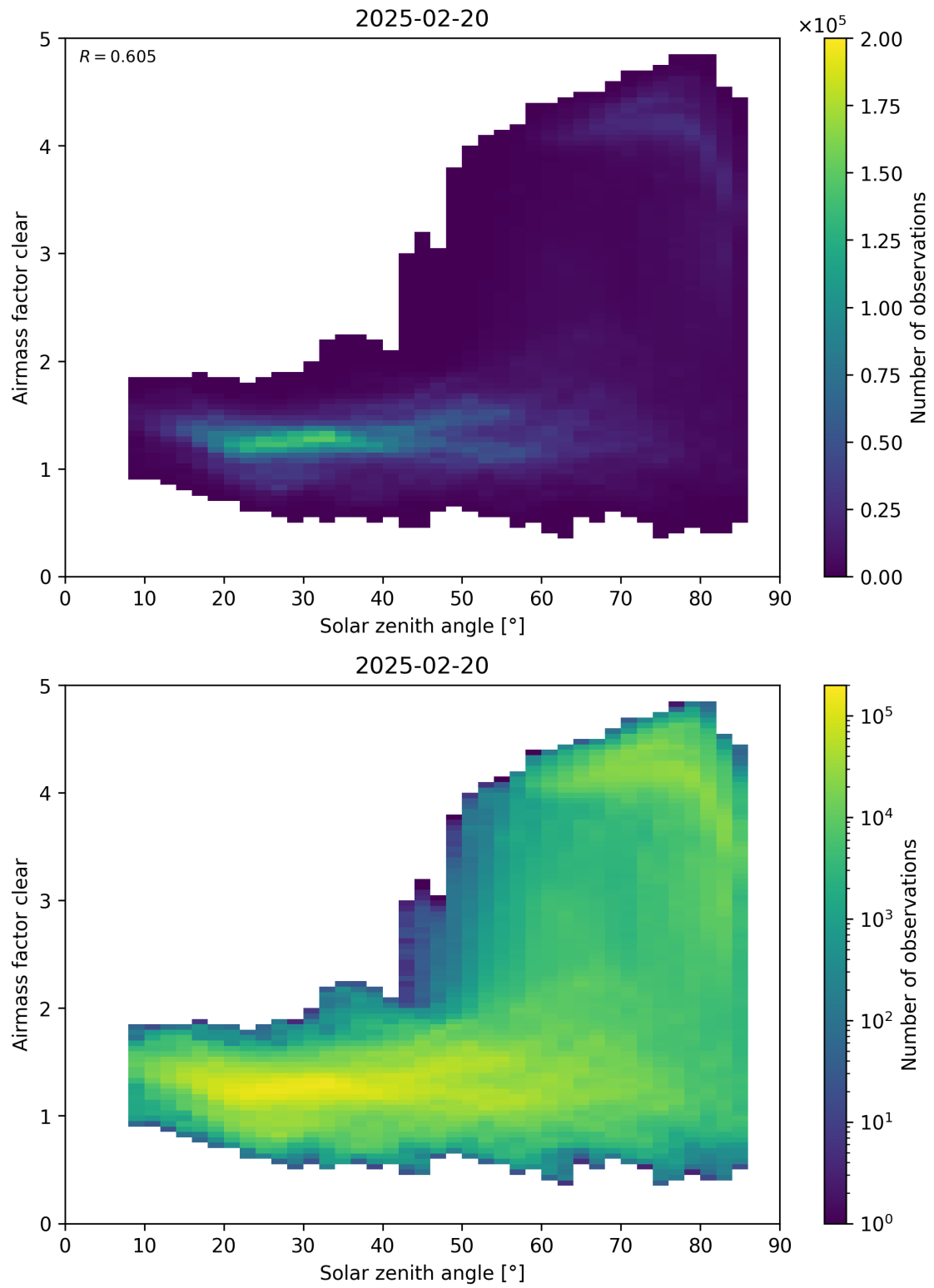
Figure 170: Scatter density plot of “Solar zenith angle” against “Airmass factor clear” for 2025-02-19 to 2025-02-21.
