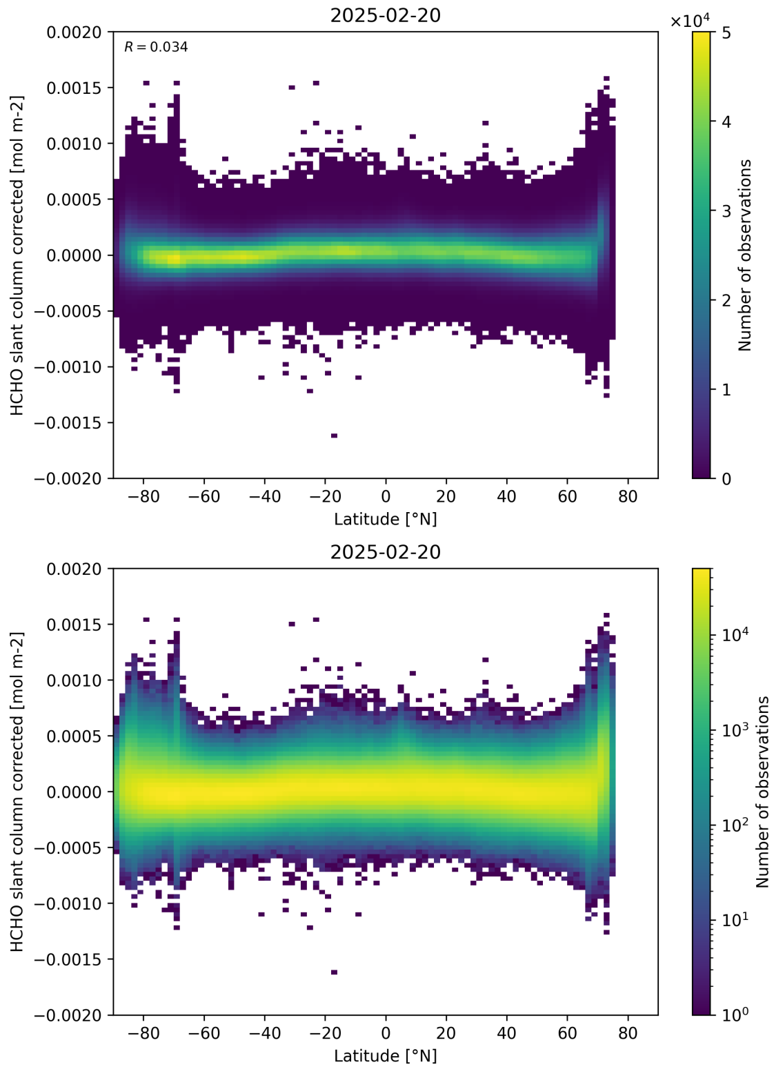
Figure 157: Scatter density plot of “Latitude” against “HCHO slant column corrected” for 2025-02-19 to 2025-02-21.
