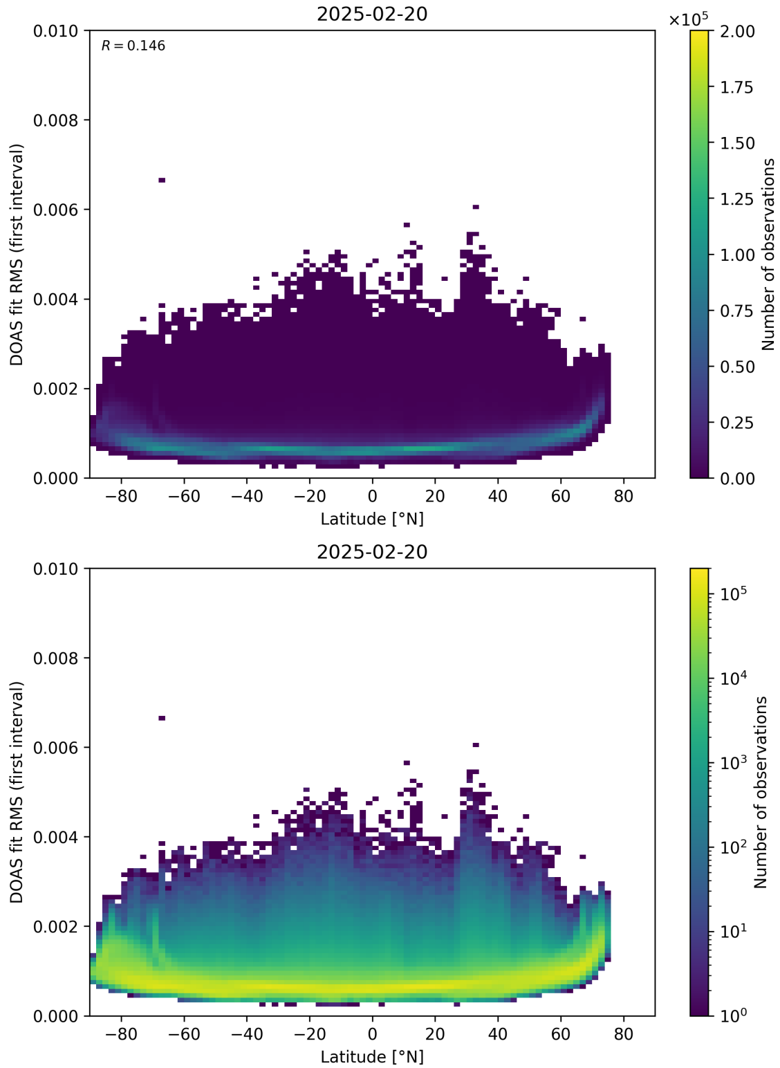
Figure 153: Scatter density plot of “Latitude” against “DOAS fit RMS (first interval)” for 2025-02-19 to 2025-02-21.
