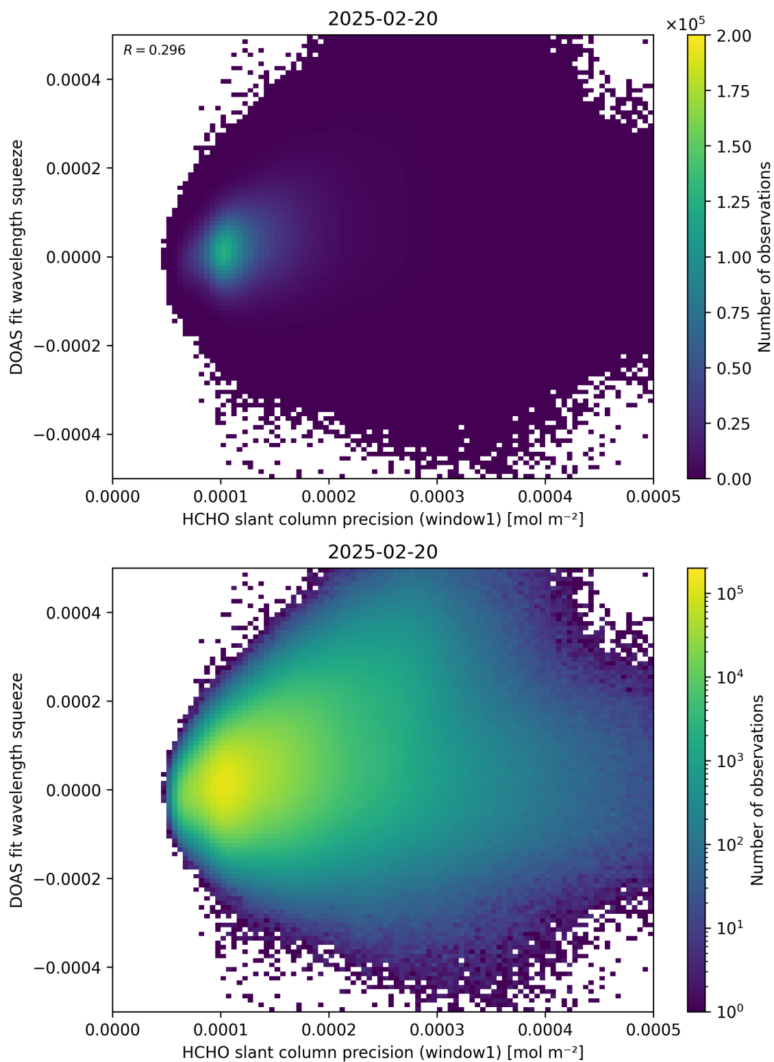
Figure 90: Scatter density plot of “HCHO slant column precision (window1)” against “DOAS fit wavelength squeeze” for 2025-02-19 to 2025-02-21.
