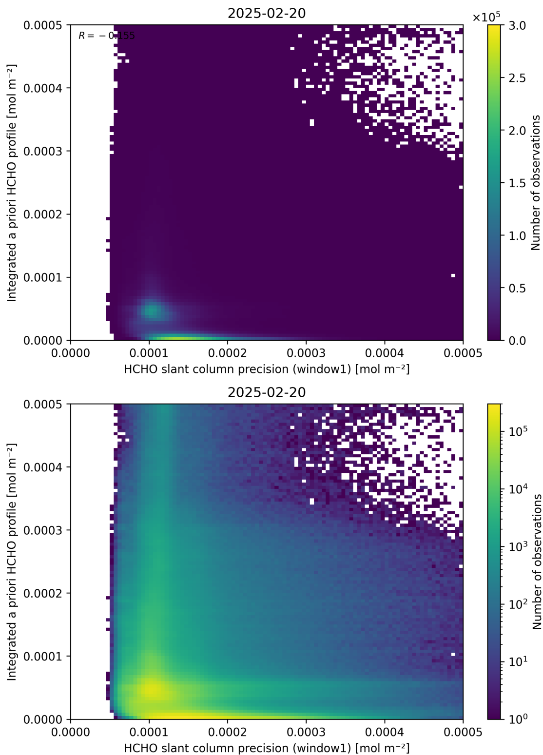
Figure 96: Scatter density plot of “HCHO slant column precision (window1)” against “Integrated a priori HCHO profile” for 2025-02-19 to 2025-02-21.
