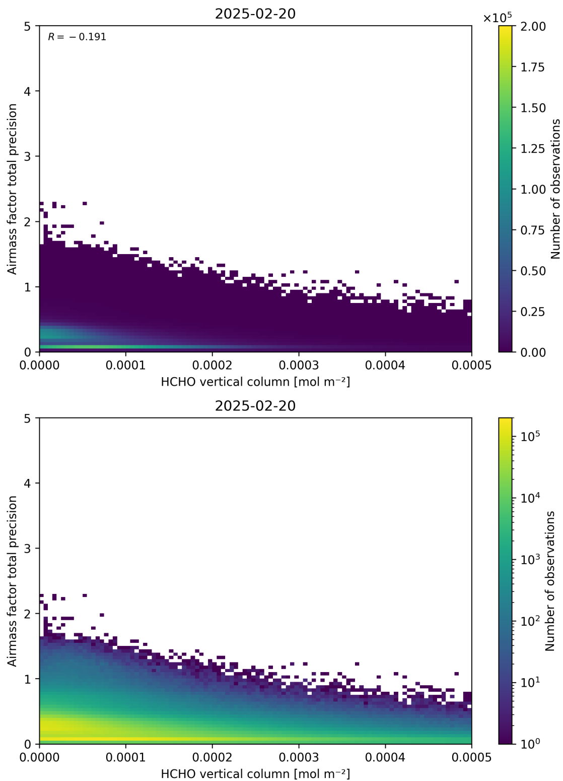
Figure 132: Scatter density plot of “HCHO vertical column” against “Airmass factor total precision” for 2025-02-19 to 2025-02-21.
