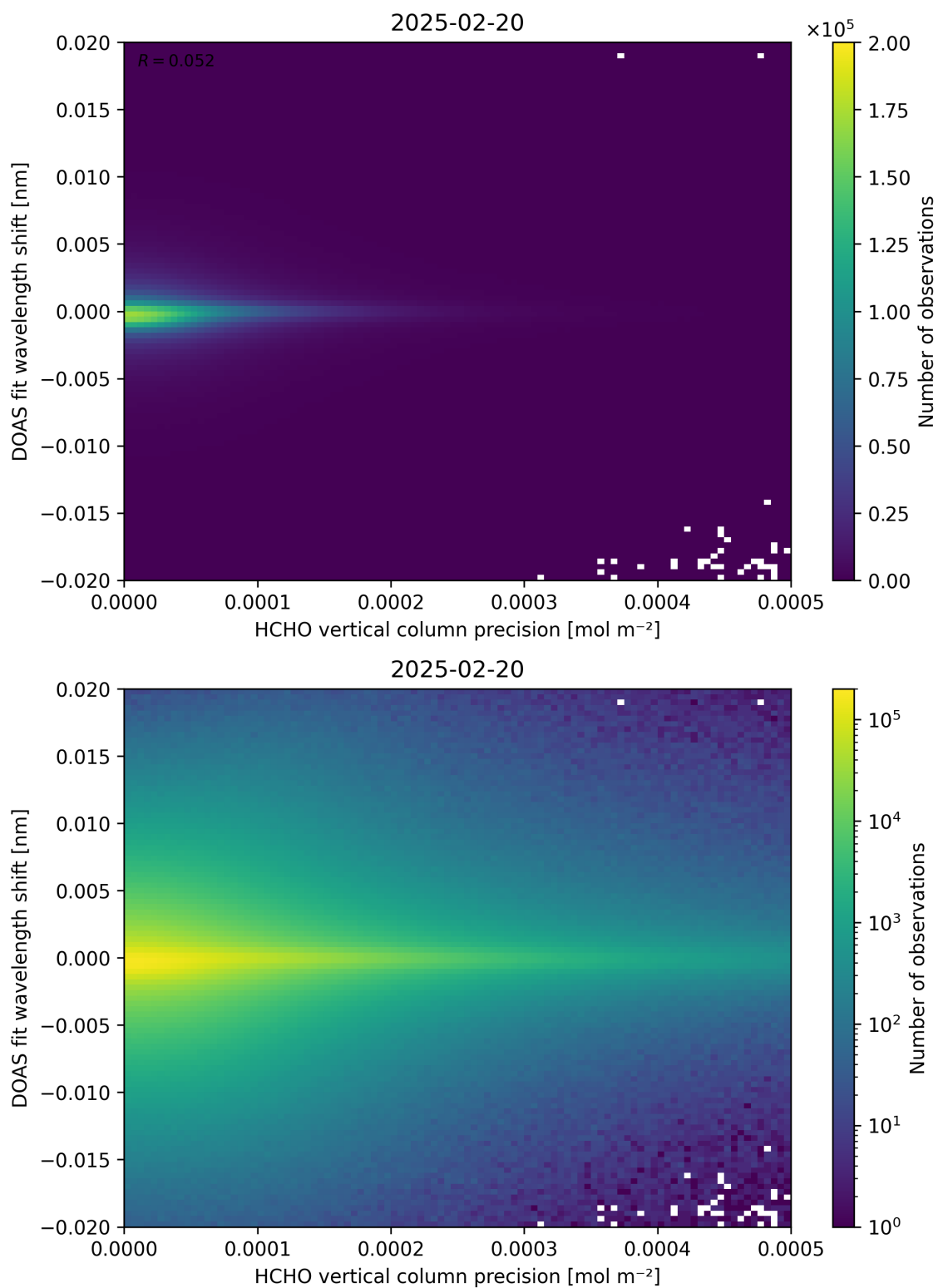
Figure 137: Scatter density plot of “HCHO vertical column precision” against “DOAS fit wavelength shift” for 2025-02-19 to 2025-02-21.
