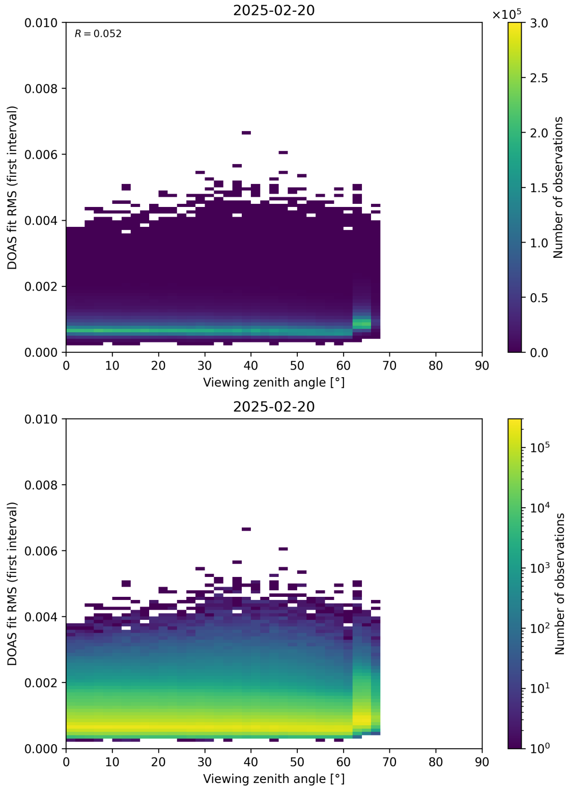
Figure 182: Scatter density plot of “Viewing zenith angle” against “DOAS fit RMS (first interval)” for 2025-02-19 to 2025-02-21.
