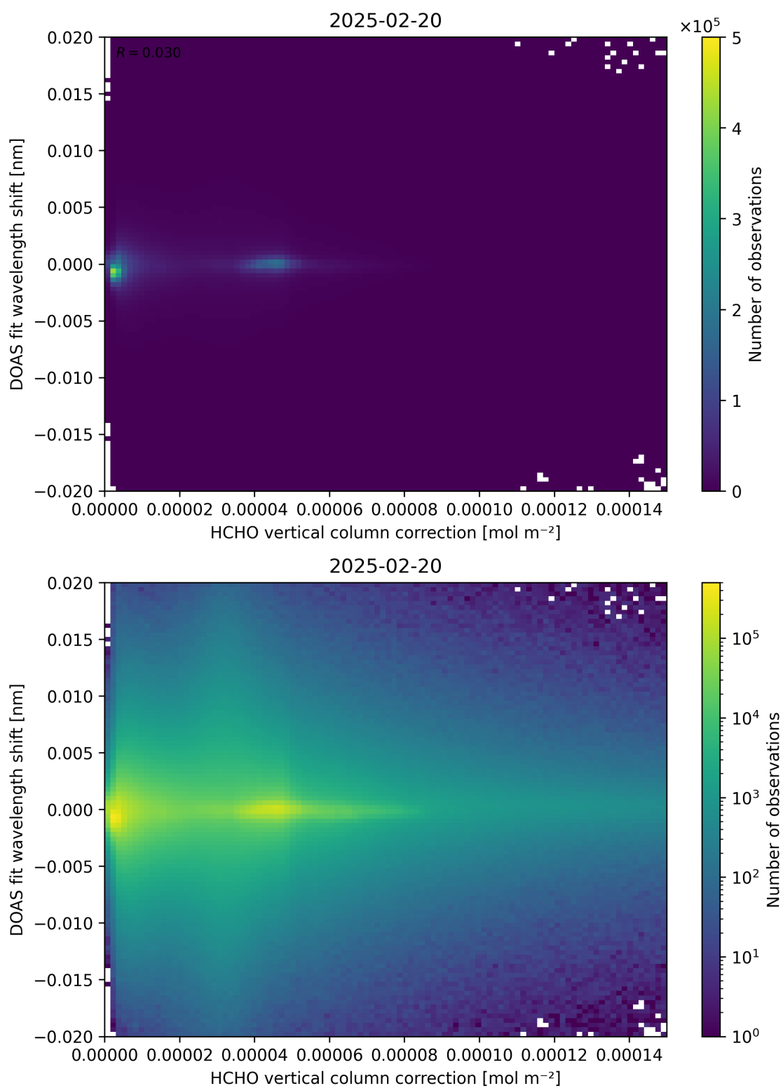
Figure 113: Scatter density plot of “HCHO vertical column correction” against “DOAS fit wavelength shift” for 2025-02-19 to 2025-02-21.
