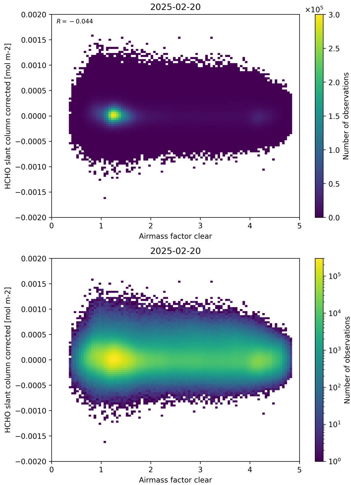
Figure 74: Scatter density plot of “Airmass factor clear” against “HCHO slant column corrected” for 2025-02-19 to 2025-02-21.
