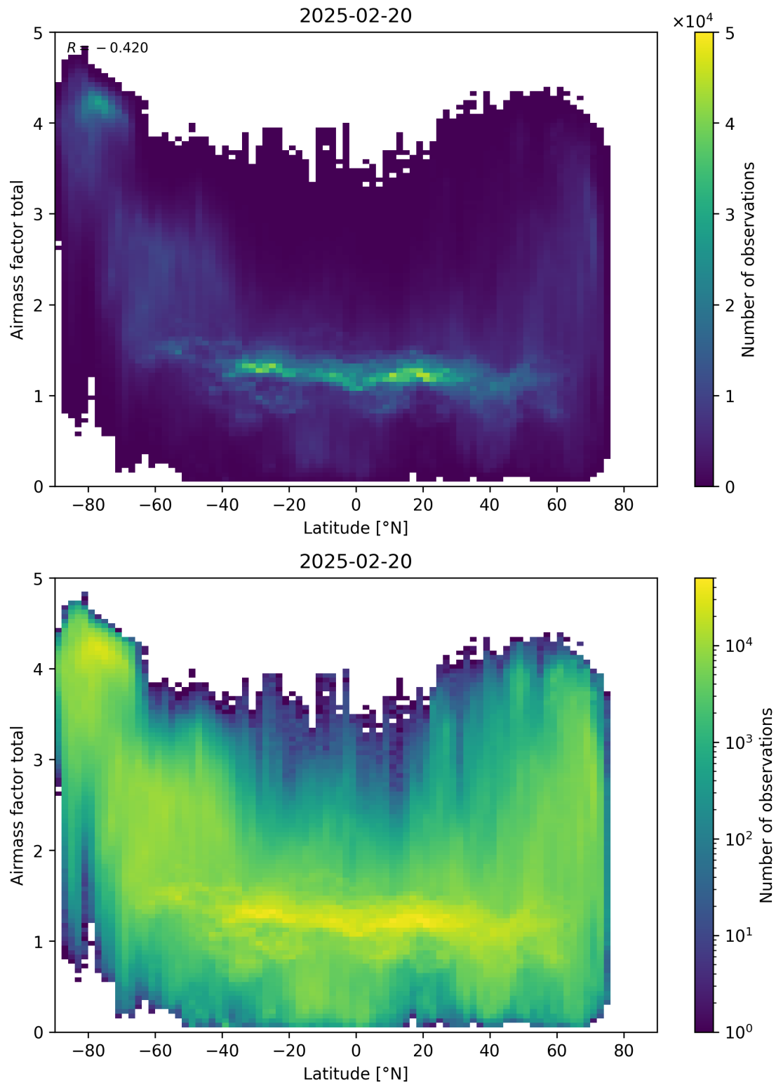
Figure 161: Scatter density plot of “Latitude” against “Airmass factor total” for 2025-02-19 to 2025-02-21.
