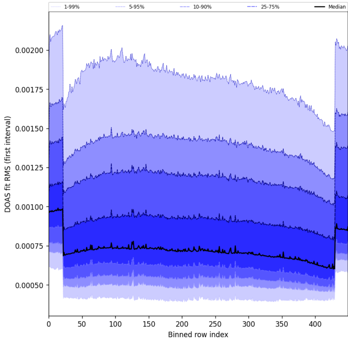
Figure 60: Along track statistics of “DOAS fit RMS (first interval)” for 2025-02-19 to 2025-02-21
