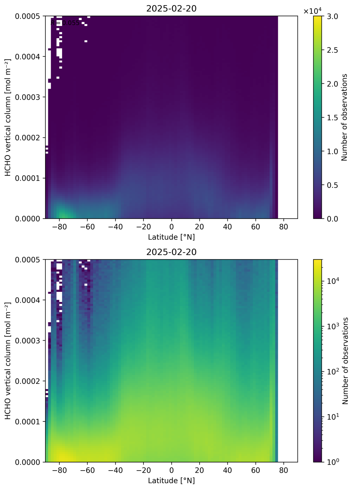
Figure 163: Scatter density plot of “Latitude” against “HCHO vertical column” for 2025-02-19 to 2025-02-21.
