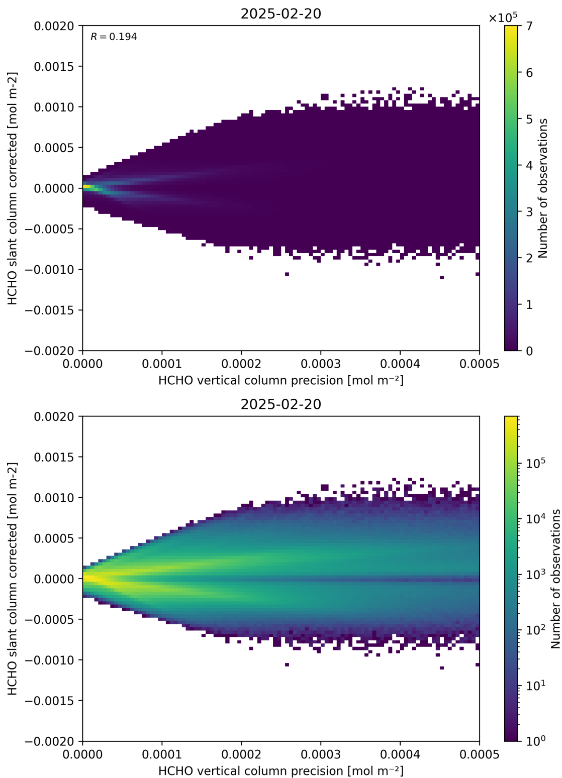
Figure 140: Scatter density plot of “HCHO vertical column precision” against “HCHO slant column corrected” for 2025-02-19 to 2025-02-21.
