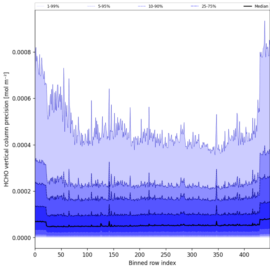
Figure 50: Along track statistics of “HCHO vertical column precision” for 2025-02-19 to 2025-02-21
