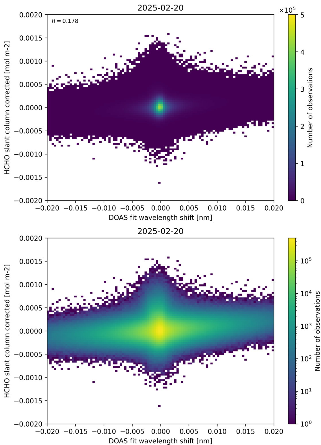
Figure 66: Scatter density plot of “DOAS fit wavelength shift” against “HCHO slant column corrected” for 2025-02-19 to 2025-02-21.
