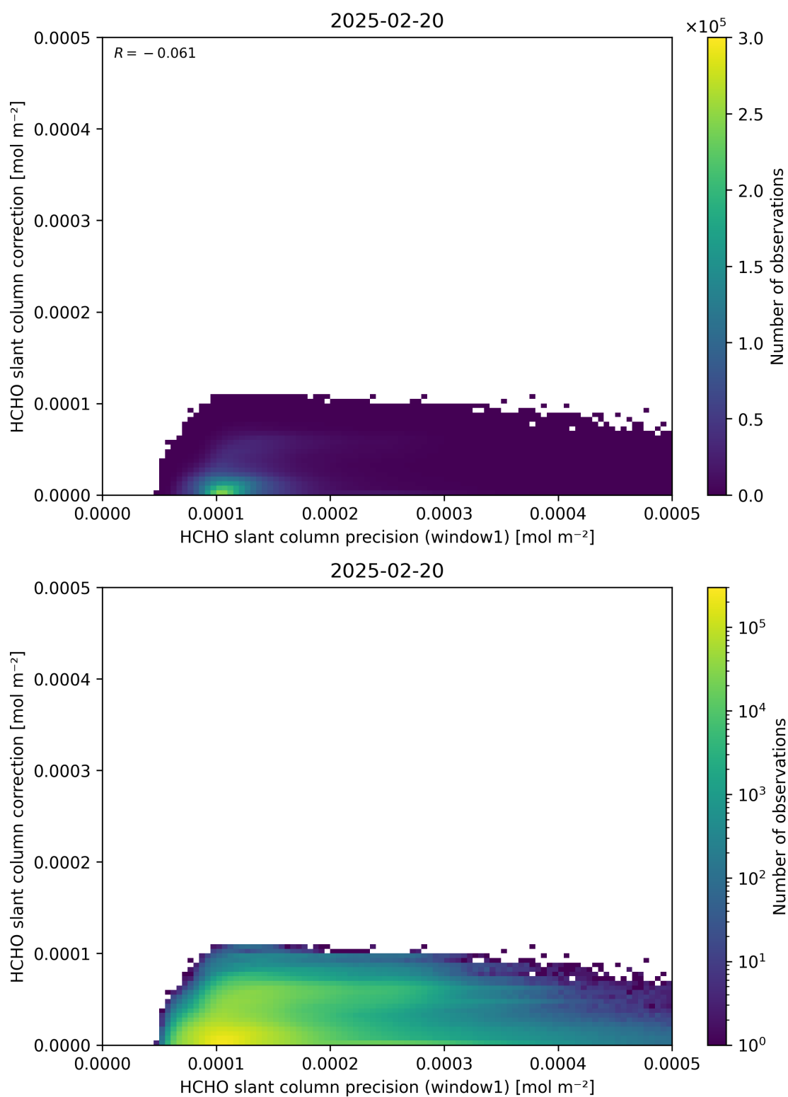
Figure 93: Scatter density plot of “HCHO slant column precision (window1)” against “HCHO slant column correction” for 2025-02-19 to 2025-02-21.
