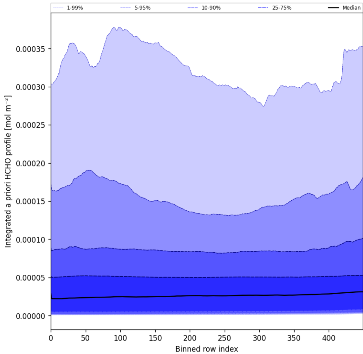
Figure 57: Along track statistics of “Integrated a priori HCHO profile” for 2025-02-19 to 2025-02-21
