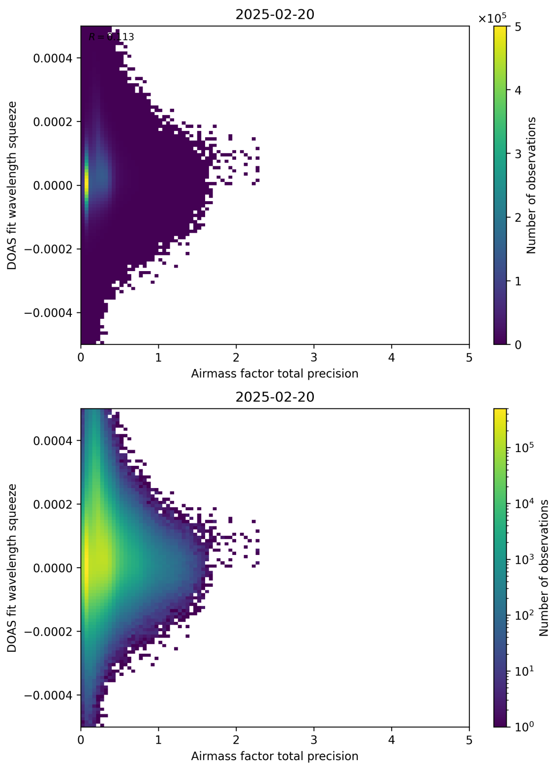
Figure 107: Scatter density plot of “Airmass factor total precision” against “DOAS fit wavelength squeeze” for 2025-02-19 to 2025-02-21.
