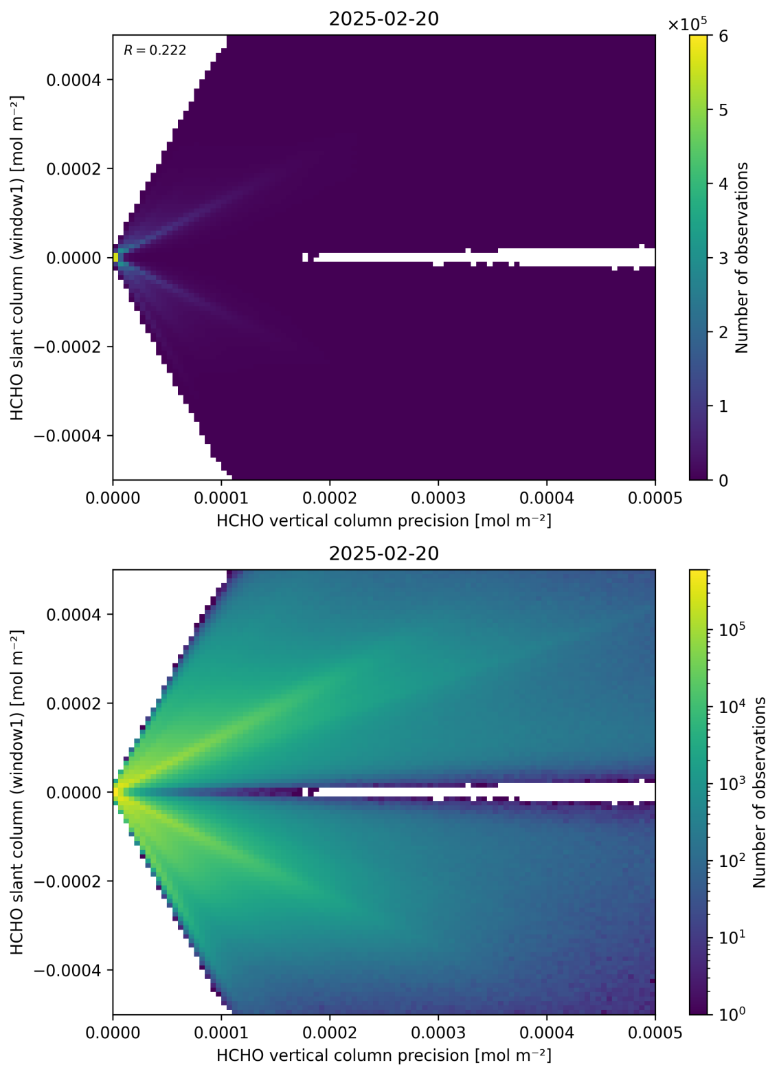
Figure 142: Scatter density plot of “HCHO vertical column precision” against “HCHO slant column (window1)” for 2025-02-19 to 2025-02-21.
