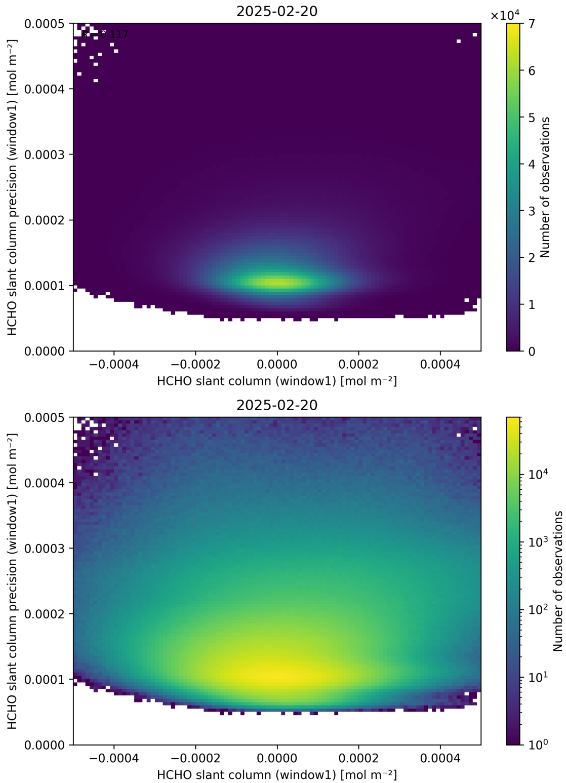
Figure 84: Scatter density plot of “HCHO slant column (window1)” against “HCHO slant column precision (window1)” for 2025-02-19 to 2025-02-21.
