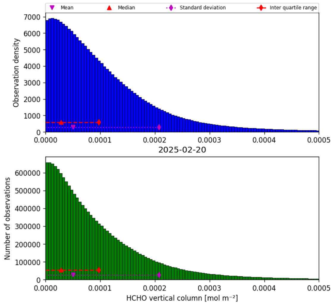
Figure 35: Histogram of “HCHO vertical column” for 2025-02-19 to 2025-02-21
