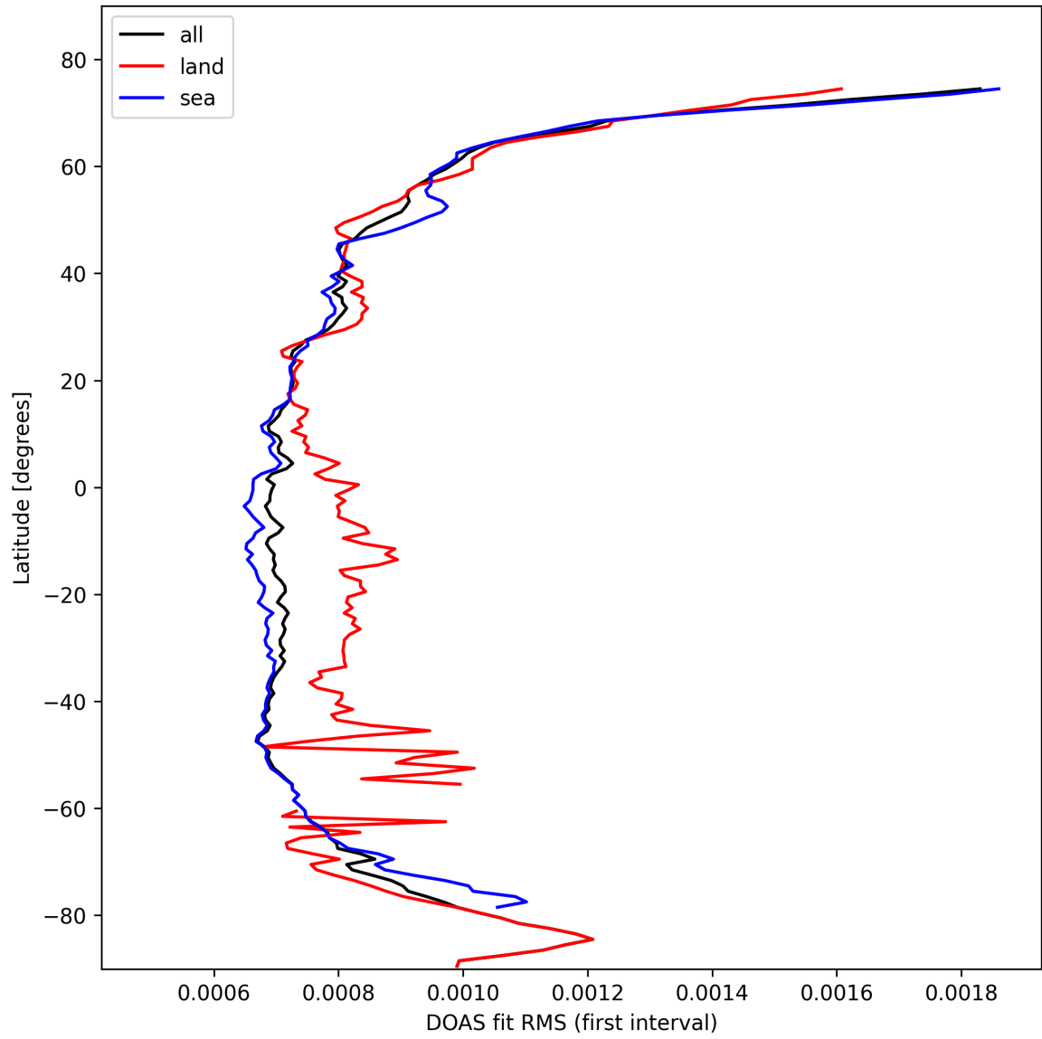
Figure 32: Zonal average of “DOAS fit RMS (first interval)” for 2025-02-19 to 2025-02-21.
