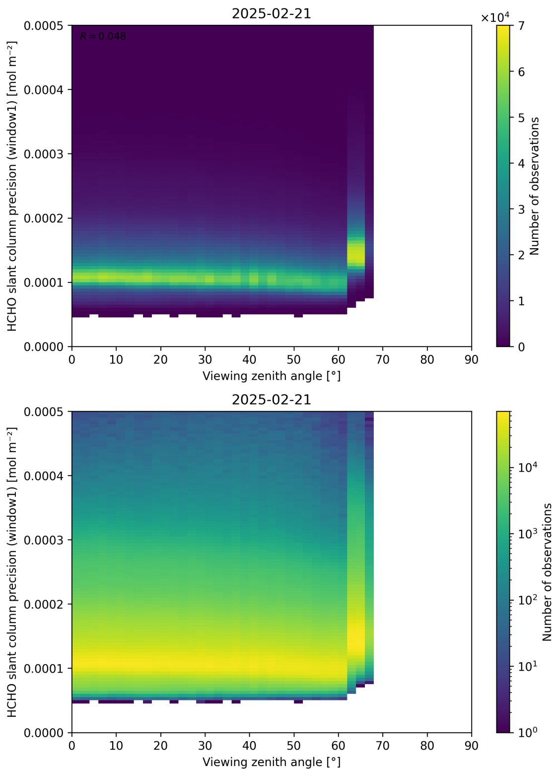
Figure 189: Scatter density plot of “Viewing zenith angle” against “HCHO slant column precision (window1)” for 2025-02-20 to 2025-02-22.
