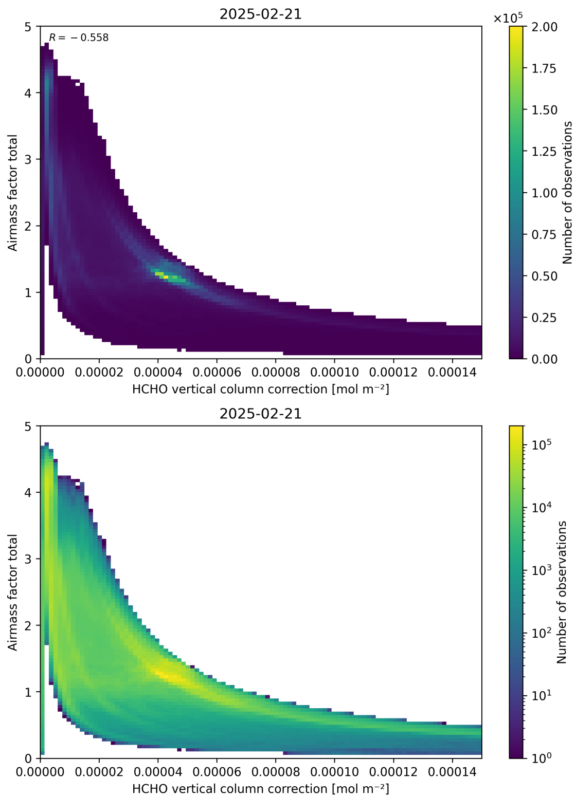
Figure 120: Scatter density plot of “HCHO vertical column correction” against “Airmass factor total” for 2025-02-20 to 2025-02-22.
