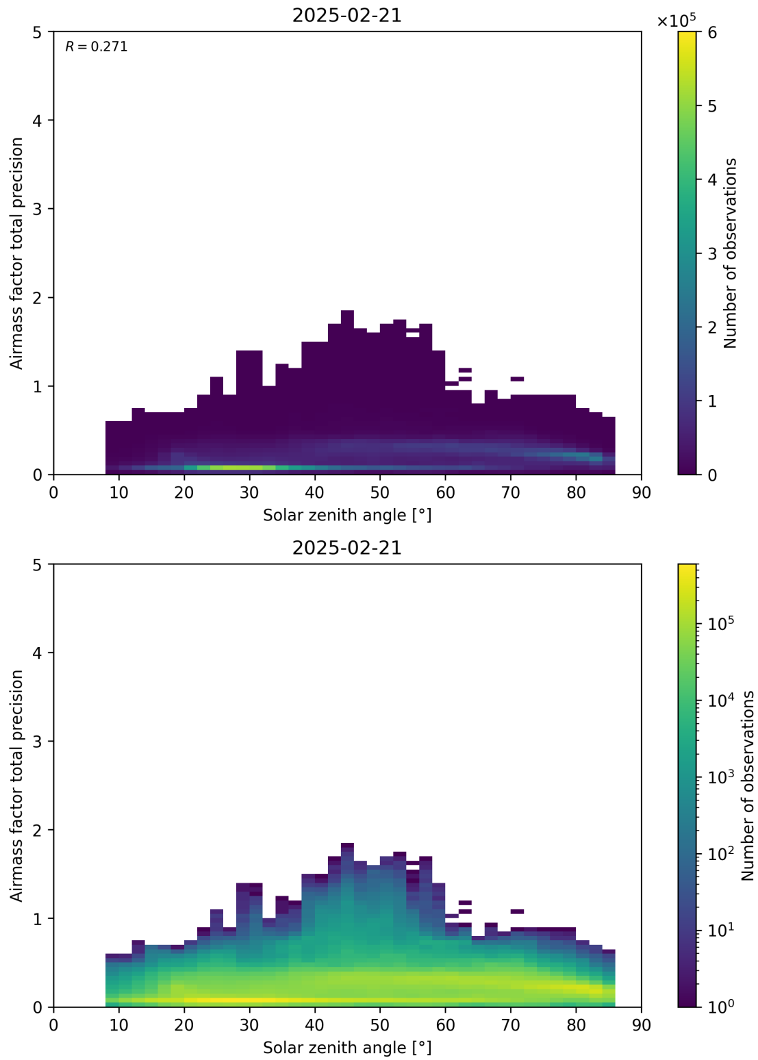
Figure 176: Scatter density plot of “Solar zenith angle” against “Airmass factor total precision” for 2025-02-20 to 2025-02-22.
