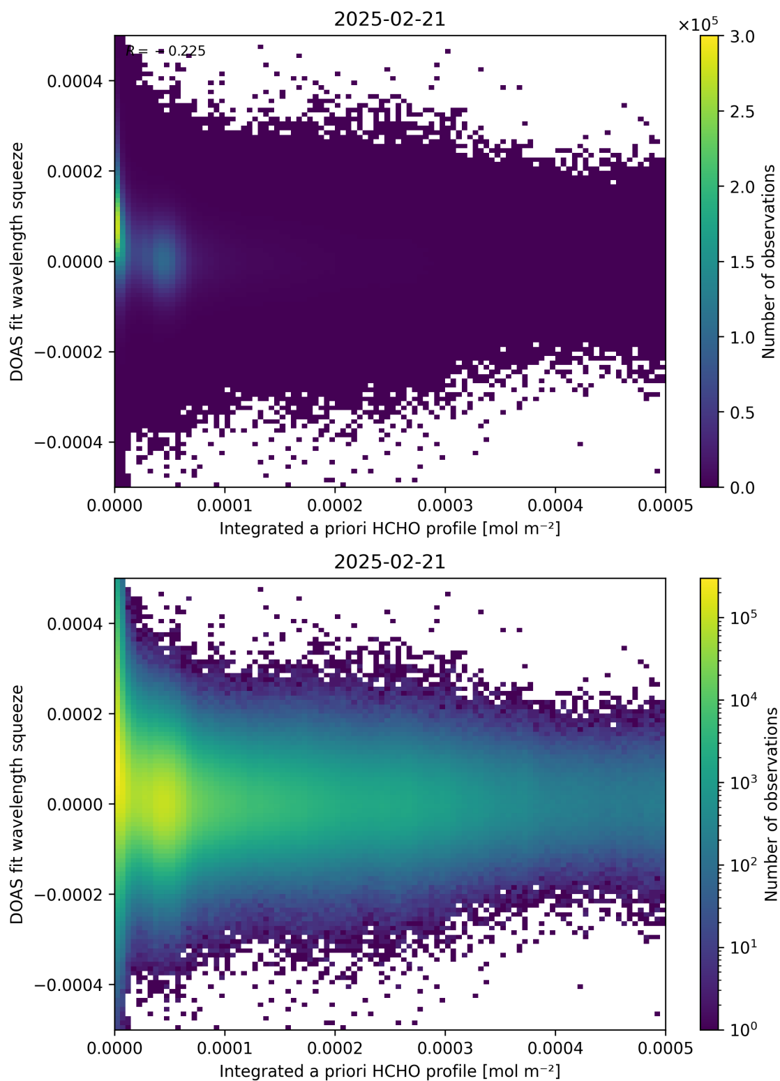
Figure 150: Scatter density plot of “Integrated a priori HCHO profile” against “DOAS fit wavelength squeeze” for 2025-02-20 to 2025-02-22.
