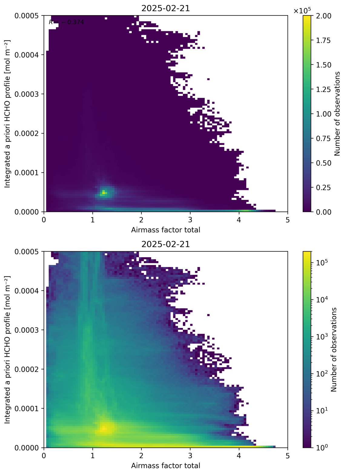
Figure 104: Scatter density plot of “Airmass factor total” against “Integrated a priori HCHO profile” for 2025-02-20 to 2025-02-22.
