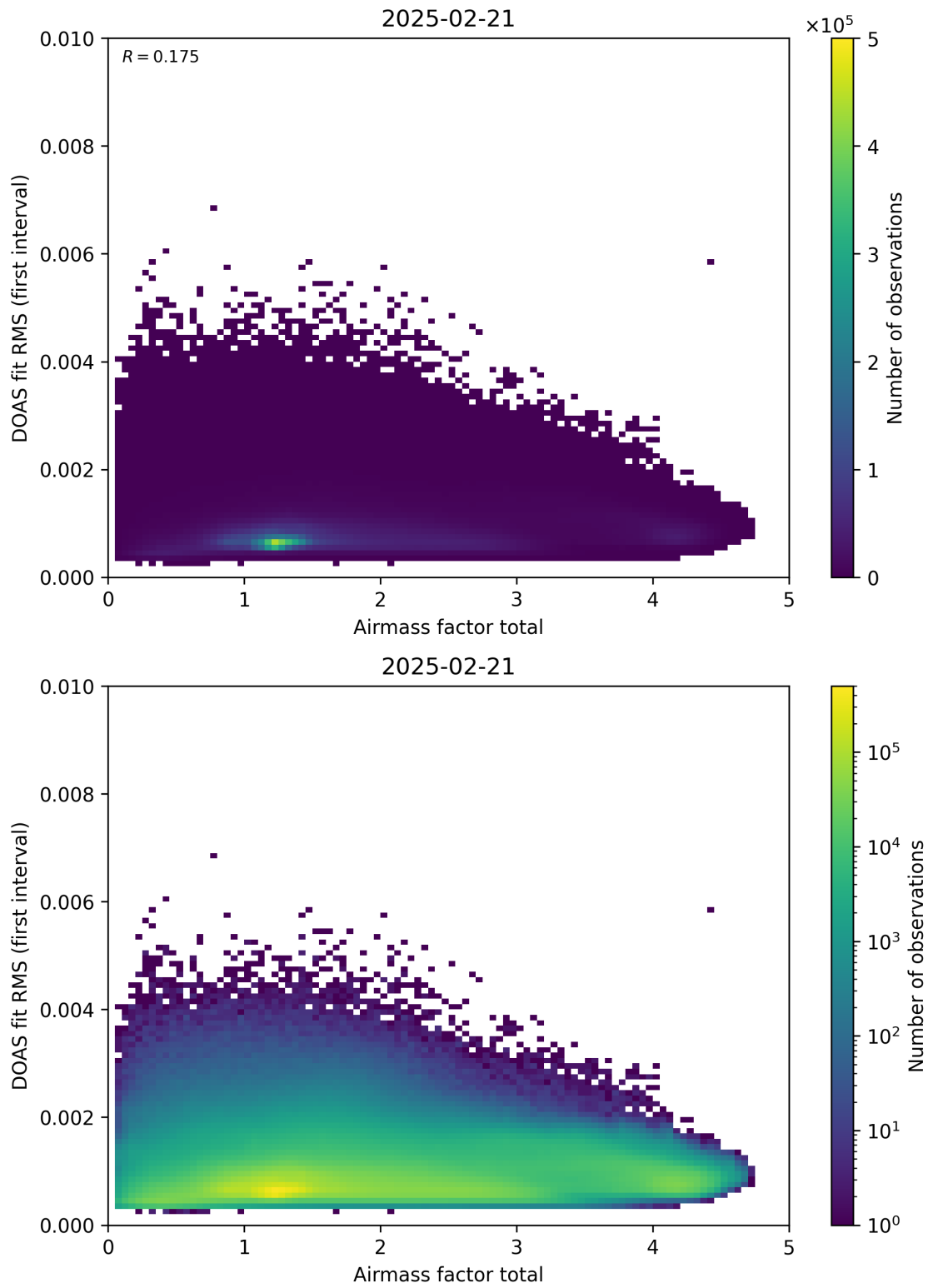
Figure 97: Scatter density plot of “Airmass factor total” against “DOAS fit RMS (first interval)” for 2025-02-20 to 2025-02-22.
