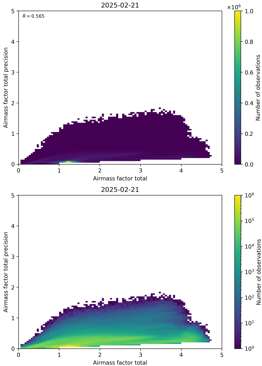
Figure 103: Scatter density plot of “Airmass factor total” against “Airmass factor total precision” for 2025-02-20 to 2025-02-22.
