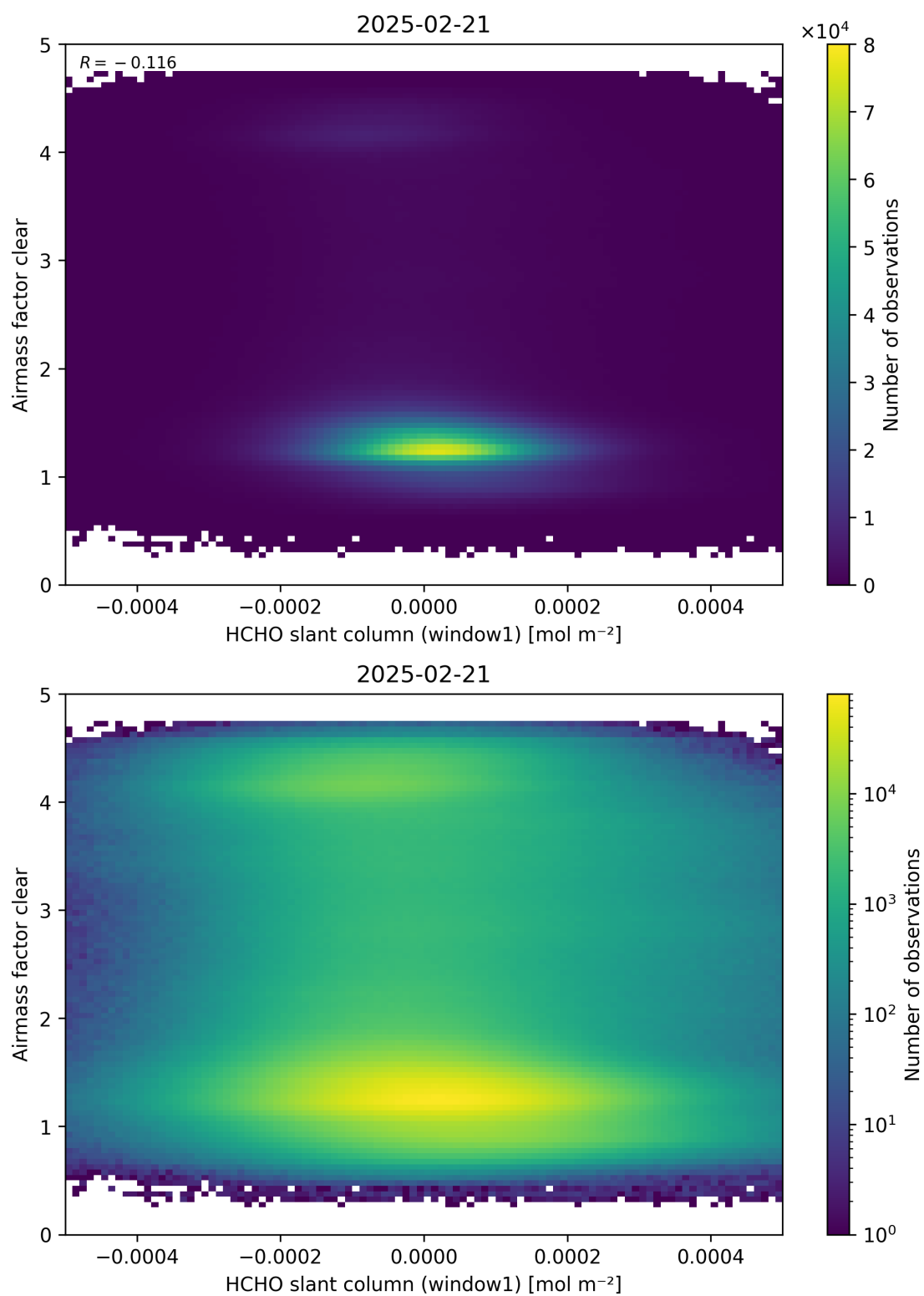
Figure 81: Scatter density plot of “HCHO slant column (window1)” against “Airmass factor clear” for 2025-02-20 to 2025-02-22.
