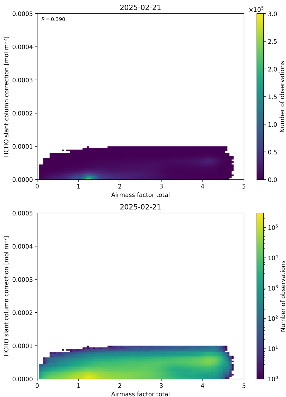
Figure 102: Scatter density plot of “Airmass factor total” against “HCHO slant column correction” for 2025-02-20 to 2025-02-22.
