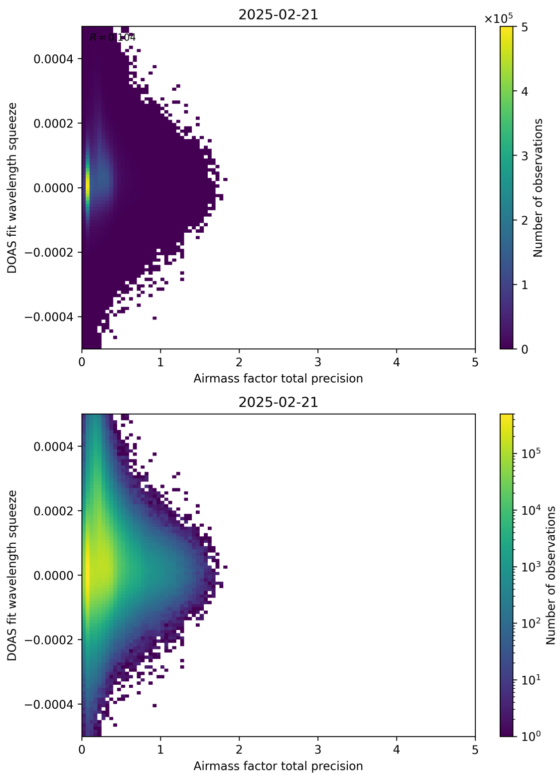
Figure 107: Scatter density plot of “Airmass factor total precision” against “DOAS fit wavelength squeeze” for 2025-02-20 to 2025-02-22.
