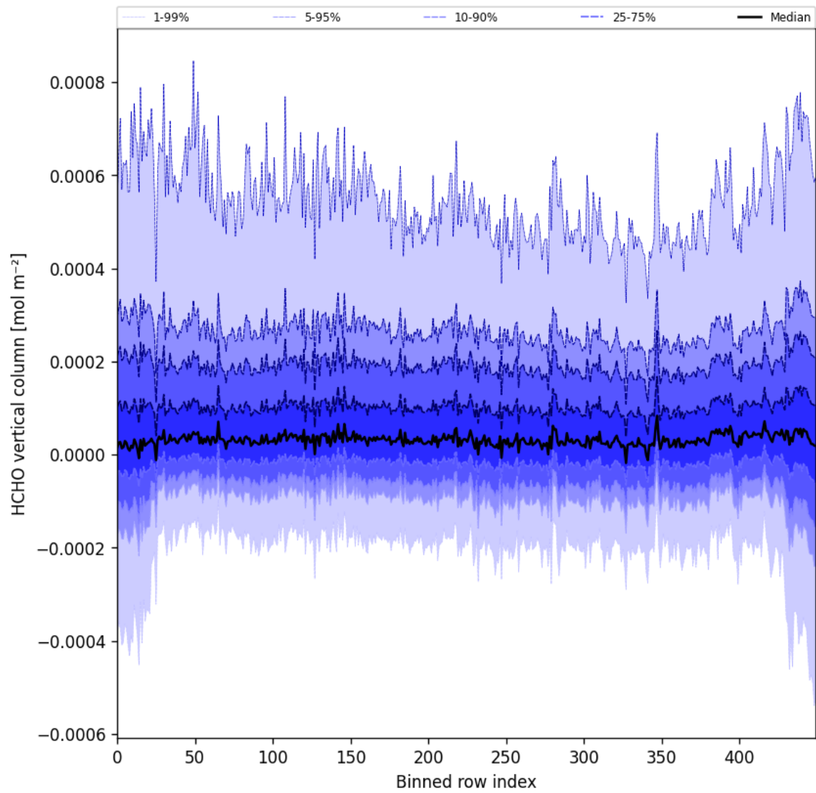
Figure 49: Along track statistics of “HCHO vertical column” for 2025-02-20 to 2025-02-22
