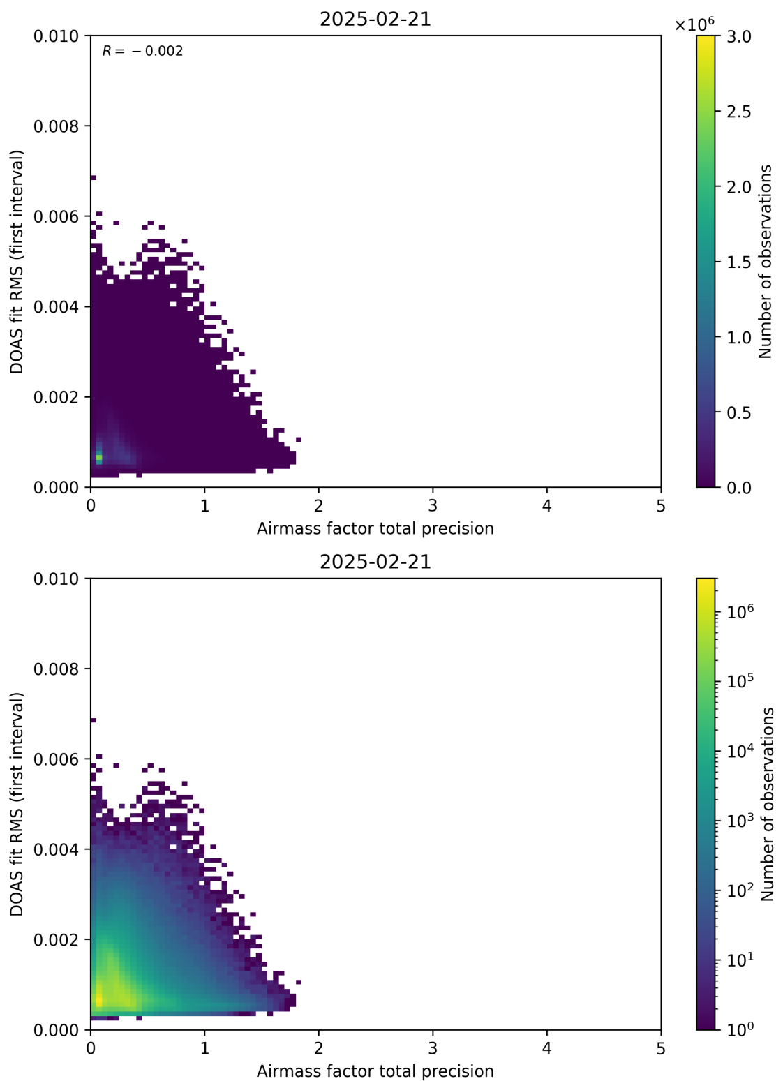
Figure 105: Scatter density plot of “Airmass factor total precision” against “DOAS fit RMS (first interval)” for 2025-02-20 to 2025-02-22.
