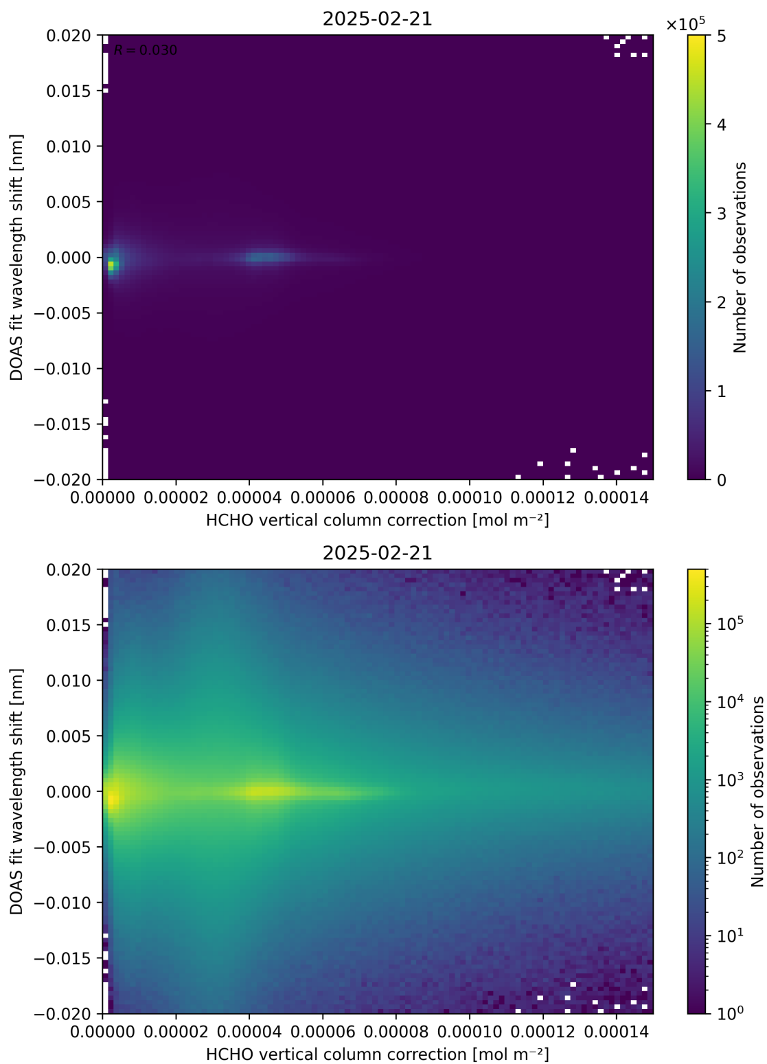
Figure 113: Scatter density plot of “HCHO vertical column correction” against “DOAS fit wavelength shift” for 2025-02-20 to 2025-02-22.
