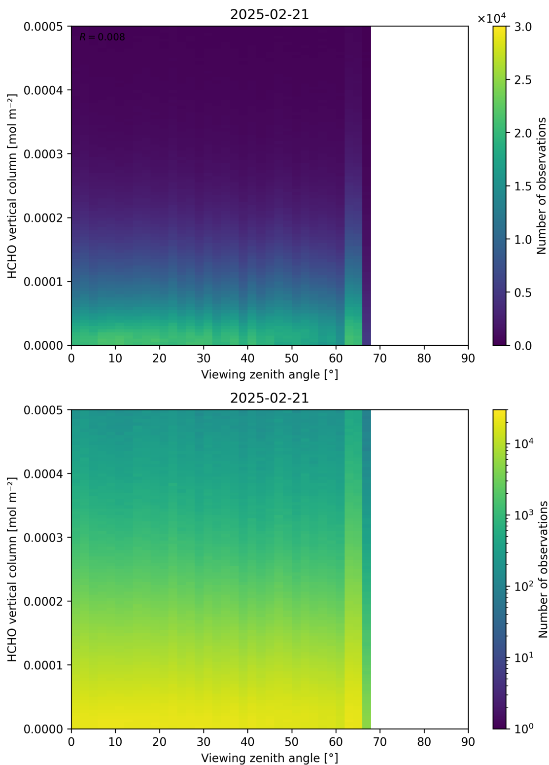
Figure 192: Scatter density plot of “Viewing zenith angle” against “HCHO vertical column” for 2025-02-20 to 2025-02-22.
