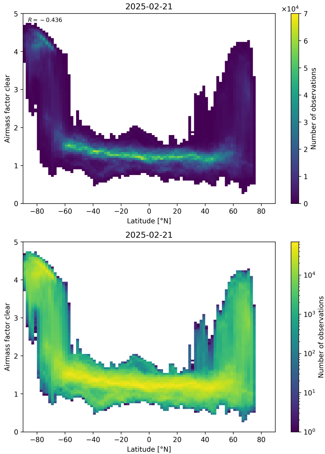
Figure 156: Scatter density plot of “Latitude” against “Airmass factor clear” for 2025-02-20 to 2025-02-22.
