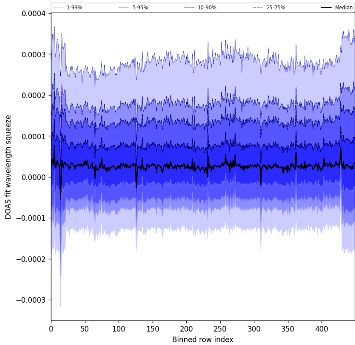
Figure 59: Along track statistics of “DOAS fit wavelength squeeze” for 2025-02-20 to 2025-02-22
