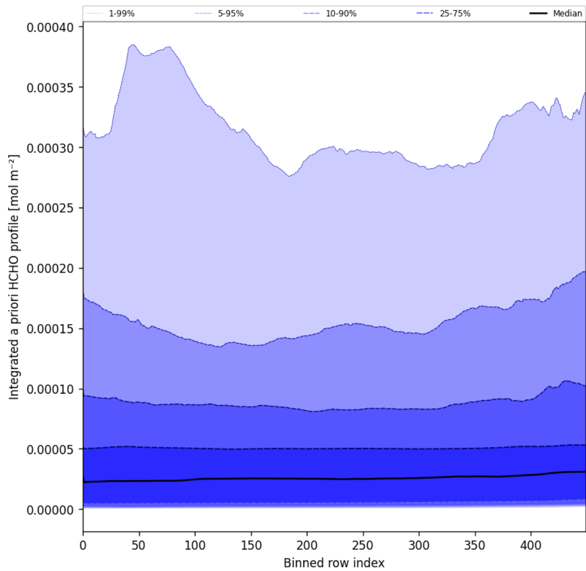
Figure 57: Along track statistics of “Integrated a priori HCHO profile” for 2025-02-20 to 2025-02-22
