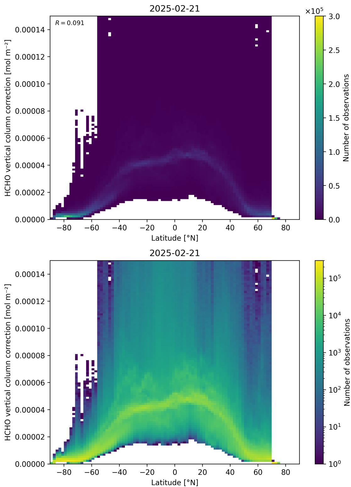
Figure 164: Scatter density plot of “Latitude” against “HCHO vertical column correction” for 2025-02-20 to 2025-02-22.
