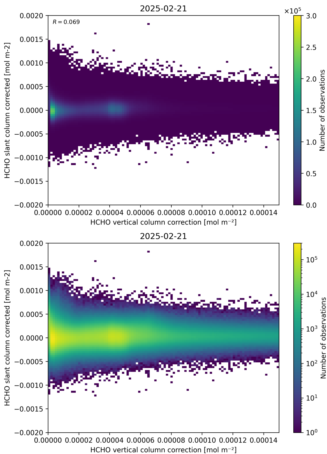
Figure 116: Scatter density plot of “HCHO vertical column correction” against “HCHO slant column corrected” for 2025-02-20 to 2025-02-22.
