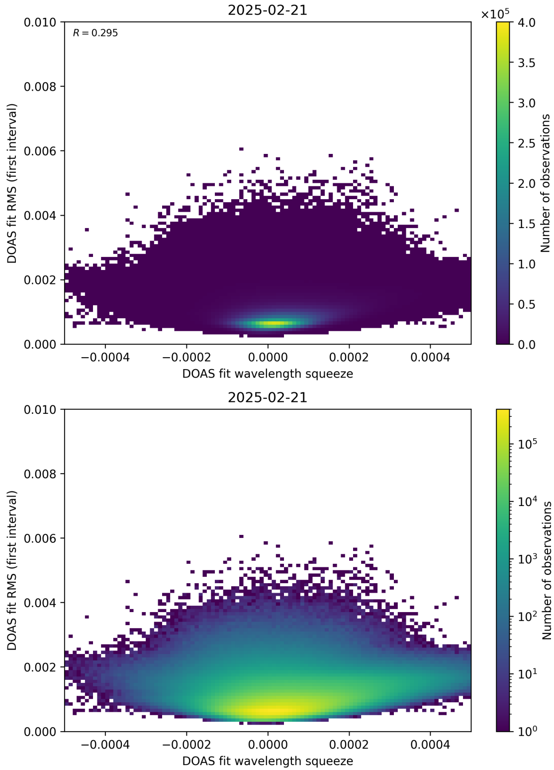
Figure 68: Scatter density plot of “DOAS fit wavelength squeeze” against “DOAS fit RMS (first interval)” for 2025-02-20 to 2025-02-22.
