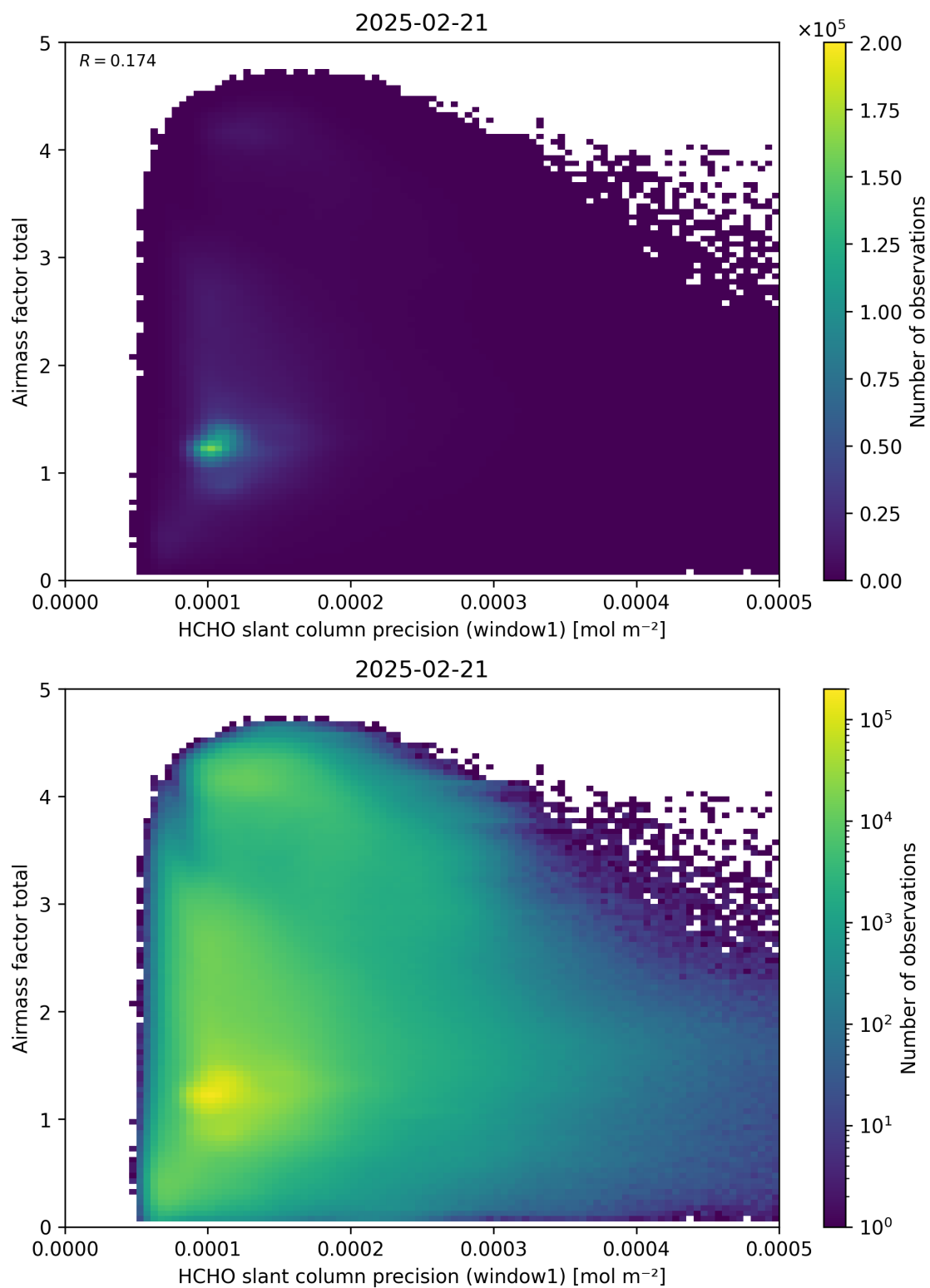
Figure 94: Scatter density plot of “HCHO slant column precision (window1)” against “Airmass factor total” for 2025-02-20 to 2025-02-22.
