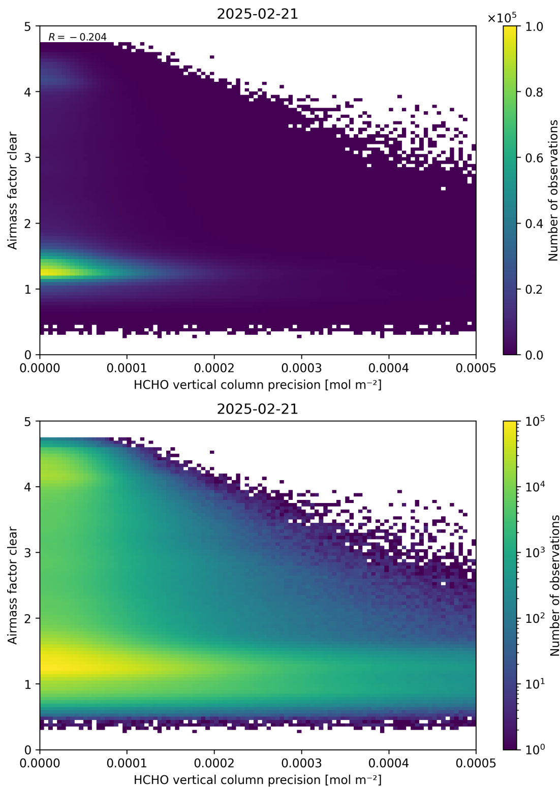
Figure 139: Scatter density plot of “HCHO vertical column precision” against “Airmass factor clear” for 2025-02-20 to 2025-02-22.
