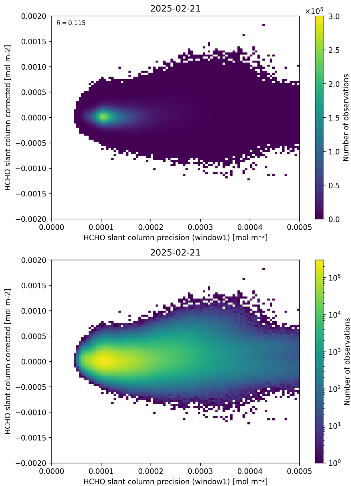
Figure 92: Scatter density plot of “HCHO slant column precision (window1)” against “HCHO slant column corrected” for 2025-02-20 to 2025-02-22.
