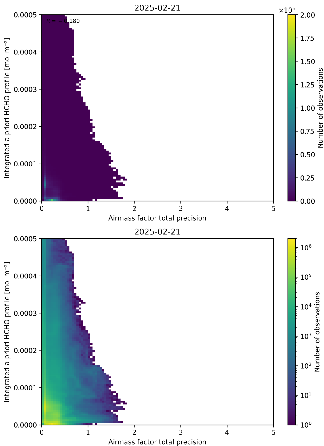
Figure 111: Scatter density plot of “Airmass factor total precision” against “Integrated a priori HCHO profile” for 2025-02-20 to 2025-02-22.
