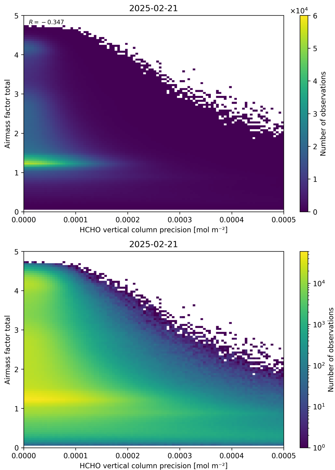
Figure 144: Scatter density plot of “HCHO vertical column precision” against “Airmass factor total” for 2025-02-20 to 2025-02-22.
