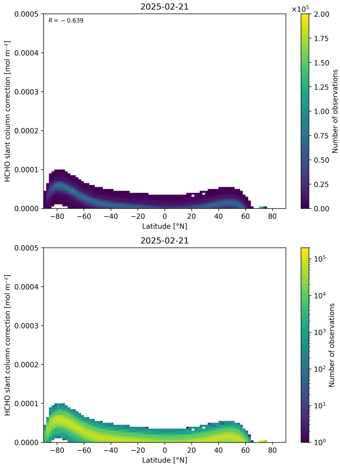
Figure 158: Scatter density plot of “Latitude” against “HCHO slant column correction” for 2025-02-20 to 2025-02-22.
