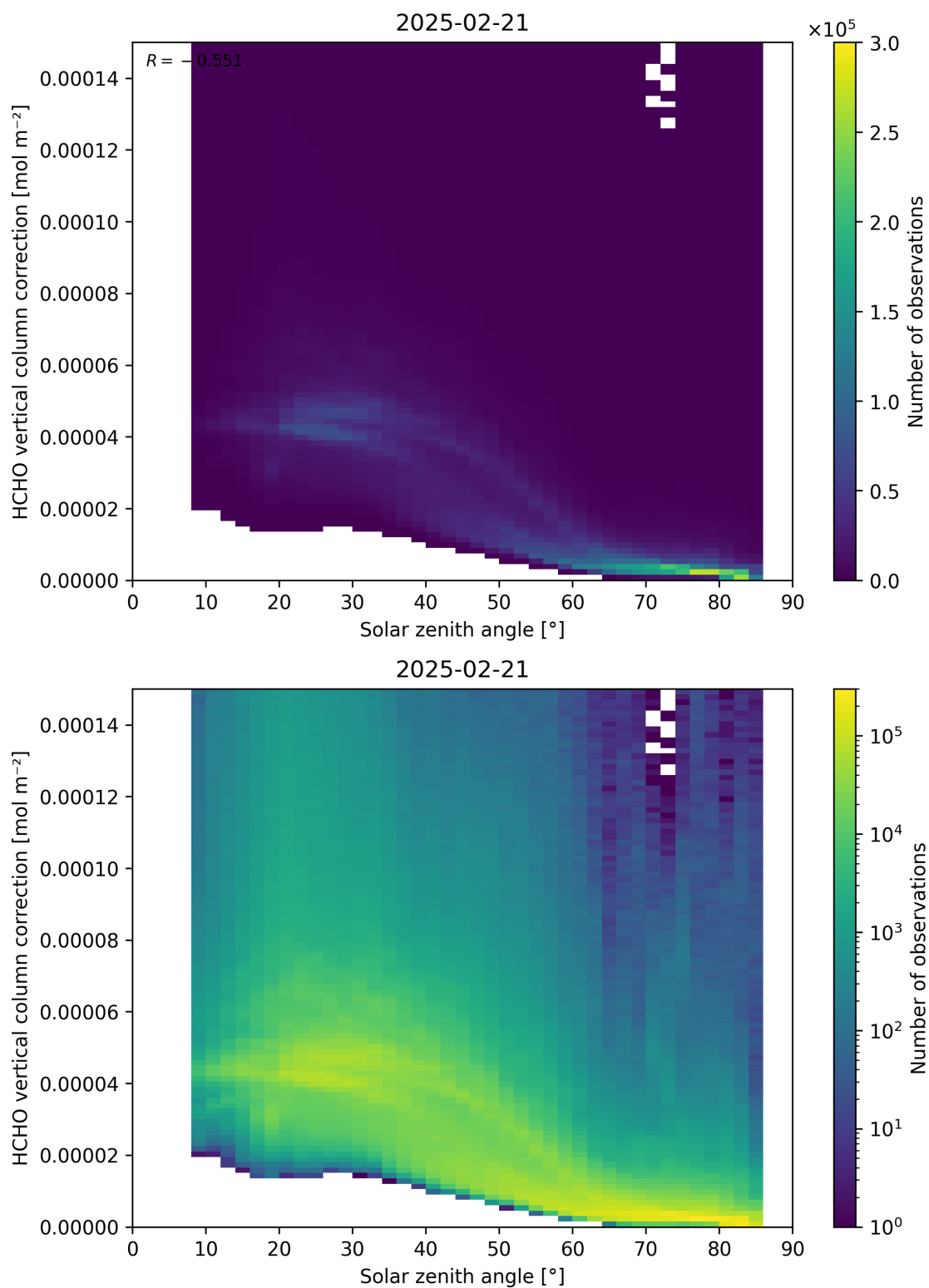
Figure 178: Scatter density plot of “Solar zenith angle” against “HCHO vertical column correction” for 2025-02-20 to 2025-02-22.
