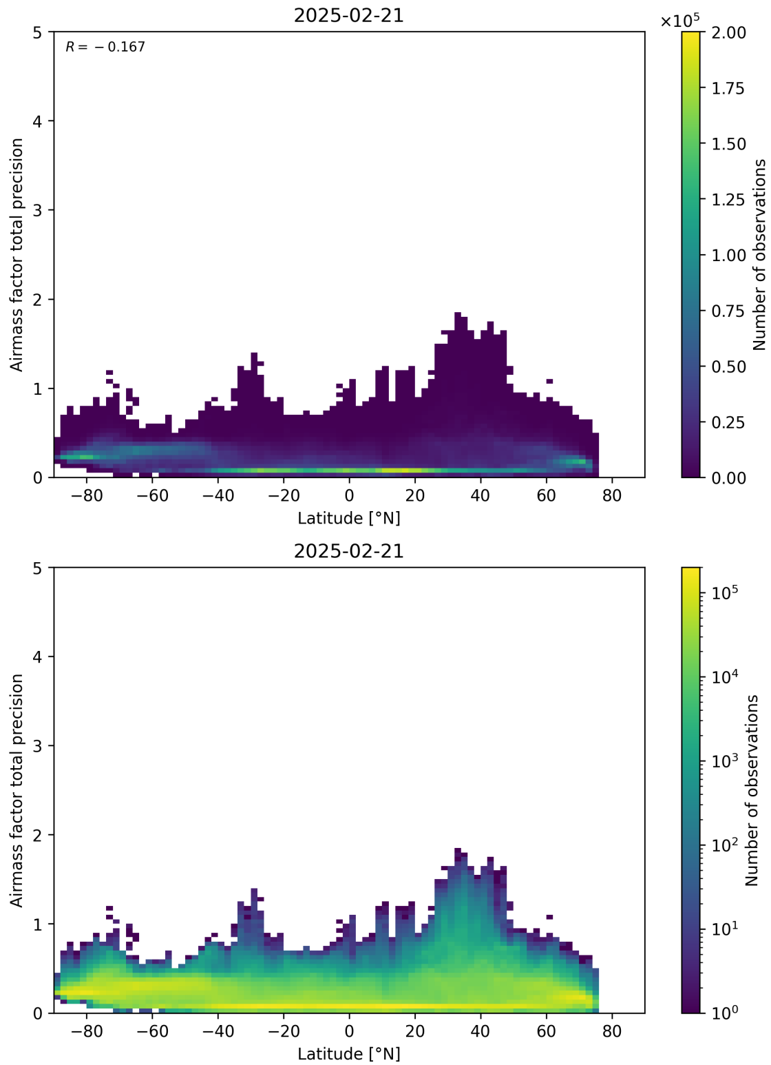
Figure 162: Scatter density plot of “Latitude” against “Airmass factor total precision” for 2025-02-20 to 2025-02-22.
