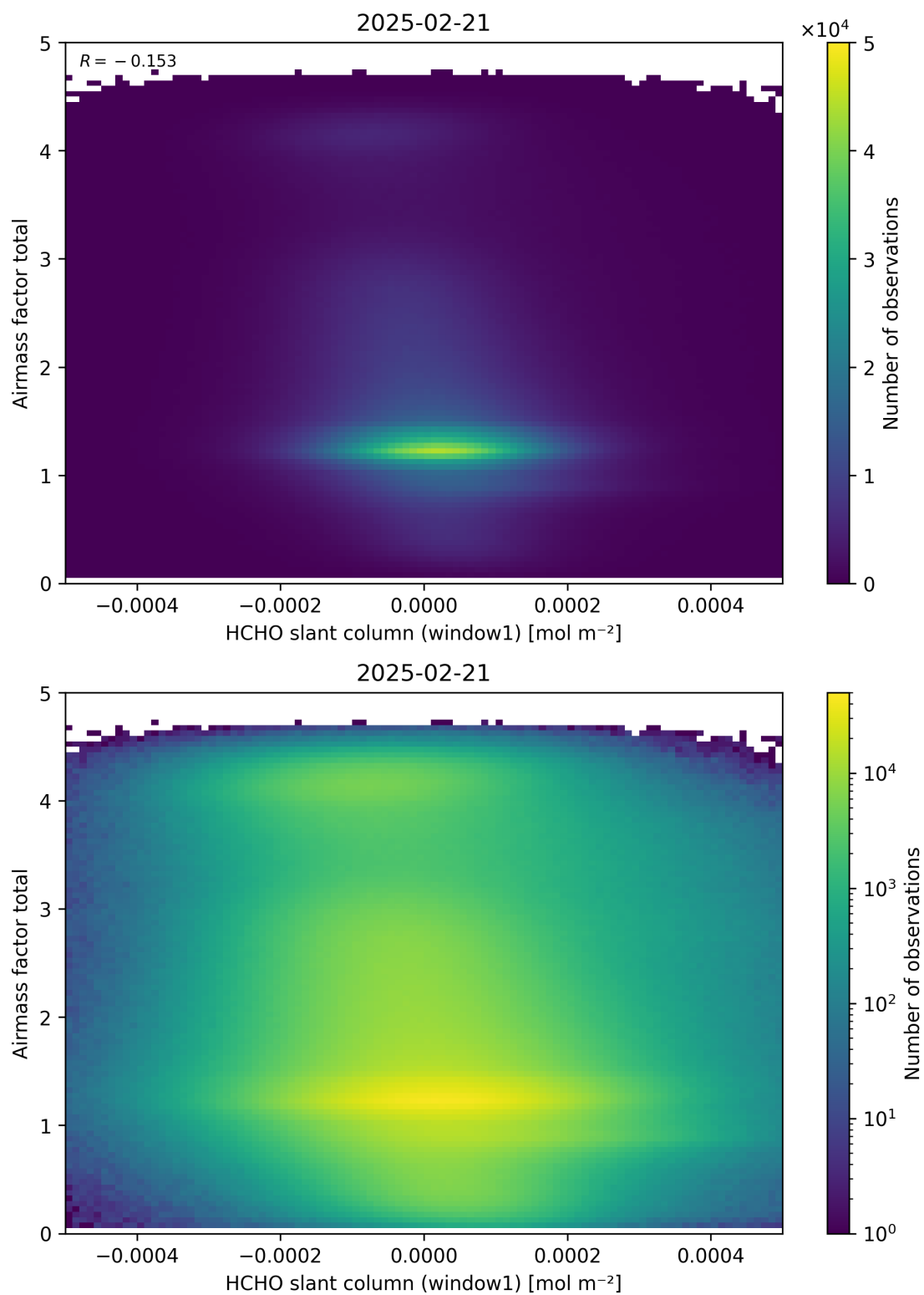
Figure 85: Scatter density plot of “HCHO slant column (window1)” against “Airmass factor total” for 2025-02-20 to 2025-02-22.
