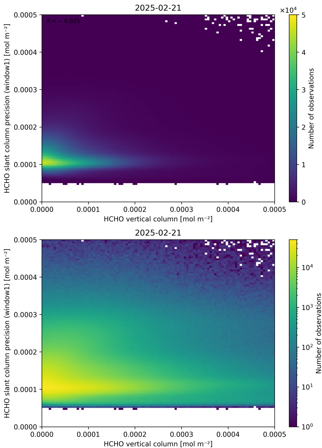
Figure 130: Scatter density plot of “HCHO vertical column” against “HCHO slant column precision (window1)” for 2025-02-20 to 2025-02-22.
