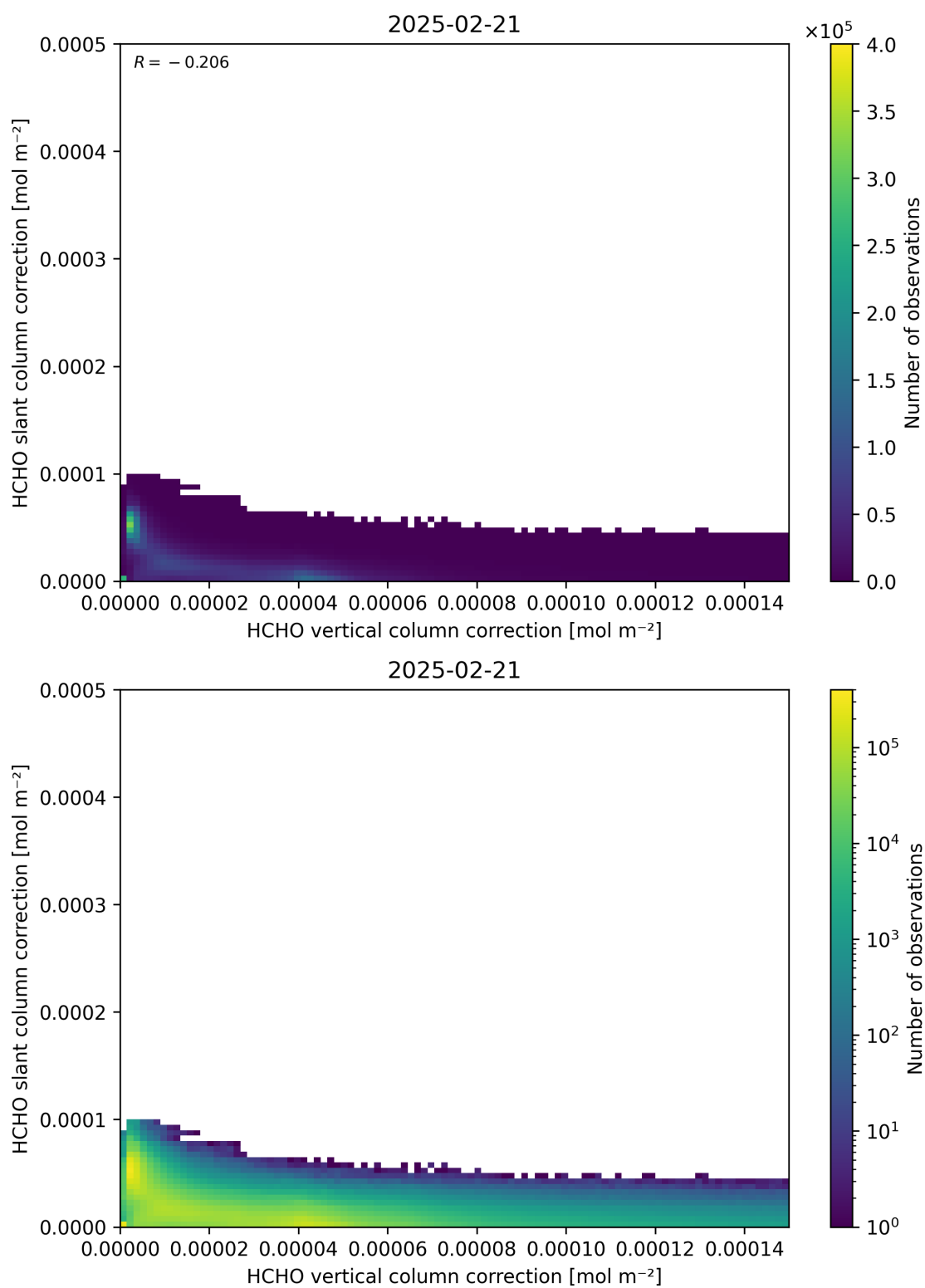
Figure 117: Scatter density plot of “HCHO vertical column correction” against “HCHO slant column correction” for 2025-02-20 to 2025-02-22.
