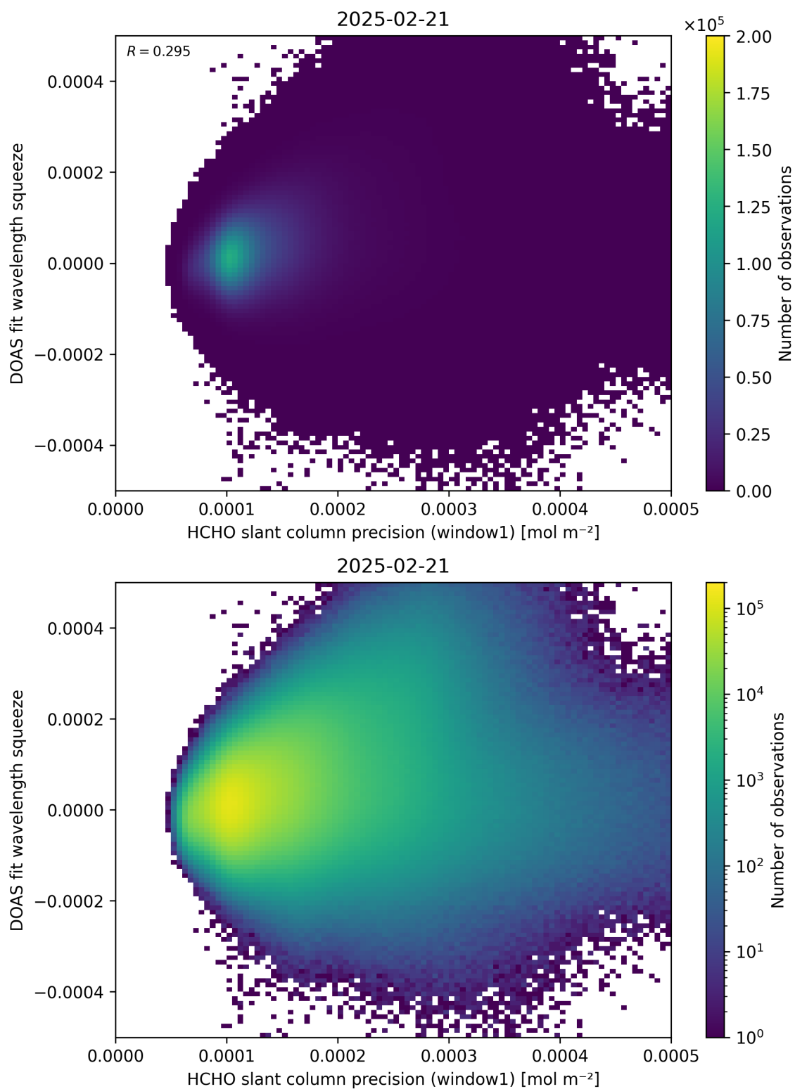
Figure 90: Scatter density plot of “HCHO slant column precision (window1)” against “DOAS fit wavelength squeeze” for 2025-02-20 to 2025-02-22.
