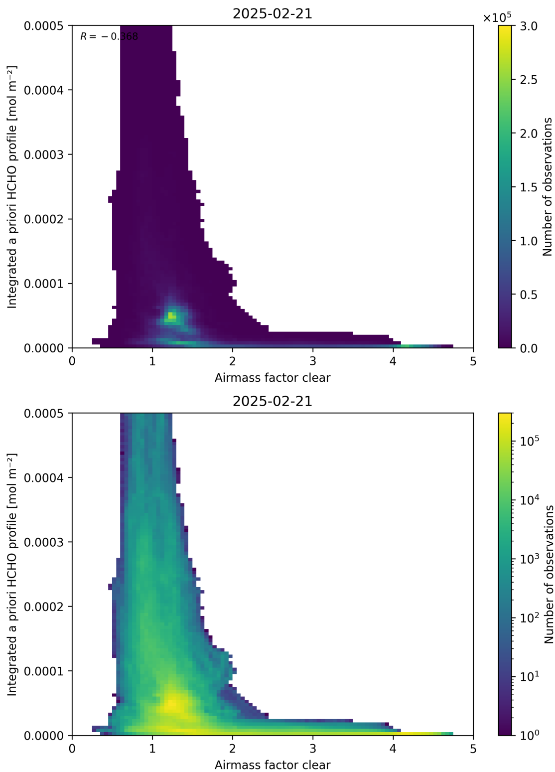
Figure 76: Scatter density plot of “Airmass factor clear” against “Integrated a priori HCHO profile” for 2025-02-20 to 2025-02-22.
