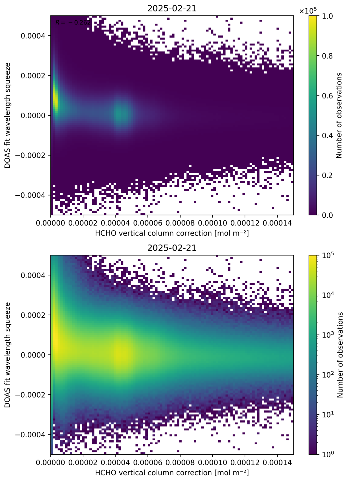
Figure 114: Scatter density plot of “HCHO vertical column correction” against “DOAS fit wavelength squeeze” for 2025-02-20 to 2025-02-22.
