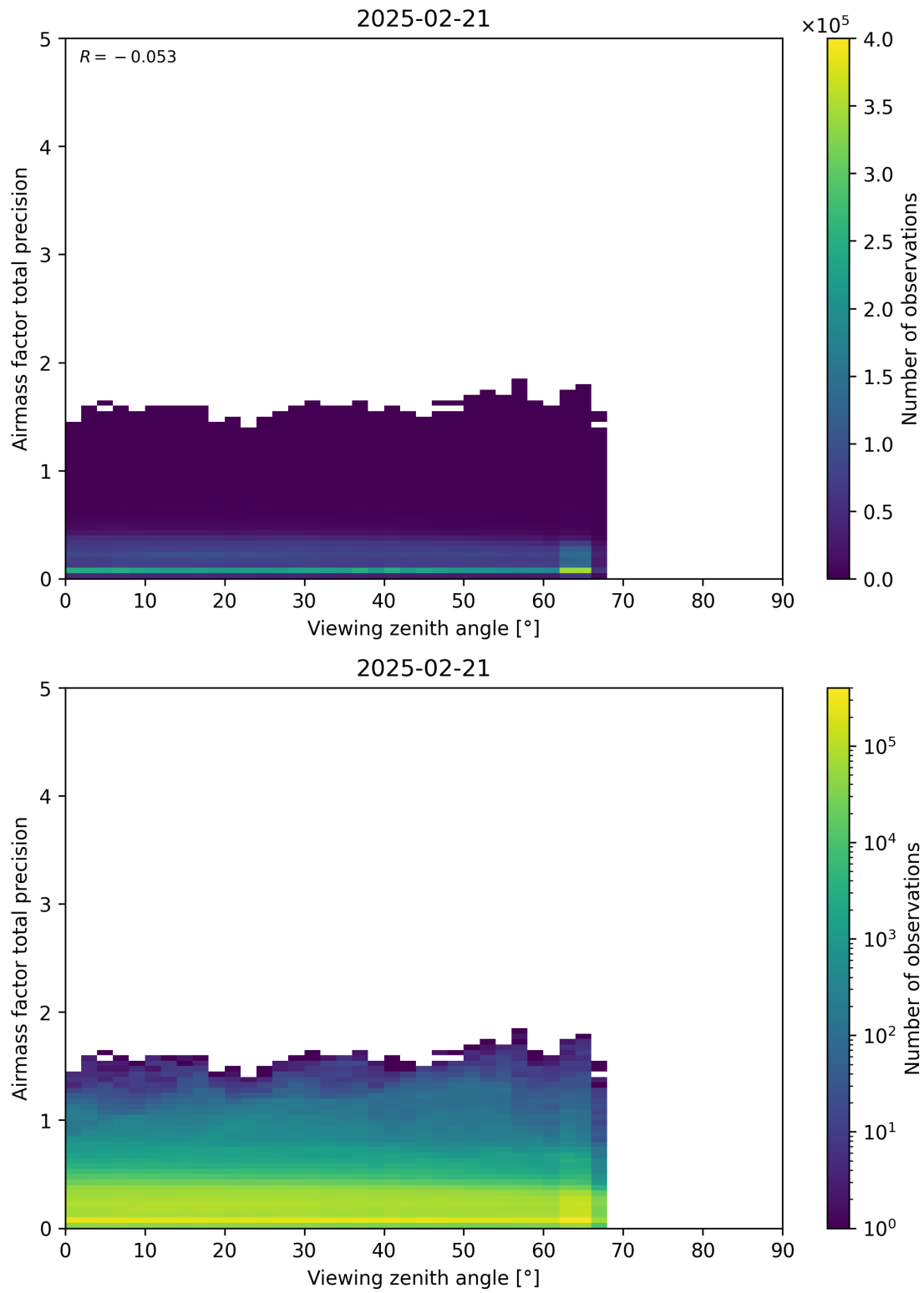
Figure 191: Scatter density plot of “Viewing zenith angle” against “Airmass factor total precision” for 2025-02-20 to 2025-02-22.
