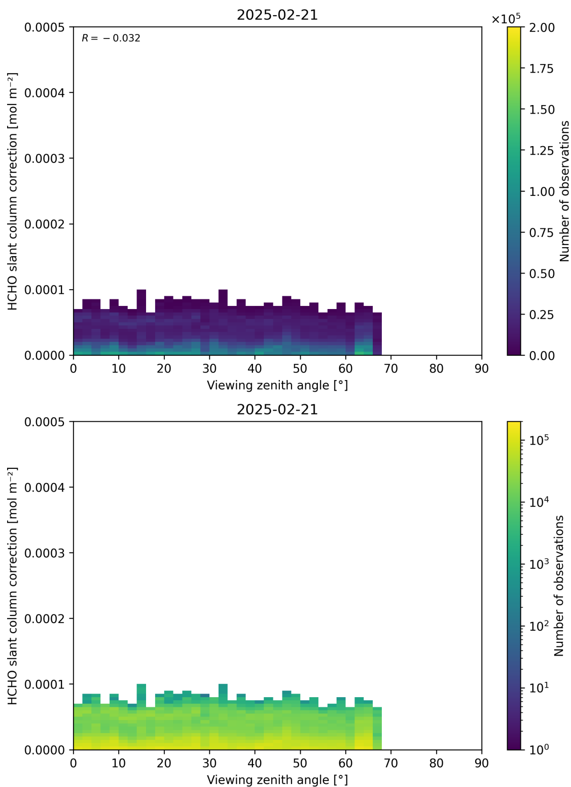
Figure 187: Scatter density plot of “Viewing zenith angle” against “HCHO slant column correction” for 2025-02-20 to 2025-02-22.
