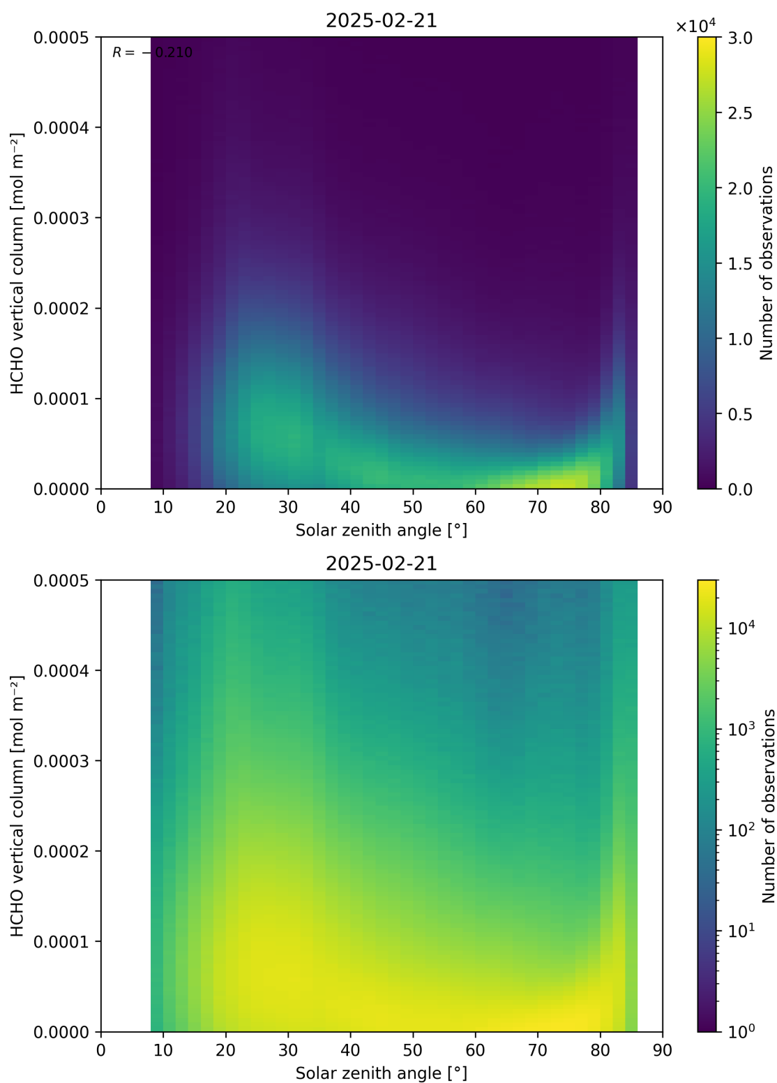
Figure 177: Scatter density plot of “Solar zenith angle” against “HCHO vertical column” for 2025-02-20 to 2025-02-22.
