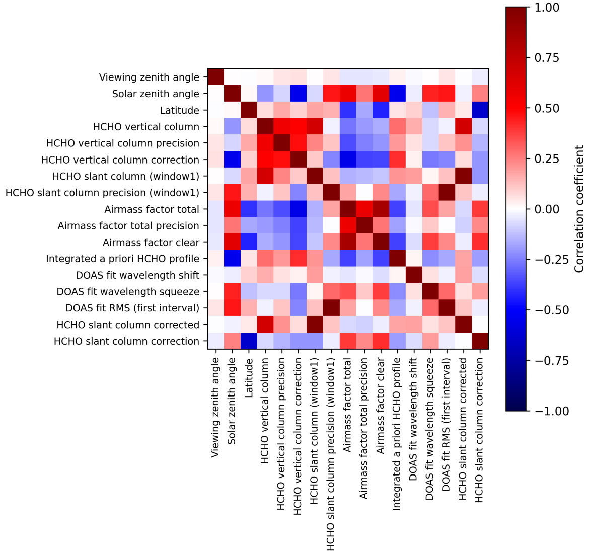
Figure 2: Map of correlation matrix for 2025-02-20 to 2025-02-22.
