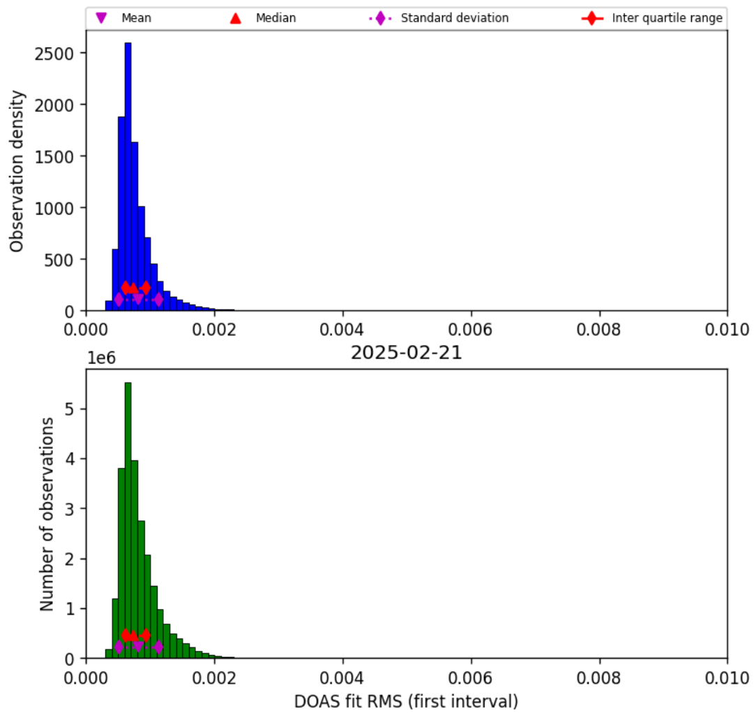
Figure 46: Histogram of “DOAS fit RMS (first interval)” for 2025-02-20 to 2025-02-22
