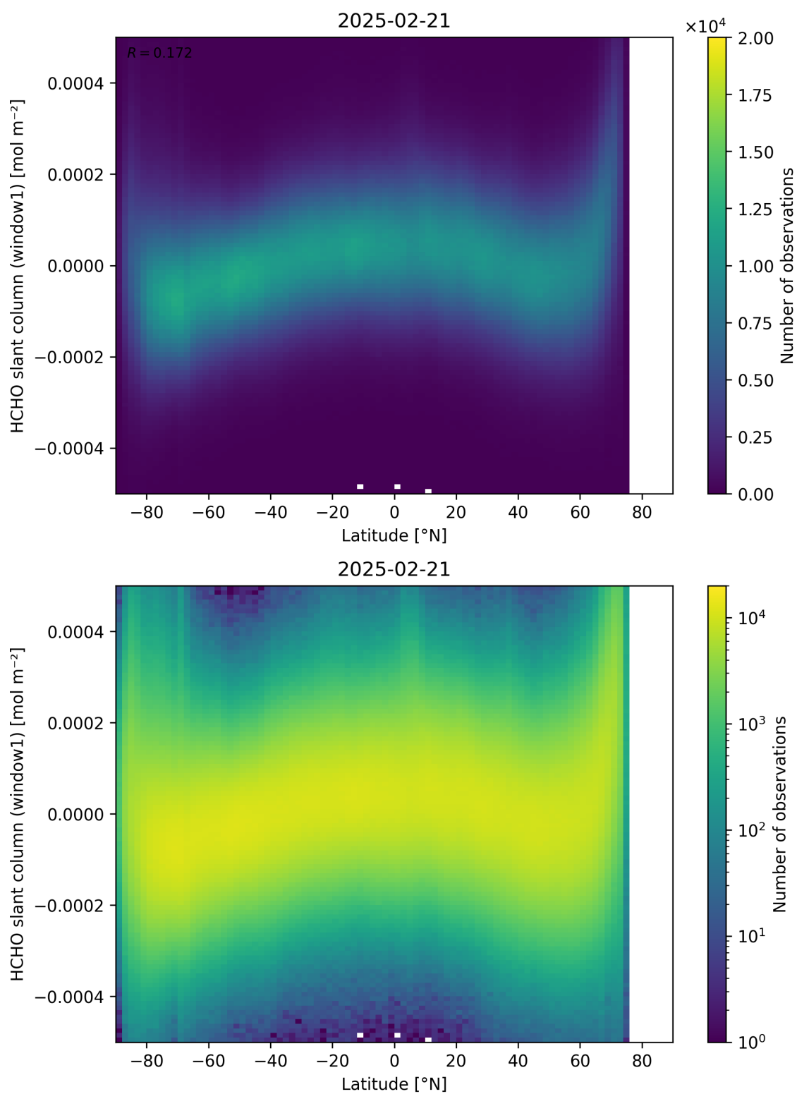
Figure 159: Scatter density plot of “Latitude” against “HCHO slant column (window1)” for 2025-02-20 to 2025-02-22.
