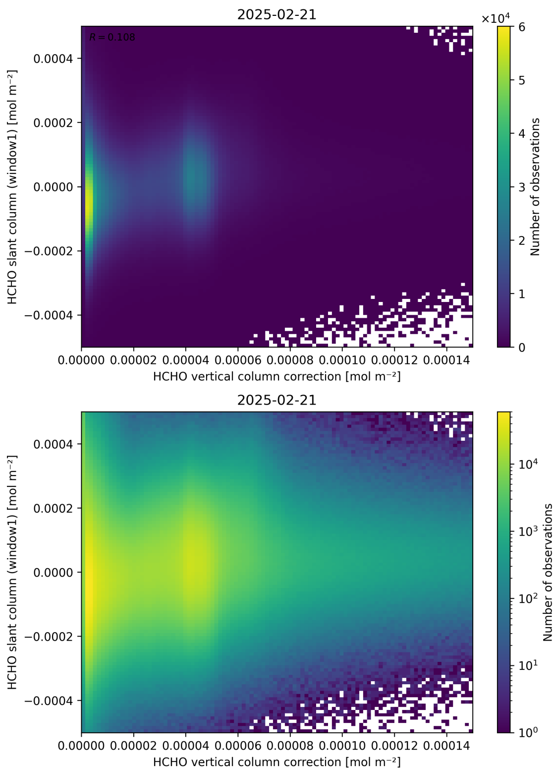
Figure 118: Scatter density plot of “HCHO vertical column correction” against “HCHO slant column (window1)” for 2025-02-20 to 2025-02-22.
