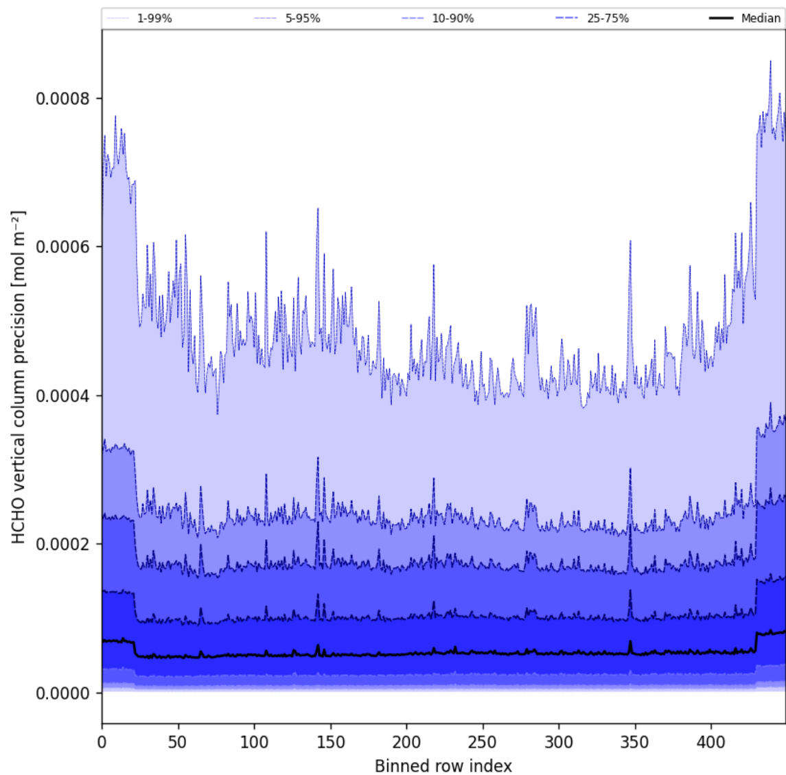
Figure 50: Along track statistics of “HCHO vertical column precision” for 2025-02-20 to 2025-02-22
