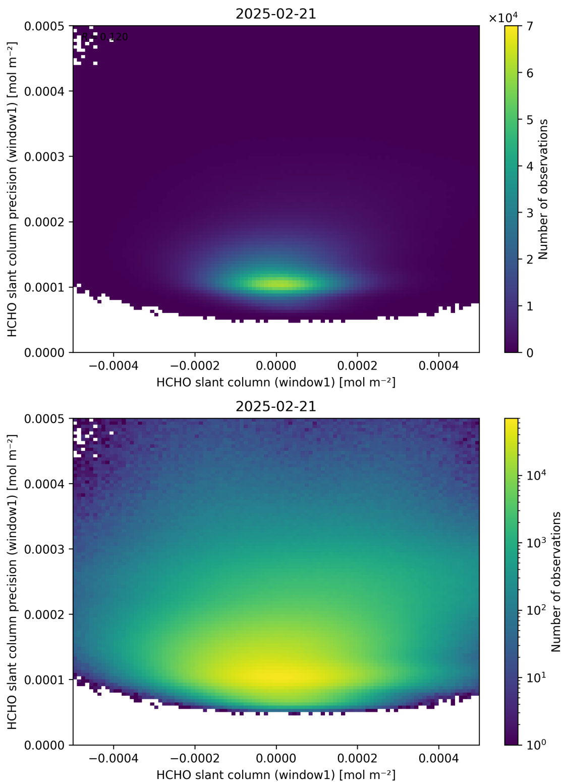
Figure 84: Scatter density plot of “HCHO slant column (window1)” against “HCHO slant column precision (window1)” for 2025-02-20 to 2025-02-22.
