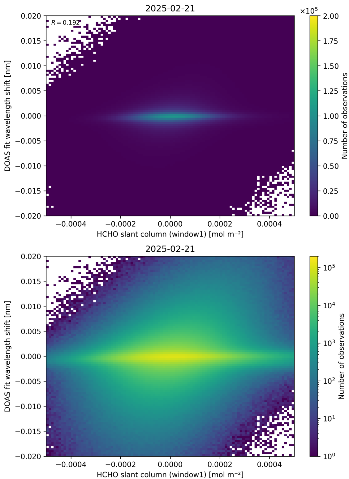
Figure 79: Scatter density plot of “HCHO slant column (window1)” against “DOAS fit wavelength shift” for 2025-02-20 to 2025-02-22.
