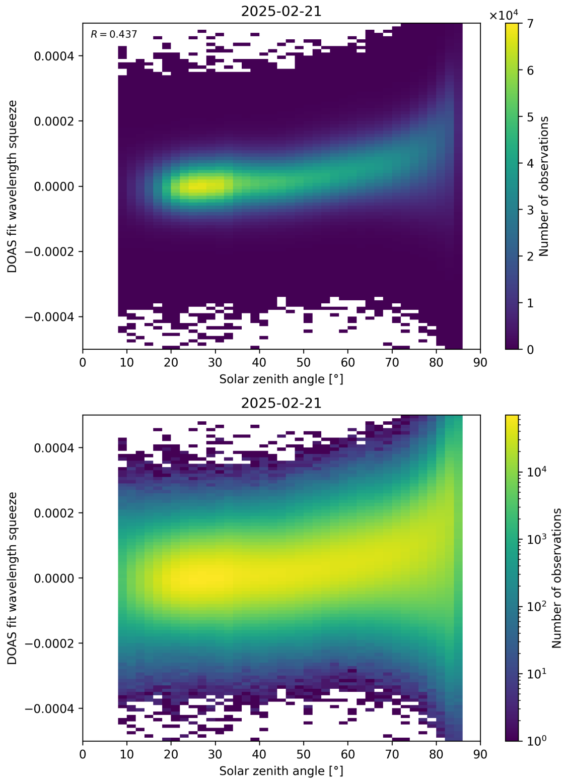
Figure 169: Scatter density plot of “Solar zenith angle” against “DOAS fit wavelength squeeze” for 2025-02-20 to 2025-02-22.
