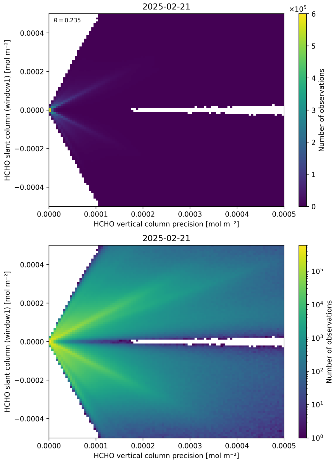
Figure 142: Scatter density plot of “HCHO vertical column precision” against “HCHO slant column (window1)” for 2025-02-20 to 2025-02-22.
