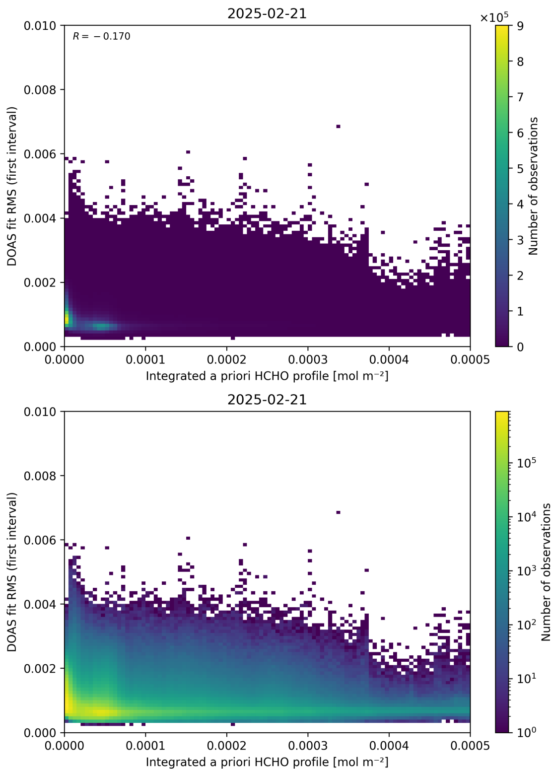
Figure 148: Scatter density plot of “Integrated a priori HCHO profile” against “DOAS fit RMS (first interval)” for 2025-02-20 to 2025-02-22.
