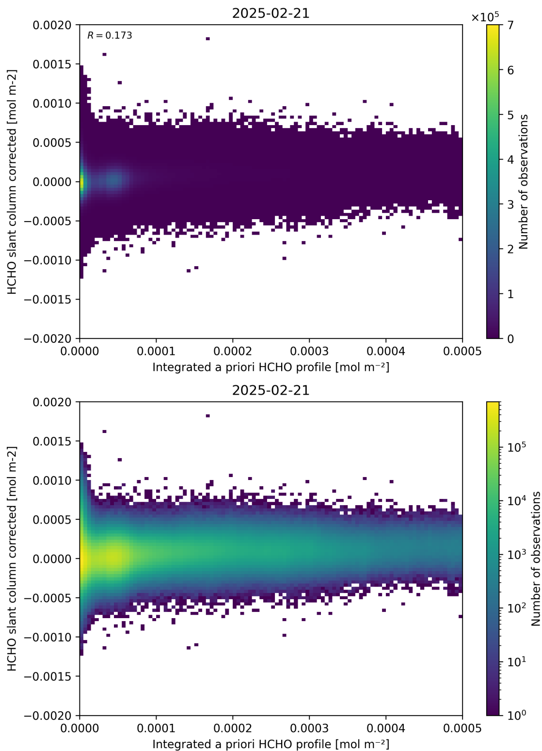
Figure 151: Scatter density plot of “Integrated a priori HCHO profile” against “HCHO slant column corrected” for 2025-02-20 to 2025-02-22.
