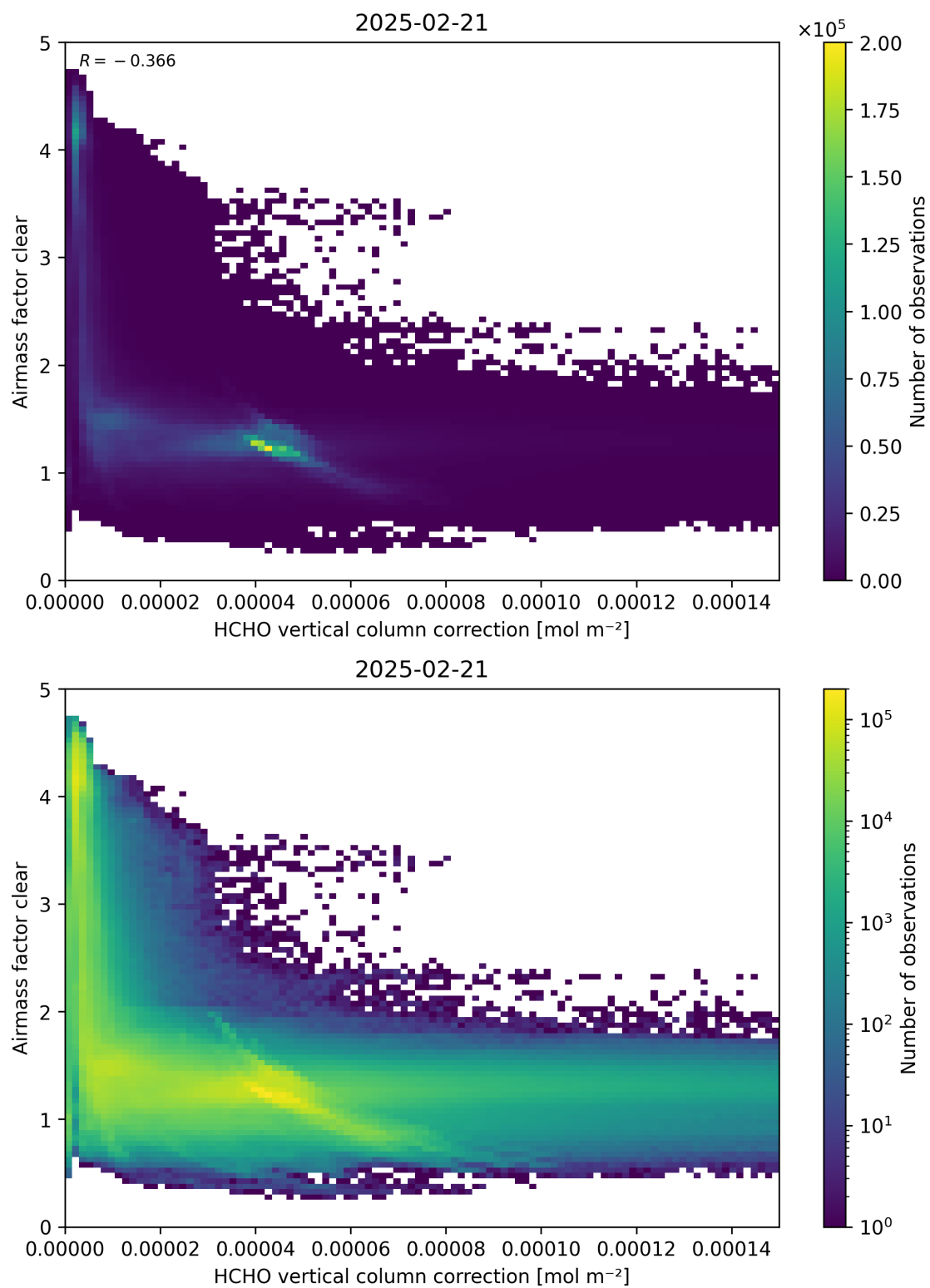
Figure 115: Scatter density plot of “HCHO vertical column correction” against “Airmass factor clear” for 2025-02-20 to 2025-02-22.
