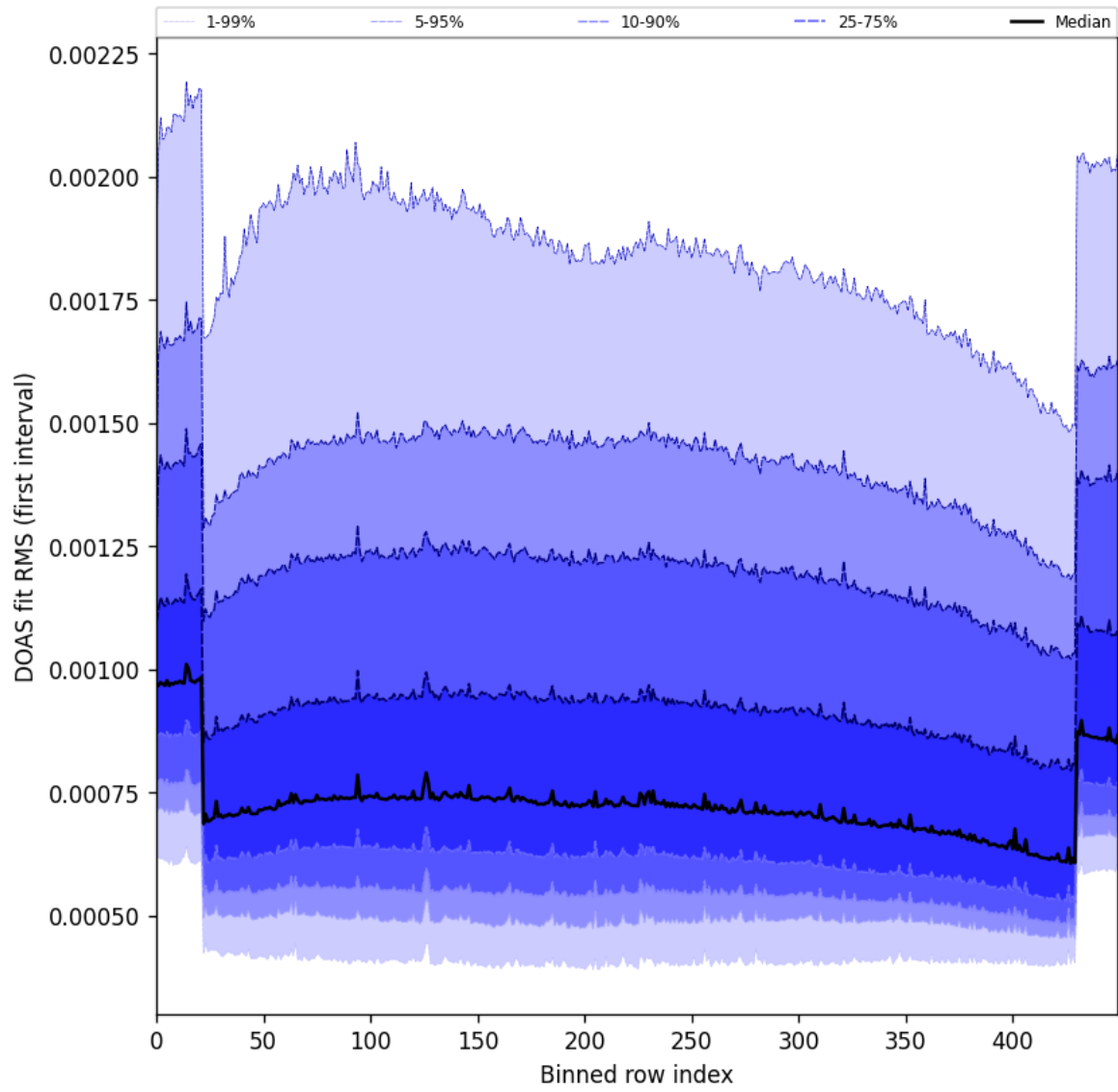
Figure 60: Along track statistics of “DOAS fit RMS (first interval)” for 2025-02-20 to 2025-02-22
