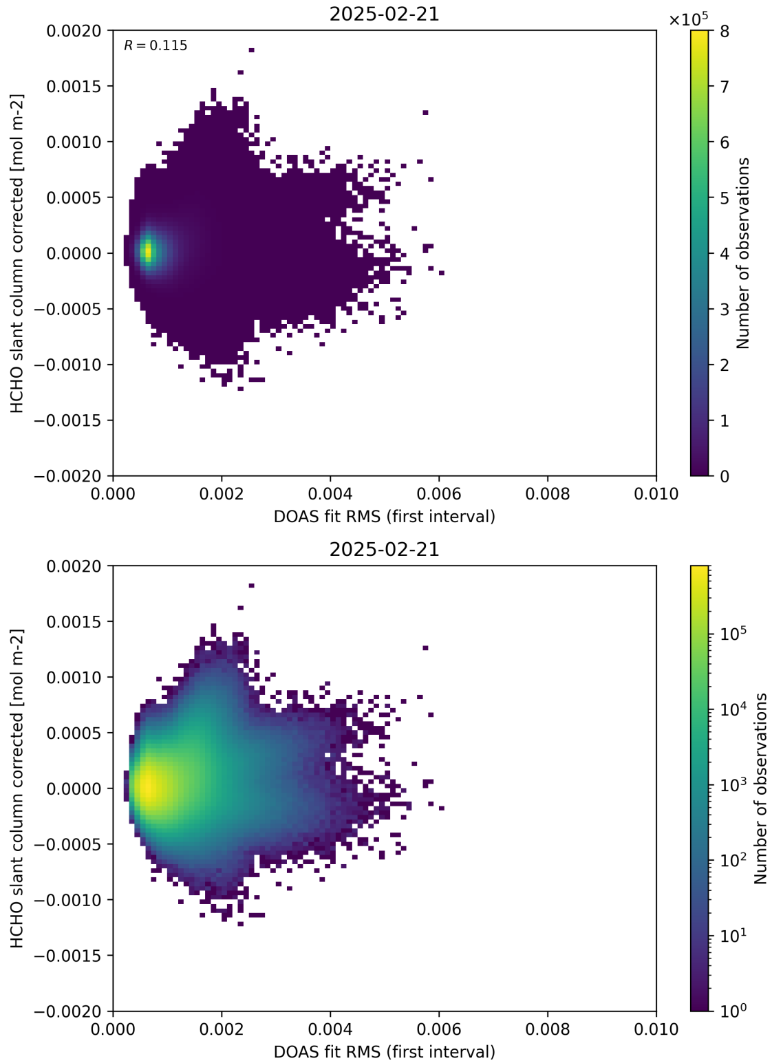
Figure 62: Scatter density plot of “DOAS fit RMS (first interval)” against “HCHO slant column corrected” for 2025-02-20 to 2025-02-22.
