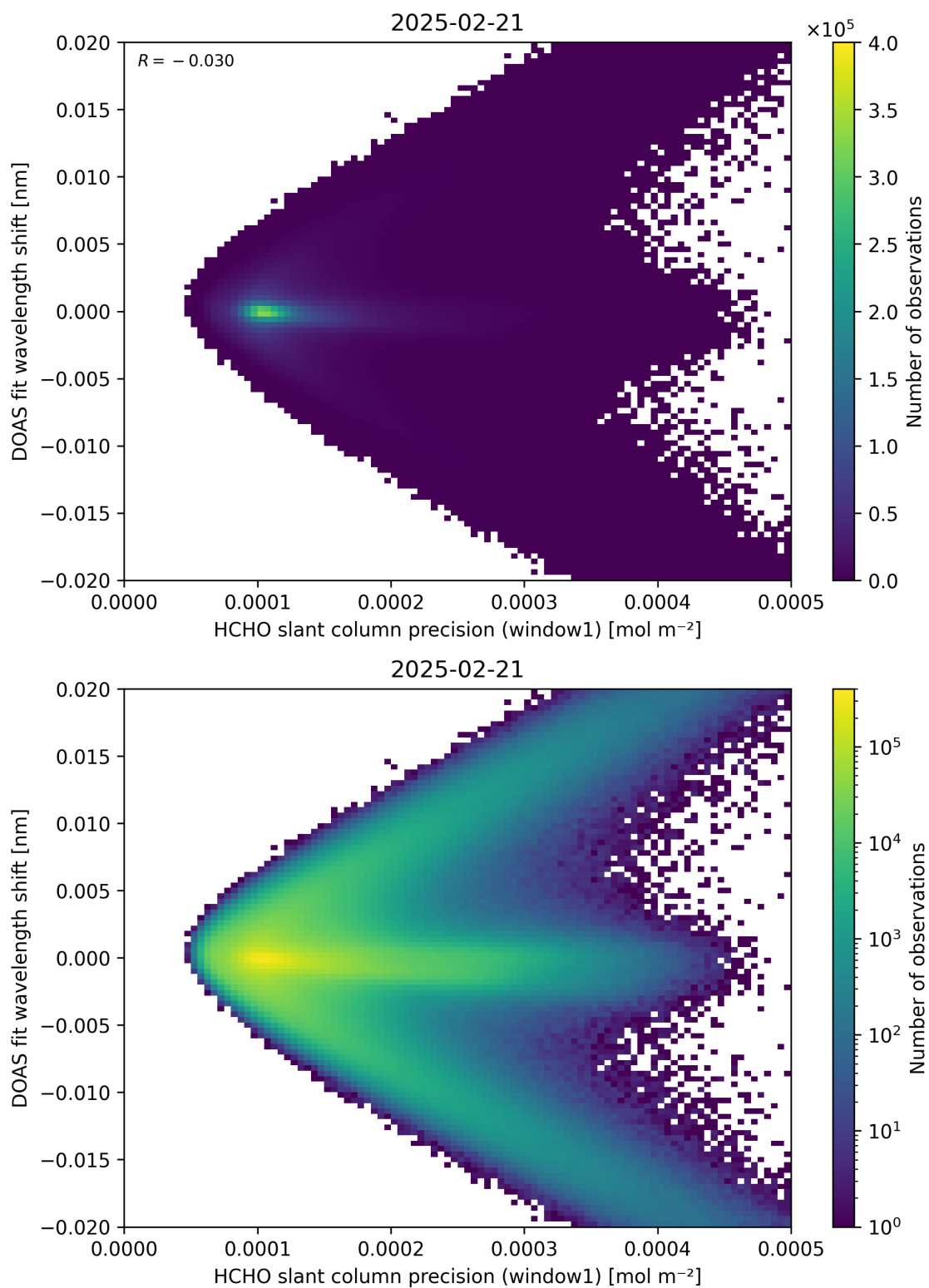
Figure 89: Scatter density plot of “HCHO slant column precision (window1)” against “DOAS fit wavelength shift” for 2025-02-20 to 2025-02-22.
