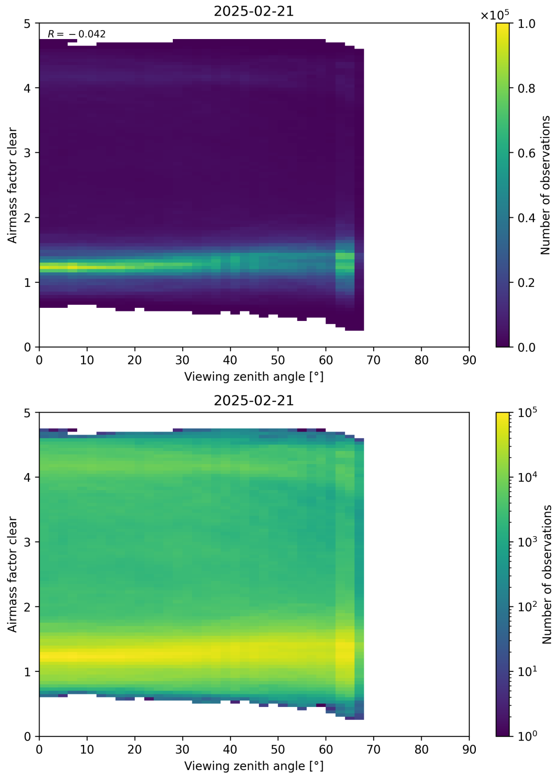
Figure 185: Scatter density plot of “Viewing zenith angle” against “Airmass factor clear” for 2025-02-20 to 2025-02-22.
