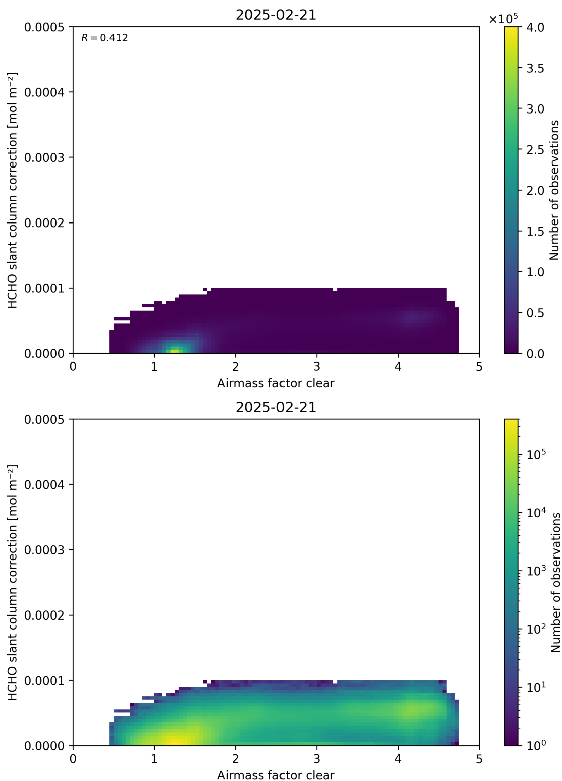
Figure 75: Scatter density plot of “Airmass factor clear” against “HCHO slant column correction” for 2025-02-20 to 2025-02-22.
