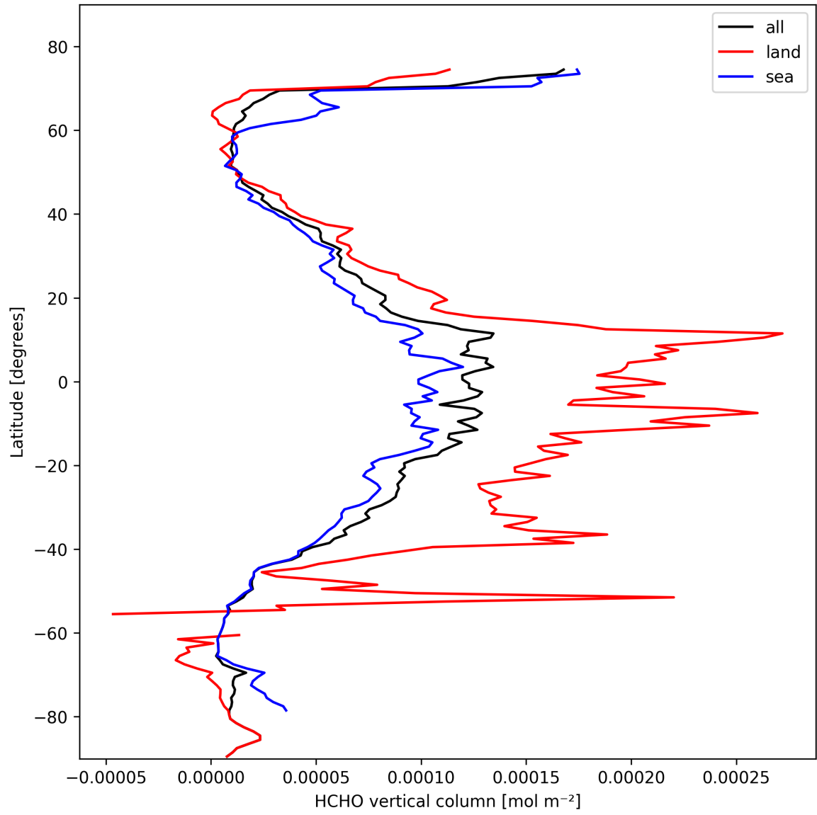
Figure 21: Zonal average of “HCHO vertical column” for 2025-02-20 to 2025-02-22.
