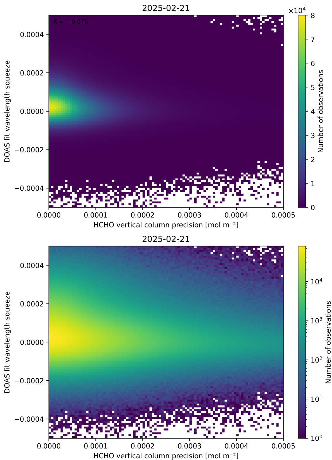
Figure 138: Scatter density plot of “HCHO vertical column precision” against “DOAS fit wavelength squeeze” for 2025-02-20 to 2025-02-22.
