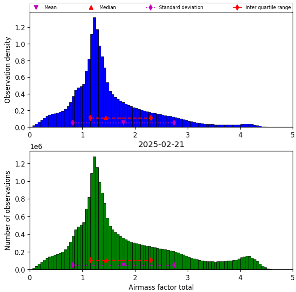
Figure 40: Histogram of “Airmass factor total” for 2025-02-20 to 2025-02-22
