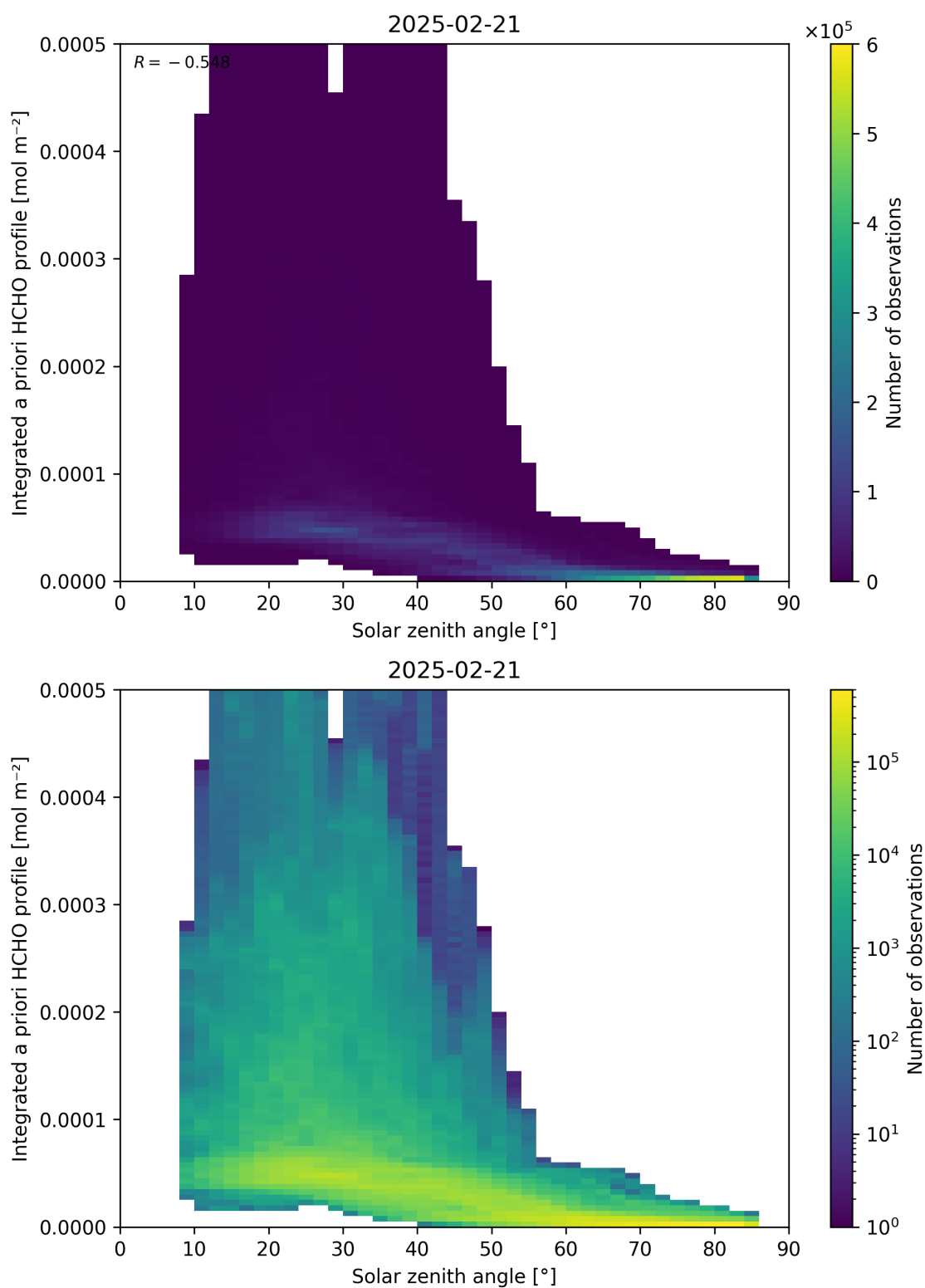
Figure 180: Scatter density plot of “Solar zenith angle” against “Integrated a priori HCHO profile” for 2025-02-20 to 2025-02-22.
