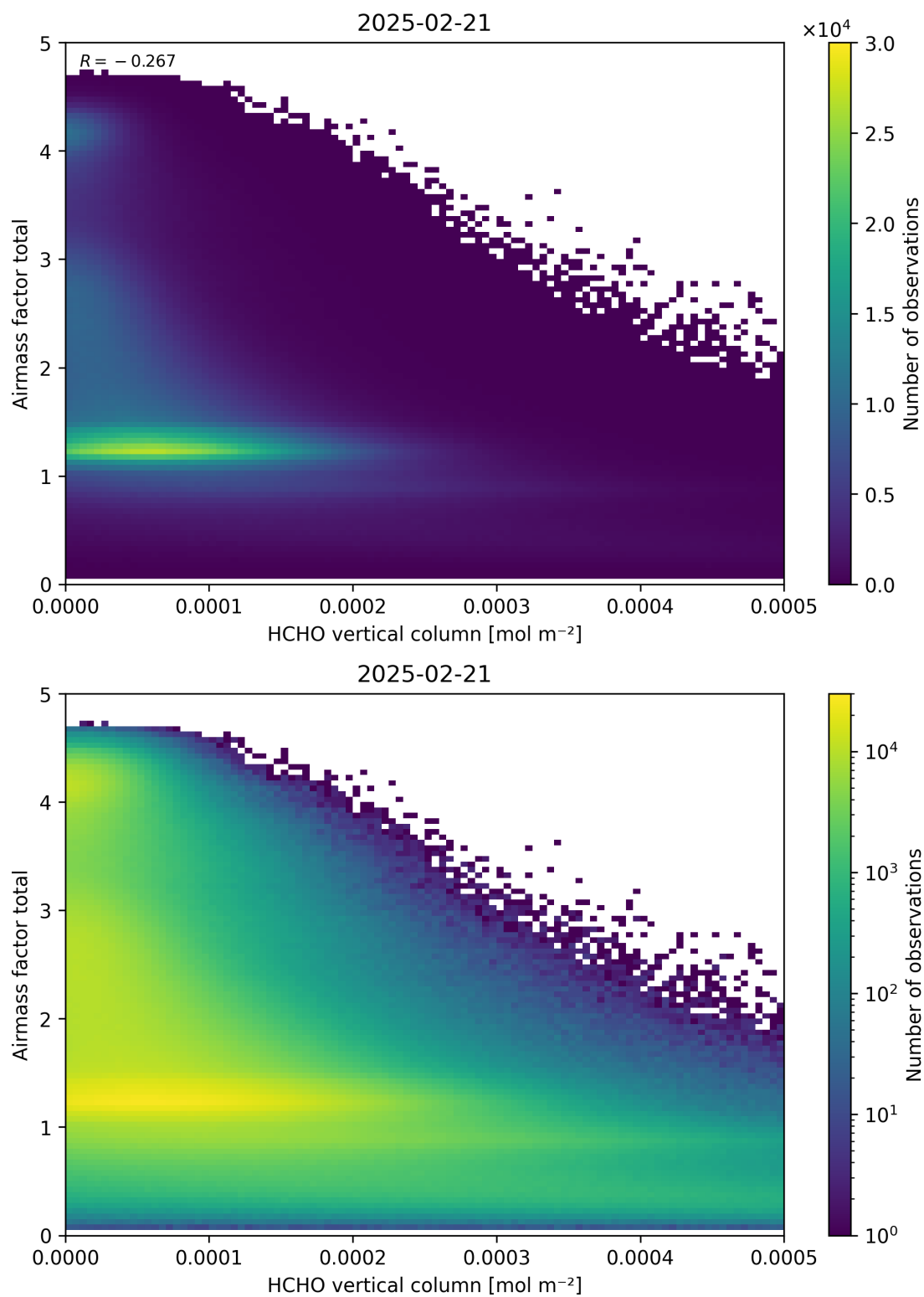
Figure 131: Scatter density plot of “HCHO vertical column” against “Airmass factor total” for 2025-02-20 to 2025-02-22.
