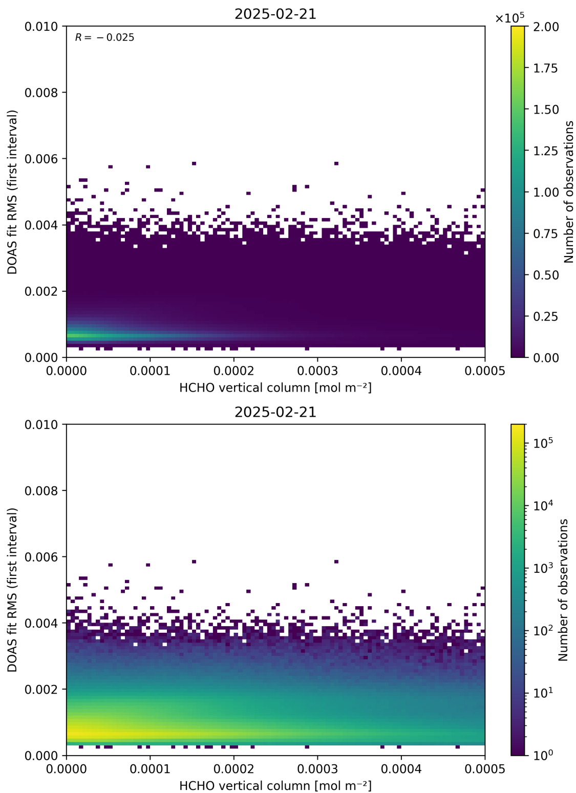
Figure 123: Scatter density plot of “HCHO vertical column” against “DOAS fit RMS (first interval)” for 2025-02-20 to 2025-02-22.
