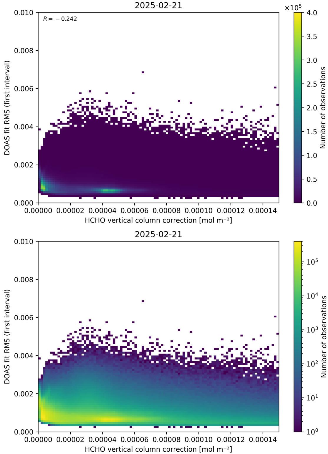
Figure 112: Scatter density plot of “HCHO vertical column correction” against “DOAS fit RMS (first interval)” for 2025-02-20 to 2025-02-22.
