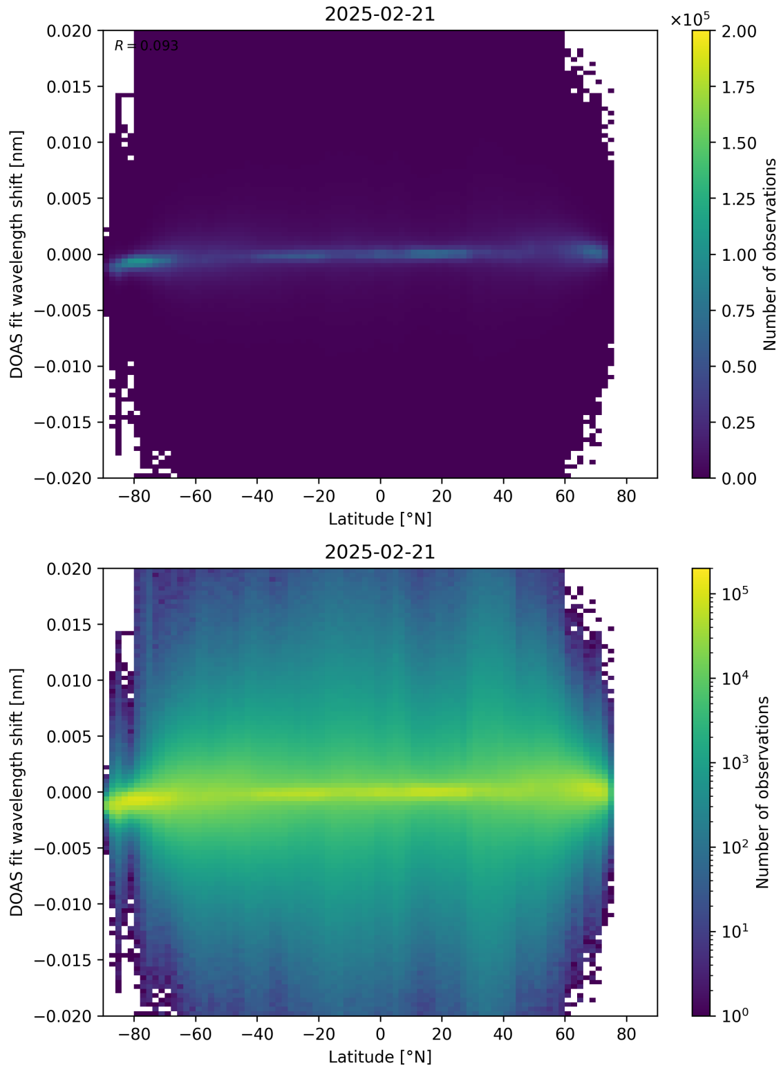
Figure 154: Scatter density plot of “Latitude” against “DOAS fit wavelength shift” for 2025-02-20 to 2025-02-22.
