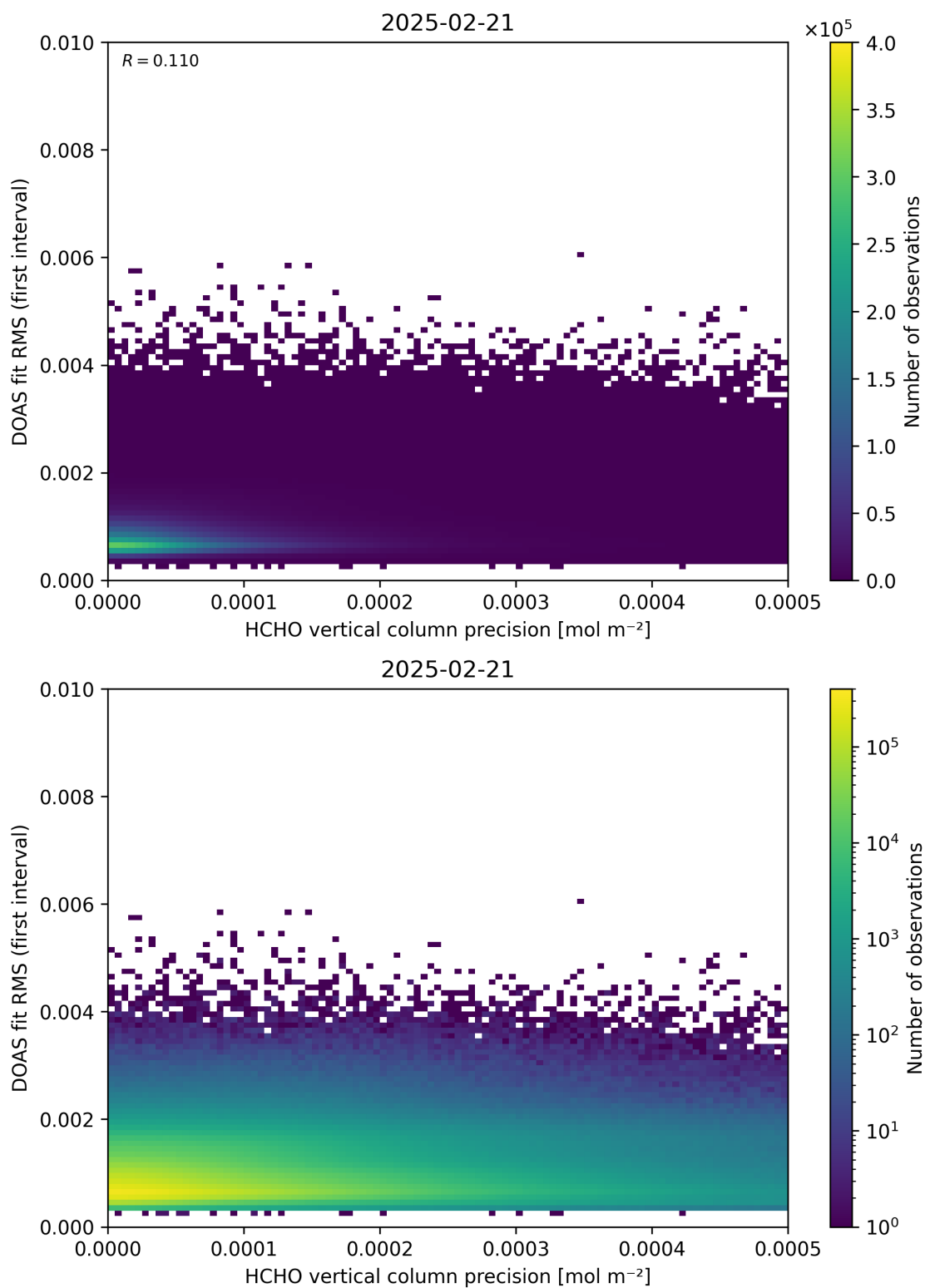
Figure 136: Scatter density plot of “HCHO vertical column precision” against “DOAS fit RMS (first interval)” for 2025-02-20 to 2025-02-22.
