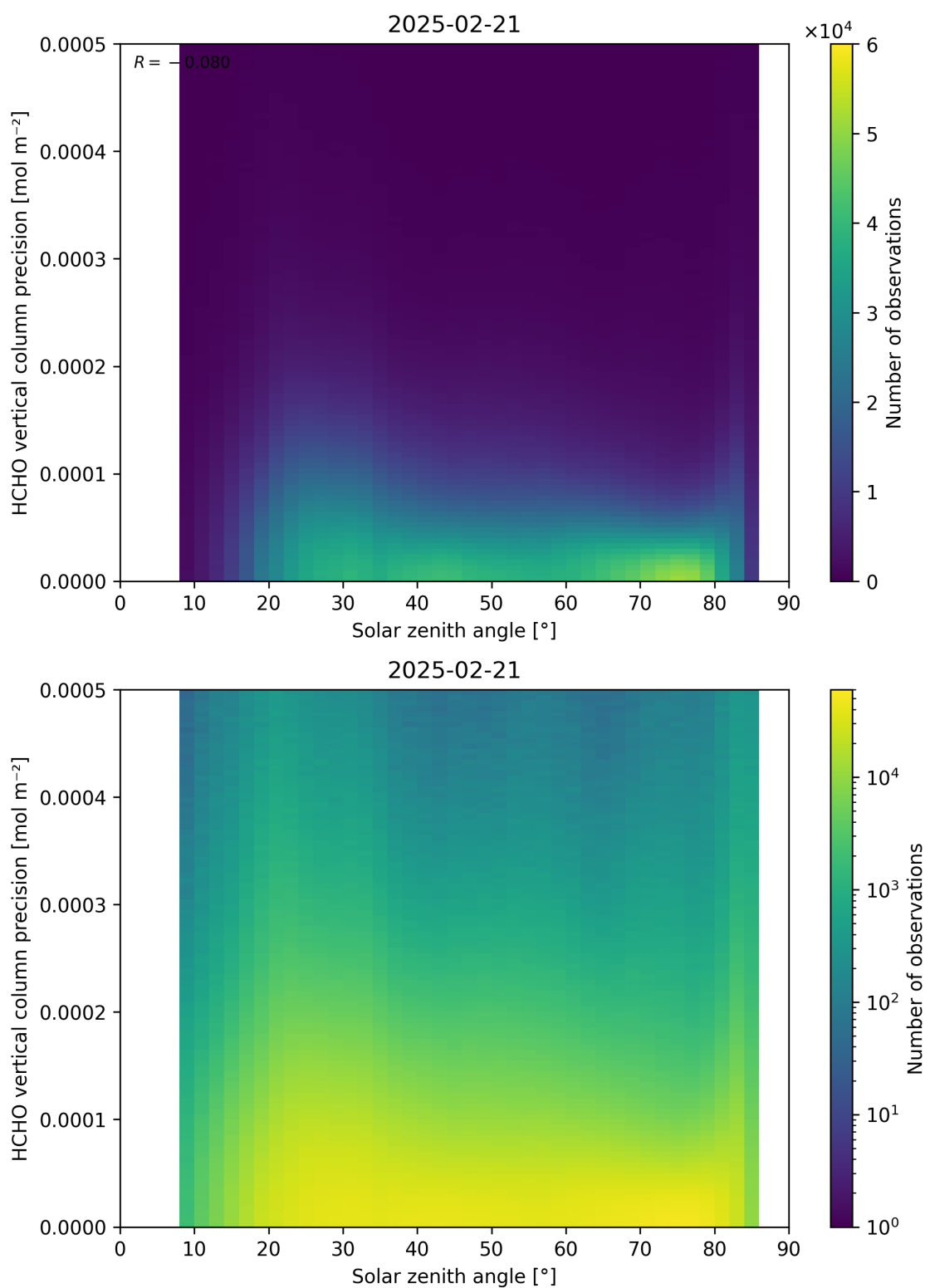
Figure 179: Scatter density plot of “Solar zenith angle” against “HCHO vertical column precision” for 2025-02-20 to 2025-02-22.
