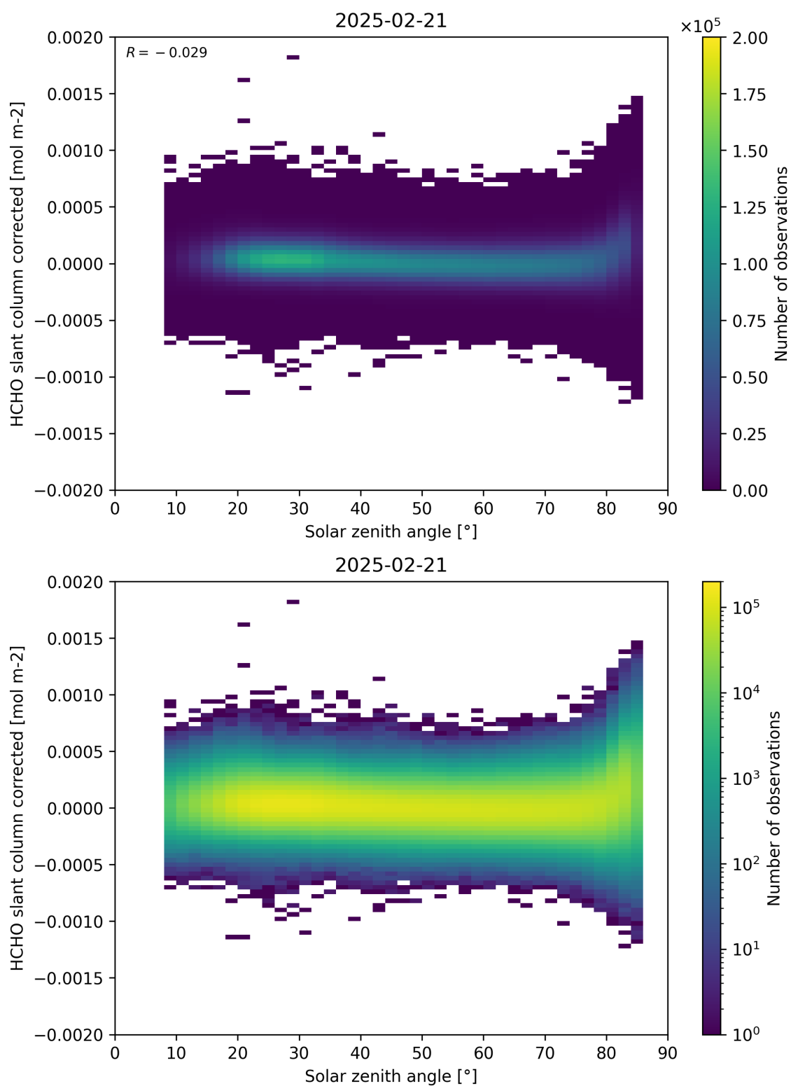
Figure 171: Scatter density plot of “Solar zenith angle” against “HCHO slant column corrected” for 2025-02-20 to 2025-02-22.
