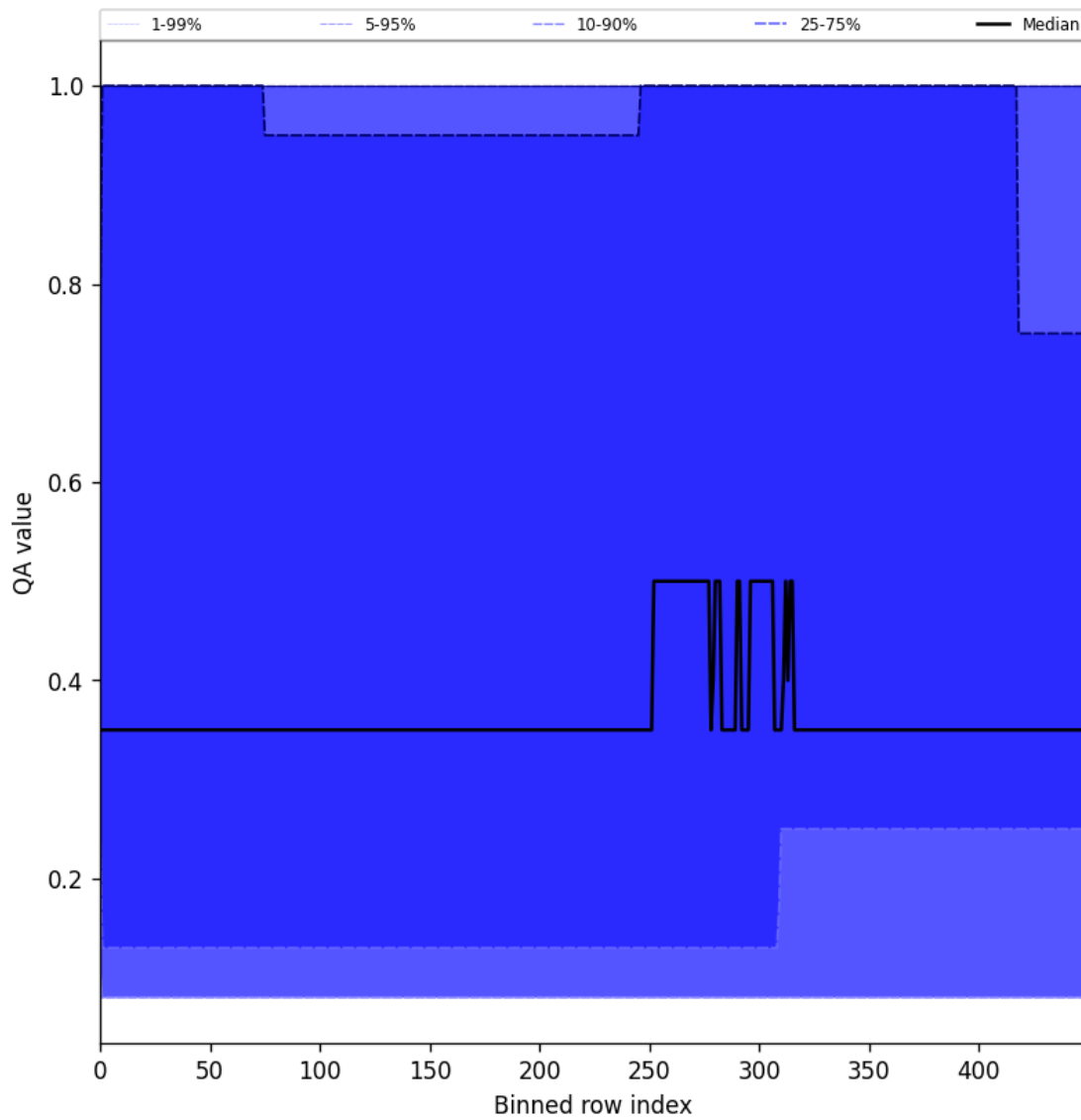
Figure 48: Along track statistics of “QA value” for 2025-02-20 to 2025-02-22
