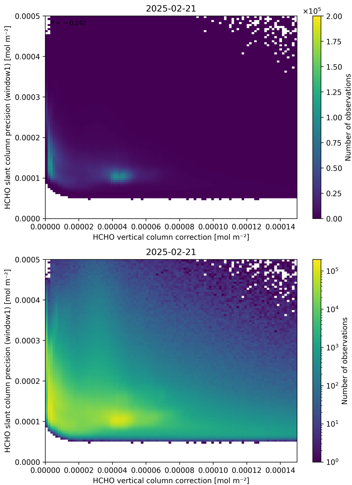
Figure 119: Scatter density plot of “HCHO vertical column correction” against “HCHO slant column precision (window1)” for 2025-02-20 to 2025-02-22.
