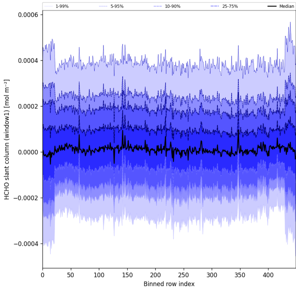
Figure 52: Along track statistics of “HCHO slant column (window1)” for 2025-02-20 to 2025-02-22
