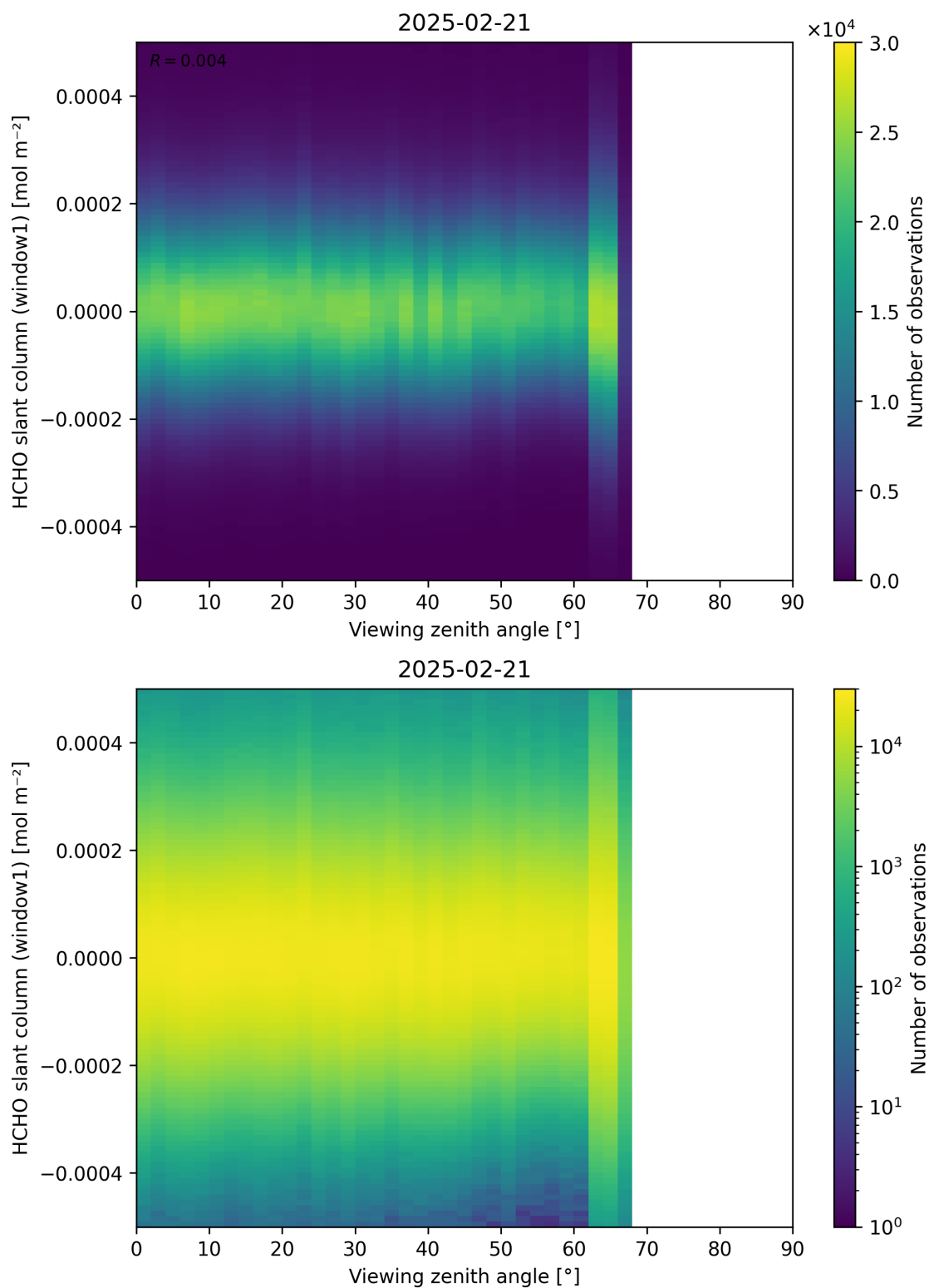
Figure 188: Scatter density plot of “Viewing zenith angle” against “HCHO slant column (window1)” for 2025-02-20 to 2025-02-22.
