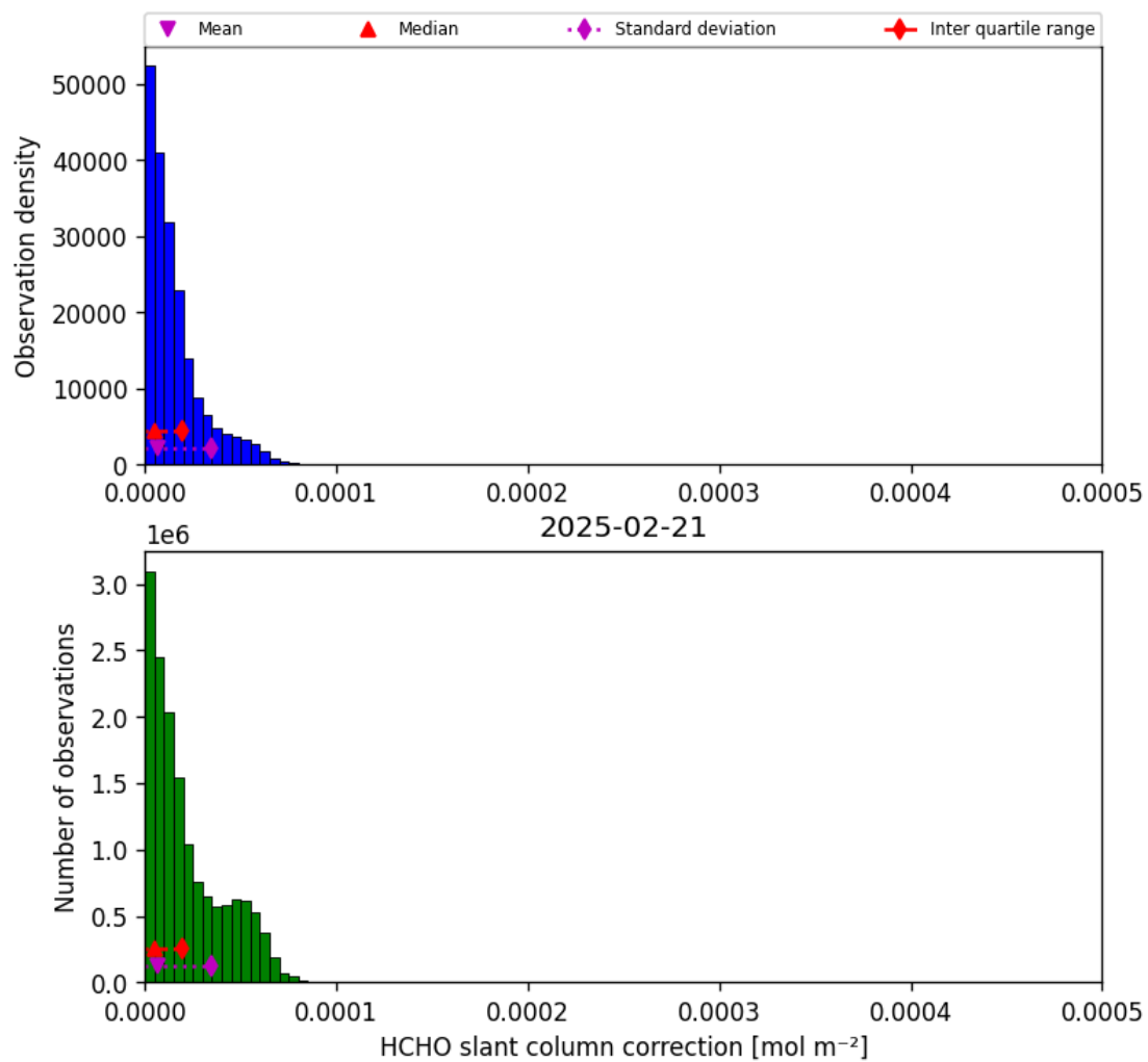
Figure 47: Histogram of “HCHO slant column correction” for 2025-02-20 to 2025-02-22
