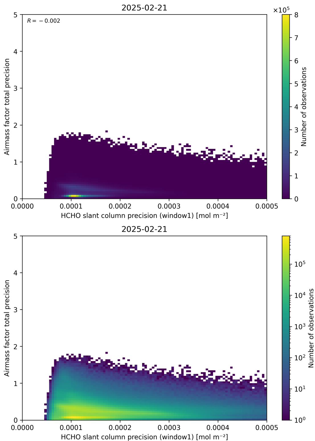
Figure 95: Scatter density plot of “HCHO slant column precision (window1)” against “Airmass factor total precision” for 2025-02-20 to 2025-02-22.
