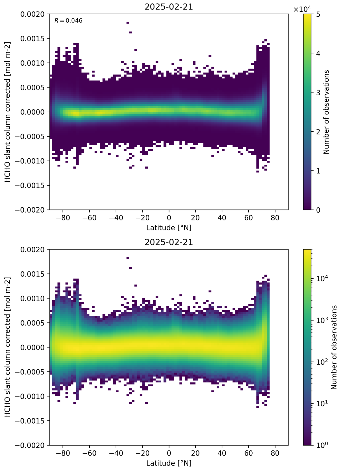
Figure 157: Scatter density plot of “Latitude” against “HCHO slant column corrected” for 2025-02-20 to 2025-02-22.
