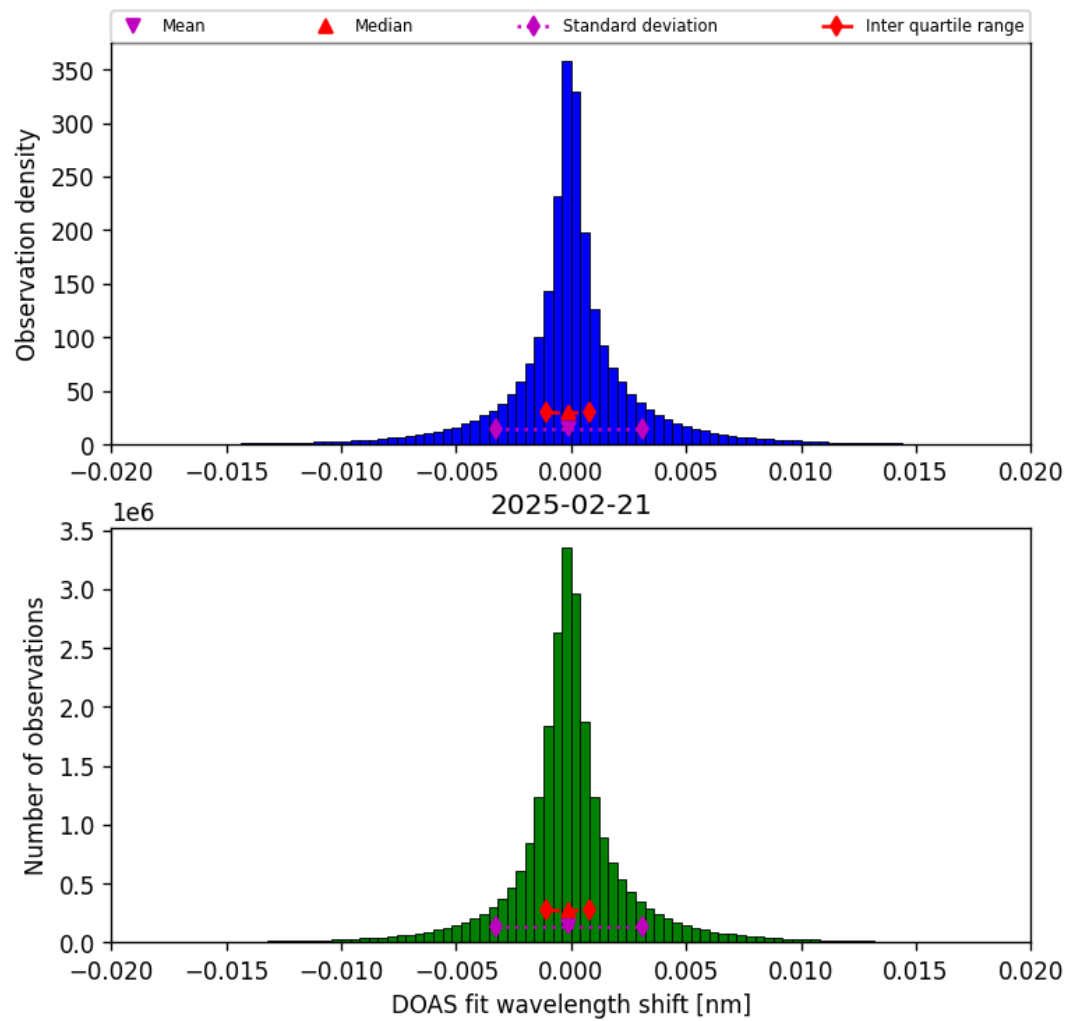
Figure 44: Histogram of “DOAS fit wavelength shift” for 2025-02-20 to 2025-02-22
