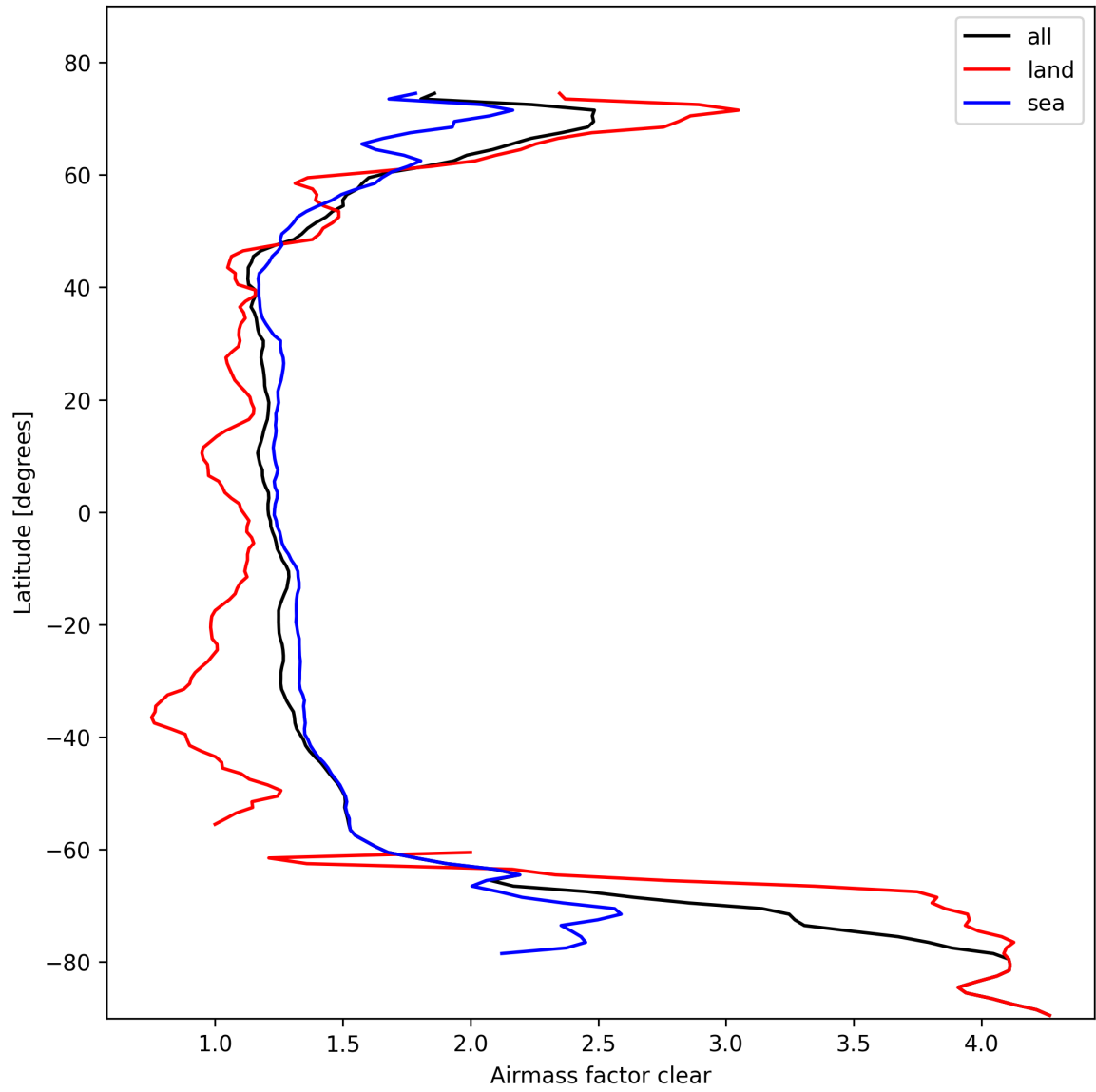
Figure 28: Zonal average of “Airmass factor clear” for 2025-02-20 to 2025-02-22.
