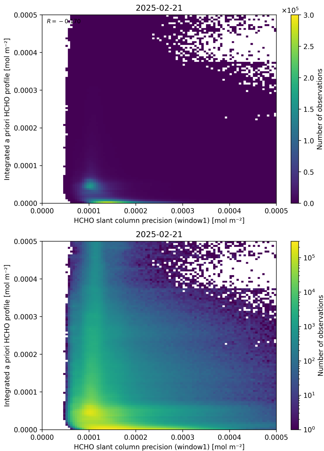
Figure 96: Scatter density plot of “HCHO slant column precision (window1)” against “Integrated a priori HCHO profile” for 2025-02-20 to 2025-02-22.
