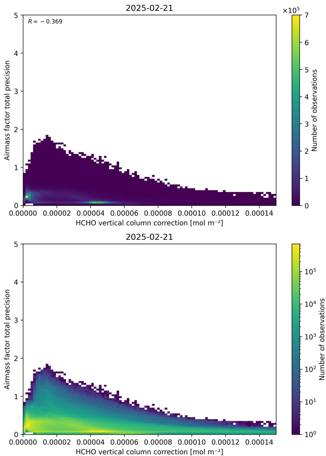
Figure 121: Scatter density plot of “HCHO vertical column correction” against “Airmass factor total precision” for 2025-02-20 to 2025-02-22.
