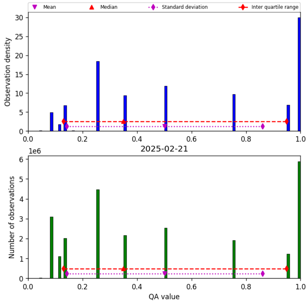
Figure 34: Histogram of “QA value” for 2025-02-20 to 2025-02-22
