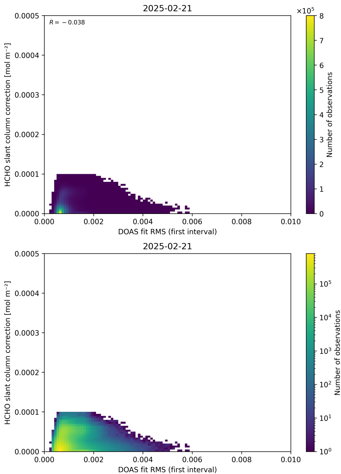
Figure 63: Scatter density plot of “DOAS fit RMS (first interval)” against “HCHO slant column correction” for 2025-02-20 to 2025-02-22.
