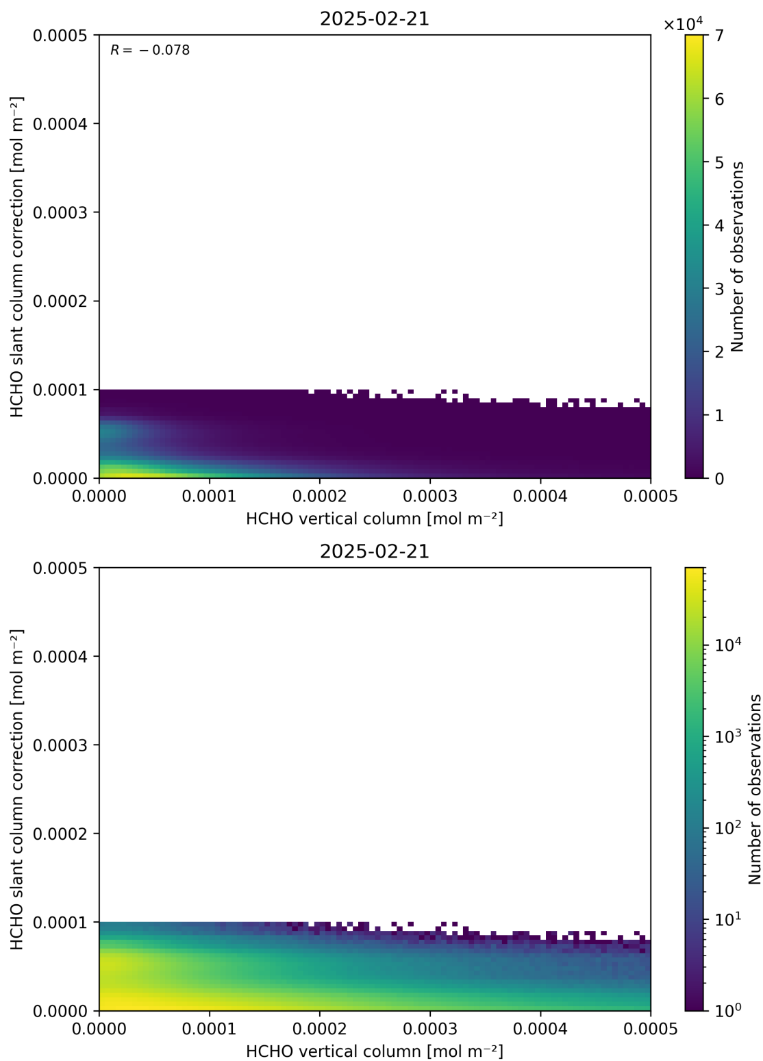
Figure 128: Scatter density plot of “HCHO vertical column” against “HCHO slant column correction” for 2025-02-20 to 2025-02-22.
