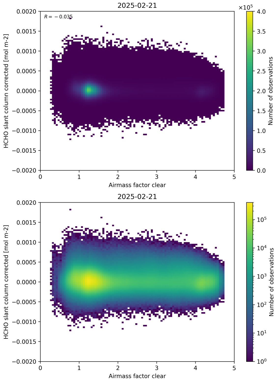
Figure 74: Scatter density plot of “Airmass factor clear” against “HCHO slant column corrected” for 2025-02-20 to 2025-02-22.
