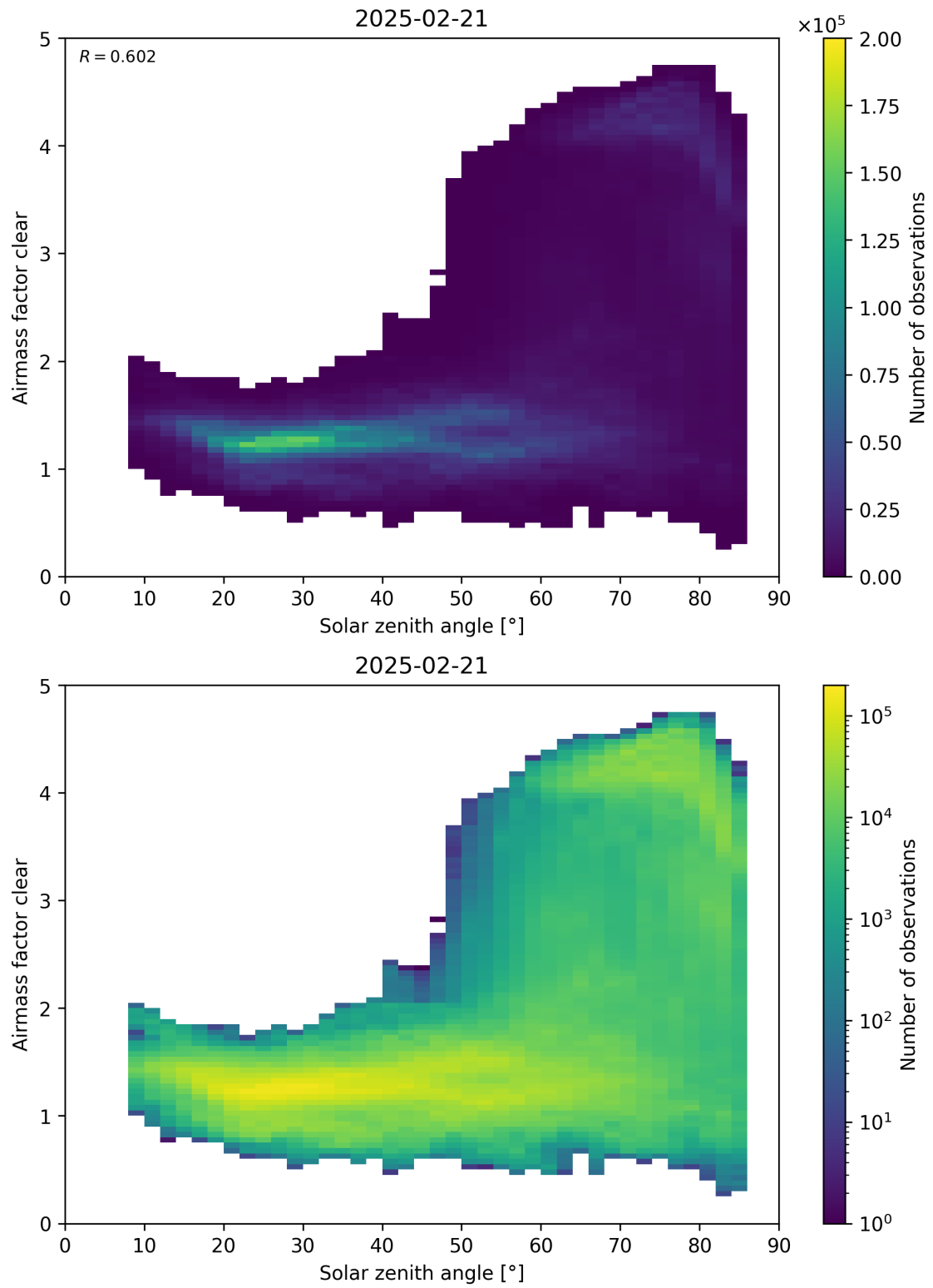
Figure 170: Scatter density plot of “Solar zenith angle” against “Airmass factor clear” for 2025-02-20 to 2025-02-22.
