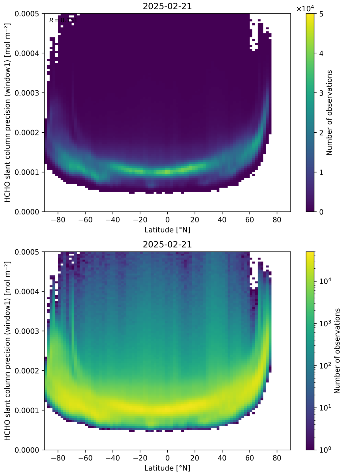
Figure 160: Scatter density plot of “Latitude” against “HCHO slant column precision (window1)” for 2025-02-20 to 2025-02-22.
