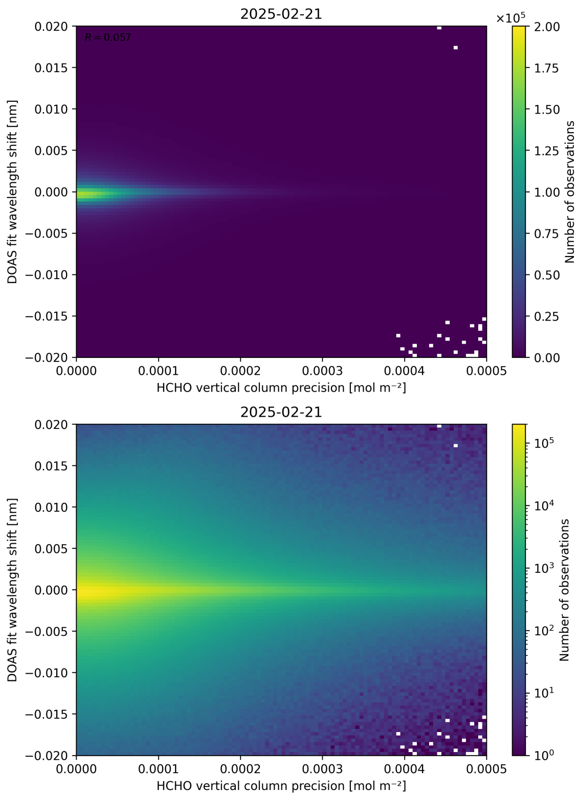
Figure 137: Scatter density plot of “HCHO vertical column precision” against “DOAS fit wavelength shift” for 2025-02-20 to 2025-02-22.
