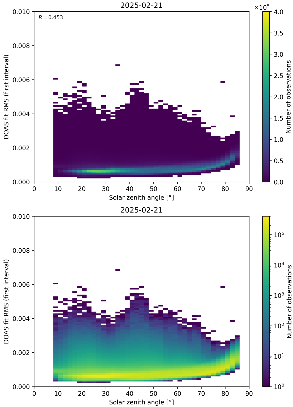
Figure 167: Scatter density plot of “Solar zenith angle” against “DOAS fit RMS (first interval)” for 2025-02-20 to 2025-02-22.
