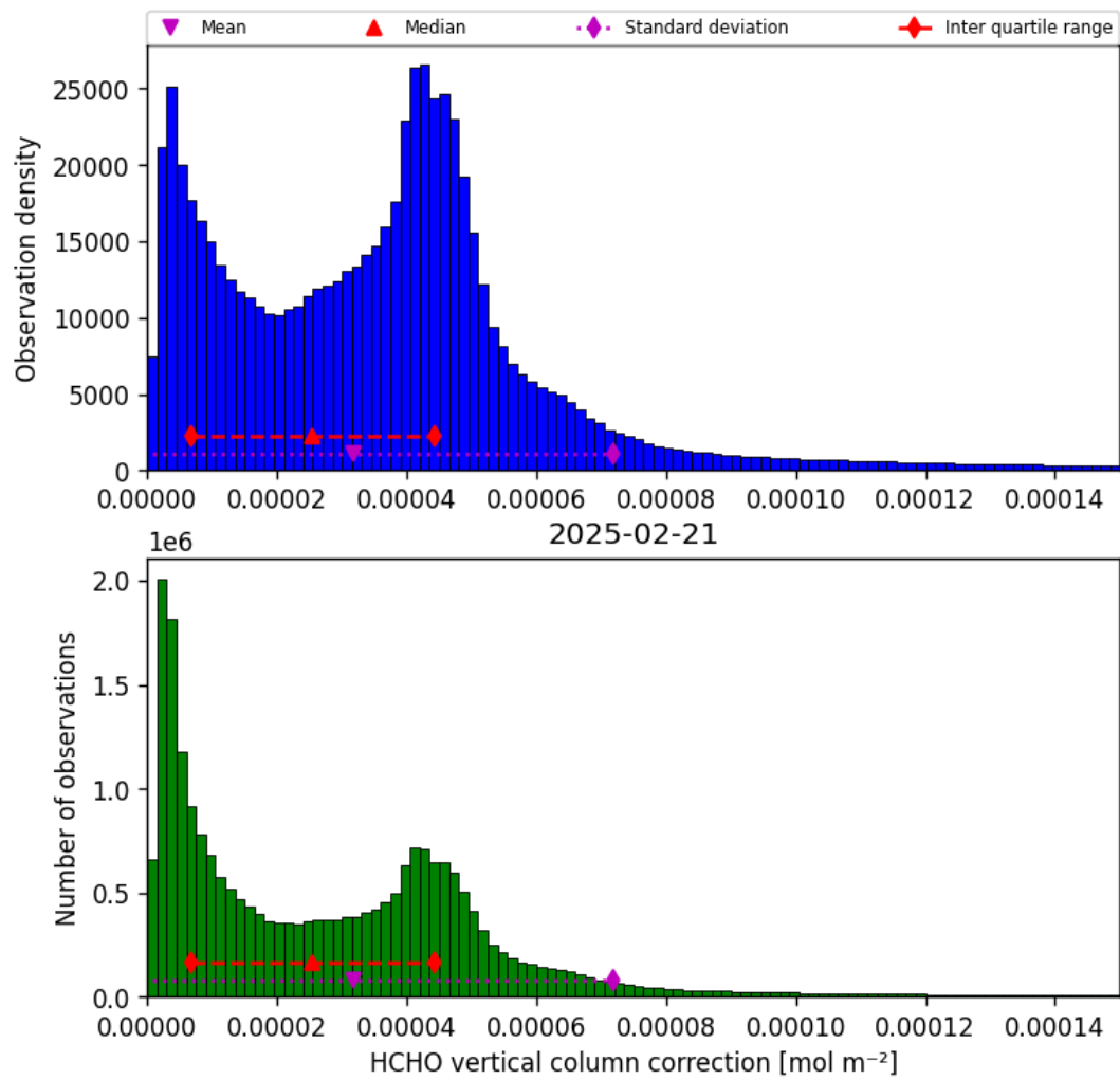
Figure 37: Histogram of “HCHO vertical column correction” for 2025-02-20 to 2025-02-22
