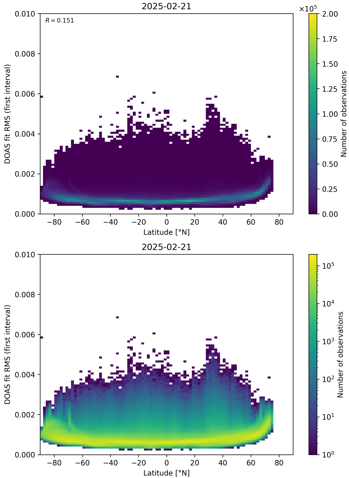
Figure 153: Scatter density plot of “Latitude” against “DOAS fit RMS (first interval)” for 2025-02-20 to 2025-02-22.
