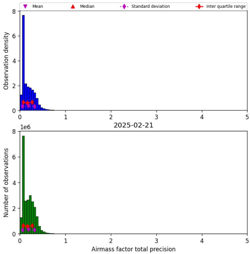
Figure 41: Histogram of “Airmass factor total precision” for 2025-02-20 to 2025-02-22
