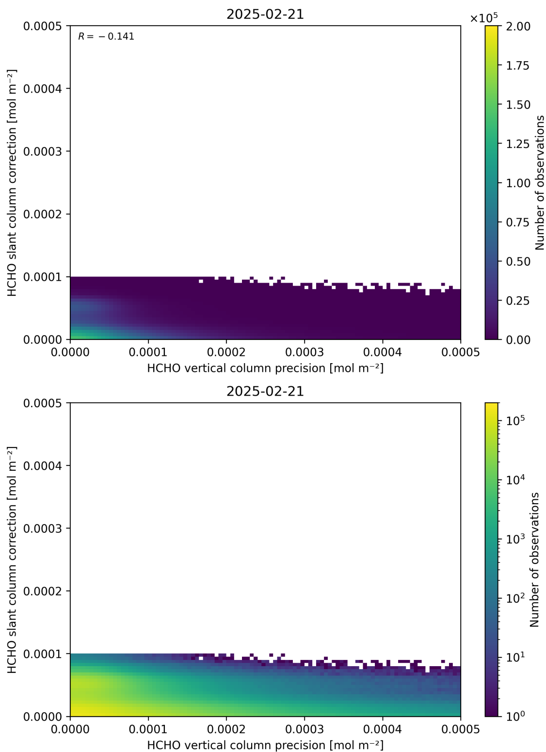
Figure 141: Scatter density plot of “HCHO vertical column precision” against “HCHO slant column correction” for 2025-02-20 to 2025-02-22.
