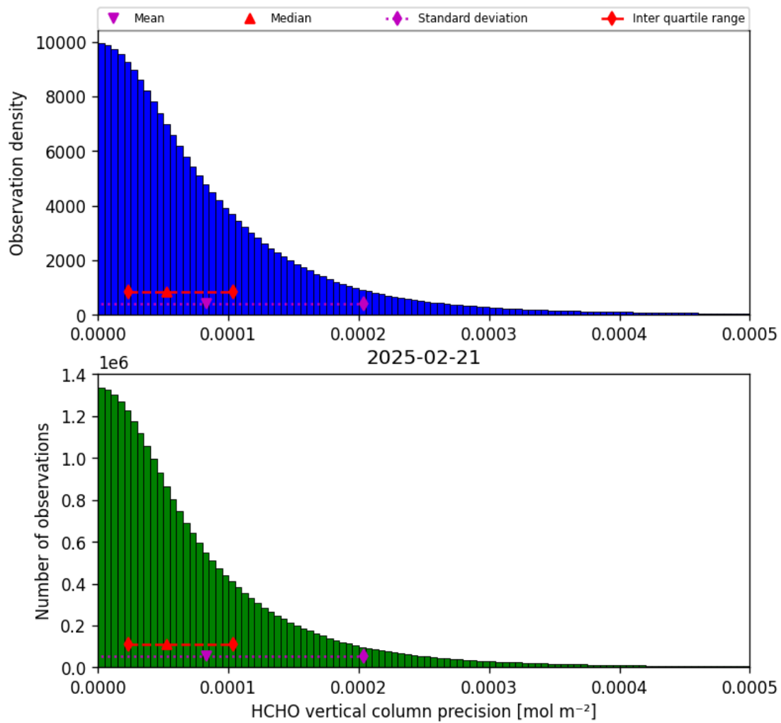
Figure 36: Histogram of “HCHO vertical column precision” for 2025-02-20 to 2025-02-22
