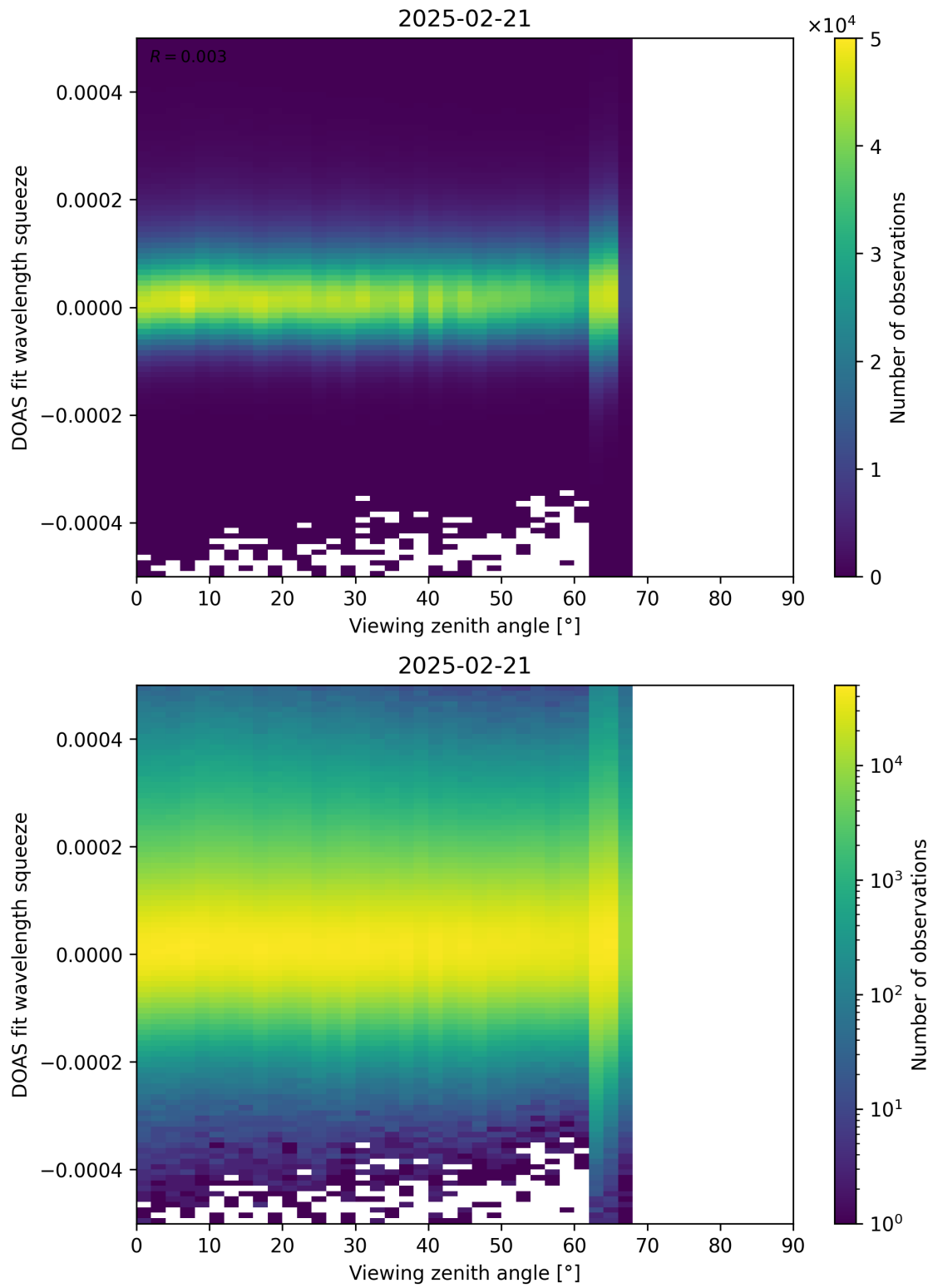
Figure 184: Scatter density plot of “Viewing zenith angle” against “DOAS fit wavelength squeeze” for 2025-02-20 to 2025-02-22.
