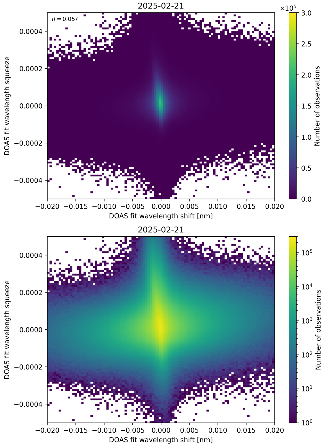
Figure 65: Scatter density plot of “DOAS fit wavelength shift” against “DOAS fit wavelength squeeze” for 2025-02-20 to 2025-02-22.
