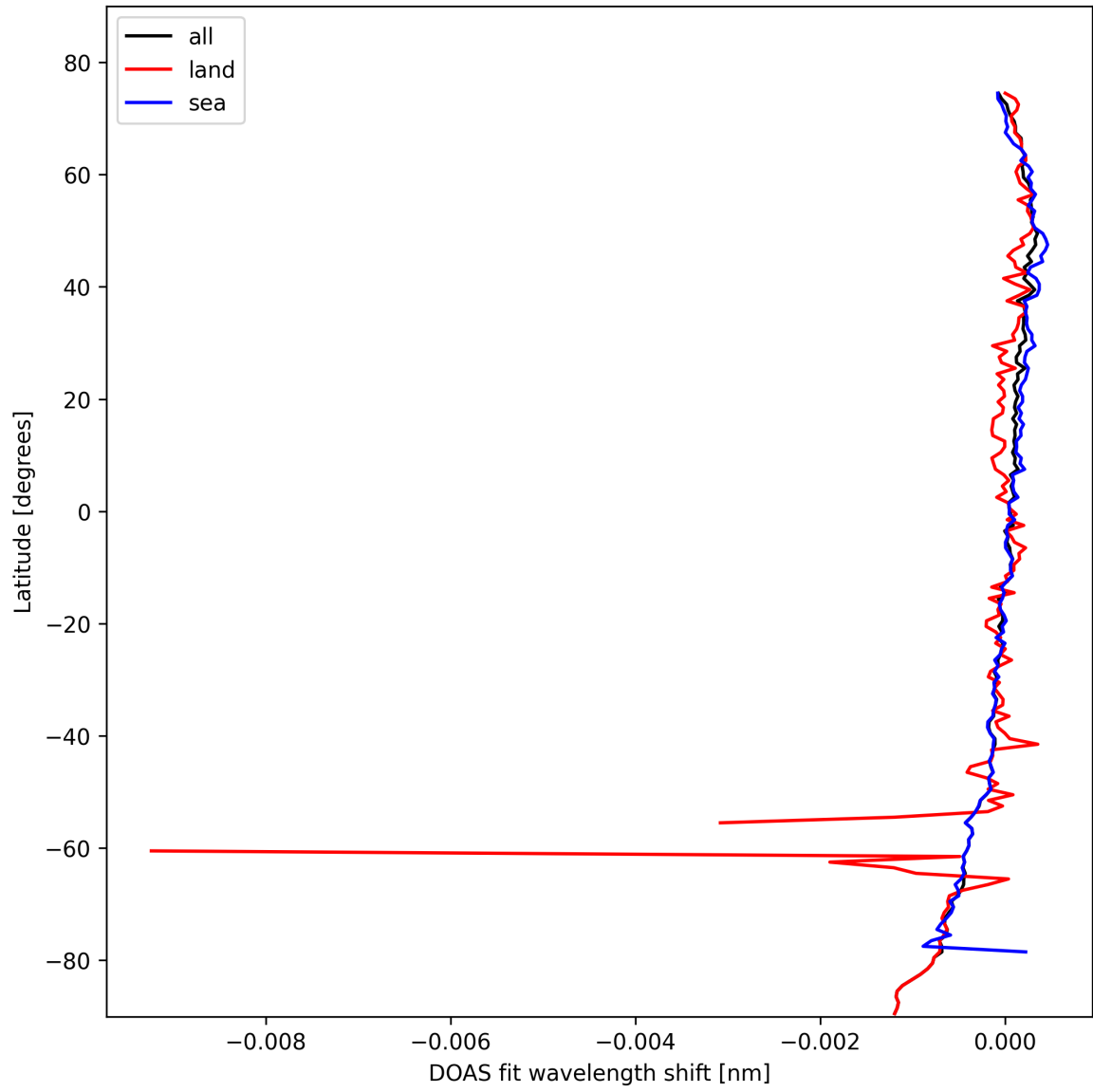
Figure 30: Zonal average of “DOAS fit wavelength shift” for 2025-02-20 to 2025-02-22.
