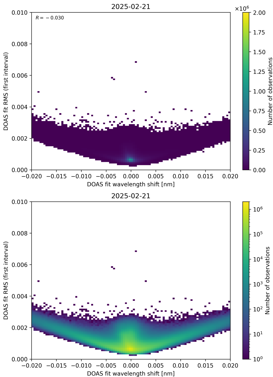
Figure 64: Scatter density plot of “DOAS fit wavelength shift” against “DOAS fit RMS (first interval)” for 2025-02-20 to 2025-02-22.
