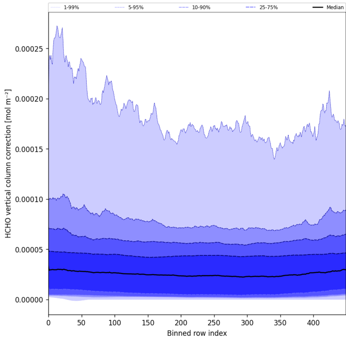
Figure 51: Along track statistics of “HCHO vertical column correction” for 2025-02-20 to 2025-02-22
