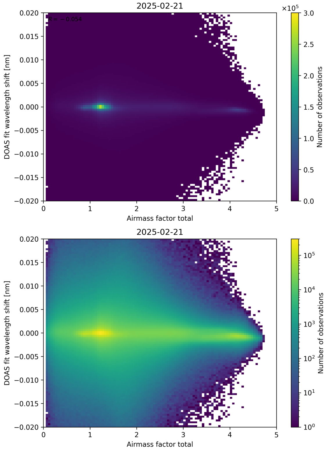
Figure 98: Scatter density plot of “Airmass factor total” against “DOAS fit wavelength shift” for 2025-02-20 to 2025-02-22.
