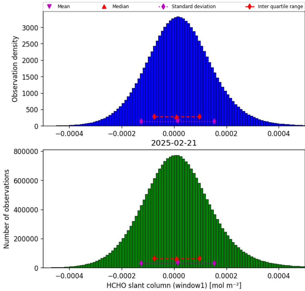
Figure 38: Histogram of “HCHO slant column (window1)” for 2025-02-20 to 2025-02-22
