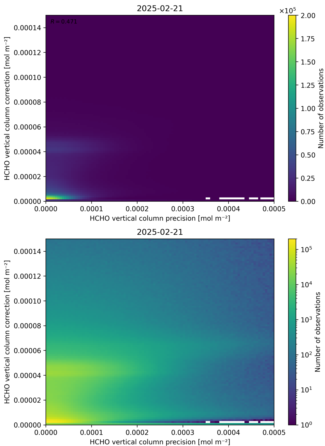
Figure 146: Scatter density plot of “HCHO vertical column precision” against “HCHO vertical column correction” for 2025-02-20 to 2025-02-22.
