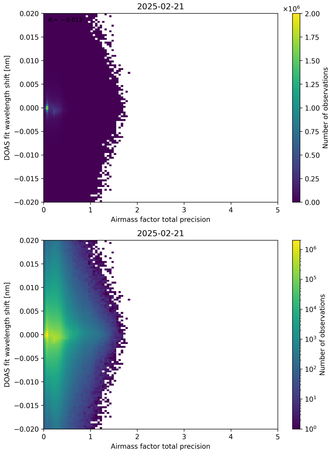
Figure 106: Scatter density plot of “Airmass factor total precision” against “DOAS fit wavelength shift” for 2025-02-20 to 2025-02-22.
