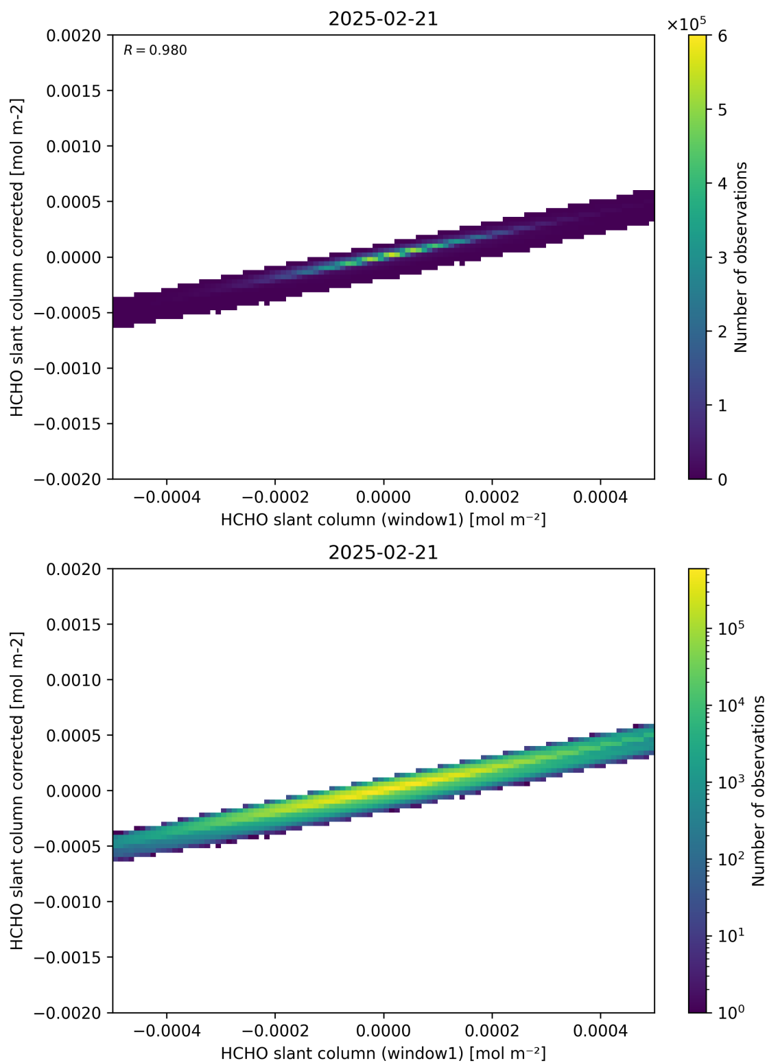
Figure 82: Scatter density plot of “HCHO slant column (window1)” against “HCHO slant column corrected” for 2025-02-20 to 2025-02-22.
