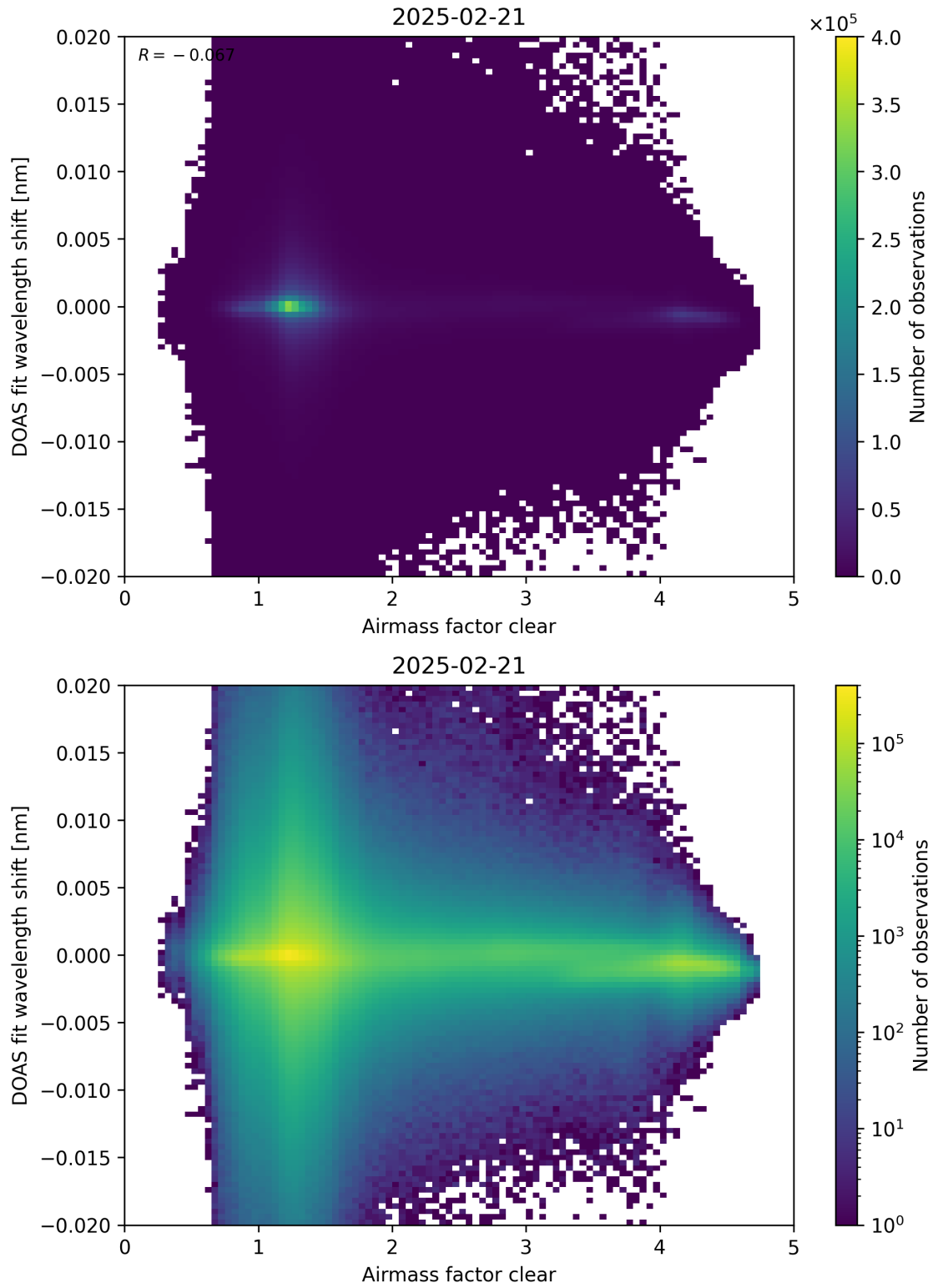
Figure 72: Scatter density plot of “Airmass factor clear” against “DOAS fit wavelength shift” for 2025-02-20 to 2025-02-22.
