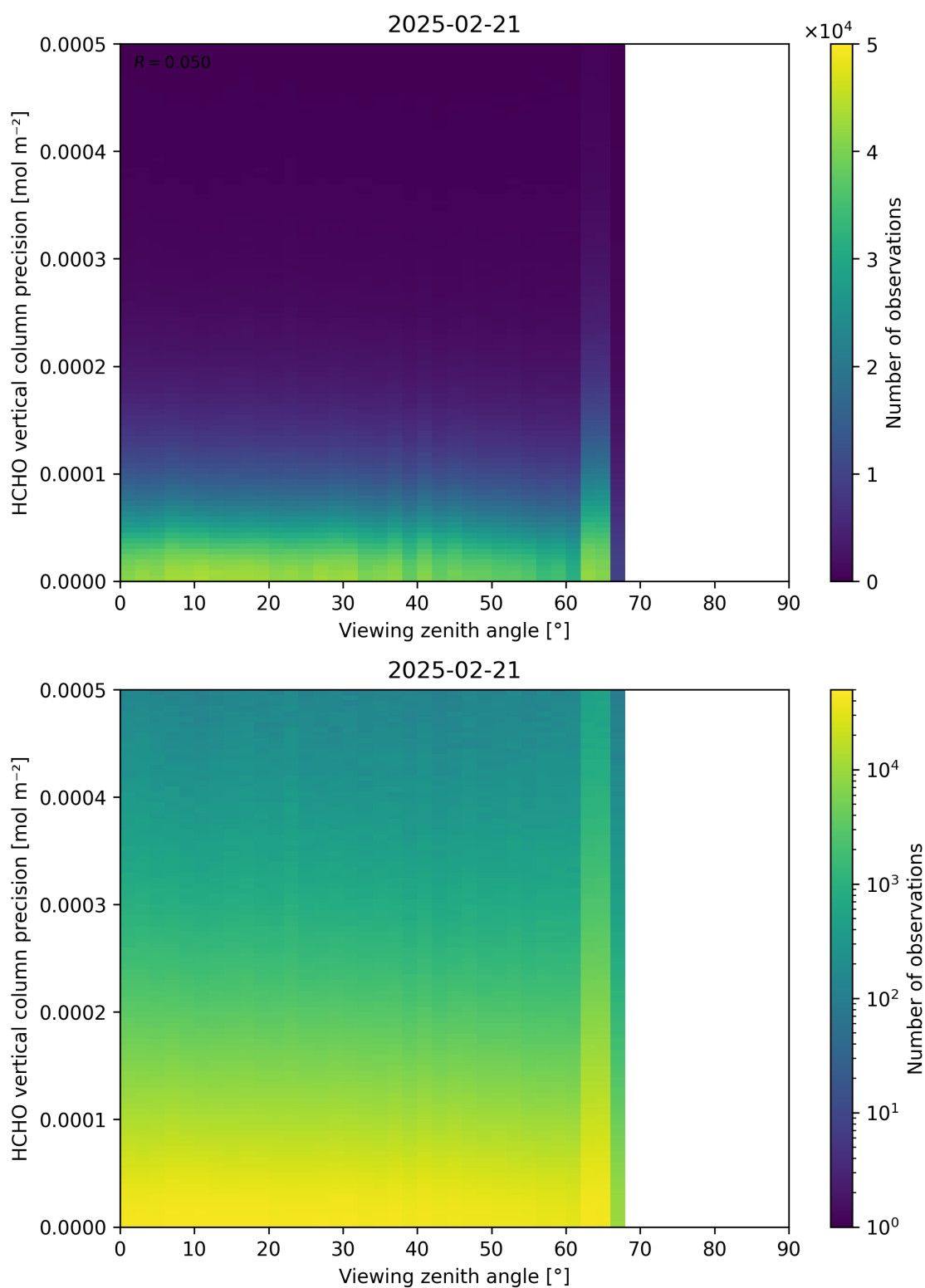
Figure 194: Scatter density plot of “Viewing zenith angle” against “HCHO vertical column precision” for 2025-02-20 to 2025-02-22.
