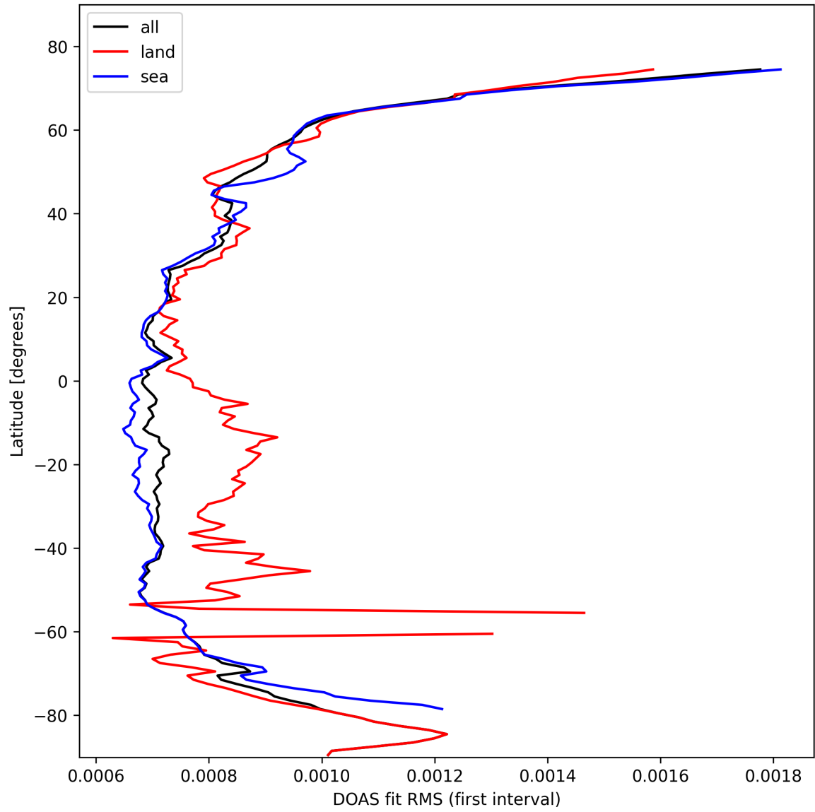
Figure 32: Zonal average of “DOAS fit RMS (first interval)” for 2025-02-20 to 2025-02-22.
