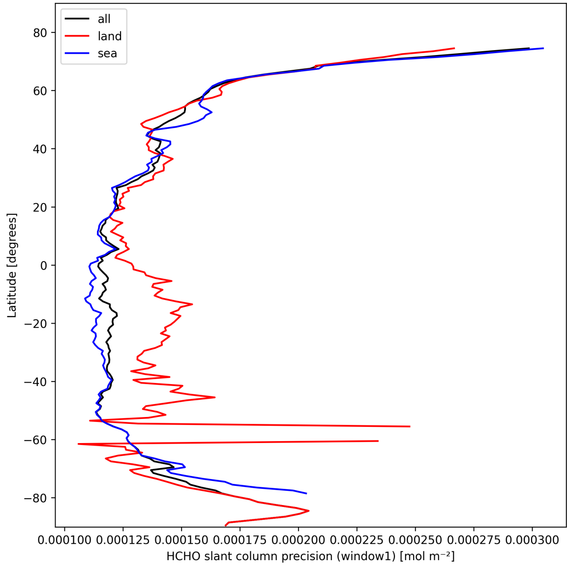
Figure 25: Zonal average of “HCHO slant column precision (window1)” for 2025-02-20 to 2025-02-22.
