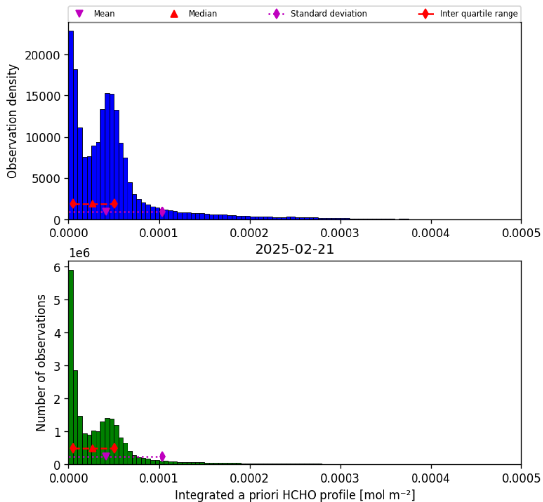
Figure 43: Histogram of “Integrated a priori HCHO profile” for 2025-02-20 to 2025-02-22
