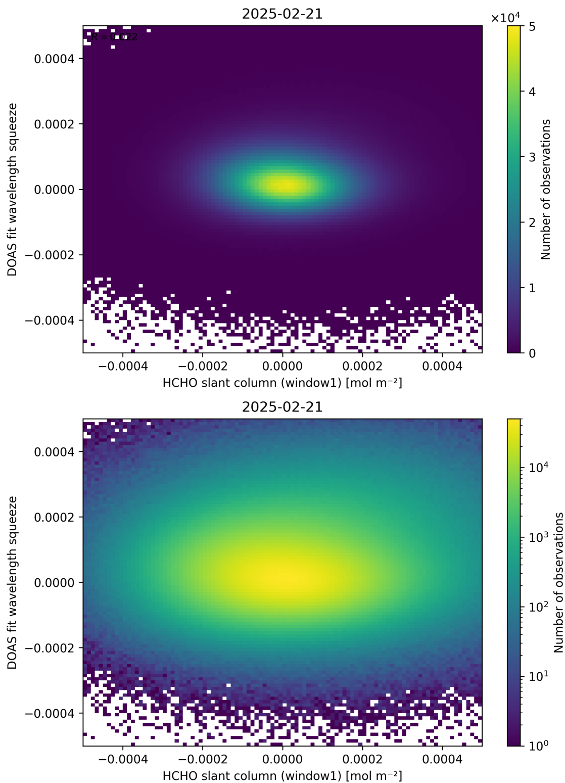
Figure 80: Scatter density plot of “HCHO slant column (window1)” against “DOAS fit wavelength squeeze” for 2025-02-20 to 2025-02-22.
