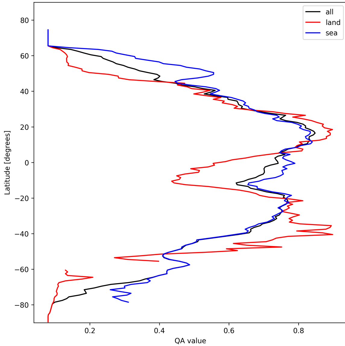
Figure 20: Zonal average of “QA value” for 2025-02-20 to 2025-02-22.
