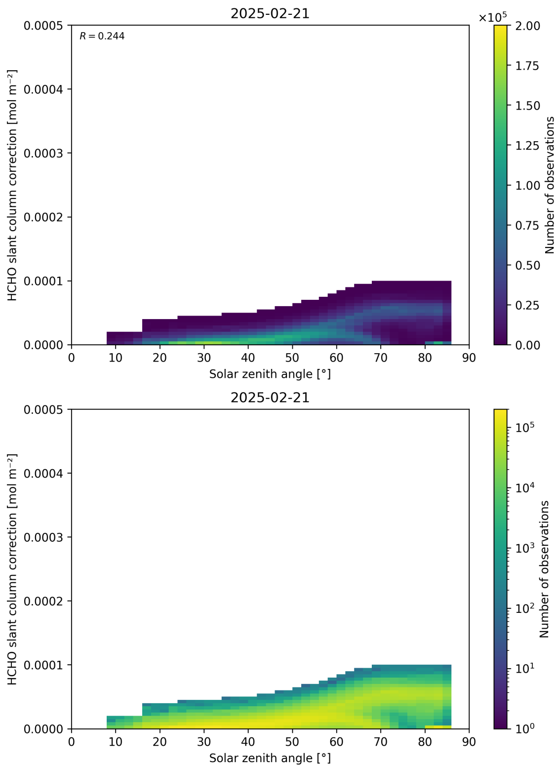
Figure 172: Scatter density plot of “Solar zenith angle” against “HCHO slant column correction” for 2025-02-20 to 2025-02-22.
