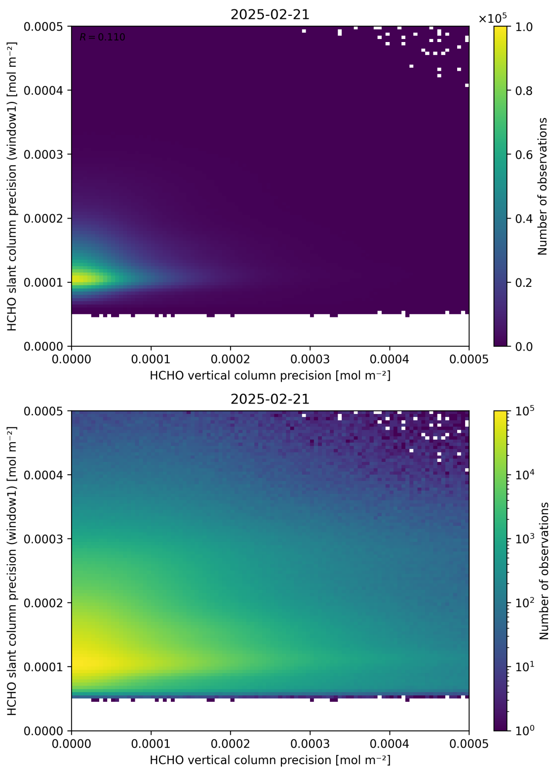
Figure 143: Scatter density plot of “HCHO vertical column precision” against “HCHO slant column precision (window1)” for 2025-02-20 to 2025-02-22.
