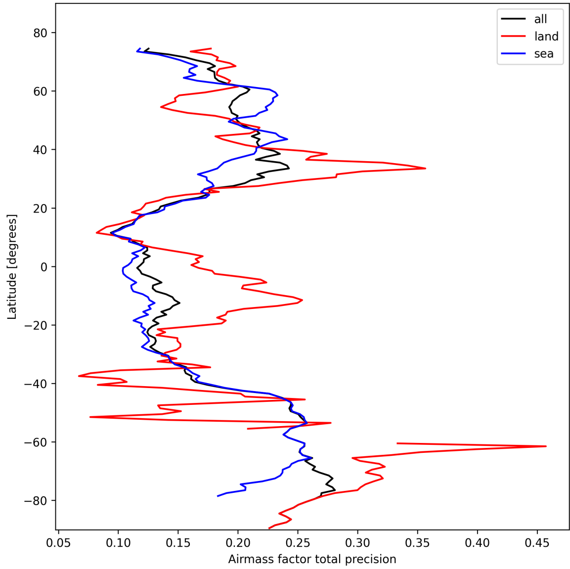
Figure 27: Zonal average of “Airmass factor total precision” for 2025-02-20 to 2025-02-22.
