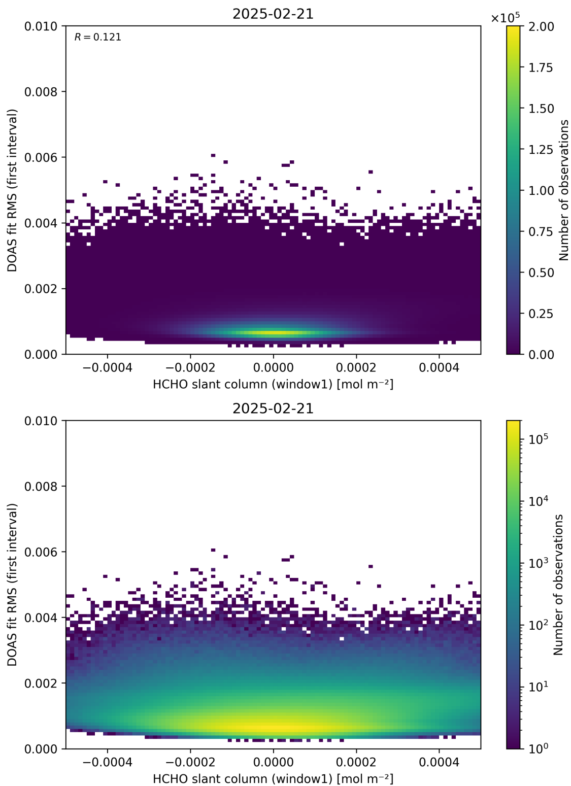
Figure 78: Scatter density plot of “HCHO slant column (window1)” against “DOAS fit RMS (first interval)” for 2025-02-20 to 2025-02-22.
