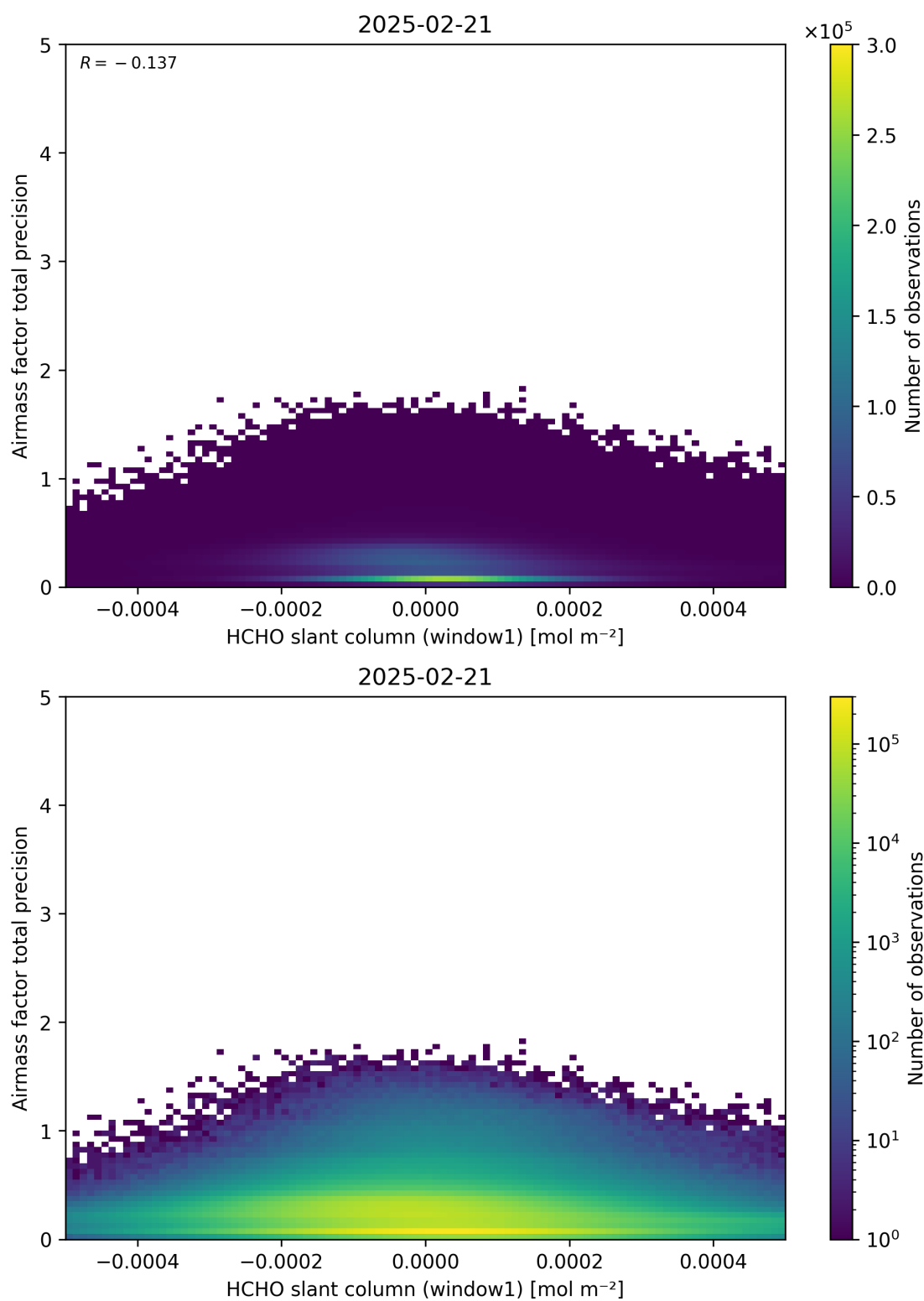
Figure 86: Scatter density plot of “HCHO slant column (window1)” against “Airmass factor total precision” for 2025-02-20 to 2025-02-22.
