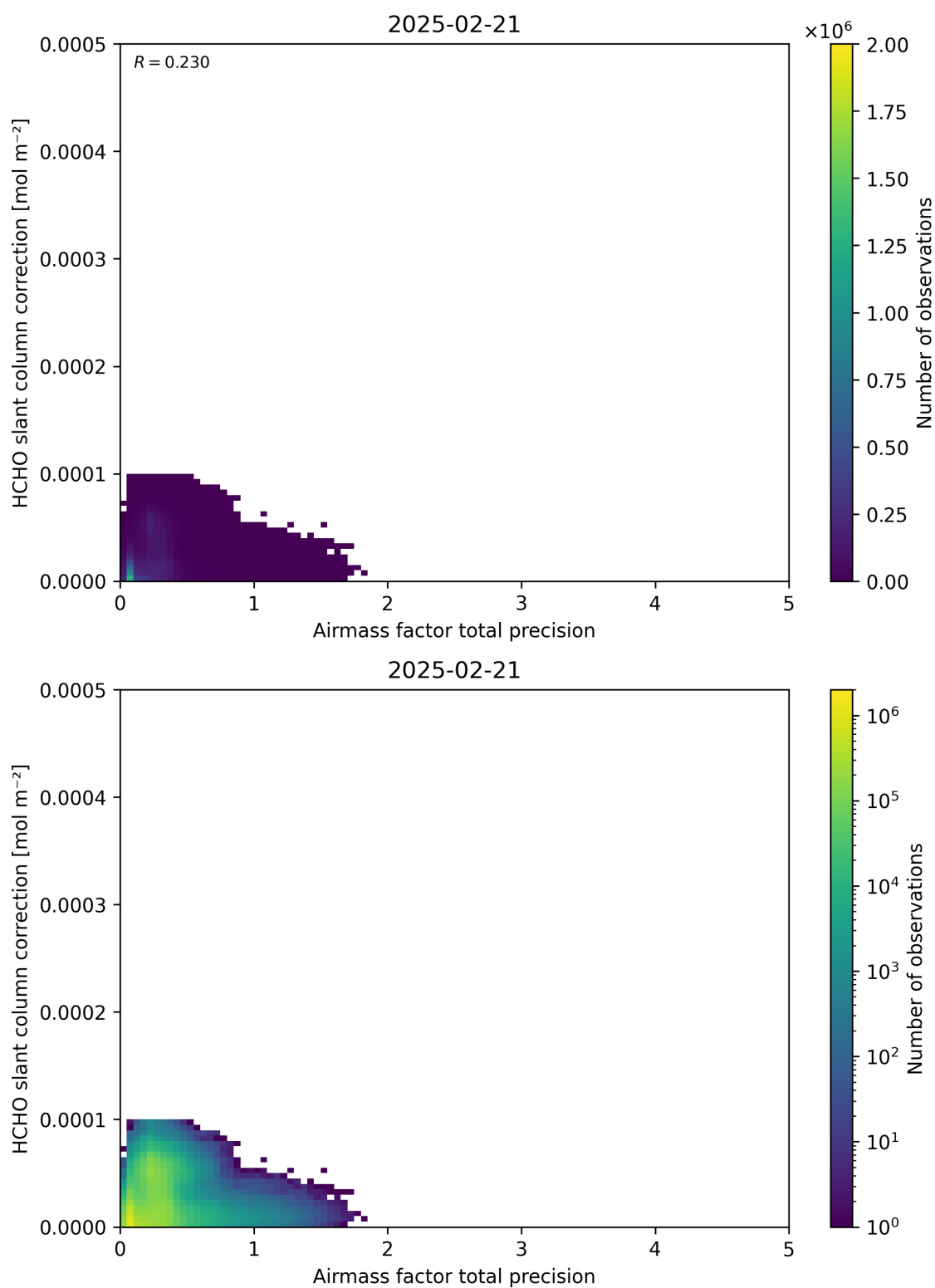
Figure 110: Scatter density plot of “Airmass factor total precision” against “HCHO slant column correction” for 2025-02-20 to 2025-02-22.
