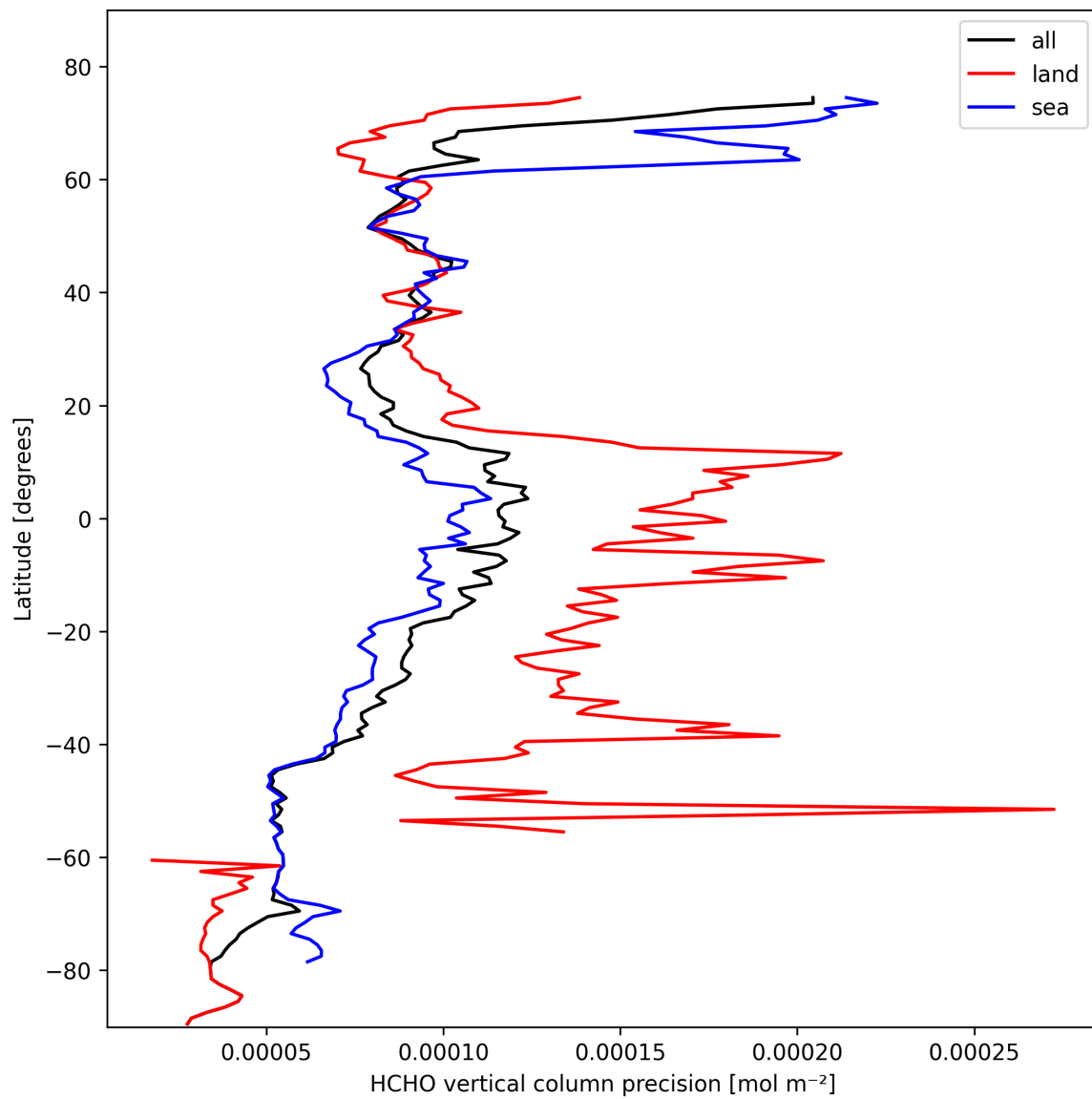
Figure 22: Zonal average of “HCHO vertical column precision” for 2025-02-20 to 2025-02-22.
