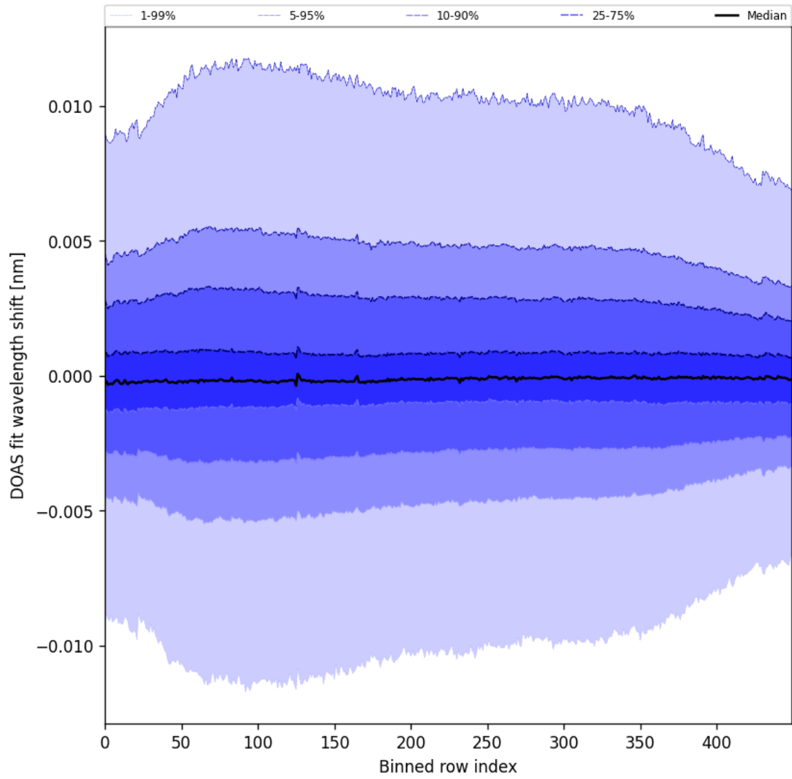
Figure 58: Along track statistics of “DOAS fit wavelength shift” for 2025-02-20 to 2025-02-22
