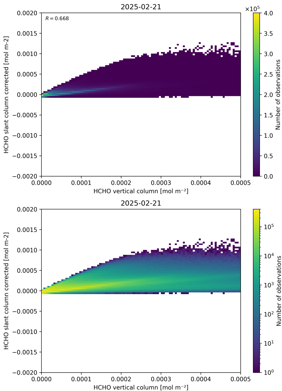
Figure 127: Scatter density plot of “HCHO vertical column” against “HCHO slant column corrected” for 2025-02-20 to 2025-02-22.
