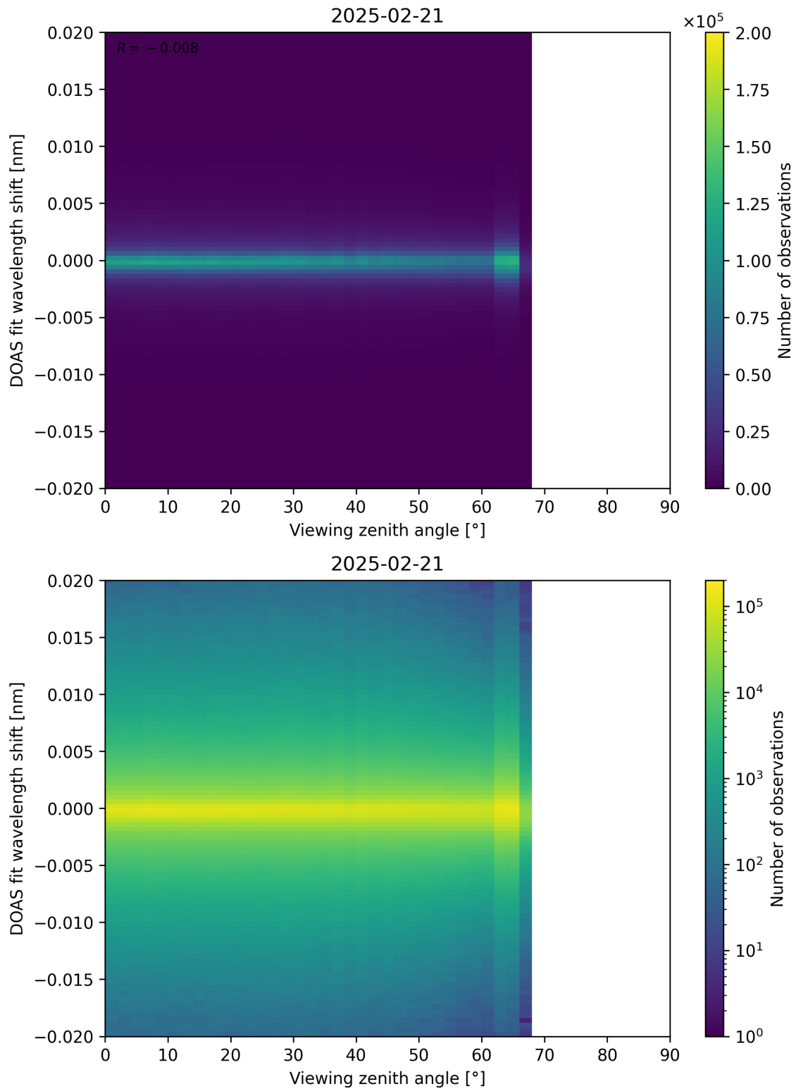
Figure 183: Scatter density plot of “Viewing zenith angle” against “DOAS fit wavelength shift” for 2025-02-20 to 2025-02-22.
