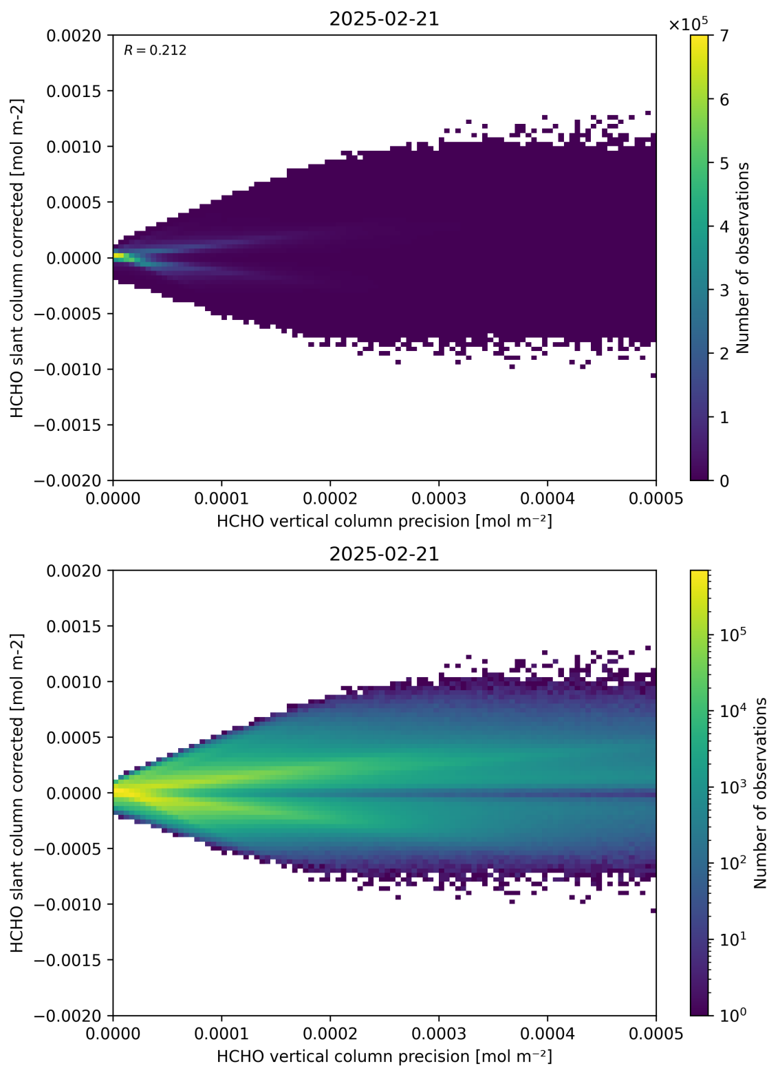
Figure 140: Scatter density plot of “HCHO vertical column precision” against “HCHO slant column corrected” for 2025-02-20 to 2025-02-22.
