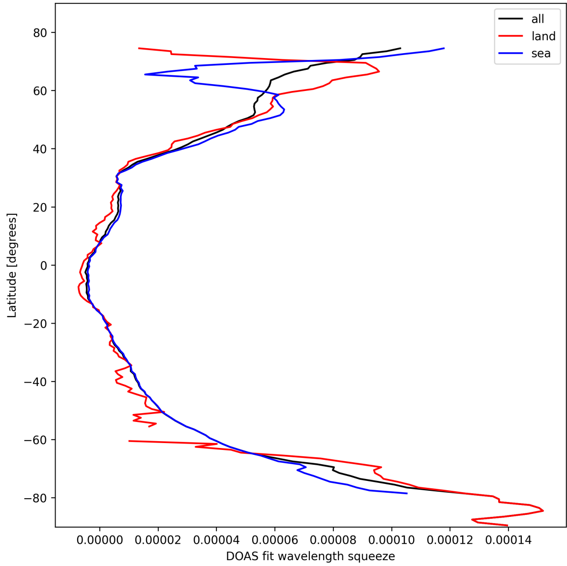
Figure 31: Zonal average of “DOAS fit wavelength squeeze” for 2025-02-20 to 2025-02-22.
