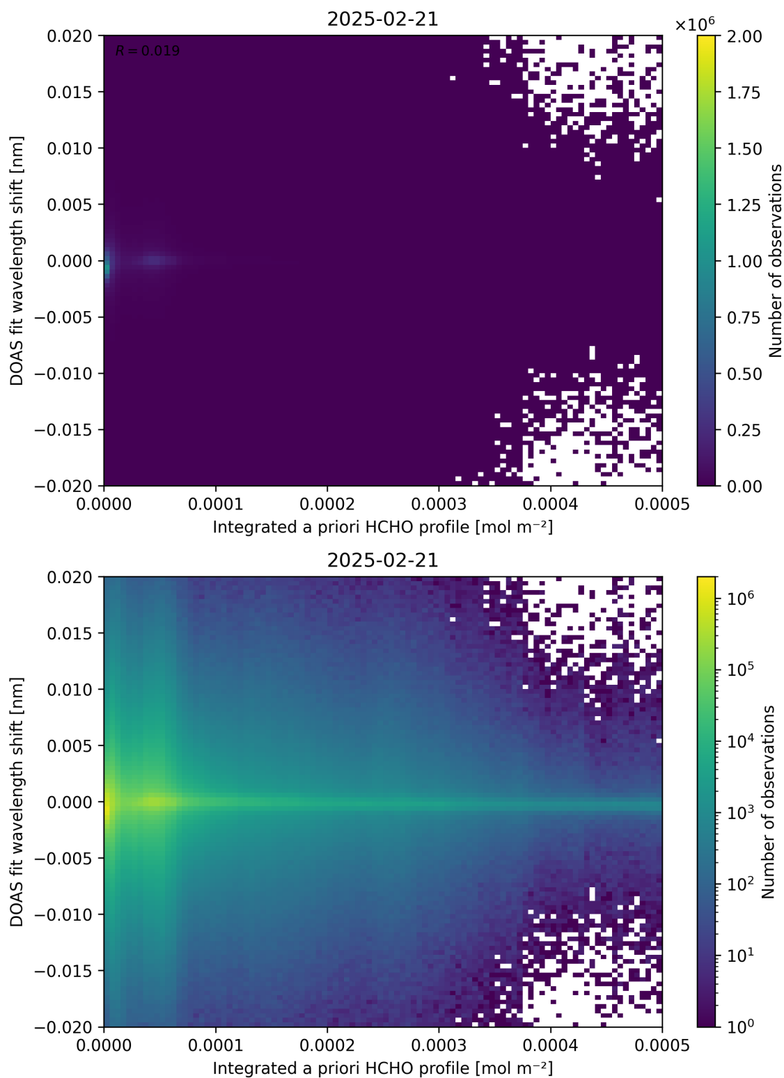
Figure 149: Scatter density plot of “Integrated a priori HCHO profile” against “DOAS fit wavelength shift” for 2025-02-20 to 2025-02-22.
