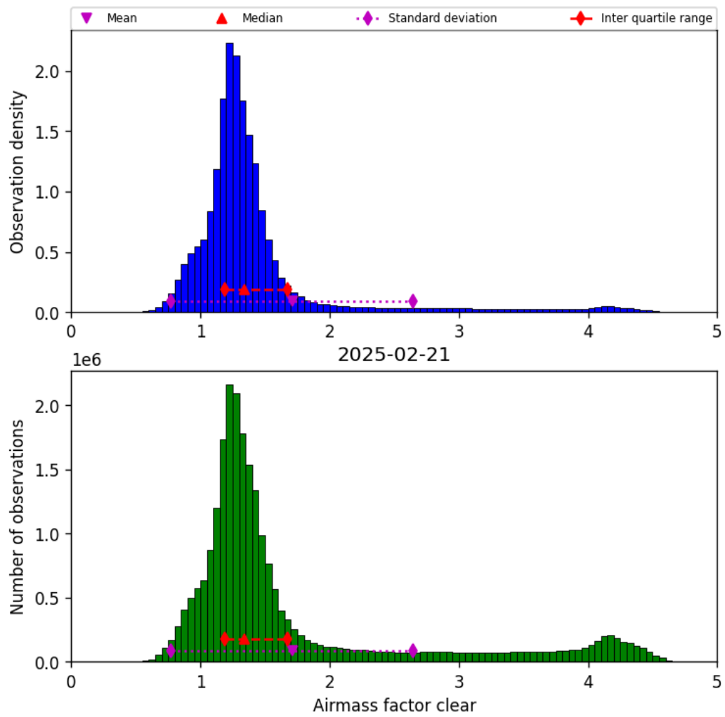
Figure 42: Histogram of “Airmass factor clear” for 2025-02-20 to 2025-02-22
