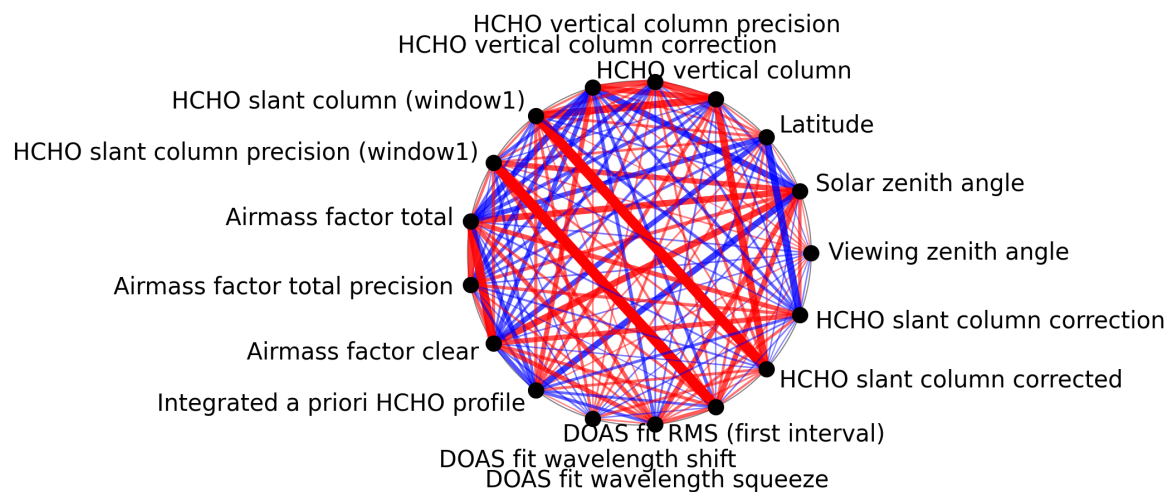
Figure 1: Map of correlation graph for 2025-02-20 to 2025-02-22.
