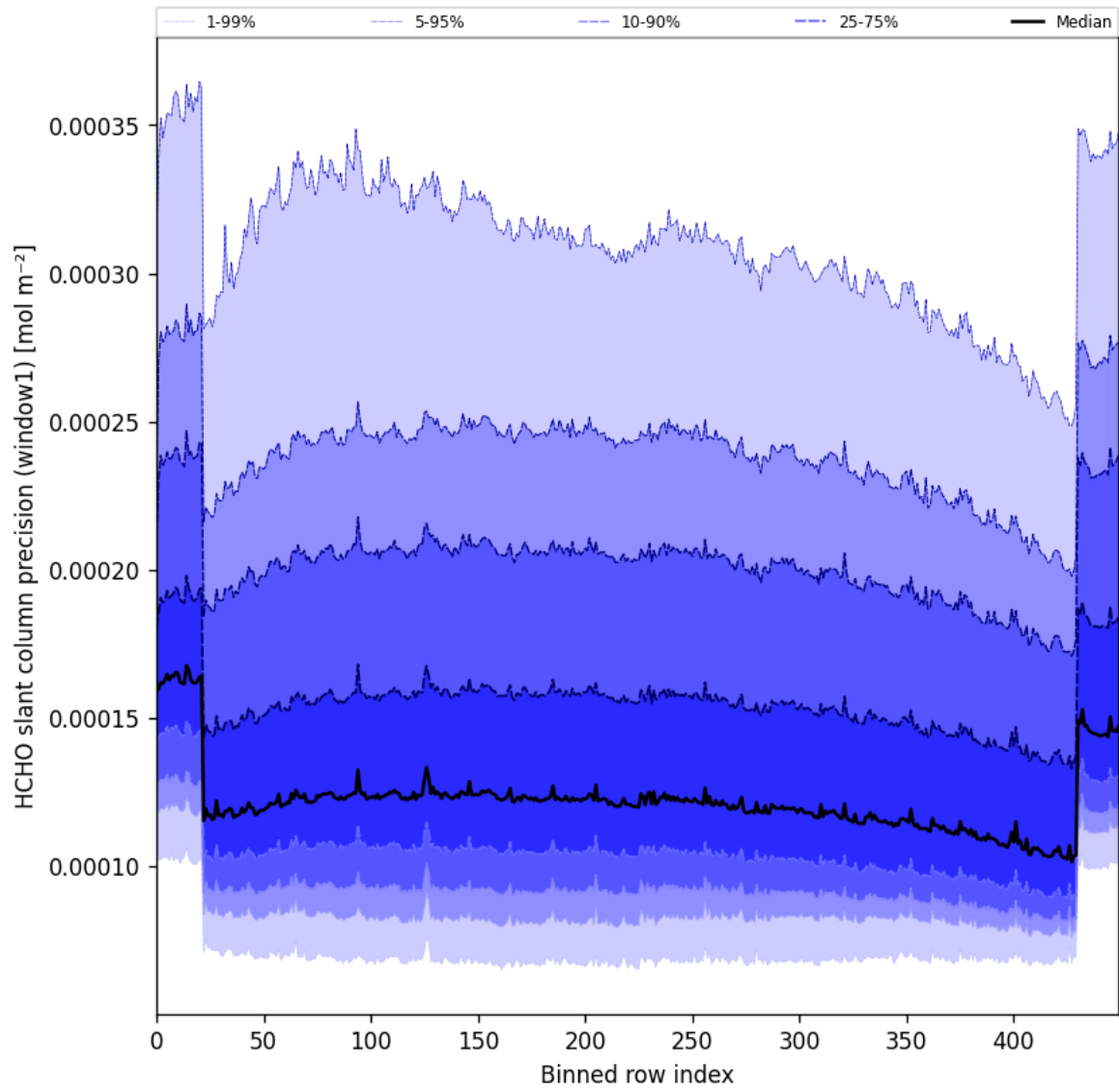
Figure 53: Along track statistics of “HCHO slant column precision (window1)” for 2025-02-20 to 2025-02-22
