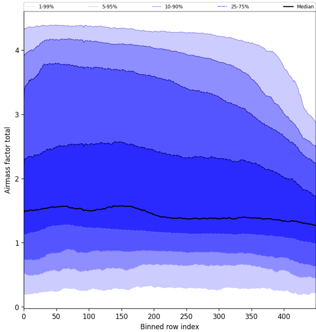
Figure 54: Along track statistics of “Airmass factor total” for 2025-02-20 to 2025-02-22
