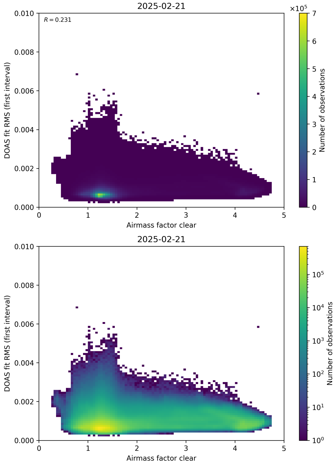
Figure 71: Scatter density plot of “Airmass factor clear” against “DOAS fit RMS (first interval)” for 2025-02-20 to 2025-02-22.
