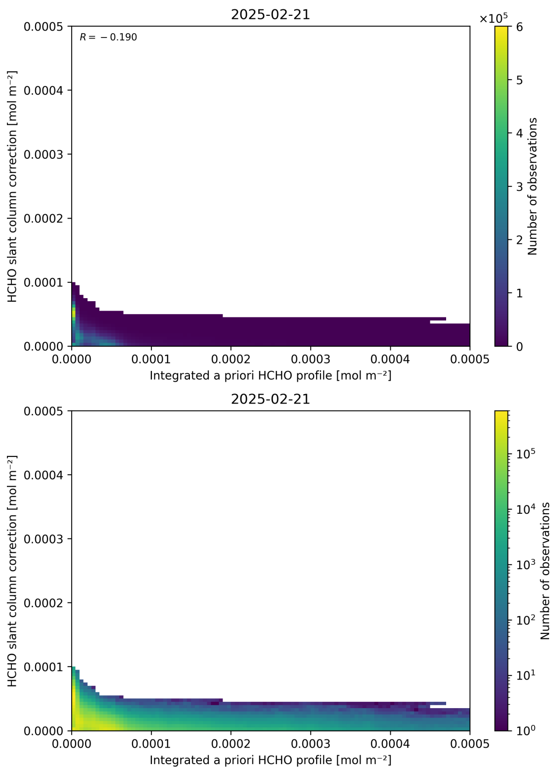
Figure 152: Scatter density plot of “Integrated a priori HCHO profile” against “HCHO slant column correction” for 2025-02-20 to 2025-02-22.
