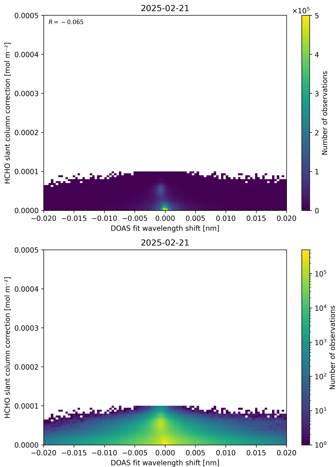
Figure 67: Scatter density plot of “DOAS fit wavelength shift” against “HCHO slant column correction” for 2025-02-20 to 2025-02-22.
