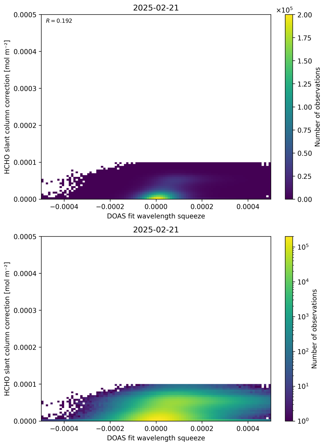
Figure 70: Scatter density plot of “DOAS fit wavelength squeeze” against “HCHO slant column correction” for 2025-02-20 to 2025-02-22.
