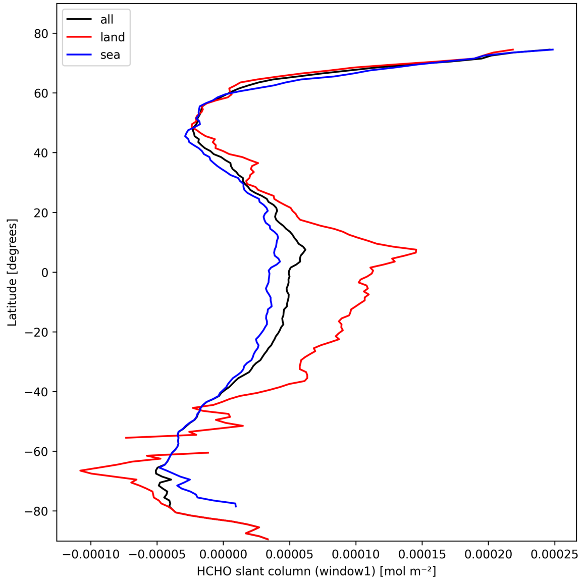
Figure 24: Zonal average of “HCHO slant column (window1)” for 2025-02-20 to 2025-02-22.
