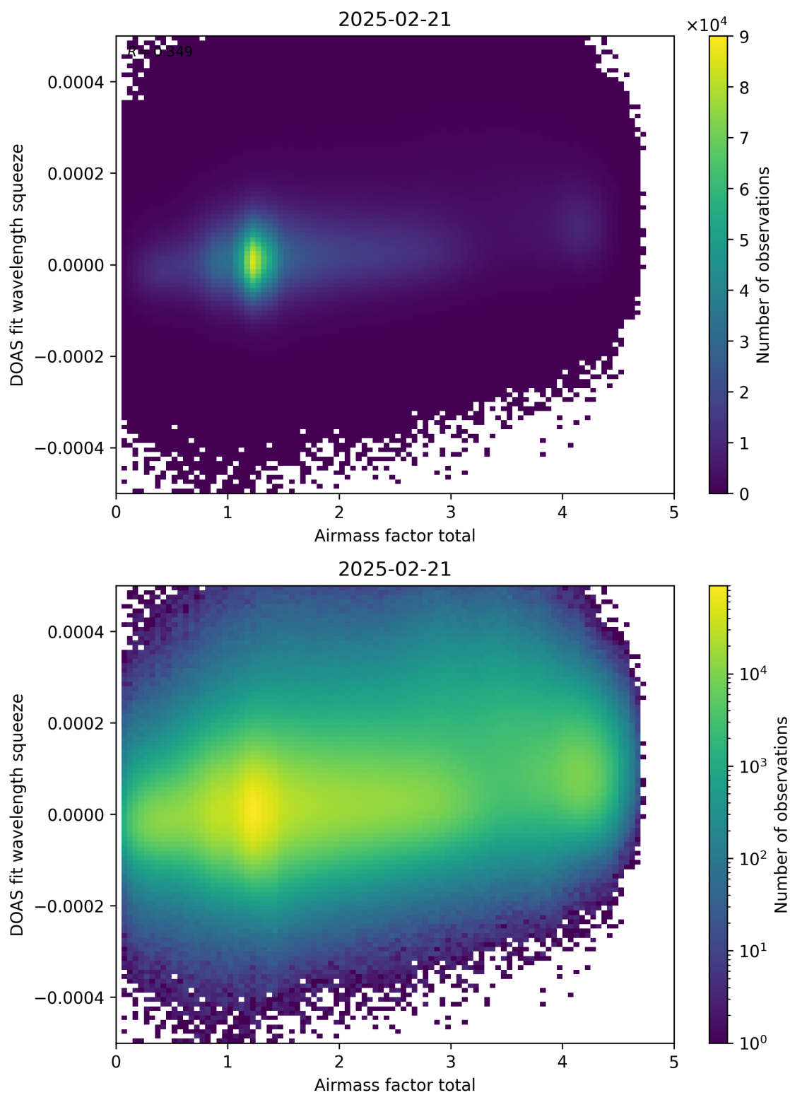
Figure 99: Scatter density plot of “Airmass factor total” against “DOAS fit wavelength squeeze” for 2025-02-20 to 2025-02-22.
