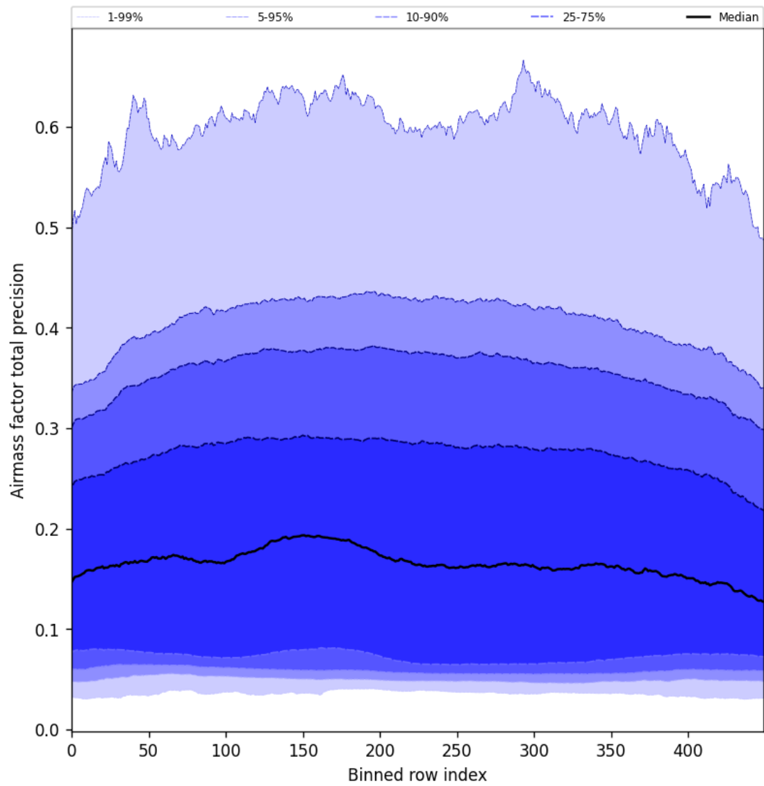
Figure 55: Along track statistics of “Airmass factor total precision” for 2025-02-20 to 2025-02-22
