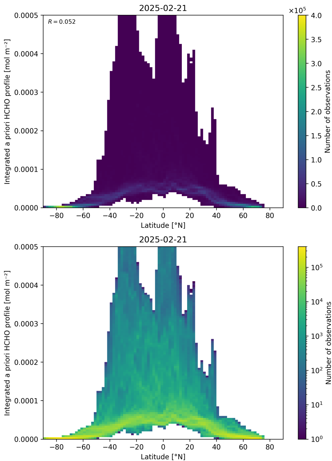
Figure 166: Scatter density plot of “Latitude” against “Integrated a priori HCHO profile” for 2025-02-20 to 2025-02-22.
