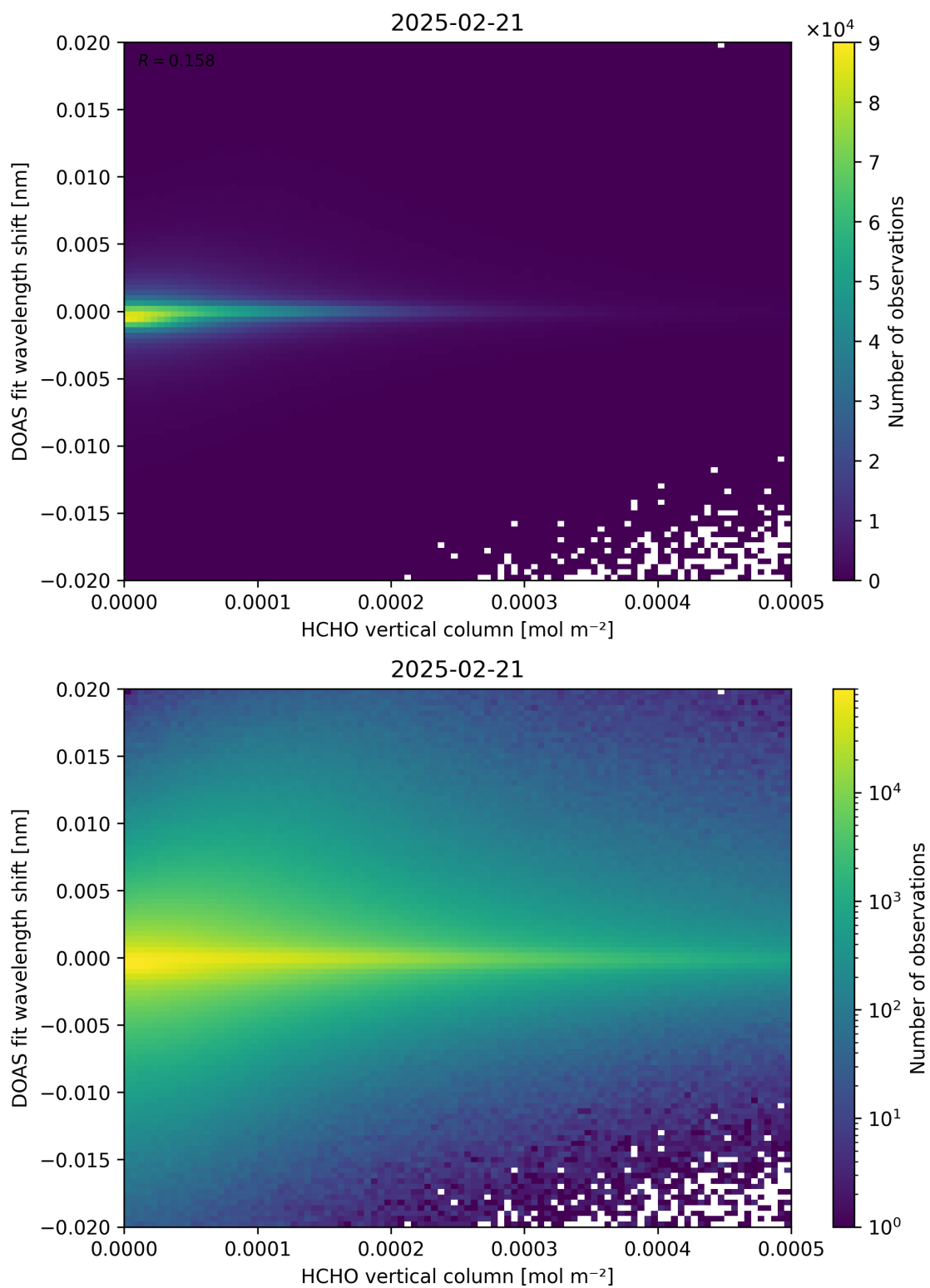
Figure 124: Scatter density plot of “HCHO vertical column” against “DOAS fit wavelength shift” for 2025-02-20 to 2025-02-22.
