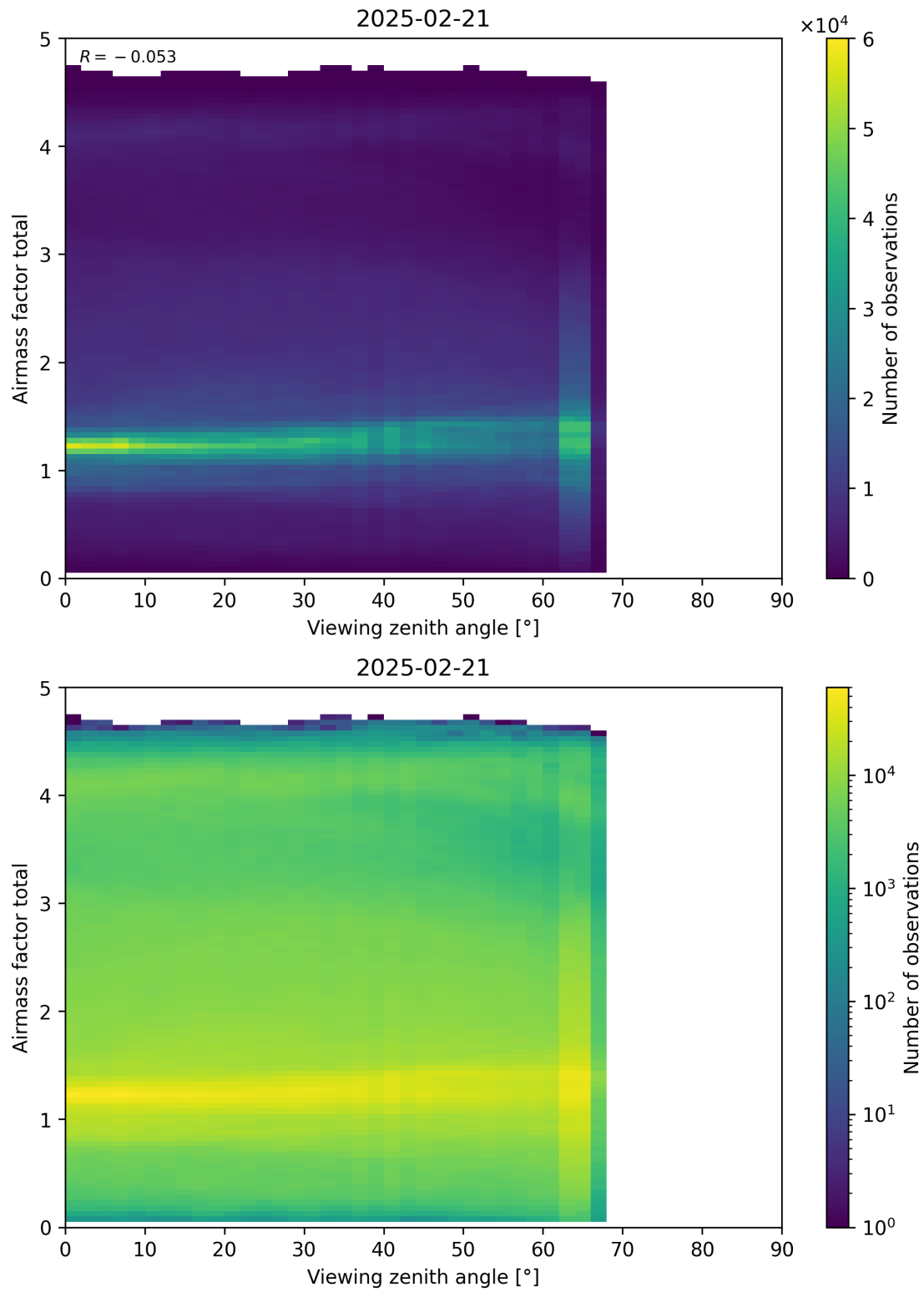
Figure 190: Scatter density plot of “Viewing zenith angle” against “Airmass factor total” for 2025-02-20 to 2025-02-22.
