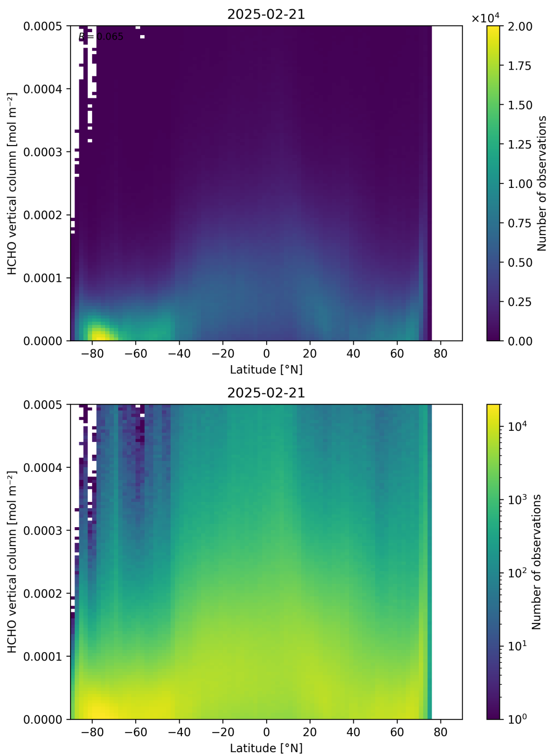
Figure 163: Scatter density plot of “Latitude” against “HCHO vertical column” for 2025-02-20 to 2025-02-22.
