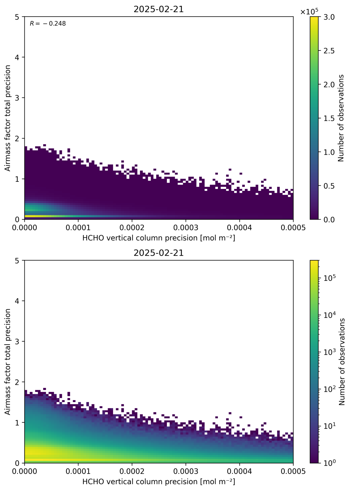
Figure 145: Scatter density plot of “HCHO vertical column precision” against “Airmass factor total precision” for 2025-02-20 to 2025-02-22.
