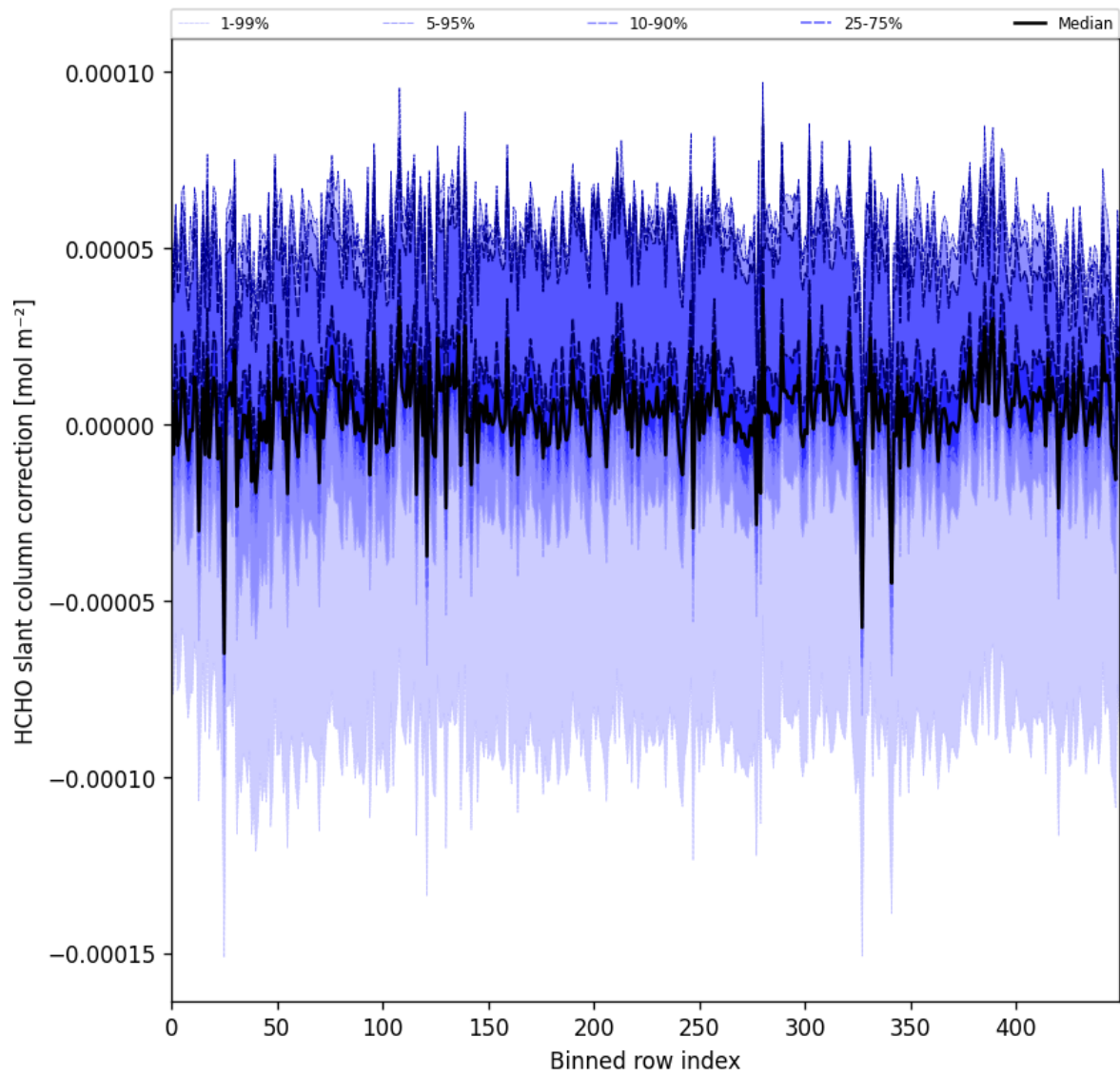
Figure 61: Along track statistics of “HCHO slant column correction” for 2025-02-20 to 2025-02-22
