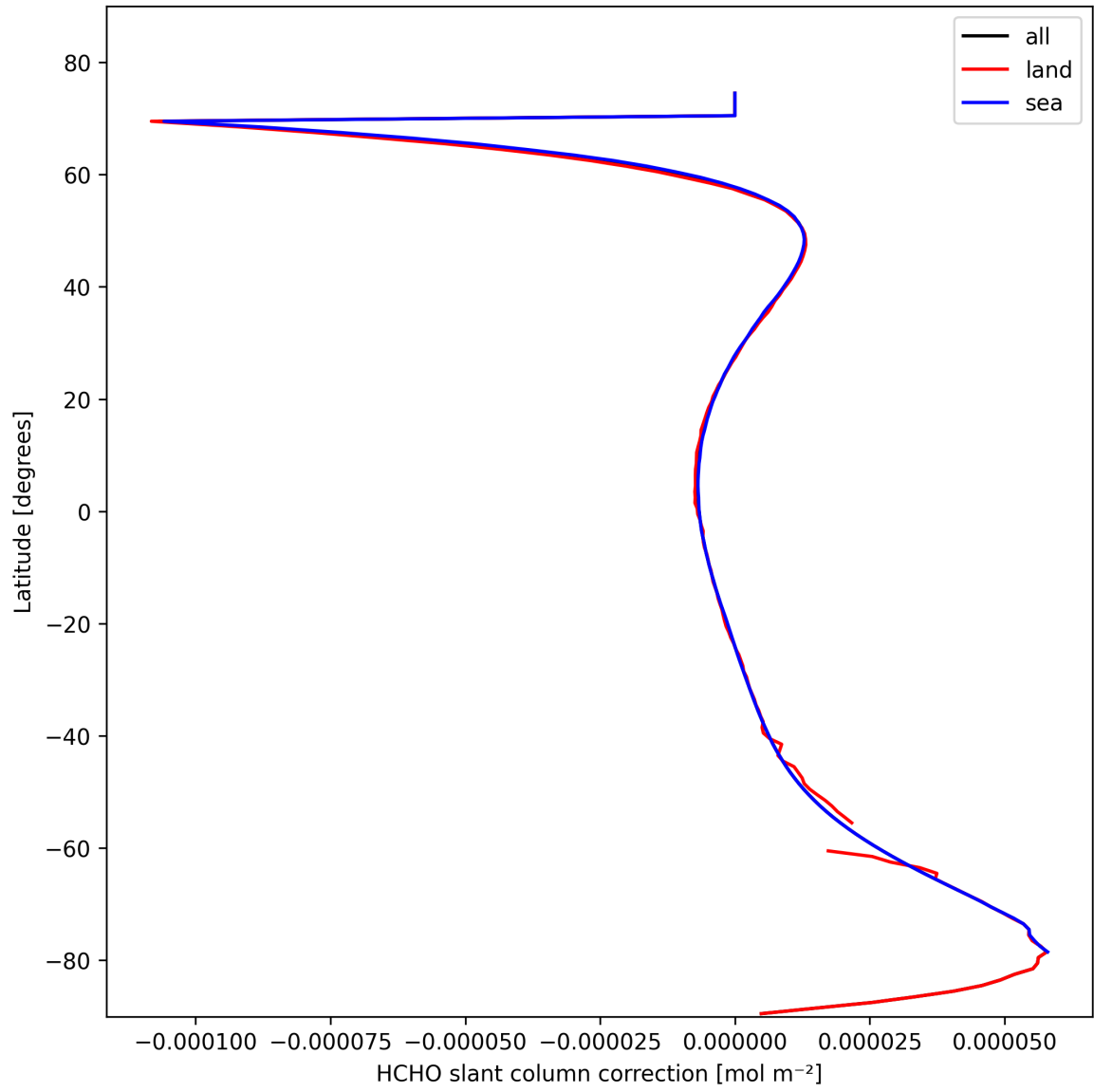
Figure 33: Zonal average of “HCHO slant column correction” for 2025-02-20 to 2025-02-22.
