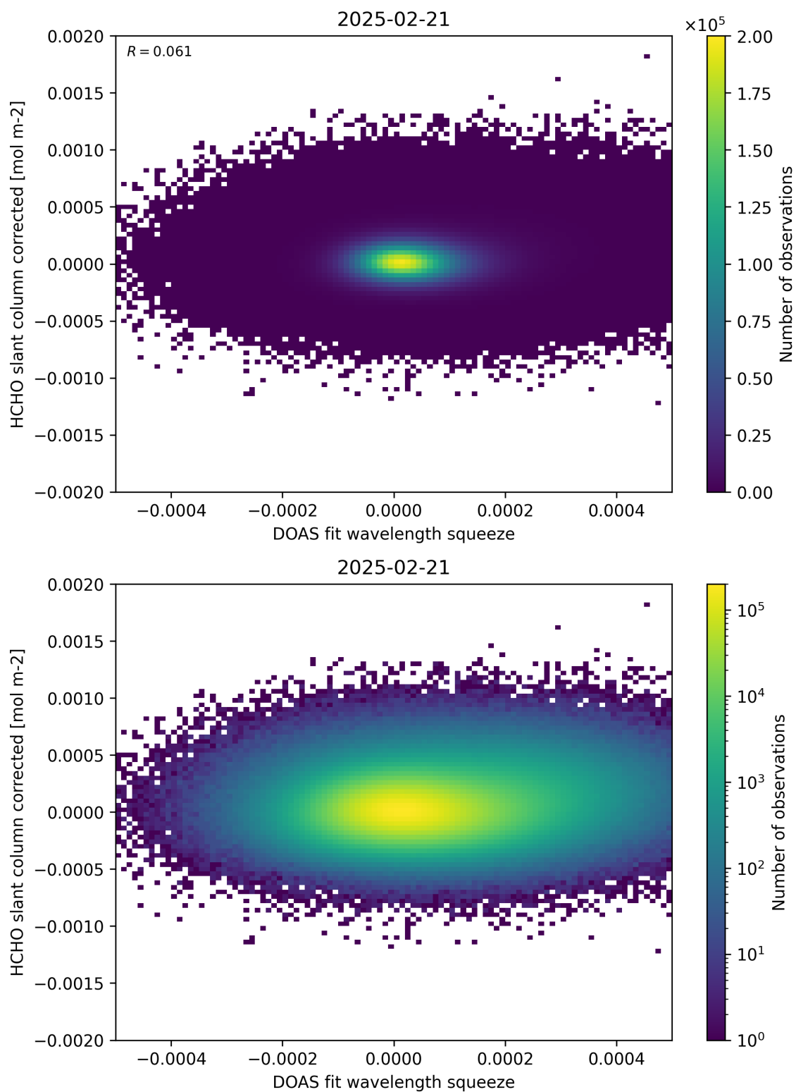
Figure 69: Scatter density plot of “DOAS fit wavelength squeeze” against “HCHO slant column corrected” for 2025-02-20 to 2025-02-22.
