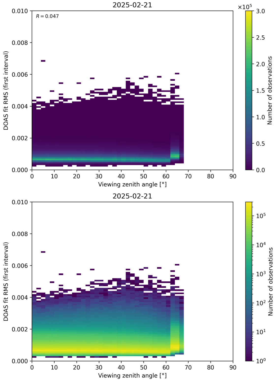
Figure 182: Scatter density plot of “Viewing zenith angle” against “DOAS fit RMS (first interval)” for 2025-02-20 to 2025-02-22.
