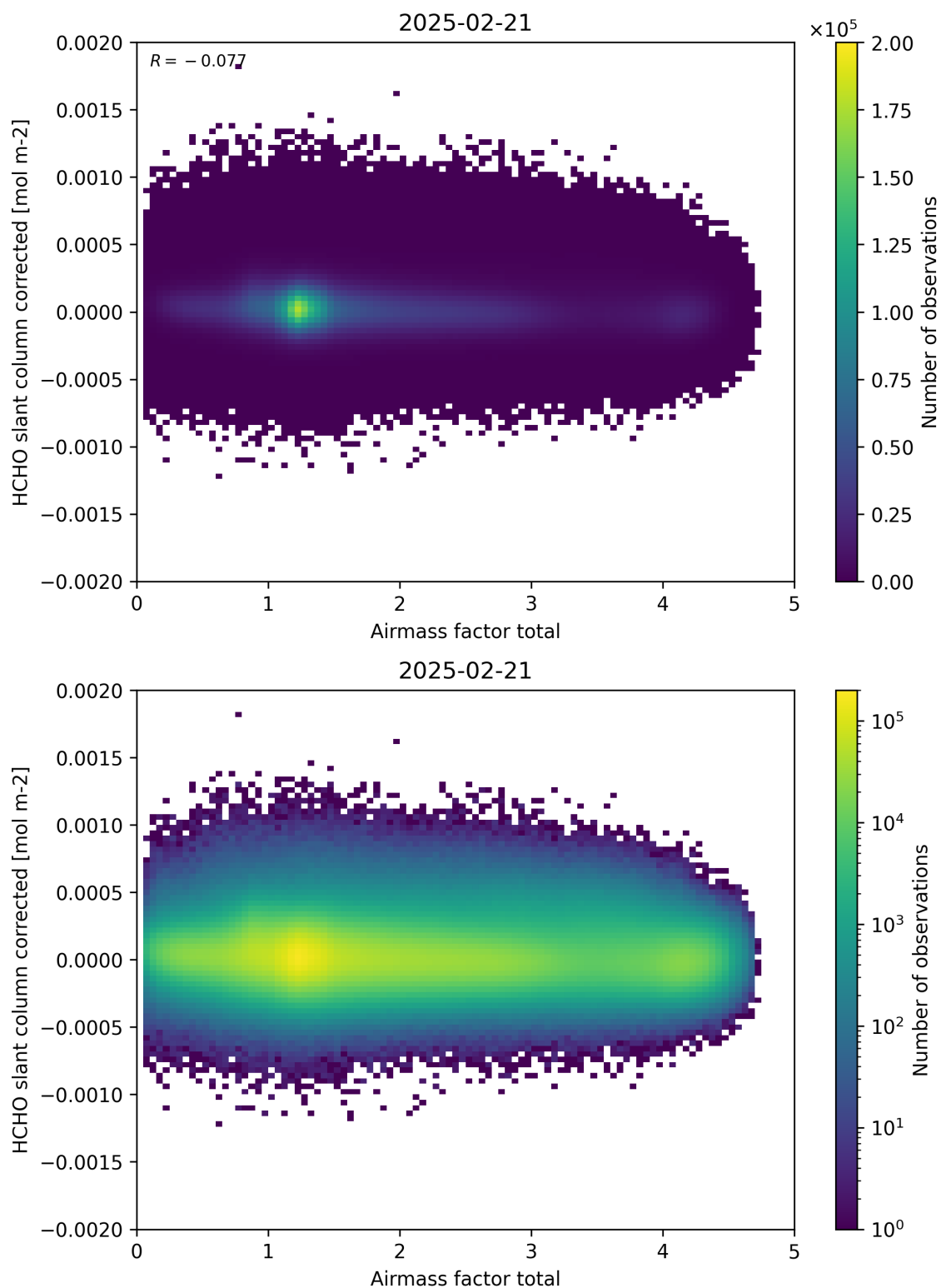
Figure 101: Scatter density plot of “Airmass factor total” against “HCHO slant column corrected” for 2025-02-20 to 2025-02-22.
