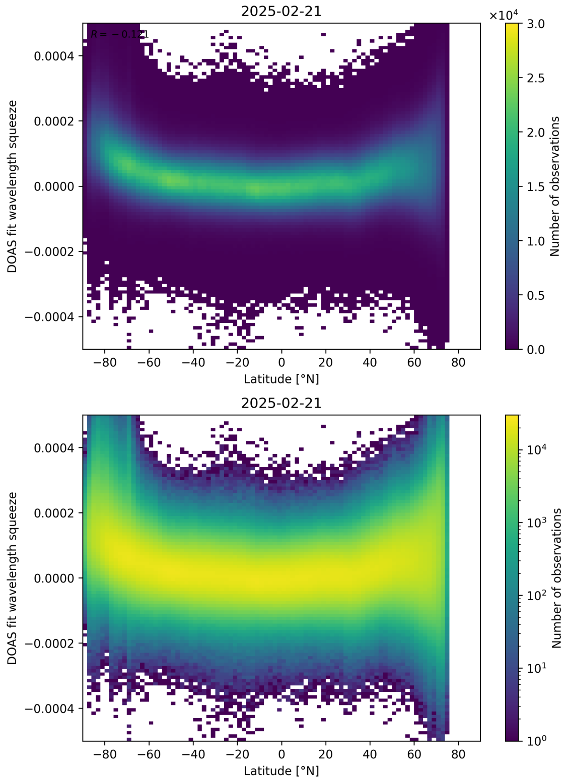
Figure 155: Scatter density plot of “Latitude” against “DOAS fit wavelength squeeze” for 2025-02-20 to 2025-02-22.
