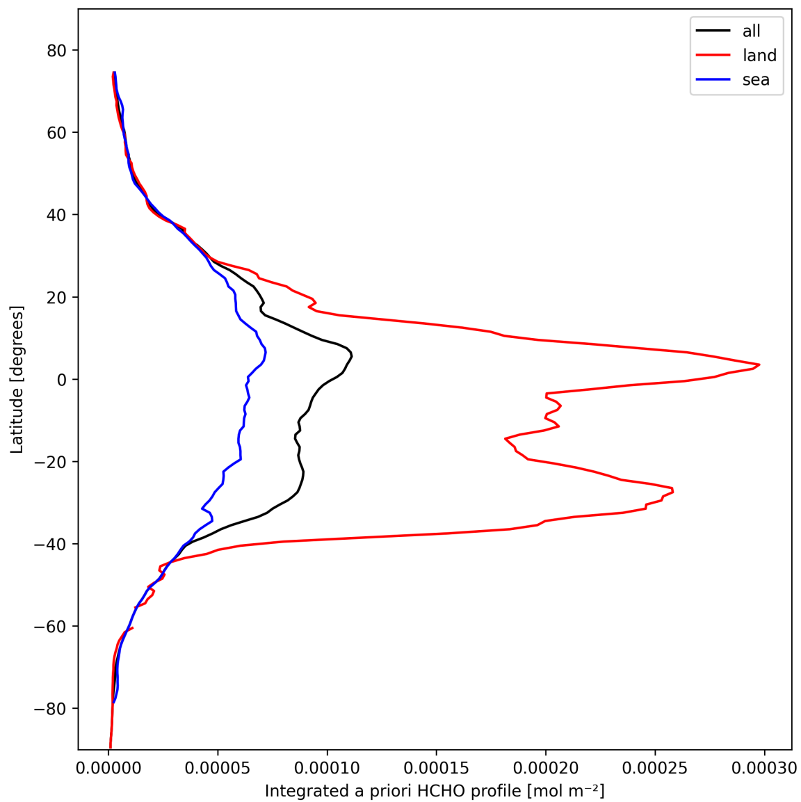
Figure 29: Zonal average of “Integrated a priori HCHO profile” for 2025-02-20 to 2025-02-22.
