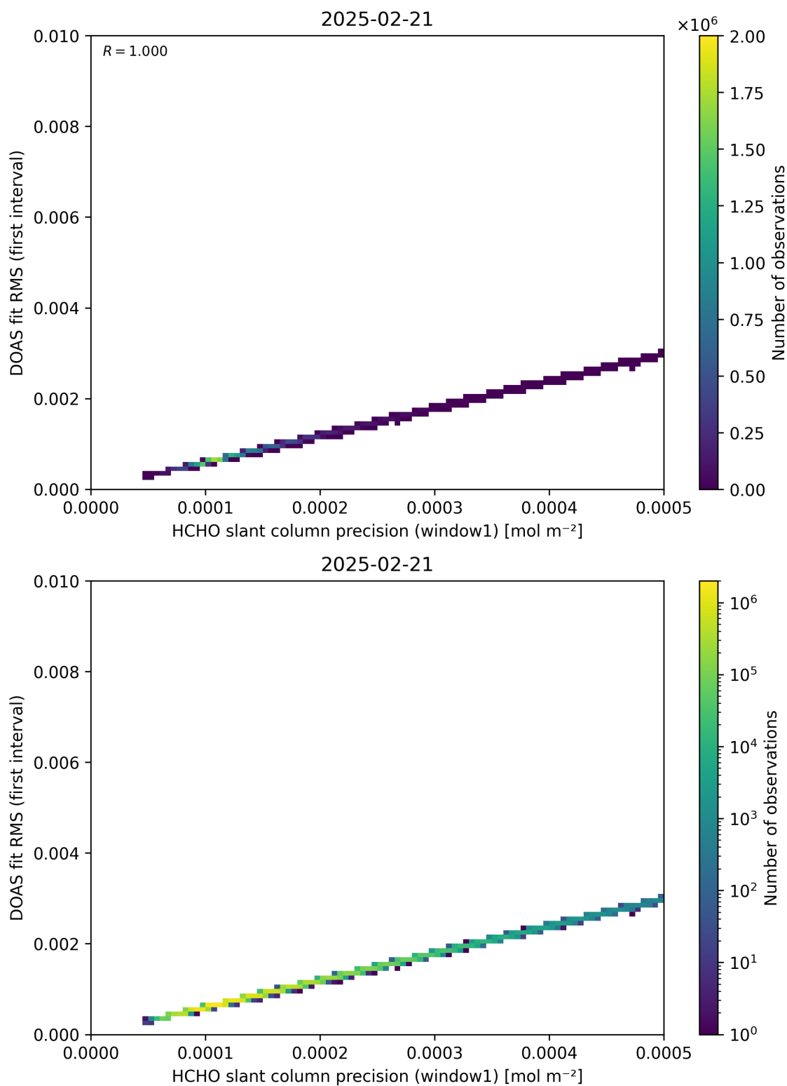
Figure 88: Scatter density plot of “HCHO slant column precision (window1)” against “DOAS fit RMS (first interval)” for 2025-02-20 to 2025-02-22.
