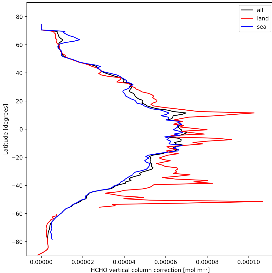
Figure 23: Zonal average of “HCHO vertical column correction” for 2025-02-20 to 2025-02-22.
