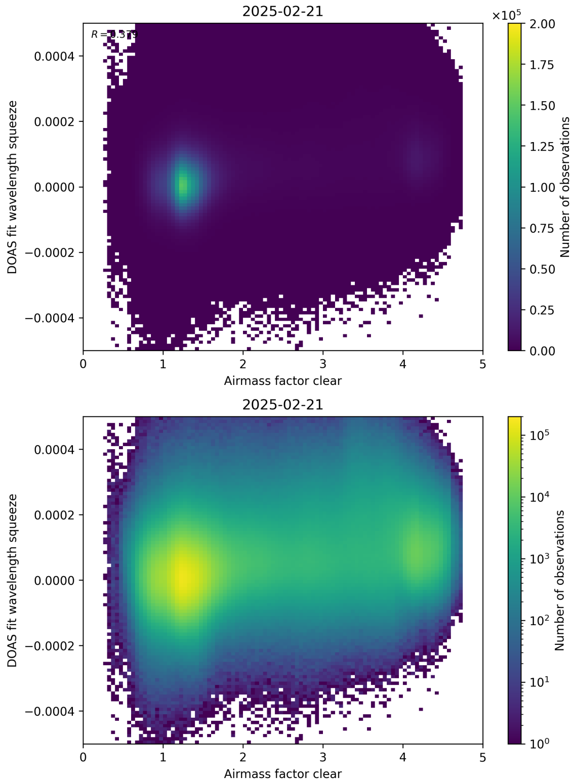
Figure 73: Scatter density plot of “Airmass factor clear” against “DOAS fit wavelength squeeze” for 2025-02-20 to 2025-02-22.
