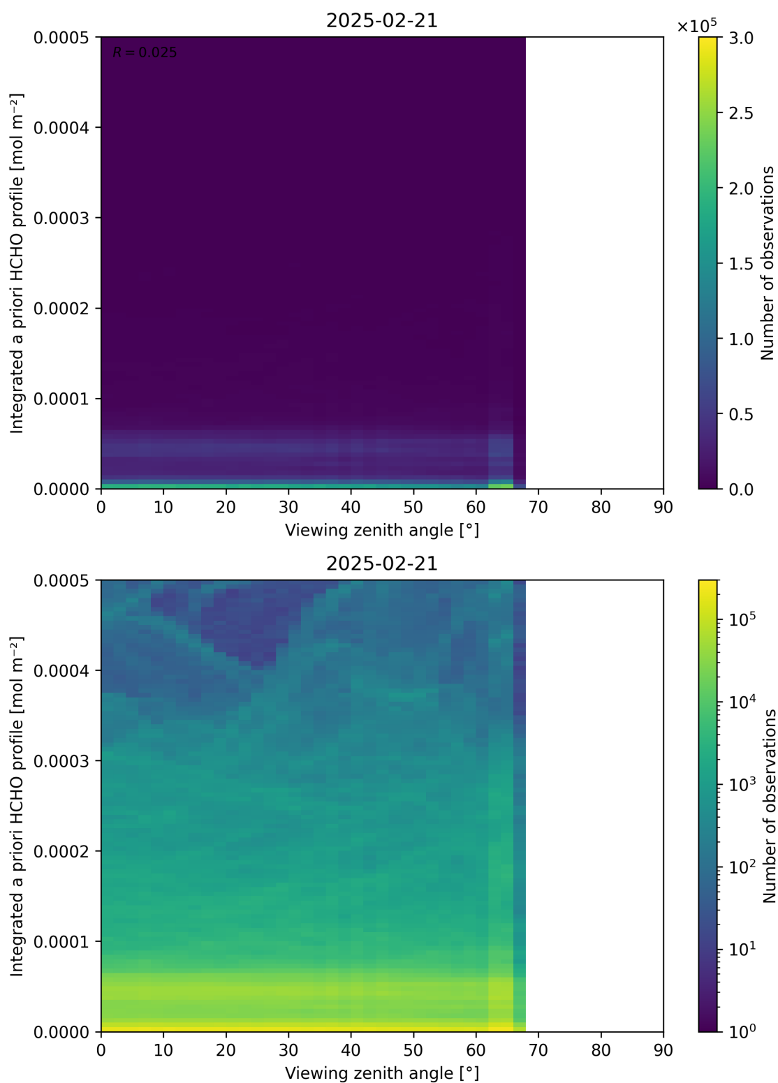
Figure 195: Scatter density plot of “Viewing zenith angle” against “Integrated a priori HCHO profile” for 2025-02-20 to 2025-02-22.
