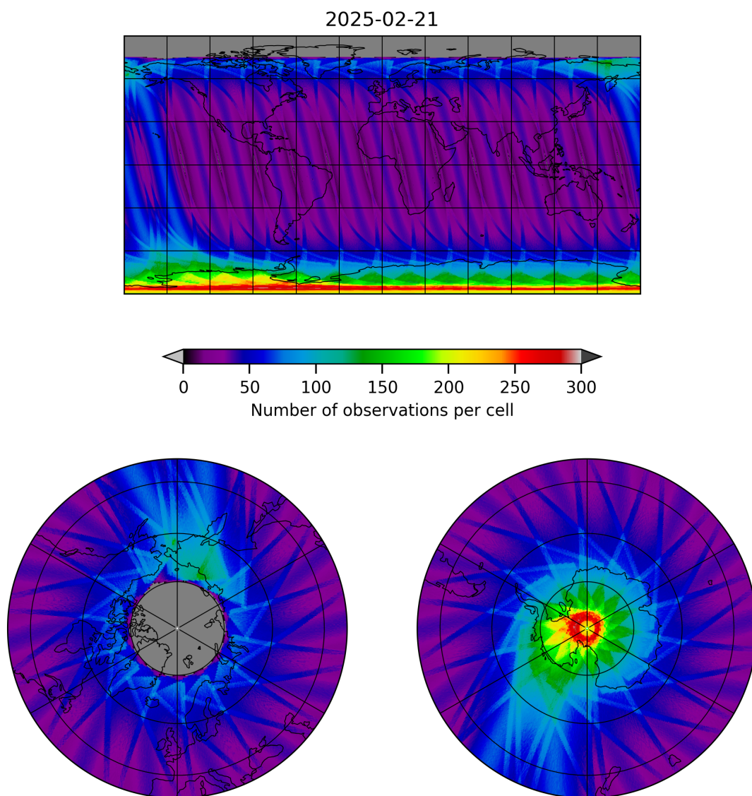
Figure 19: Map of the number of observations for 2025-02-20 to 2025-02-22
