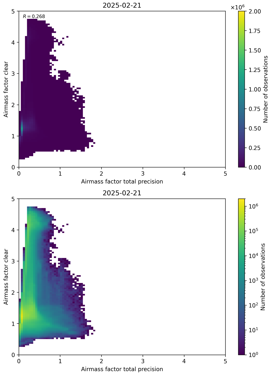
Figure 108: Scatter density plot of “Airmass factor total precision” against “Airmass factor clear” for 2025-02-20 to 2025-02-22.
