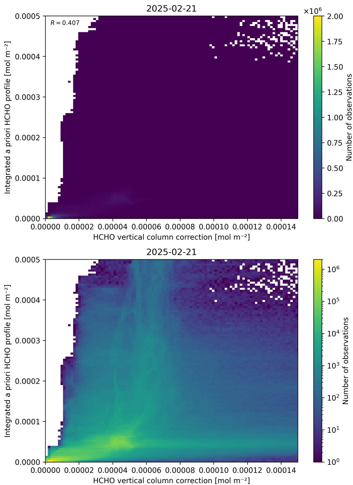
Figure 122: Scatter density plot of “HCHO vertical column correction” against “Integrated a priori HCHO profile” for 2025-02-20 to 2025-02-22.
