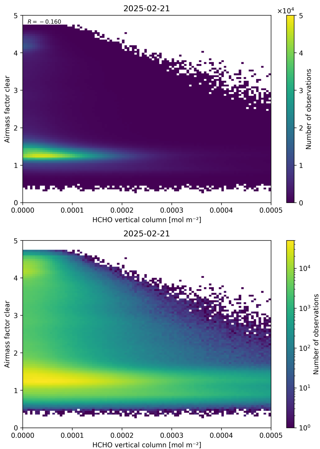
Figure 126: Scatter density plot of “HCHO vertical column” against “Airmass factor clear” for 2025-02-20 to 2025-02-22.
