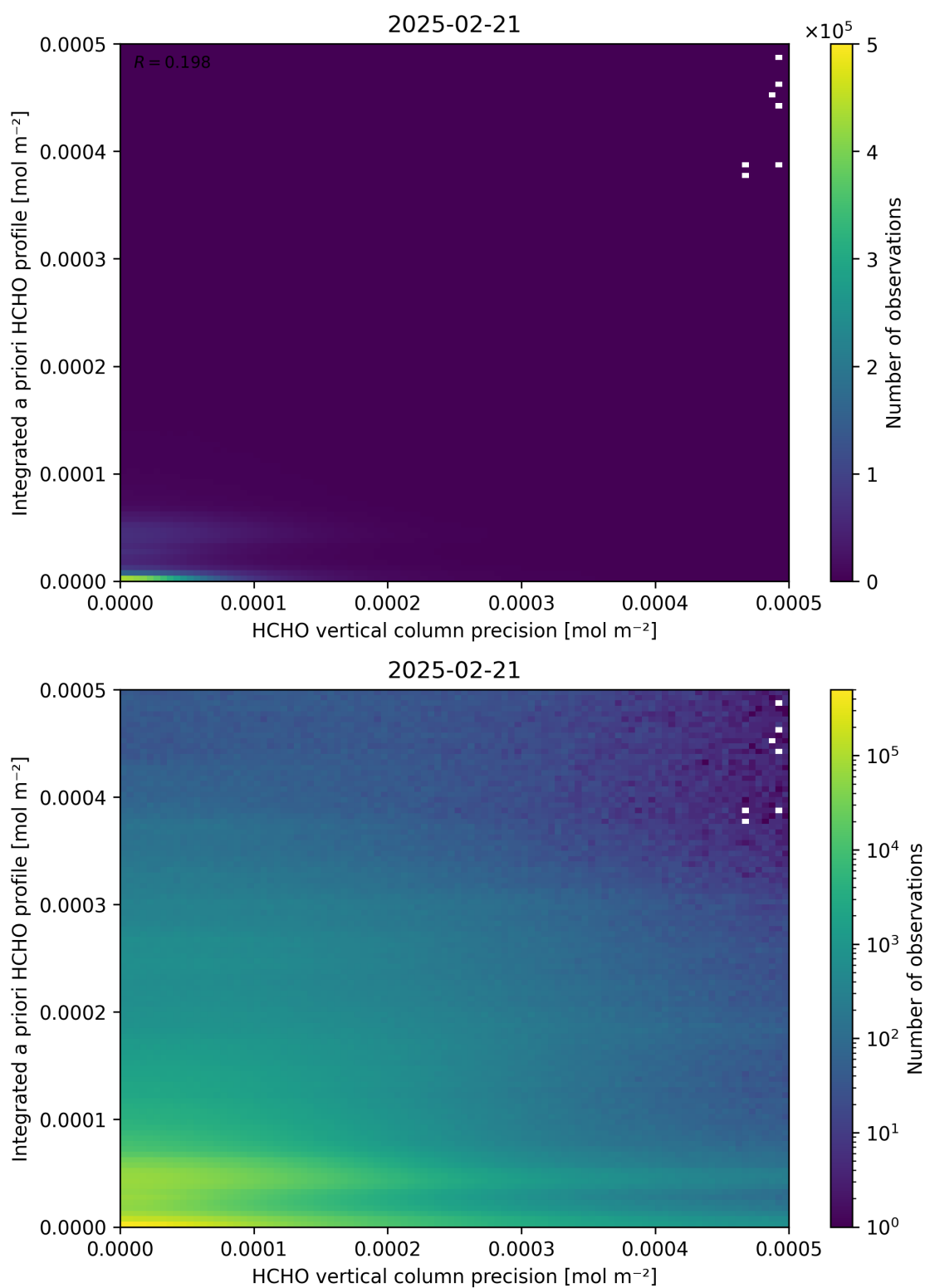
Figure 147: Scatter density plot of “HCHO vertical column precision” against “Integrated a priori HCHO profile” for 2025-02-20 to 2025-02-22.
