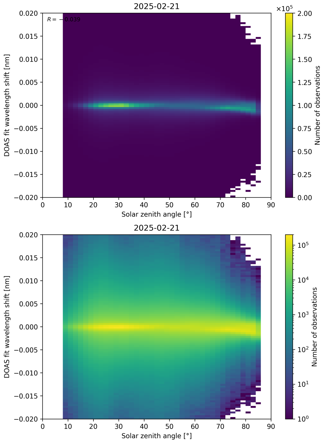
Figure 168: Scatter density plot of “Solar zenith angle” against “DOAS fit wavelength shift” for 2025-02-20 to 2025-02-22.
