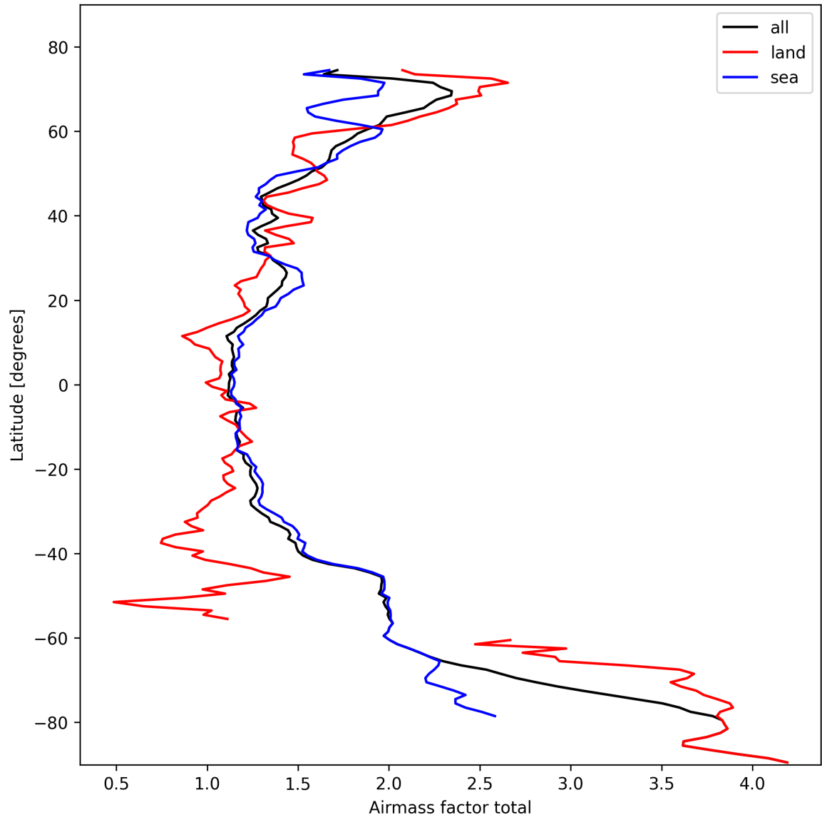
Figure 26: Zonal average of “Airmass factor total” for 2025-02-20 to 2025-02-22.
