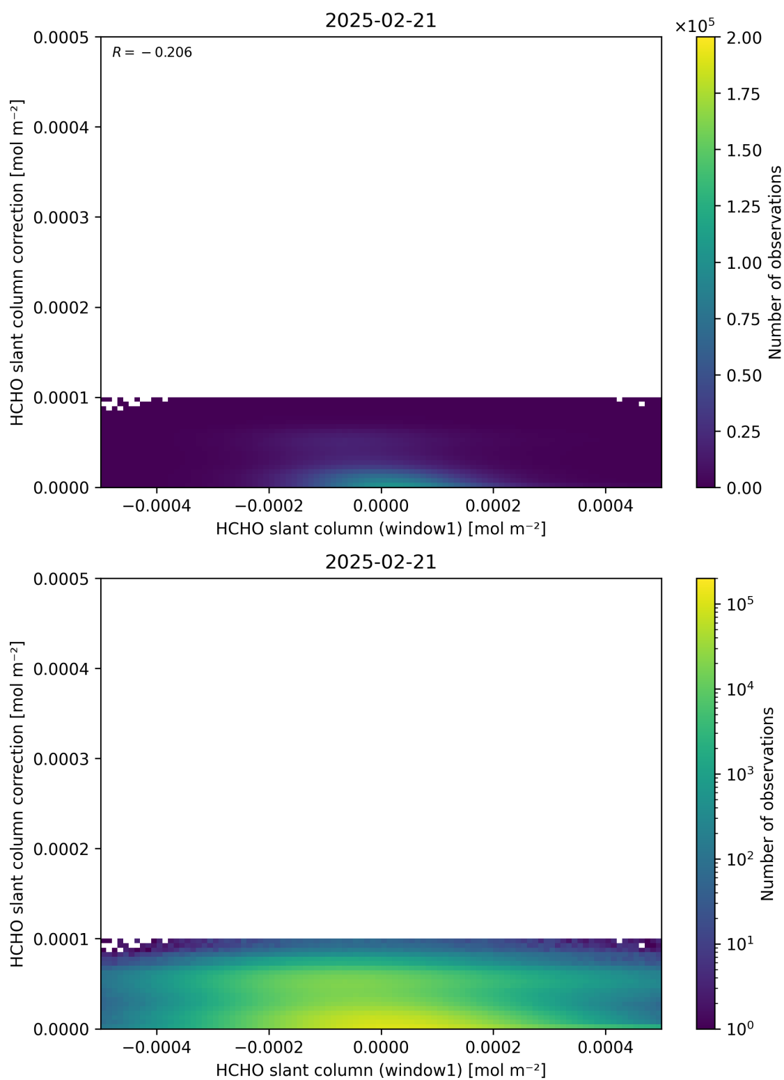
Figure 83: Scatter density plot of “HCHO slant column (window1)” against “HCHO slant column correction” for 2025-02-20 to 2025-02-22.
