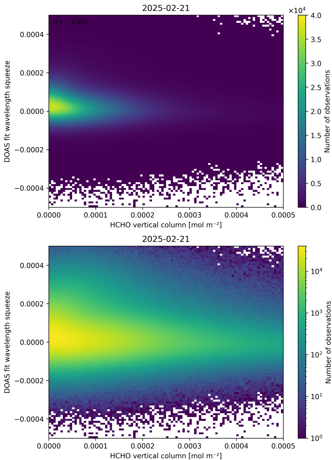
Figure 125: Scatter density plot of “HCHO vertical column” against “DOAS fit wavelength squeeze” for 2025-02-20 to 2025-02-22.
