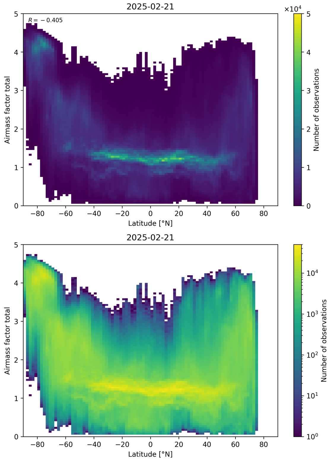
Figure 161: Scatter density plot of “Latitude” against “Airmass factor total” for 2025-02-20 to 2025-02-22.
