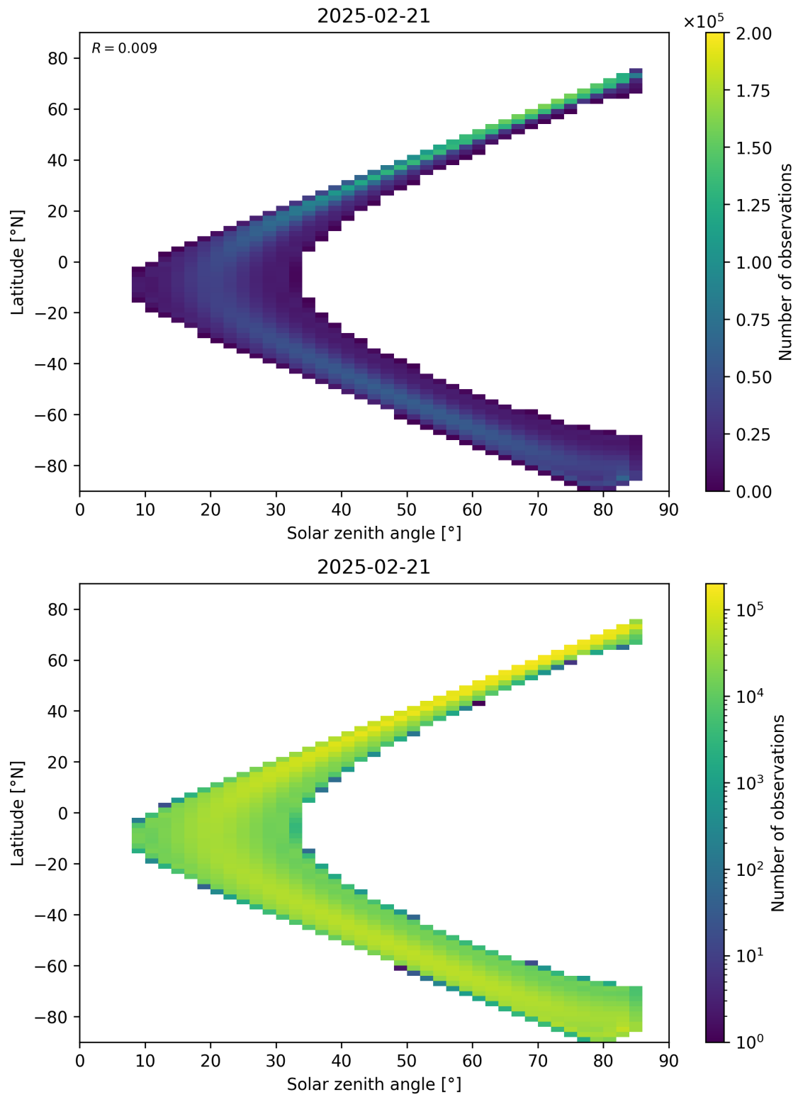
Figure 181: Scatter density plot of “Solar zenith angle” against “Latitude” for 2025-02-20 to 2025-02-22.
