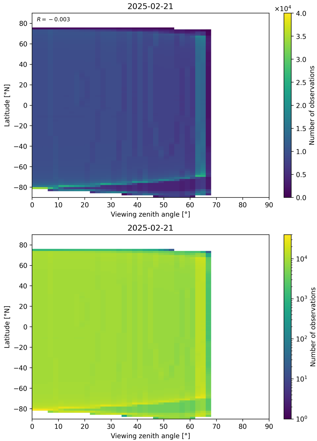
Figure 196: Scatter density plot of “Viewing zenith angle” against “Latitude” for 2025-02-20 to 2025-02-22.
