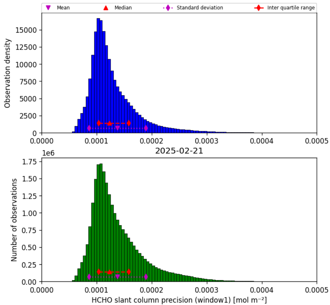
Figure 39: Histogram of “HCHO slant column precision (window1)” for 2025-02-20 to 2025-02-22
