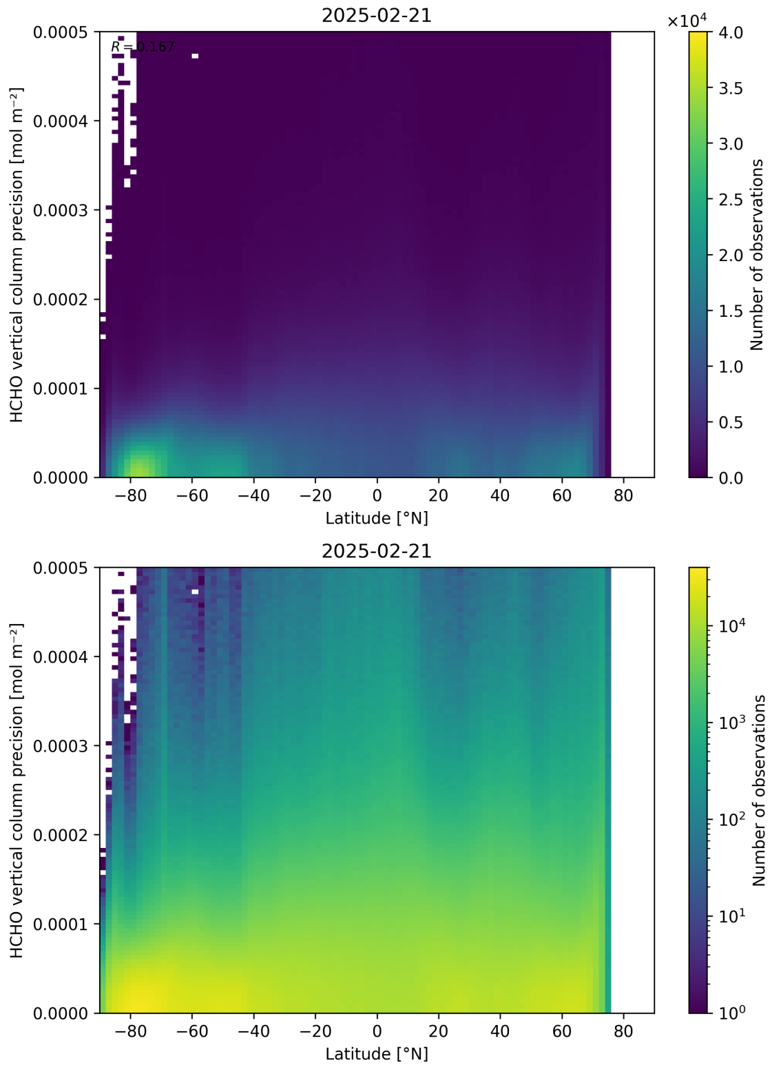
Figure 165: Scatter density plot of “Latitude” against “HCHO vertical column precision” for 2025-02-20 to 2025-02-22.
