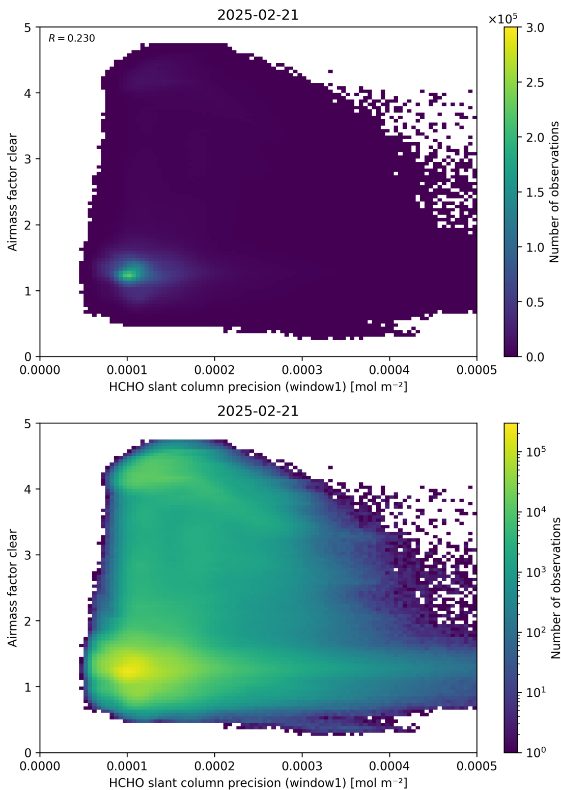
Figure 91: Scatter density plot of “HCHO slant column precision (window1)” against “Airmass factor clear” for 2025-02-20 to 2025-02-22.
