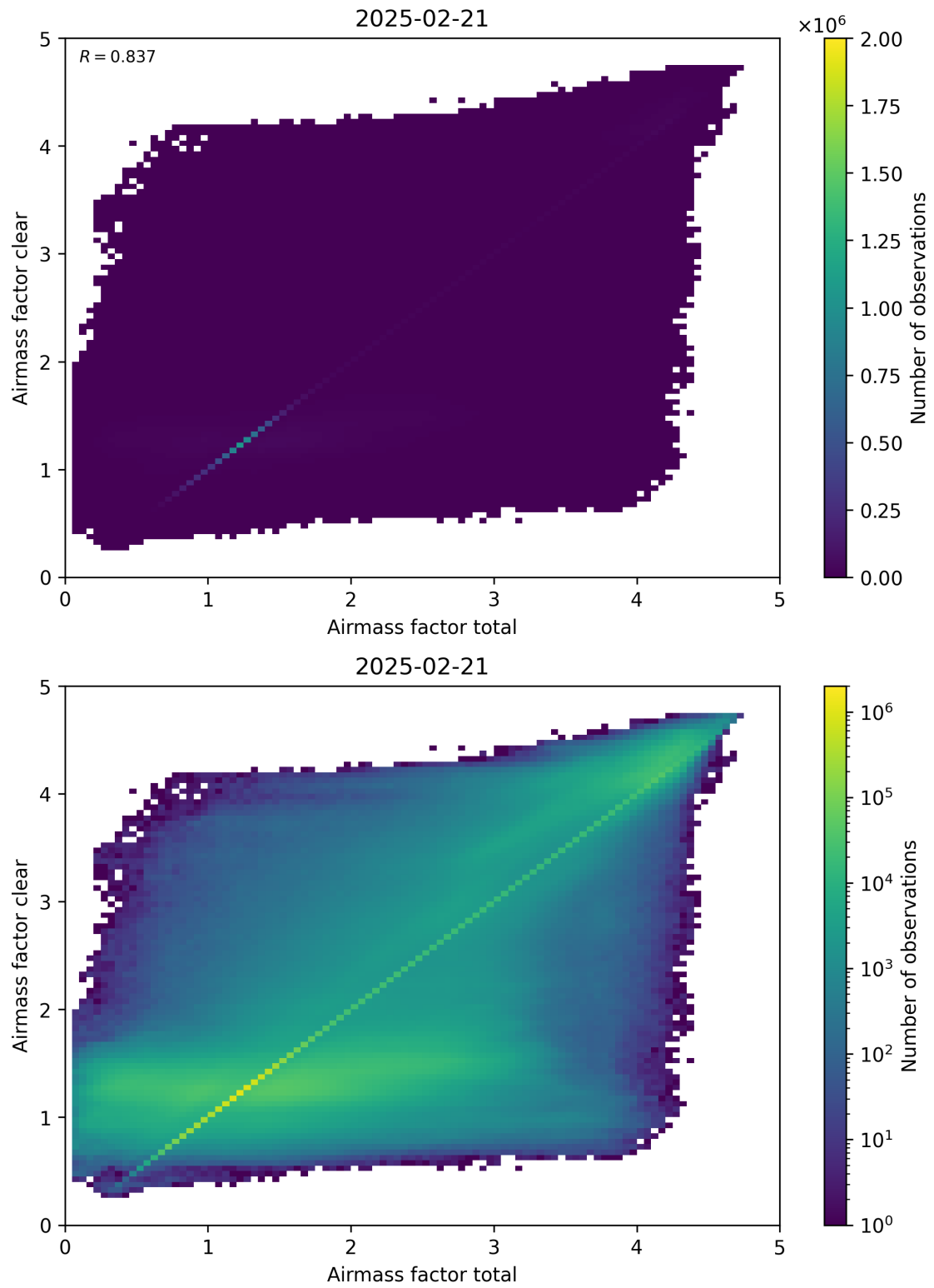
Figure 100: Scatter density plot of “Airmass factor total” against “Airmass factor clear” for 2025-02-20 to 2025-02-22.
