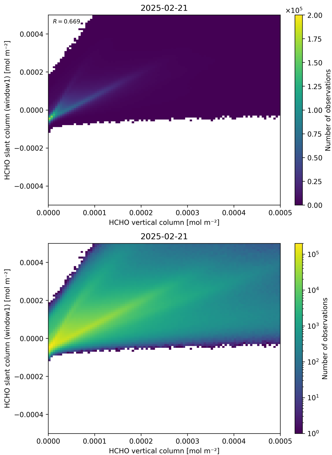
Figure 129: Scatter density plot of “HCHO vertical column” against “HCHO slant column (window1)” for 2025-02-20 to 2025-02-22.
