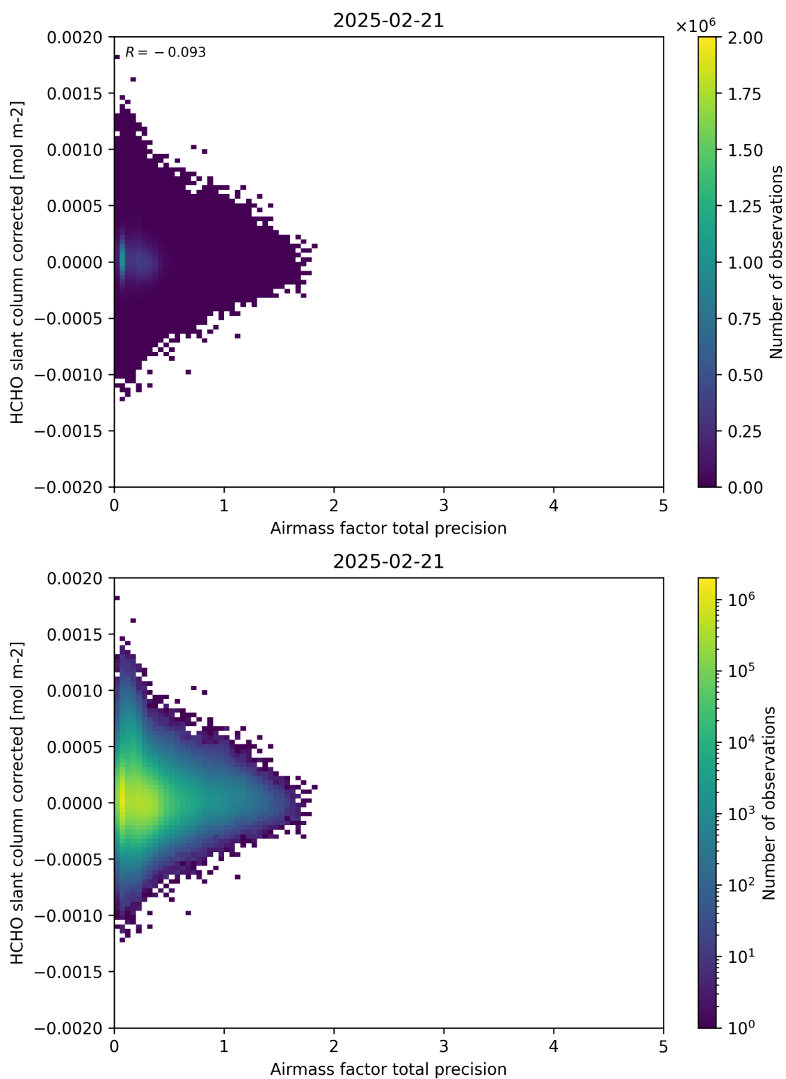
Figure 109: Scatter density plot of “Airmass factor total precision” against “HCHO slant column corrected” for 2025-02-20 to 2025-02-22.
