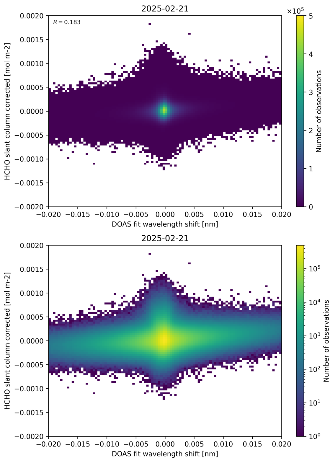
Figure 66: Scatter density plot of “DOAS fit wavelength shift” against “HCHO slant column corrected” for 2025-02-20 to 2025-02-22.
