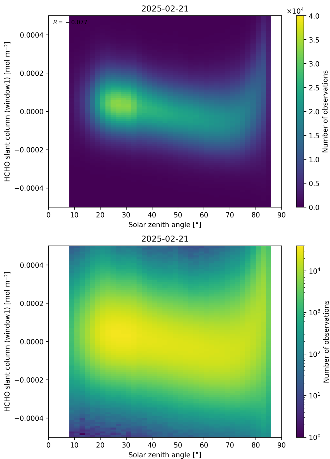
Figure 173: Scatter density plot of “Solar zenith angle” against “HCHO slant column (window1)” for 2025-02-20 to 2025-02-22.
