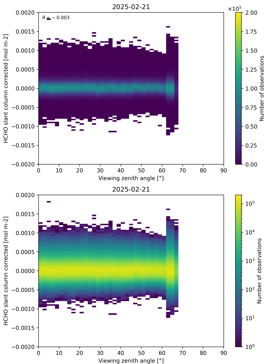
Figure 186: Scatter density plot of “Viewing zenith angle” against “HCHO slant column corrected” for 2025-02-20 to 2025-02-22.
