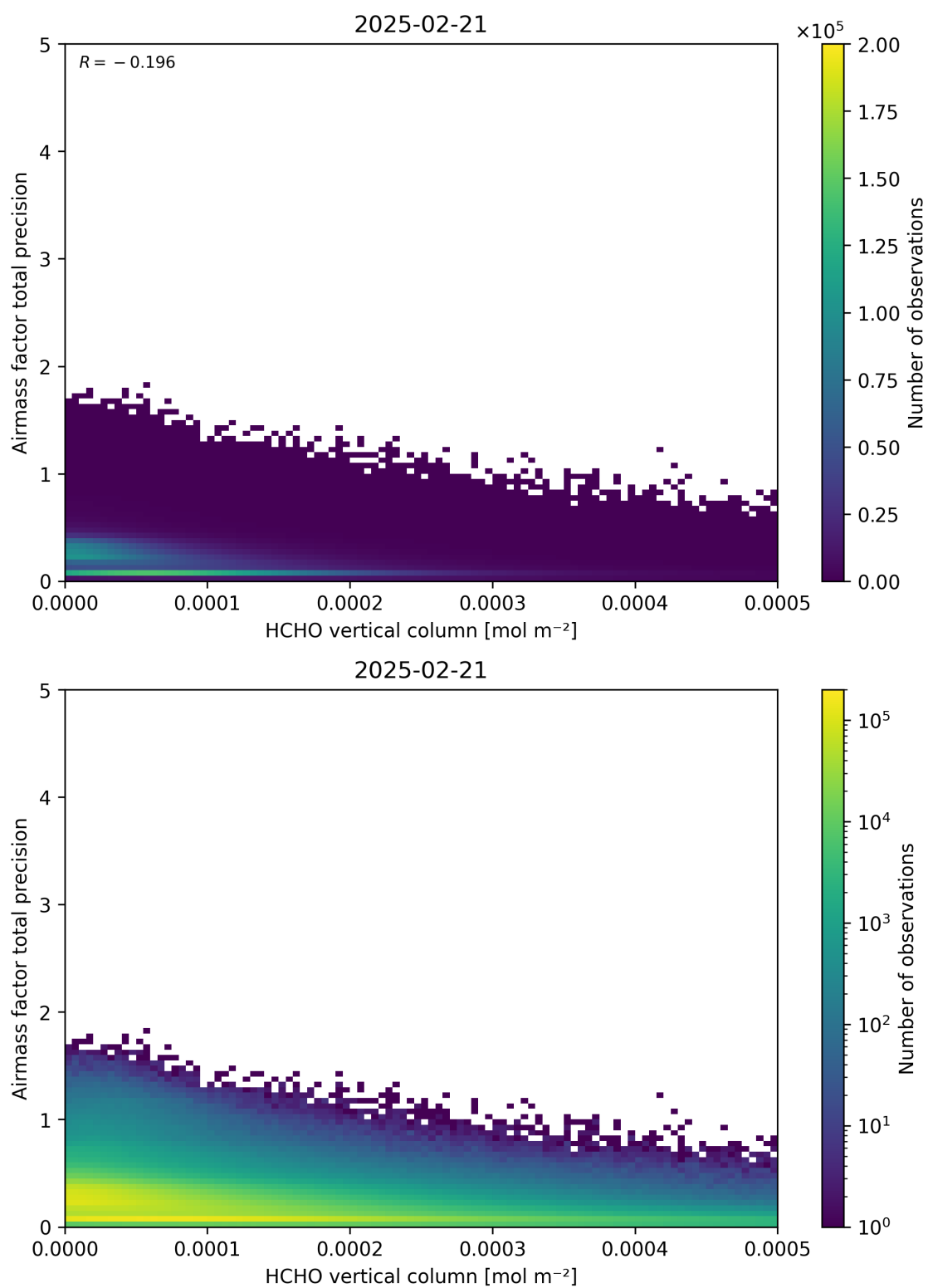
Figure 132: Scatter density plot of “HCHO vertical column” against “Airmass factor total precision” for 2025-02-20 to 2025-02-22.
