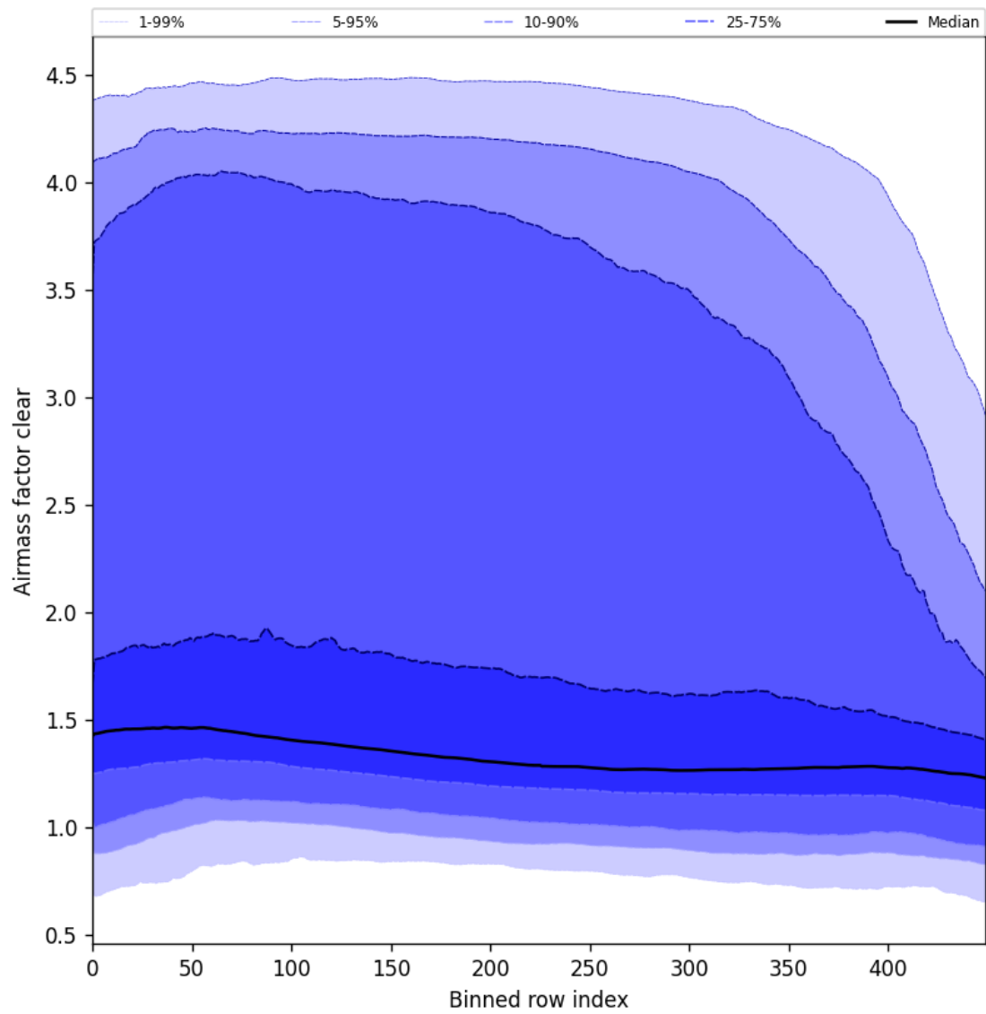
Figure 56: Along track statistics of “Airmass factor clear” for 2025-02-20 to 2025-02-22
