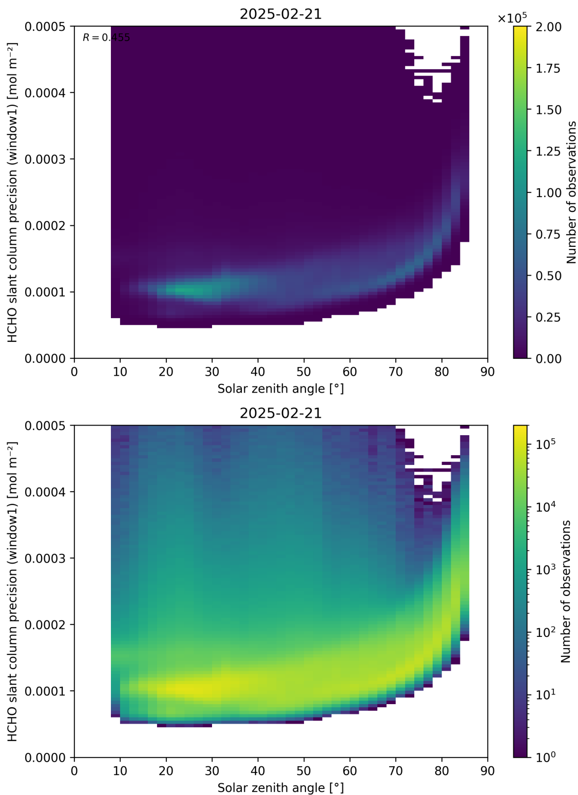
Figure 174: Scatter density plot of “Solar zenith angle” against “HCHO slant column precision (window1)” for 2025-02-20 to 2025-02-22.
