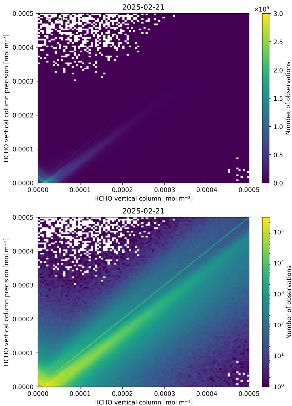
Figure 134: Scatter density plot of “HCHO vertical column” against “HCHO vertical column precision” for 2025-02-20 to 2025-02-22.
