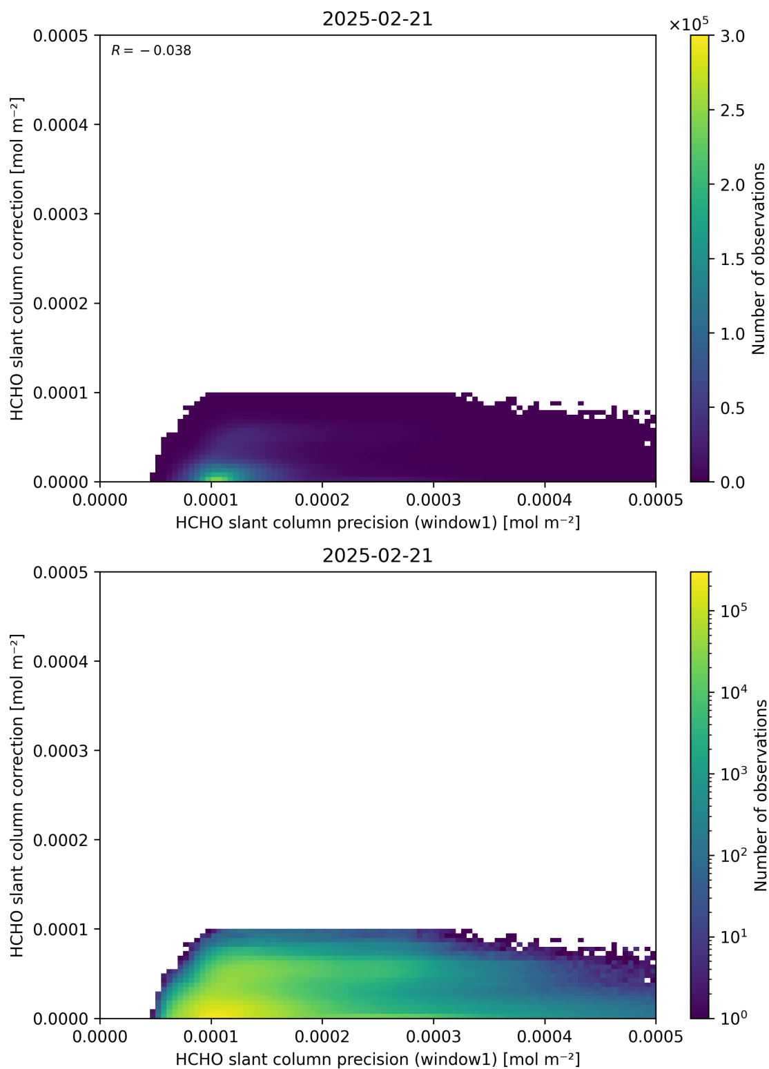
Figure 93: Scatter density plot of “HCHO slant column precision (window1)” against “HCHO slant column correction” for 2025-02-20 to 2025-02-22.
