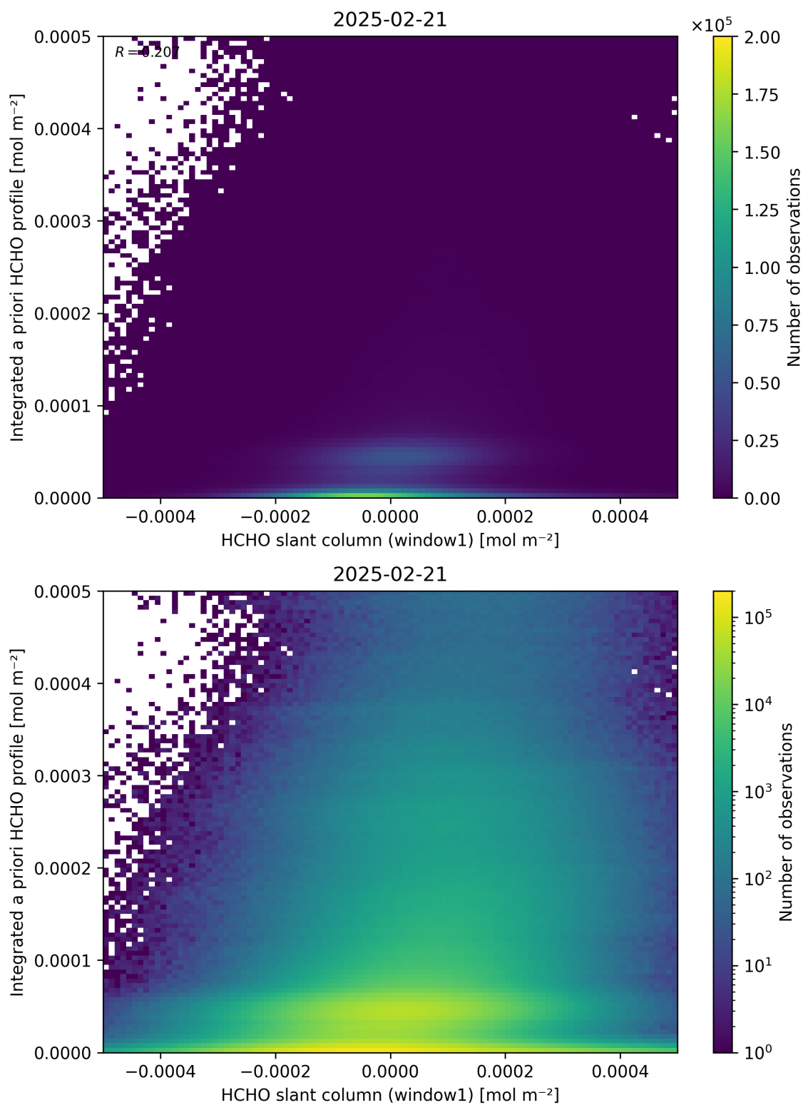
Figure 87: Scatter density plot of “HCHO slant column (window1)” against “Integrated a priori HCHO profile” for 2025-02-20 to 2025-02-22.
