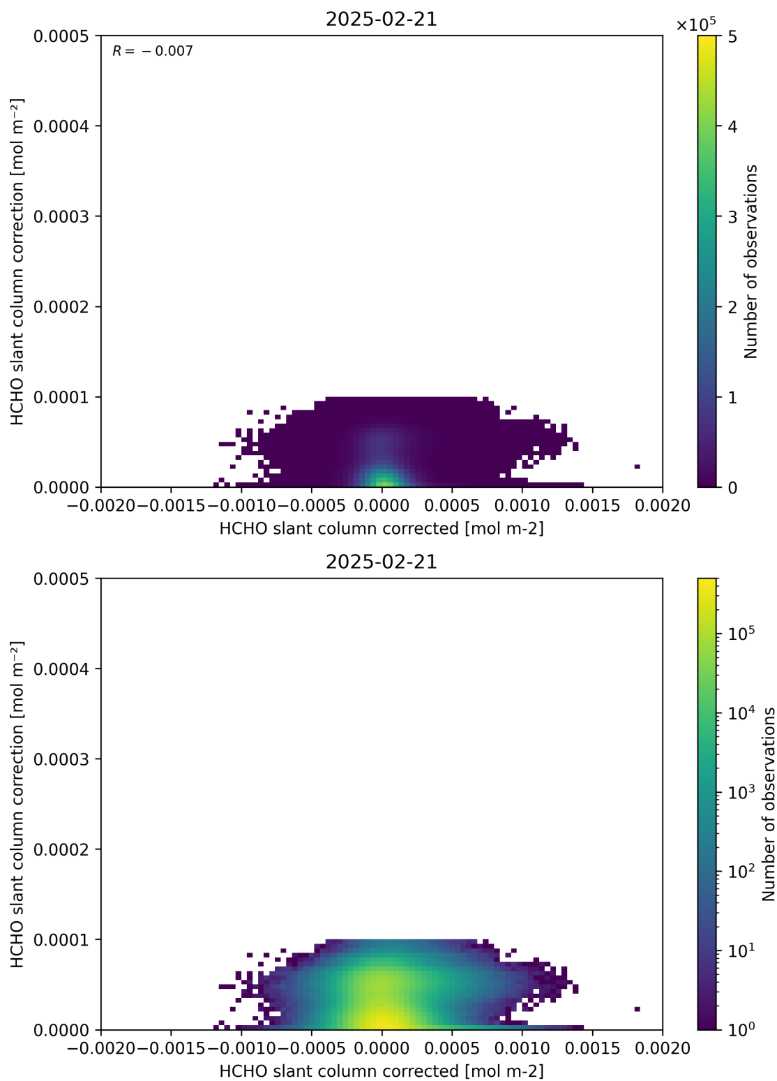
Figure 77: Scatter density plot of “HCHO slant column corrected” against “HCHO slant column correction” for 2025-02-20 to 2025-02-22.
