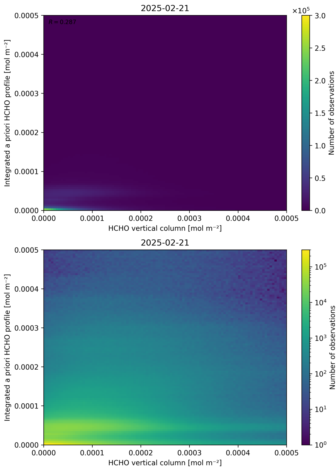
Figure 135: Scatter density plot of “HCHO vertical column” against “Integrated a priori HCHO profile” for 2025-02-20 to 2025-02-22.
