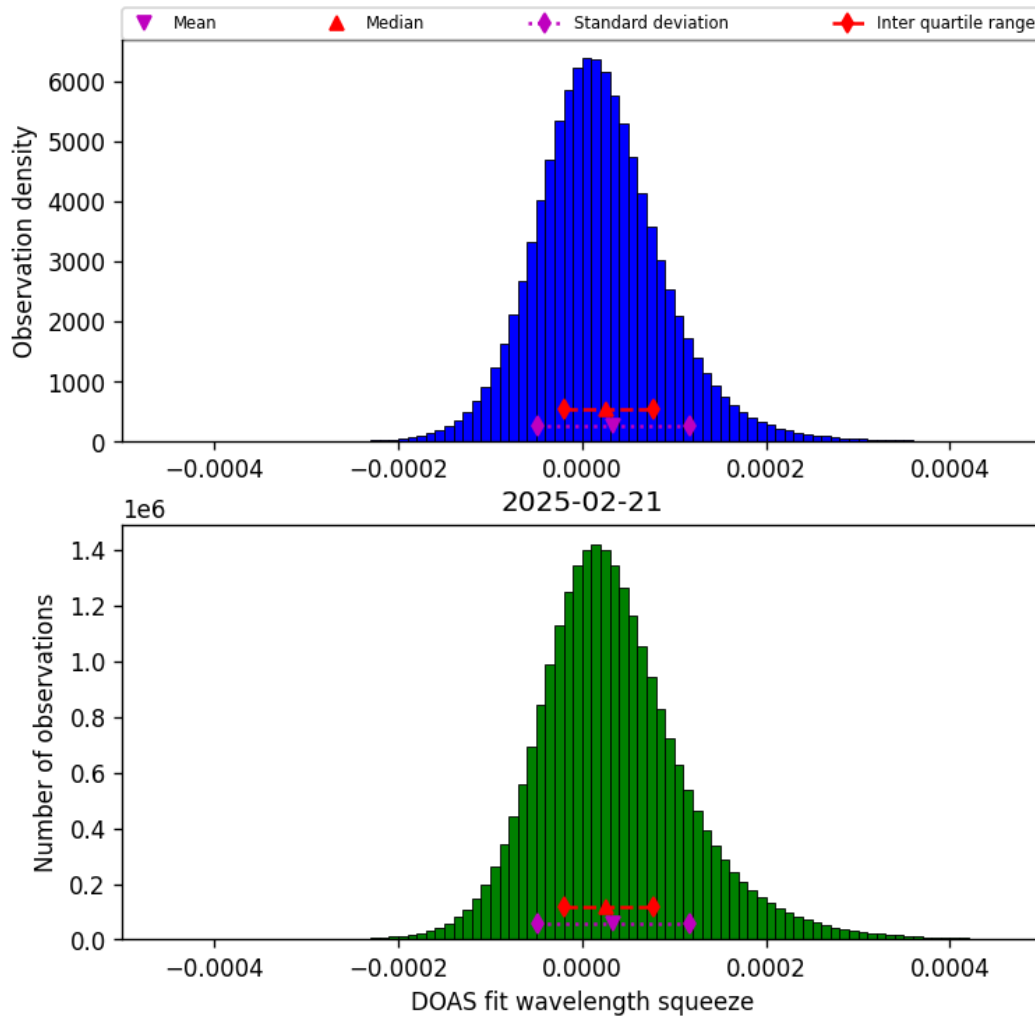
Figure 45: Histogram of “DOAS fit wavelength squeeze” for 2025-02-20 to 2025-02-22
