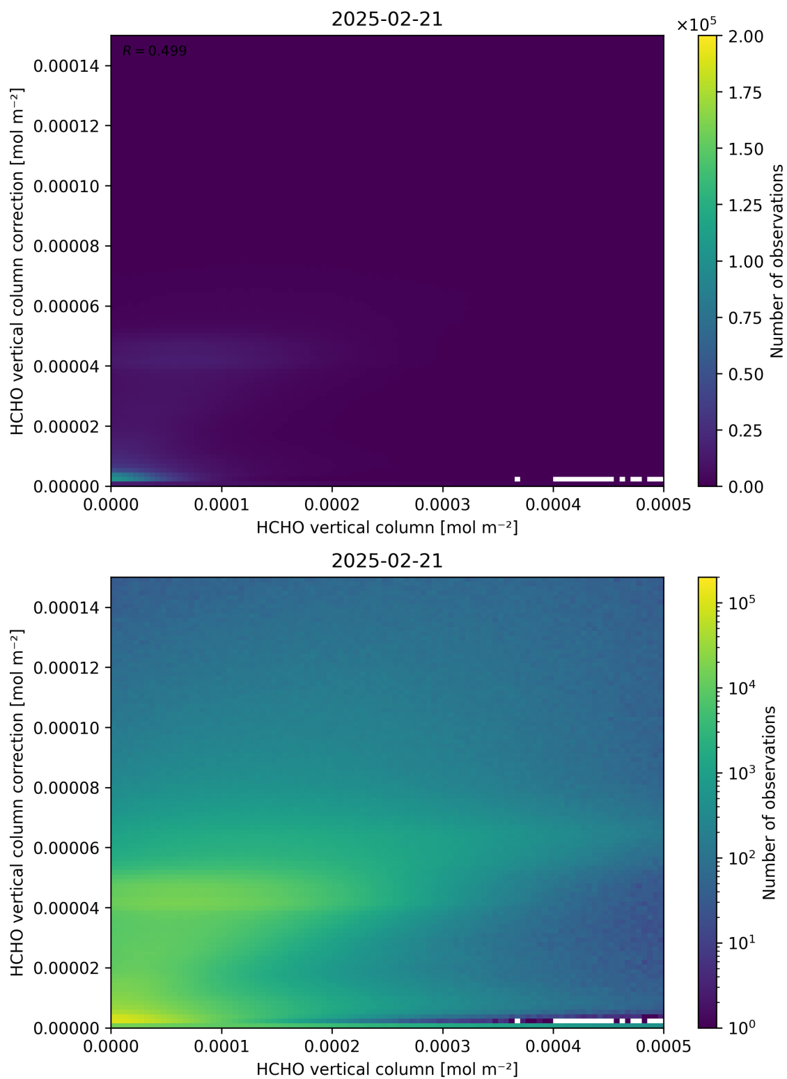
Figure 133: Scatter density plot of “HCHO vertical column” against “HCHO vertical column correction” for 2025-02-20 to 2025-02-22.
