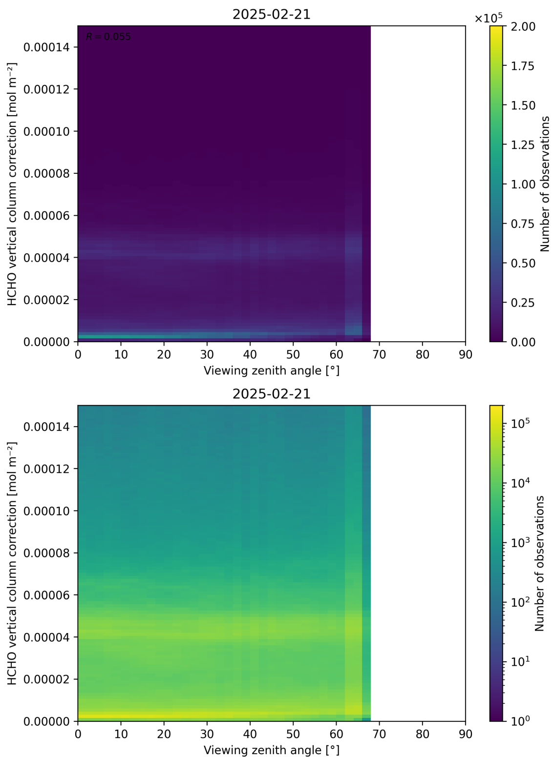
Figure 193: Scatter density plot of “Viewing zenith angle” against “HCHO vertical column correction” for 2025-02-20 to 2025-02-22.
