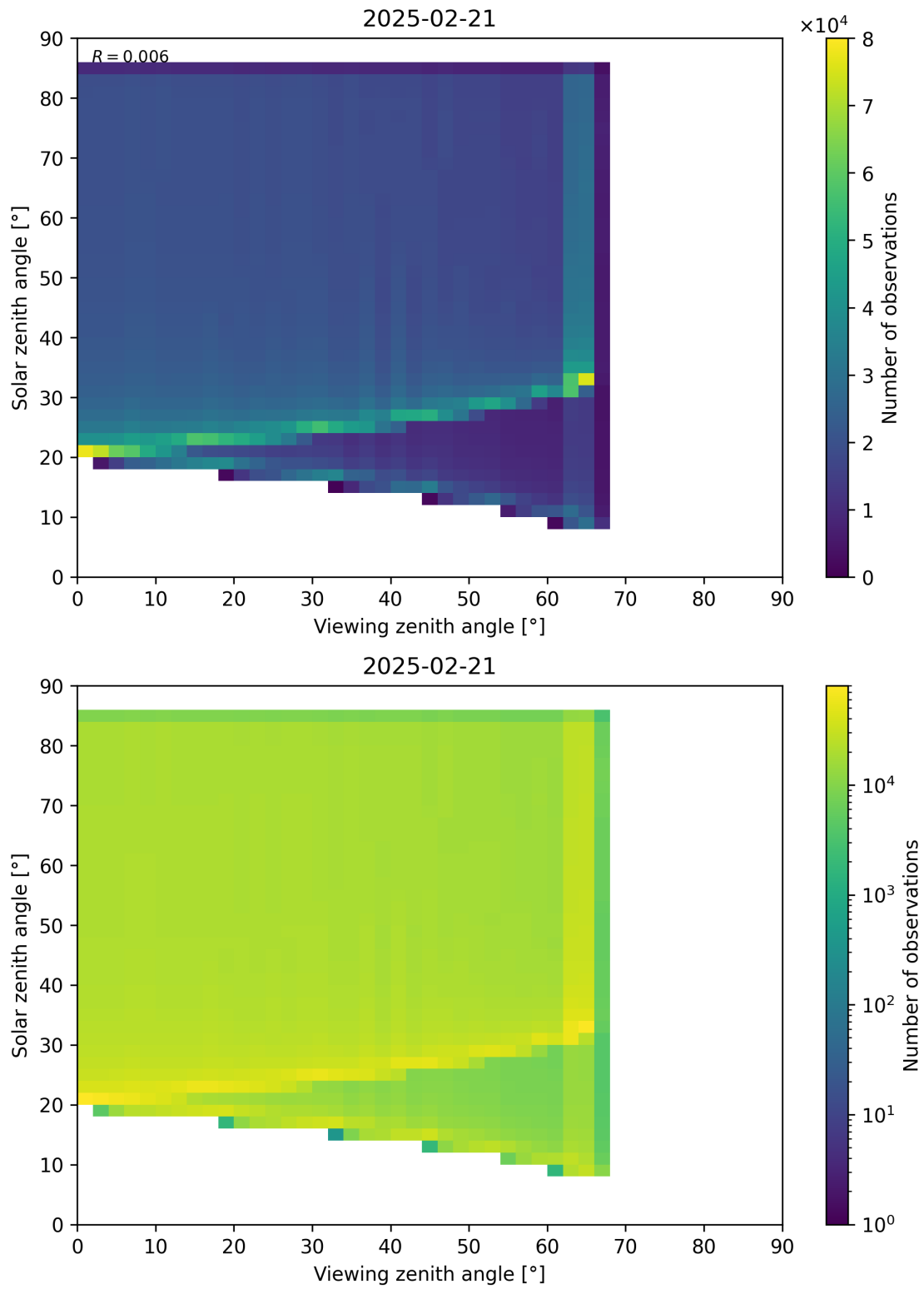
Figure 197: Scatter density plot of “Viewing zenith angle” against “Solar zenith angle” for 2025-02-20 to 2025-02-22.
