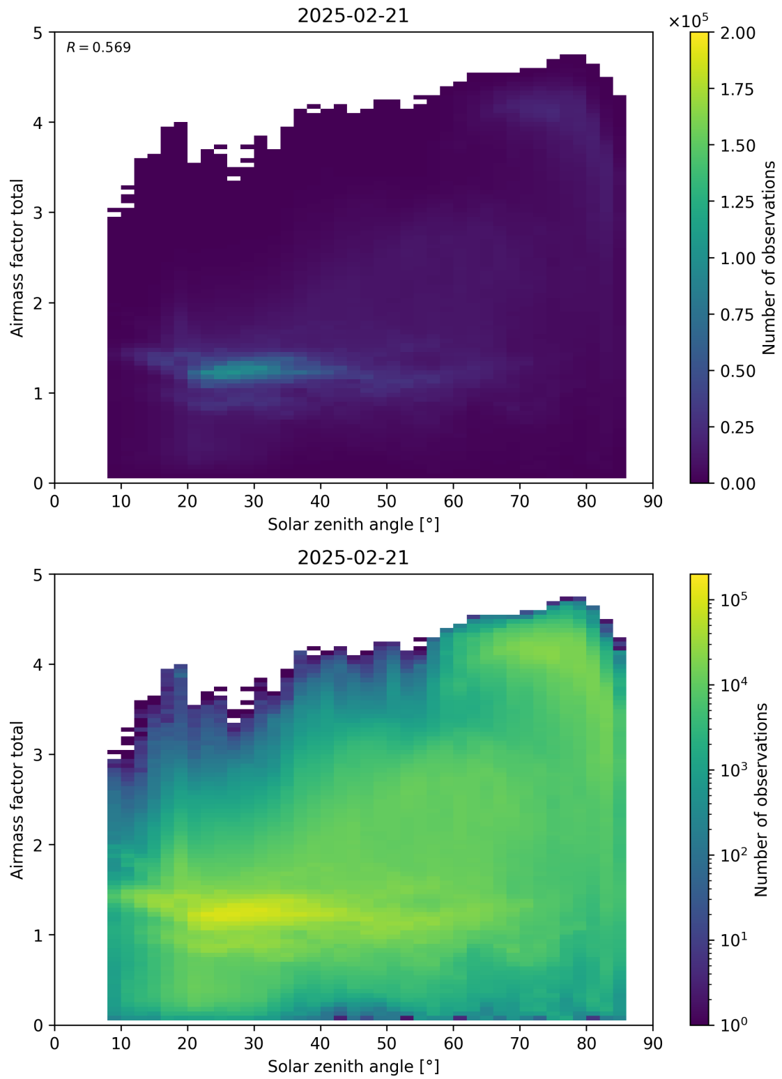
Figure 175: Scatter density plot of “Solar zenith angle” against “Airmass factor total” for 2025-02-20 to 2025-02-22.
