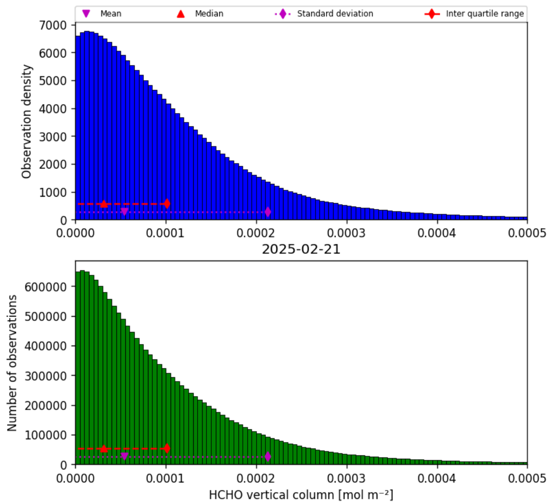
Figure 35: Histogram of “HCHO vertical column” for 2025-02-20 to 2025-02-22
