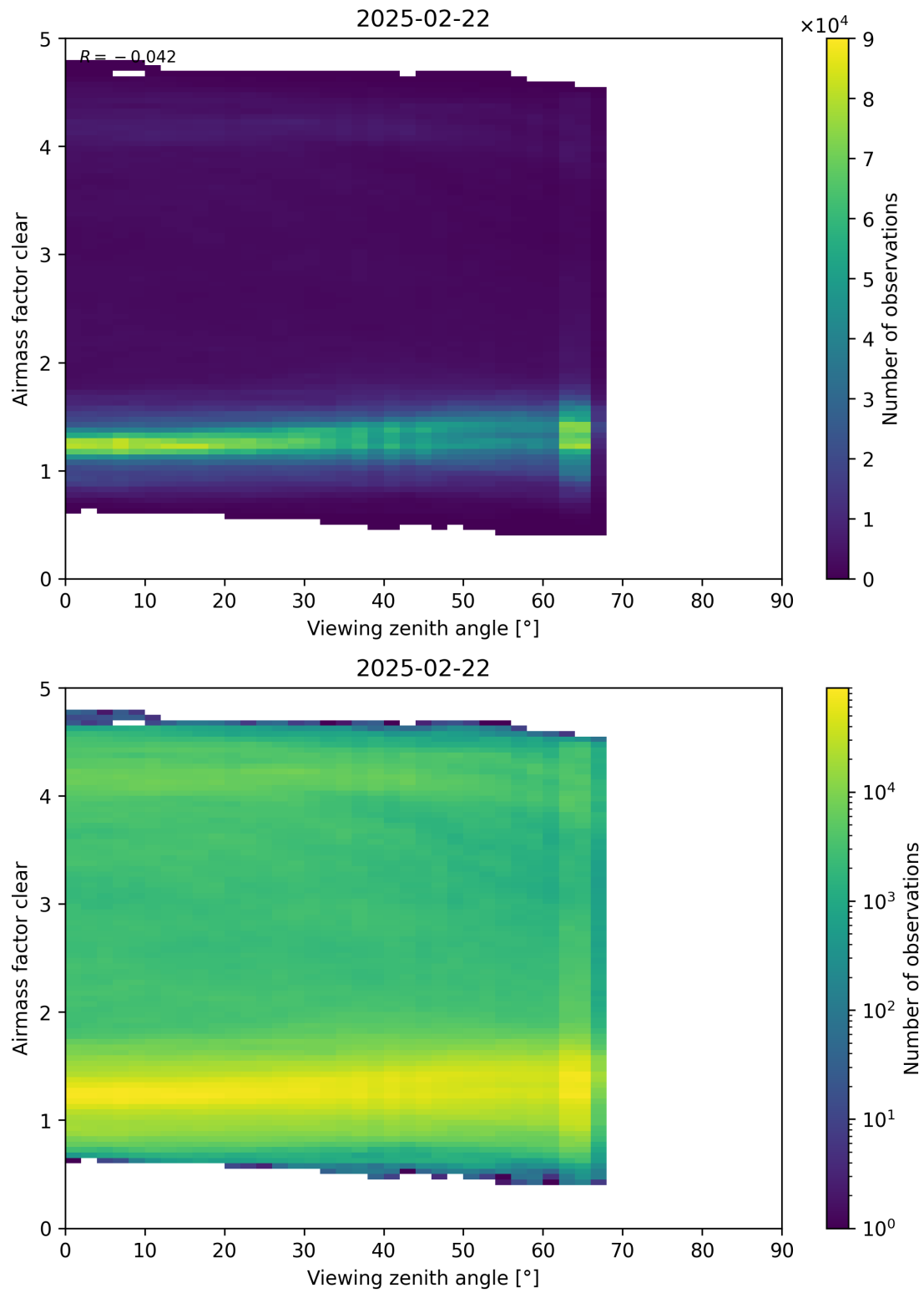
Figure 185: Scatter density plot of “Viewing zenith angle” against “Airmass factor clear” for 2025-02-21 to 2025-02-23.
