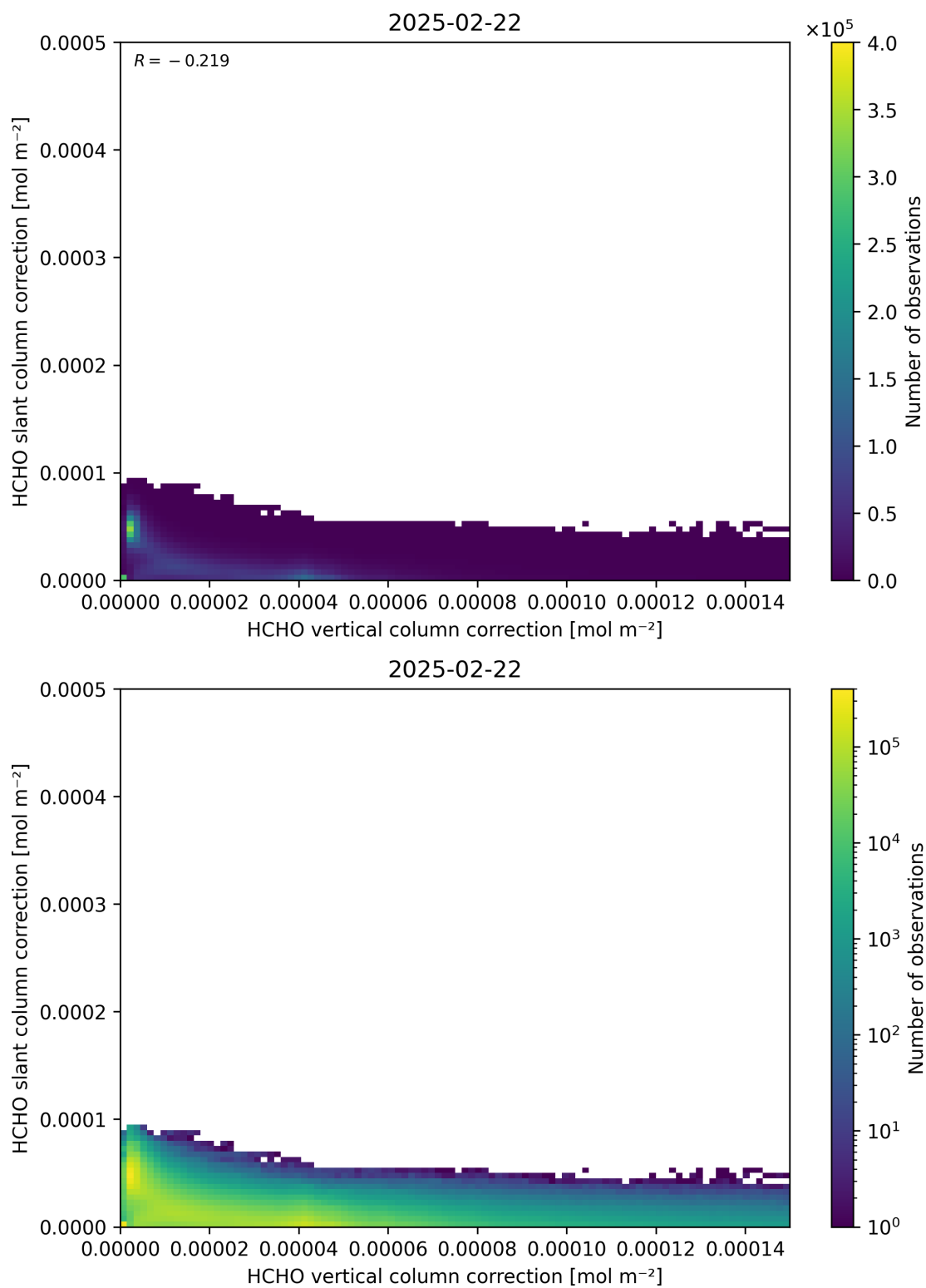
Figure 117: Scatter density plot of “HCHO vertical column correction” against “HCHO slant column correction” for 2025-02-21 to 2025-02-23.
