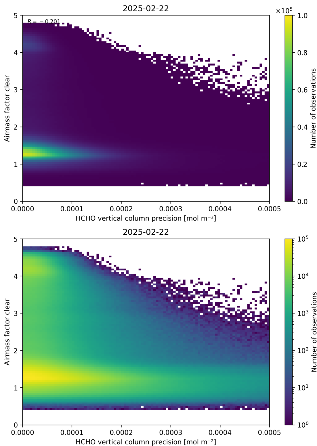
Figure 139: Scatter density plot of “HCHO vertical column precision” against “Airmass factor clear” for 2025-02-21 to 2025-02-23.
