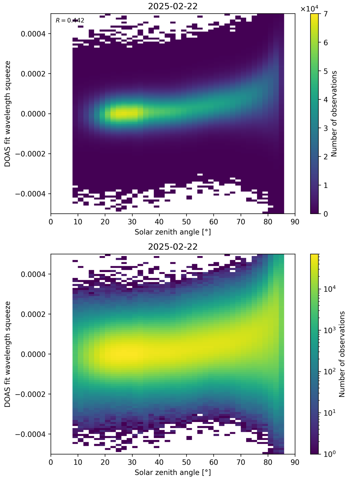
Figure 169: Scatter density plot of “Solar zenith angle” against “DOAS fit wavelength squeeze” for 2025-02-21 to 2025-02-23.
