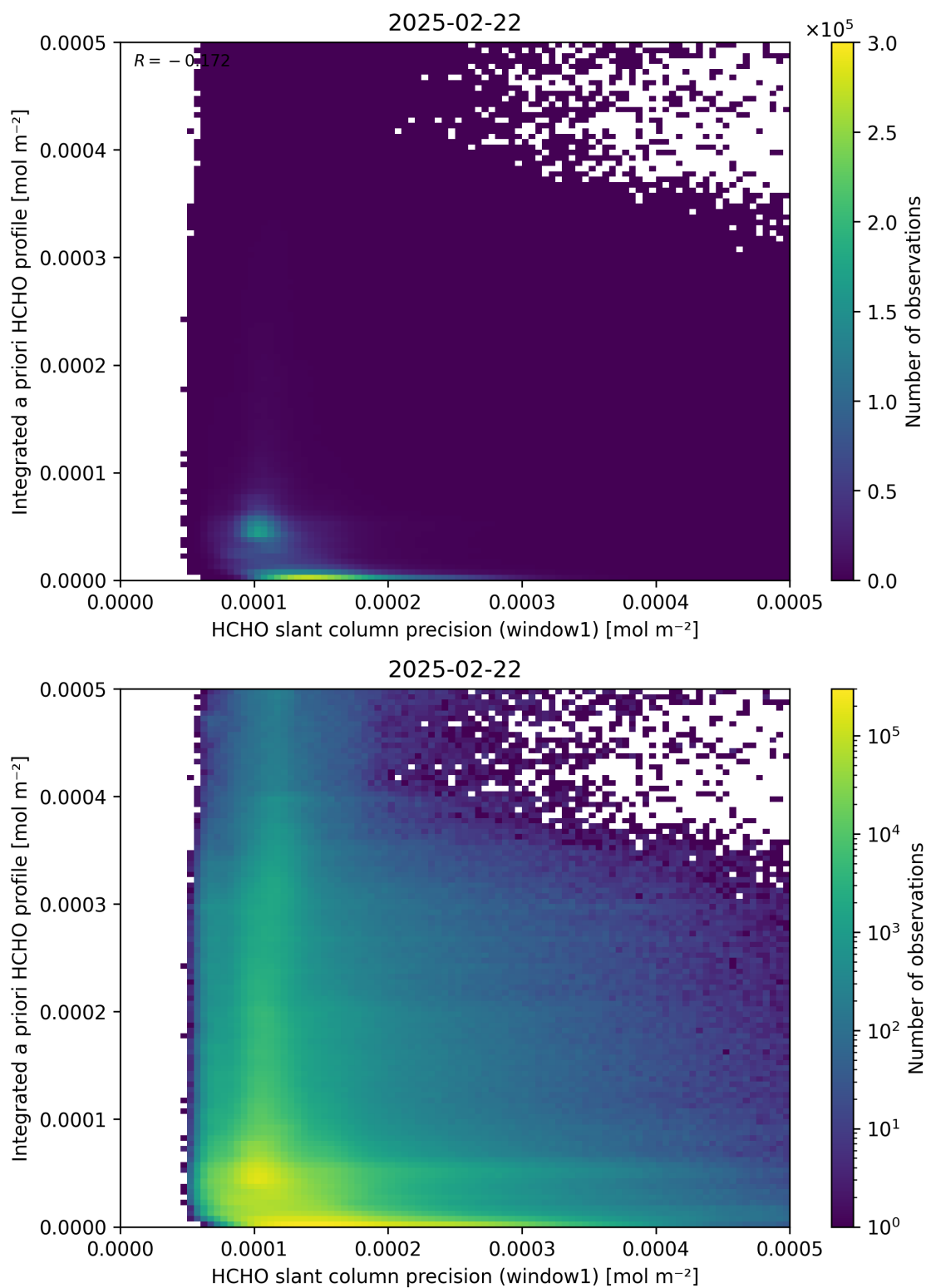
Figure 96: Scatter density plot of “HCHO slant column precision (window1)” against “Integrated a priori HCHO profile” for 2025-02-21 to 2025-02-23.
