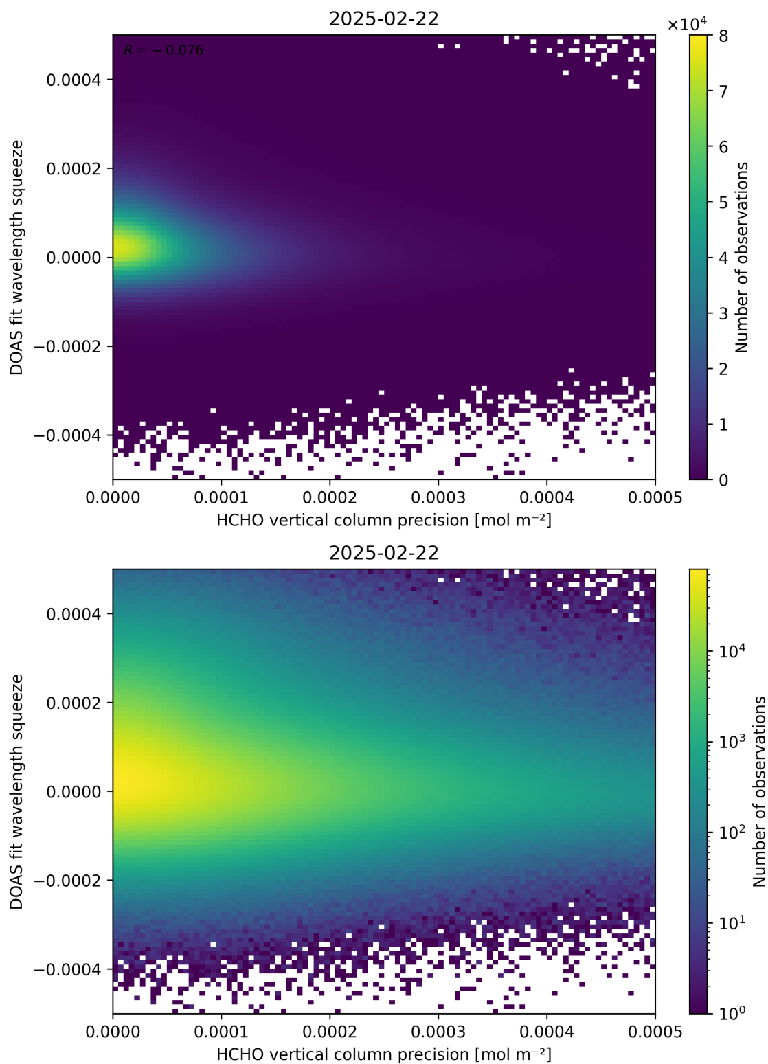
Figure 138: Scatter density plot of “HCHO vertical column precision” against “DOAS fit wavelength squeeze” for 2025-02-21 to 2025-02-23.
