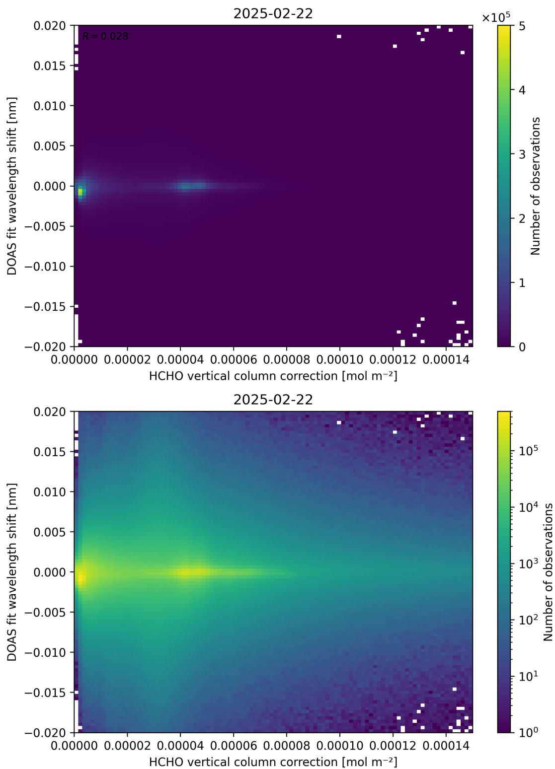
Figure 113: Scatter density plot of “HCHO vertical column correction” against “DOAS fit wavelength shift” for 2025-02-21 to 2025-02-23.
