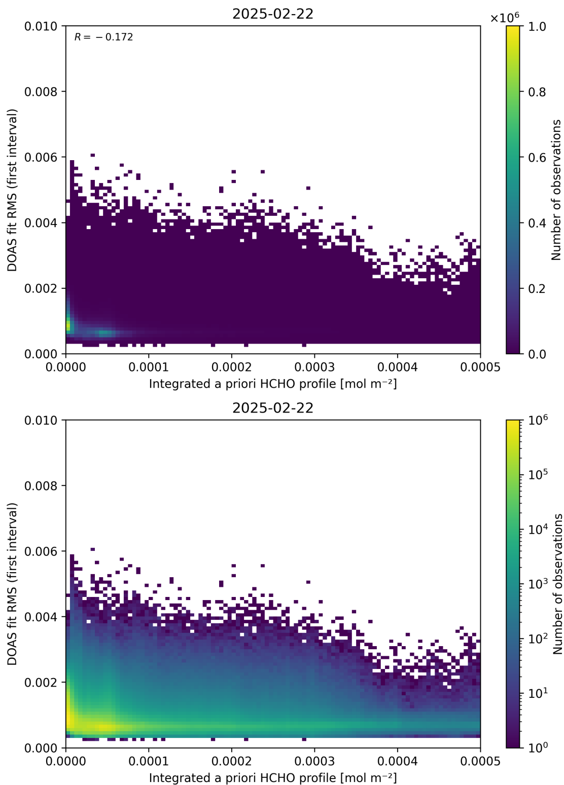
Figure 148: Scatter density plot of “Integrated a priori HCHO profile” against “DOAS fit RMS (first interval)” for 2025-02-21 to 2025-02-23.
