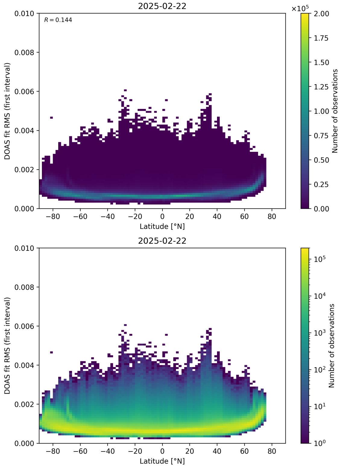
Figure 153: Scatter density plot of “Latitude” against “DOAS fit RMS (first interval)” for 2025-02-21 to 2025-02-23.
