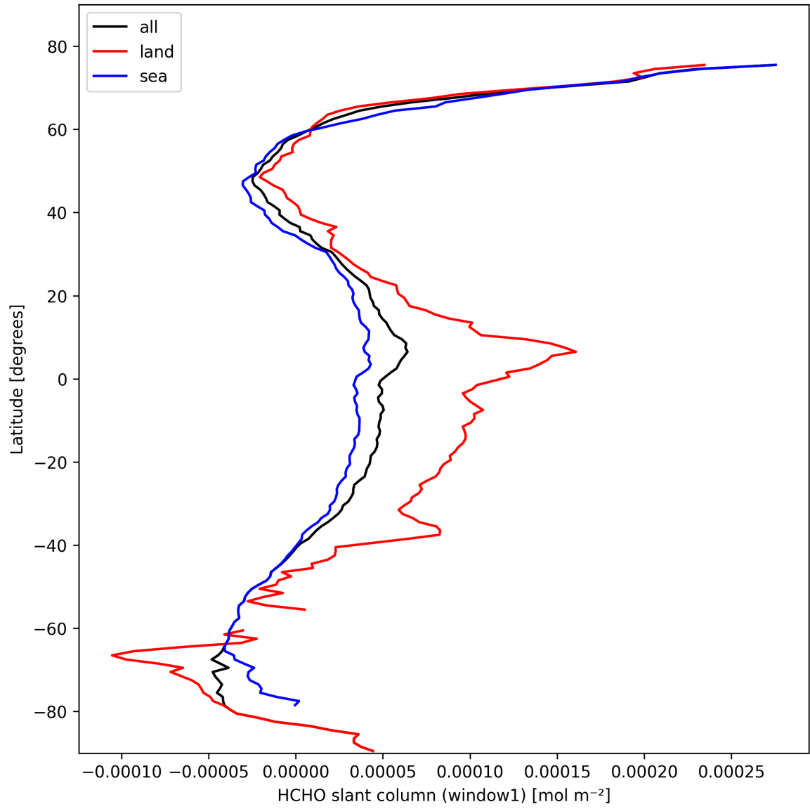
Figure 24: Zonal average of “HCHO slant column (window1)” for 2025-02-21 to 2025-02-23.
