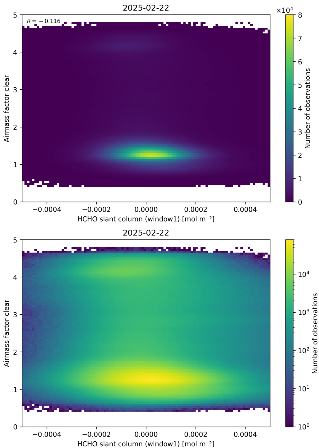
Figure 81: Scatter density plot of “HCHO slant column (window1)” against “Airmass factor clear” for 2025-02-21 to 2025-02-23.
