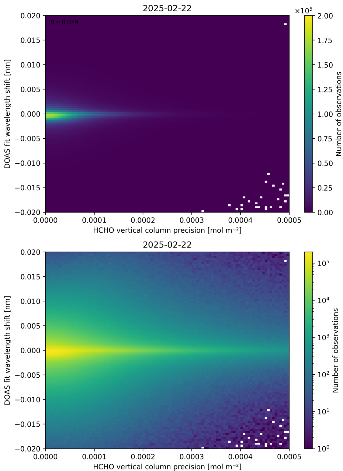
Figure 137: Scatter density plot of “HCHO vertical column precision” against “DOAS fit wavelength shift” for 2025-02-21 to 2025-02-23.
