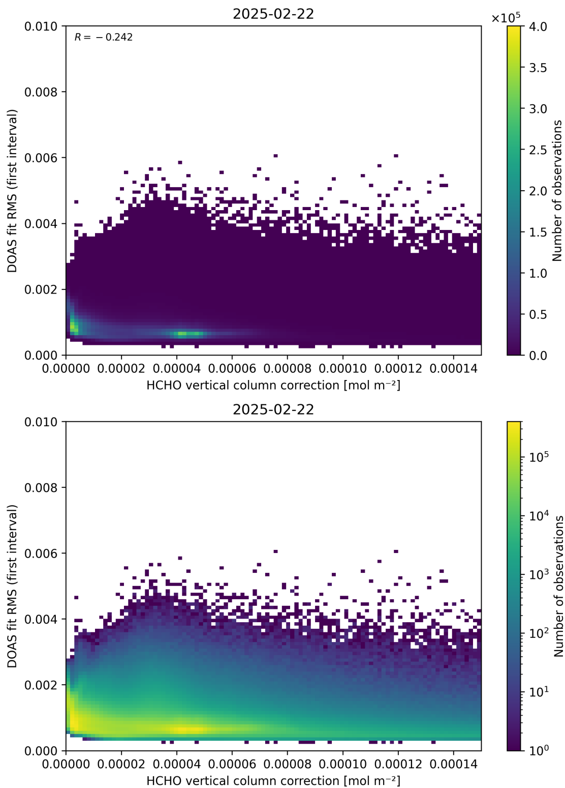
Figure 112: Scatter density plot of “HCHO vertical column correction” against “DOAS fit RMS (first interval)” for 2025-02-21 to 2025-02-23.
