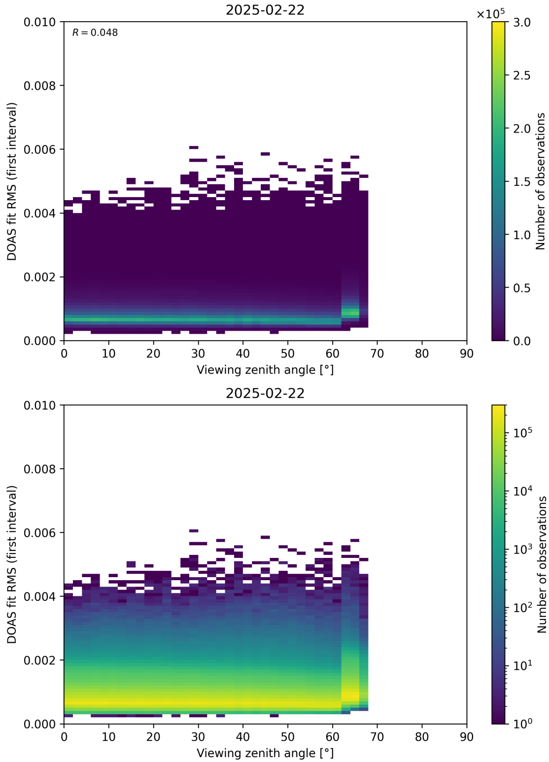
Figure 182: Scatter density plot of “Viewing zenith angle” against “DOAS fit RMS (first interval)” for 2025-02-21 to 2025-02-23.
