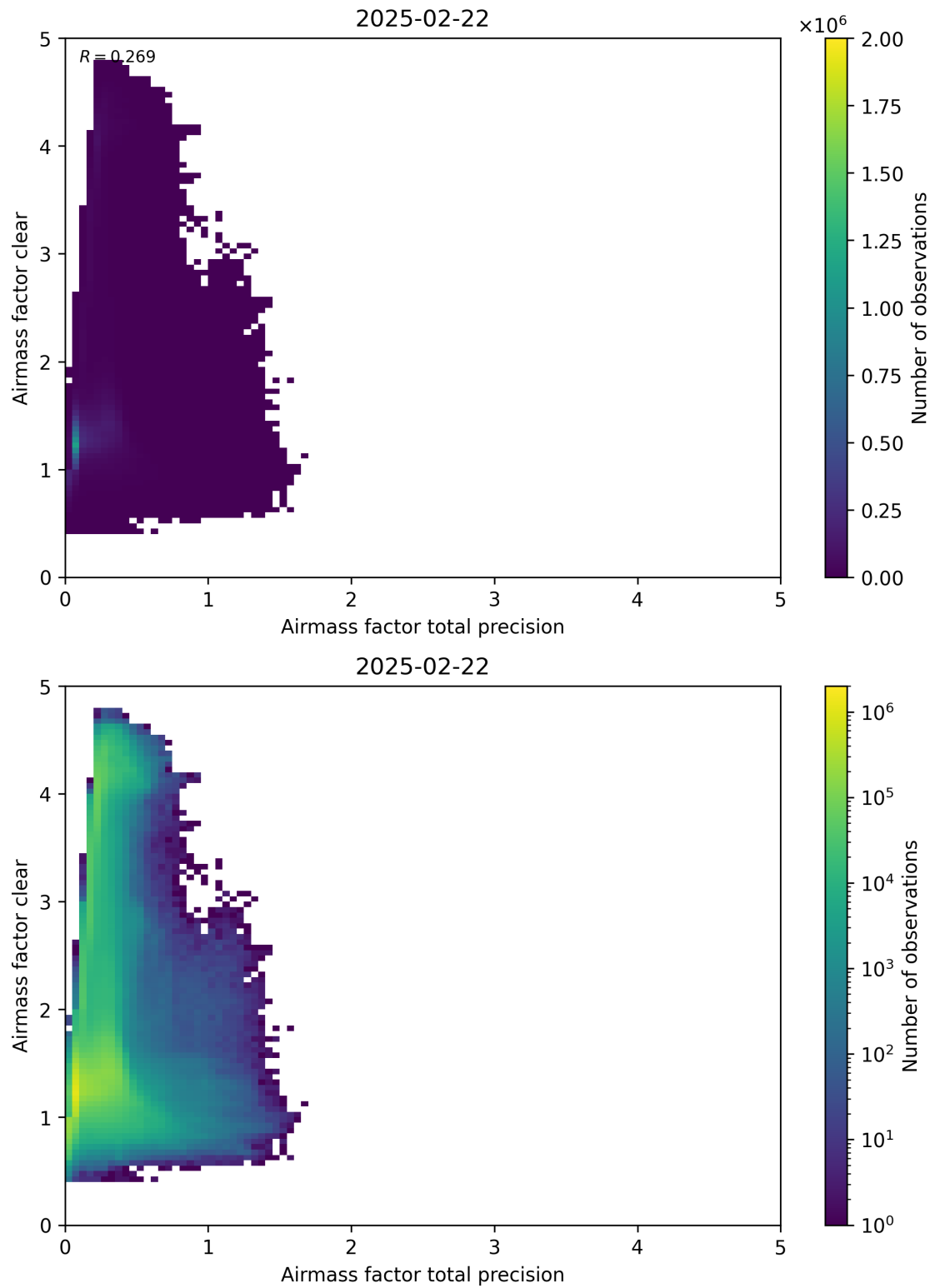
Figure 108: Scatter density plot of “Airmass factor total precision” against “Airmass factor clear” for 2025-02-21 to 2025-02-23.
