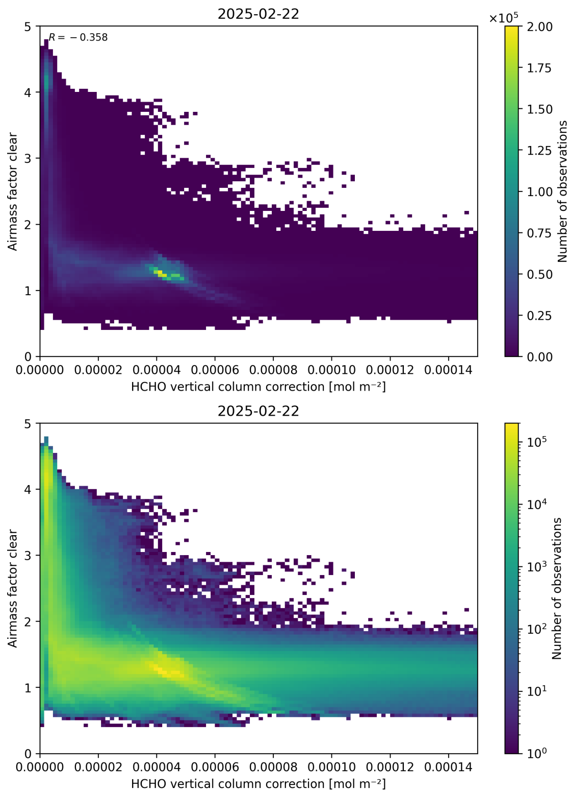
Figure 115: Scatter density plot of “HCHO vertical column correction” against “Airmass factor clear” for 2025-02-21 to 2025-02-23.
