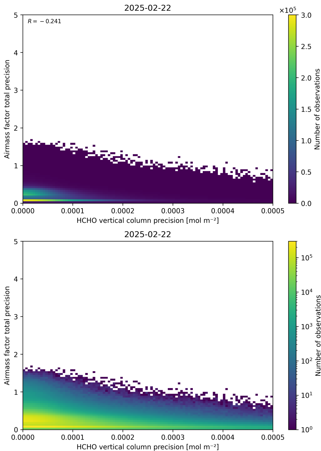
Figure 145: Scatter density plot of “HCHO vertical column precision” against “Airmass factor total precision” for 2025-02-21 to 2025-02-23.
