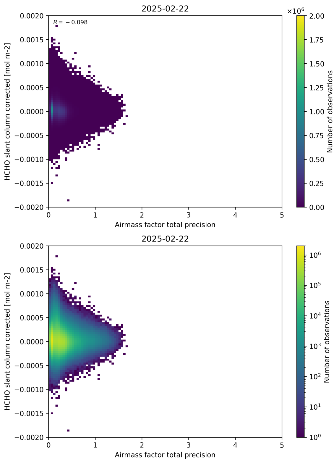
Figure 109: Scatter density plot of “Airmass factor total precision” against “HCHO slant column corrected” for 2025-02-21 to 2025-02-23.
