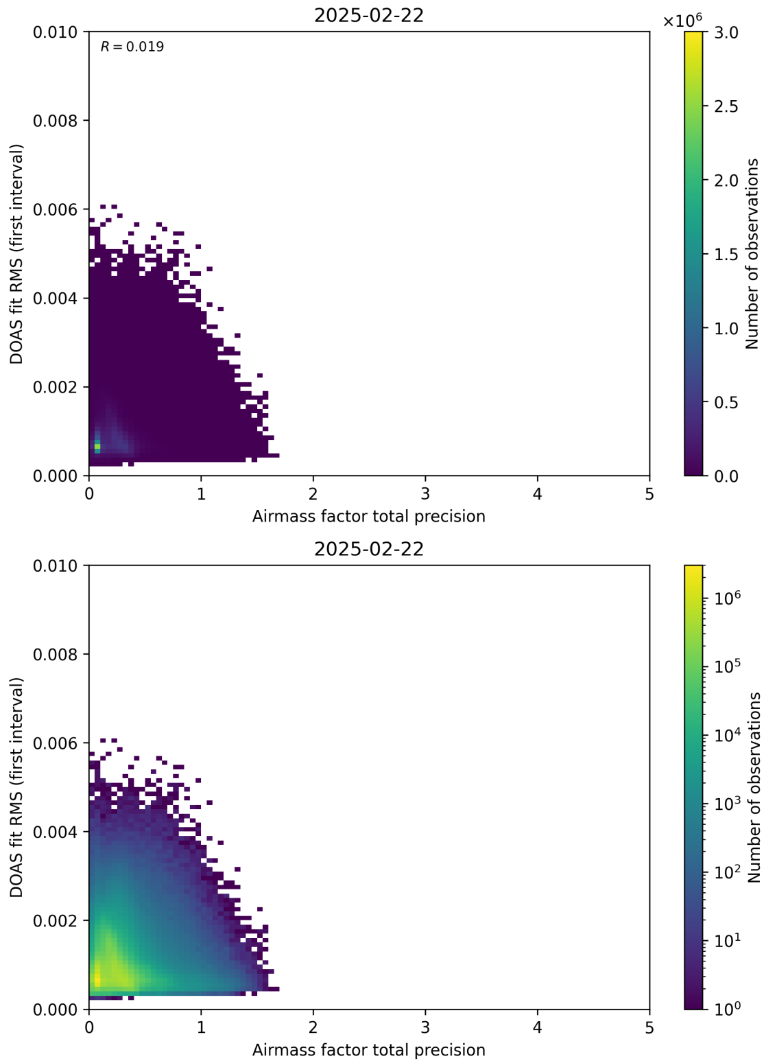
Figure 105: Scatter density plot of “Airmass factor total precision” against “DOAS fit RMS (first interval)” for 2025-02-21 to 2025-02-23.
