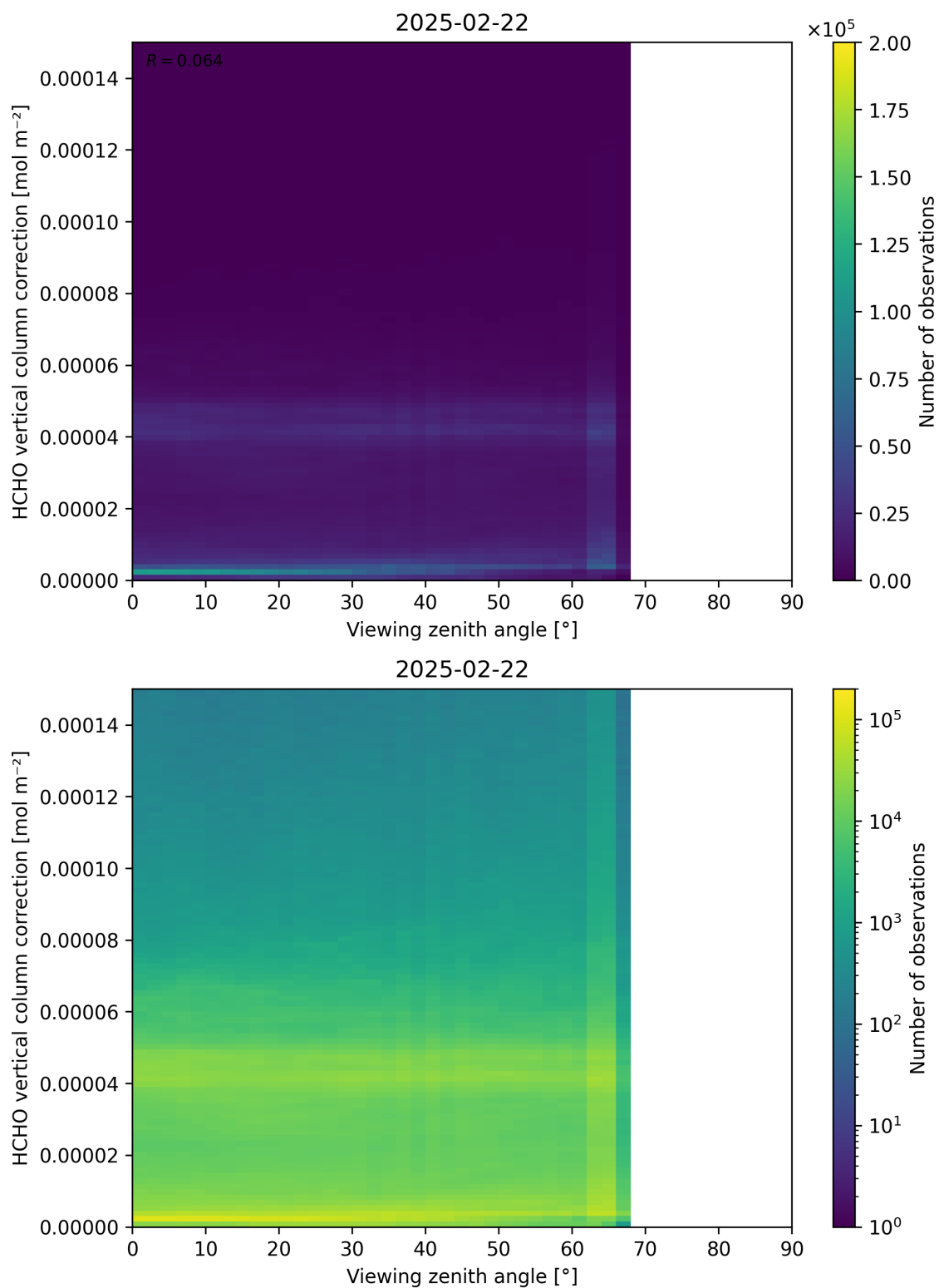
Figure 193: Scatter density plot of “Viewing zenith angle” against “HCHO vertical column correction” for 2025-02-21 to 2025-02-23.
