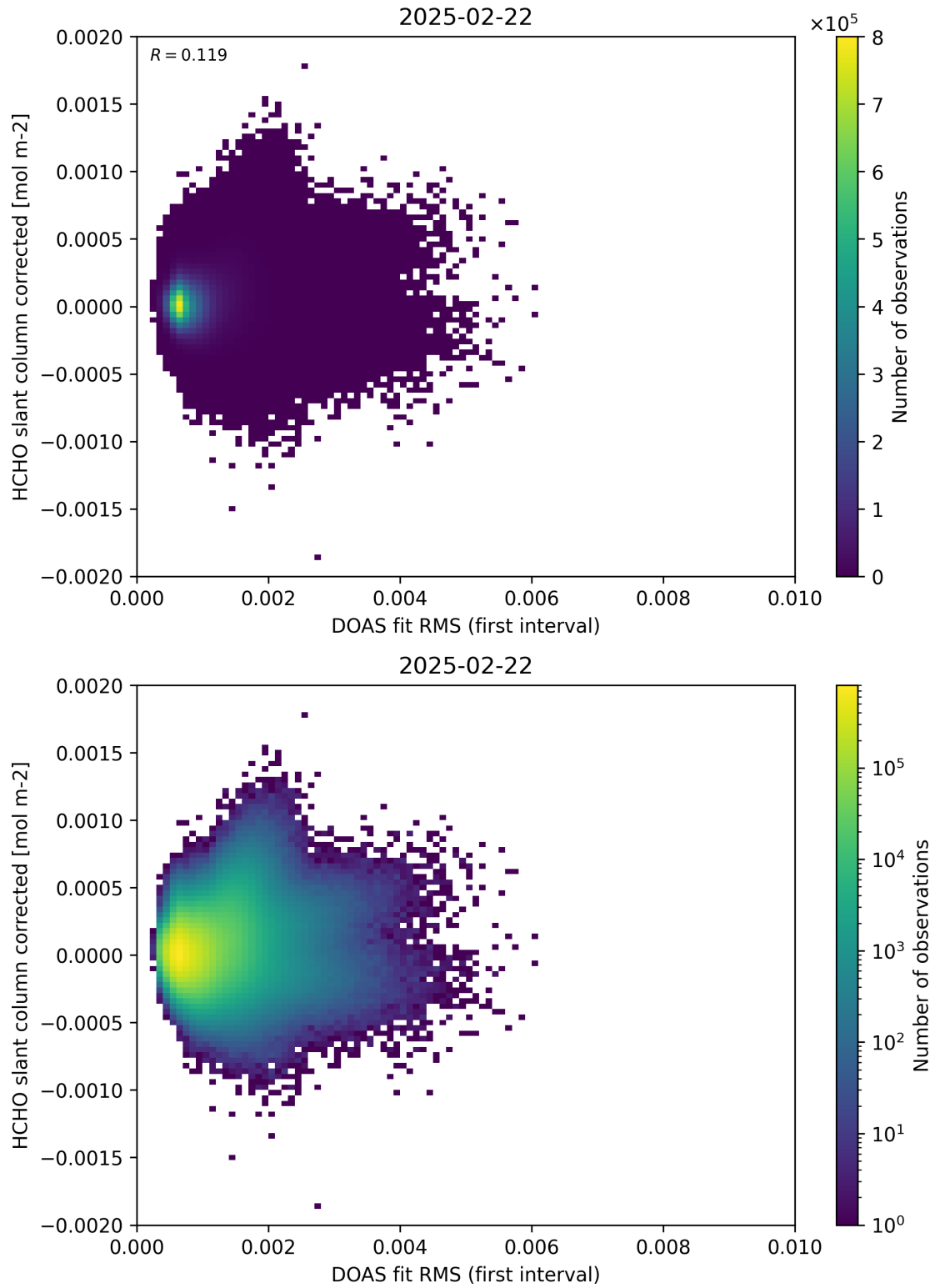
Figure 62: Scatter density plot of “DOAS fit RMS (first interval)” against “HCHO slant column corrected” for 2025-02-21 to 2025-02-23.
