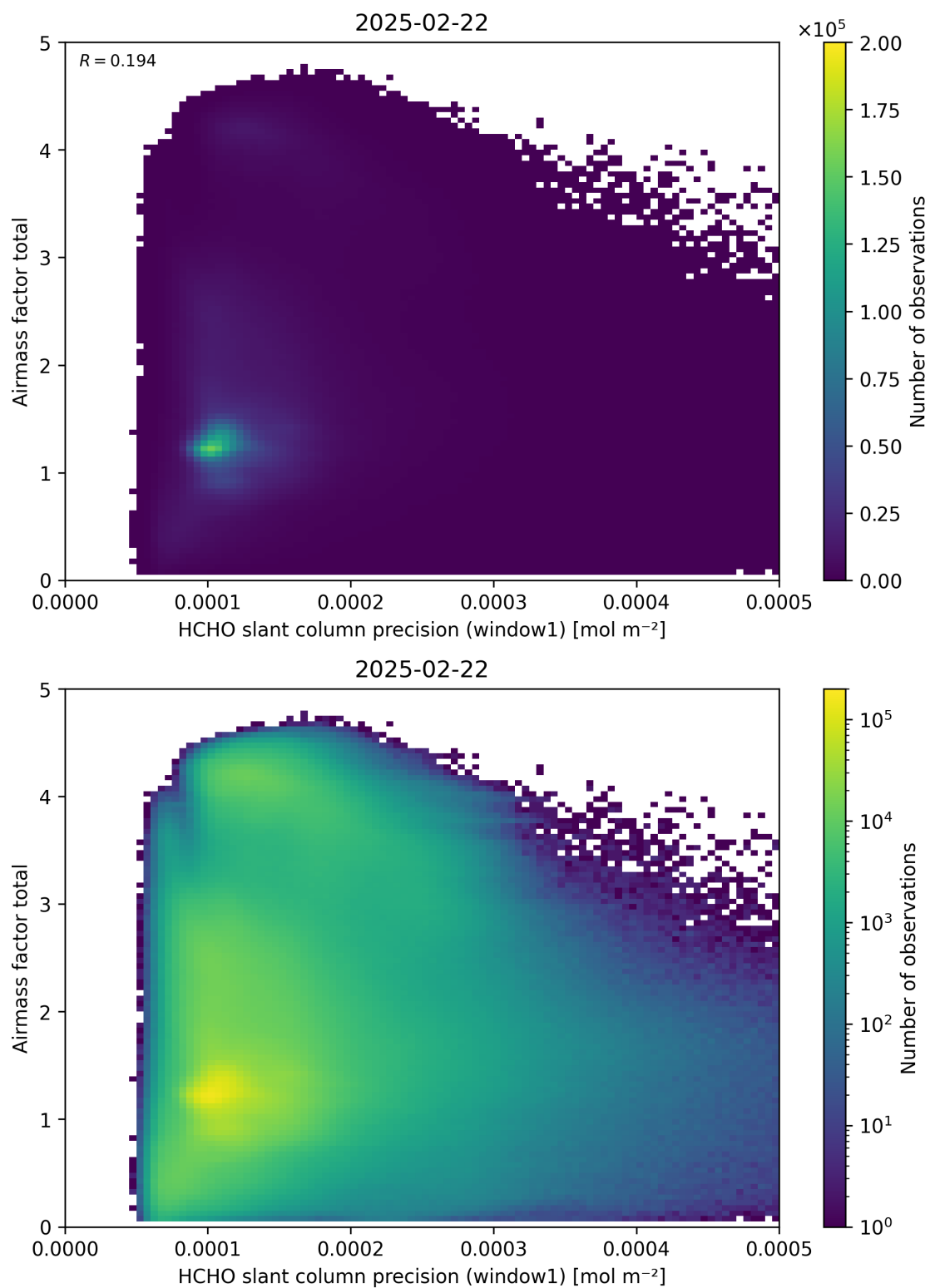
Figure 94: Scatter density plot of “HCHO slant column precision (window1)” against “Airmass factor total” for 2025-02-21 to 2025-02-23.
