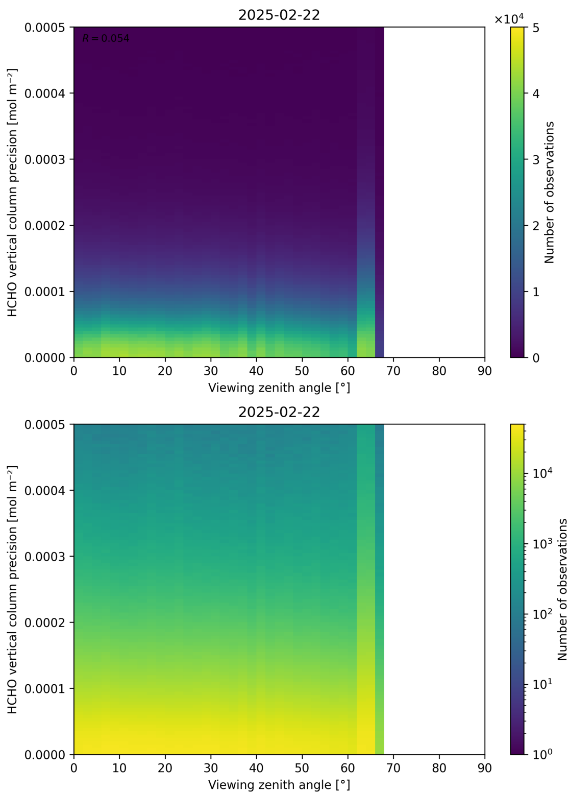
Figure 194: Scatter density plot of “Viewing zenith angle” against “HCHO vertical column precision” for 2025-02-21 to 2025-02-23.
