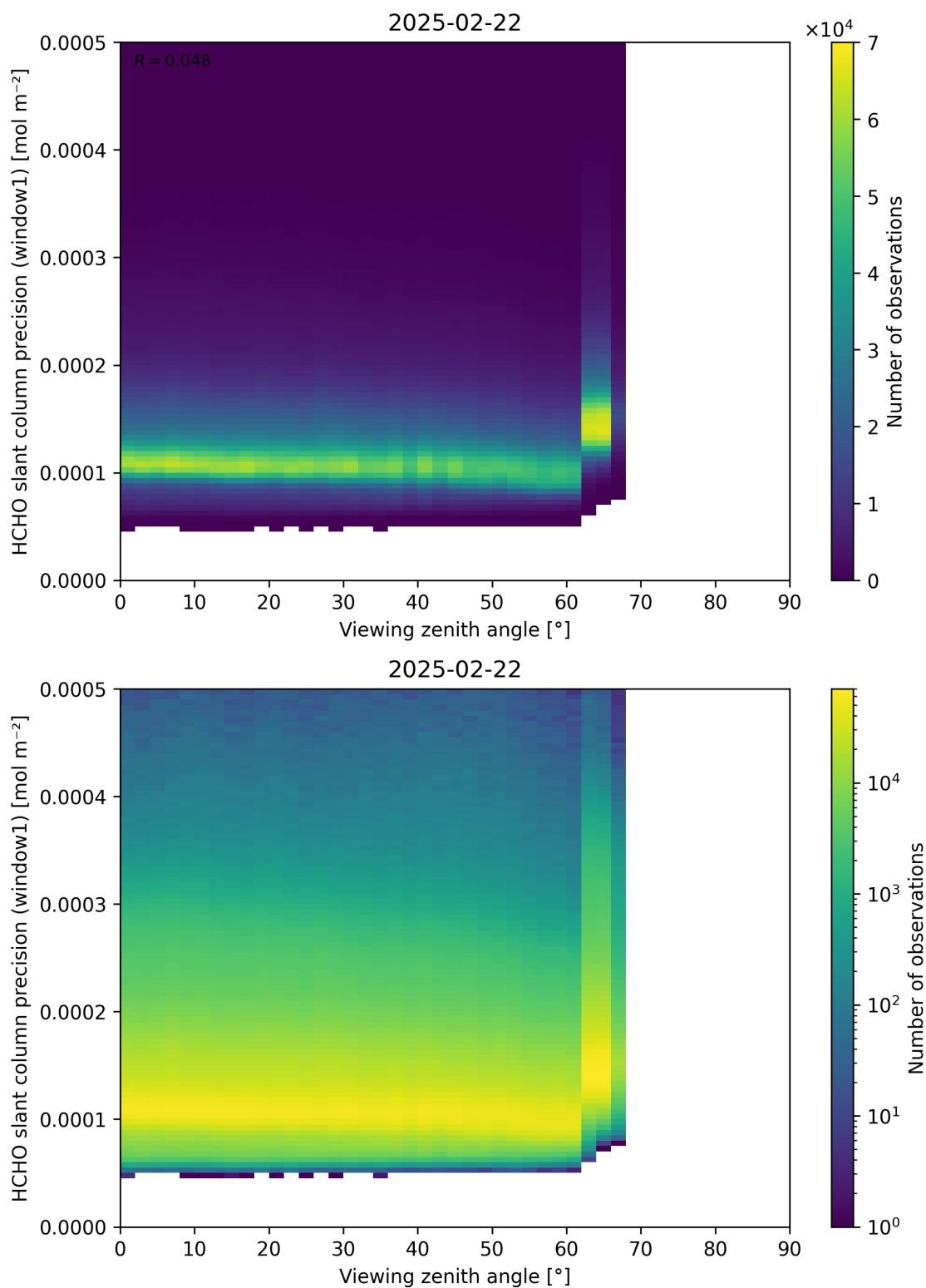
Figure 189: Scatter density plot of “Viewing zenith angle” against “HCHO slant column precision (window1)” for 2025-02-21 to 2025-02-23.
