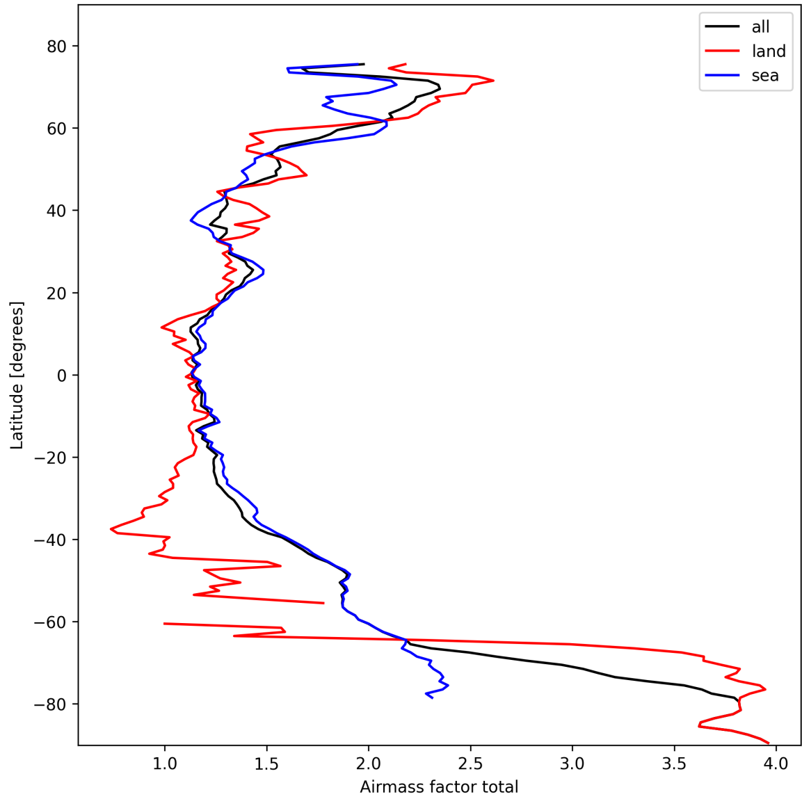
Figure 26: Zonal average of “Airmass factor total” for 2025-02-21 to 2025-02-23.
