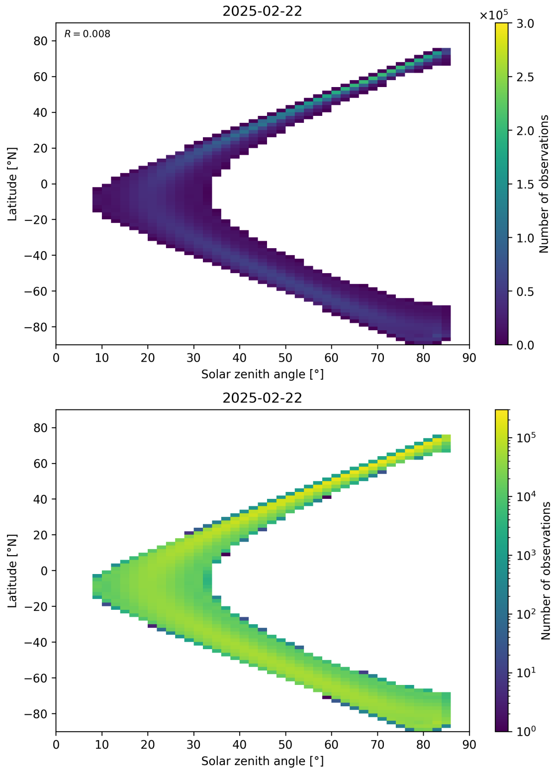
Figure 181: Scatter density plot of “Solar zenith angle” against “Latitude” for 2025-02-21 to 2025-02-23.
