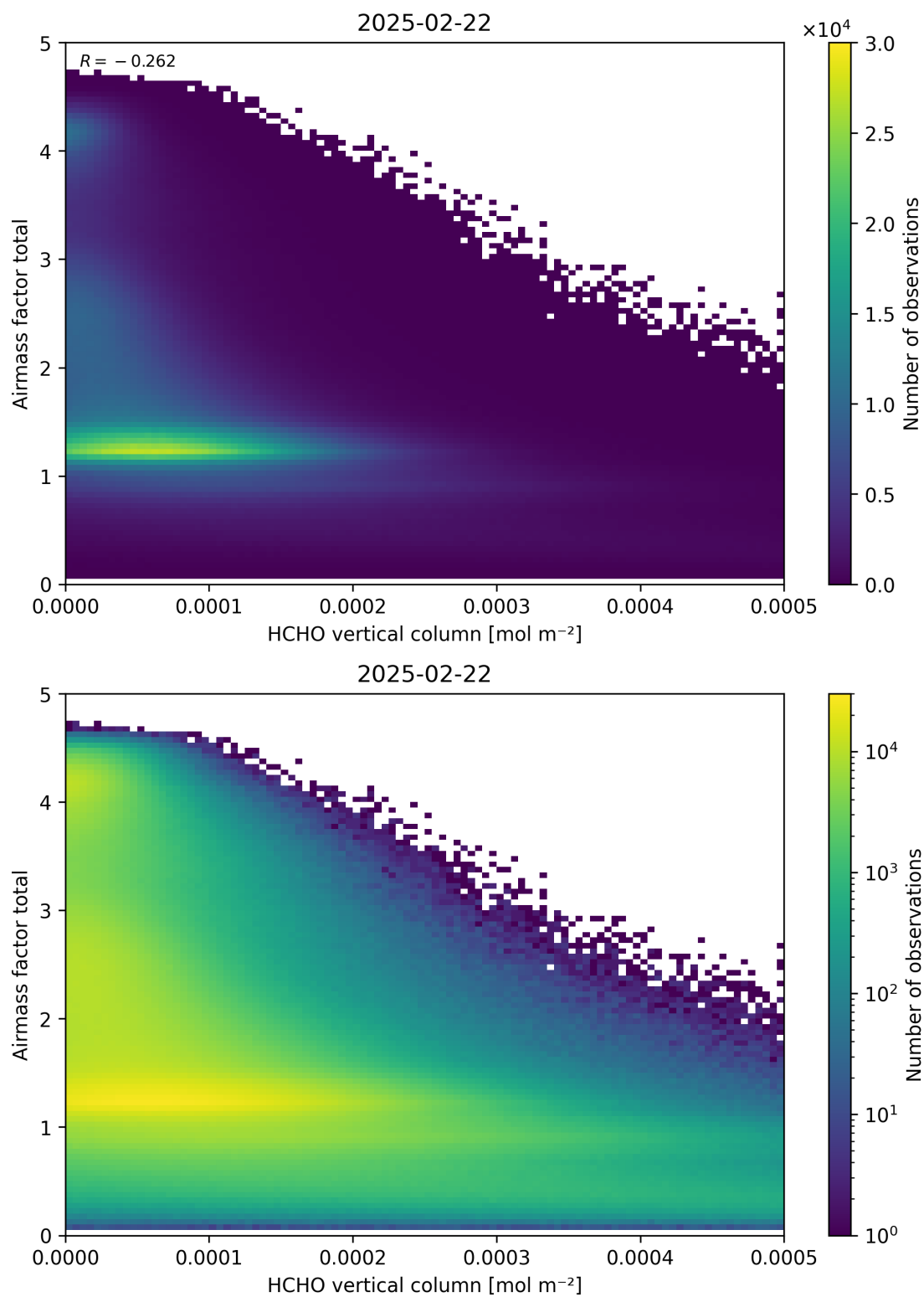
Figure 131: Scatter density plot of “HCHO vertical column” against “Airmass factor total” for 2025-02-21 to 2025-02-23.
