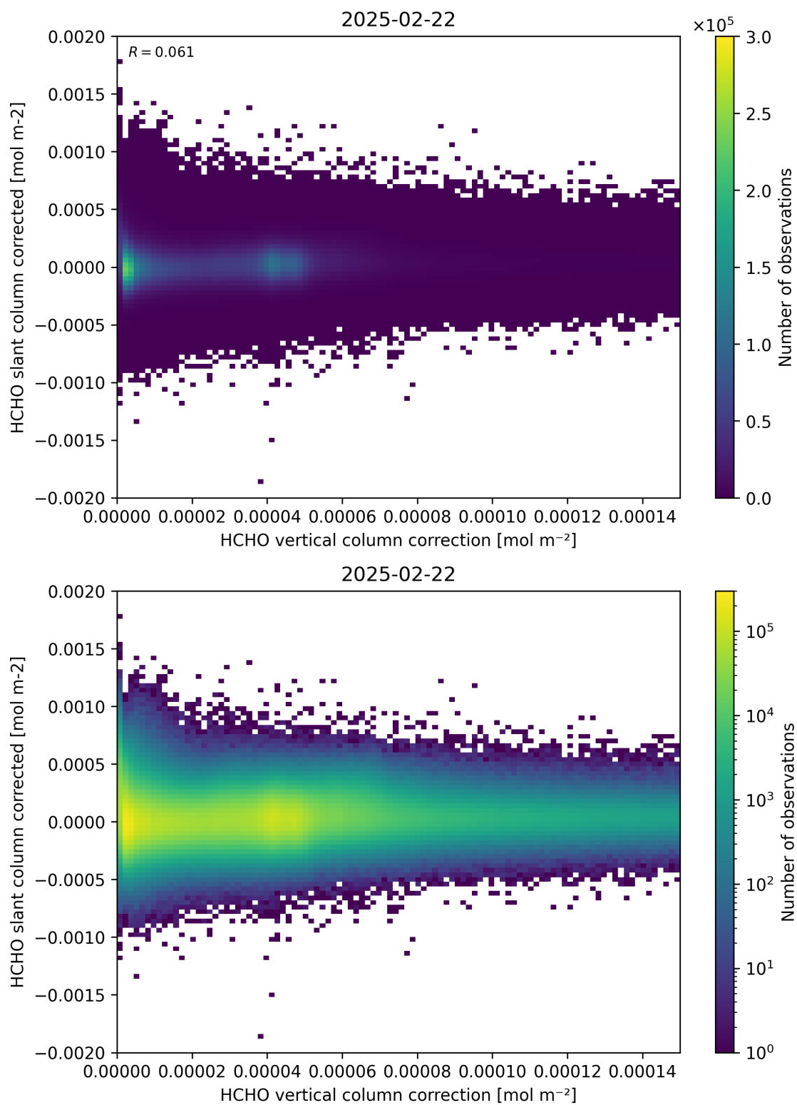
Figure 116: Scatter density plot of “HCHO vertical column correction” against “HCHO slant column corrected” for 2025-02-21 to 2025-02-23.
