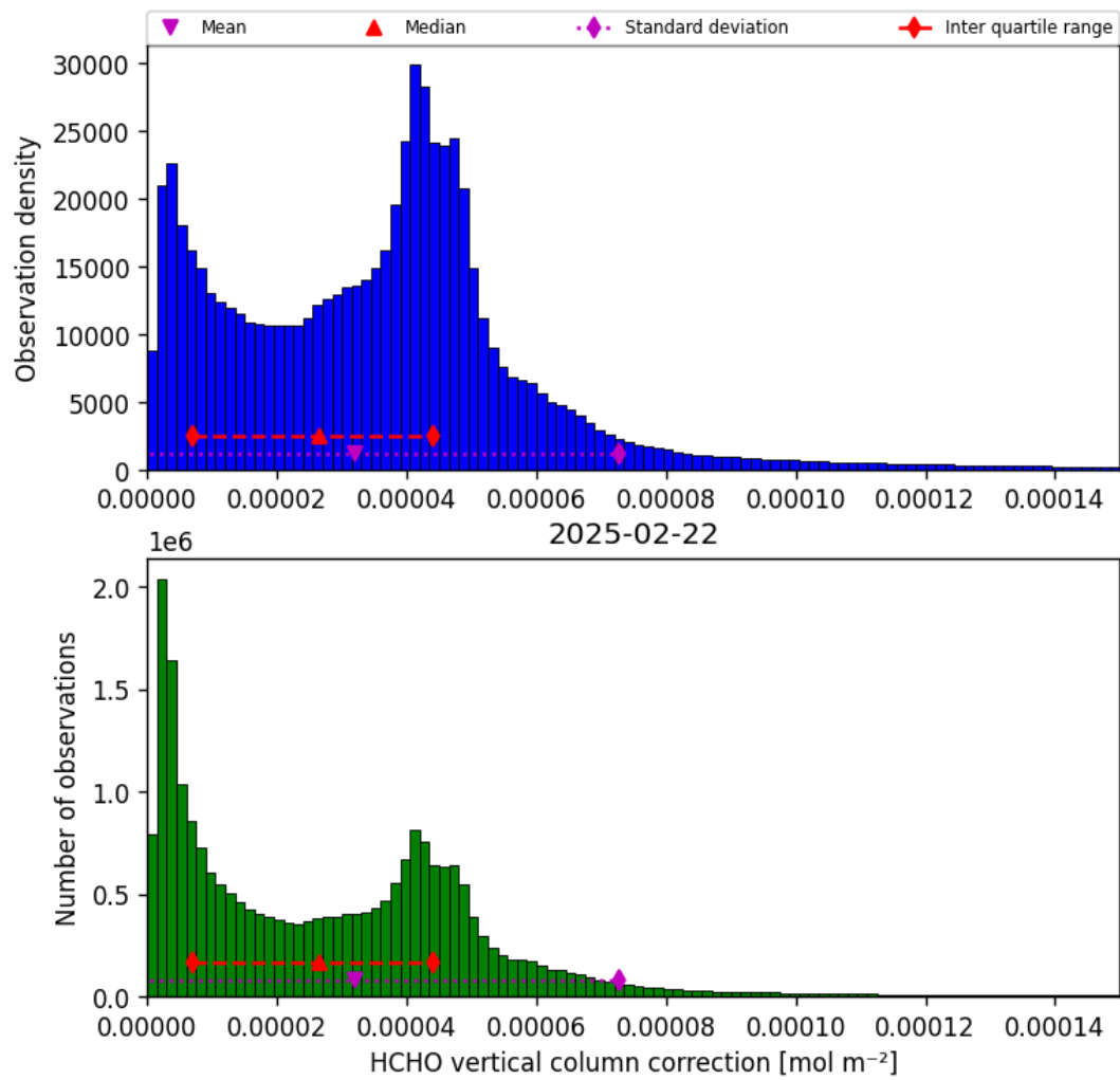
Figure 37: Histogram of “HCHO vertical column correction” for 2025-02-21 to 2025-02-23
