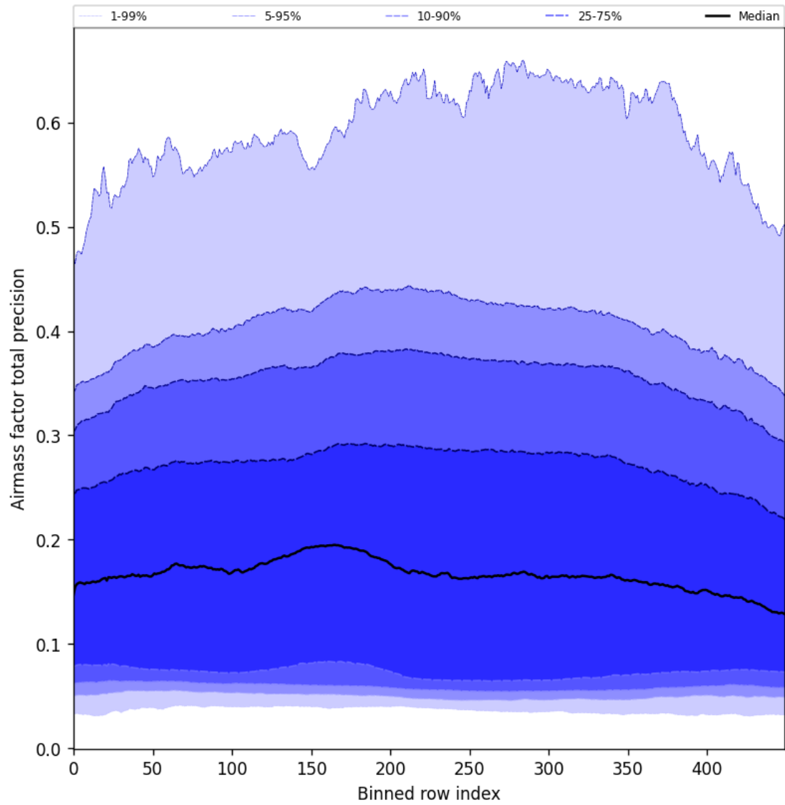
Figure 55: Along track statistics of “Airmass factor total precision” for 2025-02-21 to 2025-02-23
