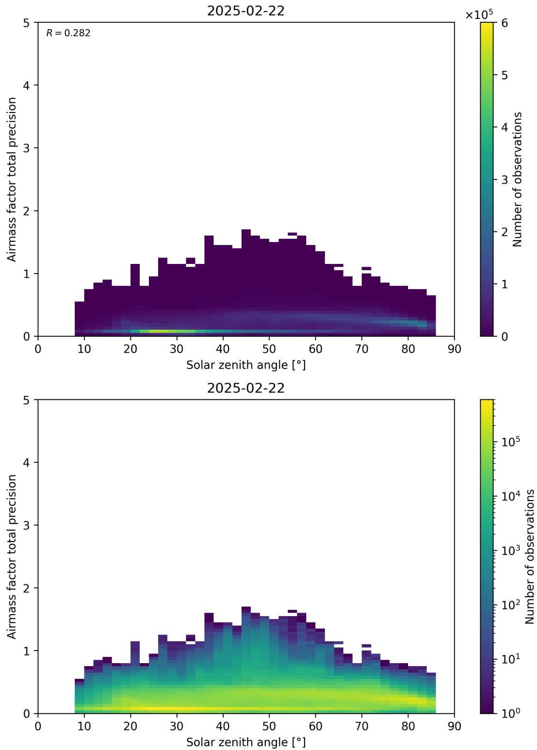
Figure 176: Scatter density plot of “Solar zenith angle” against “Airmass factor total precision” for 2025-02-21 to 2025-02-23.
