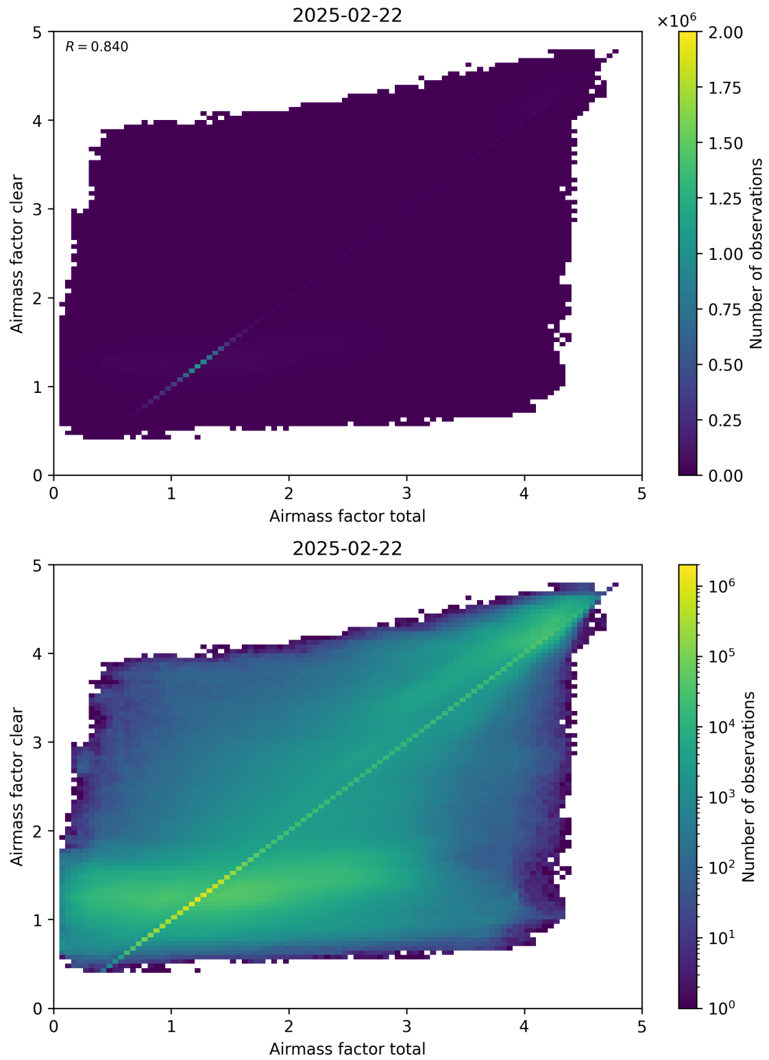
Figure 100: Scatter density plot of “Airmass factor total” against “Airmass factor clear” for 2025-02-21 to 2025-02-23.
