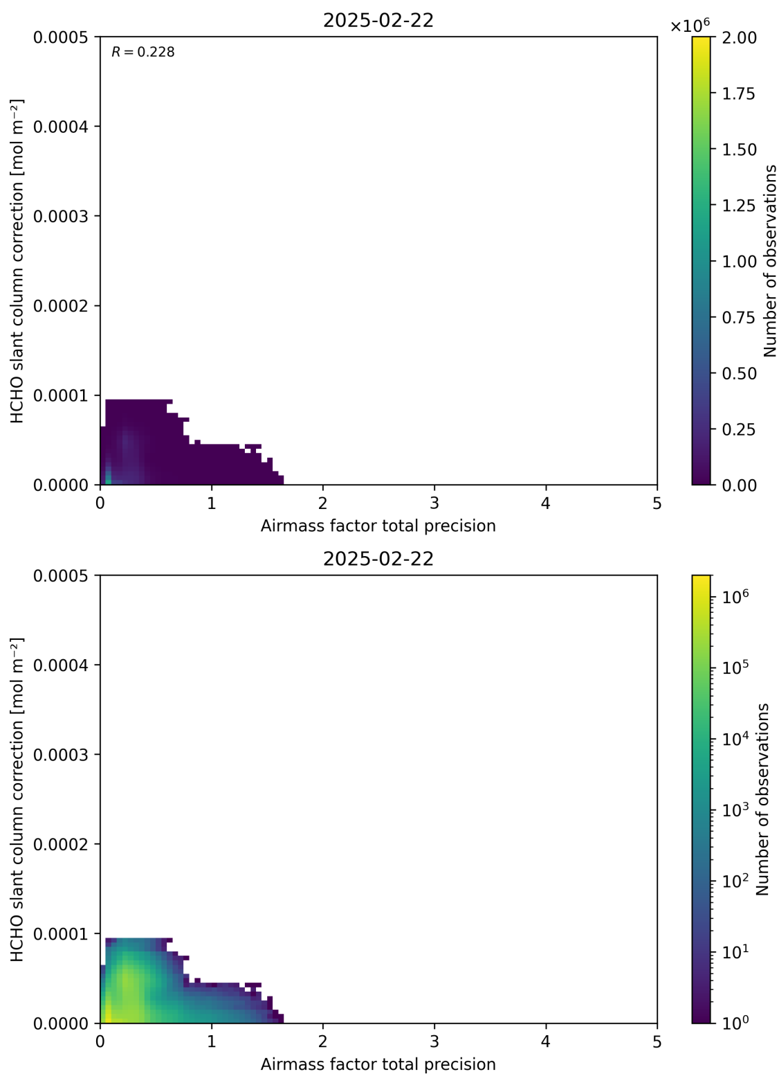
Figure 110: Scatter density plot of “Airmass factor total precision” against “HCHO slant column correction” for 2025-02-21 to 2025-02-23.
