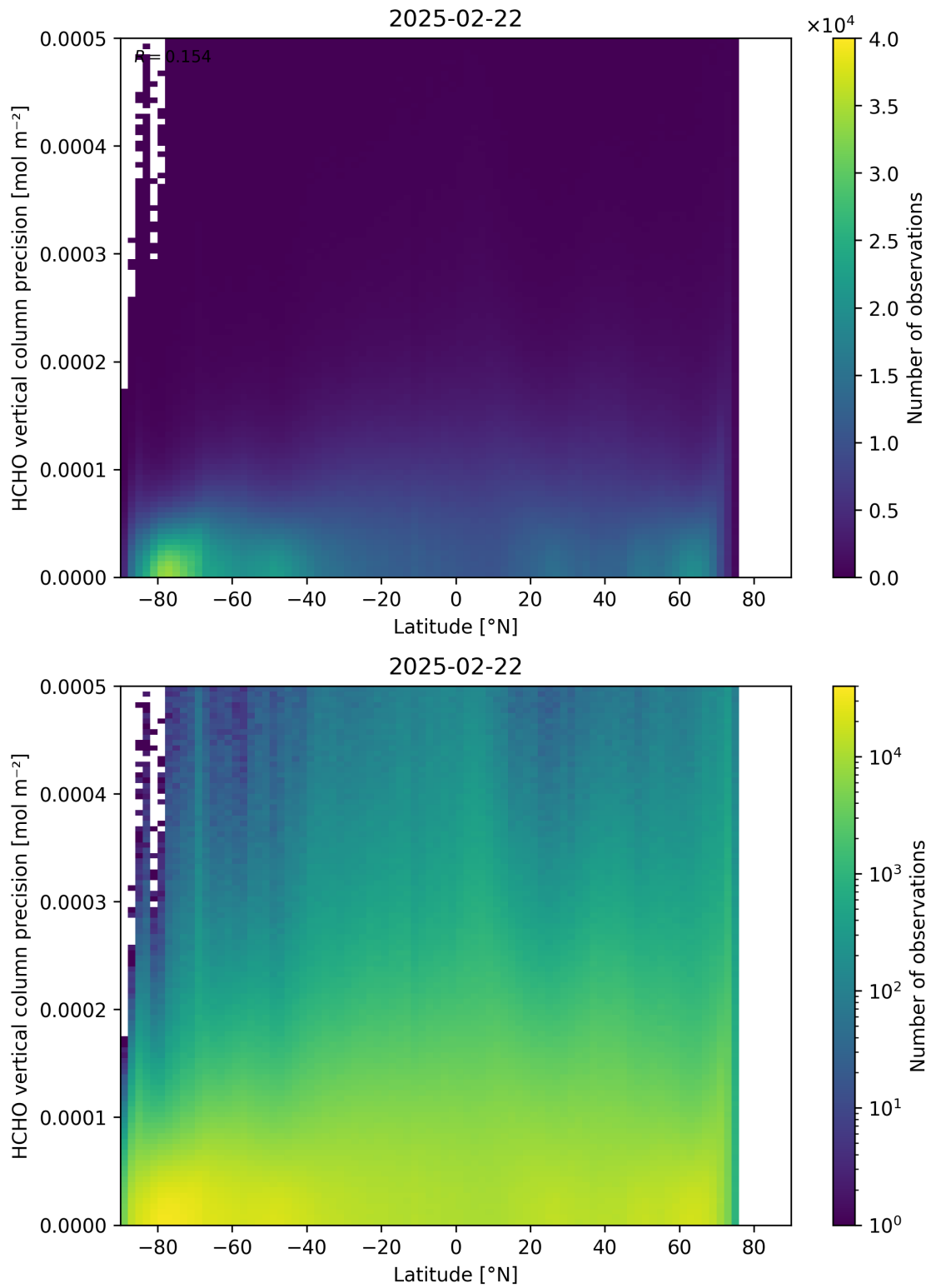
Figure 165: Scatter density plot of “Latitude” against “HCHO vertical column precision” for 2025-02-21 to 2025-02-23.
