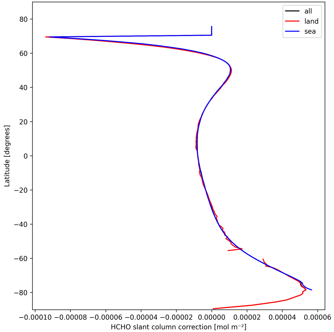
Figure 33: Zonal average of “HCHO slant column correction” for 2025-02-21 to 2025-02-23.
