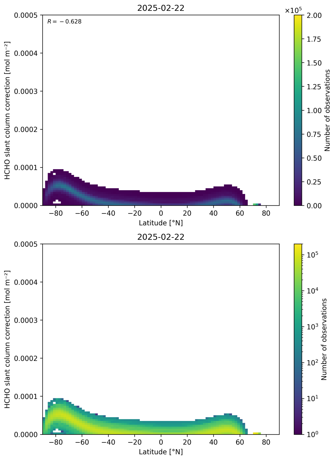
Figure 158: Scatter density plot of “Latitude” against “HCHO slant column correction” for 2025-02-21 to 2025-02-23.
