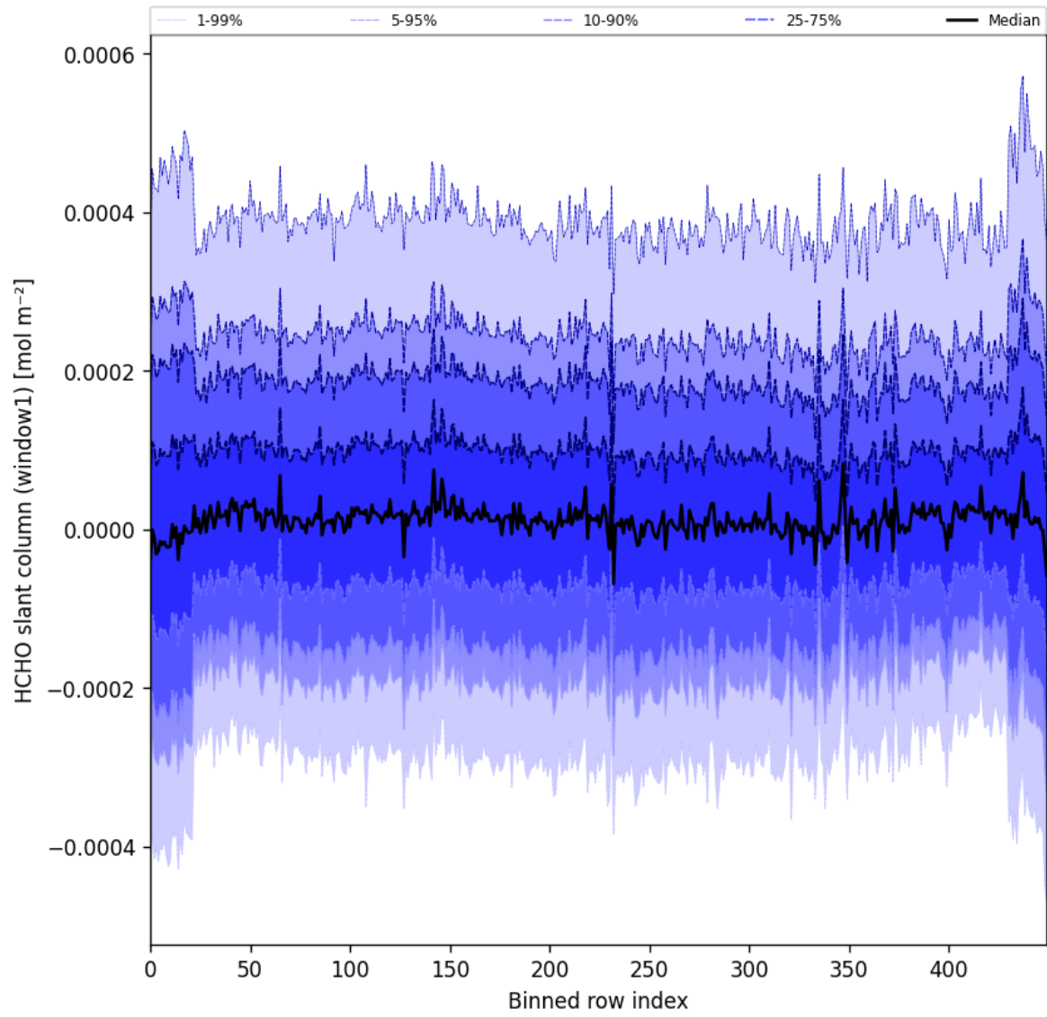
Figure 52: Along track statistics of “HCHO slant column (window1)” for 2025-02-21 to 2025-02-23
