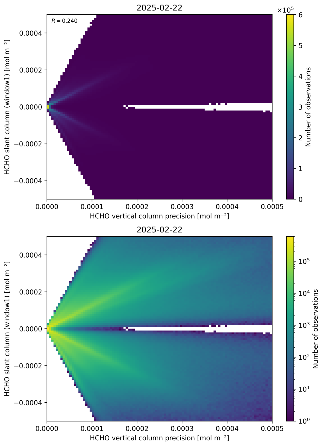
Figure 142: Scatter density plot of “HCHO vertical column precision” against “HCHO slant column (window1)” for 2025-02-21 to 2025-02-23.
