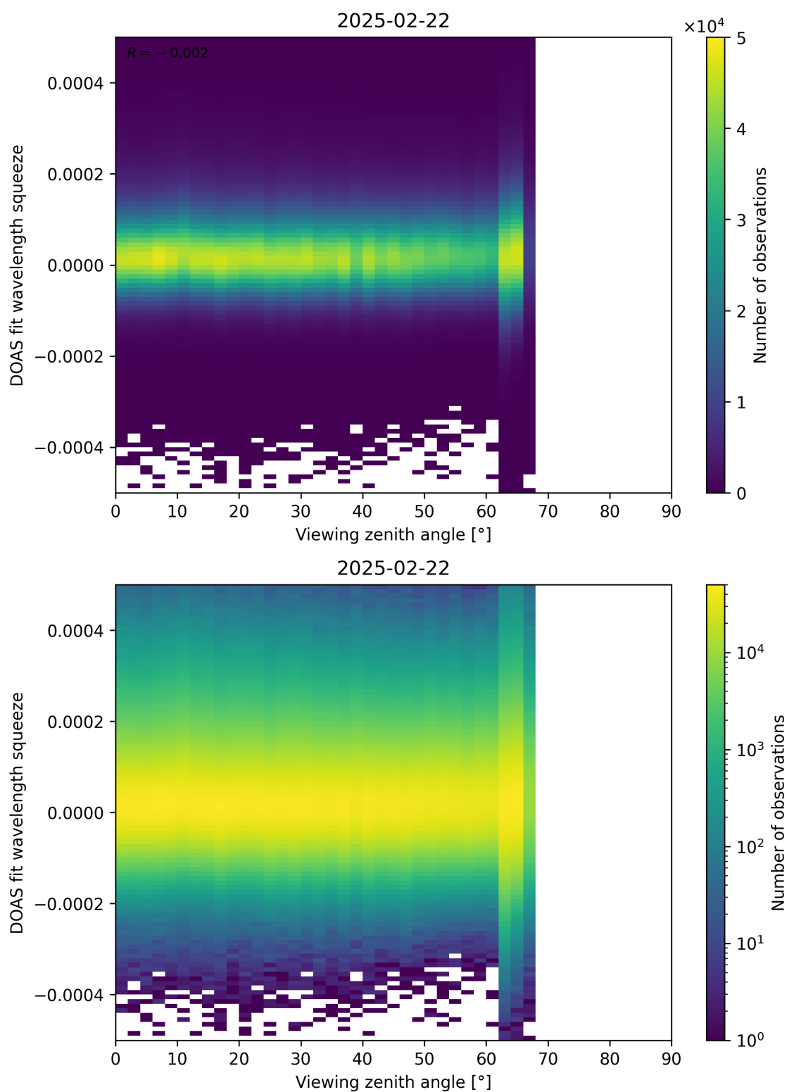
Figure 184: Scatter density plot of “Viewing zenith angle” against “DOAS fit wavelength squeeze” for 2025-02-21 to 2025-02-23.
