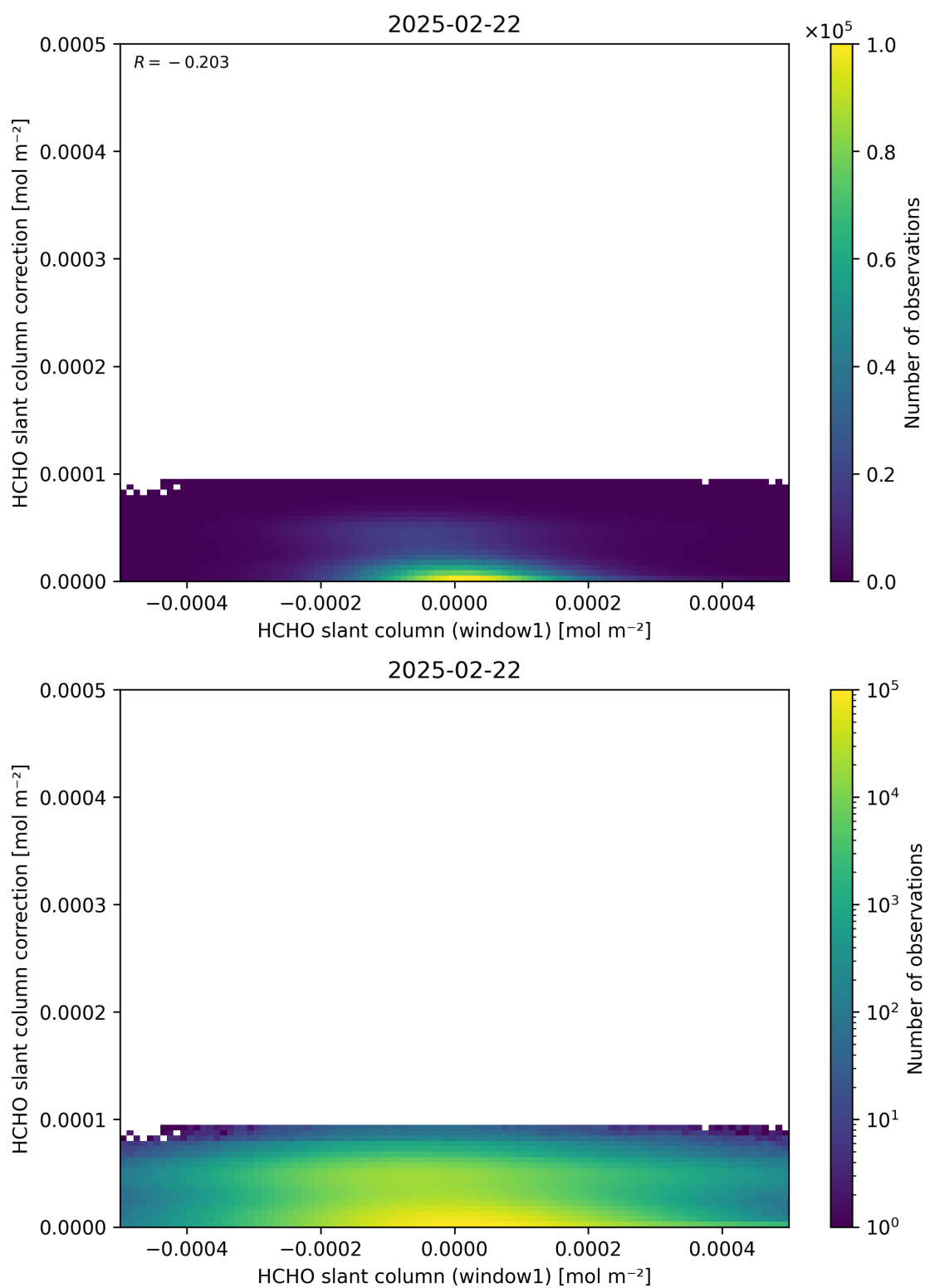
Figure 83: Scatter density plot of “HCHO slant column (window1)” against “HCHO slant column correction” for 2025-02-21 to 2025-02-23.
