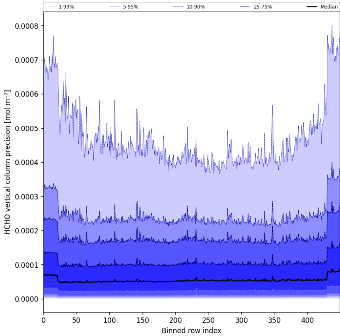
Figure 50: Along track statistics of “HCHO vertical column precision” for 2025-02-21 to 2025-02-23
