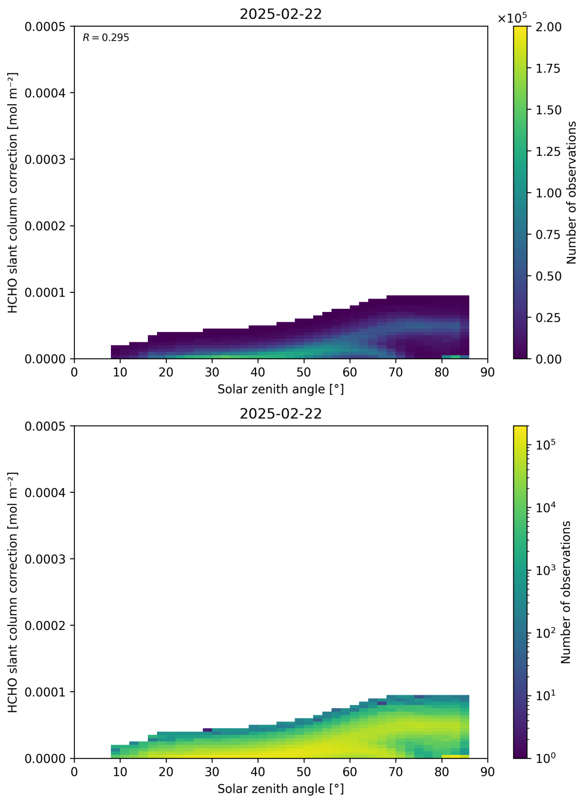
Figure 172: Scatter density plot of “Solar zenith angle” against “HCHO slant column correction” for 2025-02-21 to 2025-02-23.
