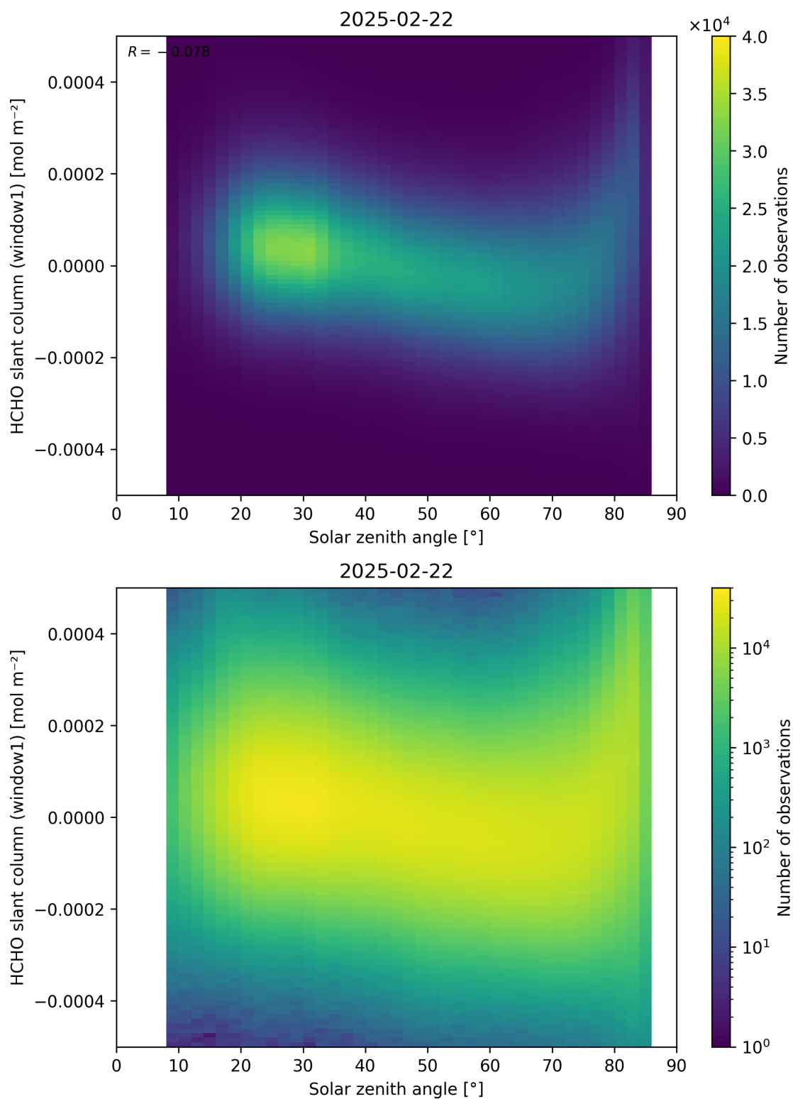
Figure 173: Scatter density plot of “Solar zenith angle” against “HCHO slant column (window1)” for 2025-02-21 to 2025-02-23.
