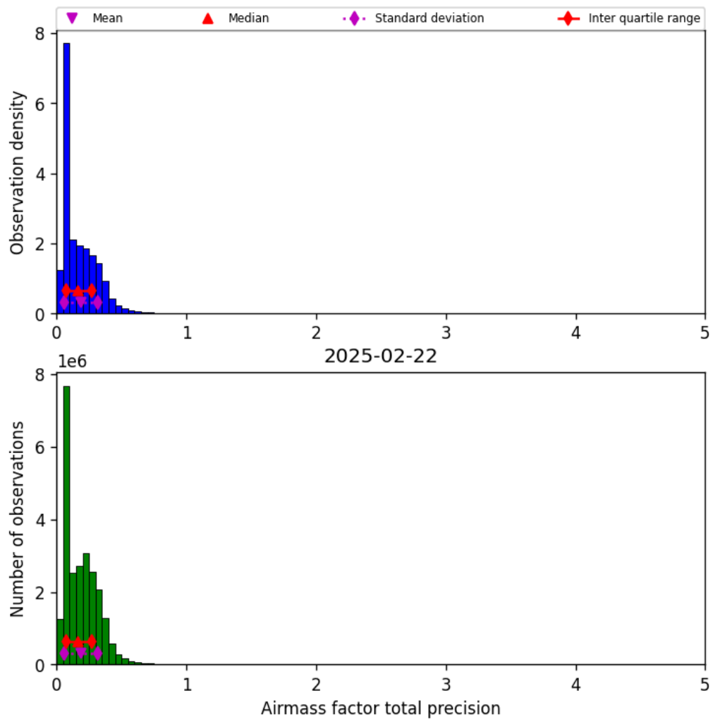
Figure 41: Histogram of “Airmass factor total precision” for 2025-02-21 to 2025-02-23
