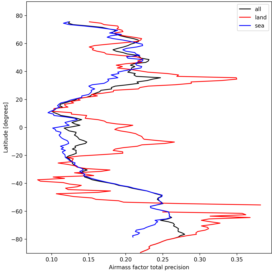
Figure 27: Zonal average of “Airmass factor total precision” for 2025-02-21 to 2025-02-23.
