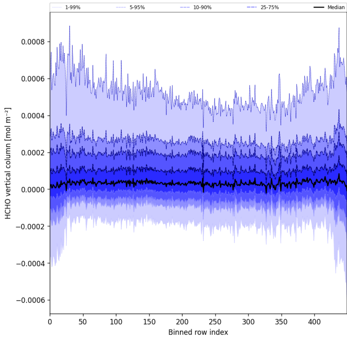
Figure 49: Along track statistics of “HCHO vertical column” for 2025-02-21 to 2025-02-23
