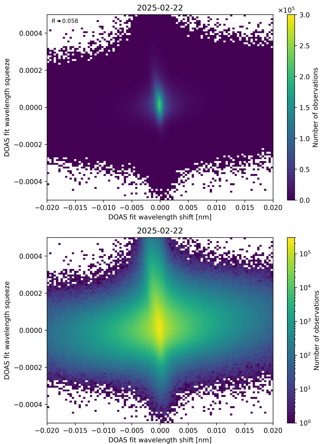
Figure 65: Scatter density plot of “DOAS fit wavelength shift” against “DOAS fit wavelength squeeze” for 2025-02-21 to 2025-02-23.
