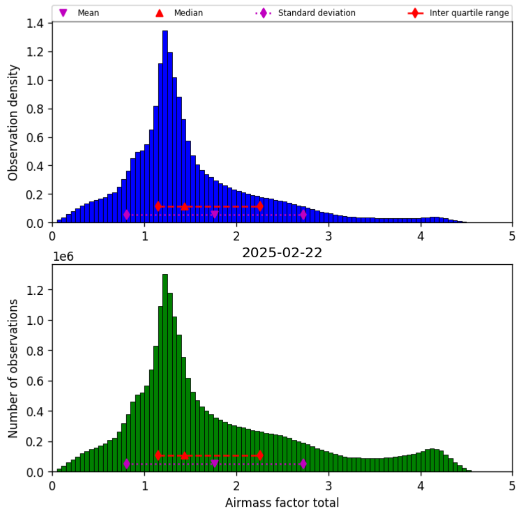
Figure 40: Histogram of “Airmass factor total” for 2025-02-21 to 2025-02-23
