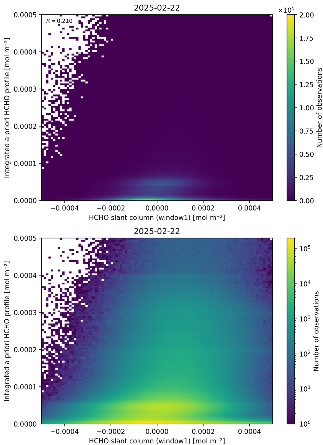
Figure 87: Scatter density plot of “HCHO slant column (window1)” against “Integrated a priori HCHO profile” for 2025-02-21 to 2025-02-23.
