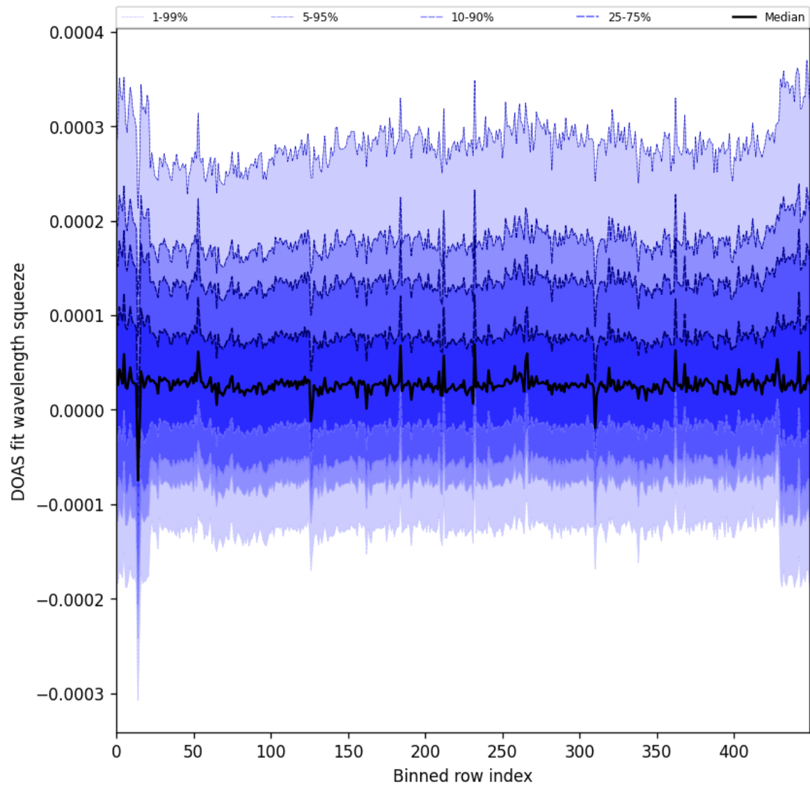
Figure 59: Along track statistics of “DOAS fit wavelength squeeze” for 2025-02-21 to 2025-02-23
