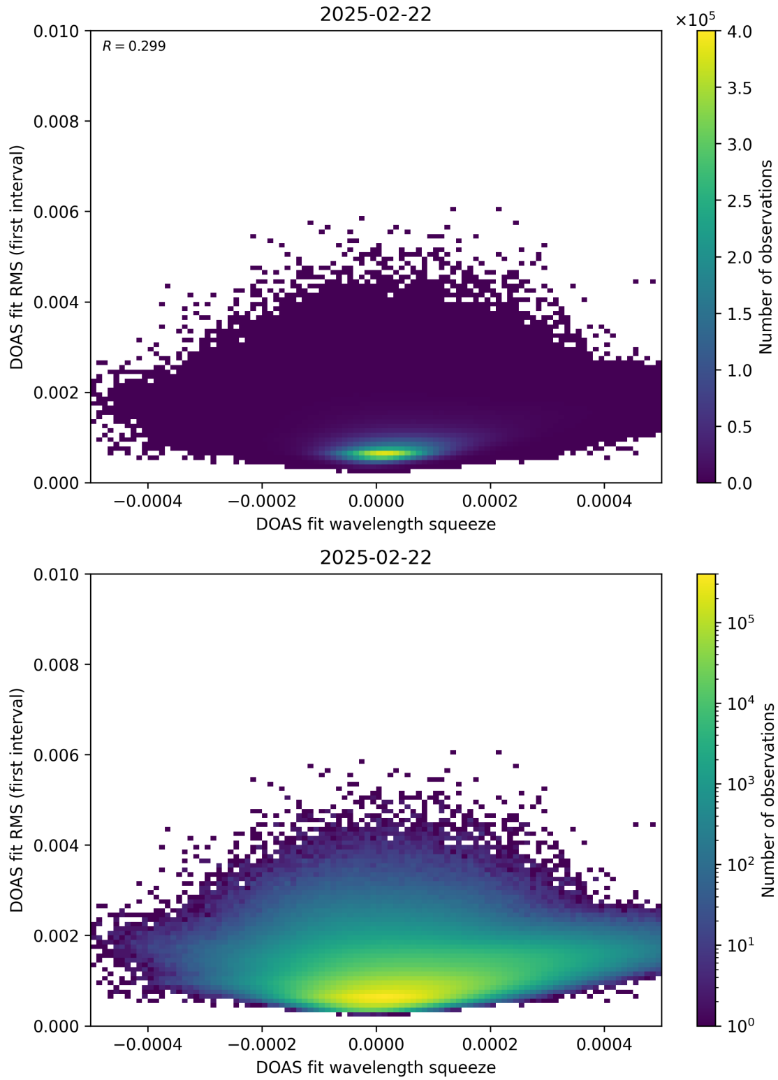
Figure 68: Scatter density plot of “DOAS fit wavelength squeeze” against “DOAS fit RMS (first interval)” for 2025-02-21 to 2025-02-23.
