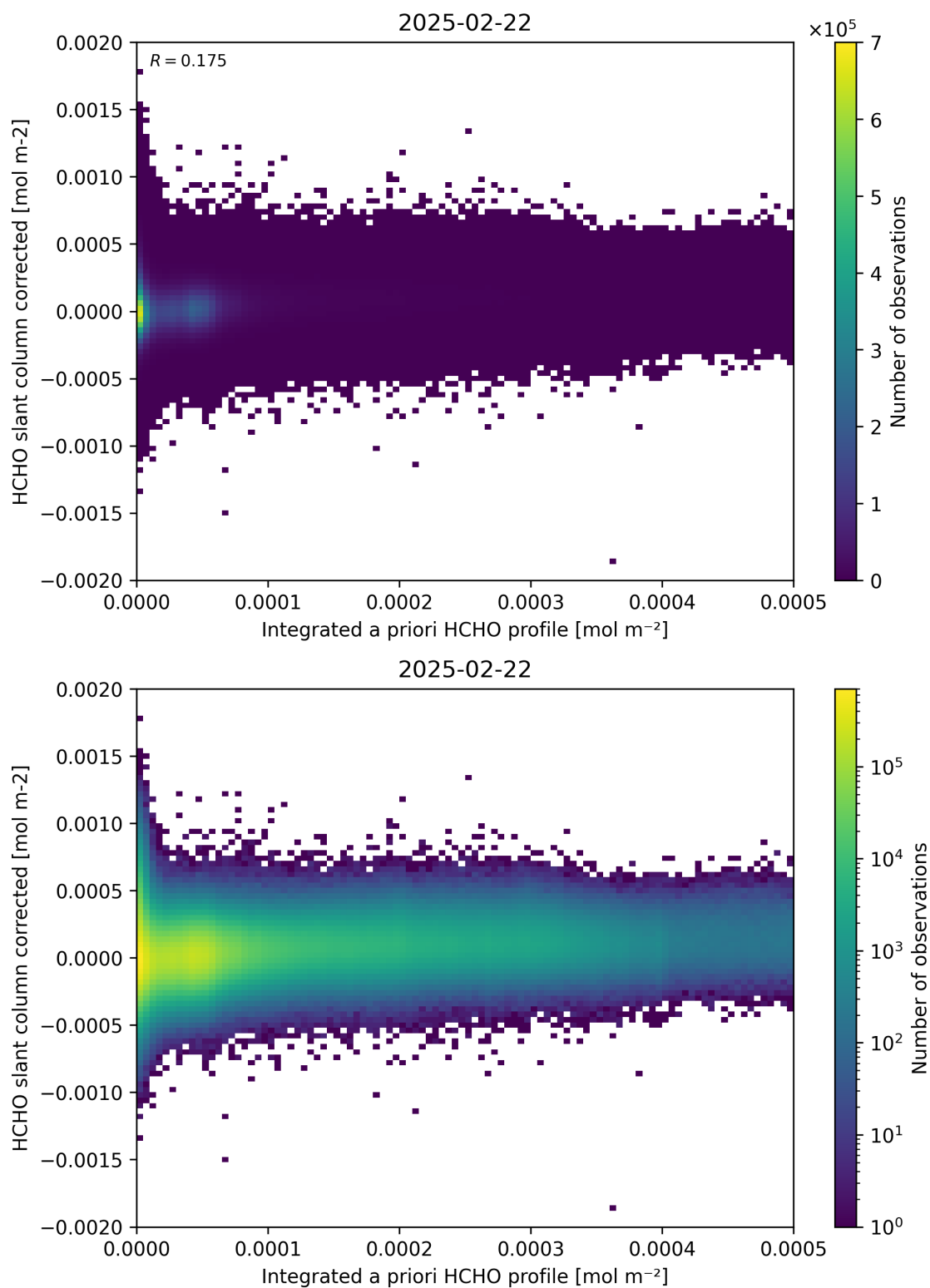
Figure 151: Scatter density plot of “Integrated a priori HCHO profile” against “HCHO slant column corrected” for 2025-02-21 to 2025-02-23.
