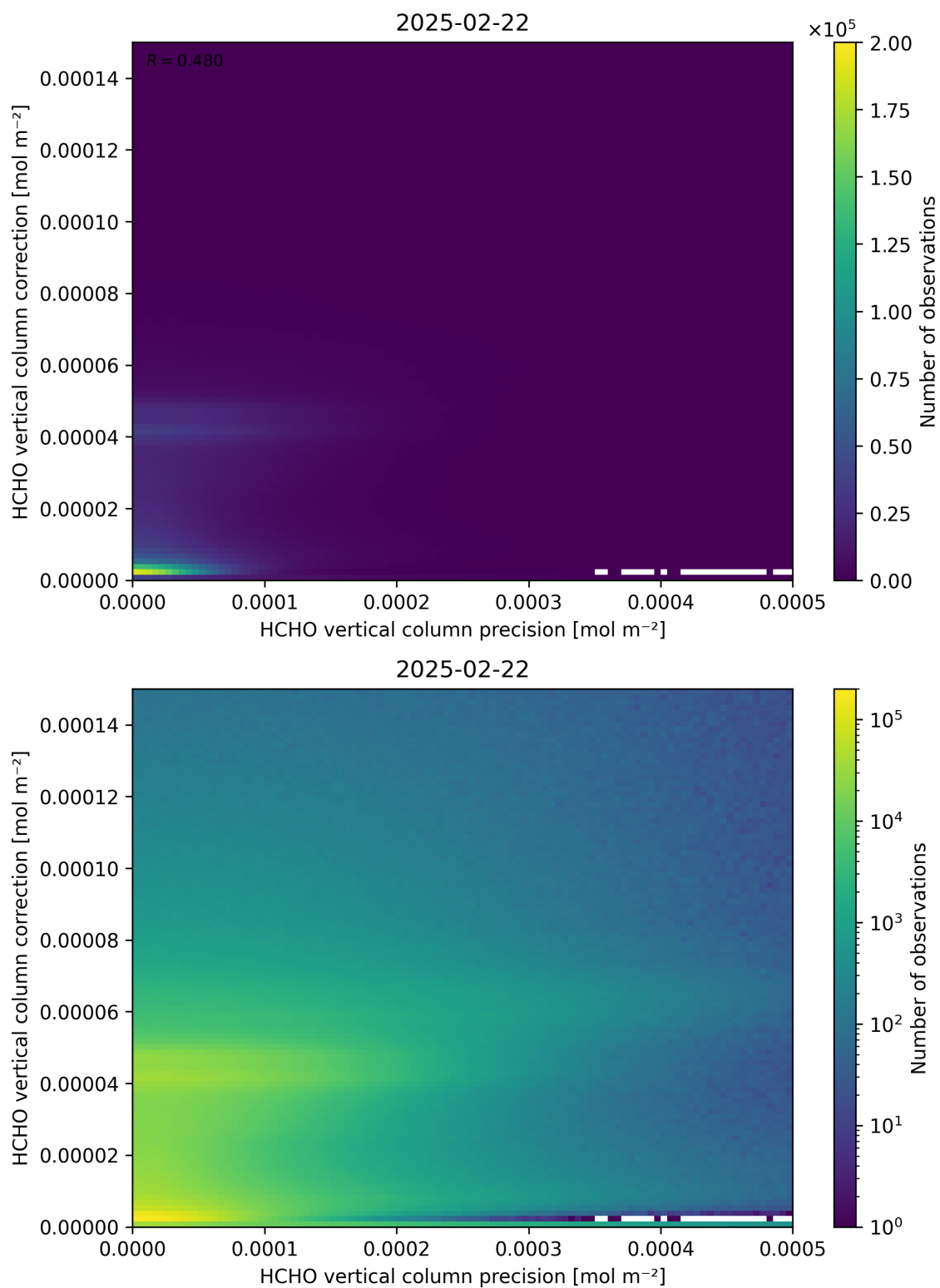
Figure 146: Scatter density plot of “HCHO vertical column precision” against “HCHO vertical column correction” for 2025-02-21 to 2025-02-23.
