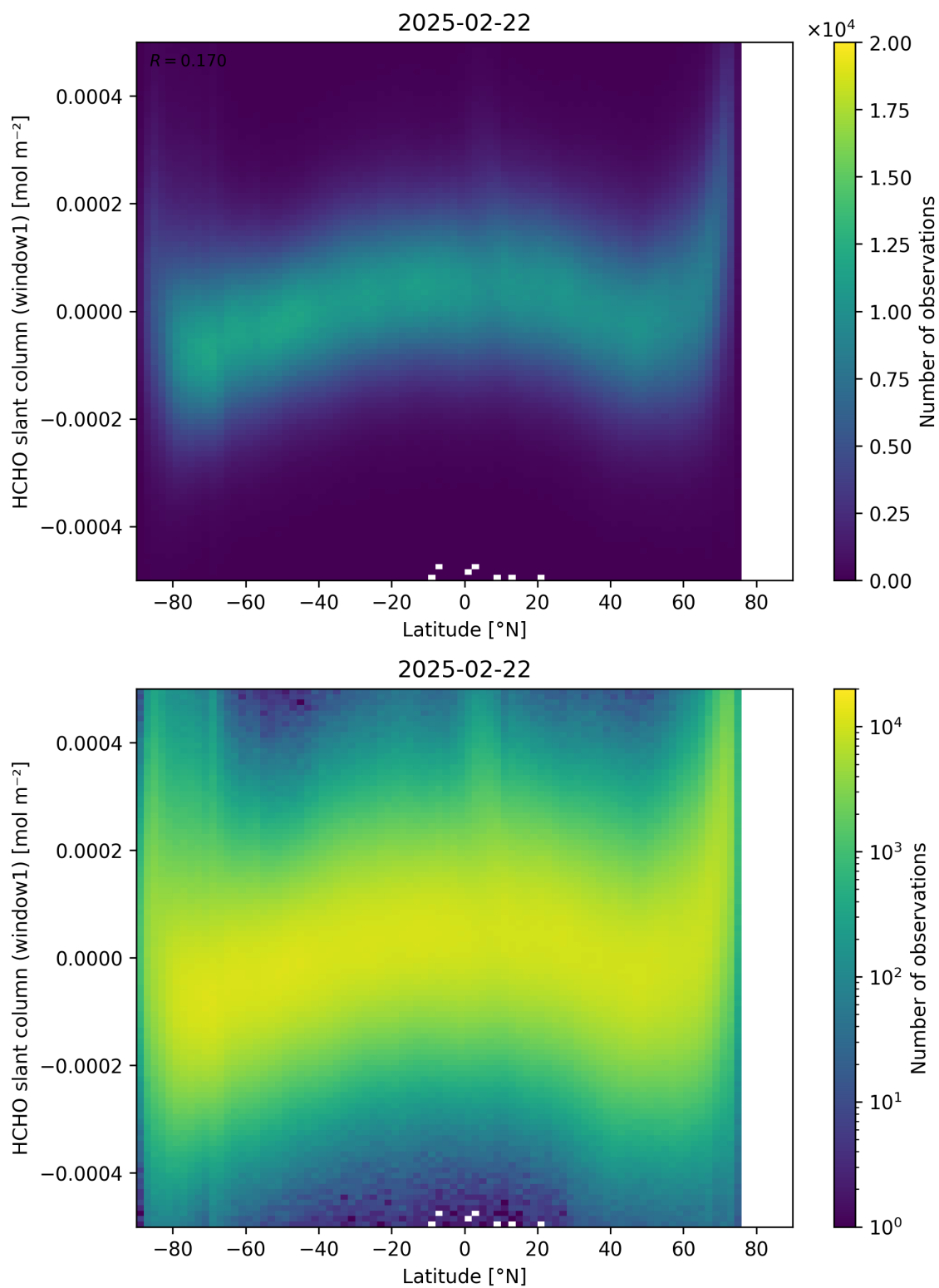
Figure 159: Scatter density plot of “Latitude” against “HCHO slant column (window1)” for 2025-02-21 to 2025-02-23.
