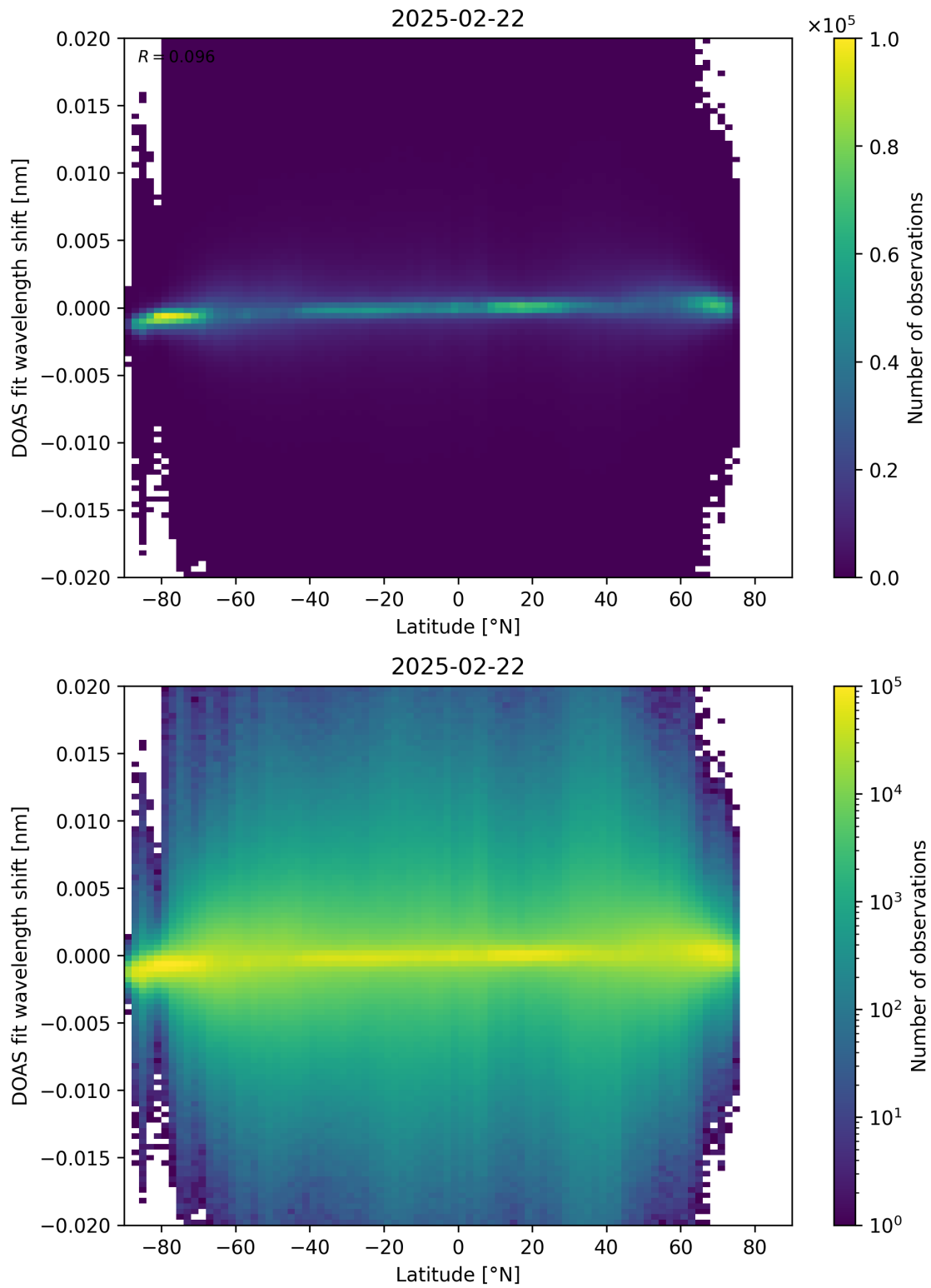
Figure 154: Scatter density plot of “Latitude” against “DOAS fit wavelength shift” for 2025-02-21 to 2025-02-23.
