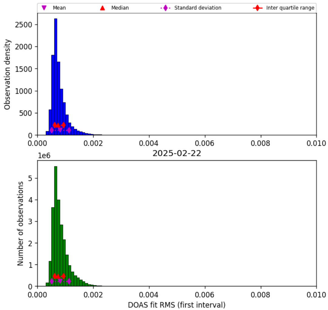
Figure 46: Histogram of “DOAS fit RMS (first interval)” for 2025-02-21 to 2025-02-23
