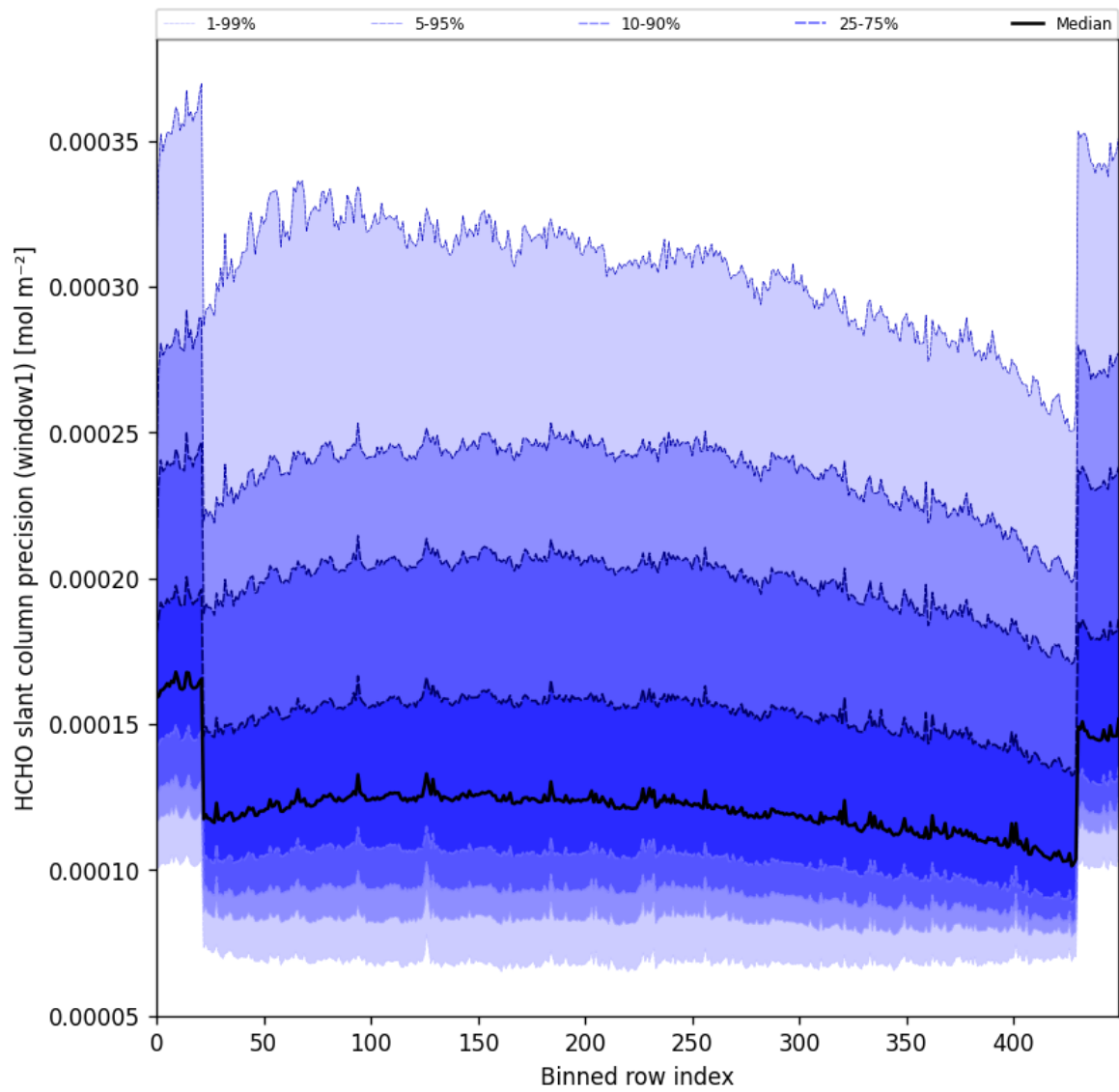
Figure 53: Along track statistics of “HCHO slant column precision (window1)” for 2025-02-21 to 2025-02-23
