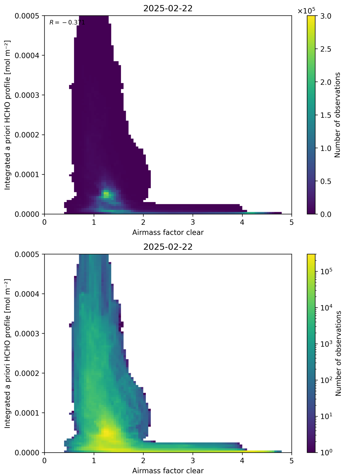
Figure 76: Scatter density plot of “Airmass factor clear” against “Integrated a priori HCHO profile” for 2025-02-21 to 2025-02-23.
