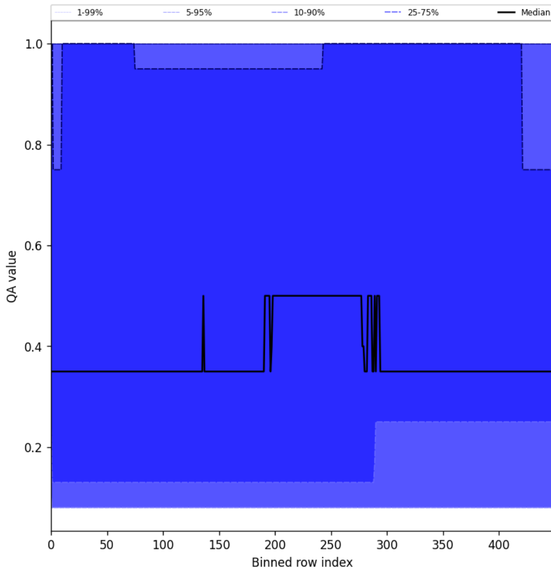
Figure 48: Along track statistics of “QA value” for 2025-02-21 to 2025-02-23
