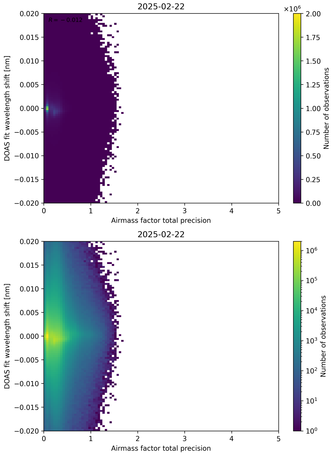
Figure 106: Scatter density plot of “Airmass factor total precision” against “DOAS fit wavelength shift” for 2025-02-21 to 2025-02-23.
