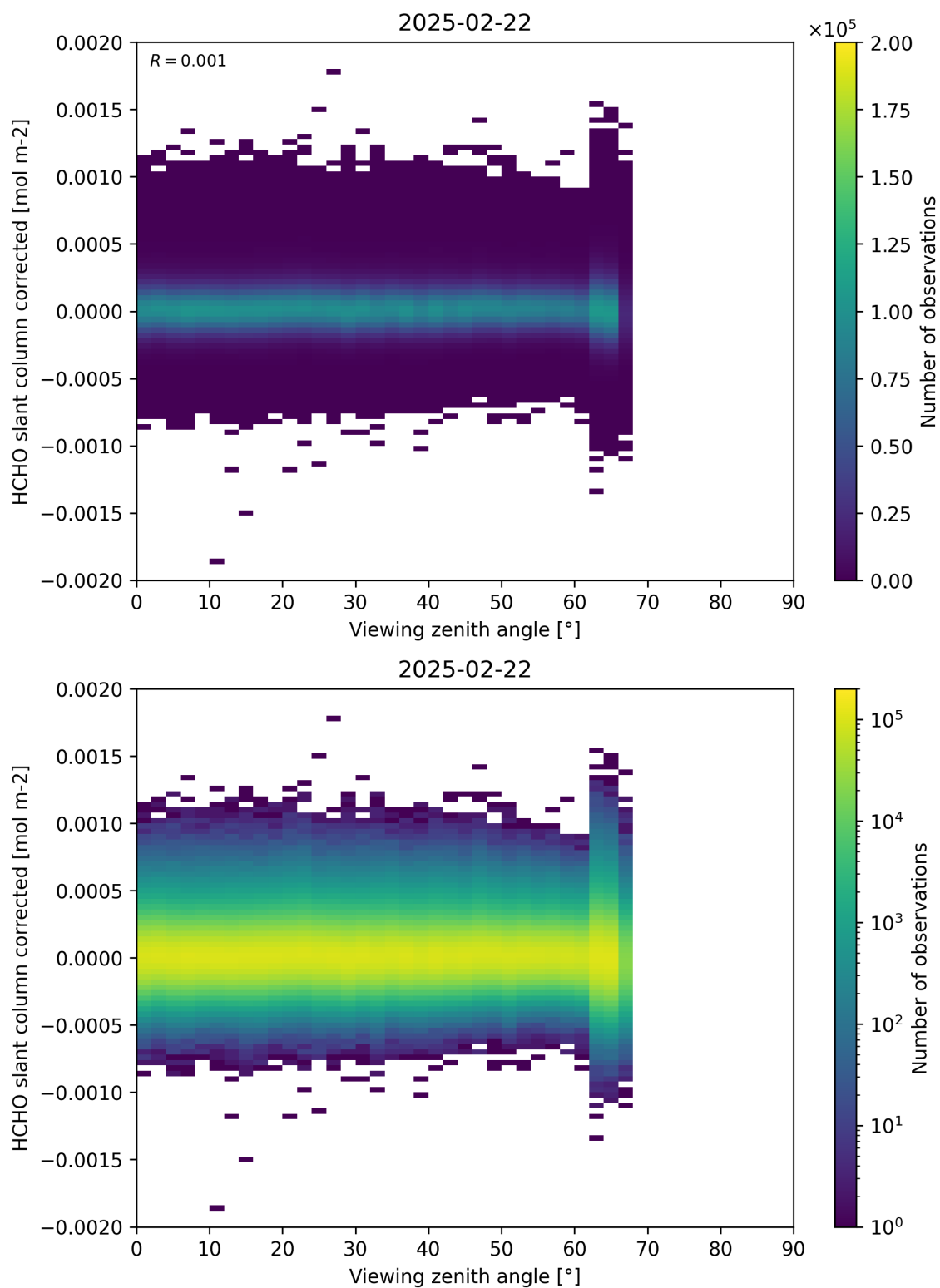
Figure 186: Scatter density plot of “Viewing zenith angle” against “HCHO slant column corrected” for 2025-02-21 to 2025-02-23.
