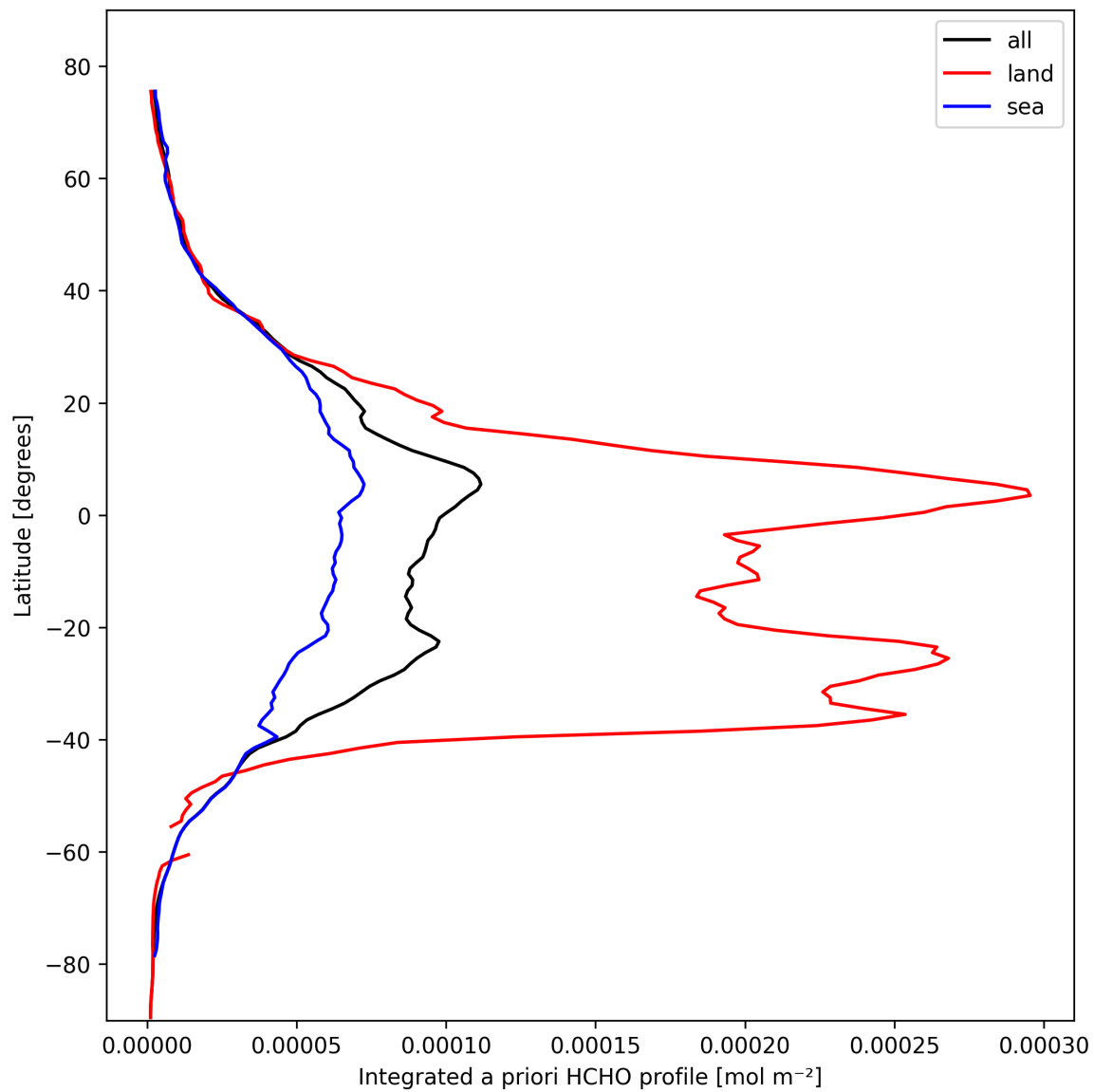
Figure 29: Zonal average of “Integrated a priori HCHO profile” for 2025-02-21 to 2025-02-23.
