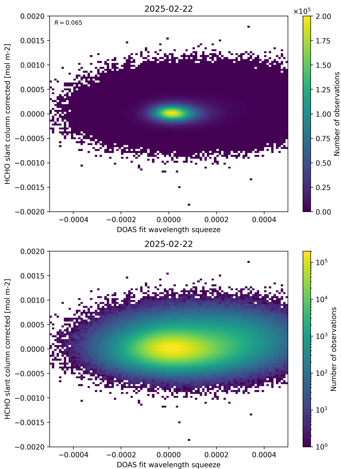
Figure 69: Scatter density plot of “DOAS fit wavelength squeeze” against “HCHO slant column corrected” for 2025-02-21 to 2025-02-23.
