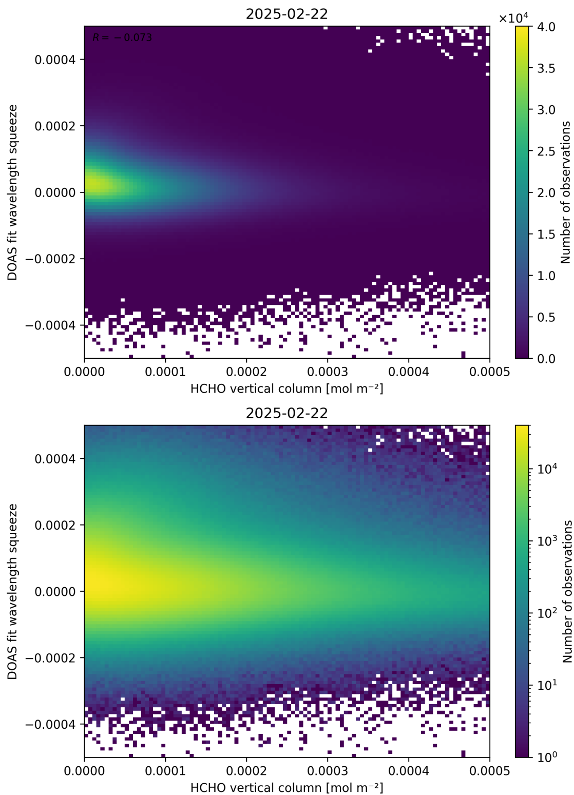
Figure 125: Scatter density plot of “HCHO vertical column” against “DOAS fit wavelength squeeze” for 2025-02-21 to 2025-02-23.
