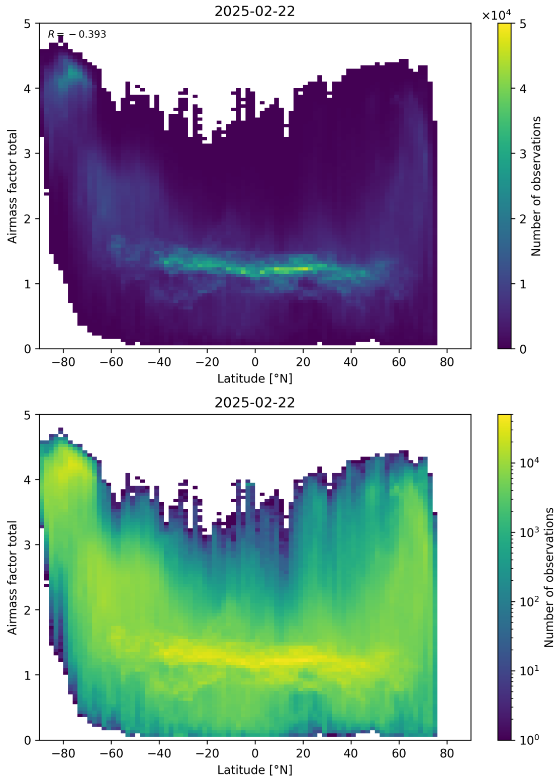
Figure 161: Scatter density plot of “Latitude” against “Airmass factor total” for 2025-02-21 to 2025-02-23.
