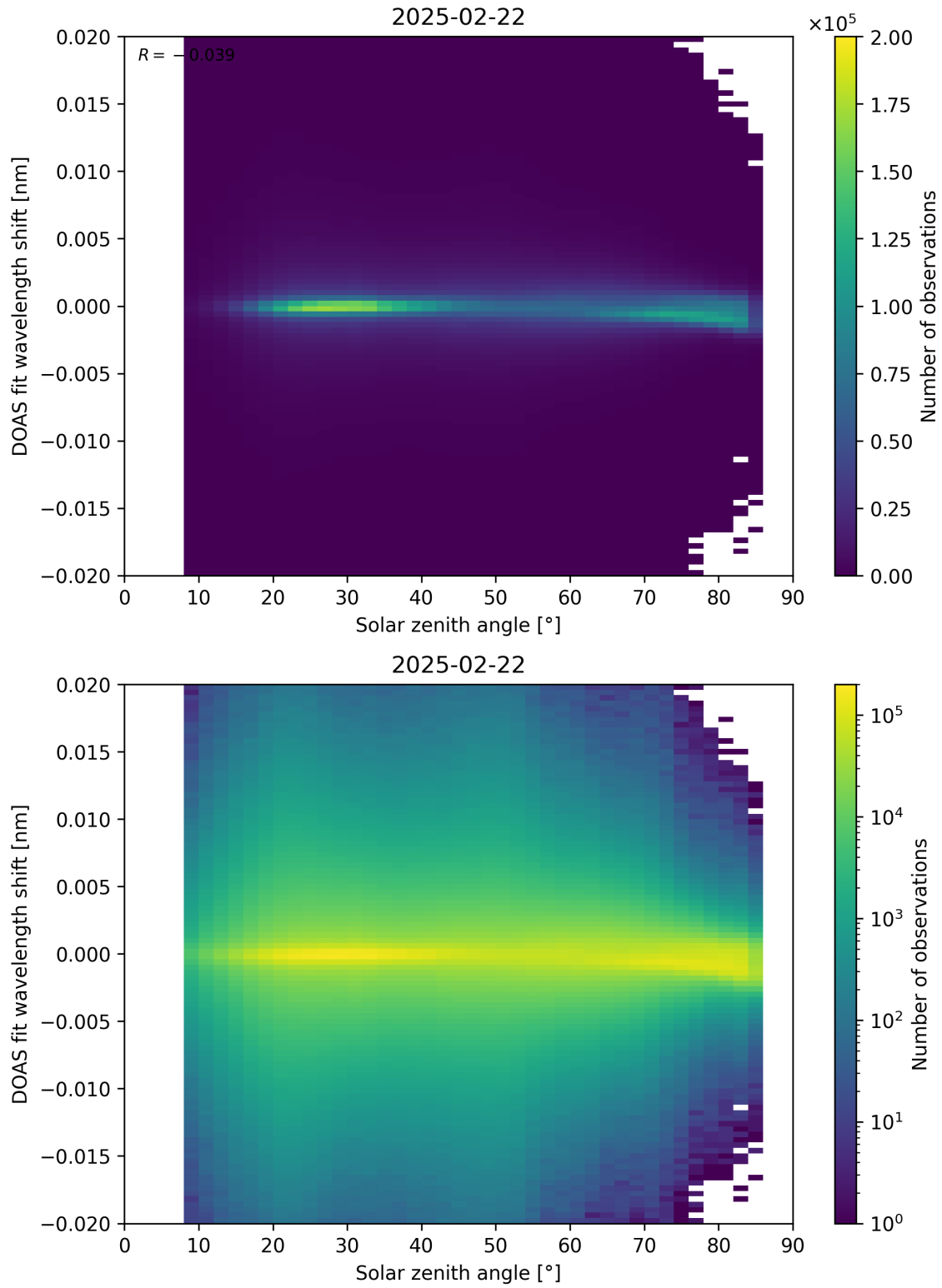
Figure 168: Scatter density plot of “Solar zenith angle” against “DOAS fit wavelength shift” for 2025-02-21 to 2025-02-23.
