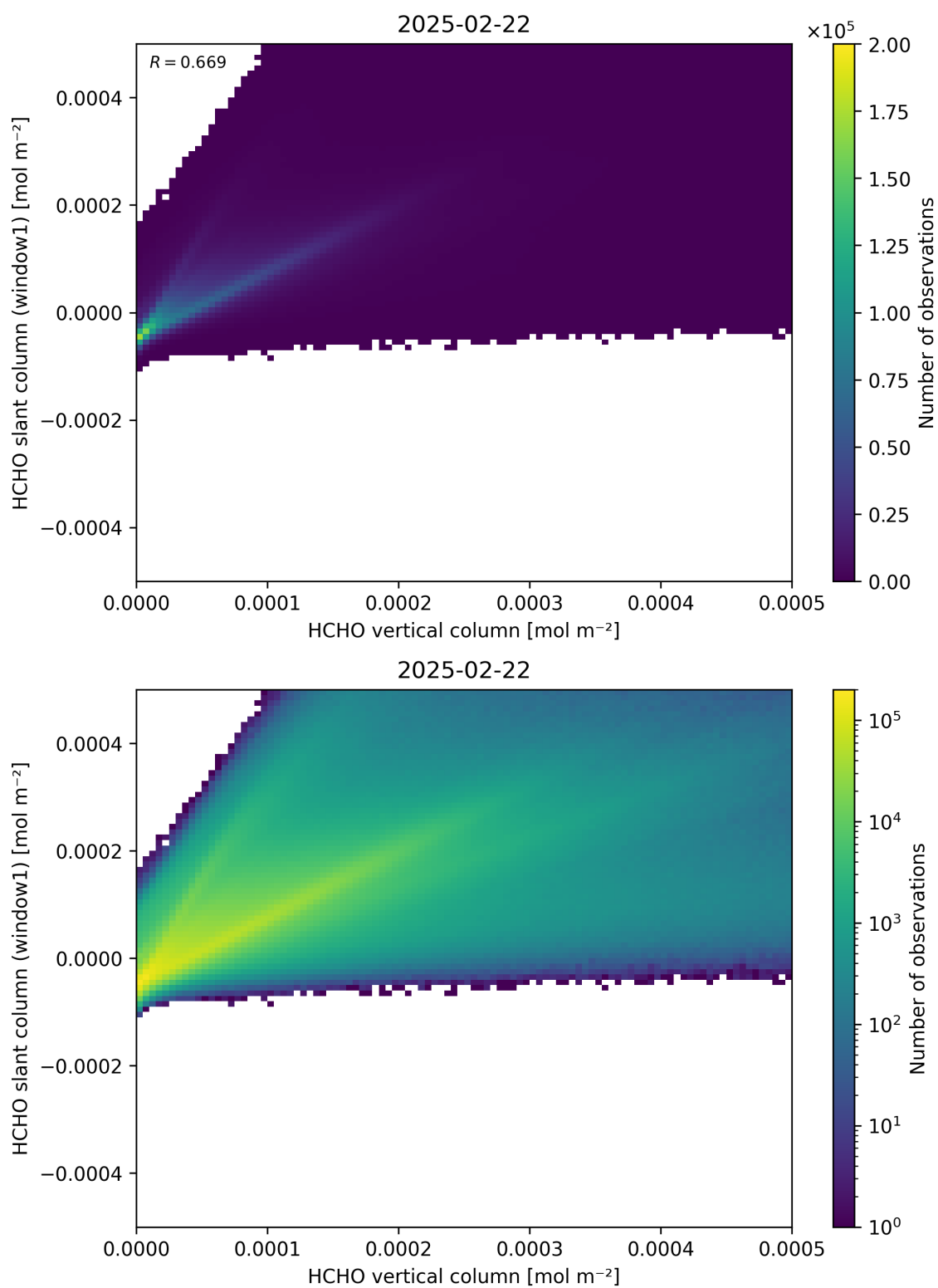
Figure 129: Scatter density plot of “HCHO vertical column” against “HCHO slant column (window1)” for 2025-02-21 to 2025-02-23.
