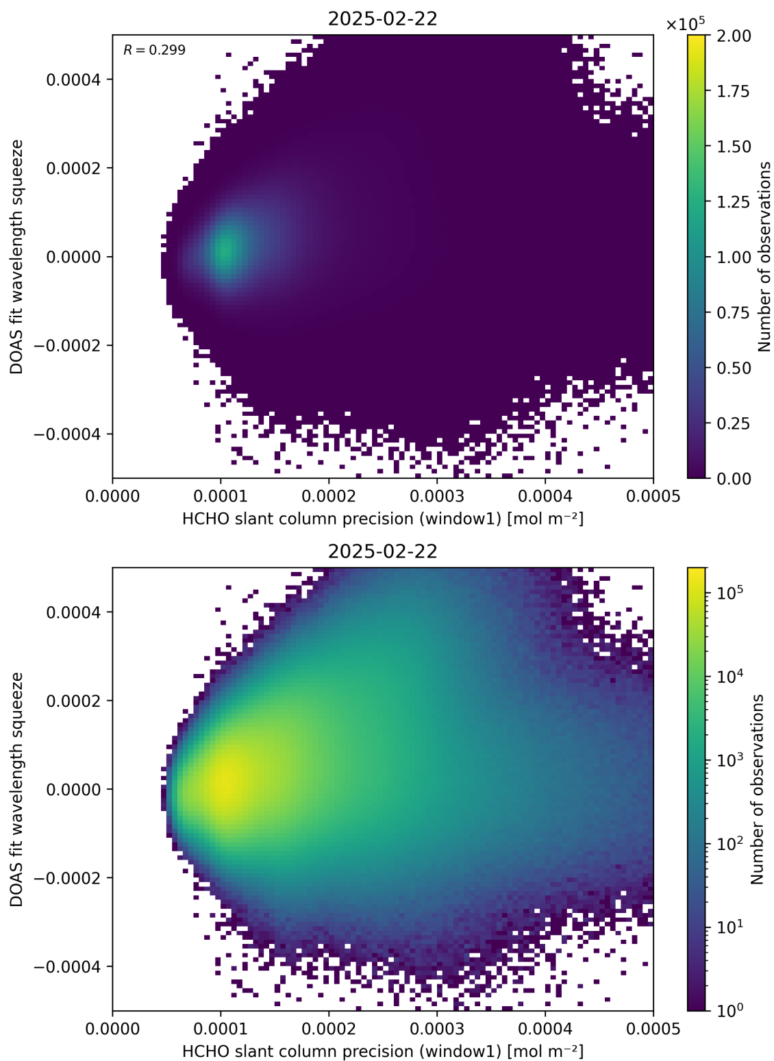
Figure 90: Scatter density plot of “HCHO slant column precision (window1)” against “DOAS fit wavelength squeeze” for 2025-02-21 to 2025-02-23.
