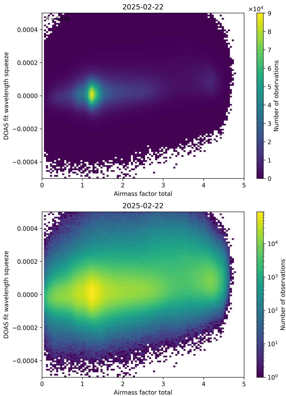
Figure 99: Scatter density plot of “Airmass factor total” against “DOAS fit wavelength squeeze” for 2025-02-21 to 2025-02-23.
