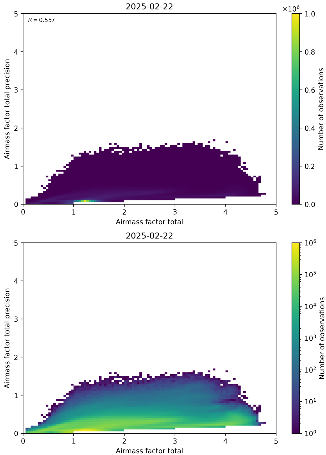
Figure 103: Scatter density plot of “Airmass factor total” against “Airmass factor total precision” for 2025-02-21 to 2025-02-23.
