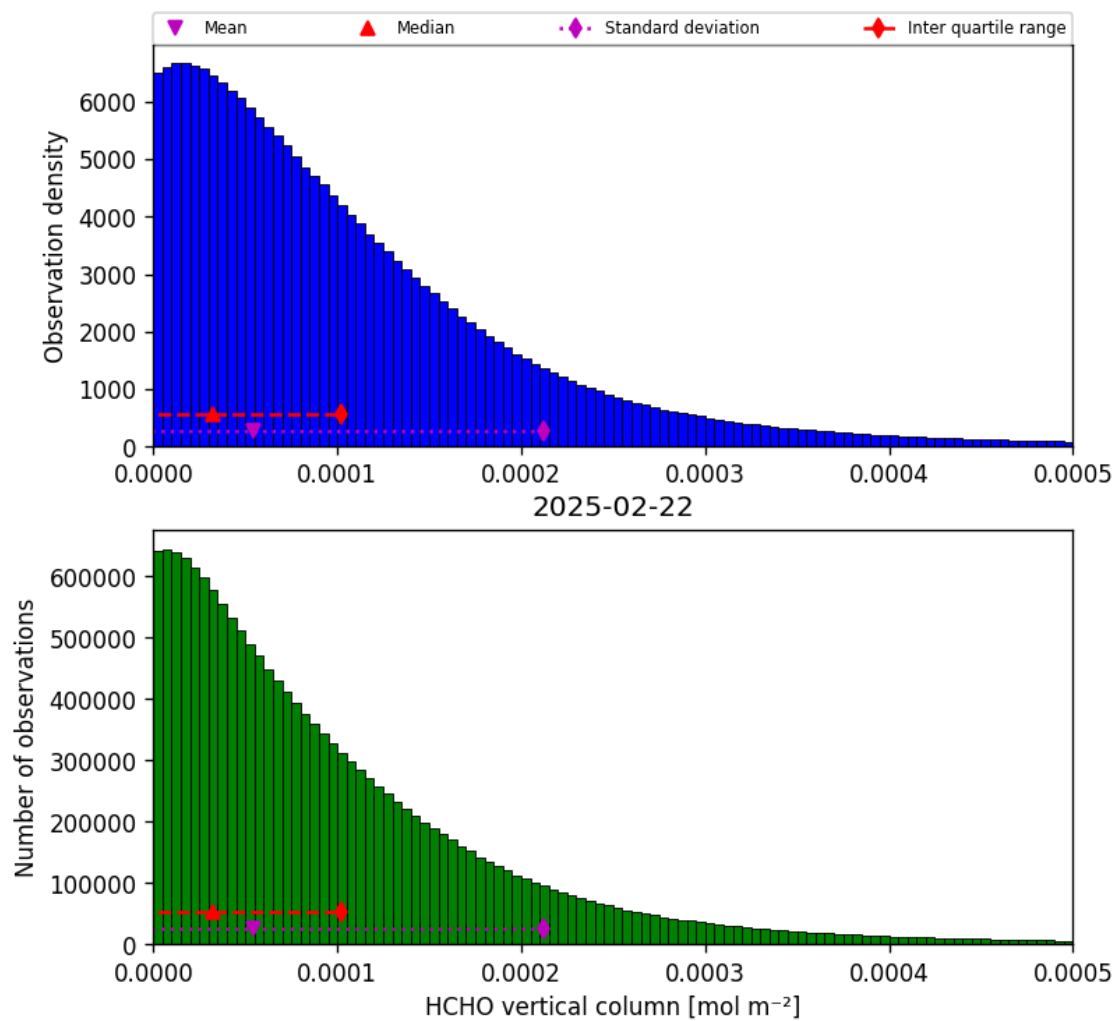
Figure 35: Histogram of “HCHO vertical column” for 2025-02-21 to 2025-02-23
