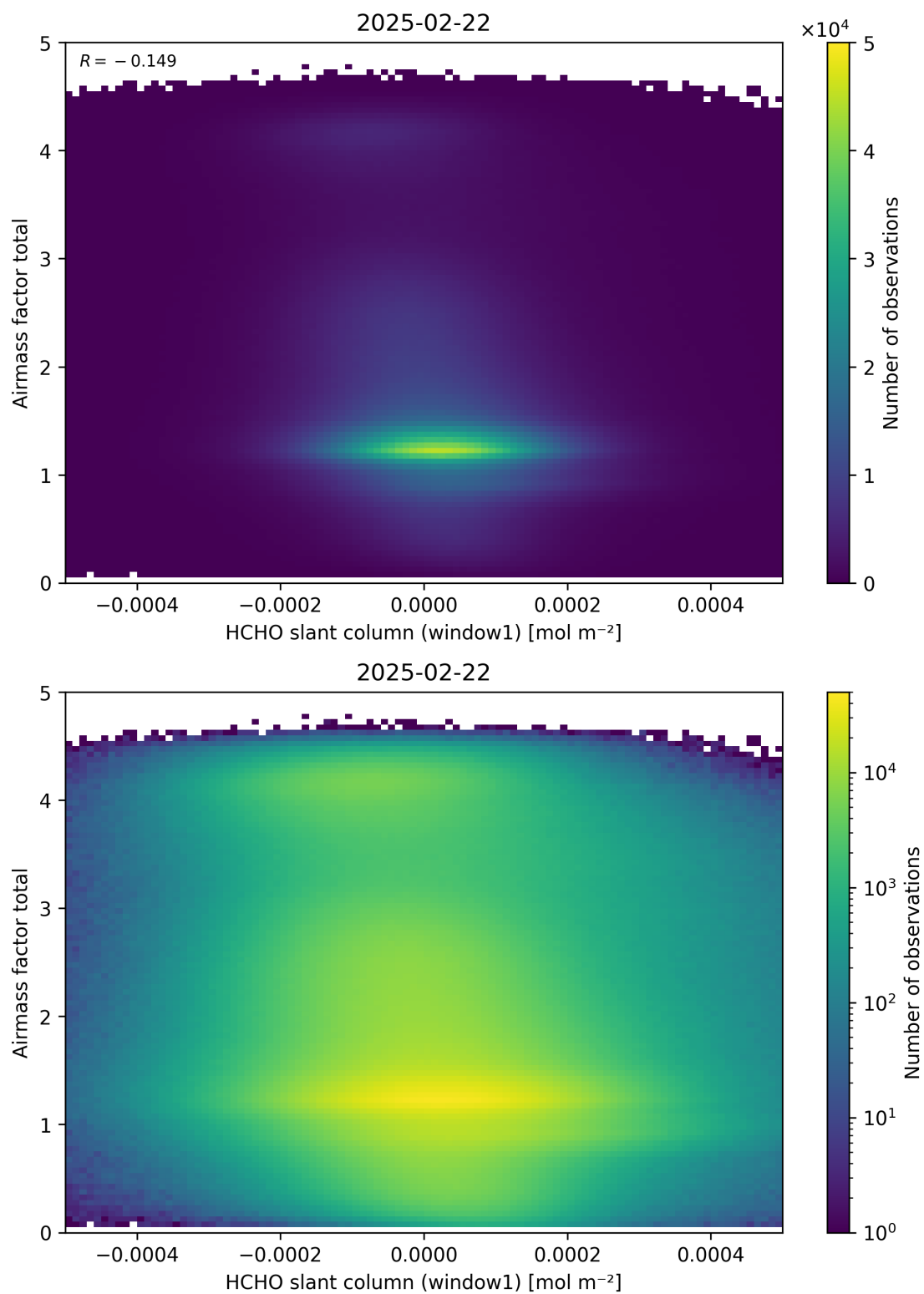
Figure 85: Scatter density plot of “HCHO slant column (window1)” against “Airmass factor total” for 2025-02-21 to 2025-02-23.
