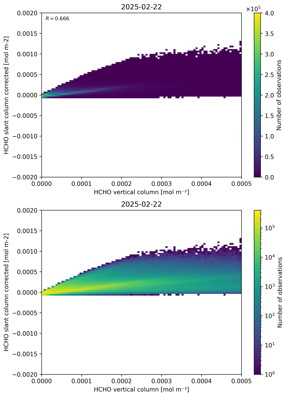
Figure 127: Scatter density plot of “HCHO vertical column” against “HCHO slant column corrected” for 2025-02-21 to 2025-02-23.
