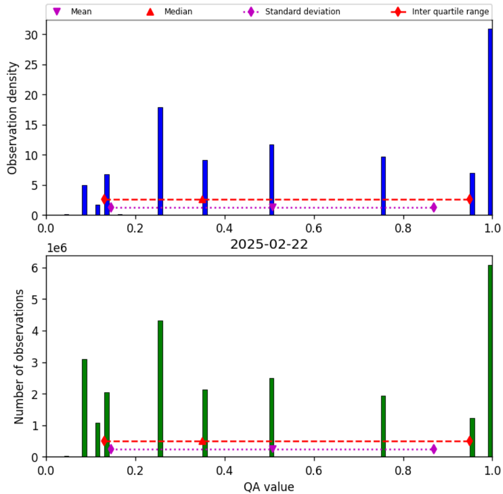
Figure 34: Histogram of “QA value” for 2025-02-21 to 2025-02-23
