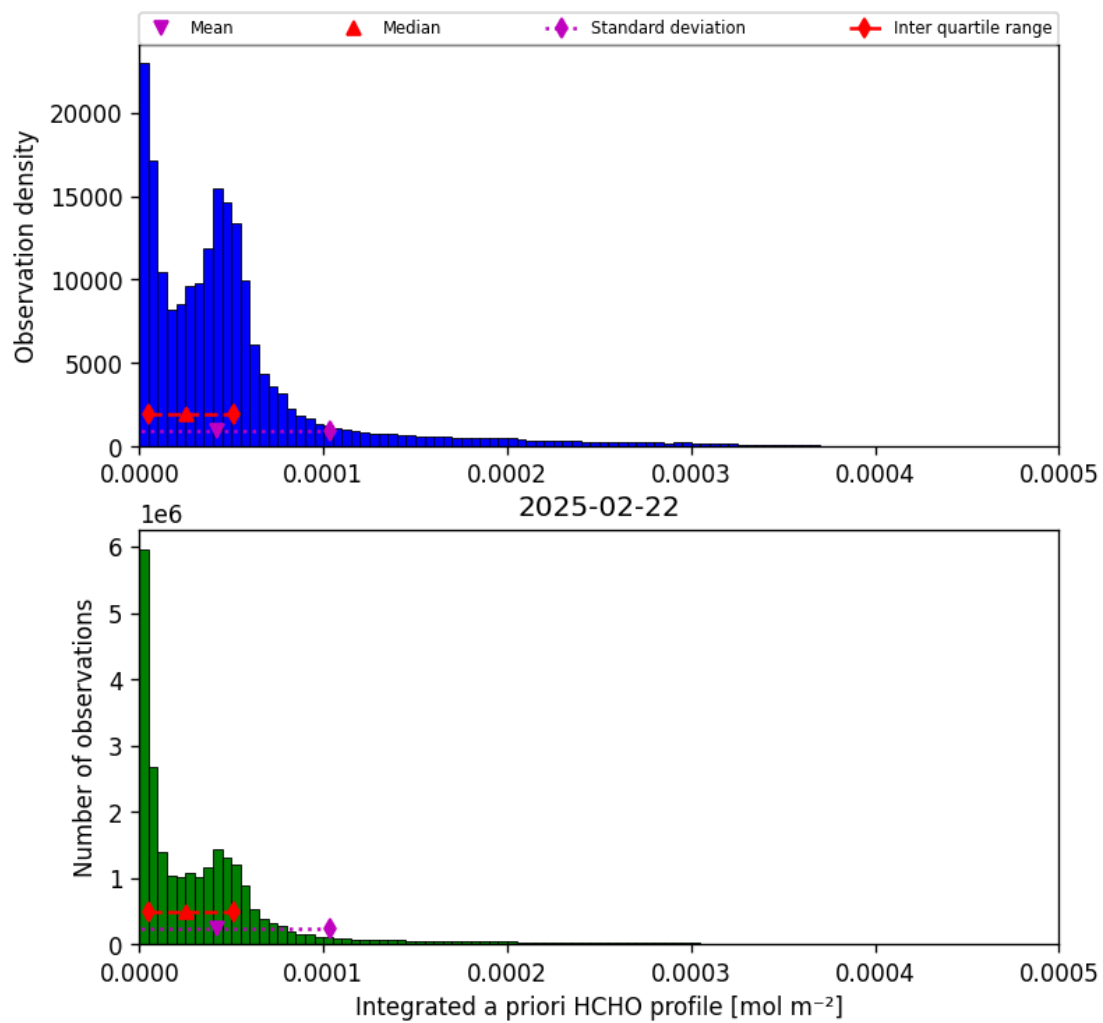
Figure 43: Histogram of “Integrated a priori HCHO profile” for 2025-02-21 to 2025-02-23
