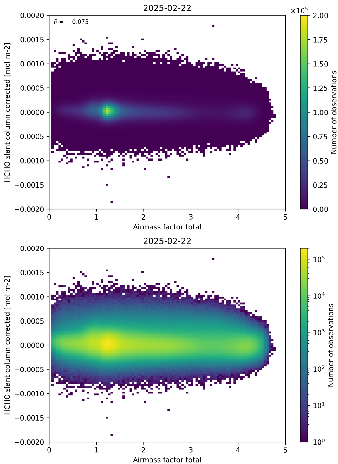
Figure 101: Scatter density plot of “Airmass factor total” against “HCHO slant column corrected” for 2025-02-21 to 2025-02-23.
