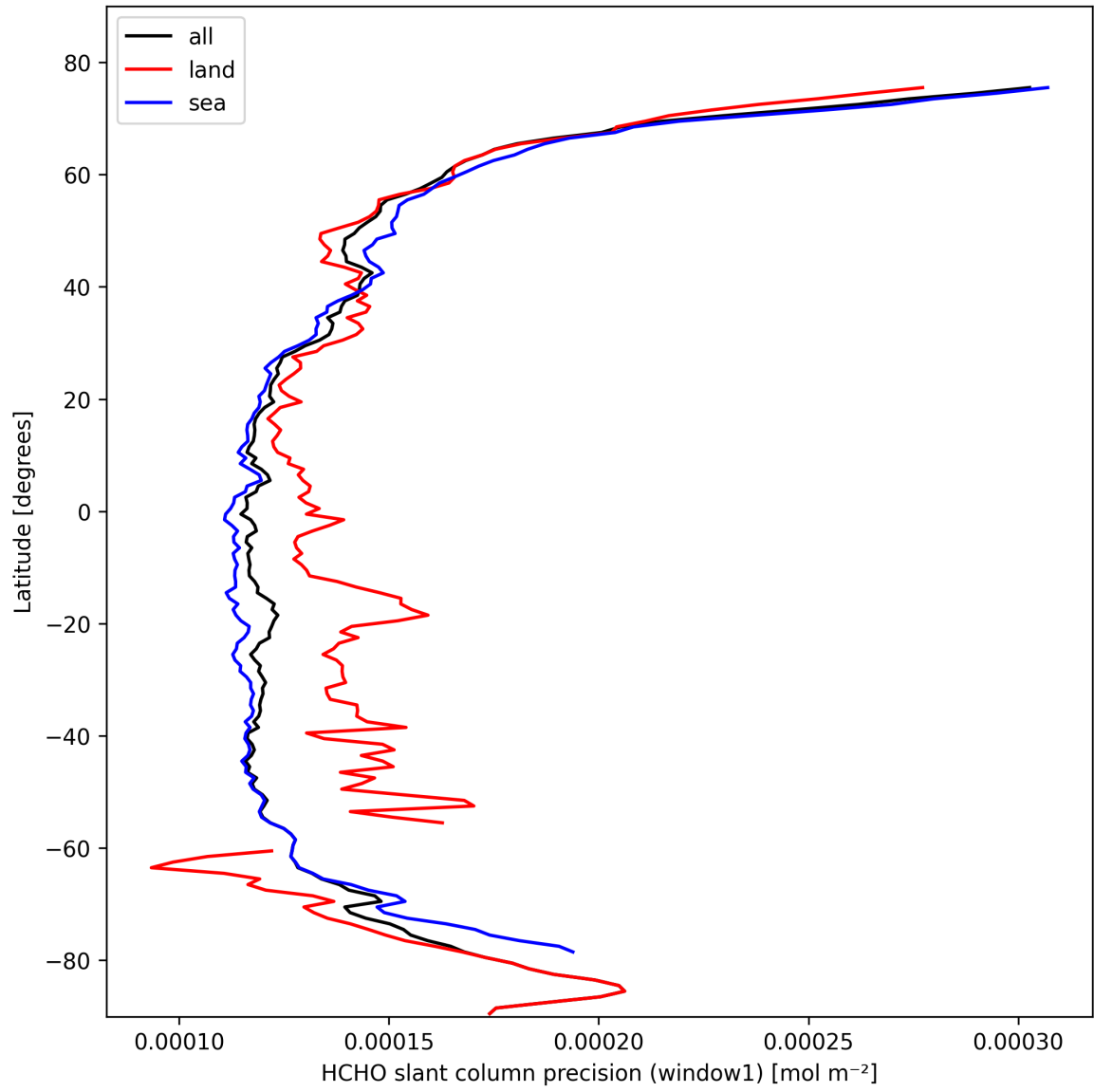
Figure 25: Zonal average of "HCHO slant column precision (window1)" for 2025-02-21 to 2025-02-23.
