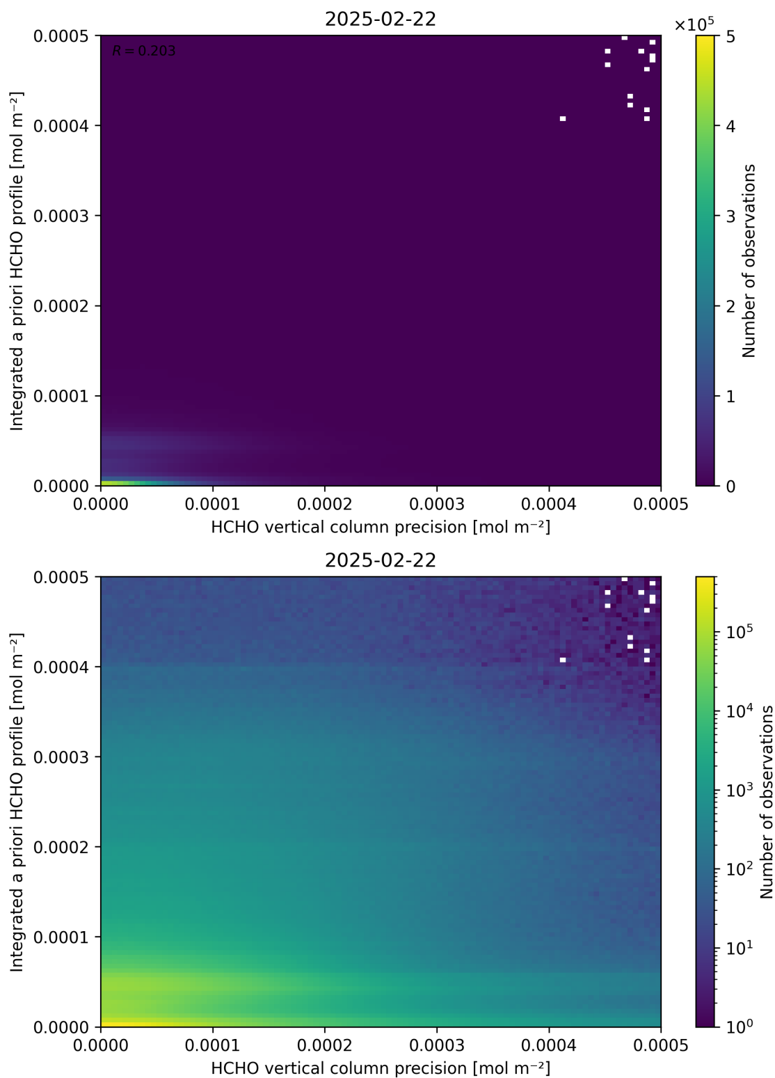
Figure 147: Scatter density plot of “HCHO vertical column precision” against “Integrated a priori HCHO profile” for 2025-02-21 to 2025-02-23.
