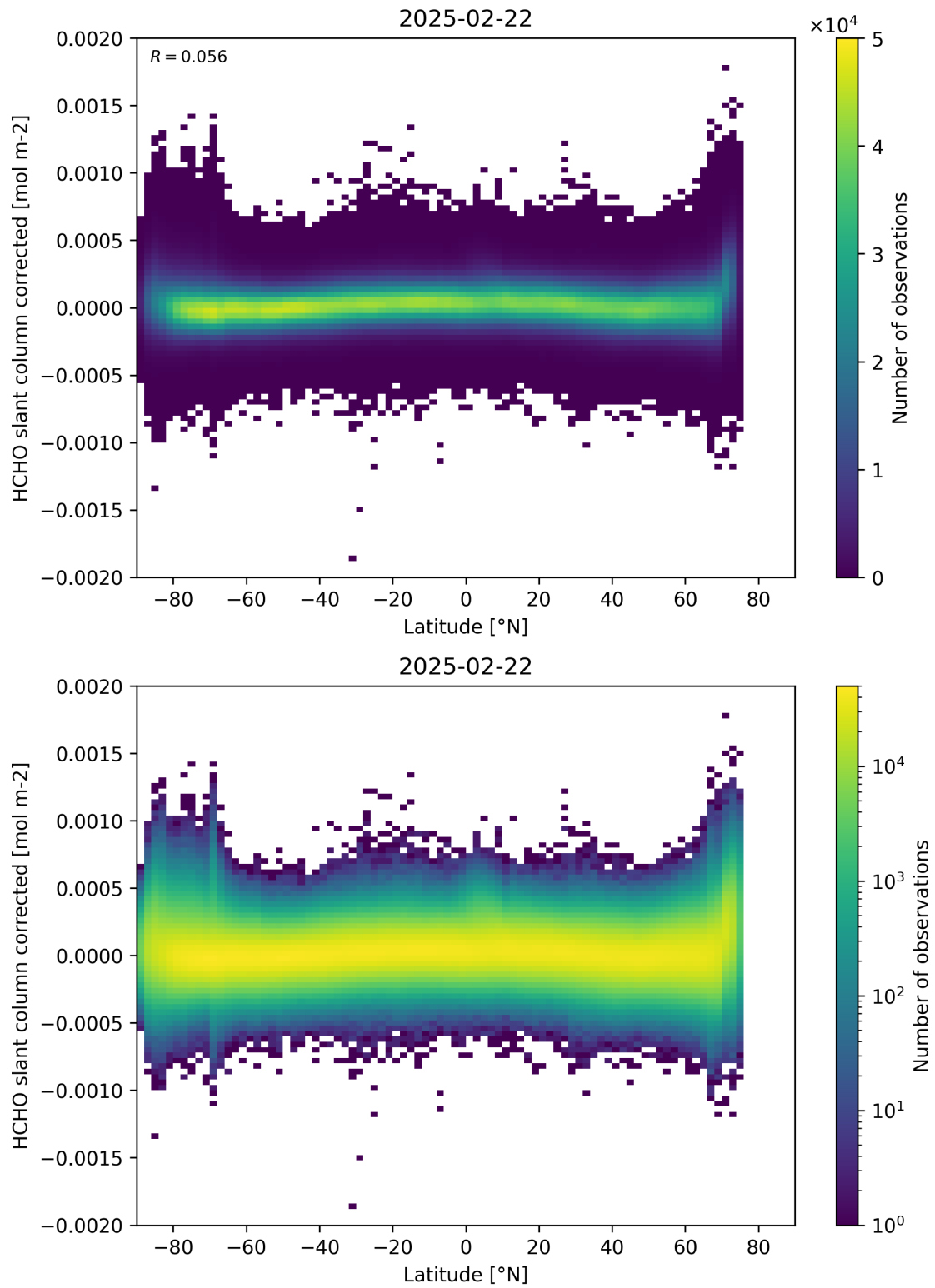
Figure 157: Scatter density plot of “Latitude” against “HCHO slant column corrected” for 2025-02-21 to 2025-02-23.
