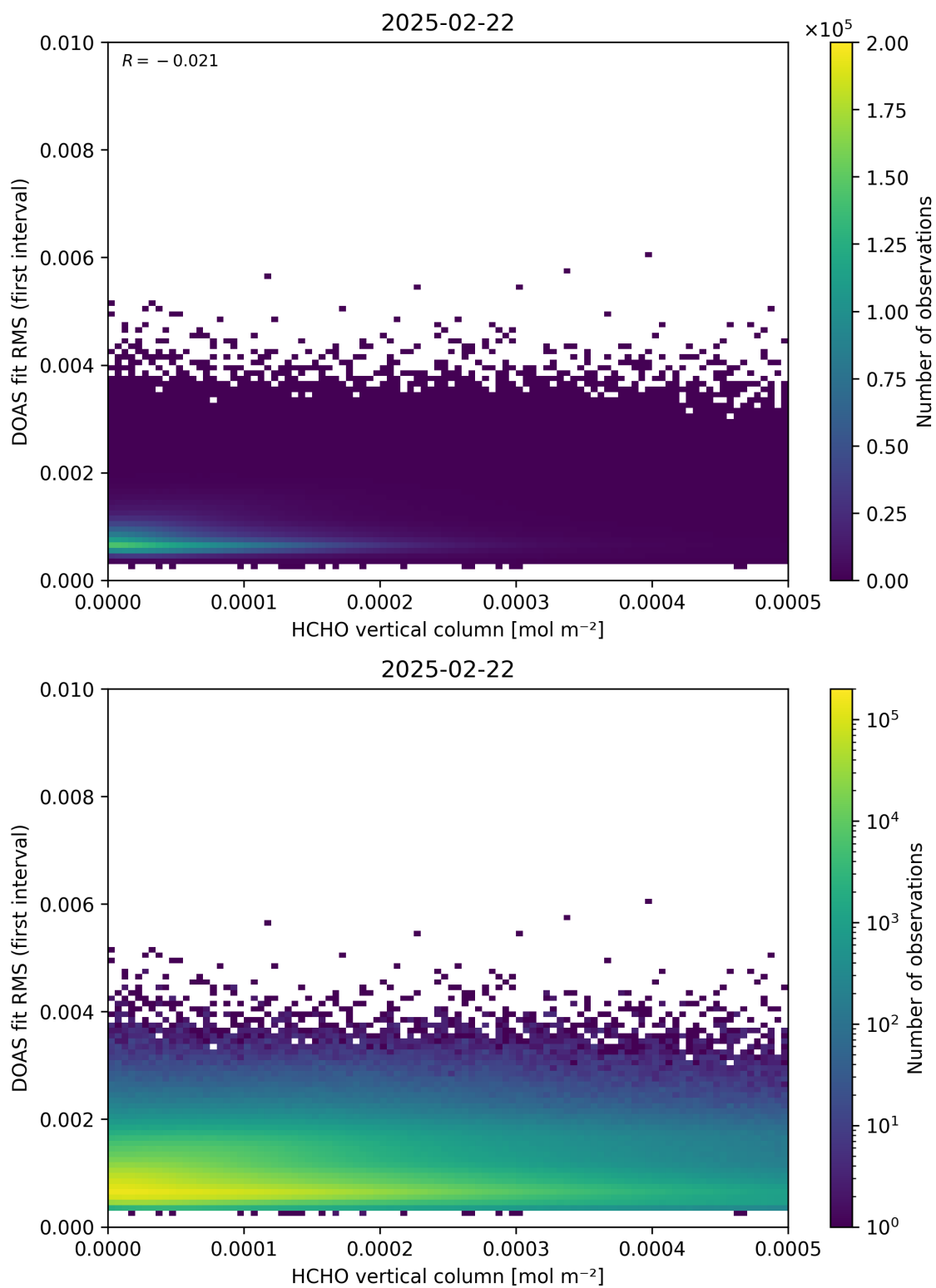
Figure 123: Scatter density plot of “HCHO vertical column” against “DOAS fit RMS (first interval)” for 2025-02-21 to 2025-02-23.
