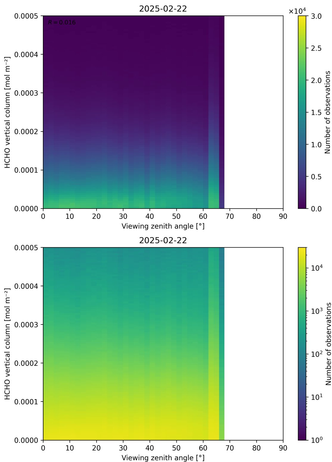
Figure 192: Scatter density plot of “Viewing zenith angle” against “HCHO vertical column” for 2025-02-21 to 2025-02-23.
