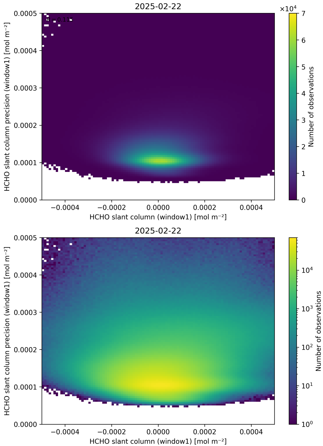
Figure 84: Scatter density plot of “HCHO slant column (window1)” against “HCHO slant column precision (window1)” for 2025-02-21 to 2025-02-23.
