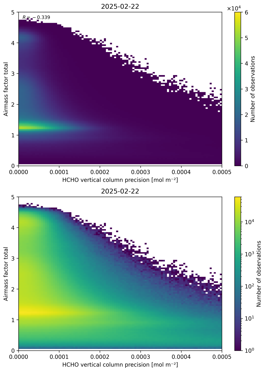
Figure 144: Scatter density plot of “HCHO vertical column precision” against “Airmass factor total” for 2025-02-21 to 2025-02-23.
