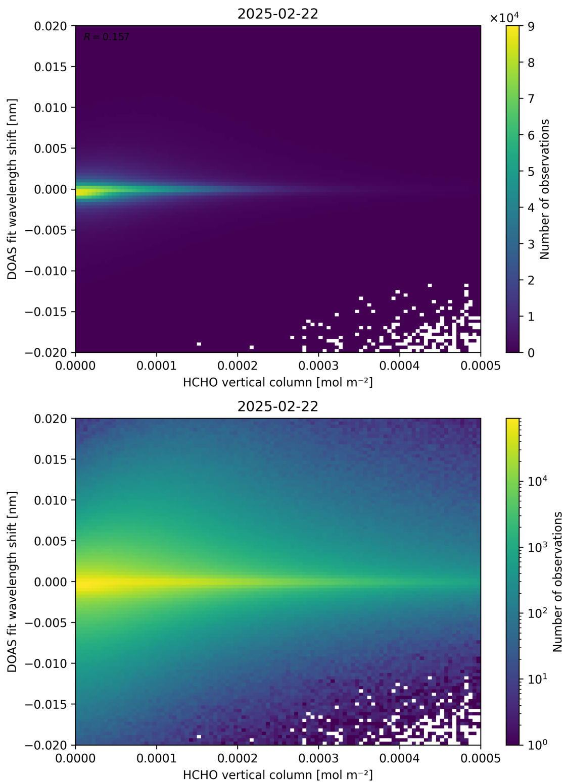
Figure 124: Scatter density plot of “HCHO vertical column” against “DOAS fit wavelength shift” for 2025-02-21 to 2025-02-23.
