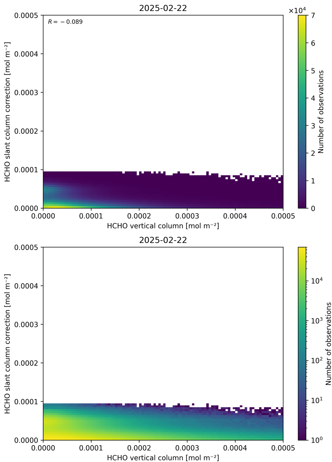
Figure 128: Scatter density plot of “HCHO vertical column” against “HCHO slant column correction” for 2025-02-21 to 2025-02-23.
