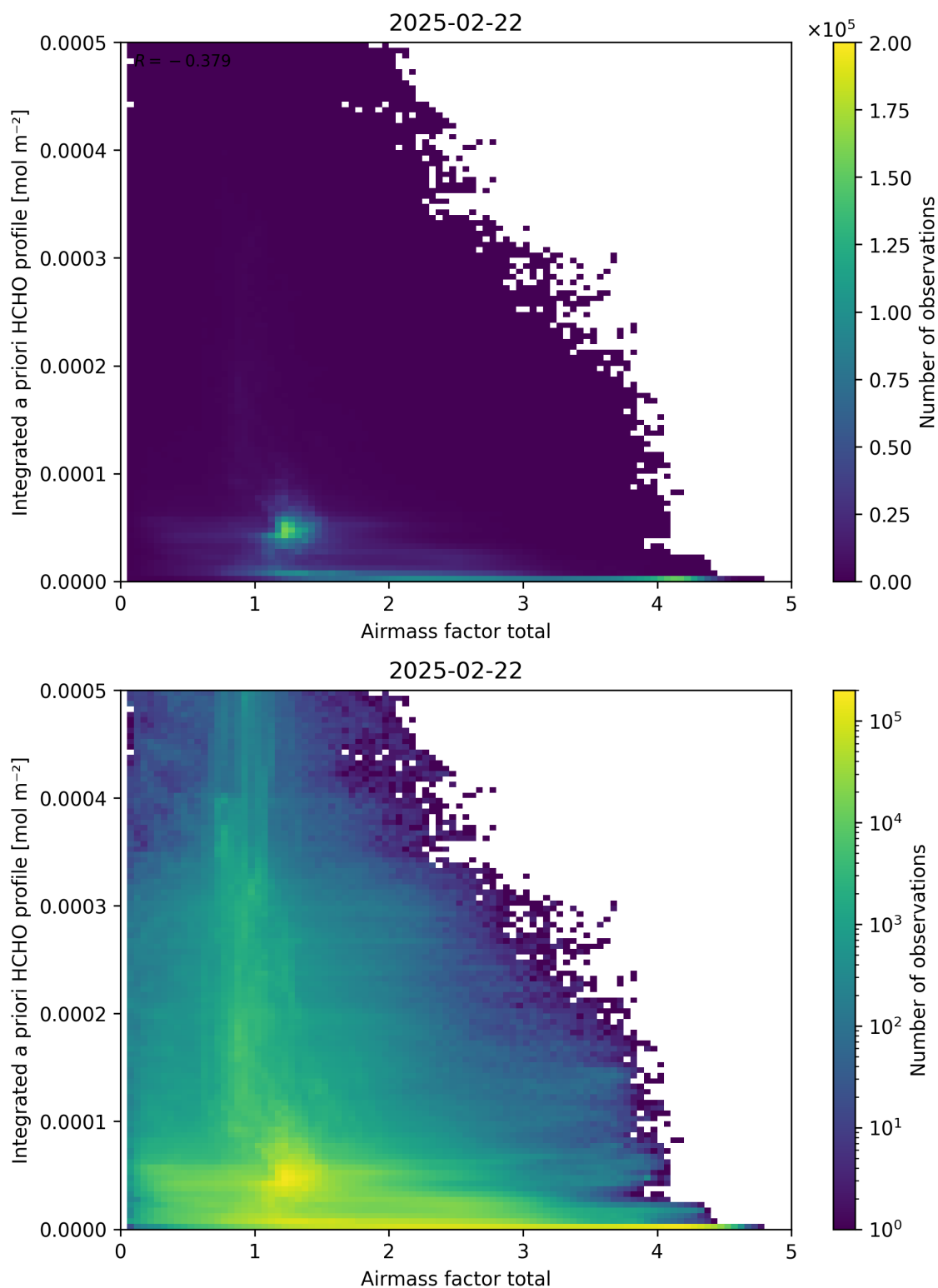
Figure 104: Scatter density plot of “Airmass factor total” against “Integrated a priori HCHO profile” for 2025-02-21 to 2025-02-23.
