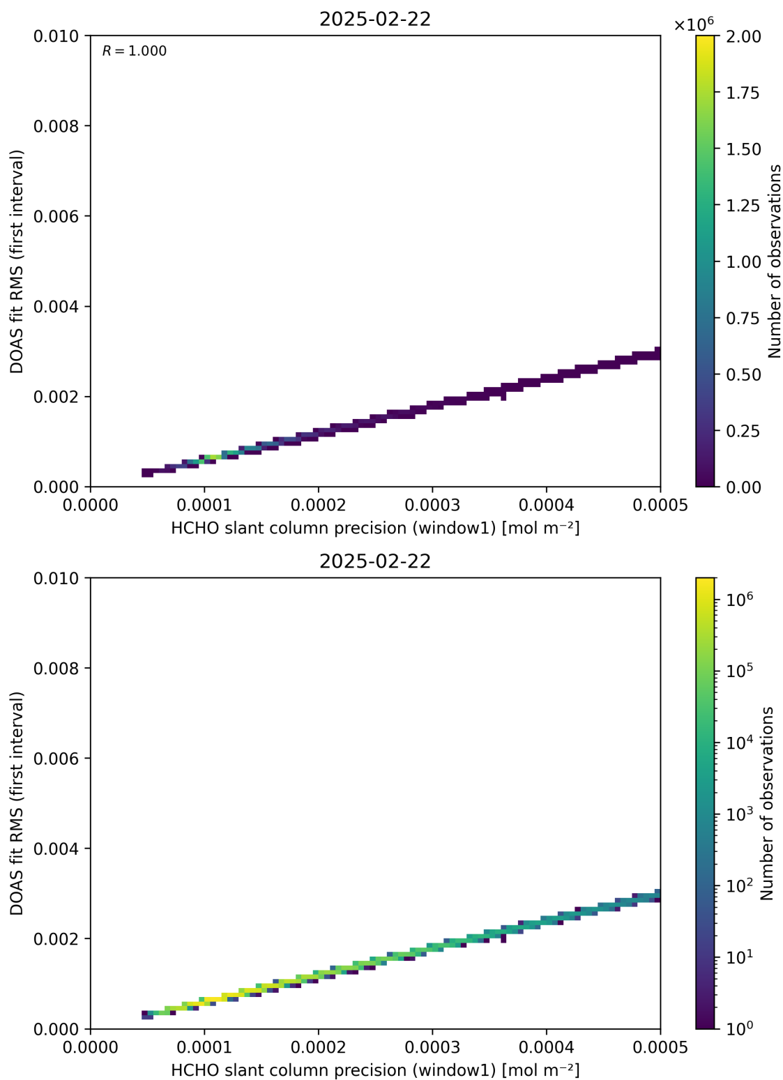
Figure 88: Scatter density plot of “HCHO slant column precision (window1)” against “DOAS fit RMS (first interval)” for 2025-02-21 to 2025-02-23.
