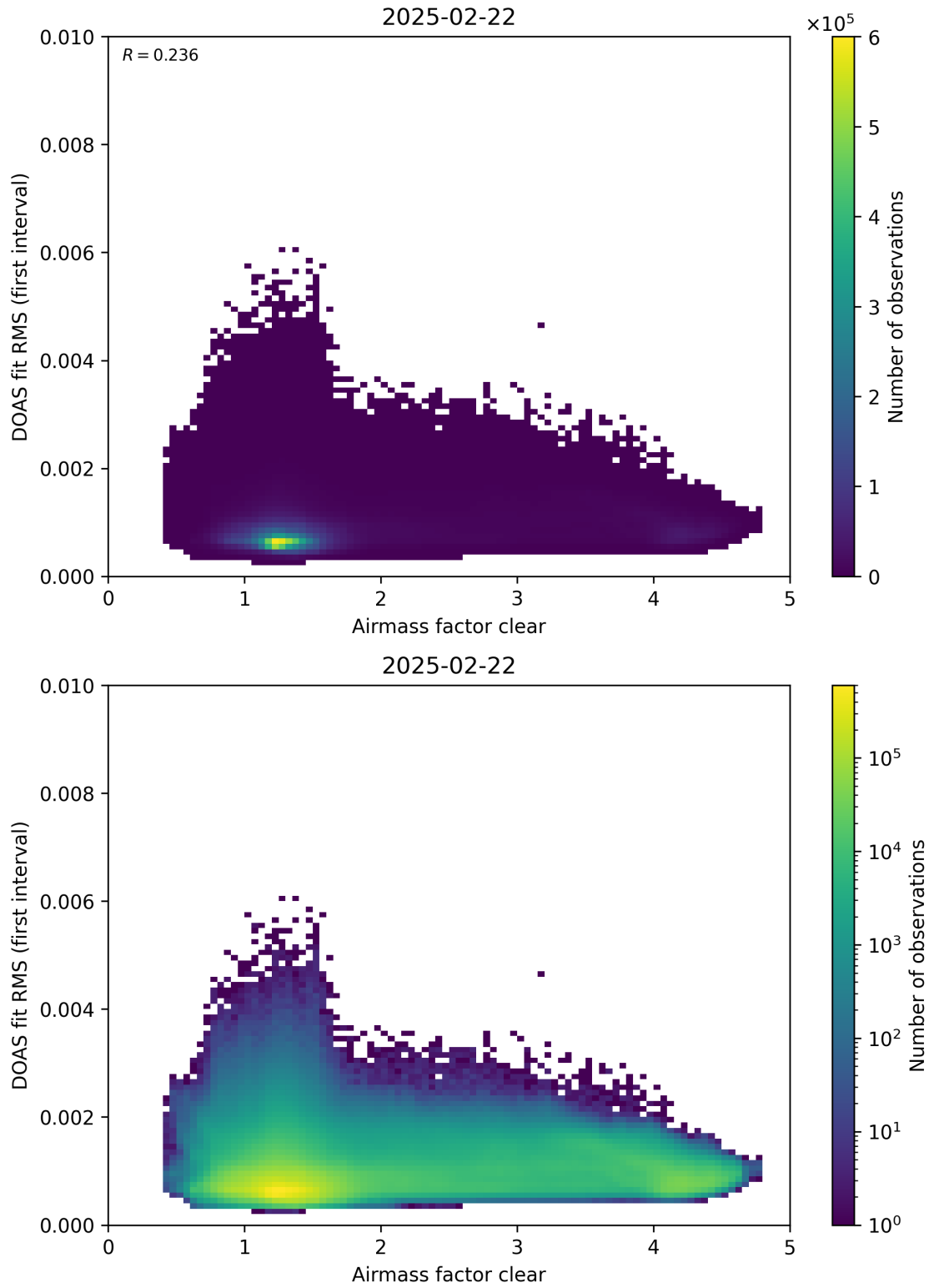
Figure 71: Scatter density plot of “Airmass factor clear” against “DOAS fit RMS (first interval)” for 2025-02-21 to 2025-02-23.
