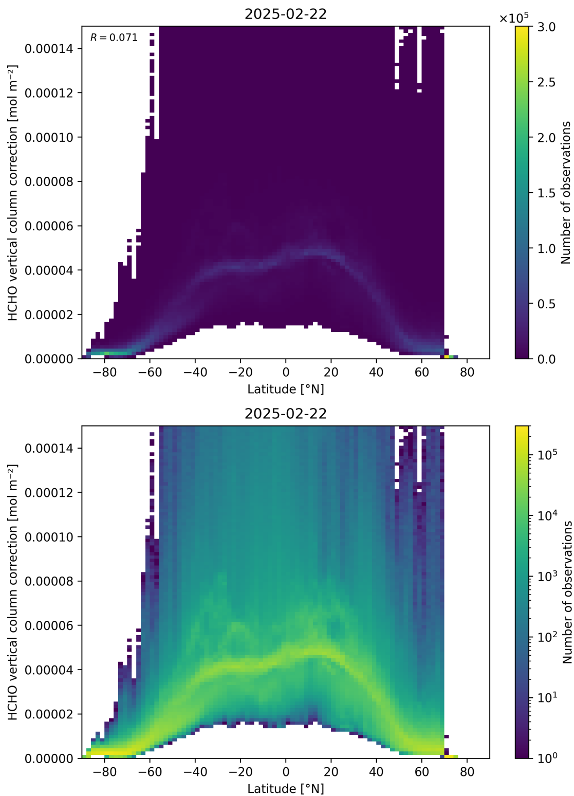
Figure 164: Scatter density plot of “Latitude” against “HCHO vertical column correction” for 2025-02-21 to 2025-02-23.
