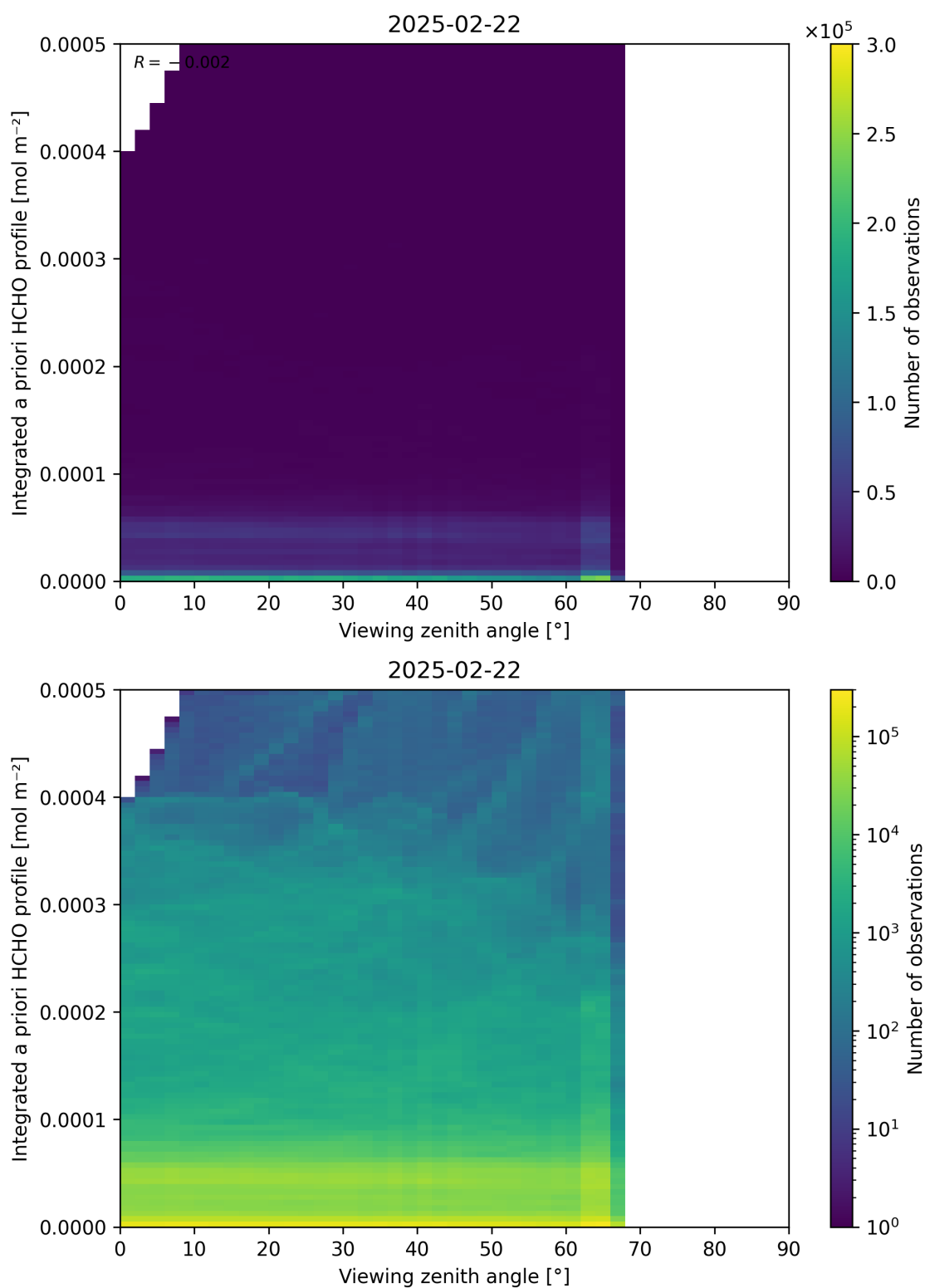
Figure 195: Scatter density plot of “Viewing zenith angle” against “Integrated a priori HCHO profile” for 2025-02-21 to 2025-02-23.
