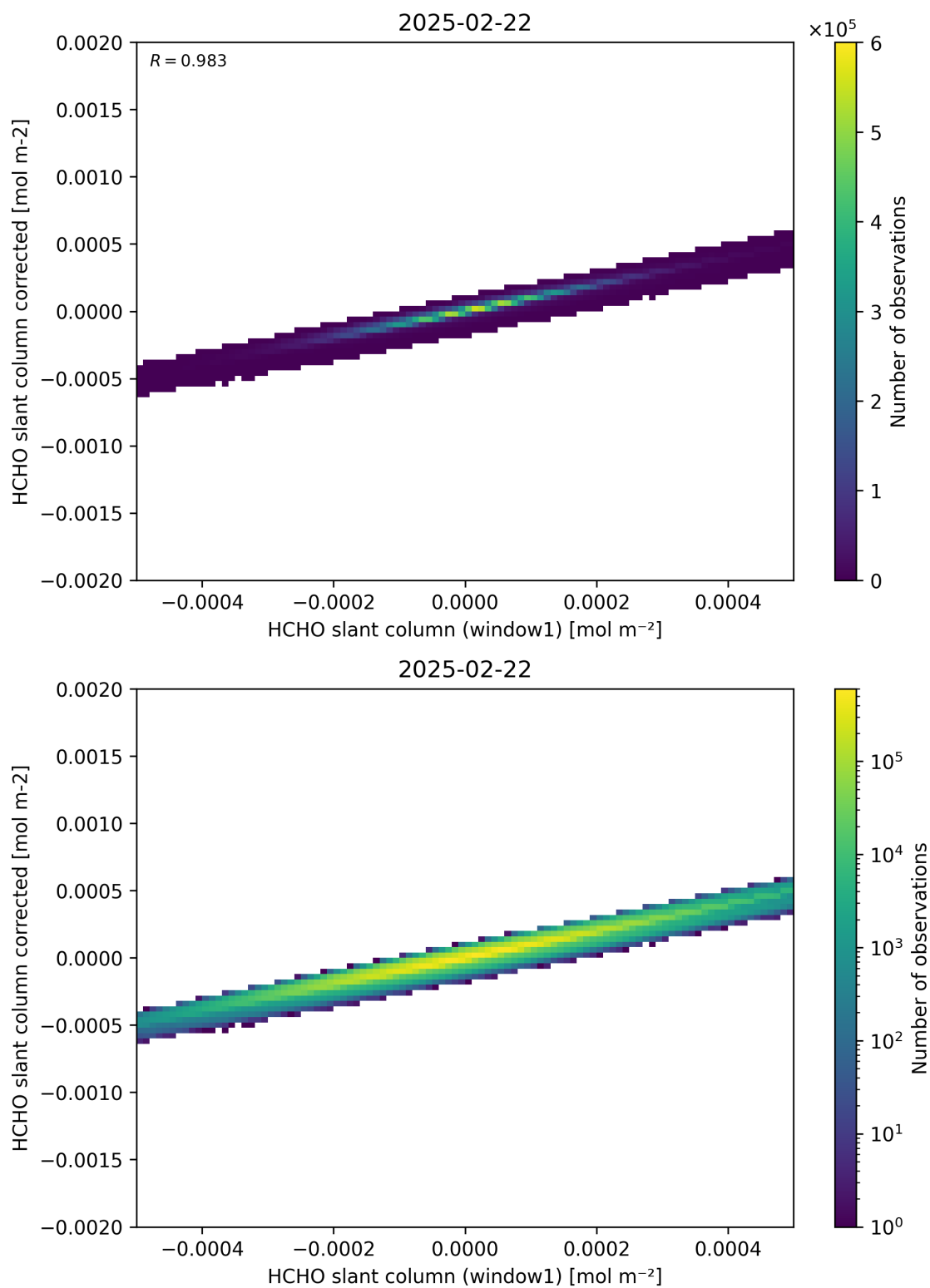
Figure 82: Scatter density plot of “HCHO slant column (window1)” against “HCHO slant column corrected” for 2025-02-21 to 2025-02-23.
