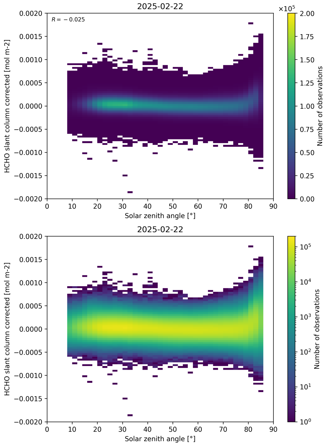
Figure 171: Scatter density plot of “Solar zenith angle” against “HCHO slant column corrected” for 2025-02-21 to 2025-02-23.
