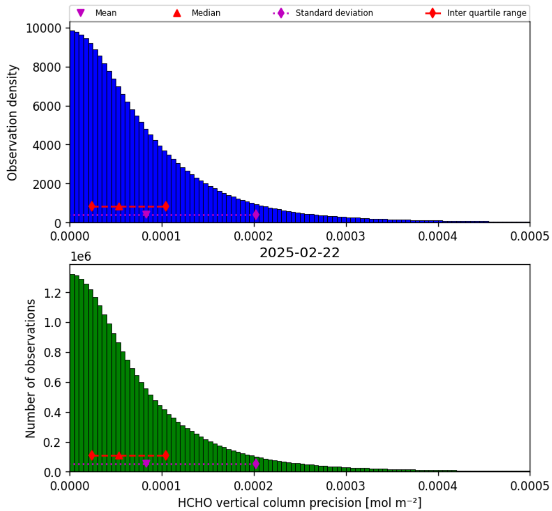
Figure 36: Histogram of “HCHO vertical column precision” for 2025-02-21 to 2025-02-23
