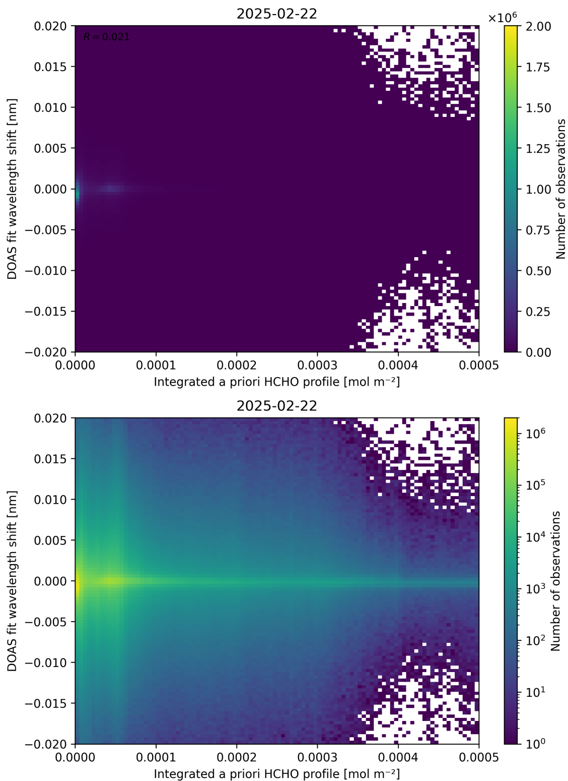
Figure 149: Scatter density plot of “Integrated a priori HCHO profile” against “DOAS fit wavelength shift” for 2025-02-21 to 2025-02-23.
