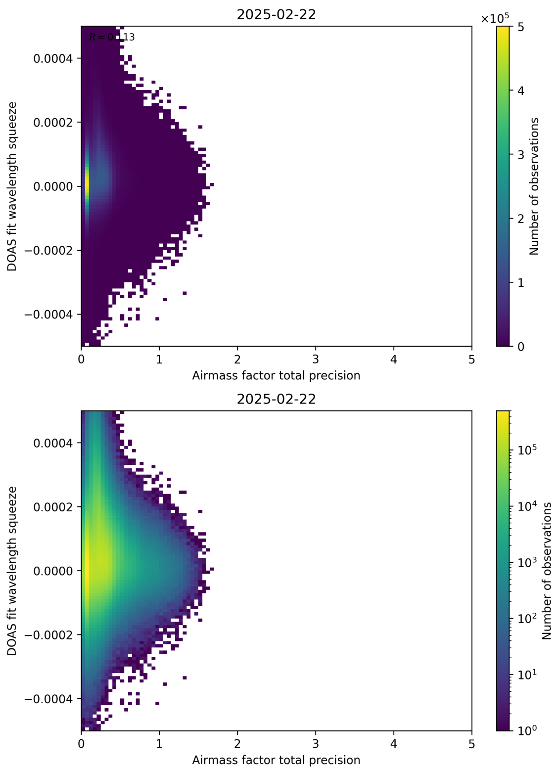
Figure 107: Scatter density plot of “Airmass factor total precision” against “DOAS fit wavelength squeeze” for 2025-02-21 to 2025-02-23.
