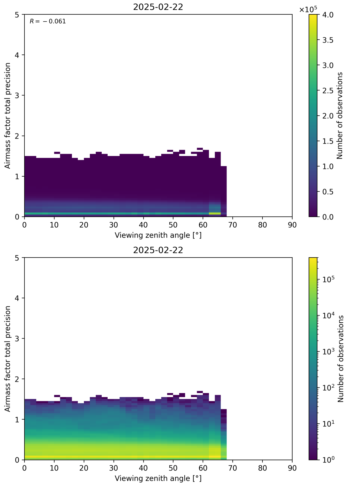
Figure 191: Scatter density plot of “Viewing zenith angle” against “Airmass factor total precision” for 2025-02-21 to 2025-02-23.
