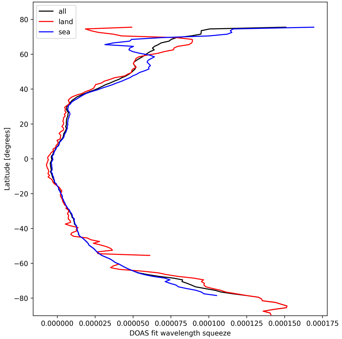
Figure 31: Zonal average of “DOAS fit wavelength squeeze” for 2025-02-21 to 2025-02-23.
