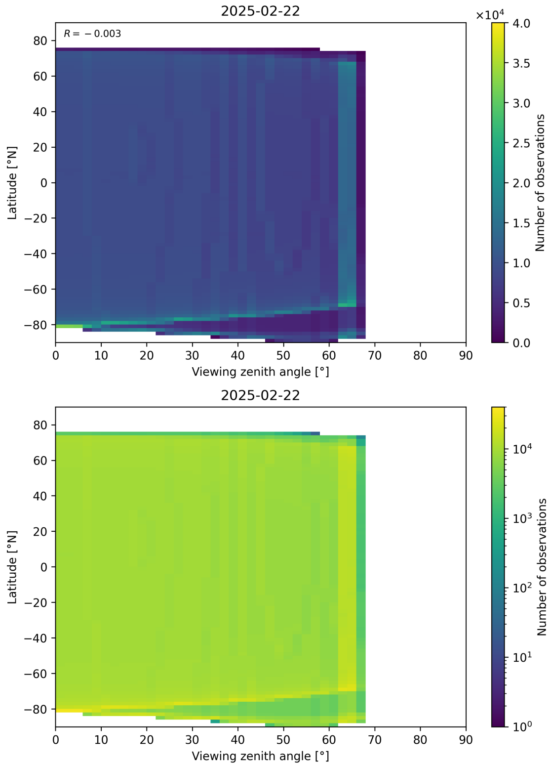
Figure 196: Scatter density plot of “Viewing zenith angle” against “Latitude” for 2025-02-21 to 2025-02-23.
