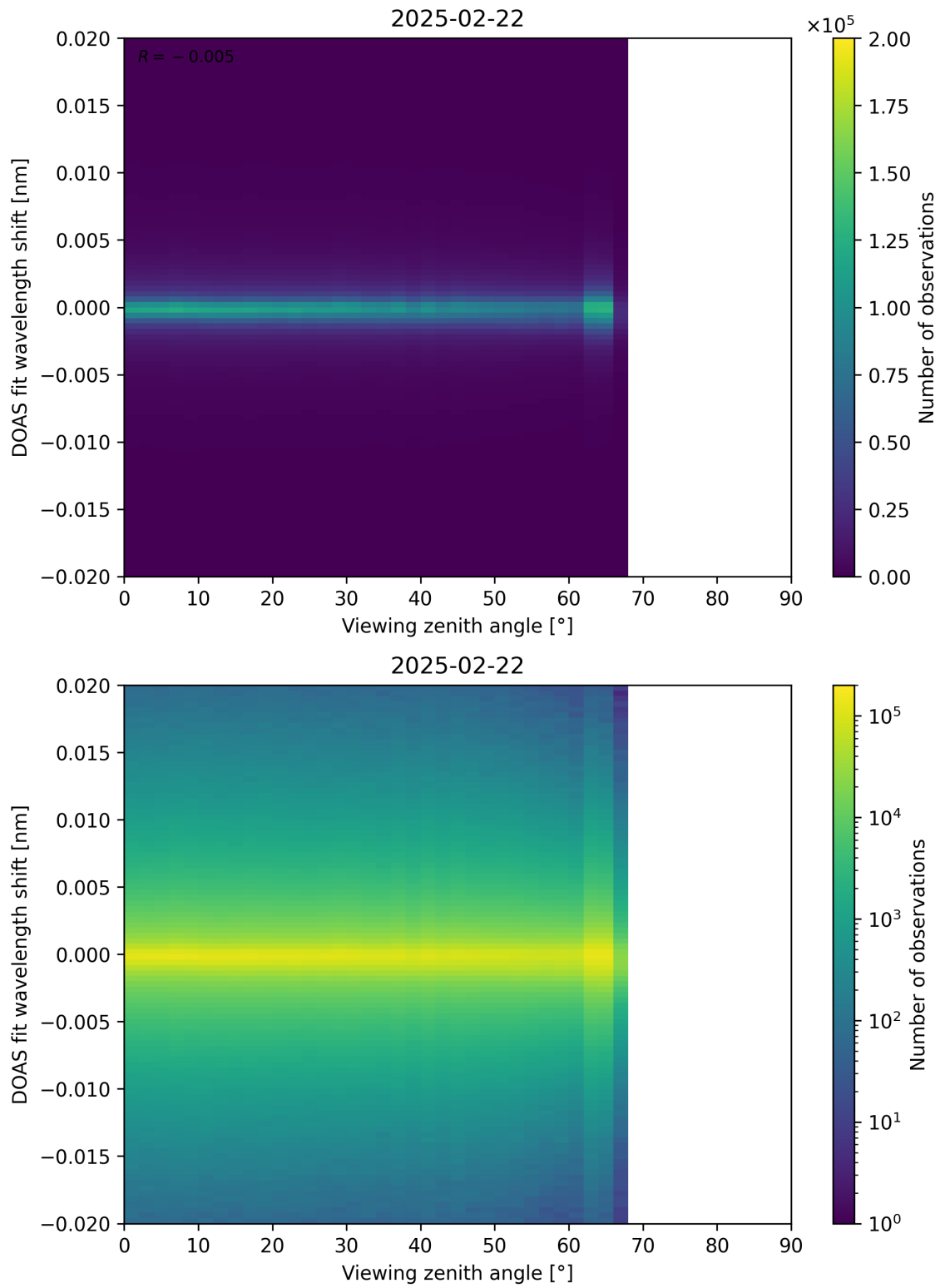
Figure 183: Scatter density plot of “Viewing zenith angle” against “DOAS fit wavelength shift” for 2025-02-21 to 2025-02-23.
