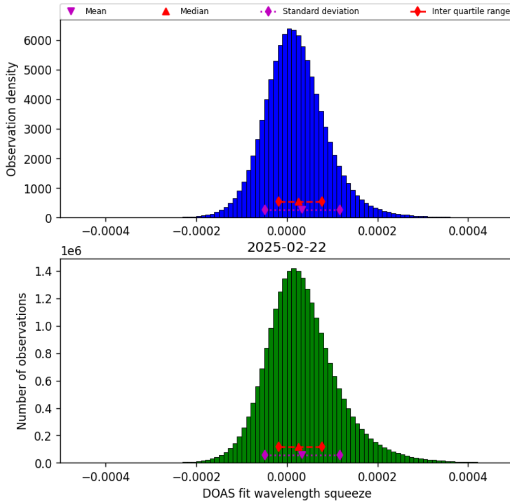
Figure 45: Histogram of “DOAS fit wavelength squeeze” for 2025-02-21 to 2025-02-23
