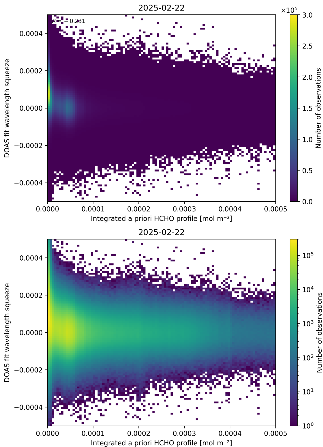
Figure 150: Scatter density plot of “Integrated a priori HCHO profile” against “DOAS fit wavelength squeeze” for 2025-02-21 to 2025-02-23.
