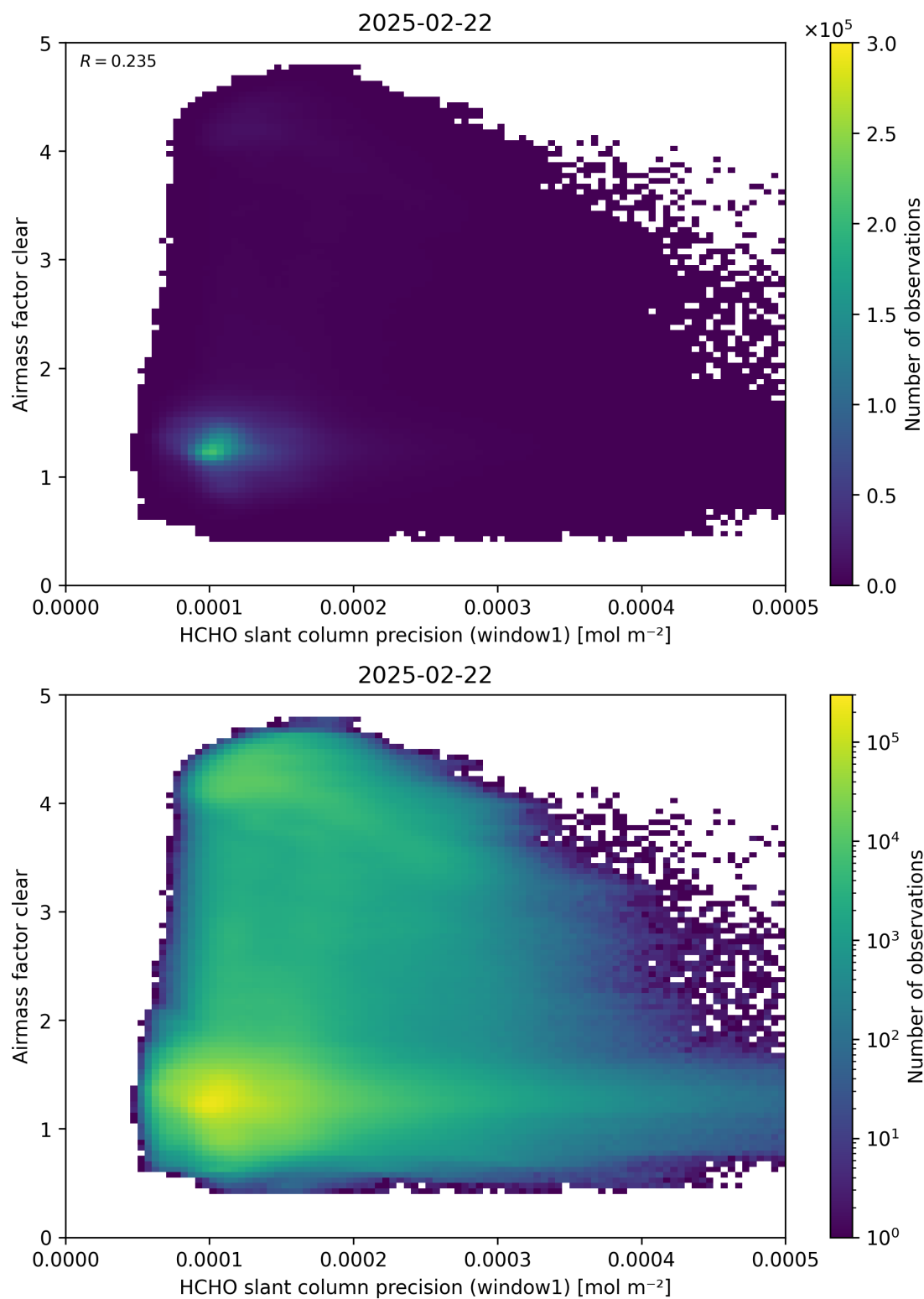
Figure 91: Scatter density plot of “HCHO slant column precision (window1)” against “Airmass factor clear” for 2025-02-21 to 2025-02-23.
