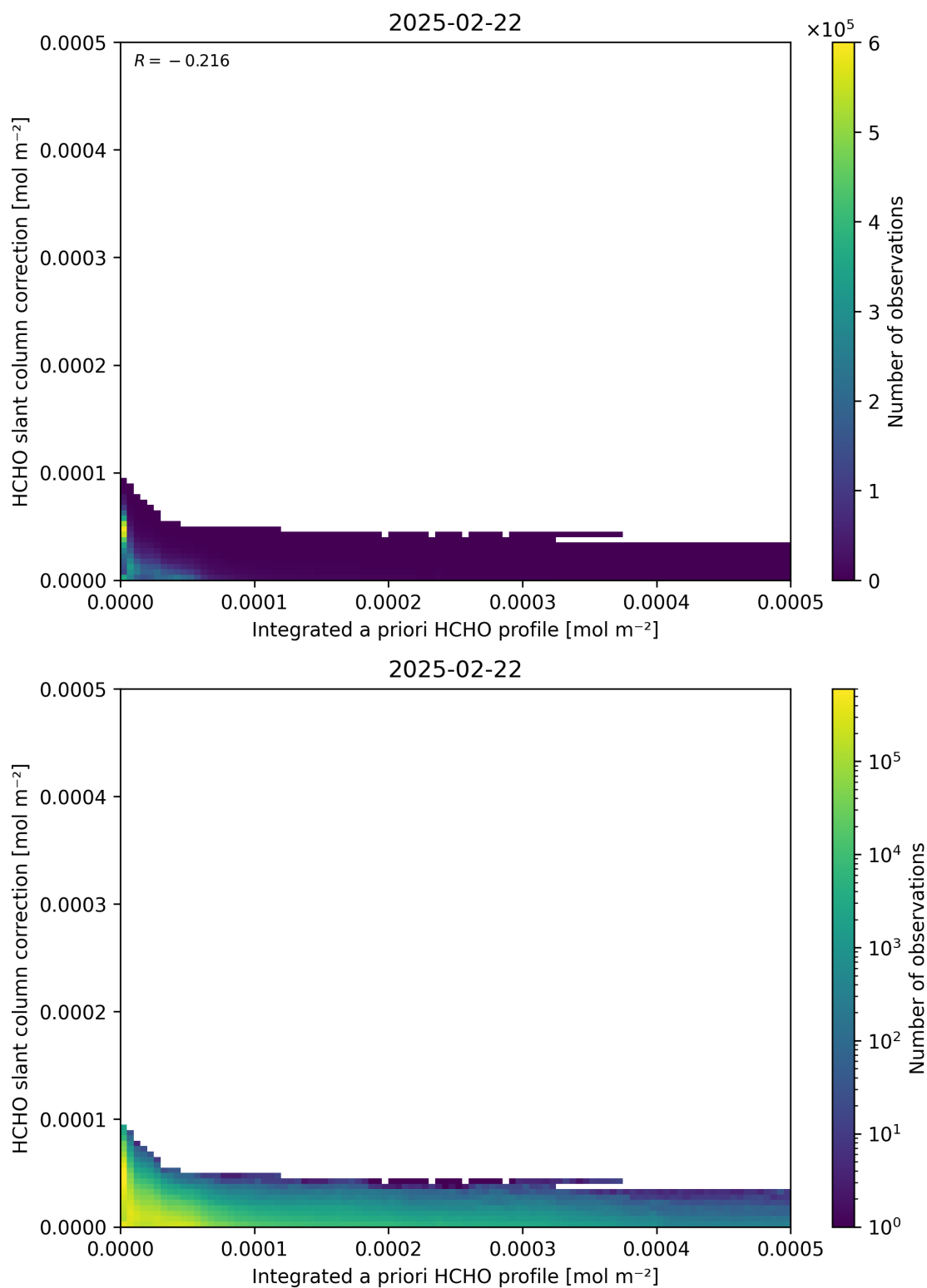
Figure 152: Scatter density plot of “Integrated a priori HCHO profile” against “HCHO slant column correction” for 2025-02-21 to 2025-02-23.
