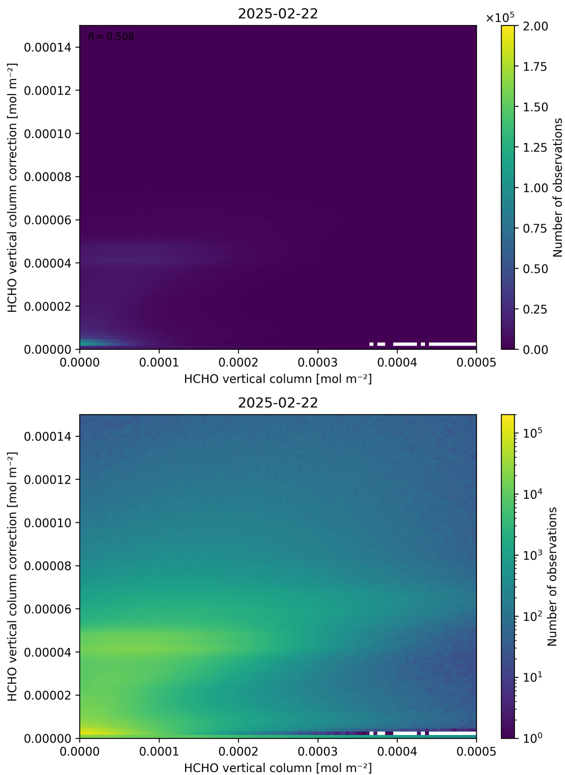
Figure 133: Scatter density plot of “HCHO vertical column” against “HCHO vertical column correction” for 2025-02-21 to 2025-02-23.
