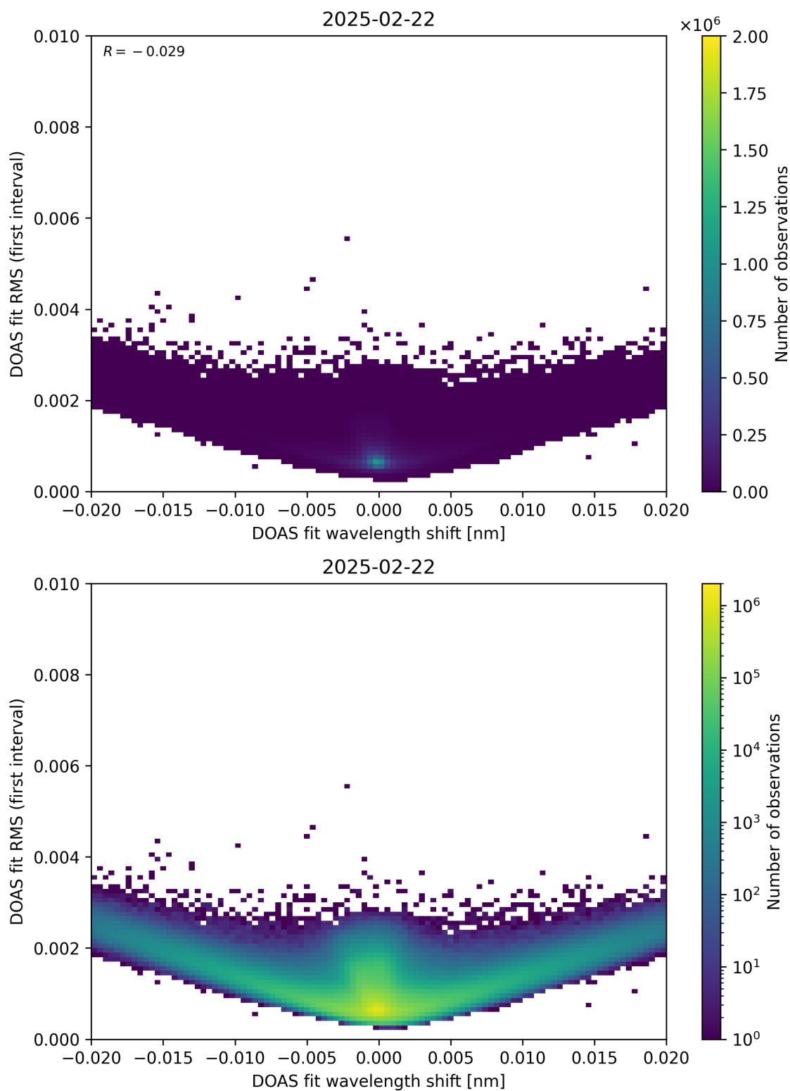
Figure 64: Scatter density plot of “DOAS fit wavelength shift” against “DOAS fit RMS (first interval)” for 2025-02-21 to 2025-02-23.
