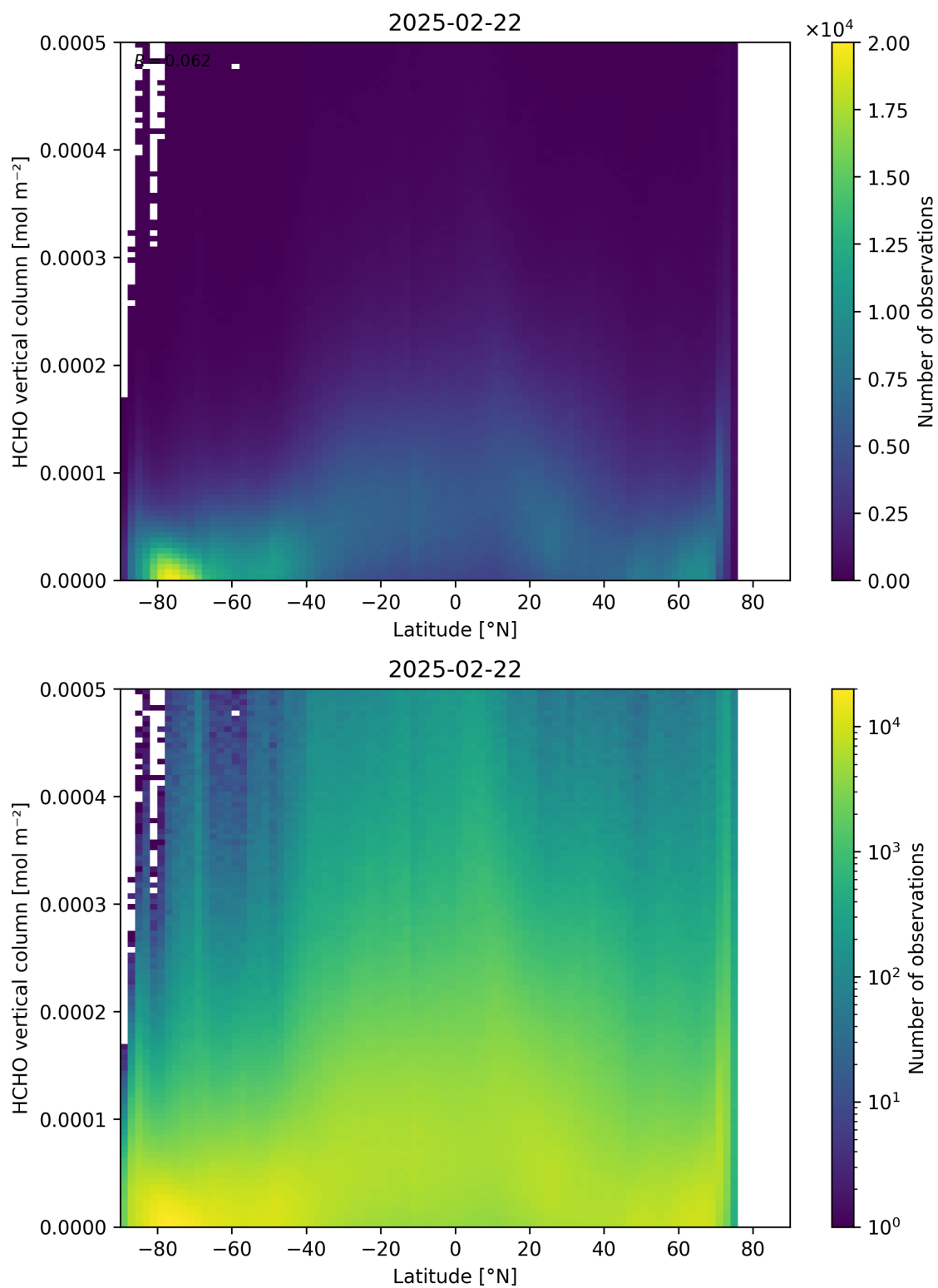
Figure 163: Scatter density plot of “Latitude” against “HCHO vertical column” for 2025-02-21 to 2025-02-23.
