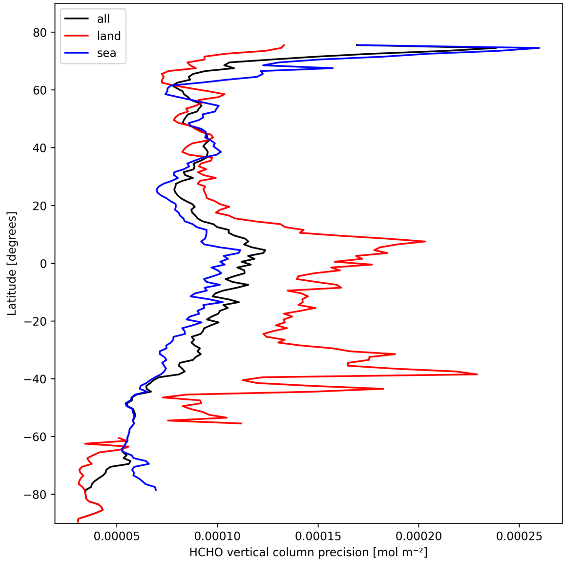
Figure 22: Zonal average of “HCHO vertical column precision” for 2025-02-21 to 2025-02-23.
