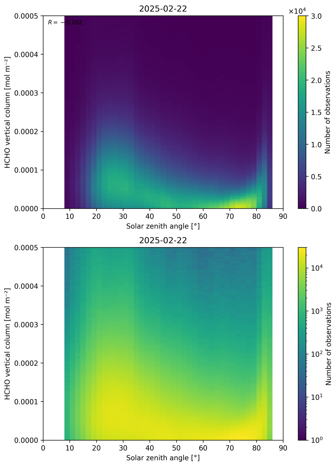
Figure 177: Scatter density plot of “Solar zenith angle” against “HCHO vertical column” for 2025-02-21 to 2025-02-23.
