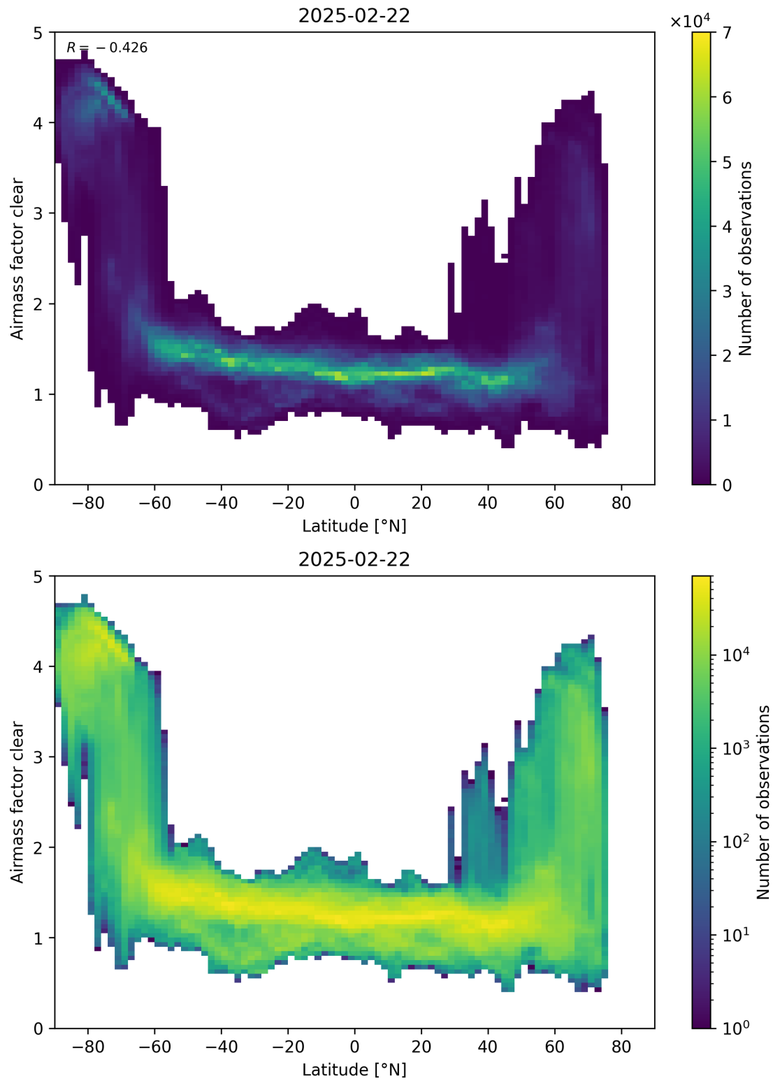
Figure 156: Scatter density plot of “Latitude” against “Airmass factor clear” for 2025-02-21 to 2025-02-23.
