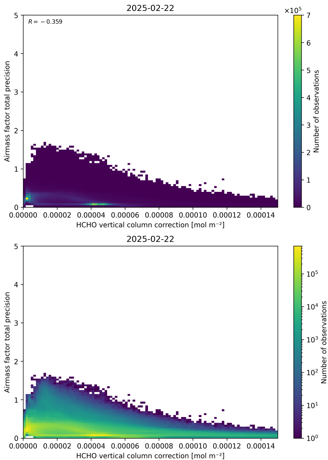
Figure 121: Scatter density plot of “HCHO vertical column correction” against “Airmass factor total precision” for 2025-02-21 to 2025-02-23.
