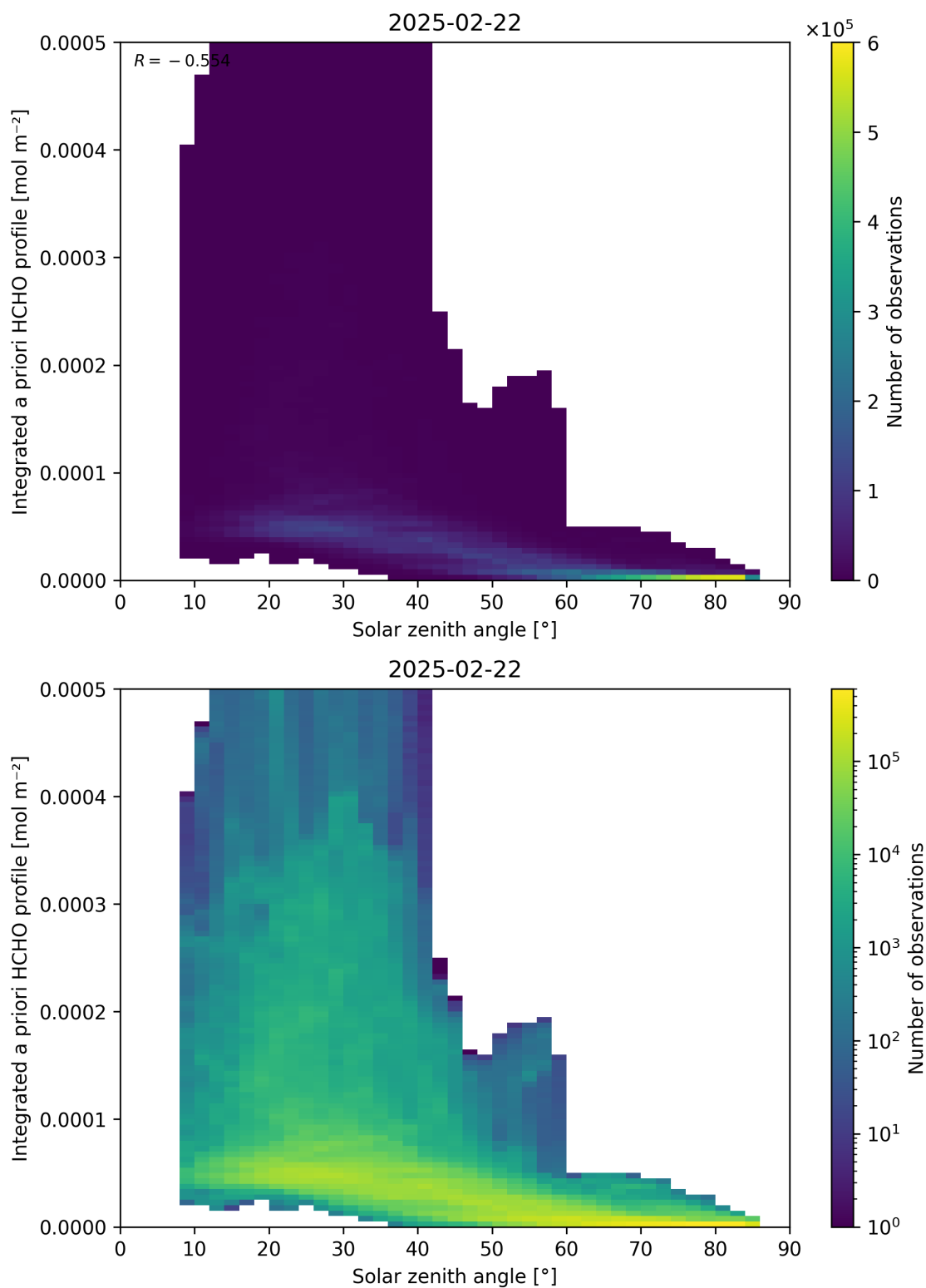
Figure 180: Scatter density plot of “Solar zenith angle” against “Integrated a priori HCHO profile” for 2025-02-21 to 2025-02-23.
