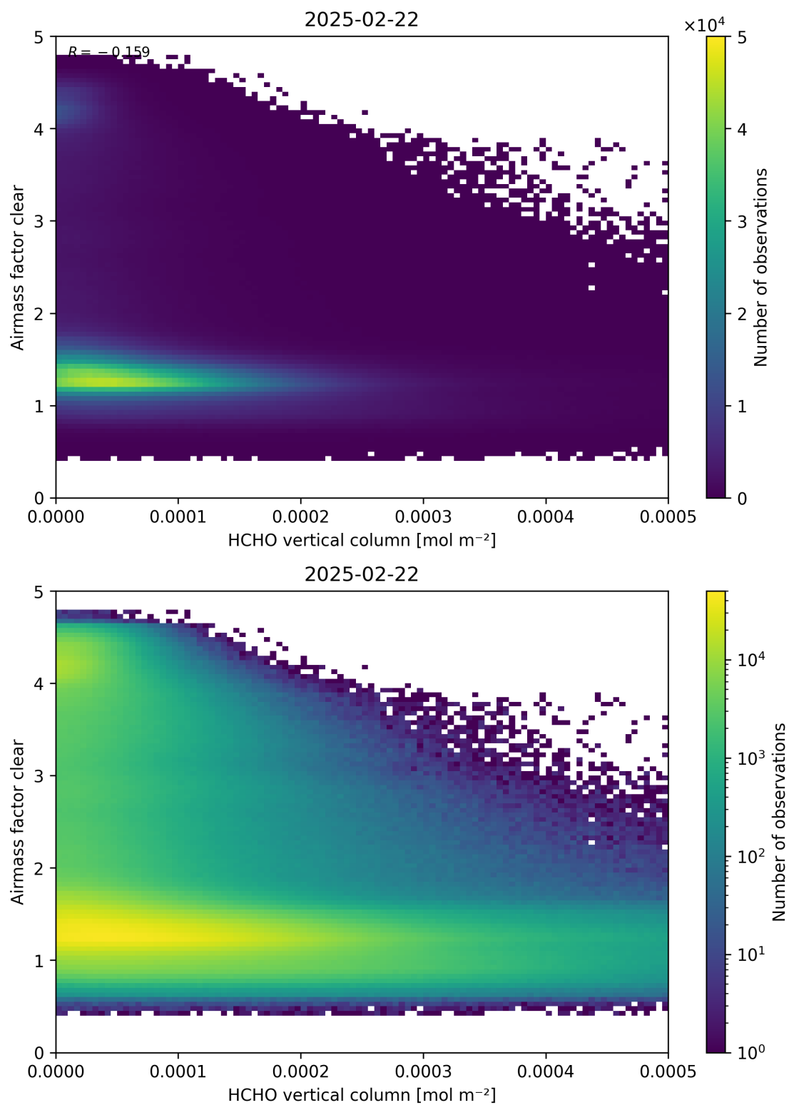
Figure 126: Scatter density plot of “HCHO vertical column” against “Airmass factor clear” for 2025-02-21 to 2025-02-23.
