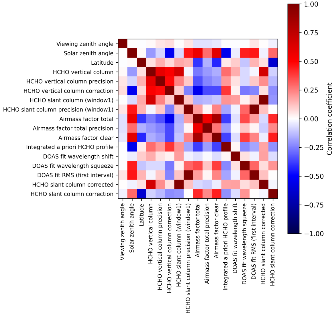
Figure 2: Map of correlation matrix for 2025-02-21 to 2025-02-23.
