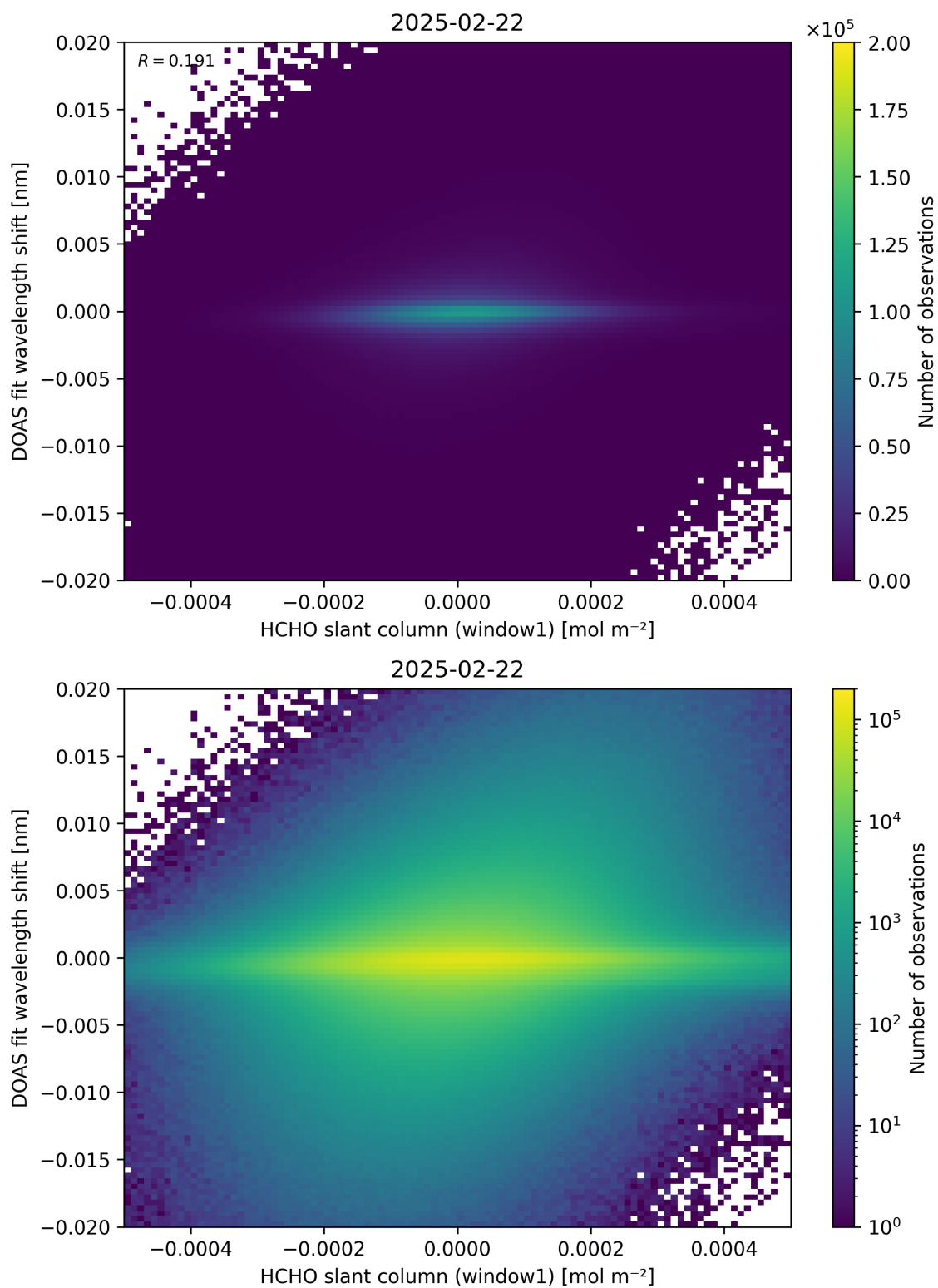
Figure 79: Scatter density plot of “HCHO slant column (window1)” against “DOAS fit wavelength shift” for 2025-02-21 to 2025-02-23.
