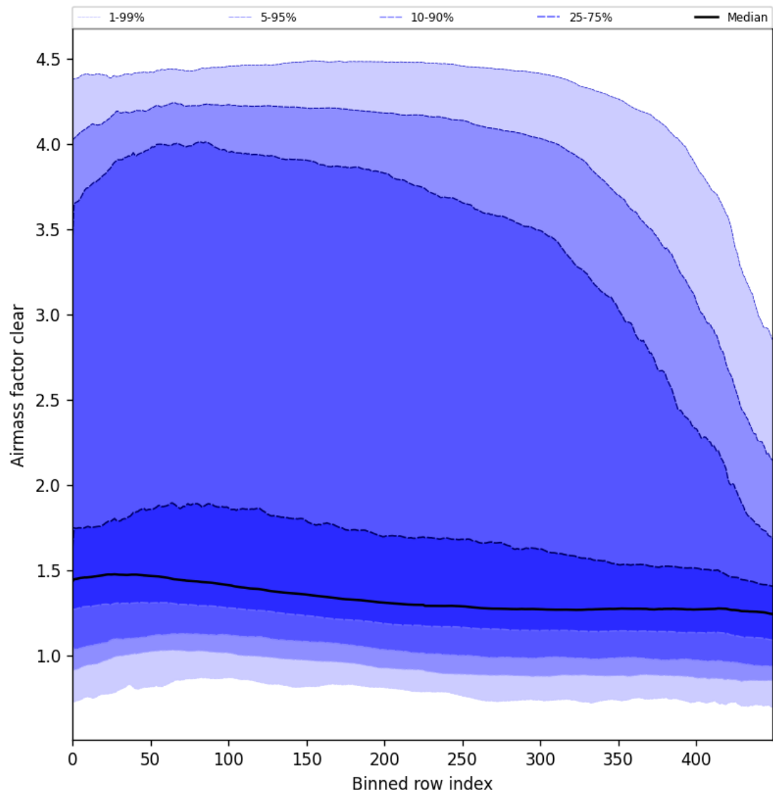
Figure 56: Along track statistics of “Airmass factor clear” for 2025-02-21 to 2025-02-23
