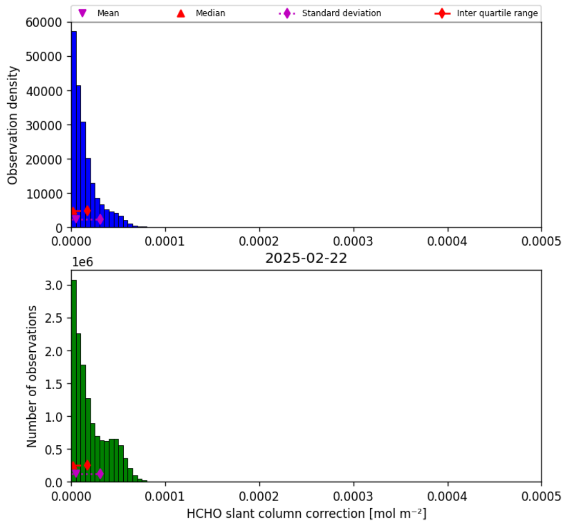
Figure 47: Histogram of “HCHO slant column correction” for 2025-02-21 to 2025-02-23
