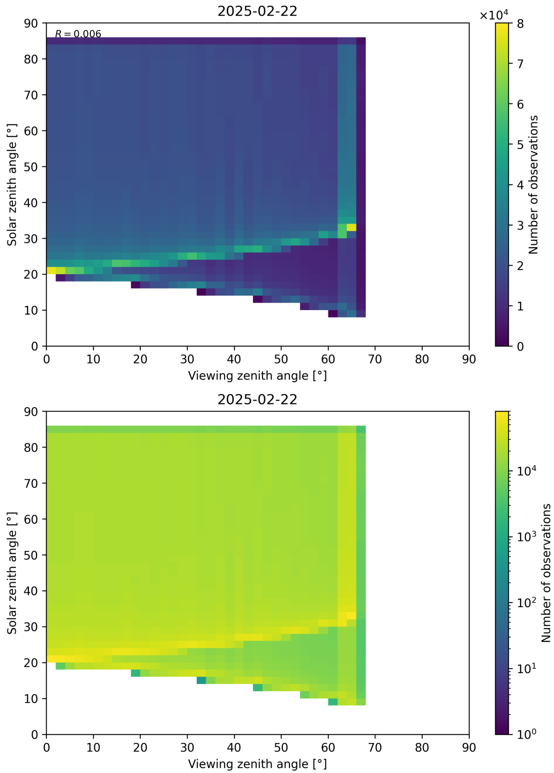
Figure 197: Scatter density plot of “Viewing zenith angle” against “Solar zenith angle” for 2025-02-21 to 2025-02-23.
