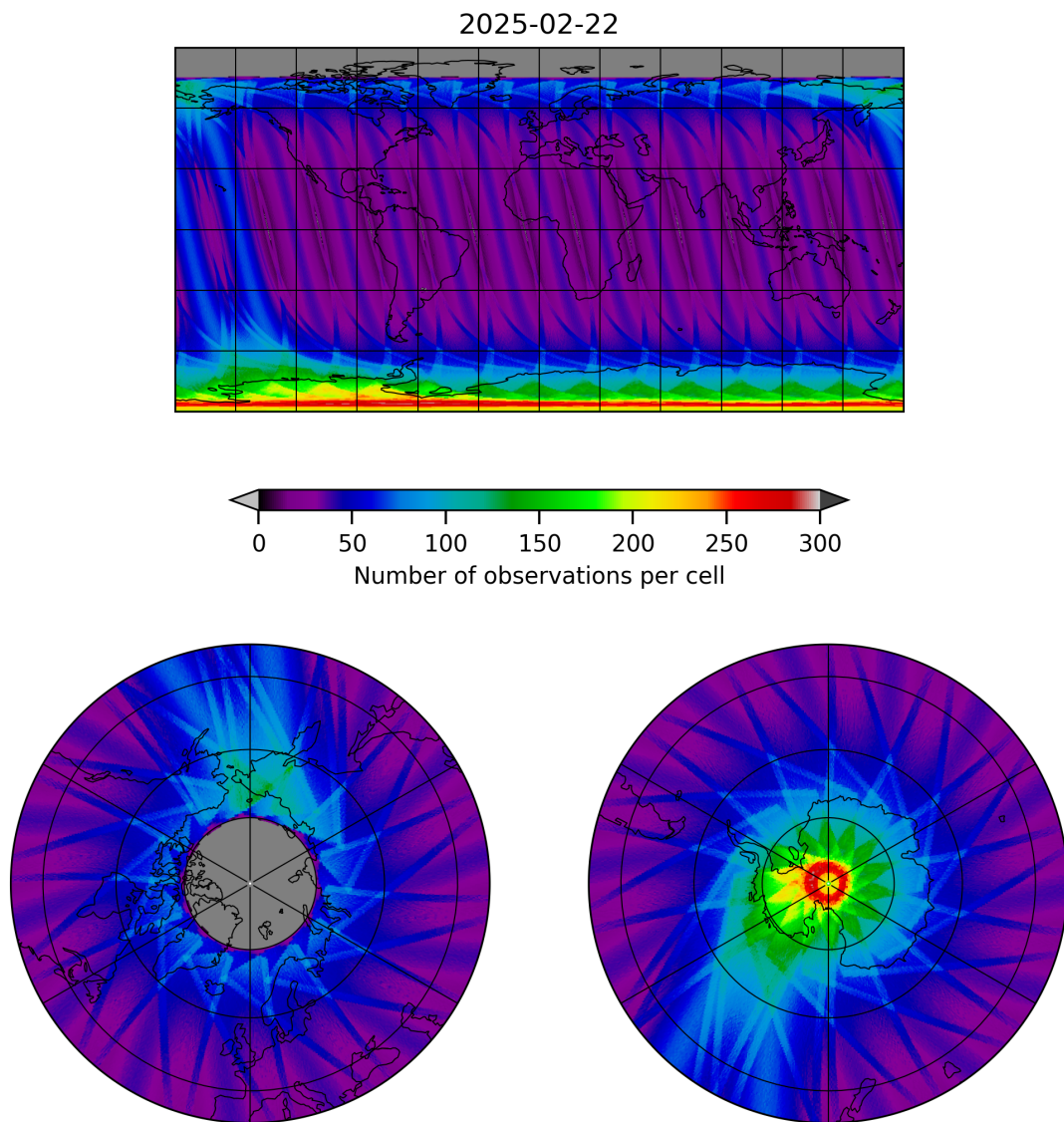
Figure 19: Map of the number of observations for 2025-02-21 to 2025-02-23
