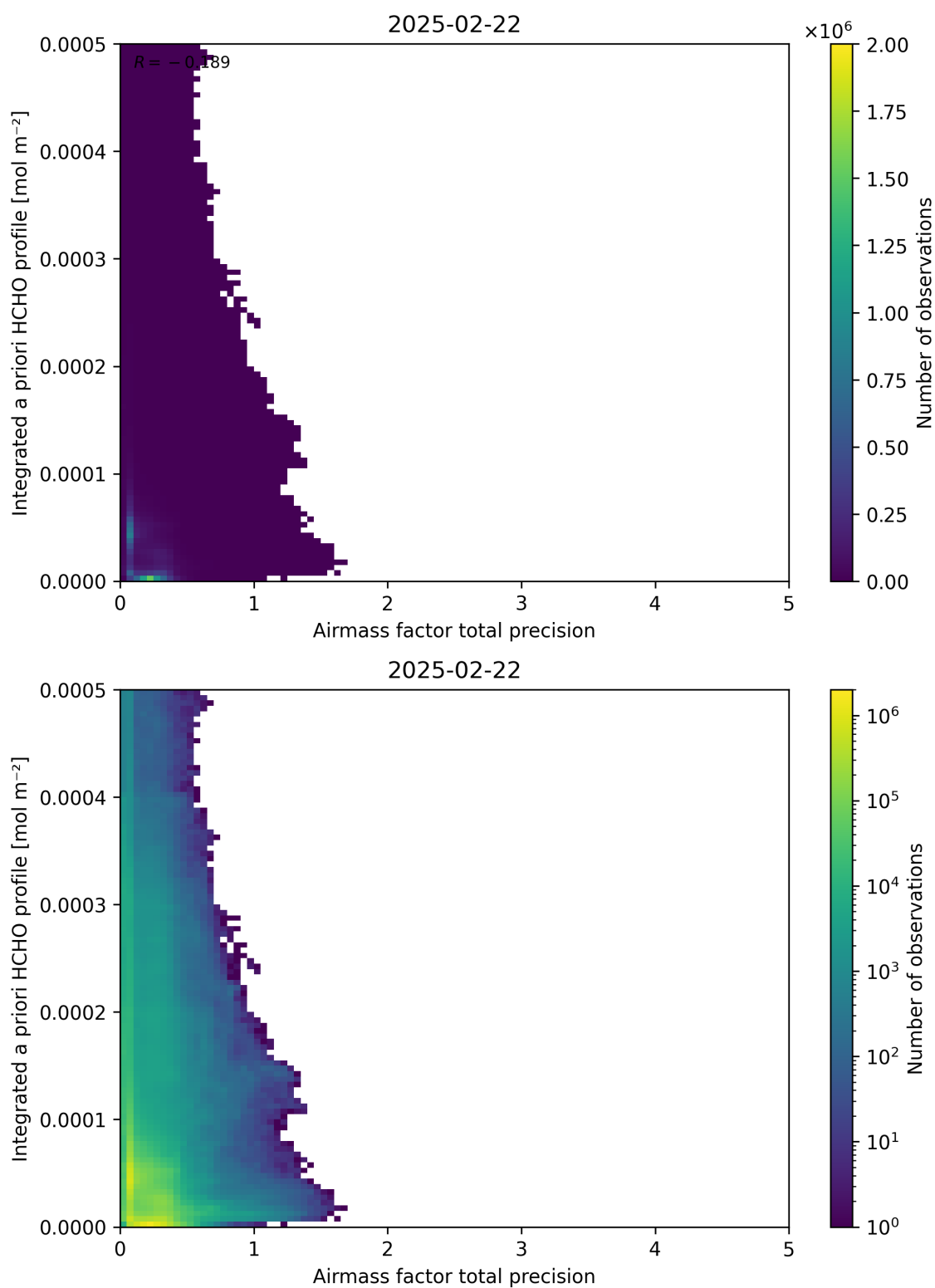
Figure 111: Scatter density plot of “Airmass factor total precision” against “Integrated a priori HCHO profile” for 2025-02-21 to 2025-02-23.
