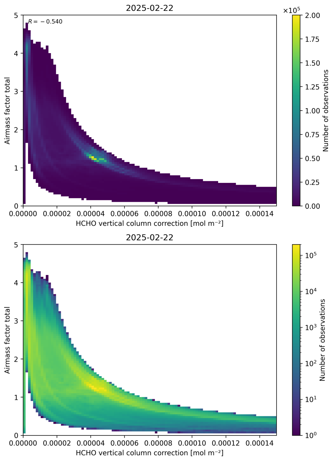
Figure 120: Scatter density plot of “HCHO vertical column correction” against “Airmass factor total” for 2025-02-21 to 2025-02-23.
