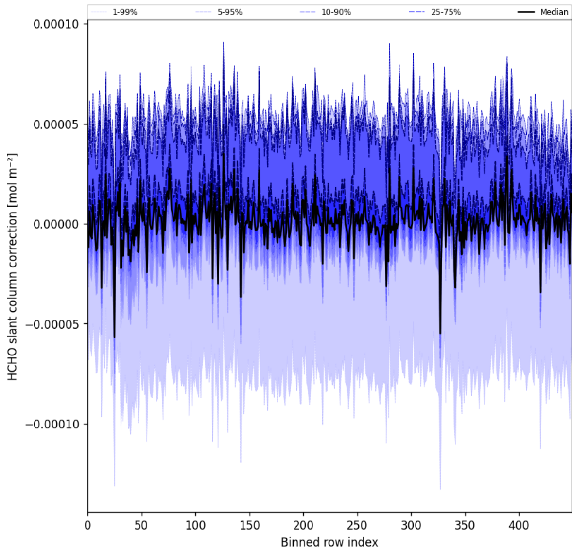
Figure 61: Along track statistics of “HCHO slant column correction” for 2025-02-21 to 2025-02-23
