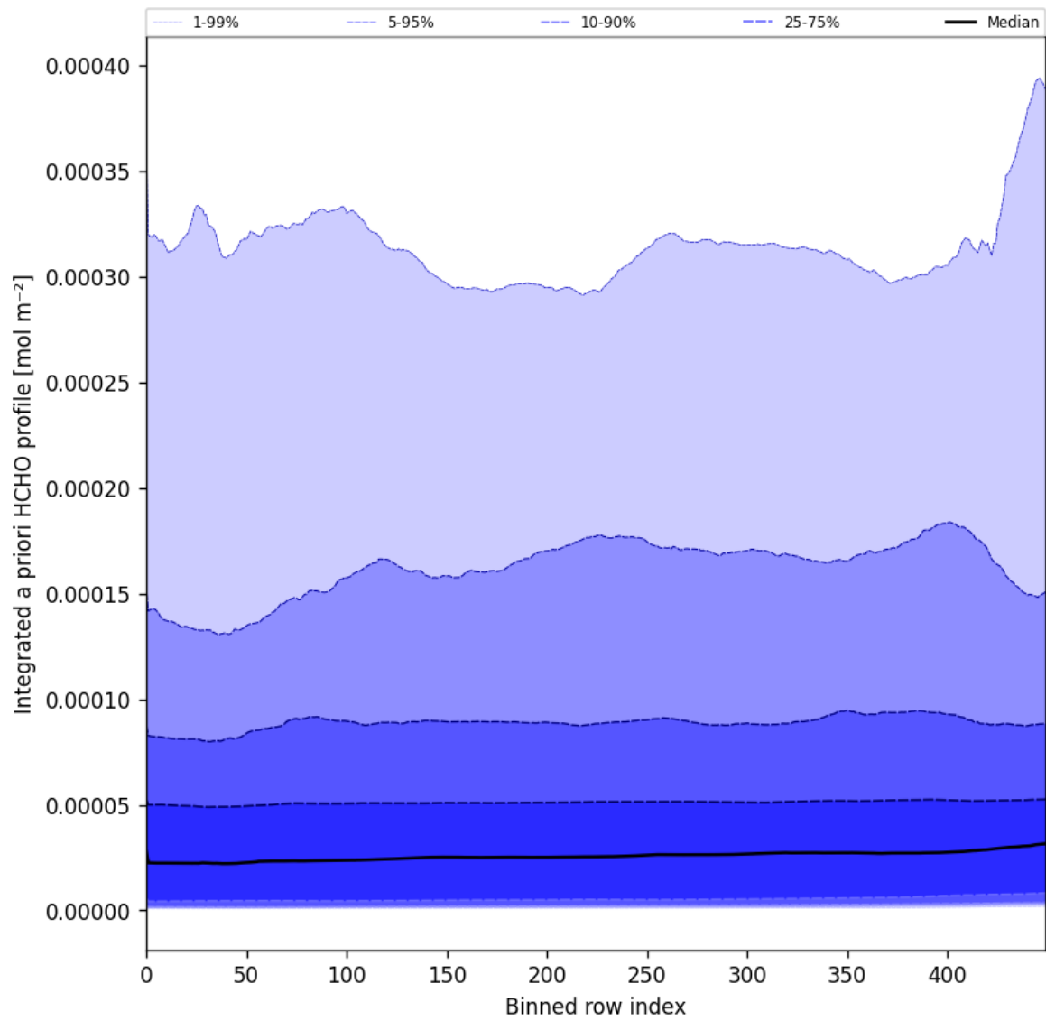
Figure 57: Along track statistics of "Integrated a priori HCHO profile" for 2025-02-21 to 2025-02-23
