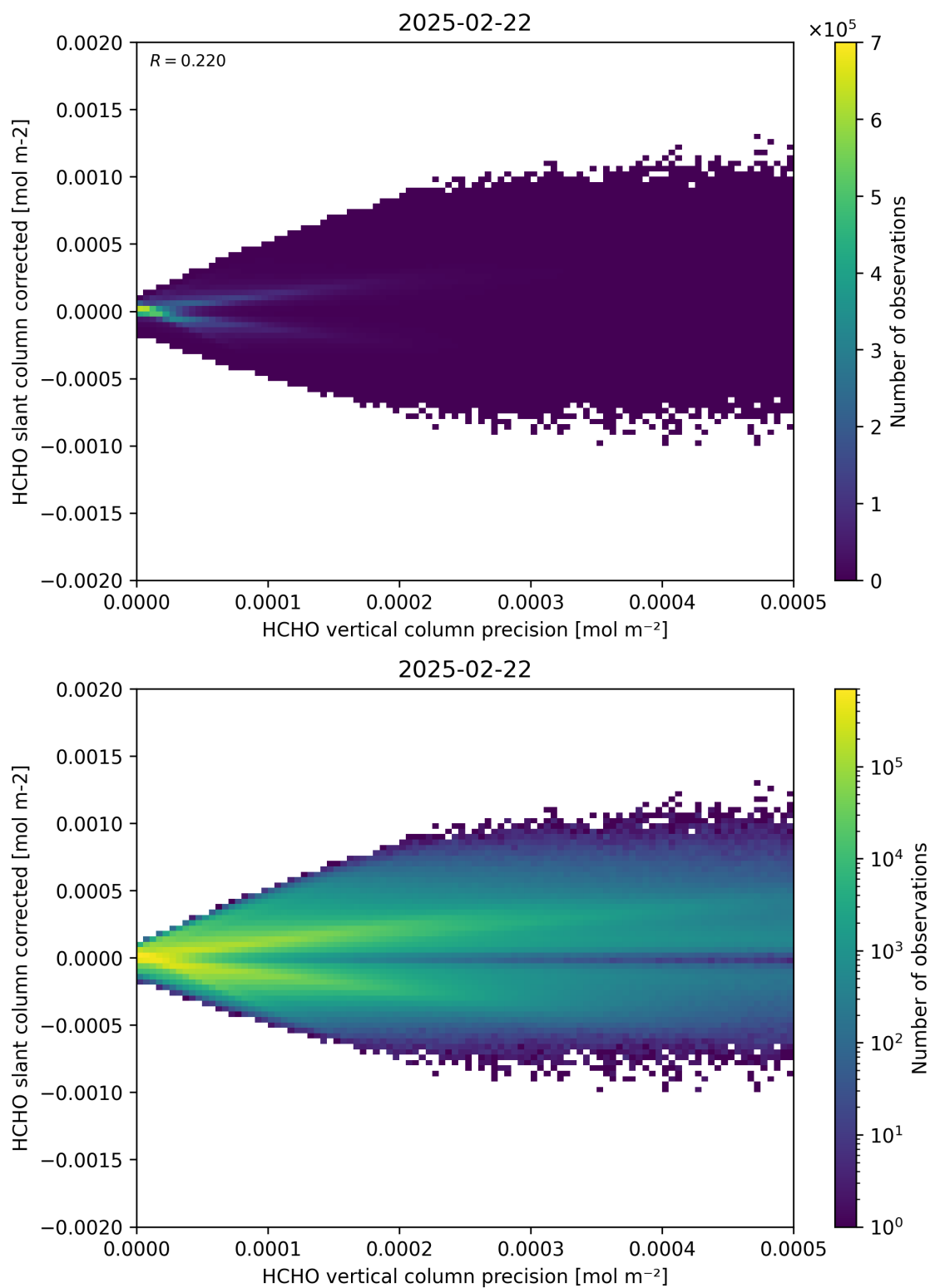
Figure 140: Scatter density plot of “HCHO vertical column precision” against “HCHO slant column corrected” for 2025-02-21 to 2025-02-23.
