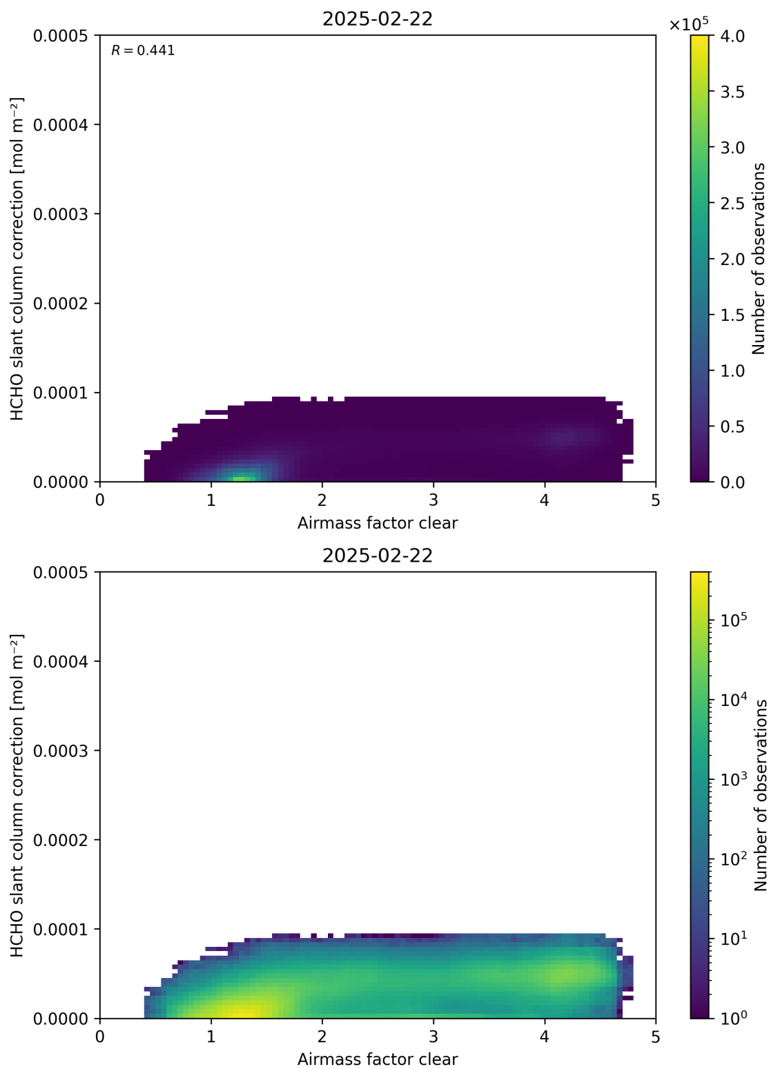
Figure 75: Scatter density plot of “Airmass factor clear” against “HCHO slant column correction” for 2025-02-21 to 2025-02-23.
