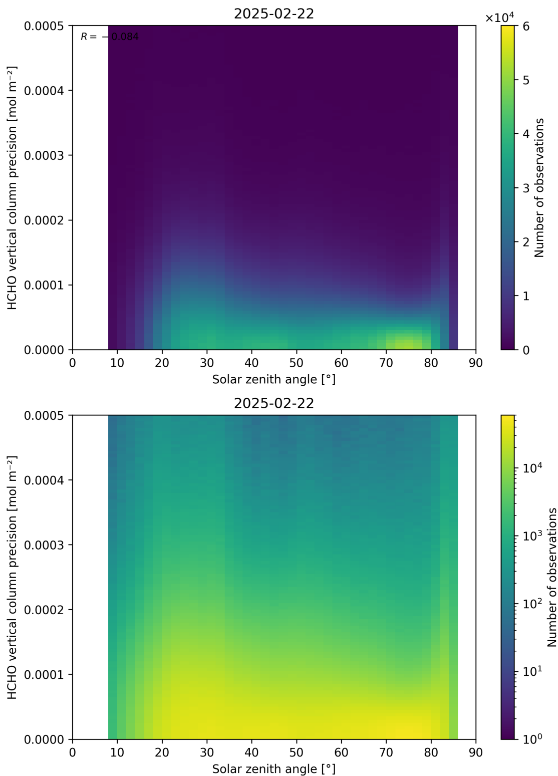
Figure 179: Scatter density plot of “Solar zenith angle” against “HCHO vertical column precision” for 2025-02-21 to 2025-02-23.
