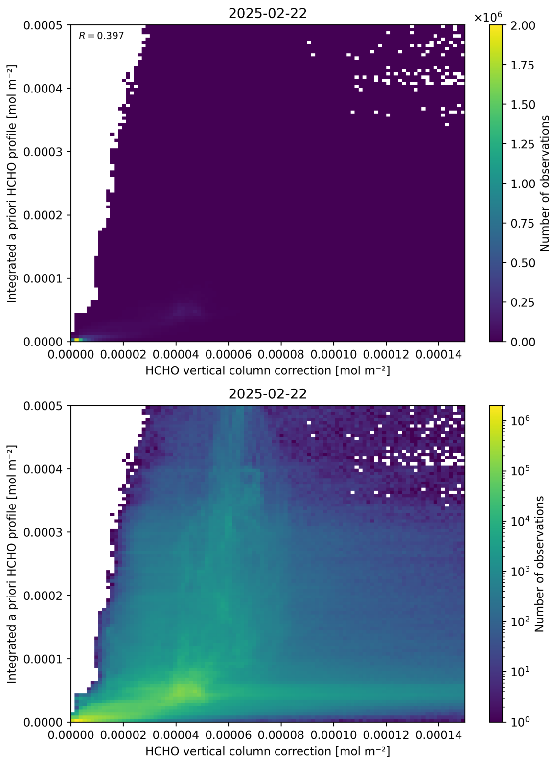
Figure 122: Scatter density plot of “HCHO vertical column correction” against “Integrated a priori HCHO profile” for 2025-02-21 to 2025-02-23.
