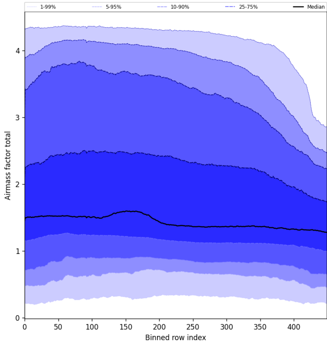
Figure 54: Along track statistics of “Airmass factor total” for 2025-02-21 to 2025-02-23
