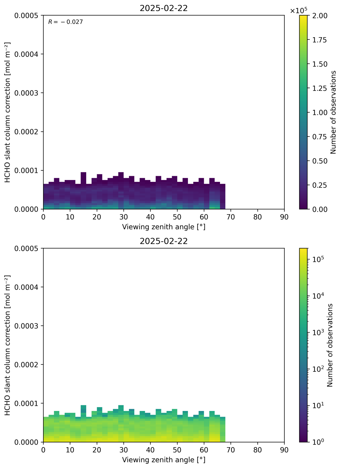
Figure 187: Scatter density plot of “Viewing zenith angle” against “HCHO slant column correction” for 2025-02-21 to 2025-02-23.
