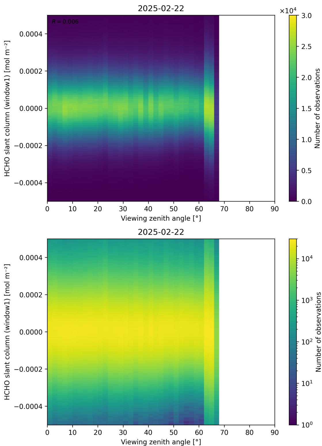
Figure 188: Scatter density plot of “Viewing zenith angle” against “HCHO slant column (window1)” for 2025-02-21 to 2025-02-23.
