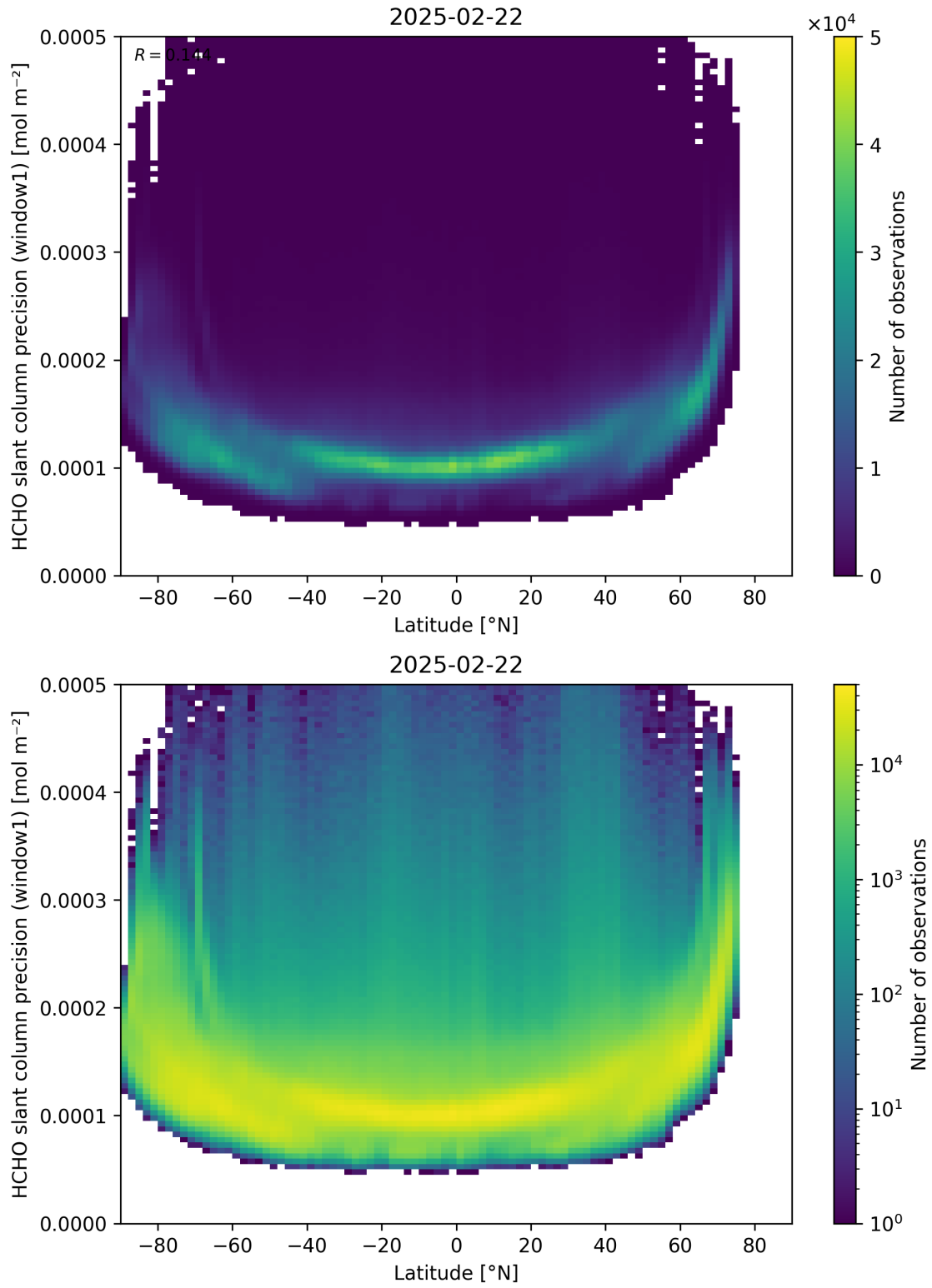
Figure 160: Scatter density plot of “Latitude” against “HCHO slant column precision (window1)” for 2025-02-21 to 2025-02-23.
