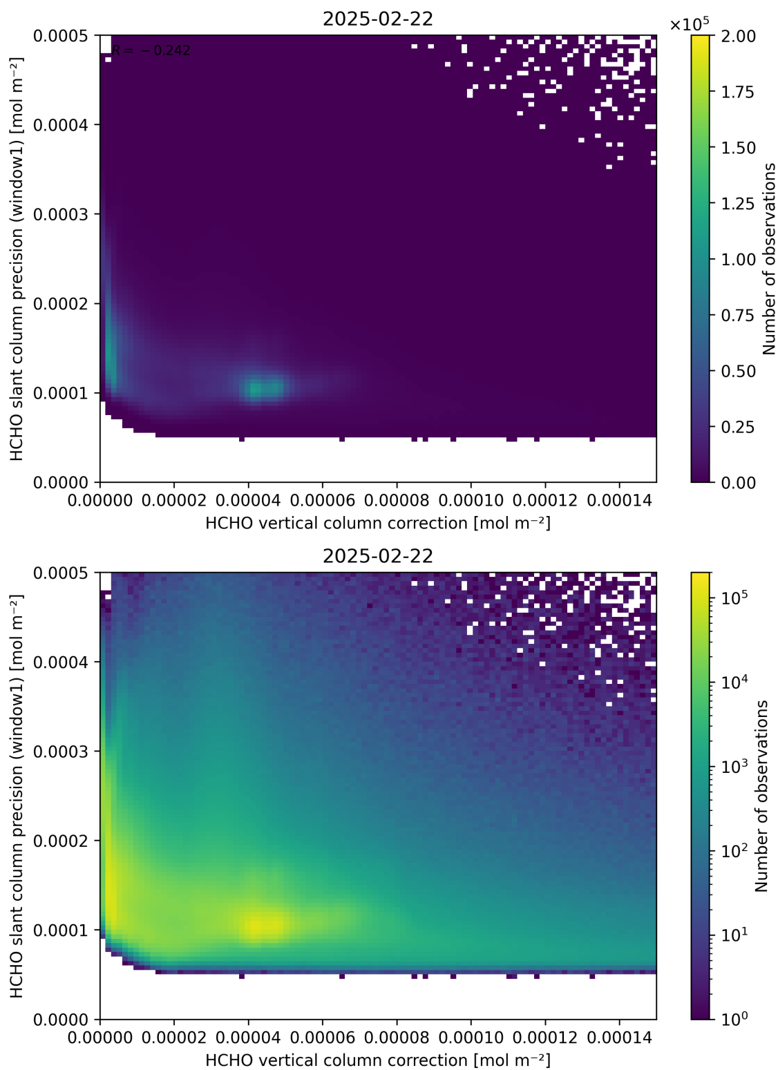
Figure 119: Scatter density plot of “HCHO vertical column correction” against “HCHO slant column precision (window1)” for 2025-02-21 to 2025-02-23.
