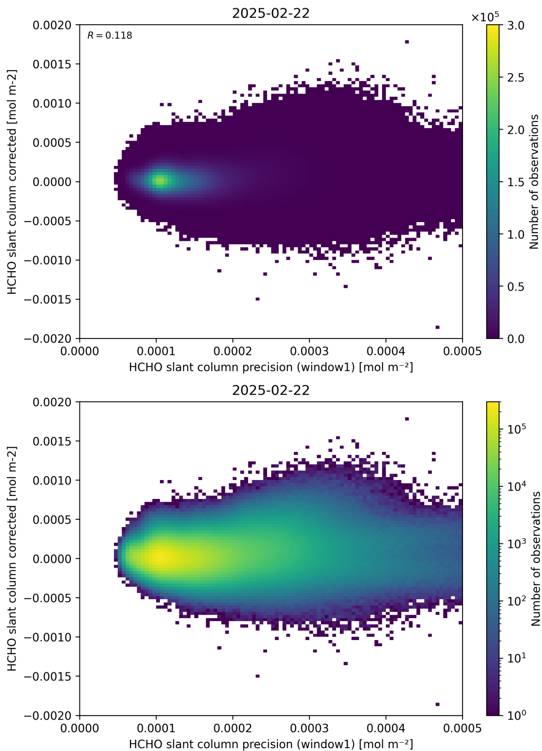
Figure 92: Scatter density plot of “HCHO slant column precision (window1)” against “HCHO slant column corrected” for 2025-02-21 to 2025-02-23.
