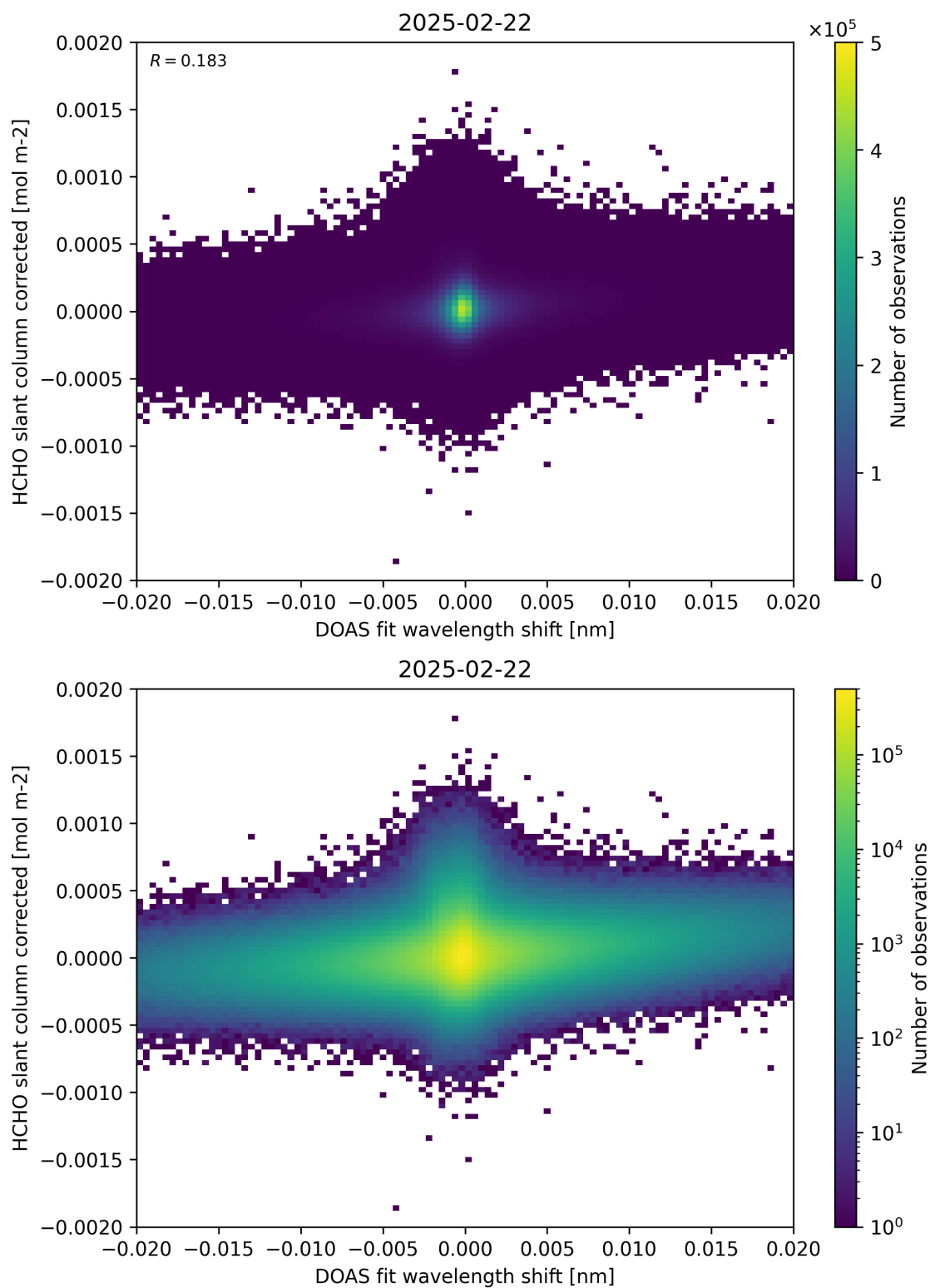
Figure 66: Scatter density plot of “DOAS fit wavelength shift” against “HCHO slant column corrected” for 2025-02-21 to 2025-02-23.
