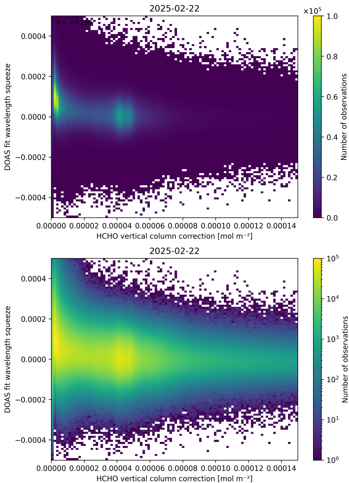
Figure 114: Scatter density plot of “HCHO vertical column correction” against “DOAS fit wavelength squeeze” for 2025-02-21 to 2025-02-23.
