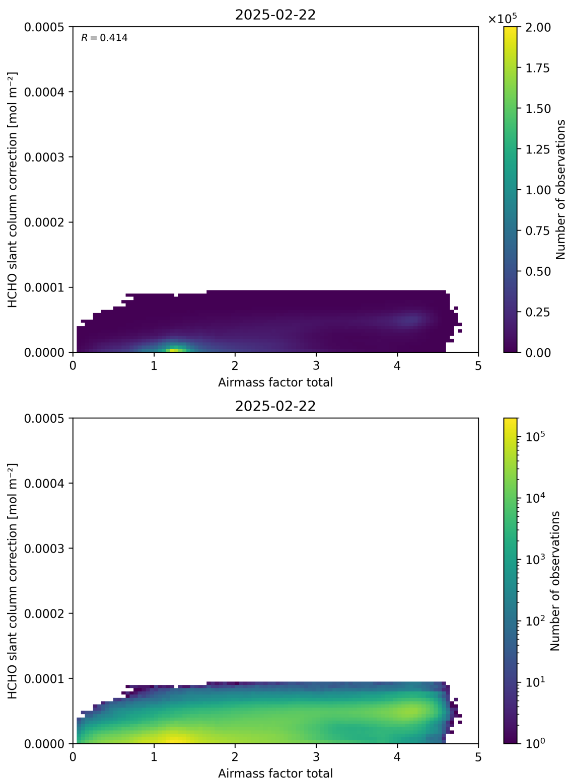
Figure 102: Scatter density plot of “Airmass factor total” against “HCHO slant column correction” for 2025-02-21 to 2025-02-23.
