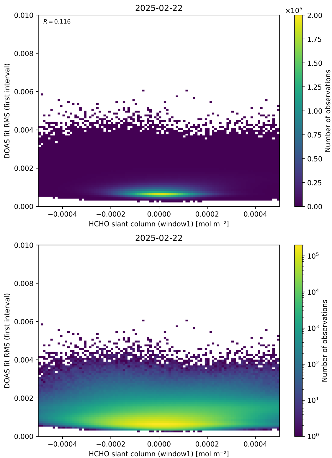
Figure 78: Scatter density plot of “HCHO slant column (window1)” against “DOAS fit RMS (first interval)” for 2025-02-21 to 2025-02-23.
