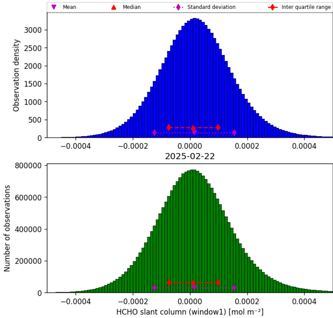
Figure 38: Histogram of “HCHO slant column (window1)” for 2025-02-21 to 2025-02-23
