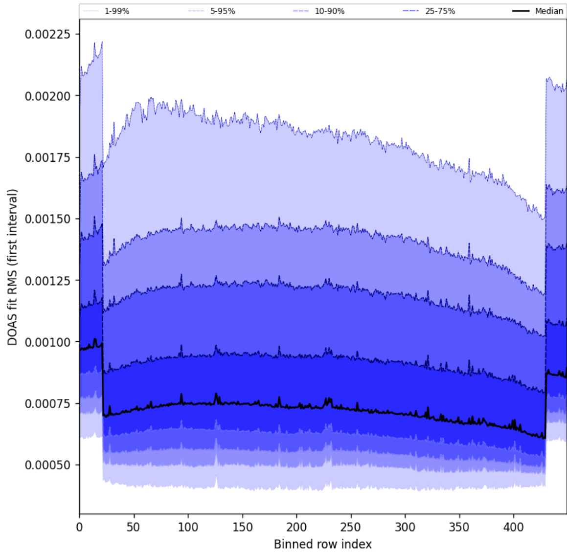
Figure 60: Along track statistics of “DOAS fit RMS (first interval)” for 2025-02-21 to 2025-02-23
