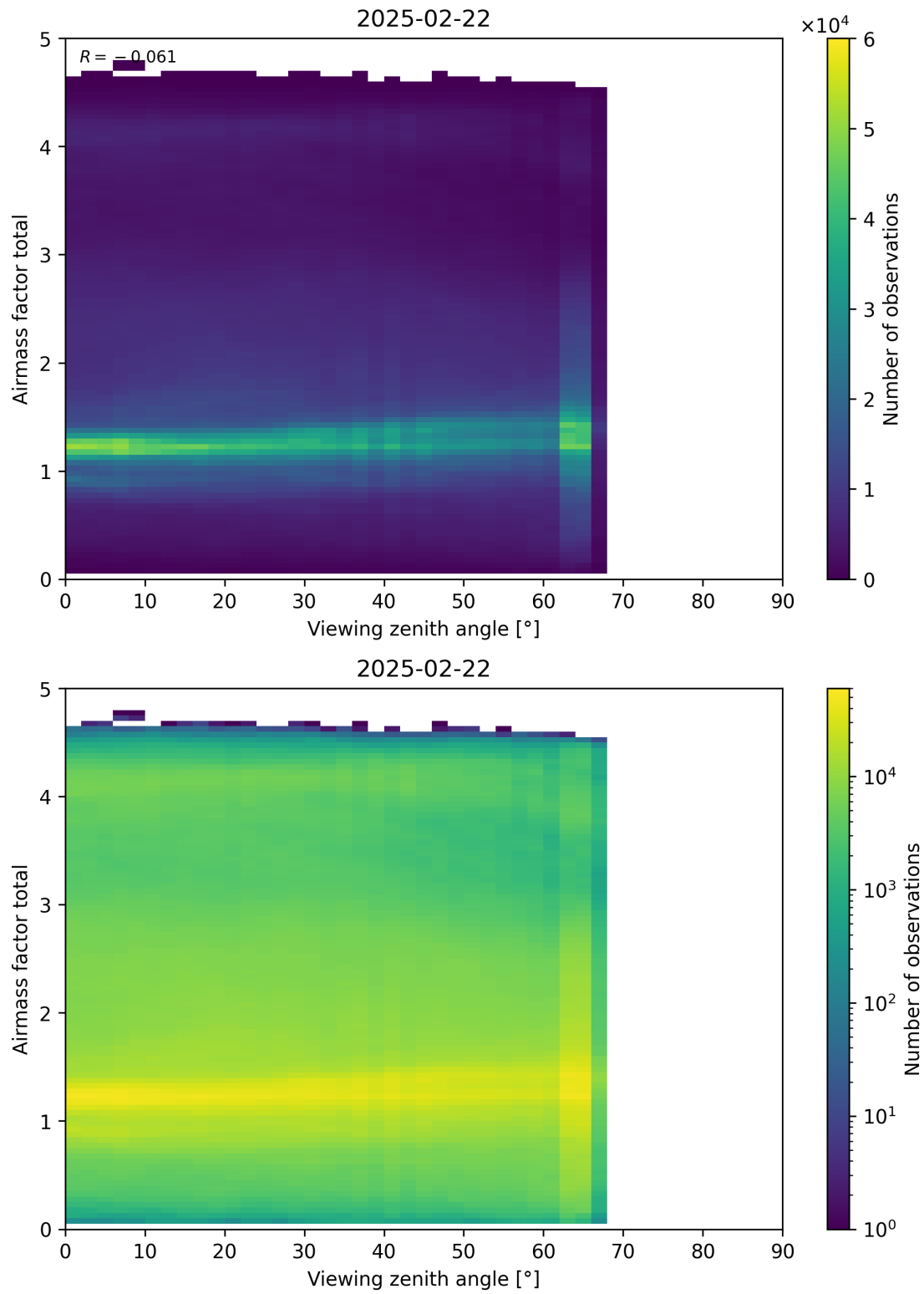
Figure 190: Scatter density plot of “Viewing zenith angle” against “Airmass factor total” for 2025-02-21 to 2025-02-23.
