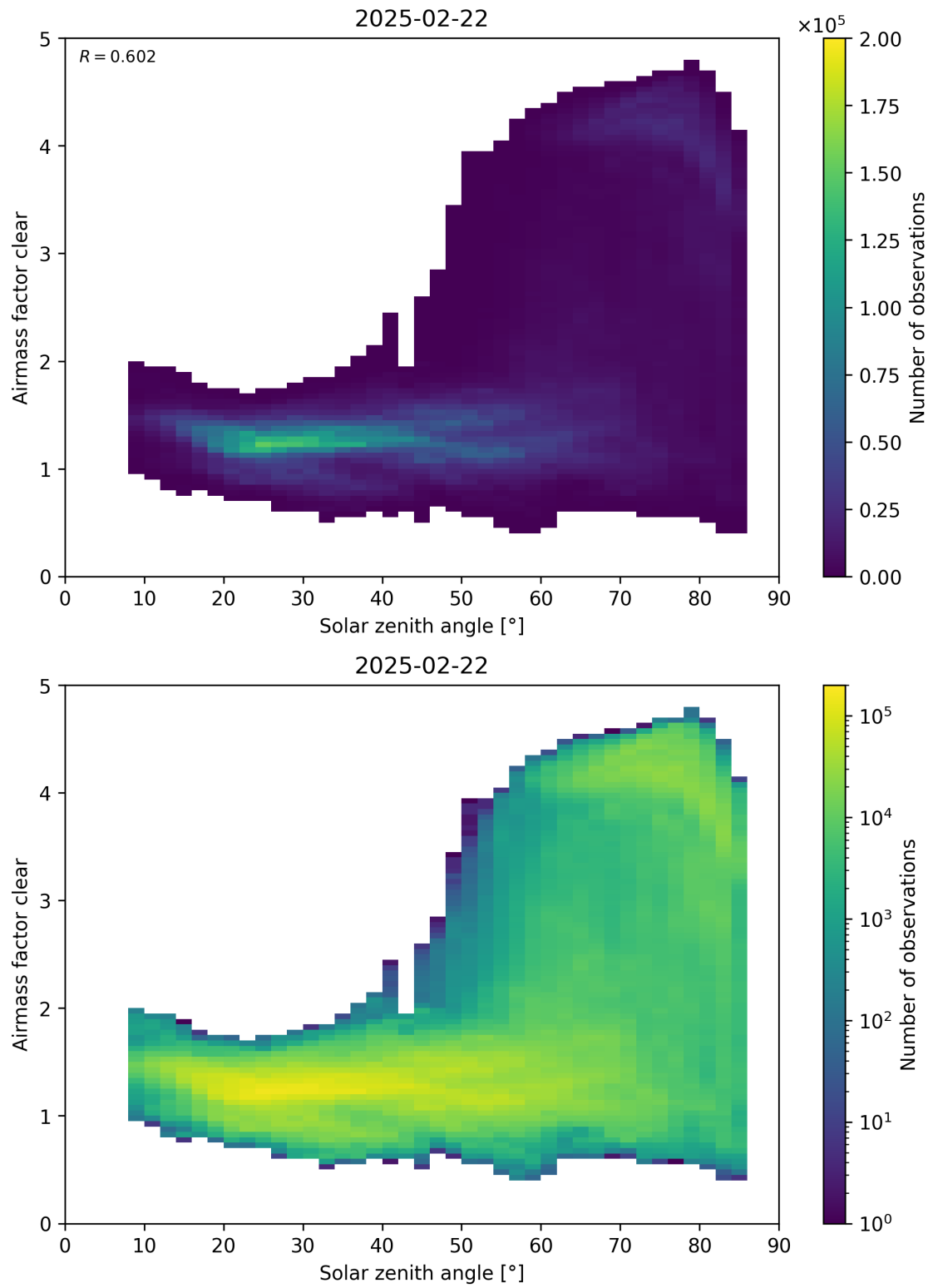
Figure 170: Scatter density plot of “Solar zenith angle” against “Airmass factor clear” for 2025-02-21 to 2025-02-23.
