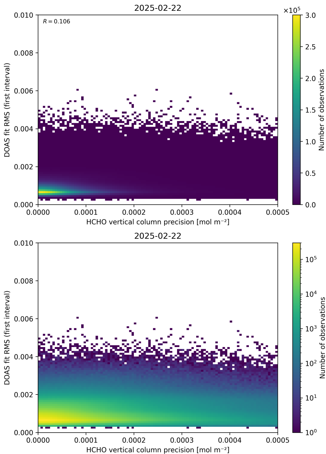
Figure 136: Scatter density plot of “HCHO vertical column precision” against “DOAS fit RMS (first interval)” for 2025-02-21 to 2025-02-23.
