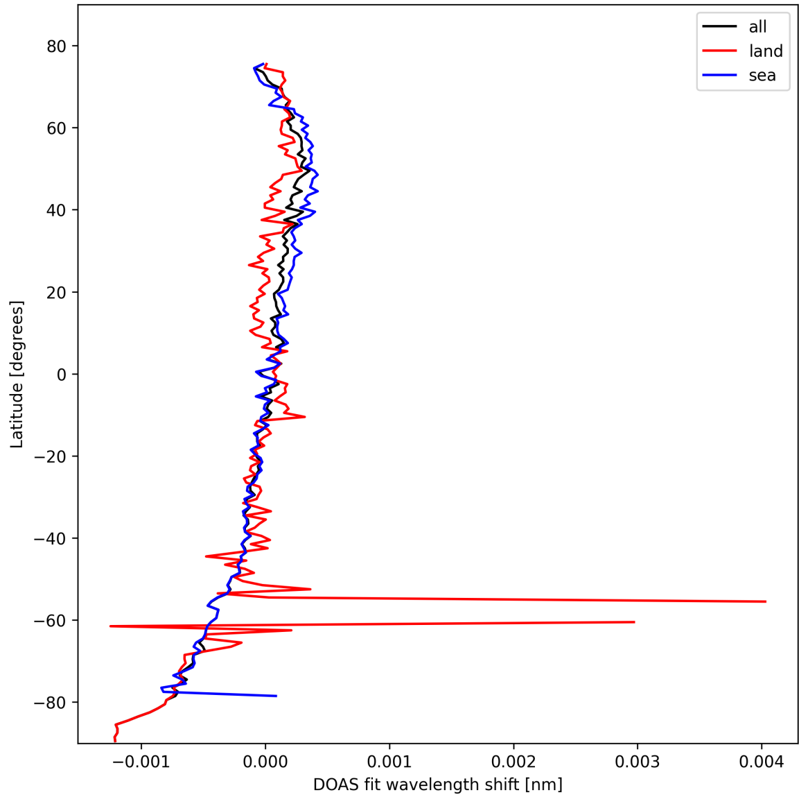
Figure 30: Zonal average of "DOAS fit wavelength shift" for 2025-02-21 to 2025-02-23.
