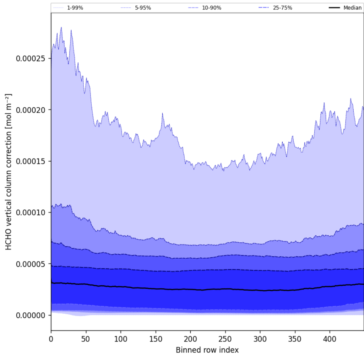
Figure 51: Along track statistics of “HCHO vertical column correction” for 2025-02-21 to 2025-02-23
