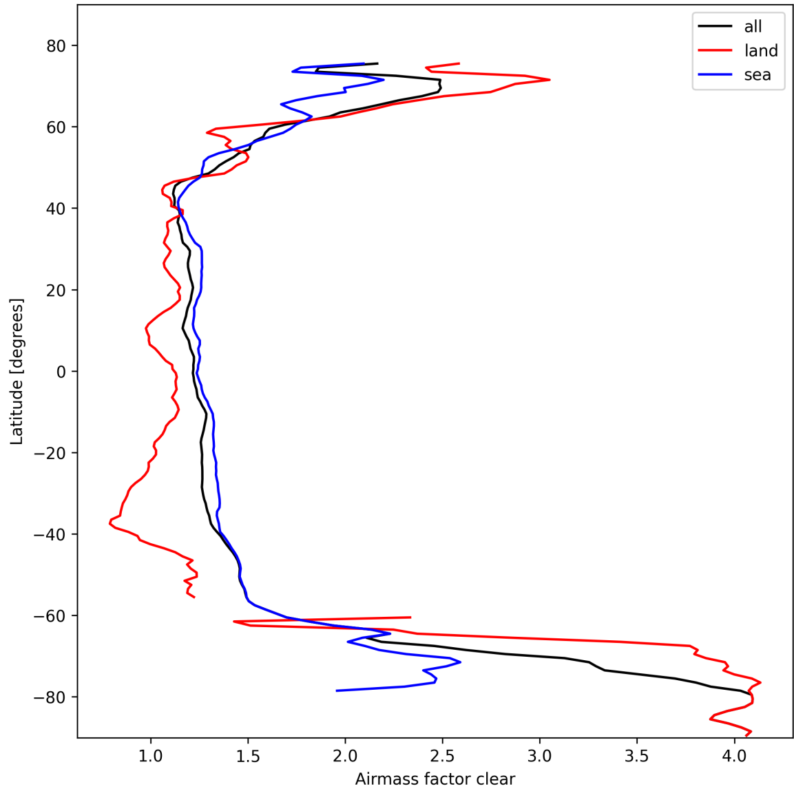
Figure 28: Zonal average of “Airmass factor clear” for 2025-02-21 to 2025-02-23.
