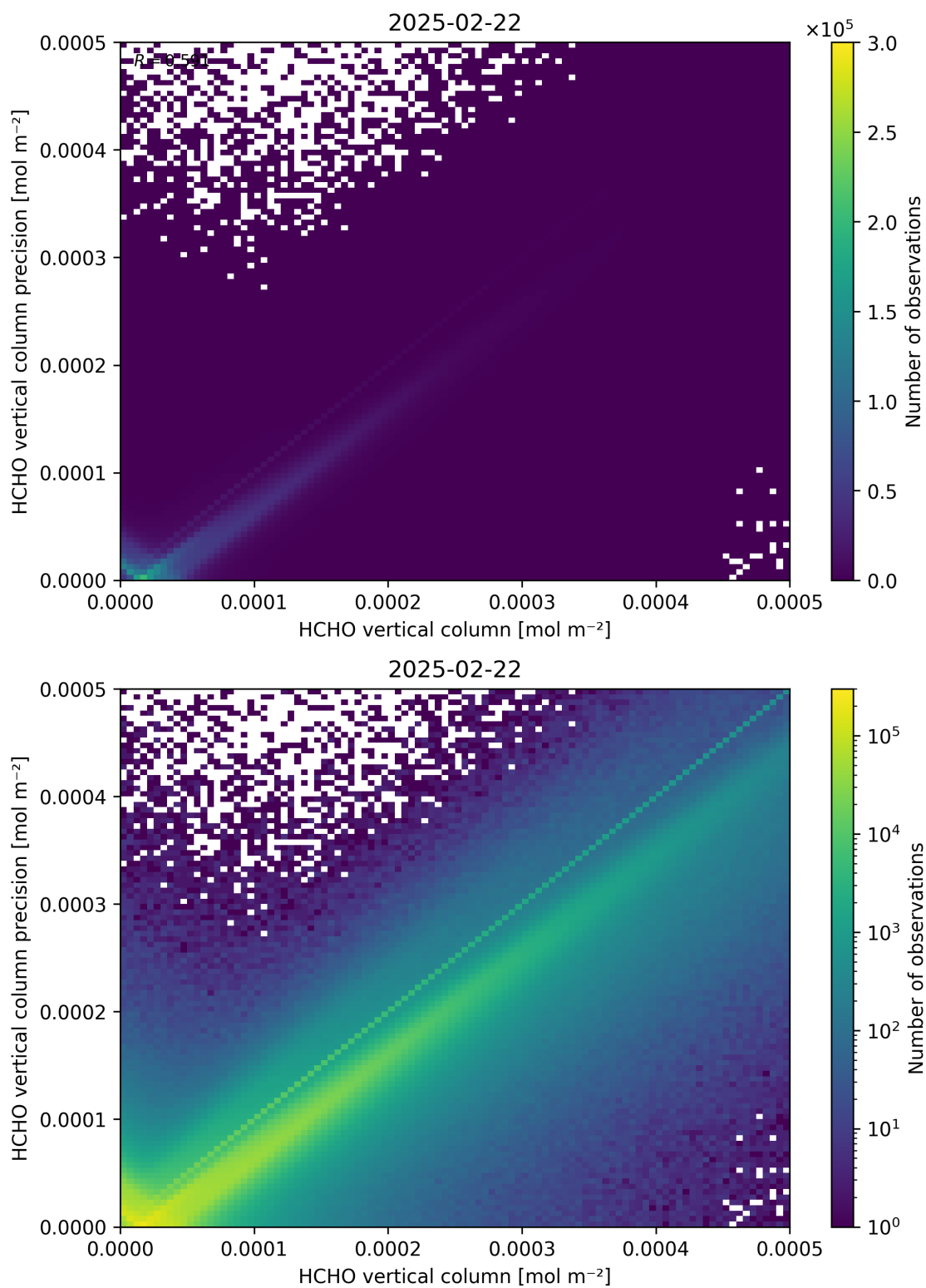
Figure 134: Scatter density plot of “HCHO vertical column” against “HCHO vertical column precision” for 2025-02-21 to 2025-02-23.
