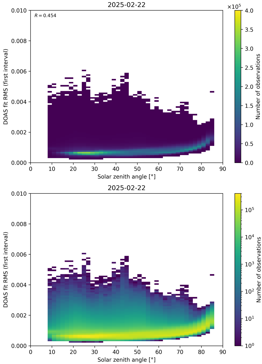
Figure 167: Scatter density plot of “Solar zenith angle” against “DOAS fit RMS (first interval)” for 2025-02-21 to 2025-02-23.
