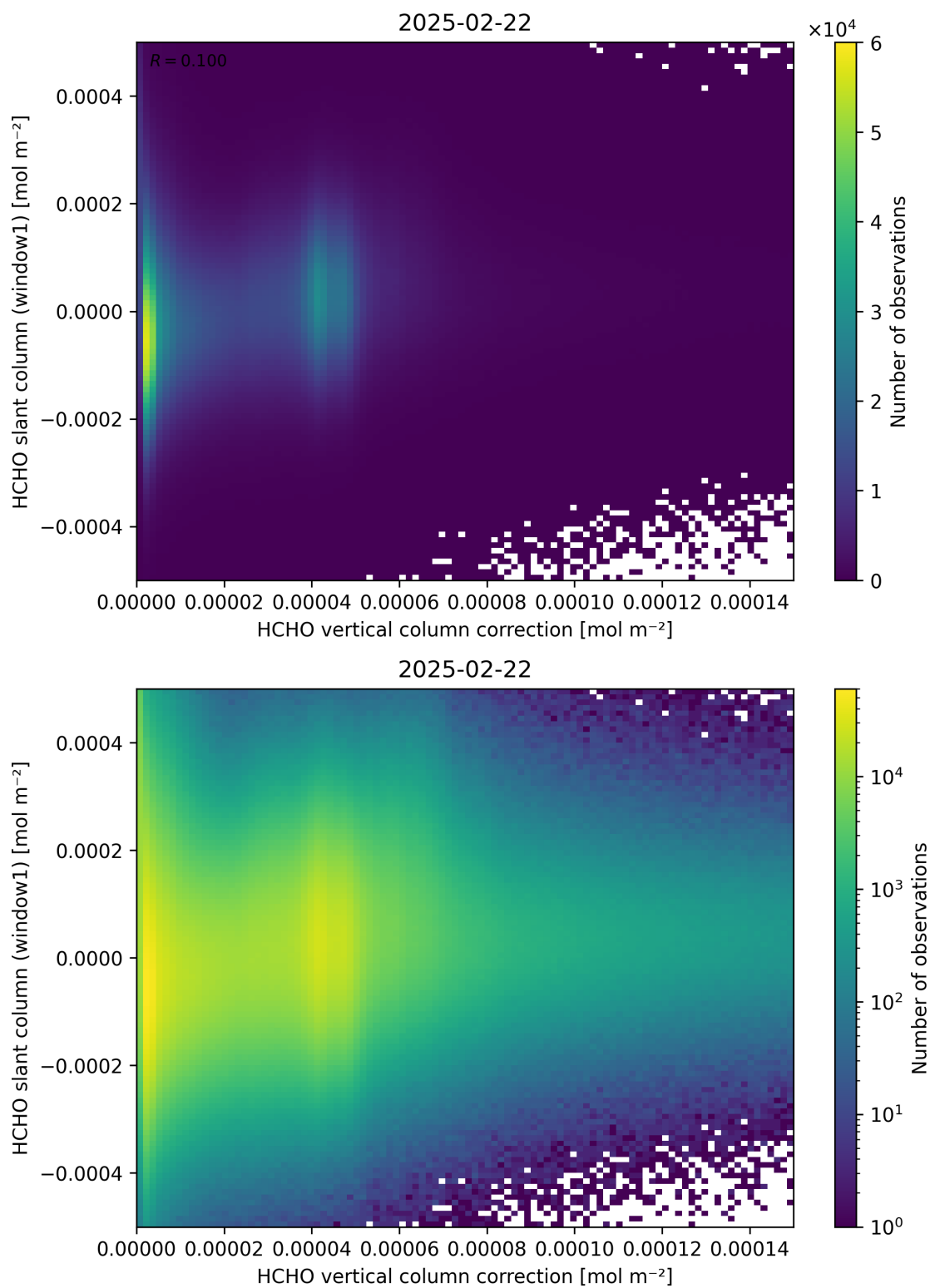
Figure 118: Scatter density plot of “HCHO vertical column correction” against “HCHO slant column (window1)” for 2025-02-21 to 2025-02-23.
