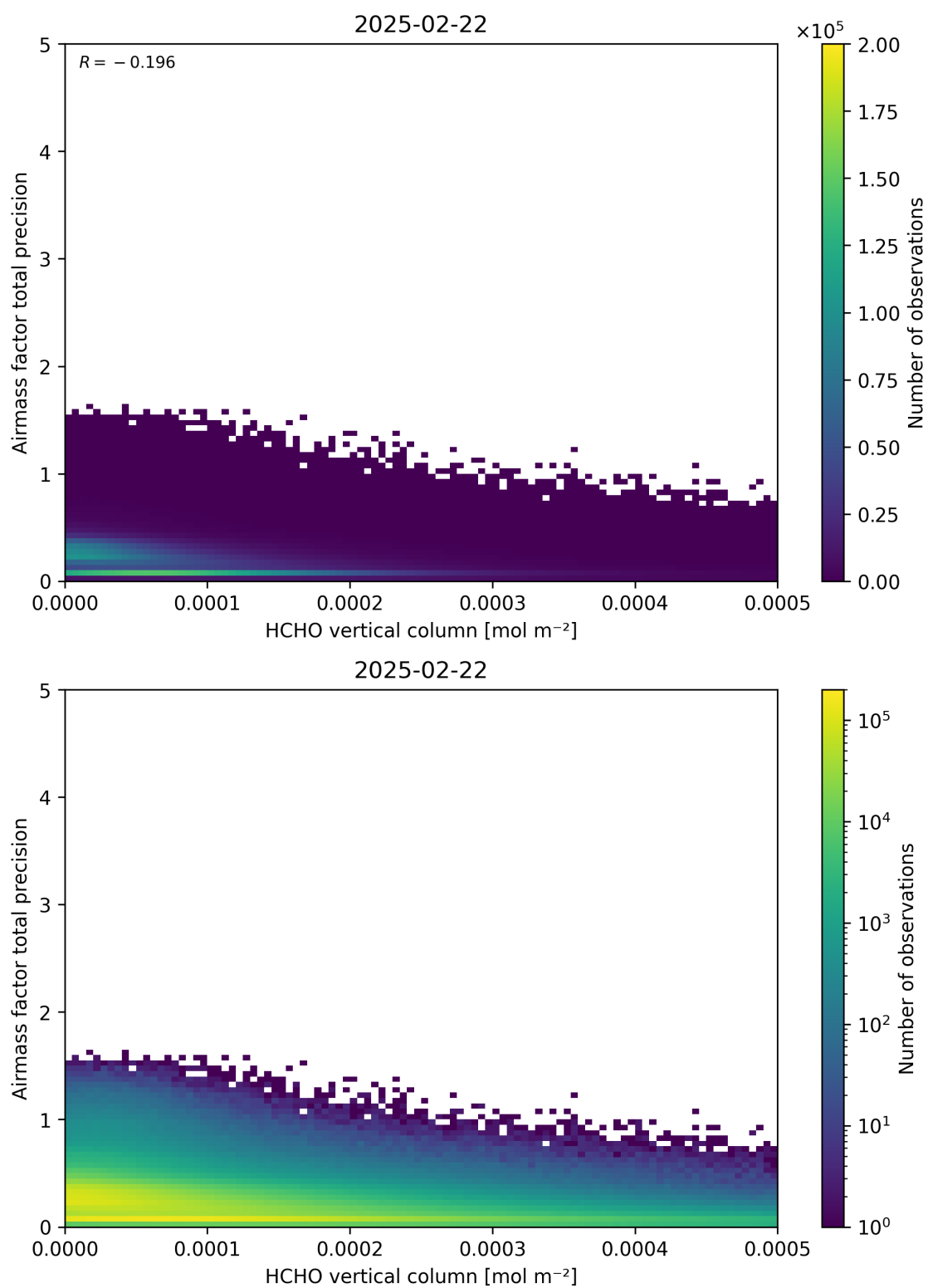
Figure 132: Scatter density plot of “HCHO vertical column” against “Airmass factor total precision” for 2025-02-21 to 2025-02-23.
