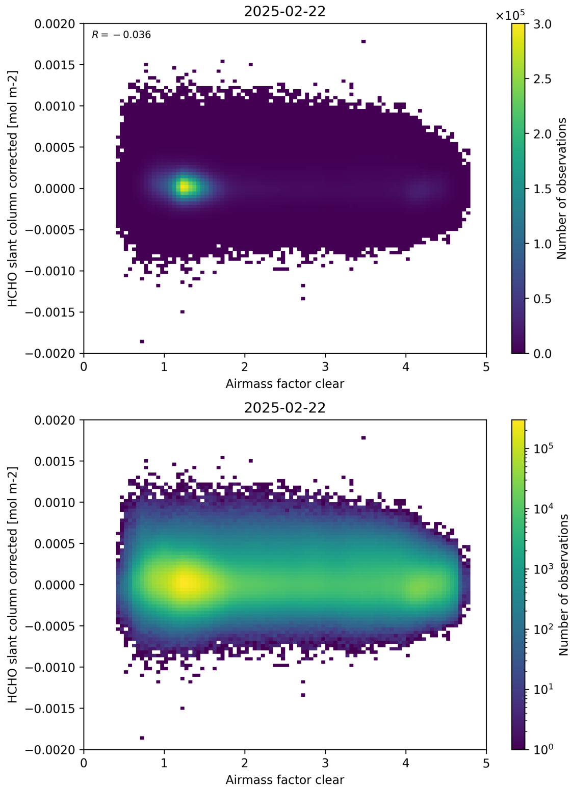
Figure 74: Scatter density plot of “Airmass factor clear” against “HCHO slant column corrected” for 2025-02-21 to 2025-02-23.
