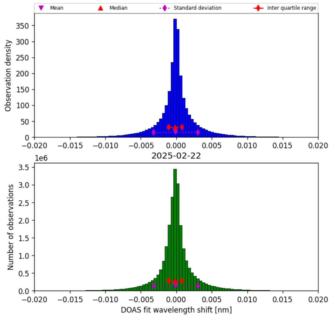
Figure 44: Histogram of “DOAS fit wavelength shift” for 2025-02-21 to 2025-02-23
