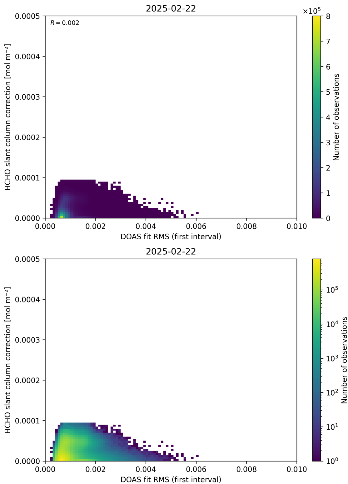
Figure 63: Scatter density plot of “DOAS fit RMS (first interval)” against “HCHO slant column correction” for 2025-02-21 to 2025-02-23.
