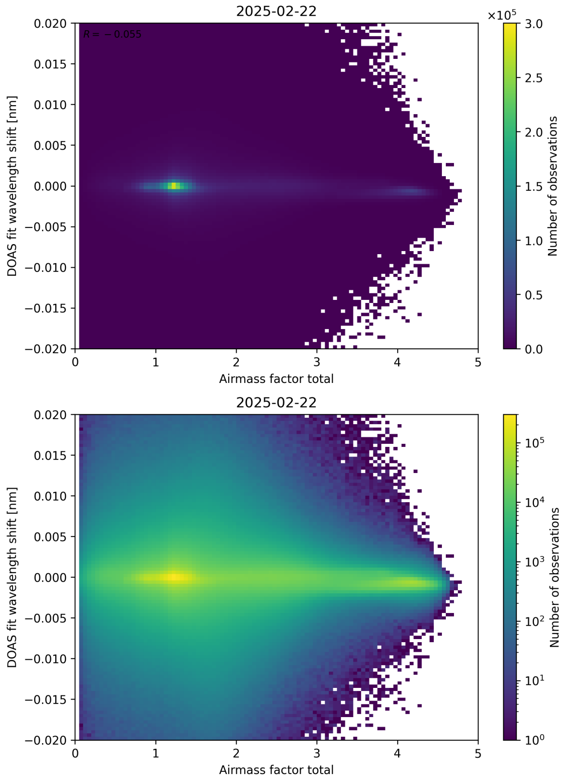
Figure 98: Scatter density plot of “Airmass factor total” against “DOAS fit wavelength shift” for 2025-02-21 to 2025-02-23.
