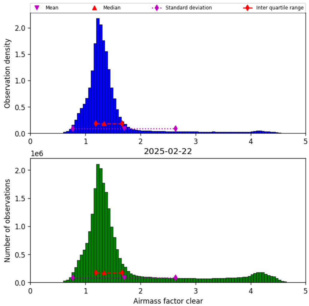
Figure 42: Histogram of “Airmass factor clear” for 2025-02-21 to 2025-02-23
