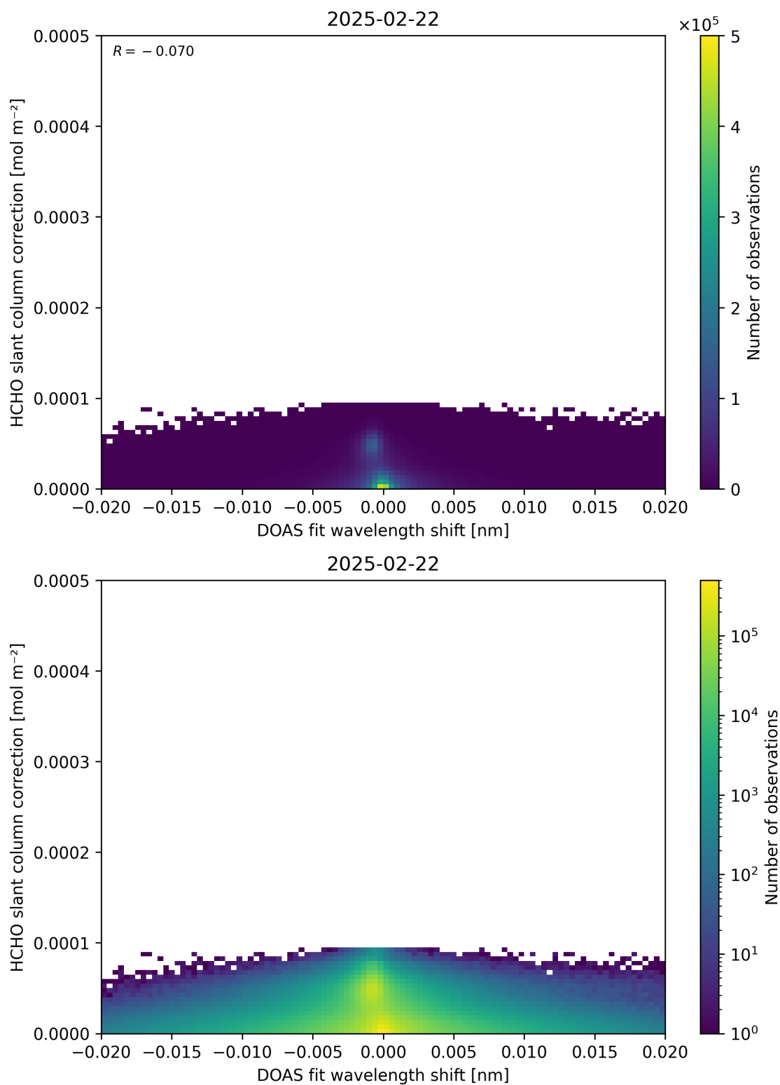
Figure 67: Scatter density plot of “DOAS fit wavelength shift” against “HCHO slant column correction” for 2025-02-21 to 2025-02-23.
