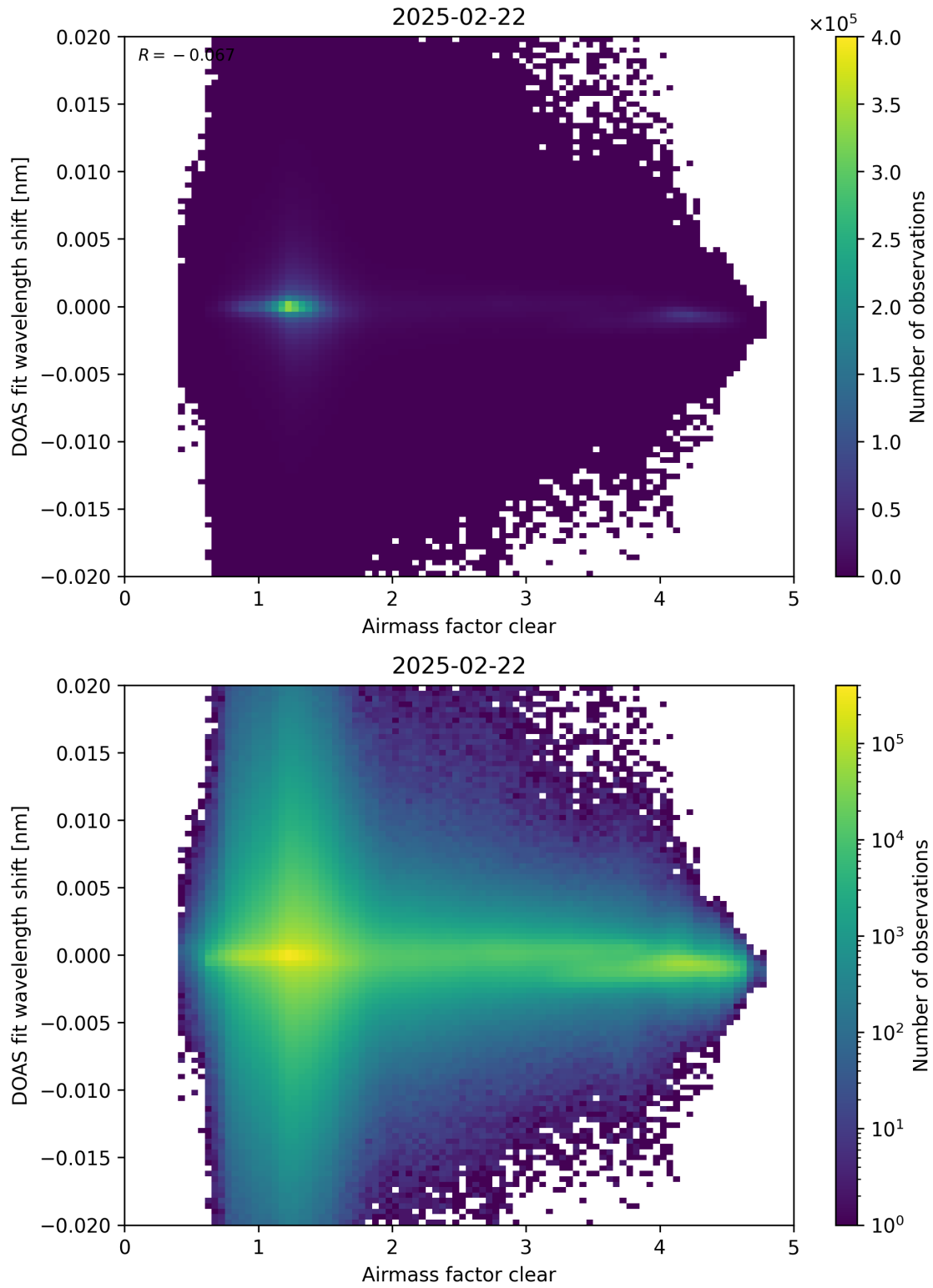
Figure 72: Scatter density plot of “Airmass factor clear” against “DOAS fit wavelength shift” for 2025-02-21 to 2025-02-23.
