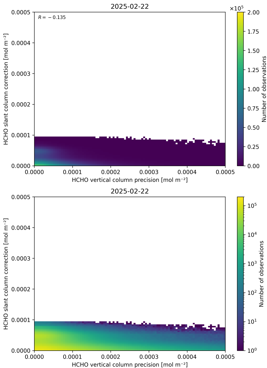
Figure 141: Scatter density plot of “HCHO vertical column precision” against “HCHO slant column correction” for 2025-02-21 to 2025-02-23.
