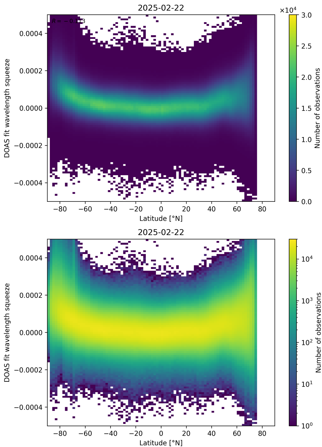
Figure 155: Scatter density plot of “Latitude” against “DOAS fit wavelength squeeze” for 2025-02-21 to 2025-02-23.
