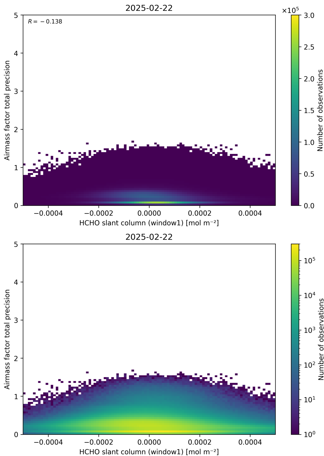
Figure 86: Scatter density plot of “HCHO slant column (window1)” against “Airmass factor total precision” for 2025-02-21 to 2025-02-23.
