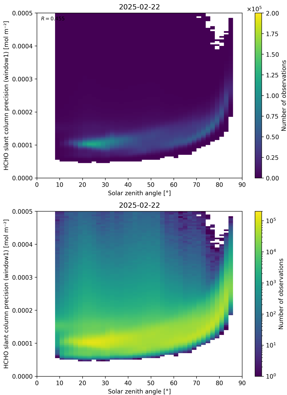
Figure 174: Scatter density plot of “Solar zenith angle” against “HCHO slant column precision (window1)” for 2025-02-21 to 2025-02-23.
