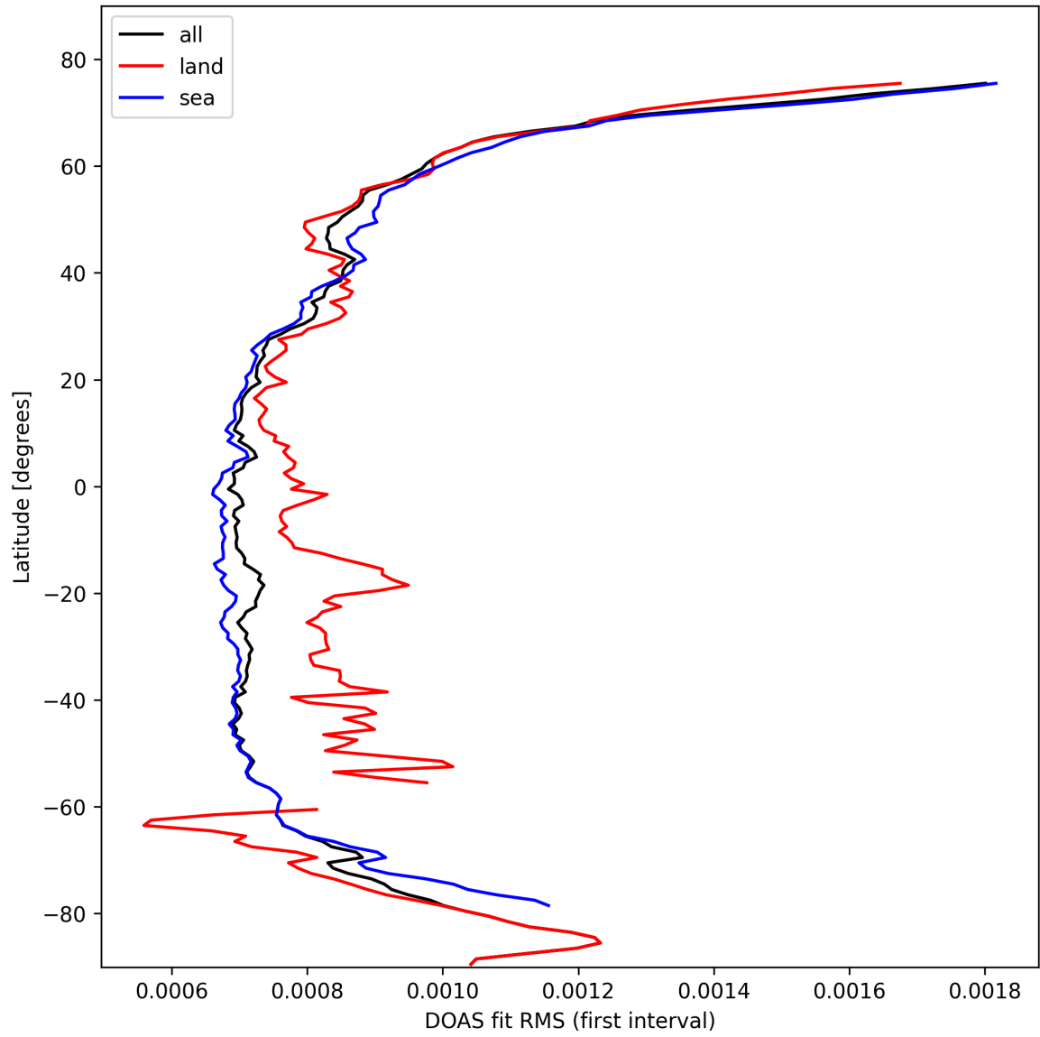
Figure 32: Zonal average of “DOAS fit RMS (first interval)” for 2025-02-21 to 2025-02-23.
