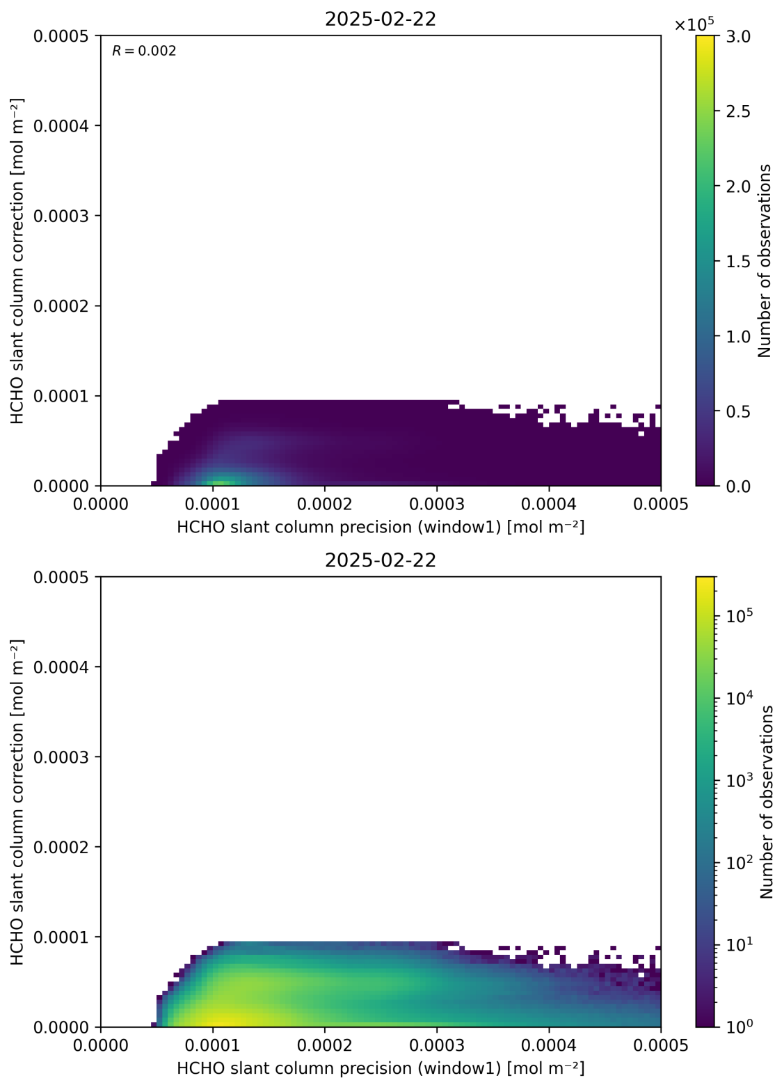
Figure 93: Scatter density plot of “HCHO slant column precision (window1)” against “HCHO slant column correction” for 2025-02-21 to 2025-02-23.
