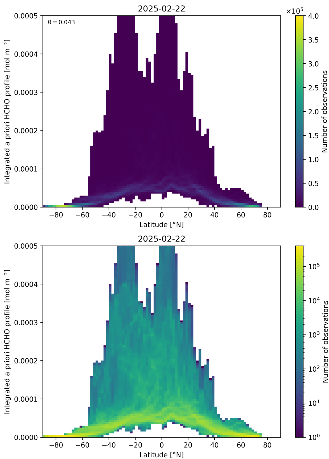
Figure 166: Scatter density plot of “Latitude” against “Integrated a priori HCHO profile” for 2025-02-21 to 2025-02-23.
