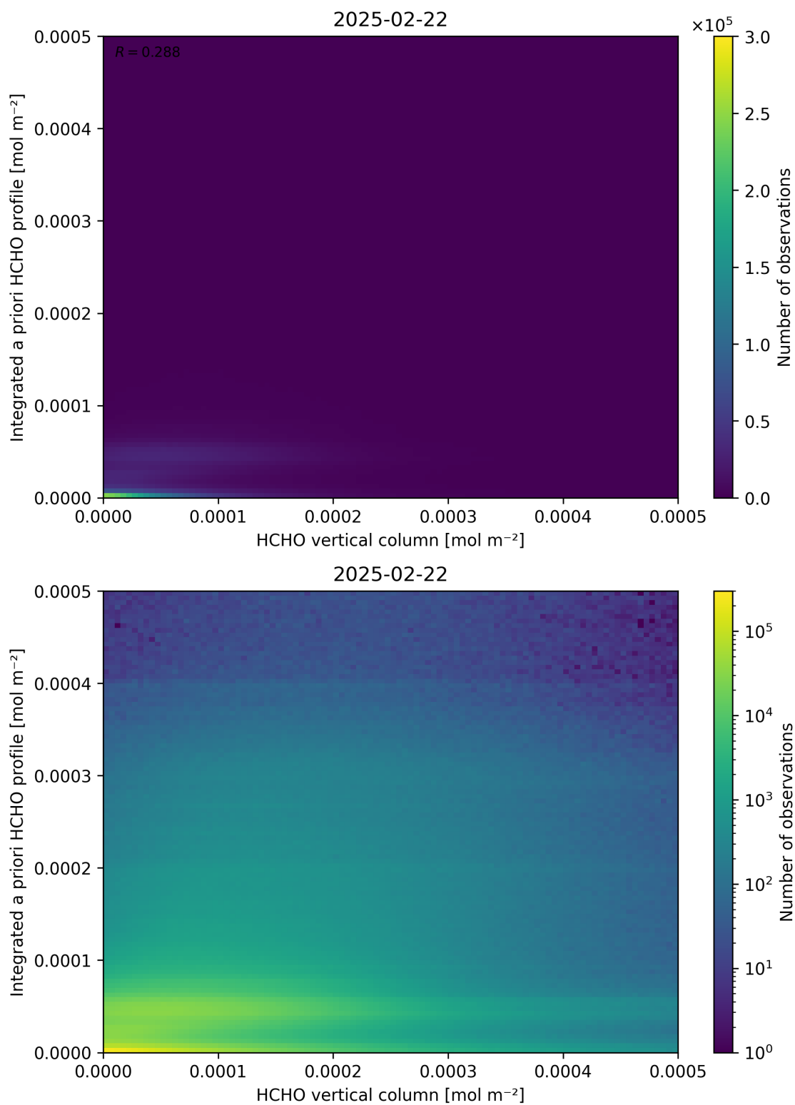
Figure 135: Scatter density plot of “HCHO vertical column” against “Integrated a priori HCHO profile” for 2025-02-21 to 2025-02-23.
