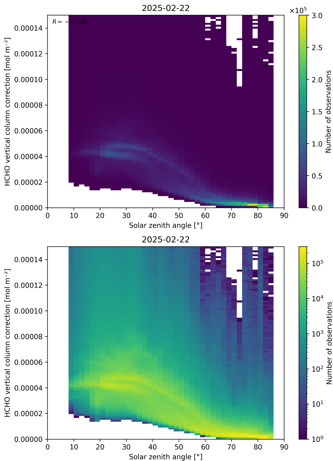
Figure 178: Scatter density plot of “Solar zenith angle” against “HCHO vertical column correction” for 2025-02-21 to 2025-02-23.
