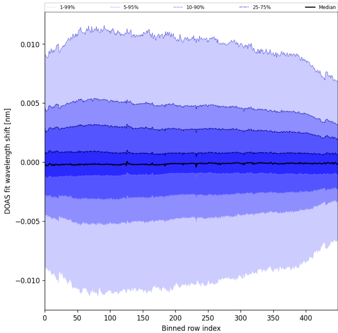
Figure 58: Along track statistics of “DOAS fit wavelength shift” for 2025-02-21 to 2025-02-23
