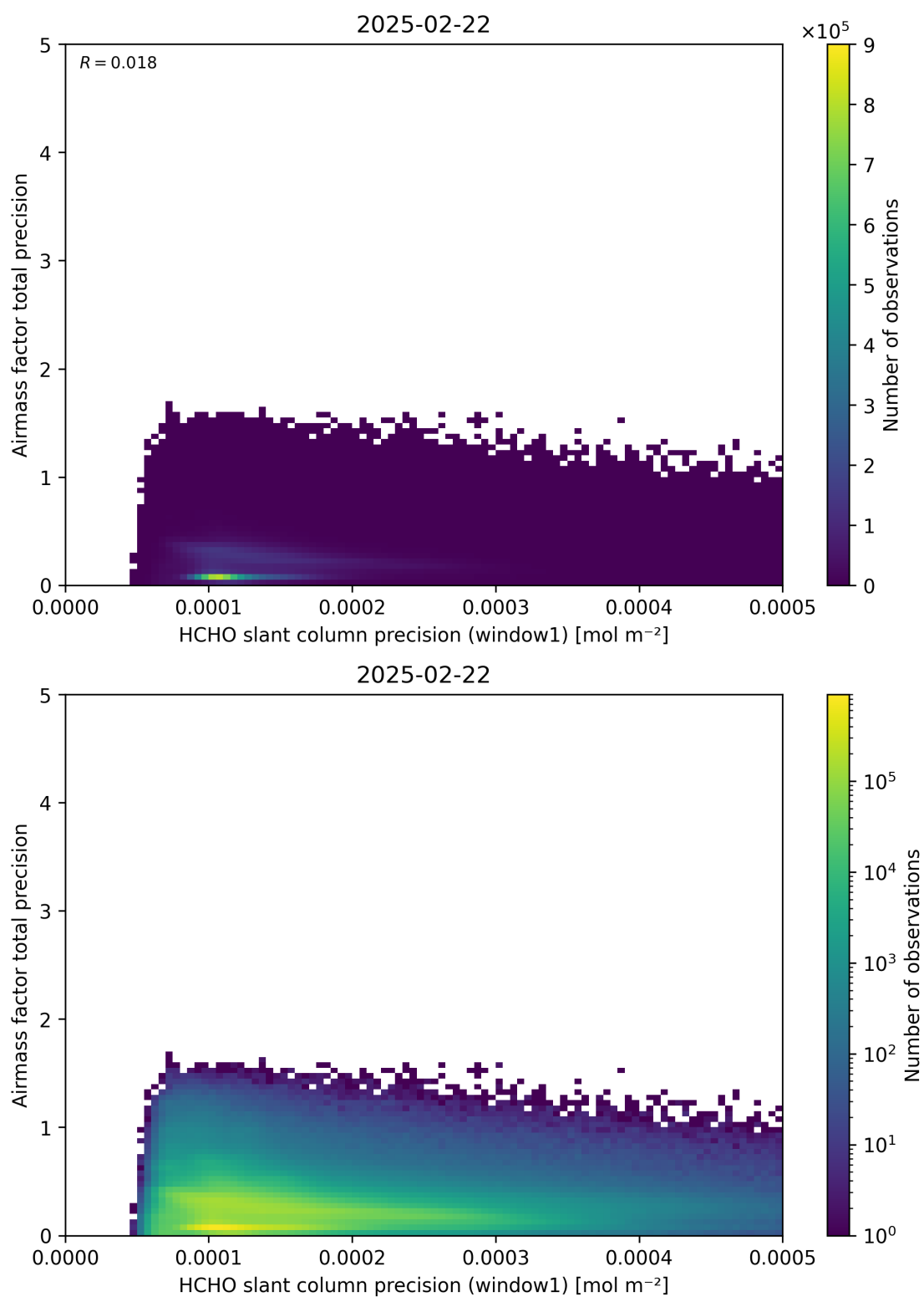
Figure 95: Scatter density plot of “HCHO slant column precision (window1)” against “Airmass factor total precision” for 2025-02-21 to 2025-02-23.
