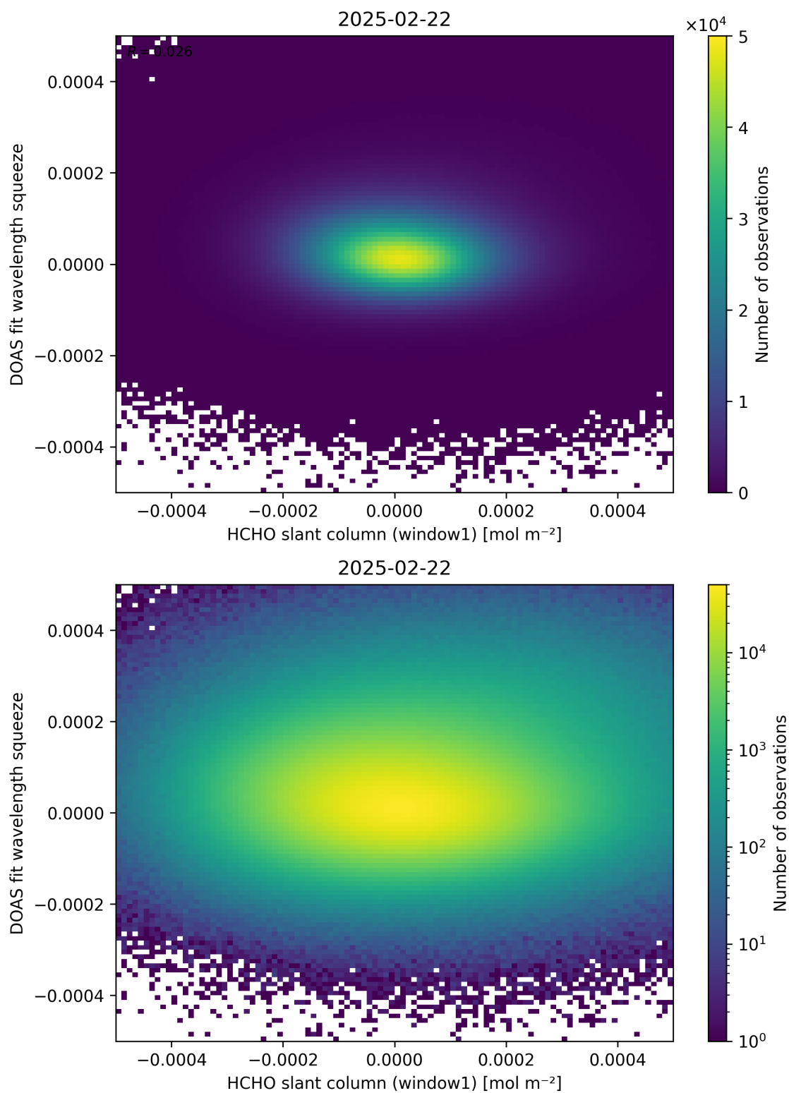
Figure 80: Scatter density plot of “HCHO slant column (window1)” against “DOAS fit wavelength squeeze” for 2025-02-21 to 2025-02-23.
