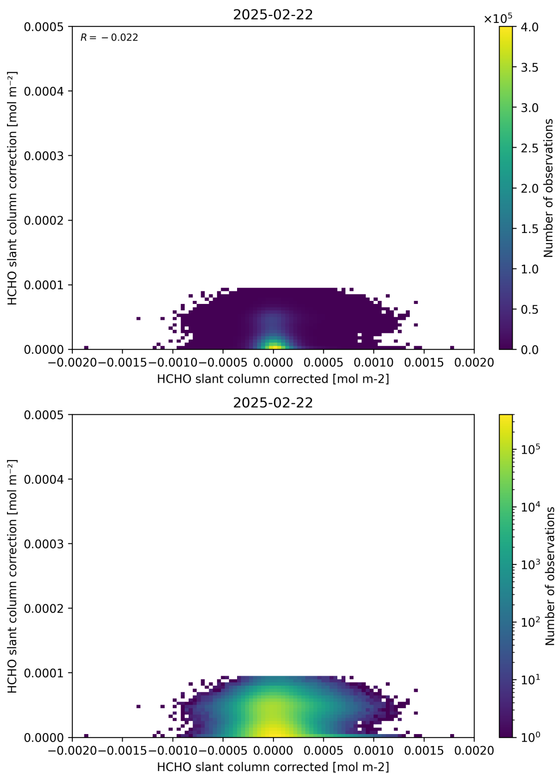
Figure 77: Scatter density plot of “HCHO slant column corrected” against “HCHO slant column correction” for 2025-02-21 to 2025-02-23.
