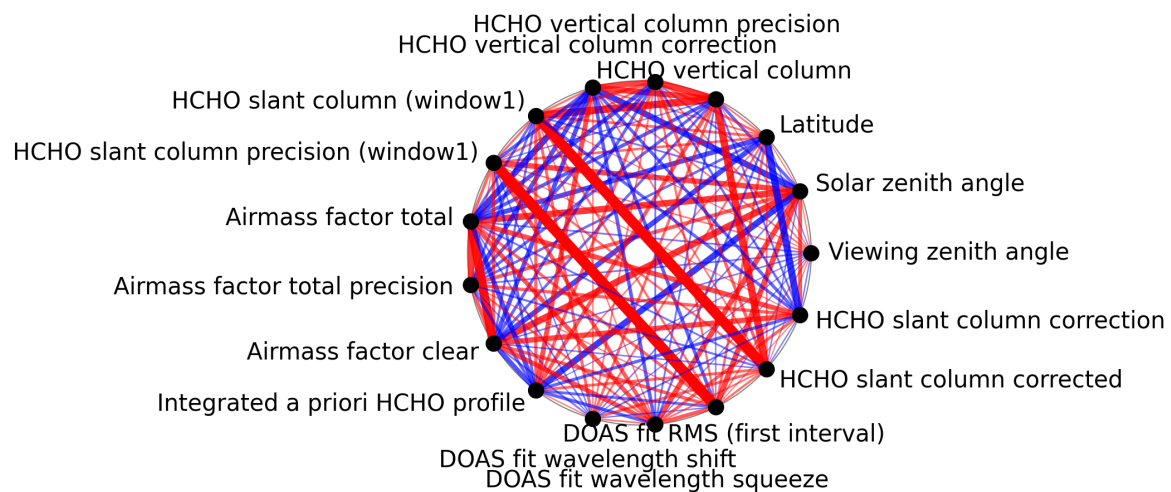
Figure 1: Map of correlation graph for 2025-02-21 to 2025-02-23.
