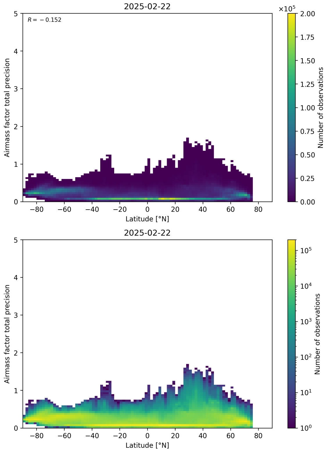
Figure 162: Scatter density plot of “Latitude” against “Airmass factor total precision” for 2025-02-21 to 2025-02-23.
