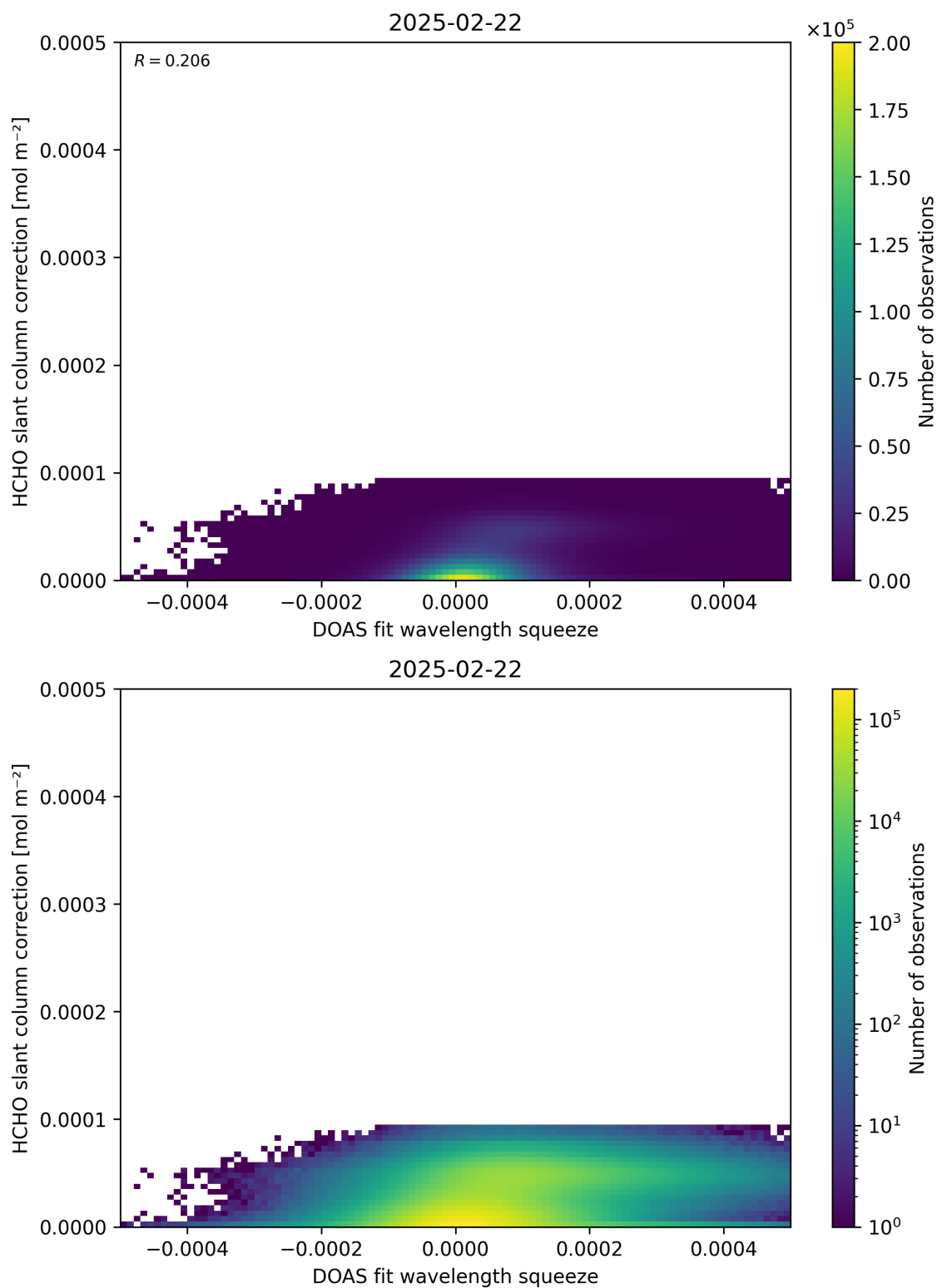
Figure 70: Scatter density plot of “DOAS fit wavelength squeeze” against “HCHO slant column correction” for 2025-02-21 to 2025-02-23.
