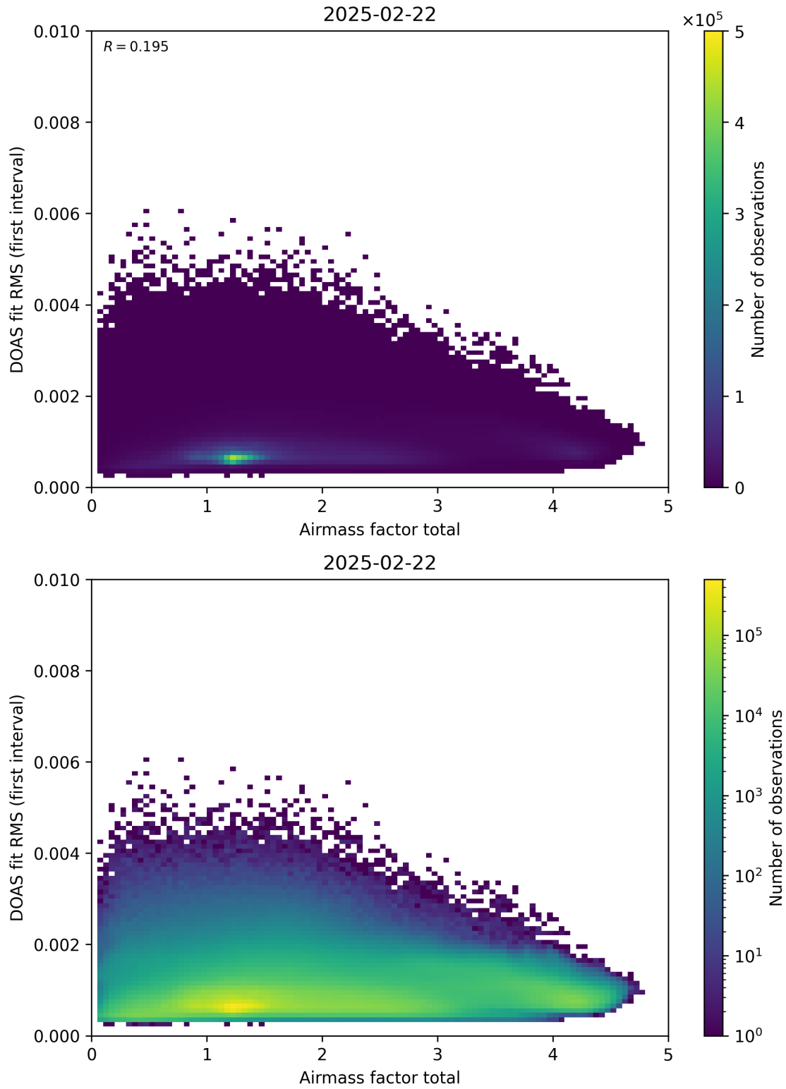
Figure 97: Scatter density plot of “Airmass factor total” against “DOAS fit RMS (first interval)” for 2025-02-21 to 2025-02-23.
