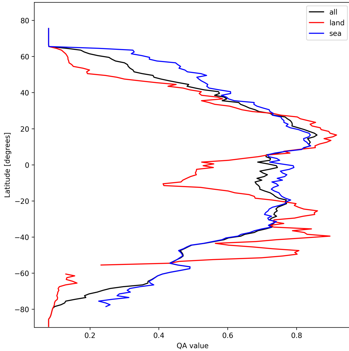
Figure 20: Zonal average of “QA value” for 2025-02-21 to 2025-02-23.
