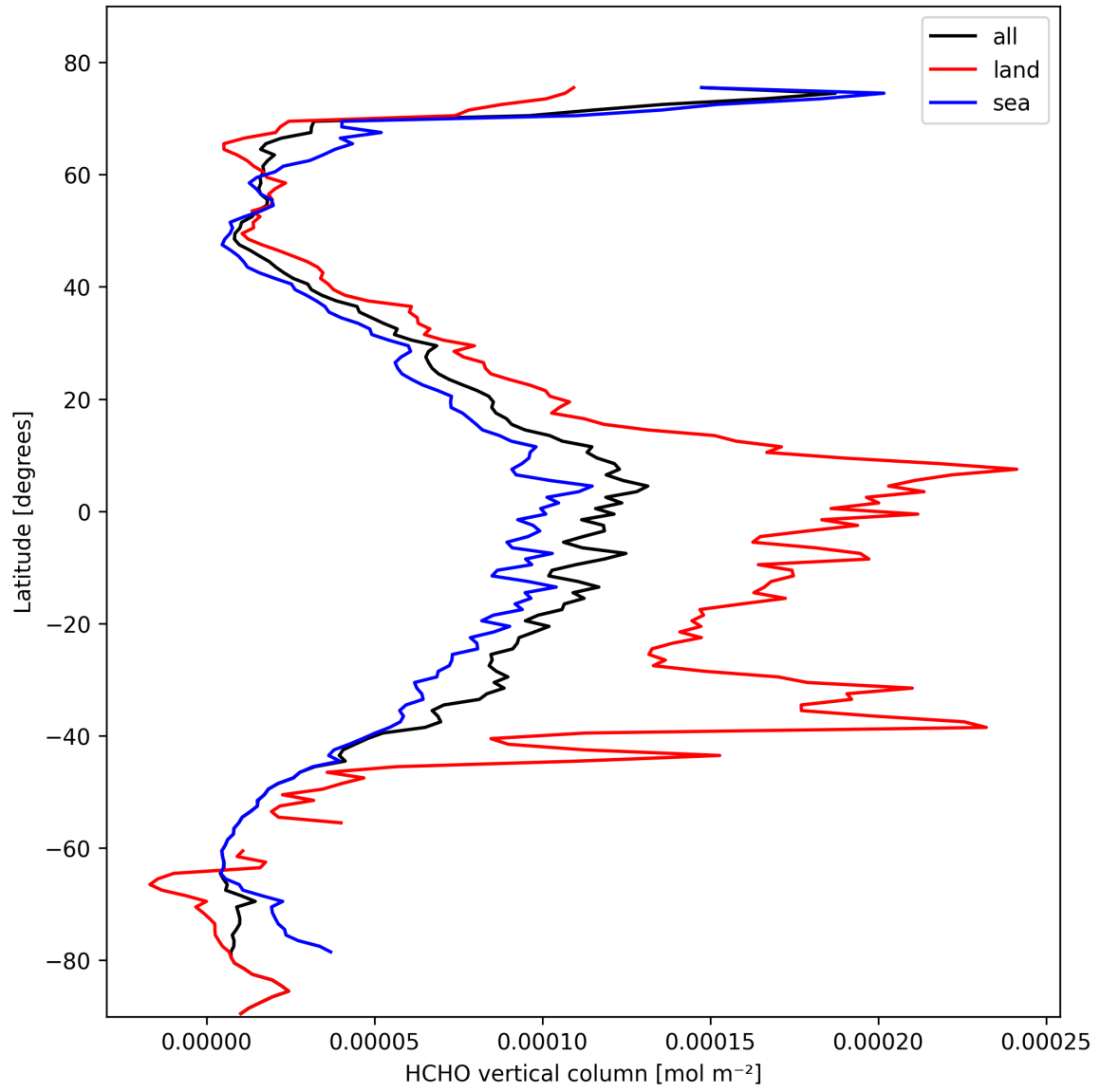
Figure 21: Zonal average of “HCHO vertical column” for 2025-02-21 to 2025-02-23.
