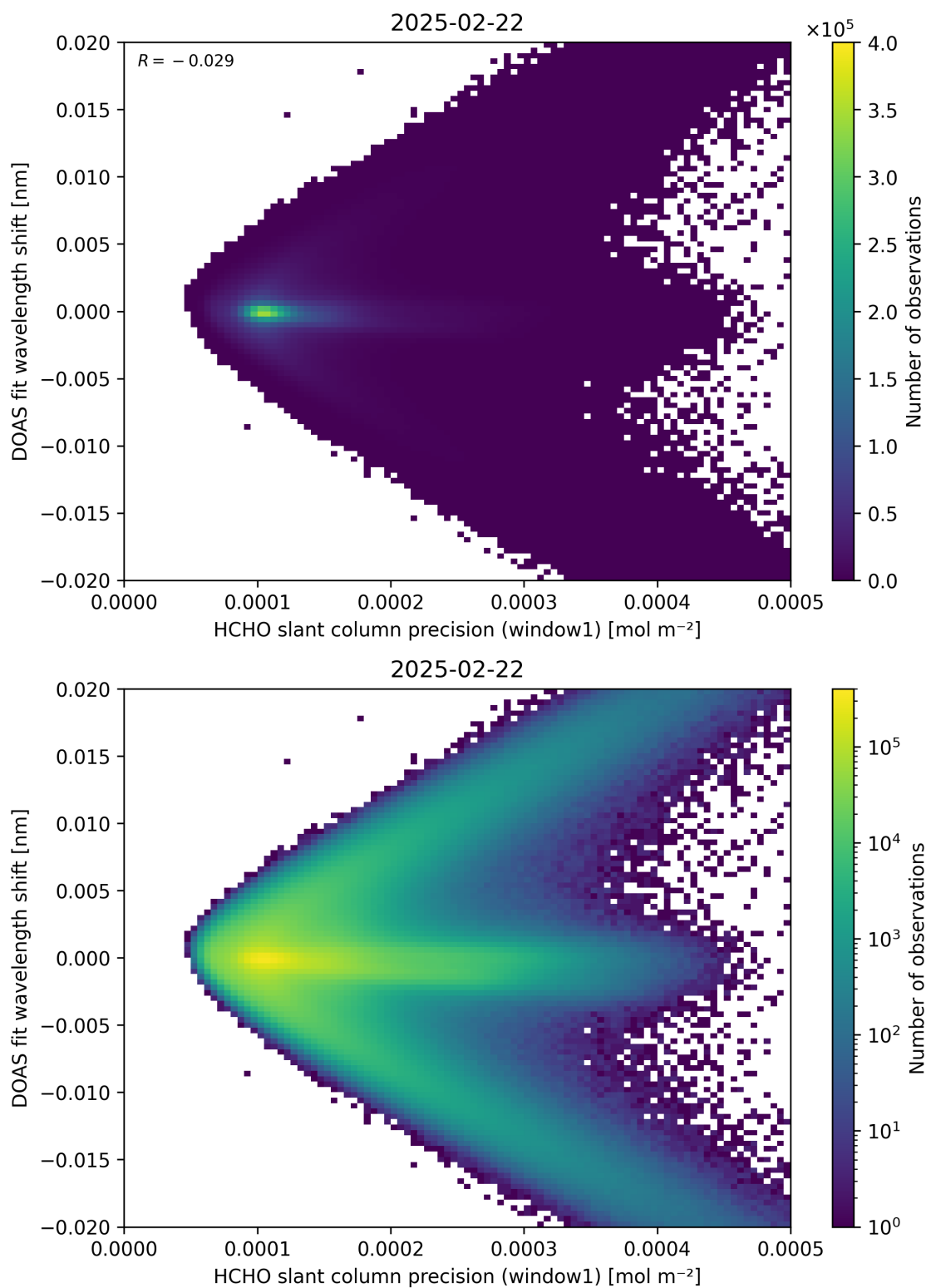
Figure 89: Scatter density plot of “HCHO slant column precision (window1)” against “DOAS fit wavelength shift” for 2025-02-21 to 2025-02-23.
