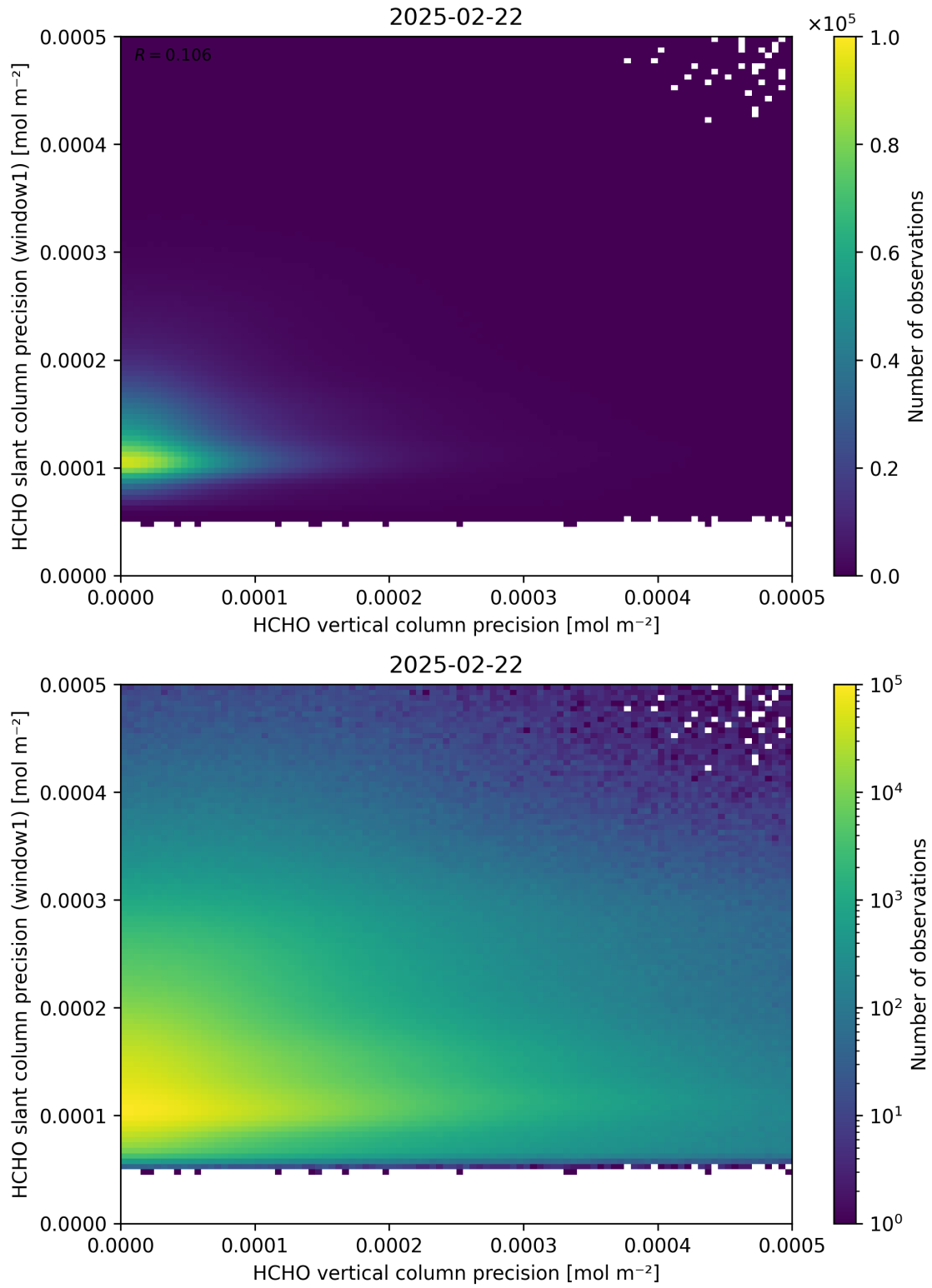
Figure 143: Scatter density plot of “HCHO vertical column precision” against “HCHO slant column precision (window1)” for 2025-02-21 to 2025-02-23.
