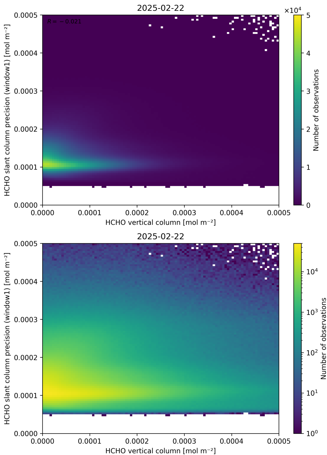
Figure 130: Scatter density plot of “HCHO vertical column” against “HCHO slant column precision (window1)” for 2025-02-21 to 2025-02-23.
