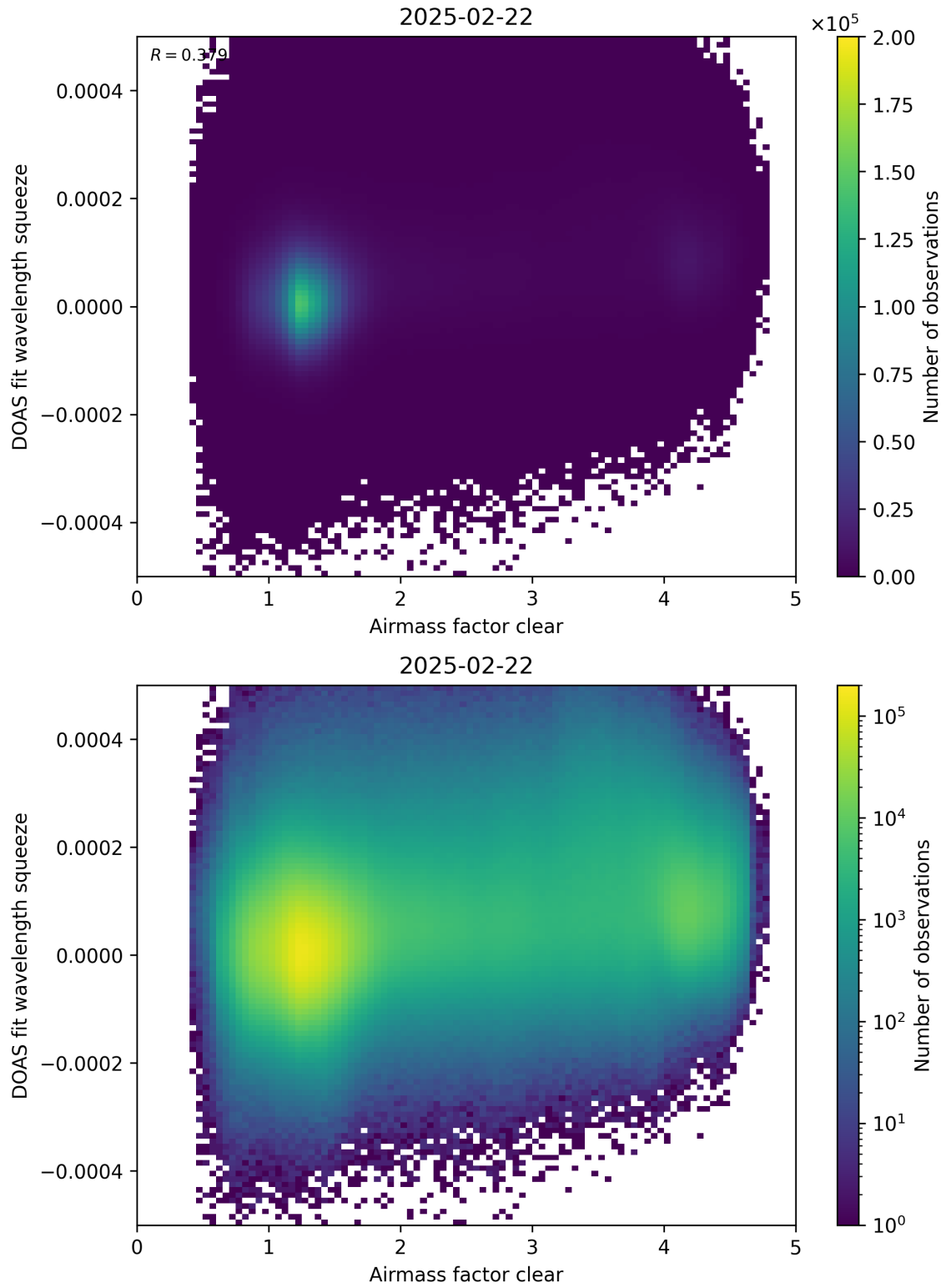
Figure 73: Scatter density plot of “Airmass factor clear” against “DOAS fit wavelength squeeze” for 2025-02-21 to 2025-02-23.
