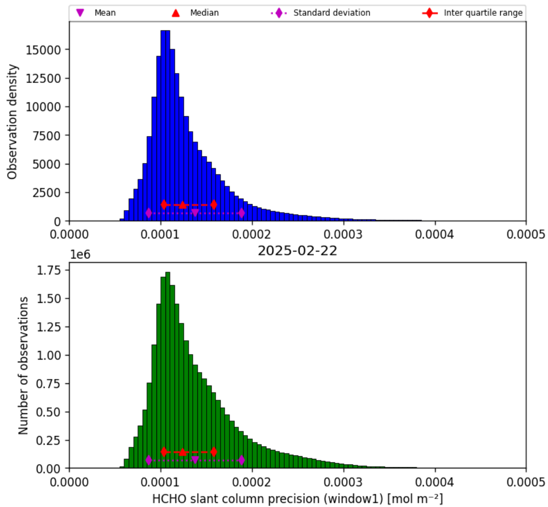
Figure 39: Histogram of “HCHO slant column precision (window1)” for 2025-02-21 to 2025-02-23
