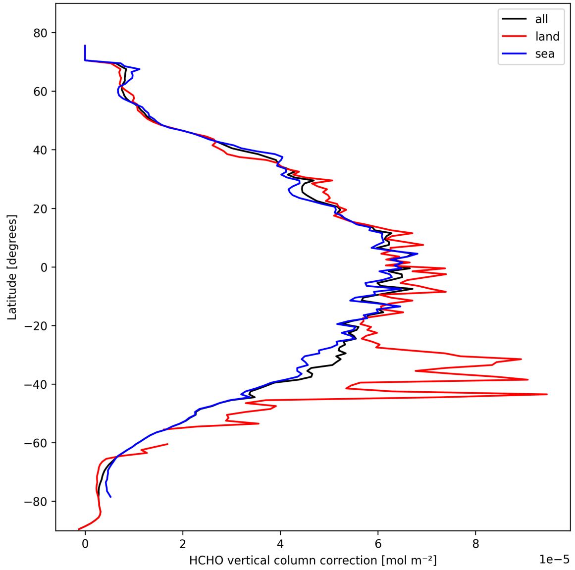
Figure 23: Zonal average of “HCHO vertical column correction” for 2025-02-21 to 2025-02-23.
