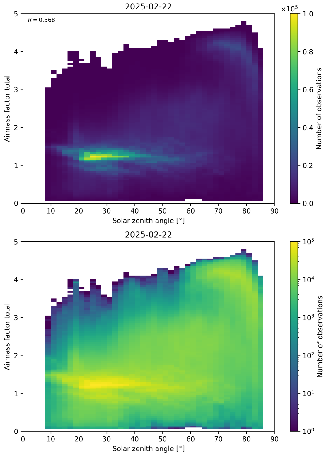
Figure 175: Scatter density plot of “Solar zenith angle” against “Airmass factor total” for 2025-02-21 to 2025-02-23.
