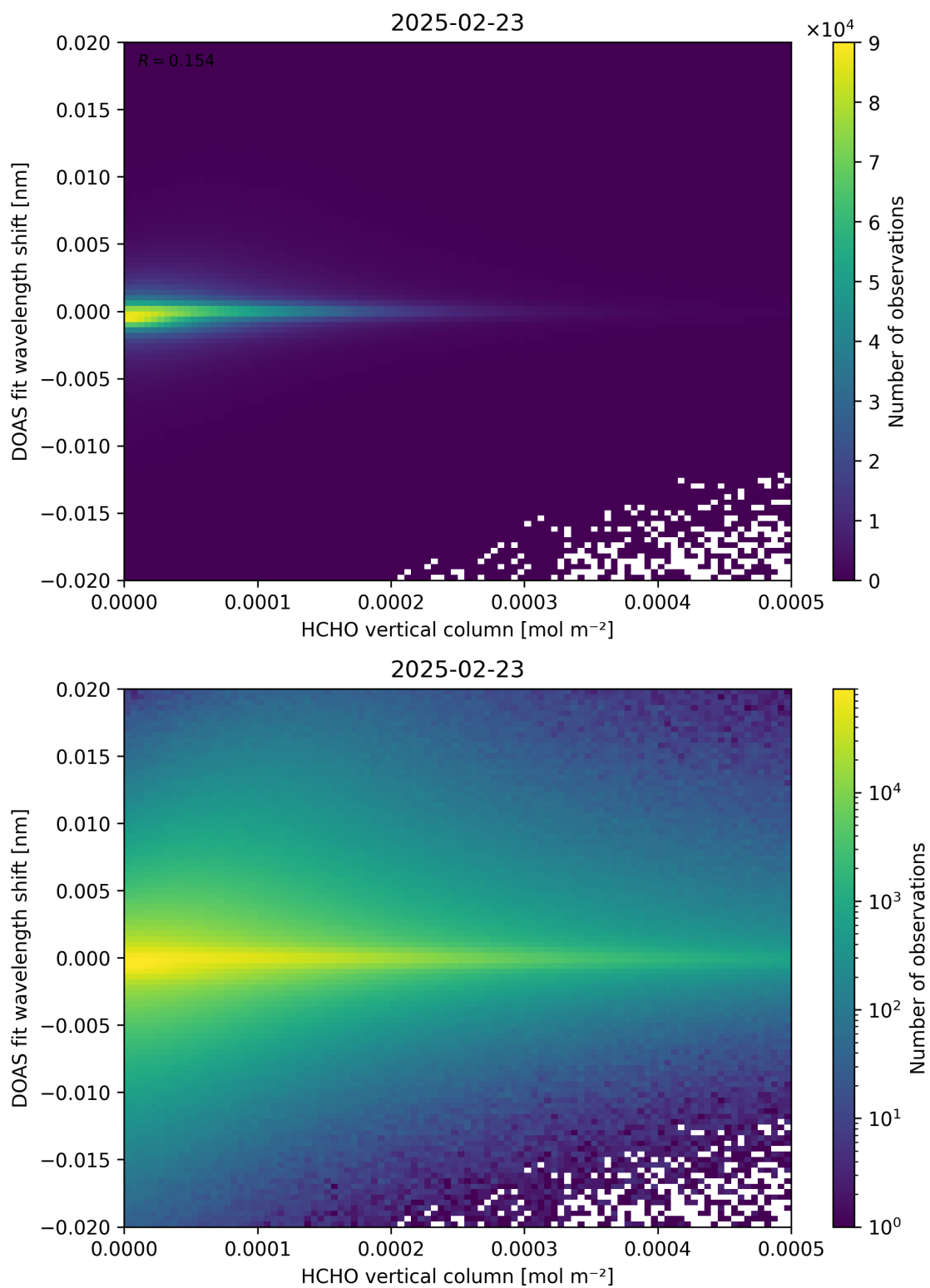
Figure 124: Scatter density plot of “HCHO vertical column” against “DOAS fit wavelength shift” for 2025-02-22 to 2025-02-24.
