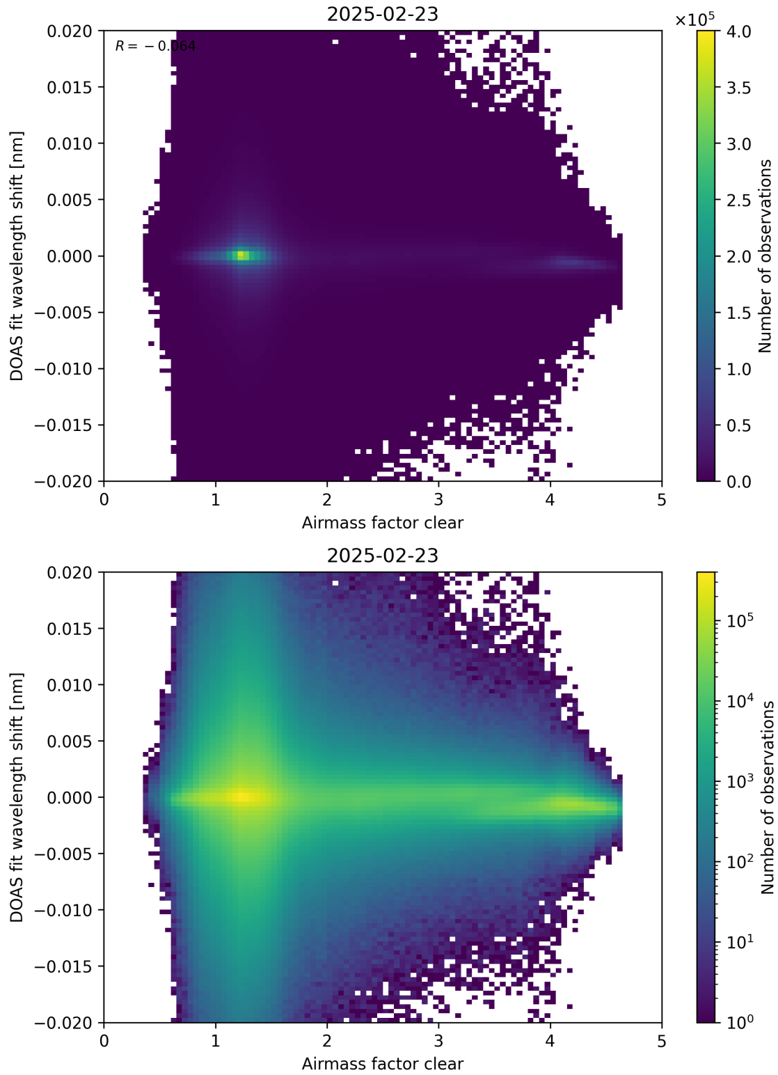
Figure 72: Scatter density plot of “Airmass factor clear” against “DOAS fit wavelength shift” for 2025-02-22 to 2025-02-24.
