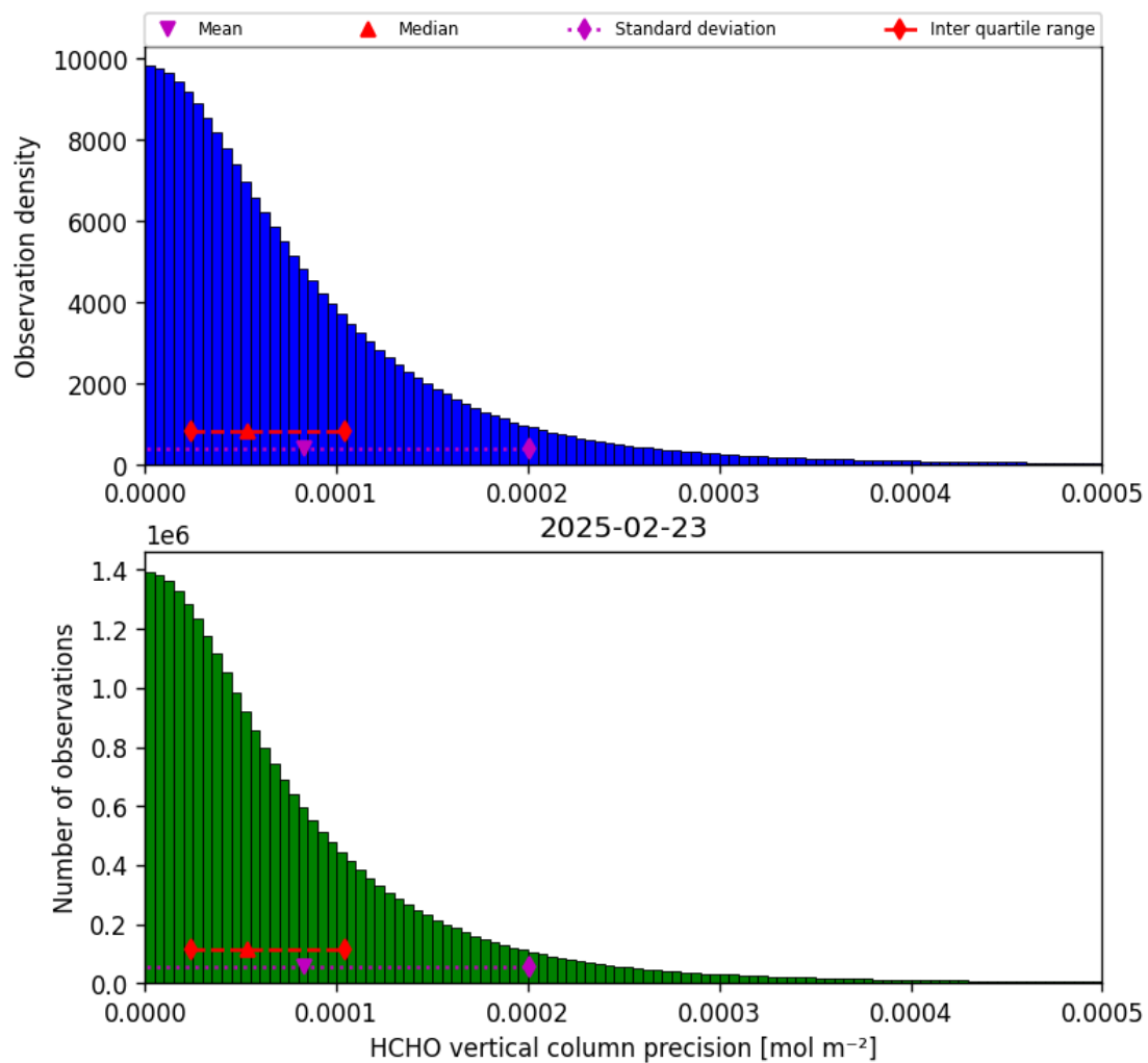
Figure 36: Histogram of “HCHO vertical column precision” for 2025-02-22 to 2025-02-24
