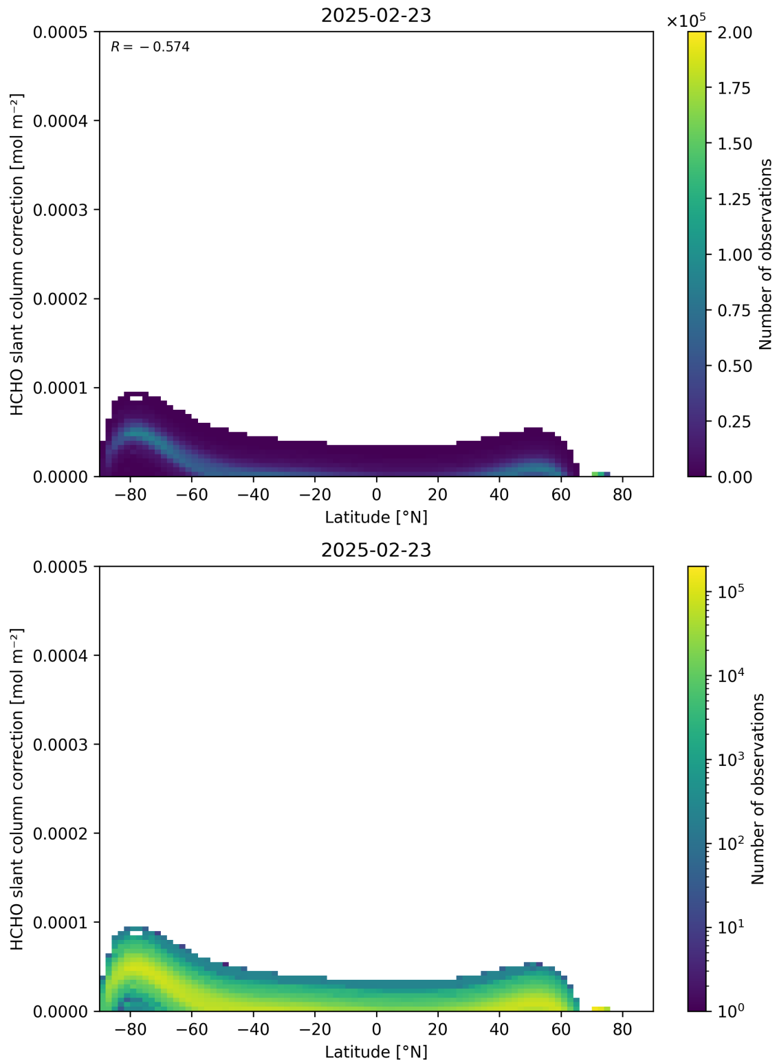
Figure 158: Scatter density plot of “Latitude” against “HCHO slant column correction” for 2025-02-22 to 2025-02-24.
