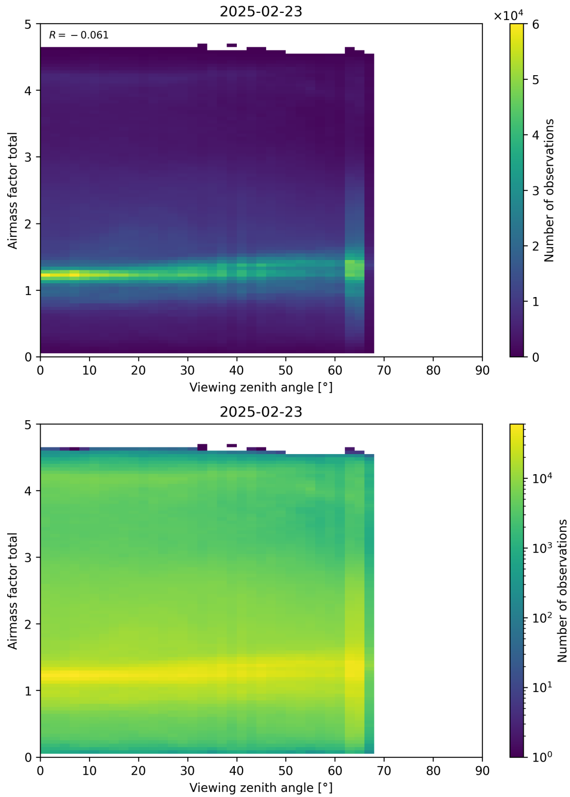
Figure 190: Scatter density plot of “Viewing zenith angle” against “Airmass factor total” for 2025-02-22 to 2025-02-24.
