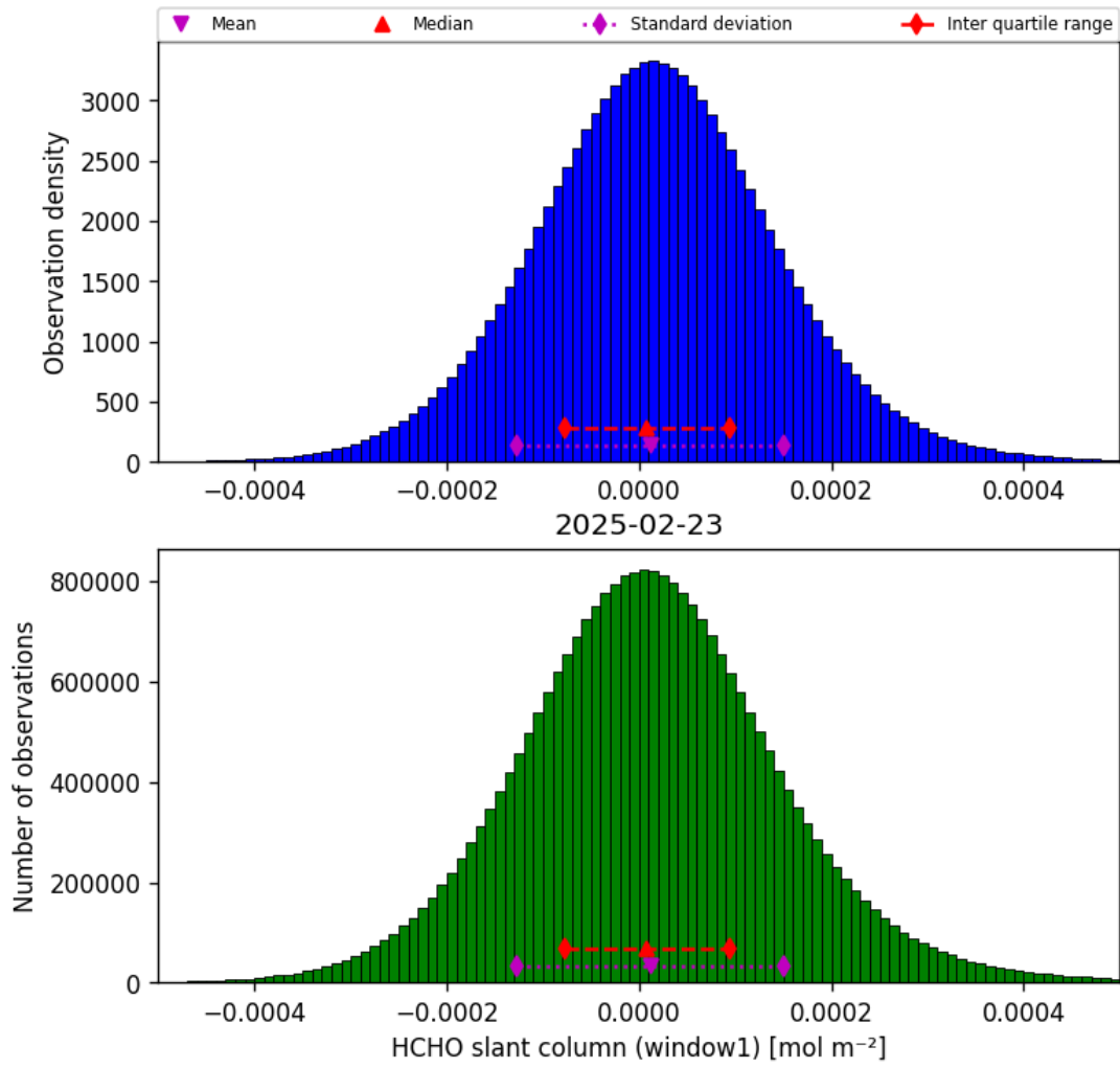
Figure 38: Histogram of “HCHO slant column (window1)” for 2025-02-22 to 2025-02-24
