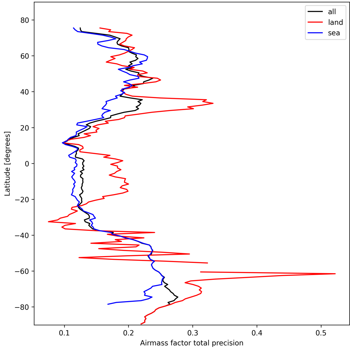
Figure 27: Zonal average of “Airmass factor total precision” for 2025-02-22 to 2025-02-24.
