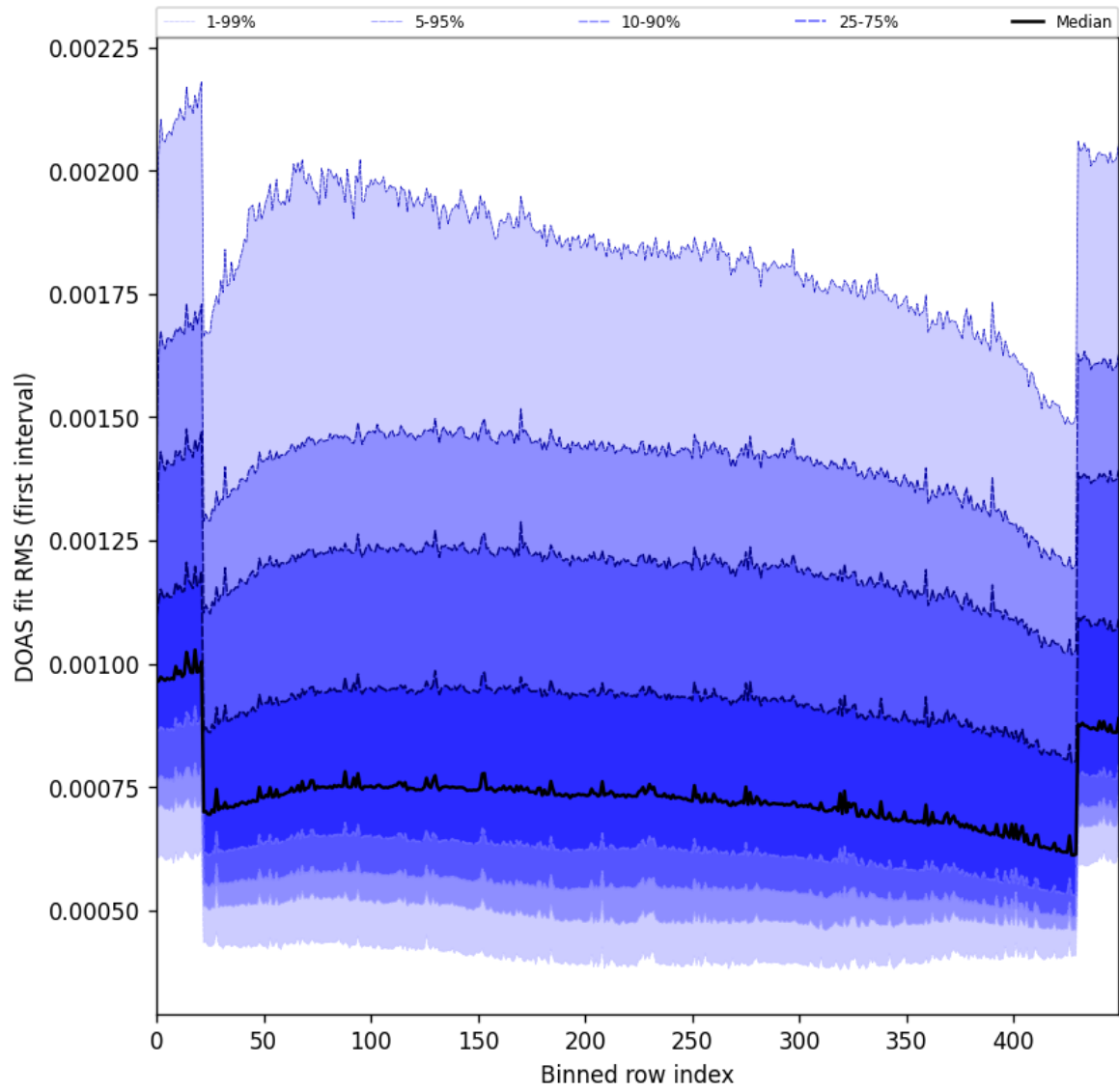
Figure 60: Along track statistics of “DOAS fit RMS (first interval)” for 2025-02-22 to 2025-02-24
