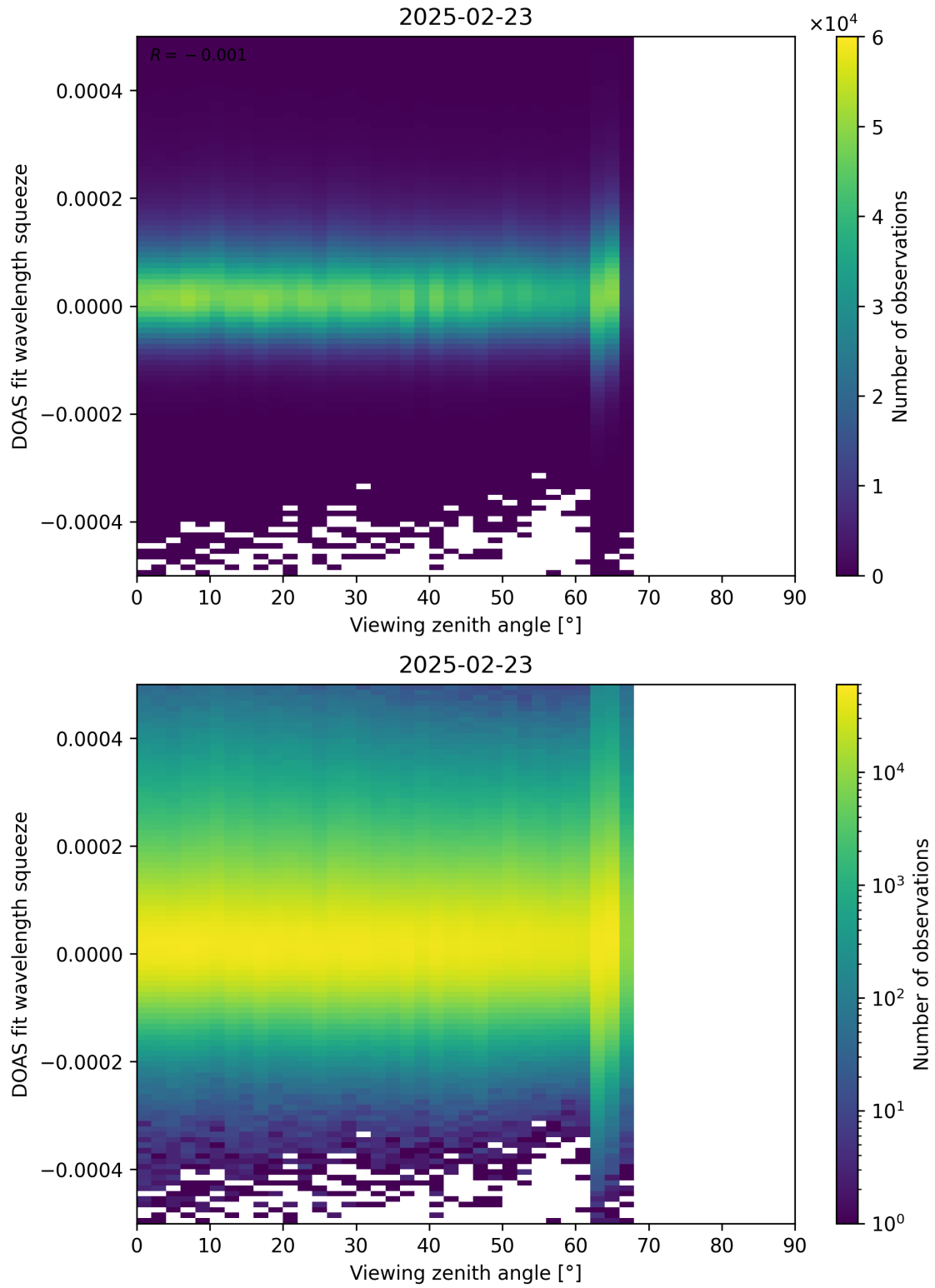
Figure 184: Scatter density plot of “Viewing zenith angle” against “DOAS fit wavelength squeeze” for 2025-02-22 to 2025-02-24.
