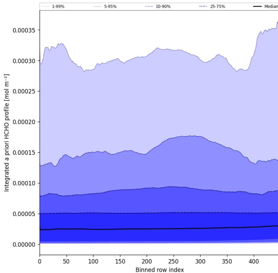
Figure 57: Along track statistics of “Integrated a priori HCHO profile” for 2025-02-22 to 2025-02-24
