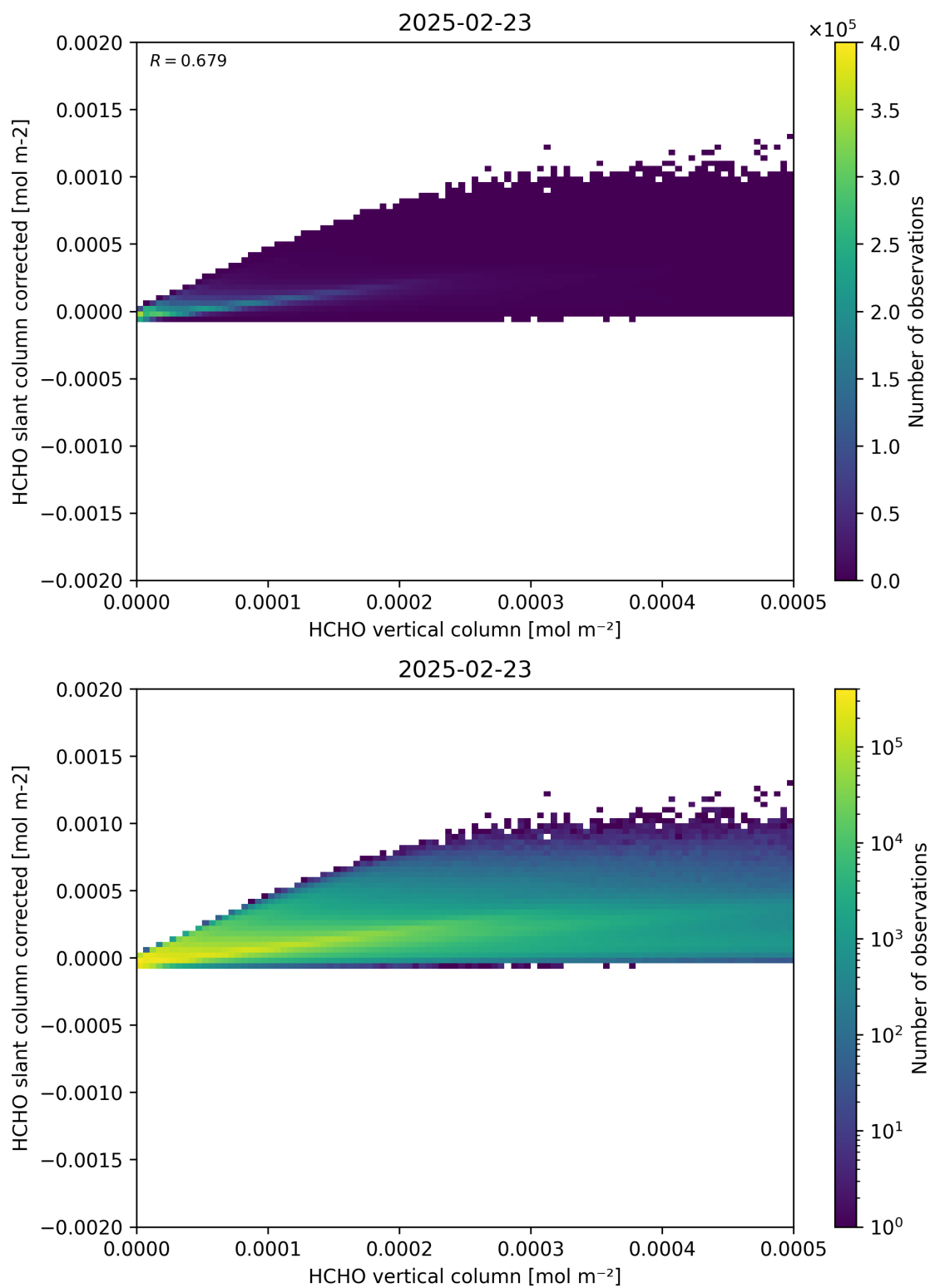
Figure 127: Scatter density plot of “HCHO vertical column” against “HCHO slant column corrected” for 2025-02-22 to 2025-02-24.
