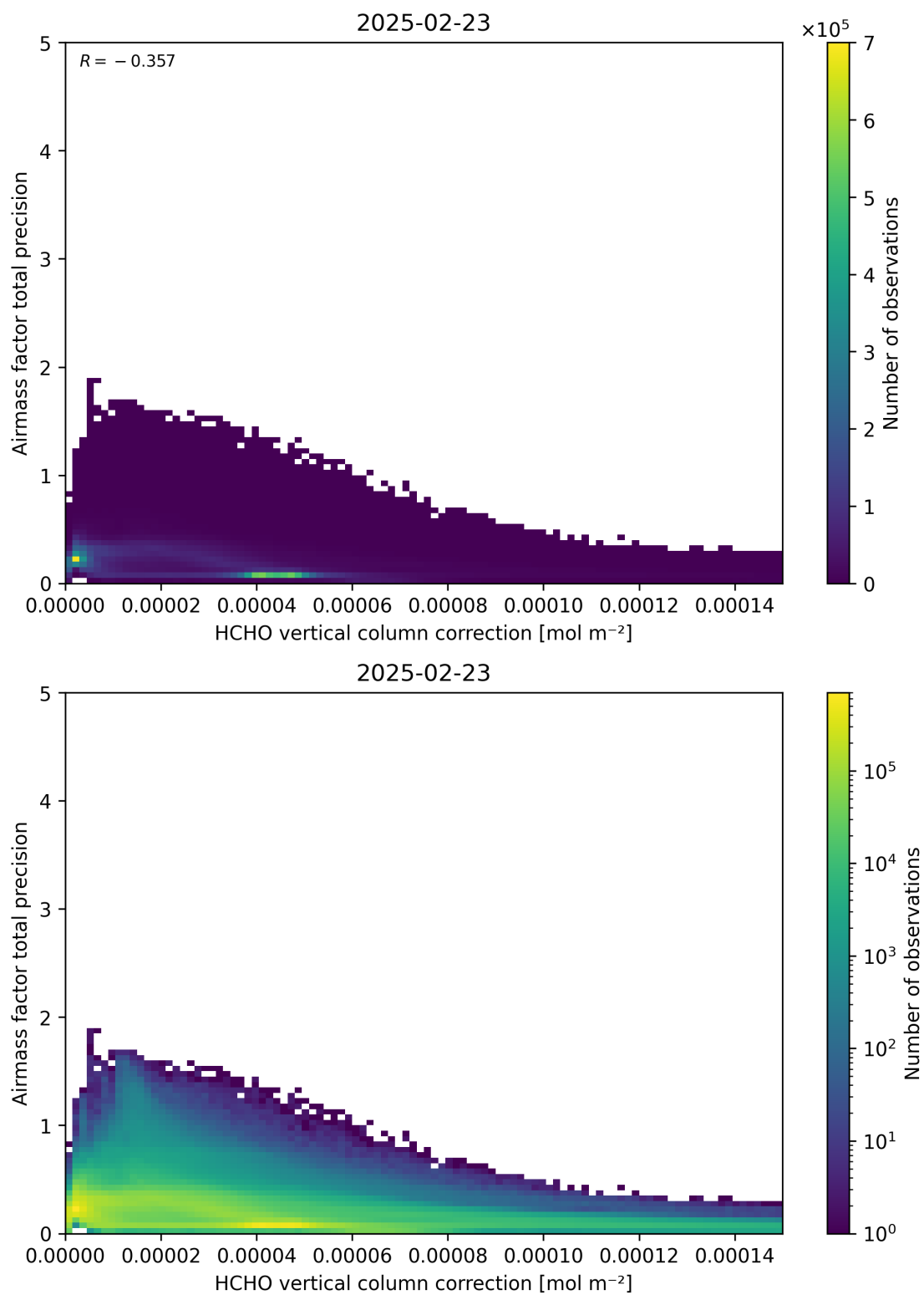
Figure 121: Scatter density plot of “HCHO vertical column correction” against “Airmass factor total precision” for 2025-02-22 to 2025-02-24.
