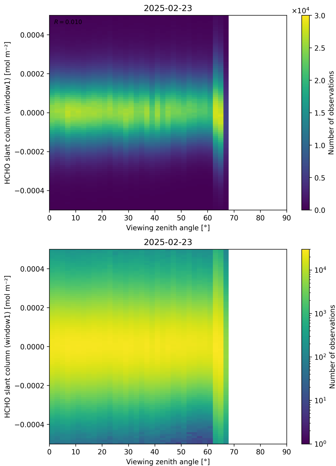
Figure 188: Scatter density plot of “Viewing zenith angle” against “HCHO slant column (window1)” for 2025-02-22 to 2025-02-24.
