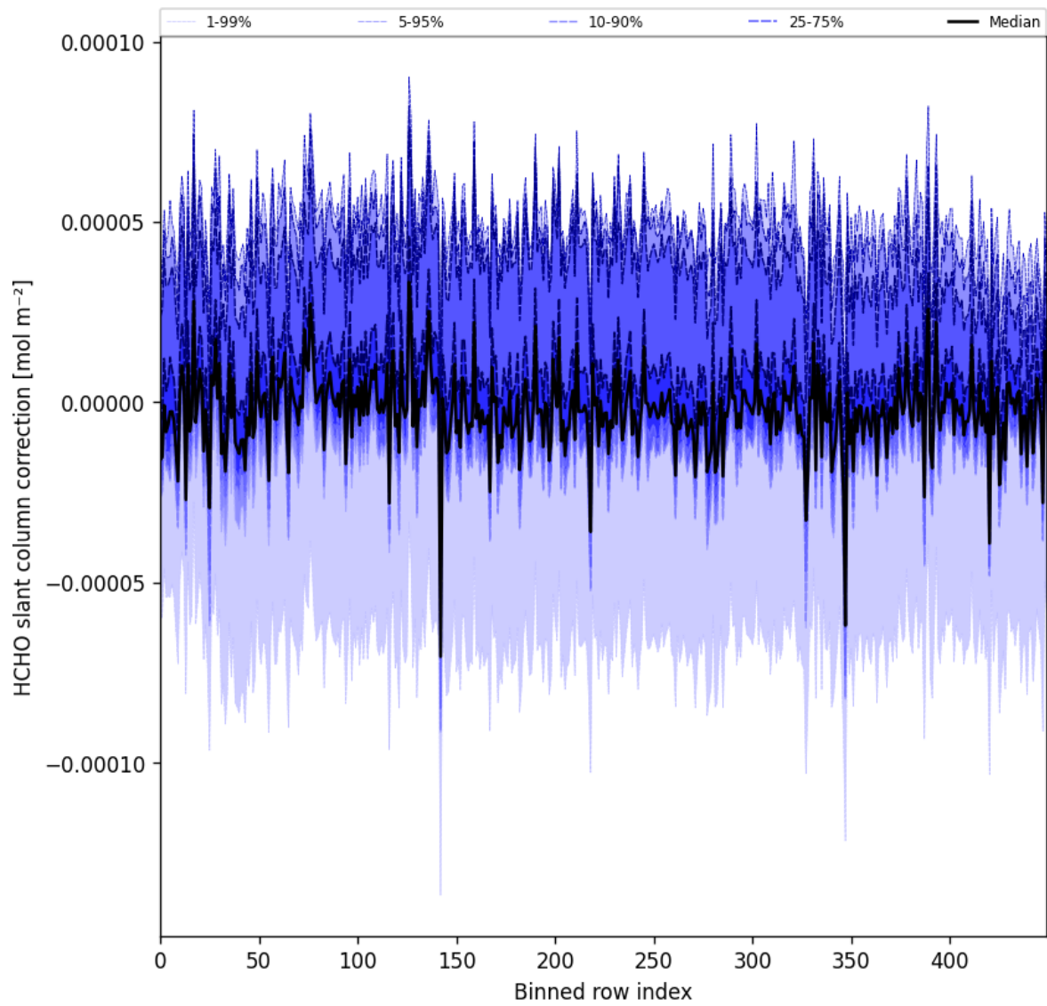
Figure 61: Along track statistics of “HCHO slant column correction” for 2025-02-22 to 2025-02-24
