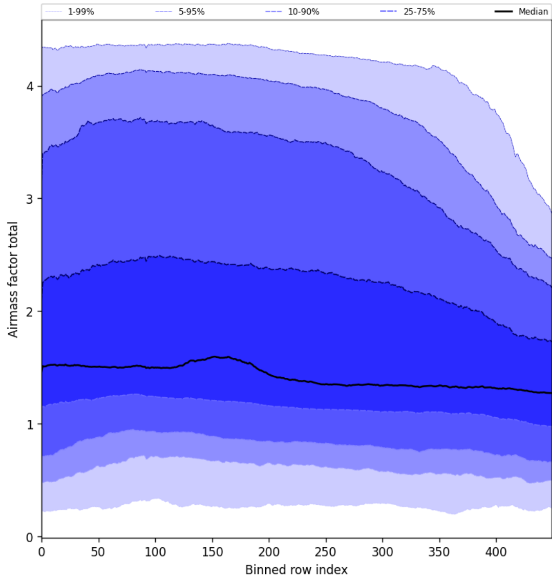
Figure 54: Along track statistics of “Airmass factor total” for 2025-02-22 to 2025-02-24
