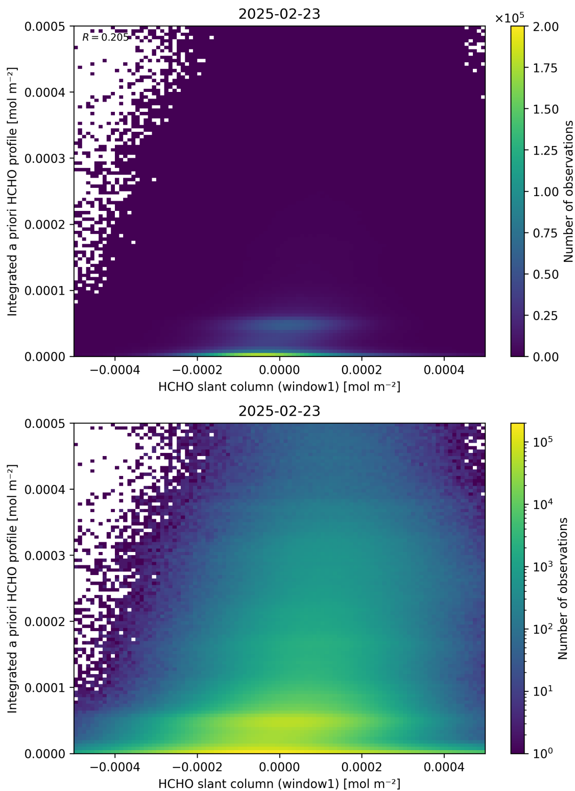
Figure 87: Scatter density plot of “HCHO slant column (window1)” against “Integrated a priori HCHO profile” for 2025-02-22 to 2025-02-24.
