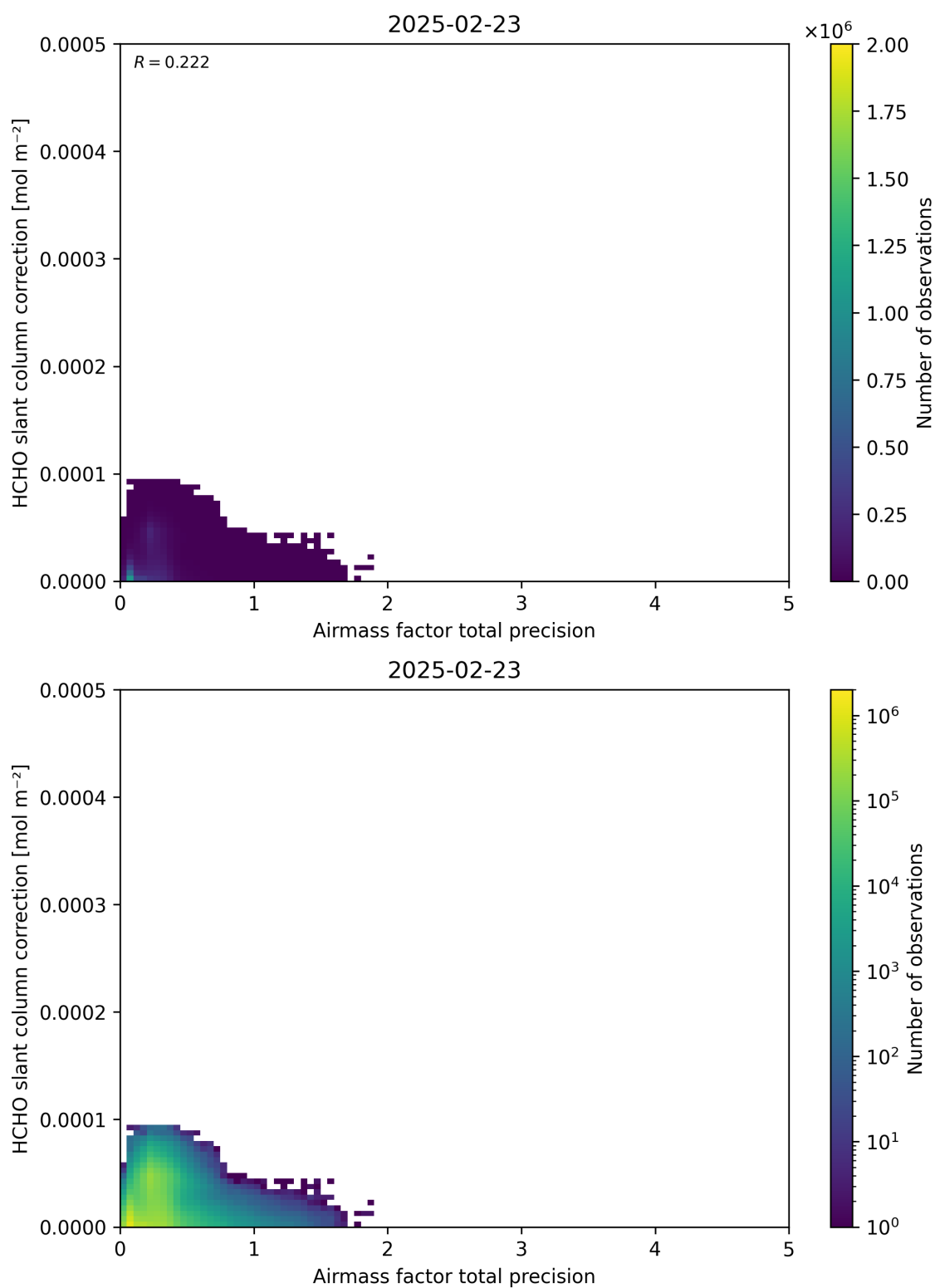
Figure 110: Scatter density plot of “Airmass factor total precision” against “HCHO slant column correction” for 2025-02-22 to 2025-02-24.
