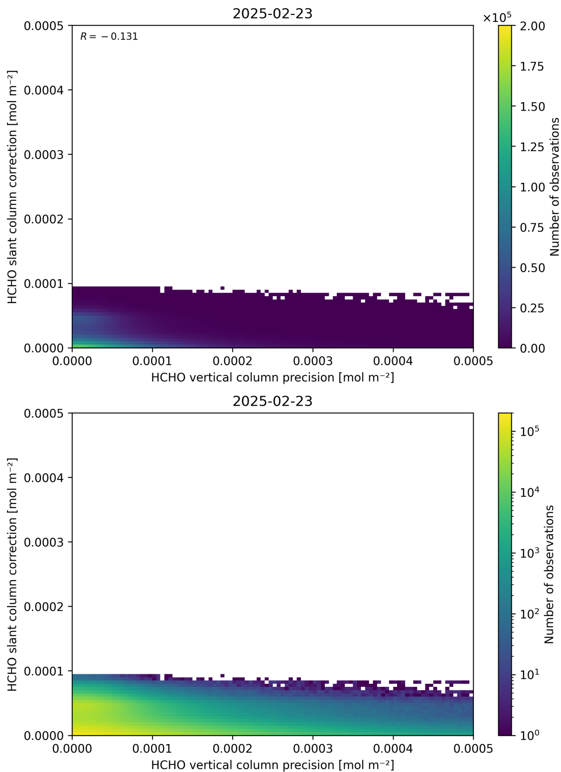
Figure 141: Scatter density plot of “HCHO vertical column precision” against “HCHO slant column correction” for 2025-02-22 to 2025-02-24.
