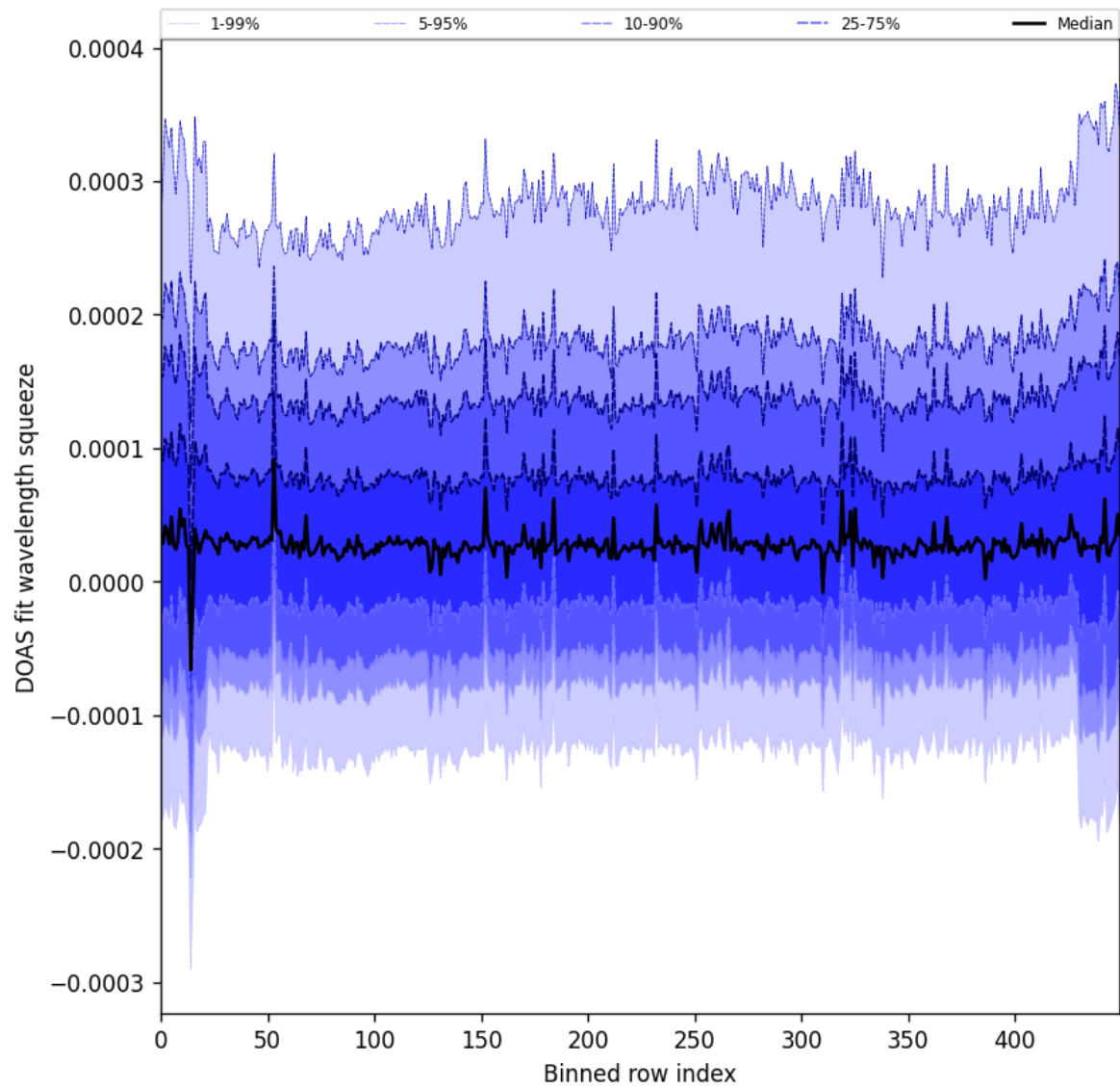
Figure 59: Along track statistics of “DOAS fit wavelength squeeze” for 2025-02-22 to 2025-02-24
