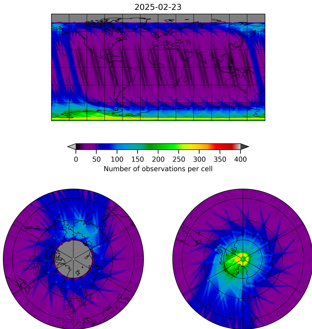
Figure 19: Map of the number of observations for 2025-02-22 to 2025-02-24
