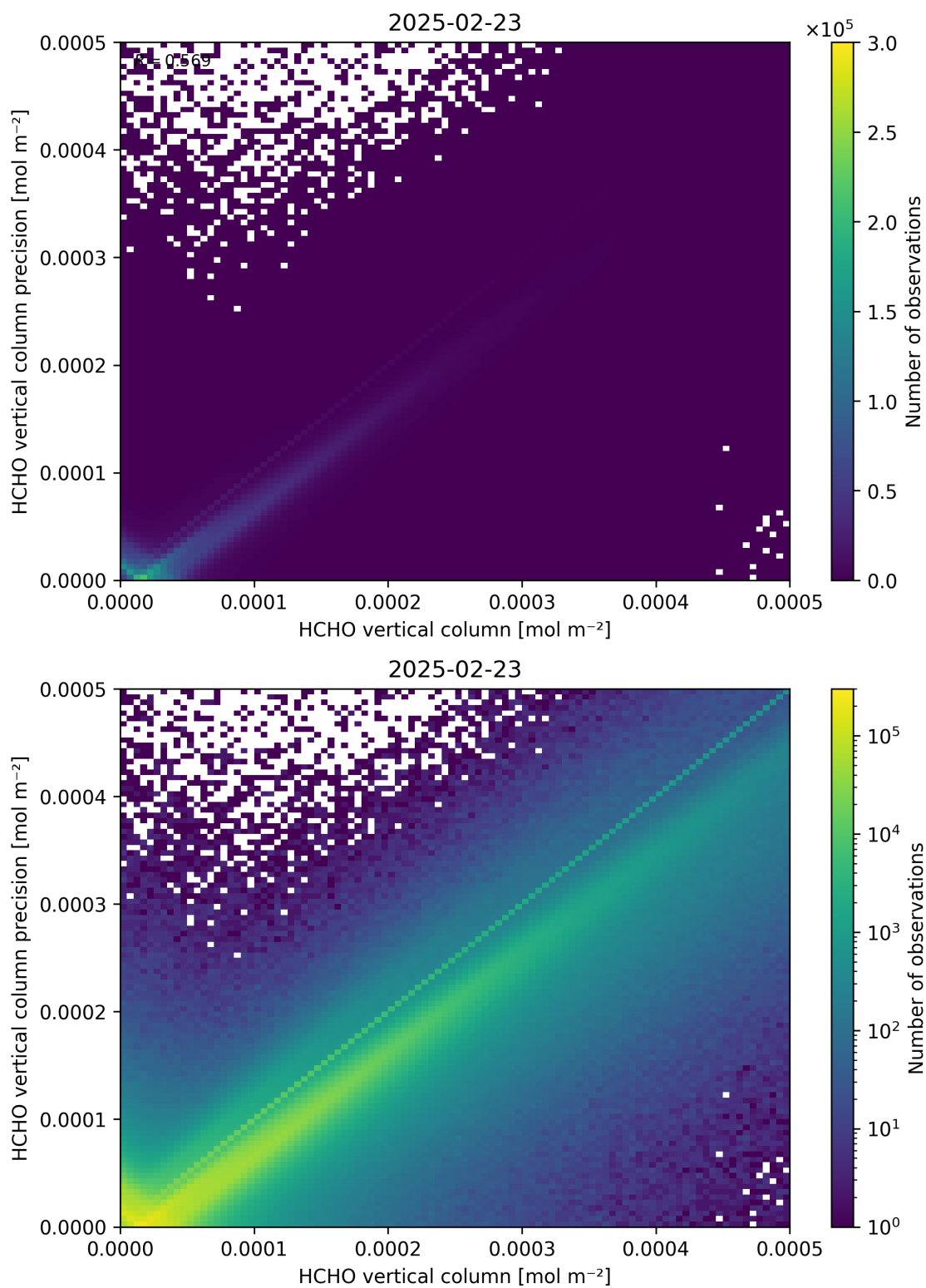
Figure 134: Scatter density plot of “HCHO vertical column” against “HCHO vertical column precision” for 2025-02-22 to 2025-02-24.
