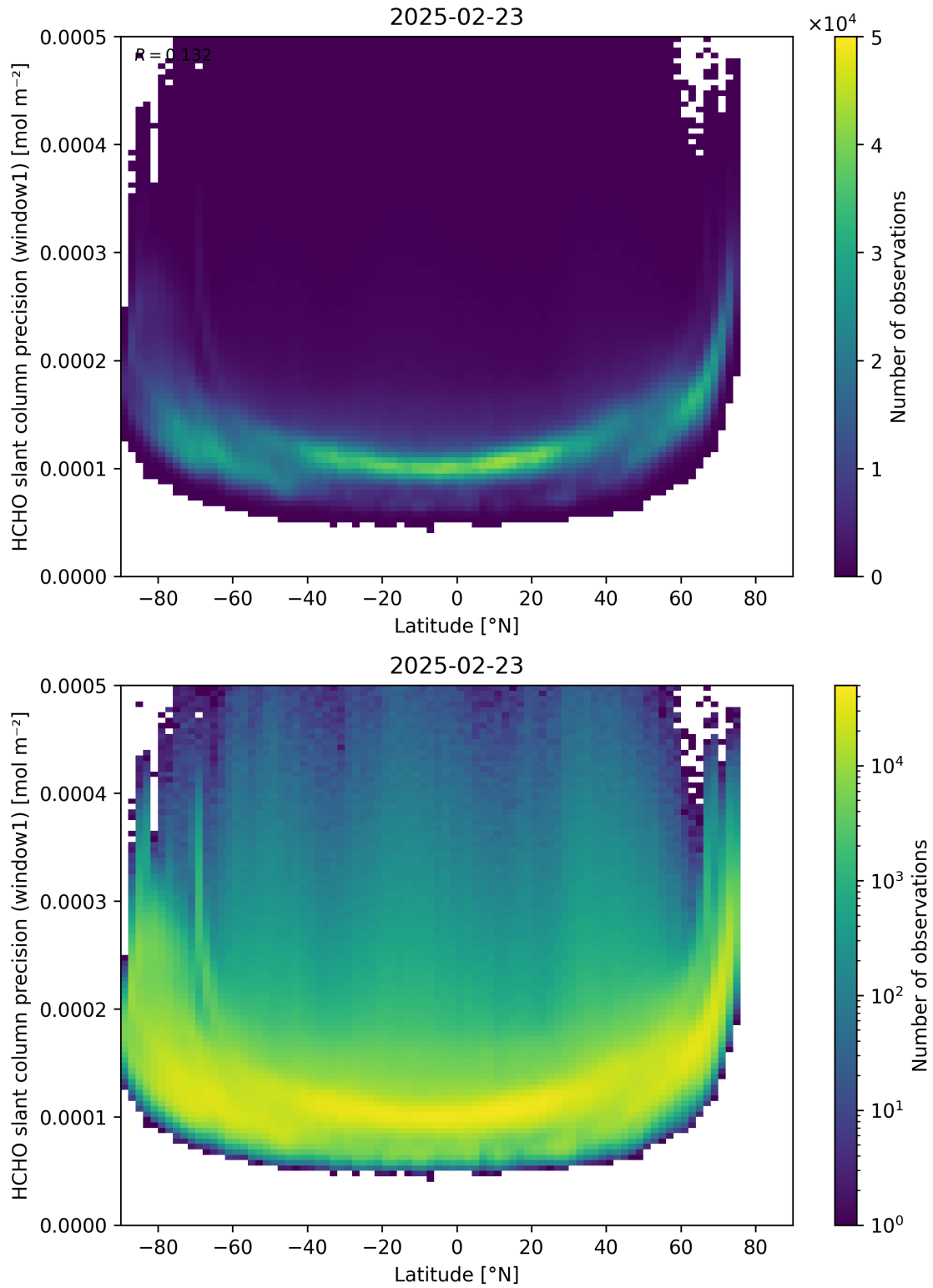
Figure 160: Scatter density plot of “Latitude” against “HCHO slant column precision (window1)” for 2025-02-22 to 2025-02-24.
