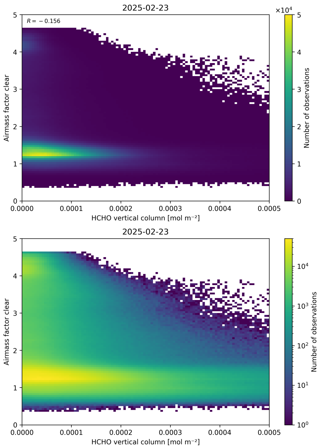
Figure 126: Scatter density plot of “HCHO vertical column” against “Airmass factor clear” for 2025-02-22 to 2025-02-24.
