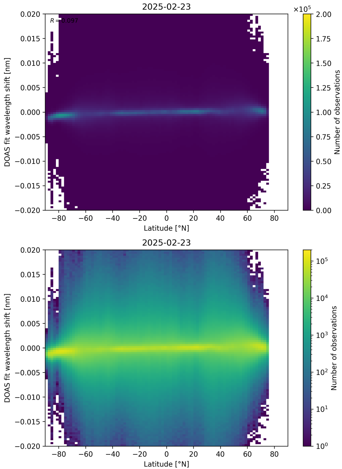
Figure 154: Scatter density plot of “Latitude” against “DOAS fit wavelength shift” for 2025-02-22 to 2025-02-24.
