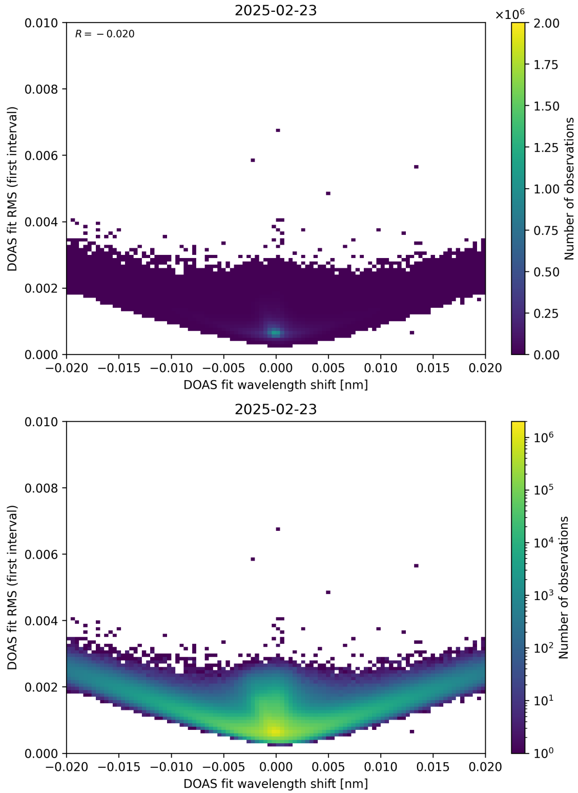
Figure 64: Scatter density plot of “DOAS fit wavelength shift” against “DOAS fit RMS (first interval)” for 2025-02-22 to 2025-02-24.
