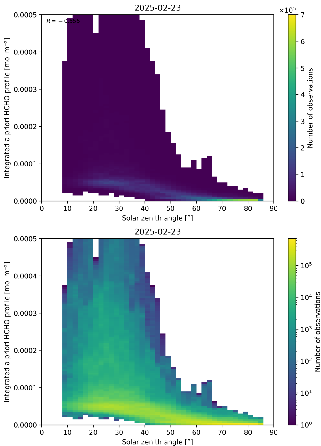
Figure 180: Scatter density plot of “Solar zenith angle” against “Integrated a priori HCHO profile” for 2025-02-22 to 2025-02-24.
