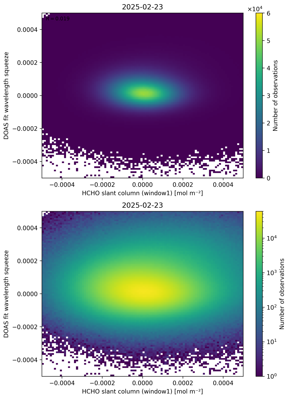
Figure 80: Scatter density plot of “HCHO slant column (window1)” against “DOAS fit wavelength squeeze” for 2025-02-22 to 2025-02-24.
