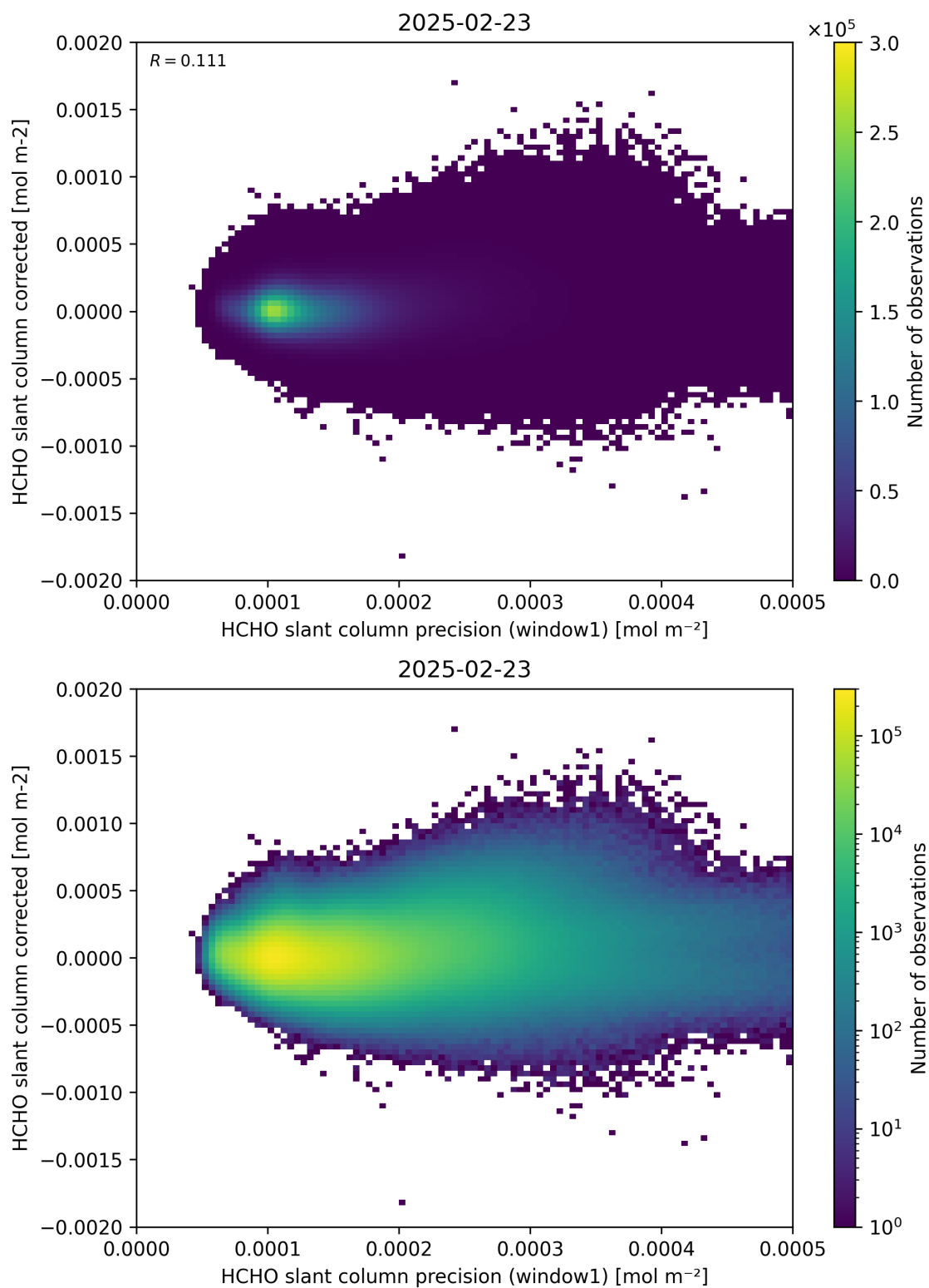
Figure 92: Scatter density plot of “HCHO slant column precision (window1)” against “HCHO slant column corrected” for 2025-02-22 to 2025-02-24.
