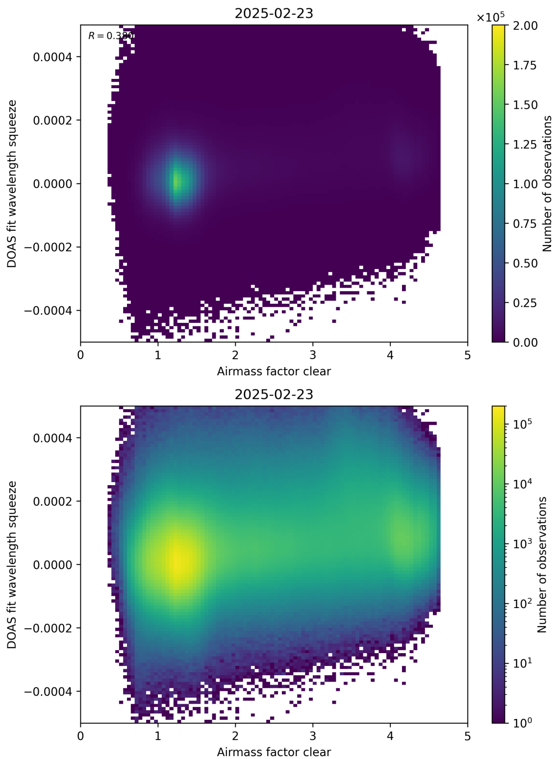
Figure 73: Scatter density plot of “Airmass factor clear” against “DOAS fit wavelength squeeze” for 2025-02-22 to 2025-02-24.
