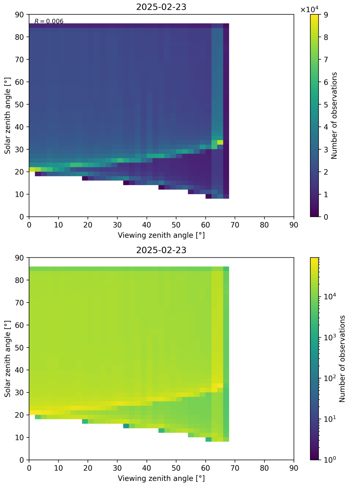
Figure 197: Scatter density plot of “Viewing zenith angle” against “Solar zenith angle” for 2025-02-22 to 2025-02-24.
