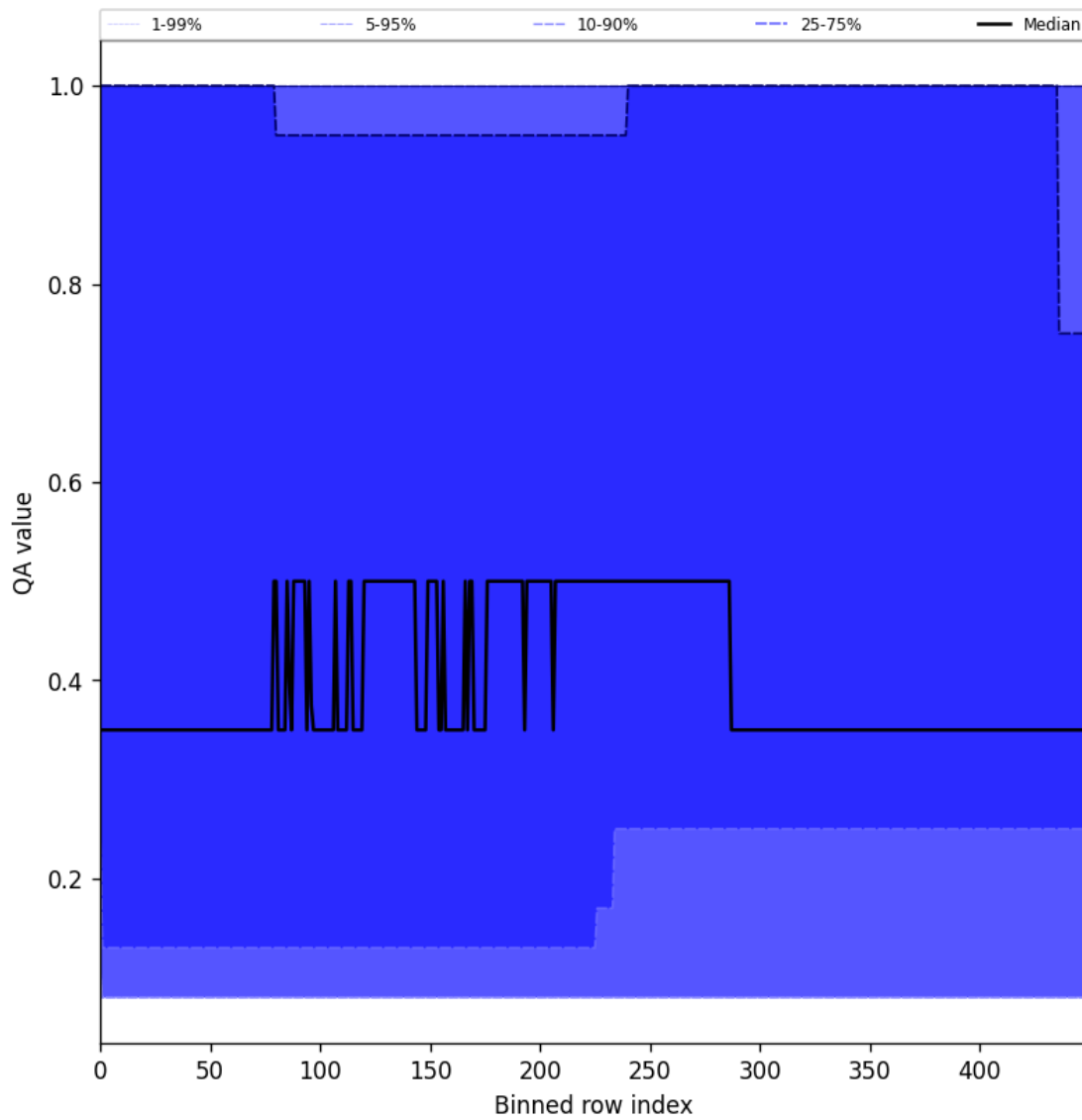
Figure 48: Along track statistics of “QA value” for 2025-02-22 to 2025-02-24
