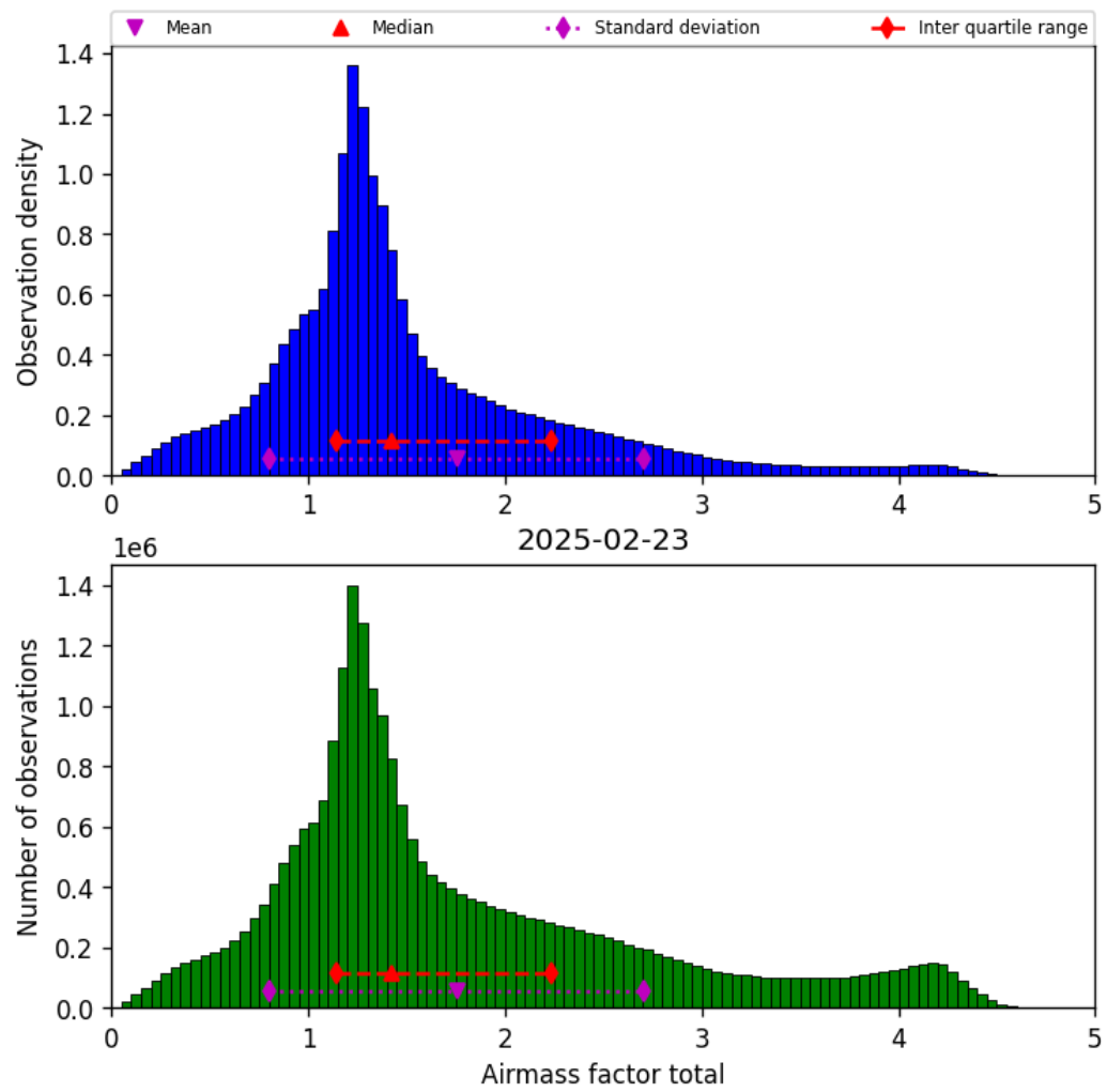
Figure 40: Histogram of “Airmass factor total” for 2025-02-22 to 2025-02-24
