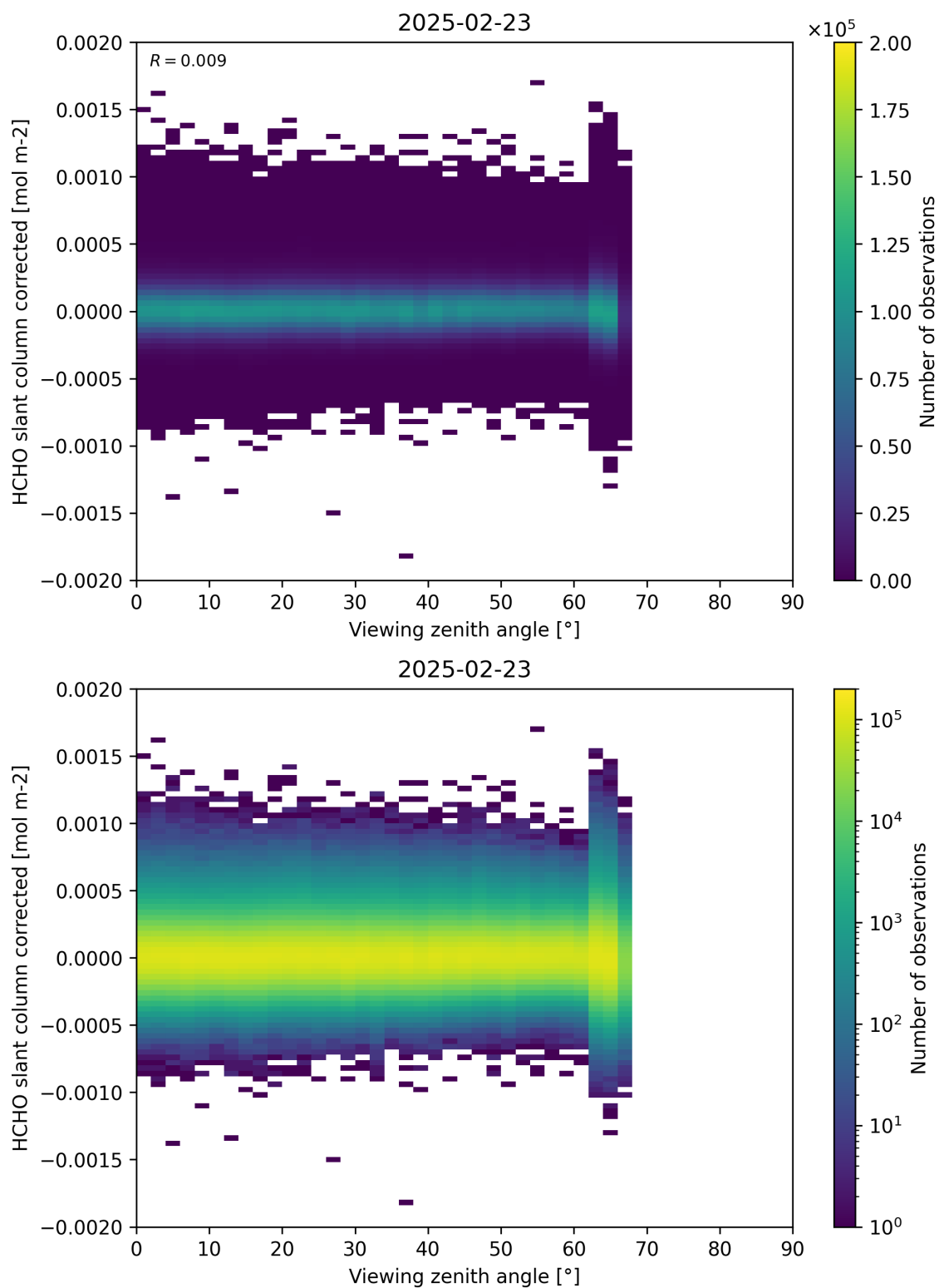
Figure 186: Scatter density plot of “Viewing zenith angle” against “HCHO slant column corrected” for 2025-02-22 to 2025-02-24.
