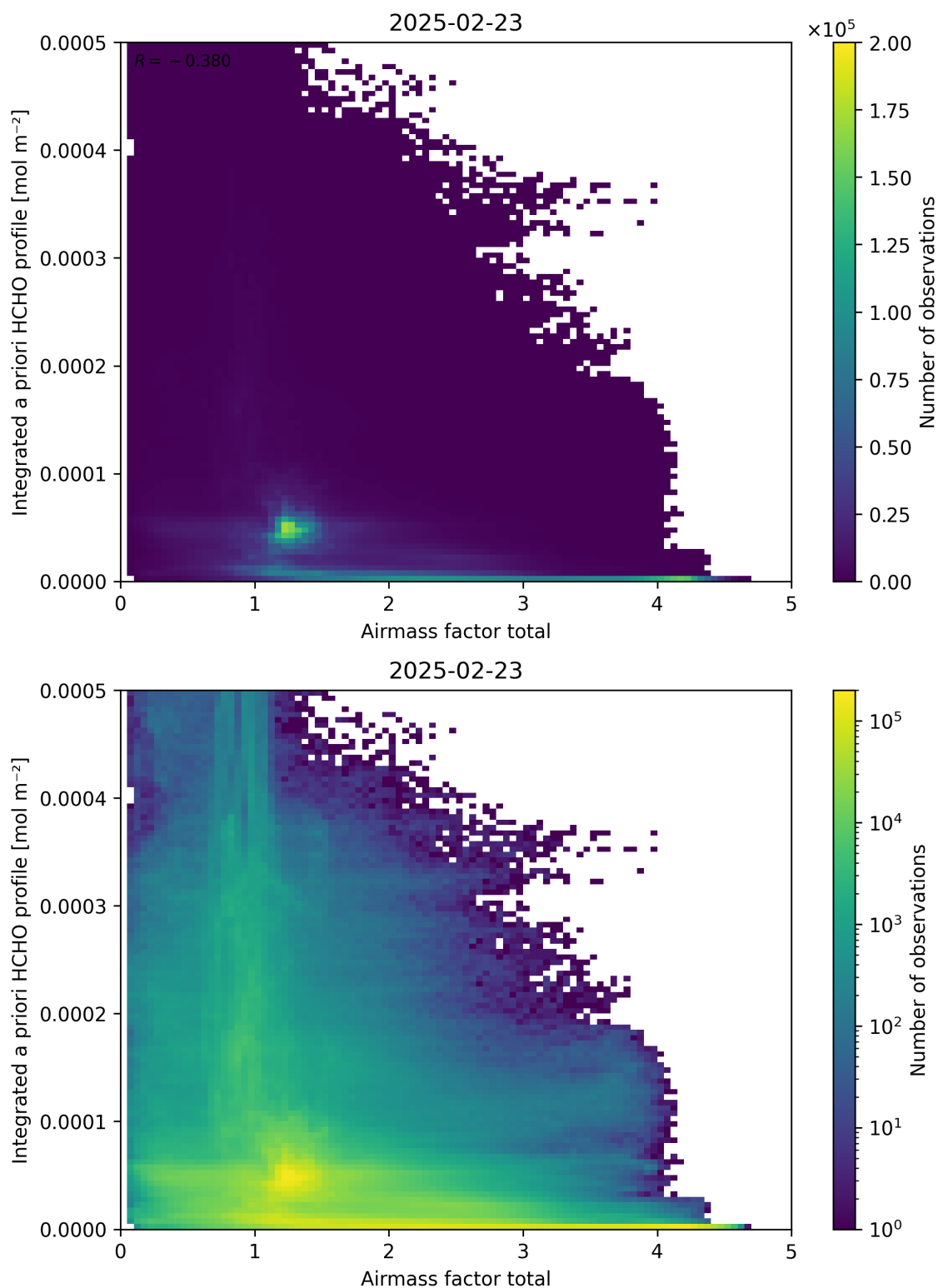
Figure 104: Scatter density plot of “Airmass factor total” against “Integrated a priori HCHO profile” for 2025-02-22 to 2025-02-24.
