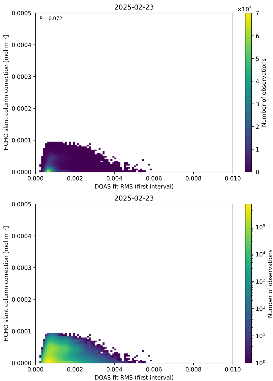
Figure 63: Scatter density plot of “DOAS fit RMS (first interval)” against “HCHO slant column correction” for 2025-02-22 to 2025-02-24.
