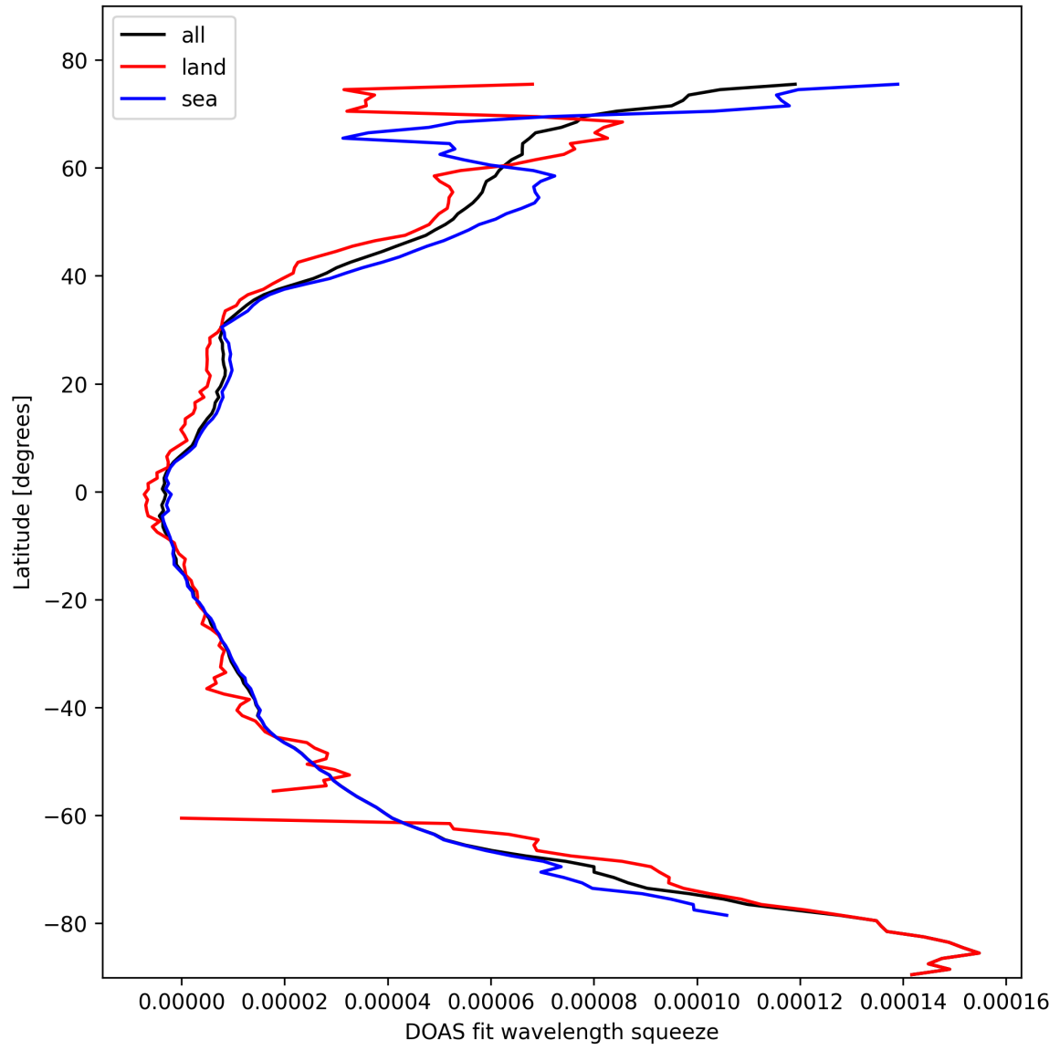
Figure 31: Zonal average of “DOAS fit wavelength squeeze” for 2025-02-22 to 2025-02-24.
