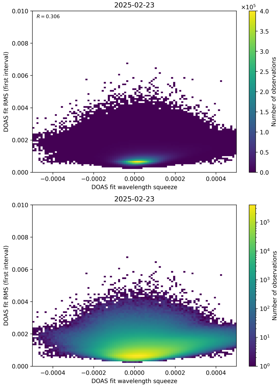
Figure 68: Scatter density plot of “DOAS fit wavelength squeeze” against “DOAS fit RMS (first interval)” for 2025-02-22 to 2025-02-24.
