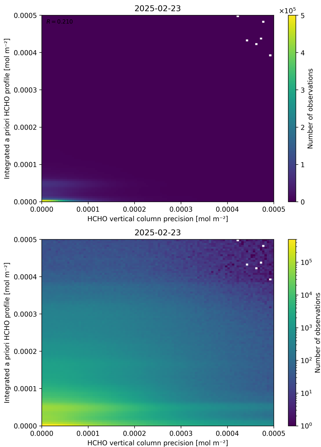
Figure 147: Scatter density plot of “HCHO vertical column precision” against “Integrated a priori HCHO profile” for 2025-02-22 to 2025-02-24.
