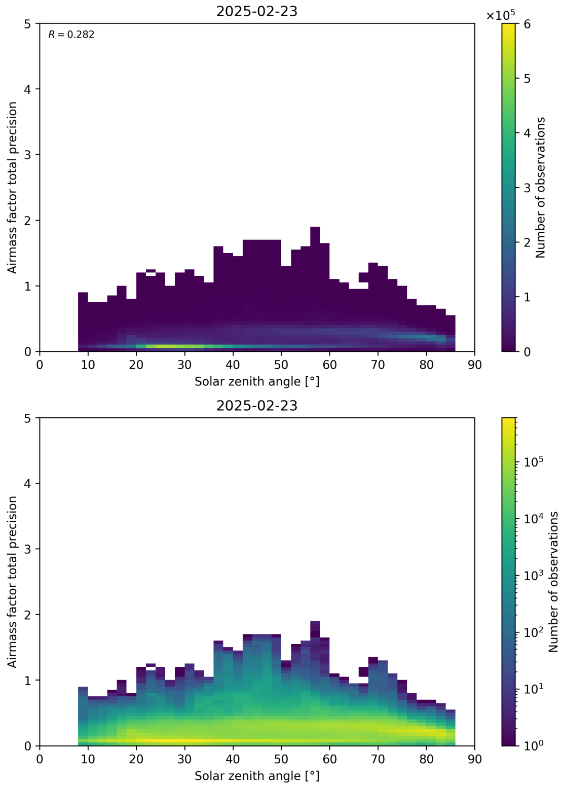
Figure 176: Scatter density plot of “Solar zenith angle” against “Airmass factor total precision” for 2025-02-22 to 2025-02-24.
