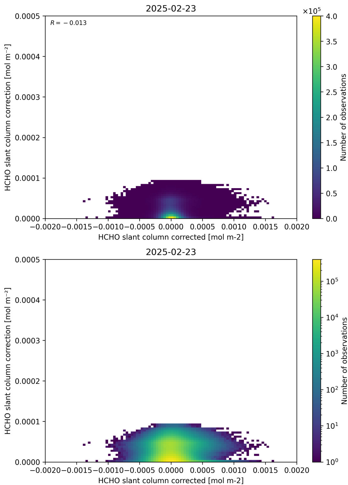
Figure 77: Scatter density plot of “HCHO slant column corrected” against “HCHO slant column correction” for 2025-02-22 to 2025-02-24.
