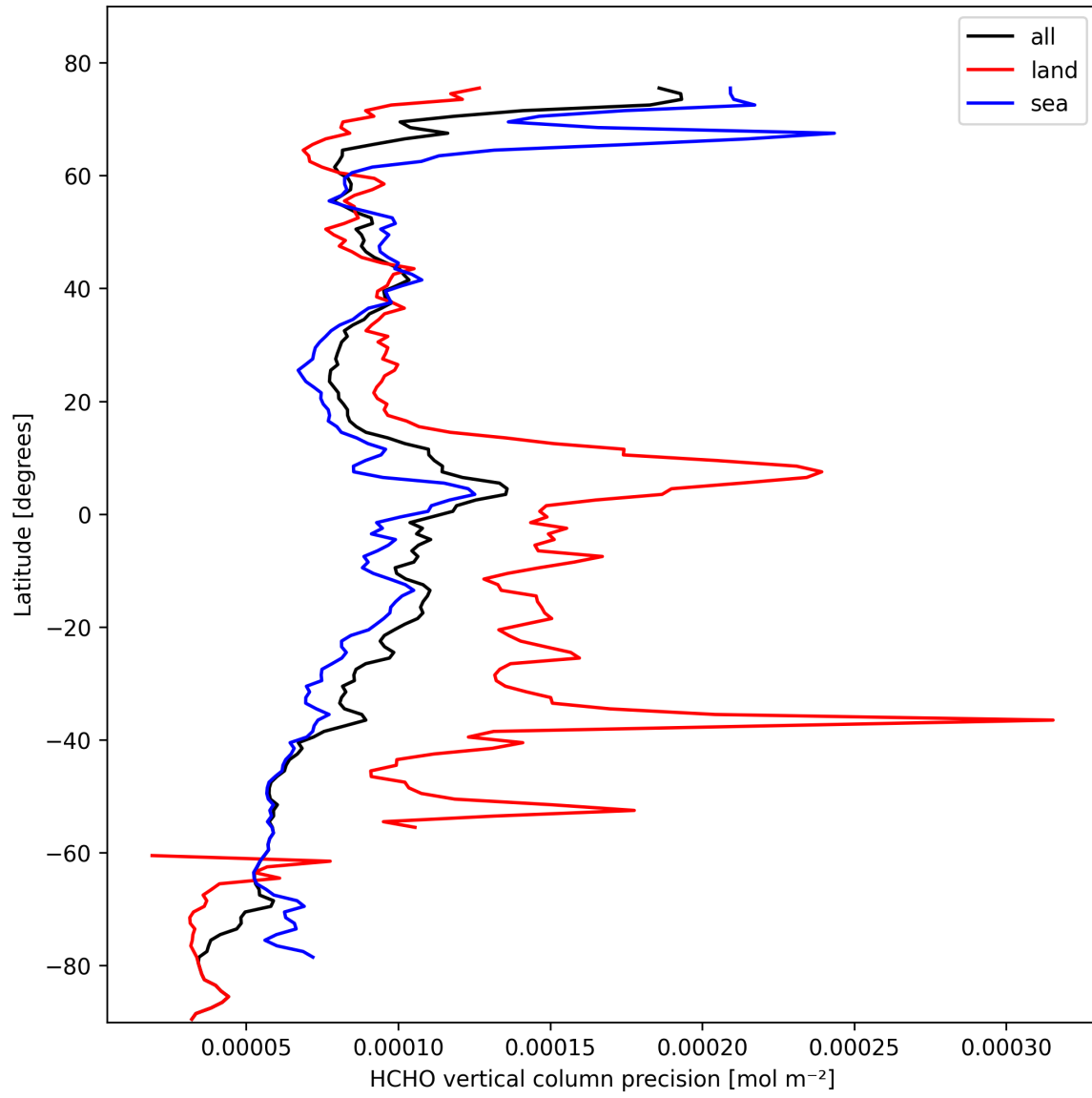
Figure 22: Zonal average of “HCHO vertical column precision” for 2025-02-22 to 2025-02-24.
