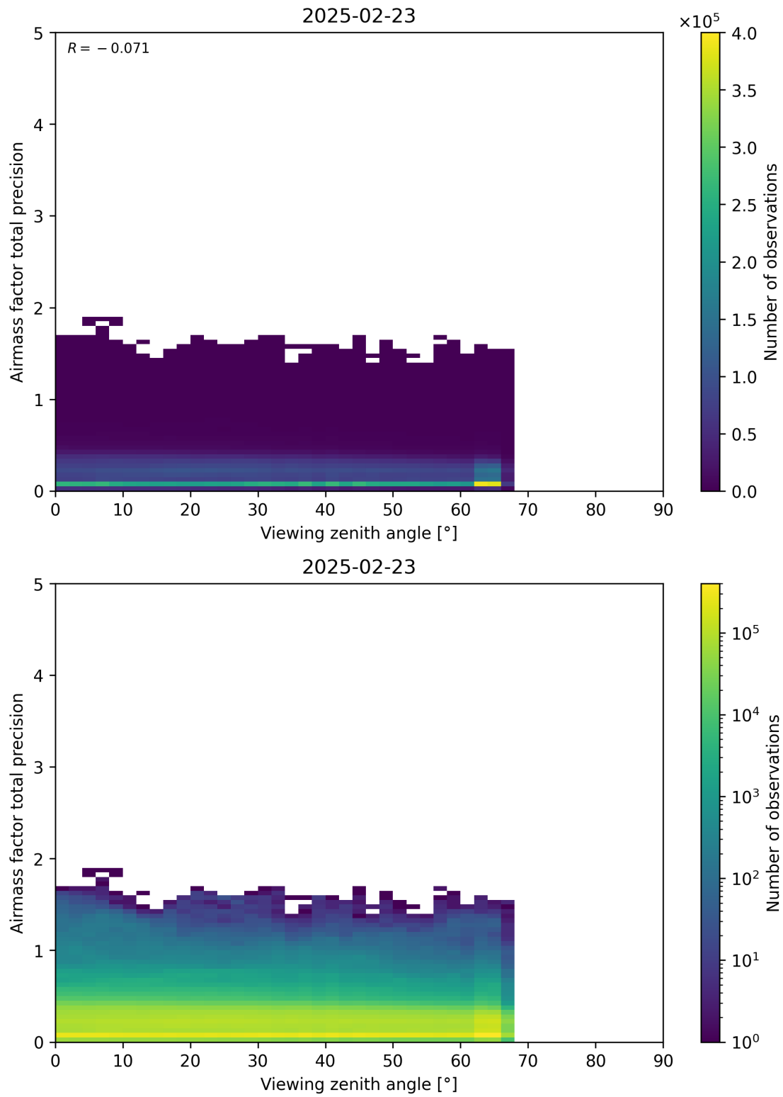
Figure 191: Scatter density plot of “Viewing zenith angle” against “Airmass factor total precision” for 2025-02-22 to 2025-02-24.
