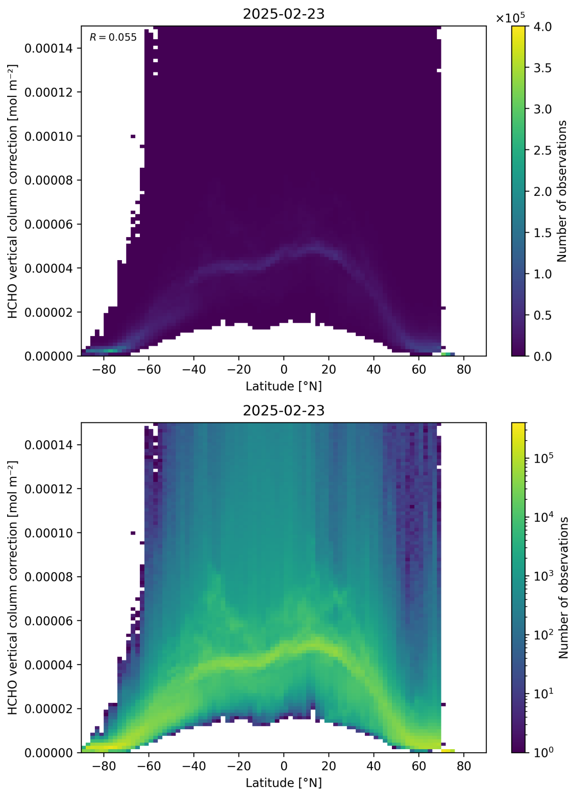
Figure 164: Scatter density plot of “Latitude” against “HCHO vertical column correction” for 2025-02-22 to 2025-02-24.
