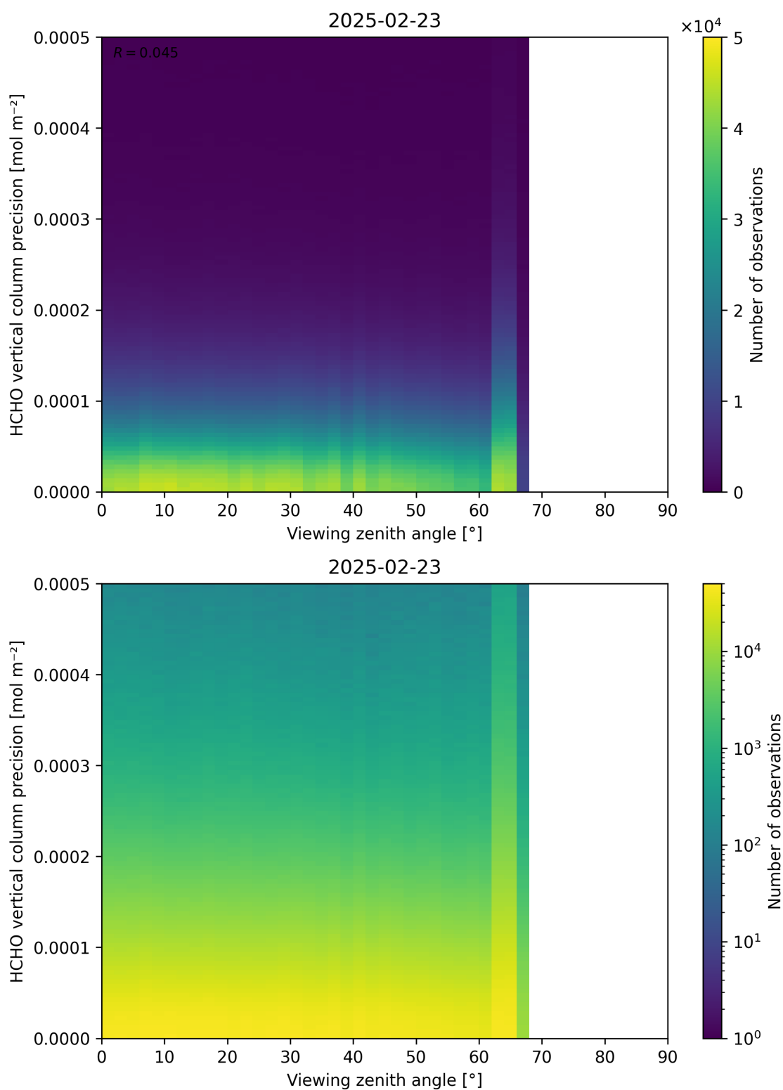
Figure 194: Scatter density plot of “Viewing zenith angle” against “HCHO vertical column precision” for 2025-02-22 to 2025-02-24.
