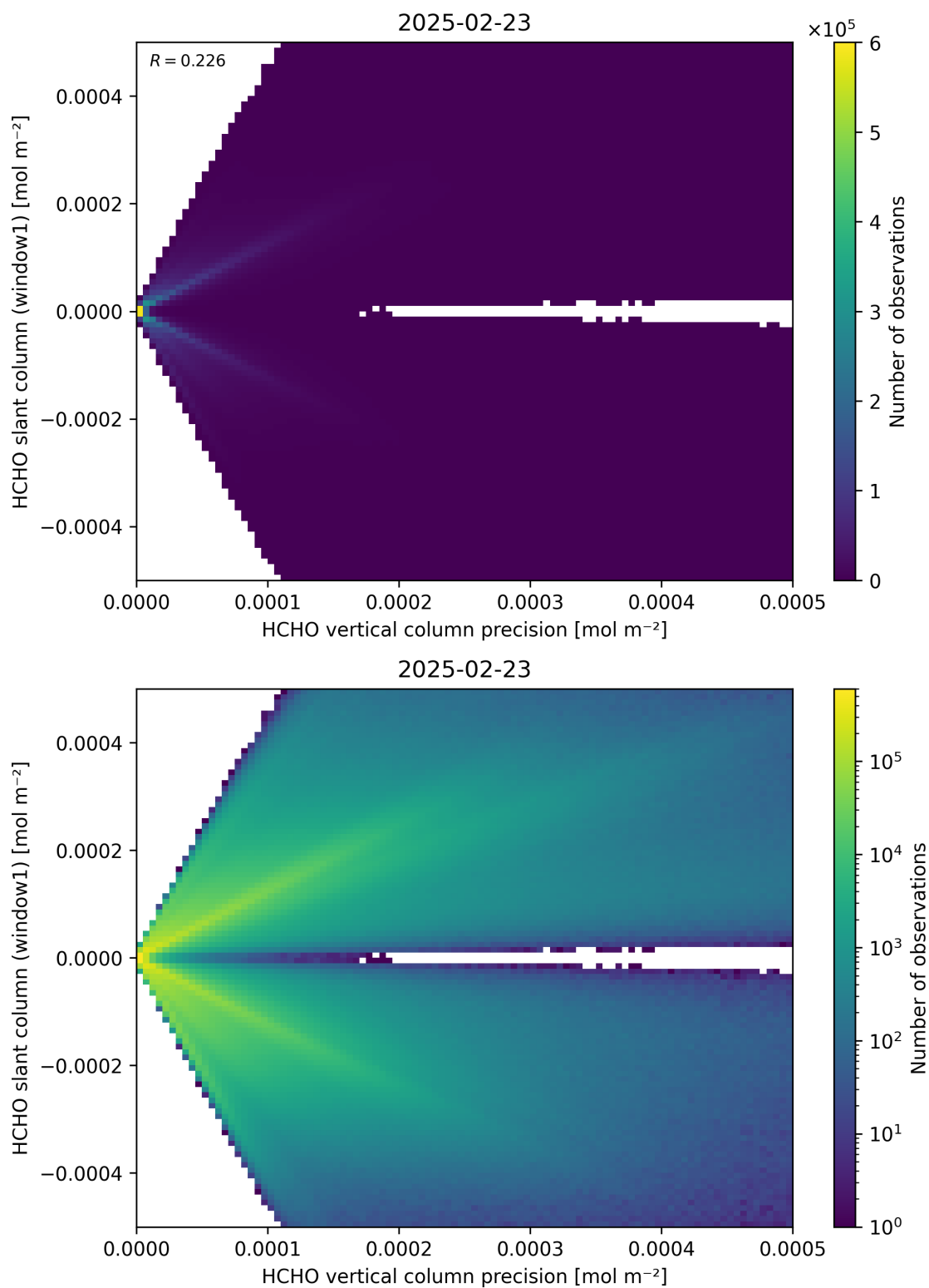
Figure 142: Scatter density plot of “HCHO vertical column precision” against “HCHO slant column (window1)” for 2025-02-22 to 2025-02-24.
