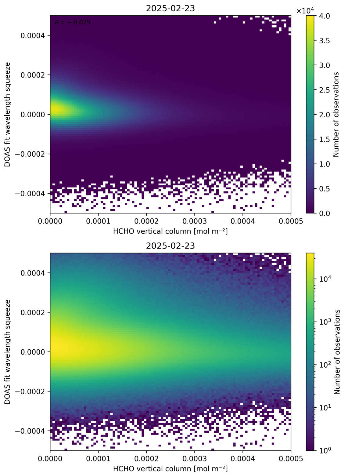
Figure 125: Scatter density plot of “HCHO vertical column” against “DOAS fit wavelength squeeze” for 2025-02-22 to 2025-02-24.
