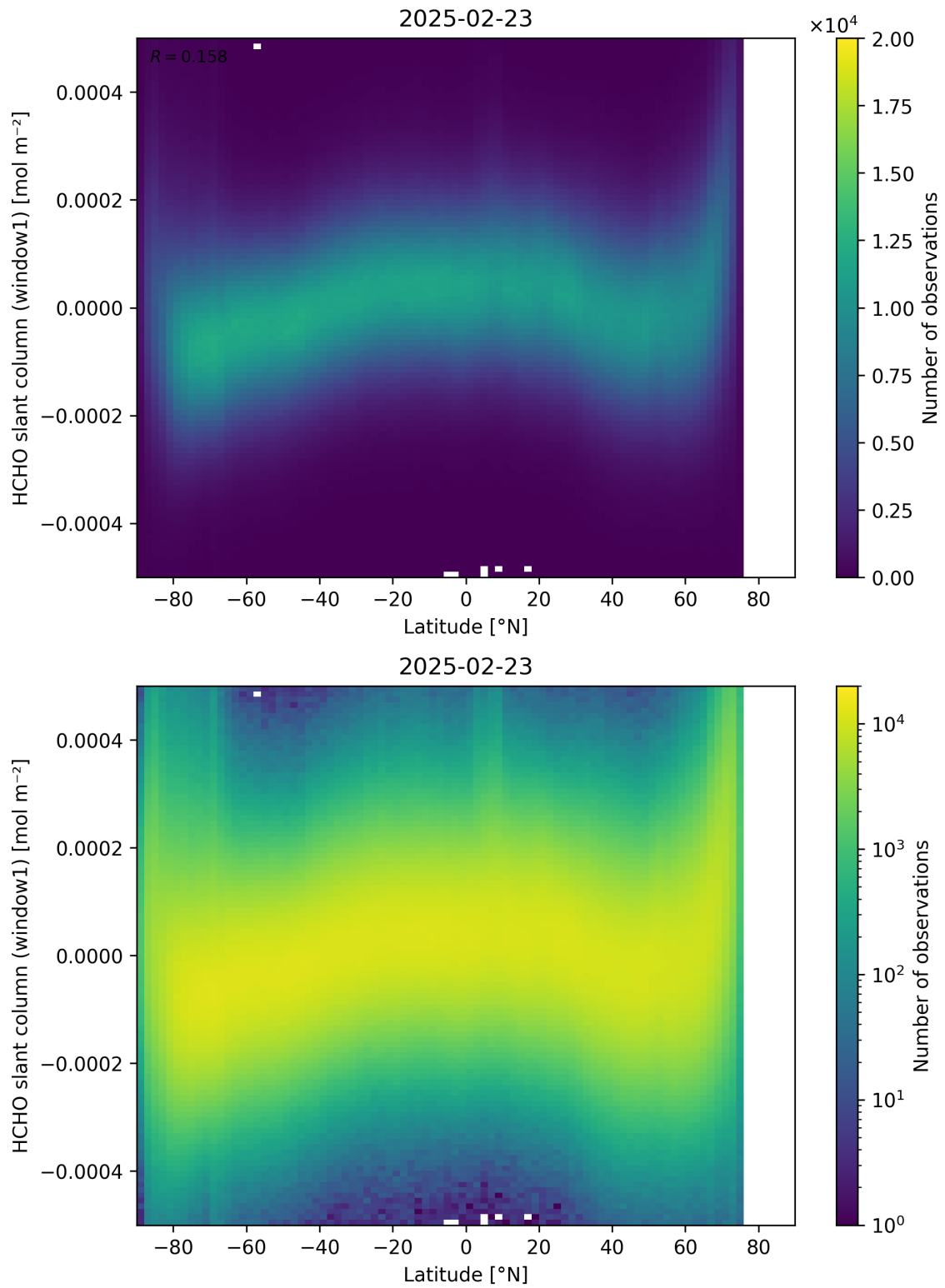
Figure 159: Scatter density plot of “Latitude” against “HCHO slant column (window1)” for 2025-02-22 to 2025-02-24.
