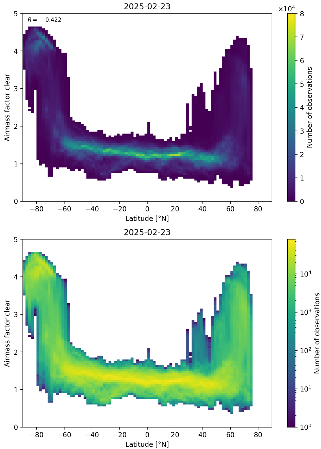
Figure 156: Scatter density plot of “Latitude” against “Airmass factor clear” for 2025-02-22 to 2025-02-24.
