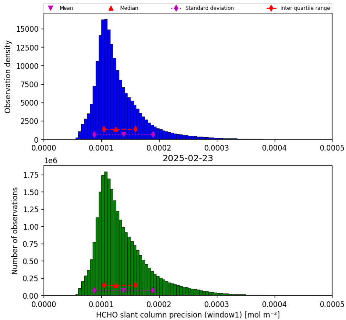
Figure 39: Histogram of “HCHO slant column precision (window1)” for 2025-02-22 to 2025-02-24
