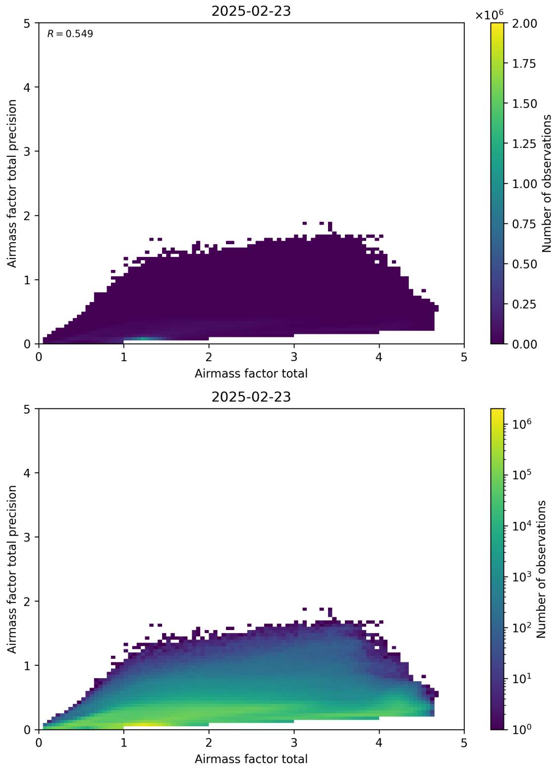
Figure 103: Scatter density plot of “Airmass factor total” against “Airmass factor total precision” for 2025-02-22 to 2025-02-24.
