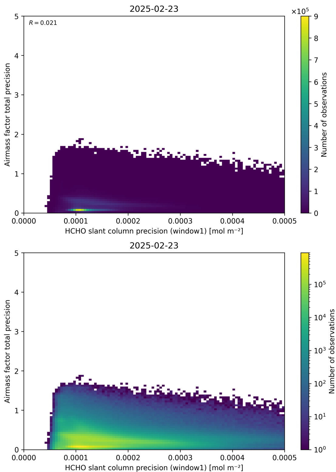
Figure 95: Scatter density plot of “HCHO slant column precision (window1)” against “Airmass factor total precision” for 2025-02-22 to 2025-02-24.
