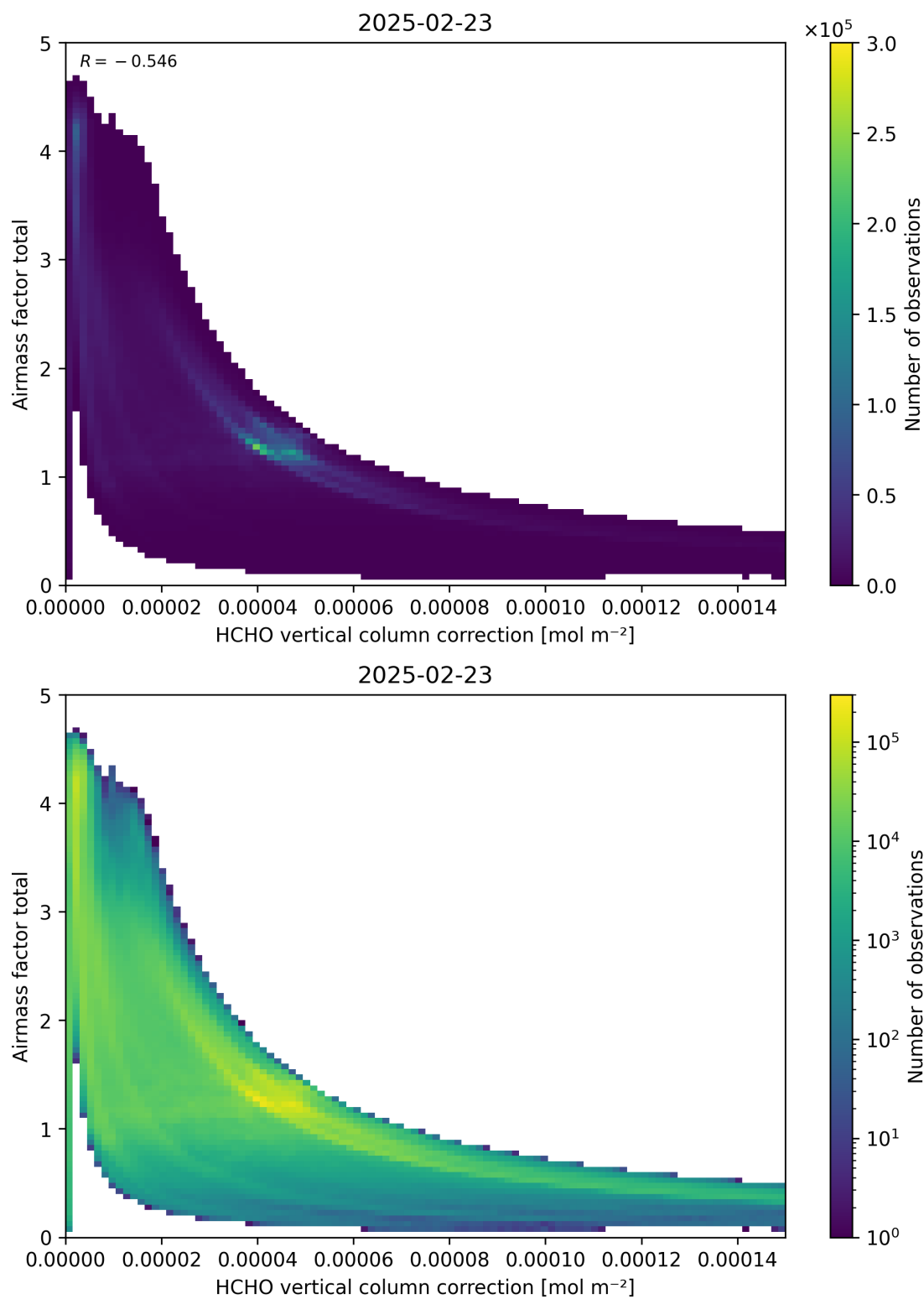
Figure 120: Scatter density plot of “HCHO vertical column correction” against “Airmass factor total” for 2025-02-22 to 2025-02-24.
