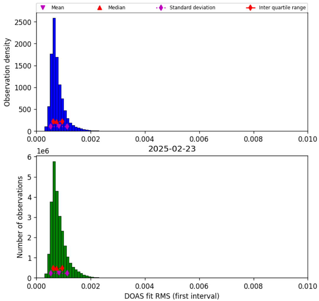
Figure 46: Histogram of “DOAS fit RMS (first interval)” for 2025-02-22 to 2025-02-24
