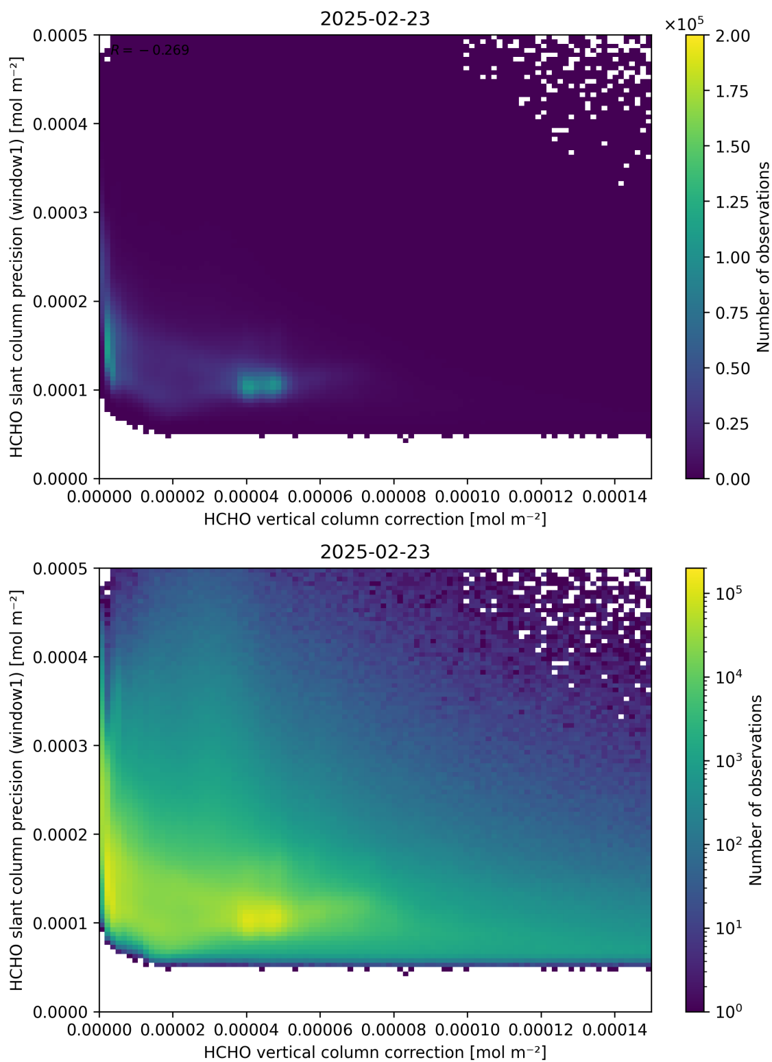
Figure 119: Scatter density plot of “HCHO vertical column correction” against “HCHO slant column precision (window1)” for 2025-02-22 to 2025-02-24.
