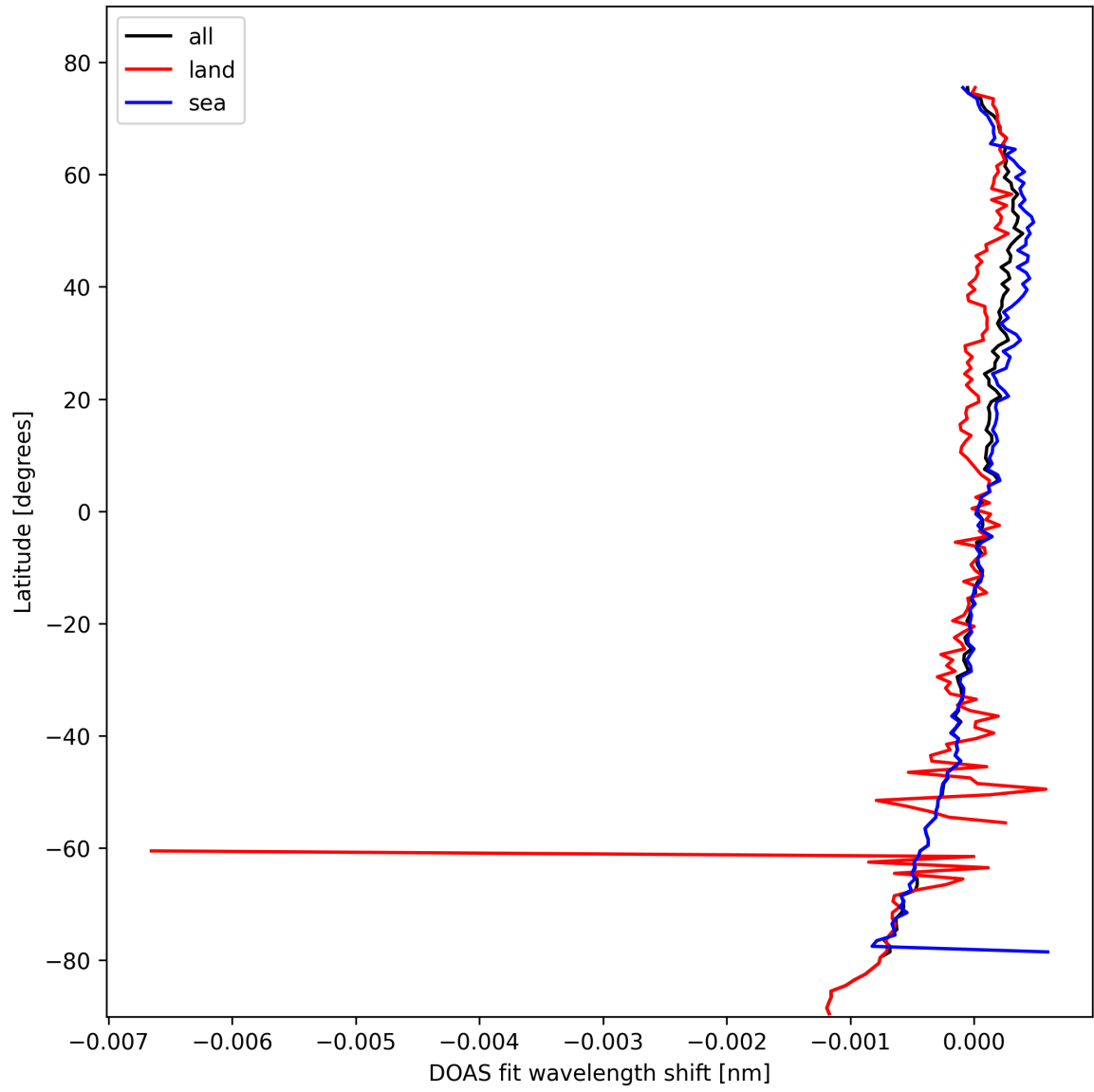
Figure 30: Zonal average of "DOAS fit wavelength shift" for 2025-02-22 to 2025-02-24.
