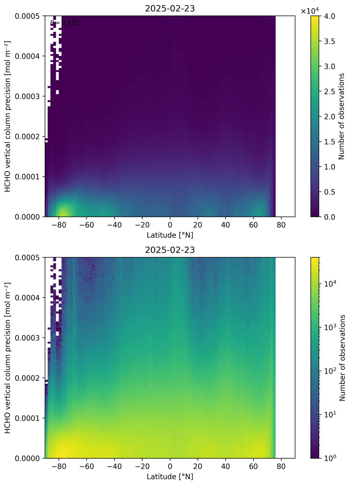
Figure 165: Scatter density plot of “Latitude” against “HCHO vertical column precision” for 2025-02-22 to 2025-02-24.
