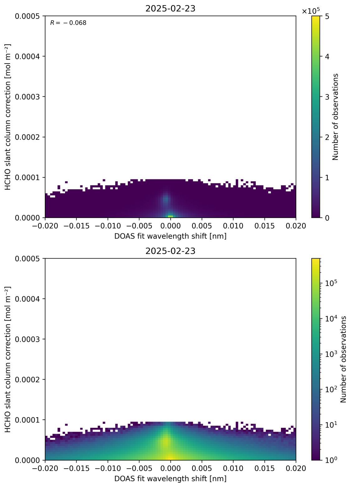
Figure 67: Scatter density plot of “DOAS fit wavelength shift” against “HCHO slant column correction” for 2025-02-22 to 2025-02-24.
