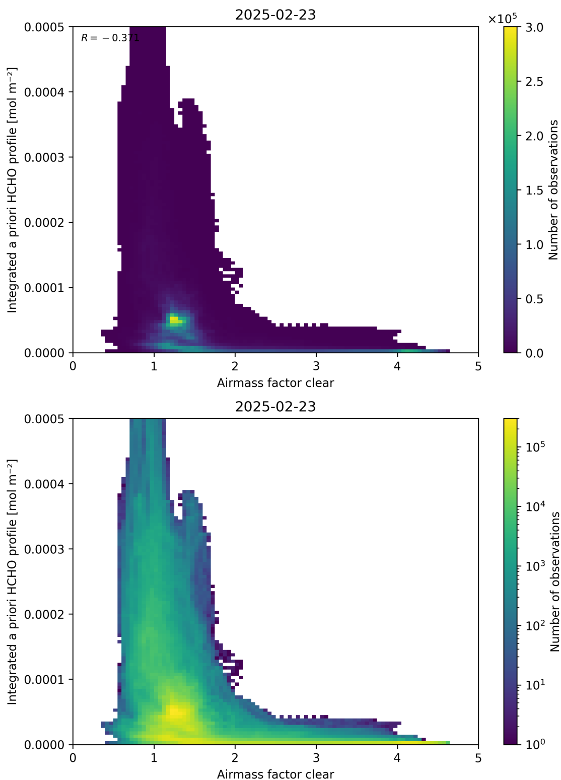
Figure 76: Scatter density plot of “Airmass factor clear” against “Integrated a priori HCHO profile” for 2025-02-22 to 2025-02-24.
