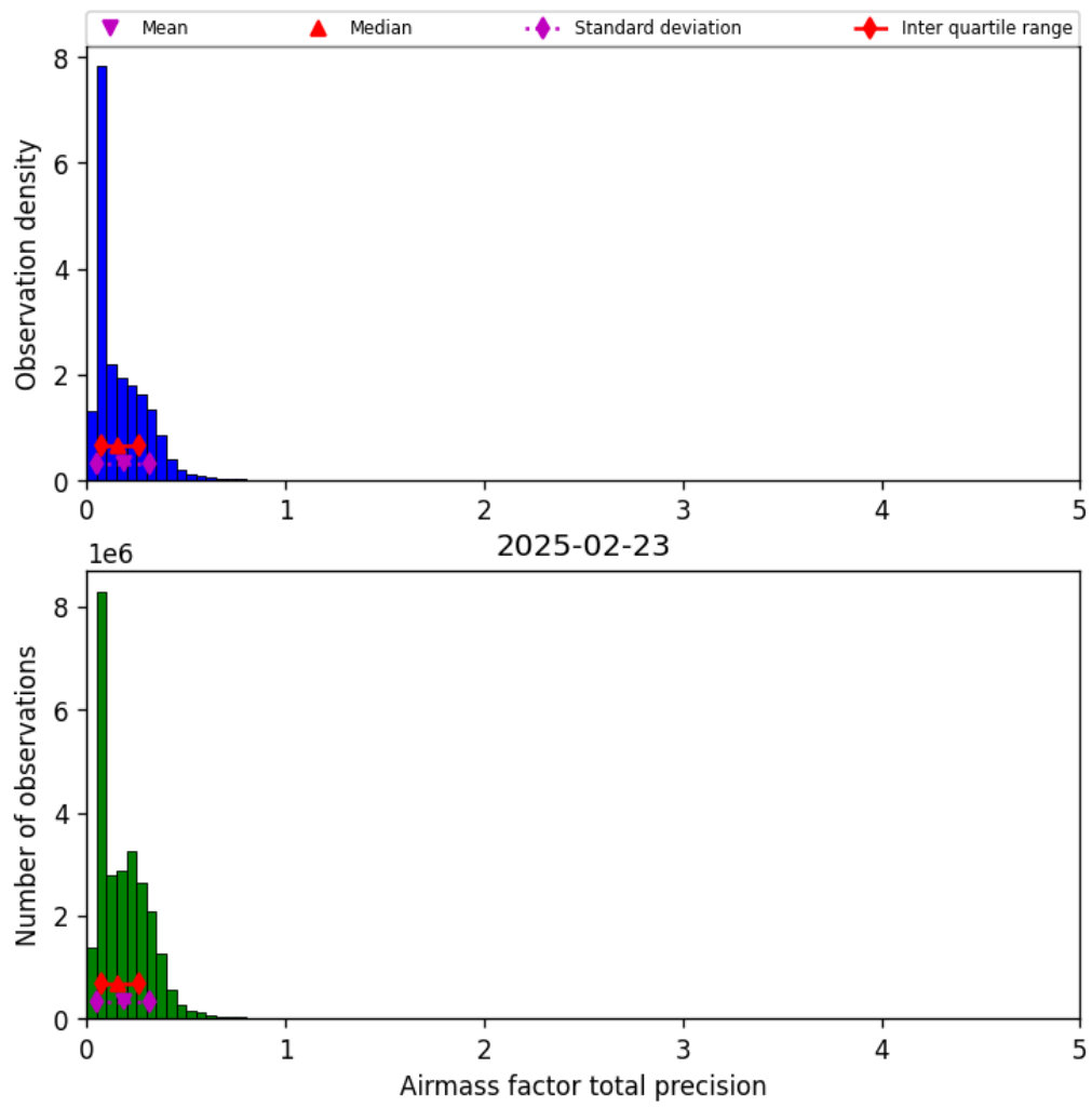
Figure 41: Histogram of “Airmass factor total precision” for 2025-02-22 to 2025-02-24
