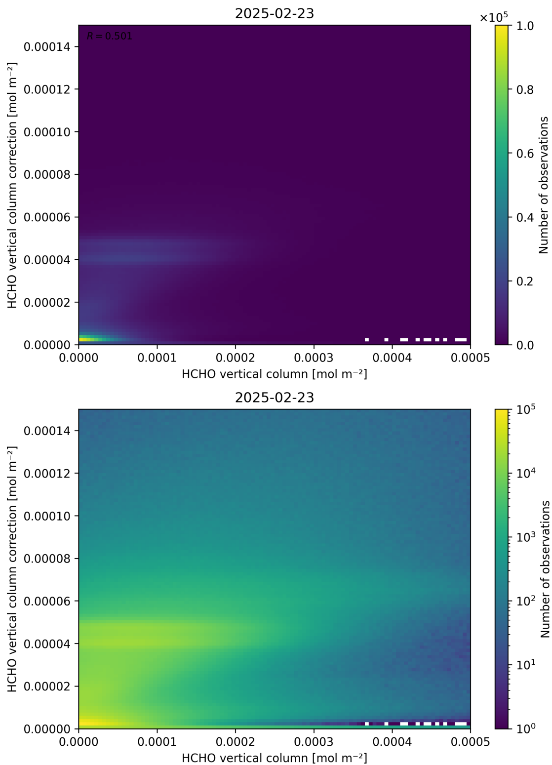
Figure 133: Scatter density plot of “HCHO vertical column” against “HCHO vertical column correction” for 2025-02-22 to 2025-02-24.
