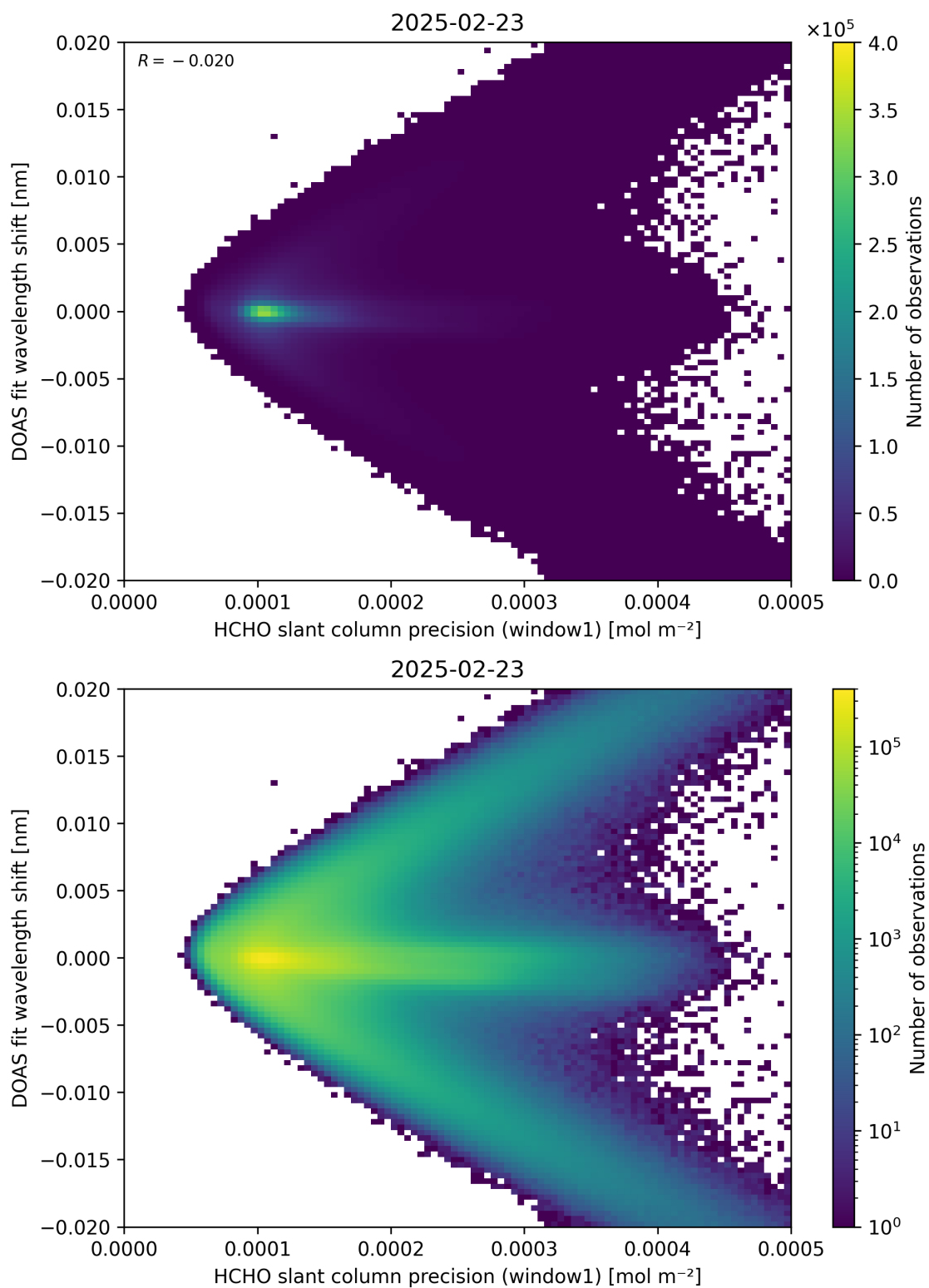
Figure 89: Scatter density plot of “HCHO slant column precision (window1)” against “DOAS fit wavelength shift” for 2025-02-22 to 2025-02-24.
