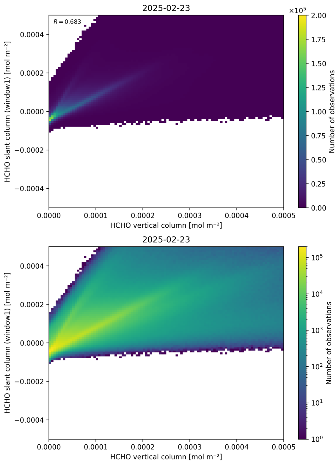
Figure 129: Scatter density plot of “HCHO vertical column” against “HCHO slant column (window1)” for 2025-02-22 to 2025-02-24.
