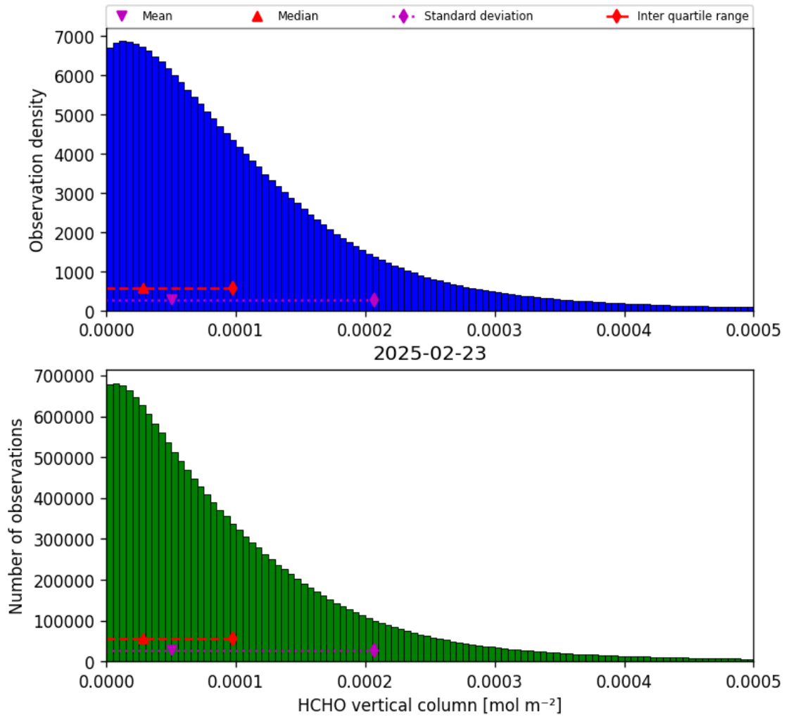
Figure 35: Histogram of “HCHO vertical column” for 2025-02-22 to 2025-02-24
