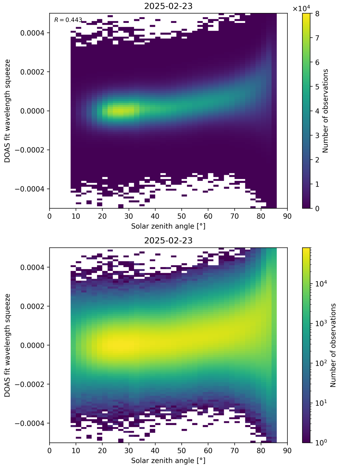
Figure 169: Scatter density plot of “Solar zenith angle” against “DOAS fit wavelength squeeze” for 2025-02-22 to 2025-02-24.
