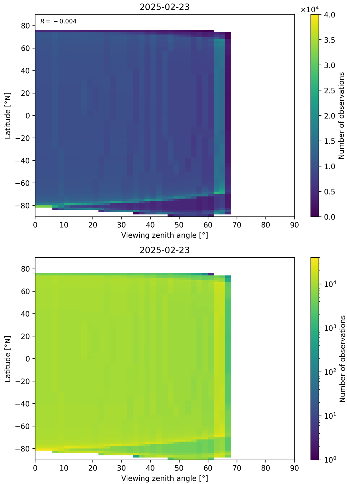
Figure 196: Scatter density plot of “Viewing zenith angle” against “Latitude” for 2025-02-22 to 2025-02-24.
