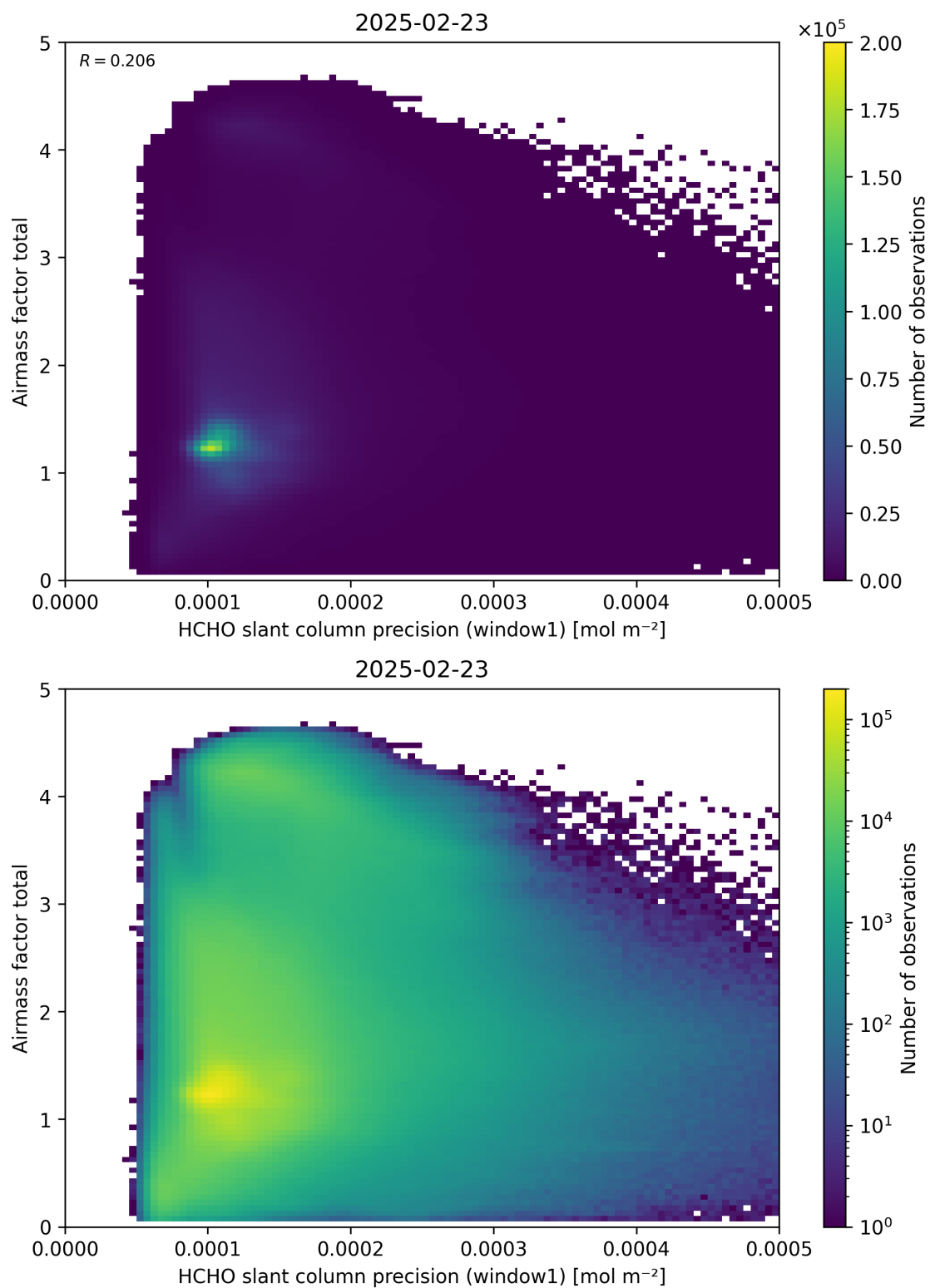
Figure 94: Scatter density plot of “HCHO slant column precision (window1)” against “Airmass factor total” for 2025-02-22 to 2025-02-24.
