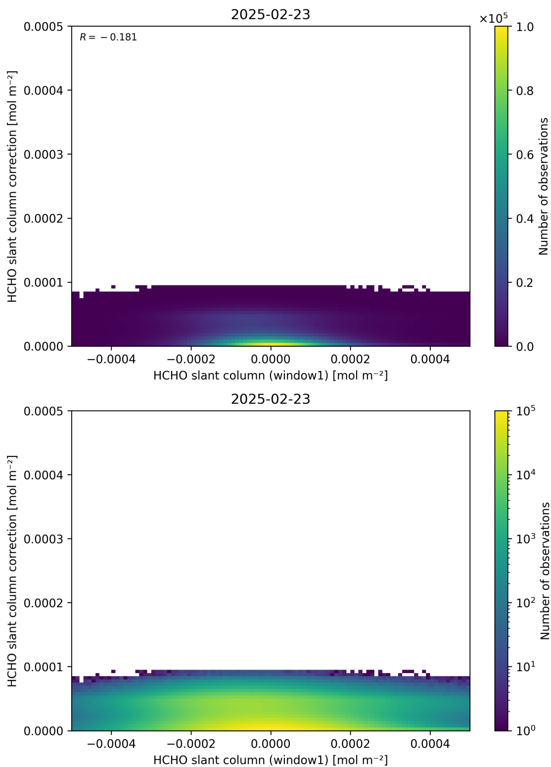
Figure 83: Scatter density plot of “HCHO slant column (window1)” against “HCHO slant column correction” for 2025-02-22 to 2025-02-24.
