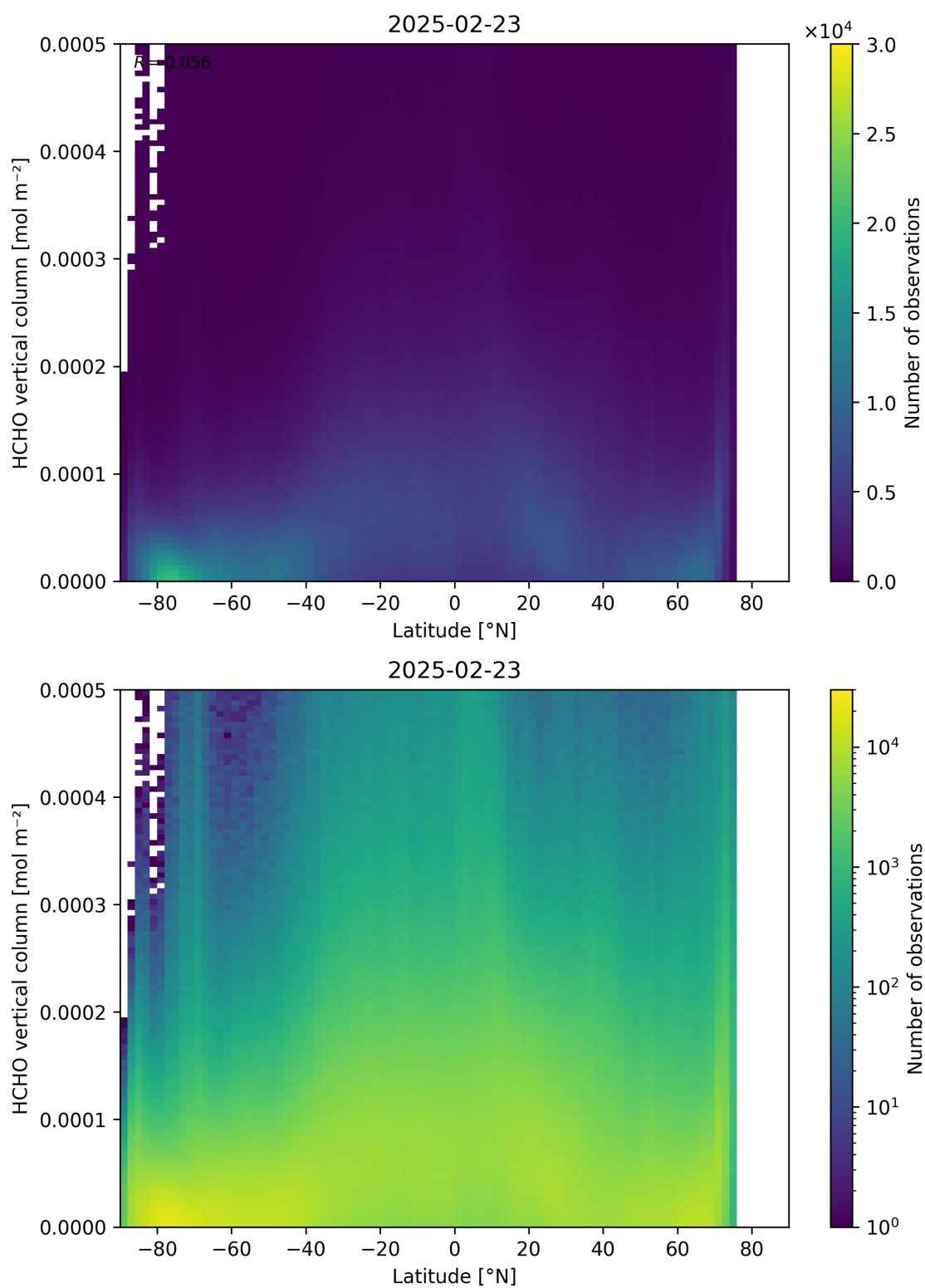
Figure 163: Scatter density plot of “Latitude” against “HCHO vertical column” for 2025-02-22 to 2025-02-24.
