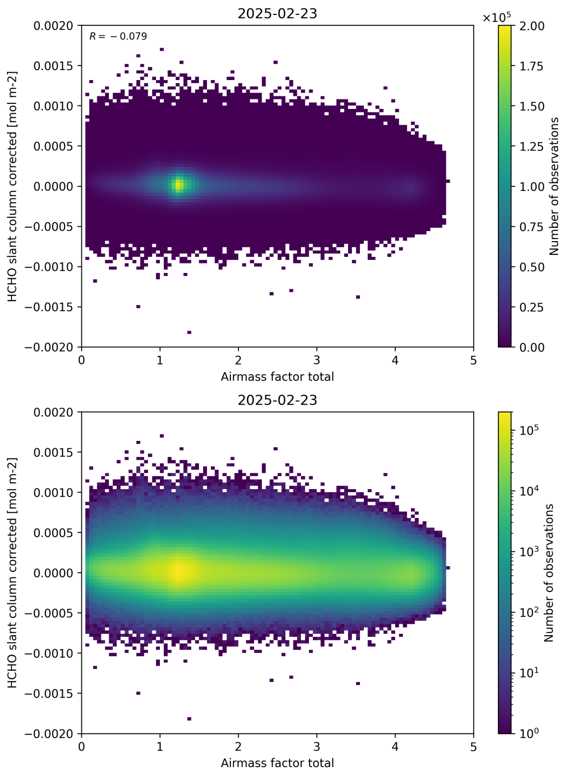
Figure 101: Scatter density plot of “Airmass factor total” against “HCHO slant column corrected” for 2025-02-22 to 2025-02-24.
