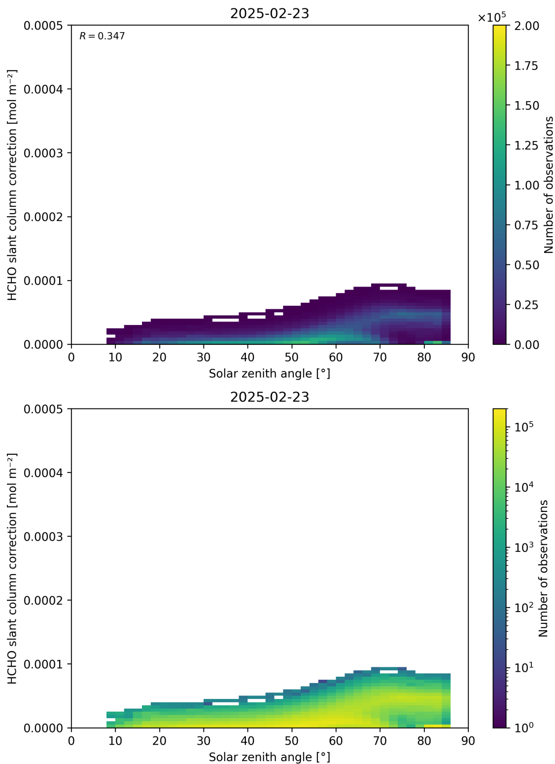
Figure 172: Scatter density plot of “Solar zenith angle” against “HCHO slant column correction” for 2025-02-22 to 2025-02-24.
