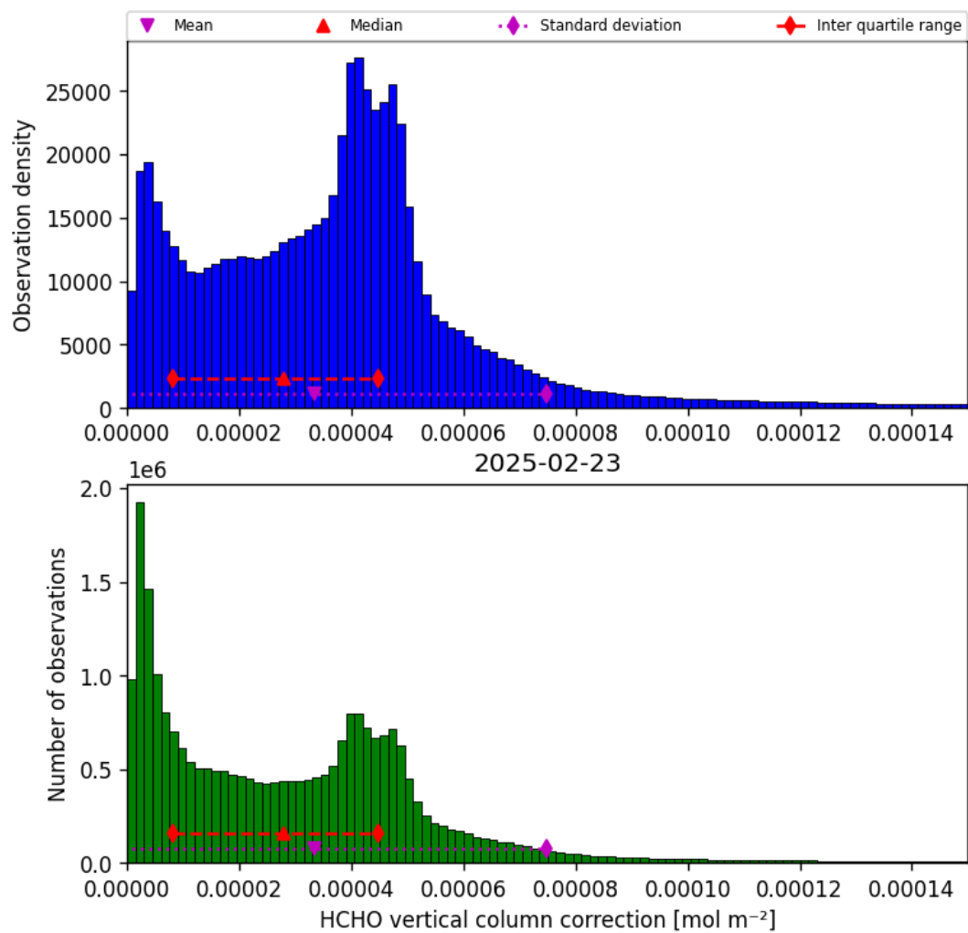
Figure 37: Histogram of “HCHO vertical column correction” for 2025-02-22 to 2025-02-24
