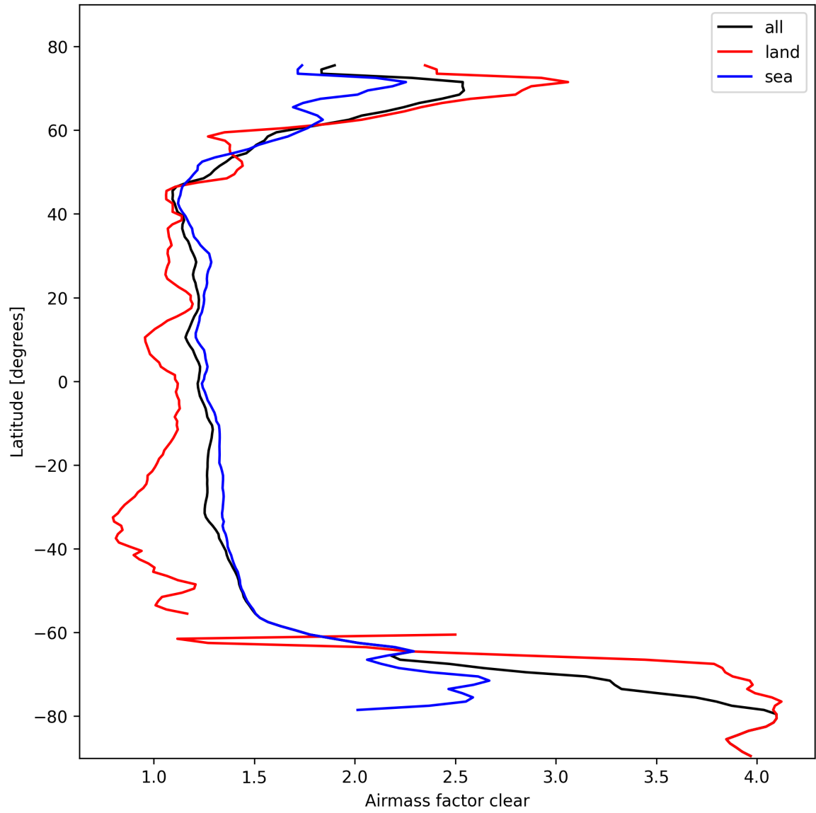
Figure 28: Zonal average of “Airmass factor clear” for 2025-02-22 to 2025-02-24.
