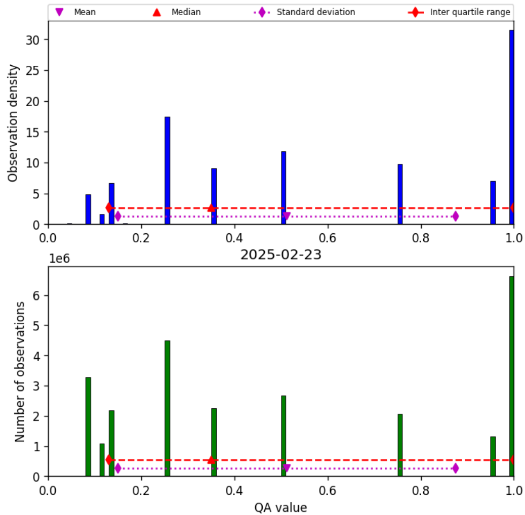
Figure 34: Histogram of “QA value” for 2025-02-22 to 2025-02-24
