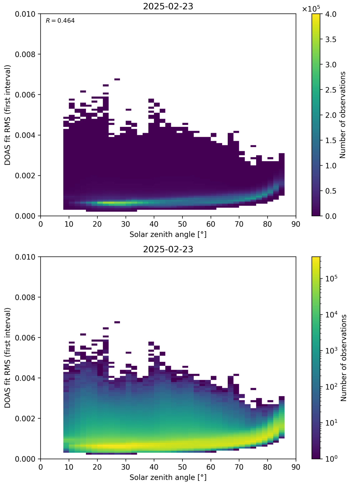
Figure 167: Scatter density plot of “Solar zenith angle” against “DOAS fit RMS (first interval)” for 2025-02-22 to 2025-02-24.
