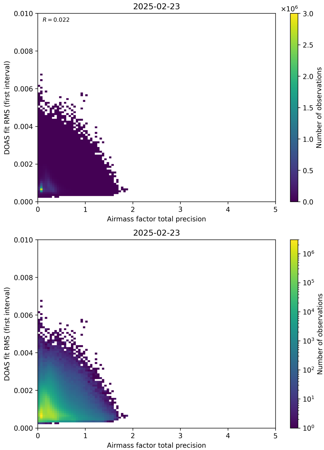
Figure 105: Scatter density plot of “Airmass factor total precision” against “DOAS fit RMS (first interval)” for 2025-02-22 to 2025-02-24.
