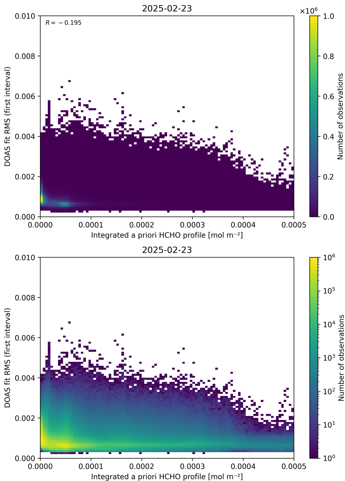
Figure 148: Scatter density plot of “Integrated a priori HCHO profile” against “DOAS fit RMS (first interval)” for 2025-02-22 to 2025-02-24.
