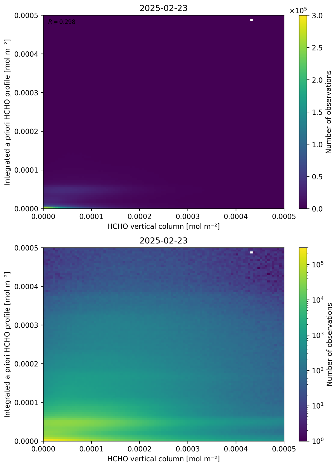
Figure 135: Scatter density plot of “HCHO vertical column” against “Integrated a priori HCHO profile” for 2025-02-22 to 2025-02-24.
