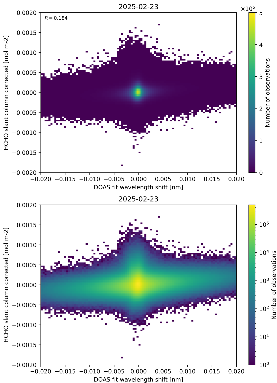
Figure 66: Scatter density plot of “DOAS fit wavelength shift” against “HCHO slant column corrected” for 2025-02-22 to 2025-02-24.
