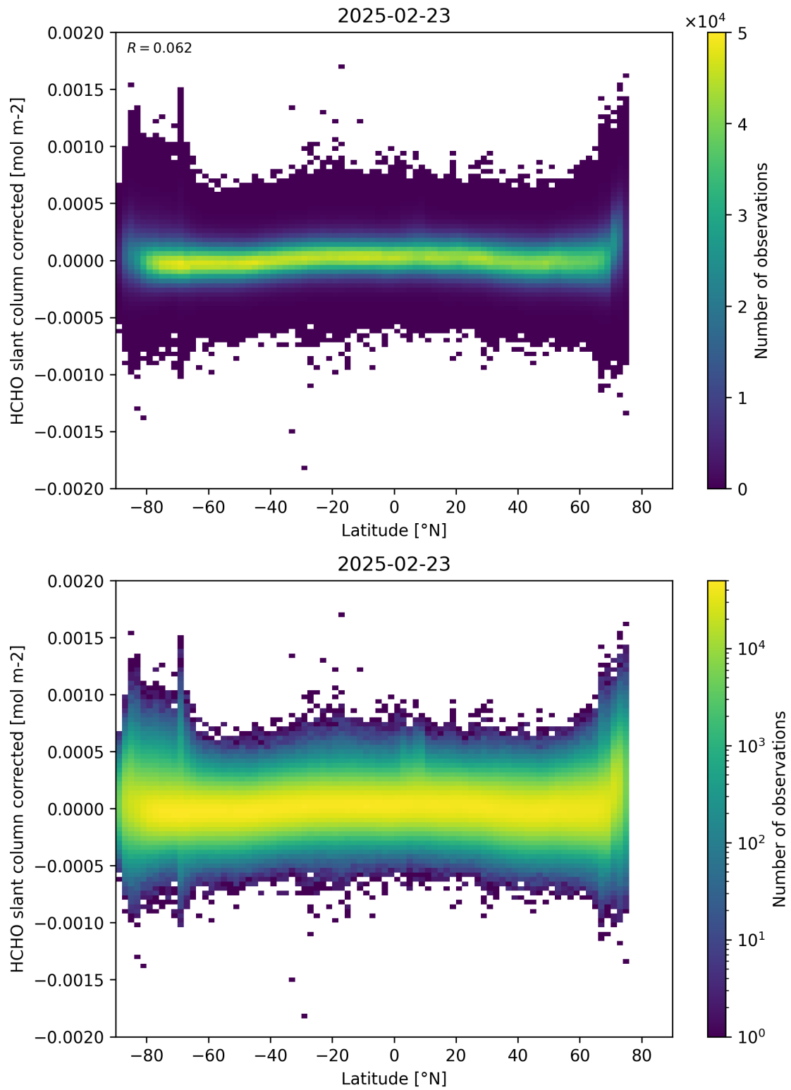
Figure 157: Scatter density plot of “Latitude” against “HCHO slant column corrected” for 2025-02-22 to 2025-02-24.
