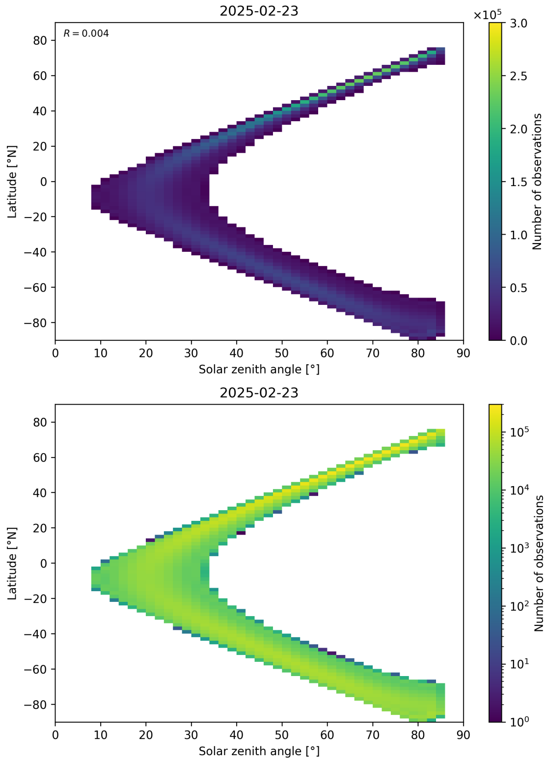
Figure 181: Scatter density plot of “Solar zenith angle” against “Latitude” for 2025-02-22 to 2025-02-24.
