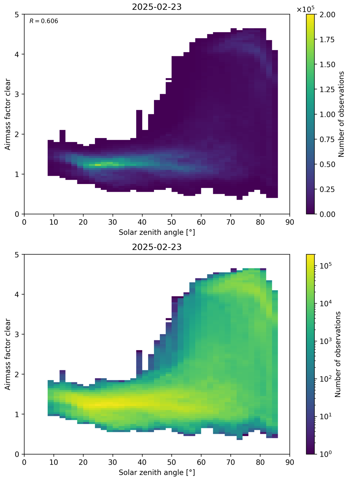
Figure 170: Scatter density plot of “Solar zenith angle” against “Airmass factor clear” for 2025-02-22 to 2025-02-24.
