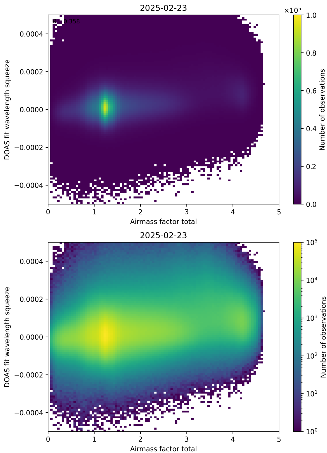
Figure 99: Scatter density plot of “Airmass factor total” against “DOAS fit wavelength squeeze” for 2025-02-22 to 2025-02-24.
