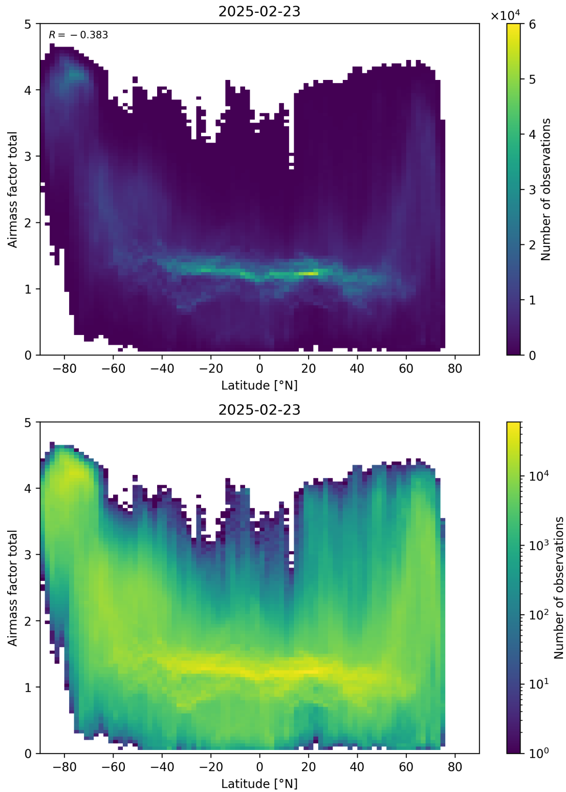
Figure 161: Scatter density plot of “Latitude” against “Airmass factor total” for 2025-02-22 to 2025-02-24.
