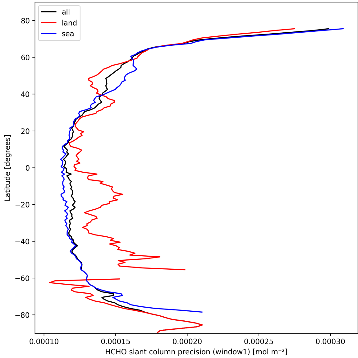
Figure 25: Zonal average of “HCHO slant column precision (window1)” for 2025-02-22 to 2025-02-24.
