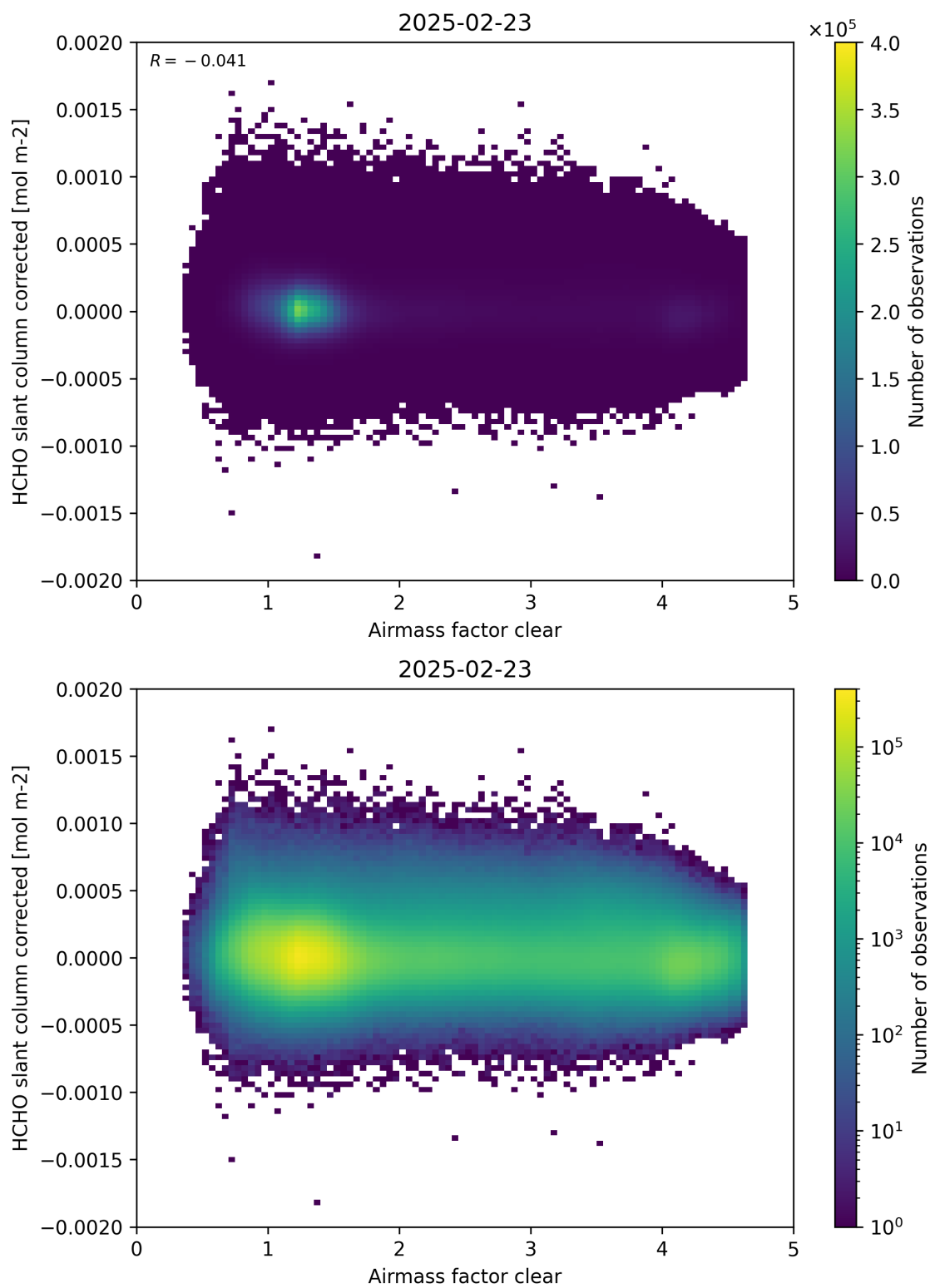
Figure 74: Scatter density plot of “Airmass factor clear” against “HCHO slant column corrected” for 2025-02-22 to 2025-02-24.
