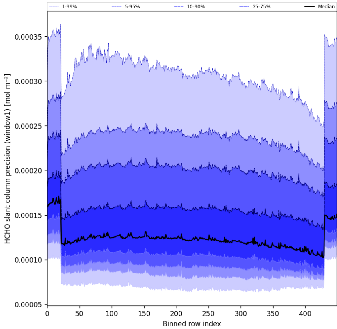
Figure 53: Along track statistics of “HCHO slant column precision (window1)” for 2025-02-22 to 2025-02-24
