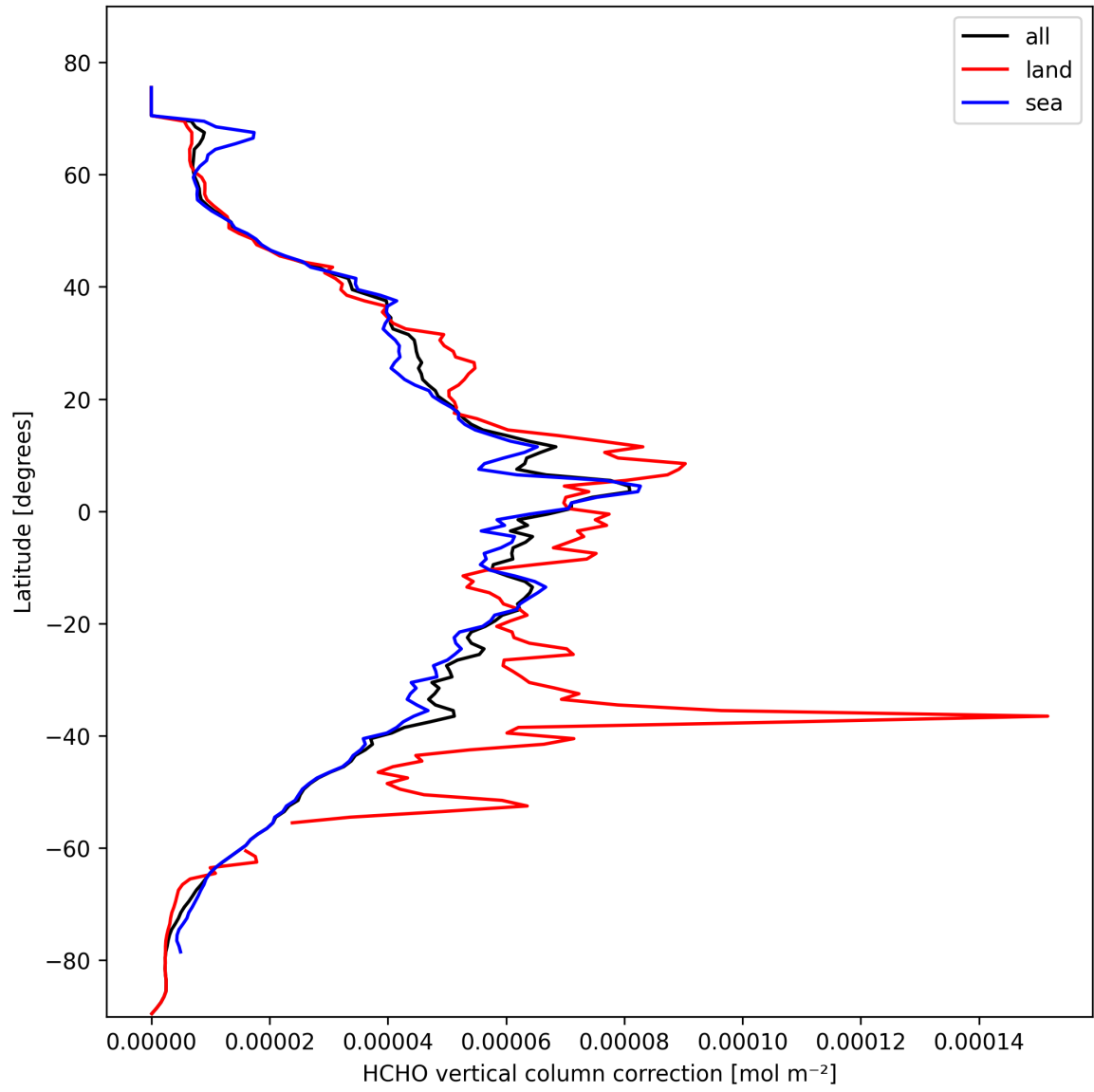
Figure 23: Zonal average of “HCHO vertical column correction” for 2025-02-22 to 2025-02-24.
