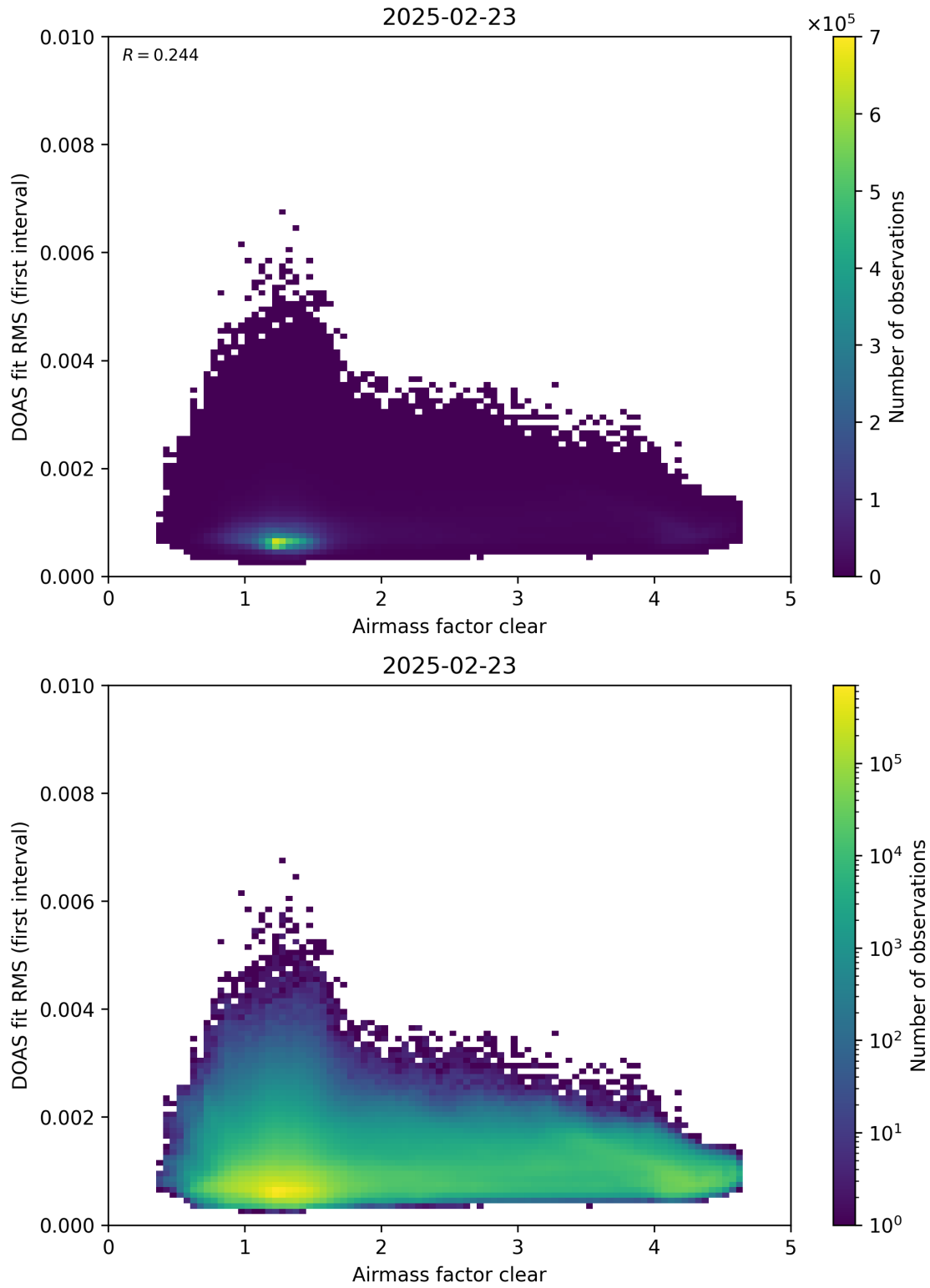
Figure 71: Scatter density plot of “Airmass factor clear” against “DOAS fit RMS (first interval)” for 2025-02-22 to 2025-02-24.
