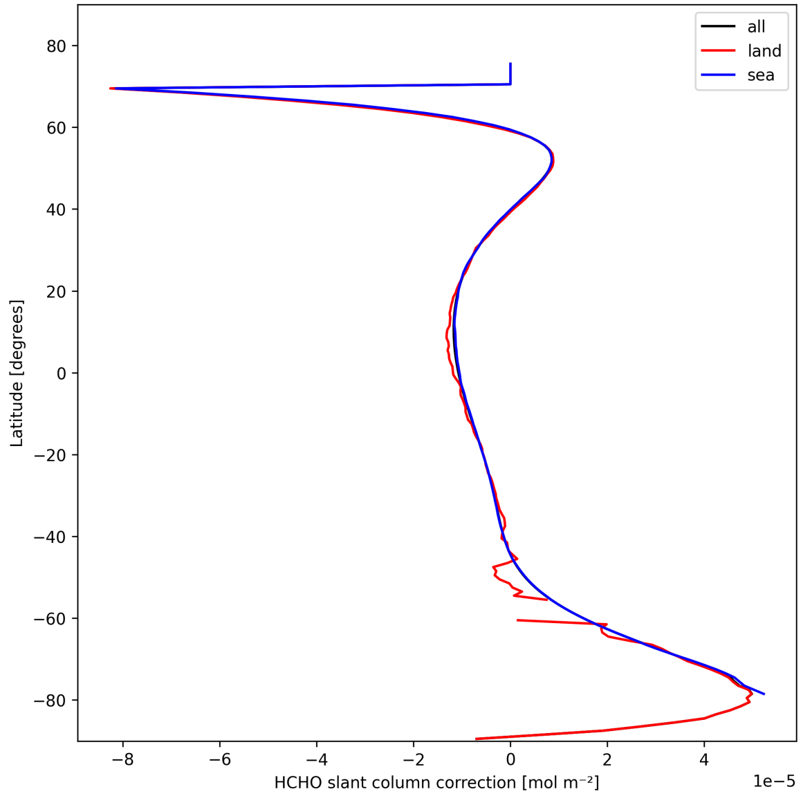
Figure 33: Zonal average of “HCHO slant column correction” for 2025-02-22 to 2025-02-24.
