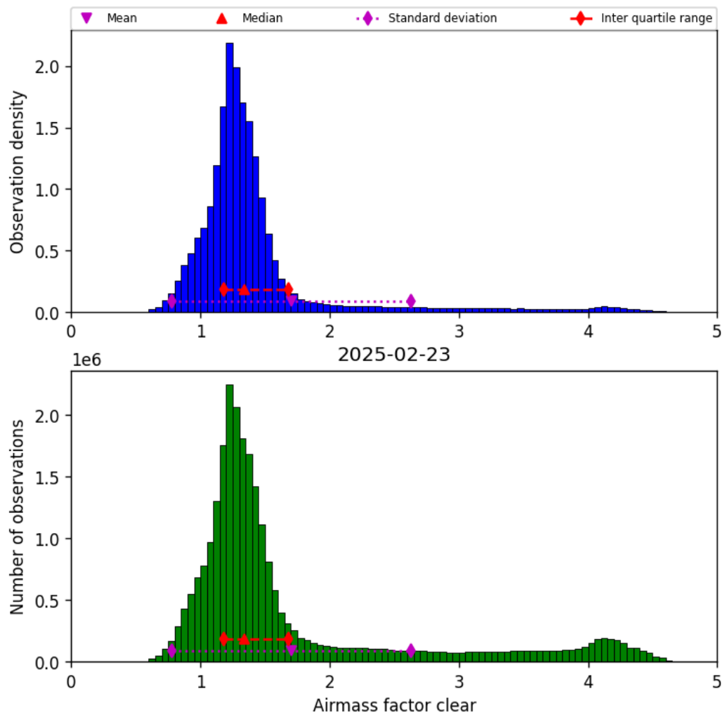
Figure 42: Histogram of “Airmass factor clear” for 2025-02-22 to 2025-02-24
