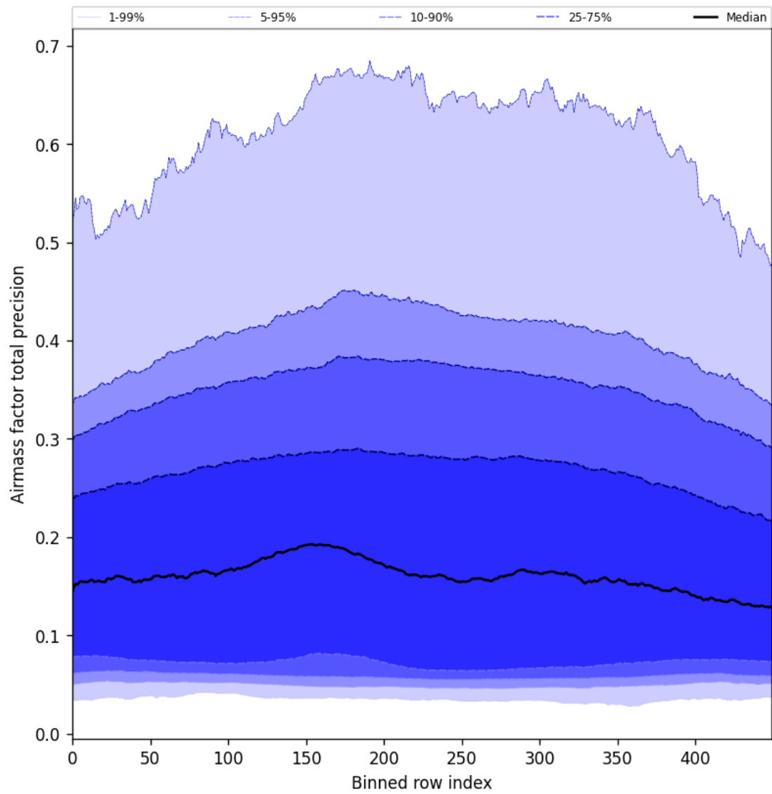
Figure 55: Along track statistics of “Airmass factor total precision” for 2025-02-22 to 2025-02-24
