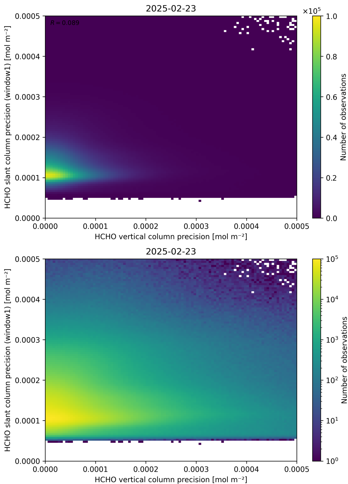
Figure 143: Scatter density plot of “HCHO vertical column precision” against “HCHO slant column precision (window1)” for 2025-02-22 to 2025-02-24.
