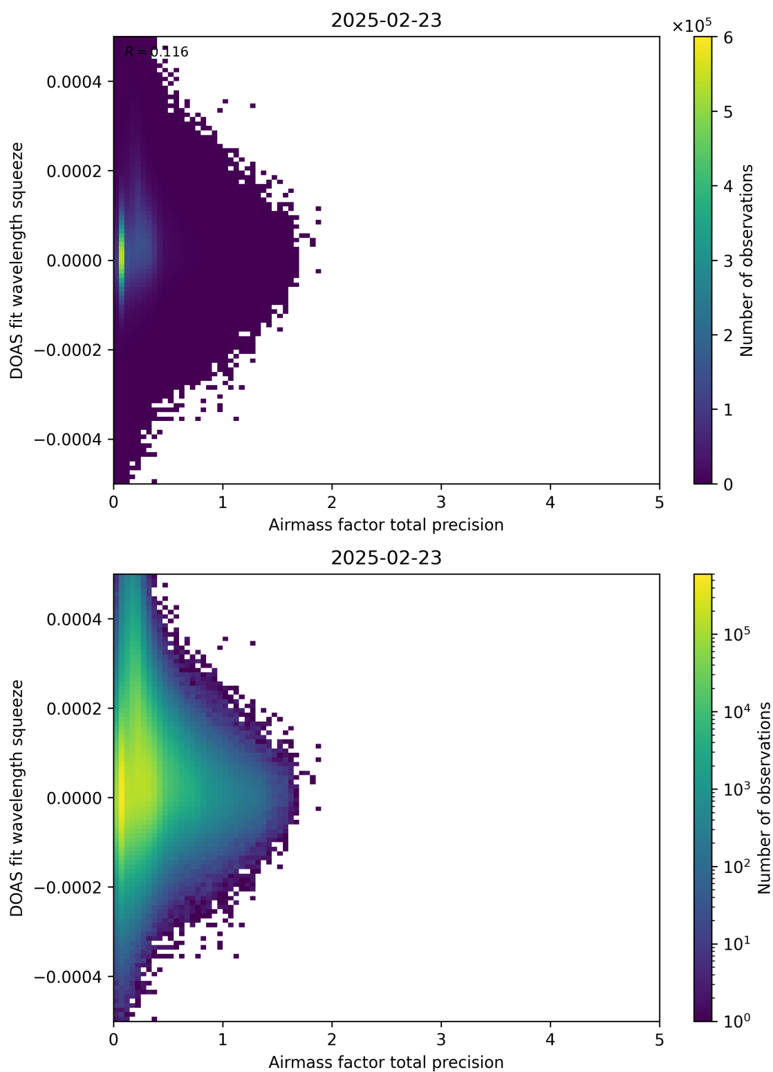
Figure 107: Scatter density plot of “Airmass factor total precision” against “DOAS fit wavelength squeeze” for 2025-02-22 to 2025-02-24.
