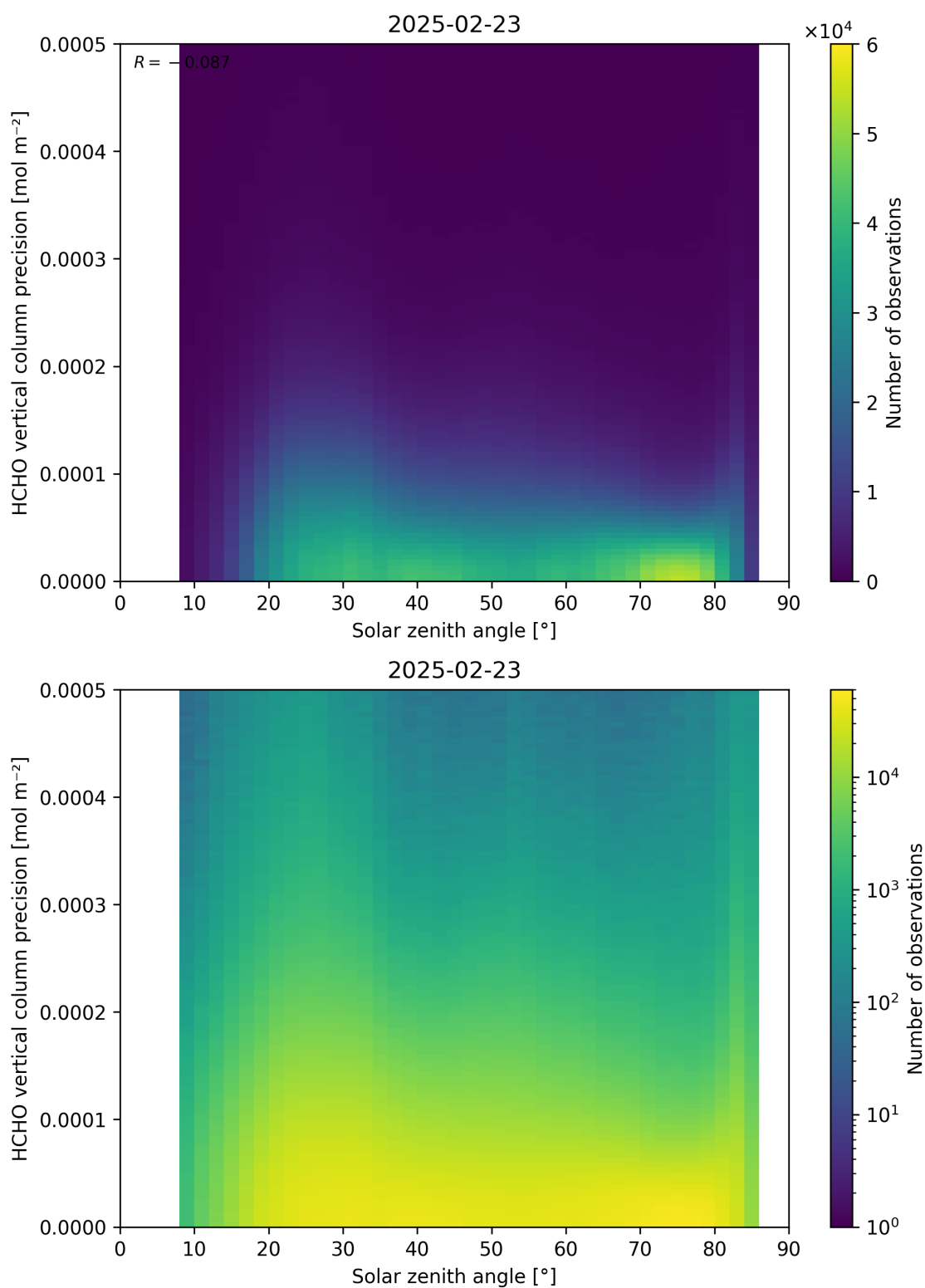
Figure 179: Scatter density plot of “Solar zenith angle” against “HCHO vertical column precision” for 2025-02-22 to 2025-02-24.
