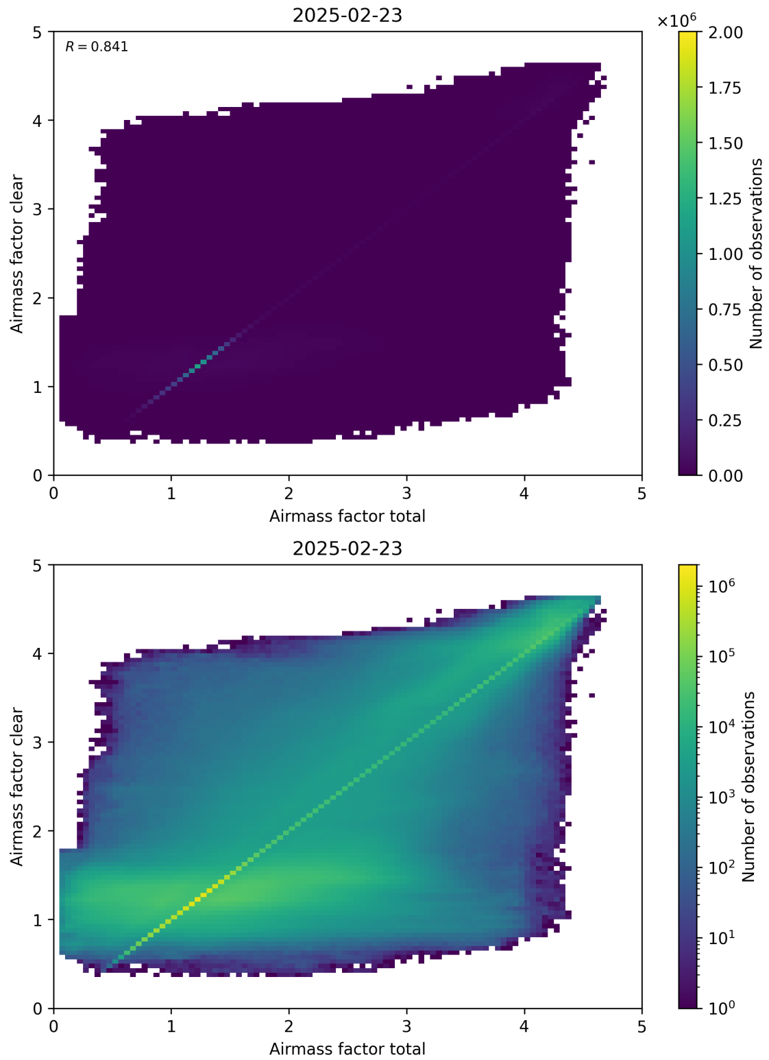
Figure 100: Scatter density plot of “Airmass factor total” against “Airmass factor clear” for 2025-02-22 to 2025-02-24.
