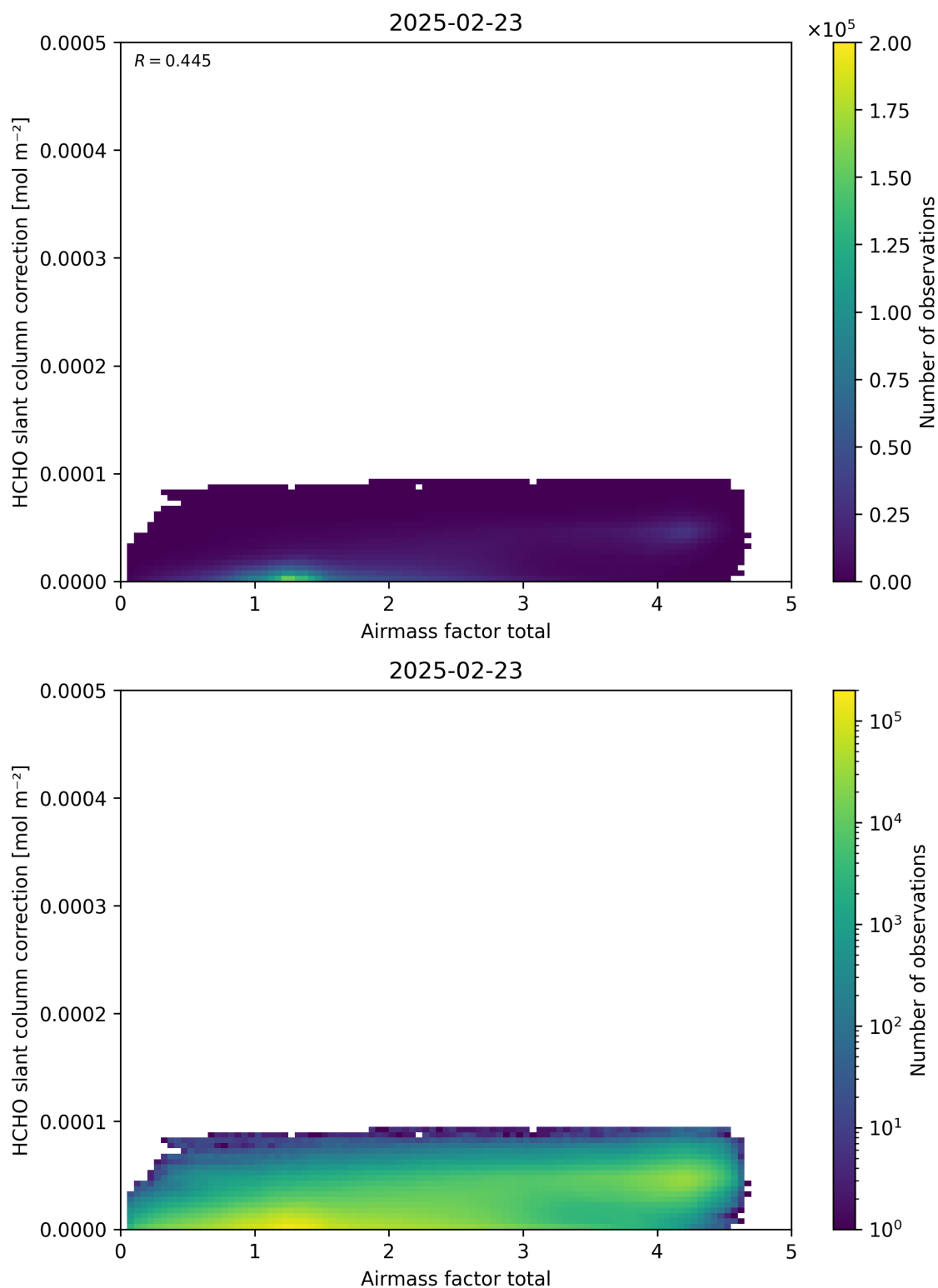
Figure 102: Scatter density plot of “Airmass factor total” against “HCHO slant column correction” for 2025-02-22 to 2025-02-24.
