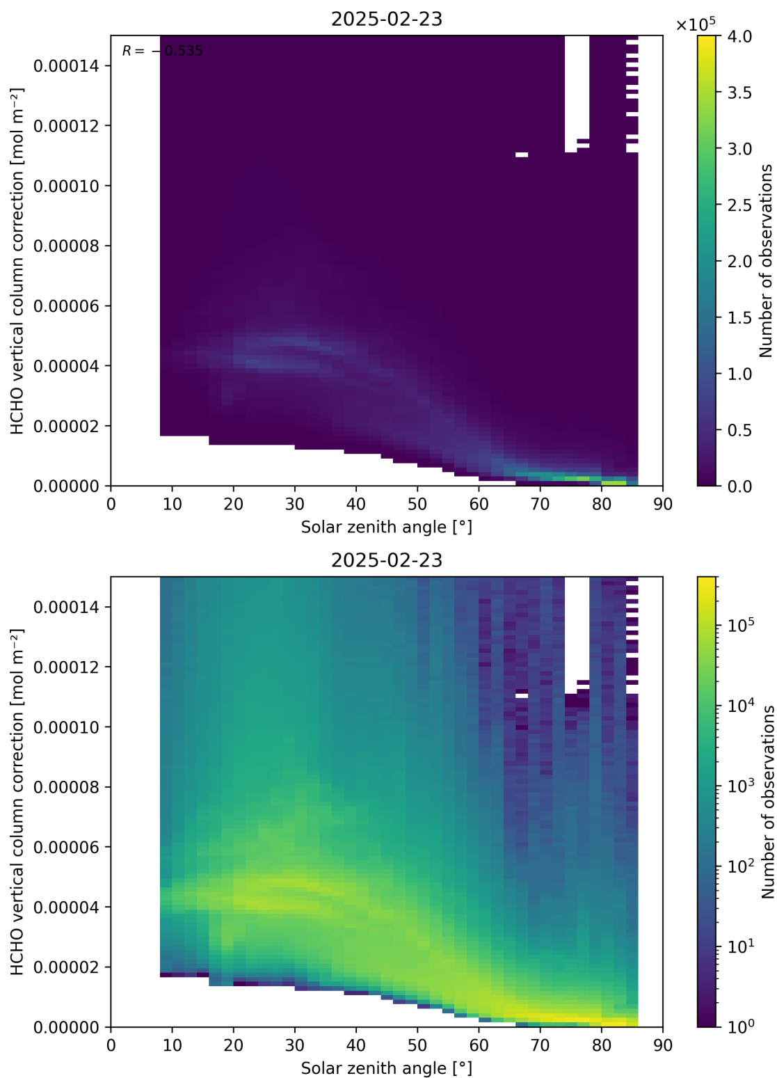
Figure 178: Scatter density plot of “Solar zenith angle” against “HCHO vertical column correction” for 2025-02-22 to 2025-02-24.
