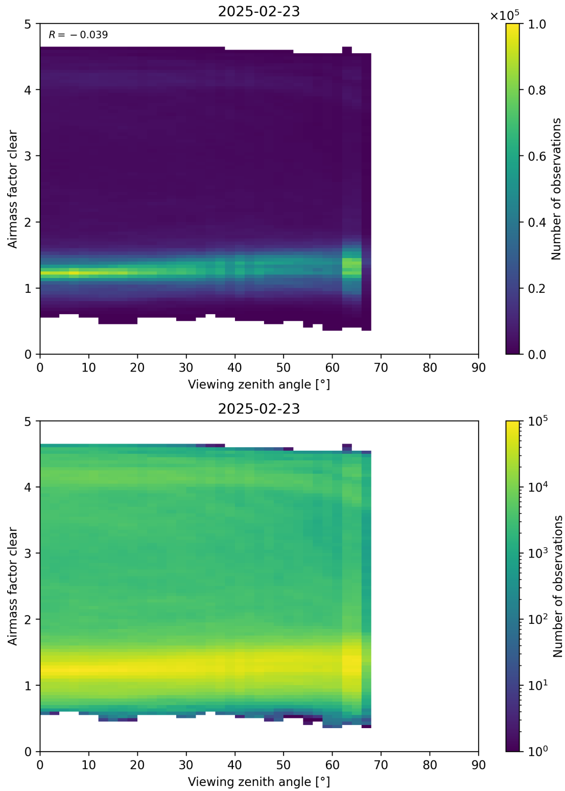
Figure 185: Scatter density plot of “Viewing zenith angle” against “Airmass factor clear” for 2025-02-22 to 2025-02-24.
