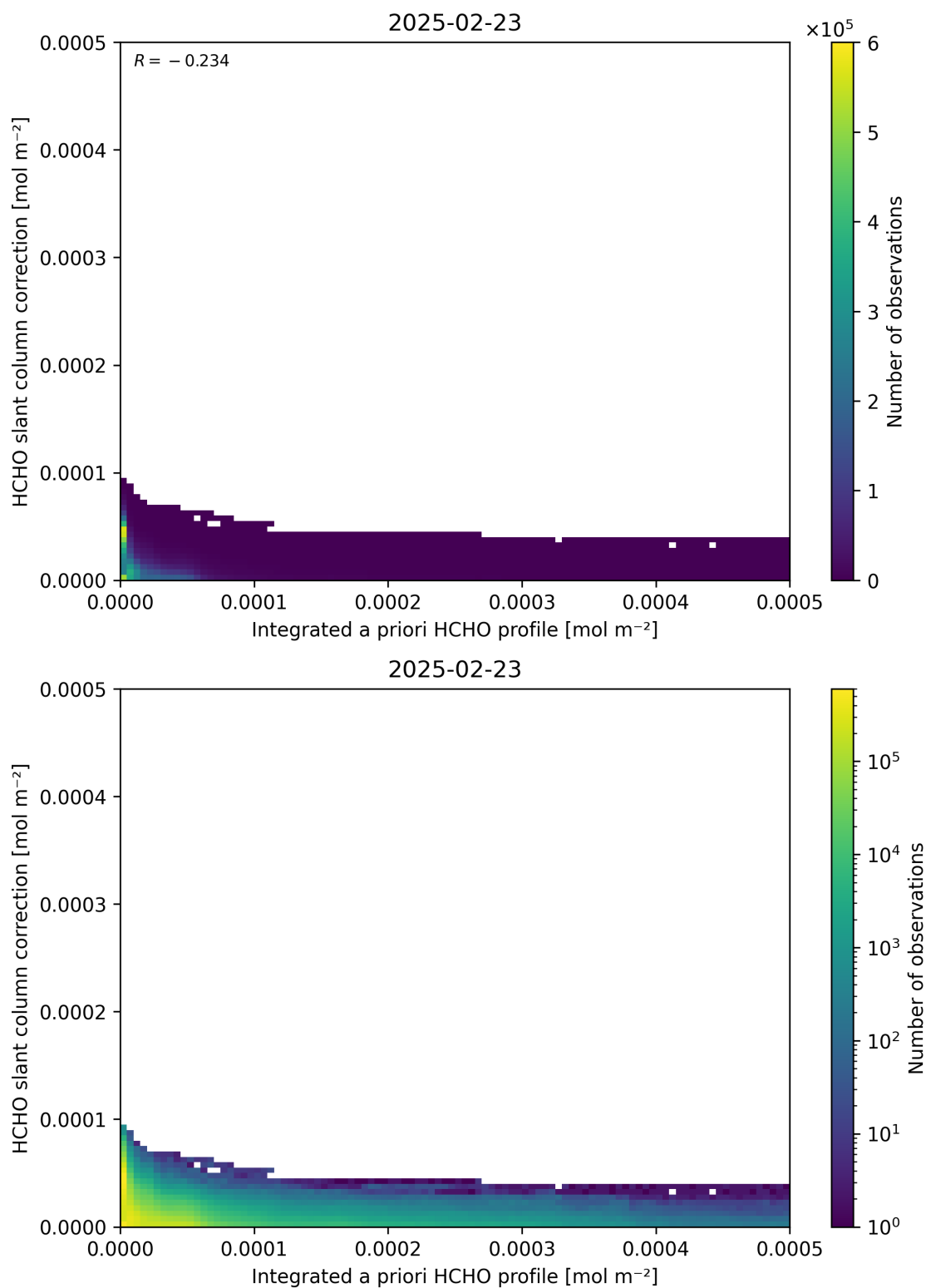
Figure 152: Scatter density plot of “Integrated a priori HCHO profile” against “HCHO slant column correction” for 2025-02-22 to 2025-02-24.
