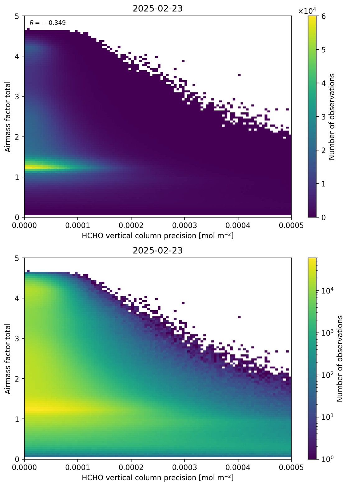
Figure 144: Scatter density plot of “HCHO vertical column precision” against “Airmass factor total” for 2025-02-22 to 2025-02-24.
