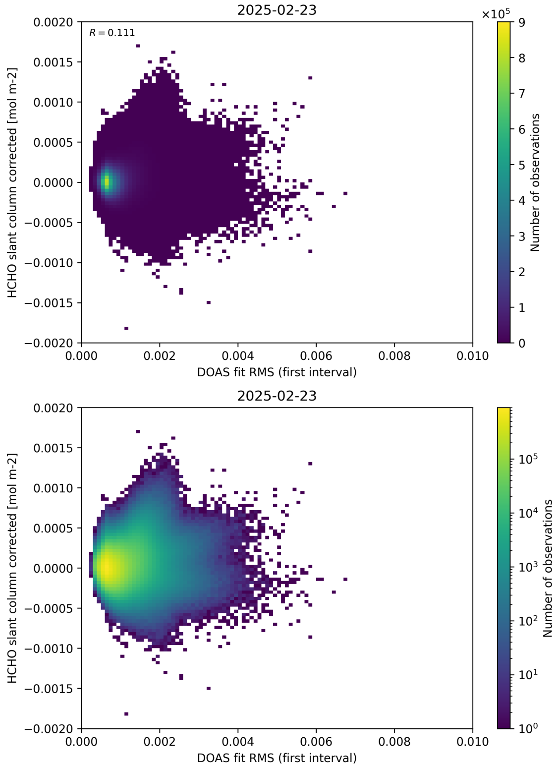
Figure 62: Scatter density plot of “DOAS fit RMS (first interval)” against “HCHO slant column corrected” for 2025-02-22 to 2025-02-24.
