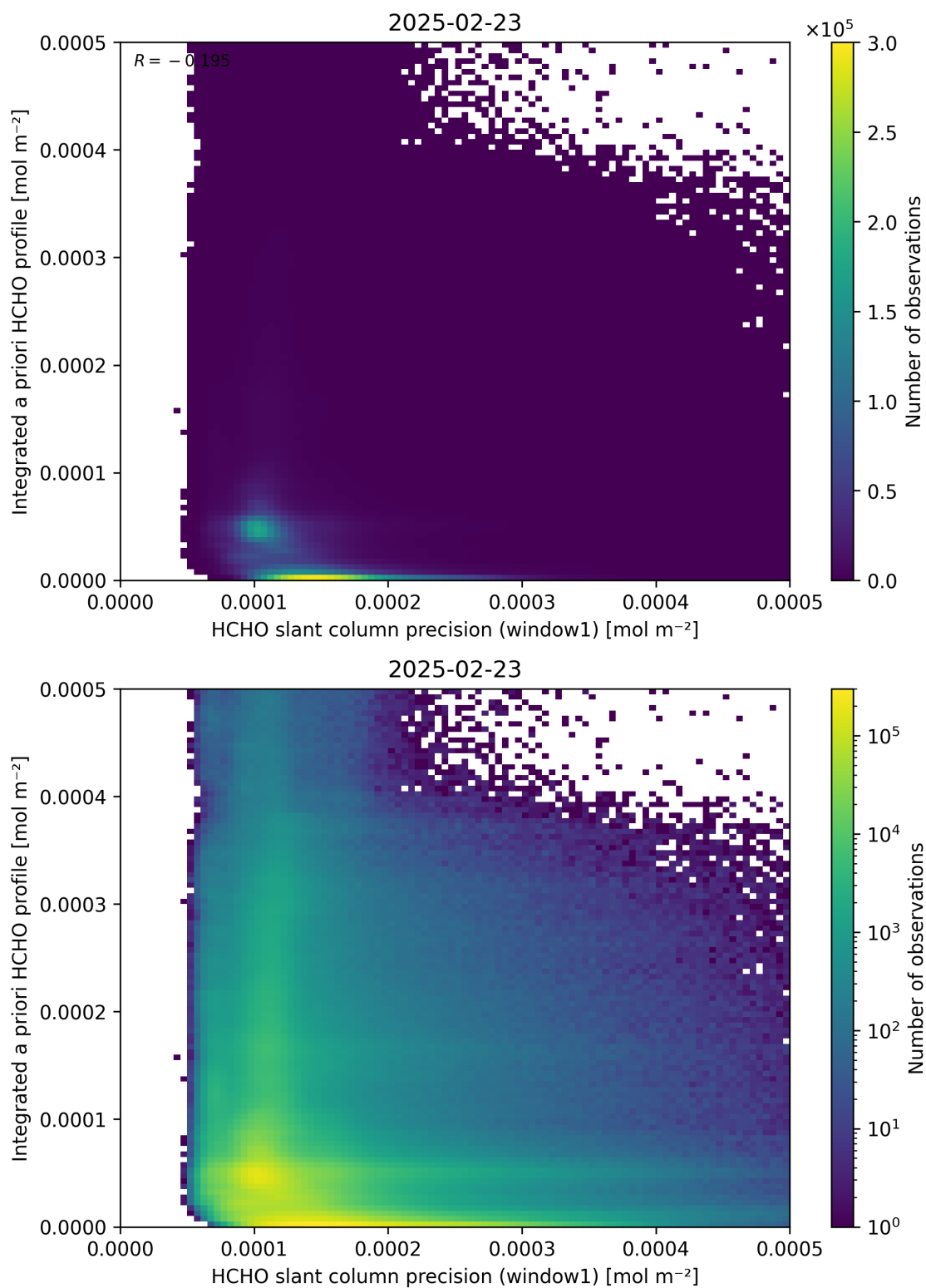
Figure 96: Scatter density plot of “HCHO slant column precision (window1)” against “Integrated a priori HCHO profile” for 2025-02-22 to 2025-02-24.
