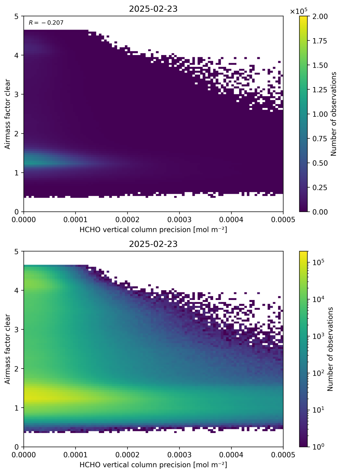
Figure 139: Scatter density plot of “HCHO vertical column precision” against “Airmass factor clear” for 2025-02-22 to 2025-02-24.
