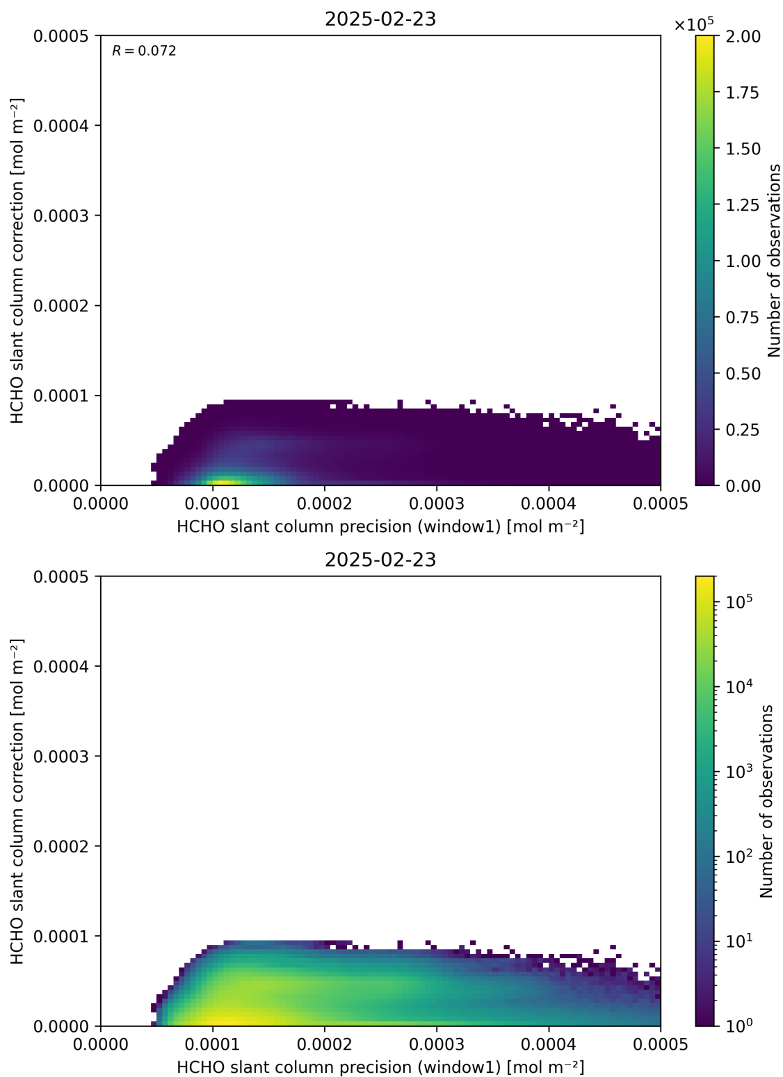
Figure 93: Scatter density plot of “HCHO slant column precision (window1)” against “HCHO slant column correction” for 2025-02-22 to 2025-02-24.
