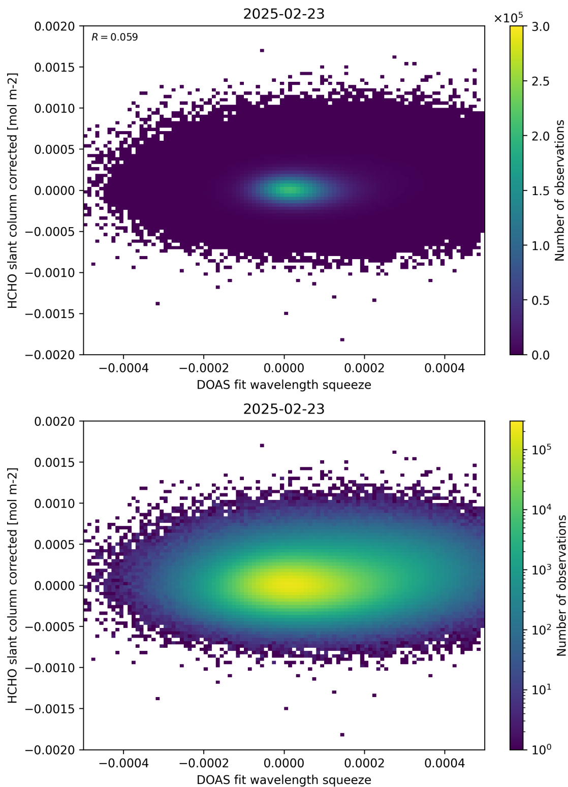
Figure 69: Scatter density plot of “DOAS fit wavelength squeeze” against “HCHO slant column corrected” for 2025-02-22 to 2025-02-24.
