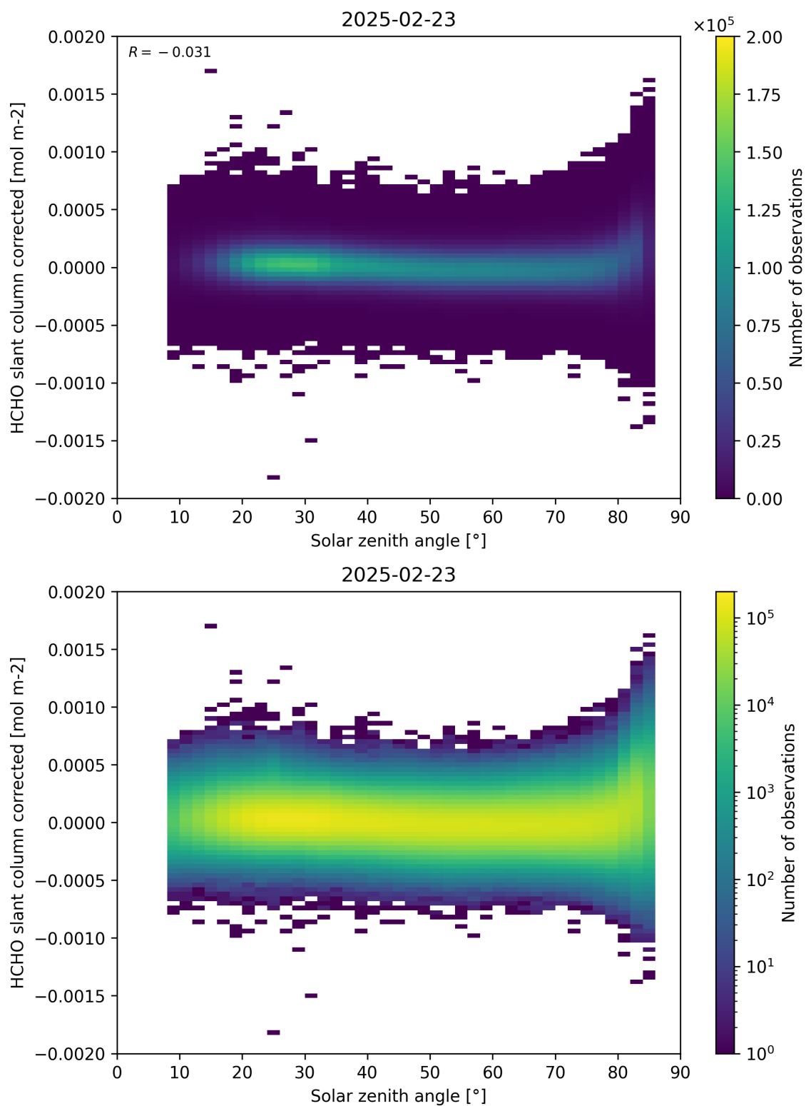
Figure 171: Scatter density plot of “Solar zenith angle” against “HCHO slant column corrected” for 2025-02-22 to 2025-02-24.
