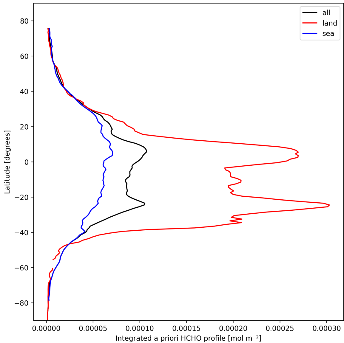
Figure 29: Zonal average of “Integrated a priori HCHO profile” for 2025-02-22 to 2025-02-24.
