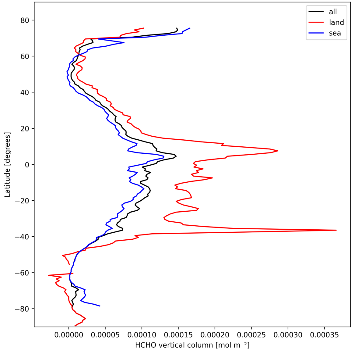
Figure 21: Zonal average of “HCHO vertical column” for 2025-02-22 to 2025-02-24.
