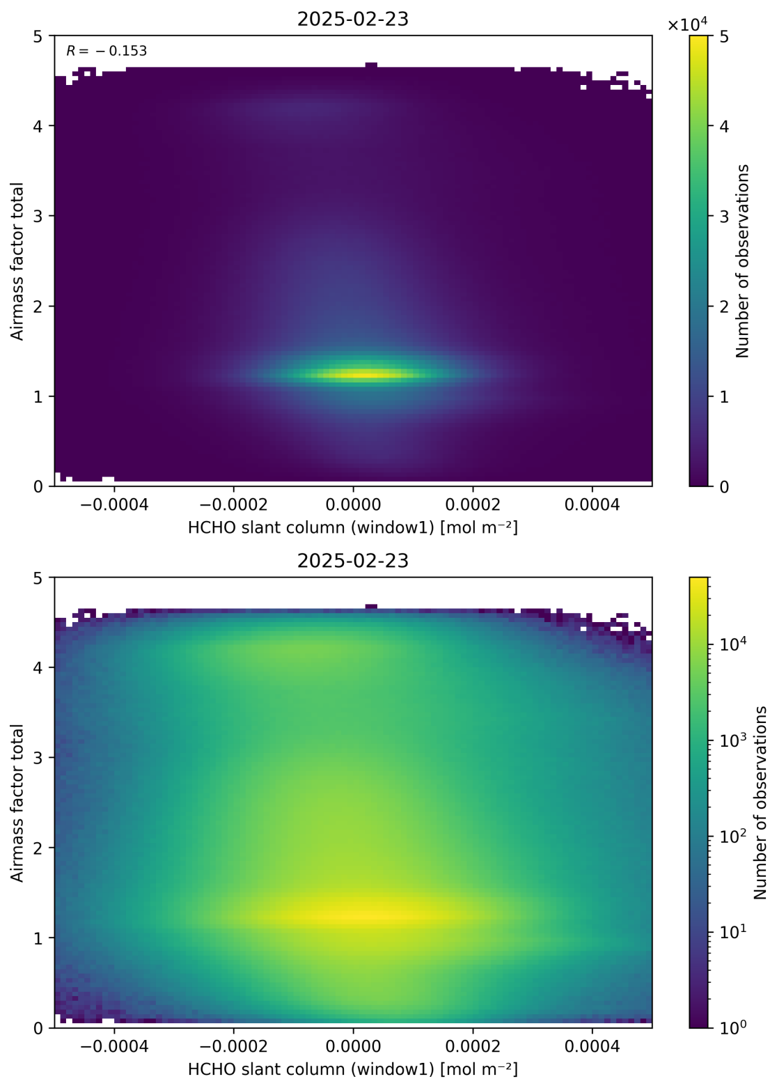
Figure 85: Scatter density plot of “HCHO slant column (window1)” against “Airmass factor total” for 2025-02-22 to 2025-02-24.
