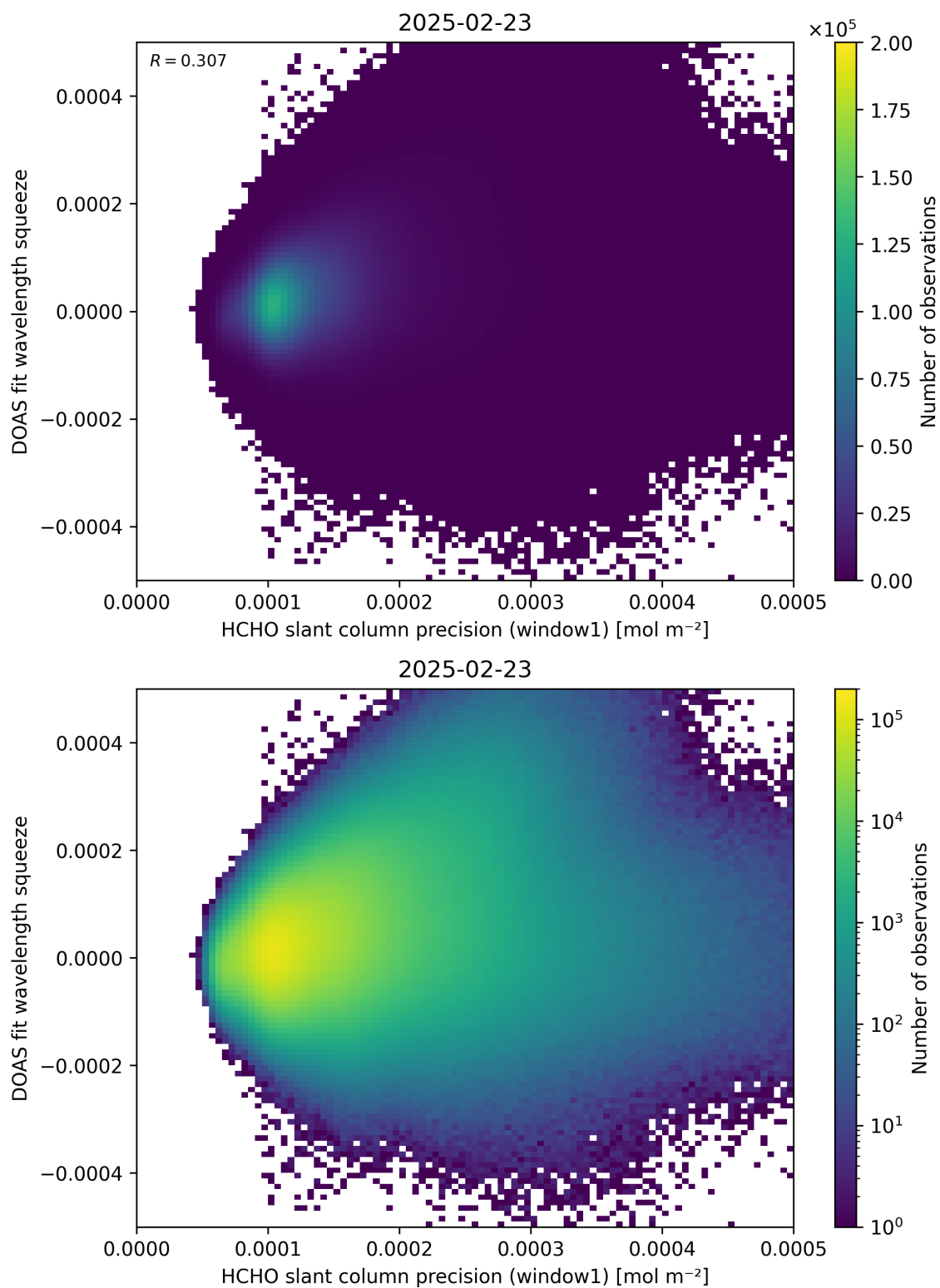
Figure 90: Scatter density plot of “HCHO slant column precision (window1)” against “DOAS fit wavelength squeeze” for 2025-02-22 to 2025-02-24.
