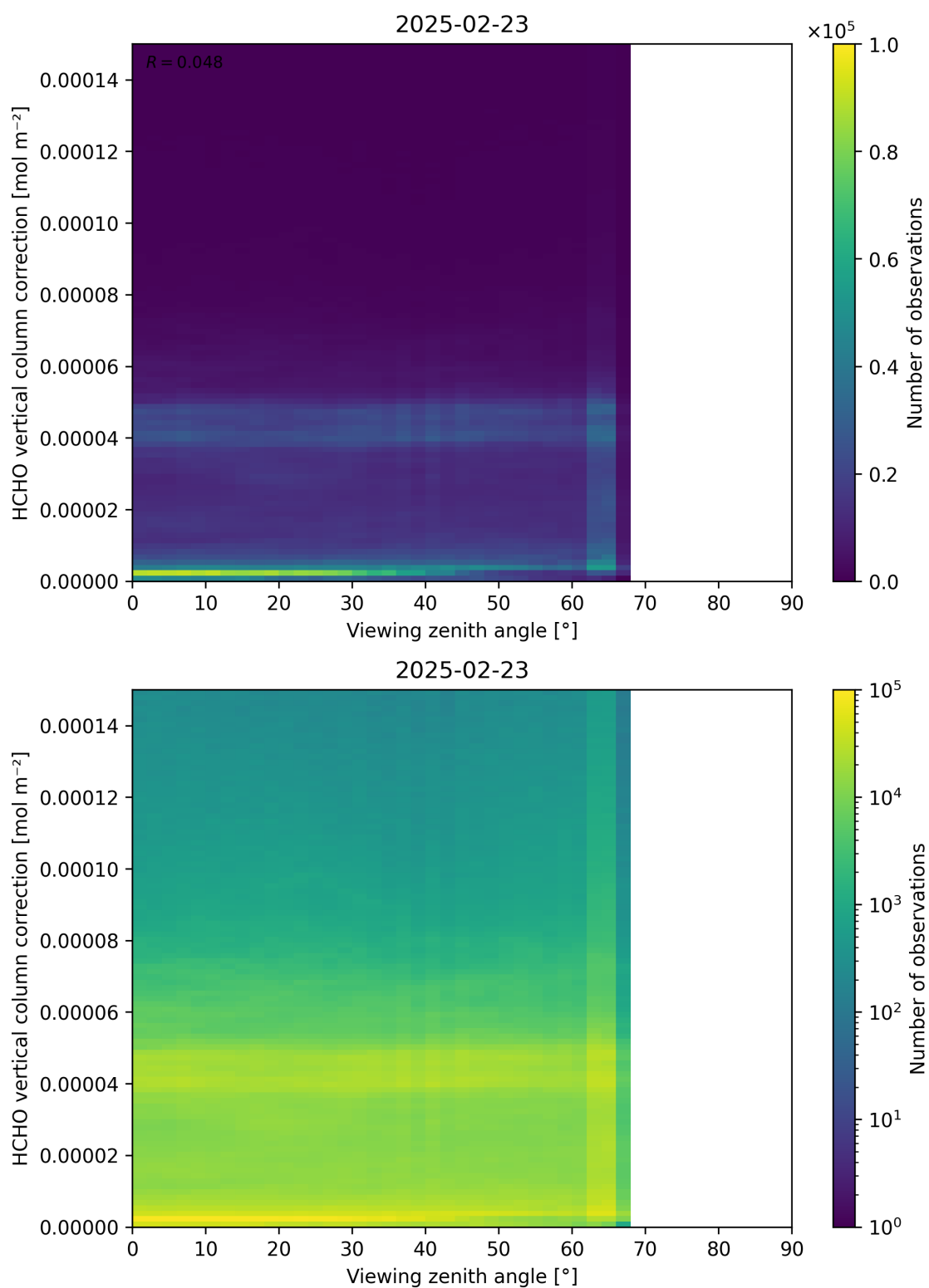
Figure 193: Scatter density plot of “Viewing zenith angle” against “HCHO vertical column correction” for 2025-02-22 to 2025-02-24.
