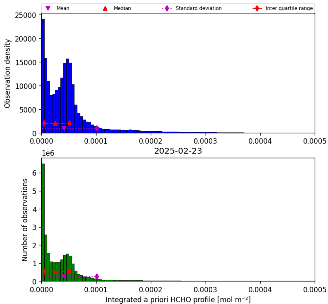
Figure 43: Histogram of “Integrated a priori HCHO profile” for 2025-02-22 to 2025-02-24
