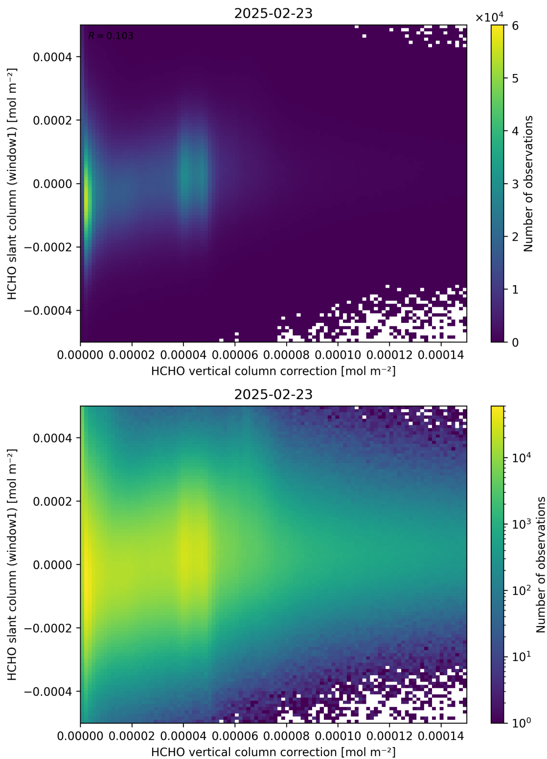
Figure 118: Scatter density plot of “HCHO vertical column correction” against “HCHO slant column (window1)” for 2025-02-22 to 2025-02-24.
