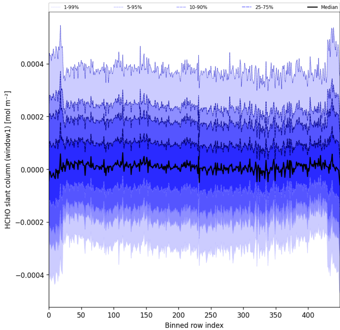
Figure 52: Along track statistics of “HCHO slant column (window1)” for 2025-02-22 to 2025-02-24
