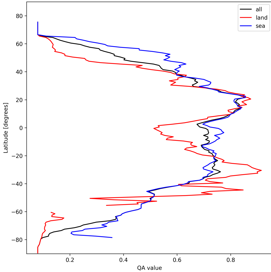
Figure 20: Zonal average of “QA value” for 2025-02-22 to 2025-02-24.
