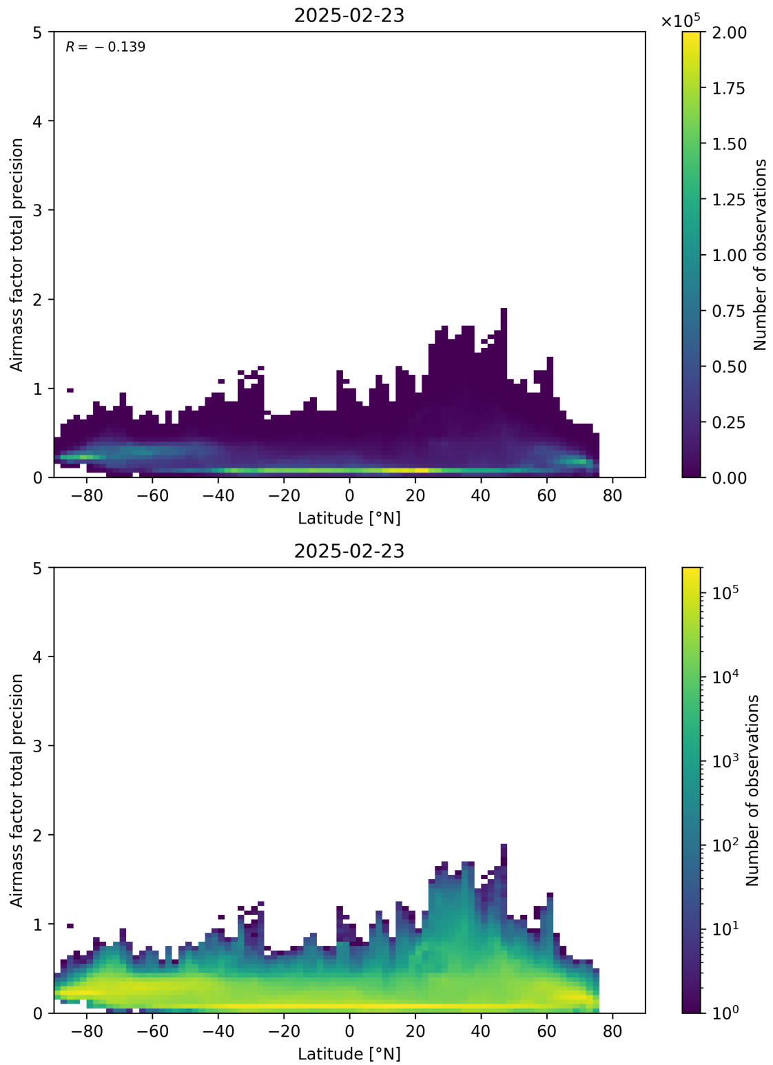
Figure 162: Scatter density plot of “Latitude” against “Airmass factor total precision” for 2025-02-22 to 2025-02-24.
