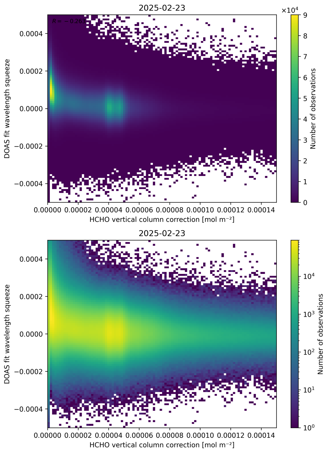
Figure 114: Scatter density plot of “HCHO vertical column correction” against “DOAS fit wavelength squeeze” for 2025-02-22 to 2025-02-24.
