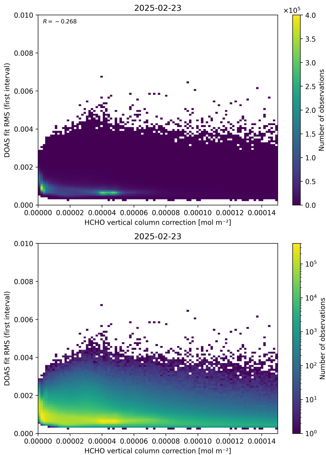
Figure 112: Scatter density plot of “HCHO vertical column correction” against “DOAS fit RMS (first interval)” for 2025-02-22 to 2025-02-24.
