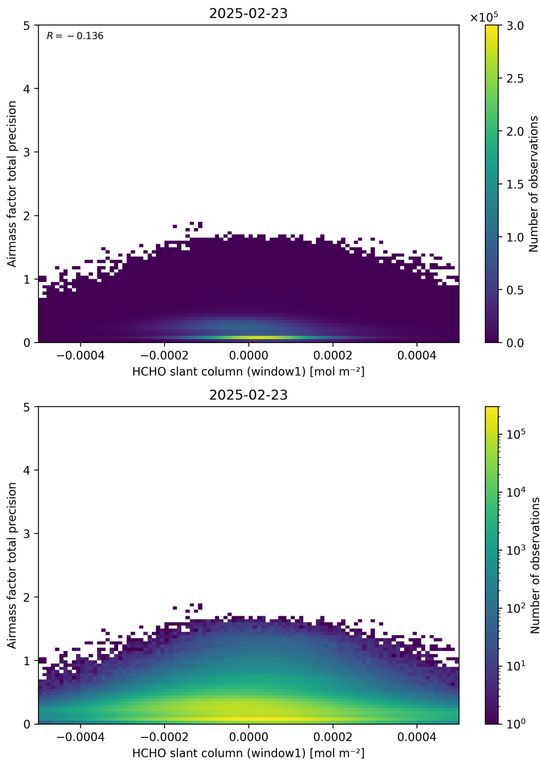
Figure 86: Scatter density plot of “HCHO slant column (window1)” against “Airmass factor total precision” for 2025-02-22 to 2025-02-24.
