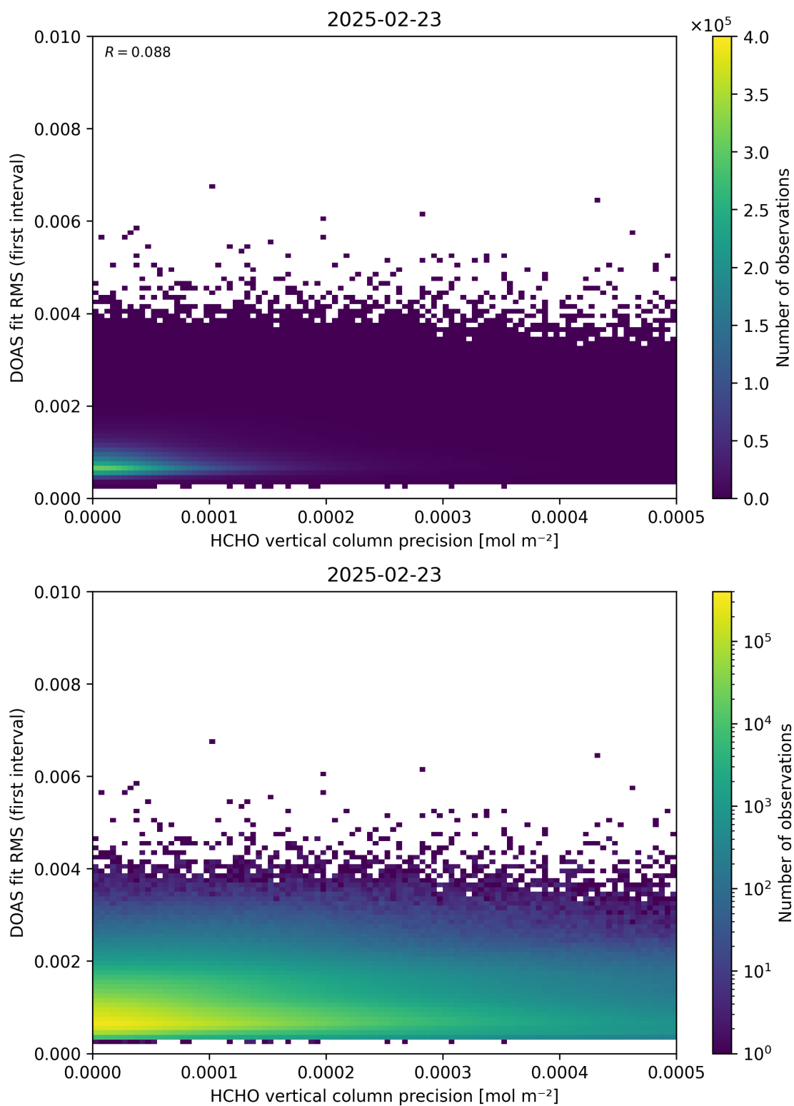
Figure 136: Scatter density plot of “HCHO vertical column precision” against “DOAS fit RMS (first interval)” for 2025-02-22 to 2025-02-24.
