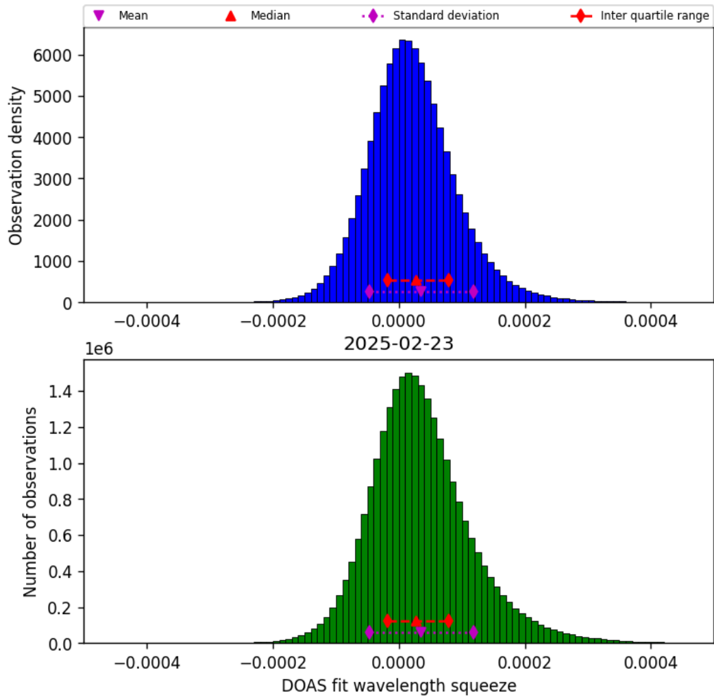
Figure 45: Histogram of “DOAS fit wavelength squeeze” for 2025-02-22 to 2025-02-24
