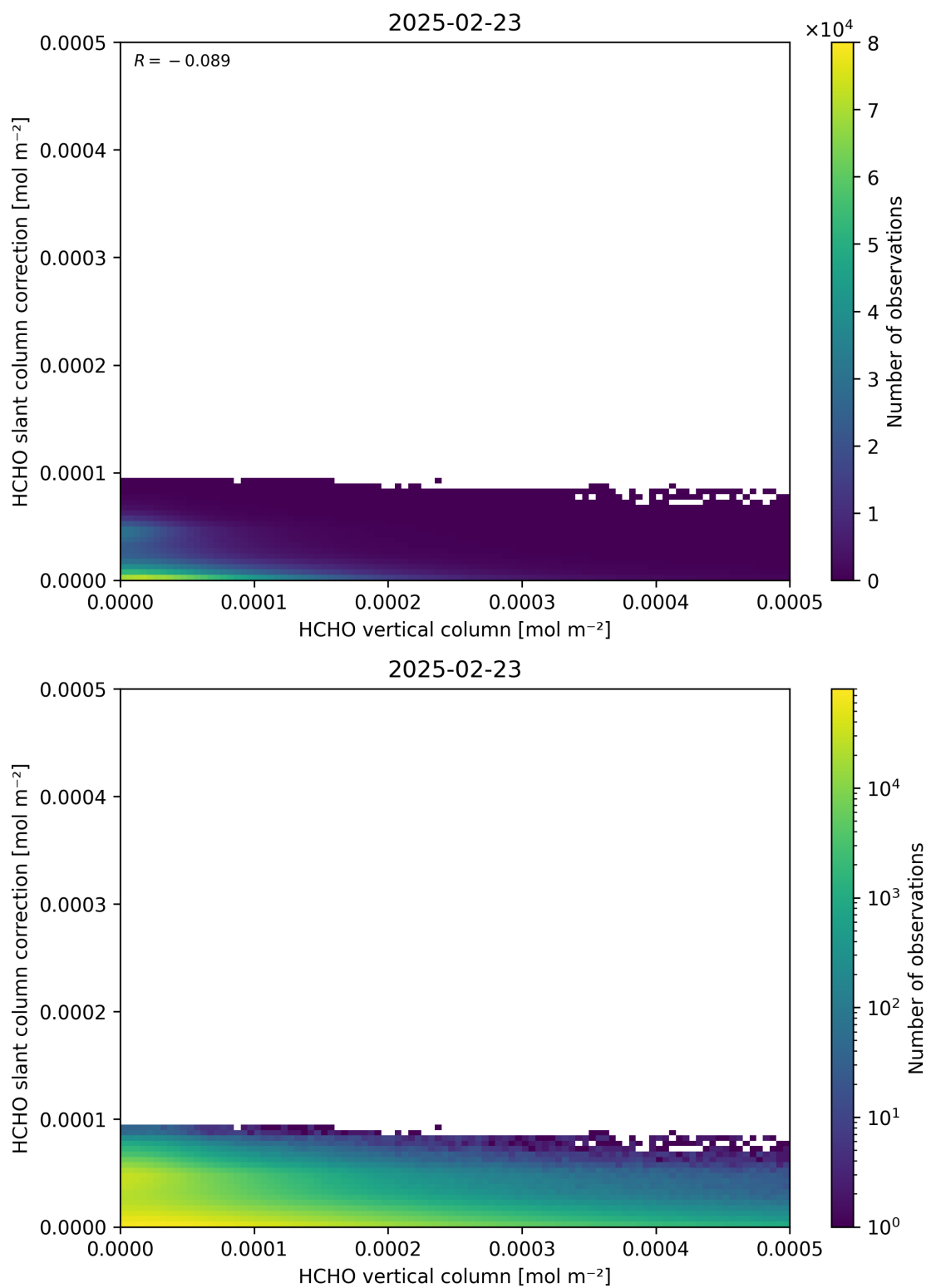
Figure 128: Scatter density plot of “HCHO vertical column” against “HCHO slant column correction” for 2025-02-22 to 2025-02-24.
