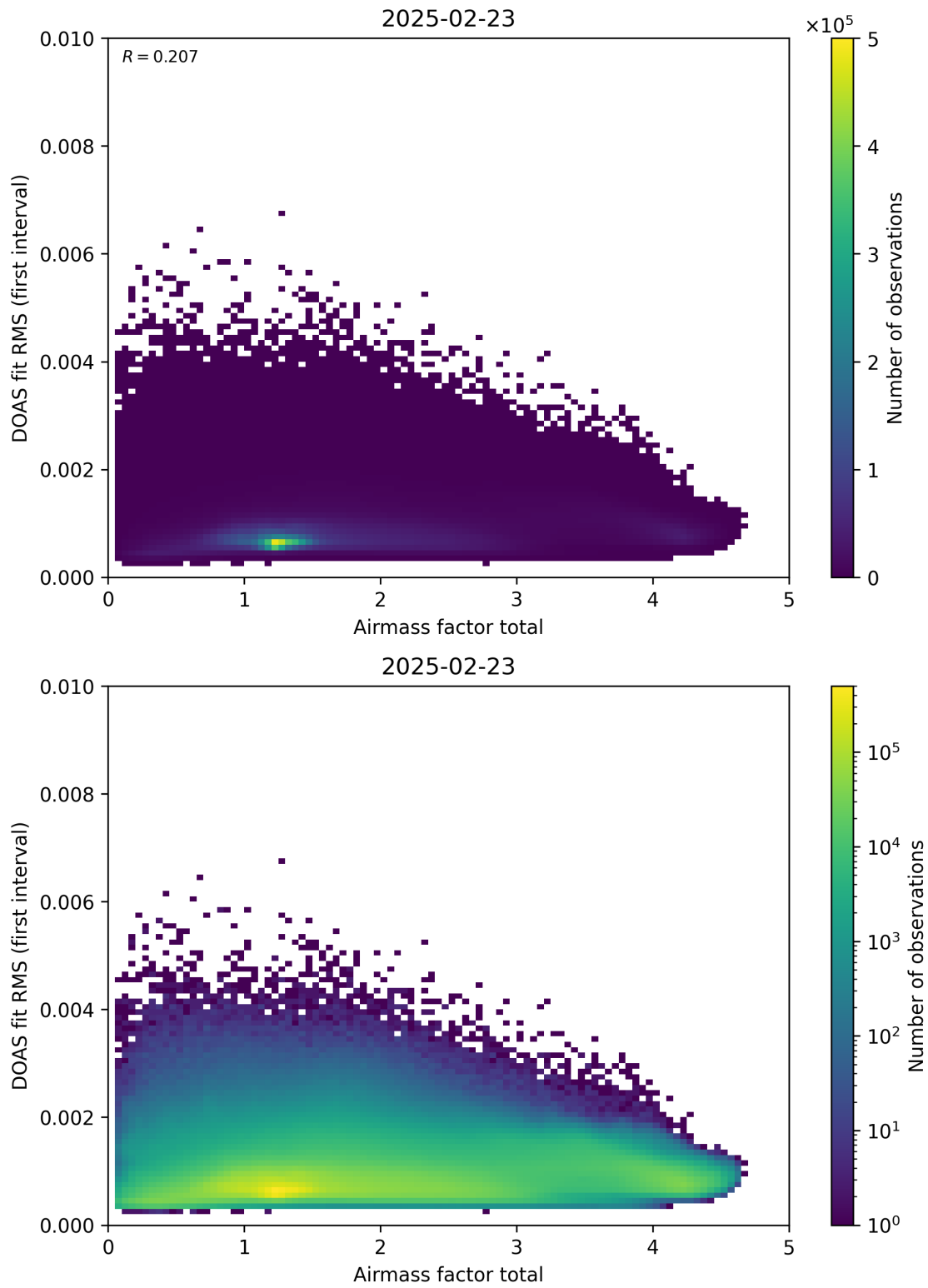
Figure 97: Scatter density plot of “Airmass factor total” against “DOAS fit RMS (first interval)” for 2025-02-22 to 2025-02-24.
