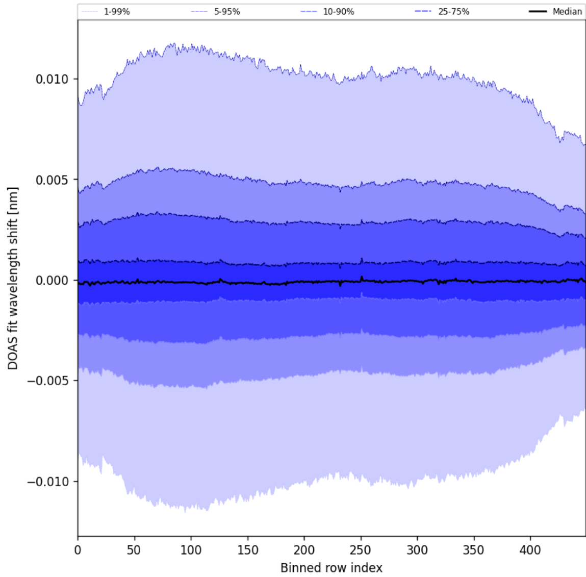
Figure 58: Along track statistics of “DOAS fit wavelength shift” for 2025-02-22 to 2025-02-24
