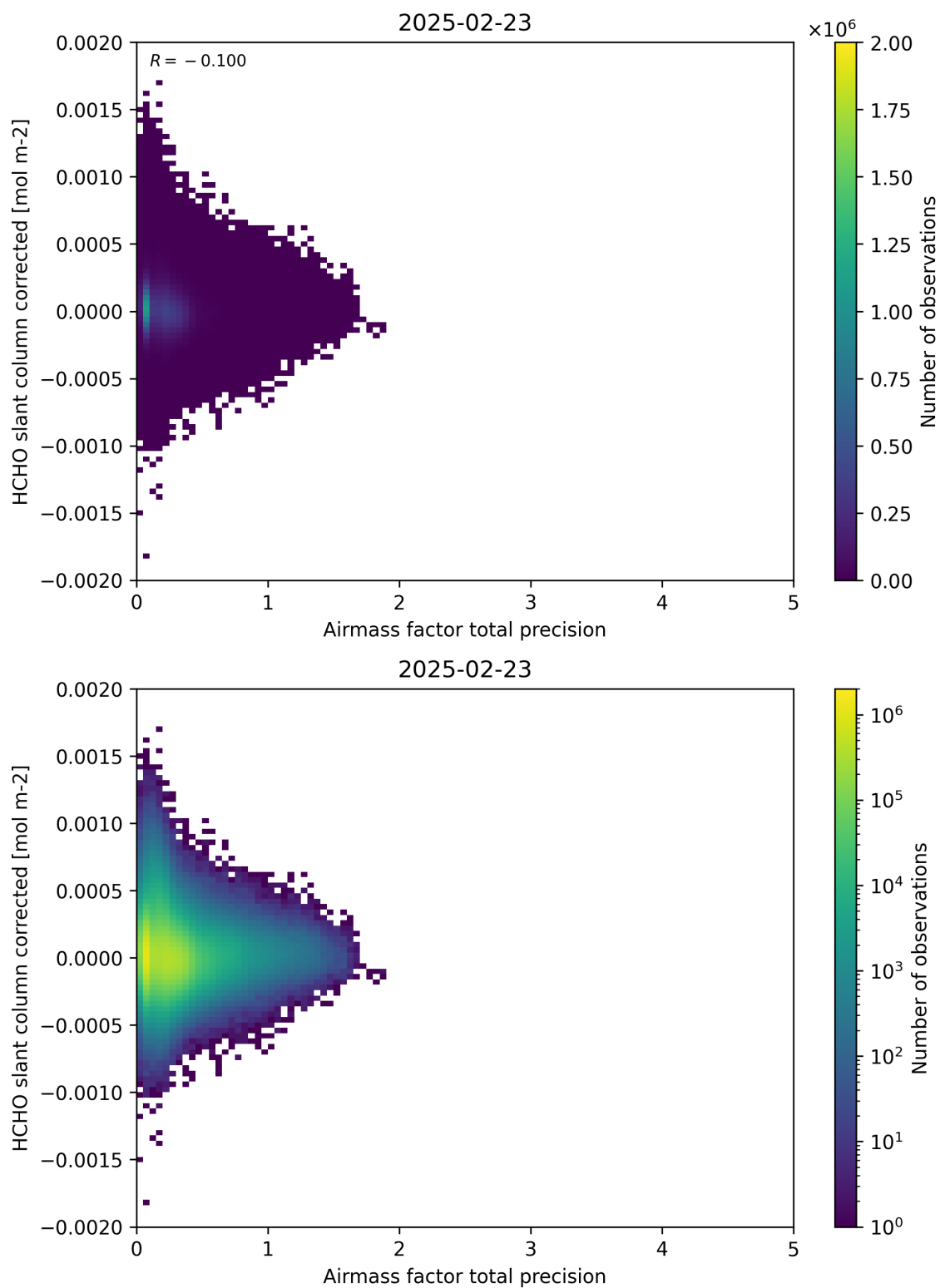
Figure 109: Scatter density plot of “Airmass factor total precision” against “HCHO slant column corrected” for 2025-02-22 to 2025-02-24.
