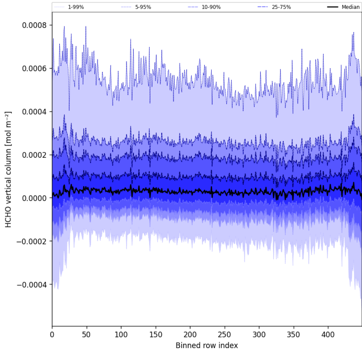
Figure 49: Along track statistics of “HCHO vertical column” for 2025-02-22 to 2025-02-24
