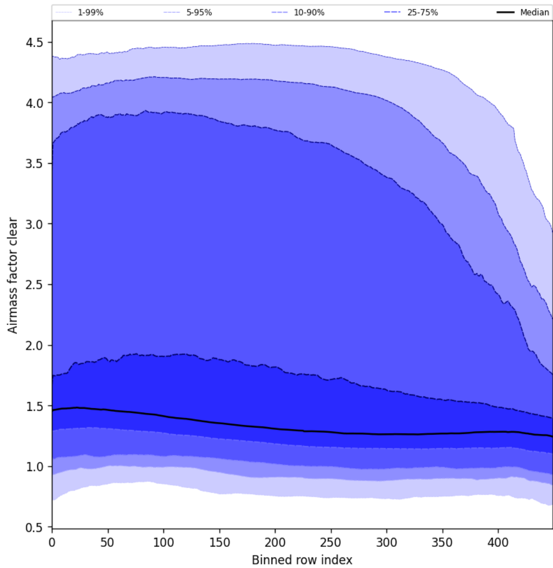
Figure 56: Along track statistics of “Air mass factor clear” for 2025-02-22 to 2025-02-24
