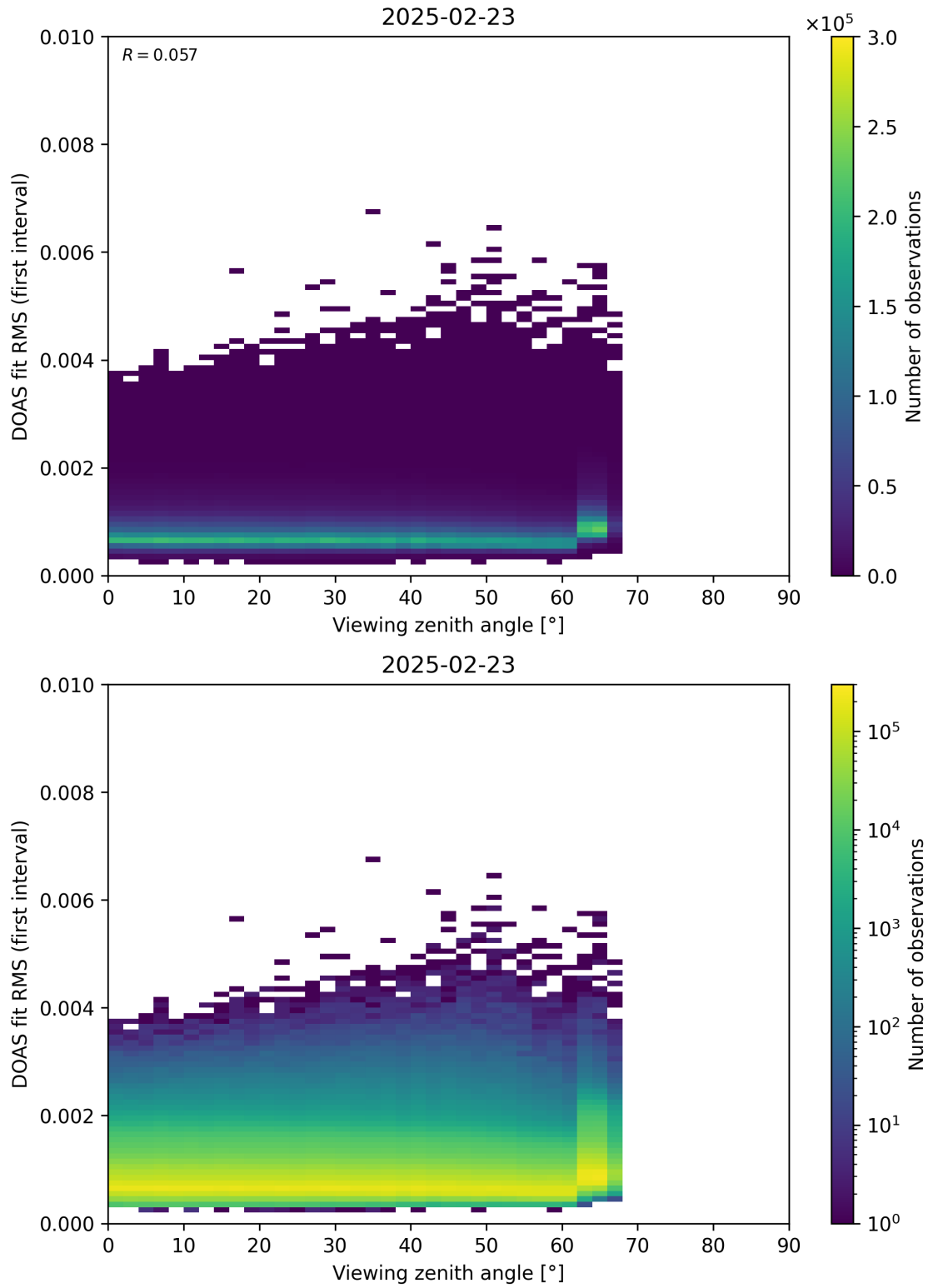
Figure 182: Scatter density plot of “Viewing zenith angle” against “DOAS fit RMS (first interval)” for 2025-02-22 to 2025-02-24.
