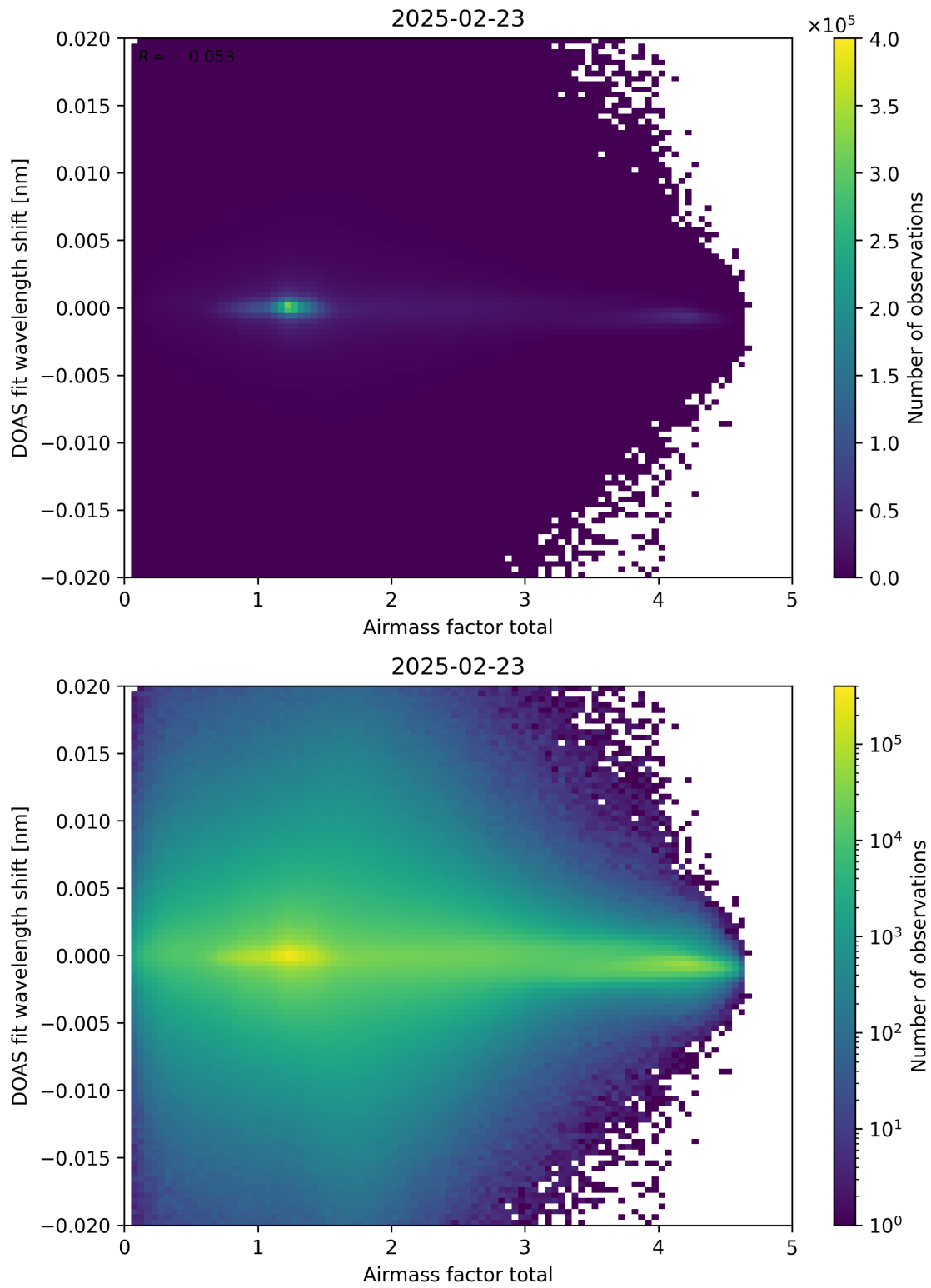
Figure 98: Scatter density plot of “Airmass factor total” against “DOAS fit wavelength shift” for 2025-02-22 to 2025-02-24.
