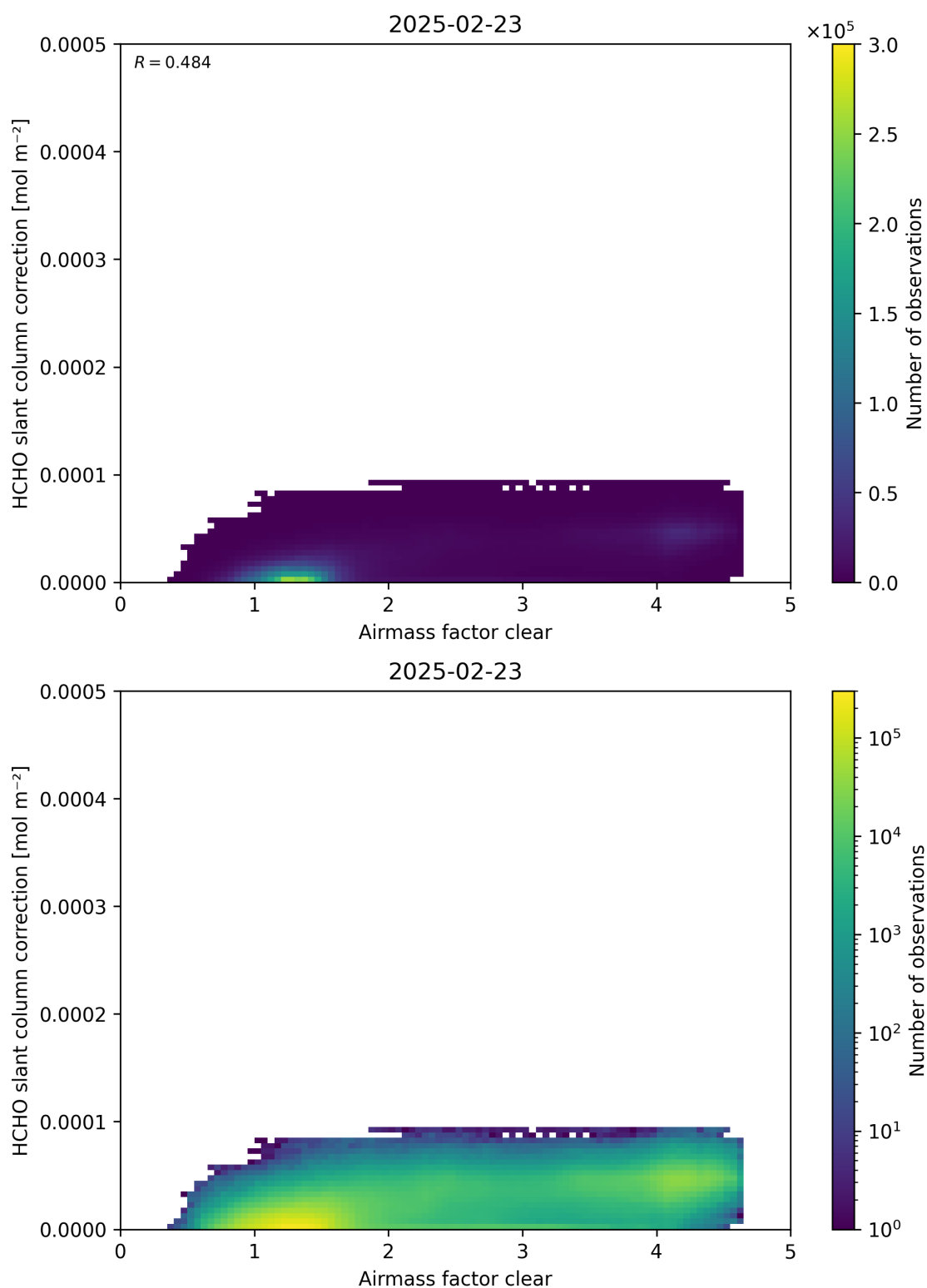
Figure 75: Scatter density plot of “Airmass factor clear” against “HCHO slant column correction” for 2025-02-22 to 2025-02-24.
