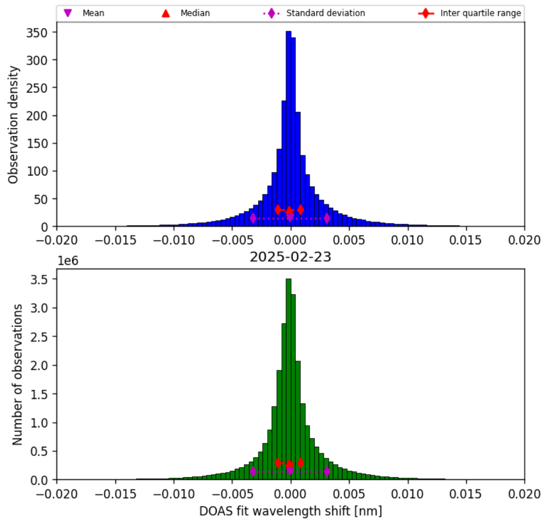
Figure 44: Histogram of “DOAS fit wavelength shift” for 2025-02-22 to 2025-02-24
