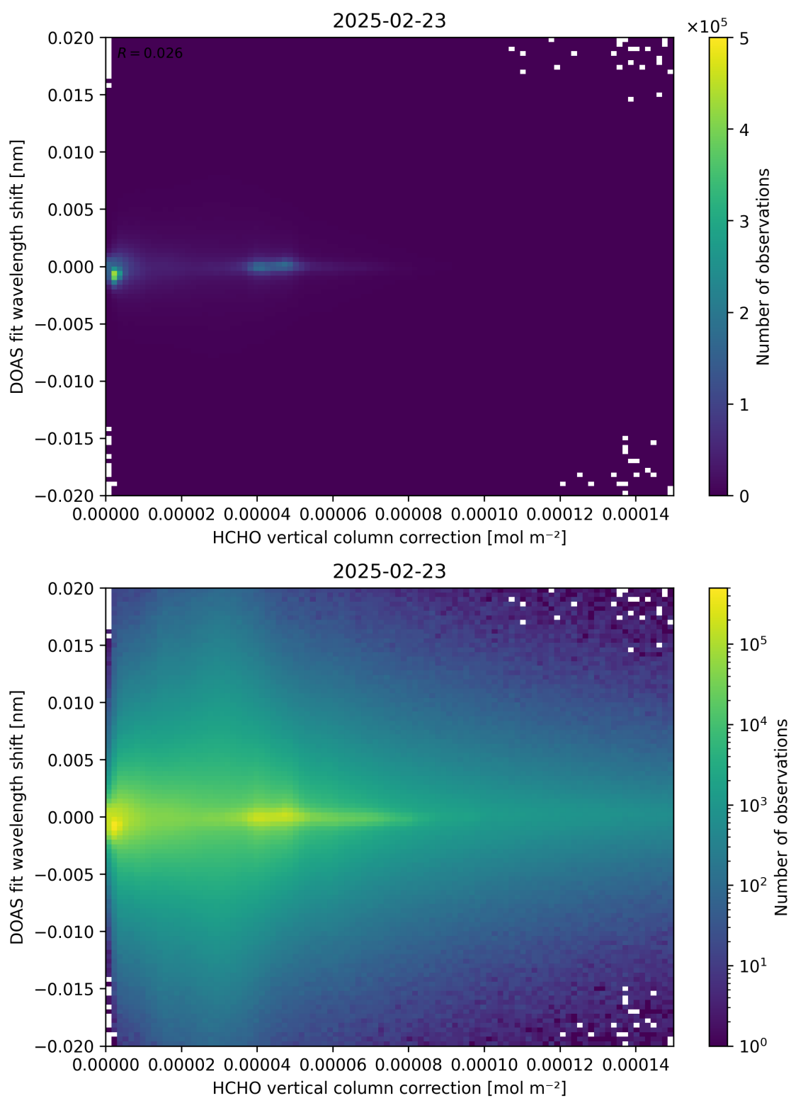
Figure 113: Scatter density plot of “HCHO vertical column correction” against “DOAS fit wavelength shift” for 2025-02-22 to 2025-02-24.
