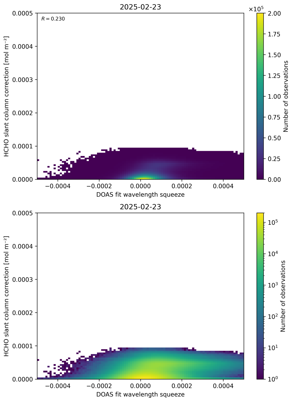
Figure 70: Scatter density plot of “DOAS fit wavelength squeeze” against “HCHO slant column correction” for 2025-02-22 to 2025-02-24.
