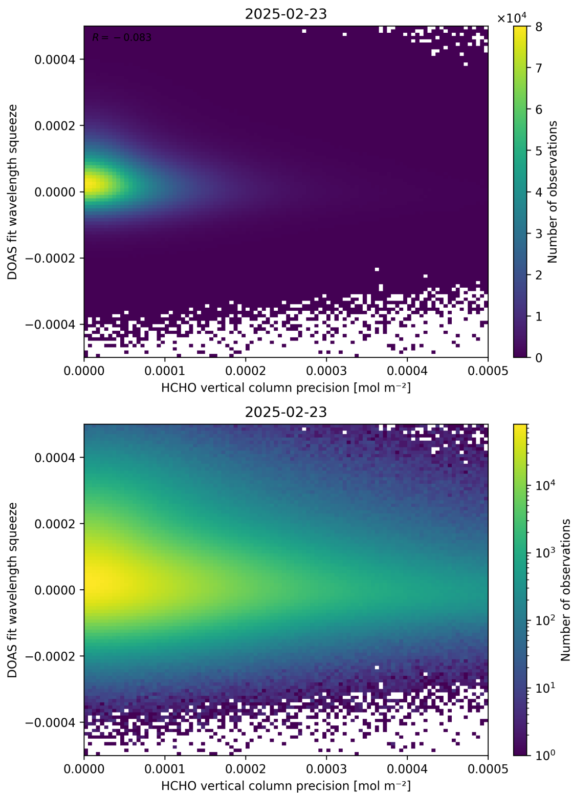
Figure 138: Scatter density plot of “HCHO vertical column precision” against “DOAS fit wavelength squeeze” for 2025-02-22 to 2025-02-24.
