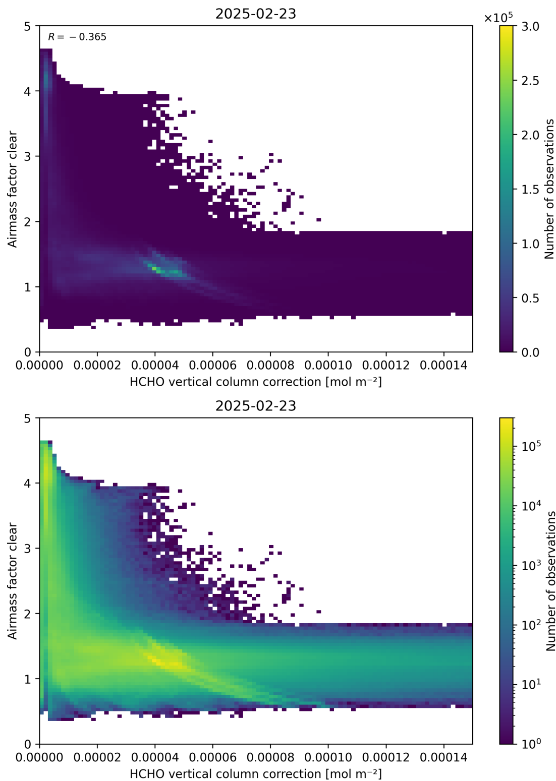
Figure 115: Scatter density plot of “HCHO vertical column correction” against “Airmass factor clear” for 2025-02-22 to 2025-02-24.
