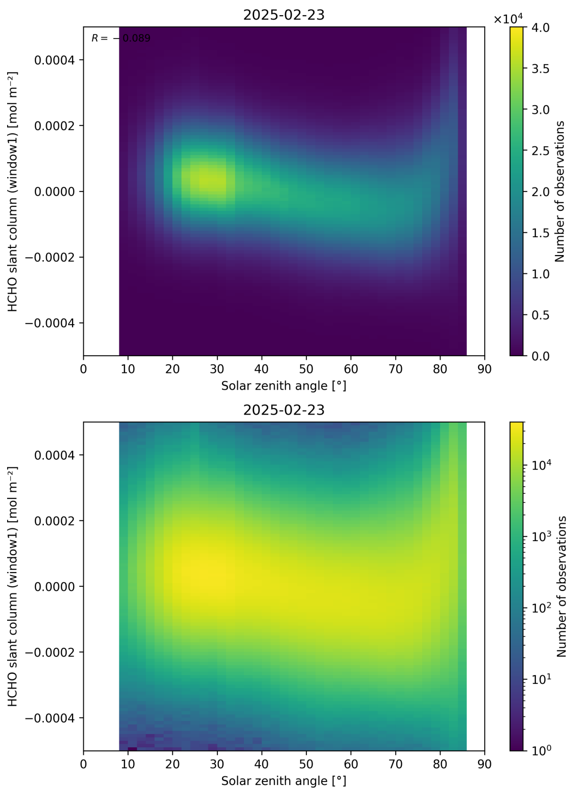
Figure 173: Scatter density plot of “Solar zenith angle” against “HCHO slant column (window1)” for 2025-02-22 to 2025-02-24.
