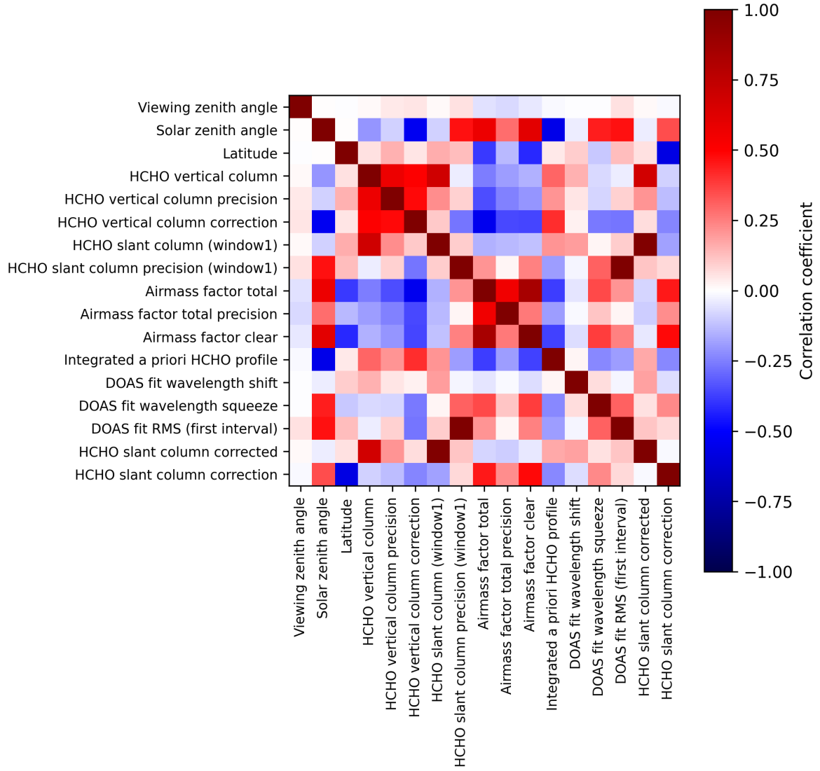
Figure 2: Map of correlation matrix for 2025-02-22 to 2025-02-24.
