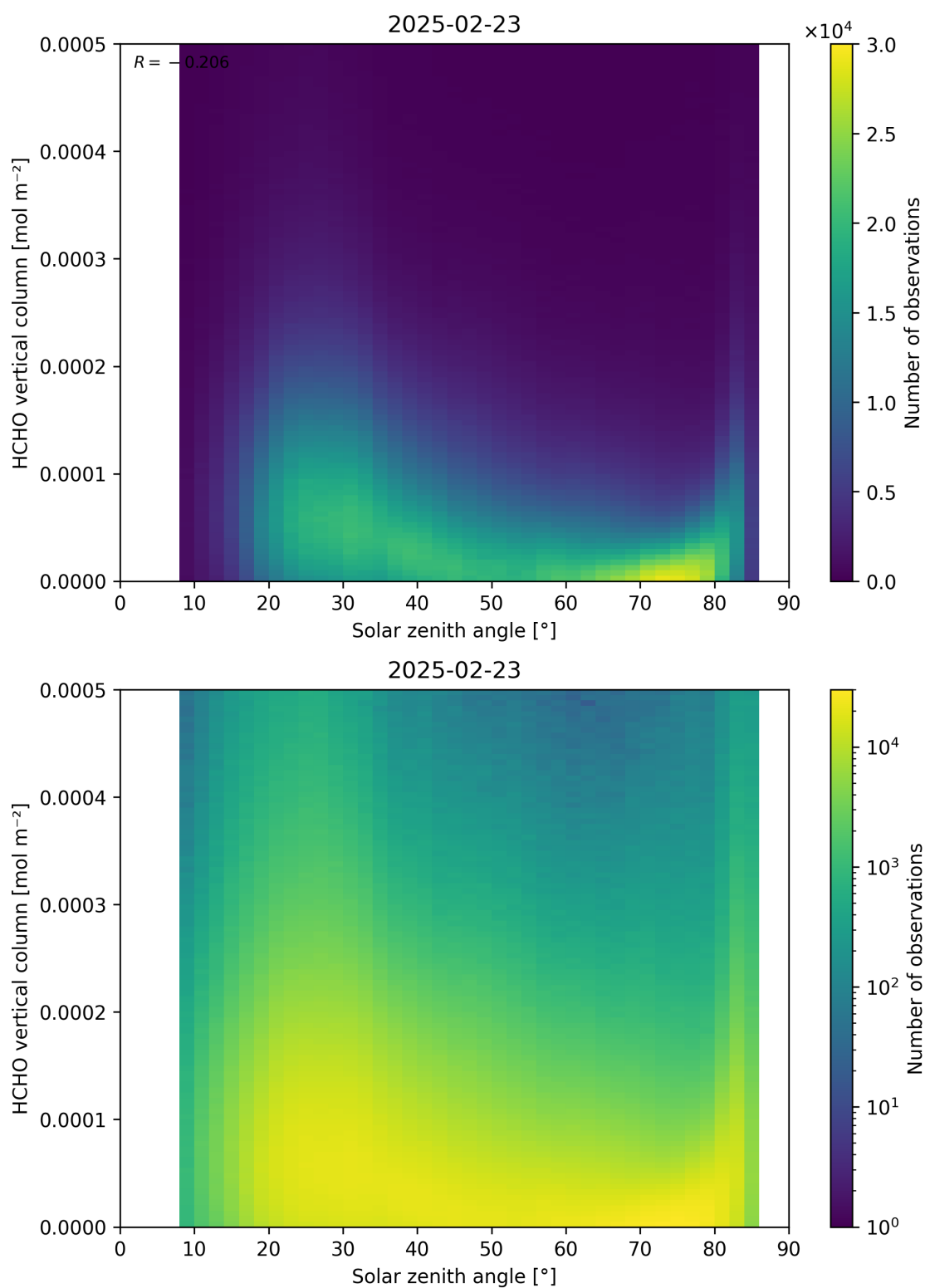
Figure 177: Scatter density plot of “Solar zenith angle” against “HCHO vertical column” for 2025-02-22 to 2025-02-24.
