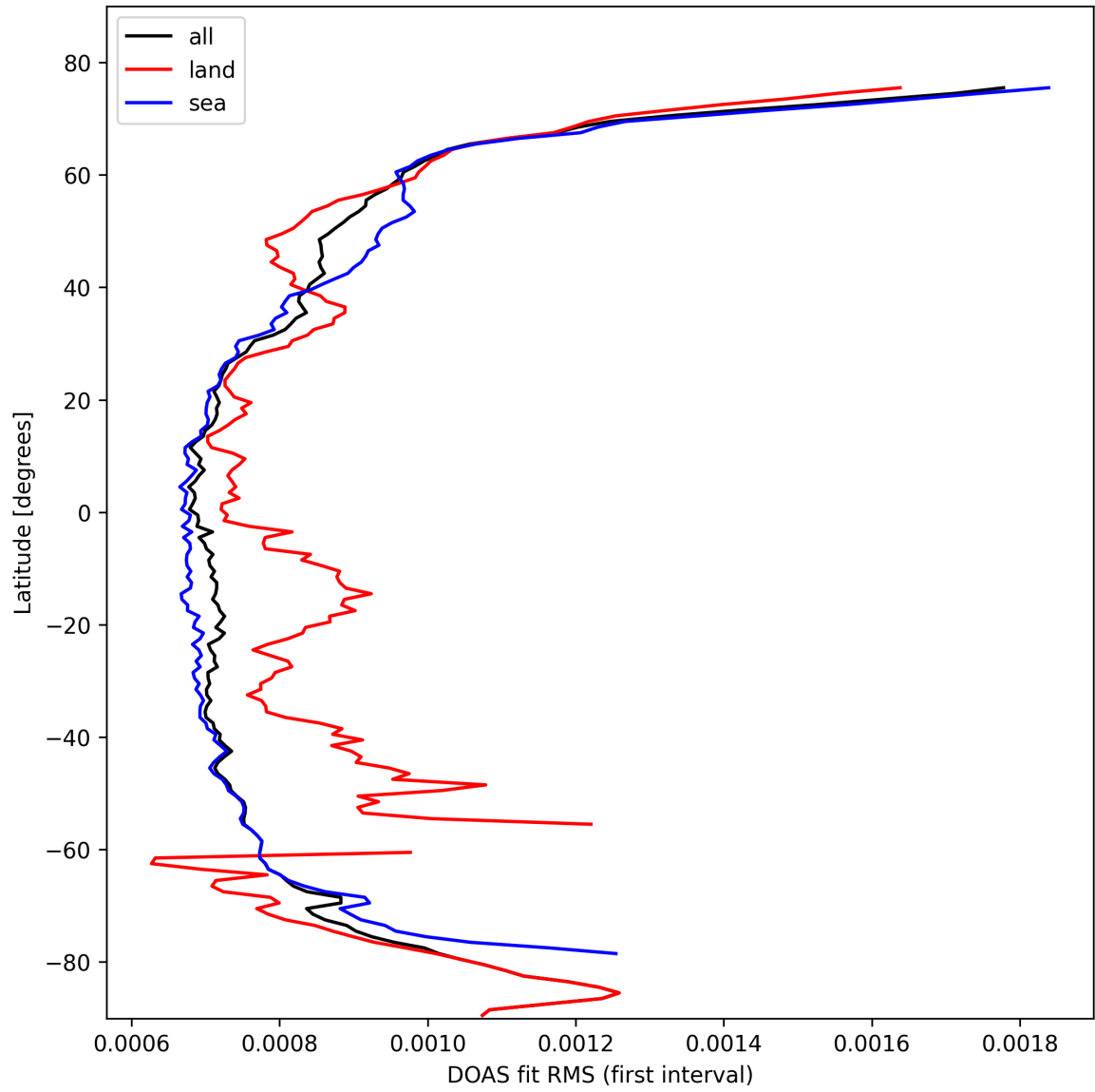
Figure 32: Zonal average of “DOAS fit RMS (first interval)” for 2025-02-22 to 2025-02-24.
