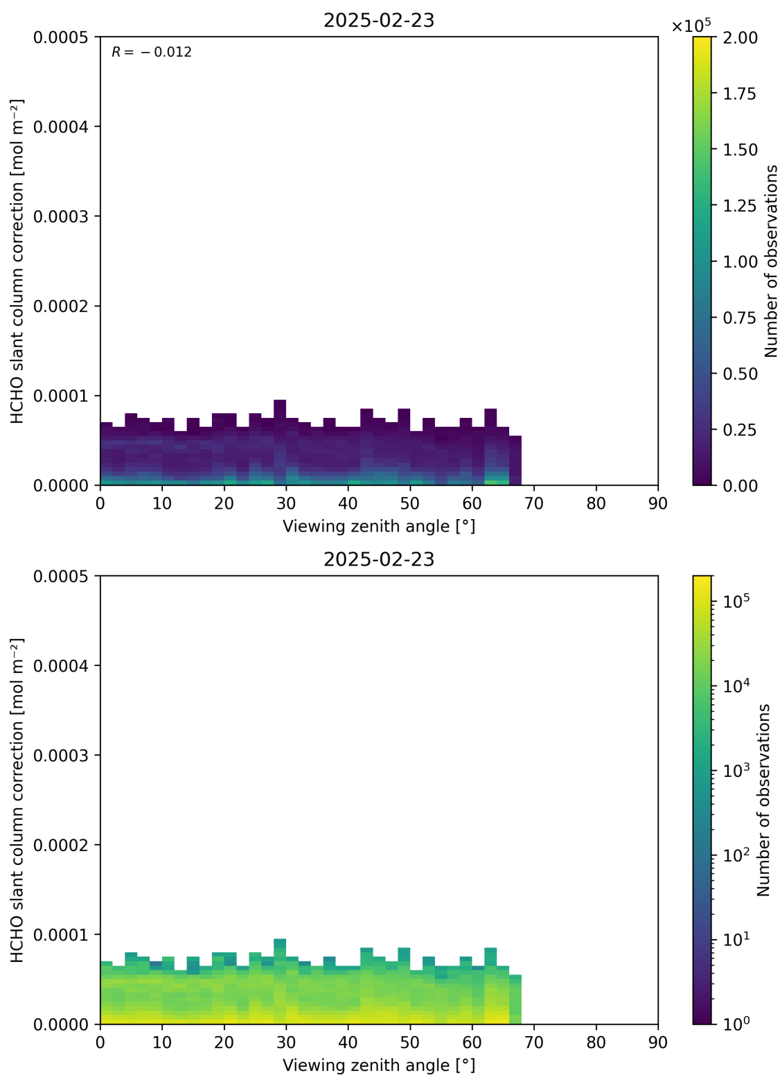
Figure 187: Scatter density plot of “Viewing zenith angle” against “HCHO slant column correction” for 2025-02-22 to 2025-02-24.
