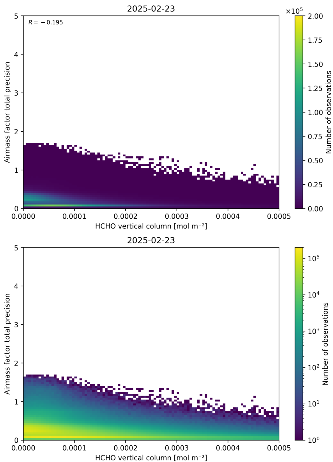
Figure 132: Scatter density plot of “HCHO vertical column” against “Airmass factor total precision” for 2025-02-22 to 2025-02-24.
