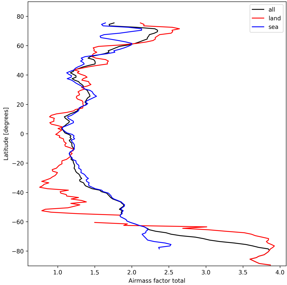
Figure 26: Zonal average of “Airmass factor total” for 2025-02-22 to 2025-02-24.
