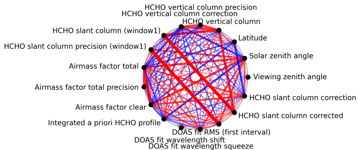
Figure 1: Map of correlation graph for 2025-02-22 to 2025-02-24.
