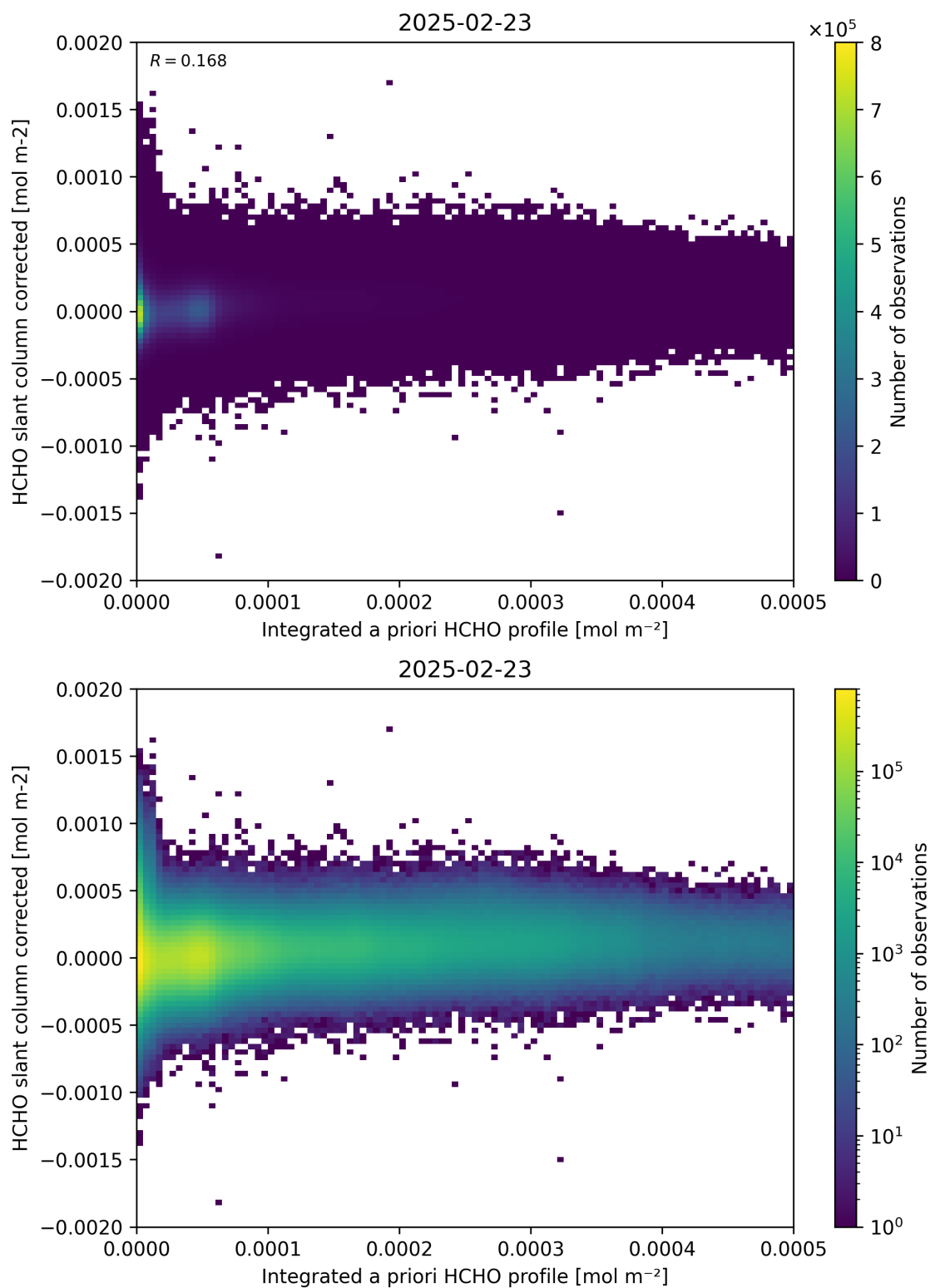
Figure 151: Scatter density plot of “Integrated a priori HCHO profile” against “HCHO slant column corrected” for 2025-02-22 to 2025-02-24.
