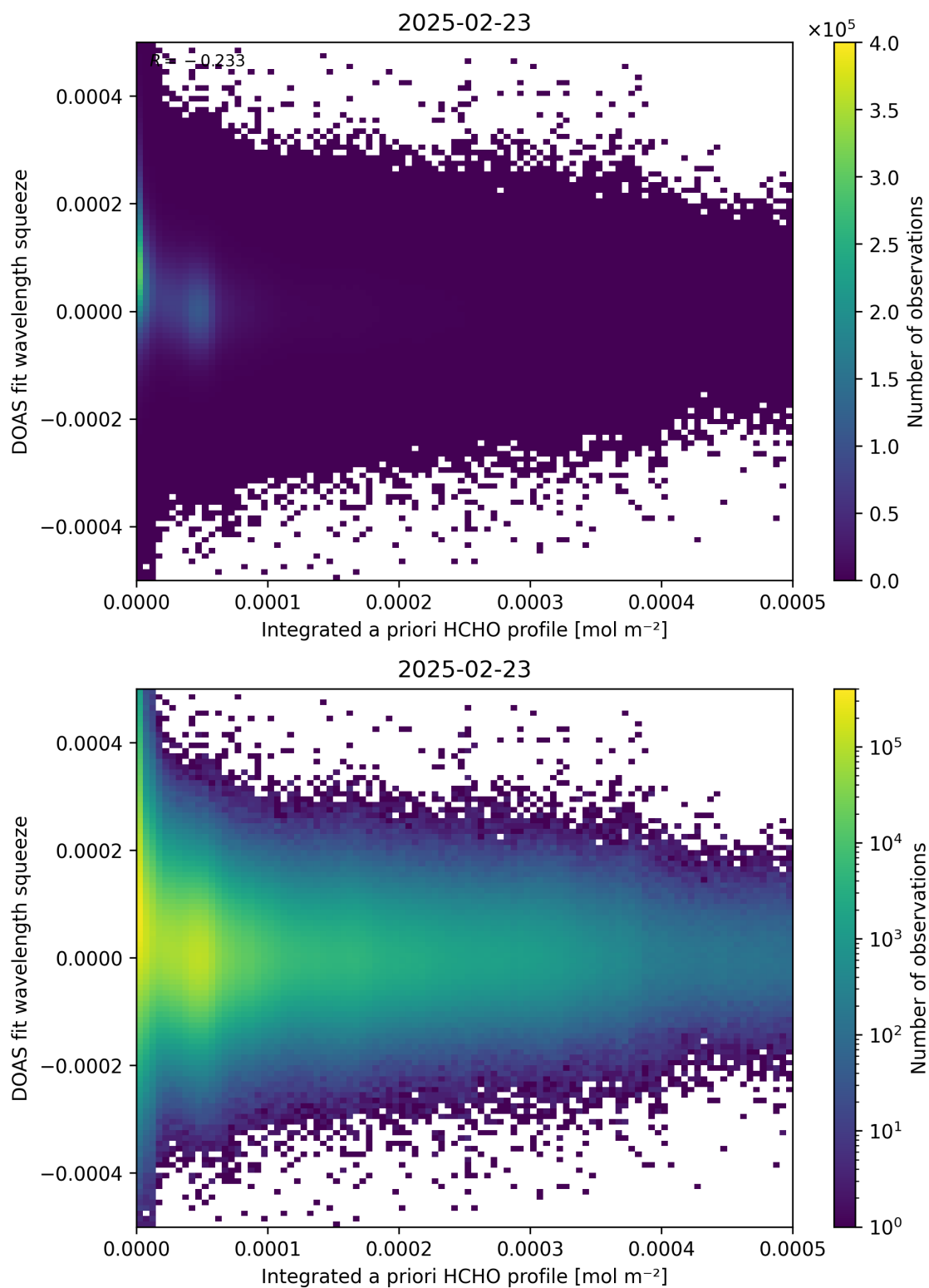
Figure 150: Scatter density plot of “Integrated a priori HCHO profile” against “DOAS fit wavelength squeeze” for 2025-02-22 to 2025-02-24.
