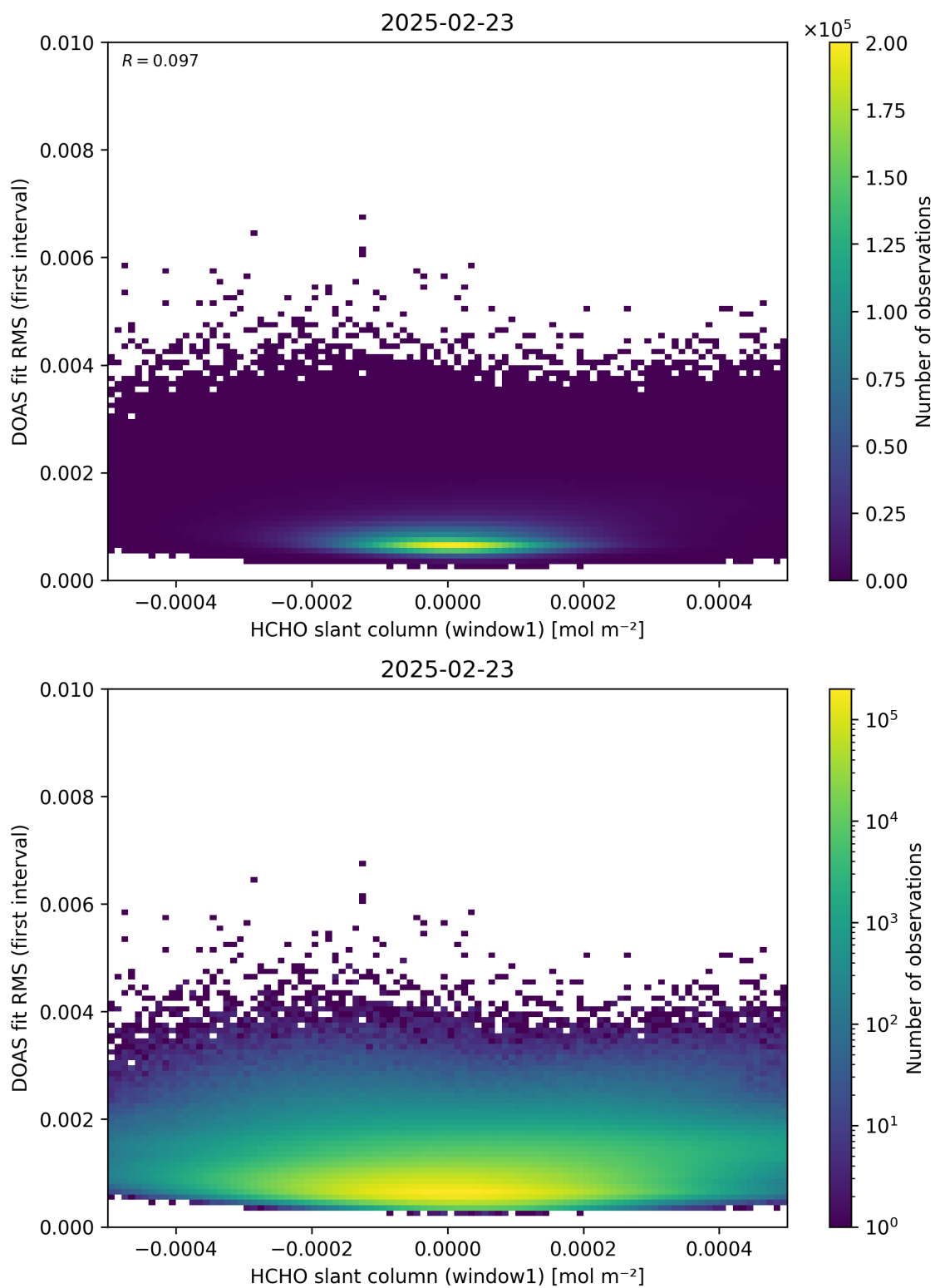
Figure 78: Scatter density plot of “HCHO slant column (window1)” against “DOAS fit RMS (first interval)” for 2025-02-22 to 2025-02-24.
