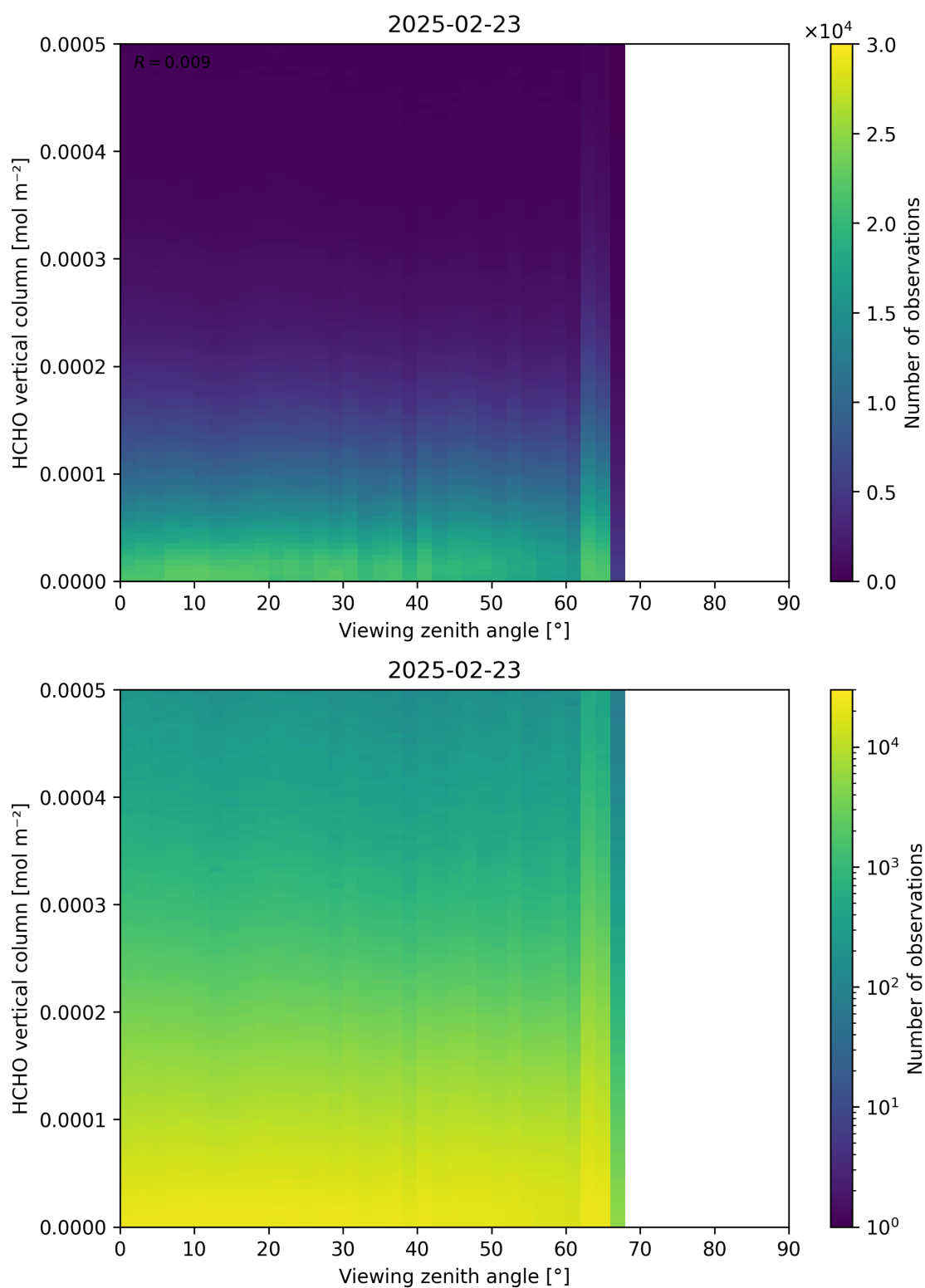
Figure 192: Scatter density plot of “Viewing zenith angle” against “HCHO vertical column” for 2025-02-22 to 2025-02-24.
