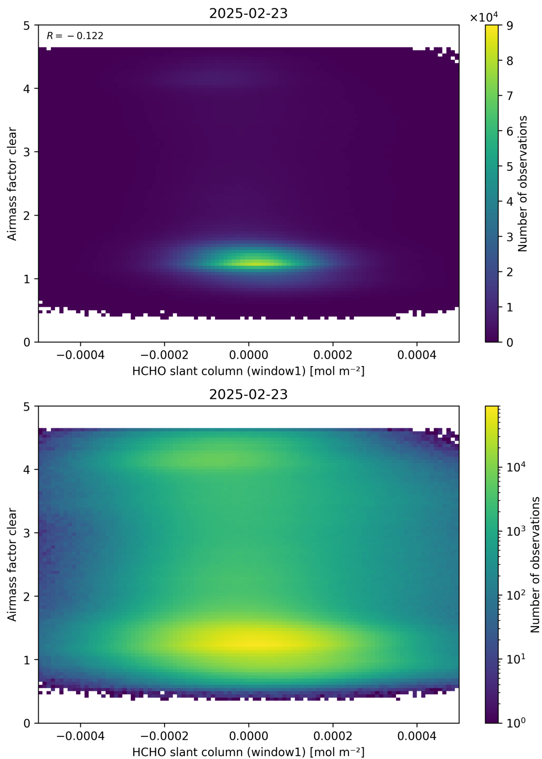
Figure 81: Scatter density plot of “HCHO slant column (window1)” against “Airmass factor clear” for 2025-02-22 to 2025-02-24.
