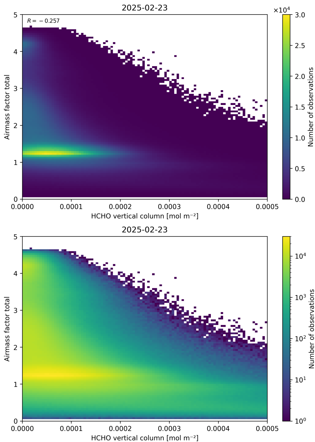
Figure 131: Scatter density plot of “HCHO vertical column” against “Airmass factor total” for 2025-02-22 to 2025-02-24.
