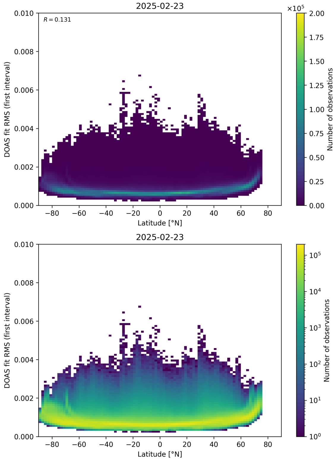
Figure 153: Scatter density plot of “Latitude” against “DOAS fit RMS (first interval)” for 2025-02-22 to 2025-02-24.
