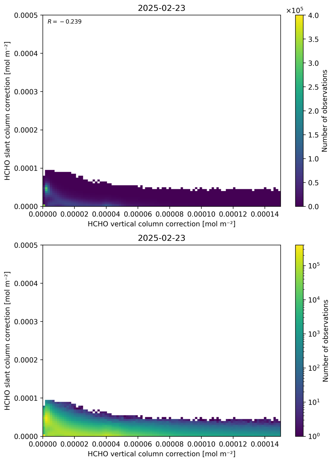
Figure 117: Scatter density plot of “HCHO vertical column correction” against “HCHO slant column correction” for 2025-02-22 to 2025-02-24.
