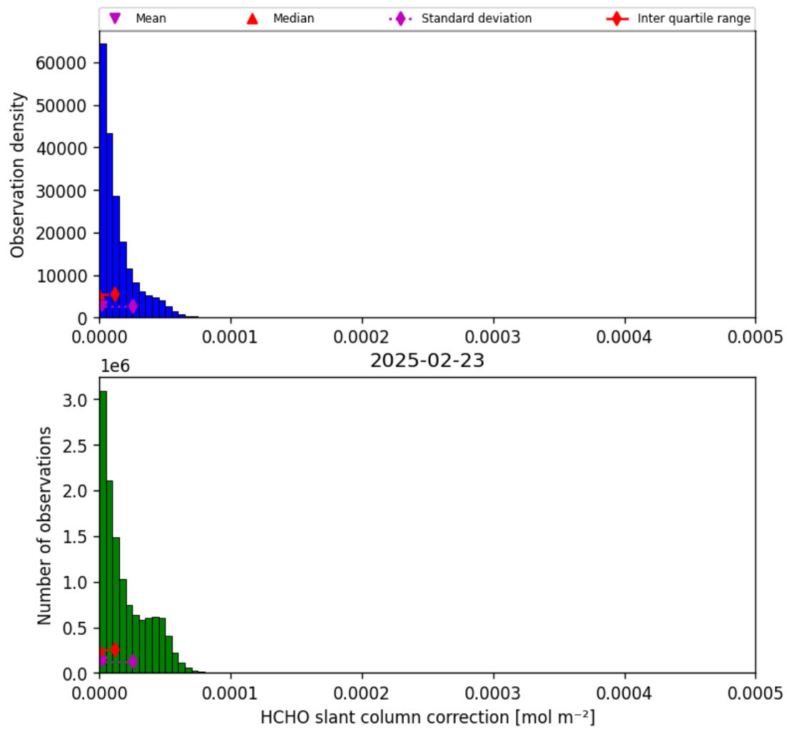
Figure 47: Histogram of “HCHO slant column correction” for 2025-02-22 to 2025-02-24
