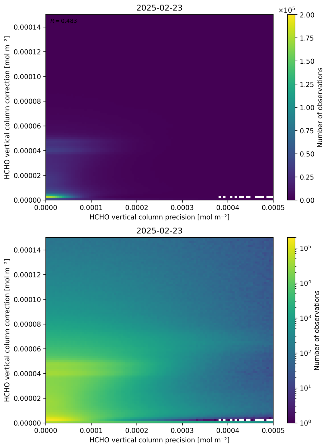
Figure 146: Scatter density plot of “HCHO vertical column precision” against “HCHO vertical column correction” for 2025-02-22 to 2025-02-24.
