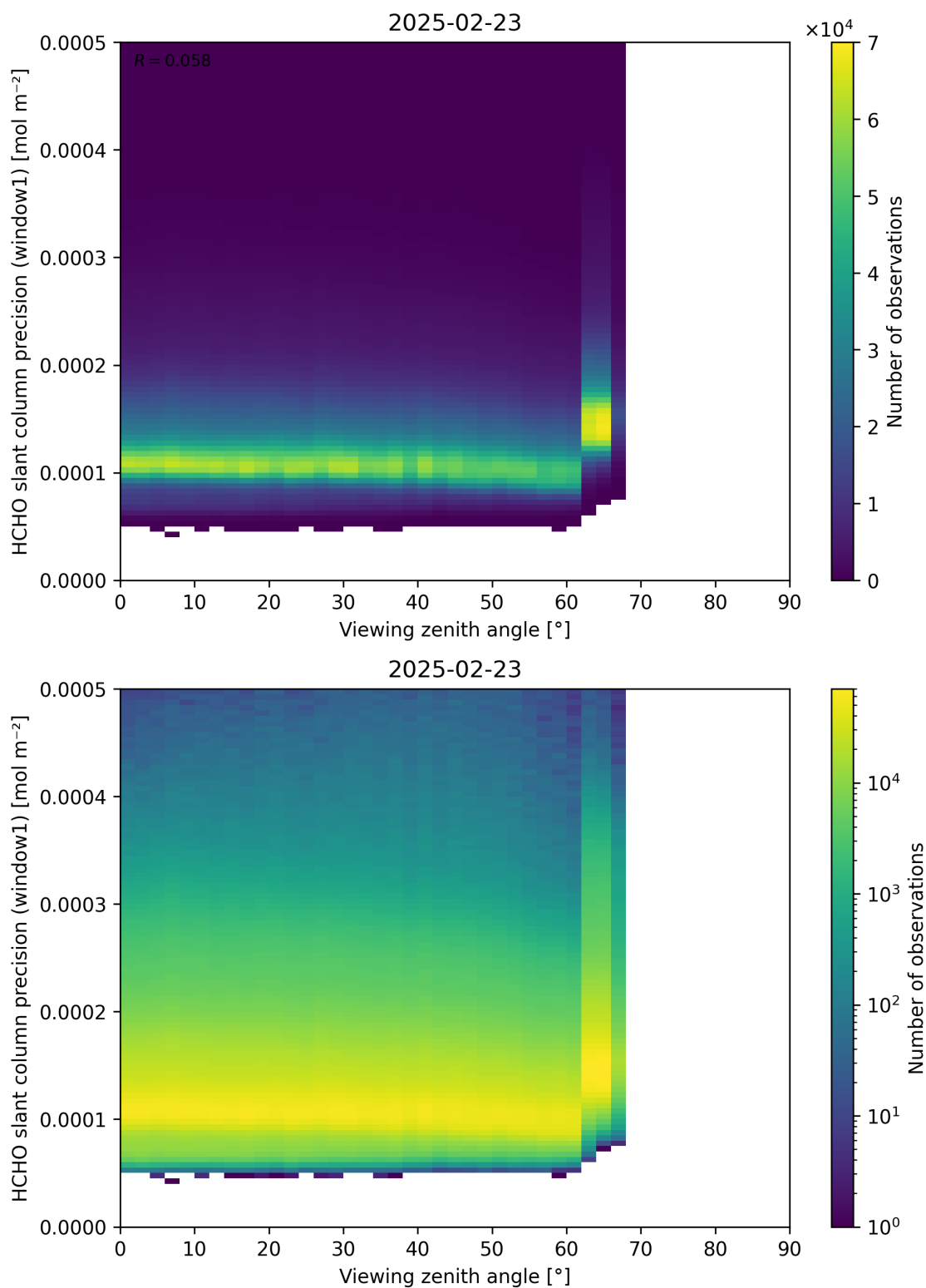
Figure 189: Scatter density plot of “Viewing zenith angle” against “HCHO slant column precision (window1)” for 2025-02-22 to 2025-02-24.
