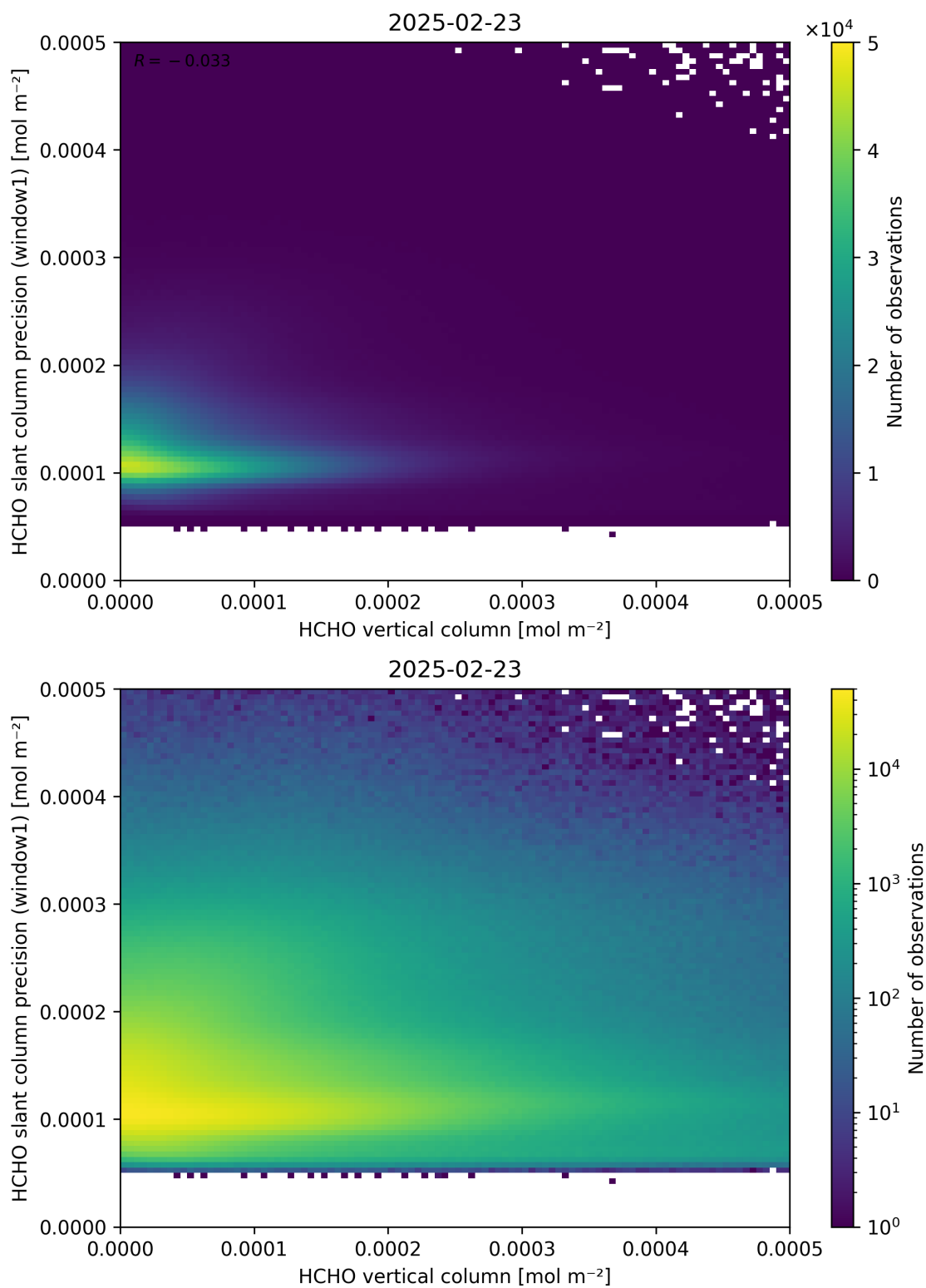
Figure 130: Scatter density plot of “HCHO vertical column” against “HCHO slant column precision (window1)” for 2025-02-22 to 2025-02-24.
