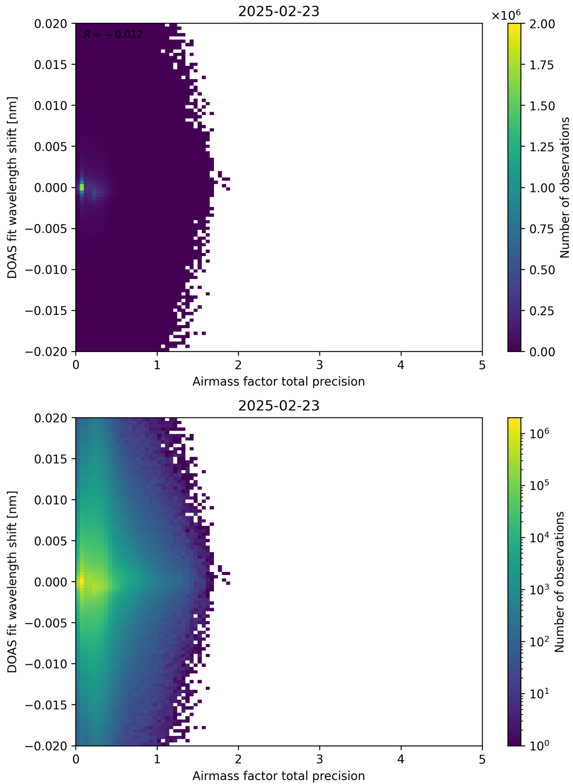
Figure 106: Scatter density plot of “Airmass factor total precision” against “DOAS fit wavelength shift” for 2025-02-22 to 2025-02-24.
