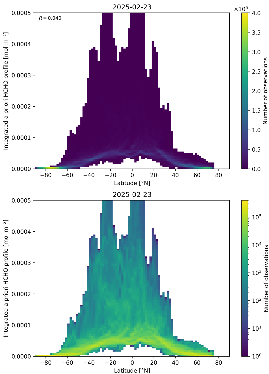
Figure 166: Scatter density plot of “Latitude” against “Integrated a priori HCHO profile” for 2025-02-22 to 2025-02-24.
