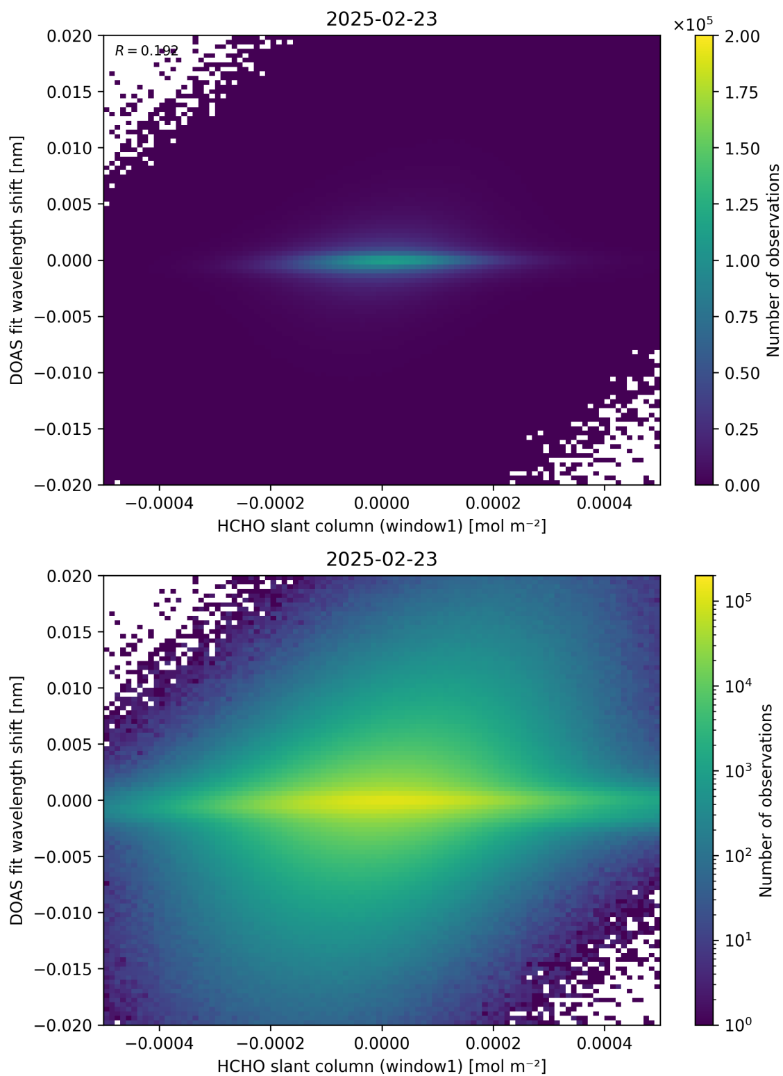
Figure 79: Scatter density plot of “HCHO slant column (window1)” against “DOAS fit wavelength shift” for 2025-02-22 to 2025-02-24.
