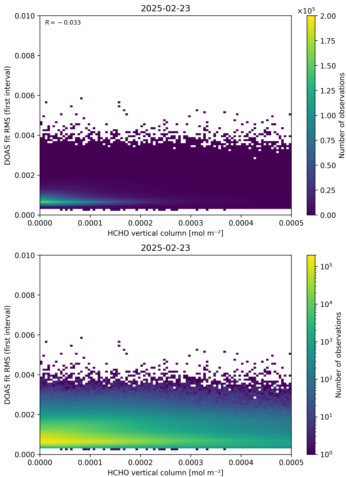
Figure 123: Scatter density plot of “HCHO vertical column” against “DOAS fit RMS (first interval)” for 2025-02-22 to 2025-02-24.
