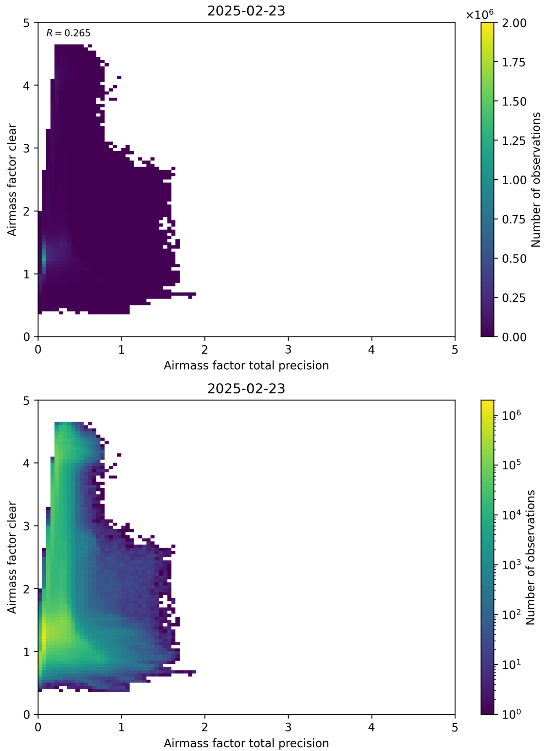
Figure 108: Scatter density plot of “Airmass factor total precision” against “Airmass factor clear” for 2025-02-22 to 2025-02-24.
