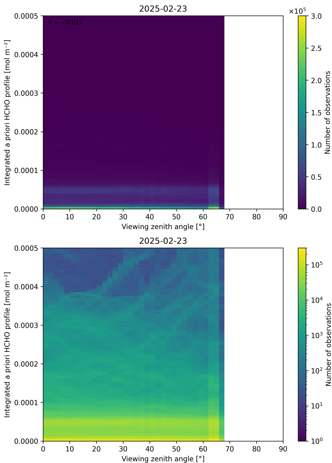
Figure 195: Scatter density plot of “Viewing zenith angle” against “Integrated a priori HCHO profile” for 2025-02-22 to 2025-02-24.
