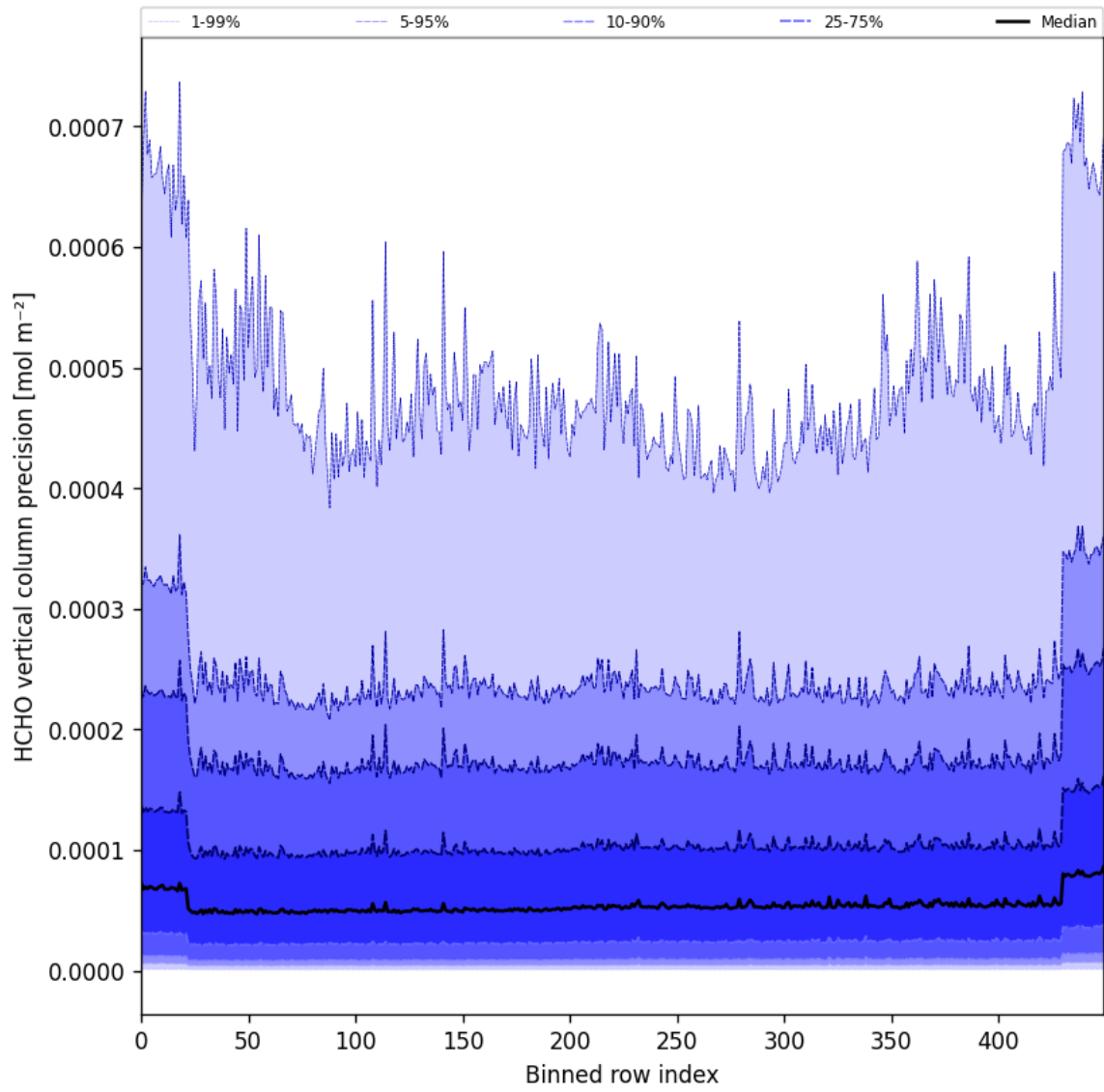
Figure 50: Along track statistics of "HCHO vertical column precision" for 2025-02-22 to 2025-02-24
