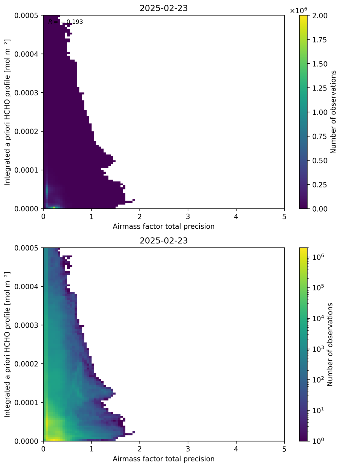
Figure 111: Scatter density plot of “Airmass factor total precision” against “Integrated a priori HCHO profile” for 2025-02-22 to 2025-02-24.
