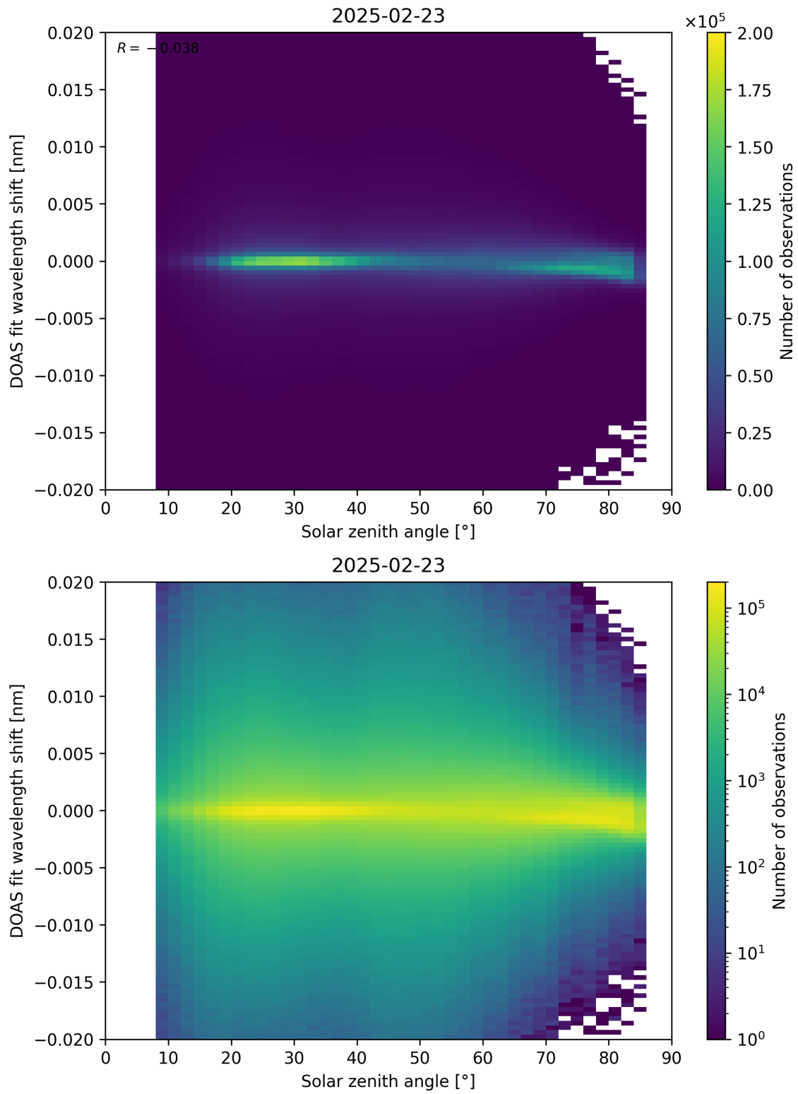
Figure 168: Scatter density plot of “Solar zenith angle” against “DOAS fit wavelength shift” for 2025-02-22 to 2025-02-24.
