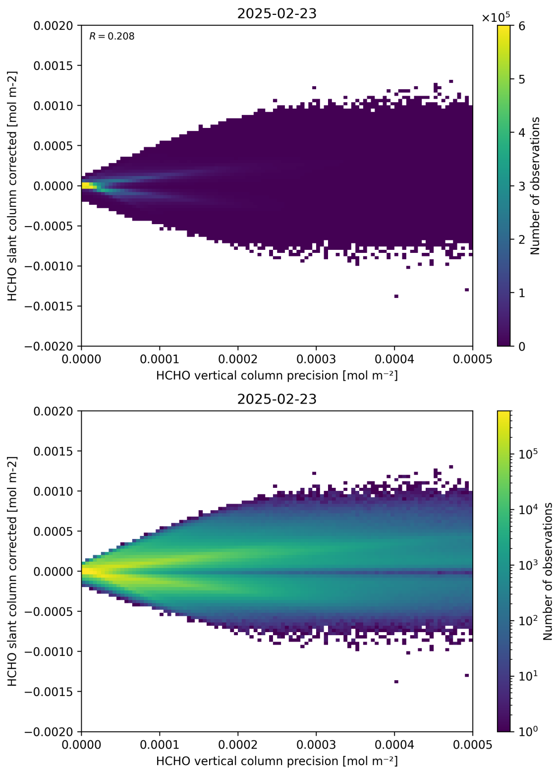
Figure 140: Scatter density plot of “HCHO vertical column precision” against “HCHO slant column corrected” for 2025-02-22 to 2025-02-24.
