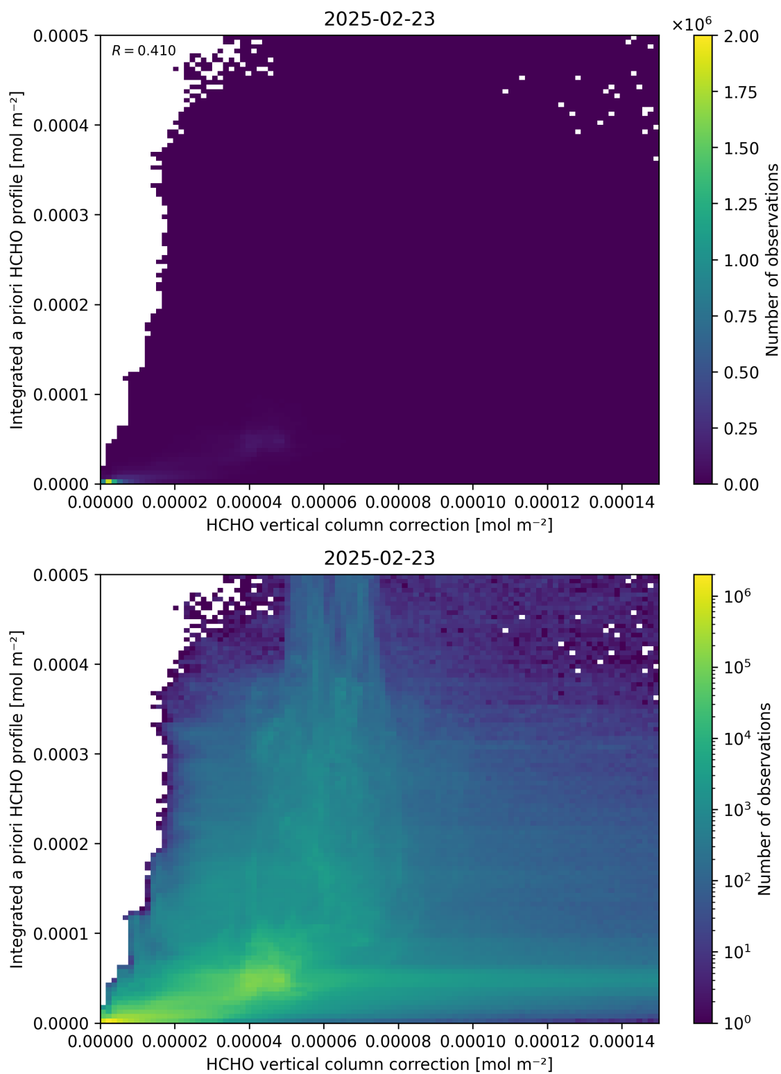
Figure 122: Scatter density plot of “HCHO vertical column correction” against “Integrated a priori HCHO profile” for 2025-02-22 to 2025-02-24.
