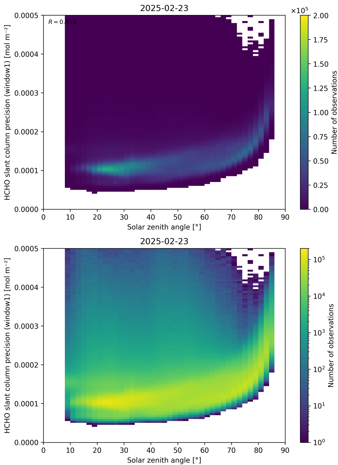
Figure 174: Scatter density plot of “Solar zenith angle” against “HCHO slant column precision (window1)” for 2025-02-22 to 2025-02-24.
