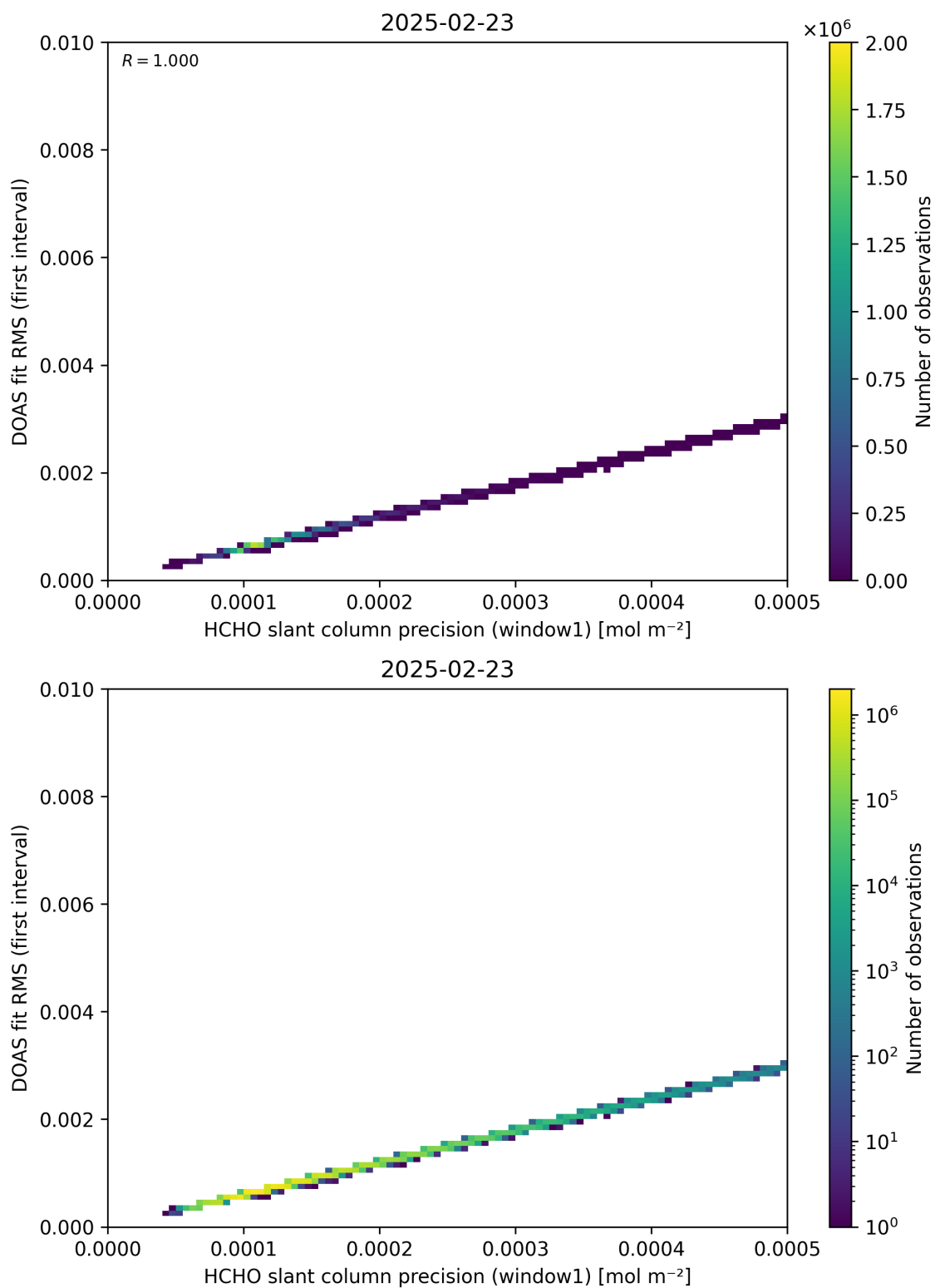
Figure 88: Scatter density plot of “HCHO slant column precision (window1)” against “DOAS fit RMS (first interval)” for 2025-02-22 to 2025-02-24.
