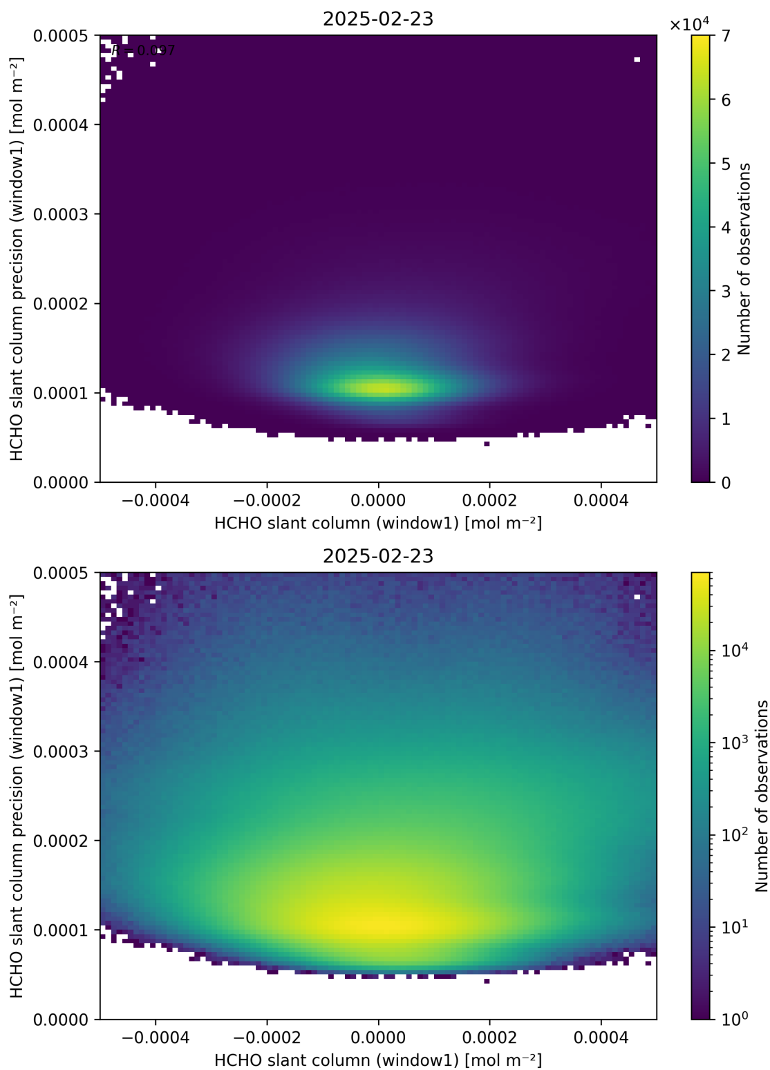
Figure 84: Scatter density plot of “HCHO slant column (window1)” against “HCHO slant column precision (window1)” for 2025-02-22 to 2025-02-24.
