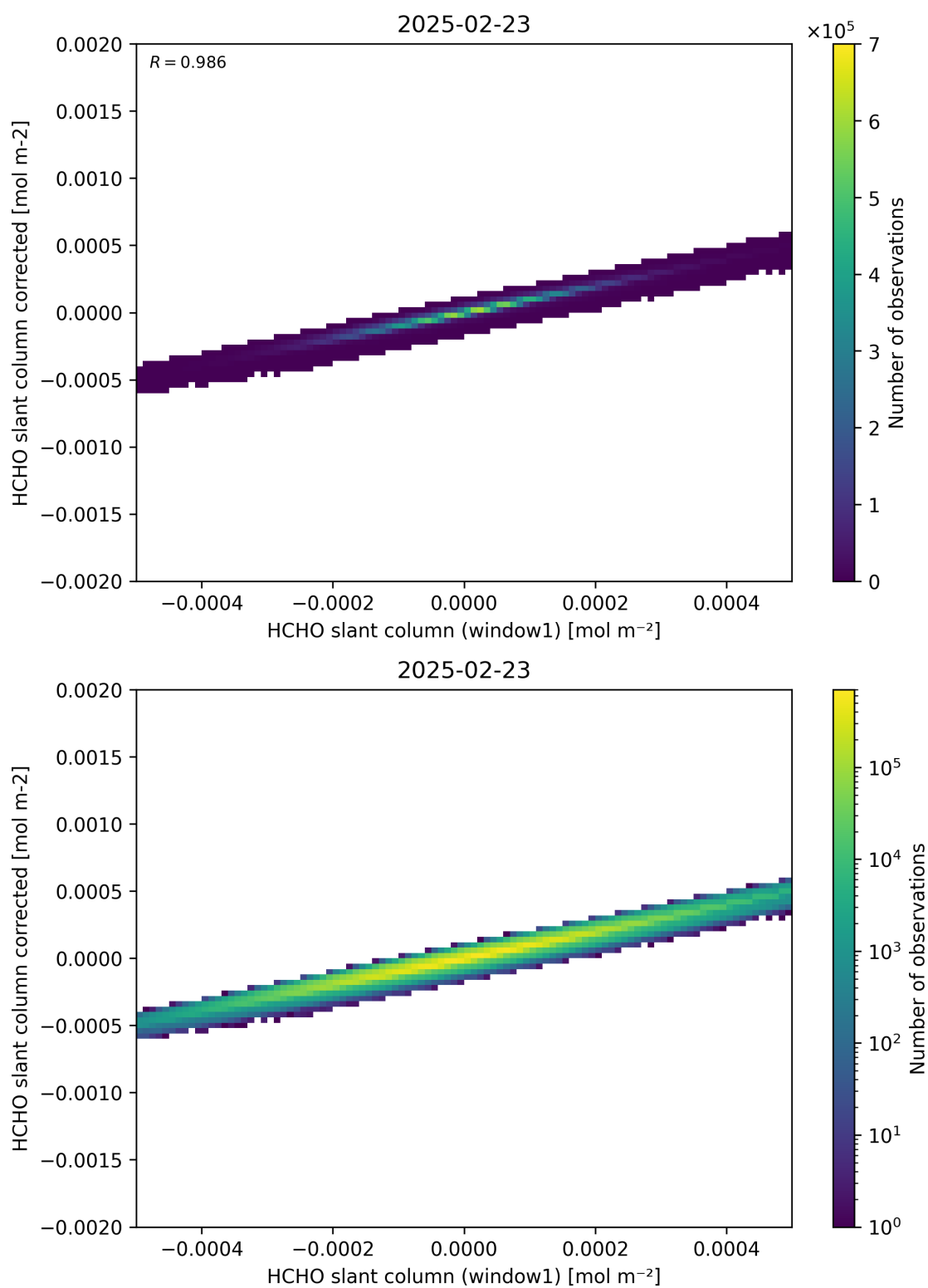
Figure 82: Scatter density plot of “HCHO slant column (window1)” against “HCHO slant column corrected” for 2025-02-22 to 2025-02-24.
