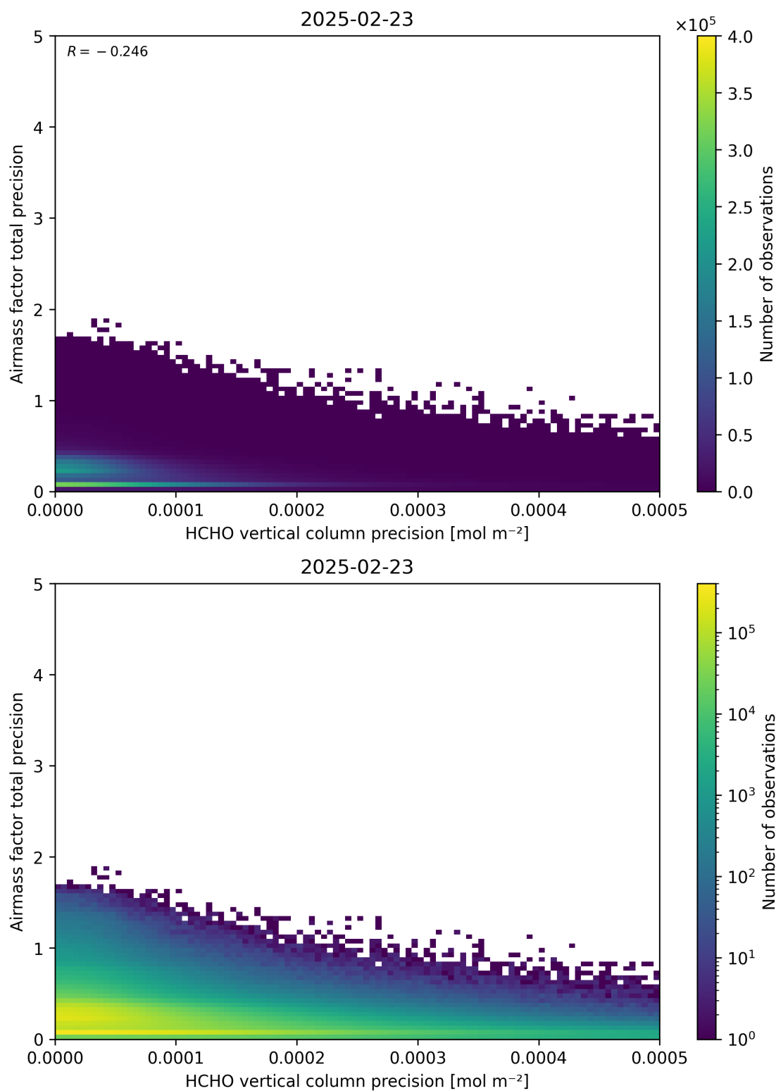
Figure 145: Scatter density plot of “HCHO vertical column precision” against “Airmass factor total precision” for 2025-02-22 to 2025-02-24.
