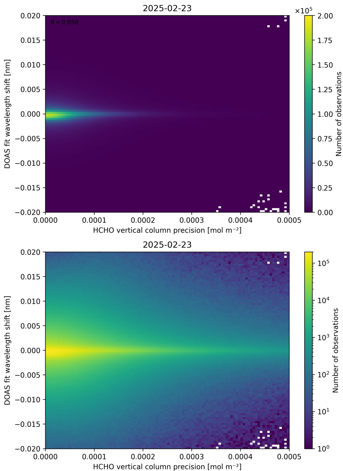
Figure 137: Scatter density plot of “HCHO vertical column precision” against “DOAS fit wavelength shift” for 2025-02-22 to 2025-02-24.
