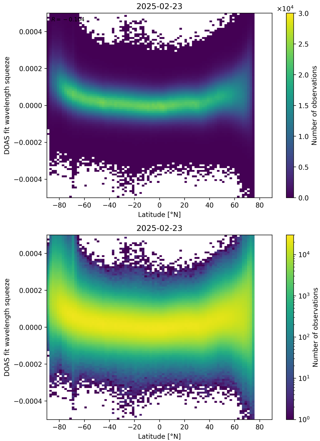
Figure 155: Scatter density plot of “Latitude” against “DOAS fit wavelength squeeze” for 2025-02-22 to 2025-02-24.
