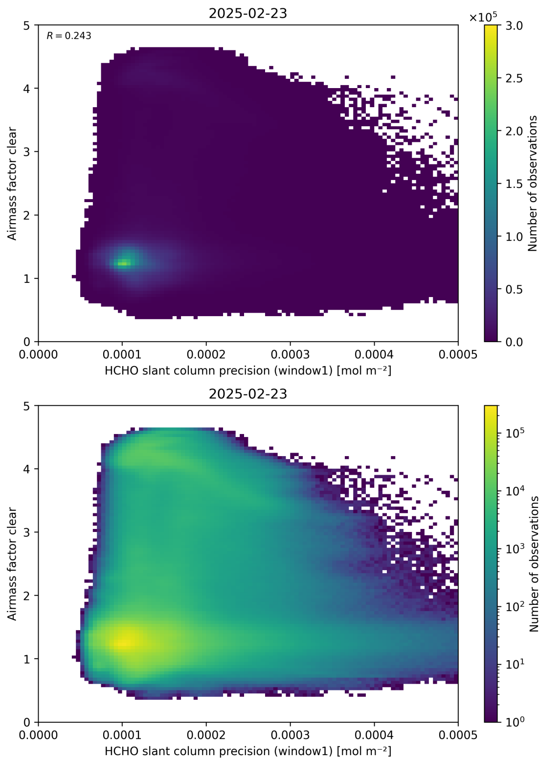
Figure 91: Scatter density plot of “HCHO slant column precision (window1)” against “Airmass factor clear” for 2025-02-22 to 2025-02-24.
