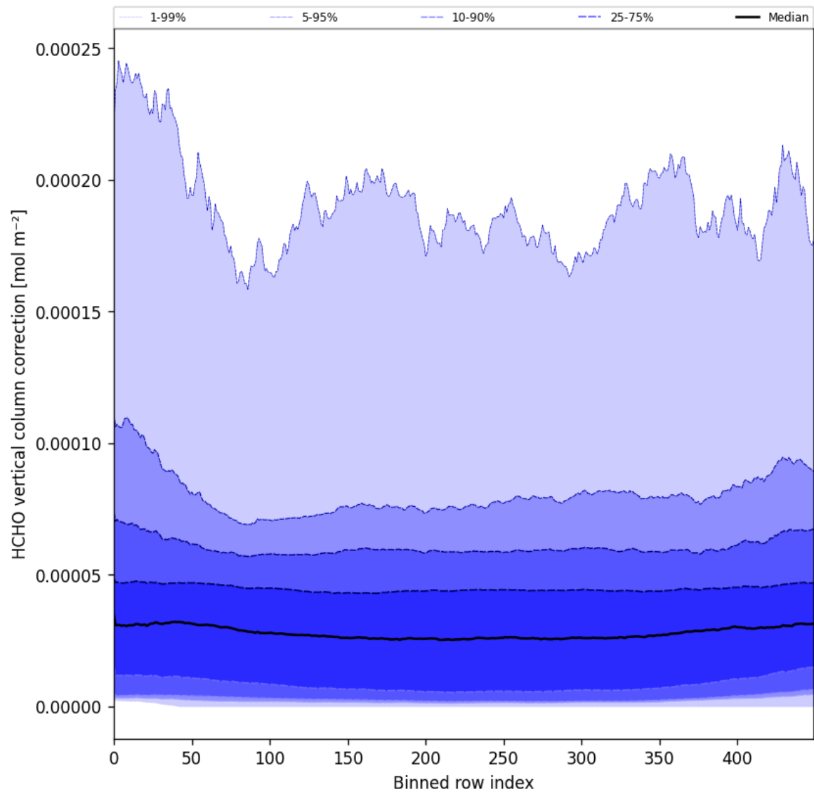
Figure 51: Along track statistics of “HCHO vertical column correction” for 2025-02-22 to 2025-02-24
