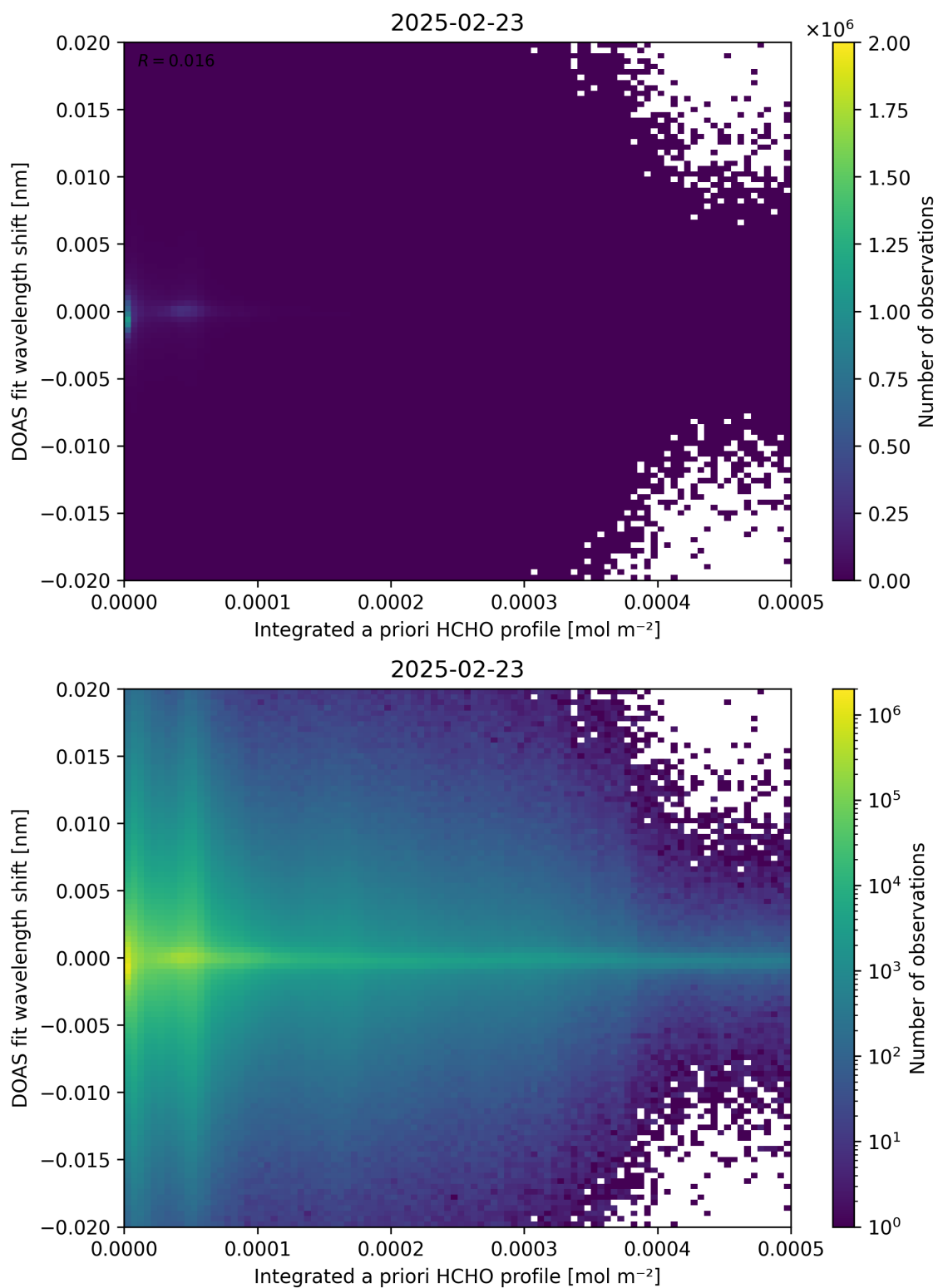
Figure 149: Scatter density plot of “Integrated a priori HCHO profile” against “DOAS fit wavelength shift” for 2025-02-22 to 2025-02-24.
