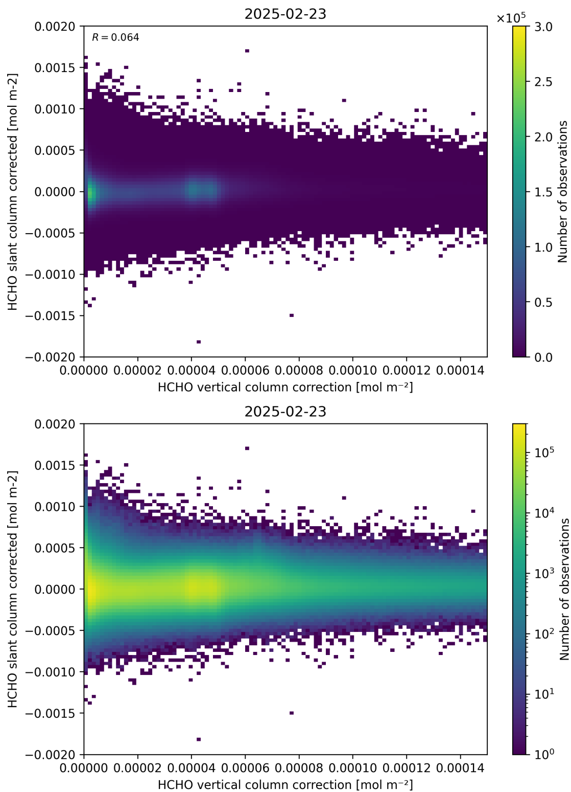
Figure 116: Scatter density plot of “HCHO vertical column correction” against “HCHO slant column corrected” for 2025-02-22 to 2025-02-24.
