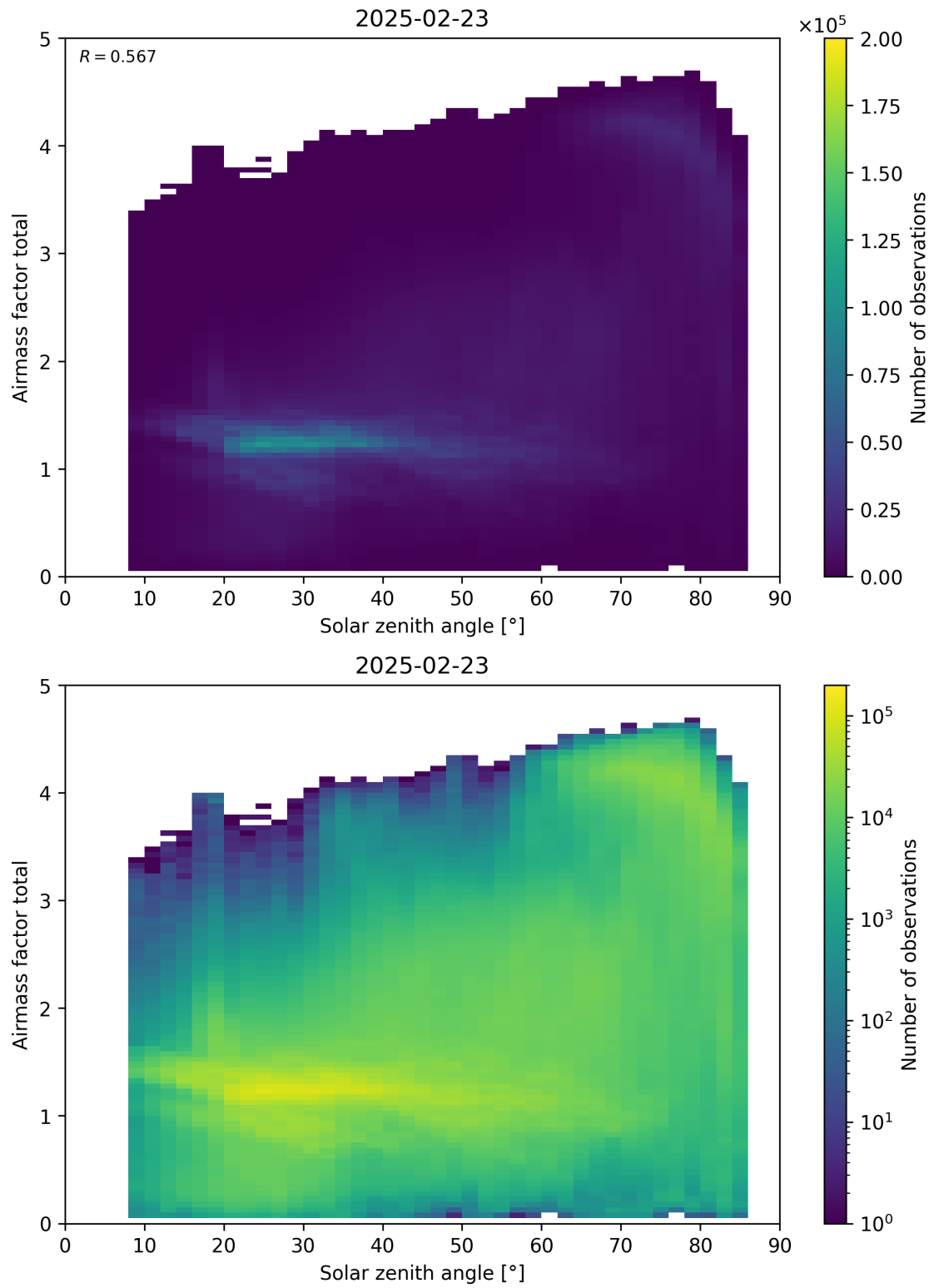
Figure 175: Scatter density plot of “Solar zenith angle” against “Airmass factor total” for 2025-02-22 to 2025-02-24.
