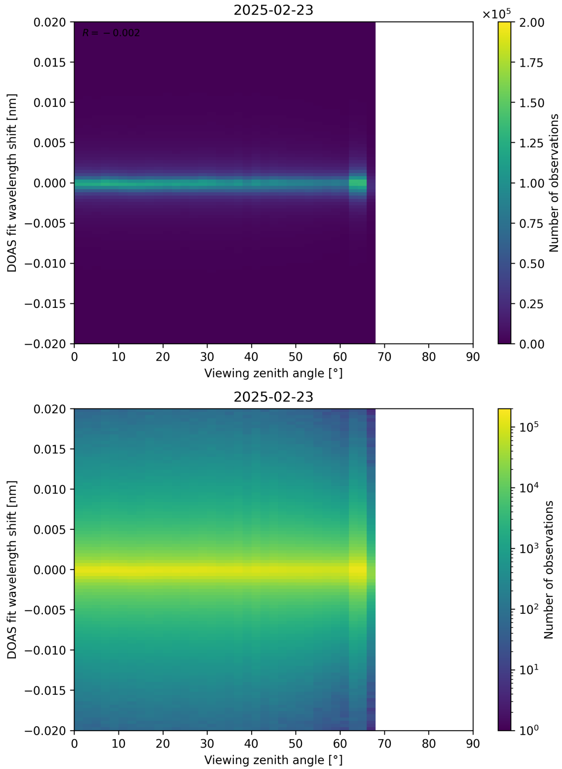
Figure 183: Scatter density plot of “Viewing zenith angle” against “DOAS fit wavelength shift” for 2025-02-22 to 2025-02-24.
