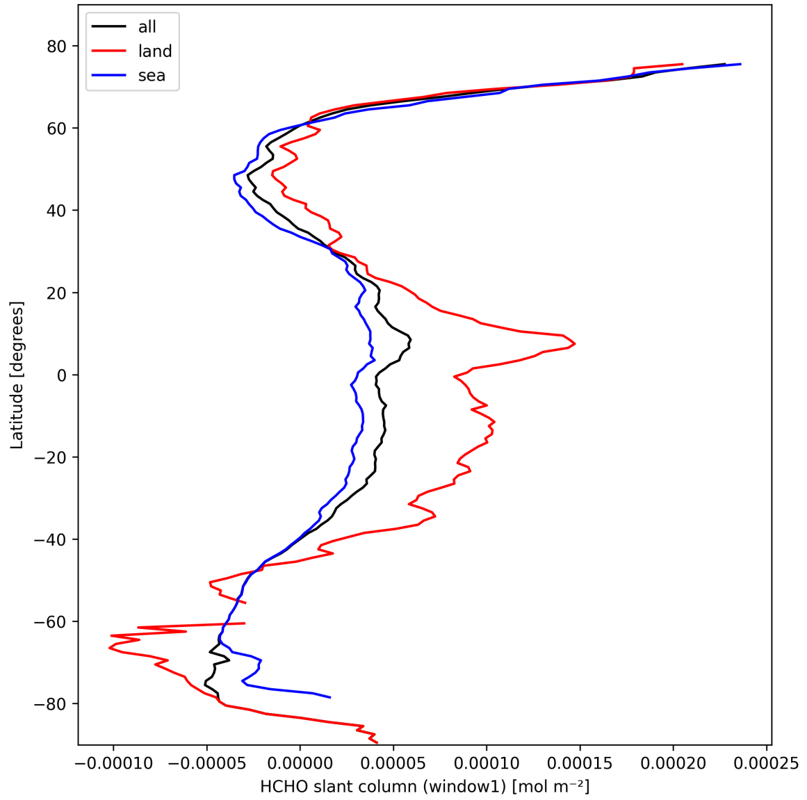
Figure 24: Zonal average of “HCHO slant column (window1)” for 2025-02-22 to 2025-02-24.
