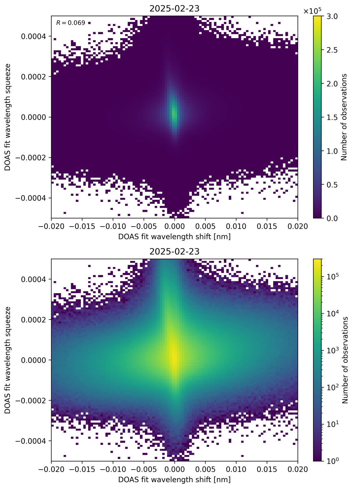
Figure 65: Scatter density plot of “DOAS fit wavelength shift” against “DOAS fit wavelength squeeze” for 2025-02-22 to 2025-02-24.
