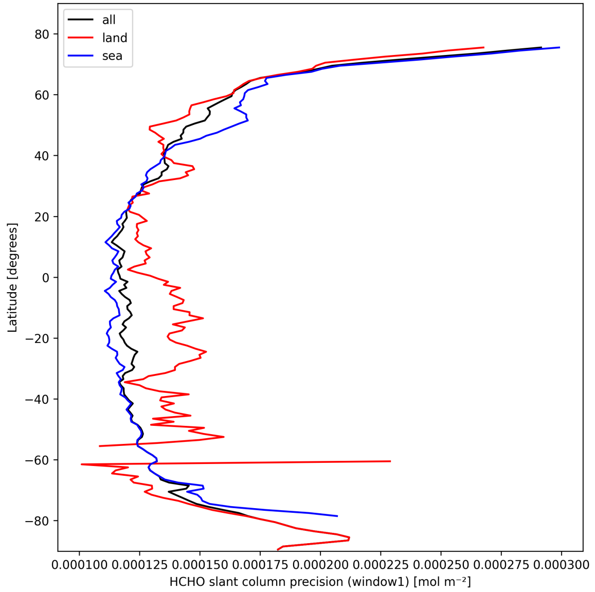
Figure 25: Zonal average of “HCHO slant column precision (window1)” for 2025-02-24 to 2025-02-25.
