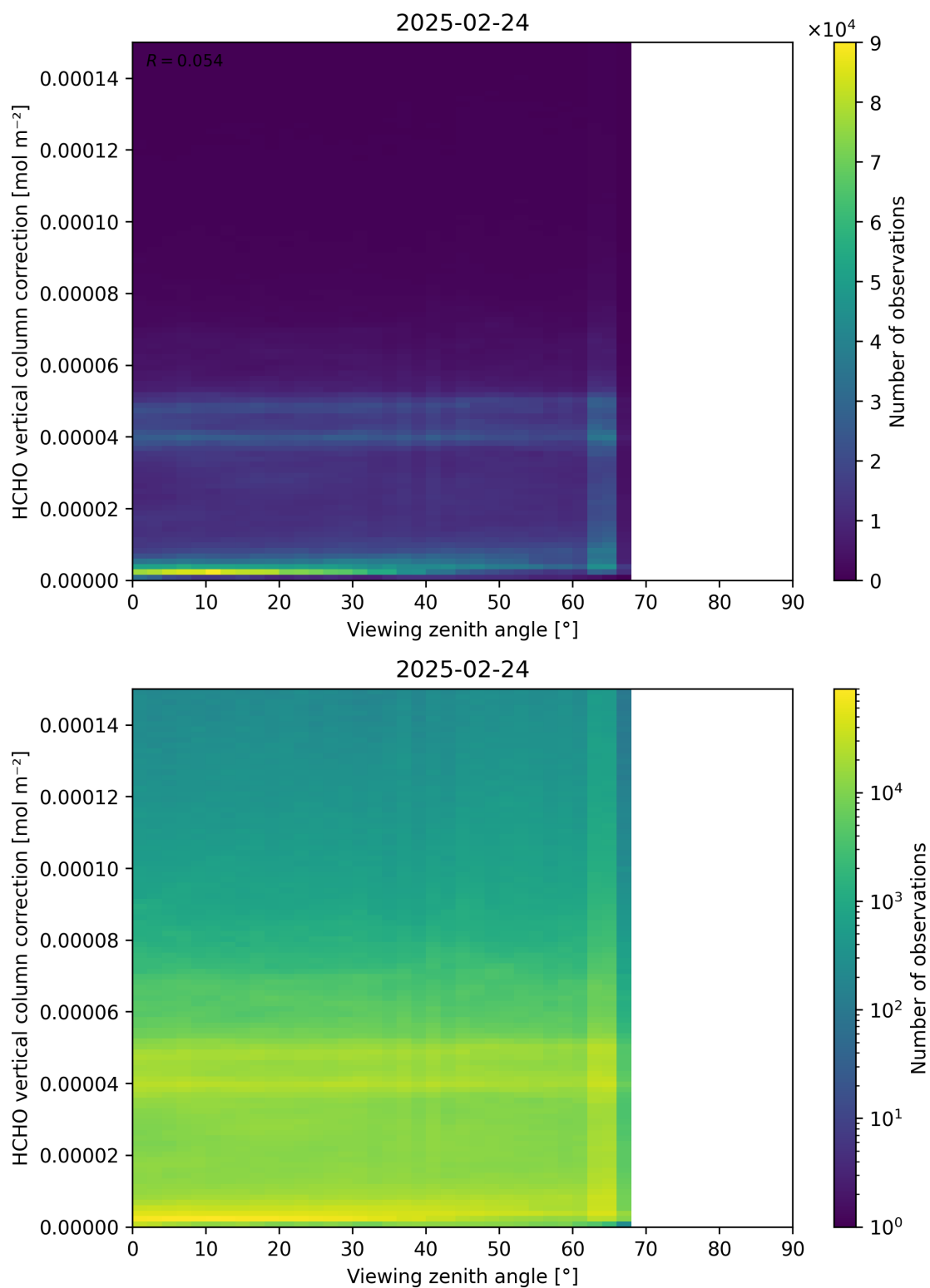
Figure 193: Scatter density plot of “Viewing zenith angle” against “HCHO vertical column correction” for 2025-02-24 to 2025-02-25.
