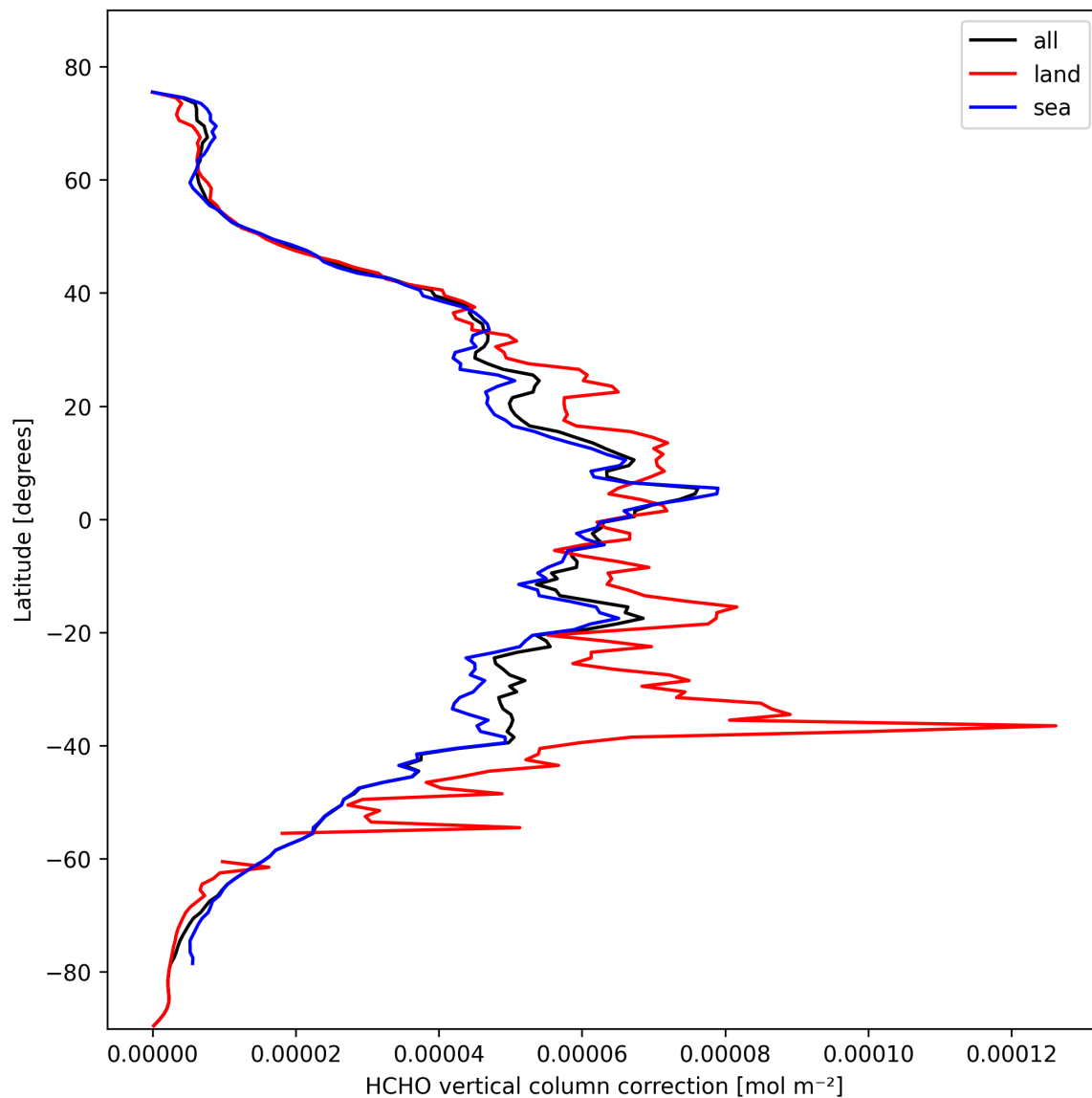
Figure 23: Zonal average of “HCHO vertical column correction” for 2025-02-24 to 2025-02-25.
