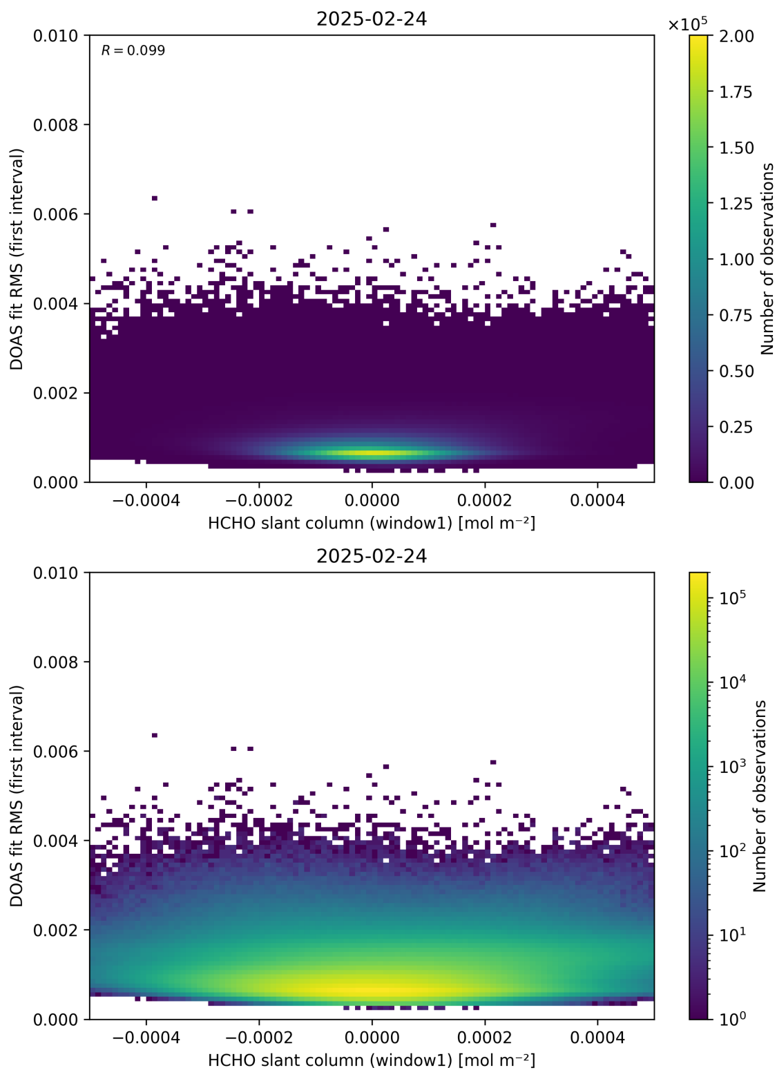
Figure 78: Scatter density plot of “HCHO slant column (window1)” against “DOAS fit RMS (first interval)” for 2025-02-24 to 2025-02-25.
