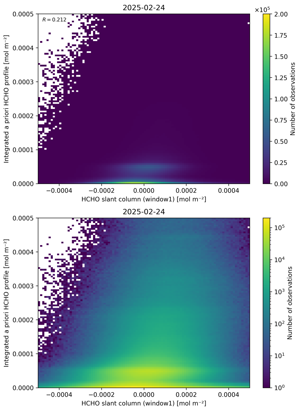
Figure 87: Scatter density plot of “HCHO slant column (window1)” against “Integrated a priori HCHO profile” for 2025-02-24 to 2025-02-25.
