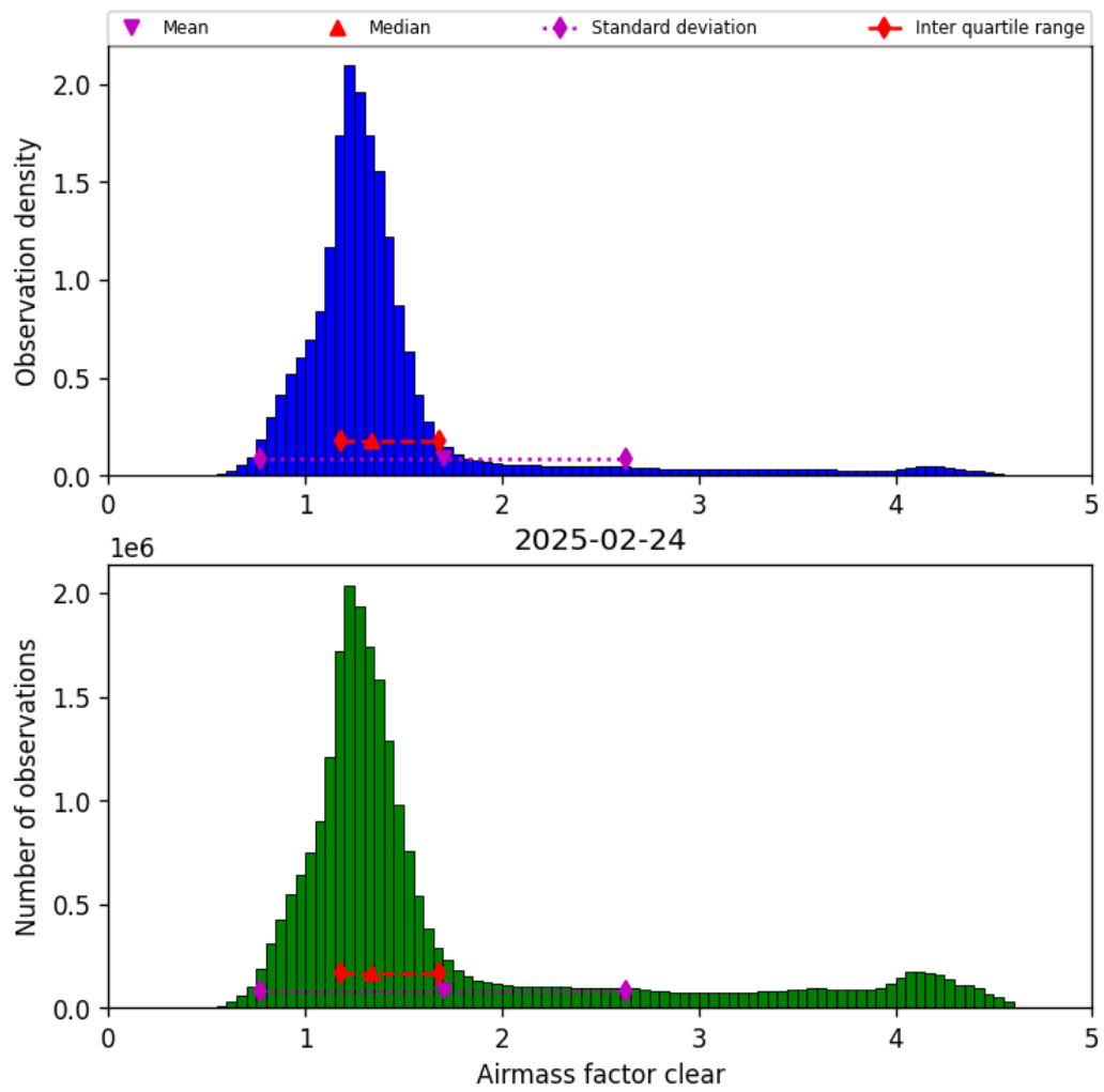
Figure 42: Histogram of “Airmass factor clear” for 2025-02-24 to 2025-02-25
