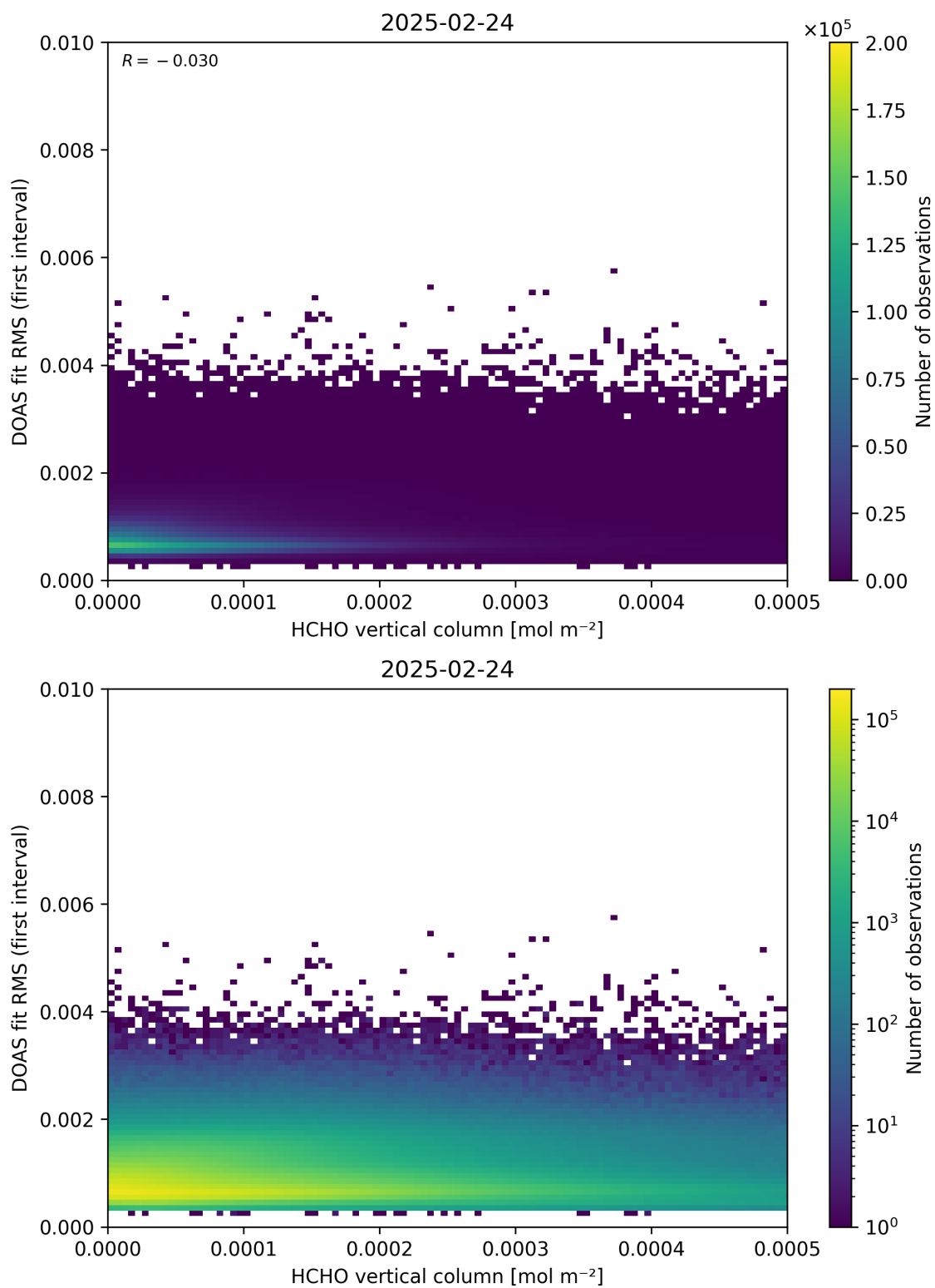
Figure 123: Scatter density plot of “HCHO vertical column” against “DOAS fit RMS (first interval)” for 2025-02-24 to 2025-02-25.
