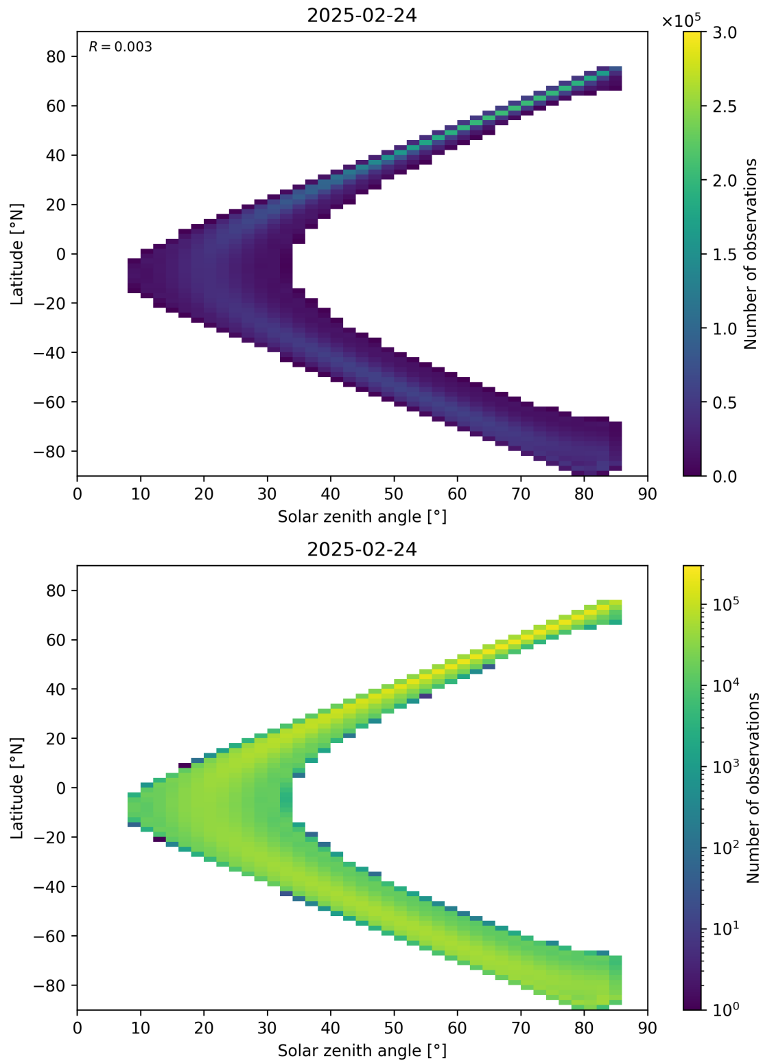
Figure 181: Scatter density plot of “Solar zenith angle” against “Latitude” for 2025-02-24 to 2025-02-25.
