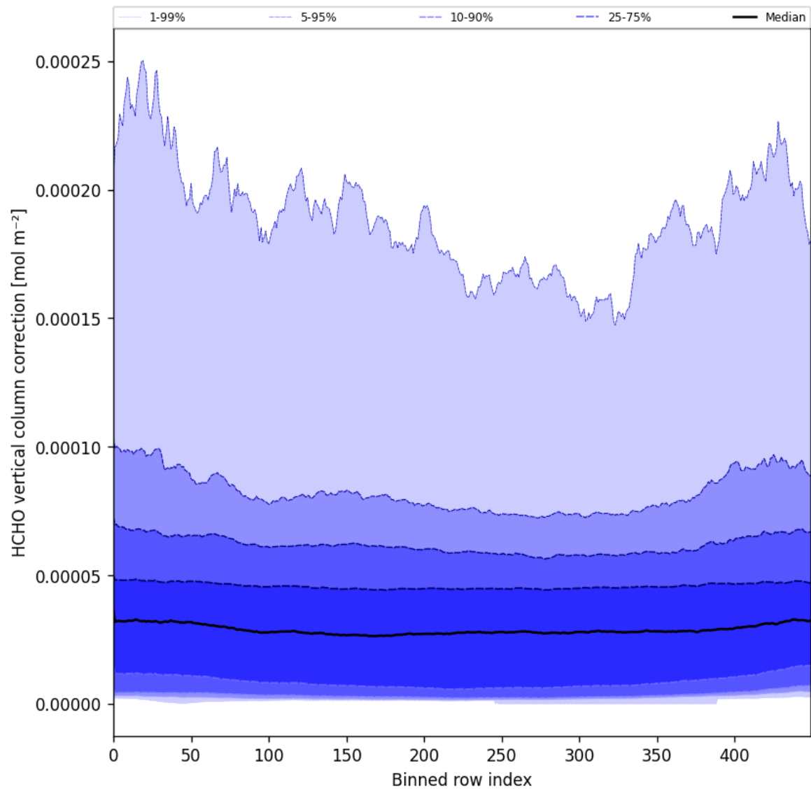
Figure 51: Along track statistics of “HCHO vertical column correction” for 2025-02-24 to 2025-02-25
