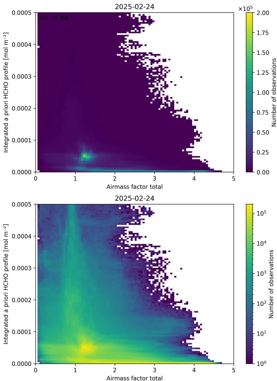
Figure 104: Scatter density plot of “Airmass factor total” against “Integrated a priori HCHO profile” for 2025-02-24 to 2025-02-25.
