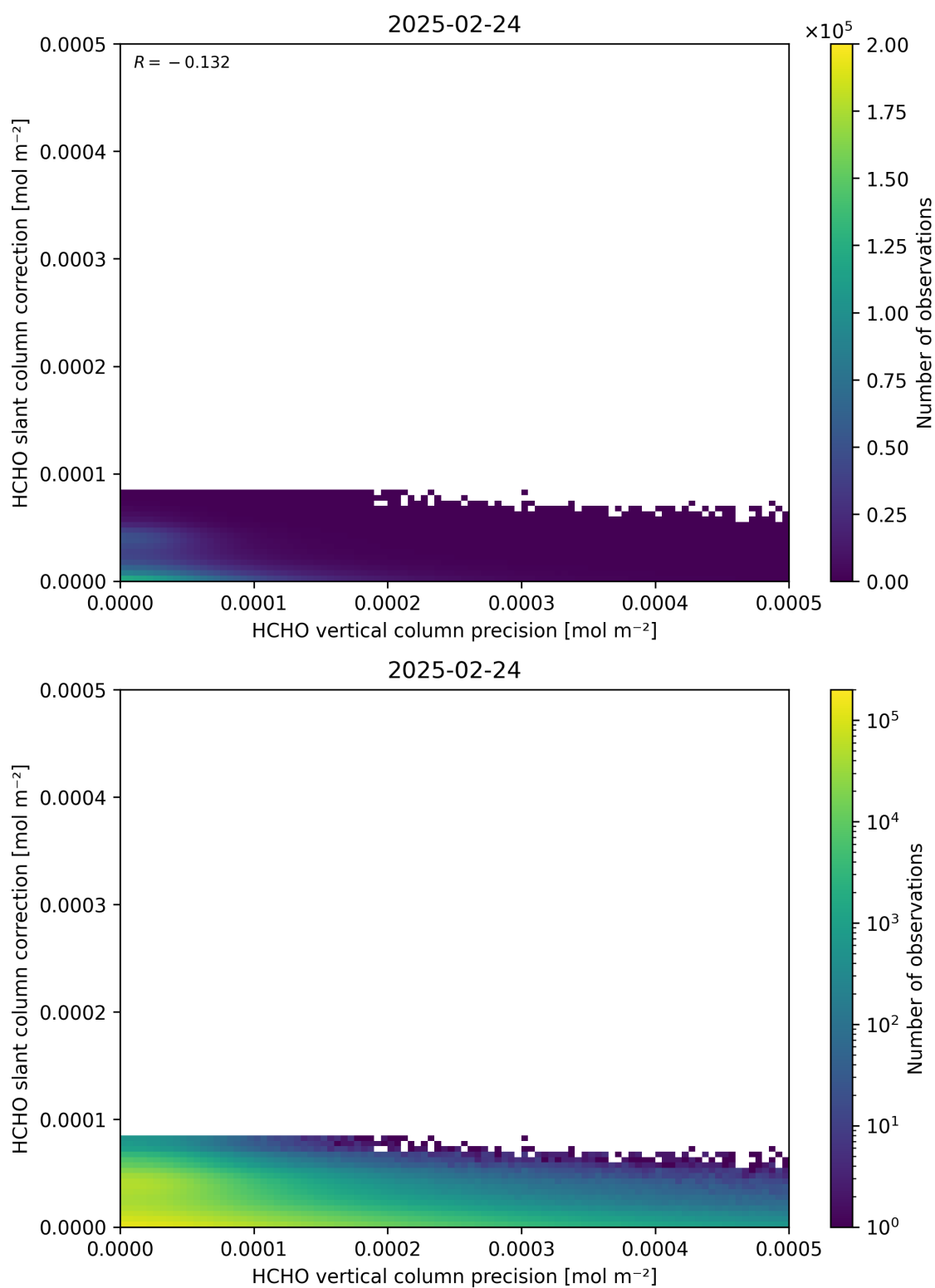
Figure 141: Scatter density plot of “HCHO vertical column precision” against “HCHO slant column correction” for 2025-02-24 to 2025-02-25.
