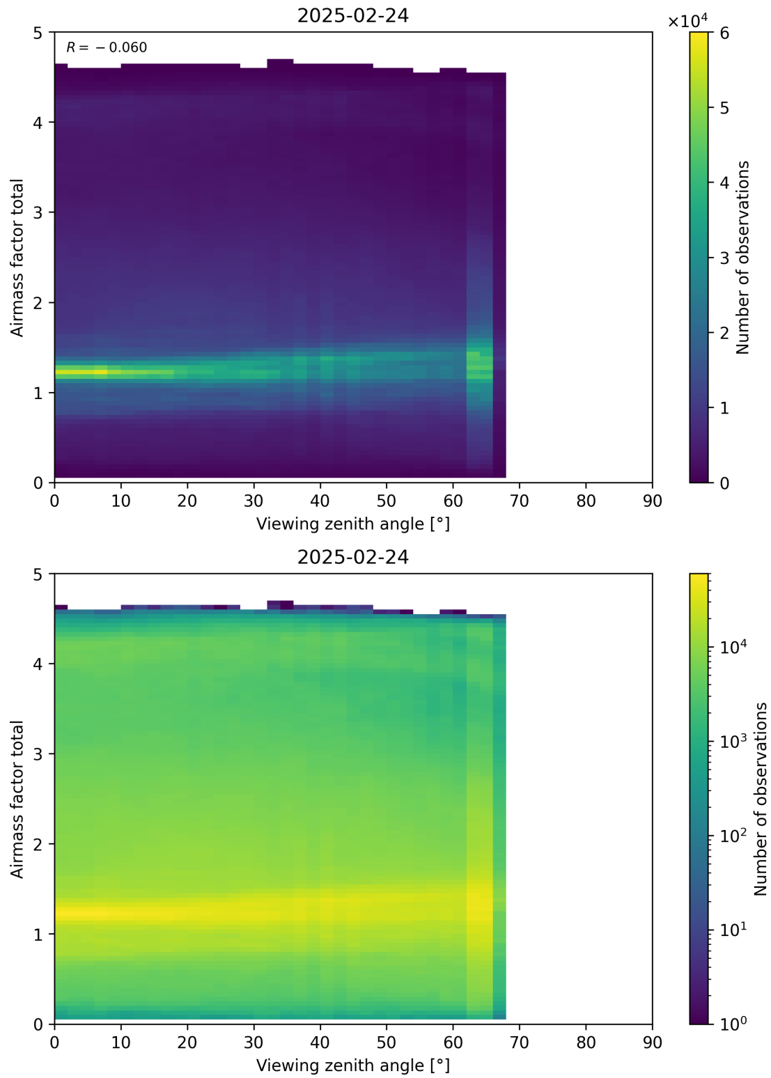
Figure 190: Scatter density plot of “Viewing zenith angle” against “Airmass factor total” for 2025-02-24 to 2025-02-25.
