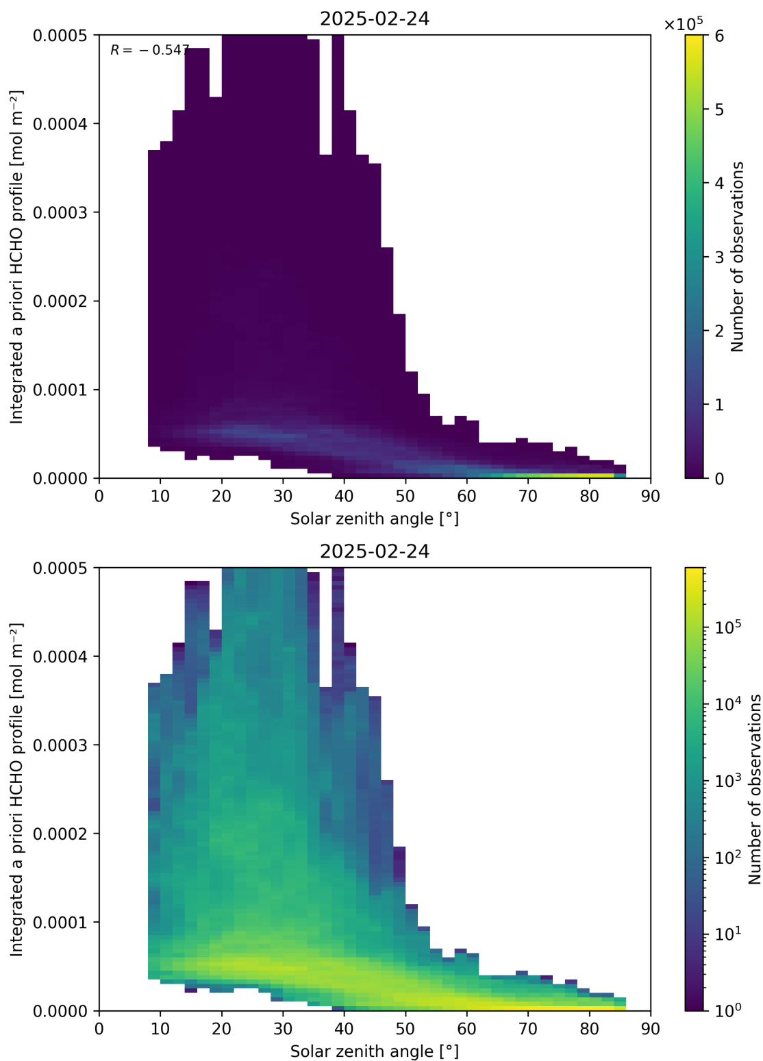
Figure 180: Scatter density plot of “Solar zenith angle” against “Integrated a priori HCHO profile” for 2025-02-24 to 2025-02-25.
