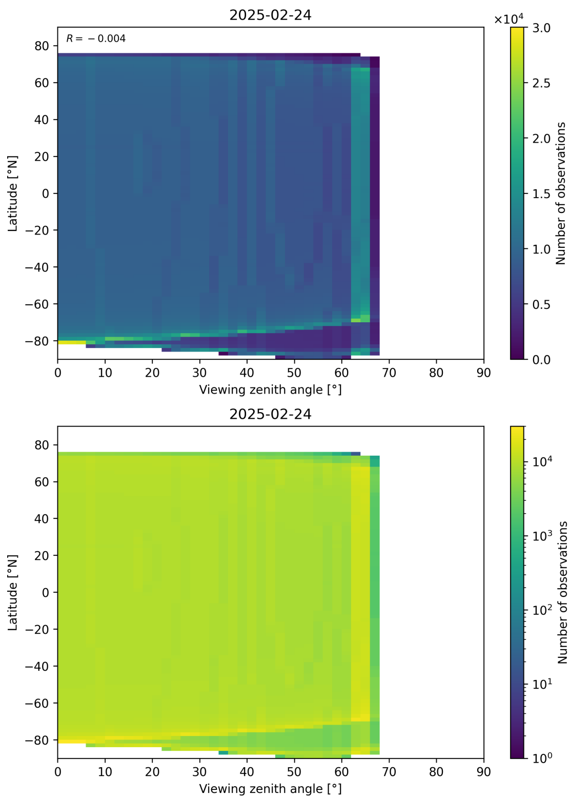
Figure 196: Scatter density plot of “Viewing zenith angle” against “Latitude” for 2025-02-24 to 2025-02-25.
