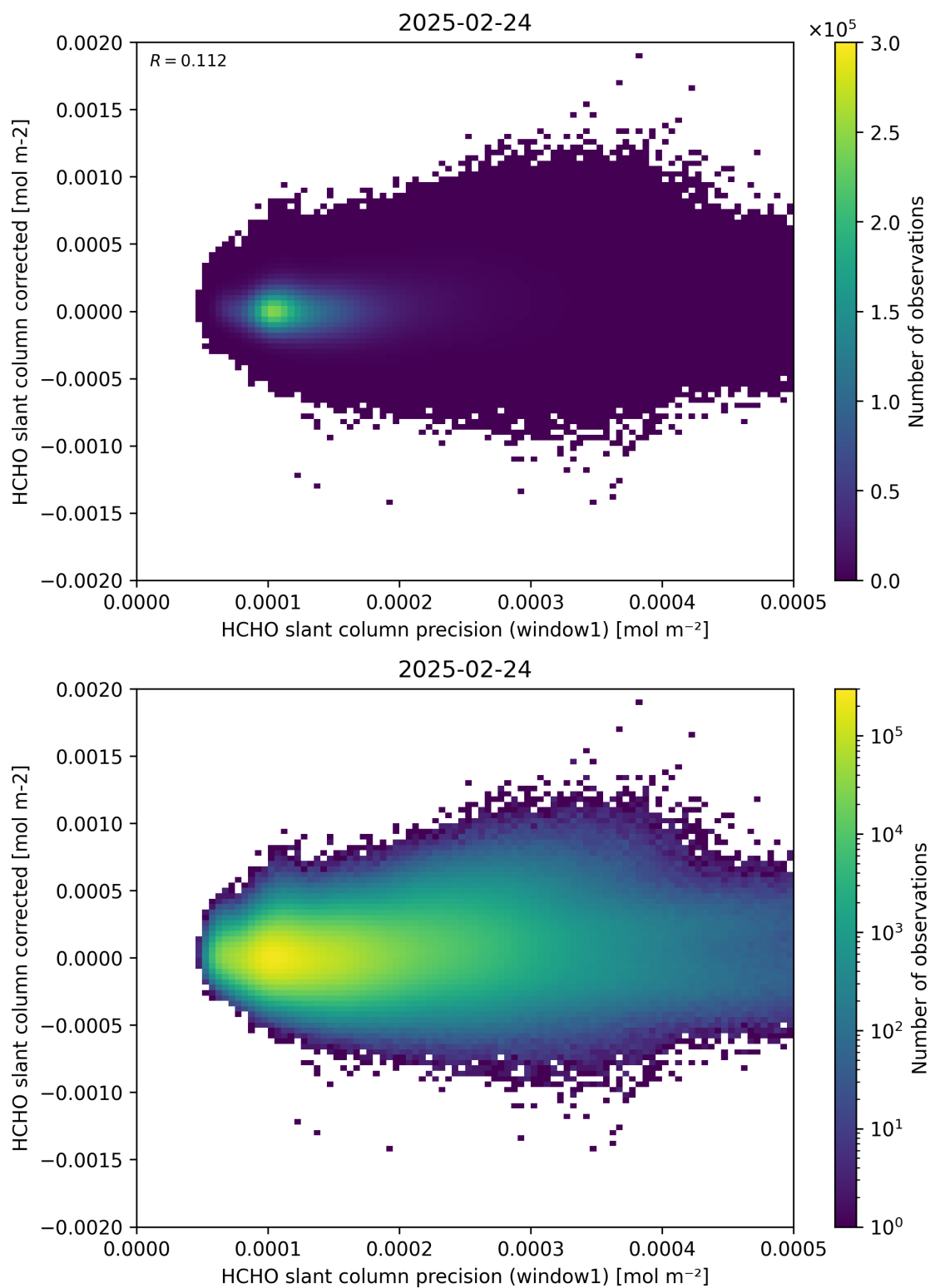
Figure 92: Scatter density plot of “HCHO slant column precision (window1)” against “HCHO slant column corrected” for 2025-02-24 to 2025-02-25.
