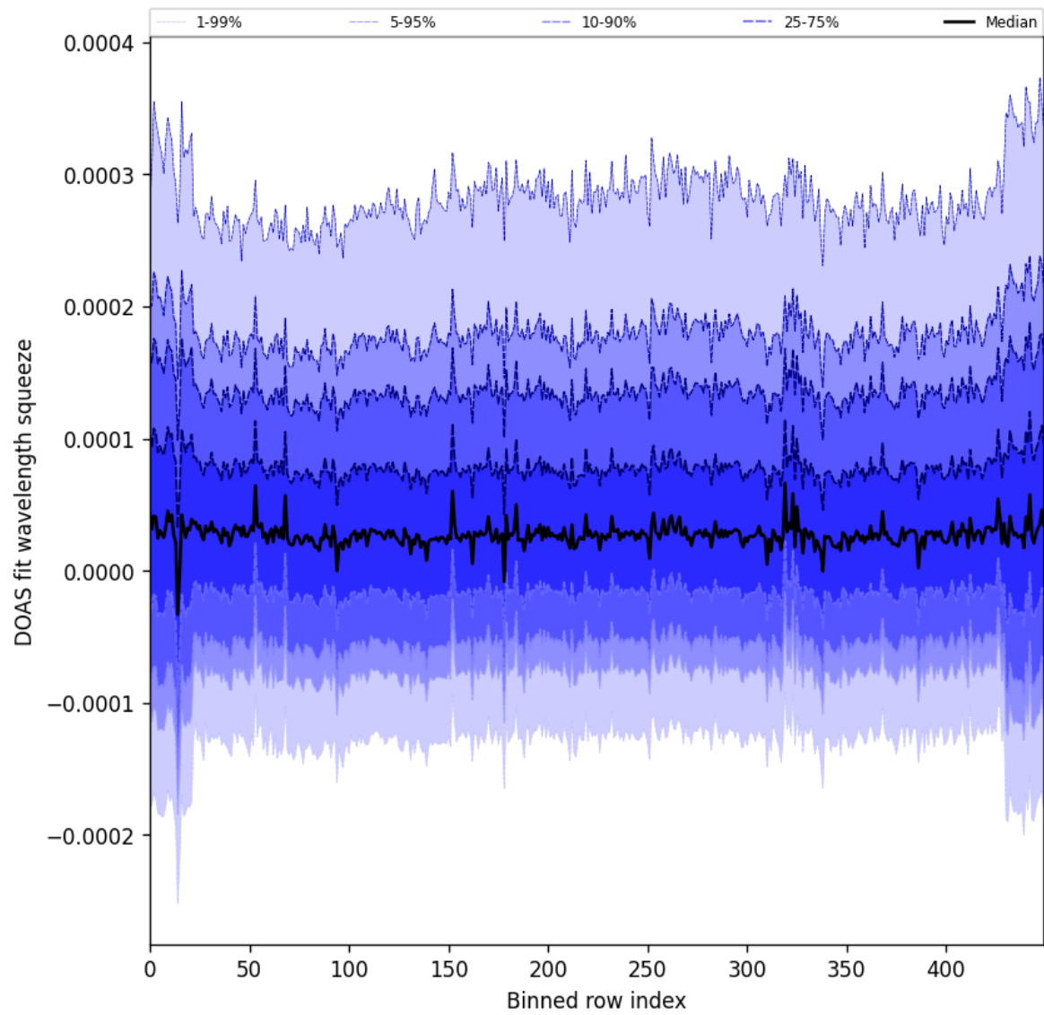
Figure 59: Along track statistics of “DOAS fit wavelength squeeze” for 2025-02-24 to 2025-02-25
