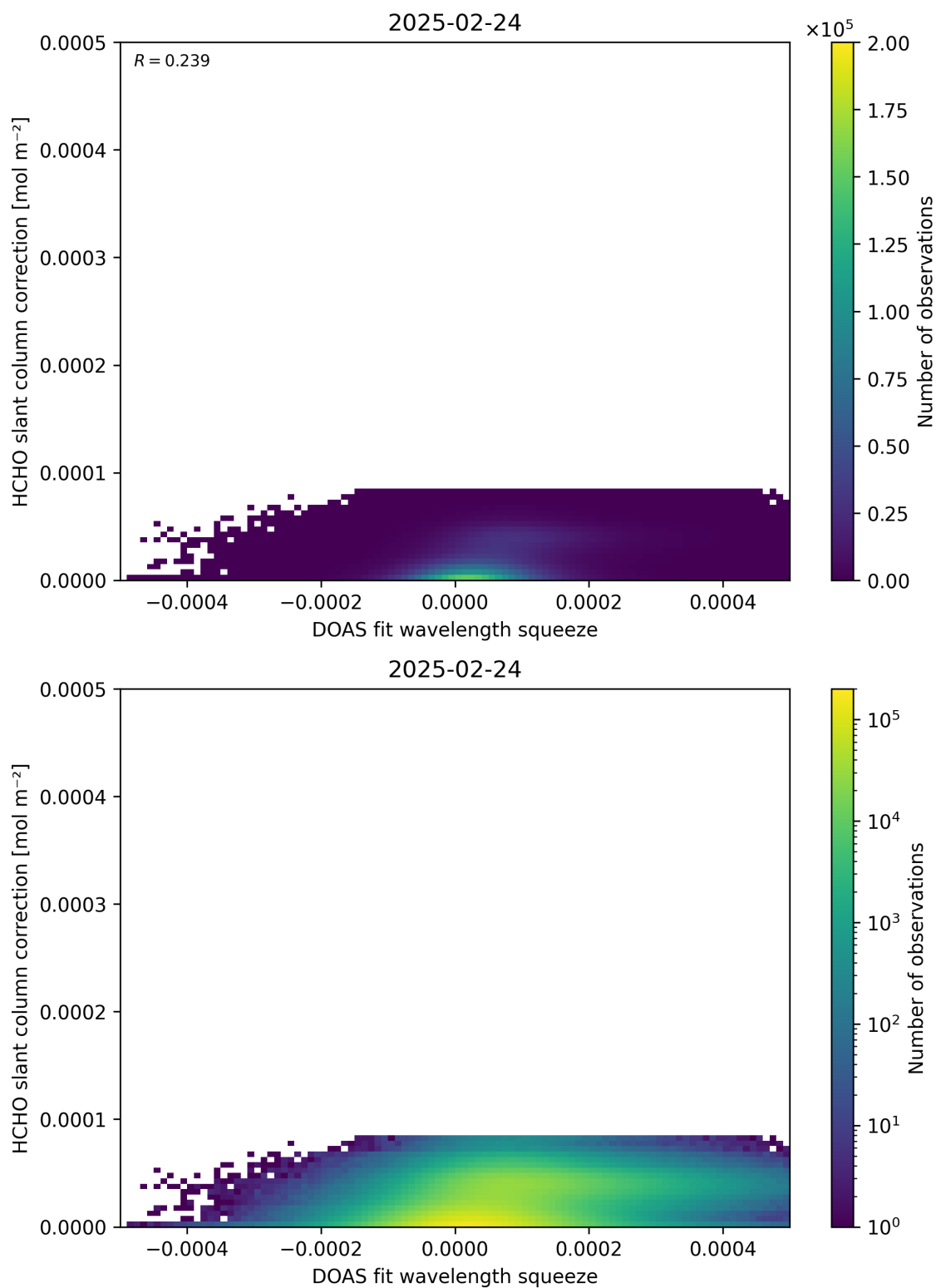
Figure 70: Scatter density plot of “DOAS fit wavelength squeeze” against “HCHO slant column correction” for 2025-02-24 to 2025-02-25.
