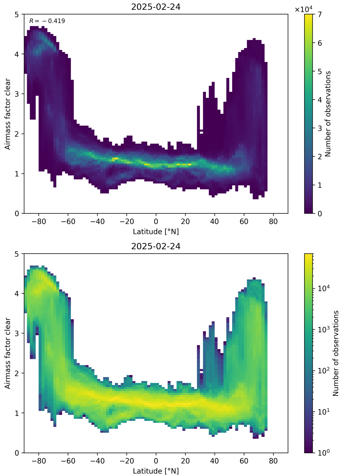
Figure 156: Scatter density plot of “Latitude” against “Airmass factor clear” for 2025-02-24 to 2025-02-25.
