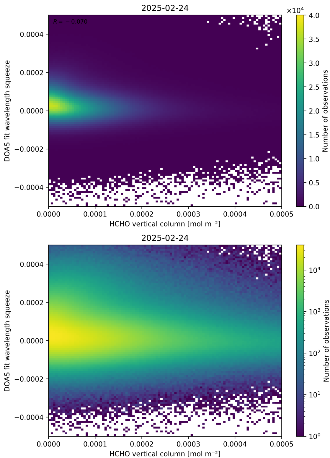
Figure 125: Scatter density plot of “HCHO vertical column” against “DOAS fit wavelength squeeze” for 2025-02-24 to 2025-02-25.
