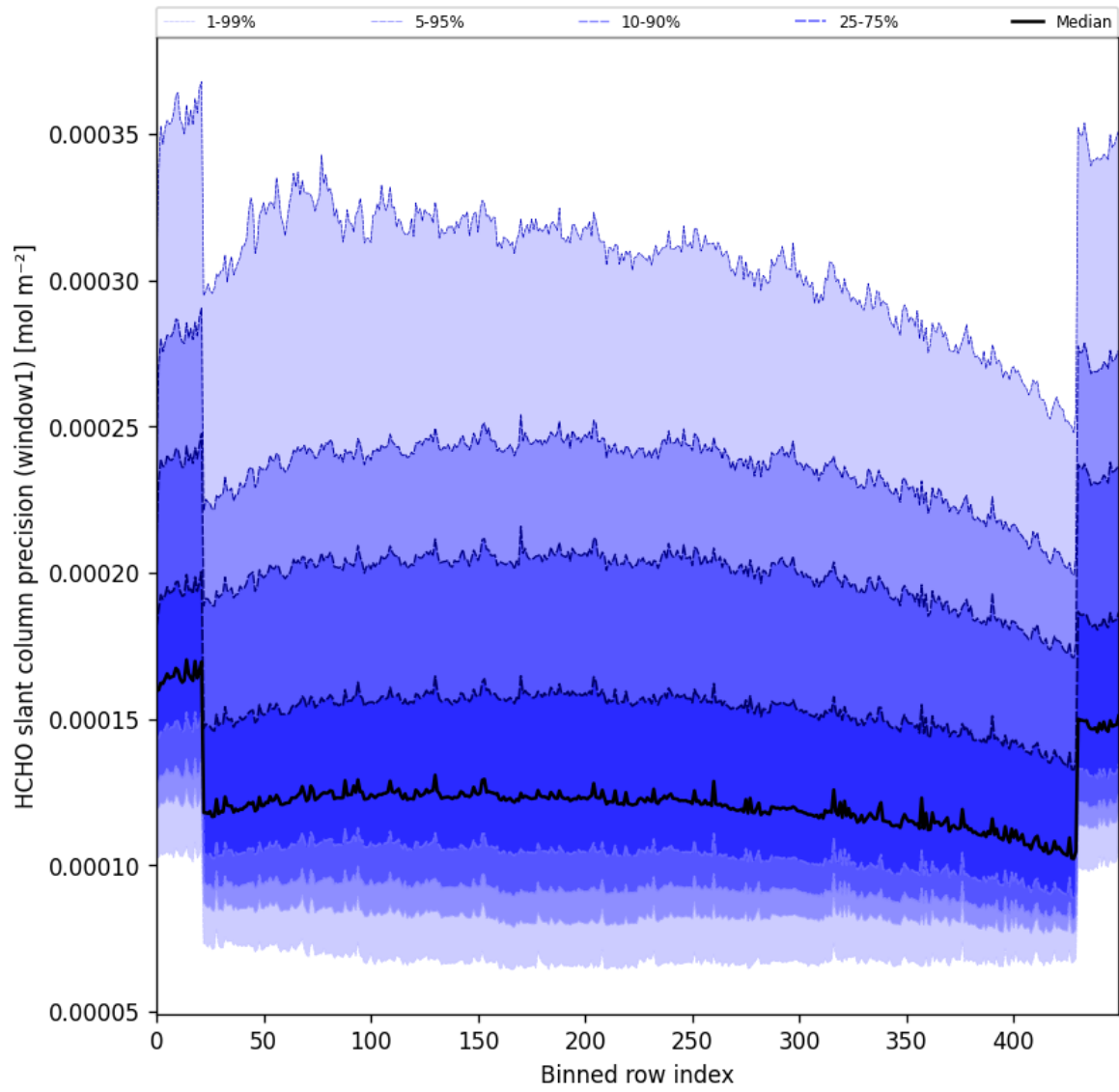
Figure 53: Along track statistics of “HCHO slant column precision (window1)” for 2025-02-24 to 2025-02-25
