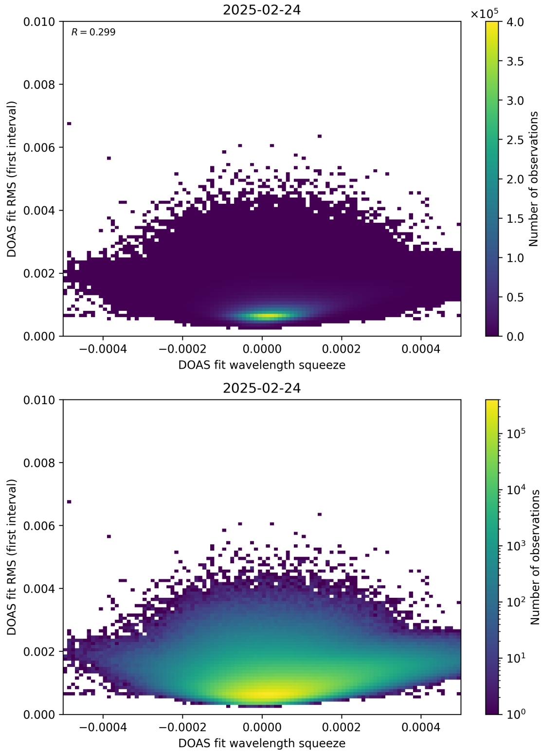
Figure 68: Scatter density plot of “DOAS fit wavelength squeeze” against “DOAS fit RMS (first interval)” for 2025-02-24 to 2025-02-25.
