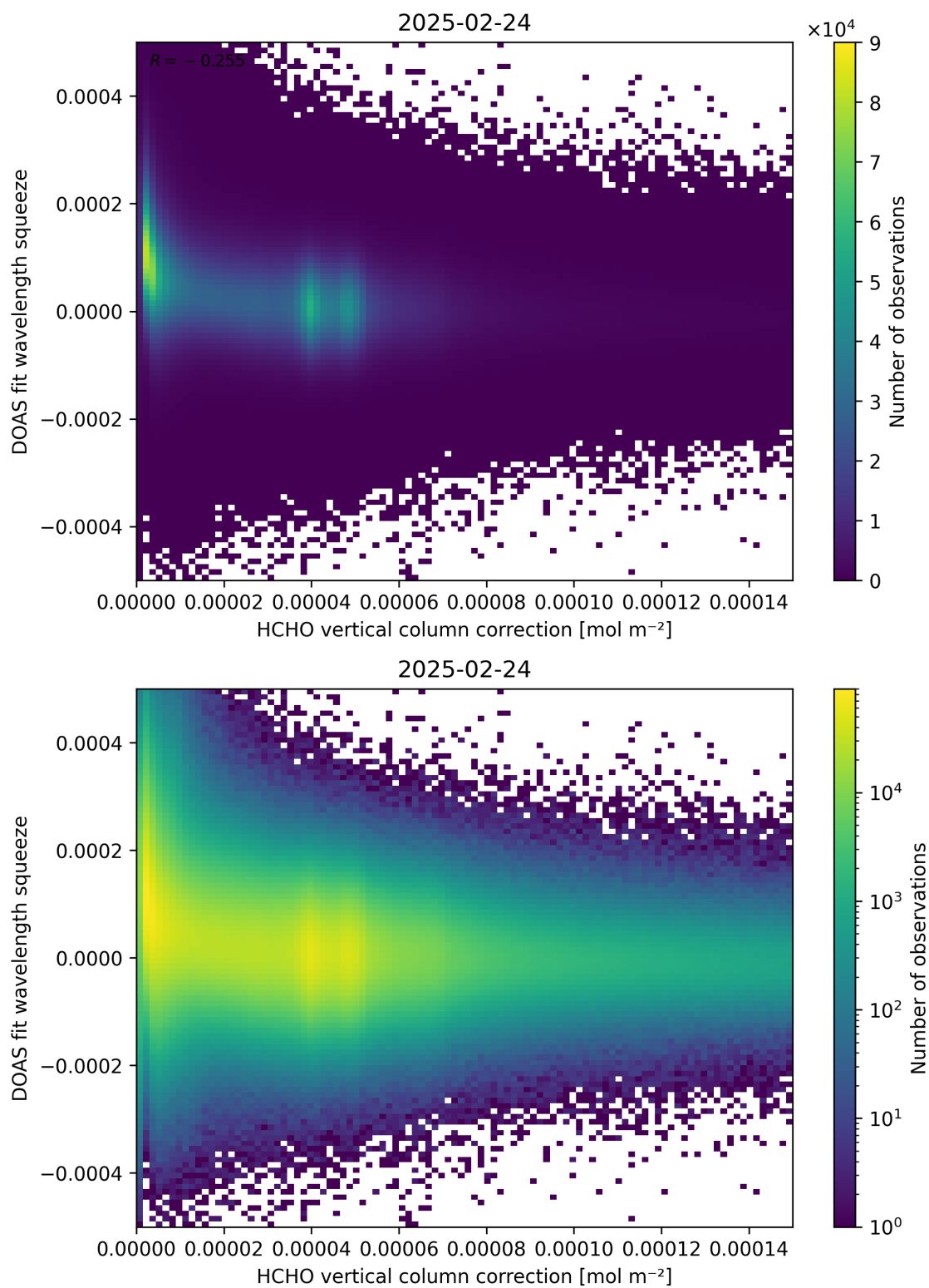
Figure 114: Scatter density plot of “HCHO vertical column correction” against “DOAS fit wavelength squeeze” for 2025-02-24 to 2025-02-25.
