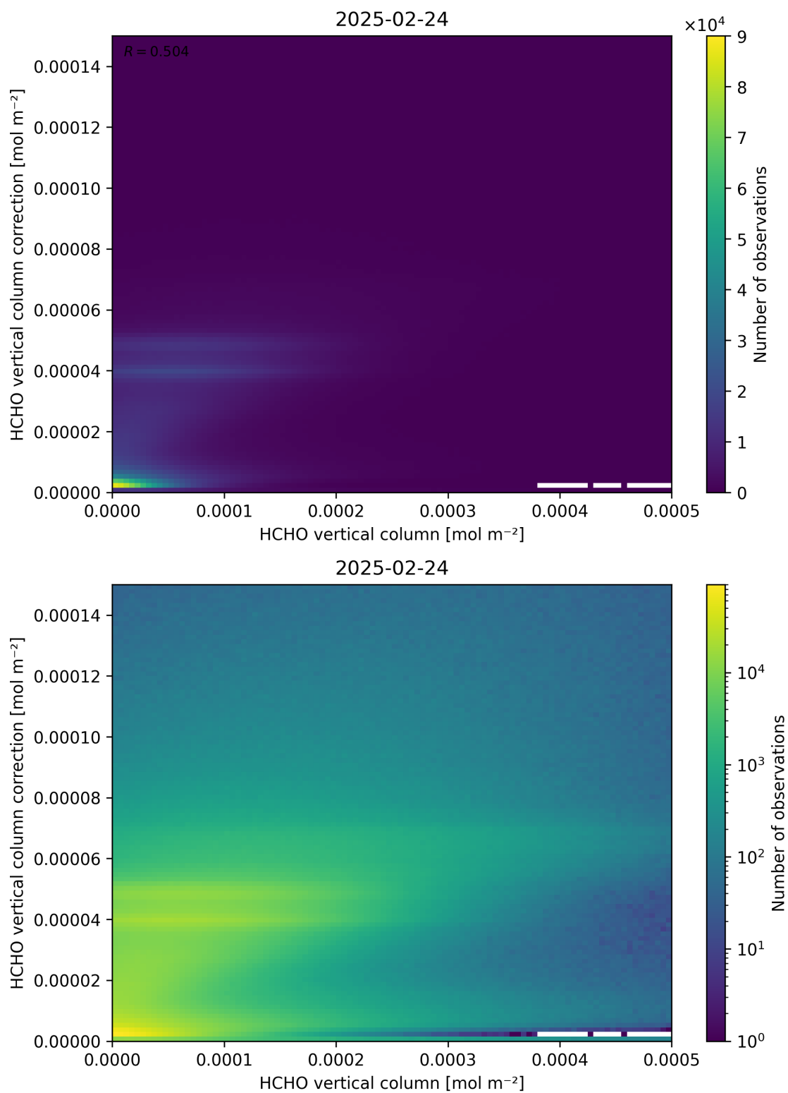
Figure 133: Scatter density plot of “HCHO vertical column” against “HCHO vertical column correction” for 2025-02-24 to 2025-02-25.
