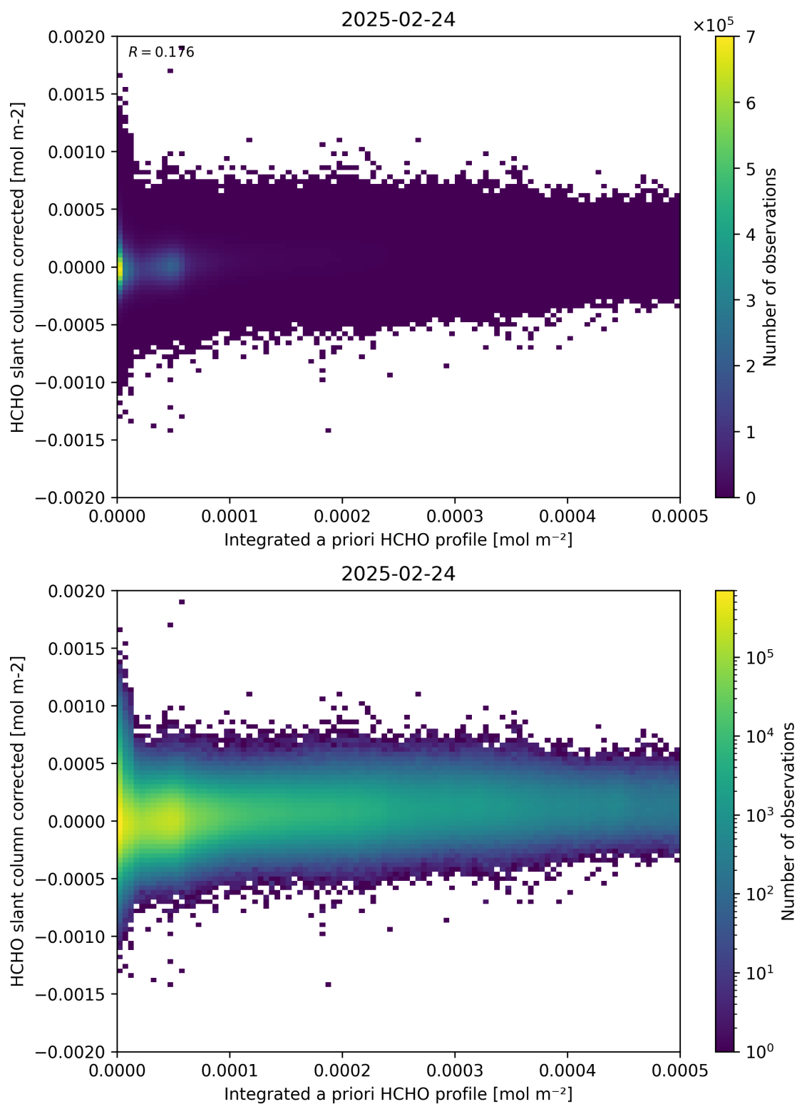
Figure 151: Scatter density plot of “Integrated a priori HCHO profile” against “HCHO slant column corrected” for 2025-02-24 to 2025-02-25.
