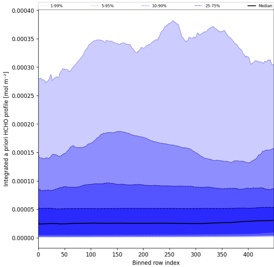
Figure 57: Along track statistics of "Integrated a priori HCHO profile" for 2025-02-24 to 2025-02-25
