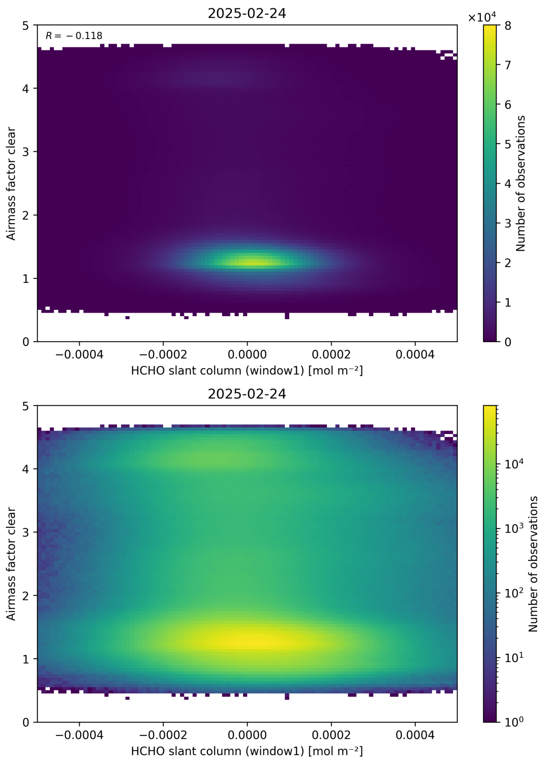
Figure 81: Scatter density plot of “HCHO slant column (window1)” against “Airmass factor clear” for 2025-02-24 to 2025-02-25.
