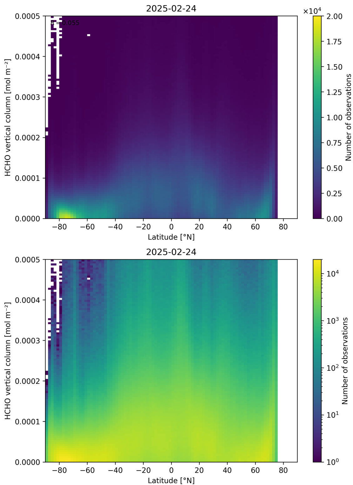
Figure 163: Scatter density plot of “Latitude” against “HCHO vertical column” for 2025-02-24 to 2025-02-25.
