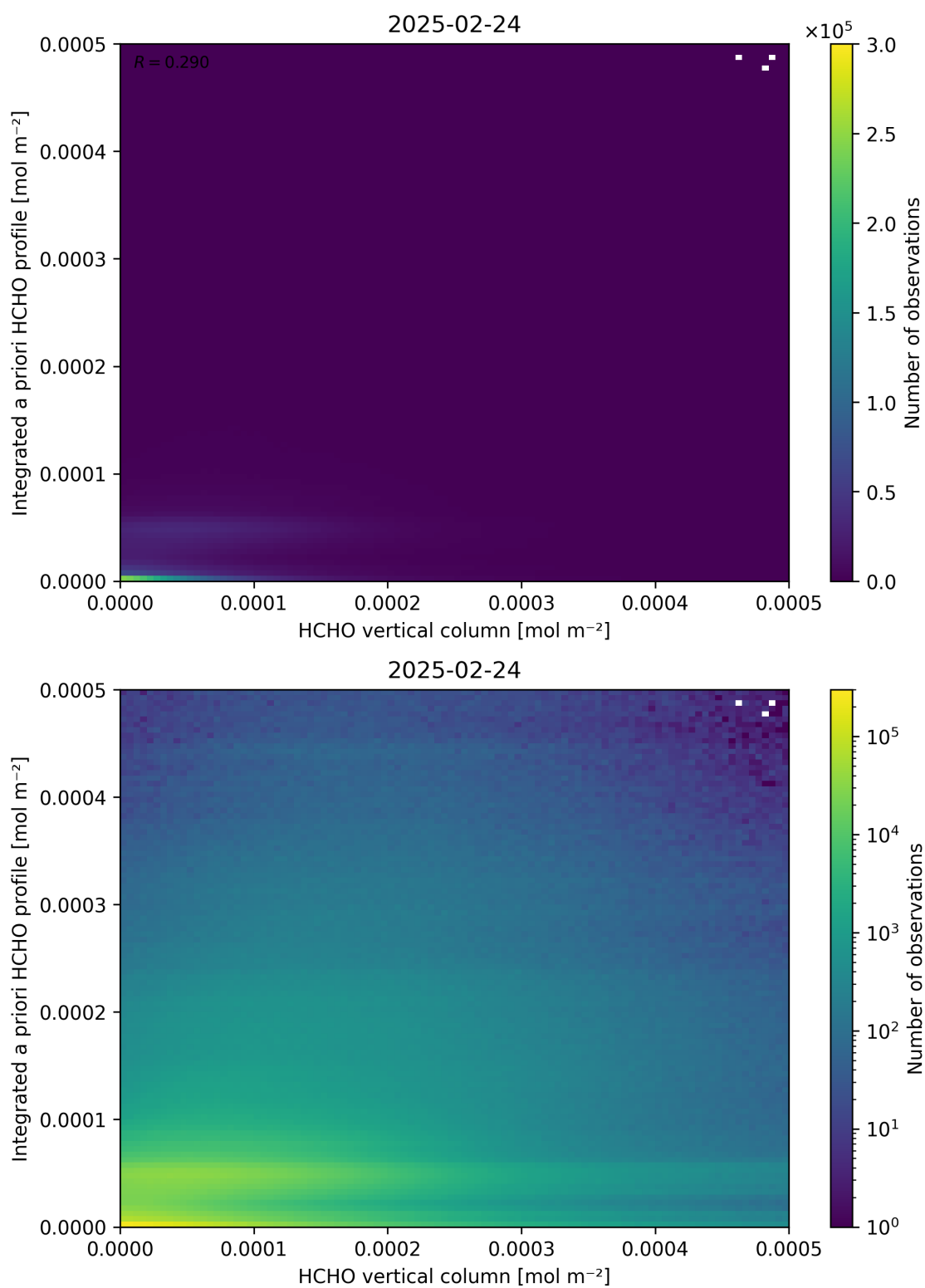
Figure 135: Scatter density plot of “HCHO vertical column” against “Integrated a priori HCHO profile” for 2025-02-24 to 2025-02-25.
