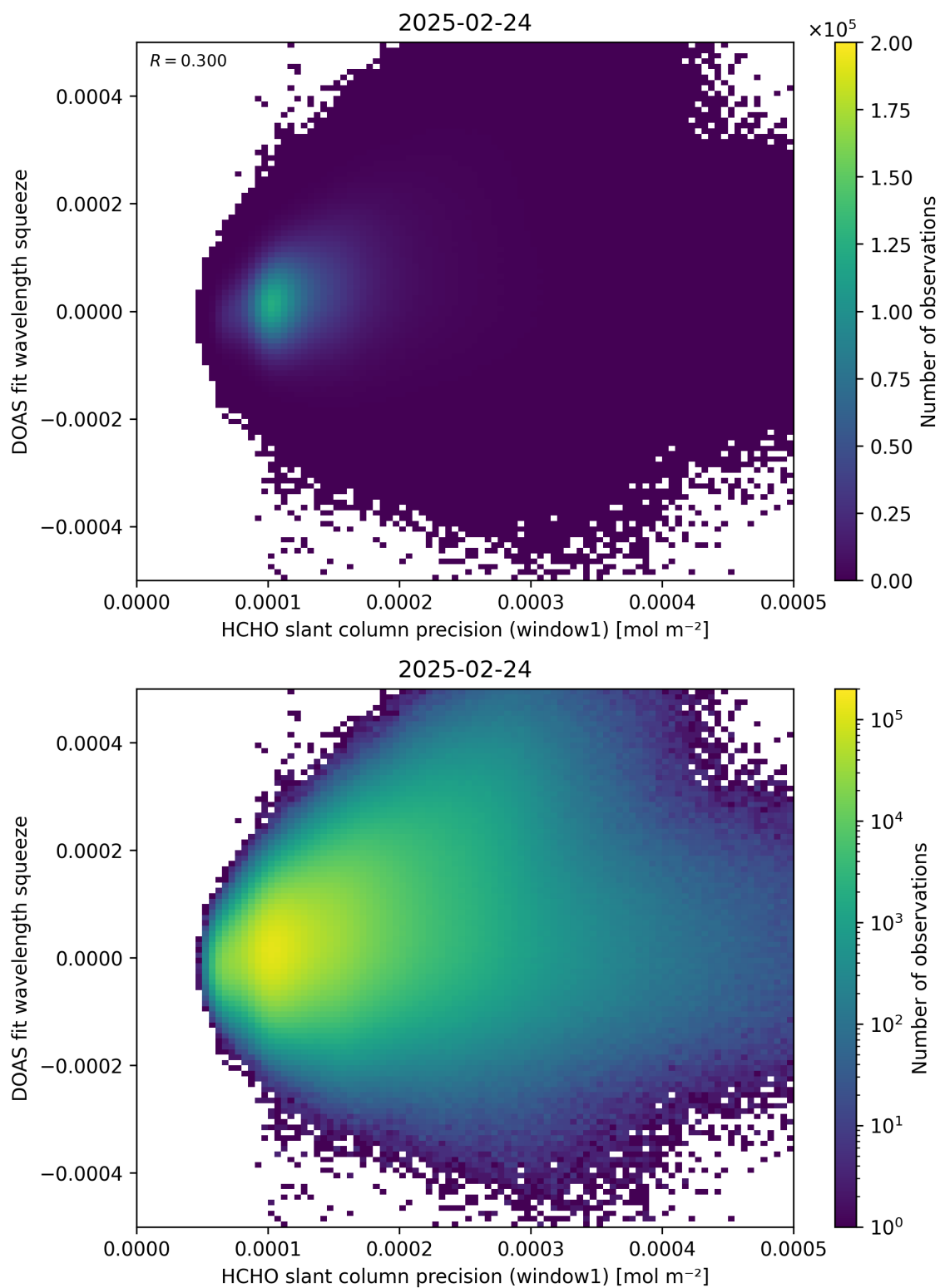
Figure 90: Scatter density plot of “HCHO slant column precision (window1)” against “DOAS fit wavelength squeeze” for 2025-02-24 to 2025-02-25.
