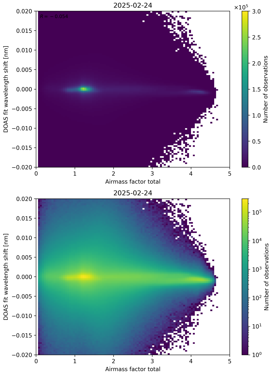
Figure 98: Scatter density plot of “Airmass factor total” against “DOAS fit wavelength shift” for 2025-02-24 to 2025-02-25.
