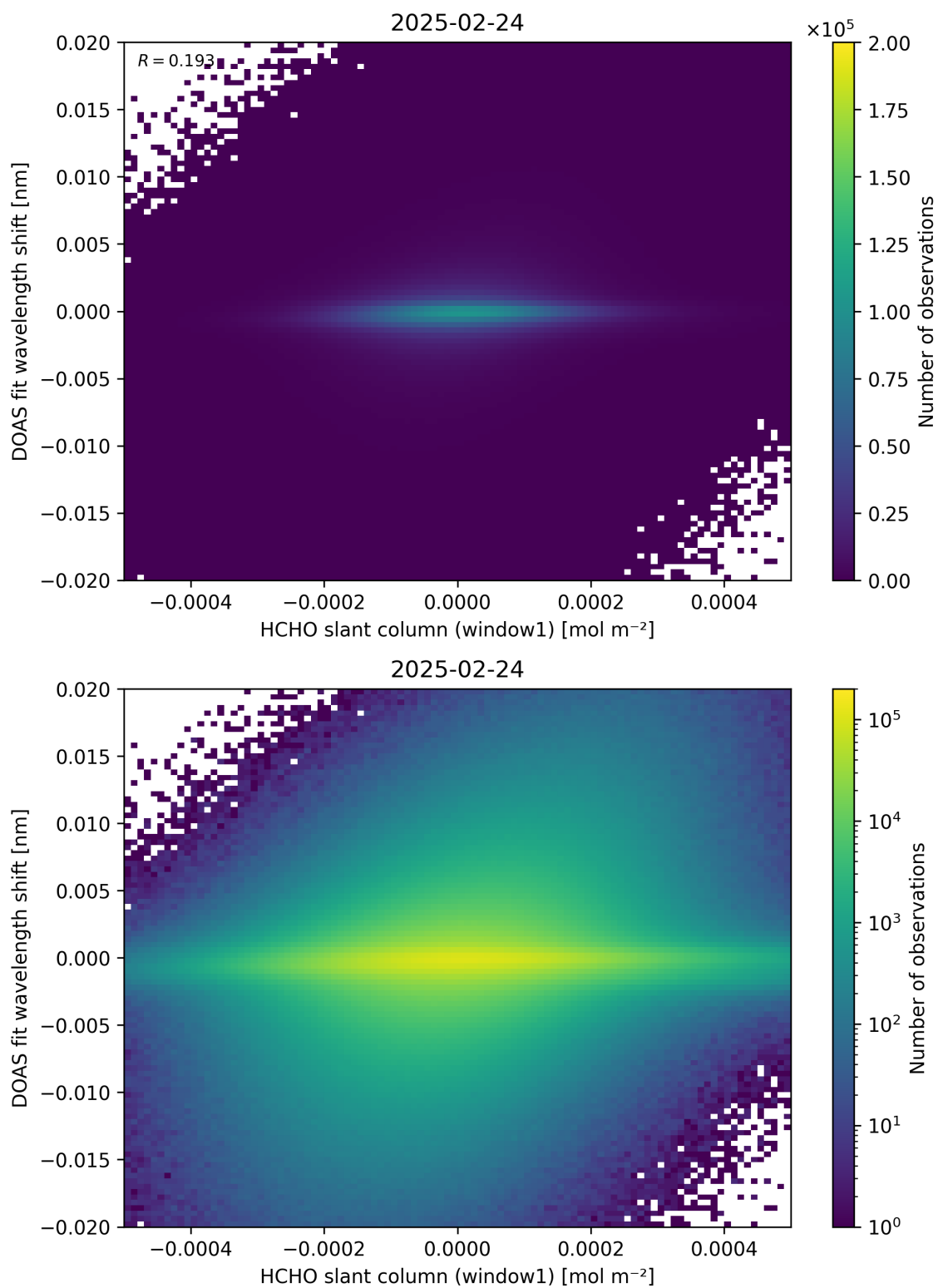
Figure 79: Scatter density plot of “HCHO slant column (window1)” against “DOAS fit wavelength shift” for 2025-02-24 to 2025-02-25.
