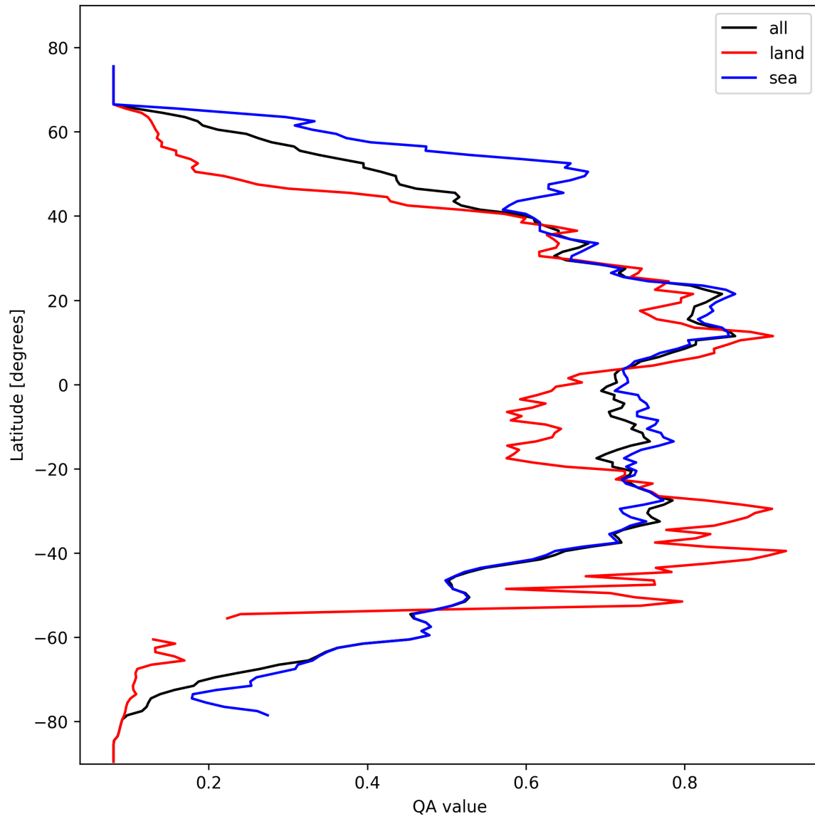
Figure 20: Zonal average of “QA value” for 2025-02-24 to 2025-02-25.
