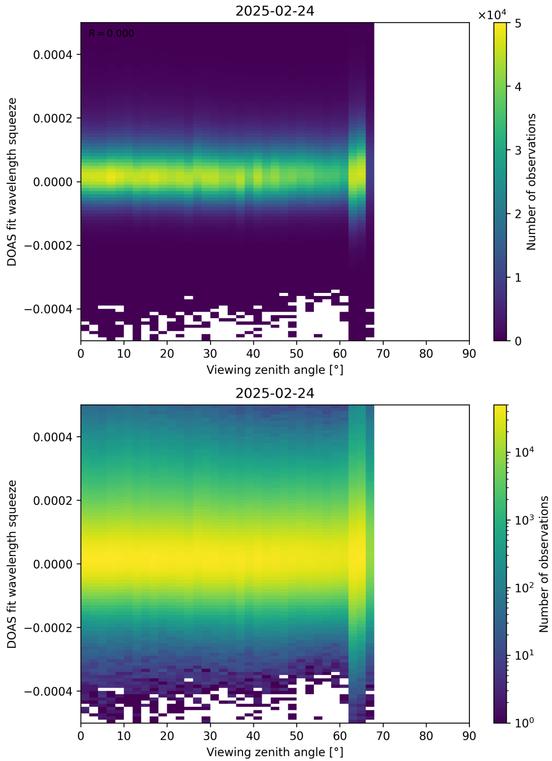
Figure 184: Scatter density plot of “Viewing zenith angle” against “DOAS fit wavelength squeeze” for 2025-02-24 to 2025-02-25.
