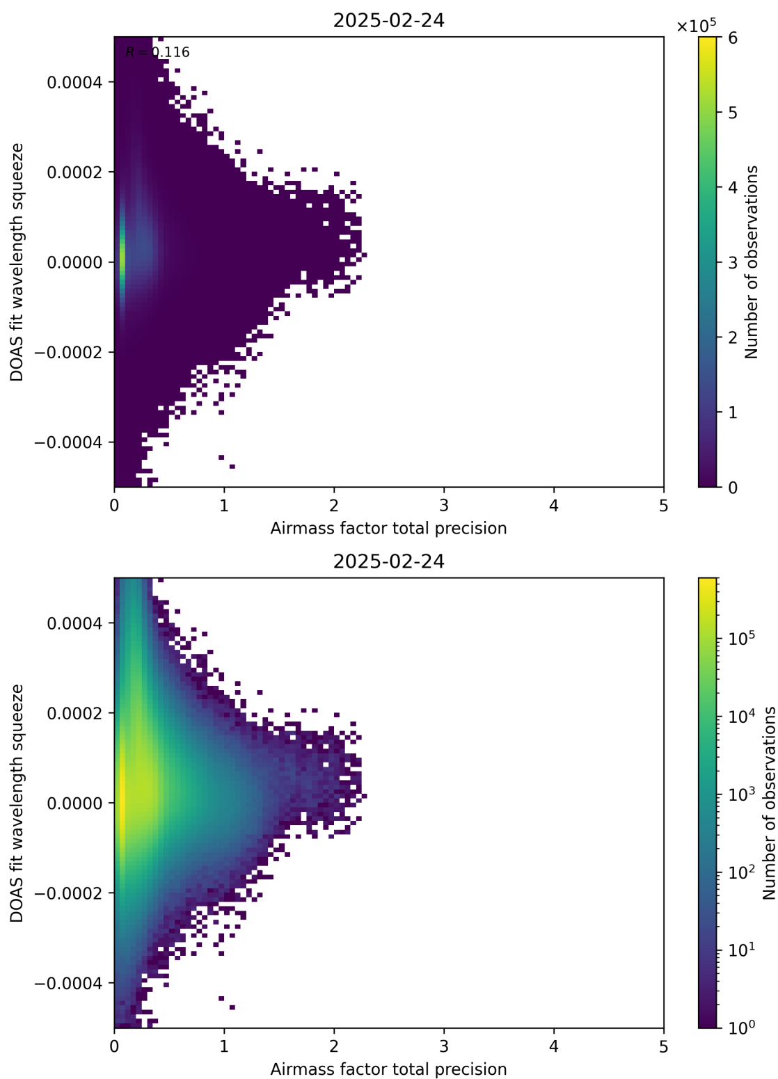
Figure 107: Scatter density plot of “Airmass factor total precision” against “DOAS fit wavelength squeeze” for 2025-02-24 to 2025-02-25.
