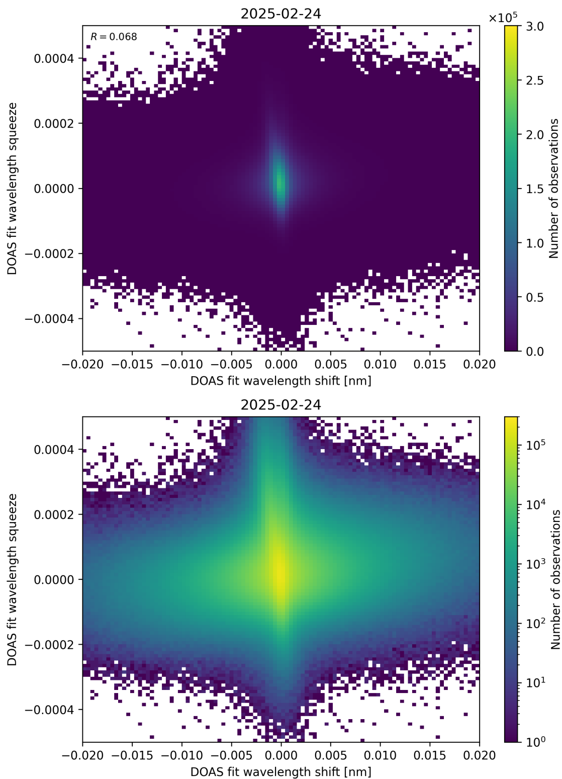
Figure 65: Scatter density plot of “DOAS fit wavelength shift” against “DOAS fit wavelength squeeze” for 2025-02-24 to 2025-02-25.
