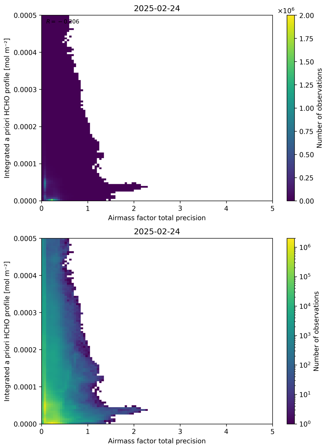
Figure 111: Scatter density plot of “Airmass factor total precision” against “Integrated a priori HCHO profile” for 2025-02-24 to 2025-02-25.
