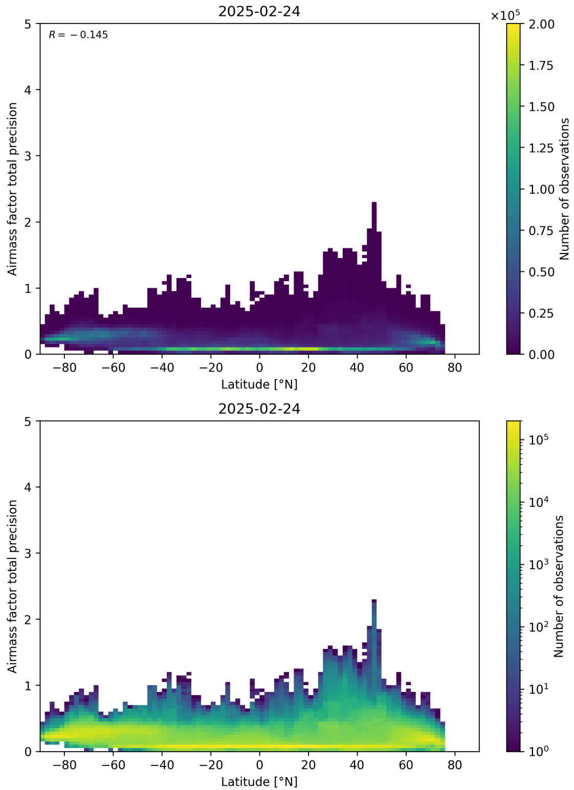
Figure 162: Scatter density plot of “Latitude” against “Airmass factor total precision” for 2025-02-24 to 2025-02-25.
