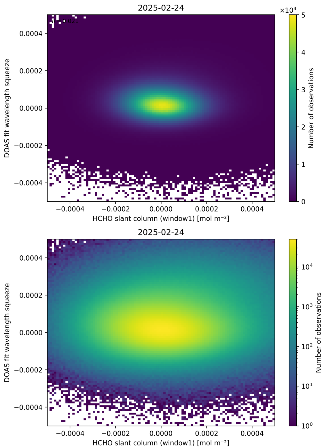
Figure 80: Scatter density plot of “HCHO slant column (window1)” against “DOAS fit wavelength squeeze” for 2025-02-24 to 2025-02-25.
