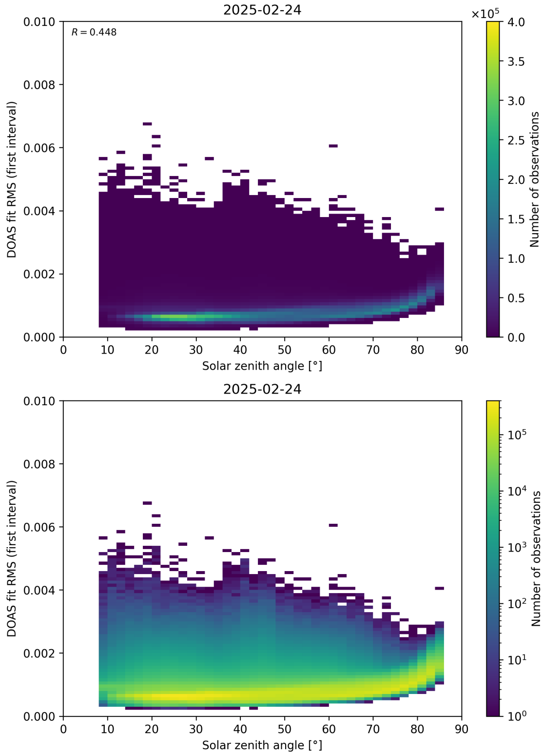
Figure 167: Scatter density plot of “Solar zenith angle” against “DOAS fit RMS (first interval)” for 2025-02-24 to 2025-02-25.
