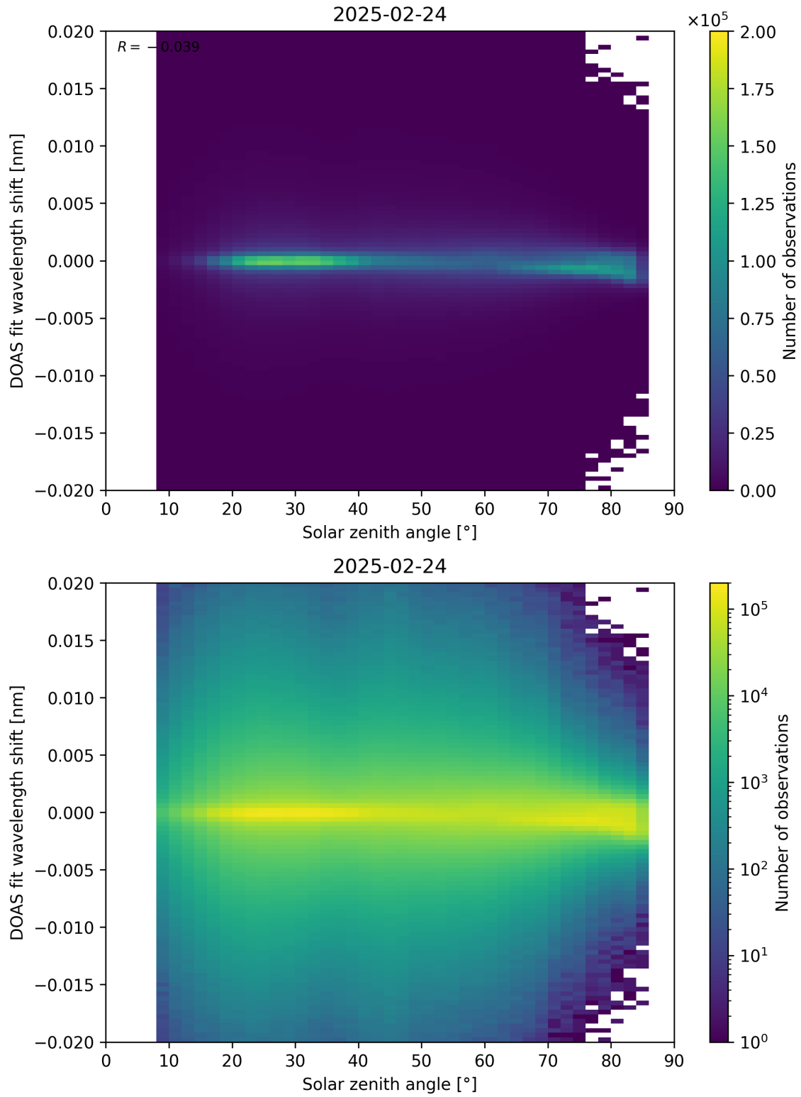
Figure 168: Scatter density plot of “Solar zenith angle” against “DOAS fit wavelength shift” for 2025-02-24 to 2025-02-25.
