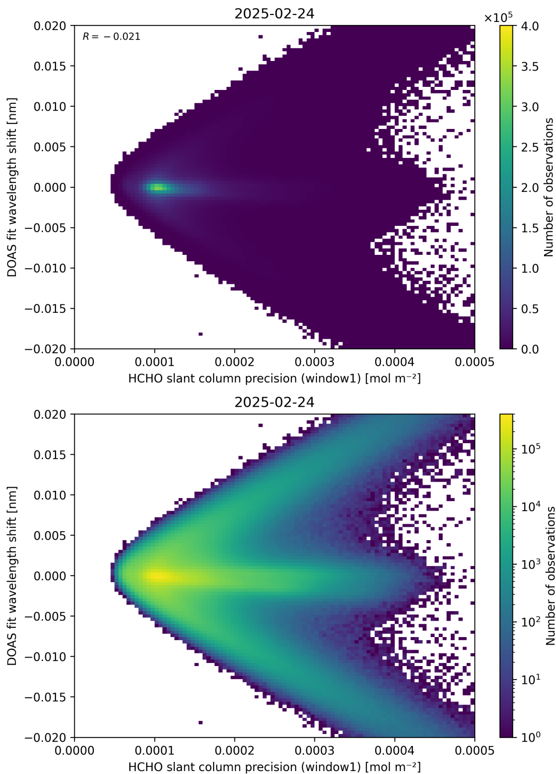
Figure 89: Scatter density plot of “HCHO slant column precision (window1)” against “DOAS fit wavelength shift” for 2025-02-24 to 2025-02-25.
