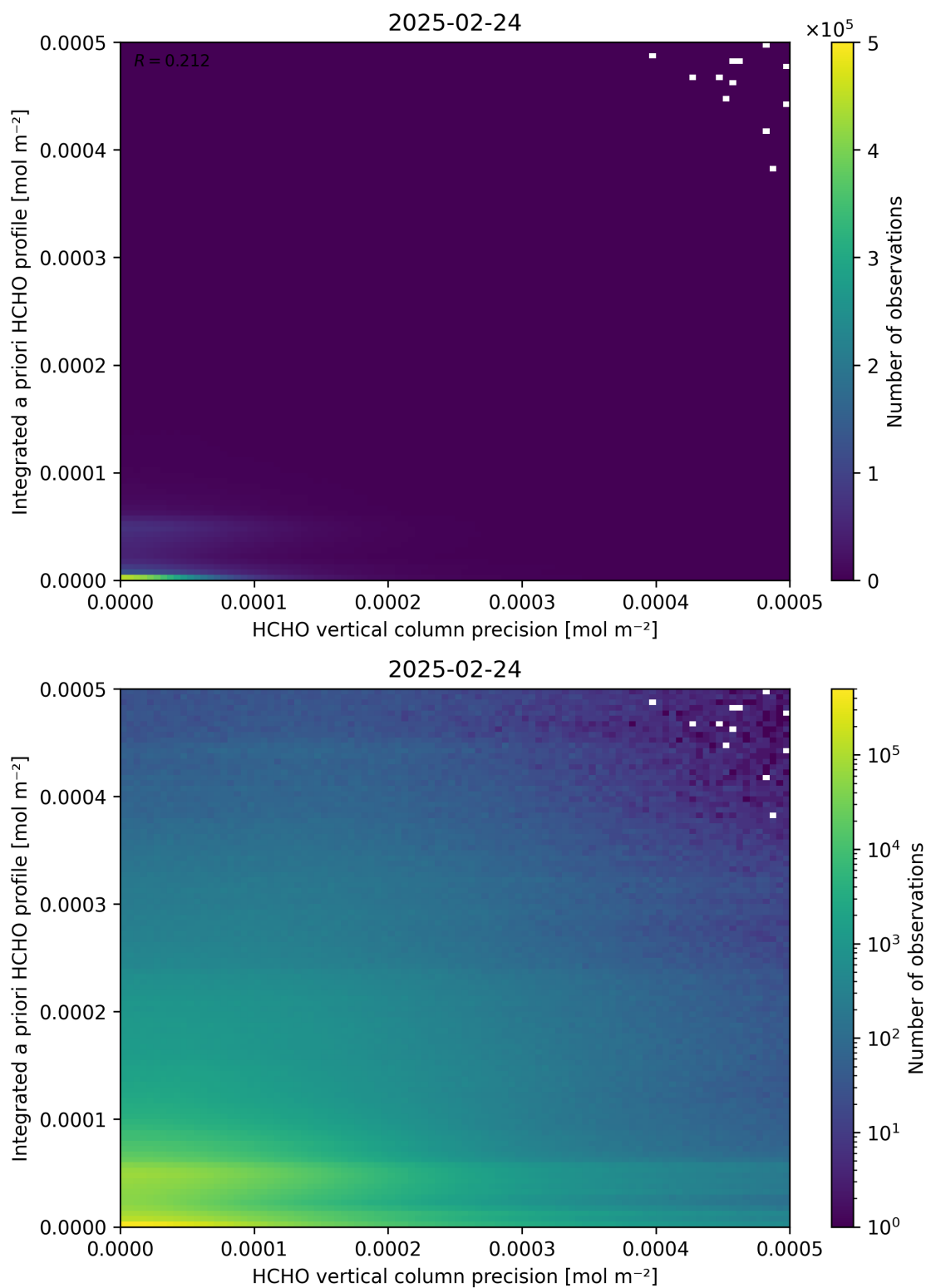
Figure 147: Scatter density plot of “HCHO vertical column precision” against “Integrated a priori HCHO profile” for 2025-02-24 to 2025-02-25.
