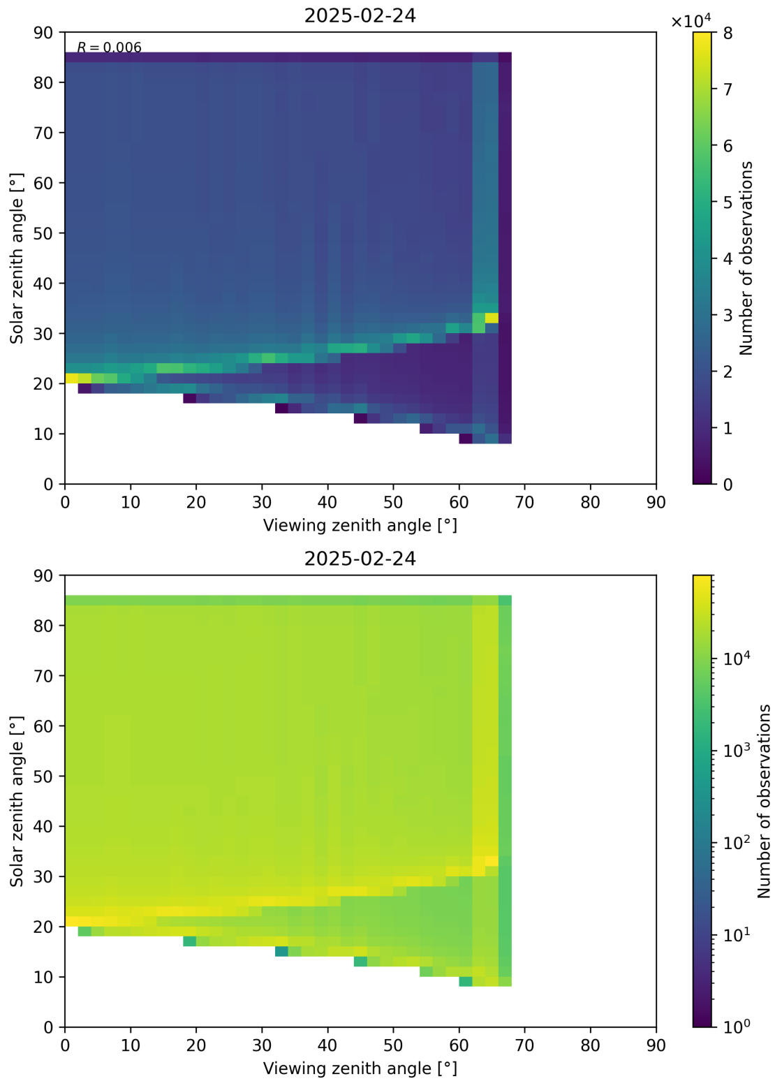
Figure 197: Scatter density plot of “Viewing zenith angle” against “Solar zenith angle” for 2025-02-24 to 2025-02-25.
