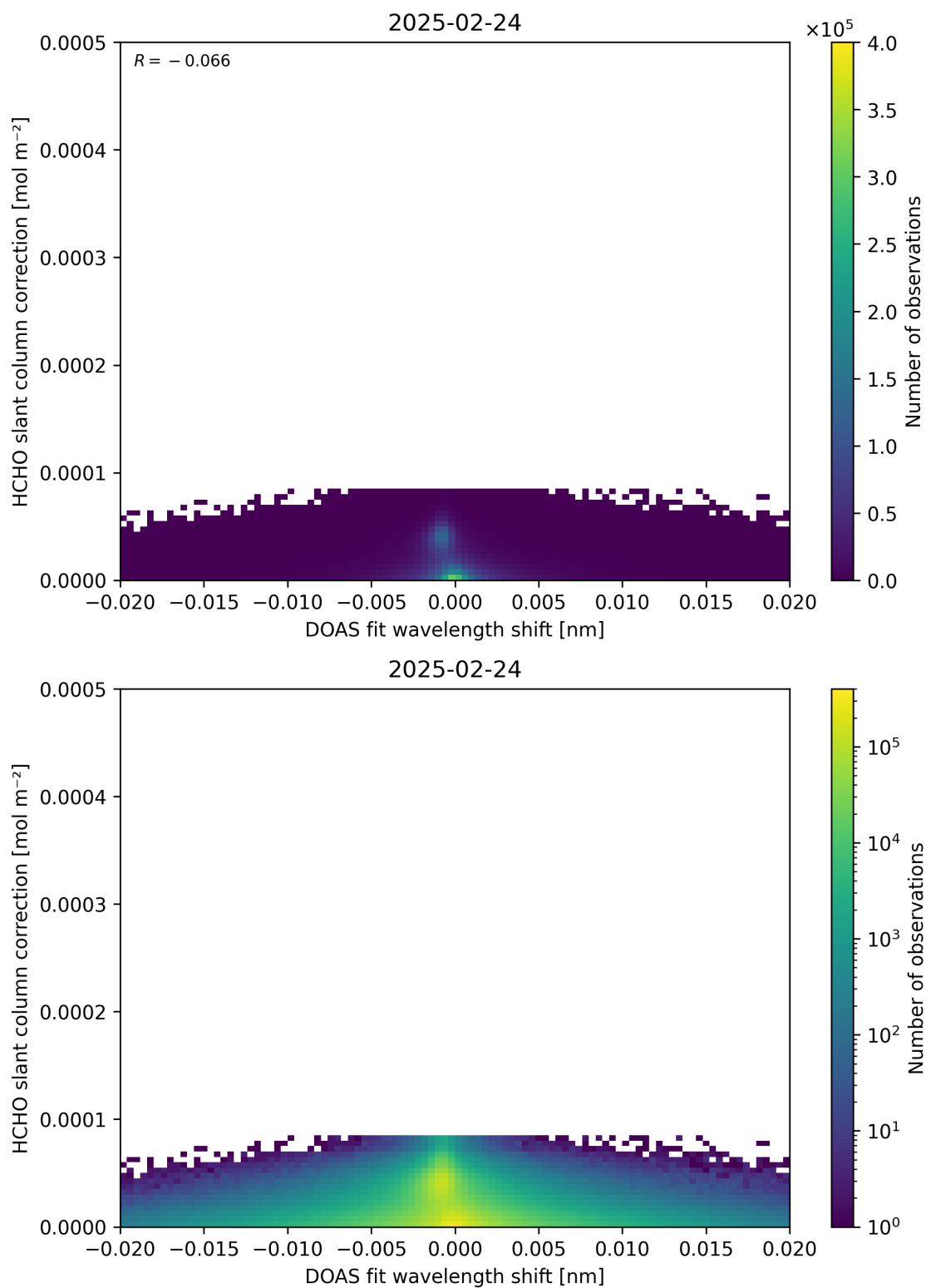
Figure 67: Scatter density plot of “DOAS fit wavelength shift” against “HCHO slant column correction” for 2025-02-24 to 2025-02-25.
