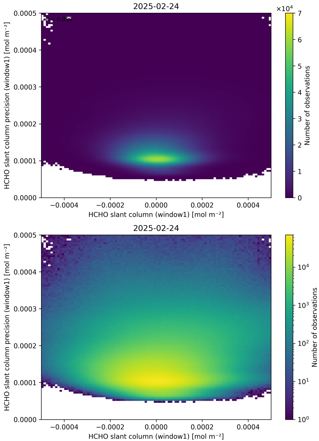
Figure 84: Scatter density plot of “HCHO slant column (window1)” against “HCHO slant column precision (window1)” for 2025-02-24 to 2025-02-25.
