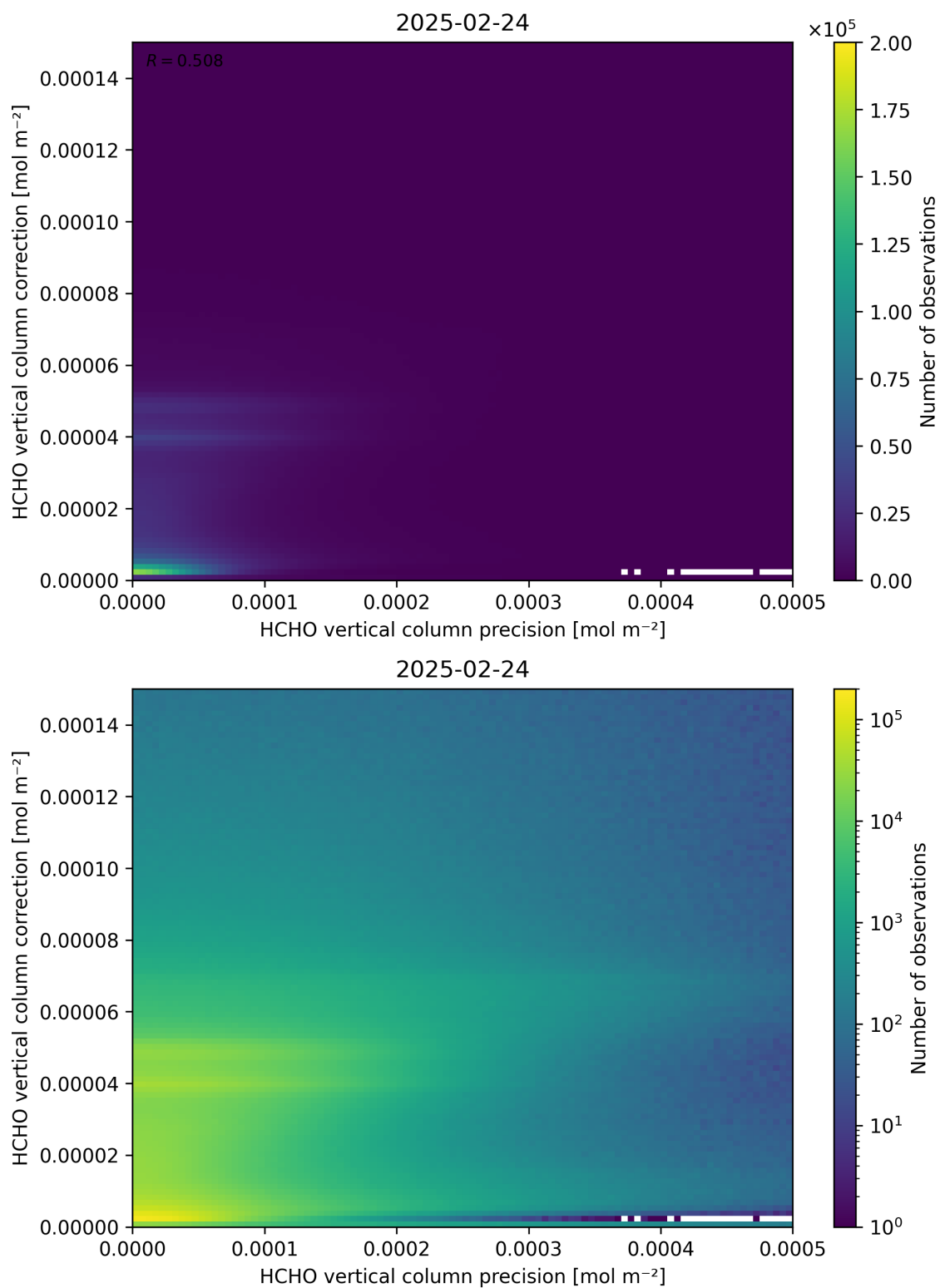
Figure 146: Scatter density plot of “HCHO vertical column precision” against “HCHO vertical column correction” for 2025-02-24 to 2025-02-25.
