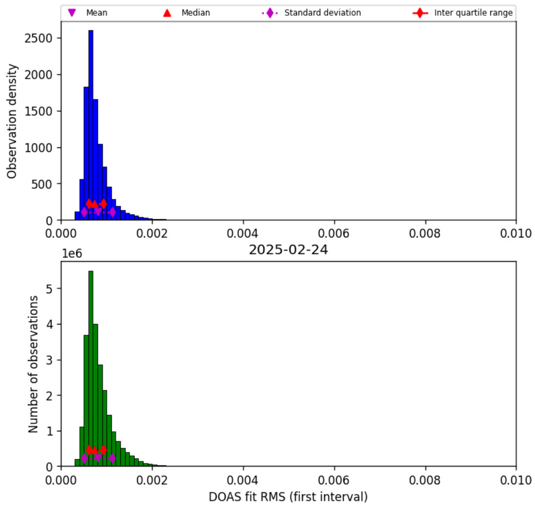
Figure 46: Histogram of “DOAS fit RMS (first interval)” for 2025-02-24 to 2025-02-25
