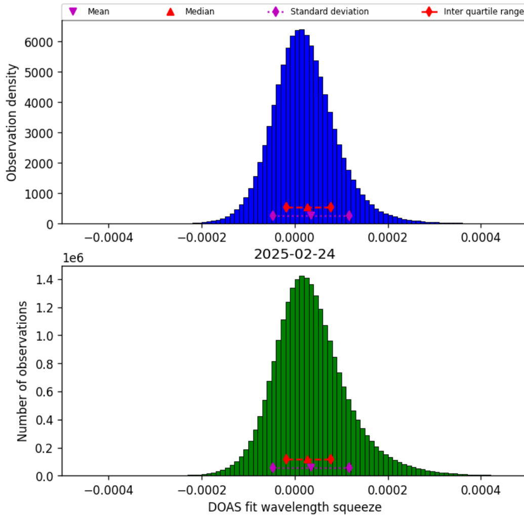
Figure 45: Histogram of “DOAS fit wavelength squeeze” for 2025-02-24 to 2025-02-25
