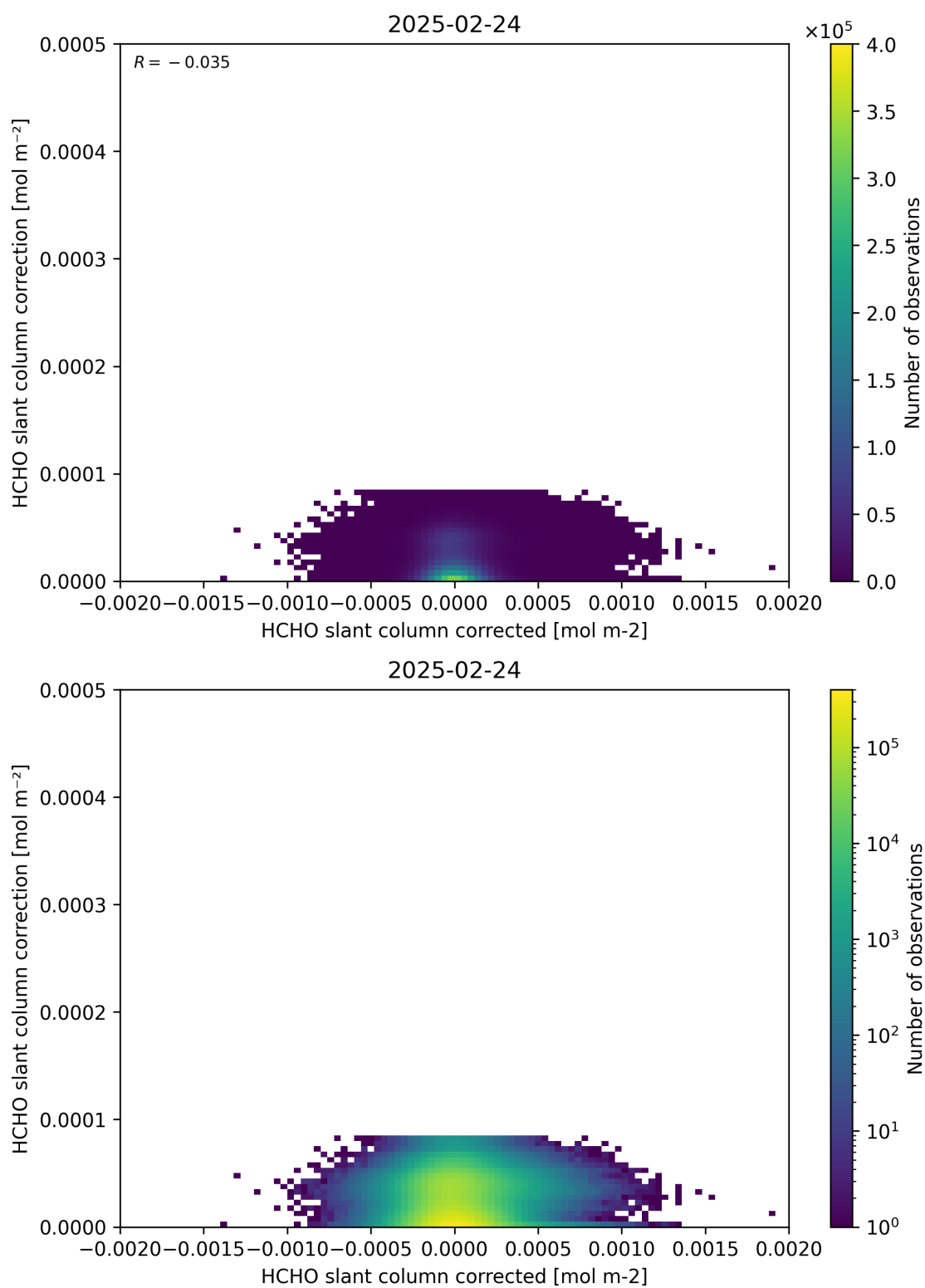
Figure 77: Scatter density plot of “HCHO slant column corrected” against “HCHO slant column correction” for 2025-02-24 to 2025-02-25.
