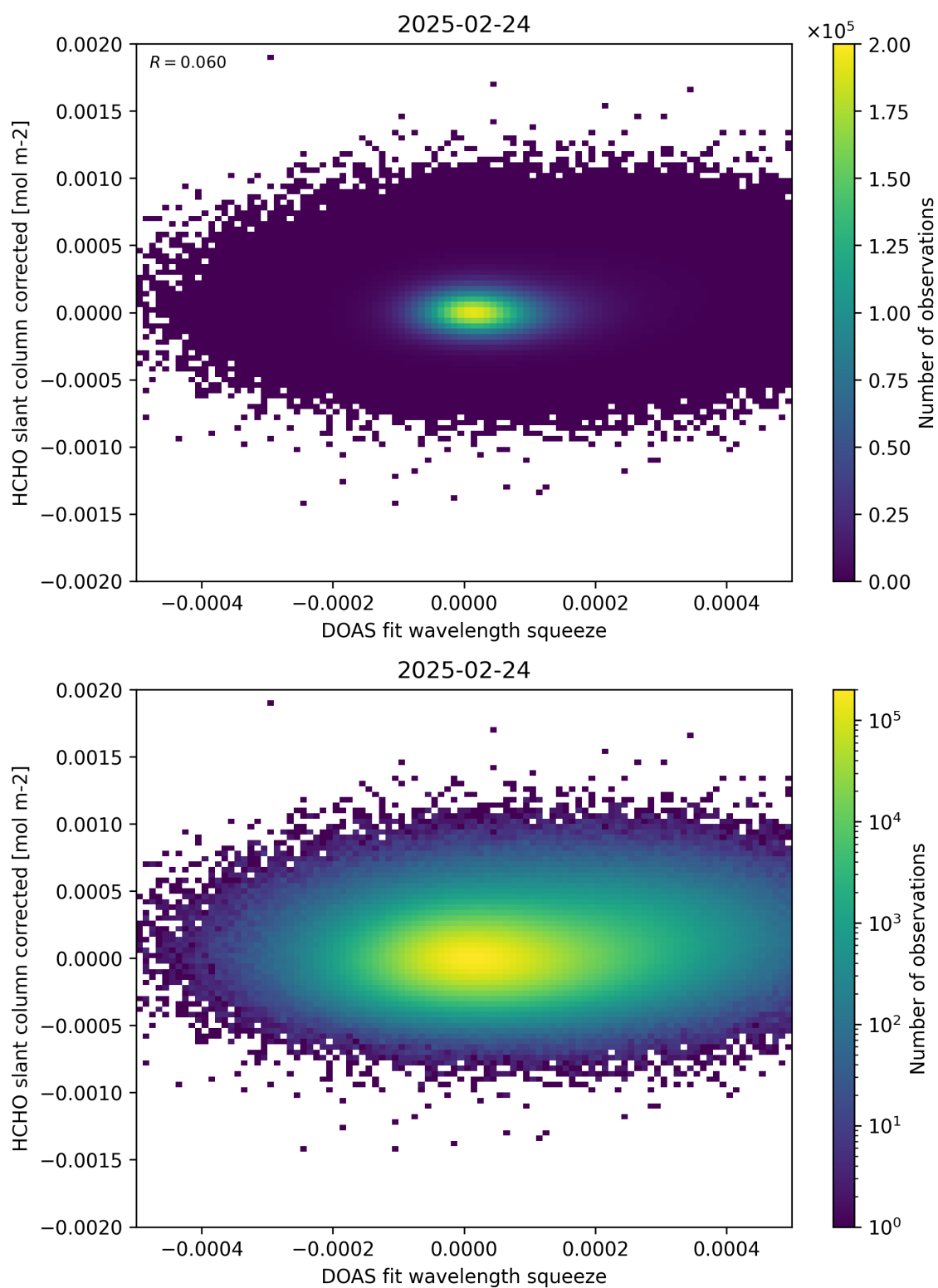
Figure 69: Scatter density plot of “DOAS fit wavelength squeeze” against “HCHO slant column corrected” for 2025-02-24 to 2025-02-25.
