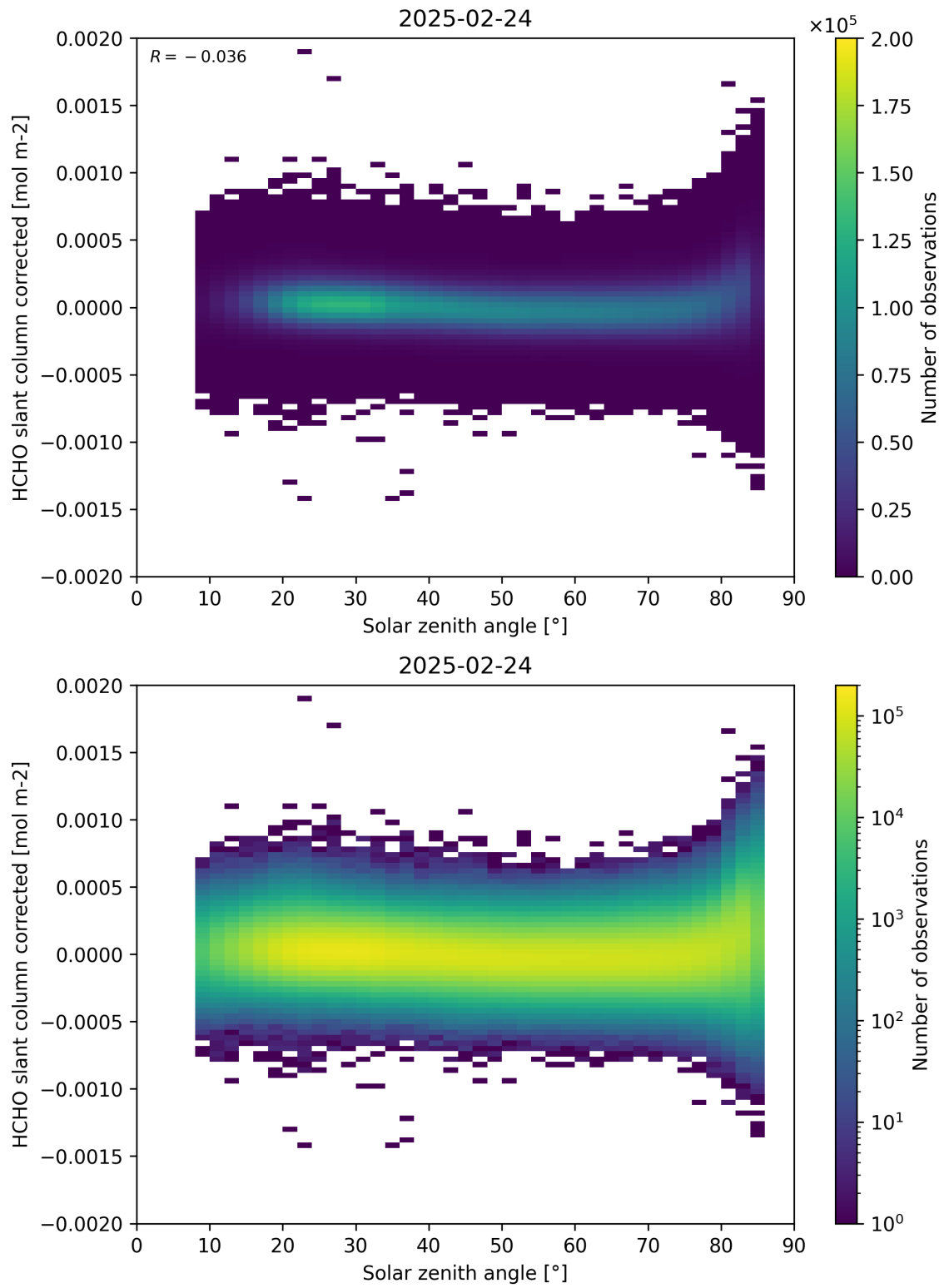
Figure 171: Scatter density plot of “Solar zenith angle” against “HCHO slant column corrected” for 2025-02-24 to 2025-02-25.
