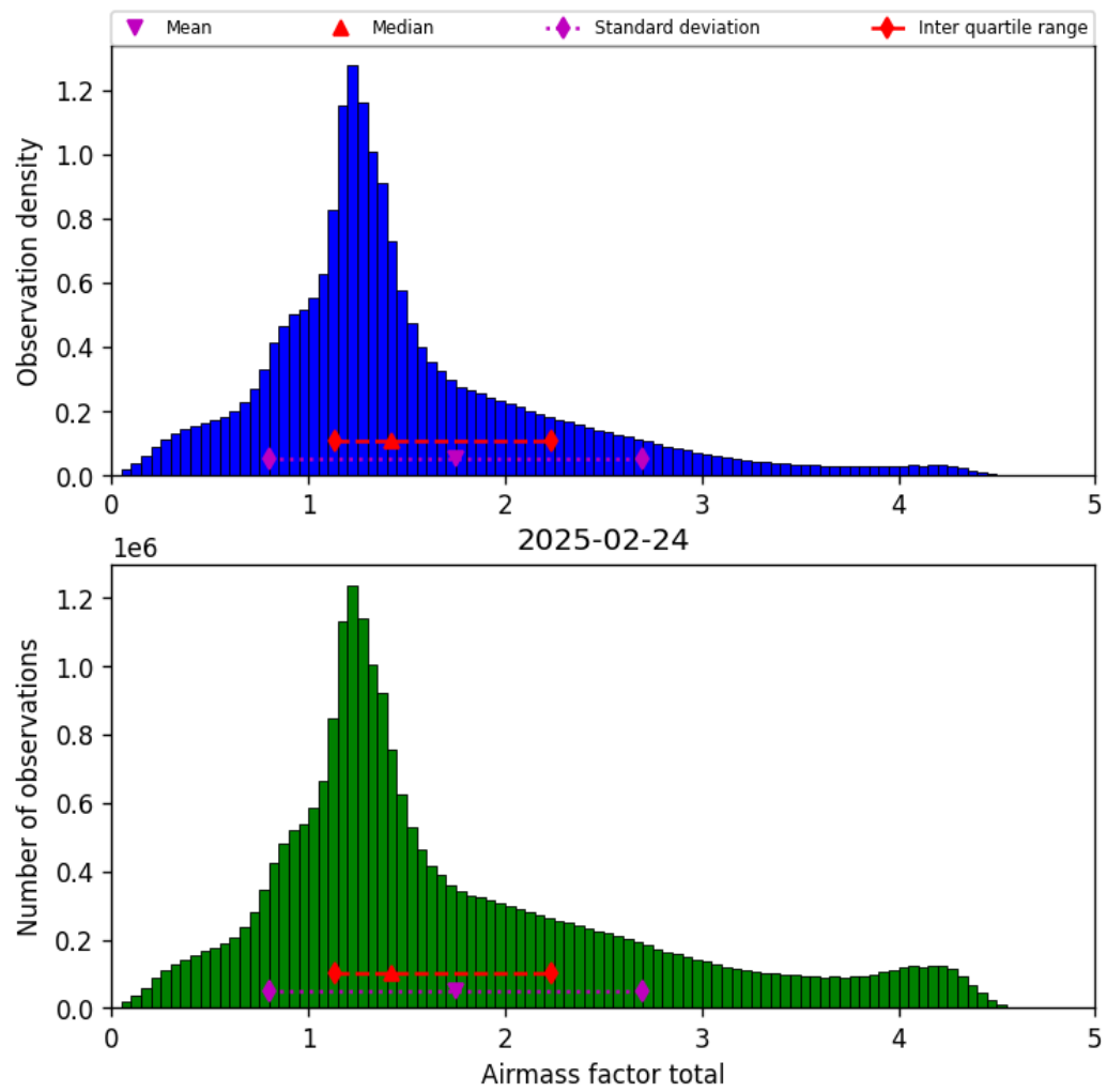
Figure 40: Histogram of “Airmass factor total” for 2025-02-24 to 2025-02-25
