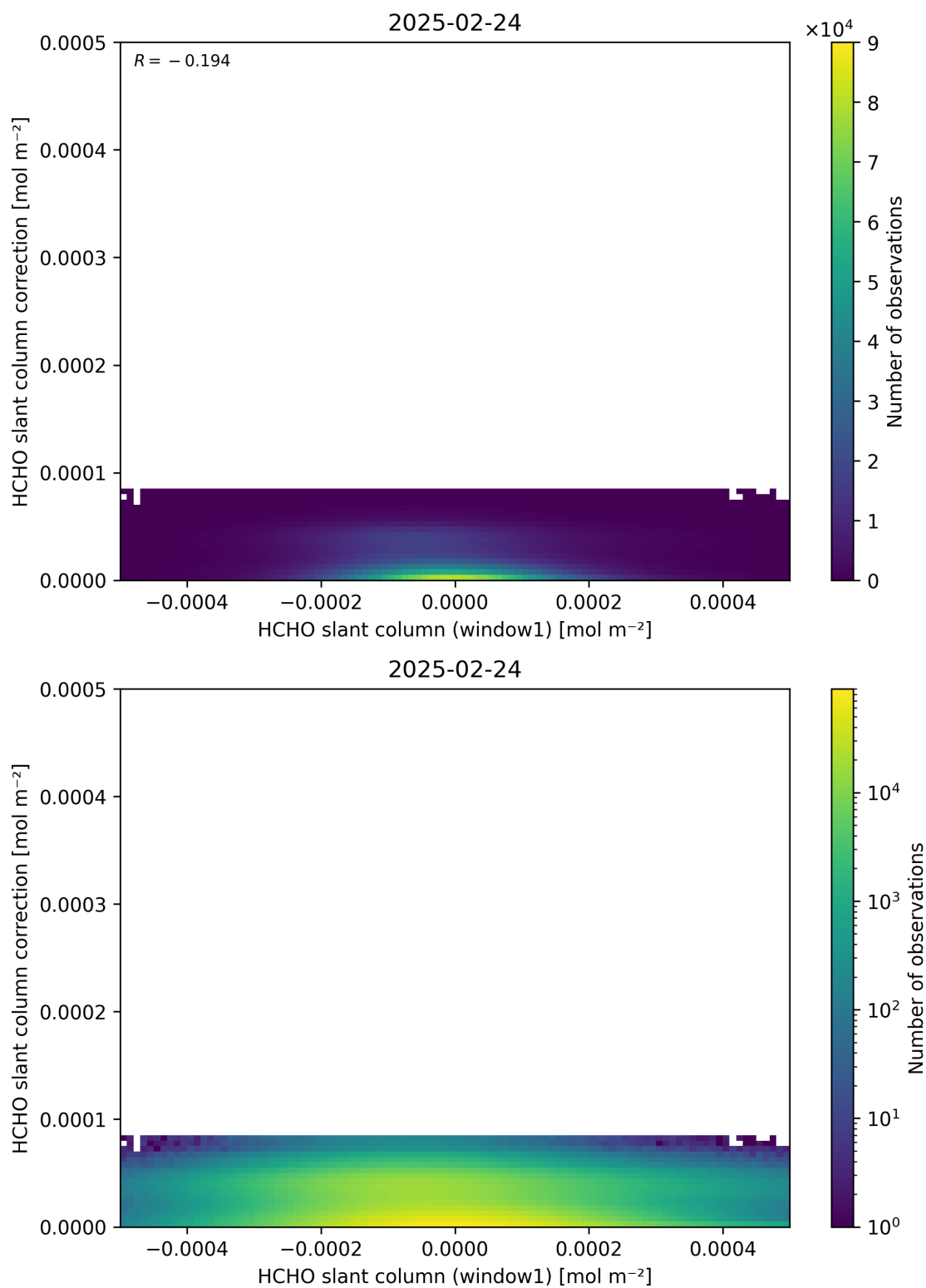
Figure 83: Scatter density plot of “HCHO slant column (window1)” against “HCHO slant column correction” for 2025-02-24 to 2025-02-25.
