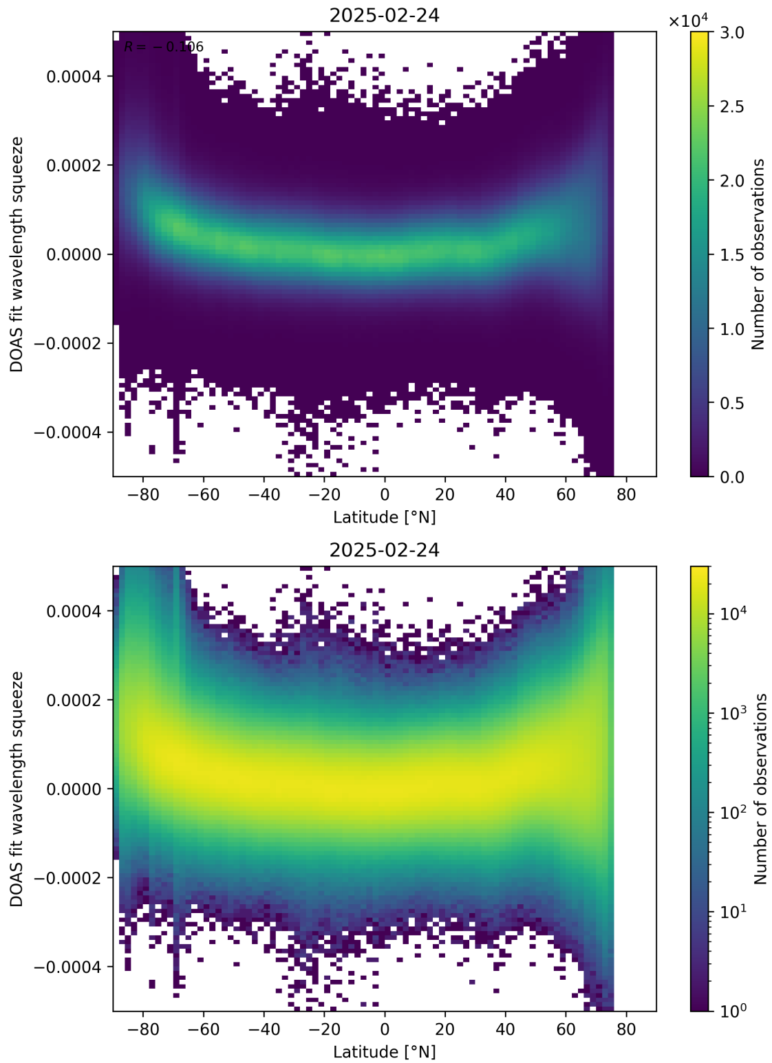
Figure 155: Scatter density plot of “Latitude” against “DOAS fit wavelength squeeze” for 2025-02-24 to 2025-02-25.
