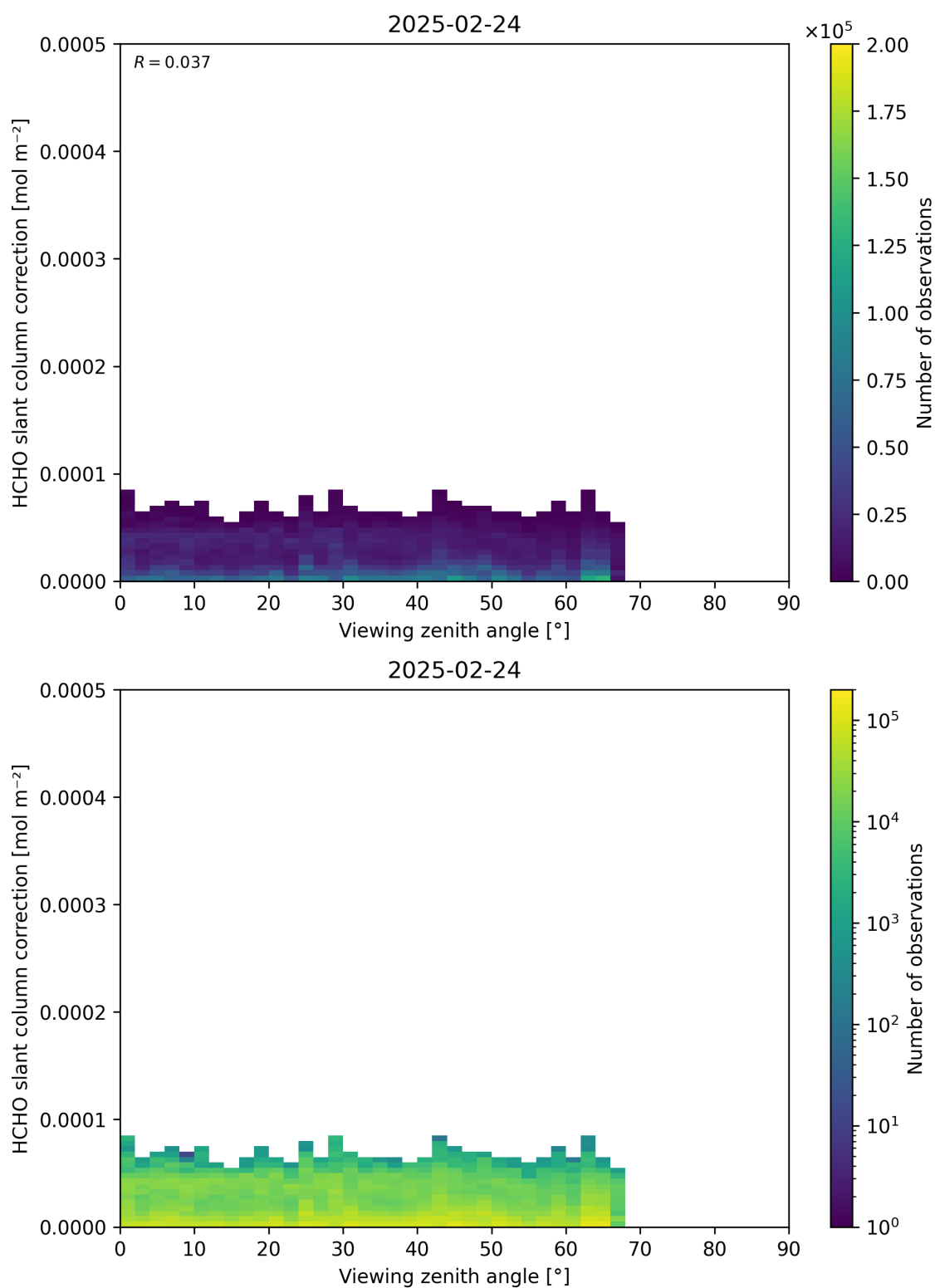
Figure 187: Scatter density plot of “Viewing zenith angle” against “HCHO slant column correction” for 2025-02-24 to 2025-02-25.
