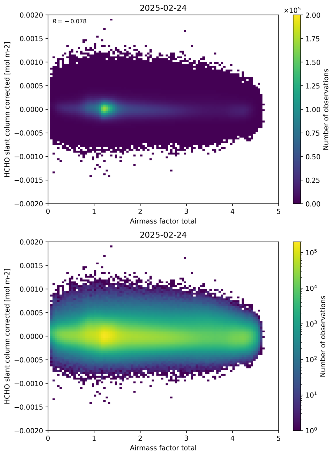
Figure 101: Scatter density plot of “Airmass factor total” against “HCHO slant column corrected” for 2025-02-24 to 2025-02-25.
