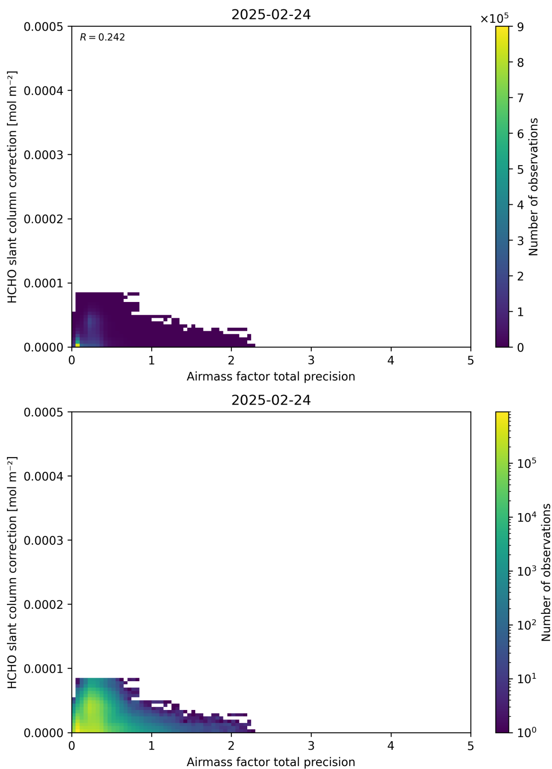
Figure 110: Scatter density plot of “Airmass factor total precision” against “HCHO slant column correction” for 2025-02-24 to 2025-02-25.
