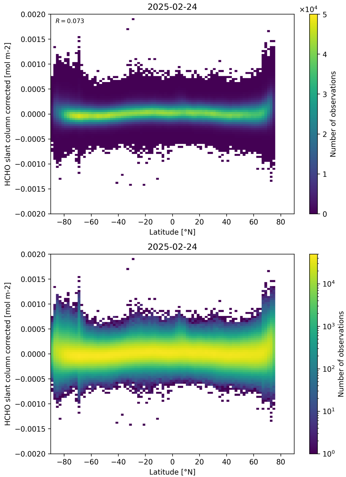
Figure 157: Scatter density plot of “Latitude” against “HCHO slant column corrected” for 2025-02-24 to 2025-02-25.
