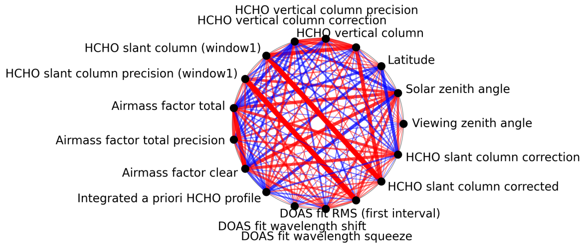
Figure 1: Map of correlation graph for 2025-02-24 to 2025-02-25.
