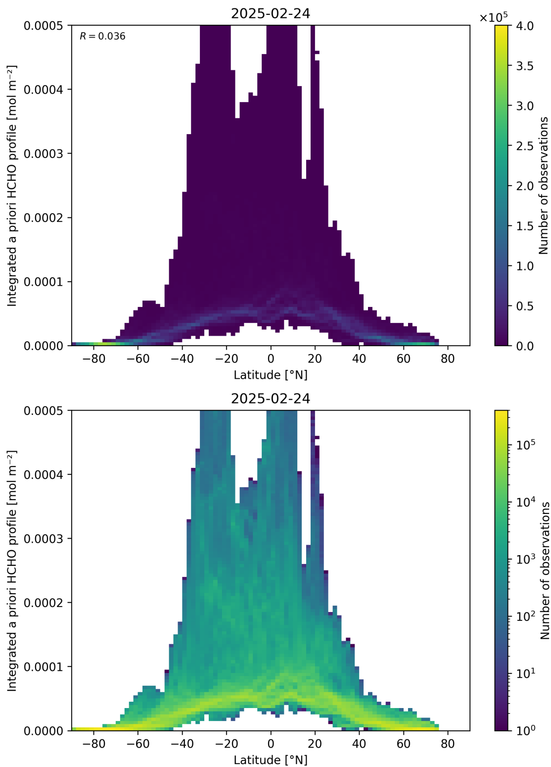
Figure 166: Scatter density plot of “Latitude” against “Integrated a priori HCHO profile” for 2025-02-24 to 2025-02-25.
