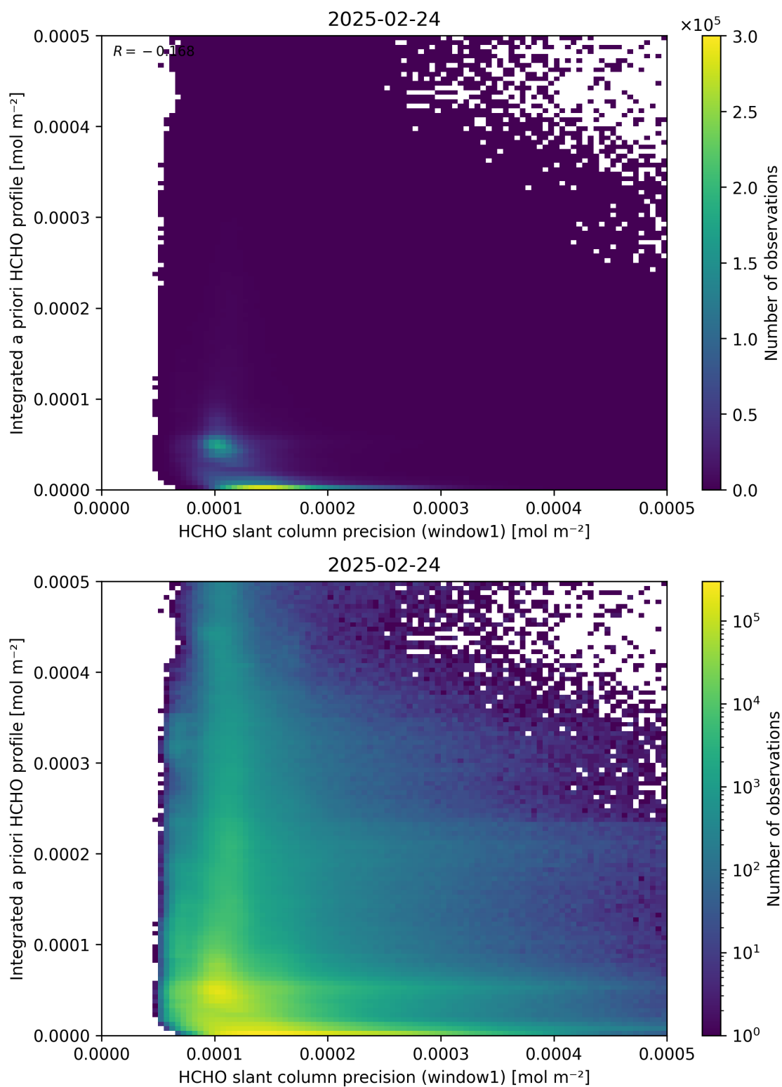
Figure 96: Scatter density plot of “HCHO slant column precision (window1)” against “Integrated a priori HCHO profile” for 2025-02-24 to 2025-02-25.
