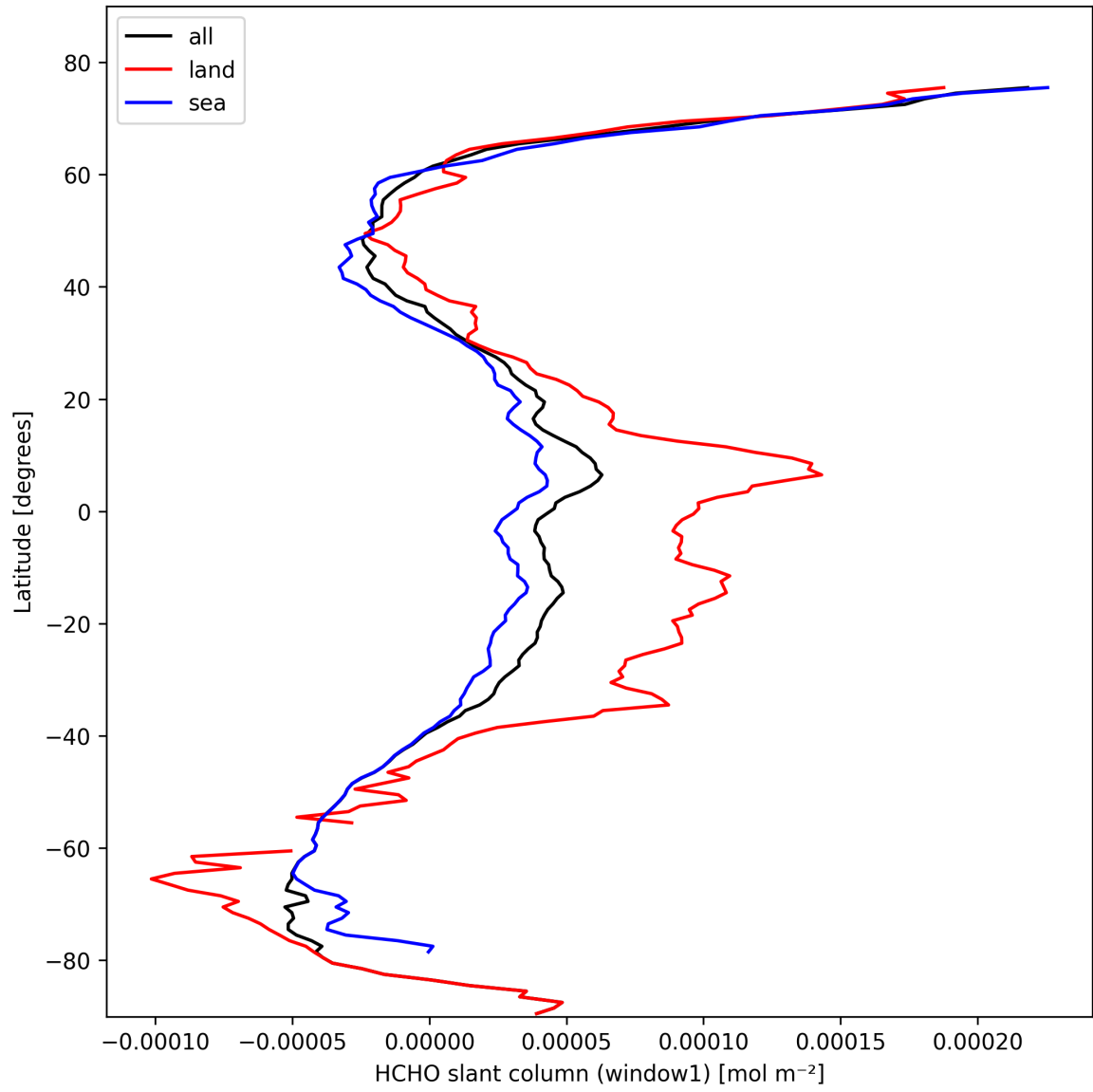
Figure 24: Zonal average of “HCHO slant column (window1)” for 2025-02-24 to 2025-02-25.
