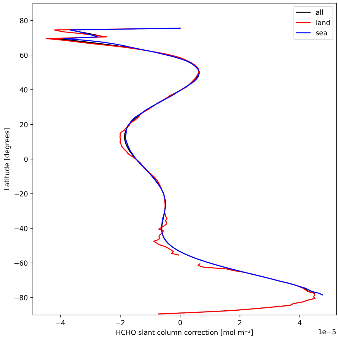
Figure 33: Zonal average of “HCHO slant column correction” for 2025-02-24 to 2025-02-25.
