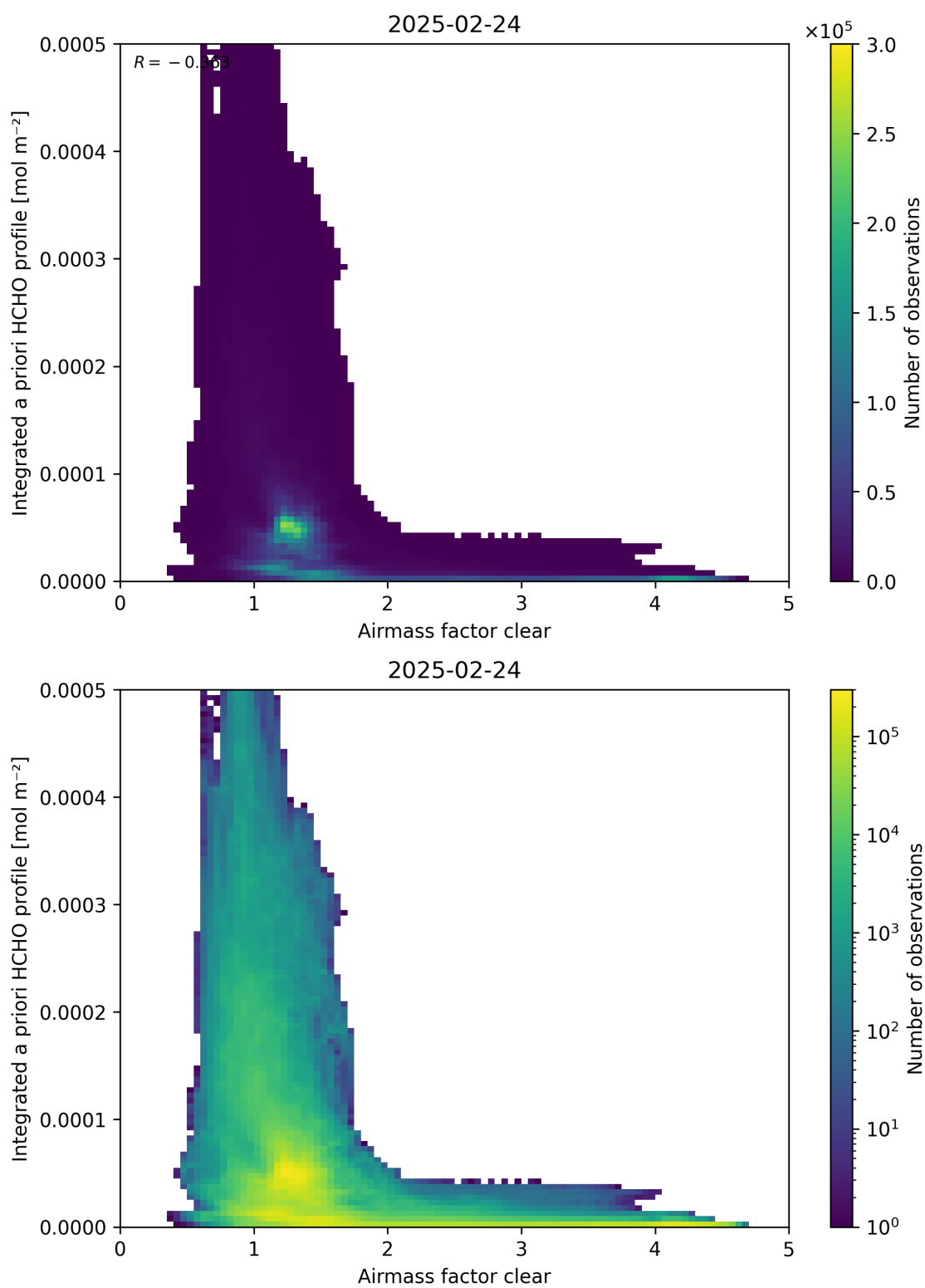
Figure 76: Scatter density plot of “Airmass factor clear” against “Integrated a priori HCHO profile” for 2025-02-24 to 2025-02-25.
