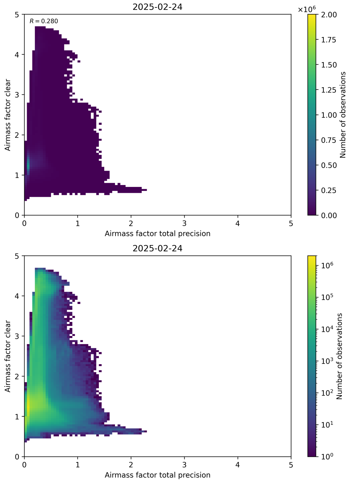
Figure 108: Scatter density plot of “Airmass factor total precision” against “Airmass factor clear” for 2025-02-24 to 2025-02-25.
