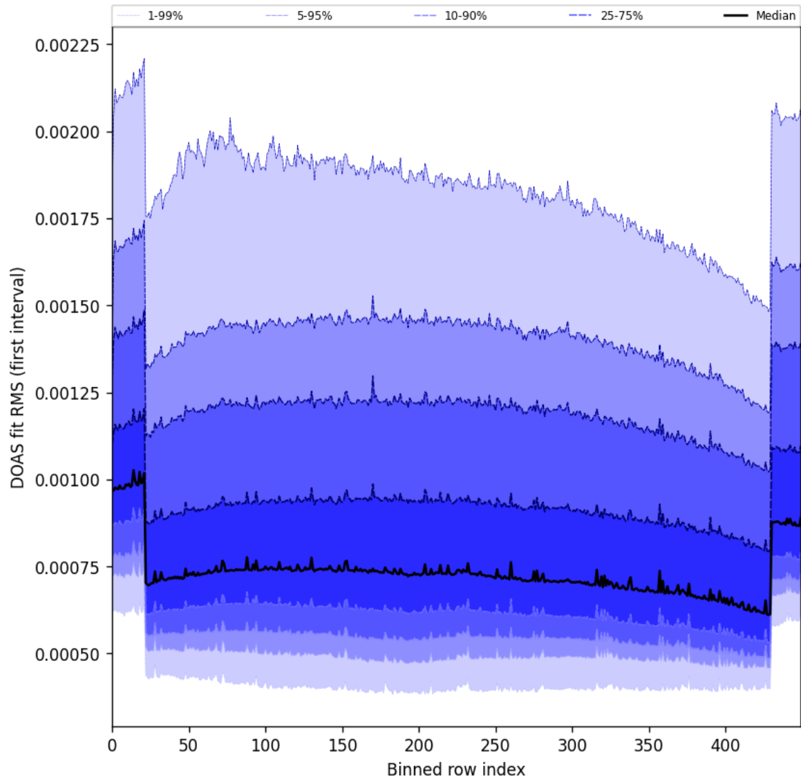
Figure 60: Along track statistics of “DOAS fit RMS (first interval)” for 2025-02-24 to 2025-02-25
