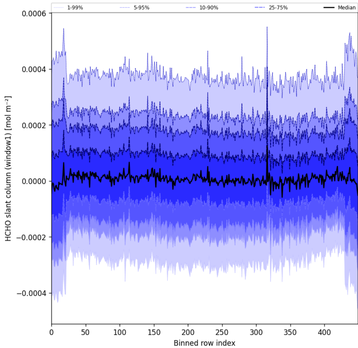
Figure 52: Along track statistics of “HCHO slant column (window1)” for 2025-02-24 to 2025-02-25
