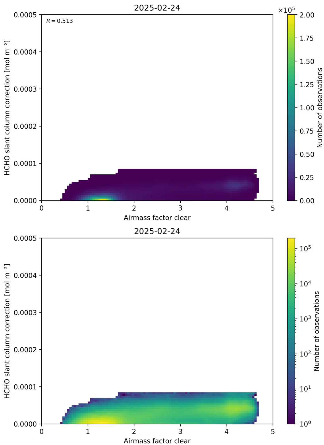
Figure 75: Scatter density plot of “Airmass factor clear” against “HCHO slant column correction” for 2025-02-24 to 2025-02-25.
