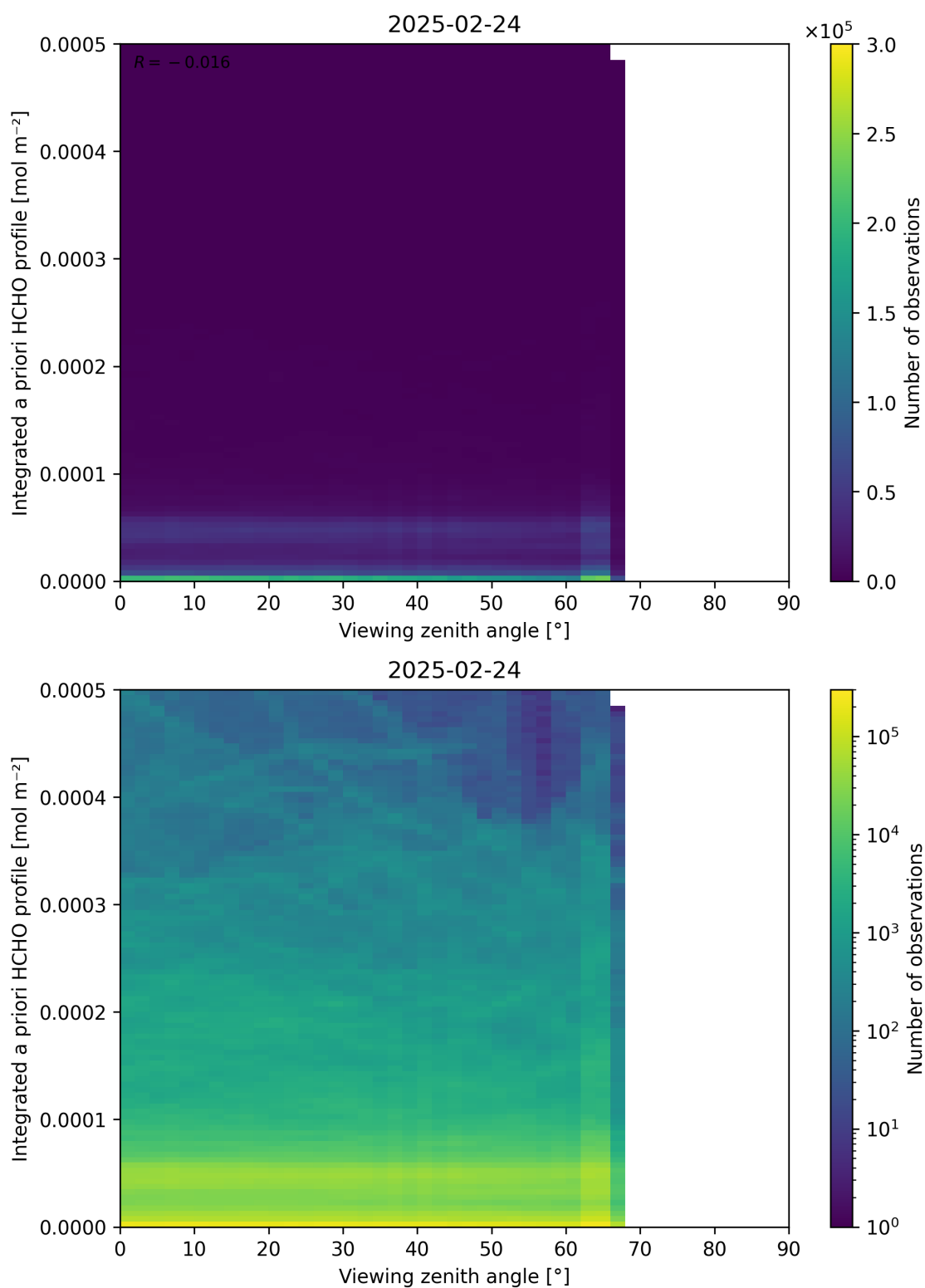
Figure 195: Scatter density plot of “Viewing zenith angle” against “Integrated a priori HCHO profile” for 2025-02-24 to 2025-02-25.
