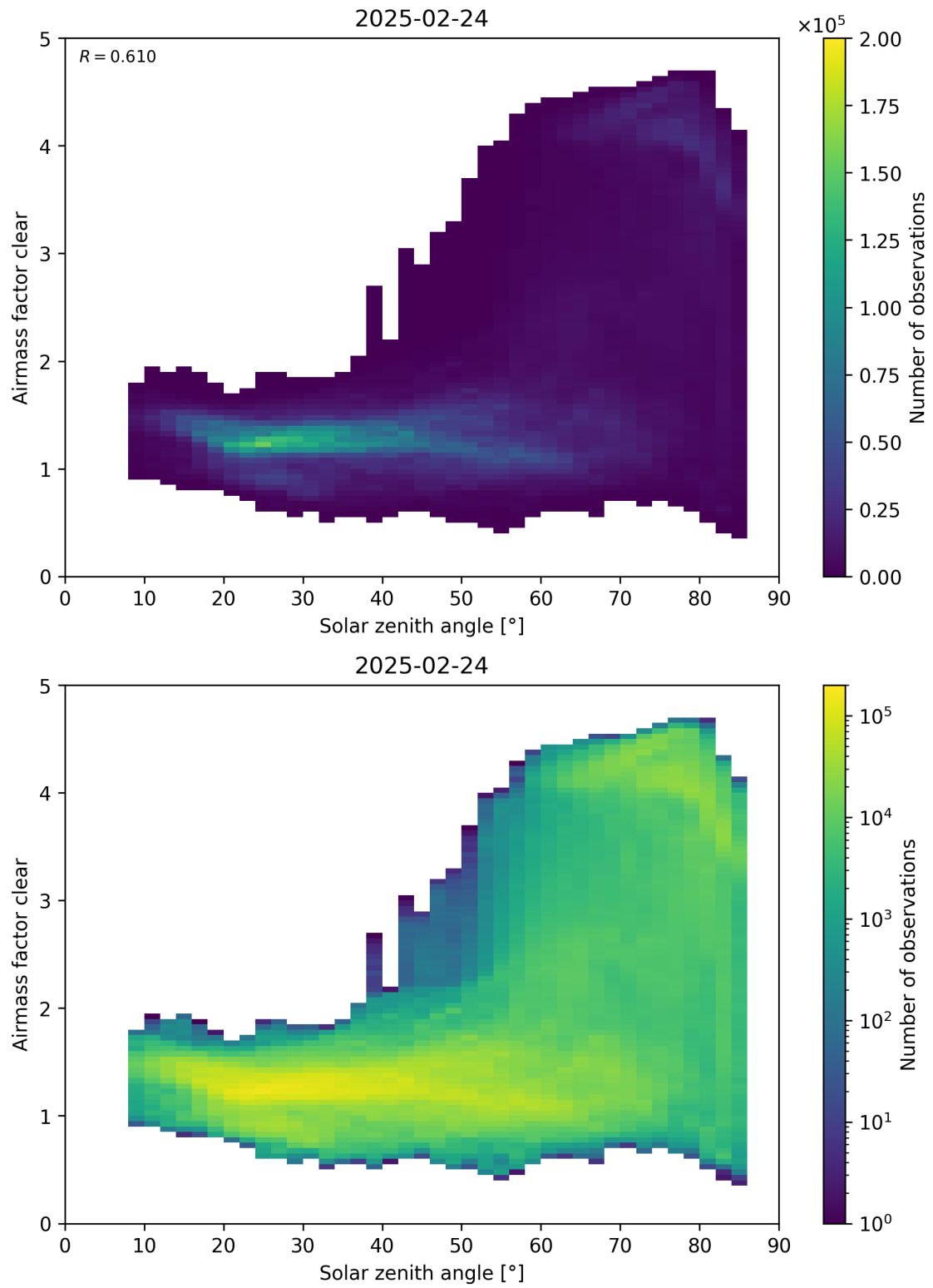
Figure 170: Scatter density plot of “Solar zenith angle” against “Airmass factor clear” for 2025-02-24 to 2025-02-25.
