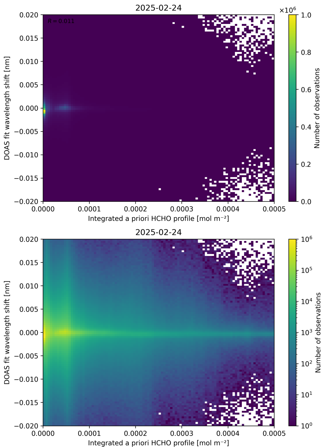
Figure 149: Scatter density plot of “Integrated a priori HCHO profile” against “DOAS fit wavelength shift” for 2025-02-24 to 2025-02-25.
