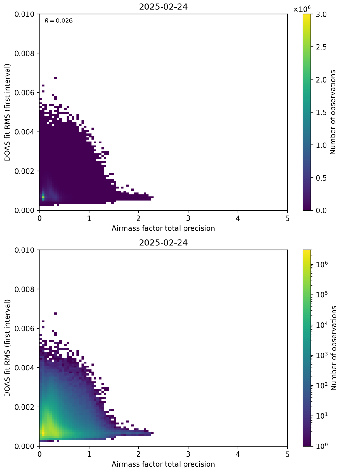
Figure 105: Scatter density plot of “Airmass factor total precision” against “DOAS fit RMS (first interval)” for 2025-02-24 to 2025-02-25.
