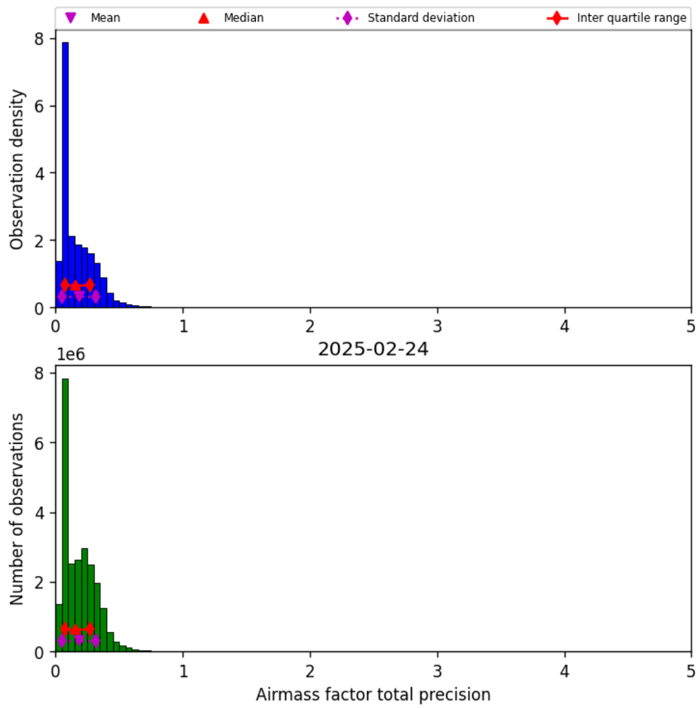
Figure 41: Histogram of “Airmass factor total precision” for 2025-02-24 to 2025-02-25
