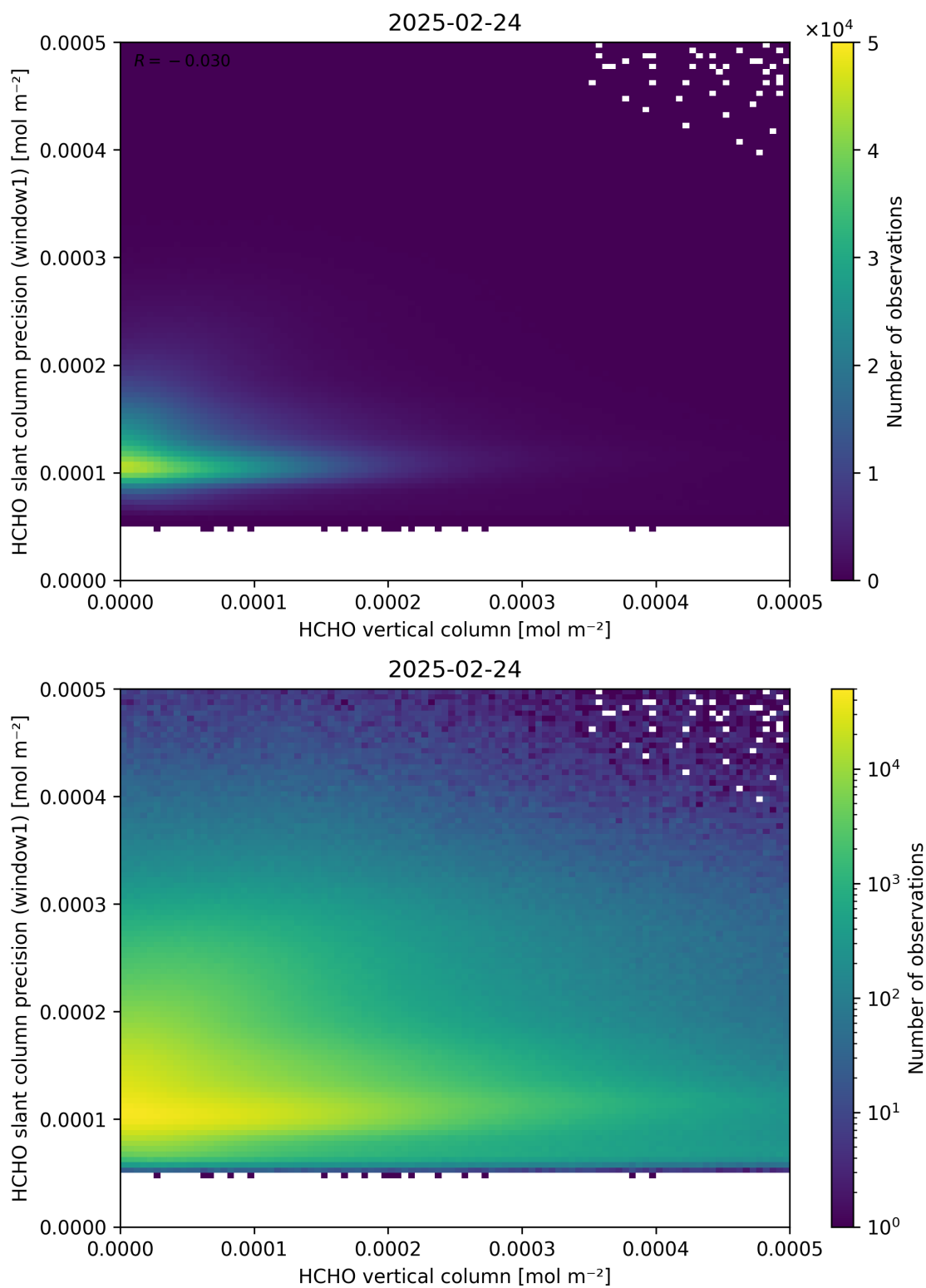
Figure 130: Scatter density plot of “HCHO vertical column” against “HCHO slant column precision (window1)” for 2025-02-24 to 2025-02-25.
