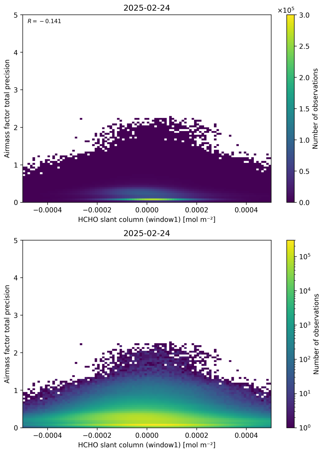
Figure 86: Scatter density plot of “HCHO slant column (window1)” against “Airmass factor total precision” for 2025-02-24 to 2025-02-25.
