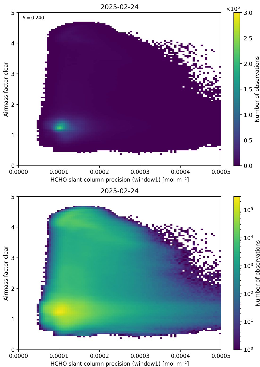
Figure 91: Scatter density plot of “HCHO slant column precision (window1)” against “Airmass factor clear” for 2025-02-24 to 2025-02-25.
