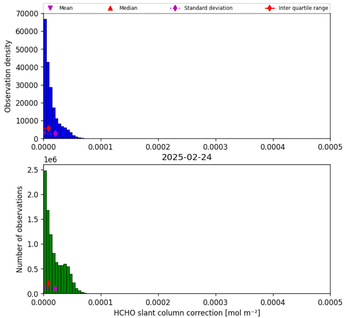
Figure 47: Histogram of “HCHO slant column correction” for 2025-02-24 to 2025-02-25
