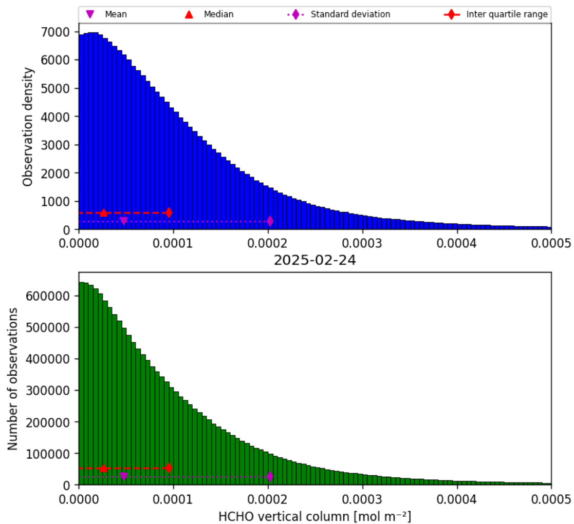
Figure 35: Histogram of “HCHO vertical column” for 2025-02-24 to 2025-02-25
