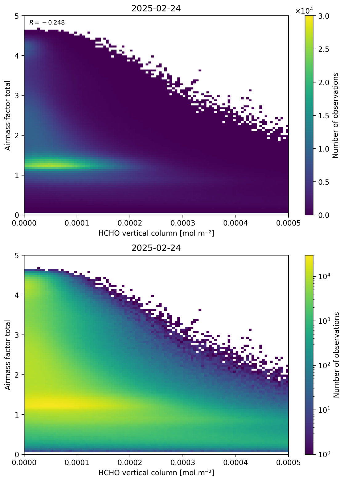
Figure 131: Scatter density plot of “HCHO vertical column” against “Airmass factor total” for 2025-02-24 to 2025-02-25.
