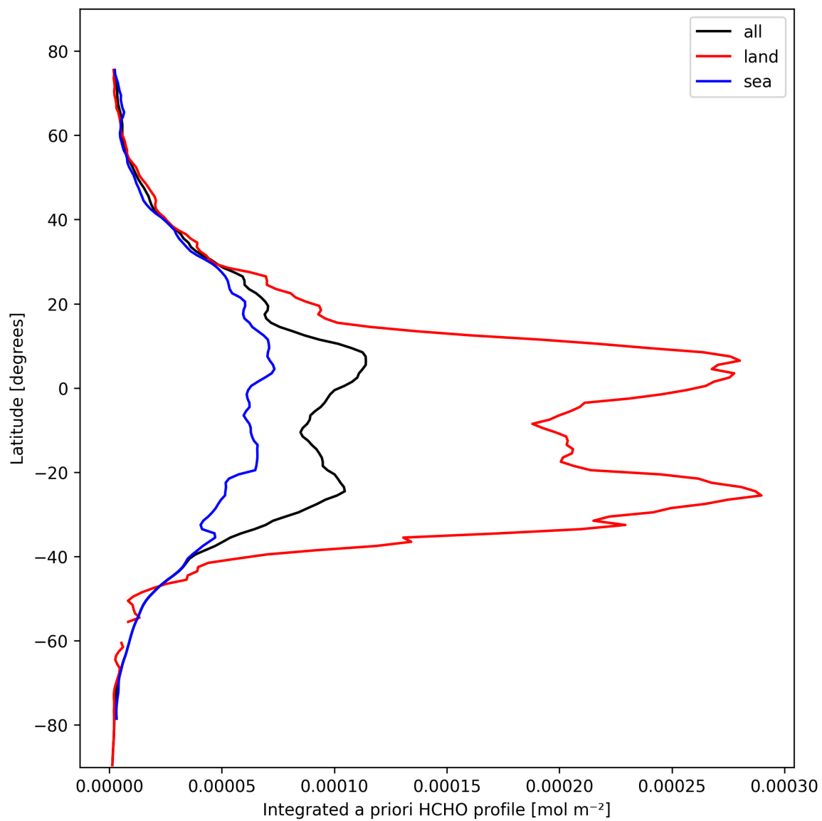
Figure 29: Zonal average of “Integrated a priori HCHO profile” for 2025-02-24 to 2025-02-25.
