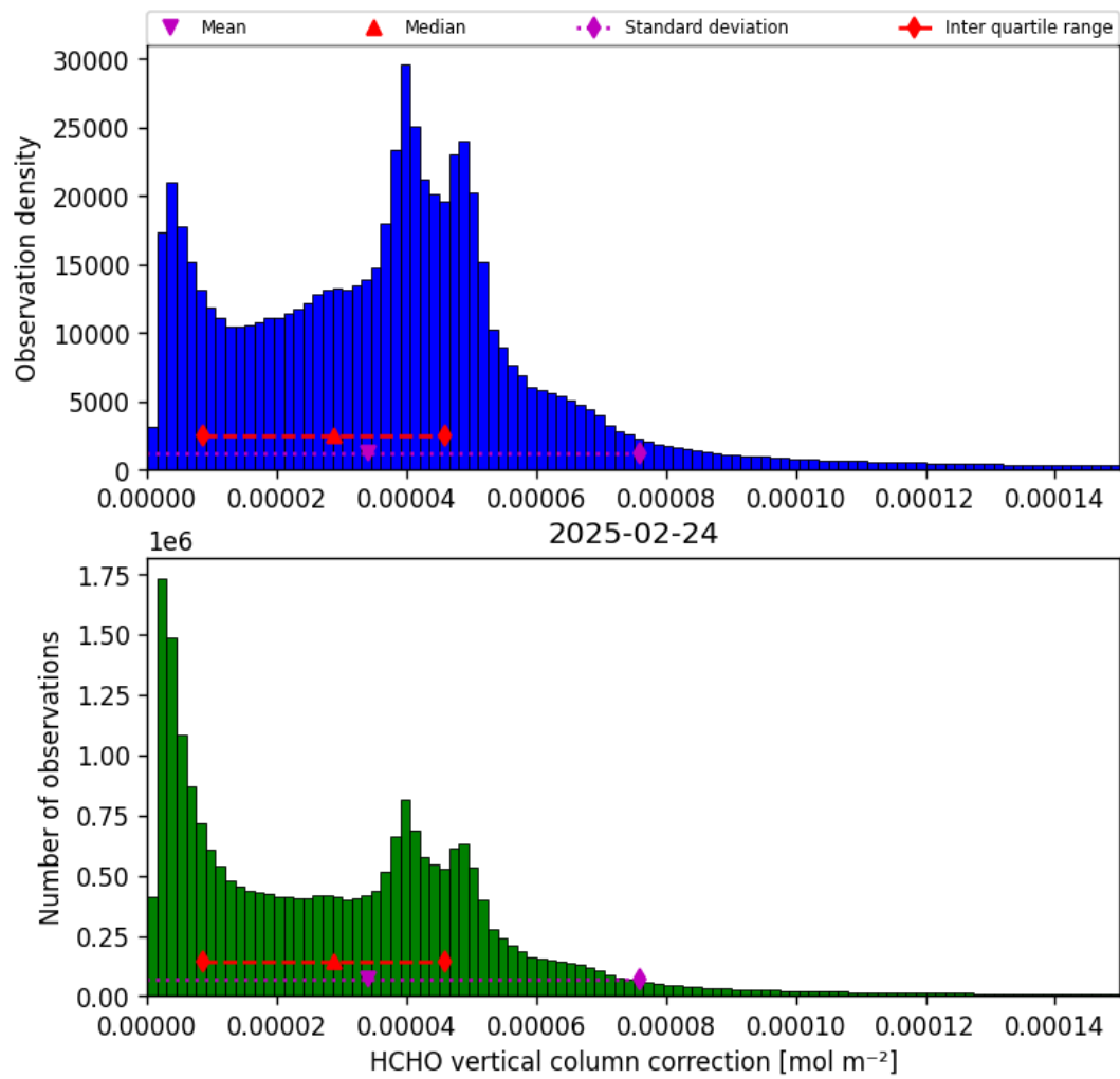
Figure 37: Histogram of “HCHO vertical column correction” for 2025-02-24 to 2025-02-25
