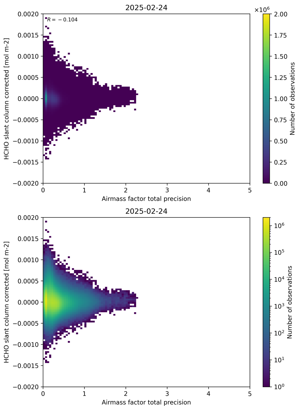
Figure 109: Scatter density plot of “Airmass factor total precision” against “HCHO slant column corrected” for 2025-02-24 to 2025-02-25.
