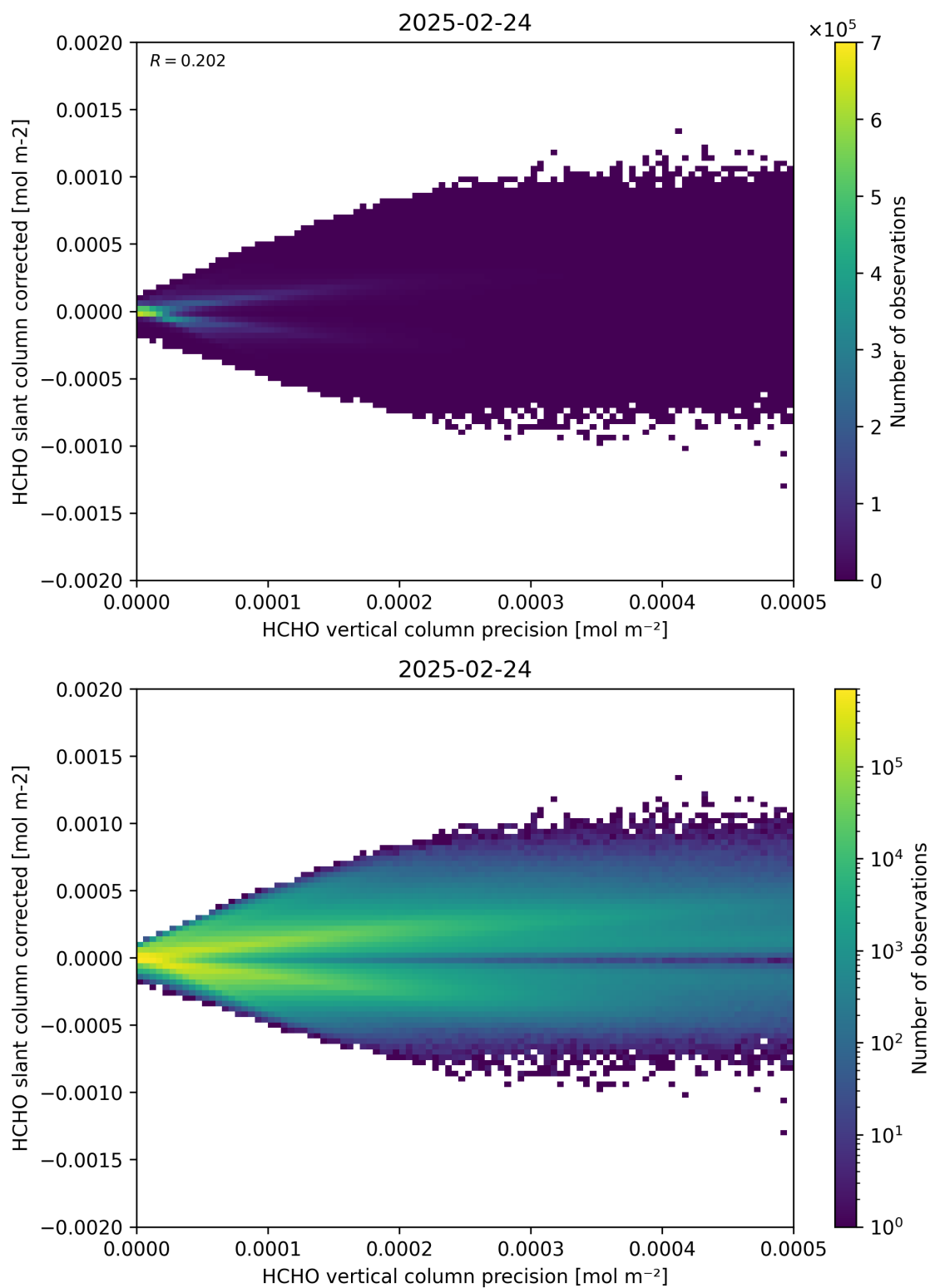
Figure 140: Scatter density plot of “HCHO vertical column precision” against “HCHO slant column corrected” for 2025-02-24 to 2025-02-25.
