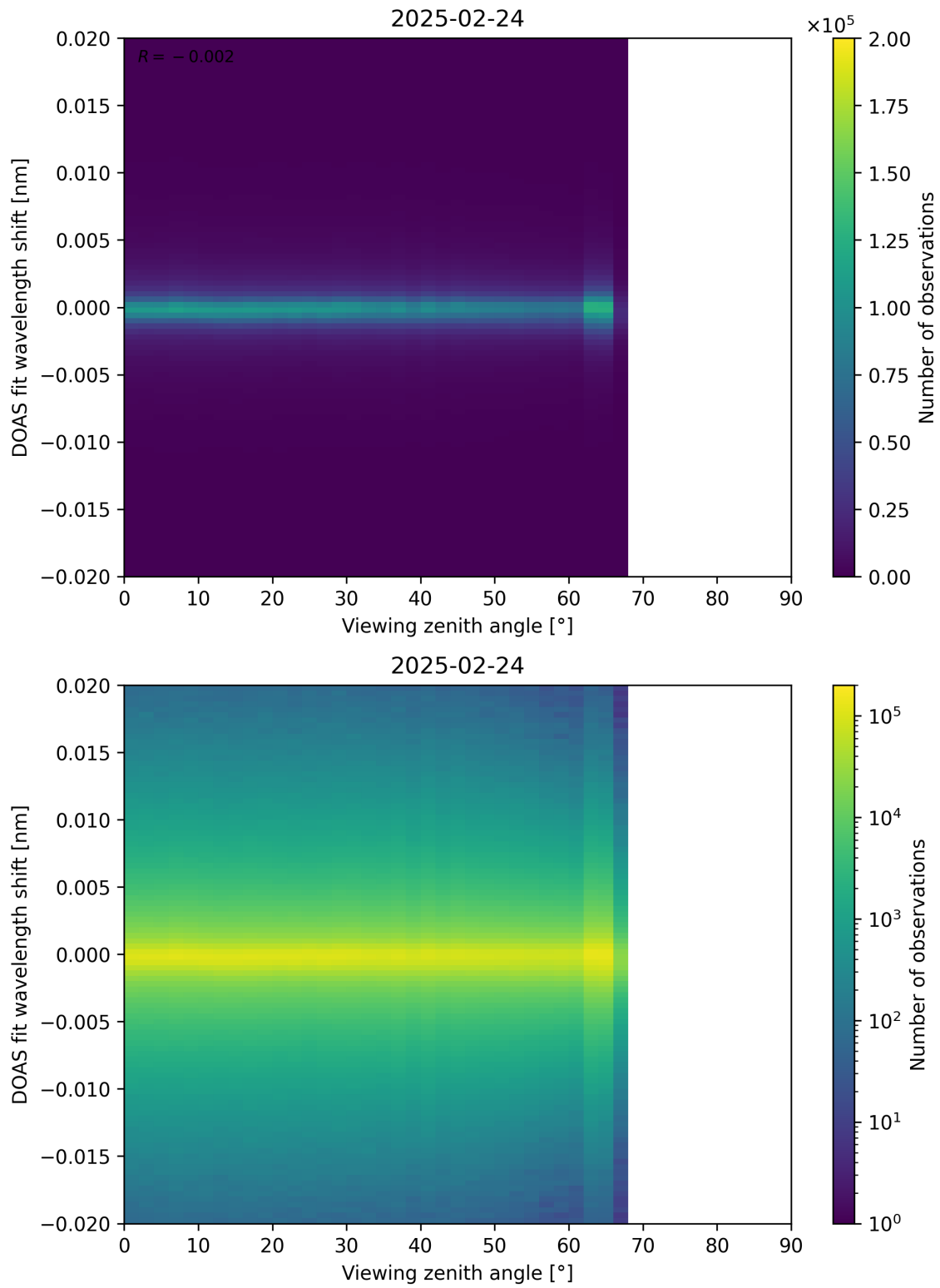
Figure 183: Scatter density plot of “Viewing zenith angle” against “DOAS fit wavelength shift” for 2025-02-24 to 2025-02-25.
