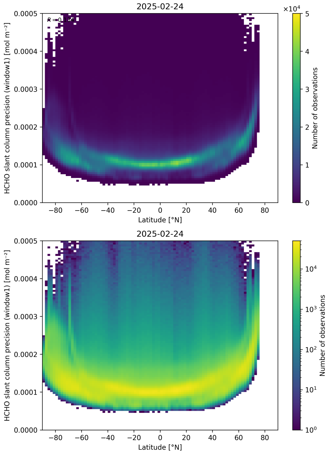
Figure 160: Scatter density plot of “Latitude” against “HCHO slant column precision (window1)” for 2025-02-24 to 2025-02-25.
