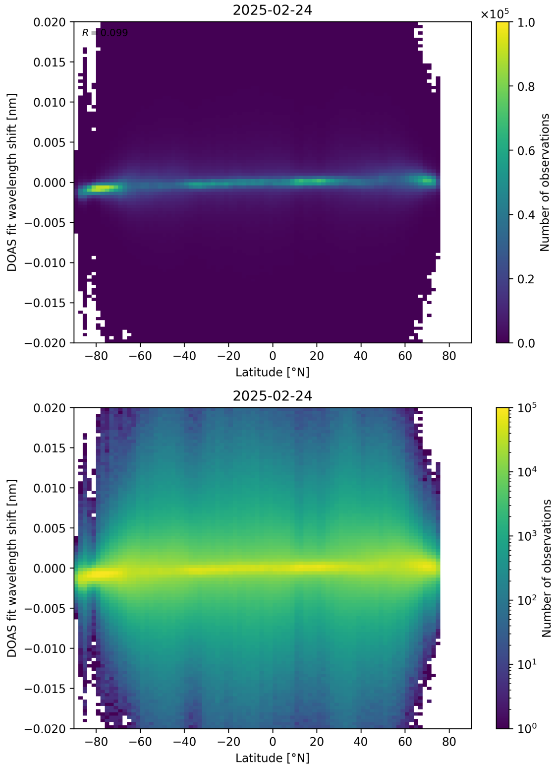
Figure 154: Scatter density plot of “Latitude” against “DOAS fit wavelength shift” for 2025-02-24 to 2025-02-25.
