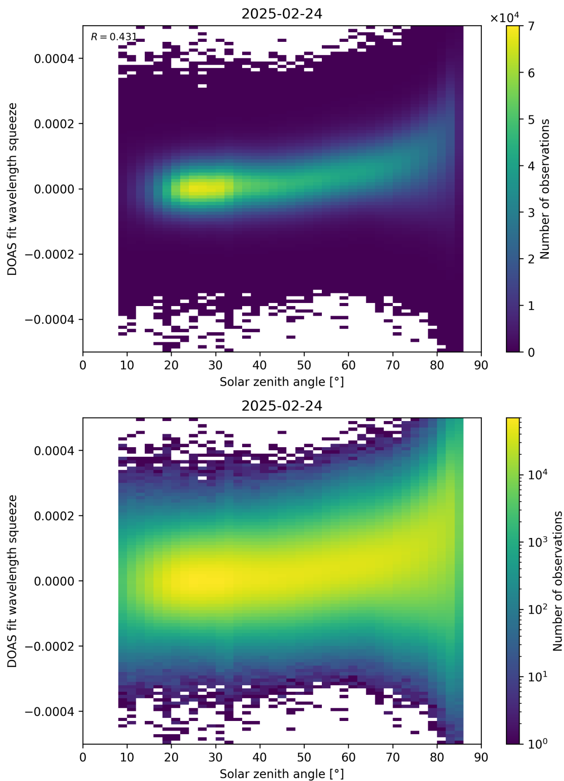
Figure 169: Scatter density plot of “Solar zenith angle” against “DOAS fit wavelength squeeze” for 2025-02-24 to 2025-02-25.
