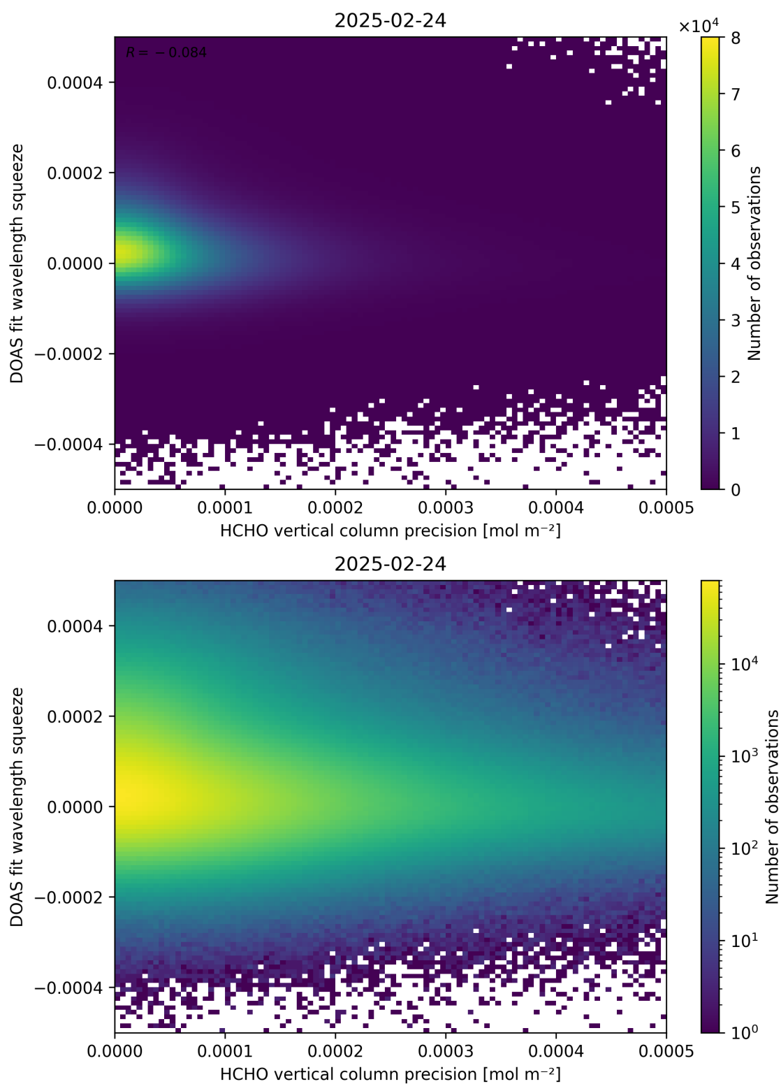
Figure 138: Scatter density plot of “HCHO vertical column precision” against “DOAS fit wavelength squeeze” for 2025-02-24 to 2025-02-25.
