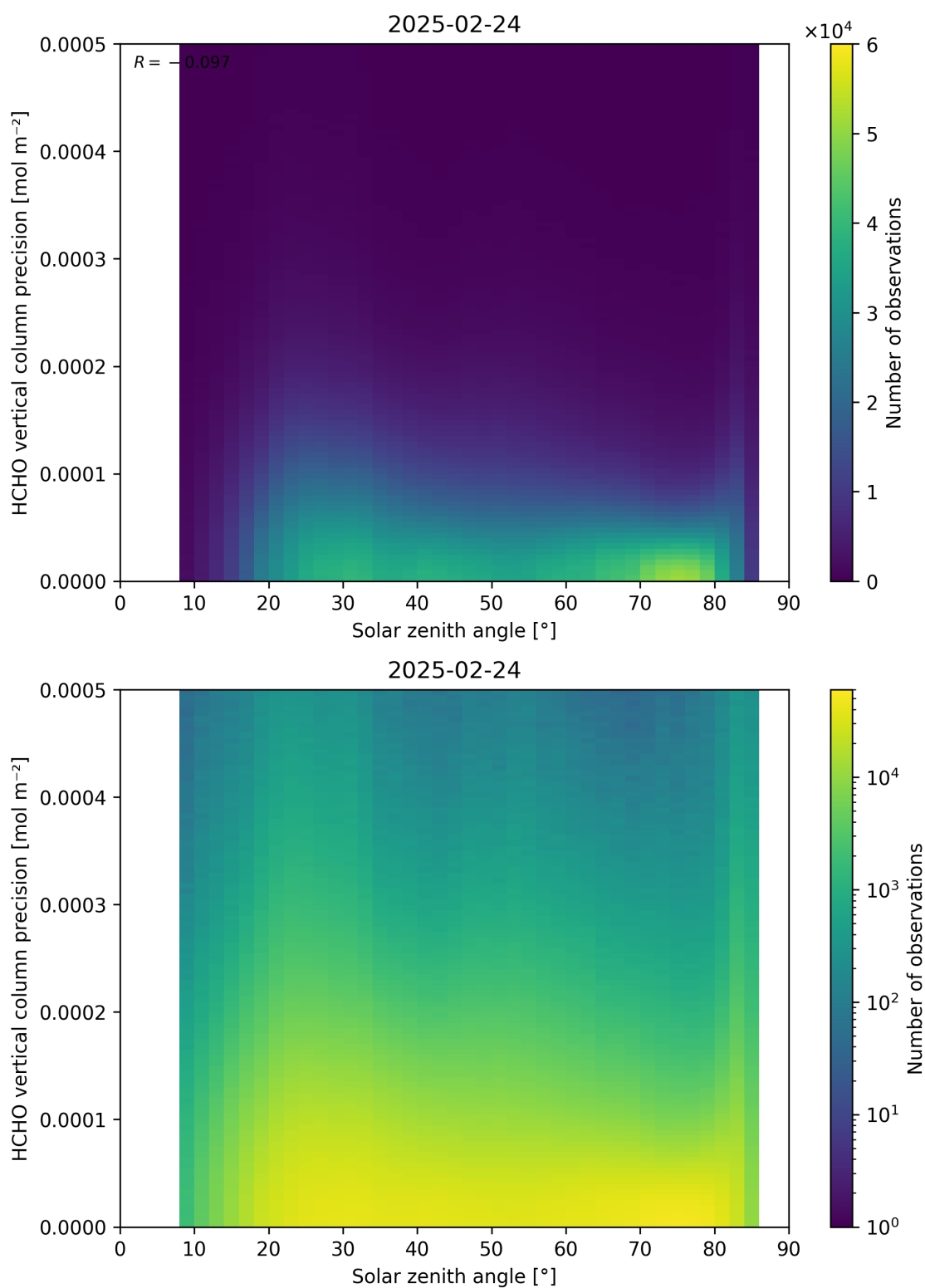
Figure 179: Scatter density plot of “Solar zenith angle” against “HCHO vertical column precision” for 2025-02-24 to 2025-02-25.
