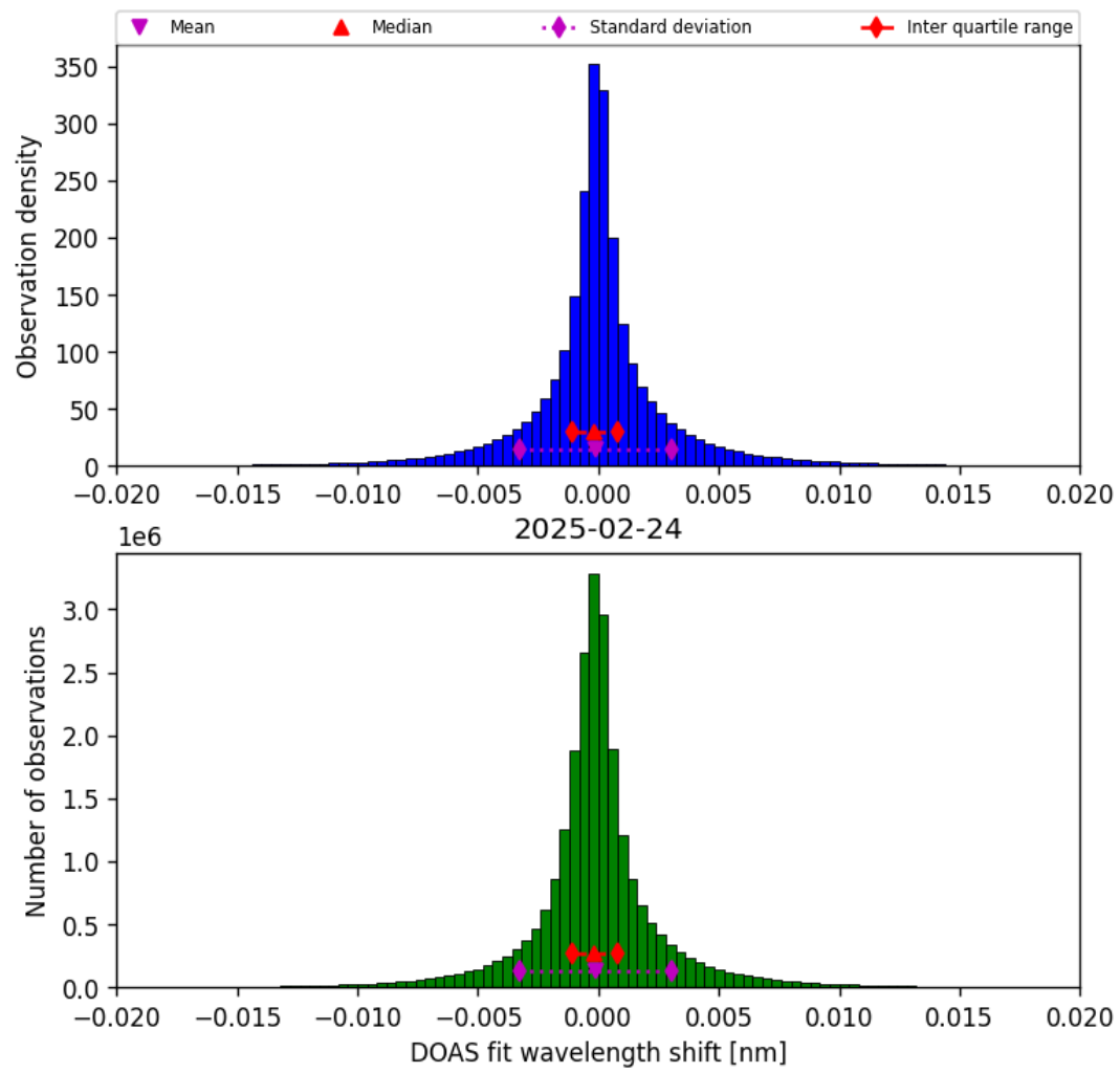
Figure 44: Histogram of “DOAS fit wavelength shift” for 2025-02-24 to 2025-02-25
