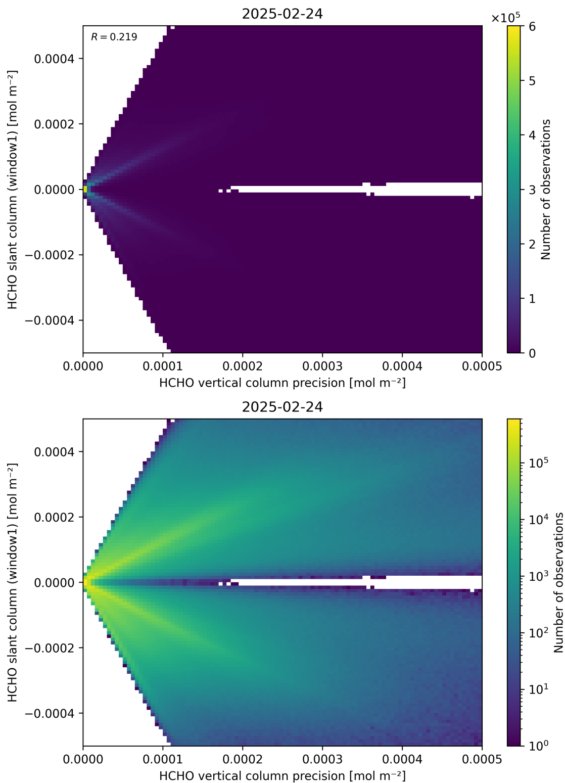
Figure 142: Scatter density plot of “HCHO vertical column precision” against “HCHO slant column (window1)” for 2025-02-24 to 2025-02-25.
