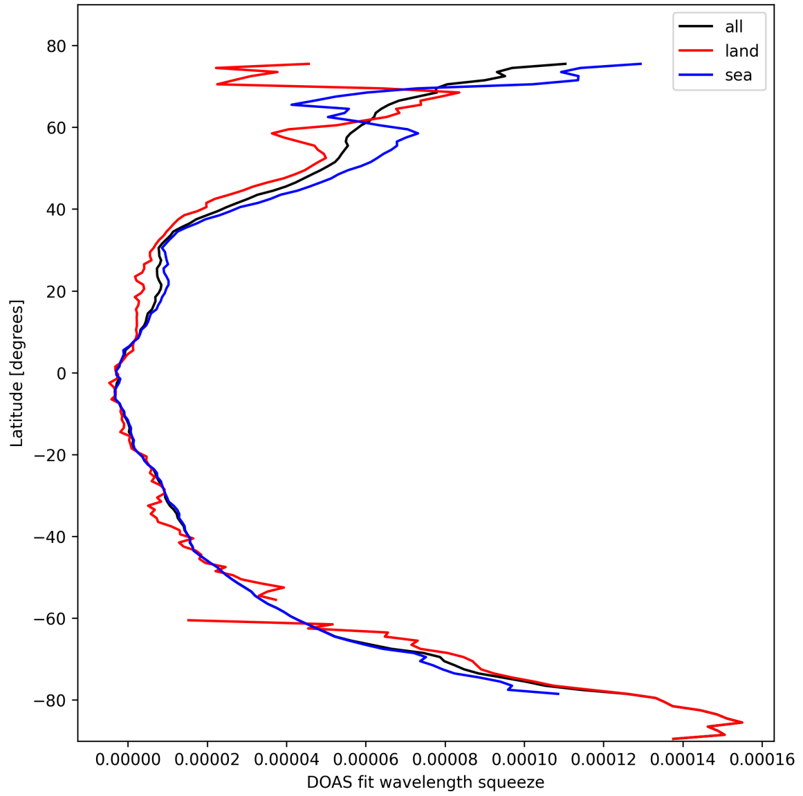
Figure 31: Zonal average of “DOAS fit wavelength squeeze” for 2025-02-24 to 2025-02-25.
