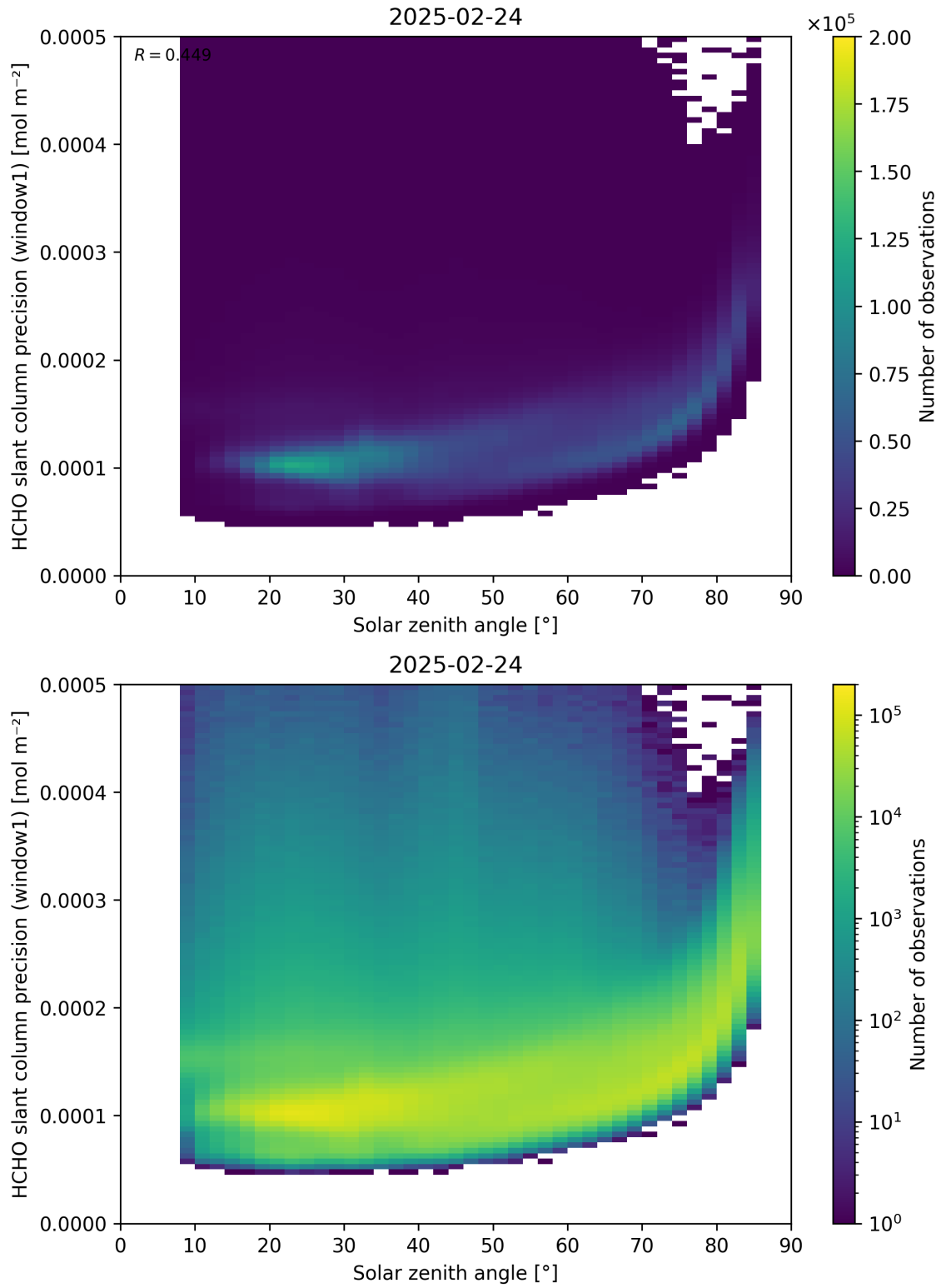
Figure 174: Scatter density plot of “Solar zenith angle” against “HCHO slant column precision (window1)” for 2025-02-24 to 2025-02-25.
