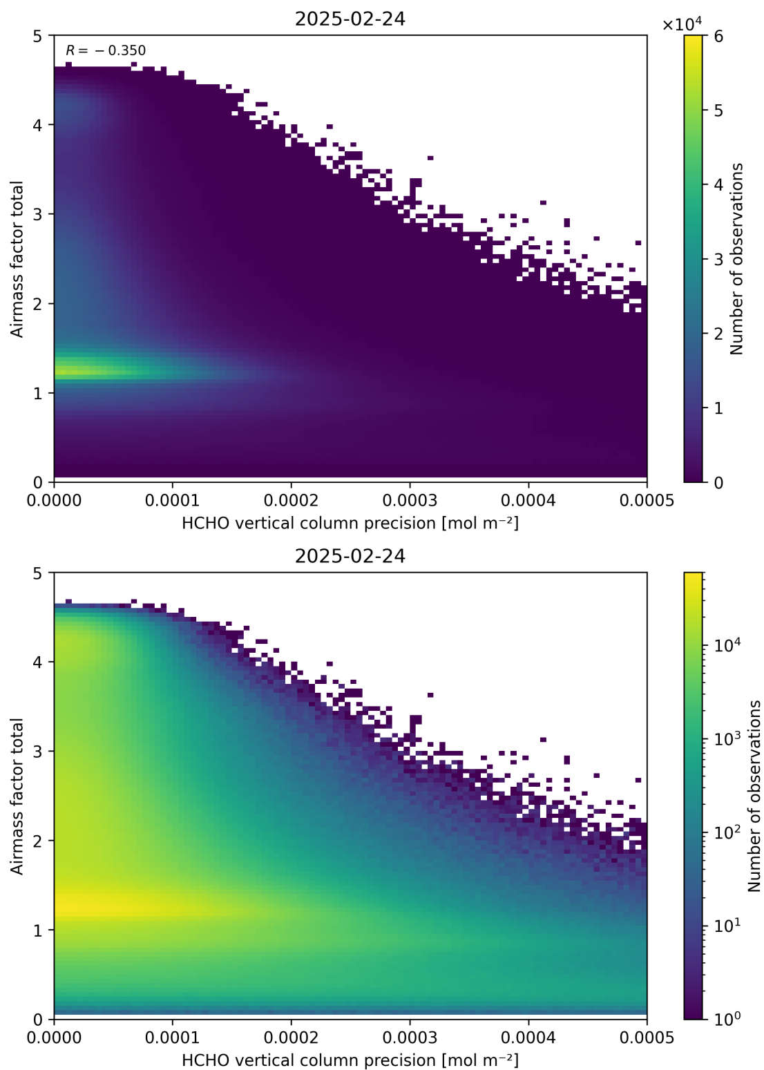
Figure 144: Scatter density plot of “HCHO vertical column precision” against “Airmass factor total” for 2025-02-24 to 2025-02-25.
