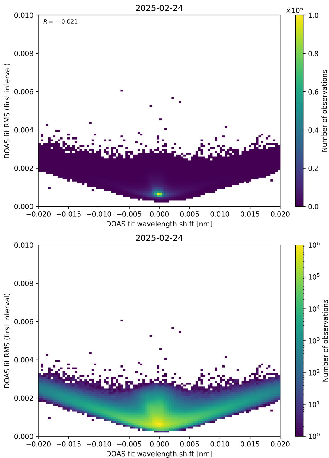
Figure 64: Scatter density plot of “DOAS fit wavelength shift” against “DOAS fit RMS (first interval)” for 2025-02-24 to 2025-02-25.
