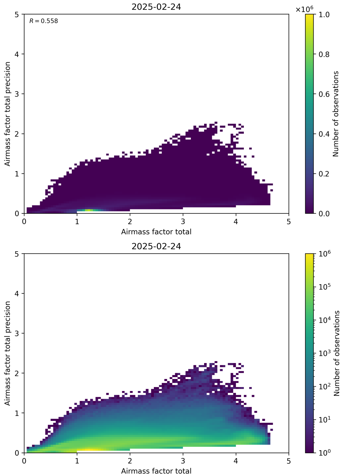
Figure 103: Scatter density plot of “Airmass factor total” against “Airmass factor total precision” for 2025-02-24 to 2025-02-25.
