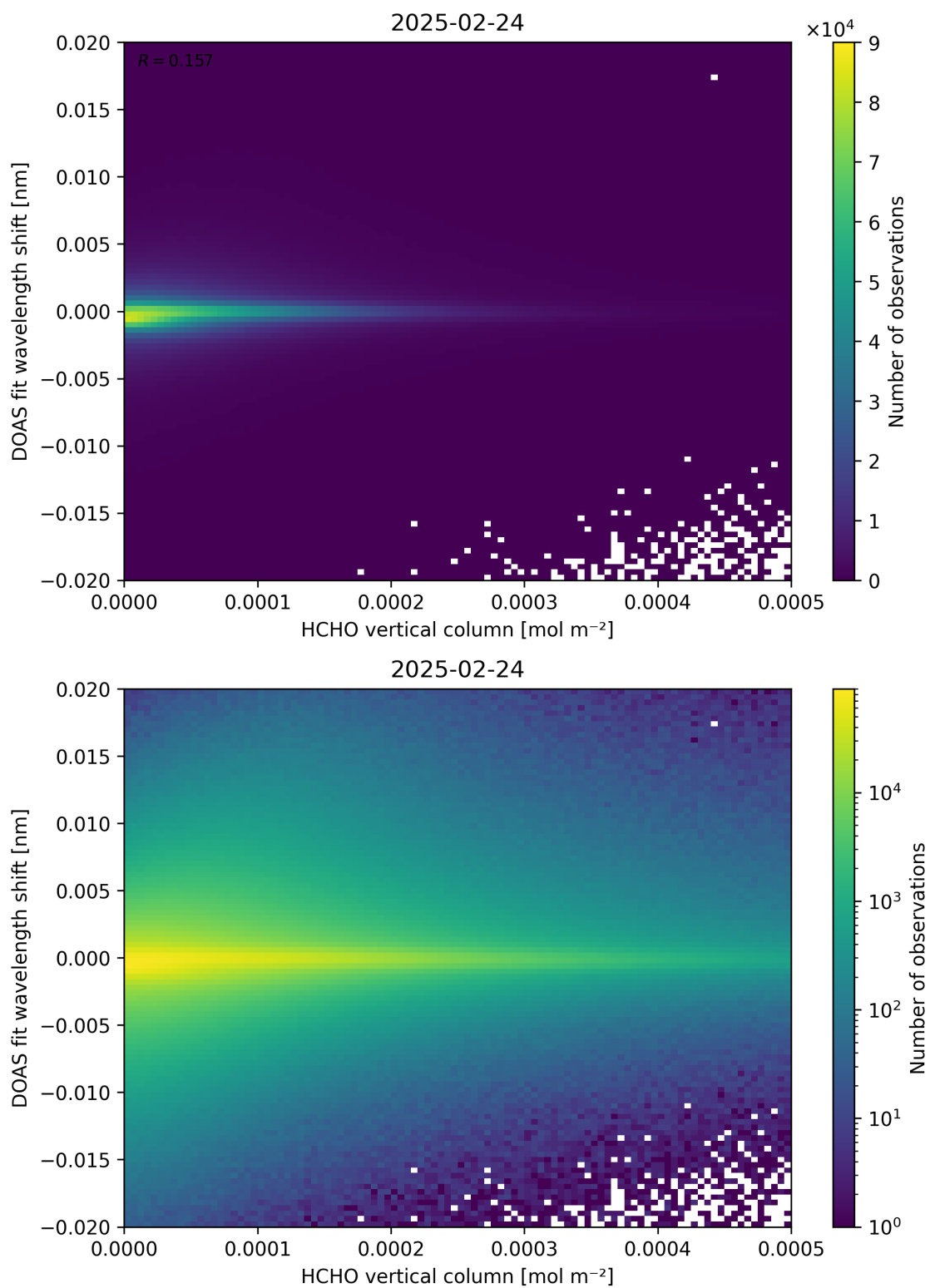
Figure 124: Scatter density plot of “HCHO vertical column” against “DOAS fit wavelength shift” for 2025-02-24 to 2025-02-25.
