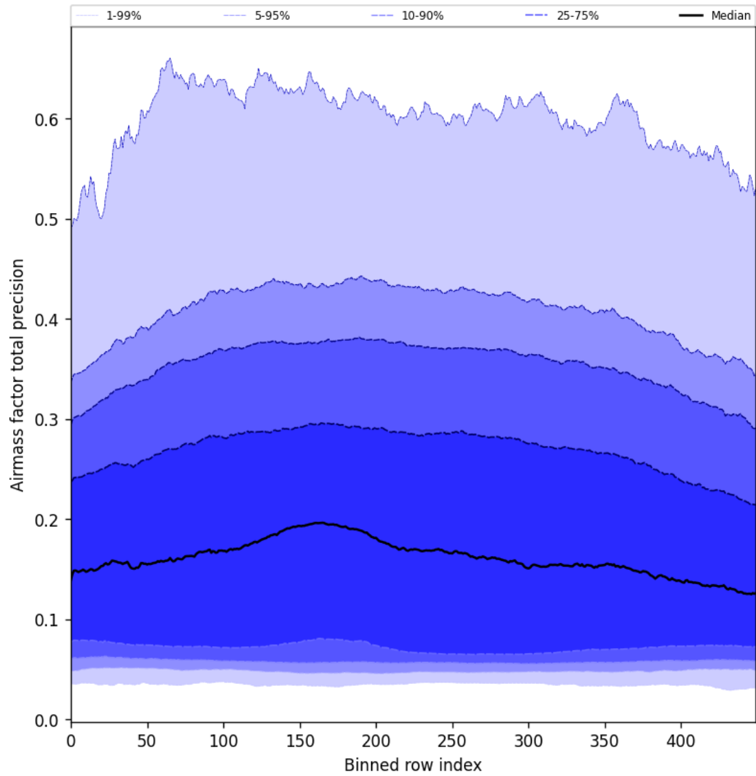
Figure 55: Along track statistics of “Airmass factor total precision” for 2025-02-24 to 2025-02-25
