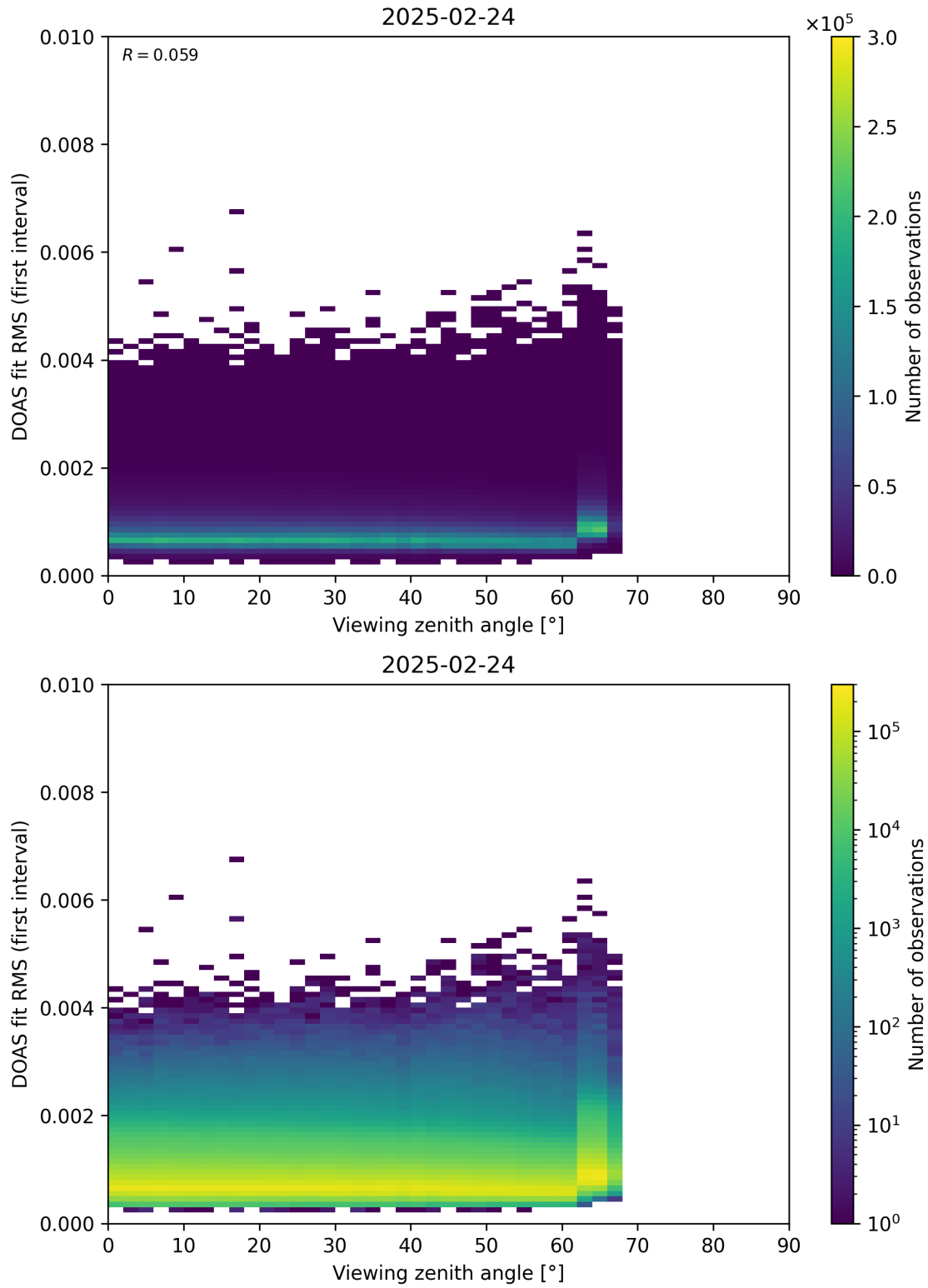
Figure 182: Scatter density plot of “Viewing zenith angle” against “DOAS fit RMS (first interval)” for 2025-02-24 to 2025-02-25.
