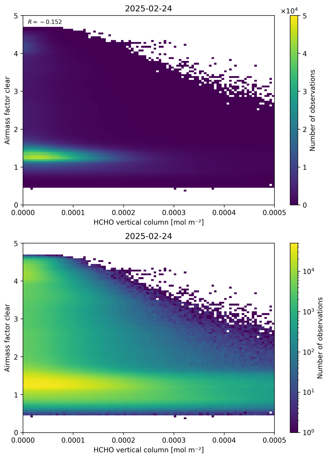
Figure 126: Scatter density plot of “HCHO vertical column” against “Airmass factor clear” for 2025-02-24 to 2025-02-25.
