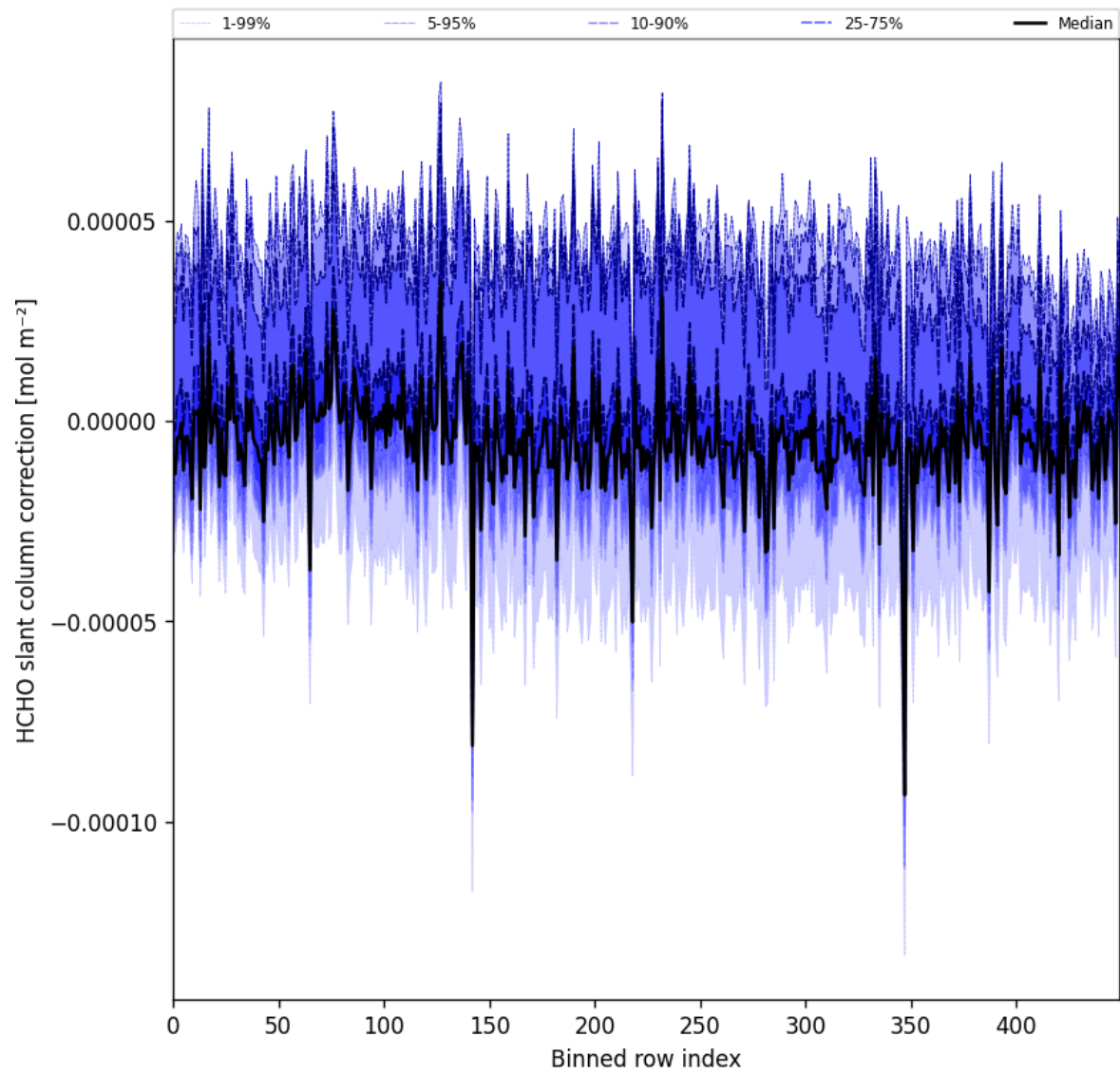
Figure 61: Along track statistics of “HCHO slant column correction” for 2025-02-24 to 2025-02-25
