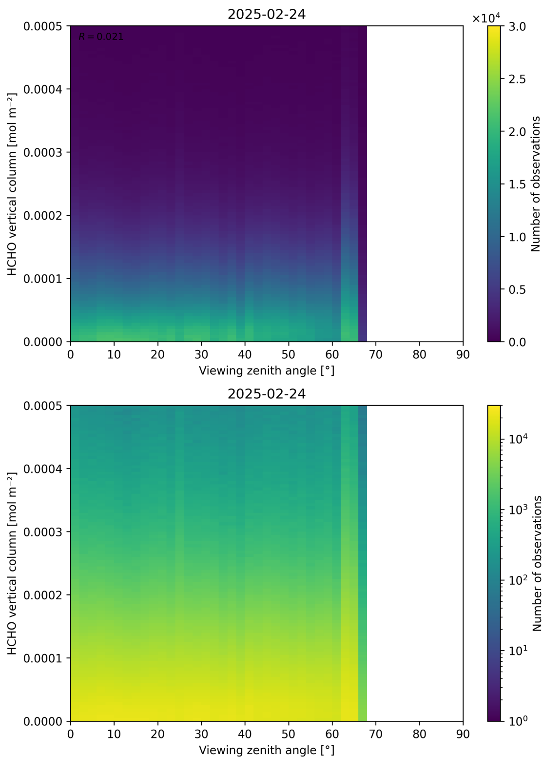
Figure 192: Scatter density plot of “Viewing zenith angle” against “HCHO vertical column” for 2025-02-24 to 2025-02-25.
