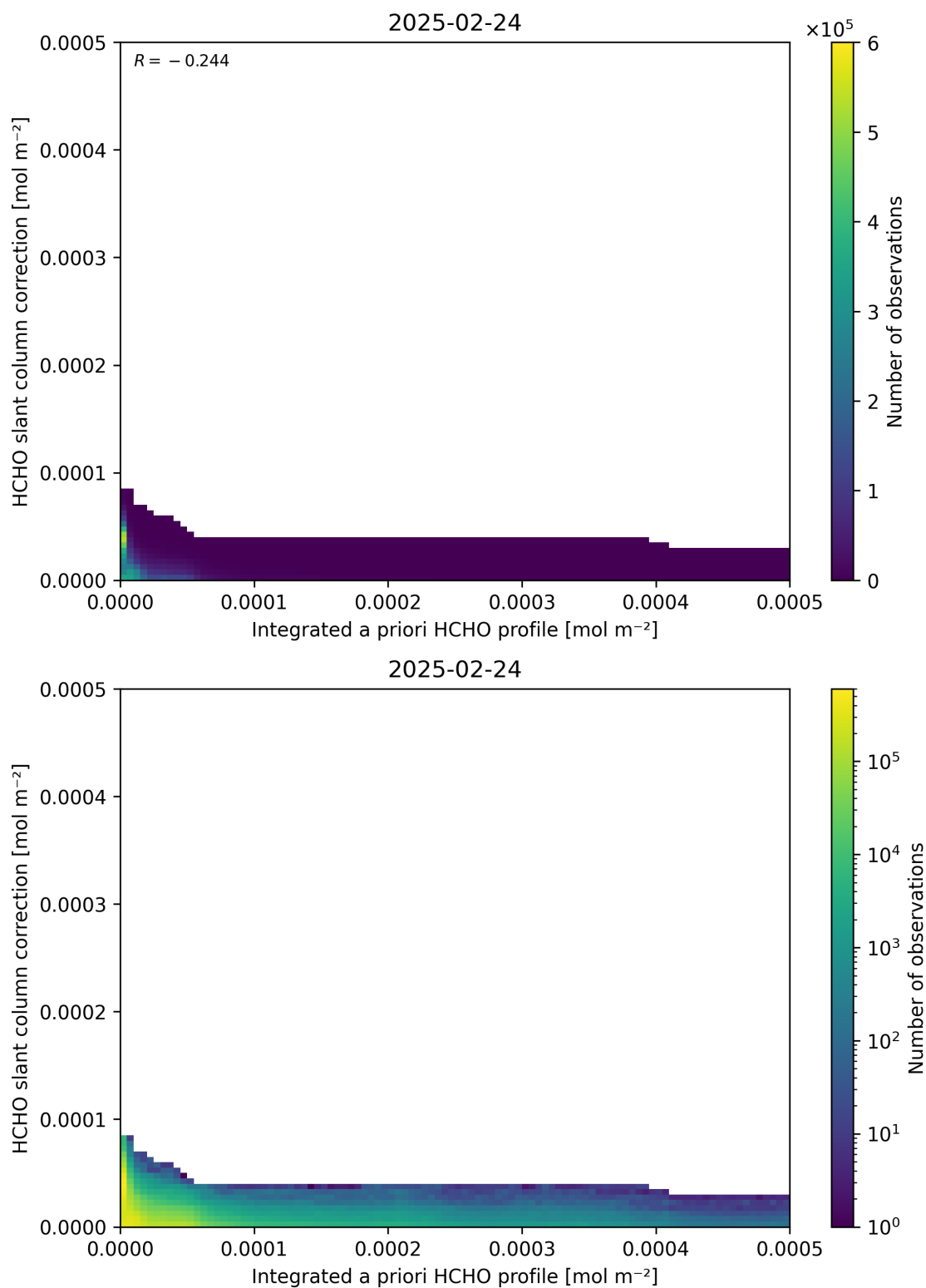
Figure 152: Scatter density plot of “Integrated a priori HCHO profile” against “HCHO slant column correction” for 2025-02-24 to 2025-02-25.
