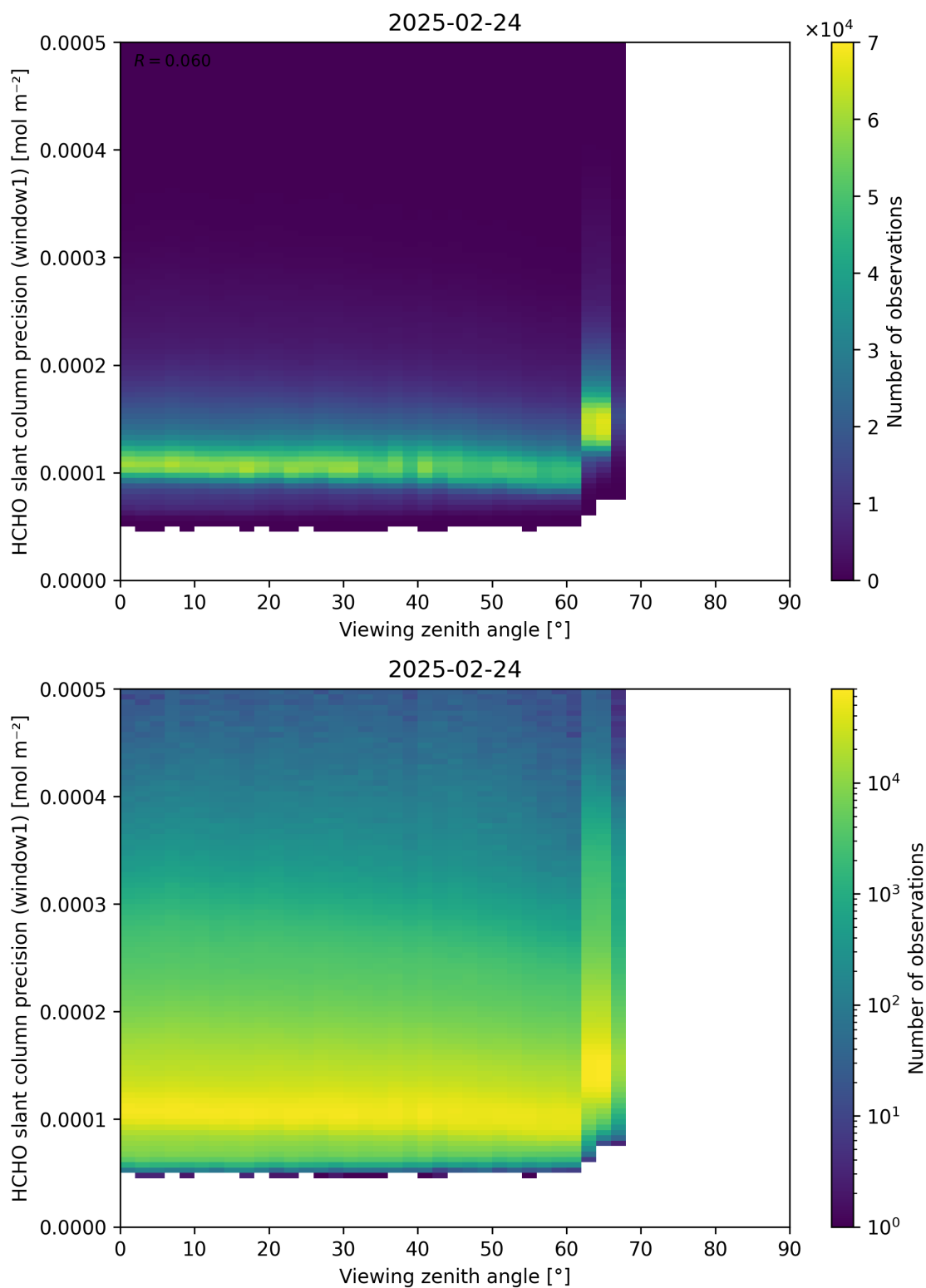
Figure 189: Scatter density plot of “Viewing zenith angle” against “HCHO slant column precision (window1)” for 2025-02-24 to 2025-02-25.
