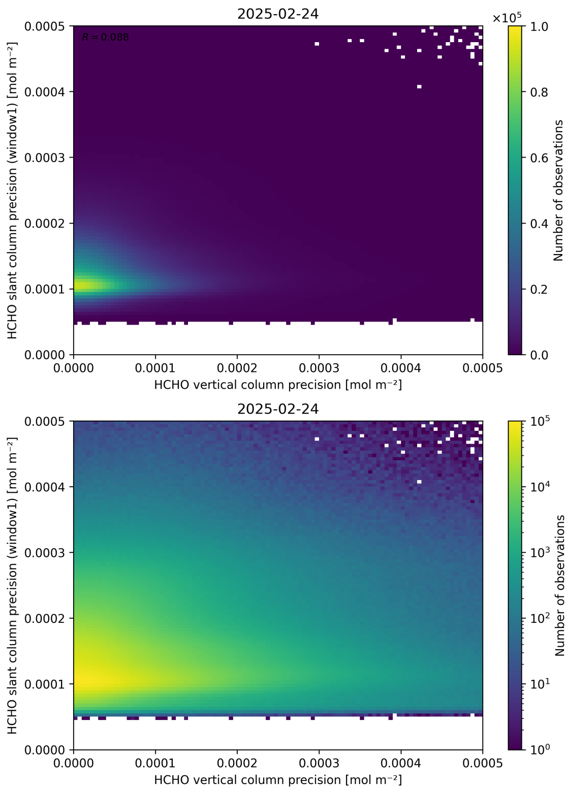
Figure 143: Scatter density plot of “HCHO vertical column precision” against “HCHO slant column precision (window1)” for 2025-02-24 to 2025-02-25.
