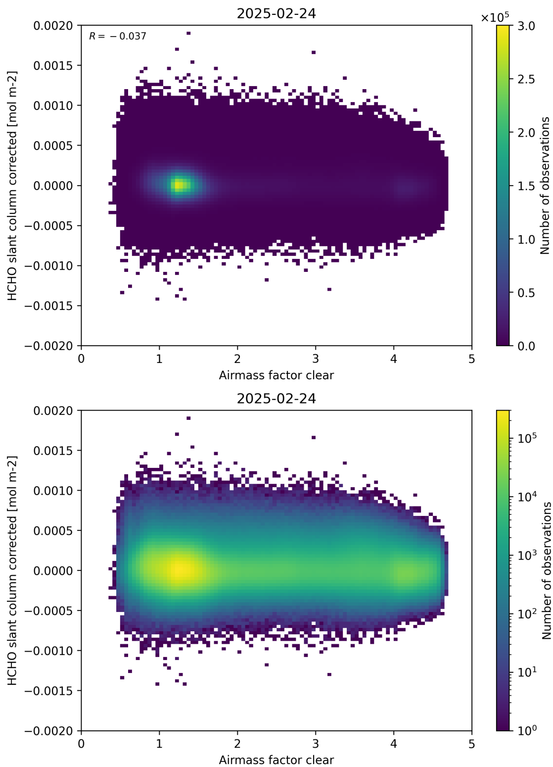
Figure 74: Scatter density plot of “Airmass factor clear” against “HCHO slant column corrected” for 2025-02-24 to 2025-02-25.
