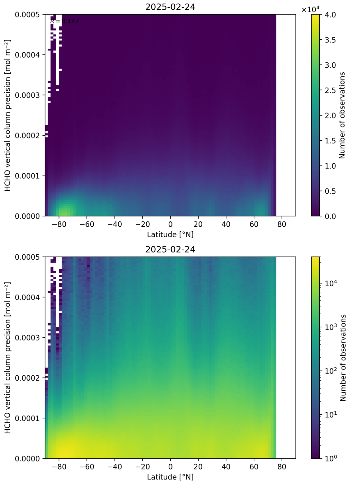
Figure 165: Scatter density plot of “Latitude” against “HCHO vertical column precision” for 2025-02-24 to 2025-02-25.
