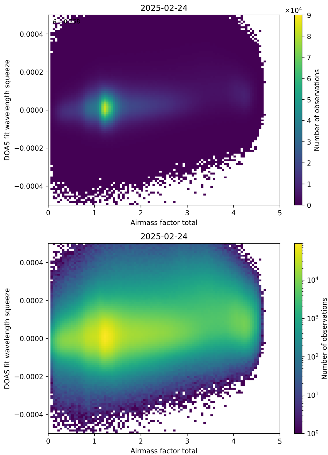
Figure 99: Scatter density plot of “Airmass factor total” against “DOAS fit wavelength squeeze” for 2025-02-24 to 2025-02-25.
