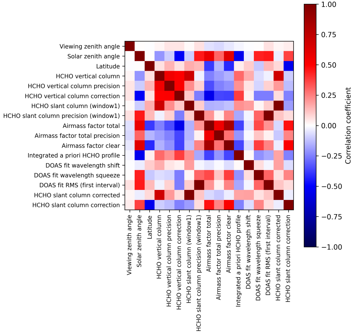
Figure 2: Map of correlation matrix for 2025-02-24 to 2025-02-25.
