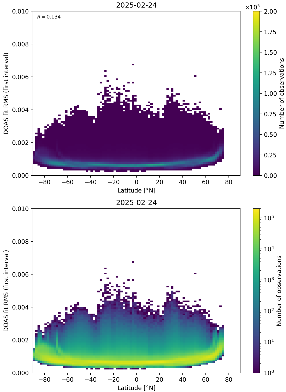
Figure 153: Scatter density plot of “Latitude” against “DOAS fit RMS (first interval)” for 2025-02-24 to 2025-02-25.
