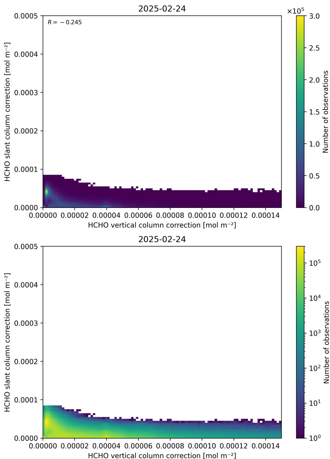
Figure 117: Scatter density plot of “HCHO vertical column correction” against “HCHO slant column correction” for 2025-02-24 to 2025-02-25.
