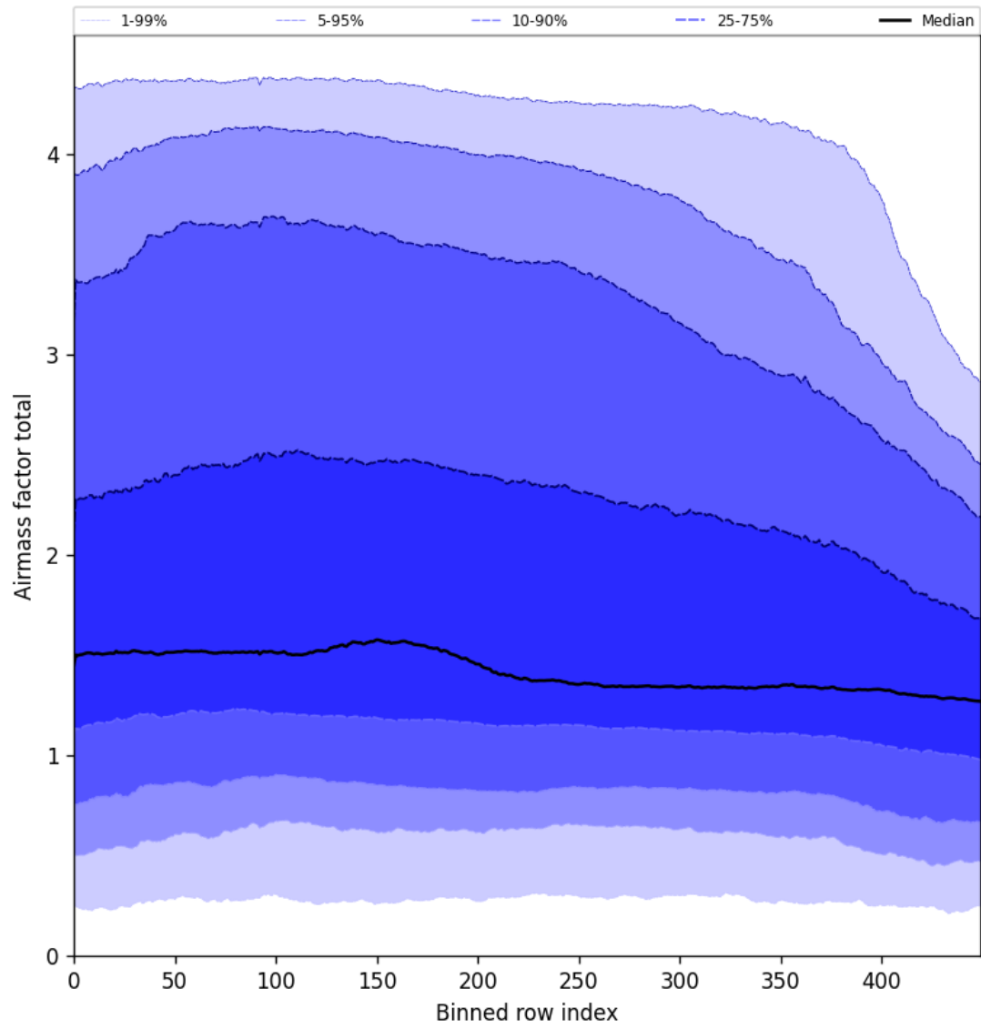
Figure 54: Along track statistics of “Airmass factor total” for 2025-02-24 to 2025-02-25
