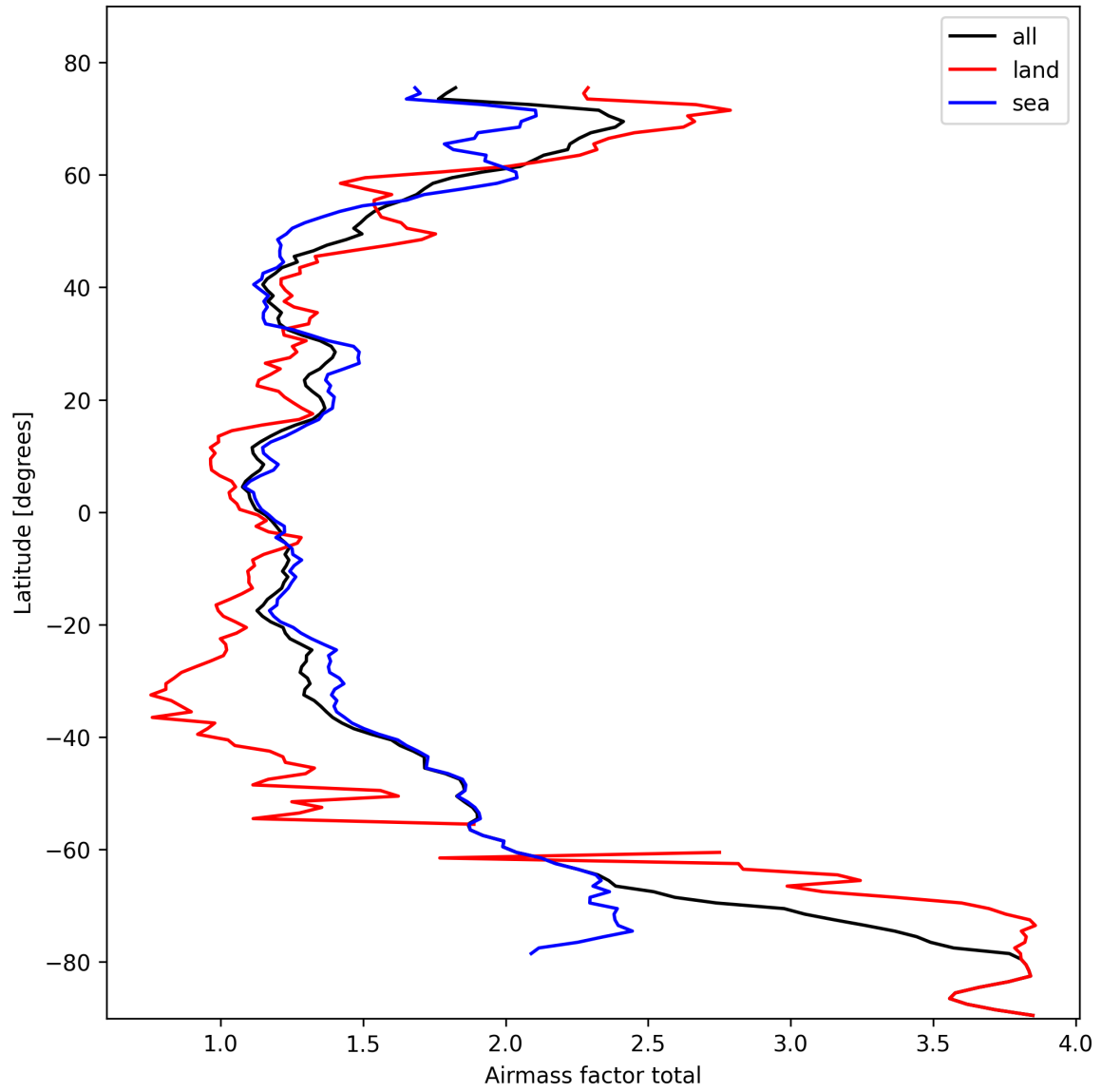
Figure 26: Zonal average of “Airmass factor total” for 2025-02-24 to 2025-02-25.
