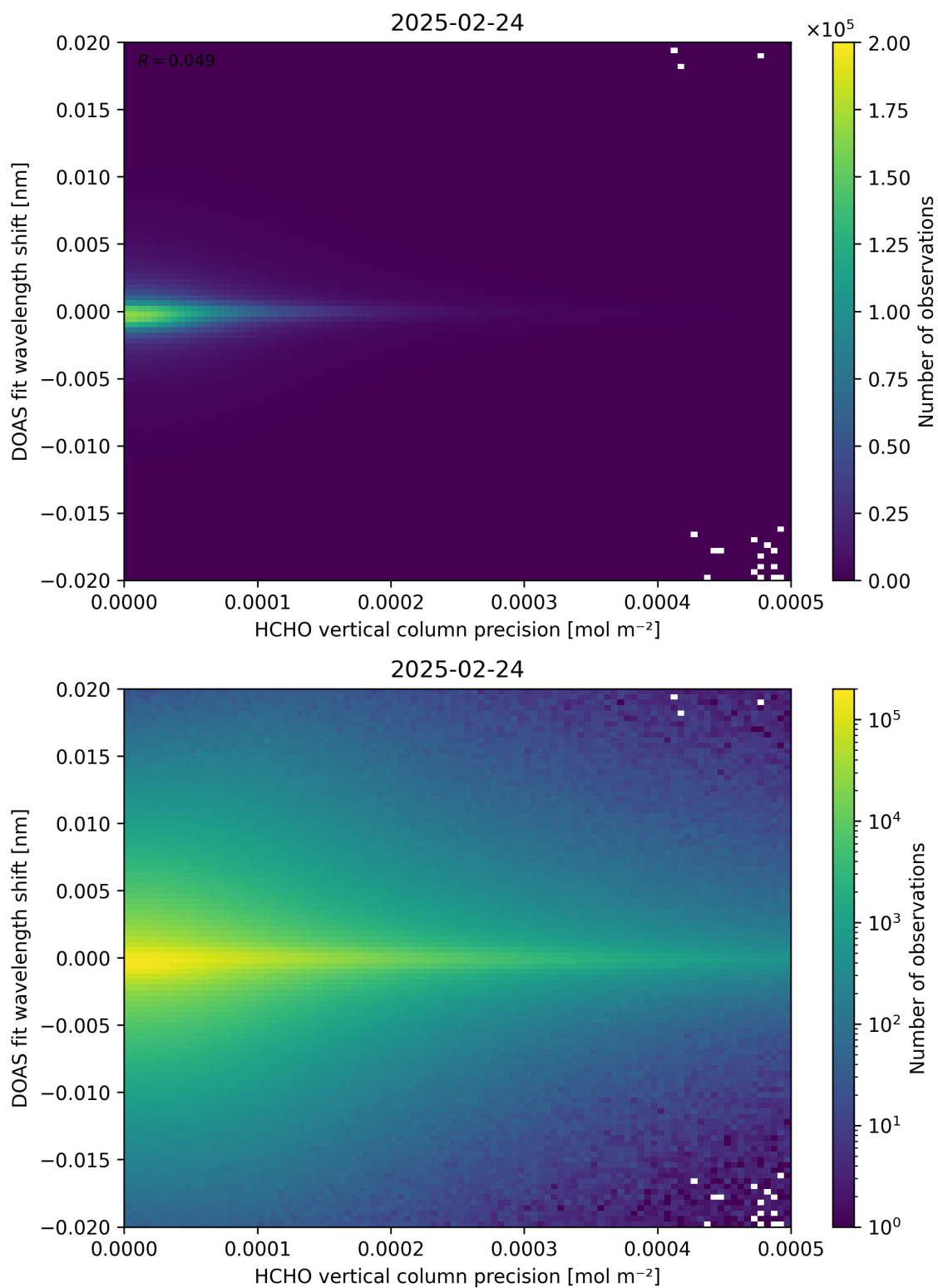
Figure 137: Scatter density plot of “HCHO vertical column precision” against “DOAS fit wavelength shift” for 2025-02-24 to 2025-02-25.
