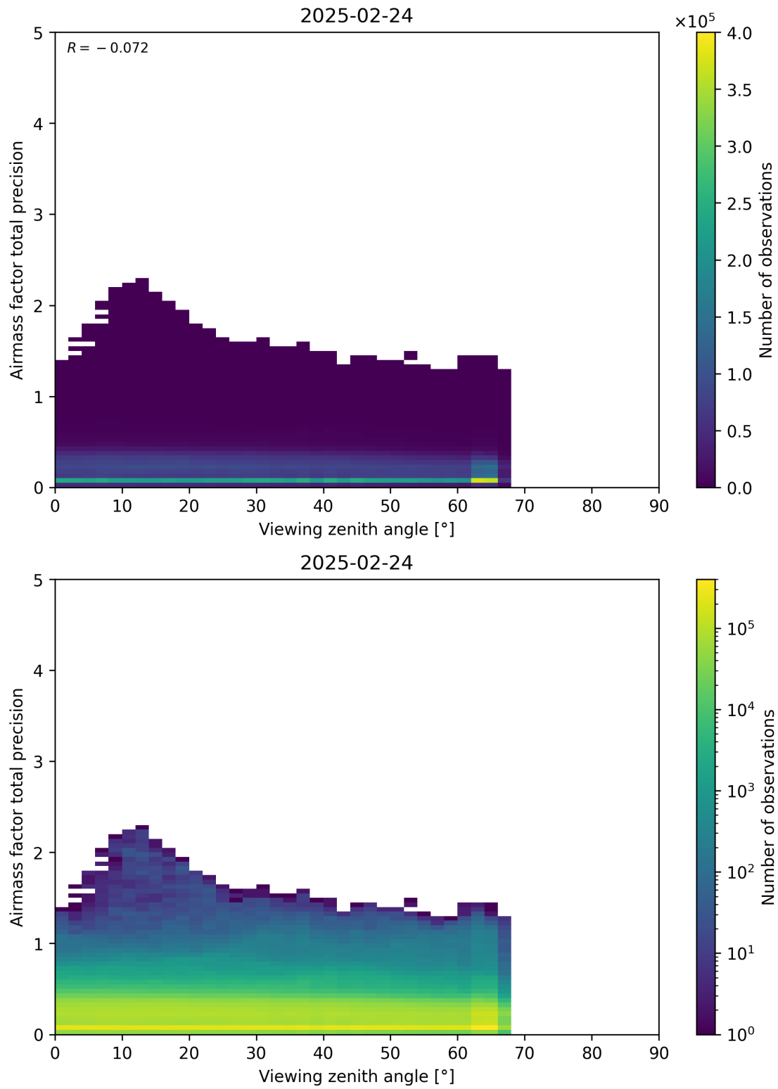
Figure 191: Scatter density plot of “Viewing zenith angle” against “Airmass factor total precision” for 2025-02-24 to 2025-02-25.
