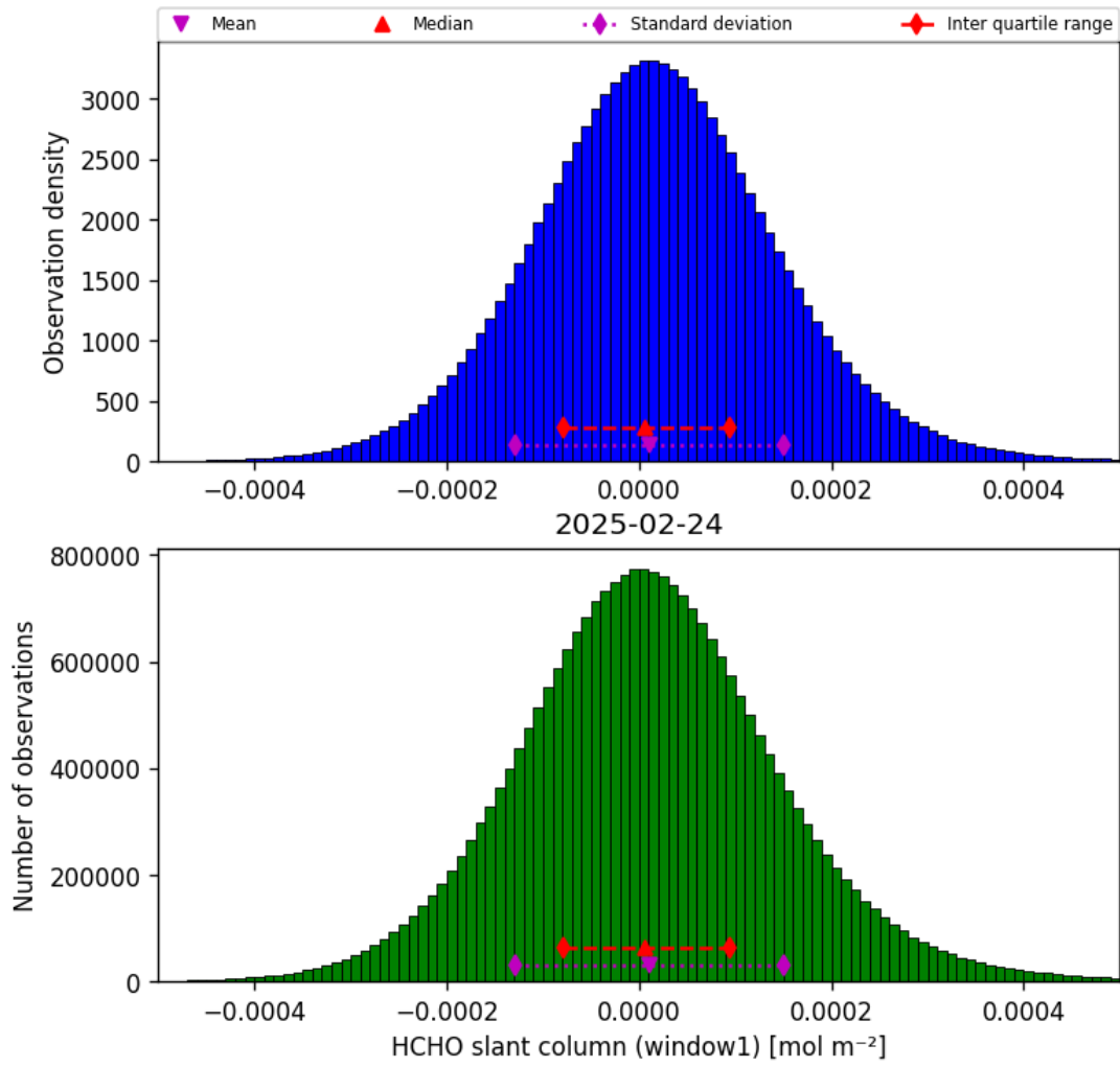
Figure 38: Histogram of “HCHO slant column (window1)” for 2025-02-24 to 2025-02-25
