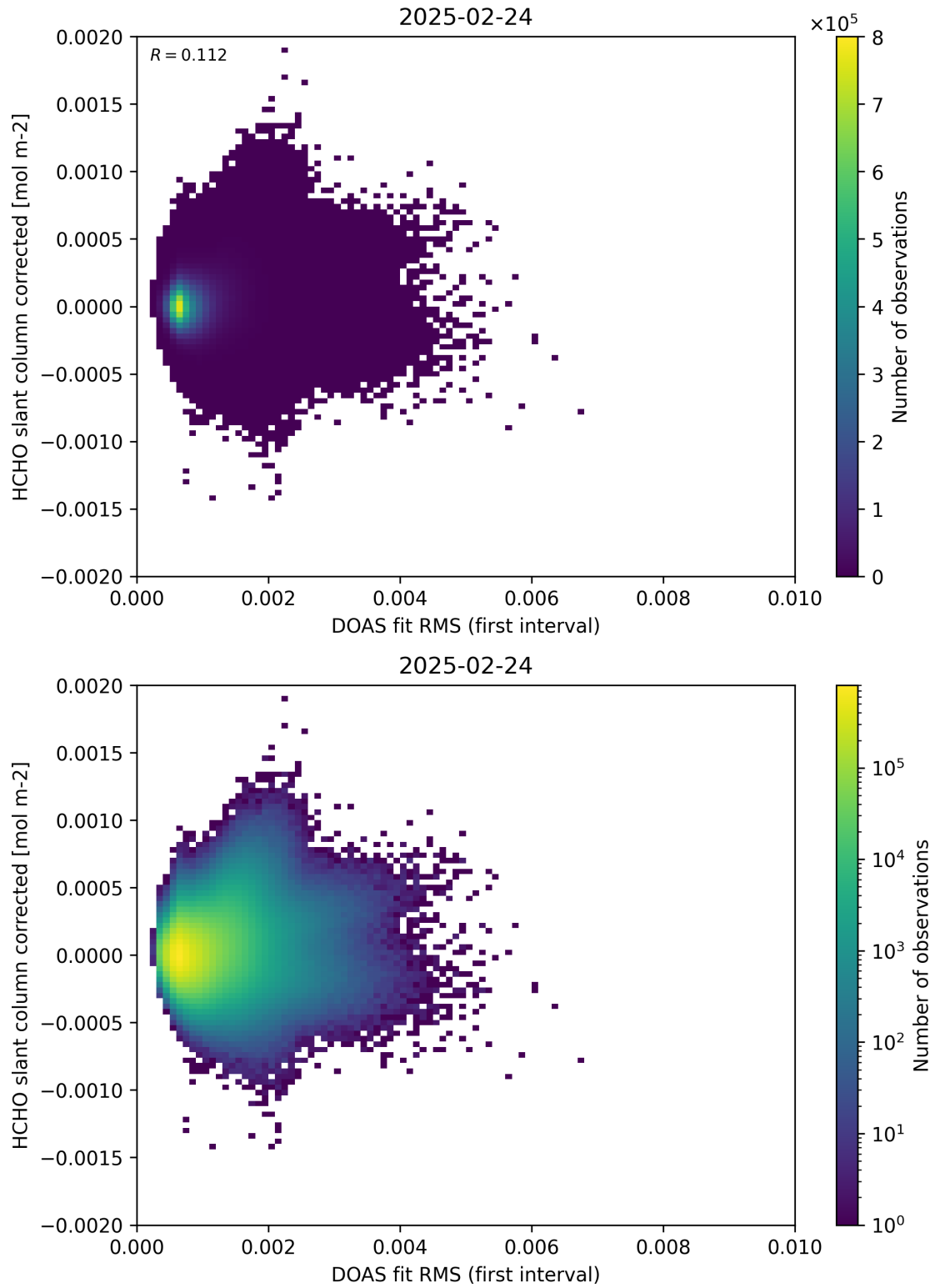
Figure 62: Scatter density plot of “DOAS fit RMS (first interval)” against “HCHO slant column corrected” for 2025-02-24 to 2025-02-25.
