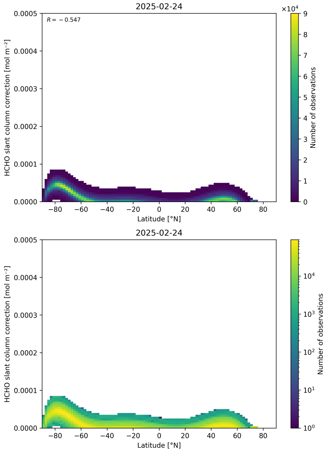
Figure 158: Scatter density plot of “Latitude” against “HCHO slant column correction” for 2025-02-24 to 2025-02-25.
