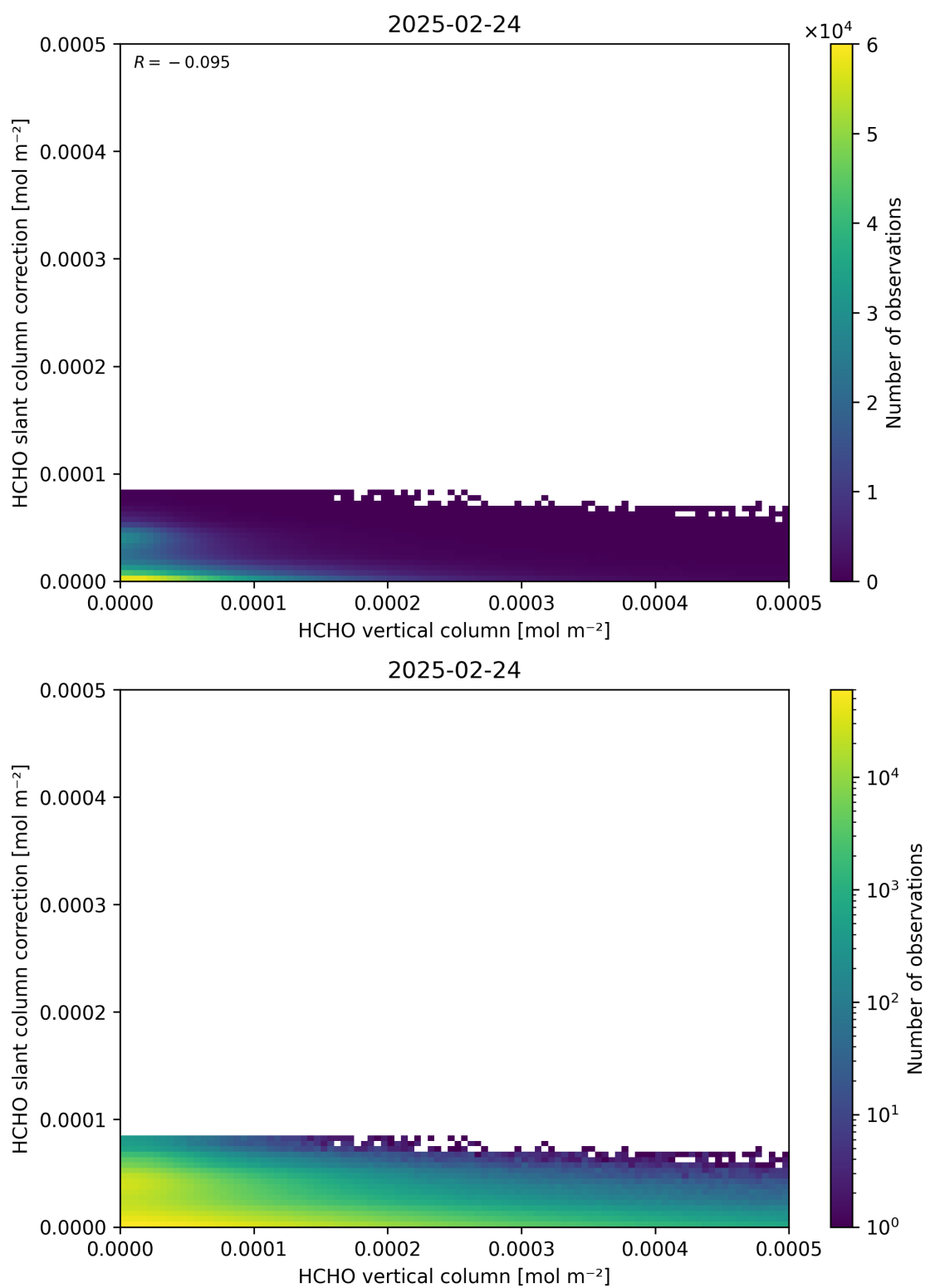
Figure 128: Scatter density plot of “HCHO vertical column” against “HCHO slant column correction” for 2025-02-24 to 2025-02-25.
