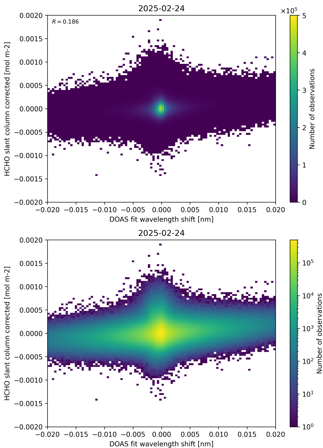
Figure 66: Scatter density plot of “DOAS fit wavelength shift” against “HCHO slant column corrected” for 2025-02-24 to 2025-02-25.
