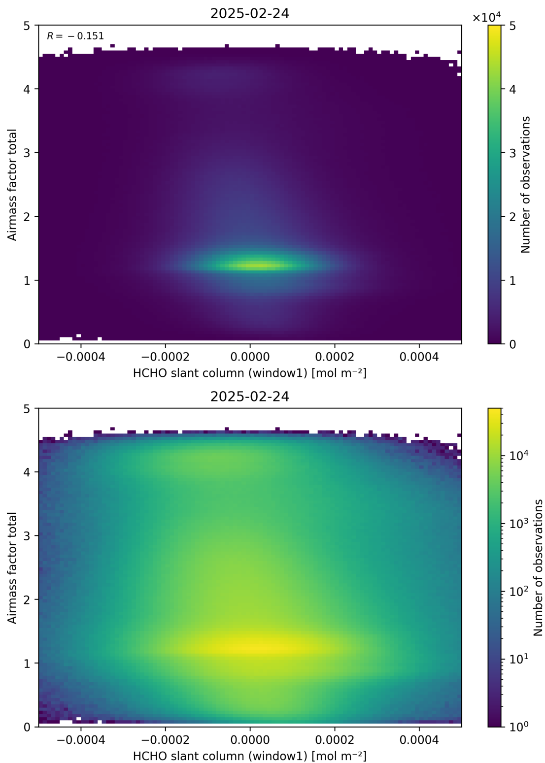
Figure 85: Scatter density plot of “HCHO slant column (window1)” against “Airmass factor total” for 2025-02-24 to 2025-02-25.
