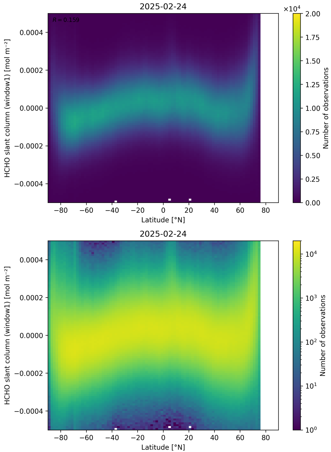
Figure 159: Scatter density plot of “Latitude” against “HCHO slant column (window1)” for 2025-02-24 to 2025-02-25.
