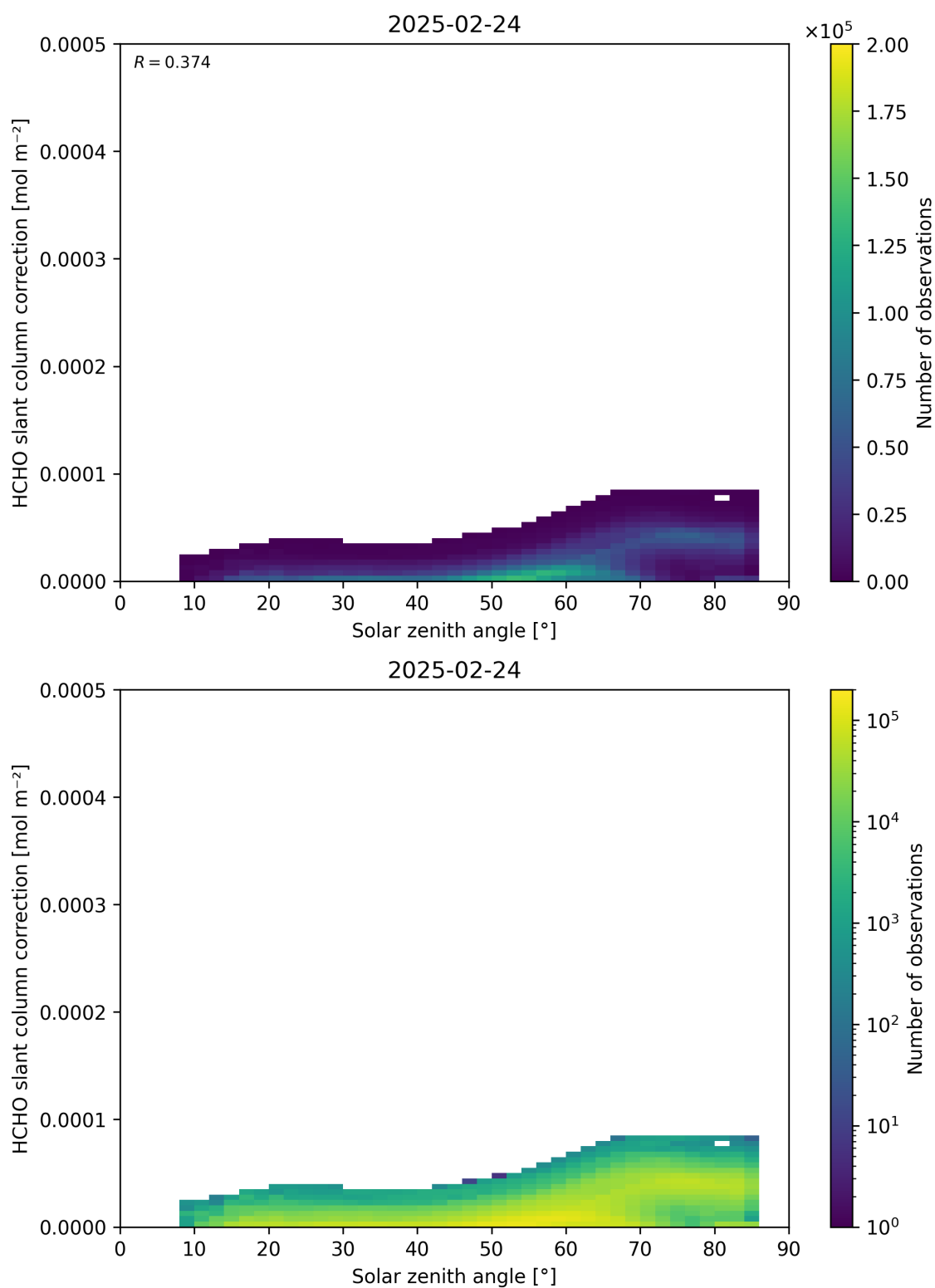
Figure 172: Scatter density plot of “Solar zenith angle” against “HCHO slant column correction” for 2025-02-24 to 2025-02-25.
