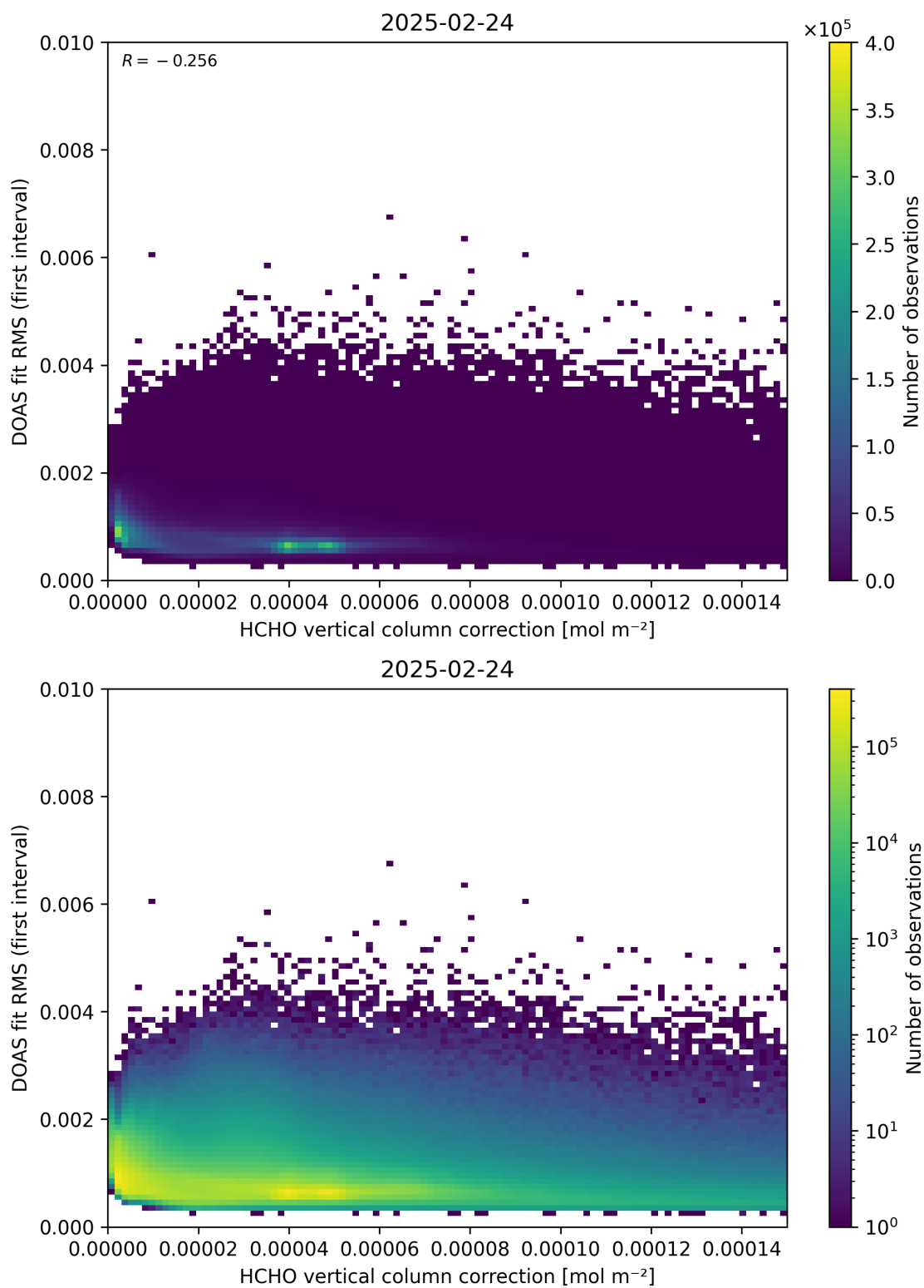
Figure 112: Scatter density plot of “HCHO vertical column correction” against “DOAS fit RMS (first interval)” for 2025-02-24 to 2025-02-25.
