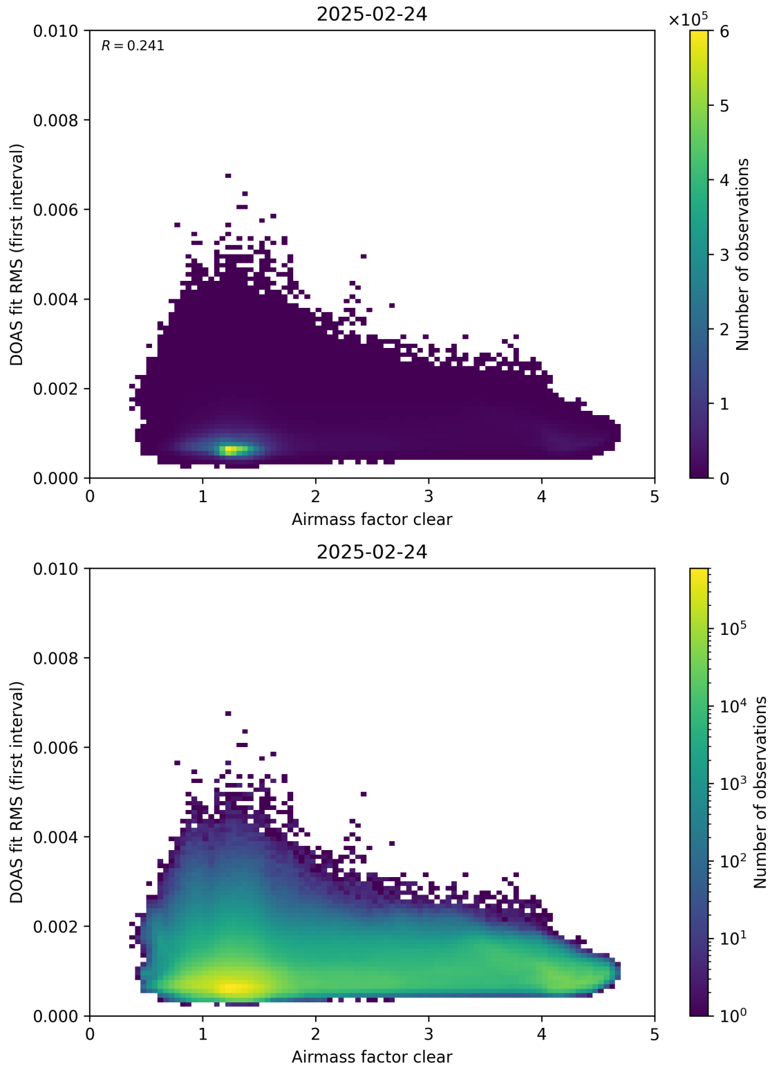
Figure 71: Scatter density plot of “Airmass factor clear” against “DOAS fit RMS (first interval)” for 2025-02-24 to 2025-02-25.
