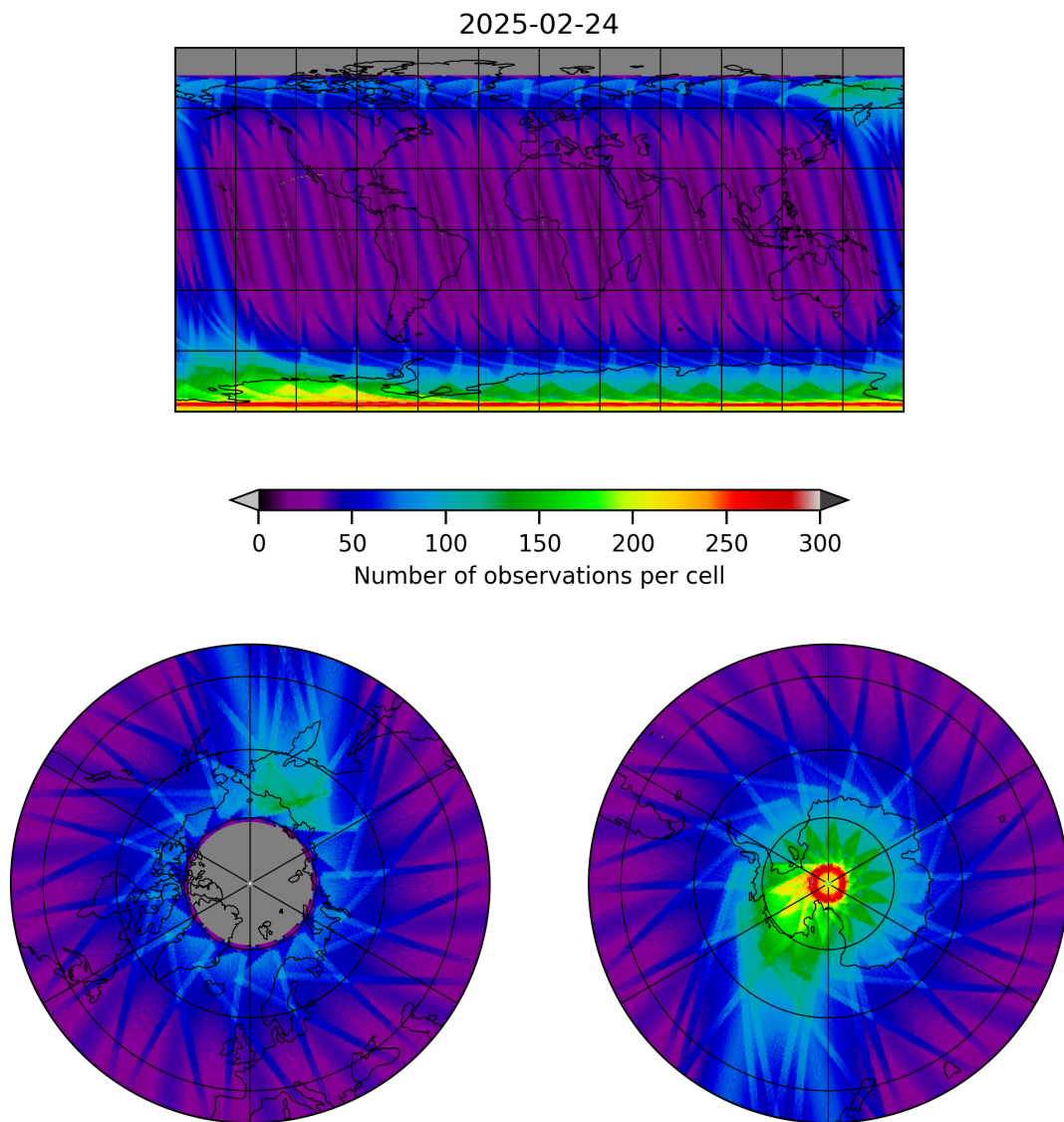
Figure 19: Map of the number of observations for 2025-02-24 to 2025-02-25
