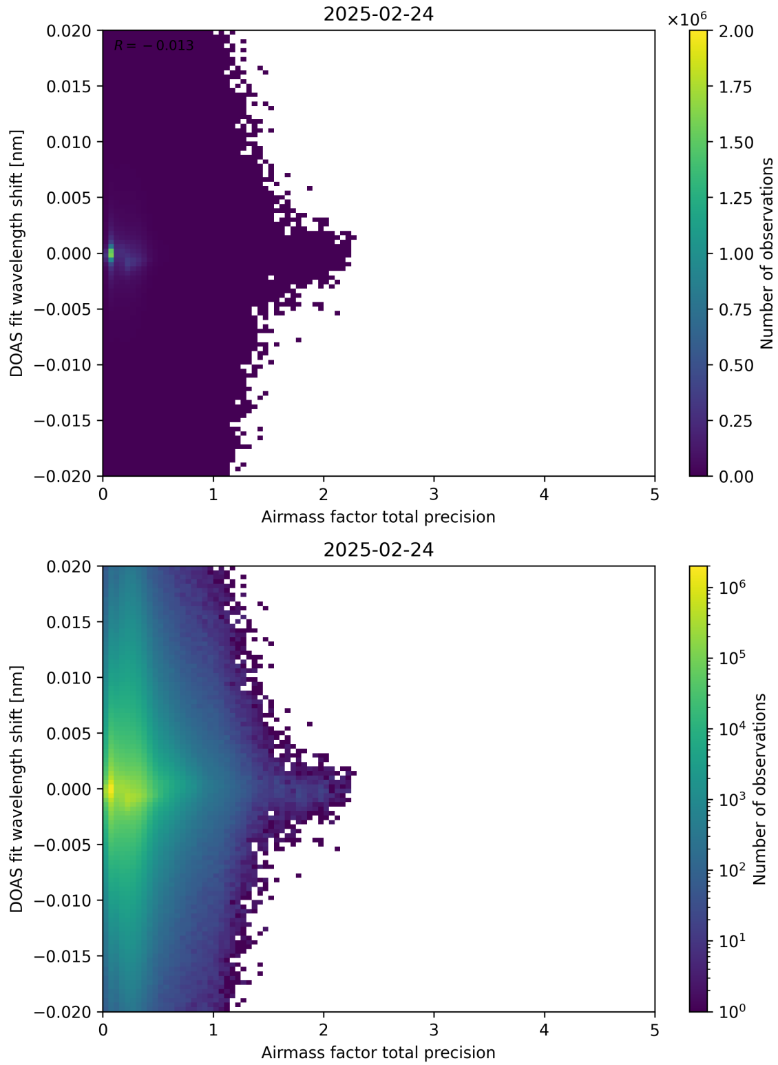
Figure 106: Scatter density plot of “Airmass factor total precision” against “DOAS fit wavelength shift” for 2025-02-24 to 2025-02-25.
