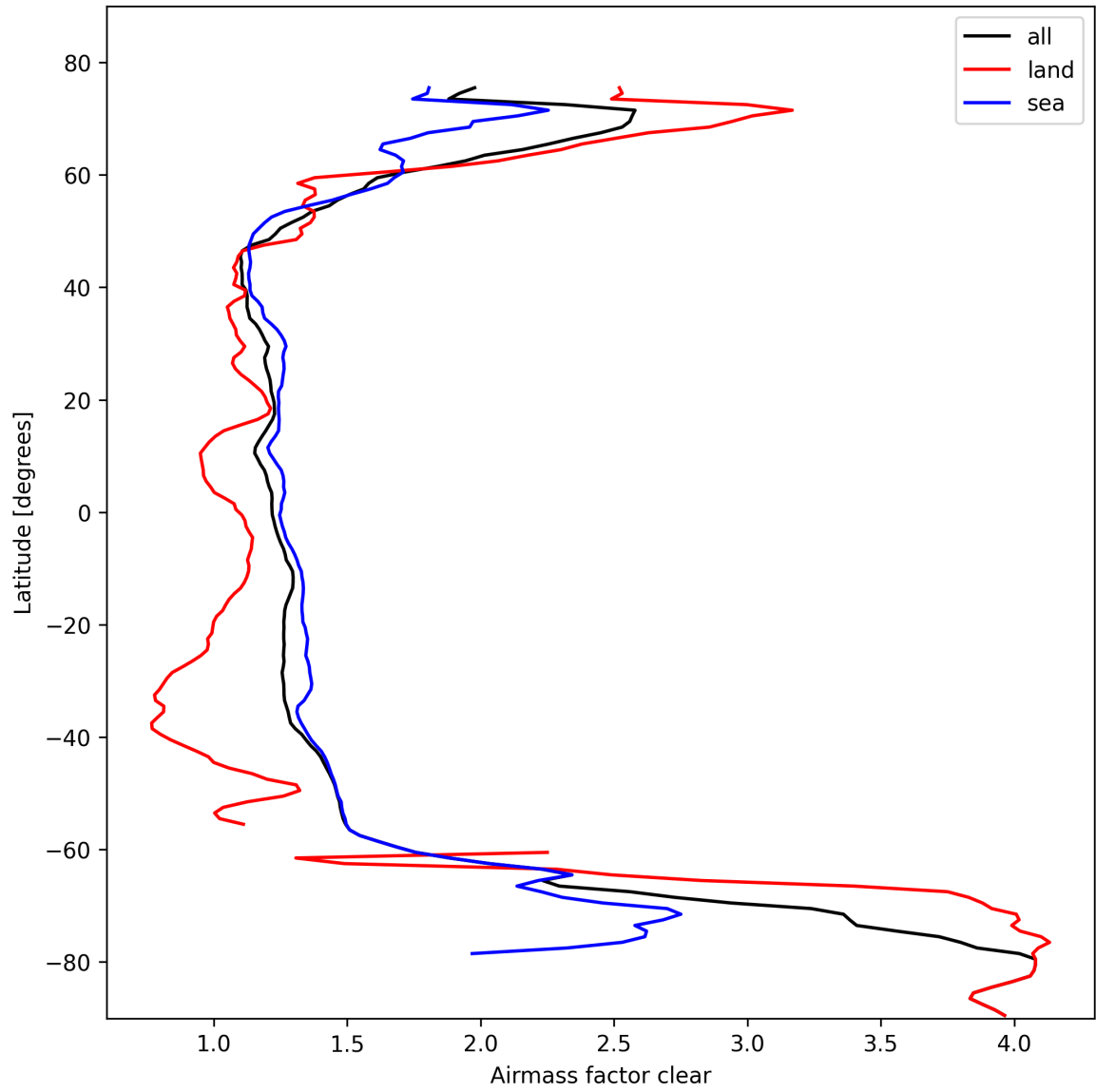
Figure 28: Zonal average of “Airmass factor clear” for 2025-02-24 to 2025-02-25.
