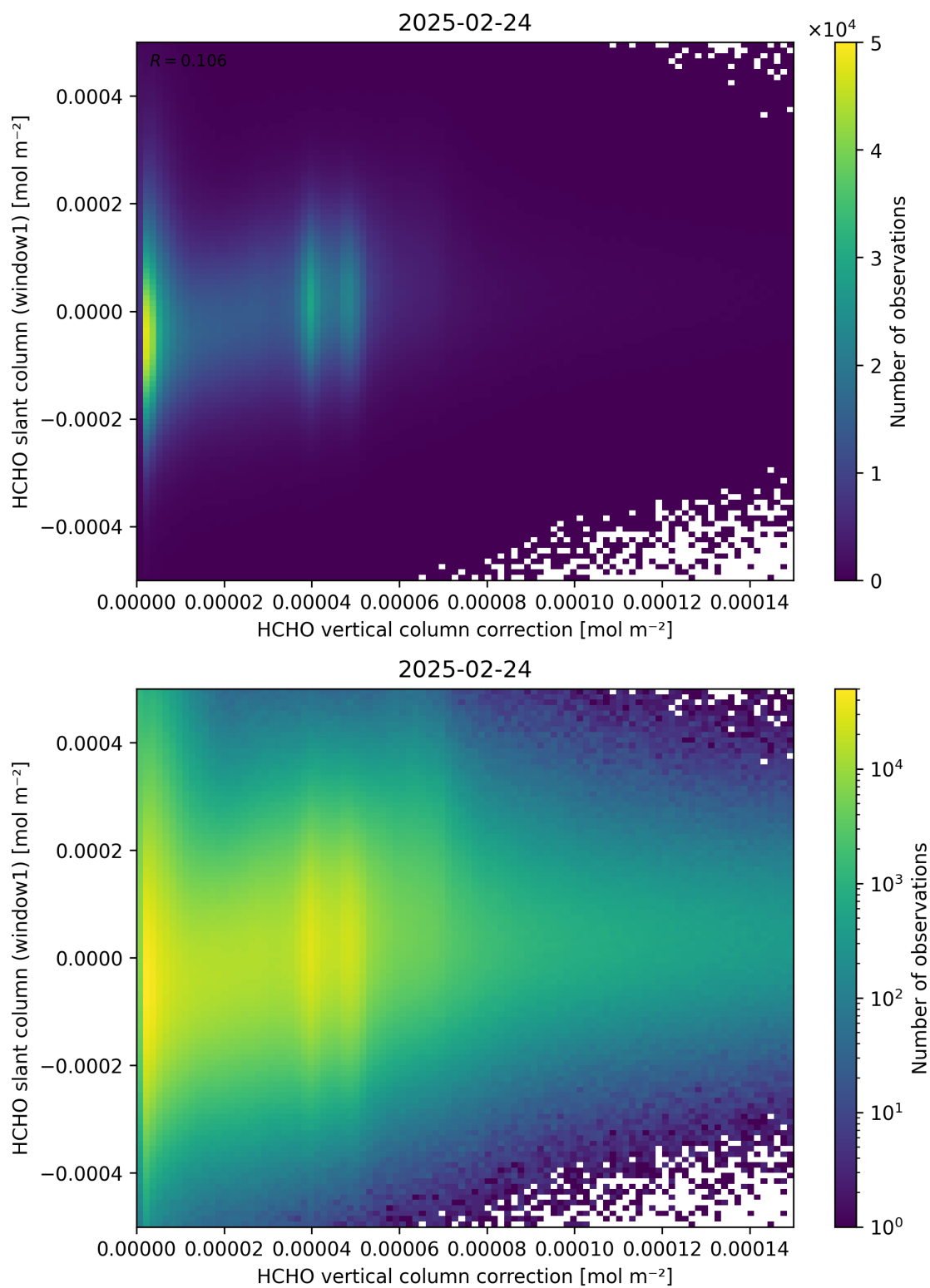
Figure 118: Scatter density plot of “HCHO vertical column correction” against “HCHO slant column (window1)” for 2025-02-24 to 2025-02-25.
