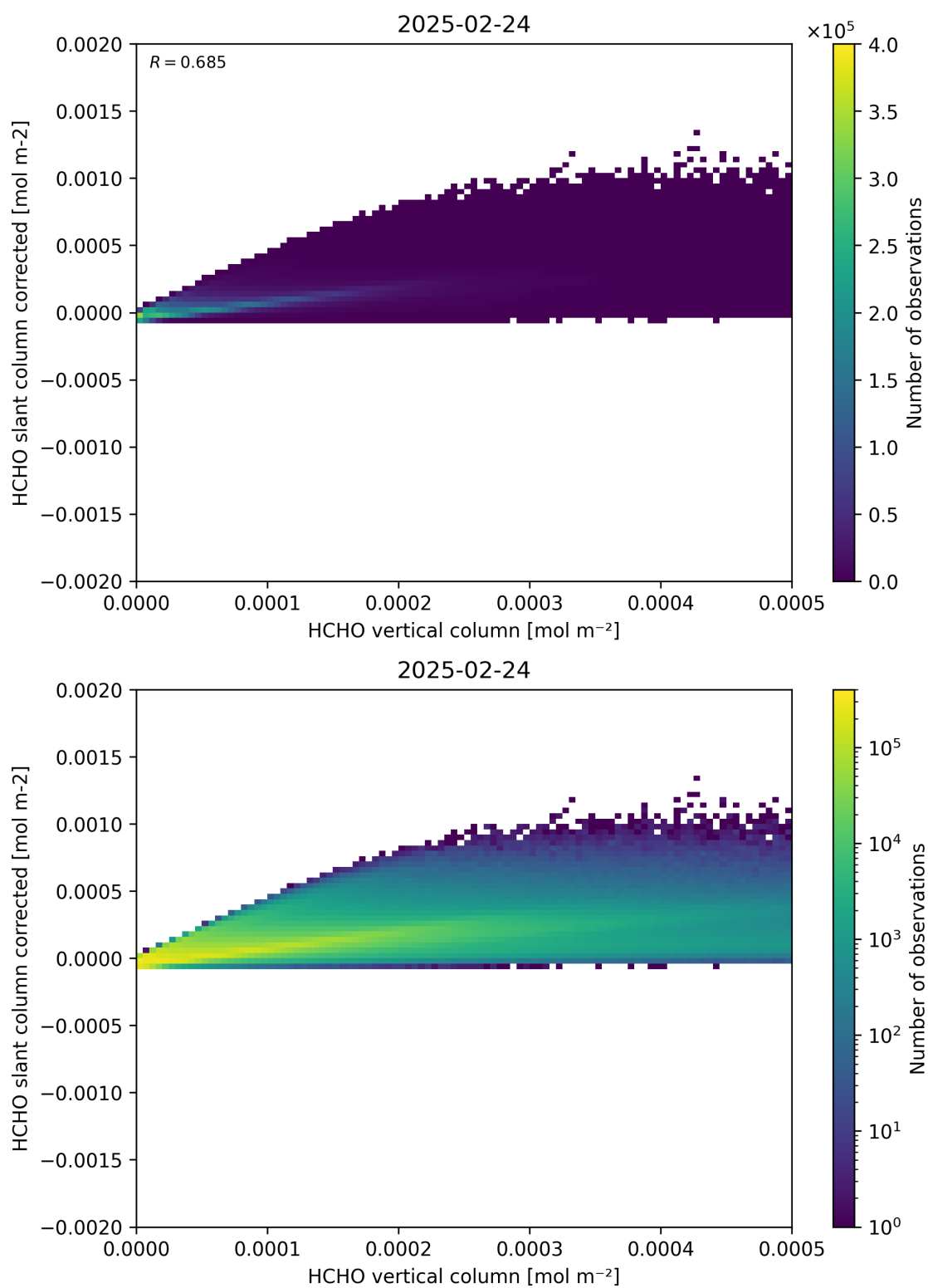
Figure 127: Scatter density plot of “HCHO vertical column” against “HCHO slant column corrected” for 2025-02-24 to 2025-02-25.
