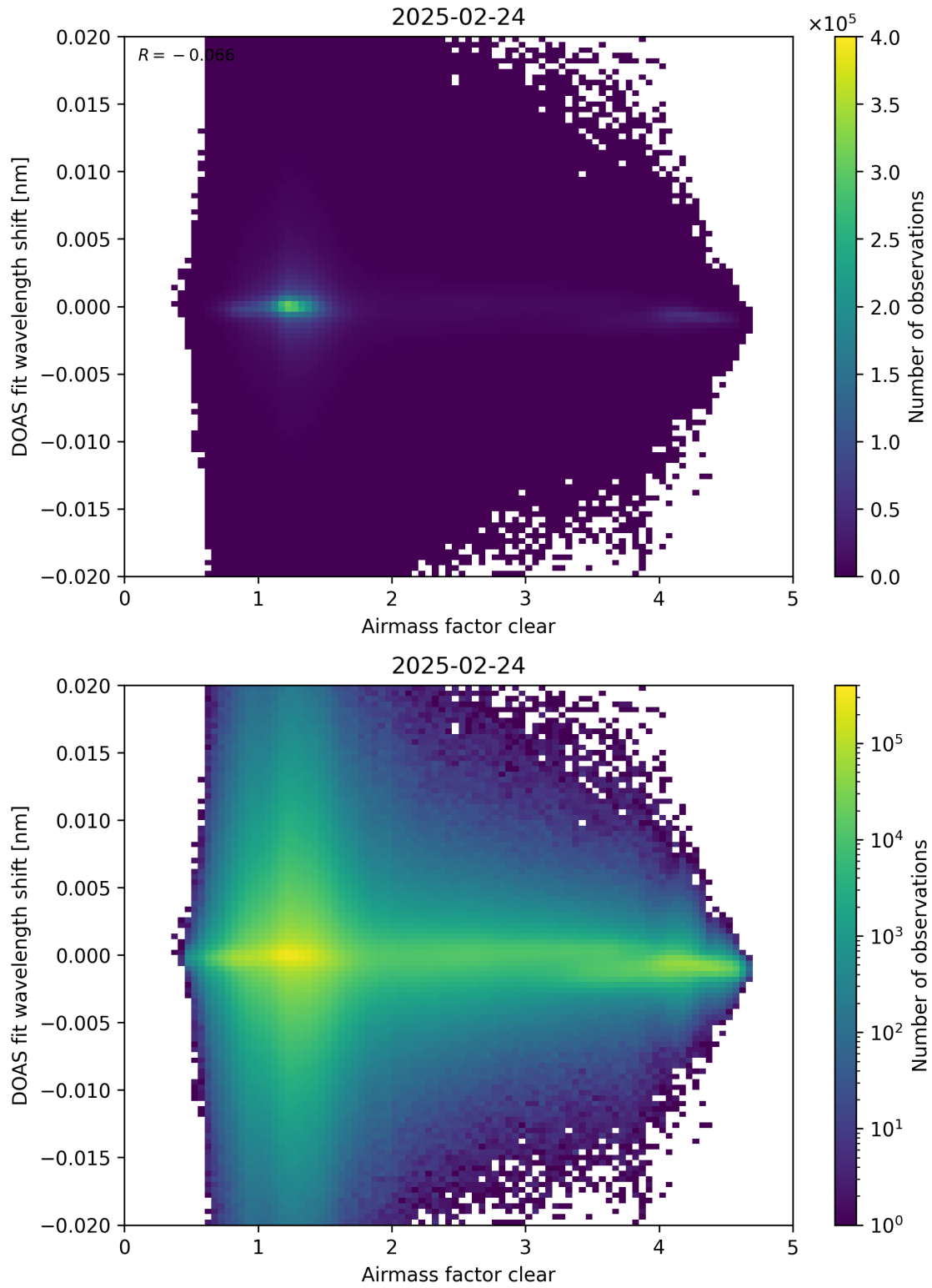
Figure 72: Scatter density plot of “Airmass factor clear” against “DOAS fit wavelength shift” for 2025-02-24 to 2025-02-25.
