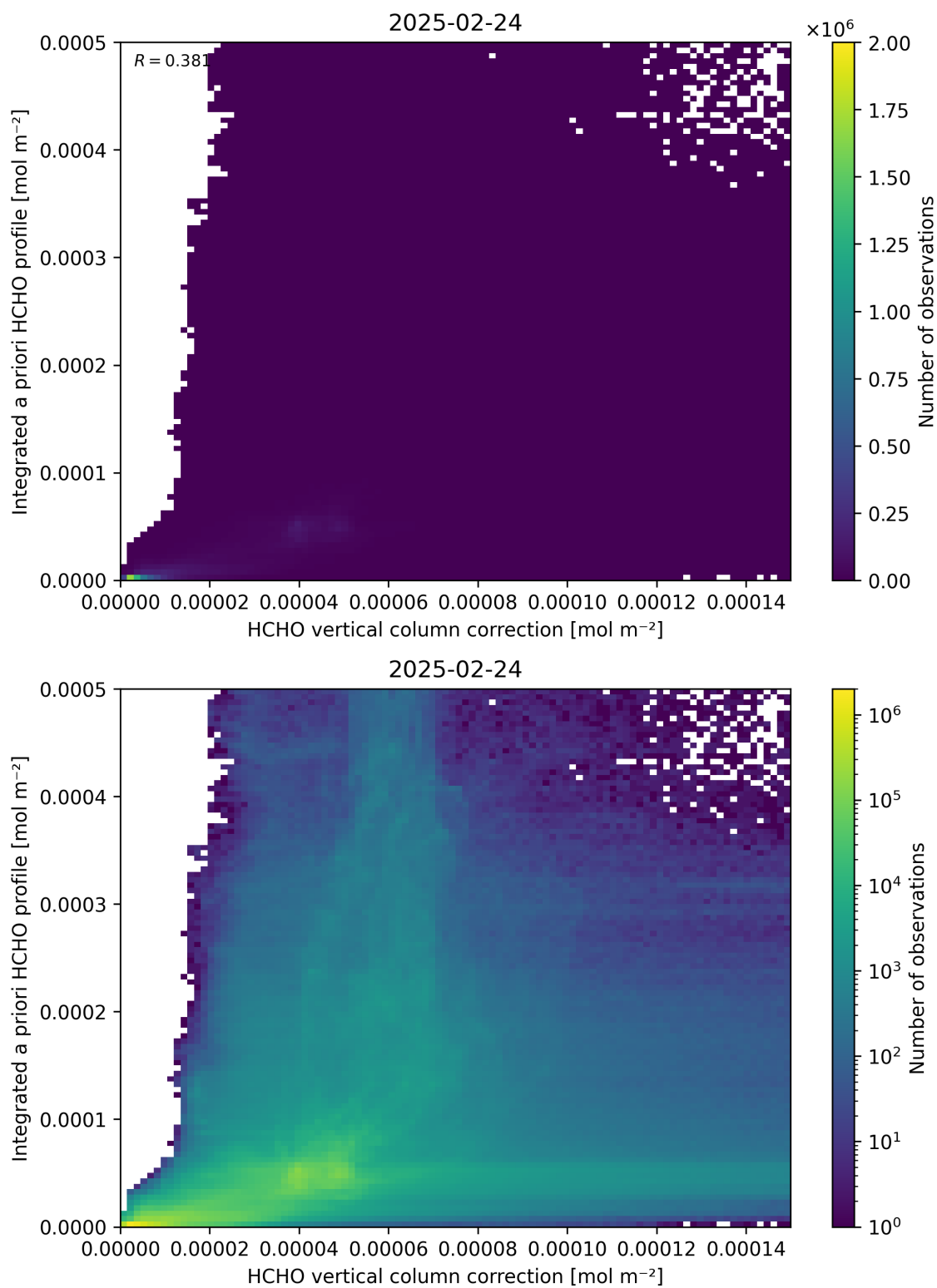
Figure 122: Scatter density plot of “HCHO vertical column correction” against “Integrated a priori HCHO profile” for 2025-02-24 to 2025-02-25.
