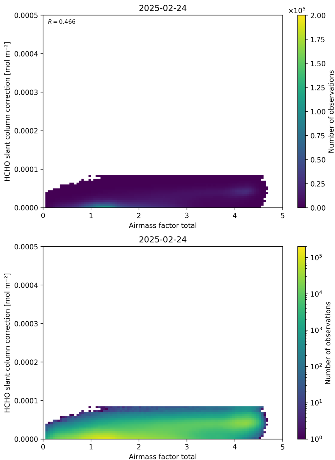
Figure 102: Scatter density plot of “Airmass factor total” against “HCHO slant column correction” for 2025-02-24 to 2025-02-25.
