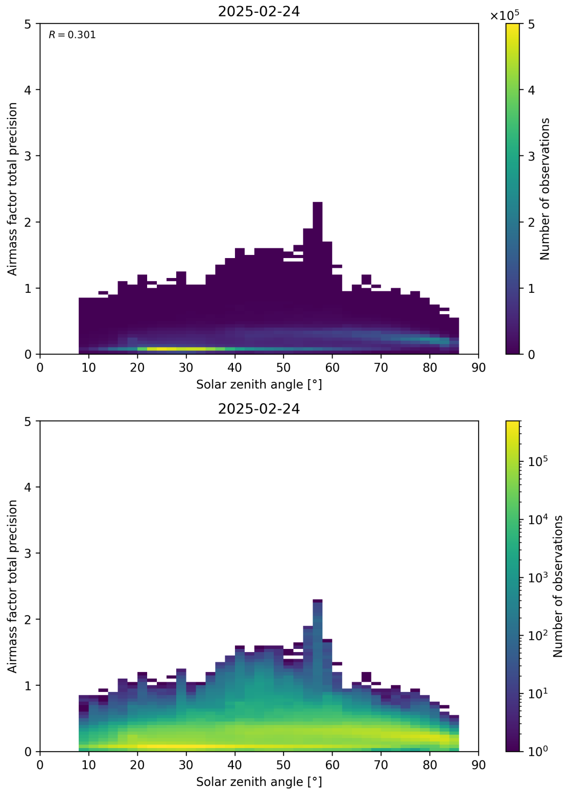
Figure 176: Scatter density plot of “Solar zenith angle” against “Airmass factor total precision” for 2025-02-24 to 2025-02-25.
