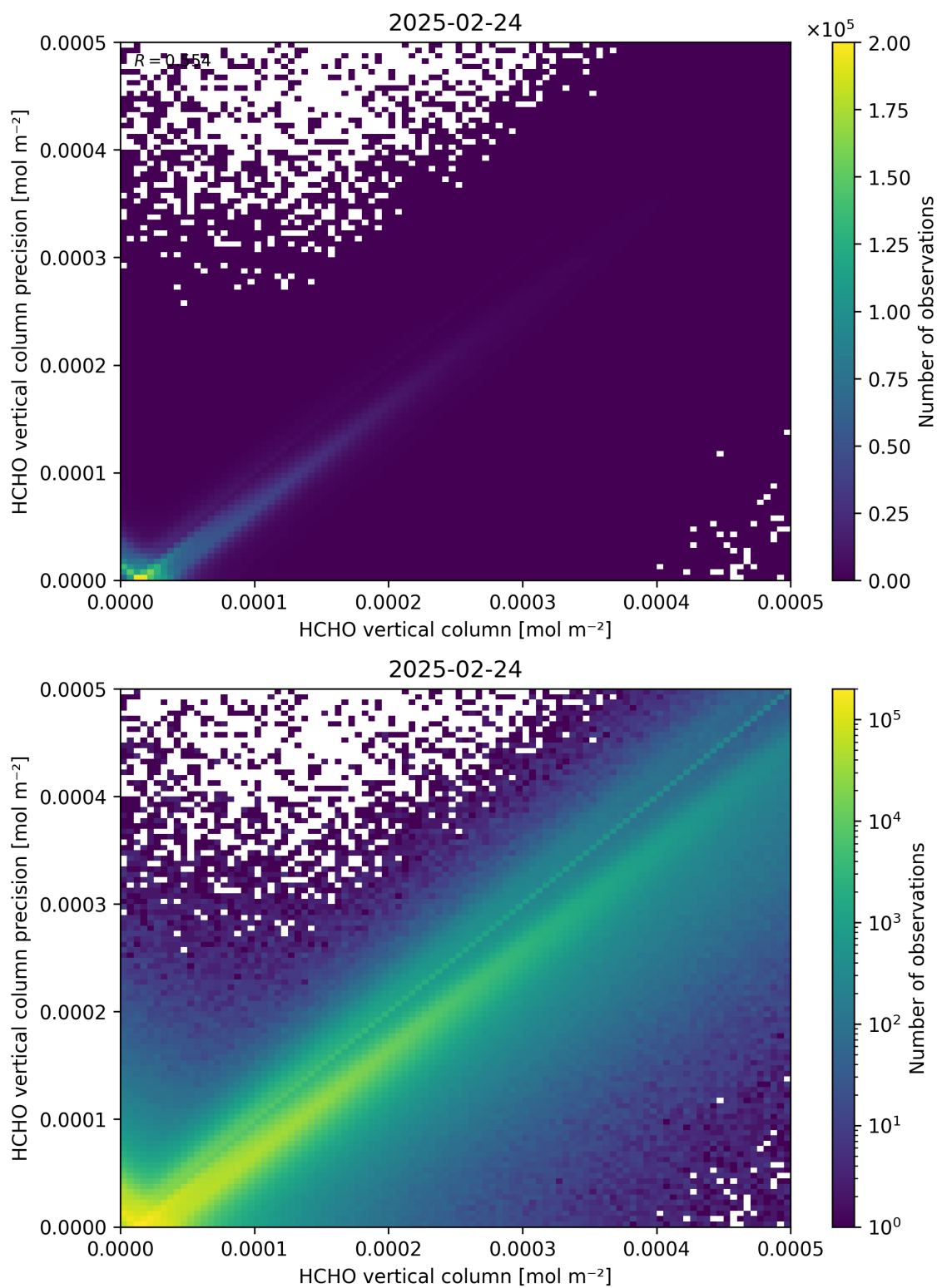
Figure 134: Scatter density plot of “HCHO vertical column” against “HCHO vertical column precision” for 2025-02-24 to 2025-02-25.
