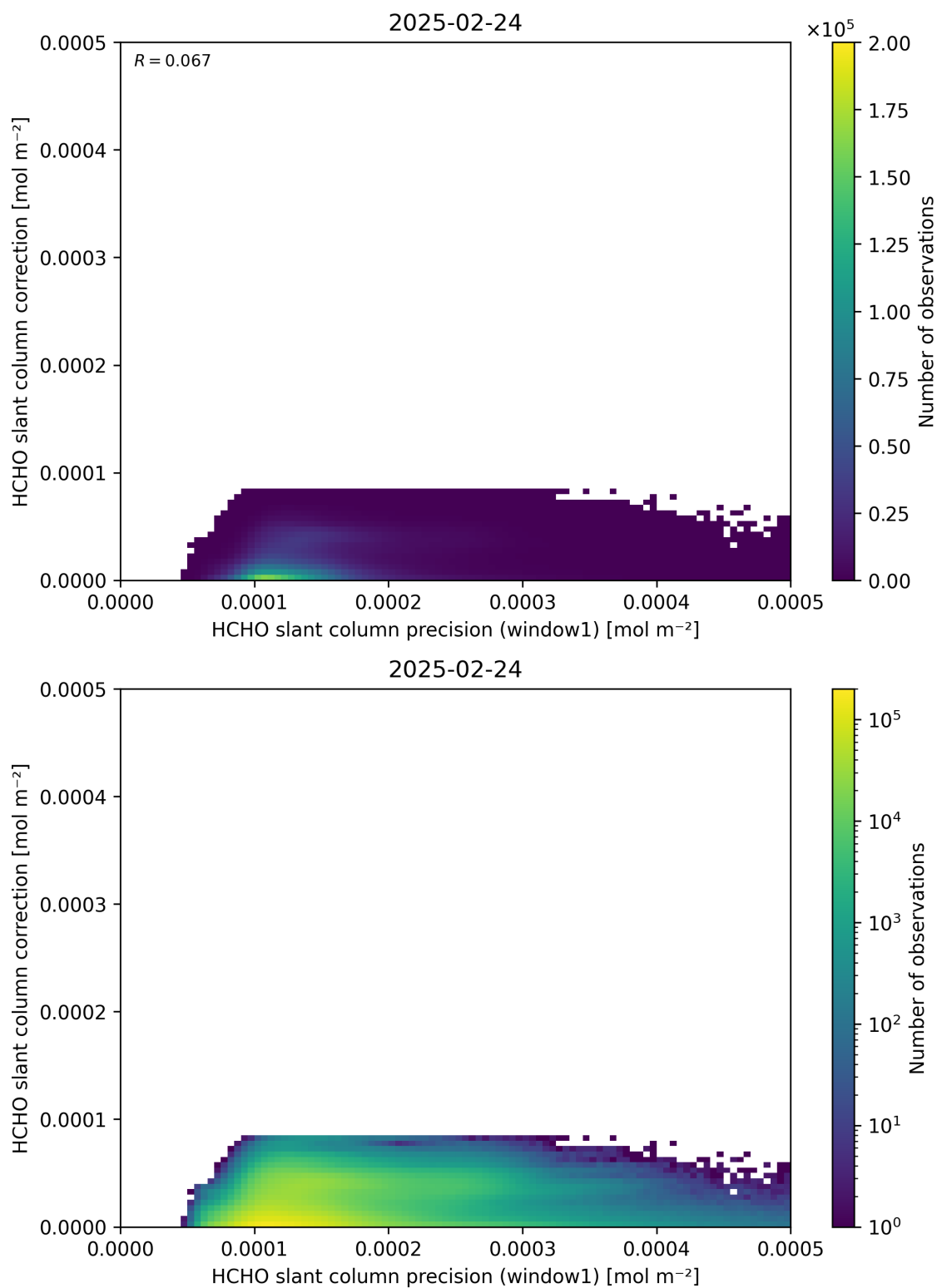
Figure 93: Scatter density plot of “HCHO slant column precision (window1)” against “HCHO slant column correction” for 2025-02-24 to 2025-02-25.
