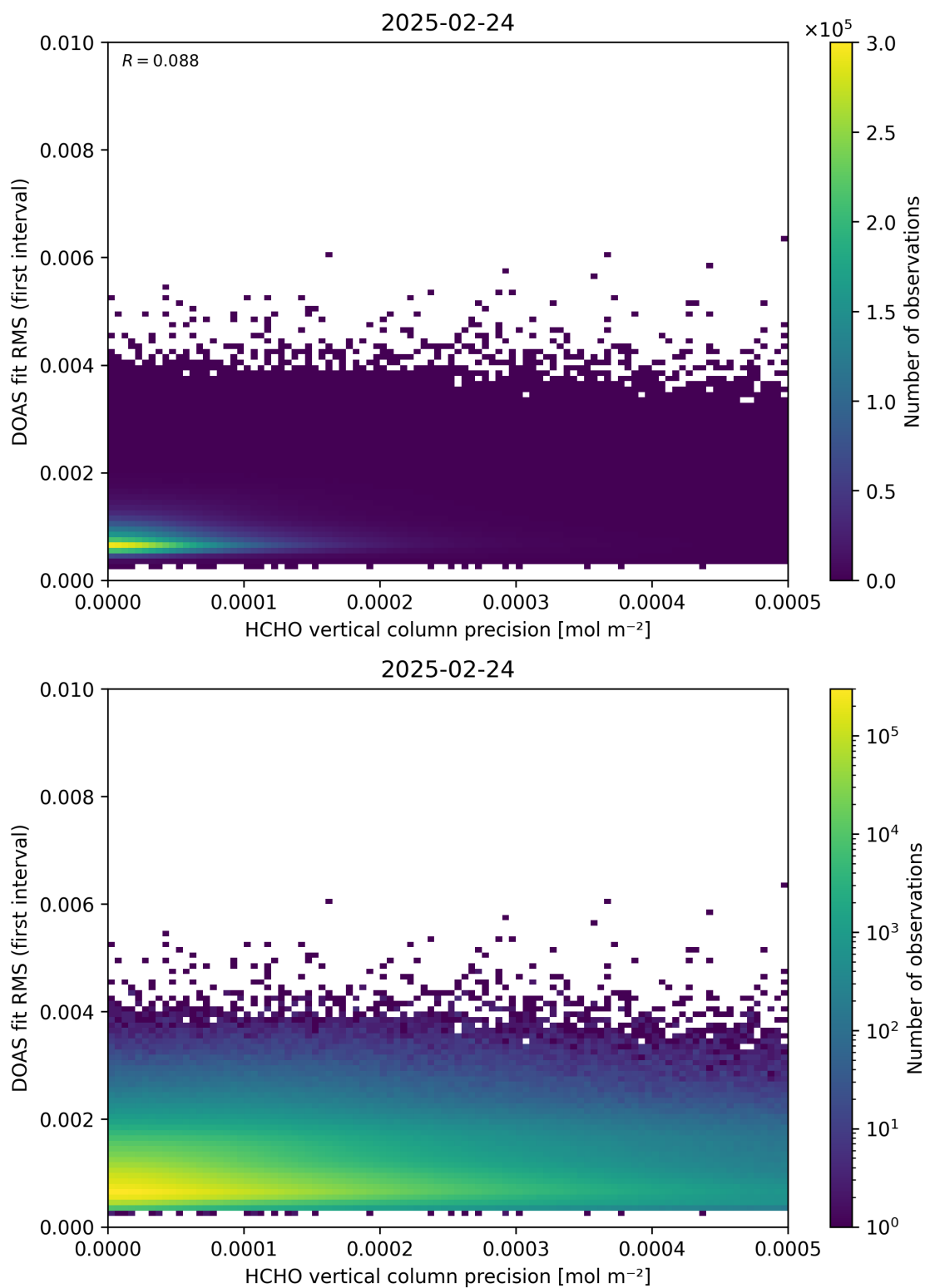
Figure 136: Scatter density plot of “HCHO vertical column precision” against “DOAS fit RMS (first interval)” for 2025-02-24 to 2025-02-25.
