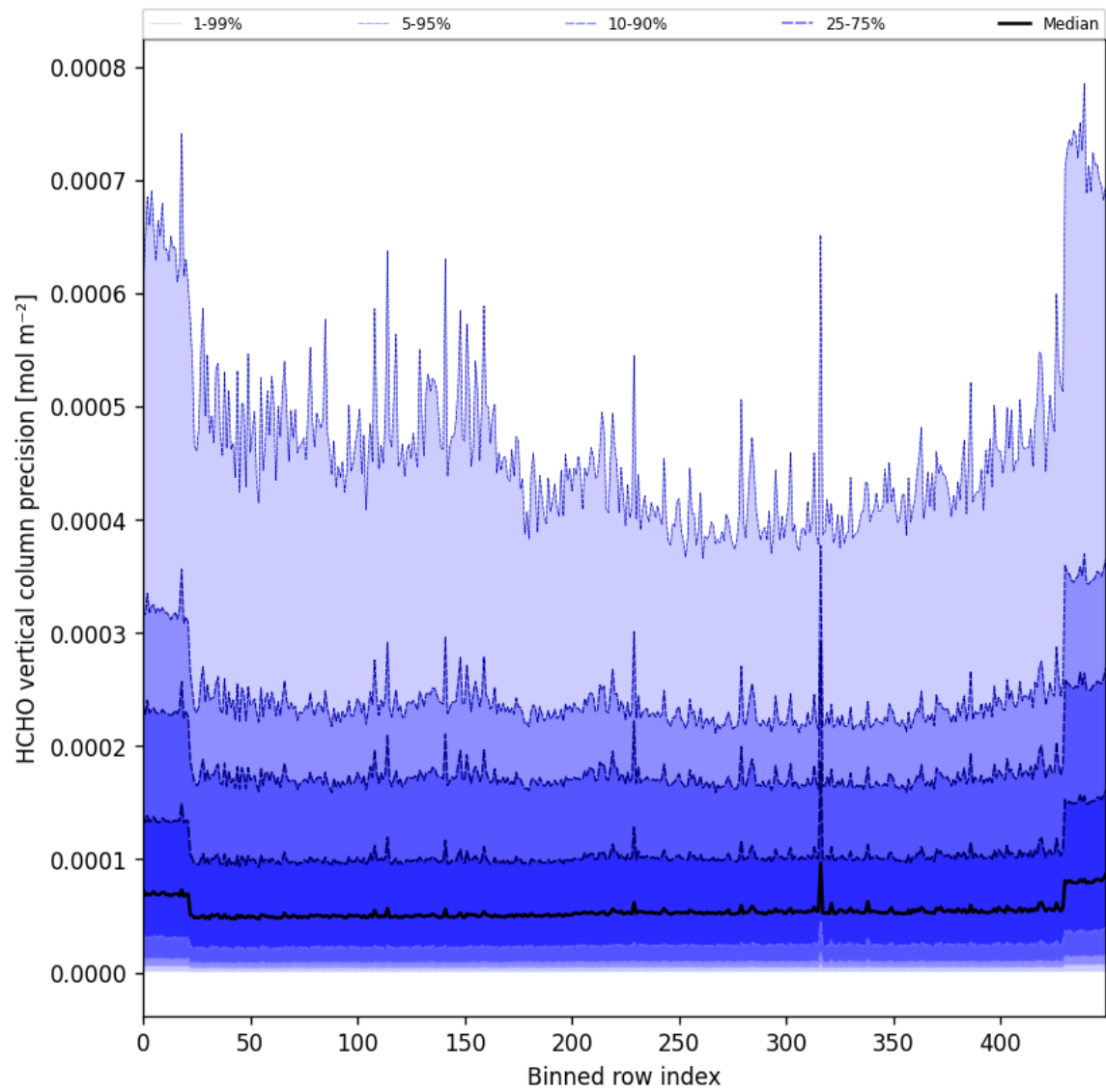
Figure 50: Along track statistics of “HCHO vertical column precision” for 2025-02-24 to 2025-02-25
