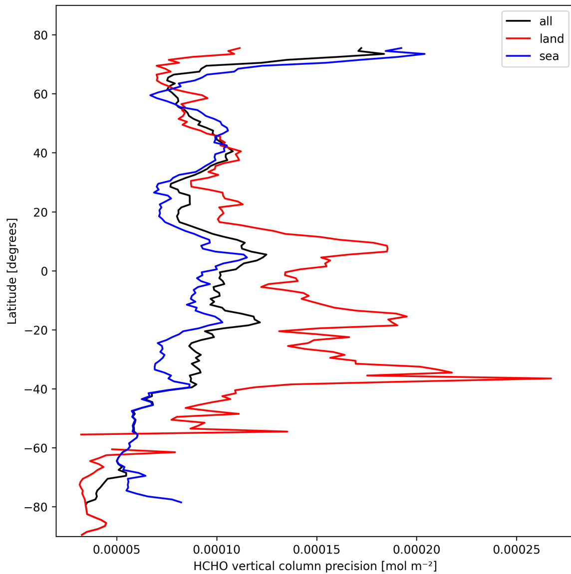
Figure 22: Zonal average of “HCHO vertical column precision” for 2025-02-24 to 2025-02-25.
