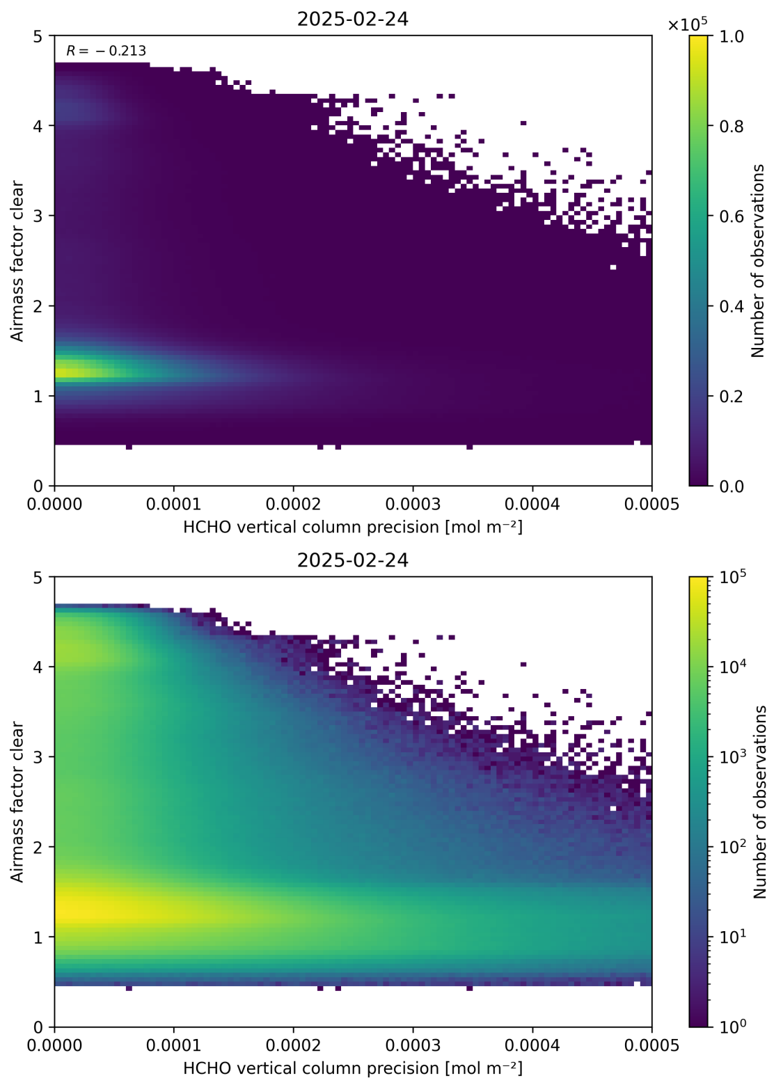
Figure 139: Scatter density plot of “HCHO vertical column precision” against “Airmass factor clear” for 2025-02-24 to 2025-02-25.
