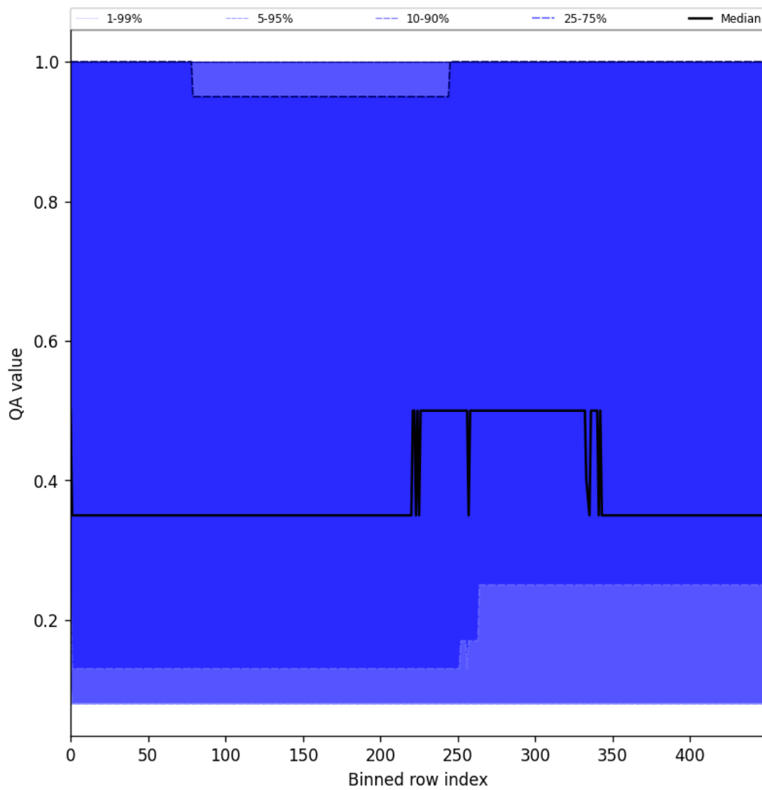
Figure 48: Along track statistics of “QA value” for 2025-02-24 to 2025-02-25
