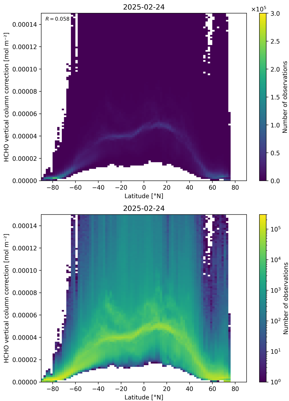
Figure 164: Scatter density plot of “Latitude” against “HCHO vertical column correction” for 2025-02-24 to 2025-02-25.
