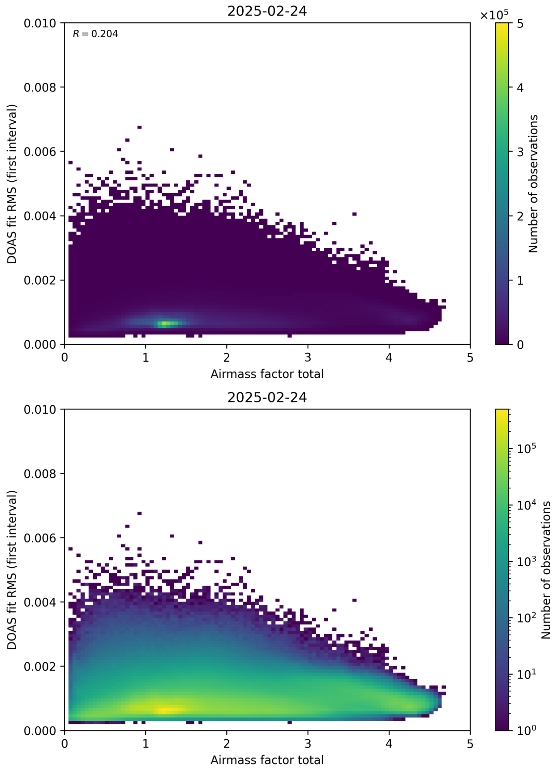
Figure 97: Scatter density plot of “Airmass factor total” against “DOAS fit RMS (first interval)” for 2025-02-24 to 2025-02-25.
