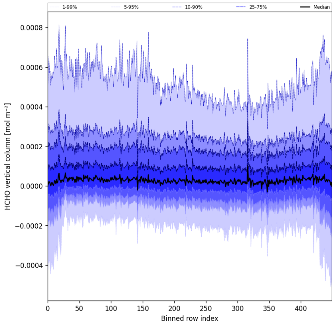
Figure 49: Along track statistics of “HCHO vertical column” for 2025-02-24 to 2025-02-25
