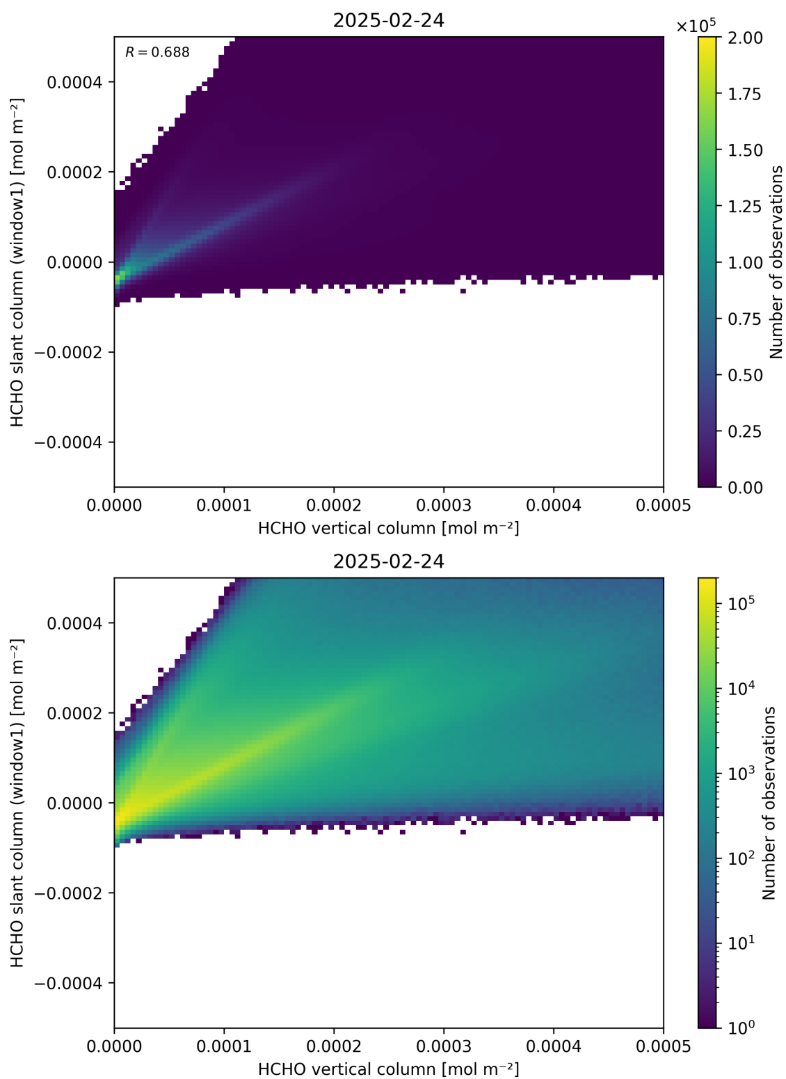
Figure 129: Scatter density plot of “HCHO vertical column” against “HCHO slant column (window1)” for 2025-02-24 to 2025-02-25.
