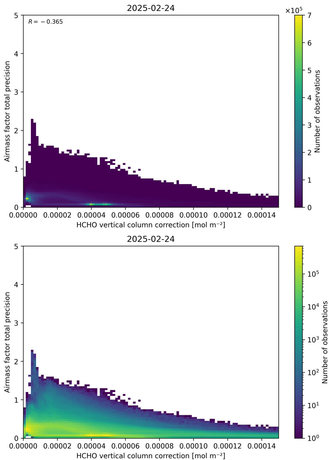
Figure 121: Scatter density plot of “HCHO vertical column correction” against “Airmass factor total precision” for 2025-02-24 to 2025-02-25.
