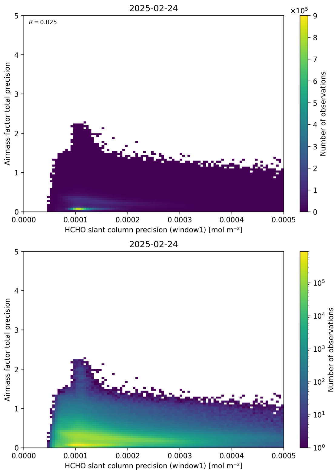
Figure 95: Scatter density plot of “HCHO slant column precision (window1)” against “Airmass factor total precision” for 2025-02-24 to 2025-02-25.
