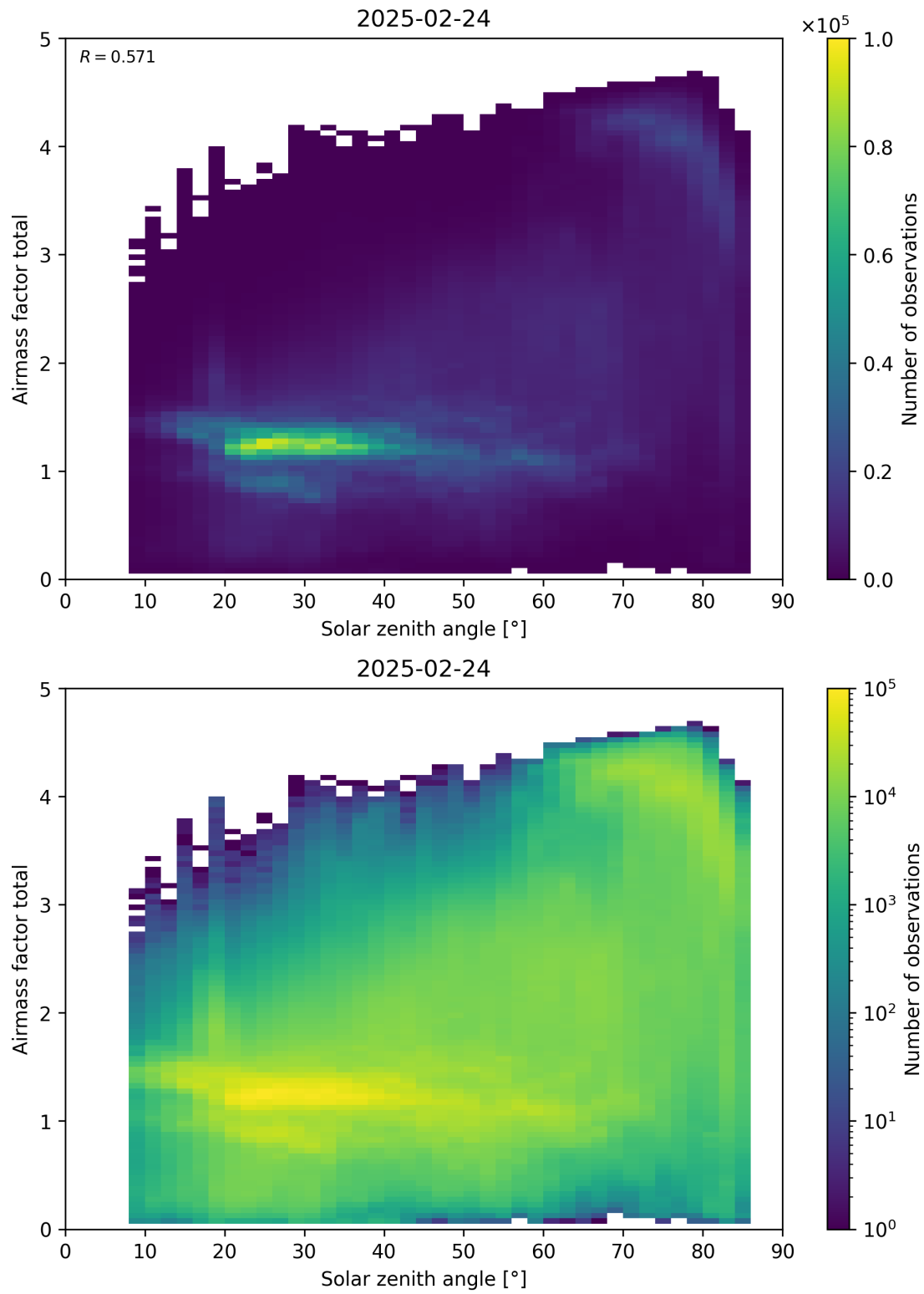
Figure 175: Scatter density plot of “Solar zenith angle” against “Airmass factor total” for 2025-02-24 to 2025-02-25.
