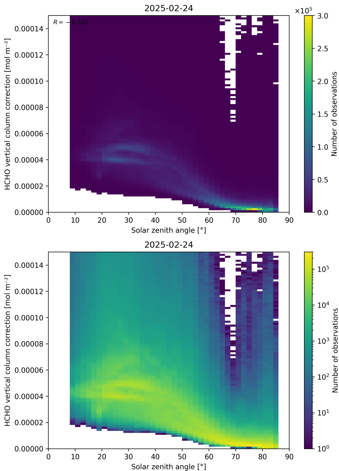
Figure 178: Scatter density plot of “Solar zenith angle” against “HCHO vertical column correction” for 2025-02-24 to 2025-02-25.
