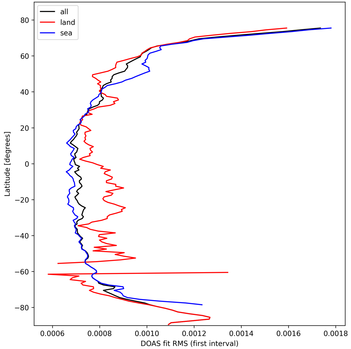
Figure 32: Zonal average of “DOAS fit RMS (first interval)” for 2025-02-24 to 2025-02-25.
