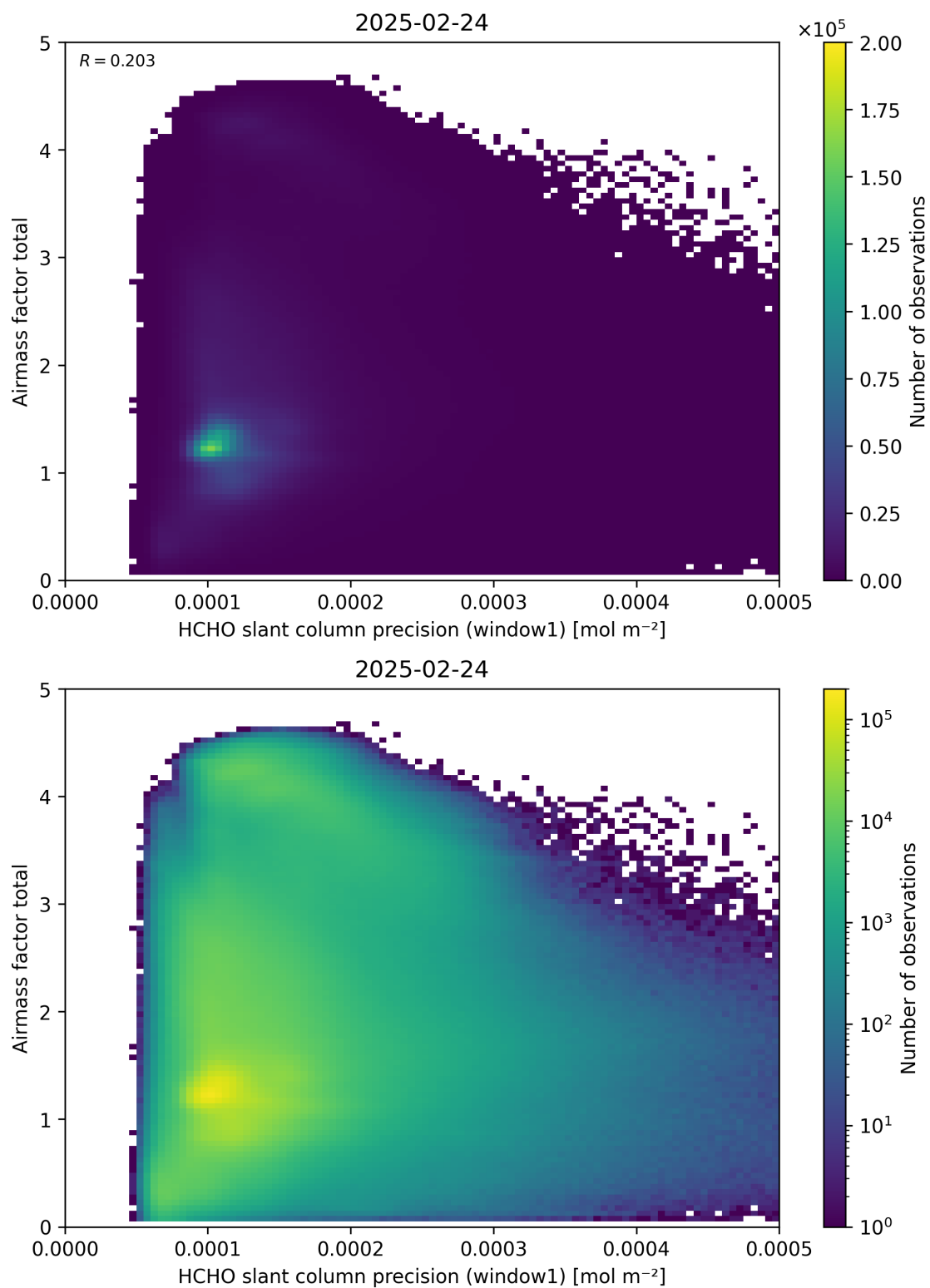
Figure 94: Scatter density plot of “HCHO slant column precision (window1)” against “Airmass factor total” for 2025-02-24 to 2025-02-25.
