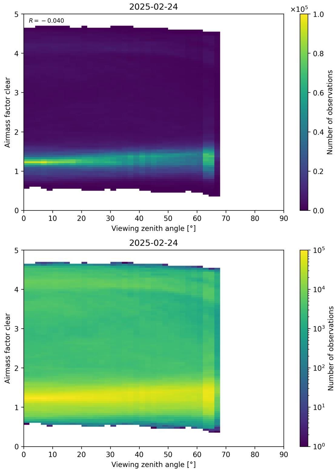
Figure 185: Scatter density plot of “Viewing zenith angle” against “Airmass factor clear” for 2025-02-24 to 2025-02-25.
