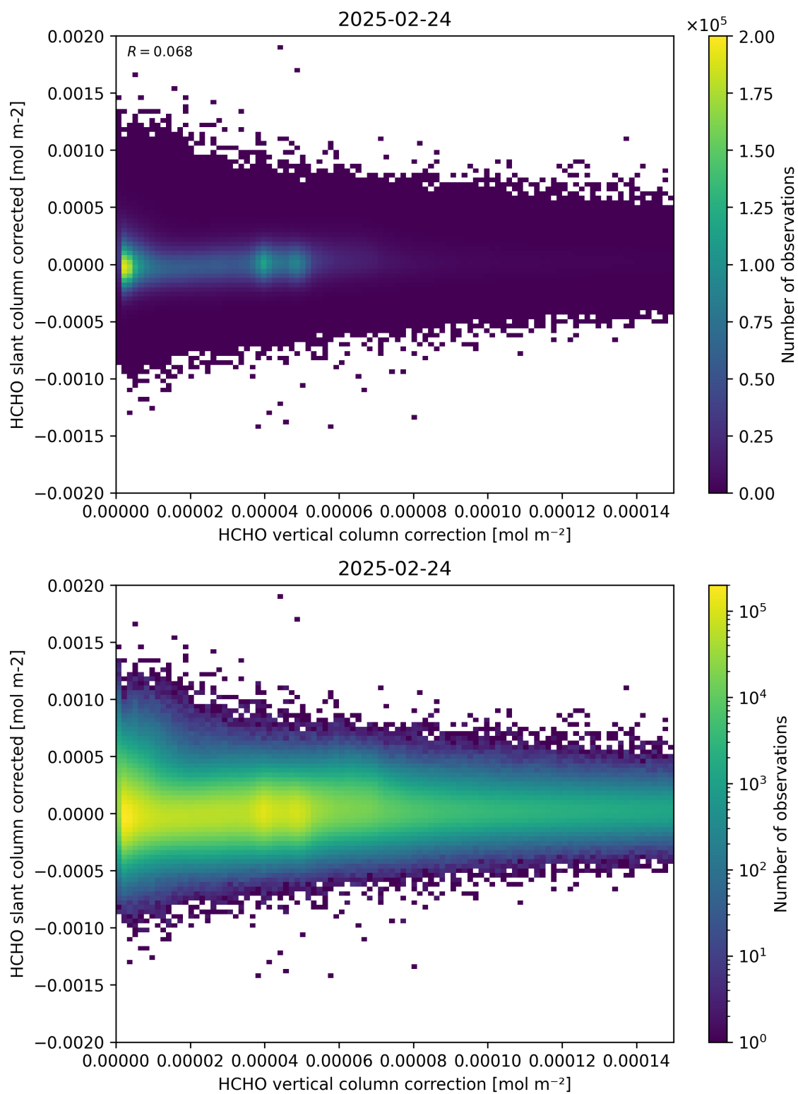
Figure 116: Scatter density plot of “HCHO vertical column correction” against “HCHO slant column corrected” for 2025-02-24 to 2025-02-25.
