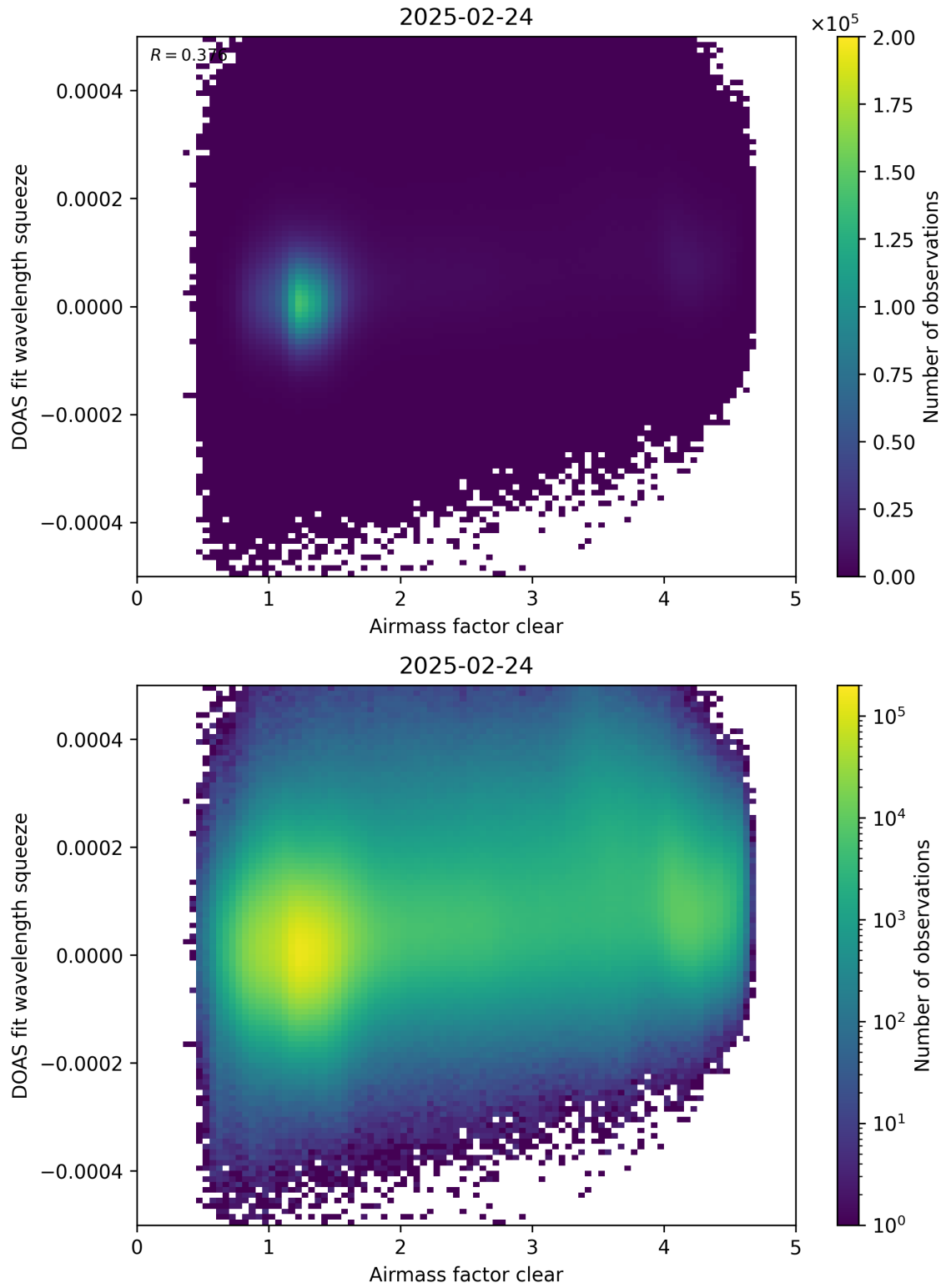
Figure 73: Scatter density plot of “Airmass factor clear” against “DOAS fit wavelength squeeze” for 2025-02-24 to 2025-02-25.
