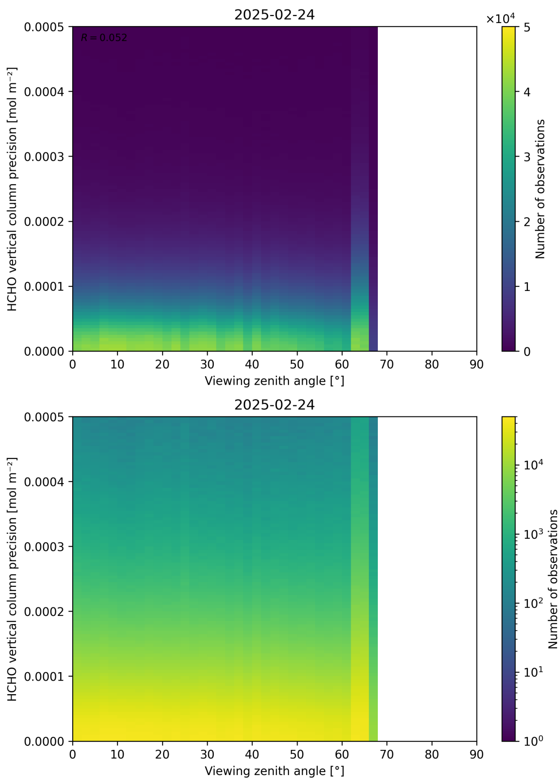
Figure 194: Scatter density plot of “Viewing zenith angle” against “HCHO vertical column precision” for 2025-02-24 to 2025-02-25.
