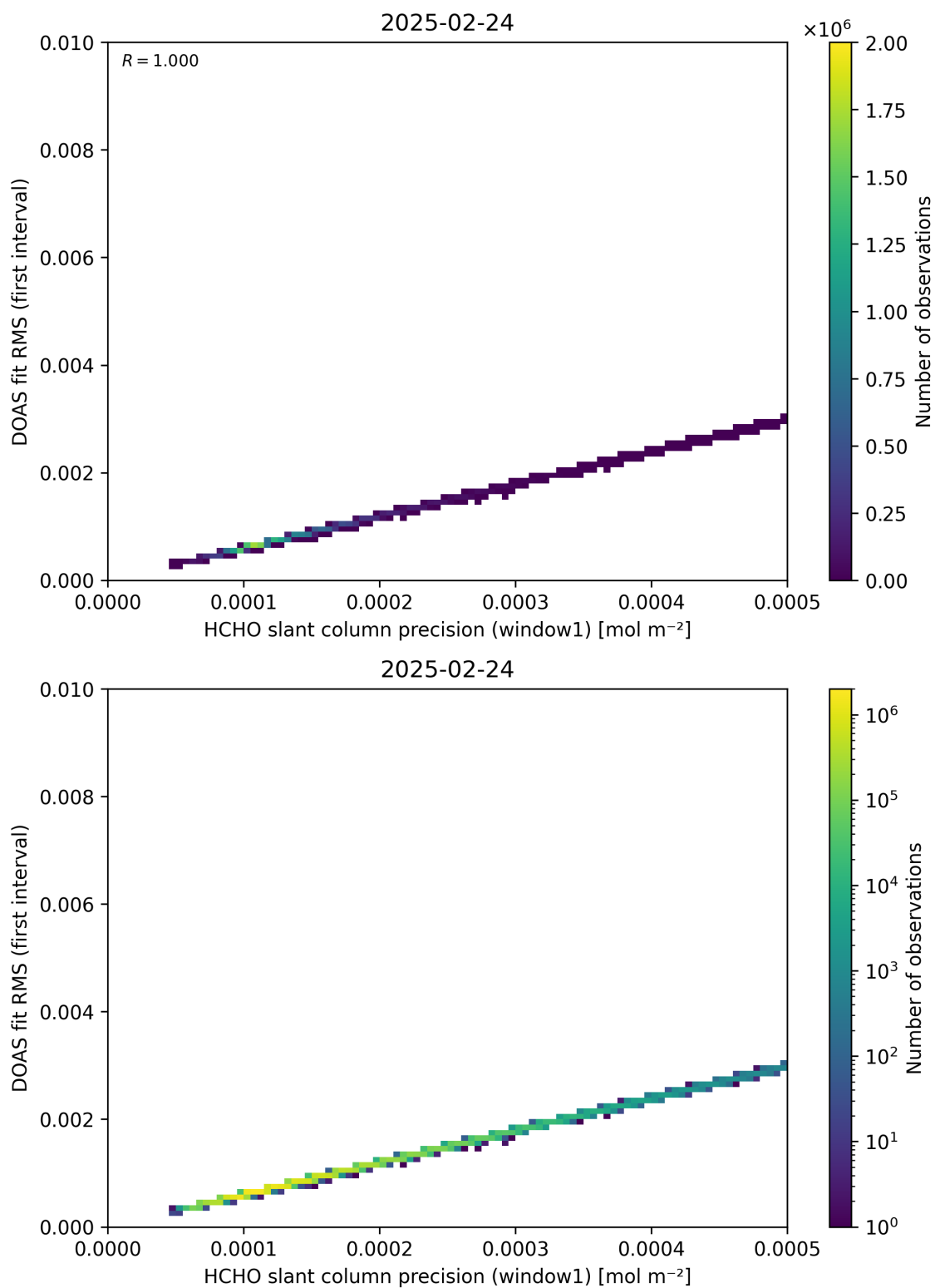
Figure 88: Scatter density plot of “HCHO slant column precision (window1)” against “DOAS fit RMS (first interval)” for 2025-02-24 to 2025-02-25.
