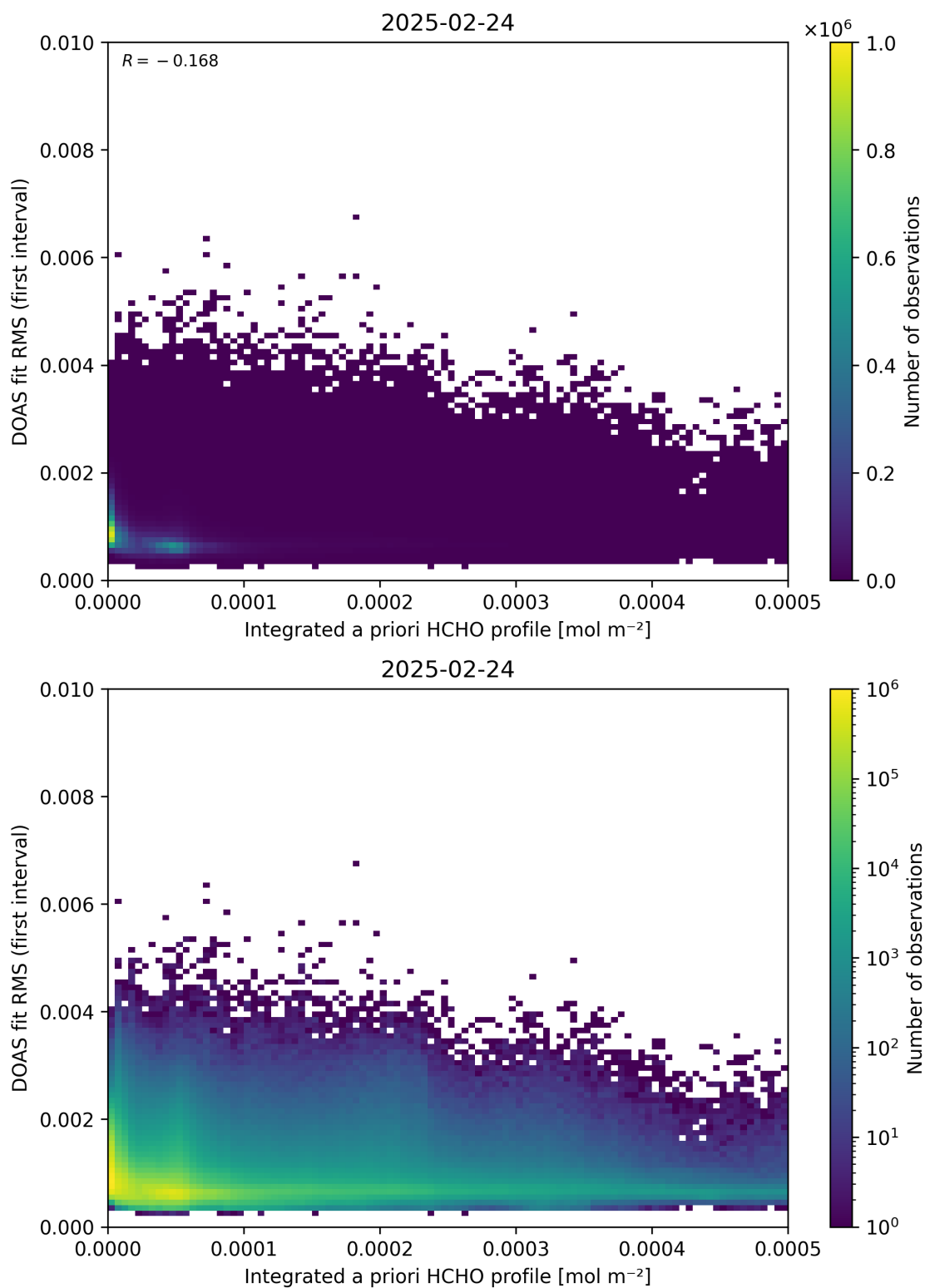
Figure 148: Scatter density plot of “Integrated a priori HCHO profile” against “DOAS fit RMS (first interval)” for 2025-02-24 to 2025-02-25.
