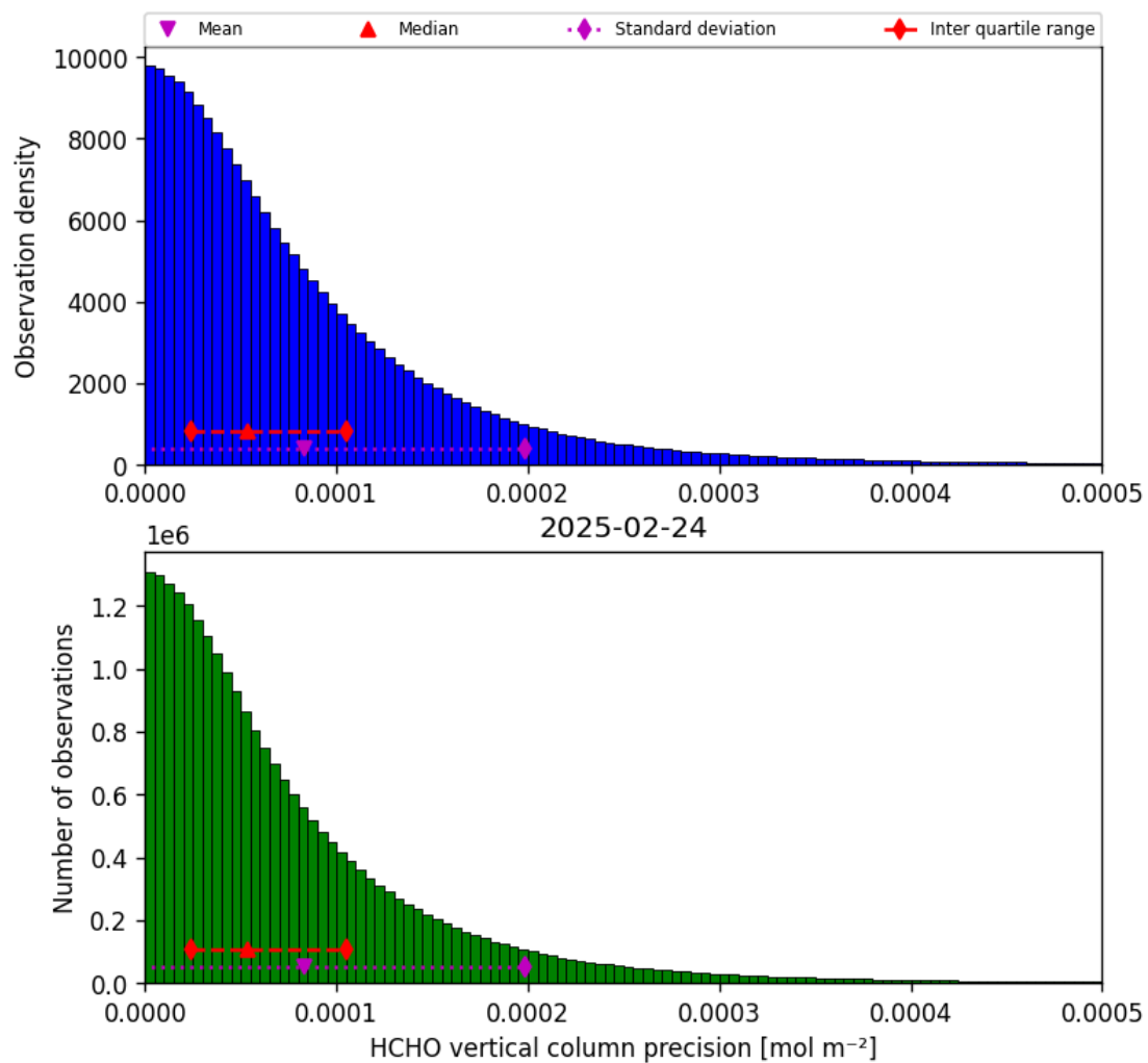
Figure 36: Histogram of “HCHO vertical column precision” for 2025-02-24 to 2025-02-25
