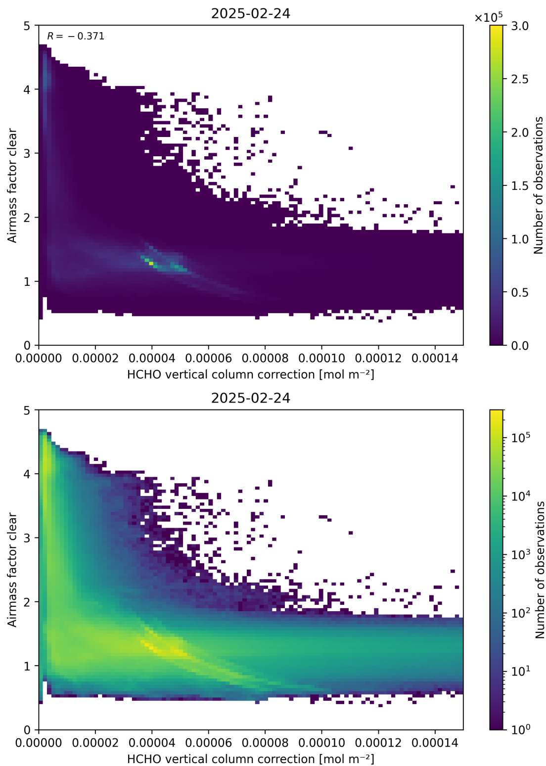
Figure 115: Scatter density plot of “HCHO vertical column correction” against “Airmass factor clear” for 2025-02-24 to 2025-02-25.
