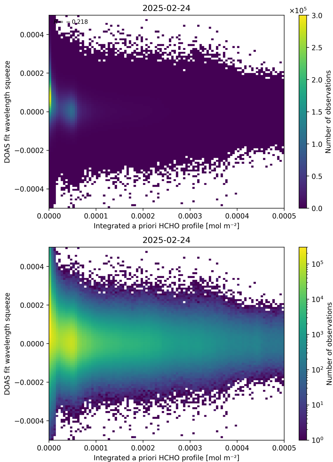
Figure 150: Scatter density plot of “Integrated a priori HCHO profile” against “DOAS fit wavelength squeeze” for 2025-02-24 to 2025-02-25.
