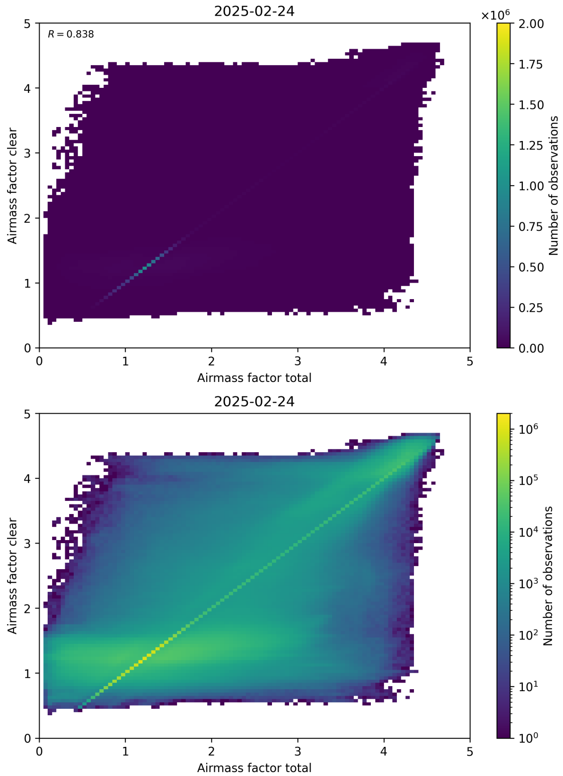
Figure 100: Scatter density plot of “Airmass factor total” against “Airmass factor clear” for 2025-02-24 to 2025-02-25.
