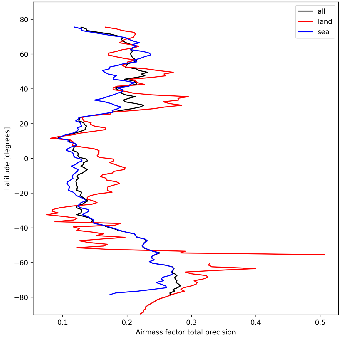
Figure 27: Zonal average of “Airmass factor total precision” for 2025-02-24 to 2025-02-25.
