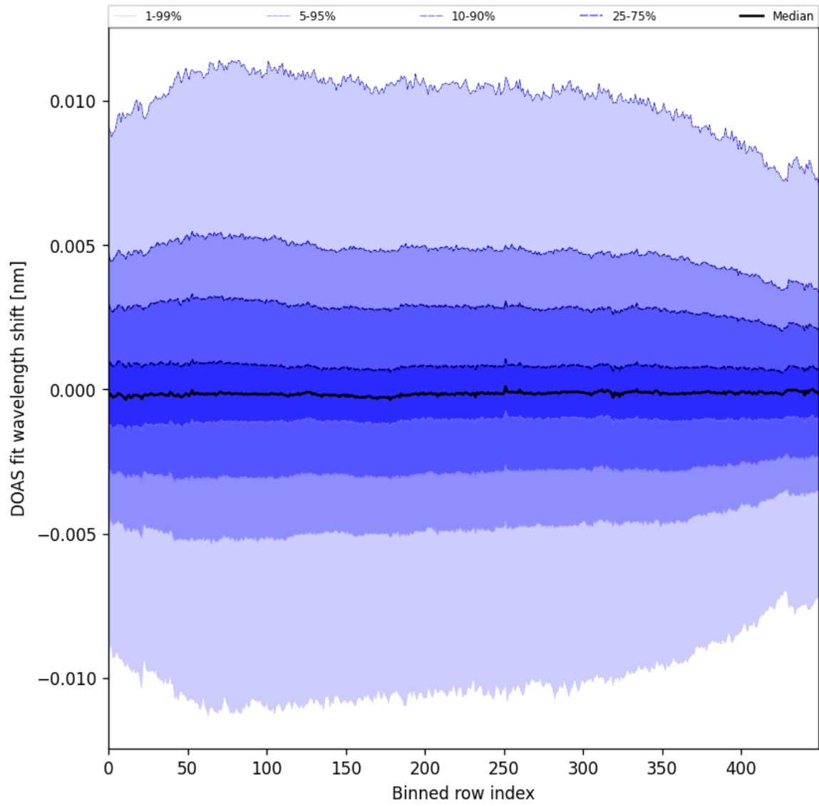
Figure 58: Along track statistics of “DOAS fit wavelength shift” for 2025-02-24 to 2025-02-25
