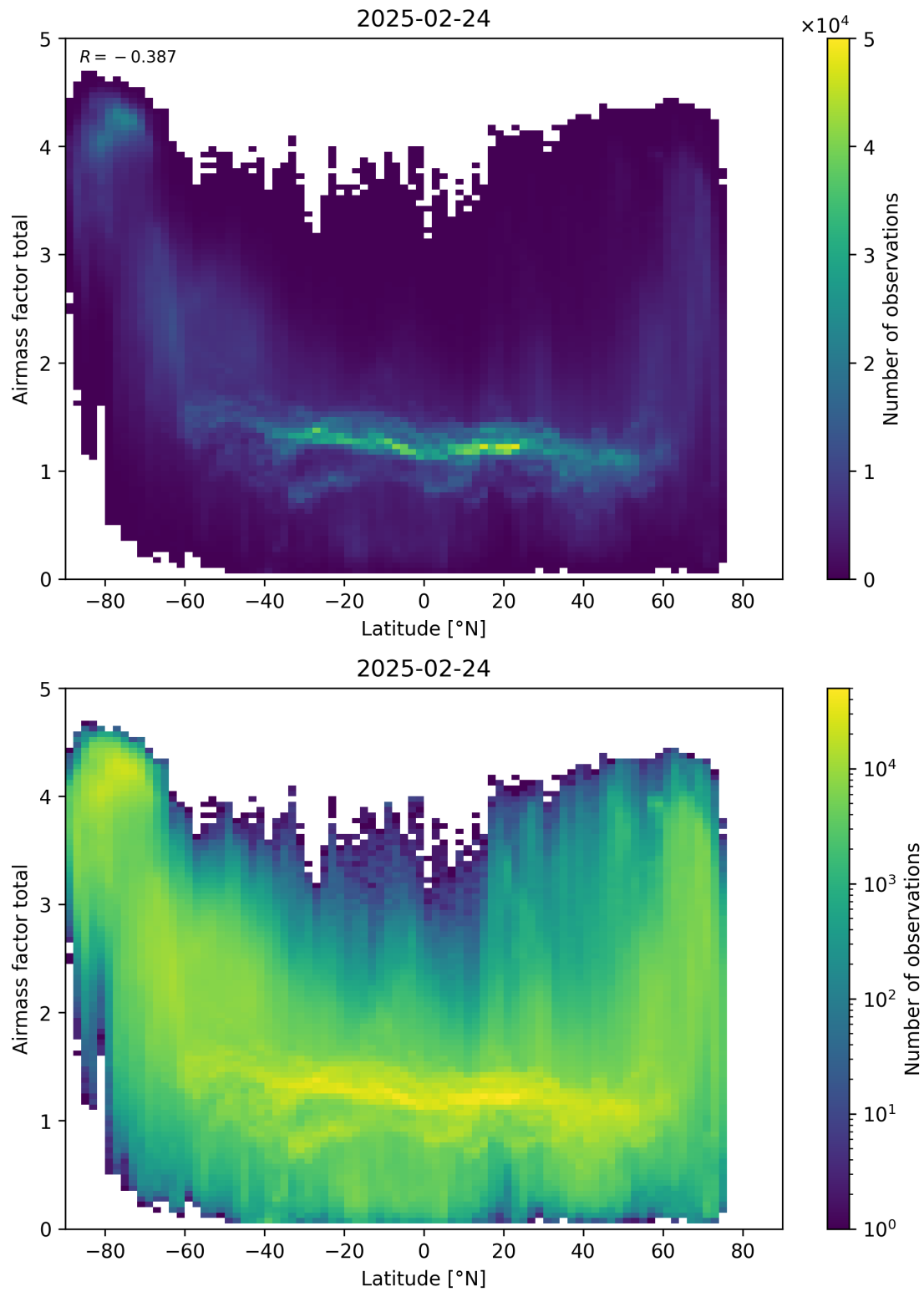
Figure 161: Scatter density plot of “Latitude” against “Airmass factor total” for 2025-02-24 to 2025-02-25.
