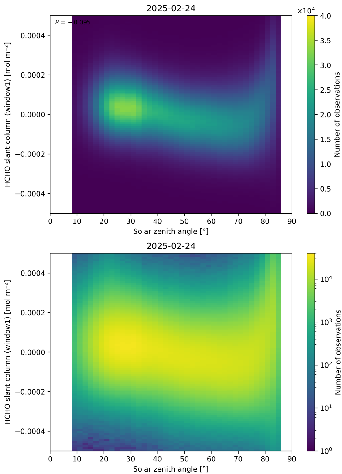
Figure 173: Scatter density plot of “Solar zenith angle” against “HCHO slant column (window1)” for 2025-02-24 to 2025-02-25.
