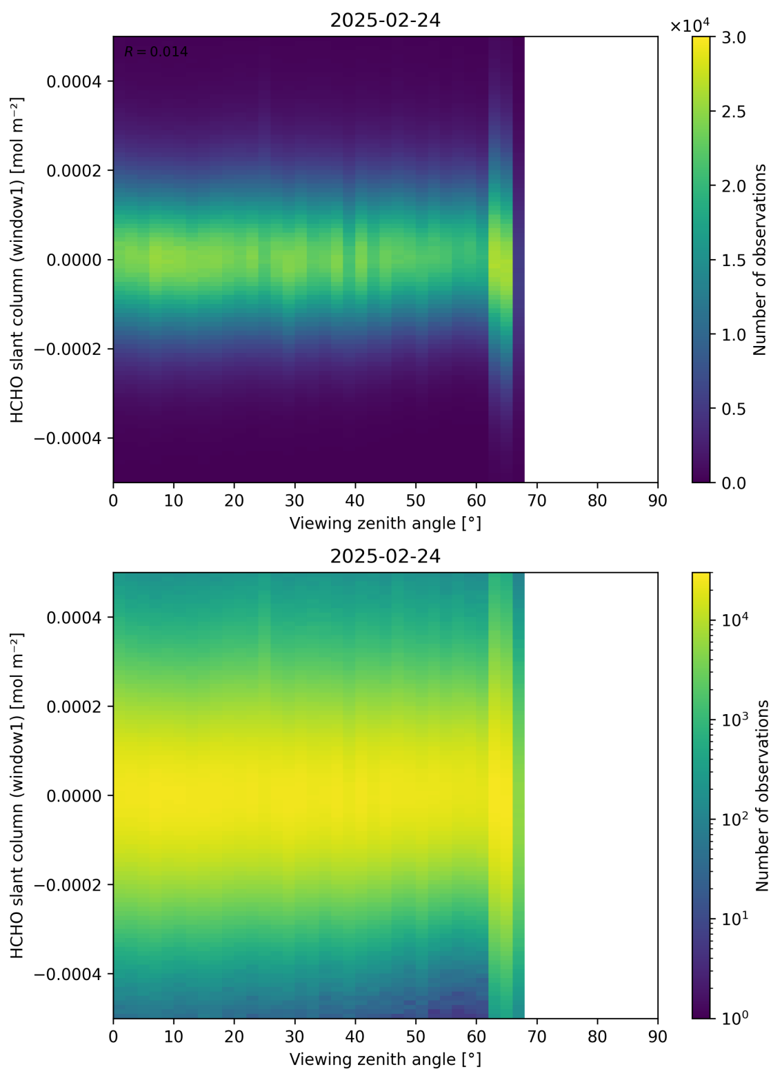
Figure 188: Scatter density plot of “Viewing zenith angle” against “HCHO slant column (window1)” for 2025-02-24 to 2025-02-25.
