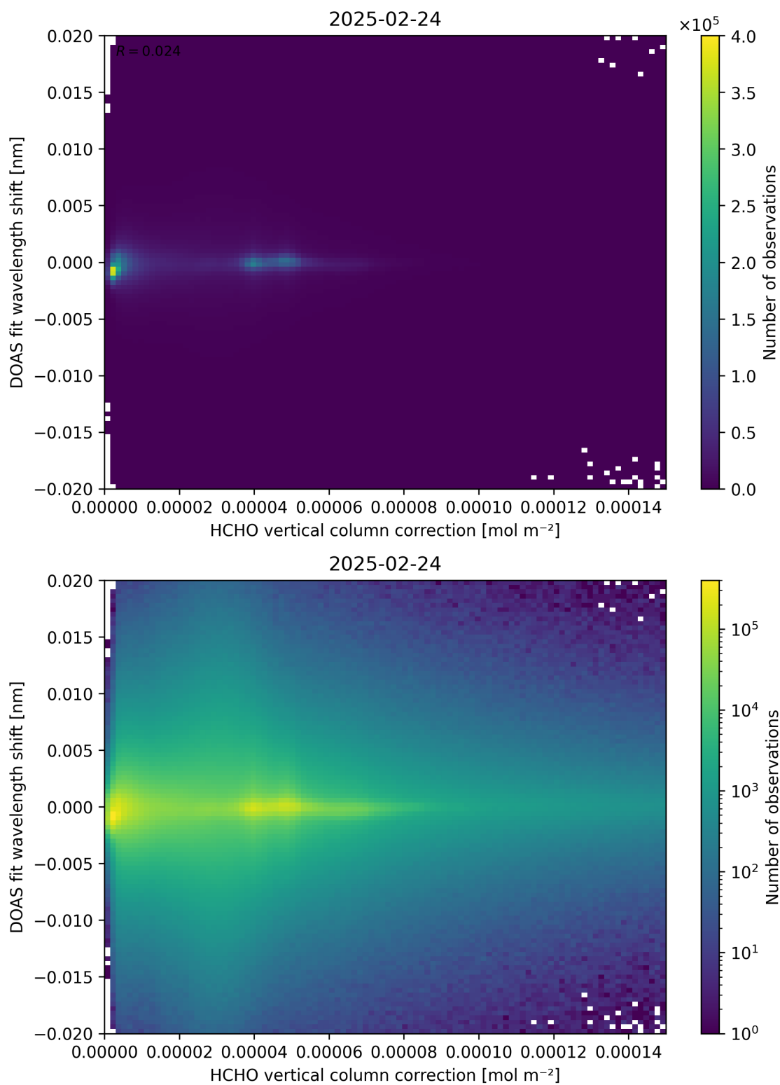
Figure 113: Scatter density plot of “HCHO vertical column correction” against “DOAS fit wavelength shift” for 2025-02-24 to 2025-02-25.
