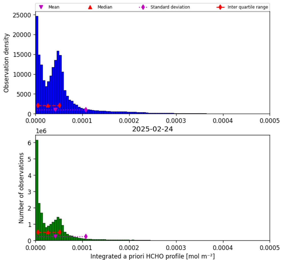
Figure 43: Histogram of “Integrated a priori HCHO profile” for 2025-02-24 to 2025-02-25
