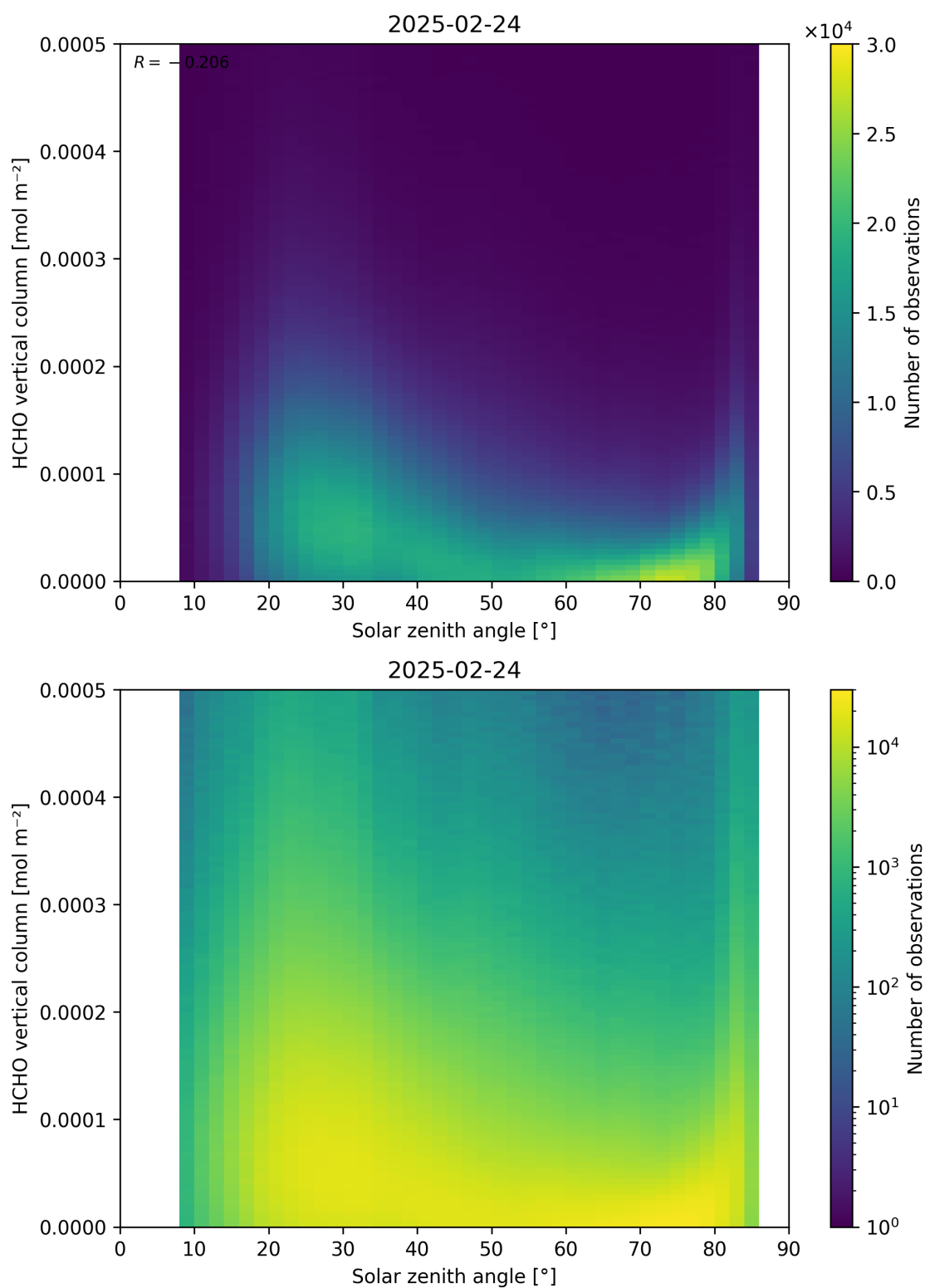
Figure 177: Scatter density plot of “Solar zenith angle” against “HCHO vertical column” for 2025-02-24 to 2025-02-25.
