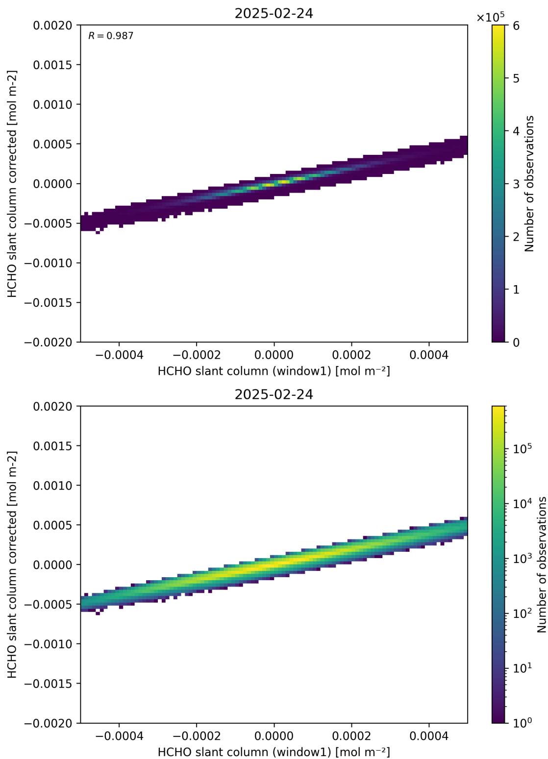
Figure 82: Scatter density plot of “HCHO slant column (window1)” against “HCHO slant column corrected” for 2025-02-24 to 2025-02-25.
