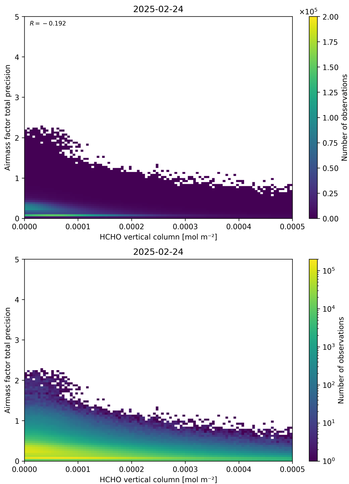
Figure 132: Scatter density plot of “HCHO vertical column” against “Airmass factor total precision” for 2025-02-24 to 2025-02-25.
