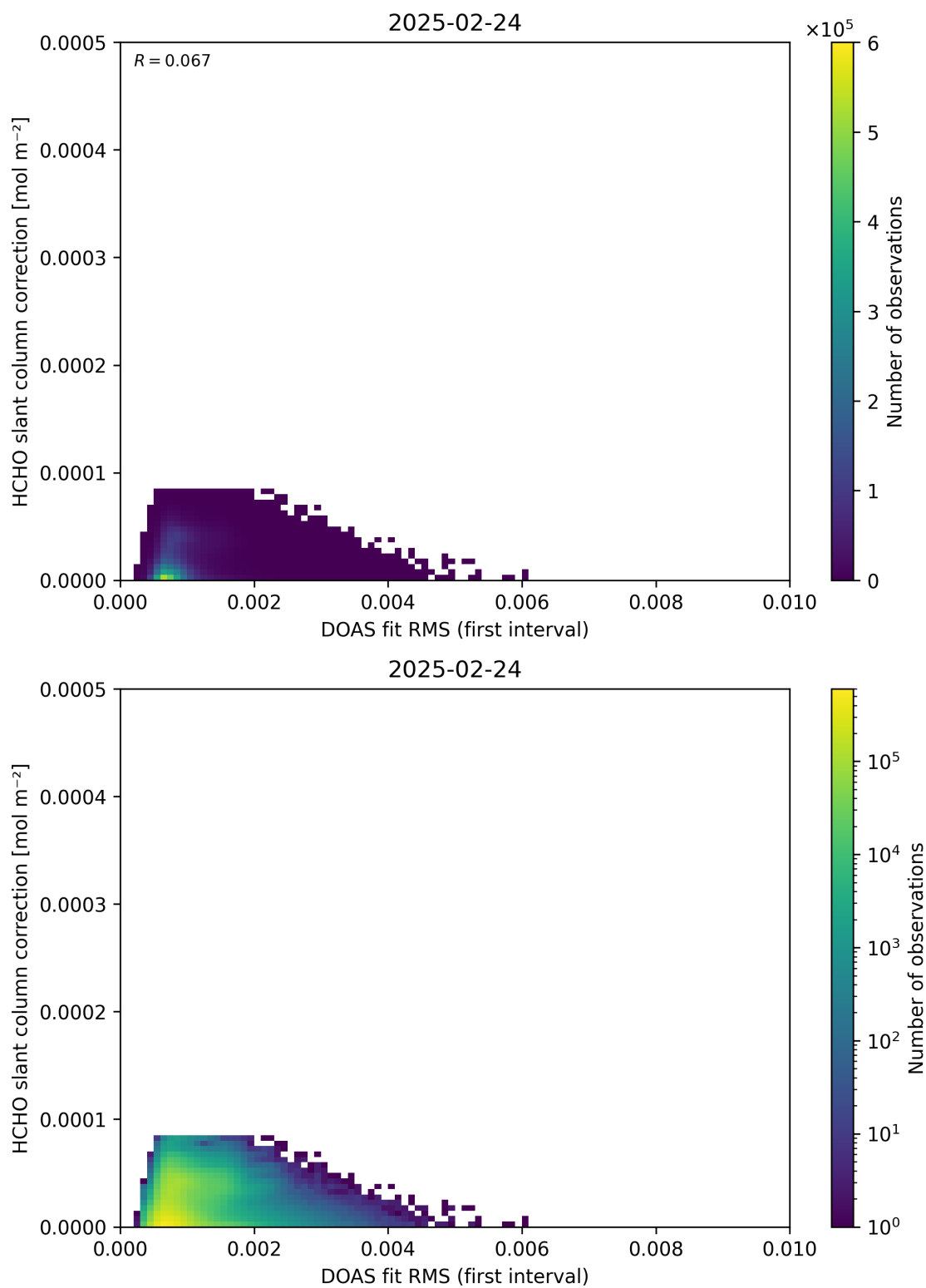
Figure 63: Scatter density plot of “DOAS fit RMS (first interval)” against “HCHO slant column correction” for 2025-02-24 to 2025-02-25.
