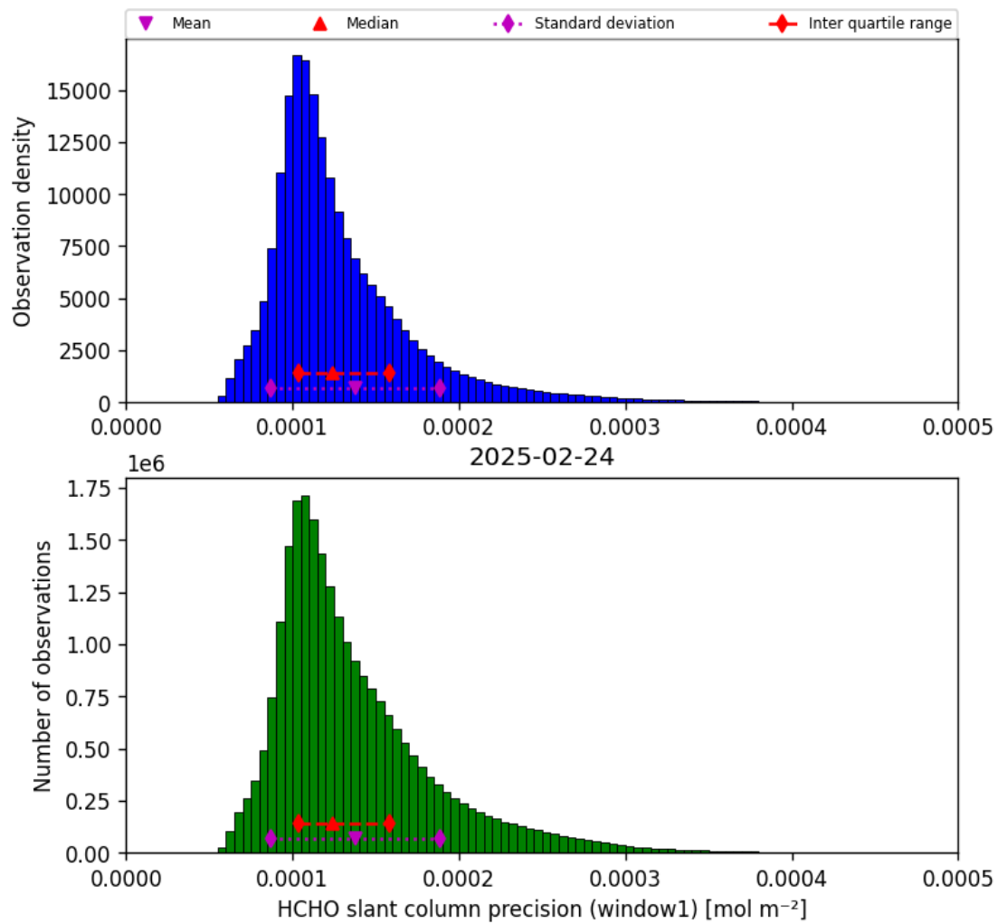
Figure 39: Histogram of “HCHO slant column precision (window1)” for 2025-02-24 to 2025-02-25
