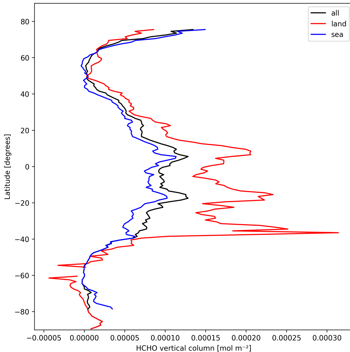
Figure 21: Zonal average of “HCHO vertical column” for 2025-02-24 to 2025-02-25.
