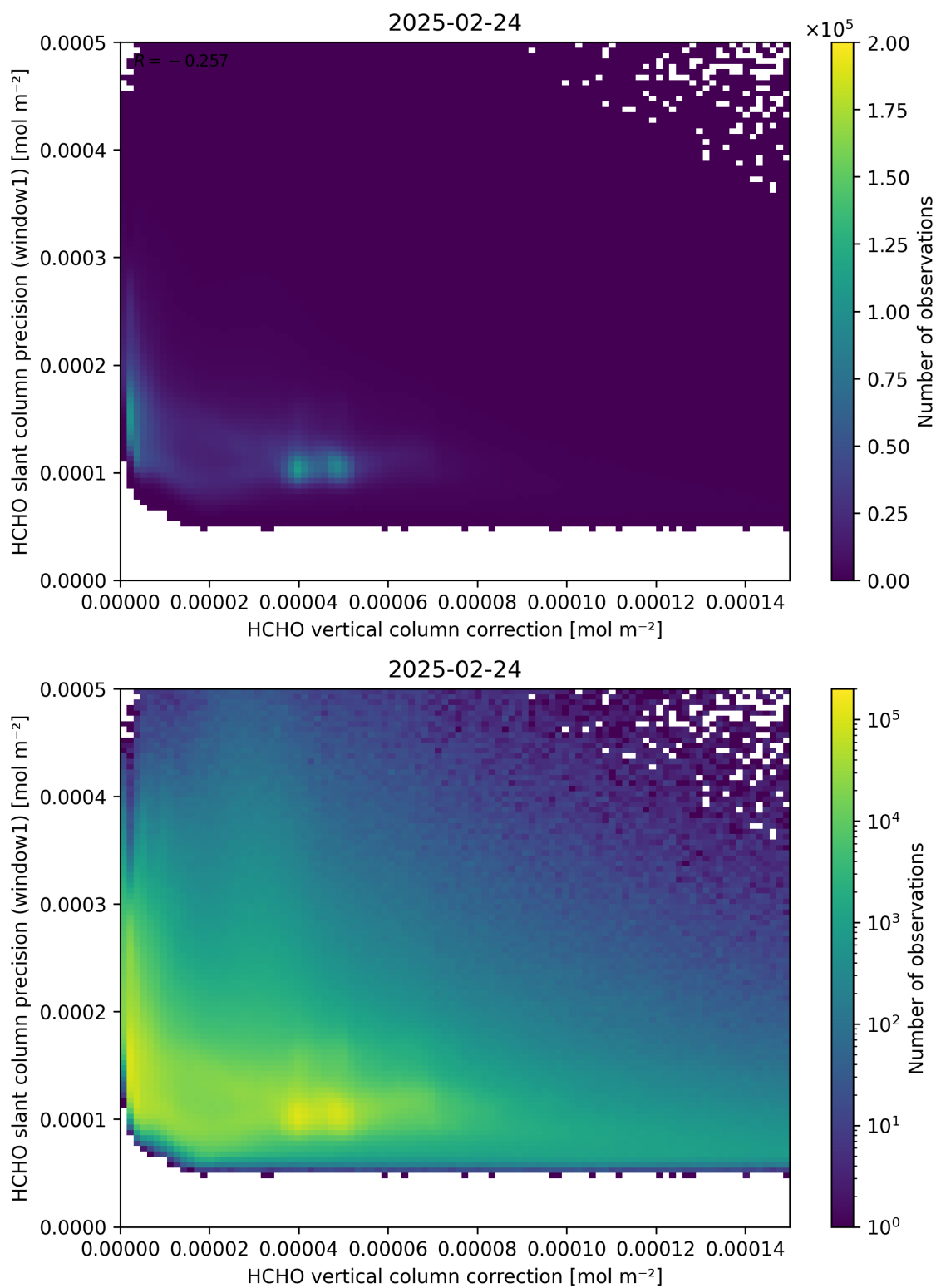
Figure 119: Scatter density plot of “HCHO vertical column correction” against “HCHO slant column precision (window1)” for 2025-02-24 to 2025-02-25.
