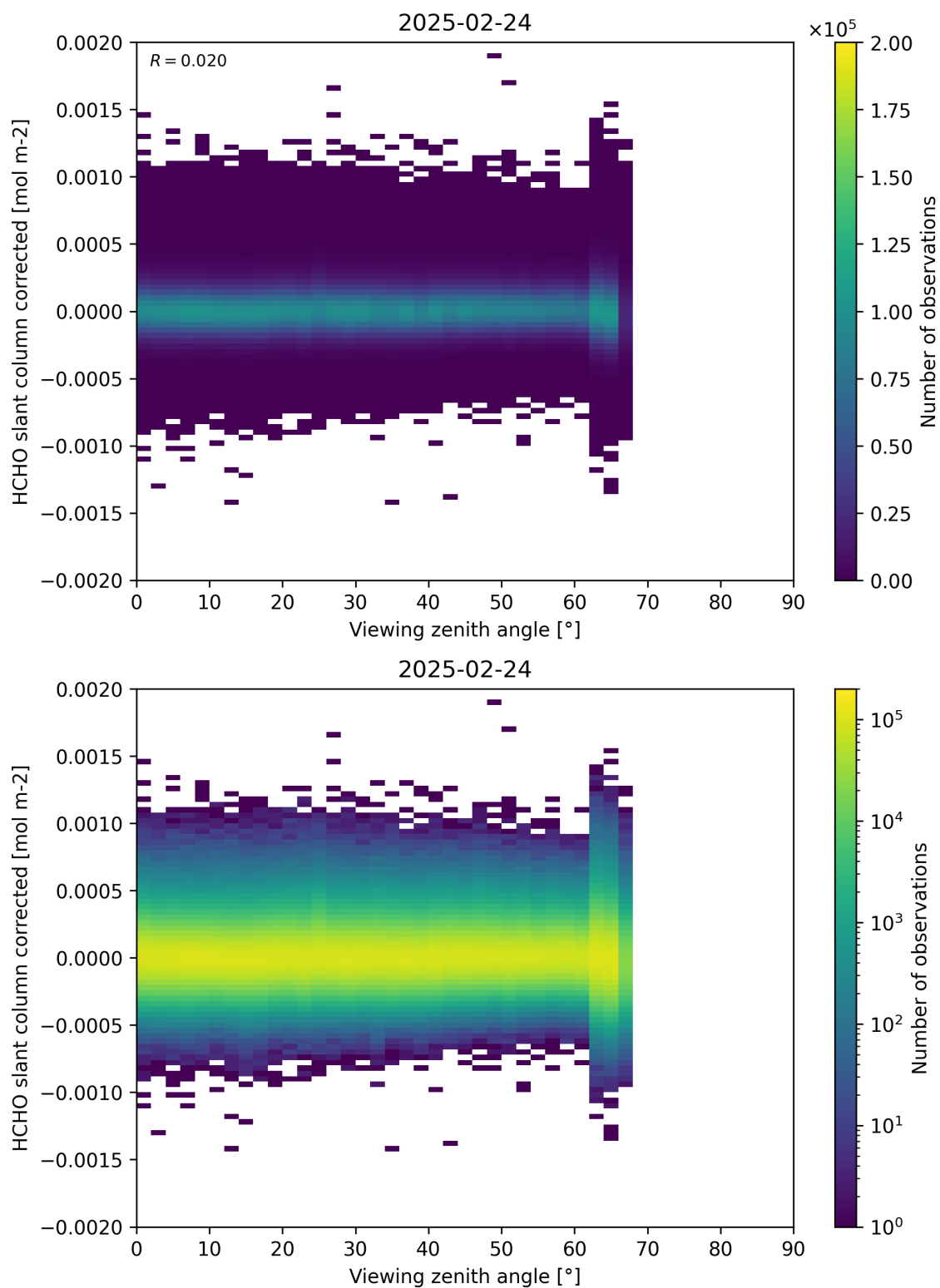
Figure 186: Scatter density plot of “Viewing zenith angle” against “HCHO slant column corrected” for 2025-02-24 to 2025-02-25.
