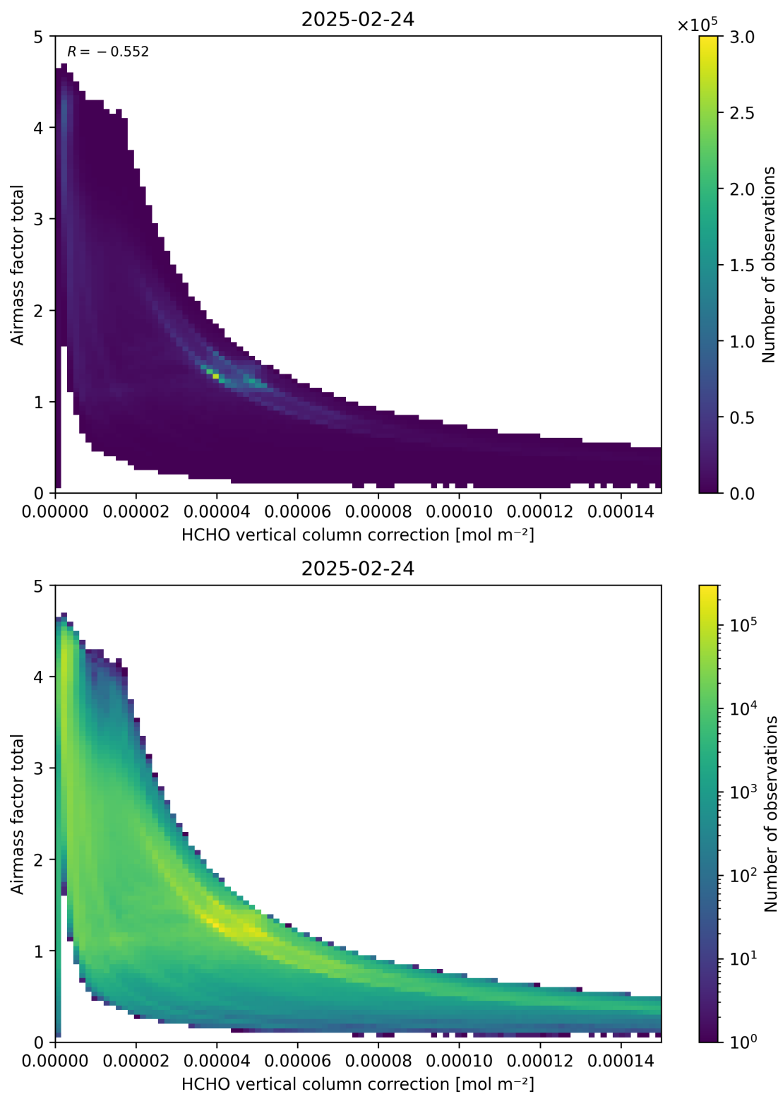
Figure 120: Scatter density plot of “HCHO vertical column correction” against “Airmass factor total” for 2025-02-24 to 2025-02-25.
