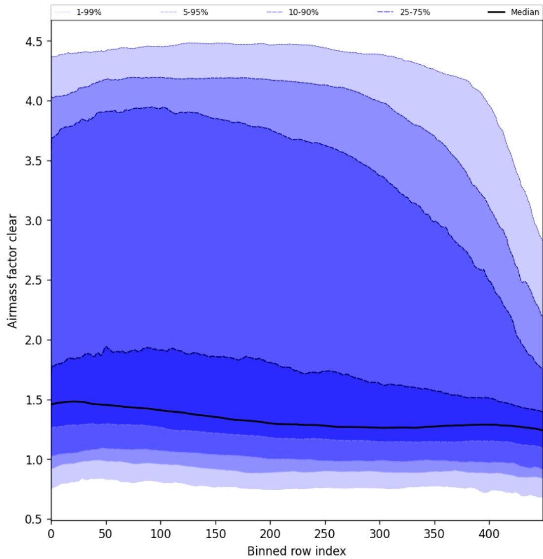
Figure 56: Along track statistics of “Airmass factor clear” for 2025-02-24 to 2025-02-25
