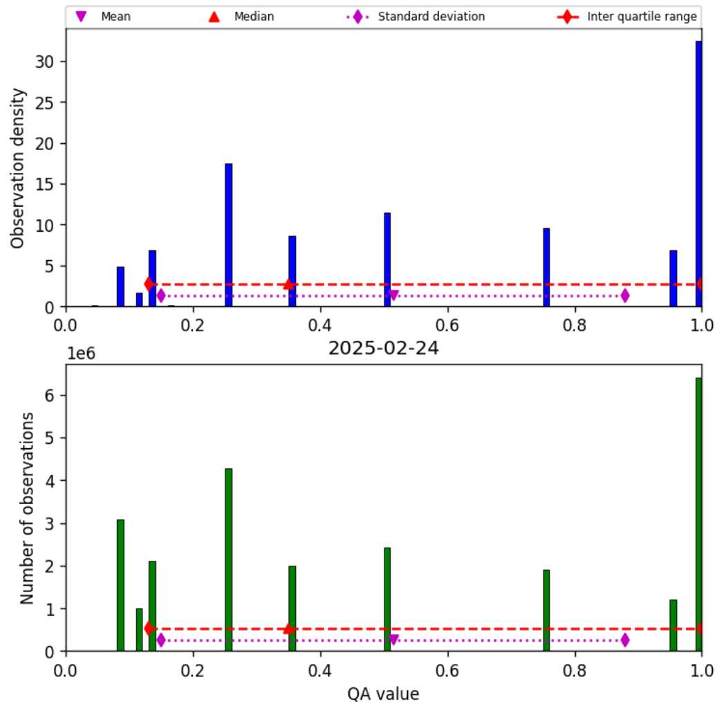
Figure 34: Histogram of “QA value” for 2025-02-24 to 2025-02-25
