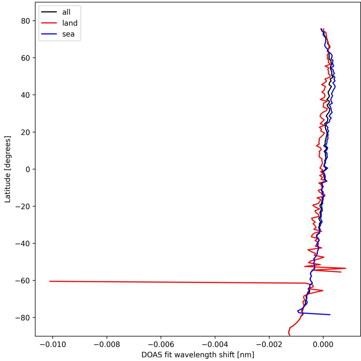
Figure 30: Zonal average of “DOAS fit wavelength shift” for 2025-02-24 to 2025-02-25.
