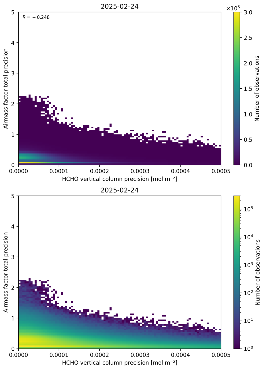
Figure 145: Scatter density plot of “HCHO vertical column precision” against “Airmass factor total precision” for 2025-02-24 to 2025-02-25.
