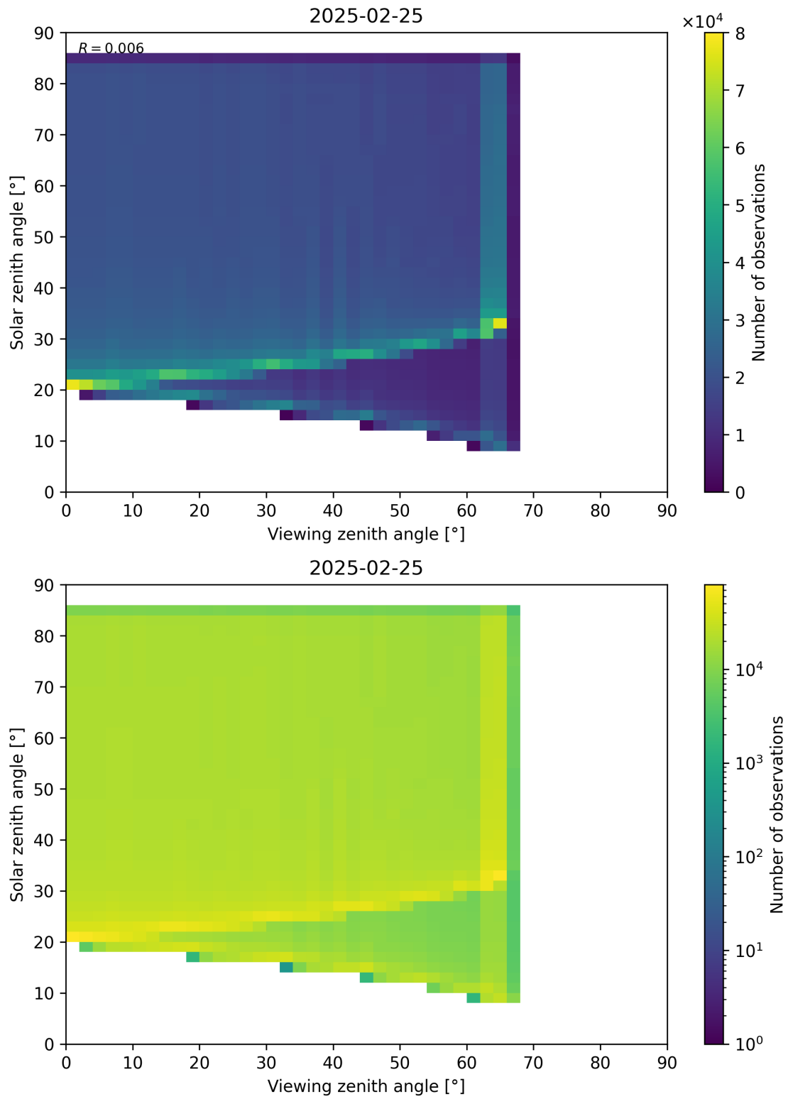
Figure 197: Scatter density plot of “Viewing zenith angle” against “Solar zenith angle” for 2025-02-24 to 2025-02-26.
