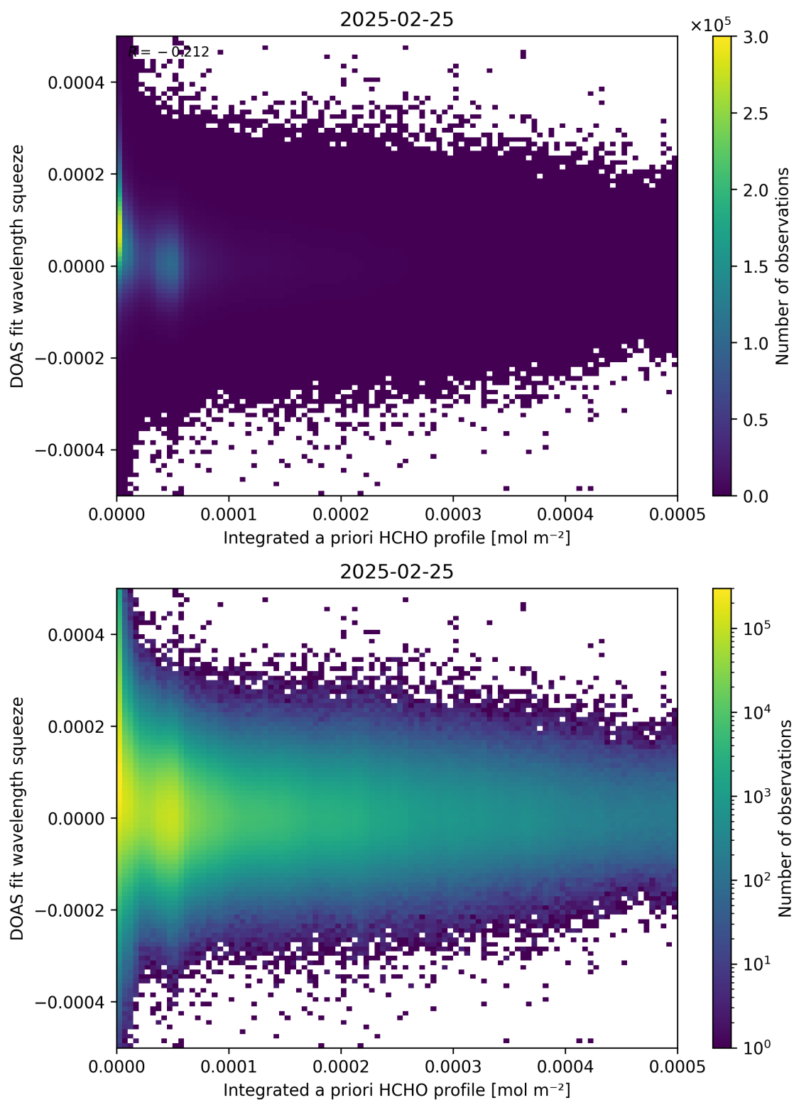
Figure 150: Scatter density plot of “Integrated a priori HCHO profile” against “DOAS fit wavelength squeeze” for 2025-02-24 to 2025-02-26.
