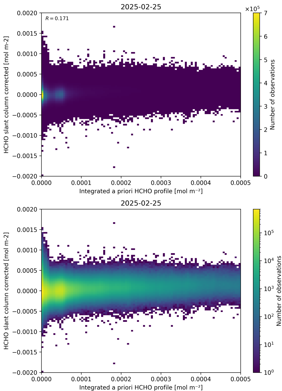
Figure 151: Scatter density plot of “Integrated a priori HCHO profile” against “HCHO slant column corrected” for 2025-02-24 to 2025-02-26.
