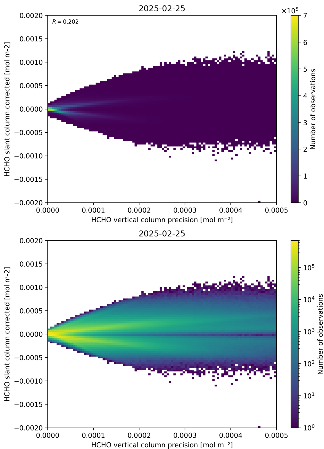
Figure 140: Scatter density plot of “HCHO vertical column precision” against “HCHO slant column corrected” for 2025-02-24 to 2025-02-26.
