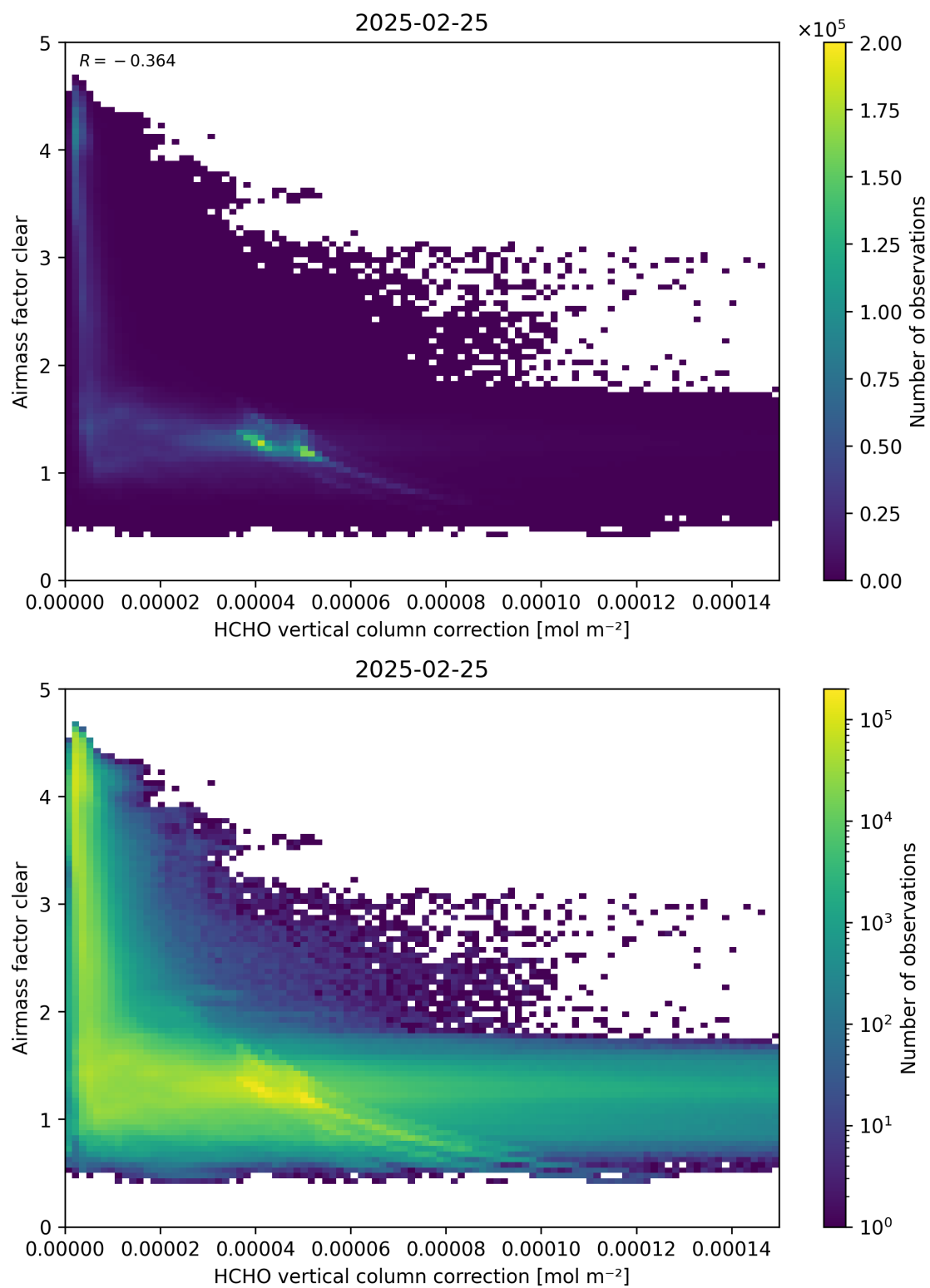
Figure 115: Scatter density plot of “HCHO vertical column correction” against “Airmass factor clear” for 2025-02-24 to 2025-02-26.
