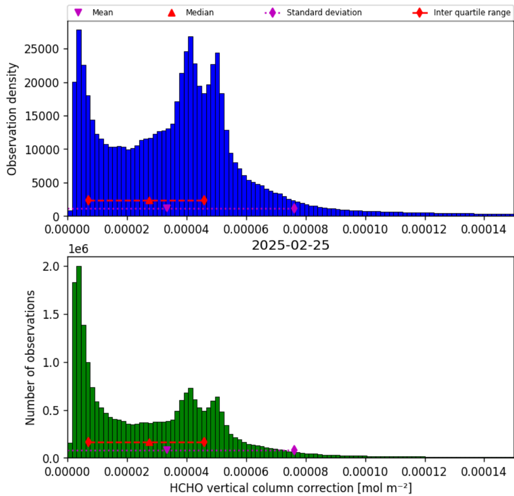
Figure 37: Histogram of “HCHO vertical column correction” for 2025-02-24 to 2025-02-26
