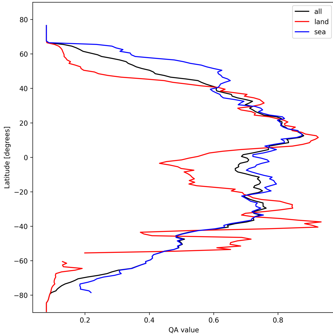
Figure 20: Zonal average of “QA value” for 2025-02-24 to 2025-02-26.
