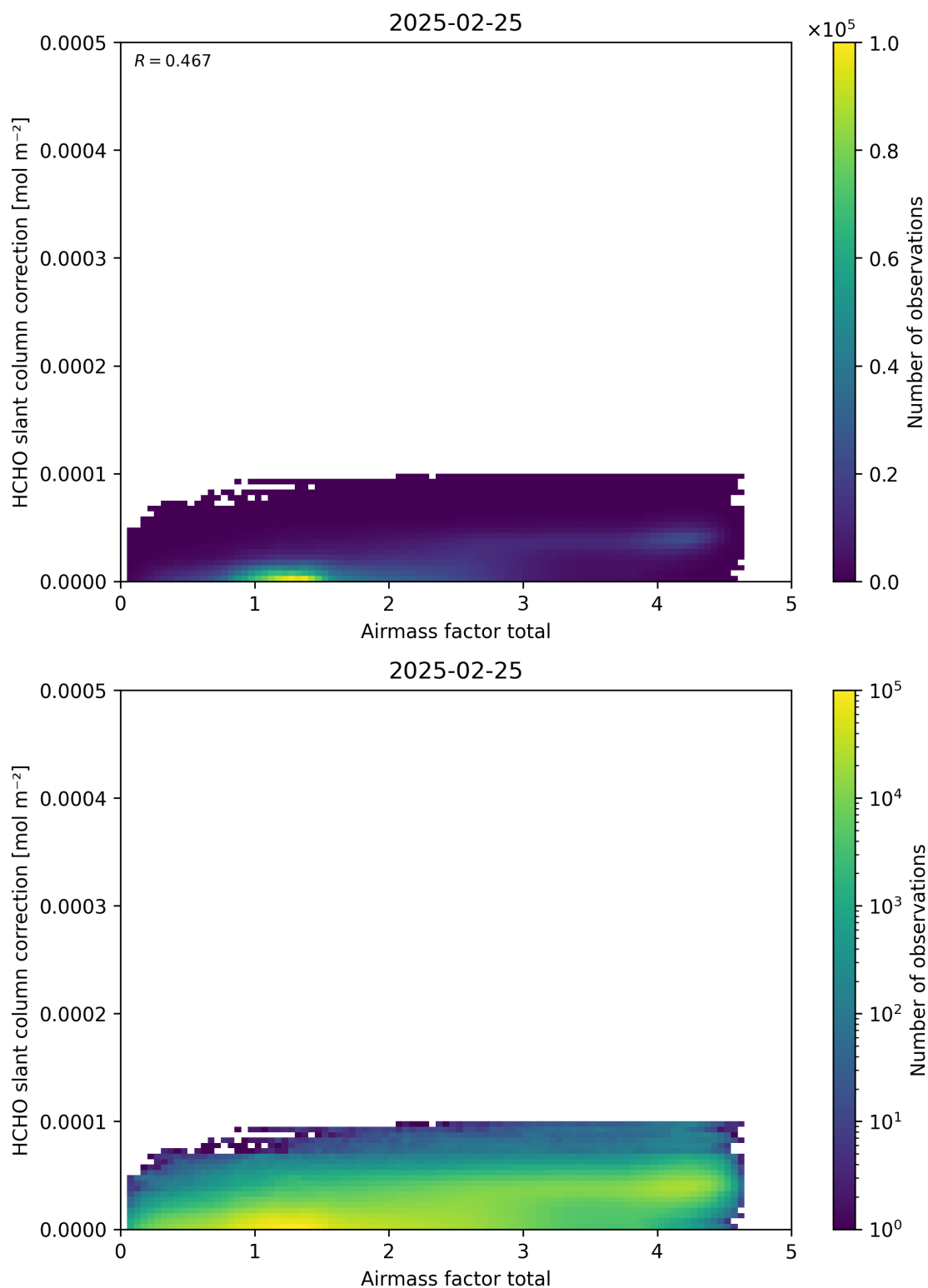
Figure 102: Scatter density plot of “Airmass factor total” against “HCHO slant column correction” for 2025-02-24 to 2025-02-26.
