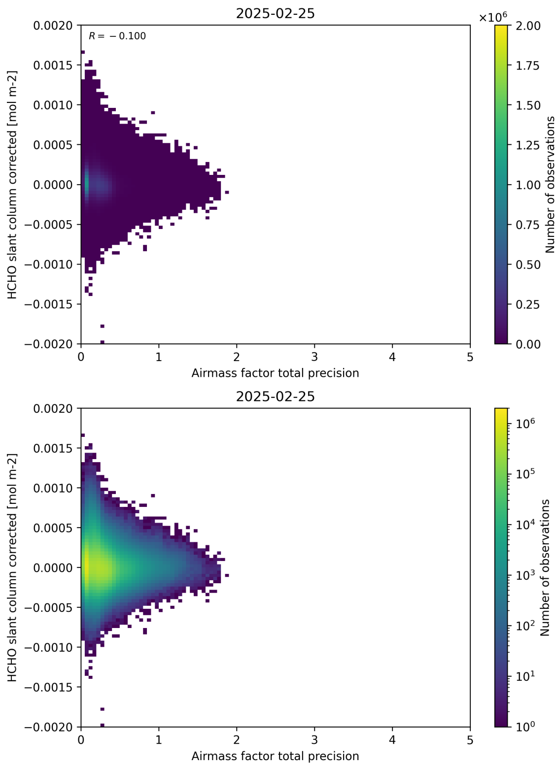
Figure 109: Scatter density plot of “Airmass factor total precision” against “HCHO slant column corrected” for 2025-02-24 to 2025-02-26.
