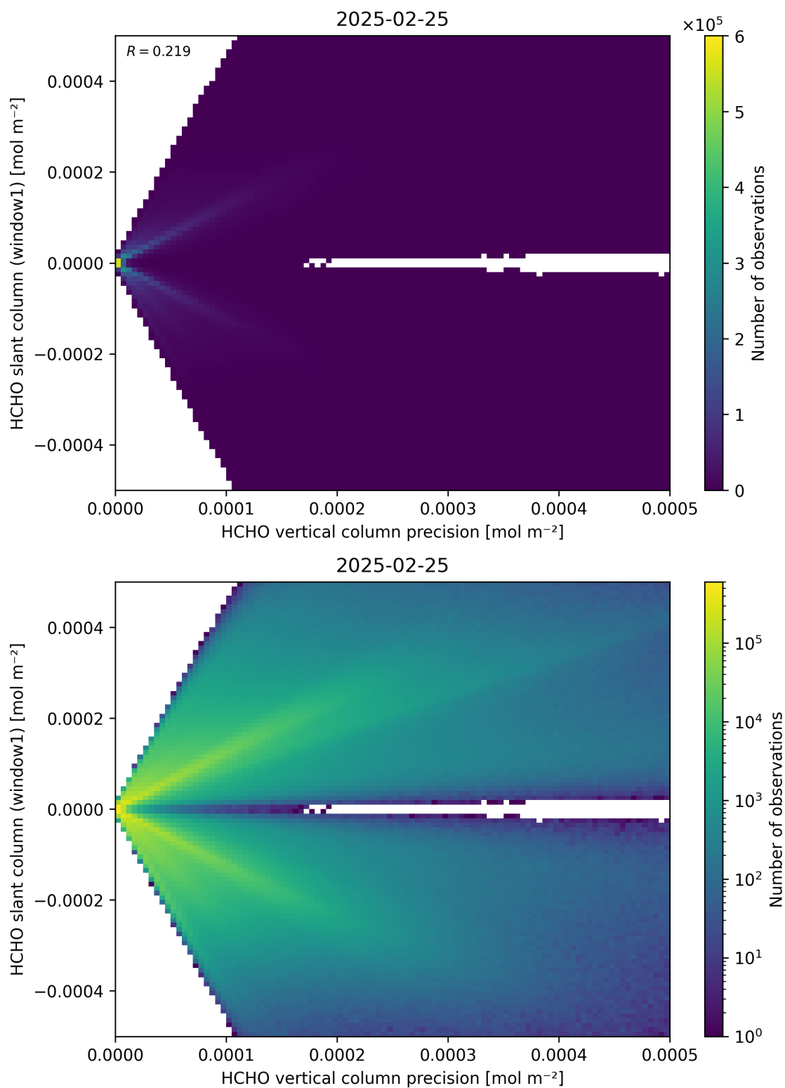
Figure 142: Scatter density plot of “HCHO vertical column precision” against “HCHO slant column (window1)” for 2025-02-24 to 2025-02-26.
