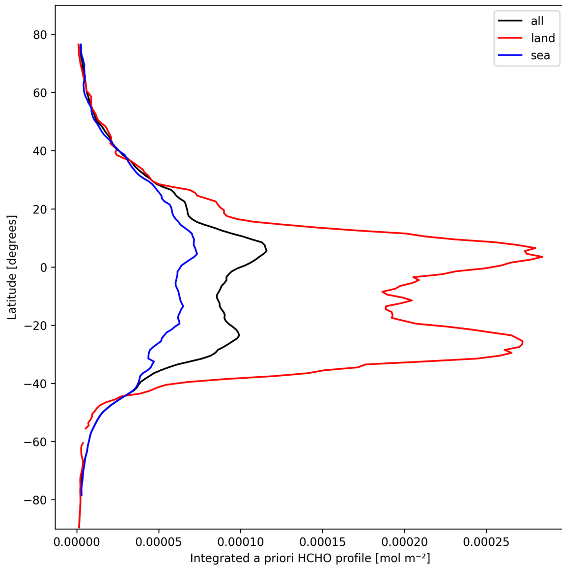
Figure 29: Zonal average of “Integrated a priori HCHO profile” for 2025-02-24 to 2025-02-26.
