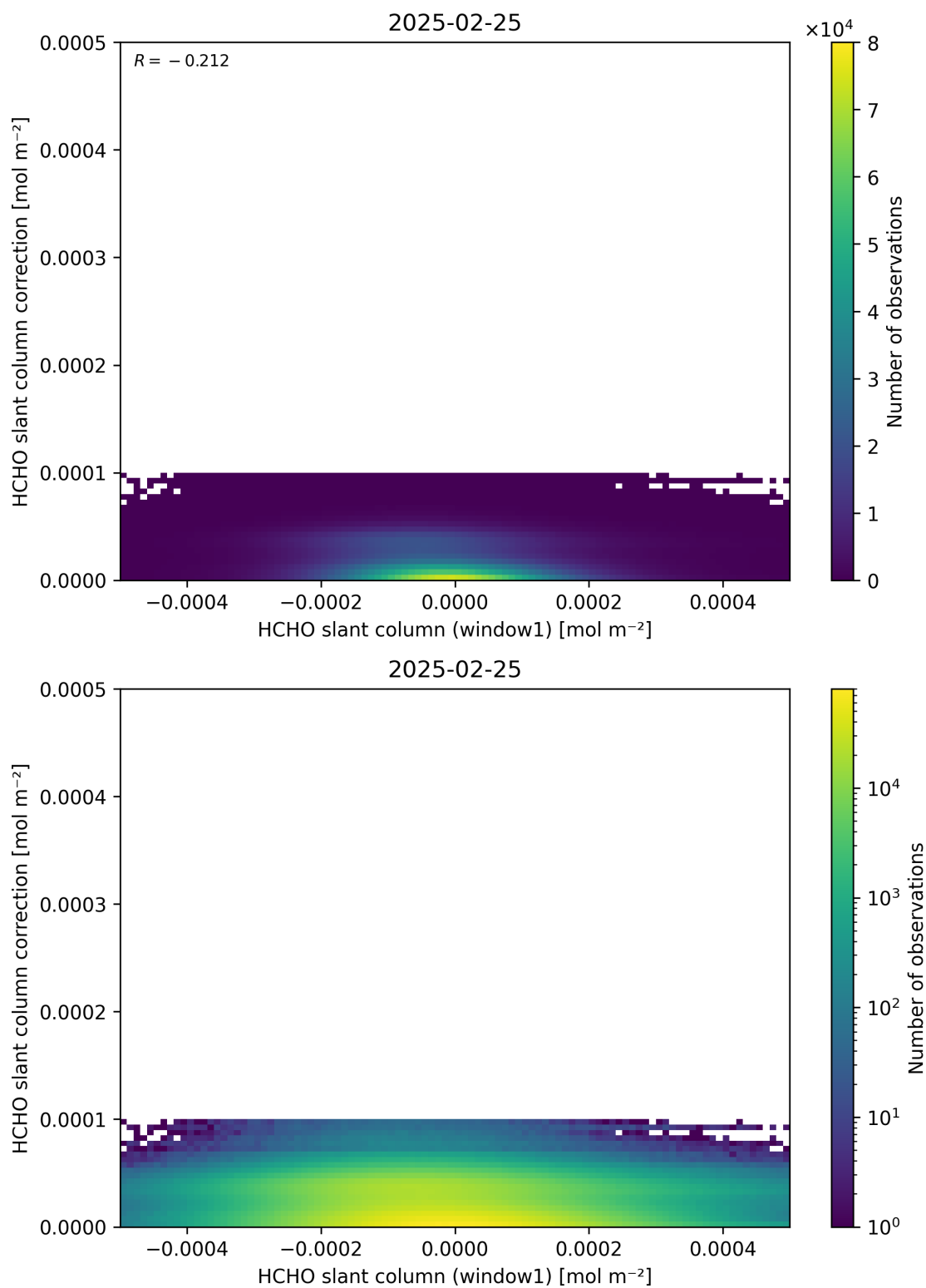
Figure 83: Scatter density plot of “HCHO slant column (window1)” against “HCHO slant column correction” for 2025-02-24 to 2025-02-26.
