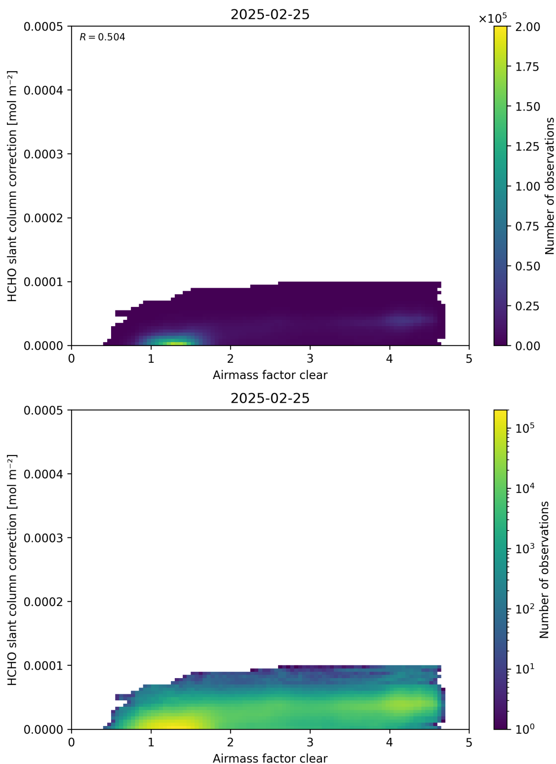
Figure 75: Scatter density plot of “Airmass factor clear” against “HCHO slant column correction” for 2025-02-24 to 2025-02-26.
