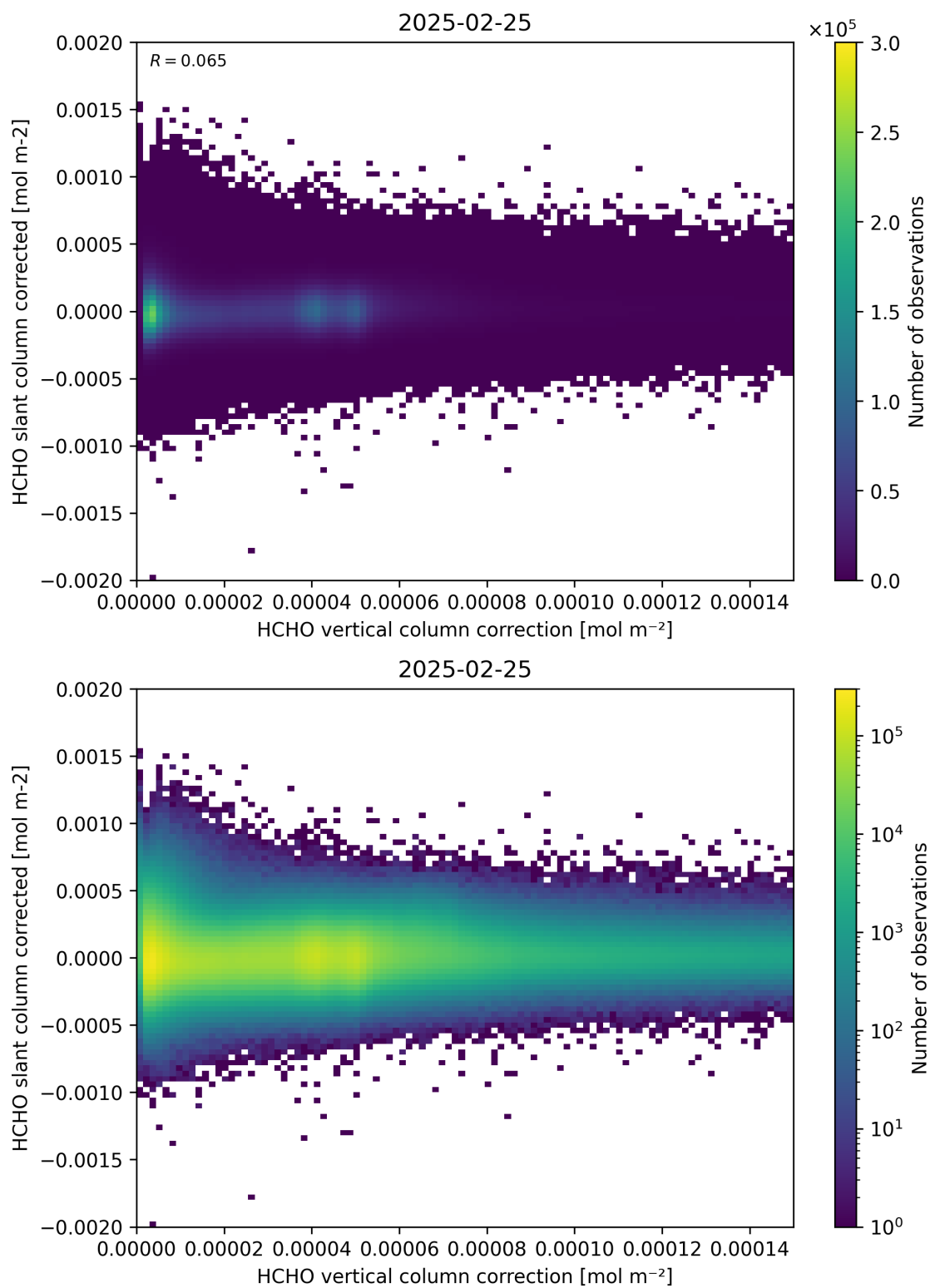
Figure 116: Scatter density plot of “HCHO vertical column correction” against “HCHO slant column corrected” for 2025-02-24 to 2025-02-26.
