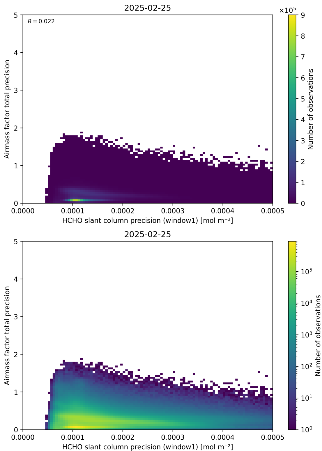
Figure 95: Scatter density plot of “HCHO slant column precision (window1)” against “Airmass factor total precision” for 2025-02-24 to 2025-02-26.
