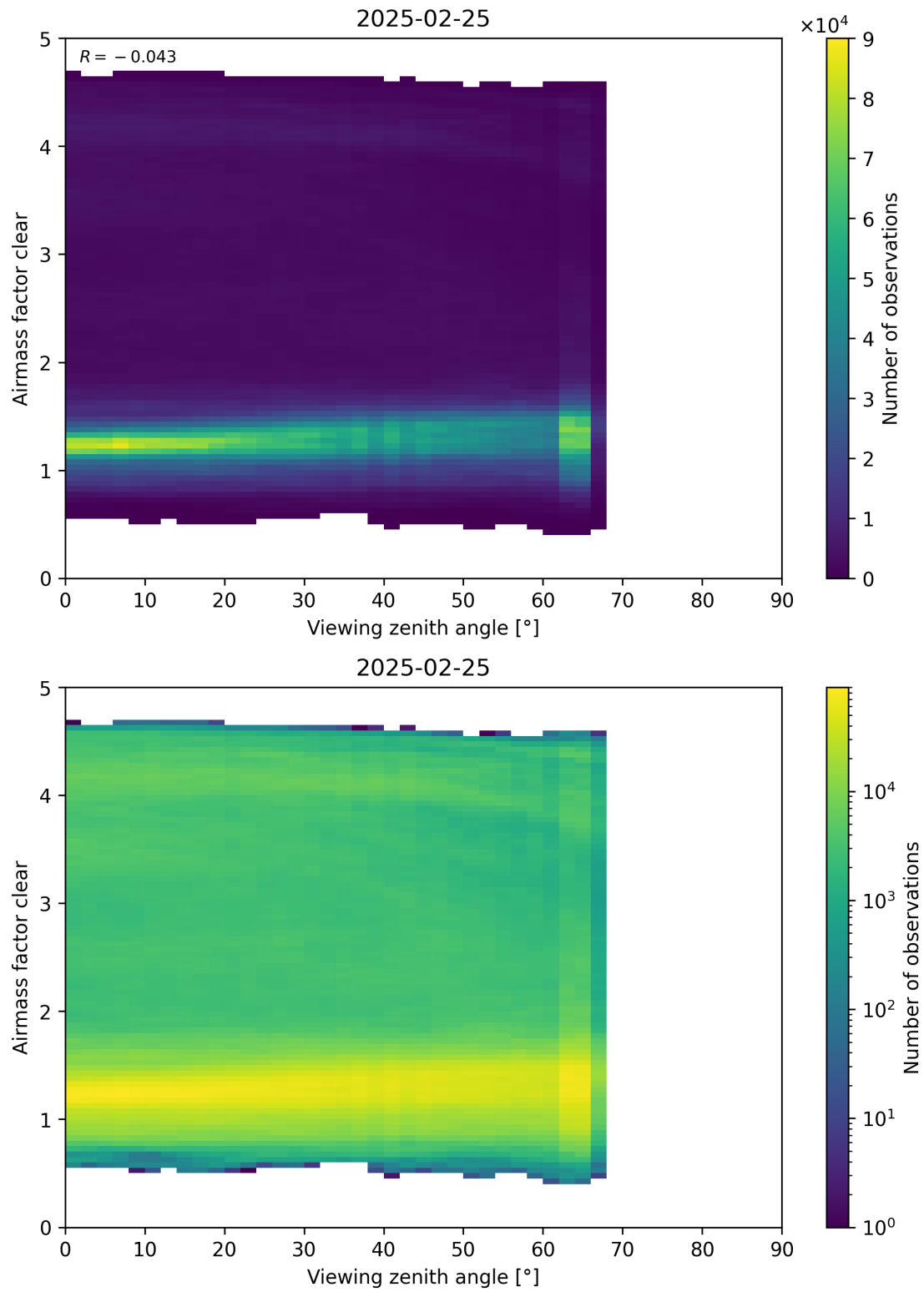
Figure 185: Scatter density plot of “Viewing zenith angle” against “Airmass factor clear” for 2025-02-24 to 2025-02-26.
