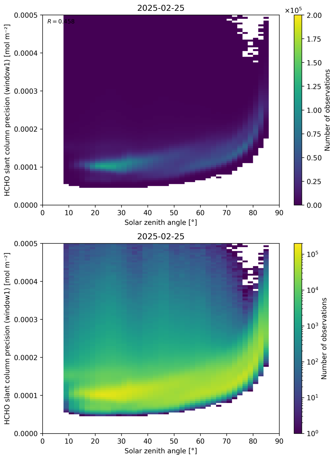
Figure 174: Scatter density plot of “Solar zenith angle” against “HCHO slant column precision (window1)” for 2025-02-24 to 2025-02-26.
