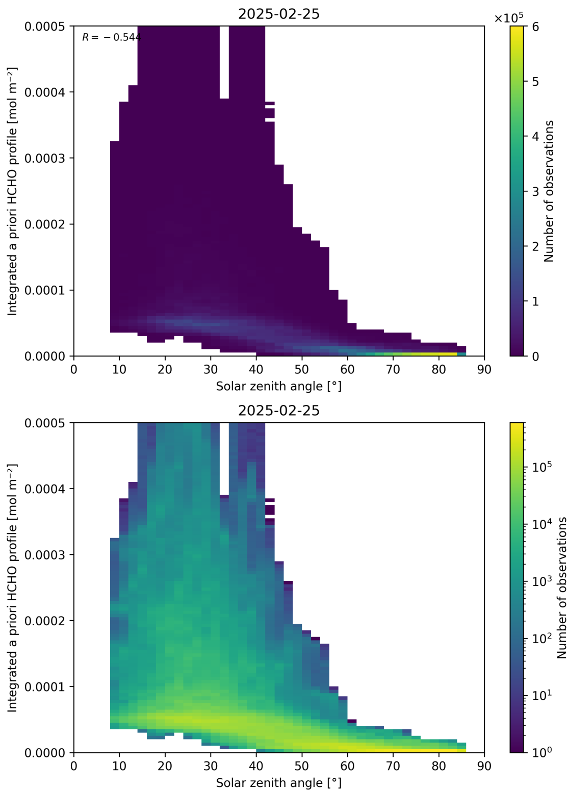
Figure 180: Scatter density plot of “Solar zenith angle” against “Integrated a priori HCHO profile” for 2025-02-24 to 2025-02-26.
