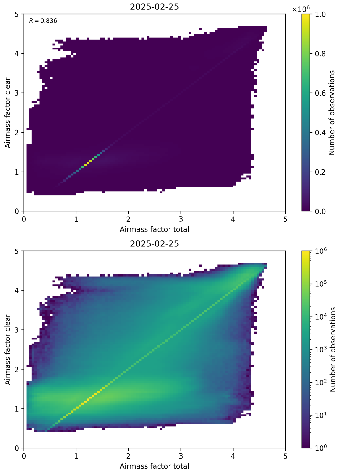
Figure 100: Scatter density plot of “Airmass factor total” against “Airmass factor clear” for 2025-02-24 to 2025-02-26.
