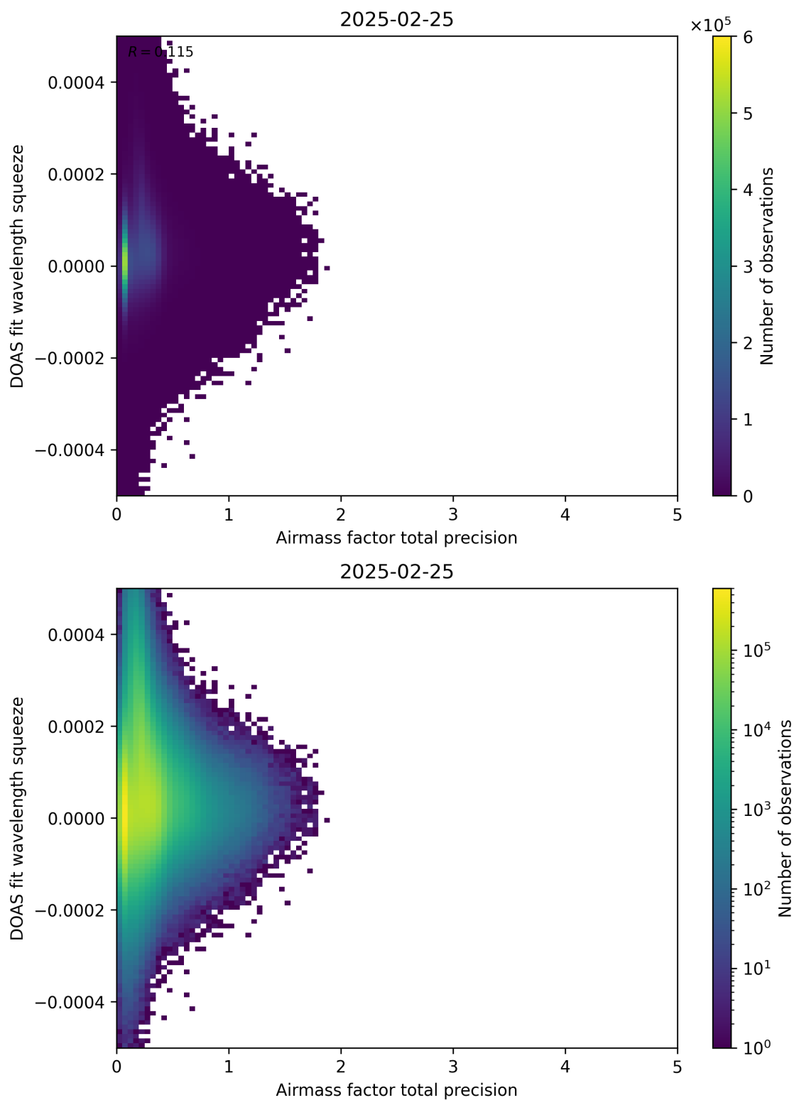
Figure 107: Scatter density plot of “Airmass factor total precision” against “DOAS fit wavelength squeeze” for 2025-02-24 to 2025-02-26.
