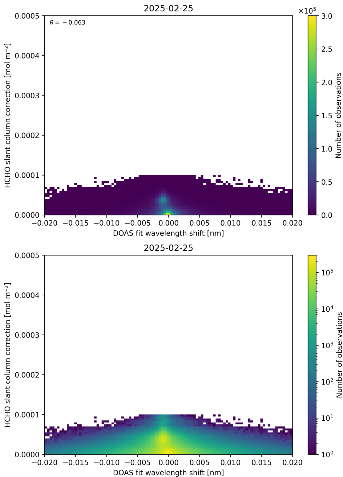
Figure 67: Scatter density plot of “DOAS fit wavelength shift” against “HCHO slant column correction” for 2025-02-24 to 2025-02-26.
