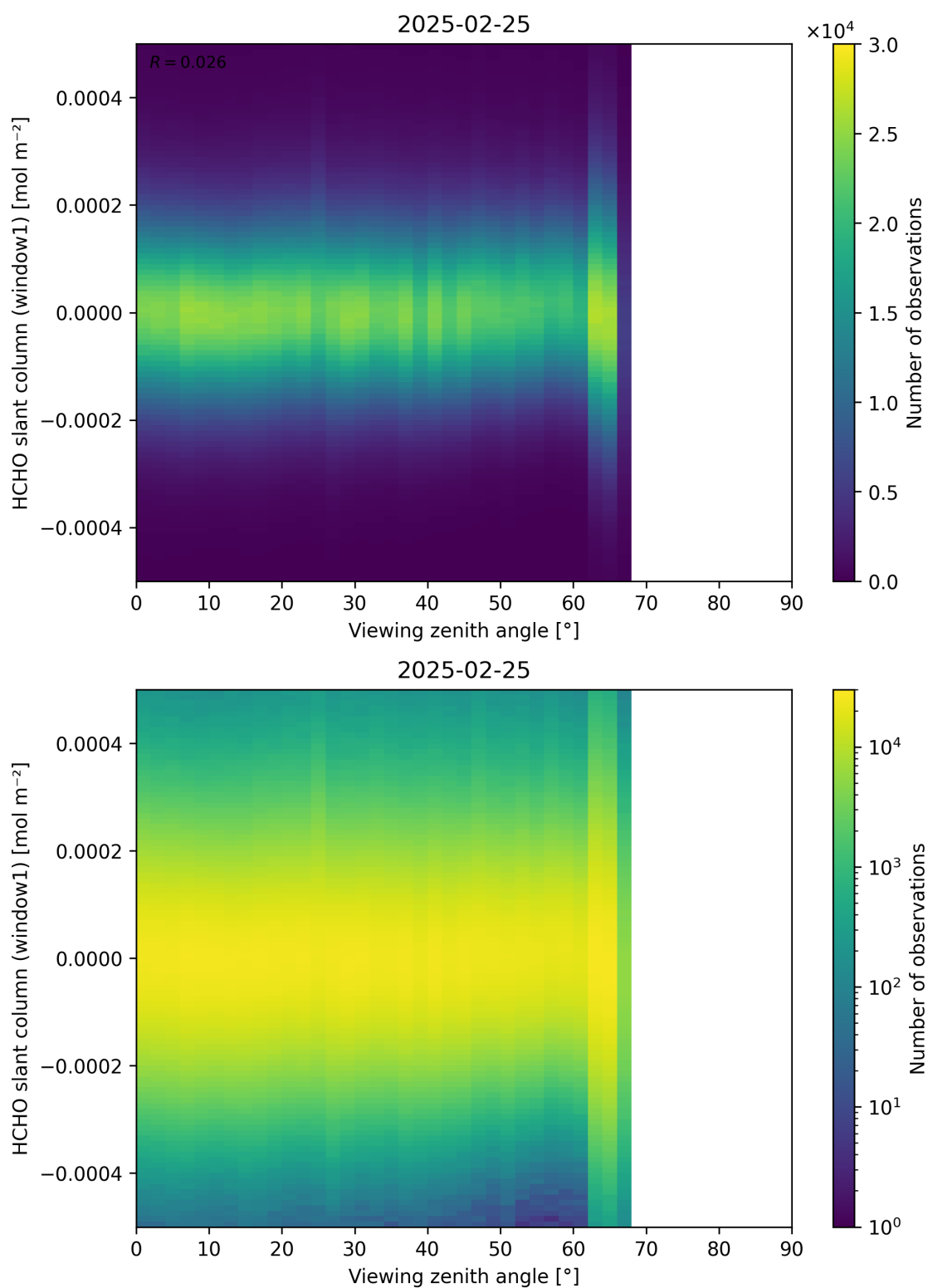
Figure 188: Scatter density plot of “Viewing zenith angle” against “HCHO slant column (window1)” for 2025-02-24 to 2025-02-26.
