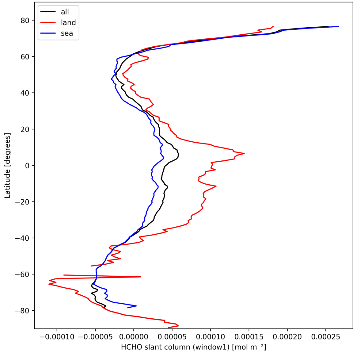
Figure 24: Zonal average of “HCHO slant column (window1)” for 2025-02-24 to 2025-02-26.
