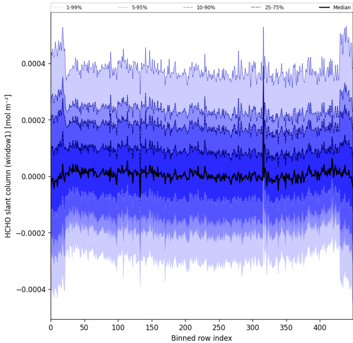
Figure 52: Along track statistics of “HCHO slant column (window1)” for 2025-02-24 to 2025-02-26
