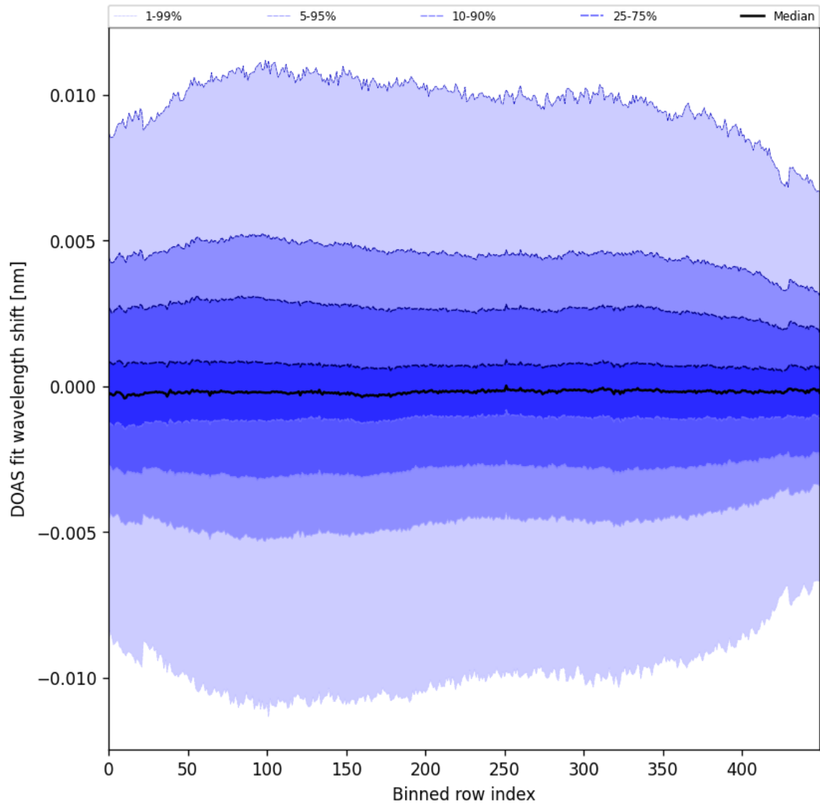
Figure 58: Along track statistics of “DOAS fit wavelength shift” for 2025-02-24 to 2025-02-26
