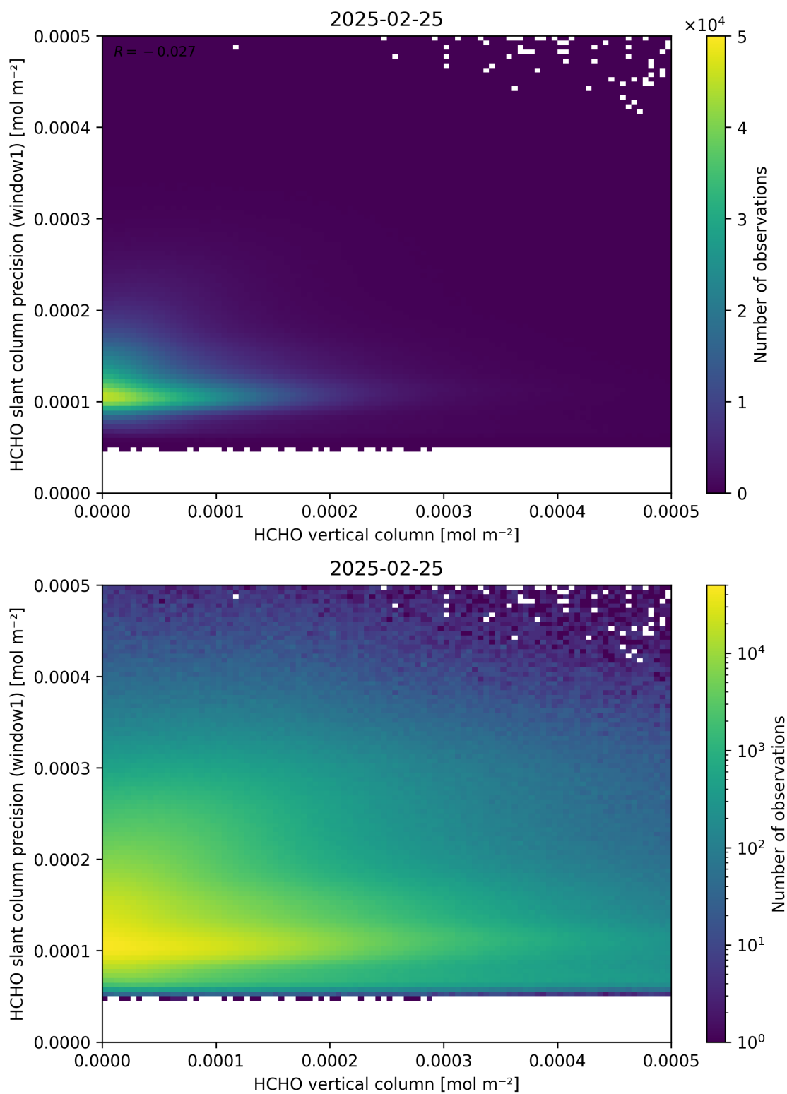
Figure 130: Scatter density plot of “HCHO vertical column” against “HCHO slant column precision (window1)” for 2025-02-24 to 2025-02-26.
