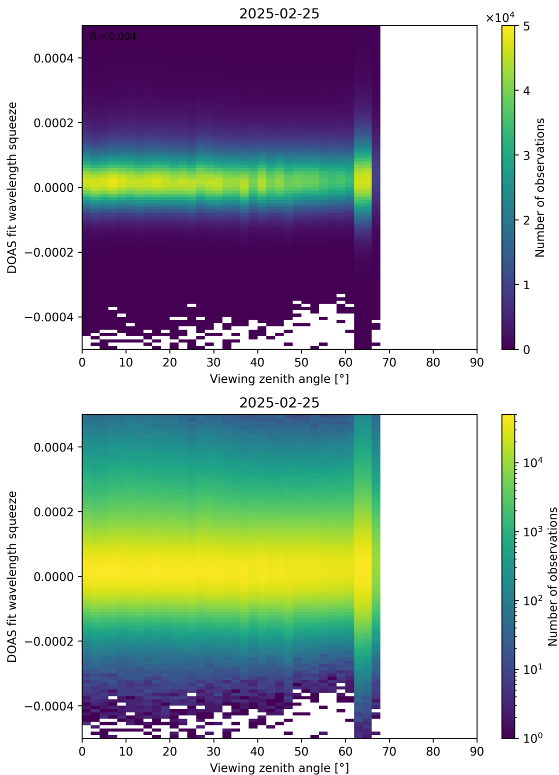
Figure 184: Scatter density plot of “Viewing zenith angle” against “DOAS fit wavelength squeeze” for 2025-02-24 to 2025-02-26.
