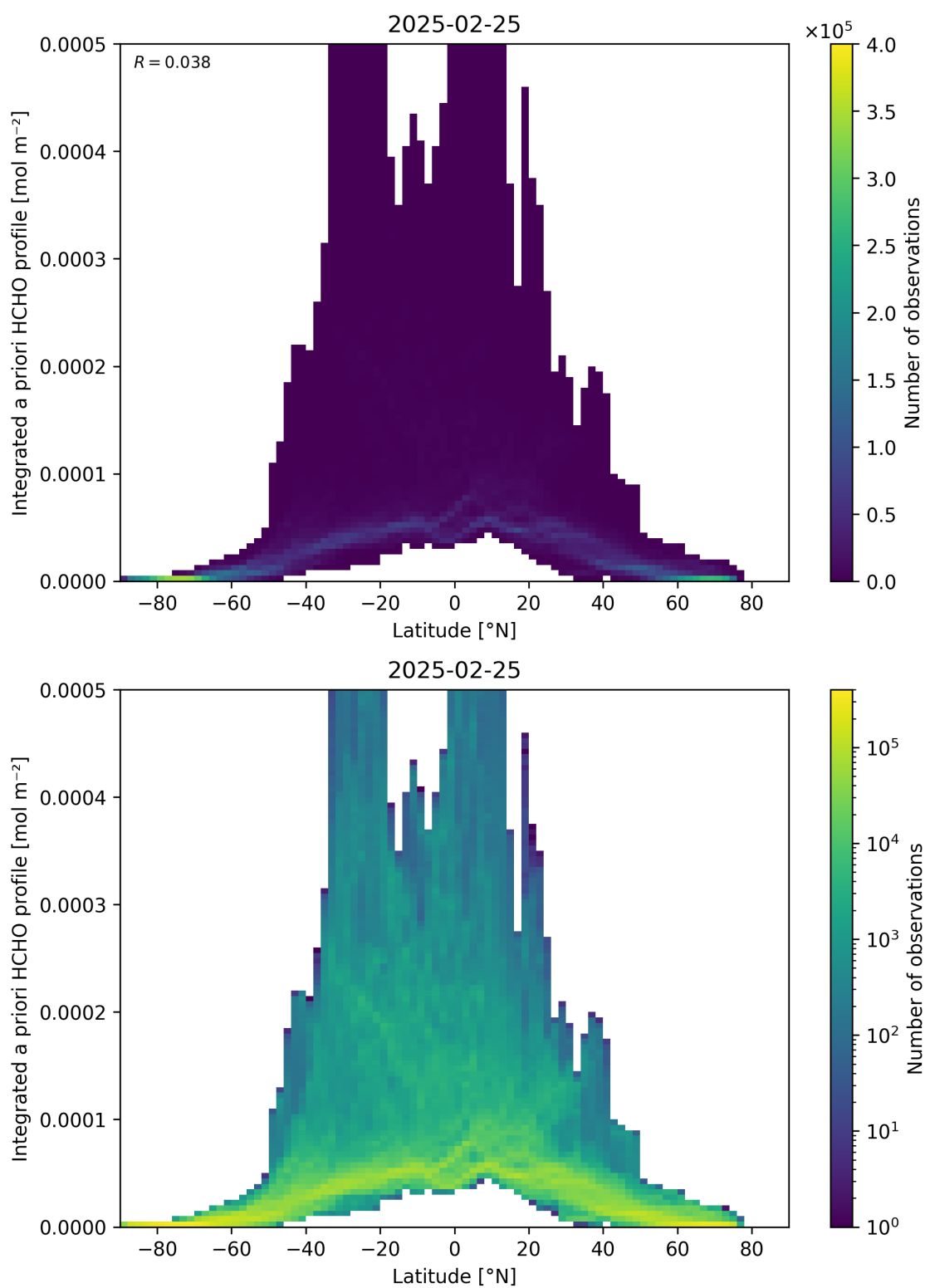
Figure 166: Scatter density plot of “Latitude” against “Integrated a priori HCHO profile” for 2025-02-24 to 2025-02-26.
