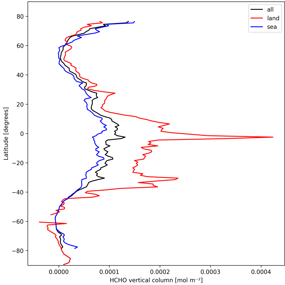
Figure 21: Zonal average of “HCHO vertical column” for 2025-02-24 to 2025-02-26.
