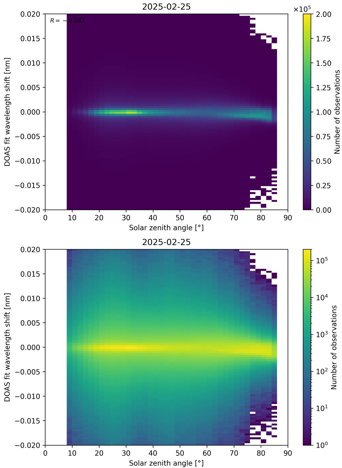
Figure 168: Scatter density plot of “Solar zenith angle” against “DOAS fit wavelength shift” for 2025-02-24 to 2025-02-26.
