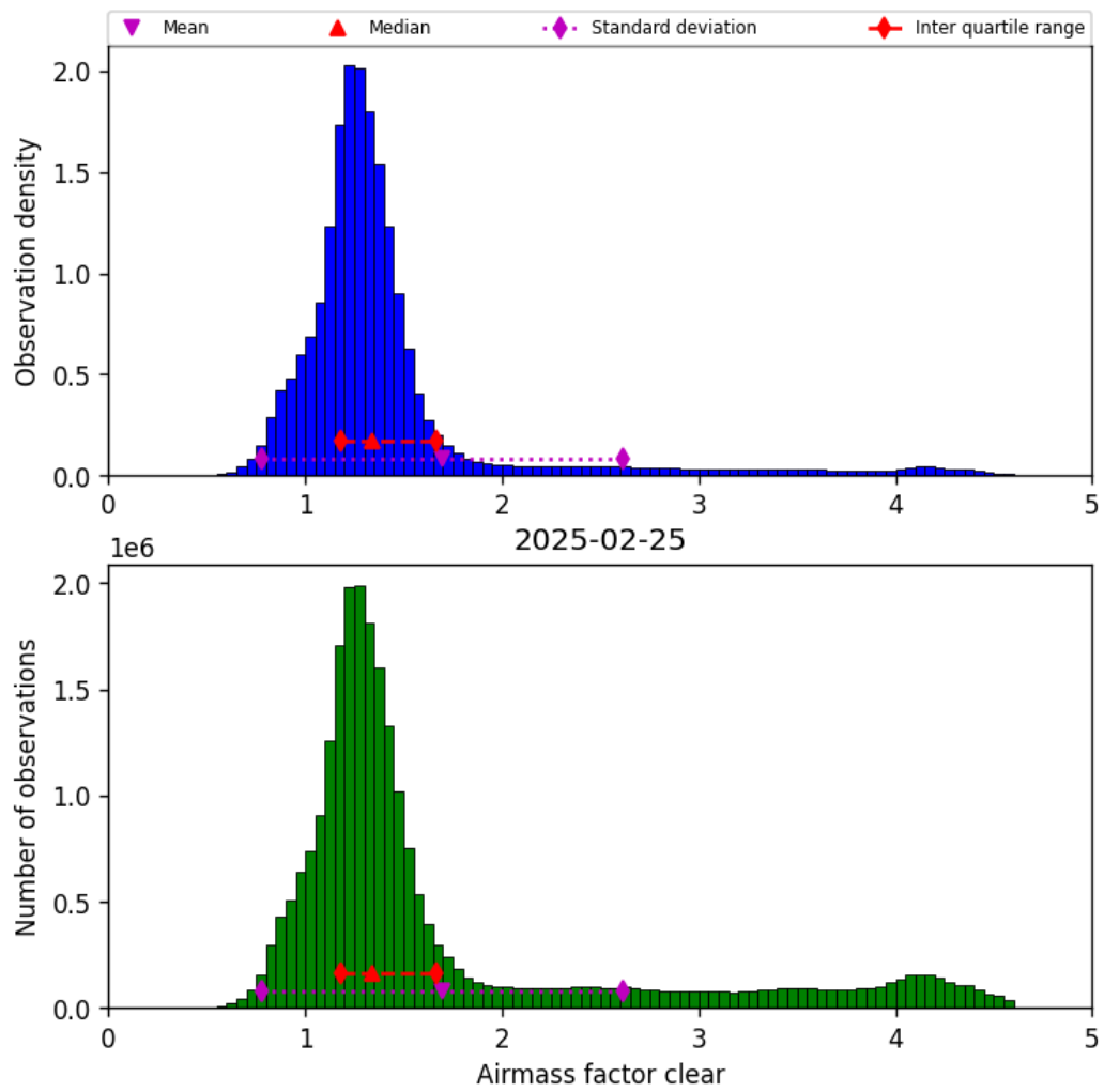
Figure 42: Histogram of “Airmass factor clear” for 2025-02-24 to 2025-02-26
