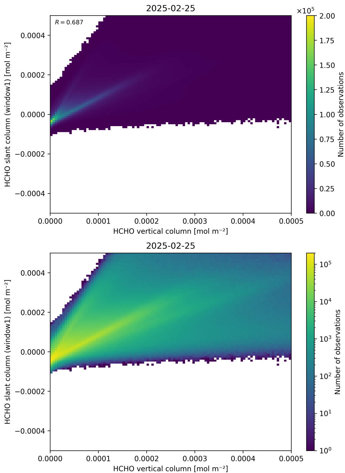
Figure 129: Scatter density plot of “HCHO vertical column” against “HCHO slant column (window1)” for 2025-02-24 to 2025-02-26.
