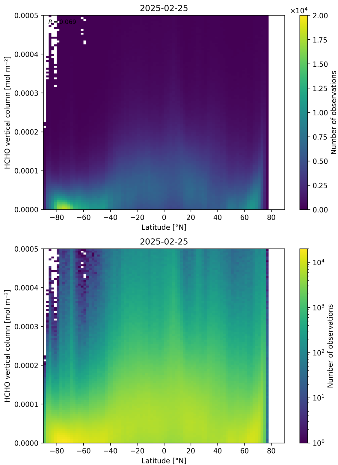
Figure 163: Scatter density plot of “Latitude” against “HCHO vertical column” for 2025-02-24 to 2025-02-26.
