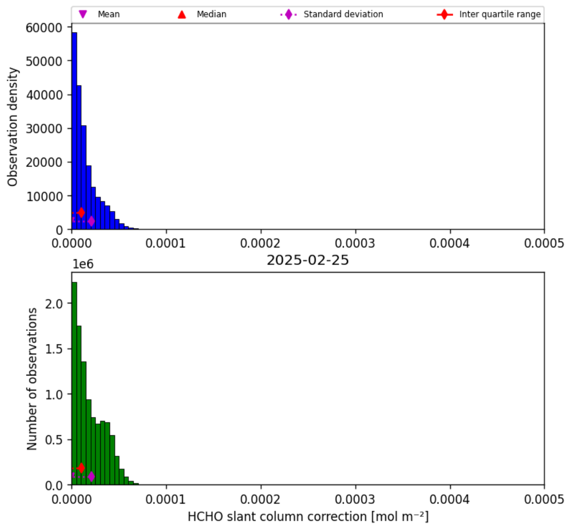
Figure 47: Histogram of “HCHO slant column correction” for 2025-02-24 to 2025-02-26
