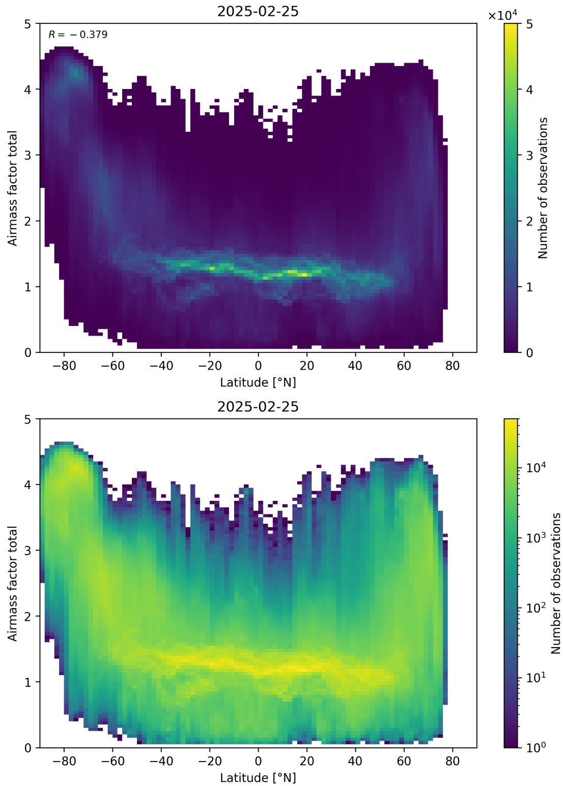
Figure 161: Scatter density plot of “Latitude” against “Airmass factor total” for 2025-02-24 to 2025-02-26.
