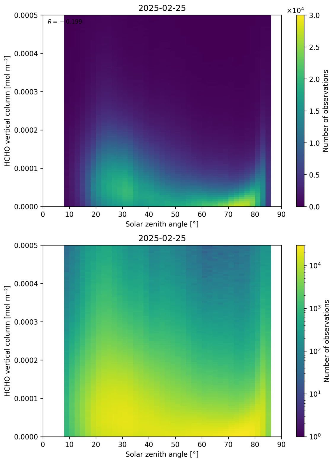
Figure 177: Scatter density plot of “Solar zenith angle” against “HCHO vertical column” for 2025-02-24 to 2025-02-26.
