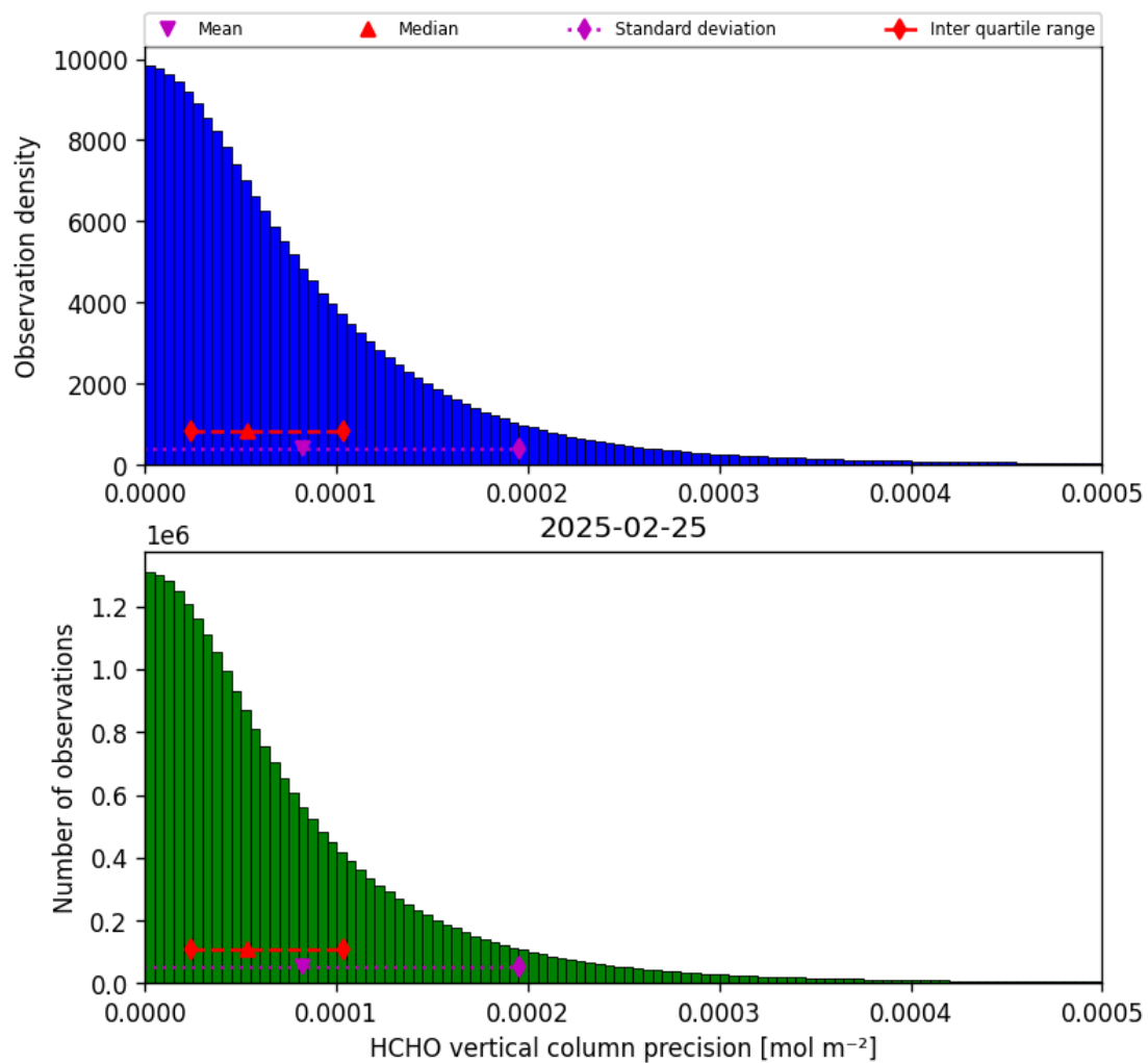
Figure 36: Histogram of “HCHO vertical column precision” for 2025-02-24 to 2025-02-26
