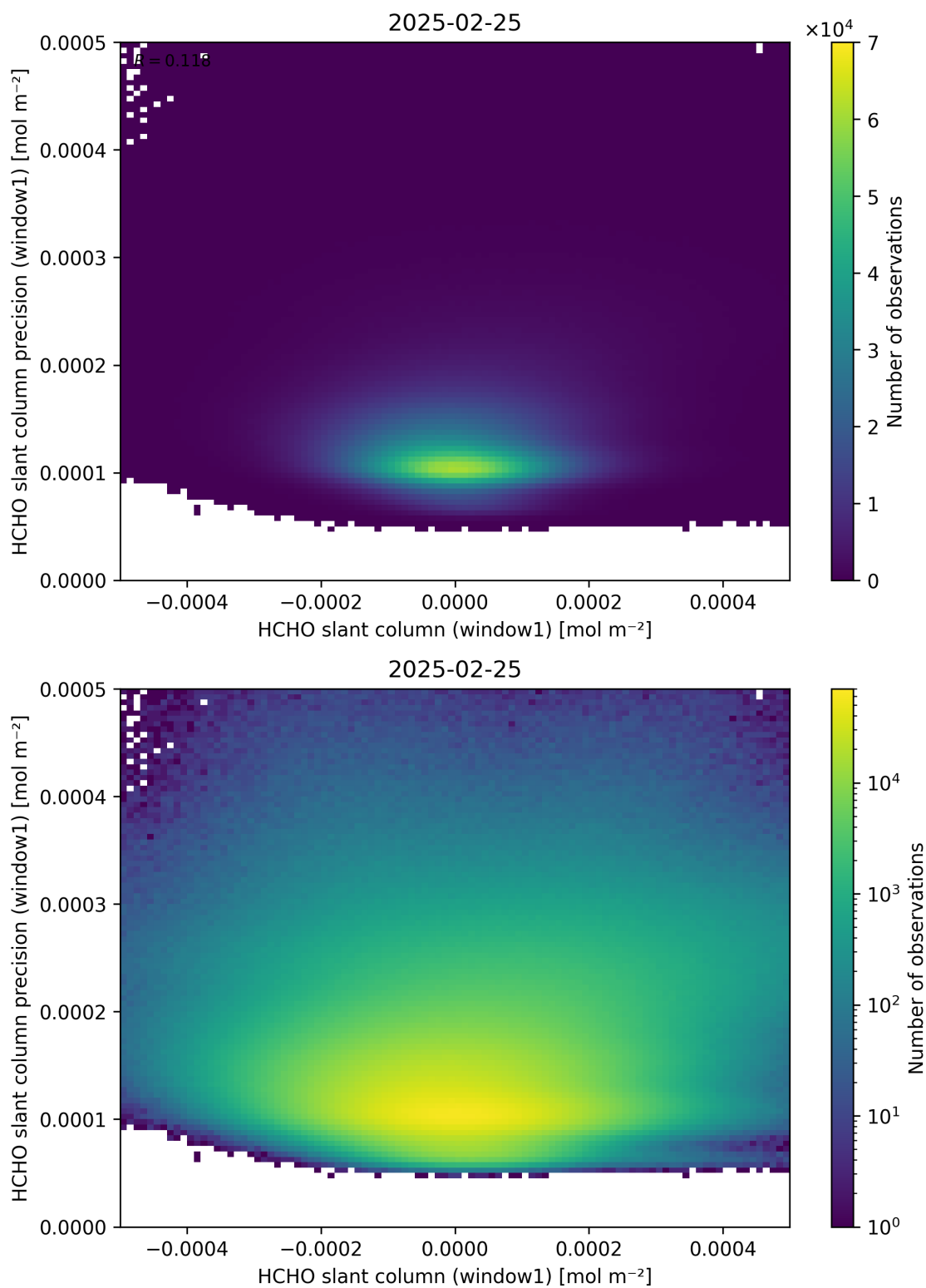
Figure 84: Scatter density plot of “HCHO slant column (window1)” against “HCHO slant column precision (window1)” for 2025-02-24 to 2025-02-26.
