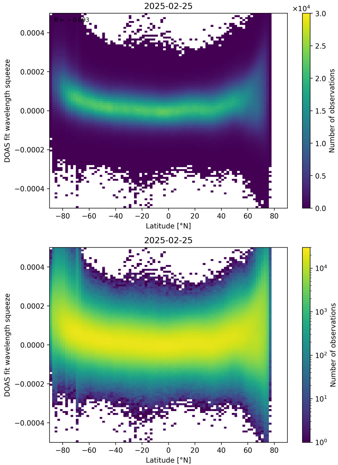
Figure 155: Scatter density plot of “Latitude” against “DOAS fit wavelength squeeze” for 2025-02-24 to 2025-02-26.
