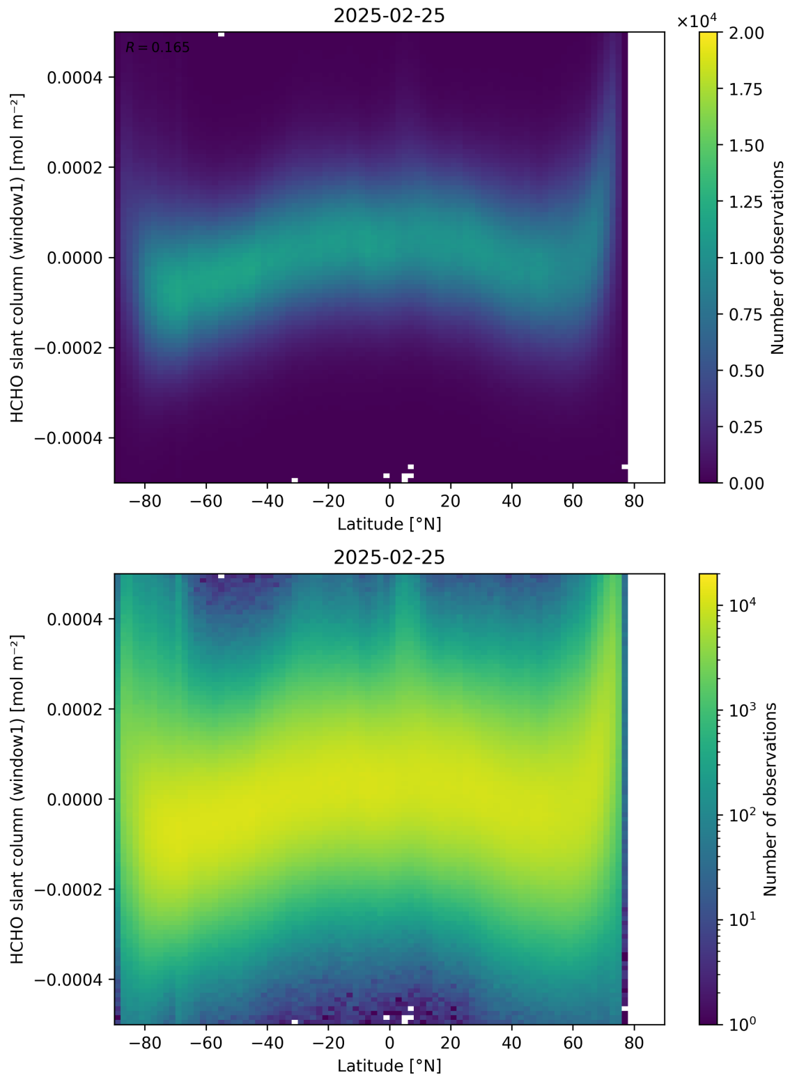
Figure 159: Scatter density plot of “Latitude” against “HCHO slant column (window1)” for 2025-02-24 to 2025-02-26.
