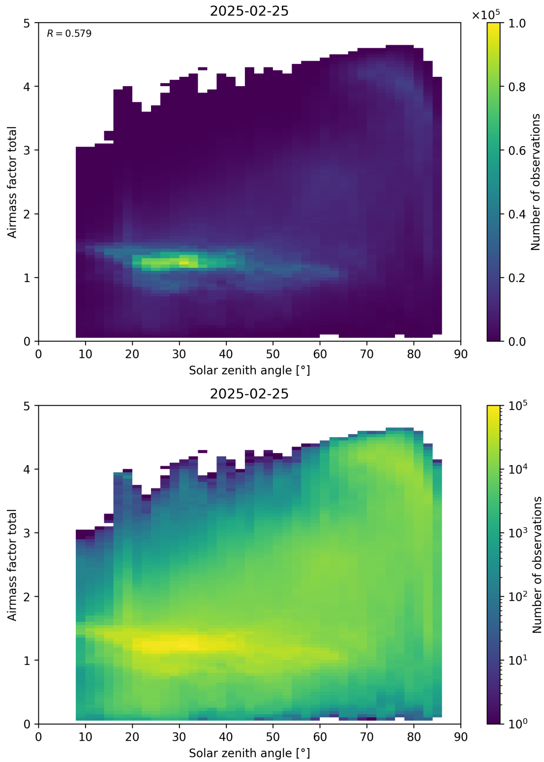
Figure 175: Scatter density plot of “Solar zenith angle” against “Airmass factor total” for 2025-02-24 to 2025-02-26.
