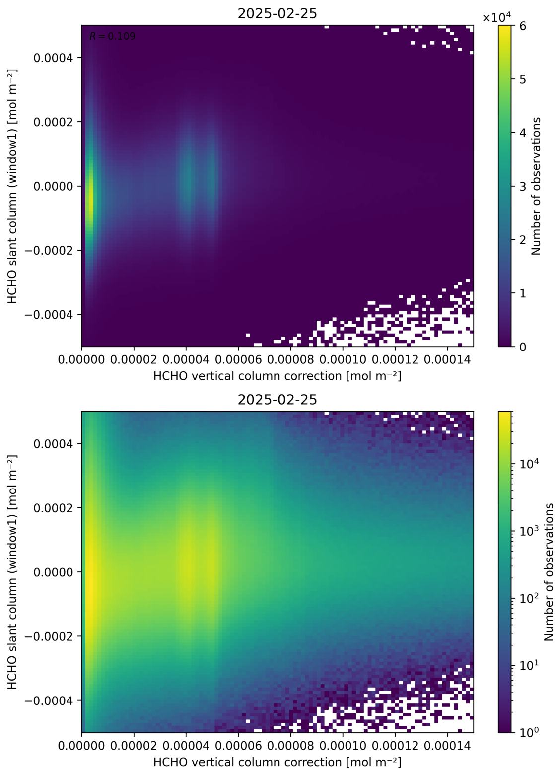
Figure 118: Scatter density plot of “HCHO vertical column correction” against “HCHO slant column (window1)” for 2025-02-24 to 2025-02-26.
