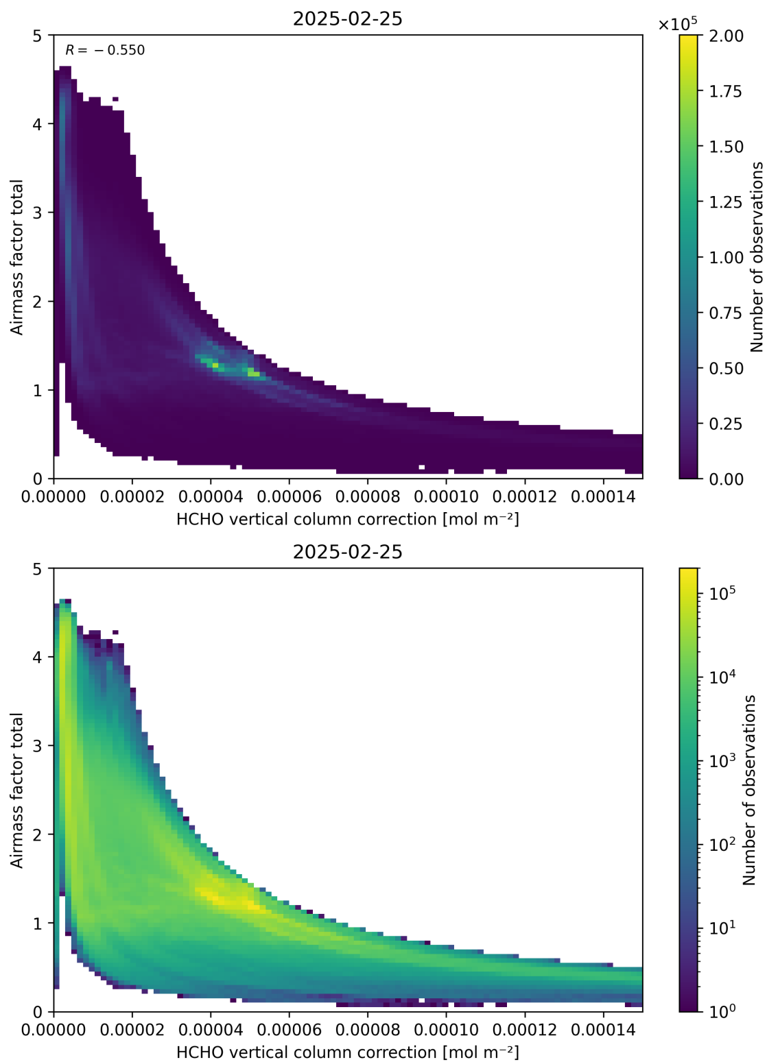
Figure 120: Scatter density plot of “HCHO vertical column correction” against “Airmass factor total” for 2025-02-24 to 2025-02-26.
