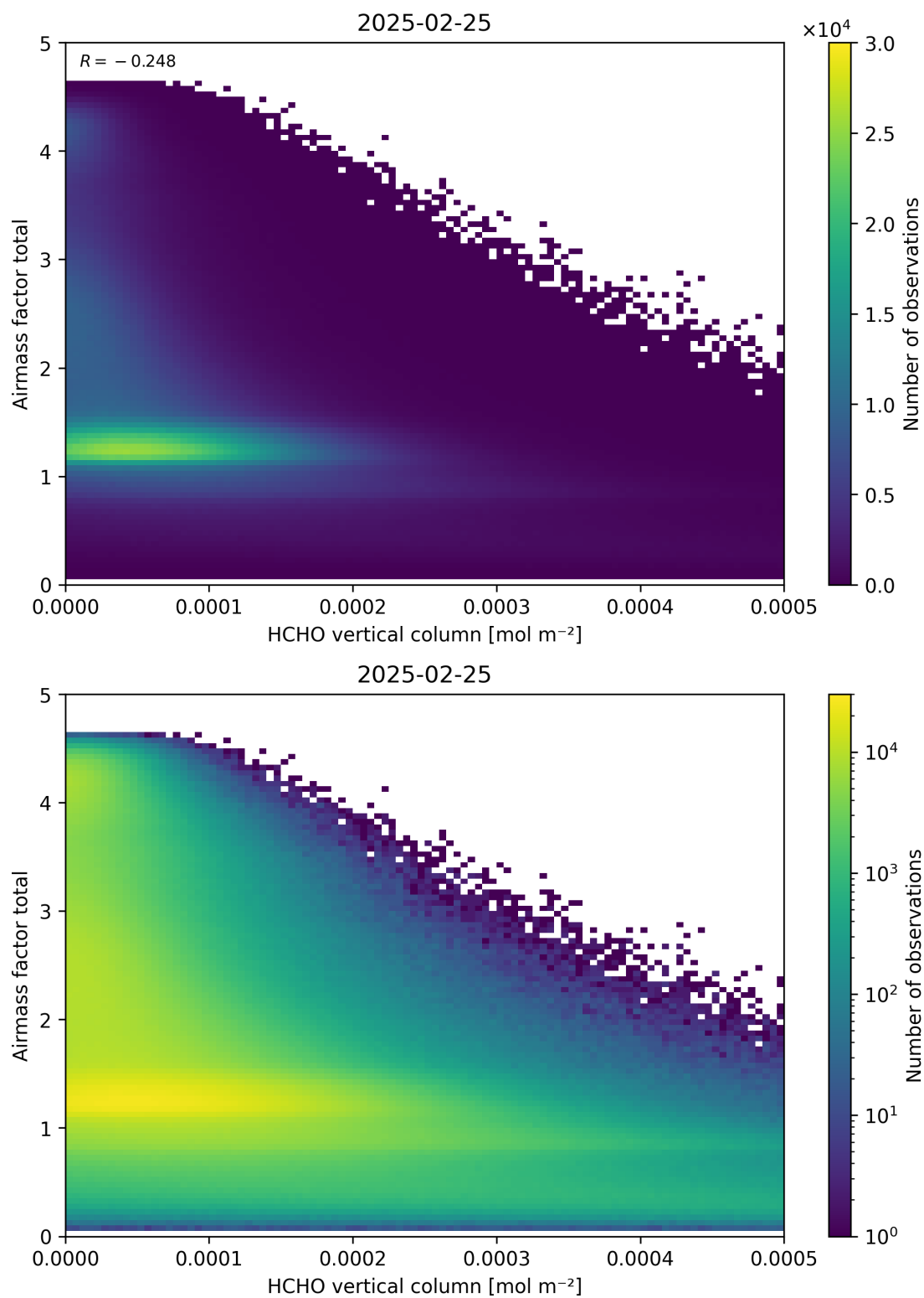
Figure 131: Scatter density plot of “HCHO vertical column” against “Airmass factor total” for 2025-02-24 to 2025-02-26.
