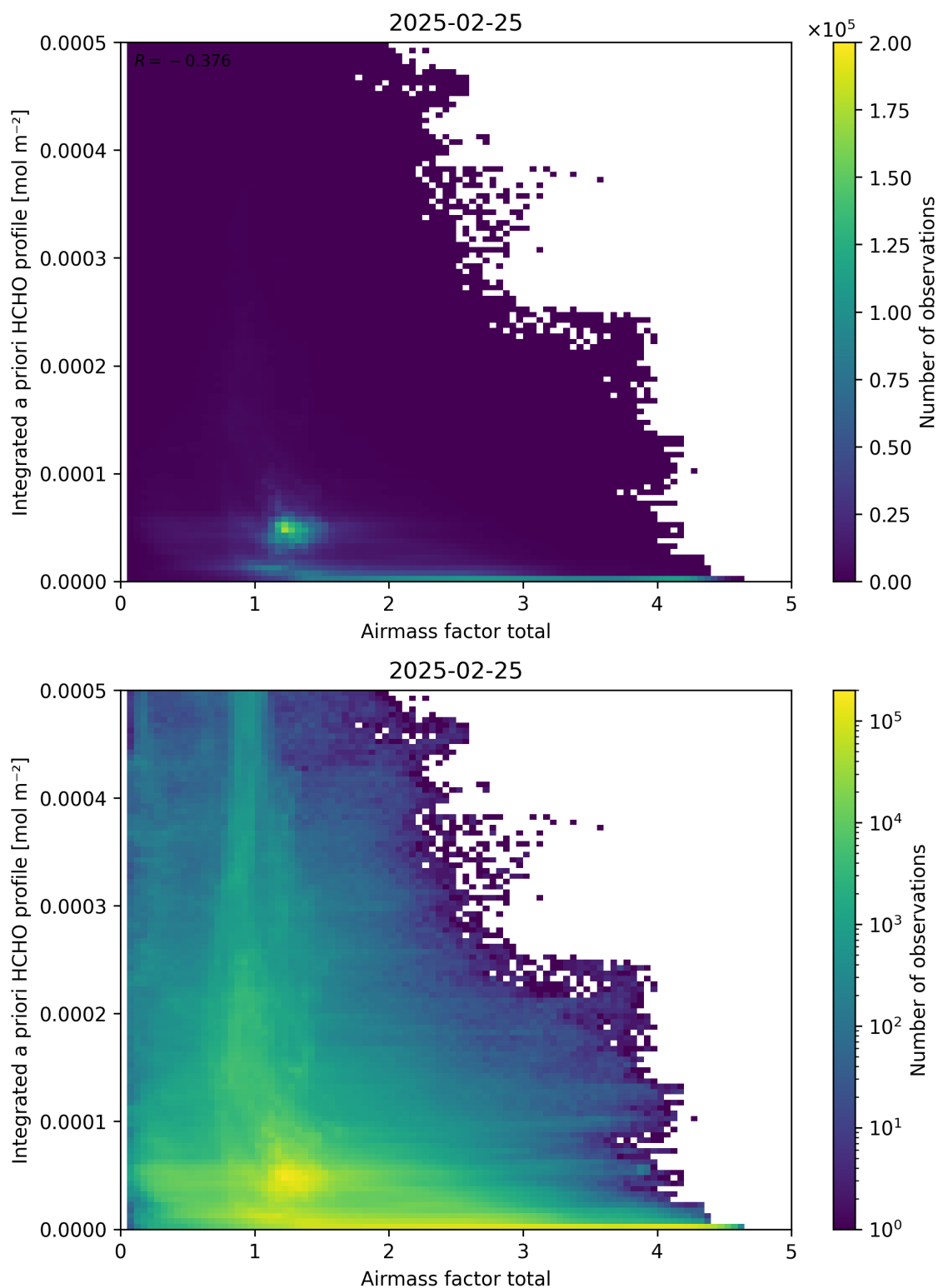
Figure 104: Scatter density plot of “Airmass factor total” against “Integrated a priori HCHO profile” for 2025-02-24 to 2025-02-26.
