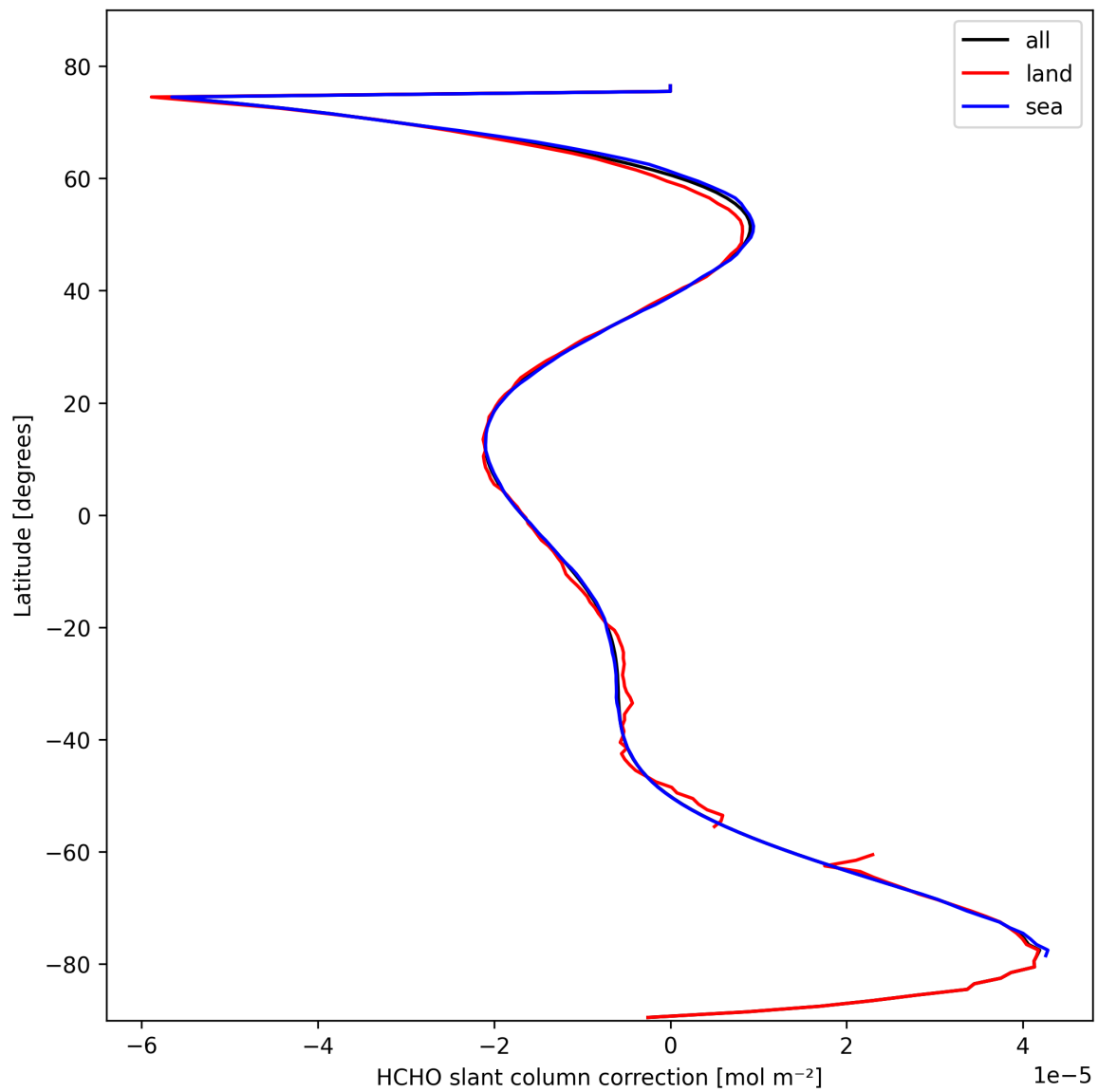
Figure 33: Zonal average of “HCHO slant column correction” for 2025-02-24 to 2025-02-26.
