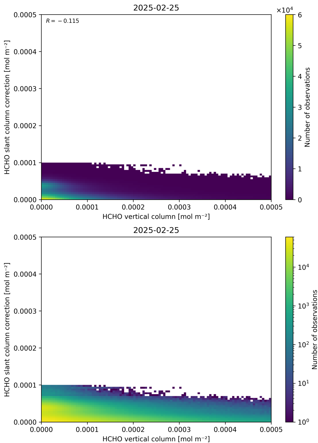
Figure 128: Scatter density plot of “HCHO vertical column” against “HCHO slant column correction” for 2025-02-24 to 2025-02-26.
