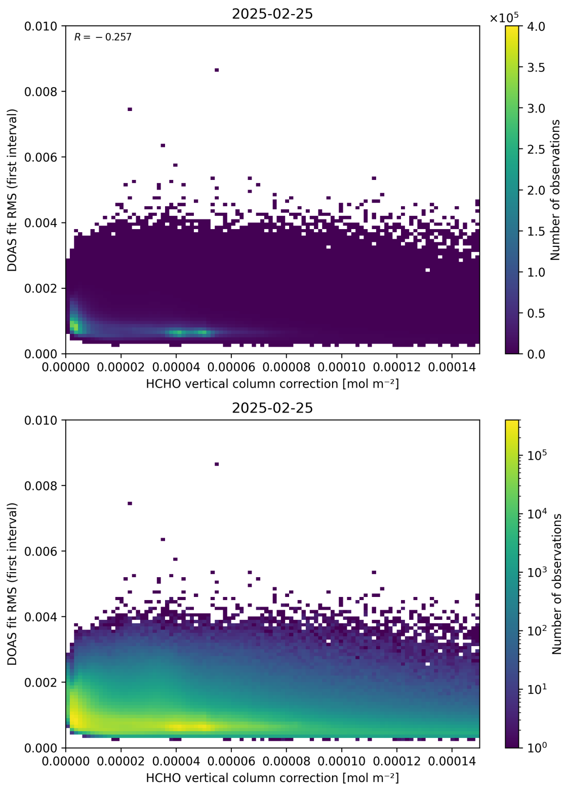
Figure 112: Scatter density plot of “HCHO vertical column correction” against “DOAS fit RMS (first interval)” for 2025-02-24 to 2025-02-26.
