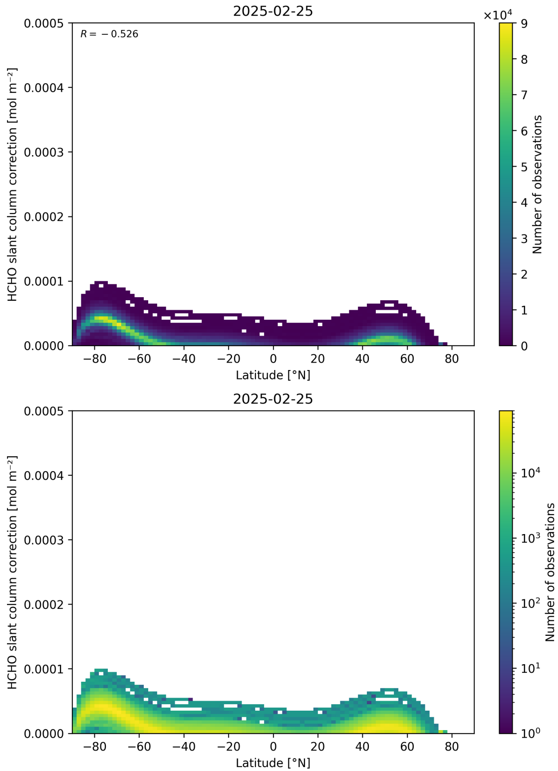
Figure 158: Scatter density plot of “Latitude” against “HCHO slant column correction” for 2025-02-24 to 2025-02-26.
