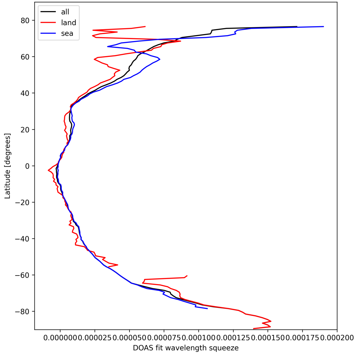
Figure 31: Zonal average of “DOAS fit wavelength squeeze” for 2025-02-24 to 2025-02-26.
