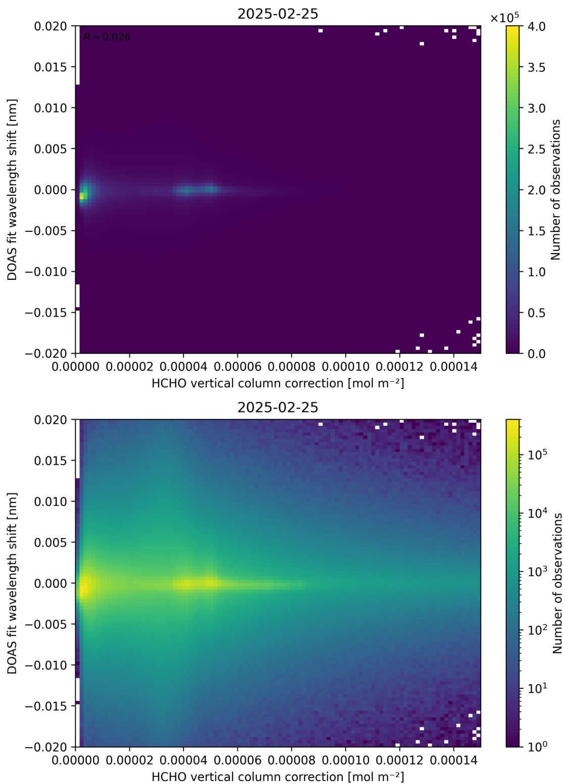
Figure 113: Scatter density plot of “HCHO vertical column correction” against “DOAS fit wavelength shift” for 2025-02-24 to 2025-02-26.
