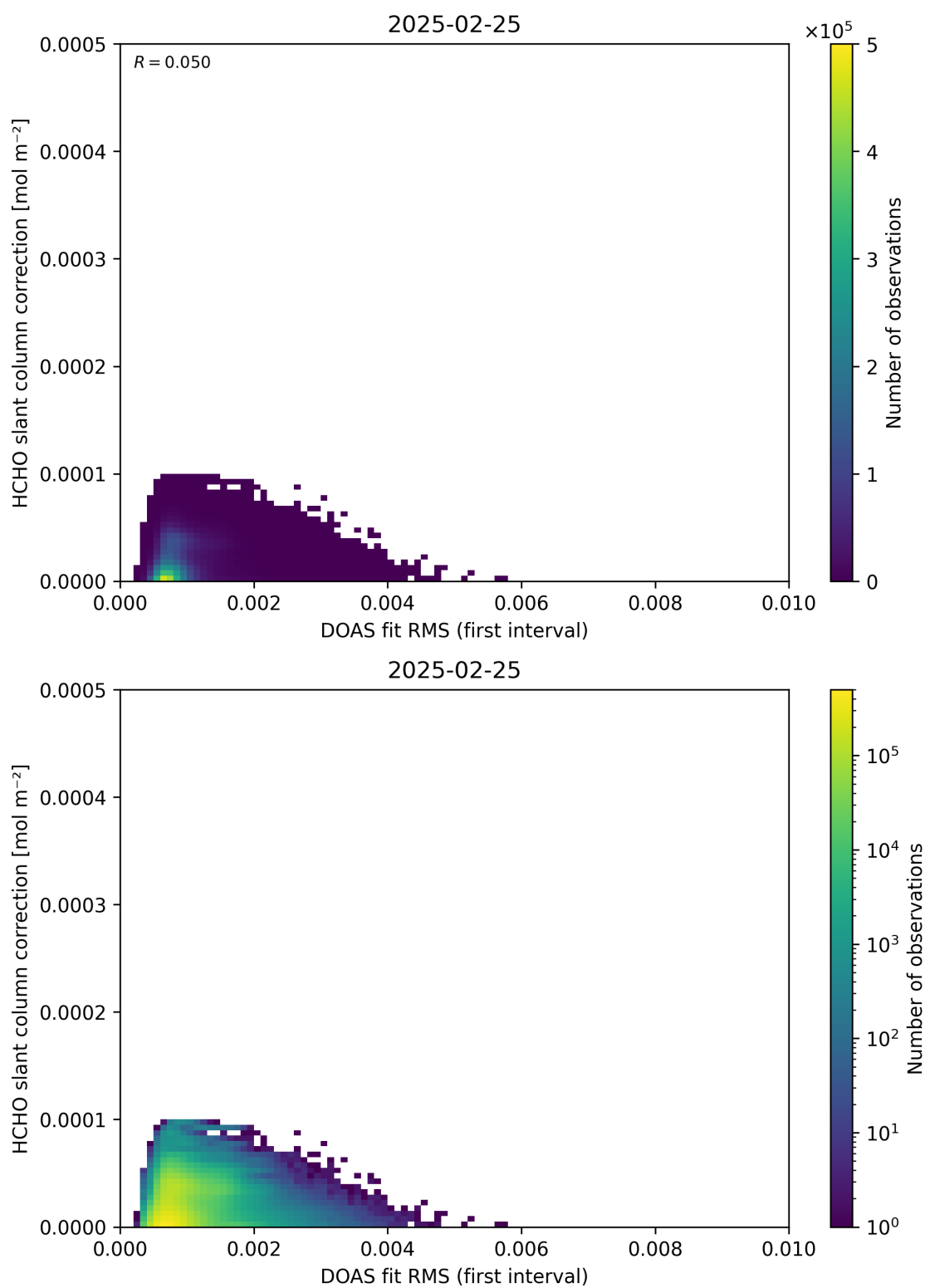
Figure 63: Scatter density plot of “DOAS fit RMS (first interval)” against “HCHO slant column correction” for 2025-02-24 to 2025-02-26.
