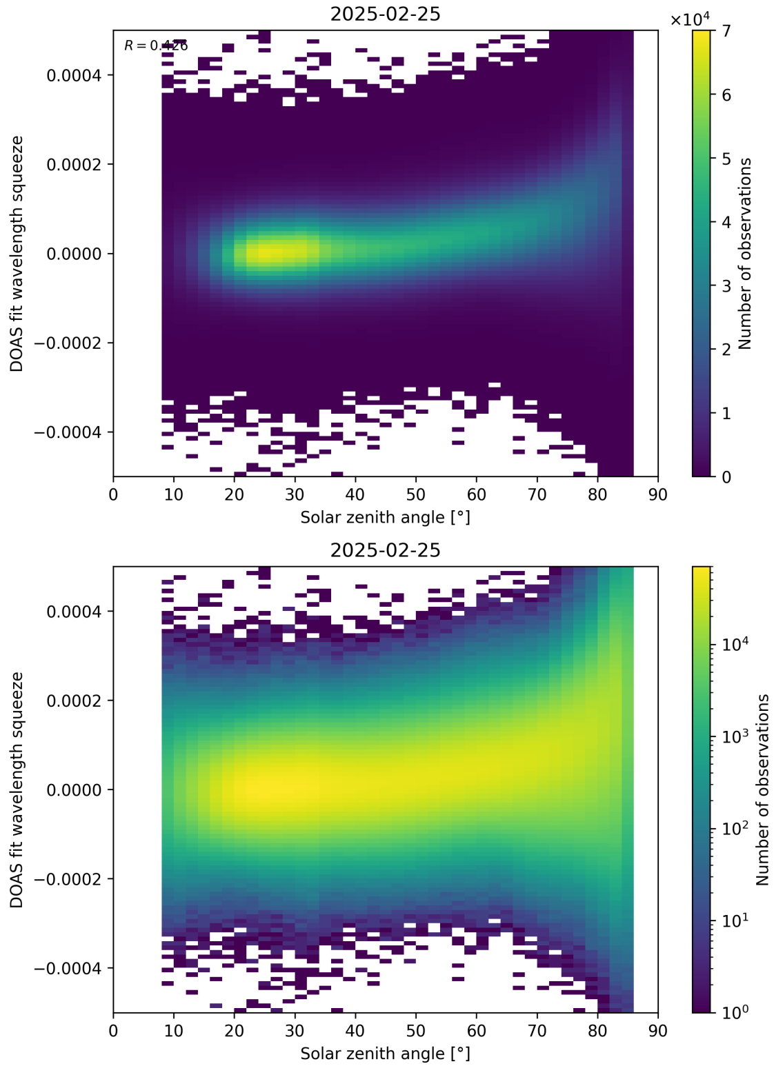
Figure 169: Scatter density plot of “Solar zenith angle” against “DOAS fit wavelength squeeze” for 2025-02-24 to 2025-02-26.
