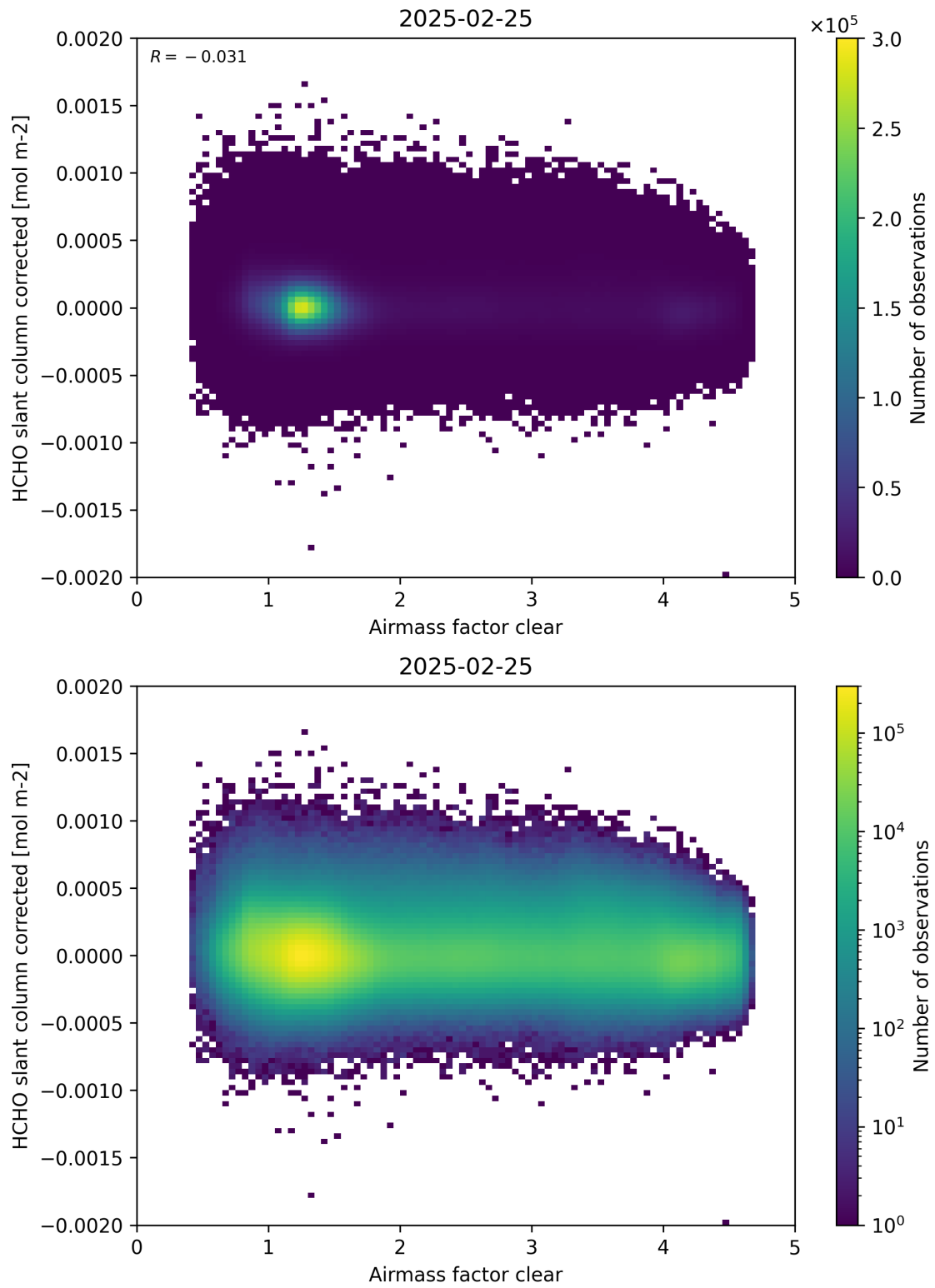
Figure 74: Scatter density plot of “Airmass factor clear” against “HCHO slant column corrected” for 2025-02-24 to 2025-02-26.
