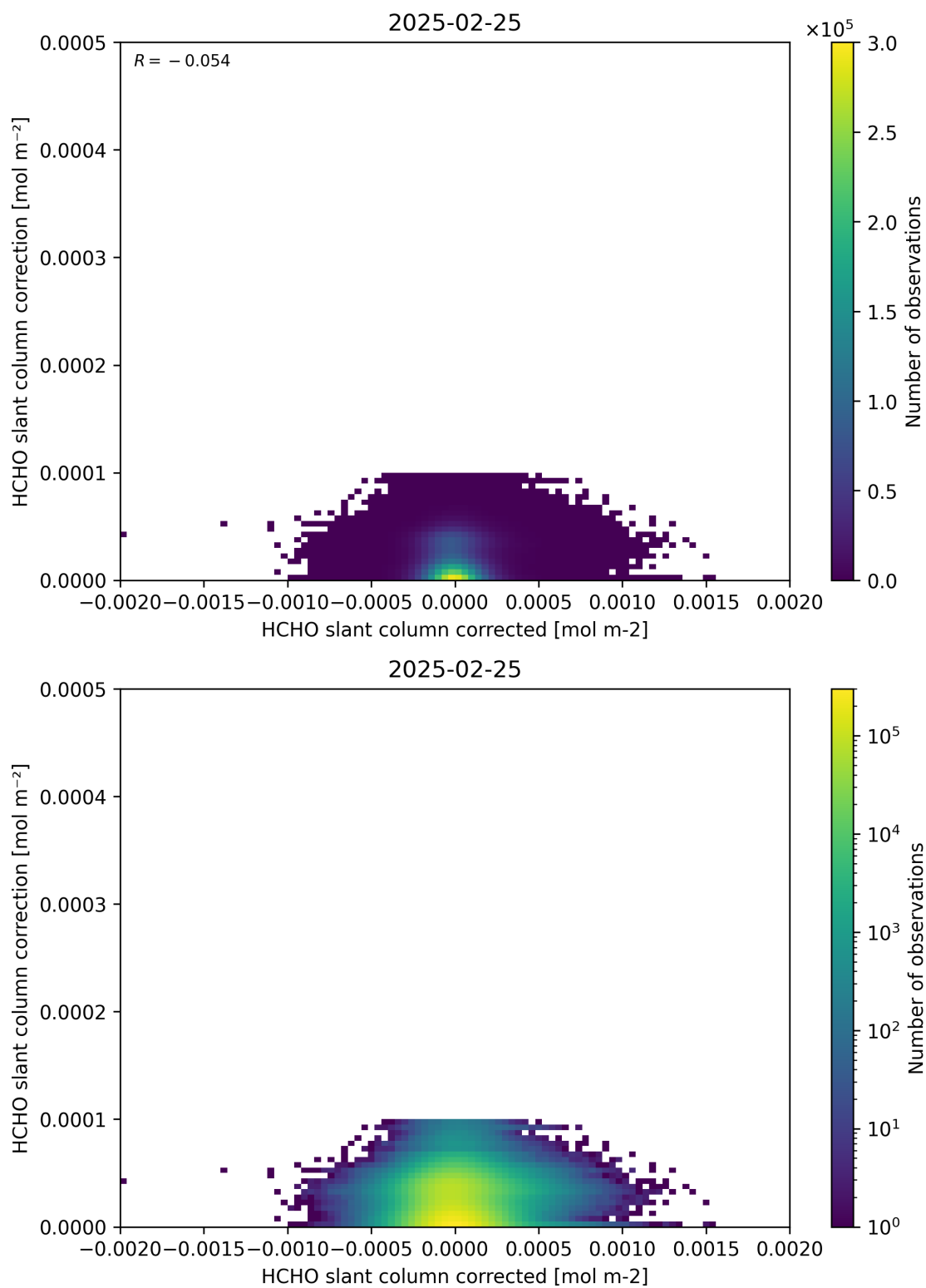
Figure 77: Scatter density plot of “HCHO slant column corrected” against “HCHO slant column correction” for 2025-02-24 to 2025-02-26.
