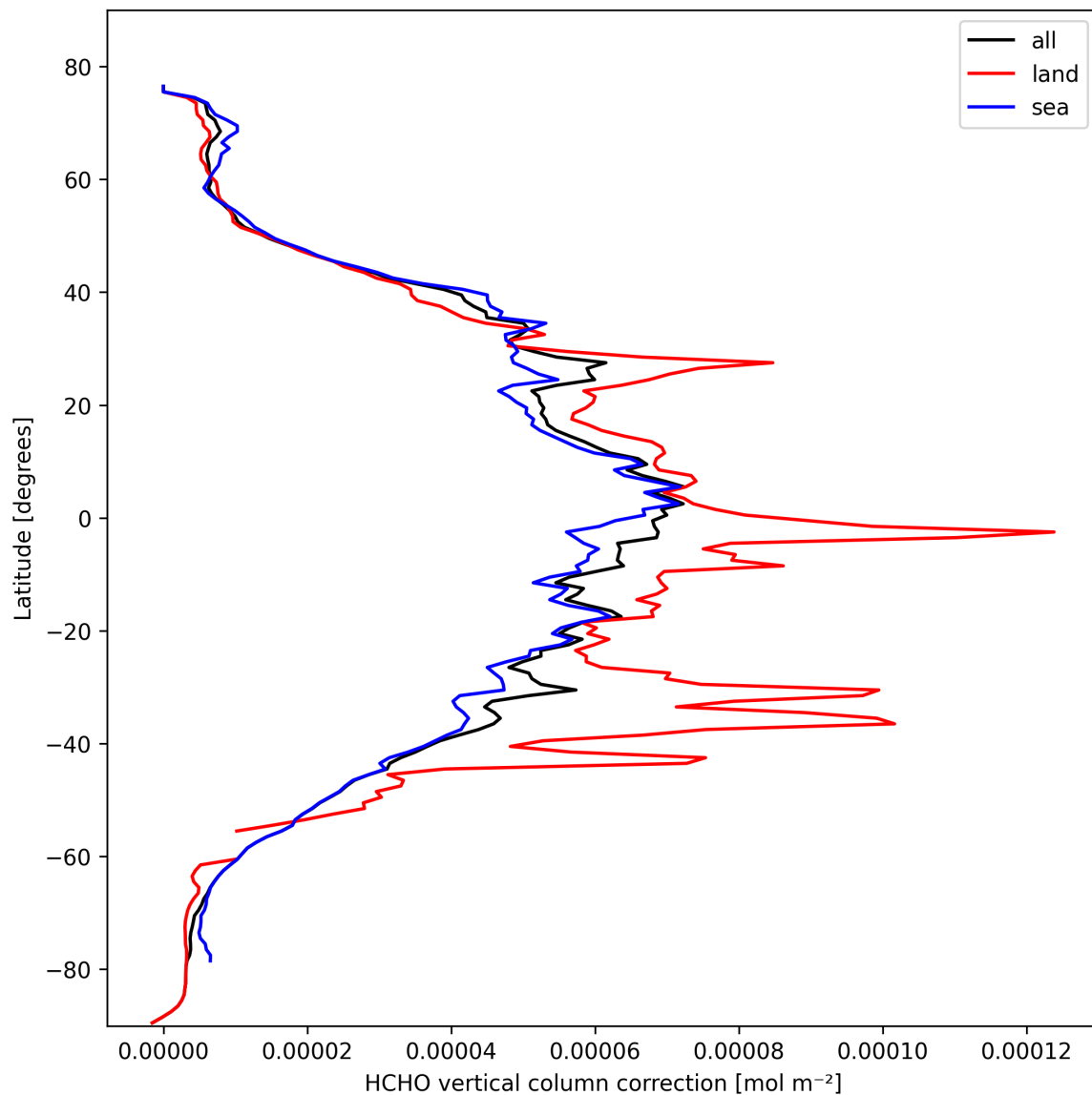
Figure 23: Zonal average of “HCHO vertical column correction” for 2025-02-24 to 2025-02-26.
