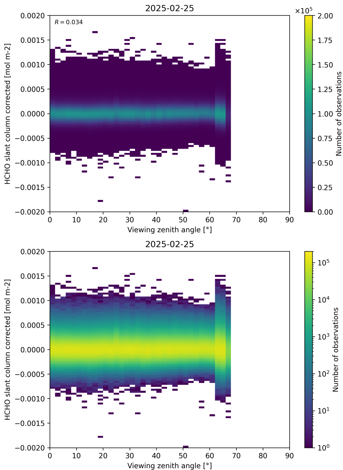
Figure 186: Scatter density plot of “Viewing zenith angle” against “HCHO slant column corrected” for 2025-02-24 to 2025-02-26.
