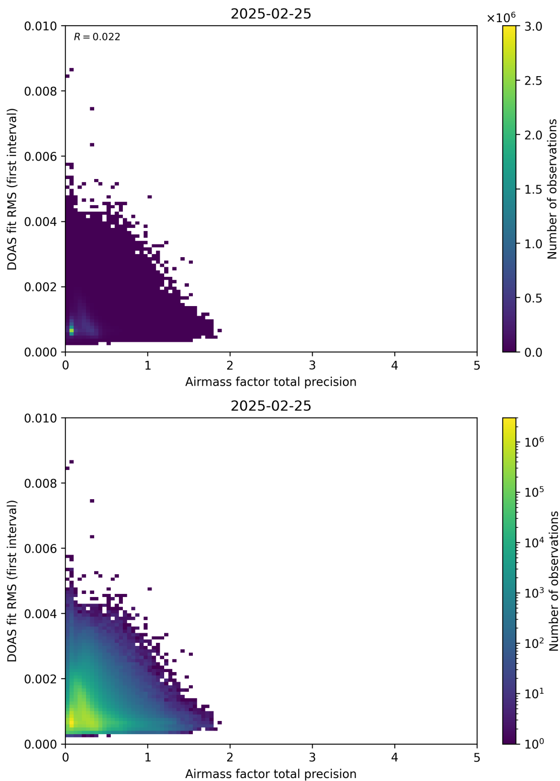
Figure 105: Scatter density plot of “Airmass factor total precision” against “DOAS fit RMS (first interval)” for 2025-02-24 to 2025-02-26.
