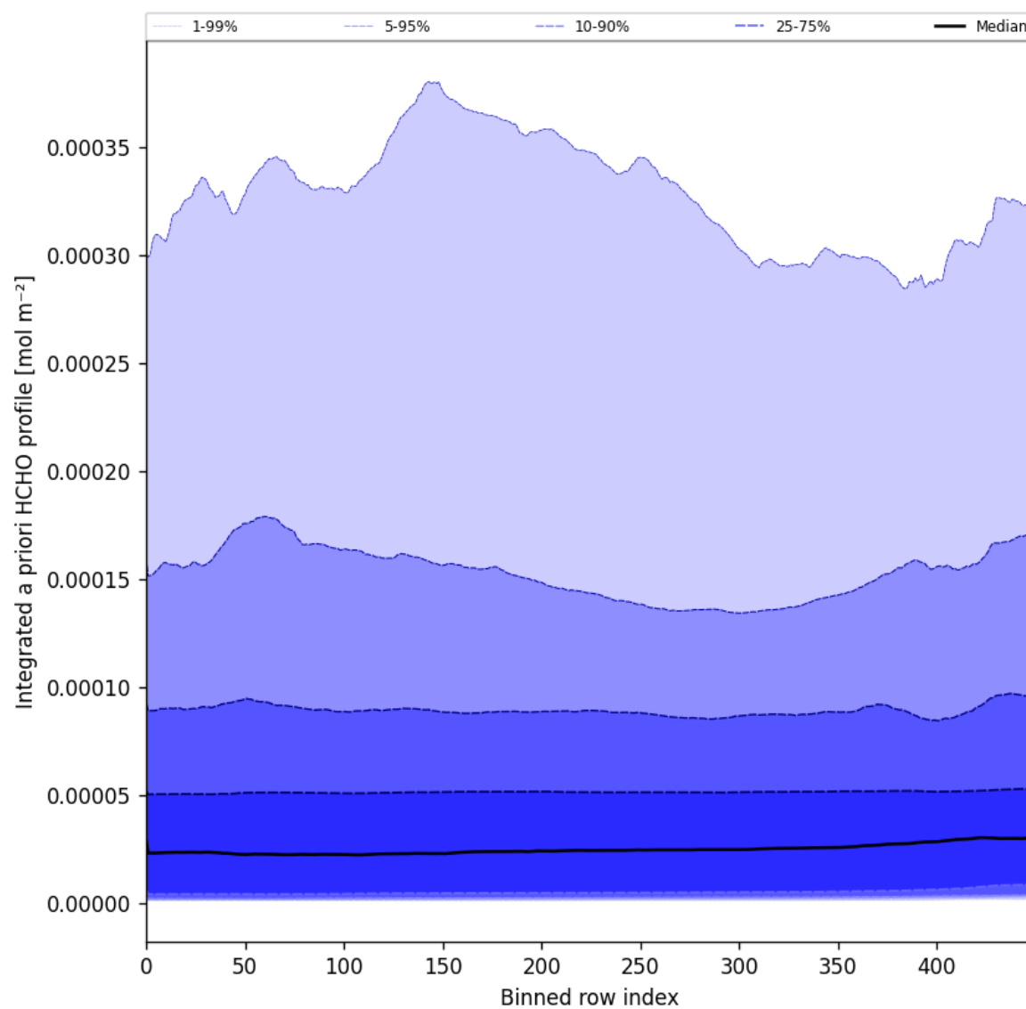
Figure 57: Along track statistics of “Integrated a priori HCHO profile” for 2025-02-24 to 2025-02-26
