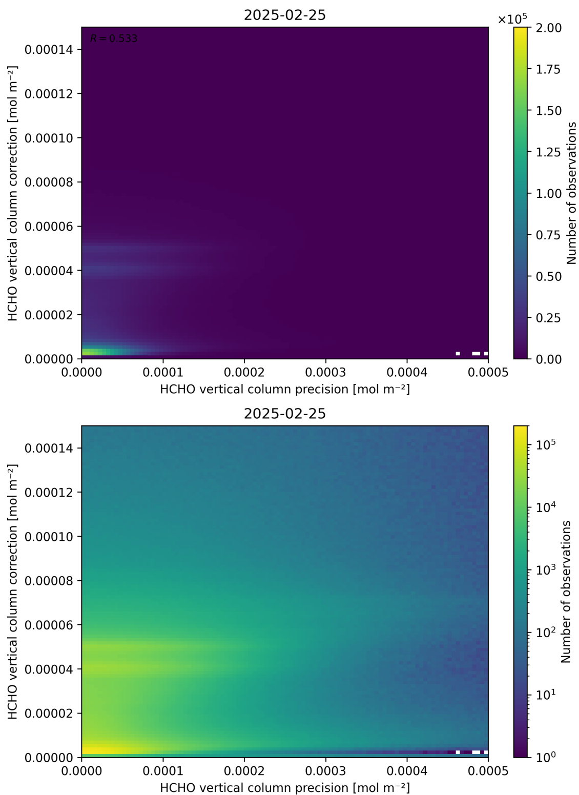
Figure 146: Scatter density plot of “HCHO vertical column precision” against “HCHO vertical column correction” for 2025-02-24 to 2025-02-26.
