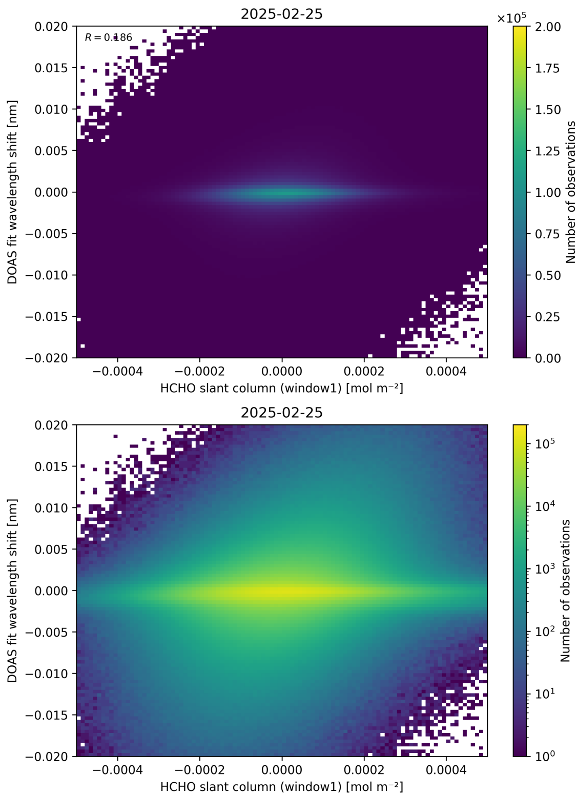
Figure 79: Scatter density plot of “HCHO slant column (window1)” against “DOAS fit wavelength shift” for 2025-02-24 to 2025-02-26.
