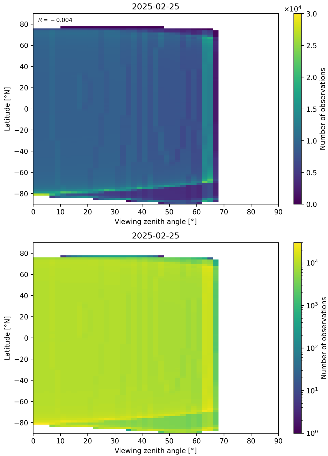
Figure 196: Scatter density plot of “Viewing zenith angle” against “Latitude” for 2025-02-24 to 2025-02-26.
