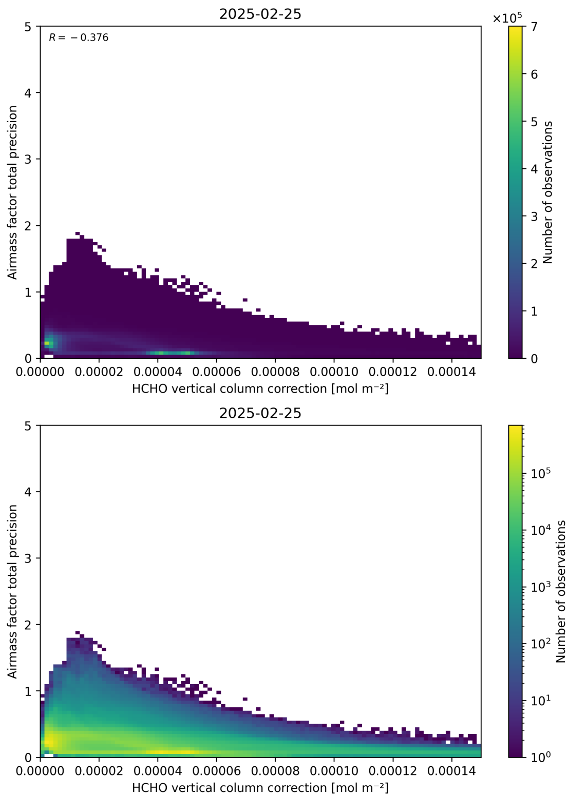
Figure 121: Scatter density plot of “HCHO vertical column correction” against “Airmass factor total precision” for 2025-02-24 to 2025-02-26.
