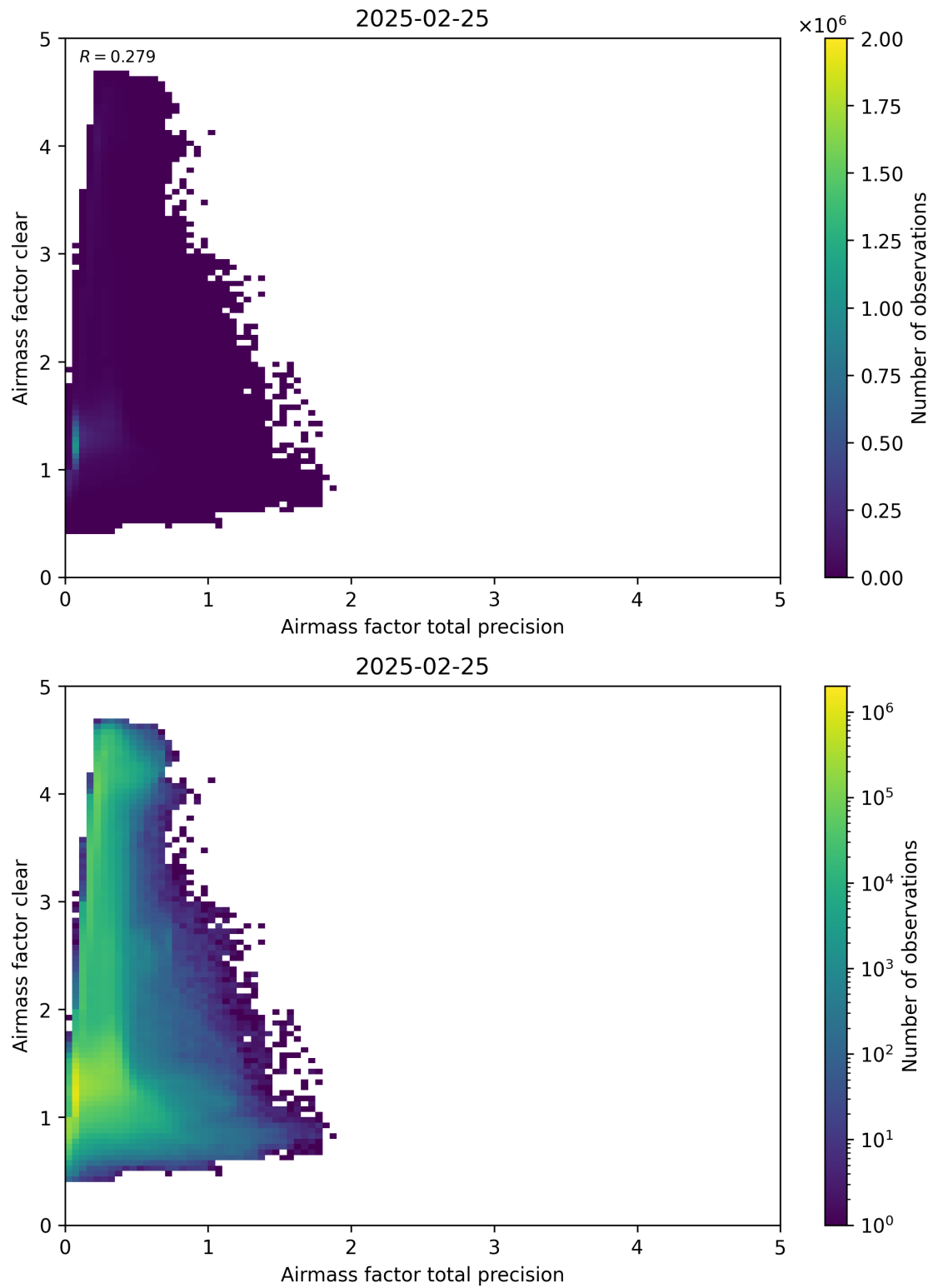
Figure 108: Scatter density plot of “Airmass factor total precision” against “Airmass factor clear” for 2025-02-24 to 2025-02-26.
