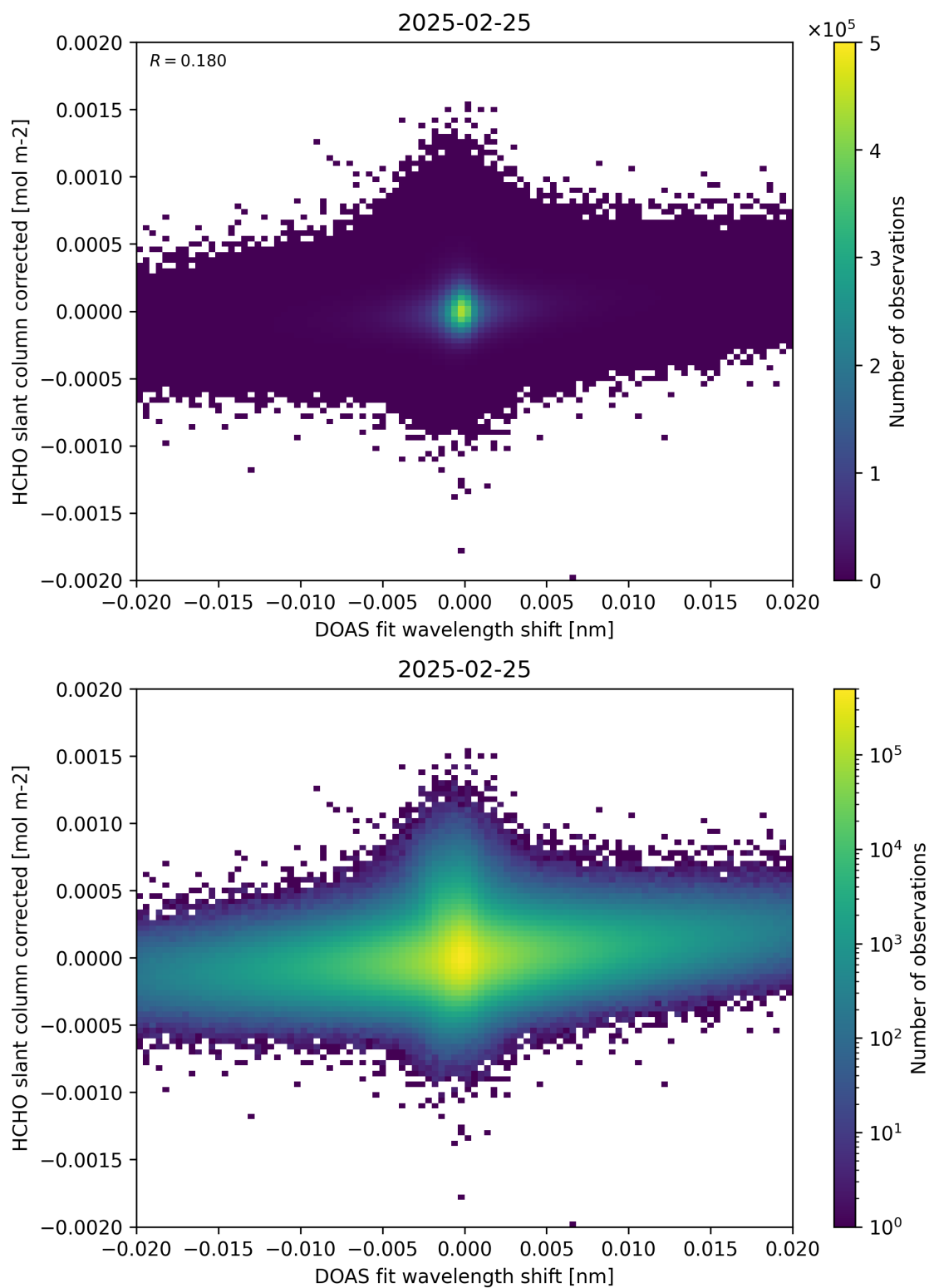
Figure 66: Scatter density plot of “DOAS fit wavelength shift” against “HCHO slant column corrected” for 2025-02-24 to 2025-02-26.
