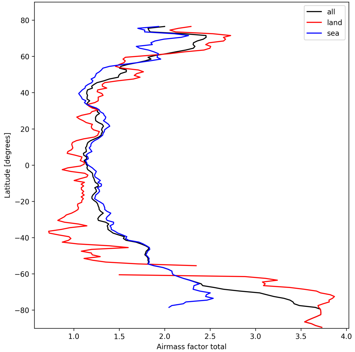
Figure 26: Zonal average of “Airmass factor total” for 2025-02-24 to 2025-02-26.
