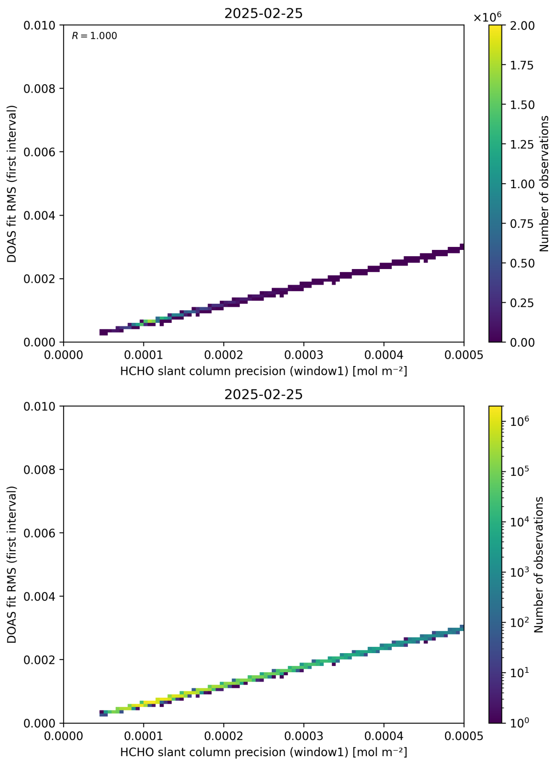
Figure 88: Scatter density plot of “HCHO slant column precision (window1)” against “DOAS fit RMS (first interval)” for 2025-02-24 to 2025-02-26.
