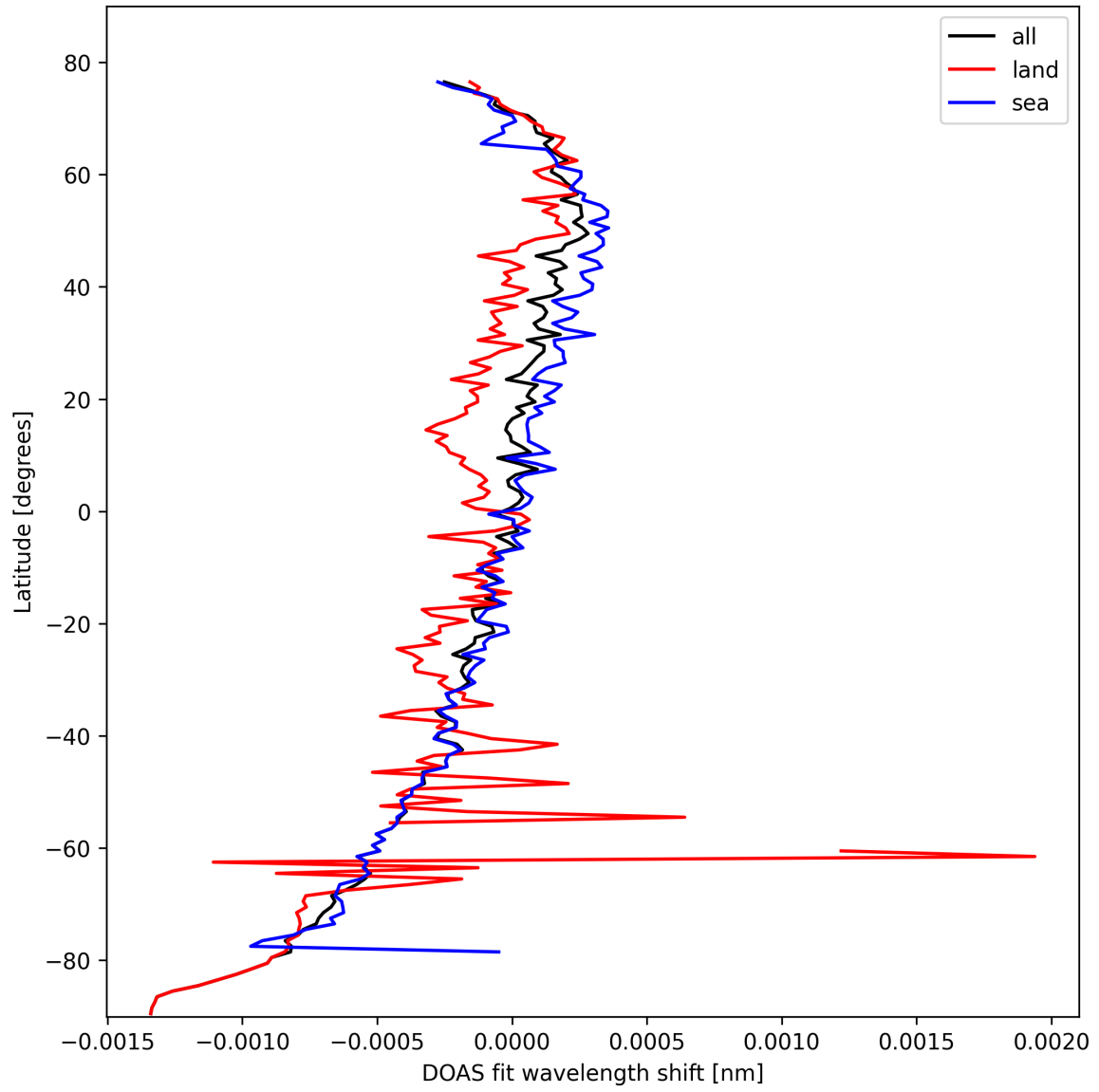
Figure 30: Zonal average of “DOAS fit wavelength shift” for 2025-02-24 to 2025-02-26.
