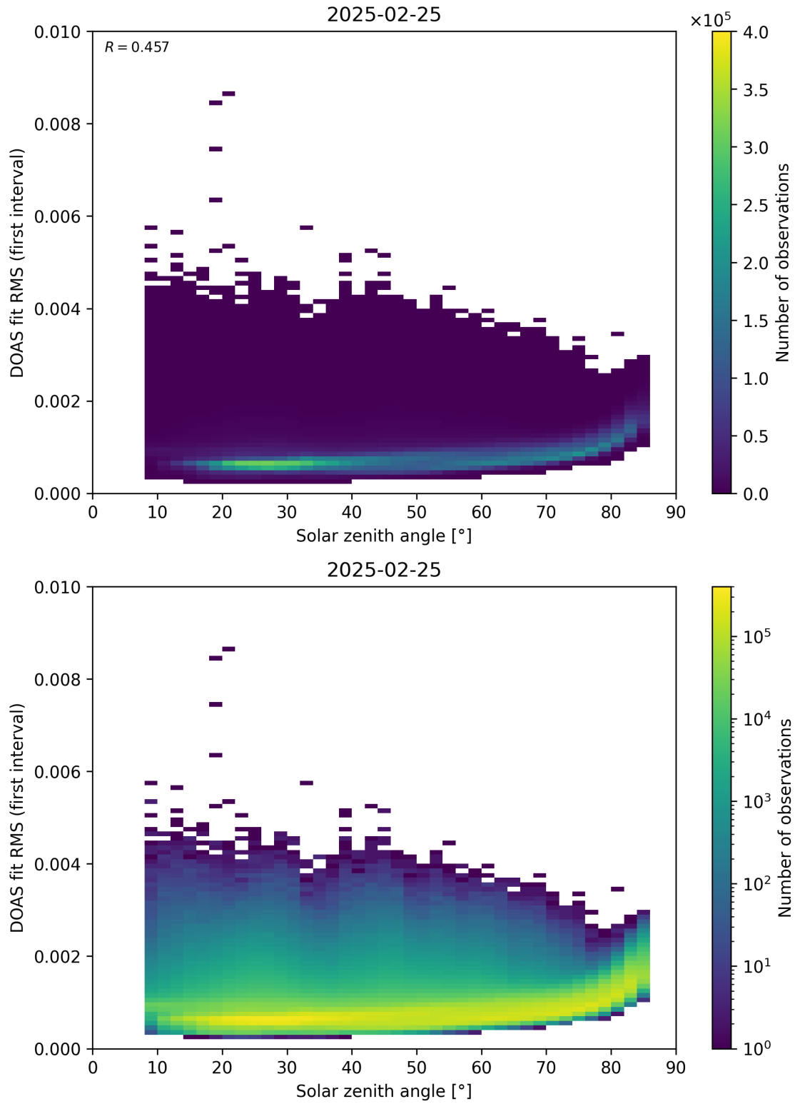
Figure 167: Scatter density plot of “Solar zenith angle” against “DOAS fit RMS (first interval)” for 2025-02-24 to 2025-02-26.
