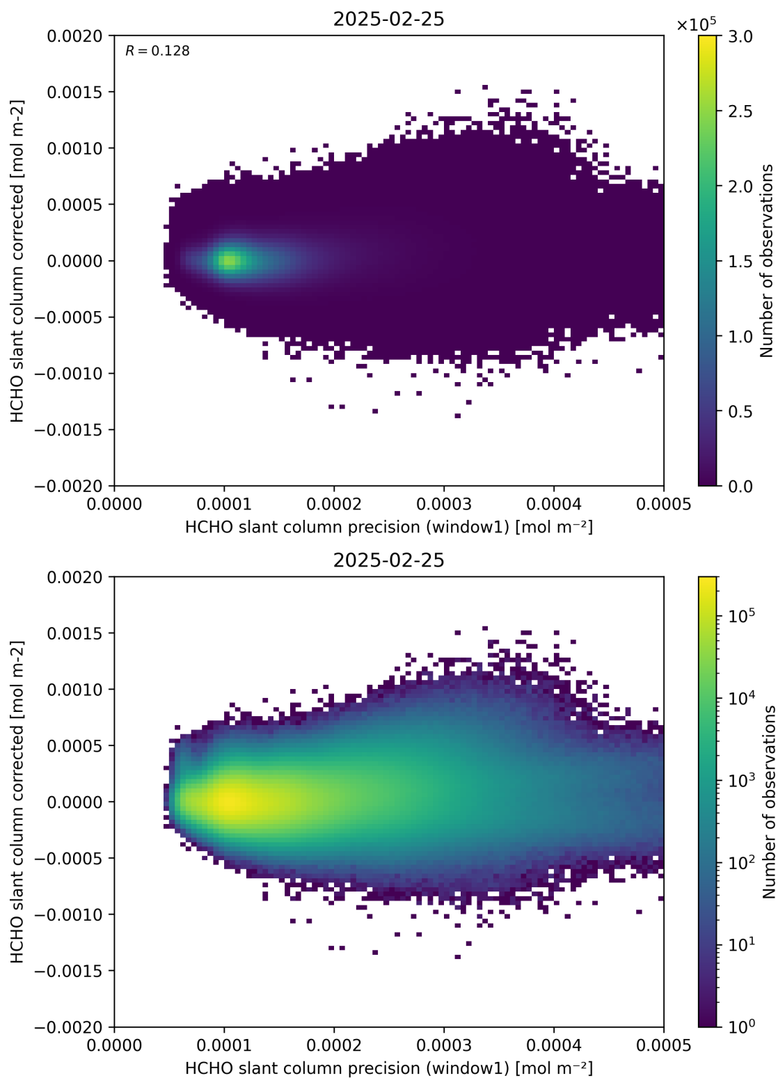
Figure 92: Scatter density plot of “HCHO slant column precision (window1)” against “HCHO slant column corrected” for 2025-02-24 to 2025-02-26.
