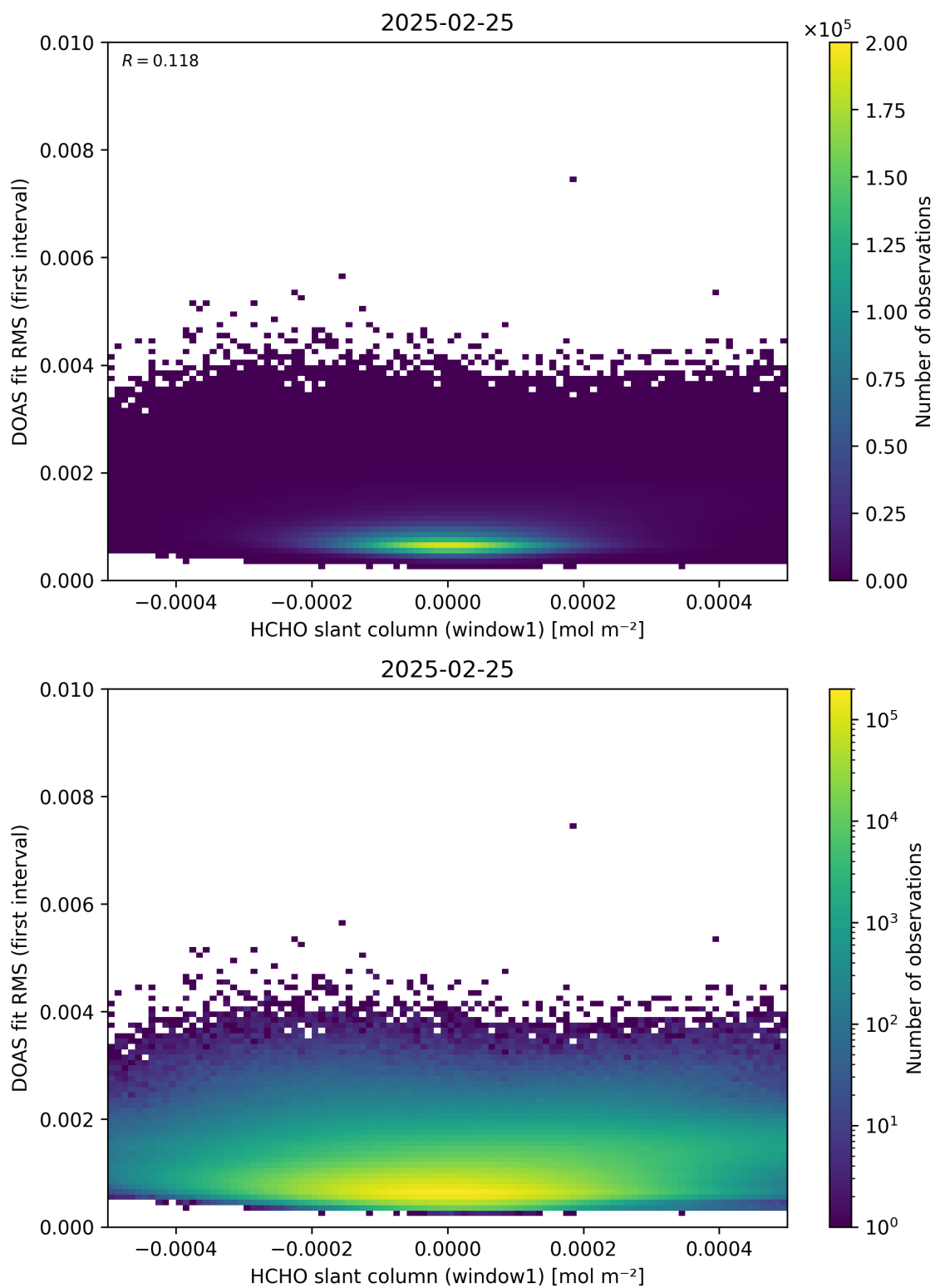
Figure 78: Scatter density plot of “HCHO slant column (window1)” against “DOAS fit RMS (first interval)” for 2025-02-24 to 2025-02-26.
