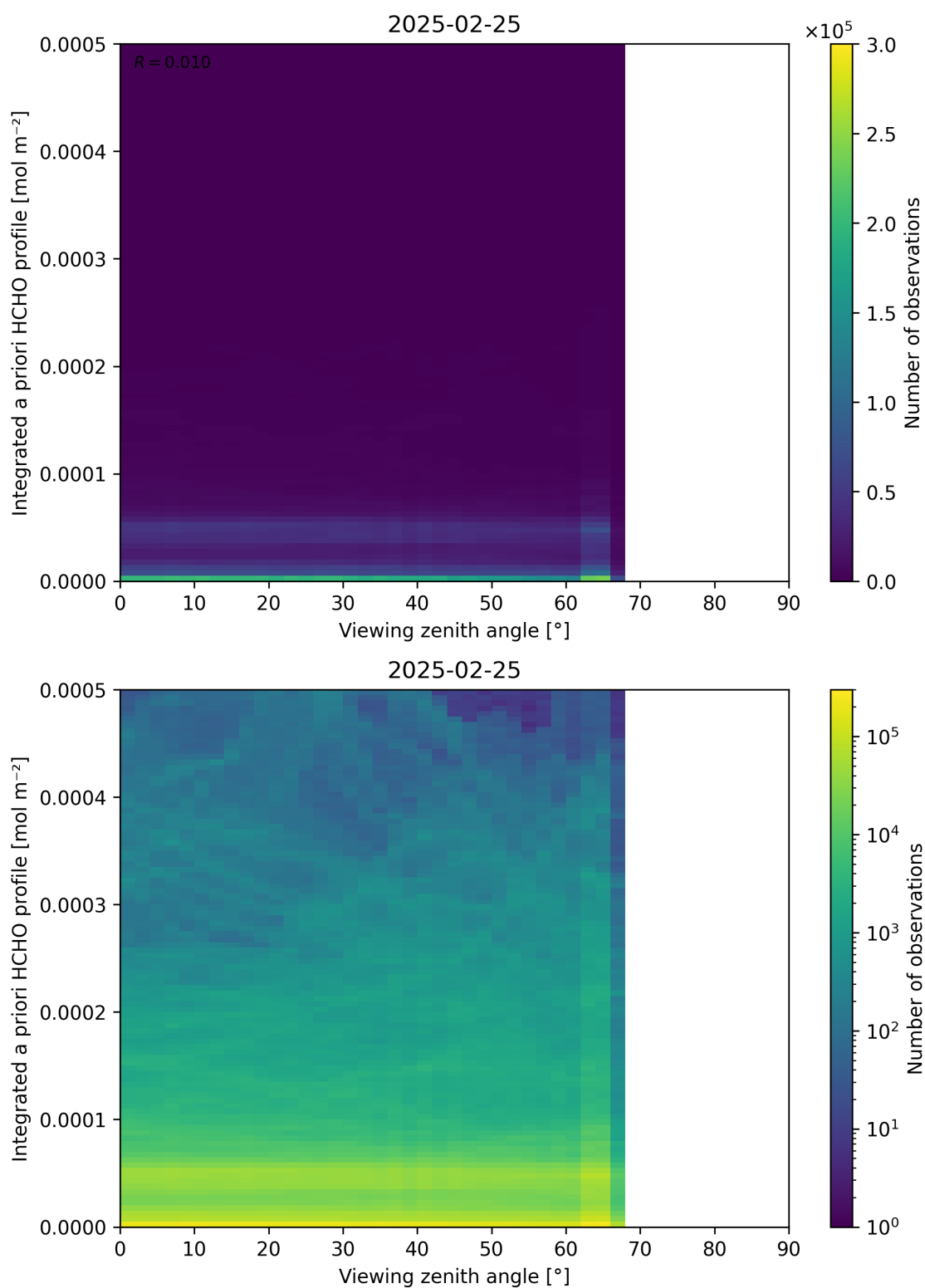
Figure 195: Scatter density plot of “Viewing zenith angle” against “Integrated a priori HCHO profile” for 2025-02-24 to 2025-02-26.
