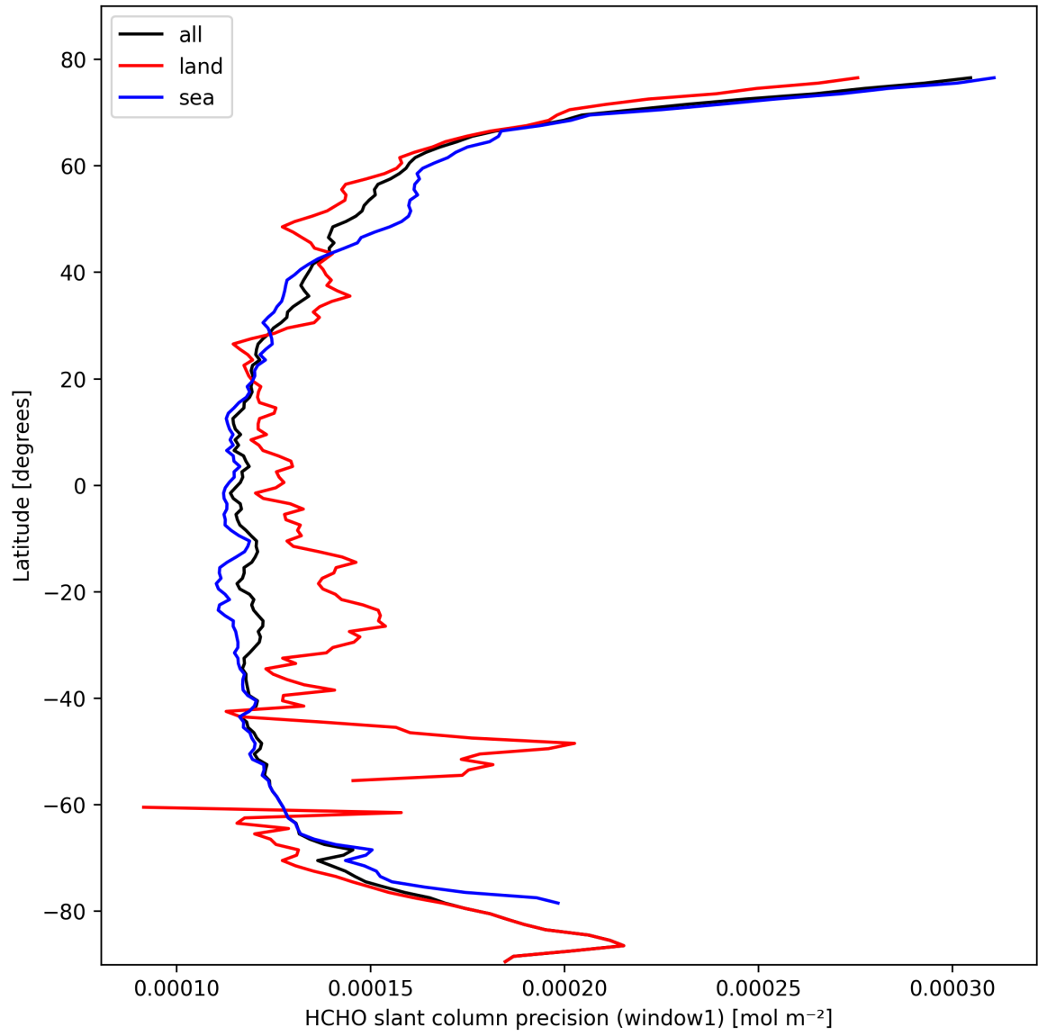
Figure 25: Zonal average of “HCHO slant column precision (window1)” for 2025-02-24 to 2025-02-26.
