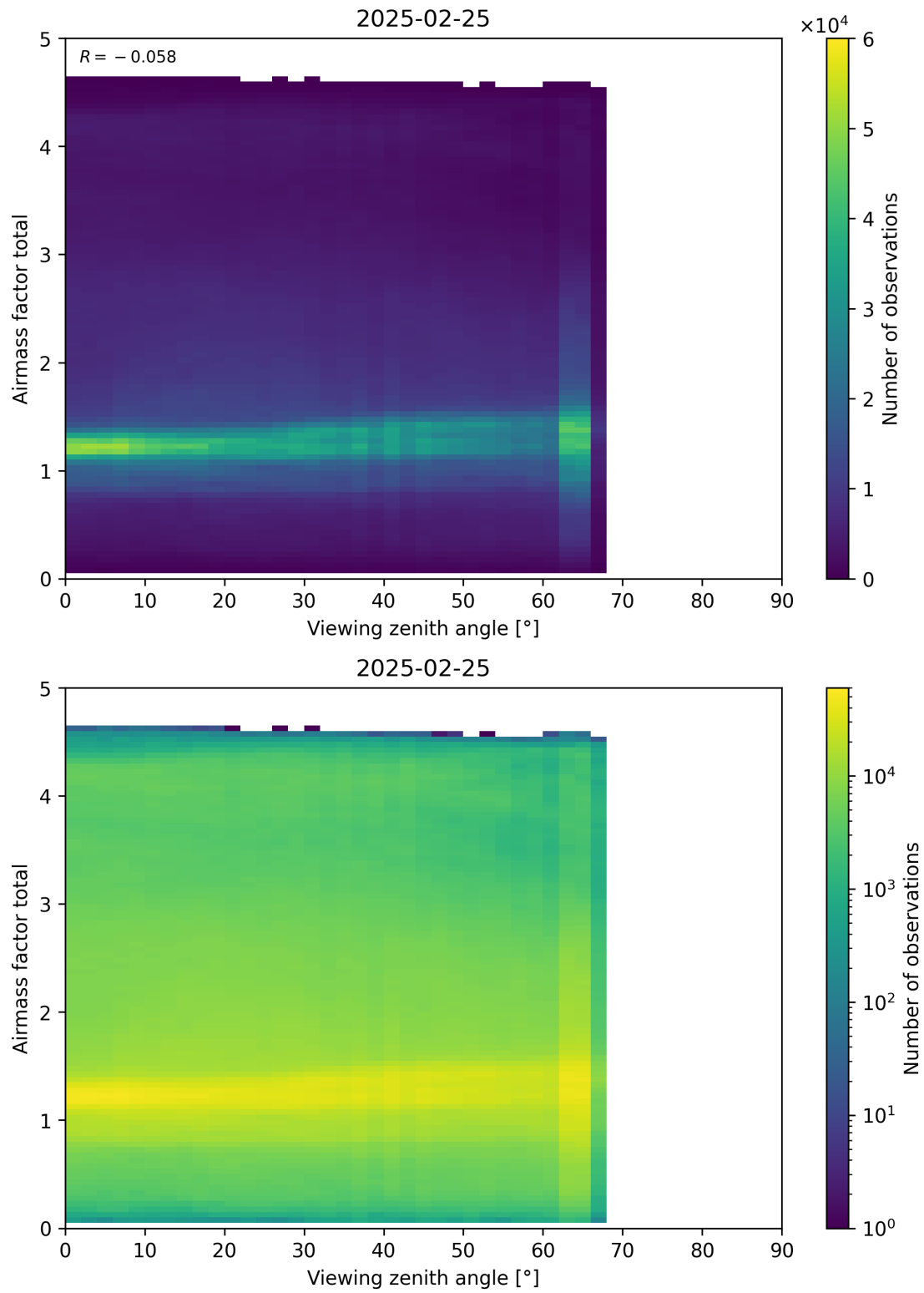
Figure 190: Scatter density plot of “Viewing zenith angle” against “Airmass factor total” for 2025-02-24 to 2025-02-26.
