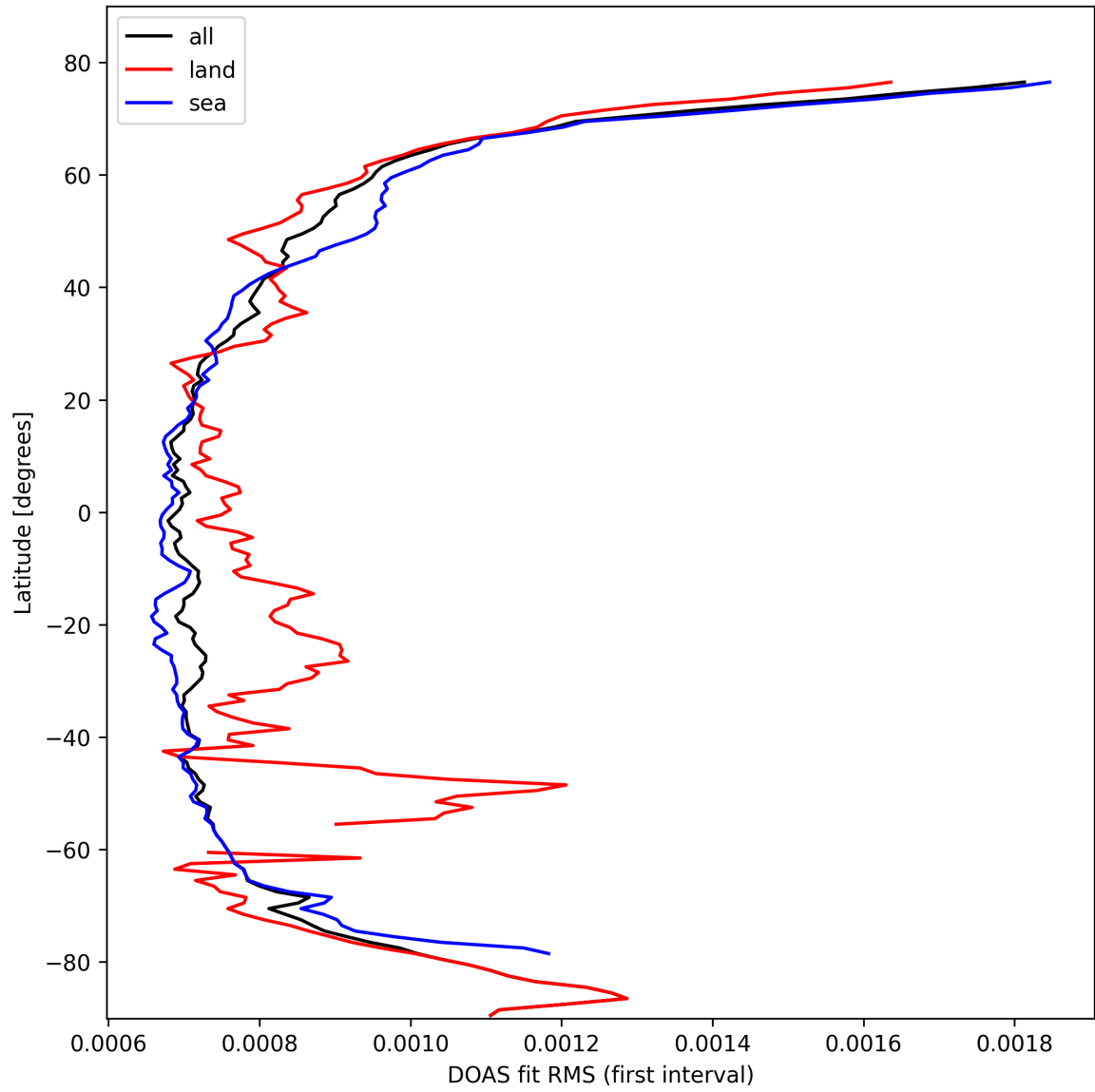
Figure 32: Zonal average of “DOAS fit RMS (first interval)” for 2025-02-24 to 2025-02-26.
