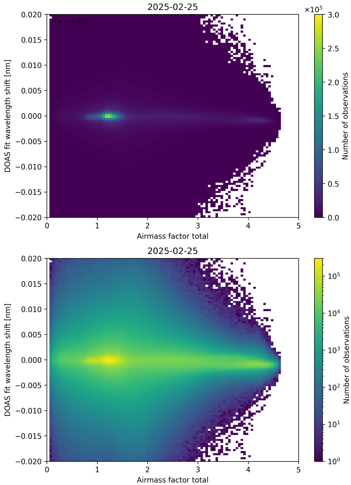
Figure 98: Scatter density plot of “Airmass factor total” against “DOAS fit wavelength shift” for 2025-02-24 to 2025-02-26.
