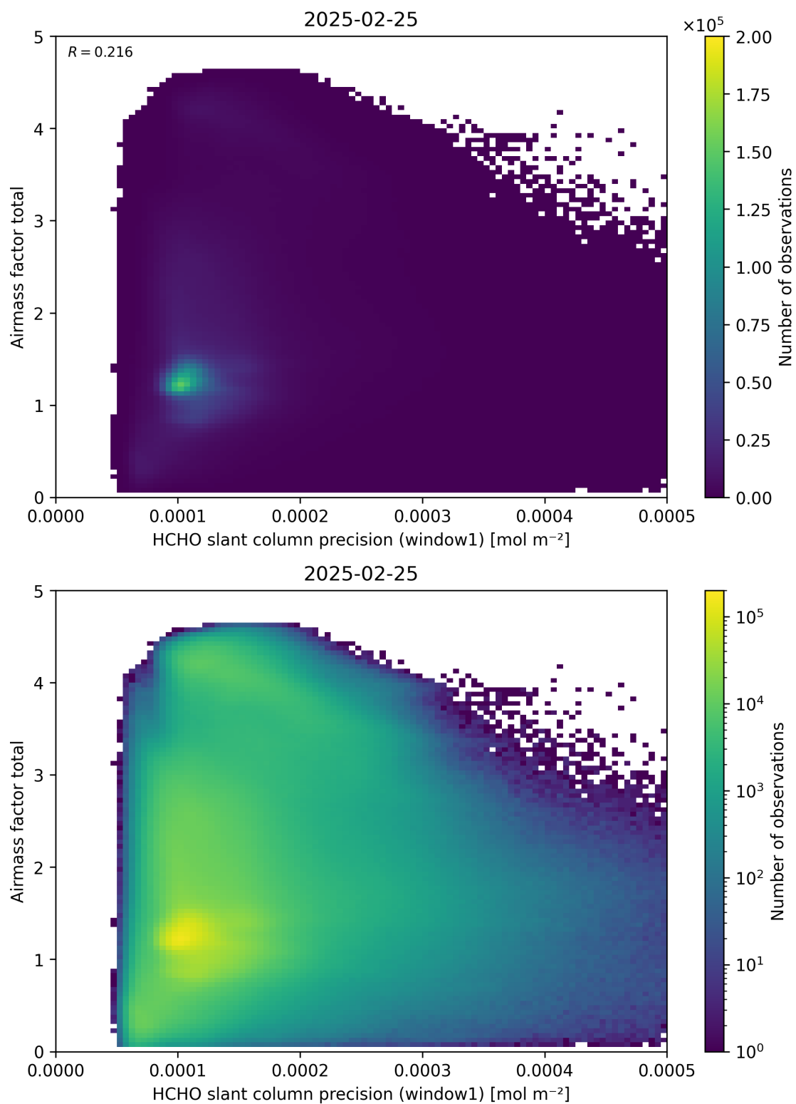
Figure 94: Scatter density plot of “HCHO slant column precision (window1)” against “Airmass factor total” for 2025-02-24 to 2025-02-26.
