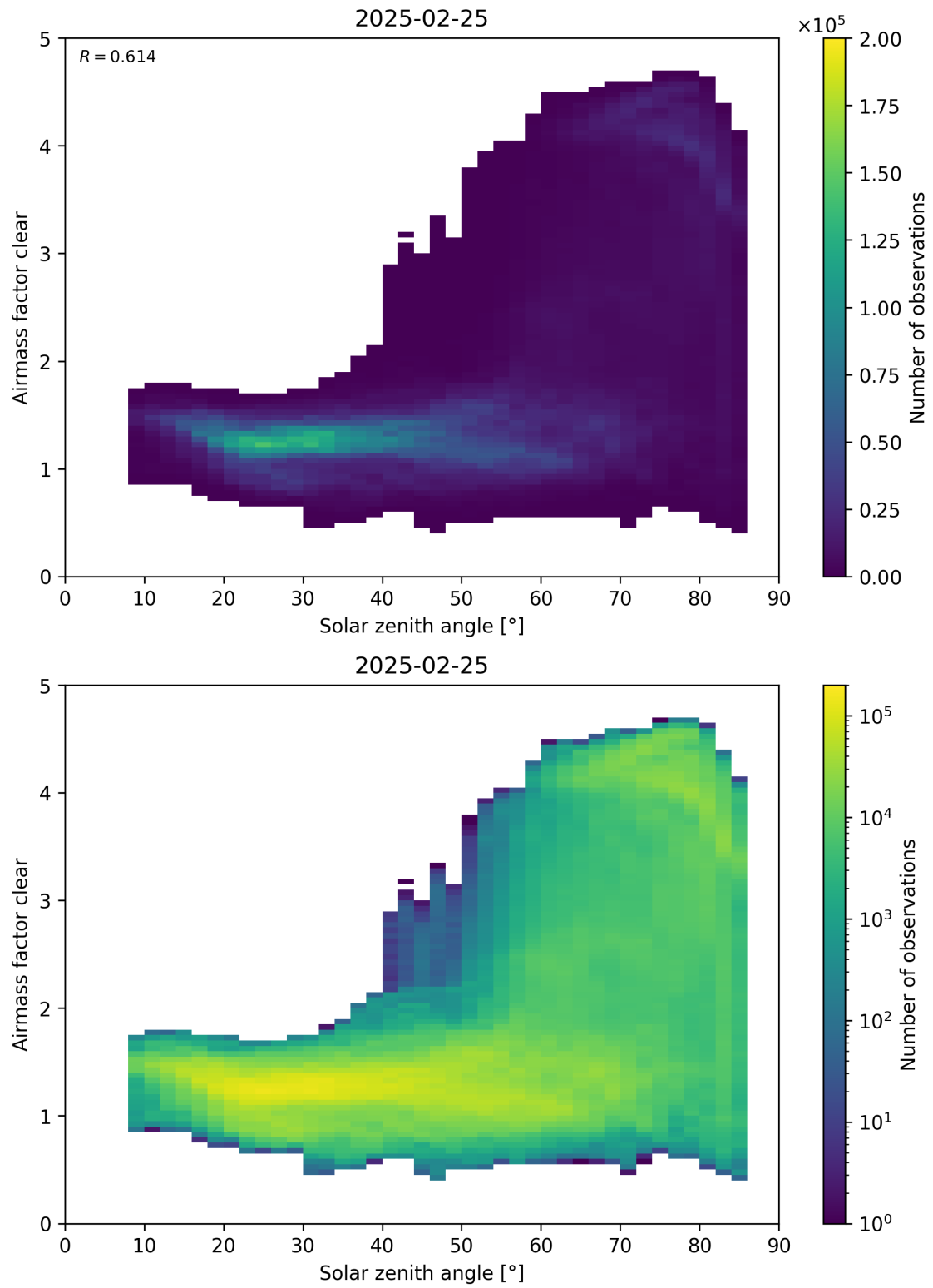
Figure 170: Scatter density plot of “Solar zenith angle” against “Airmass factor clear” for 2025-02-24 to 2025-02-26.
