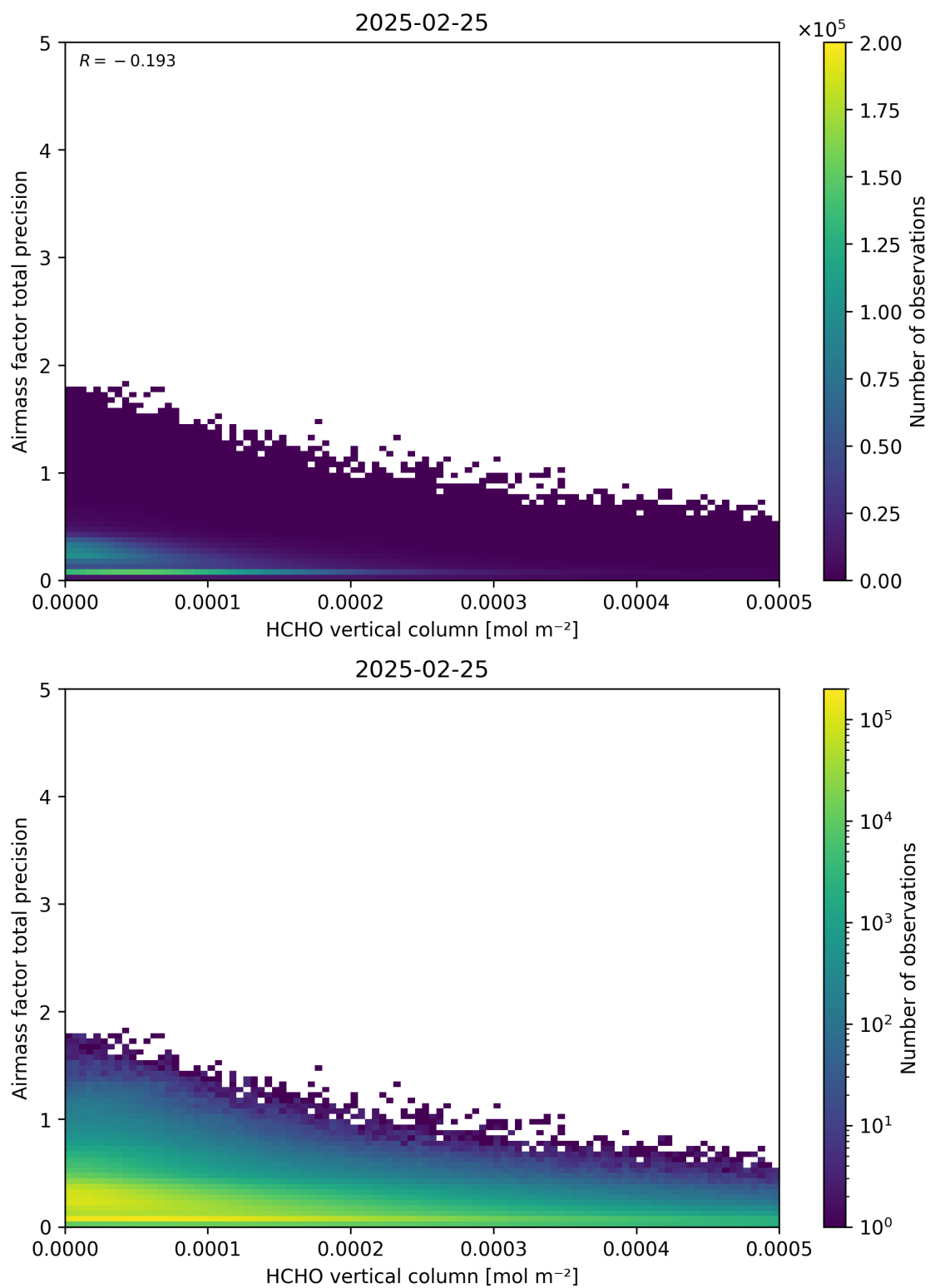
Figure 132: Scatter density plot of “HCHO vertical column” against “Airmass factor total precision” for 2025-02-24 to 2025-02-26.
