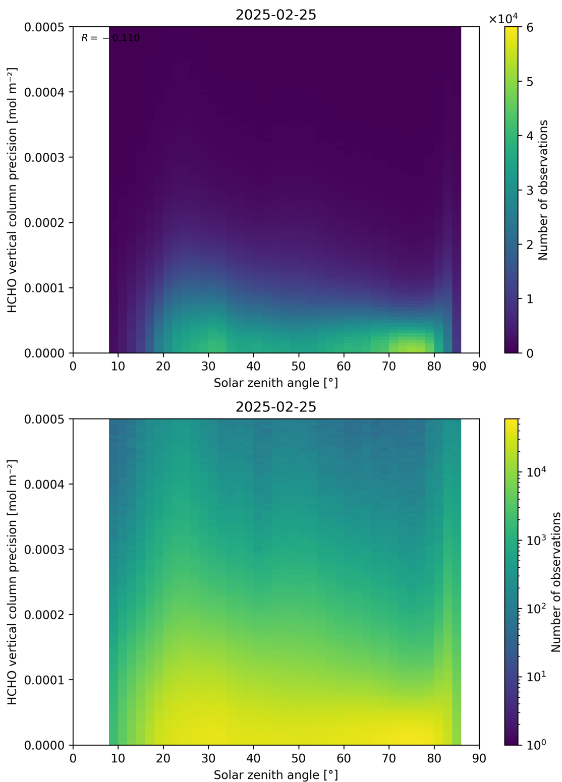
Figure 179: Scatter density plot of “Solar zenith angle” against “HCHO vertical column precision” for 2025-02-24 to 2025-02-26.
