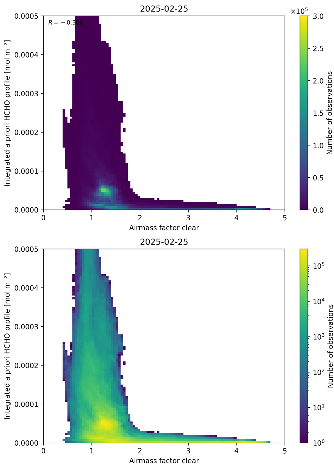
Figure 76: Scatter density plot of “Airmass factor clear” against “Integrated a priori HCHO profile” for 2025-02-24 to 2025-02-26.
