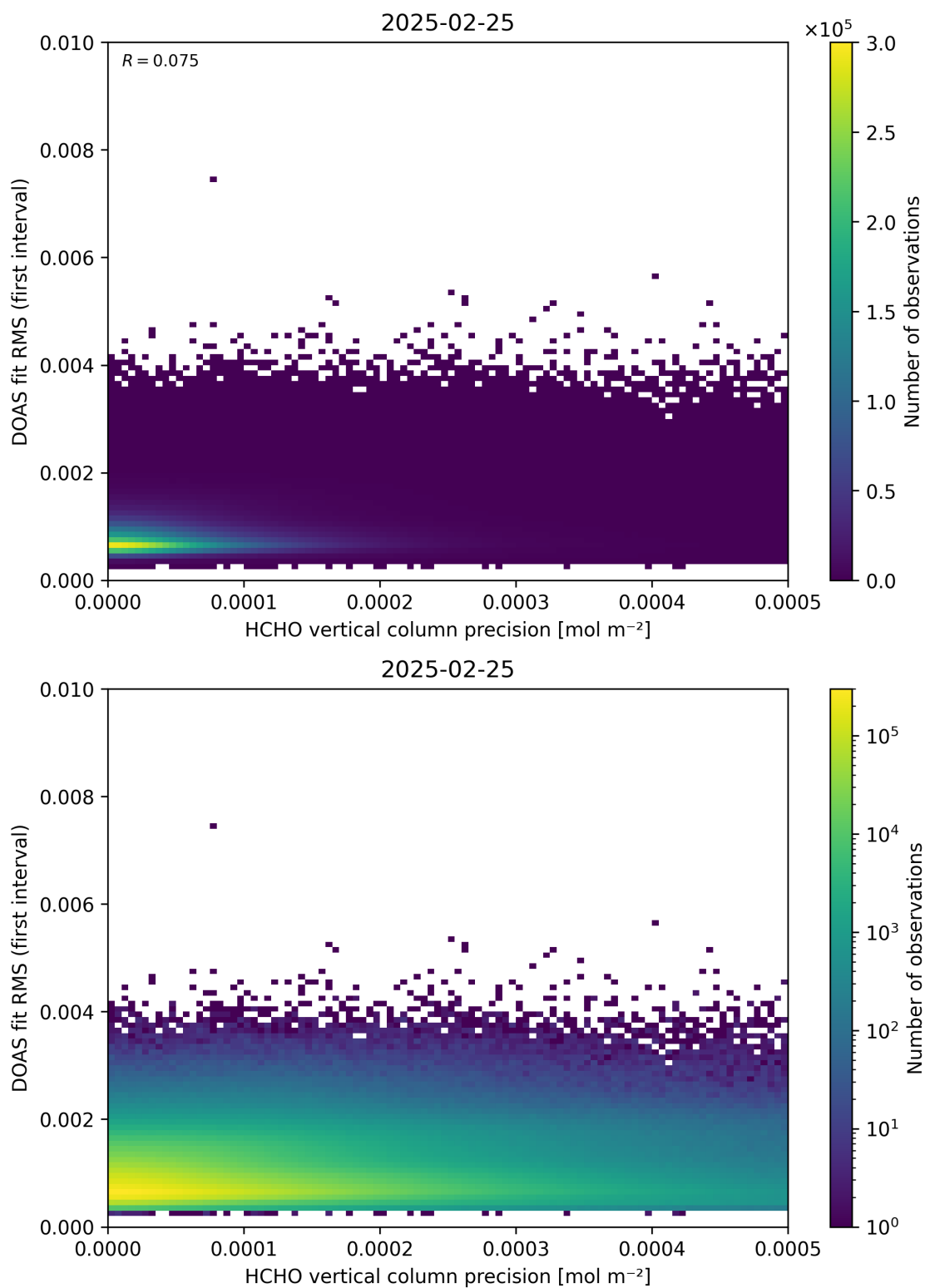
Figure 136: Scatter density plot of “HCHO vertical column precision” against “DOAS fit RMS (first interval)” for 2025-02-24 to 2025-02-26.
