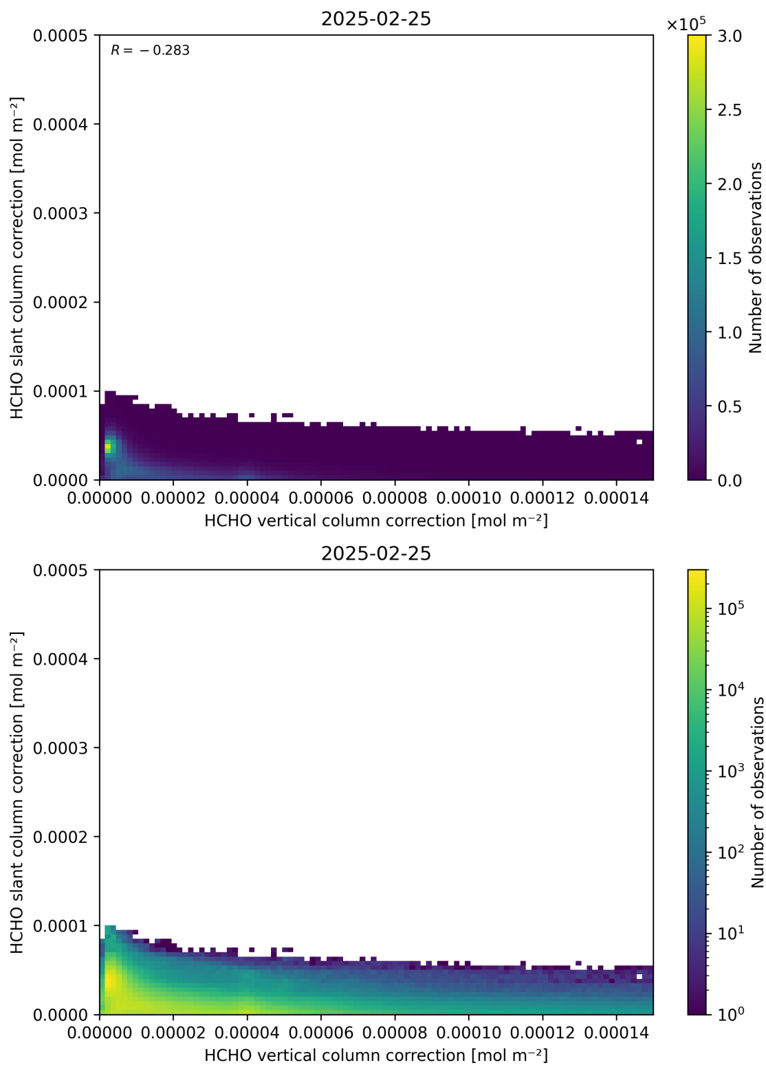
Figure 117: Scatter density plot of “HCHO vertical column correction” against “HCHO slant column correction” for 2025-02-24 to 2025-02-26.
