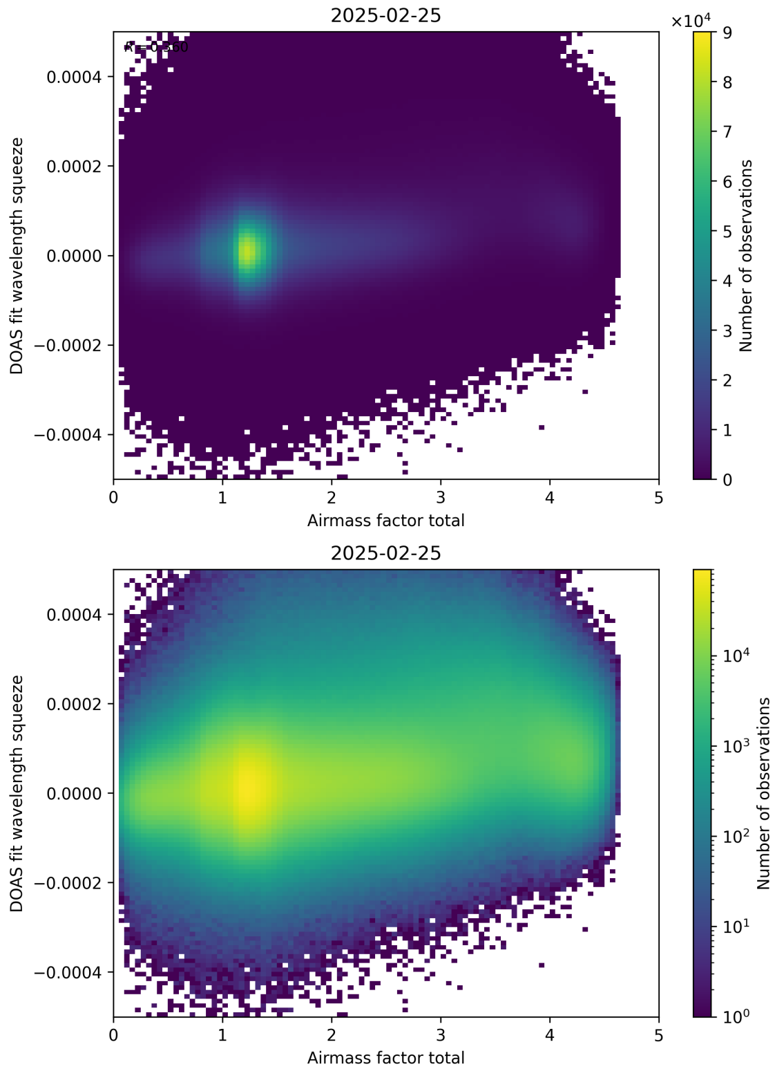
Figure 99: Scatter density plot of “Airmass factor total” against “DOAS fit wavelength squeeze” for 2025-02-24 to 2025-02-26.
