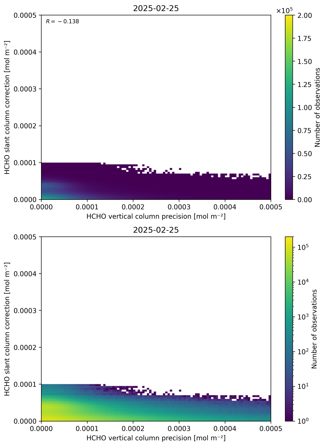
Figure 141: Scatter density plot of “HCHO vertical column precision” against “HCHO slant column correction” for 2025-02-24 to 2025-02-26.
