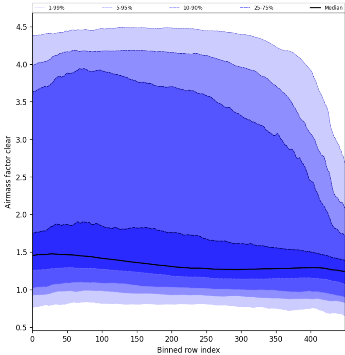
Figure 56: Along track statistics of “Airmass factor clear” for 2025-02-24 to 2025-02-26
