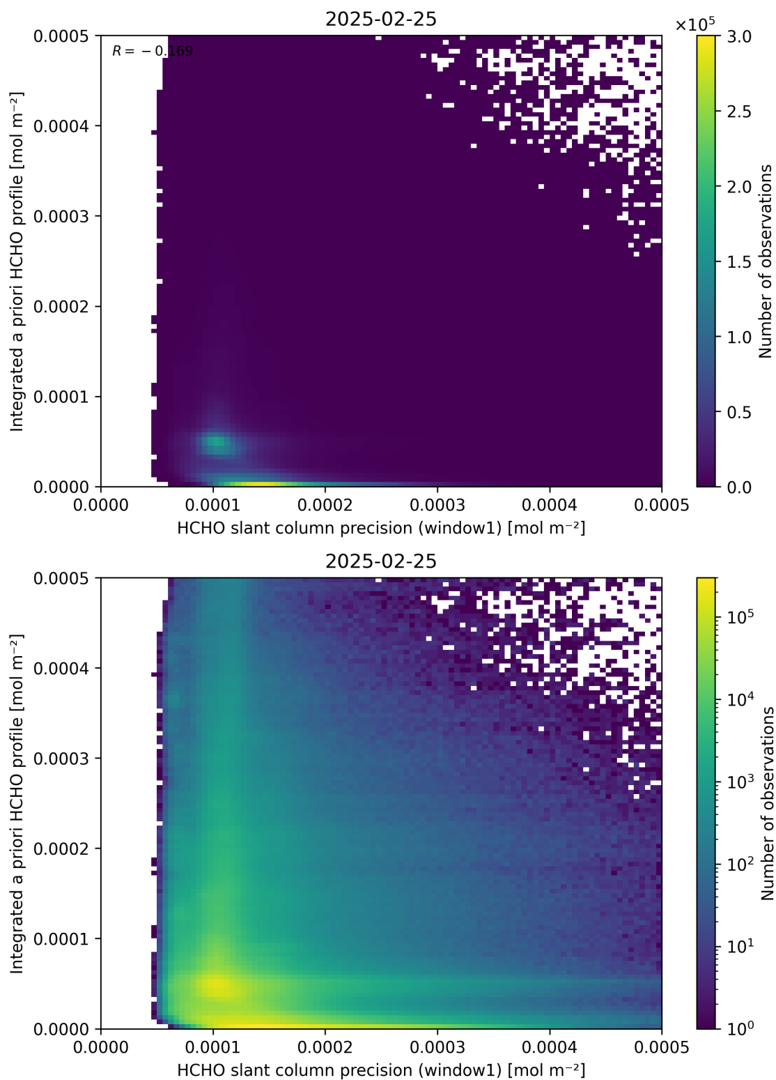
Figure 96: Scatter density plot of “HCHO slant column precision (window1)” against “Integrated a priori HCHO profile” for 2025-02-24 to 2025-02-26.
