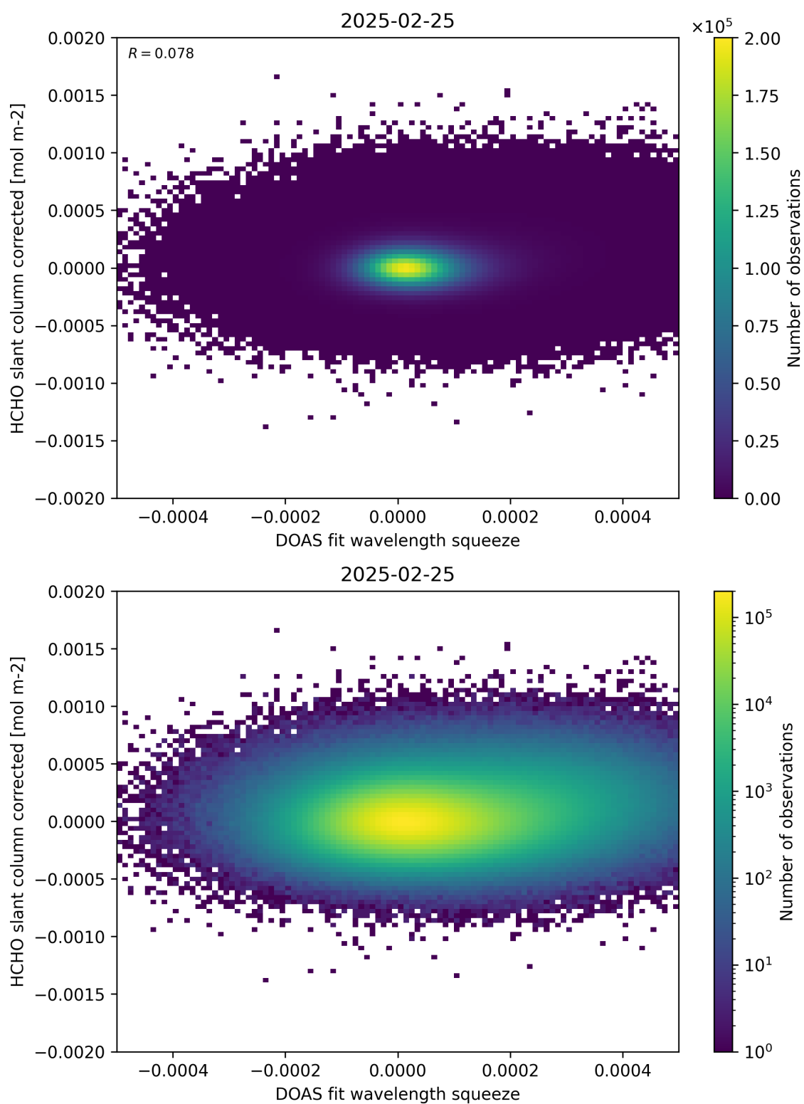
Figure 69: Scatter density plot of “DOAS fit wavelength squeeze” against “HCHO slant column corrected” for 2025-02-24 to 2025-02-26.
