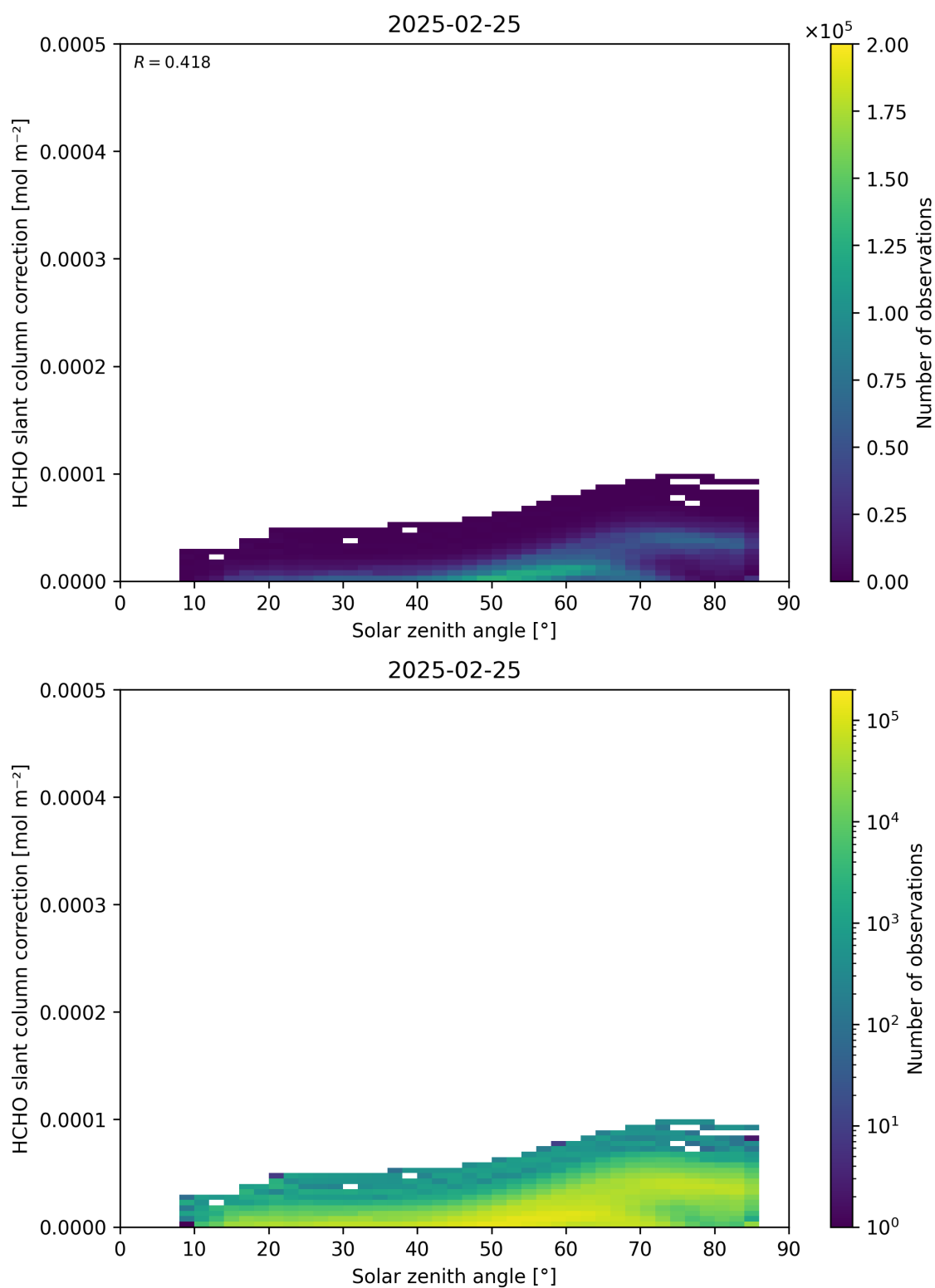
Figure 172: Scatter density plot of “Solar zenith angle” against “HCHO slant column correction” for 2025-02-24 to 2025-02-26.
