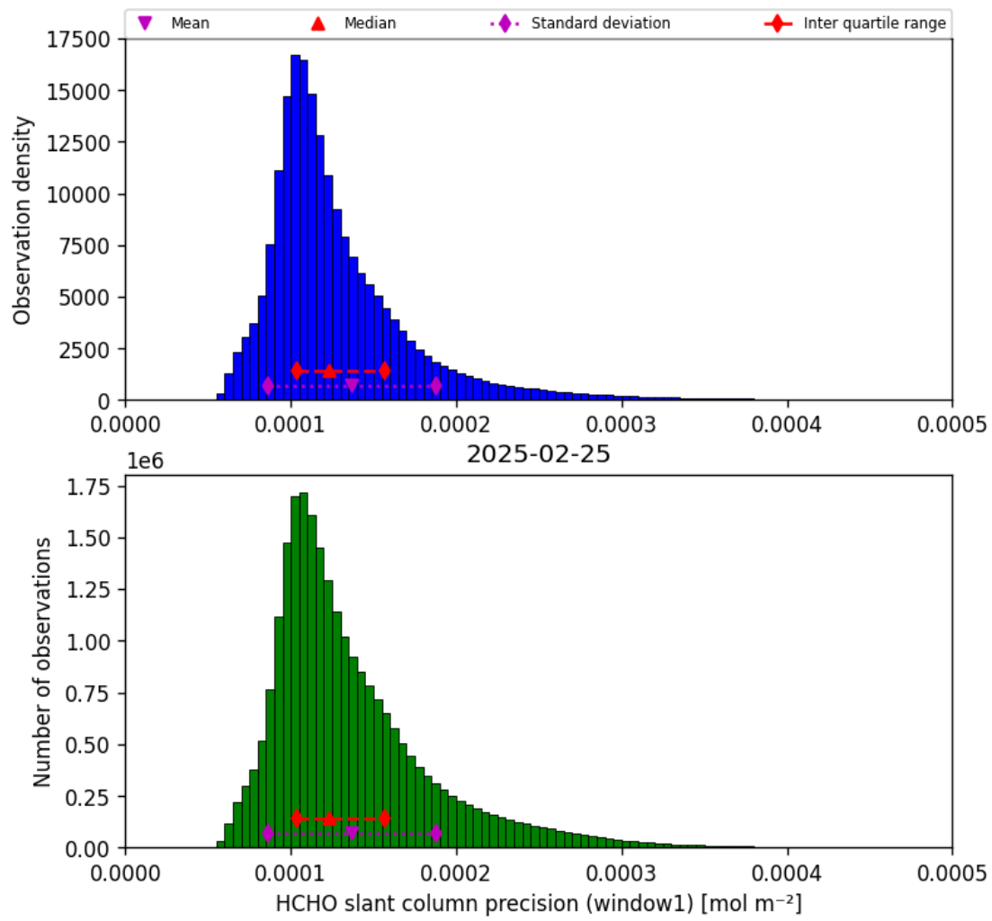
Figure 39: Histogram of “HCHO slant column precision (window1)” for 2025-02-24 to 2025-02-26
