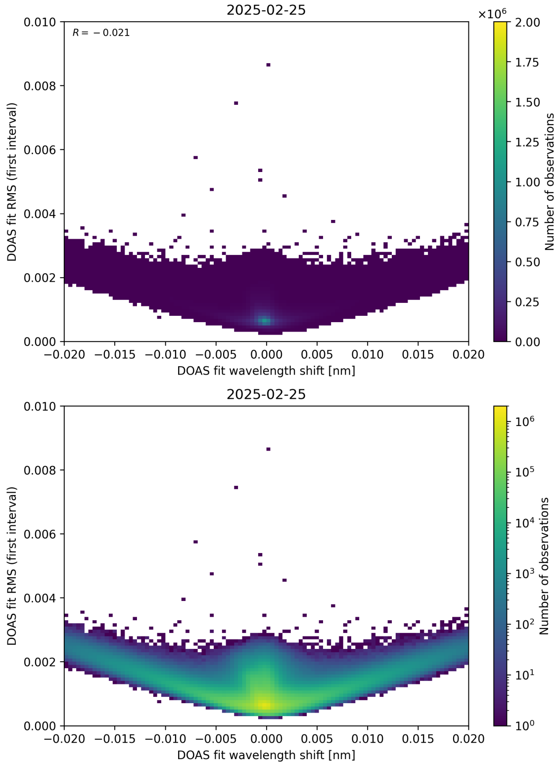
Figure 64: Scatter density plot of “DOAS fit wavelength shift” against “DOAS fit RMS (first interval)” for 2025-02-24 to 2025-02-26.
