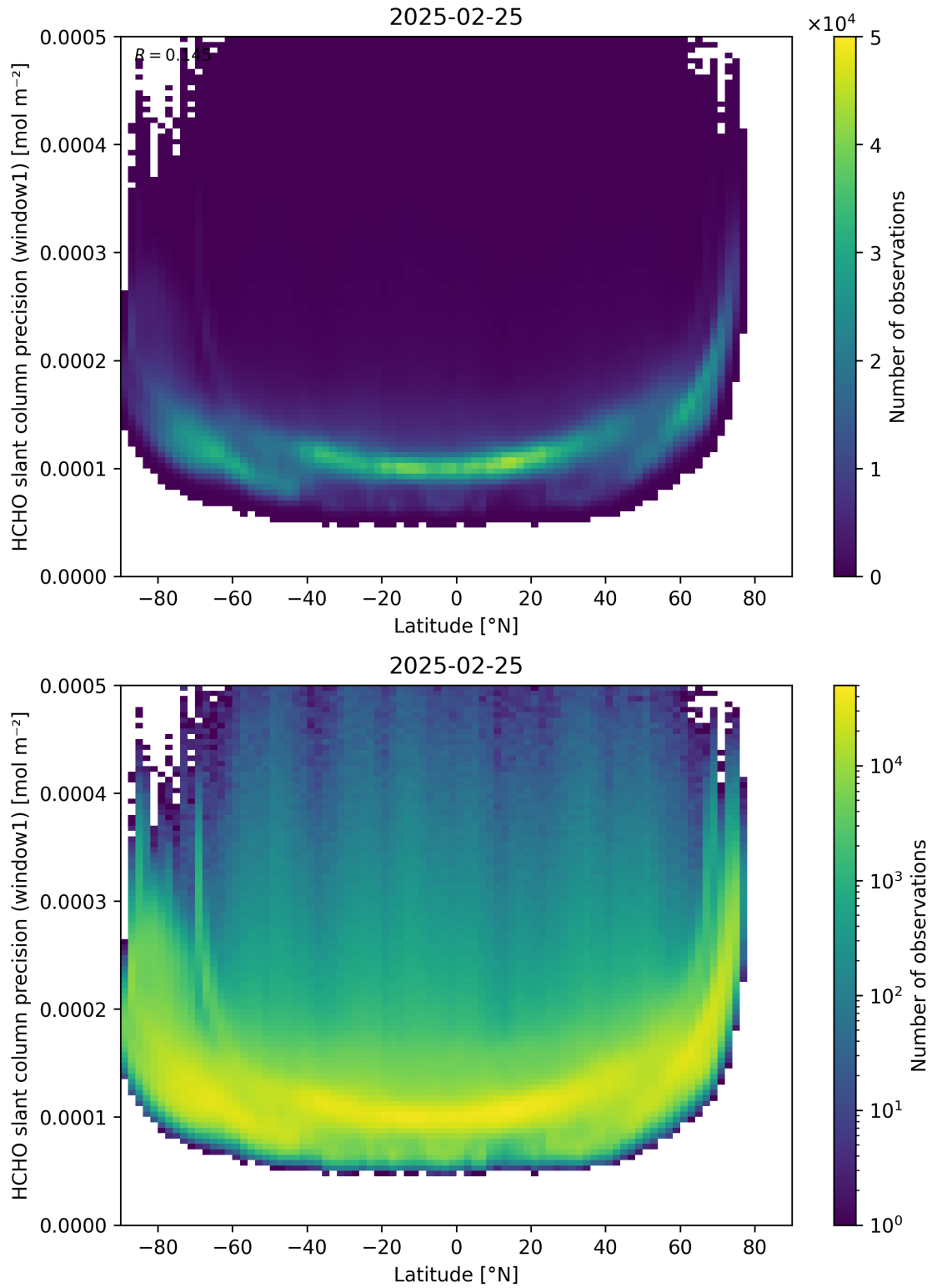
Figure 160: Scatter density plot of “Latitude” against “HCHO slant column precision (window1)” for 2025-02-24 to 2025-02-26.
