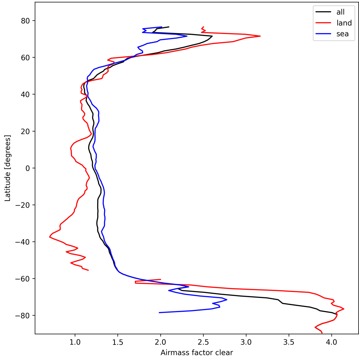
Figure 28: Zonal average of “Airmass factor clear” for 2025-02-24 to 2025-02-26.
