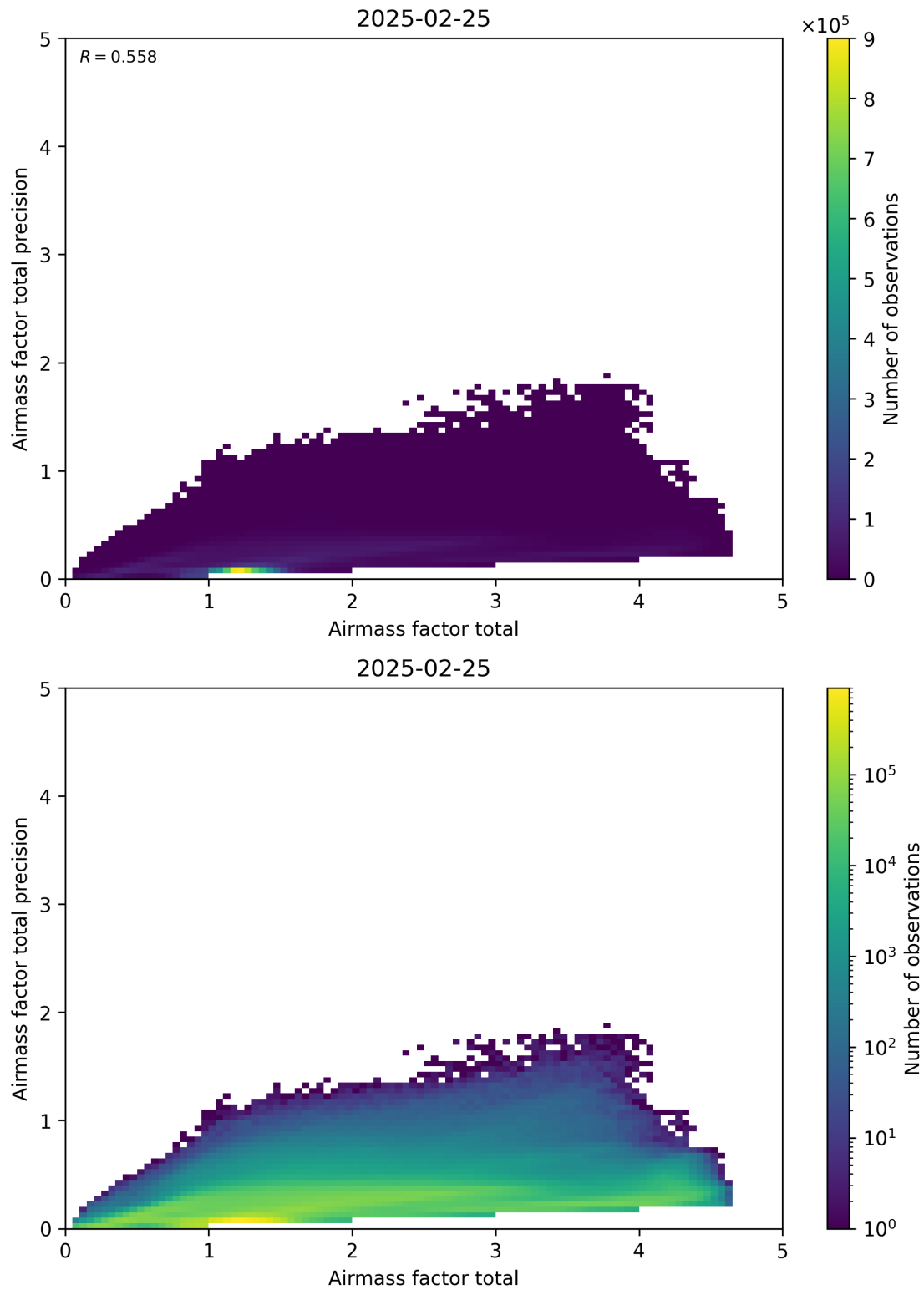
Figure 103: Scatter density plot of “Airmass factor total” against “Airmass factor total precision” for 2025-02-24 to 2025-02-26.
