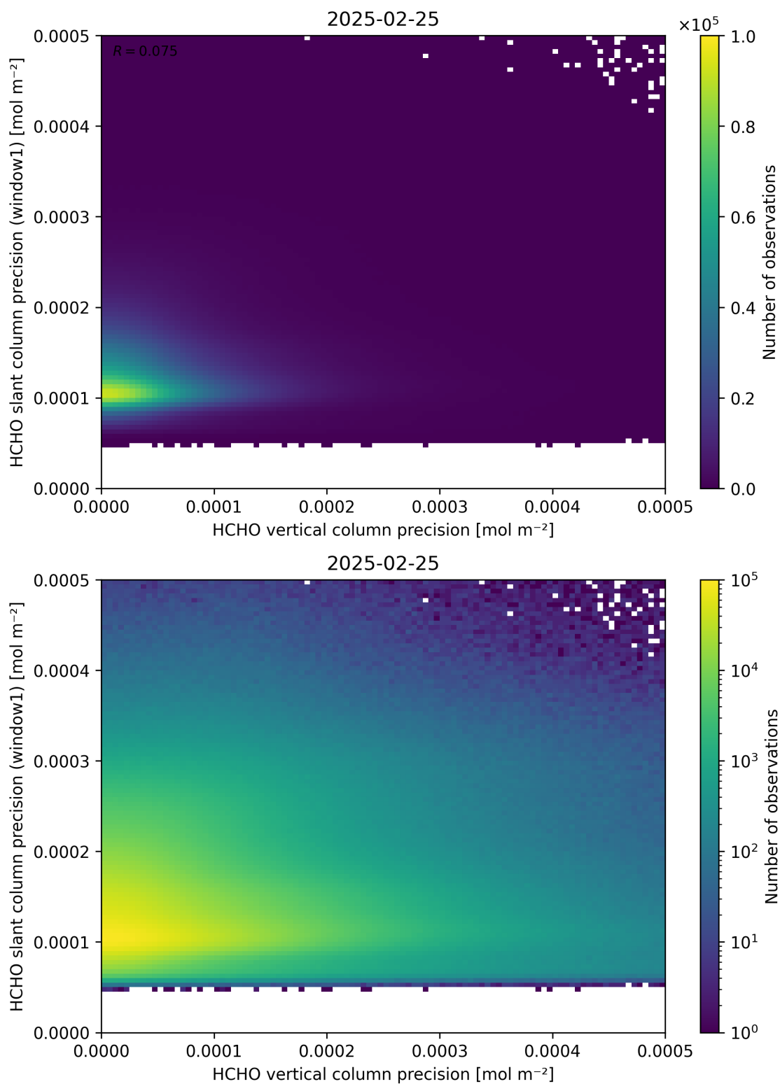
Figure 143: Scatter density plot of “HCHO vertical column precision” against “HCHO slant column precision (window1)” for 2025-02-24 to 2025-02-26.
