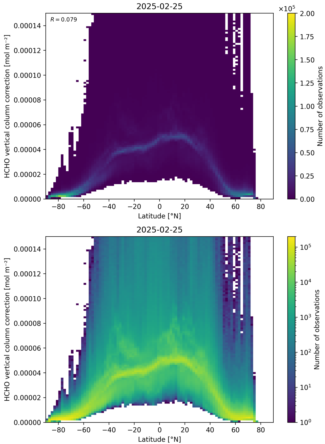
Figure 164: Scatter density plot of “Latitude” against “HCHO vertical column correction” for 2025-02-24 to 2025-02-26.
