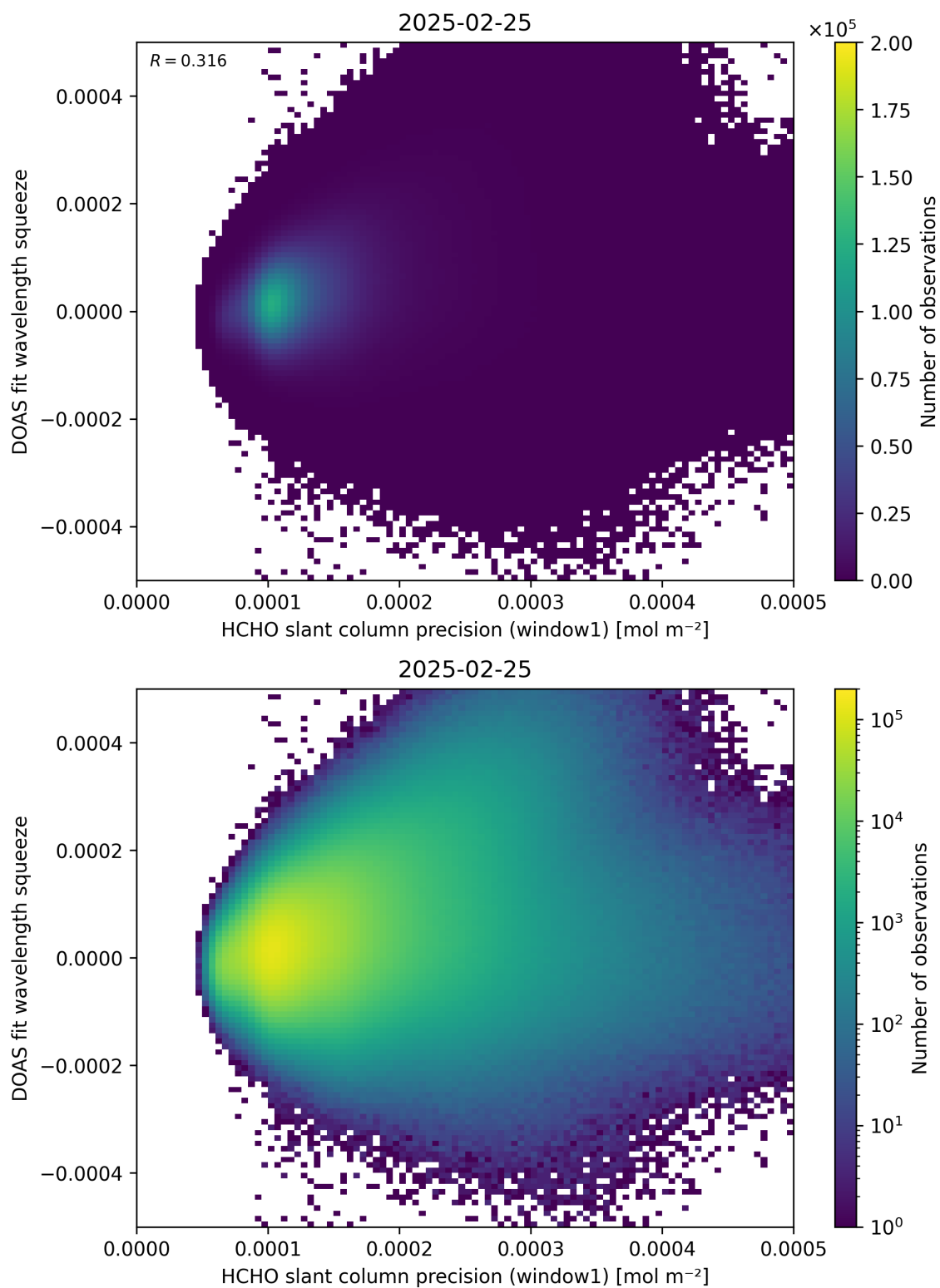
Figure 90: Scatter density plot of “HCHO slant column precision (window1)” against “DOAS fit wavelength squeeze” for 2025-02-24 to 2025-02-26.
