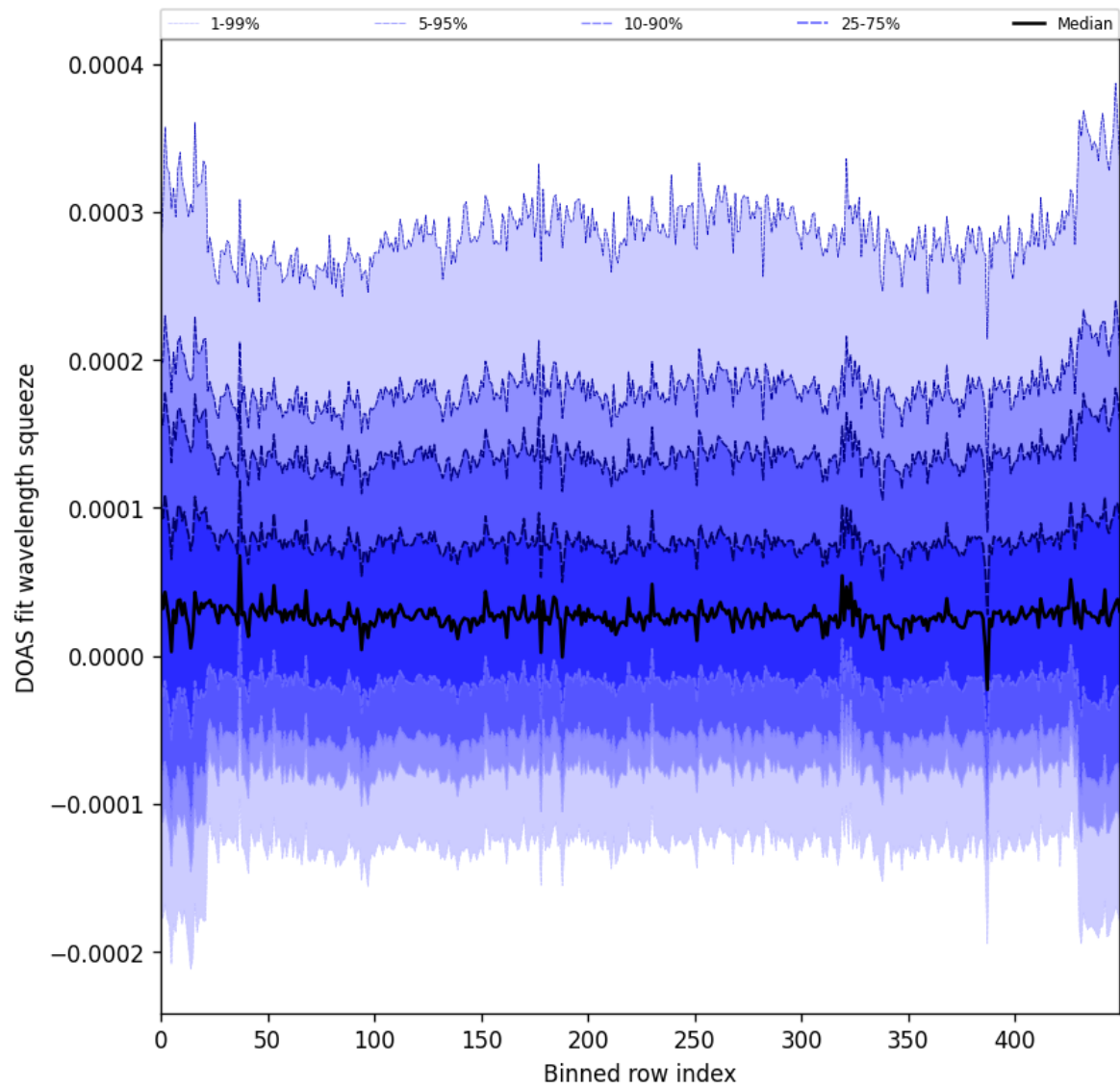
Figure 59: Along track statistics of “DOAS fit wavelength squeeze” for 2025-02-24 to 2025-02-26
