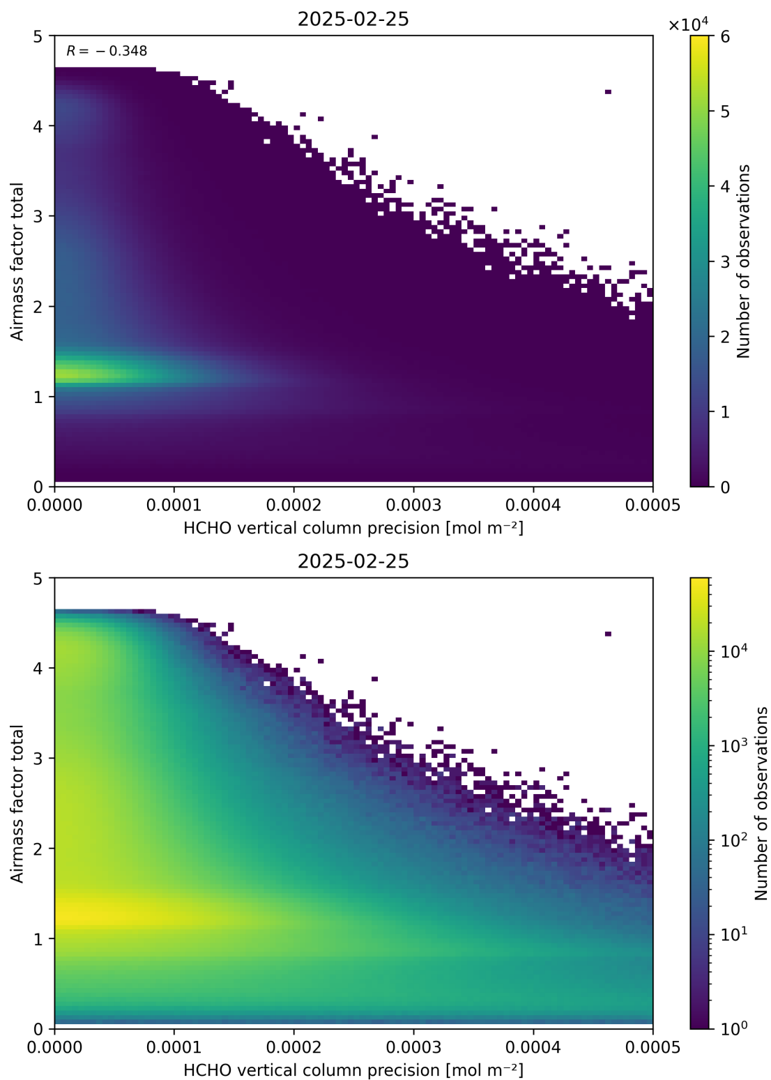
Figure 144: Scatter density plot of “HCHO vertical column precision” against “Airmass factor total” for 2025-02-24 to 2025-02-26.
