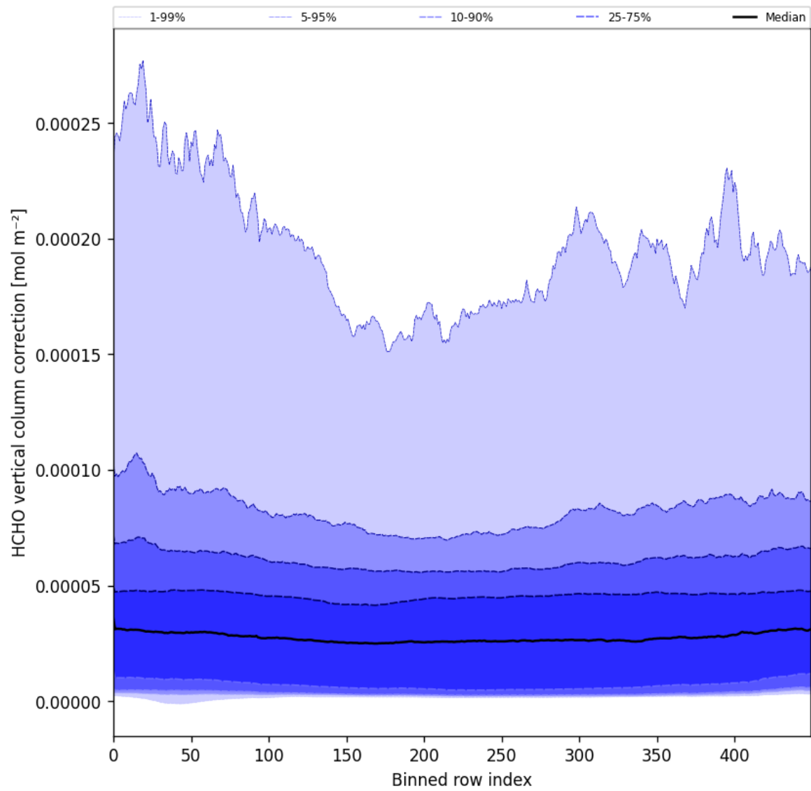
Figure 51: Along track statistics of “HCHO vertical column correction” for 2025-02-24 to 2025-02-26
