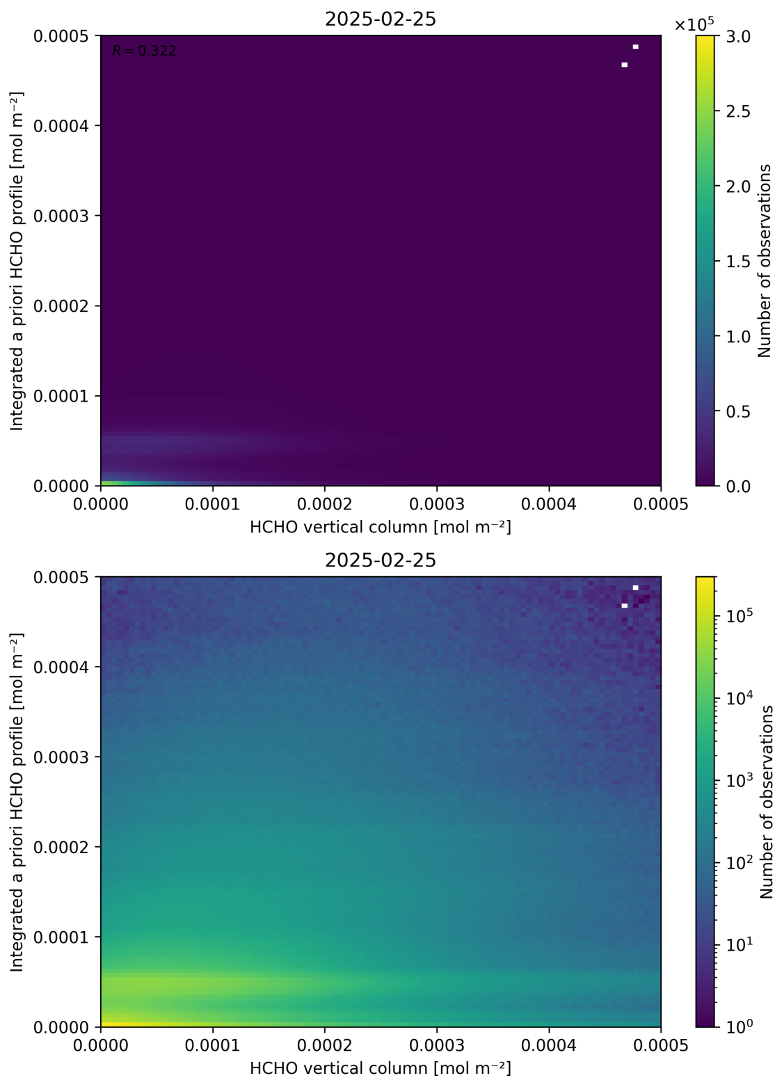
Figure 135: Scatter density plot of “HCHO vertical column” against “Integrated a priori HCHO profile” for 2025-02-24 to 2025-02-26.
