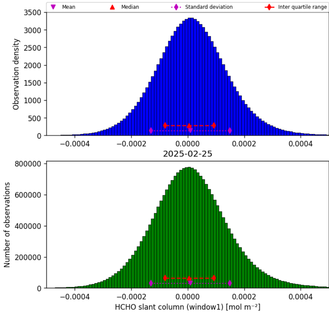
Figure 38: Histogram of “HCHO slant column (window1)” for 2025-02-24 to 2025-02-26
