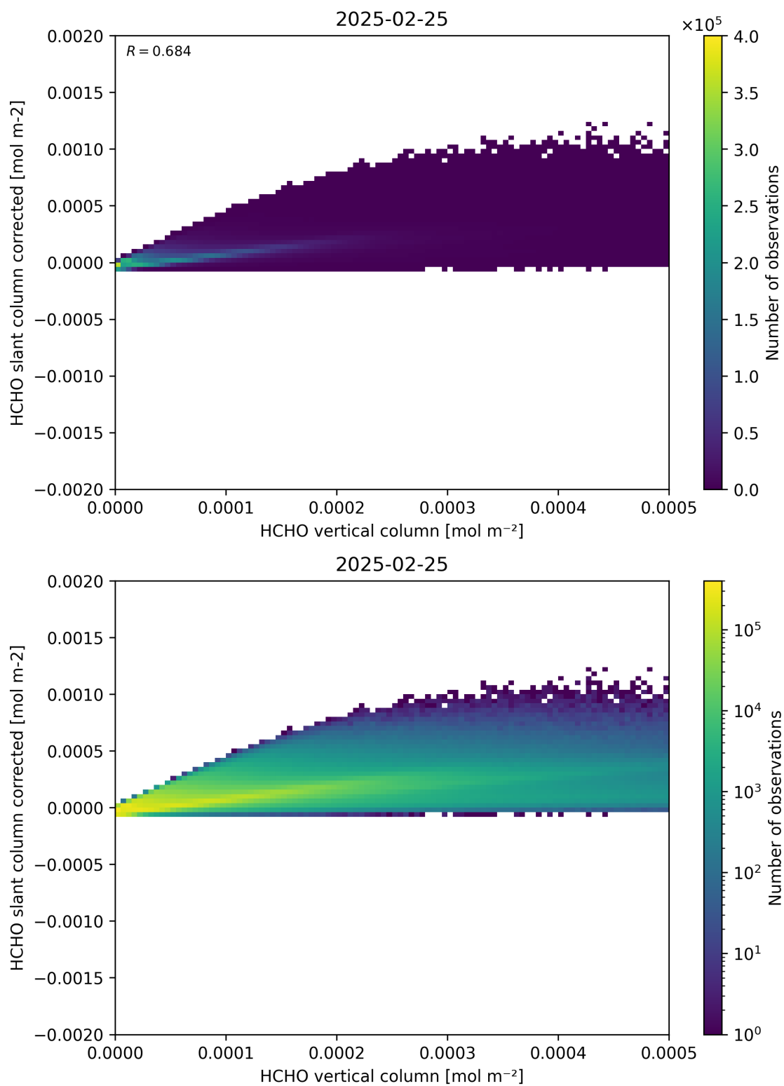
Figure 127: Scatter density plot of “HCHO vertical column” against “HCHO slant column corrected” for 2025-02-24 to 2025-02-26.
