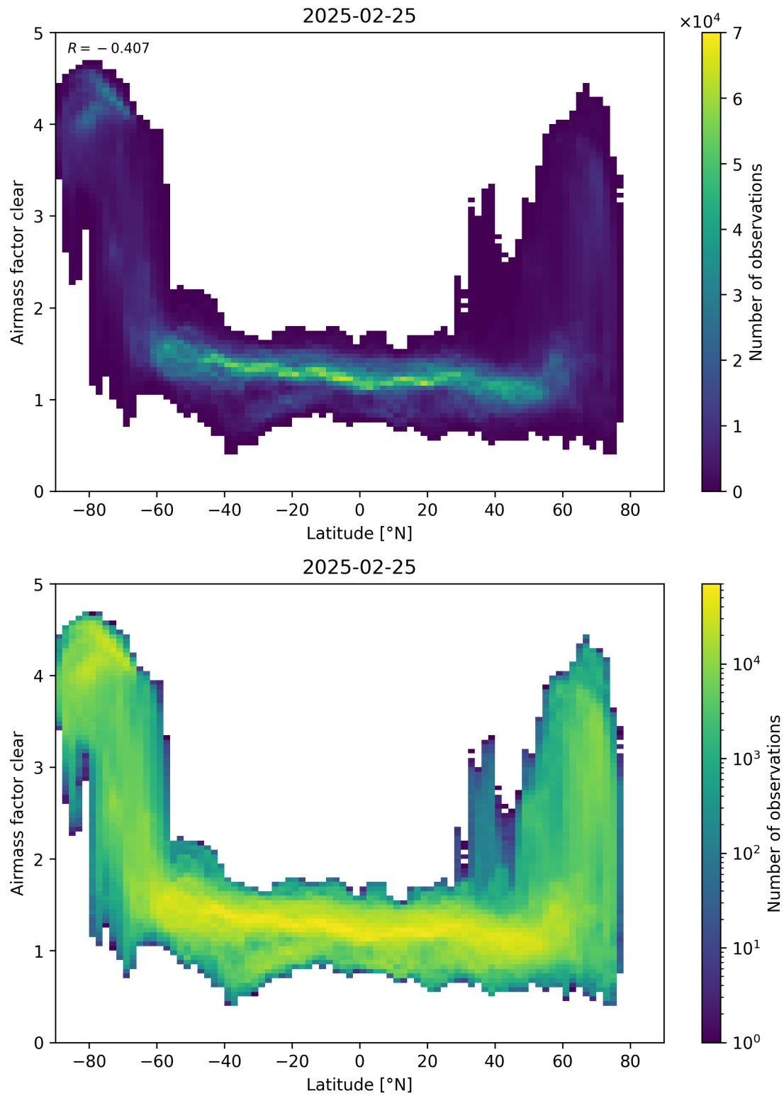
Figure 156: Scatter density plot of “Latitude” against “Airmass factor clear” for 2025-02-24 to 2025-02-26.
