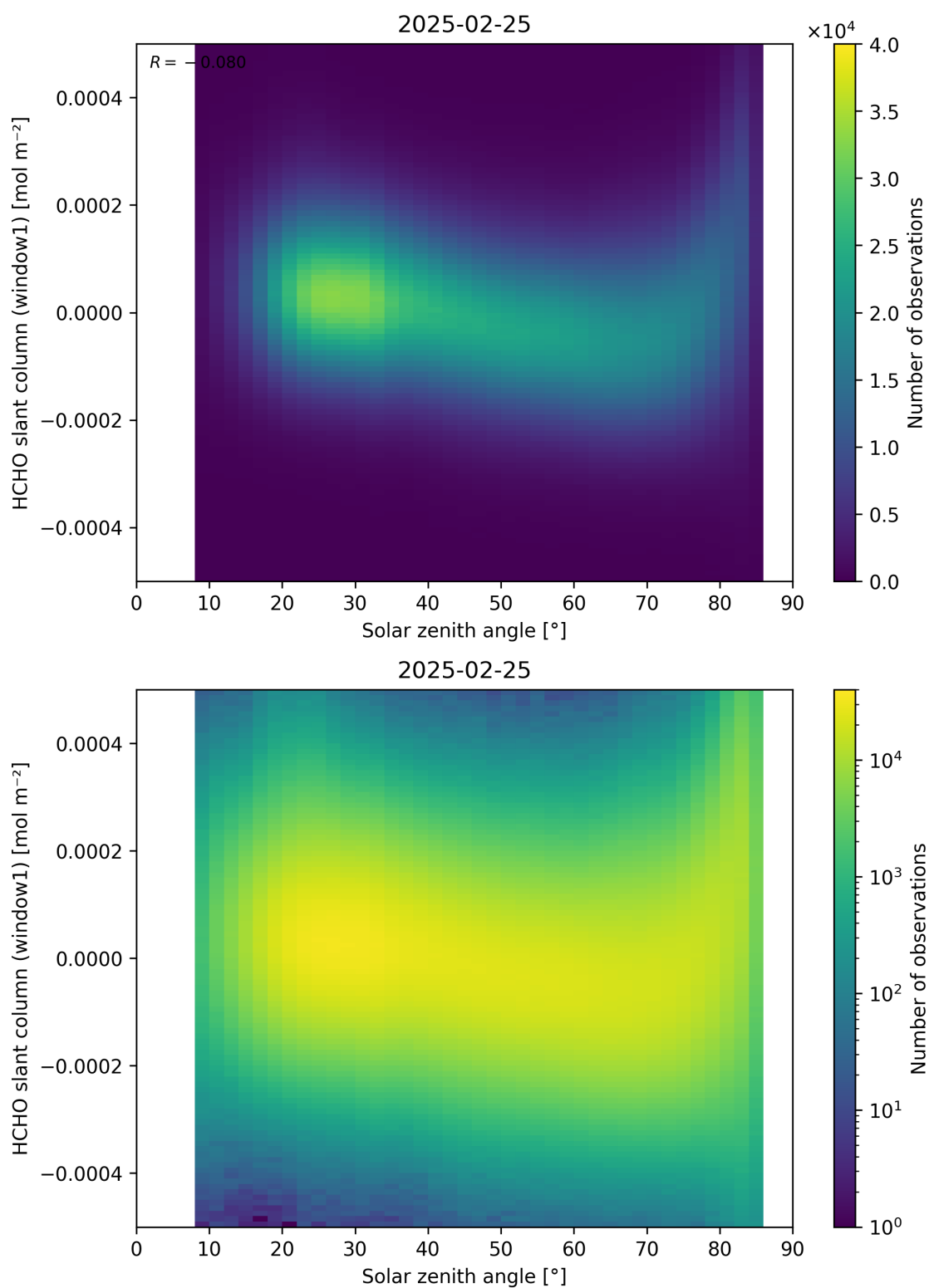
Figure 173: Scatter density plot of “Solar zenith angle” against “HCHO slant column (window1)” for 2025-02-24 to 2025-02-26.
