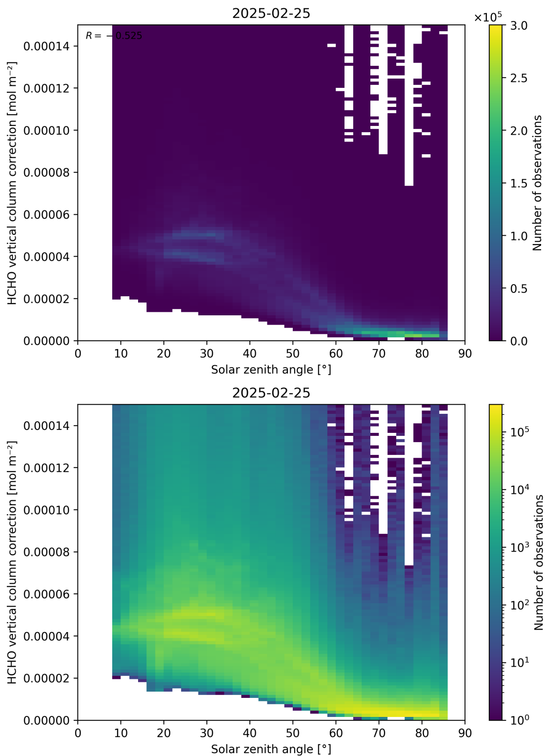
Figure 178: Scatter density plot of “Solar zenith angle” against “HCHO vertical column correction” for 2025-02-24 to 2025-02-26.
