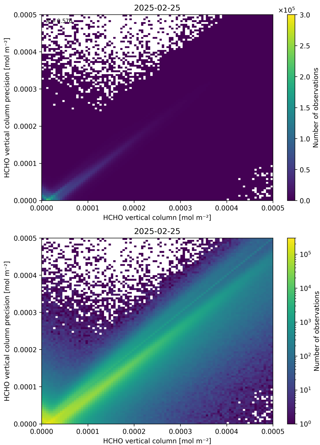
Figure 134: Scatter density plot of “HCHO vertical column” against “HCHO vertical column precision” for 2025-02-24 to 2025-02-26.
