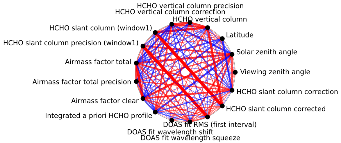
Figure 1: Map of correlation graph for 2025-02-24 to 2025-02-26.
