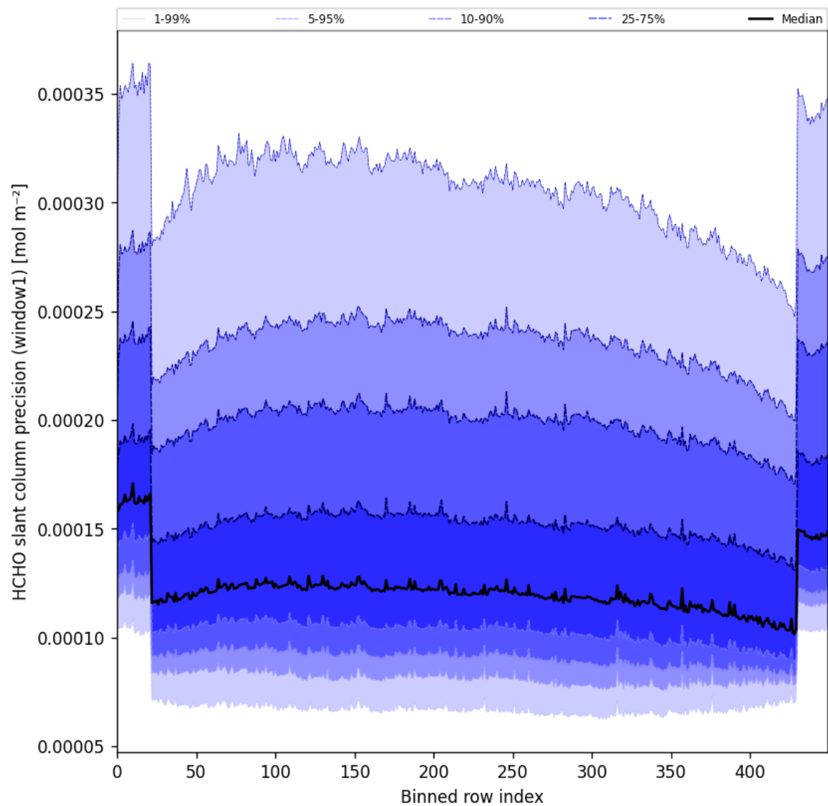
Figure 53: Along track statistics of “HCHO slant column precision (window1)” for 2025-02-24 to 2025-02-26
