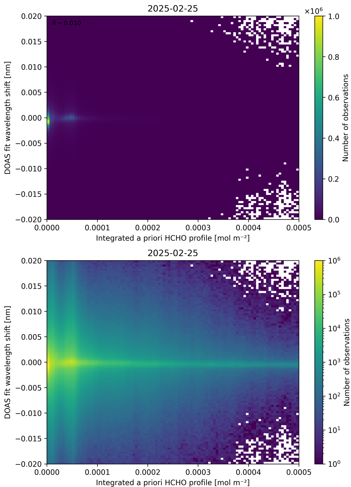
Figure 149: Scatter density plot of “Integrated a priori HCHO profile” against “DOAS fit wavelength shift” for 2025-02-24 to 2025-02-26.
