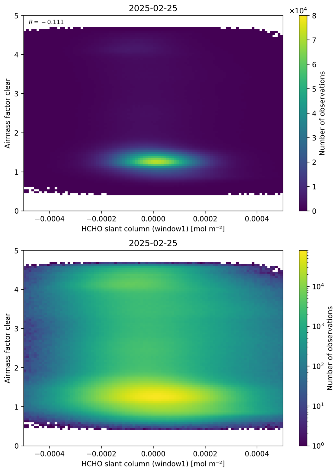
Figure 81: Scatter density plot of “HCHO slant column (window1)” against “Airmass factor clear” for 2025-02-24 to 2025-02-26.
