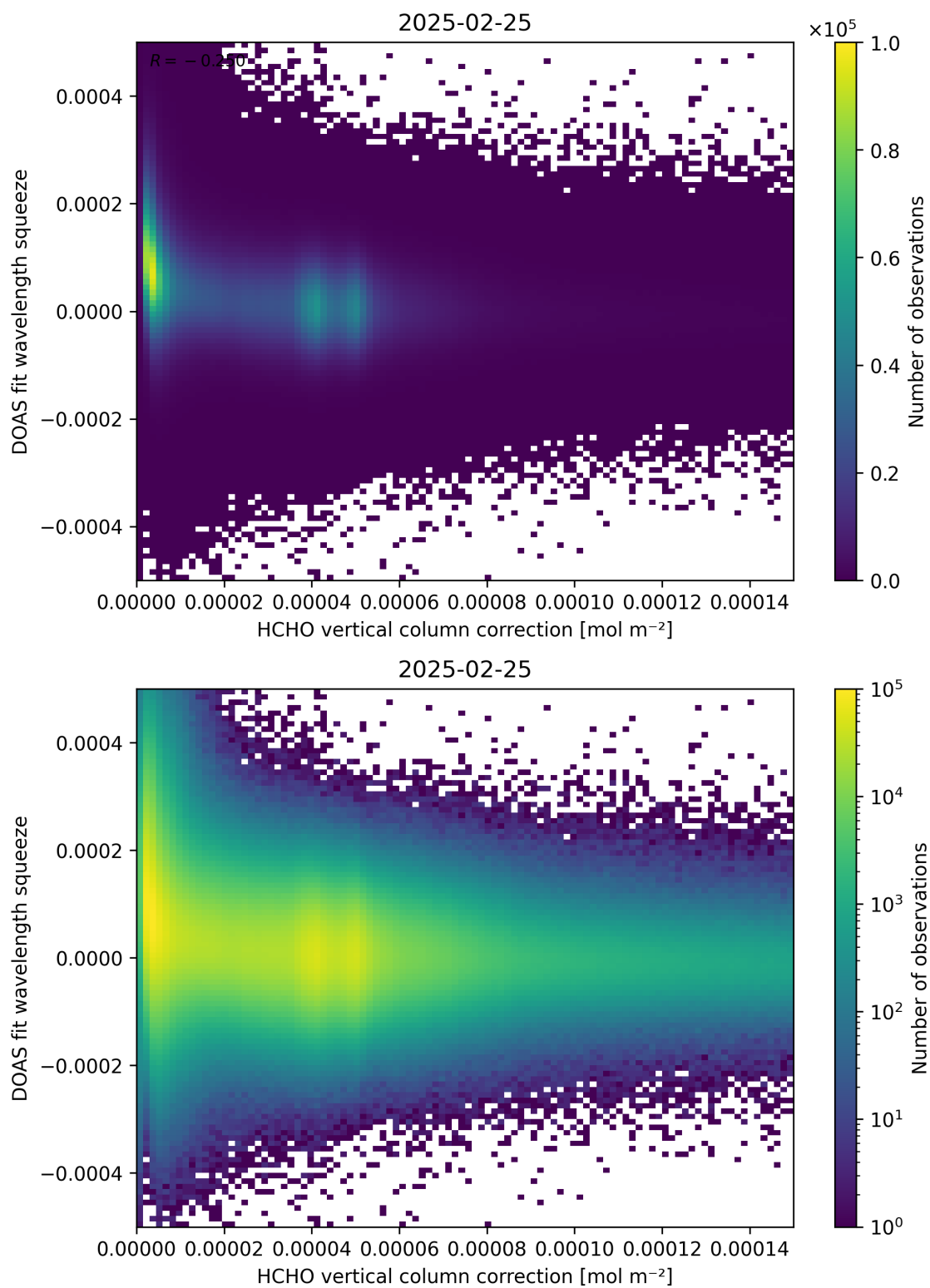
Figure 114: Scatter density plot of “HCHO vertical column correction” against “DOAS fit wavelength squeeze” for 2025-02-24 to 2025-02-26.
