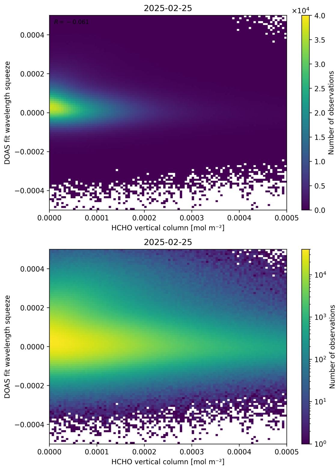
Figure 125: Scatter density plot of “HCHO vertical column” against “DOAS fit wavelength squeeze” for 2025-02-24 to 2025-02-26.
