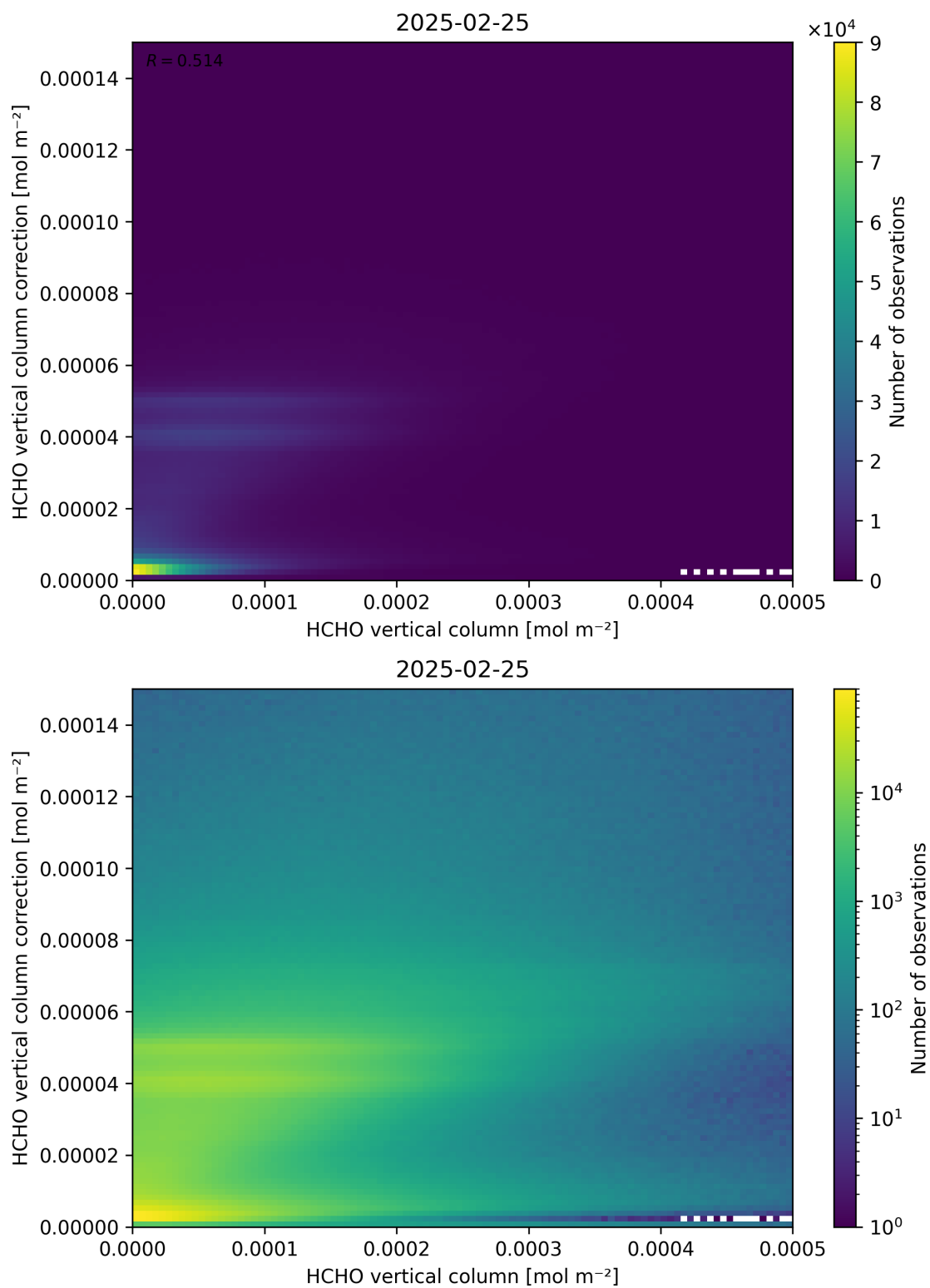
Figure 133: Scatter density plot of “HCHO vertical column” against “HCHO vertical column correction” for 2025-02-24 to 2025-02-26.
