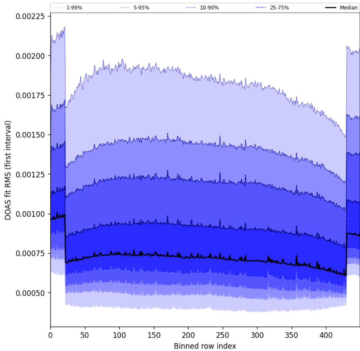
Figure 60: Along track statistics of “DOAS fit RMS (first interval)” for 2025-02-24 to 2025-02-26
