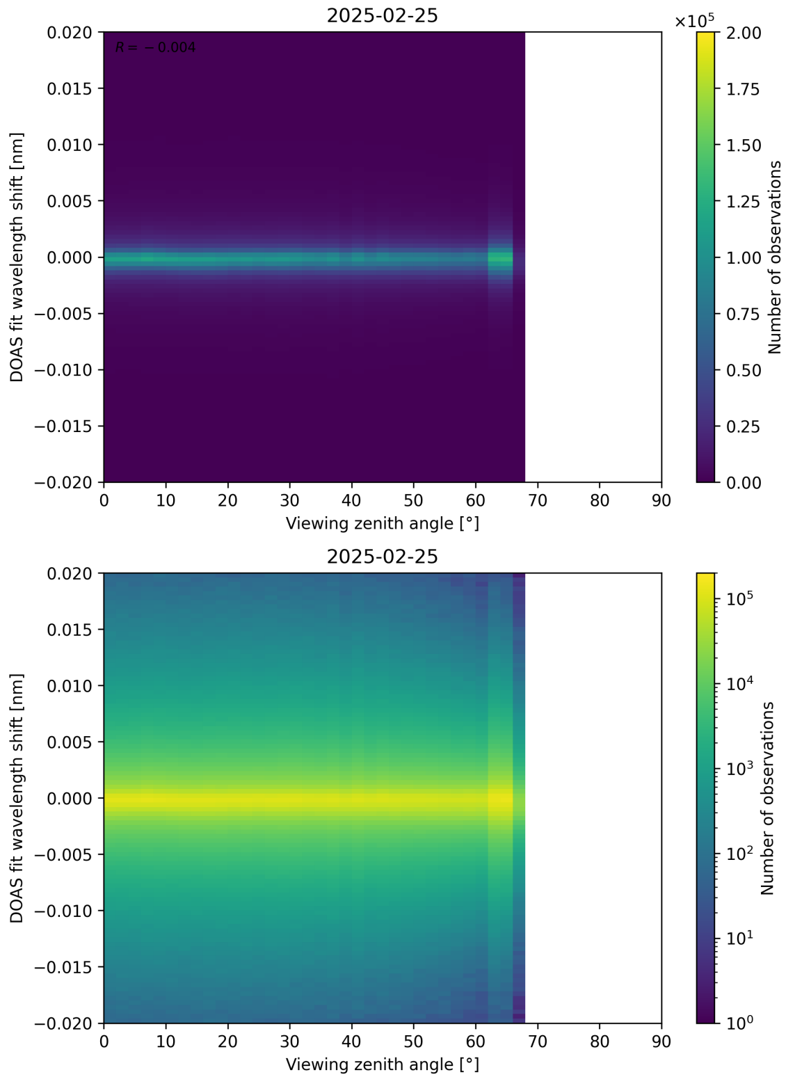
Figure 183: Scatter density plot of “Viewing zenith angle” against “DOAS fit wavelength shift” for 2025-02-24 to 2025-02-26.
