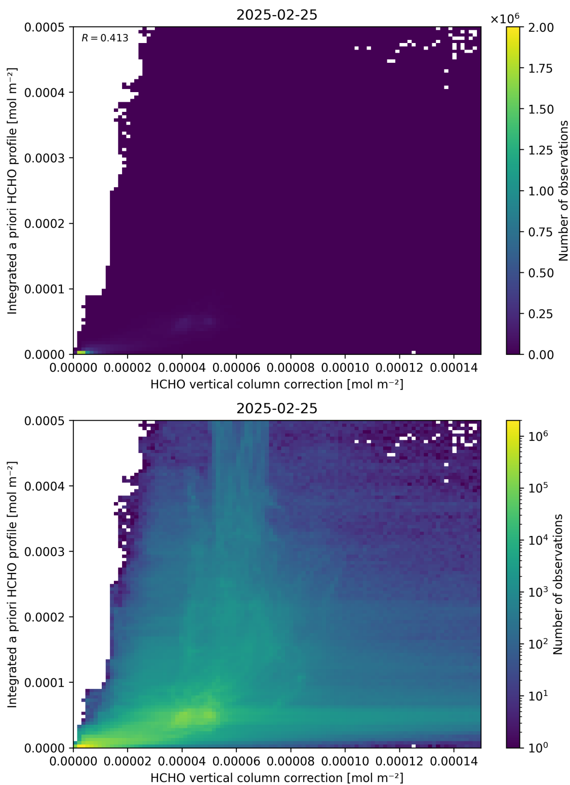
Figure 122: Scatter density plot of “HCHO vertical column correction” against “Integrated a priori HCHO profile” for 2025-02-24 to 2025-02-26.
