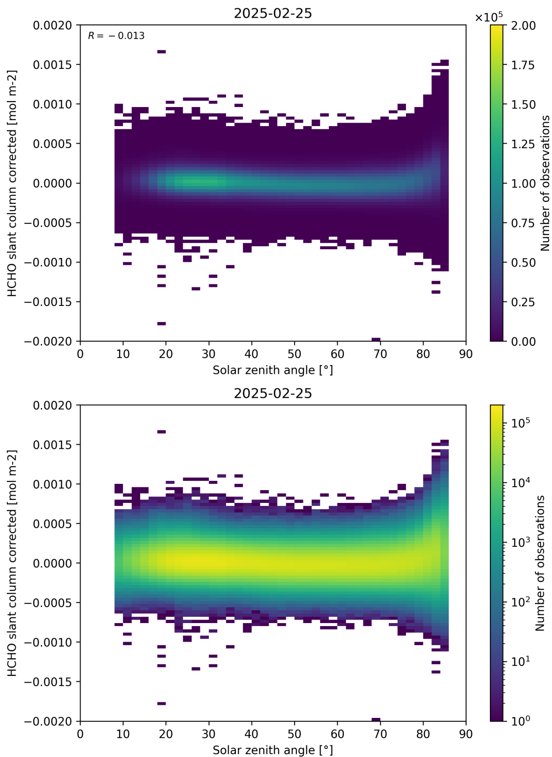
Figure 171: Scatter density plot of “Solar zenith angle” against “HCHO slant column corrected” for 2025-02-24 to 2025-02-26.
