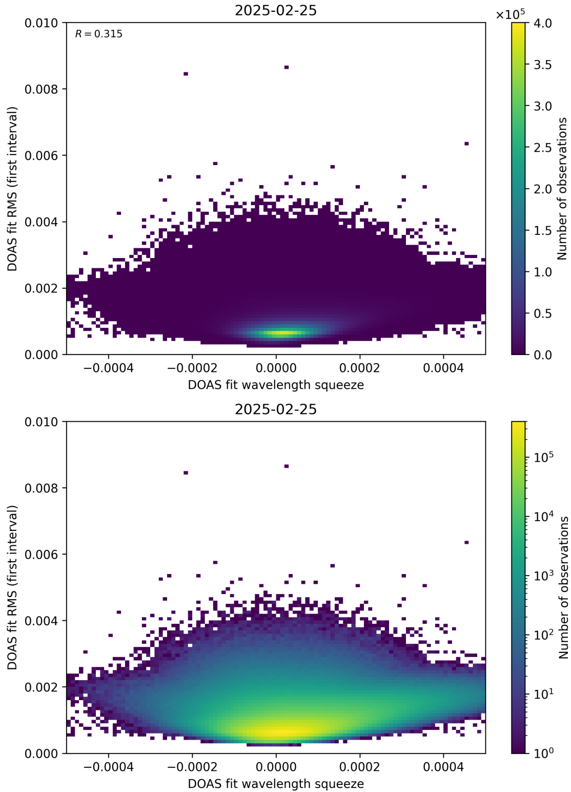
Figure 68: Scatter density plot of “DOAS fit wavelength squeeze” against “DOAS fit RMS (first interval)” for 2025-02-24 to 2025-02-26.
