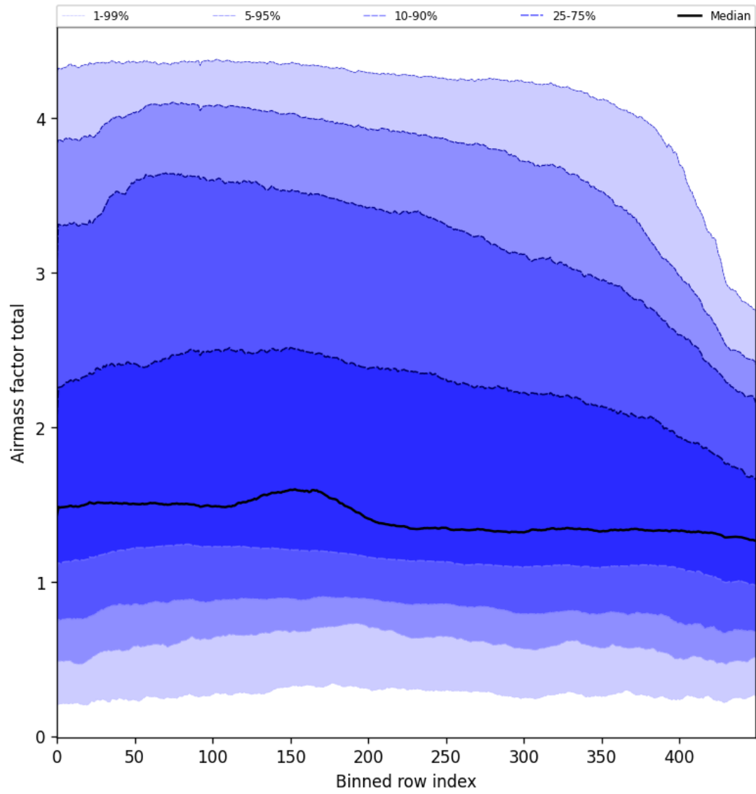
Figure 54: Along track statistics of “Airmass factor total” for 2025-02-24 to 2025-02-26
