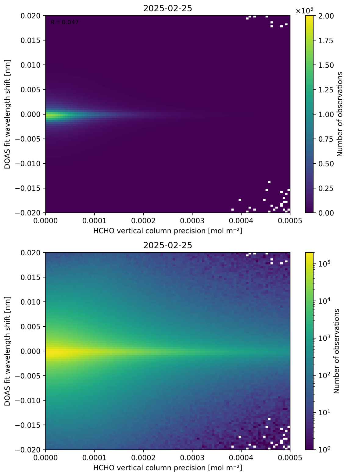
Figure 137: Scatter density plot of “HCHO vertical column precision” against “DOAS fit wavelength shift” for 2025-02-24 to 2025-02-26.
