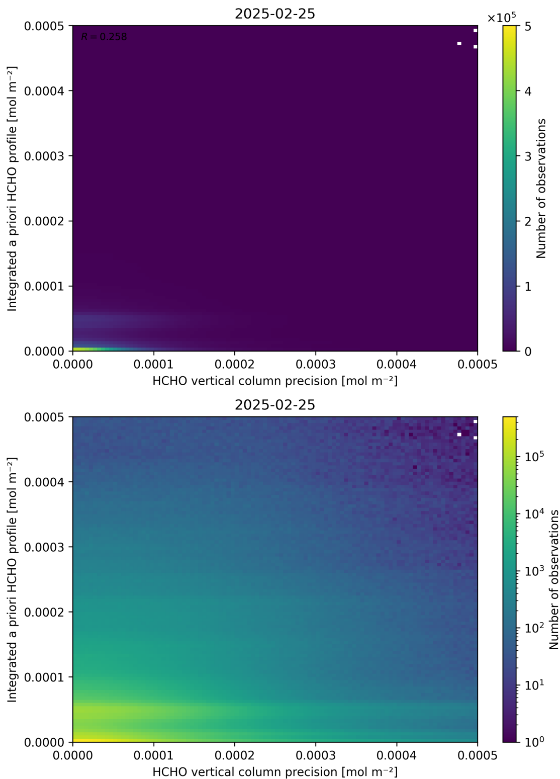
Figure 147: Scatter density plot of “HCHO vertical column precision” against “Integrated a priori HCHO profile” for 2025-02-24 to 2025-02-26.
