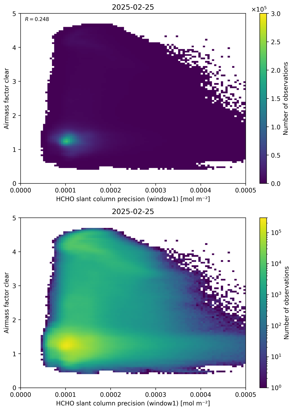
Figure 91: Scatter density plot of “HCHO slant column precision (window1)” against “Airmass factor clear” for 2025-02-24 to 2025-02-26.
