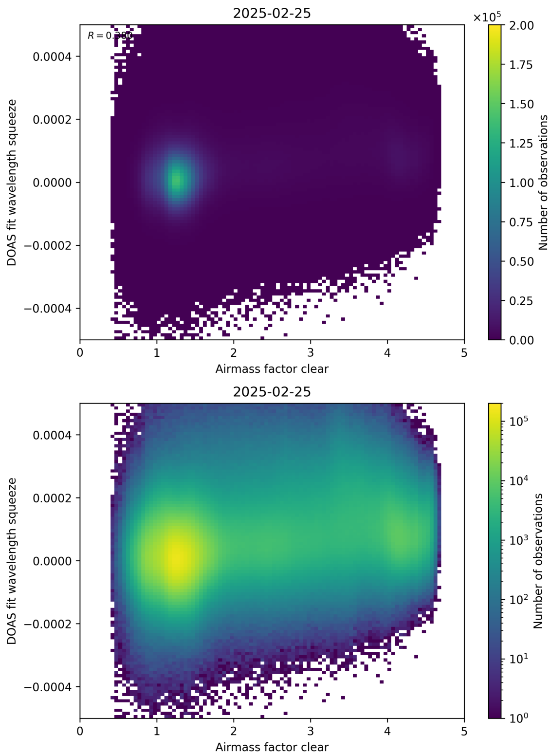
Figure 73: Scatter density plot of “Airmass factor clear” against “DOAS fit wavelength squeeze” for 2025-02-24 to 2025-02-26.
