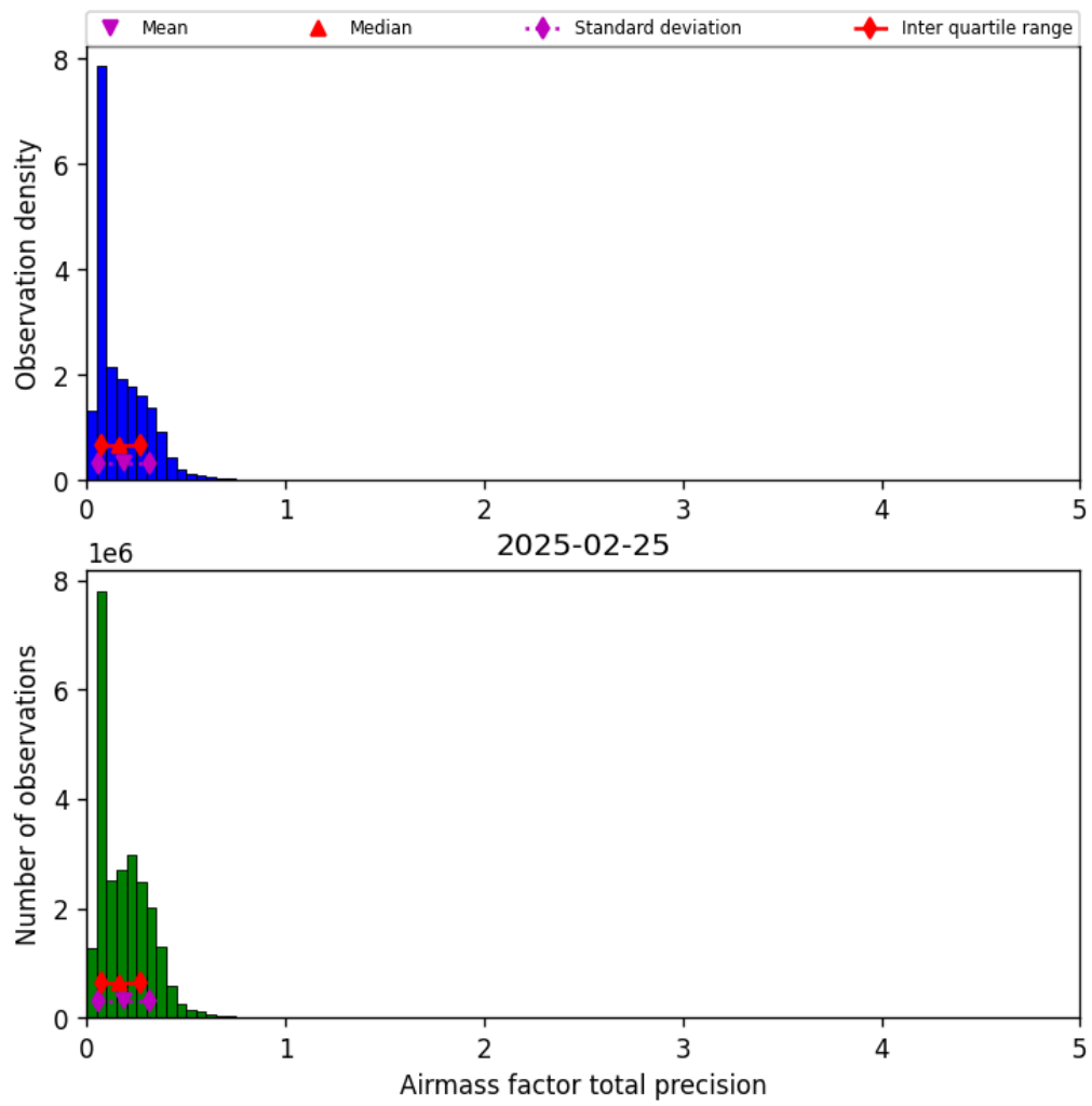
Figure 41: Histogram of “Airmass factor total precision” for 2025-02-24 to 2025-02-26
