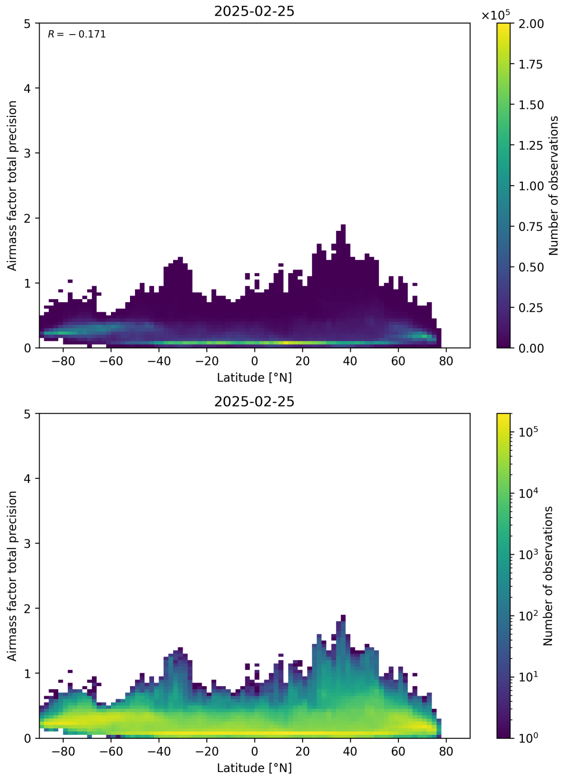
Figure 162: Scatter density plot of “Latitude” against “Airmass factor total precision” for 2025-02-24 to 2025-02-26.
