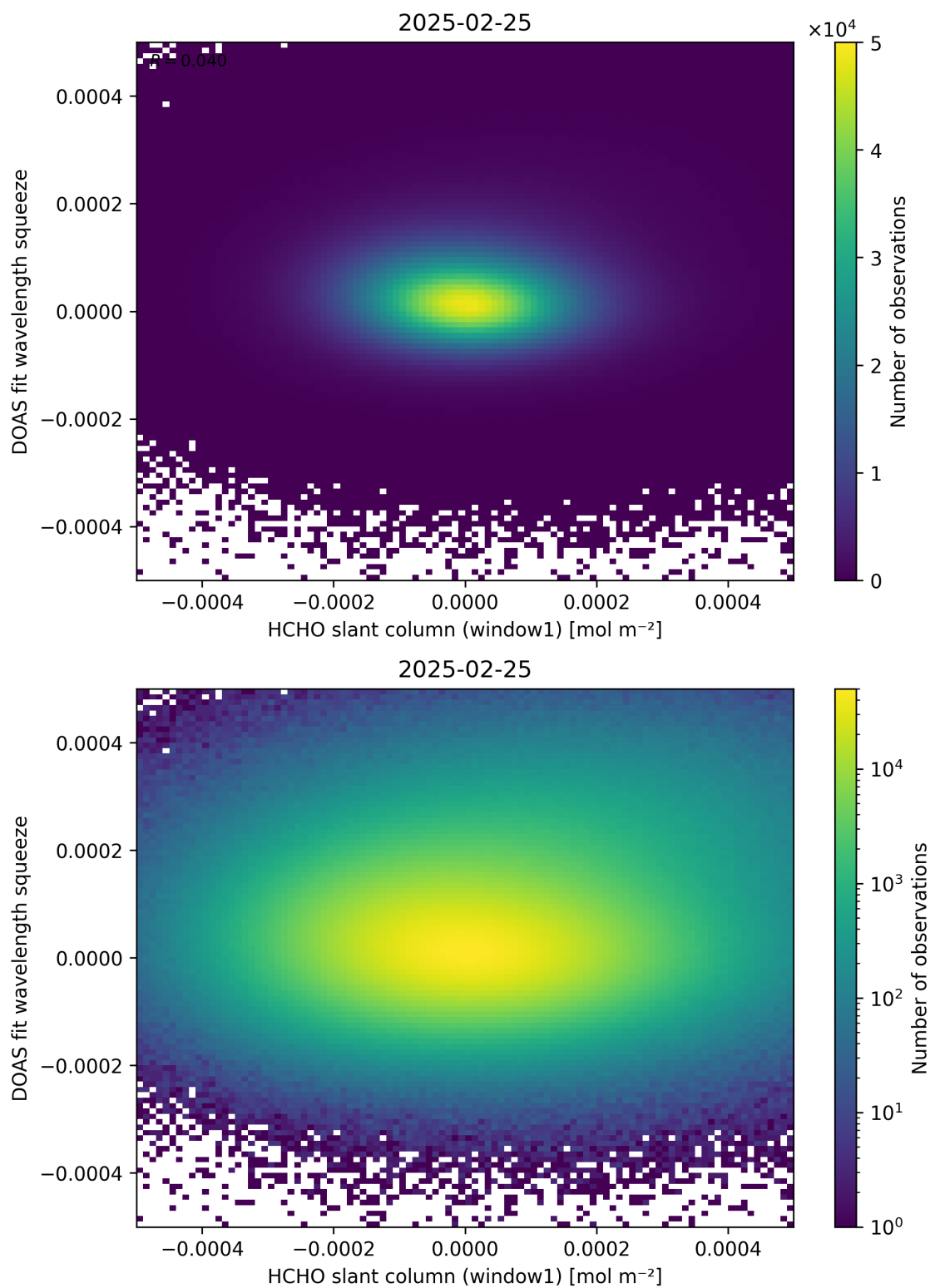
Figure 80: Scatter density plot of “HCHO slant column (window1)” against “DOAS fit wavelength squeeze” for 2025-02-24 to 2025-02-26.
