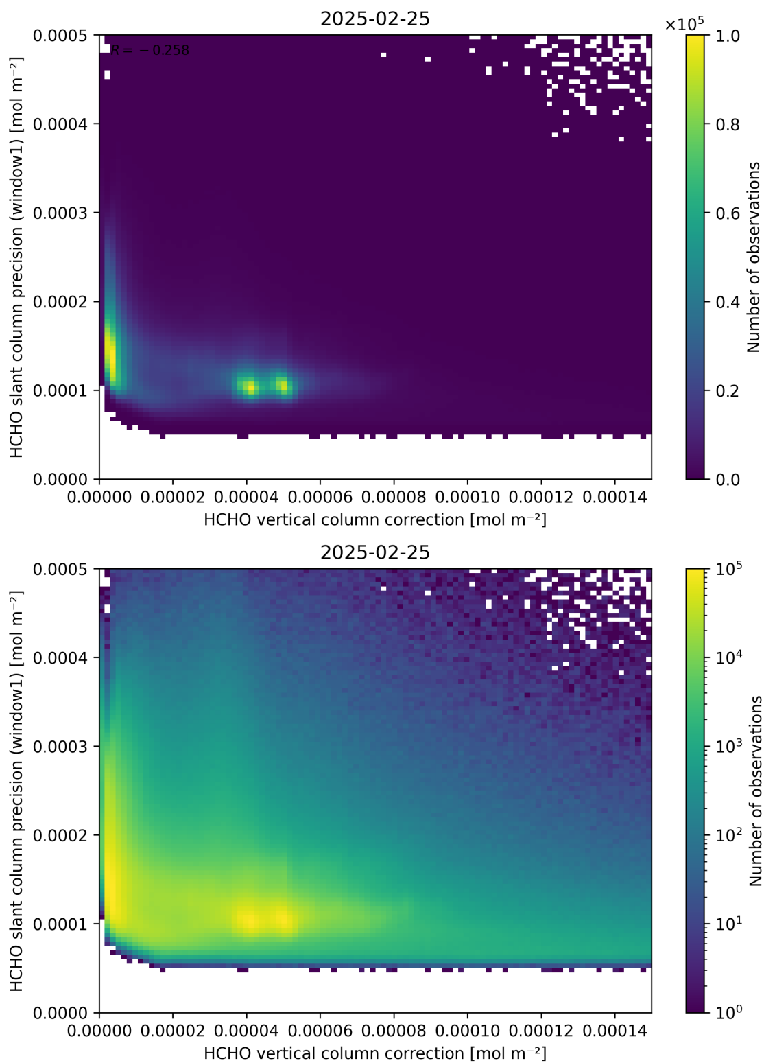
Figure 119: Scatter density plot of “HCHO vertical column correction” against “HCHO slant column precision (window1)” for 2025-02-24 to 2025-02-26.
