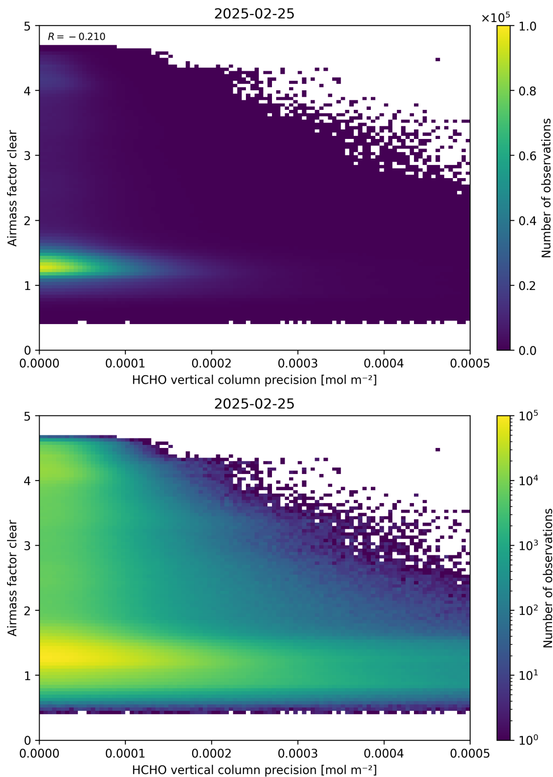
Figure 139: Scatter density plot of “HCHO vertical column precision” against “Airmass factor clear” for 2025-02-24 to 2025-02-26.
