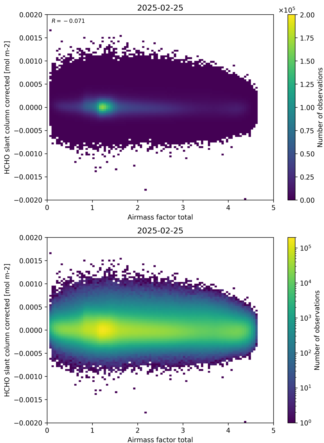
Figure 101: Scatter density plot of “Airmass factor total” against “HCHO slant column corrected” for 2025-02-24 to 2025-02-26.
