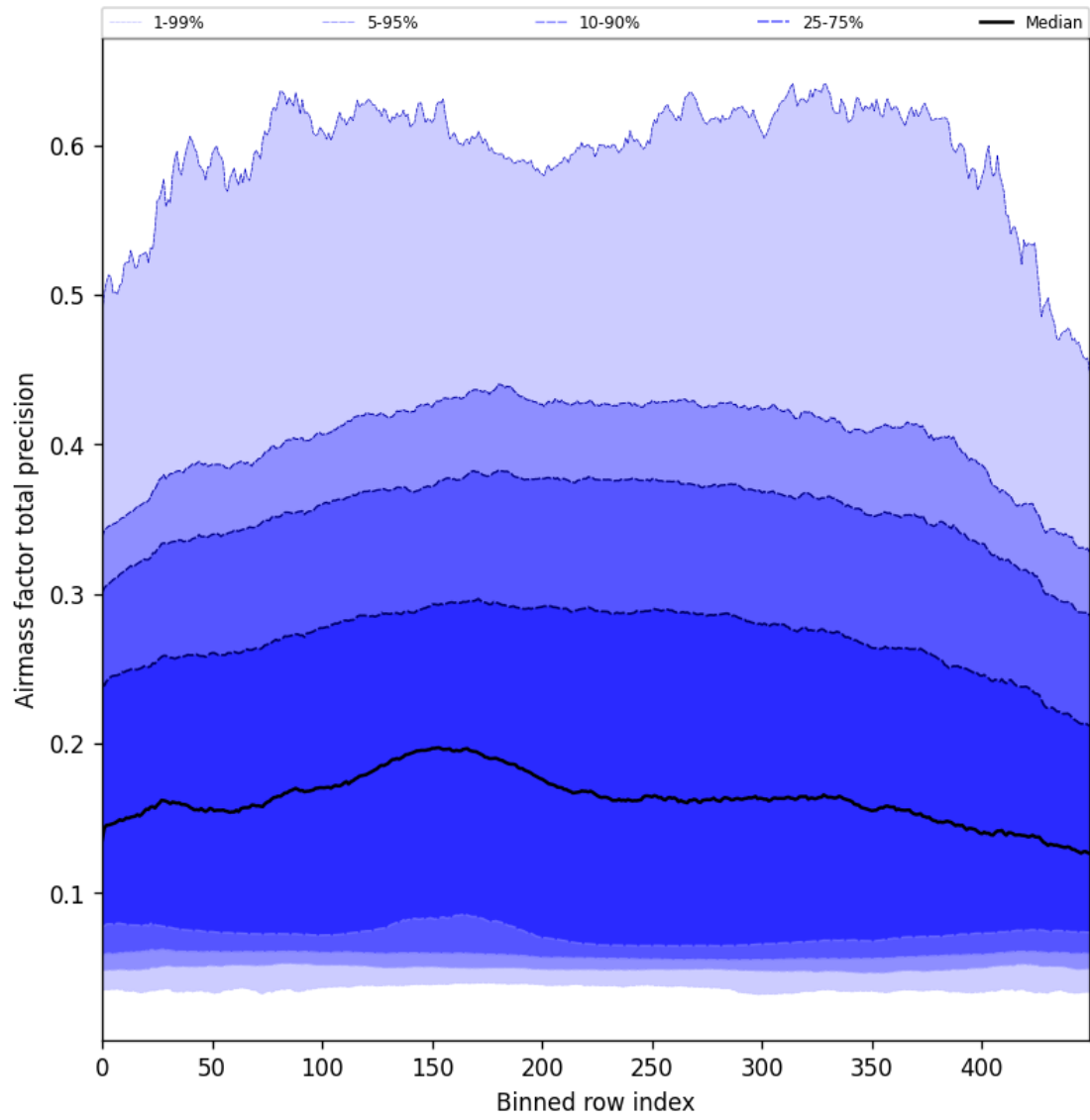
Figure 55: Along track statistics of “Airmass factor total precision” for 2025-02-24 to 2025-02-26
