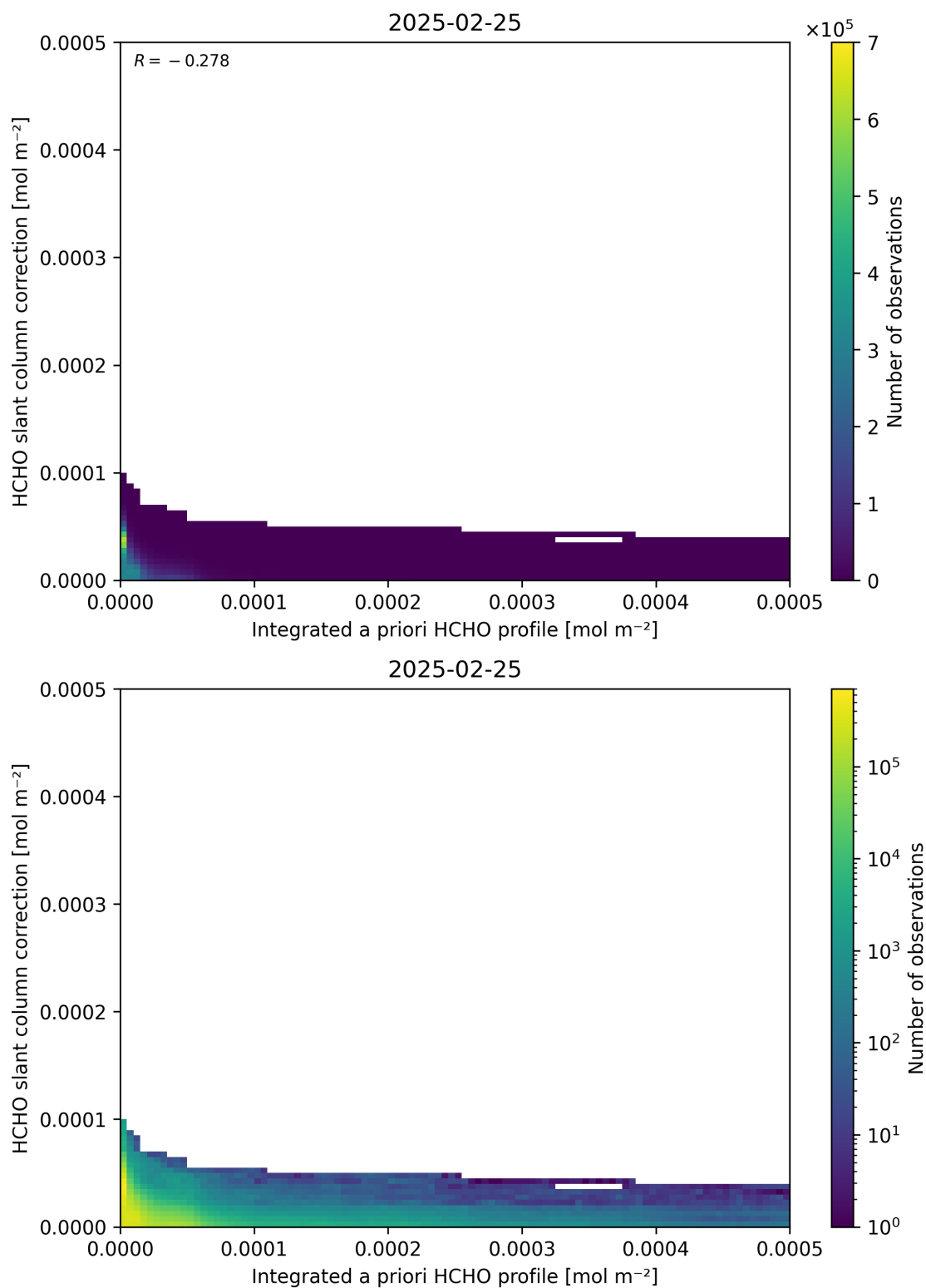
Figure 152: Scatter density plot of “Integrated a priori HCHO profile” against “HCHO slant column correction” for 2025-02-24 to 2025-02-26.
