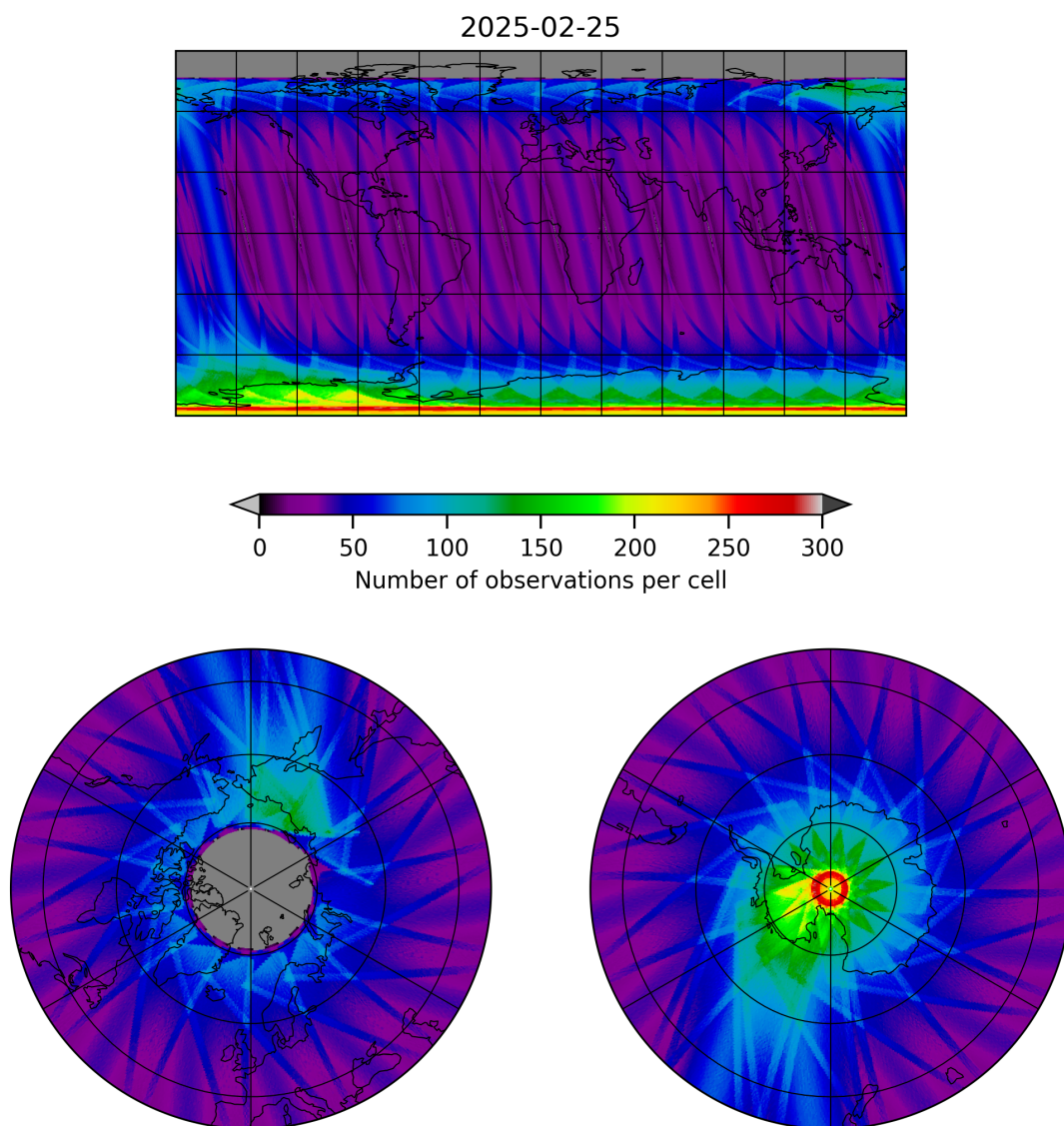
Figure 19: Map of the number of observations for 2025-02-24 to 2025-02-26
