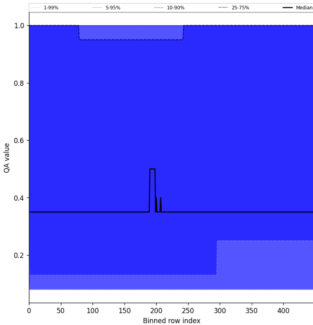
Figure 48: Along track statistics of "QA value" for 2025-02-24 to 2025-02-26
