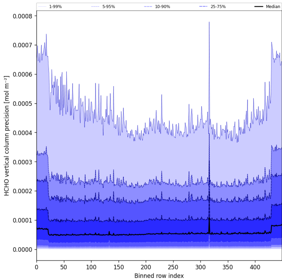
Figure 50: Along track statistics of “HCHO vertical column precision” for 2025-02-24 to 2025-02-26
