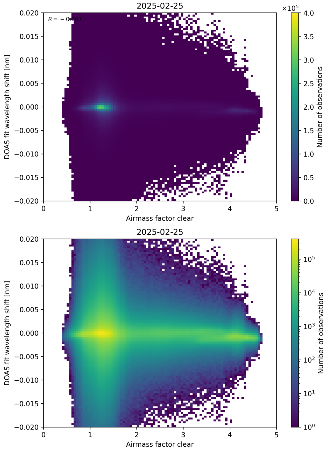
Figure 72: Scatter density plot of “Airmass factor clear” against “DOAS fit wavelength shift” for 2025-02-24 to 2025-02-26.
