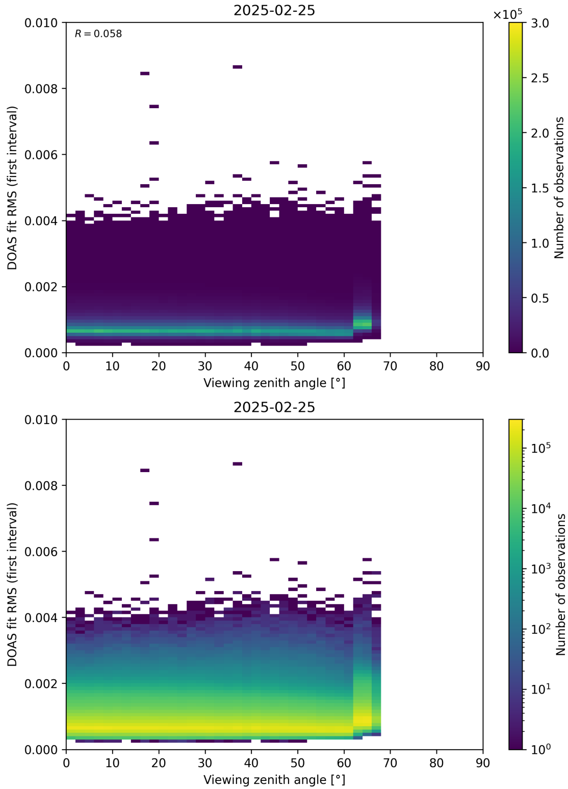
Figure 182: Scatter density plot of “Viewing zenith angle” against “DOAS fit RMS (first interval)” for 2025-02-24 to 2025-02-26.
