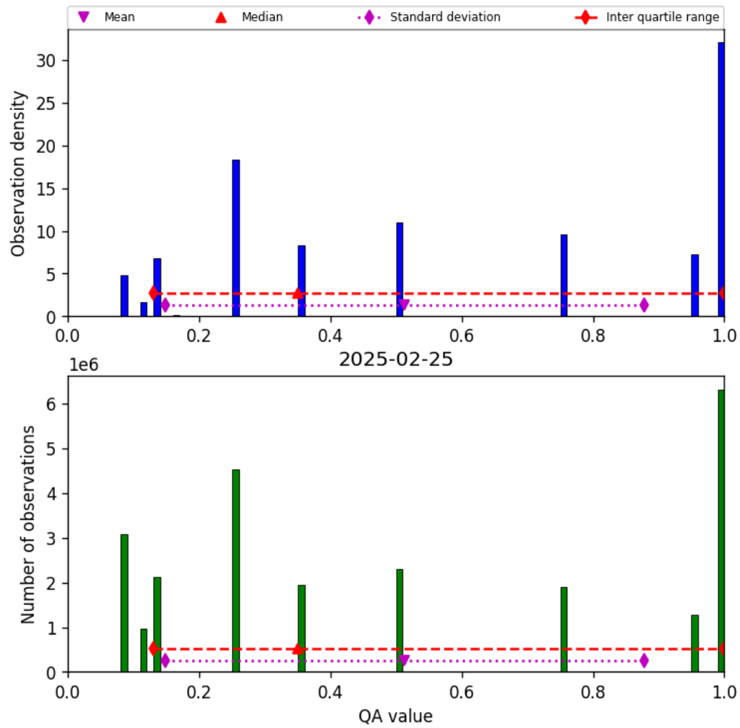
Figure 34: Histogram of “QA value” for 2025-02-24 to 2025-02-26
