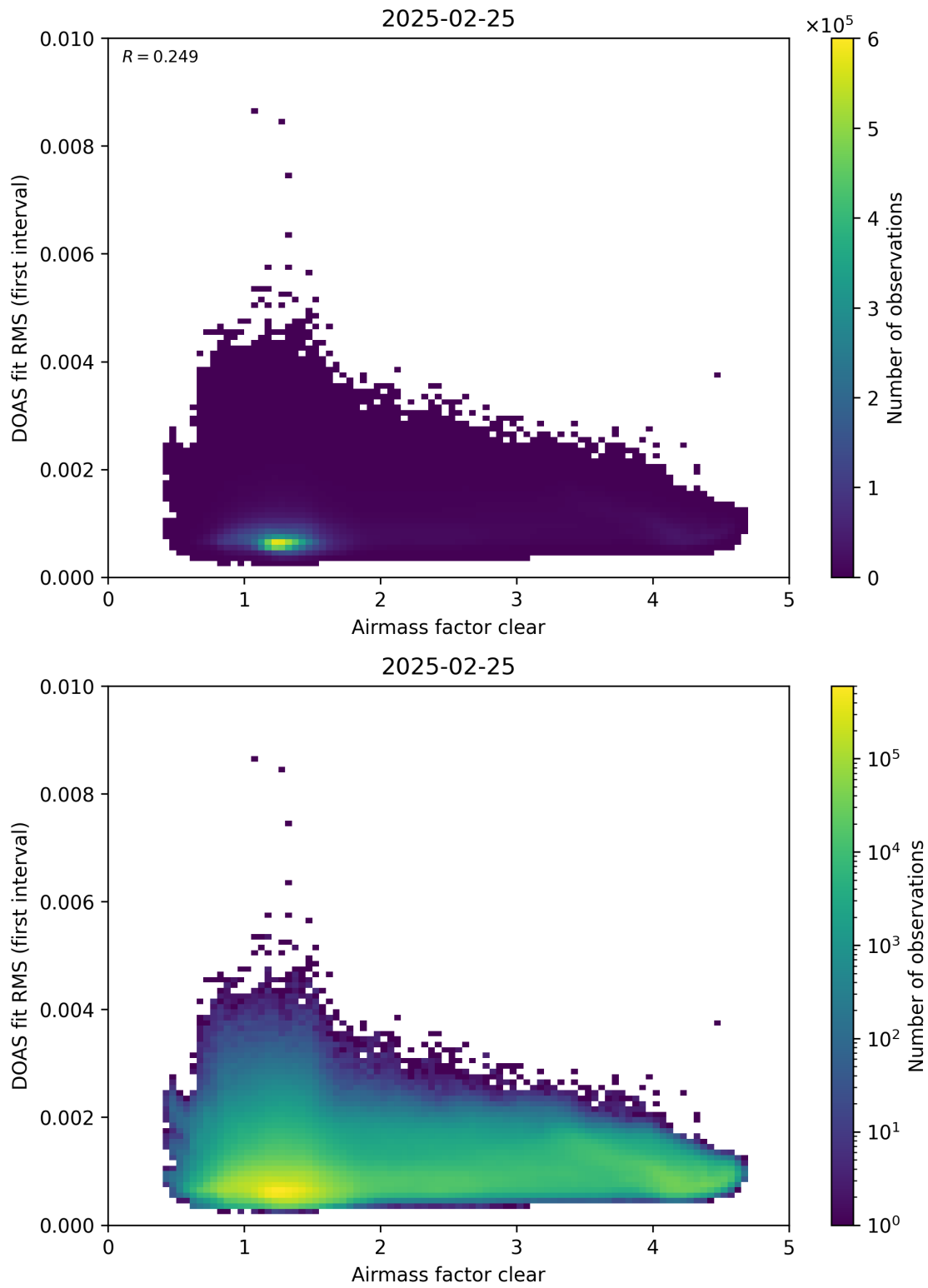
Figure 71: Scatter density plot of “Airmass factor clear” against “DOAS fit RMS (first interval)” for 2025-02-24 to 2025-02-26.
