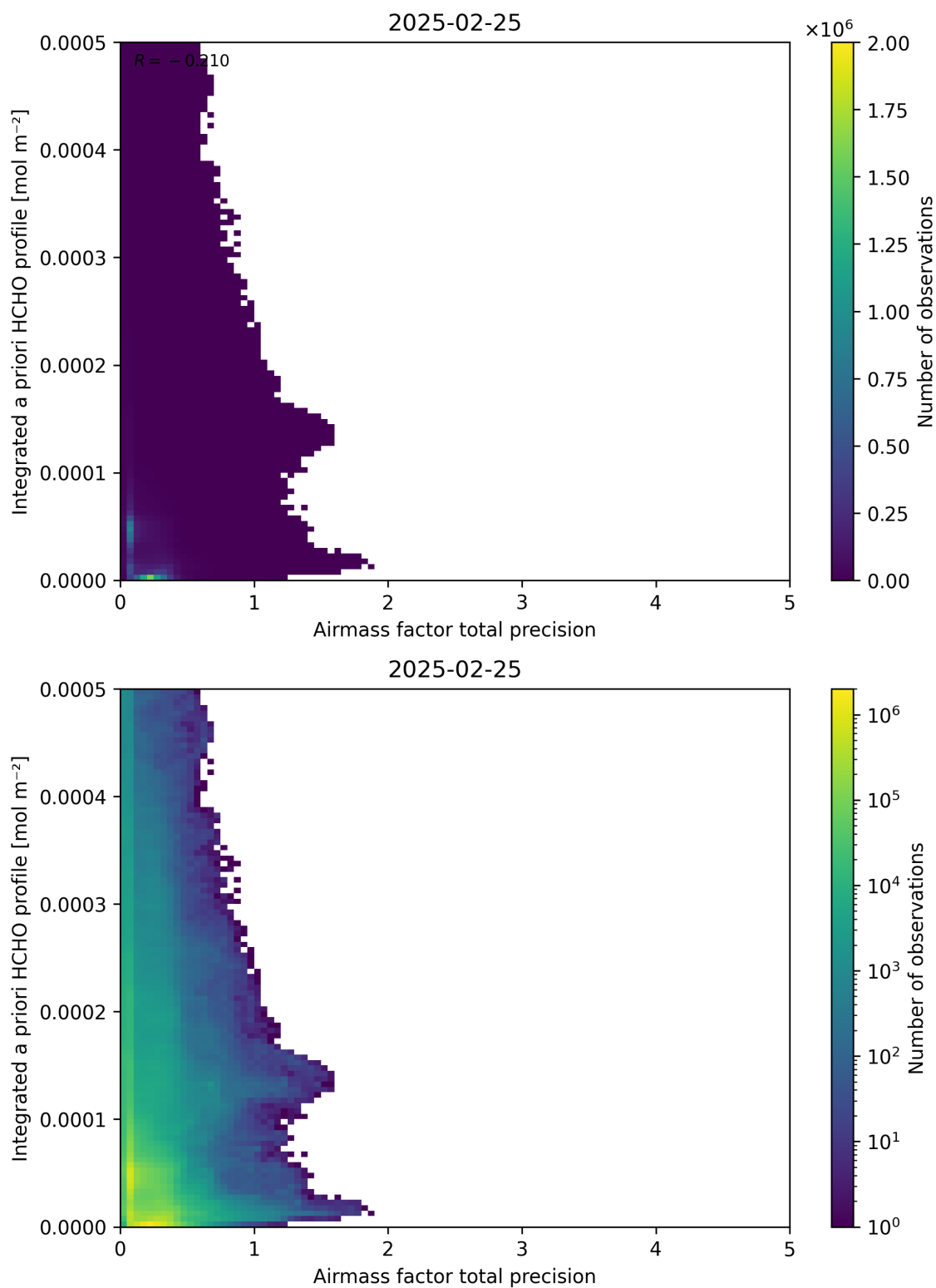
Figure 111: Scatter density plot of “Airmass factor total precision” against “Integrated a priori HCHO profile” for 2025-02-24 to 2025-02-26.
