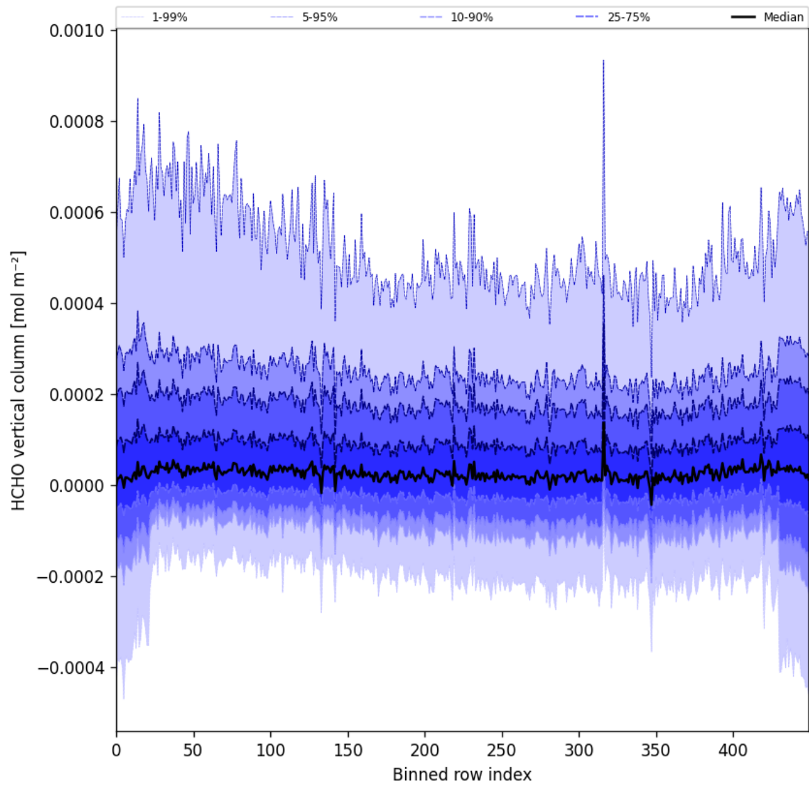
Figure 49: Along track statistics of “HCHO vertical column” for 2025-02-24 to 2025-02-26
