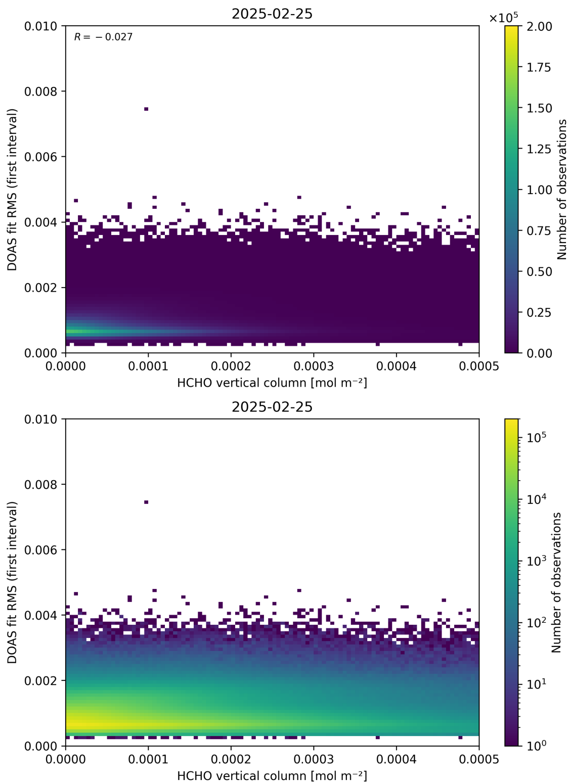
Figure 123: Scatter density plot of “HCHO vertical column” against “DOAS fit RMS (first interval)” for 2025-02-24 to 2025-02-26.
