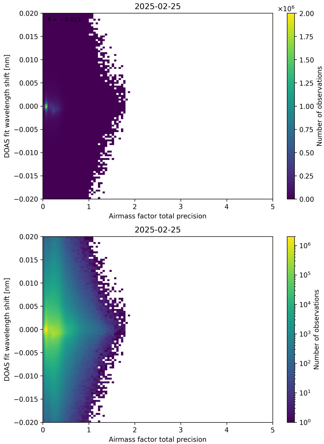
Figure 106: Scatter density plot of “Airmass factor total precision” against “DOAS fit wavelength shift” for 2025-02-24 to 2025-02-26.
