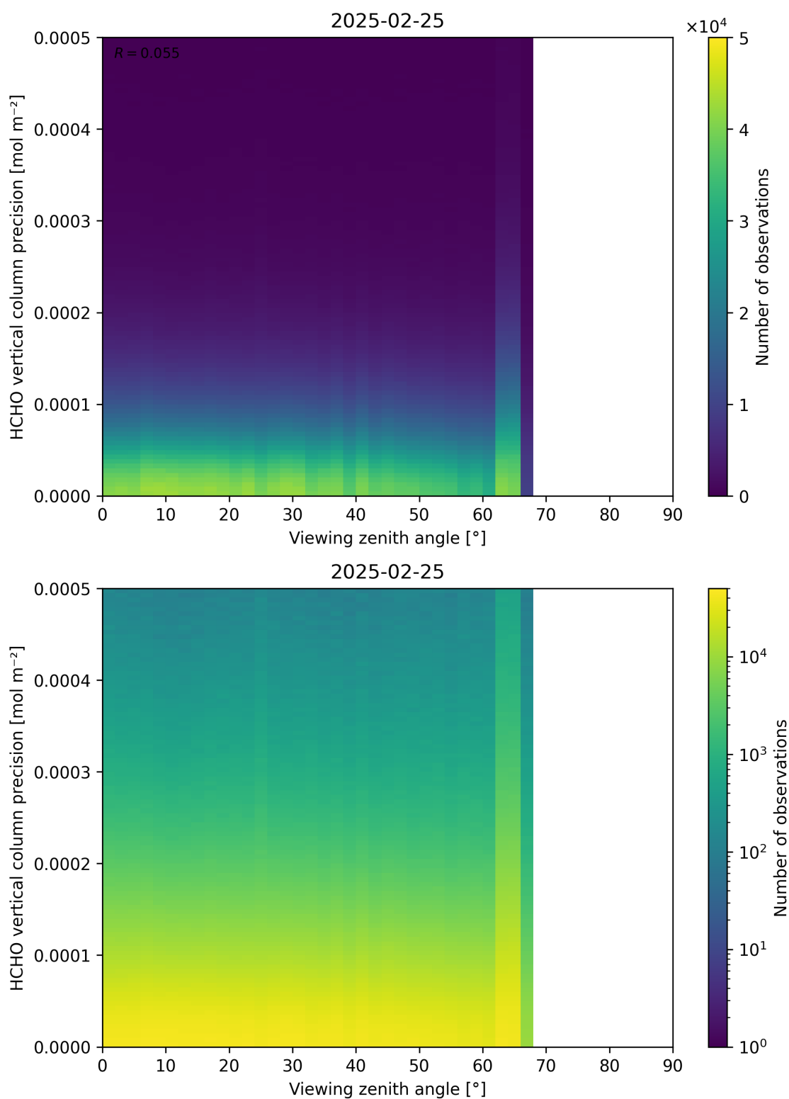
Figure 194: Scatter density plot of “Viewing zenith angle” against “HCHO vertical column precision” for 2025-02-24 to 2025-02-26.
