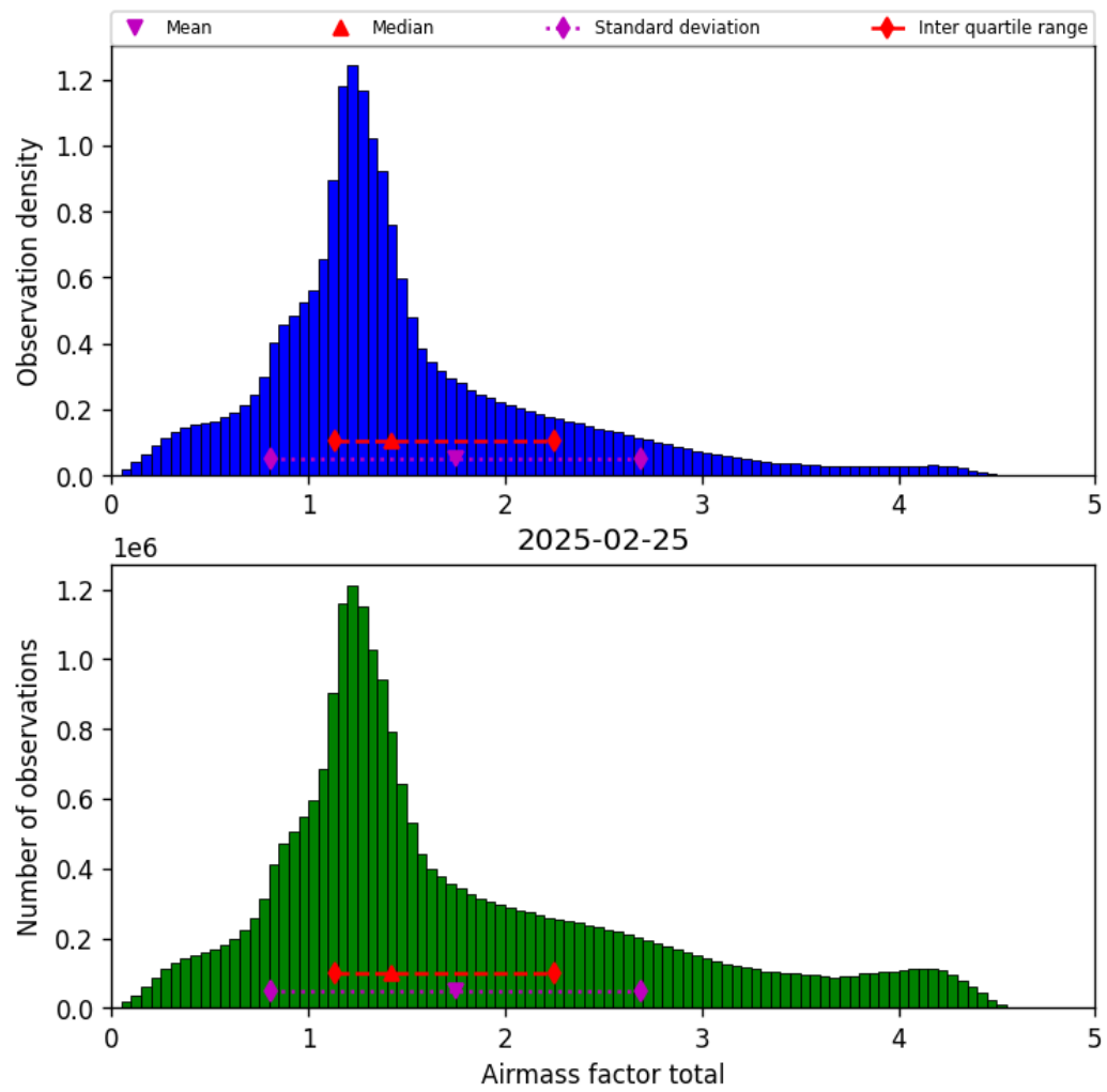
Figure 40: Histogram of “Airmass factor total” for 2025-02-24 to 2025-02-26
