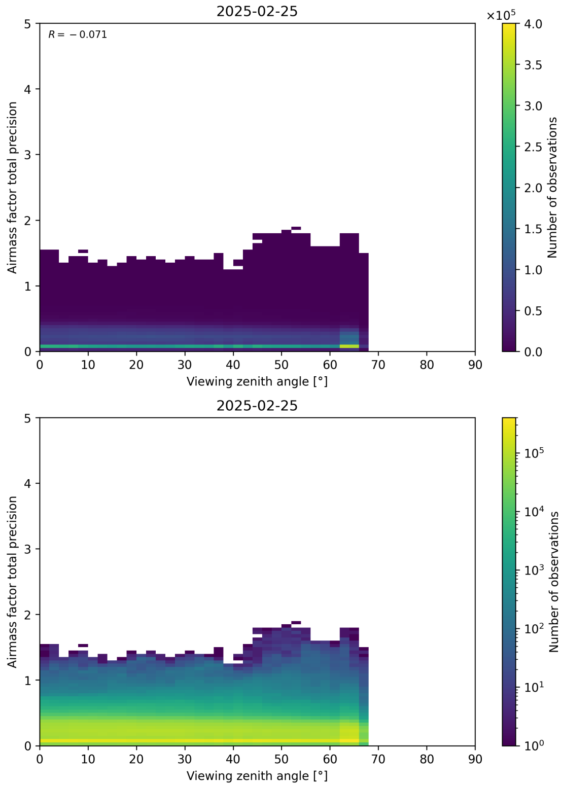
Figure 191: Scatter density plot of “Viewing zenith angle” against “Airmass factor total precision” for 2025-02-24 to 2025-02-26.
