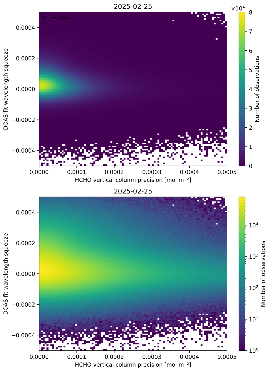
Figure 138: Scatter density plot of “HCHO vertical column precision” against “DOAS fit wavelength squeeze” for 2025-02-24 to 2025-02-26.
