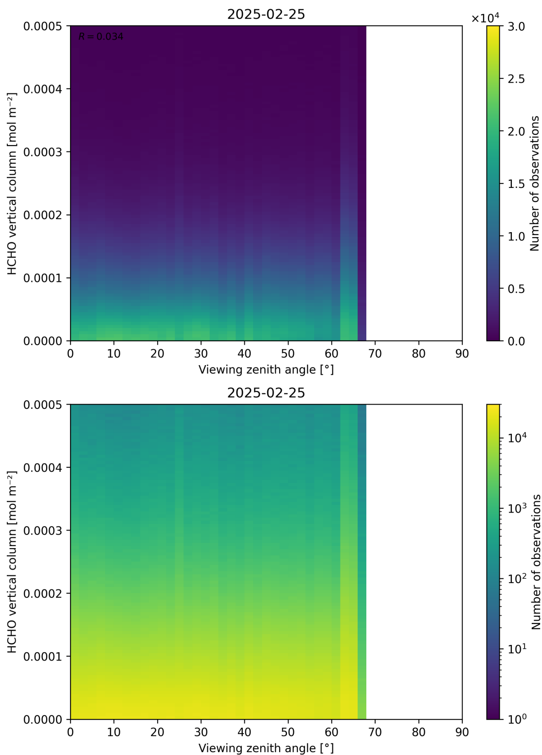
Figure 192: Scatter density plot of “Viewing zenith angle” against “HCHO vertical column” for 2025-02-24 to 2025-02-26.
