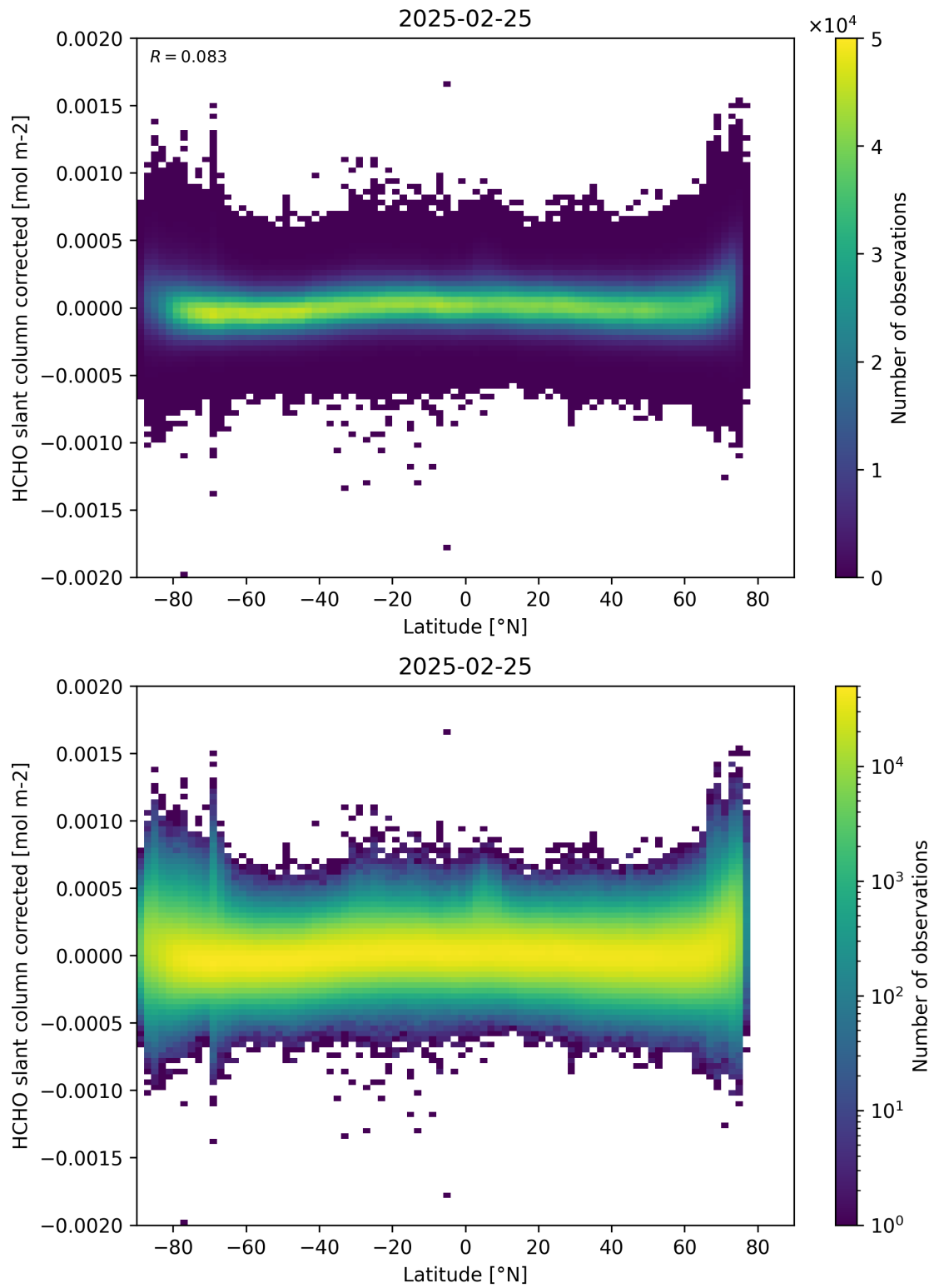
Figure 157: Scatter density plot of “Latitude” against “HCHO slant column corrected” for 2025-02-24 to 2025-02-26.
