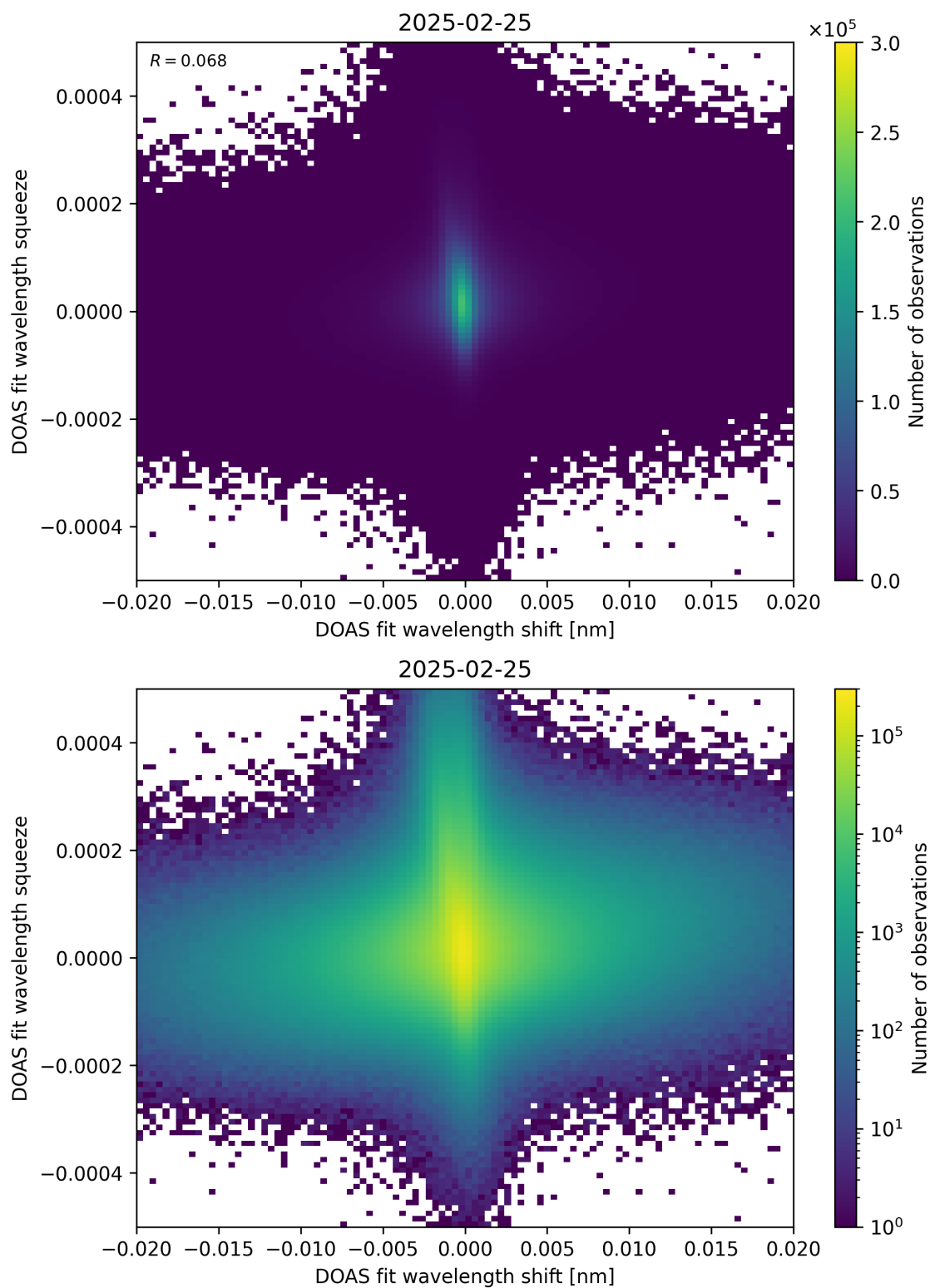
Figure 65: Scatter density plot of “DOAS fit wavelength shift” against “DOAS fit wavelength squeeze” for 2025-02-24 to 2025-02-26.
