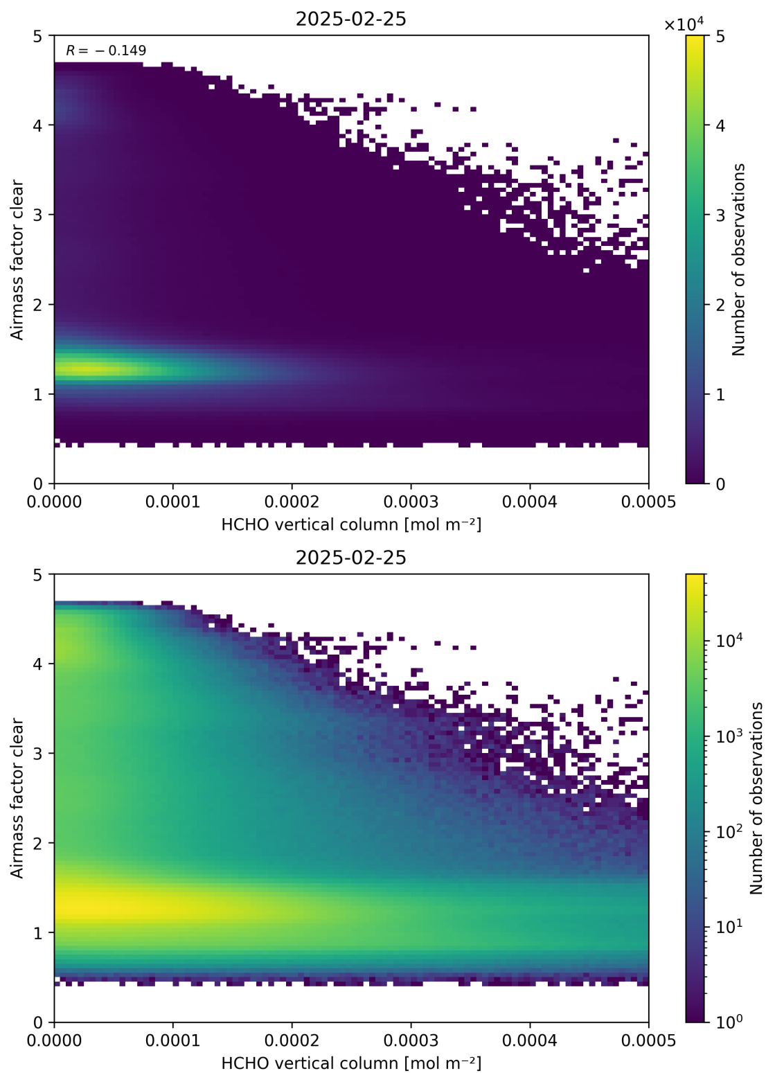
Figure 126: Scatter density plot of “HCHO vertical column” against “Airmass factor clear” for 2025-02-24 to 2025-02-26.
