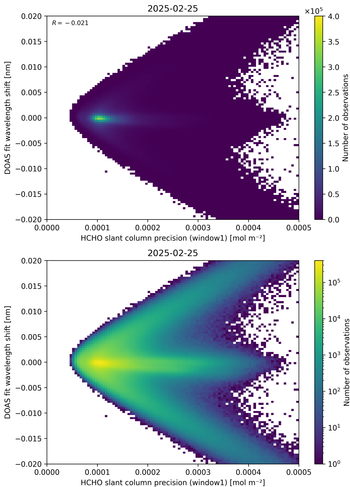
Figure 89: Scatter density plot of “HCHO slant column precision (window1)” against “DOAS fit wavelength shift” for 2025-02-24 to 2025-02-26.
