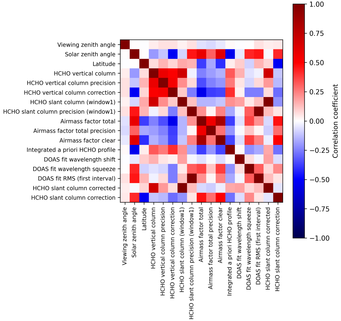
Figure 2: Map of correlation matrix for 2025-02-24 to 2025-02-26.
