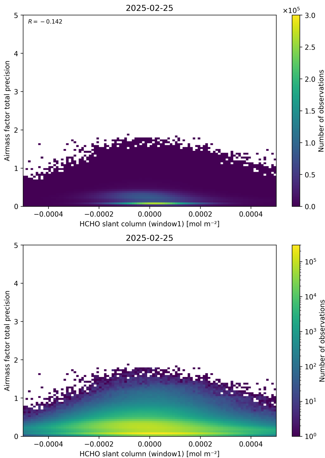
Figure 86: Scatter density plot of “HCHO slant column (window1)” against “Airmass factor total precision” for 2025-02-24 to 2025-02-26.
