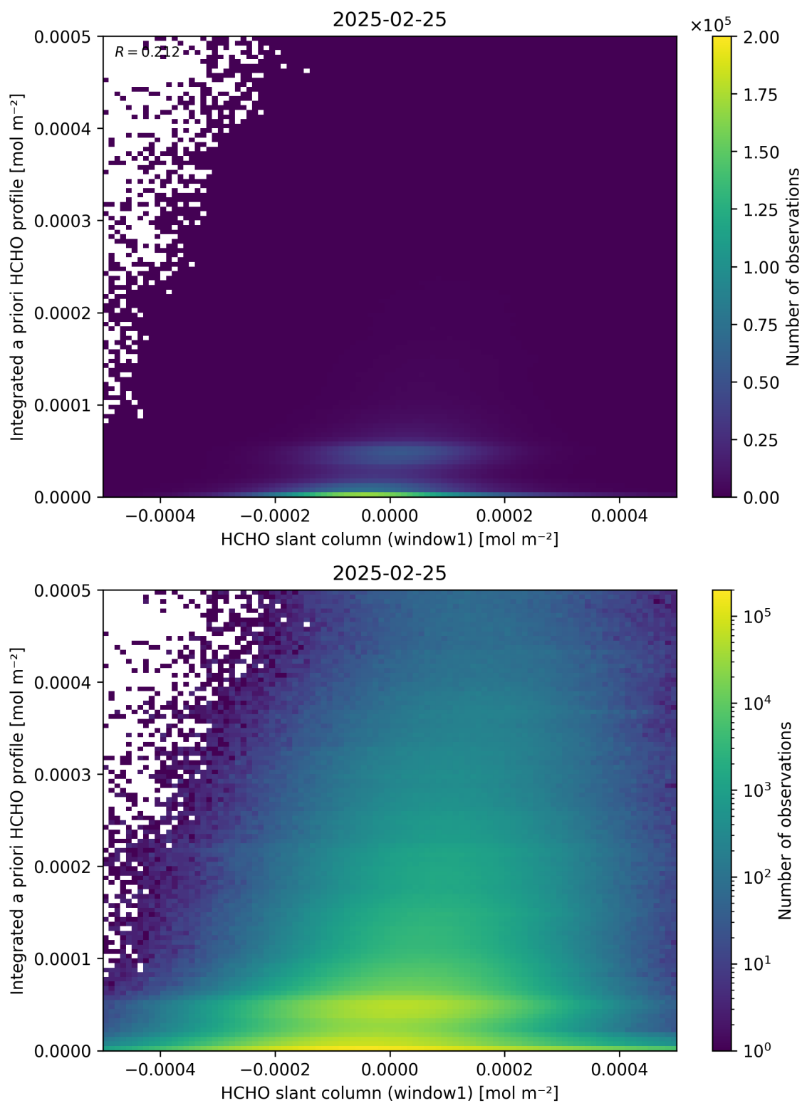
Figure 87: Scatter density plot of “HCHO slant column (window1)” against “Integrated a priori HCHO profile” for 2025-02-24 to 2025-02-26.
