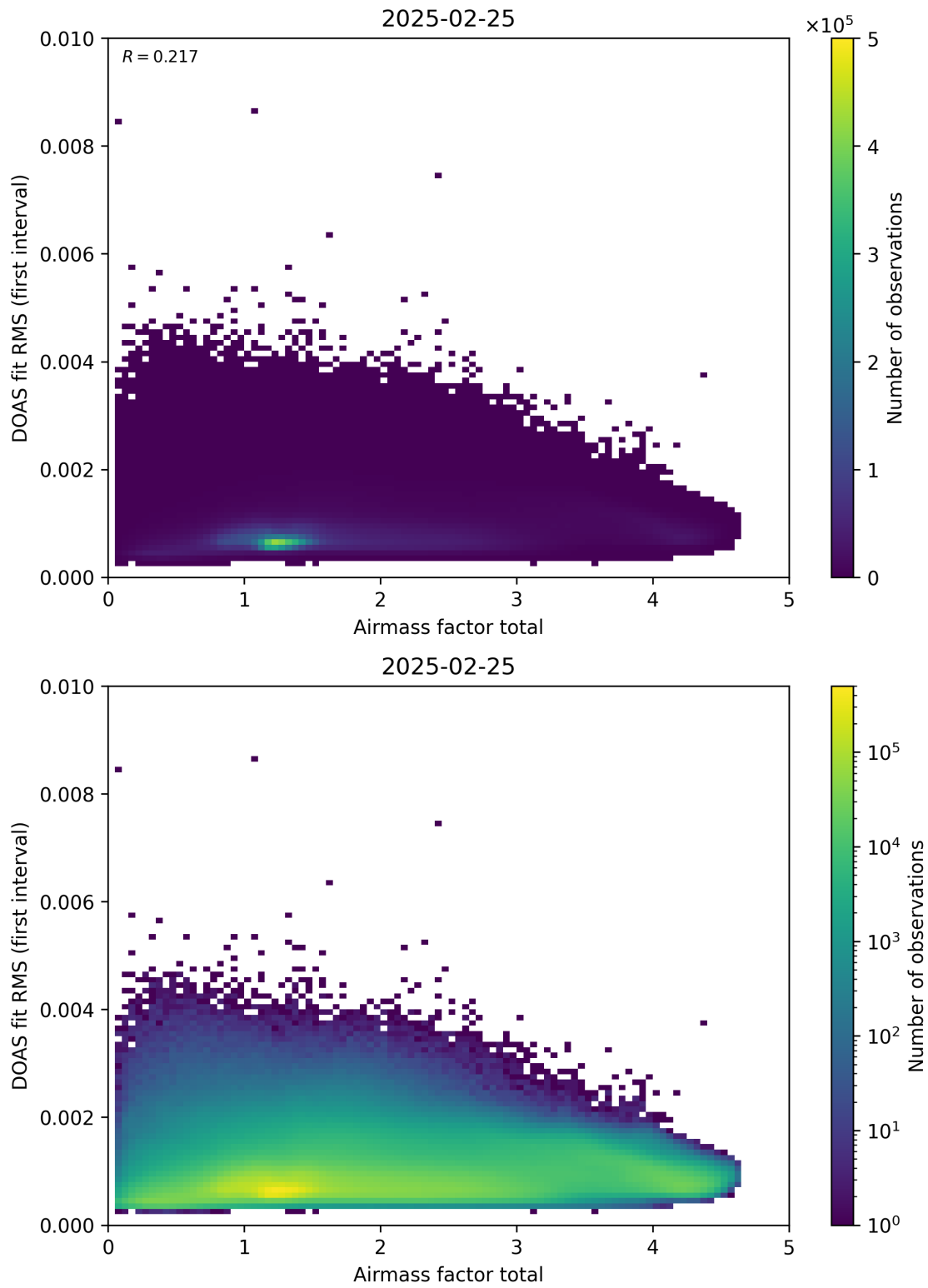
Figure 97: Scatter density plot of “Airmass factor total” against “DOAS fit RMS (first interval)” for 2025-02-24 to 2025-02-26.
