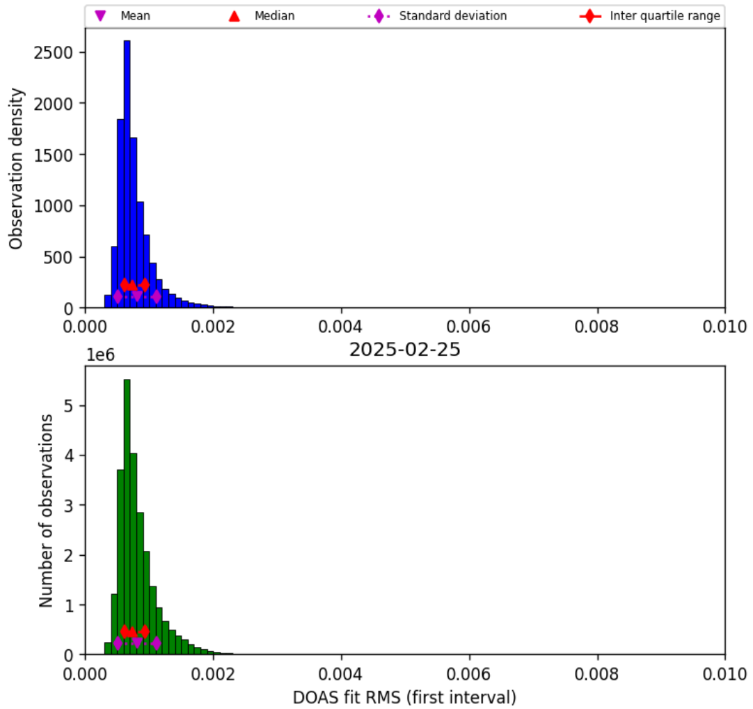
Figure 46: Histogram of “DOAS fit RMS (first interval)” for 2025-02-24 to 2025-02-26
