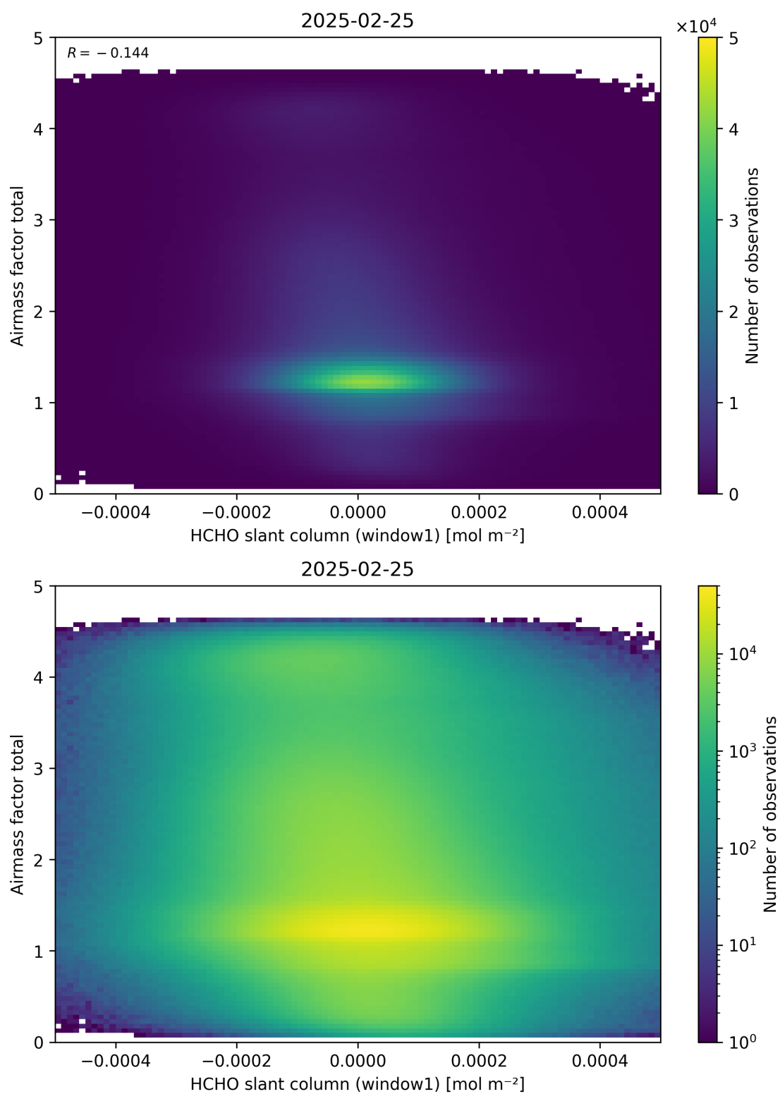
Figure 85: Scatter density plot of “HCHO slant column (window1)” against “Airmass factor total” for 2025-02-24 to 2025-02-26.
