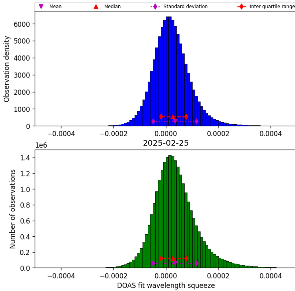
Figure 45: Histogram of “DOAS fit wavelength squeeze” for 2025-02-24 to 2025-02-26
