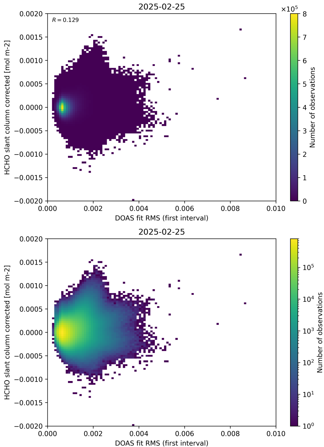
Figure 62: Scatter density plot of “DOAS fit RMS (first interval)” against “HCHO slant column corrected” for 2025-02-24 to 2025-02-26.
