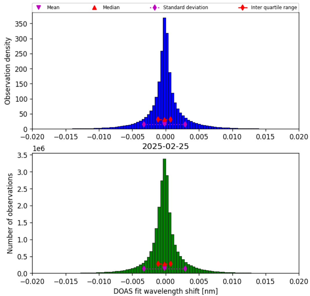
Figure 44: Histogram of “DOAS fit wavelength shift” for 2025-02-24 to 2025-02-26
