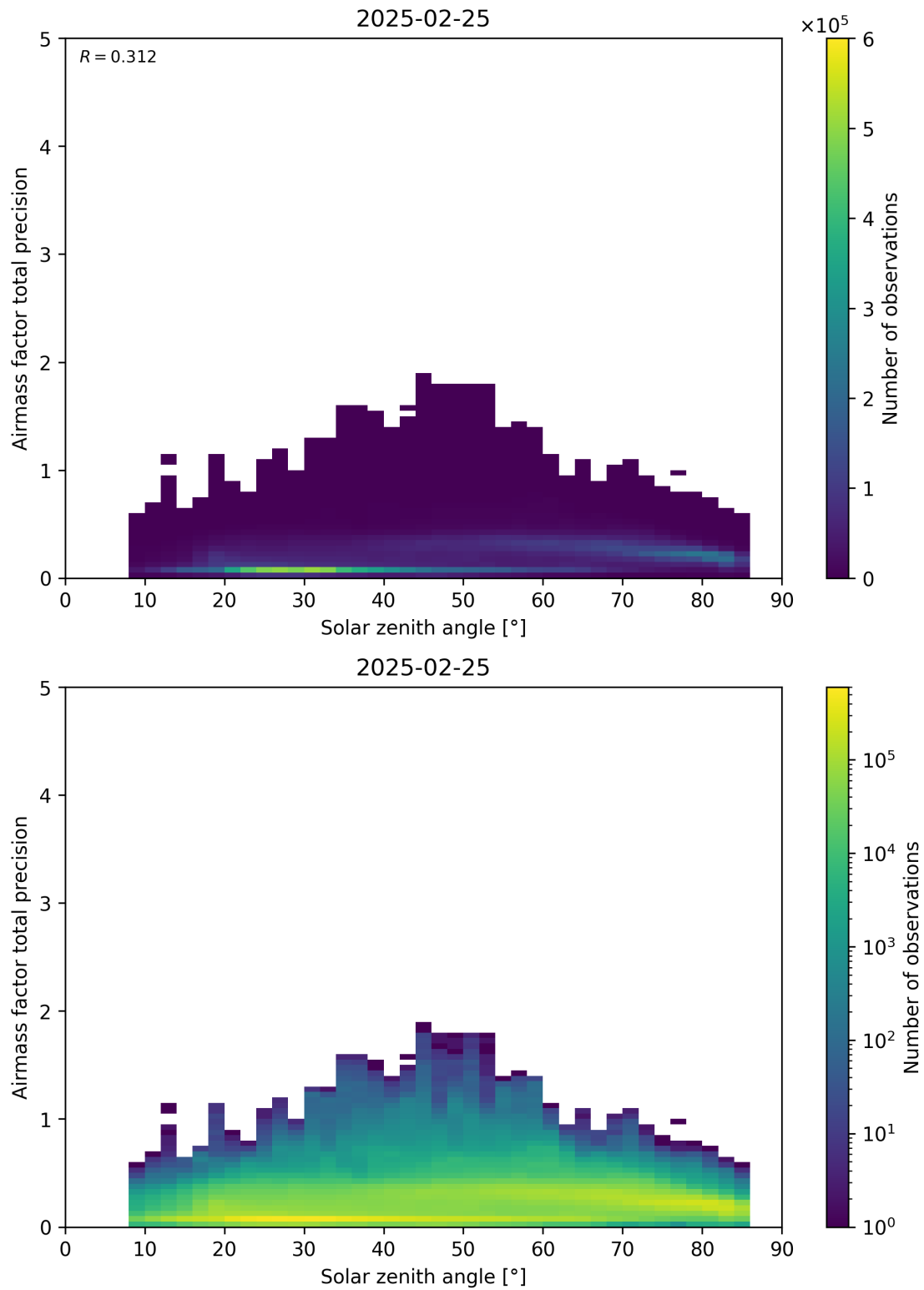
Figure 176: Scatter density plot of “Solar zenith angle” against “Airmass factor total precision” for 2025-02-24 to 2025-02-26.
