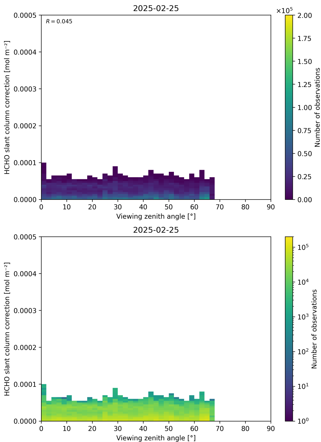
Figure 187: Scatter density plot of “Viewing zenith angle” against “HCHO slant column correction” for 2025-02-24 to 2025-02-26.
