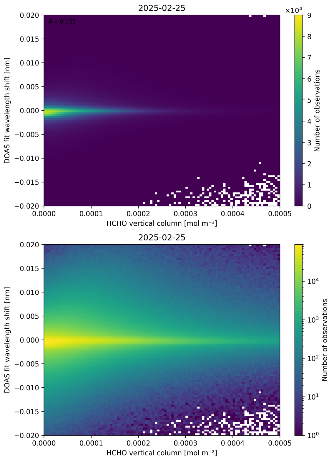
Figure 124: Scatter density plot of “HCHO vertical column” against “DOAS fit wavelength shift” for 2025-02-24 to 2025-02-26.
