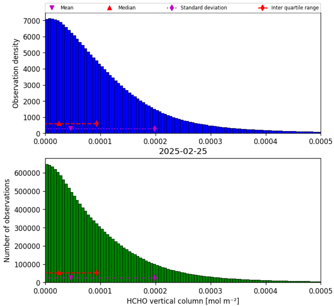
Figure 35: Histogram of “HCHO vertical column” for 2025-02-24 to 2025-02-26
