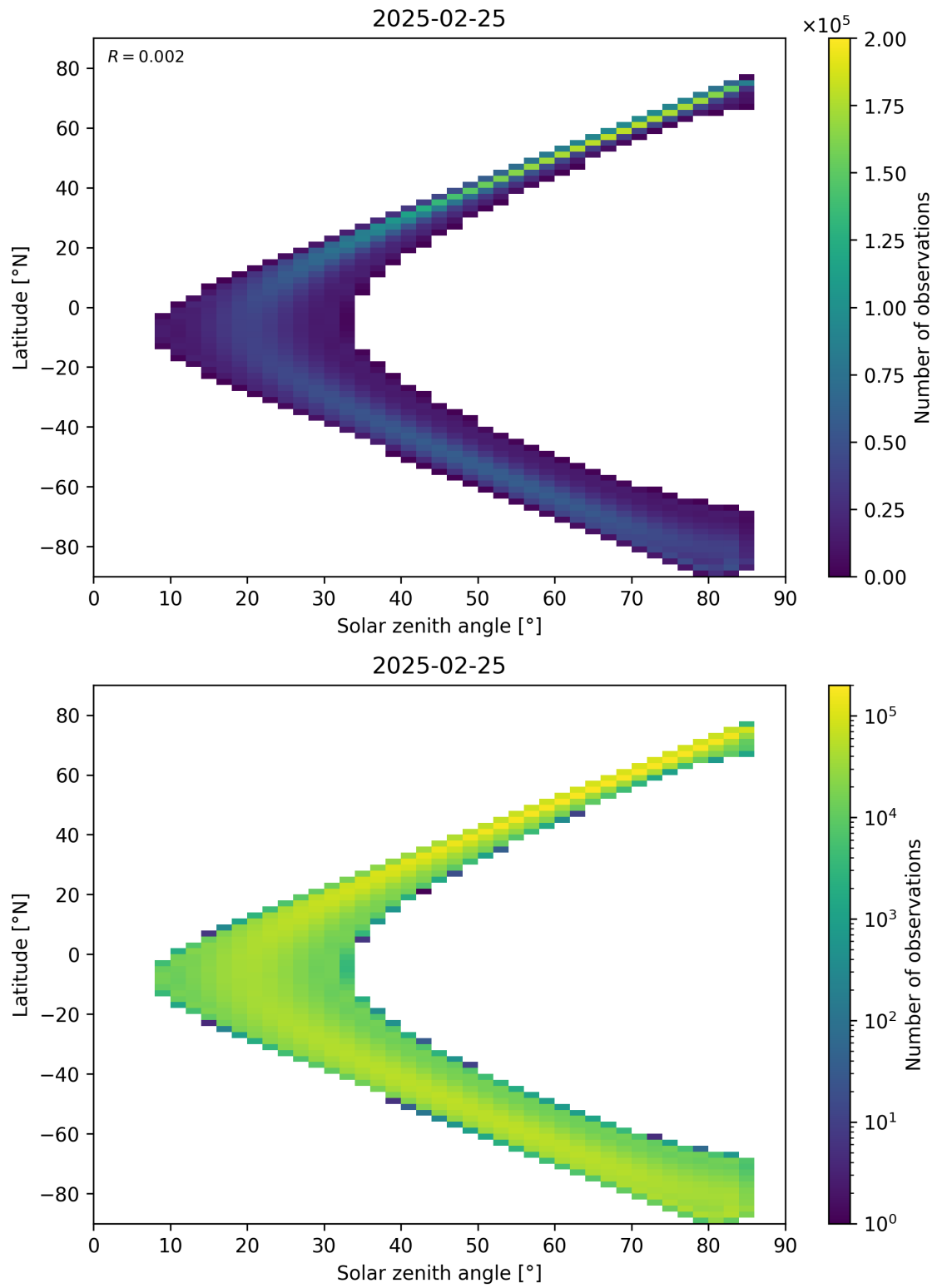
Figure 181: Scatter density plot of “Solar zenith angle” against “Latitude” for 2025-02-24 to 2025-02-26.
