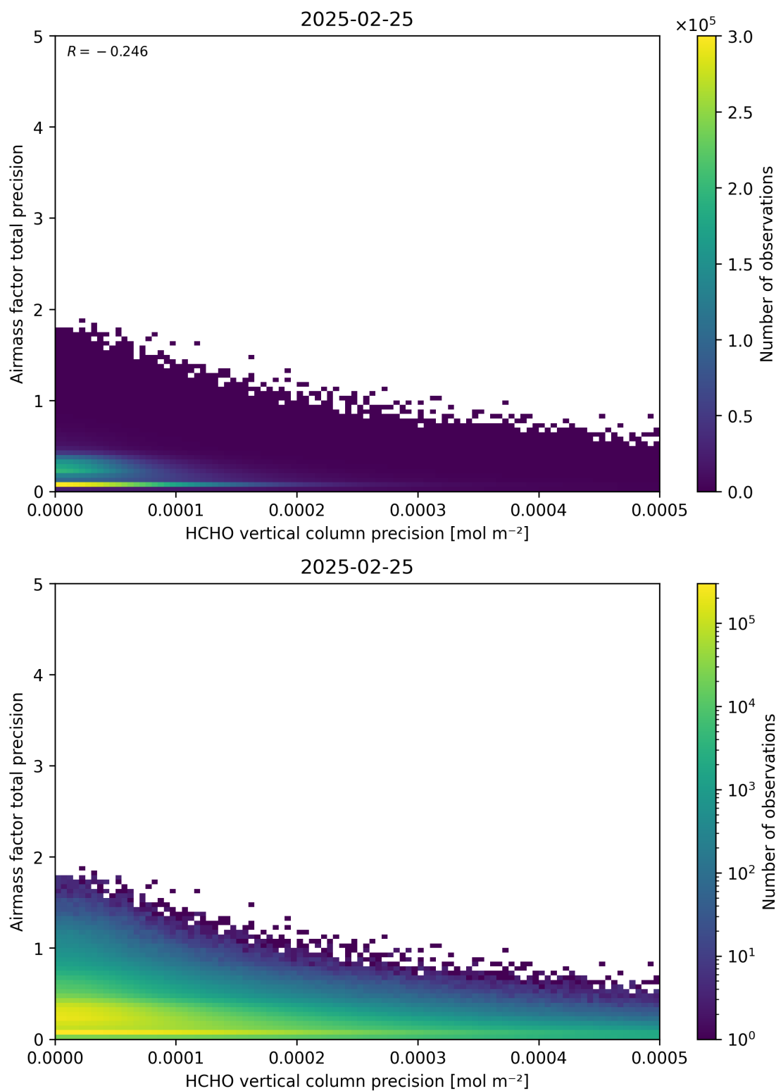
Figure 145: Scatter density plot of “HCHO vertical column precision” against “Airmass factor total precision” for 2025-02-24 to 2025-02-26.
