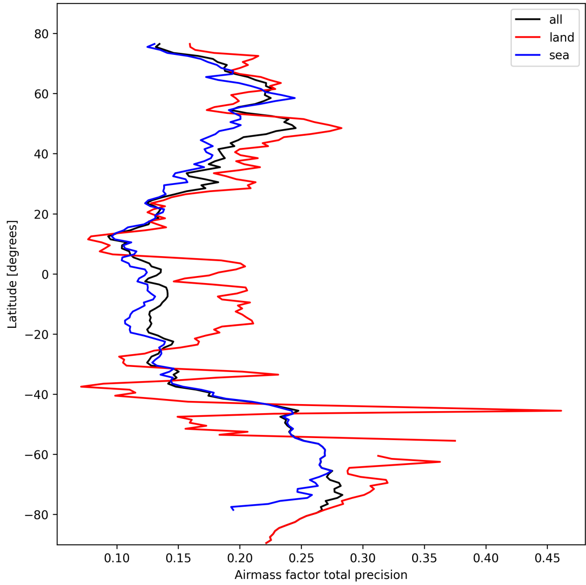
Figure 27: Zonal average of “Airmass factor total precision” for 2025-02-24 to 2025-02-26.
