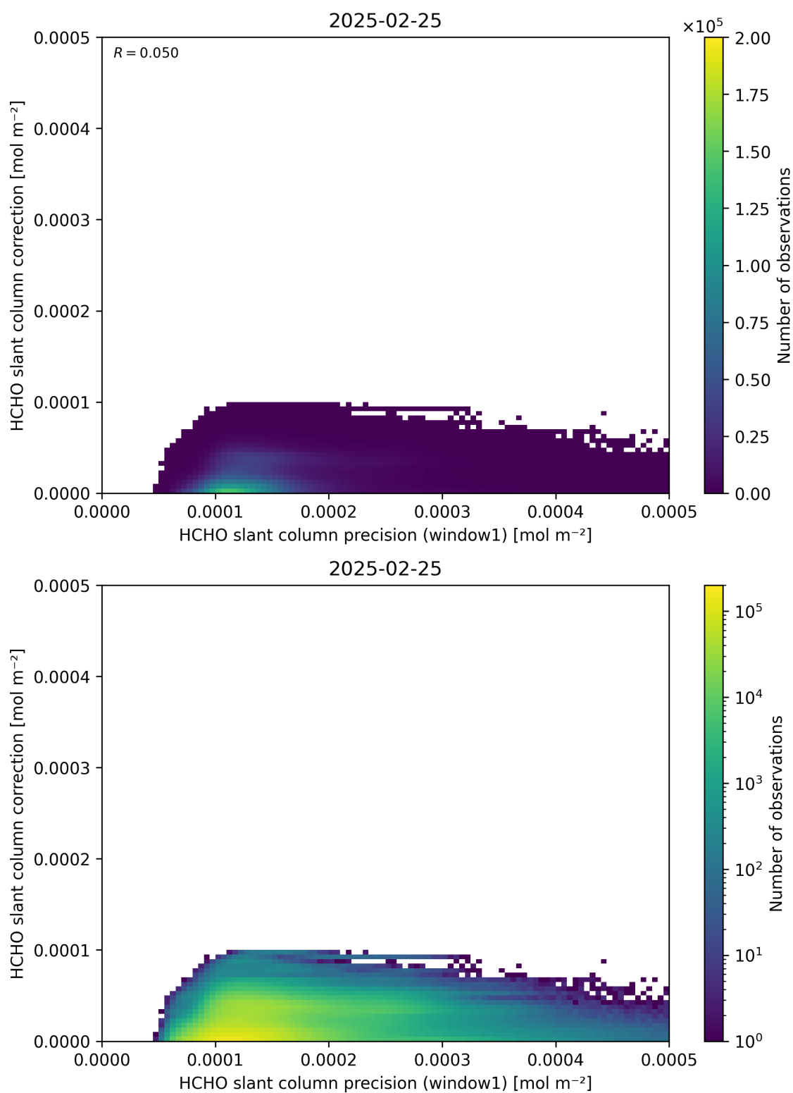
Figure 93: Scatter density plot of “HCHO slant column precision (window1)” against “HCHO slant column correction” for 2025-02-24 to 2025-02-26.
