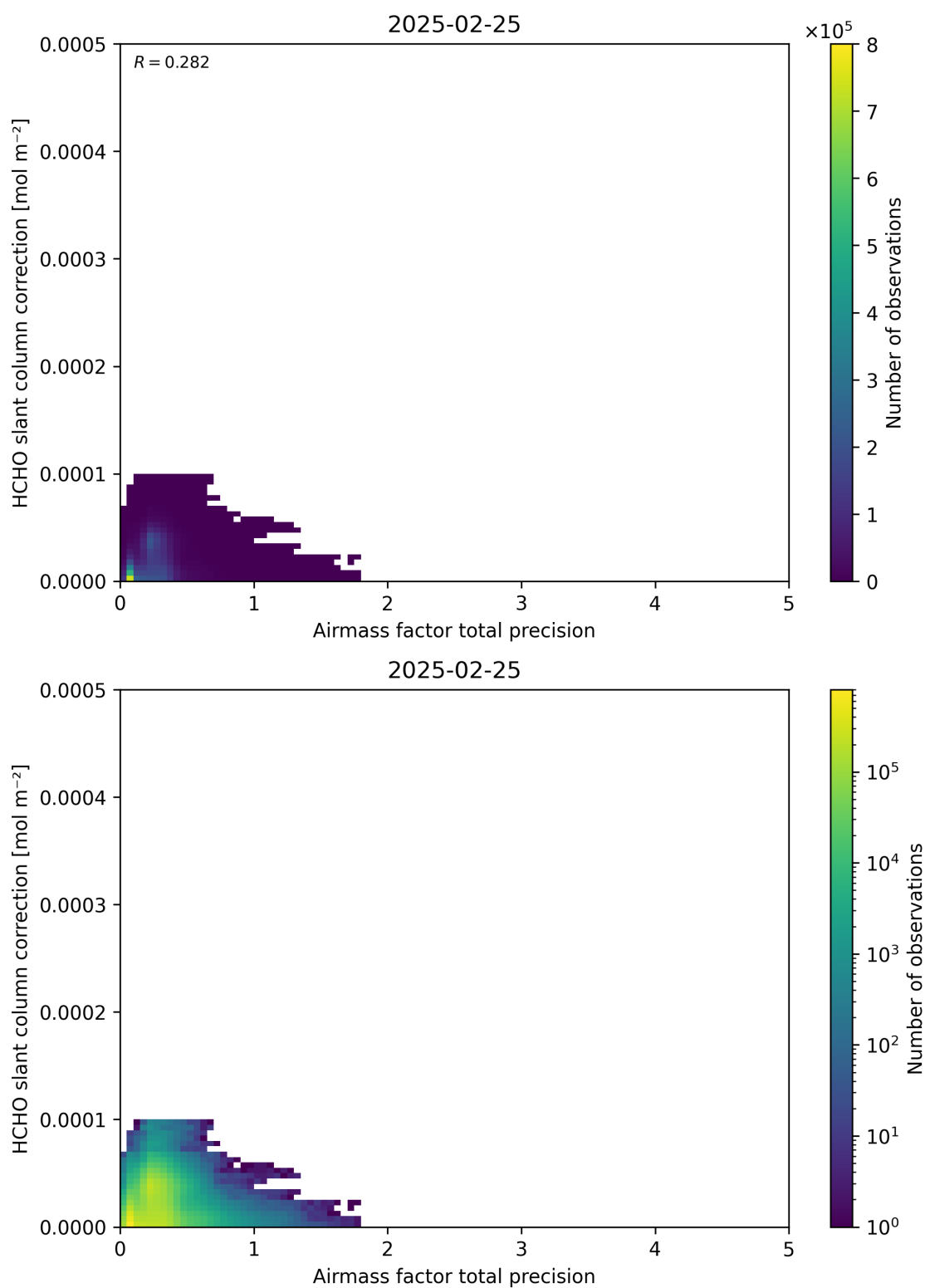
Figure 110: Scatter density plot of “Airmass factor total precision” against “HCHO slant column correction” for 2025-02-24 to 2025-02-26.
