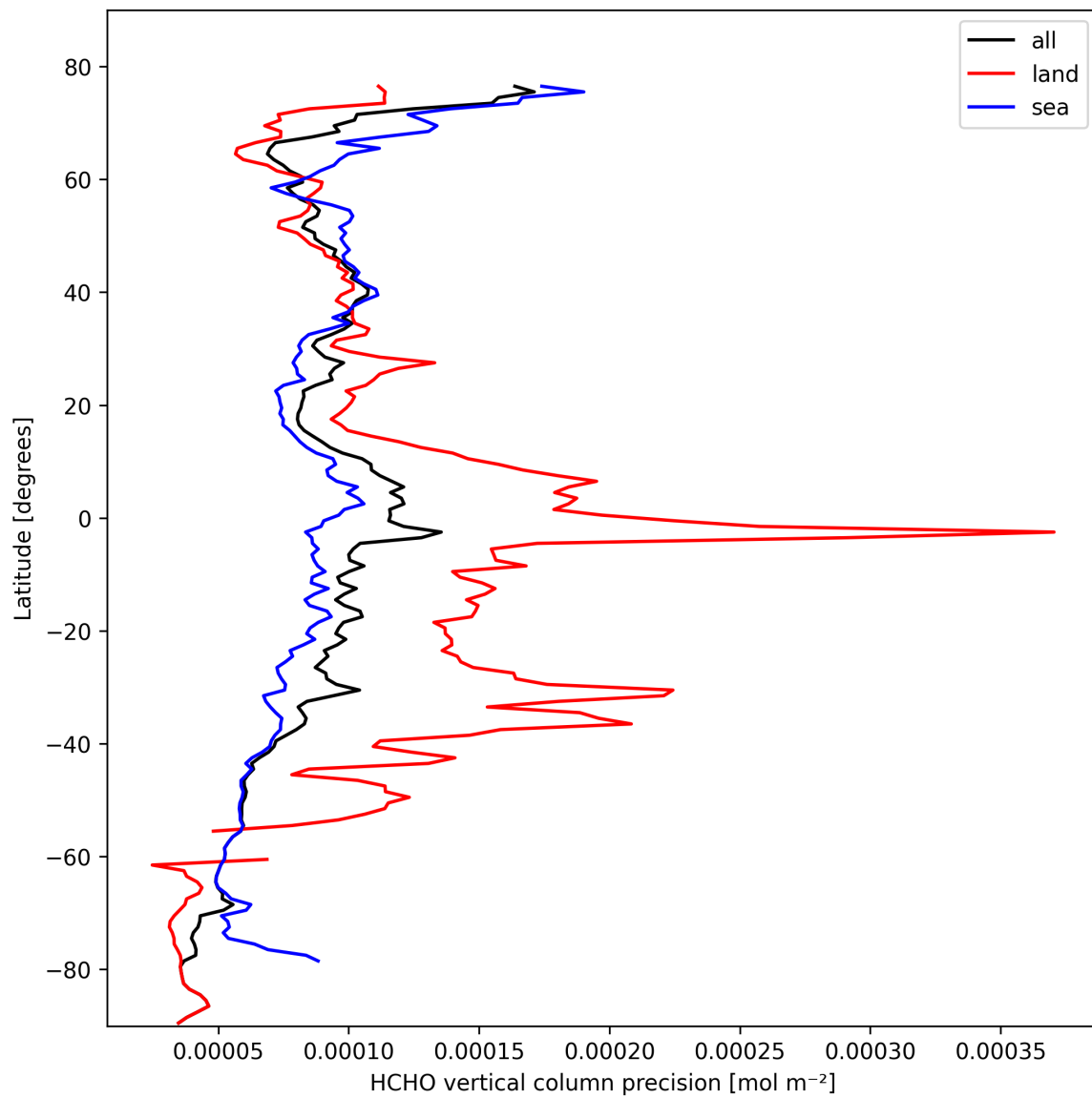
Figure 22: Zonal average of “HCHO vertical column precision” for 2025-02-24 to 2025-02-26.
