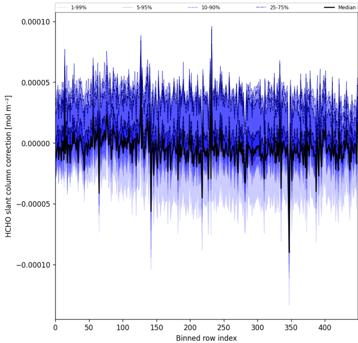
Figure 61: Along track statistics of “HCHO slant column correction” for 2025-02-24 to 2025-02-26
