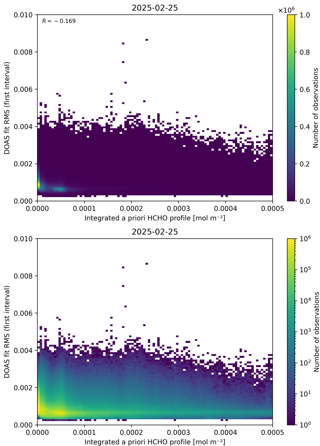
Figure 148: Scatter density plot of “Integrated a priori HCHO profile” against “DOAS fit RMS (first interval)” for 2025-02-24 to 2025-02-26.
