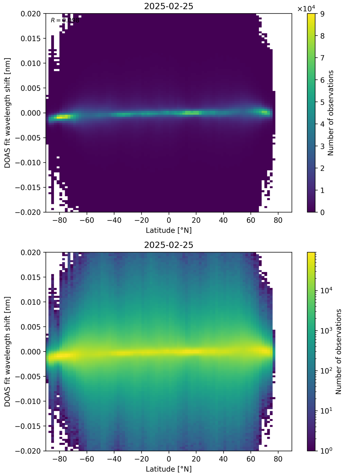
Figure 154: Scatter density plot of “Latitude” against “DOAS fit wavelength shift” for 2025-02-24 to 2025-02-26.
