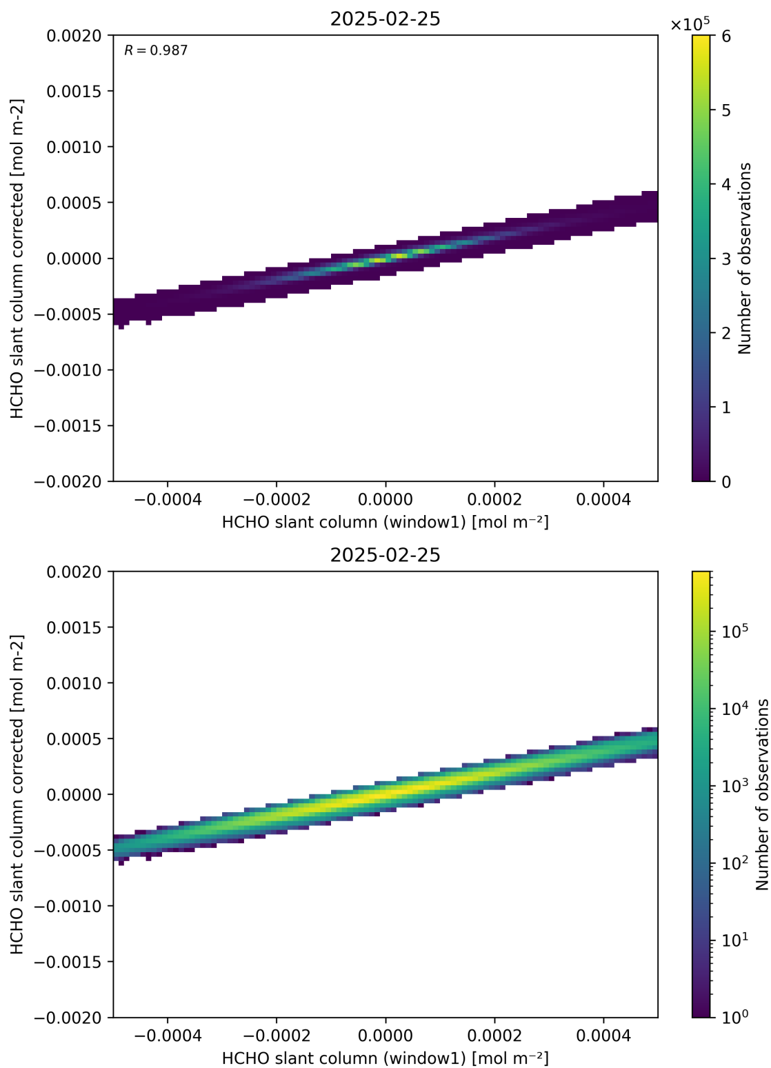
Figure 82: Scatter density plot of “HCHO slant column (window1)” against “HCHO slant column corrected” for 2025-02-24 to 2025-02-26.
