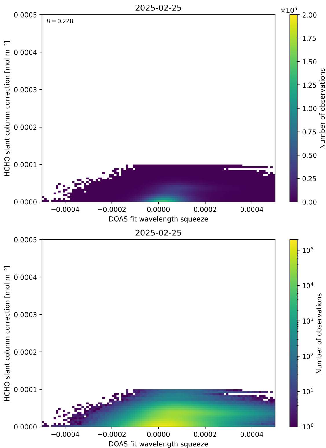
Figure 70: Scatter density plot of “DOAS fit wavelength squeeze” against “HCHO slant column correction” for 2025-02-24 to 2025-02-26.
