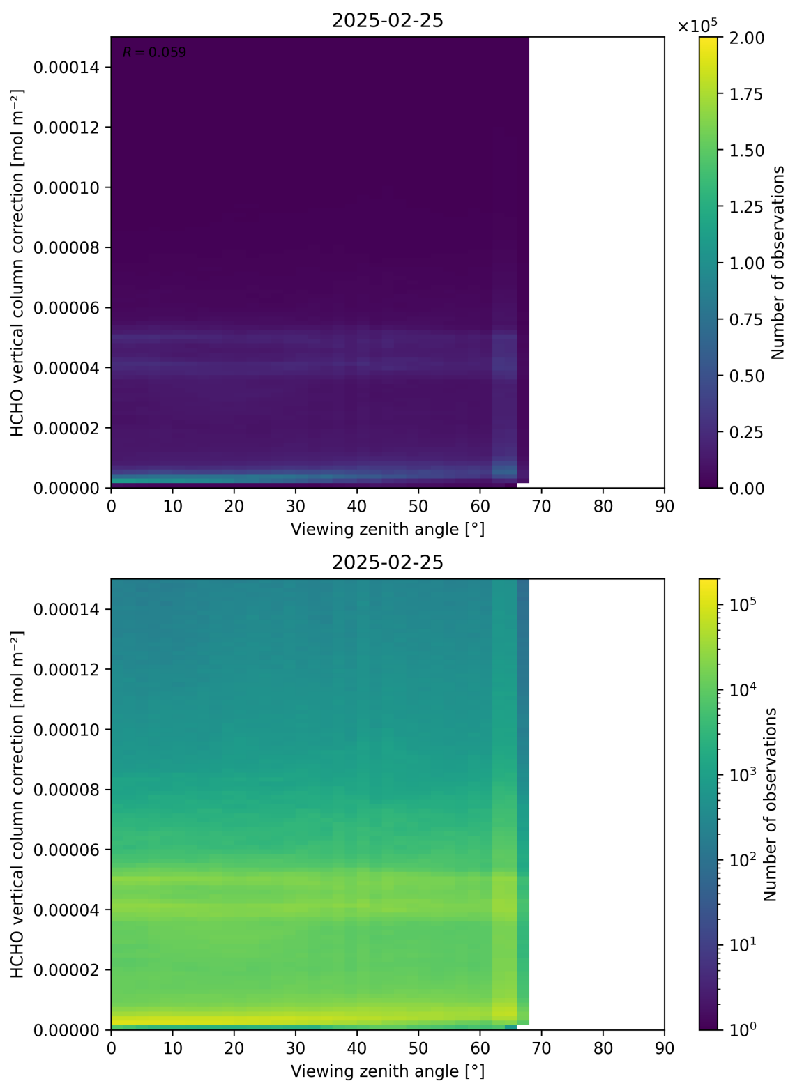
Figure 193: Scatter density plot of “Viewing zenith angle” against “HCHO vertical column correction” for 2025-02-24 to 2025-02-26.
