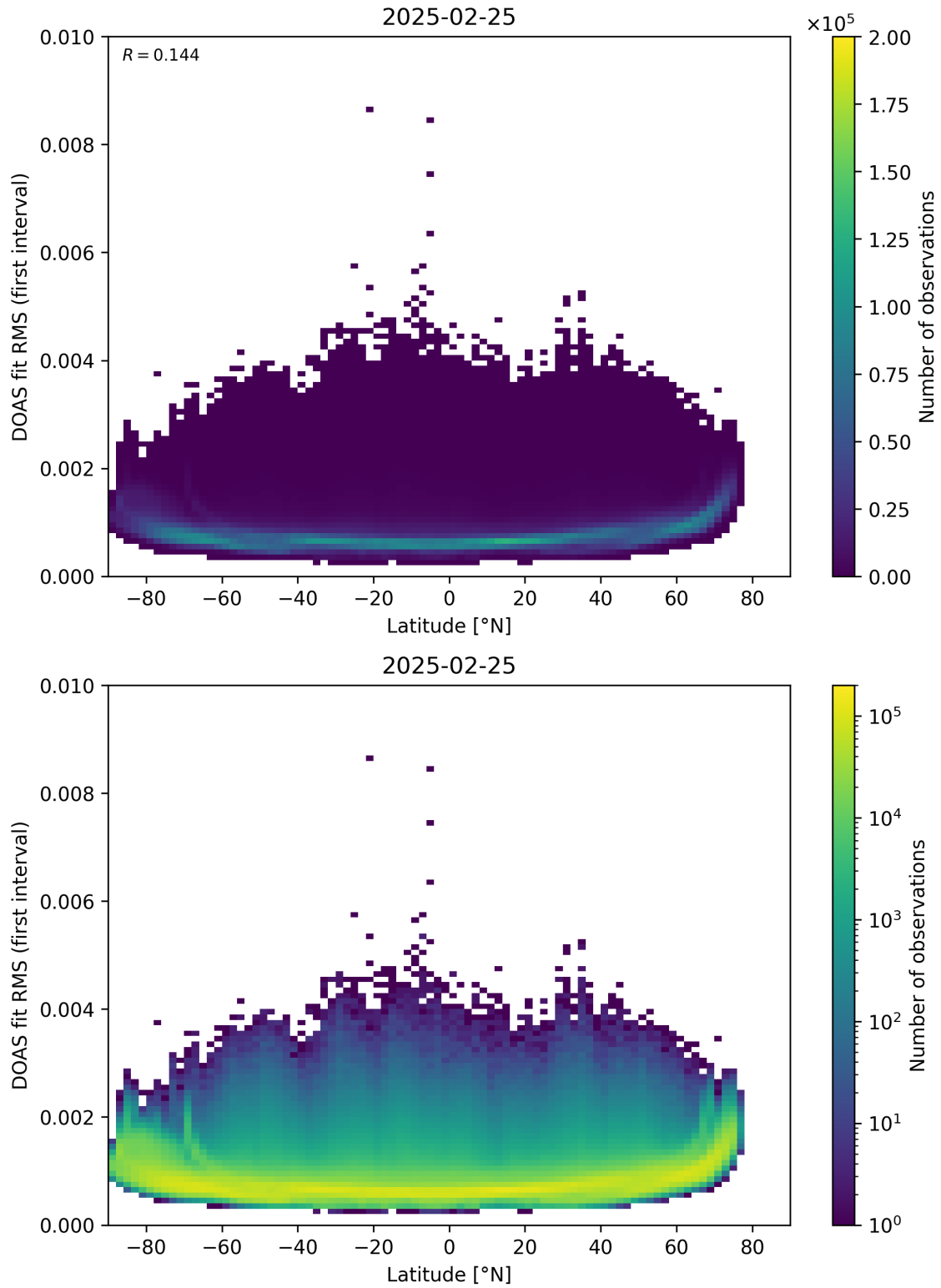
Figure 153: Scatter density plot of “Latitude” against “DOAS fit RMS (first interval)” for 2025-02-24 to 2025-02-26.
