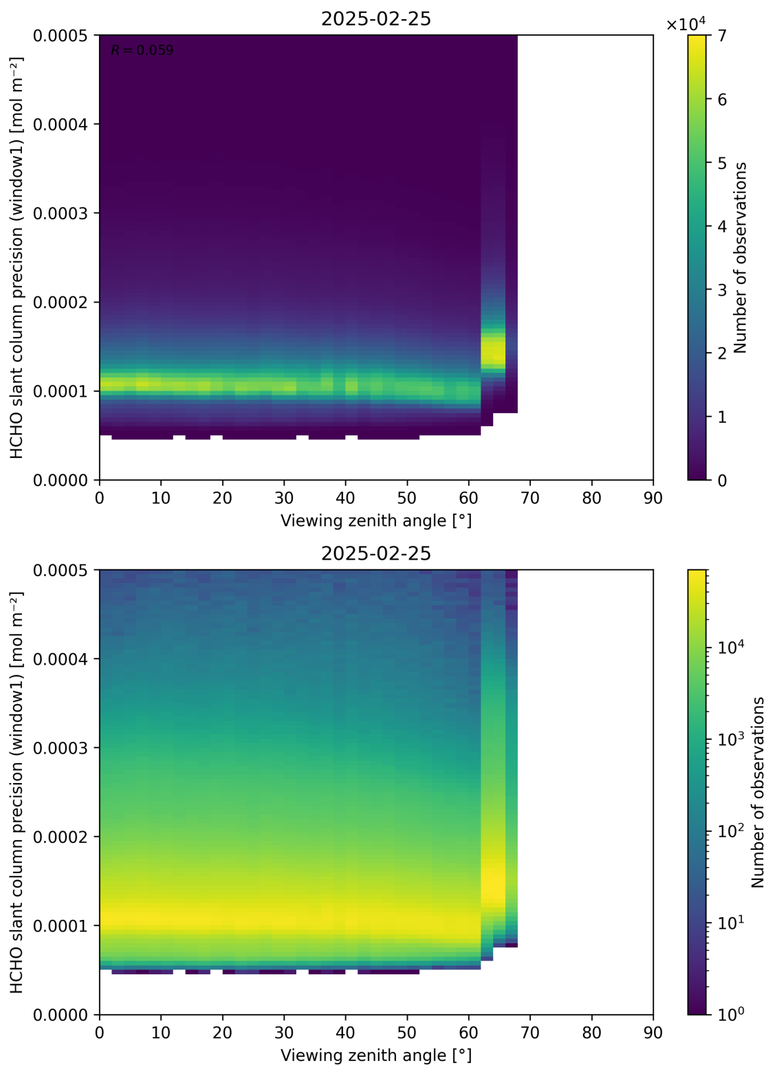
Figure 189: Scatter density plot of “Viewing zenith angle” against “HCHO slant column precision (window1)” for 2025-02-24 to 2025-02-26.
