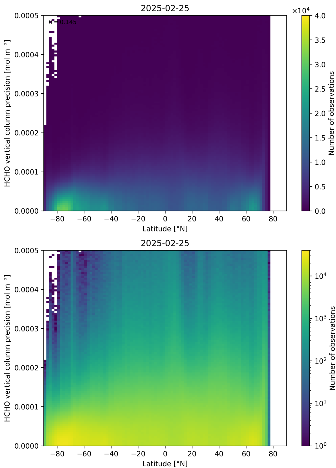
Figure 165: Scatter density plot of “Latitude” against “HCHO vertical column precision” for 2025-02-24 to 2025-02-26.
