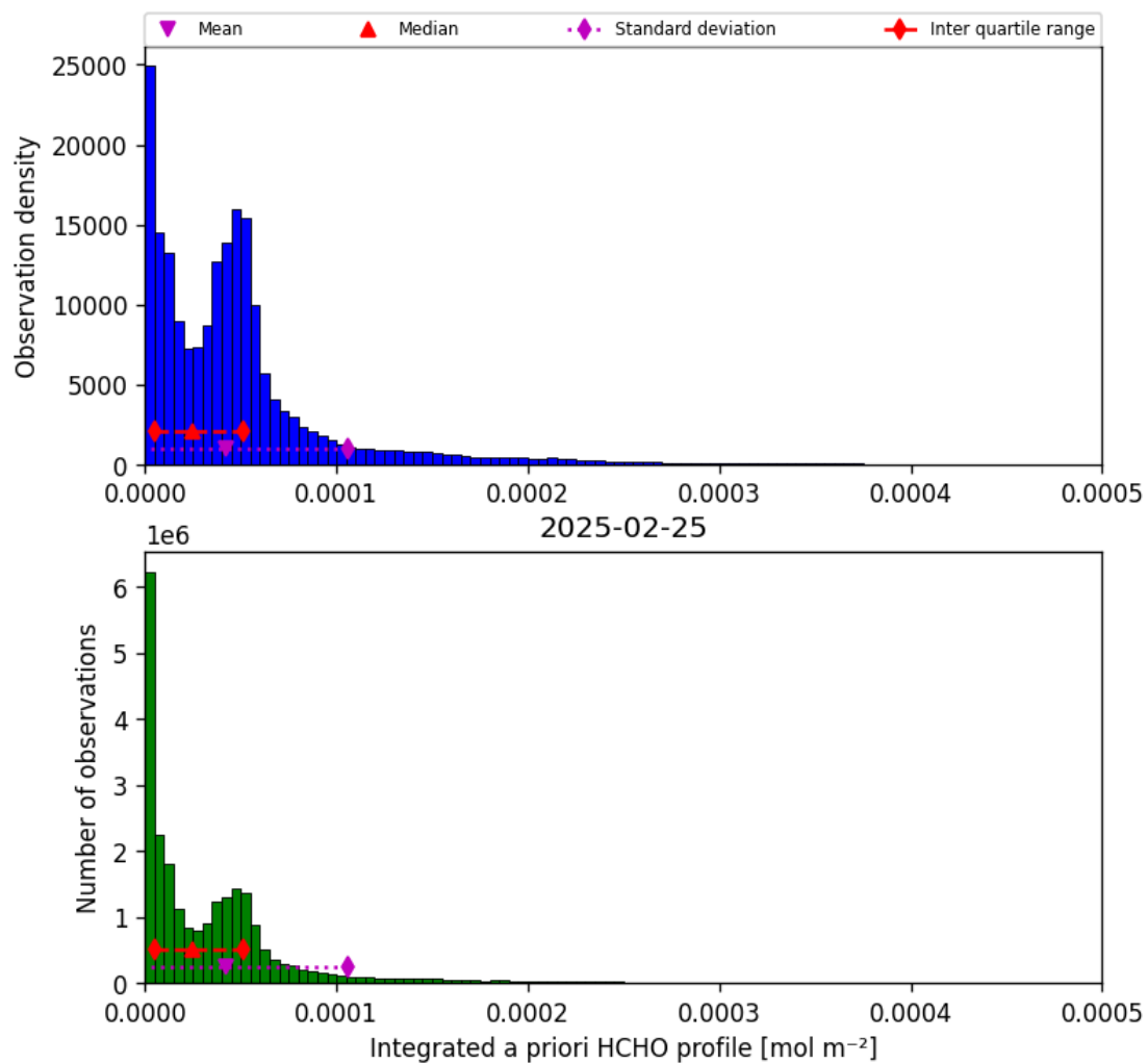
Figure 43: Histogram of “Integrated a priori HCHO profile” for 2025-02-24 to 2025-02-26
