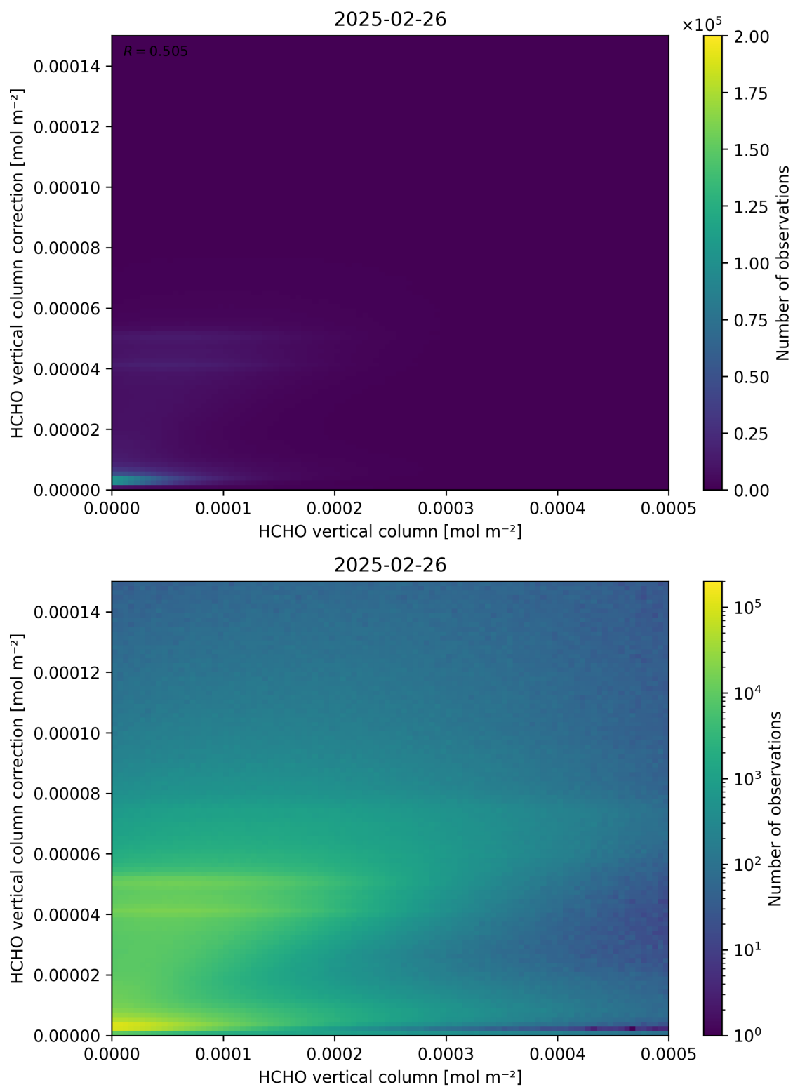
Figure 133: Scatter density plot of “HCHO vertical column” against “HCHO vertical column correction” for 2025-02-25 to 2025-02-27.
