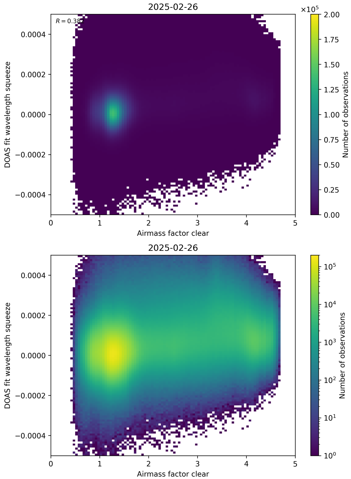
Figure 73: Scatter density plot of “Airmass factor clear” against “DOAS fit wavelength squeeze” for 2025-02-25 to 2025-02-27.
