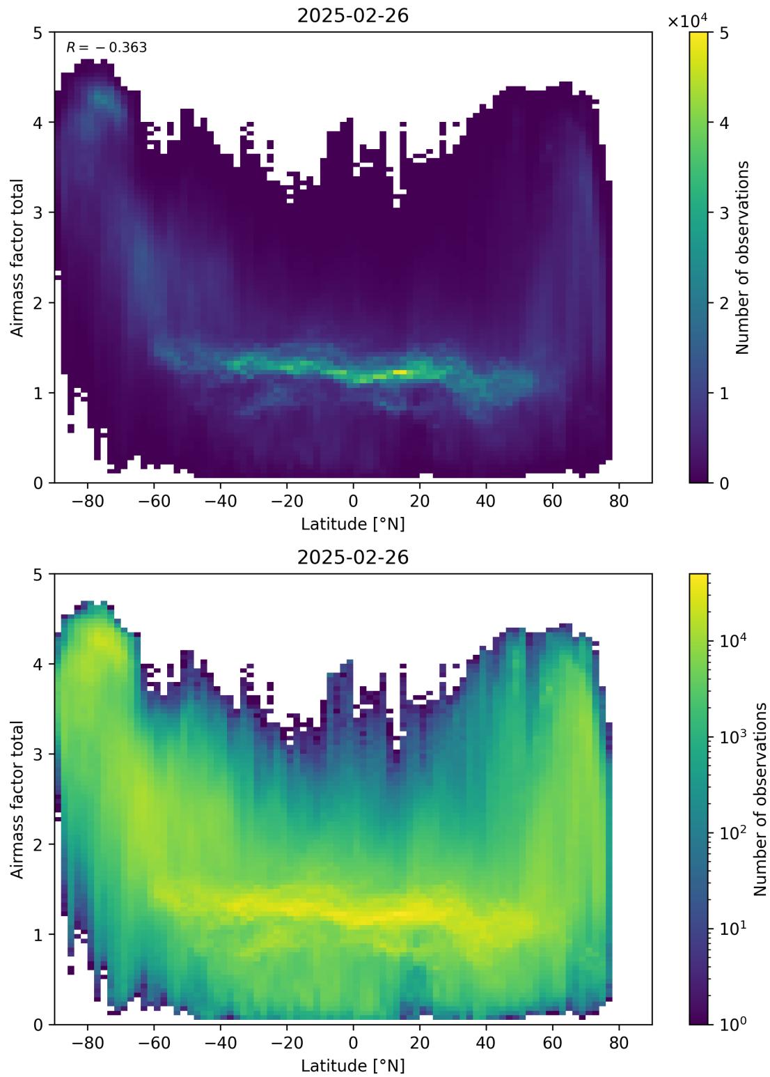
Figure 161: Scatter density plot of “Latitude” against “Airmass factor total” for 2025-02-25 to 2025-02-27.
