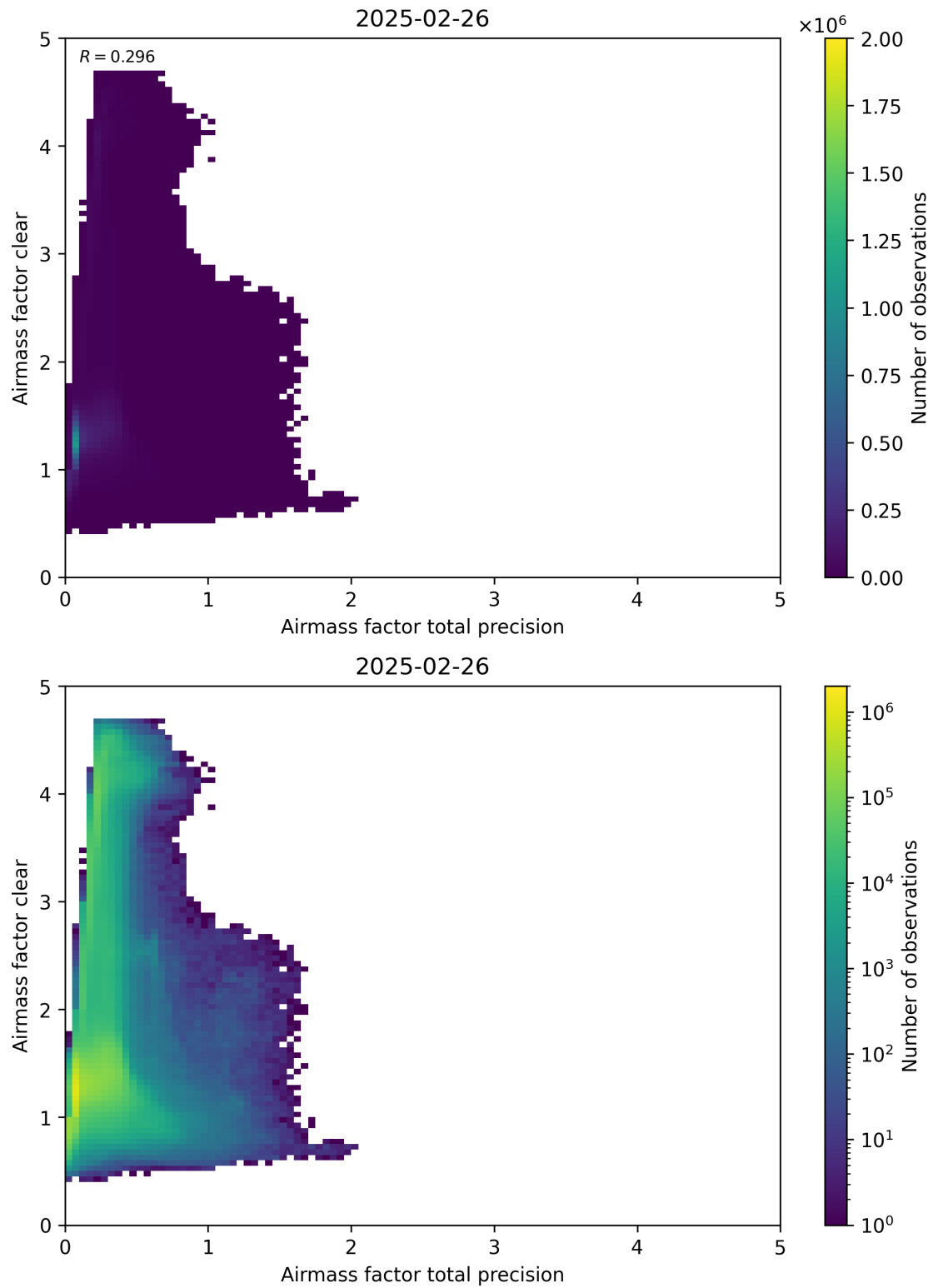
Figure 108: Scatter density plot of “Airmass factor total precision” against “Airmass factor clear” for 2025-02-25 to 2025-02-27.
