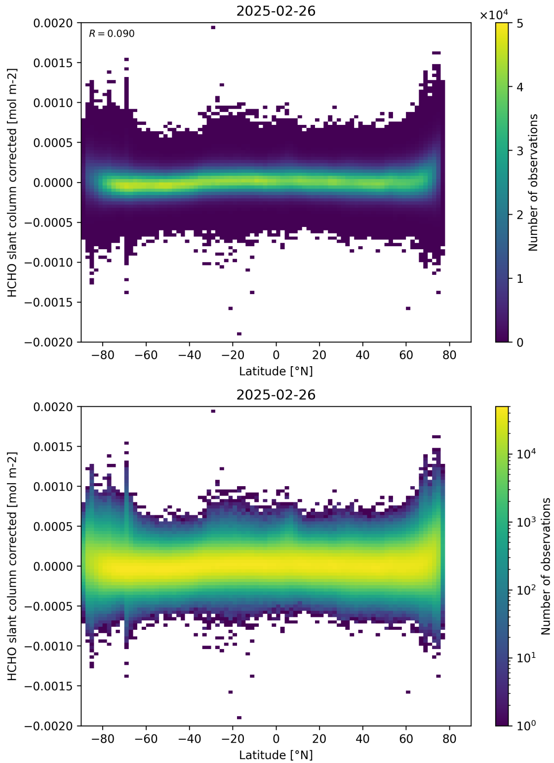
Figure 157: Scatter density plot of “Latitude” against “HCHO slant column corrected” for 2025-02-25 to 2025-02-27.
