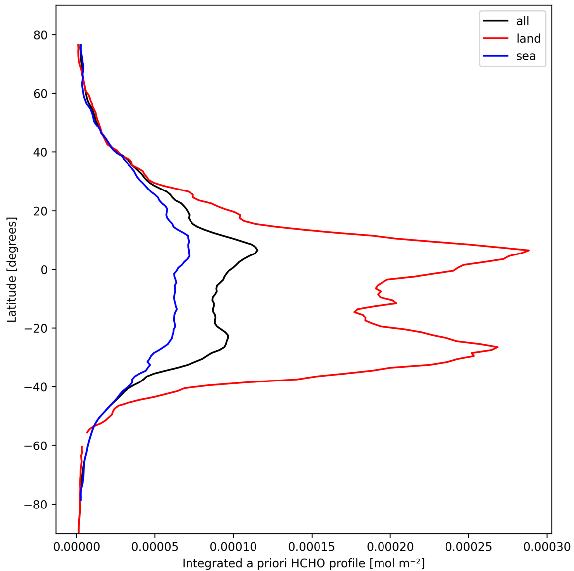
Figure 29: Zonal average of “Integrated a priori HCHO profile” for 2025-02-25 to 2025-02-27.
