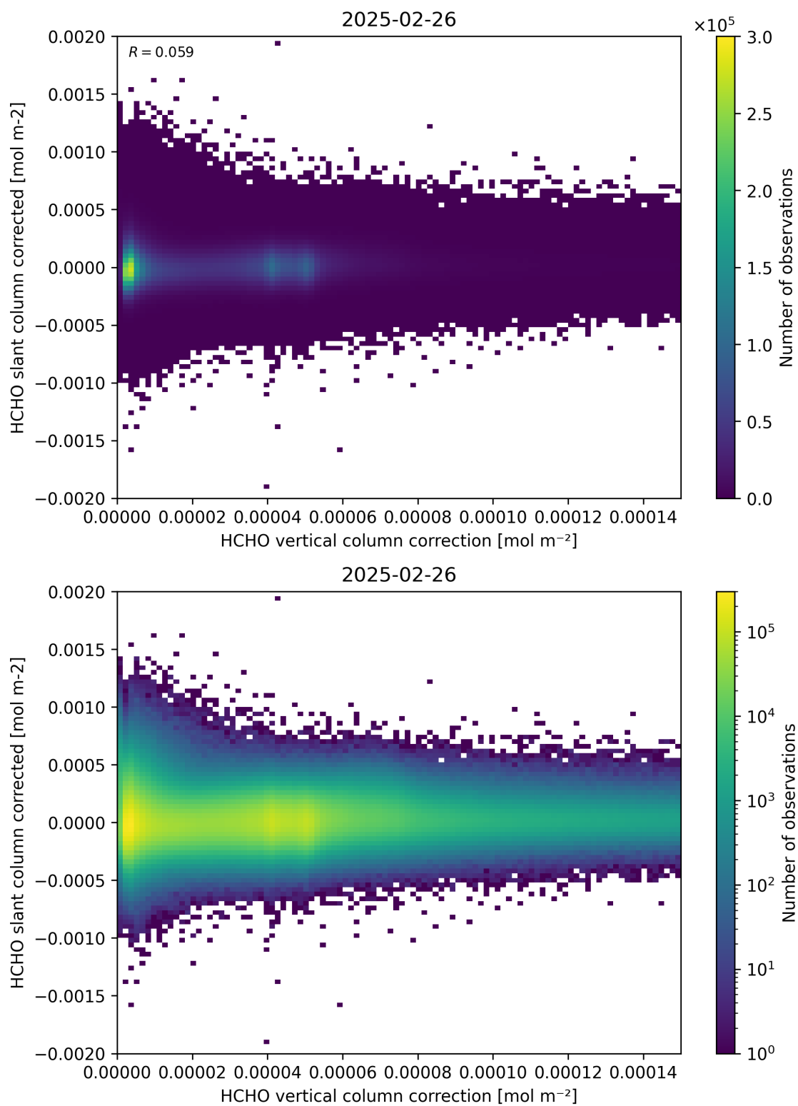
Figure 116: Scatter density plot of “HCHO vertical column correction” against “HCHO slant column corrected” for 2025-02-25 to 2025-02-27.
