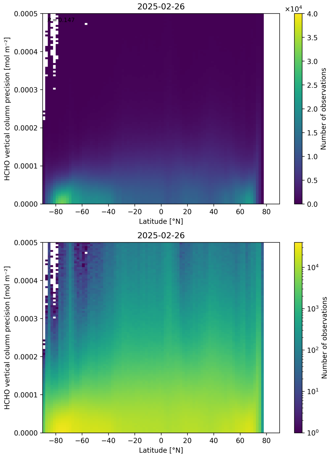
Figure 165: Scatter density plot of “Latitude” against “HCHO vertical column precision” for 2025-02-25 to 2025-02-27.
