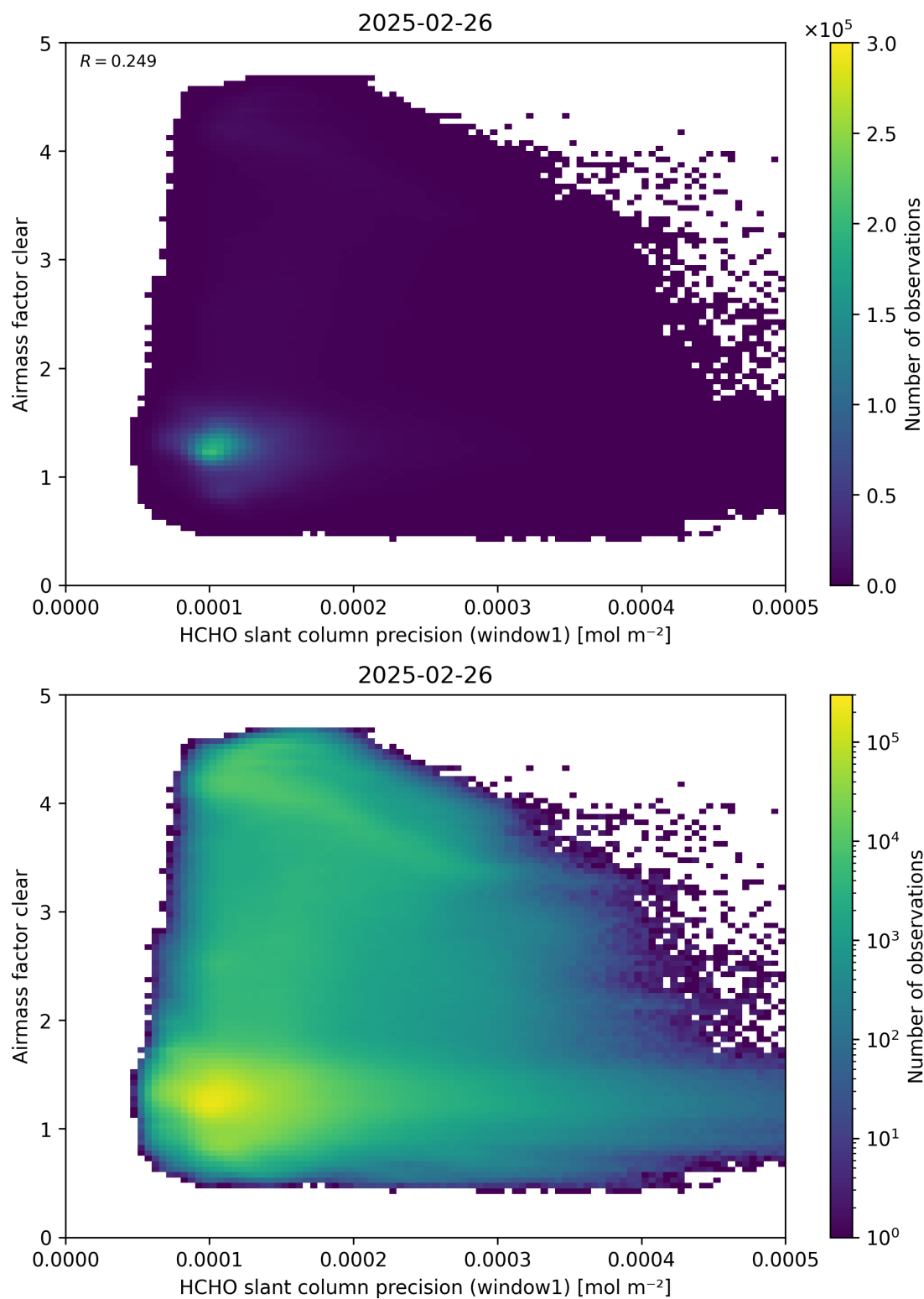
Figure 91: Scatter density plot of “HCHO slant column precision (window1)” against “Airmass factor clear” for 2025-02-25 to 2025-02-27.
