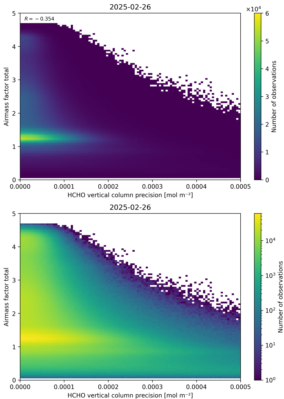
Figure 144: Scatter density plot of “HCHO vertical column precision” against “Airmass factor total” for 2025-02-25 to 2025-02-27.
