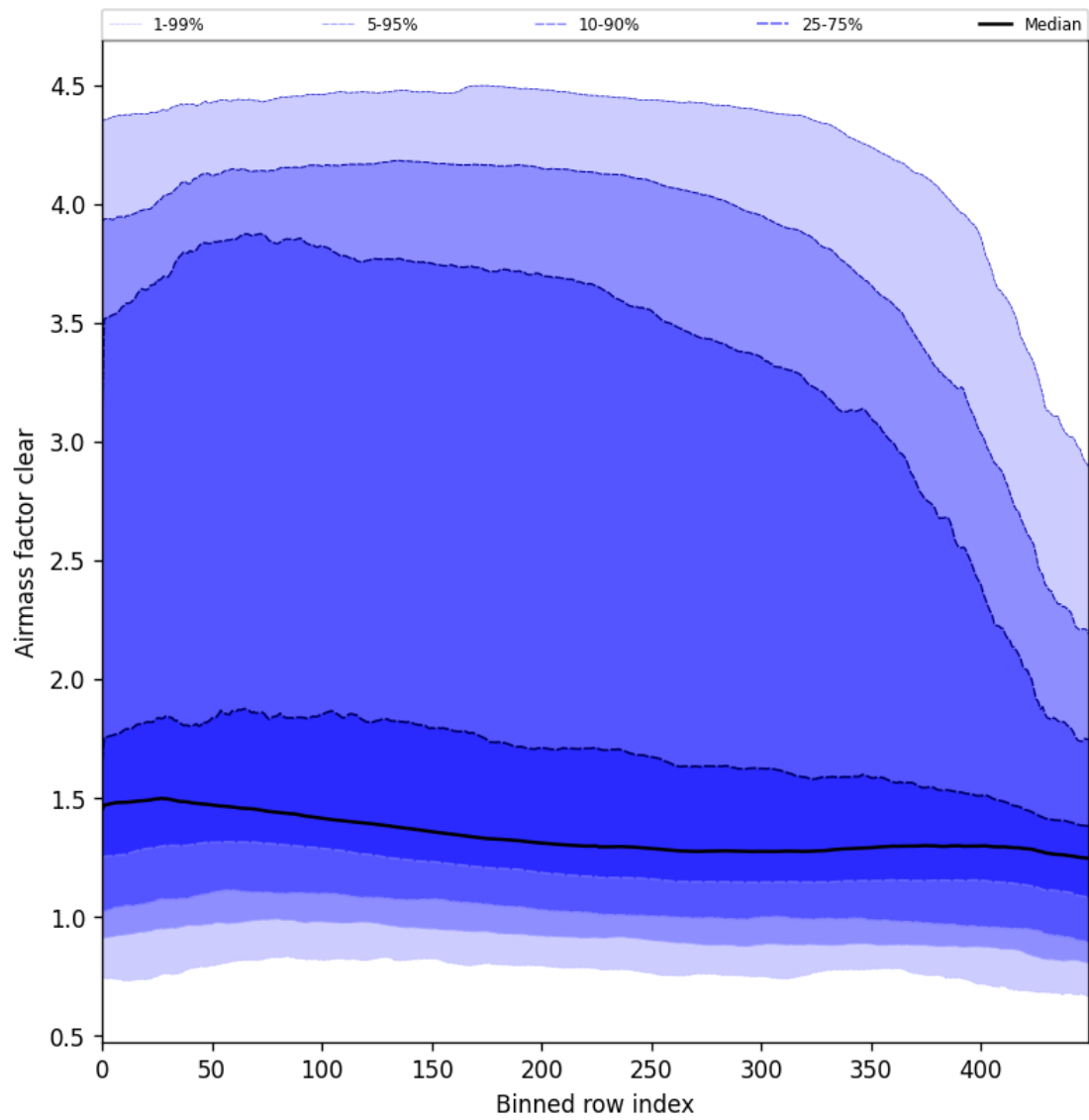
Figure 56: Along track statistics of “Airmass factor clear” for 2025-02-25 to 2025-02-27
