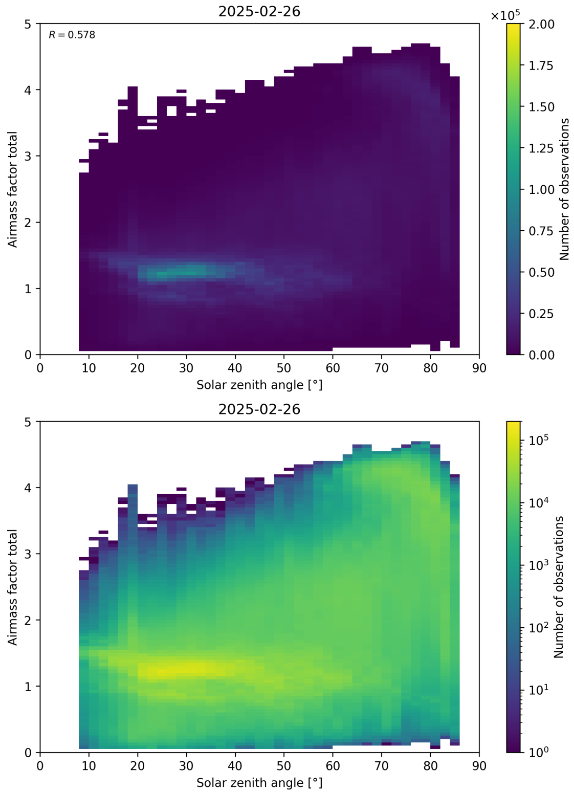
Figure 175: Scatter density plot of “Solar zenith angle” against “Airmass factor total” for 2025-02-25 to 2025-02-27.
