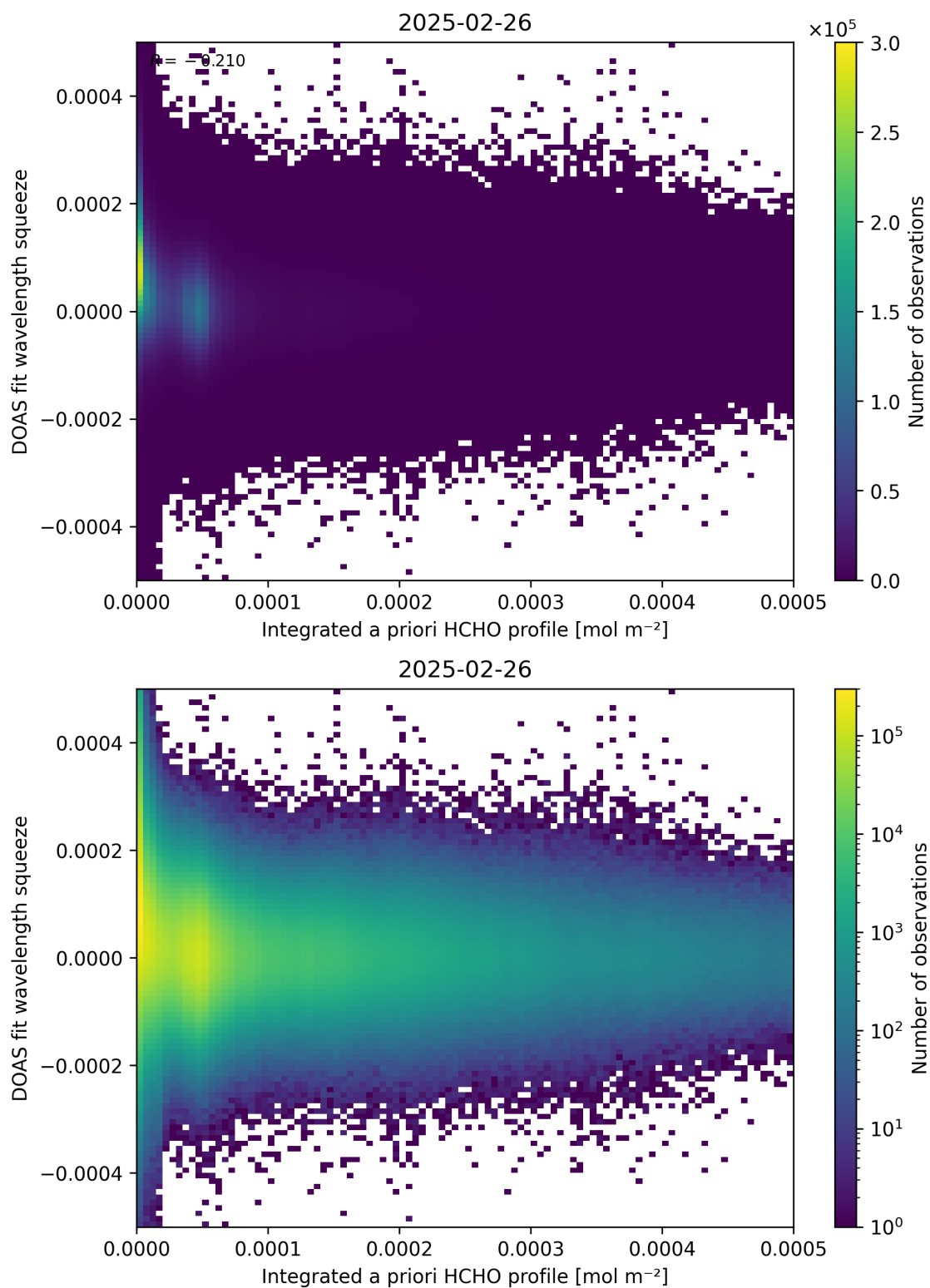
Figure 150: Scatter density plot of “Integrated a priori HCHO profile” against “DOAS fit wavelength squeeze” for 2025-02-25 to 2025-02-27.
