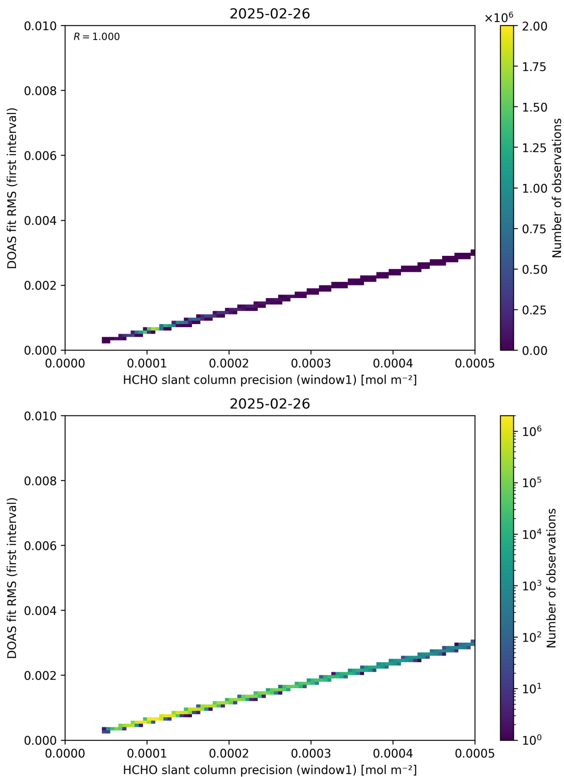
Figure 88: Scatter density plot of “HCHO slant column precision (window1)” against “DOAS fit RMS (first interval)” for 2025-02-25 to 2025-02-27.
