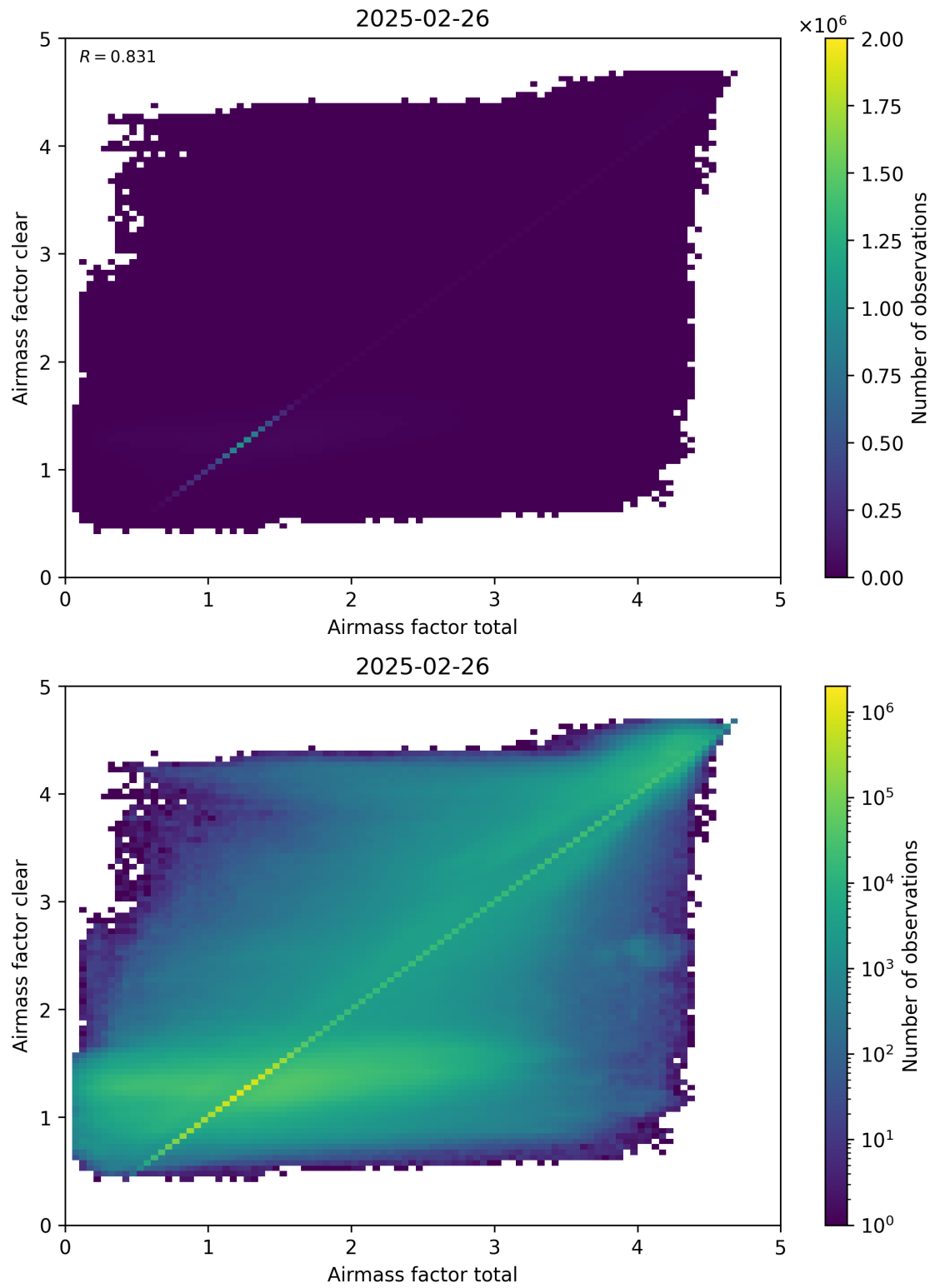
Figure 100: Scatter density plot of “Airmass factor total” against “Airmass factor clear” for 2025-02-25 to 2025-02-27.
