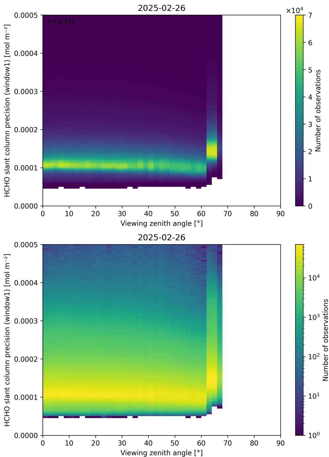
Figure 189: Scatter density plot of “Viewing zenith angle” against “HCHO slant column precision (window1)” for 2025-02-25 to 2025-02-27.
