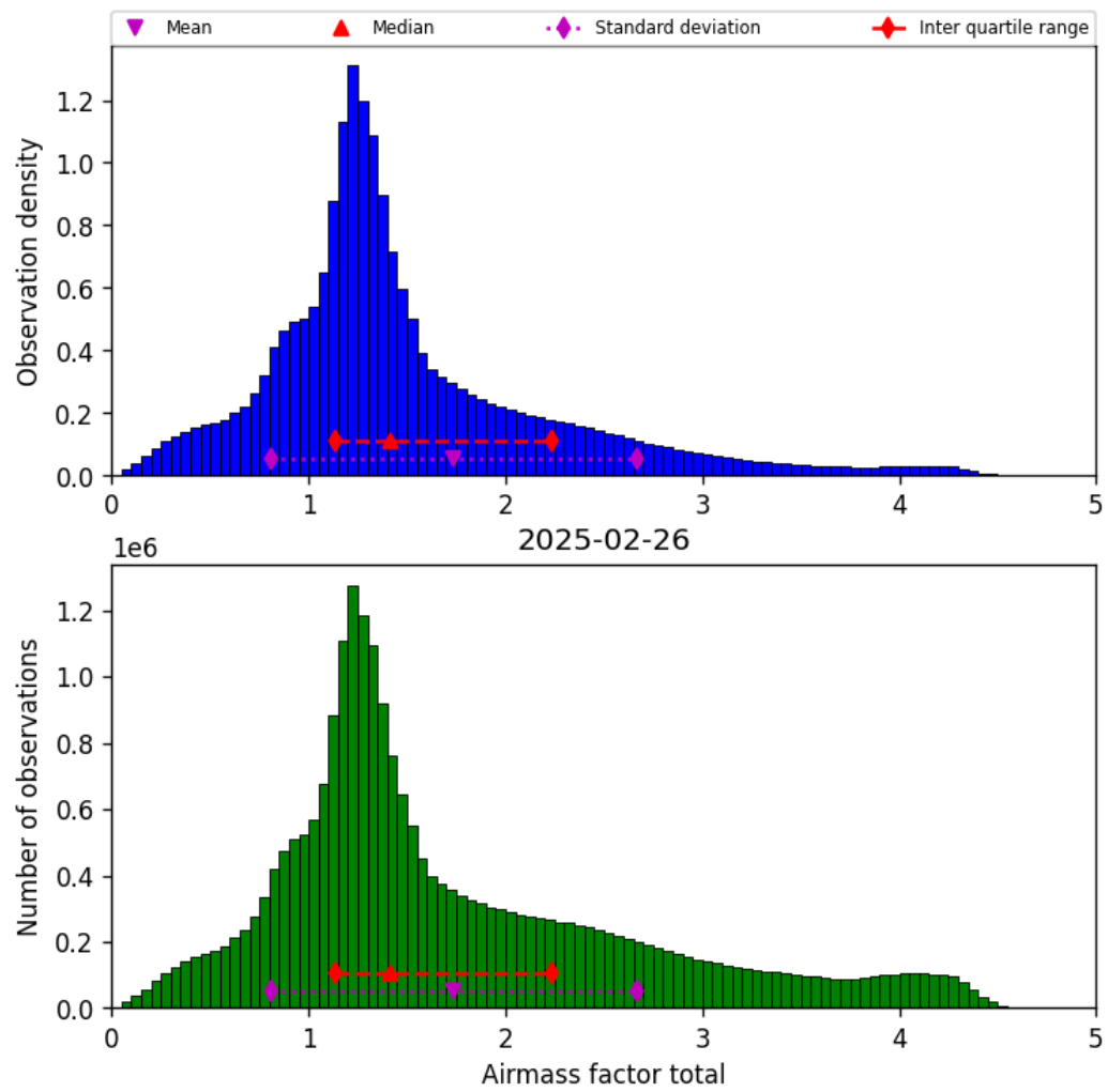
Figure 40: Histogram of “Airmass factor total” for 2025-02-25 to 2025-02-27
