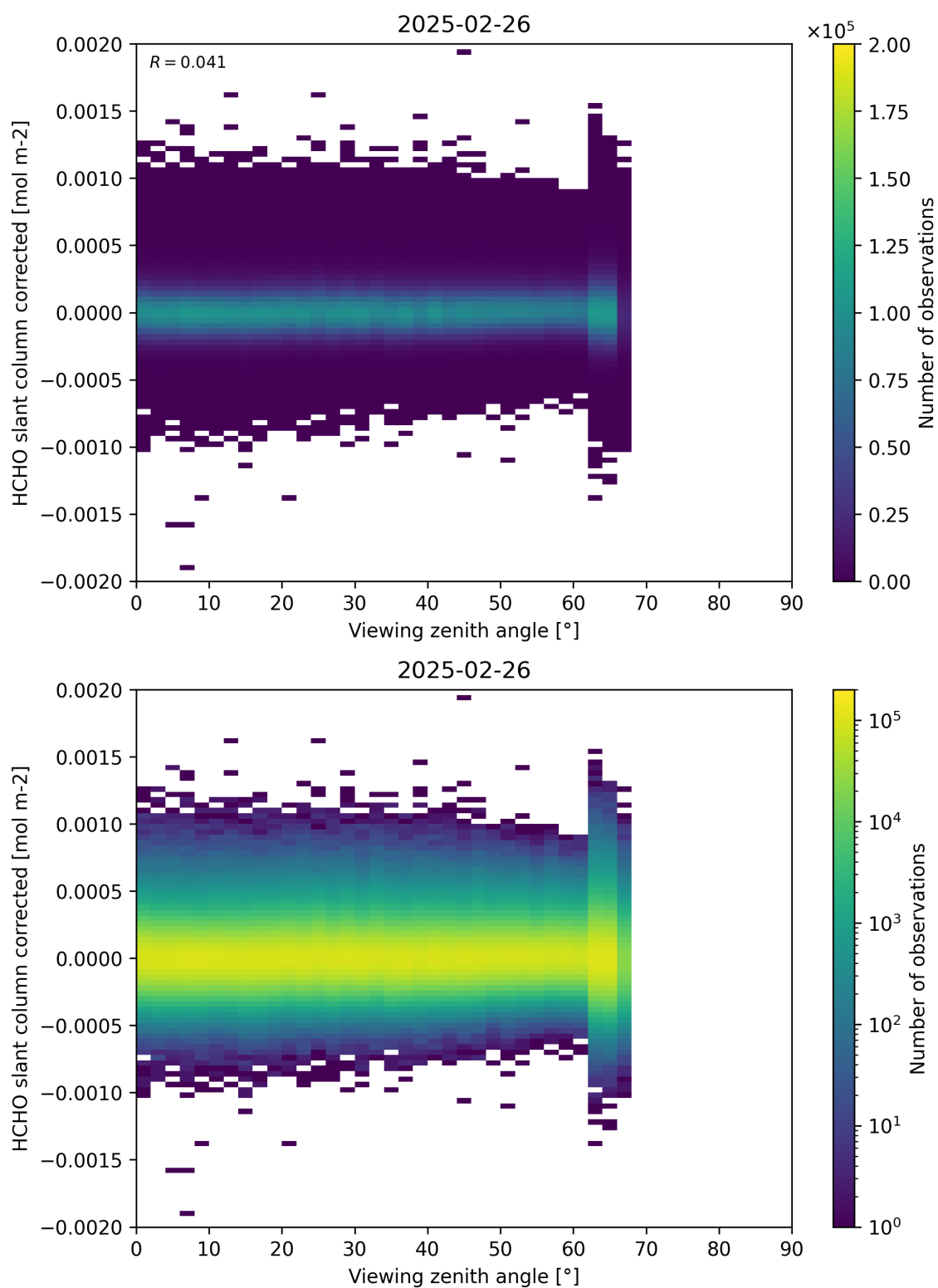
Figure 186: Scatter density plot of “Viewing zenith angle” against “HCHO slant column corrected” for 2025-02-25 to 2025-02-27.
