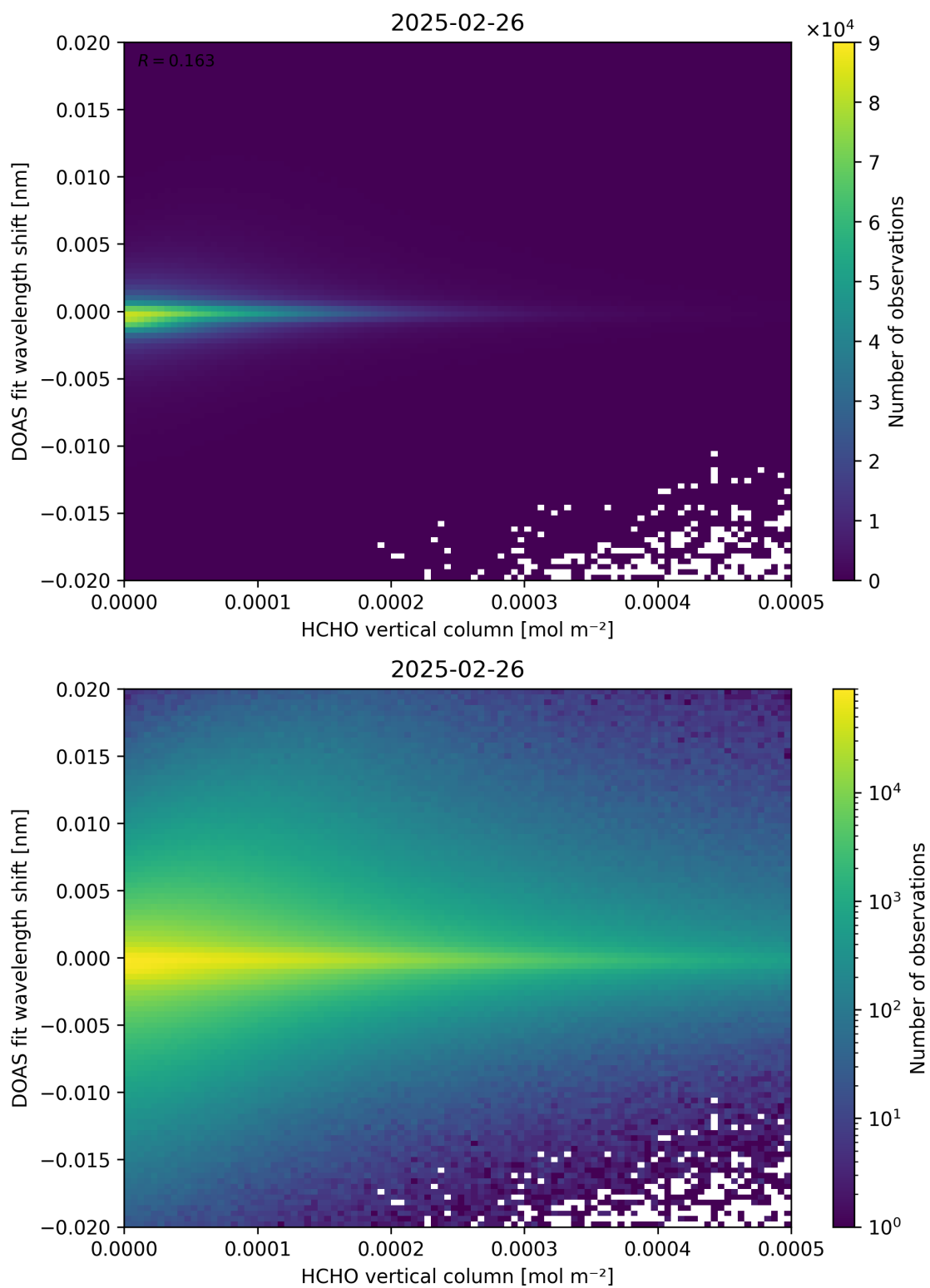
Figure 124: Scatter density plot of “HCHO vertical column” against “DOAS fit wavelength shift” for 2025-02-25 to 2025-02-27.
