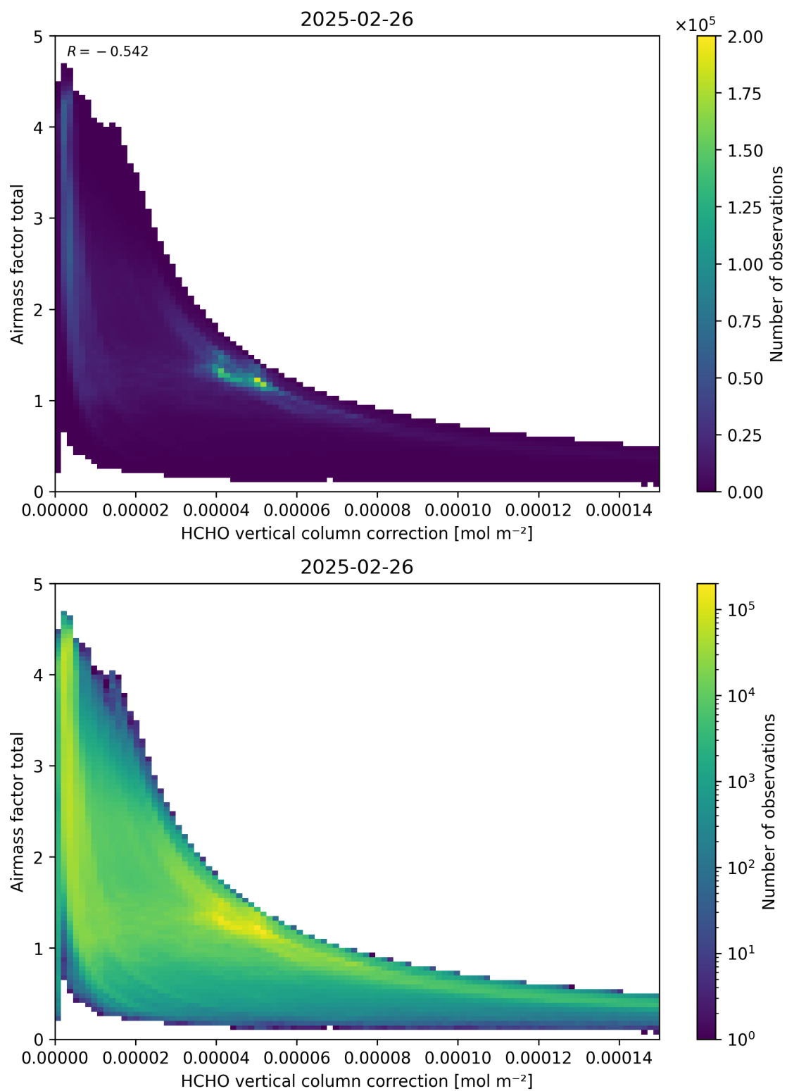
Figure 120: Scatter density plot of “HCHO vertical column correction” against “Airmass factor total” for 2025-02-25 to 2025-02-27.
