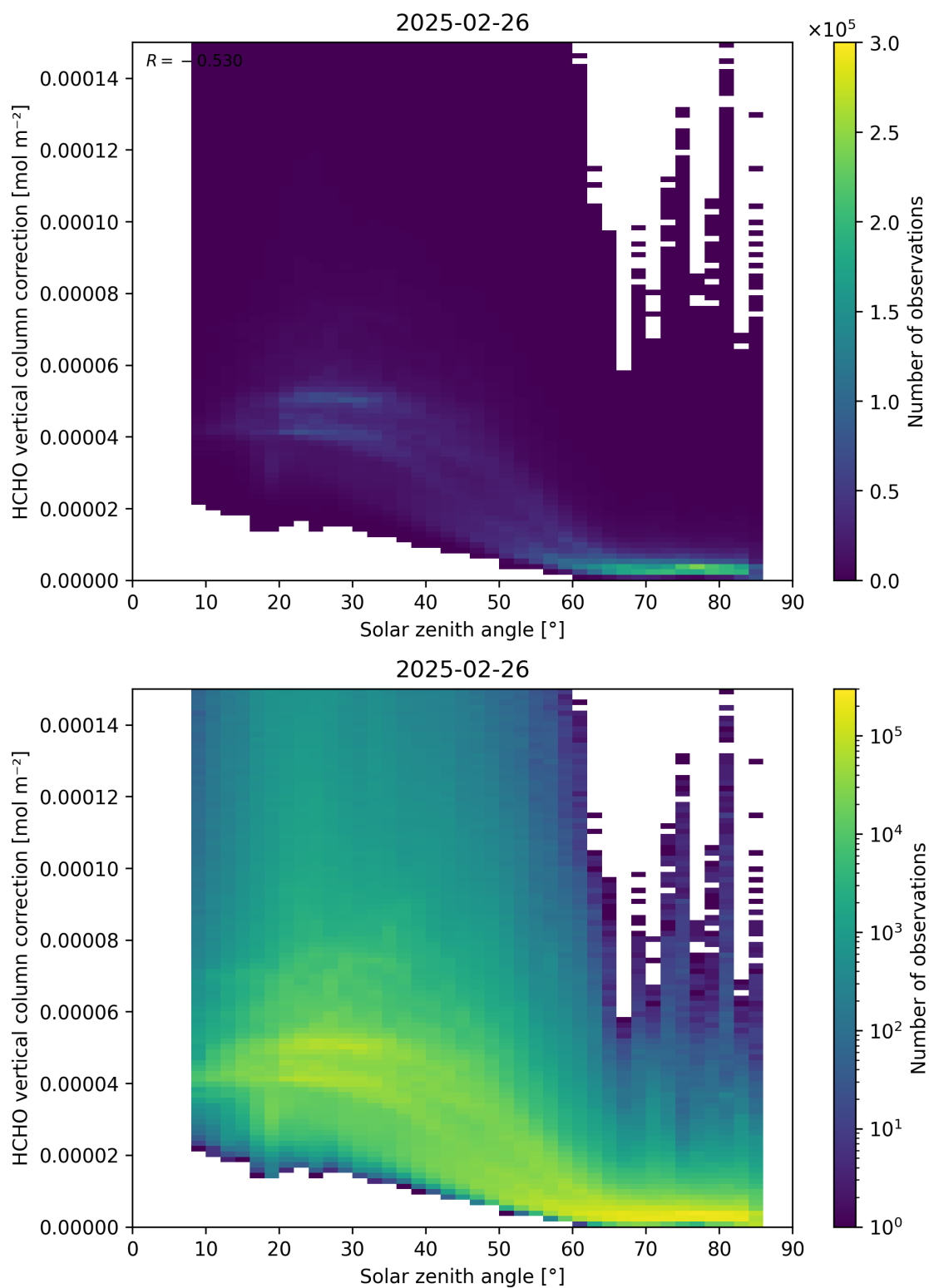
Figure 178: Scatter density plot of “Solar zenith angle” against “HCHO vertical column correction” for 2025-02-25 to 2025-02-27.
