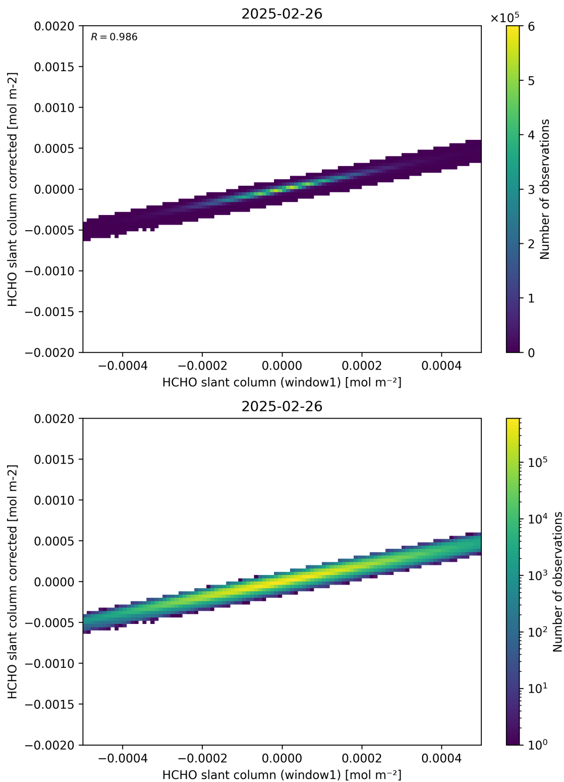
Figure 82: Scatter density plot of “HCHO slant column (window1)” against “HCHO slant column corrected” for 2025-02-25 to 2025-02-27.
