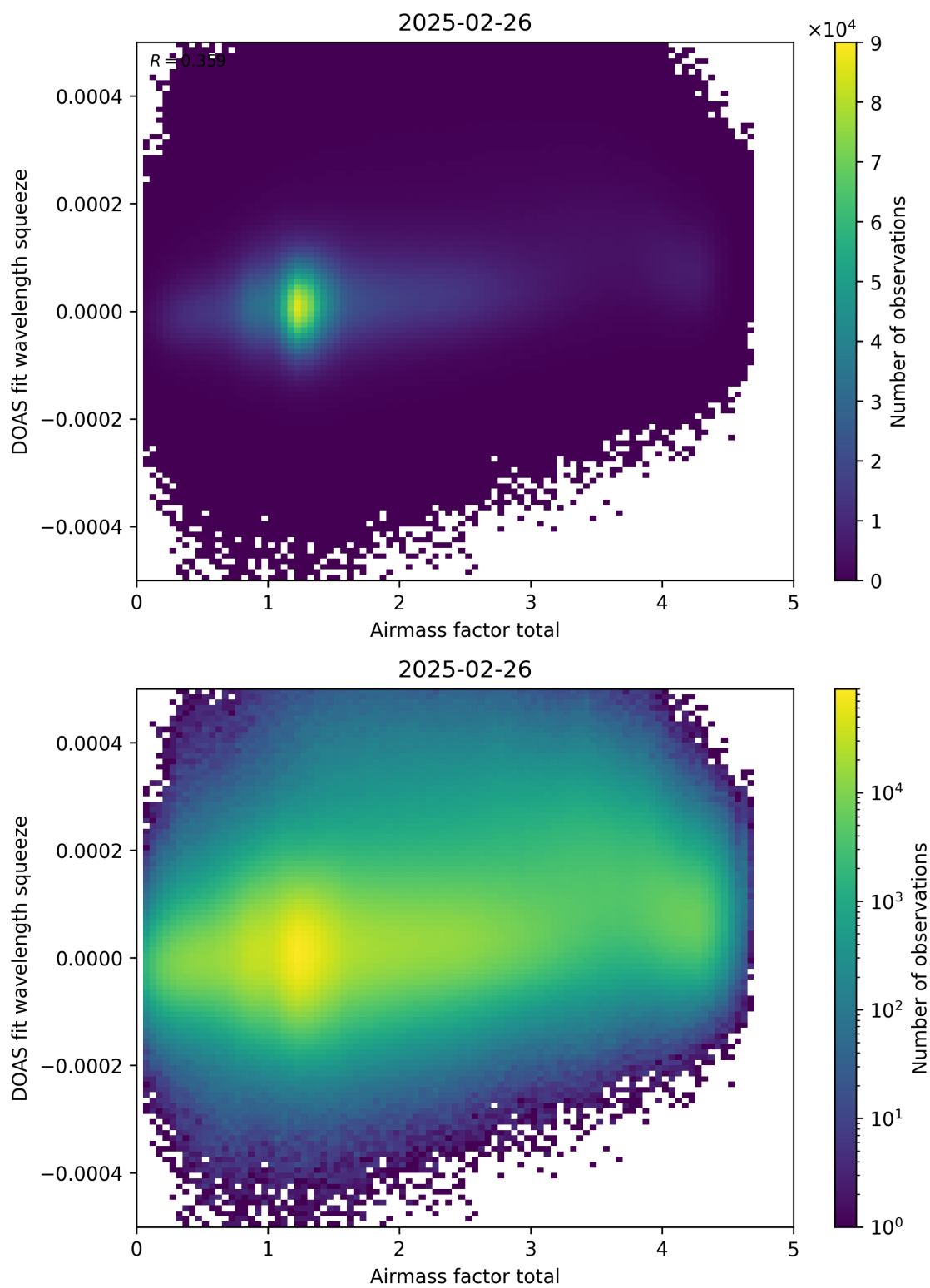
Figure 99: Scatter density plot of “Airmass factor total” against “DOAS fit wavelength squeeze” for 2025-02-25 to 2025-02-27.
