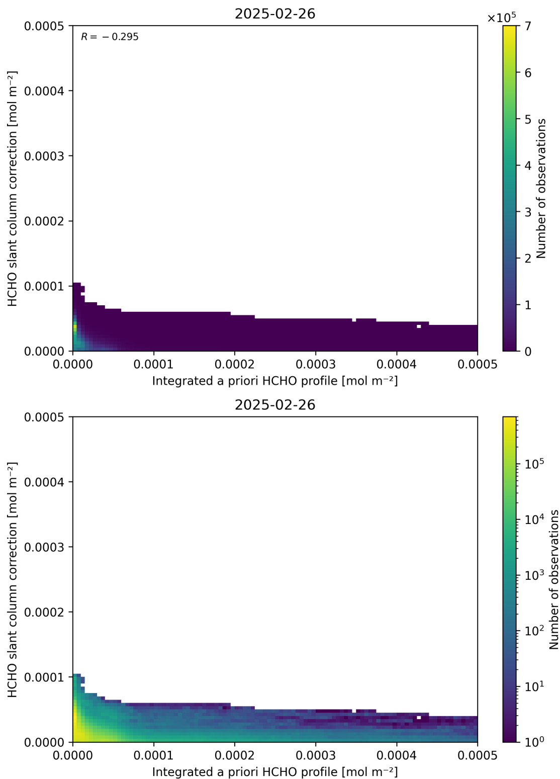
Figure 152: Scatter density plot of “Integrated a priori HCHO profile” against “HCHO slant column correction” for 2025-02-25 to 2025-02-27.
