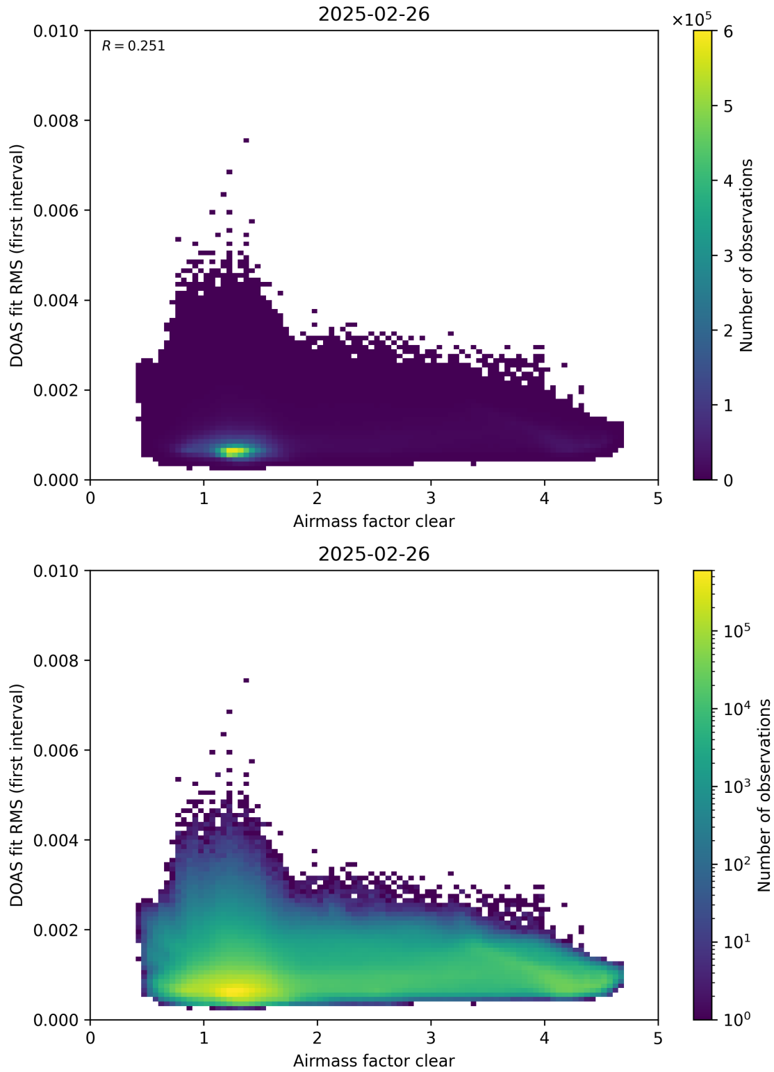
Figure 71: Scatter density plot of “Airmass factor clear” against “DOAS fit RMS (first interval)” for 2025-02-25 to 2025-02-27.
