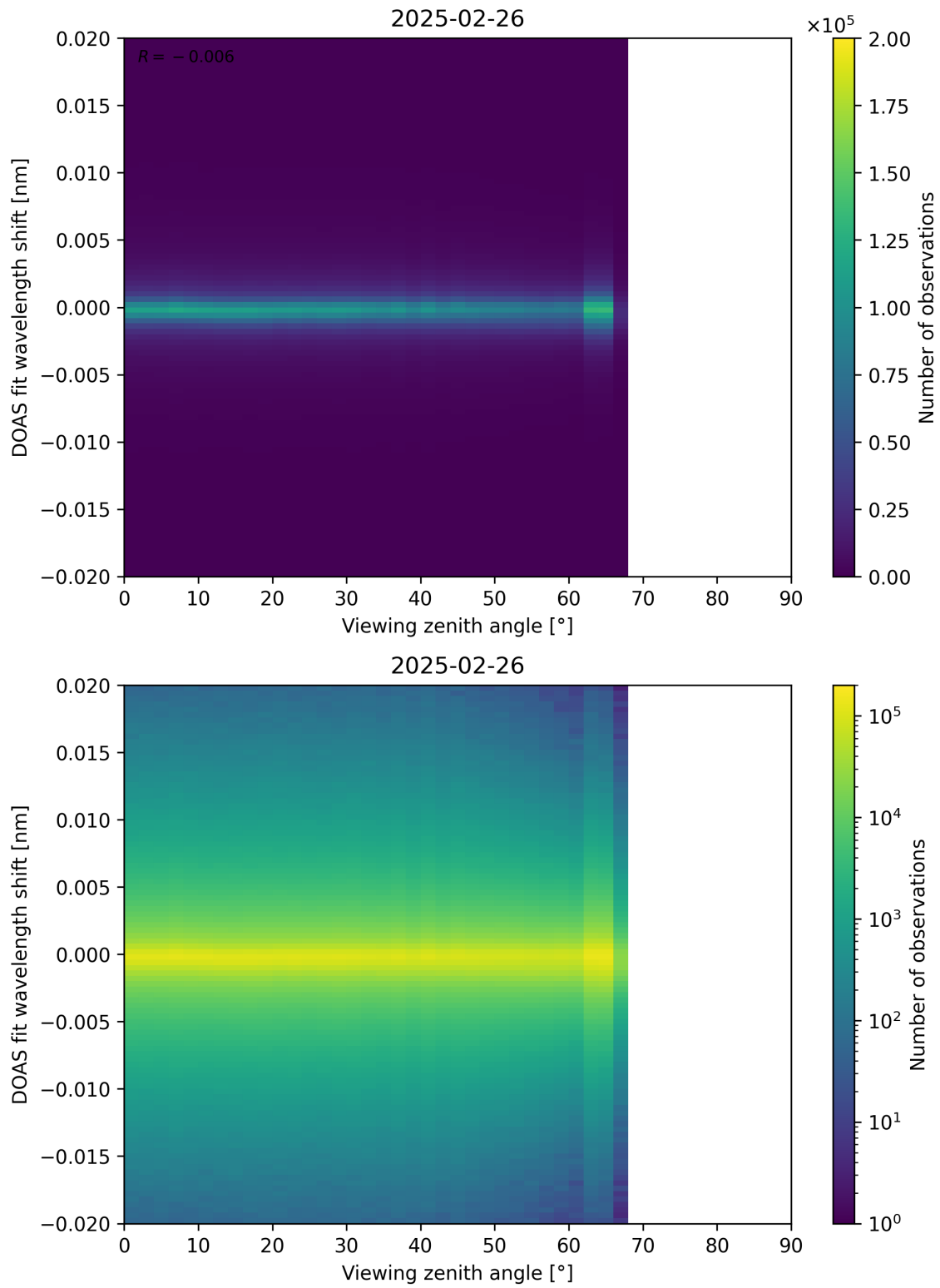
Figure 183: Scatter density plot of “Viewing zenith angle” against “DOAS fit wavelength shift” for 2025-02-25 to 2025-02-27.
