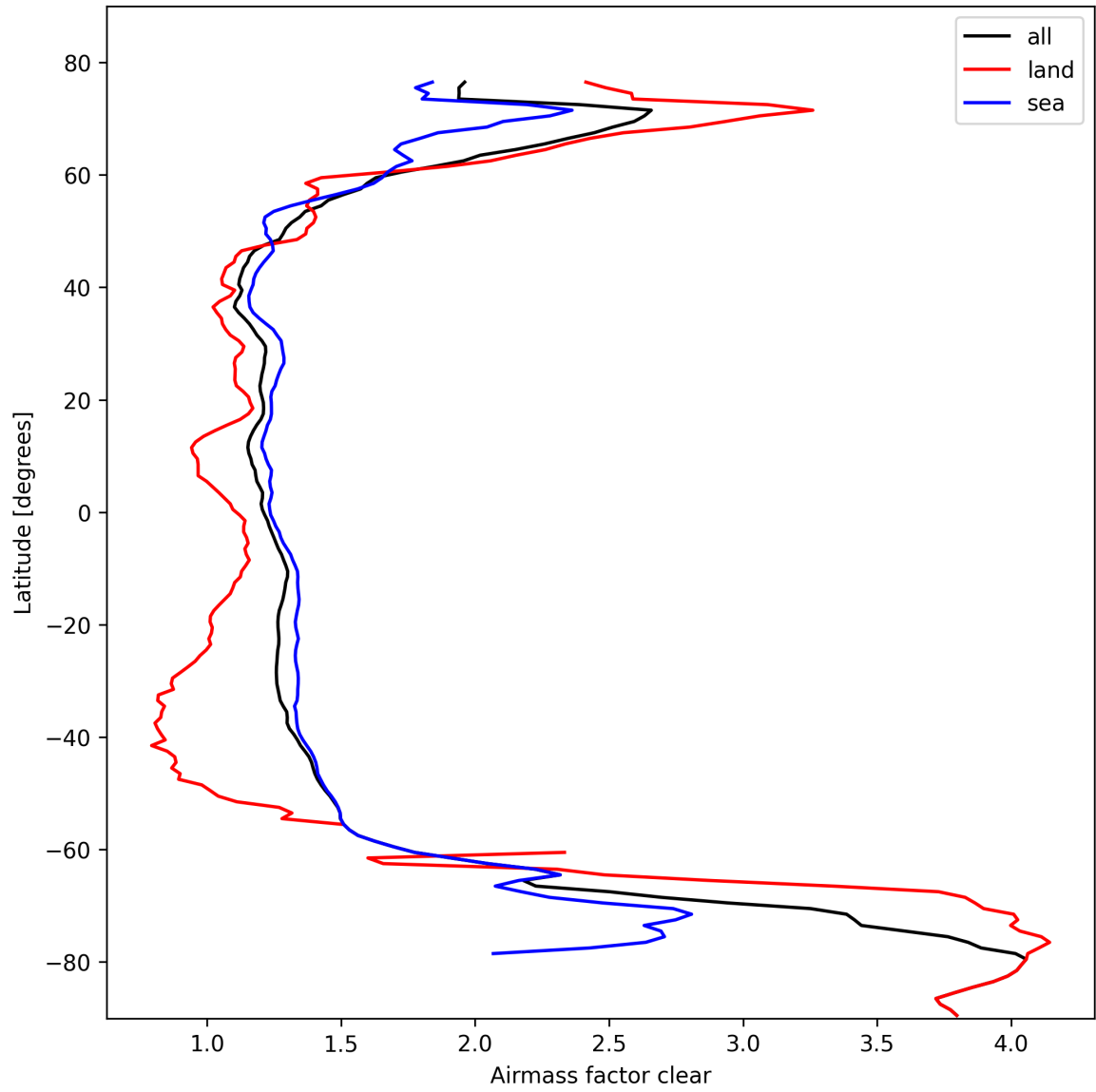
Figure 28: Zonal average of “Airmass factor clear” for 2025-02-25 to 2025-02-27.
