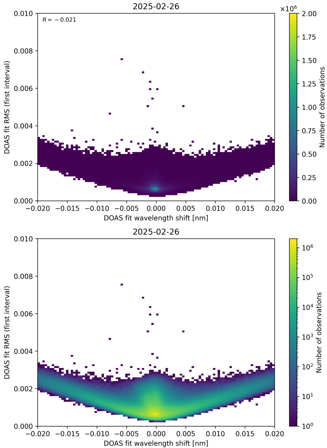
Figure 64: Scatter density plot of “DOAS fit wavelength shift” against “DOAS fit RMS (first interval)” for 2025-02-25 to 2025-02-27.
