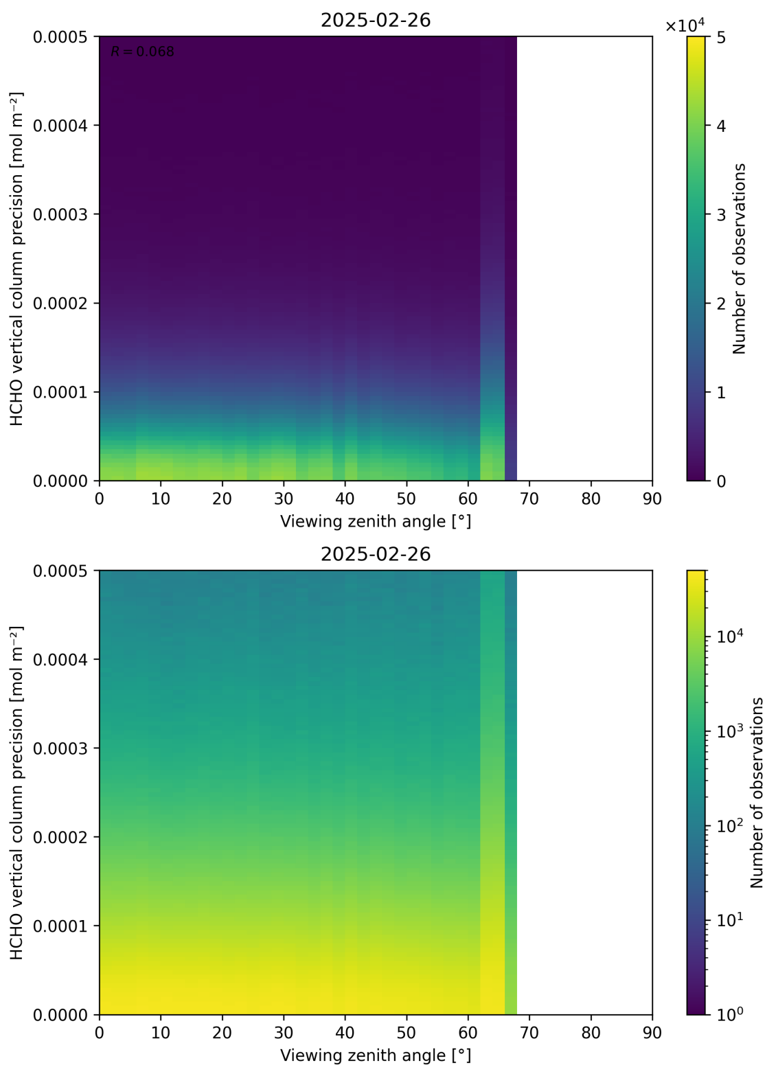
Figure 194: Scatter density plot of “Viewing zenith angle” against “HCHO vertical column precision” for 2025-02-25 to 2025-02-27.
