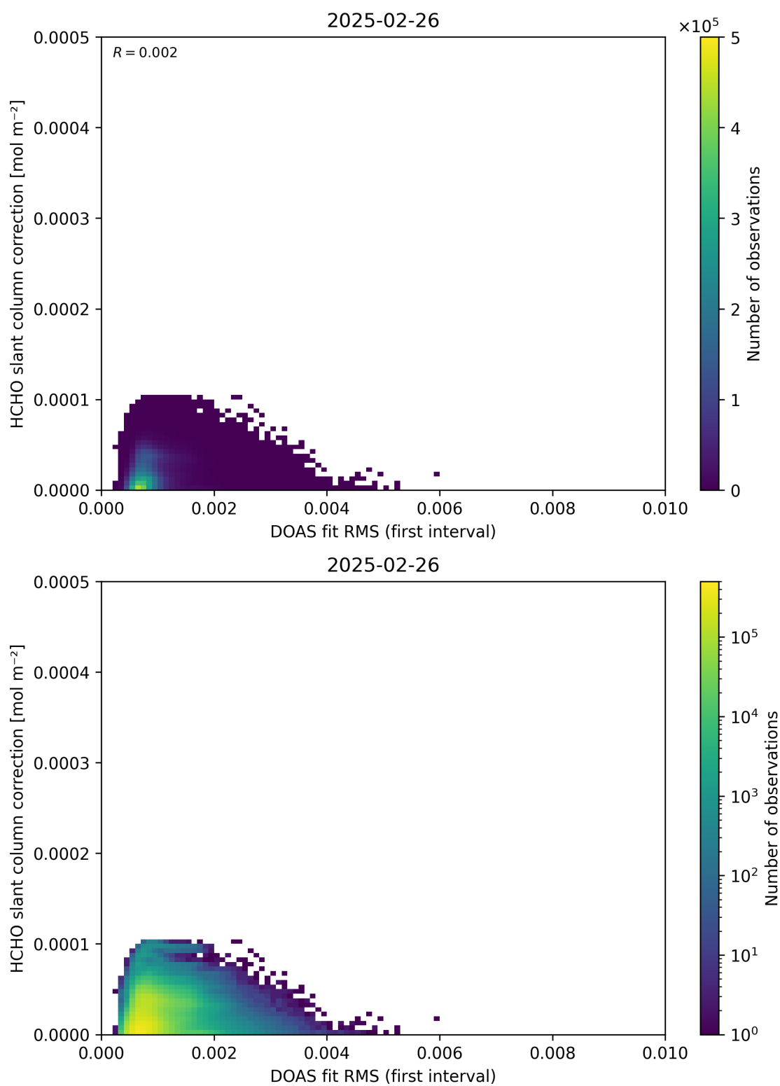
Figure 63: Scatter density plot of “DOAS fit RMS (first interval)” against “HCHO slant column correction” for 2025-02-25 to 2025-02-27.
