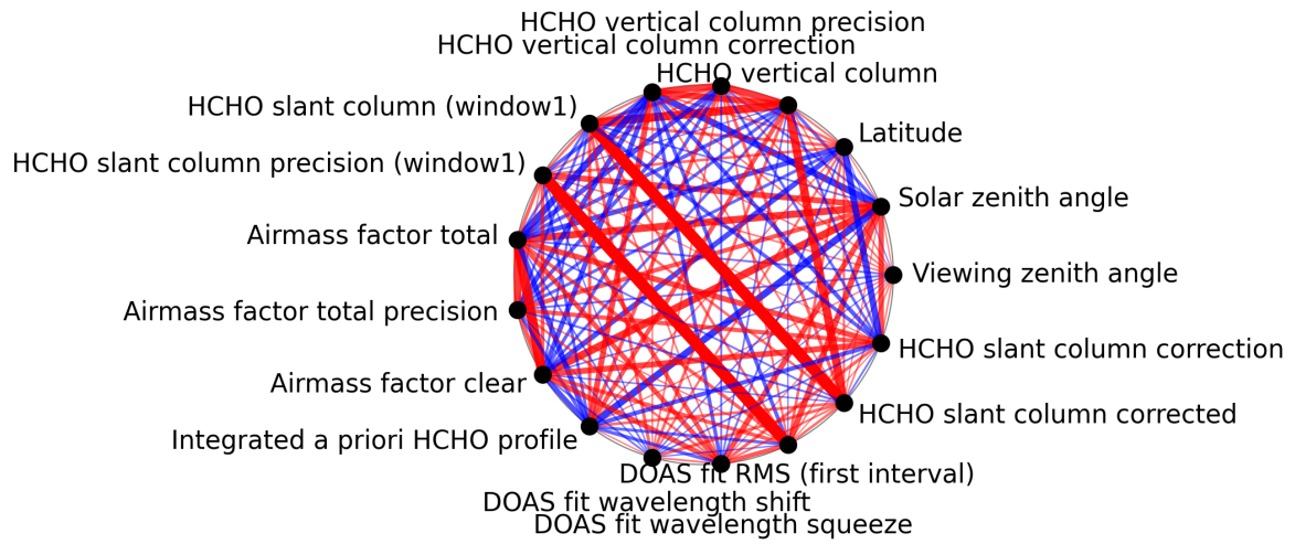
Figure 1: Map of correlation graph for 2025-02-25 to 2025-02-27.
