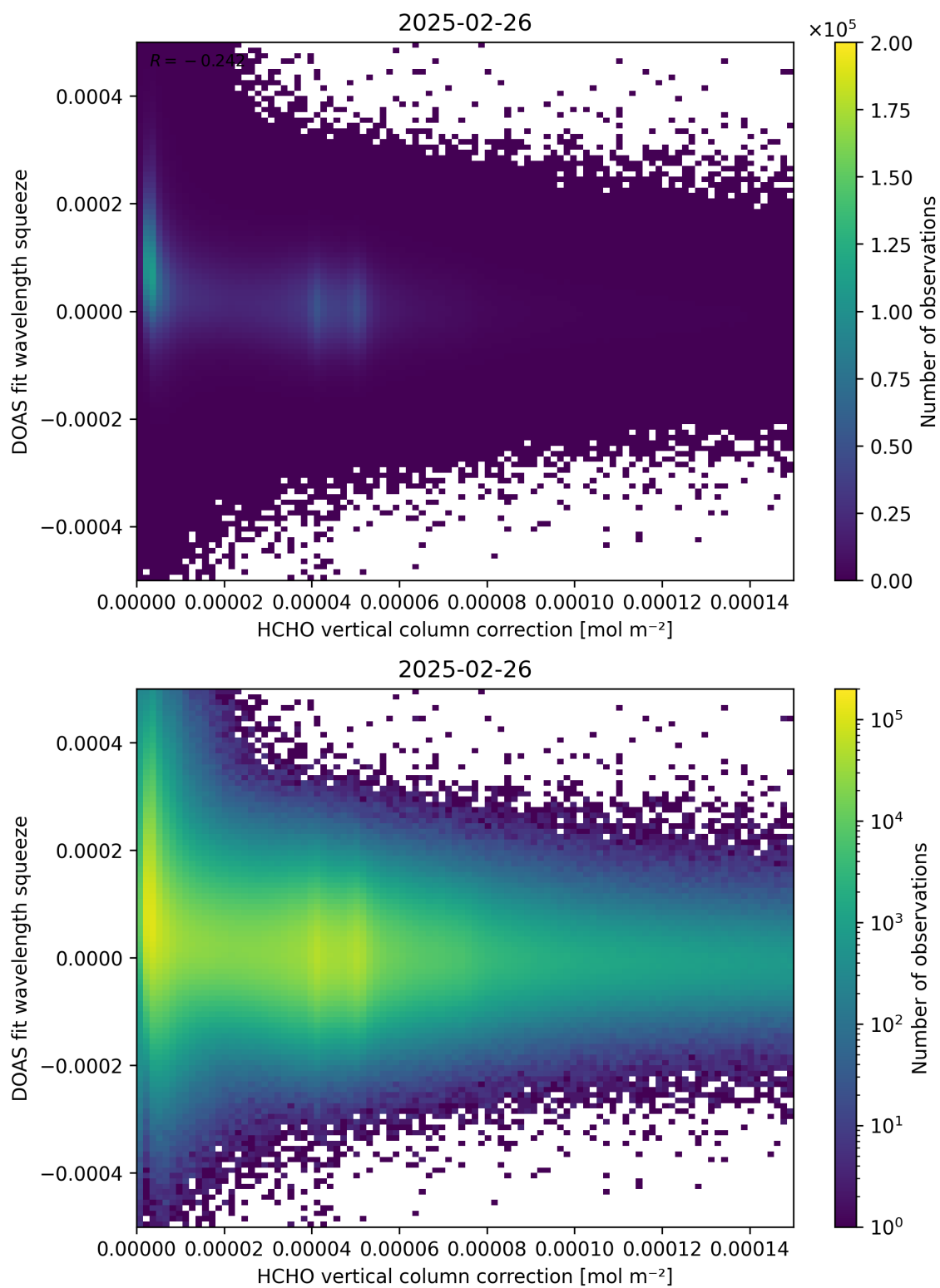
Figure 114: Scatter density plot of “HCHO vertical column correction” against “DOAS fit wavelength squeeze” for 2025-02-25 to 2025-02-27.
