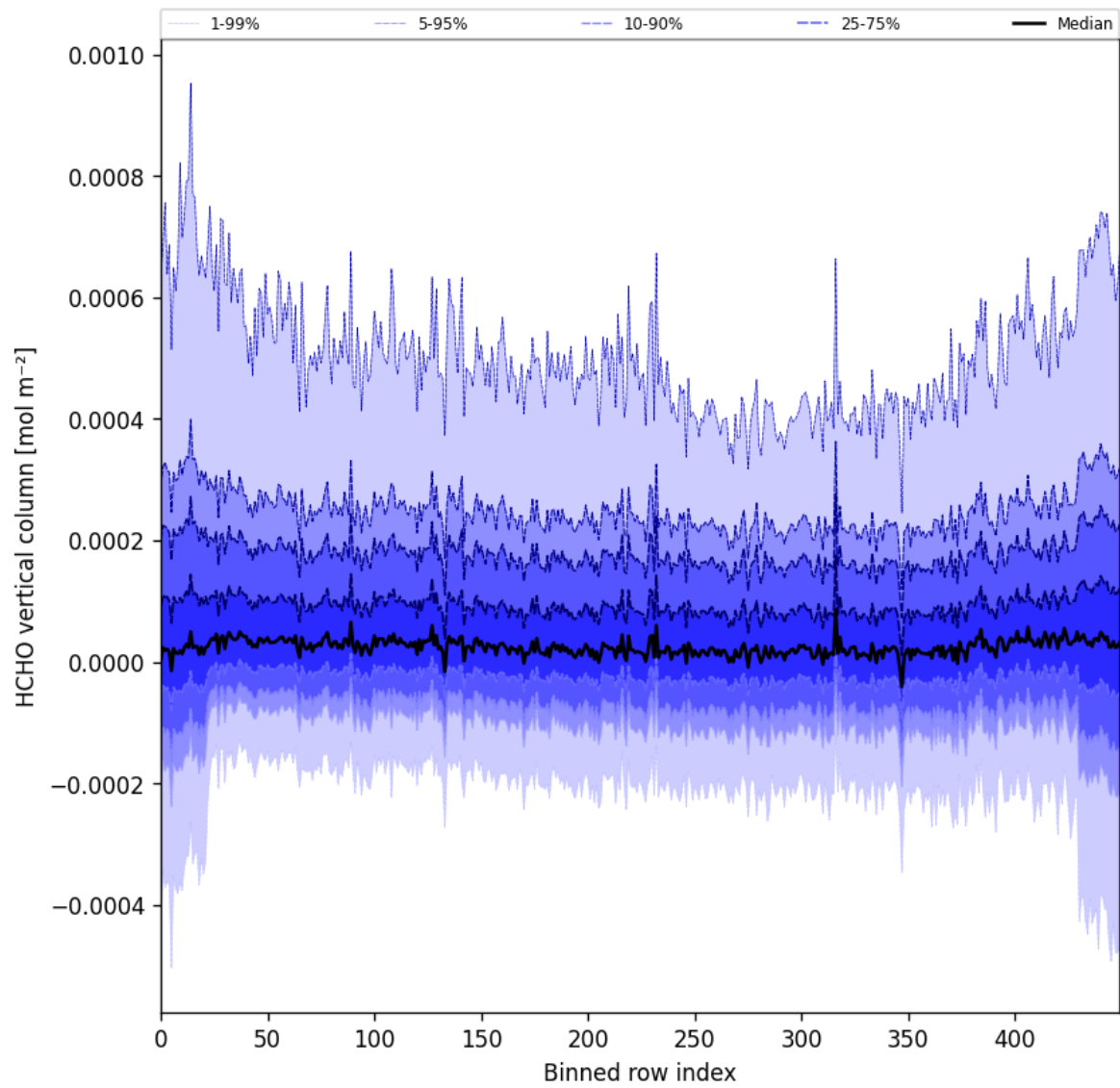
Figure 49: Along track statistics of “HCHO vertical column” for 2025-02-25 to 2025-02-27
