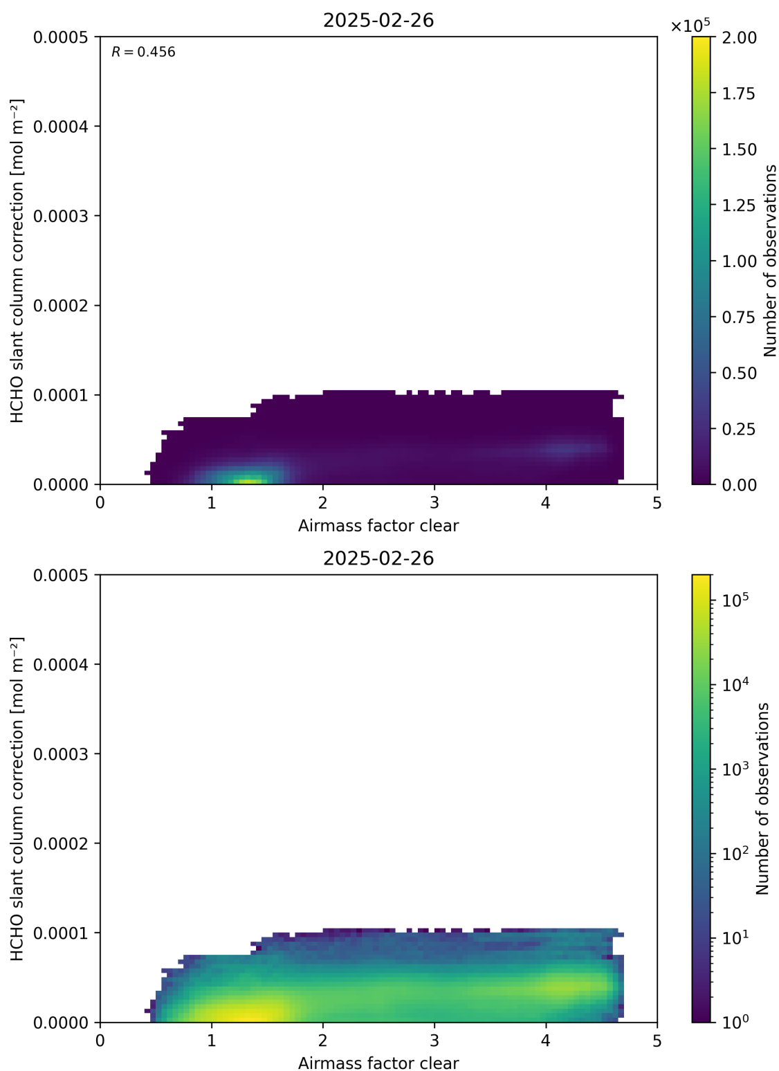
Figure 75: Scatter density plot of “Airmass factor clear” against “HCHO slant column correction” for 2025-02-25 to 2025-02-27.
