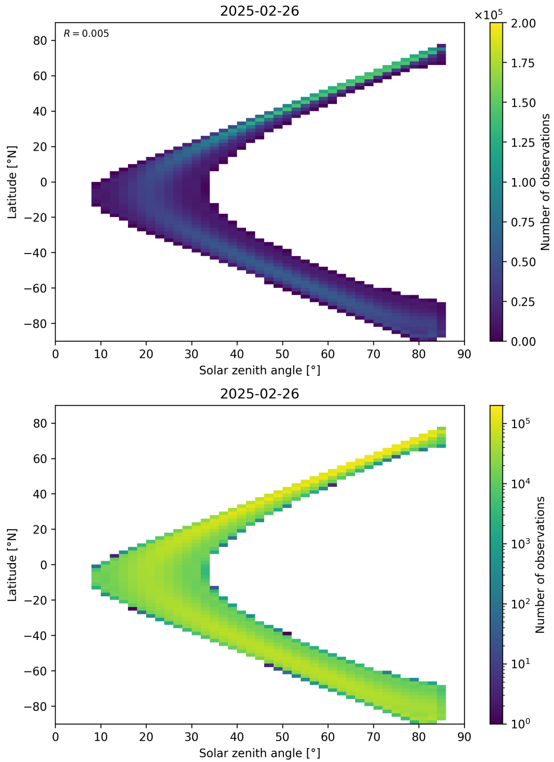
Figure 181: Scatter density plot of “Solar zenith angle” against “Latitude” for 2025-02-25 to 2025-02-27.
