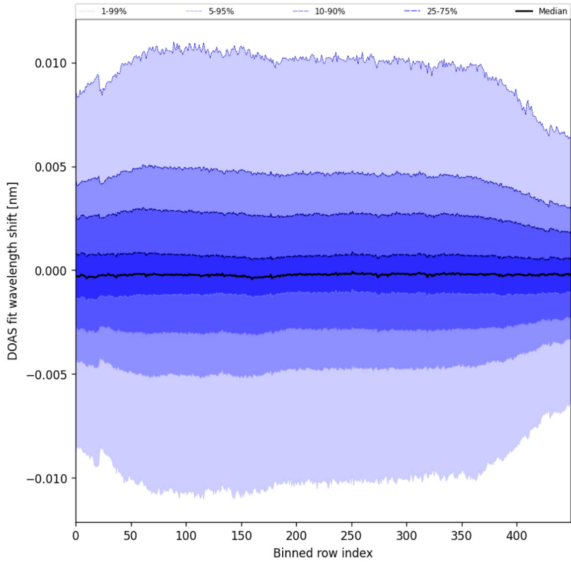
Figure 58: Along track statistics of “DOAS fit wavelength shift” for 2025-02-25 to 2025-02-27
