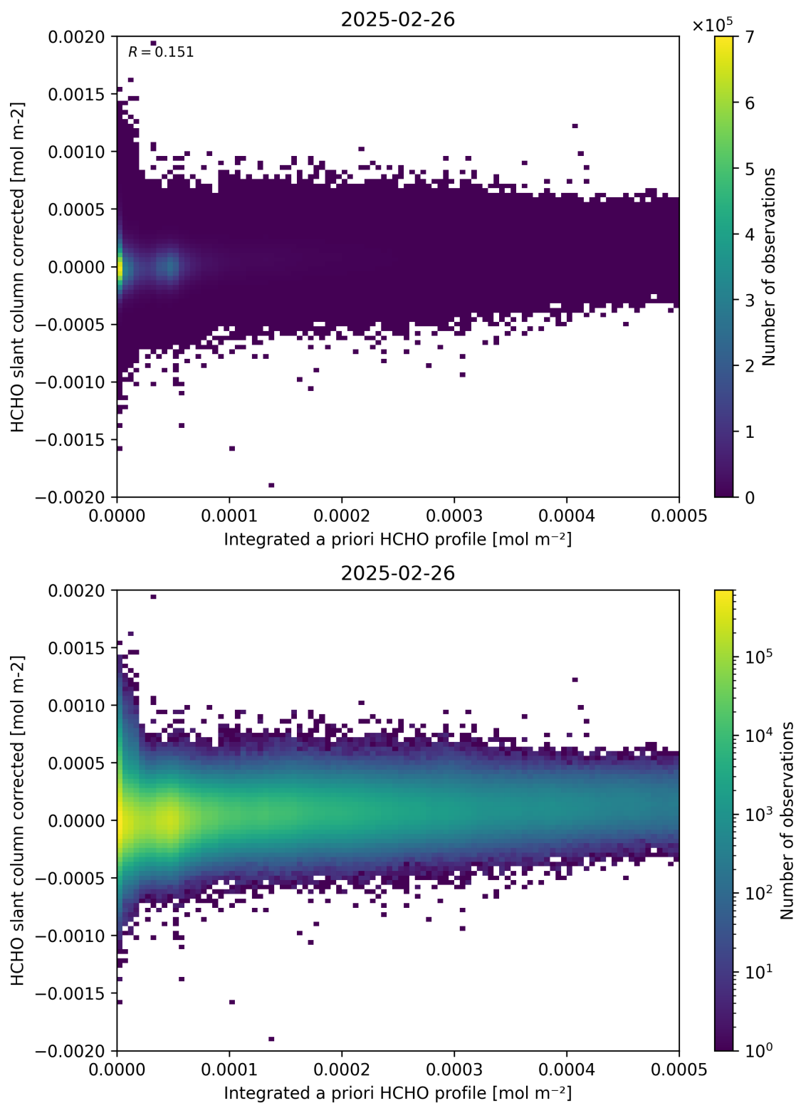
Figure 151: Scatter density plot of “Integrated a priori HCHO profile” against “HCHO slant column corrected” for 2025-02-25 to 2025-02-27.
