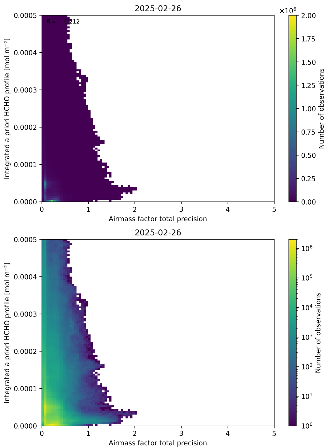
Figure 111: Scatter density plot of “Airmass factor total precision” against “Integrated a priori HCHO profile” for 2025-02-25 to 2025-02-27.
