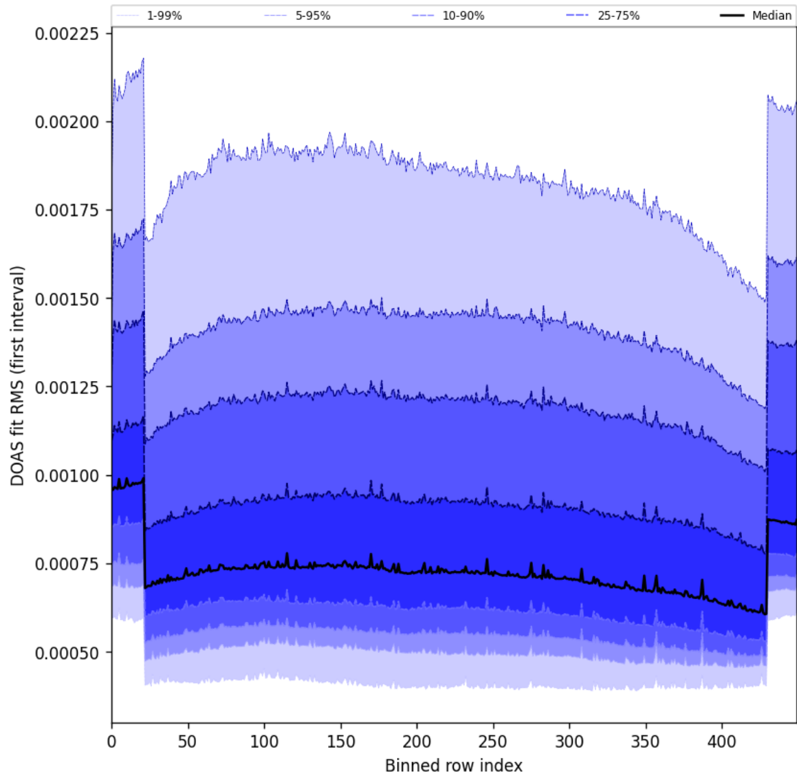
Figure 60: Along track statistics of “DOAS fit RMS (first interval)” for 2025-02-25 to 2025-02-27
