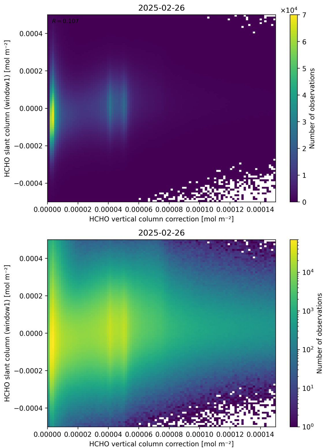
Figure 118: Scatter density plot of “HCHO vertical column correction” against “HCHO slant column (window1)” for 2025-02-25 to 2025-02-27.
