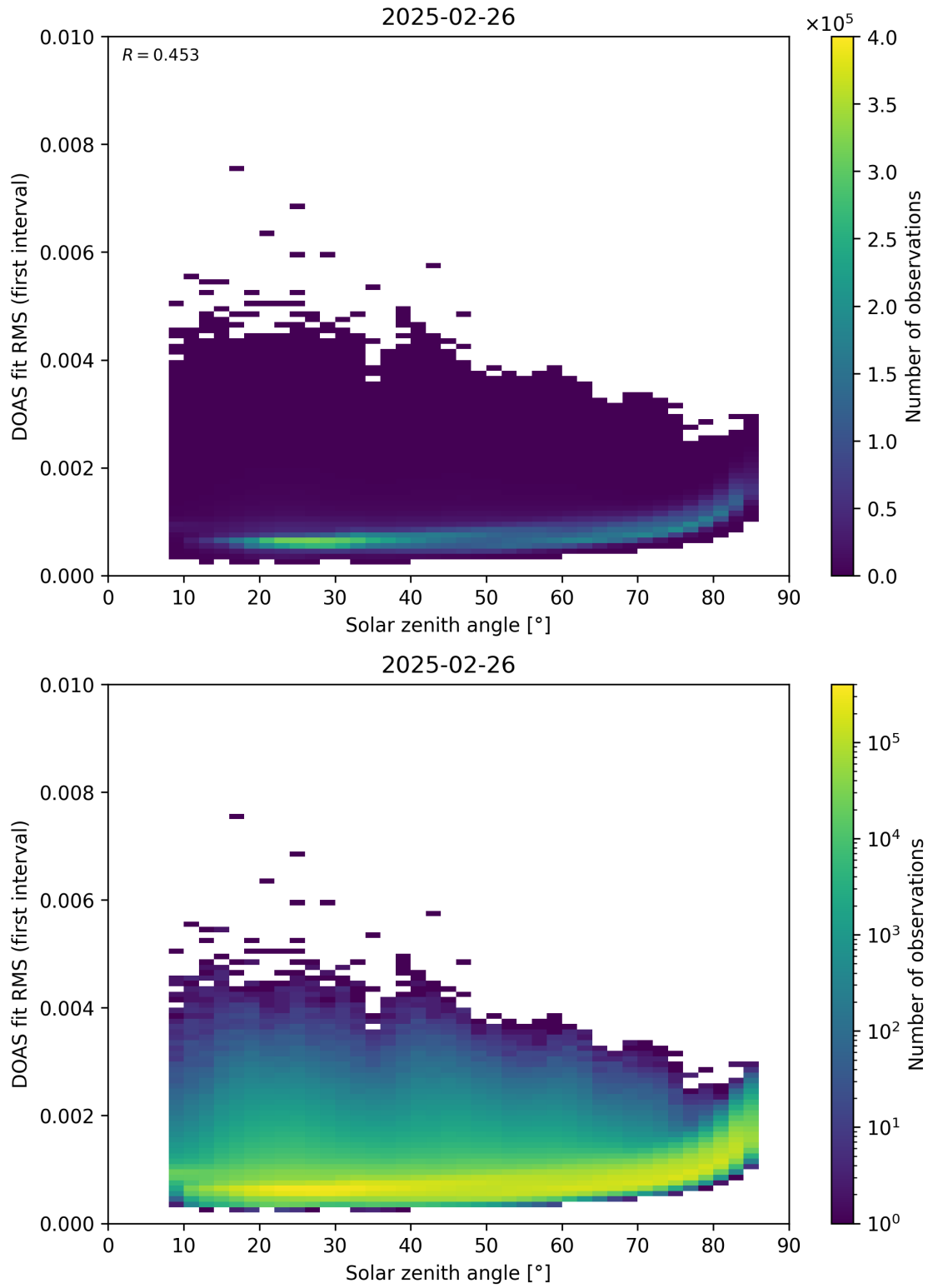
Figure 167: Scatter density plot of “Solar zenith angle” against “DOAS fit RMS (first interval)” for 2025-02-25 to 2025-02-27.
