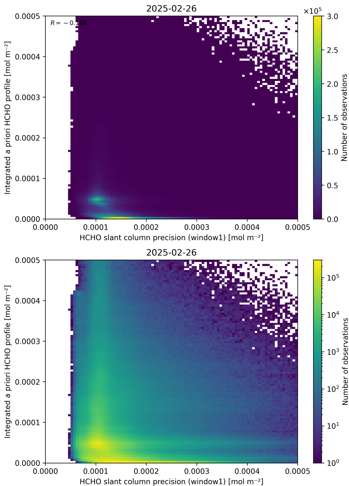
Figure 96: Scatter density plot of “HCHO slant column precision (window1)” against “Integrated a priori HCHO profile” for 2025-02-25 to 2025-02-27.
