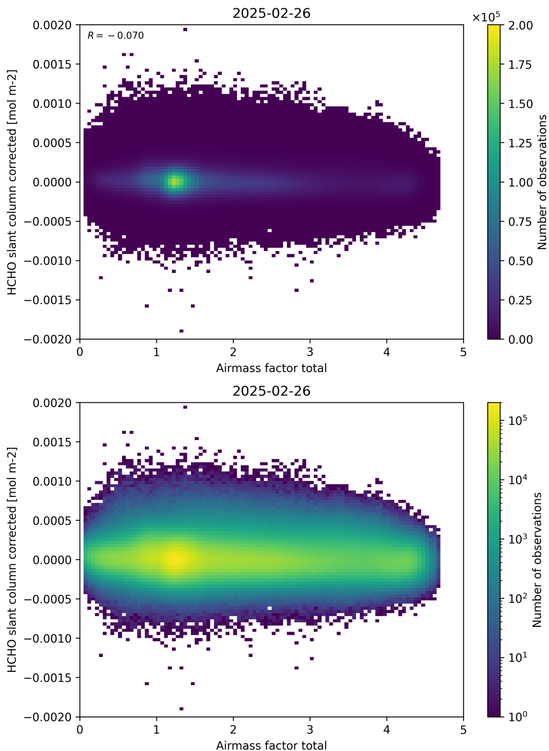
Figure 101: Scatter density plot of “Airmass factor total” against “HCHO slant column corrected” for 2025-02-25 to 2025-02-27.
