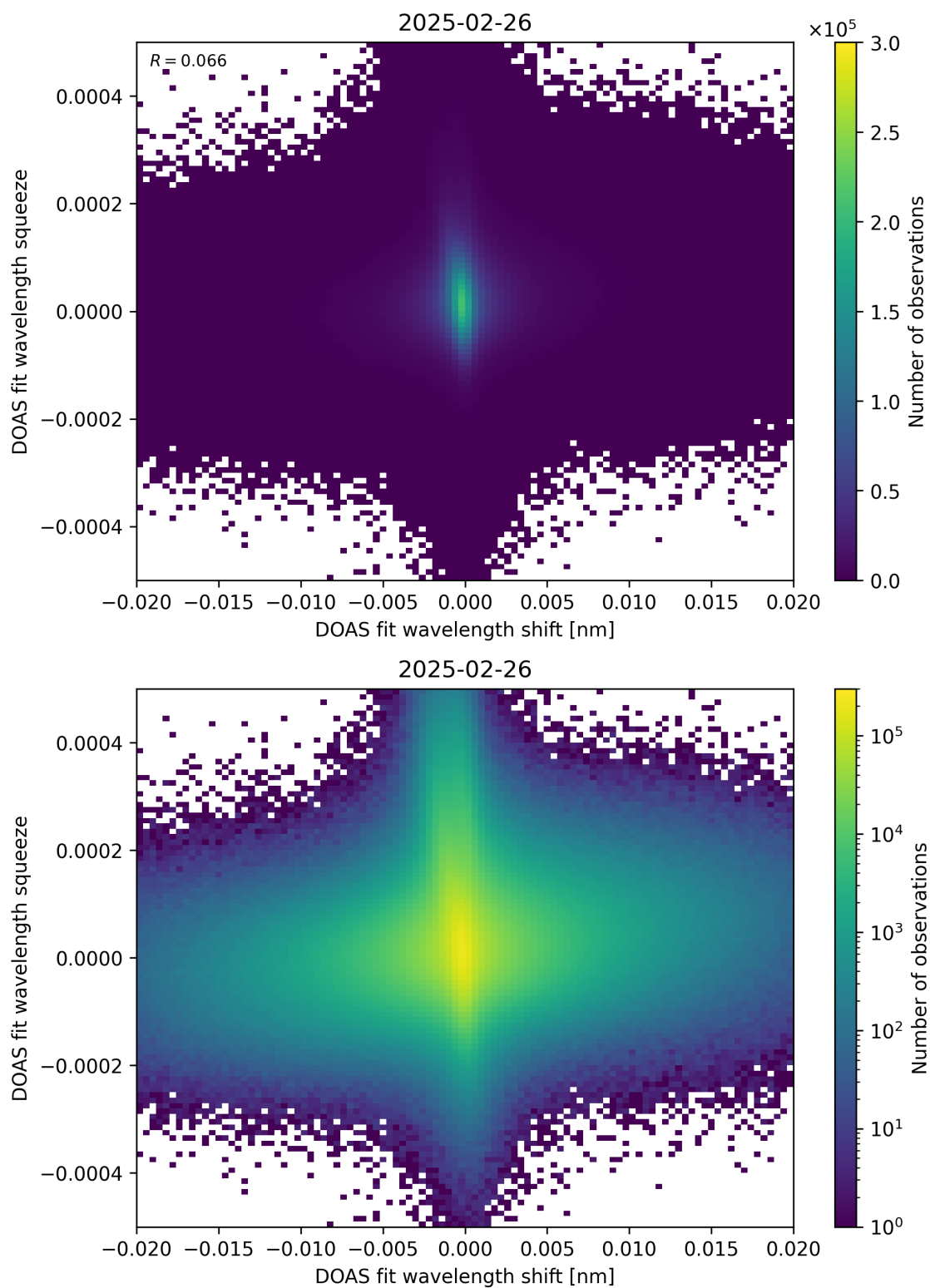
Figure 65: Scatter density plot of “DOAS fit wavelength shift” against “DOAS fit wavelength squeeze” for 2025-02-25 to 2025-02-27.
