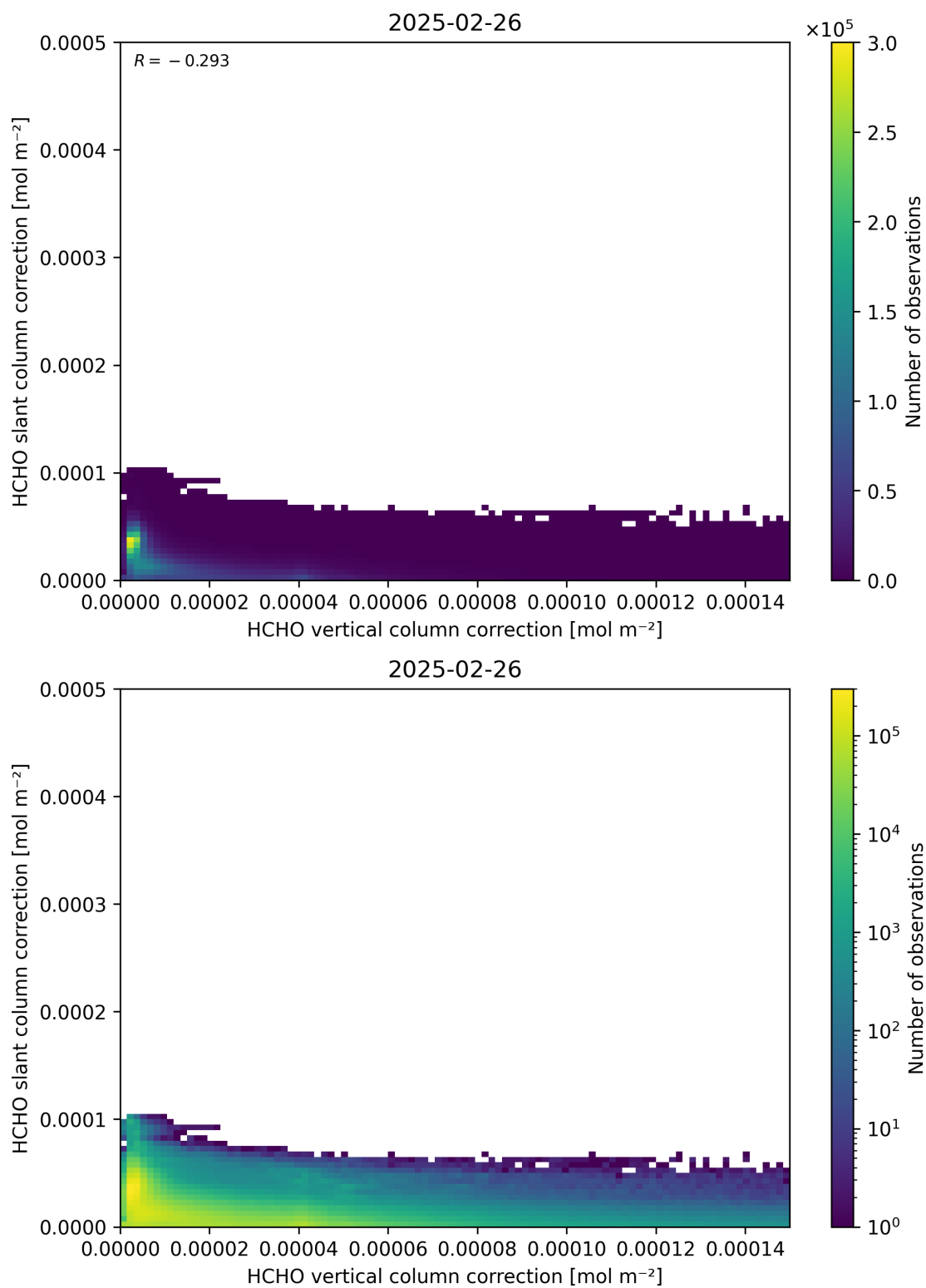
Figure 117: Scatter density plot of “HCHO vertical column correction” against “HCHO slant column correction” for 2025-02-25 to 2025-02-27.
