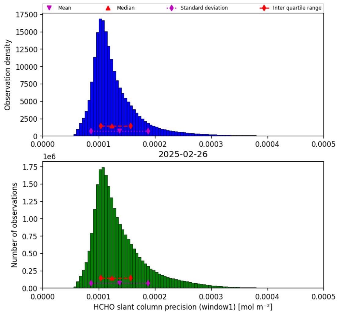
Figure 39: Histogram of “HCHO slant column precision (window1)” for 2025-02-25 to 2025-02-27
