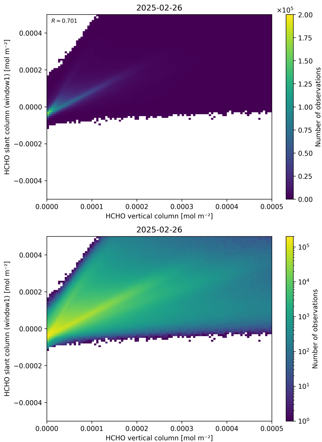
Figure 129: Scatter density plot of “HCHO vertical column” against “HCHO slant column (window1)” for 2025-02-25 to 2025-02-27.
