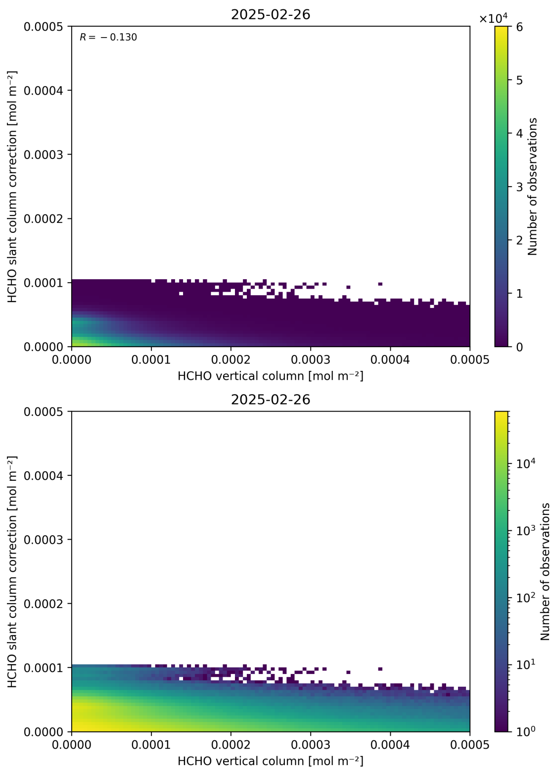
Figure 128: Scatter density plot of “HCHO vertical column” against “HCHO slant column correction” for 2025-02-25 to 2025-02-27.
