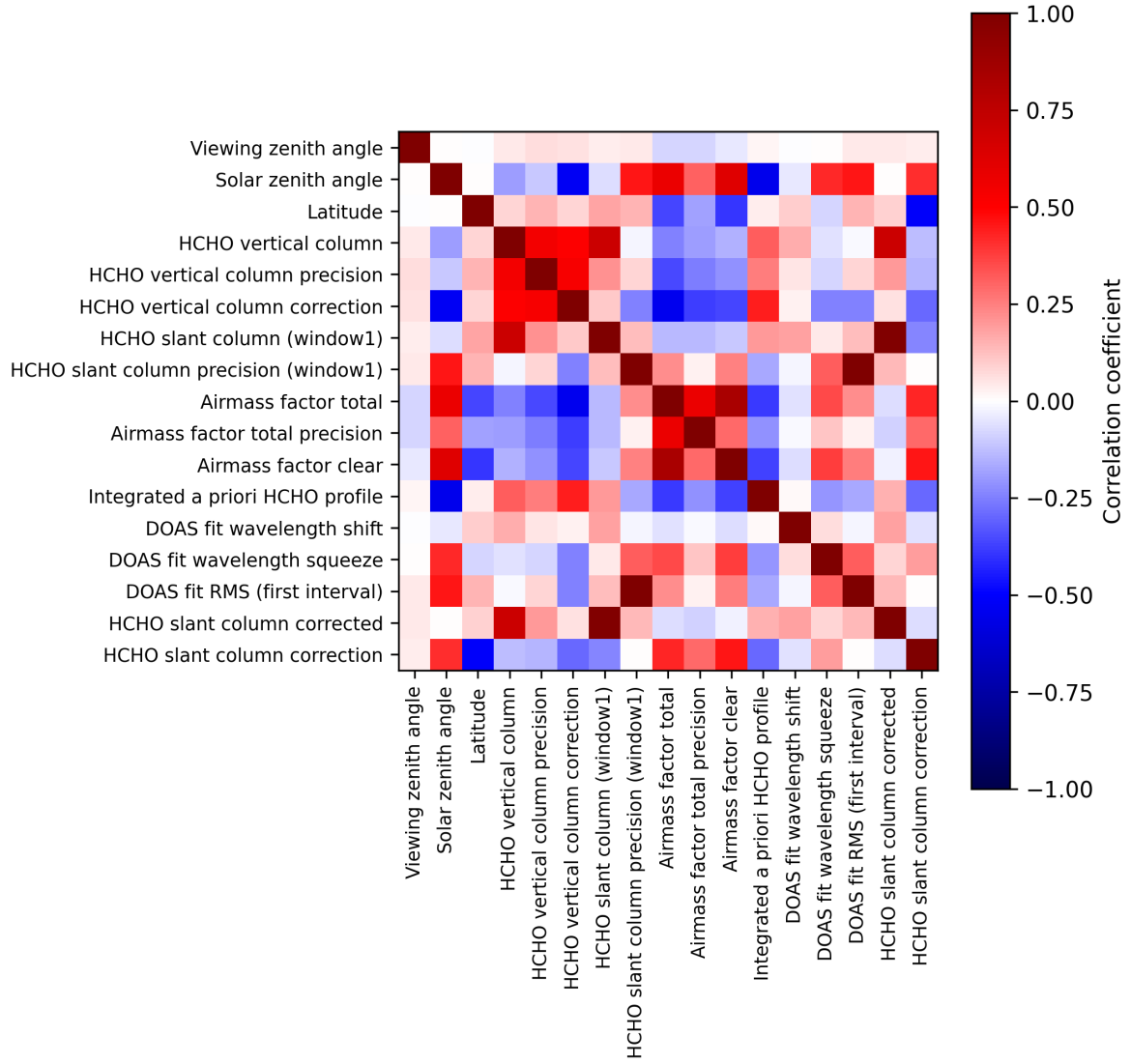
Figure 2: Map of correlation matrix for 2025-02-25 to 2025-02-27.
