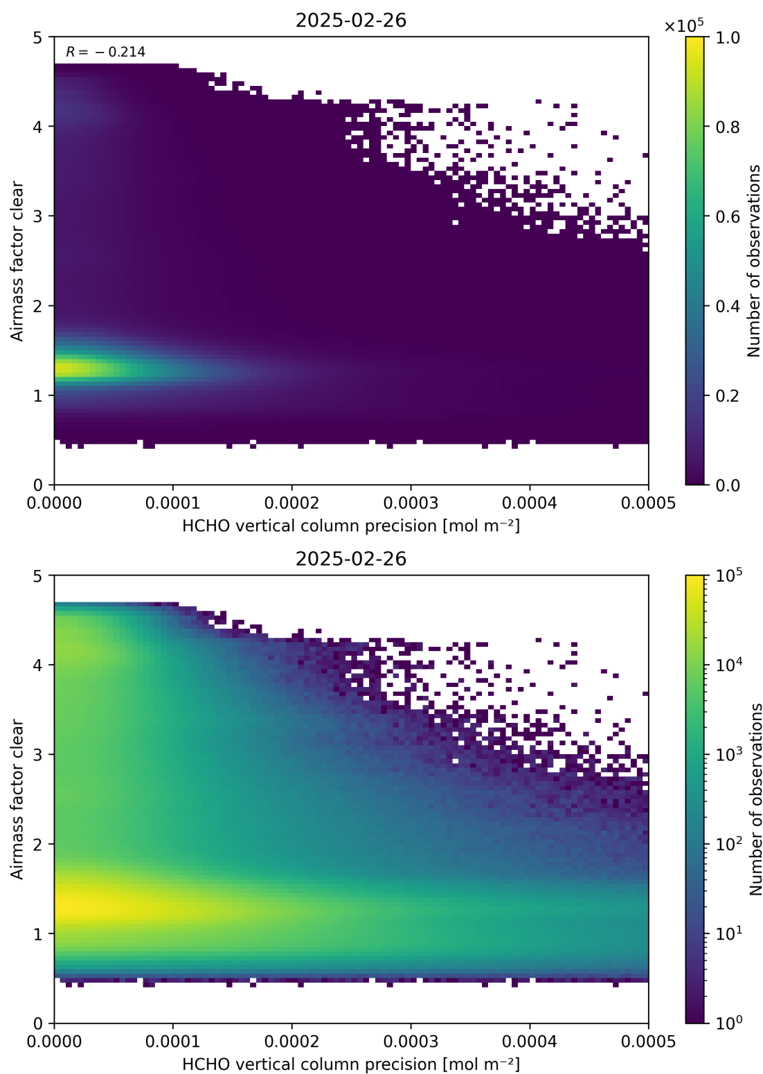
Figure 139: Scatter density plot of “HCHO vertical column precision” against “Airmass factor clear” for 2025-02-25 to 2025-02-27.
