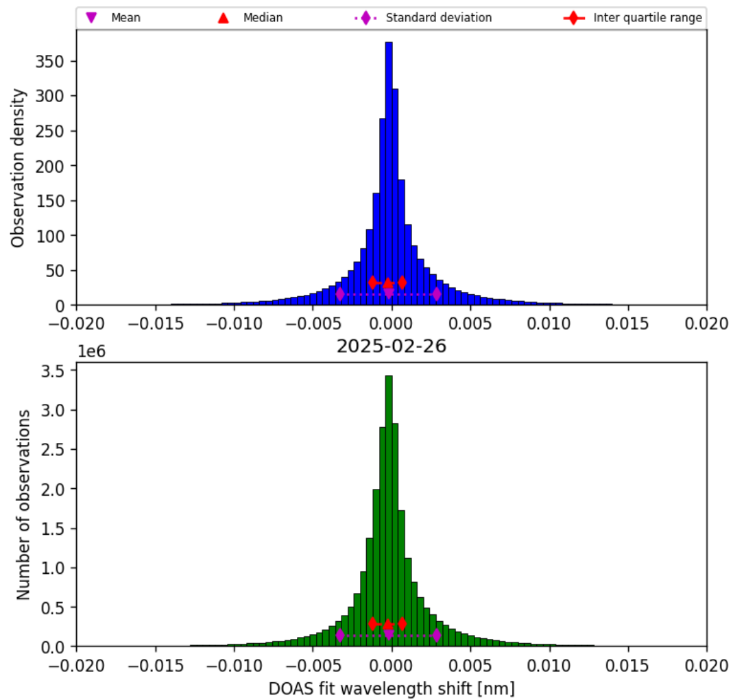
Figure 44: Histogram of “DOAS fit wavelength shift” for 2025-02-25 to 2025-02-27
