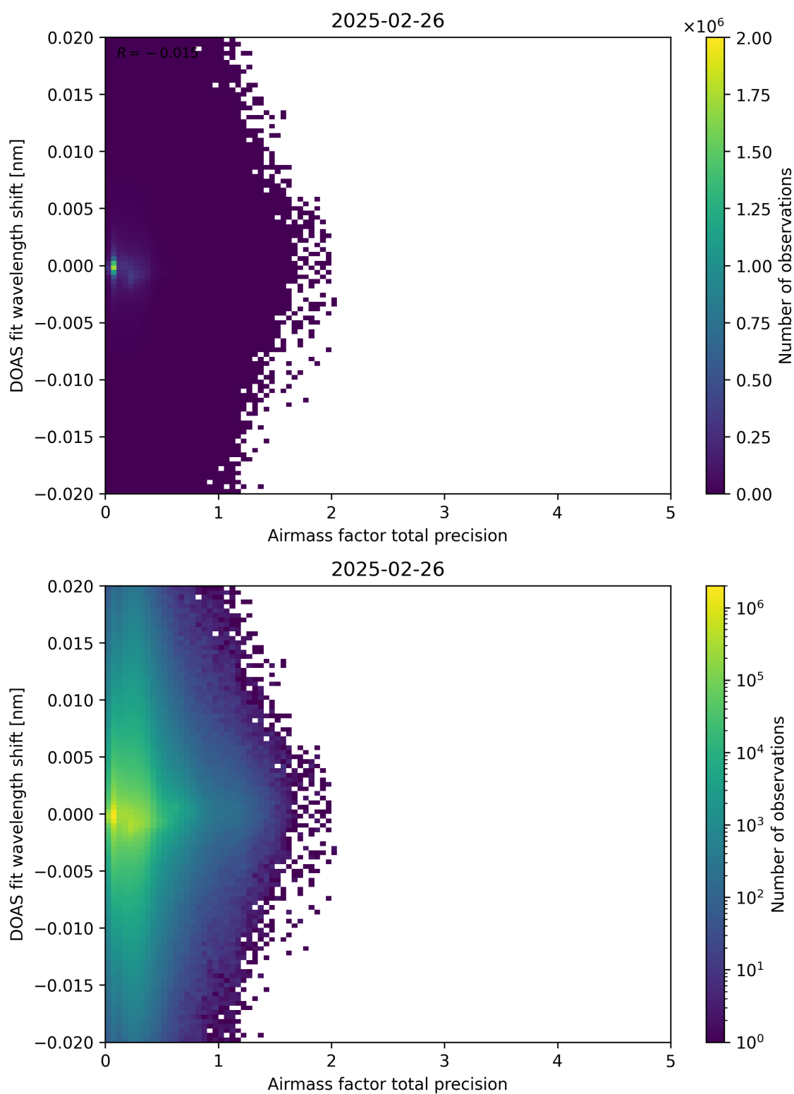
Figure 106: Scatter density plot of “Airmass factor total precision” against “DOAS fit wavelength shift” for 2025-02-25 to 2025-02-27.
