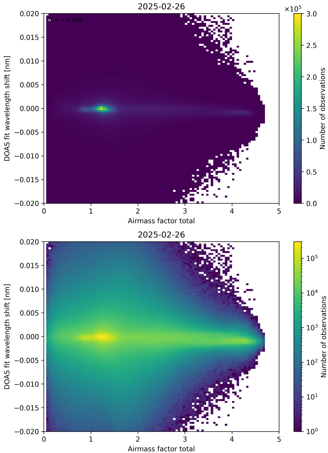
Figure 98: Scatter density plot of “Airmass factor total” against “DOAS fit wavelength shift” for 2025-02-25 to 2025-02-27.
