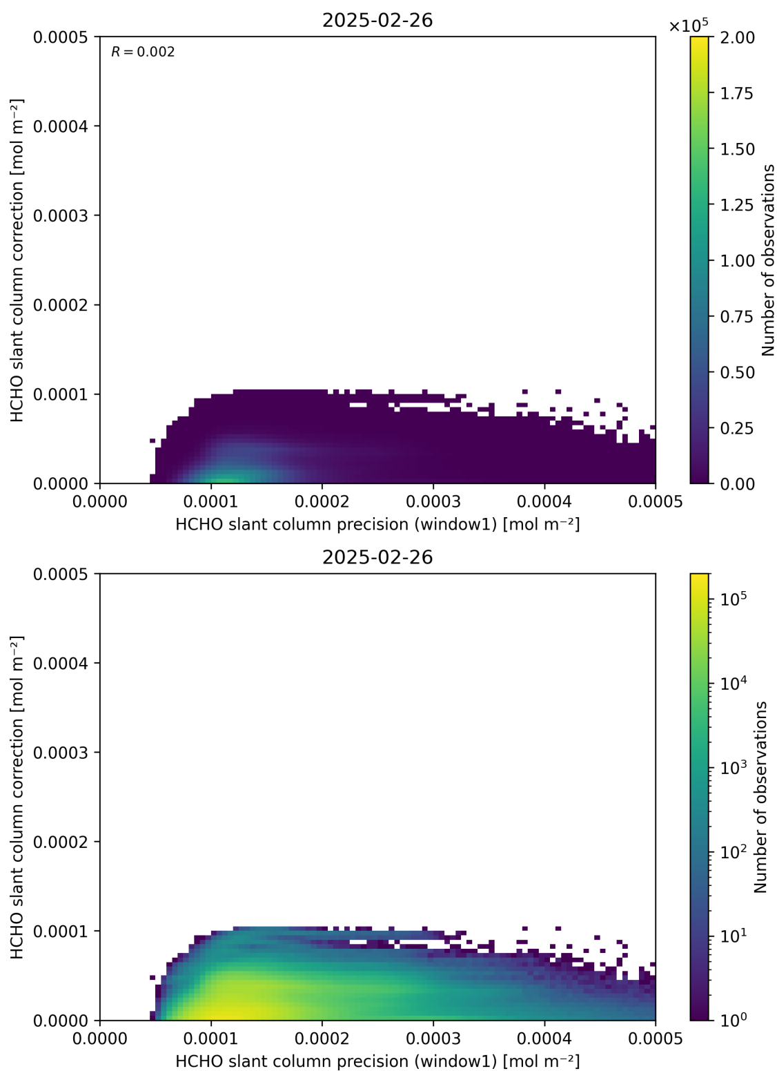
Figure 93: Scatter density plot of “HCHO slant column precision (window1)” against “HCHO slant column correction” for 2025-02-25 to 2025-02-27.
