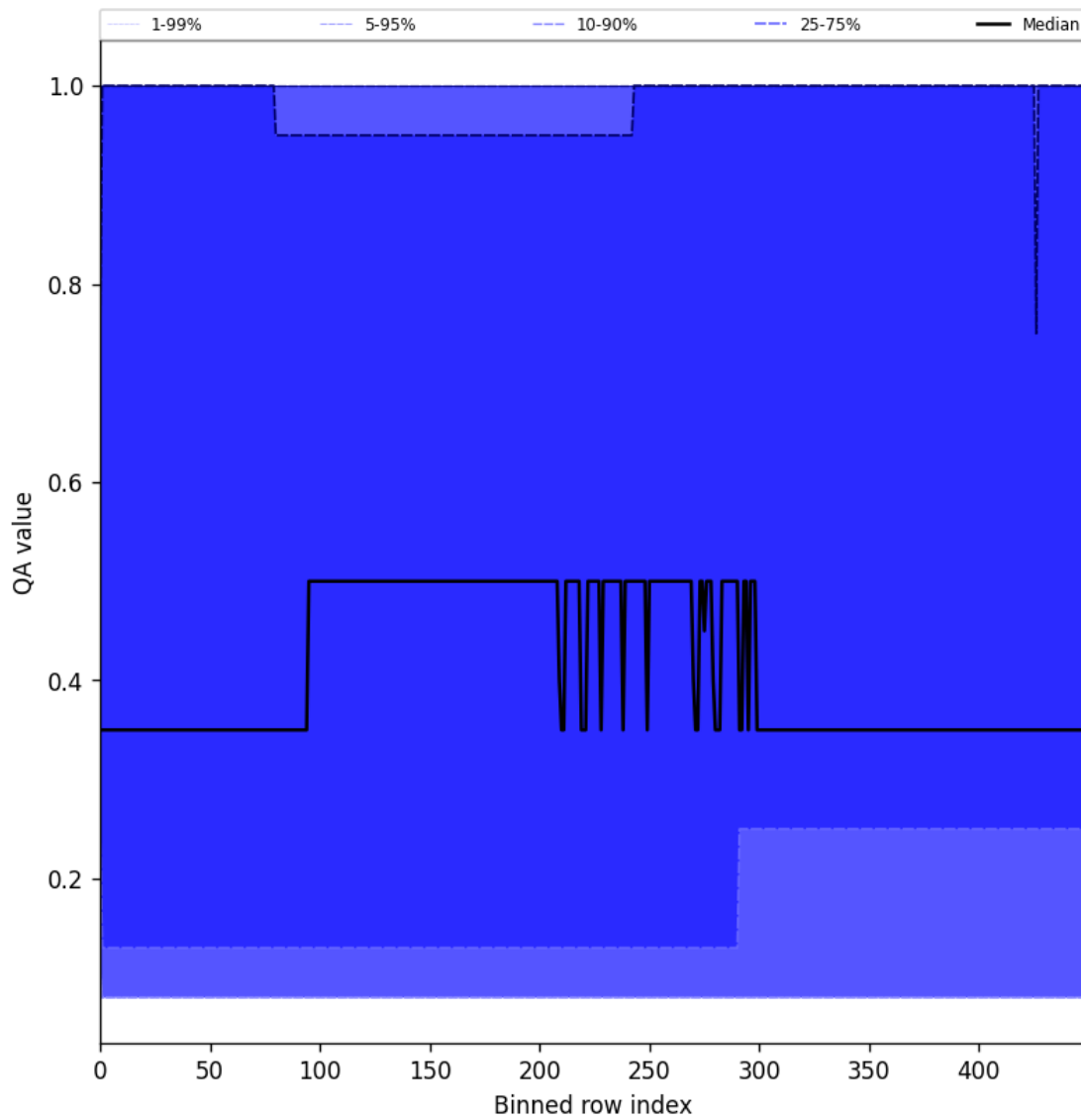
Figure 48: Along track statistics of “QA value” for 2025-02-25 to 2025-02-27
