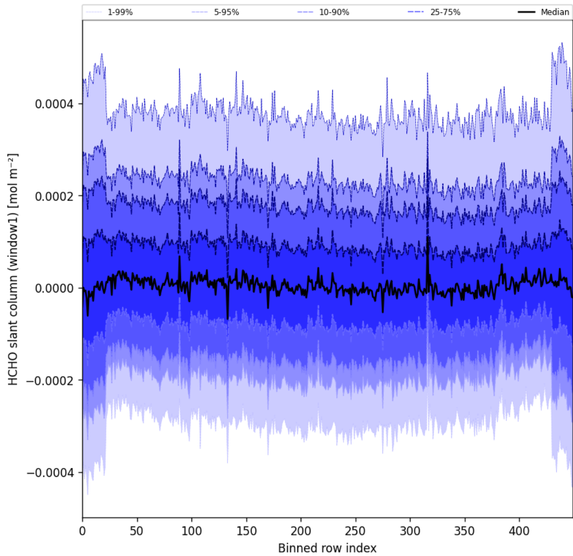
Figure 52: Along track statistics of “HCHO slant column (window1)” for 2025-02-25 to 2025-02-27
