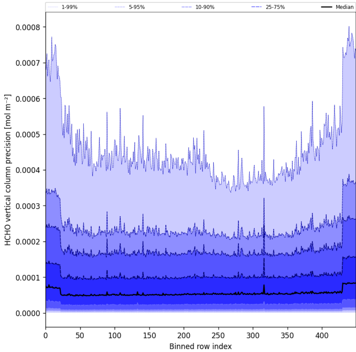
Figure 50: Along track statistics of “HCHO vertical column precision” for 2025-02-25 to 2025-02-27
