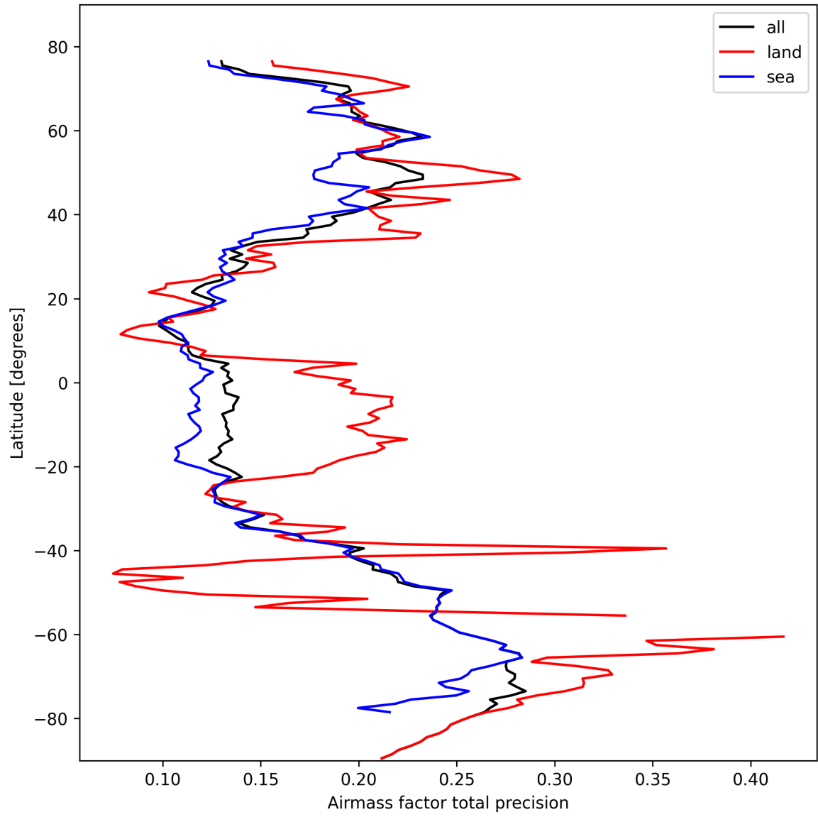
Figure 27: Zonal average of “Airmass factor total precision” for 2025-02-25 to 2025-02-27.
