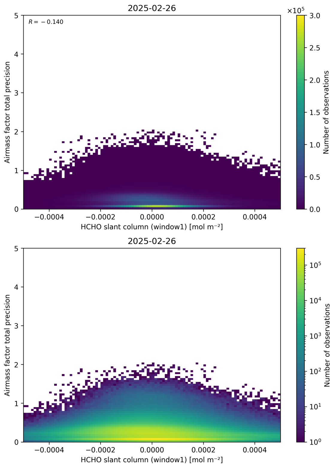
Figure 86: Scatter density plot of “HCHO slant column (window1)” against “Airmass factor total precision” for 2025-02-25 to 2025-02-27.
