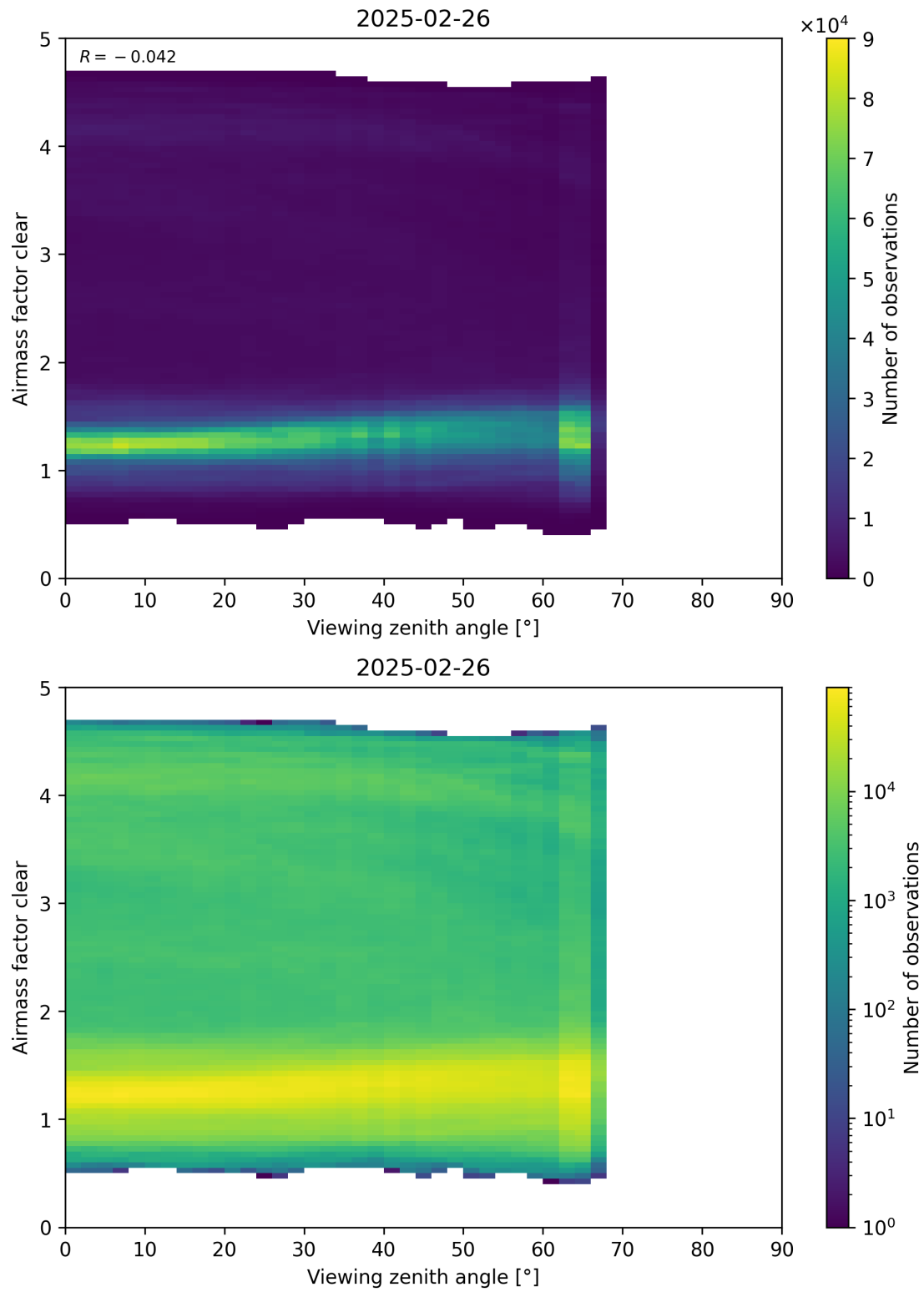
Figure 185: Scatter density plot of “Viewing zenith angle” against “Airmass factor clear” for 2025-02-25 to 2025-02-27.
