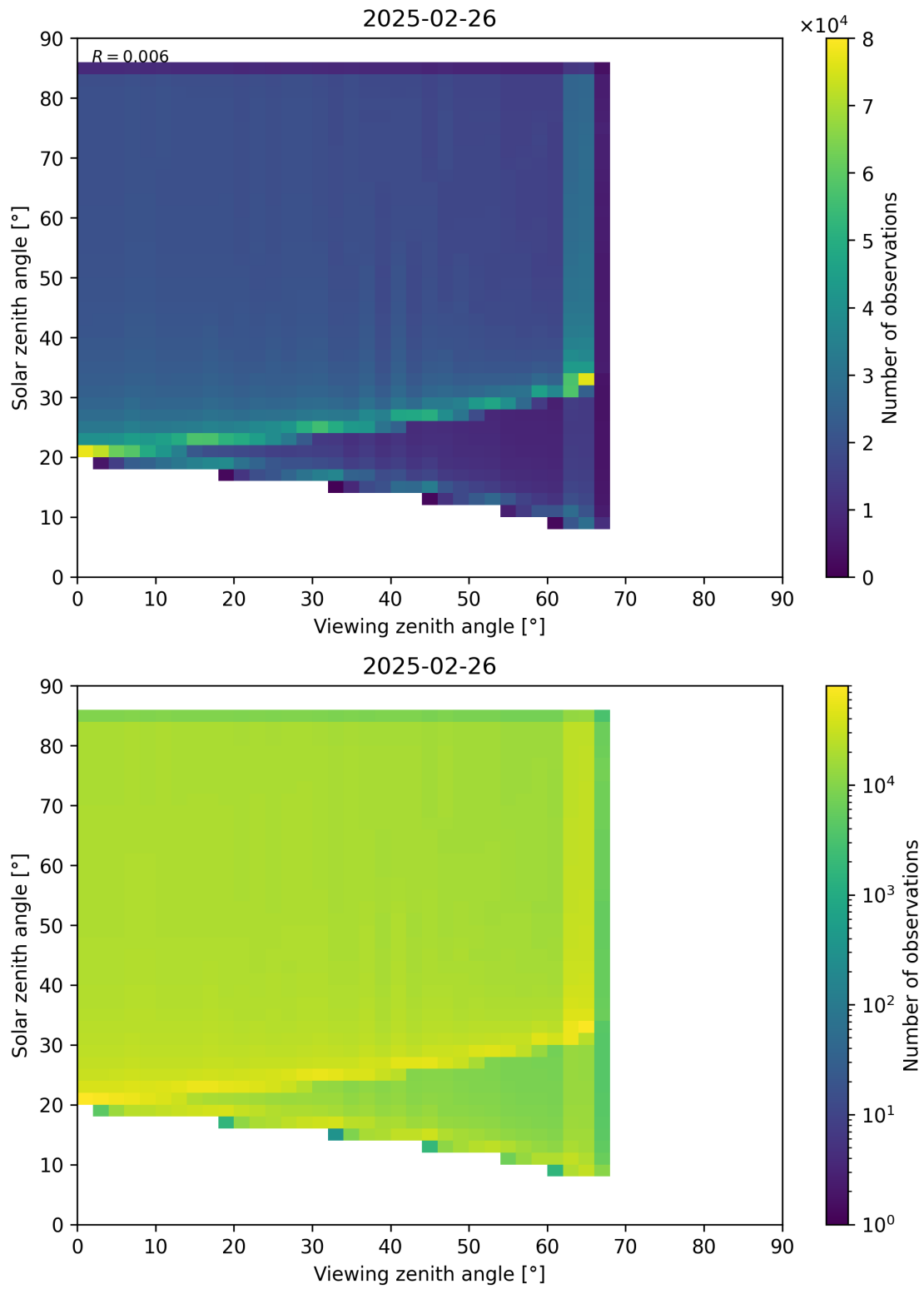
Figure 197: Scatter density plot of “Viewing zenith angle” against “Solar zenith angle” for 2025-02-25 to 2025-02-27.
