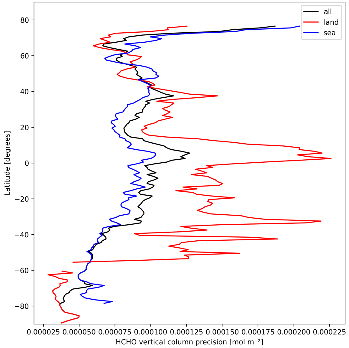
Figure 22: Zonal average of “HCHO vertical column precision” for 2025-02-25 to 2025-02-27.
