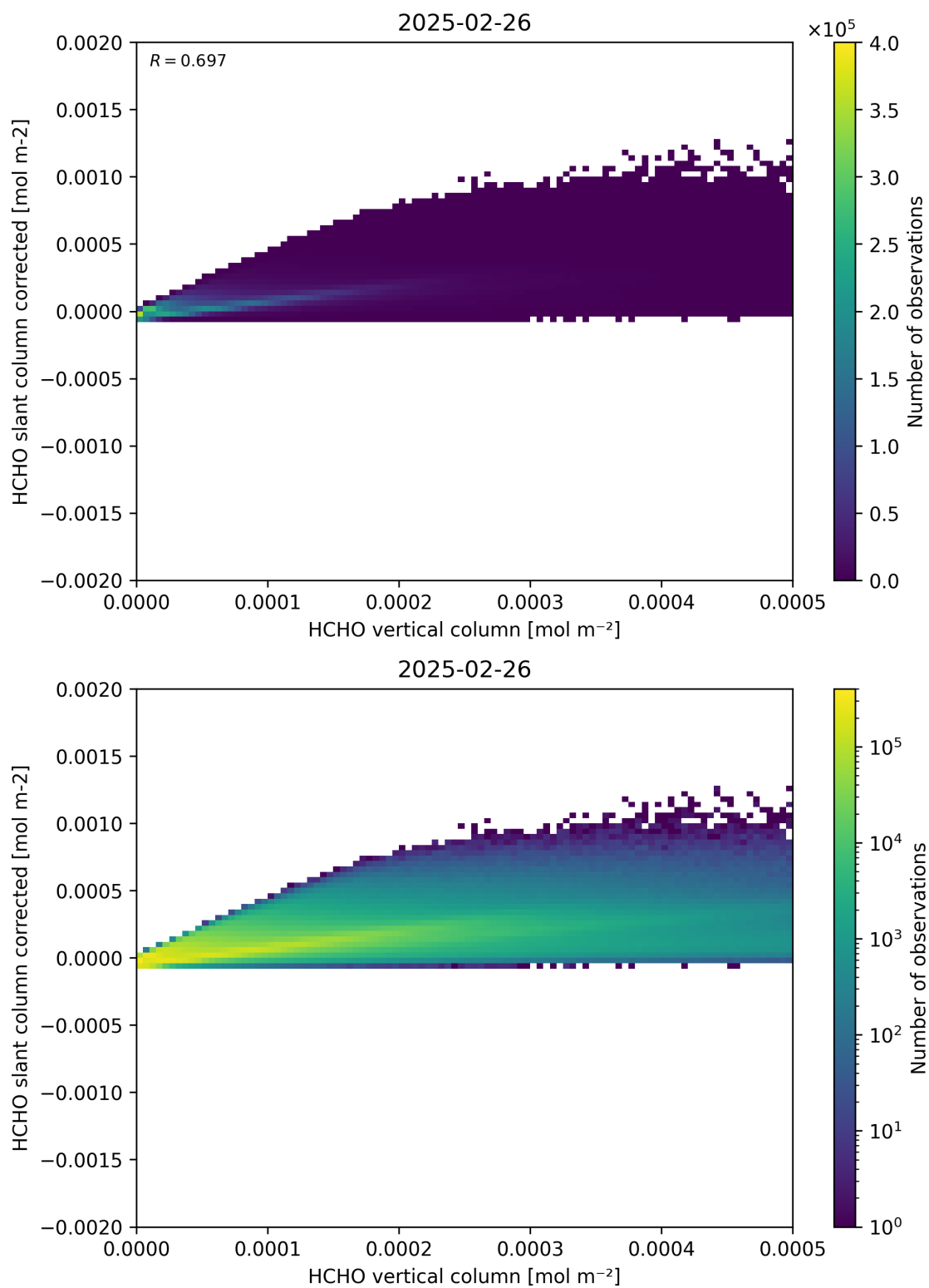
Figure 127: Scatter density plot of “HCHO vertical column” against “HCHO slant column corrected” for 2025-02-25 to 2025-02-27.
