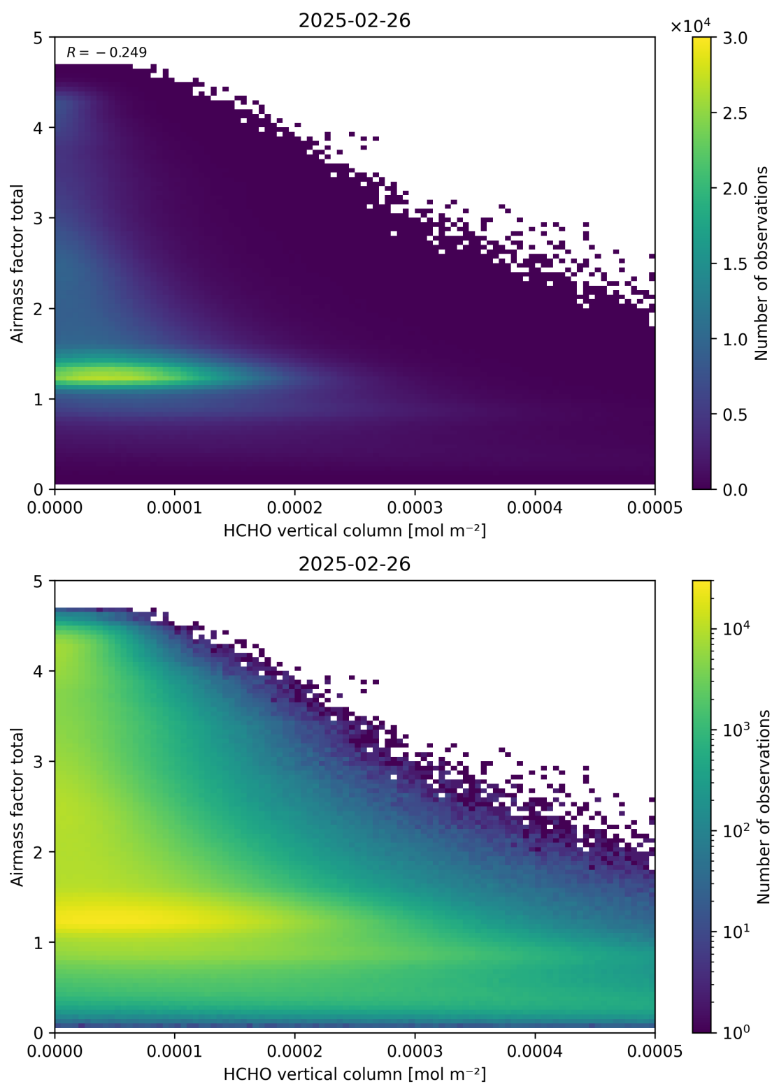
Figure 131: Scatter density plot of “HCHO vertical column” against “Airmass factor total” for 2025-02-25 to 2025-02-27.
