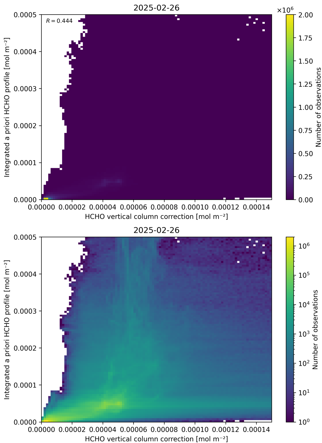
Figure 122: Scatter density plot of “HCHO vertical column correction” against “Integrated a priori HCHO profile” for 2025-02-25 to 2025-02-27.
