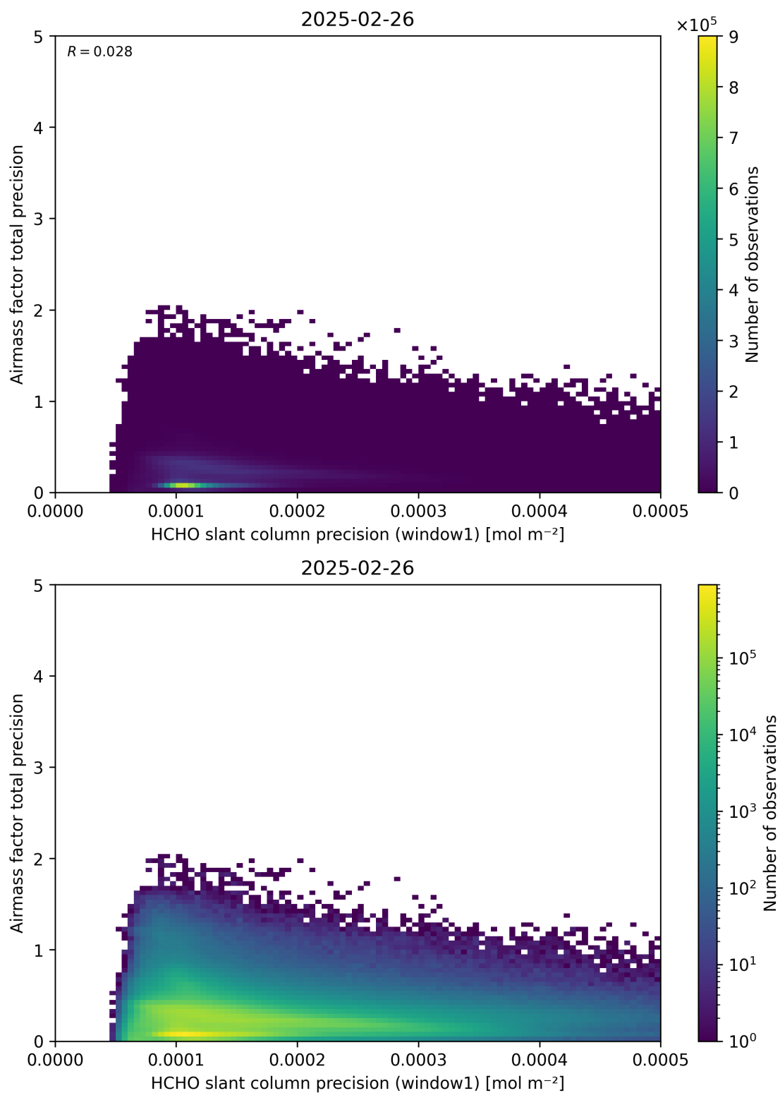
Figure 95: Scatter density plot of “HCHO slant column precision (window1)” against “Airmass factor total precision” for 2025-02-25 to 2025-02-27.
