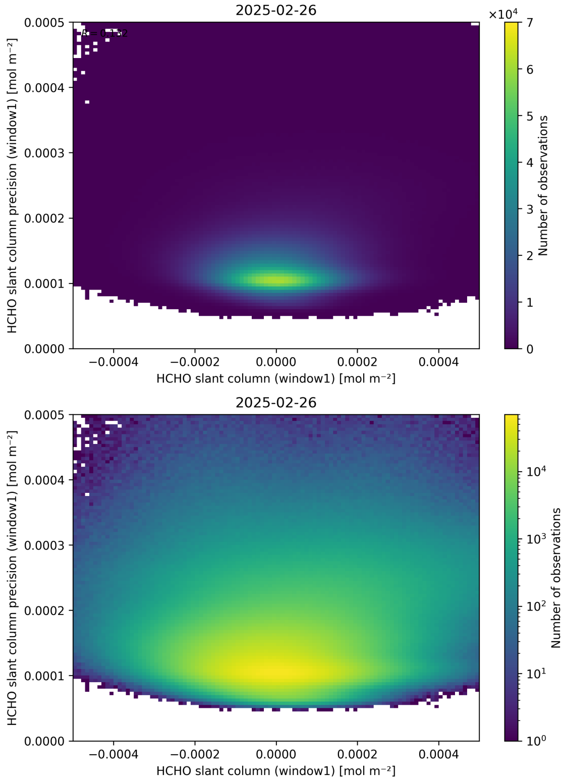
Figure 84: Scatter density plot of “HCHO slant column (window1)” against “HCHO slant column precision (window1)” for 2025-02-25 to 2025-02-27.
