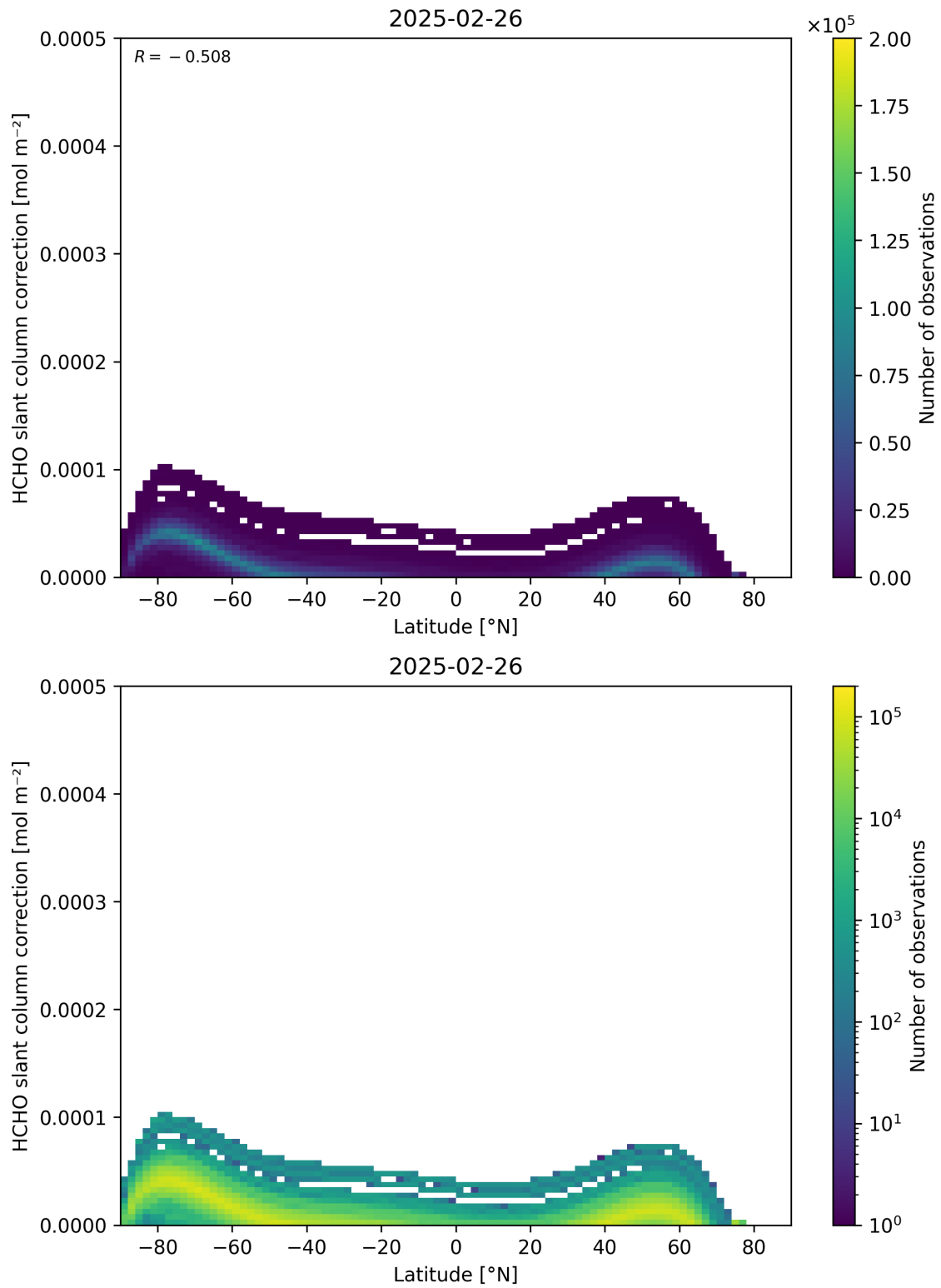
Figure 158: Scatter density plot of “Latitude” against “HCHO slant column correction” for 2025-02-25 to 2025-02-27.
