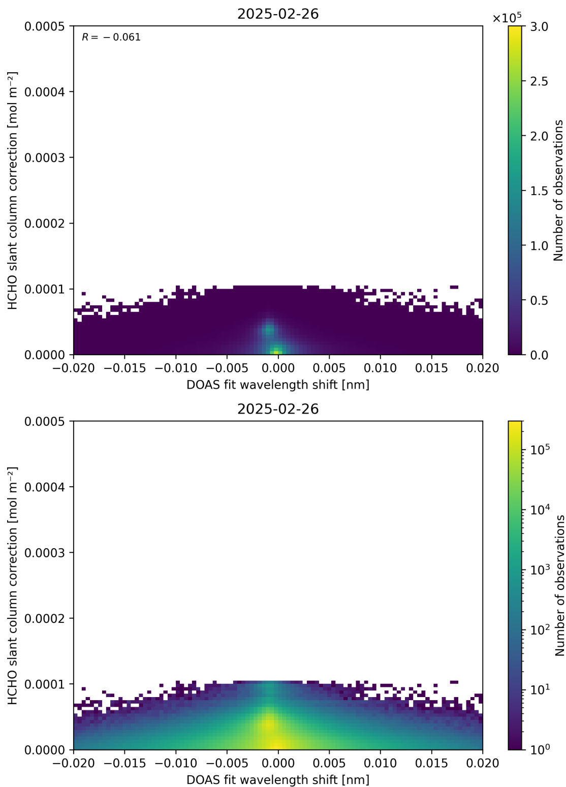
Figure 67: Scatter density plot of “DOAS fit wavelength shift” against “HCHO slant column correction” for 2025-02-25 to 2025-02-27.
