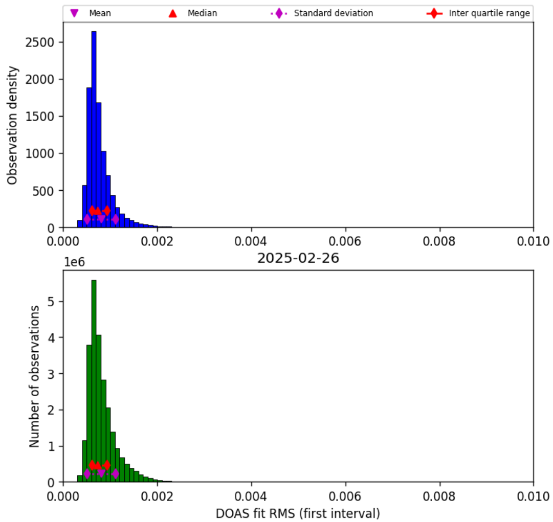
Figure 46: Histogram of “DOAS fit RMS (first interval)” for 2025-02-25 to 2025-02-27
