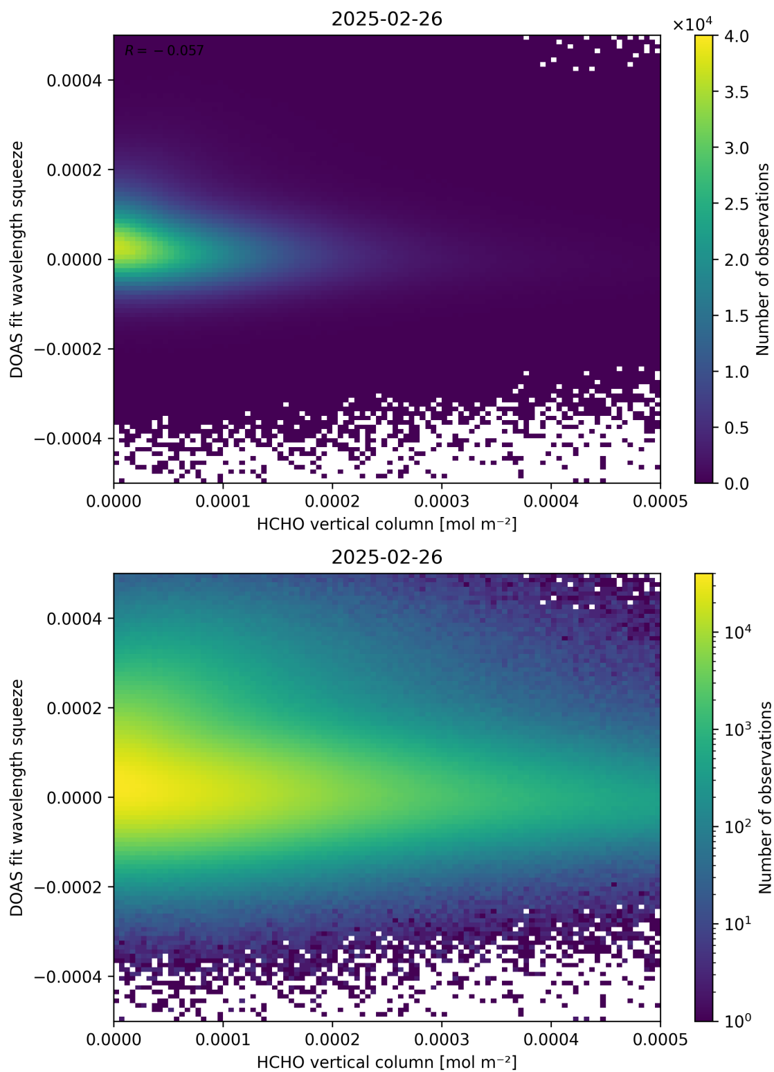
Figure 125: Scatter density plot of “HCHO vertical column” against “DOAS fit wavelength squeeze” for 2025-02-25 to 2025-02-27.
