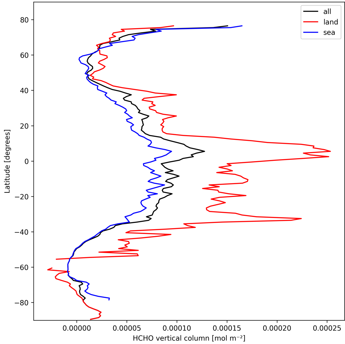
Figure 21: Zonal average of “HCHO vertical column” for 2025-02-25 to 2025-02-27.
