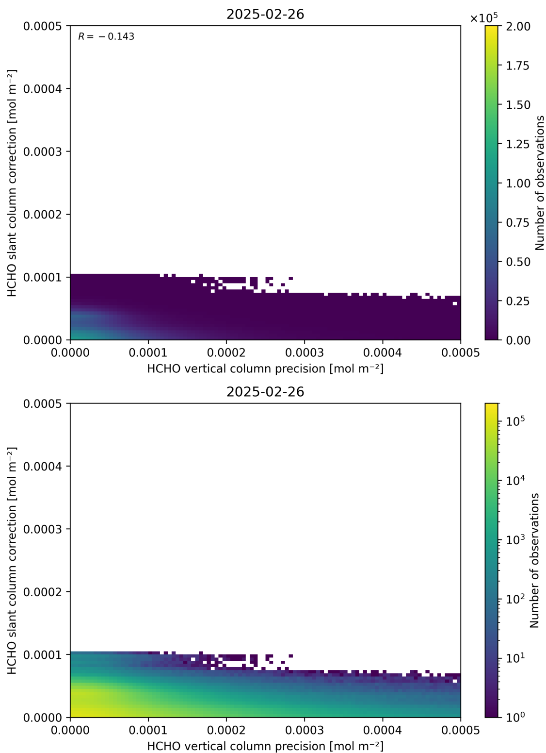
Figure 141: Scatter density plot of “HCHO vertical column precision” against “HCHO slant column correction” for 2025-02-25 to 2025-02-27.
