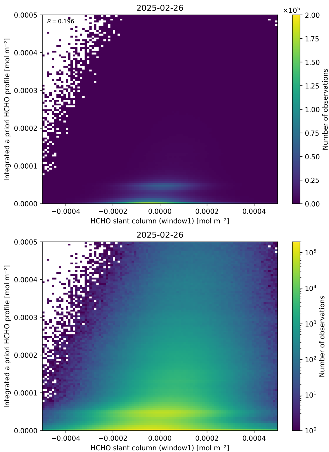
Figure 87: Scatter density plot of “HCHO slant column (window1)” against “Integrated a priori HCHO profile” for 2025-02-25 to 2025-02-27.
