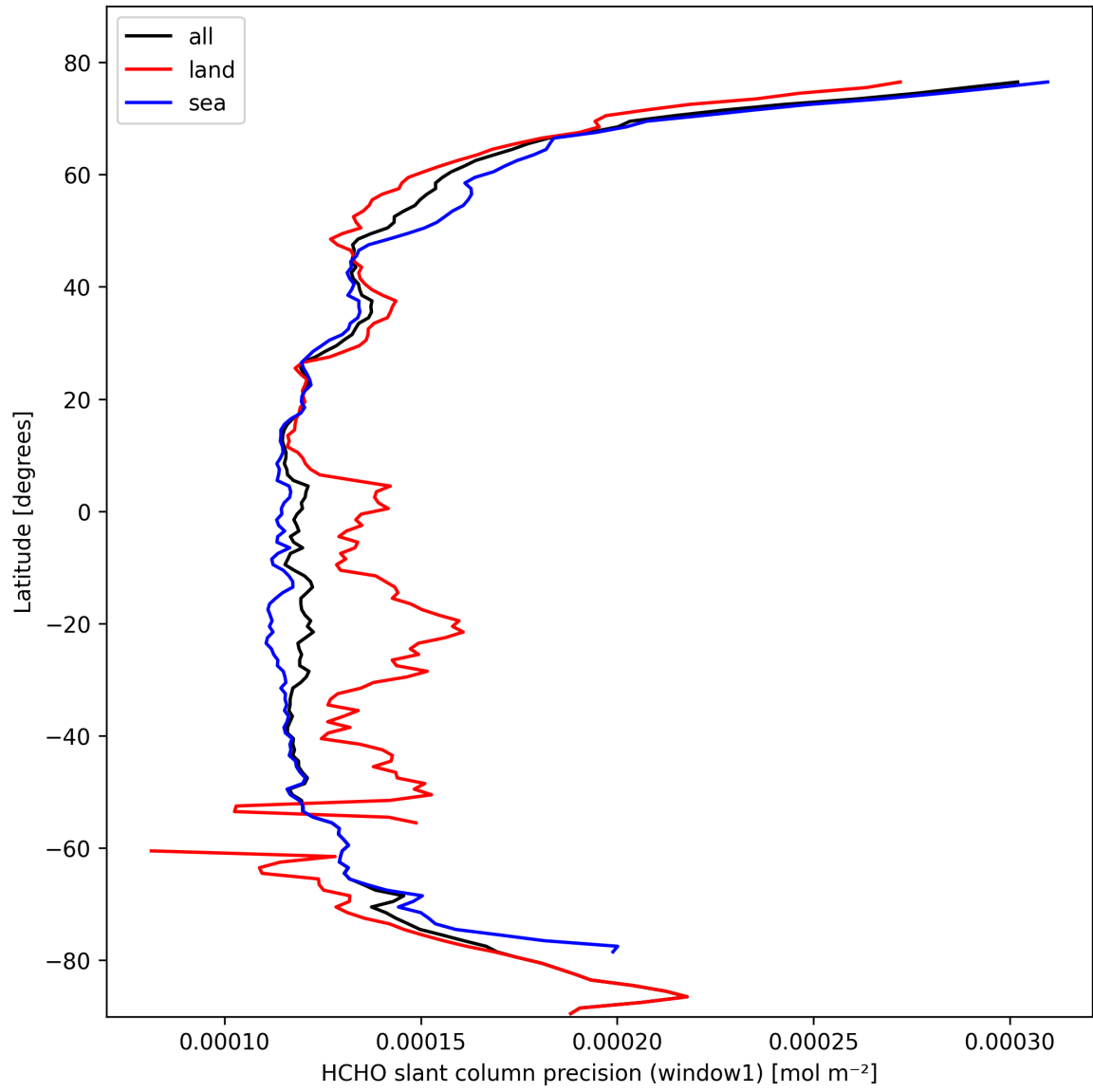
Figure 25: Zonal average of “HCHO slant column precision (window1)” for 2025-02-25 to 2025-02-27.
