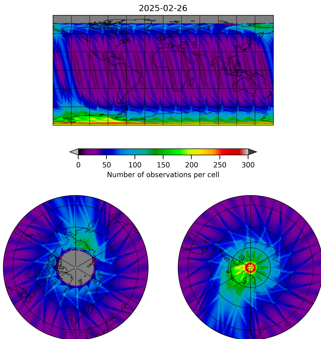
Figure 19: Map of the number of observations for 2025-02-25 to 2025-02-27
