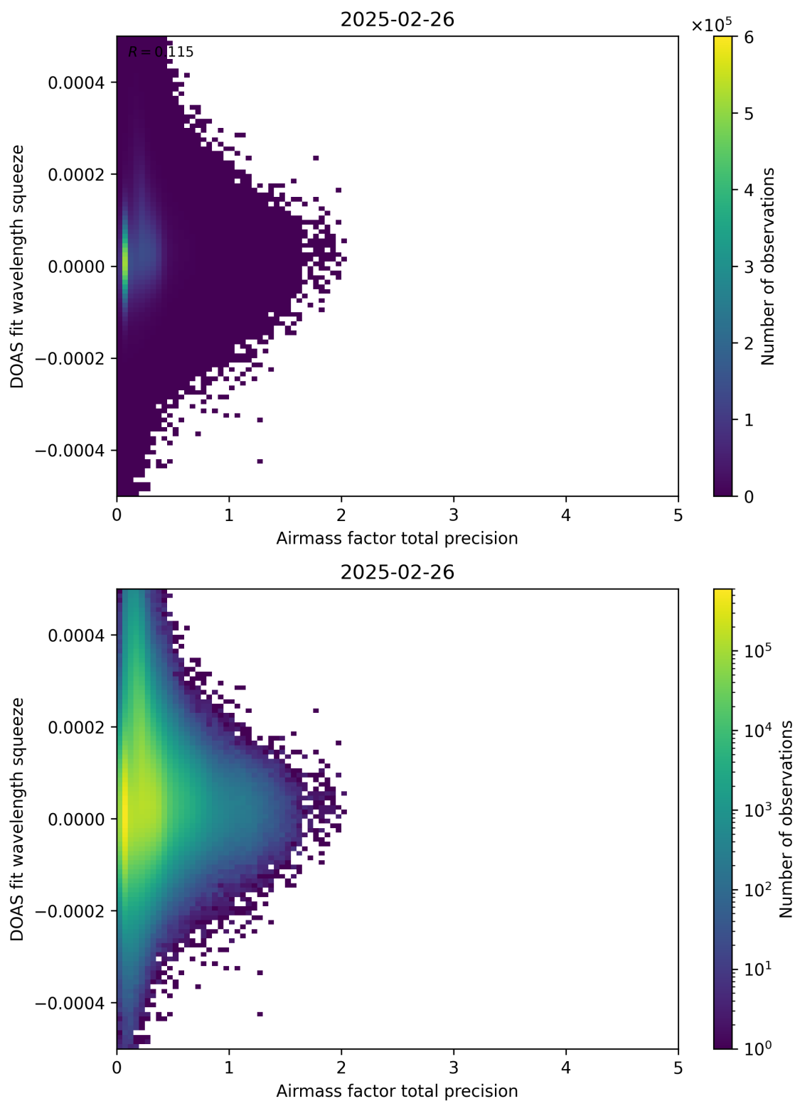
Figure 107: Scatter density plot of “Airmass factor total precision” against “DOAS fit wavelength squeeze” for 2025-02-25 to 2025-02-27.
