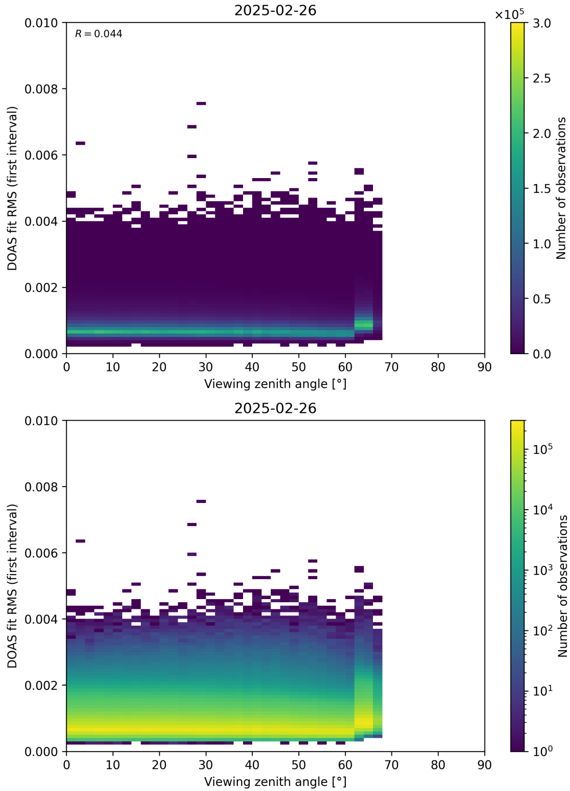
Figure 182: Scatter density plot of “Viewing zenith angle” against “DOAS fit RMS (first interval)” for 2025-02-25 to 2025-02-27.
