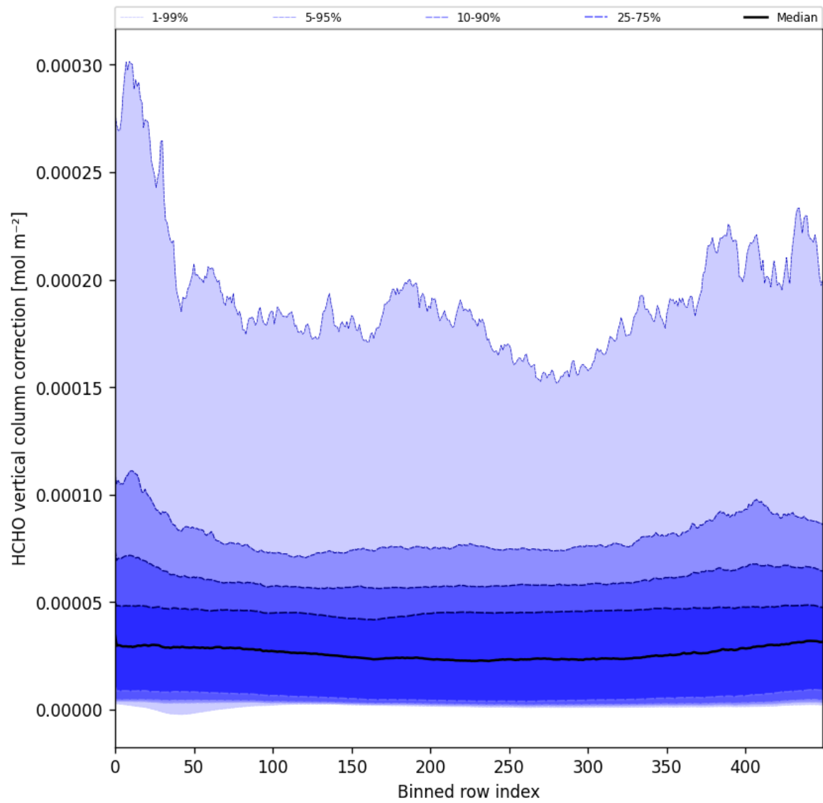
Figure 51: Along track statistics of “HCHO vertical column correction” for 2025-02-25 to 2025-02-27
