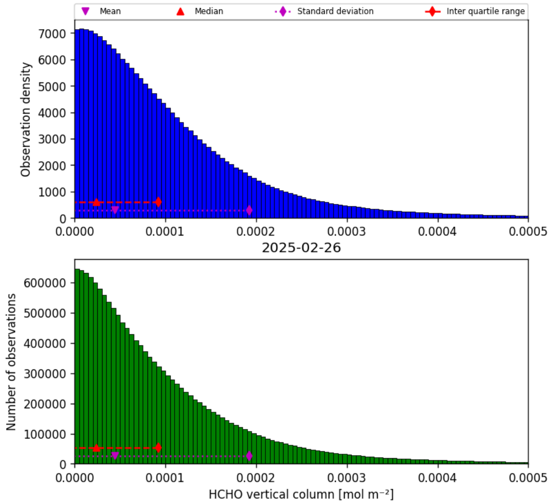
Figure 35: Histogram of “HCHO vertical column” for 2025-02-25 to 2025-02-27
