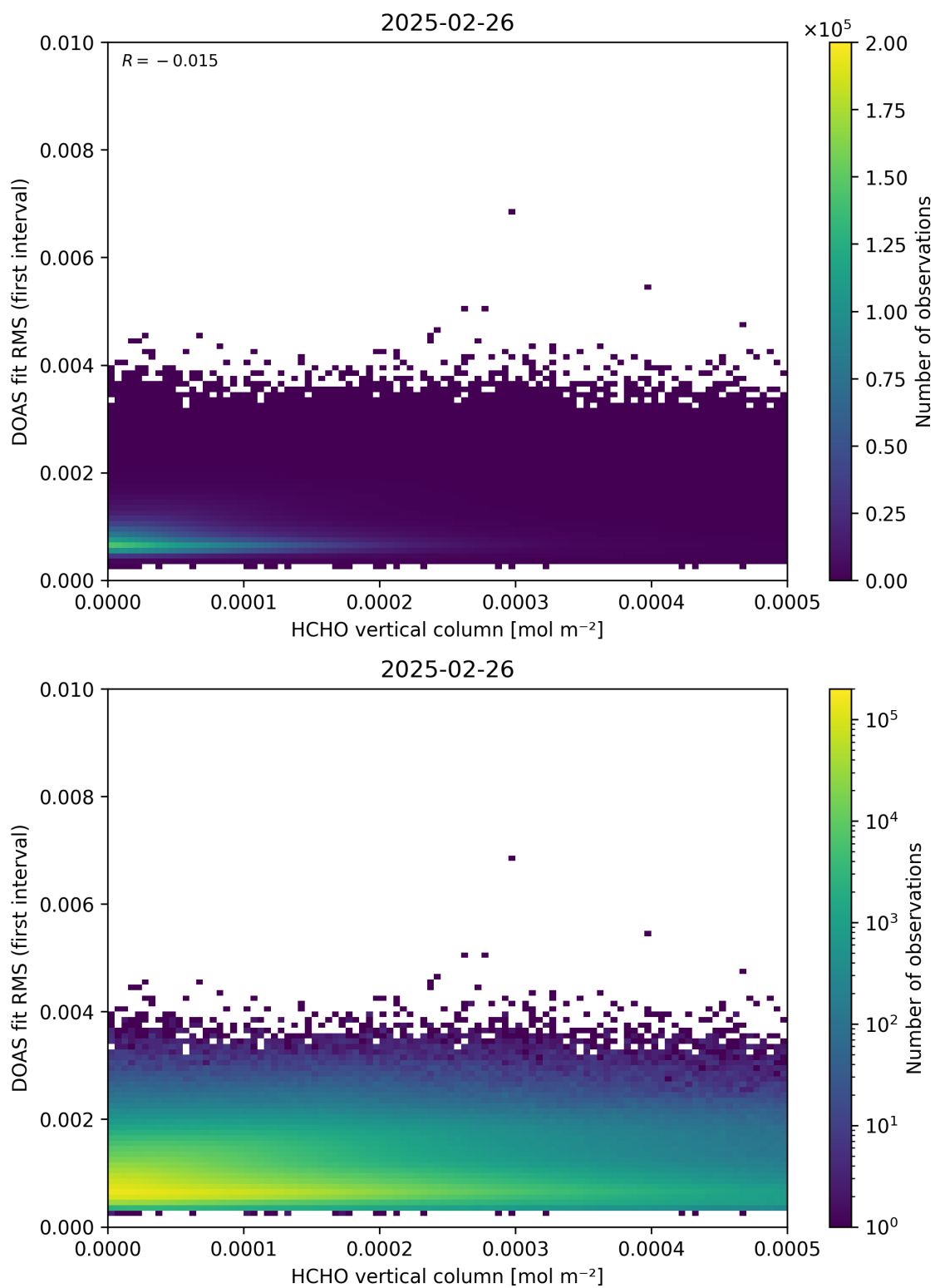
Figure 123: Scatter density plot of “HCHO vertical column” against “DOAS fit RMS (first interval)” for 2025-02-25 to 2025-02-27.
