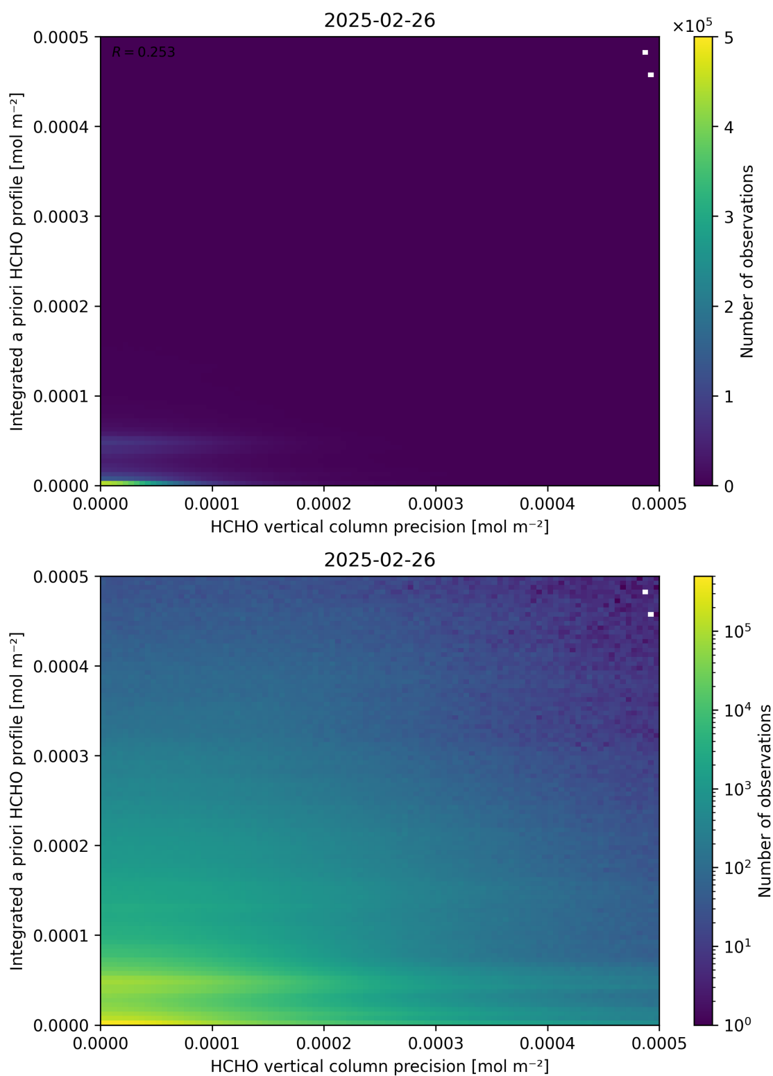
Figure 147: Scatter density plot of “HCHO vertical column precision” against “Integrated a priori HCHO profile” for 2025-02-25 to 2025-02-27.
