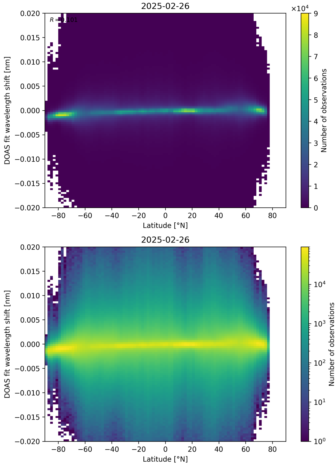
Figure 154: Scatter density plot of “Latitude” against “DOAS fit wavelength shift” for 2025-02-25 to 2025-02-27.
