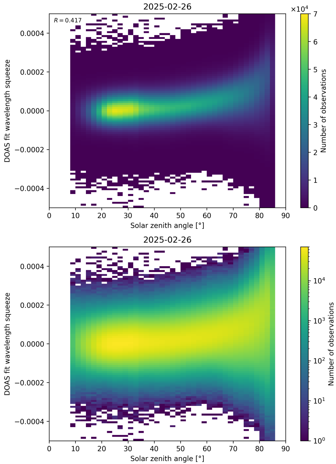
Figure 169: Scatter density plot of “Solar zenith angle” against “DOAS fit wavelength squeeze” for 2025-02-25 to 2025-02-27.
