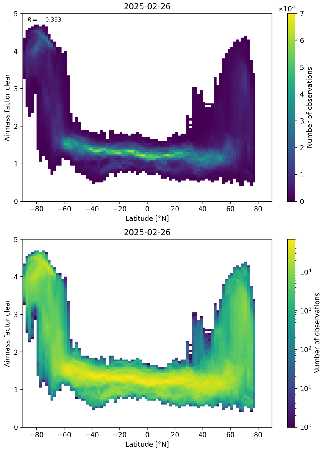
Figure 156: Scatter density plot of “Latitude” against “Airmass factor clear” for 2025-02-25 to 2025-02-27.
