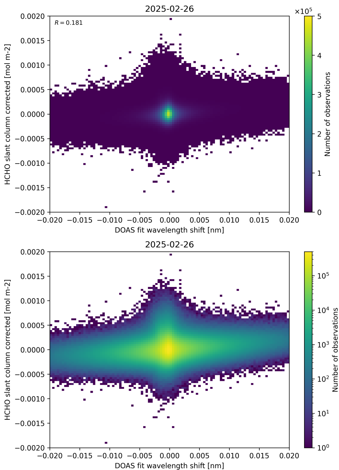
Figure 66: Scatter density plot of “DOAS fit wavelength shift” against “HCHO slant column corrected” for 2025-02-25 to 2025-02-27.
