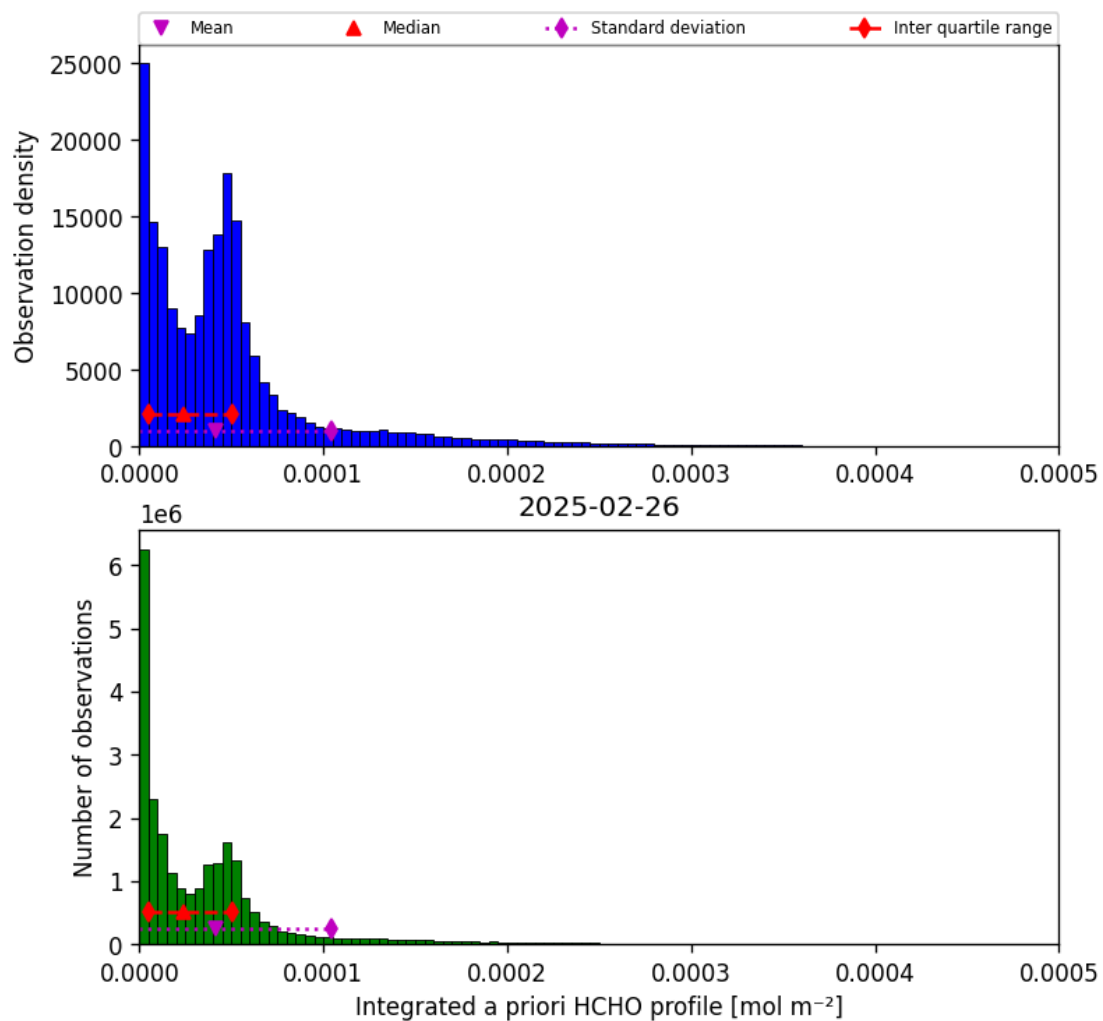
Figure 43: Histogram of “Integrated a priori HCHO profile” for 2025-02-25 to 2025-02-27
