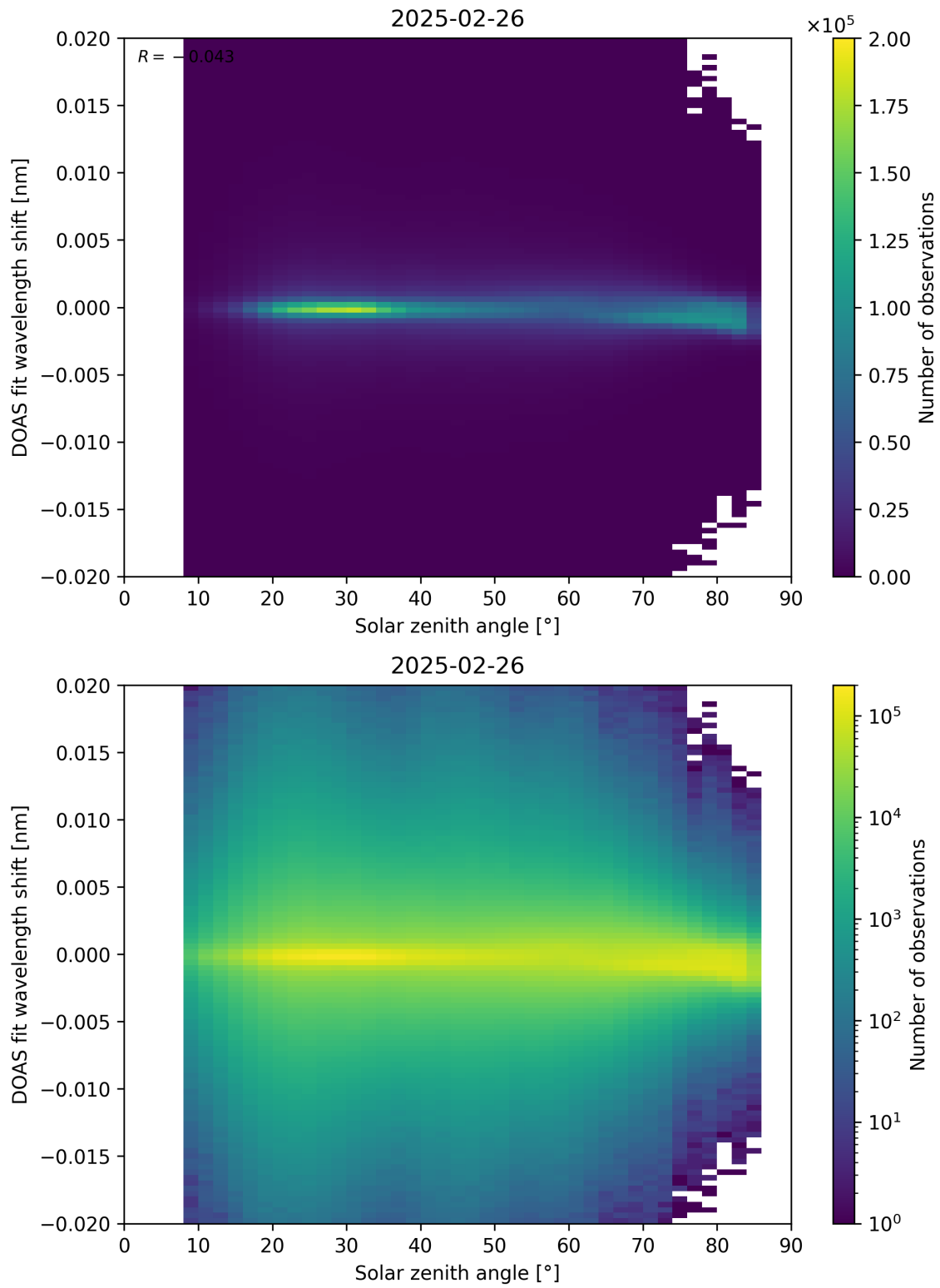
Figure 168: Scatter density plot of “Solar zenith angle” against “DOAS fit wavelength shift” for 2025-02-25 to 2025-02-27.
