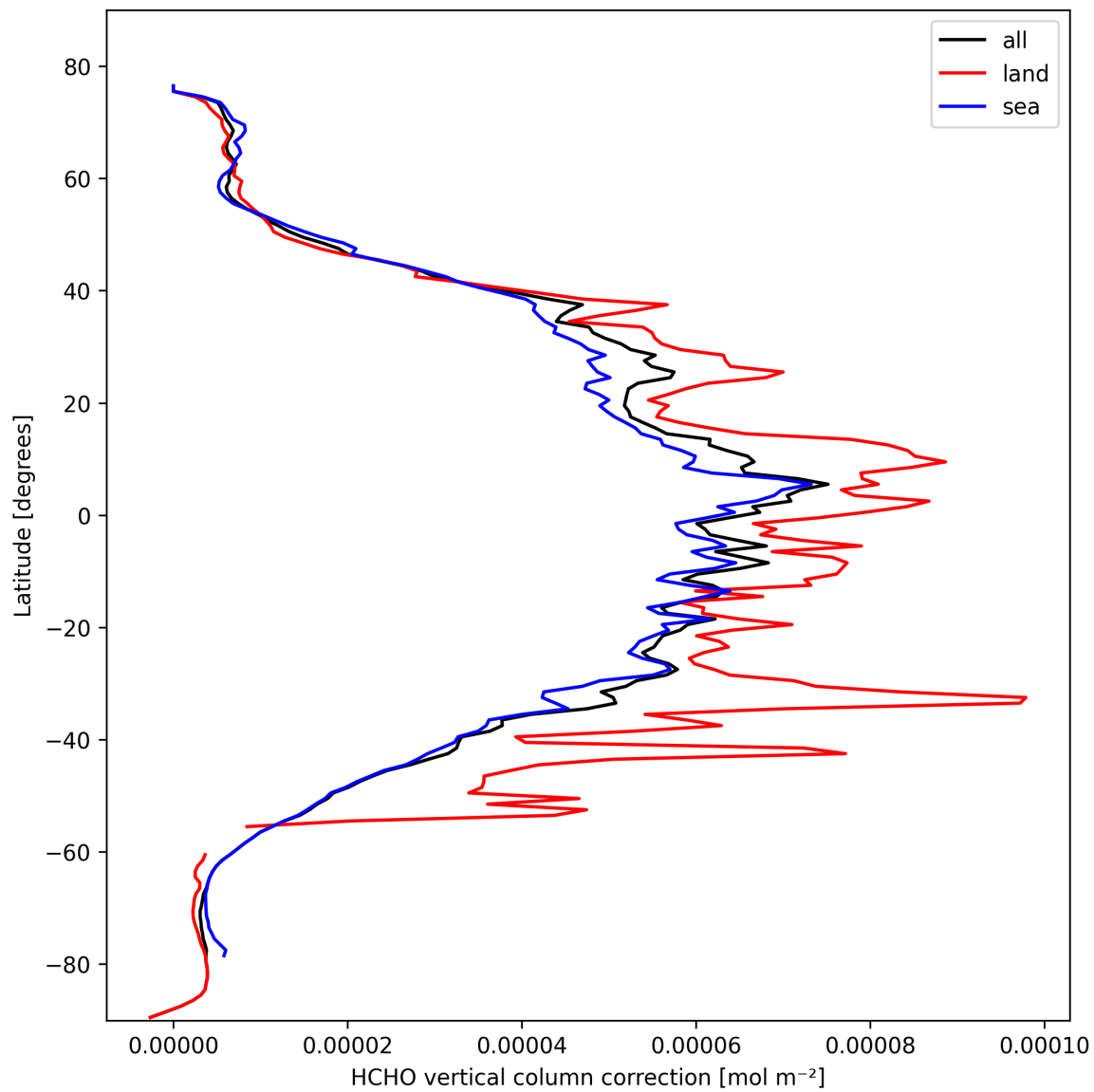
Figure 23: Zonal average of “HCHO vertical column correction” for 2025-02-25 to 2025-02-27.
