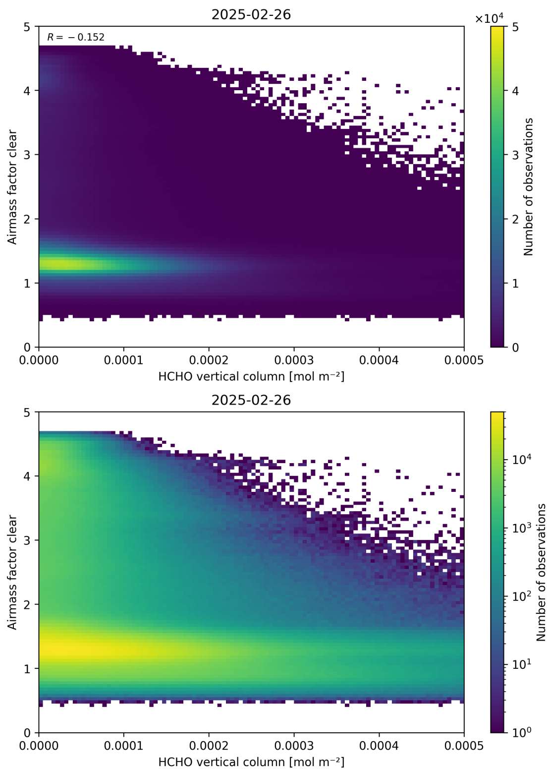
Figure 126: Scatter density plot of “HCHO vertical column” against “Airmass factor clear” for 2025-02-25 to 2025-02-27.
