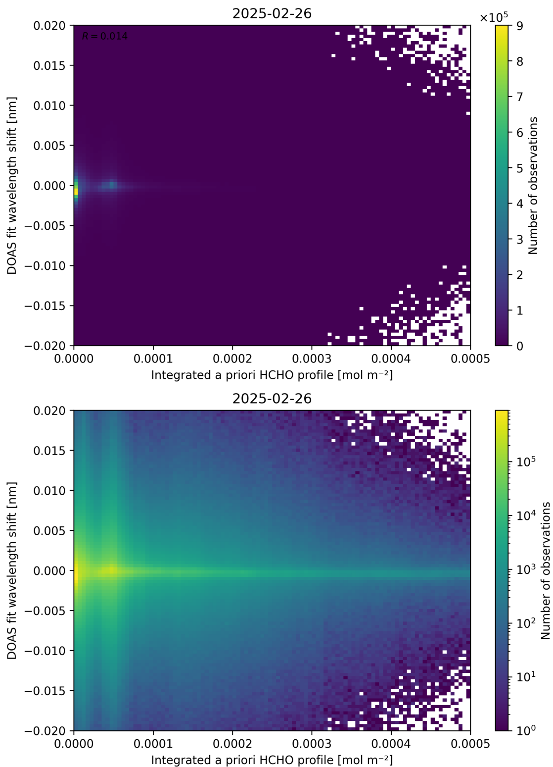
Figure 149: Scatter density plot of “Integrated a priori HCHO profile” against “DOAS fit wavelength shift” for 2025-02-25 to 2025-02-27.
