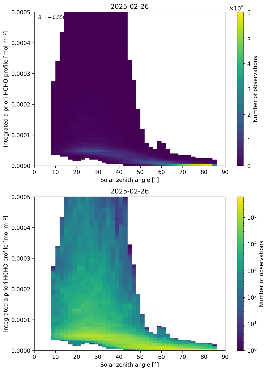
Figure 180: Scatter density plot of “Solar zenith angle” against “Integrated a priori HCHO profile” for 2025-02-25 to 2025-02-27.
