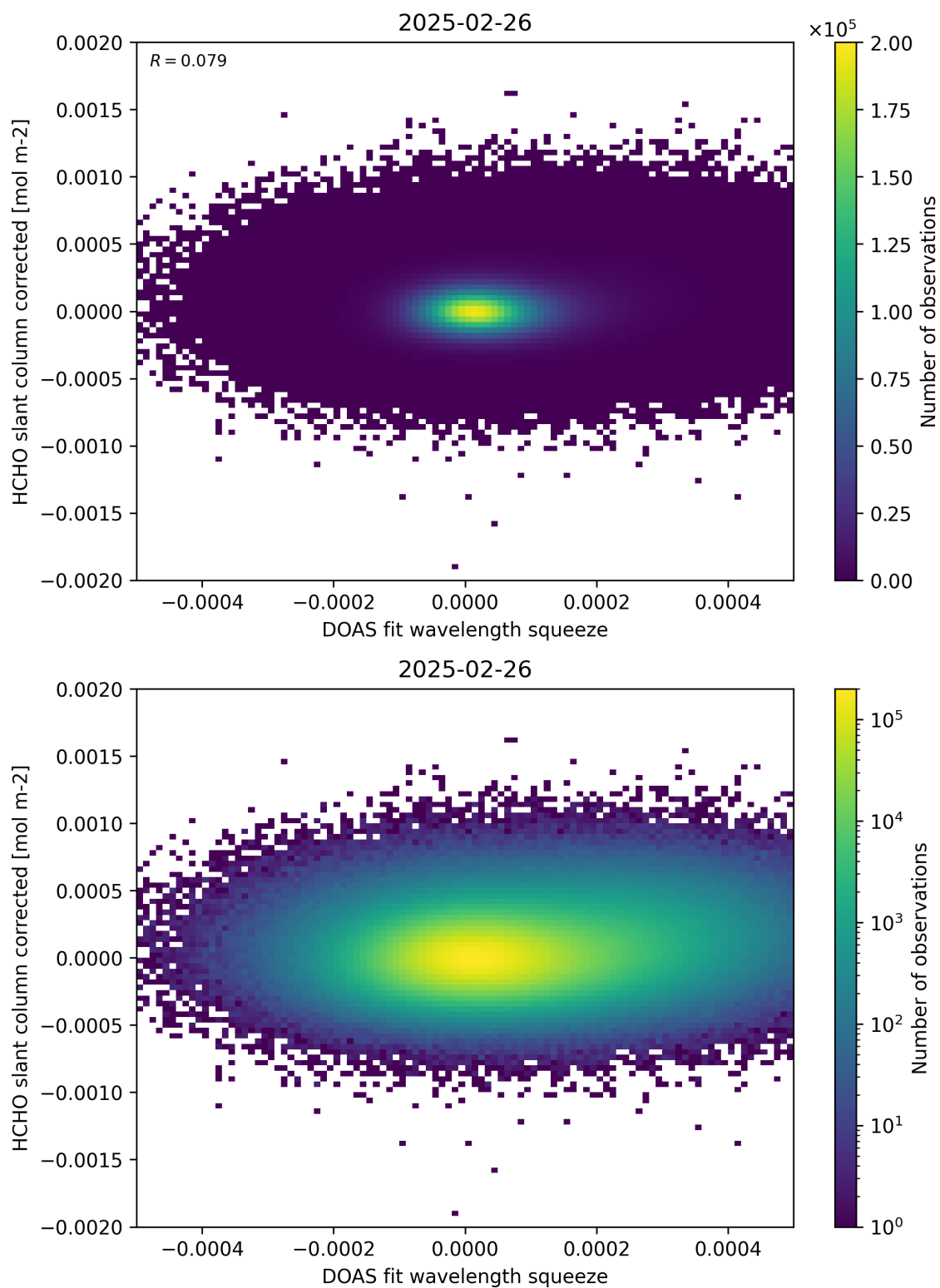
Figure 69: Scatter density plot of “DOAS fit wavelength squeeze” against “HCHO slant column corrected” for 2025-02-25 to 2025-02-27.
