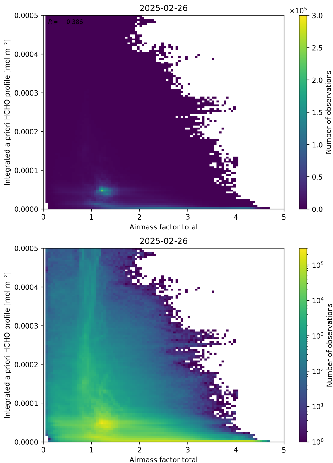
Figure 104: Scatter density plot of “Airmass factor total” against “Integrated a priori HCHO profile” for 2025-02-25 to 2025-02-27.
