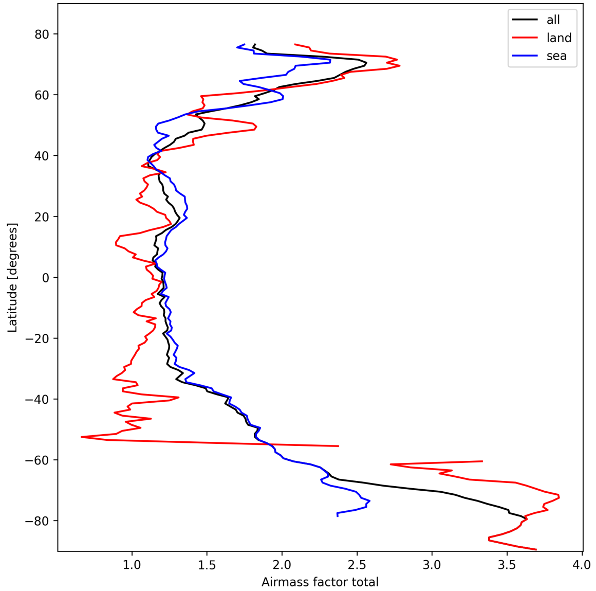
Figure 26: Zonal average of “Airmass factor total” for 2025-02-25 to 2025-02-27.
