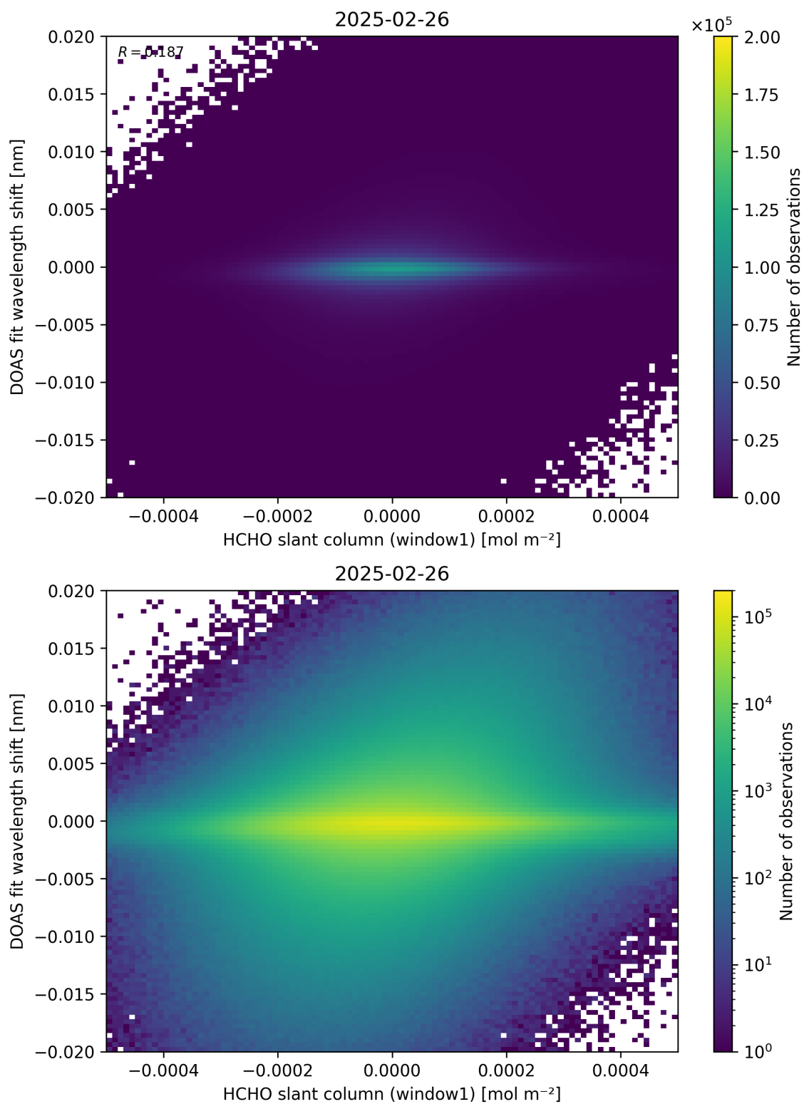
Figure 79: Scatter density plot of “HCHO slant column (window1)” against “DOAS fit wavelength shift” for 2025-02-25 to 2025-02-27.
