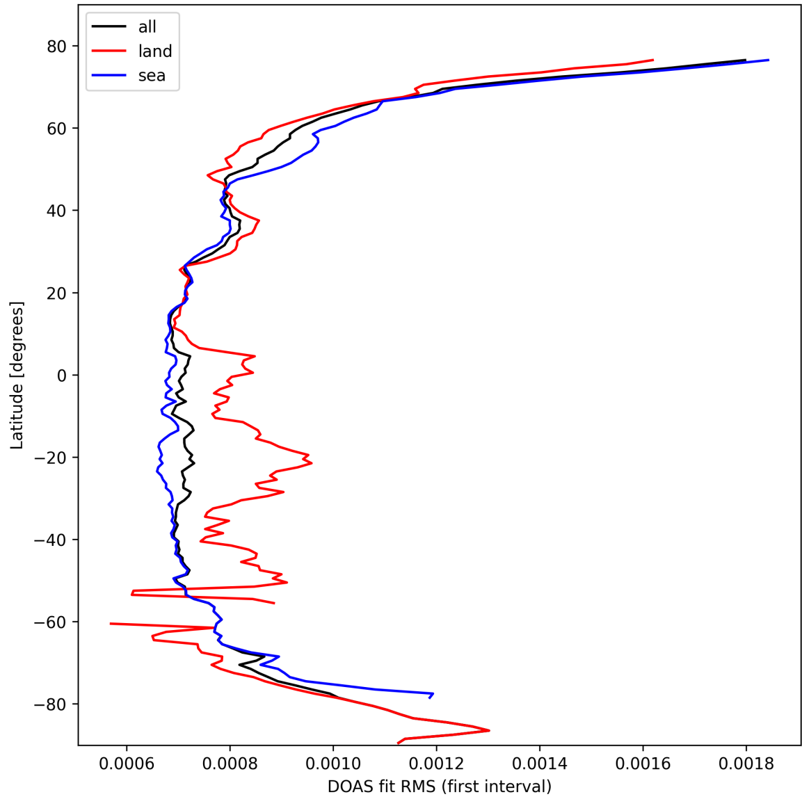
Figure 32: Zonal average of "DOAS fit RMS (first interval)" for 2025-02-25 to 2025-02-27.
