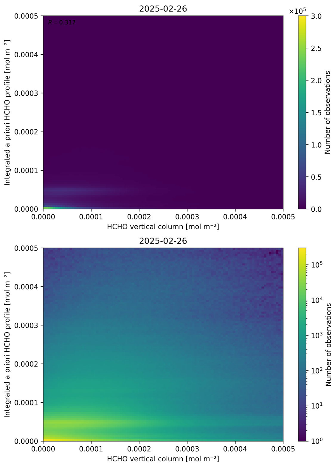
Figure 135: Scatter density plot of “HCHO vertical column” against “Integrated a priori HCHO profile” for 2025-02-25 to 2025-02-27.
