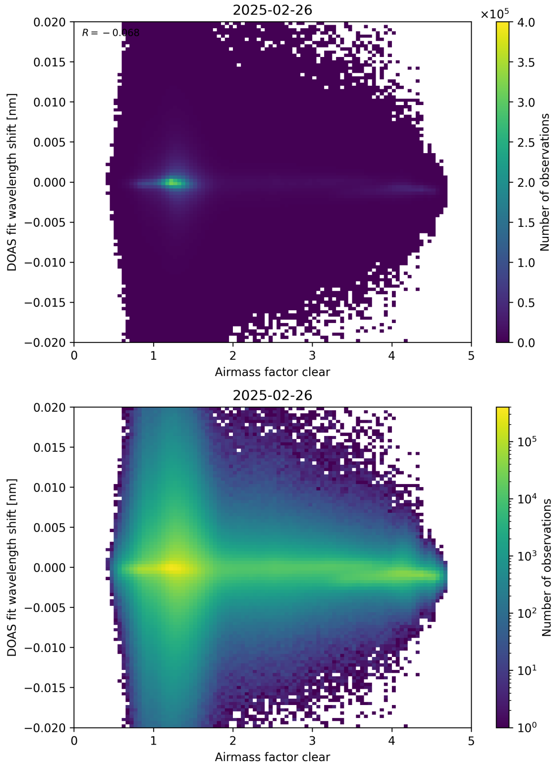
Figure 72: Scatter density plot of “Airmass factor clear” against “DOAS fit wavelength shift” for 2025-02-25 to 2025-02-27.
