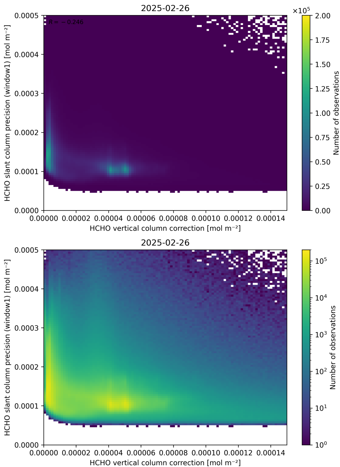
Figure 119: Scatter density plot of “HCHO vertical column correction” against “HCHO slant column precision (window1)” for 2025-02-25 to 2025-02-27.
