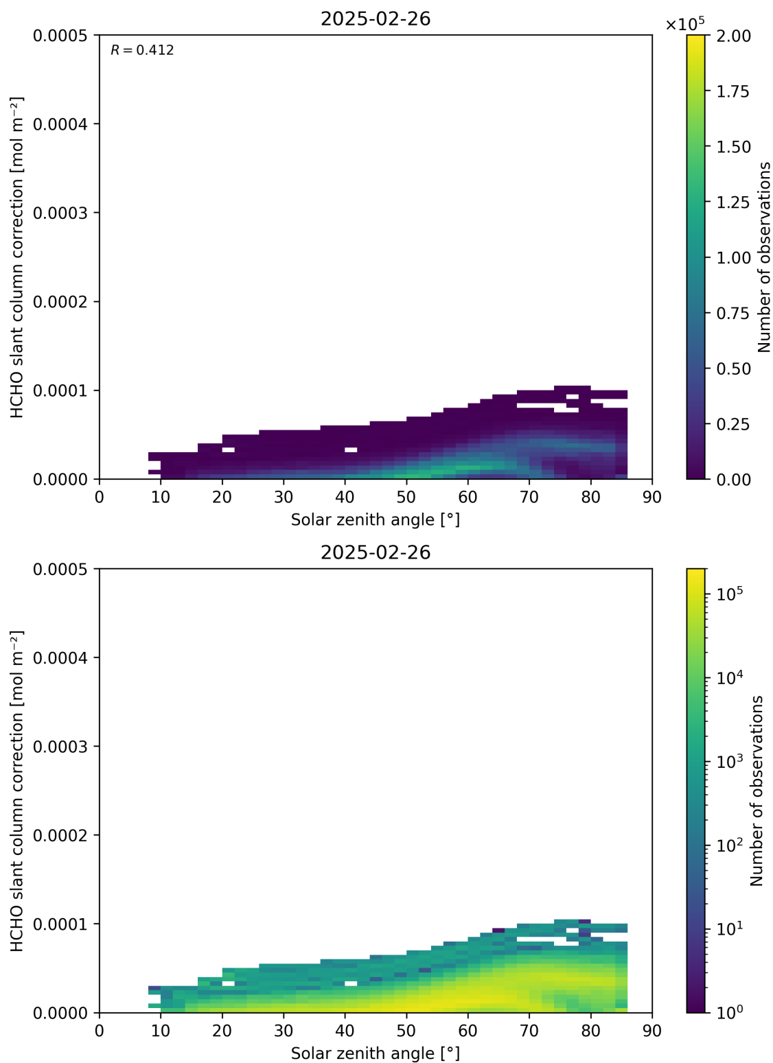
Figure 172: Scatter density plot of “Solar zenith angle” against “HCHO slant column correction” for 2025-02-25 to 2025-02-27.
