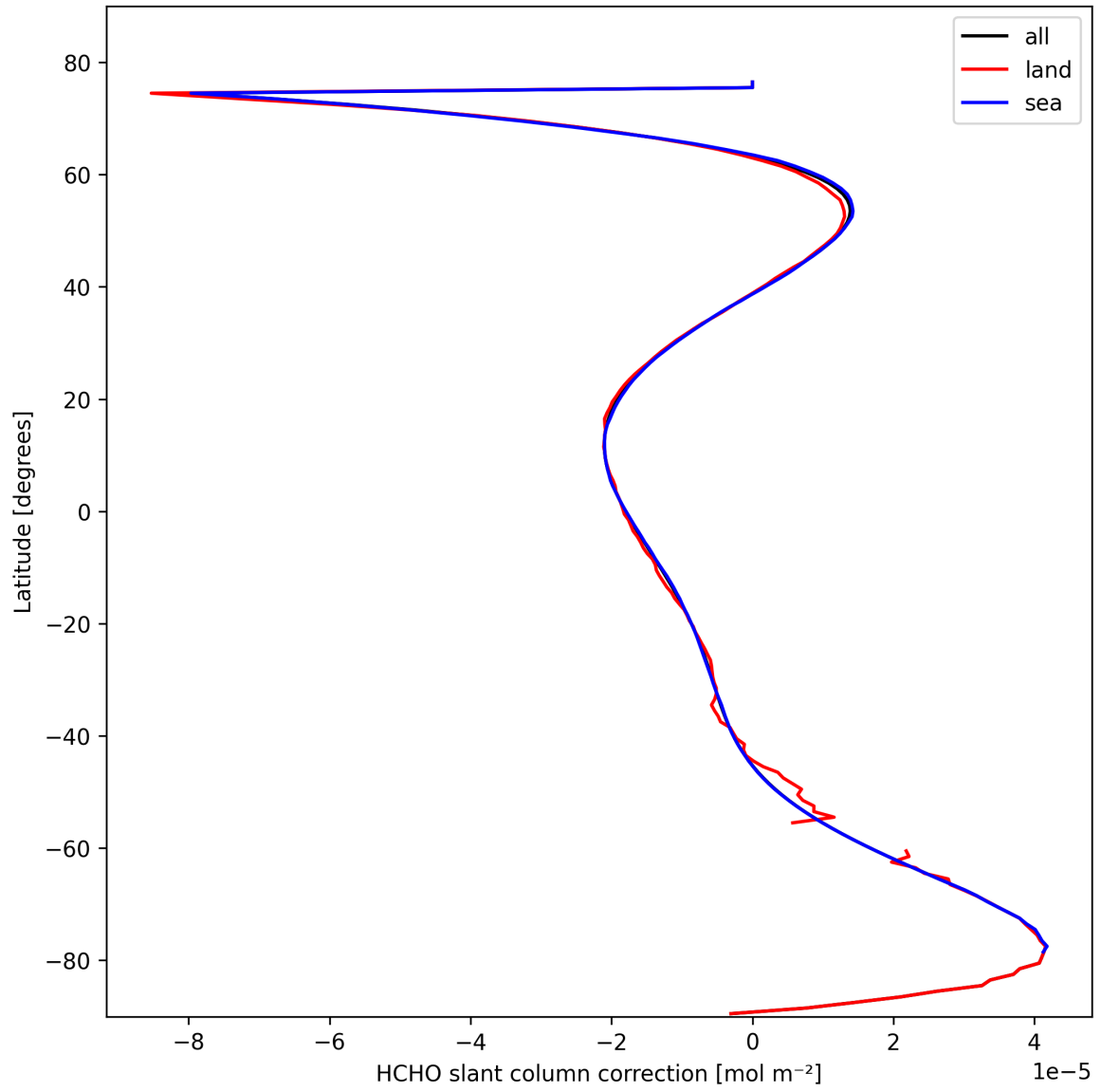
Figure 33: Zonal average of “HCHO slant column correction” for 2025-02-25 to 2025-02-27.
