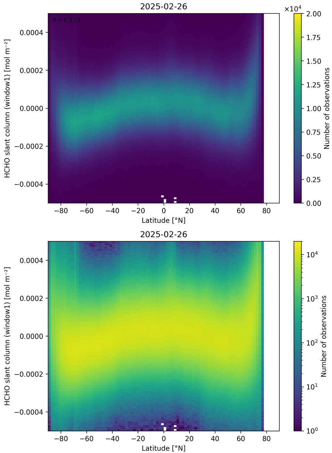
Figure 159: Scatter density plot of “Latitude” against “HCHO slant column (window1)” for 2025-02-25 to 2025-02-27.
