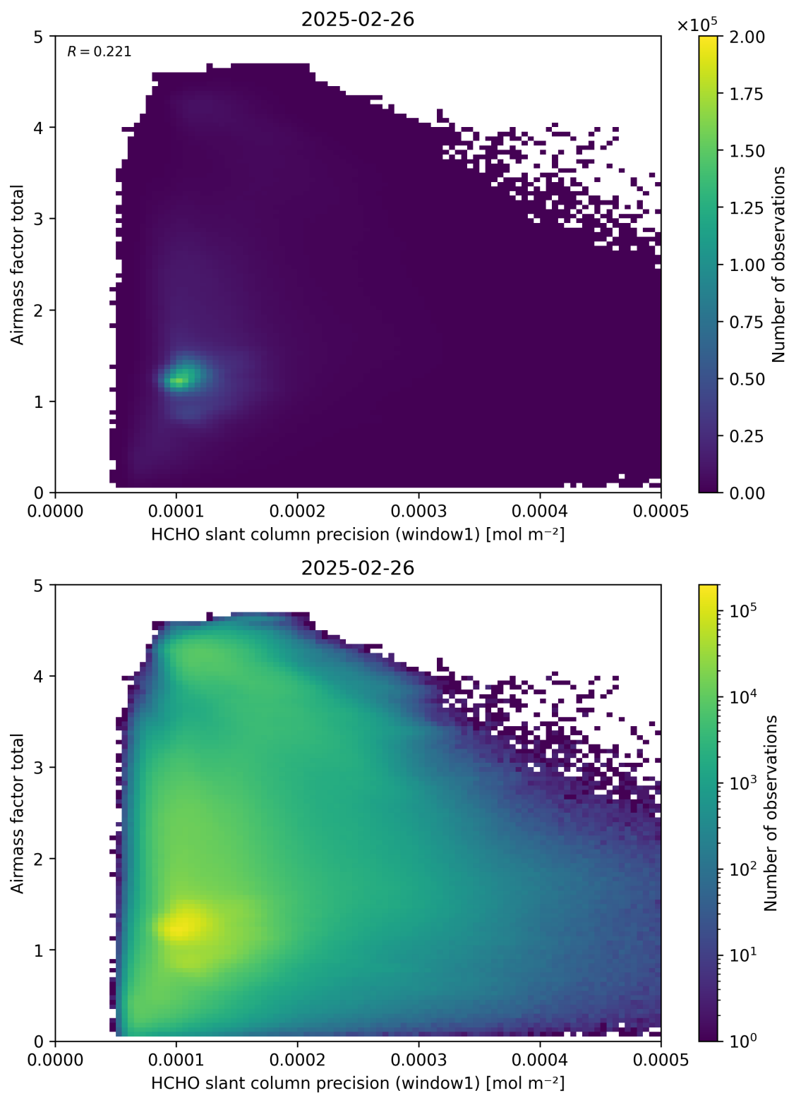
Figure 94: Scatter density plot of “HCHO slant column precision (window1)” against “Airmass factor total” for 2025-02-25 to 2025-02-27.
