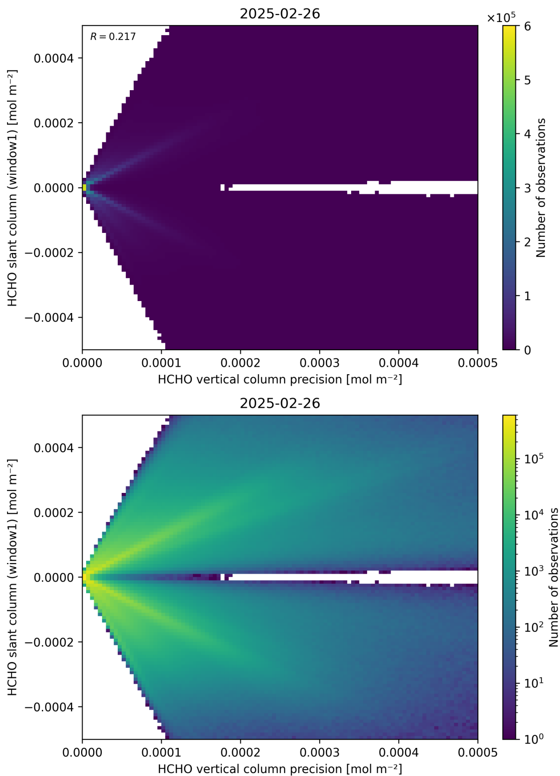
Figure 142: Scatter density plot of “HCHO vertical column precision” against “HCHO slant column (window1)” for 2025-02-25 to 2025-02-27.
