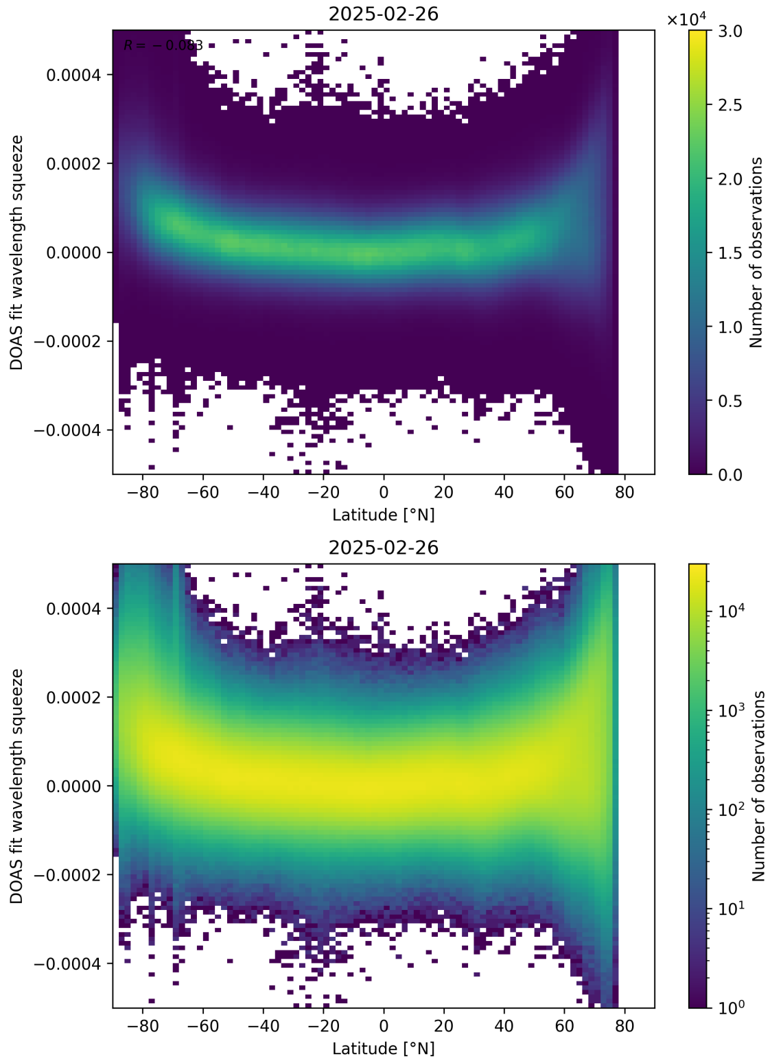
Figure 155: Scatter density plot of “Latitude” against “DOAS fit wavelength squeeze” for 2025-02-25 to 2025-02-27.
