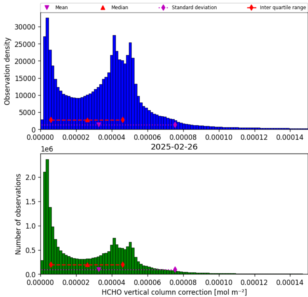
Figure 37: Histogram of “HCHO vertical column correction” for 2025-02-25 to 2025-02-27
