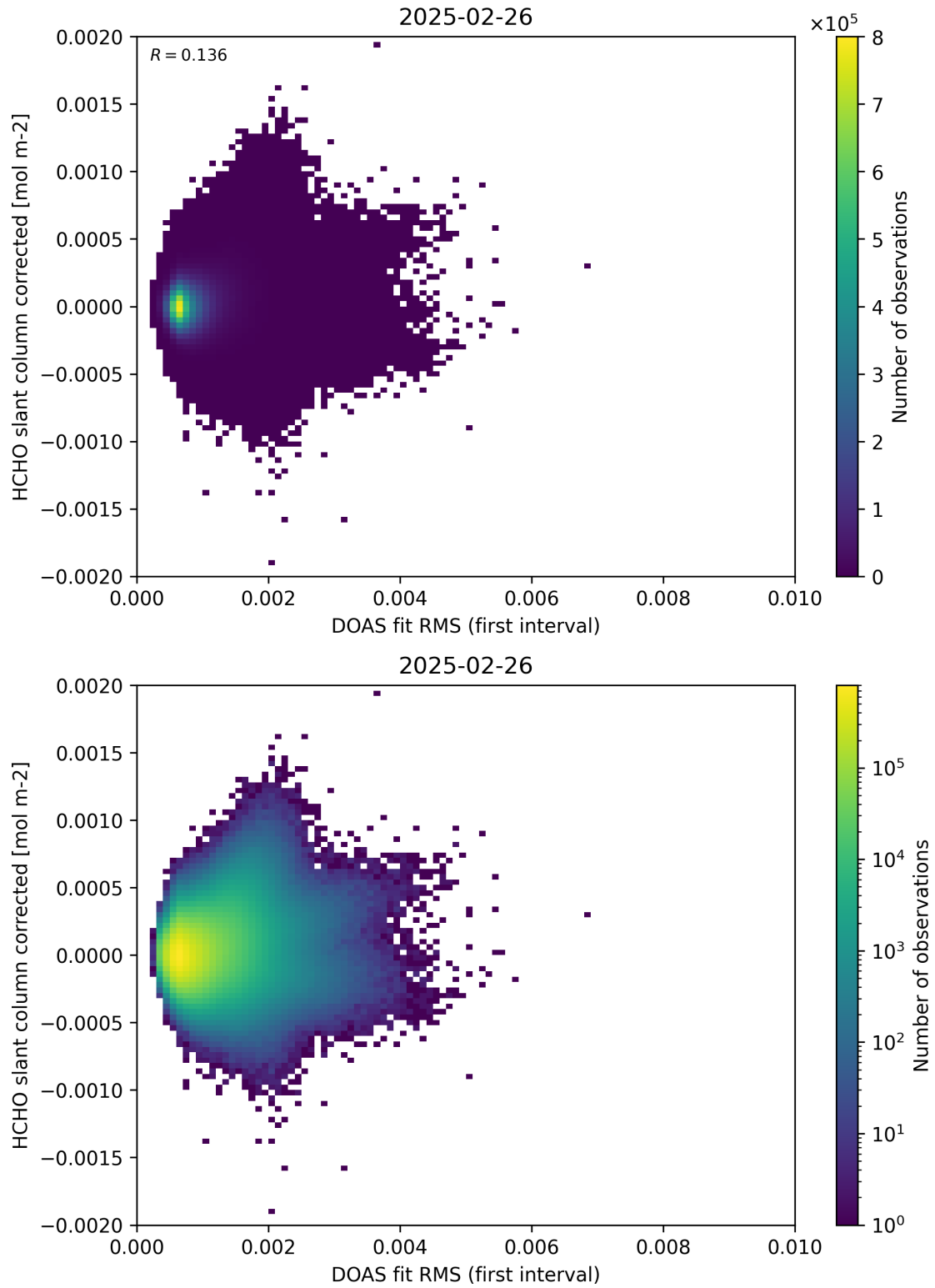
Figure 62: Scatter density plot of “DOAS fit RMS (first interval)” against “HCHO slant column corrected” for 2025-02-25 to 2025-02-27.
