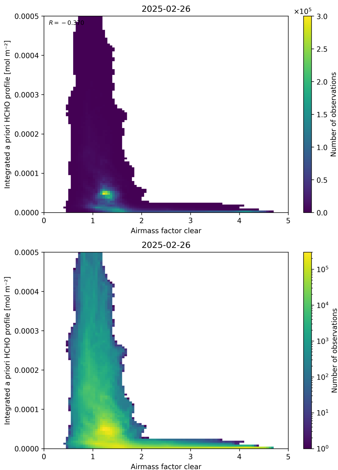
Figure 76: Scatter density plot of “Airmass factor clear” against “Integrated a priori HCHO profile” for 2025-02-25 to 2025-02-27.
