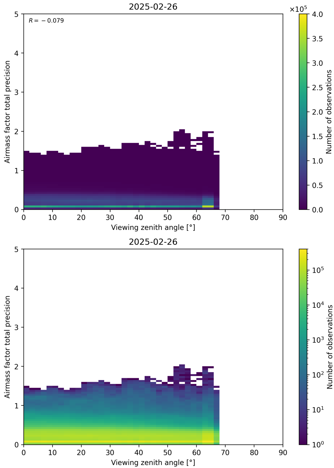
Figure 191: Scatter density plot of “Viewing zenith angle” against “Airmass factor total precision” for 2025-02-25 to 2025-02-27.
