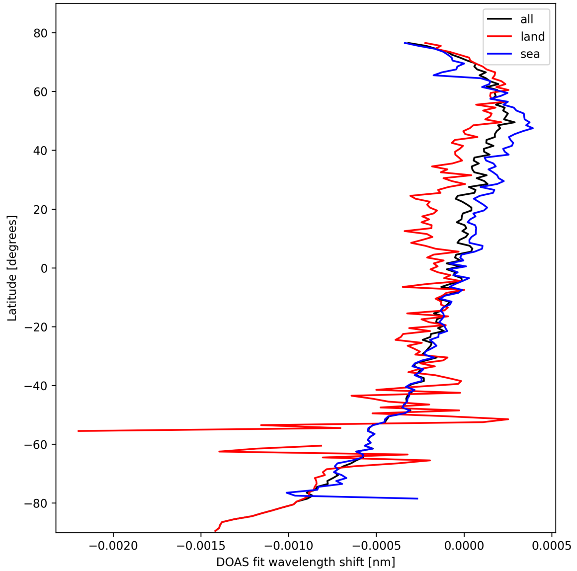
Figure 30: Zonal average of "DOAS fit wavelength shift" for 2025-02-25 to 2025-02-27.
