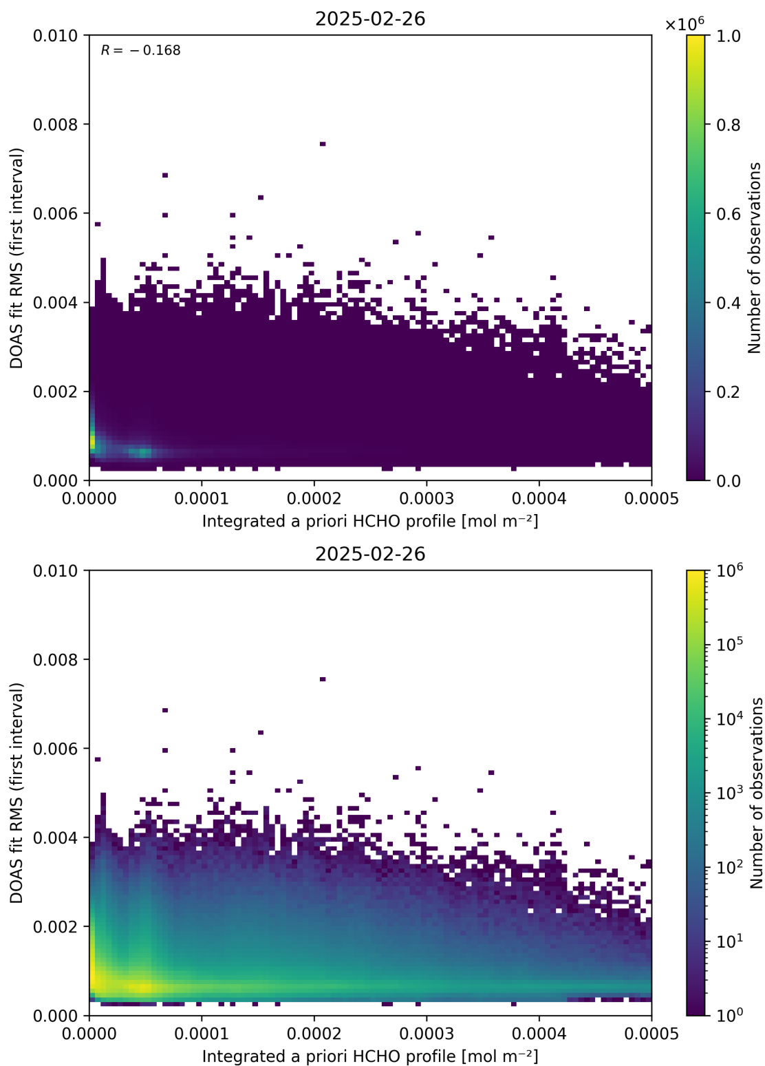
Figure 148: Scatter density plot of “Integrated a priori HCHO profile” against “DOAS fit RMS (first interval)” for 2025-02-25 to 2025-02-27.
