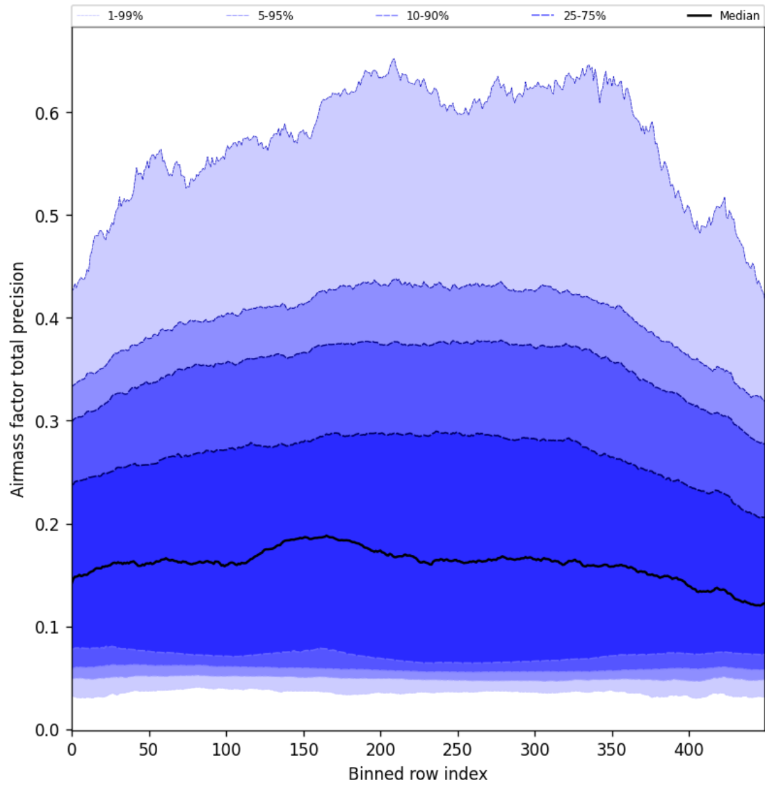
Figure 55: Along track statistics of “Airmass factor total precision” for 2025-02-25 to 2025-02-27
