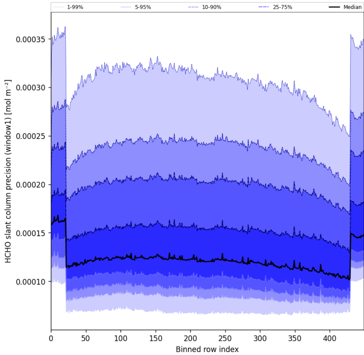
Figure 53: Along track statistics of "HCHO slant column precision (window1)" for 2025-02-25 to 2025-02-27
