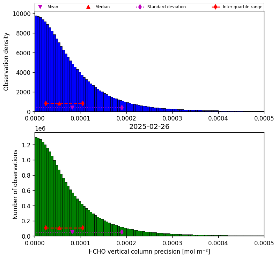
Figure 36: Histogram of “HCHO vertical column precision” for 2025-02-25 to 2025-02-27
