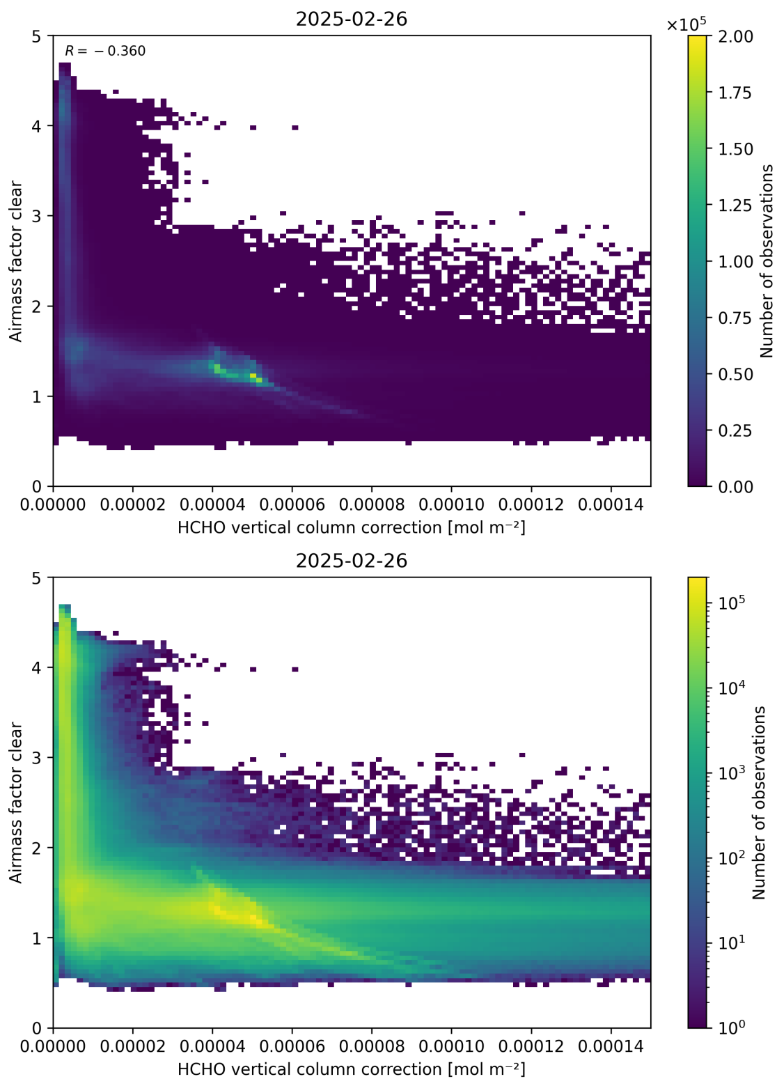
Figure 115: Scatter density plot of “HCHO vertical column correction” against “Airmass factor clear” for 2025-02-25 to 2025-02-27.
