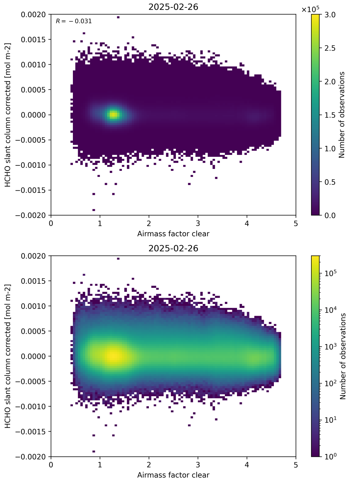
Figure 74: Scatter density plot of “Airmass factor clear” against “HCHO slant column corrected” for 2025-02-25 to 2025-02-27.
