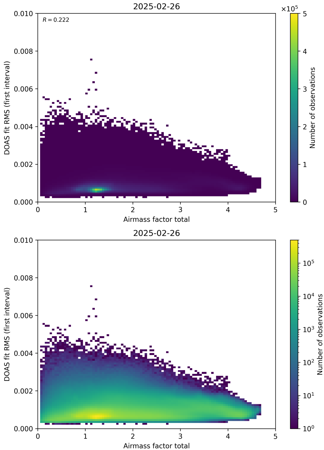
Figure 97: Scatter density plot of “Airmass factor total” against “DOAS fit RMS (first interval)” for 2025-02-25 to 2025-02-27.
