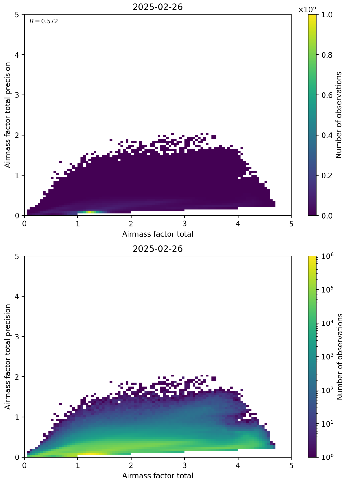
Figure 103: Scatter density plot of “Airmass factor total” against “Airmass factor total precision” for 2025-02-25 to 2025-02-27.
