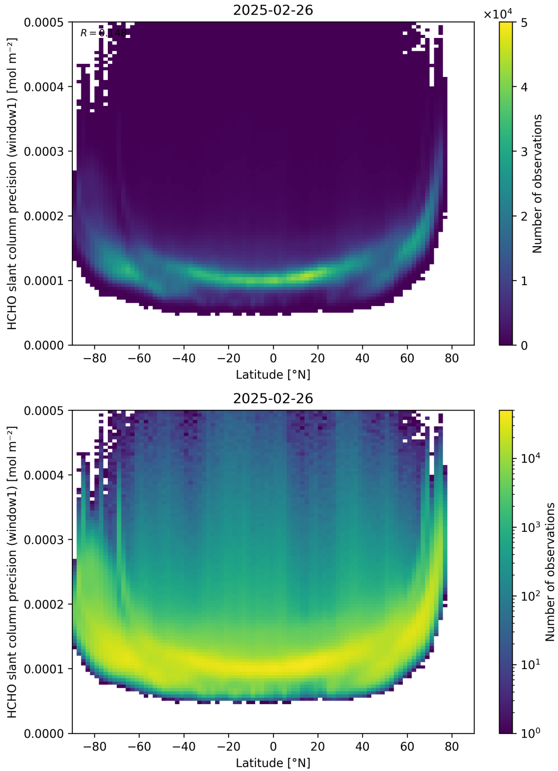
Figure 160: Scatter density plot of “Latitude” against “HCHO slant column precision (window1)” for 2025-02-25 to 2025-02-27.
