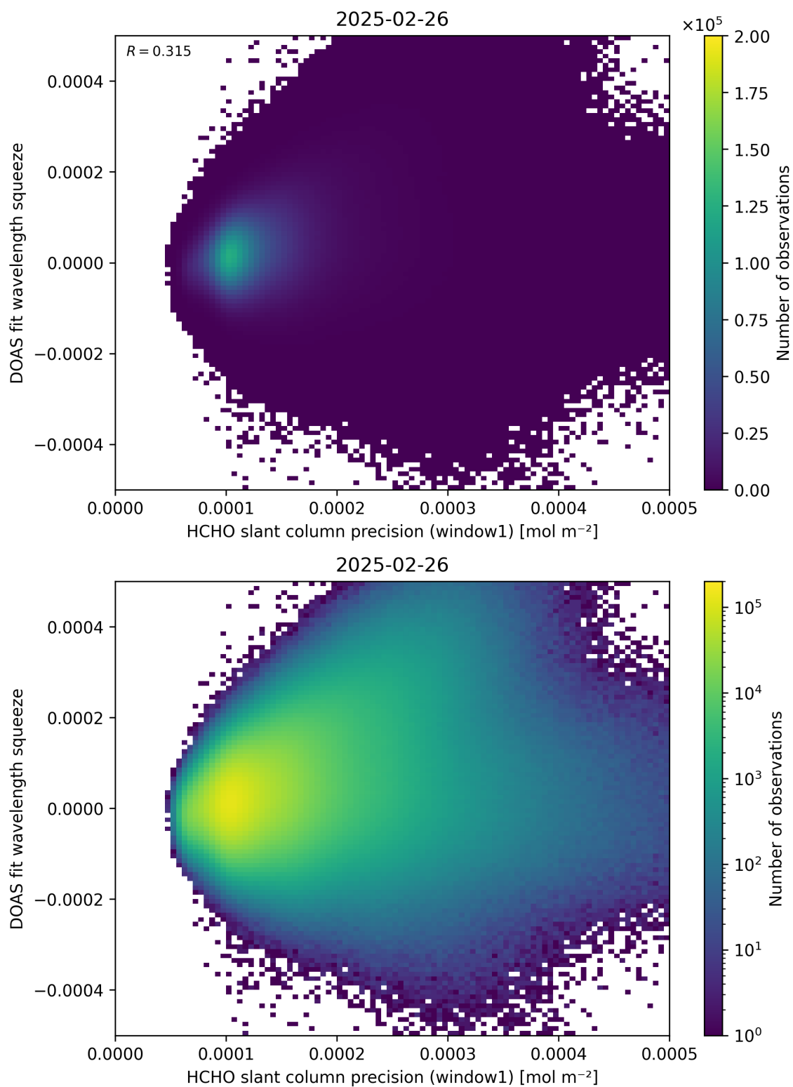
Figure 90: Scatter density plot of “HCHO slant column precision (window1)” against “DOAS fit wavelength squeeze” for 2025-02-25 to 2025-02-27.
