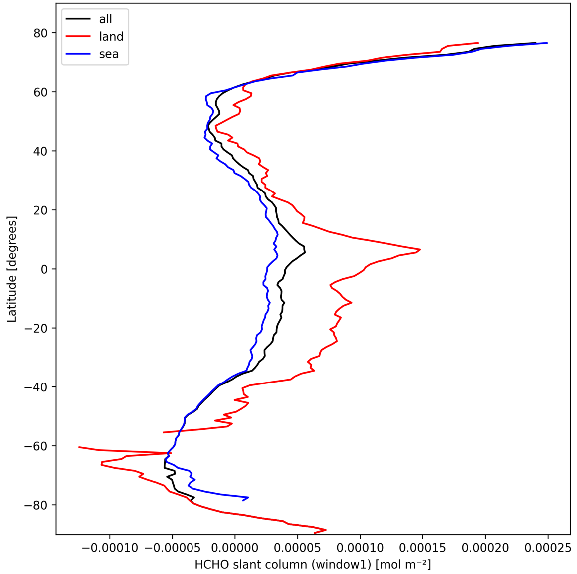
Figure 24: Zonal average of “HCHO slant column (window1)” for 2025-02-25 to 2025-02-27.
