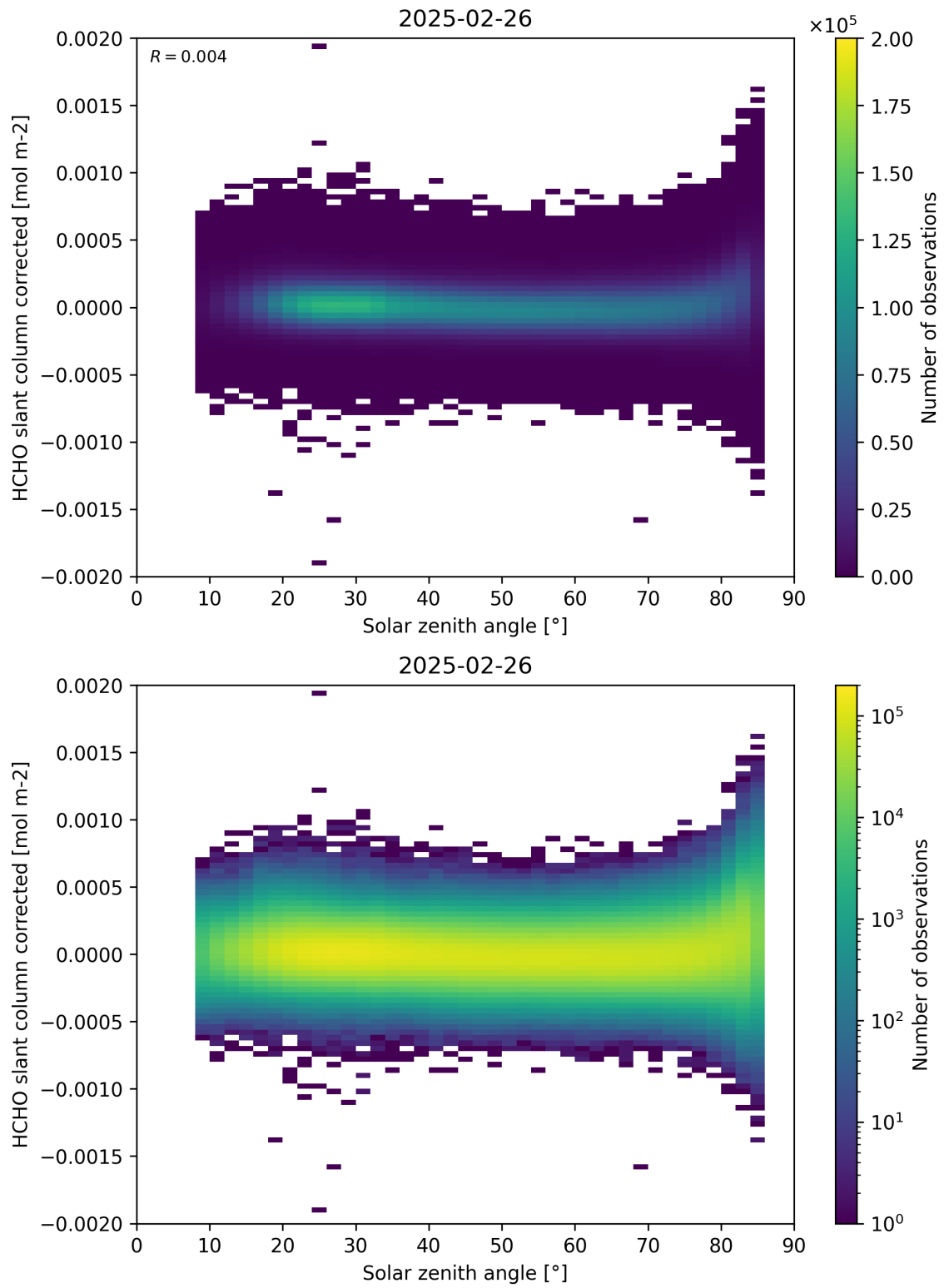
Figure 171: Scatter density plot of “Solar zenith angle” against “HCHO slant column corrected” for 2025-02-25 to 2025-02-27.
