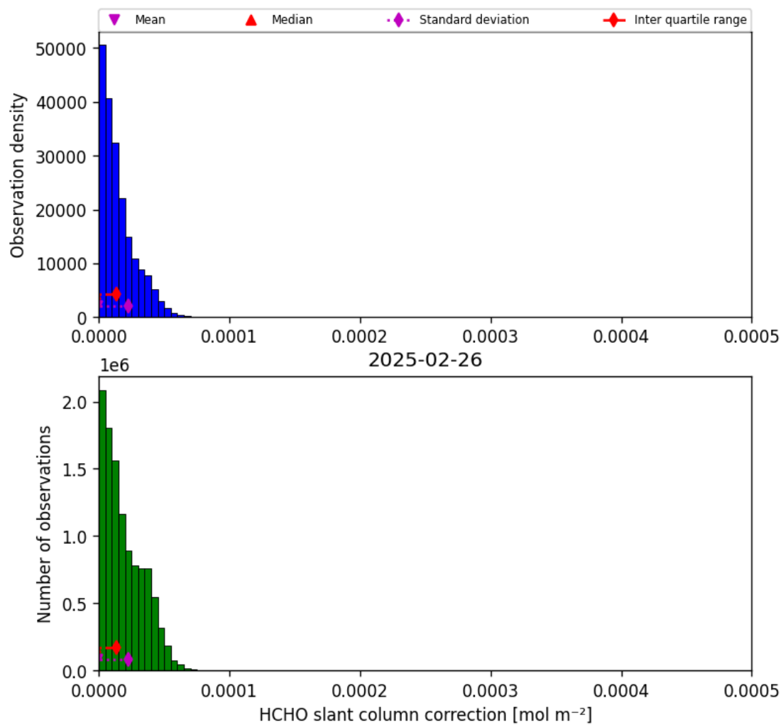
Figure 47: Histogram of “HCHO slant column correction” for 2025-02-25 to 2025-02-27
