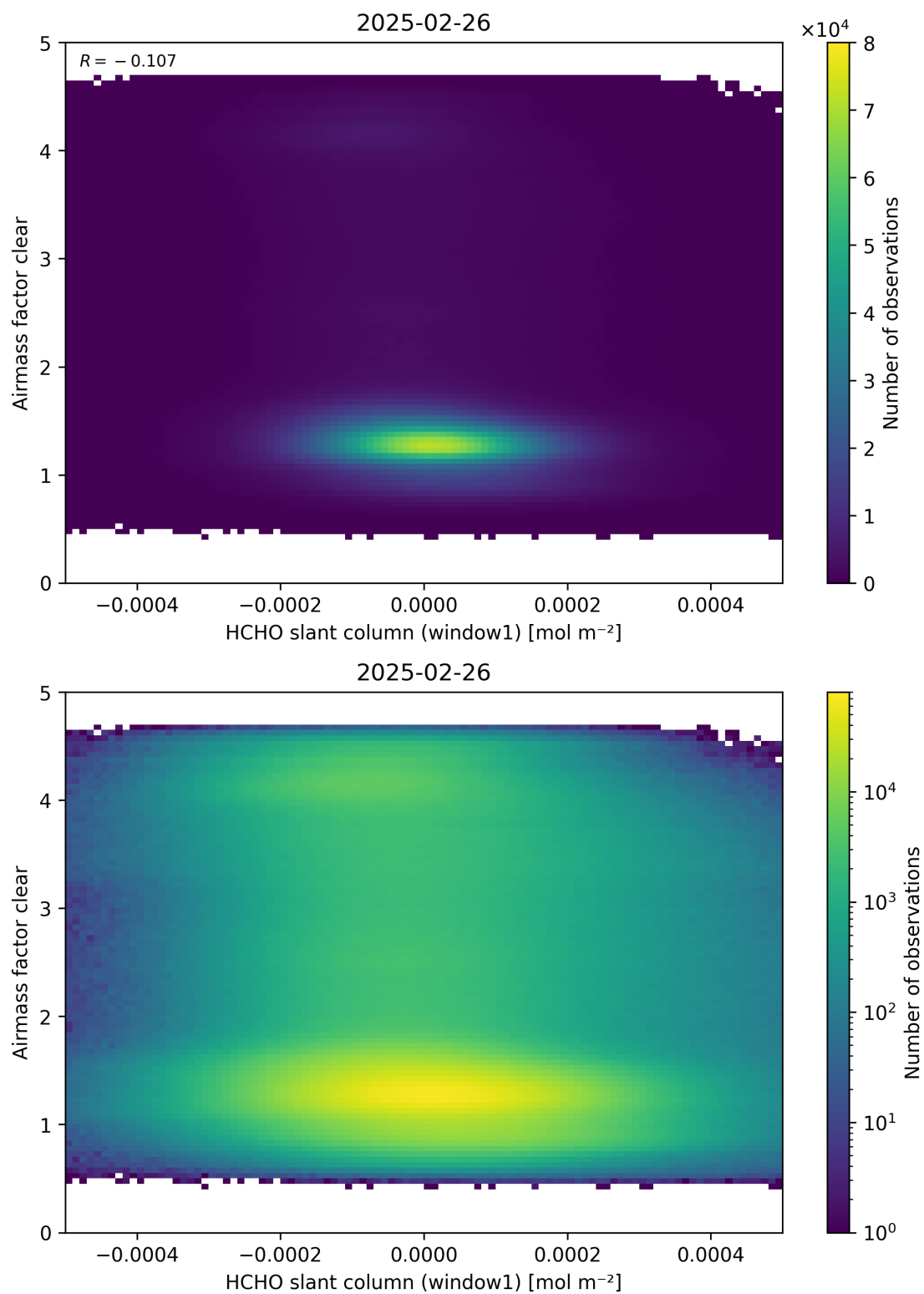
Figure 81: Scatter density plot of “HCHO slant column (window1)” against “Airmass factor clear” for 2025-02-25 to 2025-02-27.
