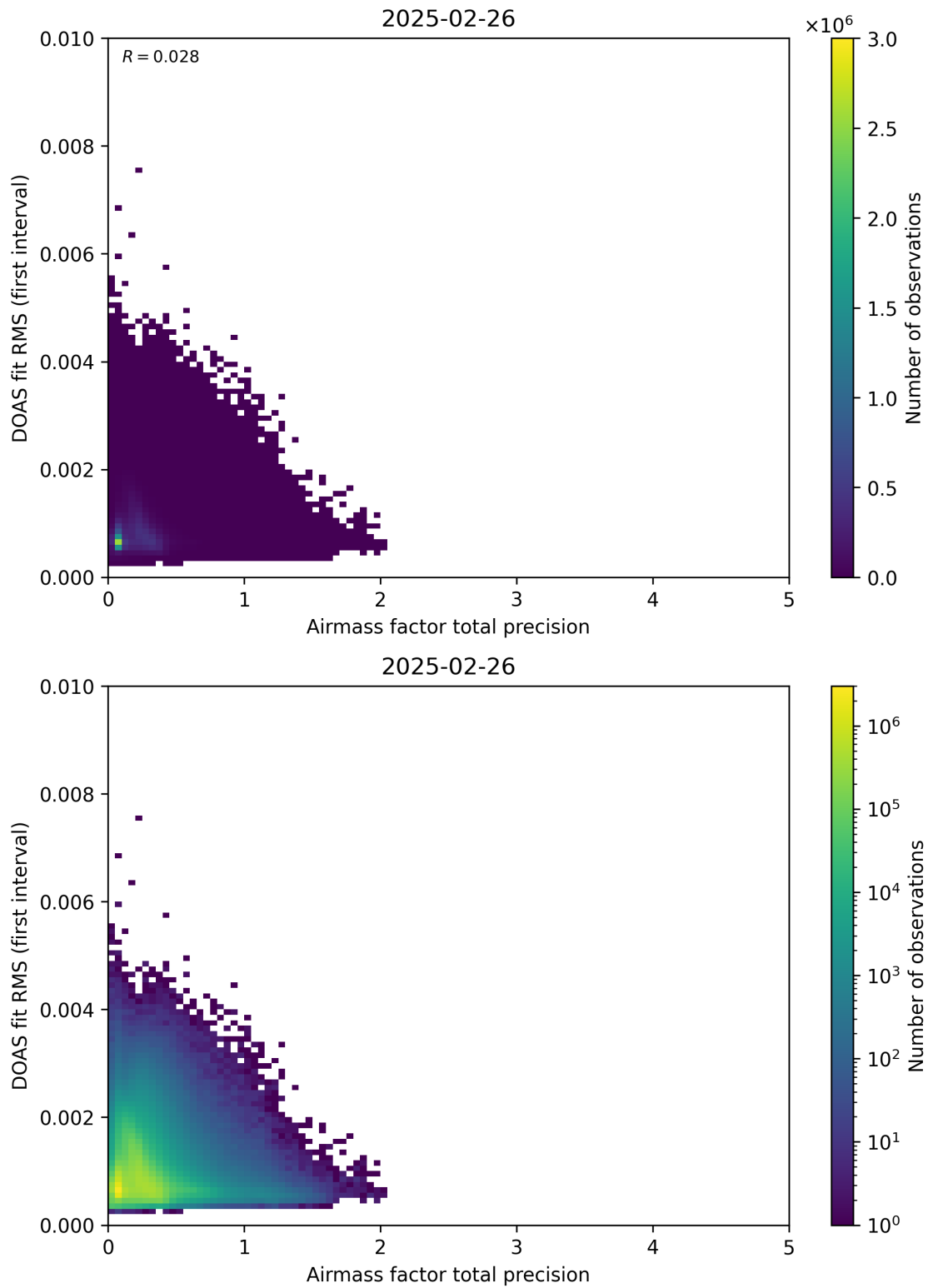
Figure 105: Scatter density plot of “Airmass factor total precision” against “DOAS fit RMS (first interval)” for 2025-02-25 to 2025-02-27.
