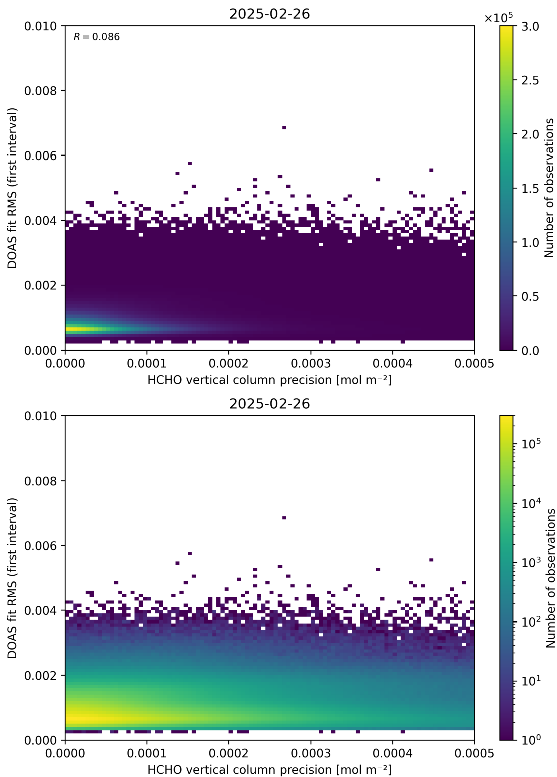
Figure 136: Scatter density plot of “HCHO vertical column precision” against “DOAS fit RMS (first interval)” for 2025-02-25 to 2025-02-27.
