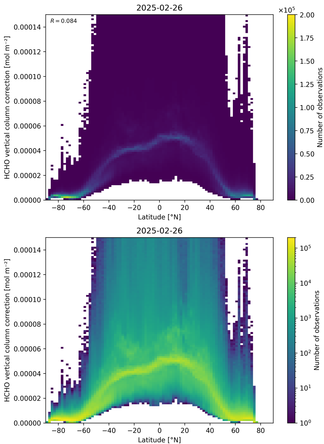
Figure 164: Scatter density plot of “Latitude” against “HCHO vertical column correction” for 2025-02-25 to 2025-02-27.
