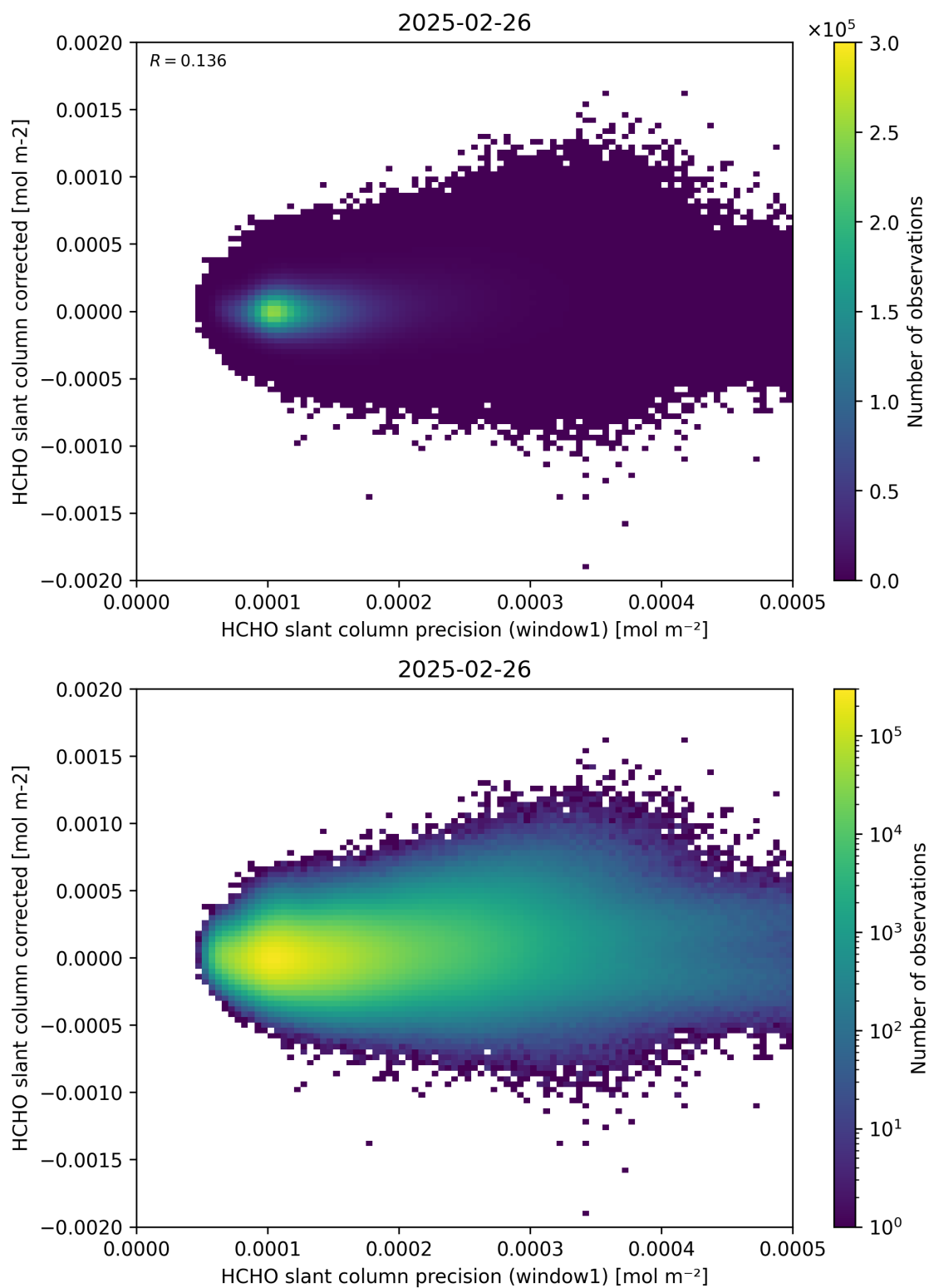
Figure 92: Scatter density plot of “HCHO slant column precision (window1)” against “HCHO slant column corrected” for 2025-02-25 to 2025-02-27.
