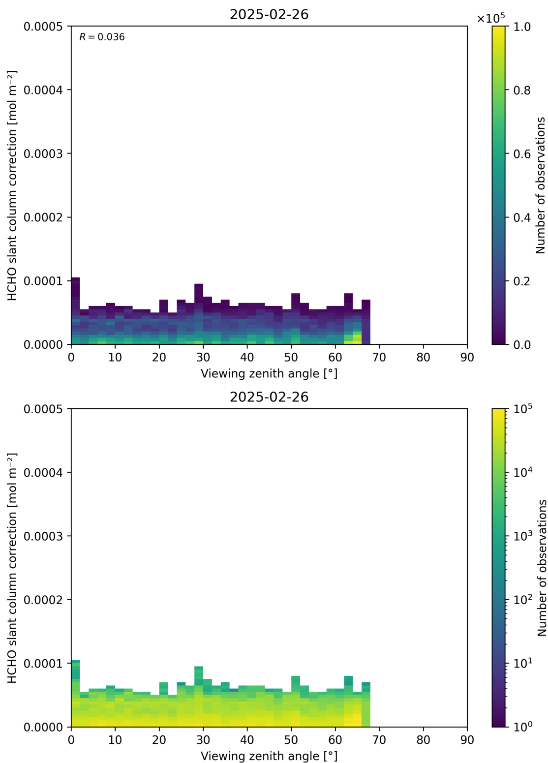
Figure 187: Scatter density plot of “Viewing zenith angle” against “HCHO slant column correction” for 2025-02-25 to 2025-02-27.
