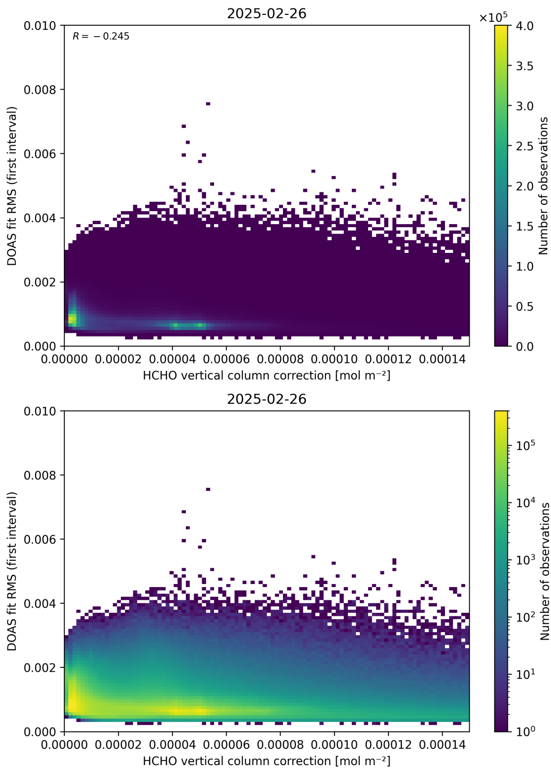
Figure 112: Scatter density plot of “HCHO vertical column correction” against “DOAS fit RMS (first interval)” for 2025-02-25 to 2025-02-27.
