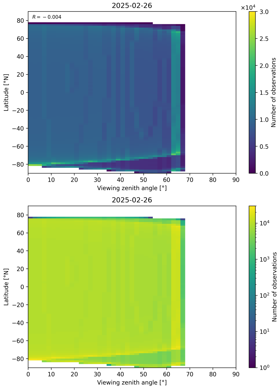
Figure 196: Scatter density plot of “Viewing zenith angle” against “Latitude” for 2025-02-25 to 2025-02-27.
