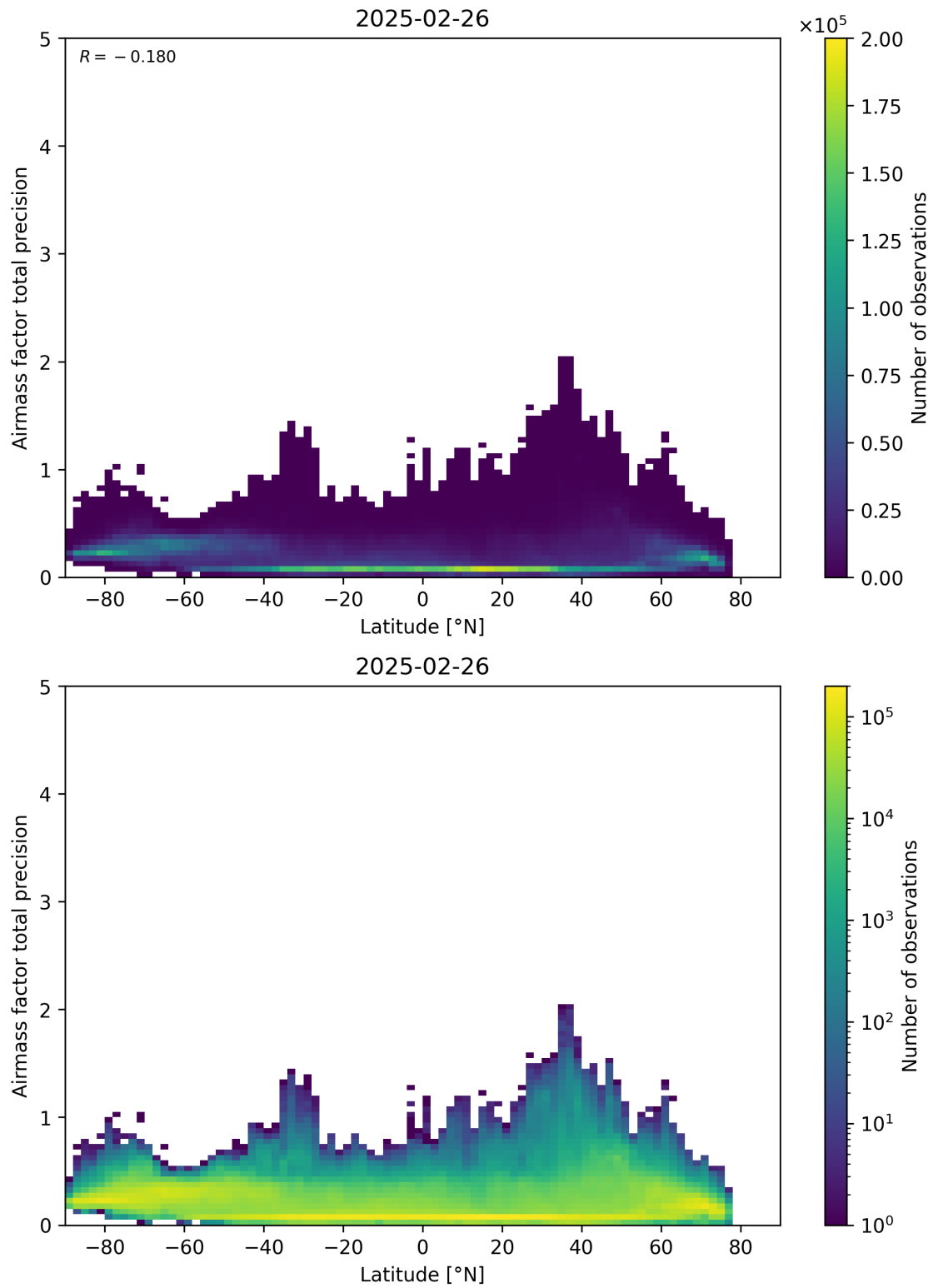
Figure 162: Scatter density plot of “Latitude” against “Airmass factor total precision” for 2025-02-25 to 2025-02-27.
