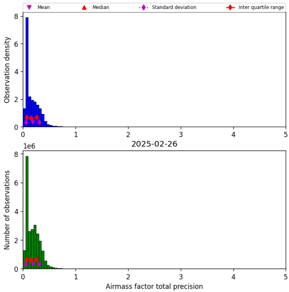
Figure 41: Histogram of “Airmass factor total precision” for 2025-02-25 to 2025-02-27
