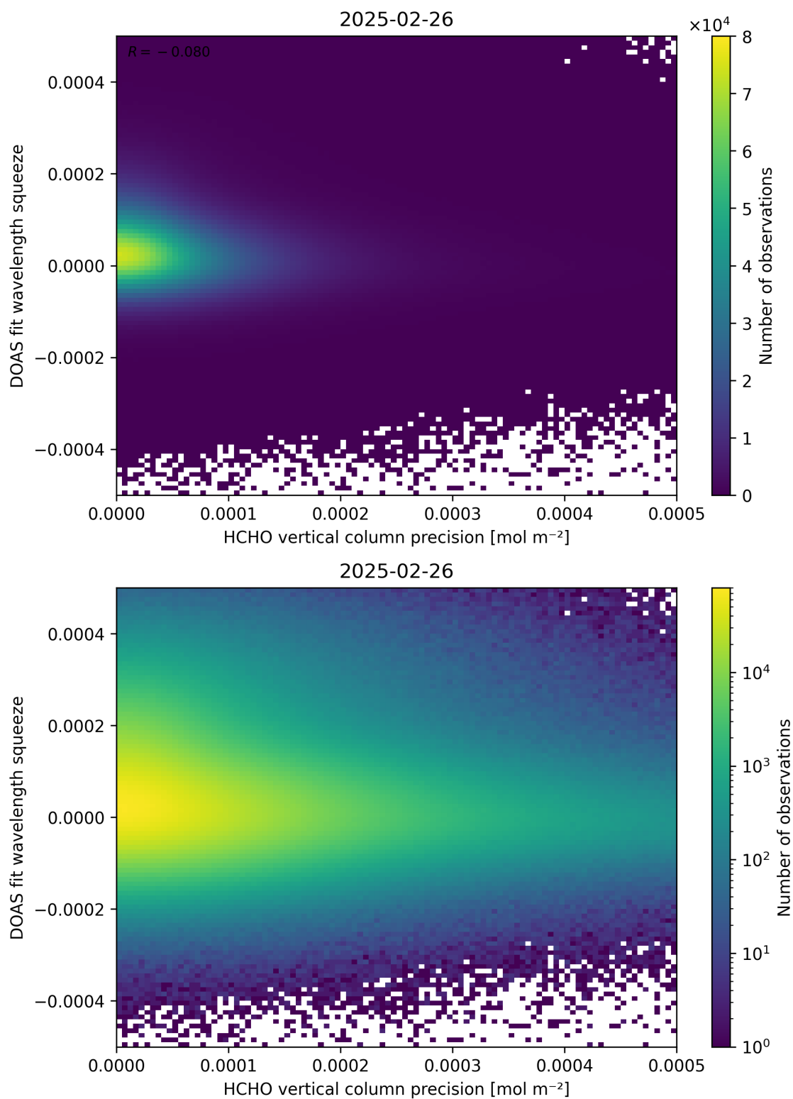
Figure 138: Scatter density plot of “HCHO vertical column precision” against “DOAS fit wavelength squeeze” for 2025-02-25 to 2025-02-27.
