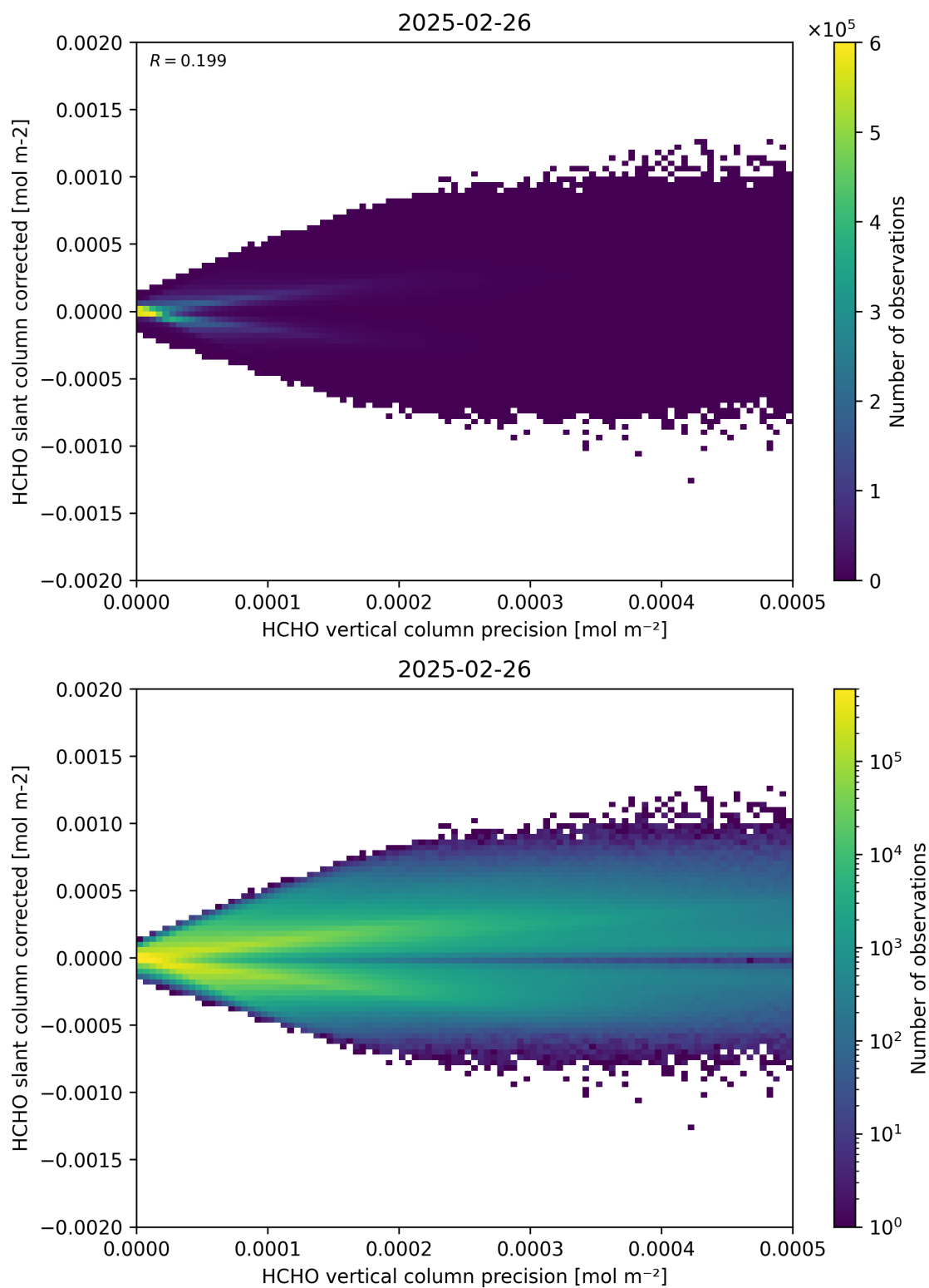
Figure 140: Scatter density plot of “HCHO vertical column precision” against “HCHO slant column corrected” for 2025-02-25 to 2025-02-27.
