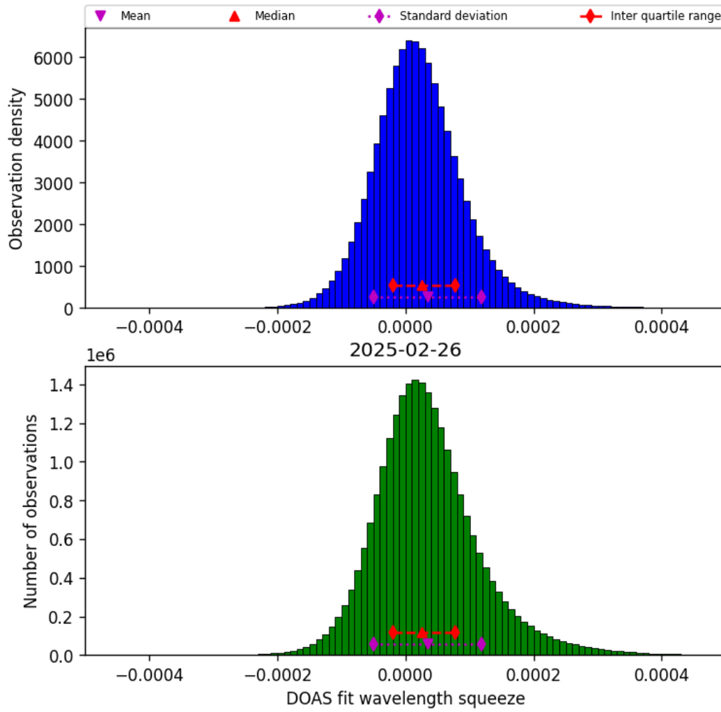
Figure 45: Histogram of “DOAS fit wavelength squeeze” for 2025-02-25 to 2025-02-27
