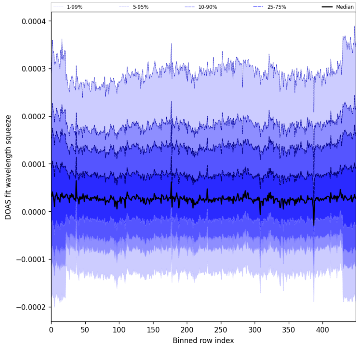
Figure 59: Along track statistics of “DOAS fit wavelength squeeze” for 2025-02-25 to 2025-02-27
