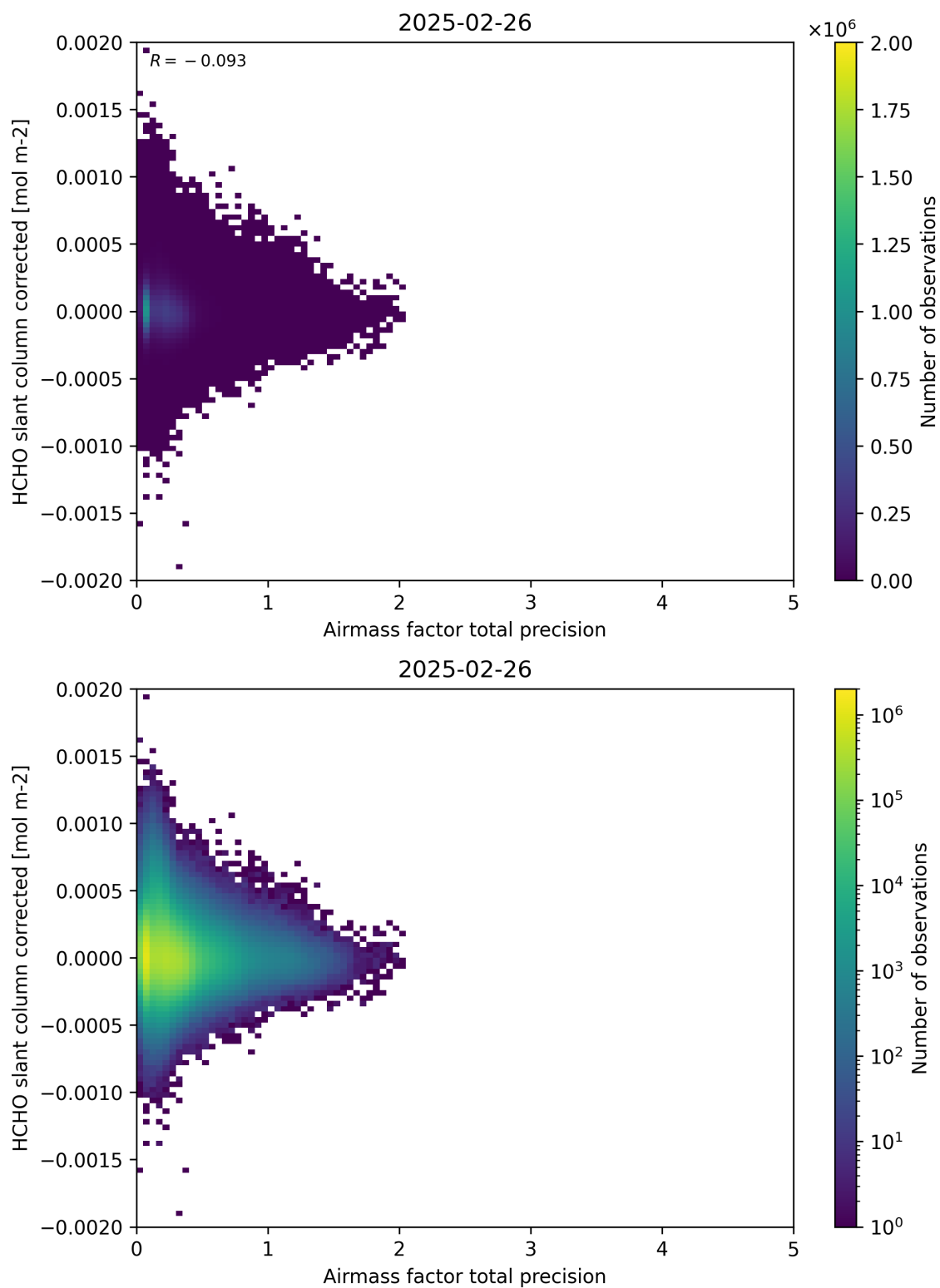
Figure 109: Scatter density plot of “Airmass factor total precision” against “HCHO slant column corrected” for 2025-02-25 to 2025-02-27.
