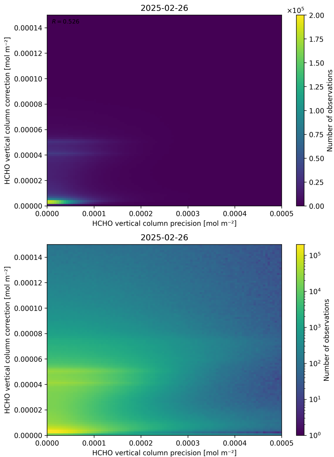
Figure 146: Scatter density plot of “HCHO vertical column precision” against “HCHO vertical column correction” for 2025-02-25 to 2025-02-27.
