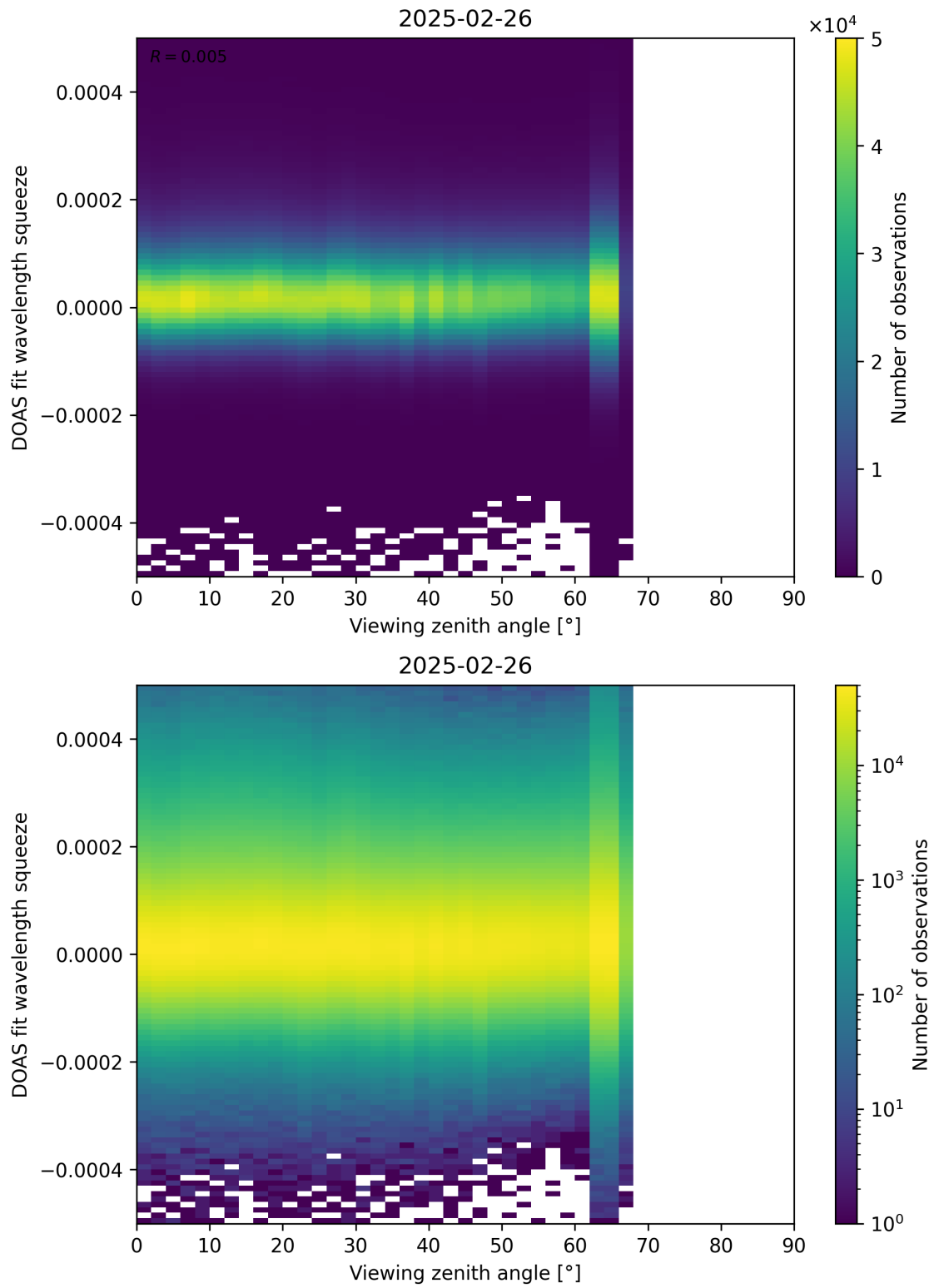
Figure 184: Scatter density plot of “Viewing zenith angle” against “DOAS fit wavelength squeeze” for 2025-02-25 to 2025-02-27.
