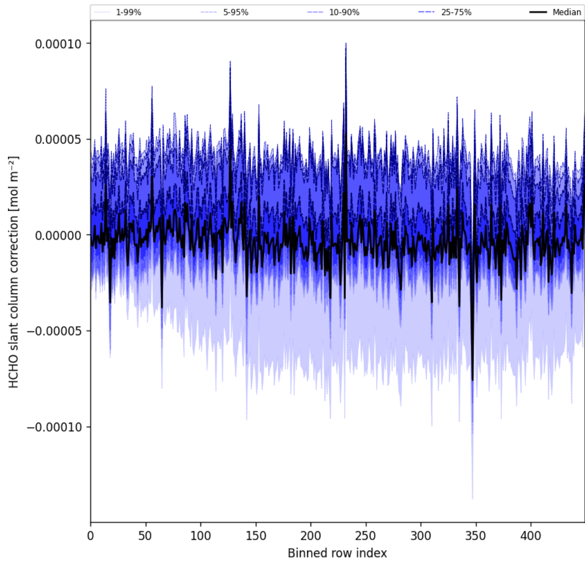
Figure 61: Along track statistics of “HCHO slant column correction” for 2025-02-25 to 2025-02-27
