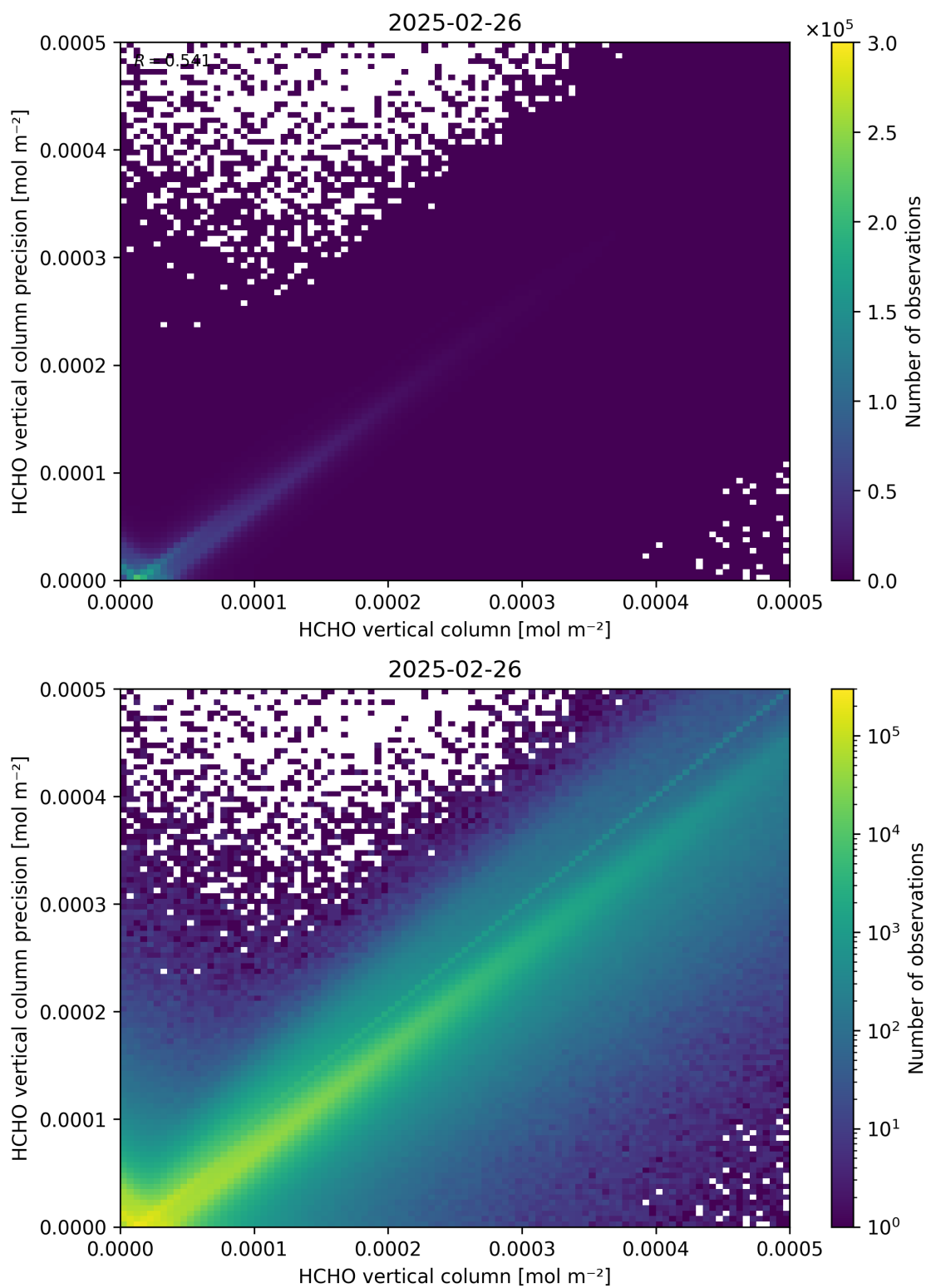
Figure 134: Scatter density plot of “HCHO vertical column” against “HCHO vertical column precision” for 2025-02-25 to 2025-02-27.
