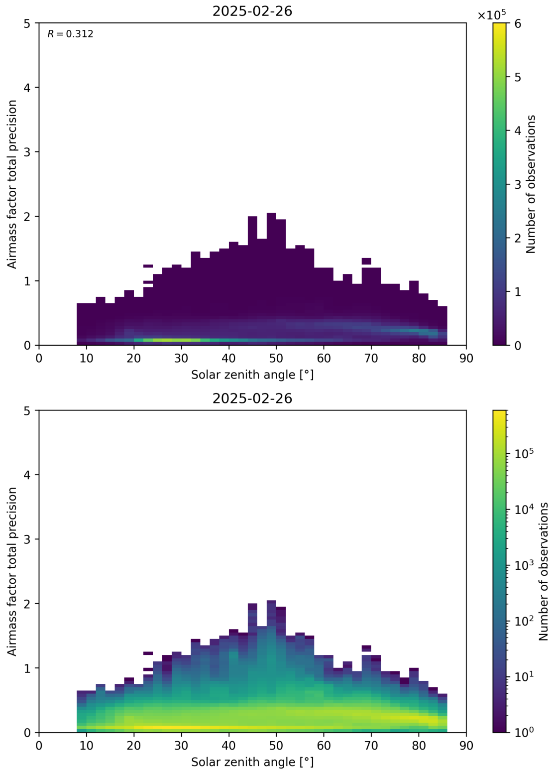
Figure 176: Scatter density plot of “Solar zenith angle” against “Airmass factor total precision” for 2025-02-25 to 2025-02-27.
