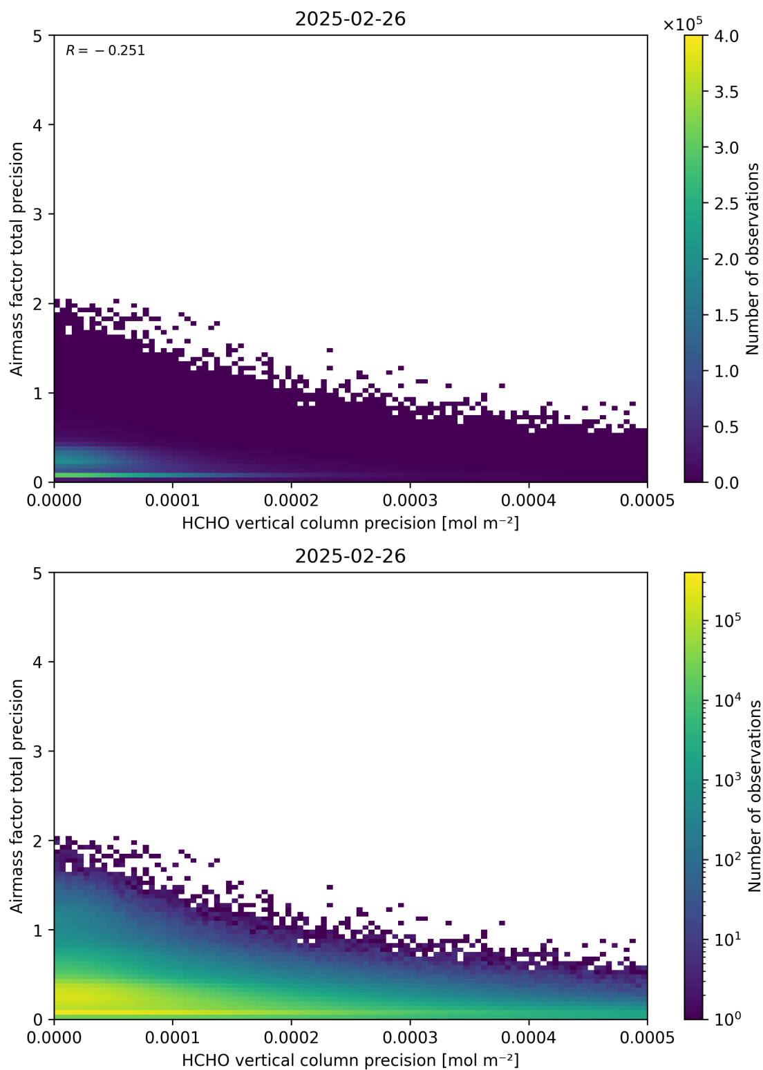
Figure 145: Scatter density plot of “HCHO vertical column precision” against “Airmass factor total precision” for 2025-02-25 to 2025-02-27.
