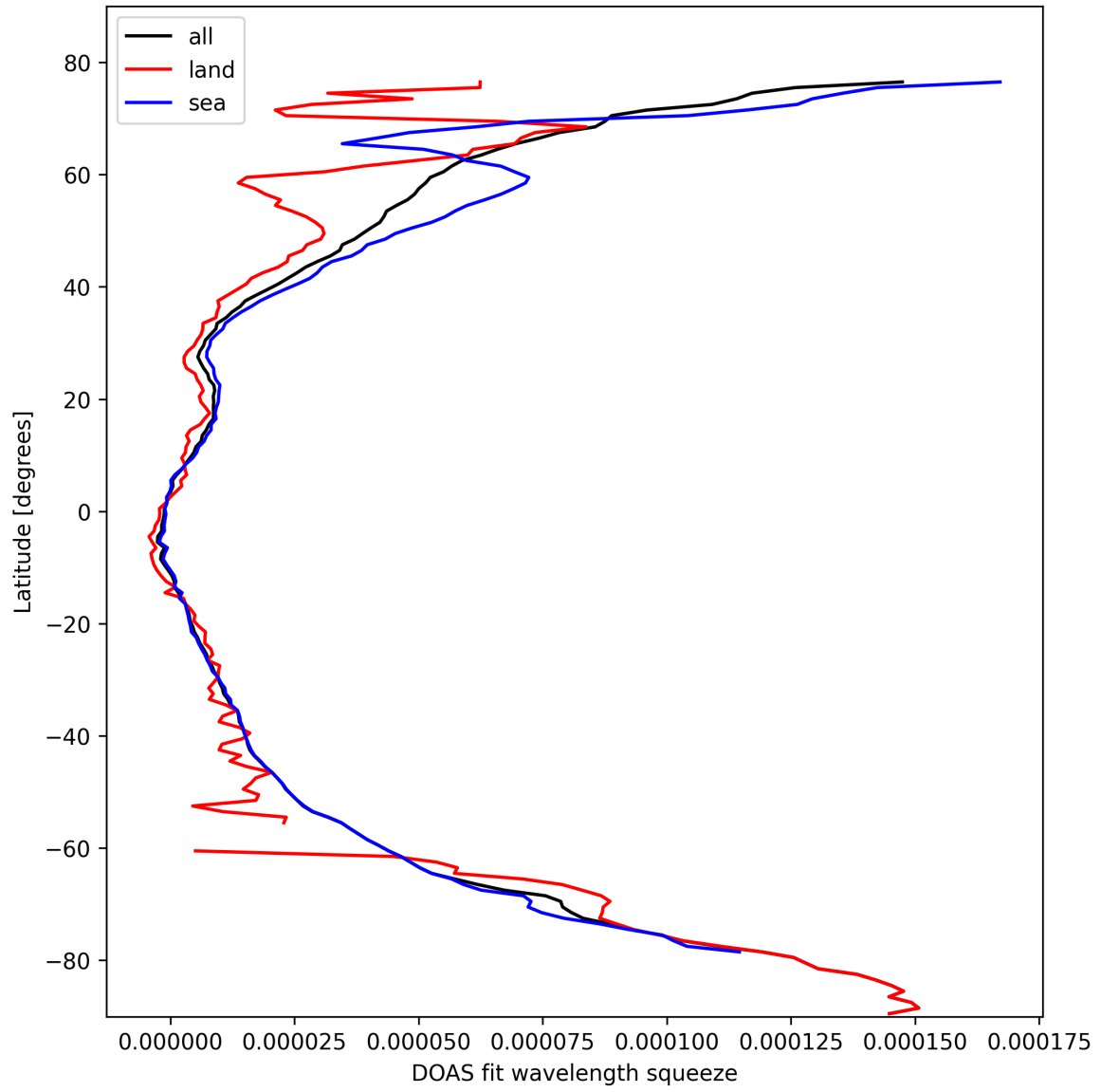
Figure 31: Zonal average of “DOAS fit wavelength squeeze” for 2025-02-25 to 2025-02-27.
