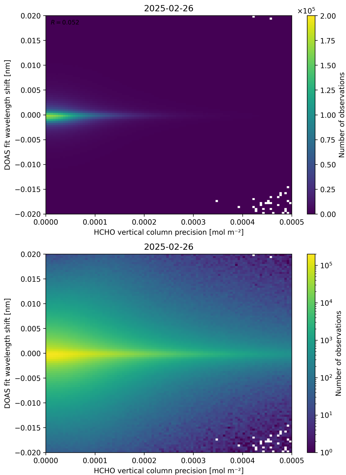
Figure 137: Scatter density plot of “HCHO vertical column precision” against “DOAS fit wavelength shift” for 2025-02-25 to 2025-02-27.
