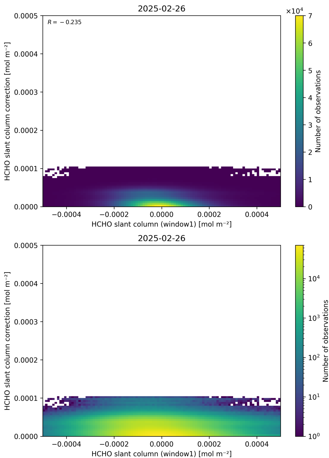
Figure 83: Scatter density plot of “HCHO slant column (window1)” against “HCHO slant column correction” for 2025-02-25 to 2025-02-27.
