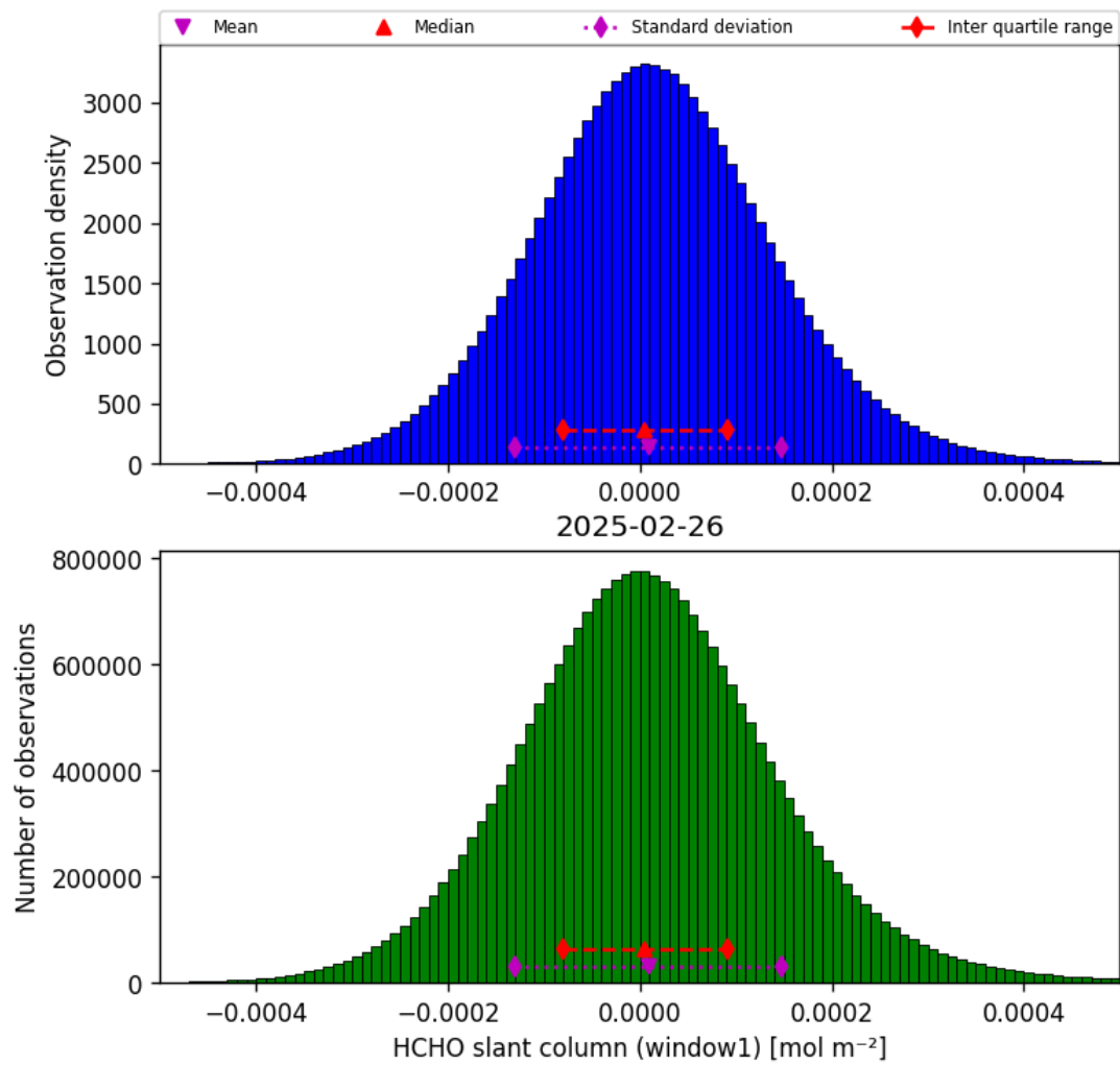
Figure 38: Histogram of “HCHO slant column (window1)” for 2025-02-25 to 2025-02-27
