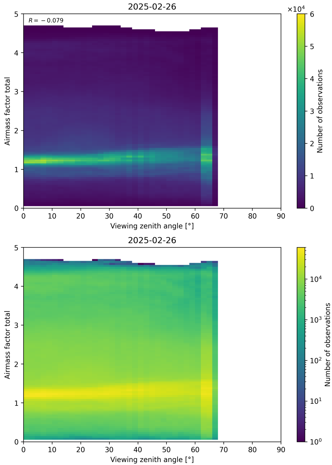
Figure 190: Scatter density plot of “Viewing zenith angle” against “Airmass factor total” for 2025-02-25 to 2025-02-27.
