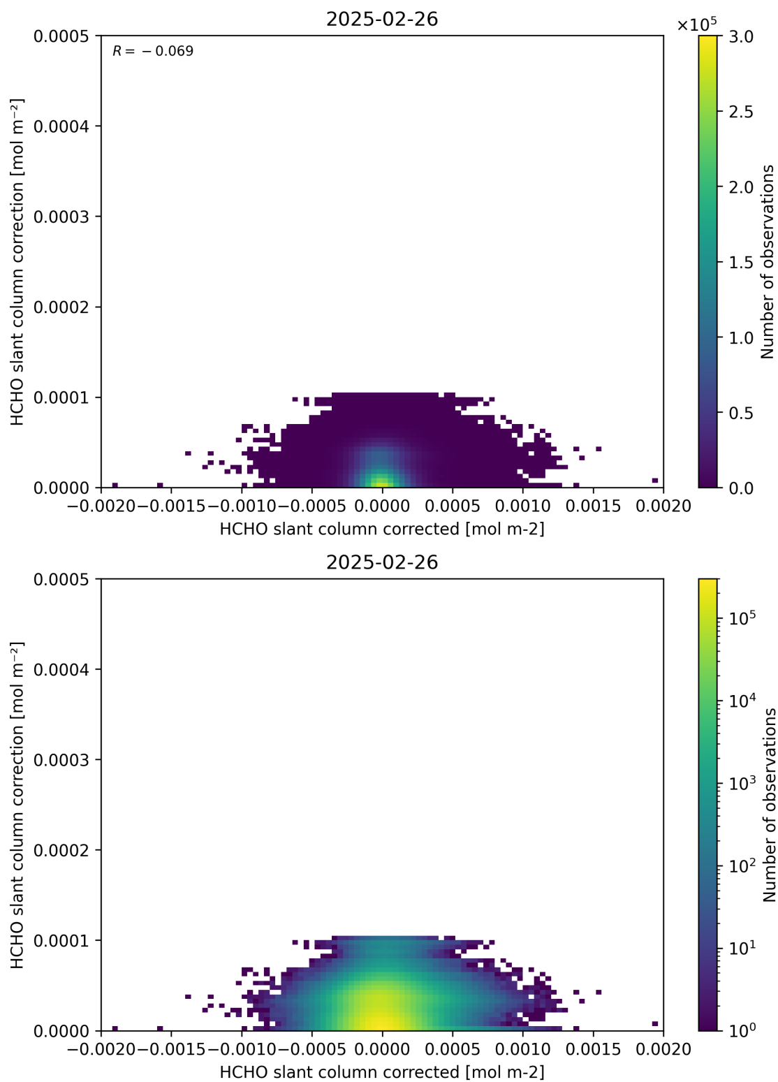
Figure 77: Scatter density plot of “HCHO slant column corrected” against “HCHO slant column correction” for 2025-02-25 to 2025-02-27.
