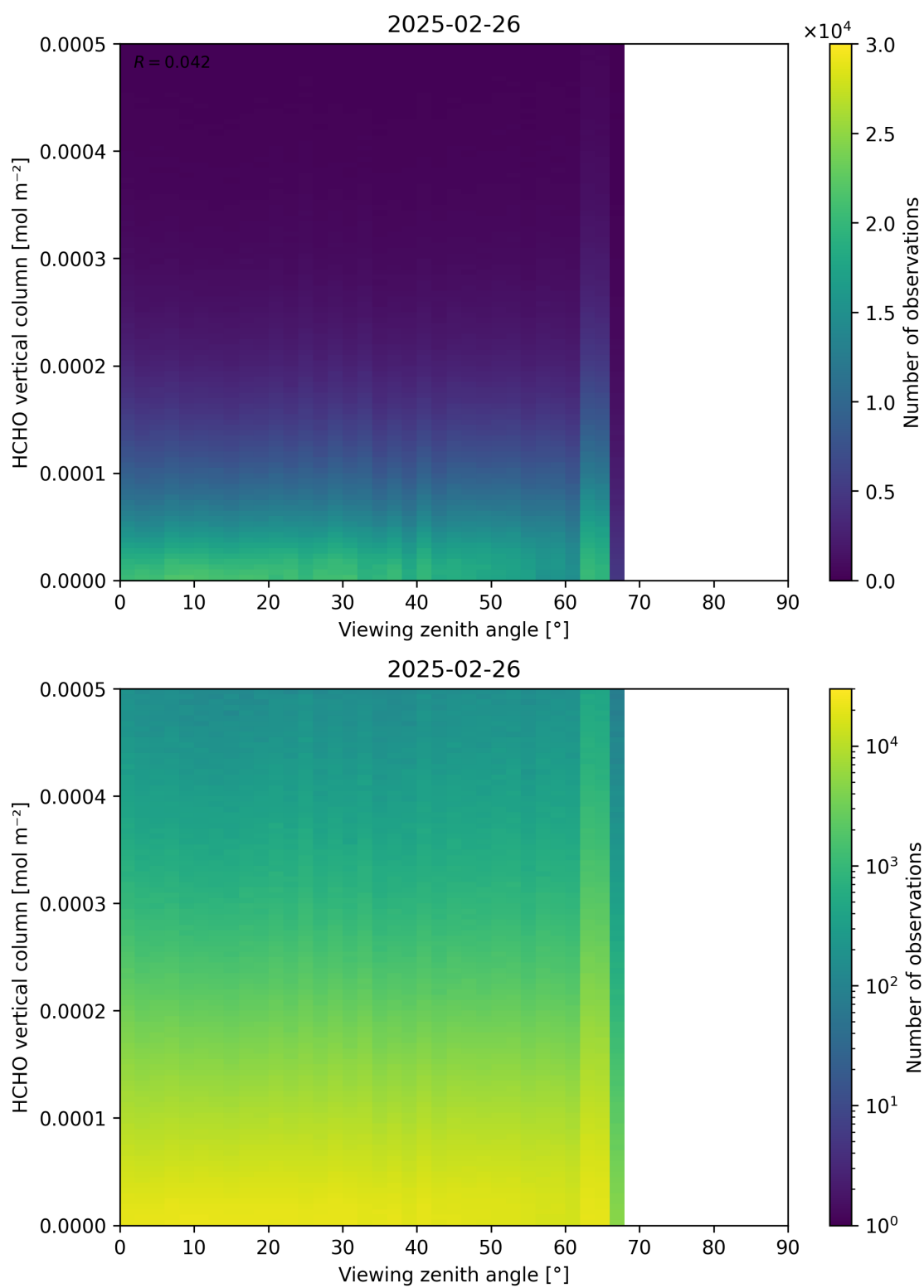
Figure 192: Scatter density plot of “Viewing zenith angle” against “HCHO vertical column” for 2025-02-25 to 2025-02-27.
