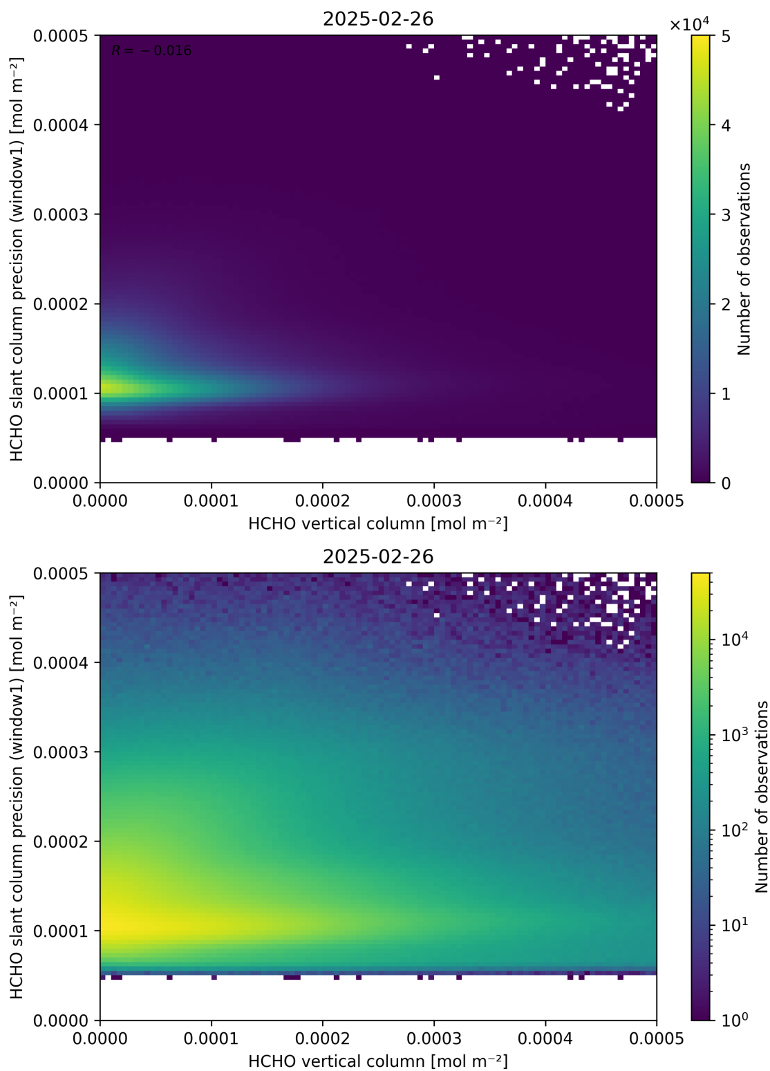
Figure 130: Scatter density plot of “HCHO vertical column” against “HCHO slant column precision (window1)” for 2025-02-25 to 2025-02-27.
