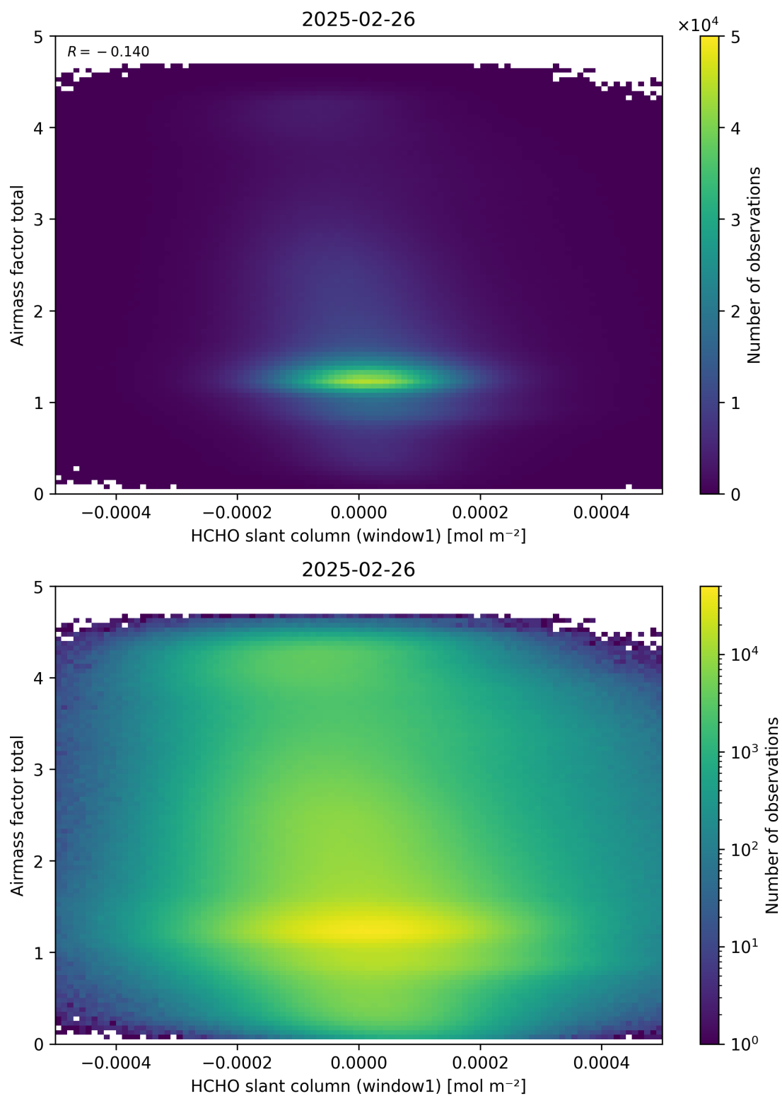
Figure 85: Scatter density plot of “HCHO slant column (window1)” against “Airmass factor total” for 2025-02-25 to 2025-02-27.
