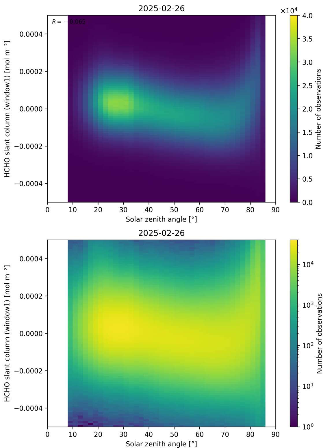
Figure 173: Scatter density plot of “Solar zenith angle” against “HCHO slant column (window1)” for 2025-02-25 to 2025-02-27.
