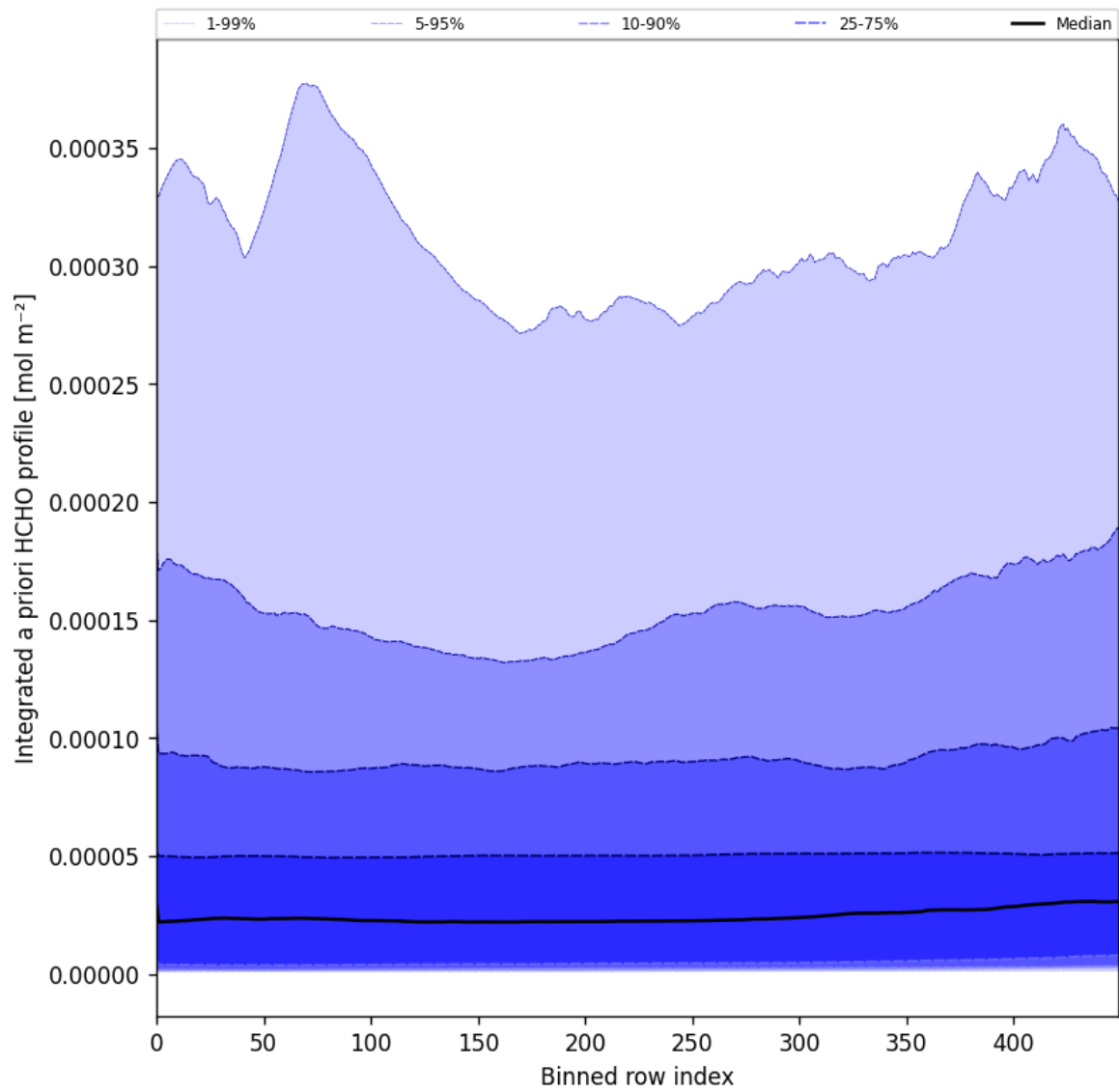
Figure 57: Along track statistics of “Integrated a priori HCHO profile” for 2025-02-25 to 2025-02-27
