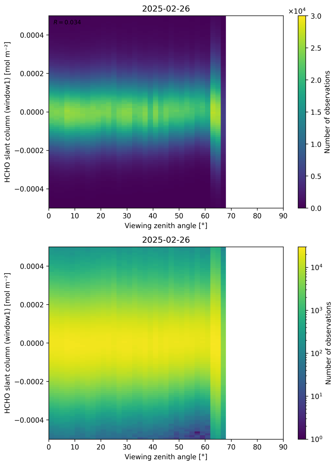
Figure 188: Scatter density plot of “Viewing zenith angle” against “HCHO slant column (window1)” for 2025-02-25 to 2025-02-27.
