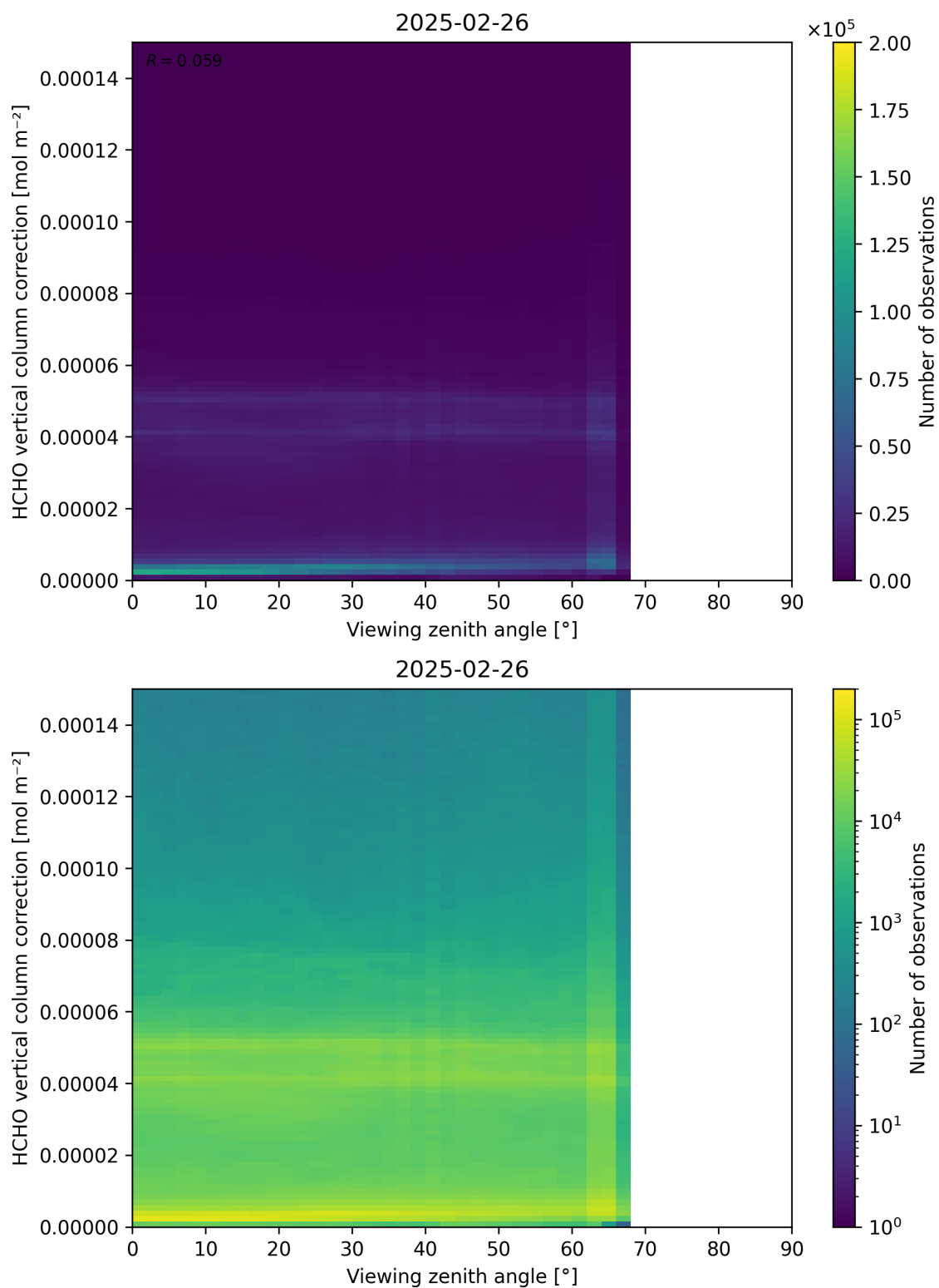
Figure 193: Scatter density plot of “Viewing zenith angle” against “HCHO vertical column correction” for 2025-02-25 to 2025-02-27.
