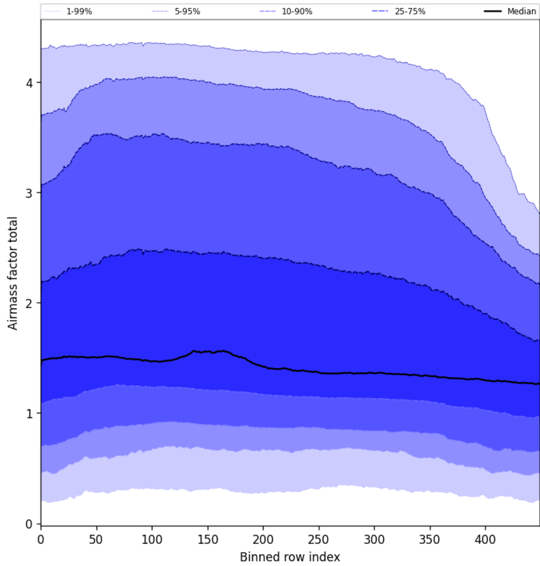
Figure 54: Along track statistics of “Airmass factor total” for 2025-02-25 to 2025-02-27
