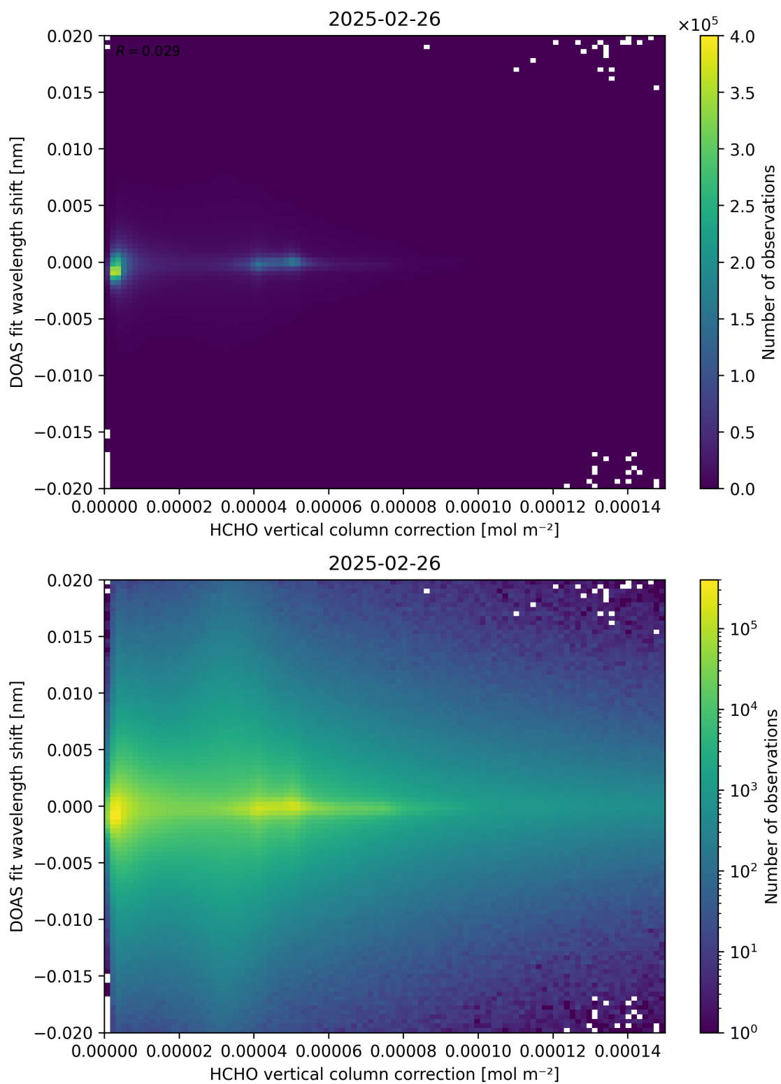
Figure 113: Scatter density plot of “HCHO vertical column correction” against “DOAS fit wavelength shift” for 2025-02-25 to 2025-02-27.
