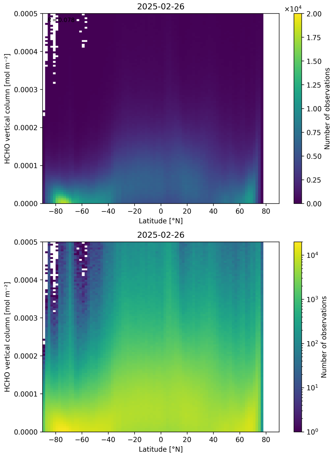
Figure 163: Scatter density plot of “Latitude” against “HCHO vertical column” for 2025-02-25 to 2025-02-27.
