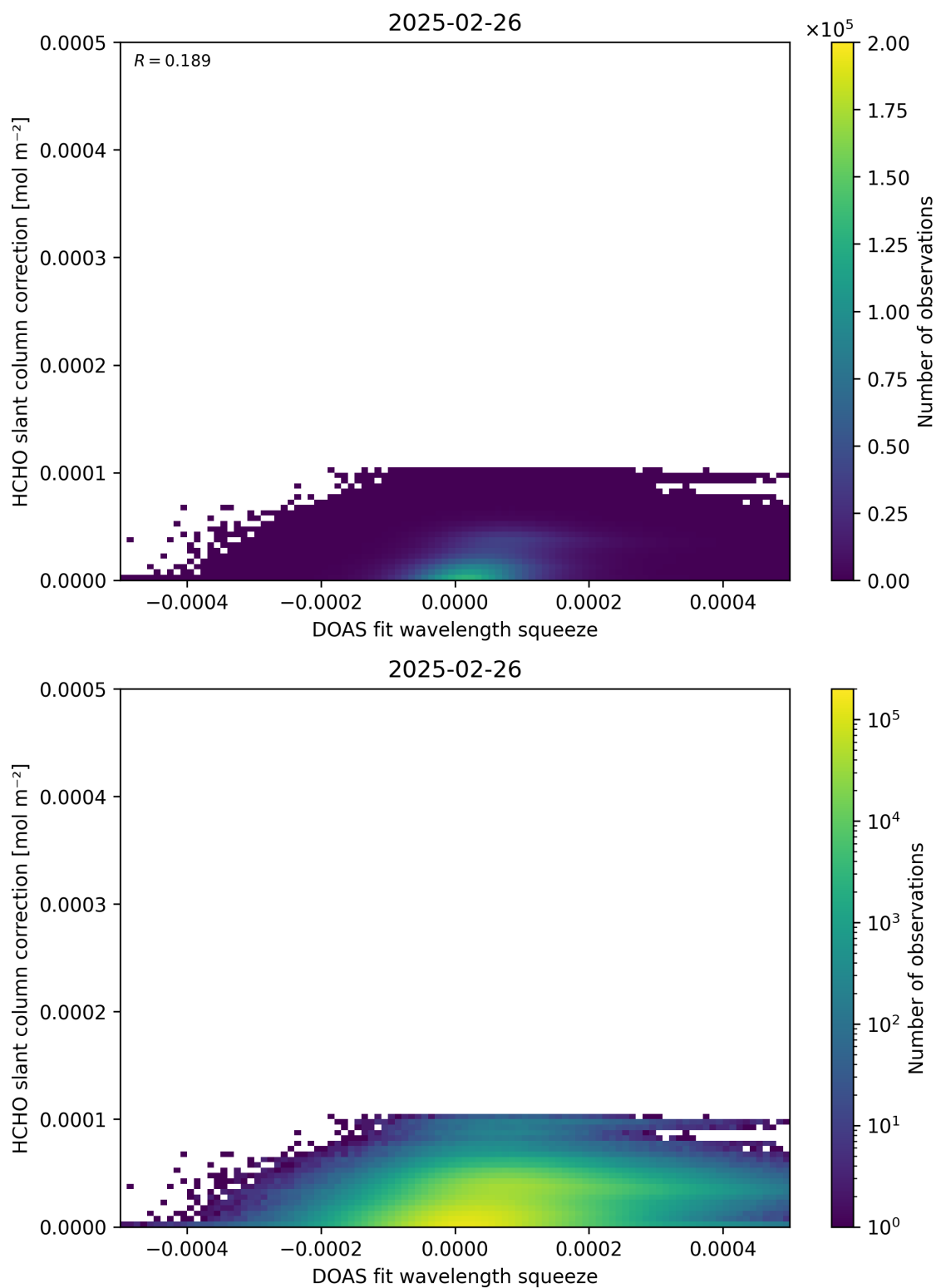
Figure 70: Scatter density plot of “DOAS fit wavelength squeeze” against “HCHO slant column correction” for 2025-02-25 to 2025-02-27.
