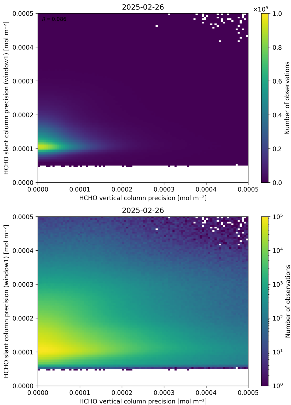
Figure 143: Scatter density plot of “HCHO vertical column precision” against “HCHO slant column precision (window1)” for 2025-02-25 to 2025-02-27.
