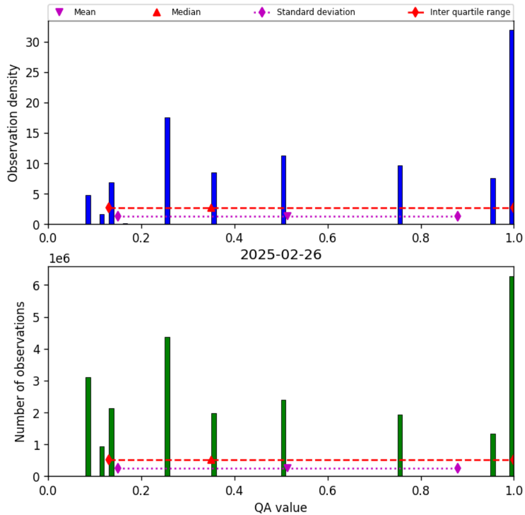
Figure 34: Histogram of “QA value” for 2025-02-25 to 2025-02-27
