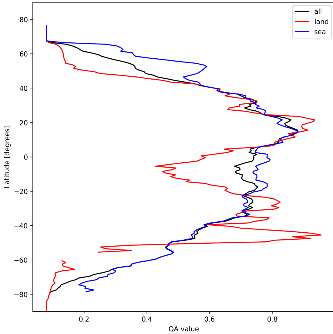
Figure 20: Zonal average of “QA value” for 2025-02-25 to 2025-02-27.
