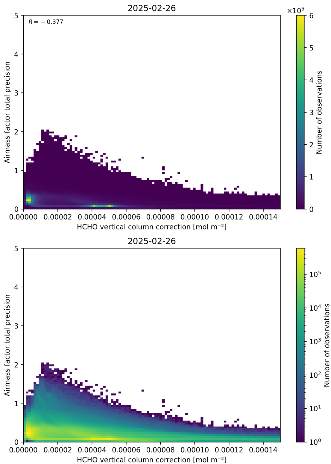
Figure 121: Scatter density plot of “HCHO vertical column correction” against “Airmass factor total precision” for 2025-02-25 to 2025-02-27.
