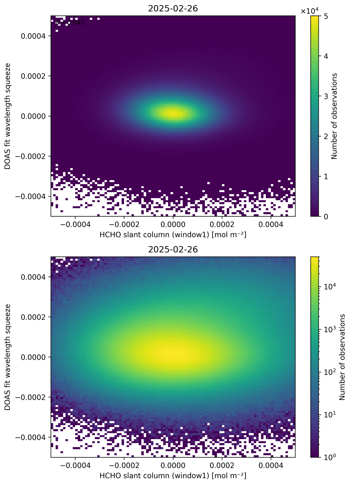
Figure 80: Scatter density plot of “HCHO slant column (window1)” against “DOAS fit wavelength squeeze” for 2025-02-25 to 2025-02-27.
