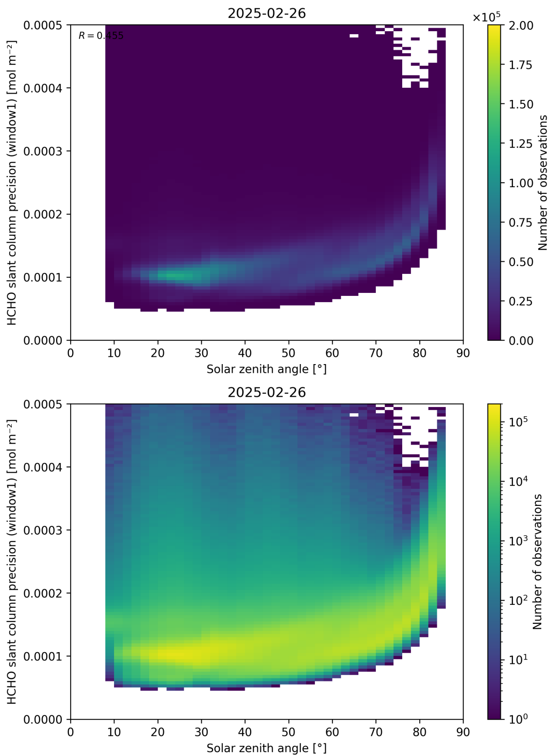
Figure 174: Scatter density plot of “Solar zenith angle” against “HCHO slant column precision (window1)” for 2025-02-25 to 2025-02-27.
