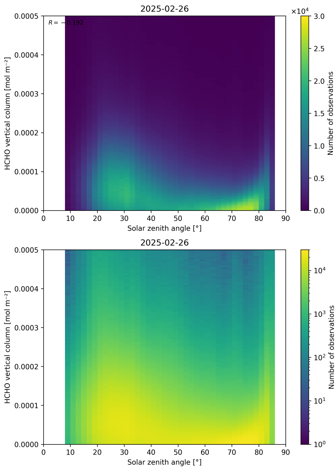
Figure 177: Scatter density plot of “Solar zenith angle” against “HCHO vertical column” for 2025-02-25 to 2025-02-27.
