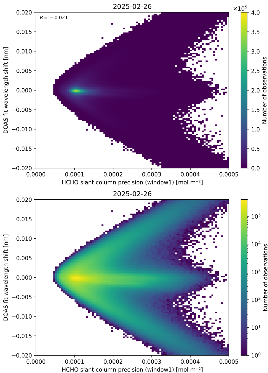
Figure 89: Scatter density plot of “HCHO slant column precision (window1)” against “DOAS fit wavelength shift” for 2025-02-25 to 2025-02-27.
