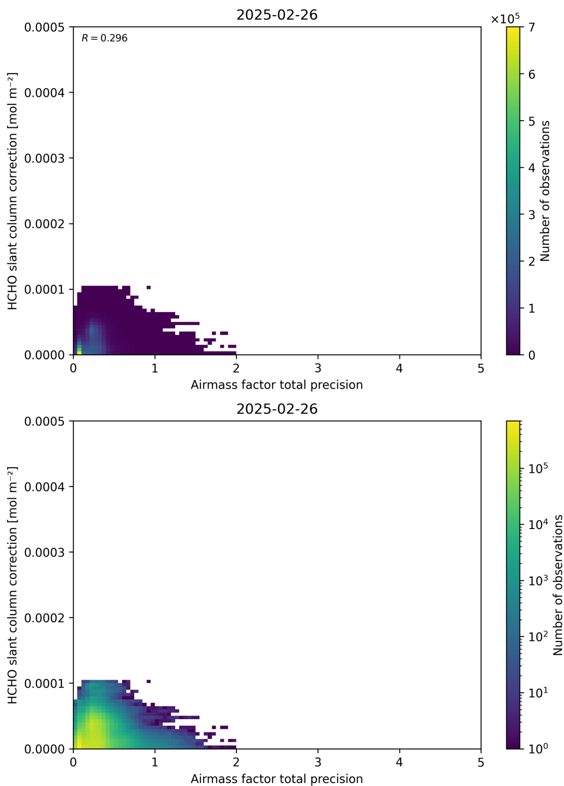
Figure 110: Scatter density plot of “Airmass factor total precision” against “HCHO slant column correction” for 2025-02-25 to 2025-02-27.
