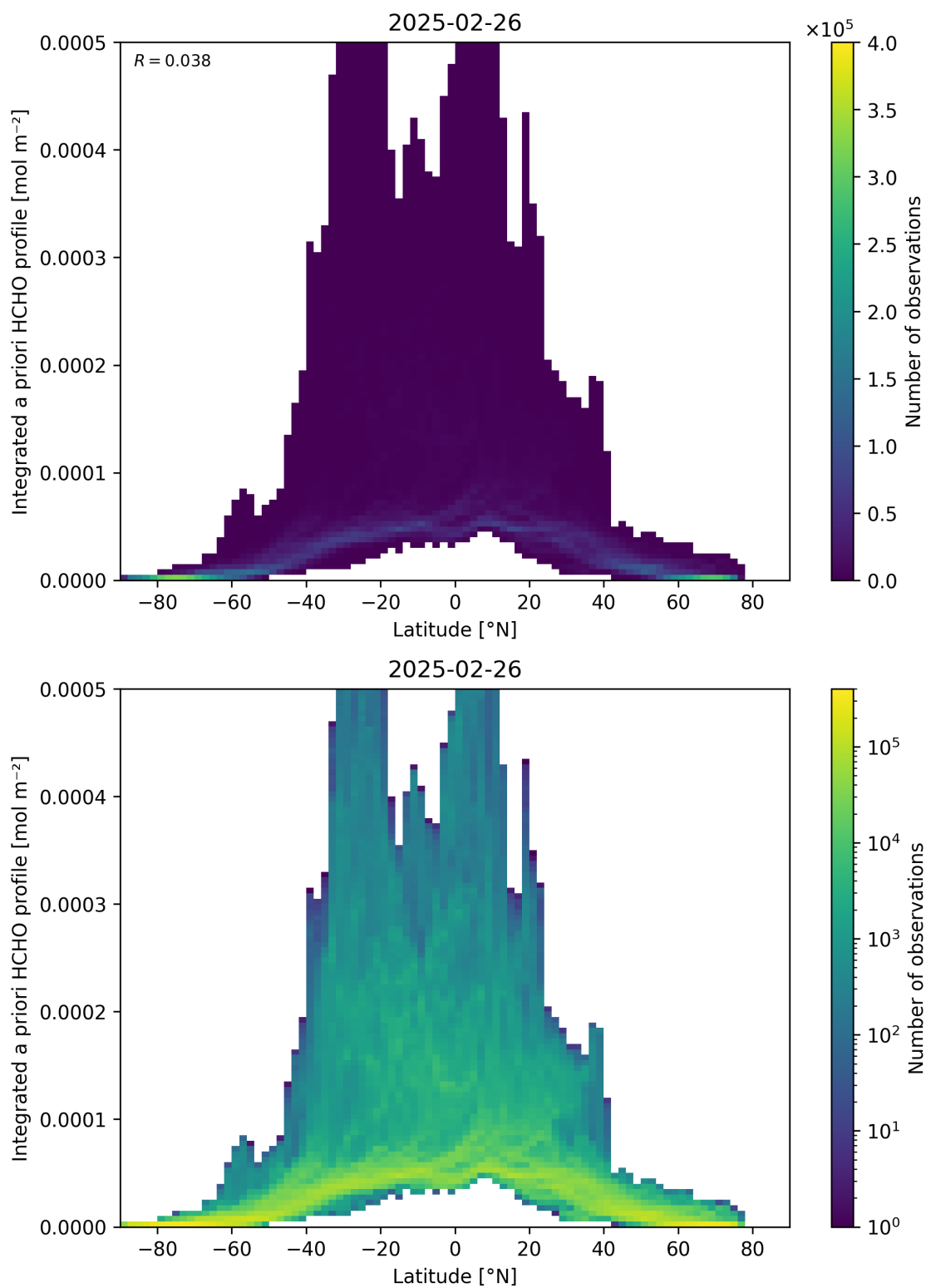
Figure 166: Scatter density plot of “Latitude” against “Integrated a priori HCHO profile” for 2025-02-25 to 2025-02-27.
