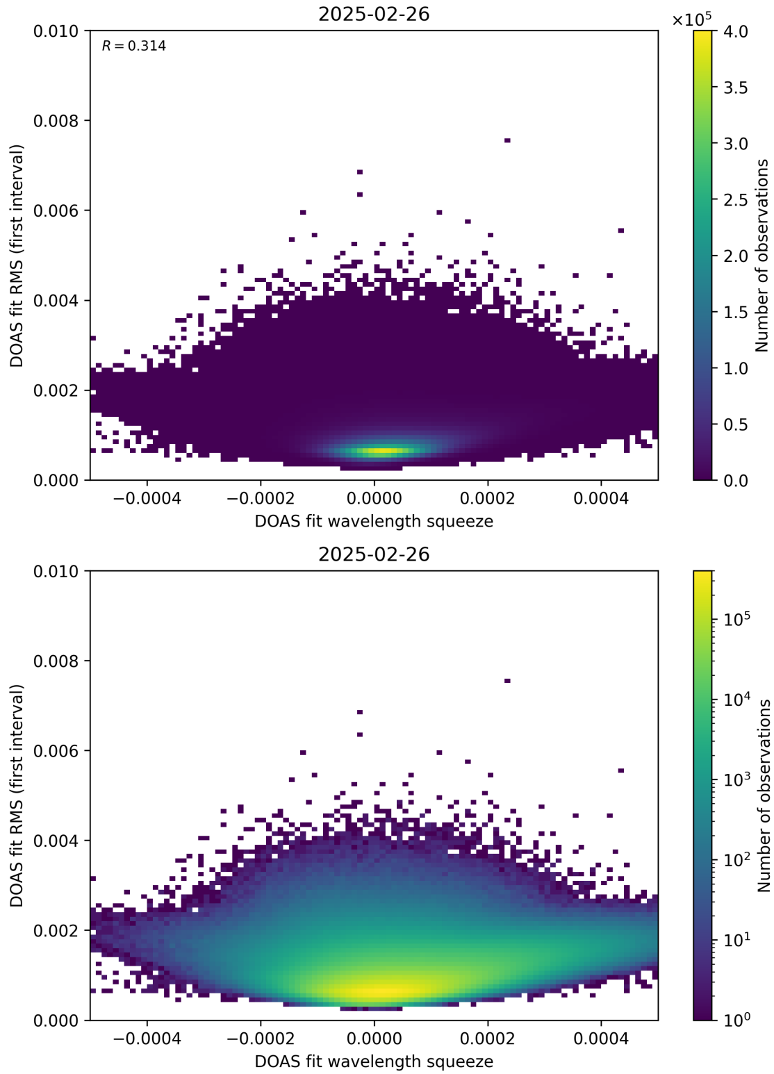
Figure 68: Scatter density plot of “DOAS fit wavelength squeeze” against “DOAS fit RMS (first interval)” for 2025-02-25 to 2025-02-27.
