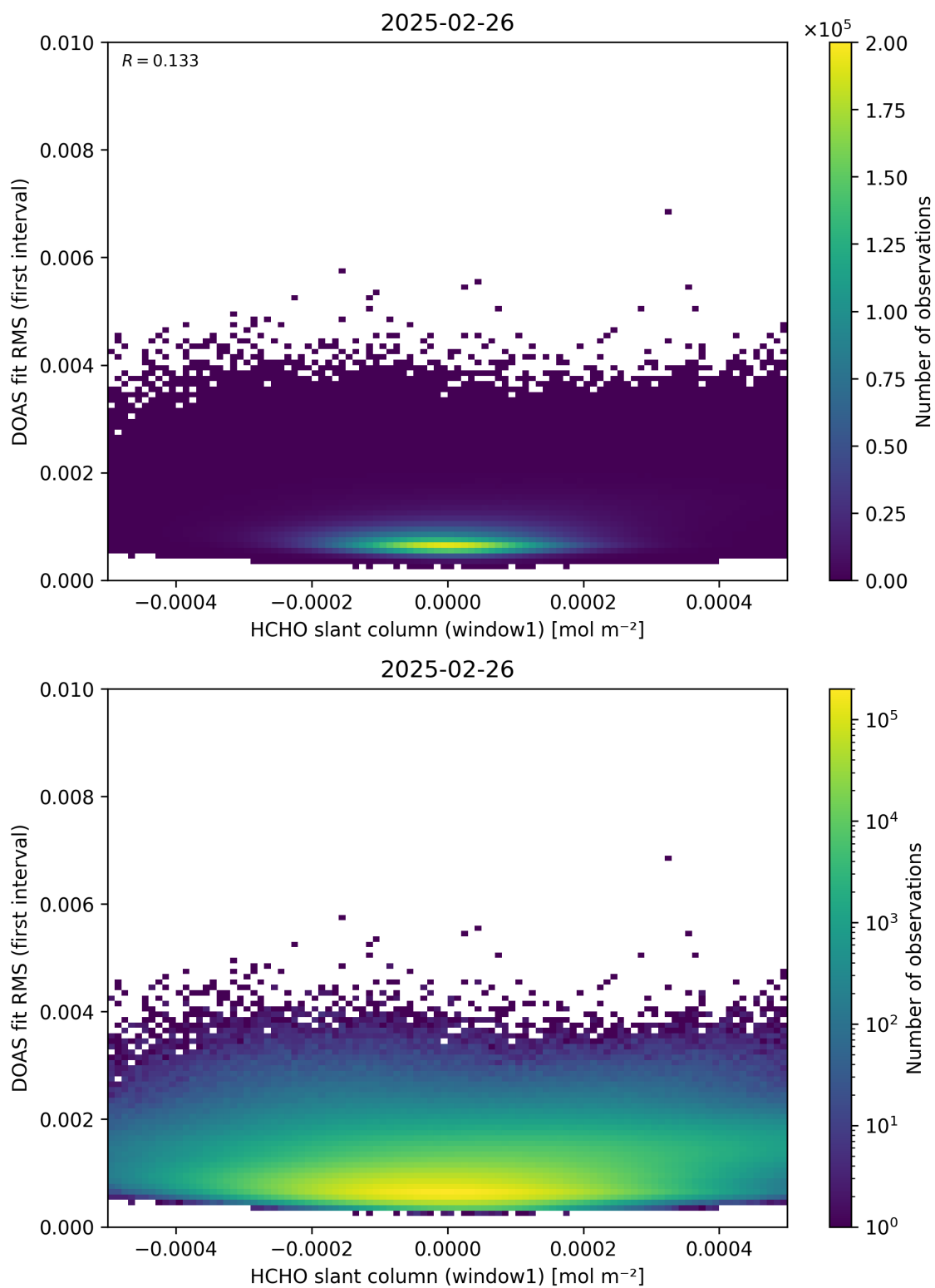
Figure 78: Scatter density plot of “HCHO slant column (window1)” against “DOAS fit RMS (first interval)” for 2025-02-25 to 2025-02-27.
