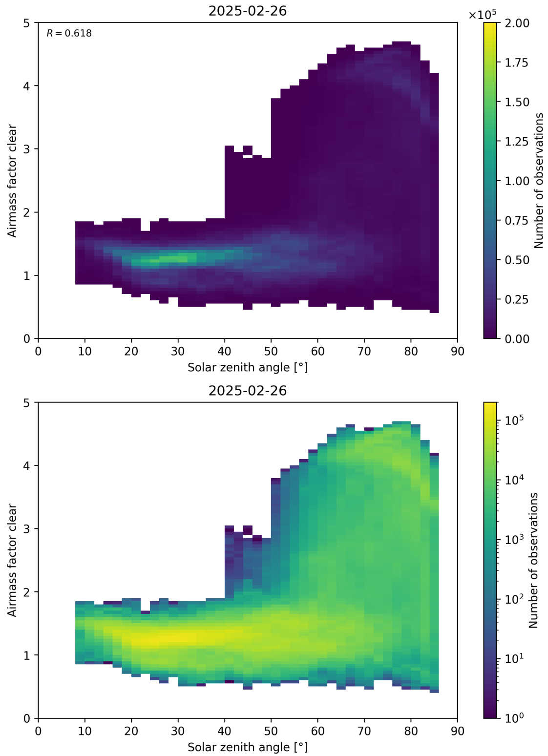
Figure 170: Scatter density plot of “Solar zenith angle” against “Airmass factor clear” for 2025-02-25 to 2025-02-27.
