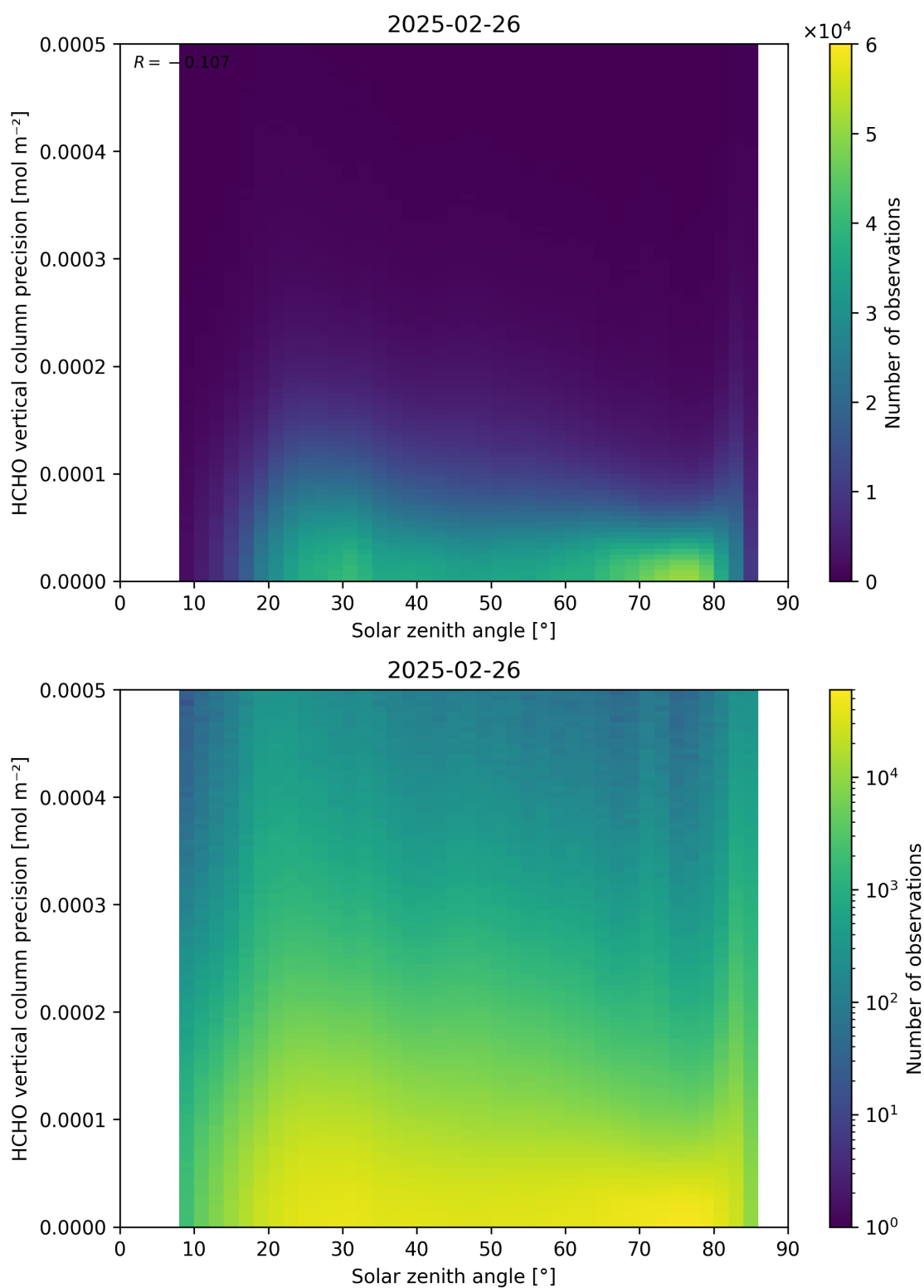
Figure 179: Scatter density plot of “Solar zenith angle” against “HCHO vertical column precision” for 2025-02-25 to 2025-02-27.
