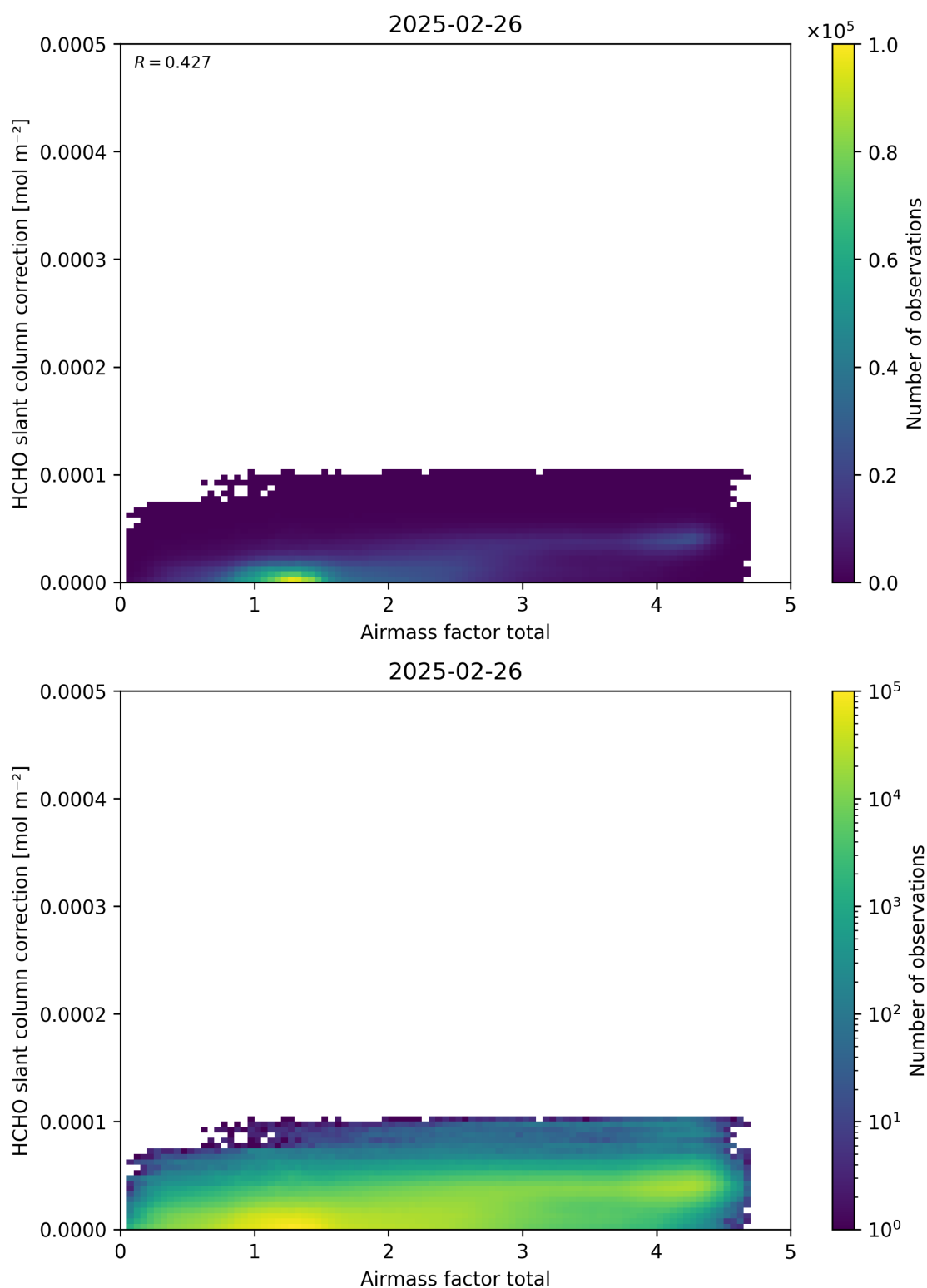
Figure 102: Scatter density plot of “Airmass factor total” against “HCHO slant column correction” for 2025-02-25 to 2025-02-27.
