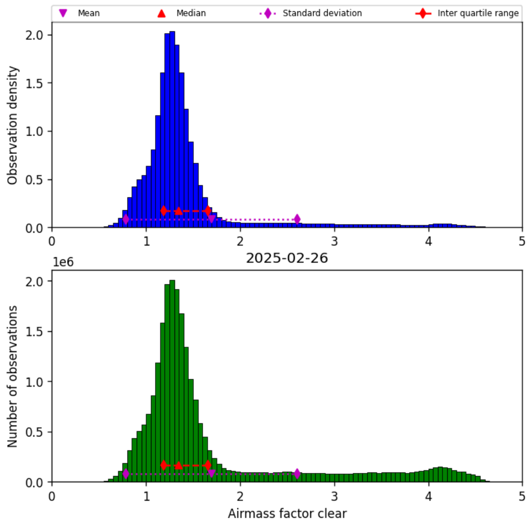
Figure 42: Histogram of “Airmass factor clear” for 2025-02-25 to 2025-02-27
