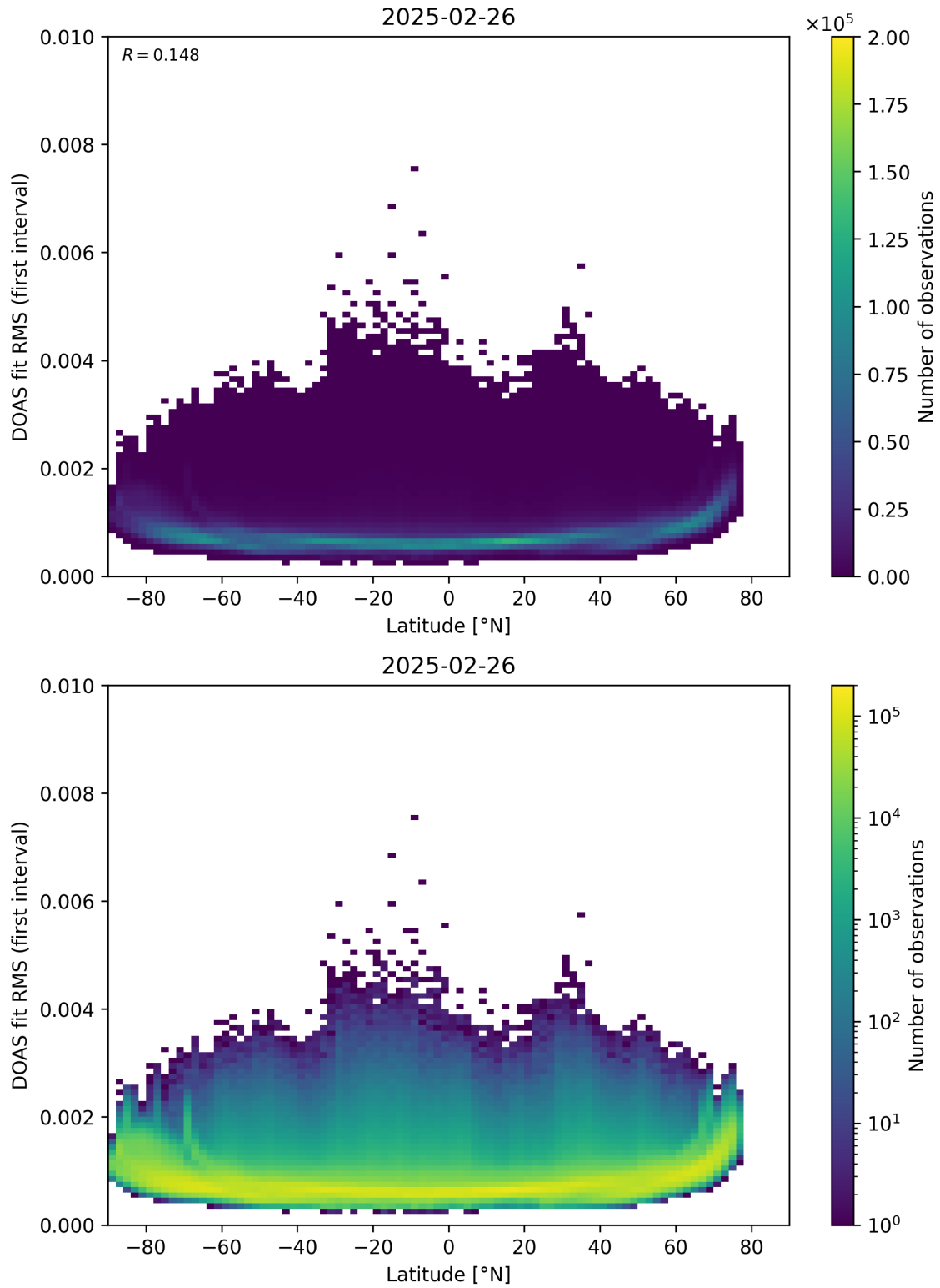
Figure 153: Scatter density plot of “Latitude” against “DOAS fit RMS (first interval)” for 2025-02-25 to 2025-02-27.
