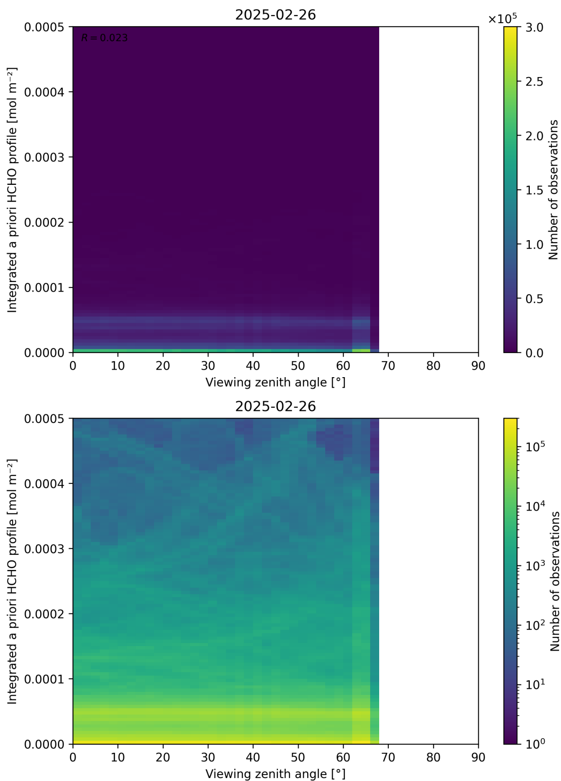
Figure 195: Scatter density plot of “Viewing zenith angle” against “Integrated a priori HCHO profile” for 2025-02-25 to 2025-02-27.
