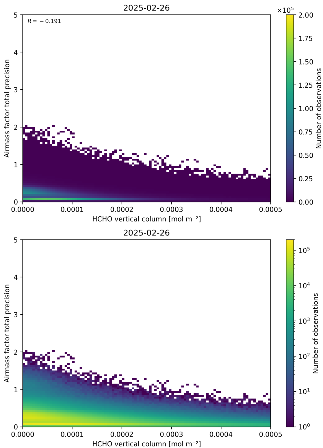
Figure 132: Scatter density plot of “HCHO vertical column” against “Airmass factor total precision” for 2025-02-25 to 2025-02-27.
