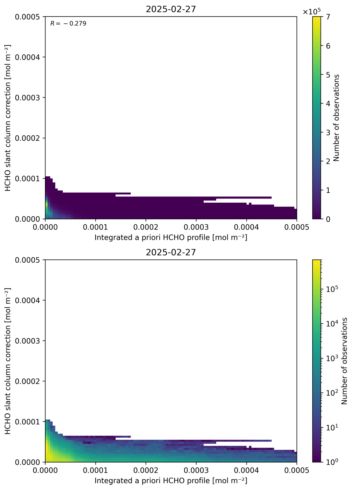
Figure 152: Scatter density plot of “Integrated a priori HCHO profile” against “HCHO slant column correction” for 2025-02-26 to 2025-02-28.
