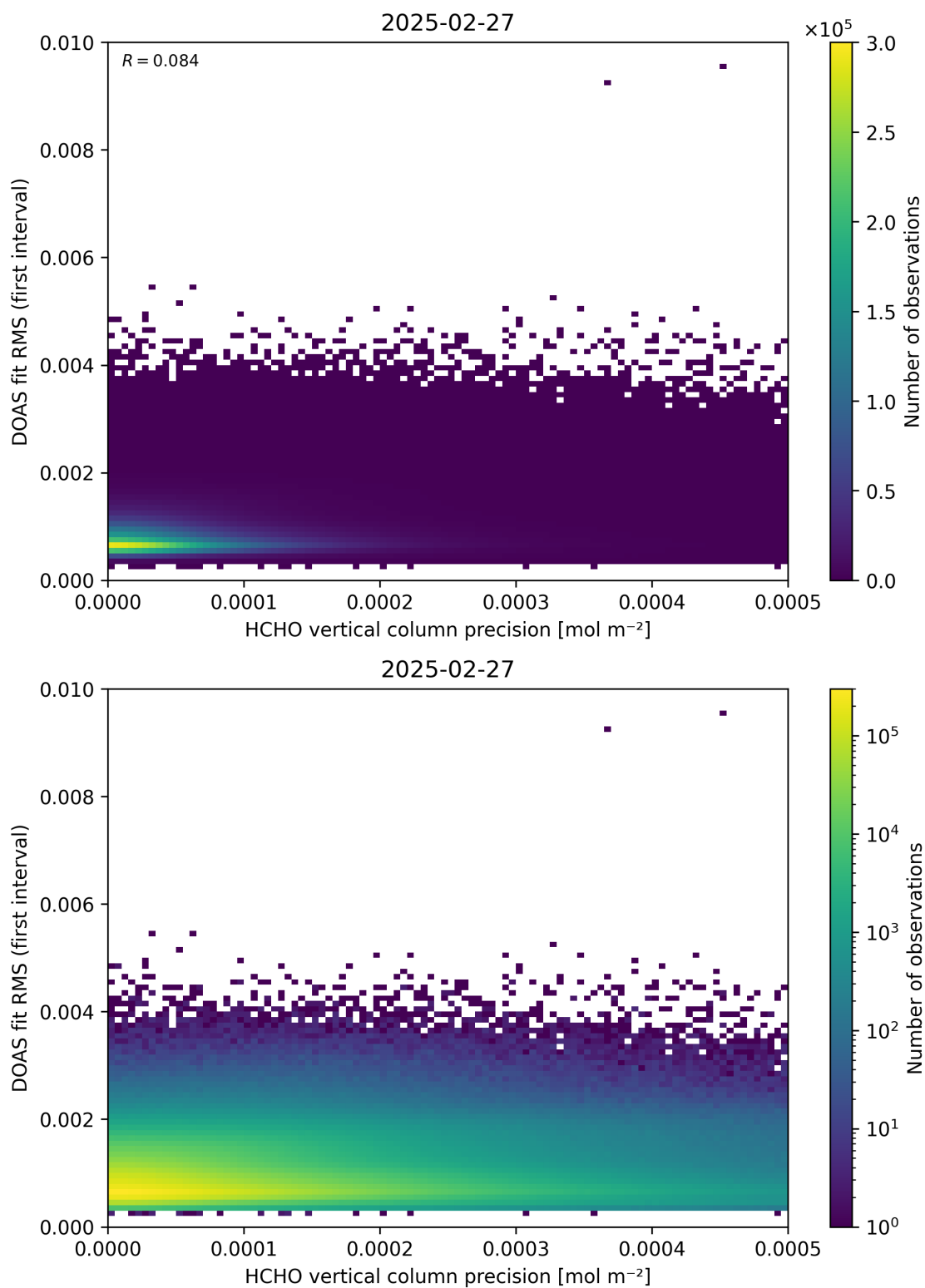
Figure 136: Scatter density plot of “HCHO vertical column precision” against “DOAS fit RMS (first interval)” for 2025-02-26 to 2025-02-28.
