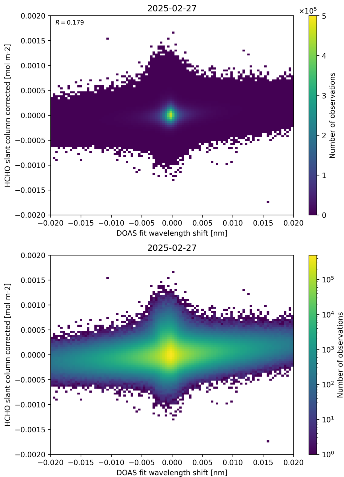
Figure 66: Scatter density plot of “DOAS fit wavelength shift” against “HCHO slant column corrected” for 2025-02-26 to 2025-02-28.
