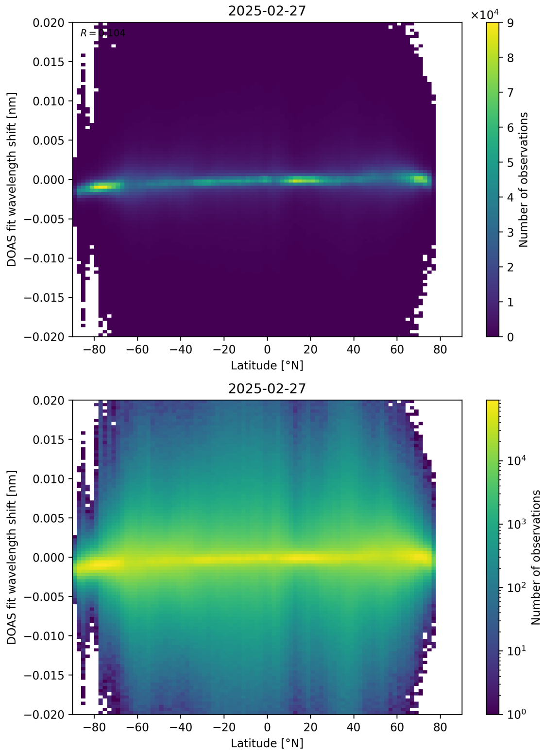
Figure 154: Scatter density plot of “Latitude” against “DOAS fit wavelength shift” for 2025-02-26 to 2025-02-28.
