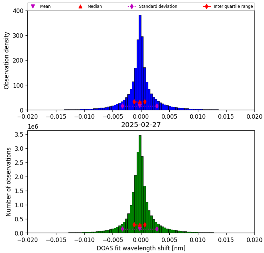
Figure 44: Histogram of “DOAS fit wavelength shift” for 2025-02-26 to 2025-02-28
