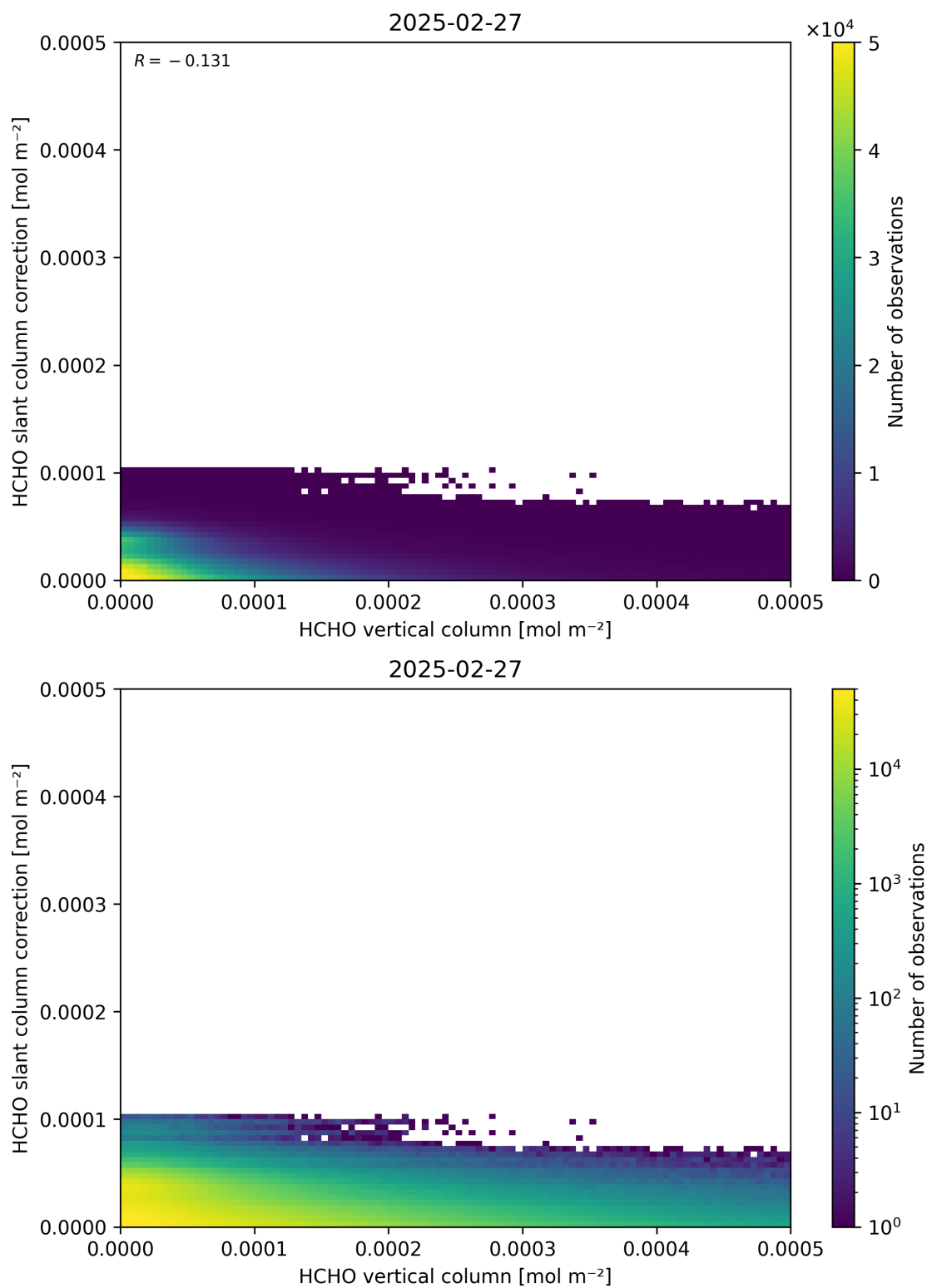
Figure 128: Scatter density plot of “HCHO vertical column” against “HCHO slant column correction” for 2025-02-26 to 2025-02-28.
