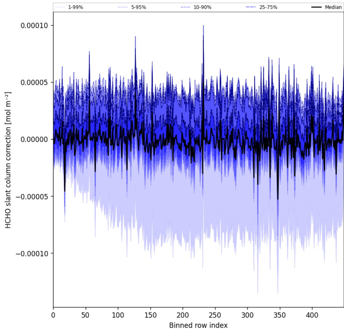
Figure 61: Along track statistics of “HCHO slant column correction” for 2025-02-26 to 2025-02-28
