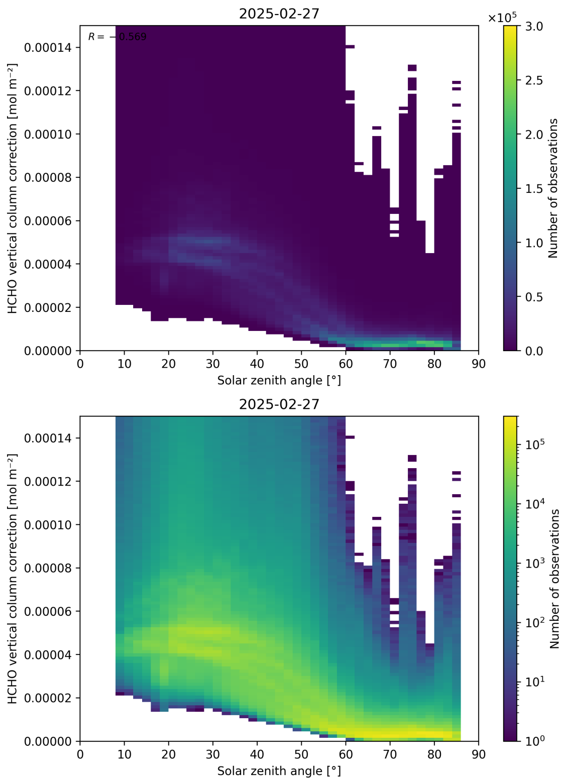
Figure 178: Scatter density plot of “Solar zenith angle” against “HCHO vertical column correction” for 2025-02-26 to 2025-02-28.
