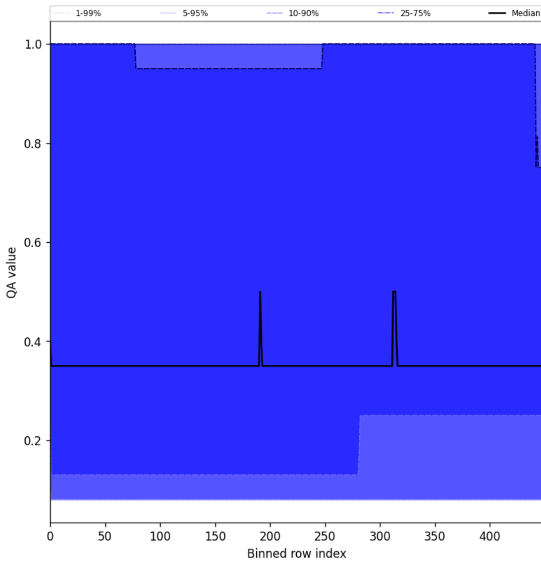
Figure 48: Along track statistics of “QA value” for 2025-02-26 to 2025-02-28
