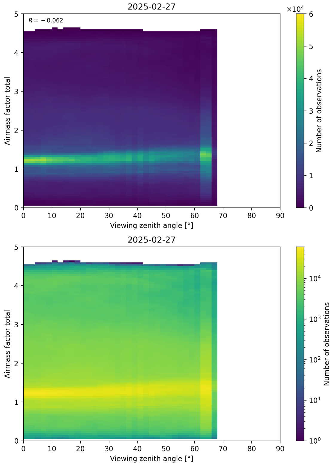
Figure 190: Scatter density plot of “Viewing zenith angle” against “Airmass factor total” for 2025-02-26 to 2025-02-28.
