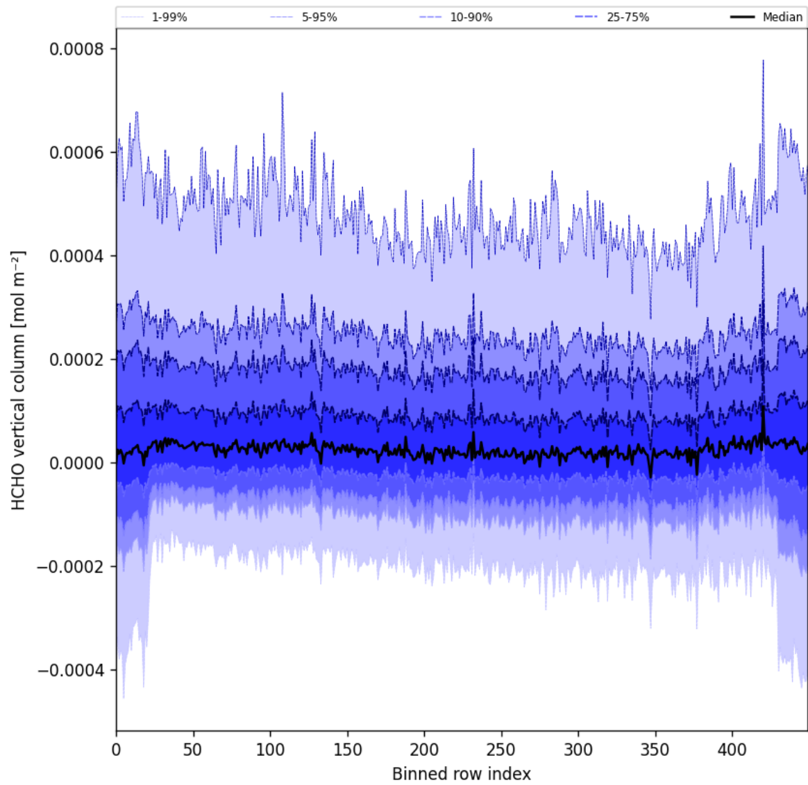
Figure 49: Along track statistics of “HCHO vertical column” for 2025-02-26 to 2025-02-28
