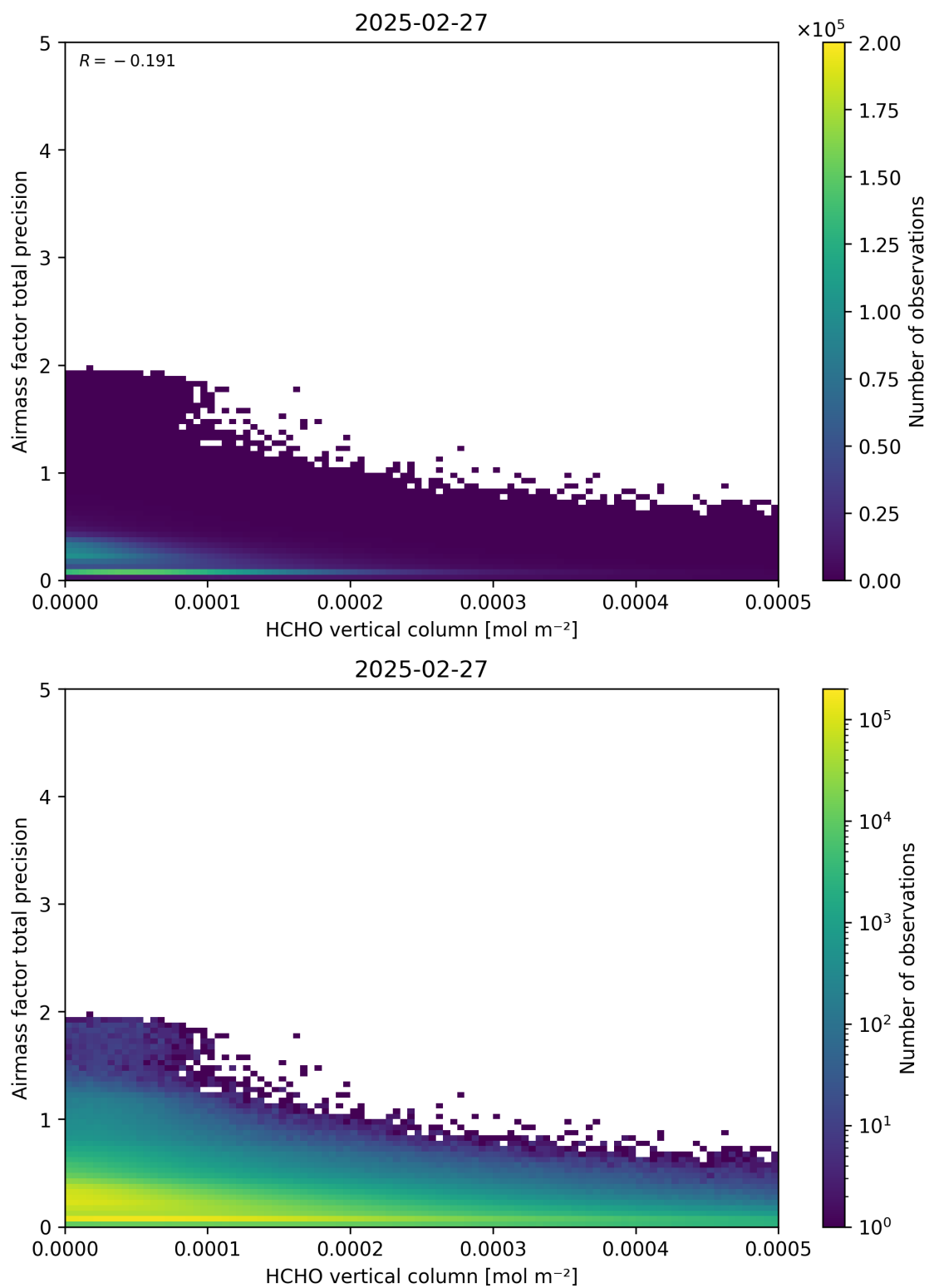
Figure 132: Scatter density plot of “HCHO vertical column” against “Airmass factor total precision” for 2025-02-26 to 2025-02-28.
