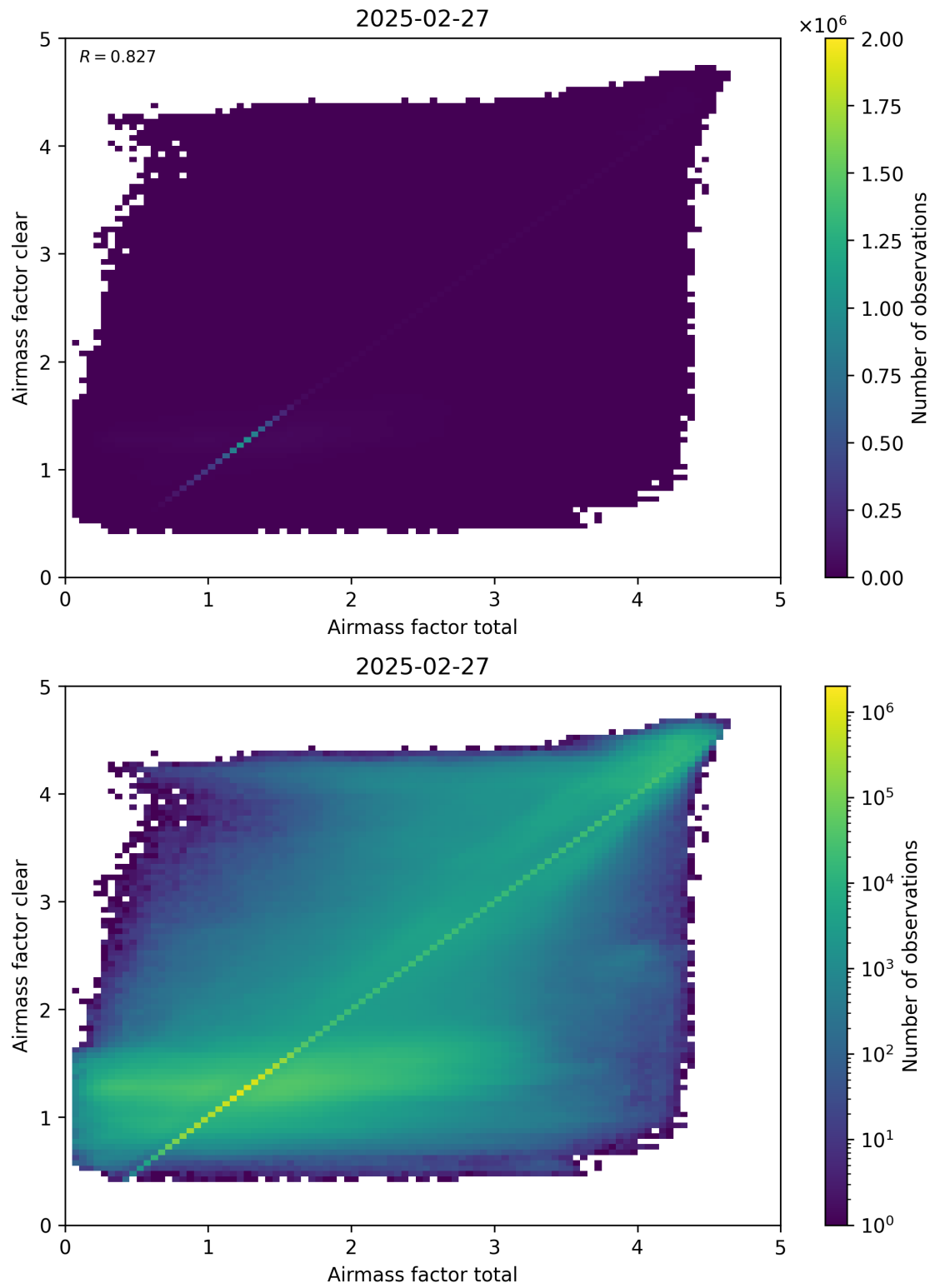
Figure 100: Scatter density plot of “Airmass factor total” against “Airmass factor clear” for 2025-02-26 to 2025-02-28.
