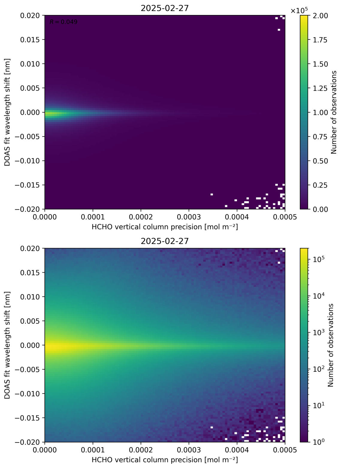
Figure 137: Scatter density plot of “HCHO vertical column precision” against “DOAS fit wavelength shift” for 2025-02-26 to 2025-02-28.
