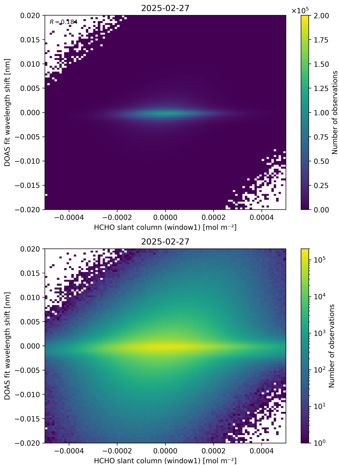
Figure 79: Scatter density plot of “HCHO slant column (window1)” against “DOAS fit wavelength shift” for 2025-02-26 to 2025-02-28.
