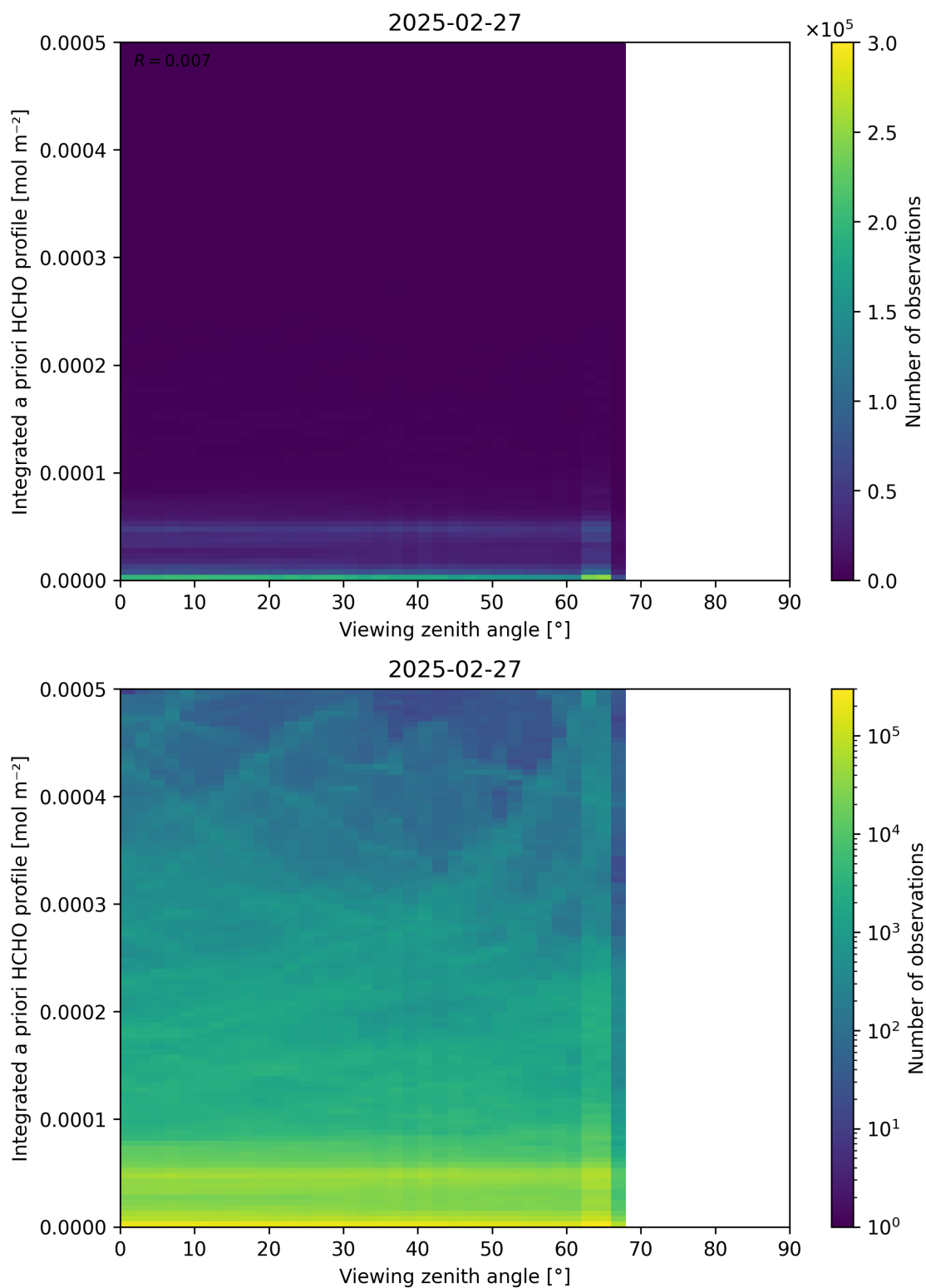
Figure 195: Scatter density plot of “Viewing zenith angle” against “Integrated a priori HCHO profile” for 2025-02-26 to 2025-02-28.
