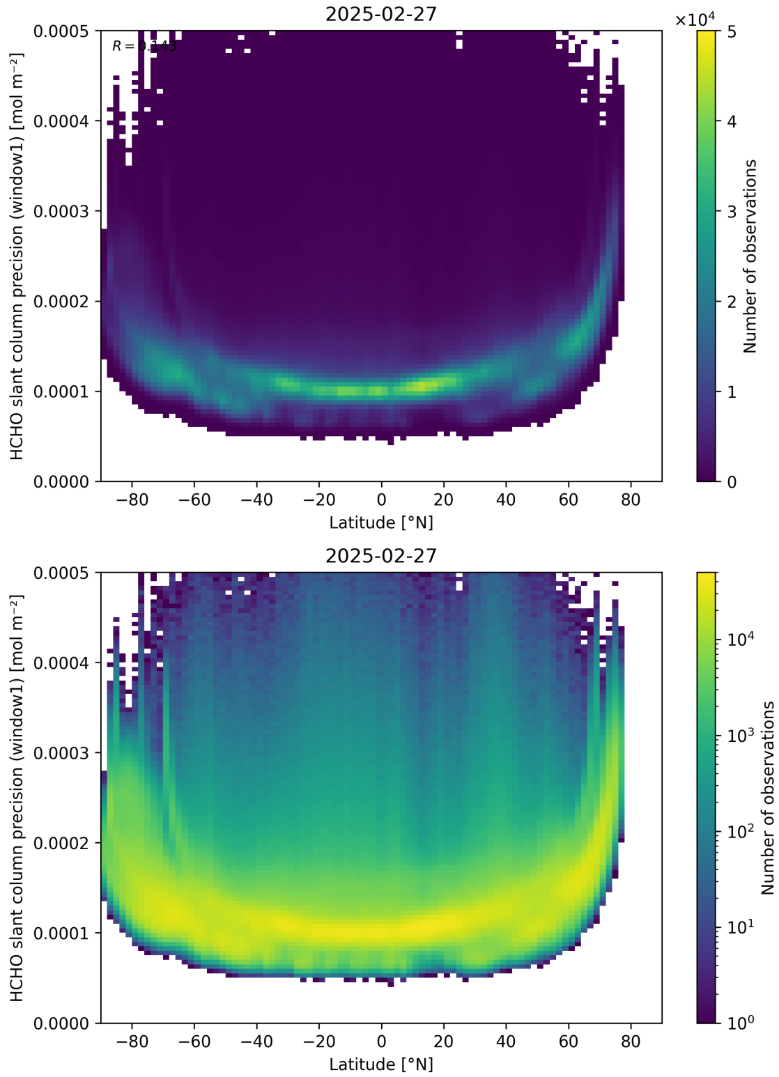
Figure 160: Scatter density plot of “Latitude” against “HCHO slant column precision (window1)” for 2025-02-26 to 2025-02-28.
