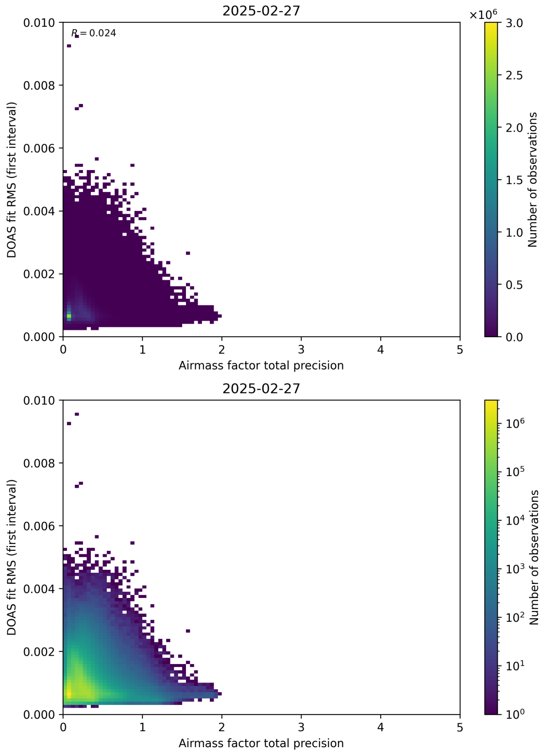
Figure 105: Scatter density plot of “Airmass factor total precision” against “DOAS fit RMS (first interval)” for 2025-02-26 to 2025-02-28.
