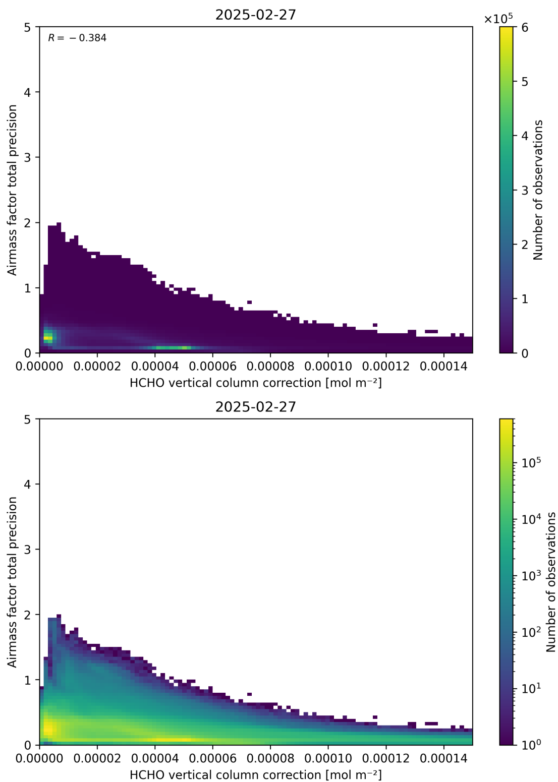
Figure 121: Scatter density plot of “HCHO vertical column correction” against “Airmass factor total precision” for 2025-02-26 to 2025-02-28.
