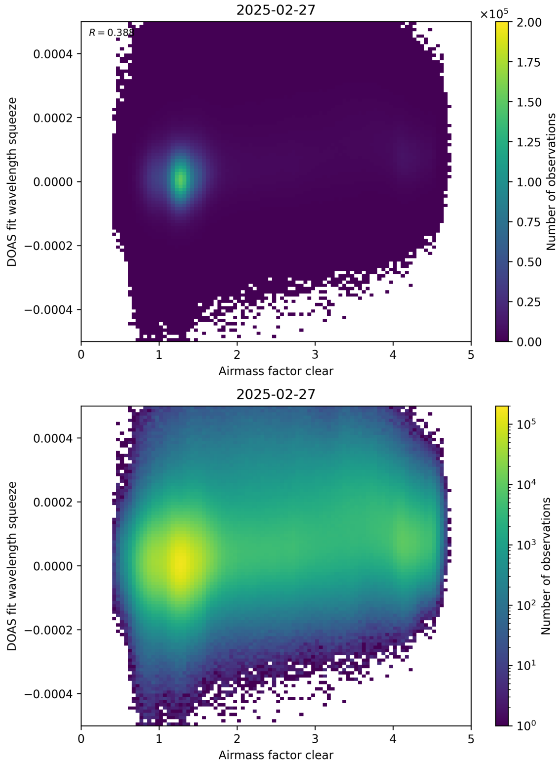
Figure 73: Scatter density plot of “Airmass factor clear” against “DOAS fit wavelength squeeze” for 2025-02-26 to 2025-02-28.
