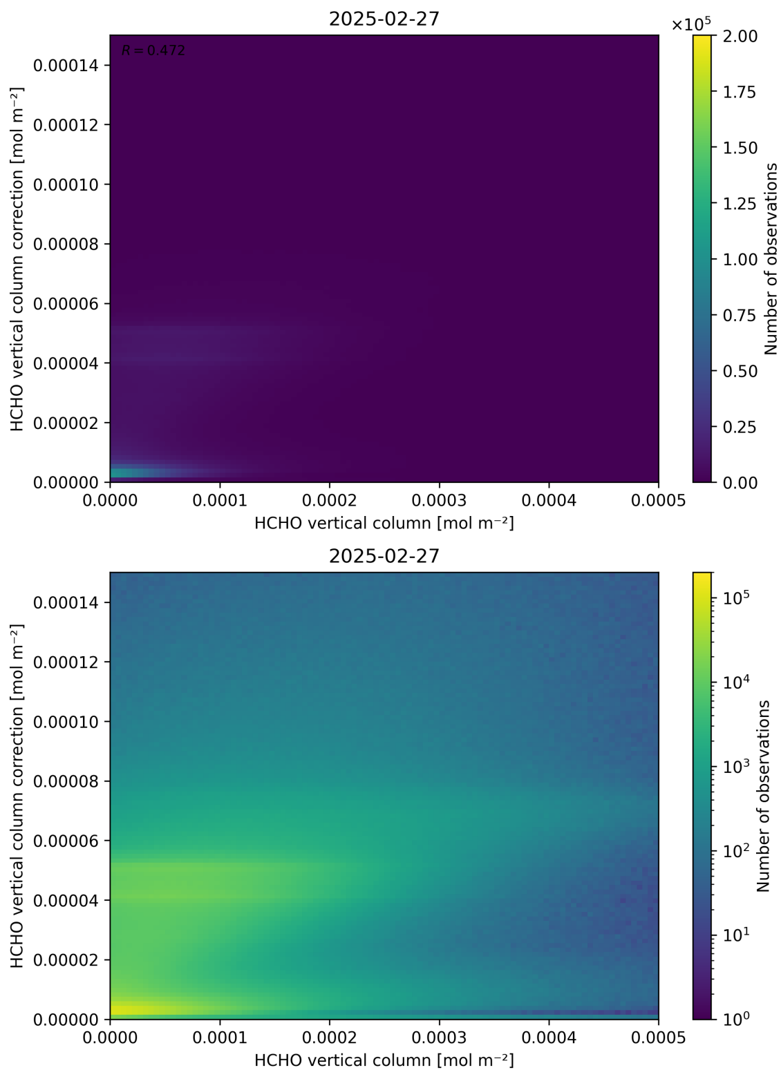
Figure 133: Scatter density plot of “HCHO vertical column” against “HCHO vertical column correction” for 2025-02-26 to 2025-02-28.
