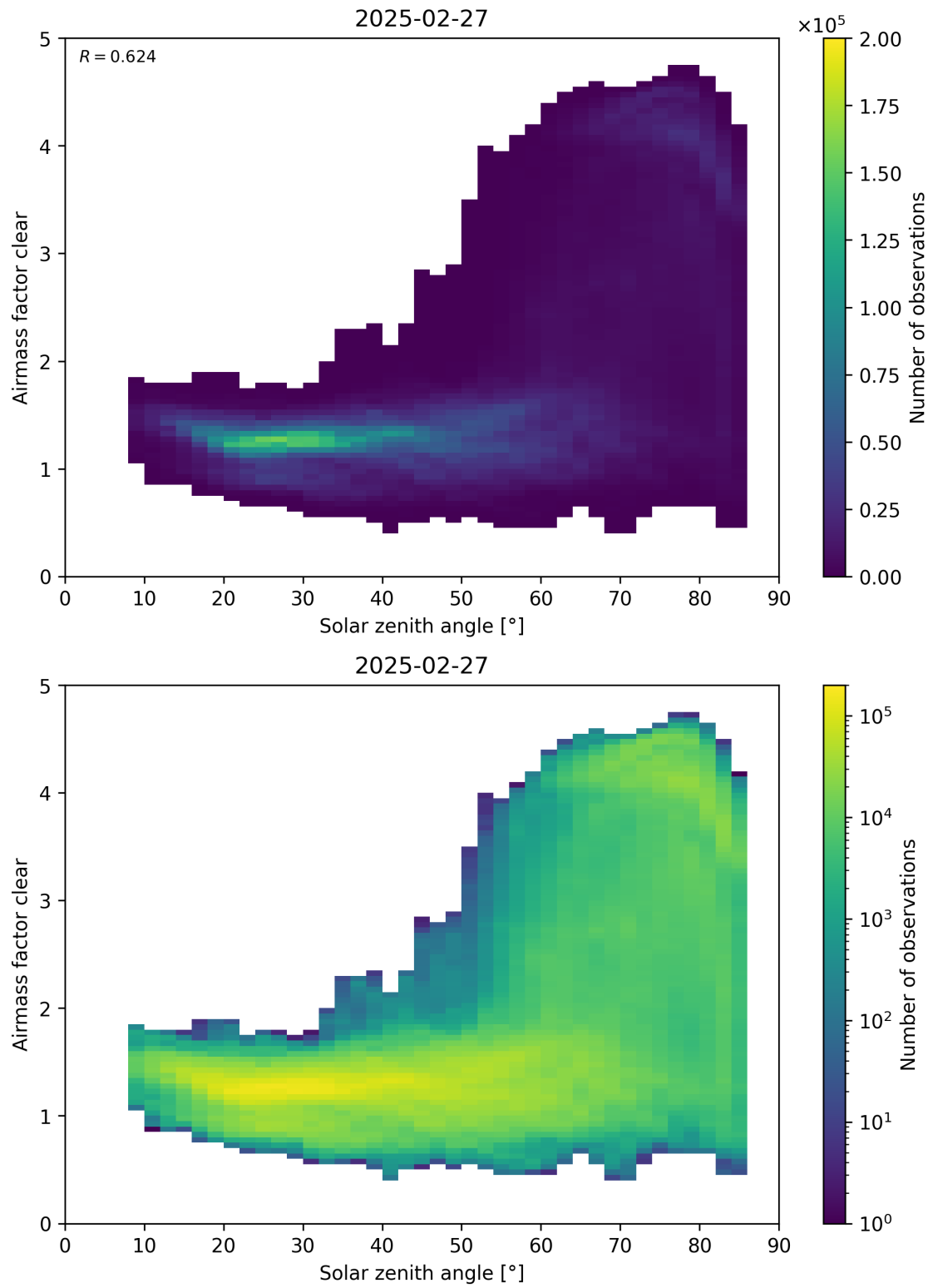
Figure 170: Scatter density plot of “Solar zenith angle” against “Airmass factor clear” for 2025-02-26 to 2025-02-28.
