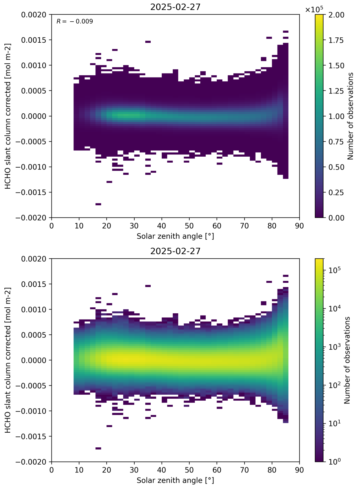
Figure 171: Scatter density plot of “Solar zenith angle” against “HCHO slant column corrected” for 2025-02-26 to 2025-02-28.
