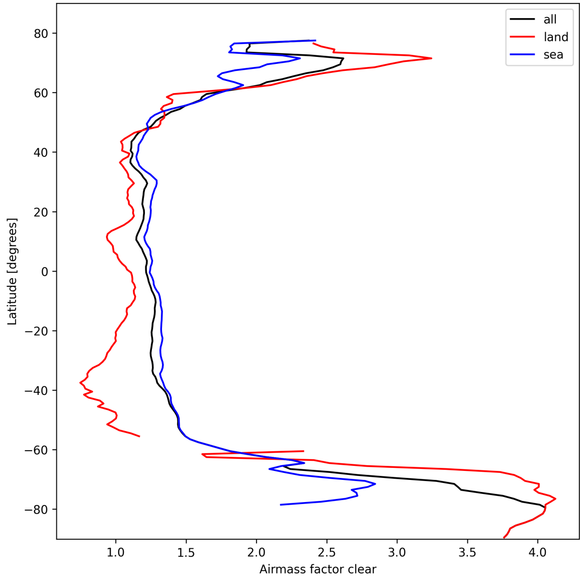
Figure 28: Zonal average of “Airmass factor clear” for 2025-02-26 to 2025-02-28.
