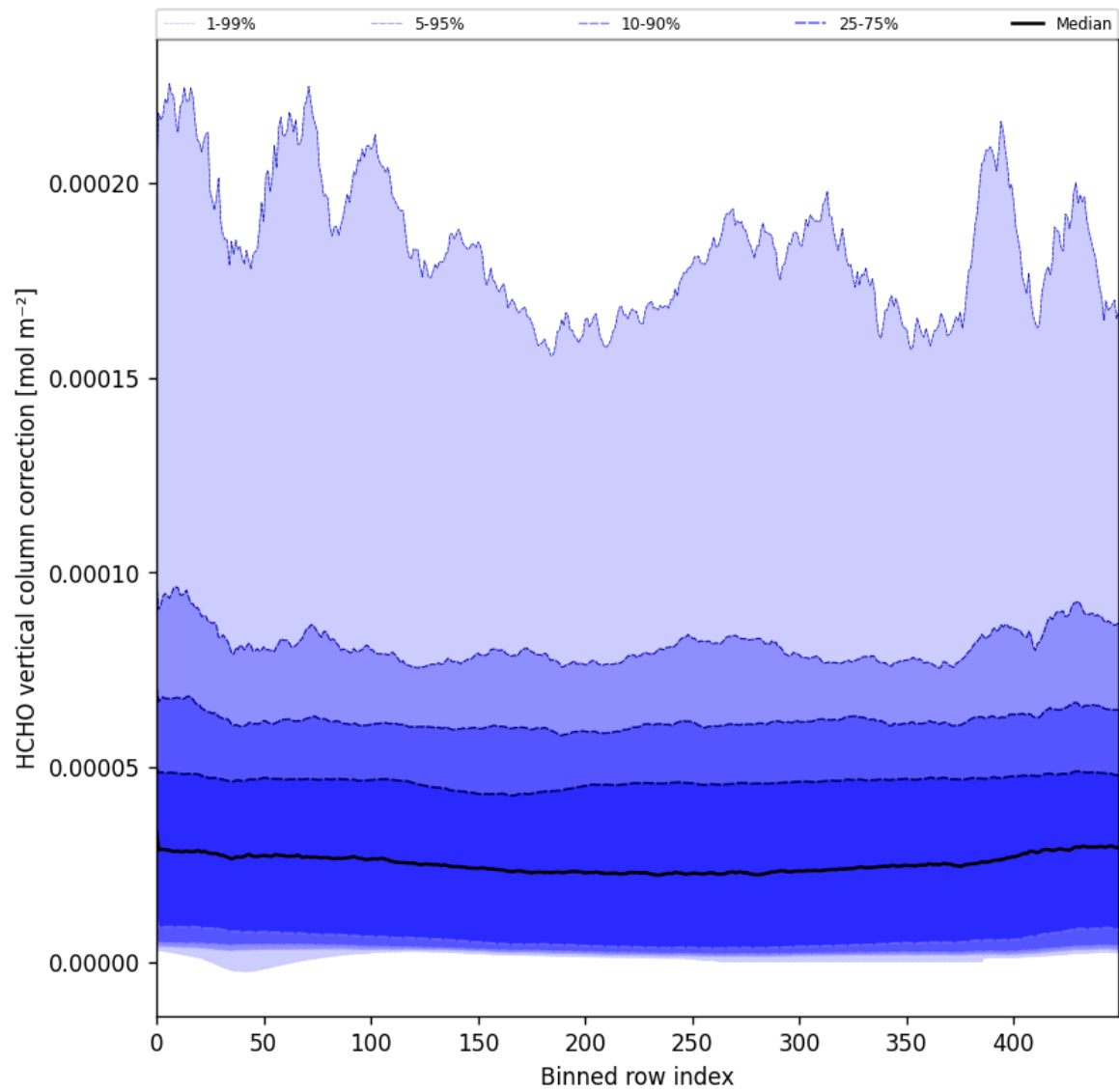
Figure 51: Along track statistics of “HCHO vertical column correction” for 2025-02-26 to 2025-02-28
