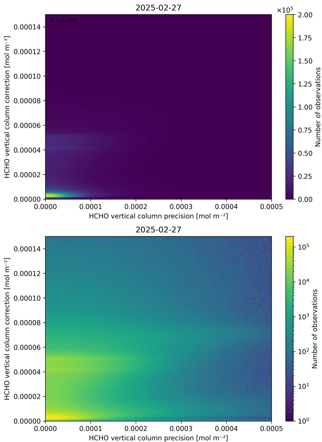
Figure 146: Scatter density plot of “HCHO vertical column precision” against “HCHO vertical column correction” for 2025-02-26 to 2025-02-28.
