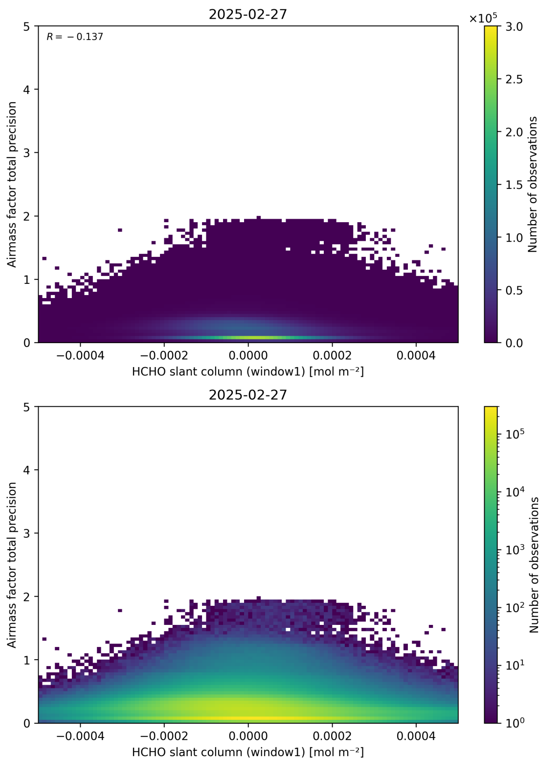
Figure 86: Scatter density plot of “HCHO slant column (window1)” against “Airmass factor total precision” for 2025-02-26 to 2025-02-28.
