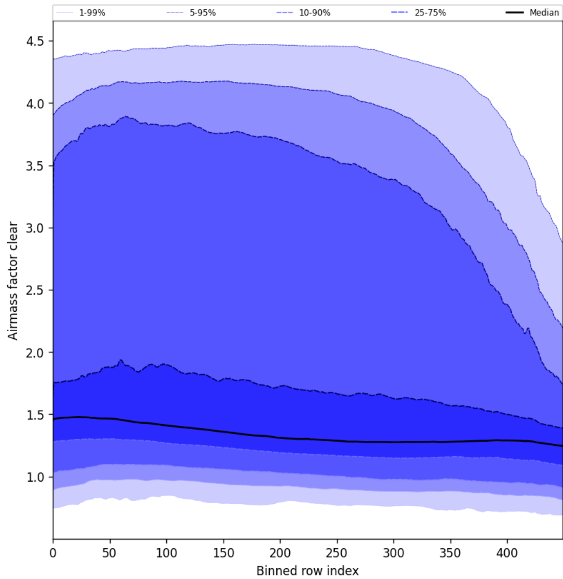
Figure 56: Along track statistics of “Airmass factor clear” for 2025-02-26 to 2025-02-28
