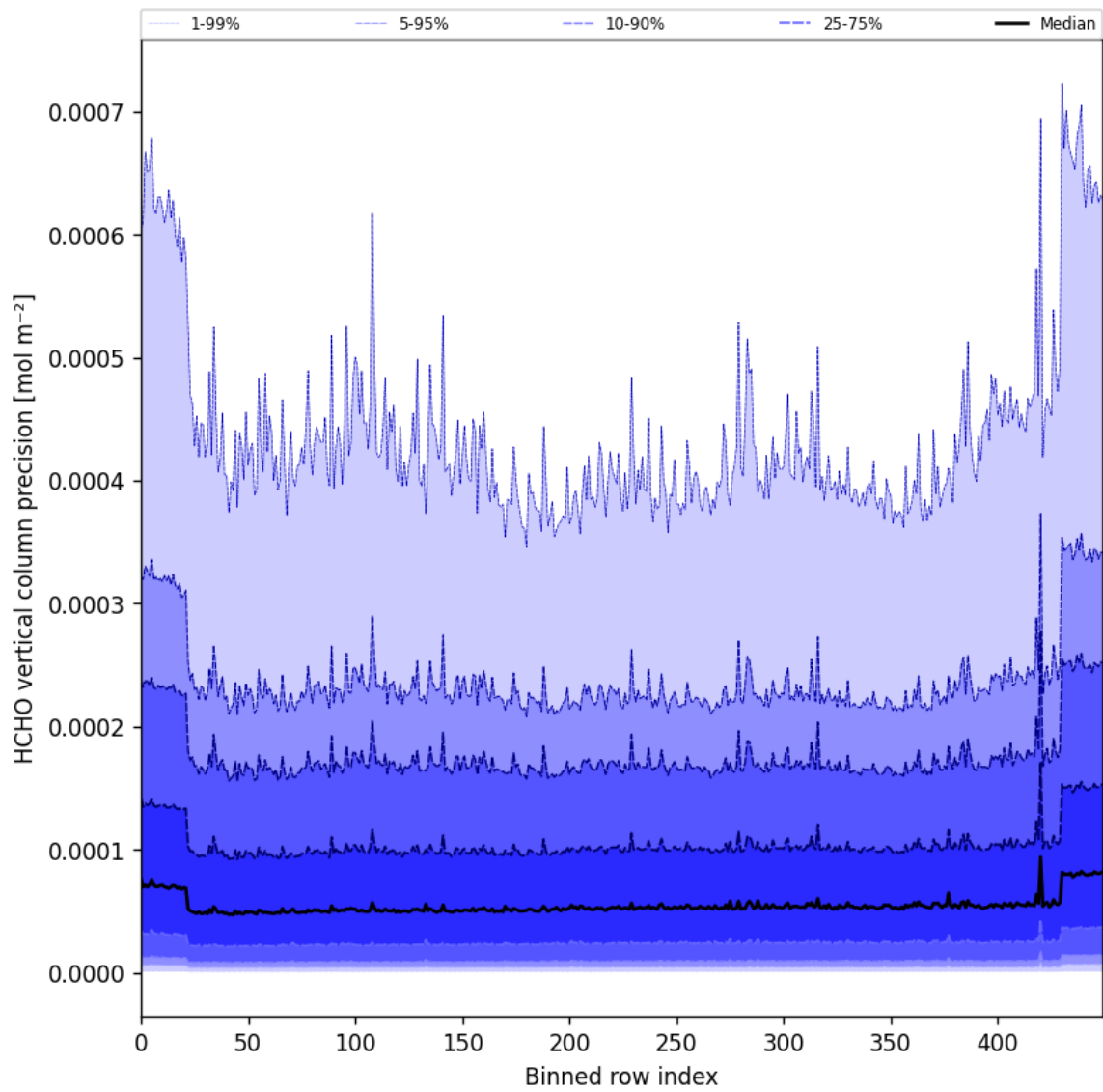
Figure 50: Along track statistics of “HCHO vertical column precision” for 2025-02-26 to 2025-02-28
