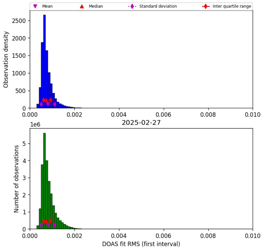
Figure 46: Histogram of “DOAS fit RMS (first interval)” for 2025-02-26 to 2025-02-28
