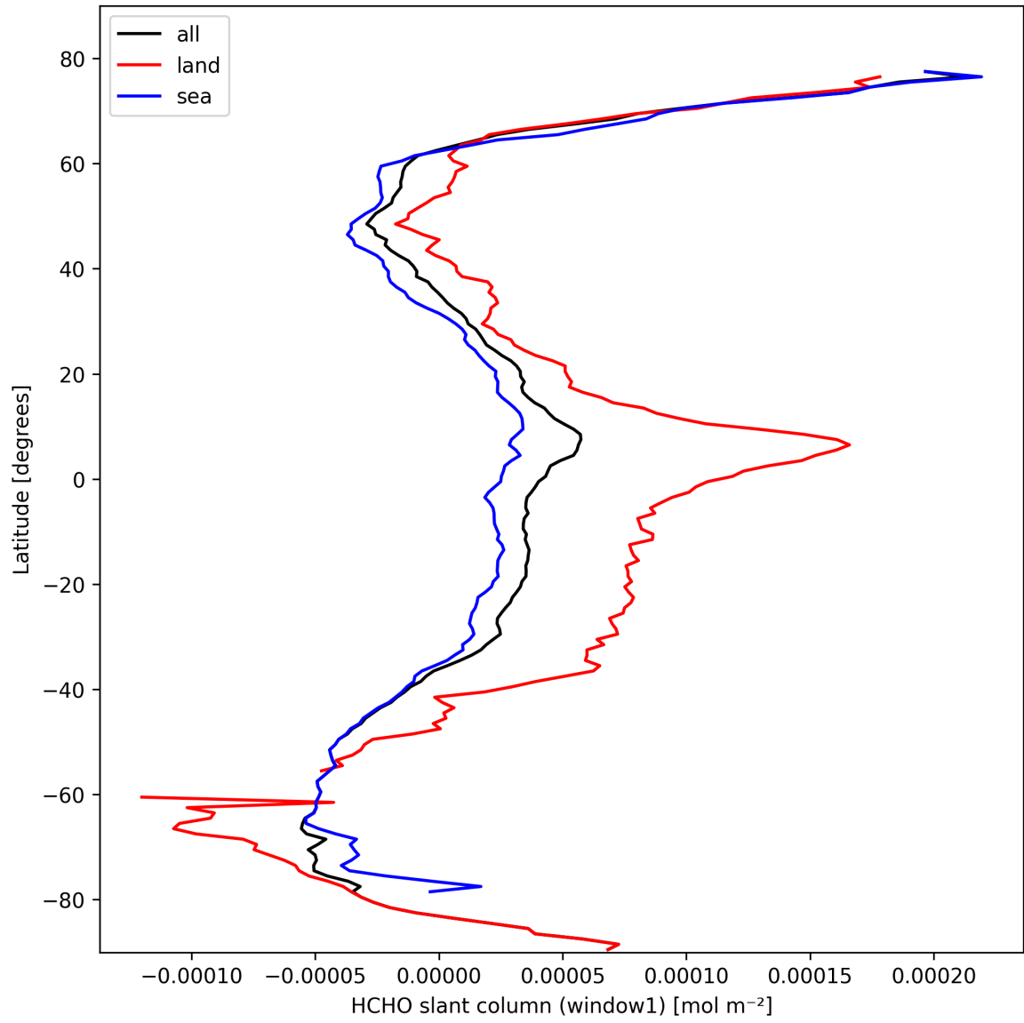
Figure 24: Zonal average of “HCHO slant column (window1)” for 2025-02-26 to 2025-02-28.
