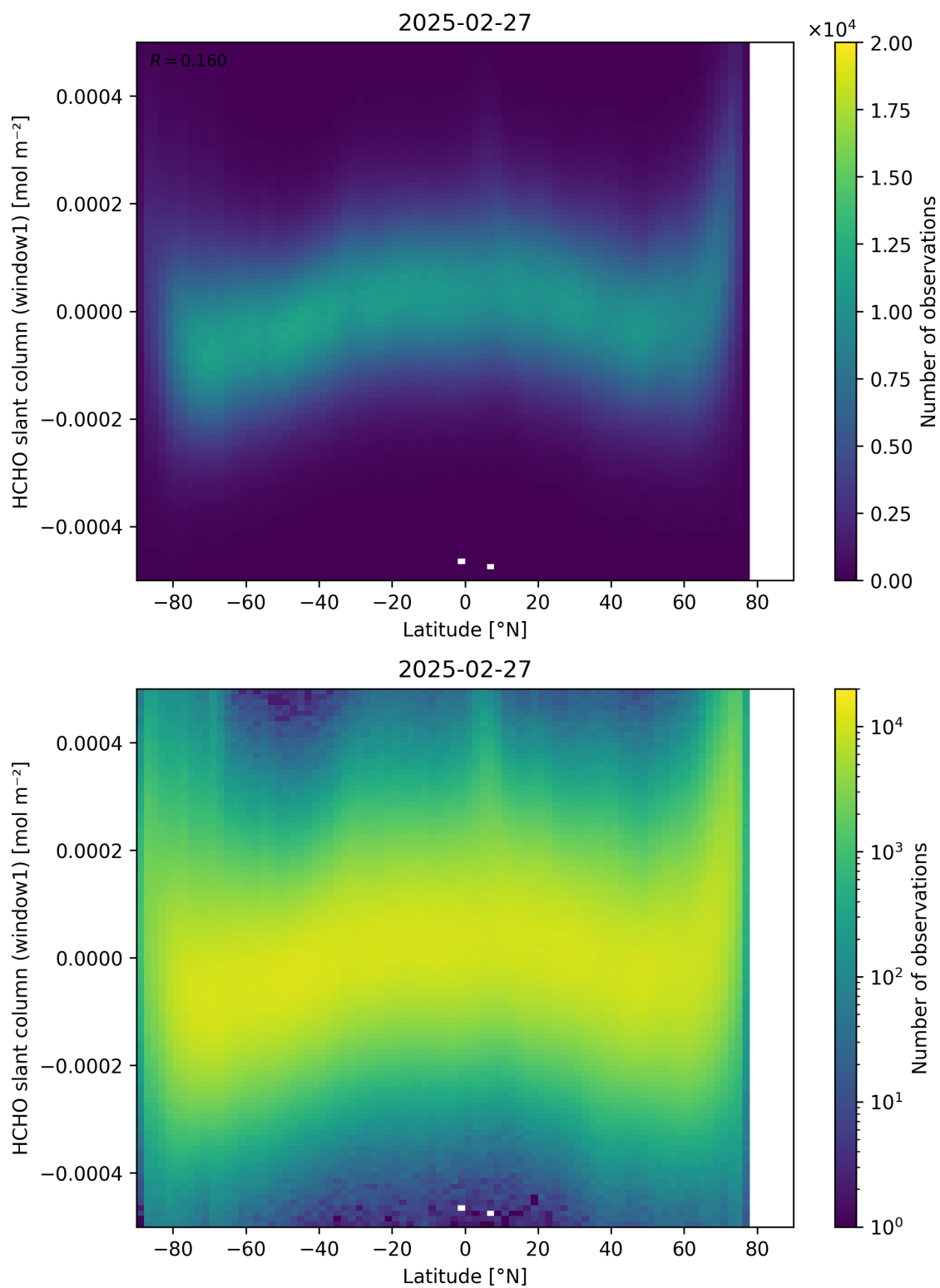
Figure 159: Scatter density plot of “Latitude” against “HCHO slant column (window1)” for 2025-02-26 to 2025-02-28.
