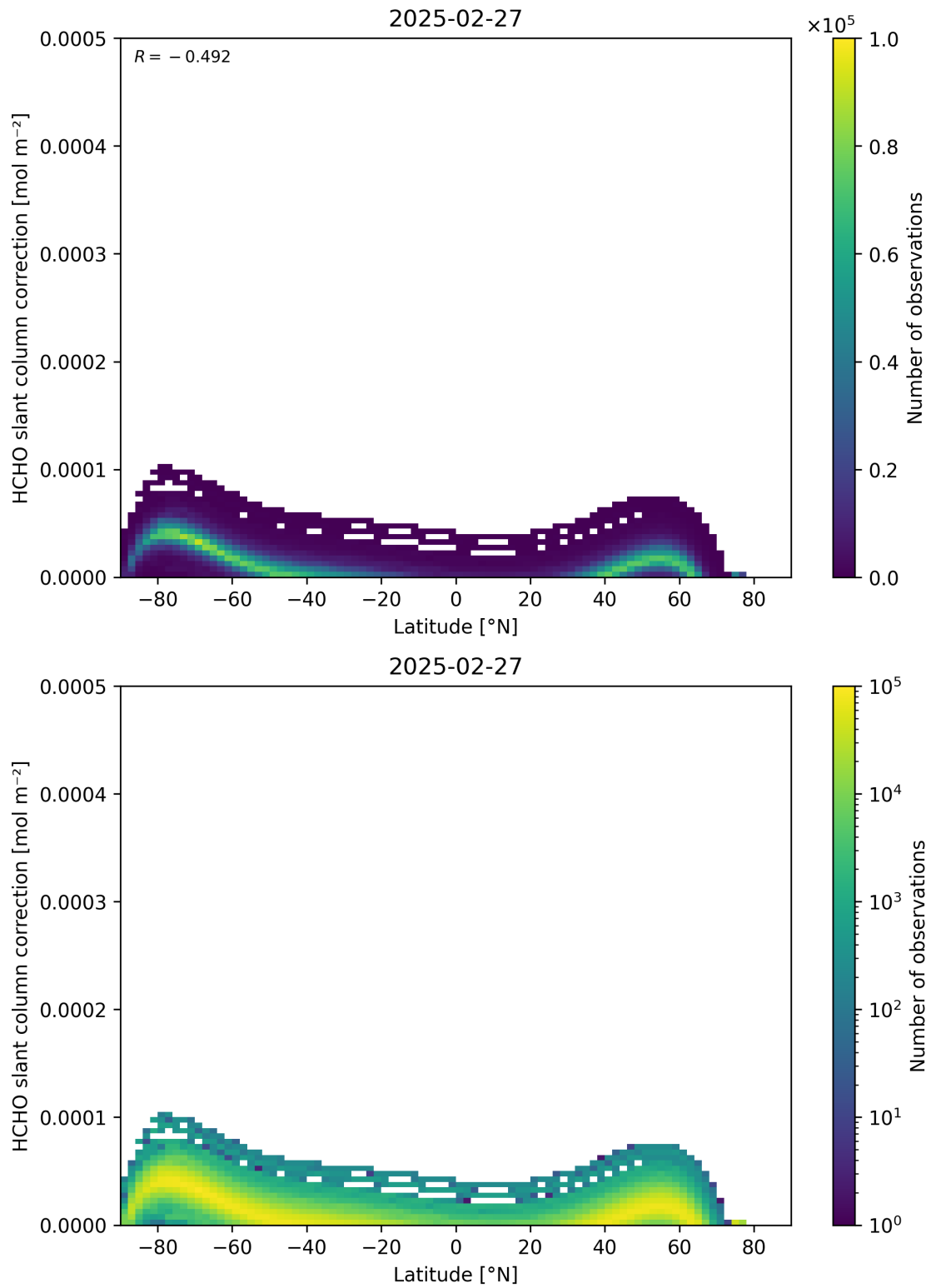
Figure 158: Scatter density plot of “Latitude” against “HCHO slant column correction” for 2025-02-26 to 2025-02-28.
