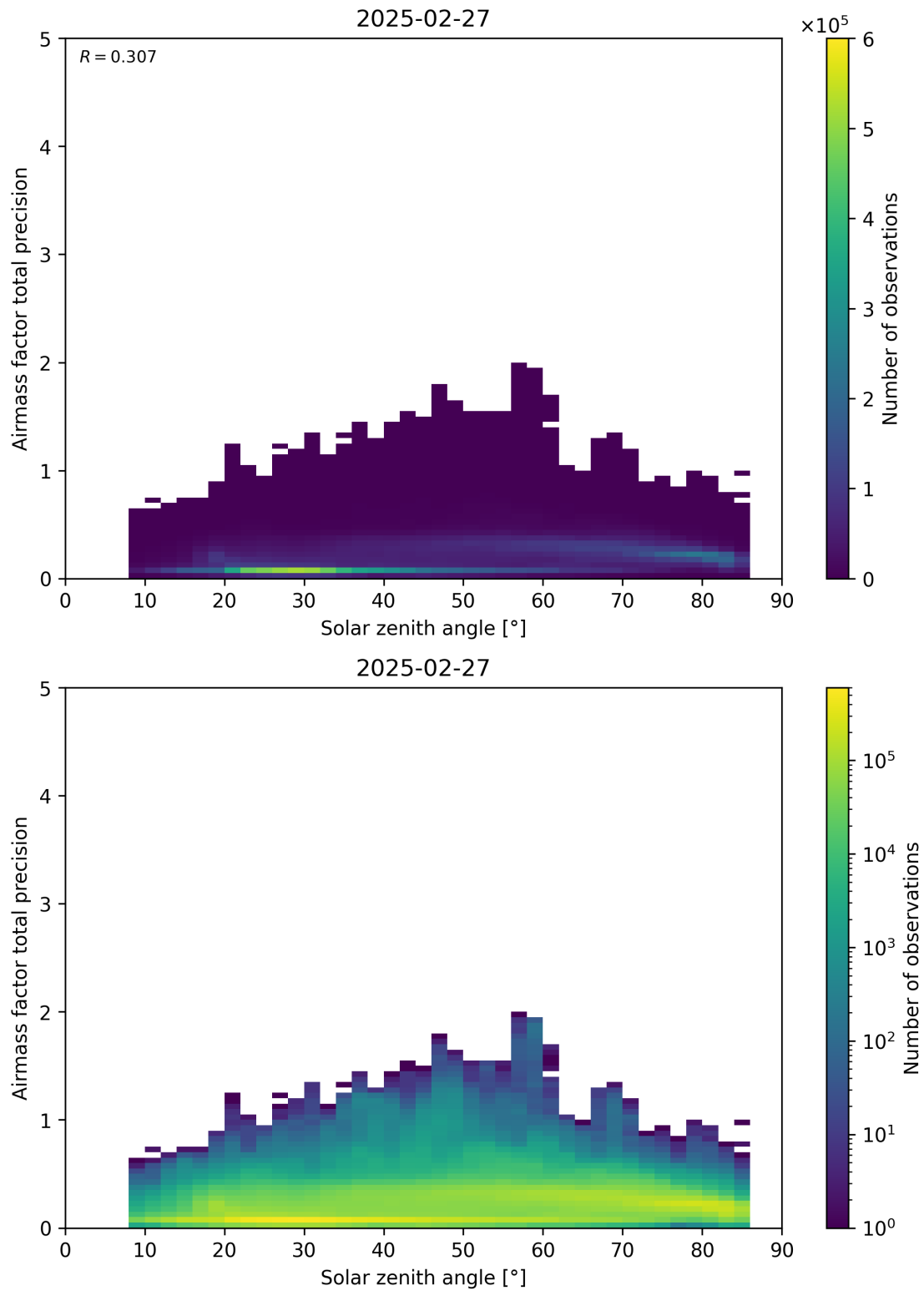
Figure 176: Scatter density plot of “Solar zenith angle” against “Airmass factor total precision” for 2025-02-26 to 2025-02-28.
