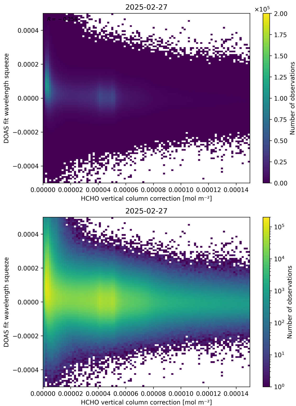
Figure 114: Scatter density plot of “HCHO vertical column correction” against “DOAS fit wavelength squeeze” for 2025-02-26 to 2025-02-28.
