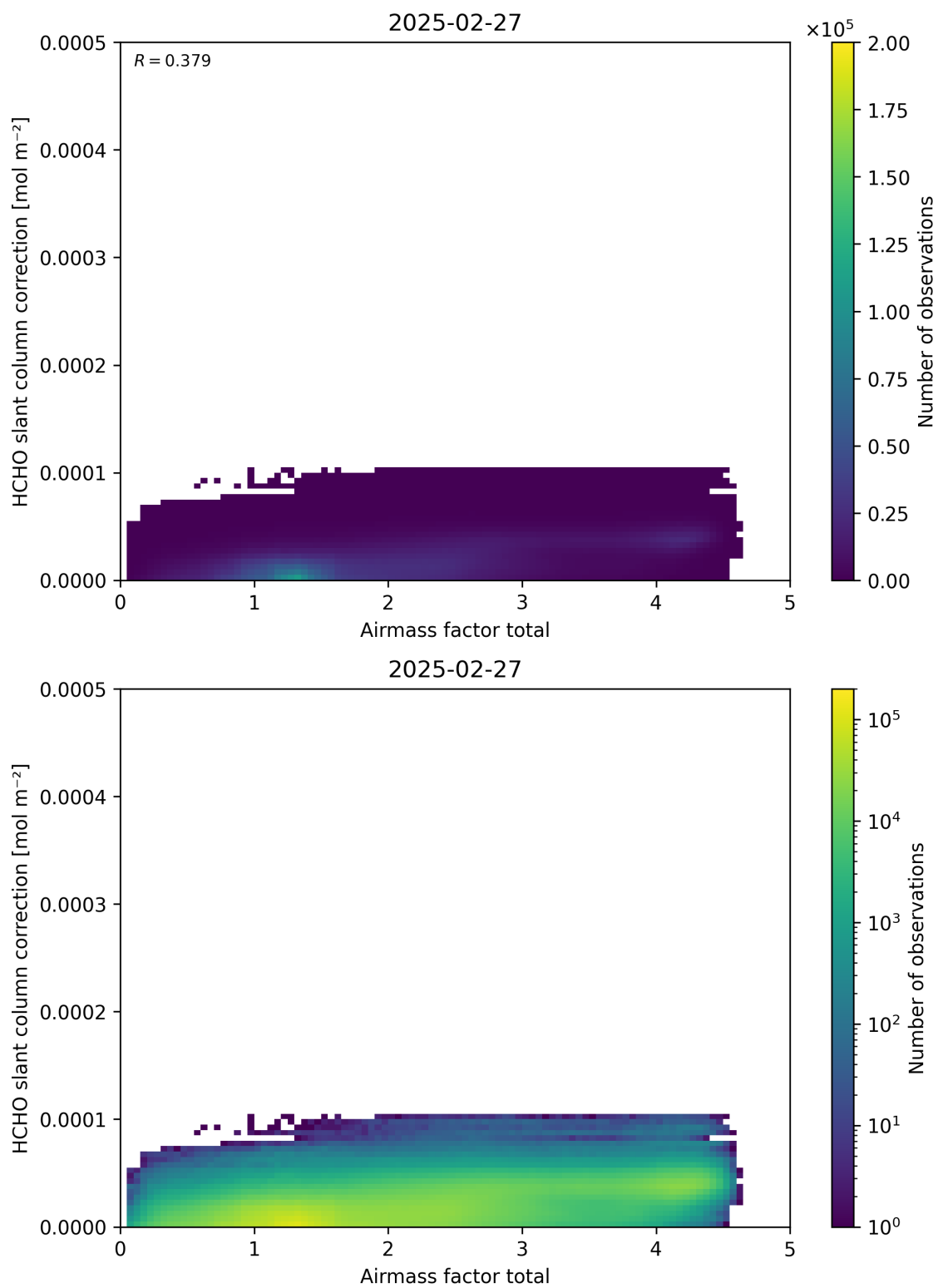
Figure 102: Scatter density plot of “Airmass factor total” against “HCHO slant column correction” for 2025-02-26 to 2025-02-28.
