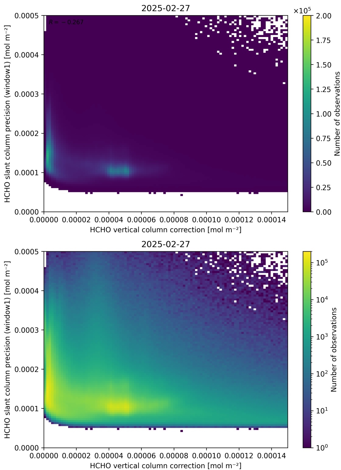
Figure 119: Scatter density plot of “HCHO vertical column correction” against “HCHO slant column precision (window1)” for 2025-02-26 to 2025-02-28.
