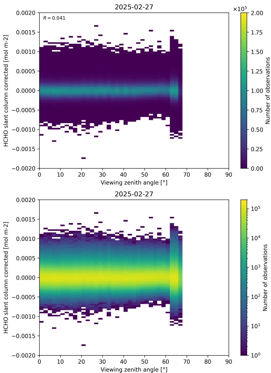
Figure 186: Scatter density plot of “Viewing zenith angle” against “HCHO slant column corrected” for 2025-02-26 to 2025-02-28.
