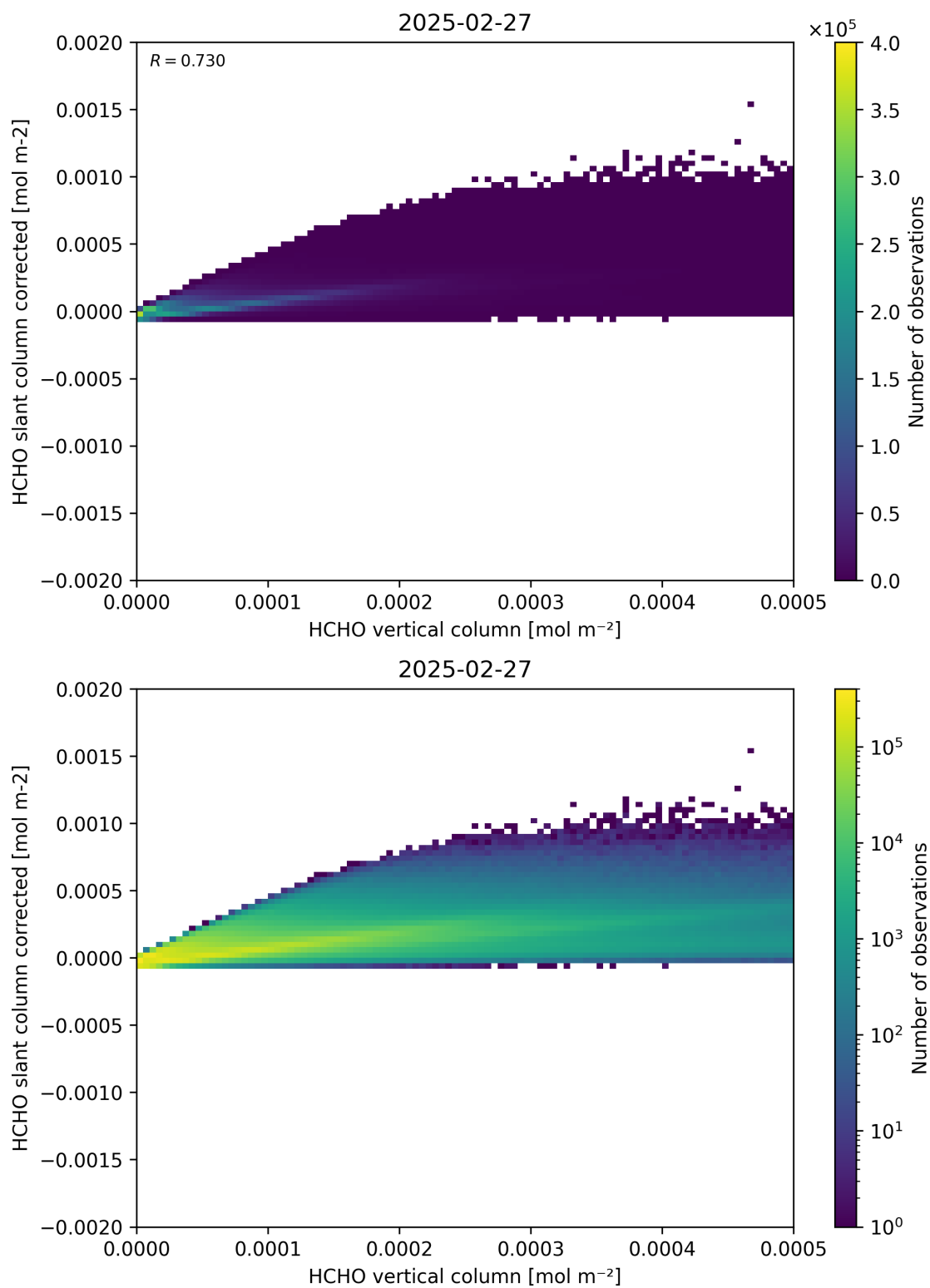
Figure 127: Scatter density plot of “HCHO vertical column” against “HCHO slant column corrected” for 2025-02-26 to 2025-02-28.
