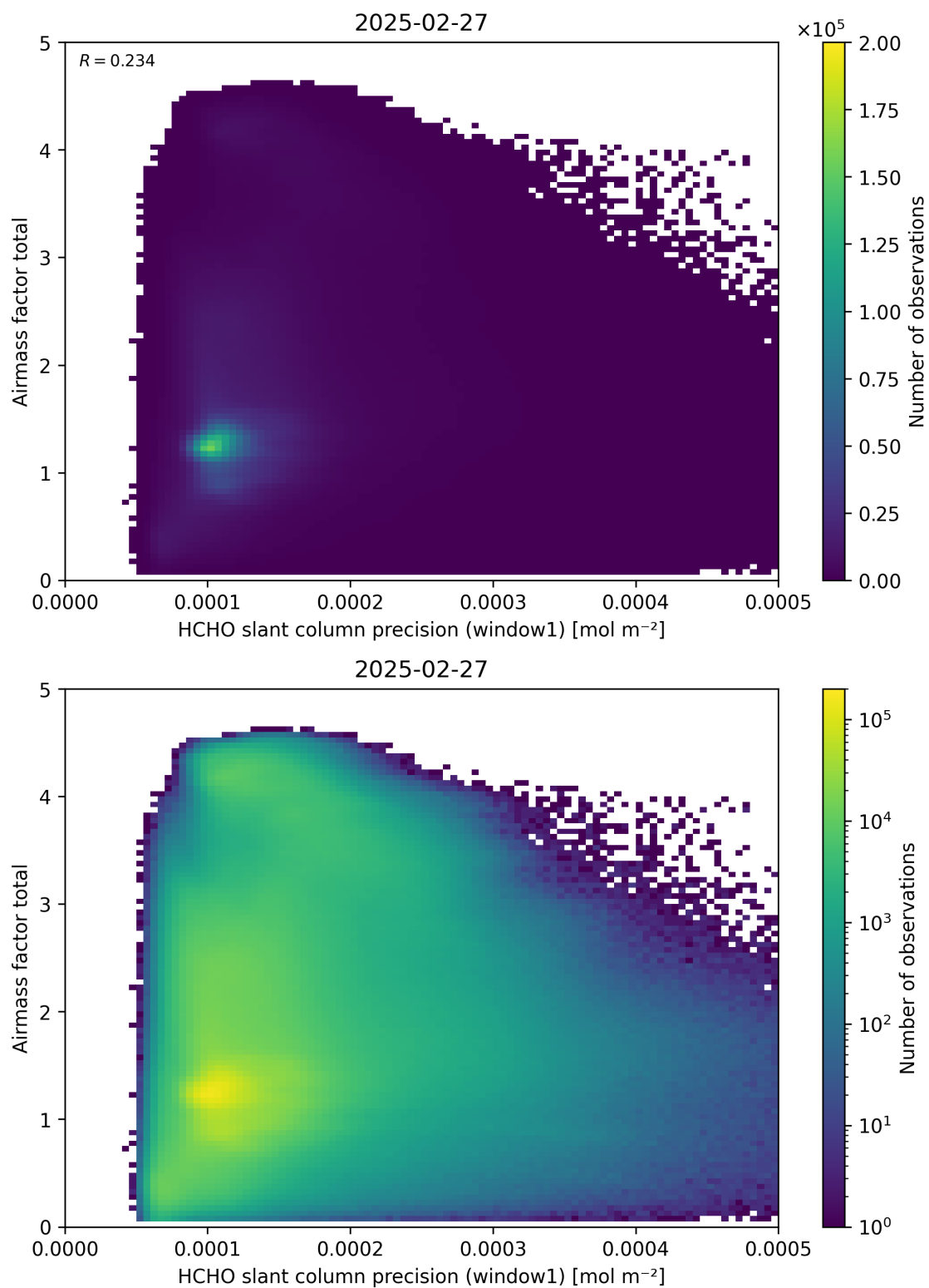
Figure 94: Scatter density plot of “HCHO slant column precision (window1)” against “Airmass factor total” for 2025-02-26 to 2025-02-28.
