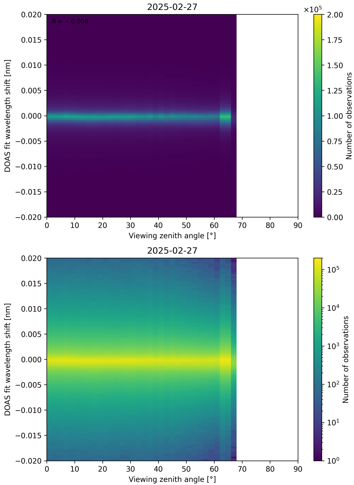
Figure 183: Scatter density plot of “Viewing zenith angle” against “DOAS fit wavelength shift” for 2025-02-26 to 2025-02-28.
