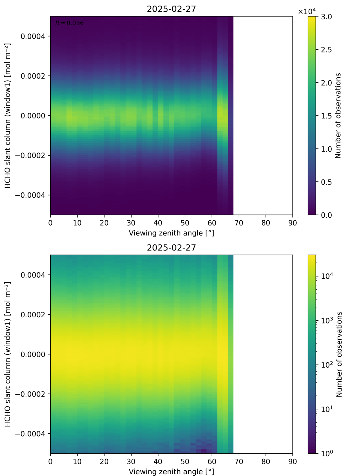
Figure 188: Scatter density plot of “Viewing zenith angle” against “HCHO slant column (window1)” for 2025-02-26 to 2025-02-28.
