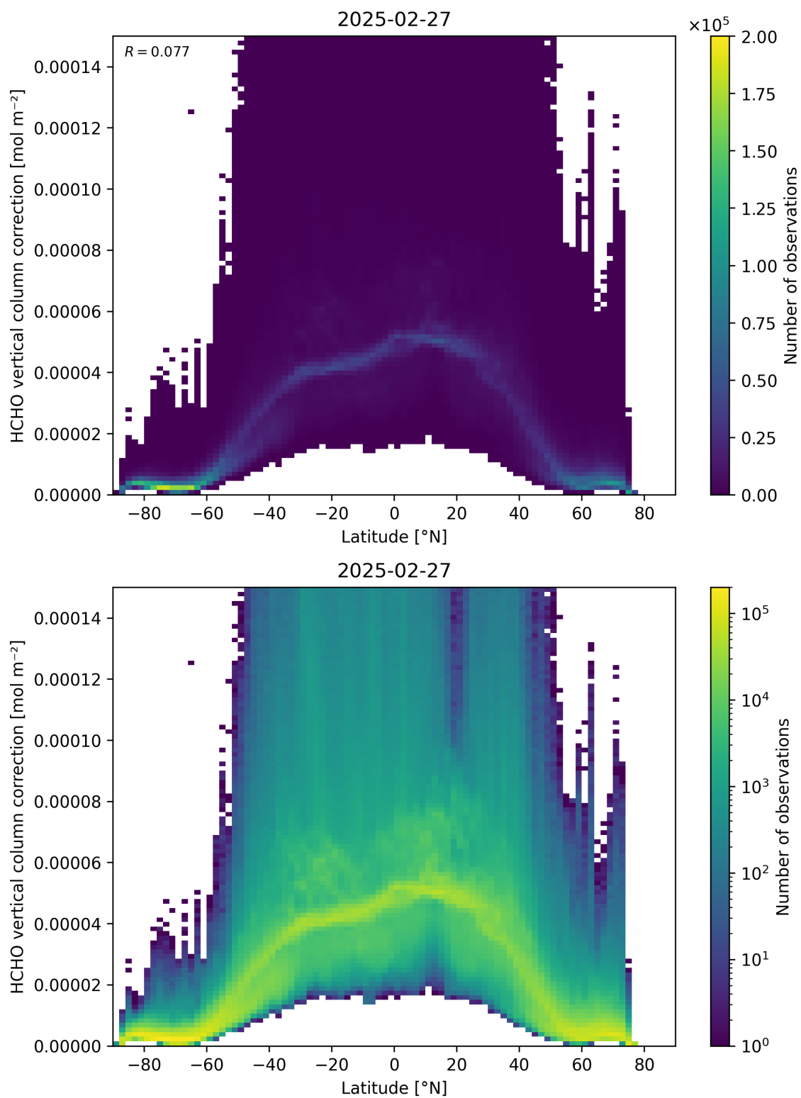
Figure 164: Scatter density plot of “Latitude” against “HCHO vertical column correction” for 2025-02-26 to 2025-02-28.
