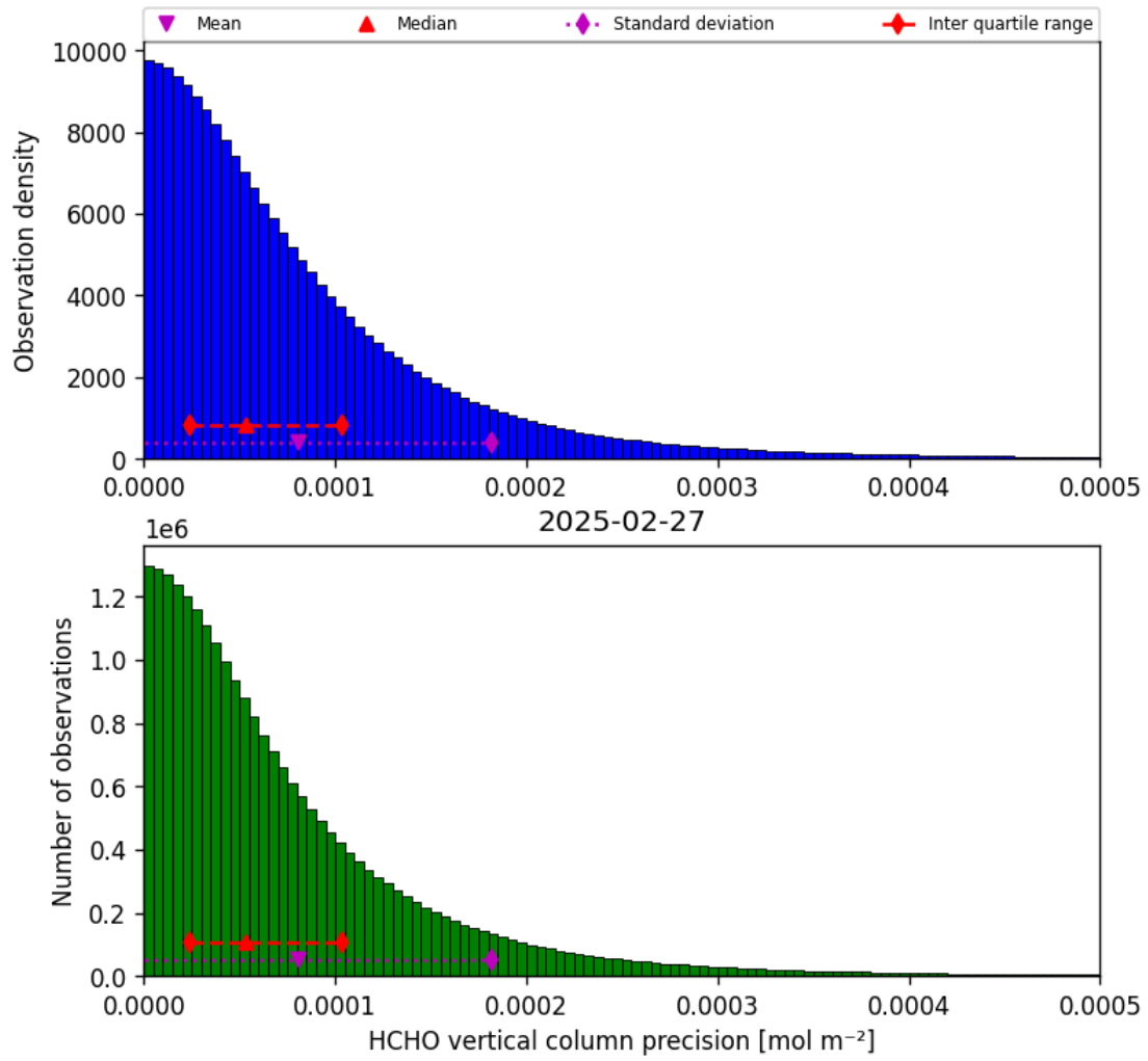
Figure 36: Histogram of “HCHO vertical column precision” for 2025-02-26 to 2025-02-28
