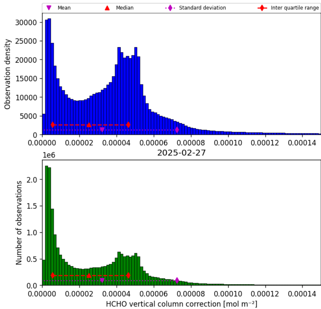
Figure 37: Histogram of “HCHO vertical column correction” for 2025-02-26 to 2025-02-28
