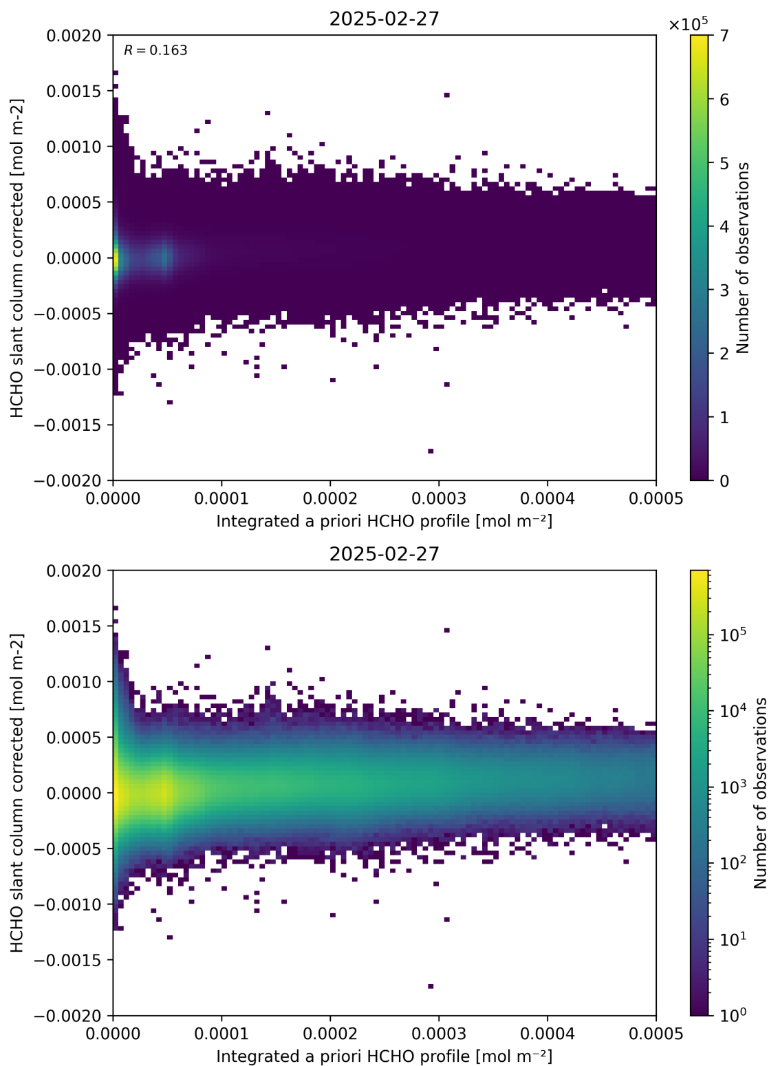
Figure 151: Scatter density plot of “Integrated a priori HCHO profile” against “HCHO slant column corrected” for 2025-02-26 to 2025-02-28.
