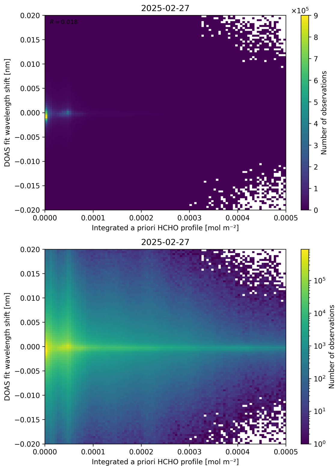
Figure 149: Scatter density plot of “Integrated a priori HCHO profile” against “DOAS fit wavelength shift” for 2025-02-26 to 2025-02-28.
