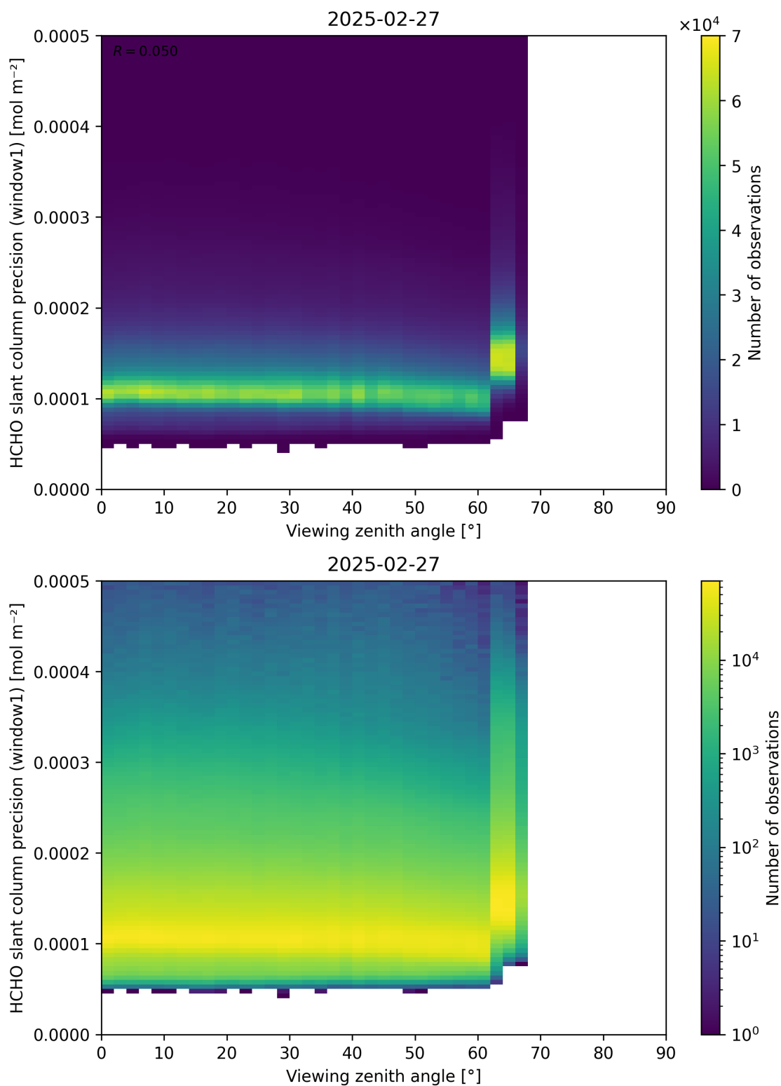
Figure 189: Scatter density plot of “Viewing zenith angle” against “HCHO slant column precision (window1)” for 2025-02-26 to 2025-02-28.
