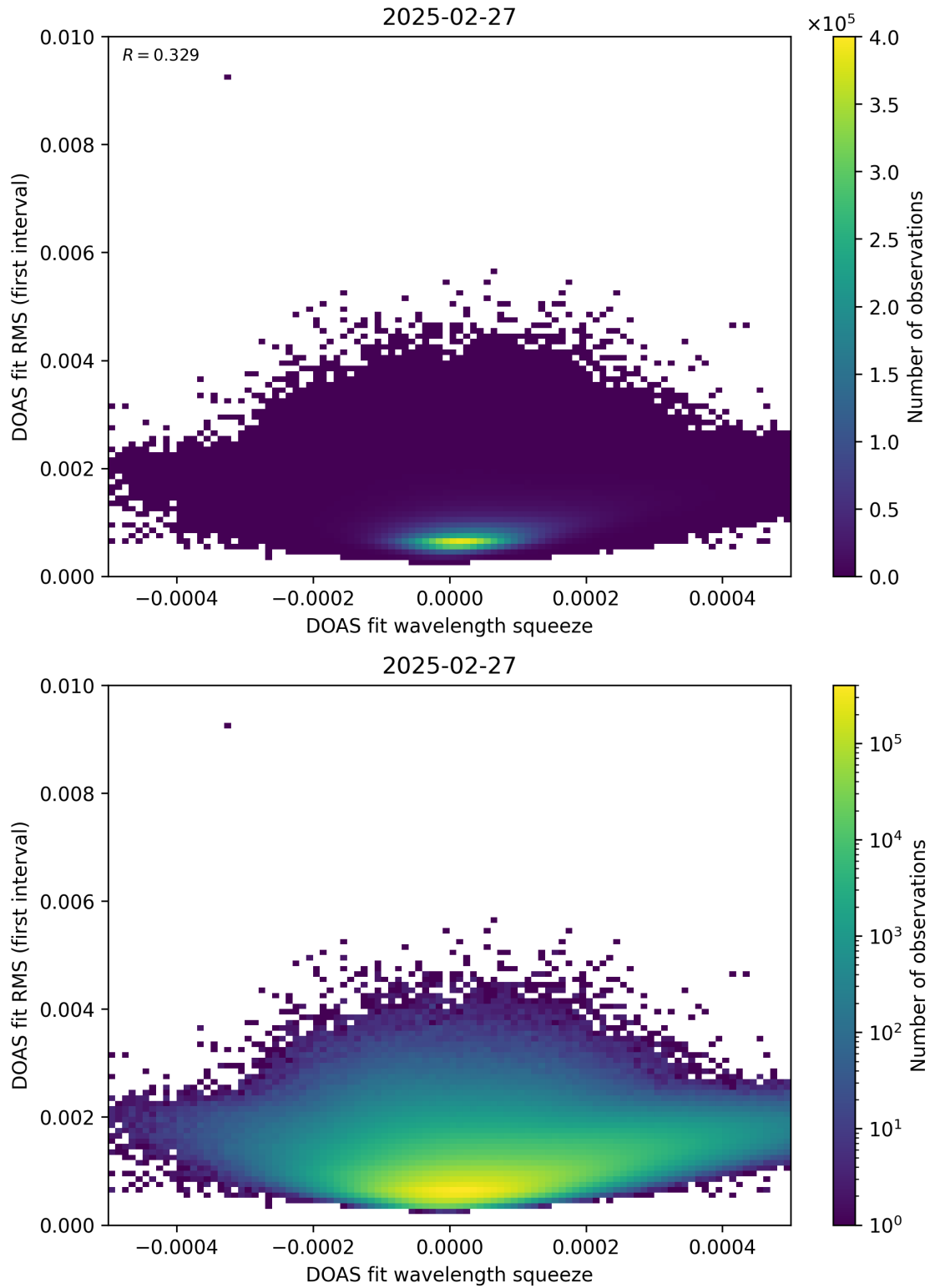
Figure 68: Scatter density plot of “DOAS fit wavelength squeeze” against “DOAS fit RMS (first interval)” for 2025-02-26 to 2025-02-28.
