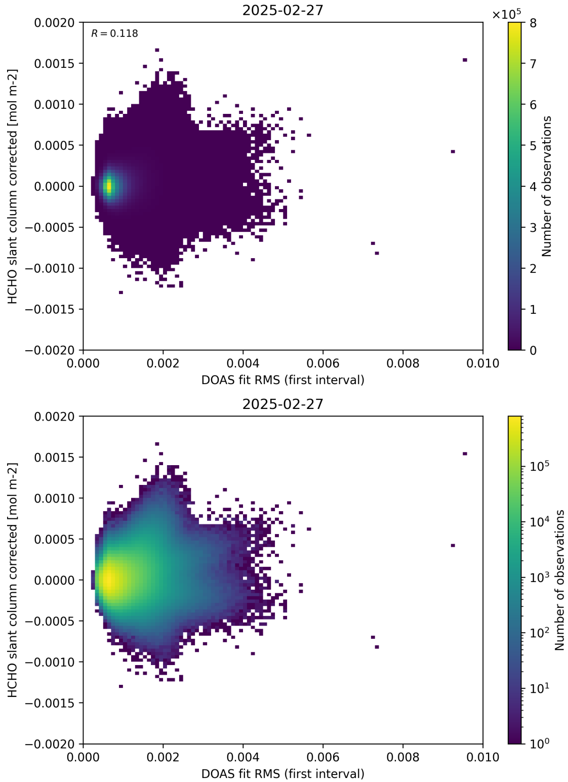
Figure 62: Scatter density plot of “DOAS fit RMS (first interval)” against “HCHO slant column corrected” for 2025-02-26 to 2025-02-28.
