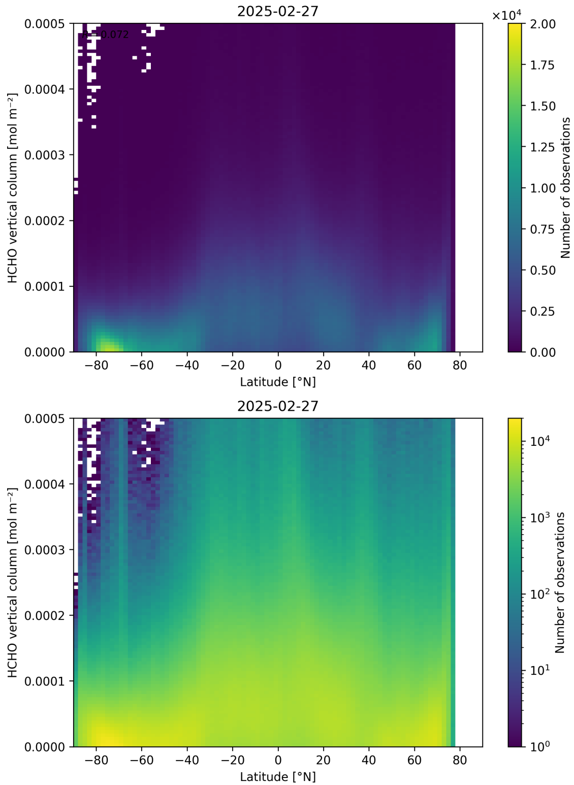
Figure 163: Scatter density plot of “Latitude” against “HCHO vertical column” for 2025-02-26 to 2025-02-28.
