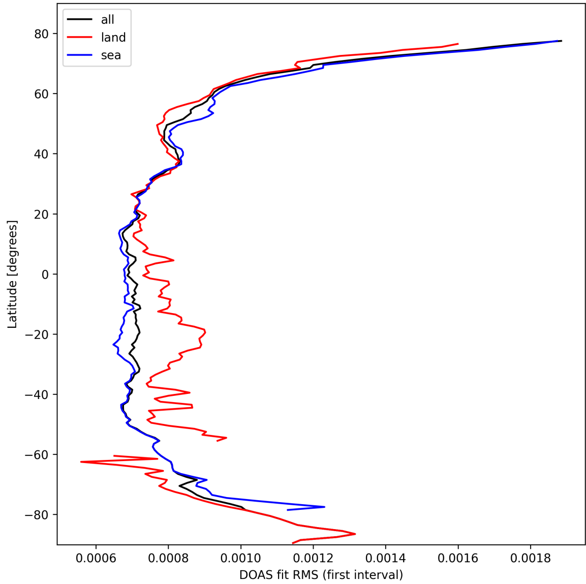
Figure 32: Zonal average of “DOAS fit RMS (first interval)” for 2025-02-26 to 2025-02-28.
