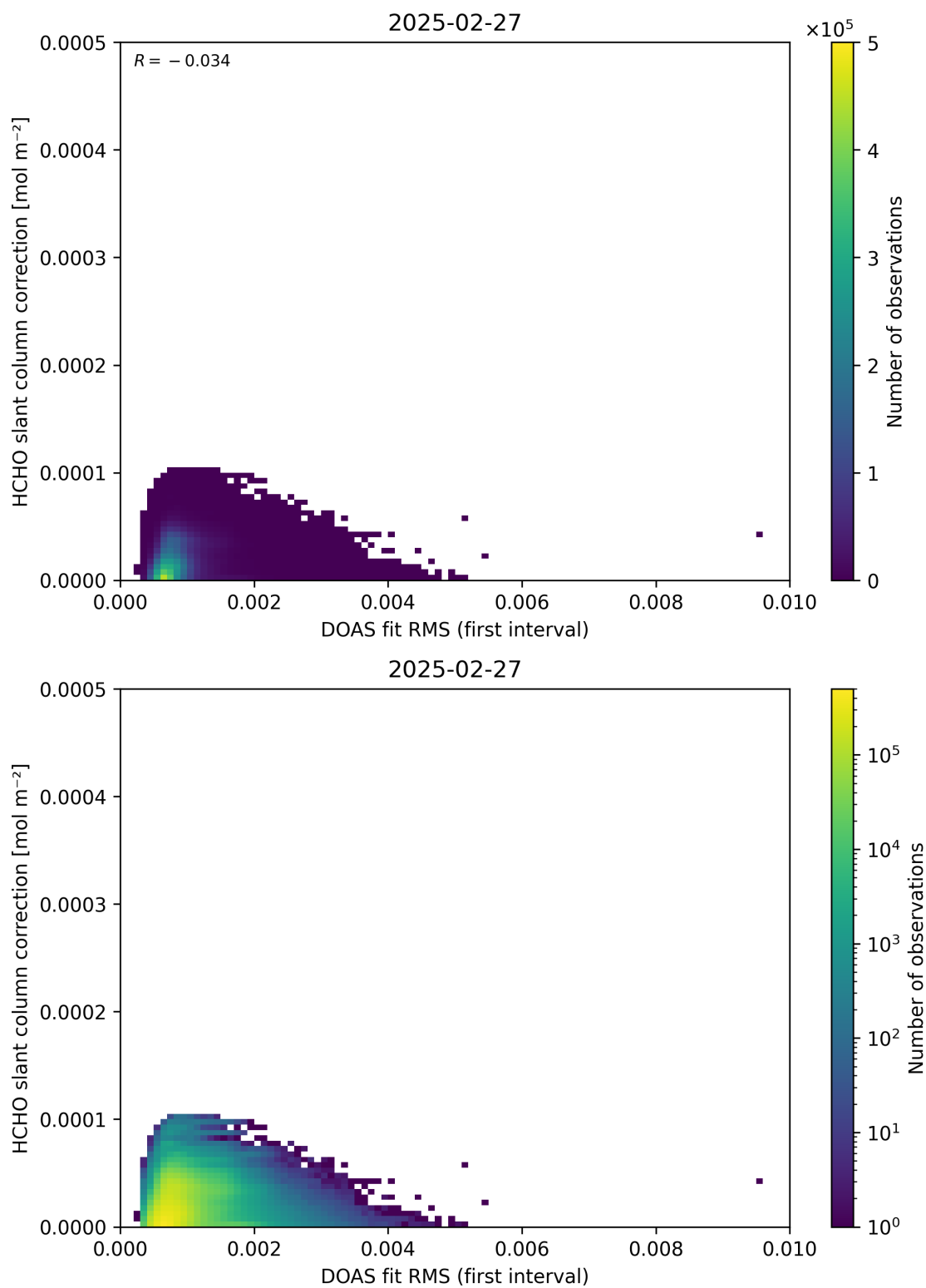
Figure 63: Scatter density plot of “DOAS fit RMS (first interval)” against “HCHO slant column correction” for 2025-02-26 to 2025-02-28.
