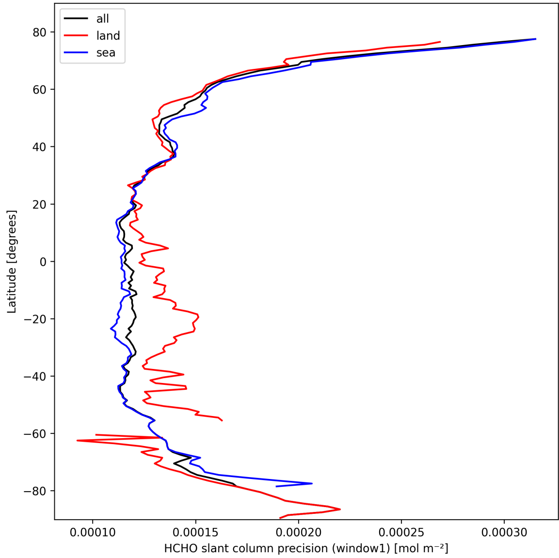
Figure 25: Zonal average of “HCHO slant column precision (window1)” for 2025-02-26 to 2025-02-28.
