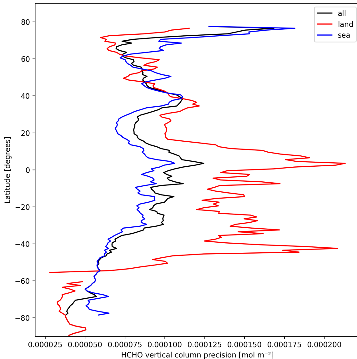
Figure 22: Zonal average of “HCHO vertical column precision” for 2025-02-26 to 2025-02-28.
