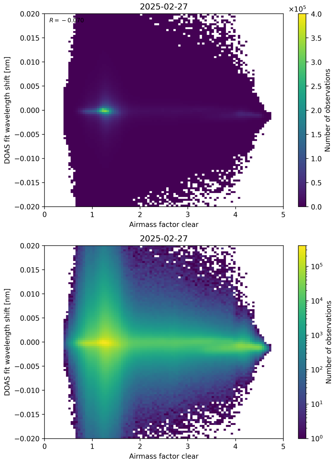
Figure 72: Scatter density plot of “Airmass factor clear” against “DOAS fit wavelength shift” for 2025-02-26 to 2025-02-28.
