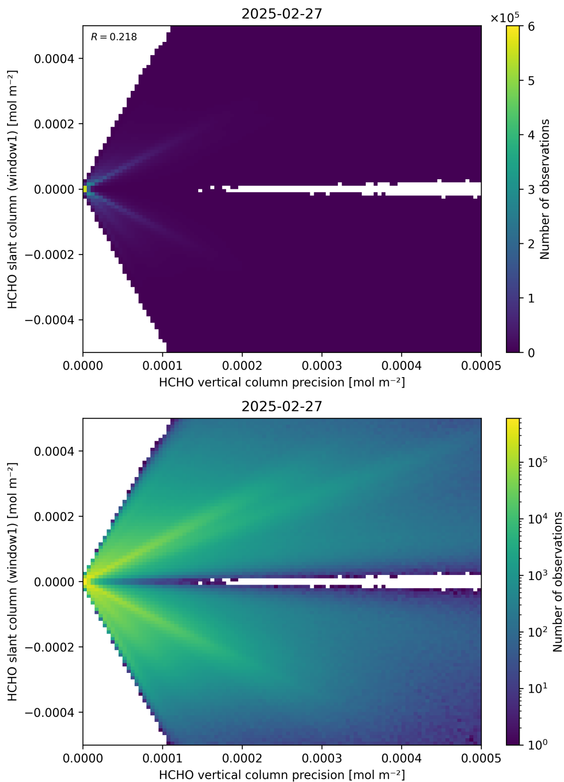
Figure 142: Scatter density plot of “HCHO vertical column precision” against “HCHO slant column (window1)” for 2025-02-26 to 2025-02-28.
