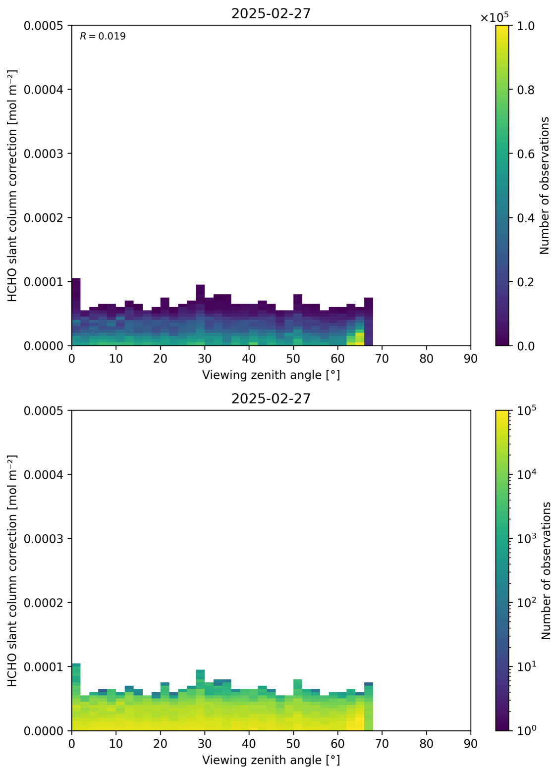
Figure 187: Scatter density plot of “Viewing zenith angle” against “HCHO slant column correction” for 2025-02-26 to 2025-02-28.
