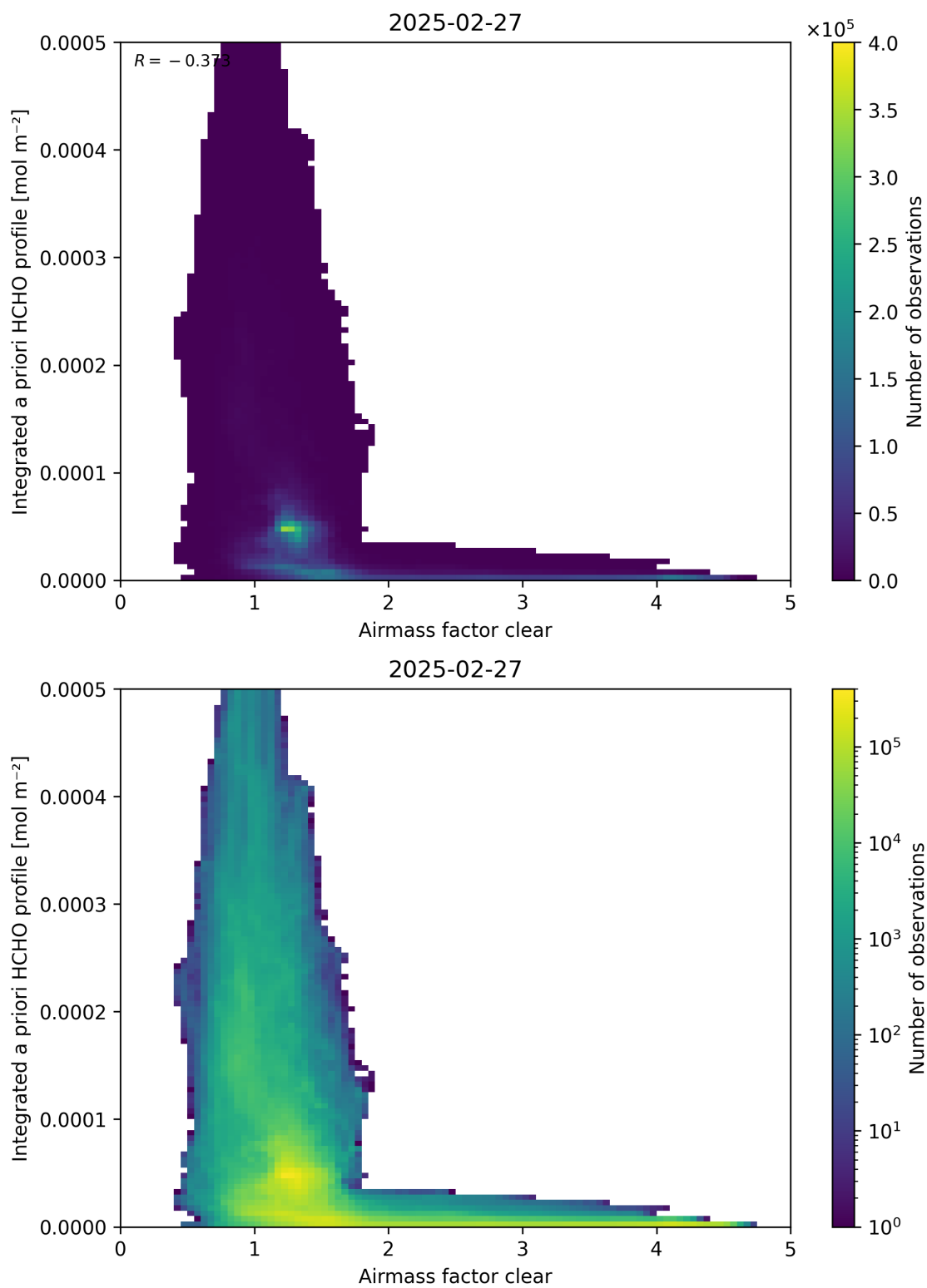
Figure 76: Scatter density plot of “Airmass factor clear” against “Integrated a priori HCHO profile” for 2025-02-26 to 2025-02-28.
