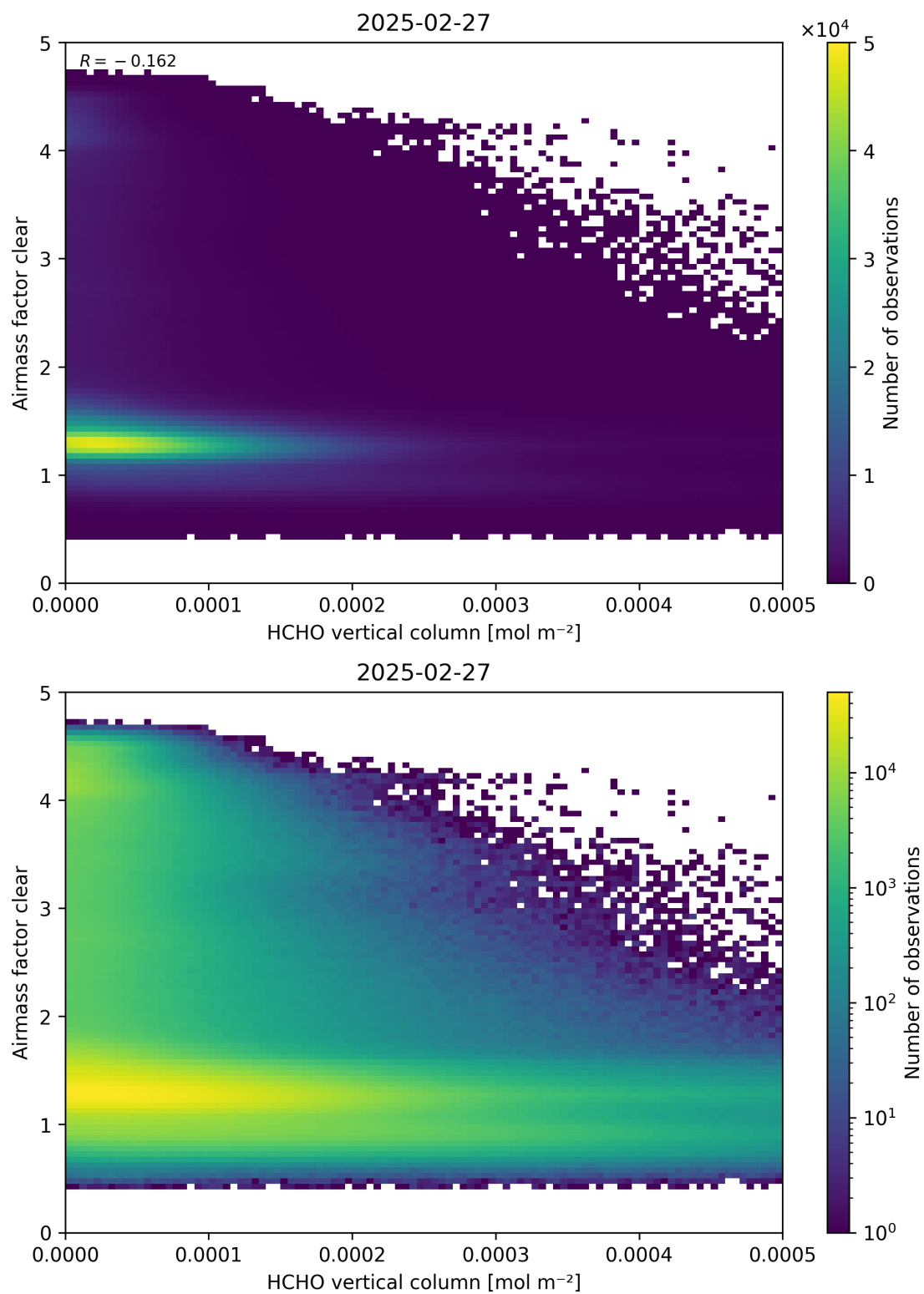
Figure 126: Scatter density plot of “HCHO vertical column” against “Airmass factor clear” for 2025-02-26 to 2025-02-28.
