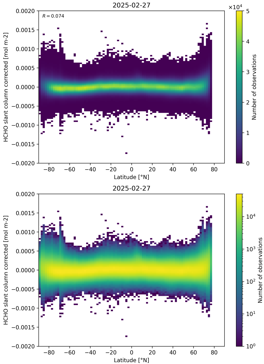
Figure 157: Scatter density plot of “Latitude” against “HCHO slant column corrected” for 2025-02-26 to 2025-02-28.
