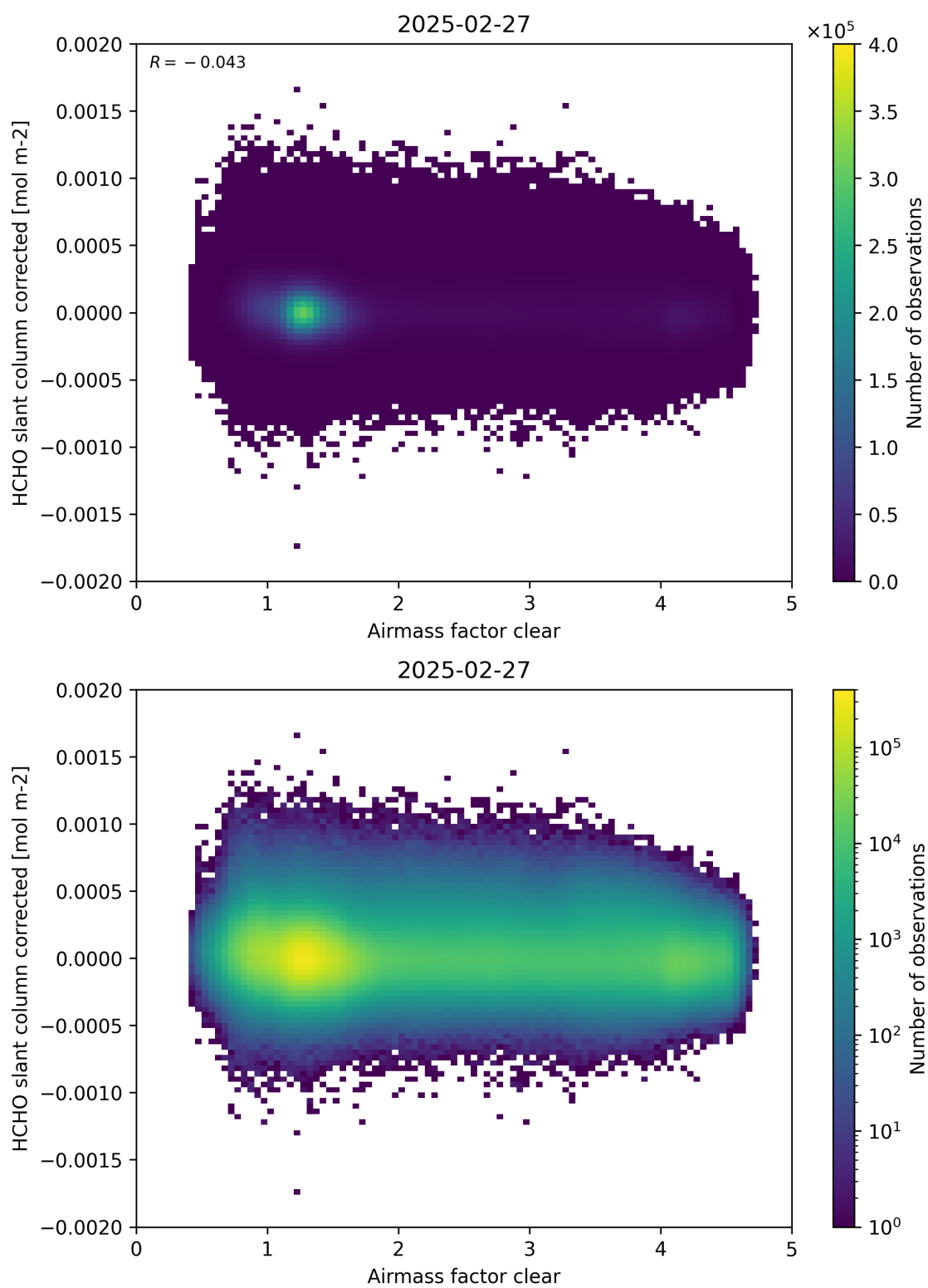
Figure 74: Scatter density plot of “Airmass factor clear” against “HCHO slant column corrected” for 2025-02-26 to 2025-02-28.
