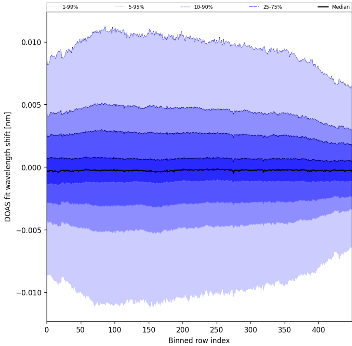
Figure 58: Along track statistics of “DOAS fit wavelength shift” for 2025-02-26 to 2025-02-28
