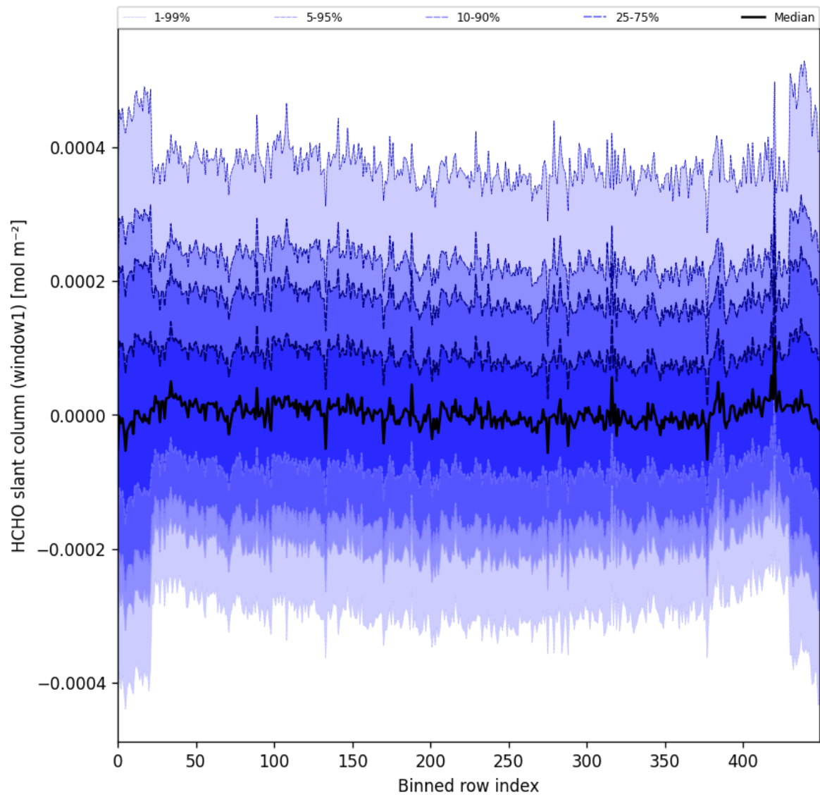
Figure 52: Along track statistics of “HCHO slant column (window1)” for 2025-02-26 to 2025-02-28
