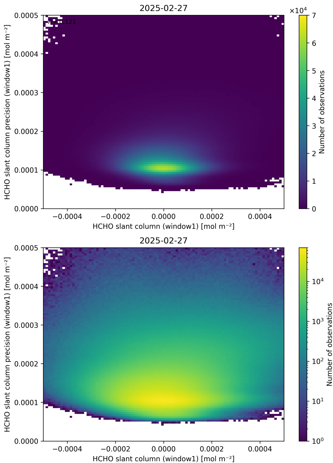
Figure 84: Scatter density plot of “HCHO slant column (window1)” against “HCHO slant column precision (window1)” for 2025-02-26 to 2025-02-28.
