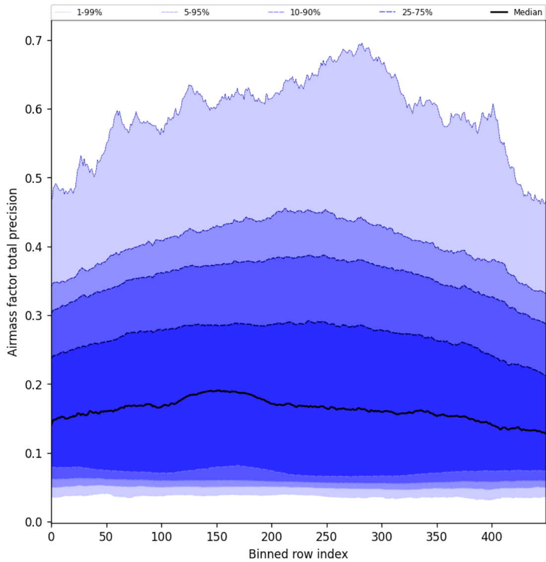
Figure 55: Along track statistics of “Airmass factor total precision” for 2025-02-26 to 2025-02-28
