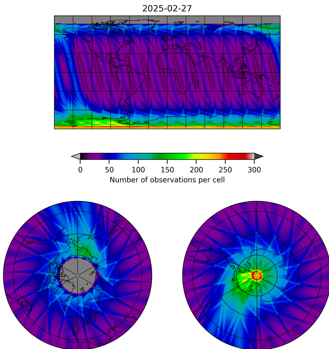
Figure 19: Map of the number of observations for 2025-02-26 to 2025-02-28
