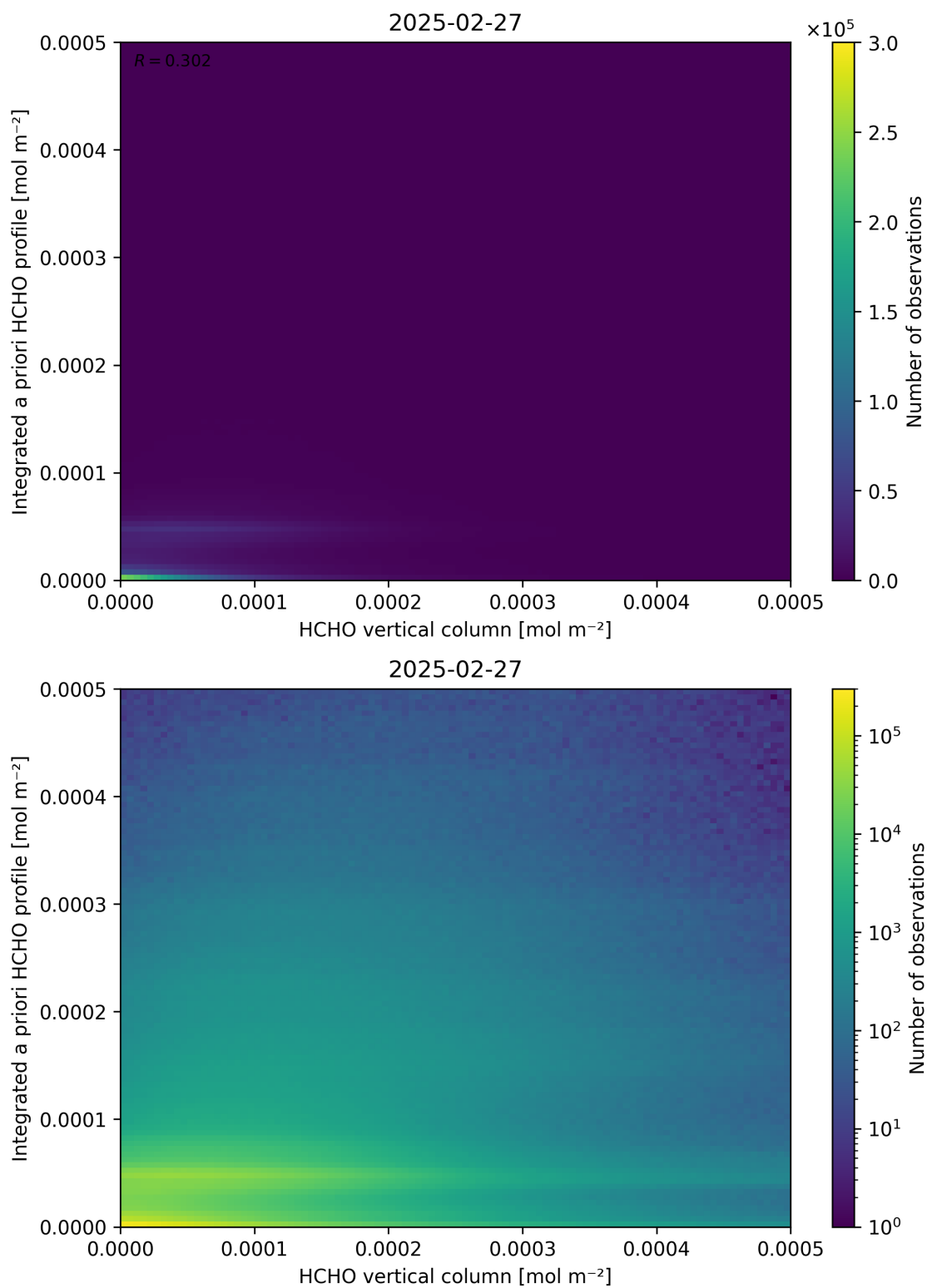
Figure 135: Scatter density plot of “HCHO vertical column” against “Integrated a priori HCHO profile” for 2025-02-26 to 2025-02-28.
