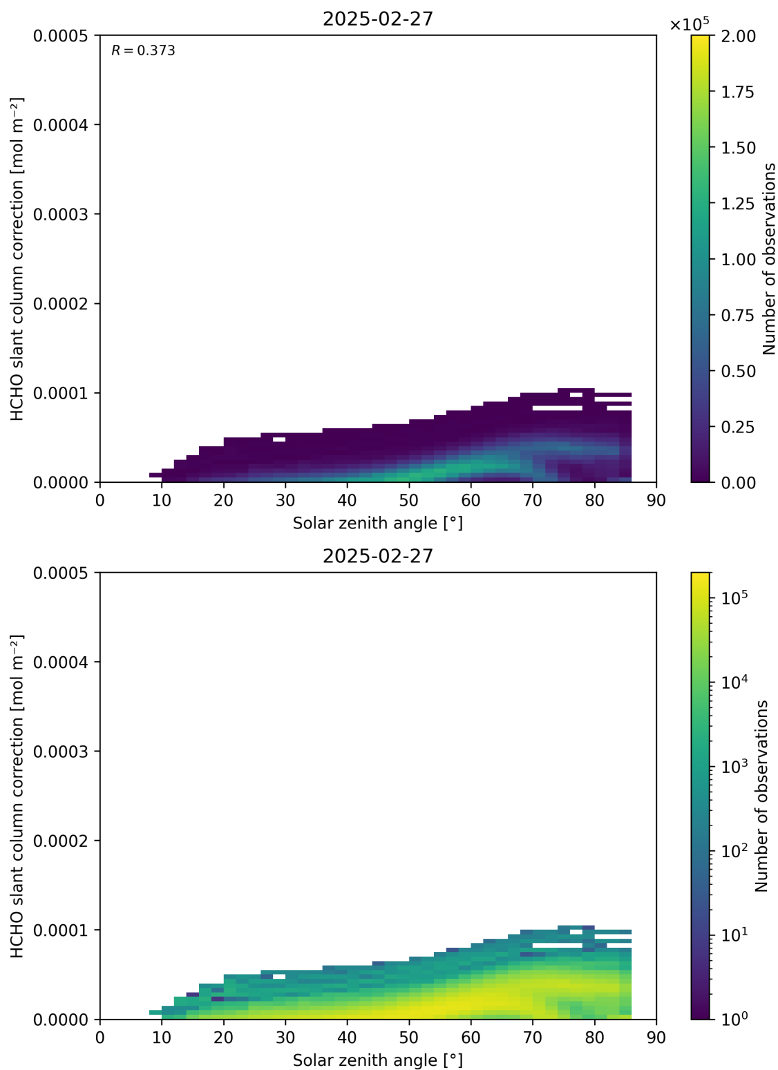
Figure 172: Scatter density plot of “Solar zenith angle” against “HCHO slant column correction” for 2025-02-26 to 2025-02-28.
