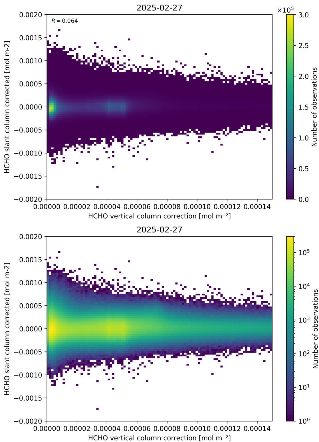
Figure 116: Scatter density plot of “HCHO vertical column correction” against “HCHO slant column corrected” for 2025-02-26 to 2025-02-28.
