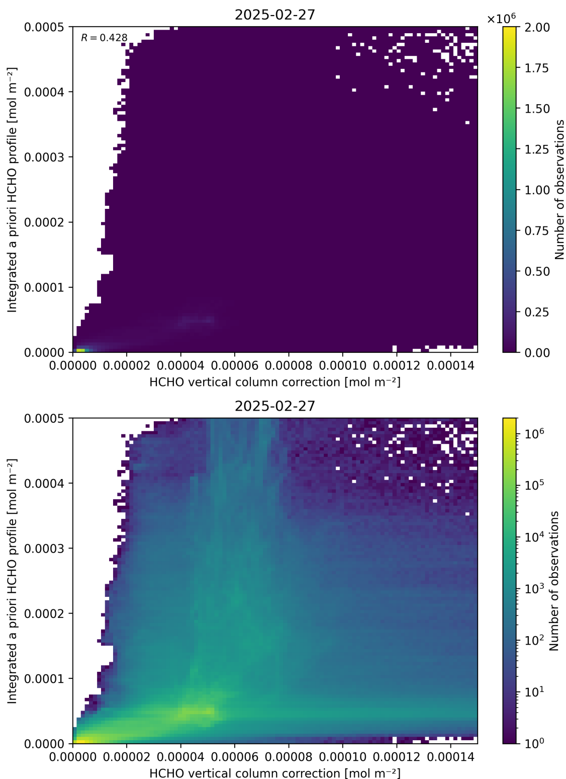
Figure 122: Scatter density plot of “HCHO vertical column correction” against “Integrated a priori HCHO profile” for 2025-02-26 to 2025-02-28.
