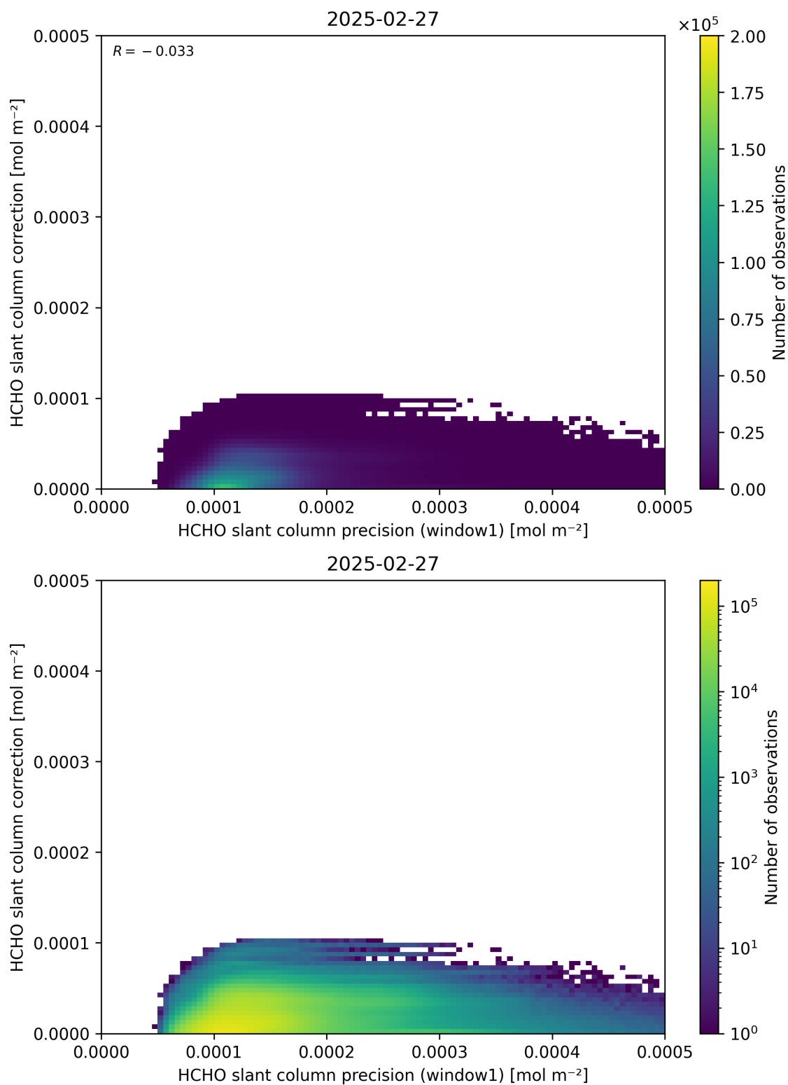
Figure 93: Scatter density plot of “HCHO slant column precision (window1)” against “HCHO slant column correction” for 2025-02-26 to 2025-02-28.
