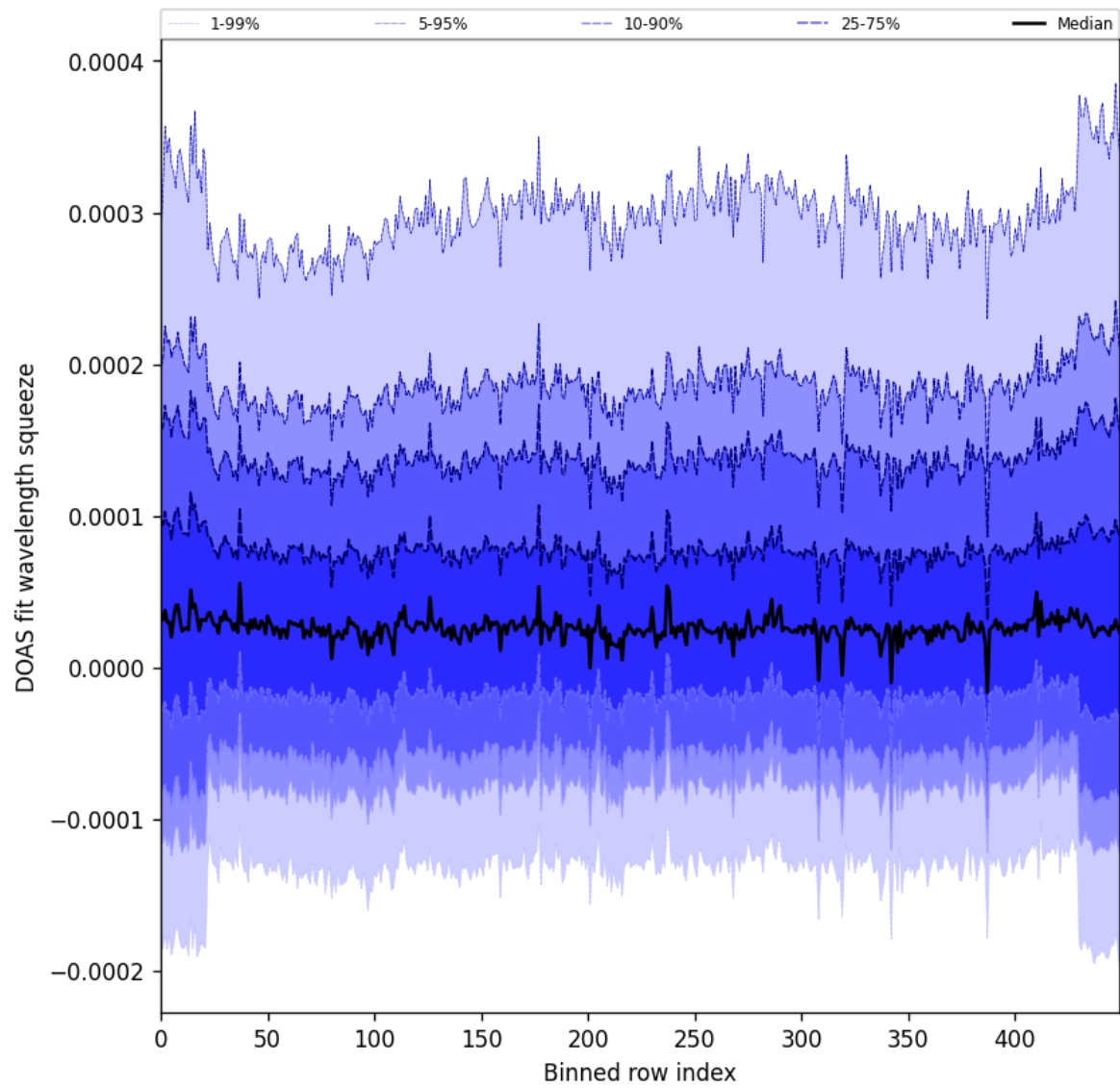
Figure 59: Along track statistics of “DOAS fit wavelength squeeze” for 2025-02-26 to 2025-02-28
