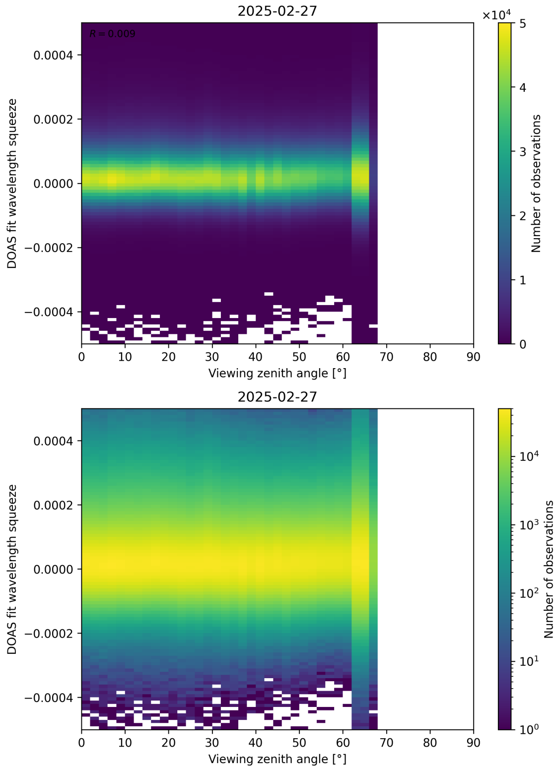
Figure 184: Scatter density plot of “Viewing zenith angle” against “DOAS fit wavelength squeeze” for 2025-02-26 to 2025-02-28.
