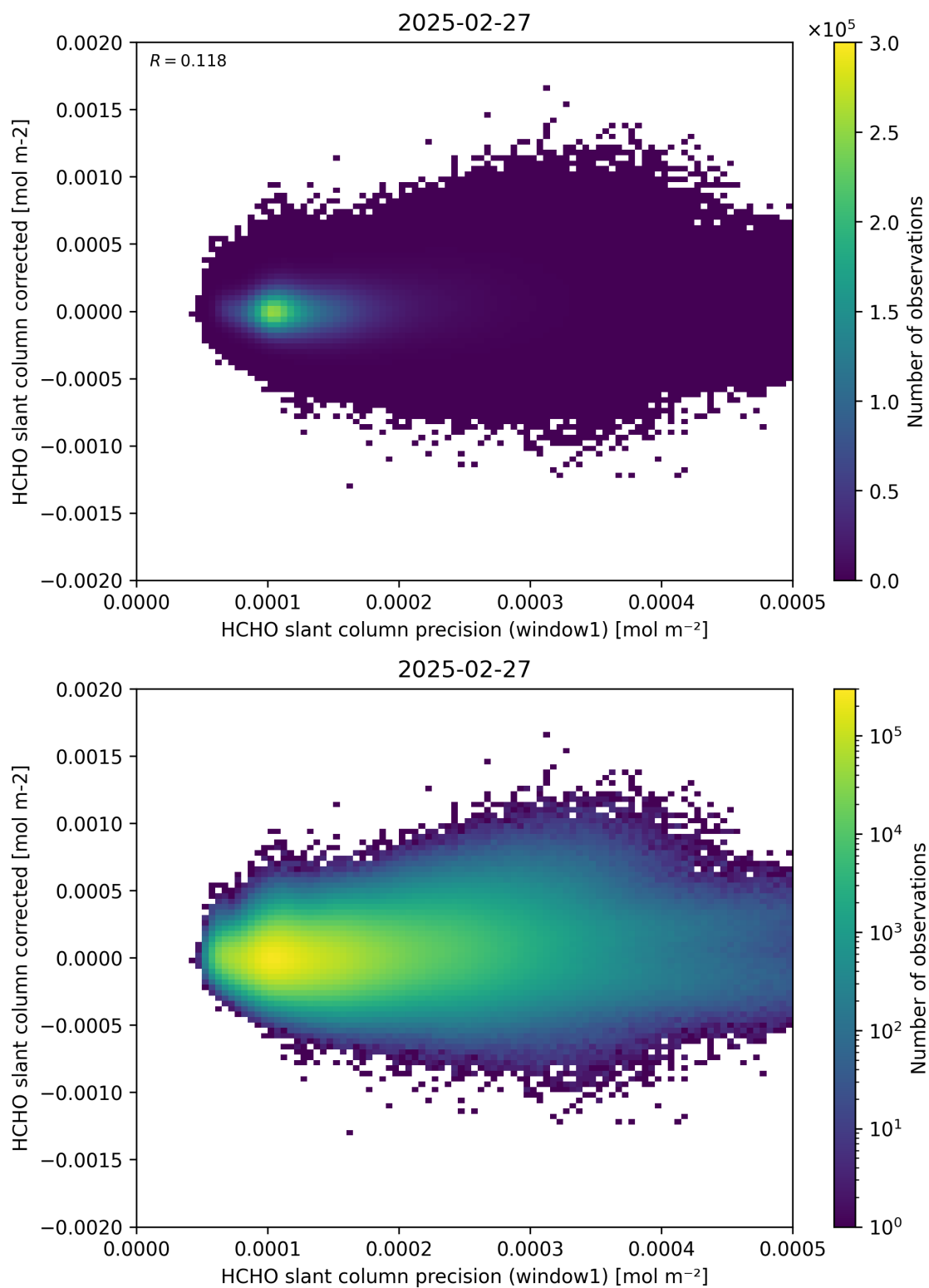
Figure 92: Scatter density plot of “HCHO slant column precision (window1)” against “HCHO slant column corrected” for 2025-02-26 to 2025-02-28.
