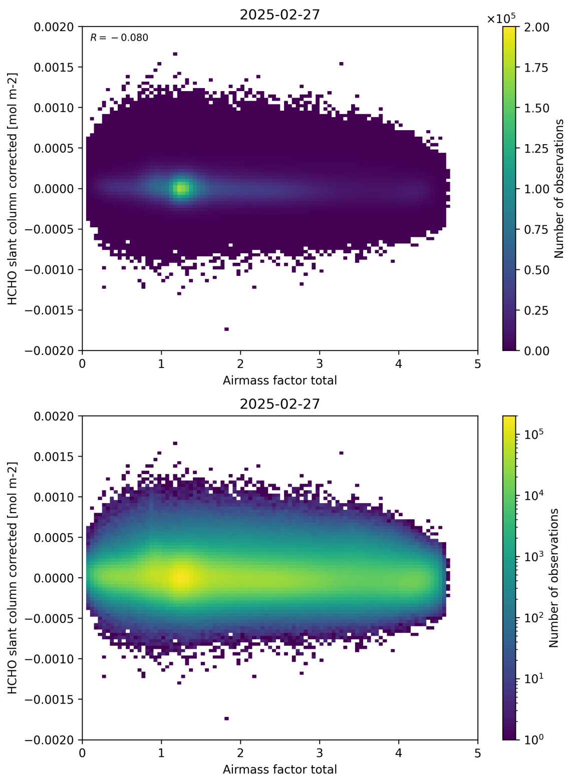
Figure 101: Scatter density plot of “Airmass factor total” against “HCHO slant column corrected” for 2025-02-26 to 2025-02-28.
