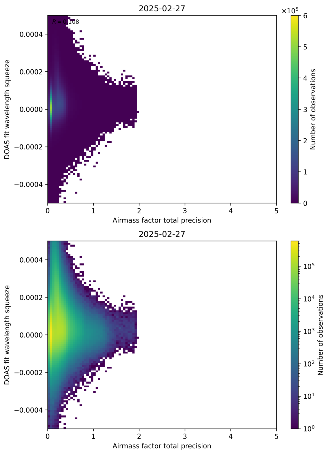
Figure 107: Scatter density plot of “Airmass factor total precision” against “DOAS fit wavelength squeeze” for 2025-02-26 to 2025-02-28.
