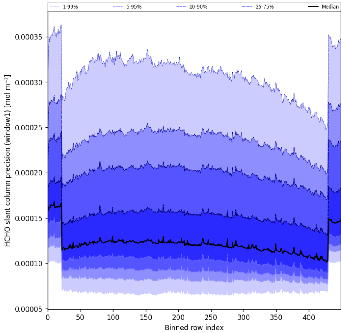
Figure 53: Along track statistics of “HCHO slant column precision (window1)” for 2025-02-26 to 2025-02-28
