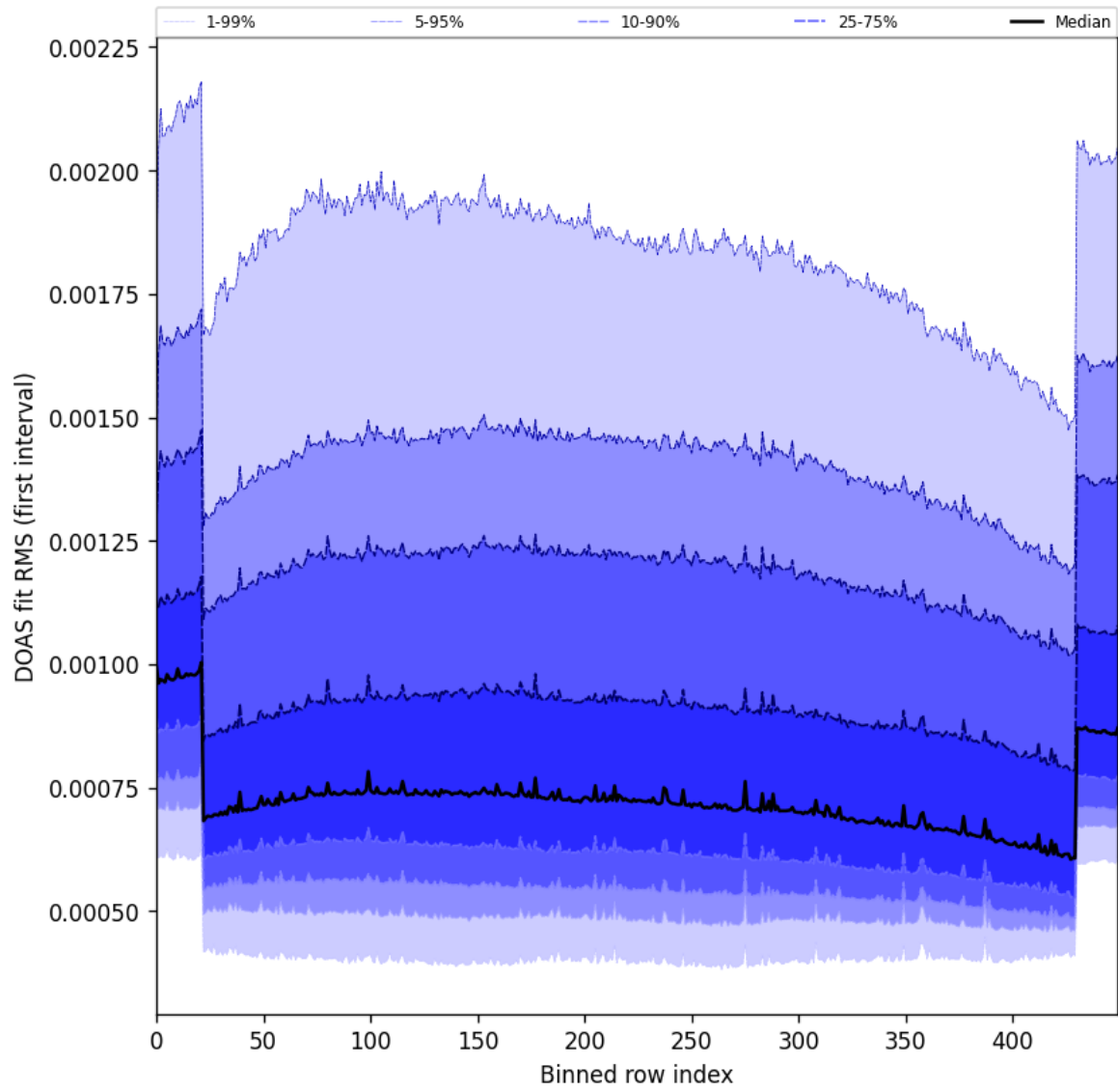
Figure 60: Along track statistics of “DOAS fit RMS (first interval)” for 2025-02-26 to 2025-02-28
