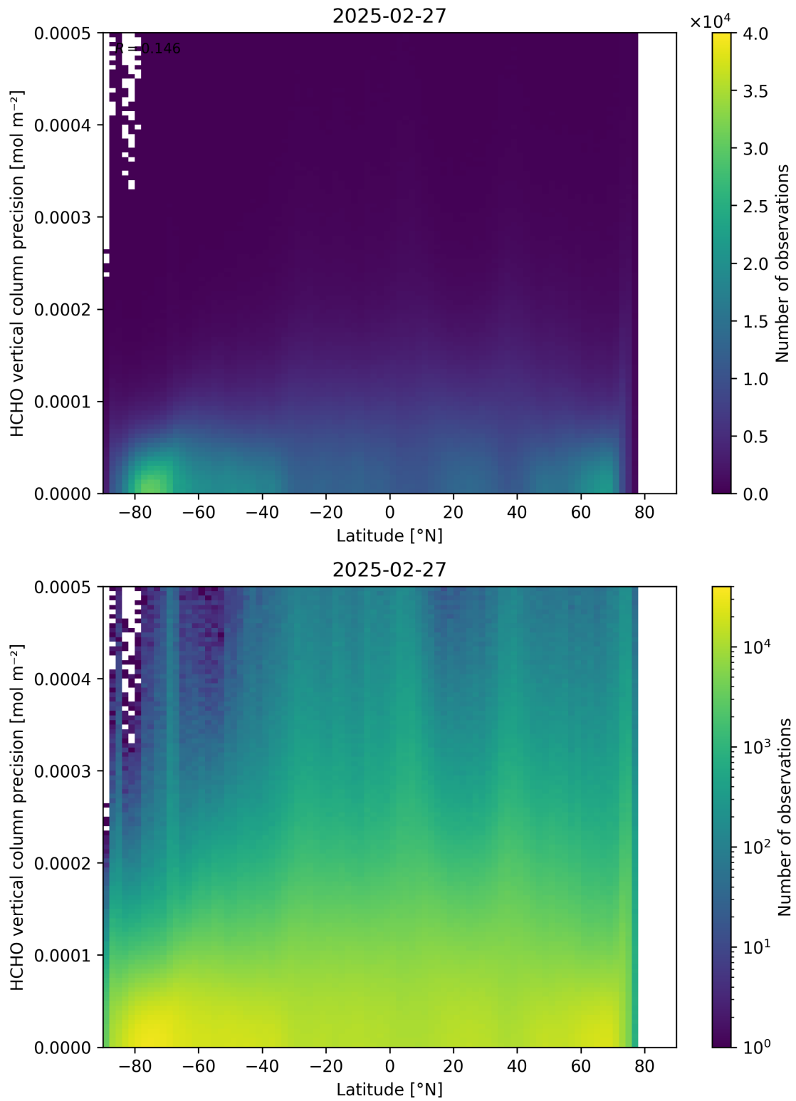
Figure 165: Scatter density plot of “Latitude” against “HCHO vertical column precision” for 2025-02-26 to 2025-02-28.
