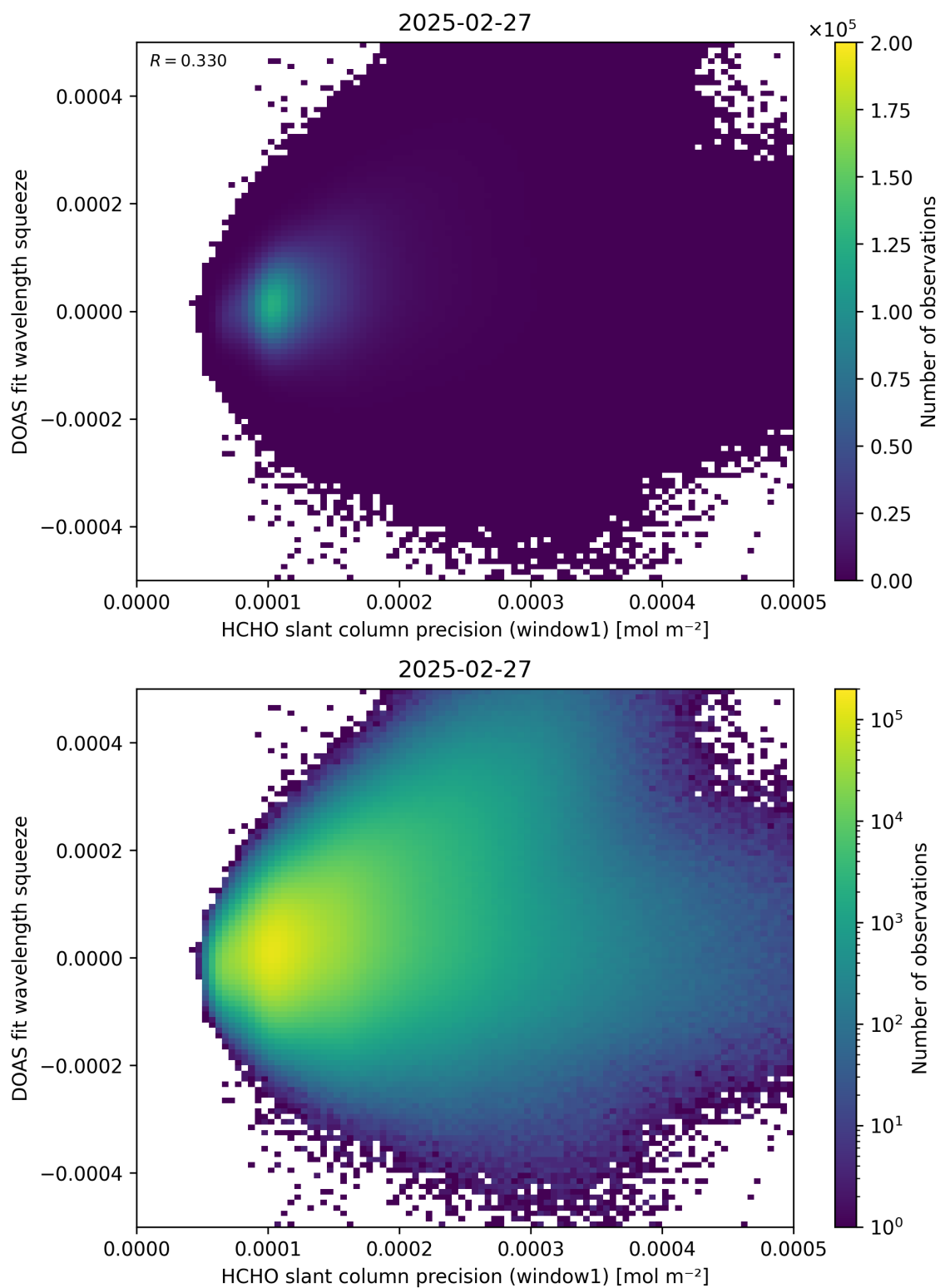
Figure 90: Scatter density plot of “HCHO slant column precision (window1)” against “DOAS fit wavelength squeeze” for 2025-02-26 to 2025-02-28.
