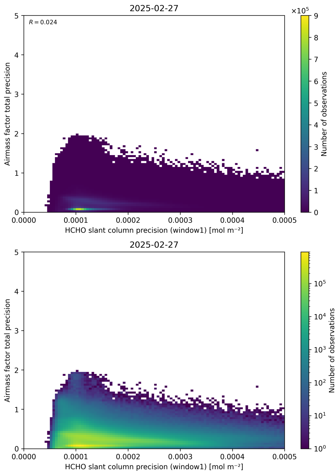
Figure 95: Scatter density plot of “HCHO slant column precision (window1)” against “Airmass factor total precision” for 2025-02-26 to 2025-02-28.
