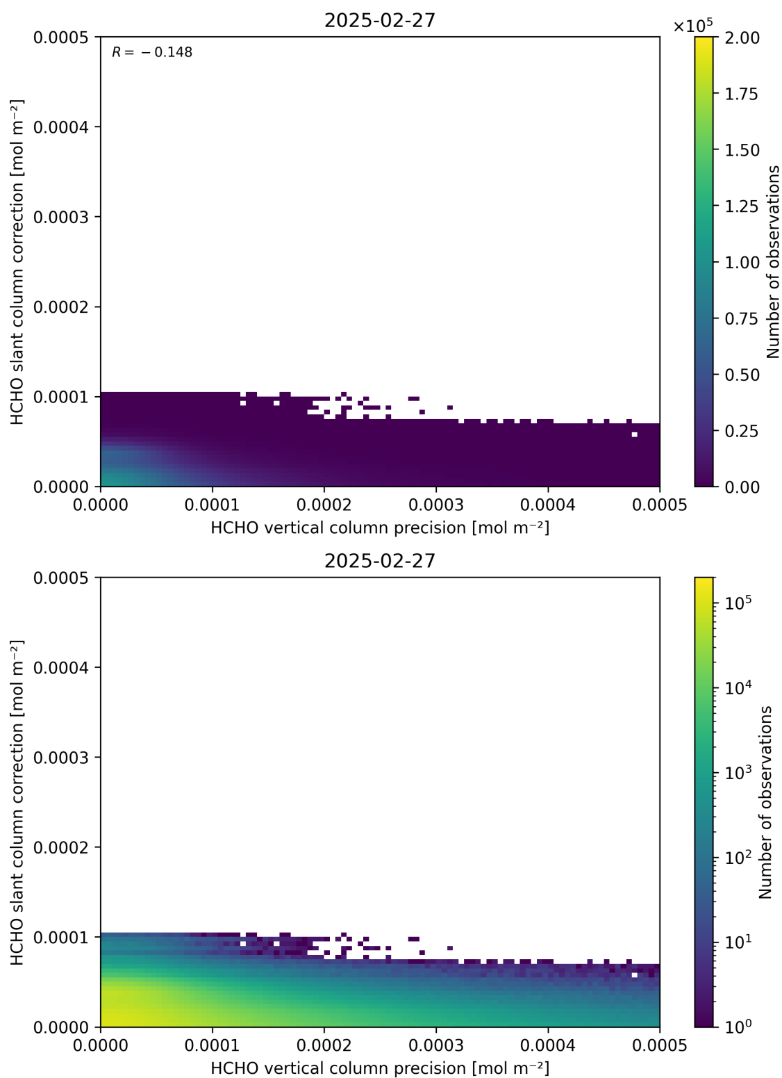
Figure 141: Scatter density plot of “HCHO vertical column precision” against “HCHO slant column correction” for 2025-02-26 to 2025-02-28.
