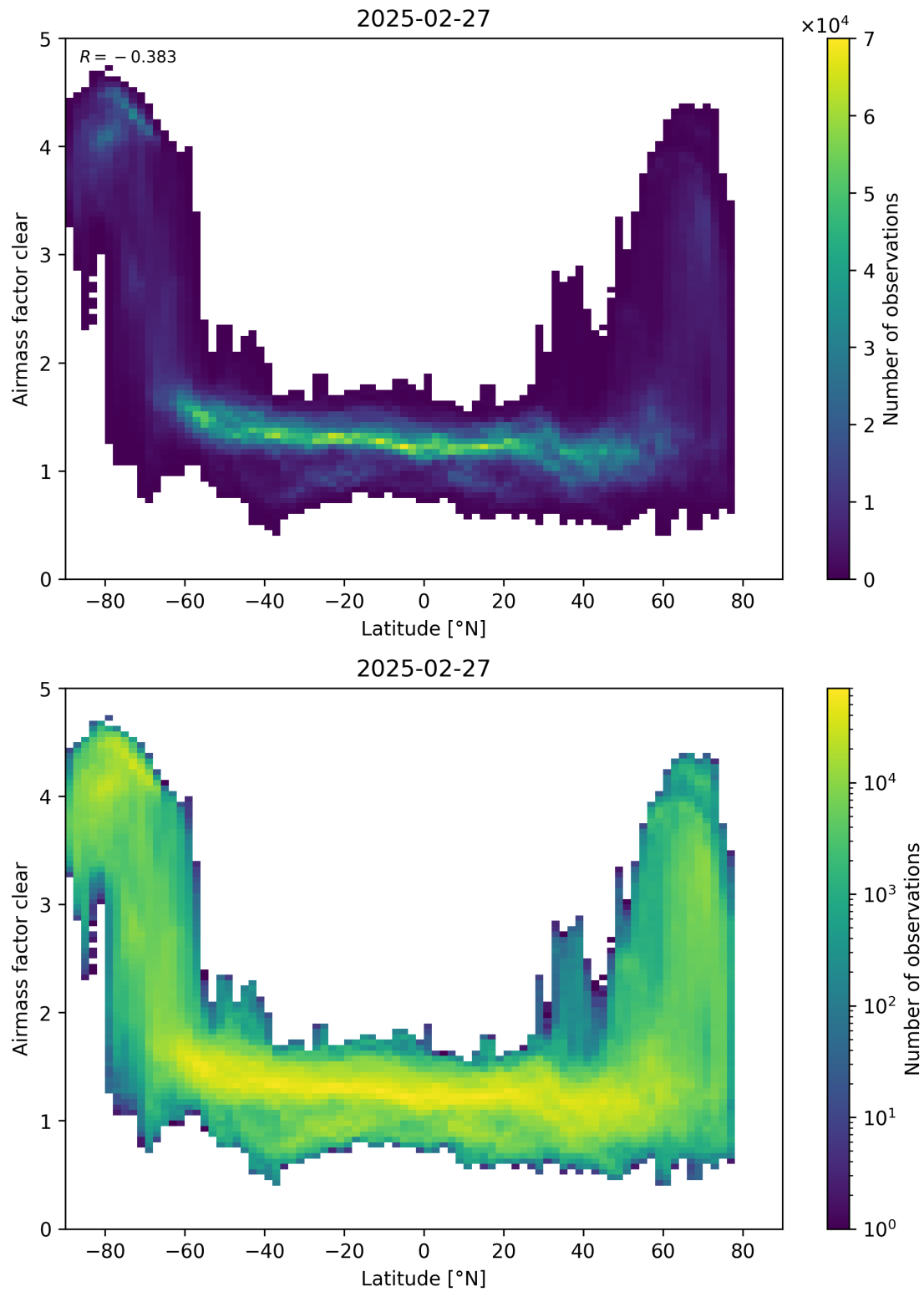
Figure 156: Scatter density plot of “Latitude” against “Airmass factor clear” for 2025-02-26 to 2025-02-28.
