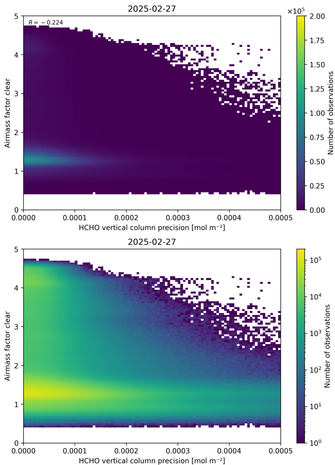
Figure 139: Scatter density plot of “HCHO vertical column precision” against “Airmass factor clear” for 2025-02-26 to 2025-02-28.
