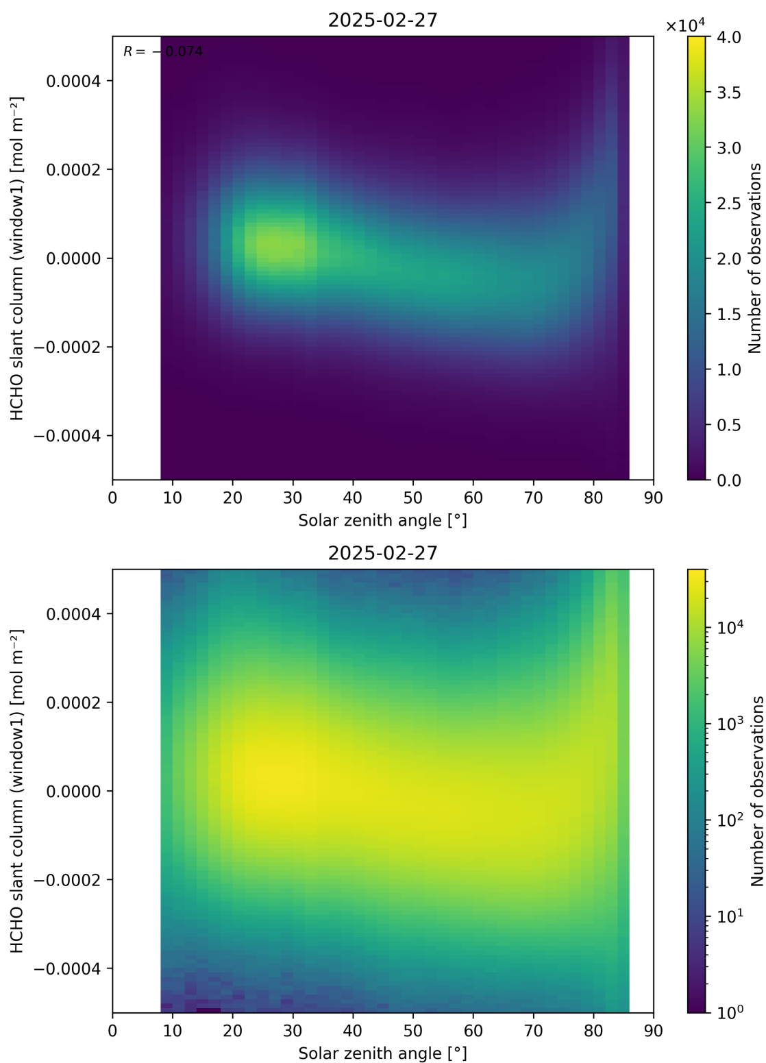
Figure 173: Scatter density plot of “Solar zenith angle” against “HCHO slant column (window1)” for 2025-02-26 to 2025-02-28.
