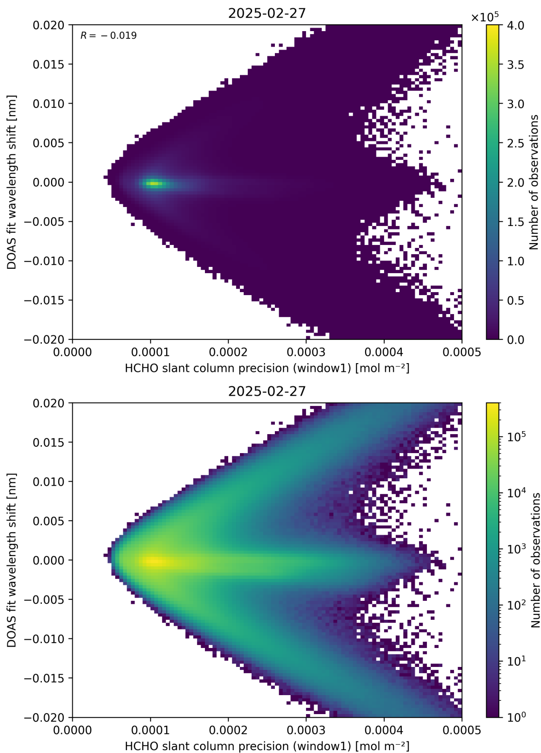
Figure 89: Scatter density plot of “HCHO slant column precision (window1)” against “DOAS fit wavelength shift” for 2025-02-26 to 2025-02-28.
