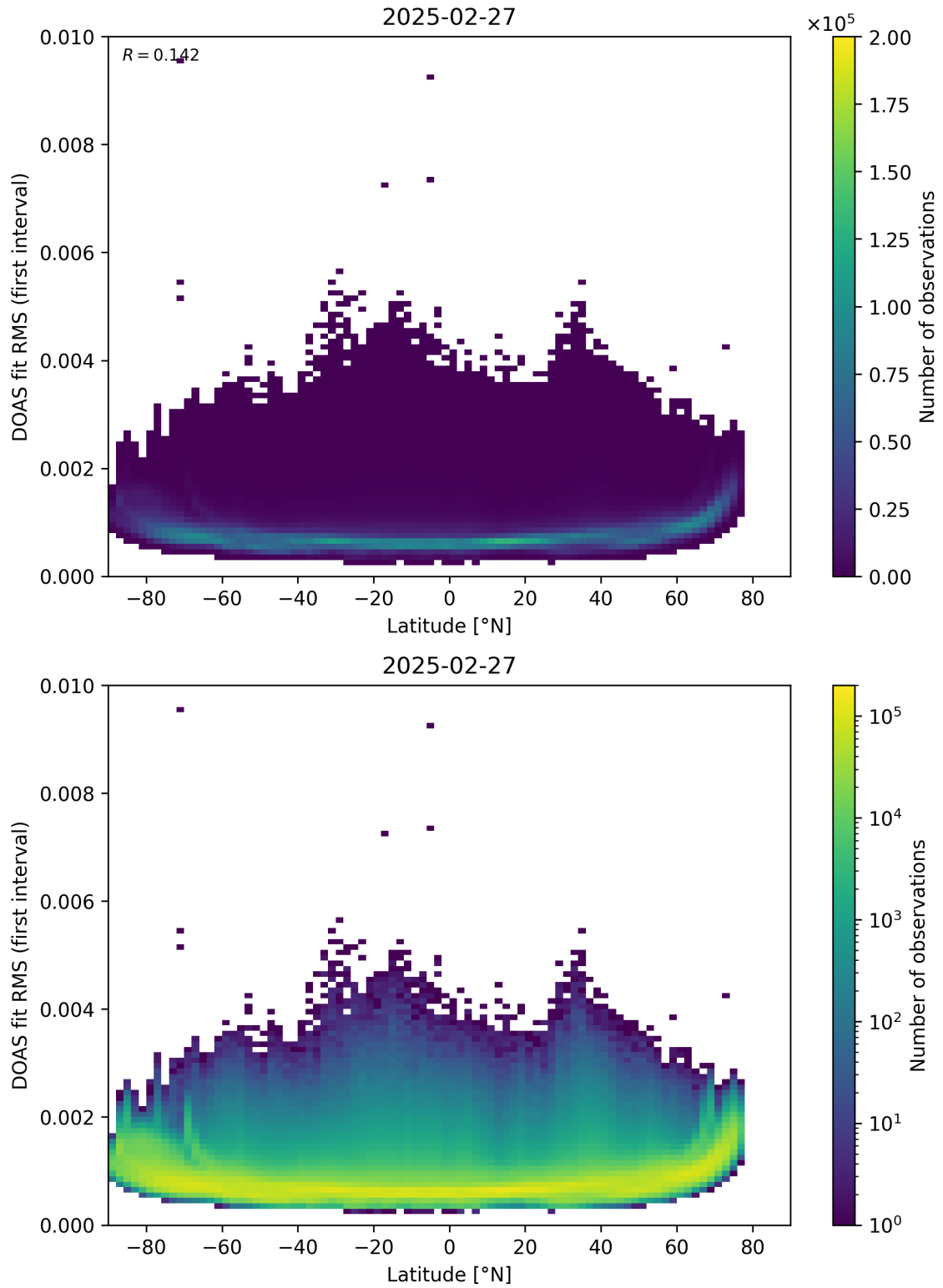
Figure 153: Scatter density plot of “Latitude” against “DOAS fit RMS (first interval)” for 2025-02-26 to 2025-02-28.
