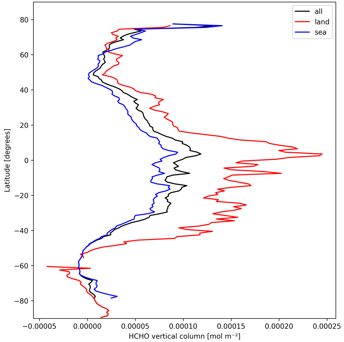
Figure 21: Zonal average of “HCHO vertical column” for 2025-02-26 to 2025-02-28.
