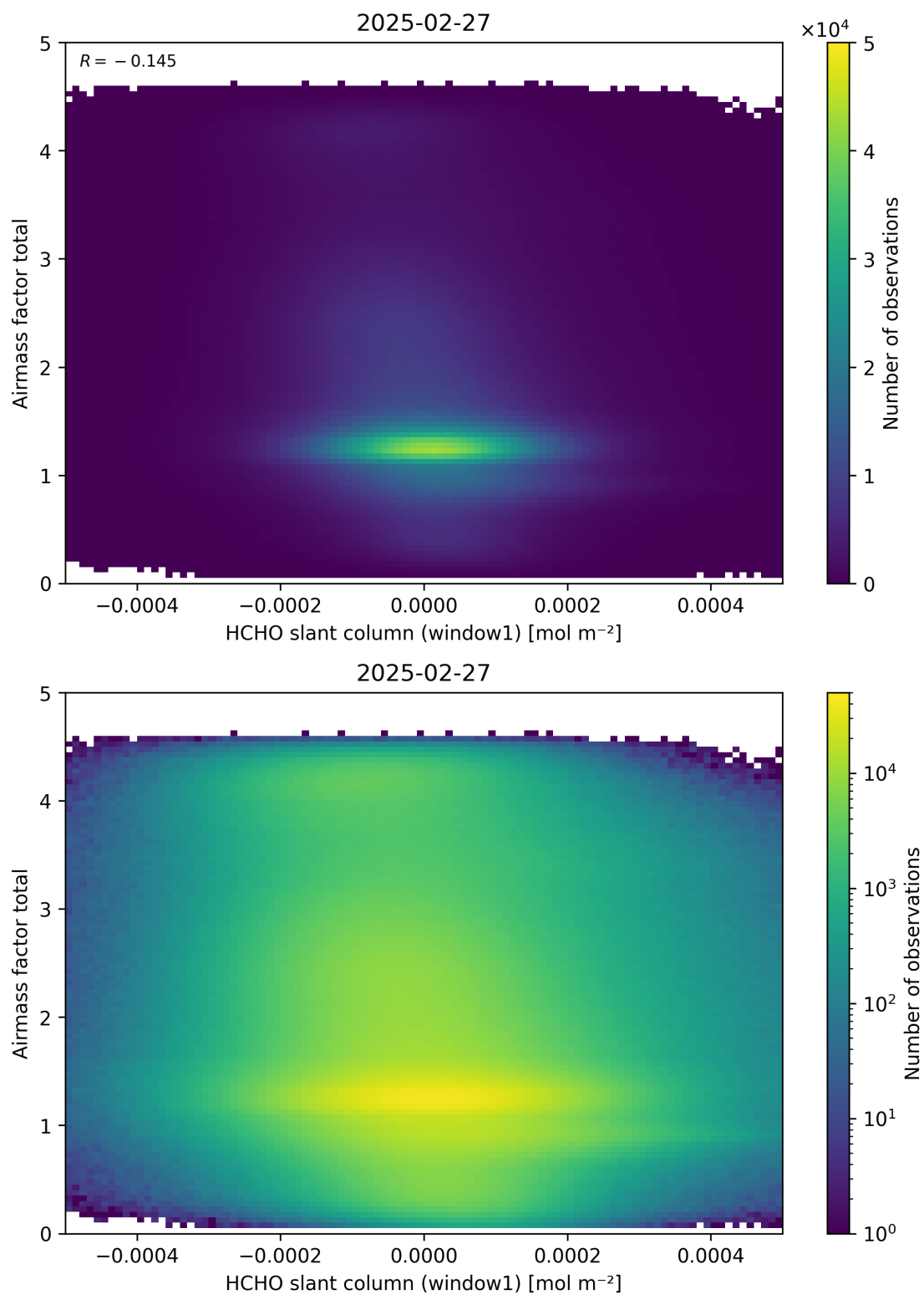
Figure 85: Scatter density plot of “HCHO slant column (window1)” against “Airmass factor total” for 2025-02-26 to 2025-02-28.
