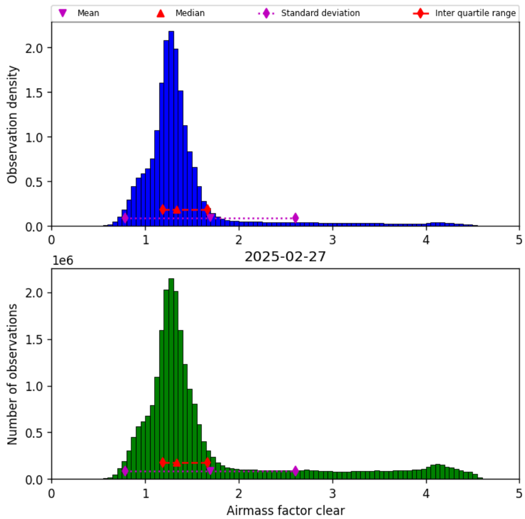
Figure 42: Histogram of “Airmass factor clear” for 2025-02-26 to 2025-02-28
