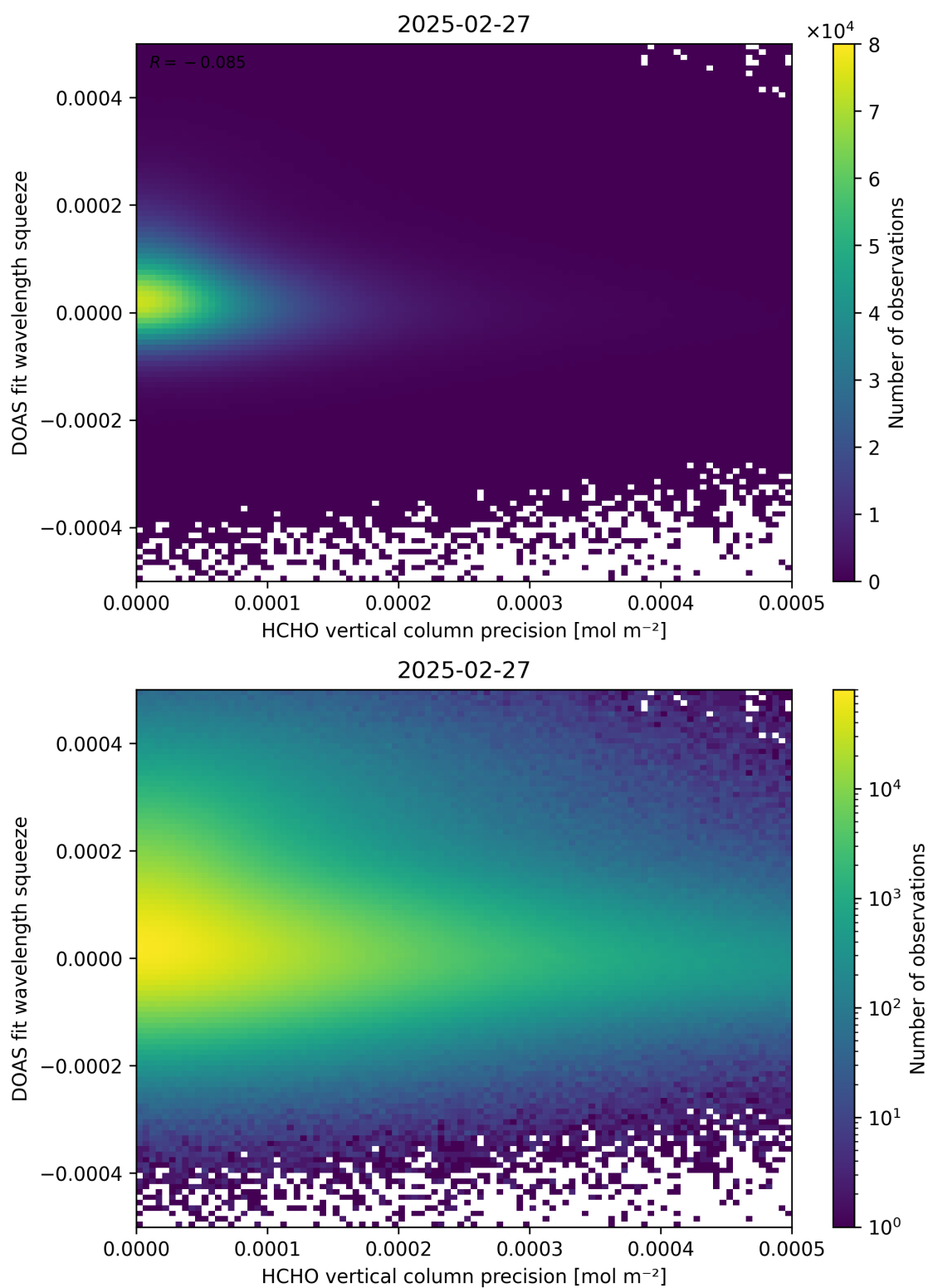
Figure 138: Scatter density plot of “HCHO vertical column precision” against “DOAS fit wavelength squeeze” for 2025-02-26 to 2025-02-28.
