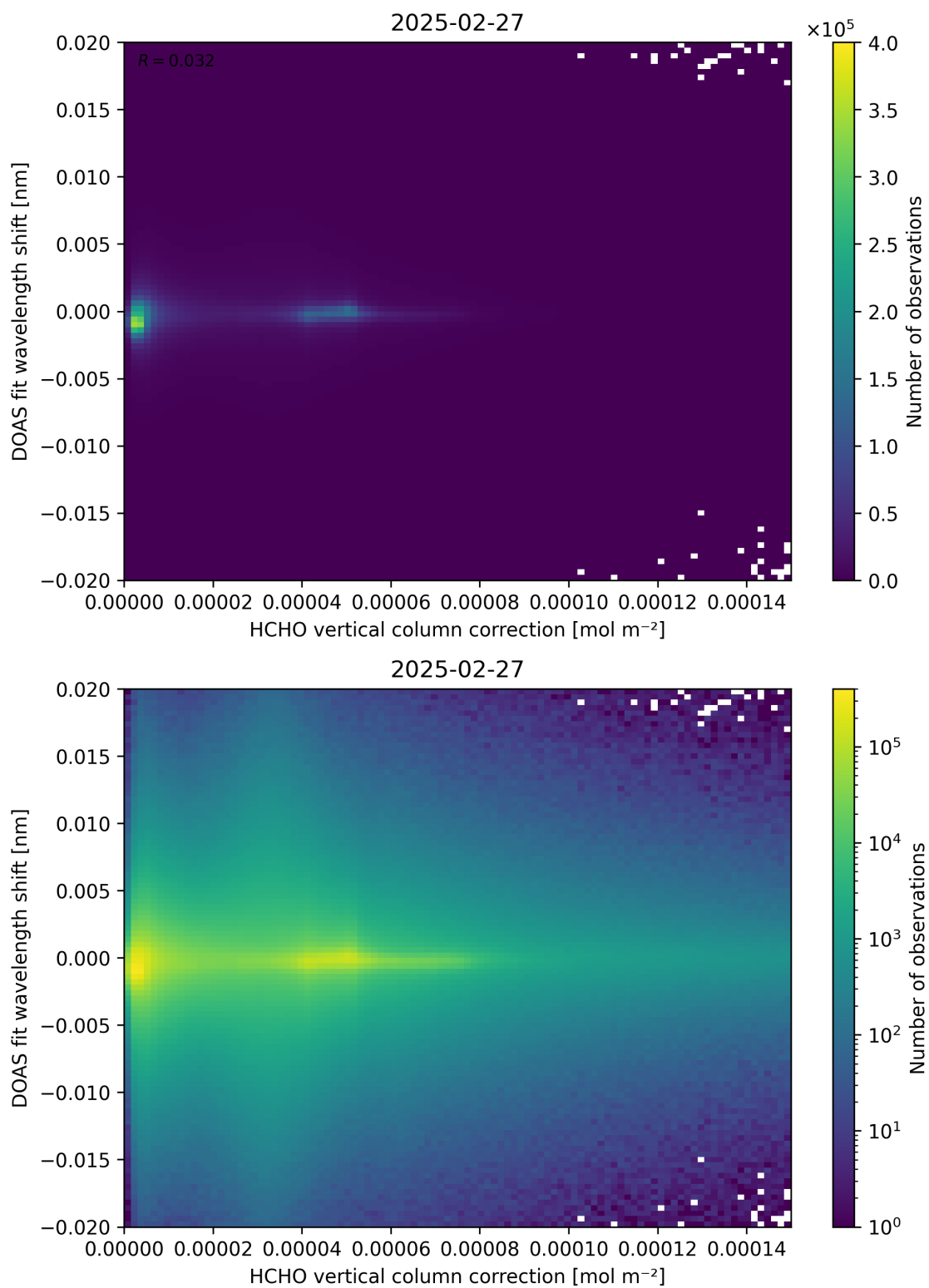
Figure 113: Scatter density plot of “HCHO vertical column correction” against “DOAS fit wavelength shift” for 2025-02-26 to 2025-02-28.
