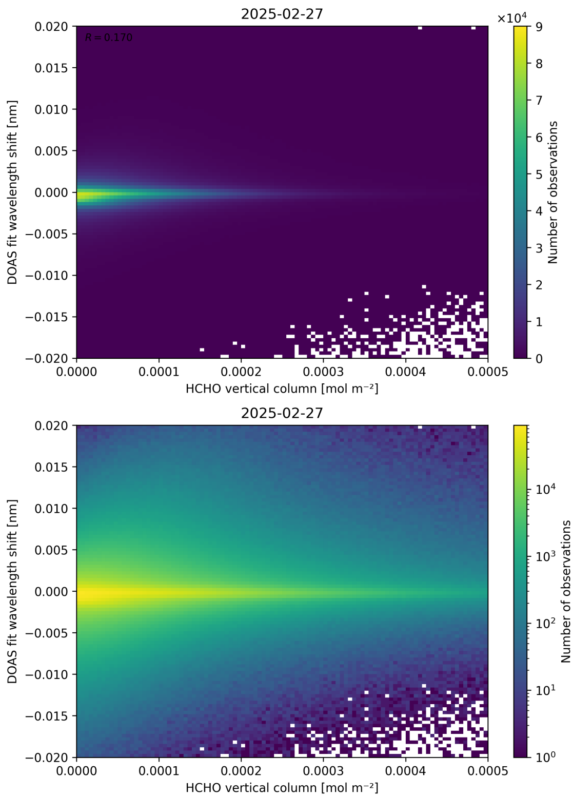
Figure 124: Scatter density plot of “HCHO vertical column” against “DOAS fit wavelength shift” for 2025-02-26 to 2025-02-28.
