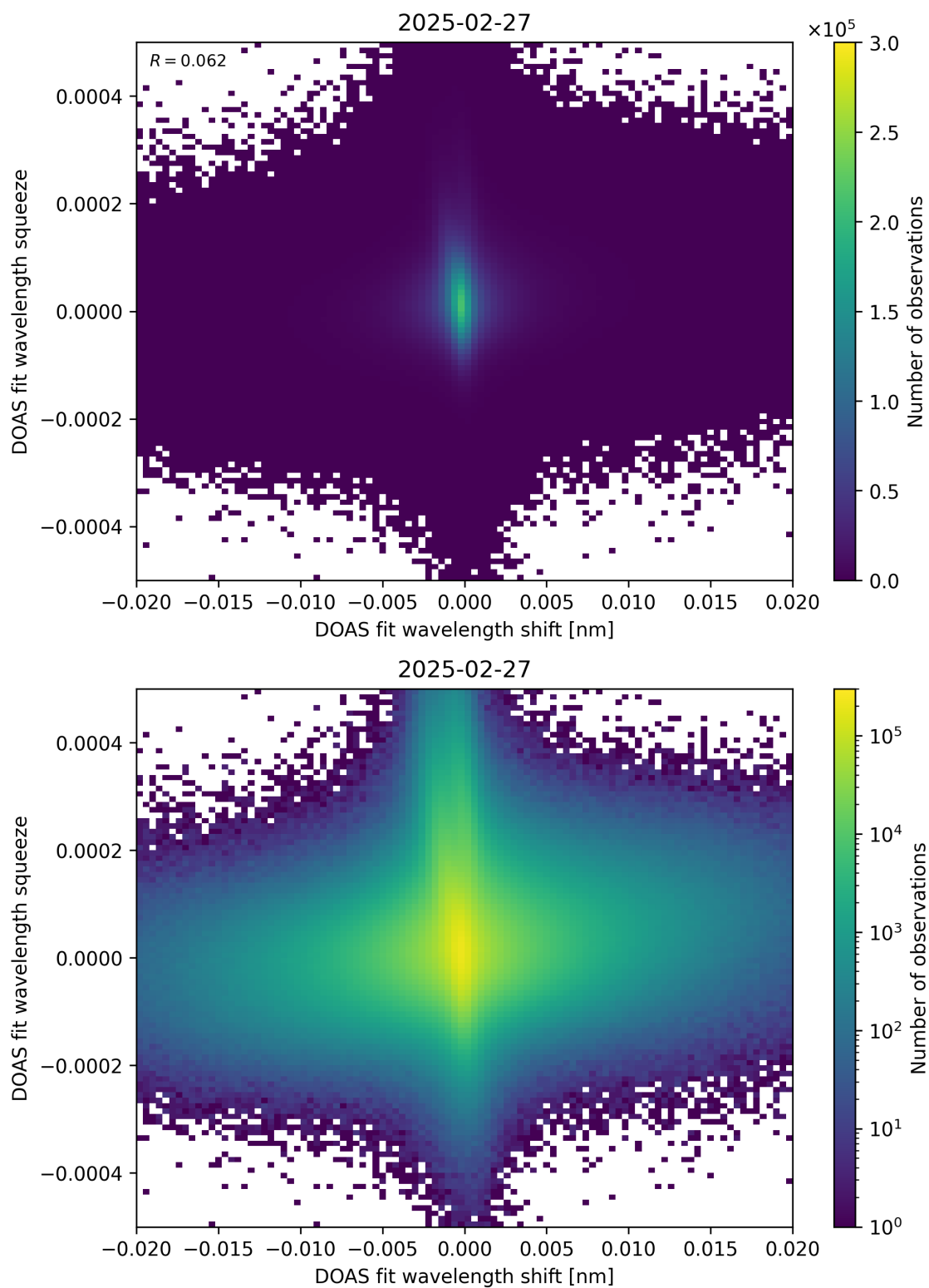
Figure 65: Scatter density plot of “DOAS fit wavelength shift” against “DOAS fit wavelength squeeze” for 2025-02-26 to 2025-02-28.
