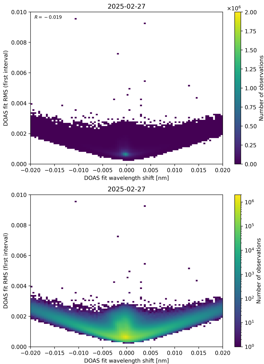
Figure 64: Scatter density plot of “DOAS fit wavelength shift” against “DOAS fit RMS (first interval)” for 2025-02-26 to 2025-02-28.
