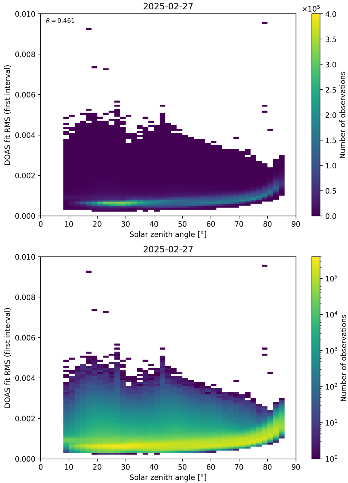
Figure 167: Scatter density plot of “Solar zenith angle” against “DOAS fit RMS (first interval)” for 2025-02-26 to 2025-02-28.
