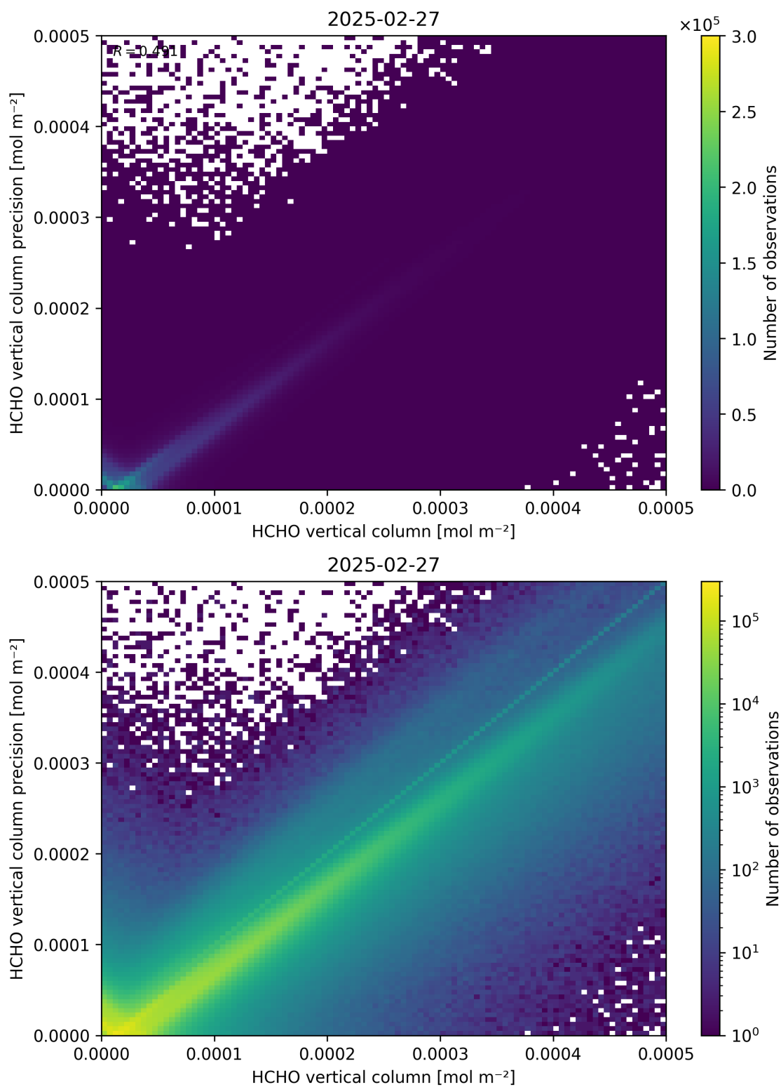
Figure 134: Scatter density plot of “HCHO vertical column” against “HCHO vertical column precision” for 2025-02-26 to 2025-02-28.
