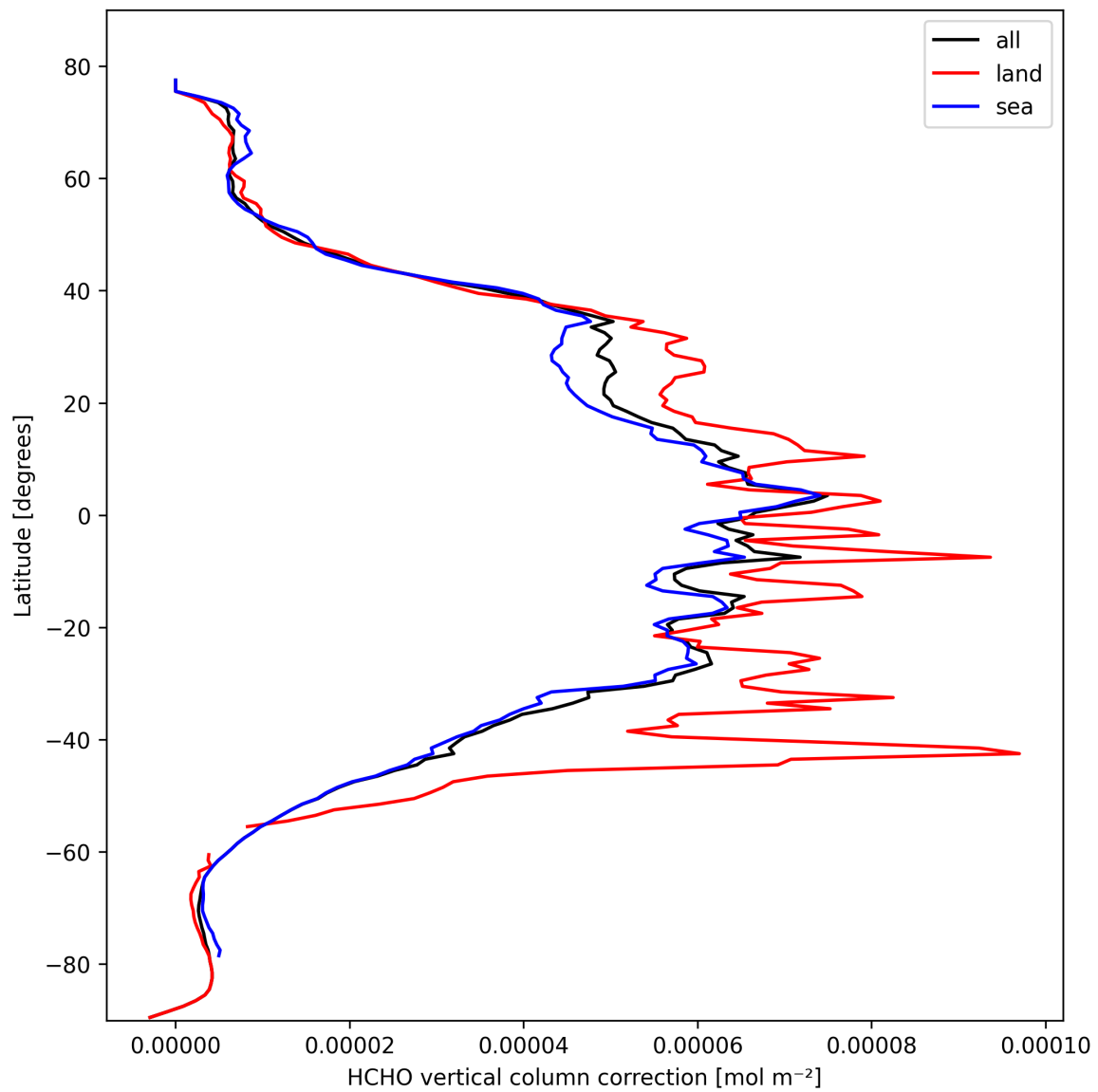
Figure 23: Zonal average of “HCHO vertical column correction” for 2025-02-26 to 2025-02-28.
