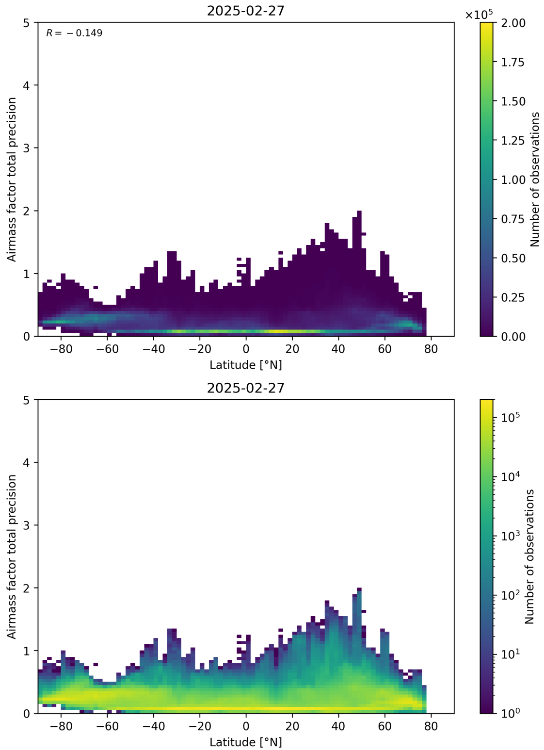
Figure 162: Scatter density plot of “Latitude” against “Airmass factor total precision” for 2025-02-26 to 2025-02-28.
