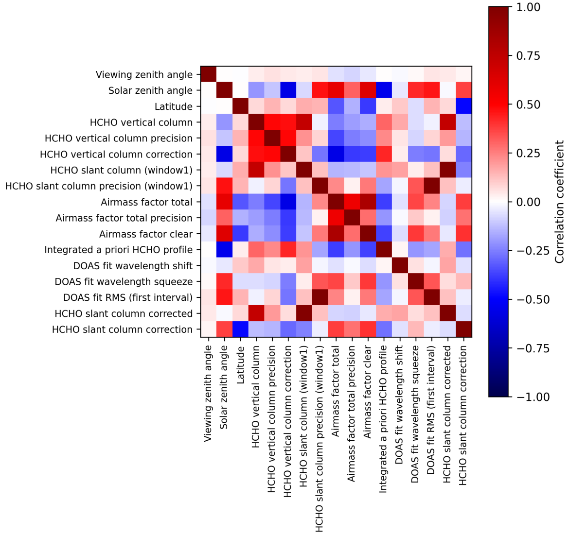
Figure 2: Map of correlation matrix for 2025-02-26 to 2025-02-28.
