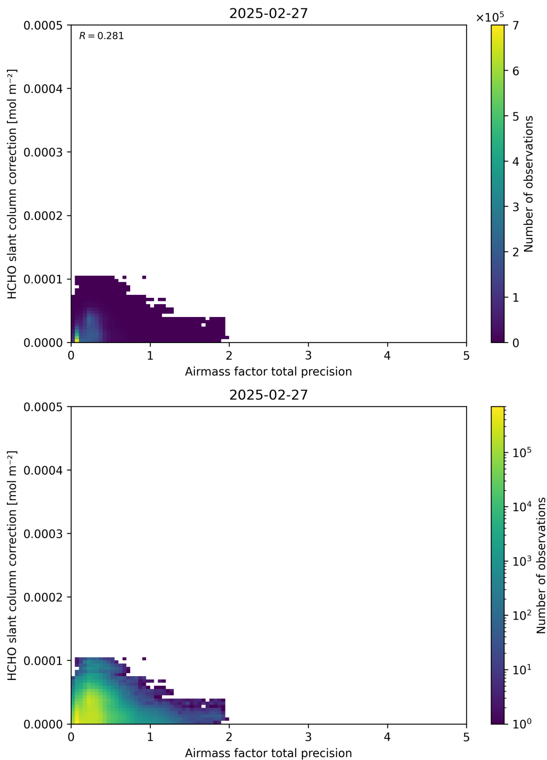
Figure 110: Scatter density plot of “Airmass factor total precision” against “HCHO slant column correction” for 2025-02-26 to 2025-02-28.
