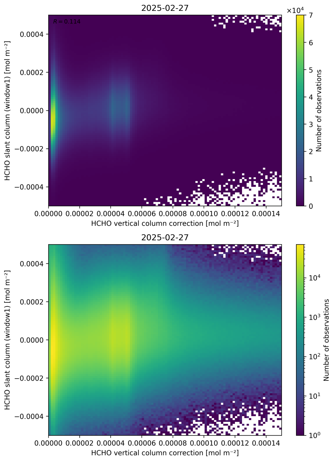
Figure 118: Scatter density plot of “HCHO vertical column correction” against “HCHO slant column (window1)” for 2025-02-26 to 2025-02-28.
