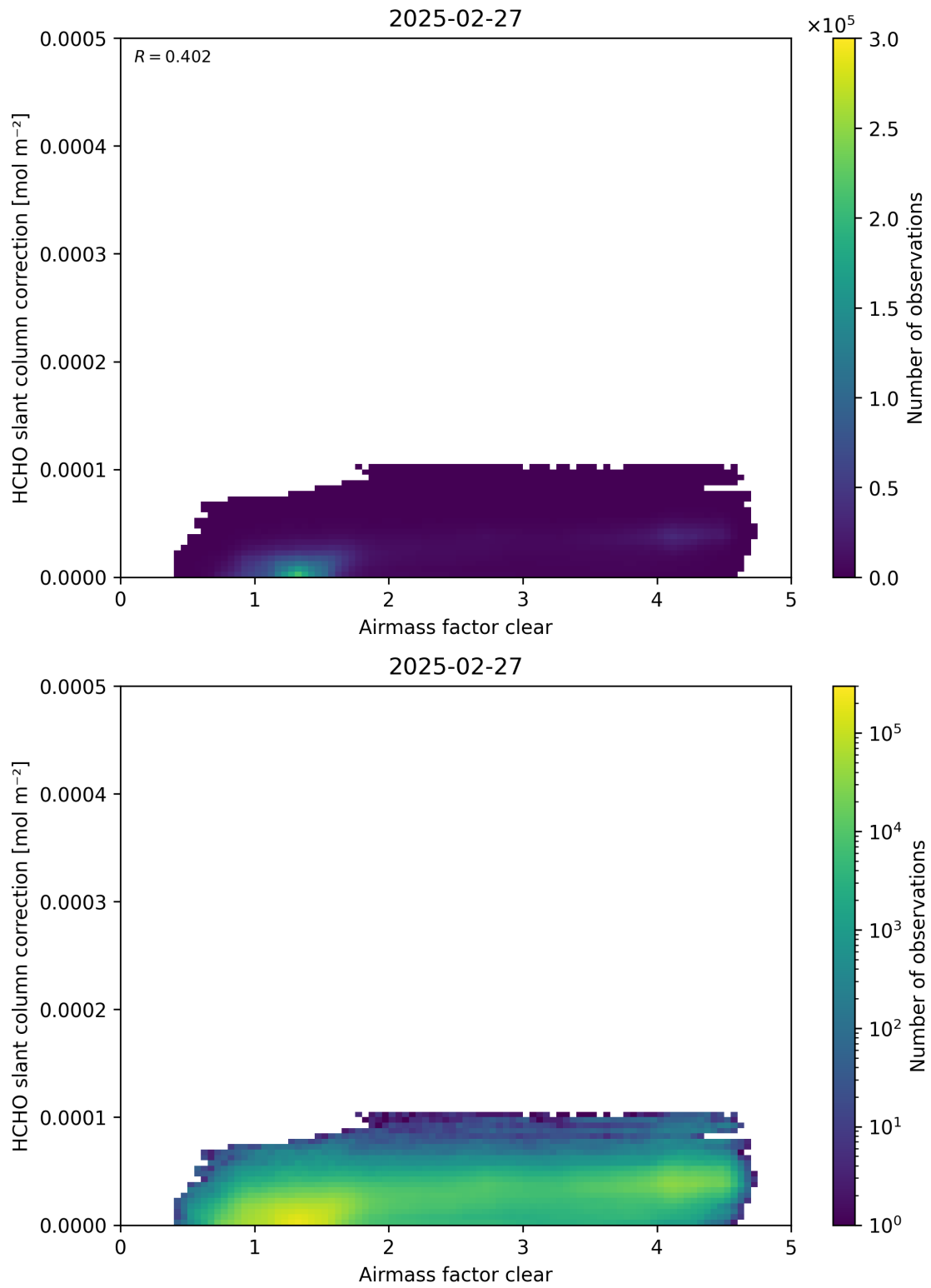
Figure 75: Scatter density plot of “Airmass factor clear” against “HCHO slant column correction” for 2025-02-26 to 2025-02-28.
