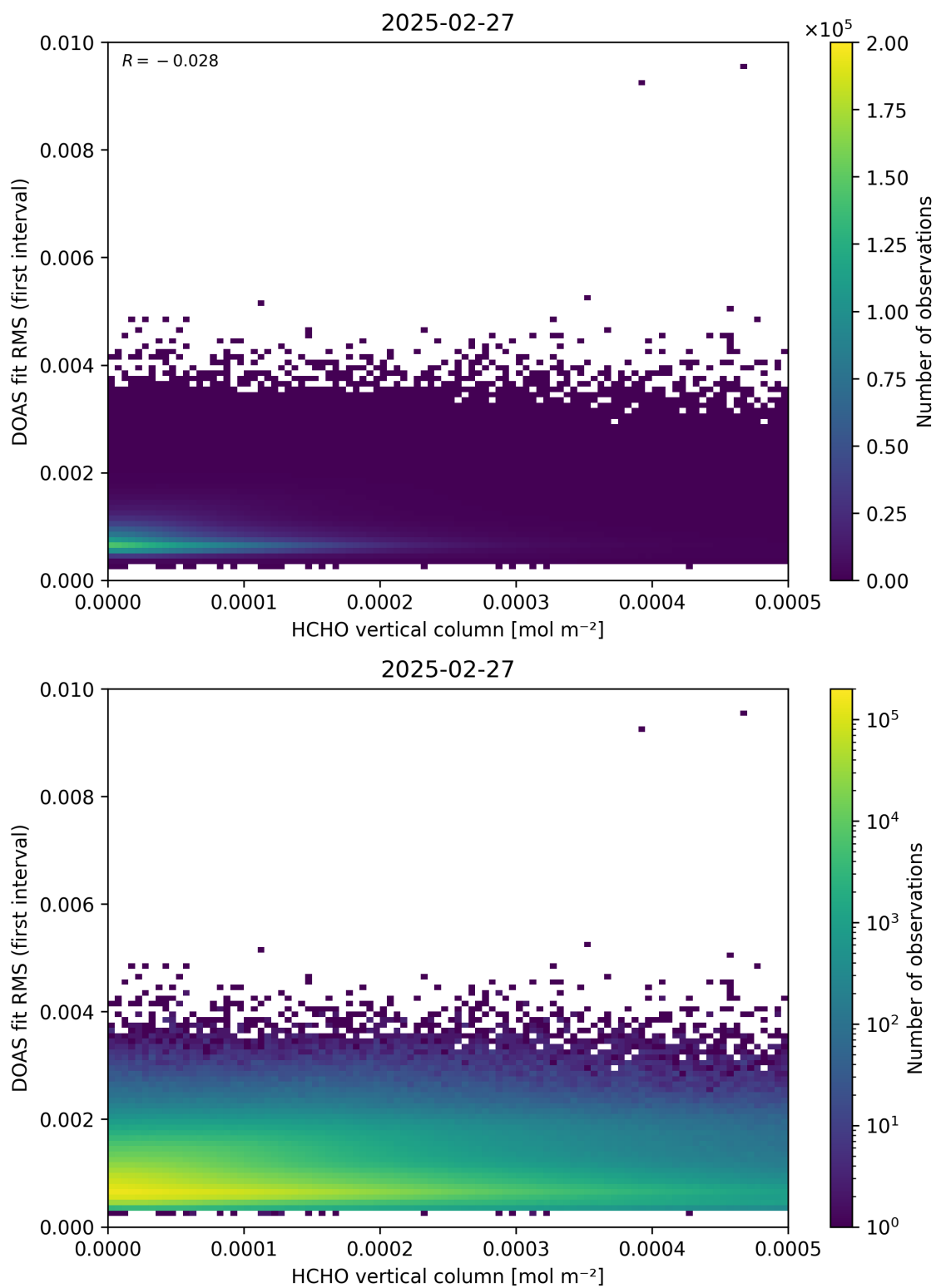
Figure 123: Scatter density plot of “HCHO vertical column” against “DOAS fit RMS (first interval)” for 2025-02-26 to 2025-02-28.
