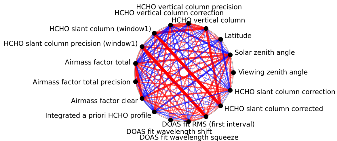
Figure 1: Map of correlation graph for 2025-02-26 to 2025-02-28.
