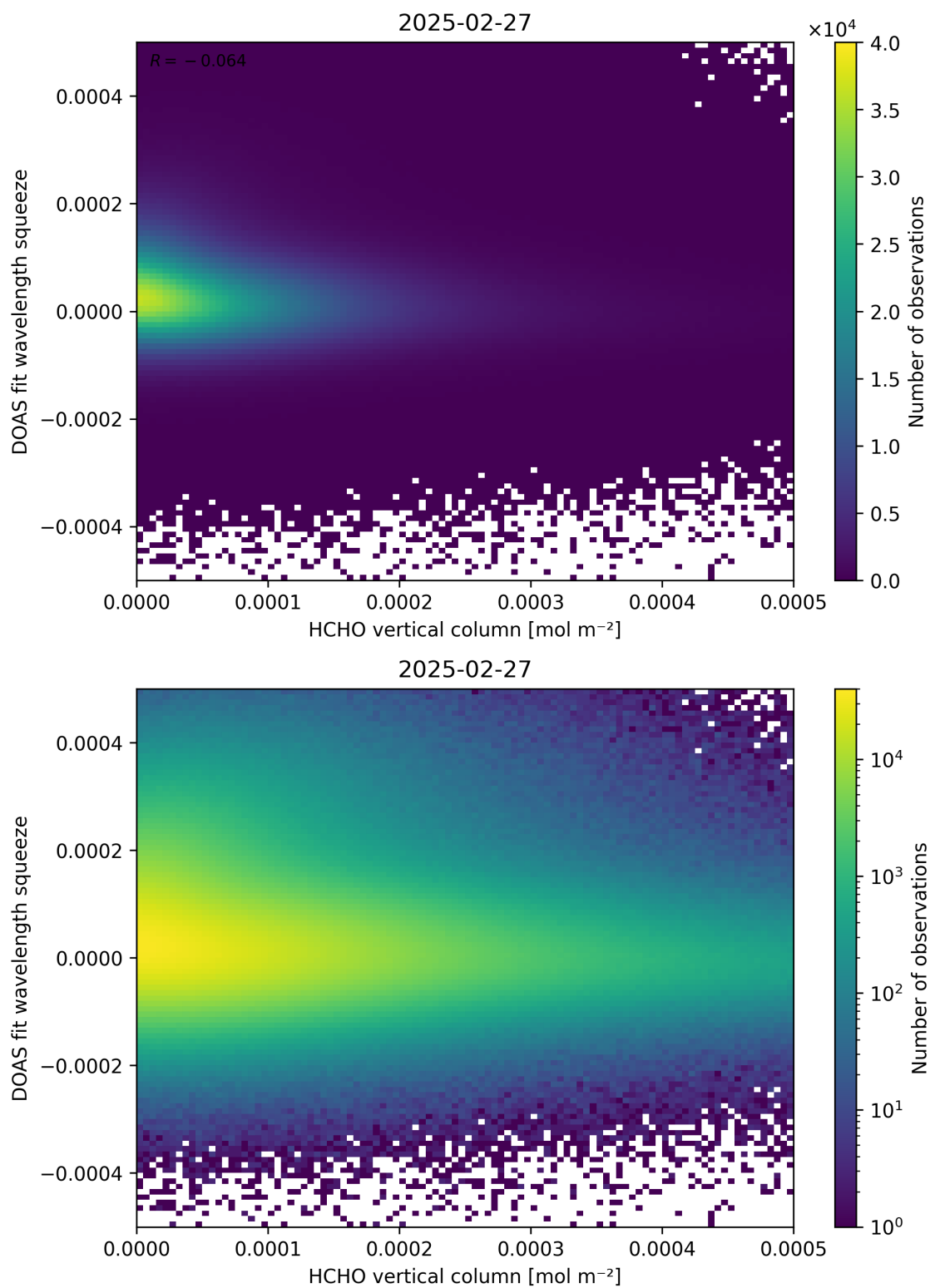
Figure 125: Scatter density plot of “HCHO vertical column” against “DOAS fit wavelength squeeze” for 2025-02-26 to 2025-02-28.
