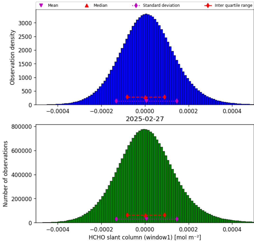
Figure 38: Histogram of “HCHO slant column (window1)” for 2025-02-26 to 2025-02-28
