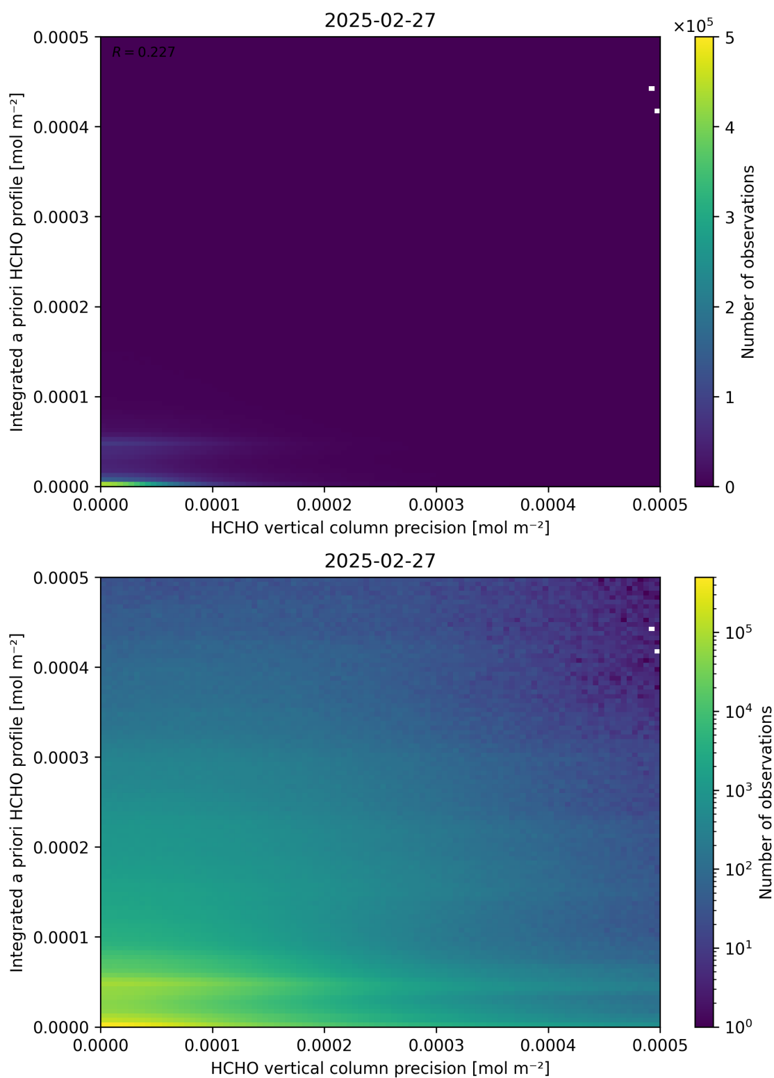
Figure 147: Scatter density plot of “HCHO vertical column precision” against “Integrated a priori HCHO profile” for 2025-02-26 to 2025-02-28.
