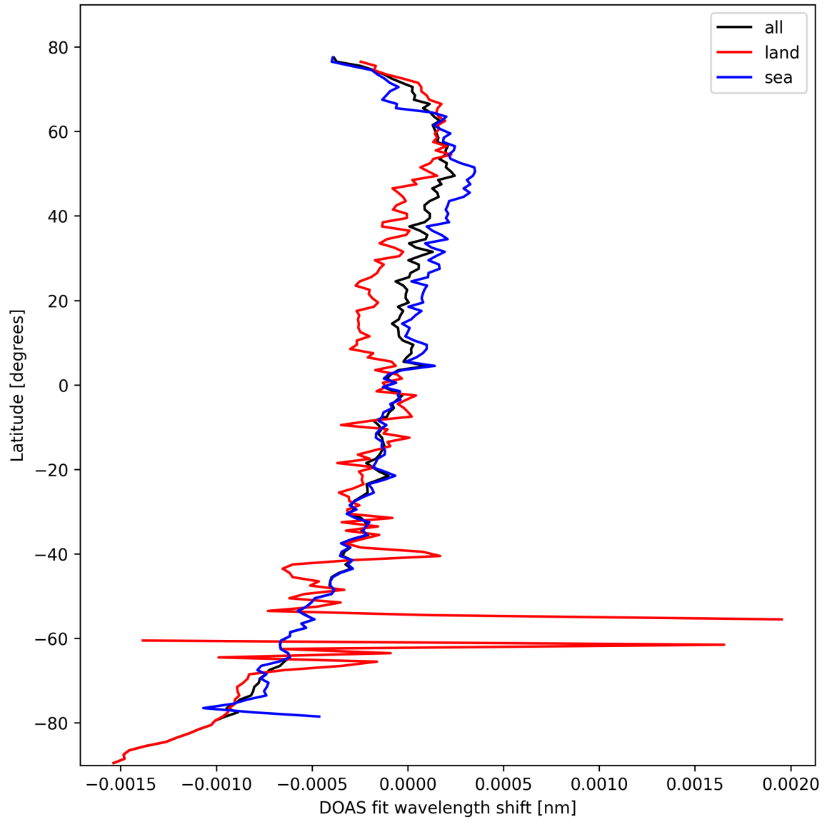
Figure 30: Zonal average of "DOAS fit wavelength shift" for 2025-02-26 to 2025-02-28.
