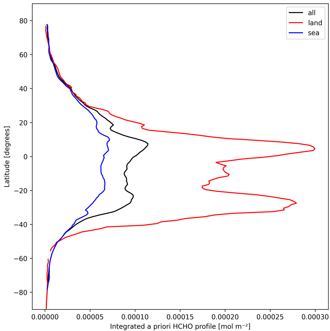
Figure 29: Zonal average of “Integrated a priori HCHO profile” for 2025-02-26 to 2025-02-28.
