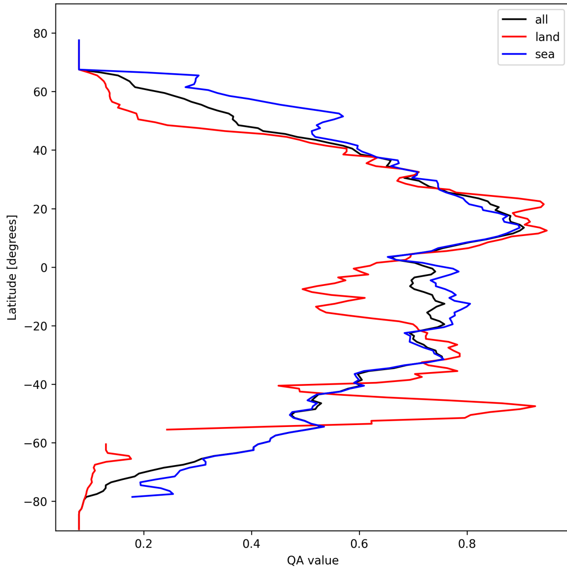
Figure 20: Zonal average of “QA value” for 2025-02-26 to 2025-02-28.
