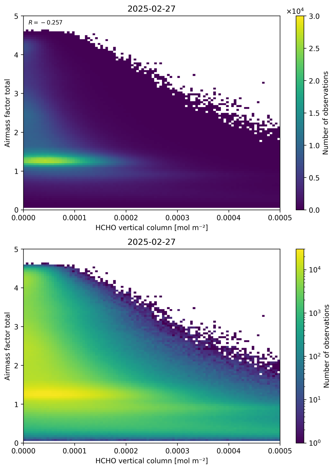
Figure 131: Scatter density plot of “HCHO vertical column” against “Airmass factor total” for 2025-02-26 to 2025-02-28.
