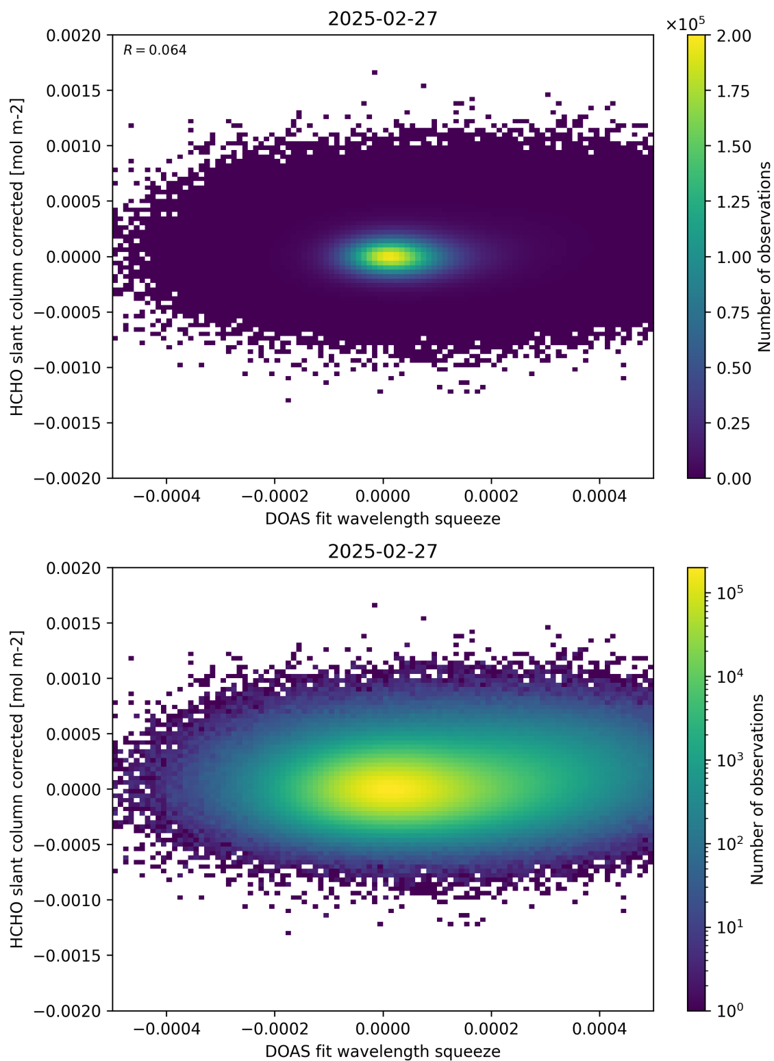
Figure 69: Scatter density plot of “DOAS fit wavelength squeeze” against “HCHO slant column corrected” for 2025-02-26 to 2025-02-28.
