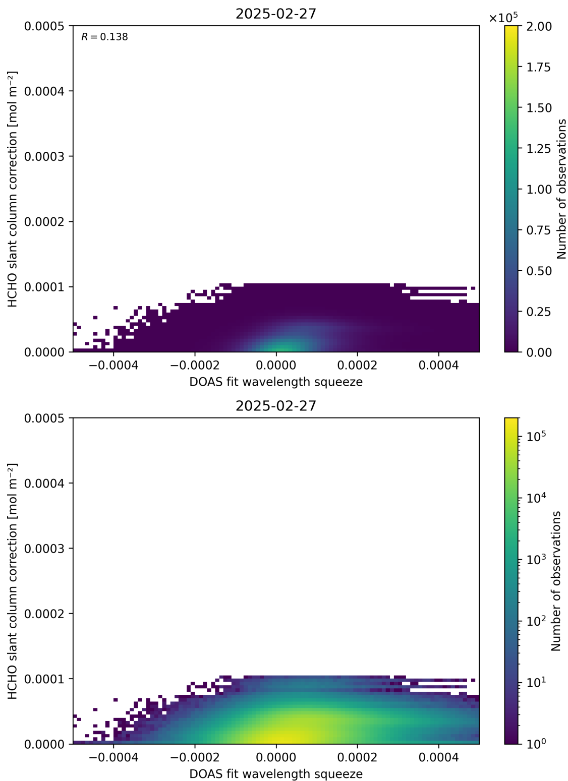
Figure 70: Scatter density plot of “DOAS fit wavelength squeeze” against “HCHO slant column correction” for 2025-02-26 to 2025-02-28.
