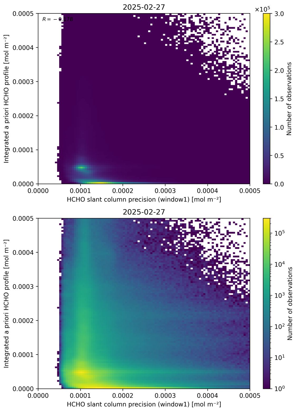
Figure 96: Scatter density plot of “HCHO slant column precision (window1)” against “Integrated a priori HCHO profile” for 2025-02-26 to 2025-02-28.
