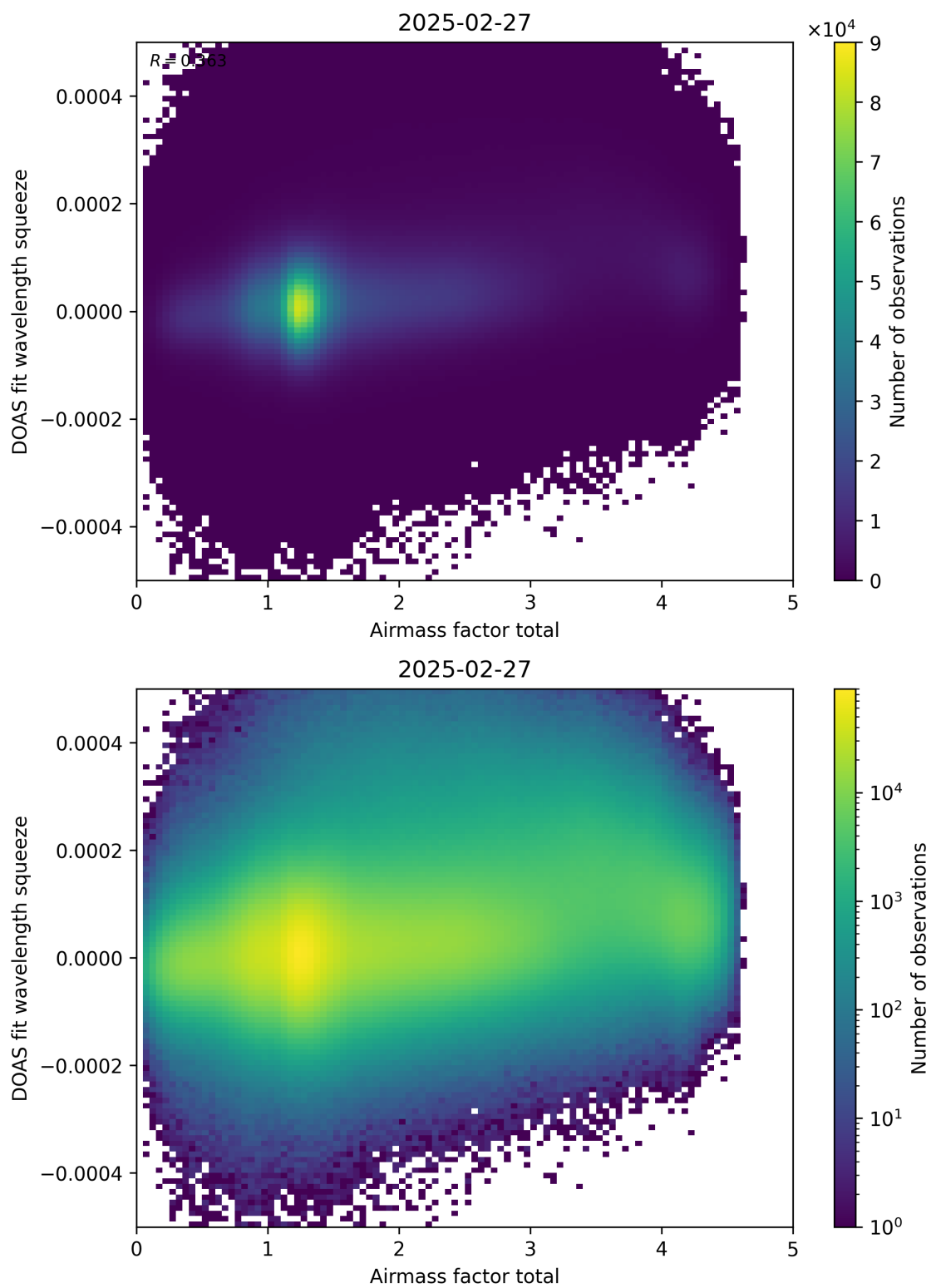
Figure 99: Scatter density plot of “Airmass factor total” against “DOAS fit wavelength squeeze” for 2025-02-26 to 2025-02-28.
