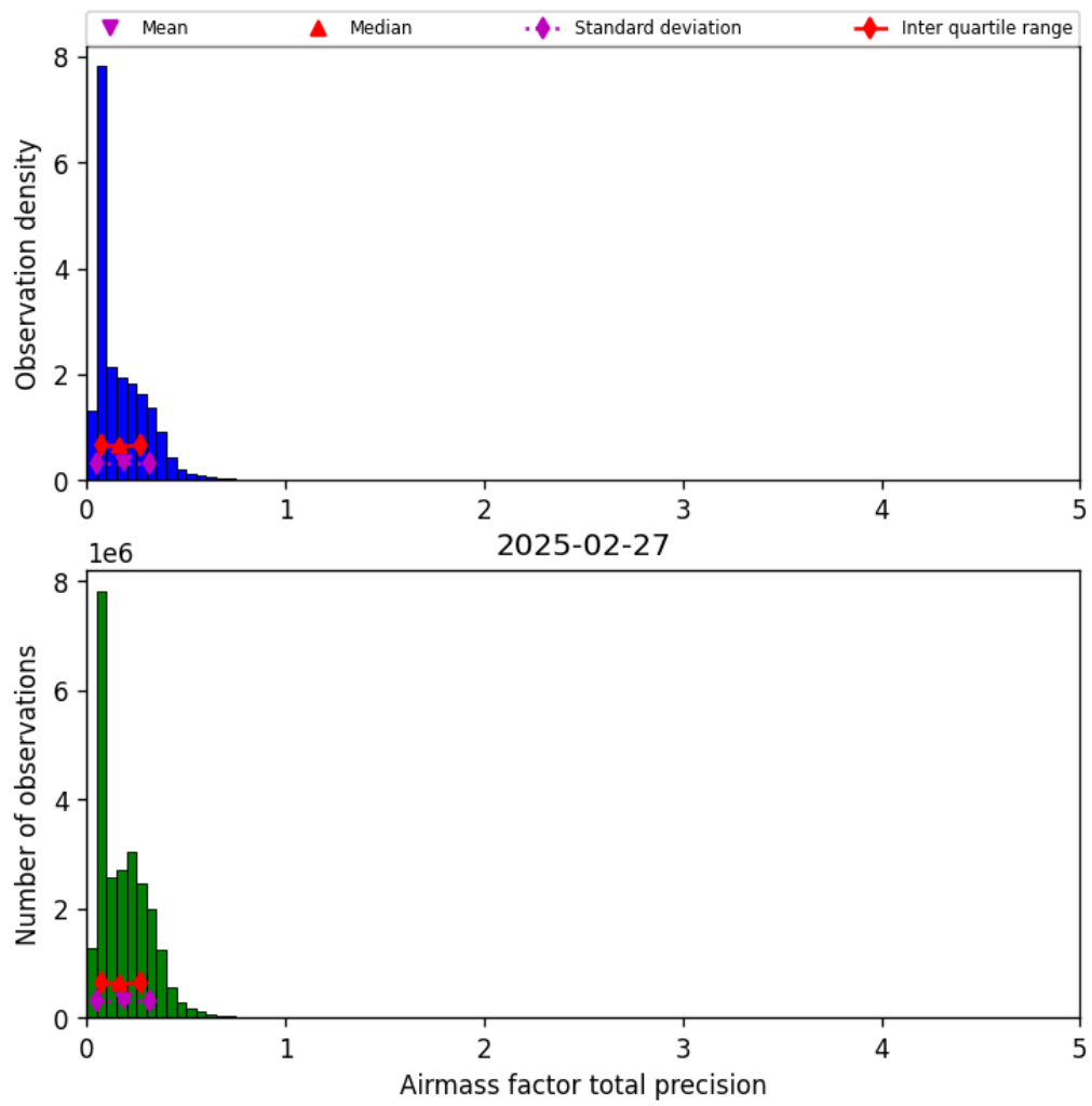
Figure 41: Histogram of “Airmass factor total precision” for 2025-02-26 to 2025-02-28
