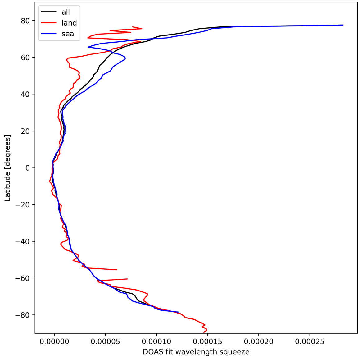
Figure 31: Zonal average of “DOAS fit wavelength squeeze” for 2025-02-26 to 2025-02-28.
