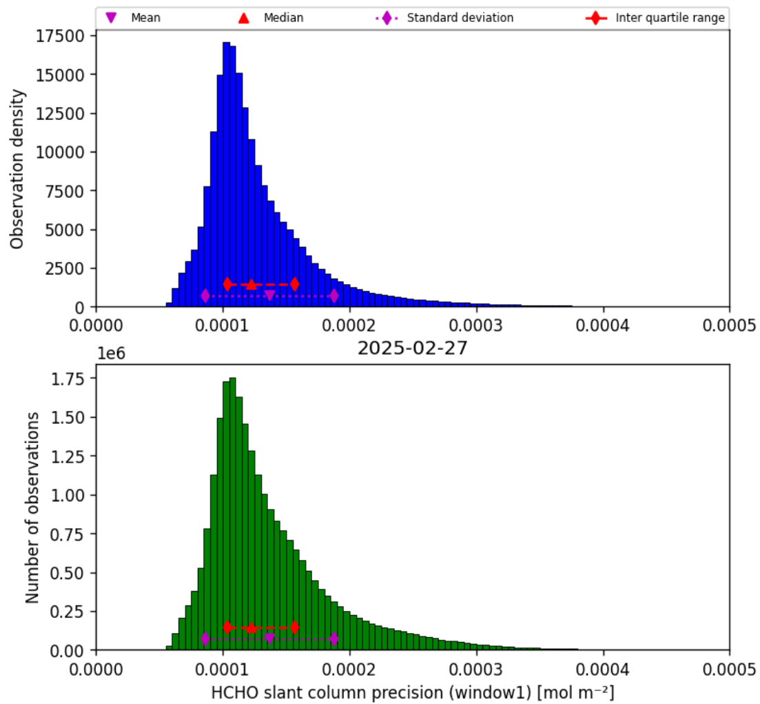
Figure 39: Histogram of “HCHO slant column precision (window1)” for 2025-02-26 to 2025-02-28
