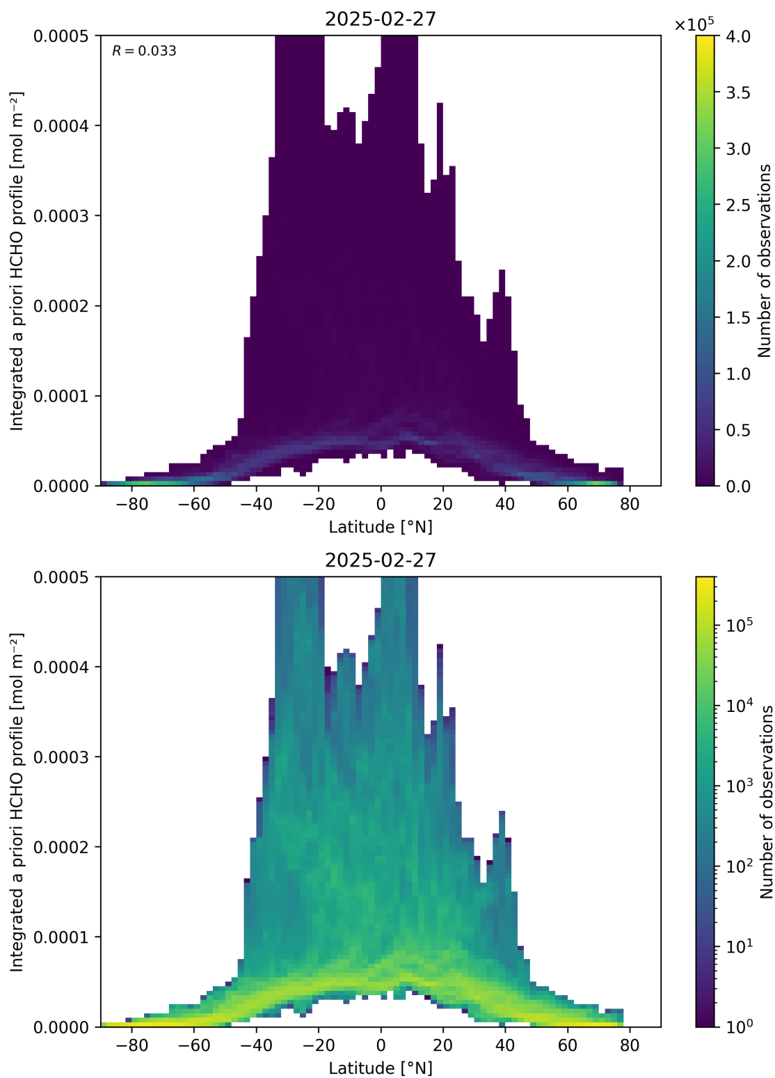
Figure 166: Scatter density plot of “Latitude” against “Integrated a priori HCHO profile” for 2025-02-26 to 2025-02-28.
