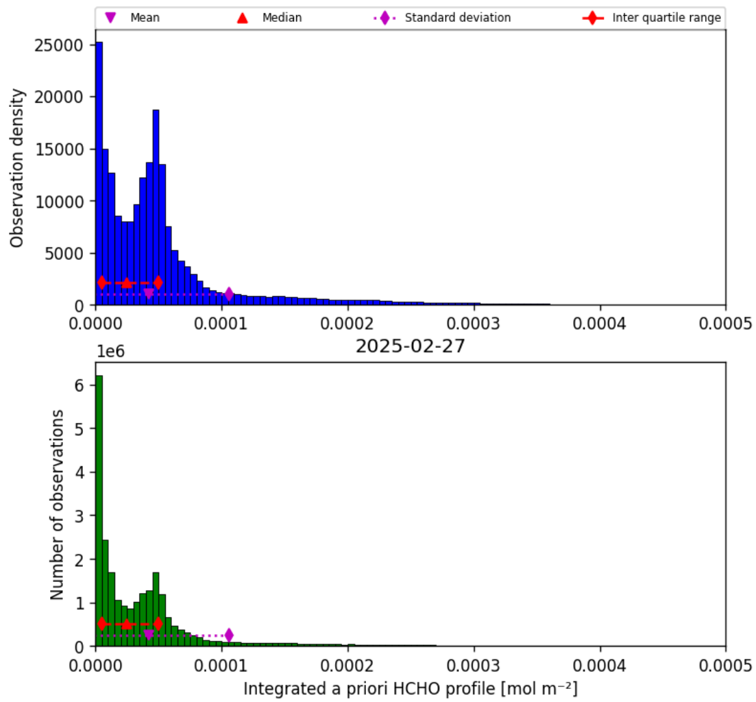
Figure 43: Histogram of “Integrated a priori HCHO profile” for 2025-02-26 to 2025-02-28
