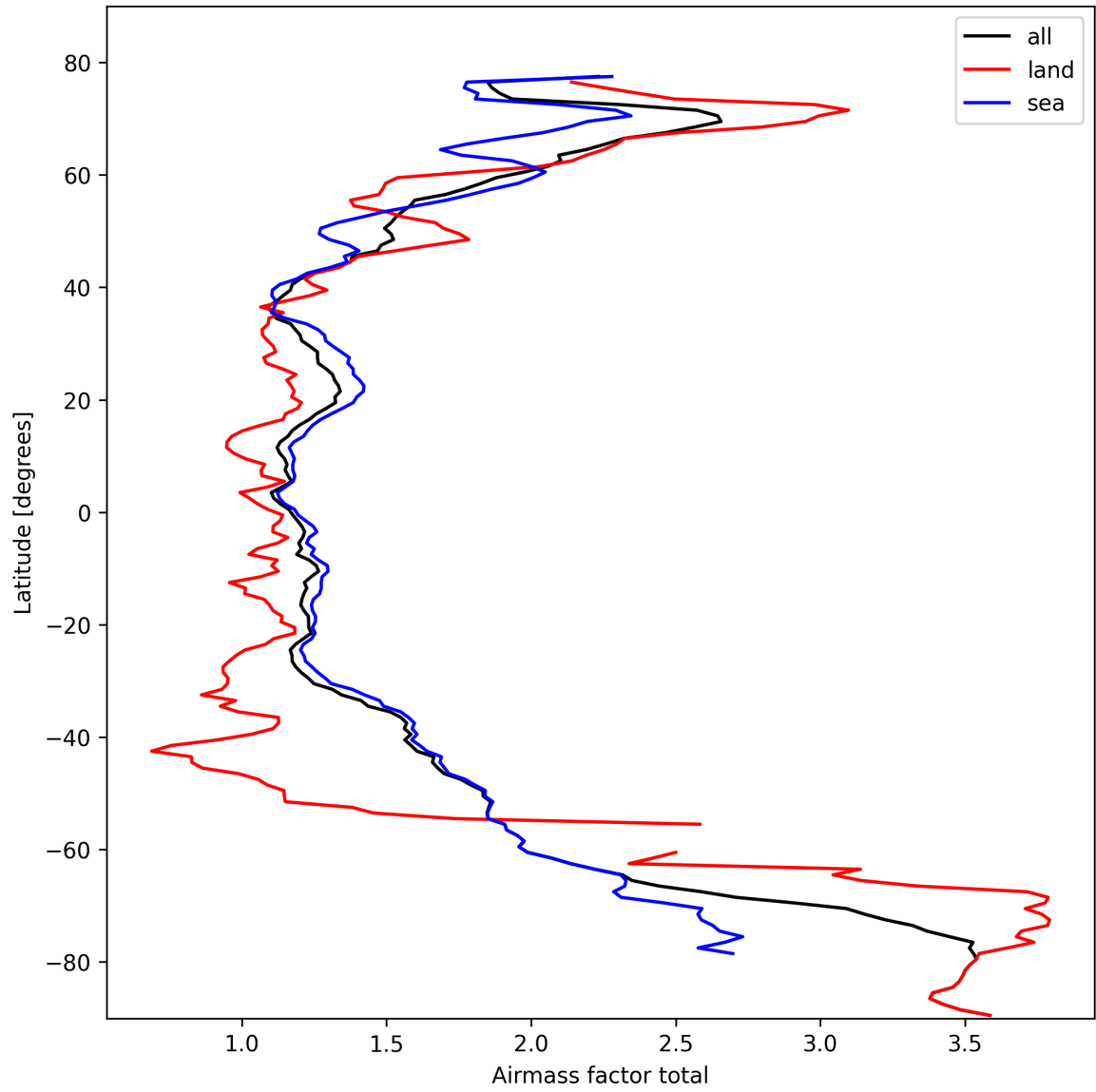
Figure 26: Zonal average of “Airmass factor total” for 2025-02-26 to 2025-02-28.
