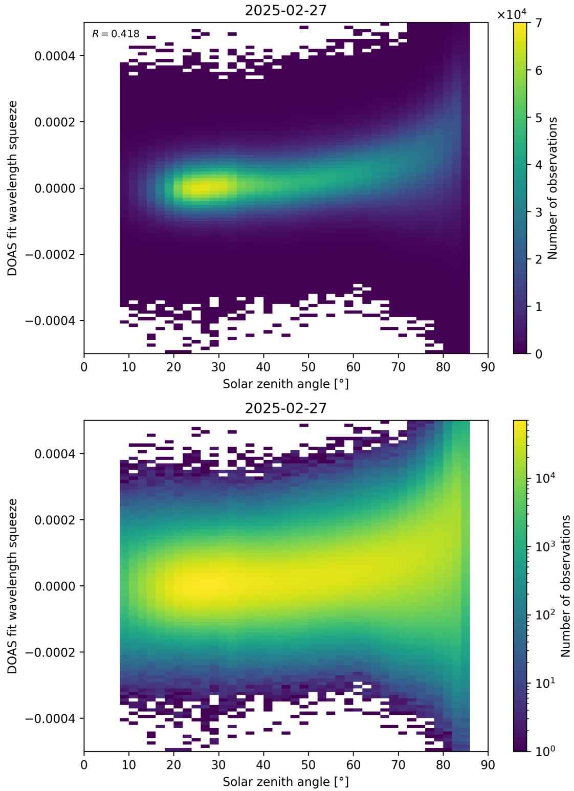
Figure 169: Scatter density plot of “Solar zenith angle” against “DOAS fit wavelength squeeze” for 2025-02-26 to 2025-02-28.
