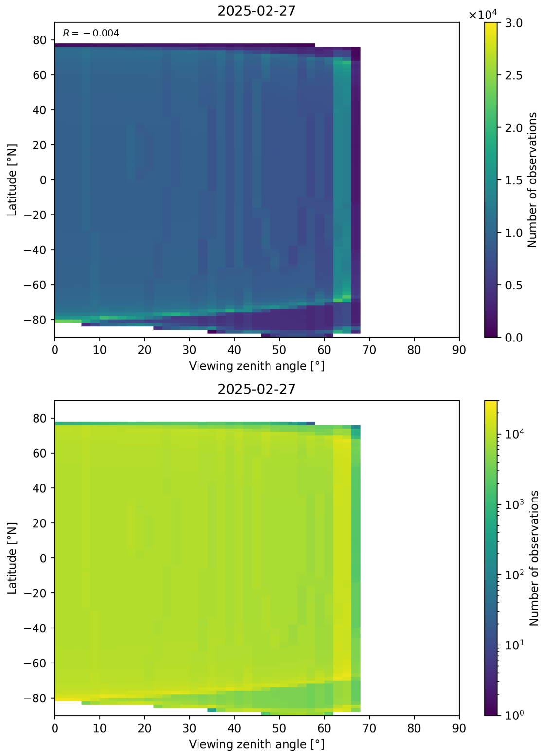
Figure 196: Scatter density plot of “Viewing zenith angle” against “Latitude” for 2025-02-26 to 2025-02-28.
