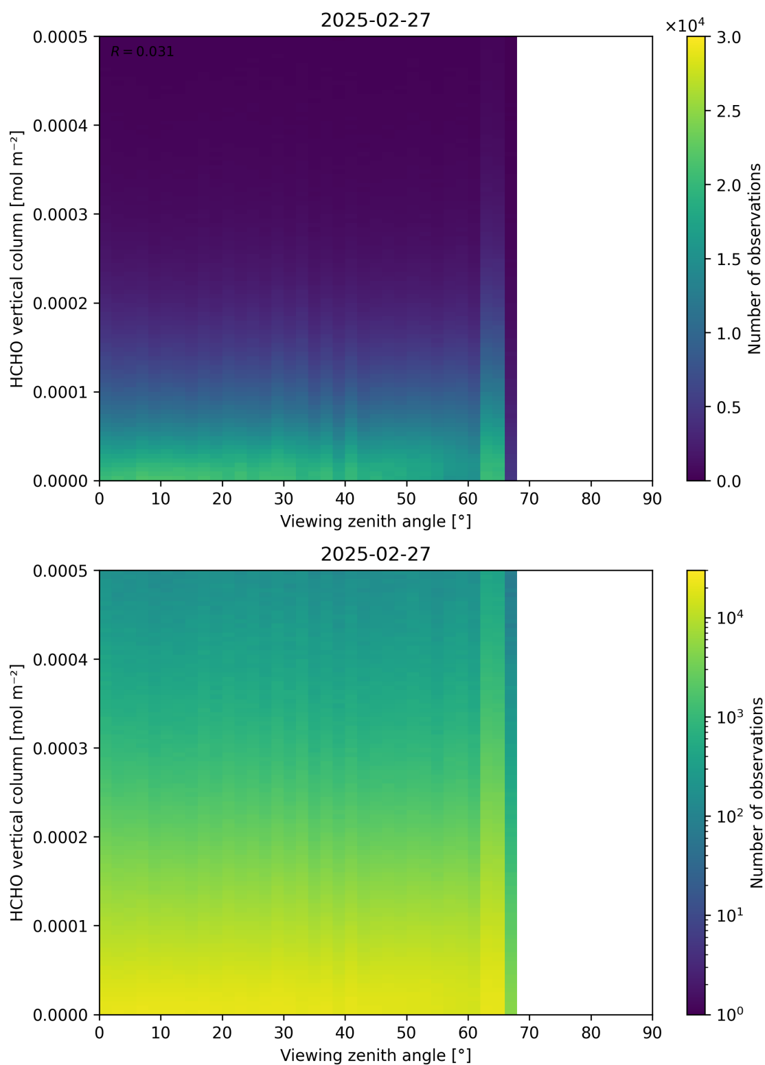
Figure 192: Scatter density plot of “Viewing zenith angle” against “HCHO vertical column” for 2025-02-26 to 2025-02-28.
