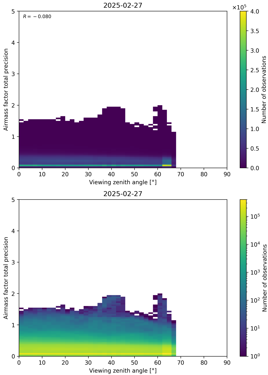
Figure 191: Scatter density plot of “Viewing zenith angle” against “Airmass factor total precision” for 2025-02-26 to 2025-02-28.
