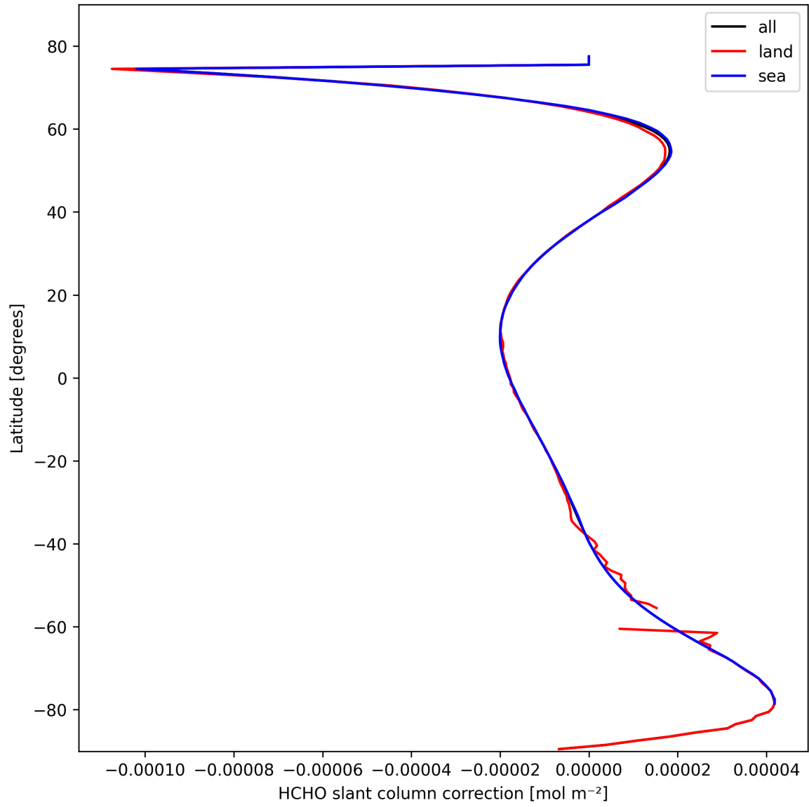
Figure 33: Zonal average of “HCHO slant column correction” for 2025-02-26 to 2025-02-28.
