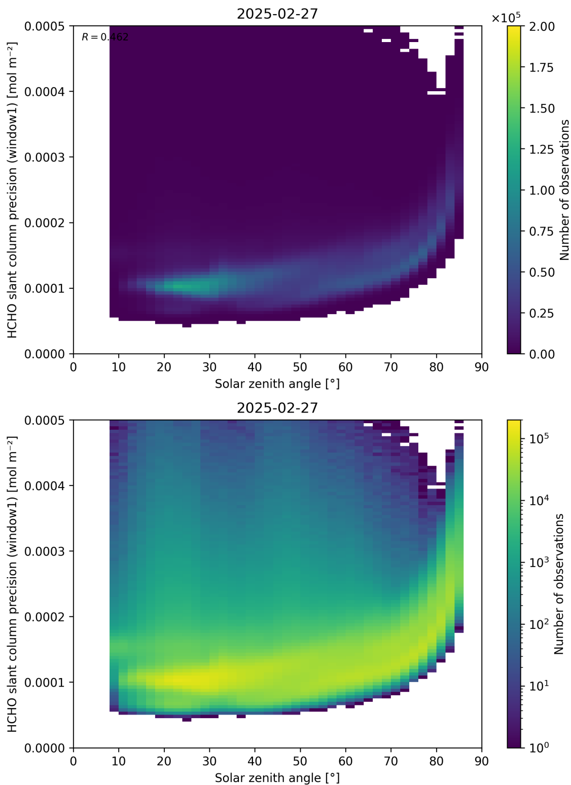
Figure 174: Scatter density plot of “Solar zenith angle” against “HCHO slant column precision (window1)” for 2025-02-26 to 2025-02-28.
