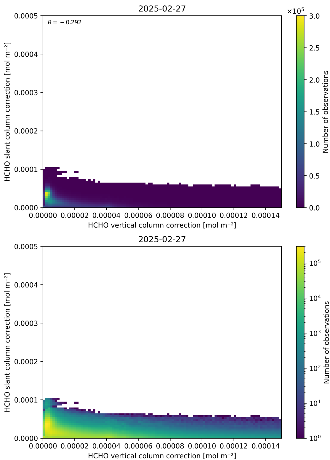
Figure 117: Scatter density plot of “HCHO vertical column correction” against “HCHO slant column correction” for 2025-02-26 to 2025-02-28.
