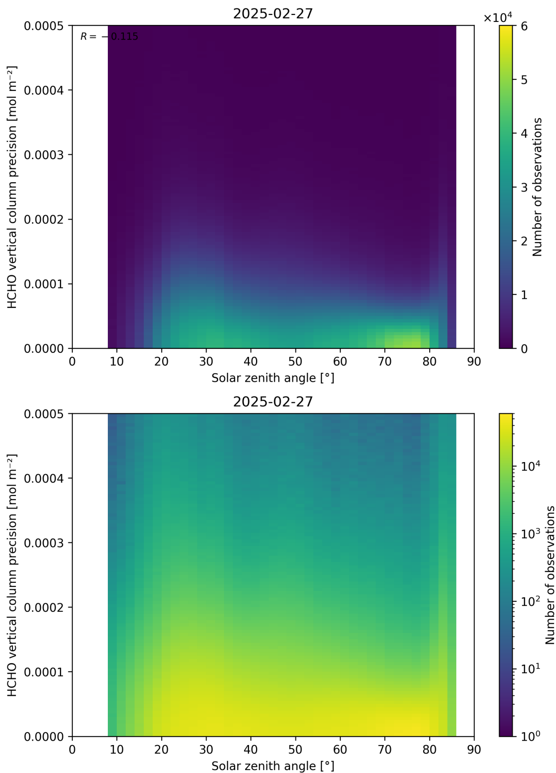
Figure 179: Scatter density plot of “Solar zenith angle” against “HCHO vertical column precision” for 2025-02-26 to 2025-02-28.
