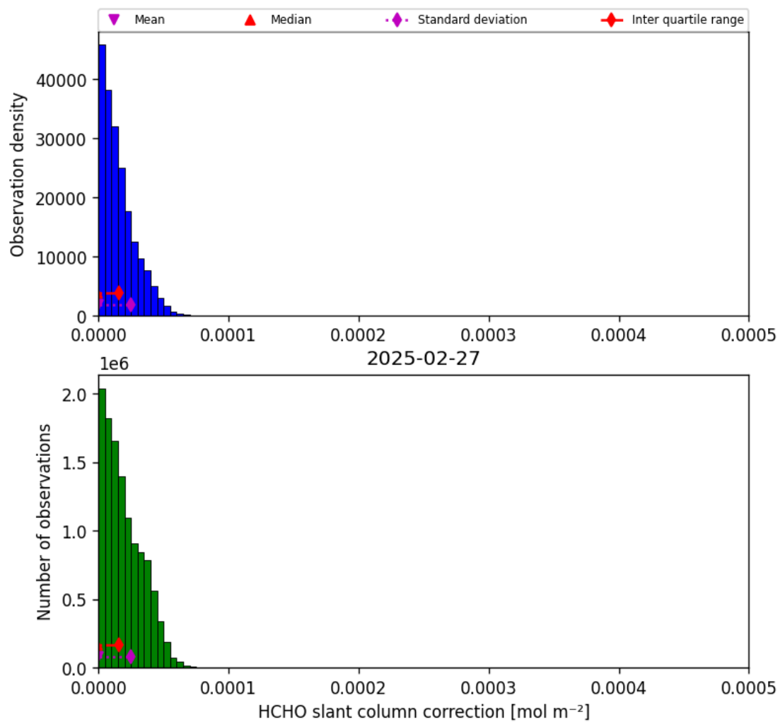
Figure 47: Histogram of “HCHO slant column correction” for 2025-02-26 to 2025-02-28
