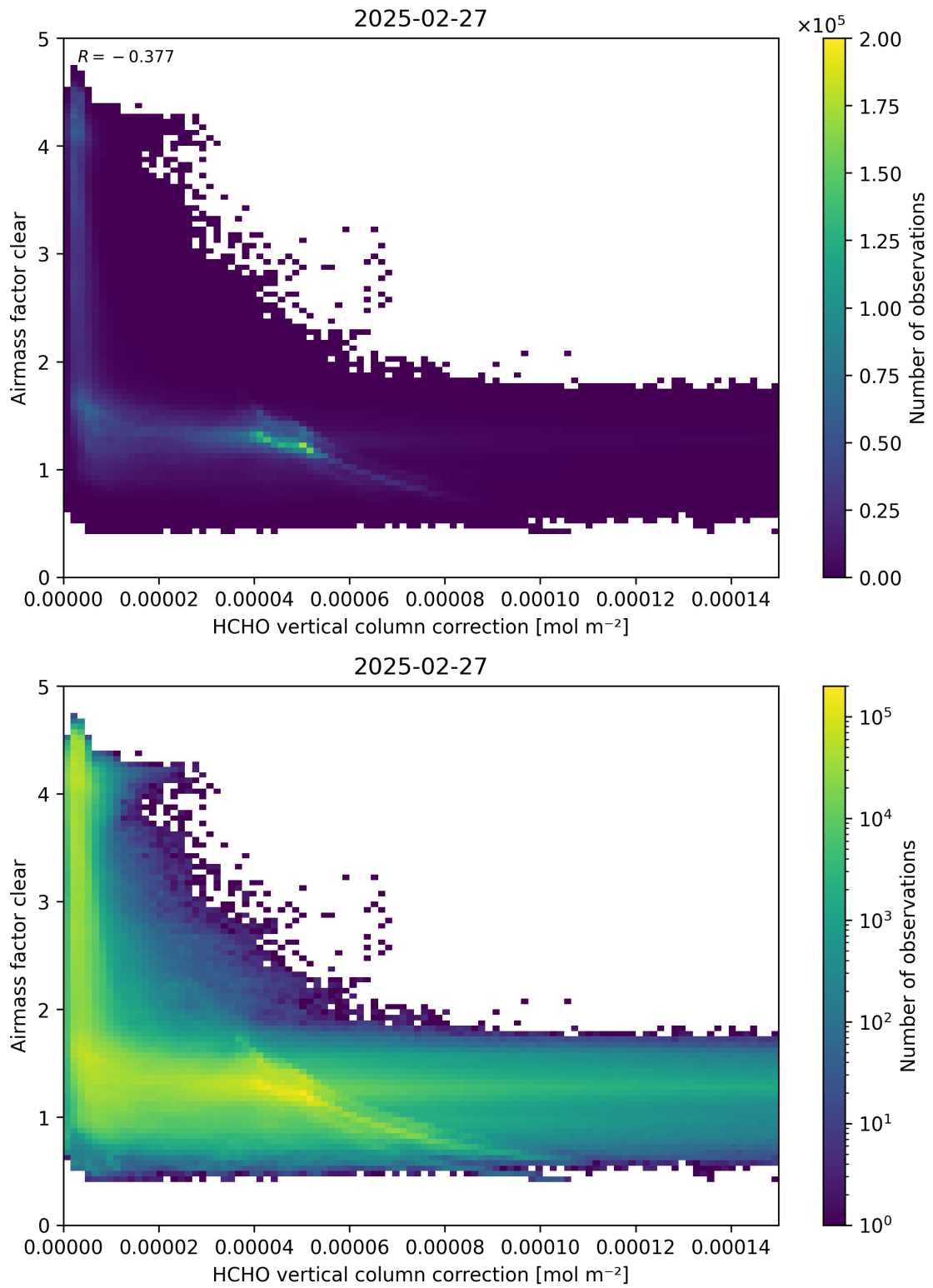
Figure 115: Scatter density plot of “HCHO vertical column correction” against “Airmass factor clear” for 2025-02-26 to 2025-02-28.
