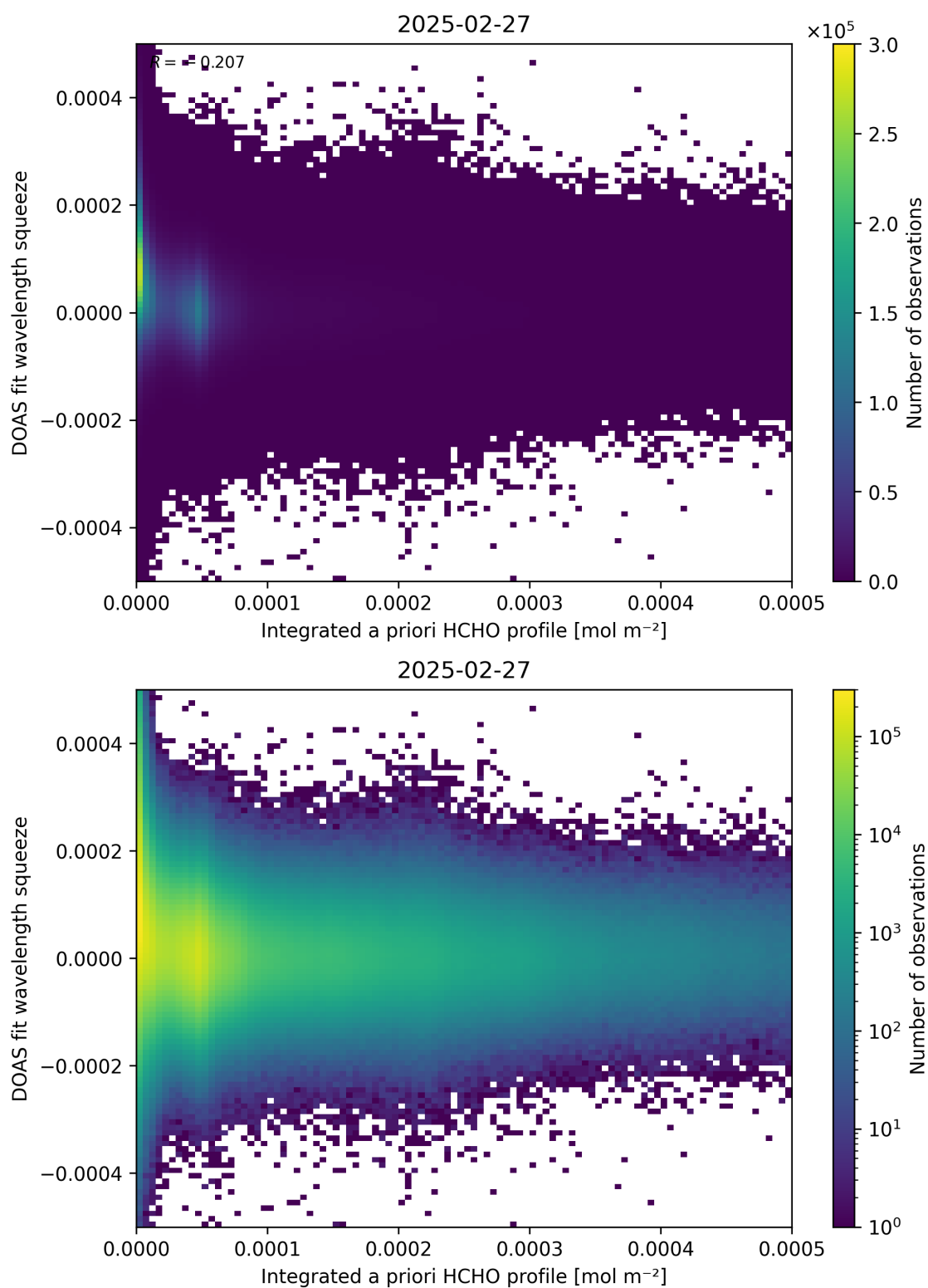
Figure 150: Scatter density plot of “Integrated a priori HCHO profile” against “DOAS fit wavelength squeeze” for 2025-02-26 to 2025-02-28.
