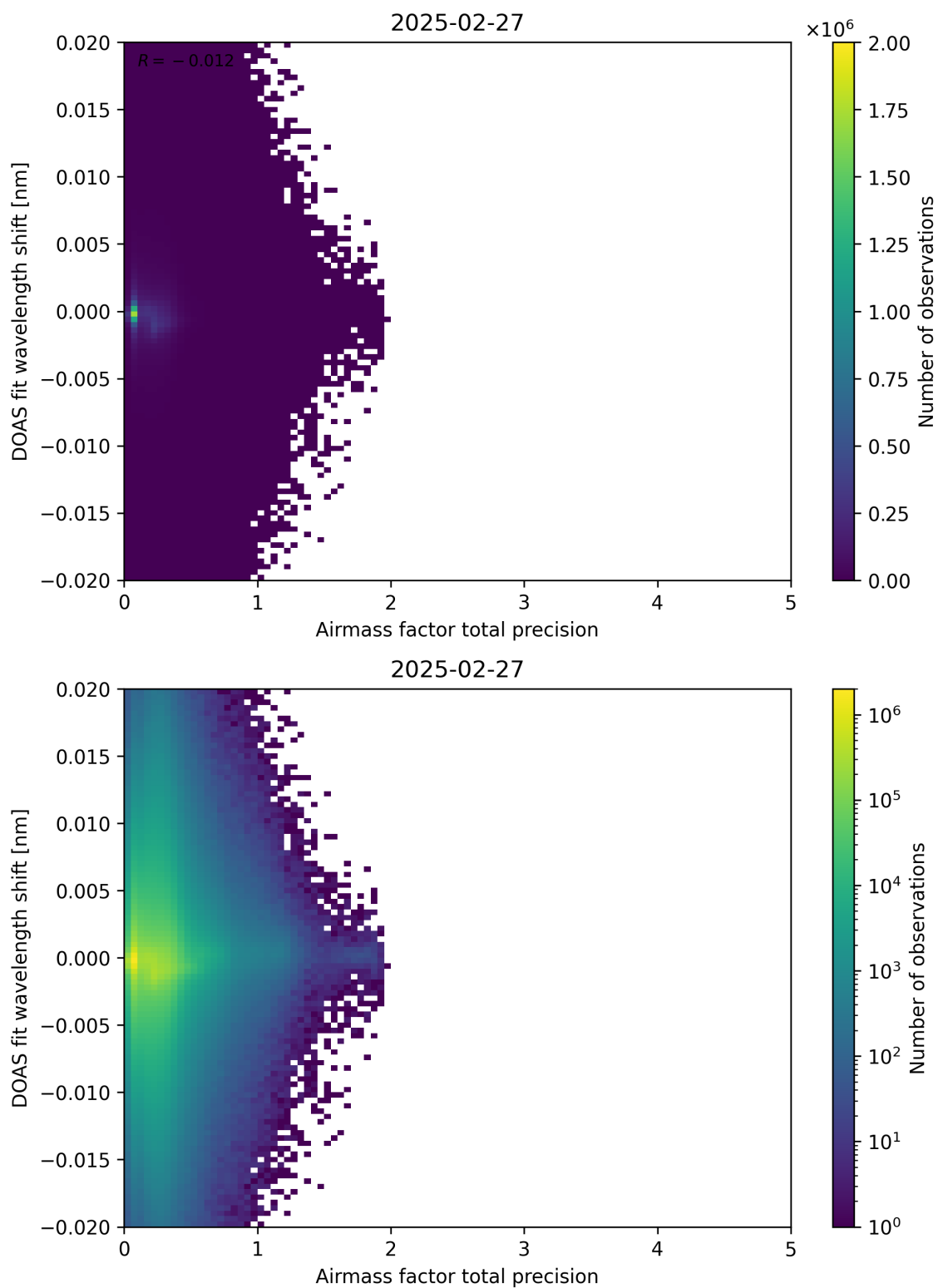
Figure 106: Scatter density plot of “Airmass factor total precision” against “DOAS fit wavelength shift” for 2025-02-26 to 2025-02-28.
