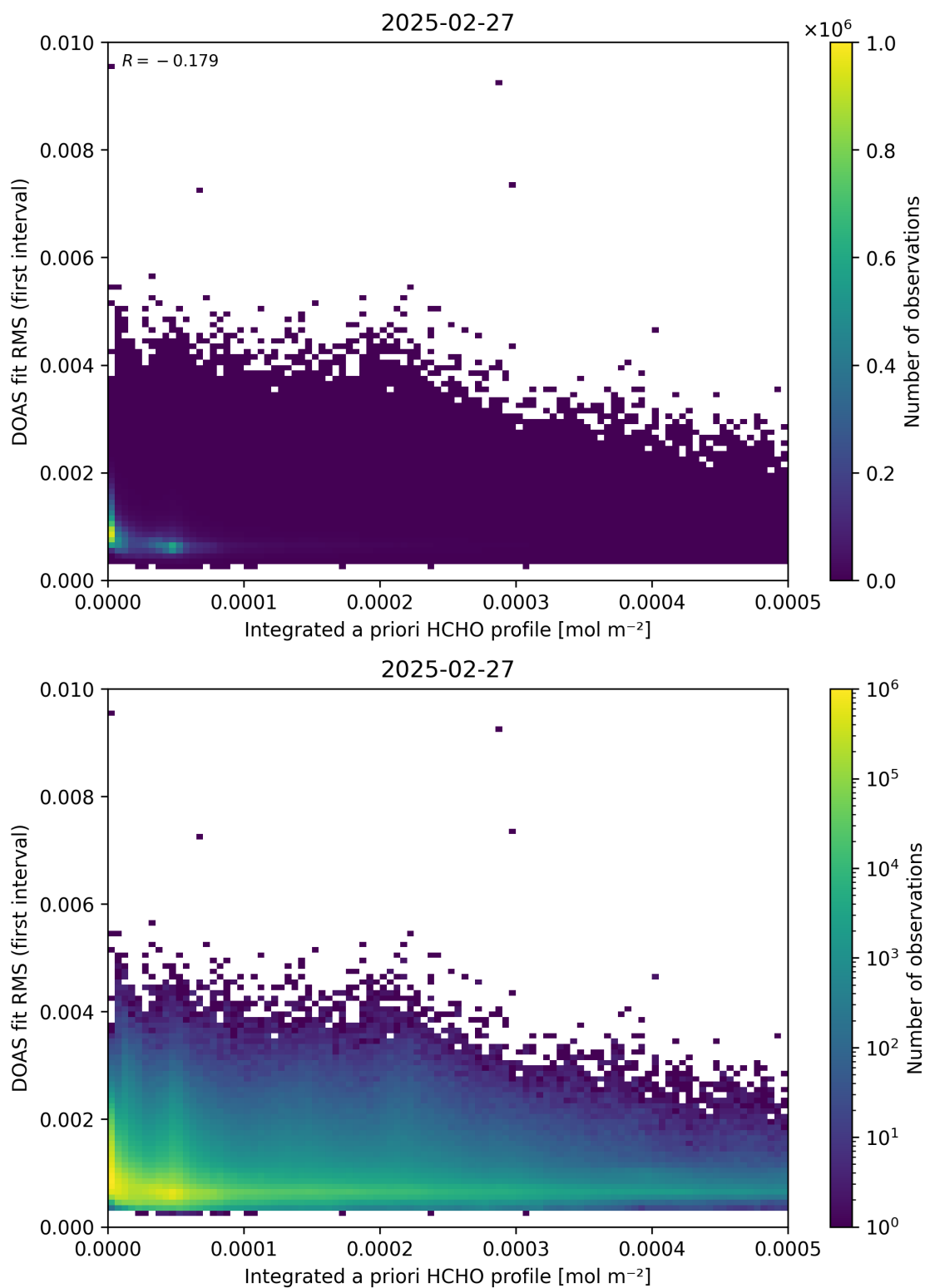
Figure 148: Scatter density plot of “Integrated a priori HCHO profile” against “DOAS fit RMS (first interval)” for 2025-02-26 to 2025-02-28.
