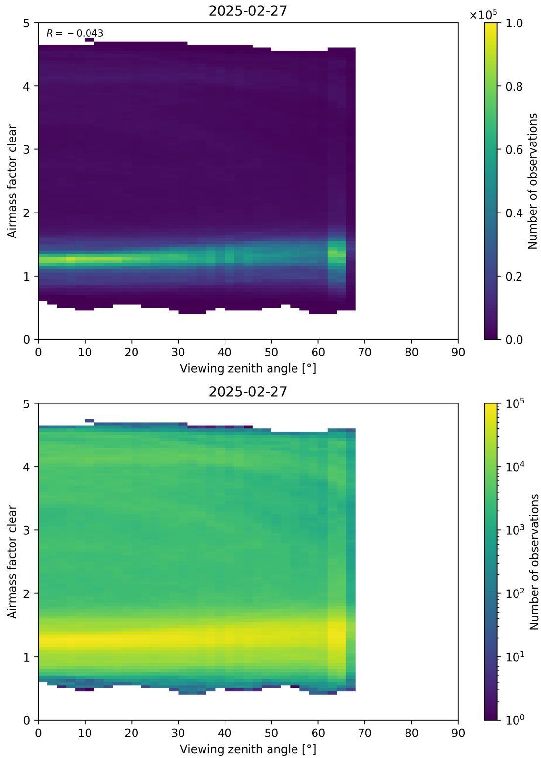
Figure 185: Scatter density plot of “Viewing zenith angle” against “Airmass factor clear” for 2025-02-26 to 2025-02-28.
