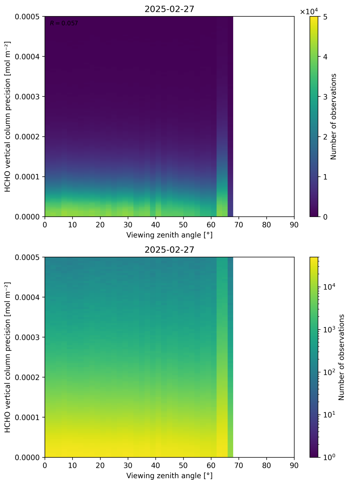
Figure 194: Scatter density plot of “Viewing zenith angle” against “HCHO vertical column precision” for 2025-02-26 to 2025-02-28.
