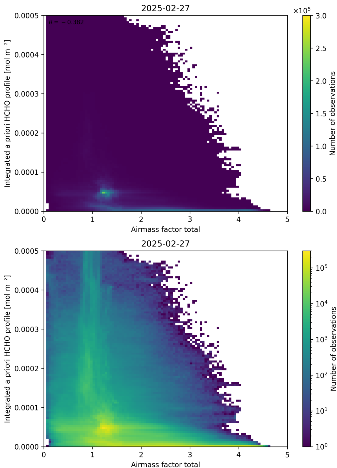
Figure 104: Scatter density plot of “Airmass factor total” against “Integrated a priori HCHO profile” for 2025-02-26 to 2025-02-28.
