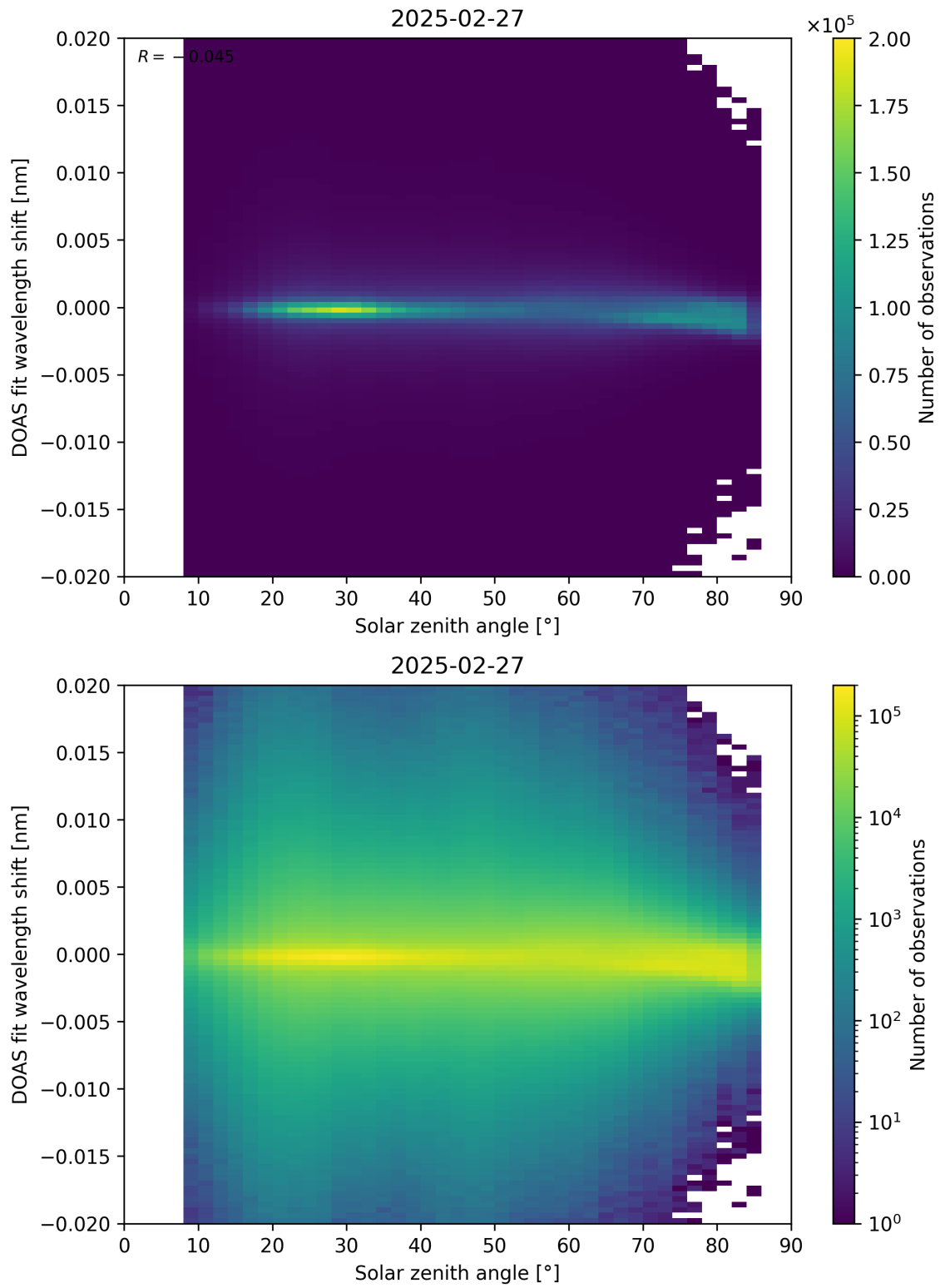
Figure 168: Scatter density plot of “Solar zenith angle” against “DOAS fit wavelength shift” for 2025-02-26 to 2025-02-28.
