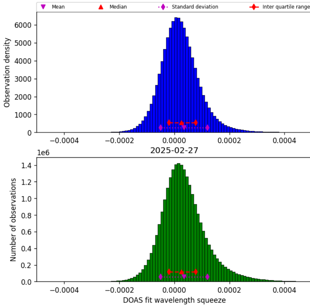
Figure 45: Histogram of “DOAS fit wavelength squeeze” for 2025-02-26 to 2025-02-28
