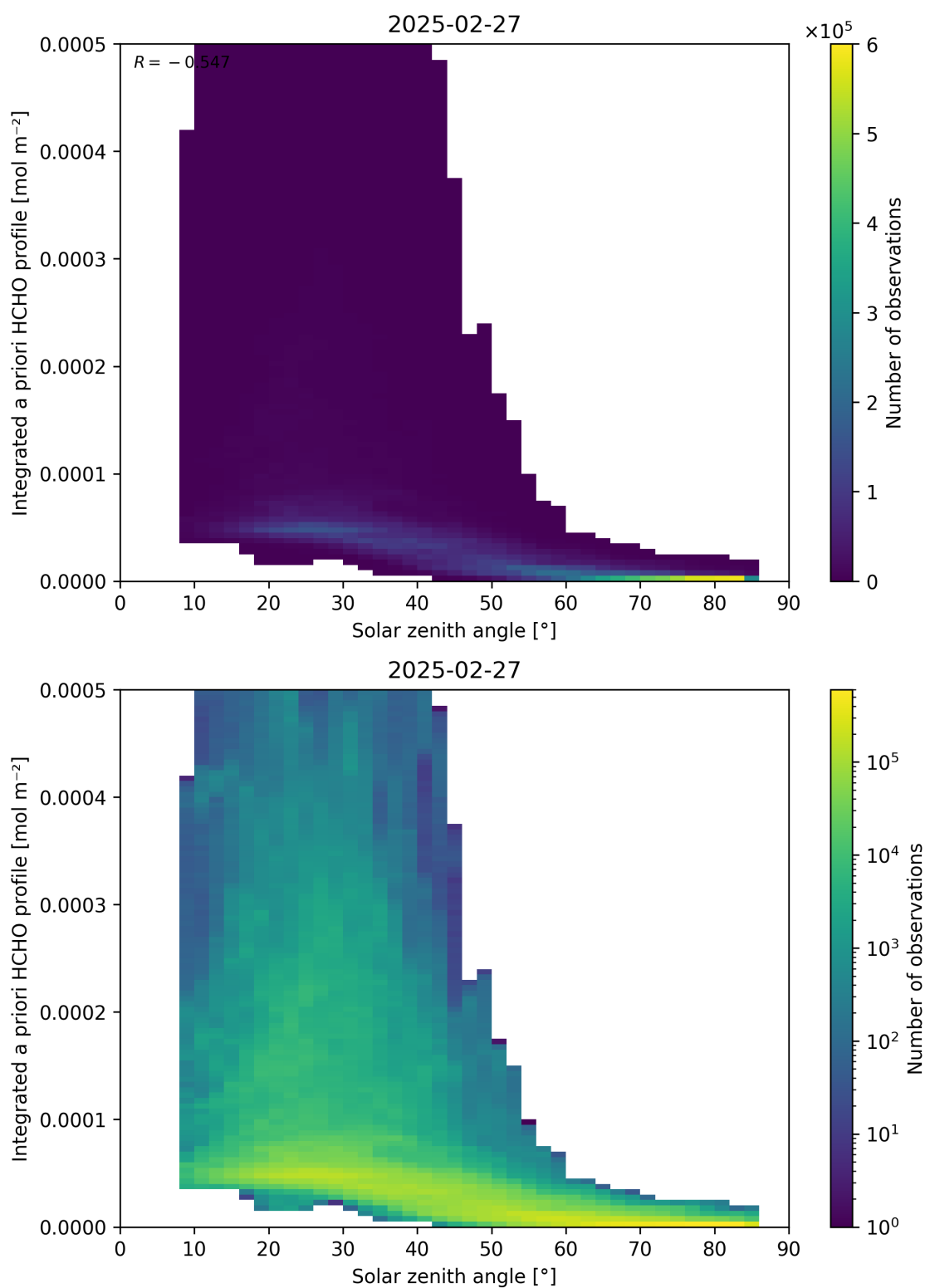
Figure 180: Scatter density plot of “Solar zenith angle” against “Integrated a priori HCHO profile” for 2025-02-26 to 2025-02-28.
