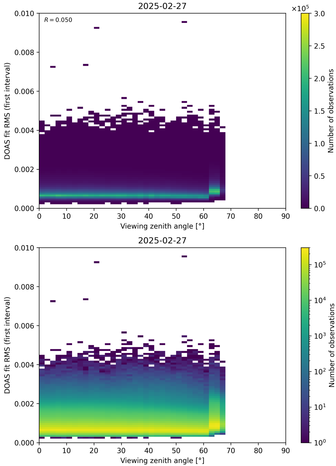
Figure 182: Scatter density plot of “Viewing zenith angle” against “DOAS fit RMS (first interval)” for 2025-02-26 to 2025-02-28.
