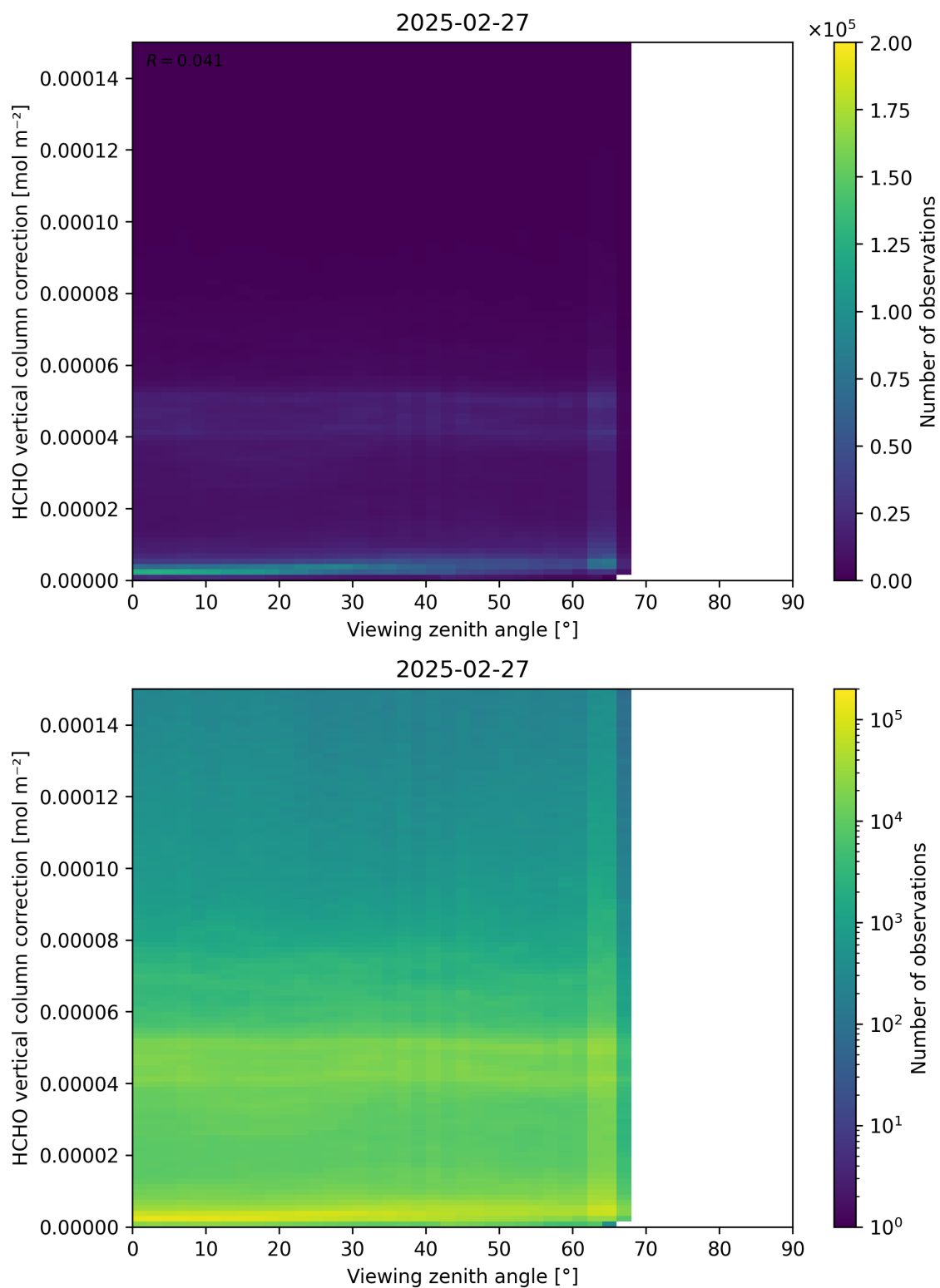
Figure 193: Scatter density plot of “Viewing zenith angle” against “HCHO vertical column correction” for 2025-02-26 to 2025-02-28.
