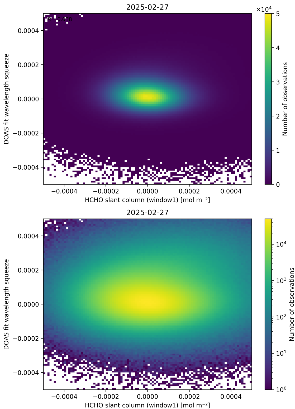
Figure 80: Scatter density plot of “HCHO slant column (window1)” against “DOAS fit wavelength squeeze” for 2025-02-26 to 2025-02-28.
