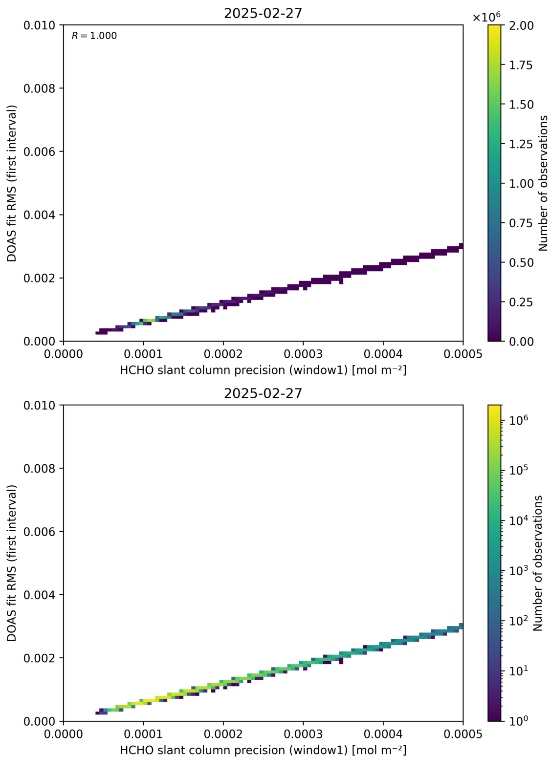
Figure 88: Scatter density plot of “HCHO slant column precision (window1)” against “DOAS fit RMS (first interval)” for 2025-02-26 to 2025-02-28.
