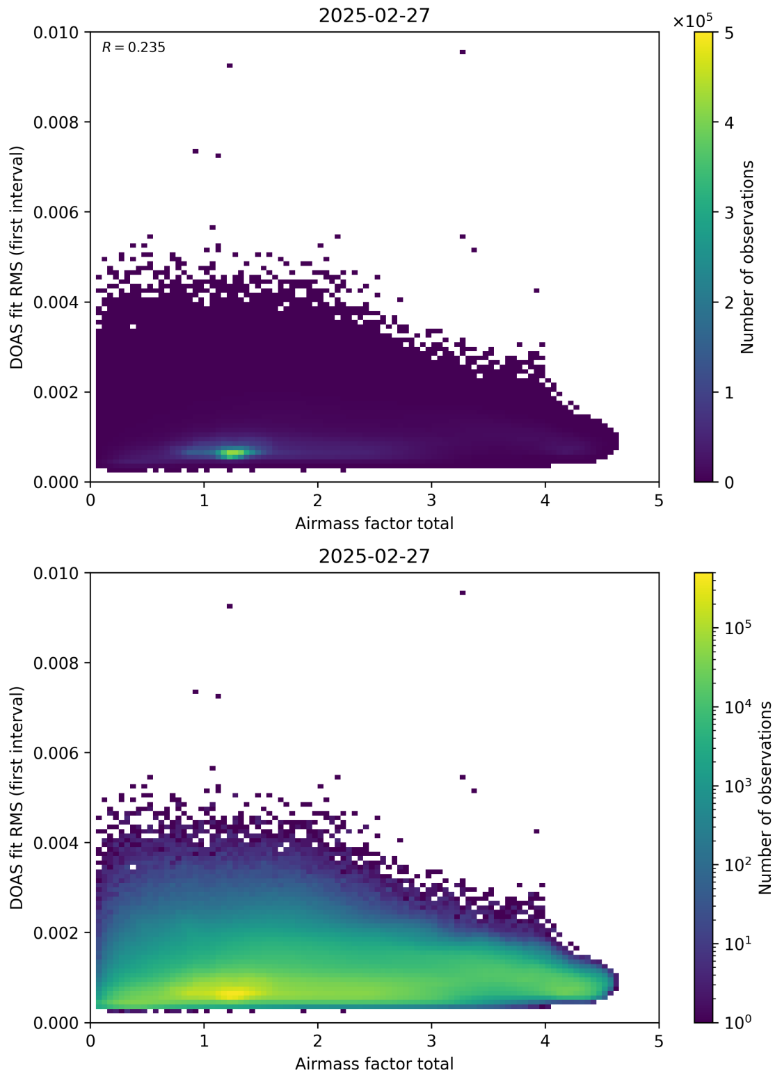
Figure 97: Scatter density plot of “Airmass factor total” against “DOAS fit RMS (first interval)” for 2025-02-26 to 2025-02-28.
