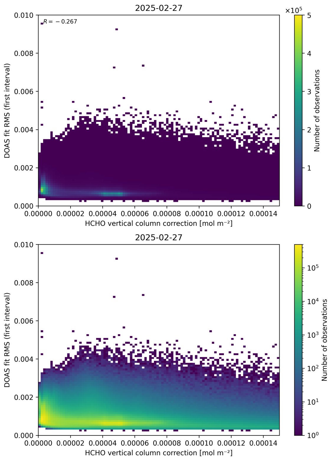
Figure 112: Scatter density plot of “HCHO vertical column correction” against “DOAS fit RMS (first interval)” for 2025-02-26 to 2025-02-28.
