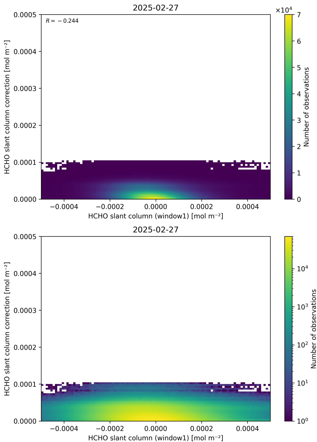
Figure 83: Scatter density plot of “HCHO slant column (window1)” against “HCHO slant column correction” for 2025-02-26 to 2025-02-28.
