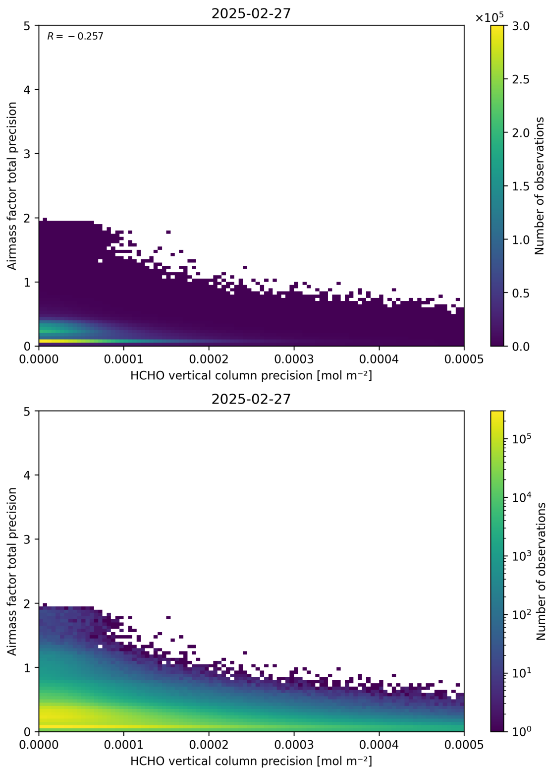
Figure 145: Scatter density plot of “HCHO vertical column precision” against “Airmass factor total precision” for 2025-02-26 to 2025-02-28.
