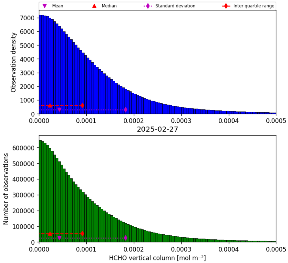
Figure 35: Histogram of “HCHO vertical column” for 2025-02-26 to 2025-02-28
