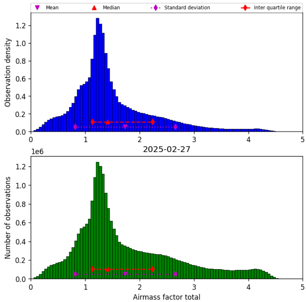
Figure 40: Histogram of “Airmass factor total” for 2025-02-26 to 2025-02-28
