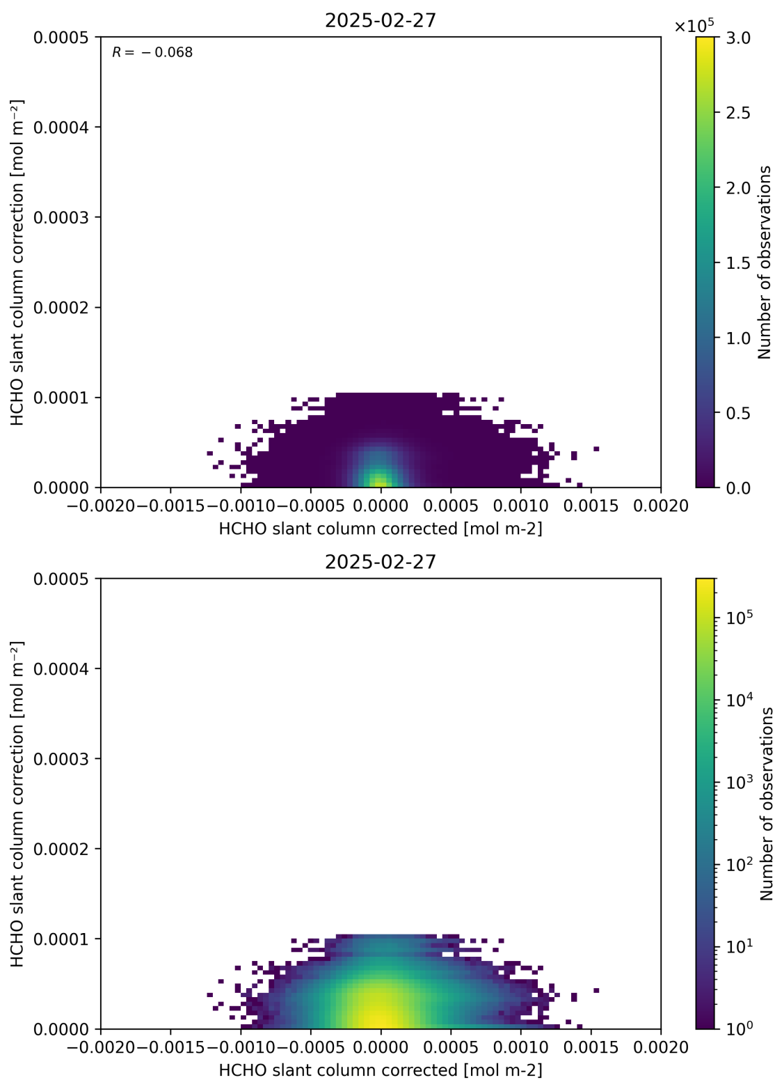
Figure 77: Scatter density plot of “HCHO slant column corrected” against “HCHO slant column correction” for 2025-02-26 to 2025-02-28.
