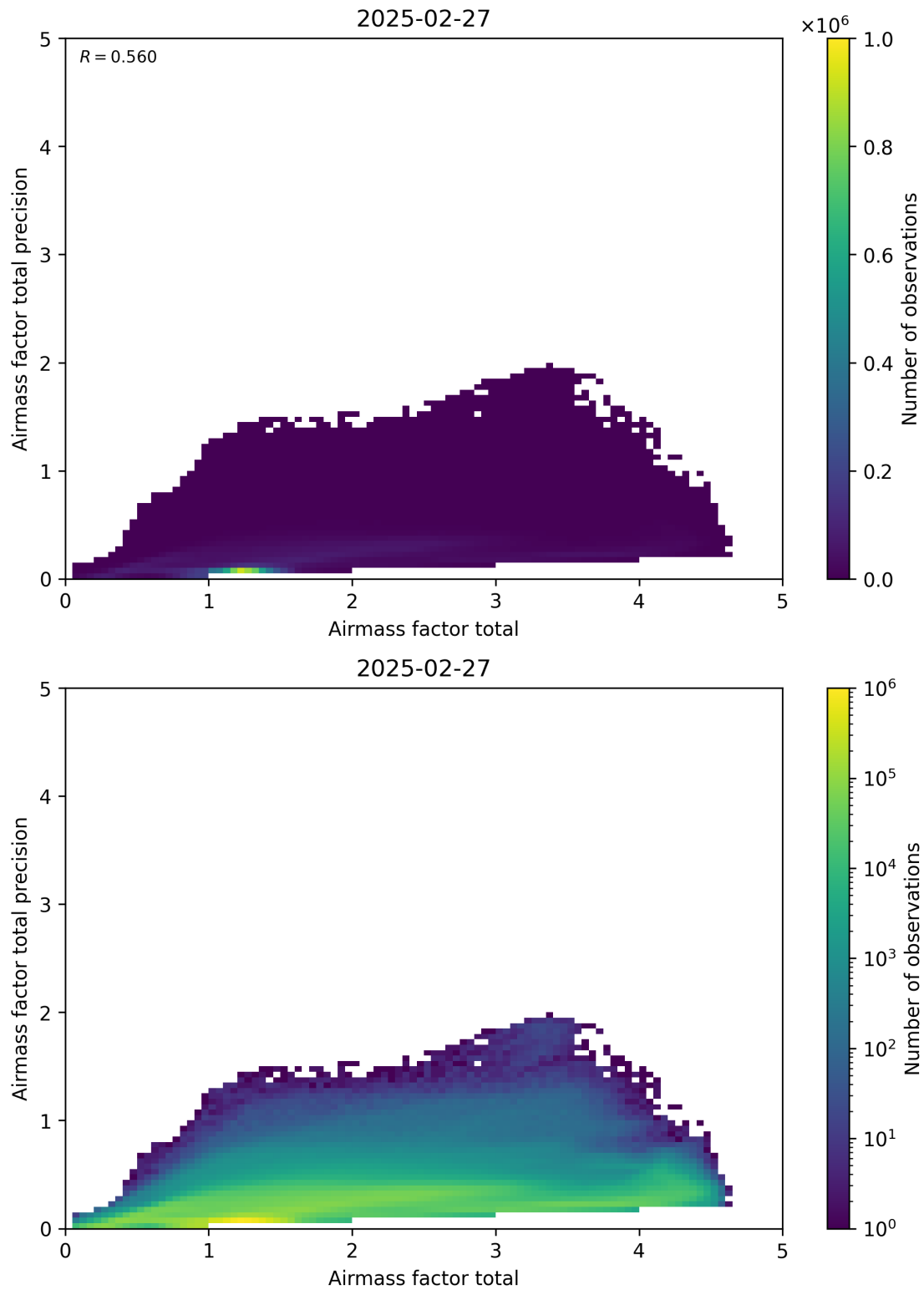
Figure 103: Scatter density plot of “Airmass factor total” against “Airmass factor total precision” for 2025-02-26 to 2025-02-28.
