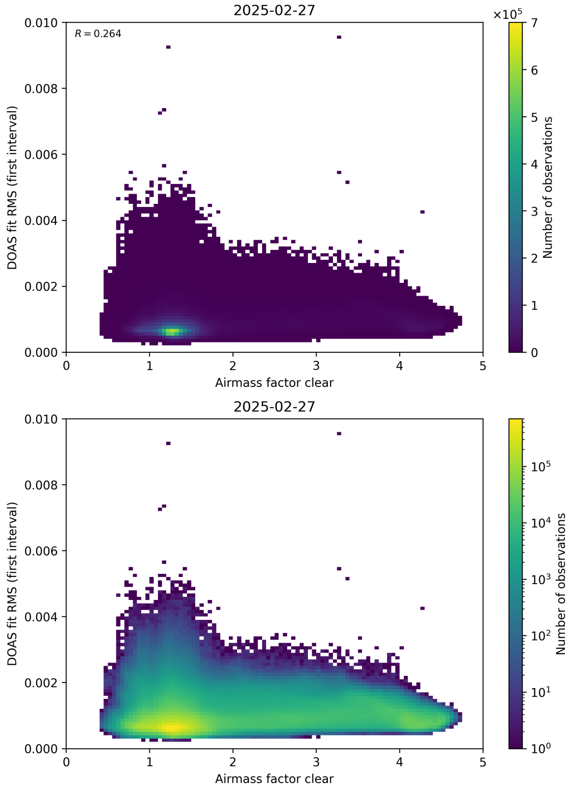
Figure 71: Scatter density plot of “Airmass factor clear” against “DOAS fit RMS (first interval)” for 2025-02-26 to 2025-02-28.
