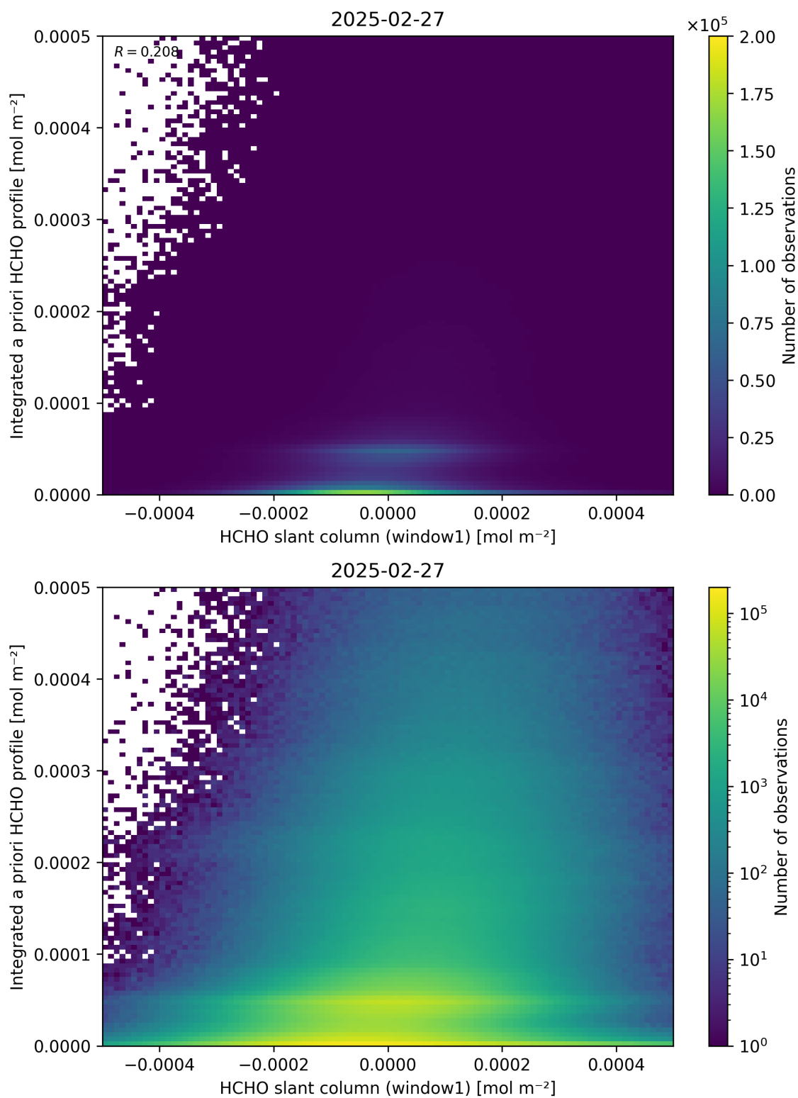
Figure 87: Scatter density plot of “HCHO slant column (window1)” against “Integrated a priori HCHO profile” for 2025-02-26 to 2025-02-28.
