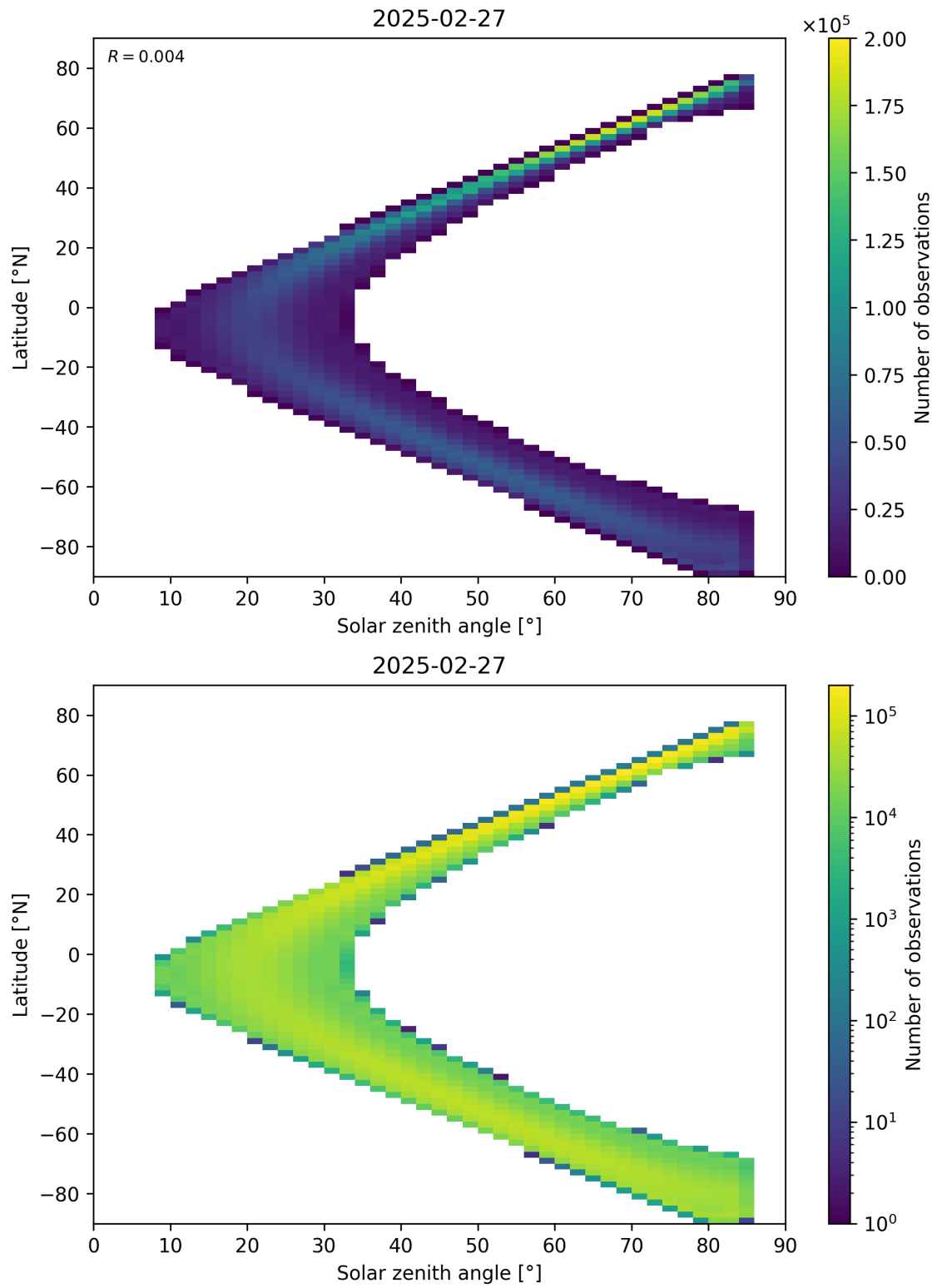
Figure 181: Scatter density plot of “Solar zenith angle” against “Latitude” for 2025-02-26 to 2025-02-28.
