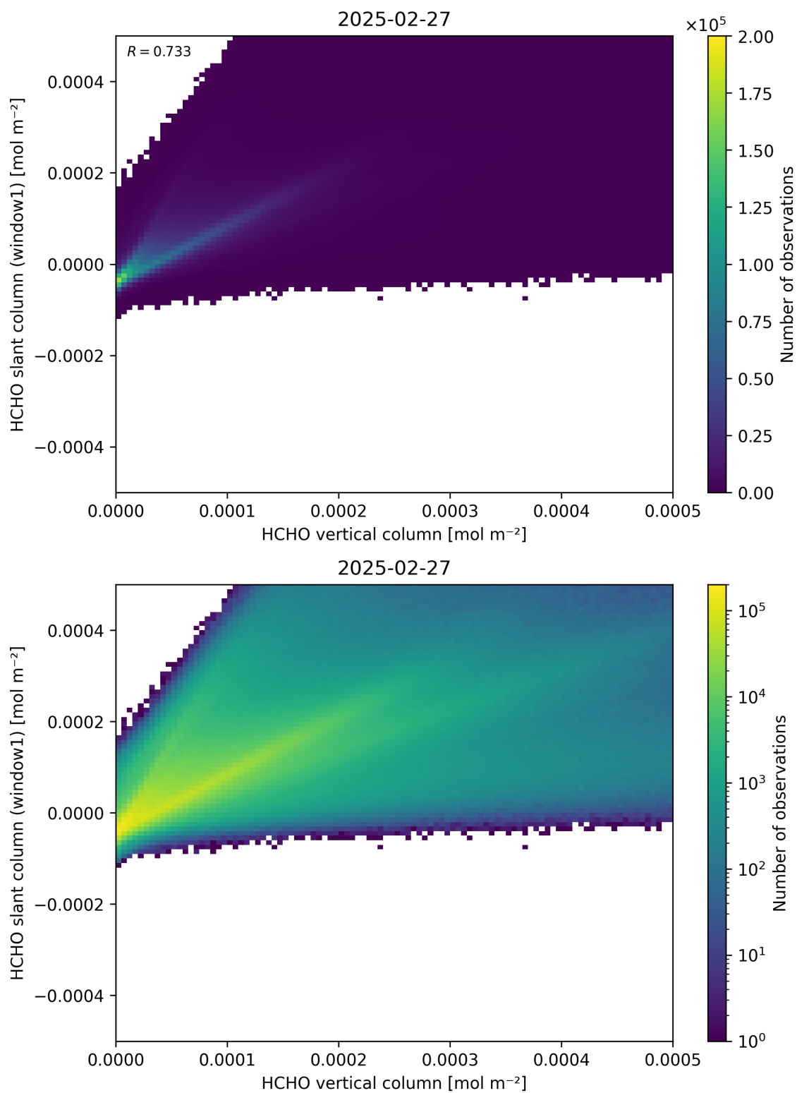
Figure 129: Scatter density plot of “HCHO vertical column” against “HCHO slant column (window1)” for 2025-02-26 to 2025-02-28.
