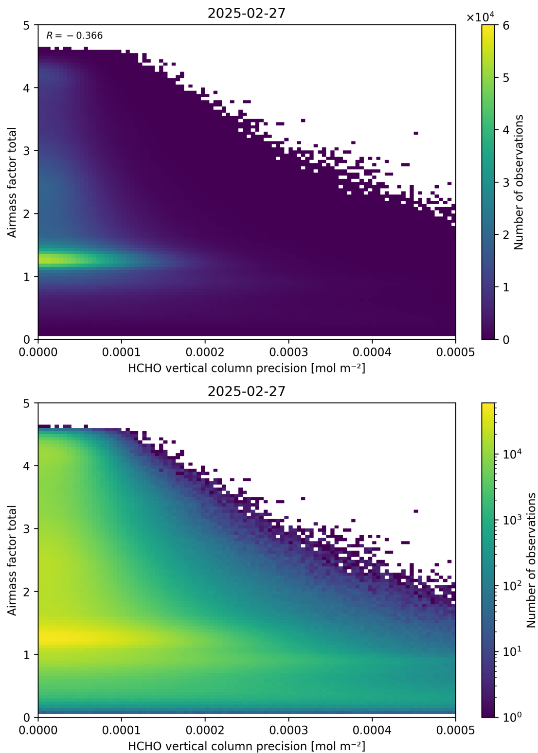
Figure 144: Scatter density plot of “HCHO vertical column precision” against “Airmass factor total” for 2025-02-26 to 2025-02-28.
