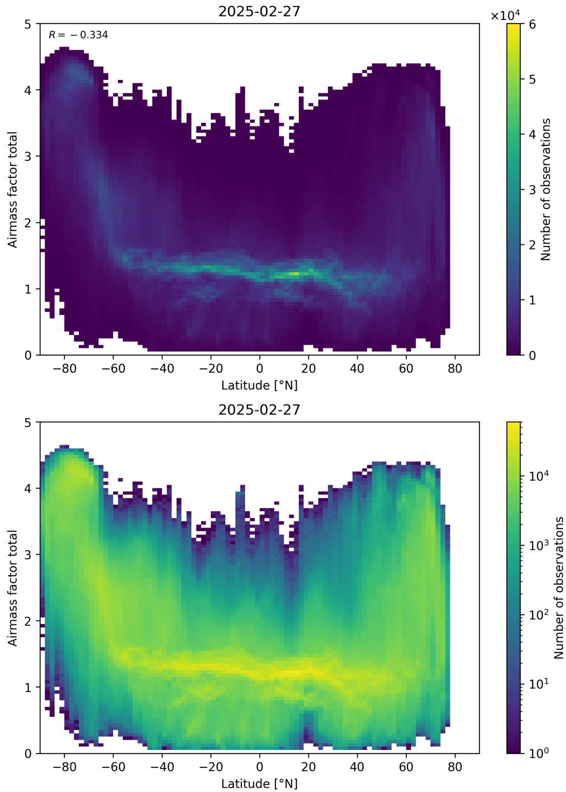
Figure 161: Scatter density plot of “Latitude” against “Airmass factor total” for 2025-02-26 to 2025-02-28.
