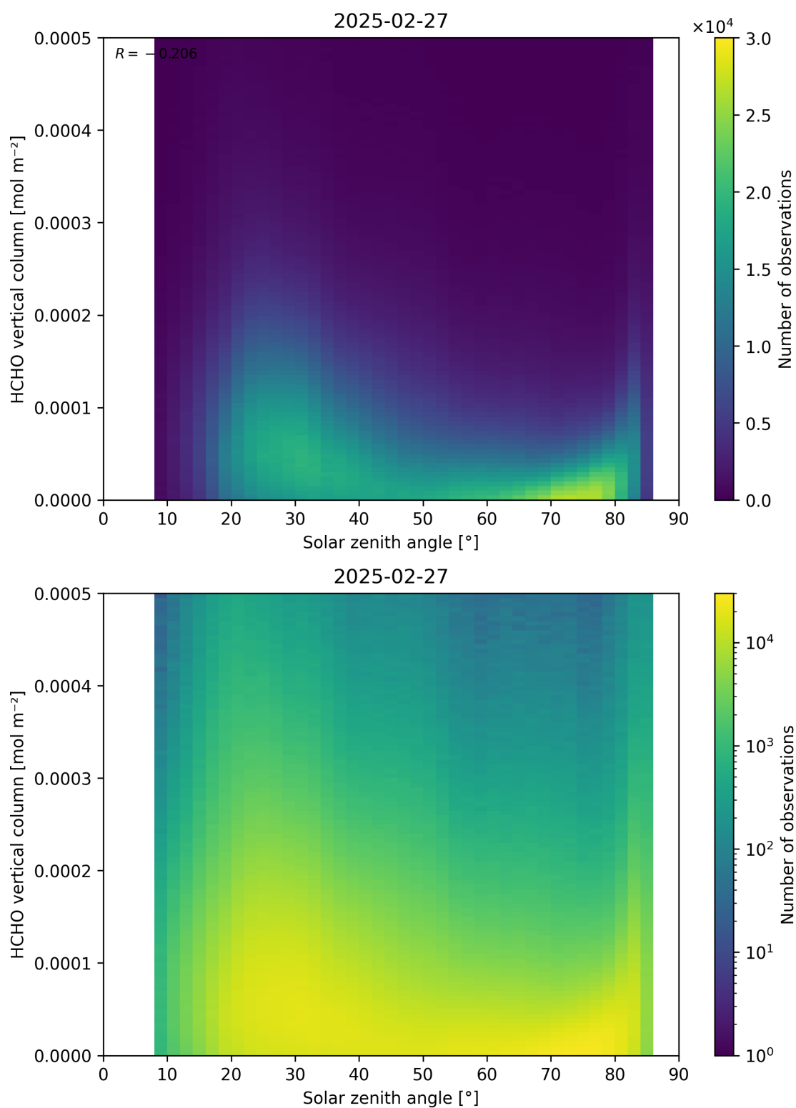
Figure 177: Scatter density plot of “Solar zenith angle” against “HCHO vertical column” for 2025-02-26 to 2025-02-28.
