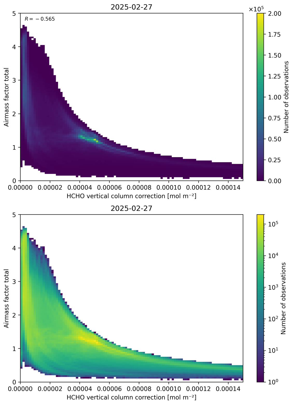
Figure 120: Scatter density plot of “HCHO vertical column correction” against “Airmass factor total” for 2025-02-26 to 2025-02-28.
