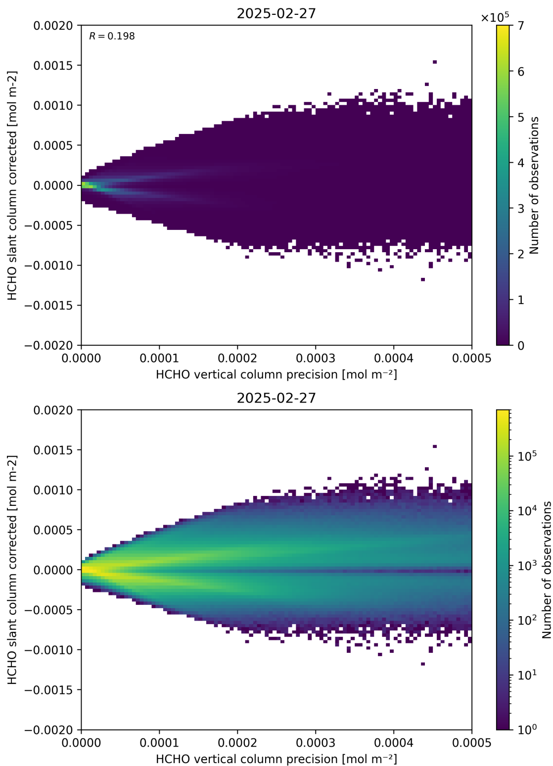
Figure 140: Scatter density plot of “HCHO vertical column precision” against “HCHO slant column corrected” for 2025-02-26 to 2025-02-28.
