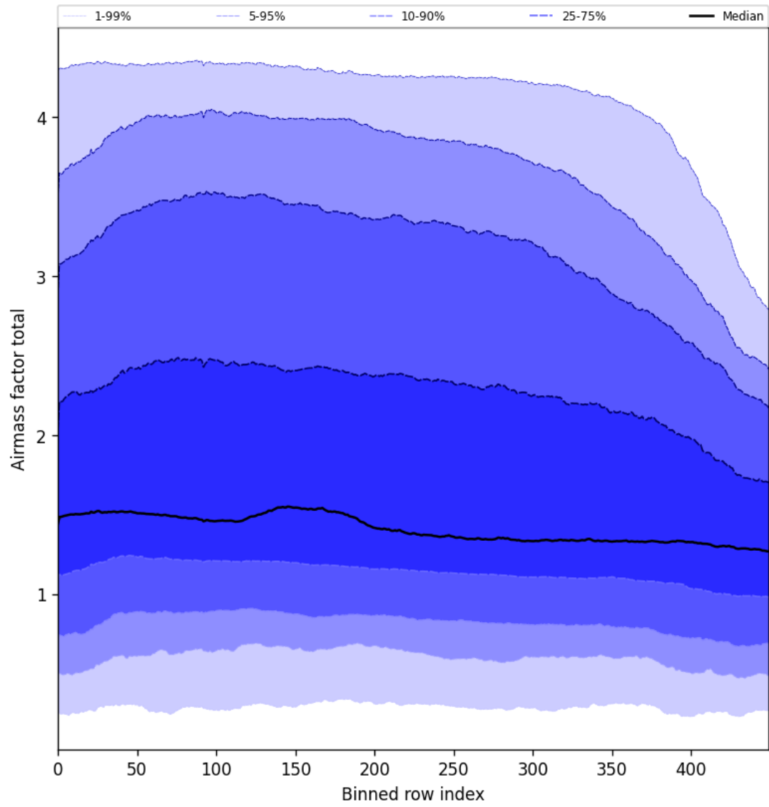
Figure 54: Along track statistics of “Airmass factor total” for 2025-02-26 to 2025-02-28
