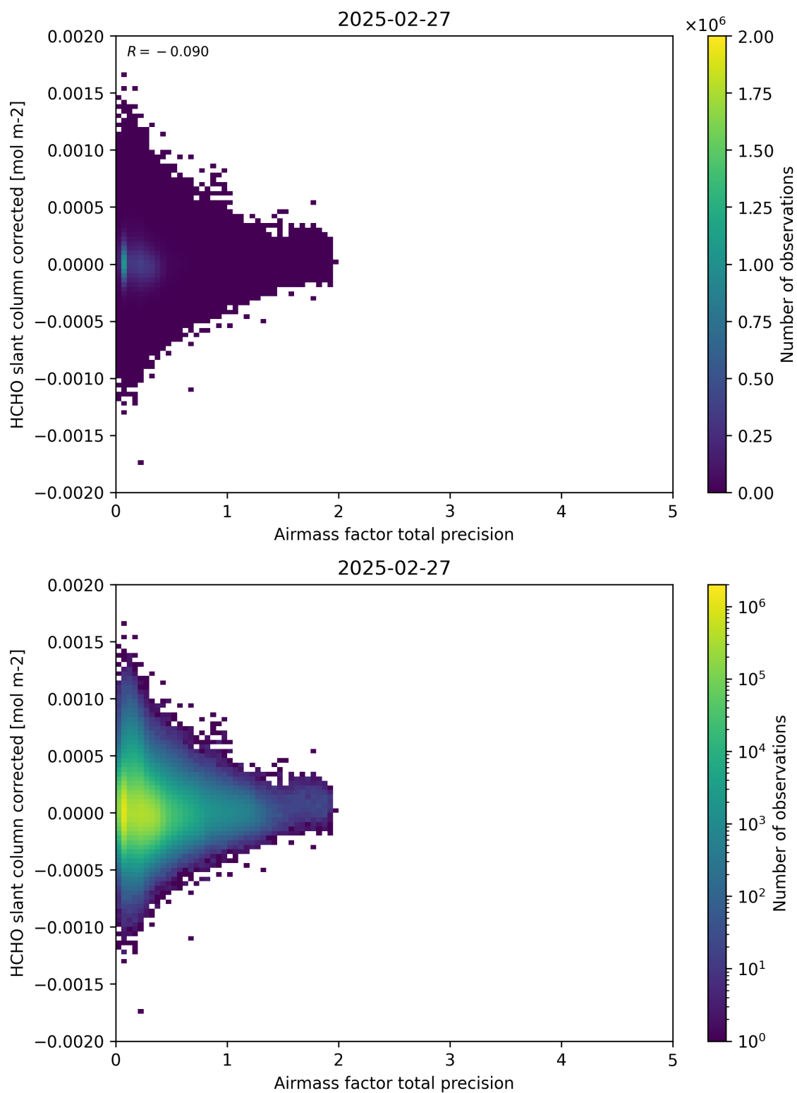
Figure 109: Scatter density plot of “Airmass factor total precision” against “HCHO slant column corrected” for 2025-02-26 to 2025-02-28.
