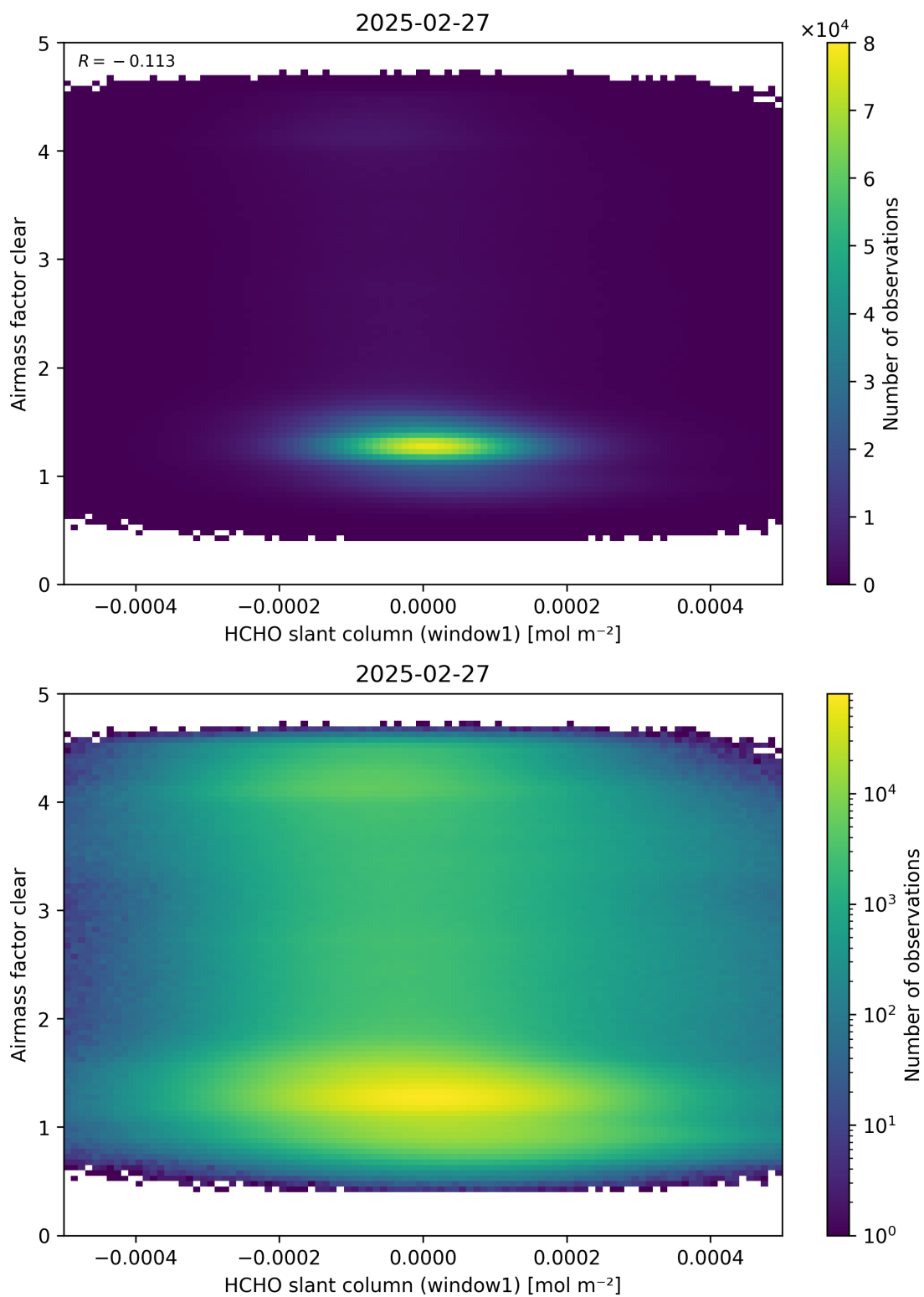
Figure 81: Scatter density plot of “HCHO slant column (window1)” against “Airmass factor clear” for 2025-02-26 to 2025-02-28.
