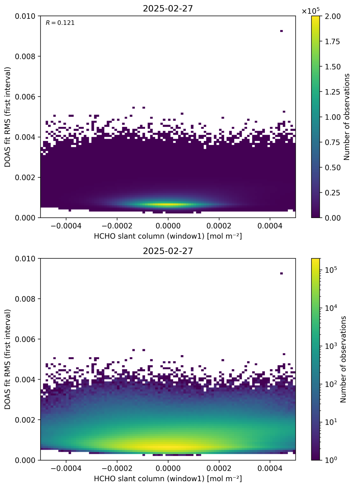
Figure 78: Scatter density plot of “HCHO slant column (window1)” against “DOAS fit RMS (first interval)” for 2025-02-26 to 2025-02-28.
