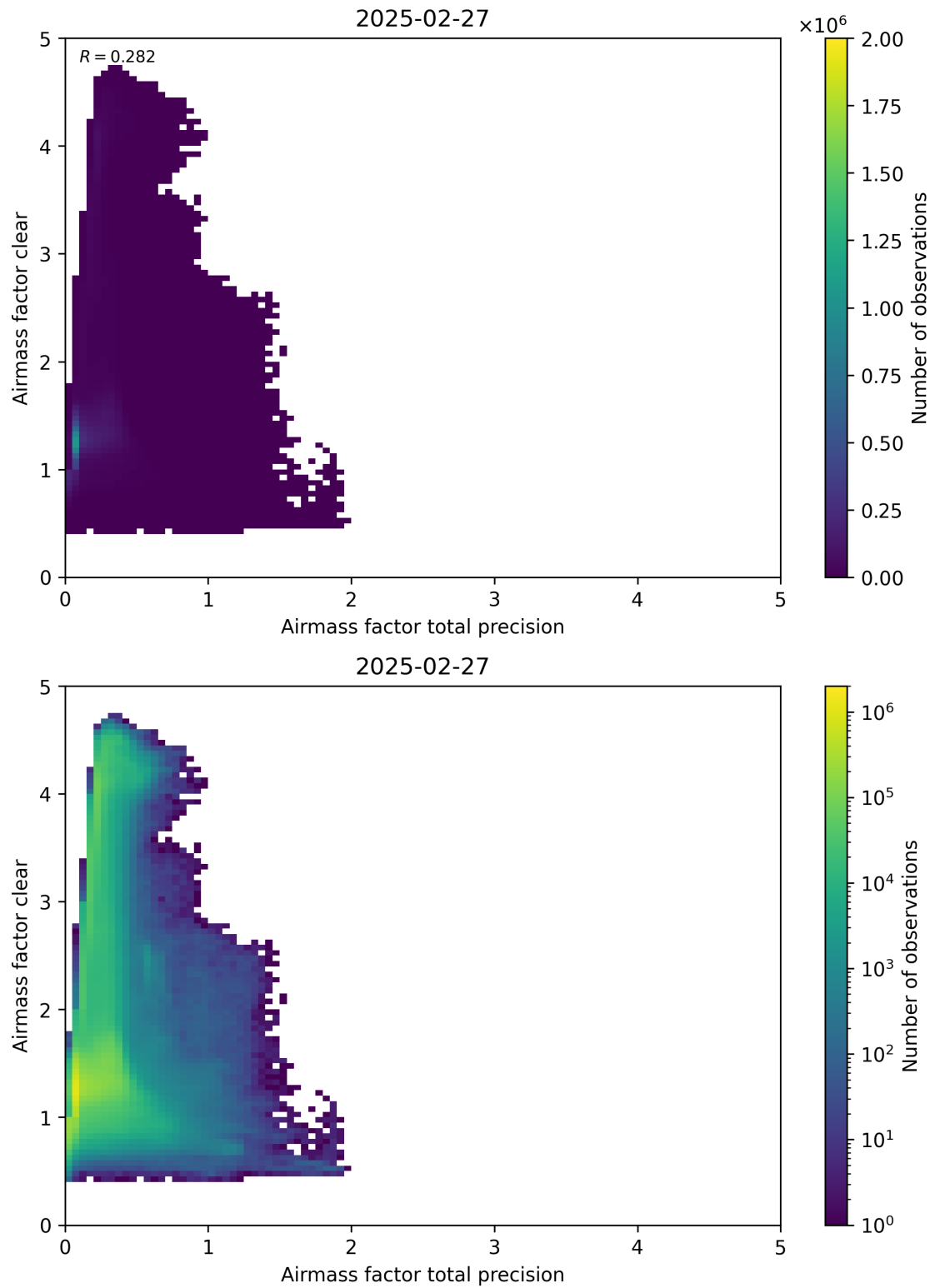
Figure 108: Scatter density plot of “Airmass factor total precision” against “Airmass factor clear” for 2025-02-26 to 2025-02-28.
