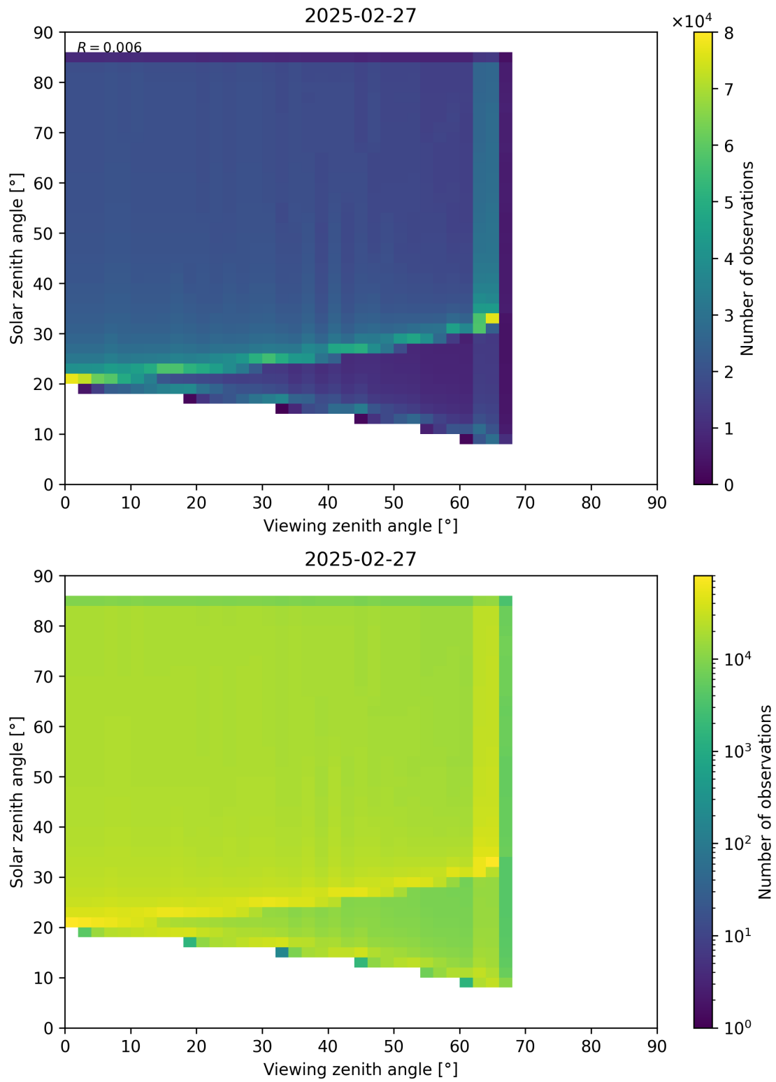
Figure 197: Scatter density plot of “Viewing zenith angle” against “Solar zenith angle” for 2025-02-26 to 2025-02-28.
