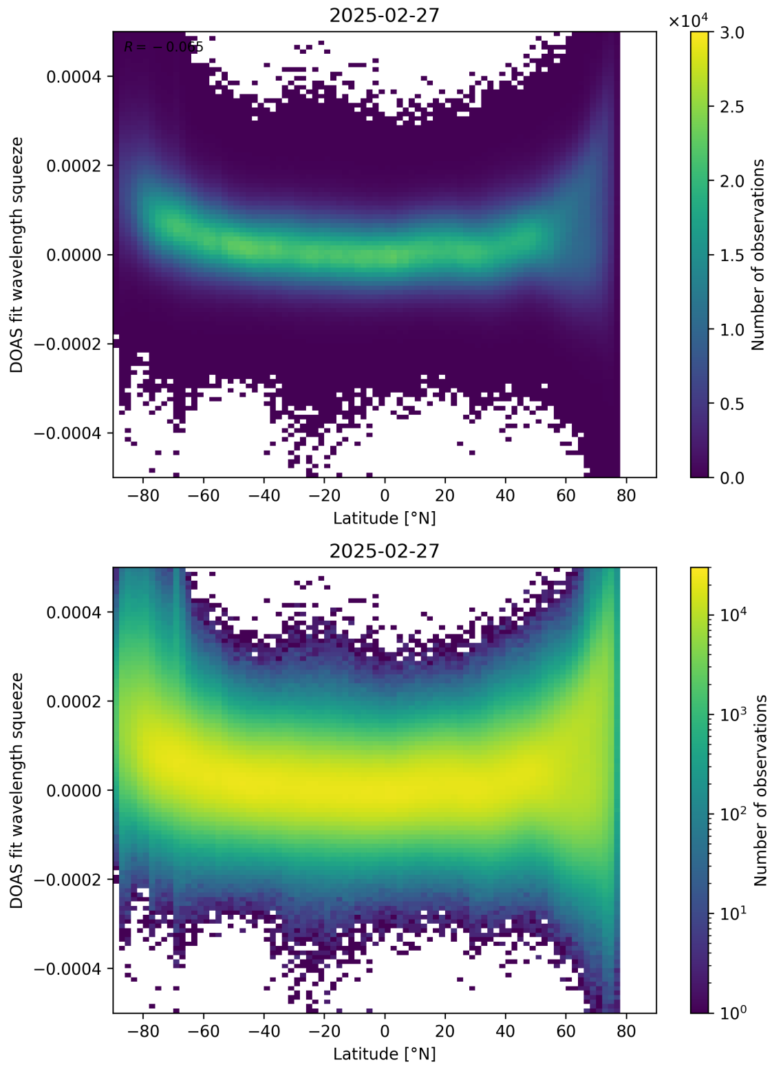
Figure 155: Scatter density plot of “Latitude” against “DOAS fit wavelength squeeze” for 2025-02-26 to 2025-02-28.
