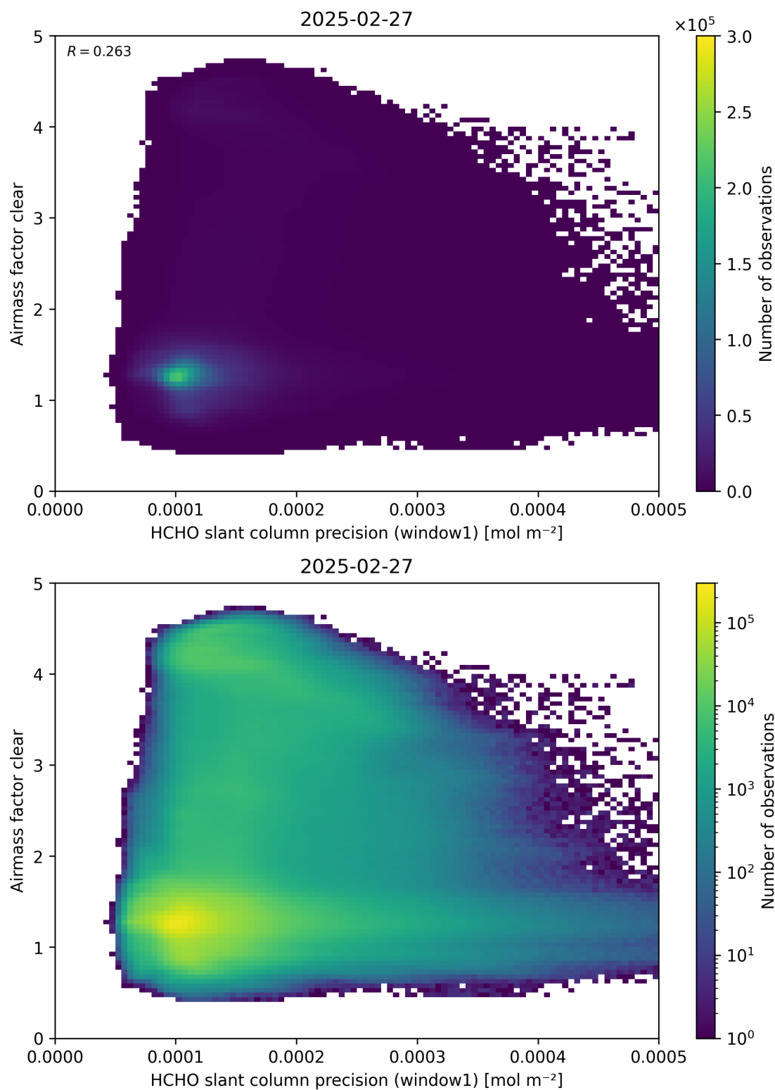
Figure 91: Scatter density plot of “HCHO slant column precision (window1)” against “Airmass factor clear” for 2025-02-26 to 2025-02-28.
