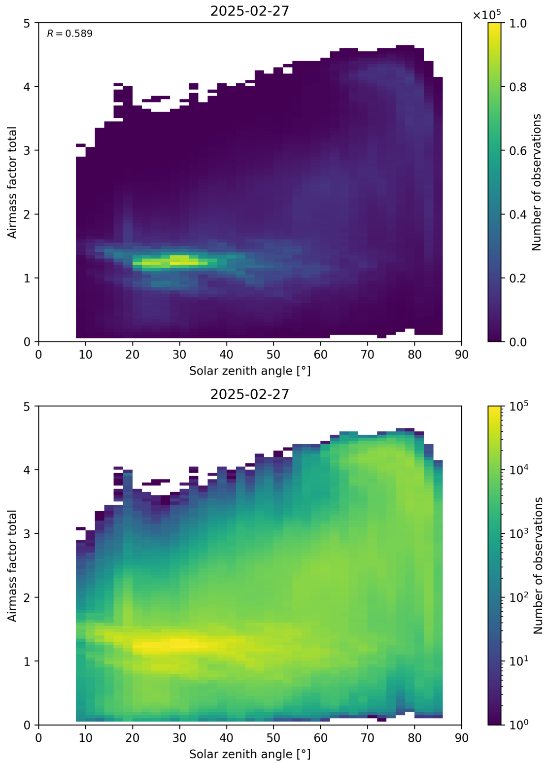
Figure 175: Scatter density plot of “Solar zenith angle” against “Airmass factor total” for 2025-02-26 to 2025-02-28.
