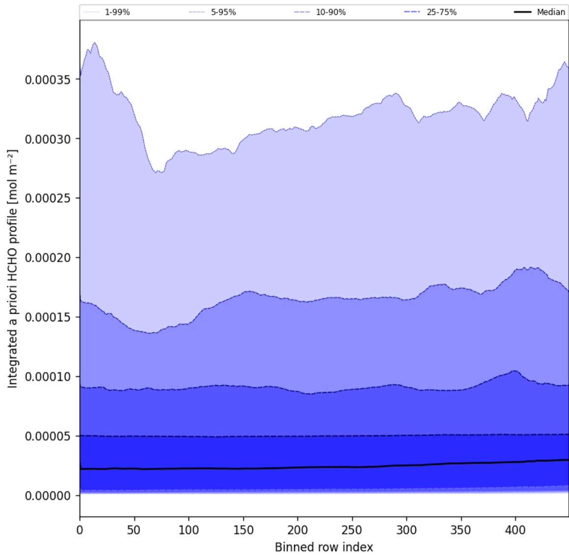
Figure 57: Along track statistics of “Integrated a priori HCHO profile” for 2025-02-26 to 2025-02-28
