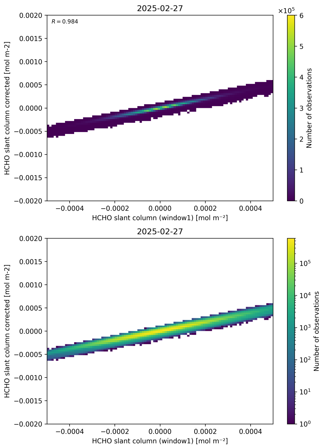
Figure 82: Scatter density plot of “HCHO slant column (window1)” against “HCHO slant column corrected” for 2025-02-26 to 2025-02-28.
