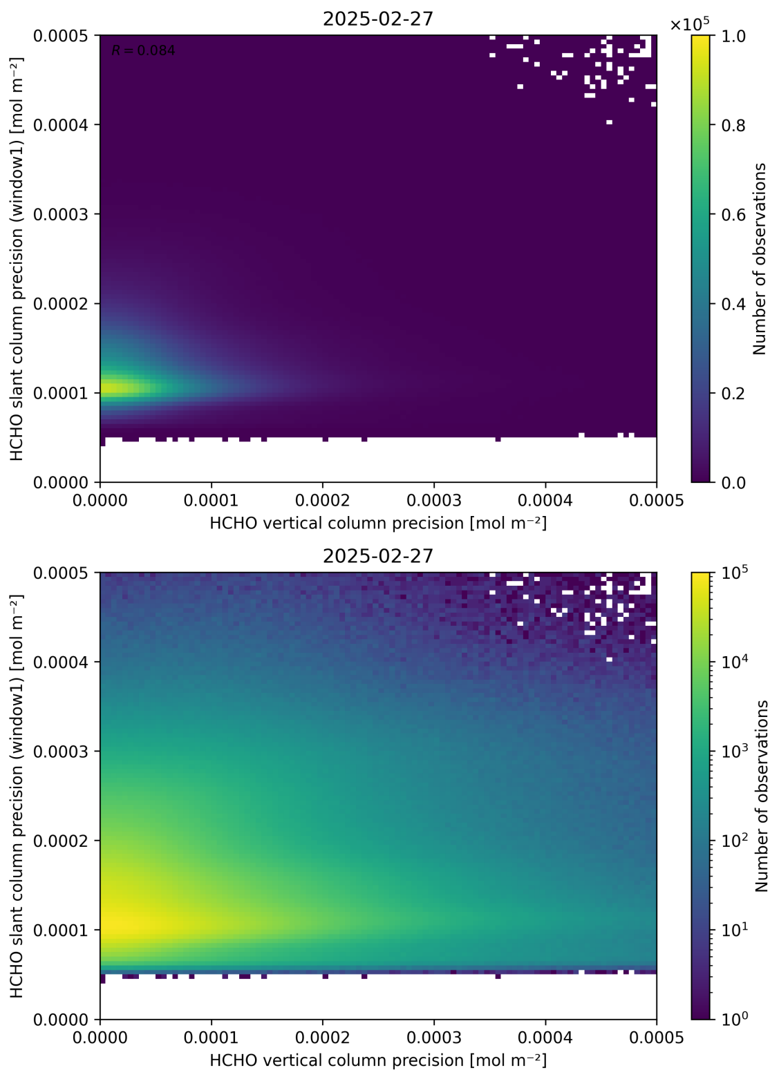
Figure 143: Scatter density plot of “HCHO vertical column precision” against “HCHO slant column precision (window1)” for 2025-02-26 to 2025-02-28.
