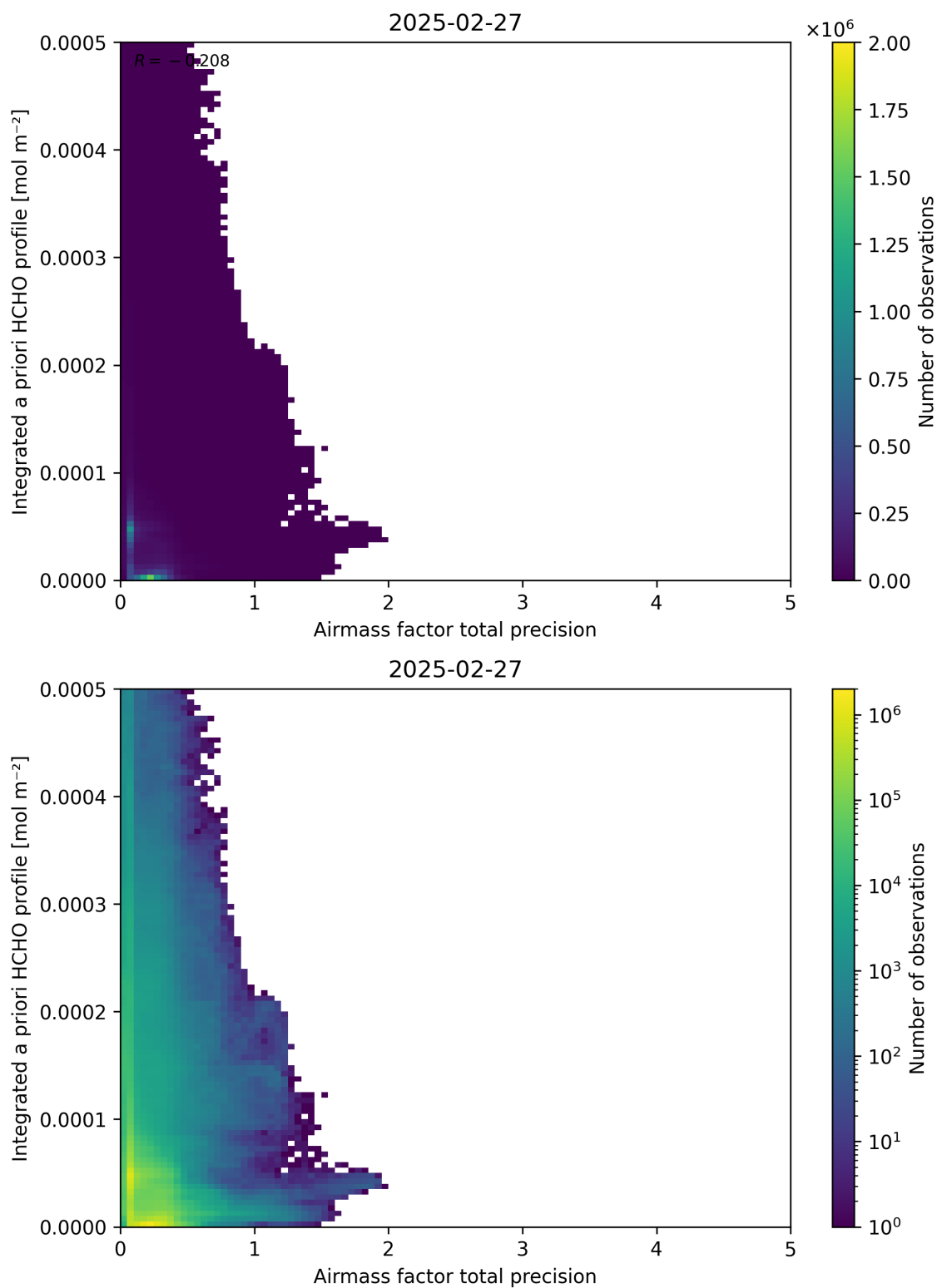
Figure 111: Scatter density plot of “Airmass factor total precision” against “Integrated a priori HCHO profile” for 2025-02-26 to 2025-02-28.
