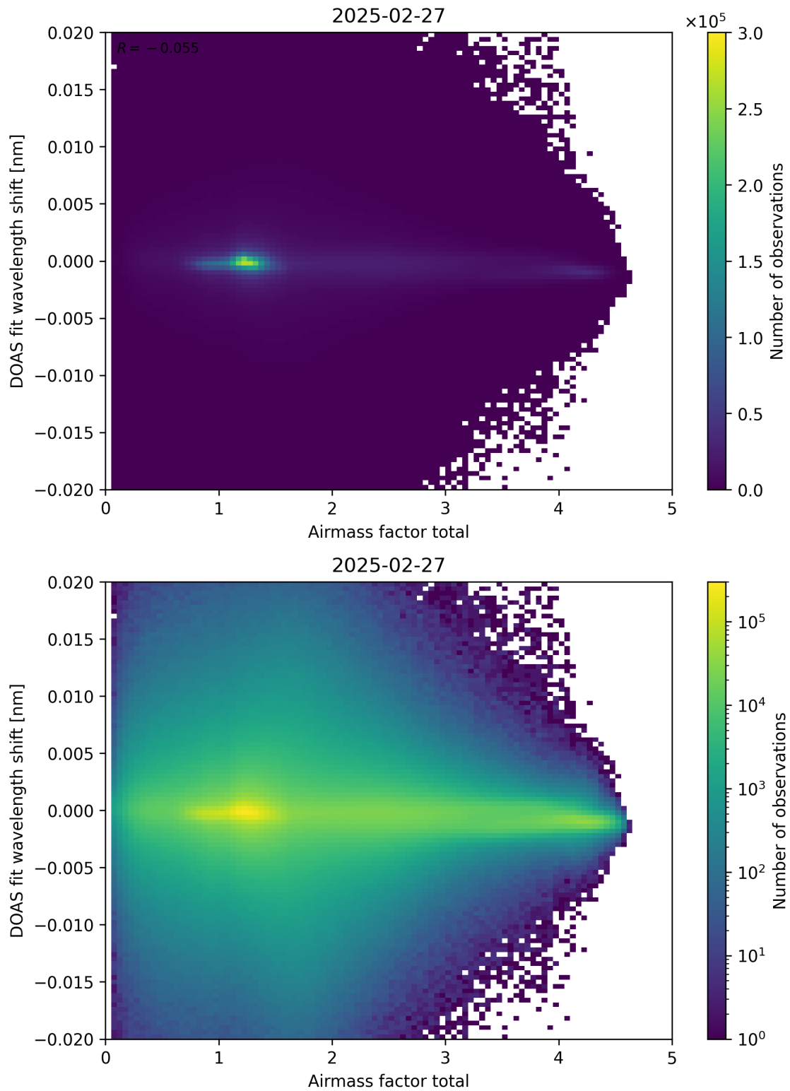
Figure 98: Scatter density plot of “Airmass factor total” against “DOAS fit wavelength shift” for 2025-02-26 to 2025-02-28.
