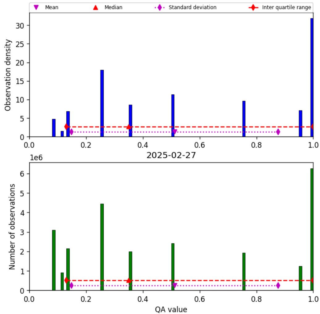
Figure 34: Histogram of “QA value” for 2025-02-26 to 2025-02-28
