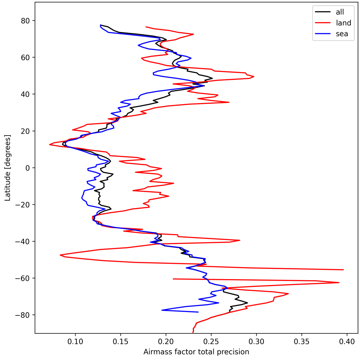
Figure 27: Zonal average of “Airmass factor total precision” for 2025-02-26 to 2025-02-28.
