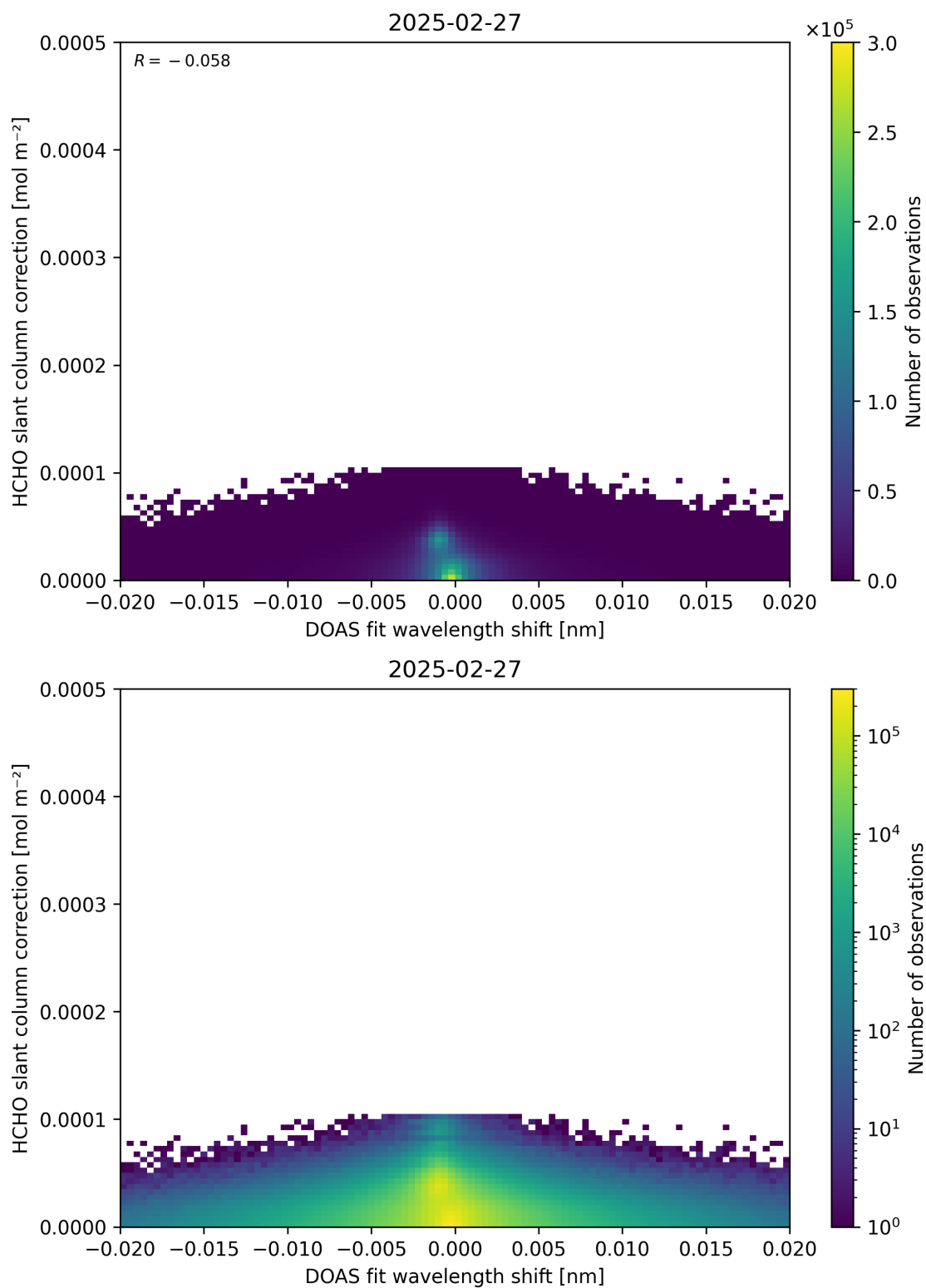
Figure 67: Scatter density plot of “DOAS fit wavelength shift” against “HCHO slant column correction” for 2025-02-26 to 2025-02-28.
