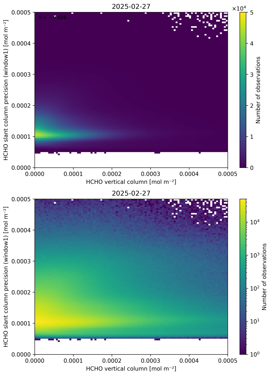
Figure 130: Scatter density plot of “HCHO vertical column” against “HCHO slant column precision (window1)” for 2025-02-26 to 2025-02-28.
