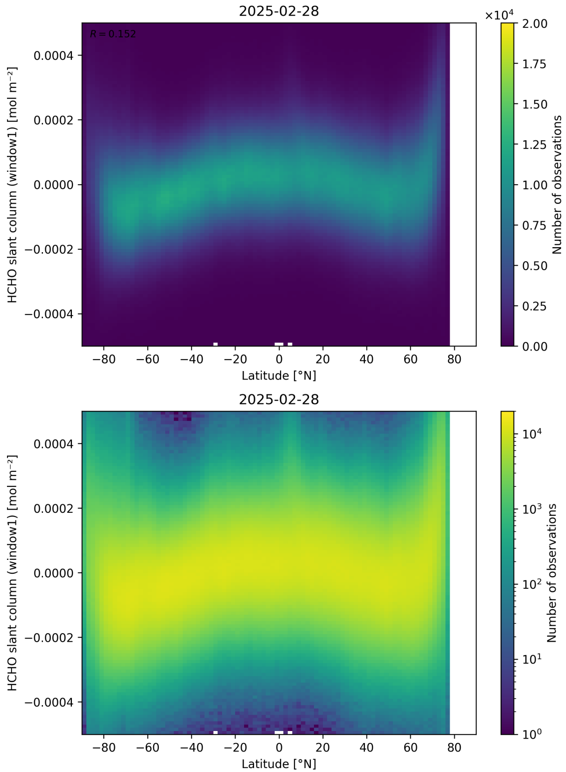
Figure 159: Scatter density plot of “Latitude” against “HCHO slant column (window1)” for 2025-02-27 to 2025-03-01.
