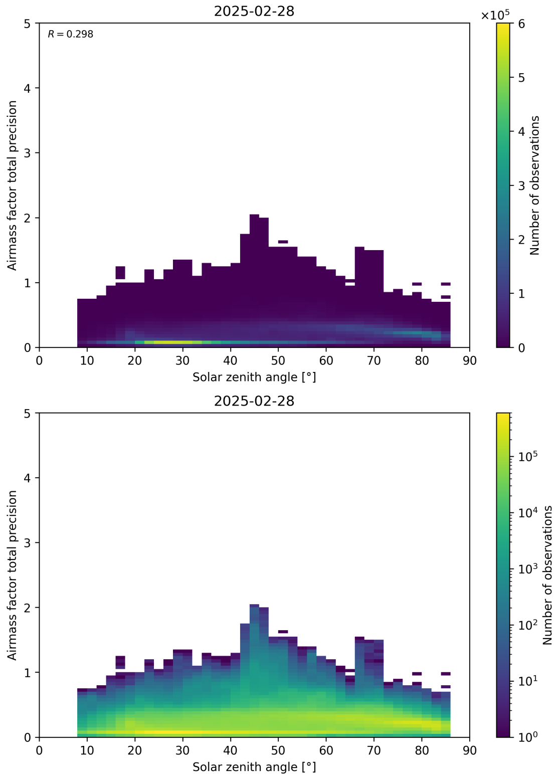
Figure 176: Scatter density plot of “Solar zenith angle” against “Airmass factor total precision” for 2025-02-27 to 2025-03-01.
