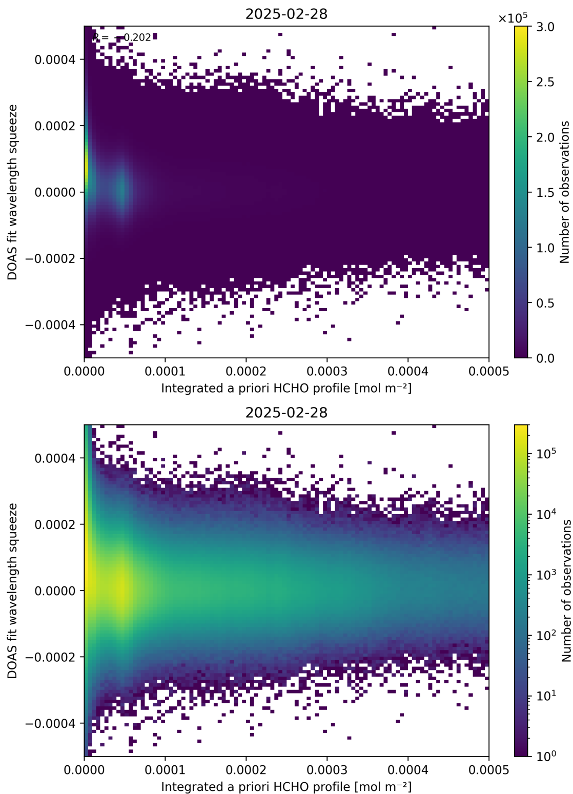
Figure 150: Scatter density plot of “Integrated a priori HCHO profile” against “DOAS fit wavelength squeeze” for 2025-02-27 to 2025-03-01.
