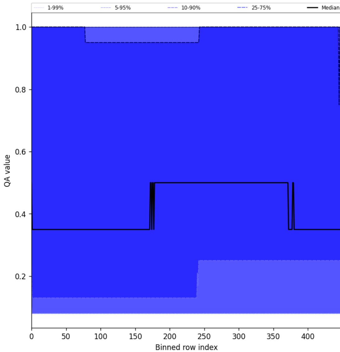
Figure 48: Along track statistics of “QA value” for 2025-02-27 to 2025-03-01
