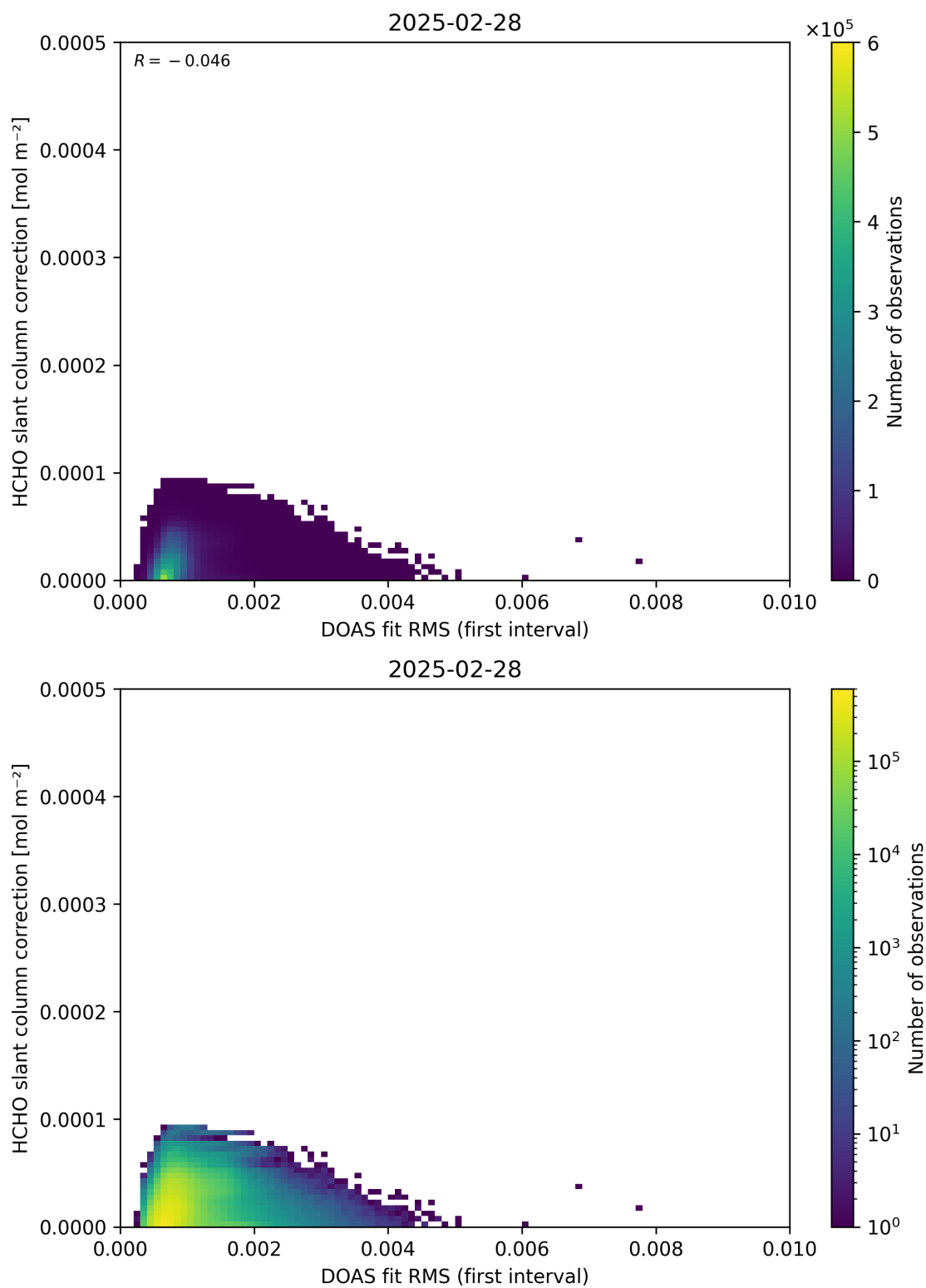
Figure 63: Scatter density plot of “DOAS fit RMS (first interval)” against “HCHO slant column correction” for 2025-02-27 to 2025-03-01.
