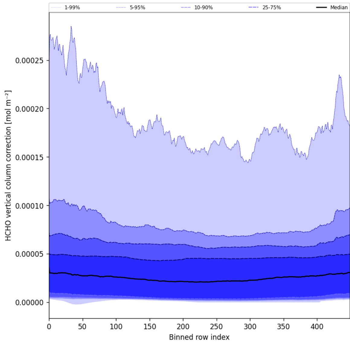
Figure 51: Along track statistics of “HCHO vertical column correction” for 2025-02-27 to 2025-03-01
