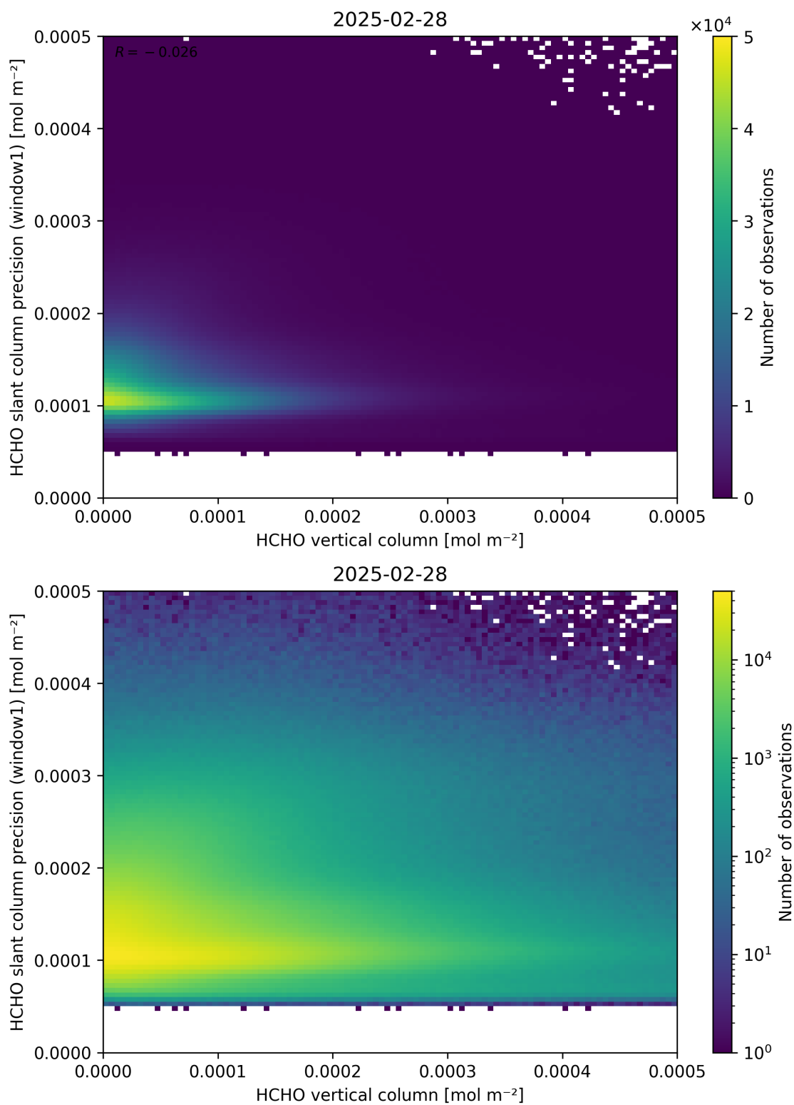
Figure 130: Scatter density plot of “HCHO vertical column” against “HCHO slant column precision (window1)” for 2025-02-27 to 2025-03-01.
