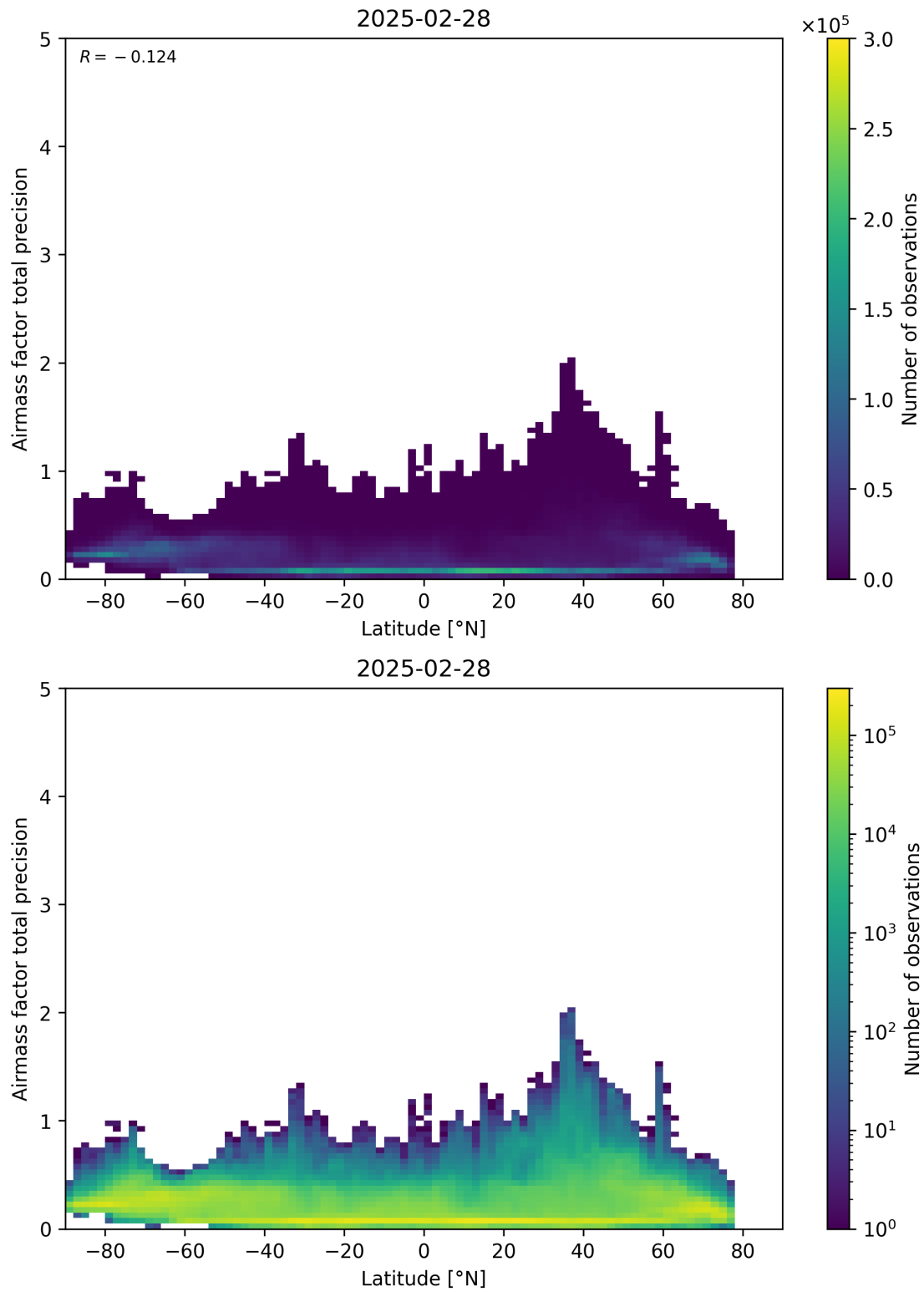
Figure 162: Scatter density plot of “Latitude” against “Airmass factor total precision” for 2025-02-27 to 2025-03-01.
