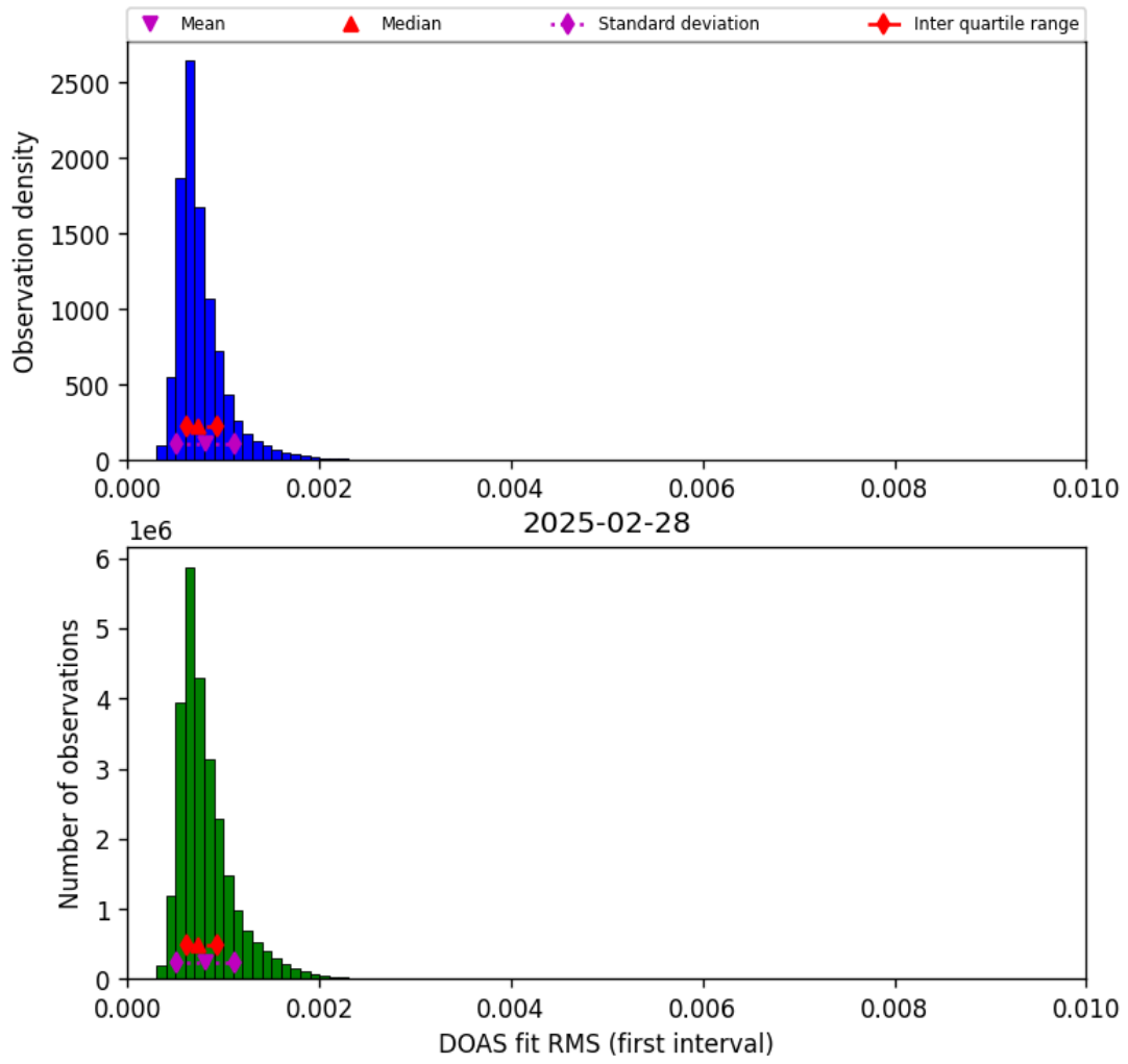
Figure 46: Histogram of “DOAS fit RMS (first interval)” for 2025-02-27 to 2025-03-01
