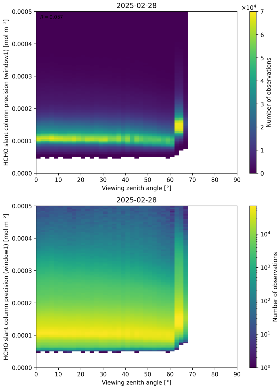
Figure 189: Scatter density plot of “Viewing zenith angle” against “HCHO slant column precision (window1)” for 2025-02-27 to 2025-03-01.
