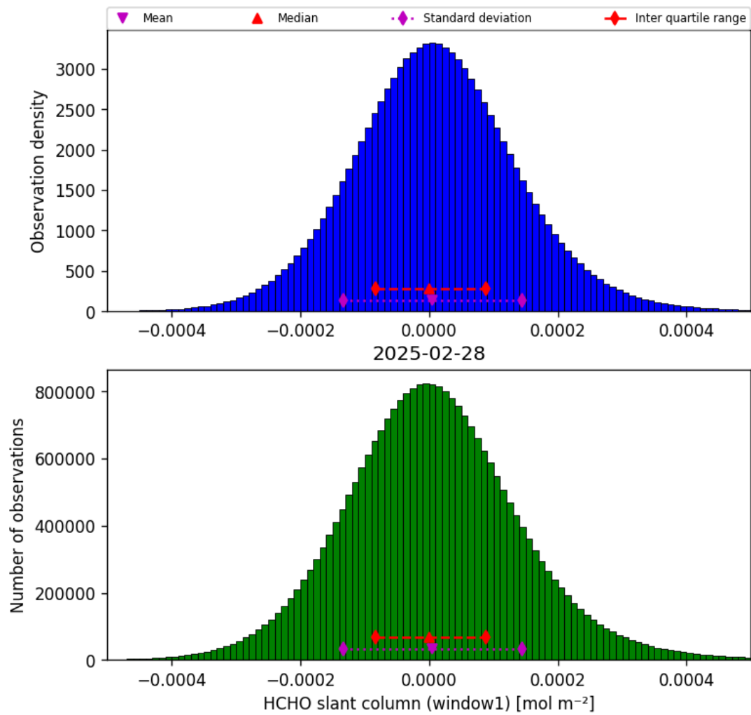
Figure 38: Histogram of “HCHO slant column (window1)” for 2025-02-27 to 2025-03-01
