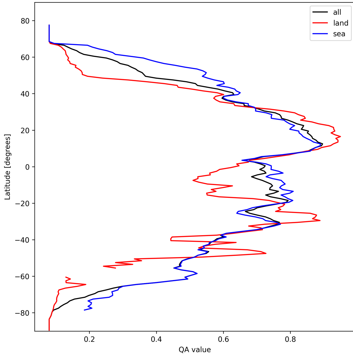
Figure 20: Zonal average of “QA value” for 2025-02-27 to 2025-03-01.
