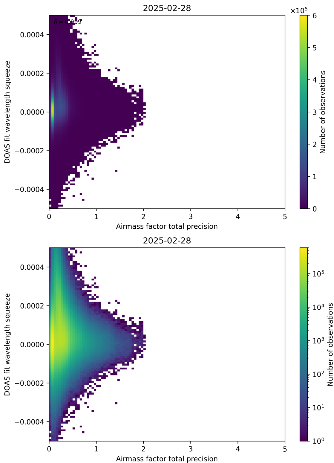
Figure 107: Scatter density plot of “Airmass factor total precision” against “DOAS fit wavelength squeeze” for 2025-02-27 to 2025-03-01.
