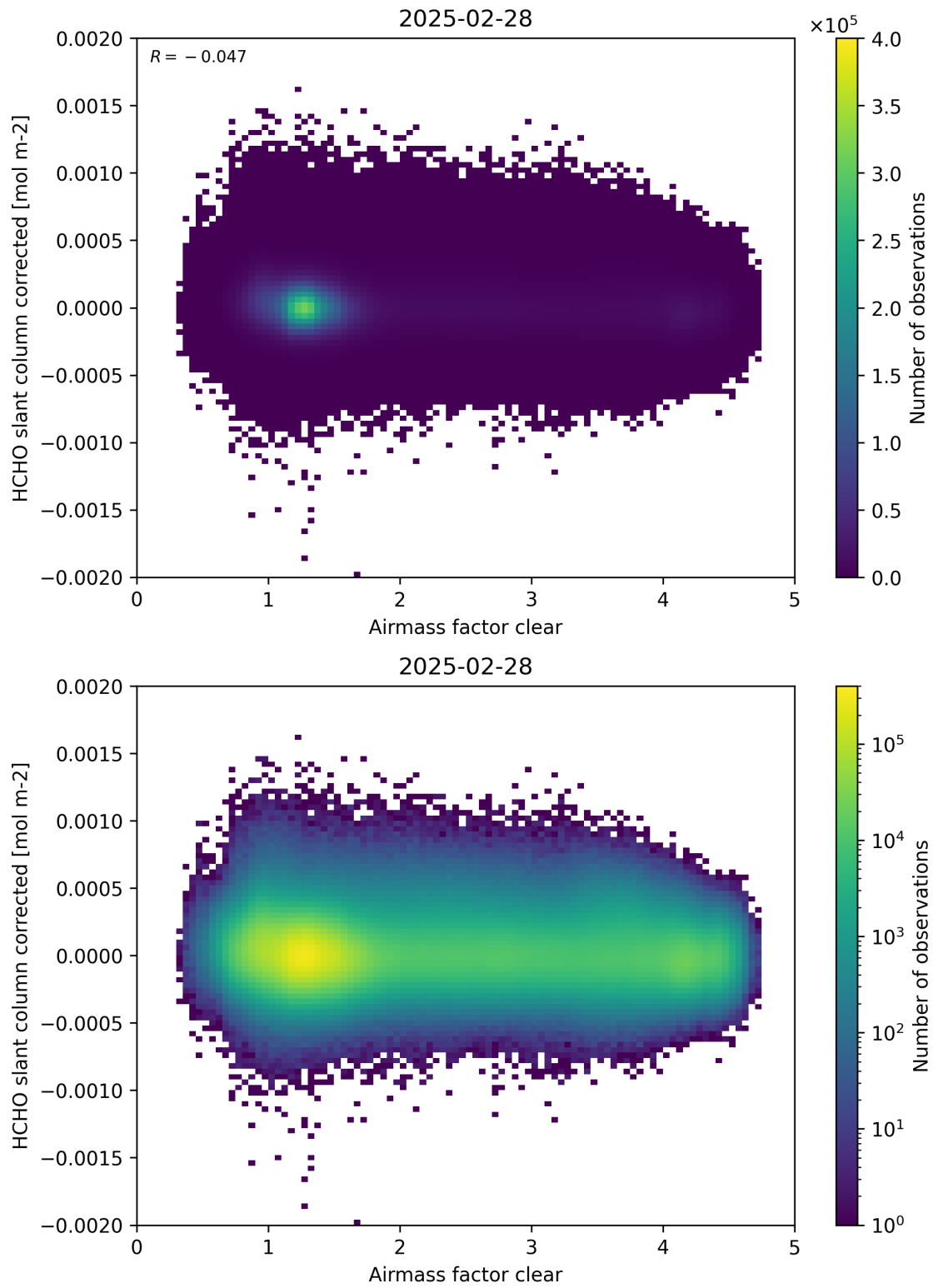
Figure 74: Scatter density plot of “Airmass factor clear” against “HCHO slant column corrected” for 2025-02-27 to 2025-03-01.
