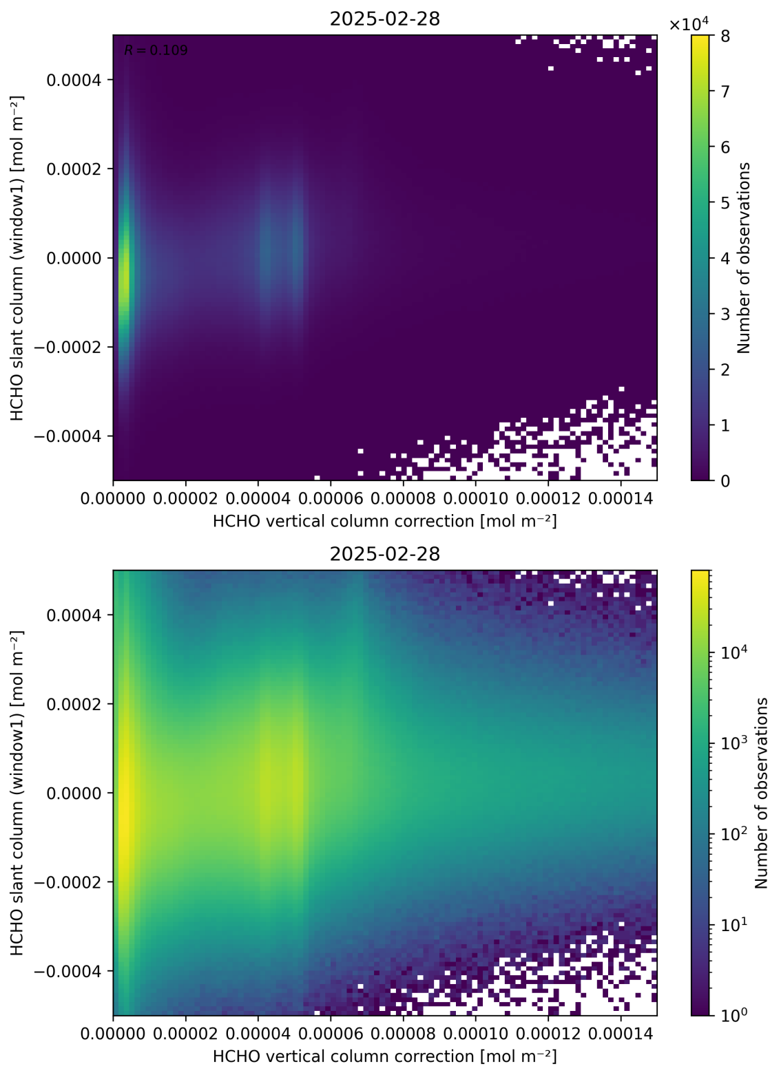
Figure 118: Scatter density plot of “HCHO vertical column correction” against “HCHO slant column (window1)” for 2025-02-27 to 2025-03-01.
