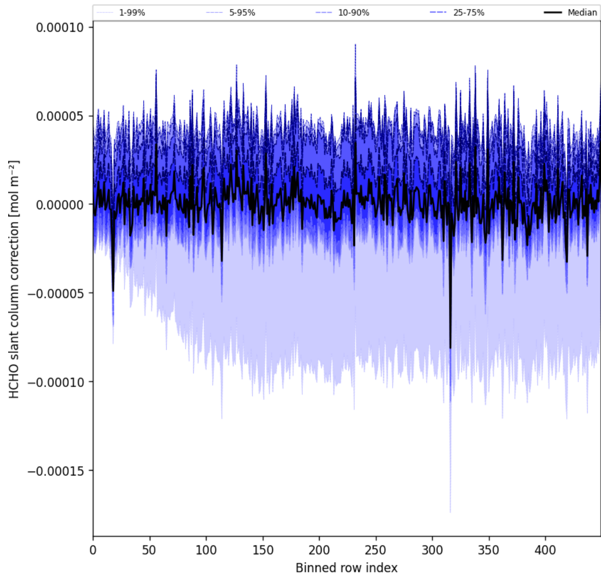
Figure 61: Along track statistics of “HCHO slant column correction” for 2025-02-27 to 2025-03-01
