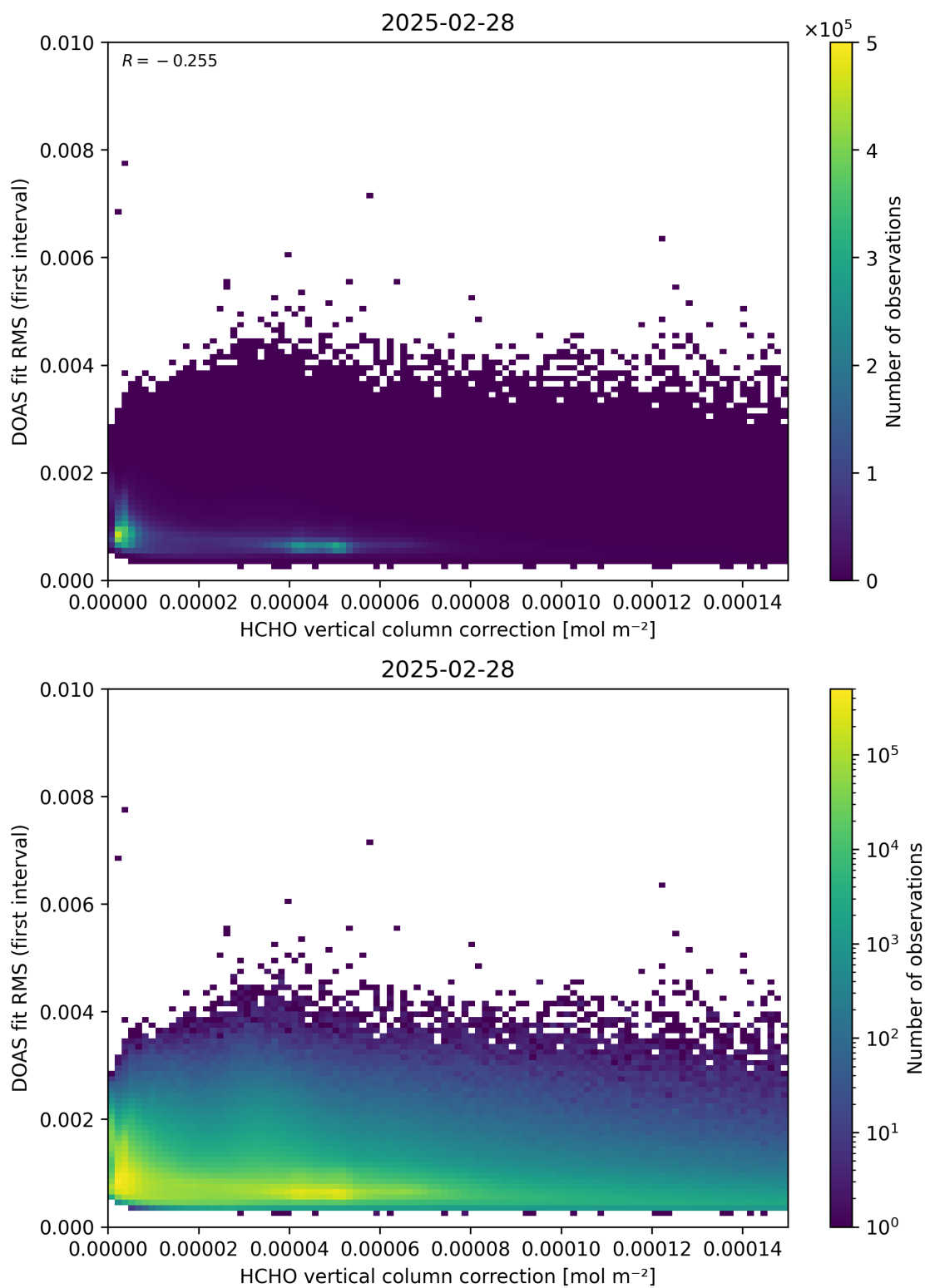
Figure 112: Scatter density plot of “HCHO vertical column correction” against “DOAS fit RMS (first interval)” for 2025-02-27 to 2025-03-01.
