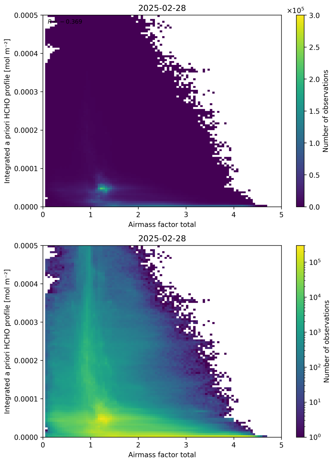
Figure 104: Scatter density plot of “Airmass factor total” against “Integrated a priori HCHO profile” for 2025-02-27 to 2025-03-01.
