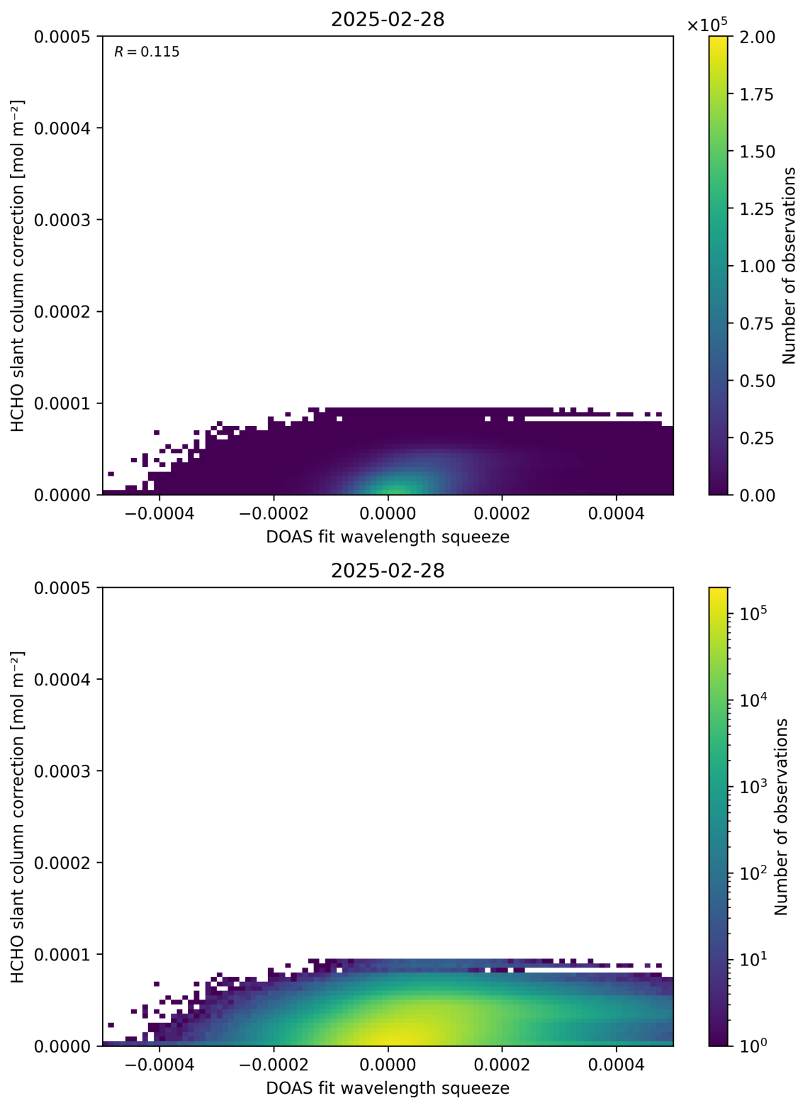
Figure 70: Scatter density plot of “DOAS fit wavelength squeeze” against “HCHO slant column correction” for 2025-02-27 to 2025-03-01.
