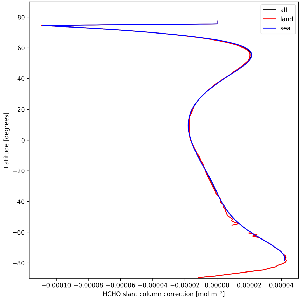
Figure 33: Zonal average of “HCHO slant column correction” for 2025-02-27 to 2025-03-01.
