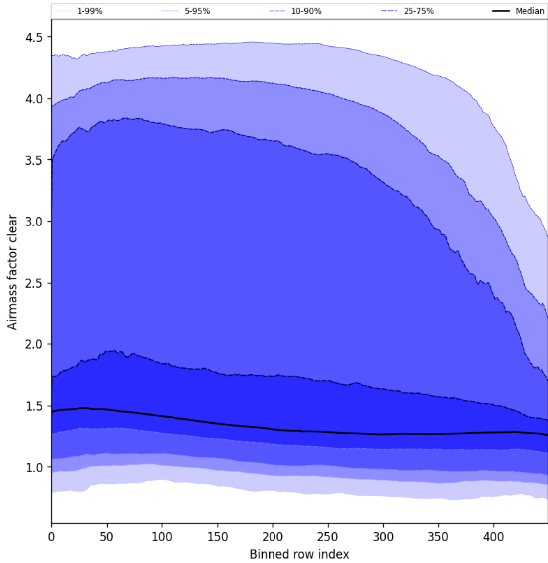
Figure 56: Along track statistics of “Airmass factor clear” for 2025-02-27 to 2025-03-01
