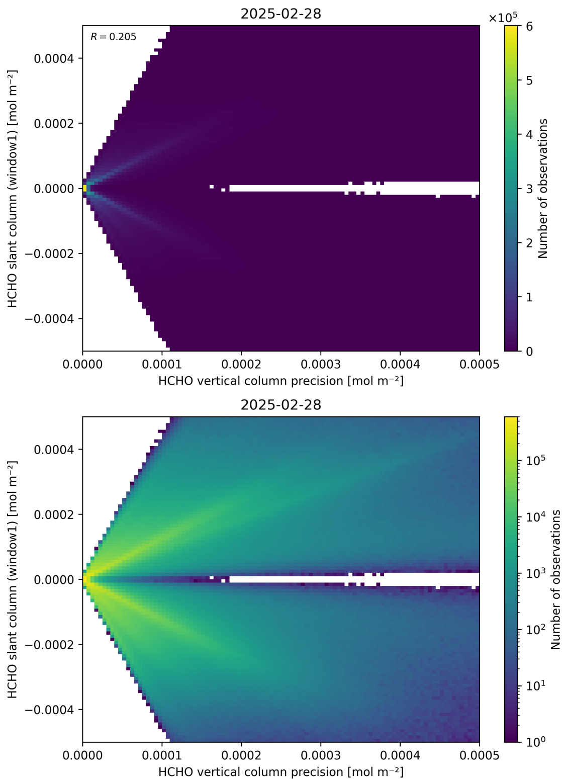
Figure 142: Scatter density plot of “HCHO vertical column precision” against “HCHO slant column (window1)” for 2025-02-27 to 2025-03-01.
