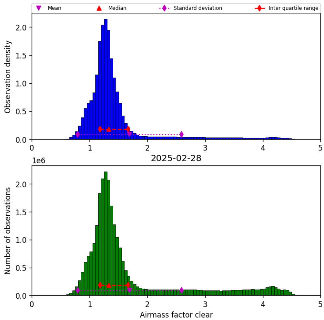
Figure 42: Histogram of “Airmass factor clear” for 2025-02-27 to 2025-03-01
