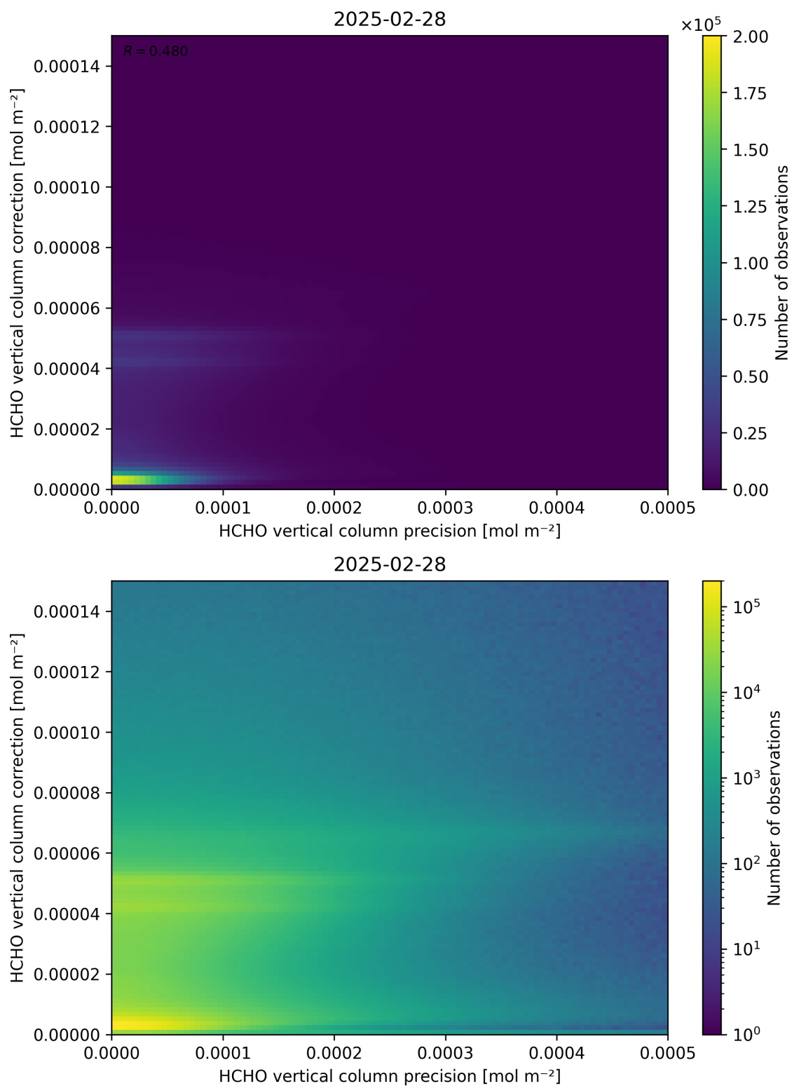
Figure 146: Scatter density plot of “HCHO vertical column precision” against “HCHO vertical column correction” for 2025-02-27 to 2025-03-01.
