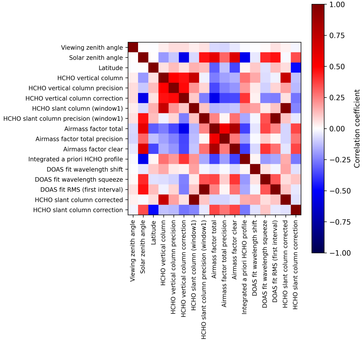
Figure 2: Map of correlation matrix for 2025-02-27 to 2025-03-01.
