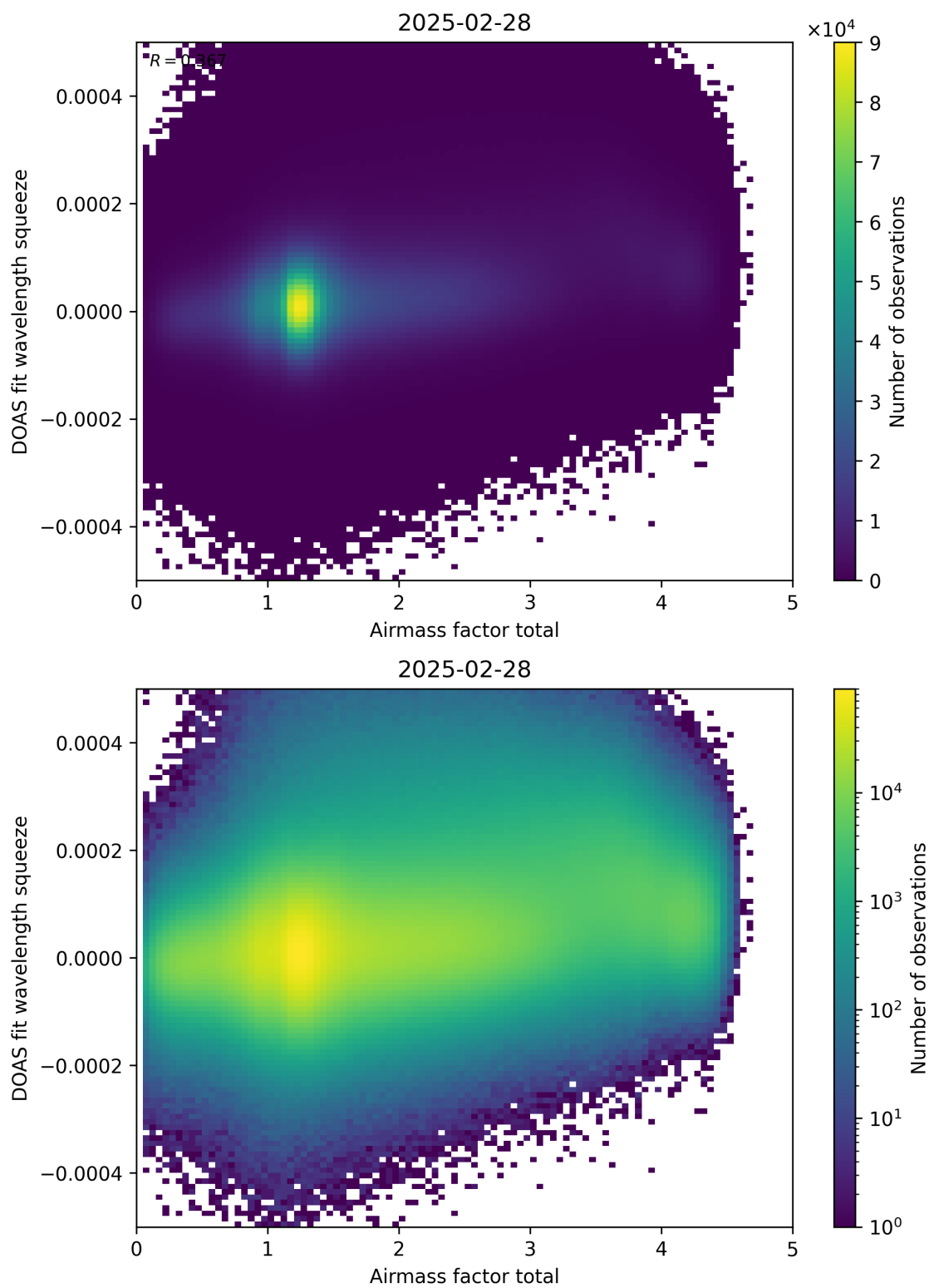
Figure 99: Scatter density plot of “Airmass factor total” against “DOAS fit wavelength squeeze” for 2025-02-27 to 2025-03-01.
