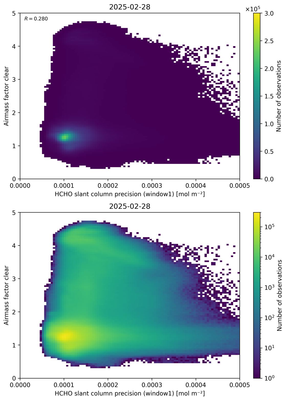
Figure 91: Scatter density plot of “HCHO slant column precision (window1)” against “Airmass factor clear” for 2025-02-27 to 2025-03-01.
