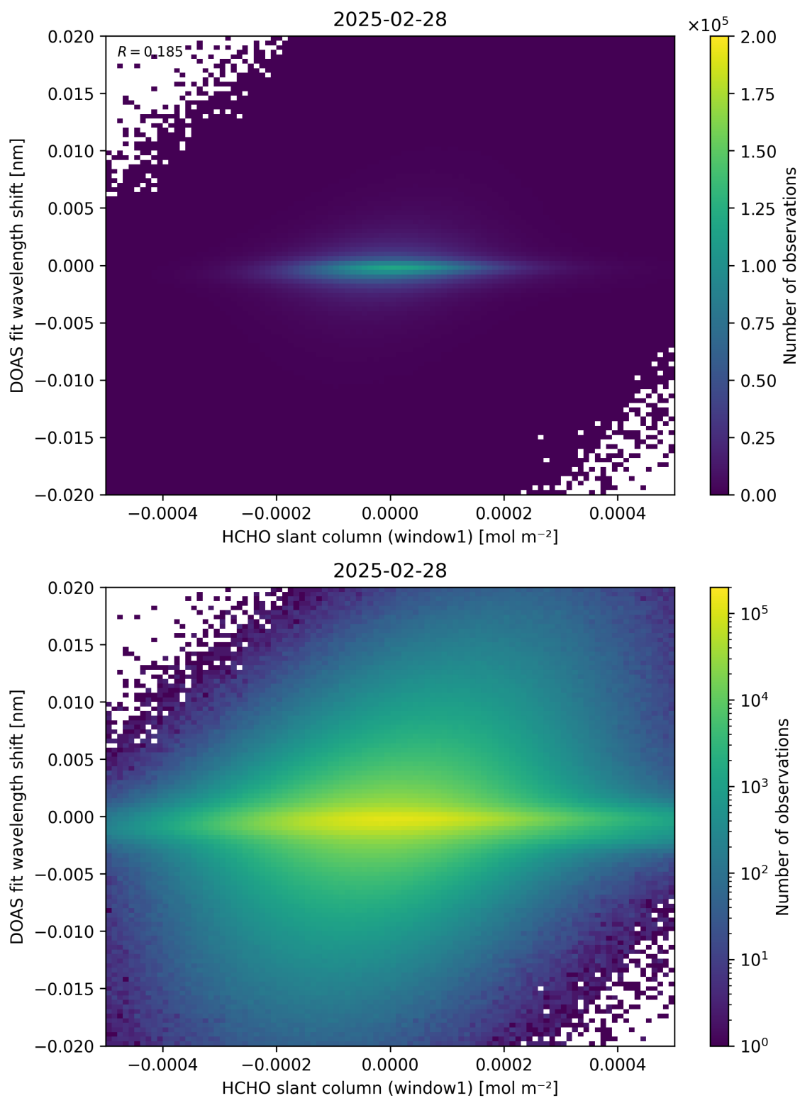
Figure 79: Scatter density plot of “HCHO slant column (window1)” against “DOAS fit wavelength shift” for 2025-02-27 to 2025-03-01.
