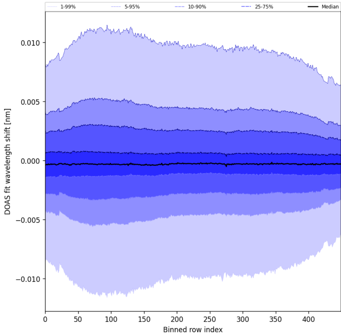
Figure 58: Along track statistics of “DOAS fit wavelength shift” for 2025-02-27 to 2025-03-01
