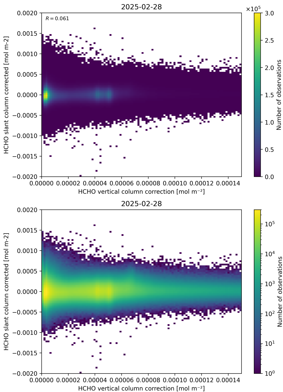
Figure 116: Scatter density plot of “HCHO vertical column correction” against “HCHO slant column corrected” for 2025-02-27 to 2025-03-01.
