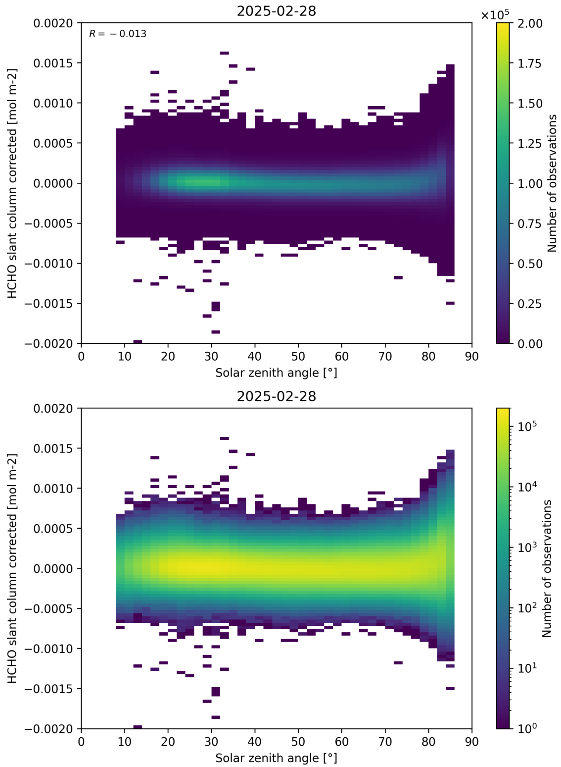
Figure 171: Scatter density plot of “Solar zenith angle” against “HCHO slant column corrected” for 2025-02-27 to 2025-03-01.
