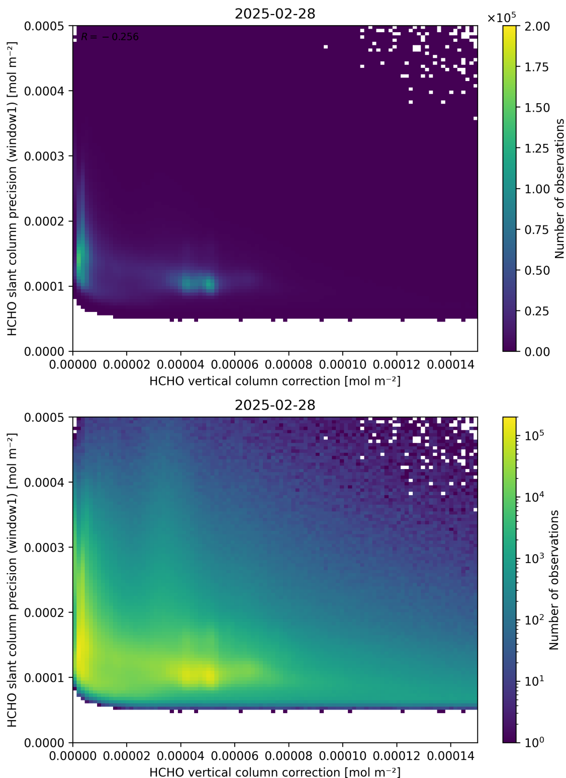
Figure 119: Scatter density plot of “HCHO vertical column correction” against “HCHO slant column precision (window1)” for 2025-02-27 to 2025-03-01.
