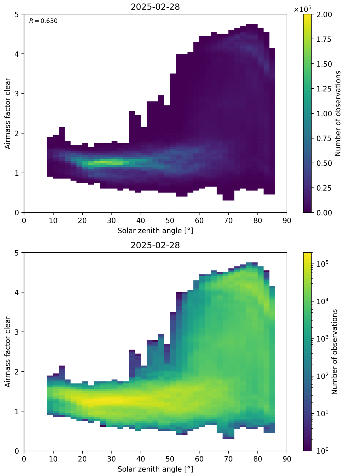
Figure 170: Scatter density plot of “Solar zenith angle” against “Airmass factor clear” for 2025-02-27 to 2025-03-01.
