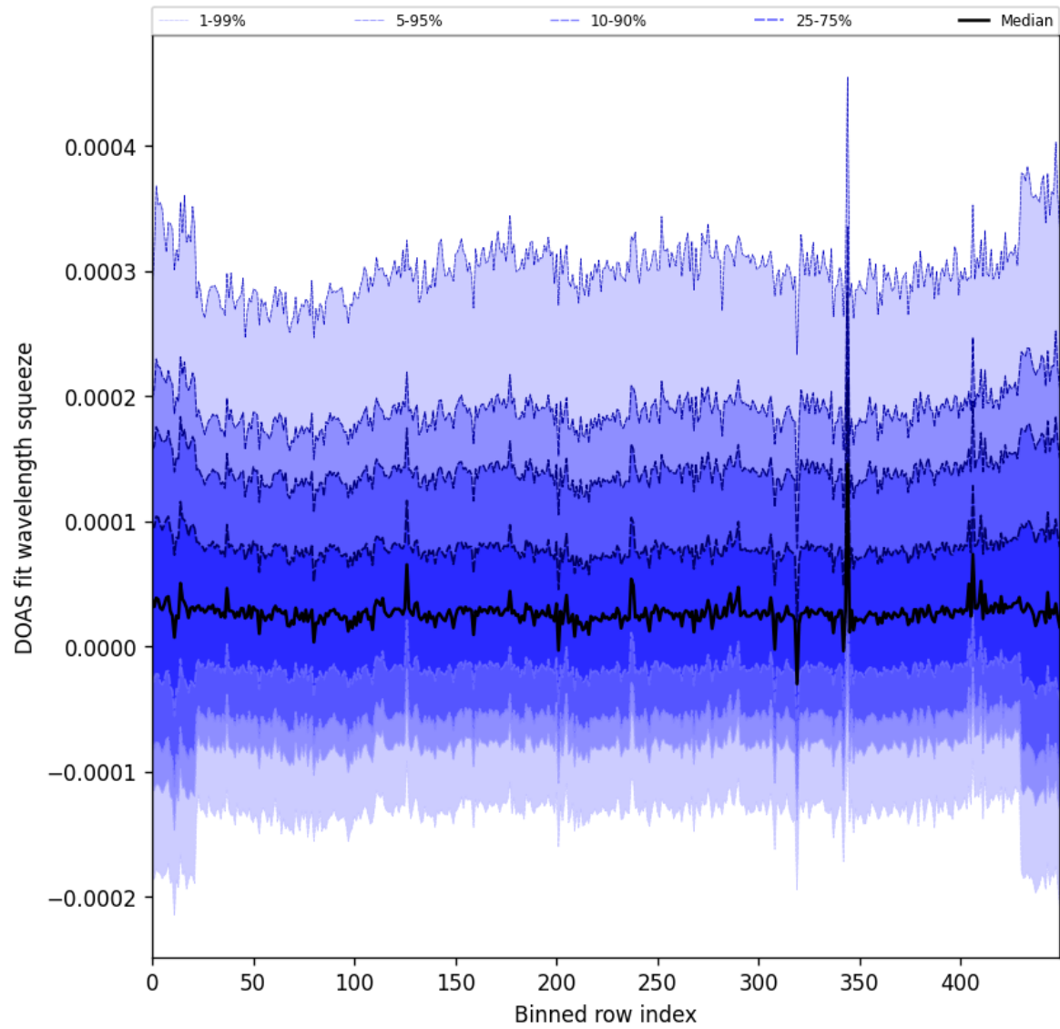
Figure 59: Along track statistics of “DOAS fit wavelength squeeze” for 2025-02-27 to 2025-03-01
