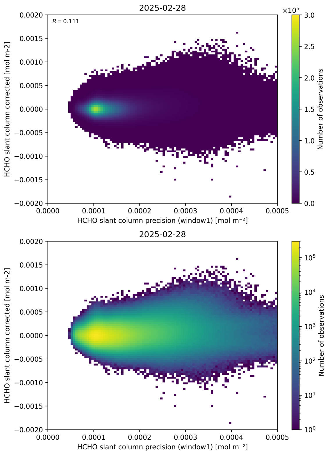
Figure 92: Scatter density plot of “HCHO slant column precision (window1)” against “HCHO slant column corrected” for 2025-02-27 to 2025-03-01.
