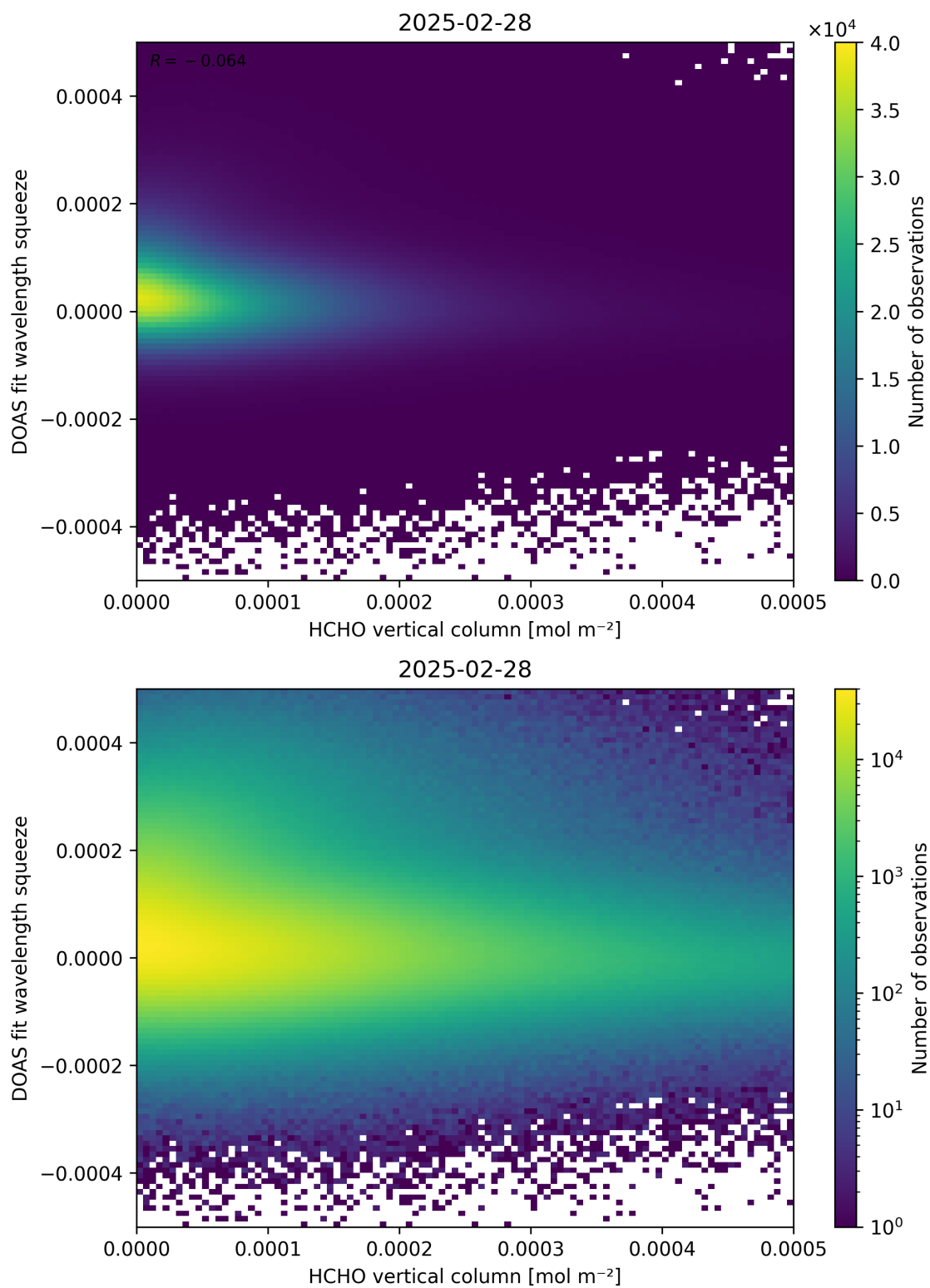
Figure 125: Scatter density plot of “HCHO vertical column” against “DOAS fit wavelength squeeze” for 2025-02-27 to 2025-03-01.
