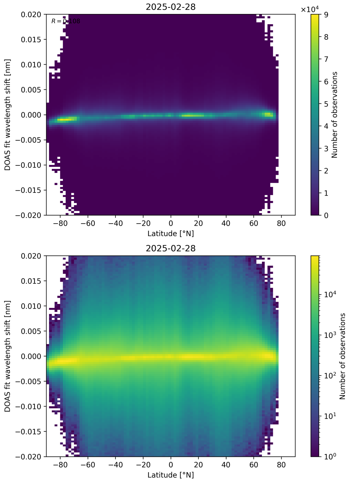
Figure 154: Scatter density plot of “Latitude” against “DOAS fit wavelength shift” for 2025-02-27 to 2025-03-01.
