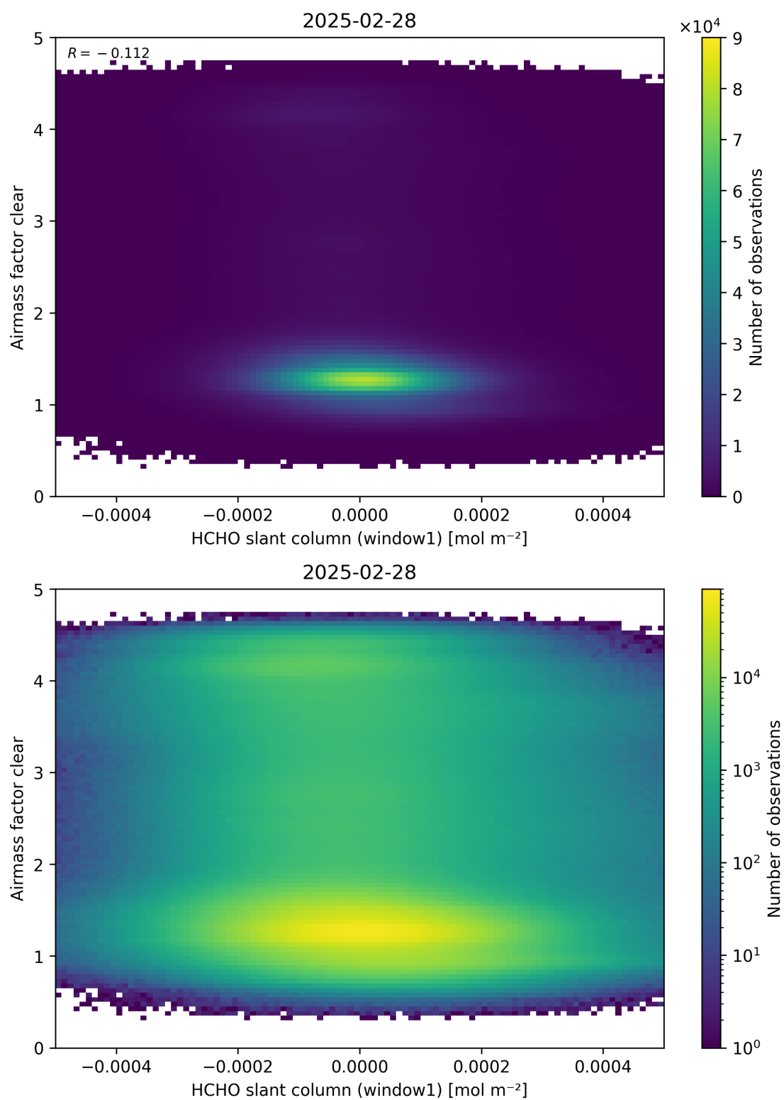
Figure 81: Scatter density plot of “HCHO slant column (window1)” against “Airmass factor clear” for 2025-02-27 to 2025-03-01.
