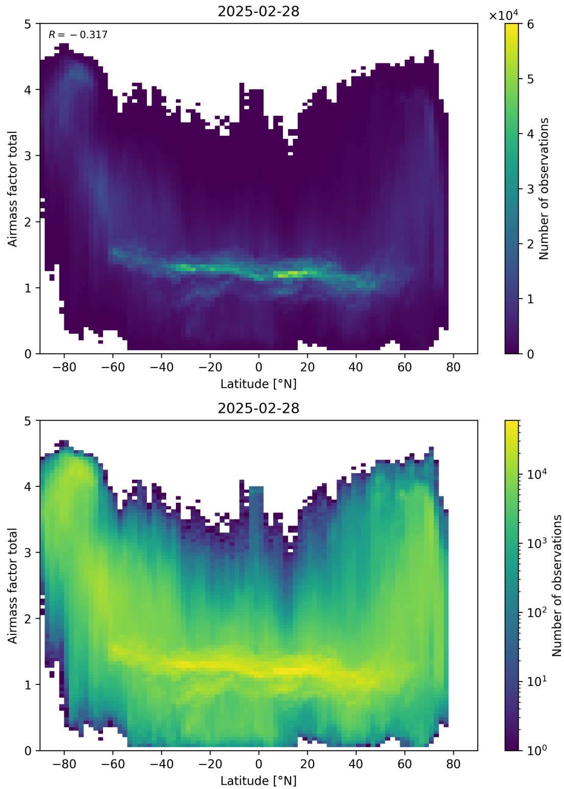
Figure 161: Scatter density plot of “Latitude” against “Airmass factor total” for 2025-02-27 to 2025-03-01.
