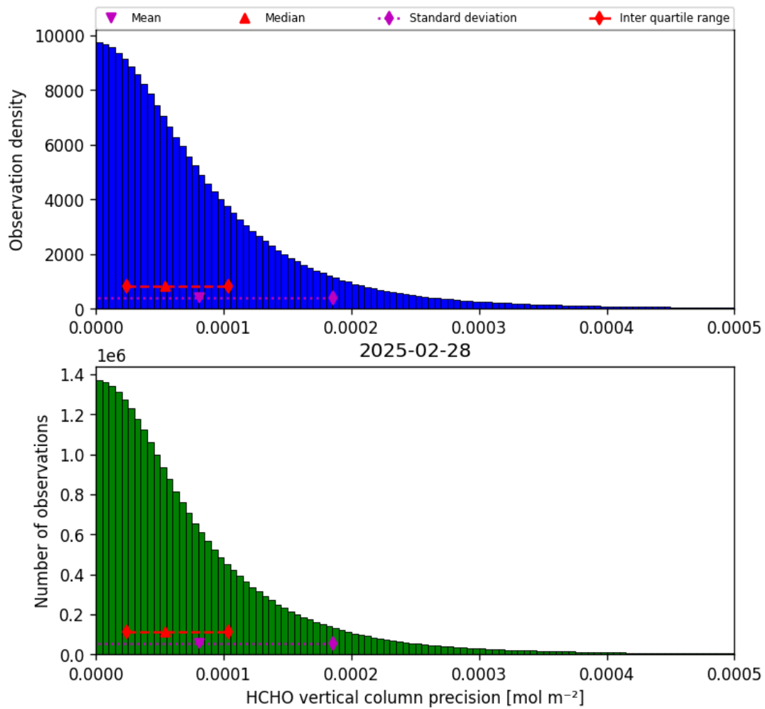
Figure 36: Histogram of “HCHO vertical column precision” for 2025-02-27 to 2025-03-01
