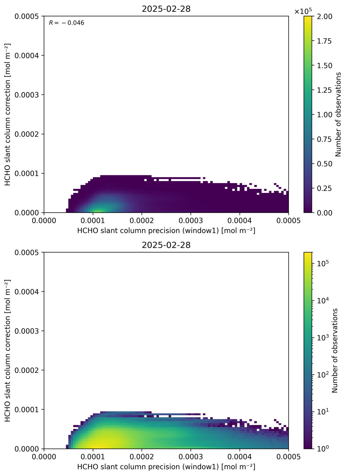
Figure 93: Scatter density plot of “HCHO slant column precision (window1)” against “HCHO slant column correction” for 2025-02-27 to 2025-03-01.
