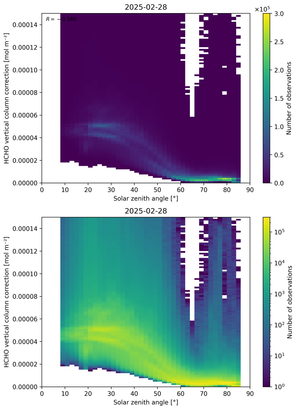
Figure 178: Scatter density plot of “Solar zenith angle” against “HCHO vertical column correction” for 2025-02-27 to 2025-03-01.
