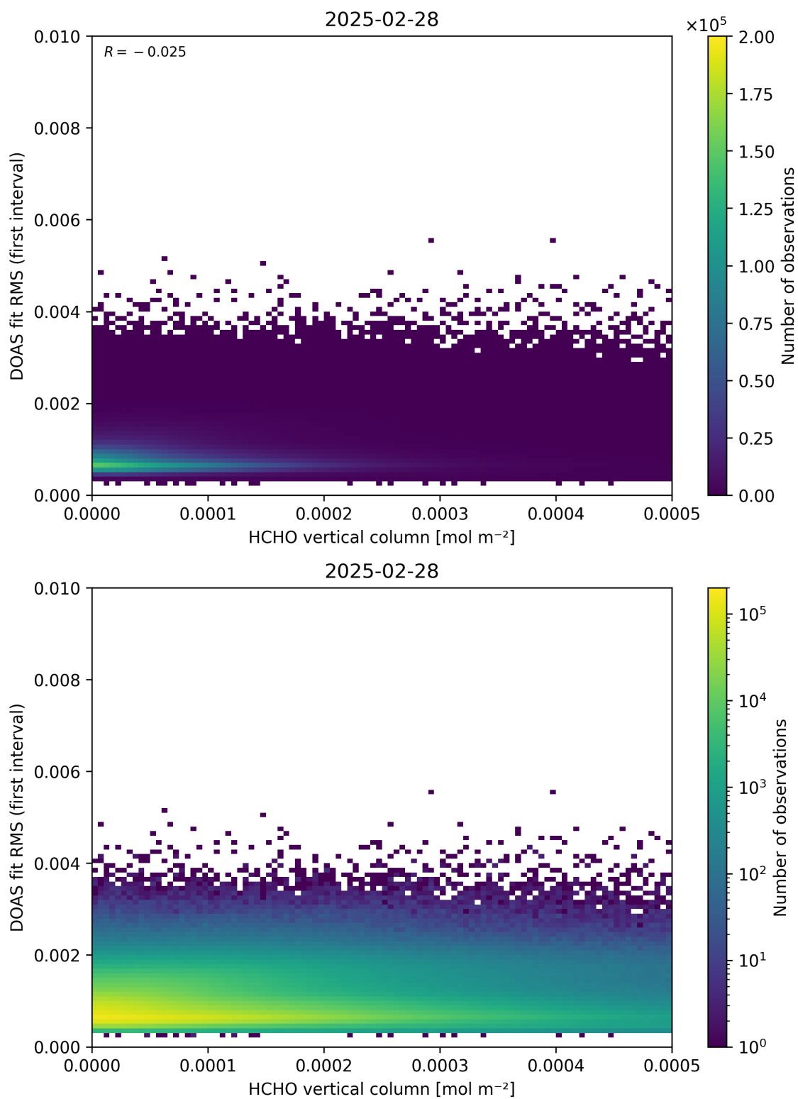
Figure 123: Scatter density plot of “HCHO vertical column” against “DOAS fit RMS (first interval)” for 2025-02-27 to 2025-03-01.
