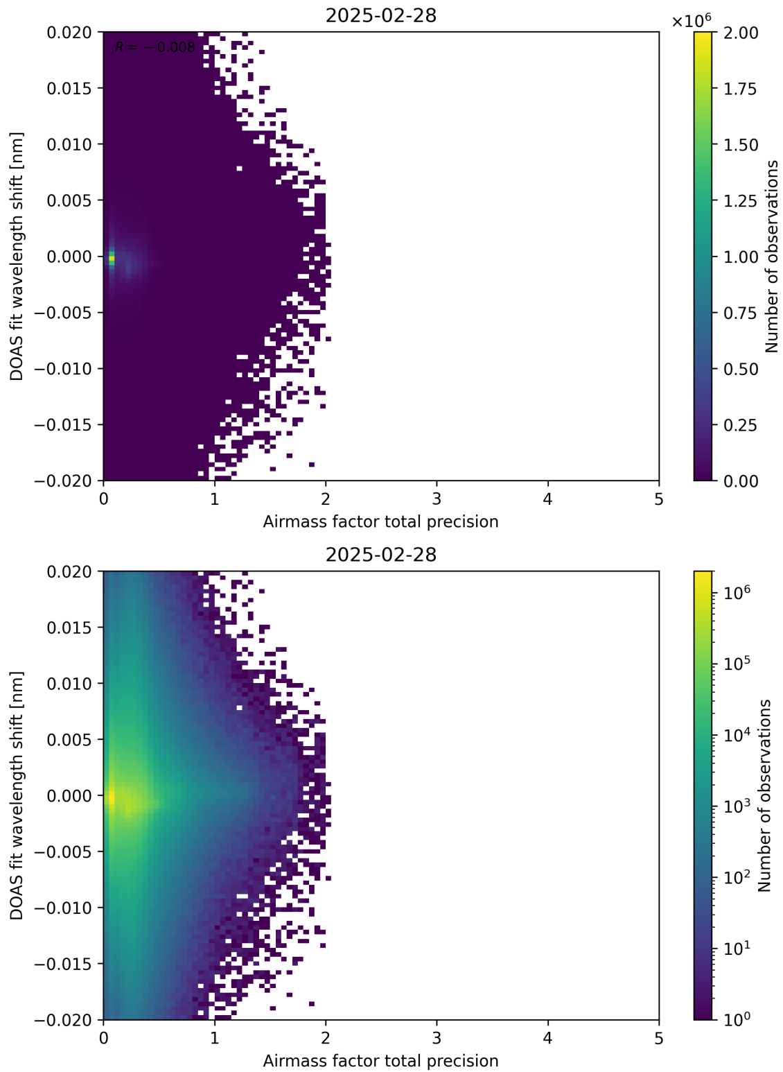
Figure 106: Scatter density plot of “Airmass factor total precision” against “DOAS fit wavelength shift” for 2025-02-27 to 2025-03-01.
