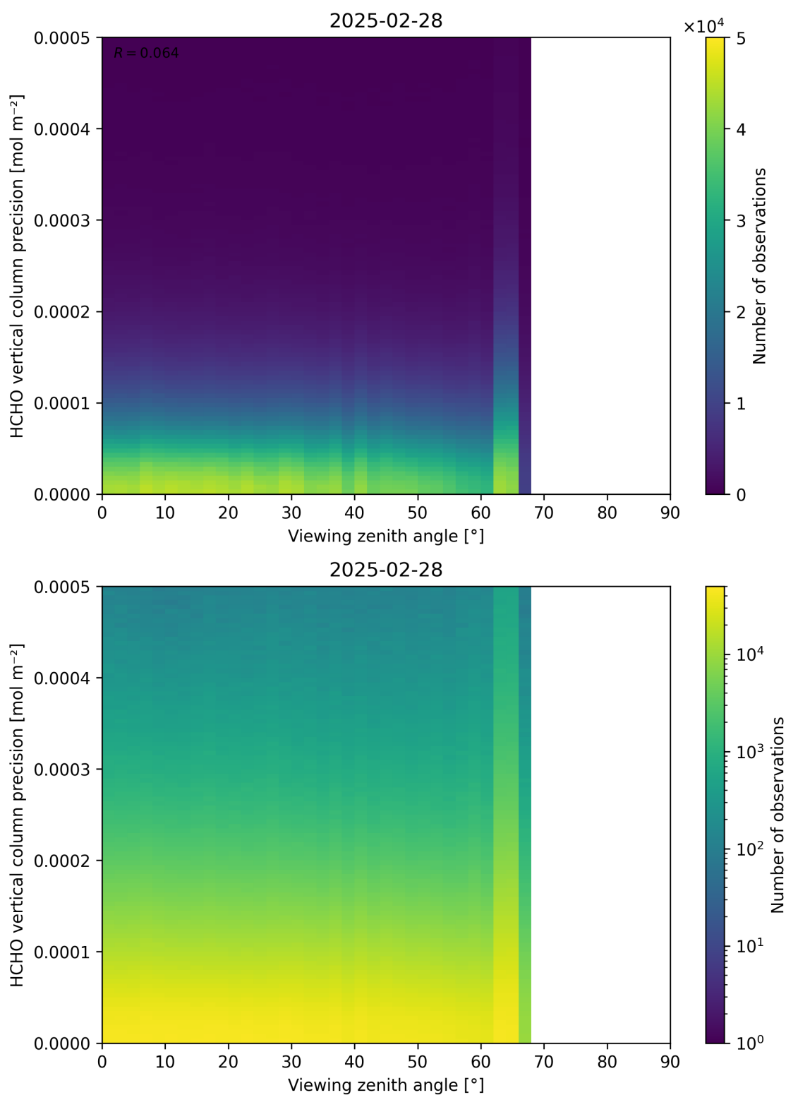
Figure 194: Scatter density plot of “Viewing zenith angle” against “HCHO vertical column precision” for 2025-02-27 to 2025-03-01.
