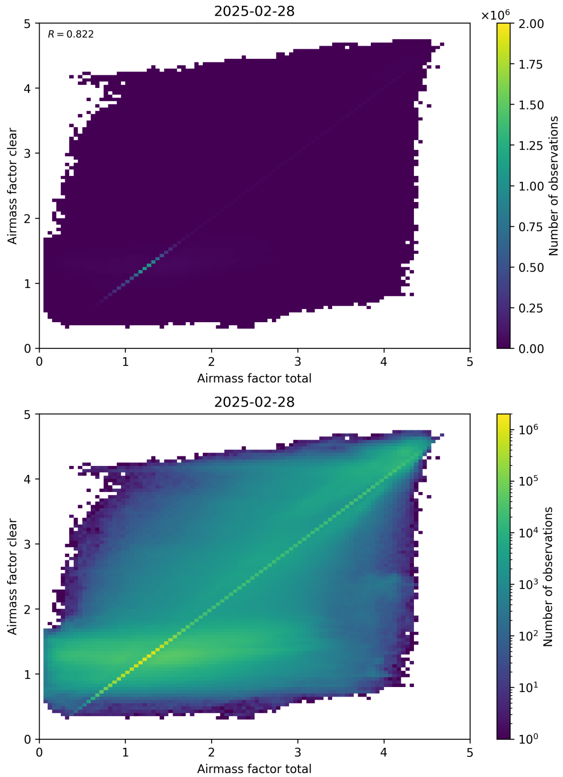
Figure 100: Scatter density plot of “Airmass factor total” against “Airmass factor clear” for 2025-02-27 to 2025-03-01.
