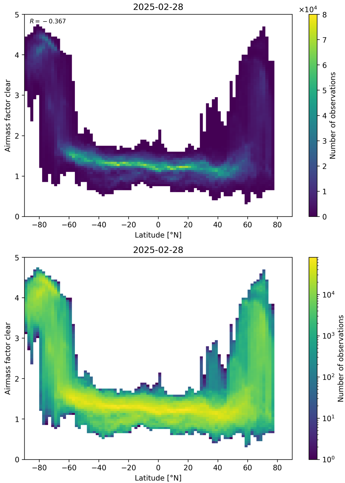
Figure 156: Scatter density plot of “Latitude” against “Airmass factor clear” for 2025-02-27 to 2025-03-01.
