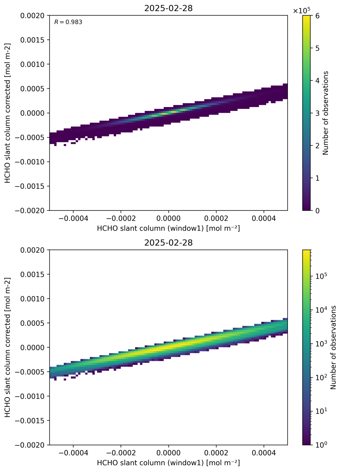
Figure 82: Scatter density plot of “HCHO slant column (window1)” against “HCHO slant column corrected” for 2025-02-27 to 2025-03-01.
