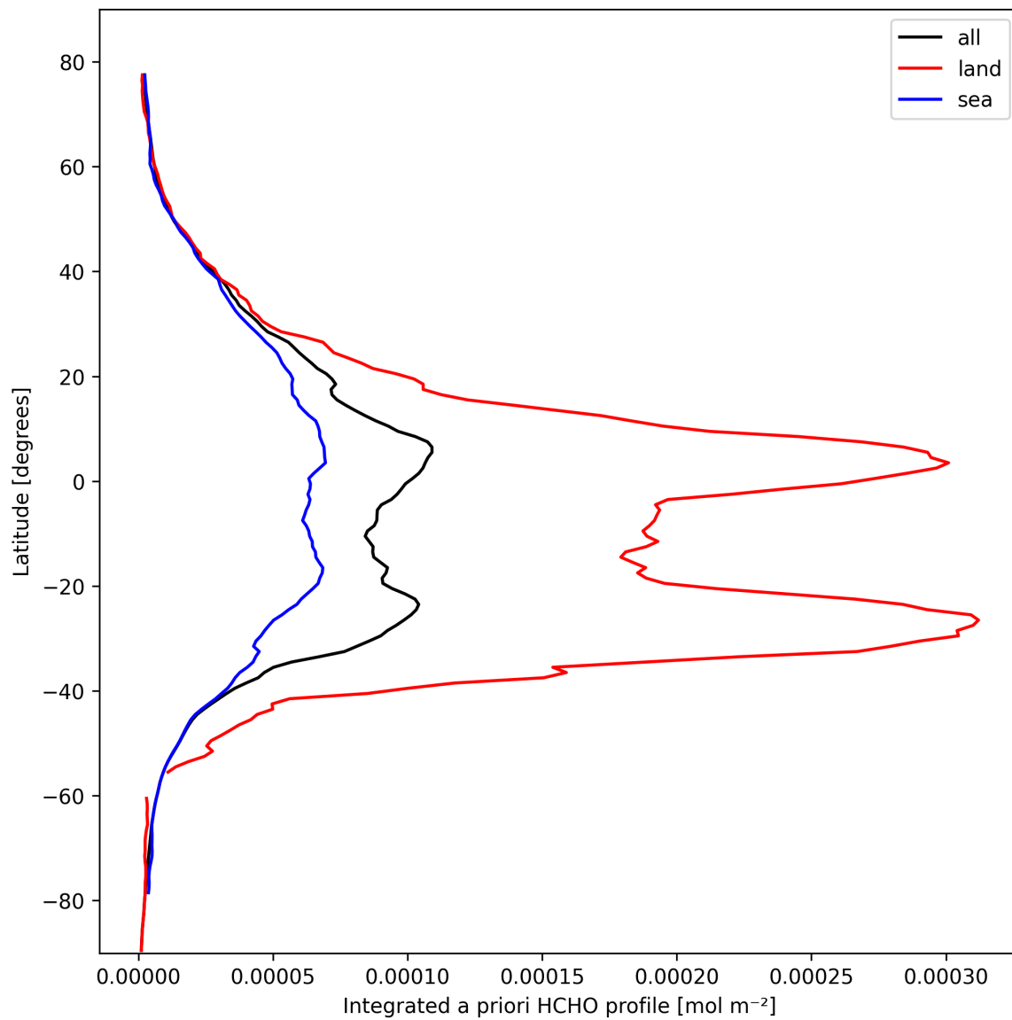
Figure 29: Zonal average of “Integrated a priori HCHO profile” for 2025-02-27 to 2025-03-01.
