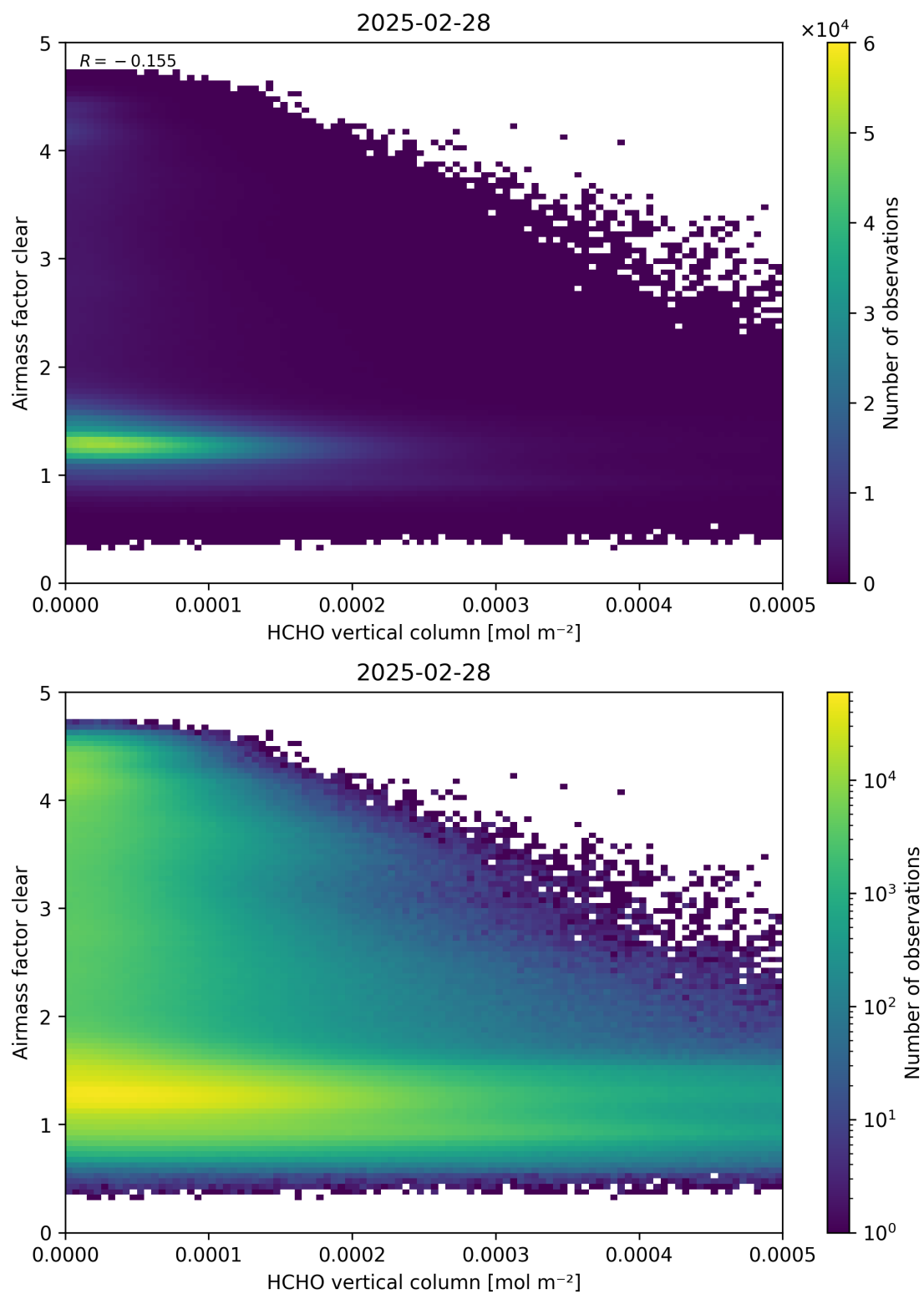
Figure 126: Scatter density plot of “HCHO vertical column” against “Airmass factor clear” for 2025-02-27 to 2025-03-01.
