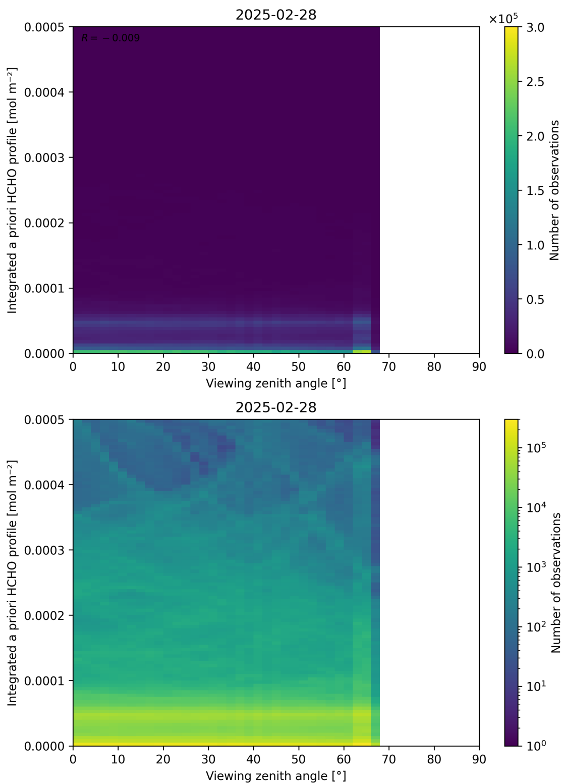
Figure 195: Scatter density plot of “Viewing zenith angle” against “Integrated a priori HCHO profile” for 2025-02-27 to 2025-03-01.
