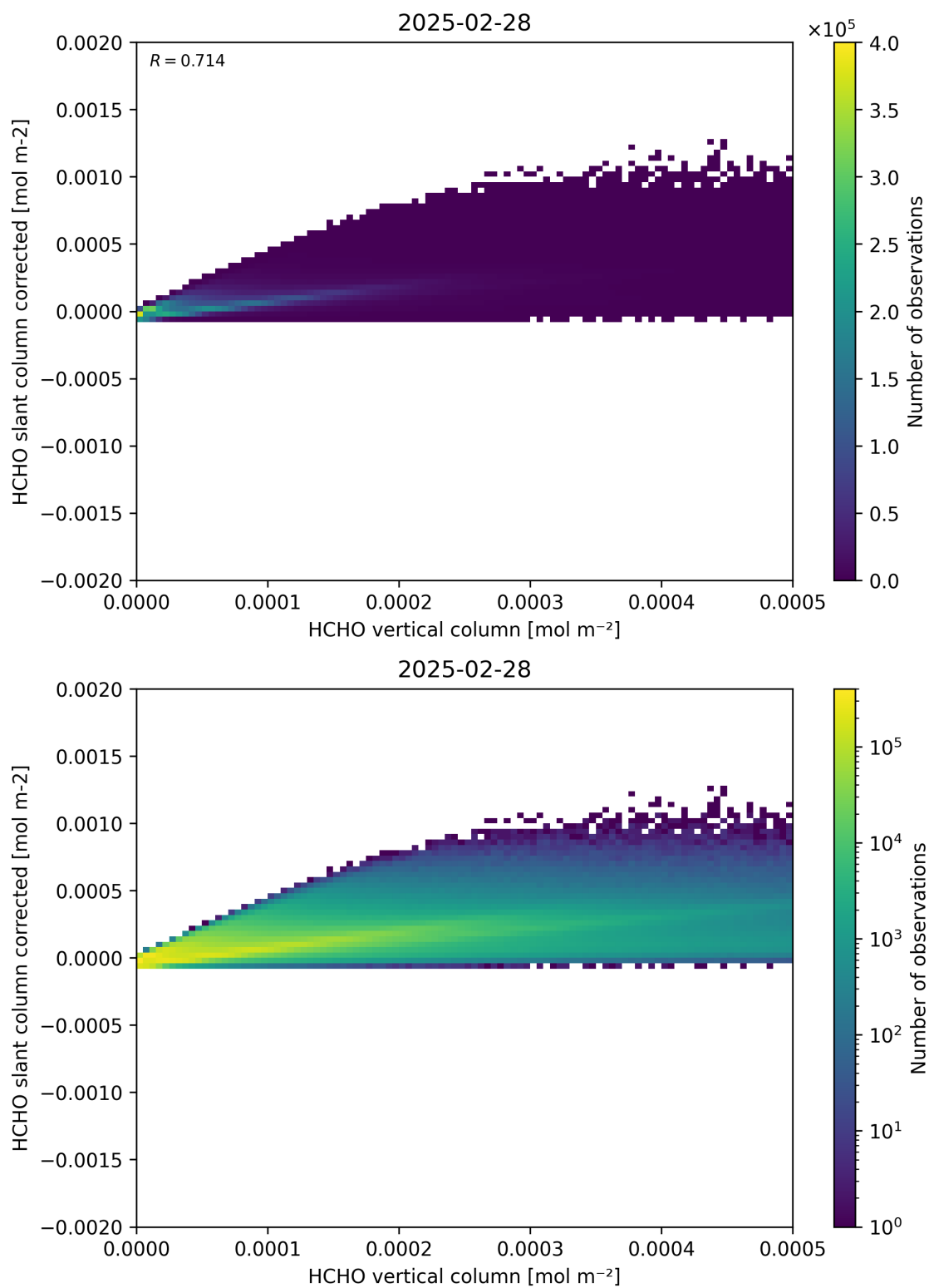
Figure 127: Scatter density plot of “HCHO vertical column” against “HCHO slant column corrected” for 2025-02-27 to 2025-03-01.
