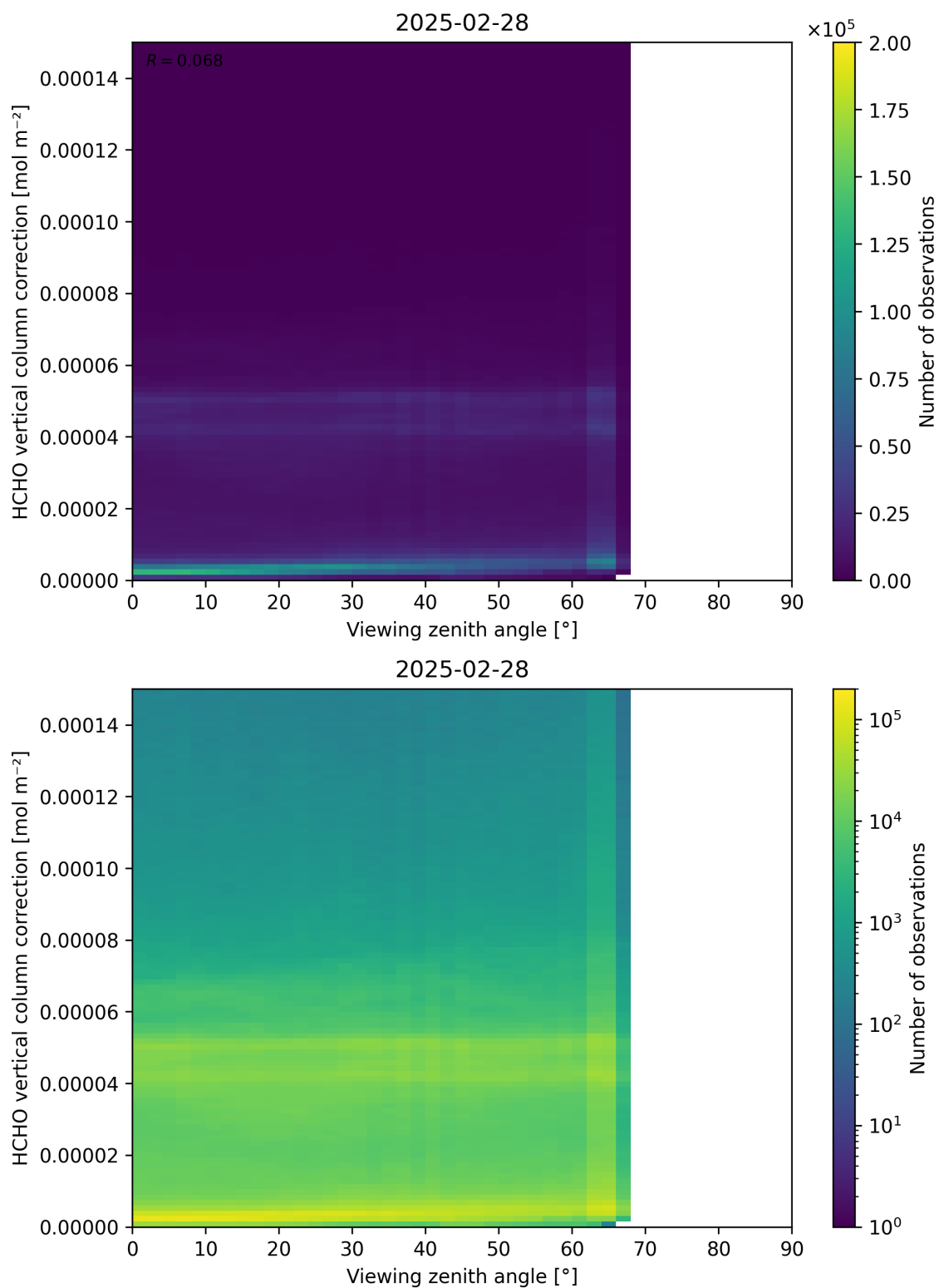
Figure 193: Scatter density plot of “Viewing zenith angle” against “HCHO vertical column correction” for 2025-02-27 to 2025-03-01.
