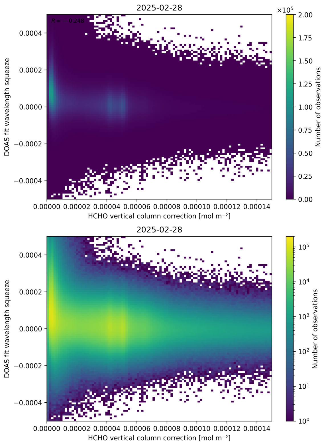
Figure 114: Scatter density plot of “HCHO vertical column correction” against “DOAS fit wavelength squeeze” for 2025-02-27 to 2025-03-01.
