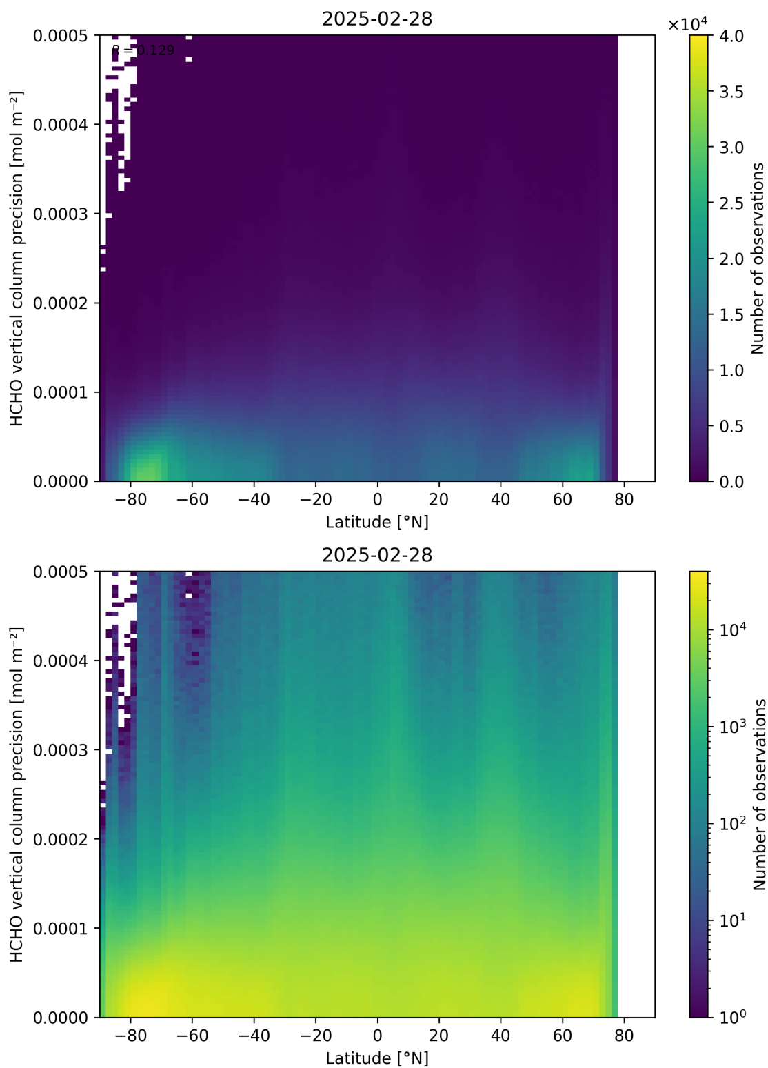
Figure 165: Scatter density plot of “Latitude” against “HCHO vertical column precision” for 2025-02-27 to 2025-03-01.
