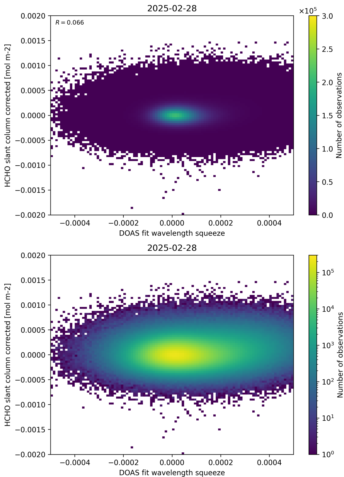
Figure 69: Scatter density plot of “DOAS fit wavelength squeeze” against “HCHO slant column corrected” for 2025-02-27 to 2025-03-01.
