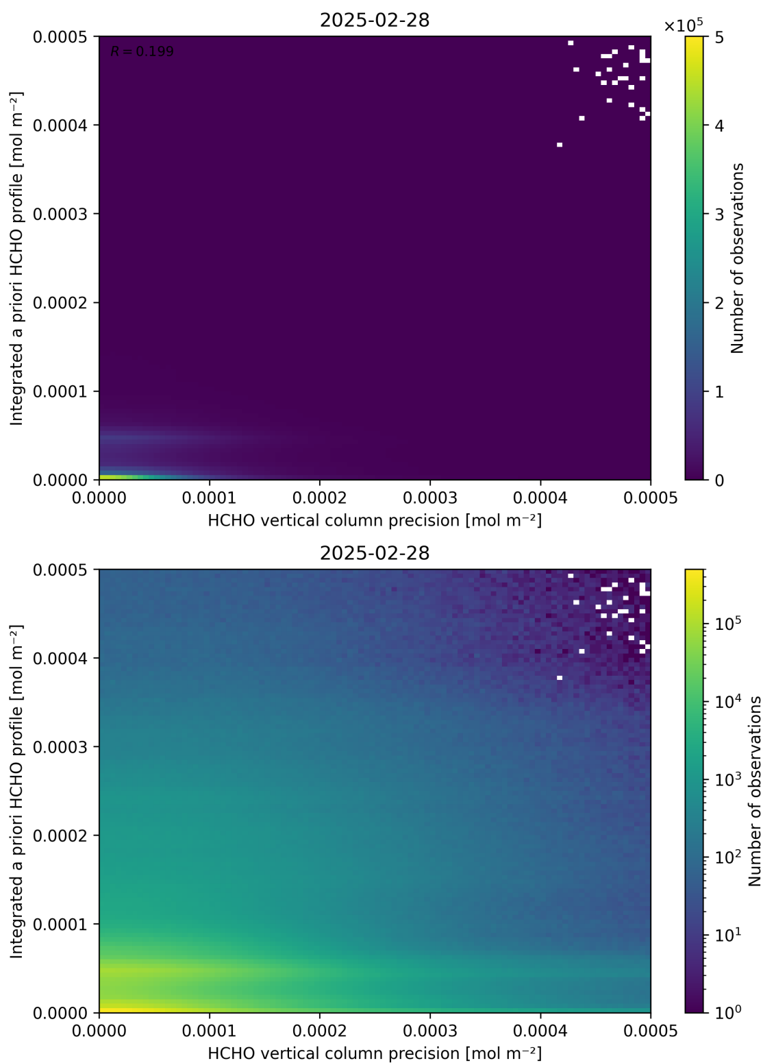
Figure 147: Scatter density plot of “HCHO vertical column precision” against “Integrated a priori HCHO profile” for 2025-02-27 to 2025-03-01.
