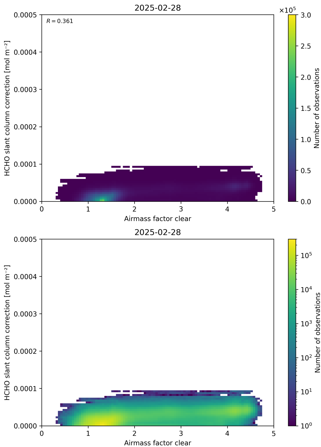
Figure 75: Scatter density plot of “Airmass factor clear” against “HCHO slant column correction” for 2025-02-27 to 2025-03-01.
