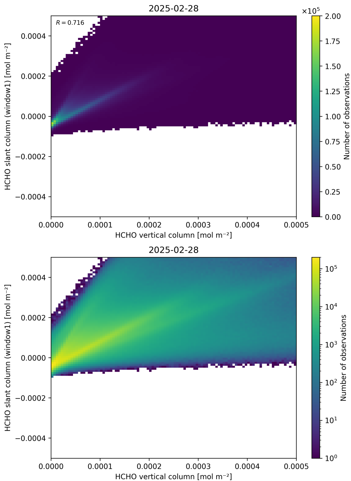
Figure 129: Scatter density plot of “HCHO vertical column” against “HCHO slant column (window1)” for 2025-02-27 to 2025-03-01.
