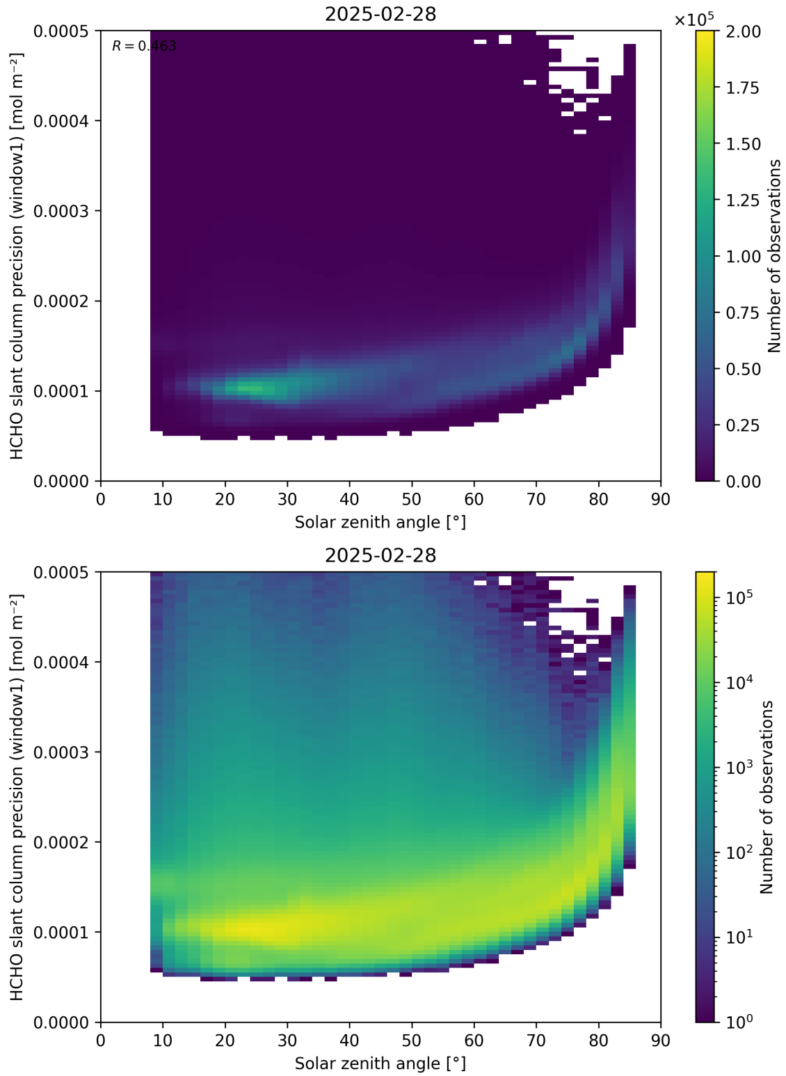
Figure 174: Scatter density plot of “Solar zenith angle” against “HCHO slant column precision (window1)” for 2025-02-27 to 2025-03-01.
