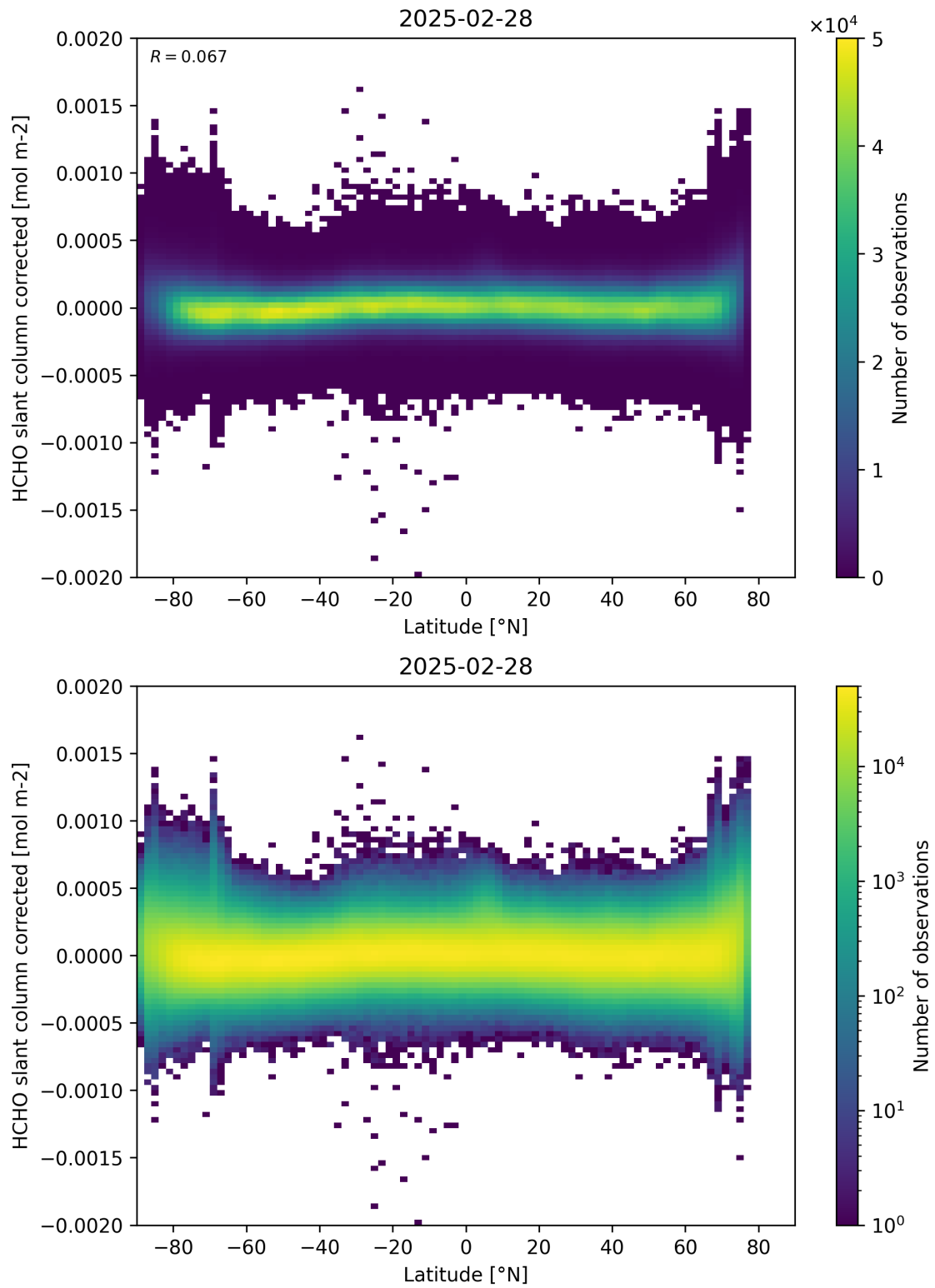
Figure 157: Scatter density plot of “Latitude” against “HCHO slant column corrected” for 2025-02-27 to 2025-03-01.
