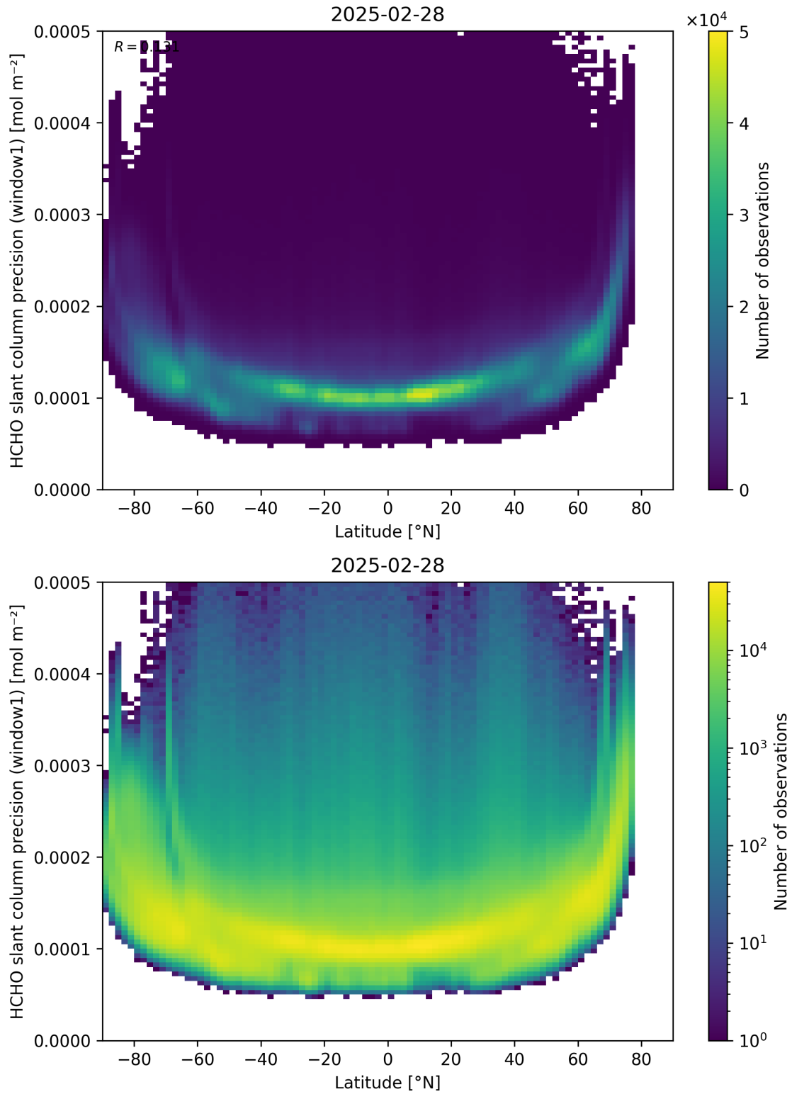
Figure 160: Scatter density plot of “Latitude” against “HCHO slant column precision (window1)” for 2025-02-27 to 2025-03-01.
