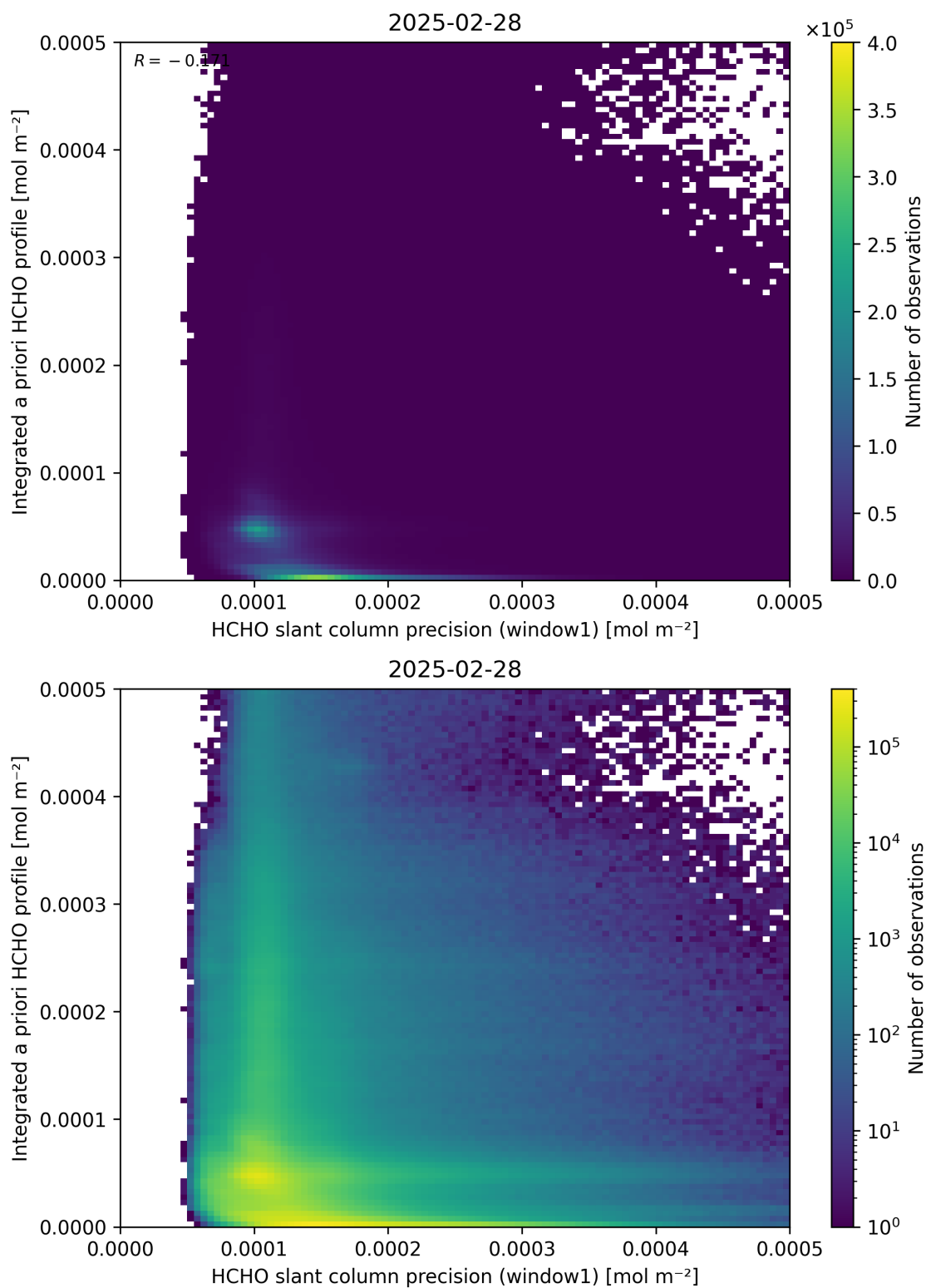
Figure 96: Scatter density plot of “HCHO slant column precision (window1)” against “Integrated a priori HCHO profile” for 2025-02-27 to 2025-03-01.
