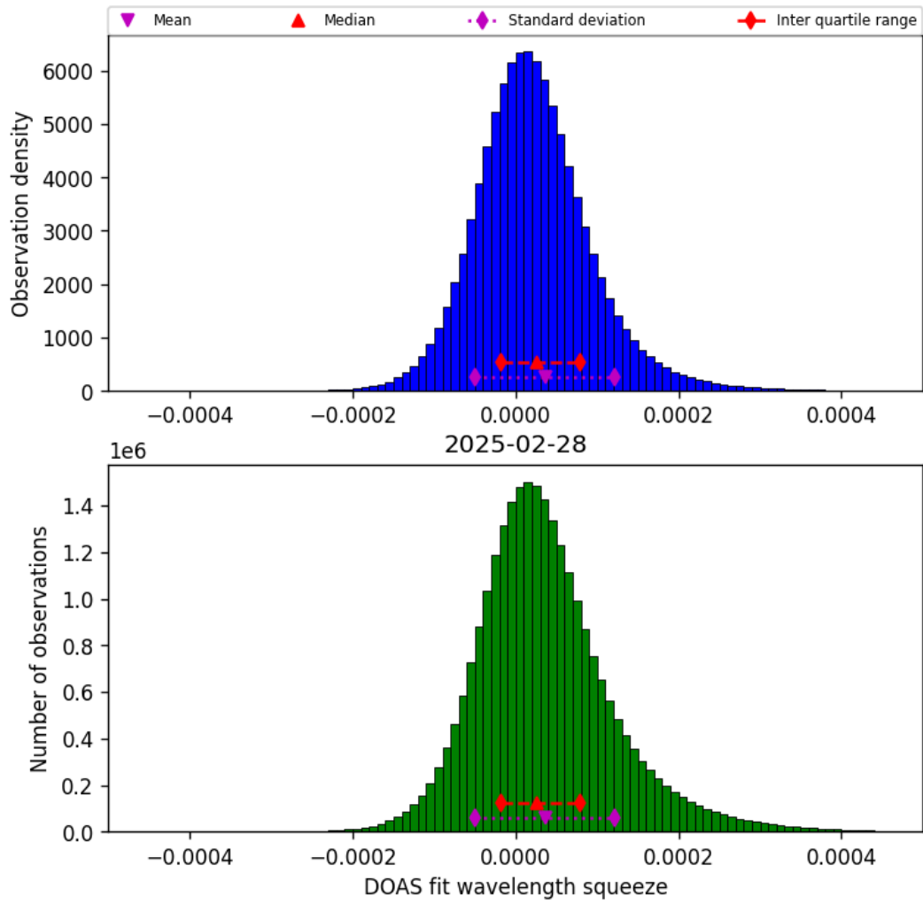
Figure 45: Histogram of “DOAS fit wavelength squeeze” for 2025-02-27 to 2025-03-01
