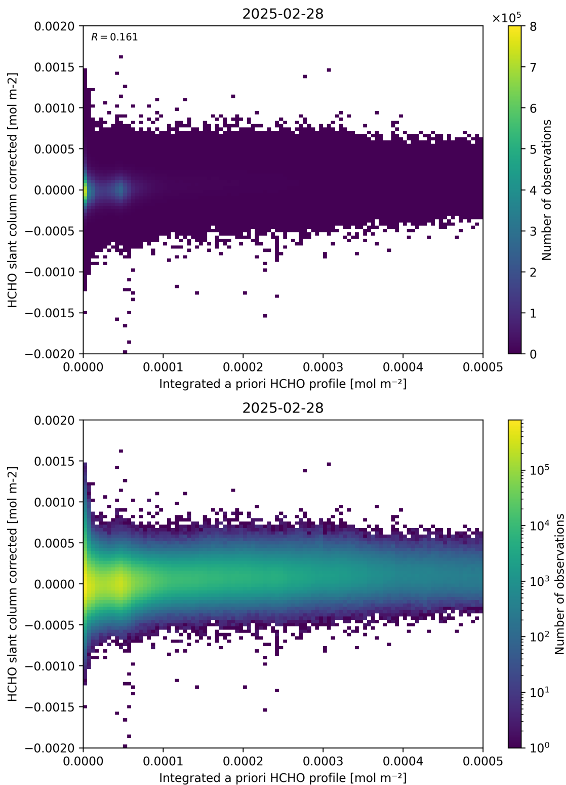
Figure 151: Scatter density plot of “Integrated a priori HCHO profile” against “HCHO slant column corrected” for 2025-02-27 to 2025-03-01.
