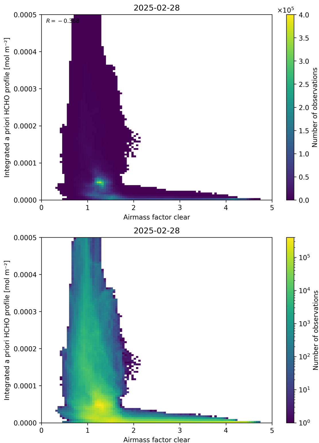
Figure 76: Scatter density plot of “Airmass factor clear” against “Integrated a priori HCHO profile” for 2025-02-27 to 2025-03-01.
