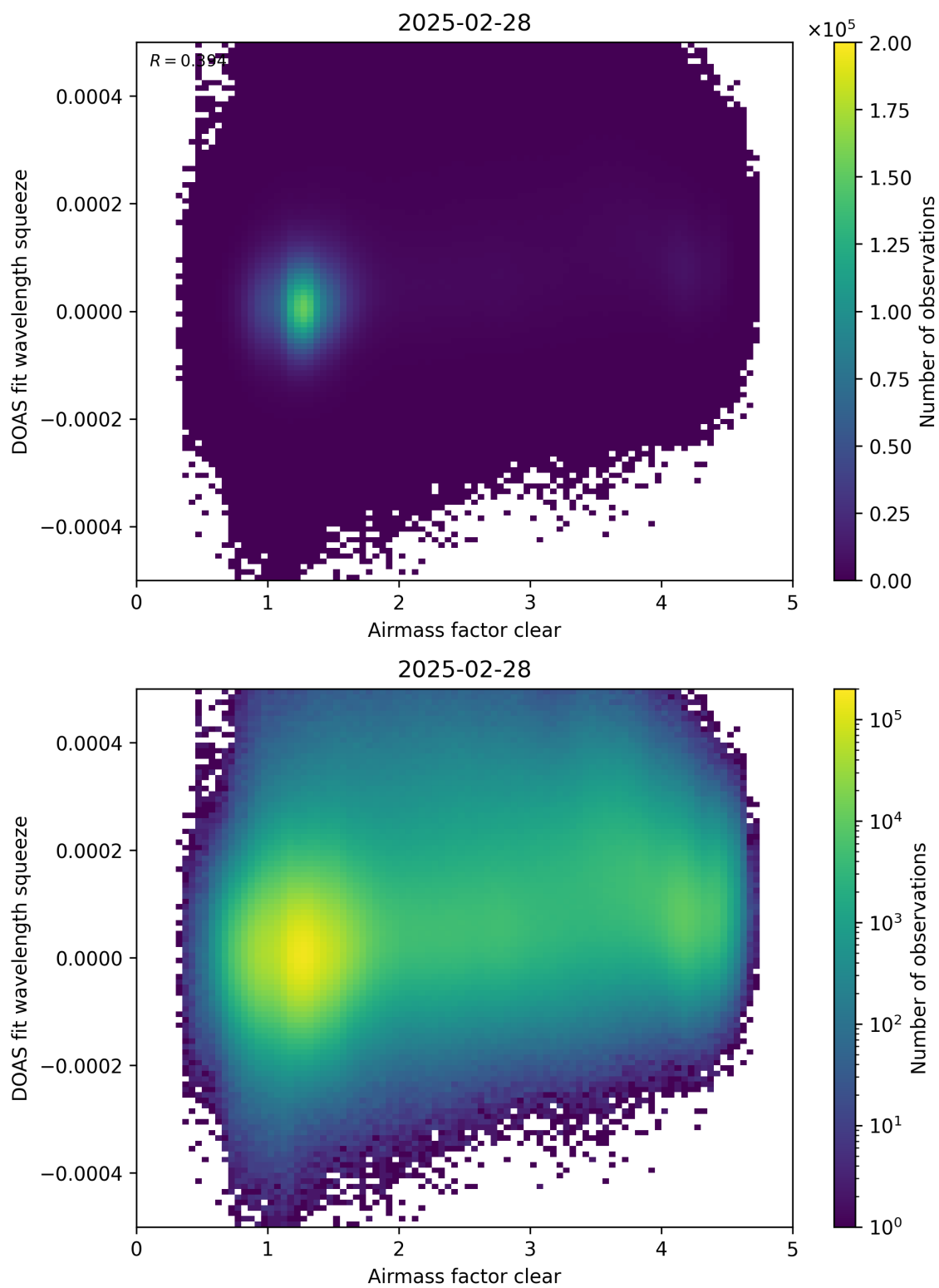
Figure 73: Scatter density plot of “Airmass factor clear” against “DOAS fit wavelength squeeze” for 2025-02-27 to 2025-03-01.
