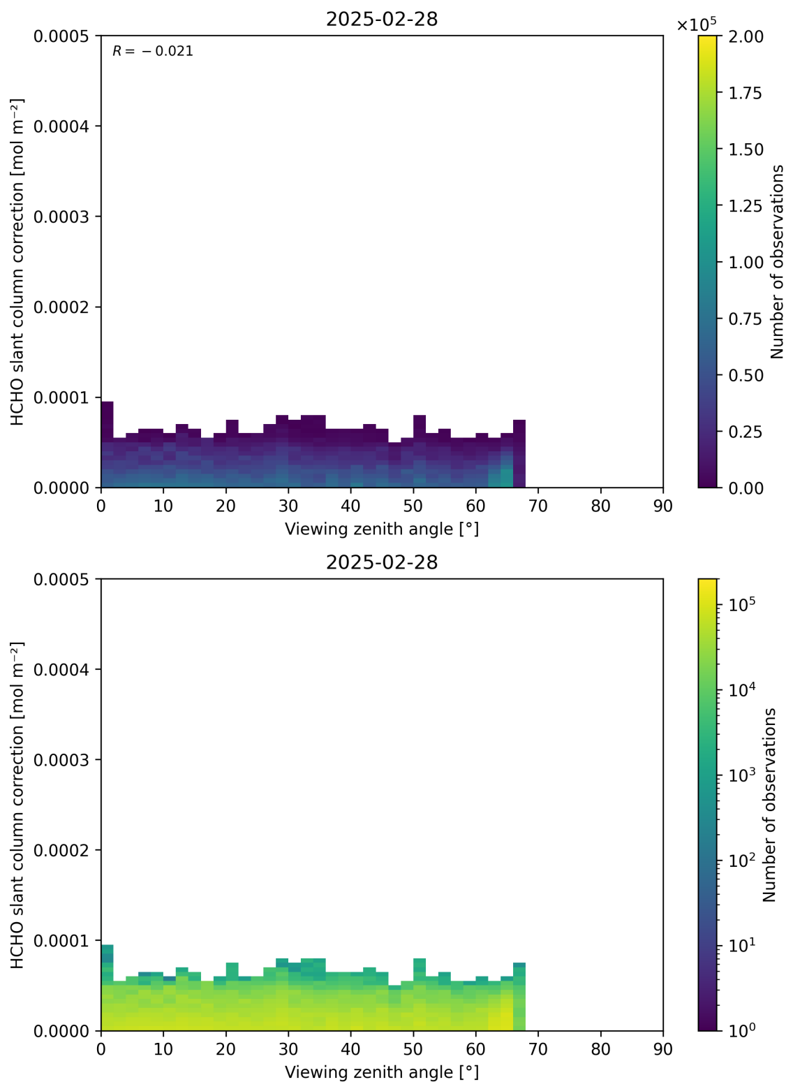
Figure 187: Scatter density plot of “Viewing zenith angle” against “HCHO slant column correction” for 2025-02-27 to 2025-03-01.
