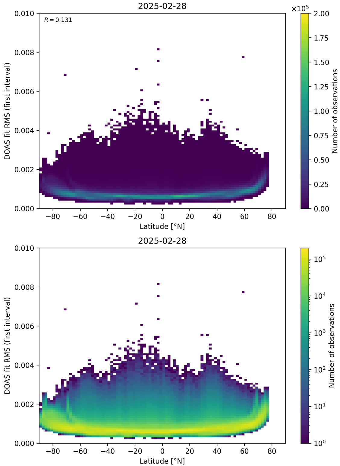
Figure 153: Scatter density plot of “Latitude” against “DOAS fit RMS (first interval)” for 2025-02-27 to 2025-03-01.
