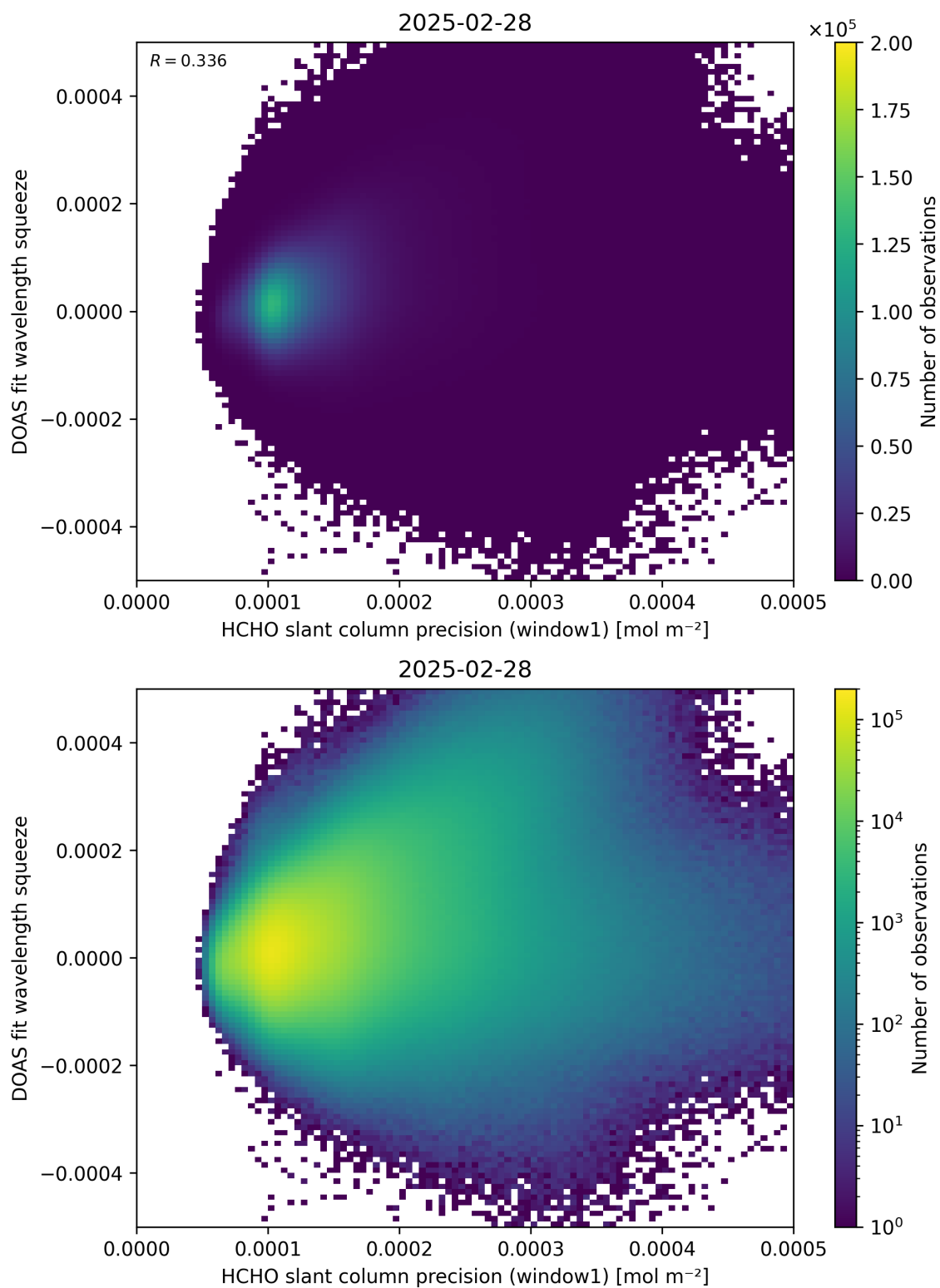
Figure 90: Scatter density plot of “HCHO slant column precision (window1)” against “DOAS fit wavelength squeeze” for 2025-02-27 to 2025-03-01.
