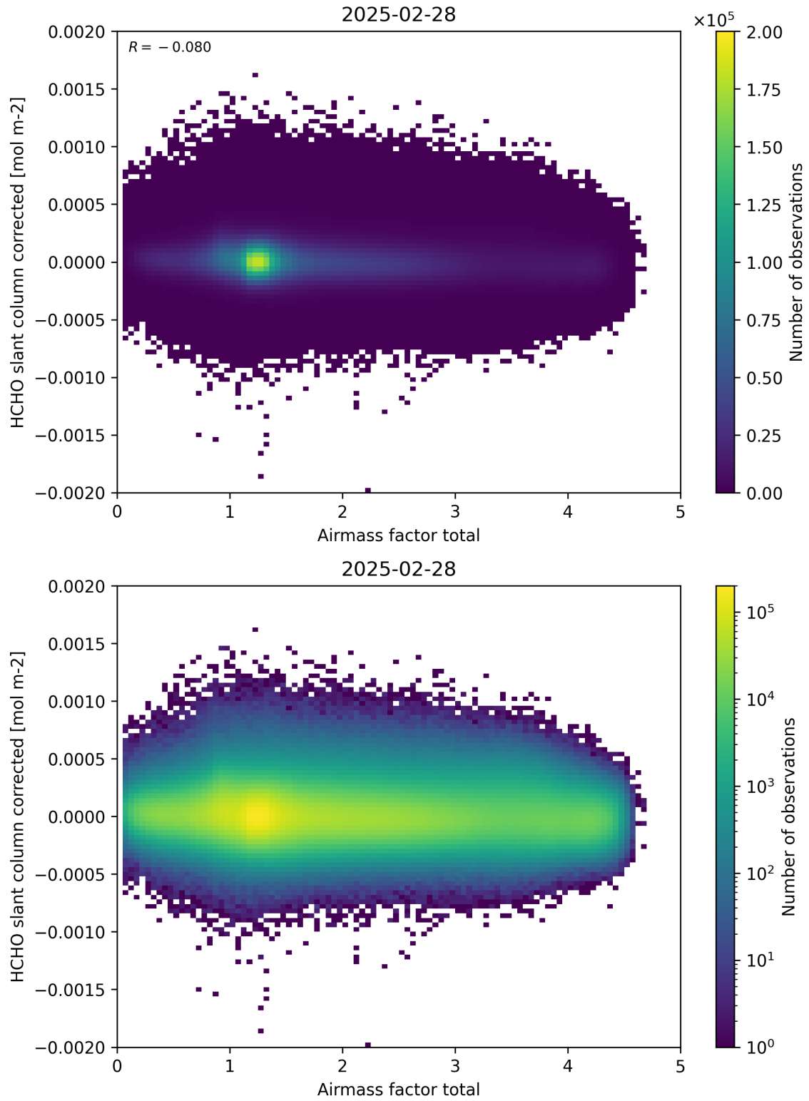
Figure 101: Scatter density plot of “Airmass factor total” against “HCHO slant column corrected” for 2025-02-27 to 2025-03-01.
