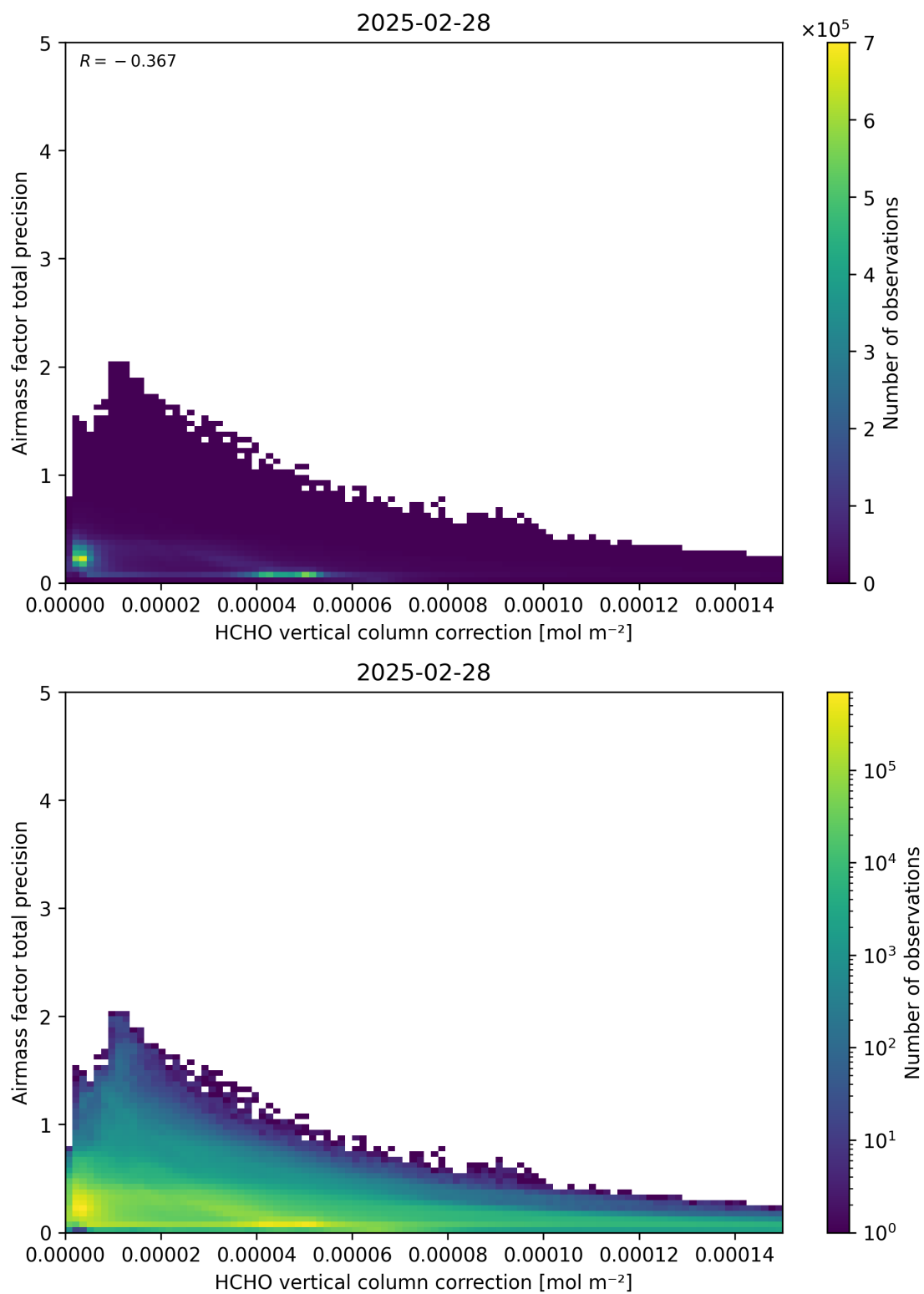
Figure 121: Scatter density plot of “HCHO vertical column correction” against “Airmass factor total precision” for 2025-02-27 to 2025-03-01.
