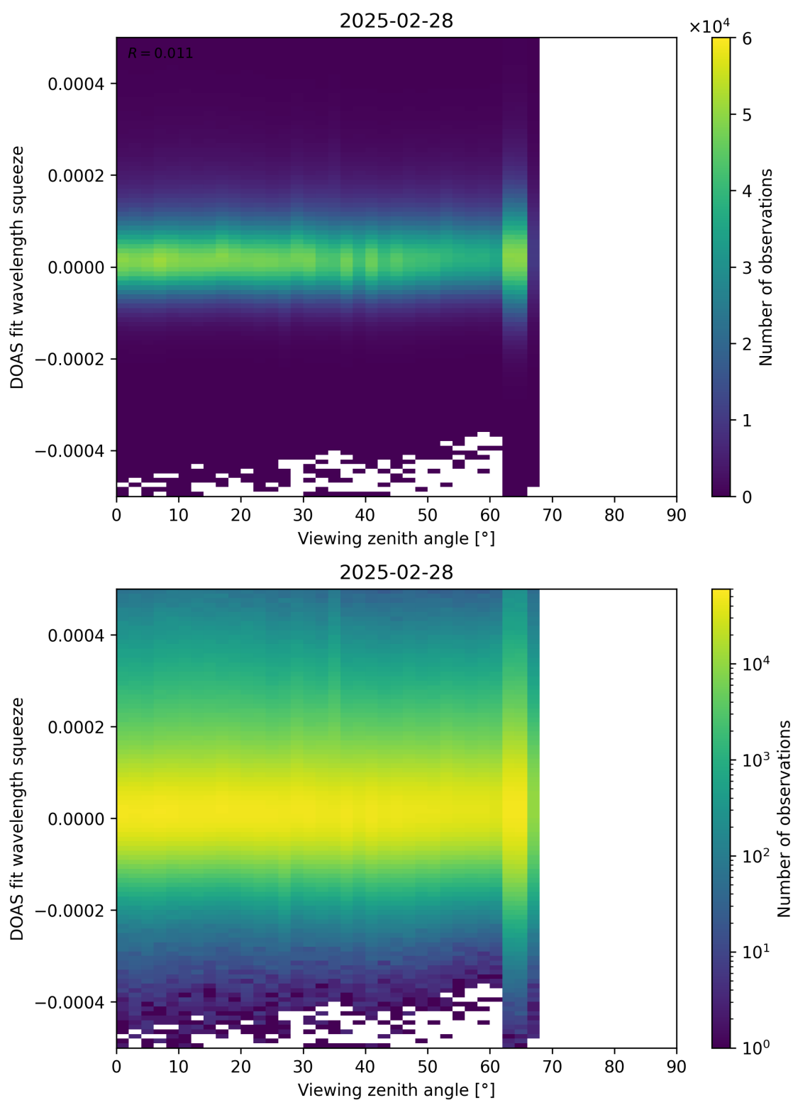
Figure 184: Scatter density plot of “Viewing zenith angle” against “DOAS fit wavelength squeeze” for 2025-02-27 to 2025-03-01.
