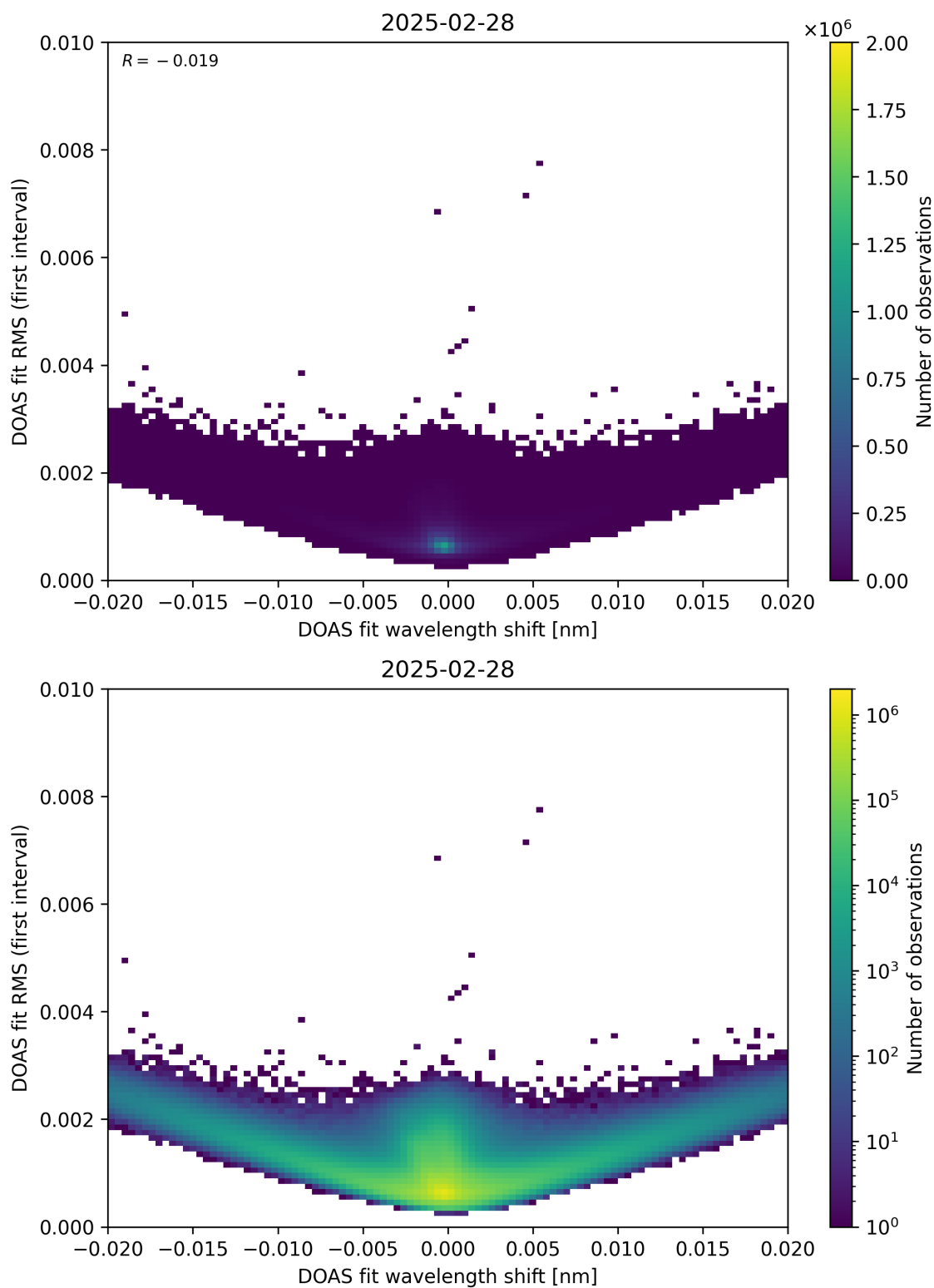
Figure 64: Scatter density plot of “DOAS fit wavelength shift” against “DOAS fit RMS (first interval)” for 2025-02-27 to 2025-03-01.
