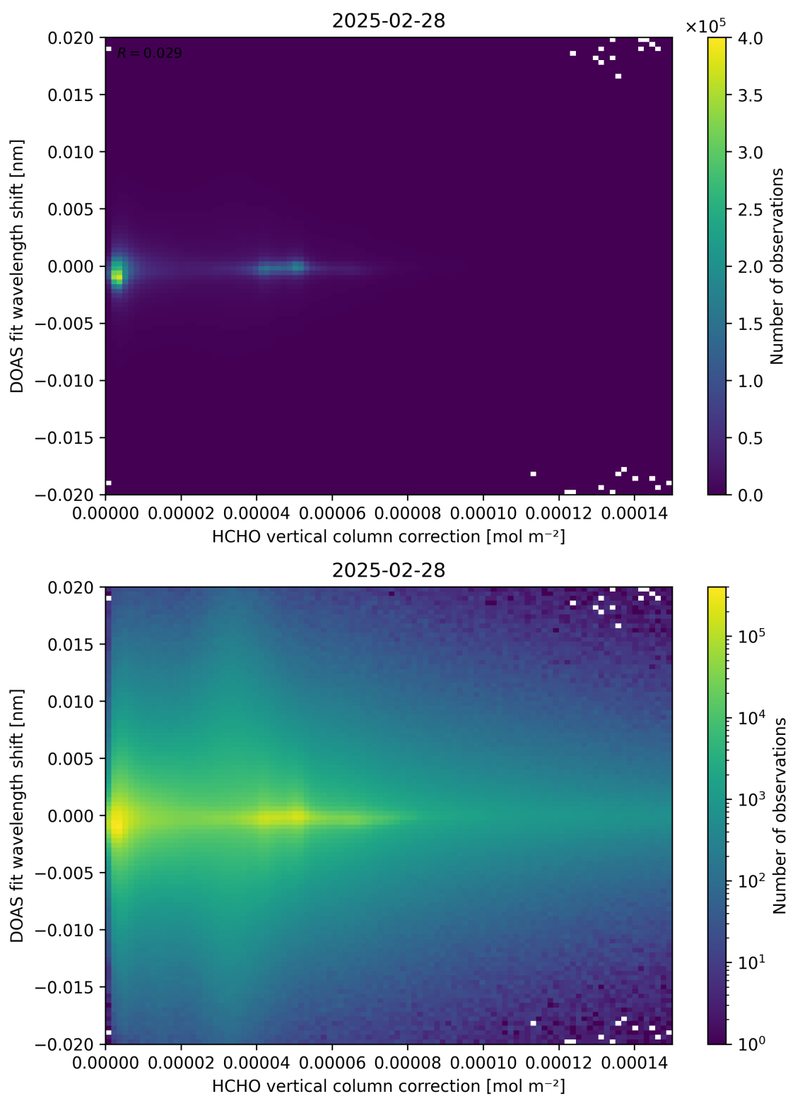
Figure 113: Scatter density plot of “HCHO vertical column correction” against “DOAS fit wavelength shift” for 2025-02-27 to 2025-03-01.
