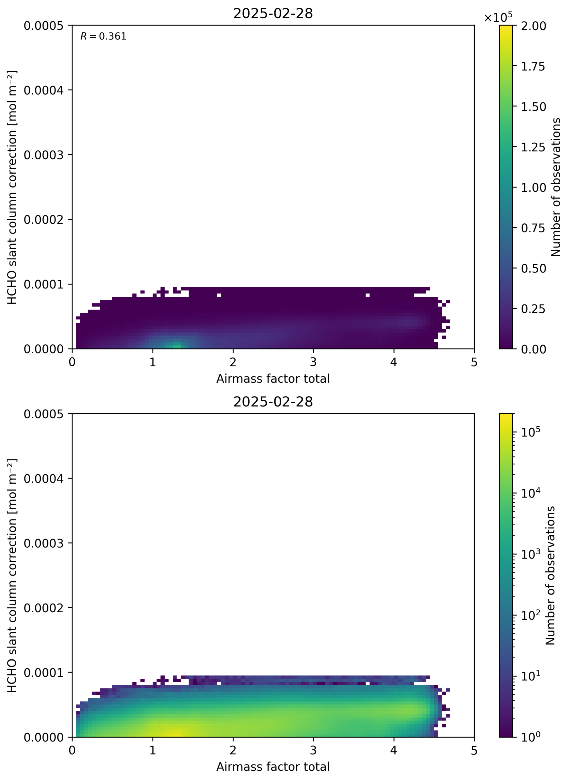
Figure 102: Scatter density plot of “Airmass factor total” against “HCHO slant column correction” for 2025-02-27 to 2025-03-01.
