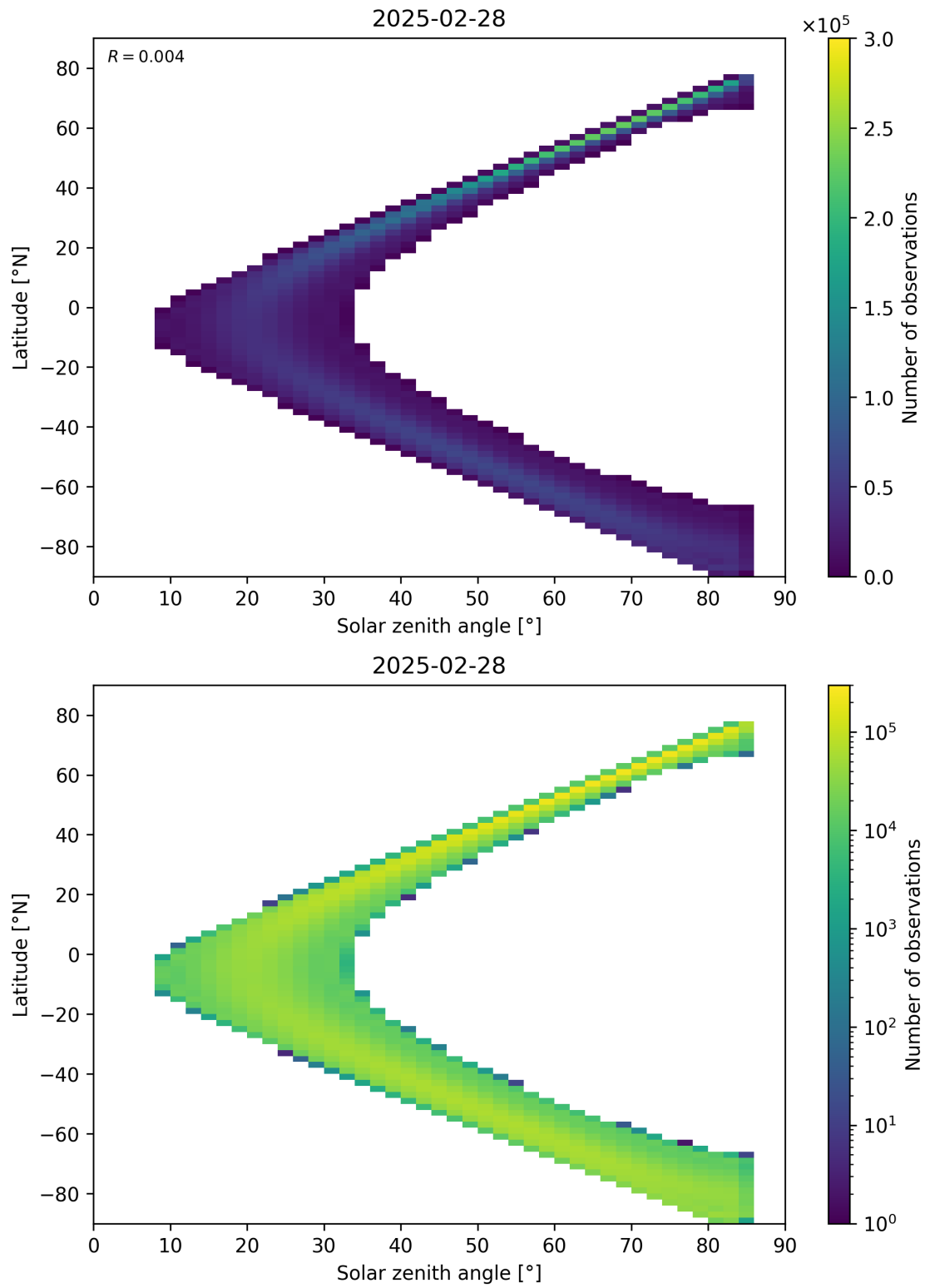
Figure 181: Scatter density plot of “Solar zenith angle” against “Latitude” for 2025-02-27 to 2025-03-01.
