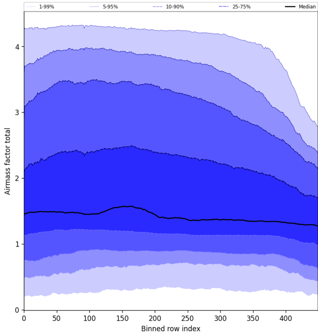
Figure 54: Along track statistics of “Airmass factor total” for 2025-02-27 to 2025-03-01
