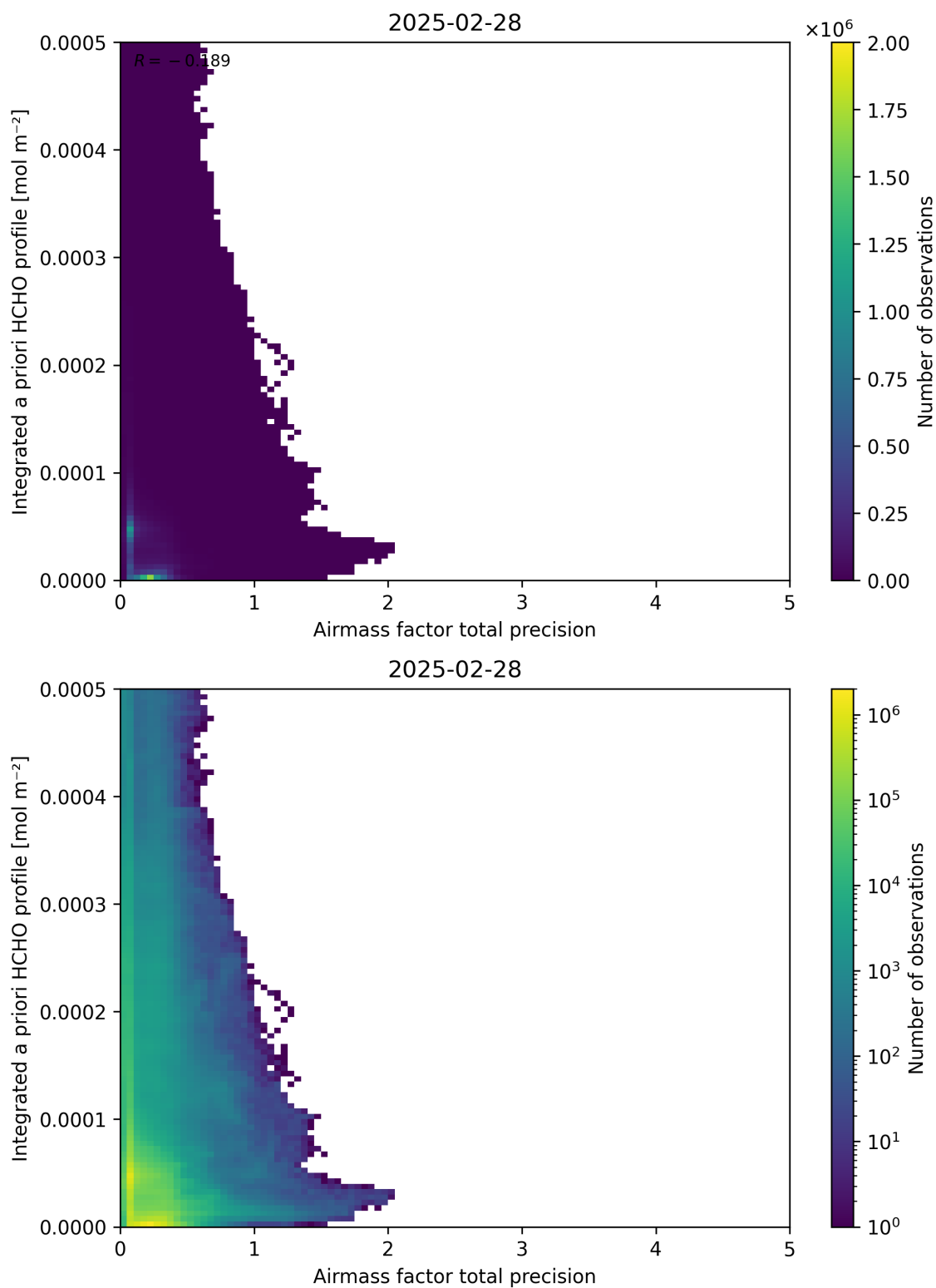
Figure 111: Scatter density plot of “Airmass factor total precision” against “Integrated a priori HCHO profile” for 2025-02-27 to 2025-03-01.
