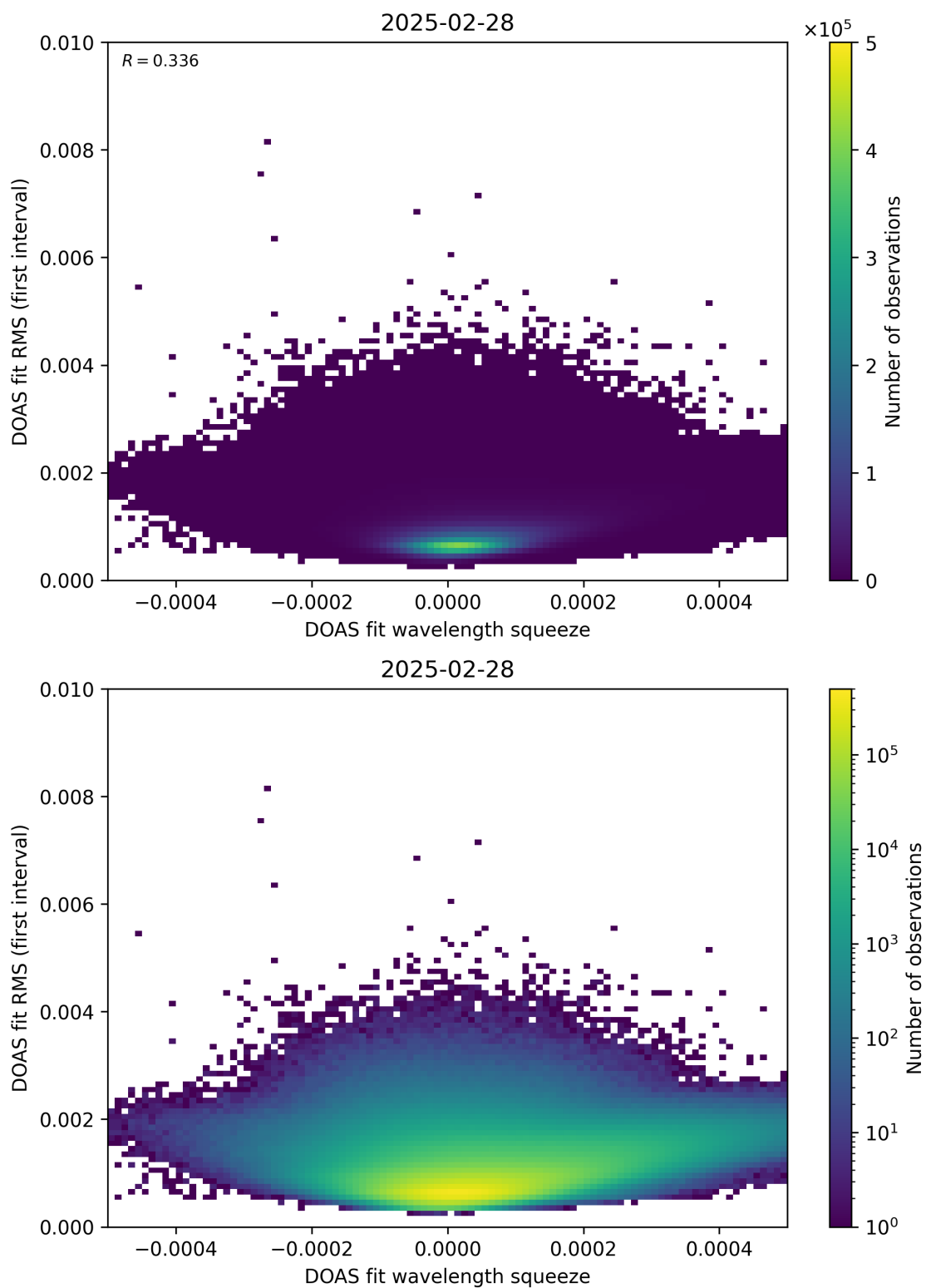
Figure 68: Scatter density plot of “DOAS fit wavelength squeeze” against “DOAS fit RMS (first interval)” for 2025-02-27 to 2025-03-01.
