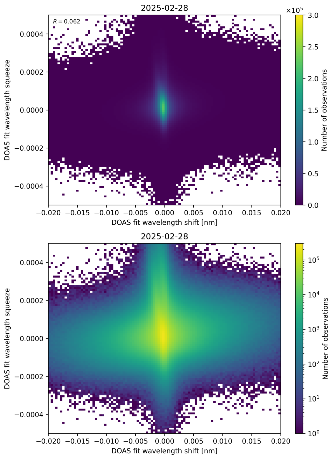
Figure 65: Scatter density plot of “DOAS fit wavelength shift” against “DOAS fit wavelength squeeze” for 2025-02-27 to 2025-03-01.
