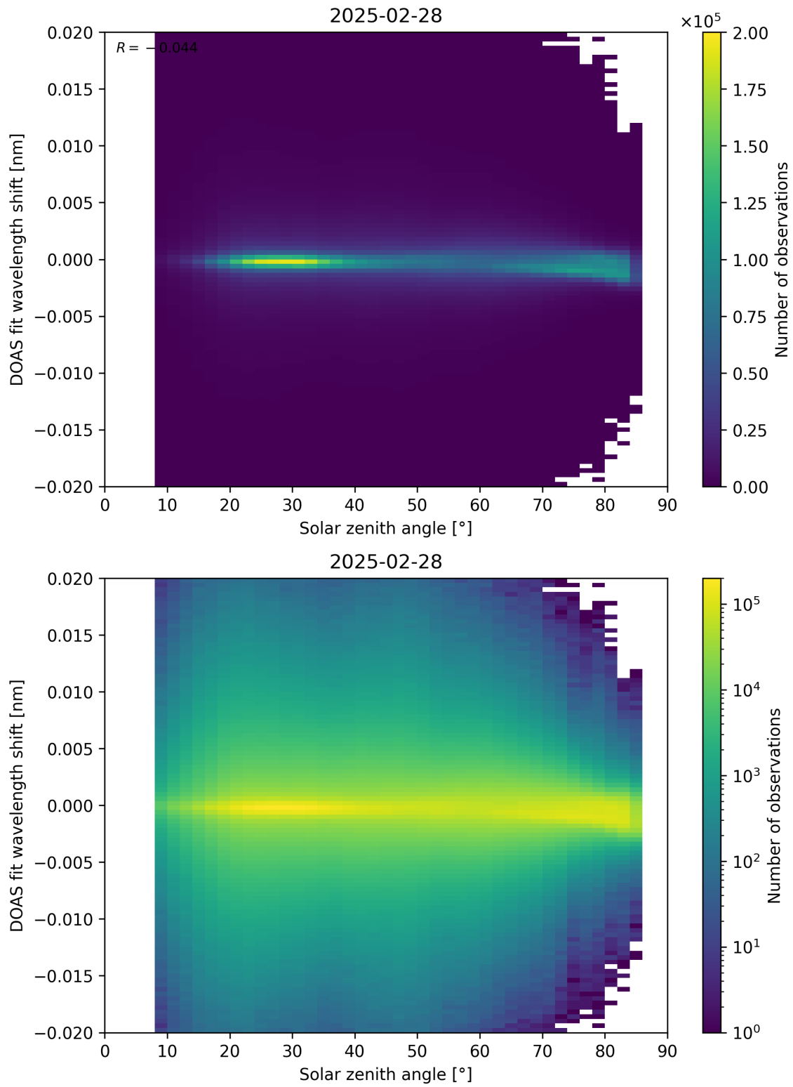
Figure 168: Scatter density plot of “Solar zenith angle” against “DOAS fit wavelength shift” for 2025-02-27 to 2025-03-01.
