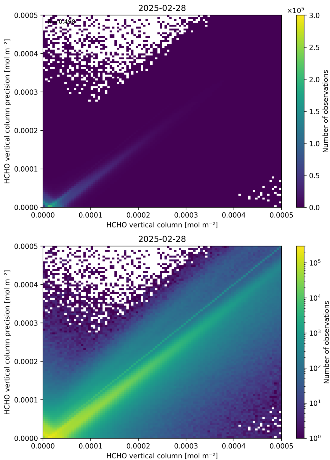
Figure 134: Scatter density plot of “HCHO vertical column” against “HCHO vertical column precision” for 2025-02-27 to 2025-03-01.
