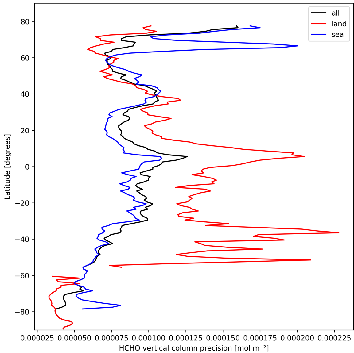
Figure 22: Zonal average of “HCHO vertical column precision” for 2025-02-27 to 2025-03-01.
