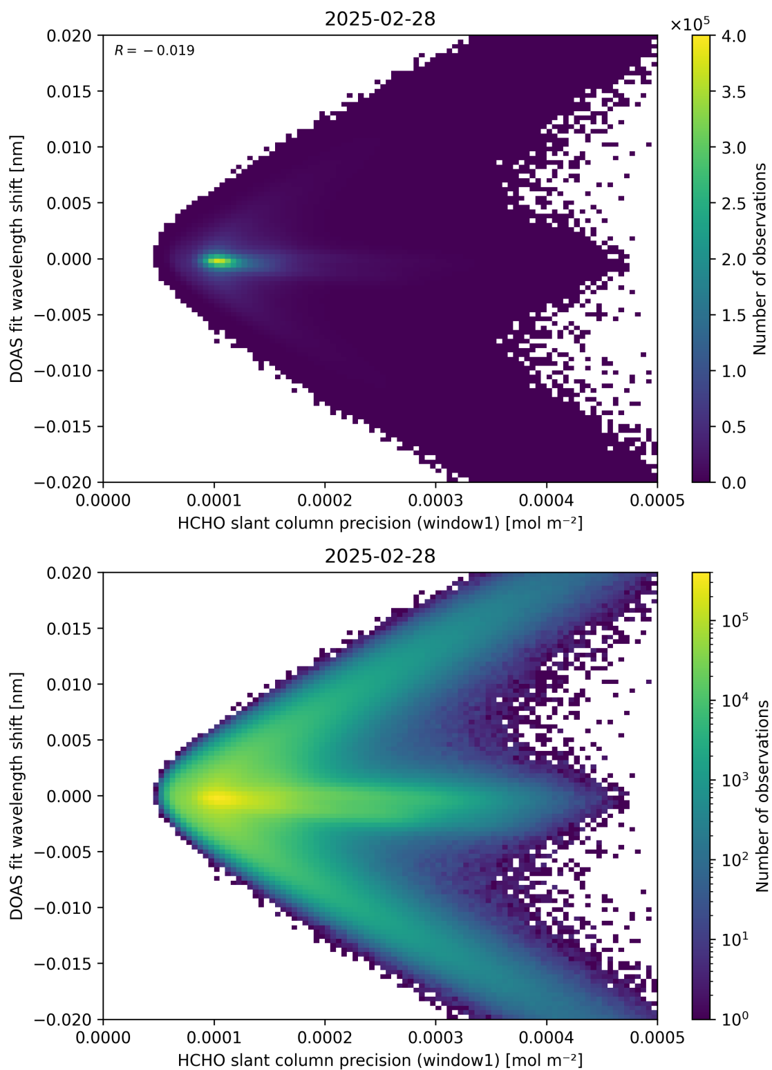
Figure 89: Scatter density plot of “HCHO slant column precision (window1)” against “DOAS fit wavelength shift” for 2025-02-27 to 2025-03-01.
