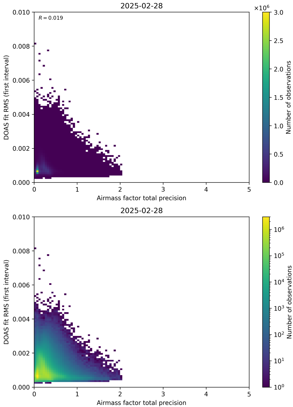
Figure 105: Scatter density plot of “Airmass factor total precision” against “DOAS fit RMS (first interval)” for 2025-02-27 to 2025-03-01.
