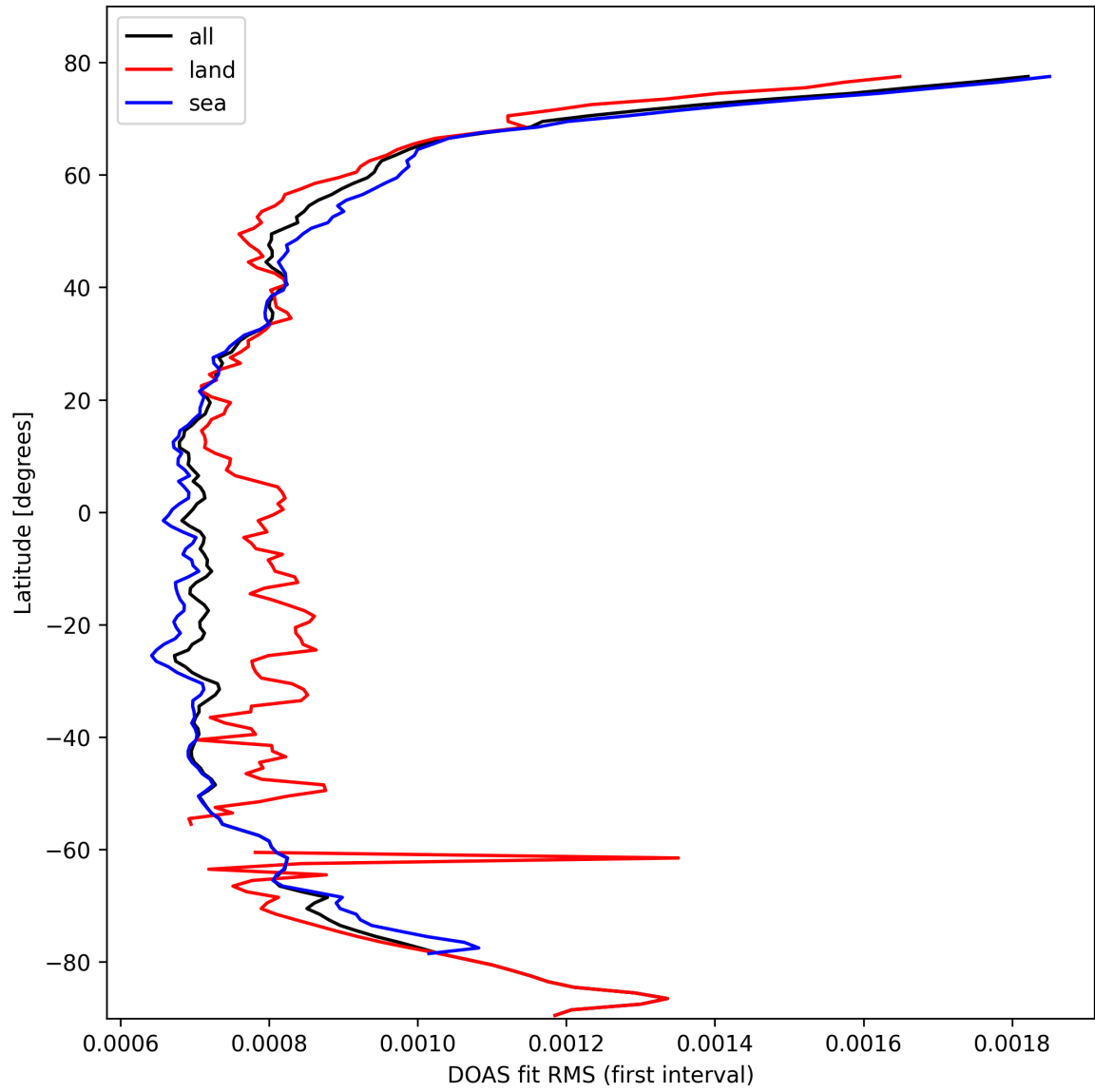
Figure 32: Zonal average of “DOAS fit RMS (first interval)” for 2025-02-27 to 2025-03-01.
