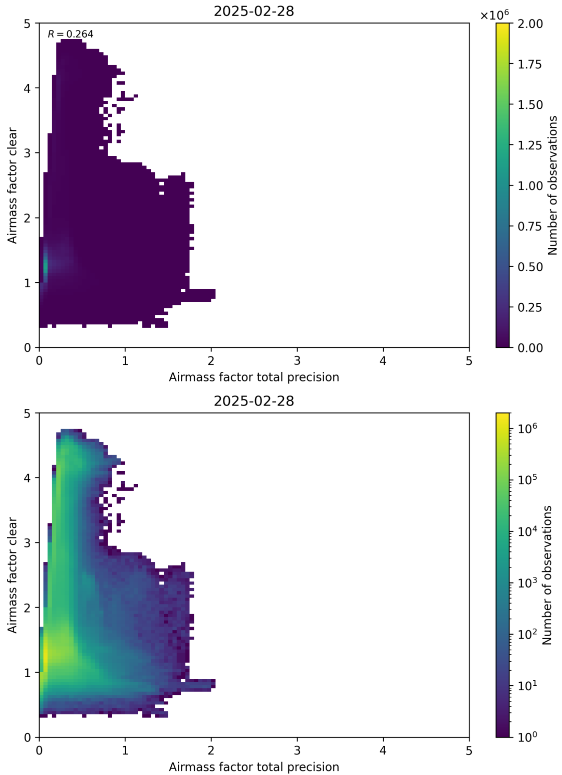
Figure 108: Scatter density plot of “Airmass factor total precision” against “Airmass factor clear” for 2025-02-27 to 2025-03-01.
