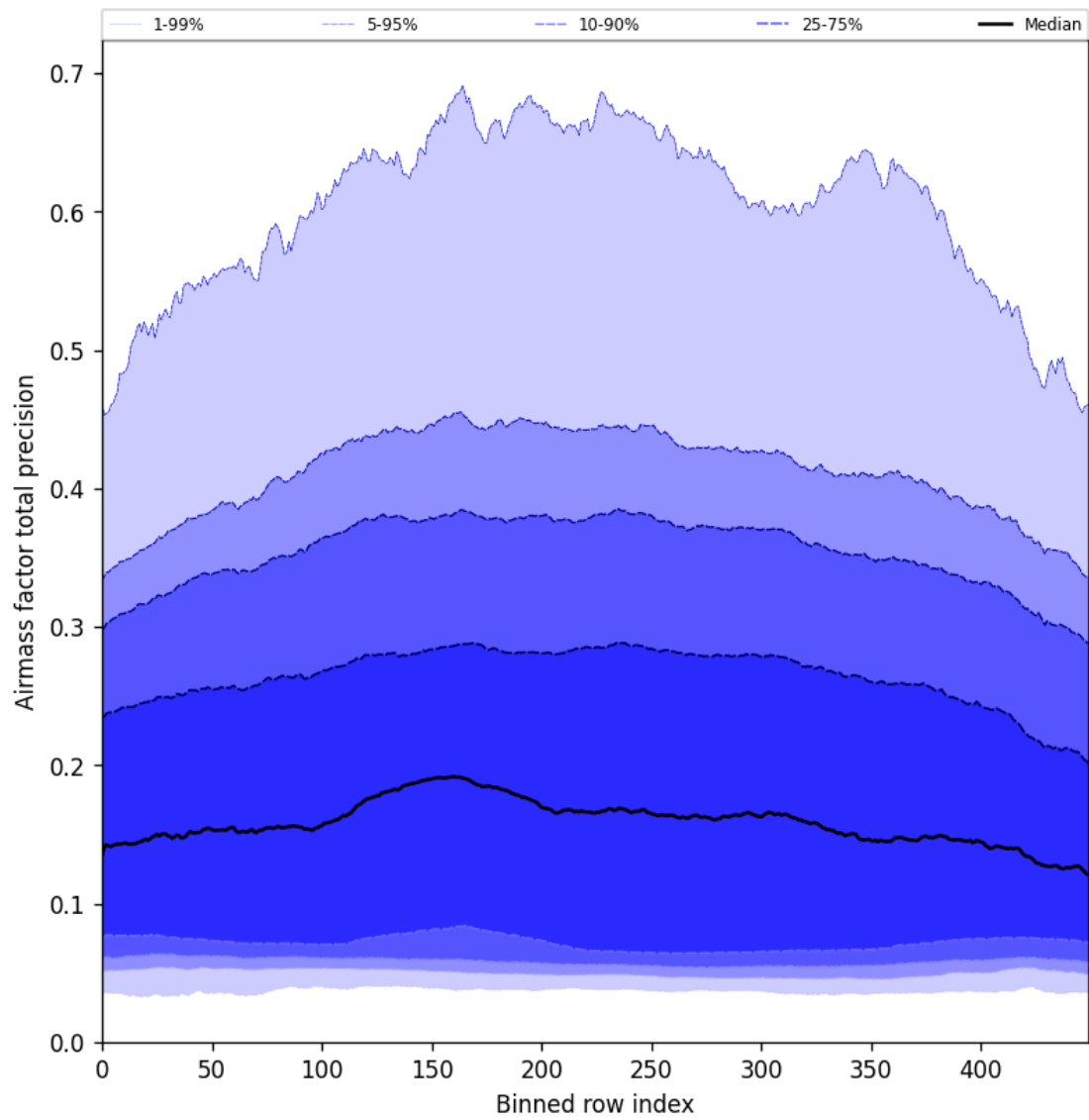
Figure 55: Along track statistics of “Airmass factor total precision” for 2025-02-27 to 2025-03-01
