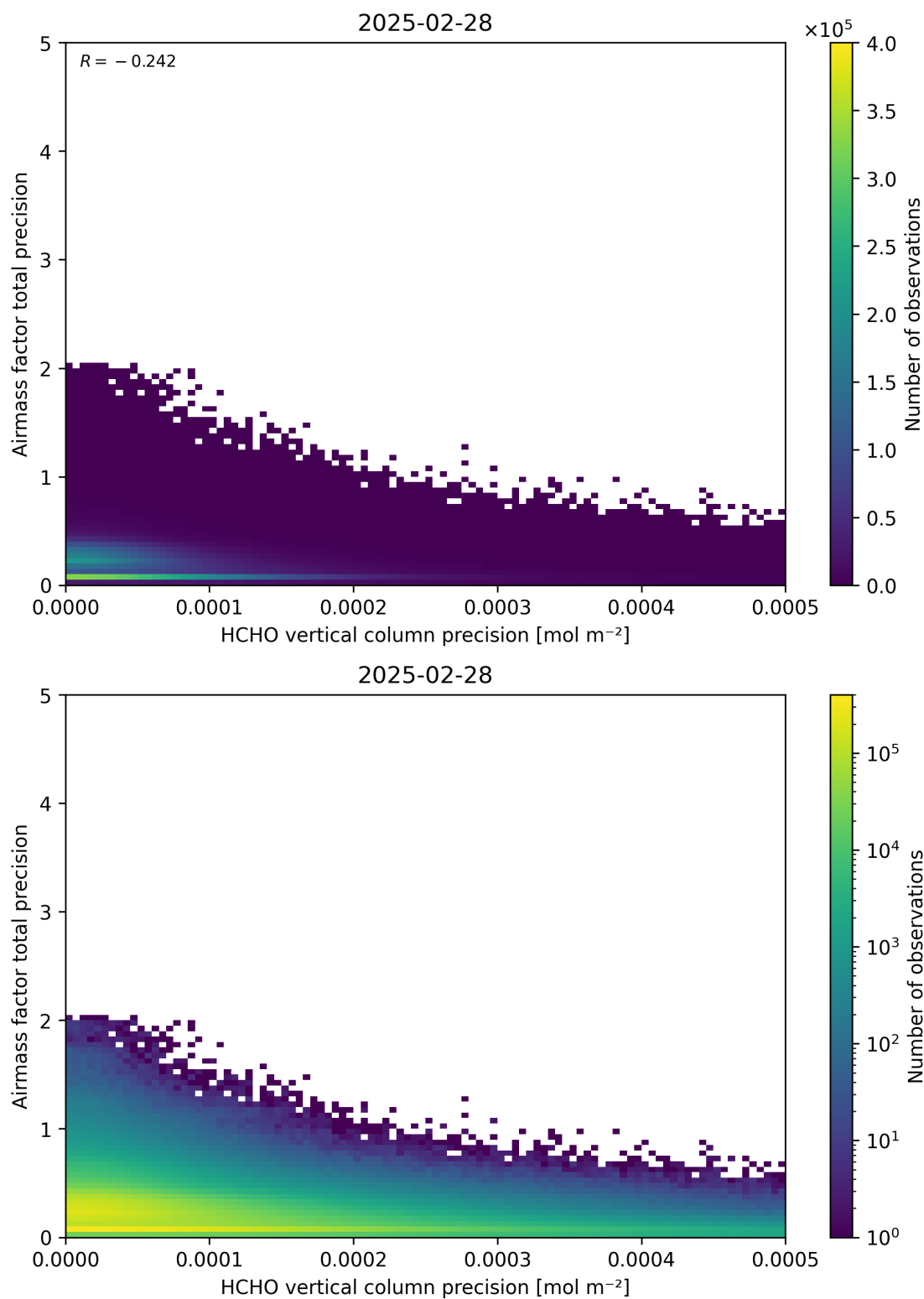
Figure 145: Scatter density plot of “HCHO vertical column precision” against “Airmass factor total precision” for 2025-02-27 to 2025-03-01.
