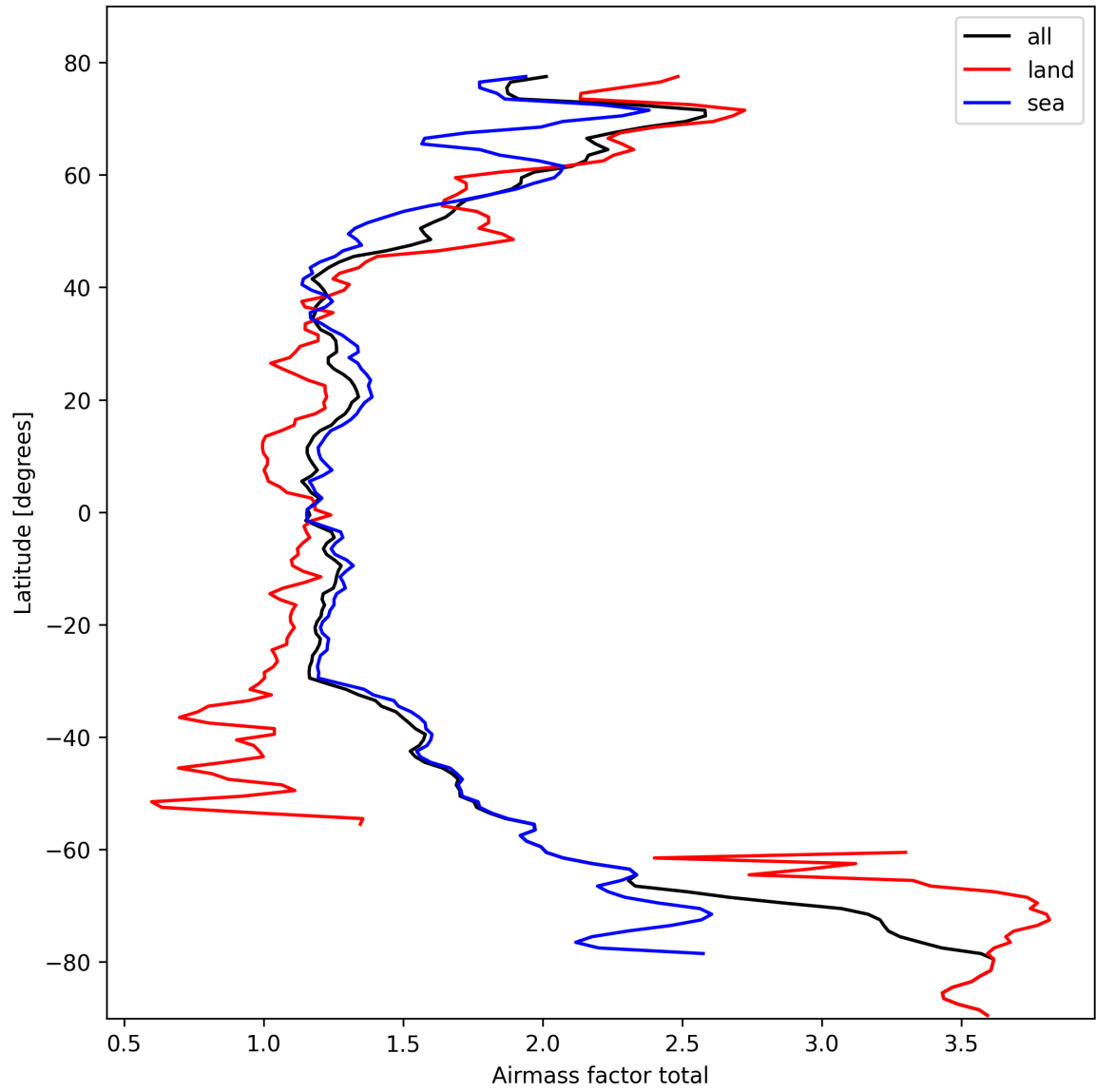
Figure 26: Zonal average of “Airmass factor total” for 2025-02-27 to 2025-03-01.
