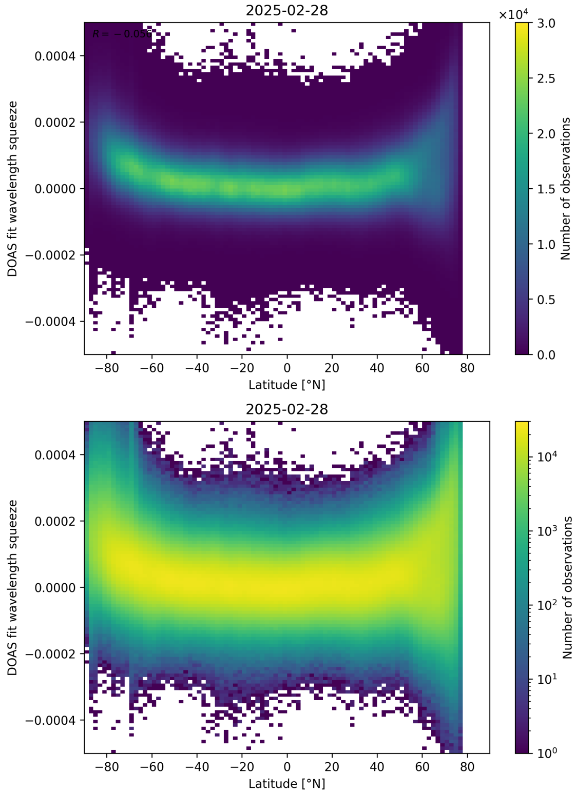
Figure 155: Scatter density plot of “Latitude” against “DOAS fit wavelength squeeze” for 2025-02-27 to 2025-03-01.
