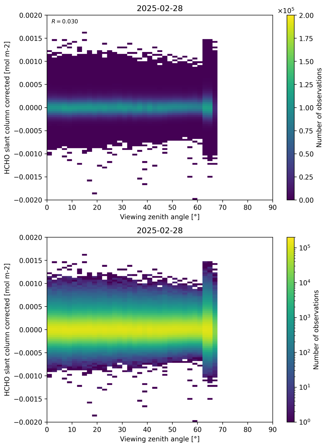
Figure 186: Scatter density plot of “Viewing zenith angle” against “HCHO slant column corrected” for 2025-02-27 to 2025-03-01.
