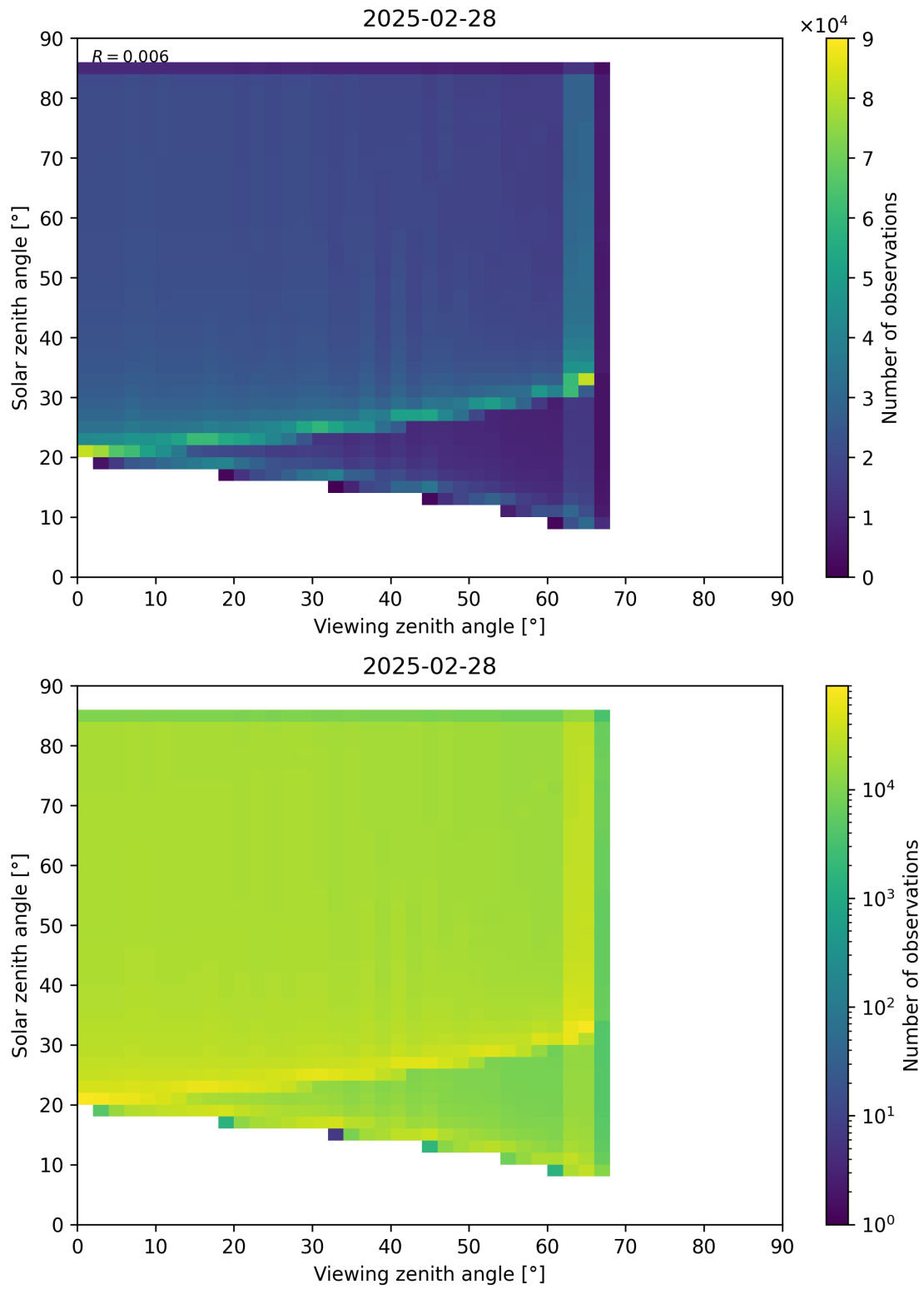
Figure 197: Scatter density plot of “Viewing zenith angle” against “Solar zenith angle” for 2025-02-27 to 2025-03-01.
