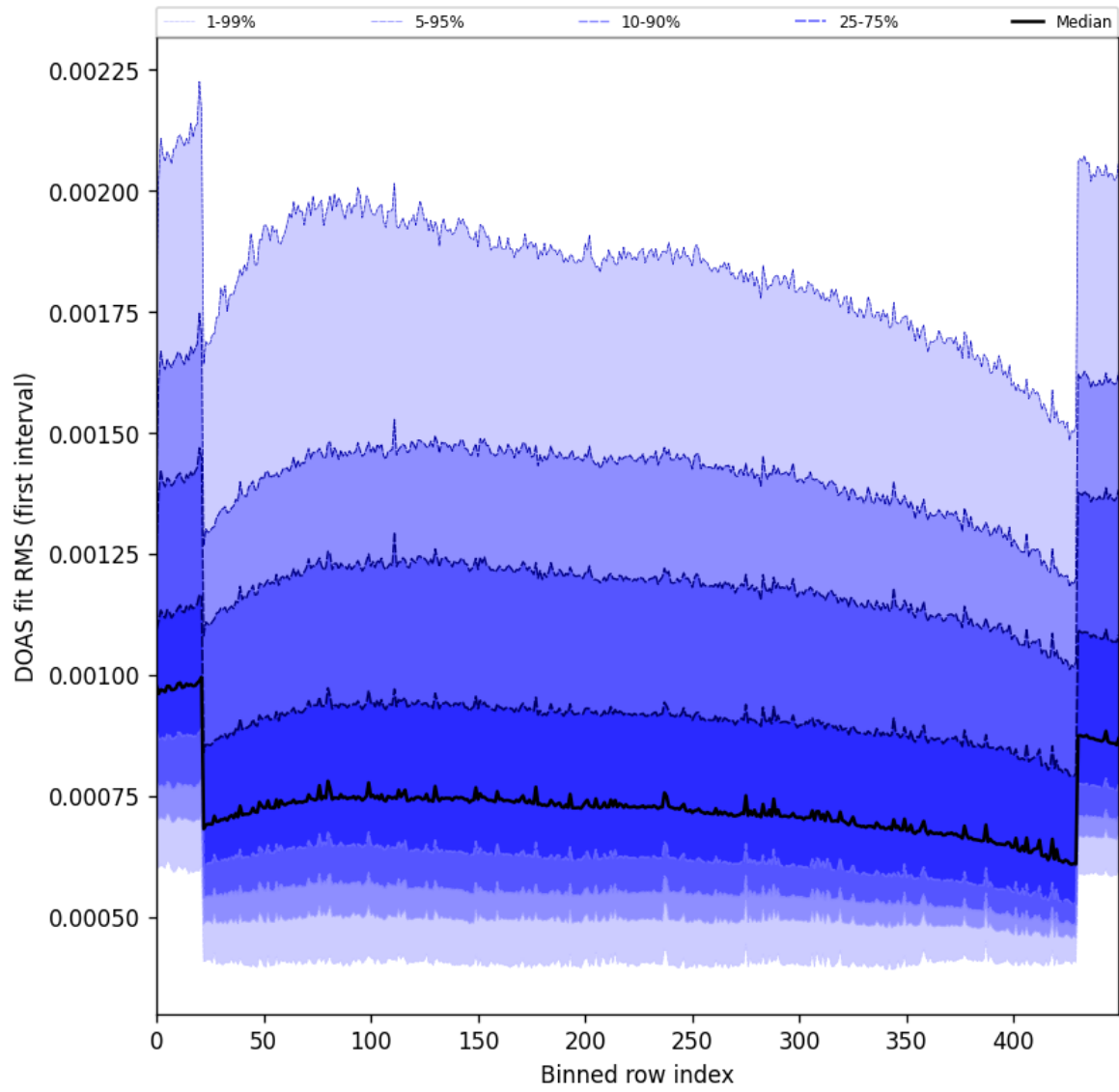
Figure 60: Along track statistics of “DOAS fit RMS (first interval)” for 2025-02-27 to 2025-03-01
