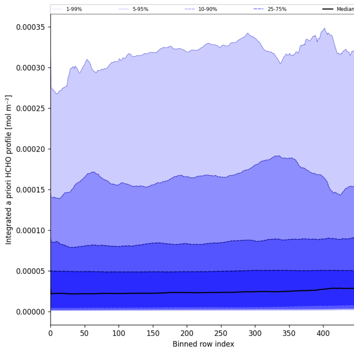
Figure 57: Along track statistics of "Integrated a priori HCHO profile" for 2025-02-27 to 2025-03-01
