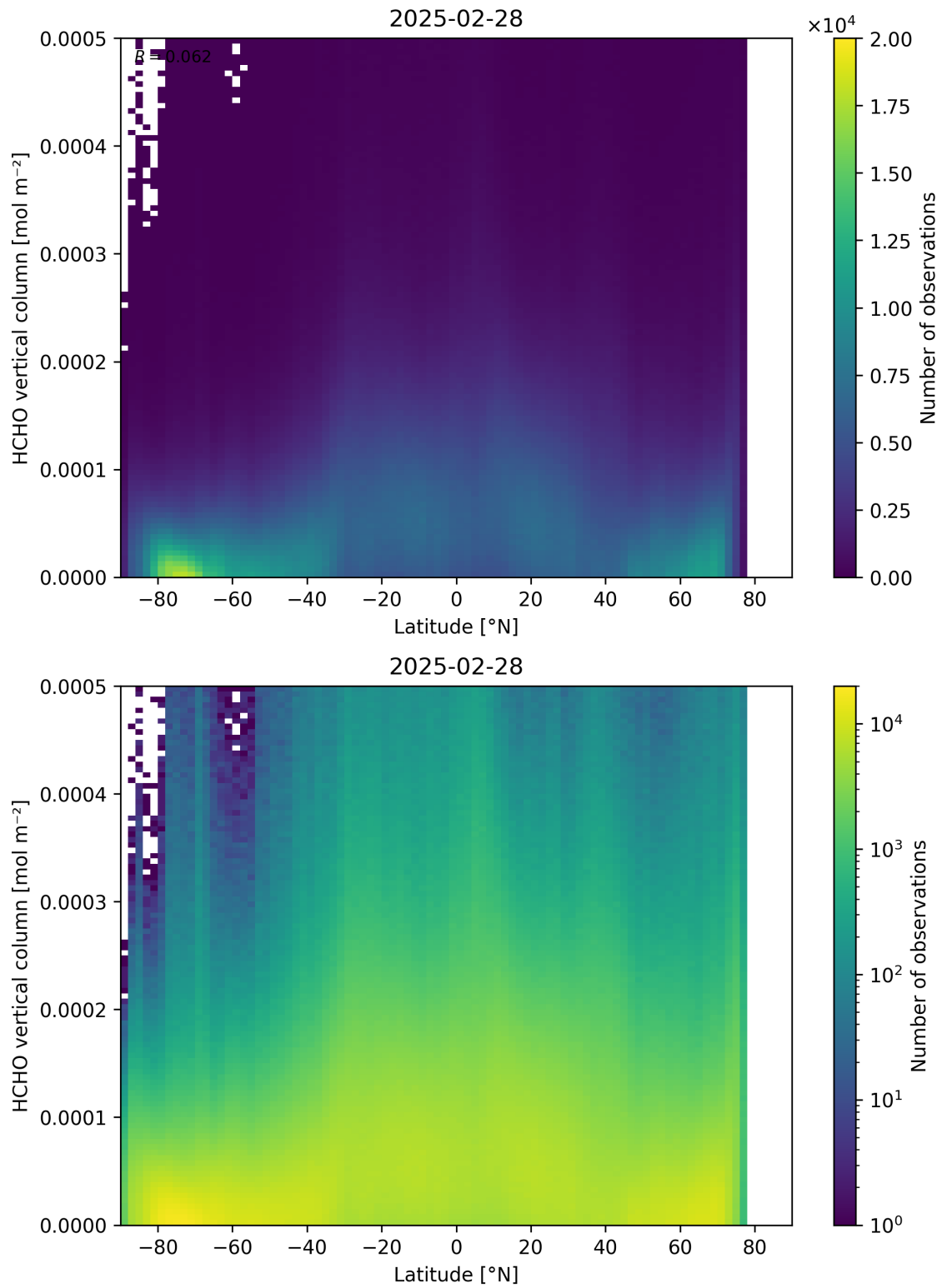
Figure 163: Scatter density plot of “Latitude” against “HCHO vertical column” for 2025-02-27 to 2025-03-01.
