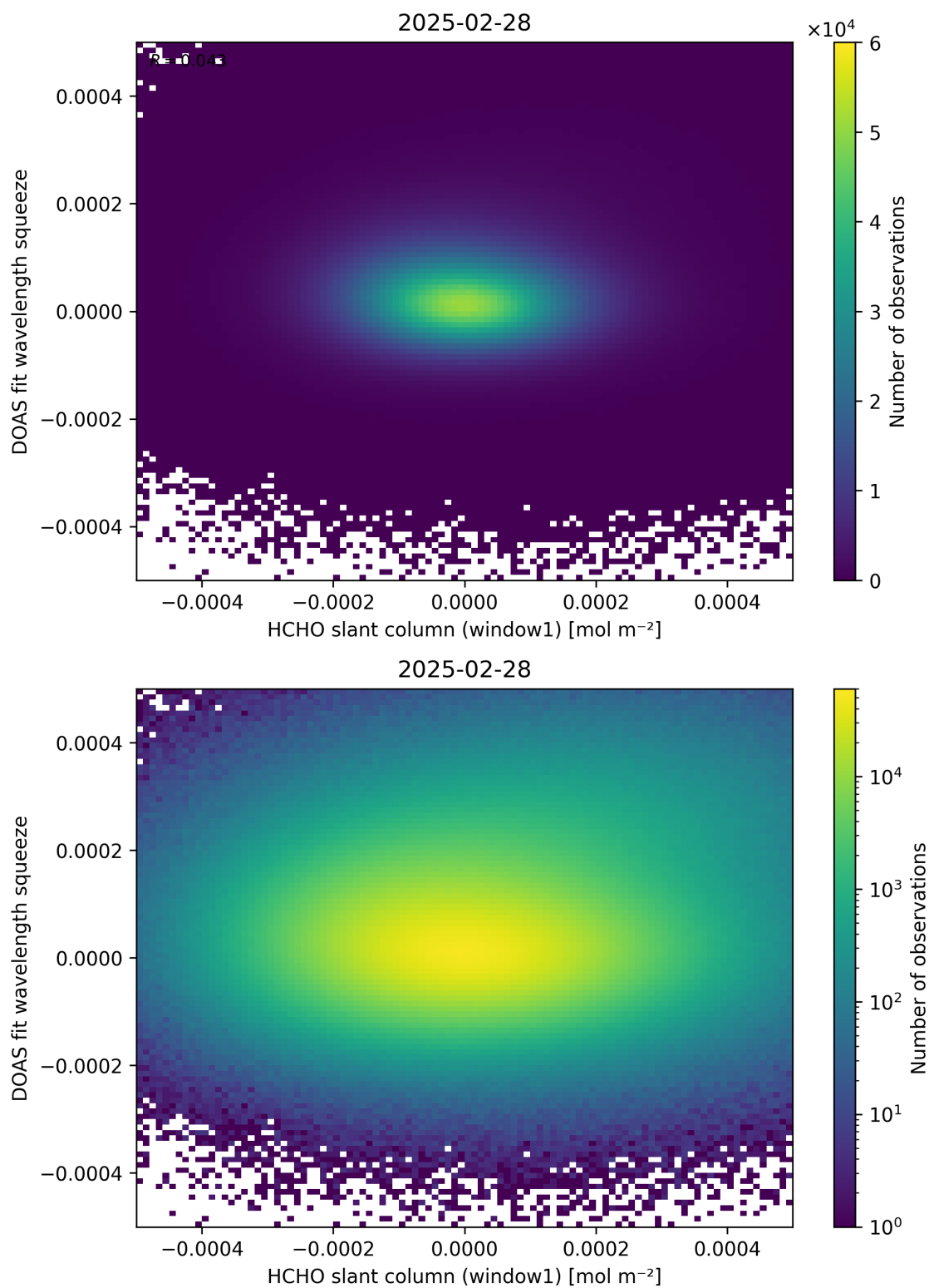
Figure 80: Scatter density plot of “HCHO slant column (window1)” against “DOAS fit wavelength squeeze” for 2025-02-27 to 2025-03-01.
