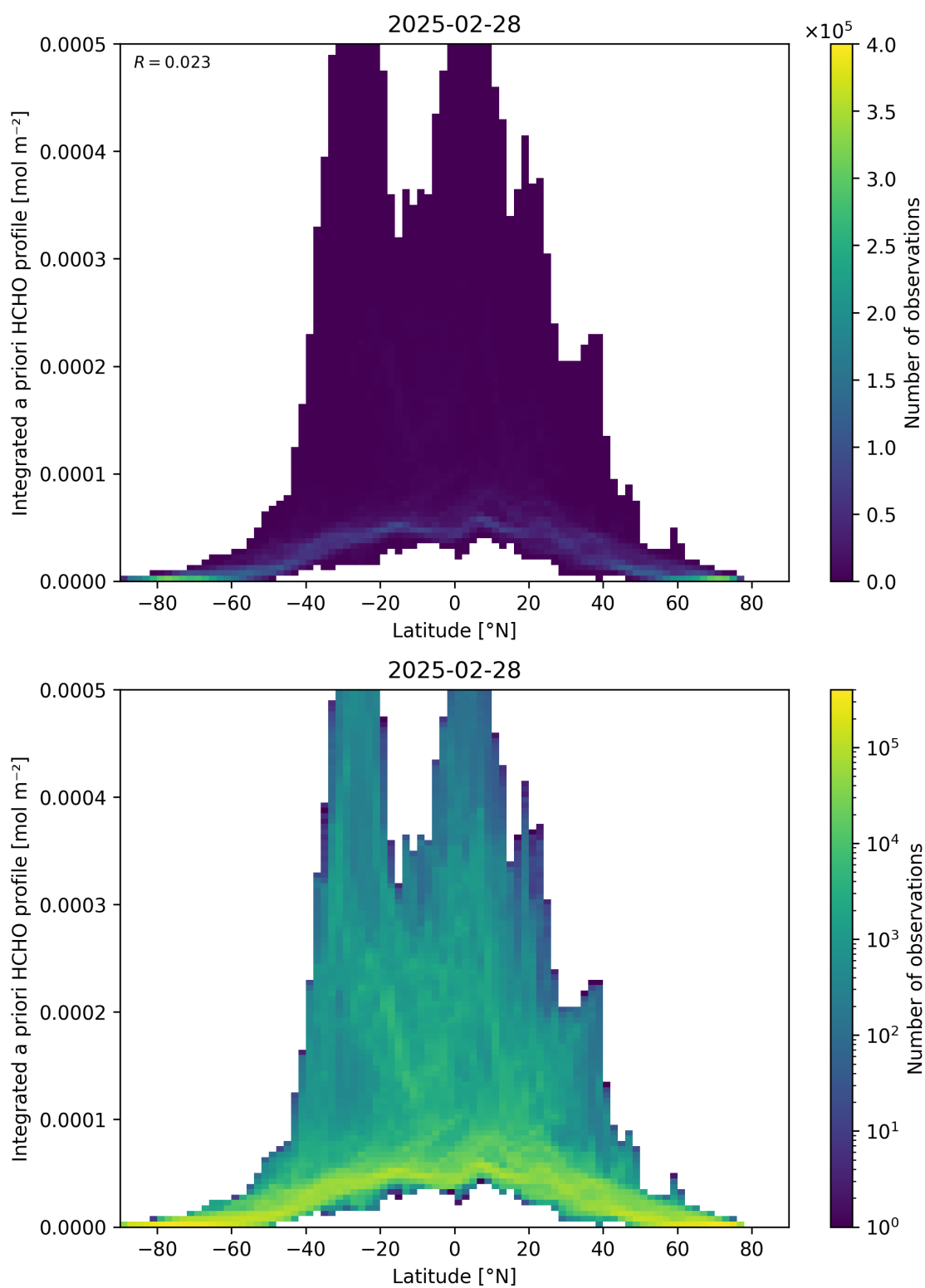
Figure 166: Scatter density plot of “Latitude” against “Integrated a priori HCHO profile” for 2025-02-27 to 2025-03-01.
