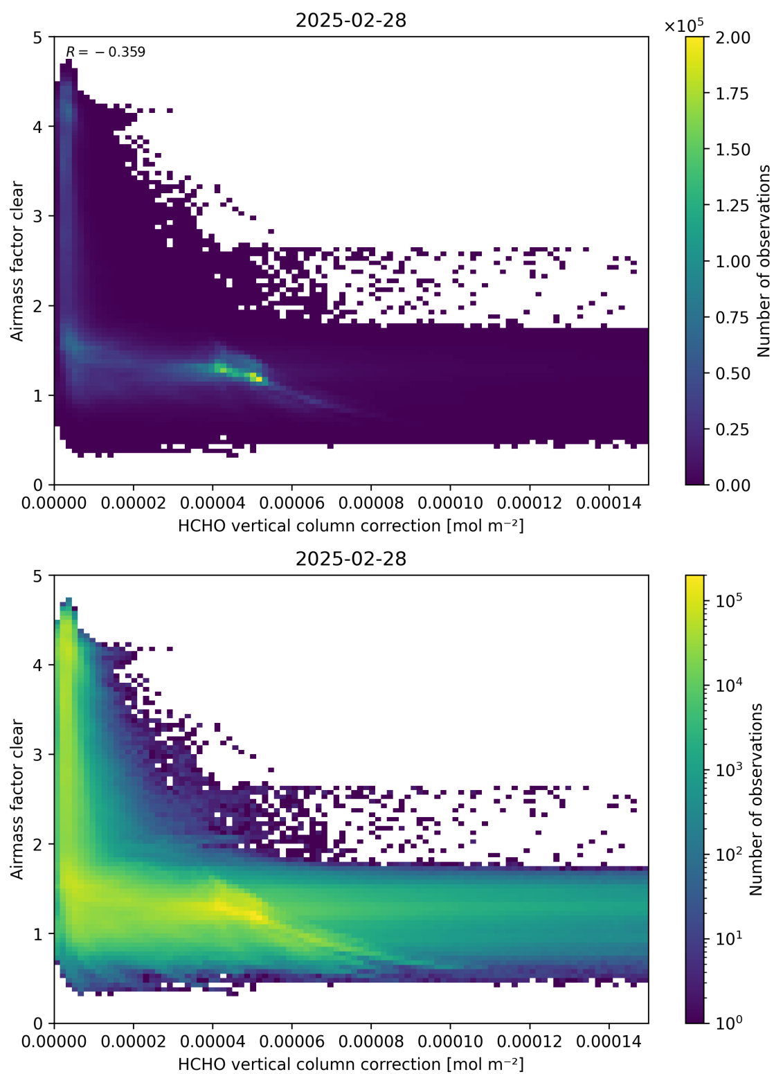
Figure 115: Scatter density plot of “HCHO vertical column correction” against “Airmass factor clear” for 2025-02-27 to 2025-03-01.
