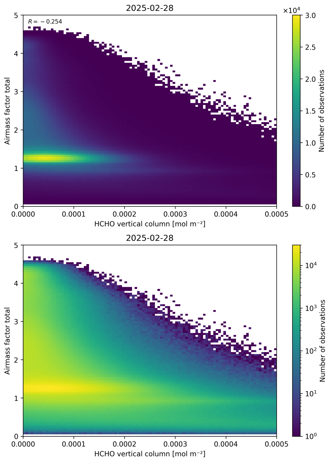
Figure 131: Scatter density plot of “HCHO vertical column” against “Airmass factor total” for 2025-02-27 to 2025-03-01.
