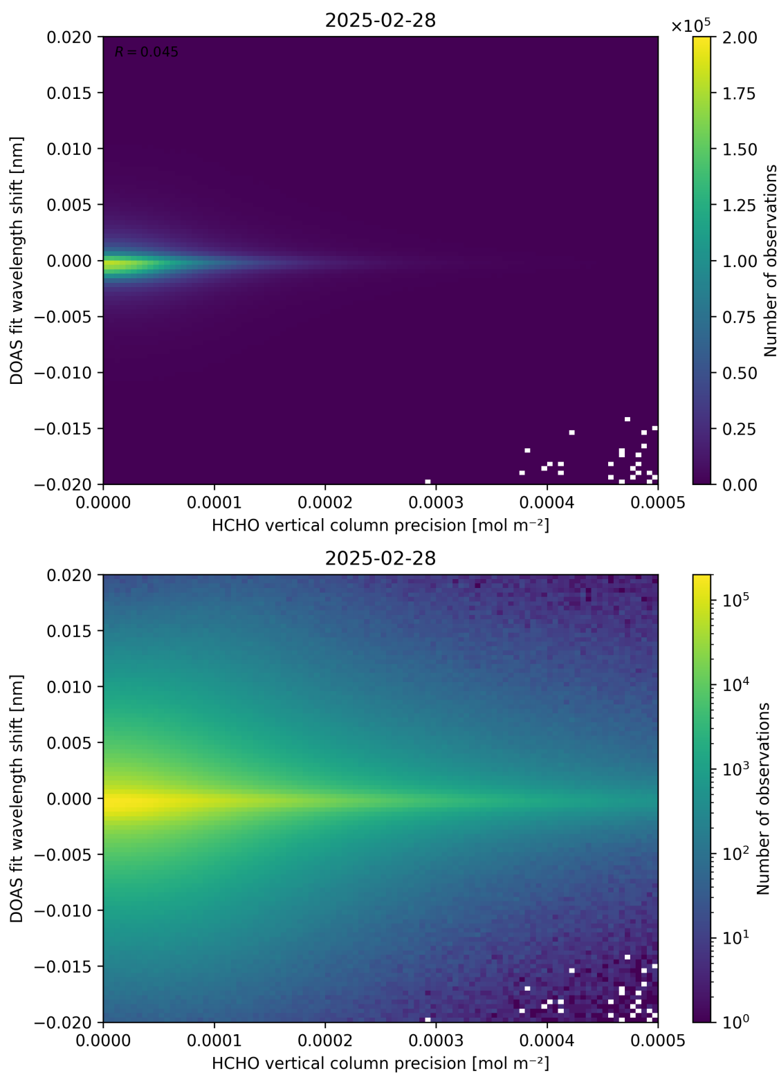
Figure 137: Scatter density plot of “HCHO vertical column precision” against “DOAS fit wavelength shift” for 2025-02-27 to 2025-03-01.
