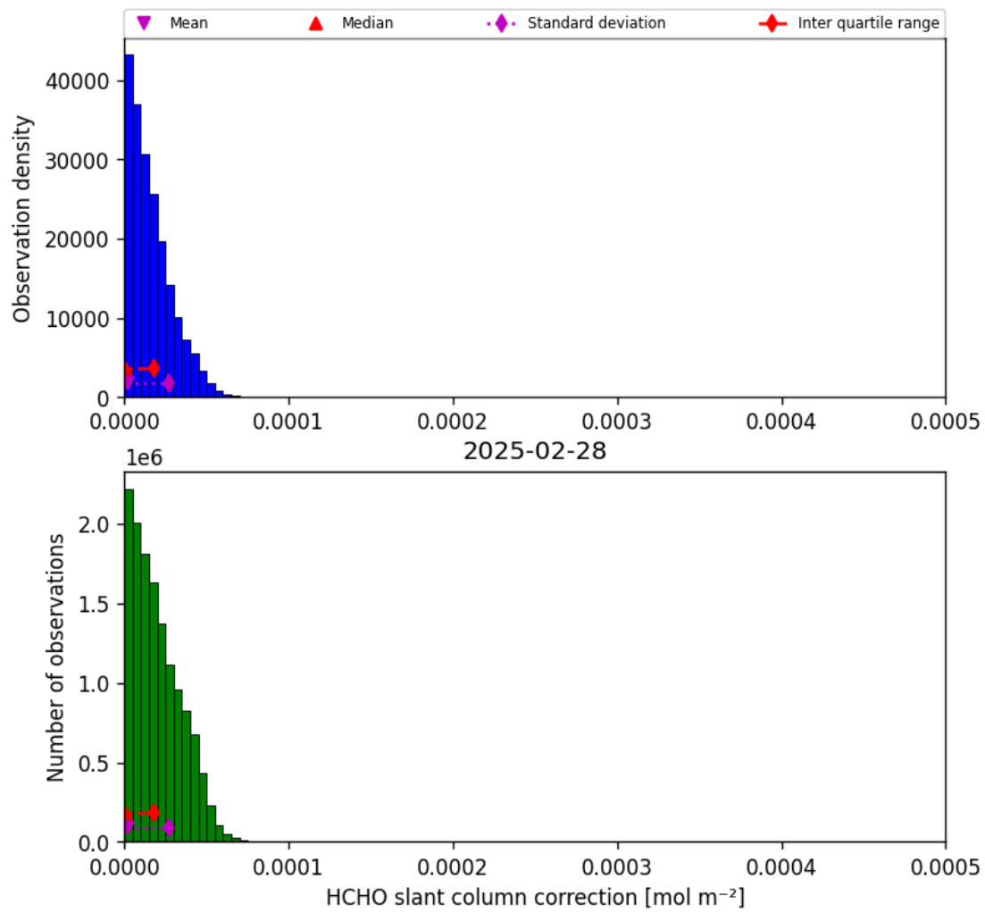
Figure 47: Histogram of “HCHO slant column correction” for 2025-02-27 to 2025-03-01
