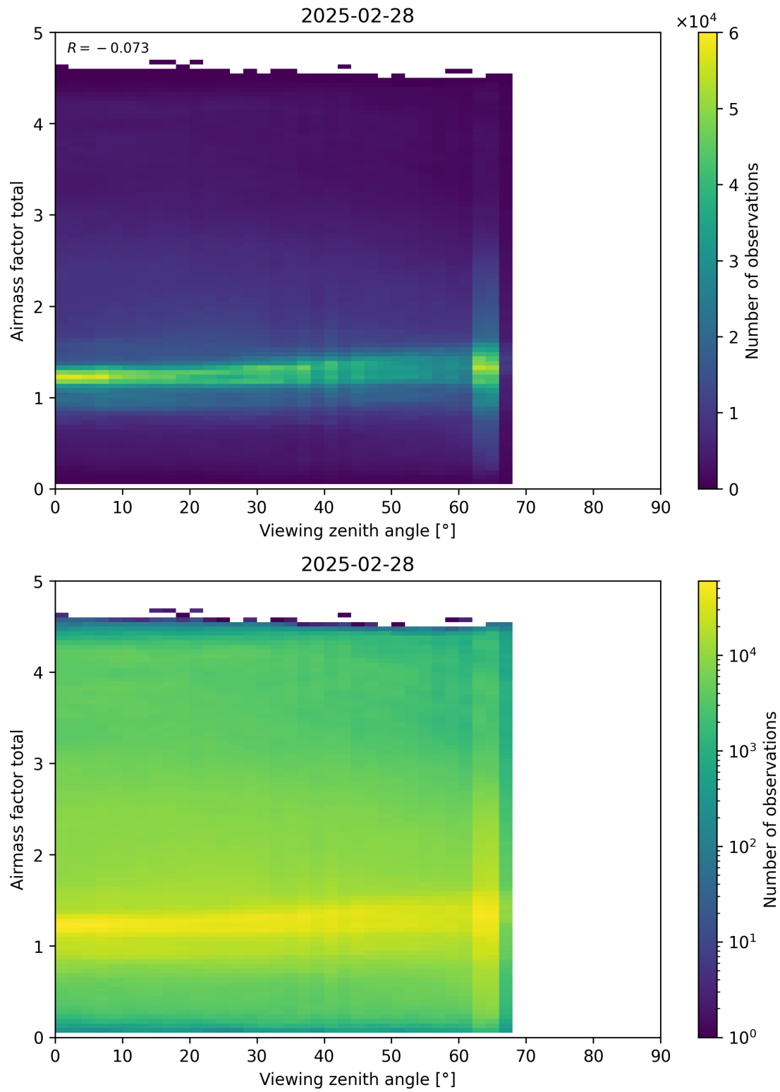
Figure 190: Scatter density plot of “Viewing zenith angle” against “Airmass factor total” for 2025-02-27 to 2025-03-01.
