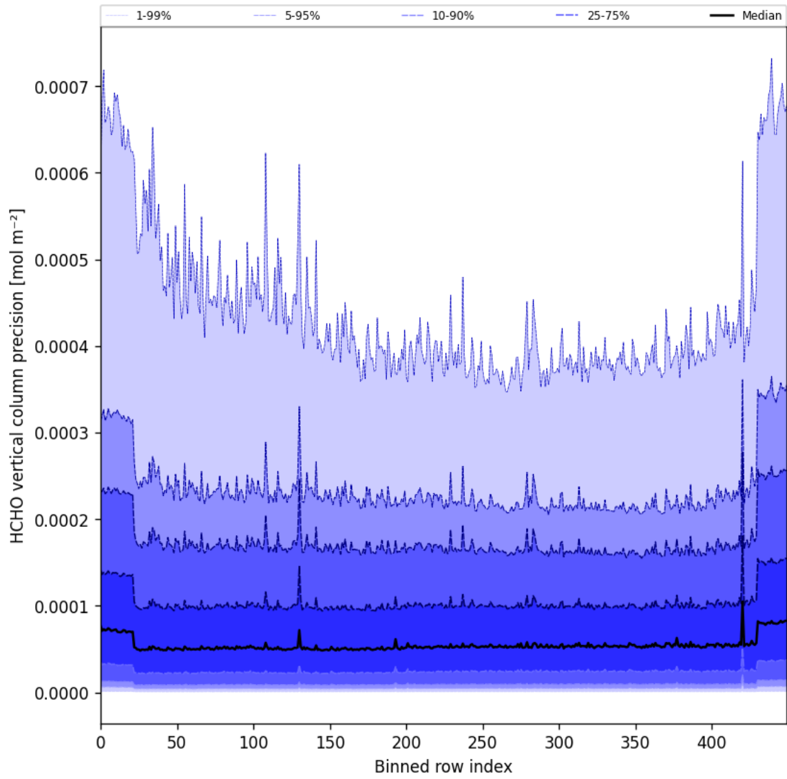
Figure 50: Along track statistics of “HCHO vertical column precision” for 2025-02-27 to 2025-03-01
