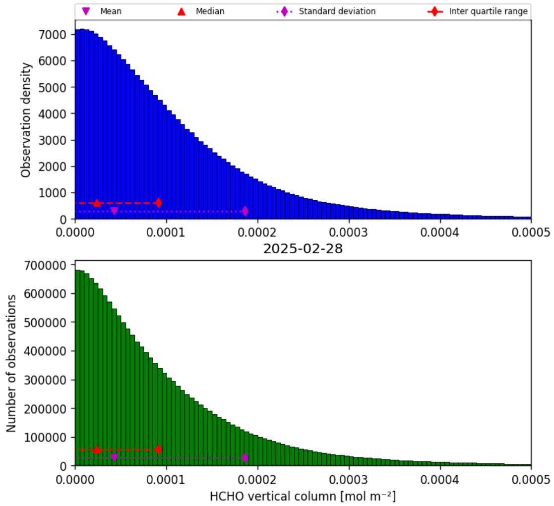
Figure 35: Histogram of “HCHO vertical column” for 2025-02-27 to 2025-03-01
