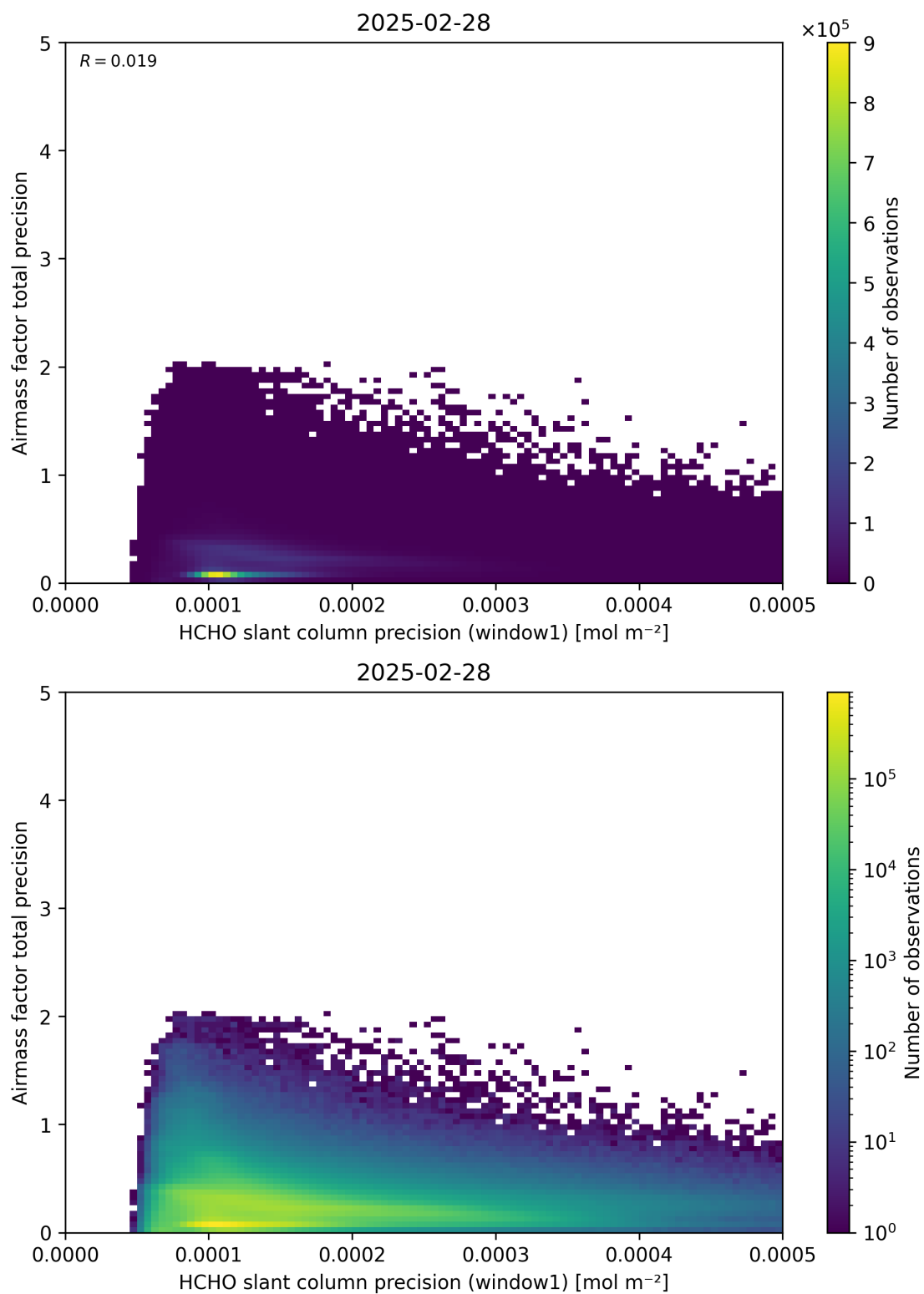
Figure 95: Scatter density plot of “HCHO slant column precision (window1)” against “Airmass factor total precision” for 2025-02-27 to 2025-03-01.
