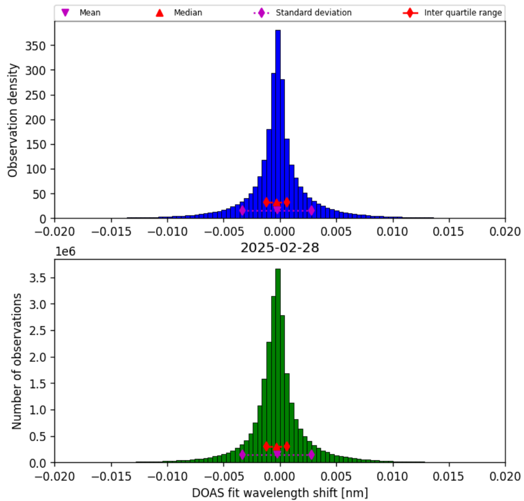
Figure 44: Histogram of “DOAS fit wavelength shift” for 2025-02-27 to 2025-03-01
