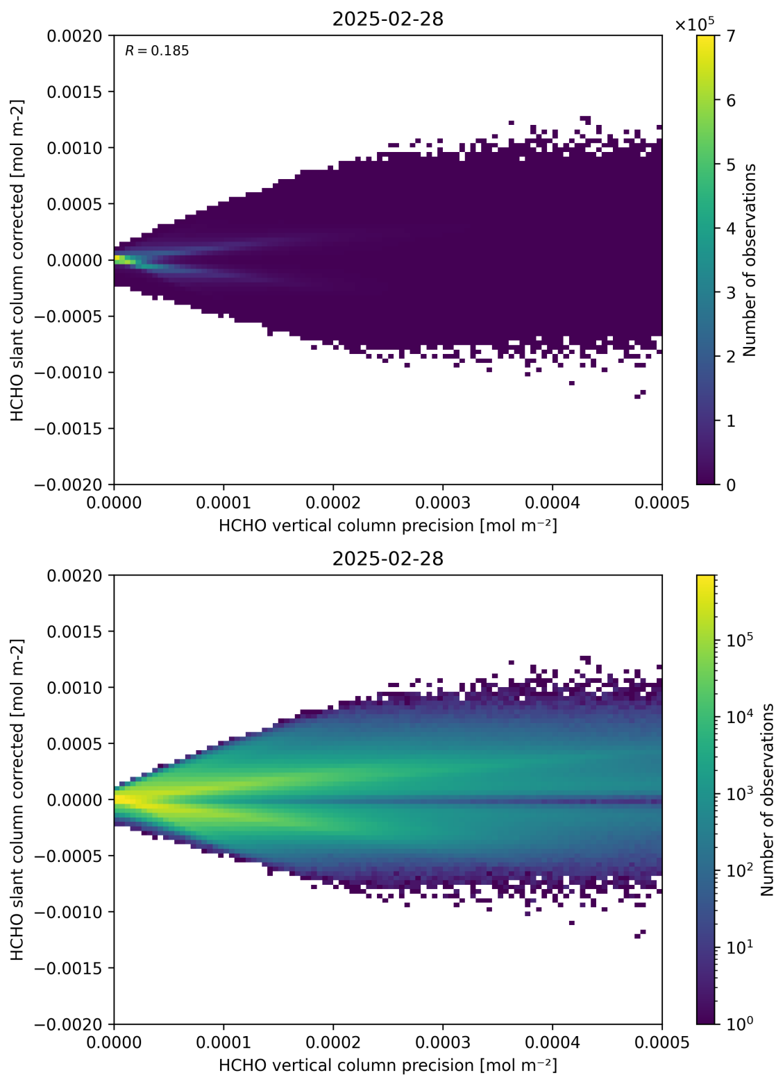
Figure 140: Scatter density plot of “HCHO vertical column precision” against “HCHO slant column corrected” for 2025-02-27 to 2025-03-01.
