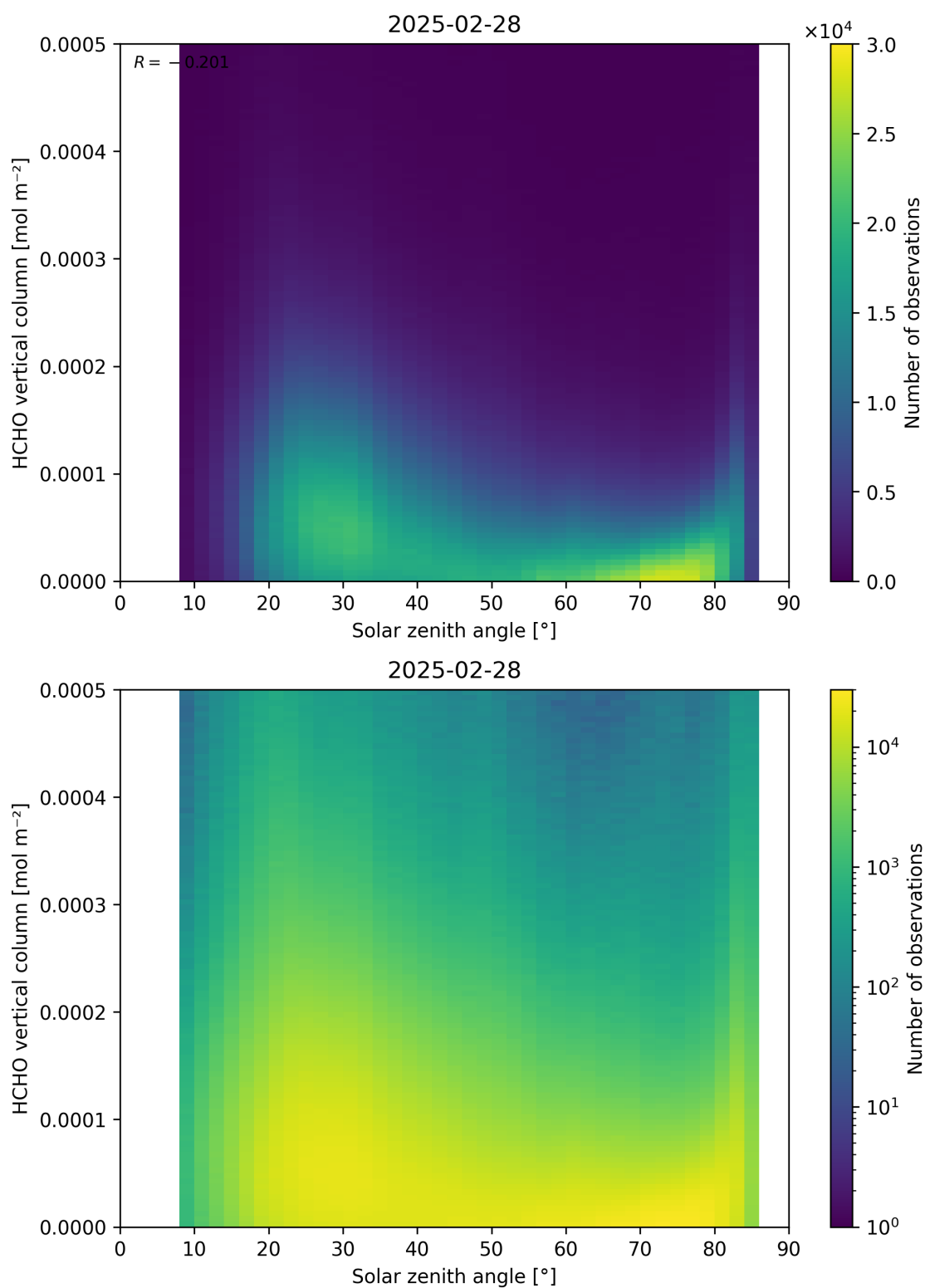
Figure 177: Scatter density plot of “Solar zenith angle” against “HCHO vertical column” for 2025-02-27 to 2025-03-01.
