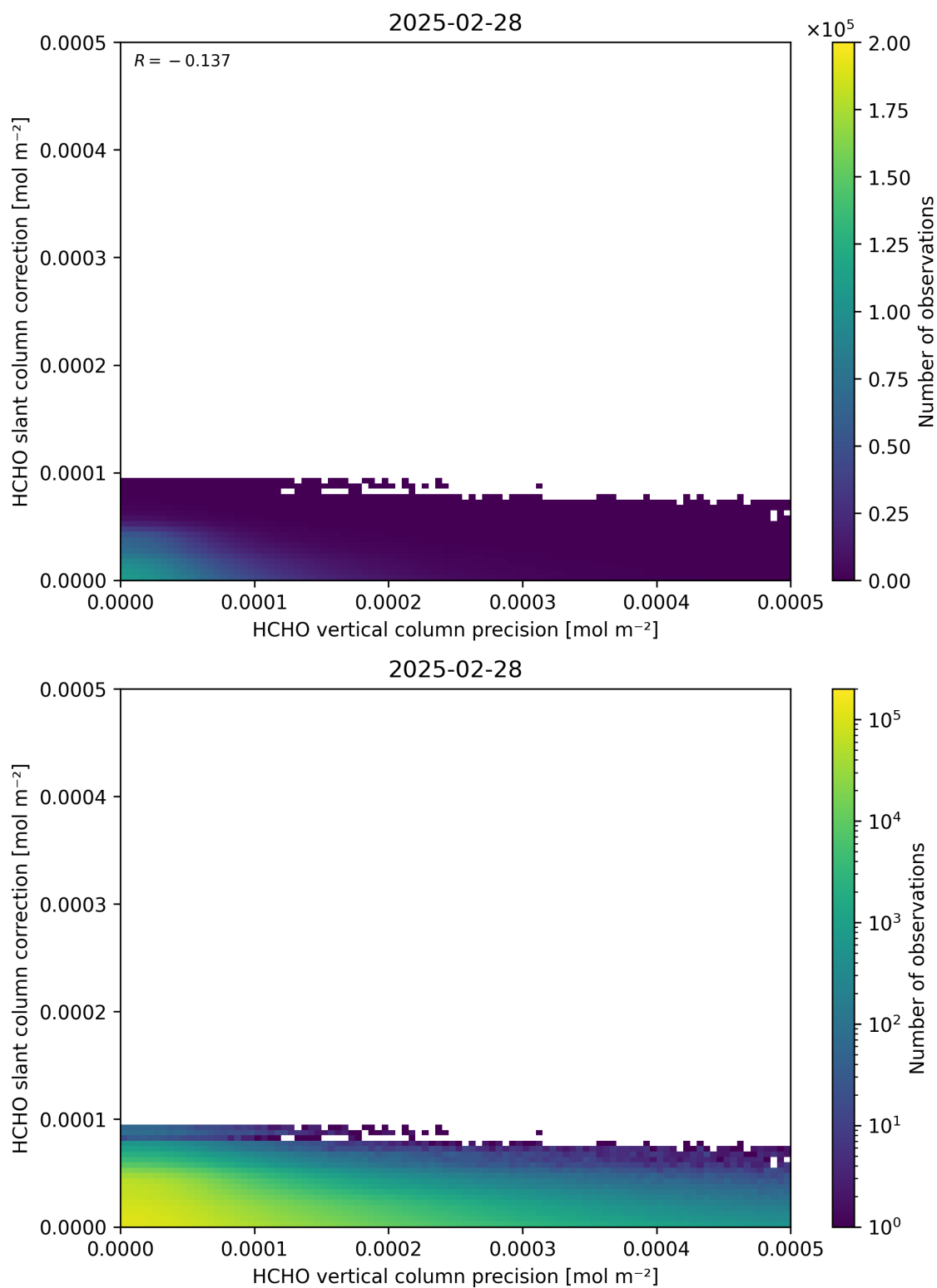
Figure 141: Scatter density plot of “HCHO vertical column precision” against “HCHO slant column correction” for 2025-02-27 to 2025-03-01.
