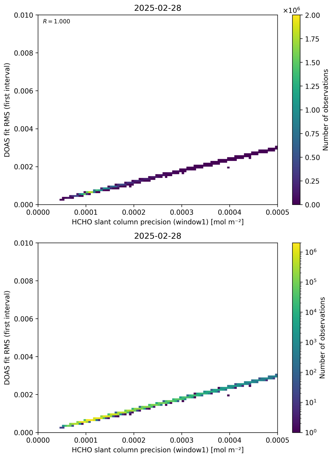
Figure 88: Scatter density plot of “HCHO slant column precision (window1)” against “DOAS fit RMS (first interval)” for 2025-02-27 to 2025-03-01.
