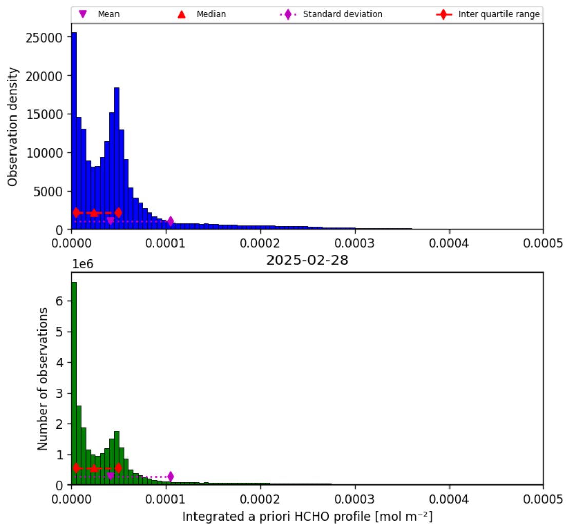
Figure 43: Histogram of “Integrated a priori HCHO profile” for 2025-02-27 to 2025-03-01
