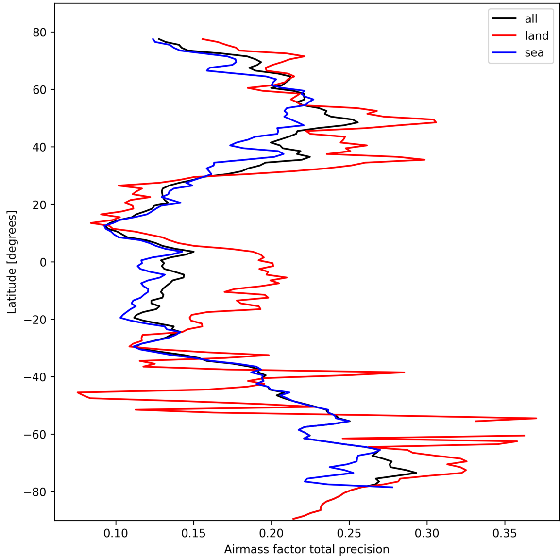
Figure 27: Zonal average of “Airmass factor total precision” for 2025-02-27 to 2025-03-01.
