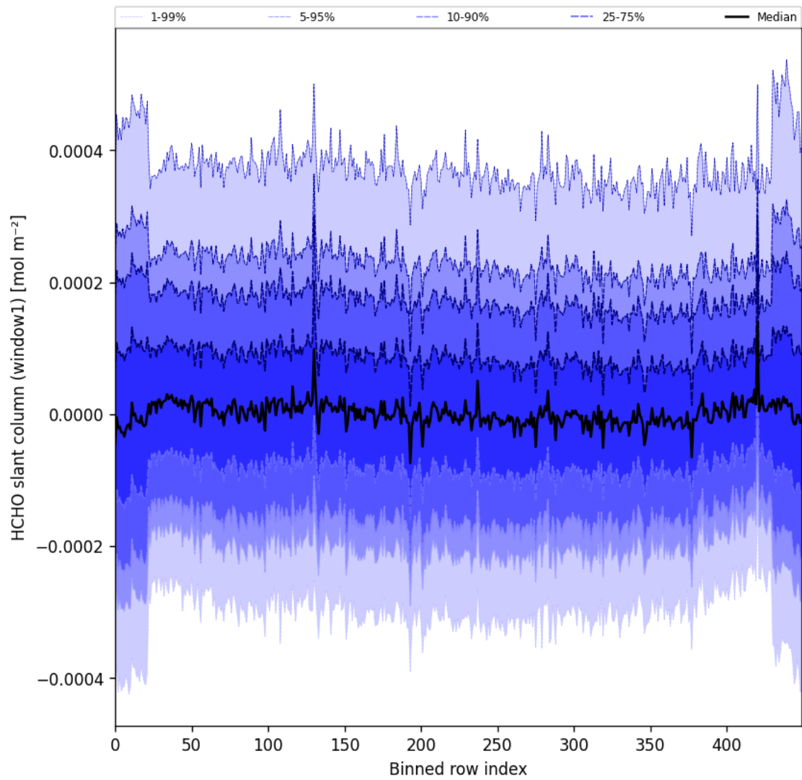
Figure 52: Along track statistics of “HCHO slant column (window1)” for 2025-02-27 to 2025-03-01
