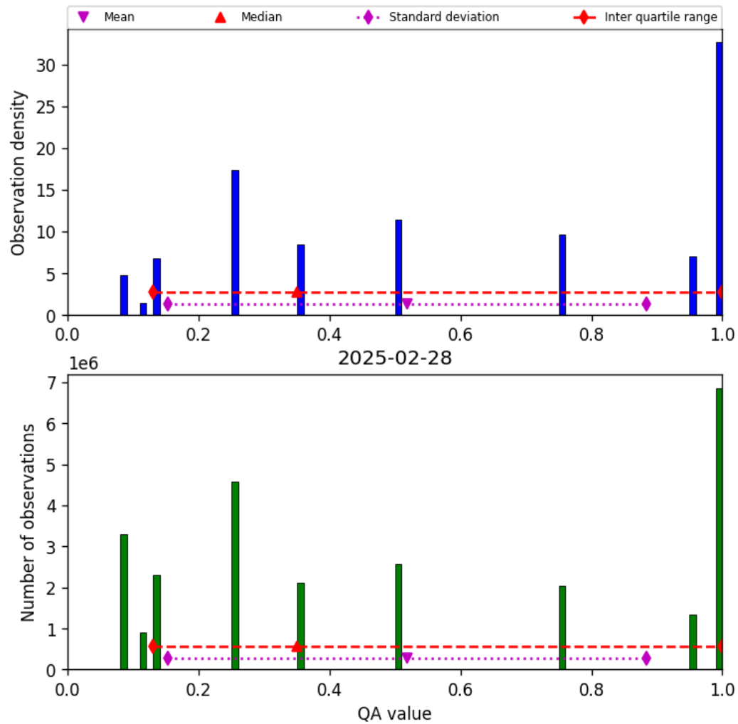
Figure 34: Histogram of “QA value” for 2025-02-27 to 2025-03-01
