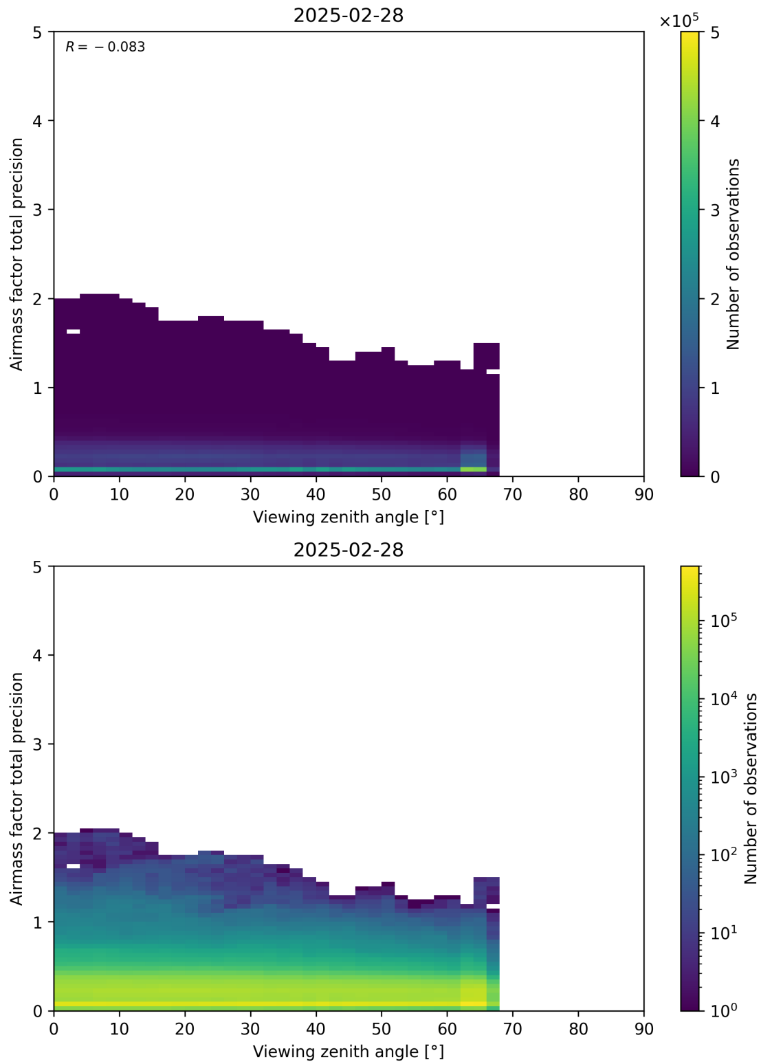
Figure 191: Scatter density plot of “Viewing zenith angle” against “Airmass factor total precision” for 2025-02-27 to 2025-03-01.
