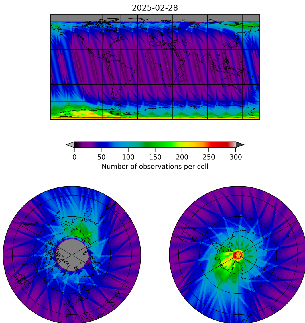
Figure 19: Map of the number of observations for 2025-02-27 to 2025-03-01
