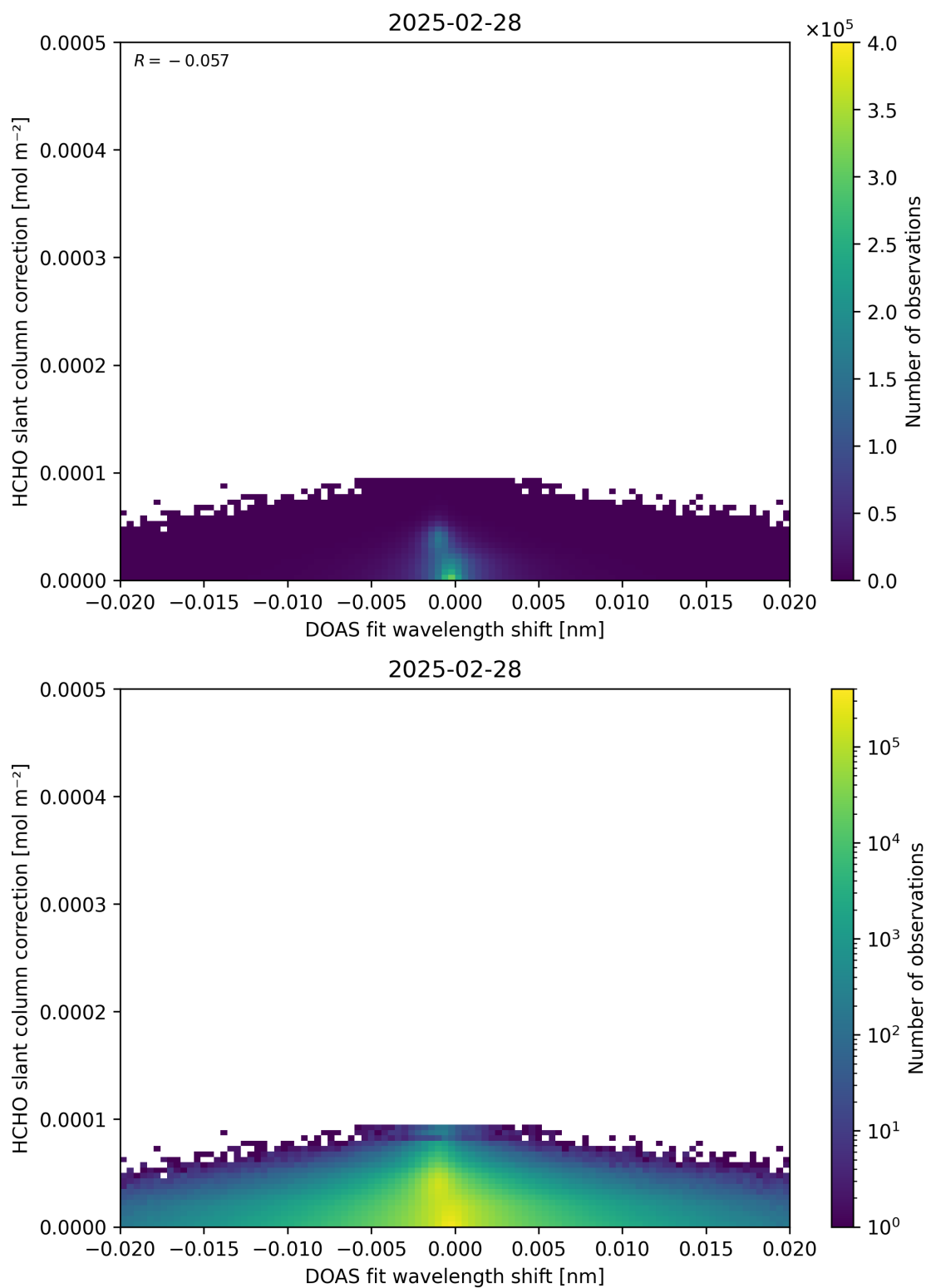
Figure 67: Scatter density plot of “DOAS fit wavelength shift” against “HCHO slant column correction” for 2025-02-27 to 2025-03-01.
