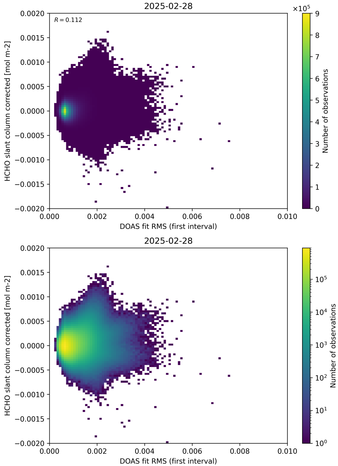
Figure 62: Scatter density plot of “DOAS fit RMS (first interval)” against “HCHO slant column corrected” for 2025-02-27 to 2025-03-01.
