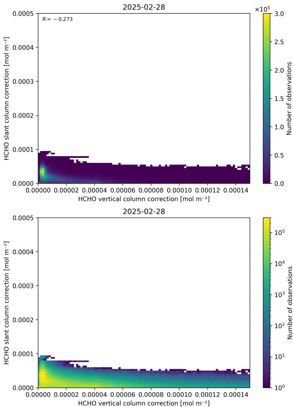
Figure 117: Scatter density plot of “HCHO vertical column correction” against “HCHO slant column correction” for 2025-02-27 to 2025-03-01.
