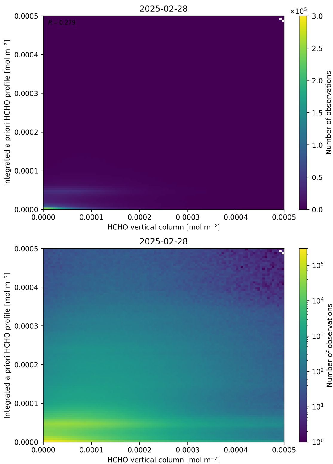
Figure 135: Scatter density plot of “HCHO vertical column” against “Integrated a priori HCHO profile” for 2025-02-27 to 2025-03-01.
