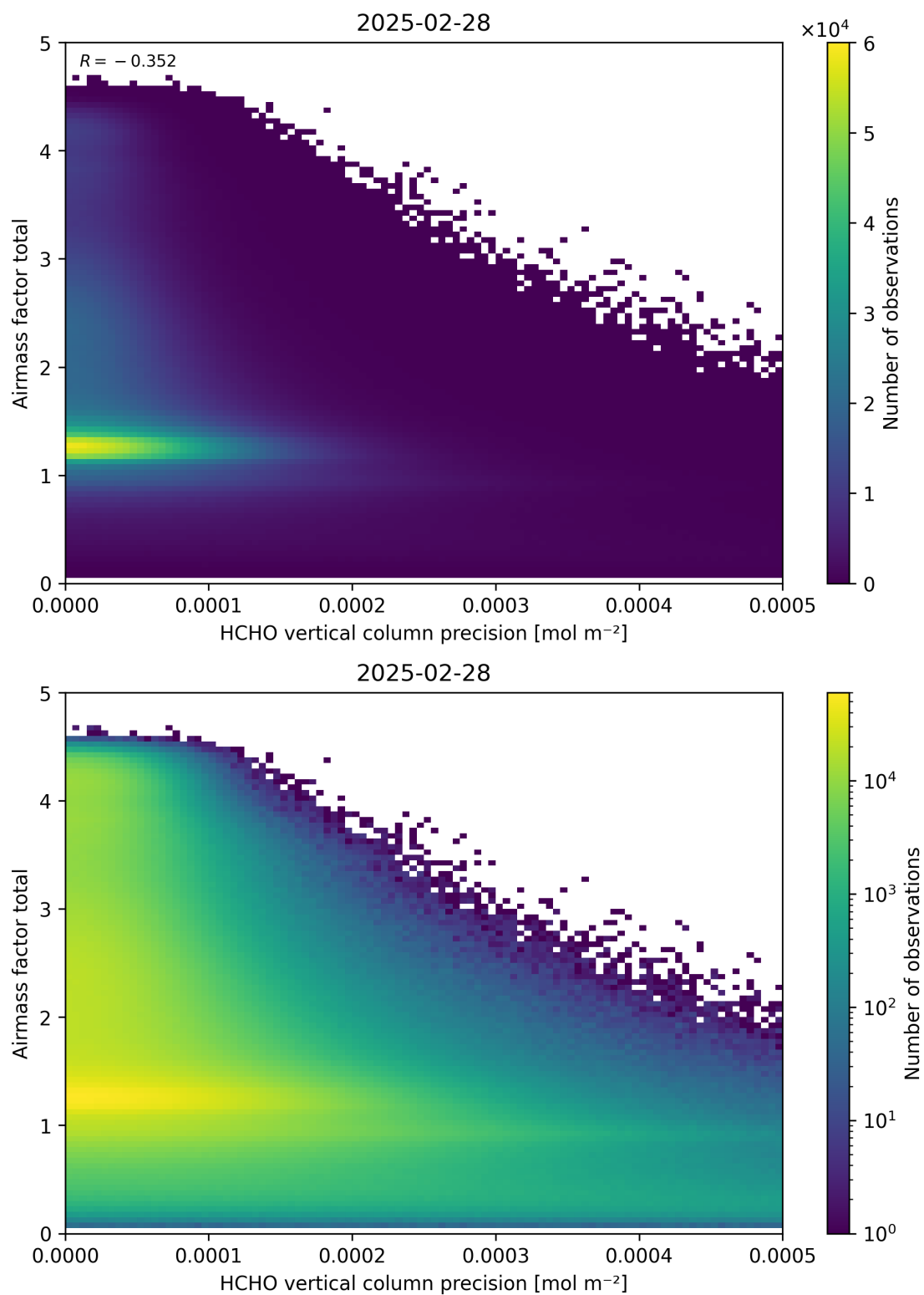
Figure 144: Scatter density plot of “HCHO vertical column precision” against “Airmass factor total” for 2025-02-27 to 2025-03-01.
