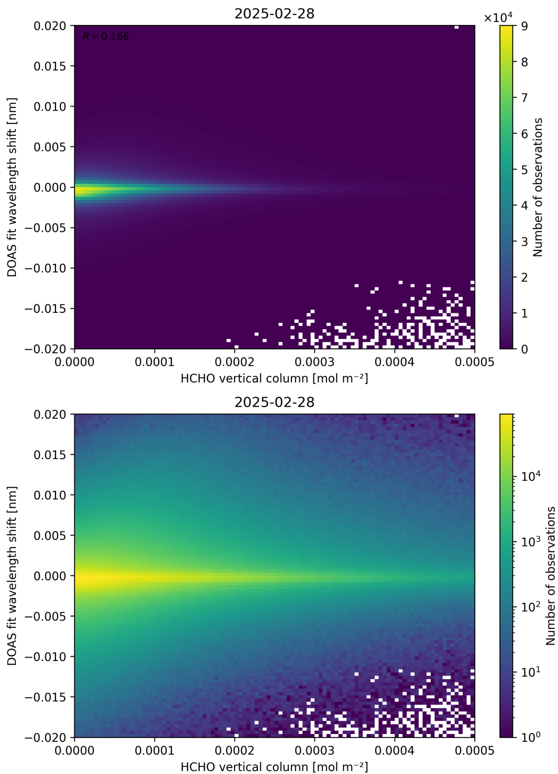
Figure 124: Scatter density plot of “HCHO vertical column” against “DOAS fit wavelength shift” for 2025-02-27 to 2025-03-01.
