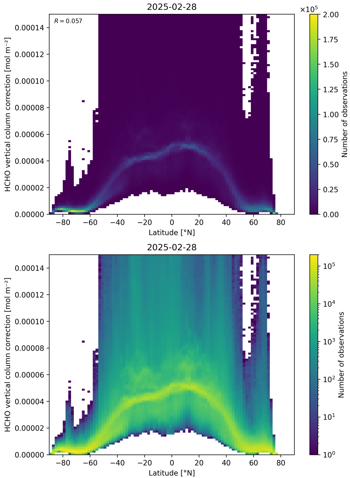
Figure 164: Scatter density plot of “Latitude” against “HCHO vertical column correction” for 2025-02-27 to 2025-03-01.
