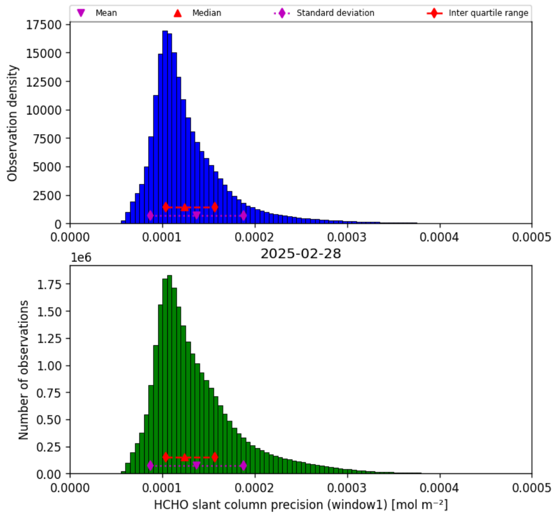
Figure 39: Histogram of “HCHO slant column precision (window1)” for 2025-02-27 to 2025-03-01
