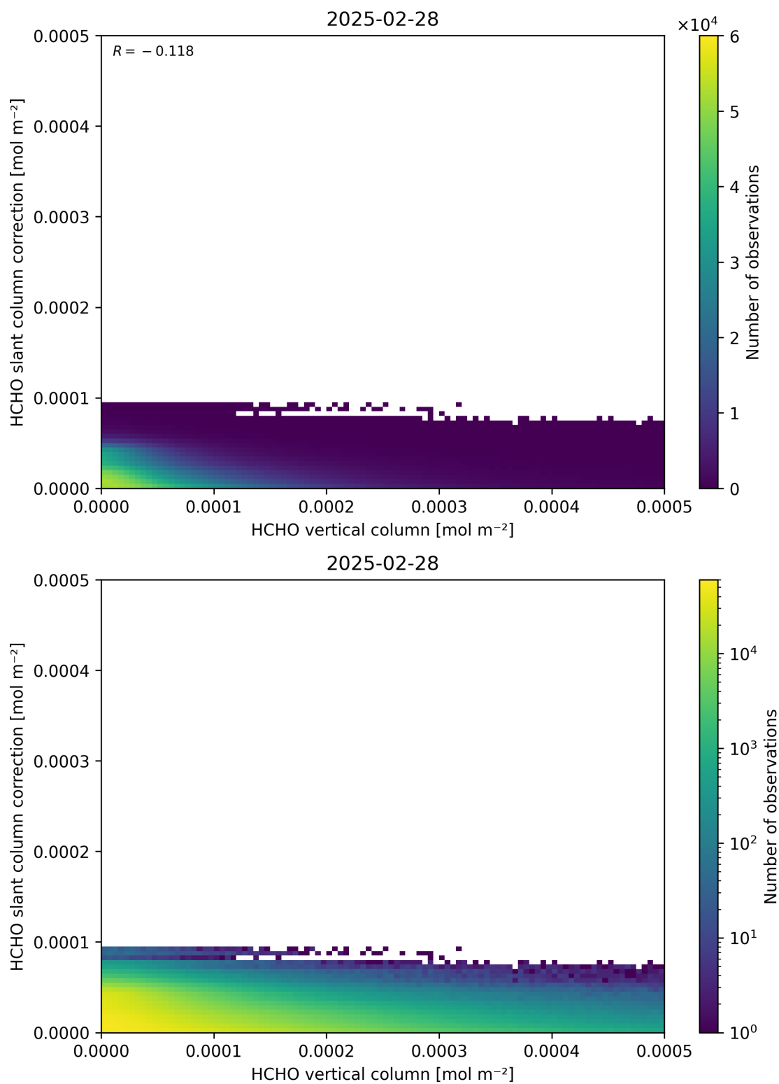
Figure 128: Scatter density plot of “HCHO vertical column” against “HCHO slant column correction” for 2025-02-27 to 2025-03-01.
