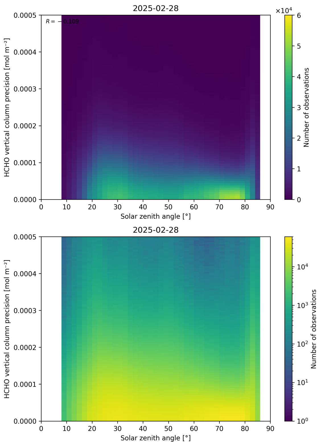
Figure 179: Scatter density plot of “Solar zenith angle” against “HCHO vertical column precision” for 2025-02-27 to 2025-03-01.
