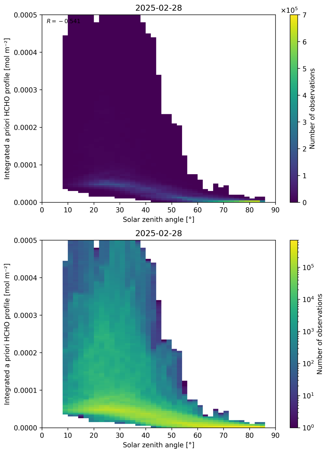
Figure 180: Scatter density plot of “Solar zenith angle” against “Integrated a priori HCHO profile” for 2025-02-27 to 2025-03-01.
