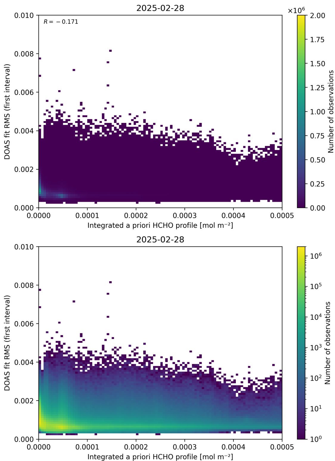
Figure 148: Scatter density plot of “Integrated a priori HCHO profile” against “DOAS fit RMS (first interval)” for 2025-02-27 to 2025-03-01.
