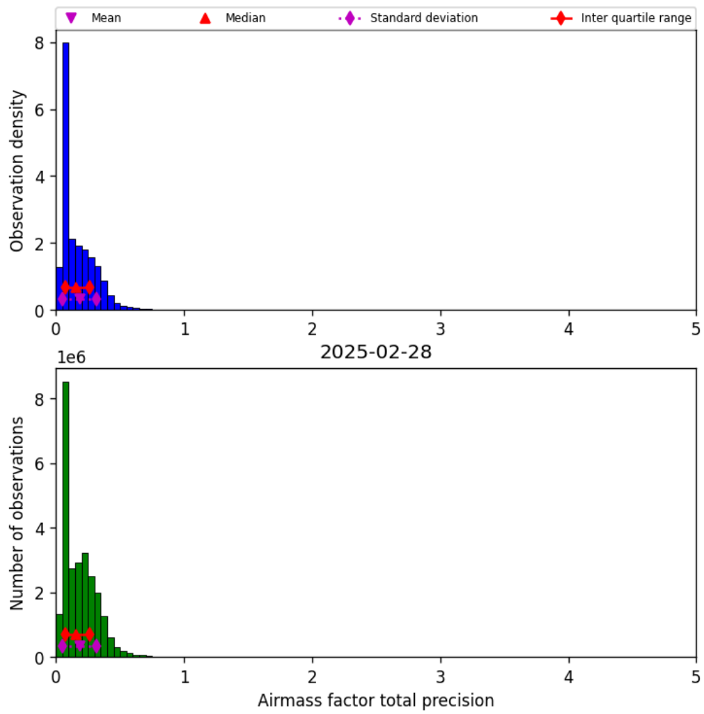
Figure 41: Histogram of “Airmass factor total precision” for 2025-02-27 to 2025-03-01
