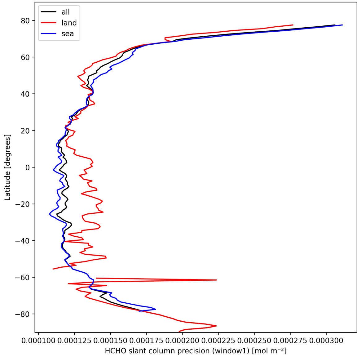
Figure 25: Zonal average of “HCHO slant column precision (window1)” for 2025-02-27 to 2025-03-01.
