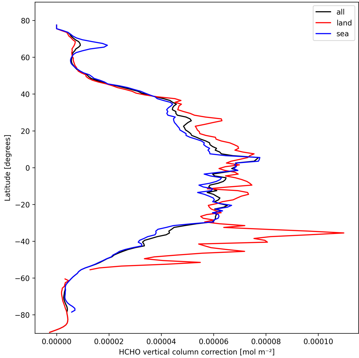
Figure 23: Zonal average of “HCHO vertical column correction” for 2025-02-27 to 2025-03-01.
