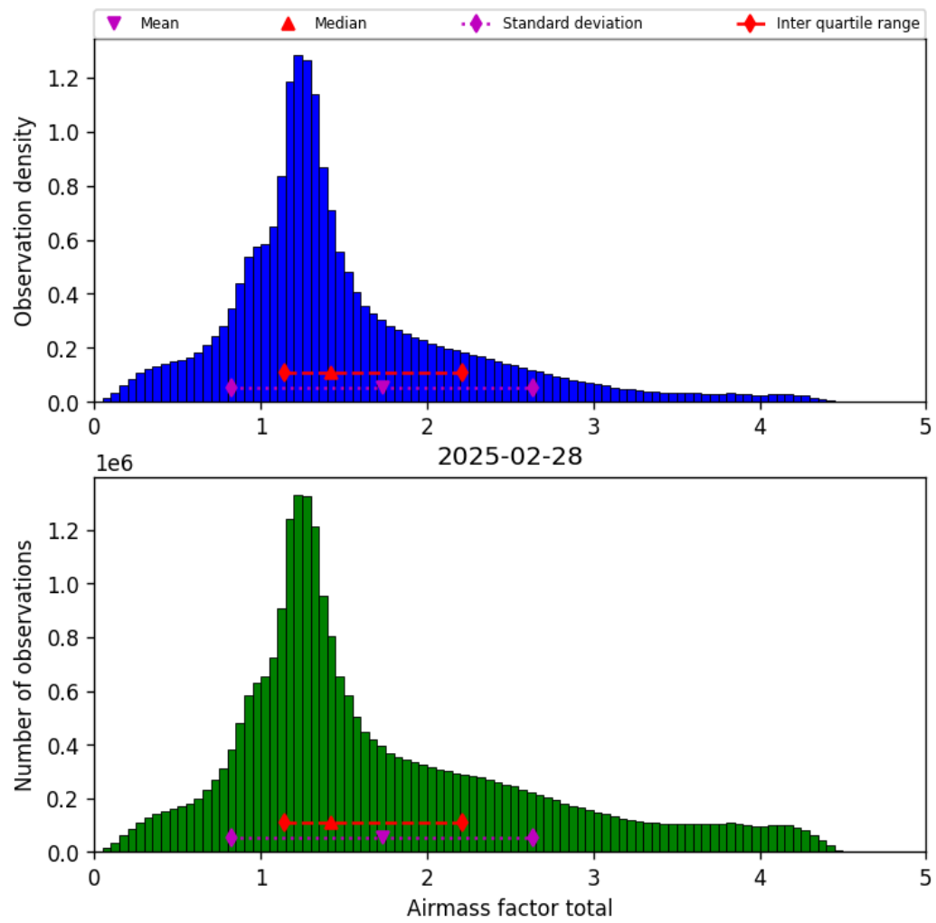
Figure 40: Histogram of “Airmass factor total” for 2025-02-27 to 2025-03-01
