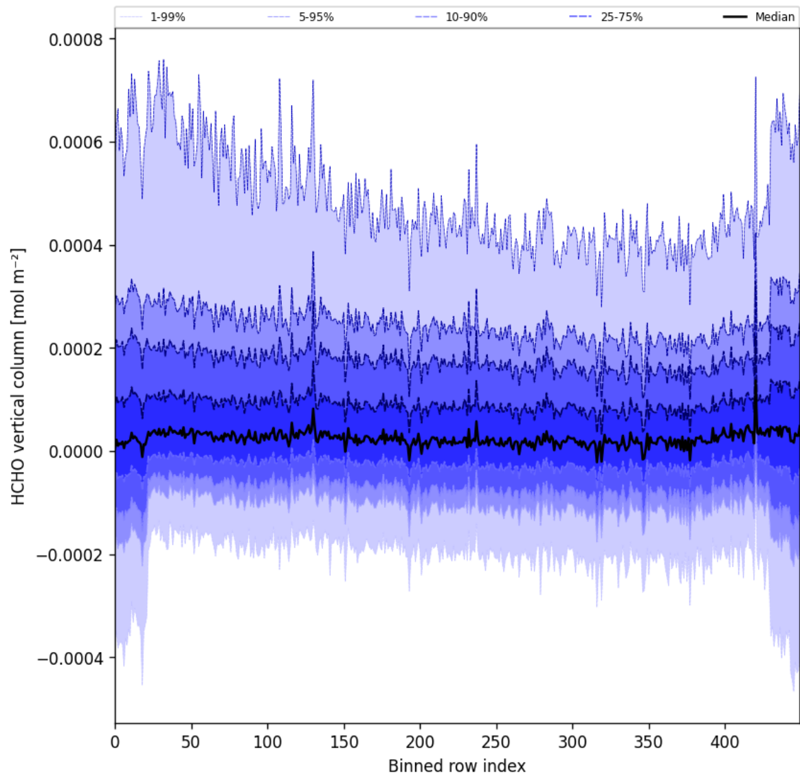
Figure 49: Along track statistics of “HCHO vertical column” for 2025-02-27 to 2025-03-01
