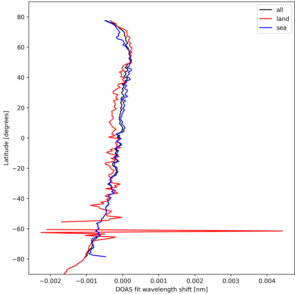
Figure 30: Zonal average of “DOAS fit wavelength shift” for 2025-02-27 to 2025-03-01.
