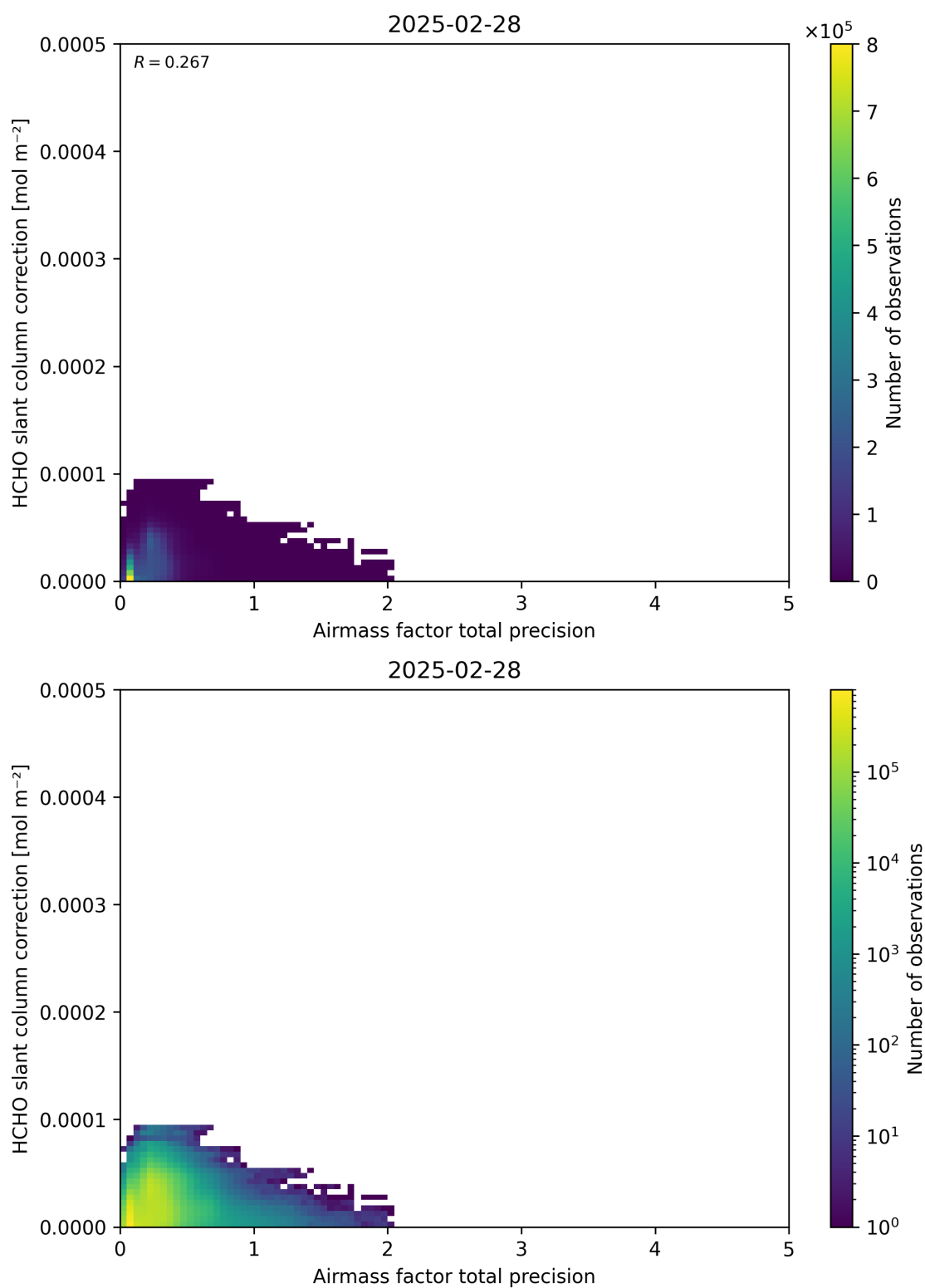
Figure 110: Scatter density plot of “Airmass factor total precision” against “HCHO slant column correction” for 2025-02-27 to 2025-03-01.
