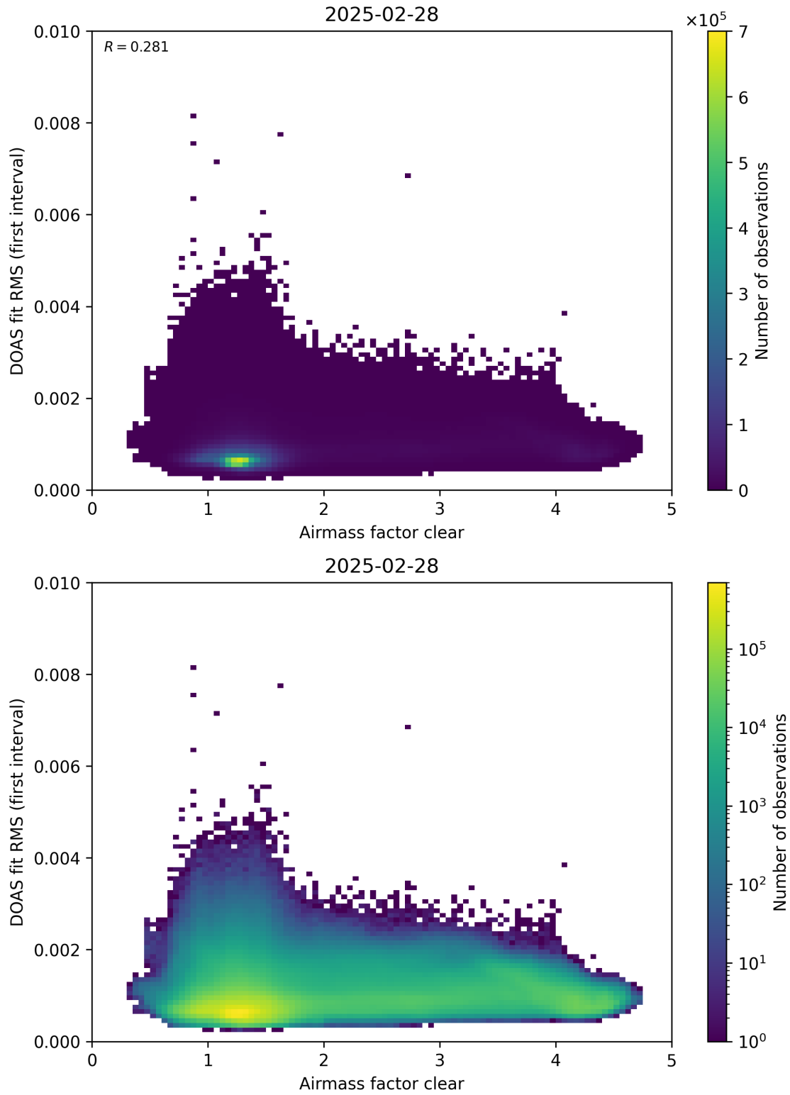
Figure 71: Scatter density plot of “Airmass factor clear” against “DOAS fit RMS (first interval)” for 2025-02-27 to 2025-03-01.
