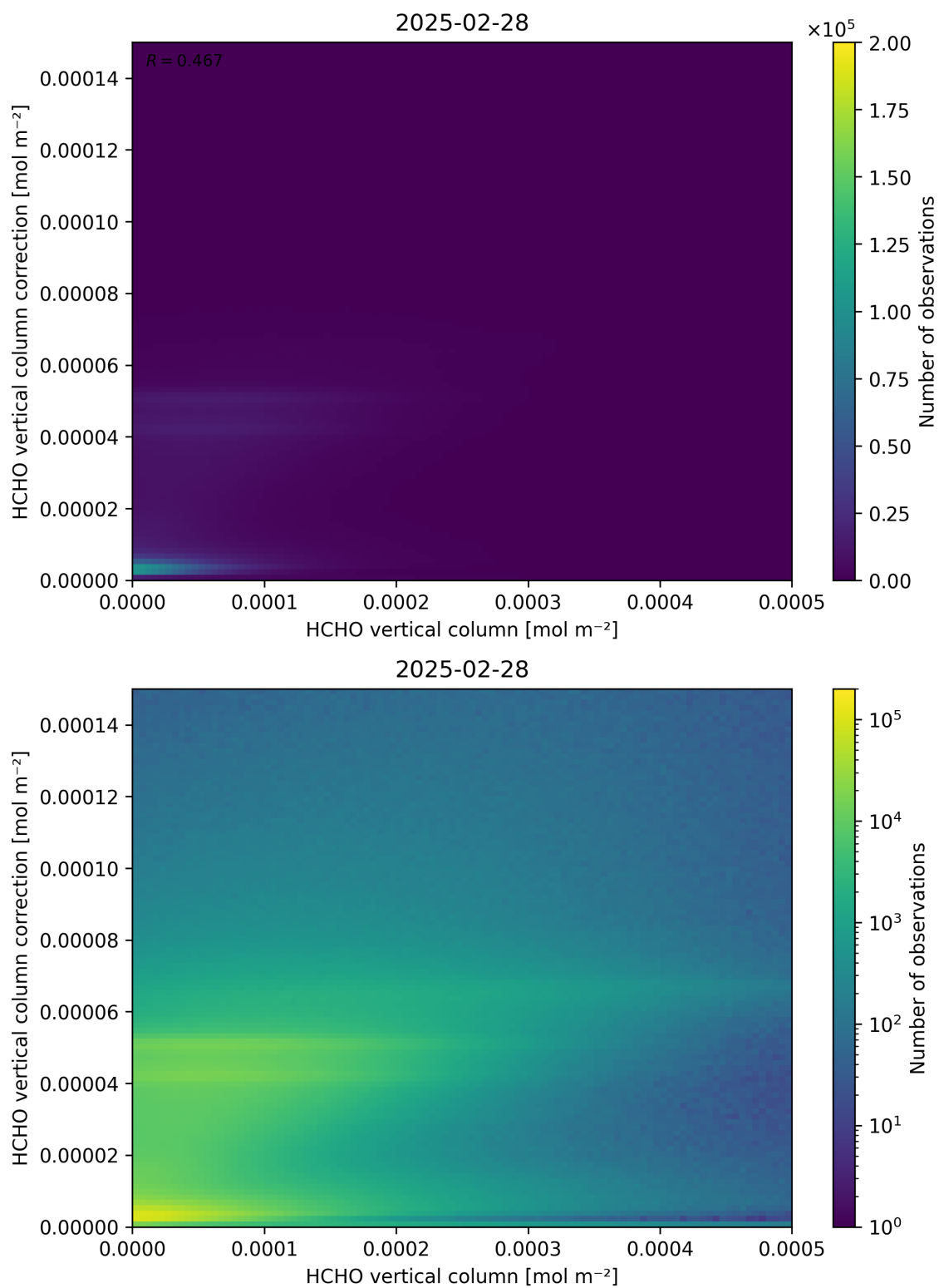
Figure 133: Scatter density plot of “HCHO vertical column” against “HCHO vertical column correction” for 2025-02-27 to 2025-03-01.
