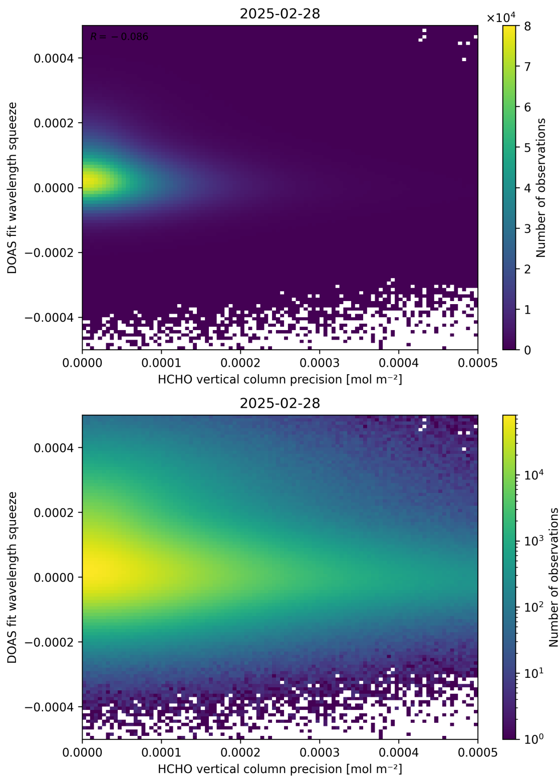
Figure 138: Scatter density plot of “HCHO vertical column precision” against “DOAS fit wavelength squeeze” for 2025-02-27 to 2025-03-01.
