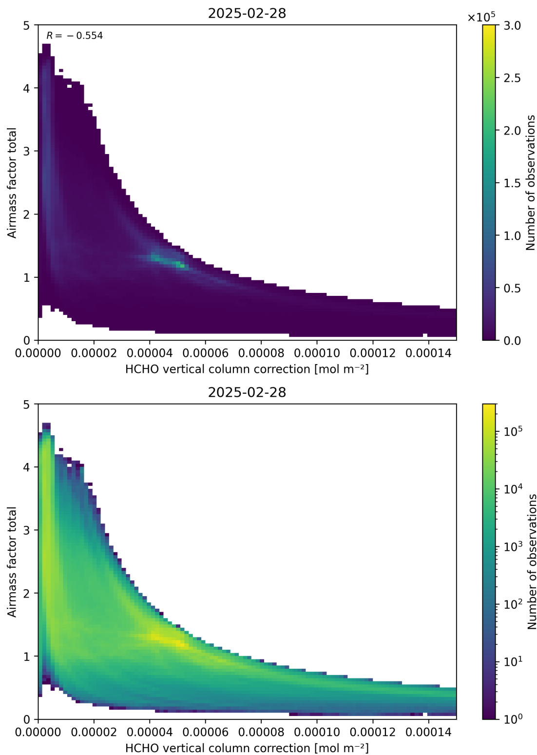
Figure 120: Scatter density plot of “HCHO vertical column correction” against “Airmass factor total” for 2025-02-27 to 2025-03-01.
