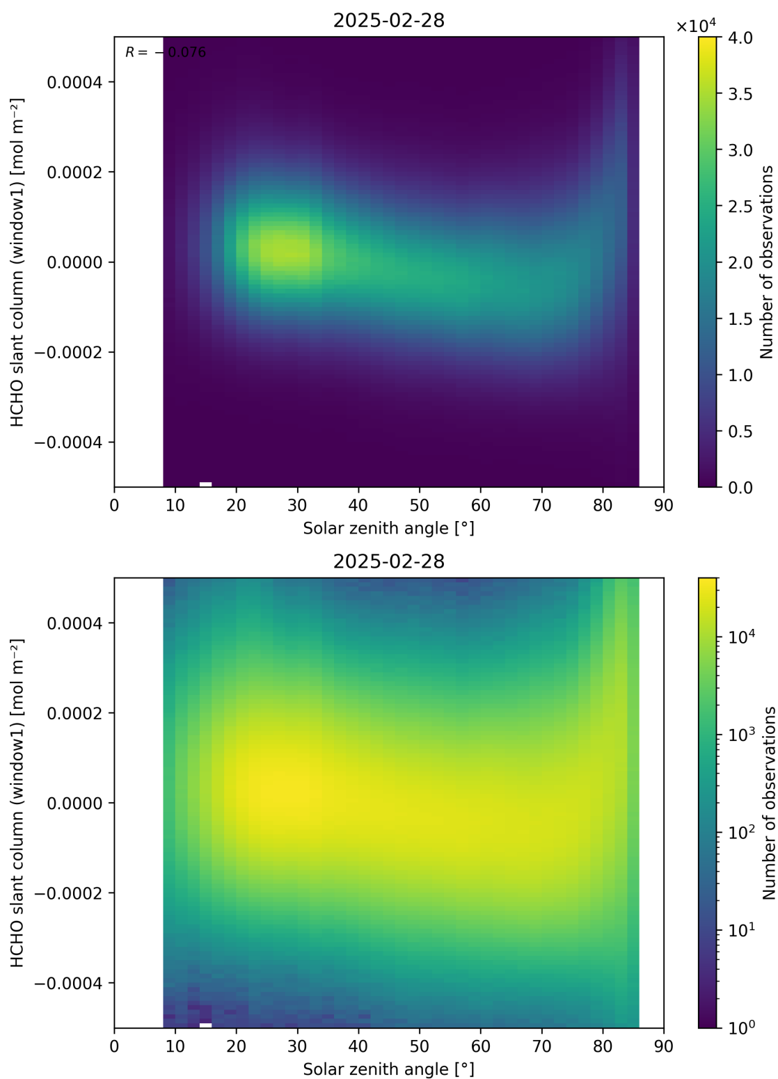
Figure 173: Scatter density plot of “Solar zenith angle” against “HCHO slant column (window1)” for 2025-02-27 to 2025-03-01.
