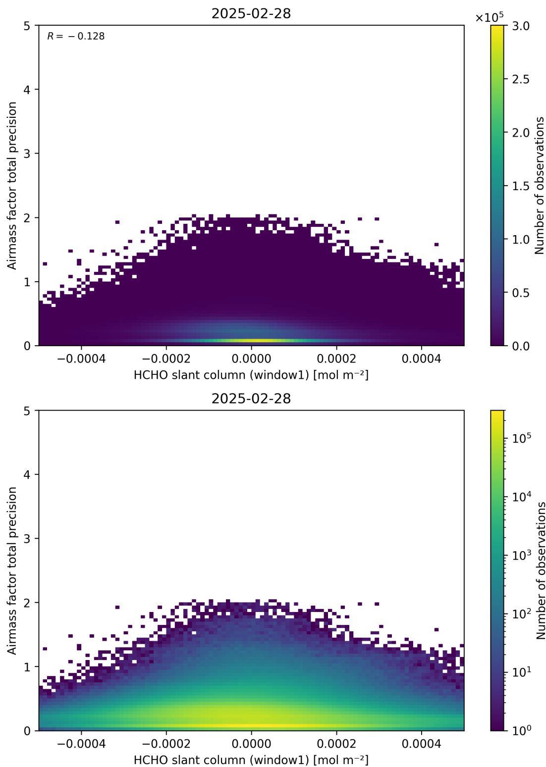
Figure 86: Scatter density plot of “HCHO slant column (window1)” against “Airmass factor total precision” for 2025-02-27 to 2025-03-01.
