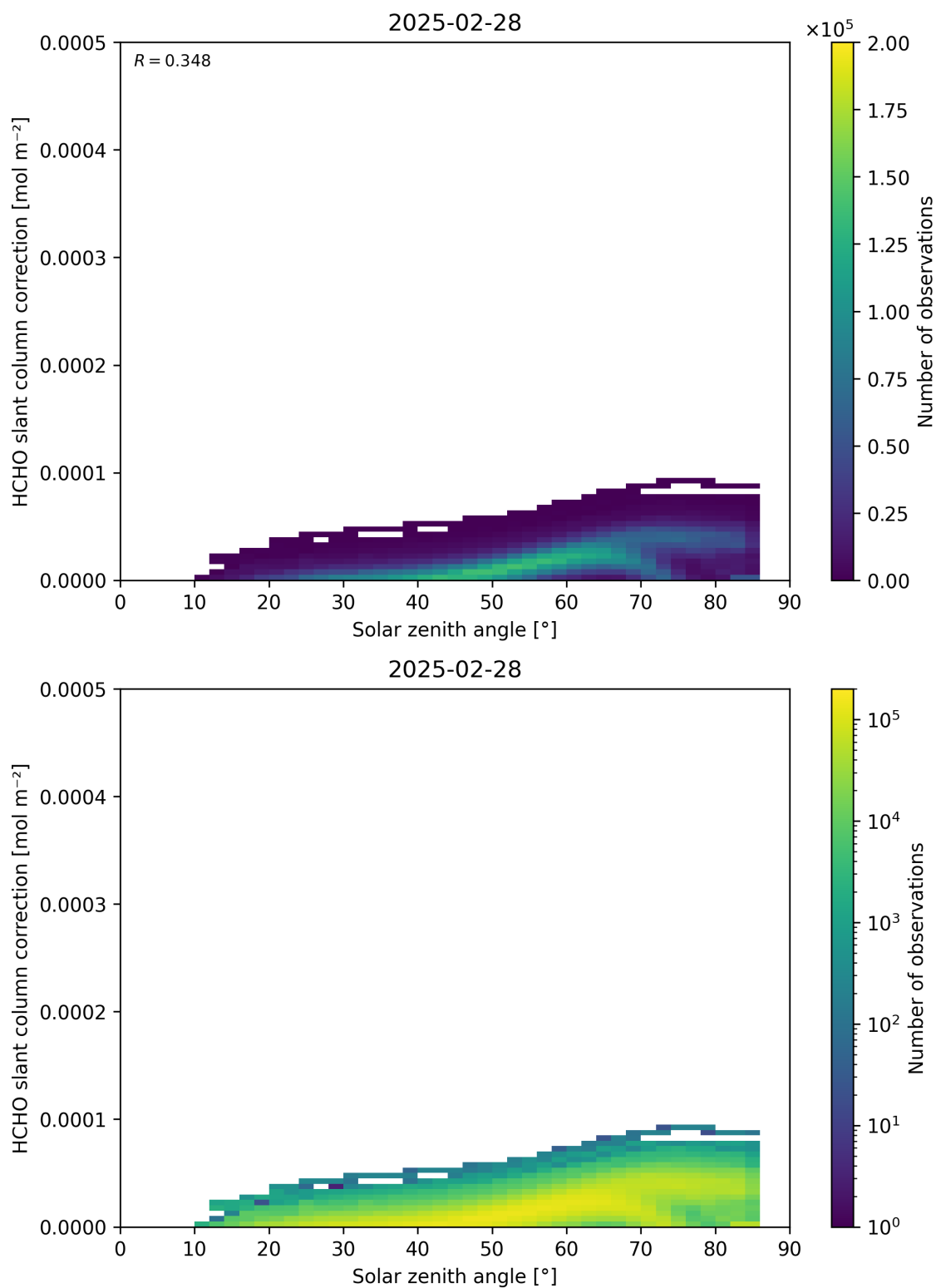
Figure 172: Scatter density plot of “Solar zenith angle” against “HCHO slant column correction” for 2025-02-27 to 2025-03-01.
