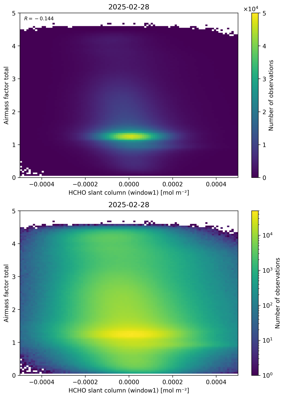
Figure 85: Scatter density plot of “HCHO slant column (window1)” against “Airmass factor total” for 2025-02-27 to 2025-03-01.
