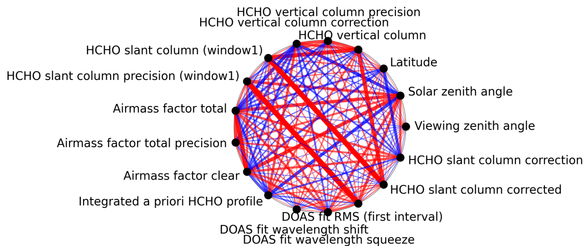
Figure 1: Map of correlation graph for 2025-02-27 to 2025-03-01.
