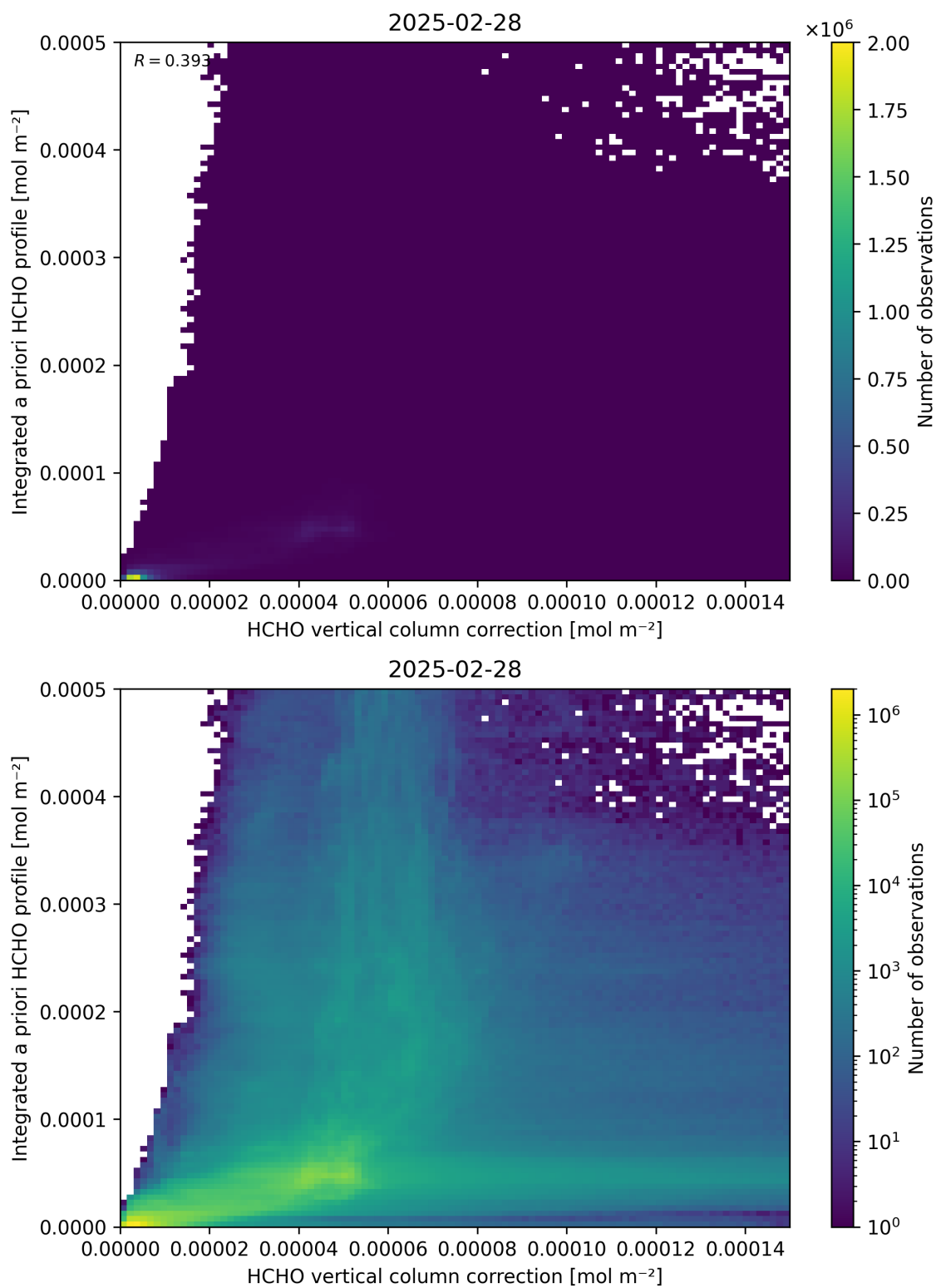
Figure 122: Scatter density plot of “HCHO vertical column correction” against “Integrated a priori HCHO profile” for 2025-02-27 to 2025-03-01.
