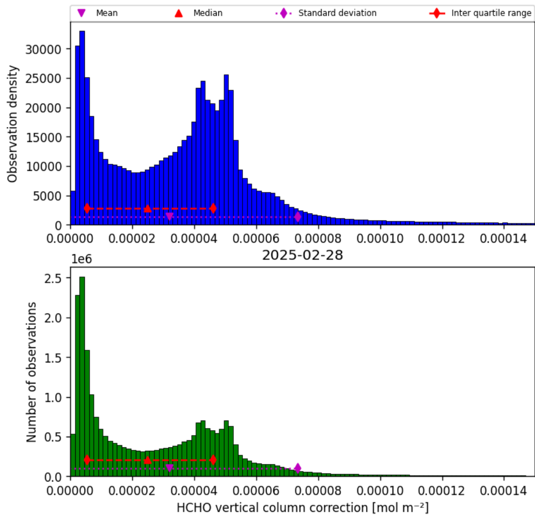
Figure 37: Histogram of “HCHO vertical column correction” for 2025-02-27 to 2025-03-01
