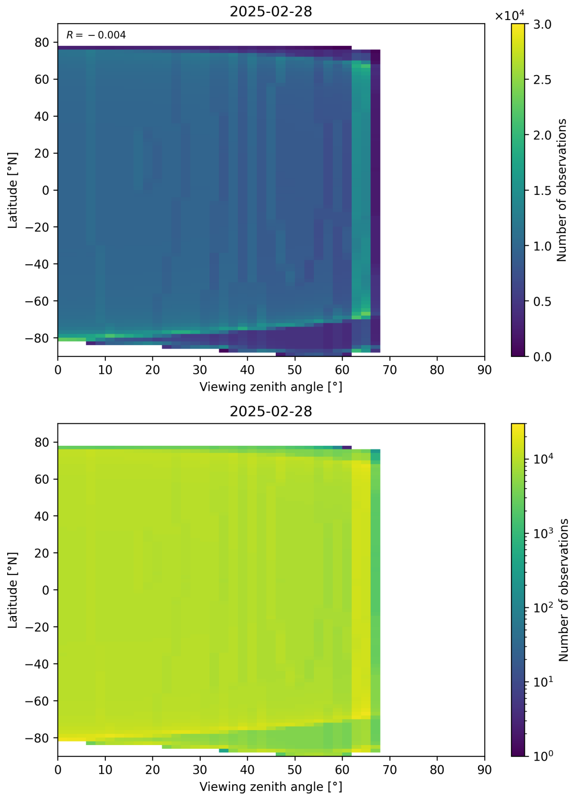
Figure 196: Scatter density plot of “Viewing zenith angle” against “Latitude” for 2025-02-27 to 2025-03-01.
