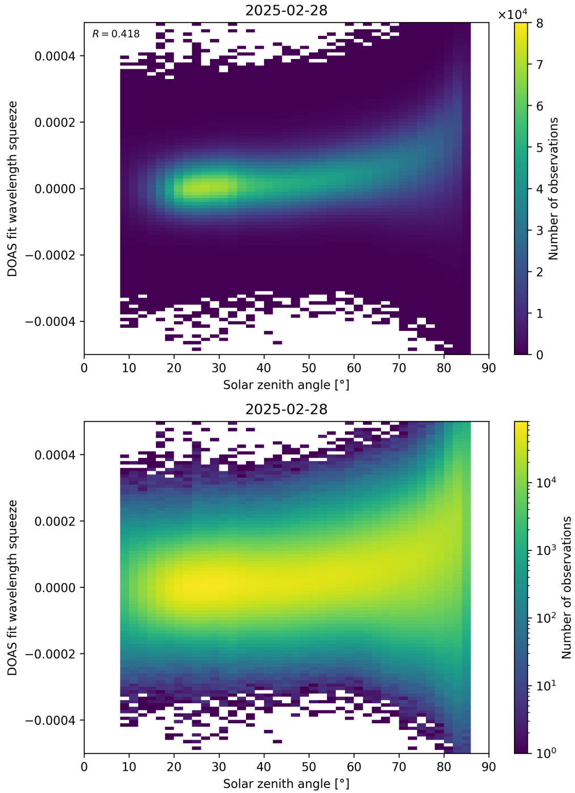
Figure 169: Scatter density plot of “Solar zenith angle” against “DOAS fit wavelength squeeze” for 2025-02-27 to 2025-03-01.
