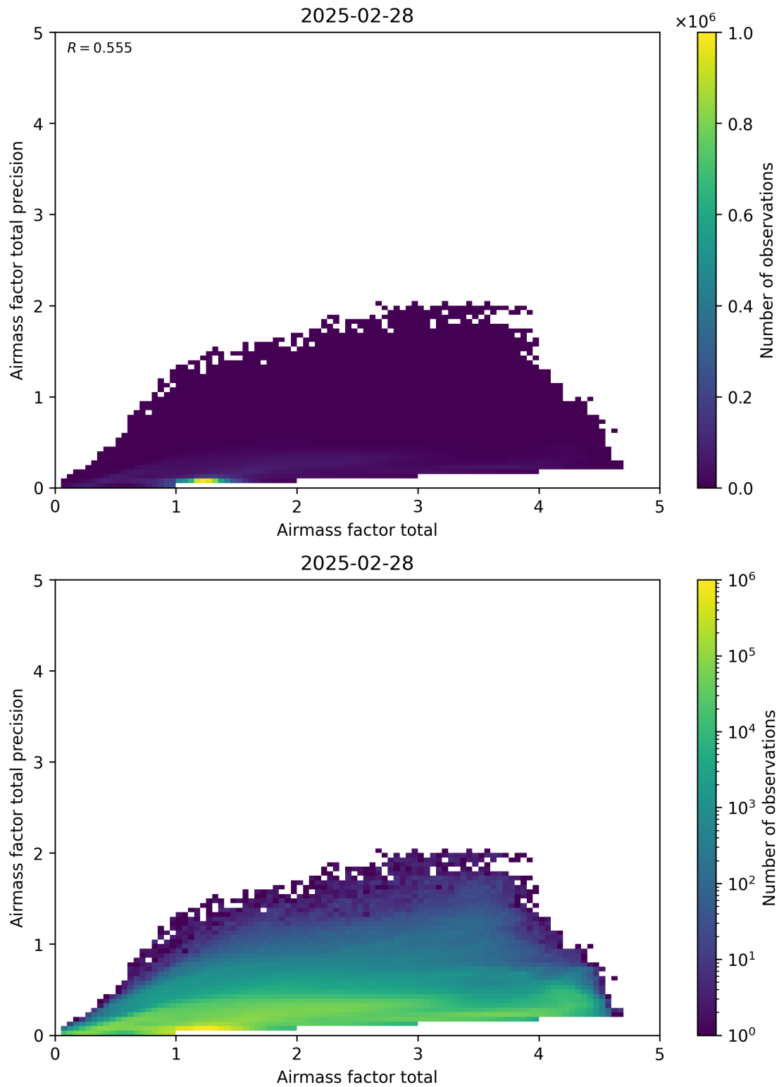
Figure 103: Scatter density plot of “Airmass factor total” against “Airmass factor total precision” for 2025-02-27 to 2025-03-01.
