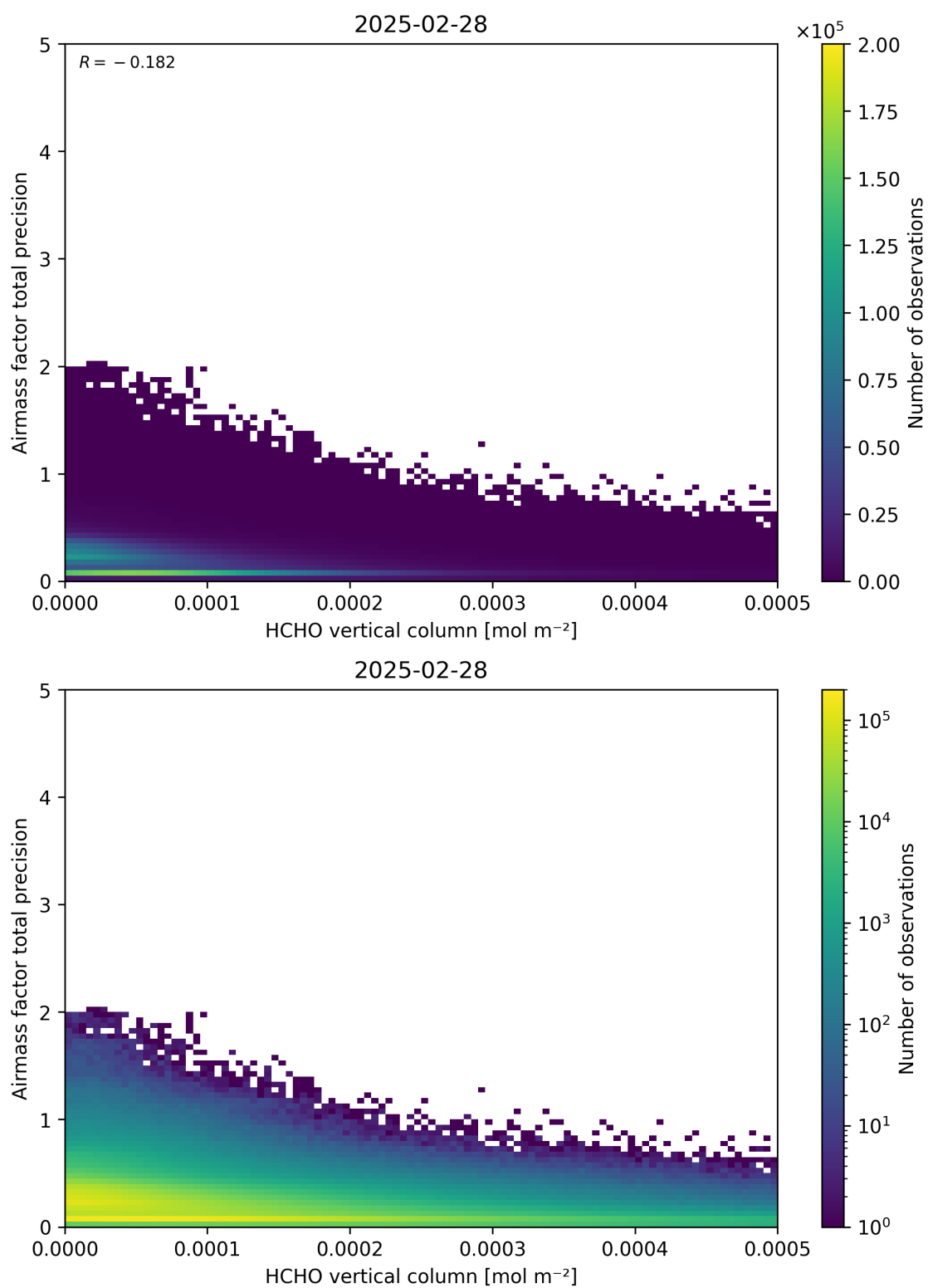
Figure 132: Scatter density plot of “HCHO vertical column” against “Airmass factor total precision” for 2025-02-27 to 2025-03-01.
