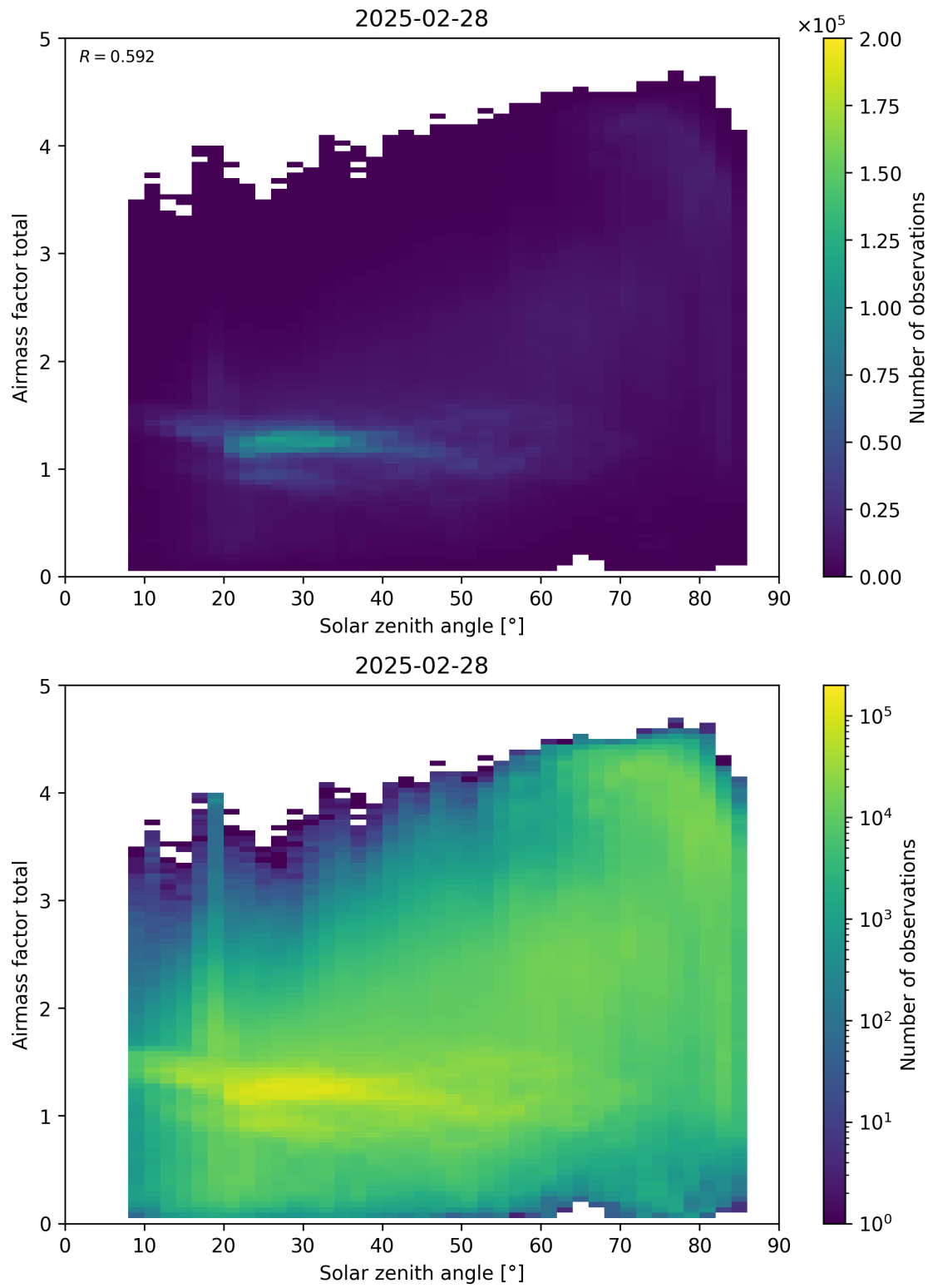
Figure 175: Scatter density plot of “Solar zenith angle” against “Airmass factor total” for 2025-02-27 to 2025-03-01.
