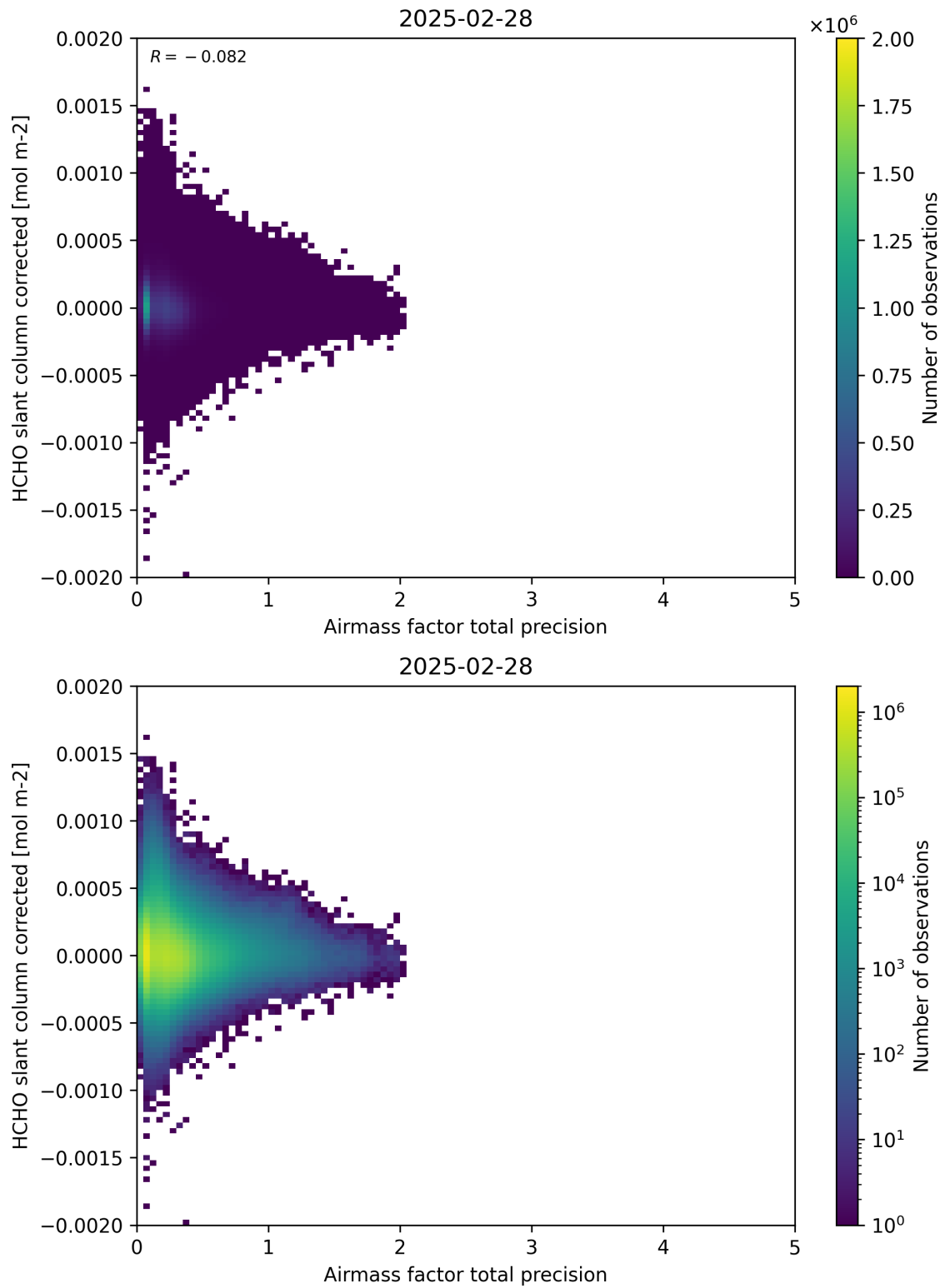
Figure 109: Scatter density plot of “Airmass factor total precision” against “HCHO slant column corrected” for 2025-02-27 to 2025-03-01.
