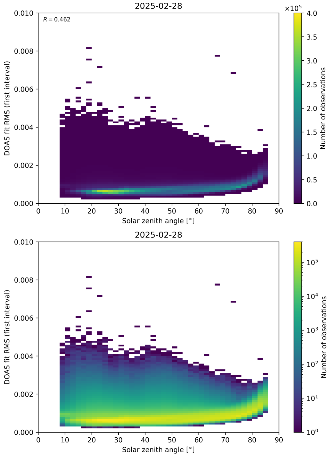
Figure 167: Scatter density plot of “Solar zenith angle” against “DOAS fit RMS (first interval)” for 2025-02-27 to 2025-03-01.
