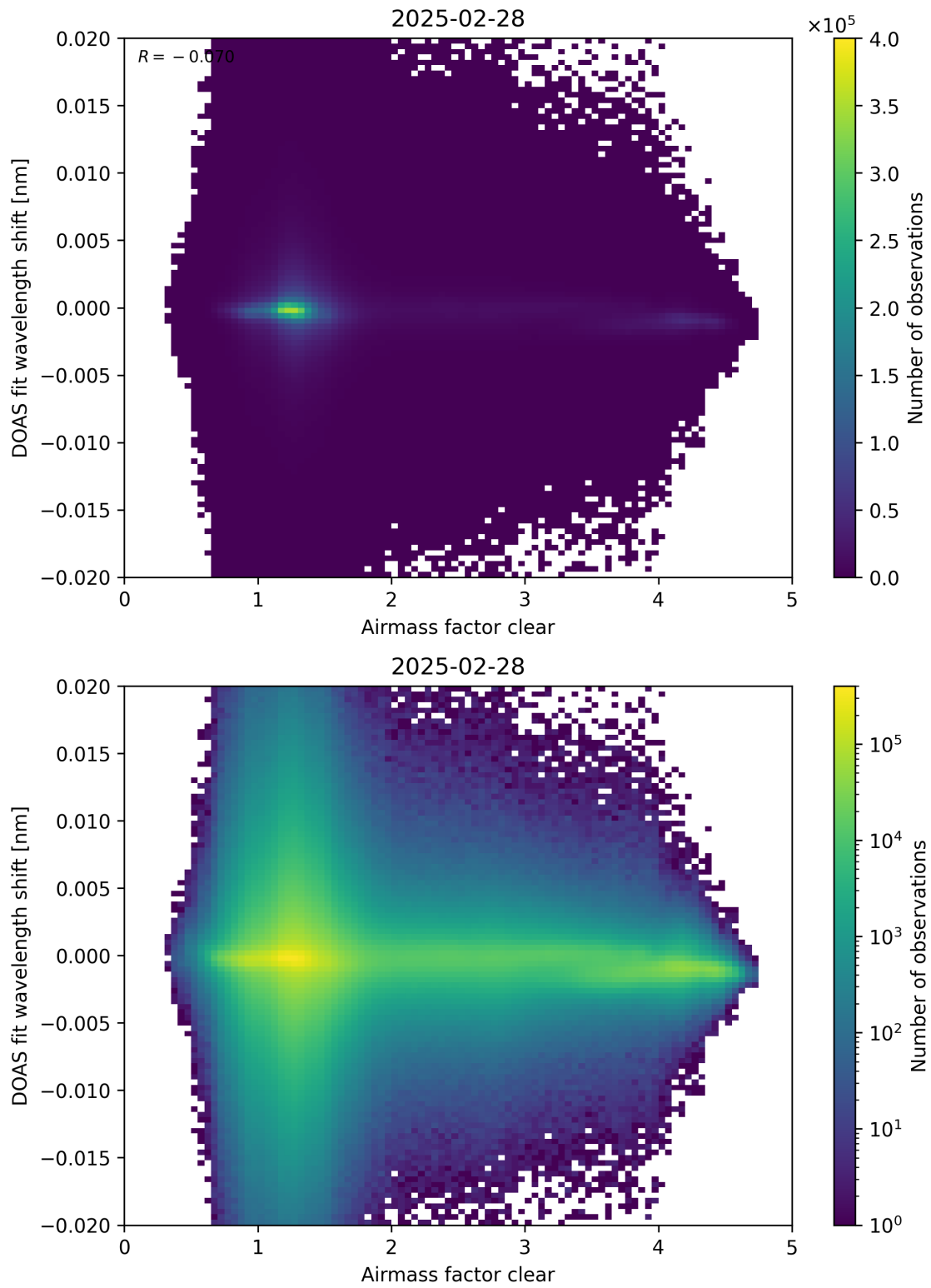
Figure 72: Scatter density plot of “Airmass factor clear” against “DOAS fit wavelength shift” for 2025-02-27 to 2025-03-01.
