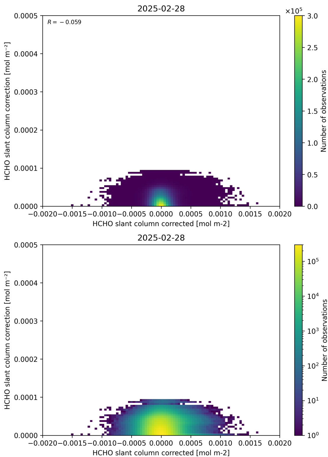
Figure 77: Scatter density plot of “HCHO slant column corrected” against “HCHO slant column correction” for 2025-02-27 to 2025-03-01.
