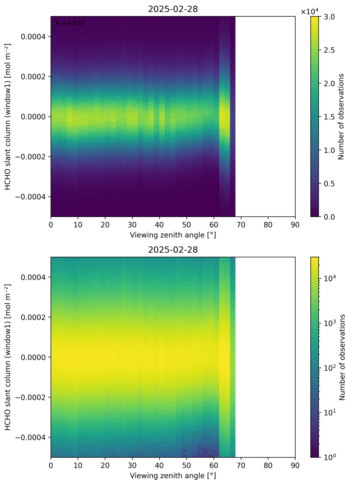
Figure 188: Scatter density plot of “Viewing zenith angle” against “HCHO slant column (window1)” for 2025-02-27 to 2025-03-01.
