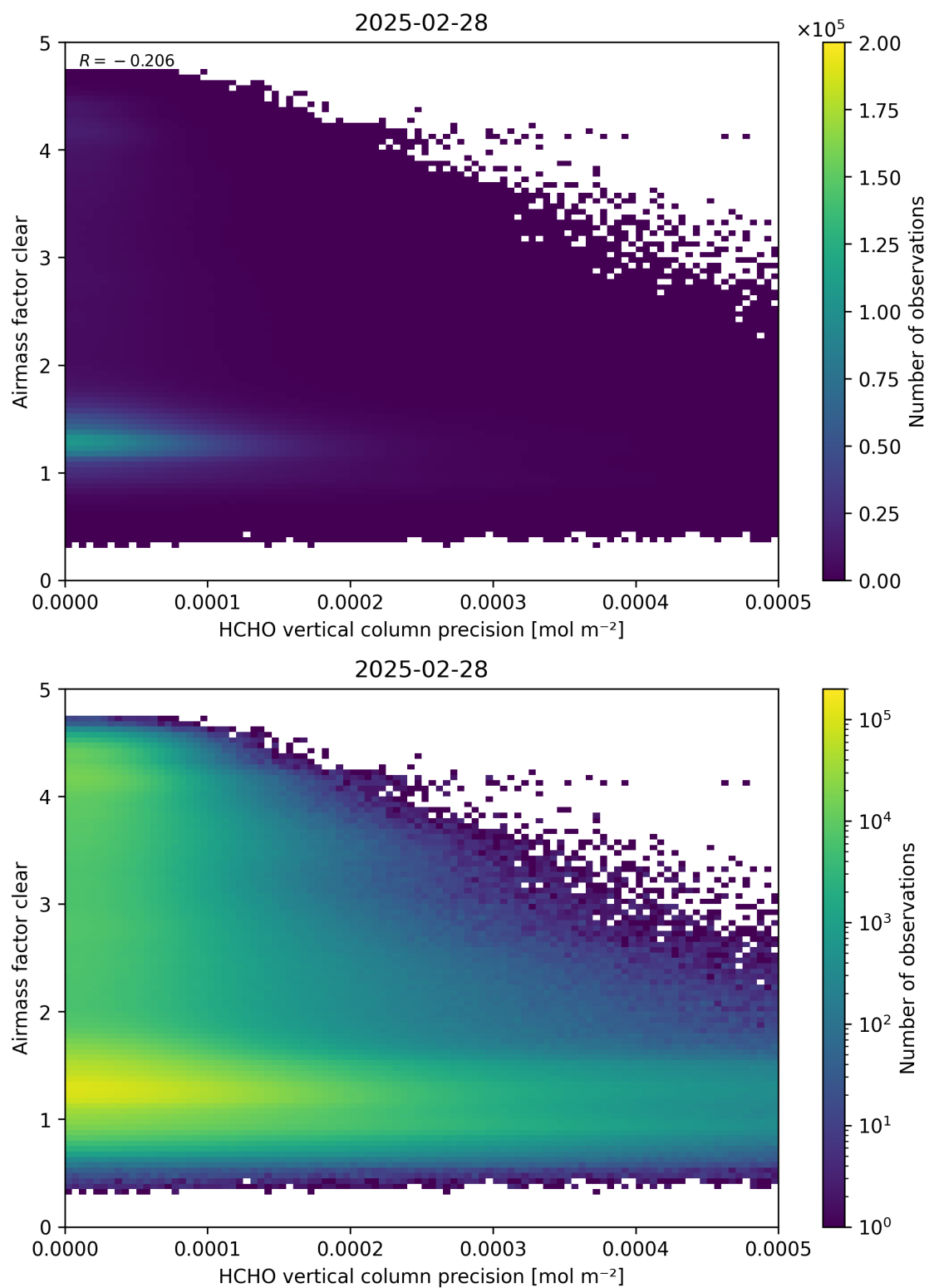
Figure 139: Scatter density plot of “HCHO vertical column precision” against “Airmass factor clear” for 2025-02-27 to 2025-03-01.
