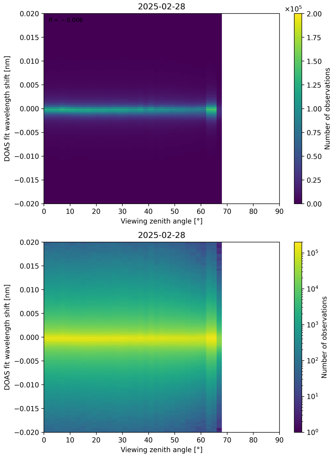
Figure 183: Scatter density plot of “Viewing zenith angle” against “DOAS fit wavelength shift” for 2025-02-27 to 2025-03-01.
