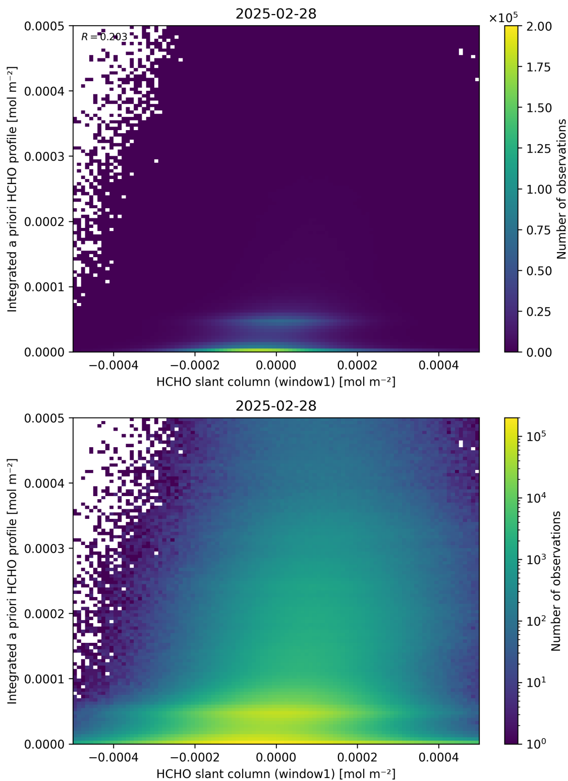
Figure 87: Scatter density plot of “HCHO slant column (window1)” against “Integrated a priori HCHO profile” for 2025-02-27 to 2025-03-01.
