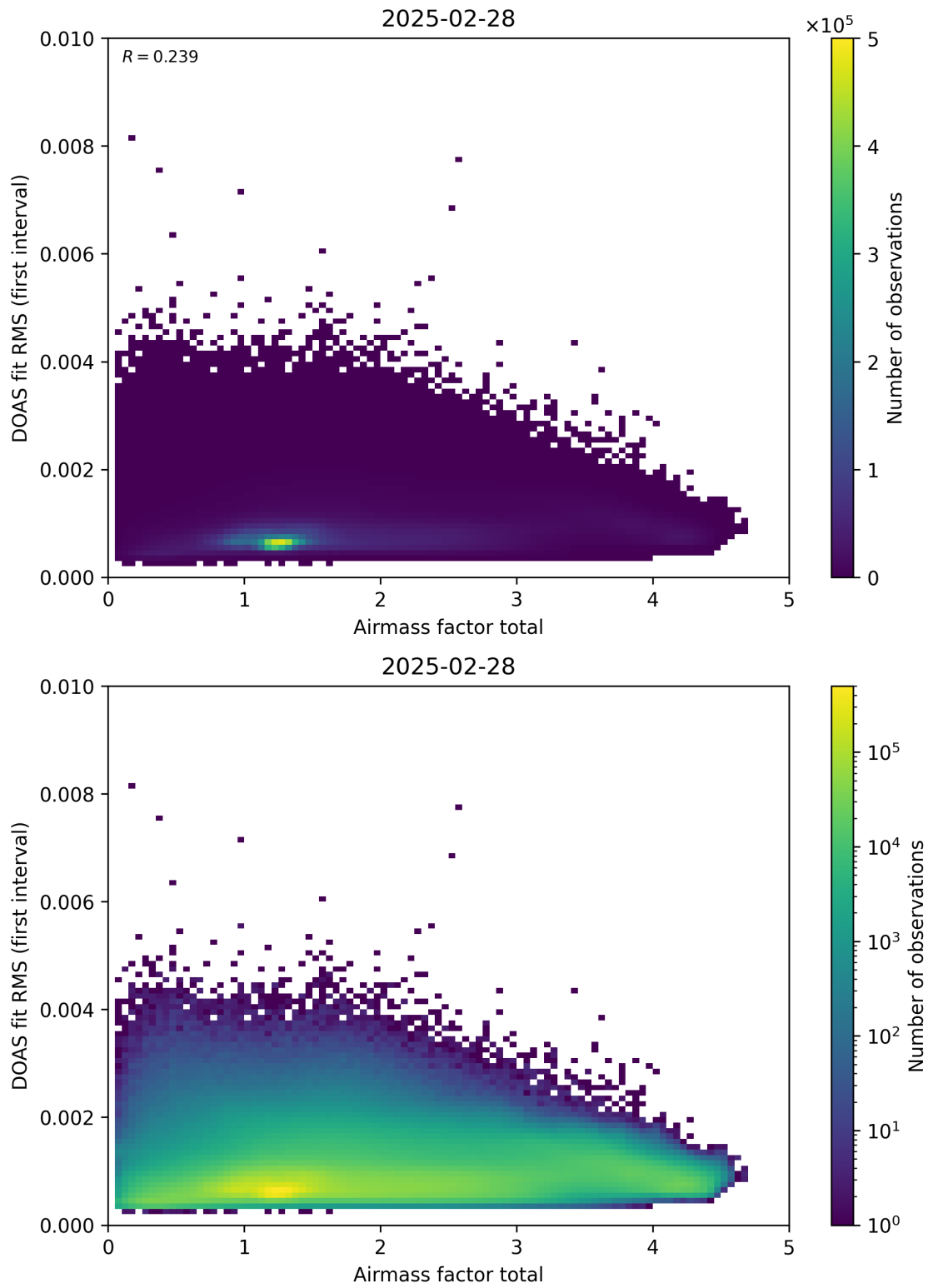
Figure 97: Scatter density plot of “Airmass factor total” against “DOAS fit RMS (first interval)” for 2025-02-27 to 2025-03-01.
