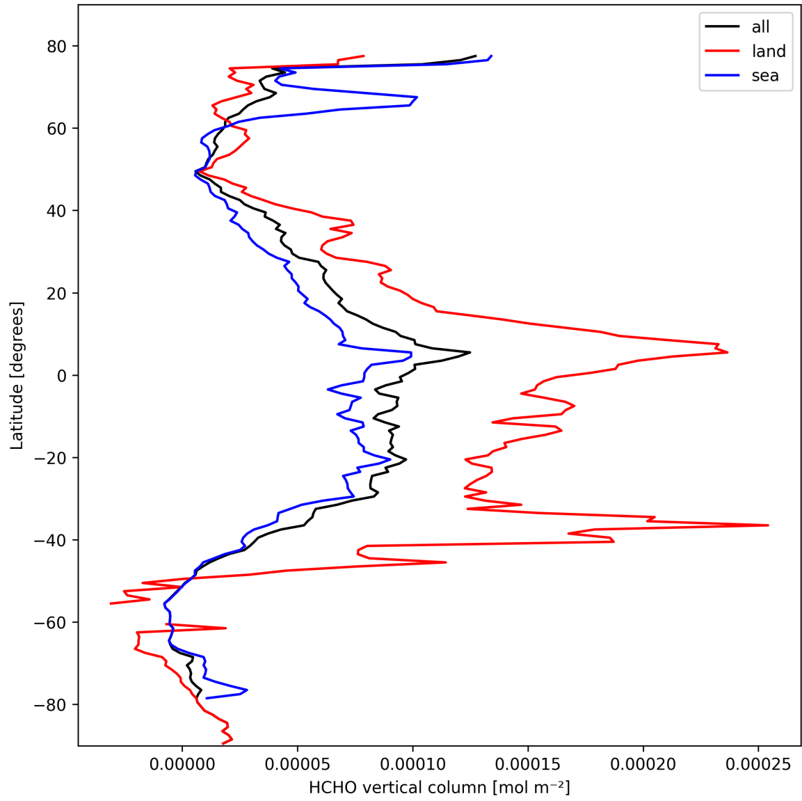
Figure 21: Zonal average of “HCHO vertical column” for 2025-02-27 to 2025-03-01.
