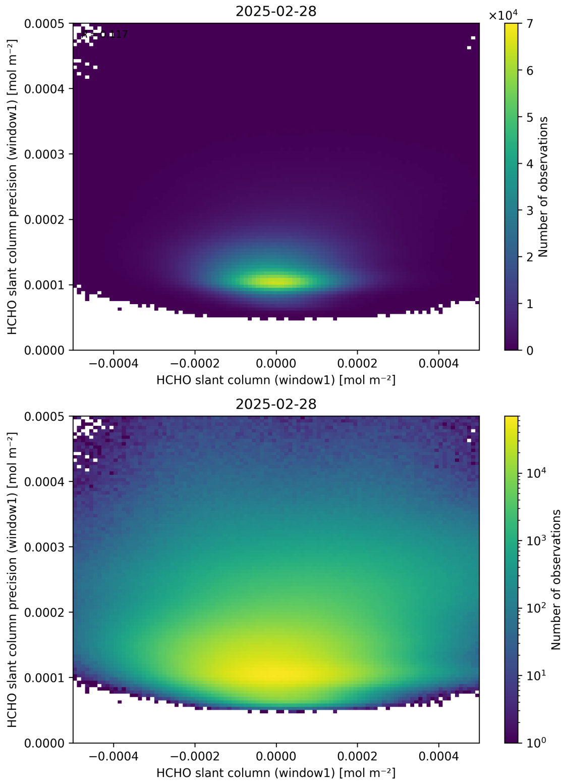
Figure 84: Scatter density plot of “HCHO slant column (window1)” against “HCHO slant column precision (window1)” for 2025-02-27 to 2025-03-01.
