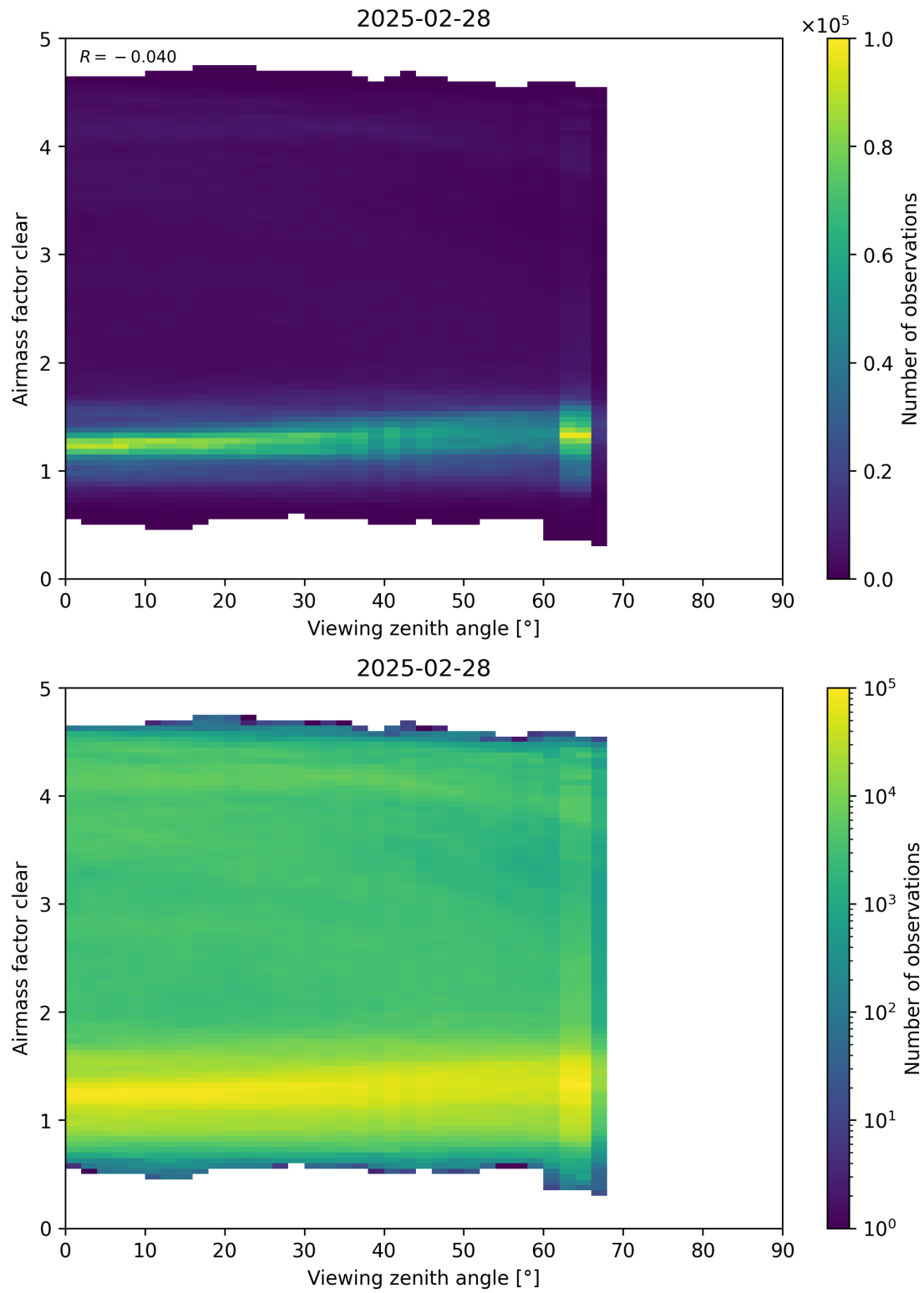
Figure 185: Scatter density plot of “Viewing zenith angle” against “Airmass factor clear” for 2025-02-27 to 2025-03-01.
