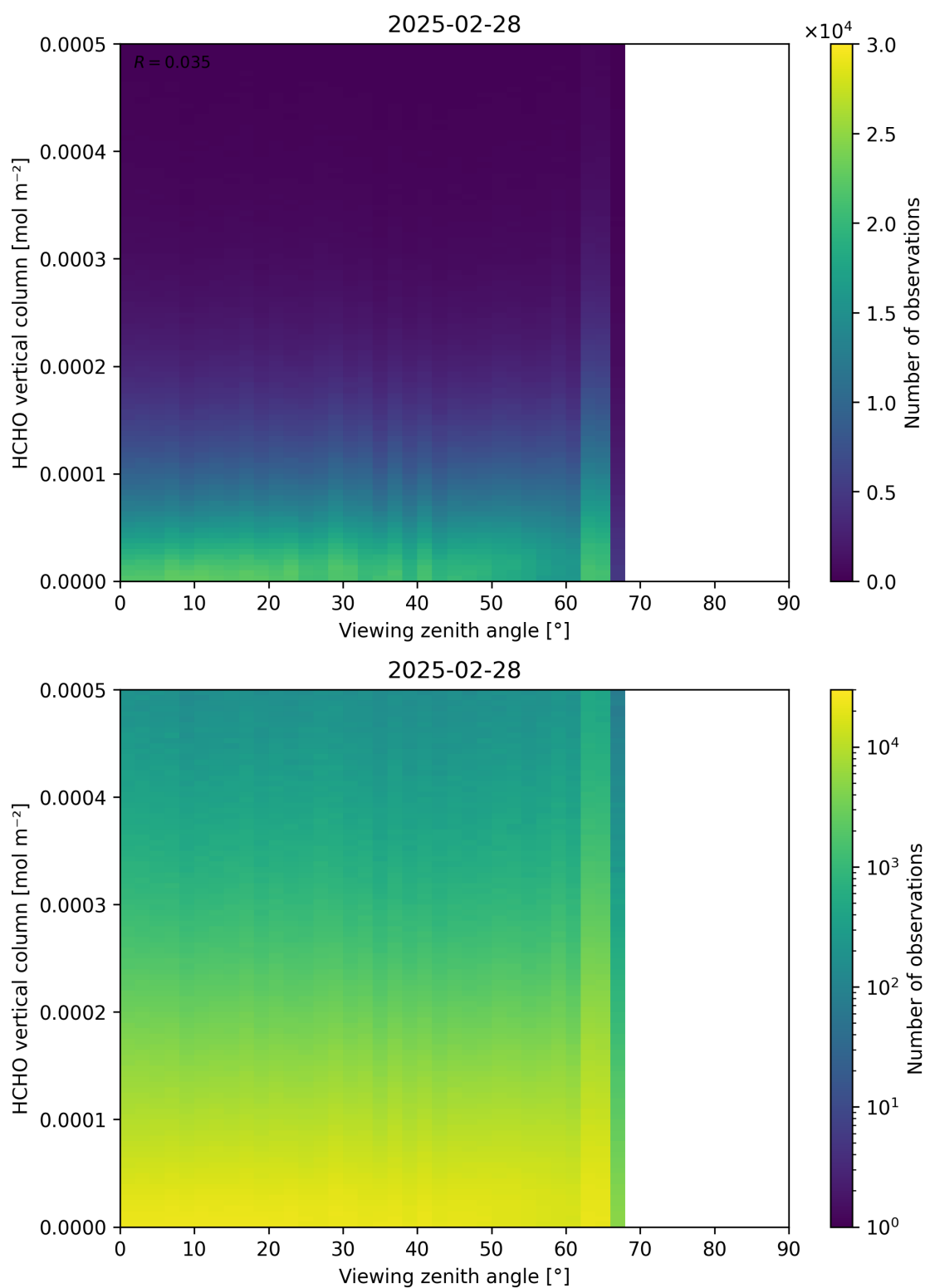
Figure 192: Scatter density plot of “Viewing zenith angle” against “HCHO vertical column” for 2025-02-27 to 2025-03-01.
