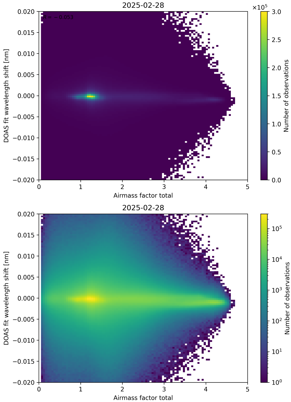
Figure 98: Scatter density plot of “Airmass factor total” against “DOAS fit wavelength shift” for 2025-02-27 to 2025-03-01.
