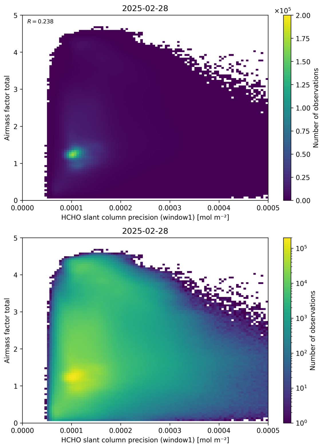
Figure 94: Scatter density plot of “HCHO slant column precision (window1)” against “Airmass factor total” for 2025-02-27 to 2025-03-01.
