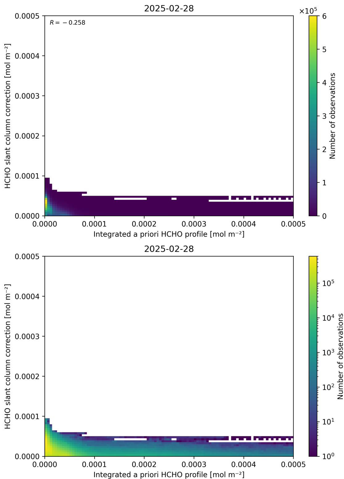
Figure 152: Scatter density plot of “Integrated a priori HCHO profile” against “HCHO slant column correction” for 2025-02-27 to 2025-03-01.
