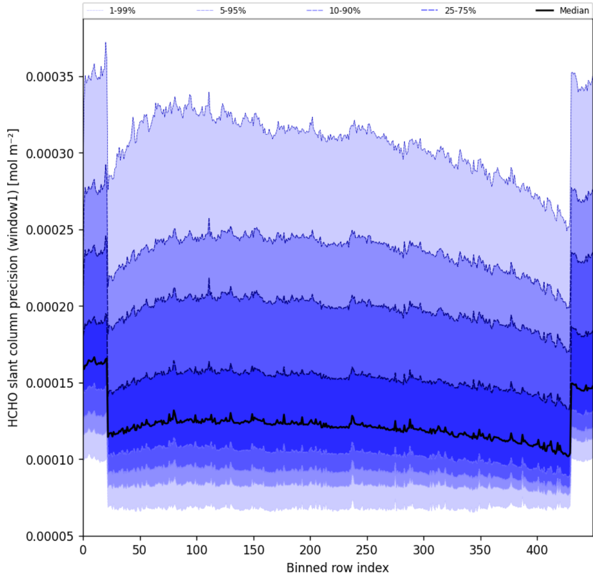
Figure 53: Along track statistics of “HCHO slant column precision (window1)” for 2025-02-27 to 2025-03-01
