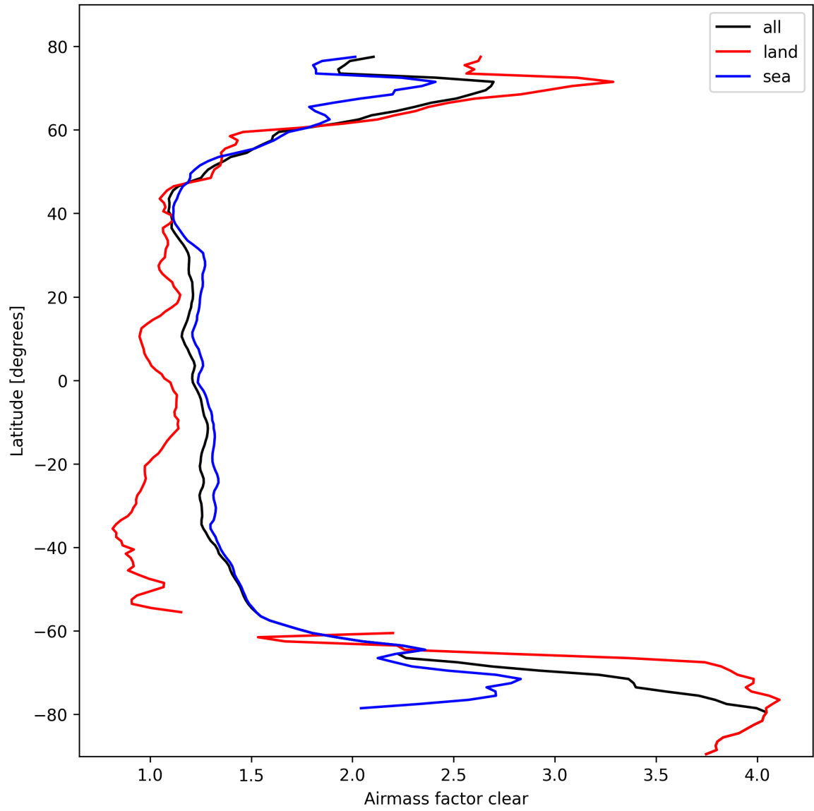
Figure 28: Zonal average of “Airmass factor clear” for 2025-02-27 to 2025-03-01.
