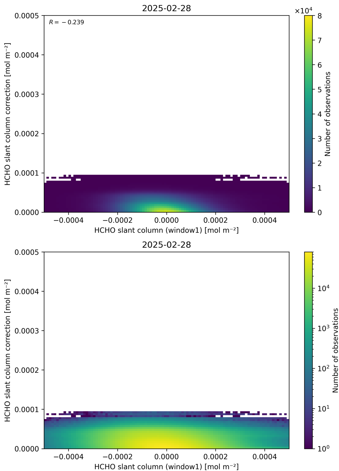
Figure 83: Scatter density plot of “HCHO slant column (window1)” against “HCHO slant column correction” for 2025-02-27 to 2025-03-01.
