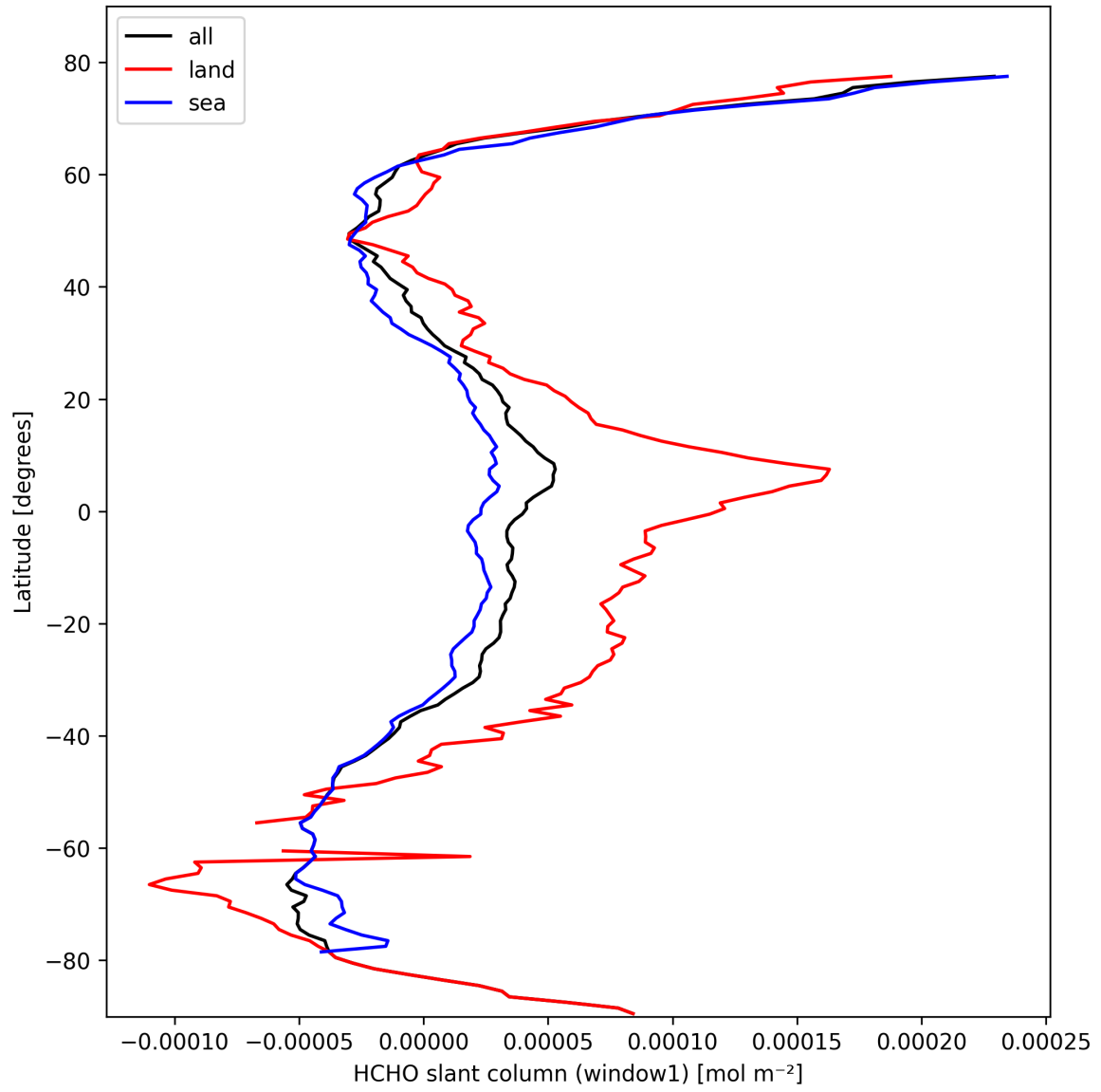
Figure 24: Zonal average of “HCHO slant column (window1)” for 2025-02-27 to 2025-03-01.
