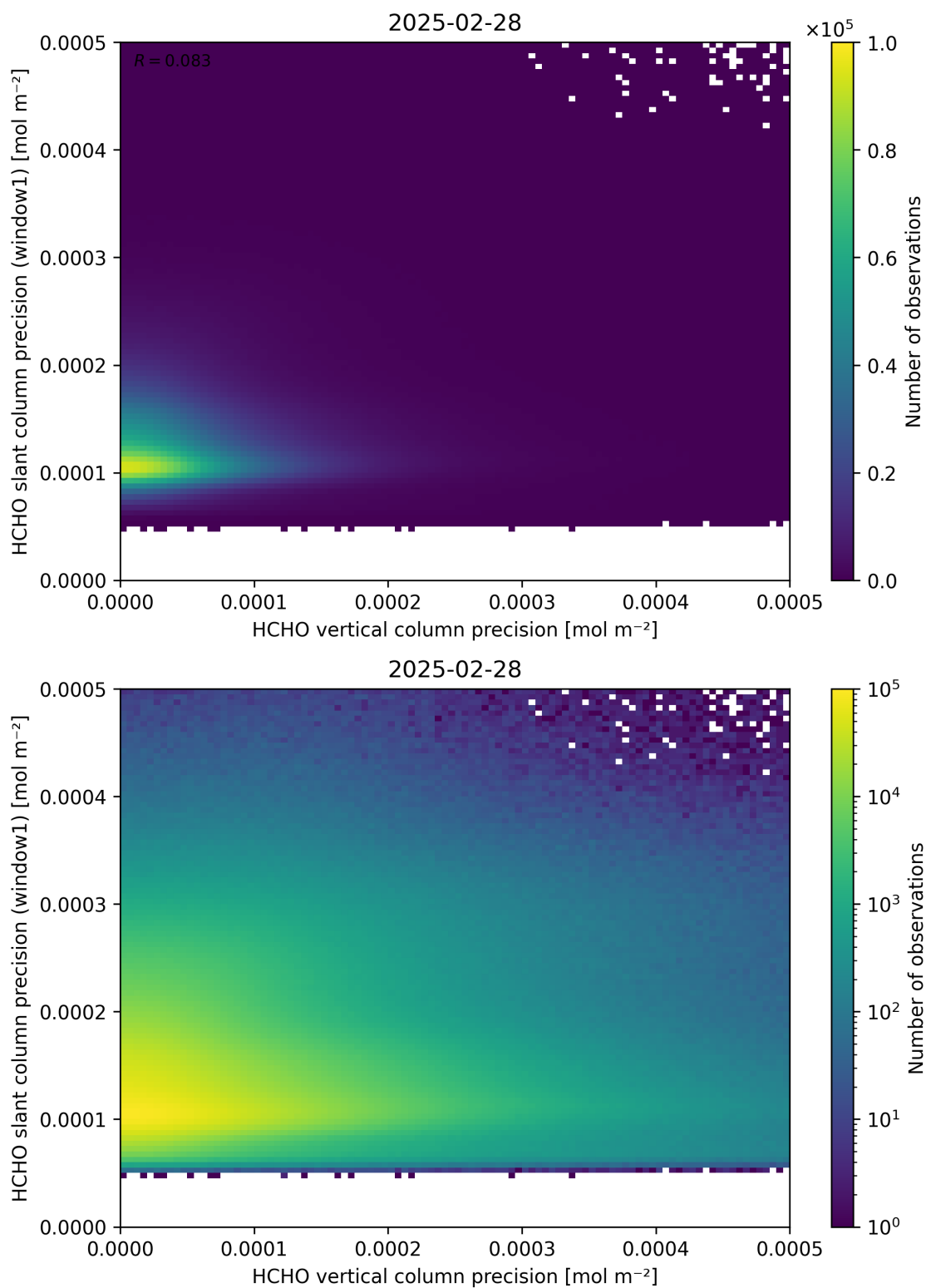
Figure 143: Scatter density plot of “HCHO vertical column precision” against “HCHO slant column precision (window1)” for 2025-02-27 to 2025-03-01.
