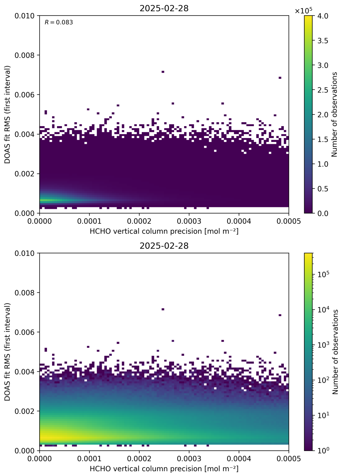
Figure 136: Scatter density plot of “HCHO vertical column precision” against “DOAS fit RMS (first interval)” for 2025-02-27 to 2025-03-01.
