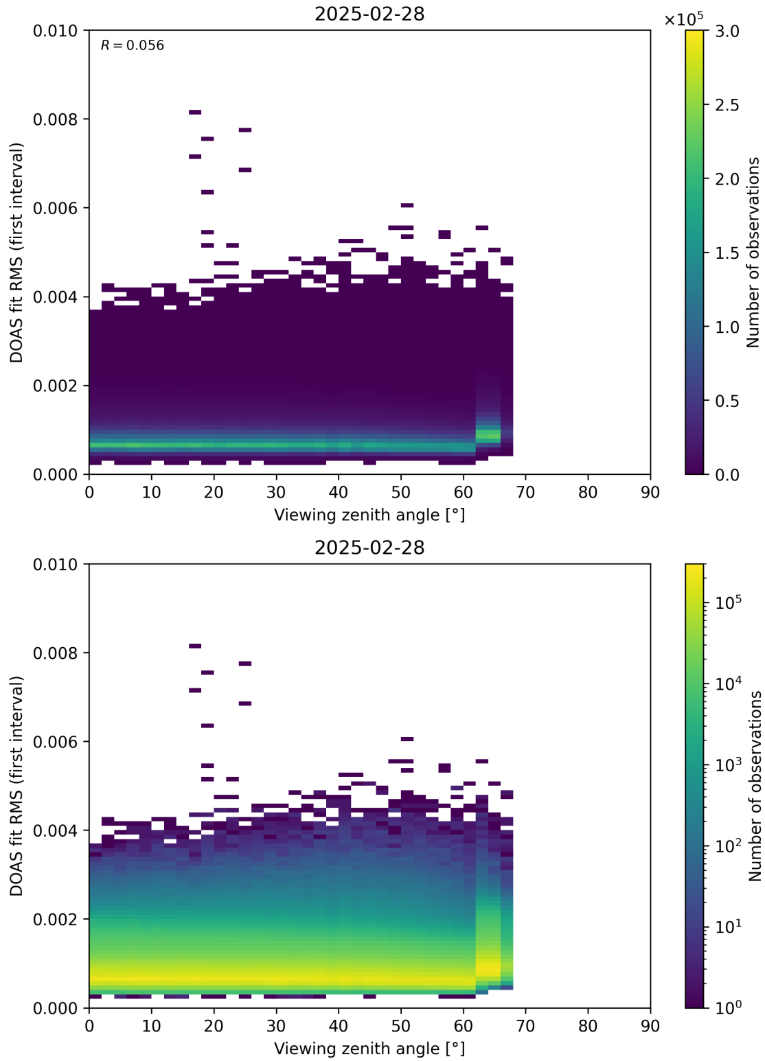
Figure 182: Scatter density plot of “Viewing zenith angle” against “DOAS fit RMS (first interval)” for 2025-02-27 to 2025-03-01.
