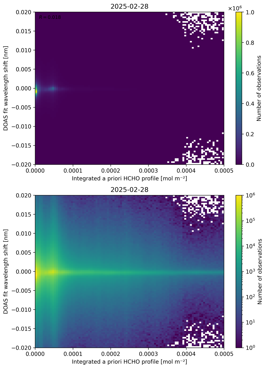
Figure 149: Scatter density plot of “Integrated a priori HCHO profile” against “DOAS fit wavelength shift” for 2025-02-27 to 2025-03-01.
