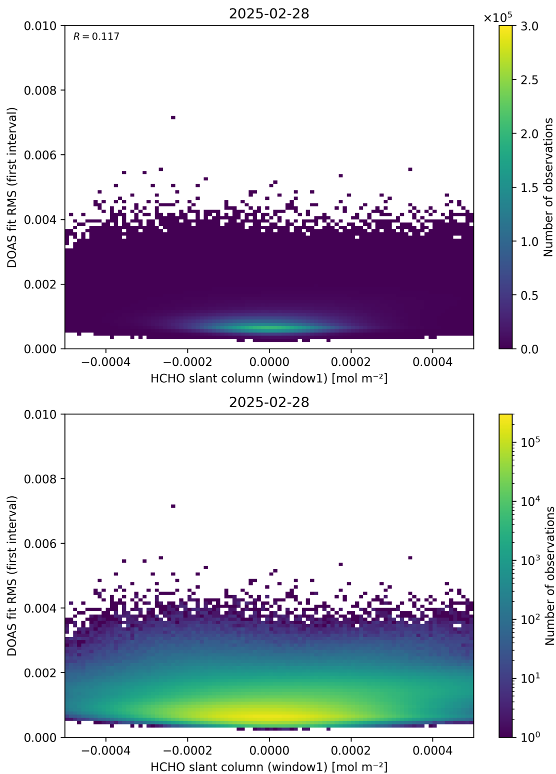
Figure 78: Scatter density plot of “HCHO slant column (window1)” against “DOAS fit RMS (first interval)” for 2025-02-27 to 2025-03-01.
