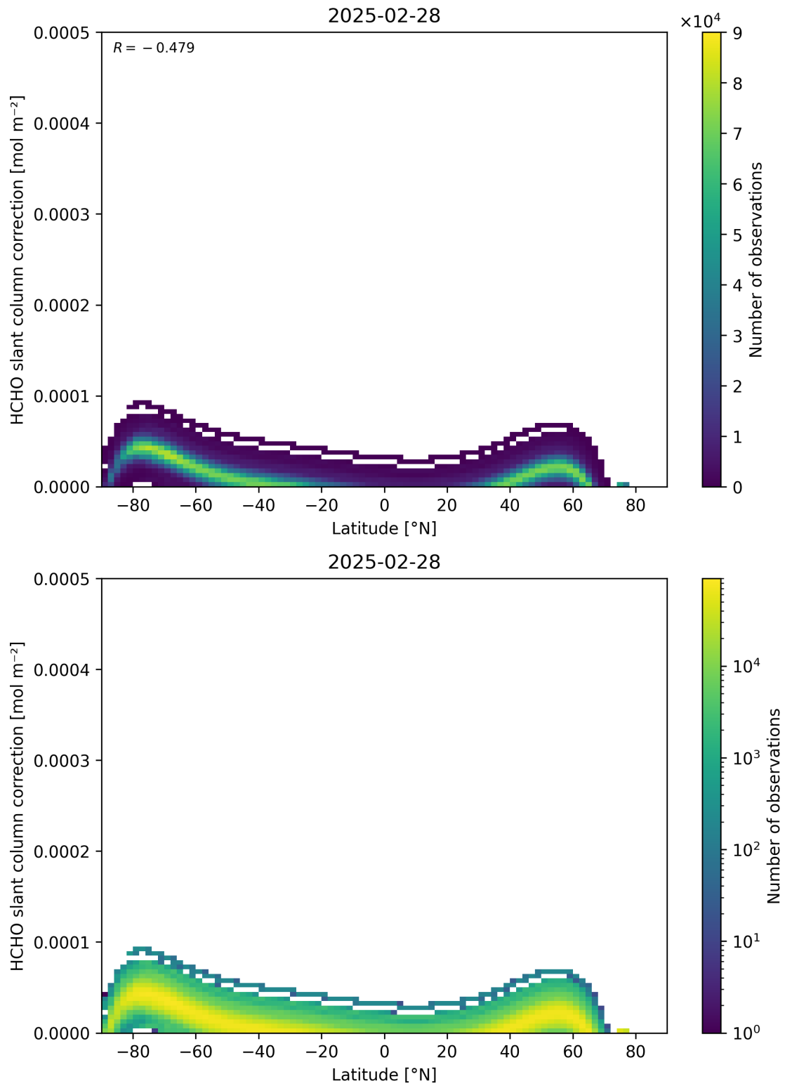
Figure 158: Scatter density plot of “Latitude” against “HCHO slant column correction” for 2025-02-27 to 2025-03-01.
