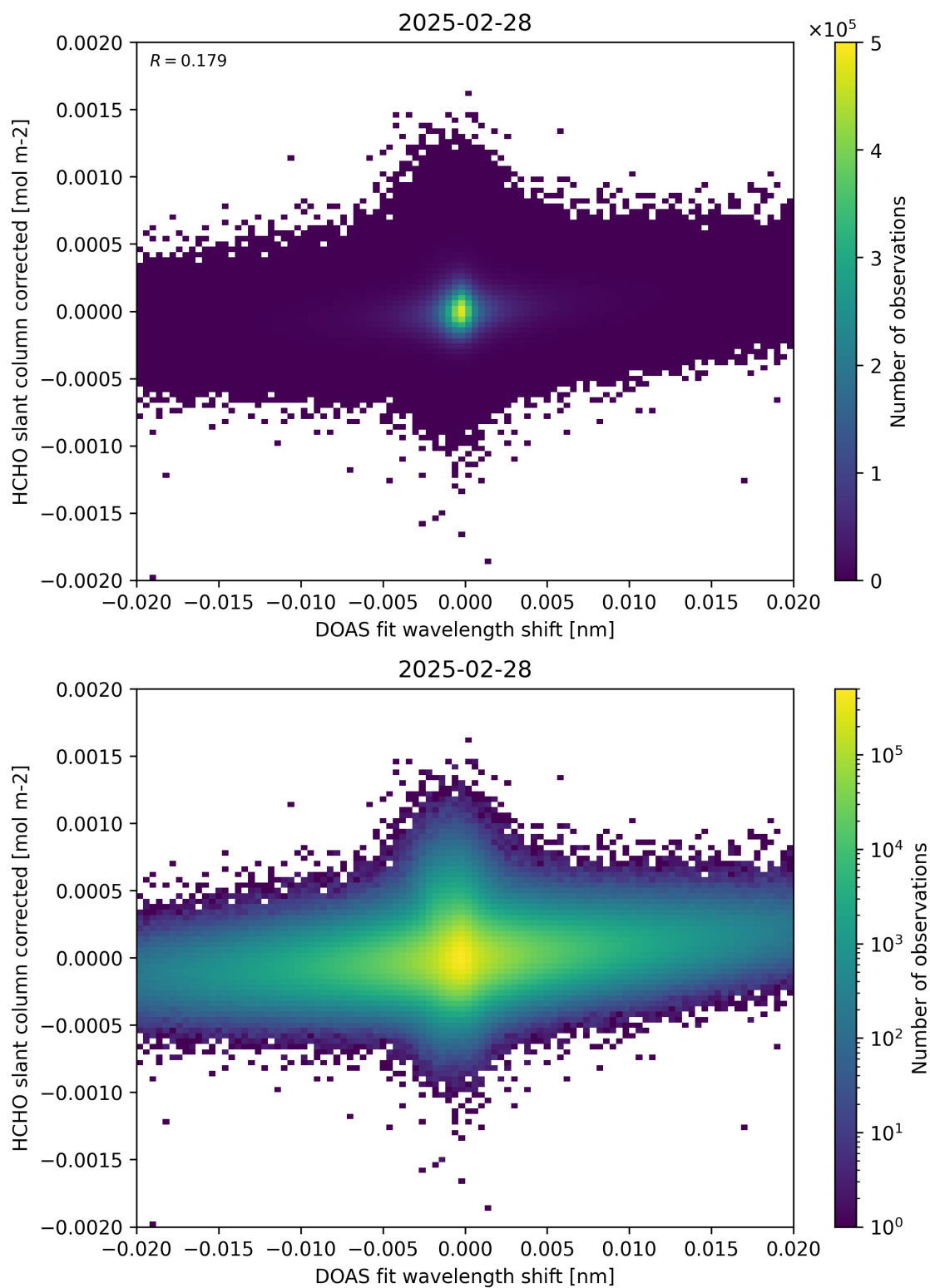
Figure 66: Scatter density plot of “DOAS fit wavelength shift” against “HCHO slant column corrected” for 2025-02-27 to 2025-03-01.
