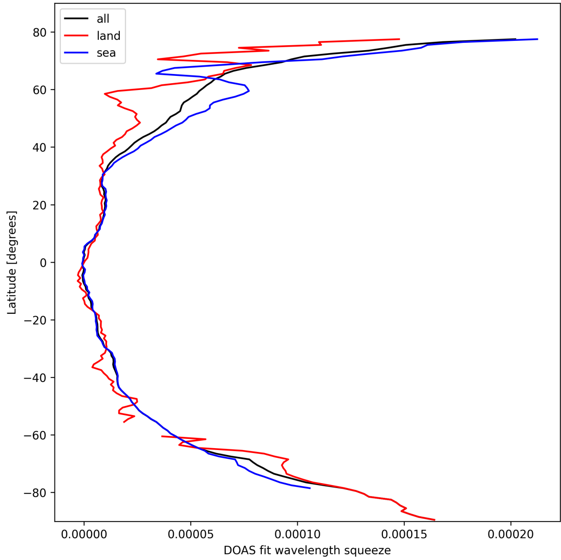
Figure 31: Zonal average of “DOAS fit wavelength squeeze” for 2025-02-27 to 2025-03-01.
