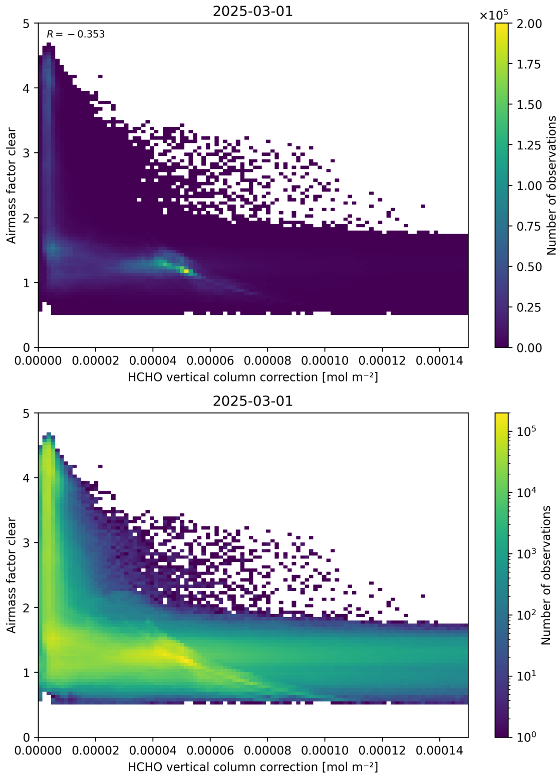
Figure 115: Scatter density plot of “HCHO vertical column correction” against “Airmass factor clear” for 2025-03-01 to 2025-03-02.
