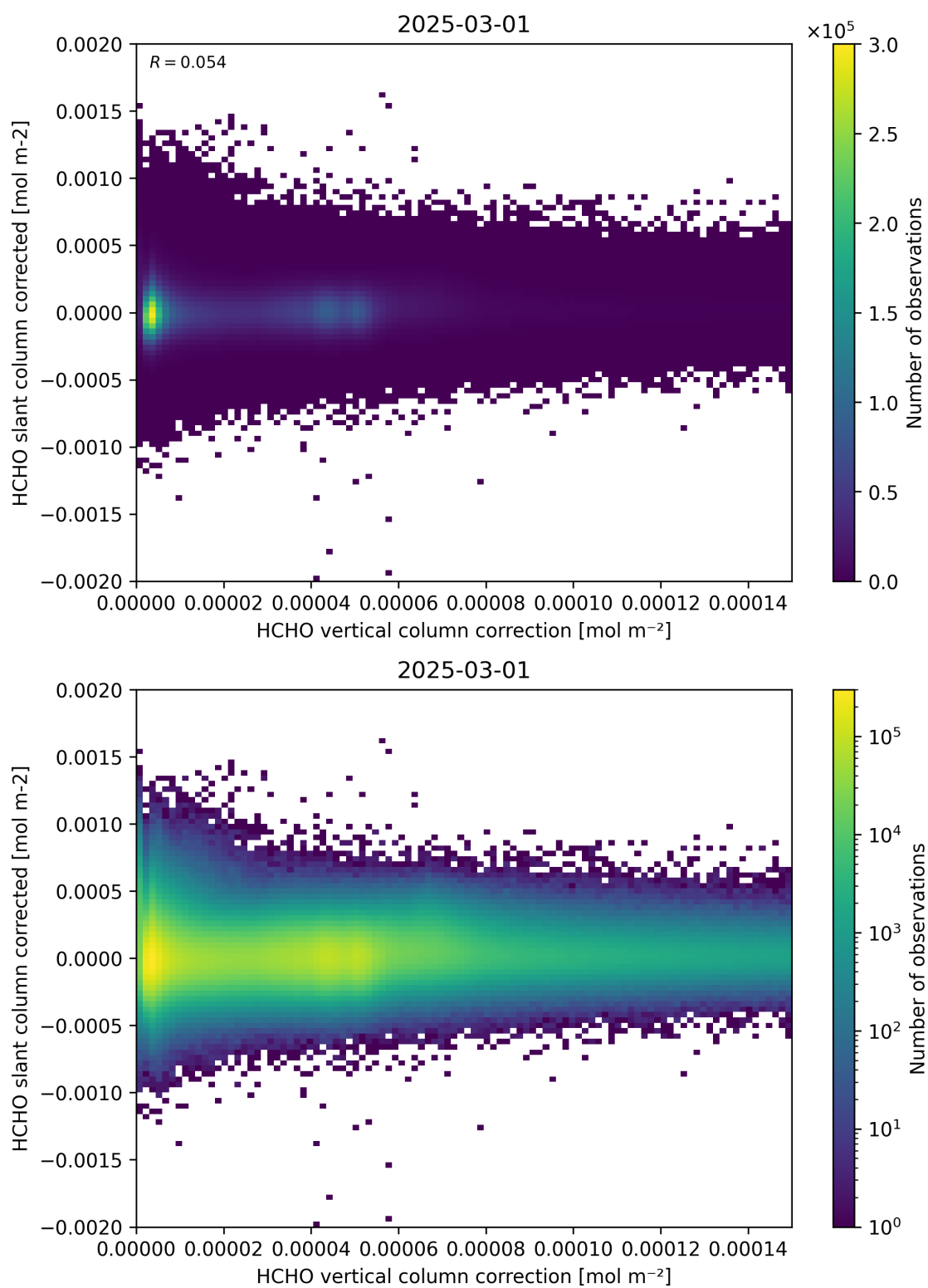
Figure 116: Scatter density plot of “HCHO vertical column correction” against “HCHO slant column corrected” for 2025-03-01 to 2025-03-02.
