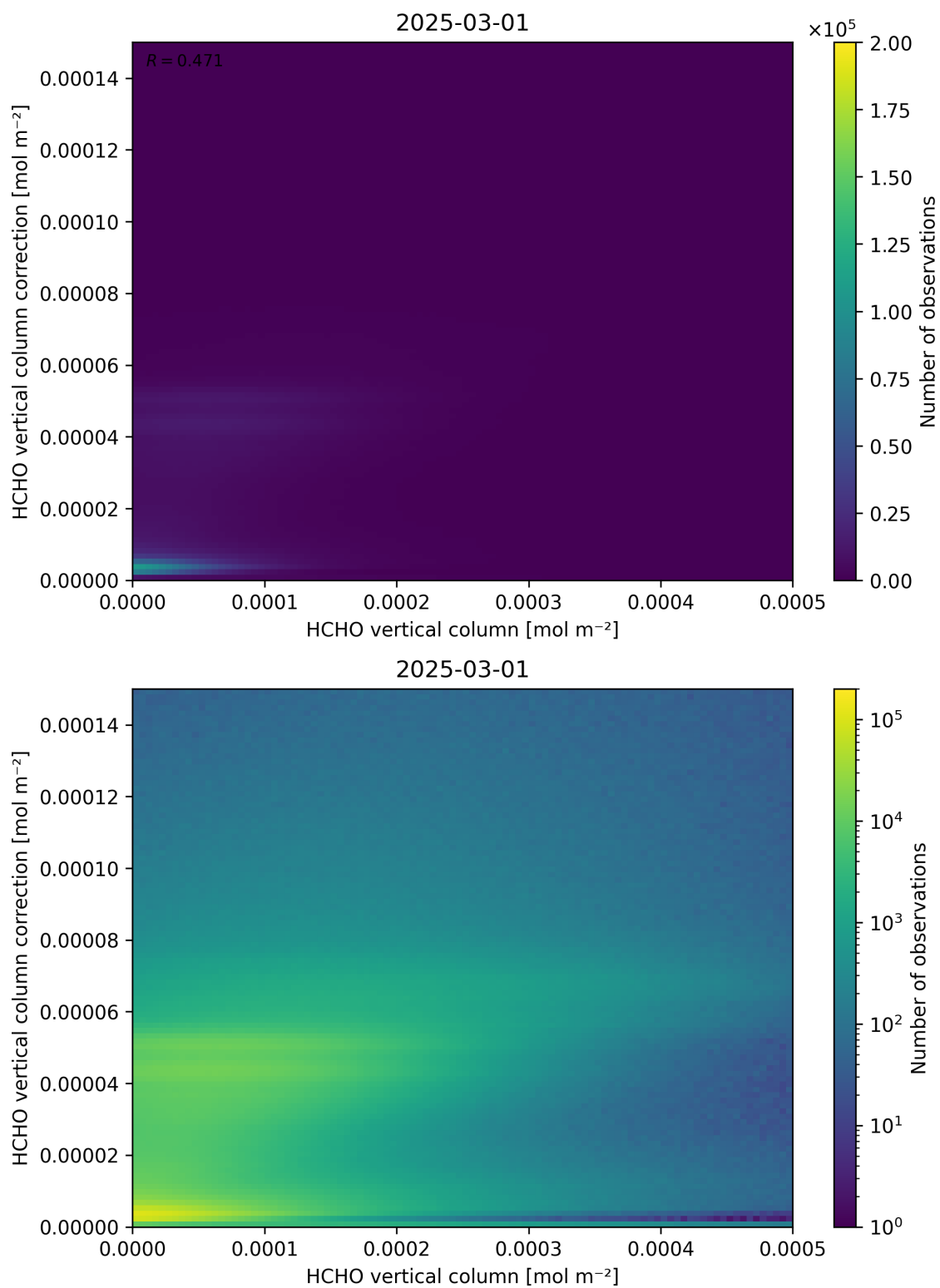
Figure 133: Scatter density plot of “HCHO vertical column” against “HCHO vertical column correction” for 2025-03-01 to 2025-03-02.
