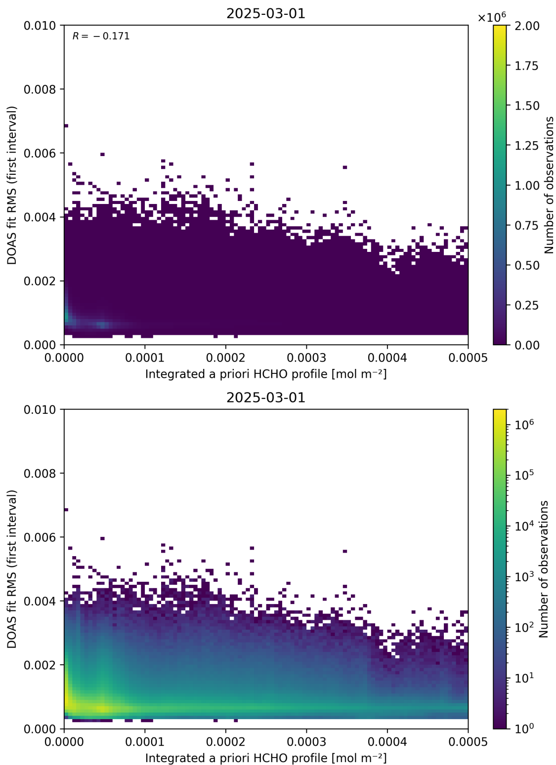
Figure 148: Scatter density plot of “Integrated a priori HCHO profile” against “DOAS fit RMS (first interval)” for 2025-03-01 to 2025-03-02.
