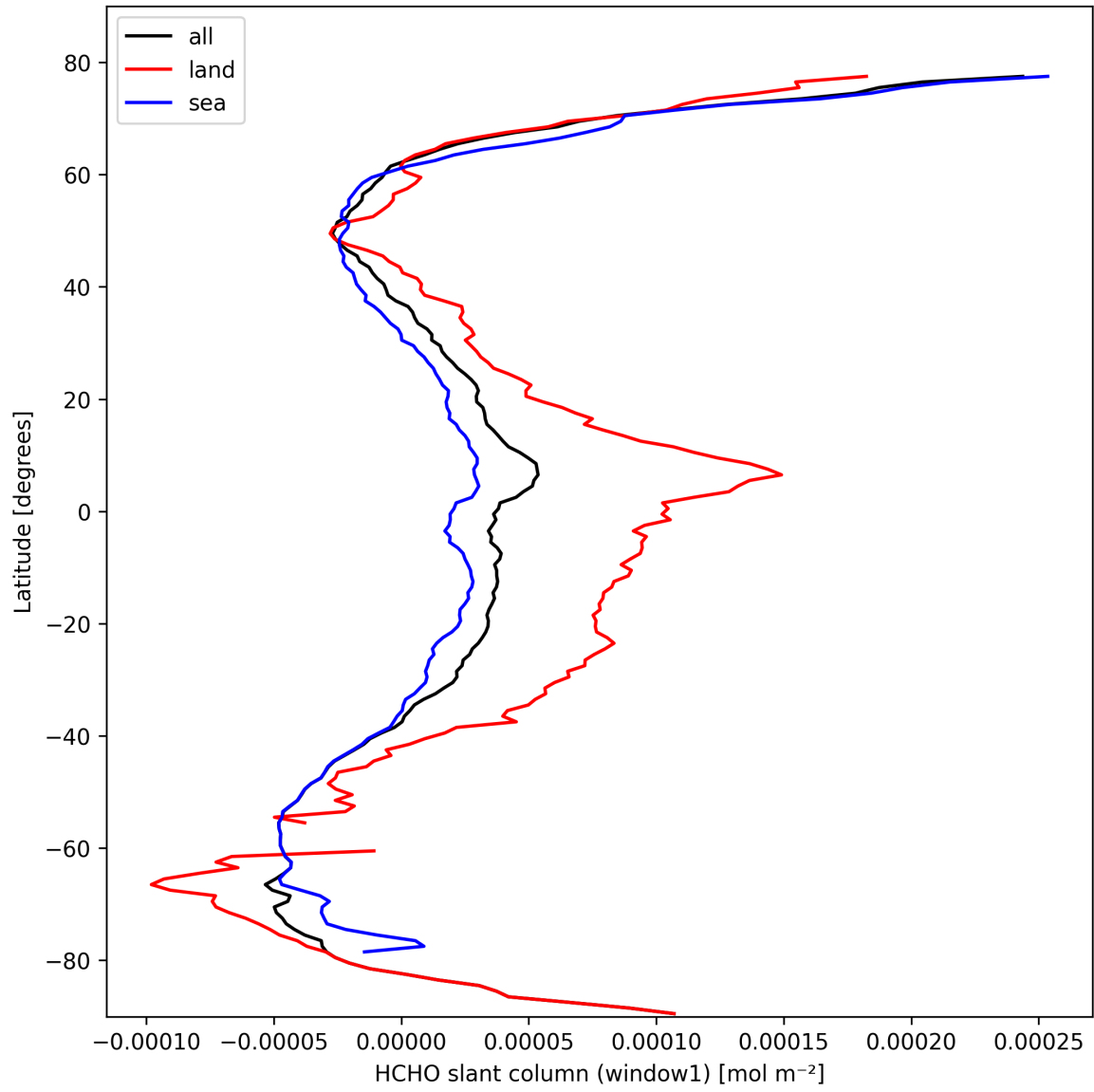
Figure 24: Zonal average of “HCHO slant column (window1)” for 2025-03-01 to 2025-03-02.
