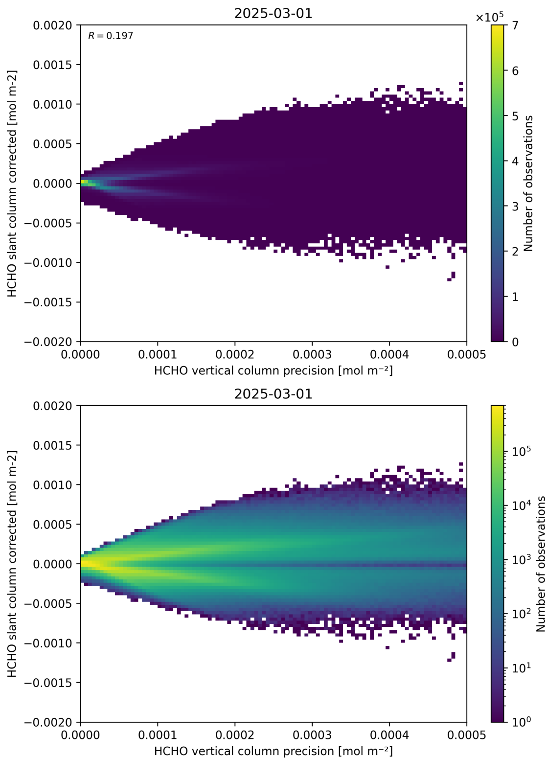
Figure 140: Scatter density plot of “HCHO vertical column precision” against “HCHO slant column corrected” for 2025-03-01 to 2025-03-02.
