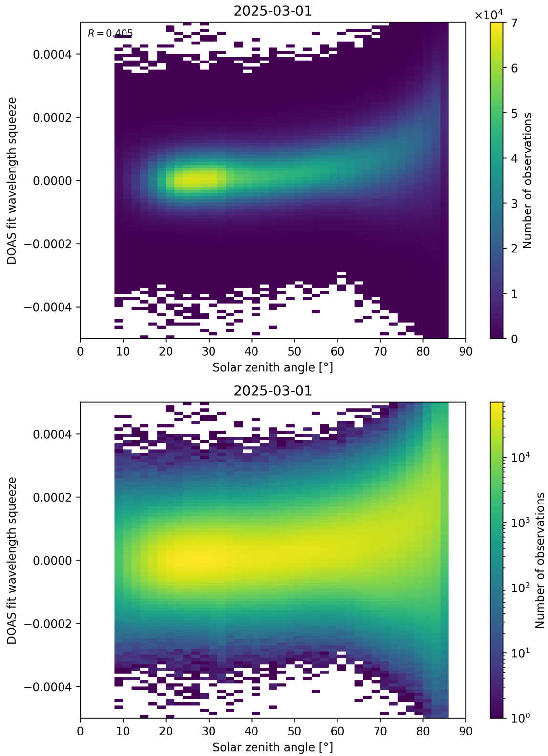
Figure 169: Scatter density plot of “Solar zenith angle” against “DOAS fit wavelength squeeze” for 2025-03-01 to 2025-03-02.
