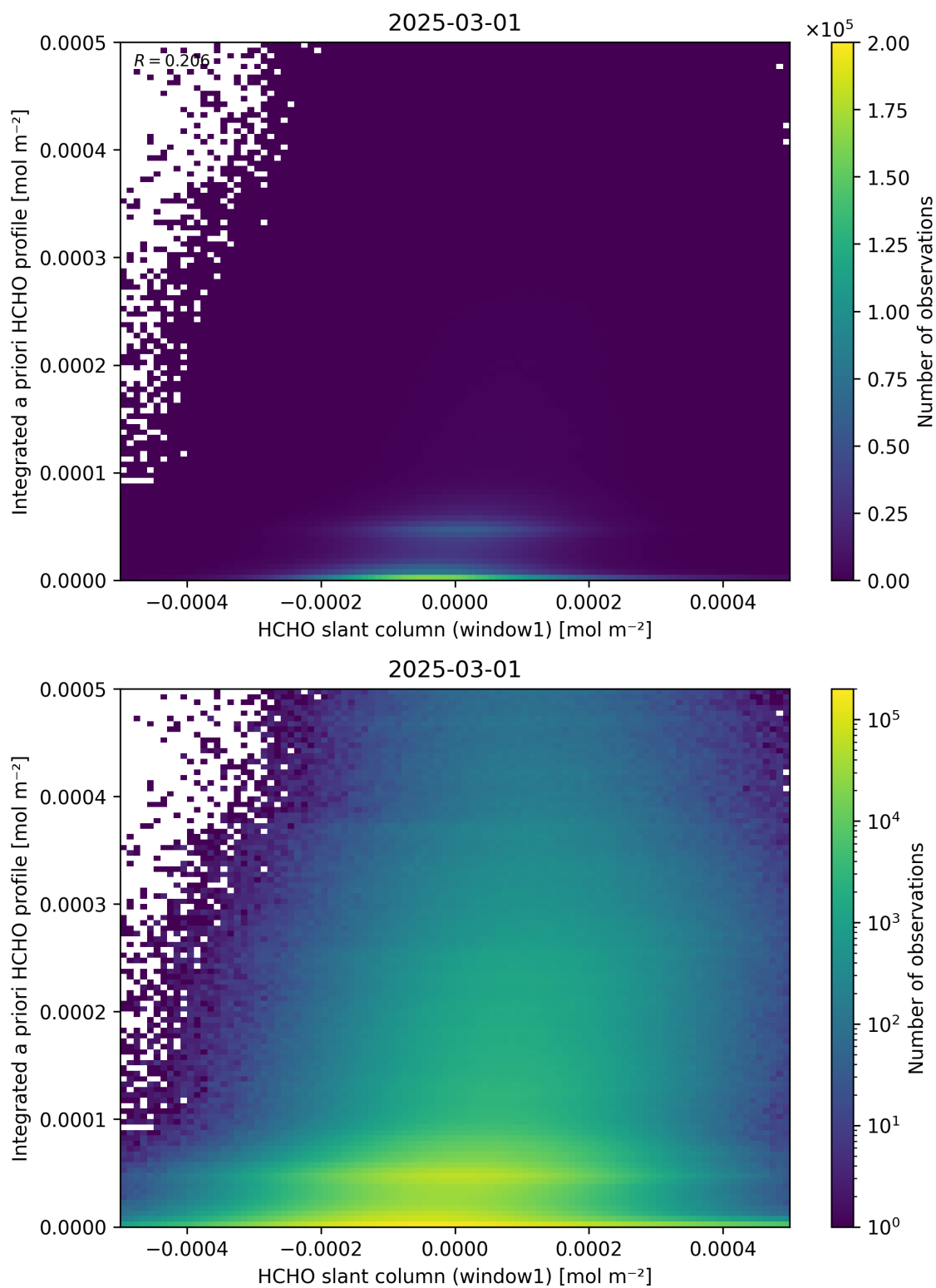
Figure 87: Scatter density plot of “HCHO slant column (window1)” against “Integrated a priori HCHO profile” for 2025-03-01 to 2025-03-02.
