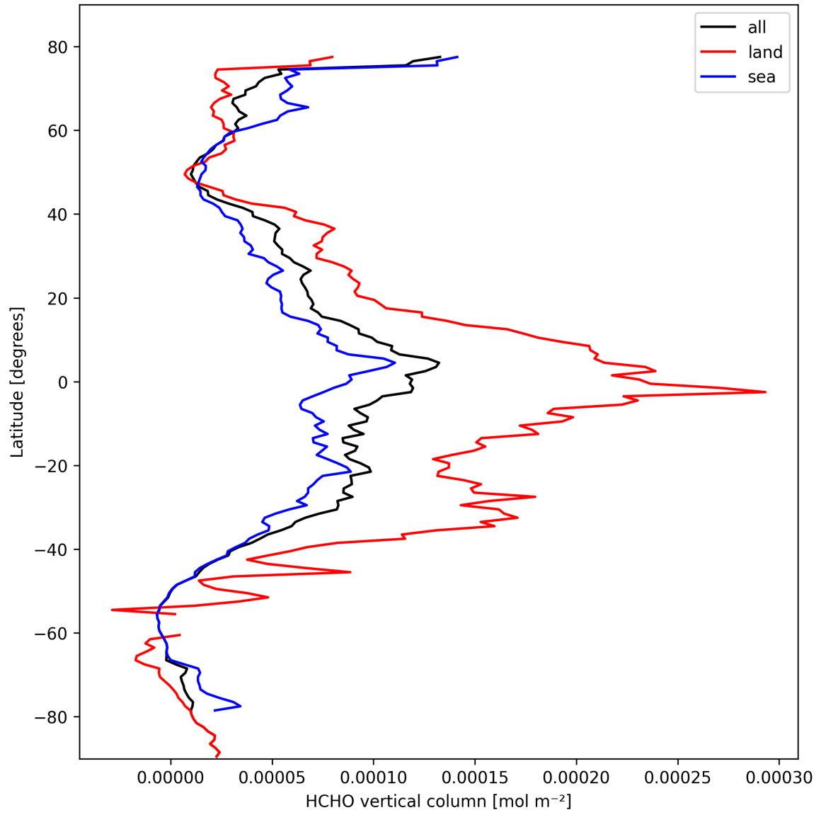
Figure 21: Zonal average of “HCHO vertical column” for 2025-03-01 to 2025-03-02.
