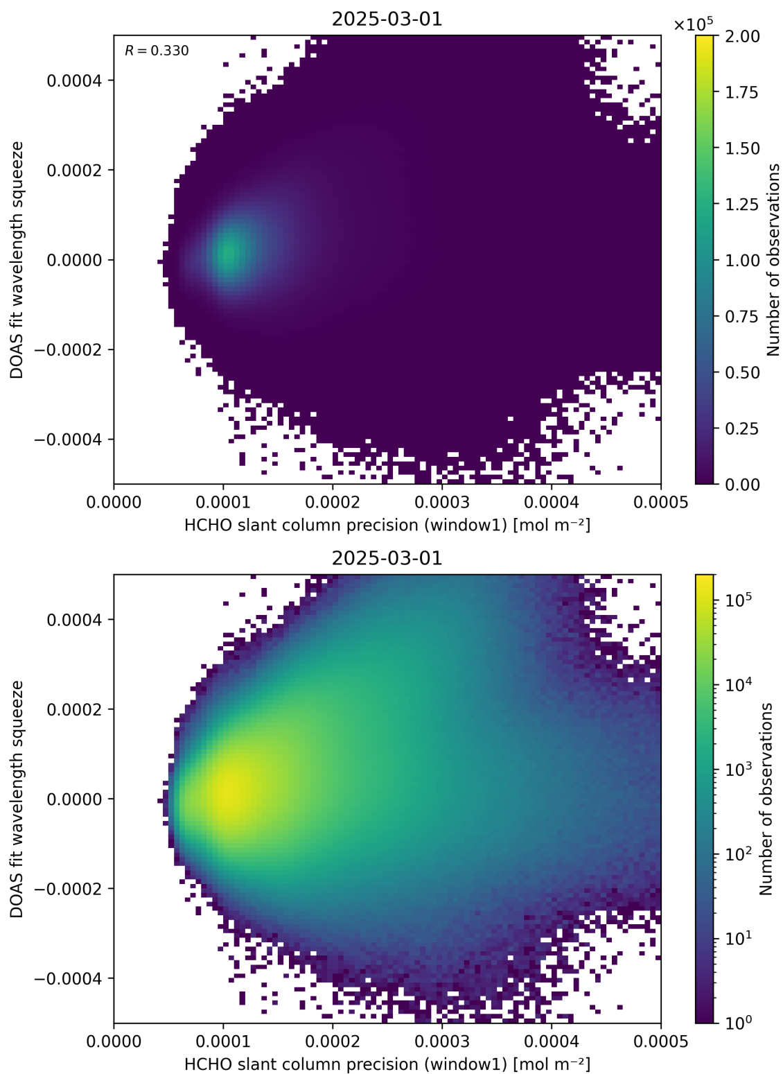
Figure 90: Scatter density plot of “HCHO slant column precision (window1)” against “DOAS fit wavelength squeeze” for 2025-03-01 to 2025-03-02.
