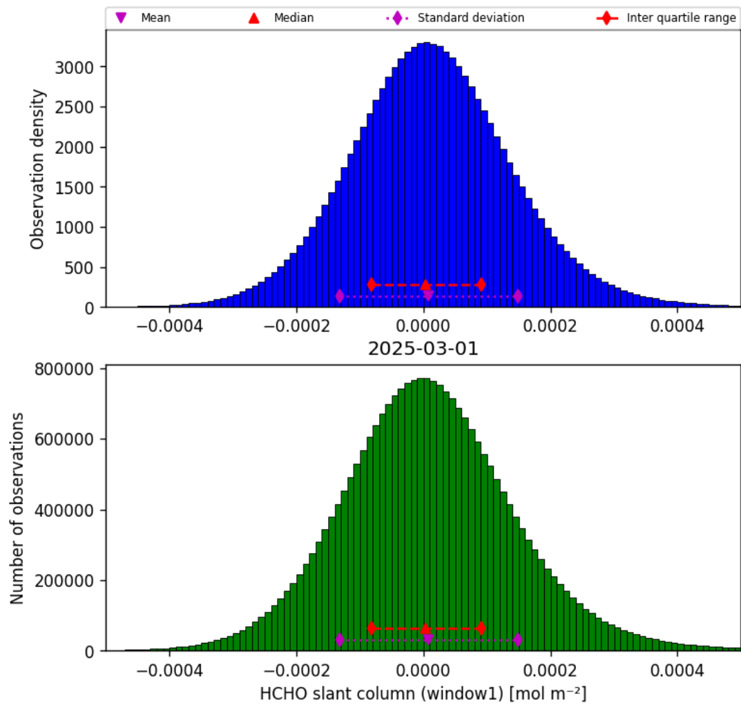
Figure 38: Histogram of “HCHO slant column (window1)” for 2025-03-01 to 2025-03-02
