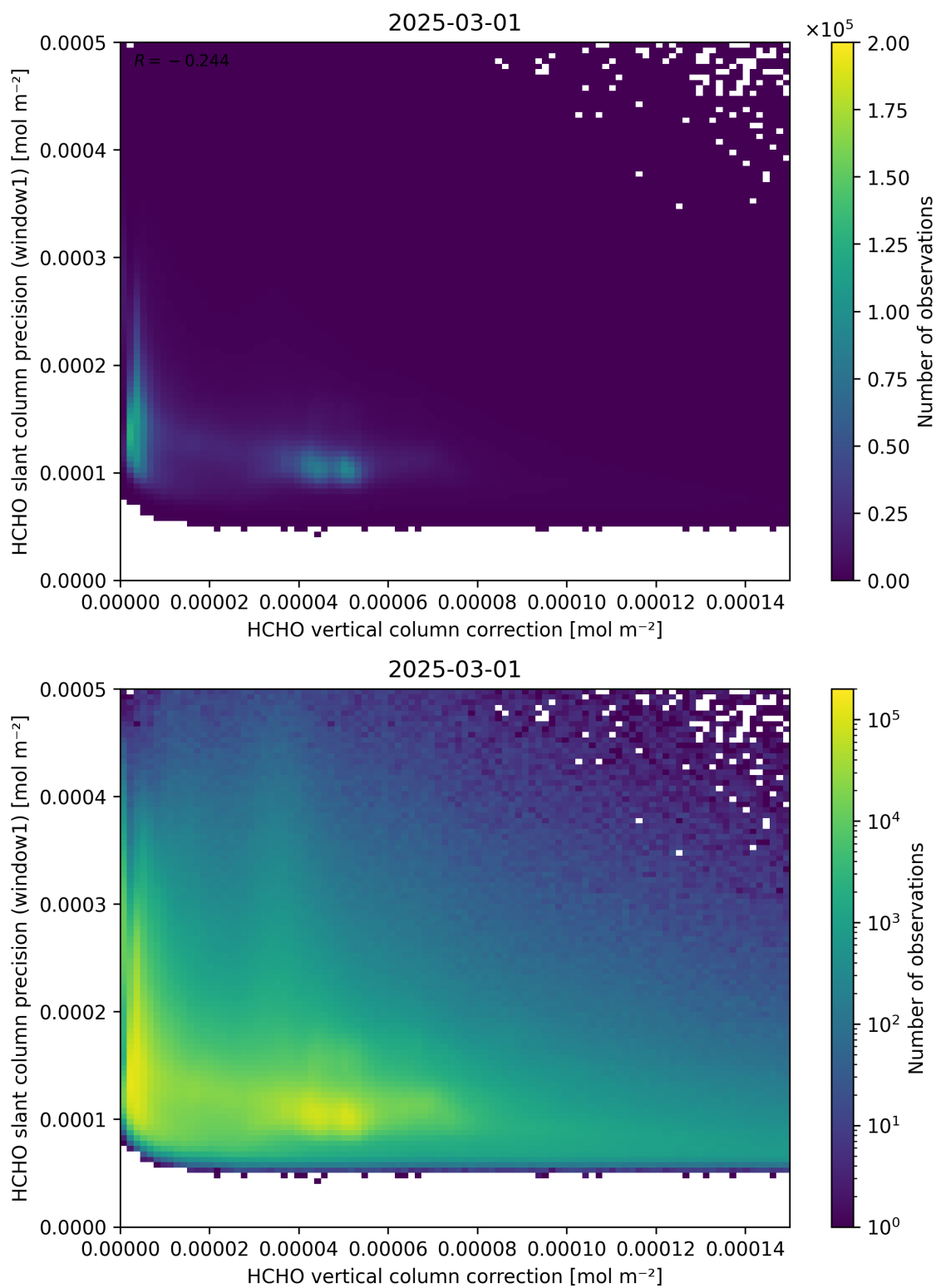
Figure 119: Scatter density plot of “HCHO vertical column correction” against “HCHO slant column precision (window1)” for 2025-03-01 to 2025-03-02.
