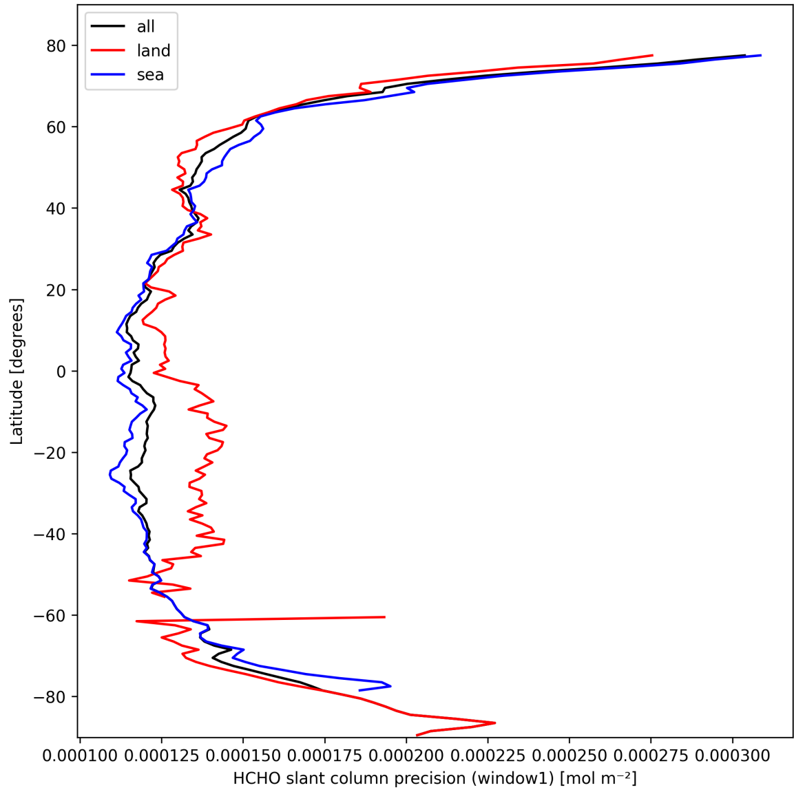
Figure 25: Zonal average of “HCHO slant column precision (window1)” for 2025-03-01 to 2025-03-02.
