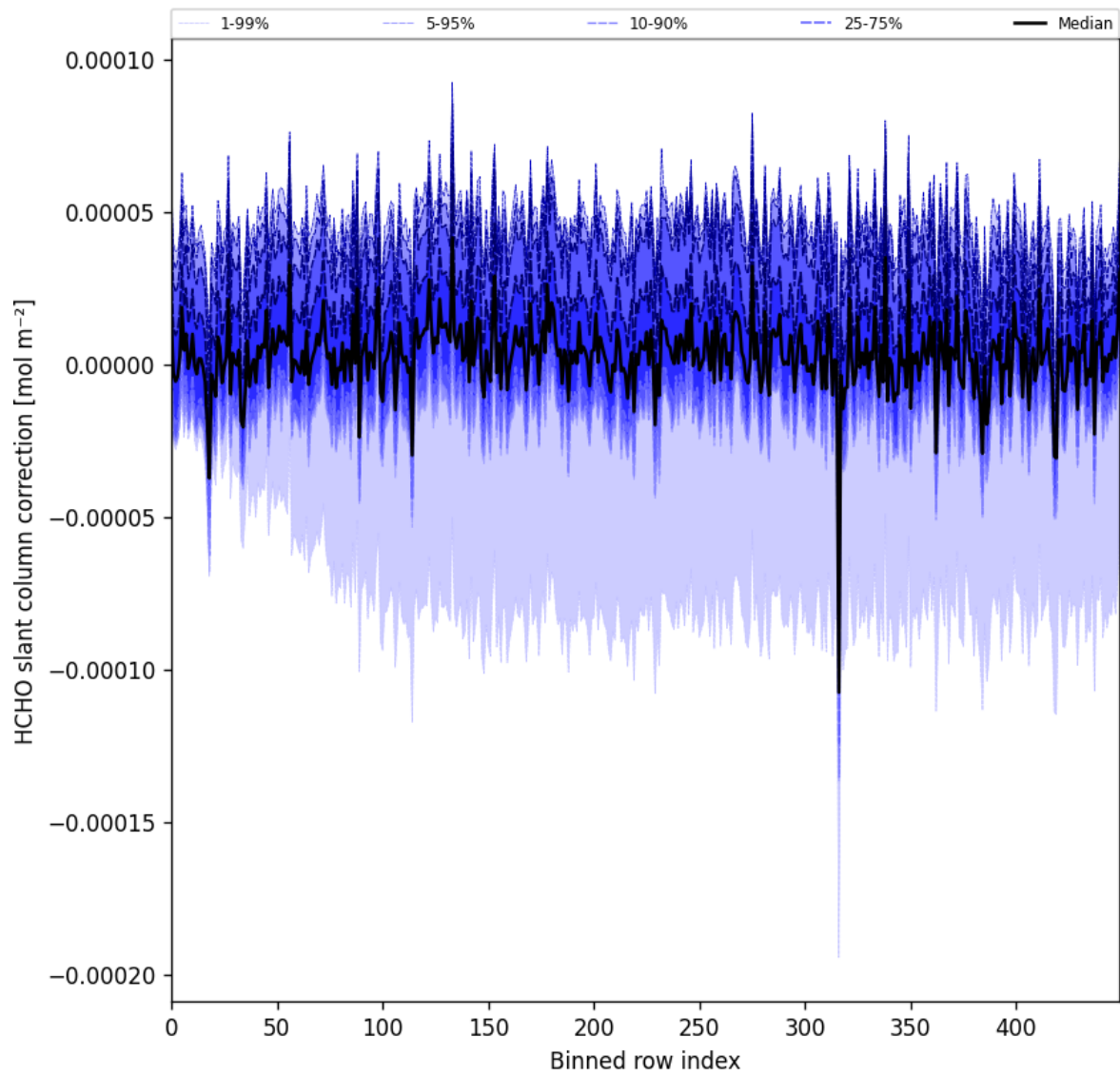
Figure 61: Along track statistics of “HCHO slant column correction” for 2025-03-01 to 2025-03-02
