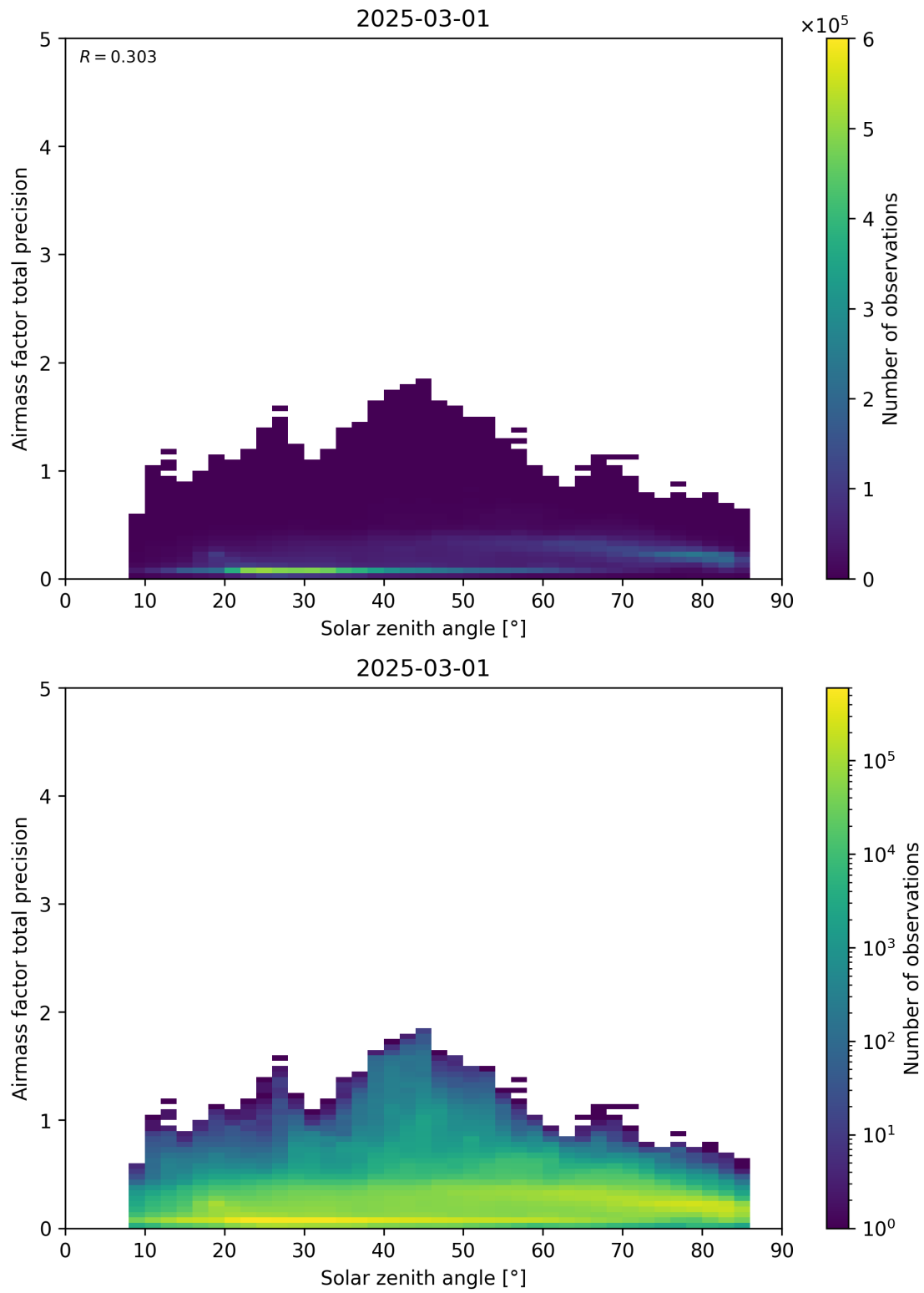
Figure 176: Scatter density plot of “Solar zenith angle” against “Airmass factor total precision” for 2025-03-01 to 2025-03-02.
