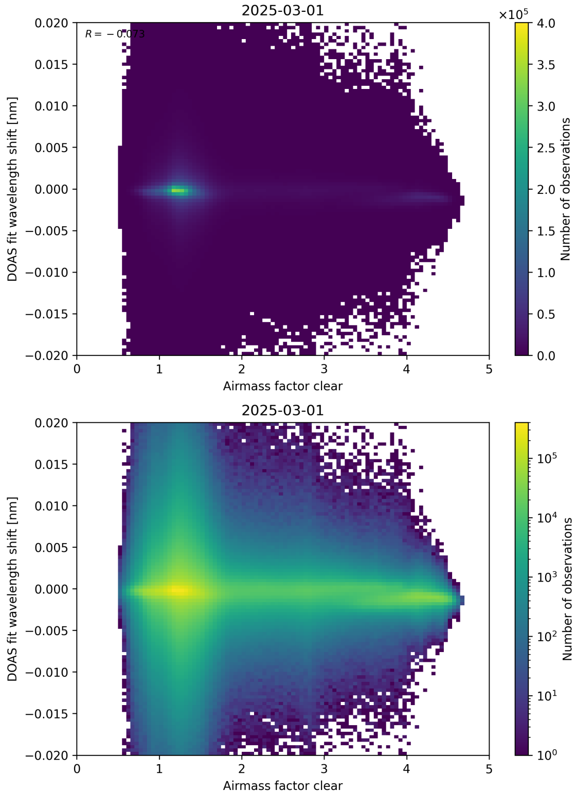
Figure 72: Scatter density plot of “Airmass factor clear” against “DOAS fit wavelength shift” for 2025-03-01 to 2025-03-02.
