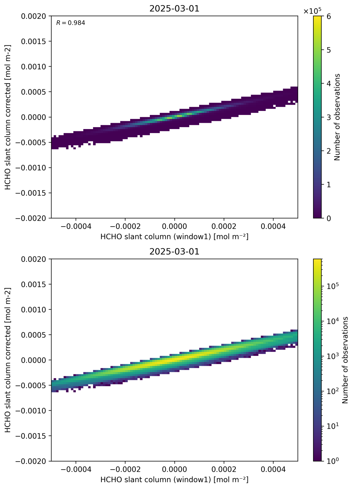
Figure 82: Scatter density plot of “HCHO slant column (window1)” against “HCHO slant column corrected” for 2025-03-01 to 2025-03-02.
