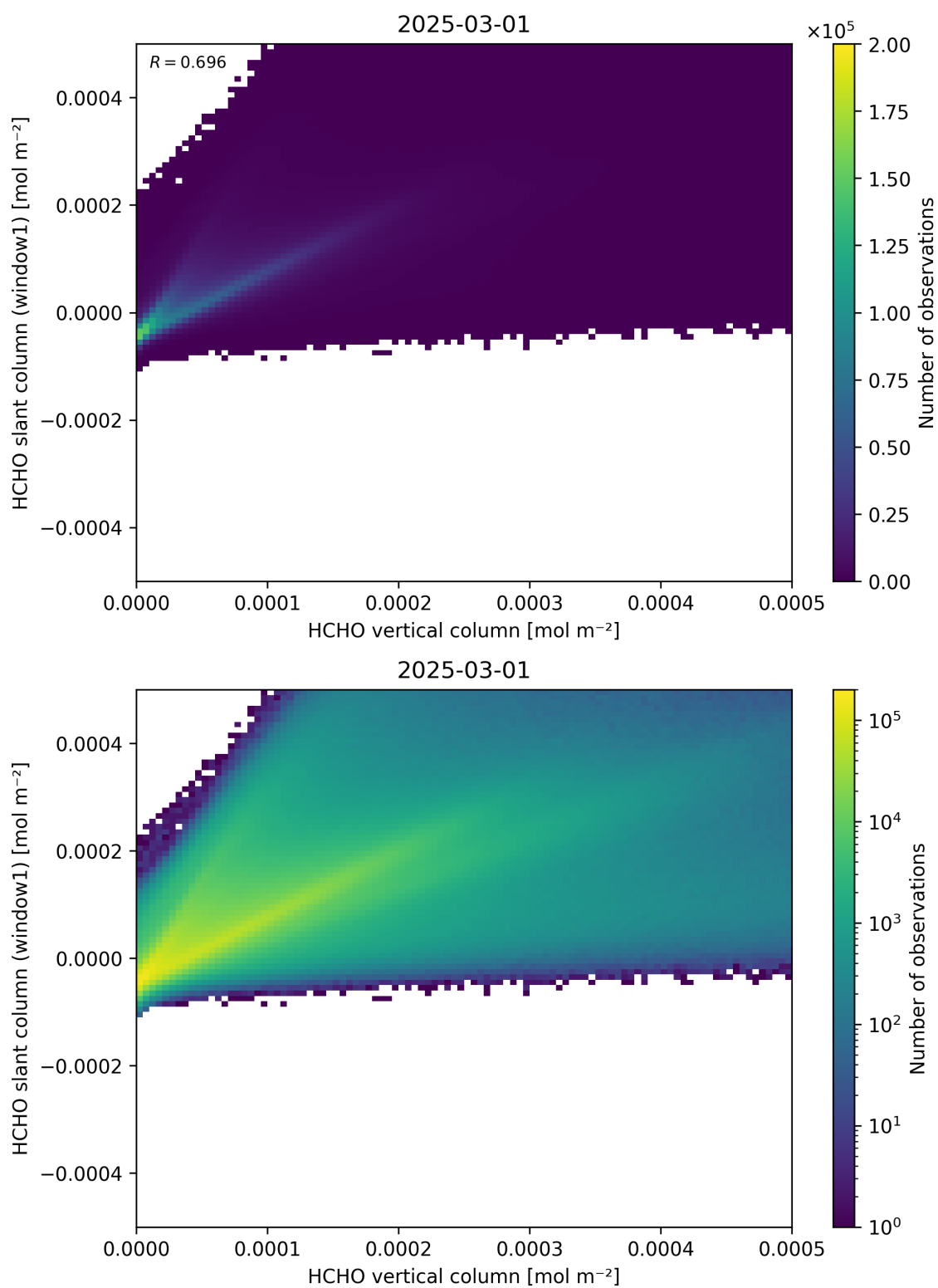
Figure 129: Scatter density plot of “HCHO vertical column” against “HCHO slant column (window1)” for 2025-03-01 to 2025-03-02.
