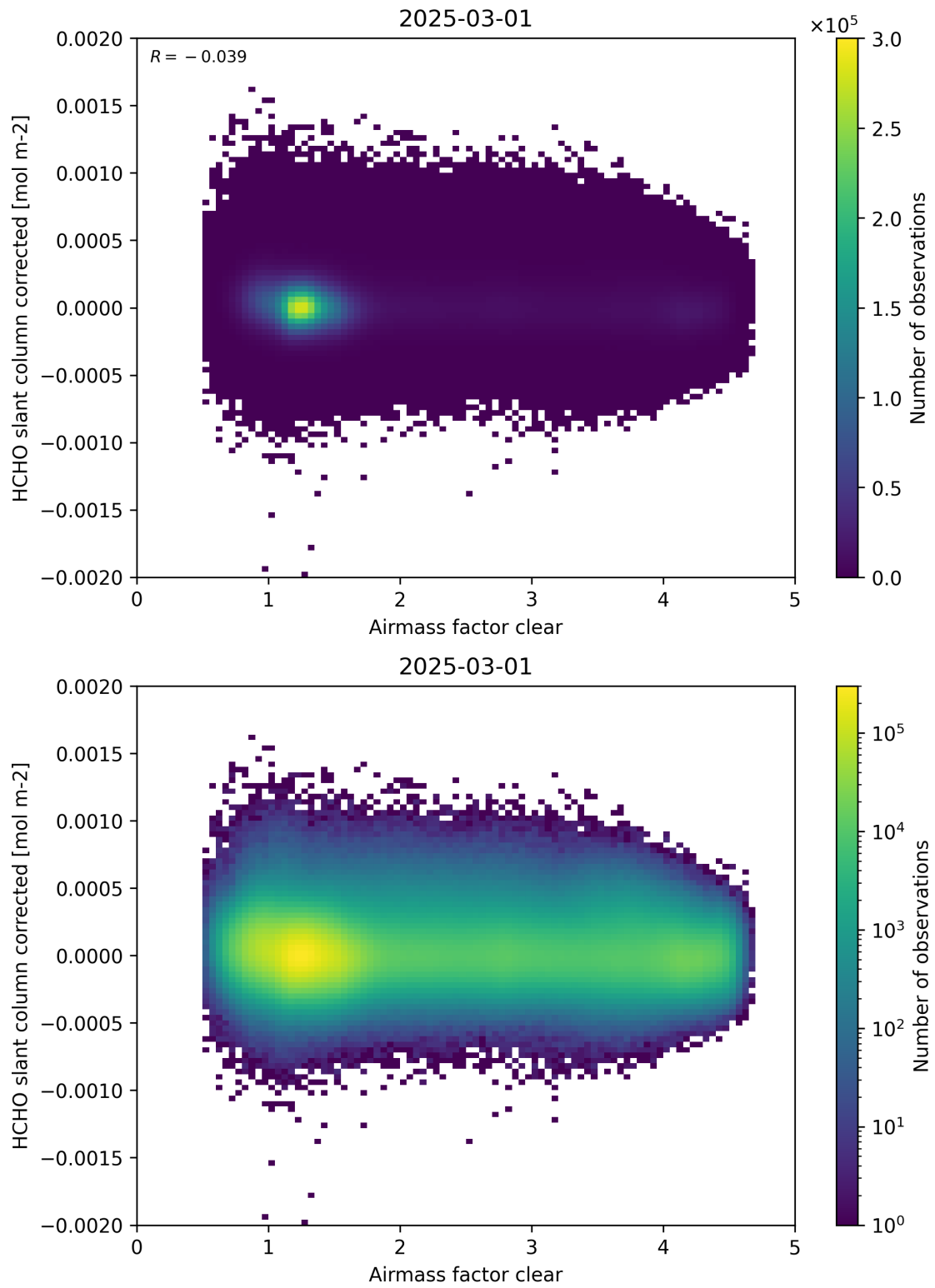
Figure 74: Scatter density plot of “Airmass factor clear” against “HCHO slant column corrected” for 2025-03-01 to 2025-03-02.
