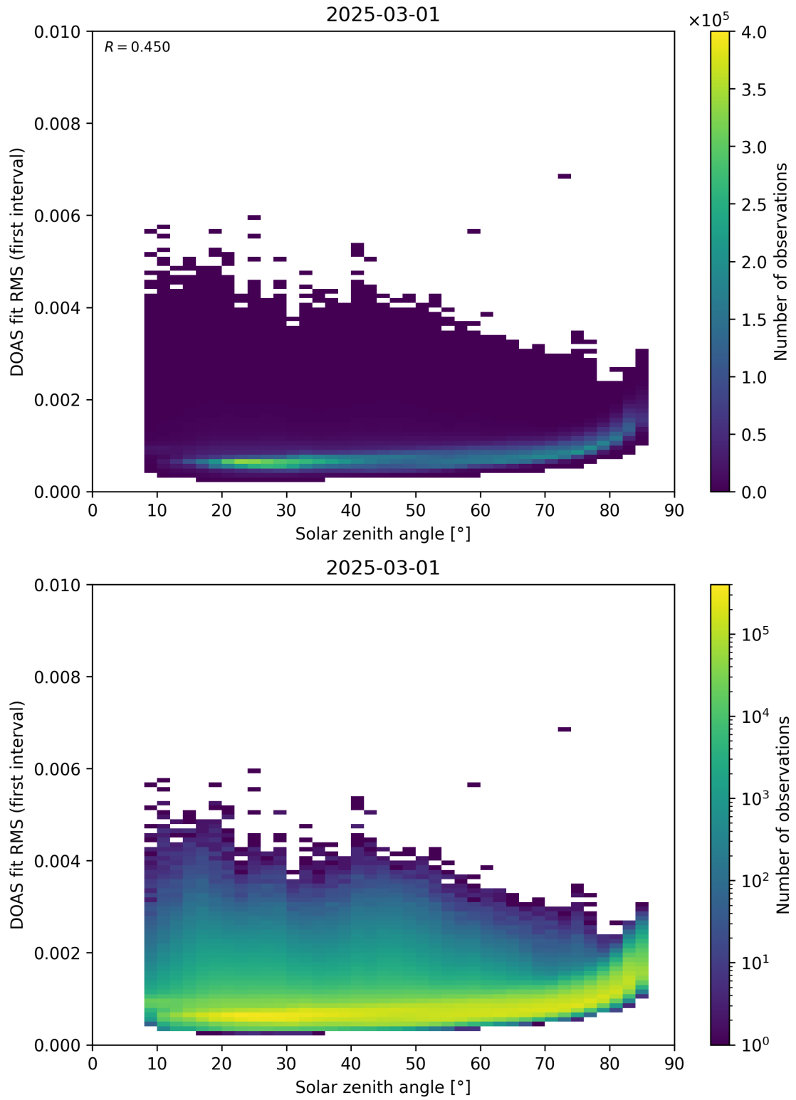
Figure 167: Scatter density plot of “Solar zenith angle” against “DOAS fit RMS (first interval)” for 2025-03-01 to 2025-03-02.
