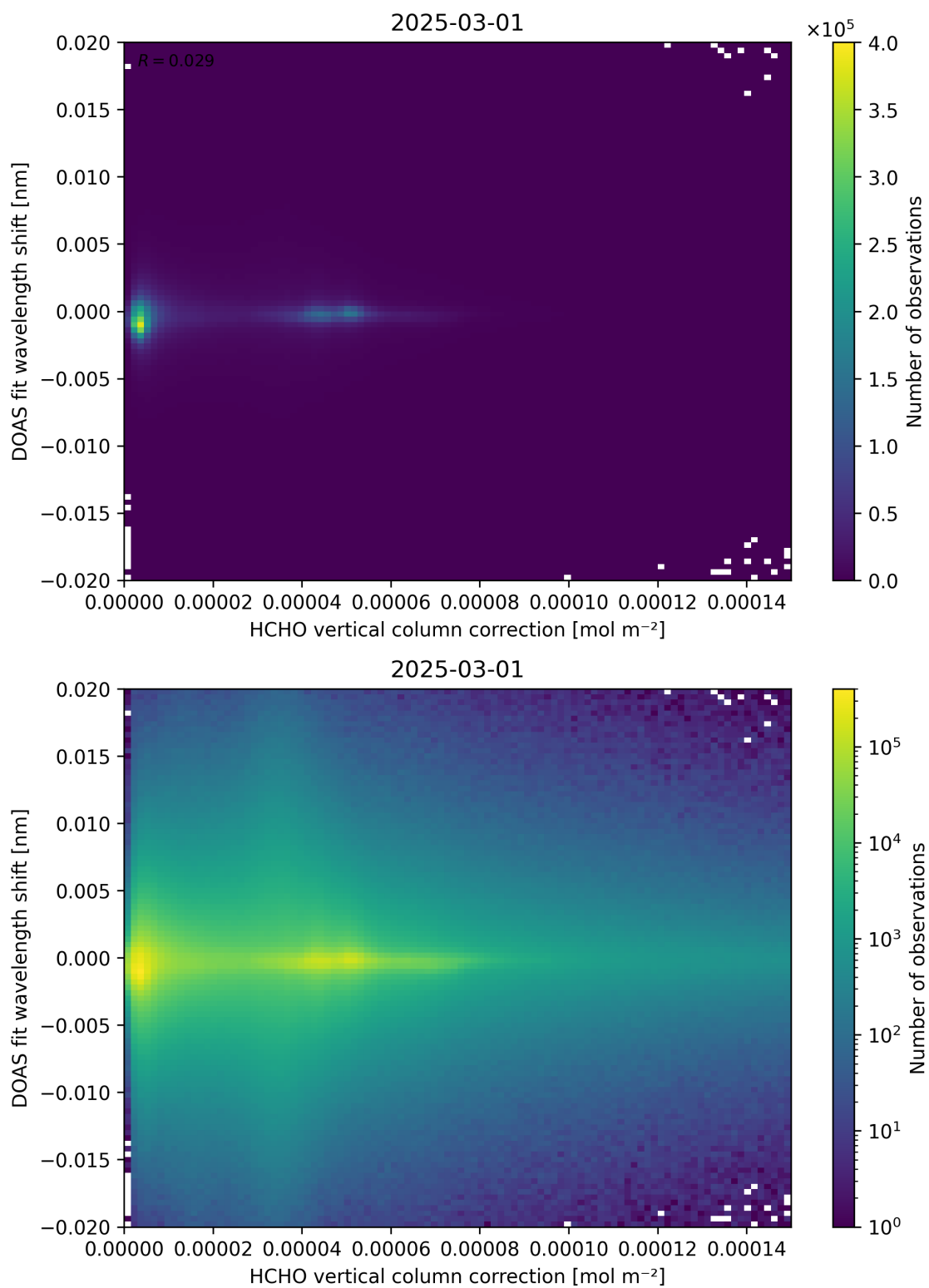
Figure 113: Scatter density plot of “HCHO vertical column correction” against “DOAS fit wavelength shift” for 2025-03-01 to 2025-03-02.
