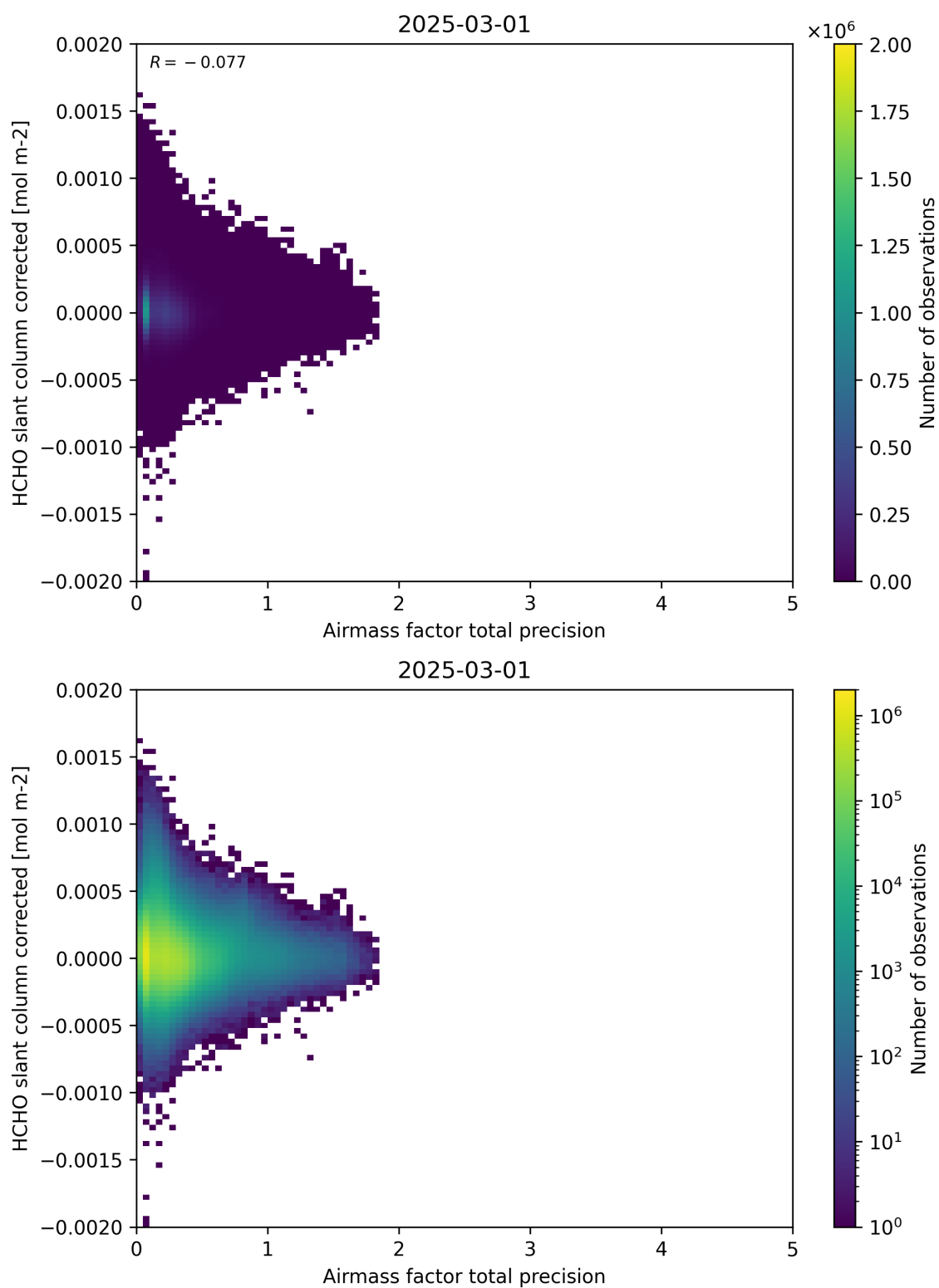
Figure 109: Scatter density plot of “Airmass factor total precision” against “HCHO slant column corrected” for 2025-03-01 to 2025-03-02.
