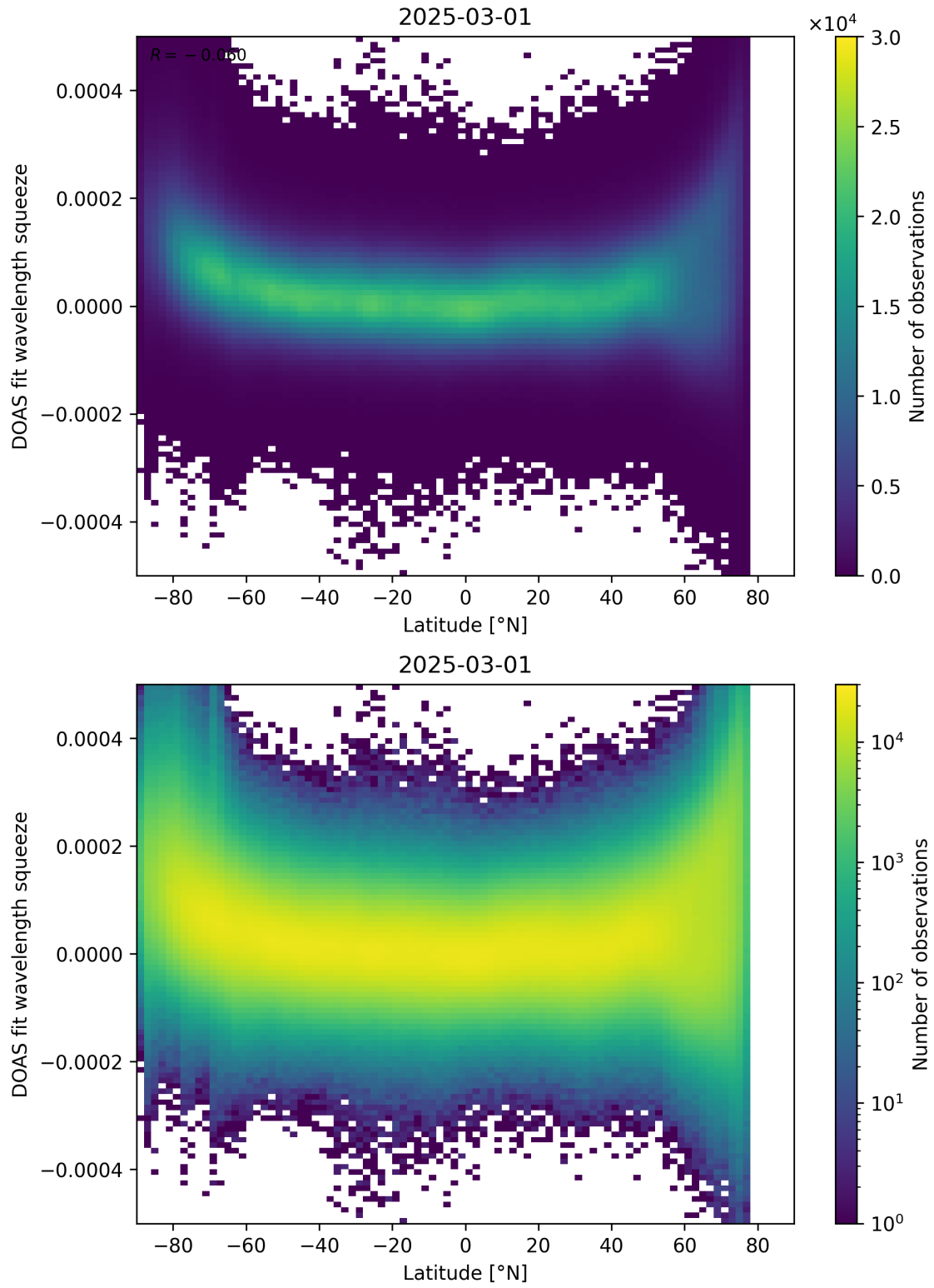
Figure 155: Scatter density plot of “Latitude” against “DOAS fit wavelength squeeze” for 2025-03-01 to 2025-03-02.
