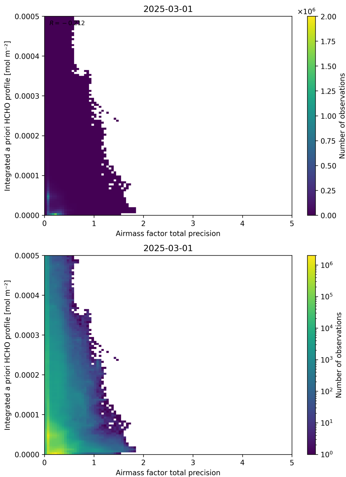
Figure 111: Scatter density plot of “Airmass factor total precision” against “Integrated a priori HCHO profile” for 2025-03-01 to 2025-03-02.
