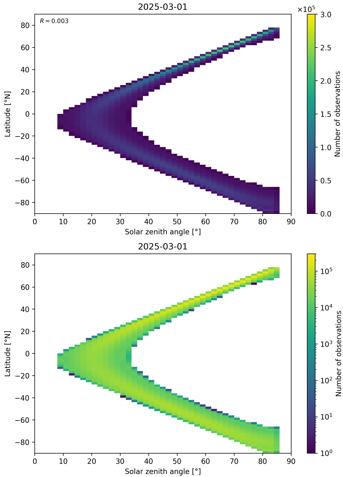
Figure 181: Scatter density plot of “Solar zenith angle” against “Latitude” for 2025-03-01 to 2025-03-02.
