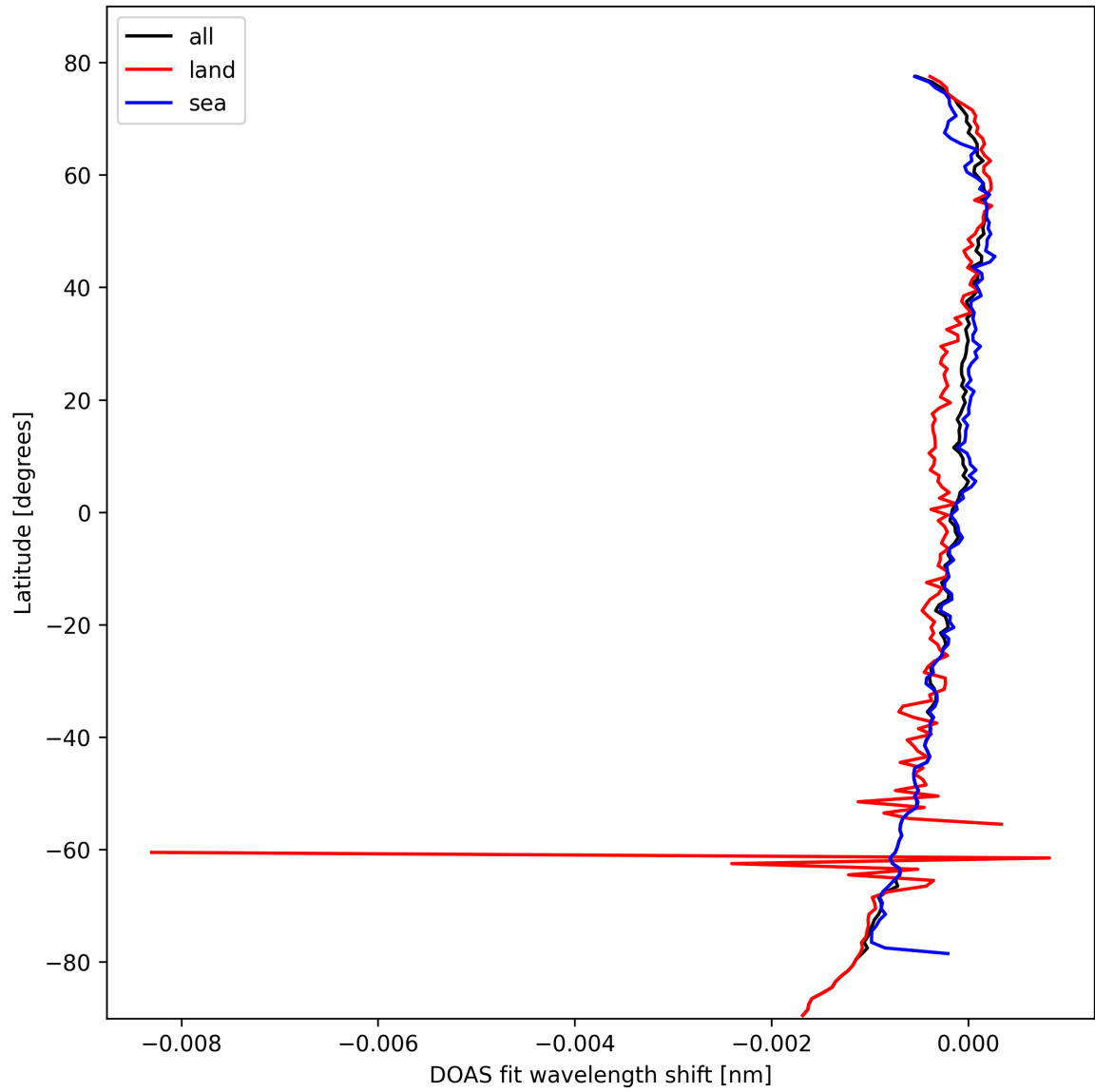
Figure 30: Zonal average of “DOAS fit wavelength shift” for 2025-03-01 to 2025-03-02.
