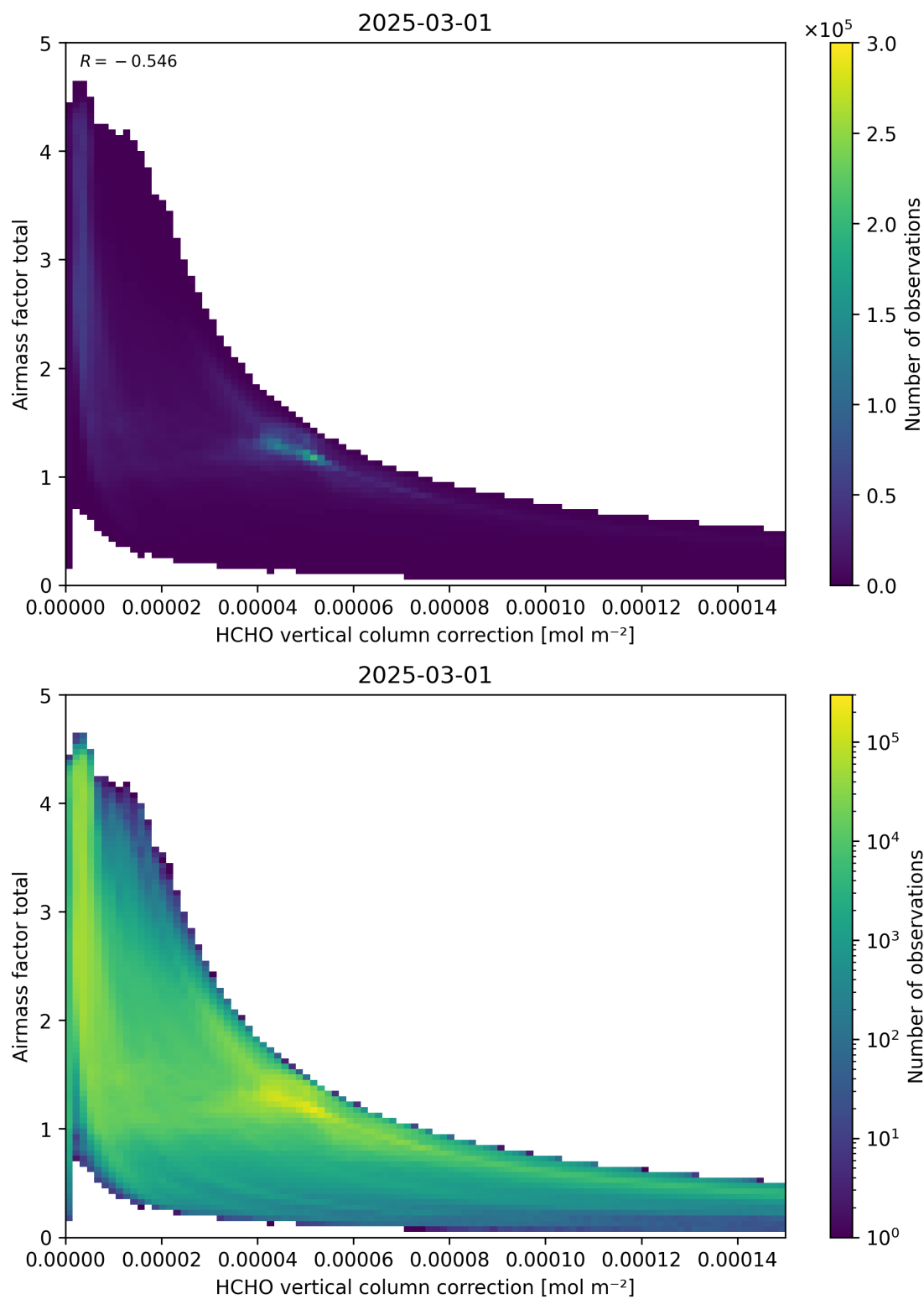
Figure 120: Scatter density plot of “HCHO vertical column correction” against “Airmass factor total” for 2025-03-01 to 2025-03-02.
