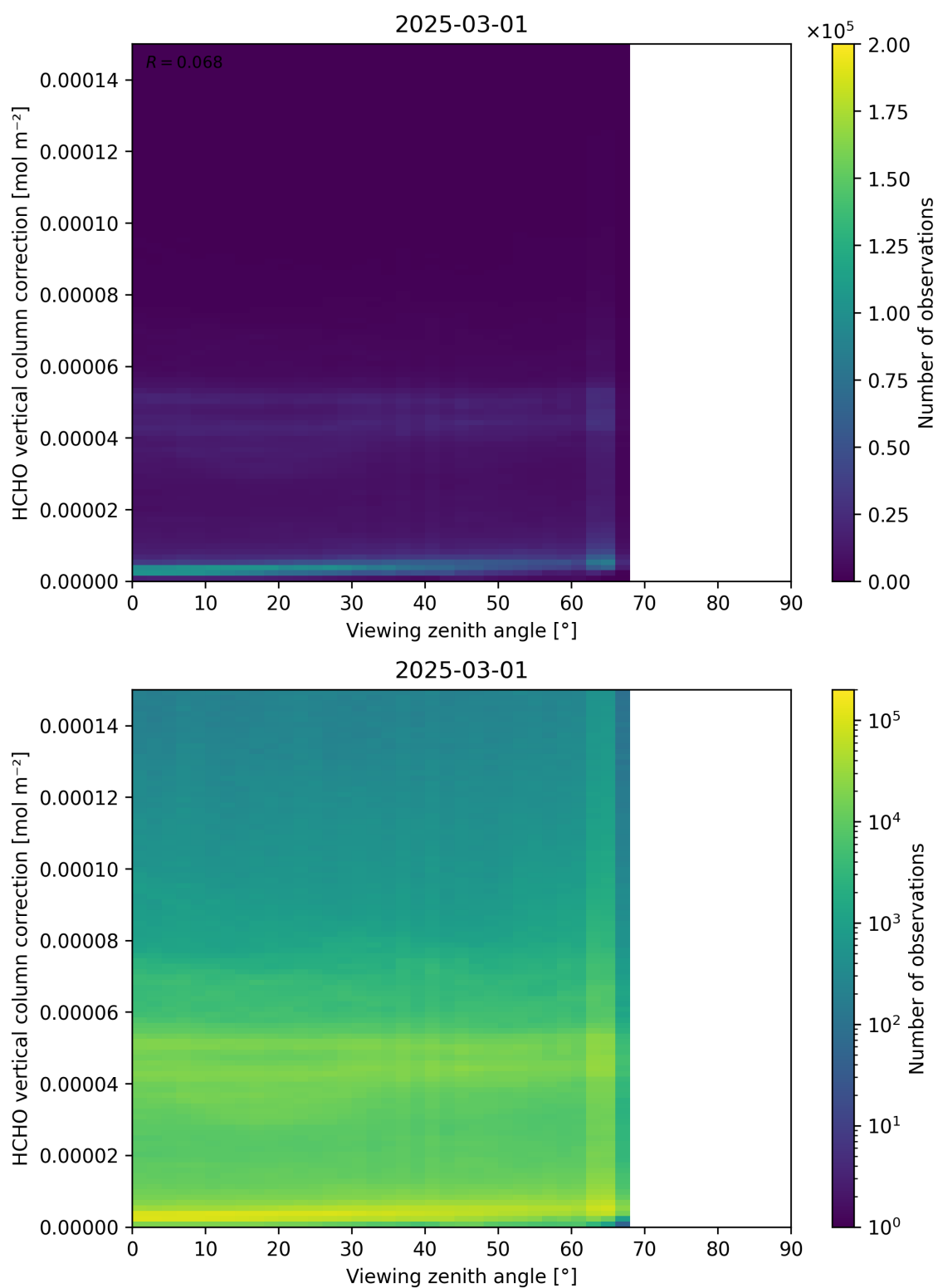
Figure 193: Scatter density plot of “Viewing zenith angle” against “HCHO vertical column correction” for 2025-03-01 to 2025-03-02.
