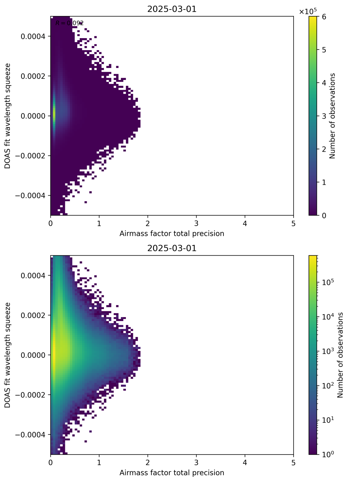
Figure 107: Scatter density plot of “Airmass factor total precision” against “DOAS fit wavelength squeeze” for 2025-03-01 to 2025-03-02.
