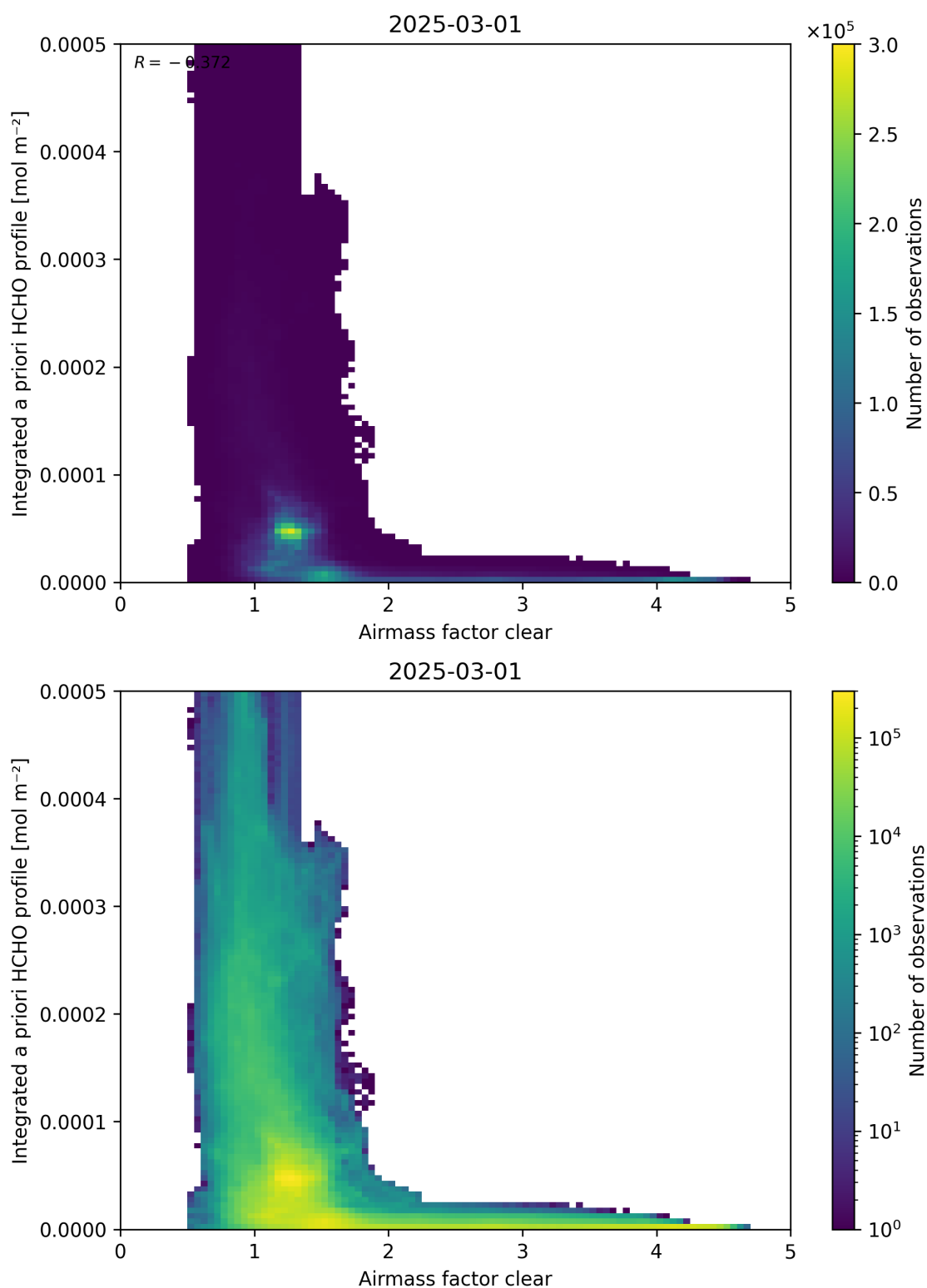
Figure 76: Scatter density plot of “Airmass factor clear” against “Integrated a priori HCHO profile” for 2025-03-01 to 2025-03-02.
