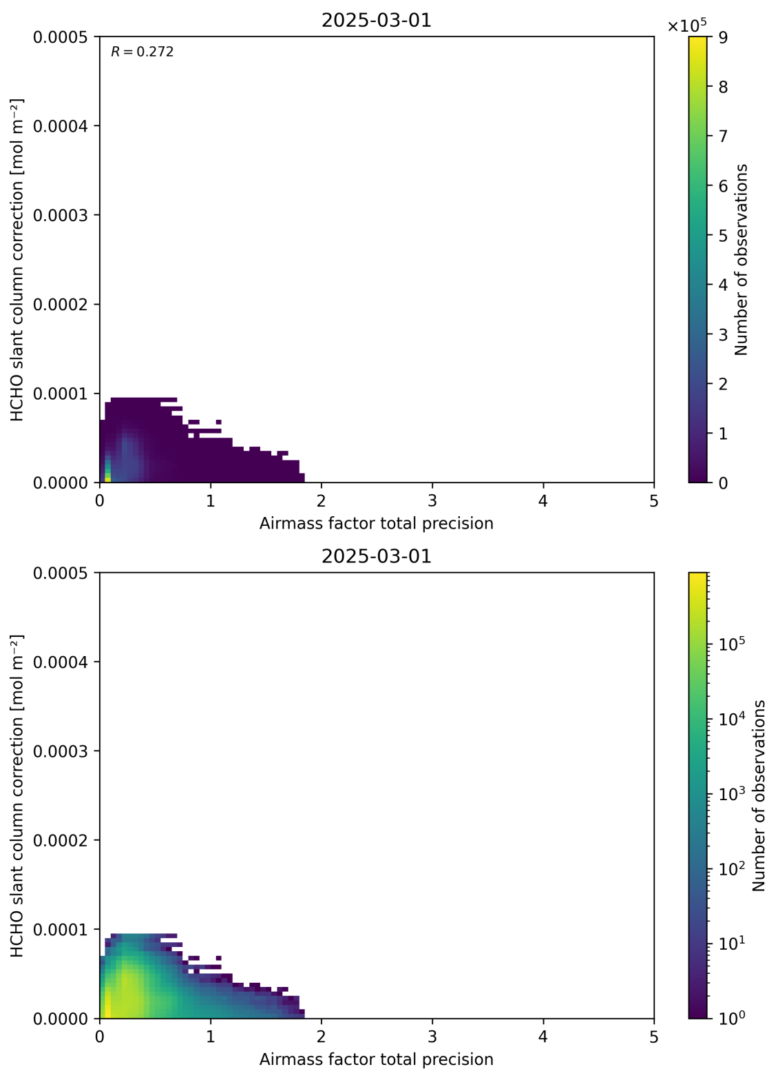
Figure 110: Scatter density plot of “Airmass factor total precision” against “HCHO slant column correction” for 2025-03-01 to 2025-03-02.
