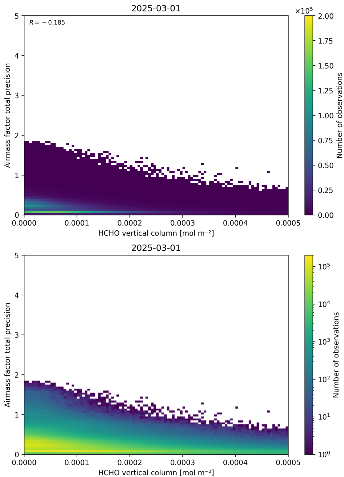
Figure 132: Scatter density plot of “HCHO vertical column” against “Airmass factor total precision” for 2025-03-01 to 2025-03-02.
