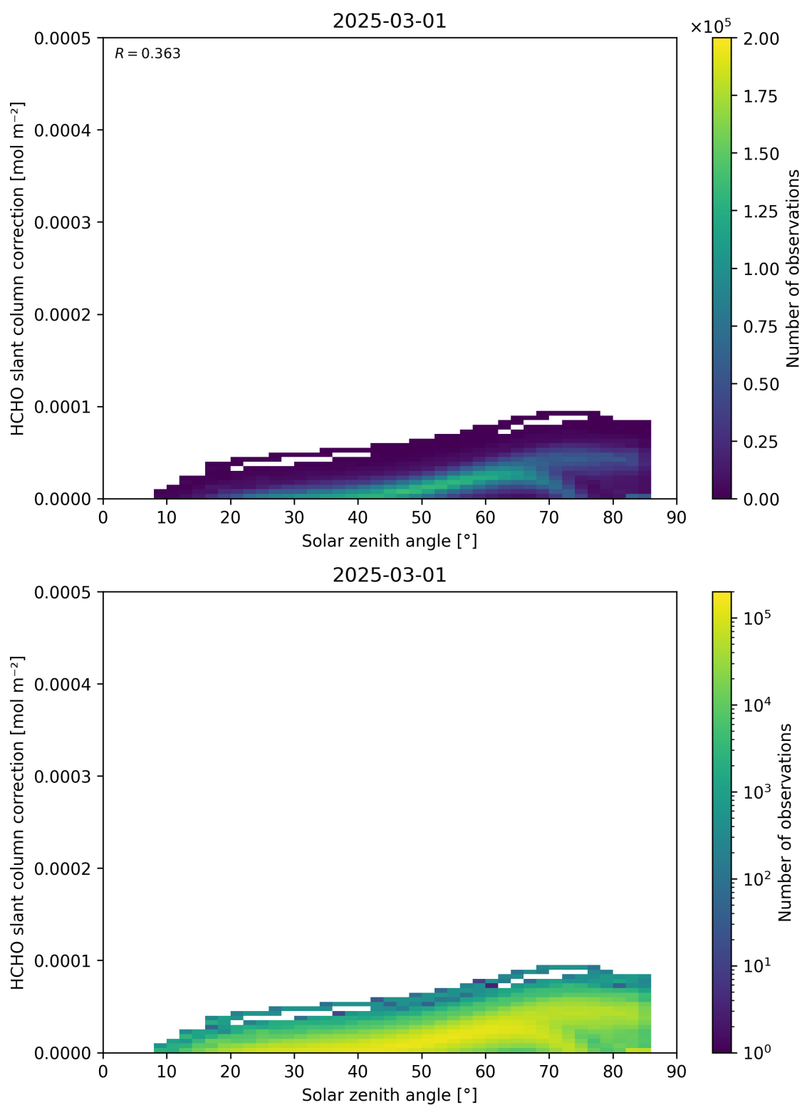
Figure 172: Scatter density plot of “Solar zenith angle” against “HCHO slant column correction” for 2025-03-01 to 2025-03-02.
