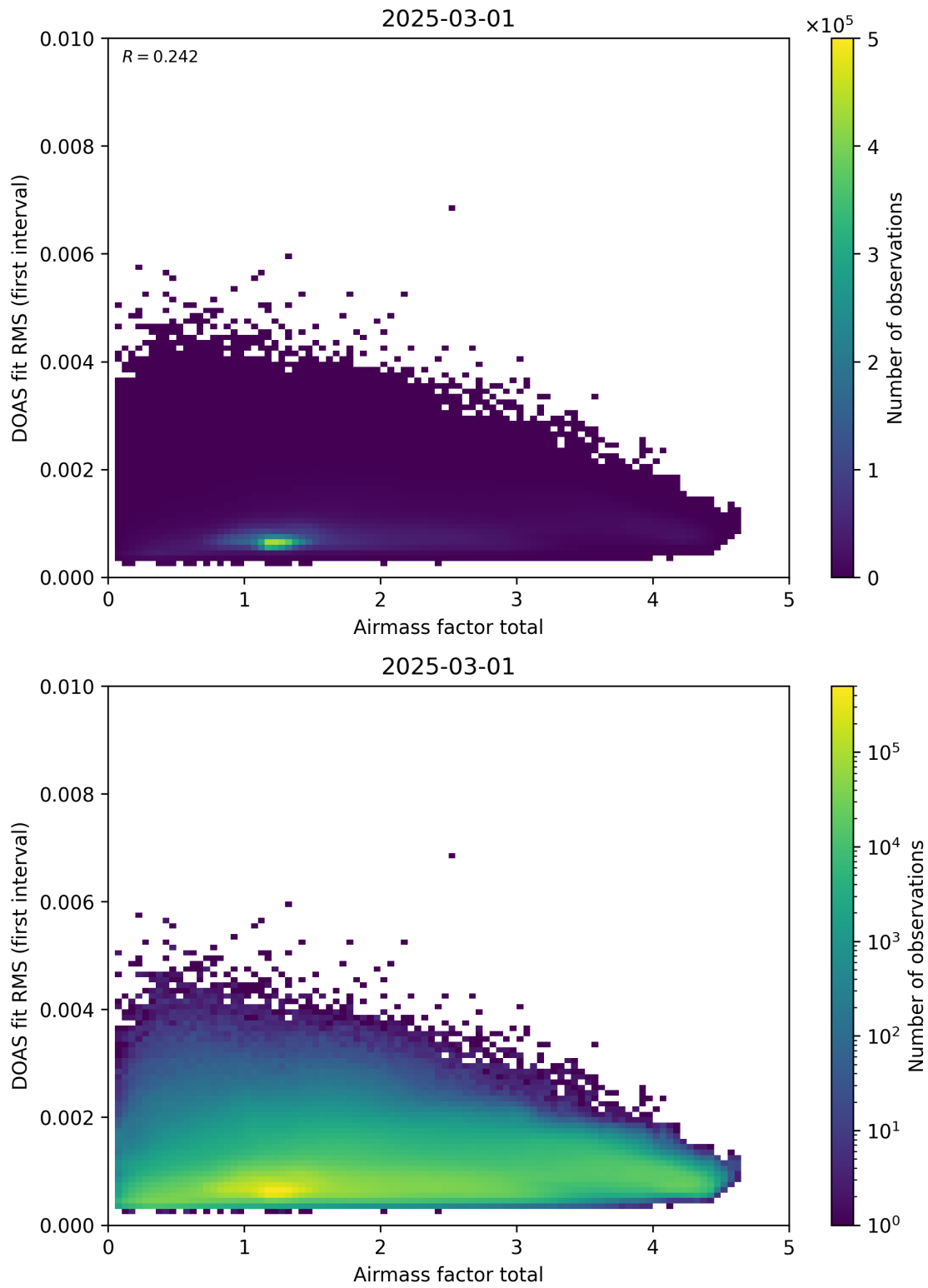
Figure 97: Scatter density plot of “Airmass factor total” against “DOAS fit RMS (first interval)” for 2025-03-01 to 2025-03-02.
