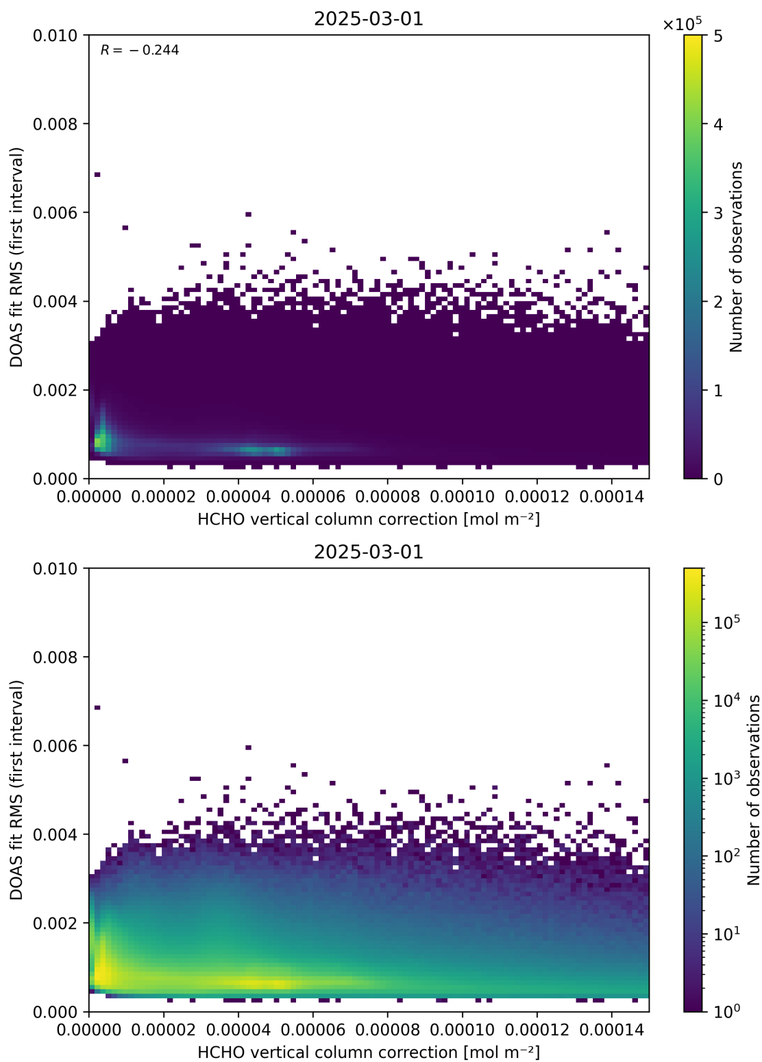
Figure 112: Scatter density plot of “HCHO vertical column correction” against “DOAS fit RMS (first interval)” for 2025-03-01 to 2025-03-02.
