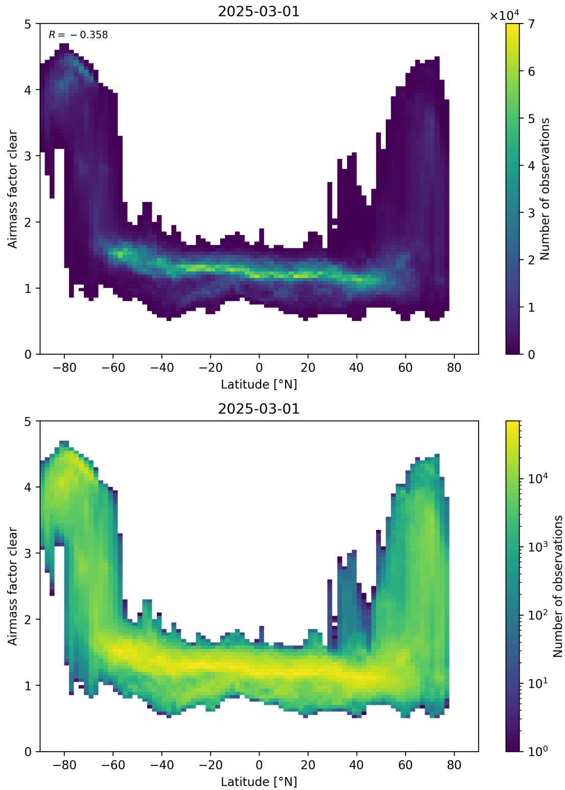
Figure 156: Scatter density plot of “Latitude” against “Airmass factor clear” for 2025-03-01 to 2025-03-02.
