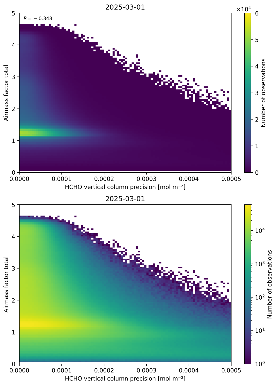
Figure 144: Scatter density plot of “HCHO vertical column precision” against “Airmass factor total” for 2025-03-01 to 2025-03-02.
