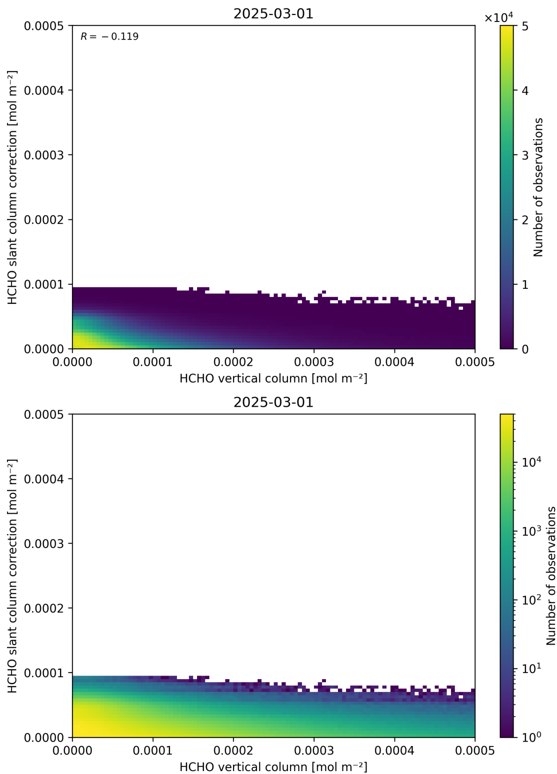
Figure 128: Scatter density plot of “HCHO vertical column” against “HCHO slant column correction” for 2025-03-01 to 2025-03-02.
