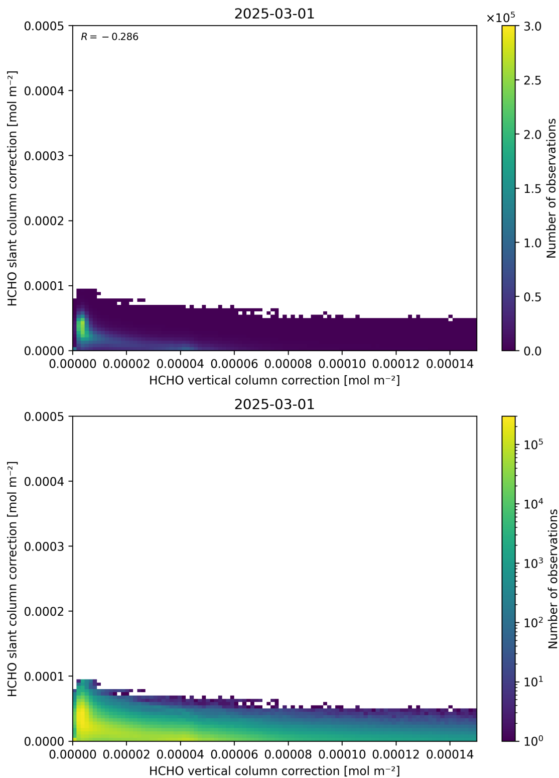
Figure 117: Scatter density plot of “HCHO vertical column correction” against “HCHO slant column correction” for 2025-03-01 to 2025-03-02.
