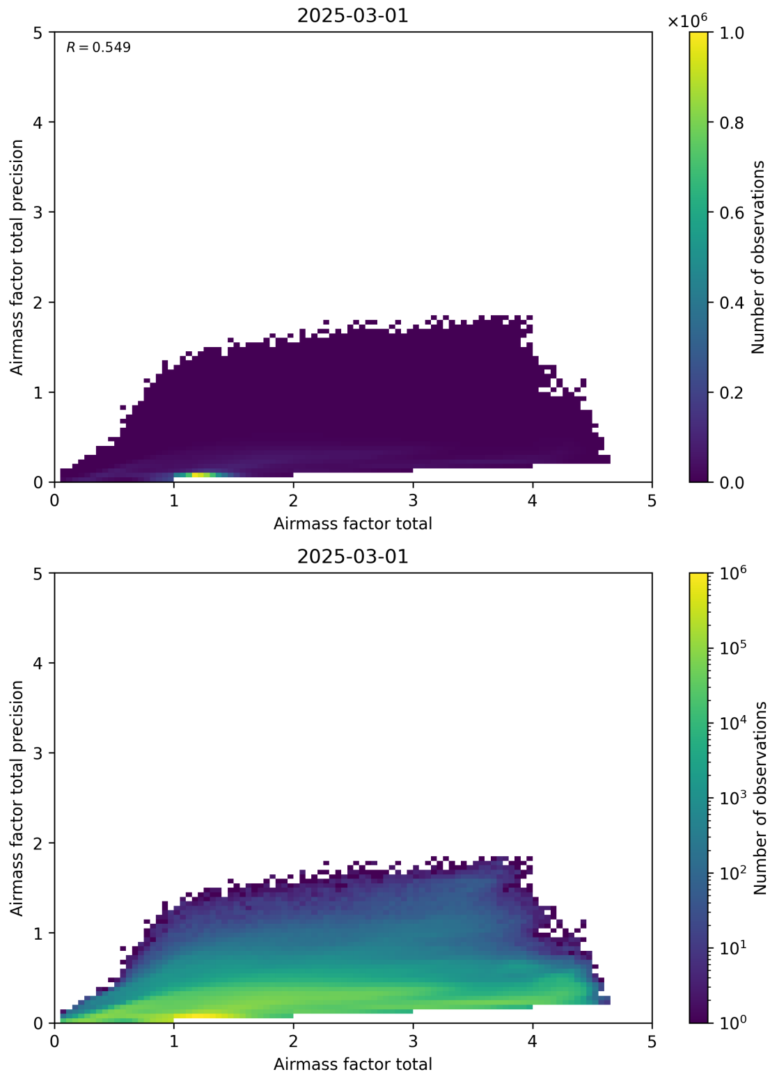
Figure 103: Scatter density plot of “Airmass factor total” against “Airmass factor total precision” for 2025-03-01 to 2025-03-02.
