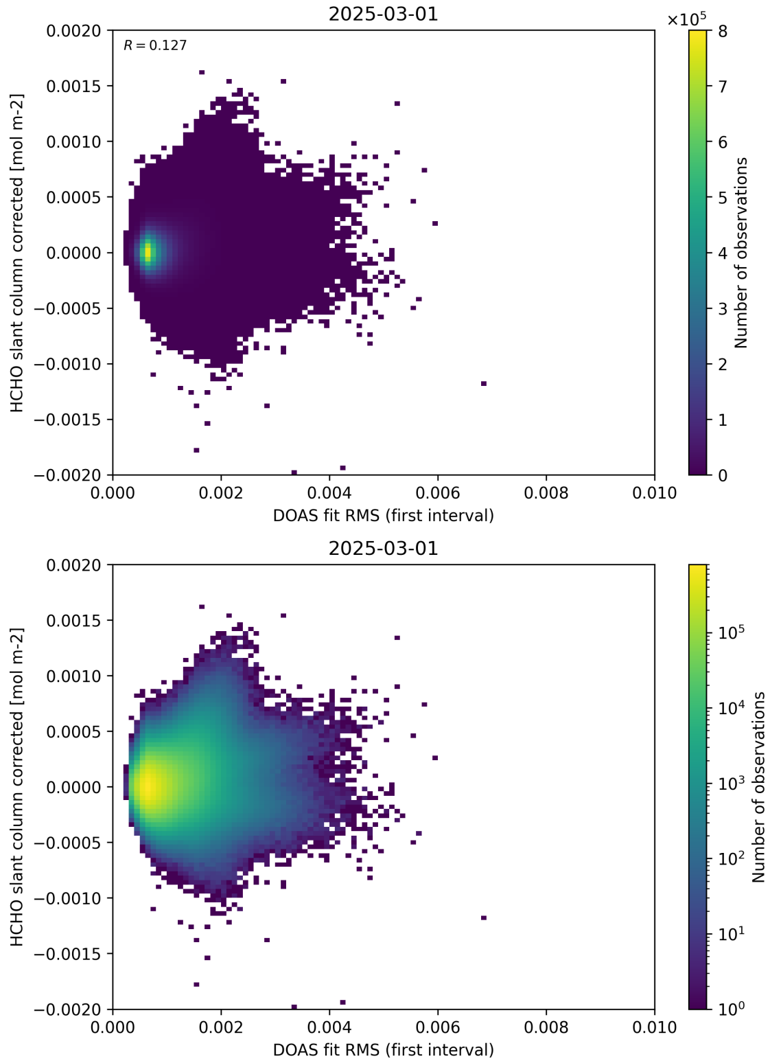
Figure 62: Scatter density plot of “DOAS fit RMS (first interval)” against “HCHO slant column corrected” for 2025-03-01 to 2025-03-02.
