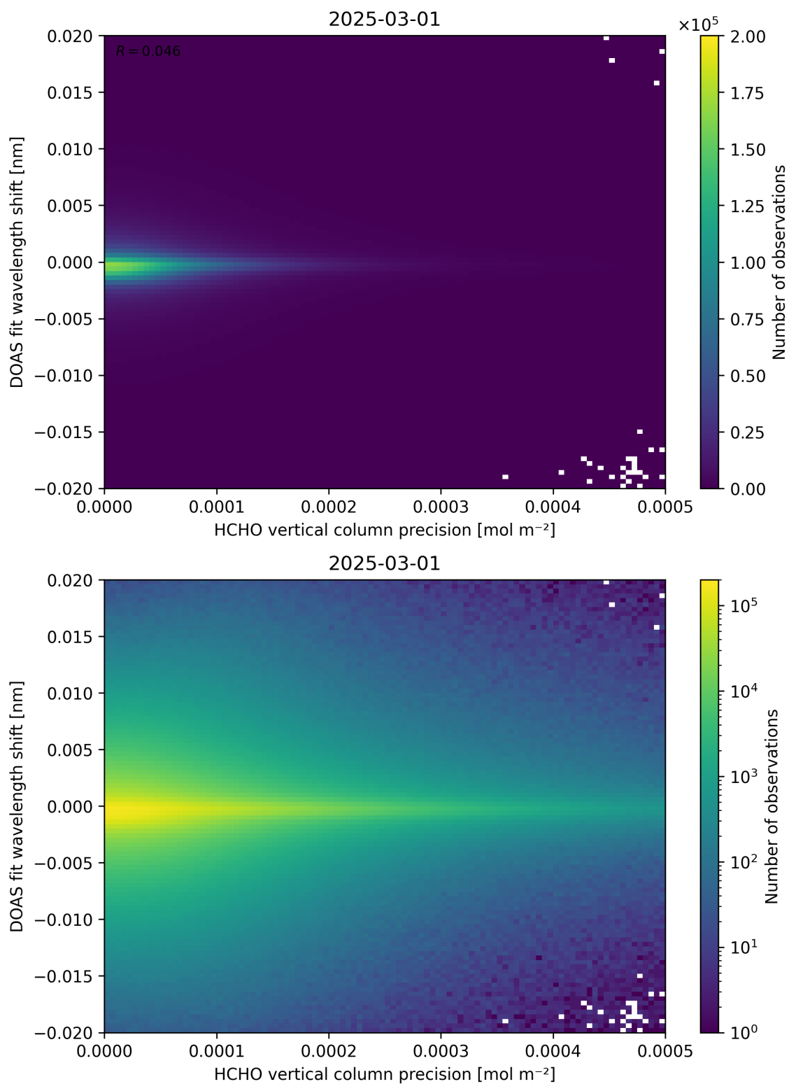
Figure 137: Scatter density plot of “HCHO vertical column precision” against “DOAS fit wavelength shift” for 2025-03-01 to 2025-03-02.
