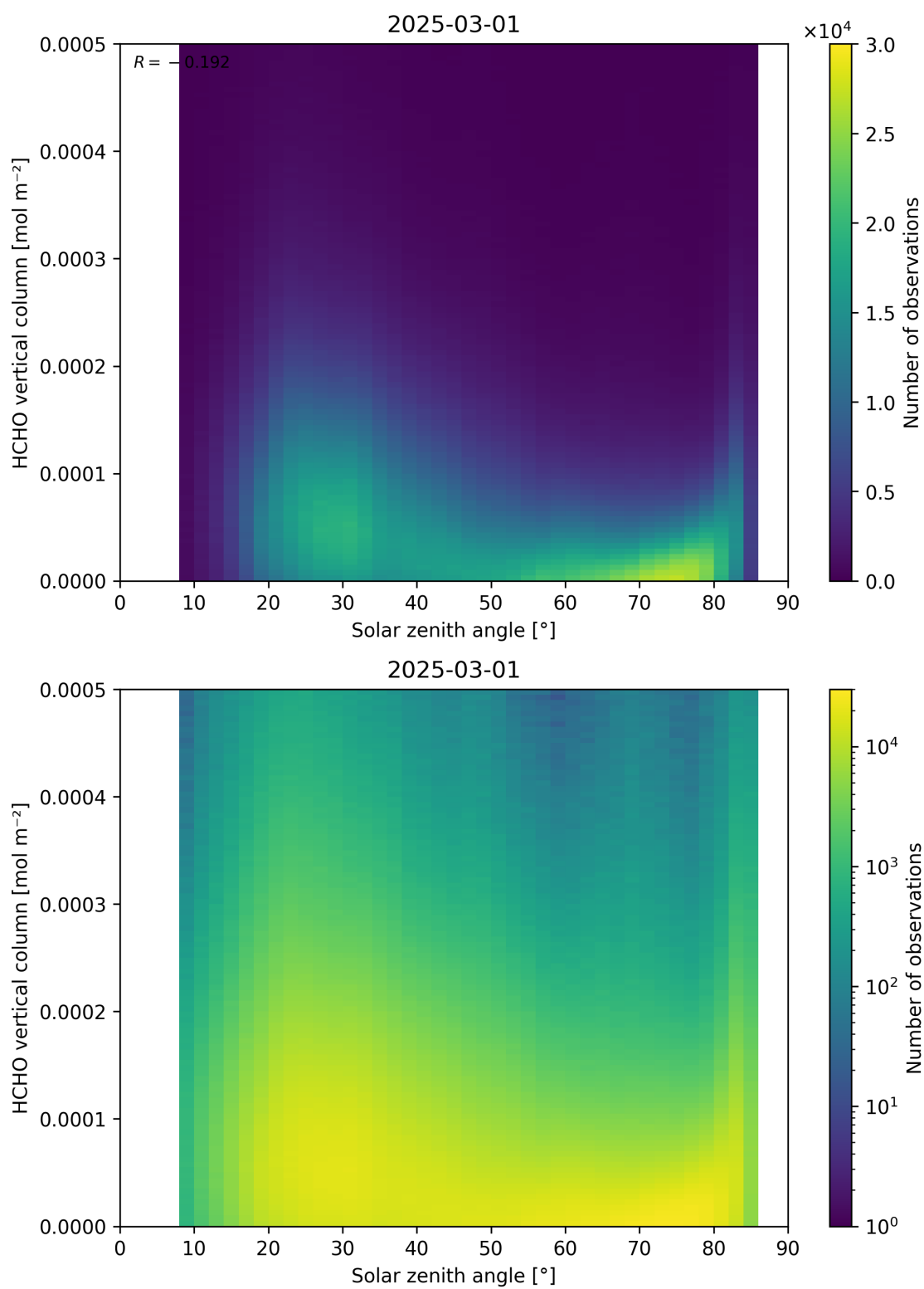
Figure 177: Scatter density plot of “Solar zenith angle” against “HCHO vertical column” for 2025-03-01 to 2025-03-02.
