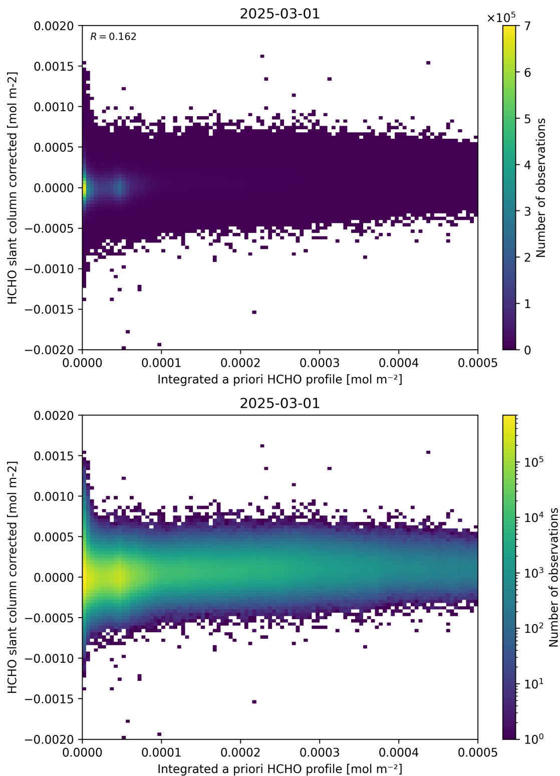
Figure 151: Scatter density plot of “Integrated a priori HCHO profile” against “HCHO slant column corrected” for 2025-03-01 to 2025-03-02.
