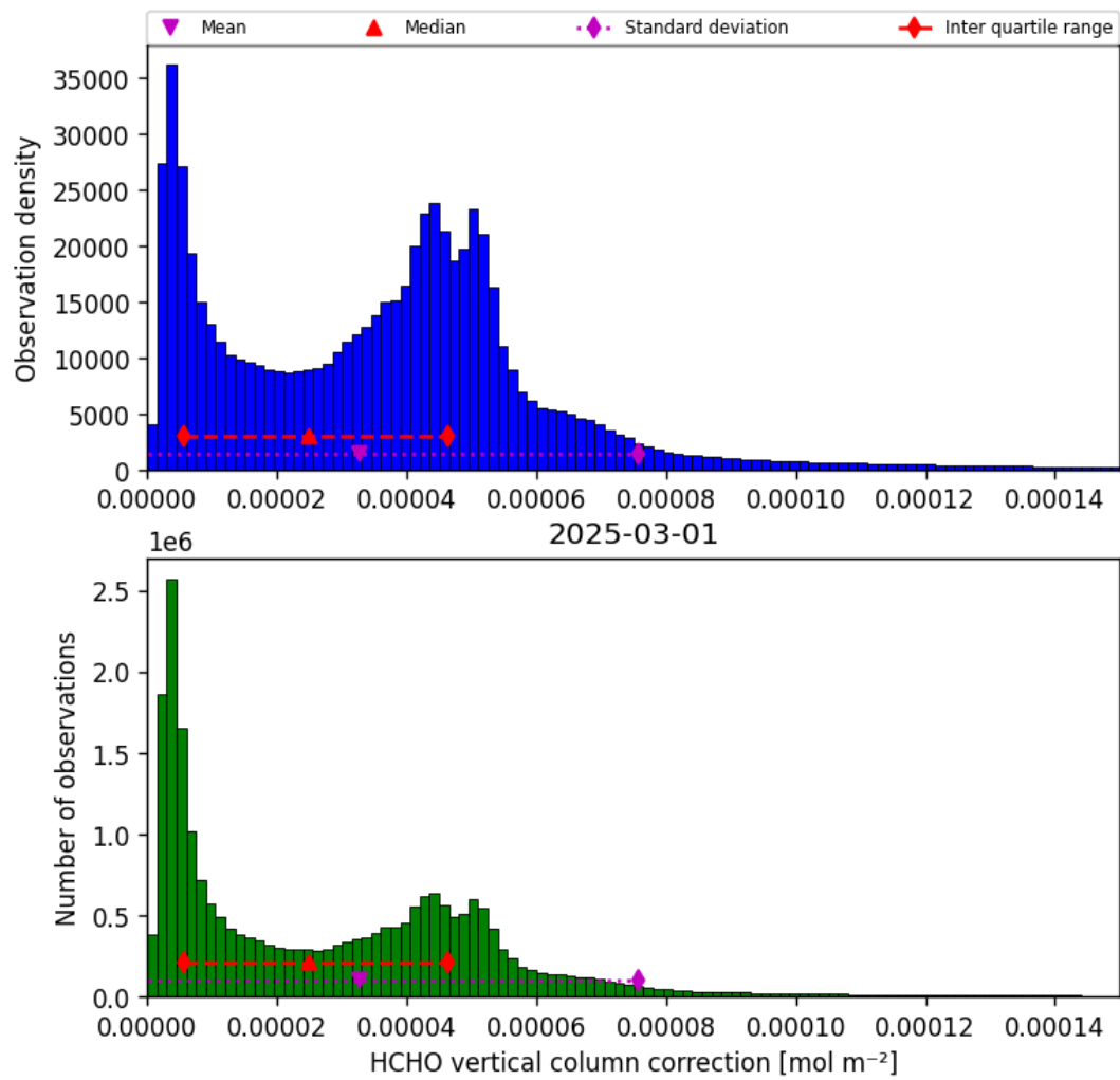
Figure 37: Histogram of “HCHO vertical column correction” for 2025-03-01 to 2025-03-02
