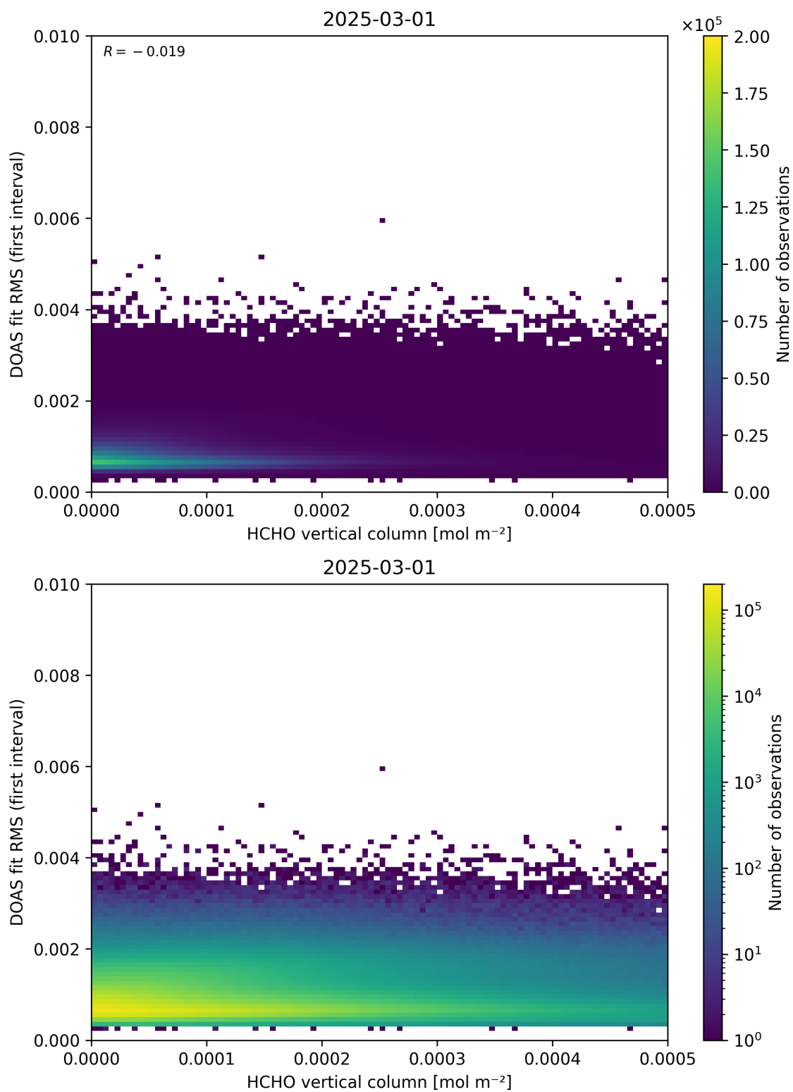
Figure 123: Scatter density plot of “HCHO vertical column” against “DOAS fit RMS (first interval)” for 2025-03-01 to 2025-03-02.
