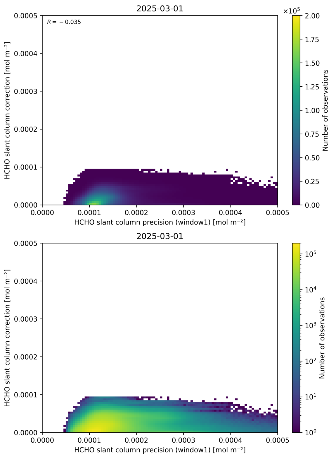
Figure 93: Scatter density plot of “HCHO slant column precision (window1)” against “HCHO slant column correction” for 2025-03-01 to 2025-03-02.
