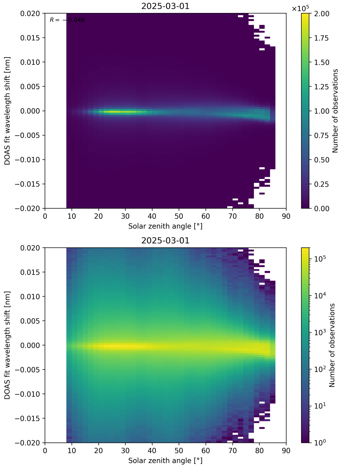
Figure 168: Scatter density plot of “Solar zenith angle” against “DOAS fit wavelength shift” for 2025-03-01 to 2025-03-02.
