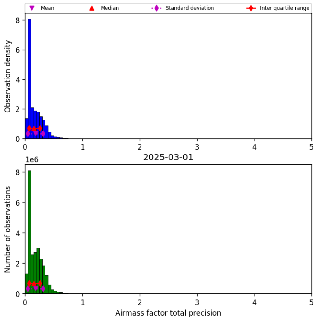
Figure 41: Histogram of “Airmass factor total precision” for 2025-03-01 to 2025-03-02
