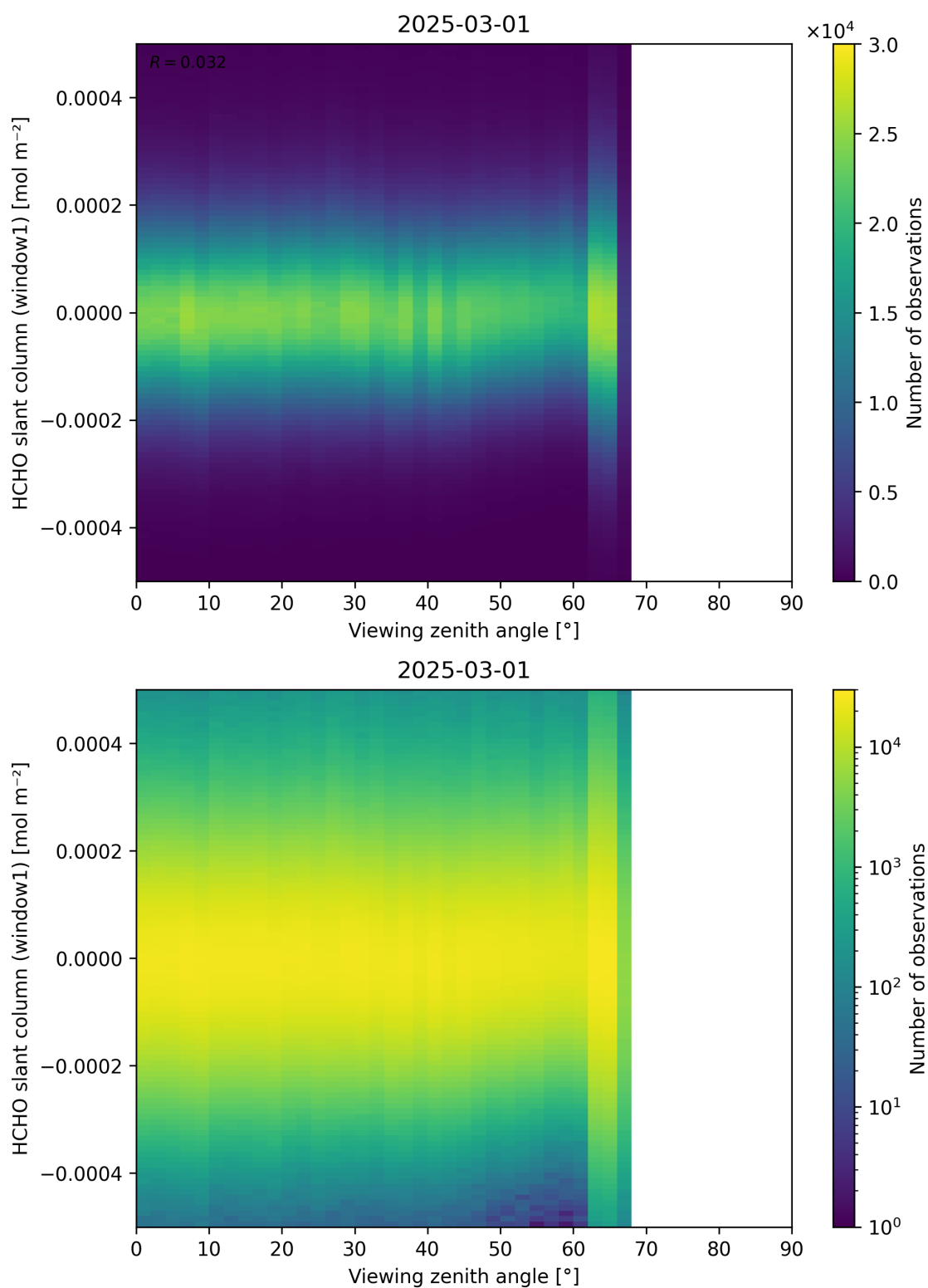
Figure 188: Scatter density plot of “Viewing zenith angle” against “HCHO slant column (window1)” for 2025-03-01 to 2025-03-02.
