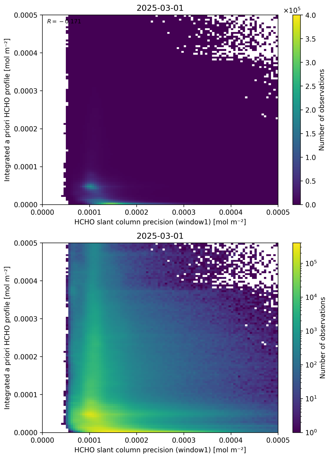
Figure 96: Scatter density plot of “HCHO slant column precision (window1)” against “Integrated a priori HCHO profile” for 2025-03-01 to 2025-03-02.
