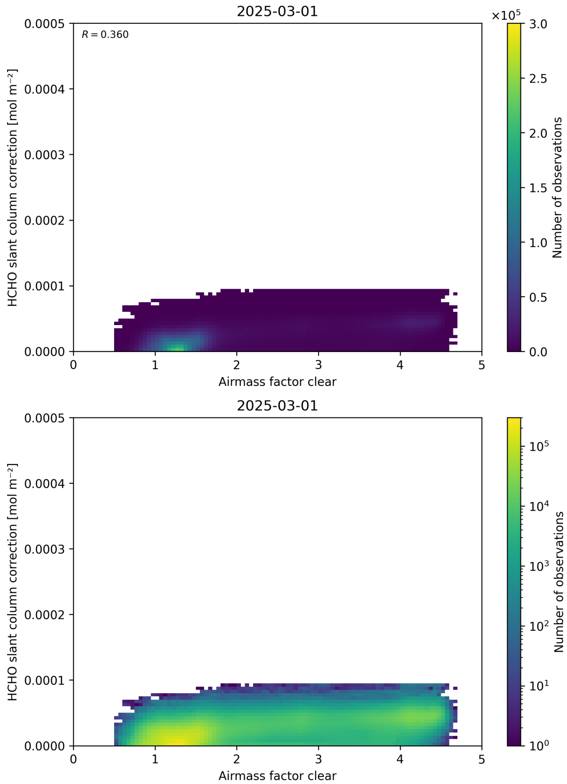
Figure 75: Scatter density plot of “Airmass factor clear” against “HCHO slant column correction” for 2025-03-01 to 2025-03-02.
