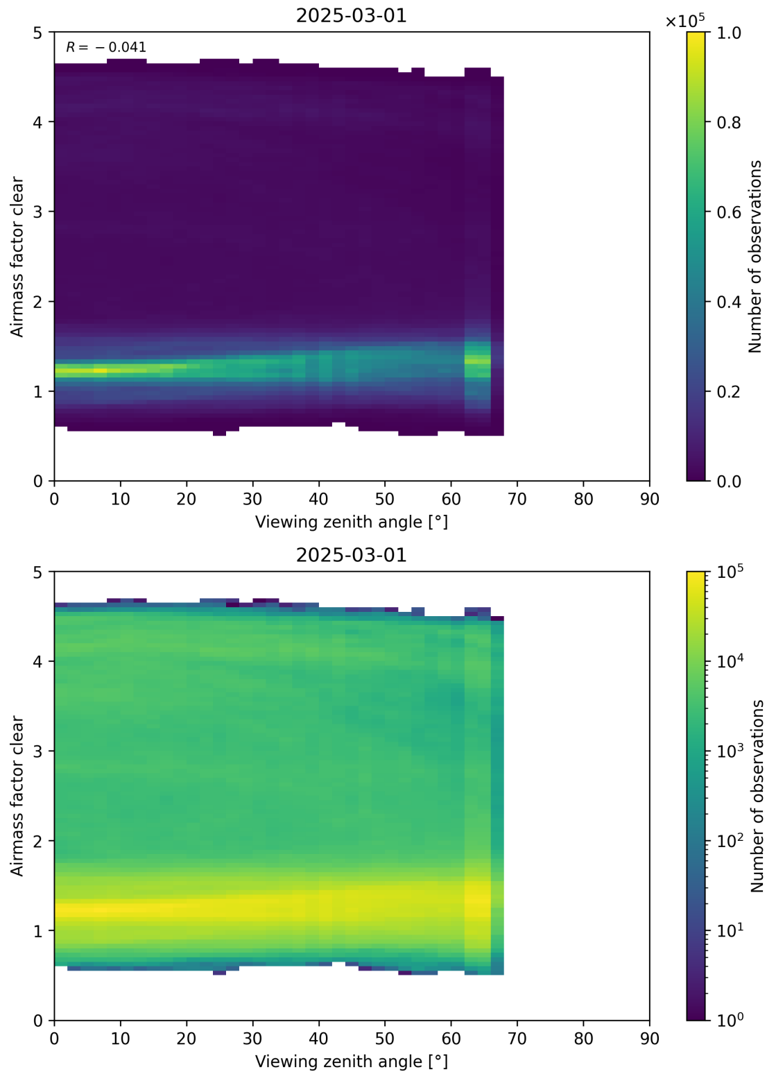
Figure 185: Scatter density plot of “Viewing zenith angle” against “Airmass factor clear” for 2025-03-01 to 2025-03-02.
