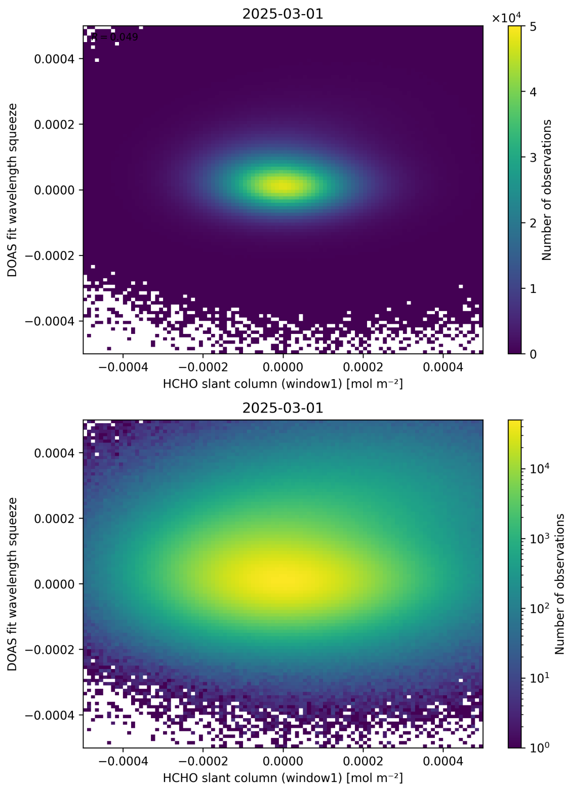
Figure 80: Scatter density plot of “HCHO slant column (window1)” against “DOAS fit wavelength squeeze” for 2025-03-01 to 2025-03-02.
