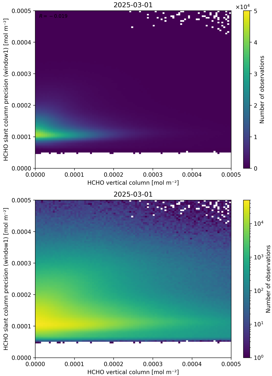
Figure 130: Scatter density plot of “HCHO vertical column” against “HCHO slant column precision (window1)” for 2025-03-01 to 2025-03-02.
