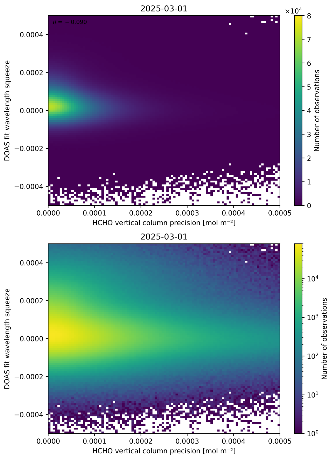
Figure 138: Scatter density plot of “HCHO vertical column precision” against “DOAS fit wavelength squeeze” for 2025-03-01 to 2025-03-02.
