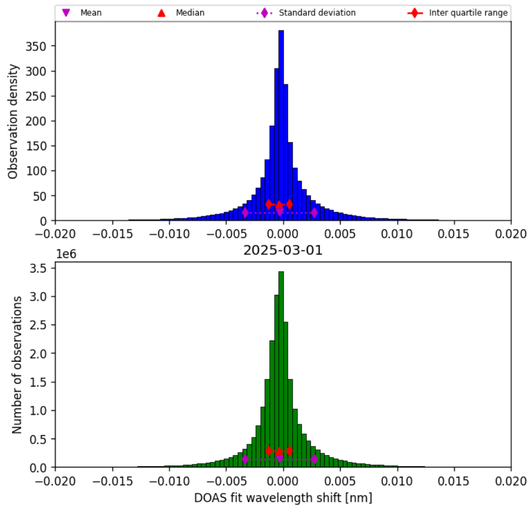
Figure 44: Histogram of “DOAS fit wavelength shift” for 2025-03-01 to 2025-03-02
