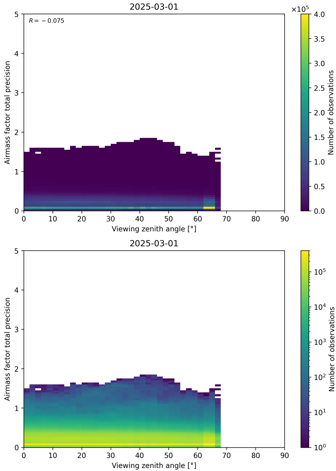
Figure 191: Scatter density plot of “Viewing zenith angle” against “Airmass factor total precision” for 2025-03-01 to 2025-03-02.
