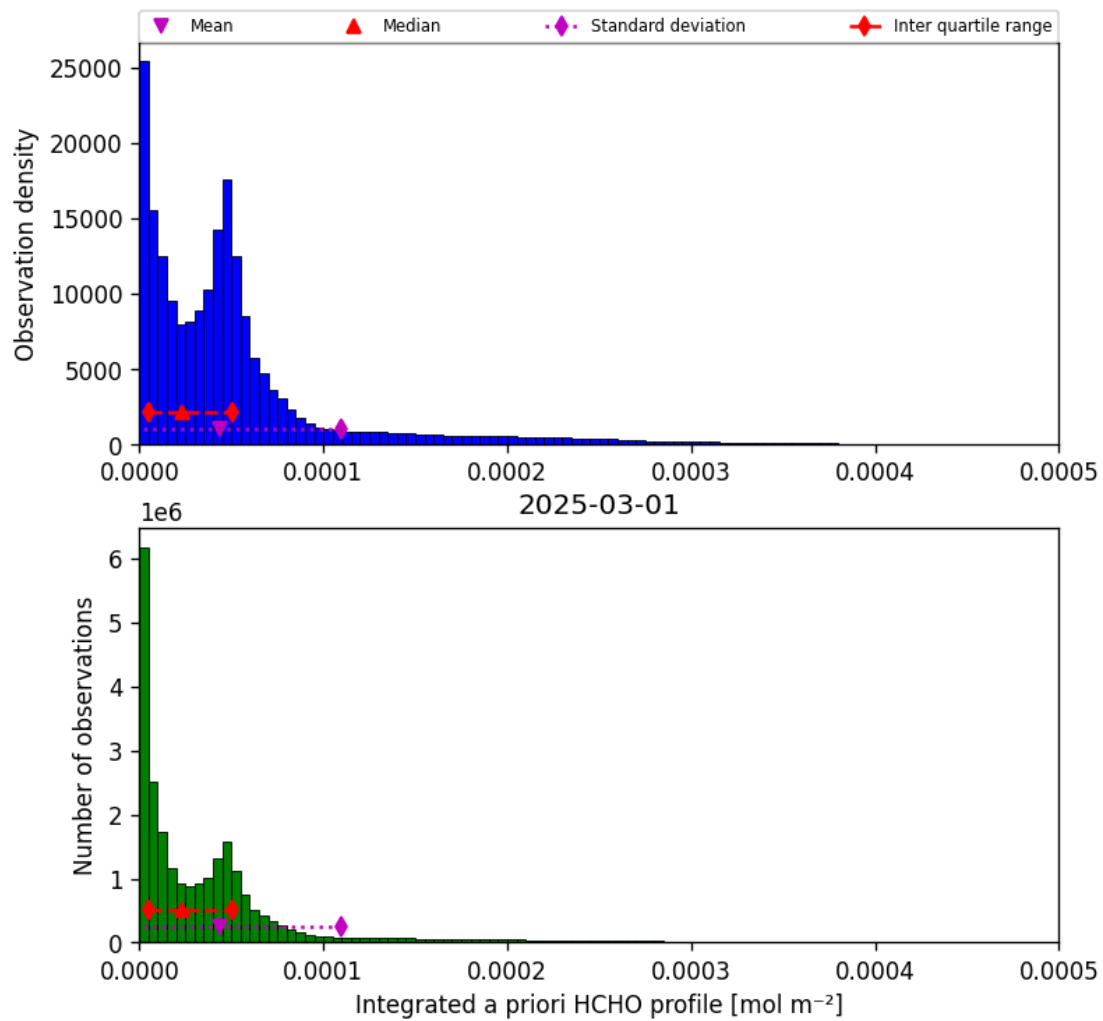
Figure 43: Histogram of “Integrated a priori HCHO profile” for 2025-03-01 to 2025-03-02
