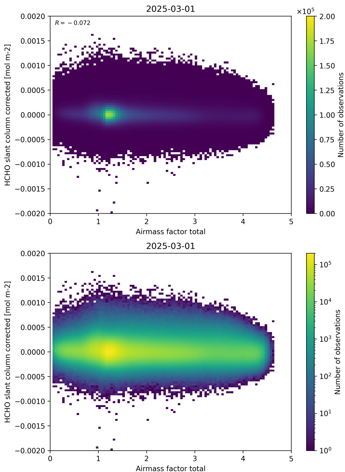
Figure 101: Scatter density plot of “Airmass factor total” against “HCHO slant column corrected” for 2025-03-01 to 2025-03-02.
