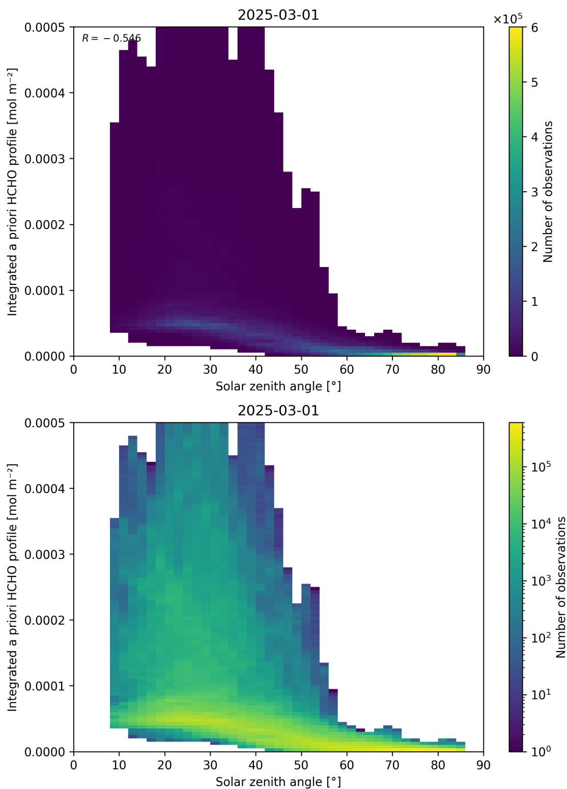
Figure 180: Scatter density plot of “Solar zenith angle” against “Integrated a priori HCHO profile” for 2025-03-01 to 2025-03-02.
