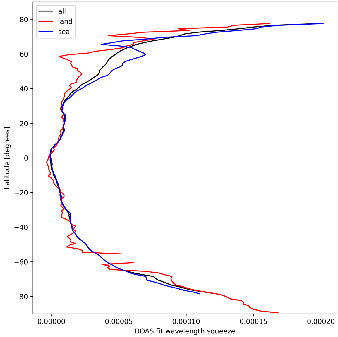
Figure 31: Zonal average of “DOAS fit wavelength squeeze” for 2025-03-01 to 2025-03-02.
