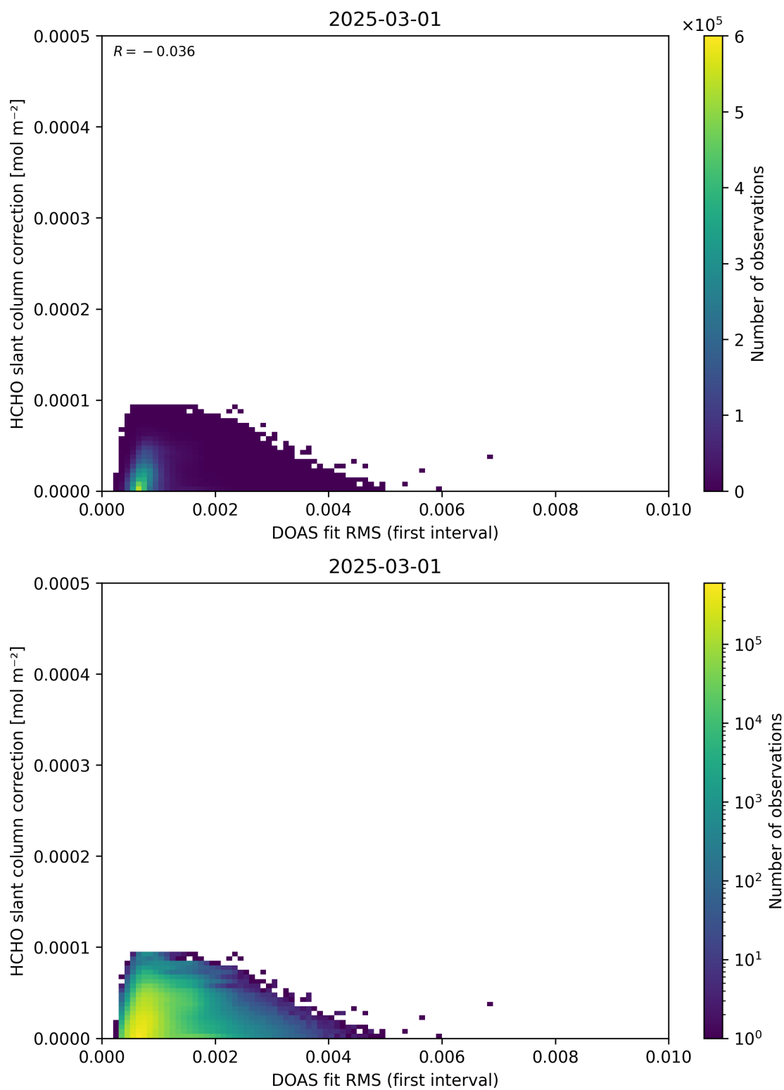
Figure 63: Scatter density plot of “DOAS fit RMS (first interval)” against “HCHO slant column correction” for 2025-03-01 to 2025-03-02.
