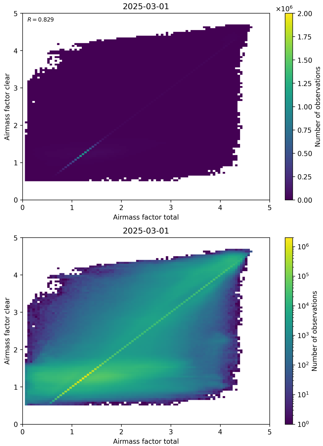
Figure 100: Scatter density plot of “Airmass factor total” against “Airmass factor clear” for 2025-03-01 to 2025-03-02.
