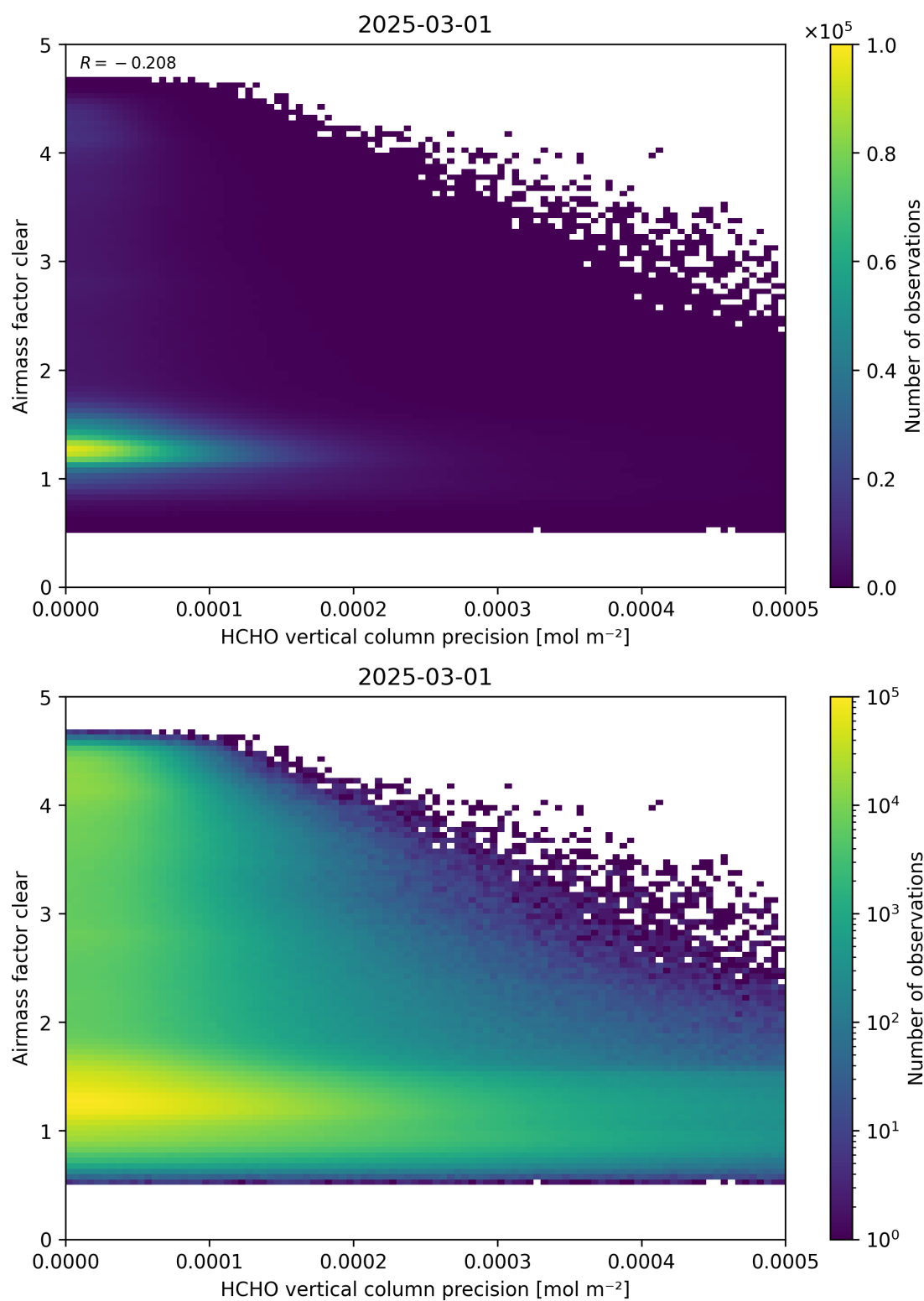
Figure 139: Scatter density plot of “HCHO vertical column precision” against “Airmass factor clear” for 2025-03-01 to 2025-03-02.
