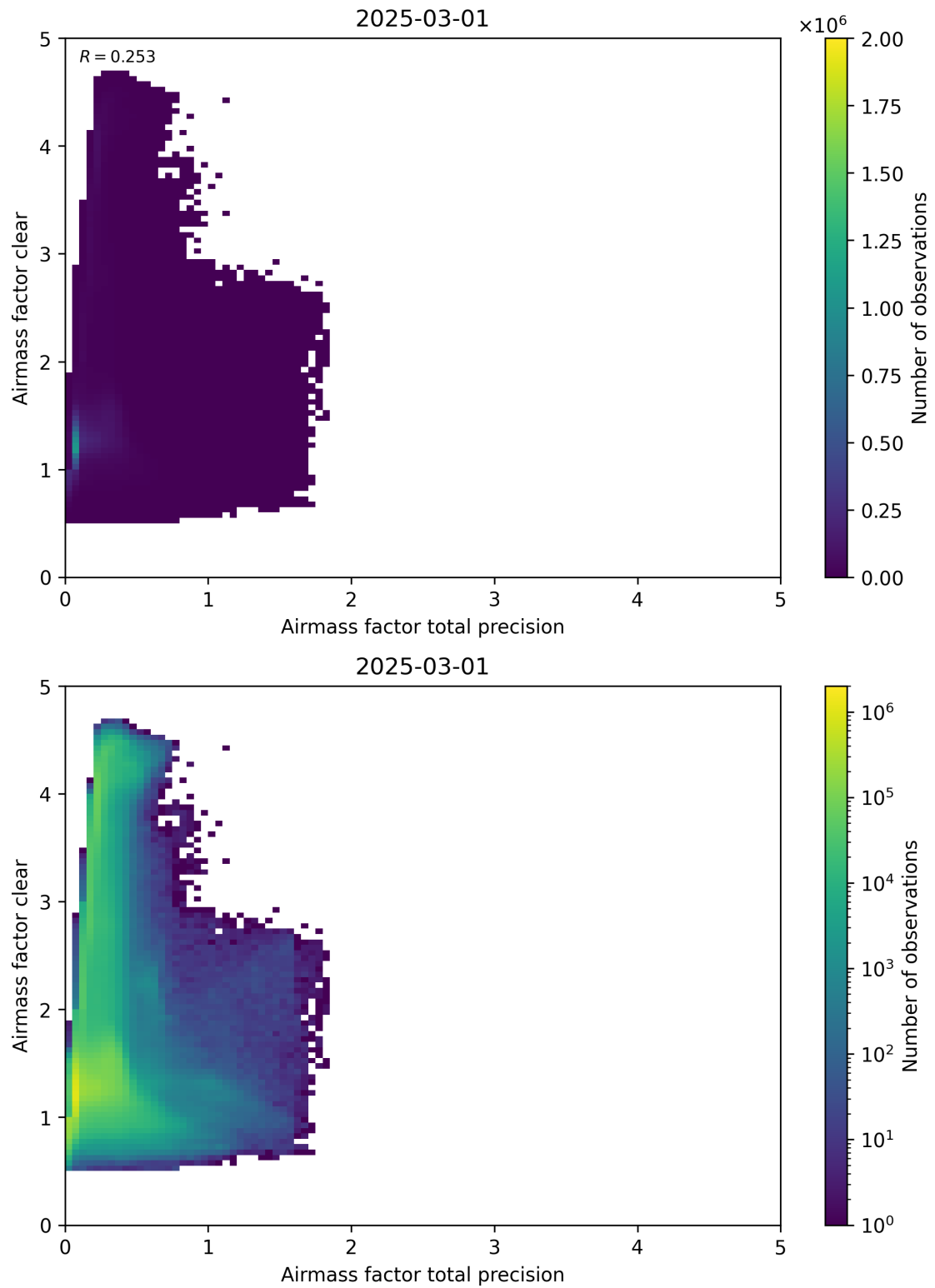
Figure 108: Scatter density plot of “Airmass factor total precision” against “Airmass factor clear” for 2025-03-01 to 2025-03-02.
