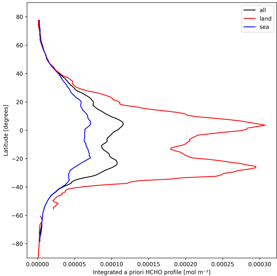
Figure 29: Zonal average of “Integrated a priori HCHO profile” for 2025-03-01 to 2025-03-02.
