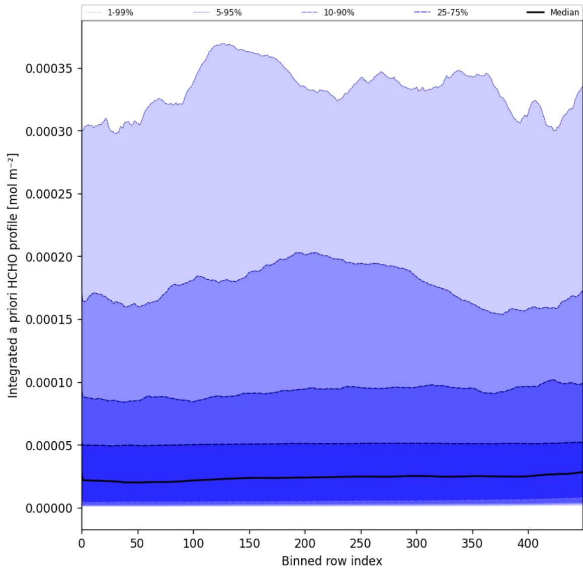
Figure 57: Along track statistics of "Integrated a priori HCHO profile" for 2025-03-01 to 2025-03-02
