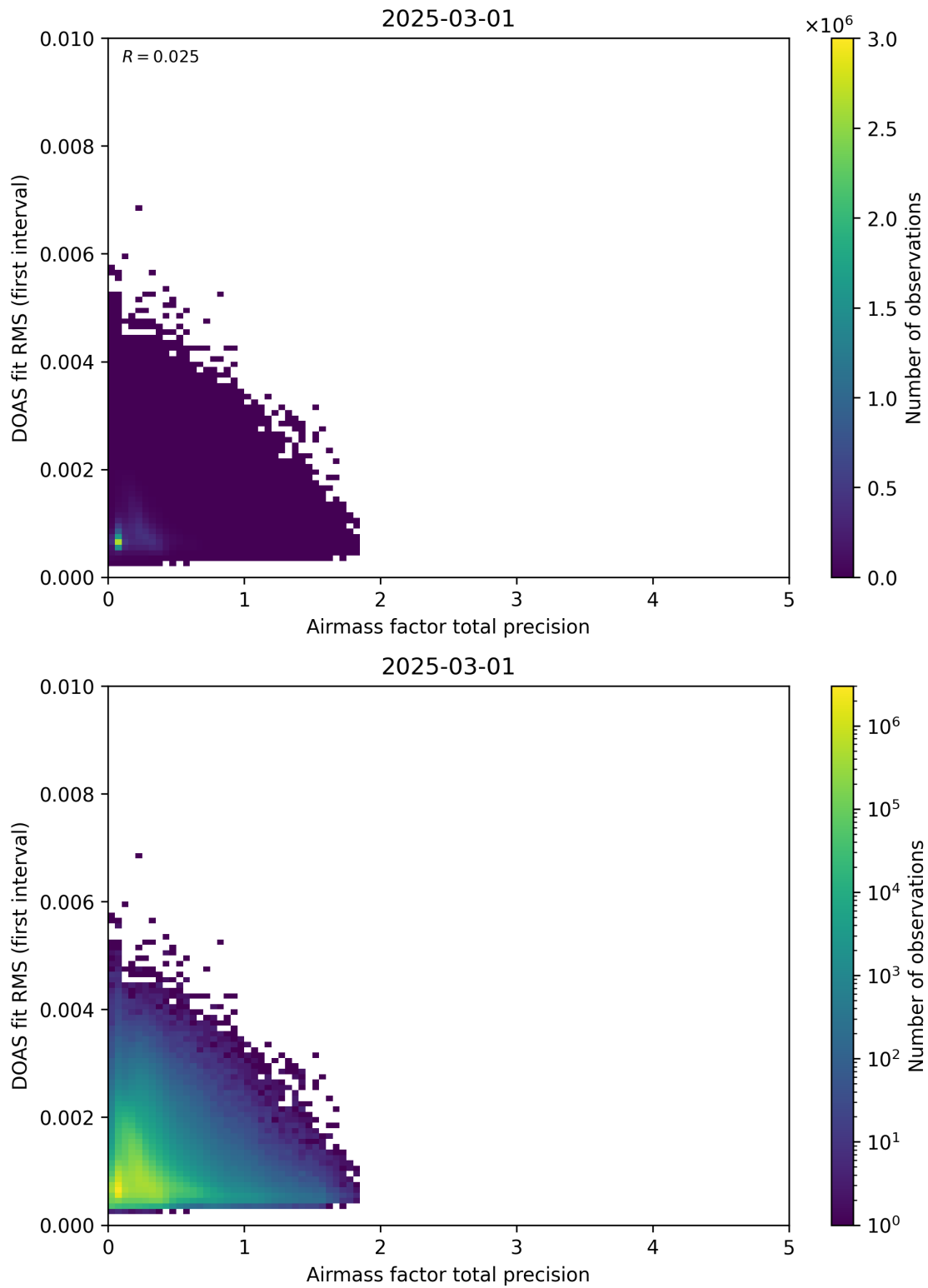
Figure 105: Scatter density plot of “Airmass factor total precision” against “DOAS fit RMS (first interval)” for 2025-03-01 to 2025-03-02.
