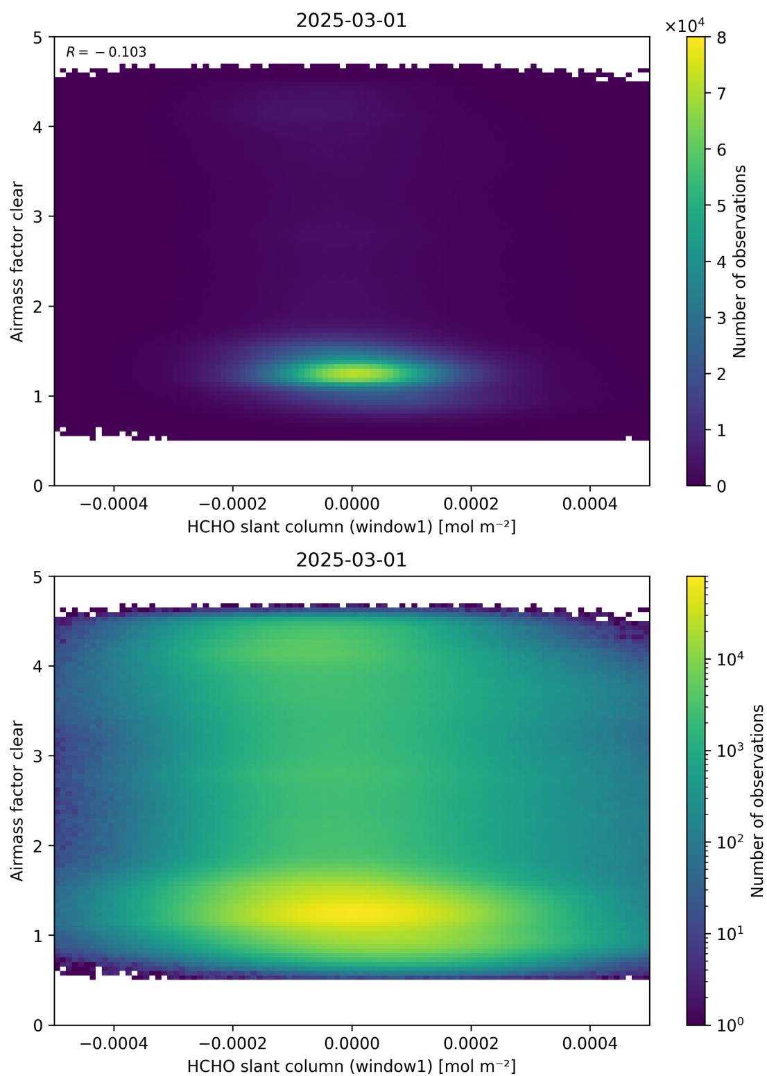
Figure 81: Scatter density plot of “HCHO slant column (window1)” against “Airmass factor clear” for 2025-03-01 to 2025-03-02.
