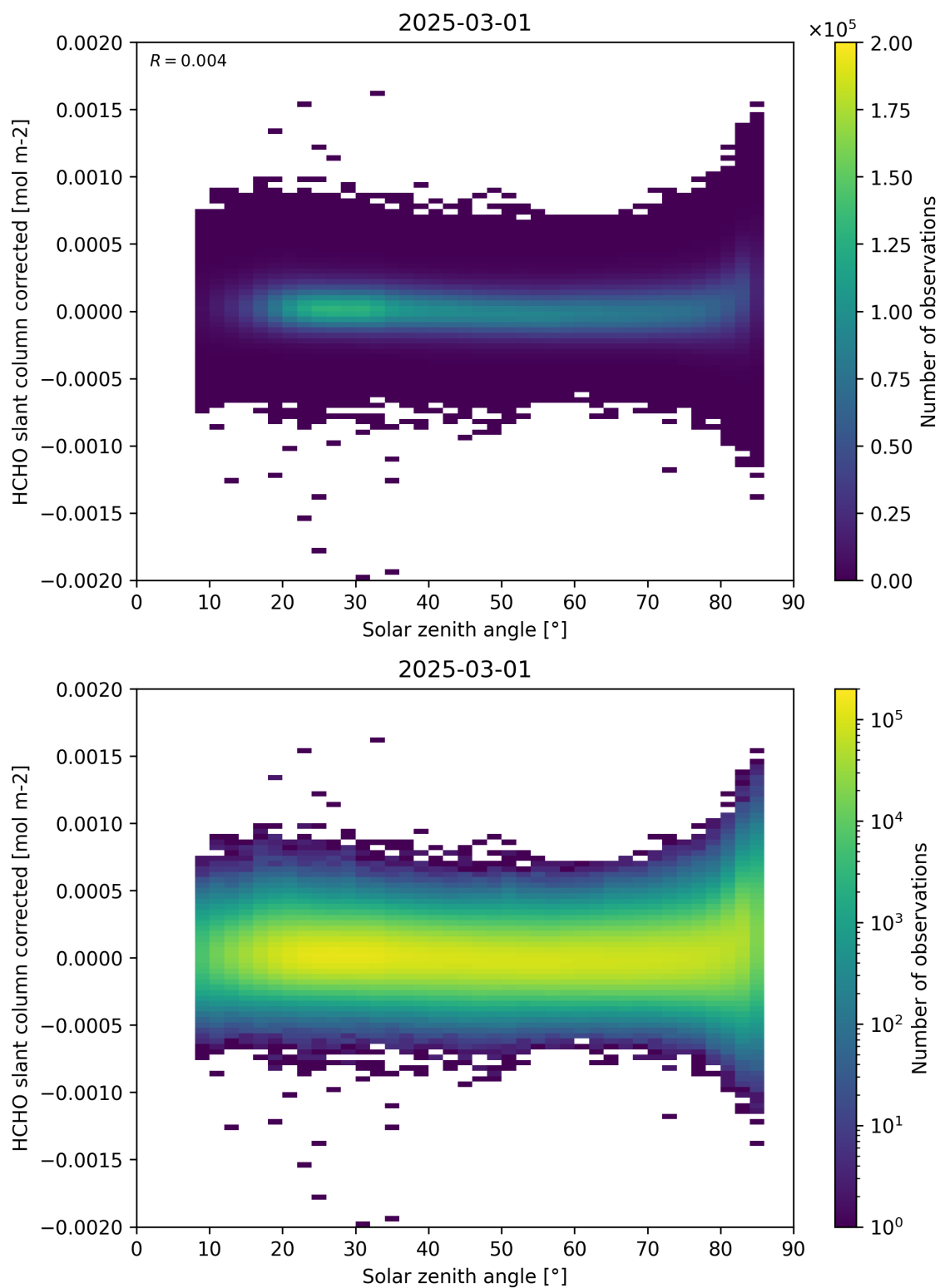
Figure 171: Scatter density plot of “Solar zenith angle” against “HCHO slant column corrected” for 2025-03-01 to 2025-03-02.
