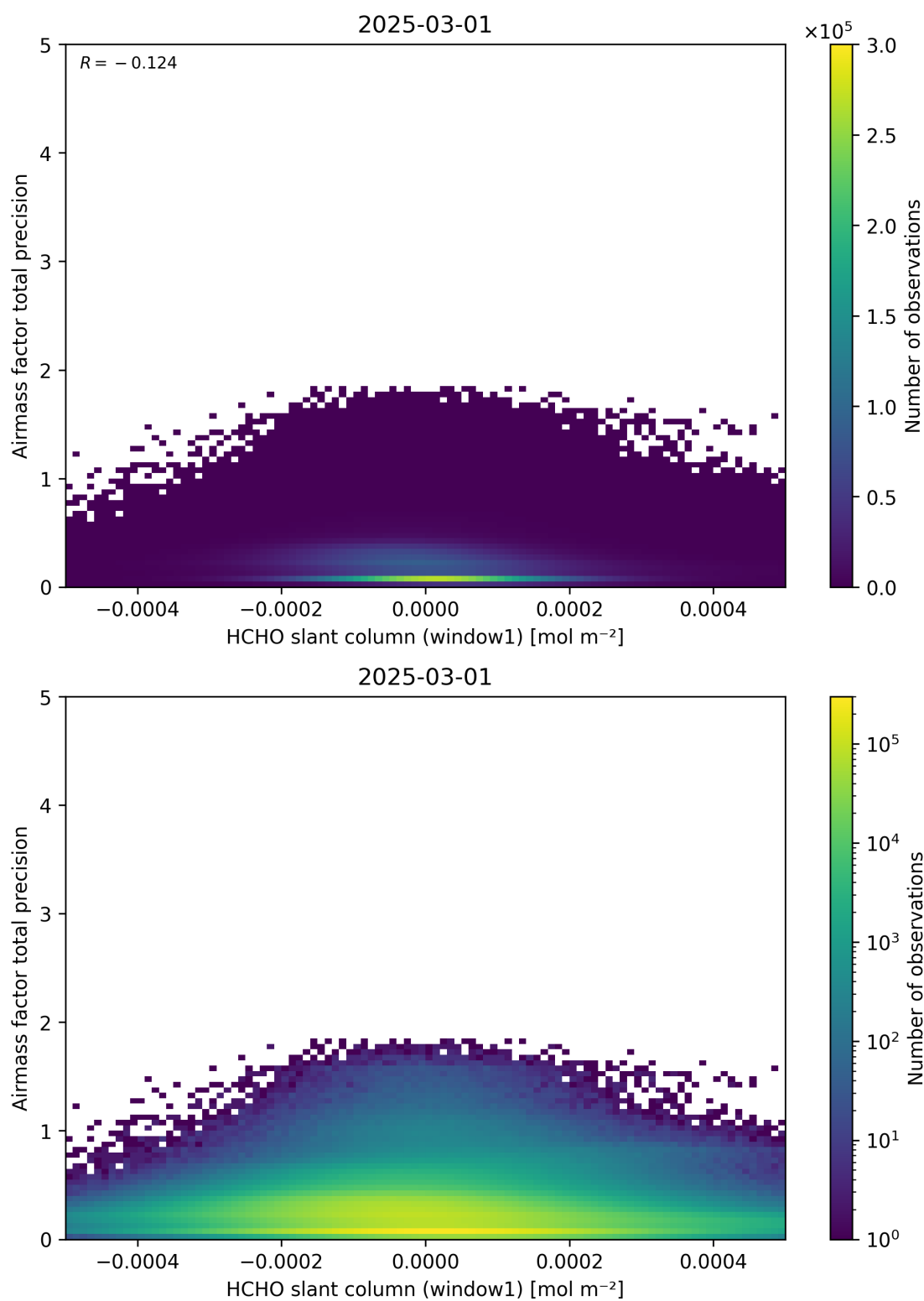
Figure 86: Scatter density plot of “HCHO slant column (window1)” against “Airmass factor total precision” for 2025-03-01 to 2025-03-02.
