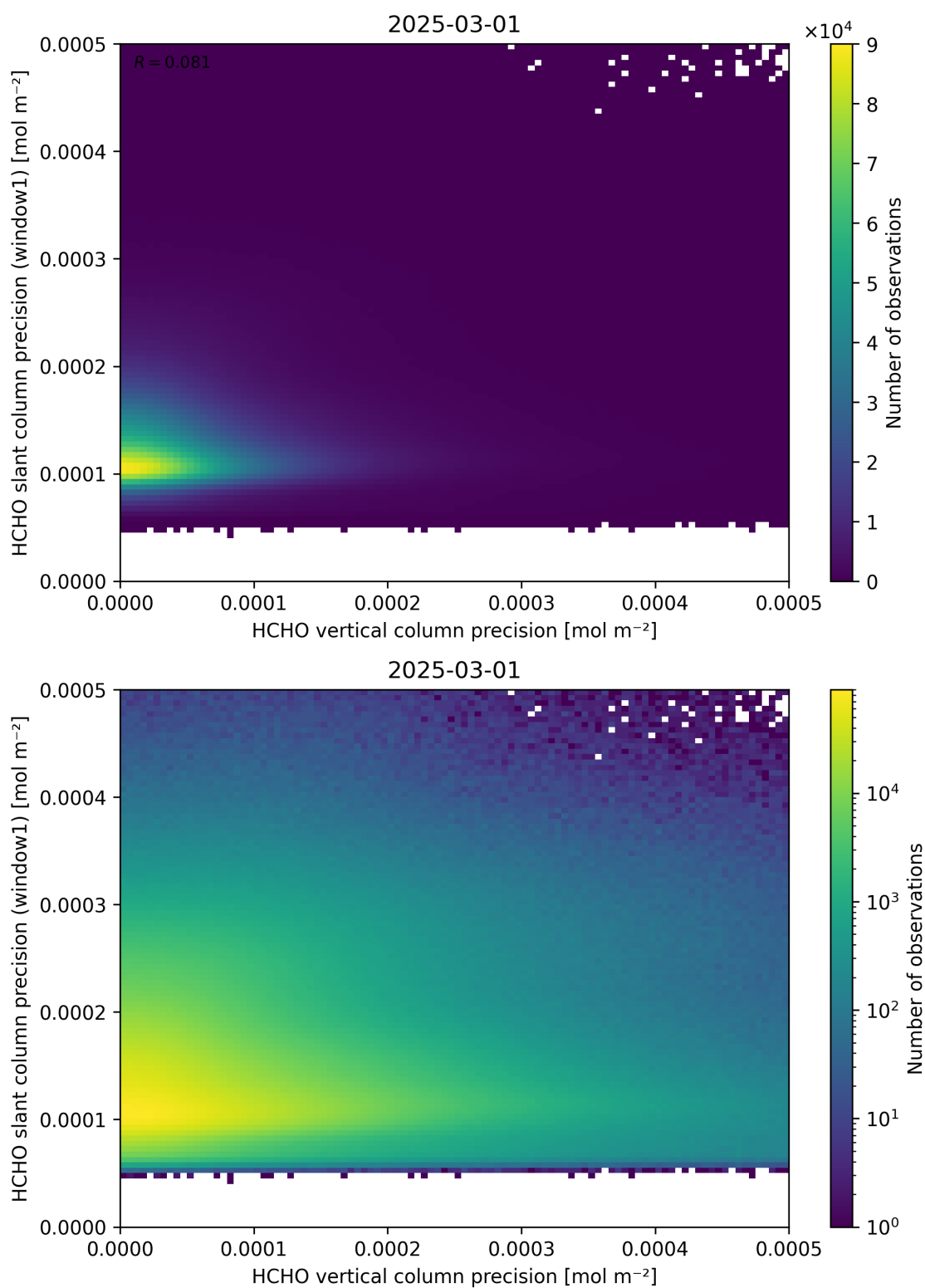
Figure 143: Scatter density plot of “HCHO vertical column precision” against “HCHO slant column precision (window1)” for 2025-03-01 to 2025-03-02.
