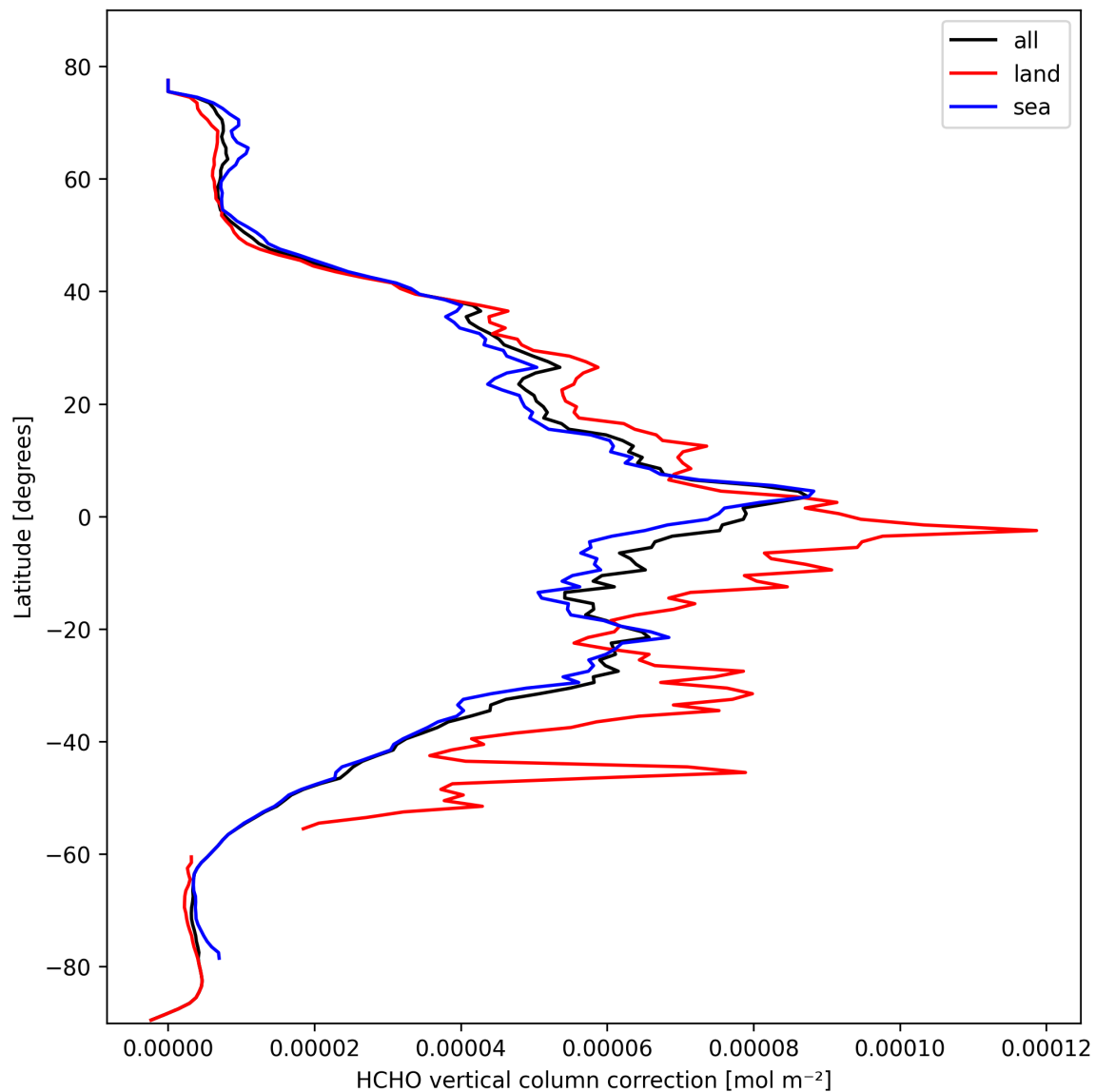
Figure 23: Zonal average of “HCHO vertical column correction” for 2025-03-01 to 2025-03-02.
