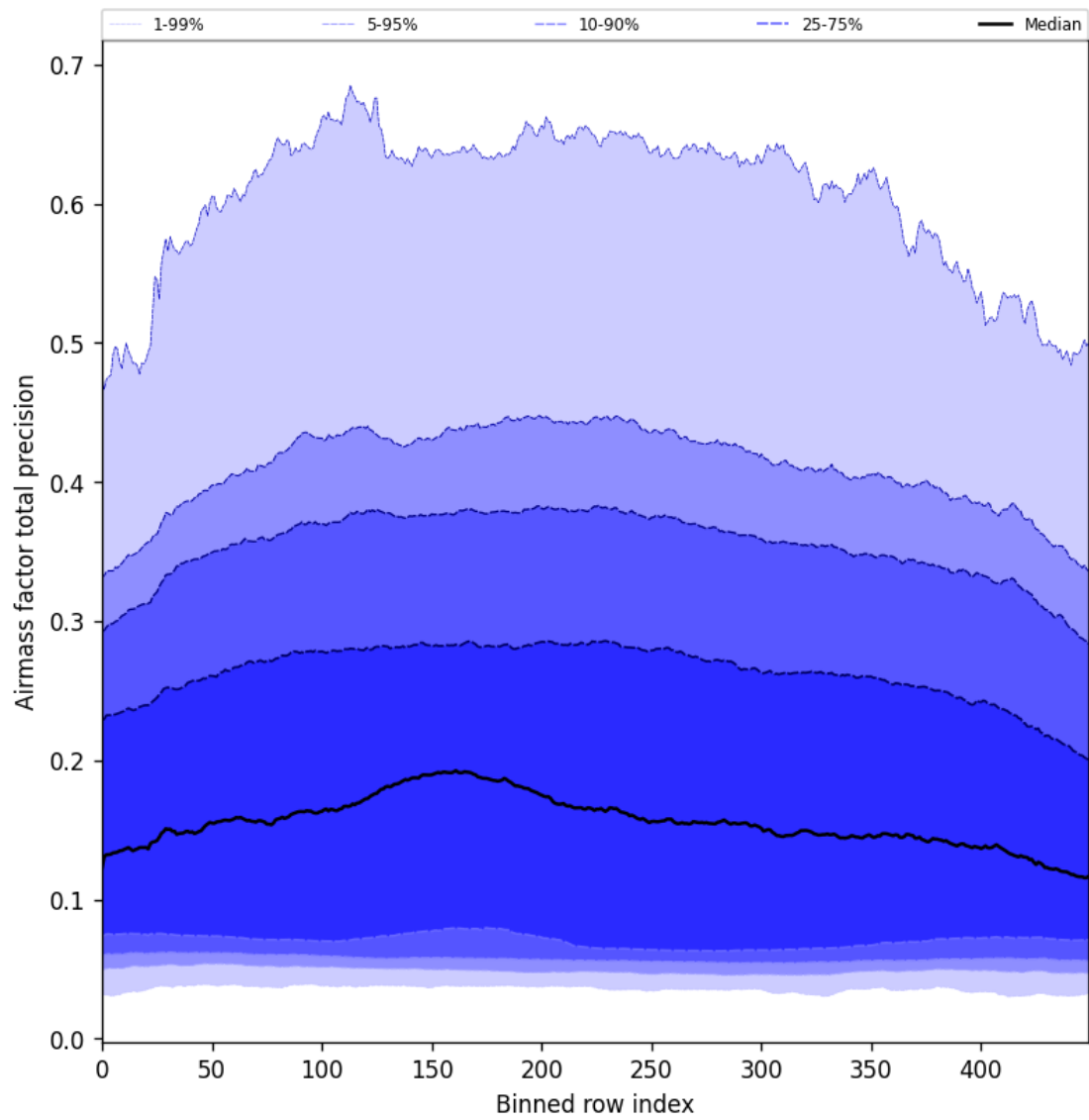
Figure 55: Along track statistics of “Airmass factor total precision” for 2025-03-01 to 2025-03-02
