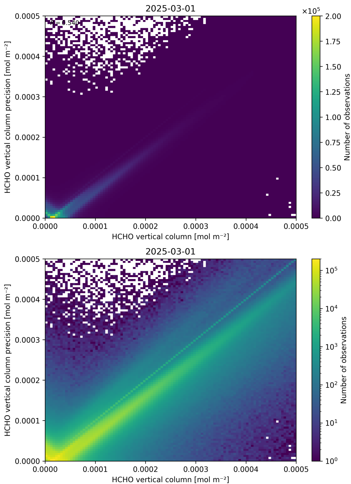
Figure 134: Scatter density plot of “HCHO vertical column” against “HCHO vertical column precision” for 2025-03-01 to 2025-03-02.
