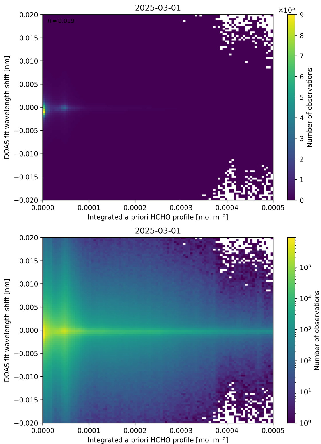
Figure 149: Scatter density plot of “Integrated a priori HCHO profile” against “DOAS fit wavelength shift” for 2025-03-01 to 2025-03-02.
