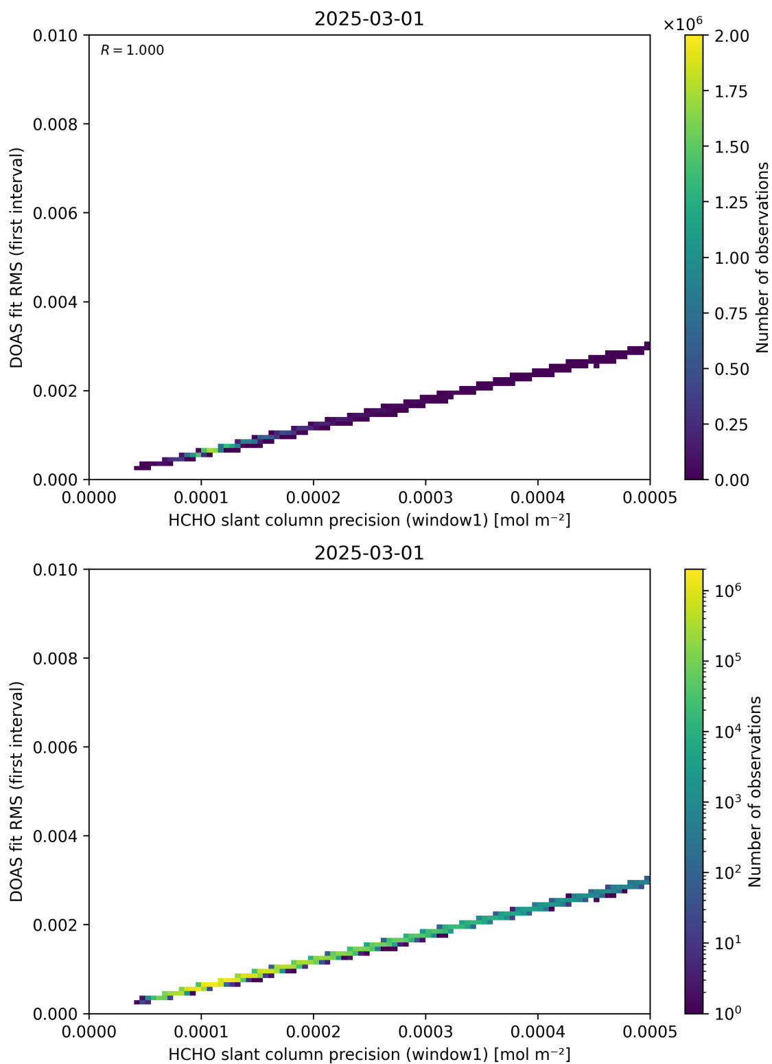
Figure 88: Scatter density plot of “HCHO slant column precision (window1)” against “DOAS fit RMS (first interval)” for 2025-03-01 to 2025-03-02.
