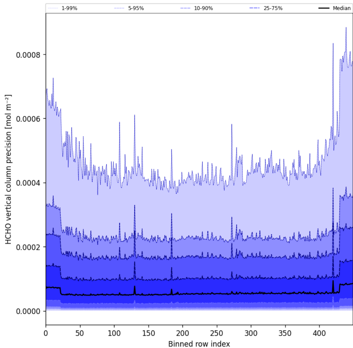
Figure 50: Along track statistics of “HCHO vertical column precision” for 2025-03-01 to 2025-03-02
