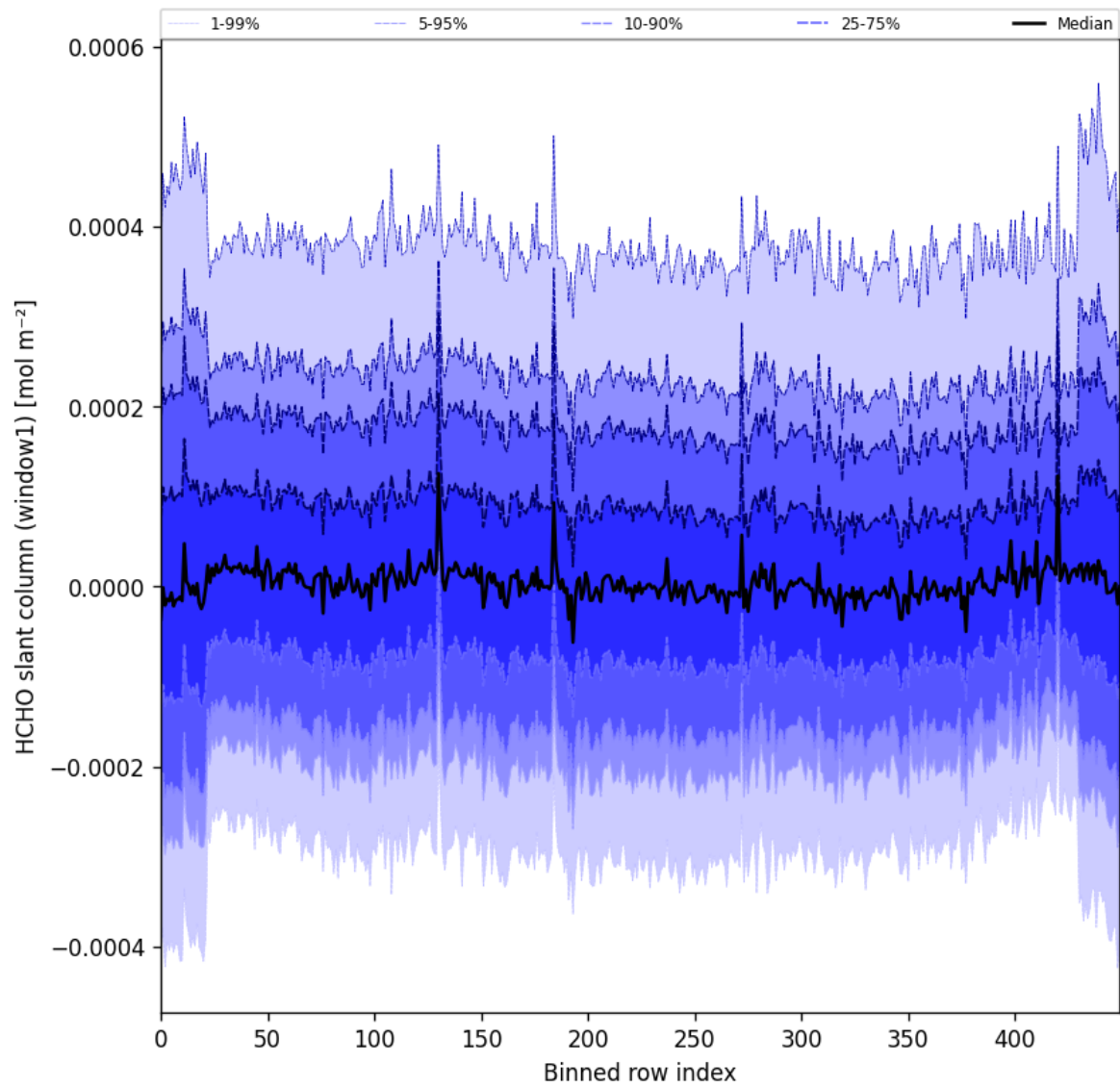
Figure 52: Along track statistics of “HCHO slant column (window1)” for 2025-03-01 to 2025-03-02
