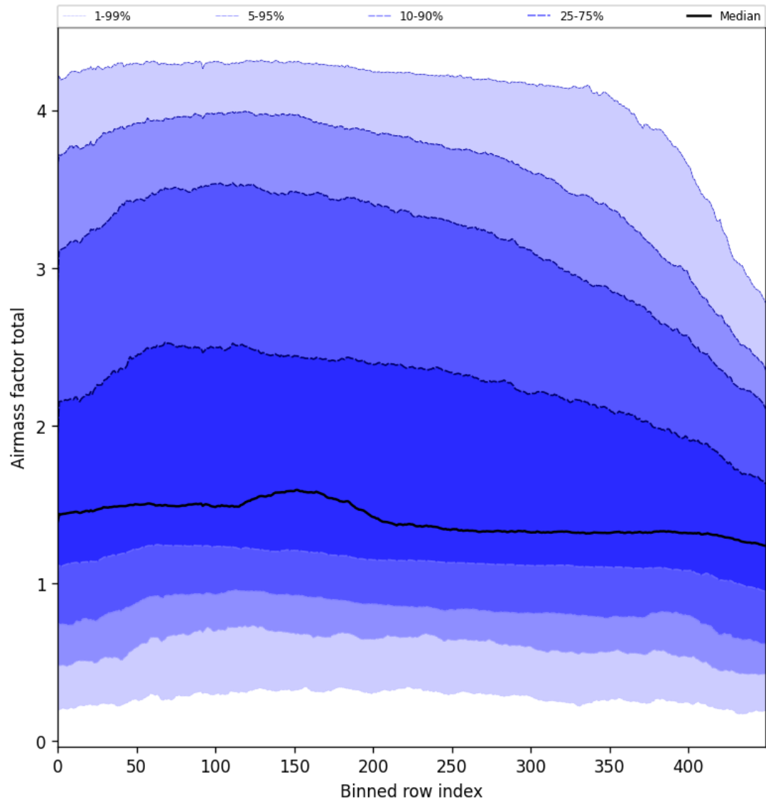
Figure 54: Along track statistics of “Airmass factor total” for 2025-03-01 to 2025-03-02
