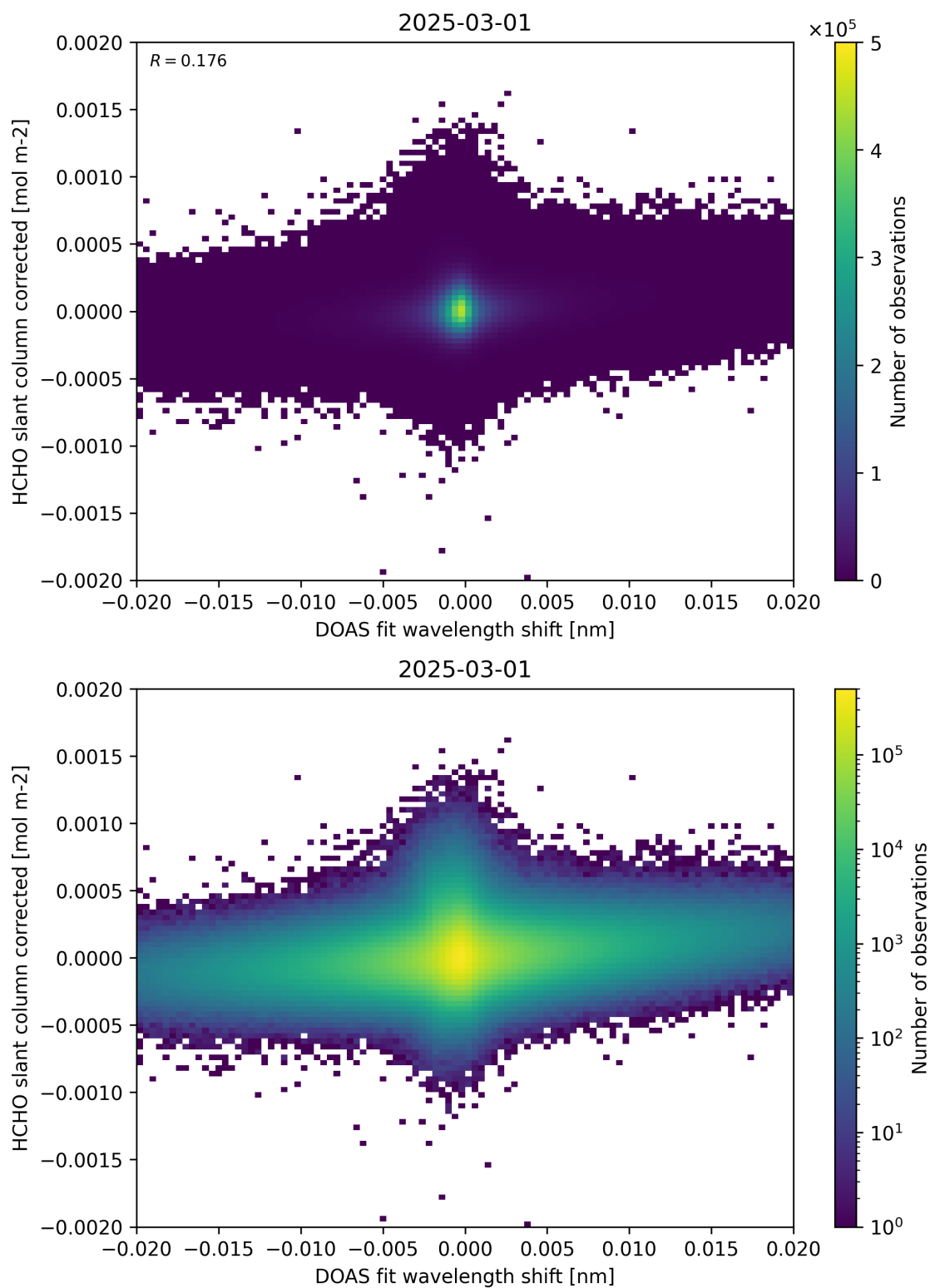
Figure 66: Scatter density plot of “DOAS fit wavelength shift” against “HCHO slant column corrected” for 2025-03-01 to 2025-03-02.
