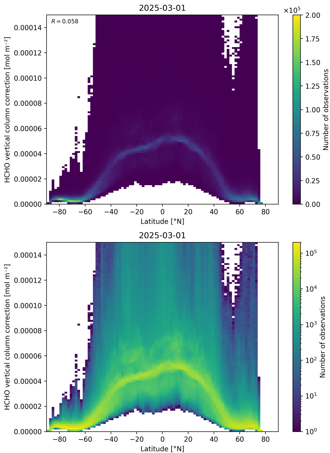
Figure 164: Scatter density plot of “Latitude” against “HCHO vertical column correction” for 2025-03-01 to 2025-03-02.
