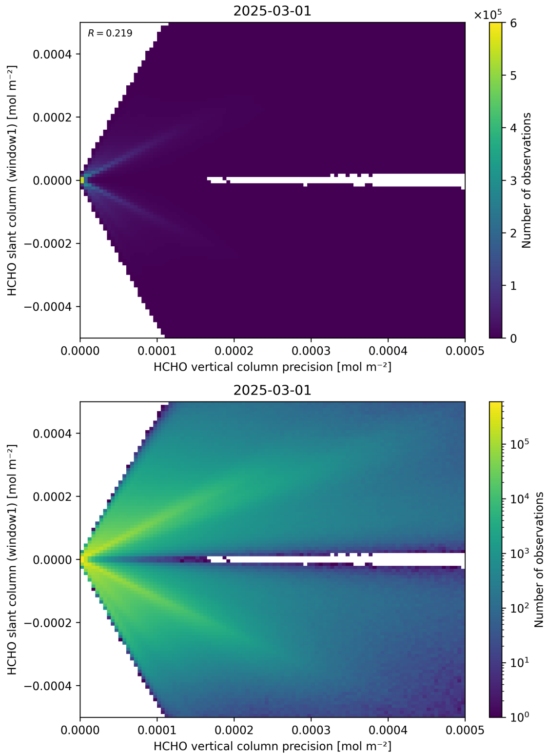
Figure 142: Scatter density plot of “HCHO vertical column precision” against “HCHO slant column (window1)” for 2025-03-01 to 2025-03-02.
