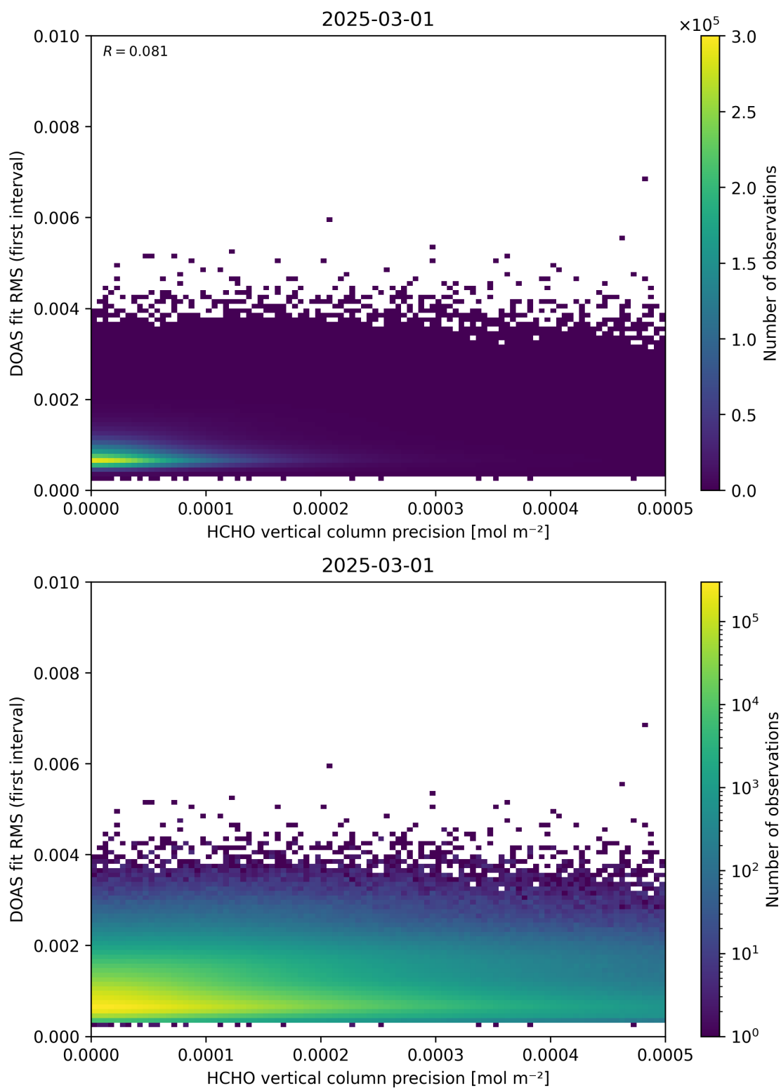
Figure 136: Scatter density plot of “HCHO vertical column precision” against “DOAS fit RMS (first interval)” for 2025-03-01 to 2025-03-02.
