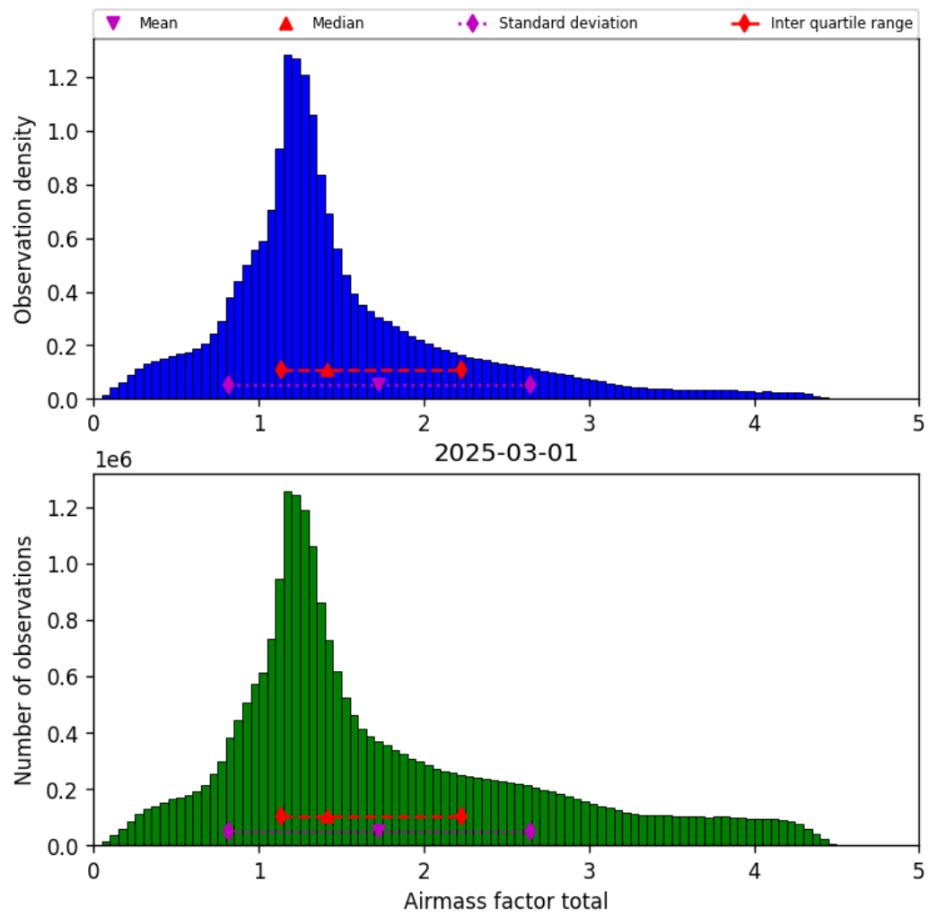
Figure 40: Histogram of “Airmass factor total” for 2025-03-01 to 2025-03-02
