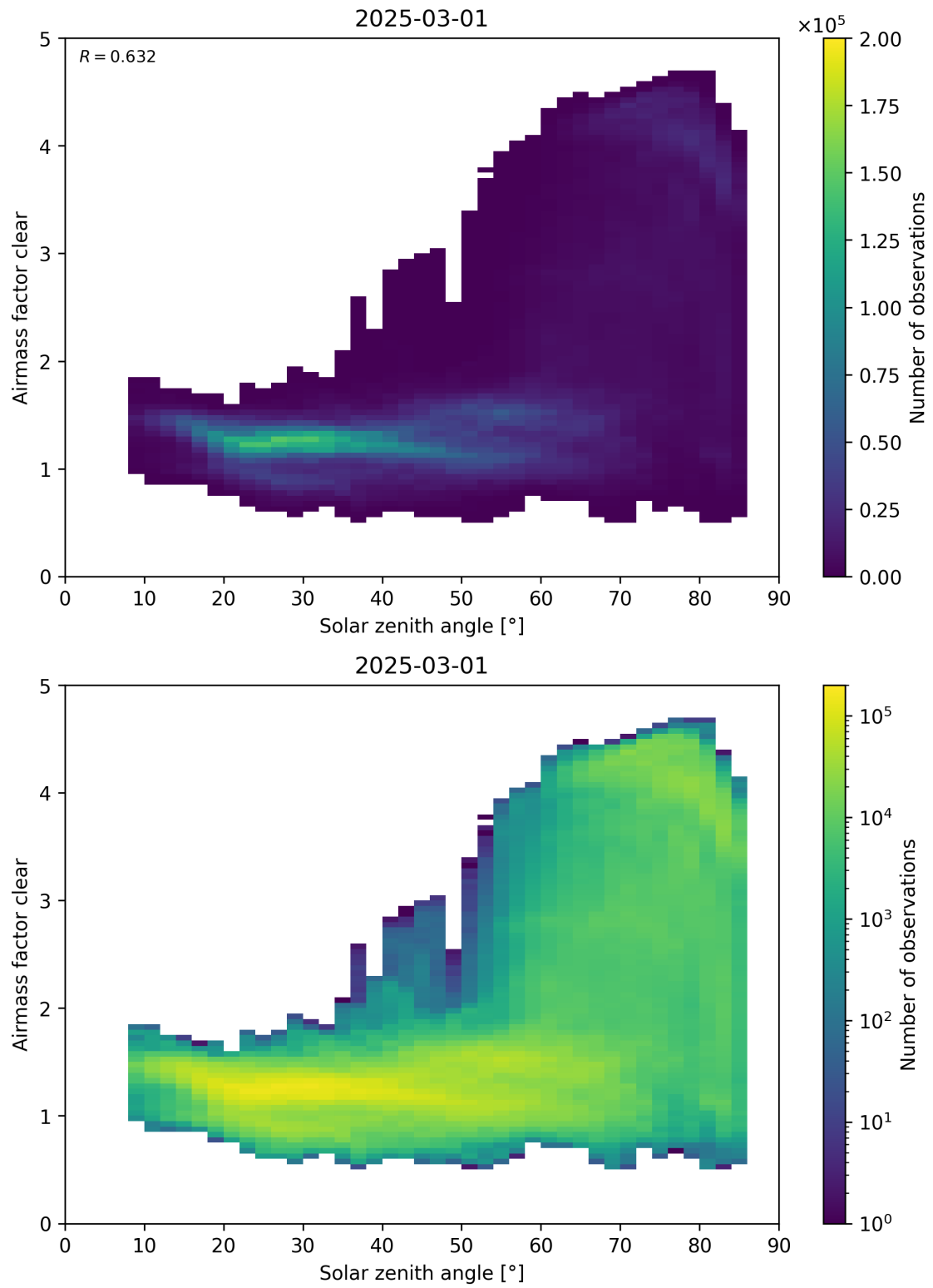
Figure 170: Scatter density plot of “Solar zenith angle” against “Airmass factor clear” for 2025-03-01 to 2025-03-02.
