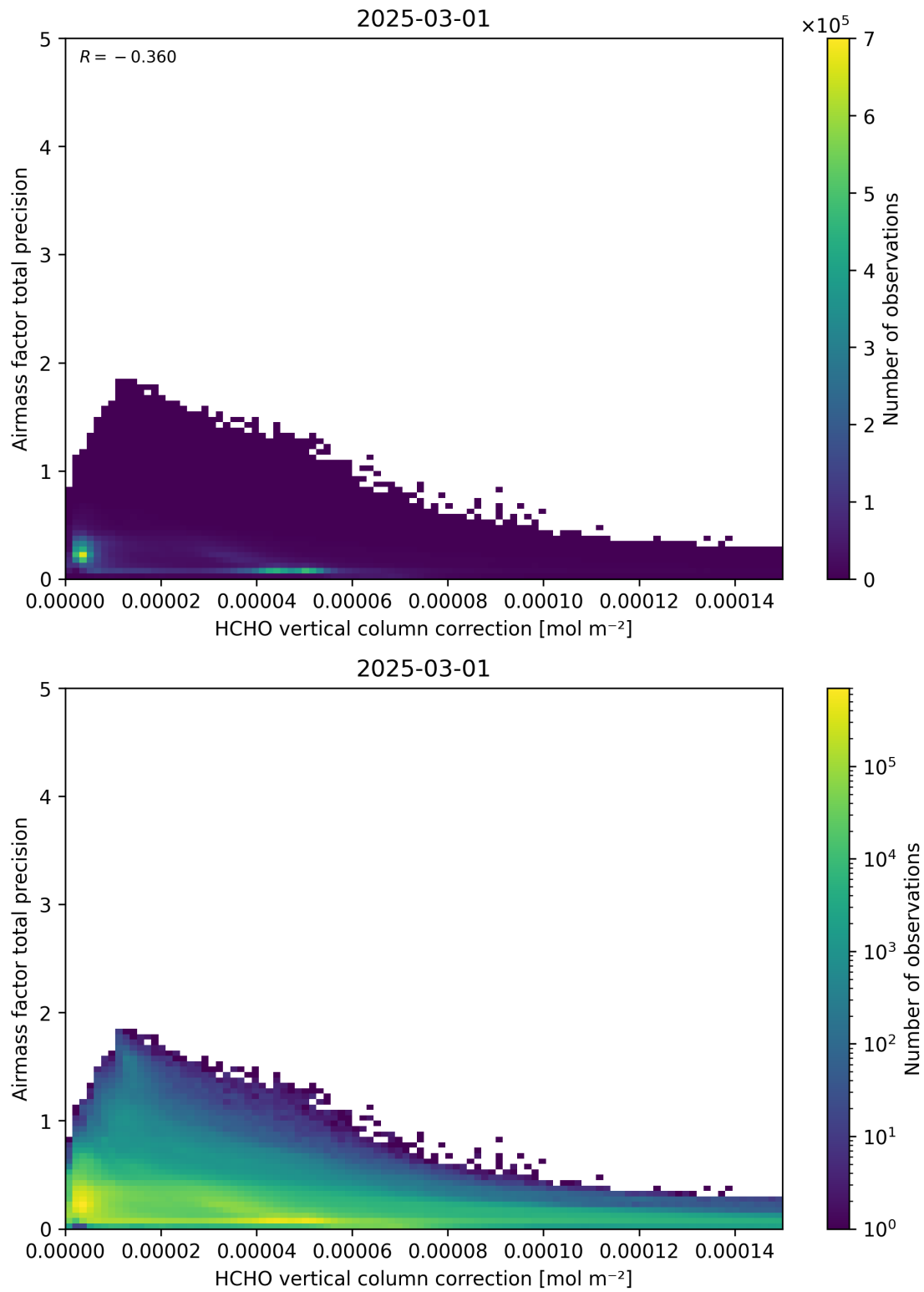
Figure 121: Scatter density plot of “HCHO vertical column correction” against “Airmass factor total precision” for 2025-03-01 to 2025-03-02.
