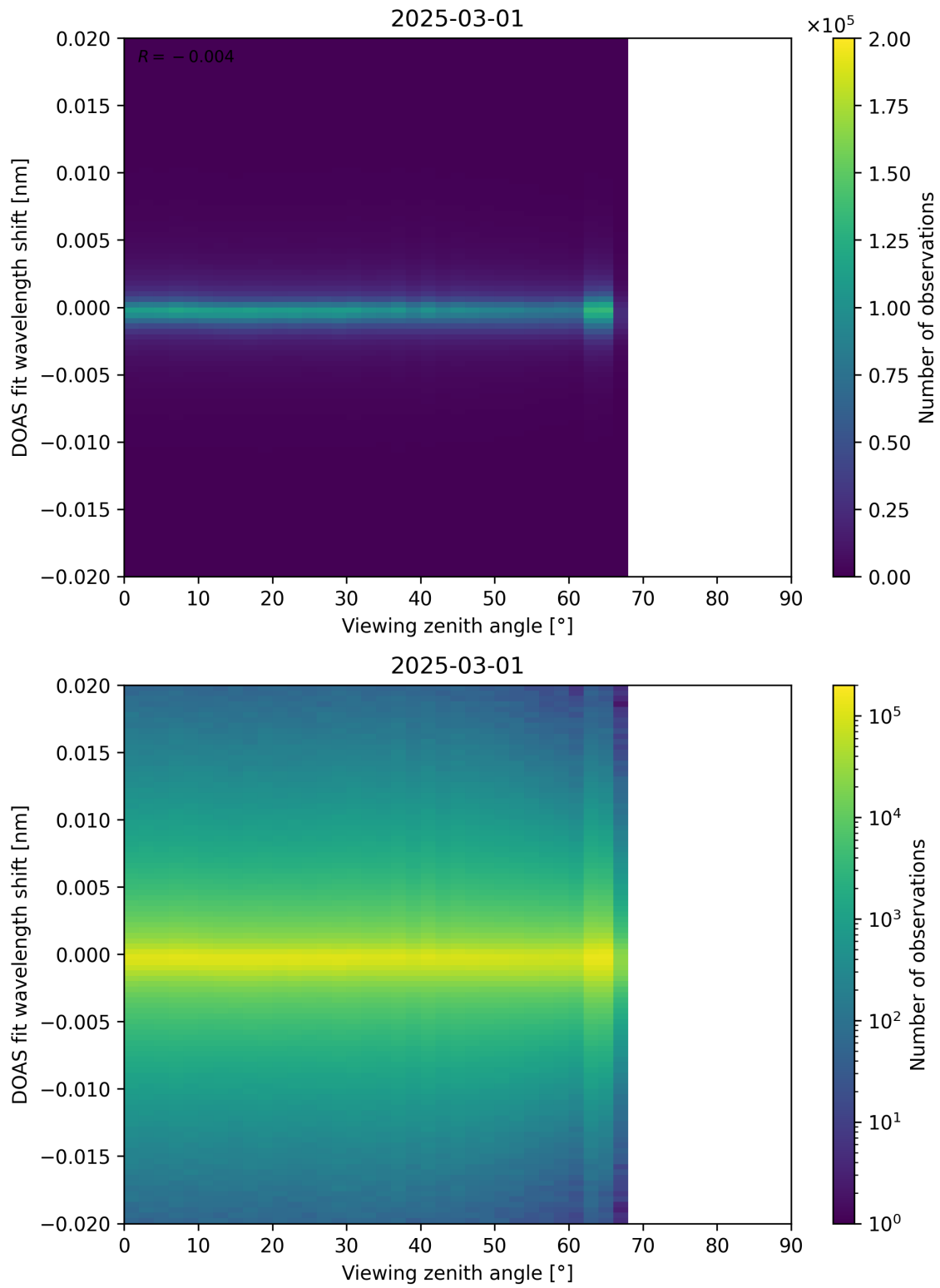
Figure 183: Scatter density plot of “Viewing zenith angle” against “DOAS fit wavelength shift” for 2025-03-01 to 2025-03-02.
