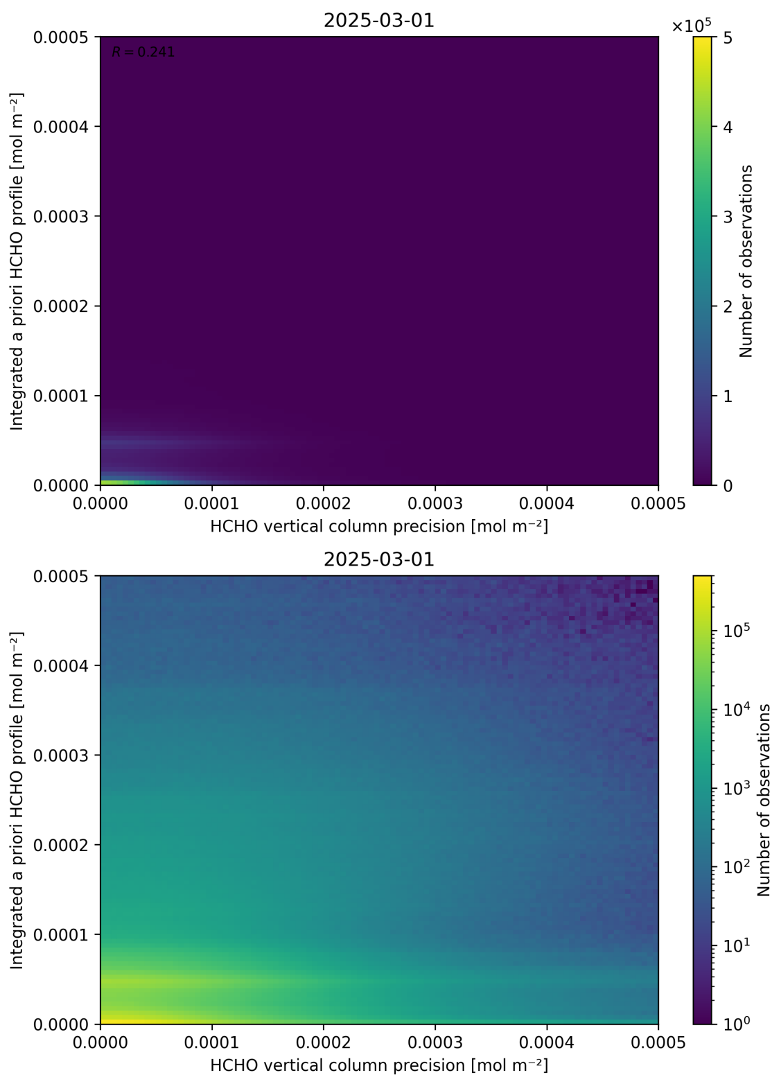
Figure 147: Scatter density plot of “HCHO vertical column precision” against “Integrated a priori HCHO profile” for 2025-03-01 to 2025-03-02.
