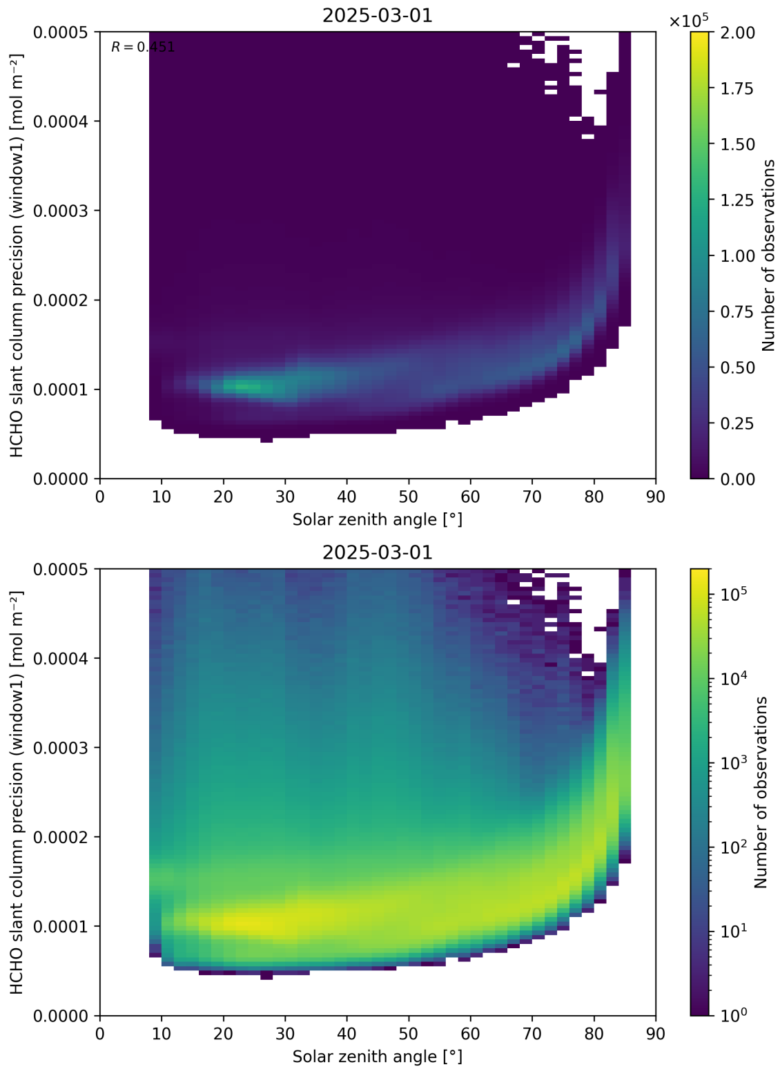
Figure 174: Scatter density plot of “Solar zenith angle” against “HCHO slant column precision (window1)” for 2025-03-01 to 2025-03-02.
