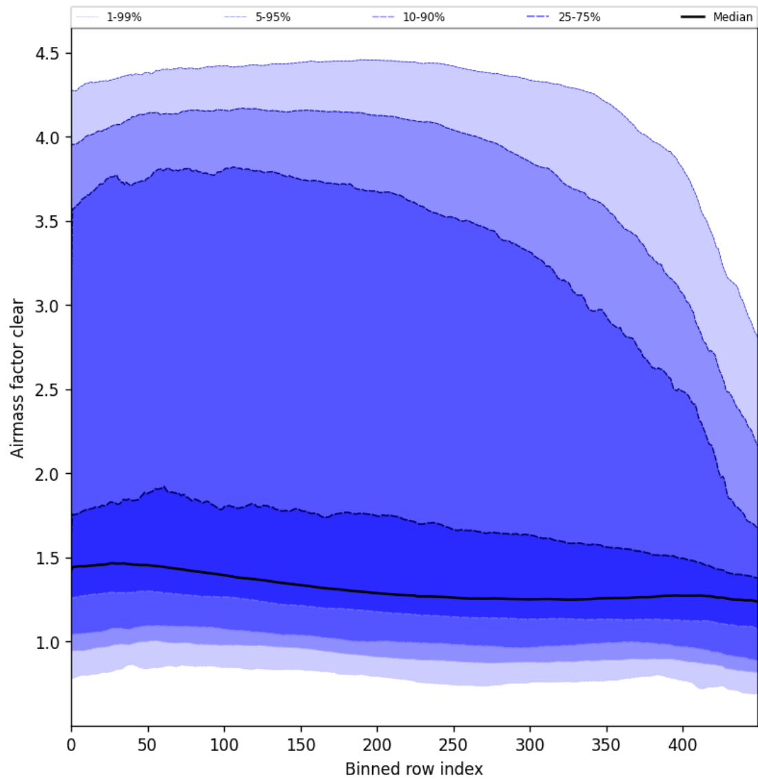
Figure 56: Along track statistics of “Air mass factor clear” for 2025-03-01 to 2025-03-02
