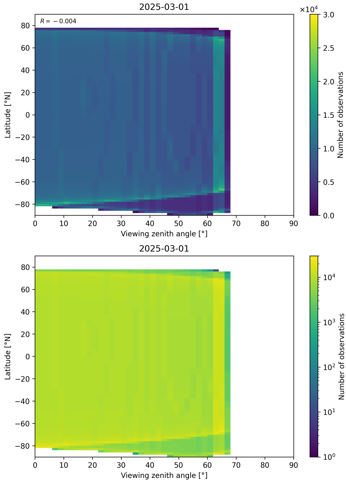
Figure 196: Scatter density plot of “Viewing zenith angle” against “Latitude” for 2025-03-01 to 2025-03-02.
