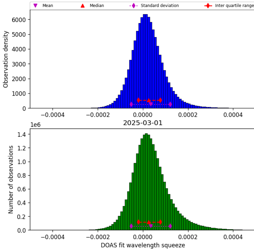
Figure 45: Histogram of “DOAS fit wavelength squeeze” for 2025-03-01 to 2025-03-02
