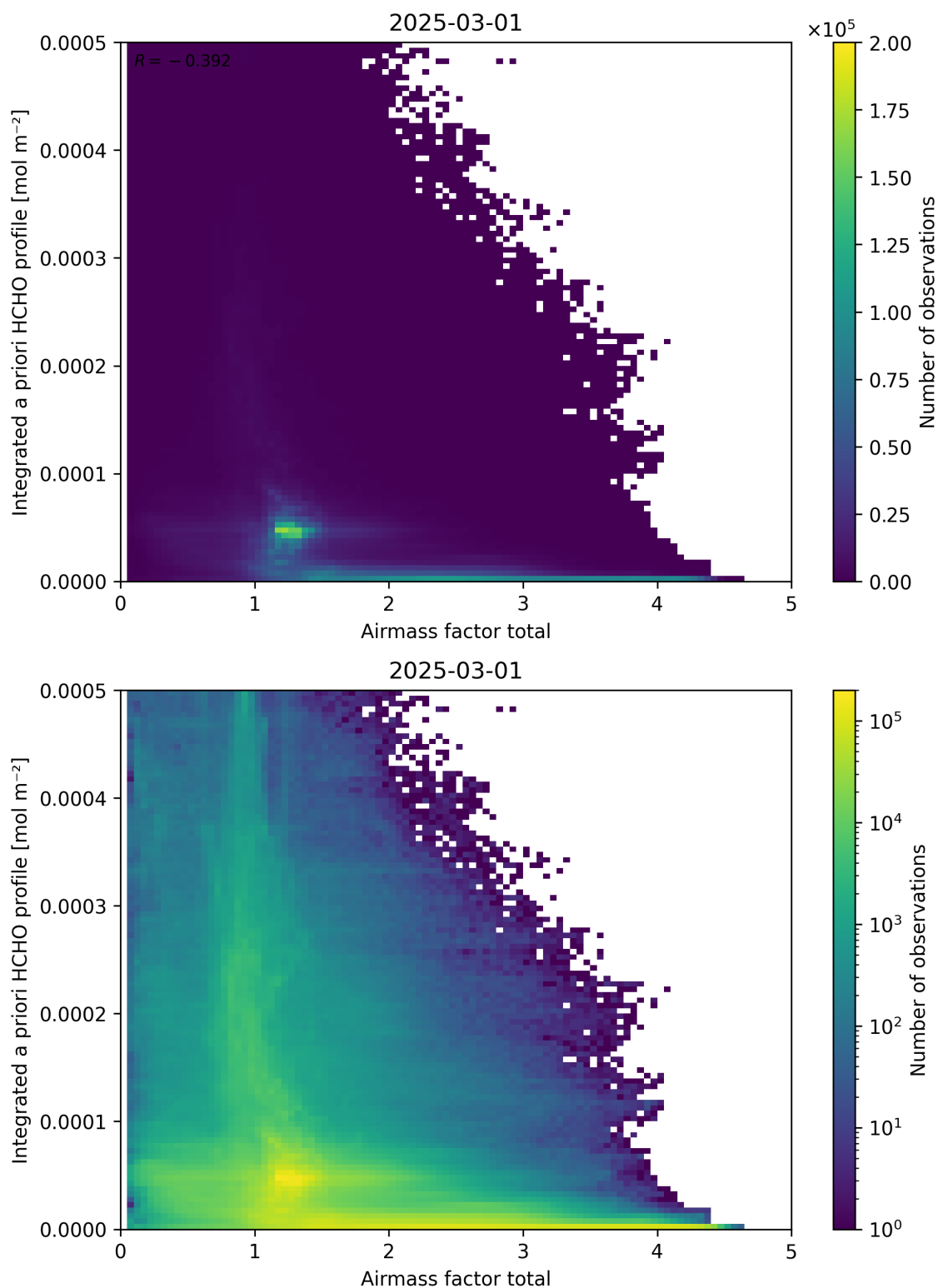
Figure 104: Scatter density plot of “Airmass factor total” against “Integrated a priori HCHO profile” for 2025-03-01 to 2025-03-02.
