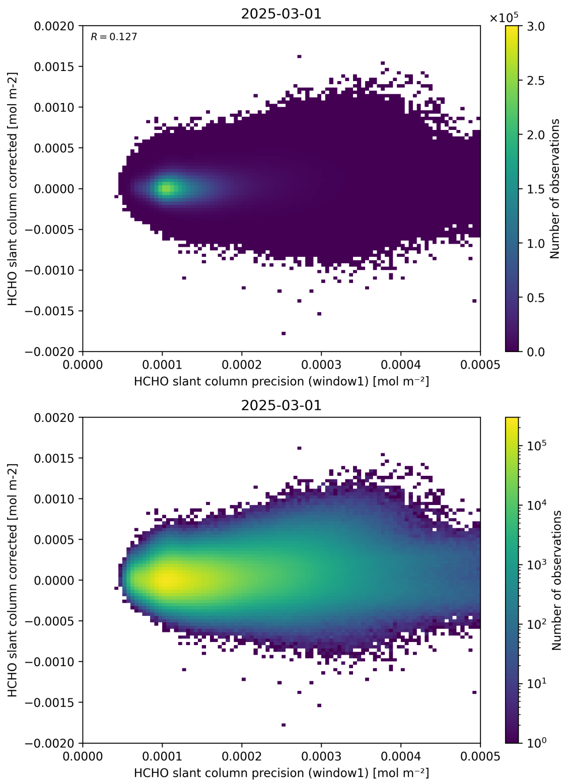
Figure 92: Scatter density plot of “HCHO slant column precision (window1)” against “HCHO slant column corrected” for 2025-03-01 to 2025-03-02.
