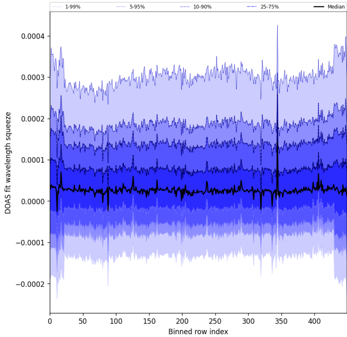
Figure 59: Along track statistics of “DOAS fit wavelength squeeze” for 2025-03-01 to 2025-03-02
