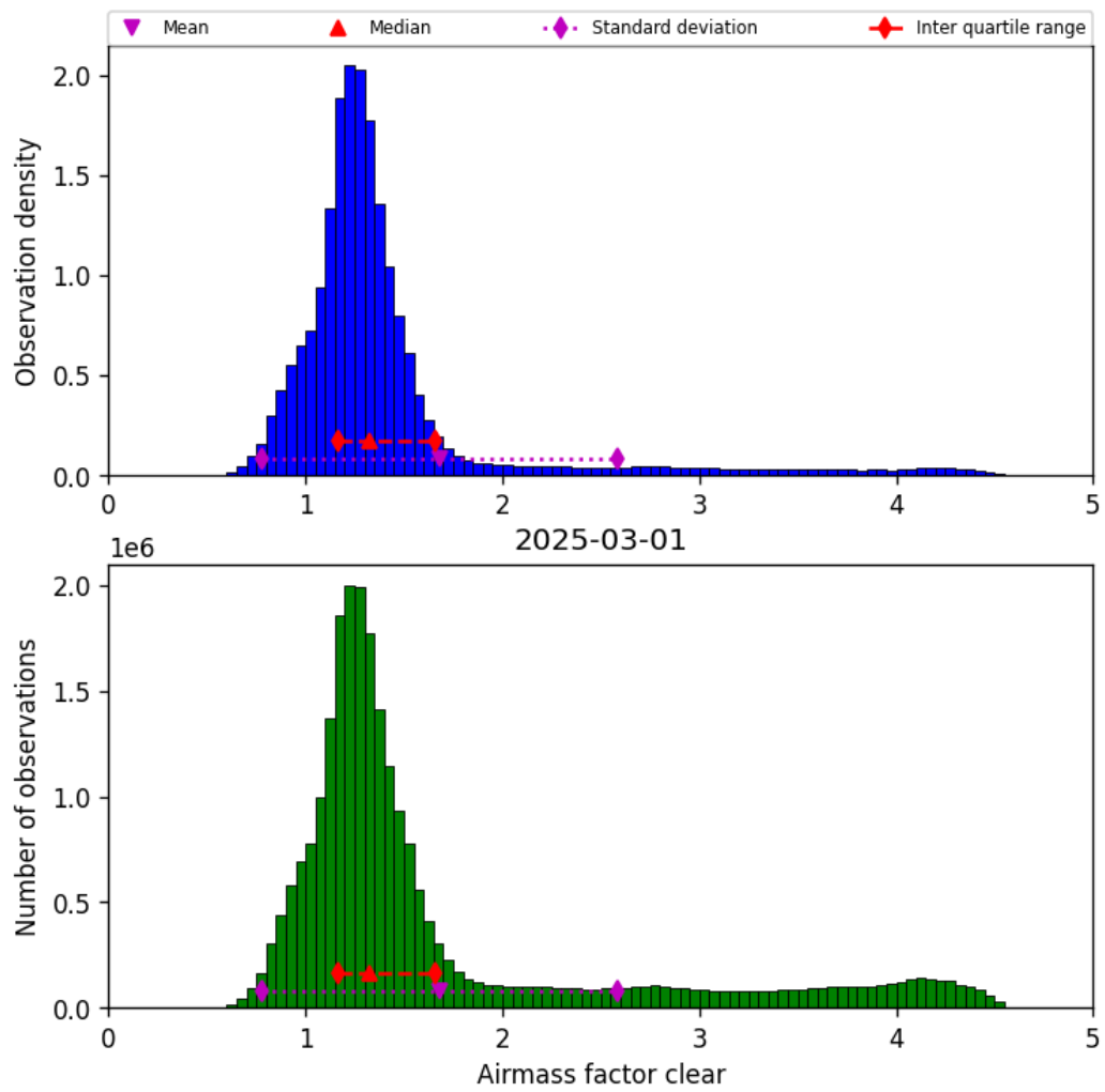
Figure 42: Histogram of “Airmass factor clear” for 2025-03-01 to 2025-03-02
