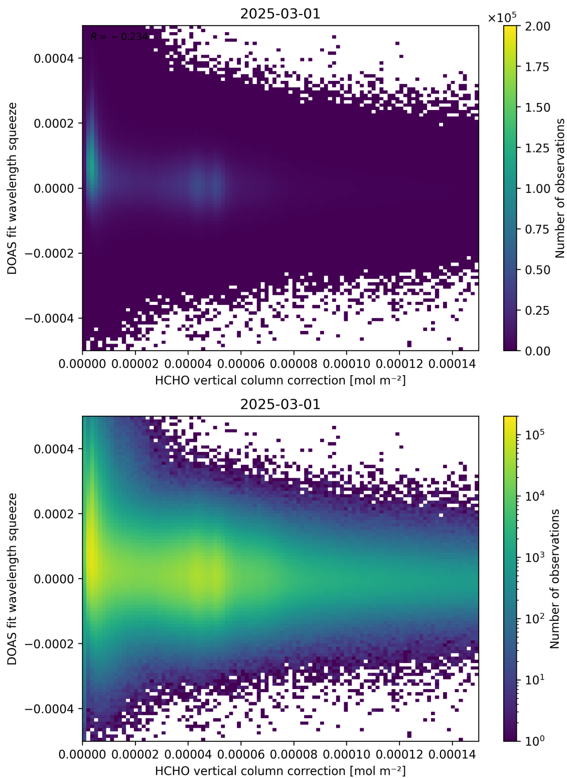
Figure 114: Scatter density plot of “HCHO vertical column correction” against “DOAS fit wavelength squeeze” for 2025-03-01 to 2025-03-02.
