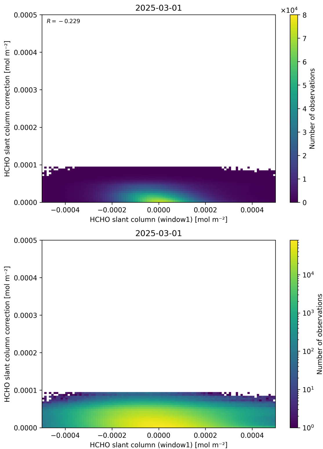
Figure 83: Scatter density plot of “HCHO slant column (window1)” against “HCHO slant column correction” for 2025-03-01 to 2025-03-02.
