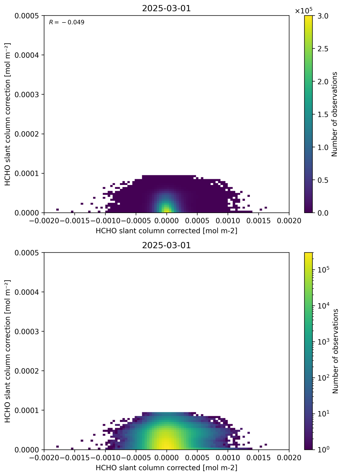
Figure 77: Scatter density plot of “HCHO slant column corrected” against “HCHO slant column correction” for 2025-03-01 to 2025-03-02.
