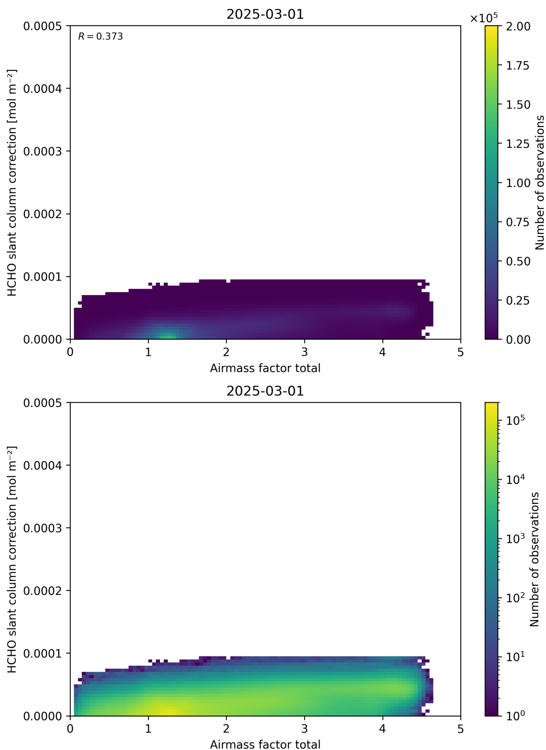
Figure 102: Scatter density plot of “Airmass factor total” against “HCHO slant column correction” for 2025-03-01 to 2025-03-02.
