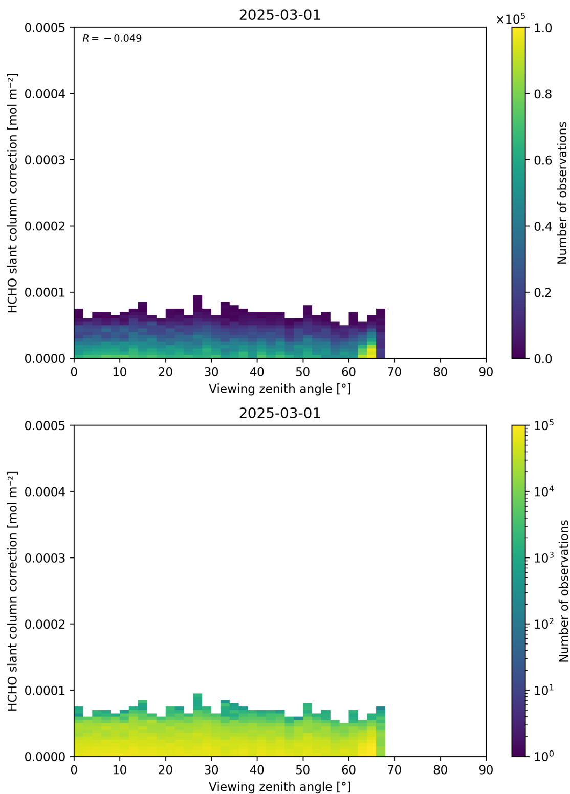
Figure 187: Scatter density plot of “Viewing zenith angle” against “HCHO slant column correction” for 2025-03-01 to 2025-03-02.
