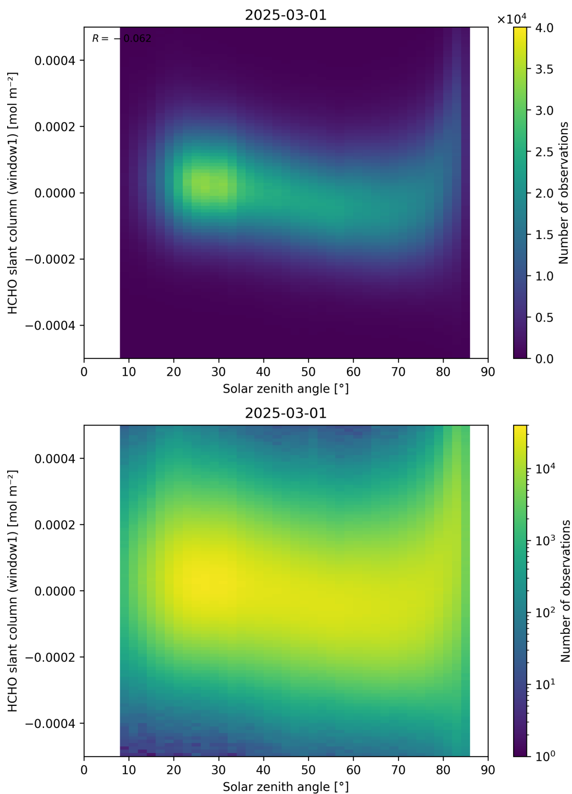
Figure 173: Scatter density plot of “Solar zenith angle” against “HCHO slant column (window1)” for 2025-03-01 to 2025-03-02.
