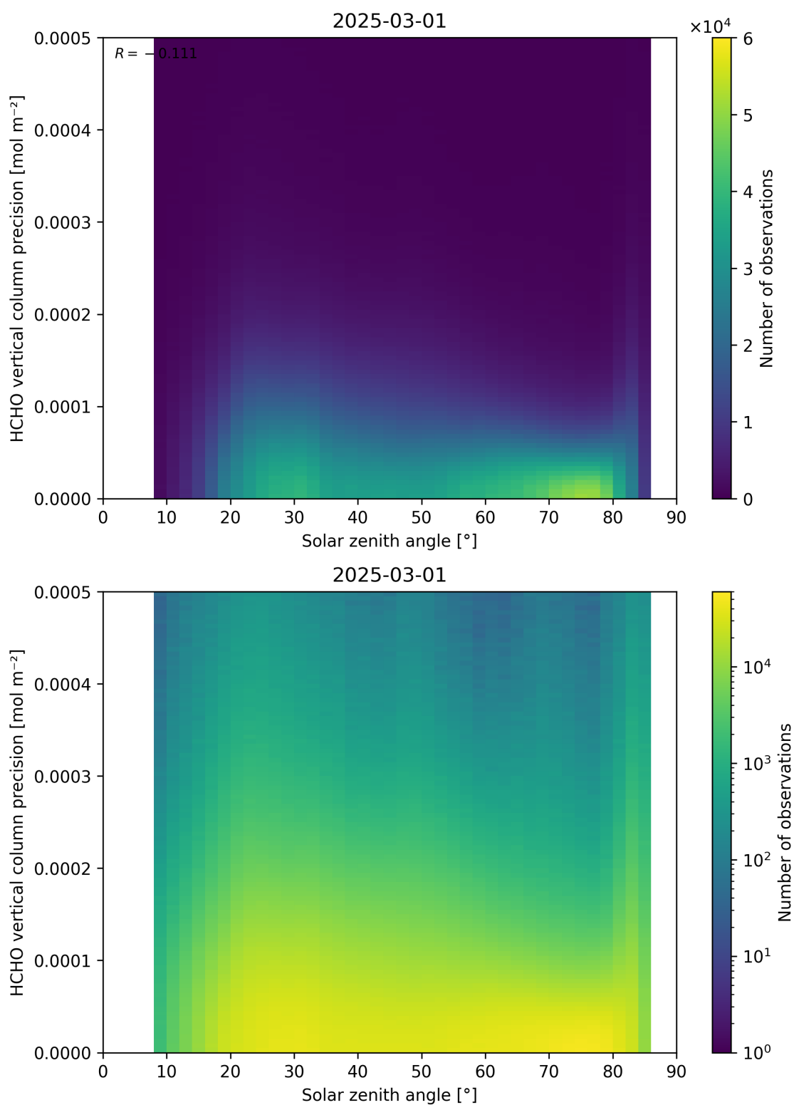
Figure 179: Scatter density plot of “Solar zenith angle” against “HCHO vertical column precision” for 2025-03-01 to 2025-03-02.
