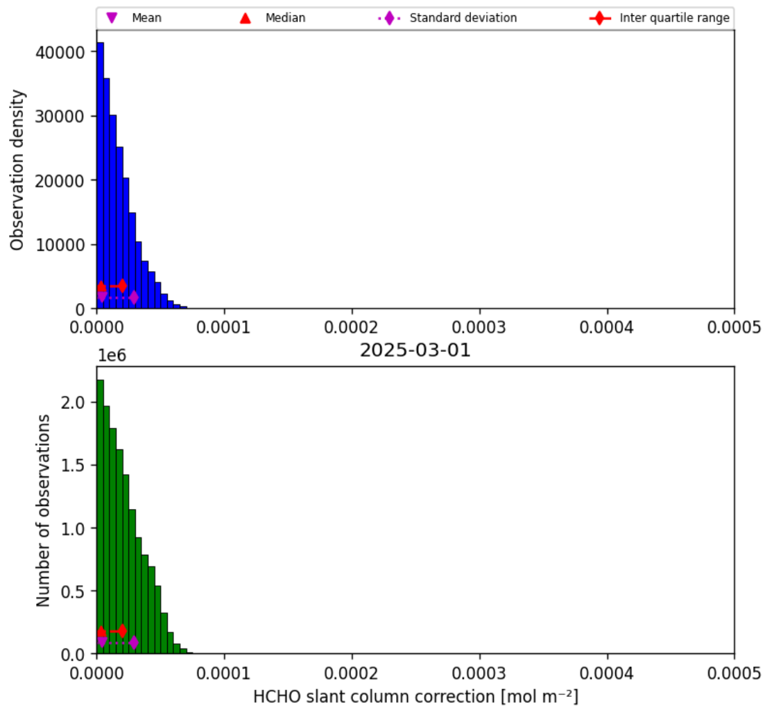
Figure 47: Histogram of “HCHO slant column correction” for 2025-03-01 to 2025-03-02
