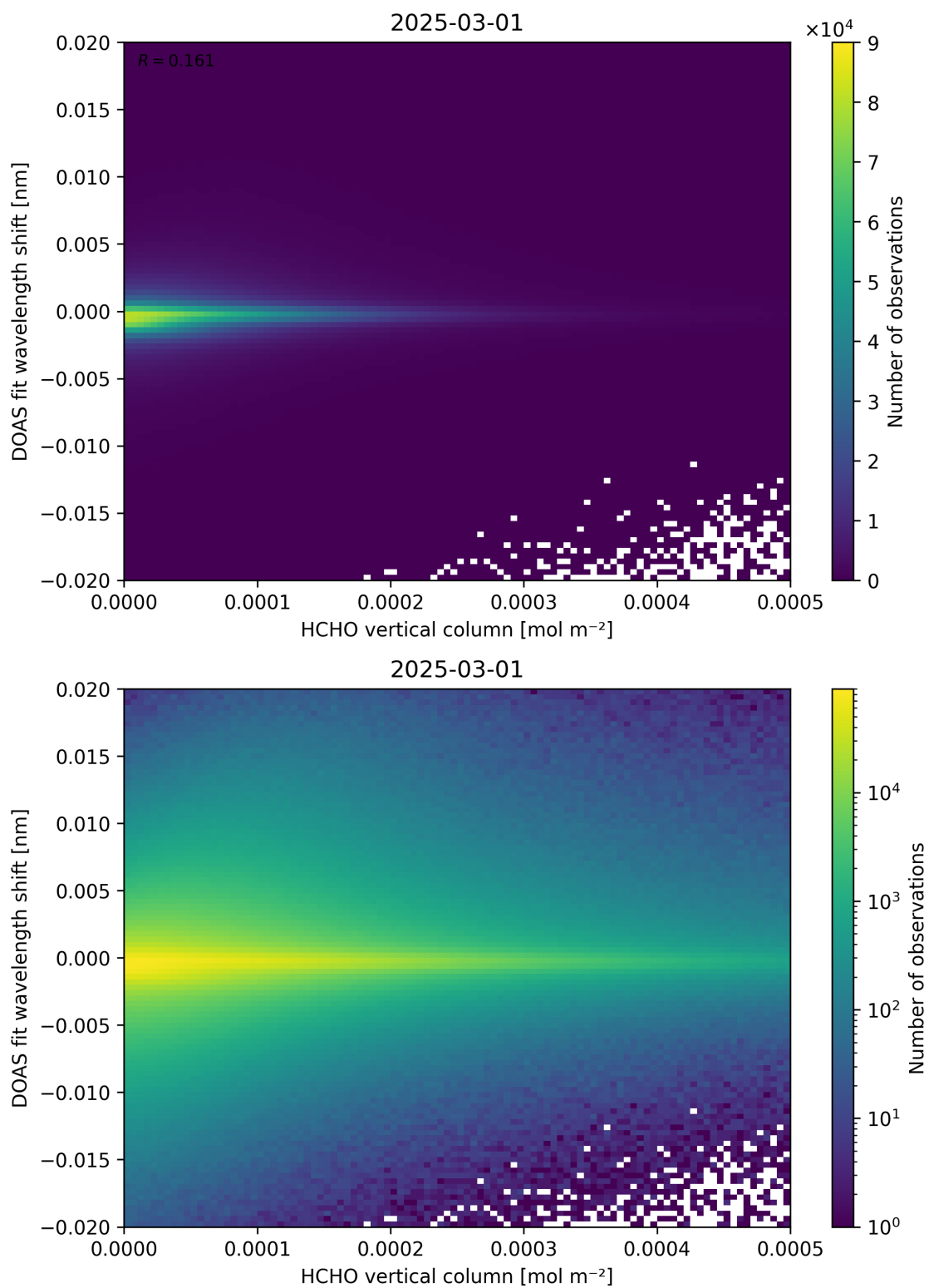
Figure 124: Scatter density plot of “HCHO vertical column” against “DOAS fit wavelength shift” for 2025-03-01 to 2025-03-02.
