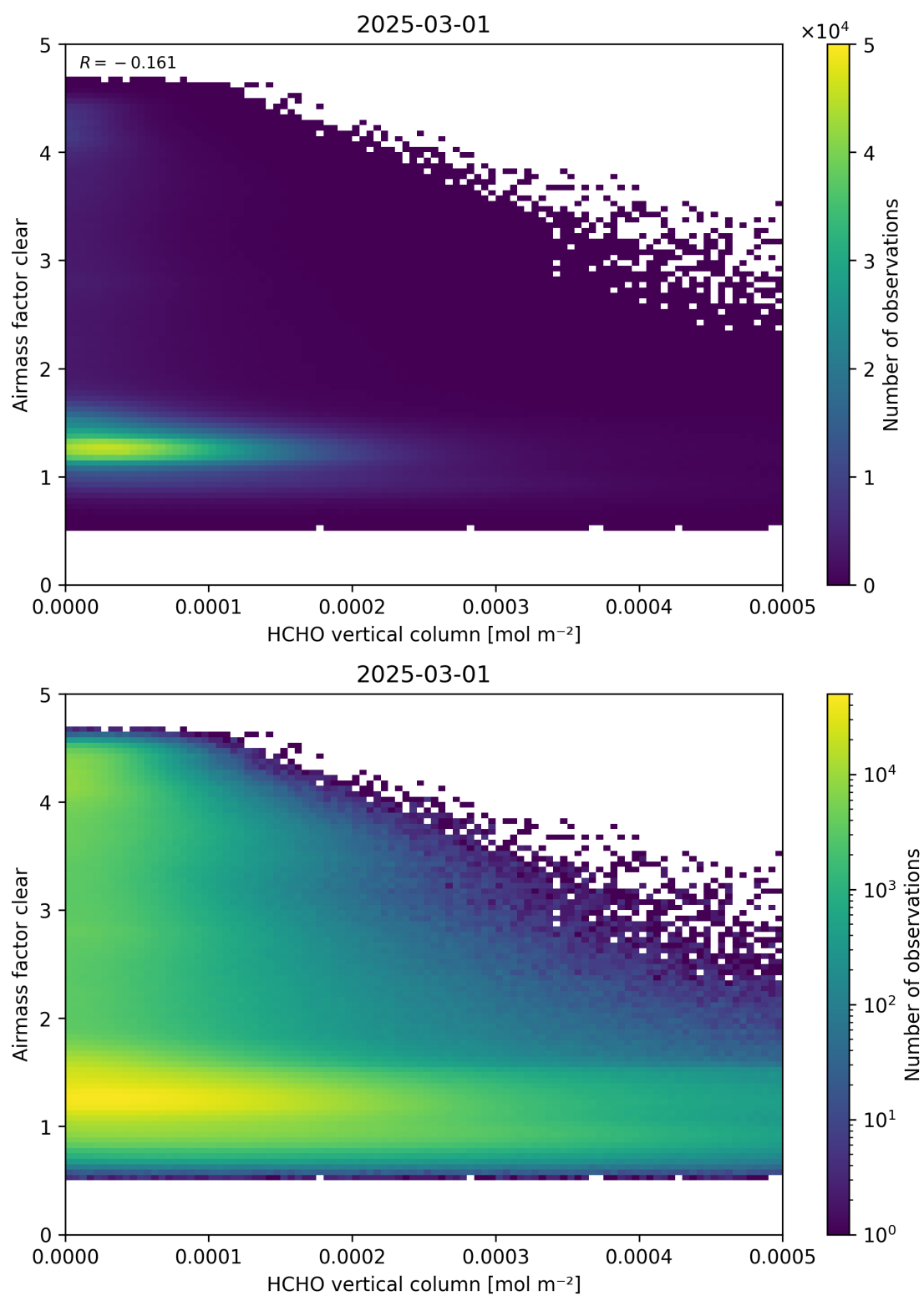
Figure 126: Scatter density plot of “HCHO vertical column” against “Airmass factor clear” for 2025-03-01 to 2025-03-02.
