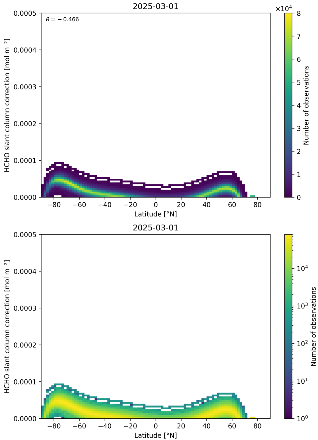
Figure 158: Scatter density plot of “Latitude” against “HCHO slant column correction” for 2025-03-01 to 2025-03-02.
