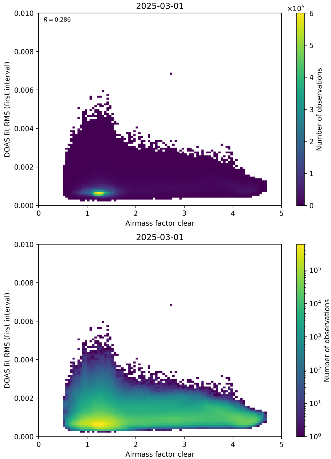
Figure 71: Scatter density plot of “Airmass factor clear” against “DOAS fit RMS (first interval)” for 2025-03-01 to 2025-03-02.
