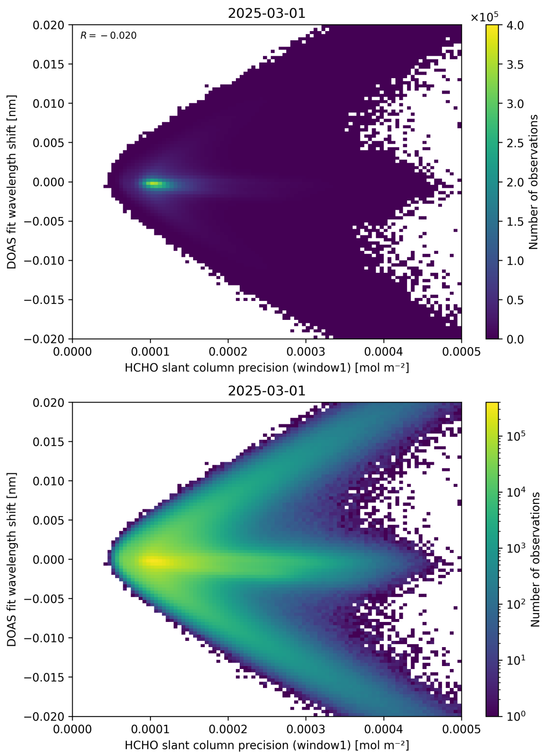
Figure 89: Scatter density plot of “HCHO slant column precision (window1)” against “DOAS fit wavelength shift” for 2025-03-01 to 2025-03-02.
