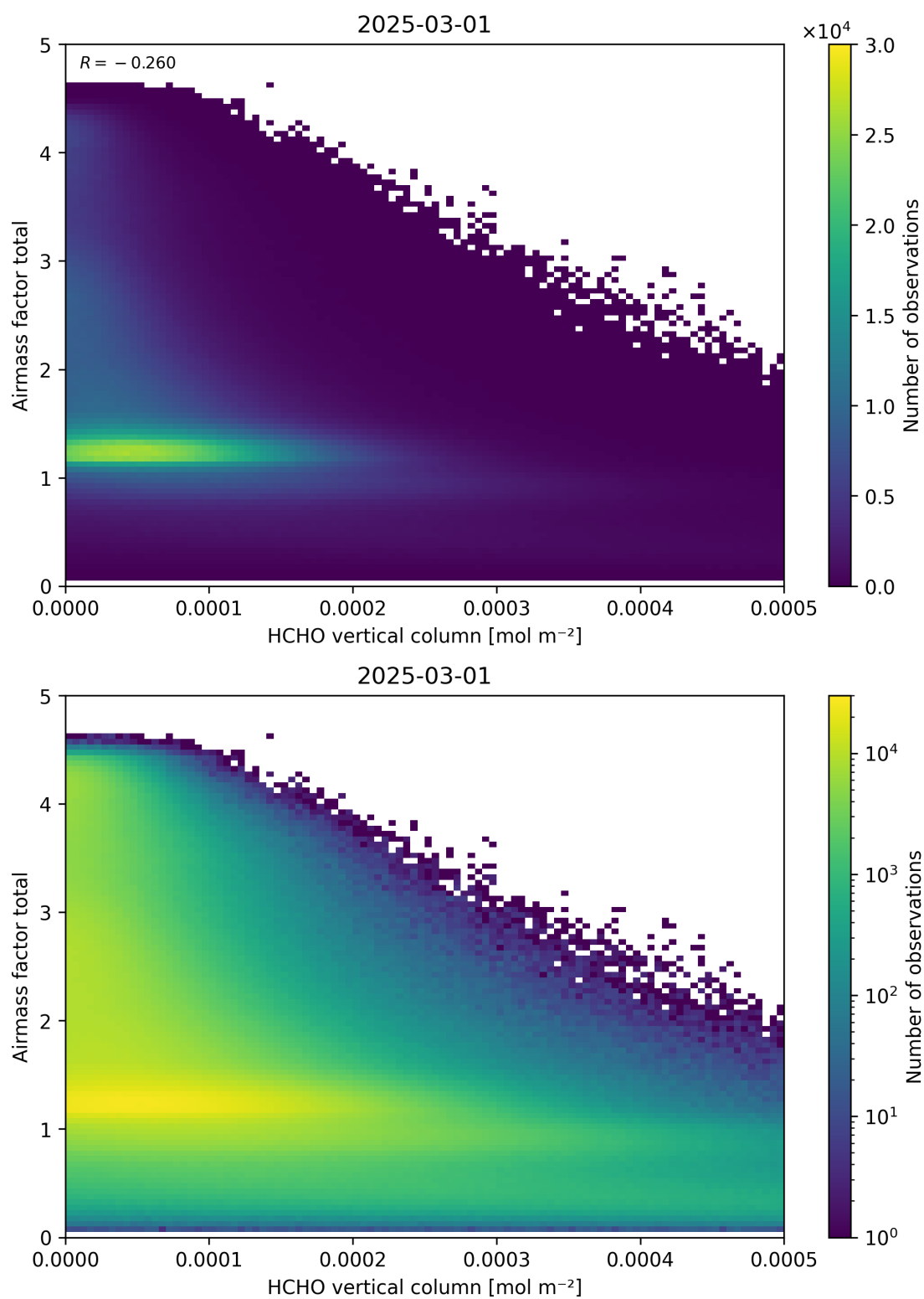
Figure 131: Scatter density plot of “HCHO vertical column” against “Airmass factor total” for 2025-03-01 to 2025-03-02.
