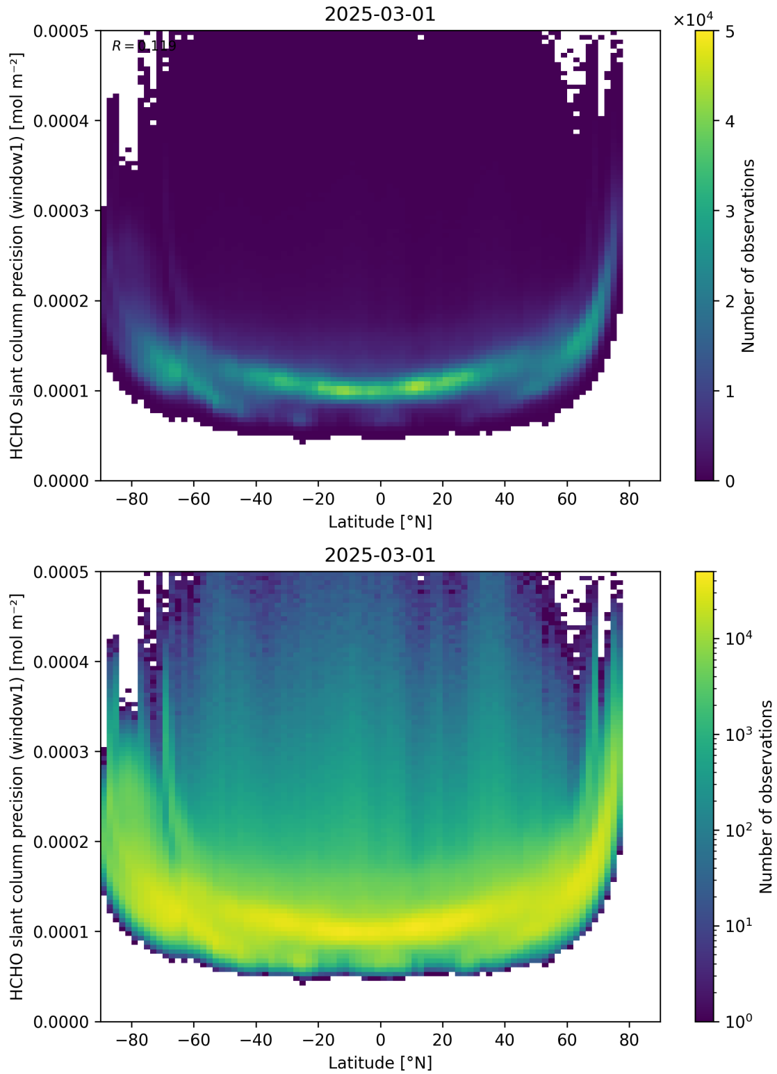
Figure 160: Scatter density plot of “Latitude” against “HCHO slant column precision (window1)” for 2025-03-01 to 2025-03-02.
