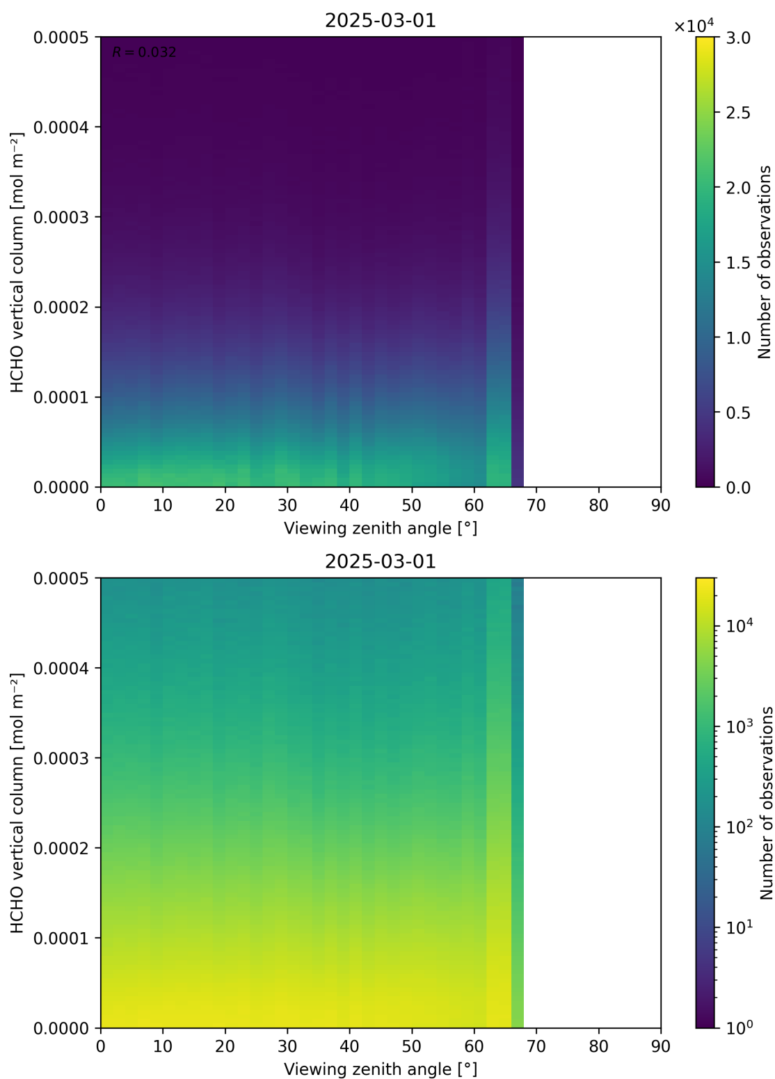
Figure 192: Scatter density plot of “Viewing zenith angle” against “HCHO vertical column” for 2025-03-01 to 2025-03-02.
