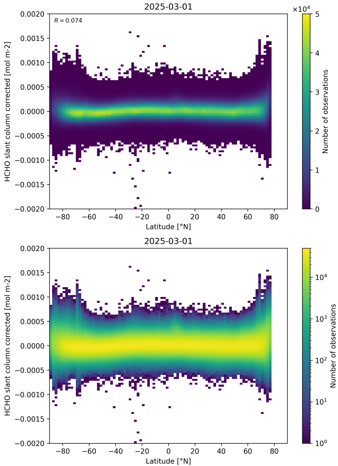
Figure 157: Scatter density plot of “Latitude” against “HCHO slant column corrected” for 2025-03-01 to 2025-03-02.
