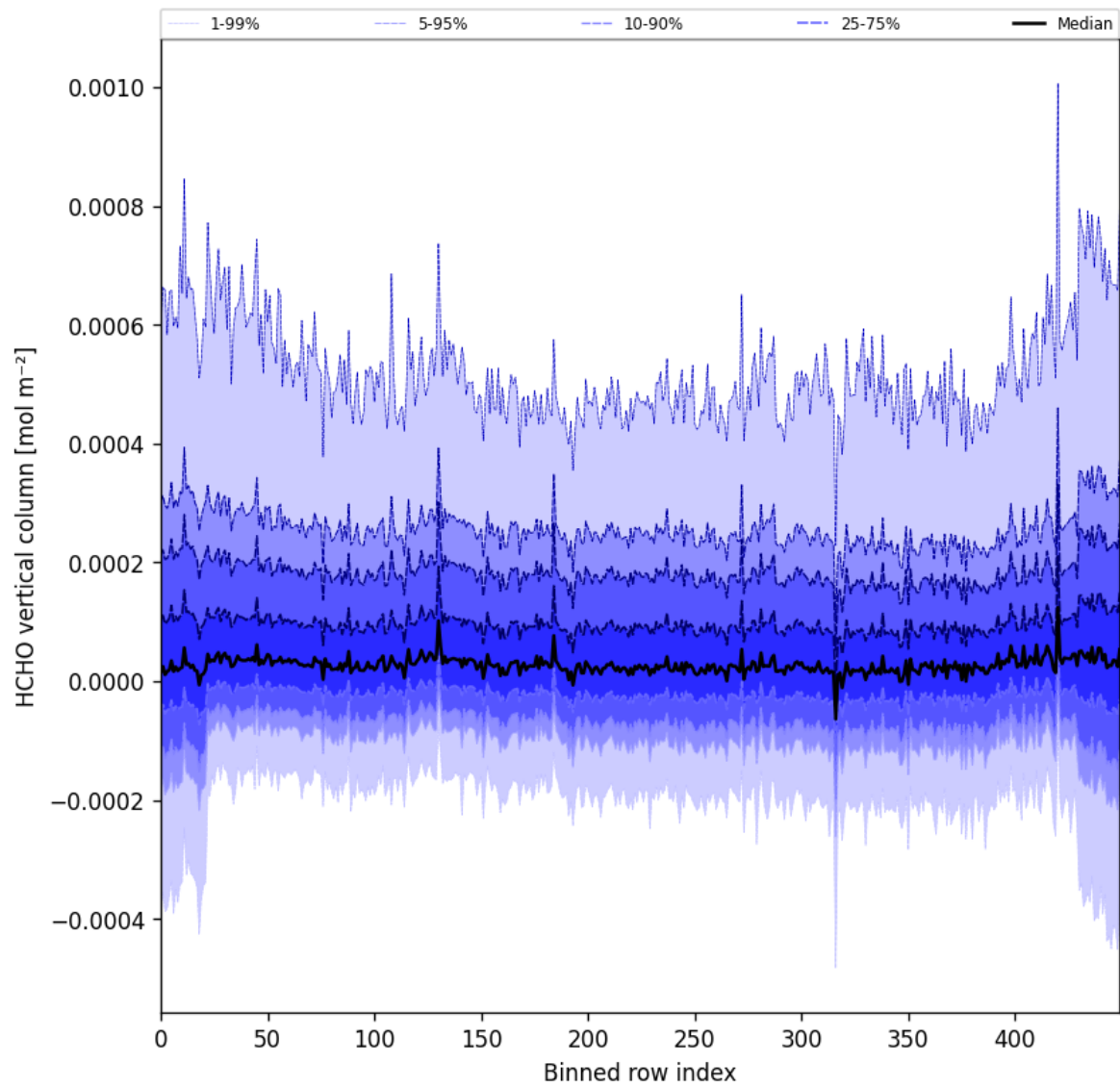
Figure 49: Along track statistics of “HCHO vertical column” for 2025-03-01 to 2025-03-02
