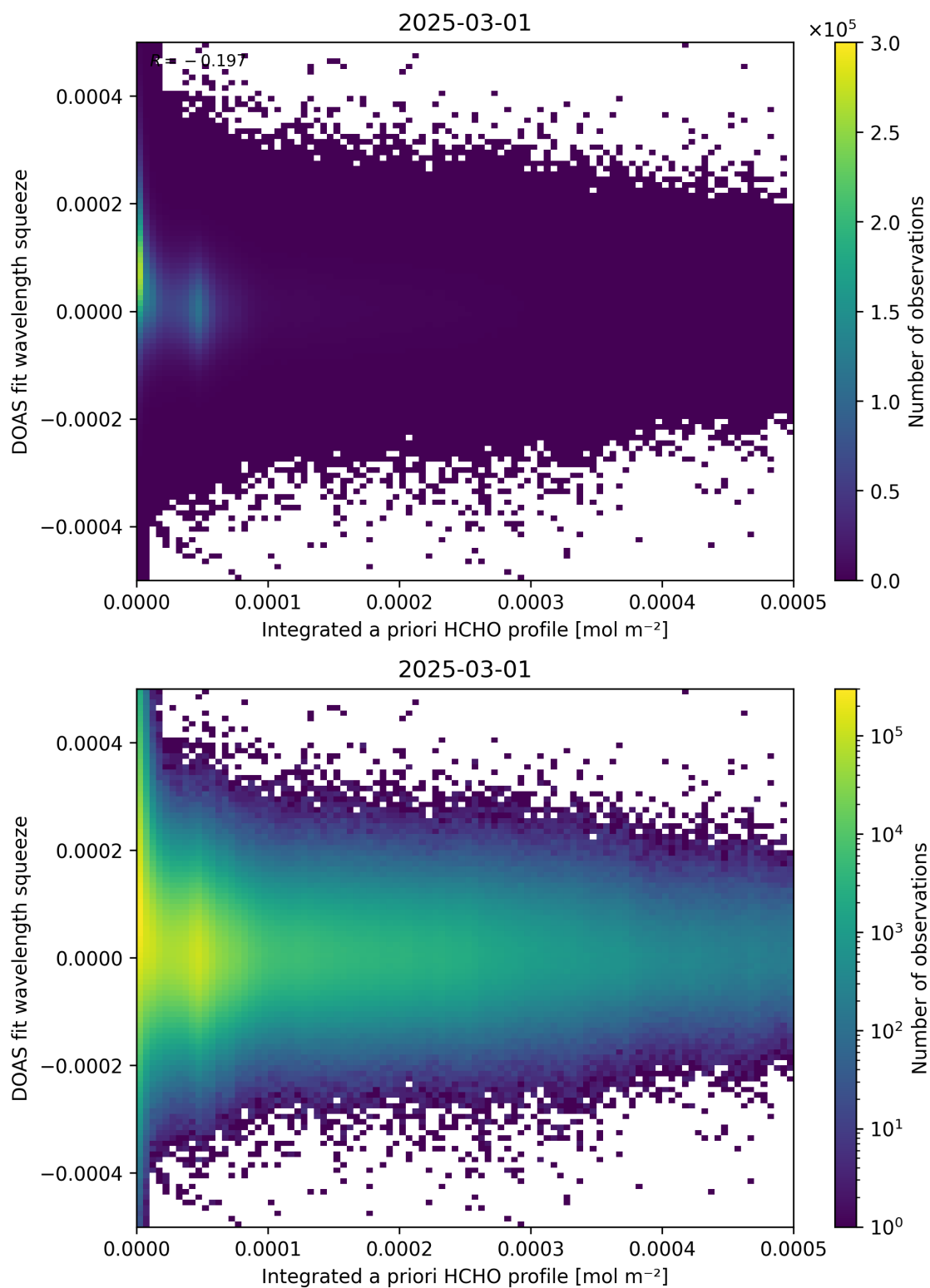
Figure 150: Scatter density plot of “Integrated a priori HCHO profile” against “DOAS fit wavelength squeeze” for 2025-03-01 to 2025-03-02.
