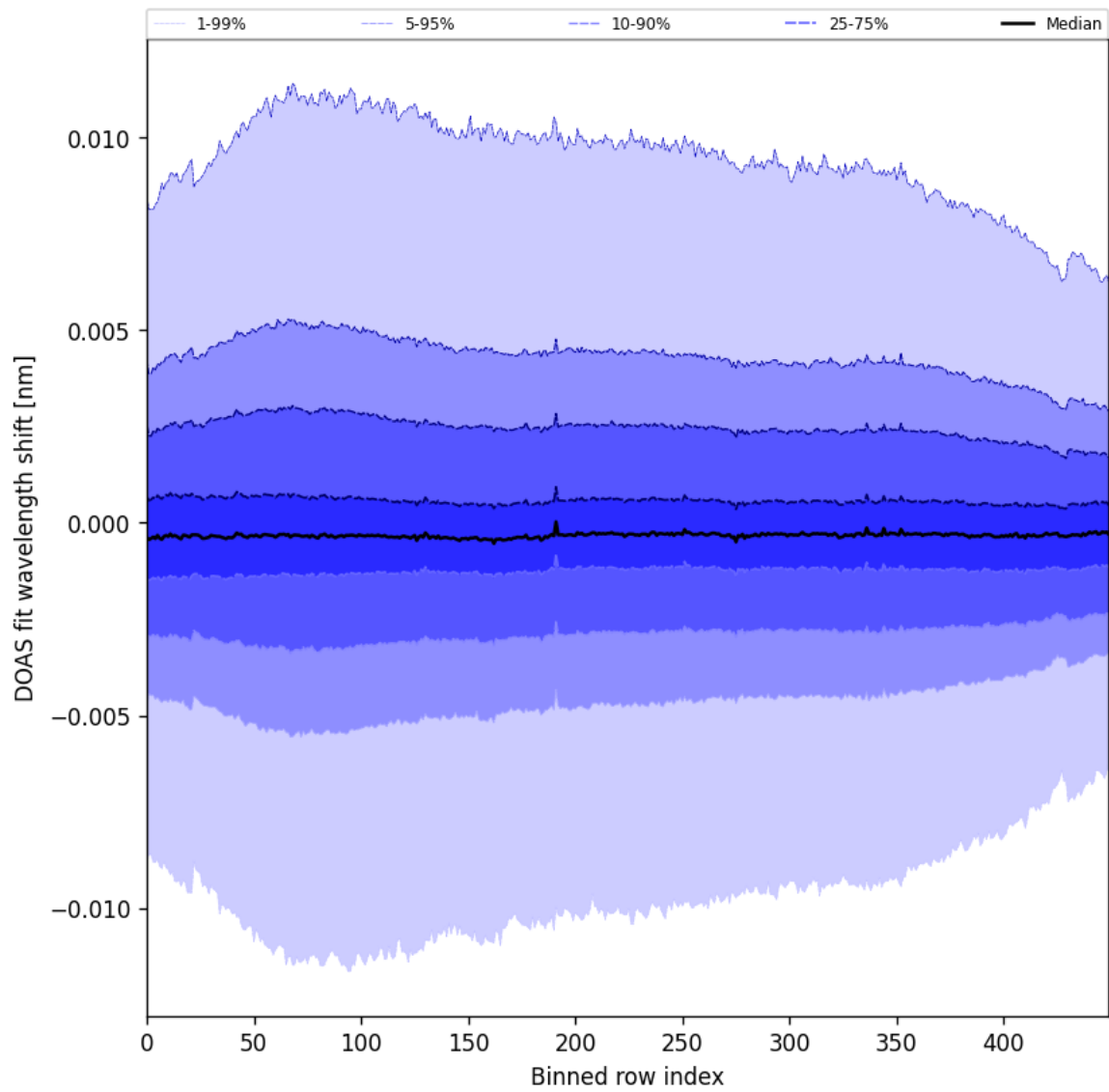
Figure 58: Along track statistics of “DOAS fit wavelength shift” for 2025-03-01 to 2025-03-02
