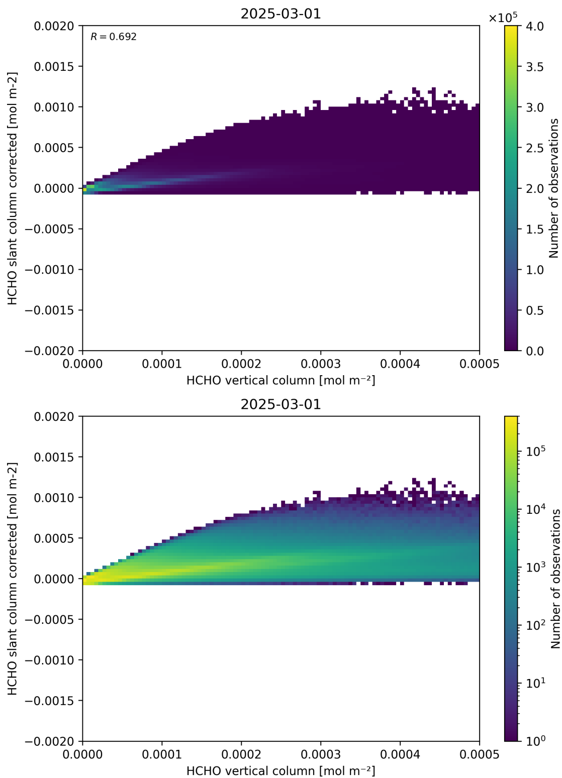
Figure 127: Scatter density plot of “HCHO vertical column” against “HCHO slant column corrected” for 2025-03-01 to 2025-03-02.
