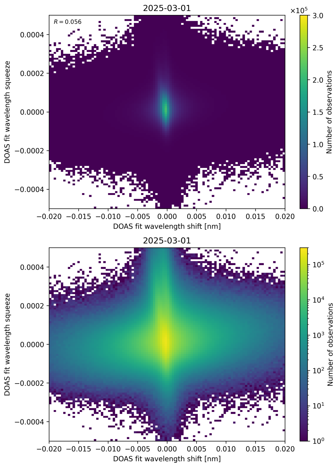
Figure 65: Scatter density plot of “DOAS fit wavelength shift” against “DOAS fit wavelength squeeze” for 2025-03-01 to 2025-03-02.
