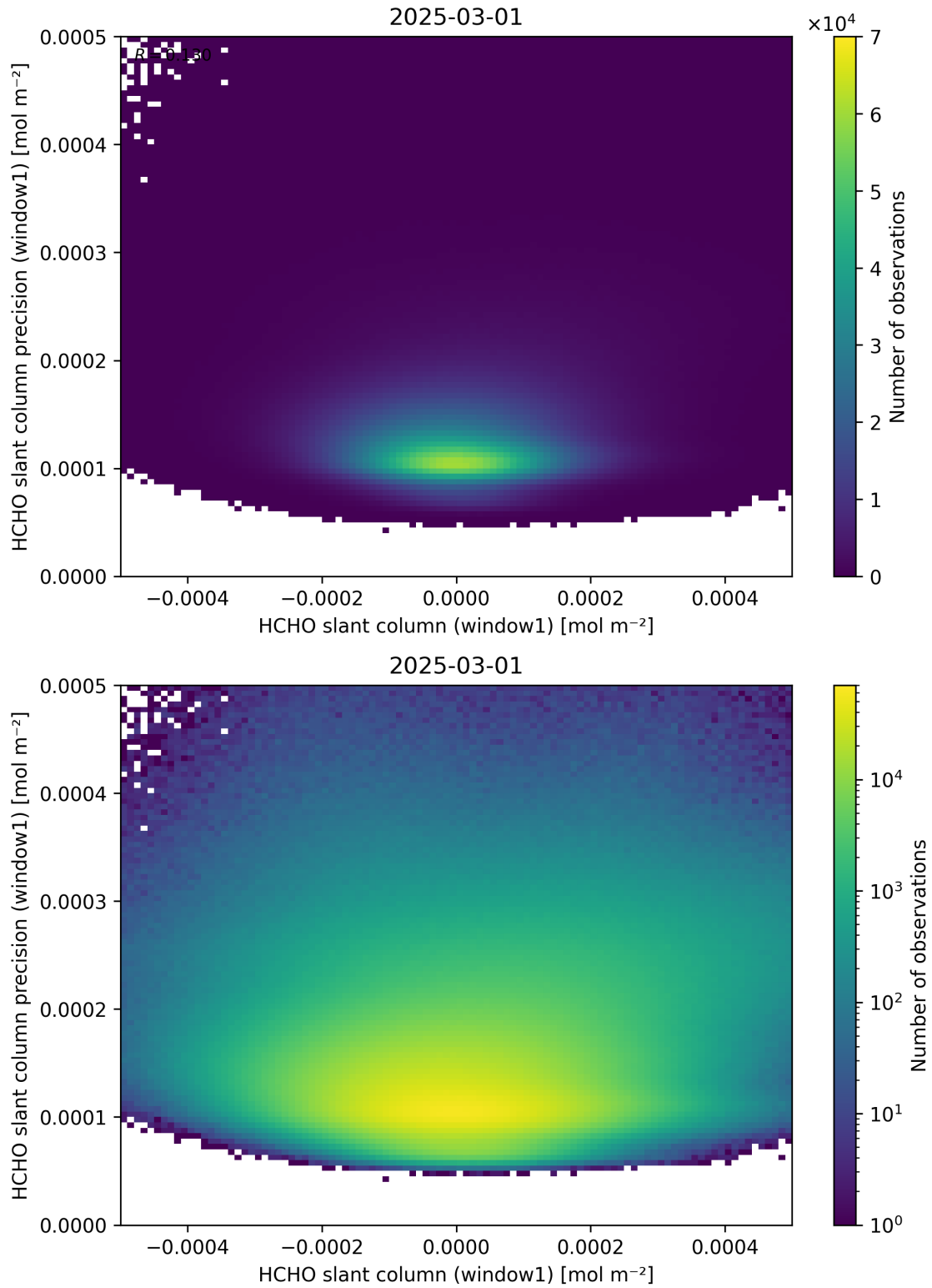
Figure 84: Scatter density plot of “HCHO slant column (window1)” against “HCHO slant column precision (window1)” for 2025-03-01 to 2025-03-02.
