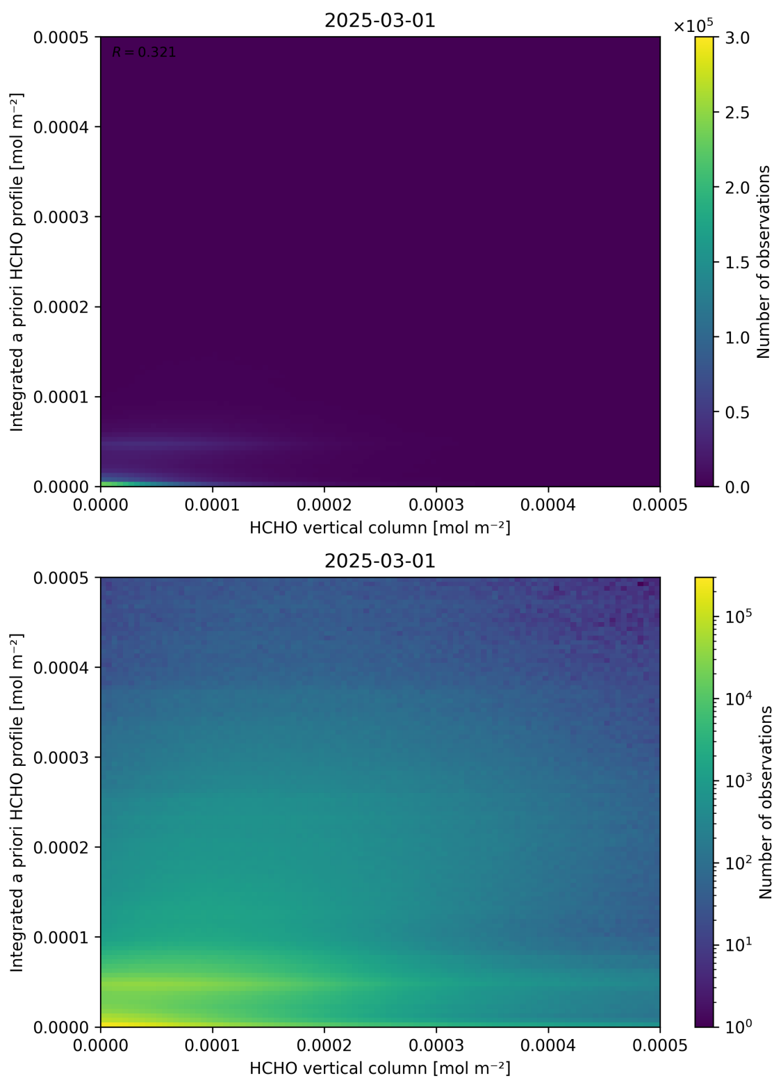
Figure 135: Scatter density plot of “HCHO vertical column” against “Integrated a priori HCHO profile” for 2025-03-01 to 2025-03-02.
