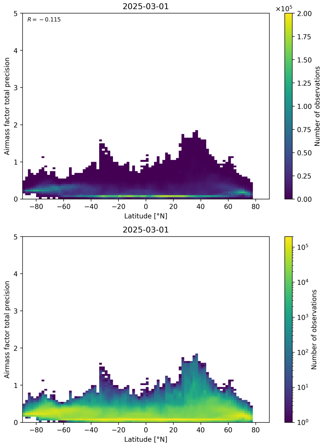
Figure 162: Scatter density plot of “Latitude” against “Airmass factor total precision” for 2025-03-01 to 2025-03-02.
