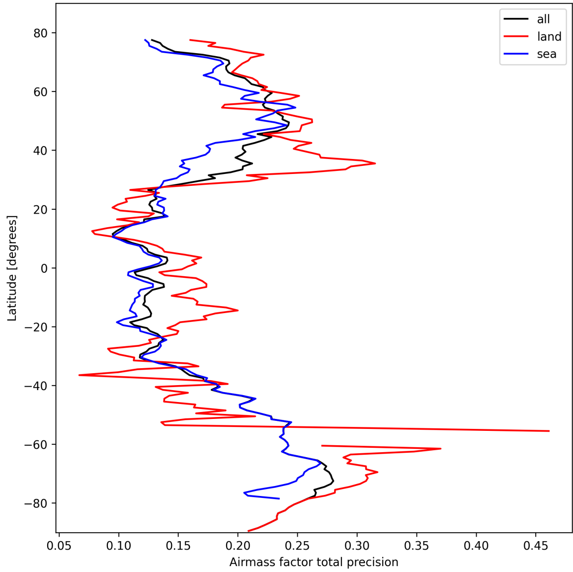
Figure 27: Zonal average of “Airmass factor total precision” for 2025-03-01 to 2025-03-02.
