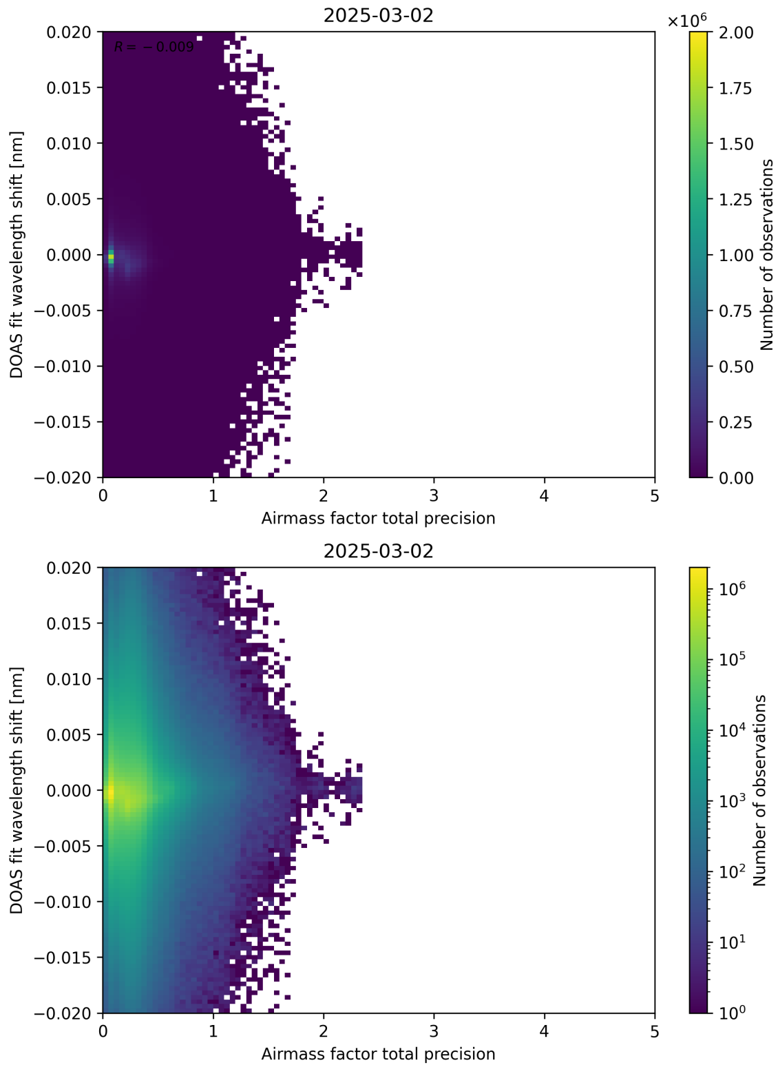
Figure 106: Scatter density plot of “Airmass factor total precision” against “DOAS fit wavelength shift” for 2025-03-01 to 2025-03-03.
