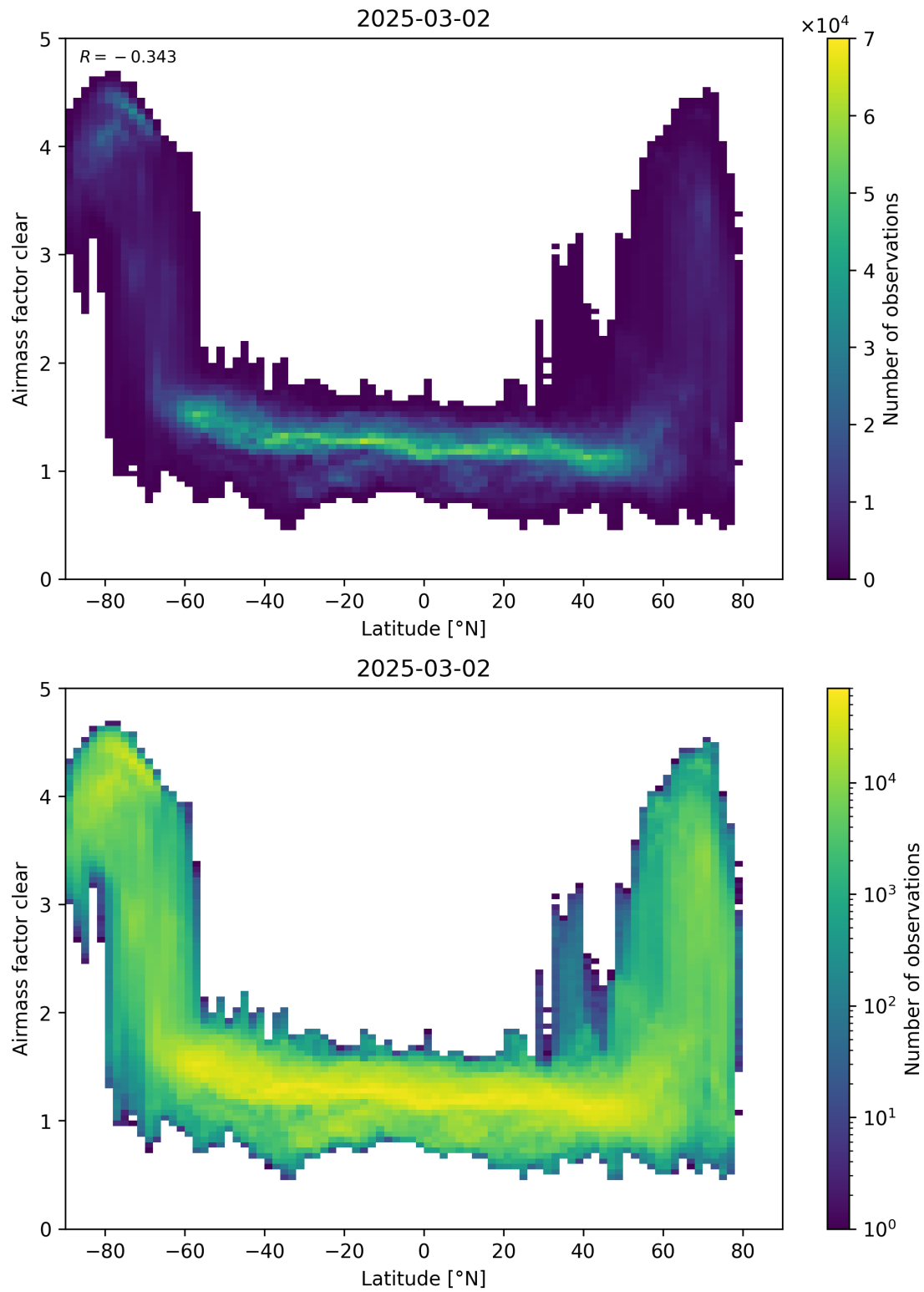
Figure 156: Scatter density plot of “Latitude” against “Airmass factor clear” for 2025-03-01 to 2025-03-03.
