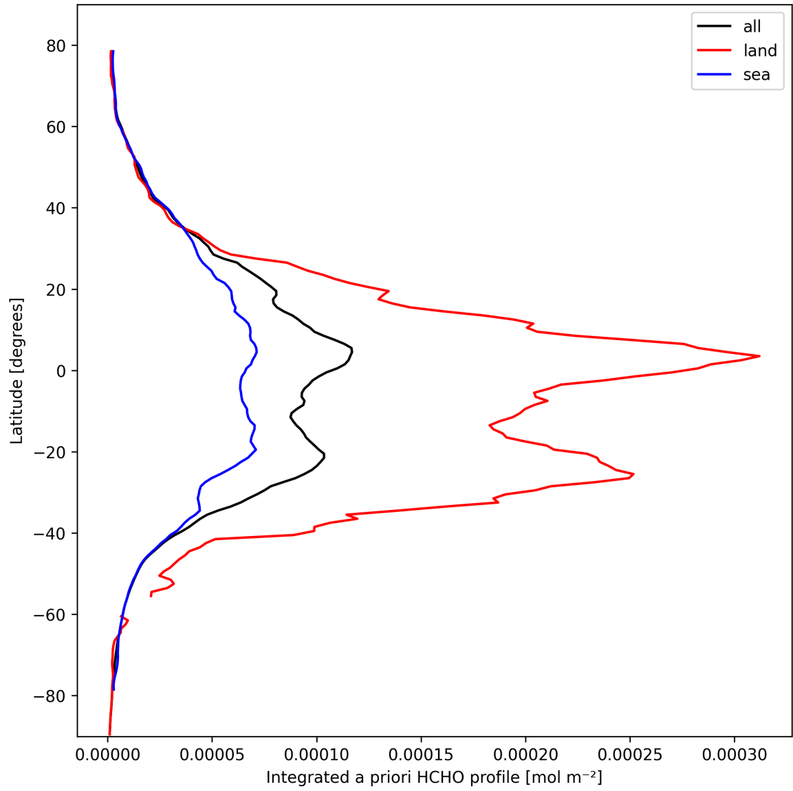
Figure 29: Zonal average of “Integrated a priori HCHO profile” for 2025-03-01 to 2025-03-03.
