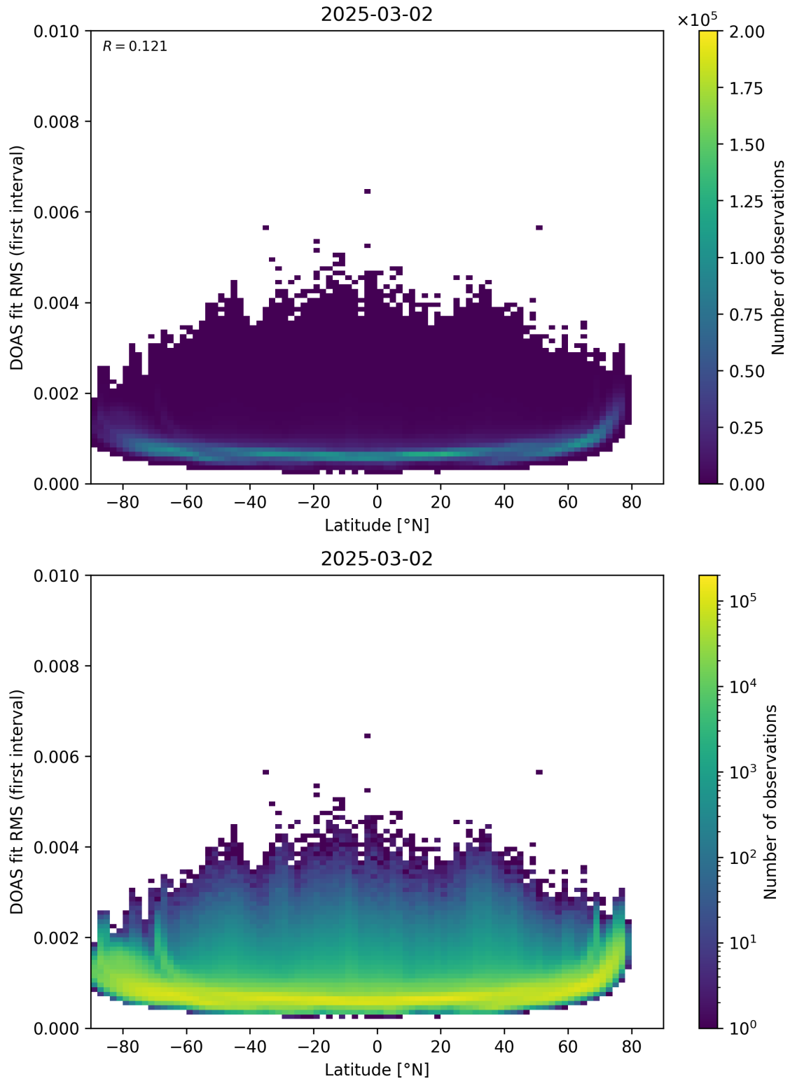
Figure 153: Scatter density plot of “Latitude” against “DOAS fit RMS (first interval)” for 2025-03-01 to 2025-03-03.
