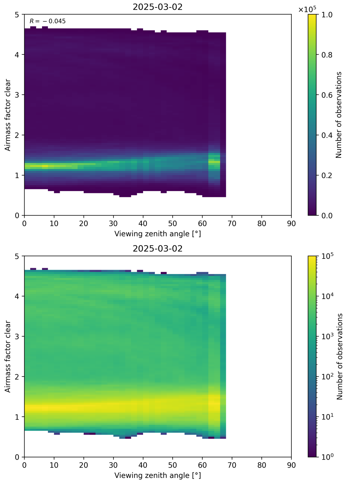
Figure 185: Scatter density plot of “Viewing zenith angle” against “Airmass factor clear” for 2025-03-01 to 2025-03-03.
