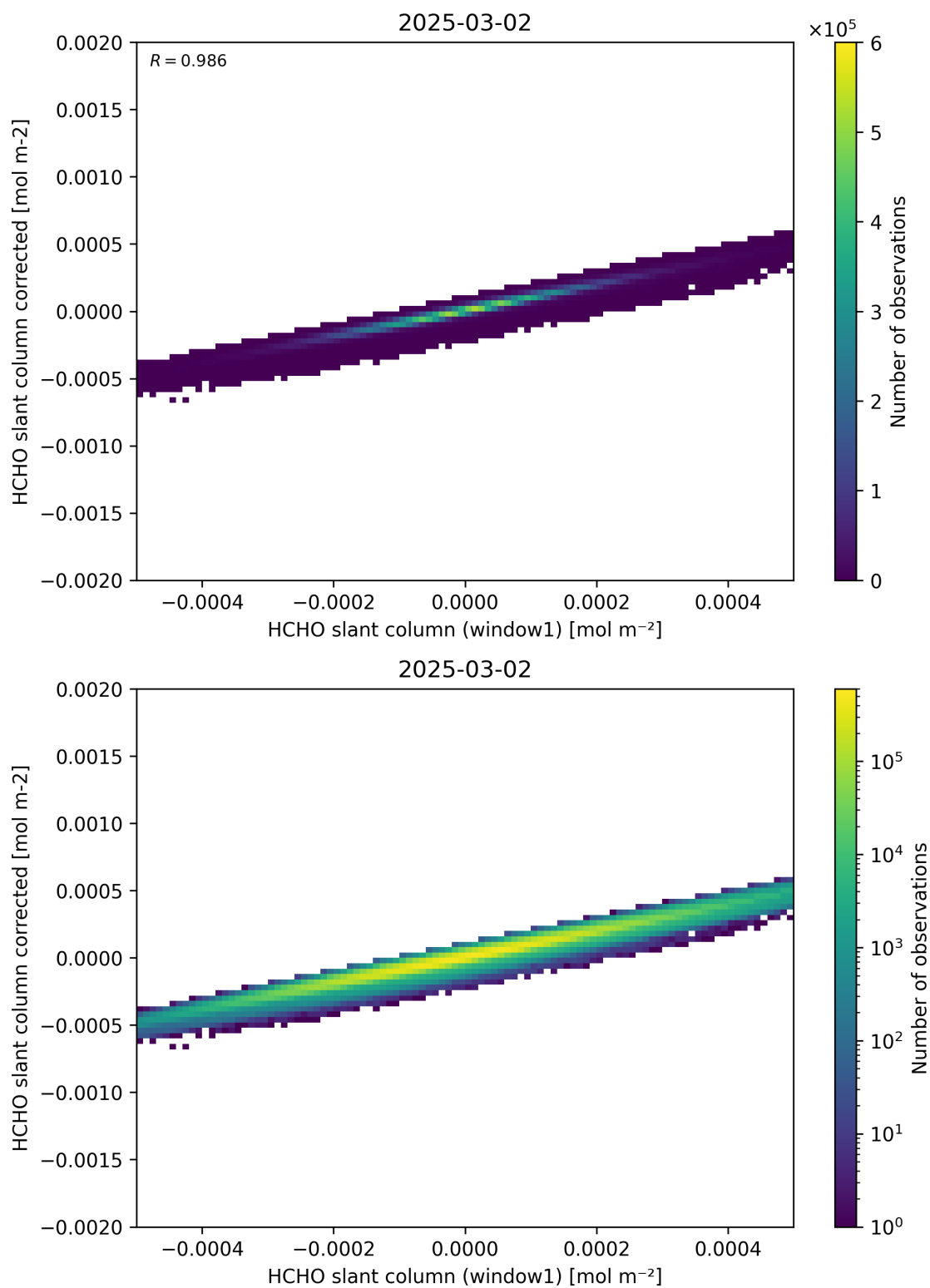
Figure 82: Scatter density plot of “HCHO slant column (window1)” against “HCHO slant column corrected” for 2025-03-01 to 2025-03-03.
