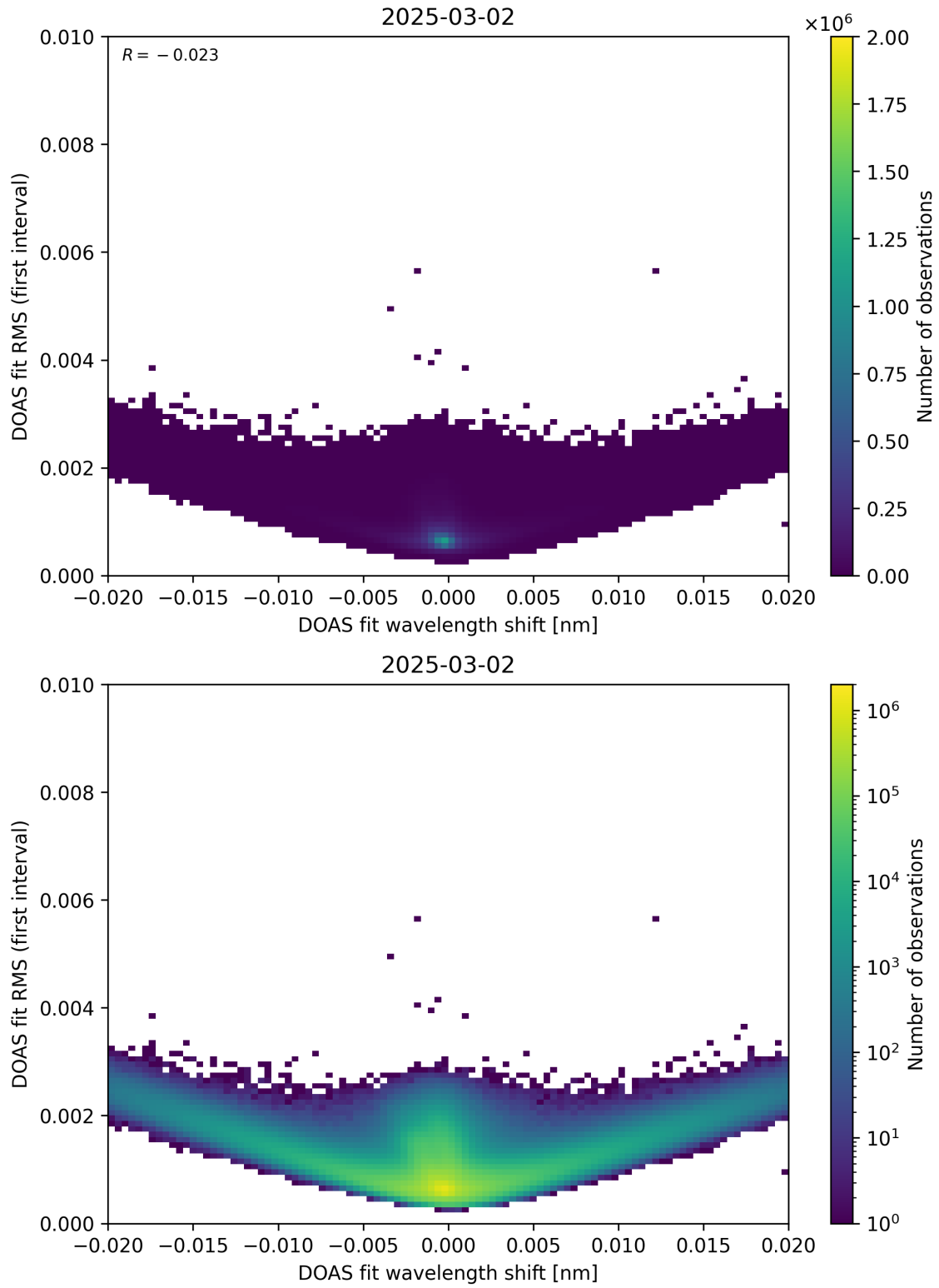
Figure 64: Scatter density plot of “DOAS fit wavelength shift” against “DOAS fit RMS (first interval)” for 2025-03-01 to 2025-03-03.
