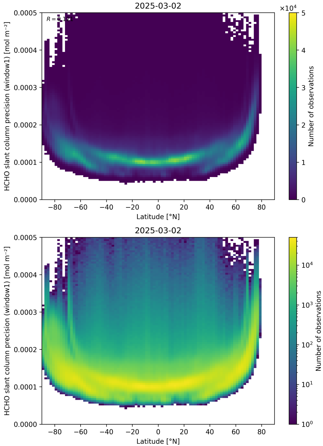
Figure 160: Scatter density plot of “Latitude” against “HCHO slant column precision (window1)” for 2025-03-01 to 2025-03-03.
