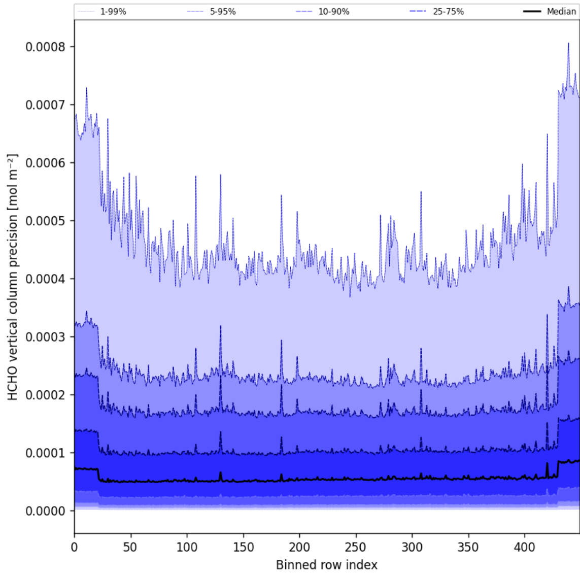
Figure 50: Along track statistics of "HCHO vertical column precision" for 2025-03-01 to 2025-03-03
