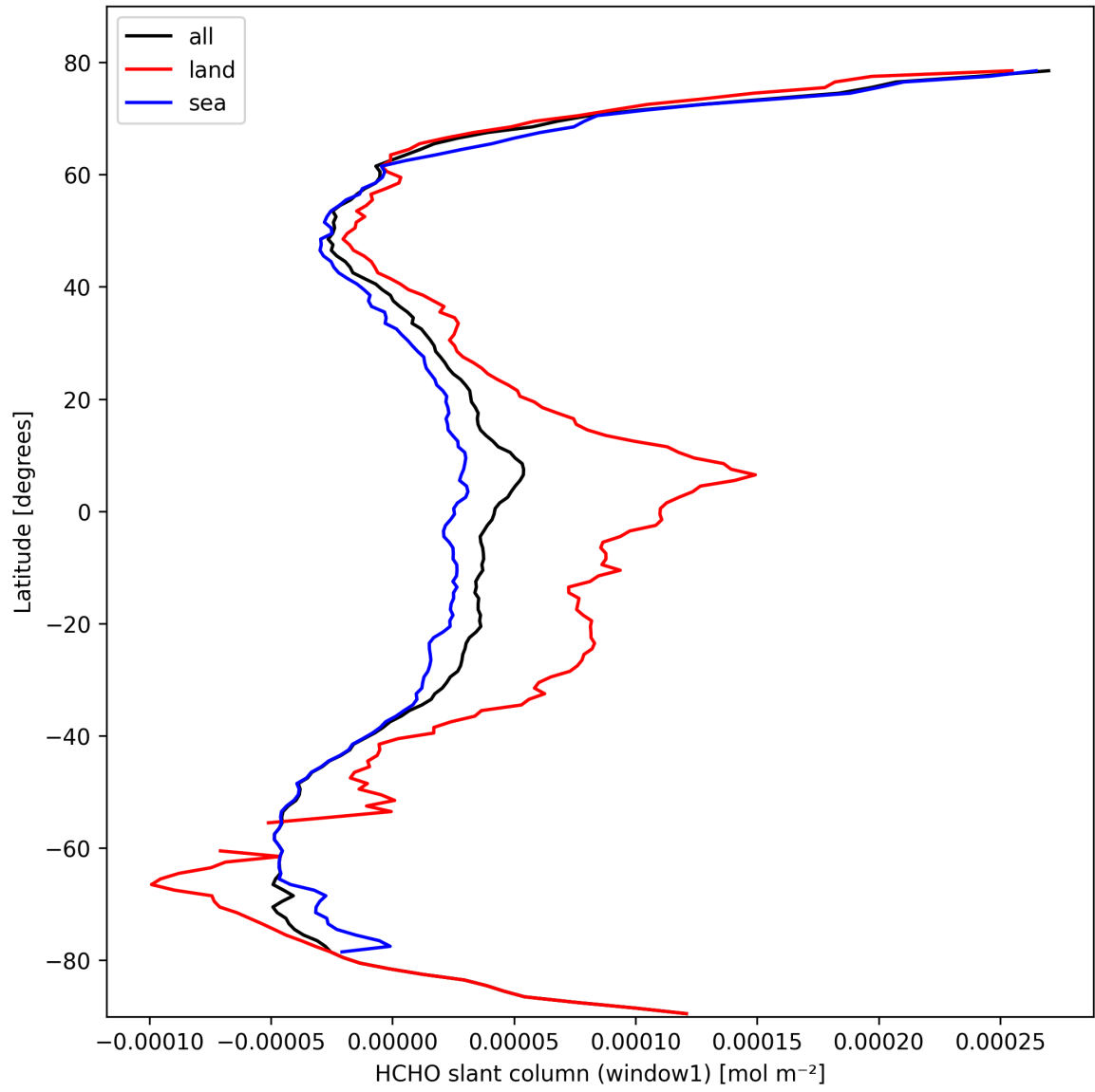
Figure 24: Zonal average of “HCHO slant column (window1)” for 2025-03-01 to 2025-03-03.
