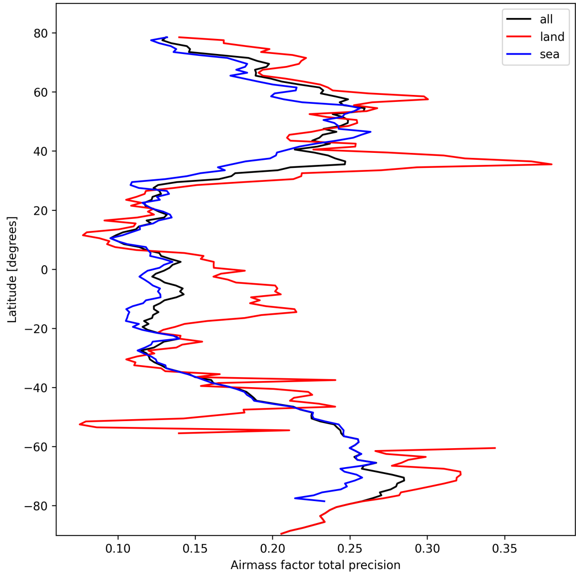
Figure 27: Zonal average of “Airmass factor total precision” for 2025-03-01 to 2025-03-03.
