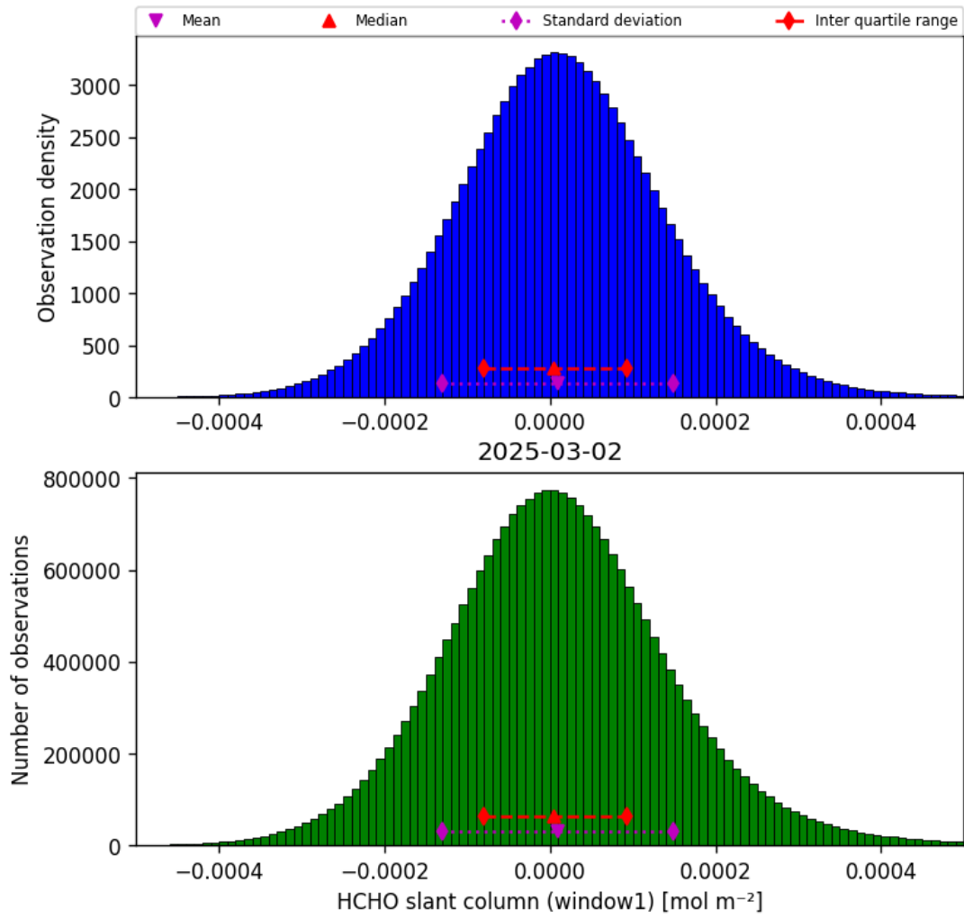
Figure 38: Histogram of “HCHO slant column (window1)” for 2025-03-01 to 2025-03-03
