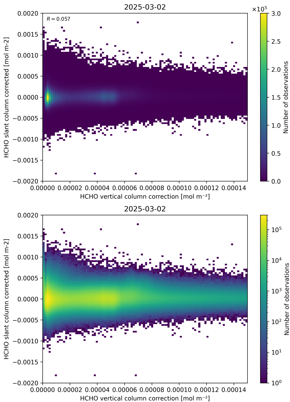
Figure 116: Scatter density plot of “HCHO vertical column correction” against “HCHO slant column corrected” for 2025-03-01 to 2025-03-03.
