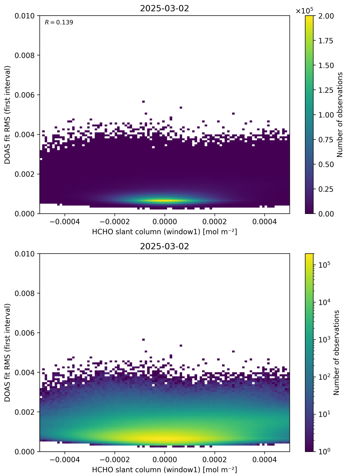
Figure 78: Scatter density plot of “HCHO slant column (window1)” against “DOAS fit RMS (first interval)” for 2025-03-01 to 2025-03-03.
