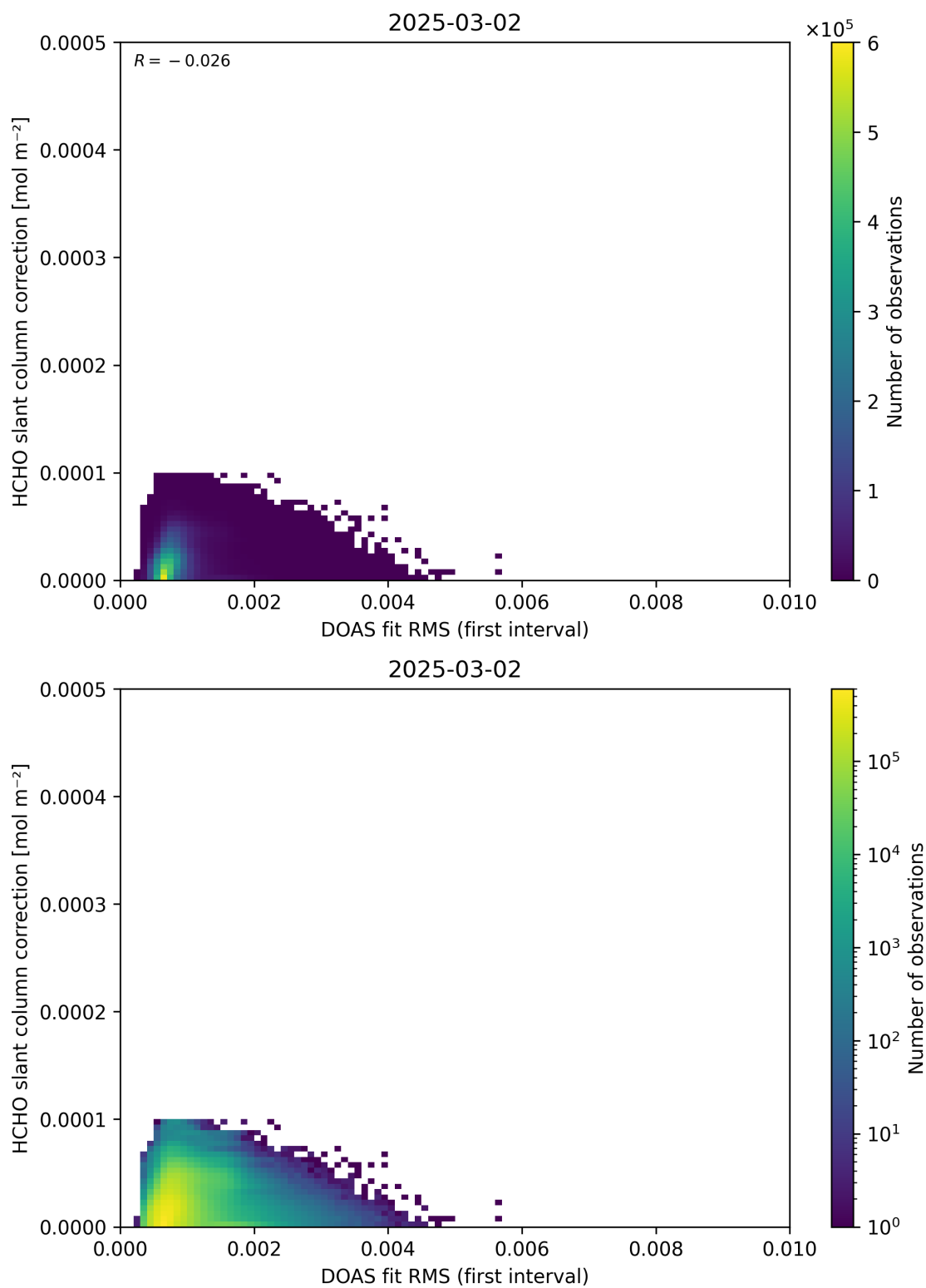
Figure 63: Scatter density plot of “DOAS fit RMS (first interval)” against “HCHO slant column correction” for 2025-03-01 to 2025-03-03.
