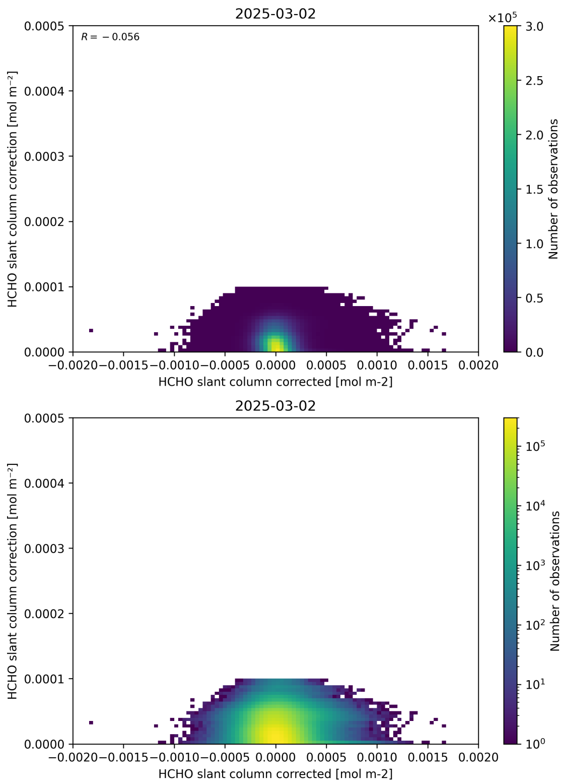
Figure 77: Scatter density plot of “HCHO slant column corrected” against “HCHO slant column correction” for 2025-03-01 to 2025-03-03.
