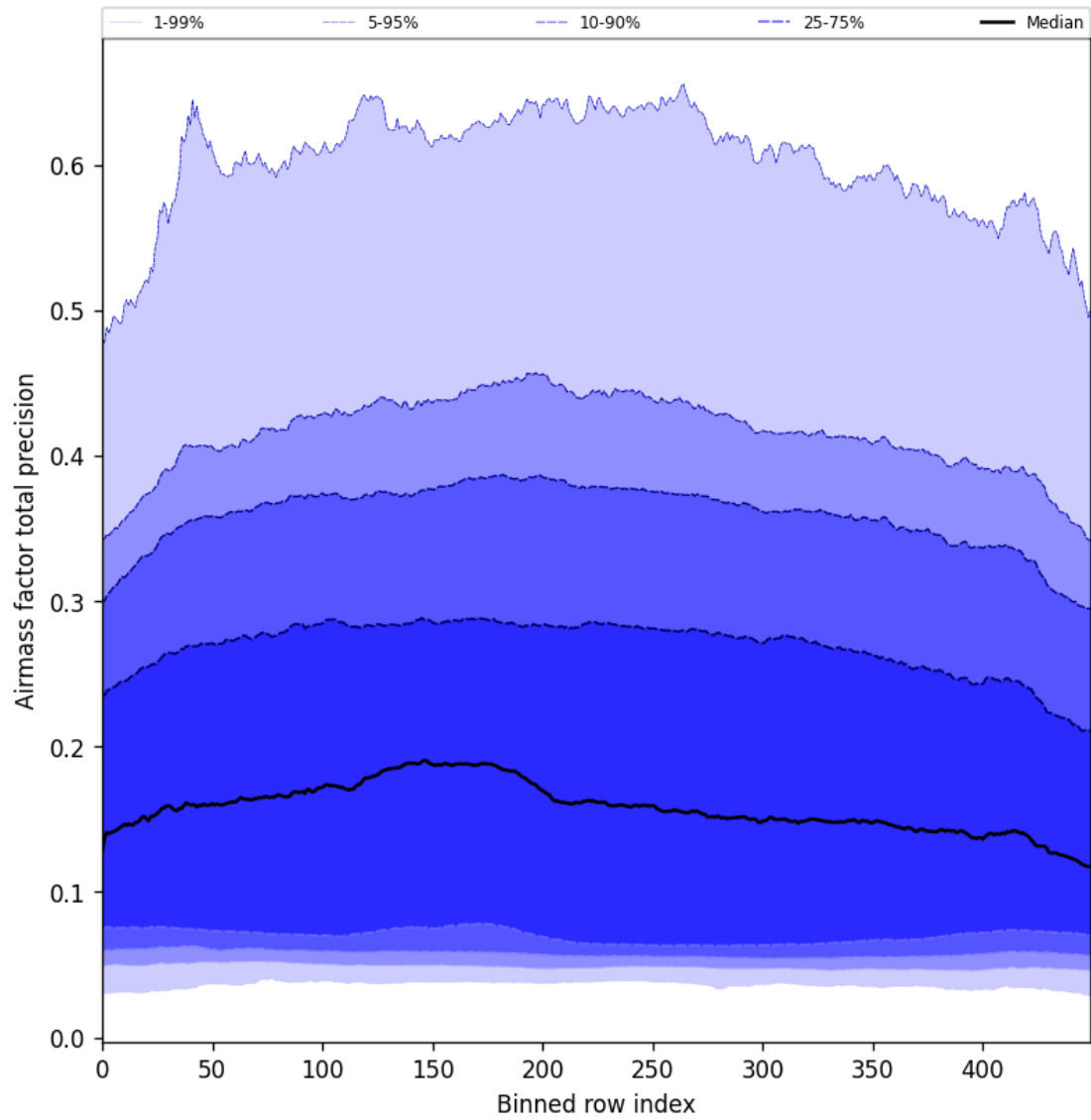
Figure 55: Along track statistics of “Airmass factor total precision” for 2025-03-01 to 2025-03-03
