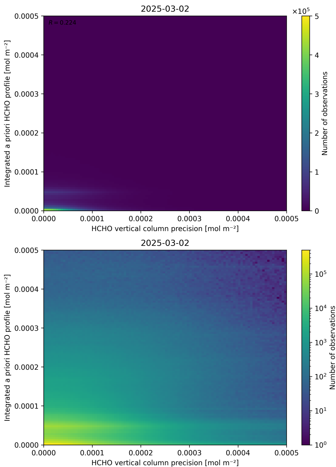
Figure 147: Scatter density plot of “HCHO vertical column precision” against “Integrated a priori HCHO profile” for 2025-03-01 to 2025-03-03.
