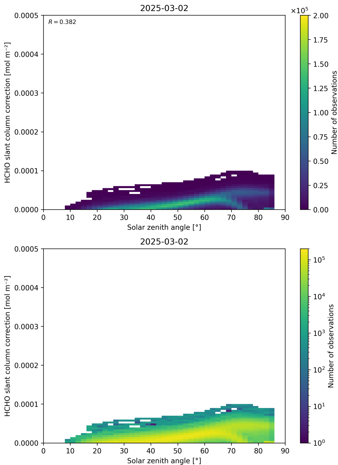
Figure 172: Scatter density plot of “Solar zenith angle” against “HCHO slant column correction” for 2025-03-01 to 2025-03-03.
