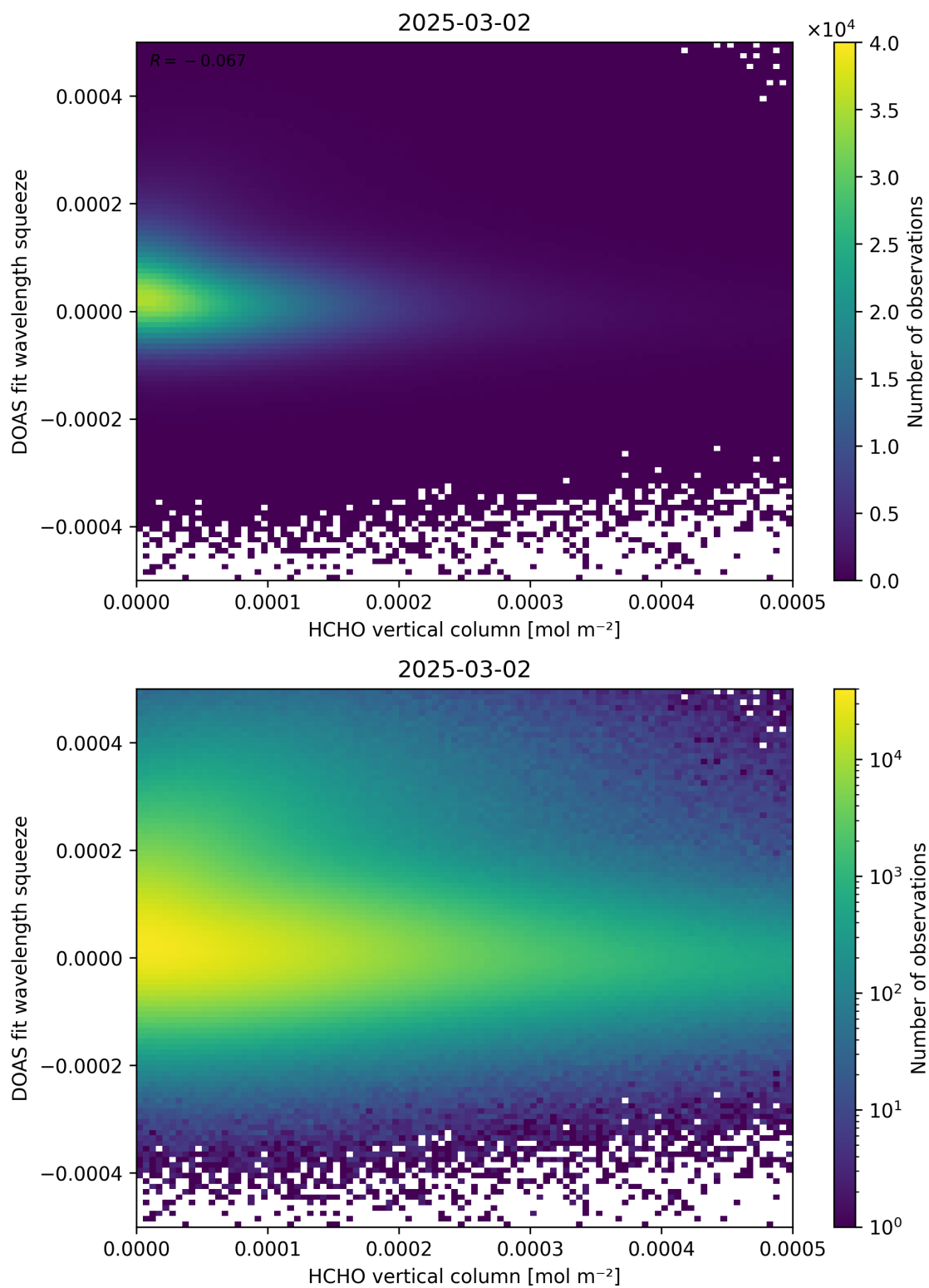
Figure 125: Scatter density plot of “HCHO vertical column” against “DOAS fit wavelength squeeze” for 2025-03-01 to 2025-03-03.
