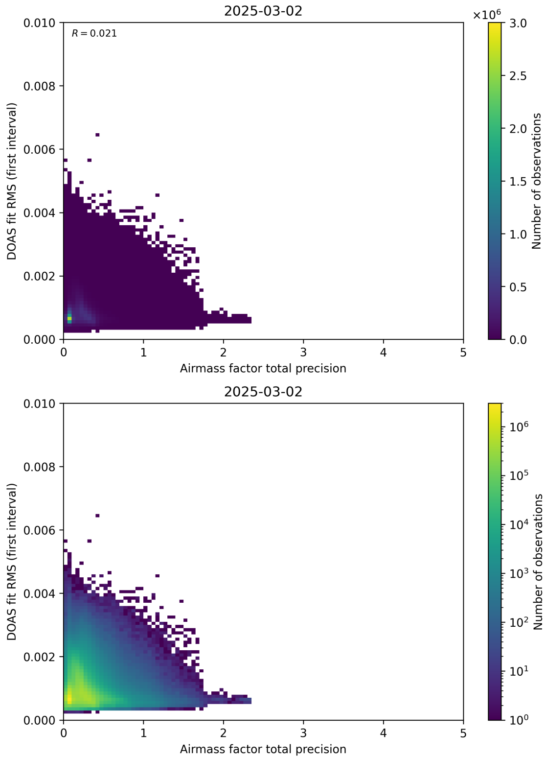
Figure 105: Scatter density plot of “Airmass factor total precision” against “DOAS fit RMS (first interval)” for 2025-03-01 to 2025-03-03.
