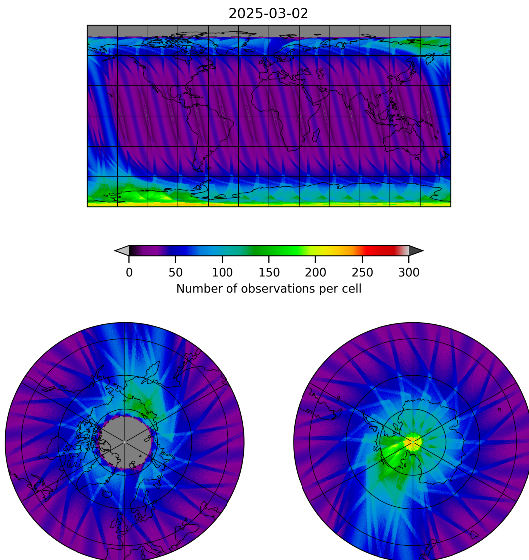
Figure 19: Map of the number of observations for 2025-03-01 to 2025-03-03
