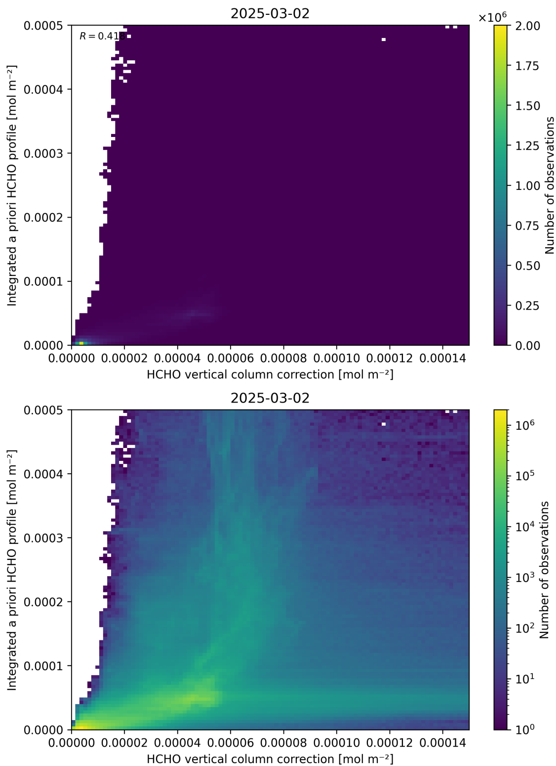
Figure 122: Scatter density plot of “HCHO vertical column correction” against “Integrated a priori HCHO profile” for 2025-03-01 to 2025-03-03.
