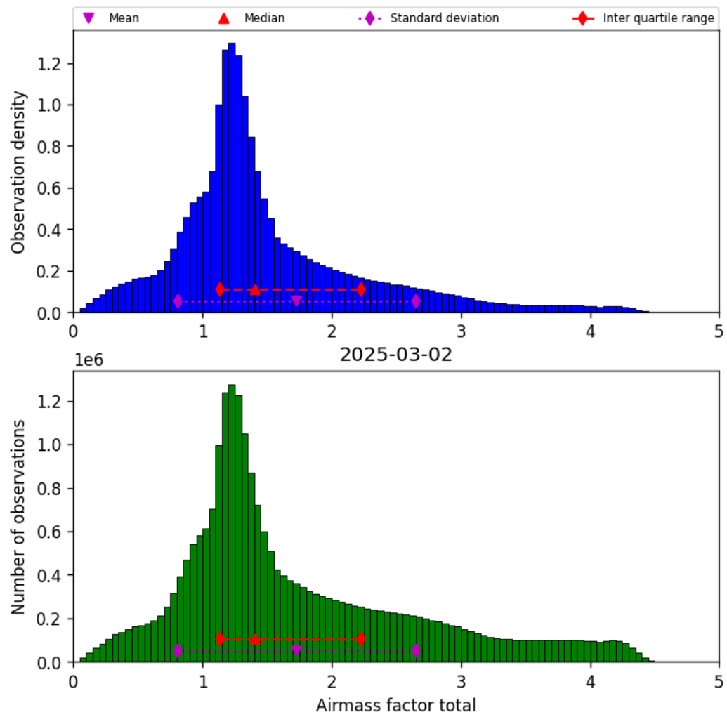
Figure 40: Histogram of “Airmass factor total” for 2025-03-01 to 2025-03-03
