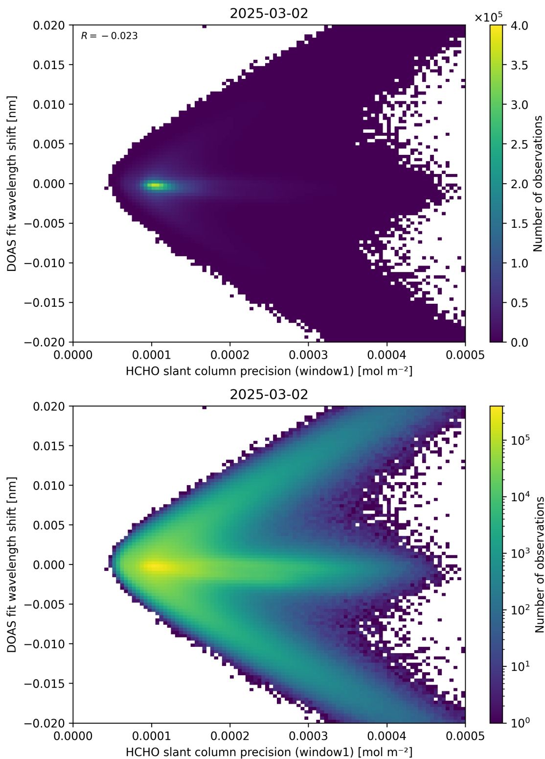
Figure 89: Scatter density plot of “HCHO slant column precision (window1)” against “DOAS fit wavelength shift” for 2025-03-01 to 2025-03-03.
