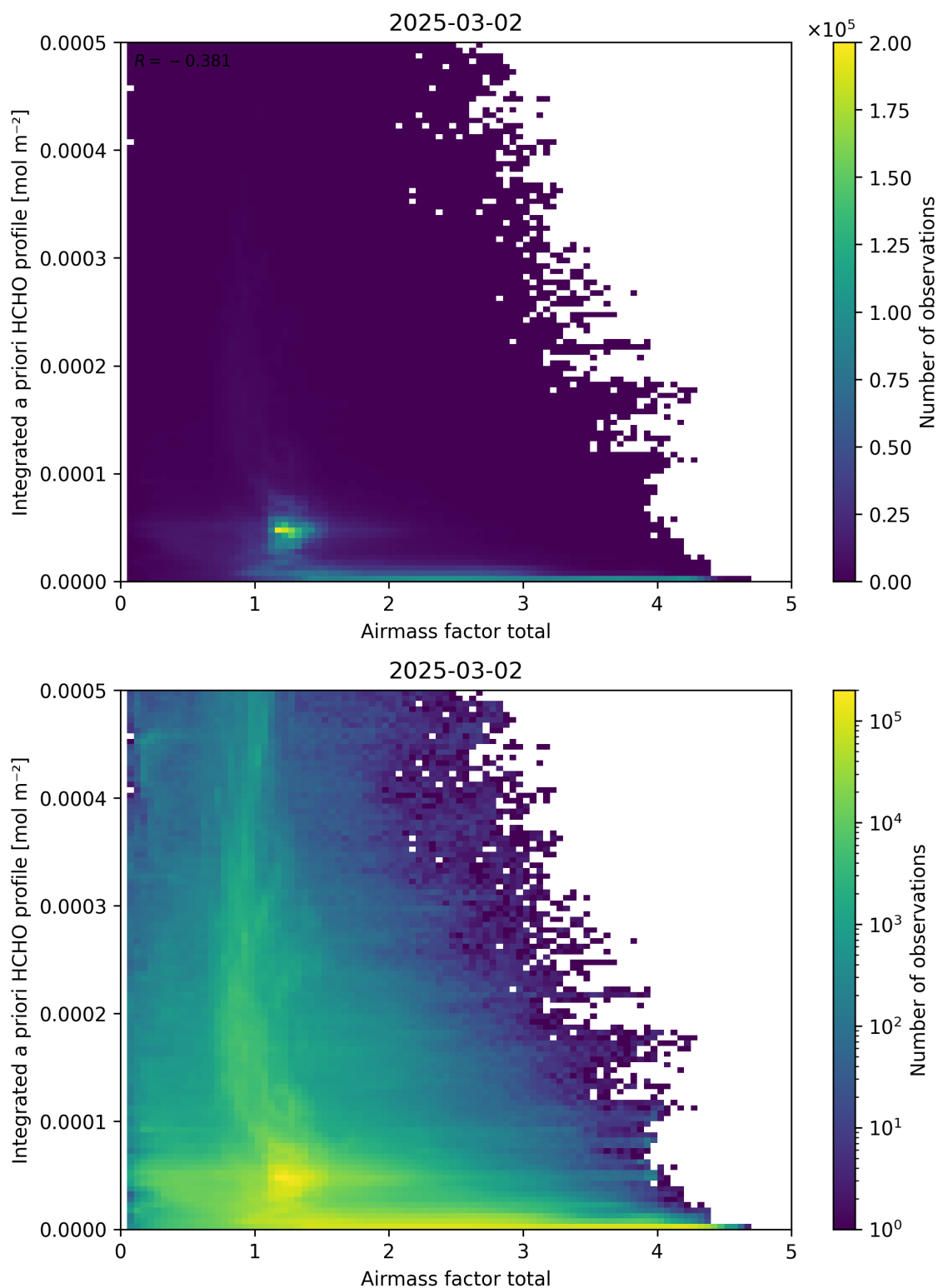
Figure 104: Scatter density plot of “Airmass factor total” against “Integrated a priori HCHO profile” for 2025-03-01 to 2025-03-03.
