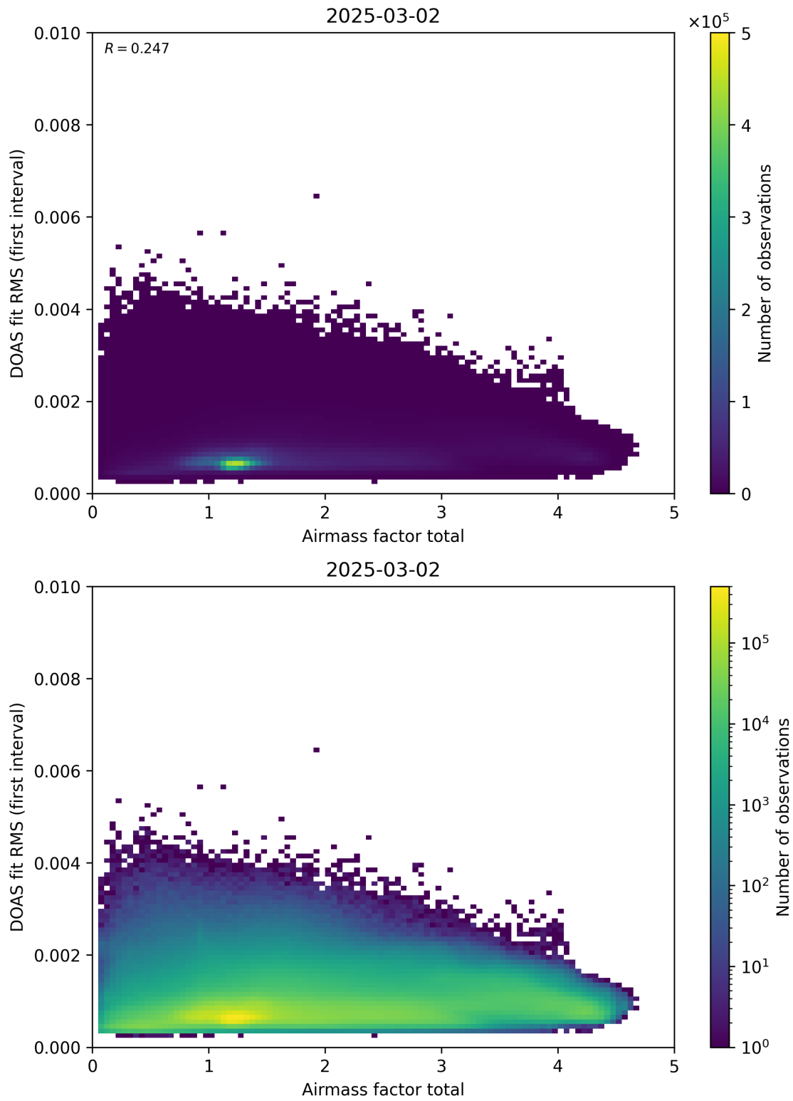
Figure 97: Scatter density plot of “Airmass factor total” against “DOAS fit RMS (first interval)” for 2025-03-01 to 2025-03-03.
