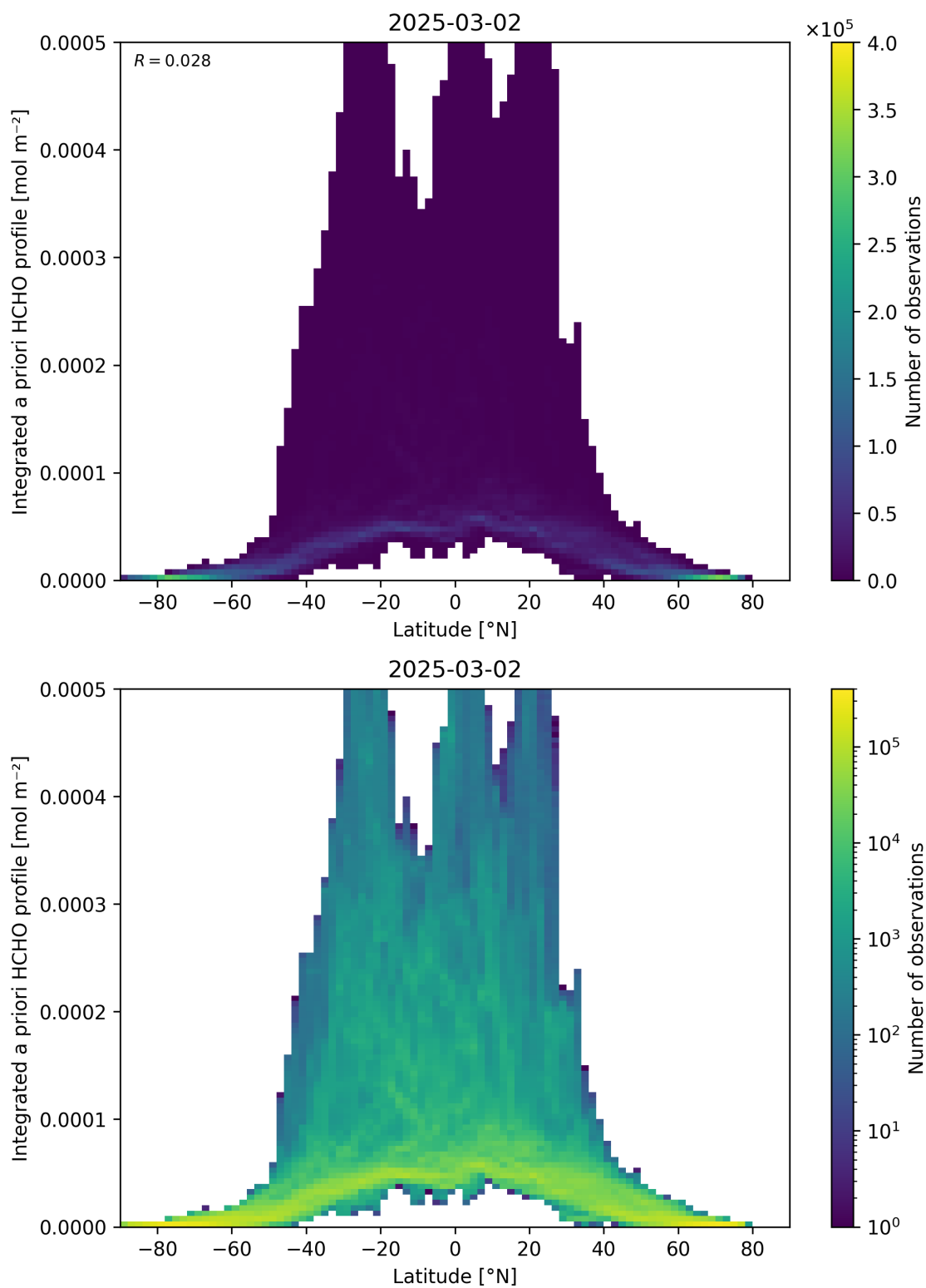
Figure 166: Scatter density plot of “Latitude” against “Integrated a priori HCHO profile” for 2025-03-01 to 2025-03-03.
