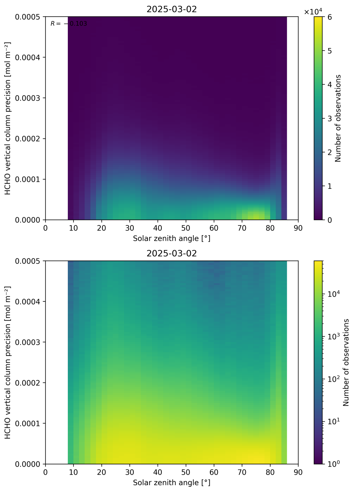
Figure 179: Scatter density plot of “Solar zenith angle” against “HCHO vertical column precision” for 2025-03-01 to 2025-03-03.
