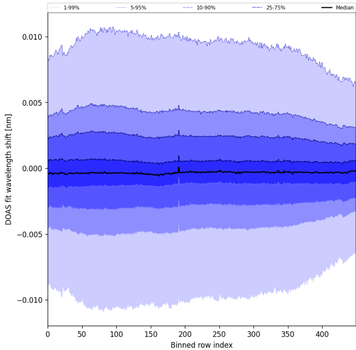
Figure 58: Along track statistics of “DOAS fit wavelength shift” for 2025-03-01 to 2025-03-03
