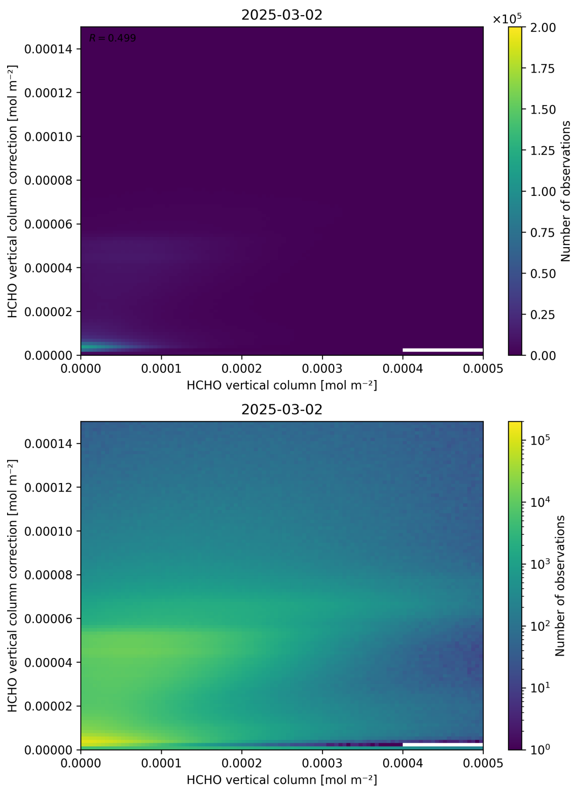
Figure 133: Scatter density plot of “HCHO vertical column” against “HCHO vertical column correction” for 2025-03-01 to 2025-03-03.
