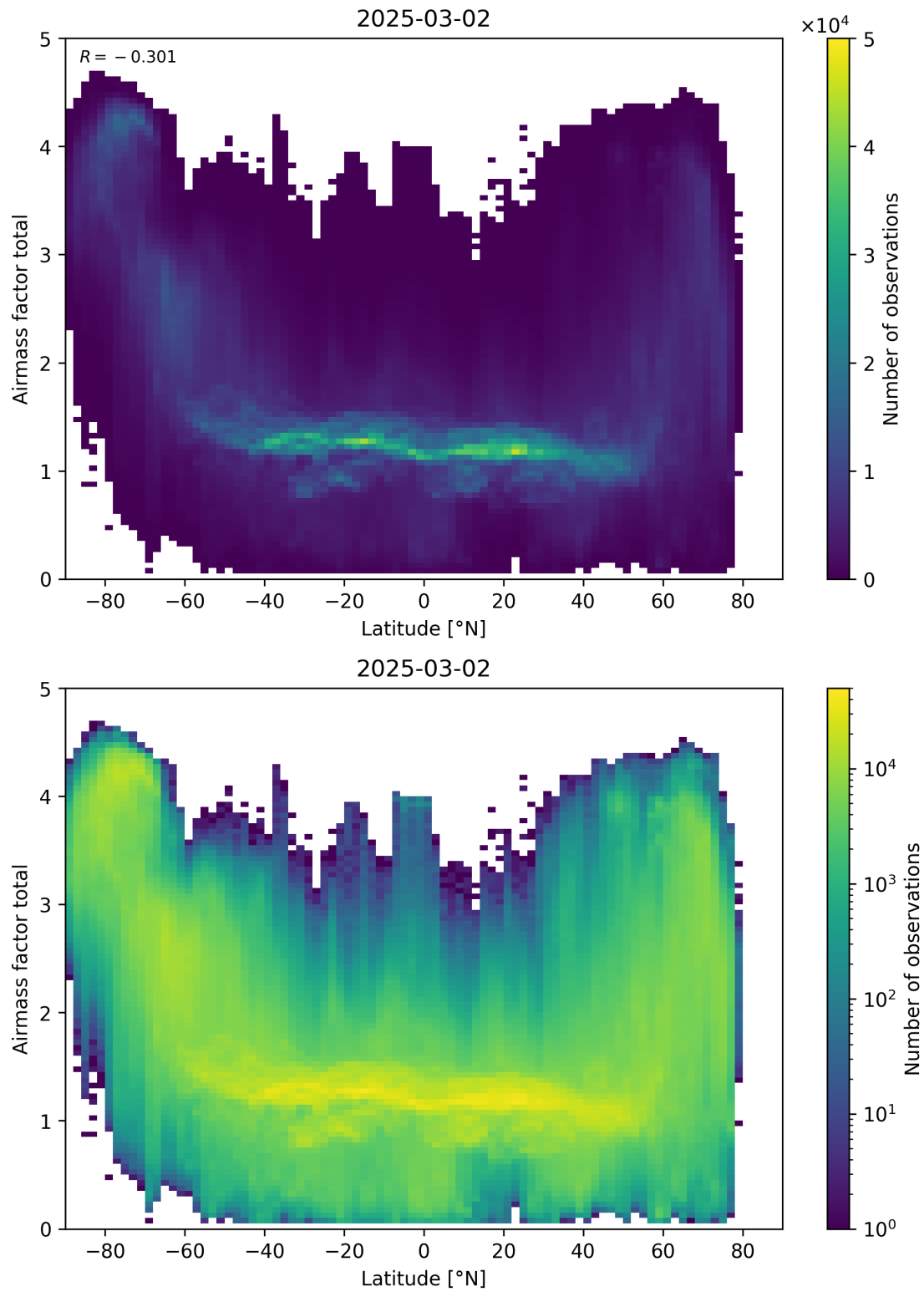
Figure 161: Scatter density plot of “Latitude” against “Airmass factor total” for 2025-03-01 to 2025-03-03.
