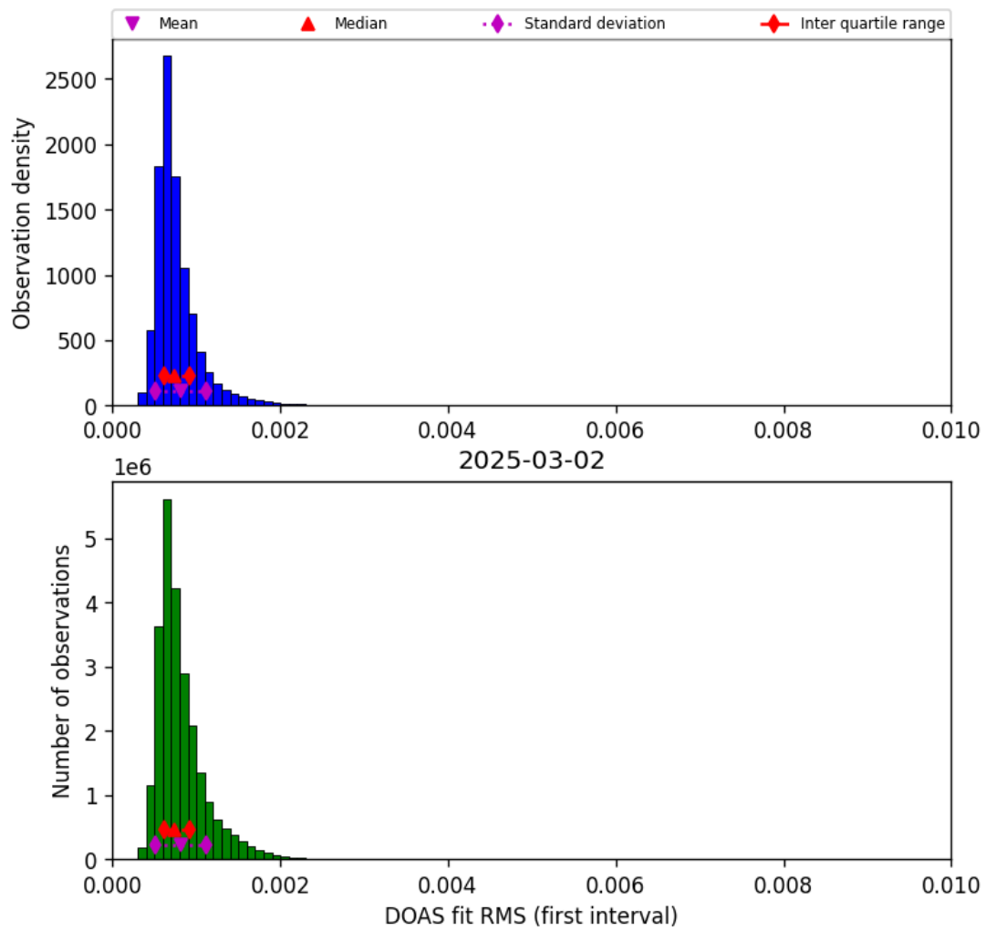
Figure 46: Histogram of “DOAS fit RMS (first interval)” for 2025-03-01 to 2025-03-03
