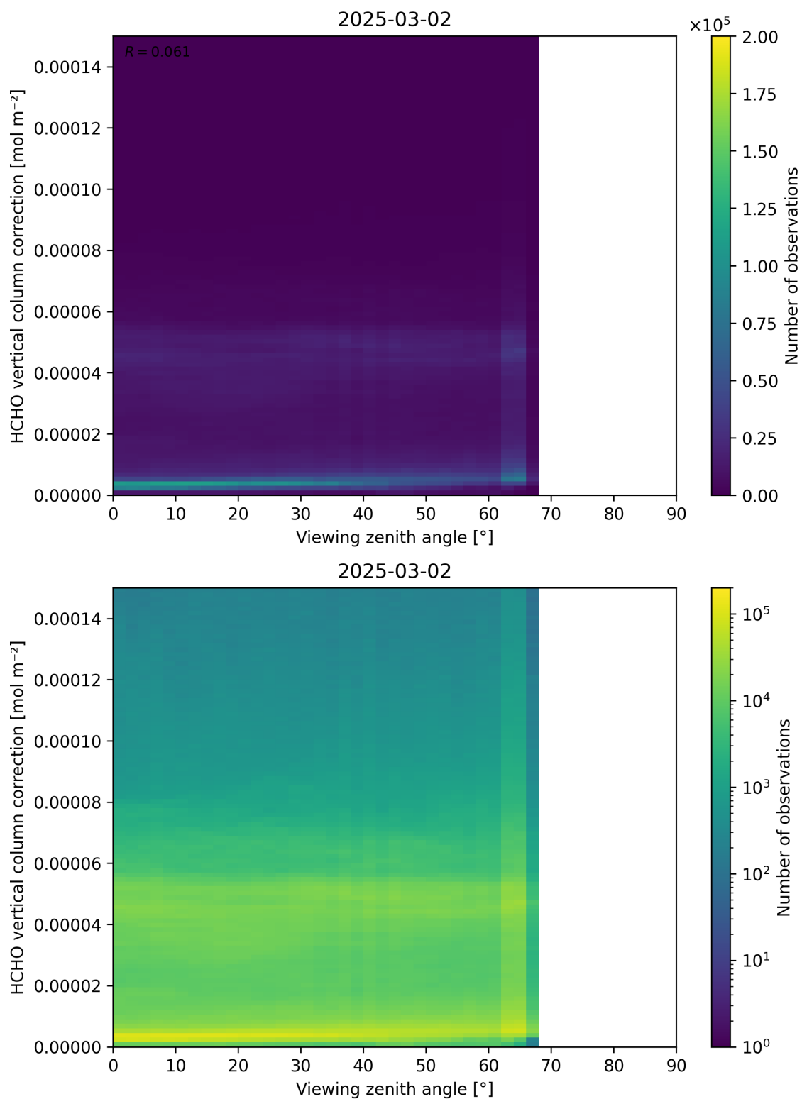
Figure 193: Scatter density plot of “Viewing zenith angle” against “HCHO vertical column correction” for 2025-03-01 to 2025-03-03.
