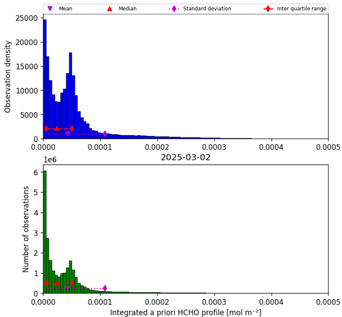
Figure 43: Histogram of “Integrated a priori HCHO profile” for 2025-03-01 to 2025-03-03
