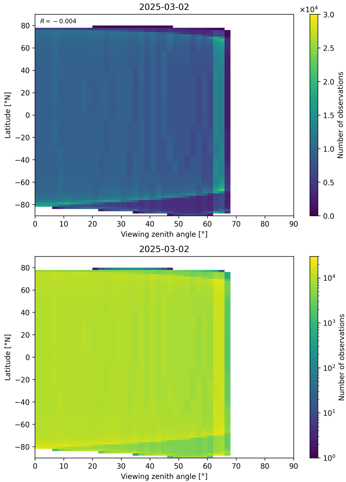
Figure 196: Scatter density plot of “Viewing zenith angle” against “Latitude” for 2025-03-01 to 2025-03-03.
