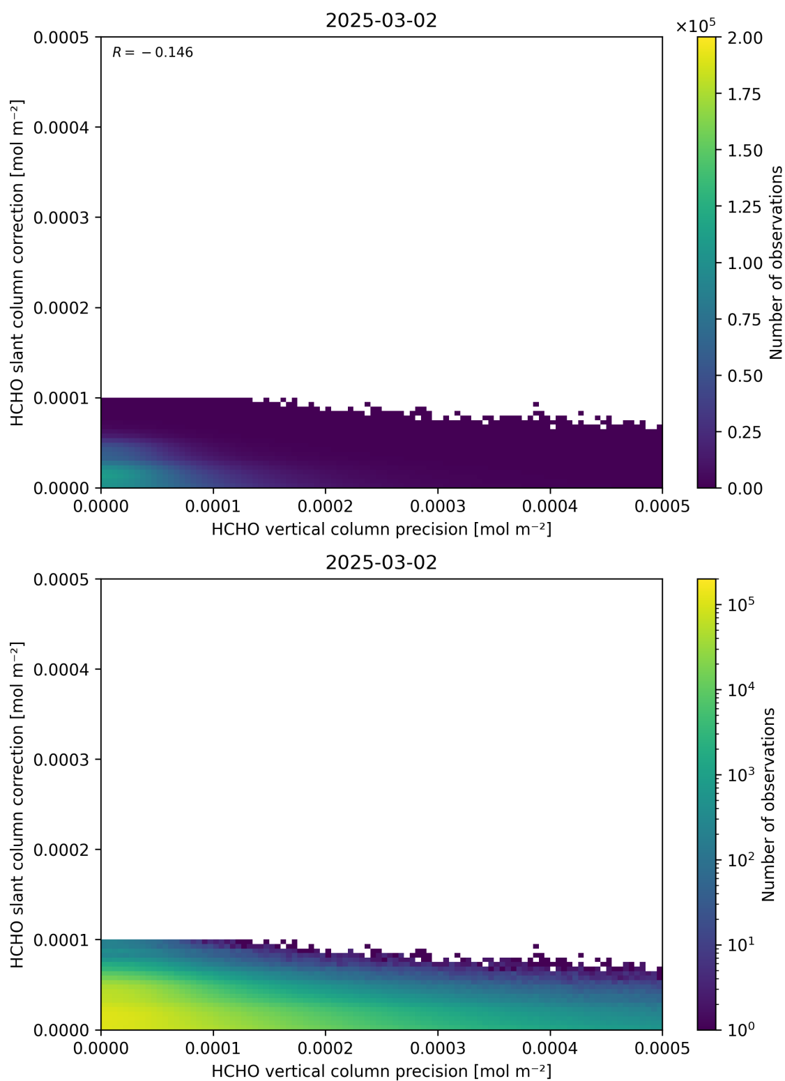
Figure 141: Scatter density plot of “HCHO vertical column precision” against “HCHO slant column correction” for 2025-03-01 to 2025-03-03.
