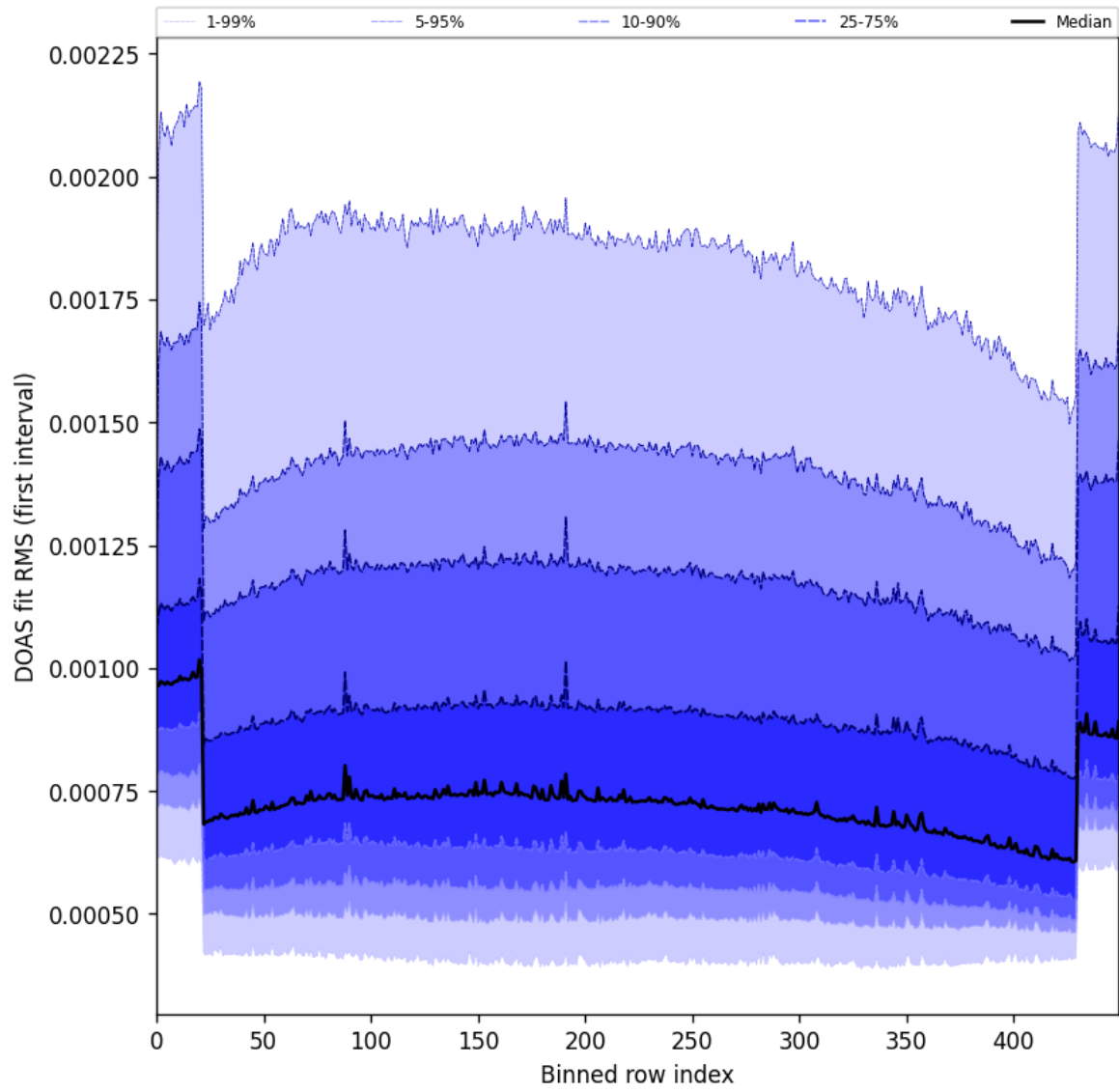
Figure 60: Along track statistics of “DOAS fit RMS (first interval)” for 2025-03-01 to 2025-03-03
