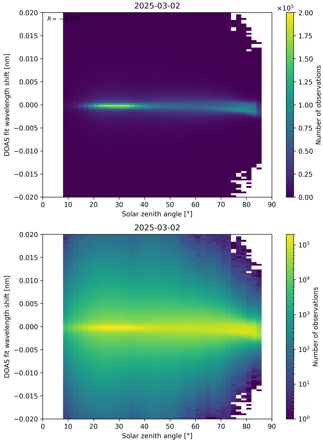
Figure 168: Scatter density plot of “Solar zenith angle” against “DOAS fit wavelength shift” for 2025-03-01 to 2025-03-03.
