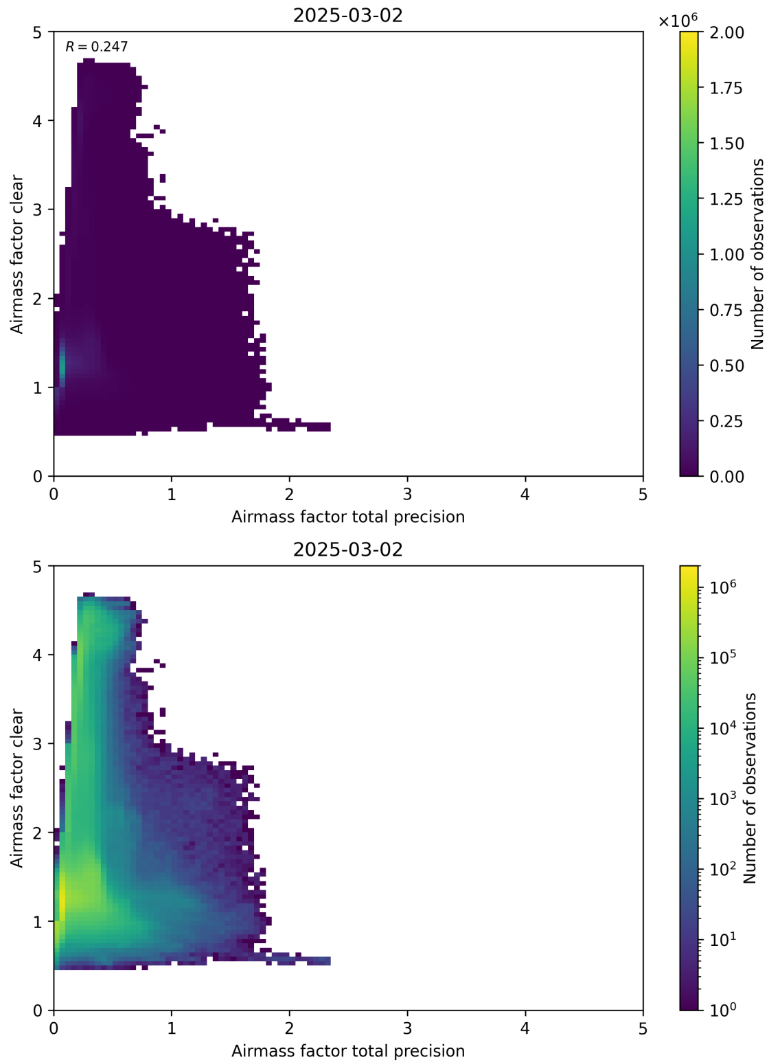
Figure 108: Scatter density plot of “Airmass factor total precision” against “Airmass factor clear” for 2025-03-01 to 2025-03-03.
