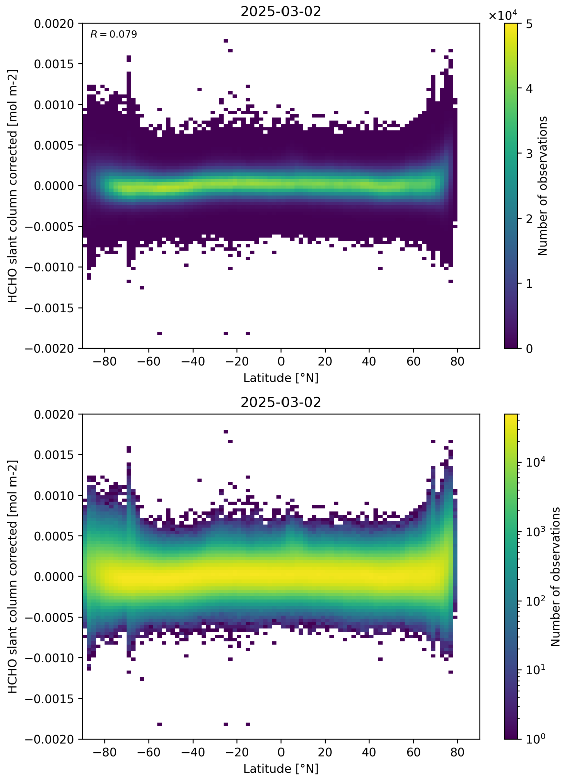
Figure 157: Scatter density plot of “Latitude” against “HCHO slant column corrected” for 2025-03-01 to 2025-03-03.
