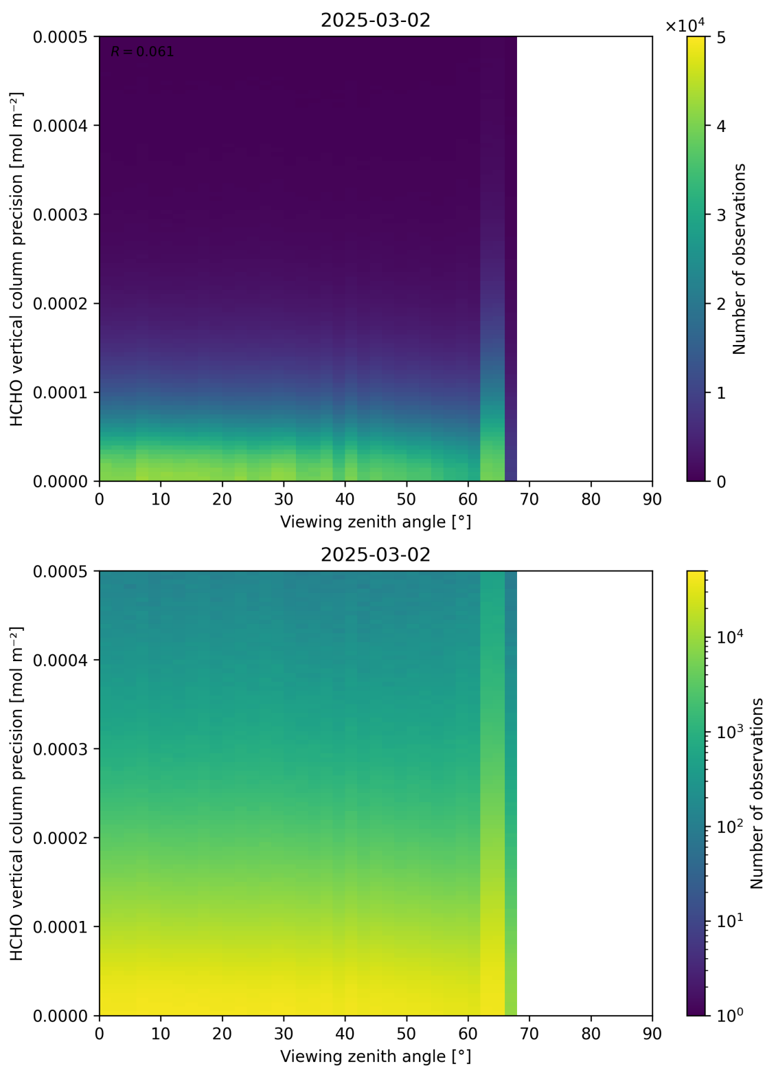
Figure 194: Scatter density plot of “Viewing zenith angle” against “HCHO vertical column precision” for 2025-03-01 to 2025-03-03.
