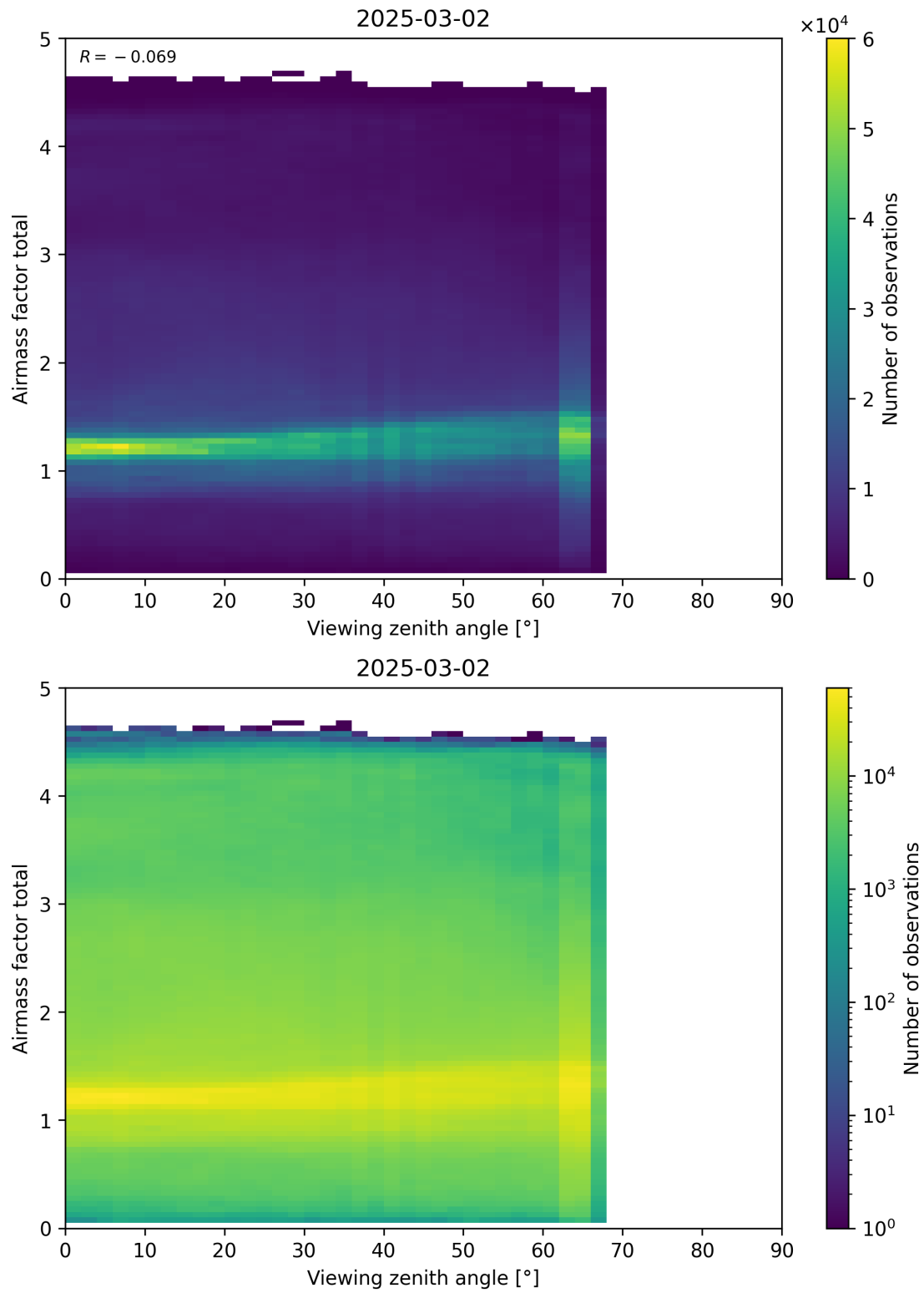
Figure 190: Scatter density plot of “Viewing zenith angle” against “Airmass factor total” for 2025-03-01 to 2025-03-03.
