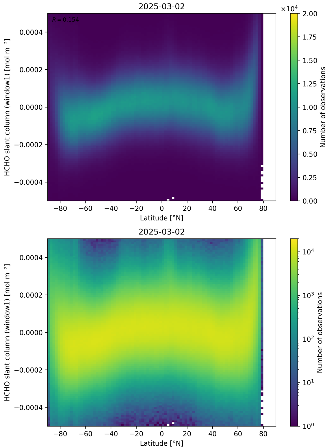
Figure 159: Scatter density plot of “Latitude” against “HCHO slant column (window1)” for 2025-03-01 to 2025-03-03.
