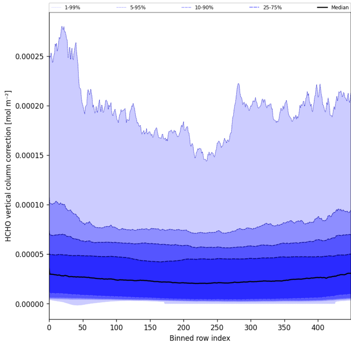
Figure 51: Along track statistics of “HCHO vertical column correction” for 2025-03-01 to 2025-03-03
