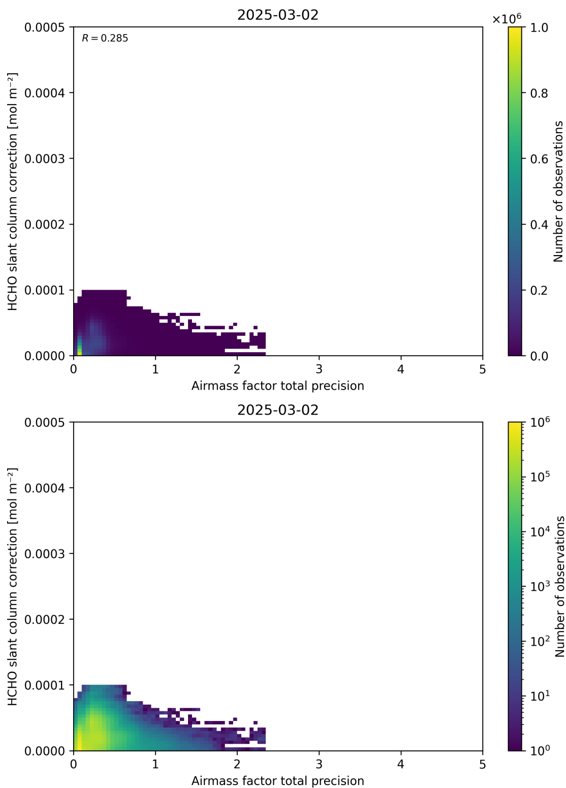
Figure 110: Scatter density plot of “Airmass factor total precision” against “HCHO slant column correction” for 2025-03-01 to 2025-03-03.
