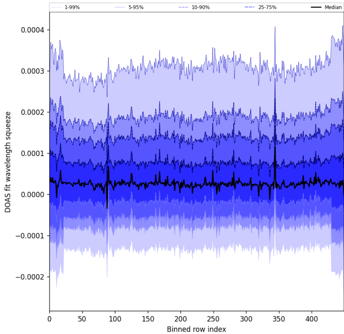
Figure 59: Along track statistics of “DOAS fit wavelength squeeze” for 2025-03-01 to 2025-03-03
