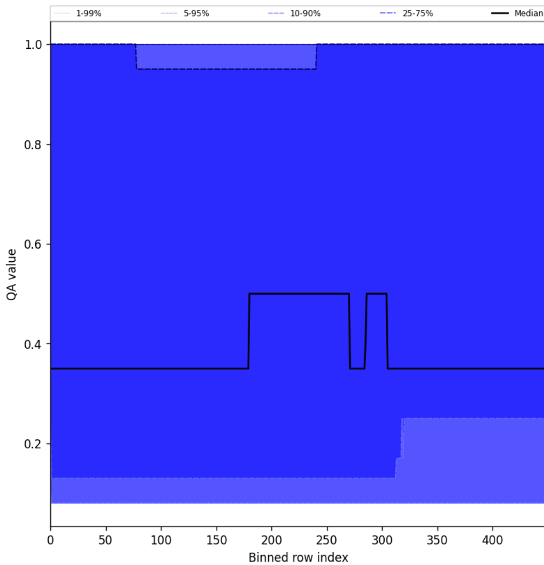
Figure 48: Along track statistics of “QA value” for 2025-03-01 to 2025-03-03
