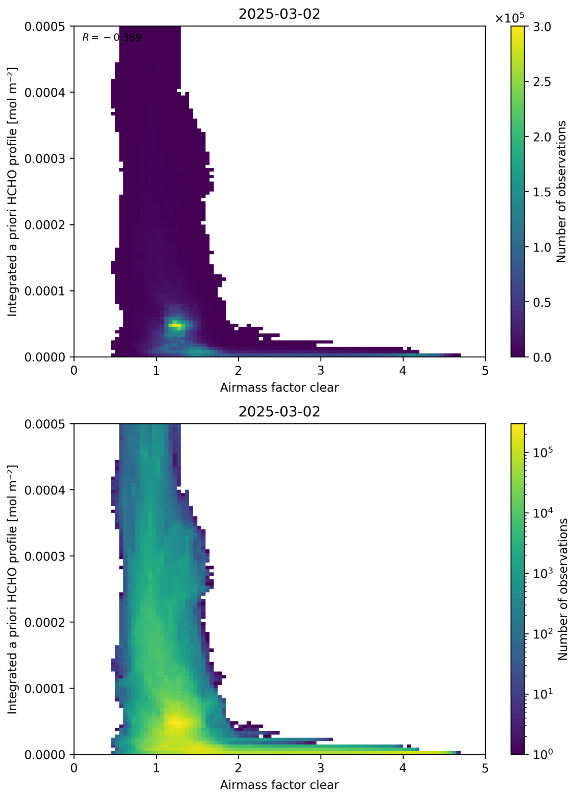
Figure 76: Scatter density plot of “Airmass factor clear” against “Integrated a priori HCHO profile” for 2025-03-01 to 2025-03-03.
