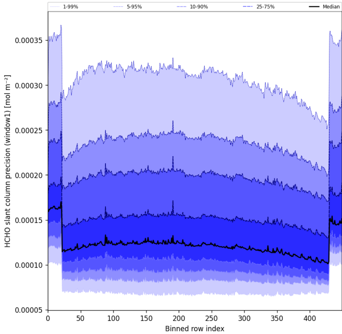
Figure 53: Along track statistics of “HCHO slant column precision (window1)” for 2025-03-01 to 2025-03-03
