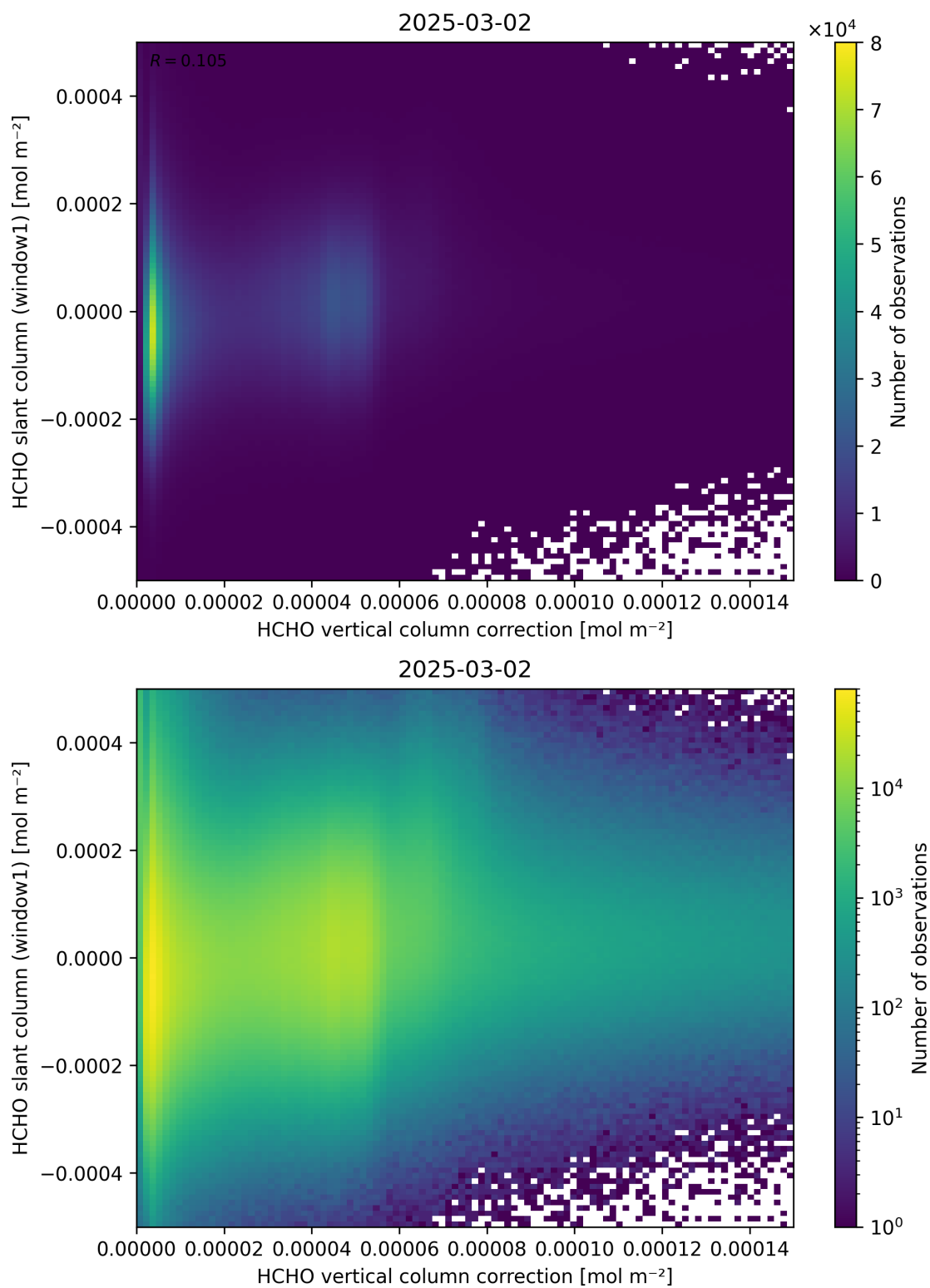
Figure 118: Scatter density plot of “HCHO vertical column correction” against “HCHO slant column (window1)” for 2025-03-01 to 2025-03-03.
