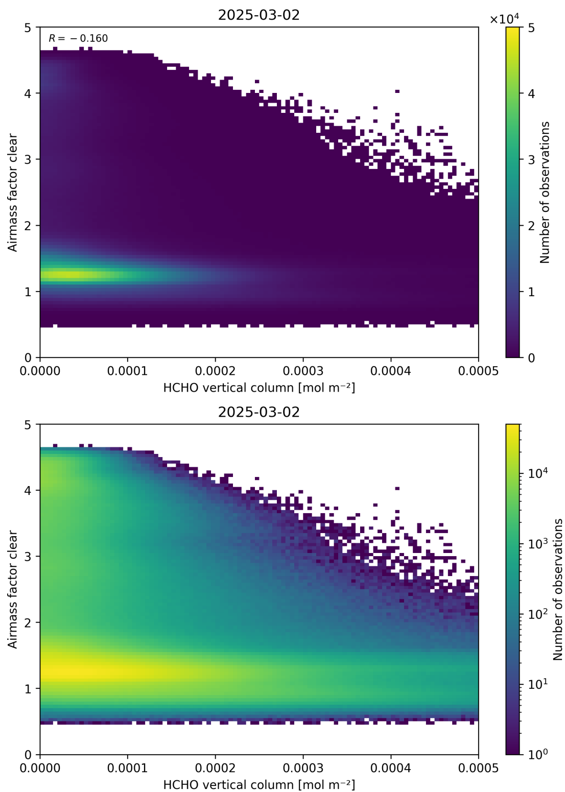
Figure 126: Scatter density plot of “HCHO vertical column” against “Airmass factor clear” for 2025-03-01 to 2025-03-03.
