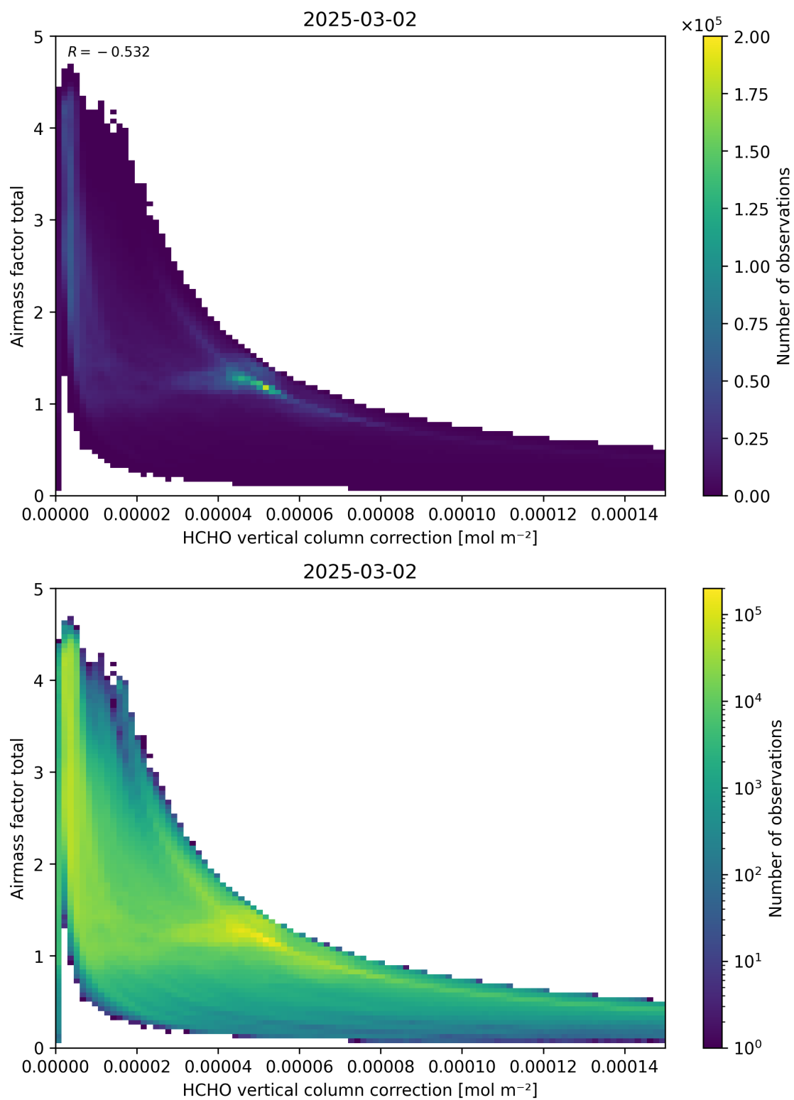
Figure 120: Scatter density plot of “HCHO vertical column correction” against “Airmass factor total” for 2025-03-01 to 2025-03-03.
