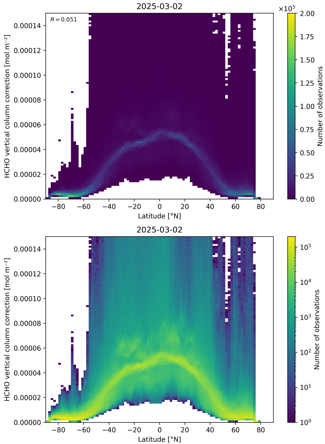
Figure 164: Scatter density plot of “Latitude” against “HCHO vertical column correction” for 2025-03-01 to 2025-03-03.
