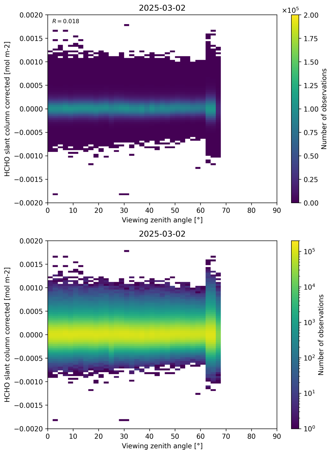
Figure 186: Scatter density plot of “Viewing zenith angle” against “HCHO slant column corrected” for 2025-03-01 to 2025-03-03.
