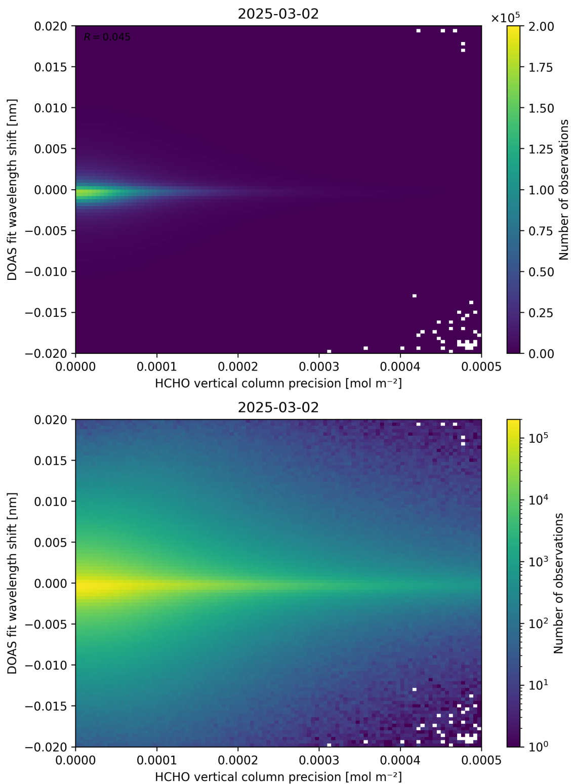
Figure 137: Scatter density plot of “HCHO vertical column precision” against “DOAS fit wavelength shift” for 2025-03-01 to 2025-03-03.
