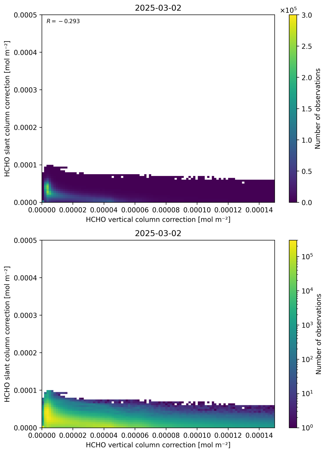
Figure 117: Scatter density plot of “HCHO vertical column correction” against “HCHO slant column correction” for 2025-03-01 to 2025-03-03.
