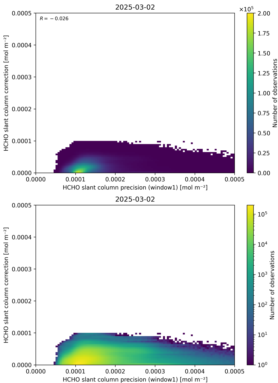
Figure 93: Scatter density plot of “HCHO slant column precision (window1)” against “HCHO slant column correction” for 2025-03-01 to 2025-03-03.
