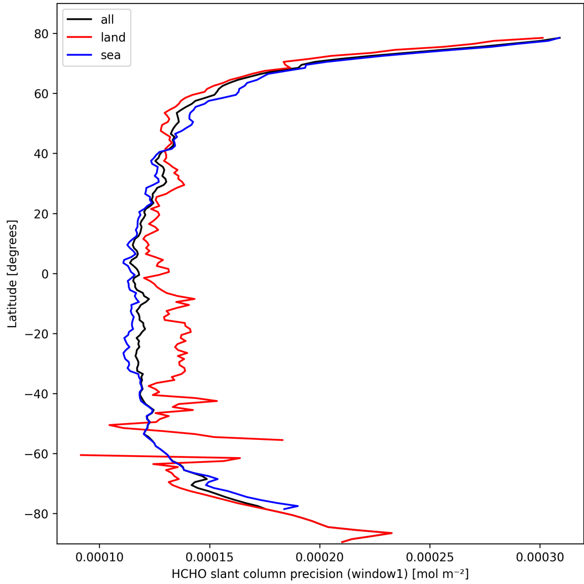
Figure 25: Zonal average of “HCHO slant column precision (window1)” for 2025-03-01 to 2025-03-03.
