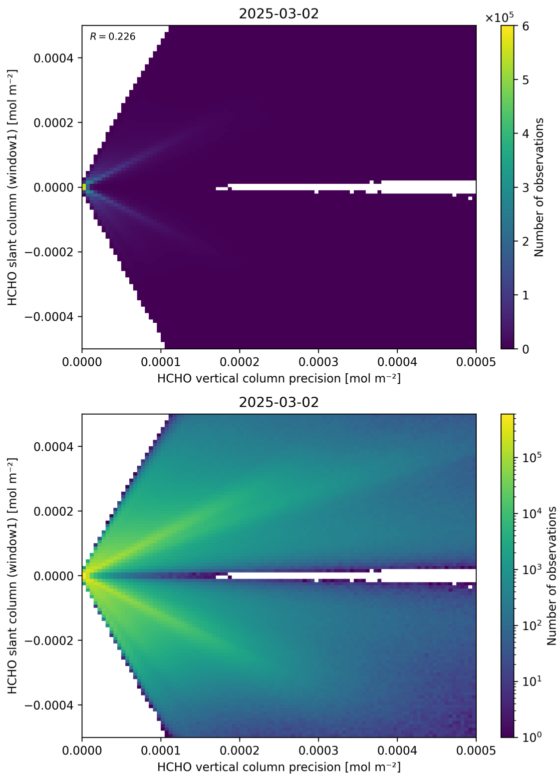
Figure 142: Scatter density plot of “HCHO vertical column precision” against “HCHO slant column (window1)” for 2025-03-01 to 2025-03-03.
