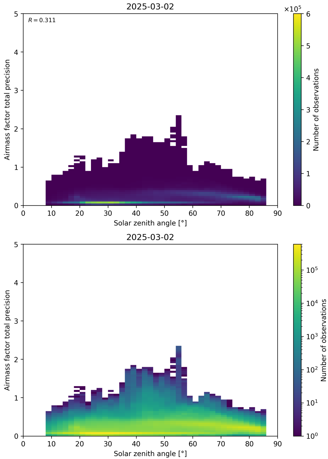
Figure 176: Scatter density plot of “Solar zenith angle” against “Airmass factor total precision” for 2025-03-01 to 2025-03-03.
