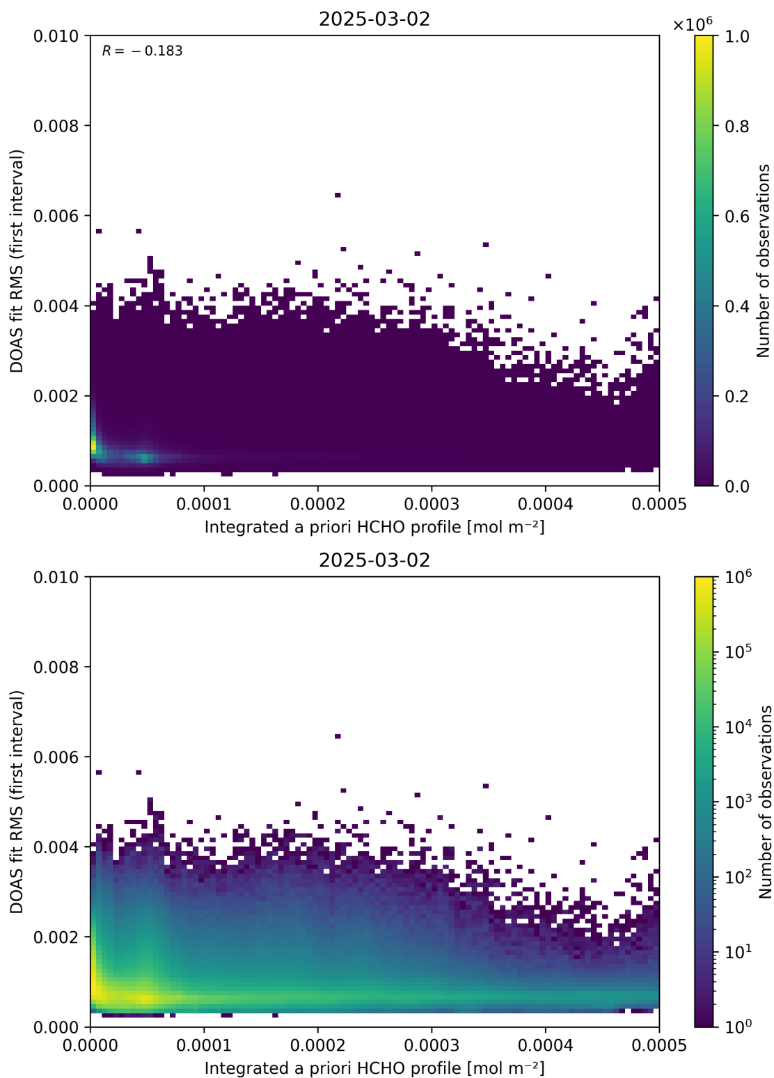
Figure 148: Scatter density plot of “Integrated a priori HCHO profile” against “DOAS fit RMS (first interval)” for 2025-03-01 to 2025-03-03.
