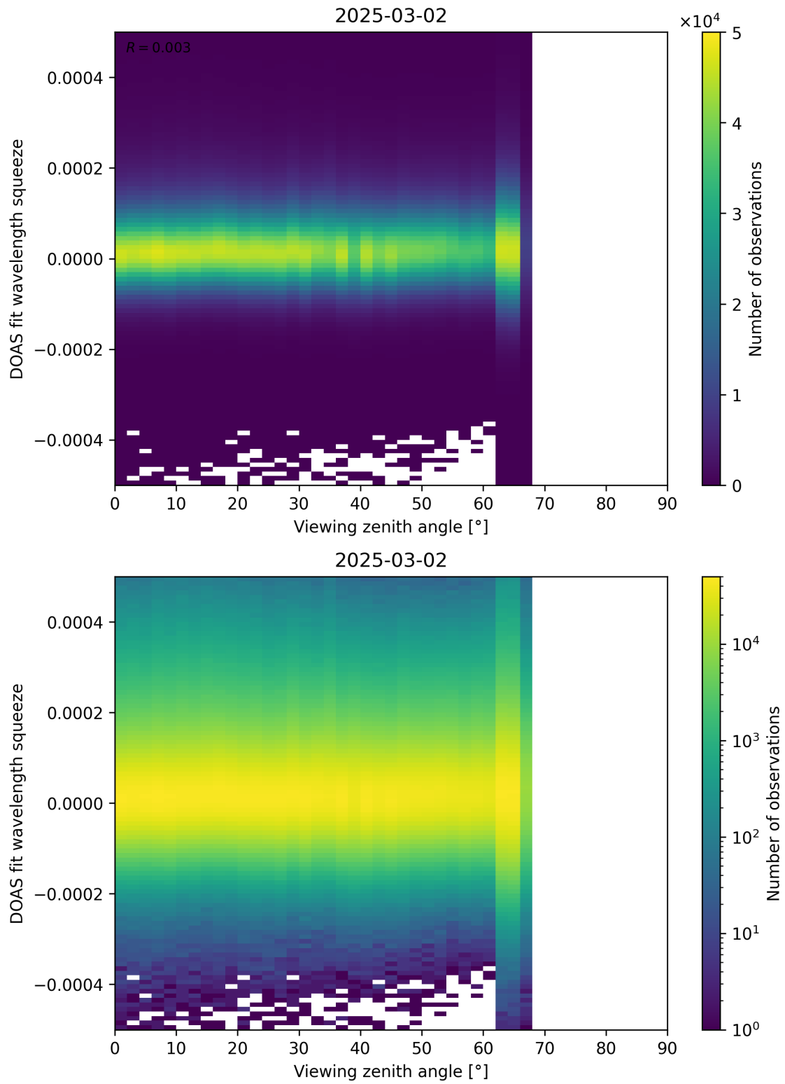
Figure 184: Scatter density plot of “Viewing zenith angle” against “DOAS fit wavelength squeeze” for 2025-03-01 to 2025-03-03.
