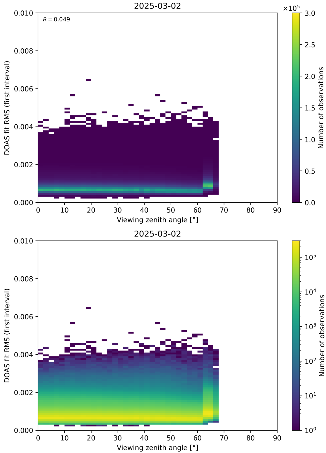
Figure 182: Scatter density plot of “Viewing zenith angle” against “DOAS fit RMS (first interval)” for 2025-03-01 to 2025-03-03.
