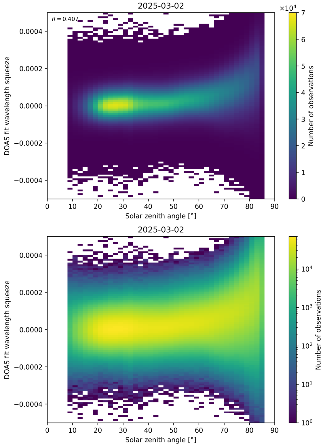
Figure 169: Scatter density plot of “Solar zenith angle” against “DOAS fit wavelength squeeze” for 2025-03-01 to 2025-03-03.
