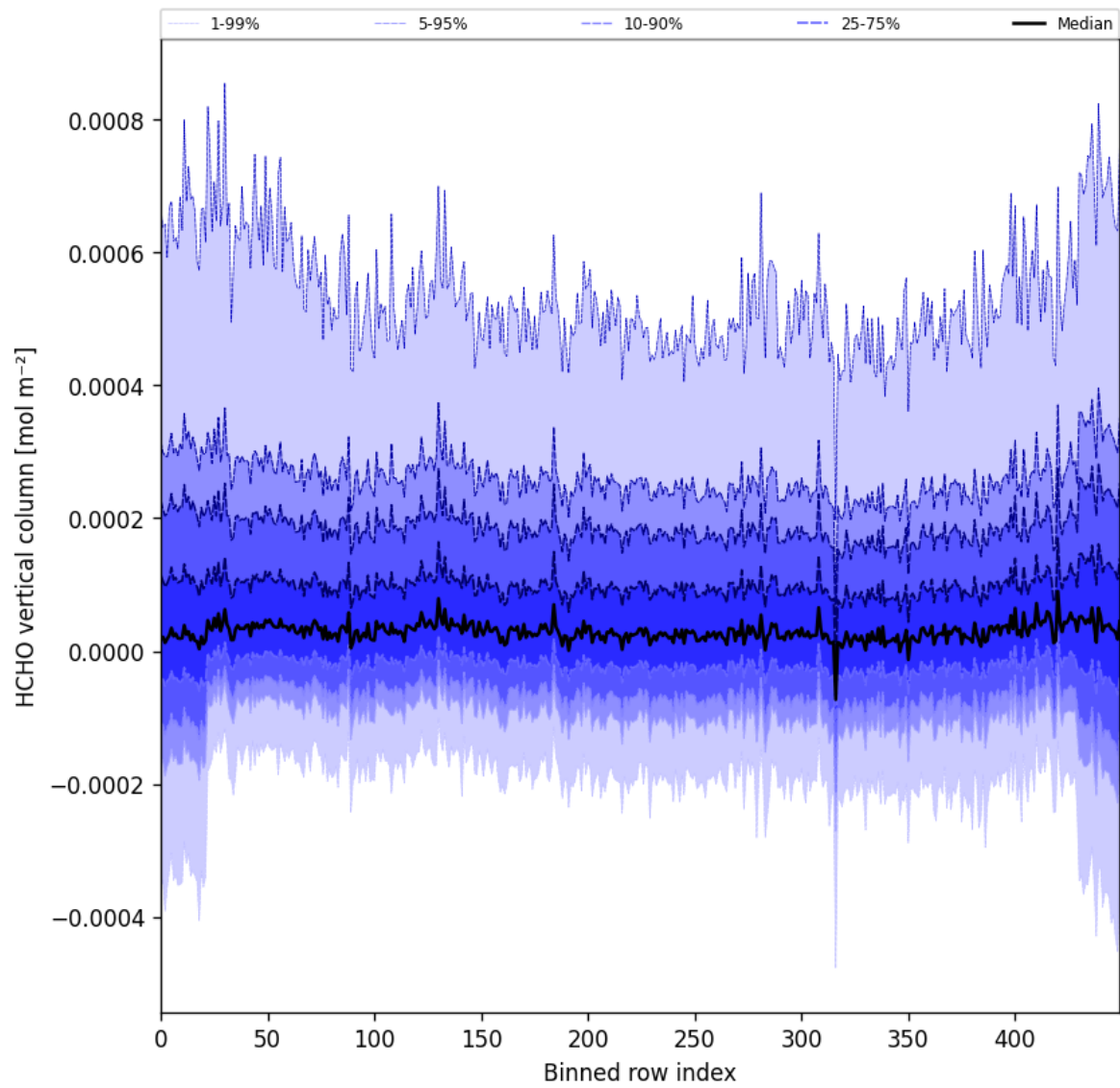
Figure 49: Along track statistics of “HCHO vertical column” for 2025-03-01 to 2025-03-03
