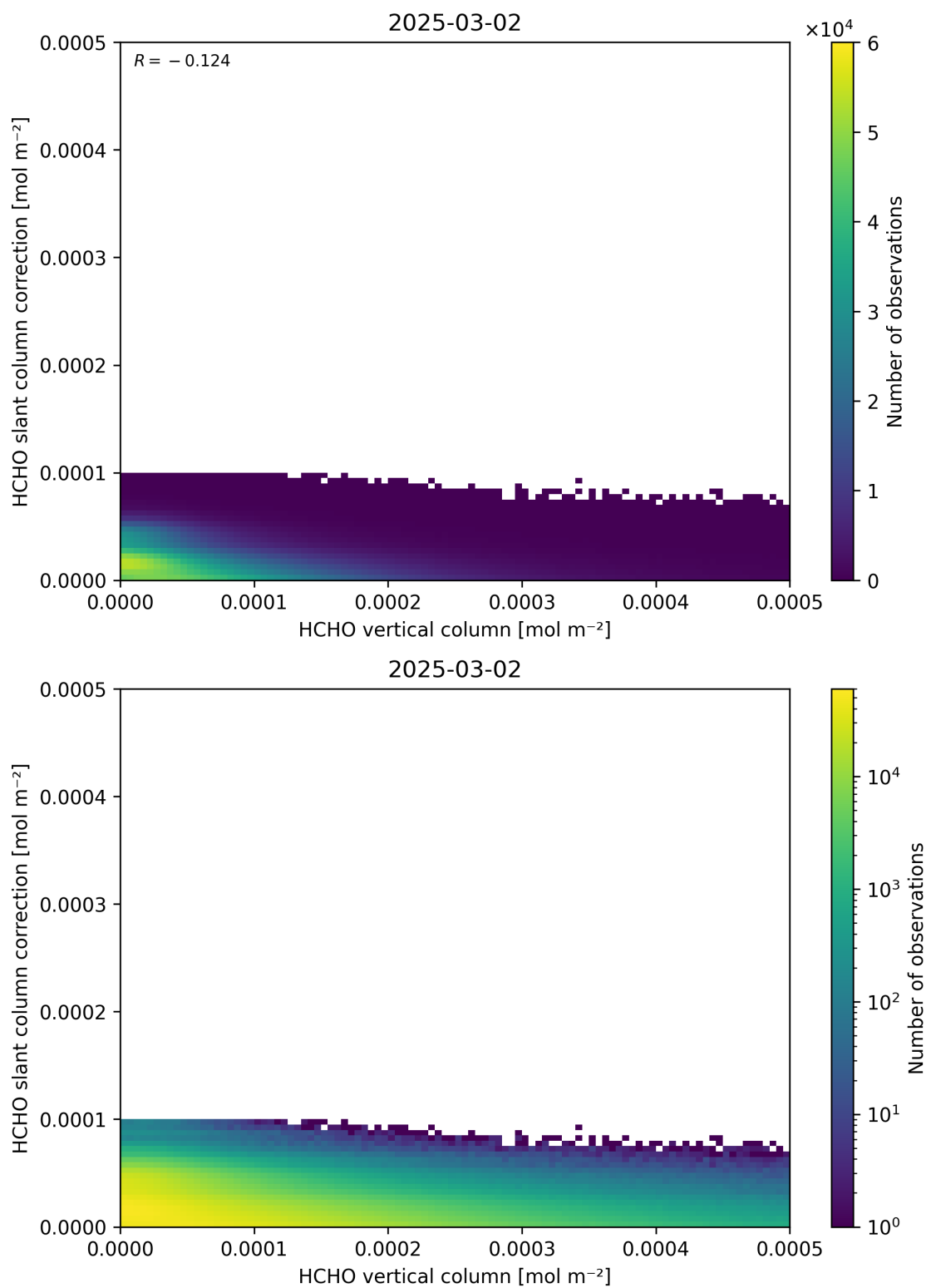
Figure 128: Scatter density plot of “HCHO vertical column” against “HCHO slant column correction” for 2025-03-01 to 2025-03-03.
