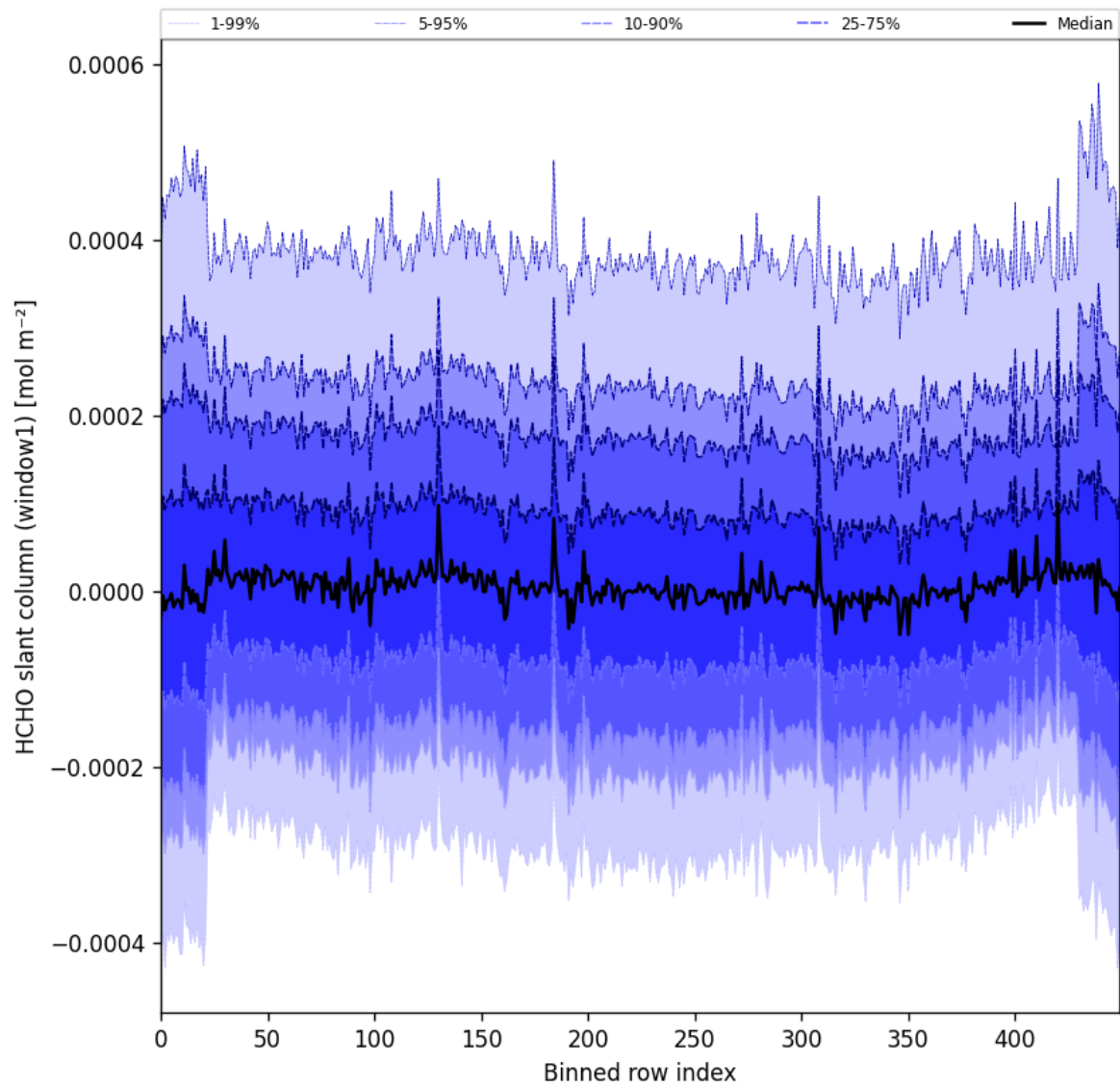
Figure 52: Along track statistics of “HCHO slant column (window1)” for 2025-03-01 to 2025-03-03
