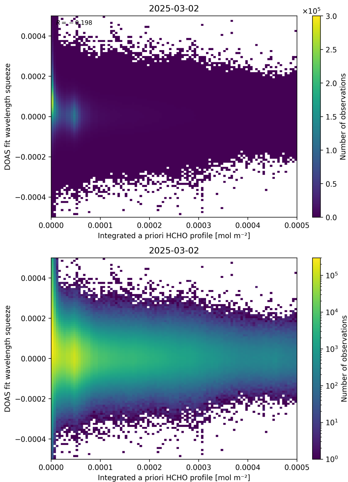
Figure 150: Scatter density plot of “Integrated a priori HCHO profile” against “DOAS fit wavelength squeeze” for 2025-03-01 to 2025-03-03.
