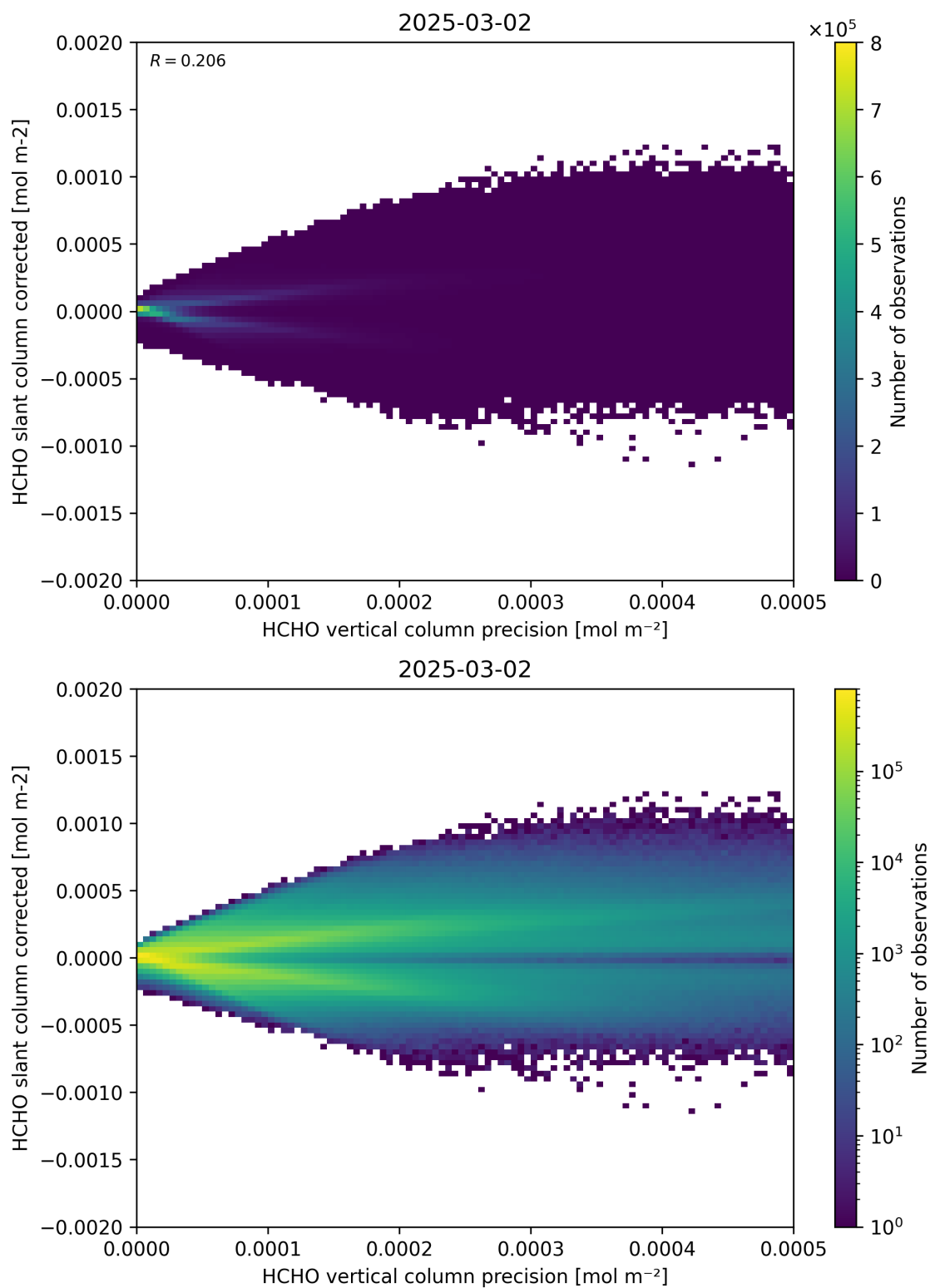
Figure 140: Scatter density plot of “HCHO vertical column precision” against “HCHO slant column corrected” for 2025-03-01 to 2025-03-03.
