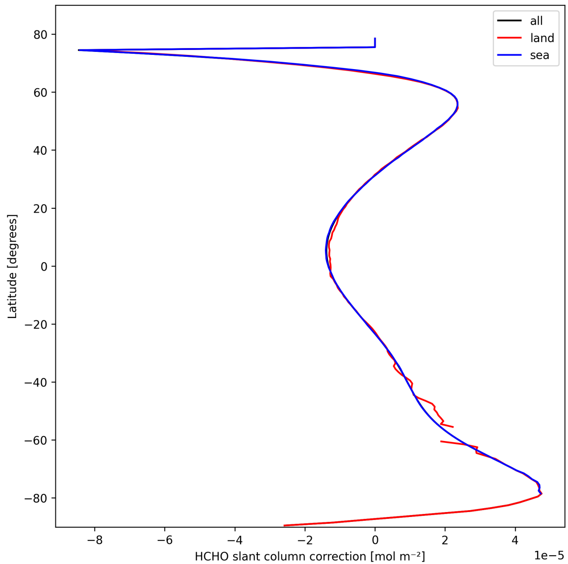
Figure 33: Zonal average of “HCHO slant column correction” for 2025-03-01 to 2025-03-03.
