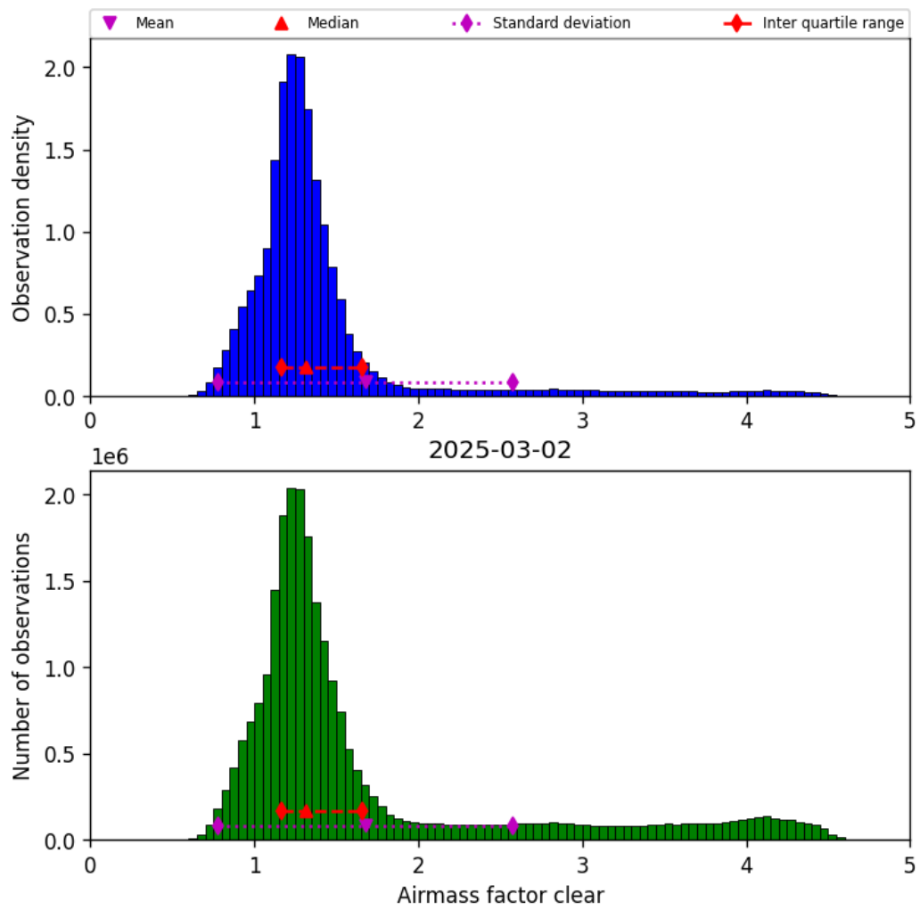
Figure 42: Histogram of “Airmass factor clear” for 2025-03-01 to 2025-03-03
