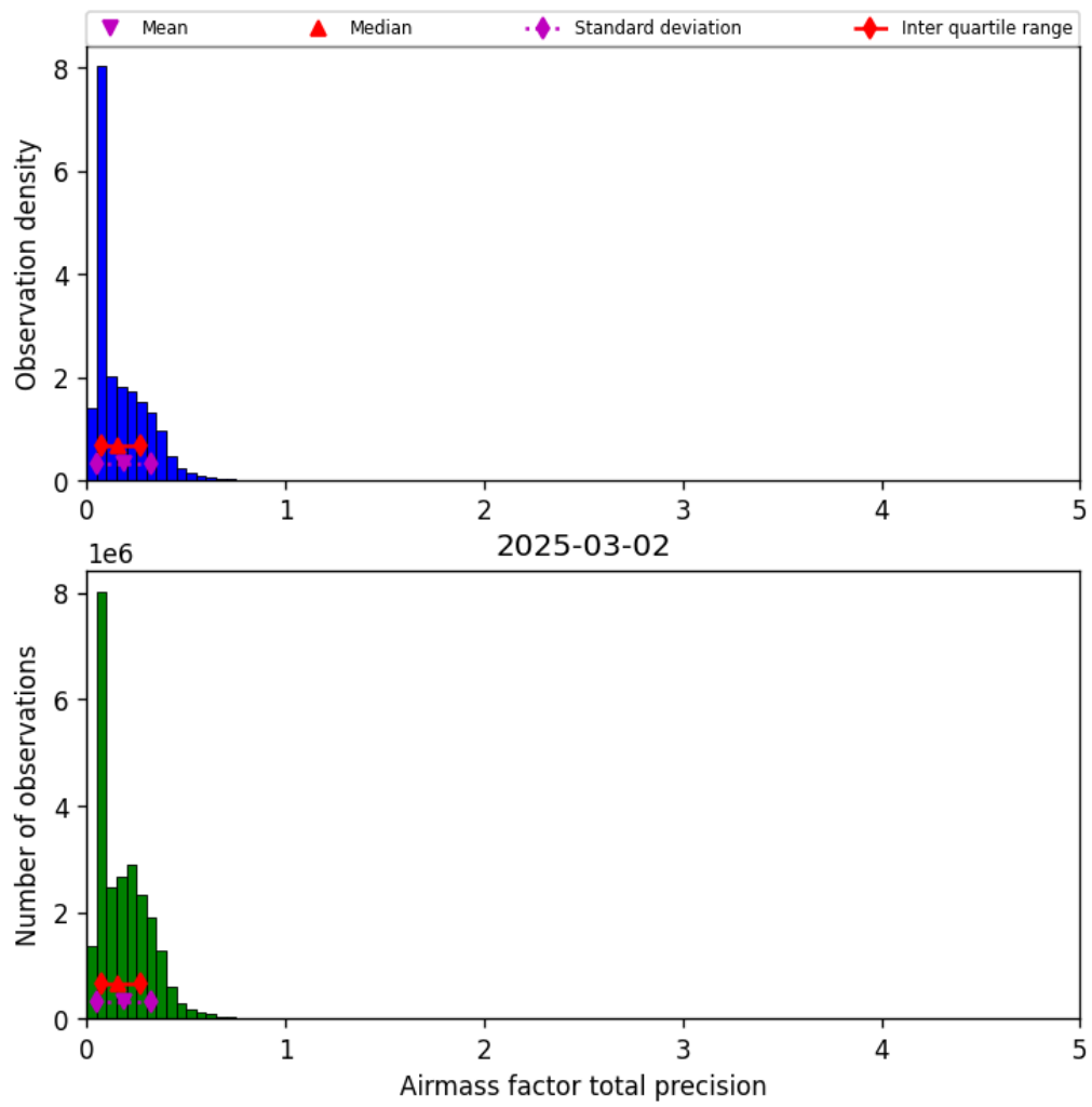
Figure 41: Histogram of “Airmass factor total precision” for 2025-03-01 to 2025-03-03
