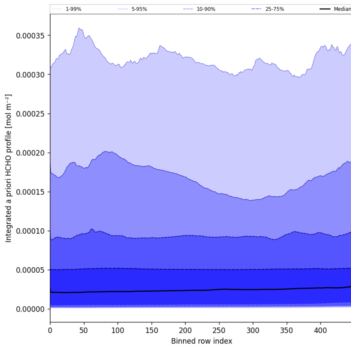
Figure 57: Along track statistics of “Integrated a priori HCHO profile” for 2025-03-01 to 2025-03-03
