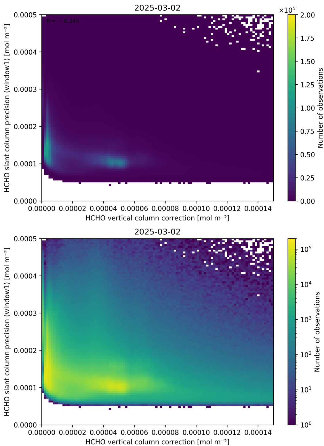
Figure 119: Scatter density plot of “HCHO vertical column correction” against “HCHO slant column precision (window1)” for 2025-03-01 to 2025-03-03.
