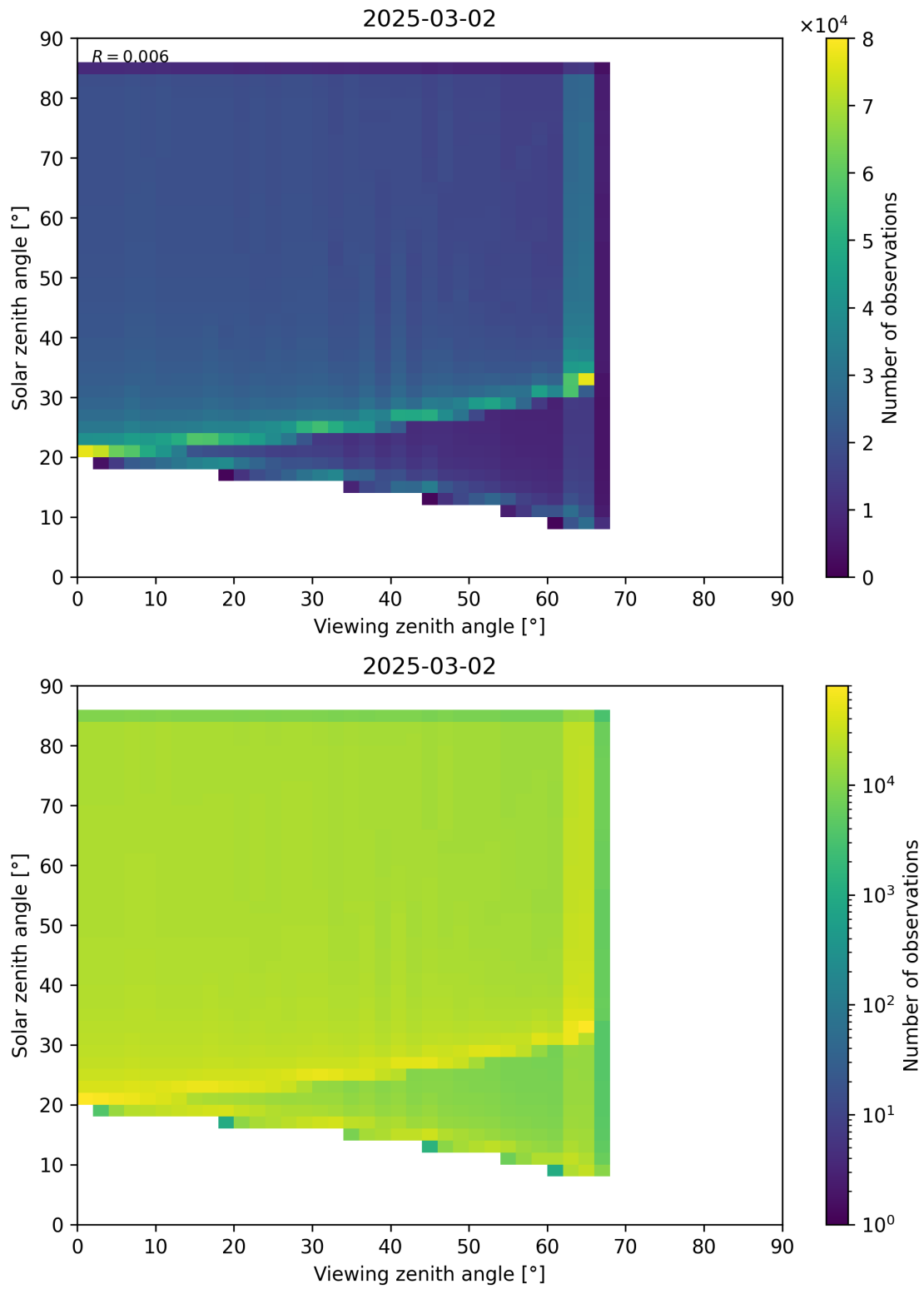
Figure 197: Scatter density plot of “Viewing zenith angle” against “Solar zenith angle” for 2025-03-01 to 2025-03-03.
