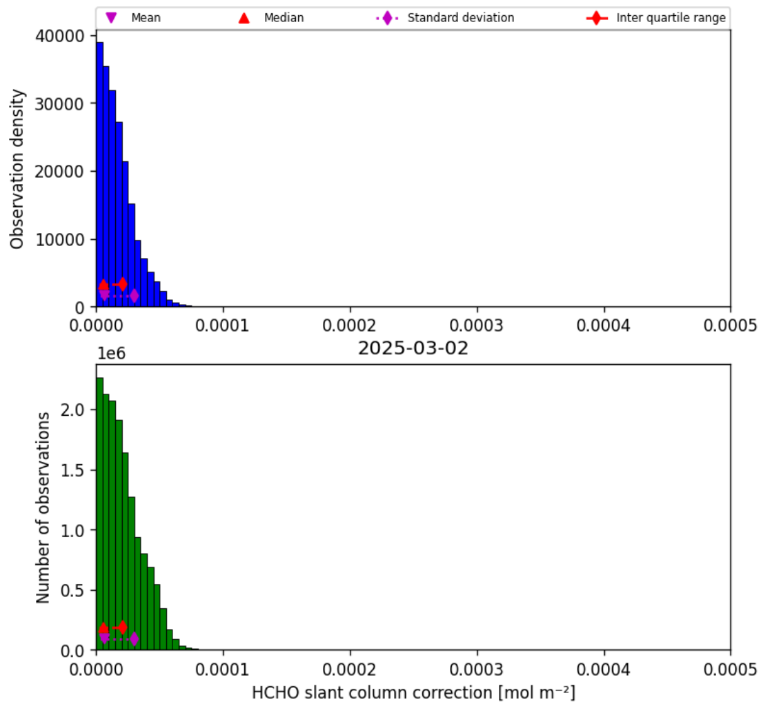
Figure 47: Histogram of “HCHO slant column correction” for 2025-03-01 to 2025-03-03
