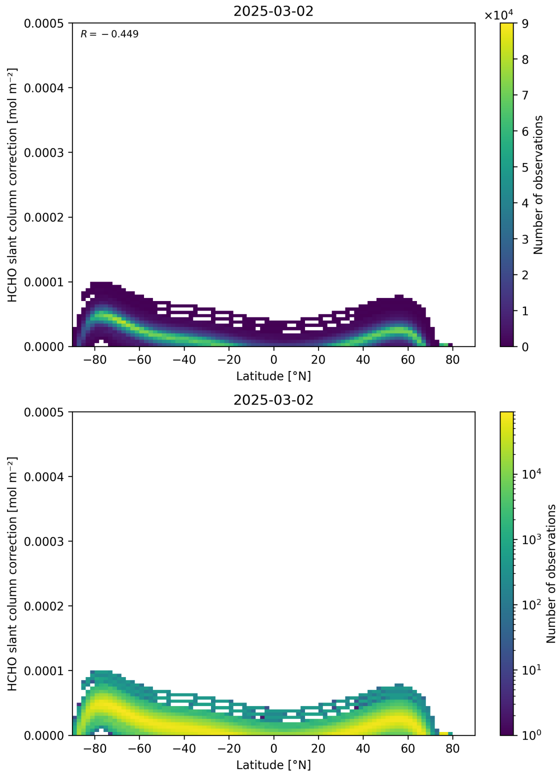
Figure 158: Scatter density plot of “Latitude” against “HCHO slant column correction” for 2025-03-01 to 2025-03-03.
