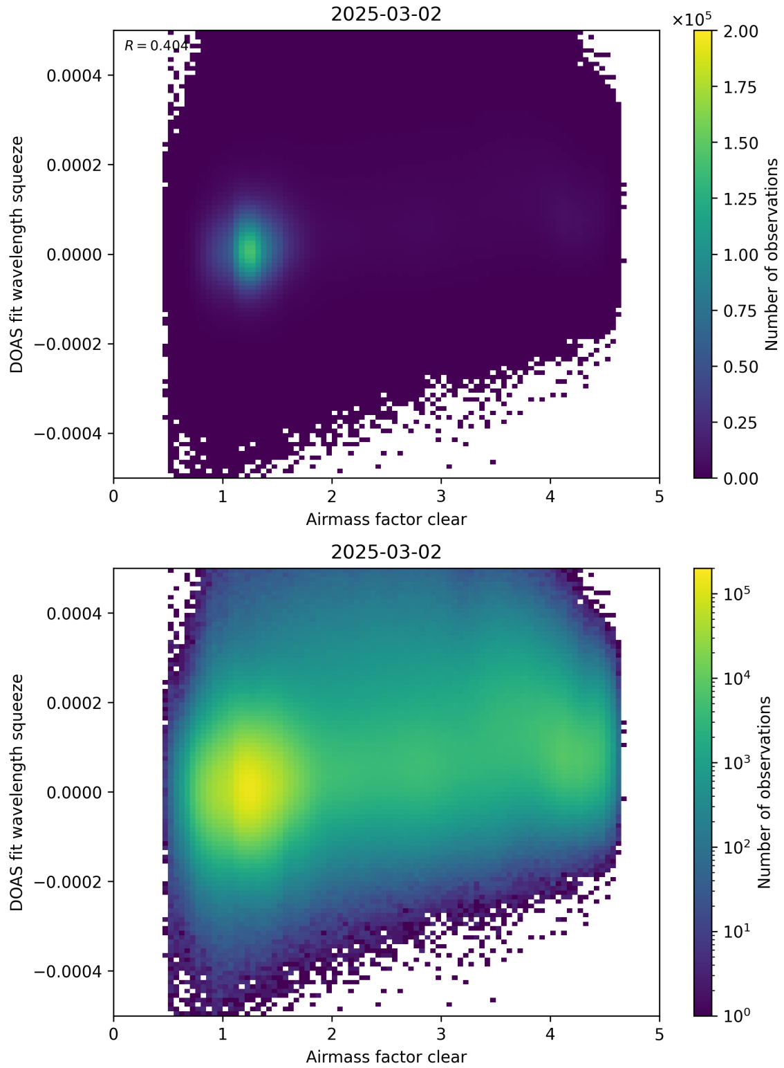
Figure 73: Scatter density plot of “Airmass factor clear” against “DOAS fit wavelength squeeze” for 2025-03-01 to 2025-03-03.
