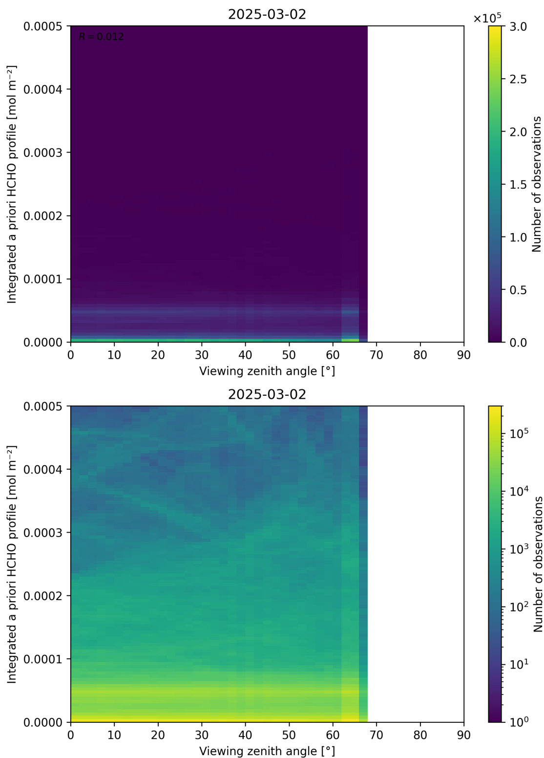
Figure 195: Scatter density plot of “Viewing zenith angle” against “Integrated a priori HCHO profile” for 2025-03-01 to 2025-03-03.
