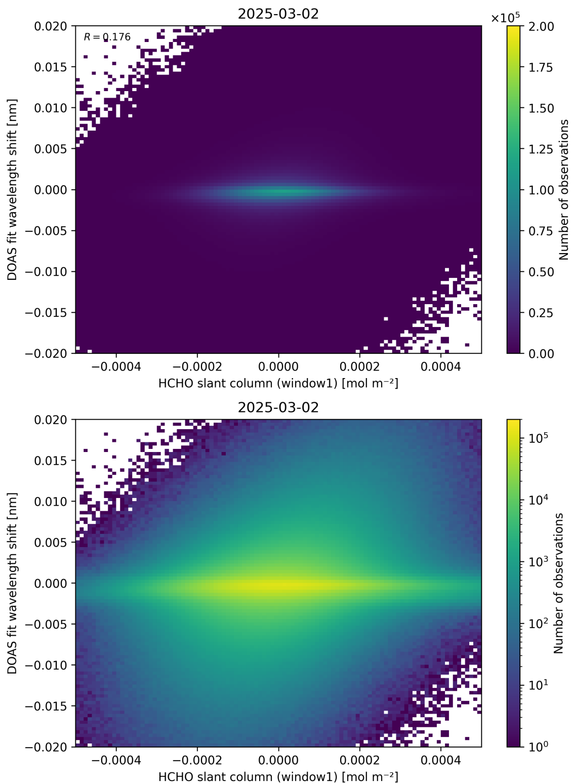
Figure 79: Scatter density plot of “HCHO slant column (window1)” against “DOAS fit wavelength shift” for 2025-03-01 to 2025-03-03.
