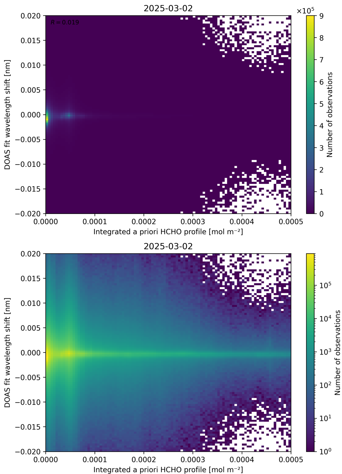
Figure 149: Scatter density plot of “Integrated a priori HCHO profile” against “DOAS fit wavelength shift” for 2025-03-01 to 2025-03-03.
