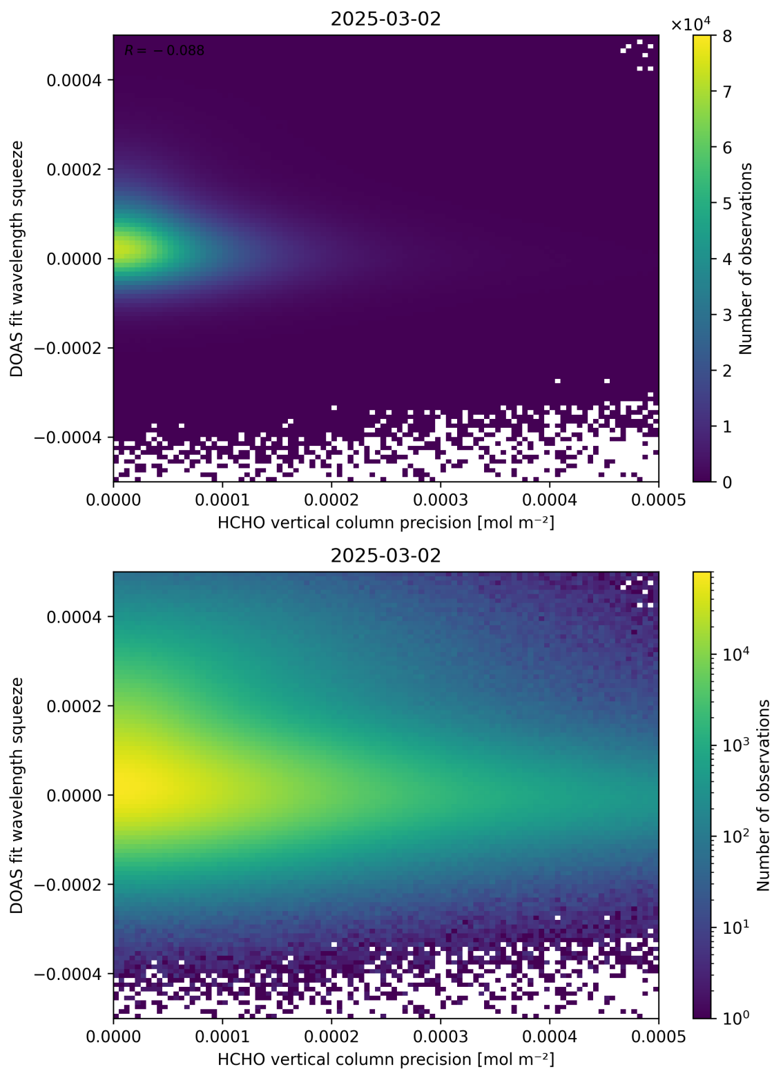
Figure 138: Scatter density plot of “HCHO vertical column precision” against “DOAS fit wavelength squeeze” for 2025-03-01 to 2025-03-03.
