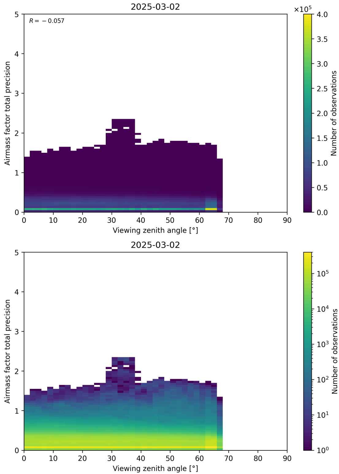
Figure 191: Scatter density plot of “Viewing zenith angle” against “Airmass factor total precision” for 2025-03-01 to 2025-03-03.
