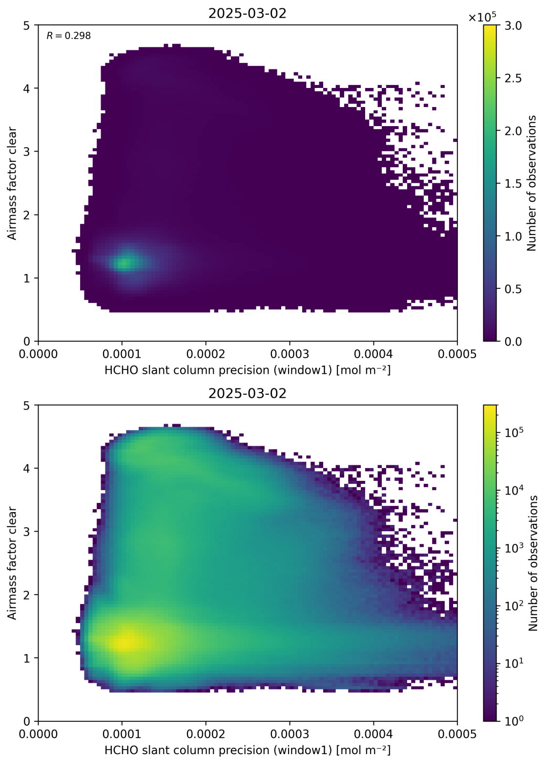
Figure 91: Scatter density plot of “HCHO slant column precision (window1)” against “Airmass factor clear” for 2025-03-01 to 2025-03-03.
