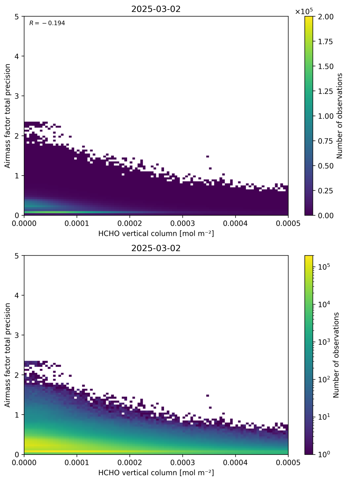
Figure 132: Scatter density plot of “HCHO vertical column” against “Airmass factor total precision” for 2025-03-01 to 2025-03-03.
