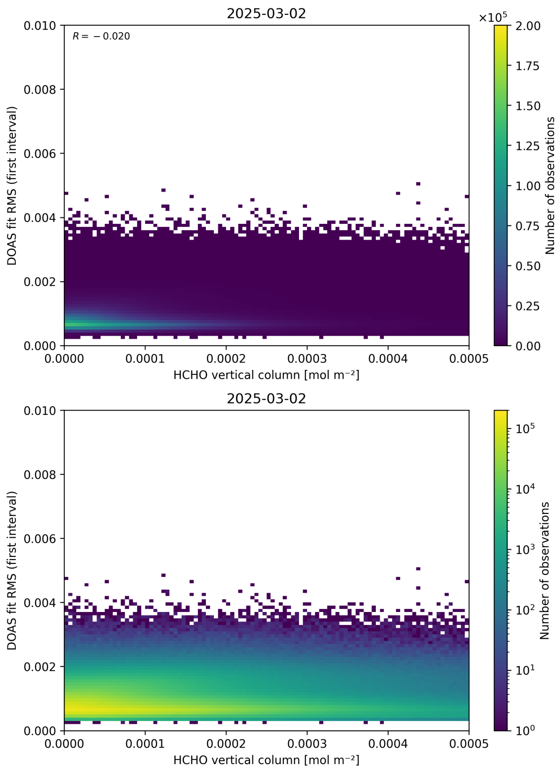
Figure 123: Scatter density plot of “HCHO vertical column” against “DOAS fit RMS (first interval)” for 2025-03-01 to 2025-03-03.
