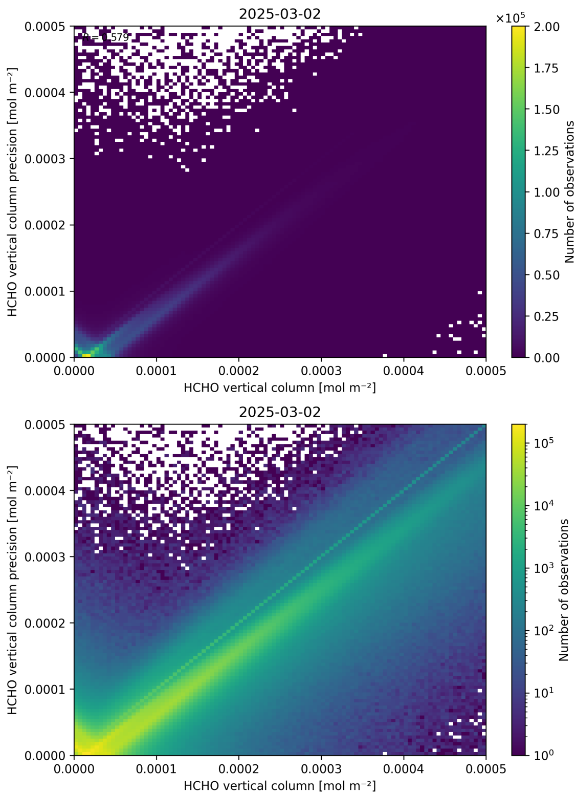
Figure 134: Scatter density plot of “HCHO vertical column” against “HCHO vertical column precision” for 2025-03-01 to 2025-03-03.
