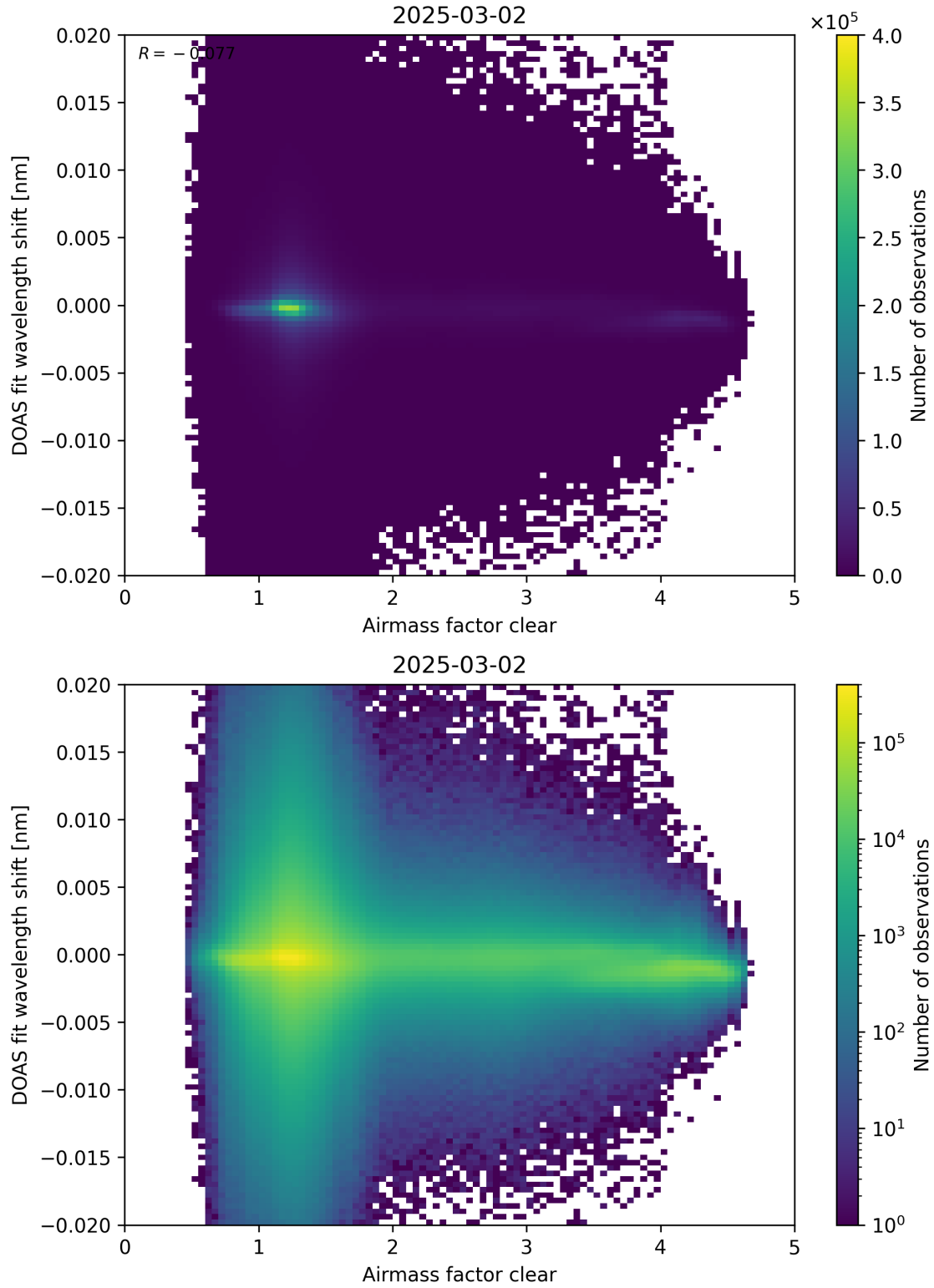
Figure 72: Scatter density plot of “Airmass factor clear” against “DOAS fit wavelength shift” for 2025-03-01 to 2025-03-03.
