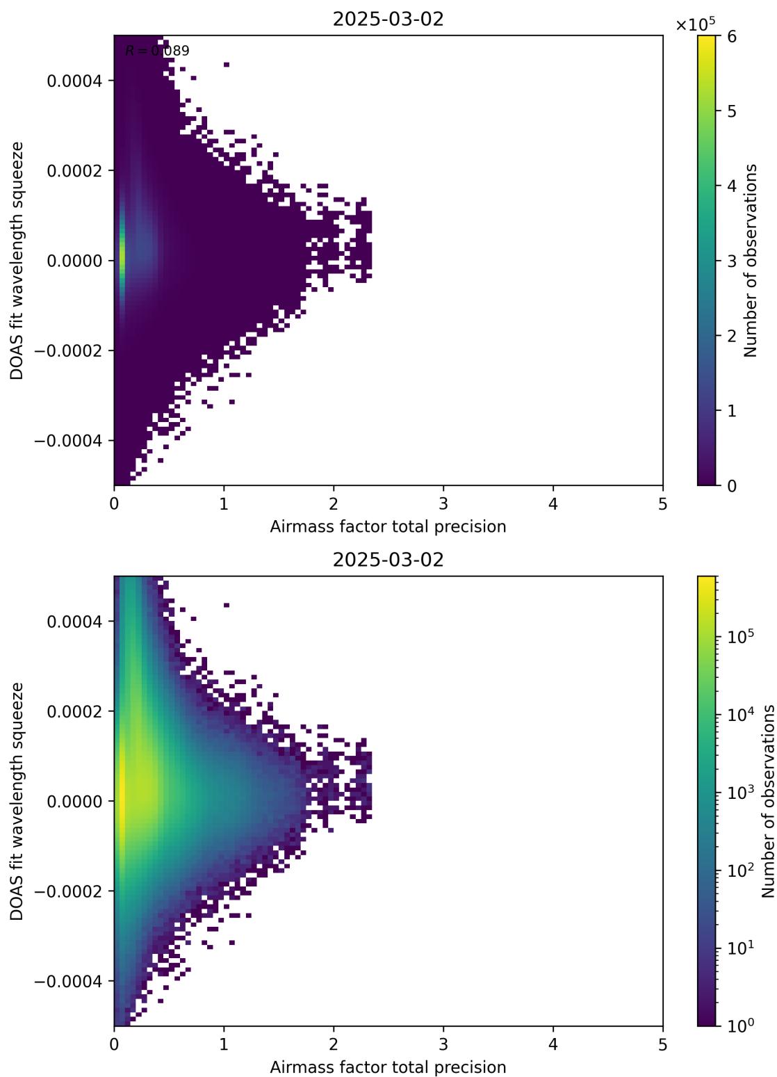
Figure 107: Scatter density plot of “Airmass factor total precision” against “DOAS fit wavelength squeeze” for 2025-03-01 to 2025-03-03.
