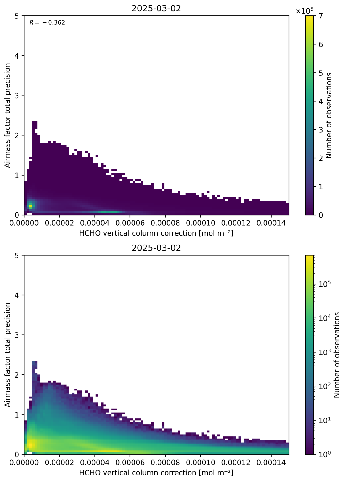
Figure 121: Scatter density plot of “HCHO vertical column correction” against “Airmass factor total precision” for 2025-03-01 to 2025-03-03.
