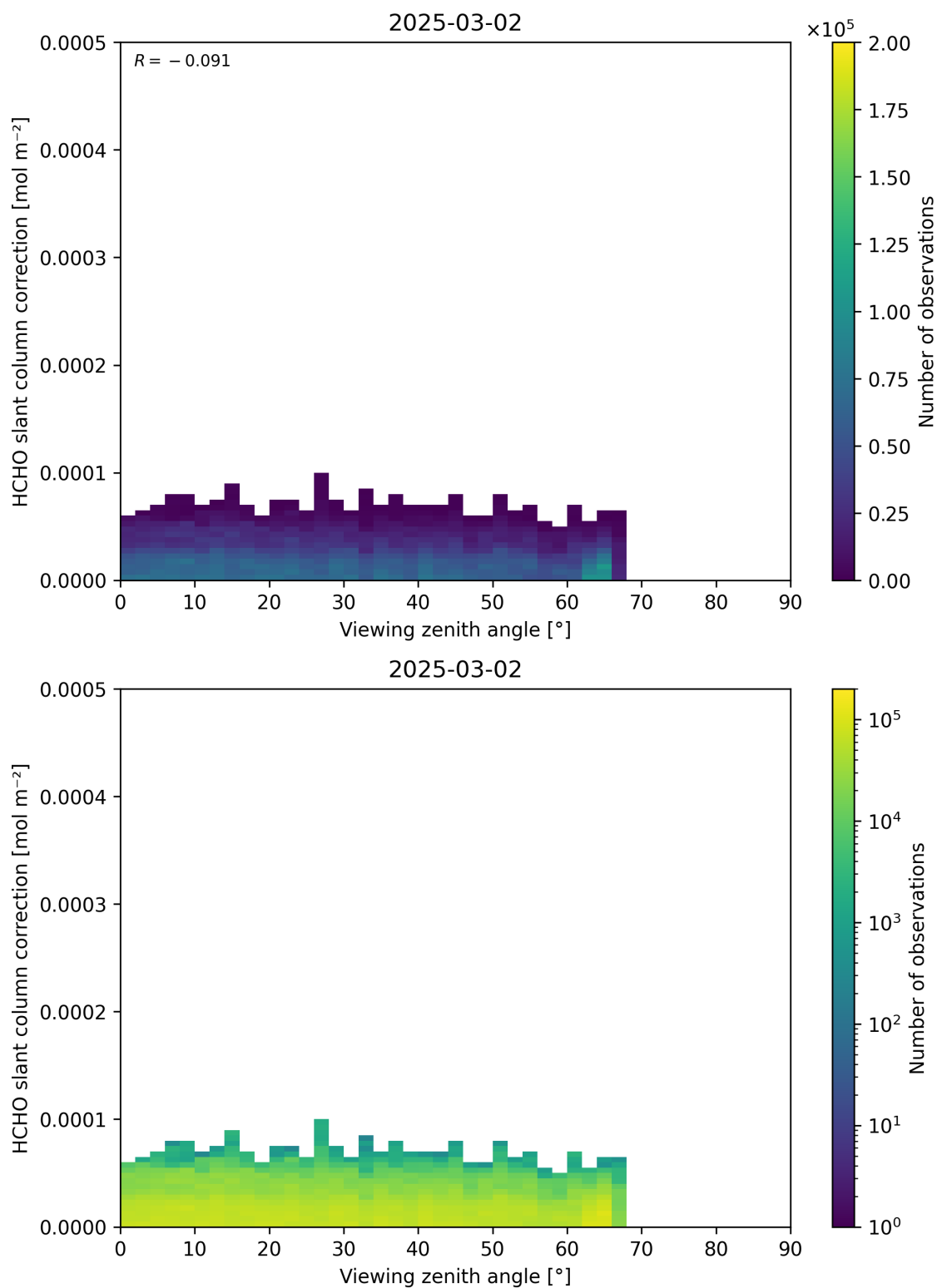
Figure 187: Scatter density plot of “Viewing zenith angle” against “HCHO slant column correction” for 2025-03-01 to 2025-03-03.
