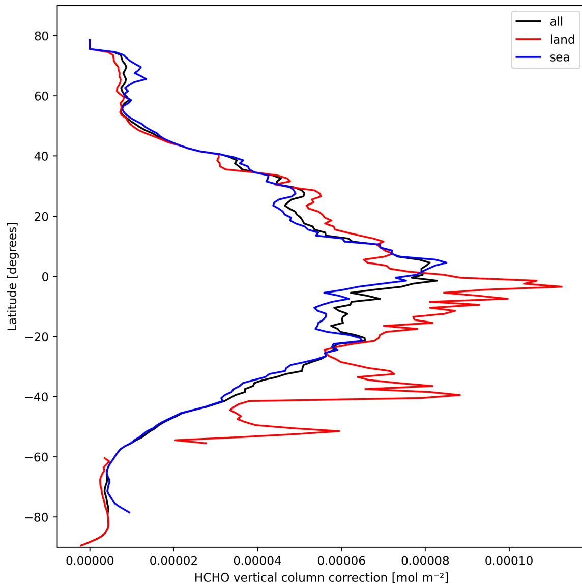
Figure 23: Zonal average of “HCHO vertical column correction” for 2025-03-01 to 2025-03-03.
