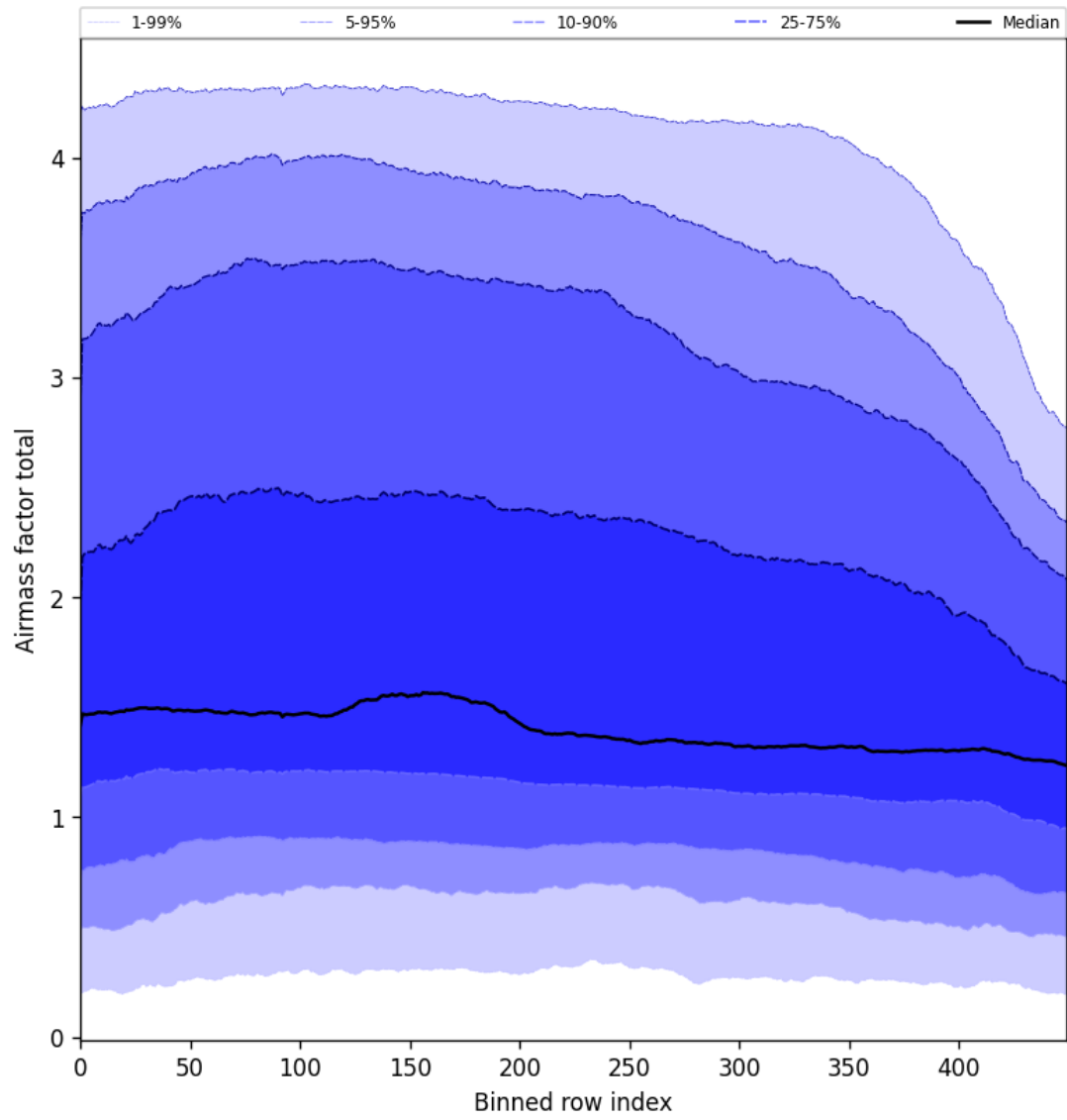
Figure 54: Along track statistics of “Airmass factor total” for 2025-03-01 to 2025-03-03
