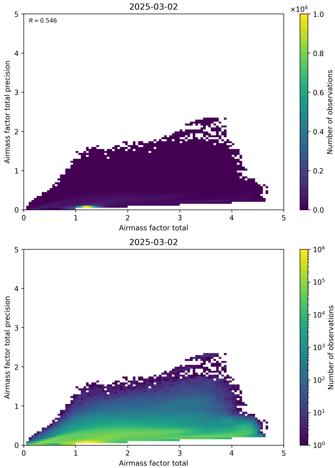
Figure 103: Scatter density plot of “Airmass factor total” against “Airmass factor total precision” for 2025-03-01 to 2025-03-03.
