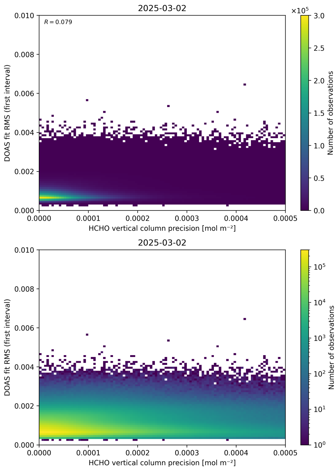
Figure 136: Scatter density plot of “HCHO vertical column precision” against “DOAS fit RMS (first interval)” for 2025-03-01 to 2025-03-03.
