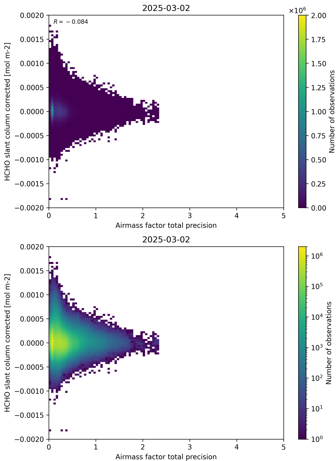
Figure 109: Scatter density plot of “Airmass factor total precision” against “HCHO slant column corrected” for 2025-03-01 to 2025-03-03.
