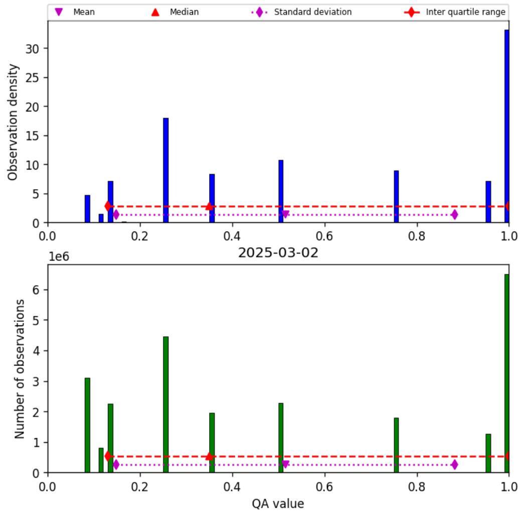
Figure 34: Histogram of “QA value” for 2025-03-01 to 2025-03-03
