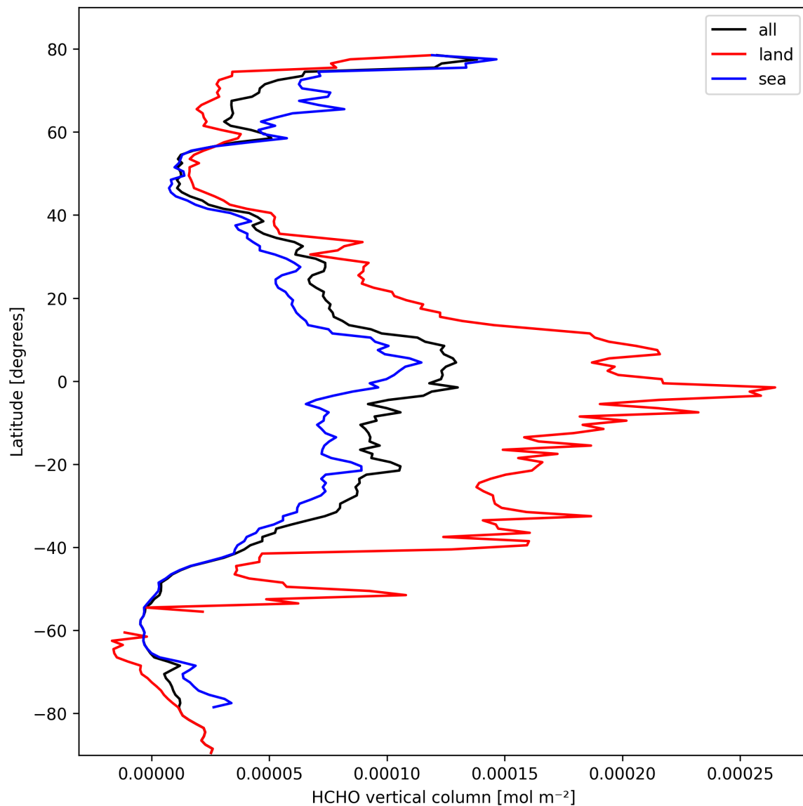
Figure 21: Zonal average of “HCHO vertical column” for 2025-03-01 to 2025-03-03.
