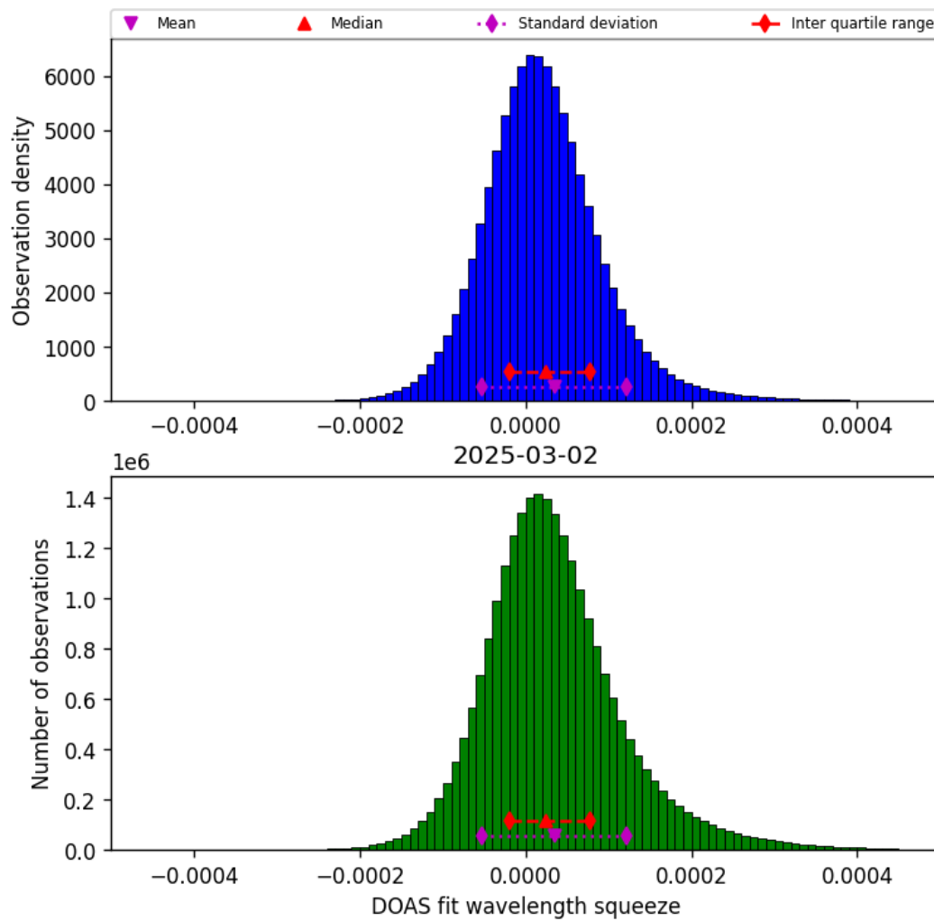
Figure 45: Histogram of “DOAS fit wavelength squeeze” for 2025-03-01 to 2025-03-03
