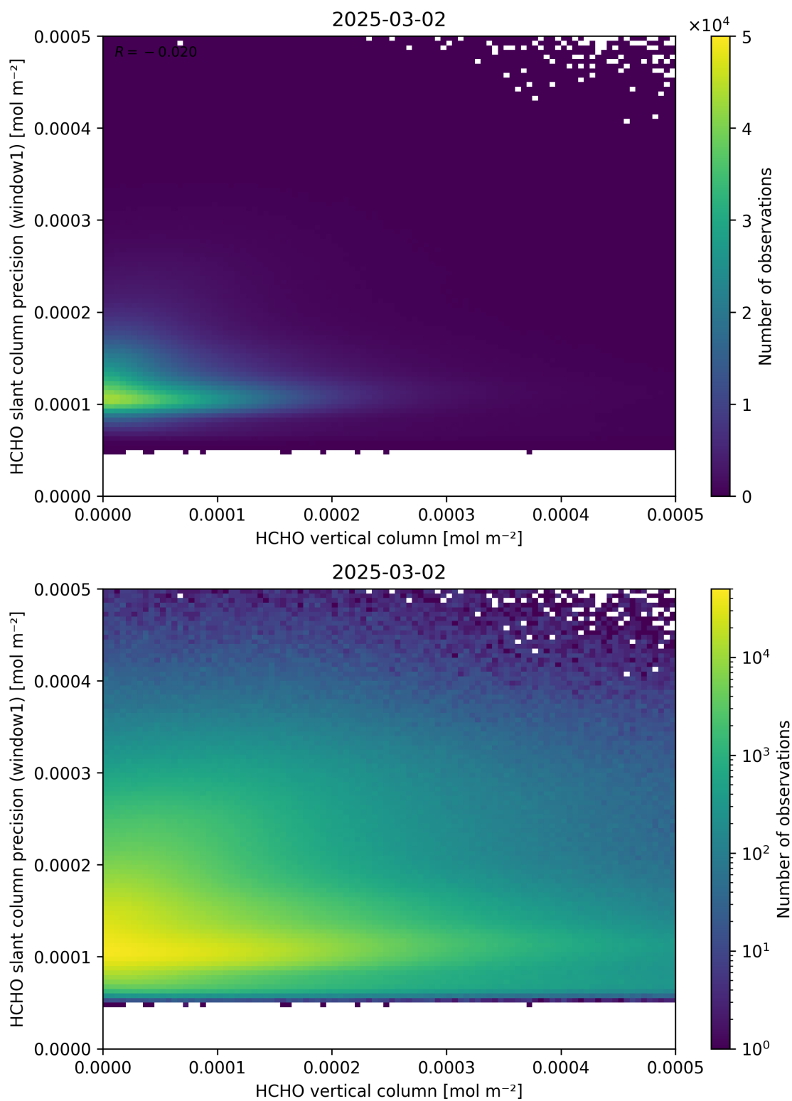
Figure 130: Scatter density plot of “HCHO vertical column” against “HCHO slant column precision (window1)” for 2025-03-01 to 2025-03-03.
