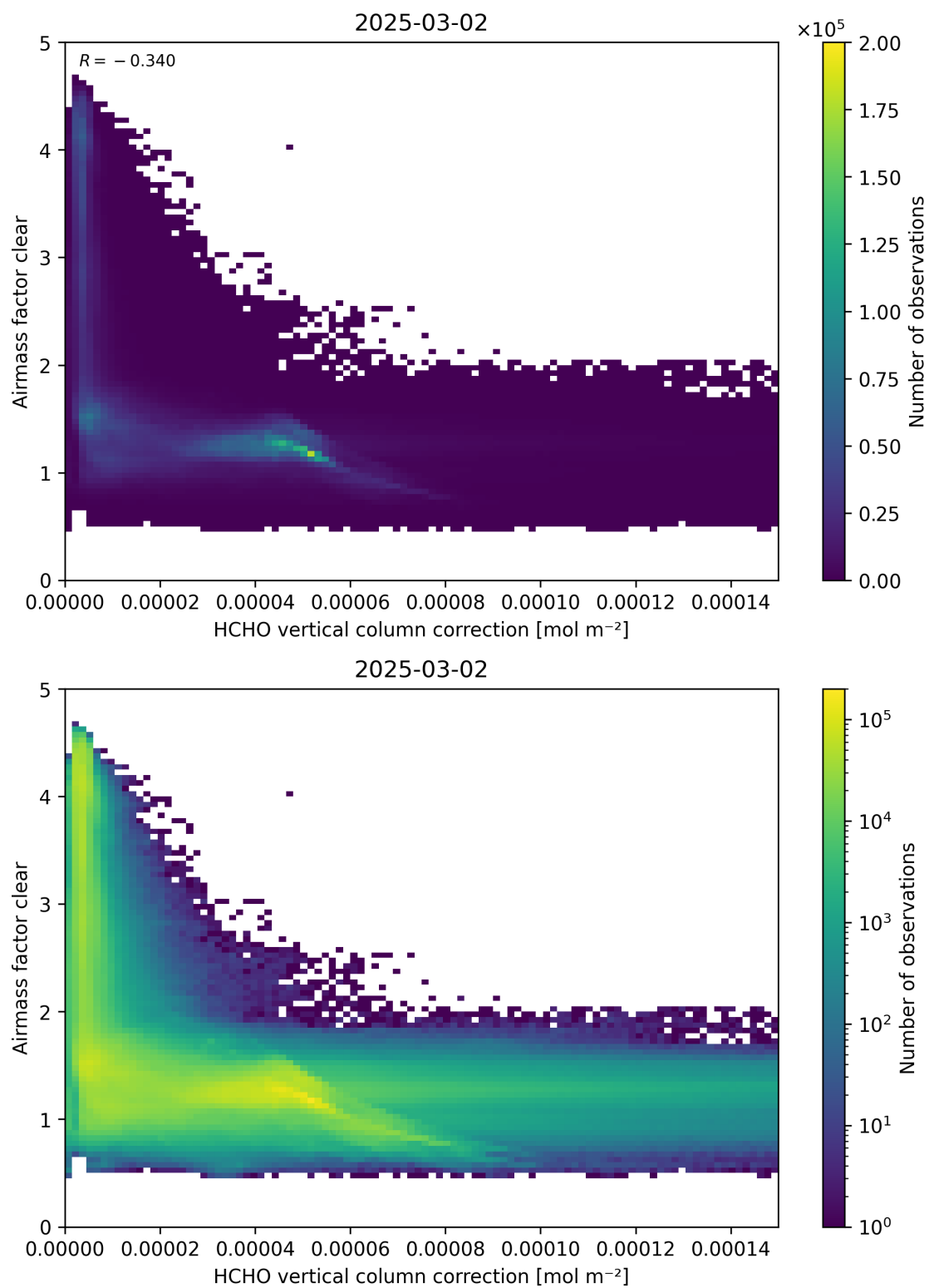
Figure 115: Scatter density plot of “HCHO vertical column correction” against “Airmass factor clear” for 2025-03-01 to 2025-03-03.
