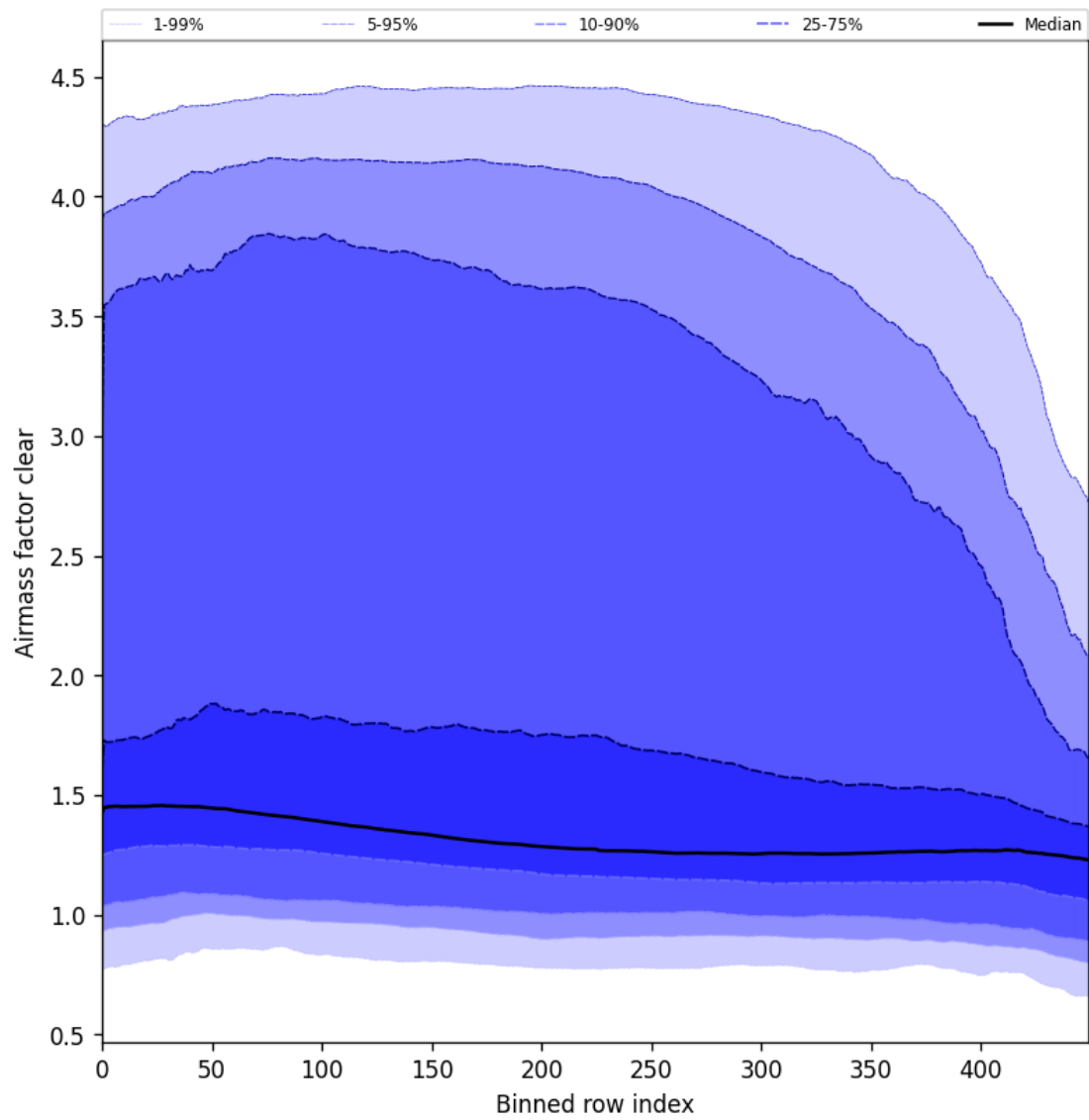
Figure 56: Along track statistics of “Airmass factor clear” for 2025-03-01 to 2025-03-03
