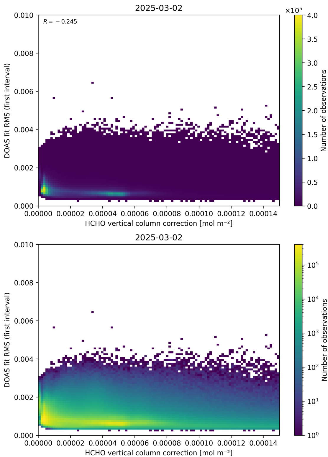
Figure 112: Scatter density plot of “HCHO vertical column correction” against “DOAS fit RMS (first interval)” for 2025-03-01 to 2025-03-03.
