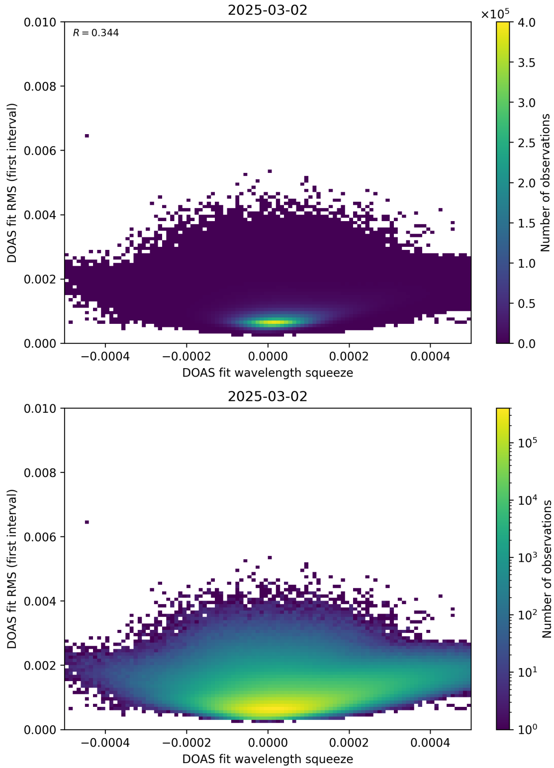
Figure 68: Scatter density plot of “DOAS fit wavelength squeeze” against “DOAS fit RMS (first interval)” for 2025-03-01 to 2025-03-03.
