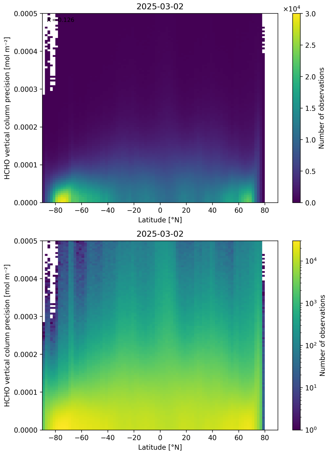
Figure 165: Scatter density plot of “Latitude” against “HCHO vertical column precision” for 2025-03-01 to 2025-03-03.
