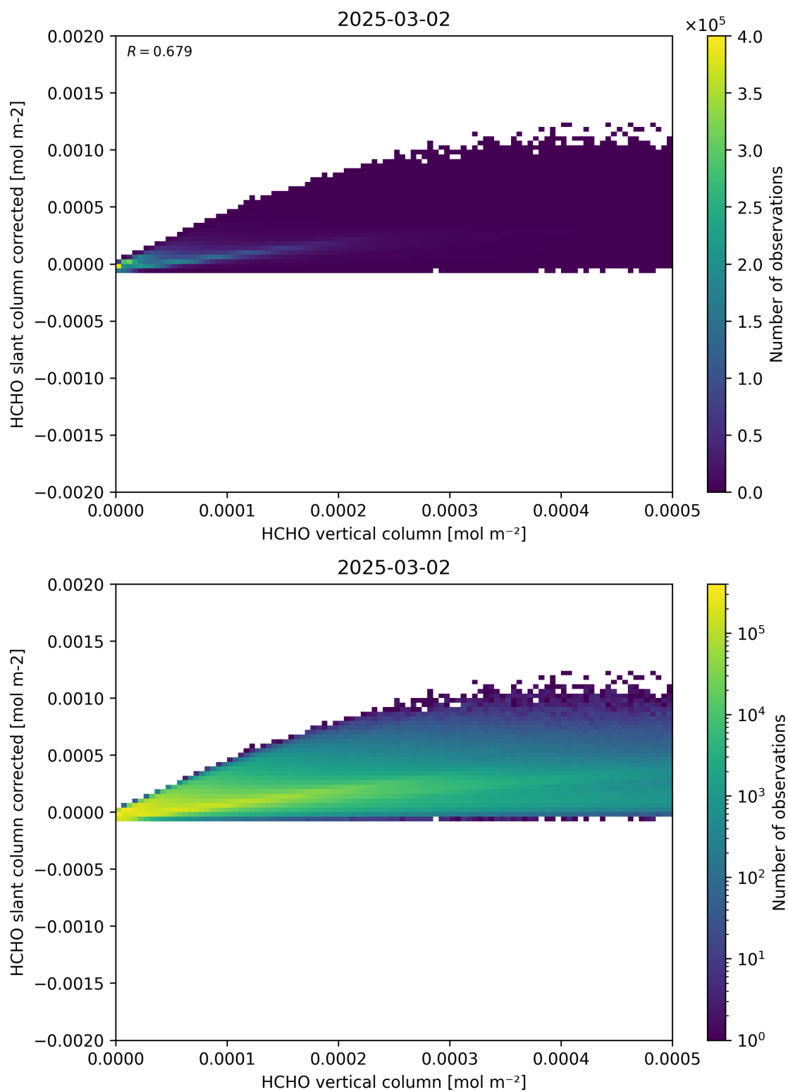
Figure 127: Scatter density plot of “HCHO vertical column” against “HCHO slant column corrected” for 2025-03-01 to 2025-03-03.
