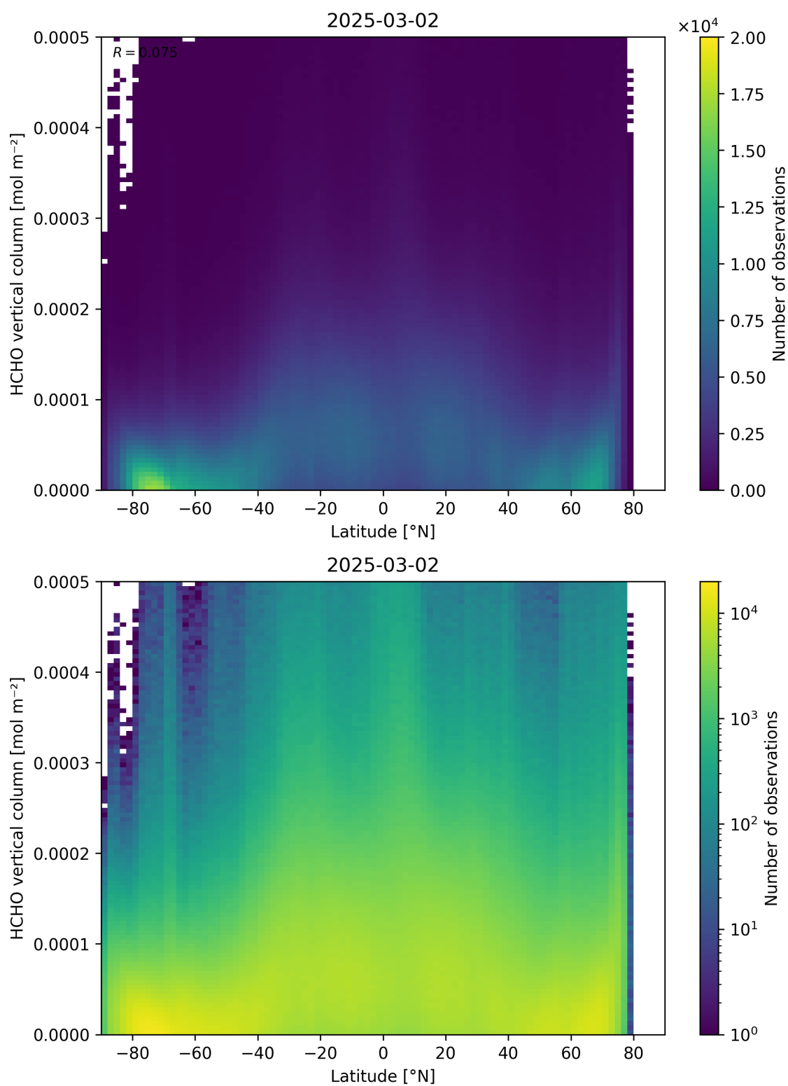
Figure 163: Scatter density plot of “Latitude” against “HCHO vertical column” for 2025-03-01 to 2025-03-03.
