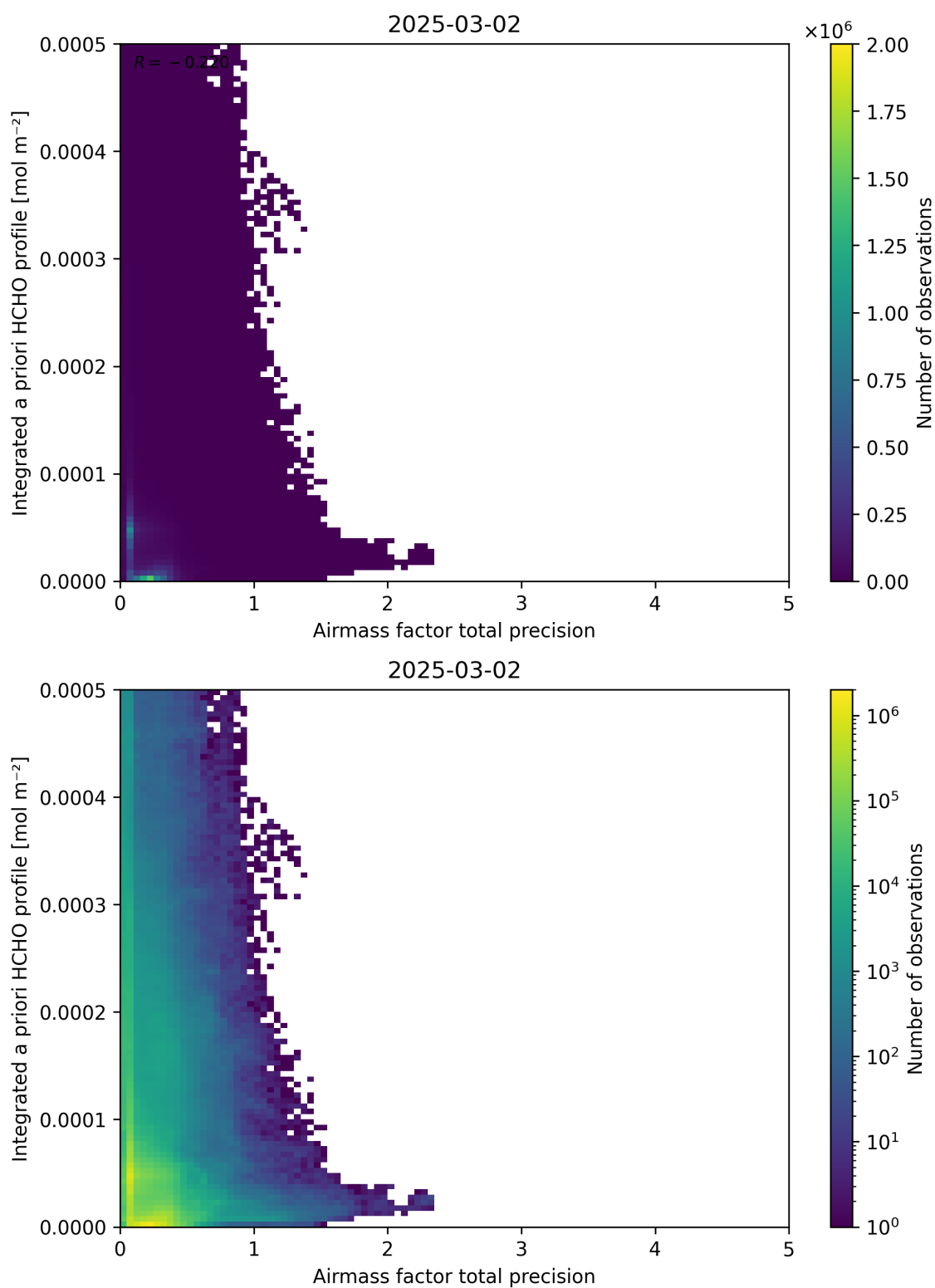
Figure 111: Scatter density plot of “Airmass factor total precision” against “Integrated a priori HCHO profile” for 2025-03-01 to 2025-03-03.
