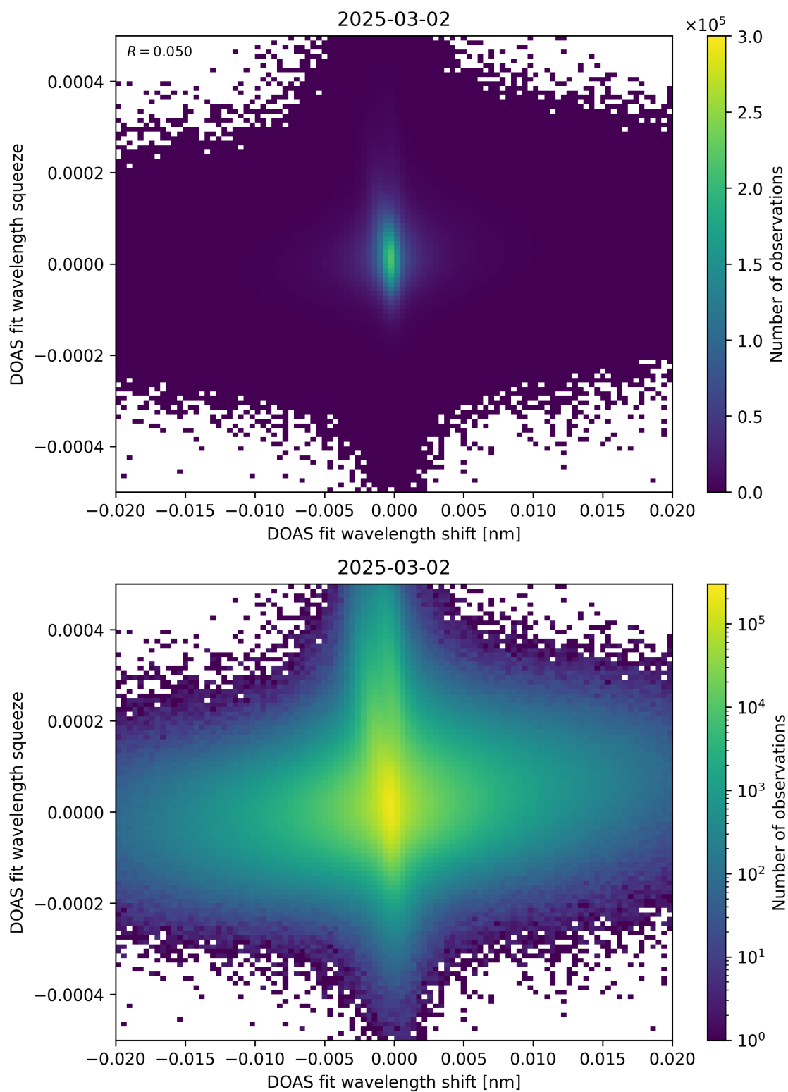
Figure 65: Scatter density plot of “DOAS fit wavelength shift” against “DOAS fit wavelength squeeze” for 2025-03-01 to 2025-03-03.
