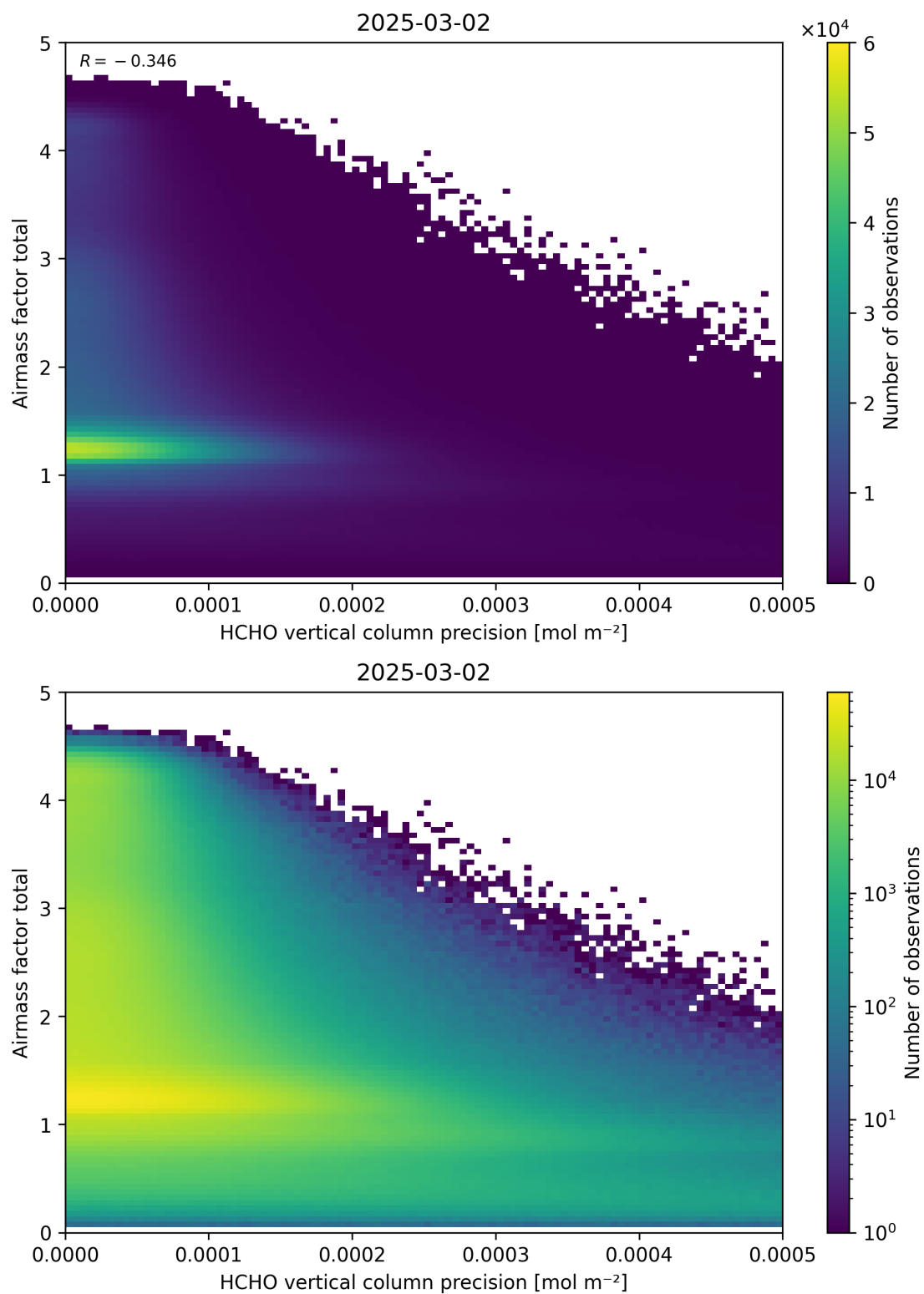
Figure 144: Scatter density plot of “HCHO vertical column precision” against “Airmass factor total” for 2025-03-01 to 2025-03-03.
