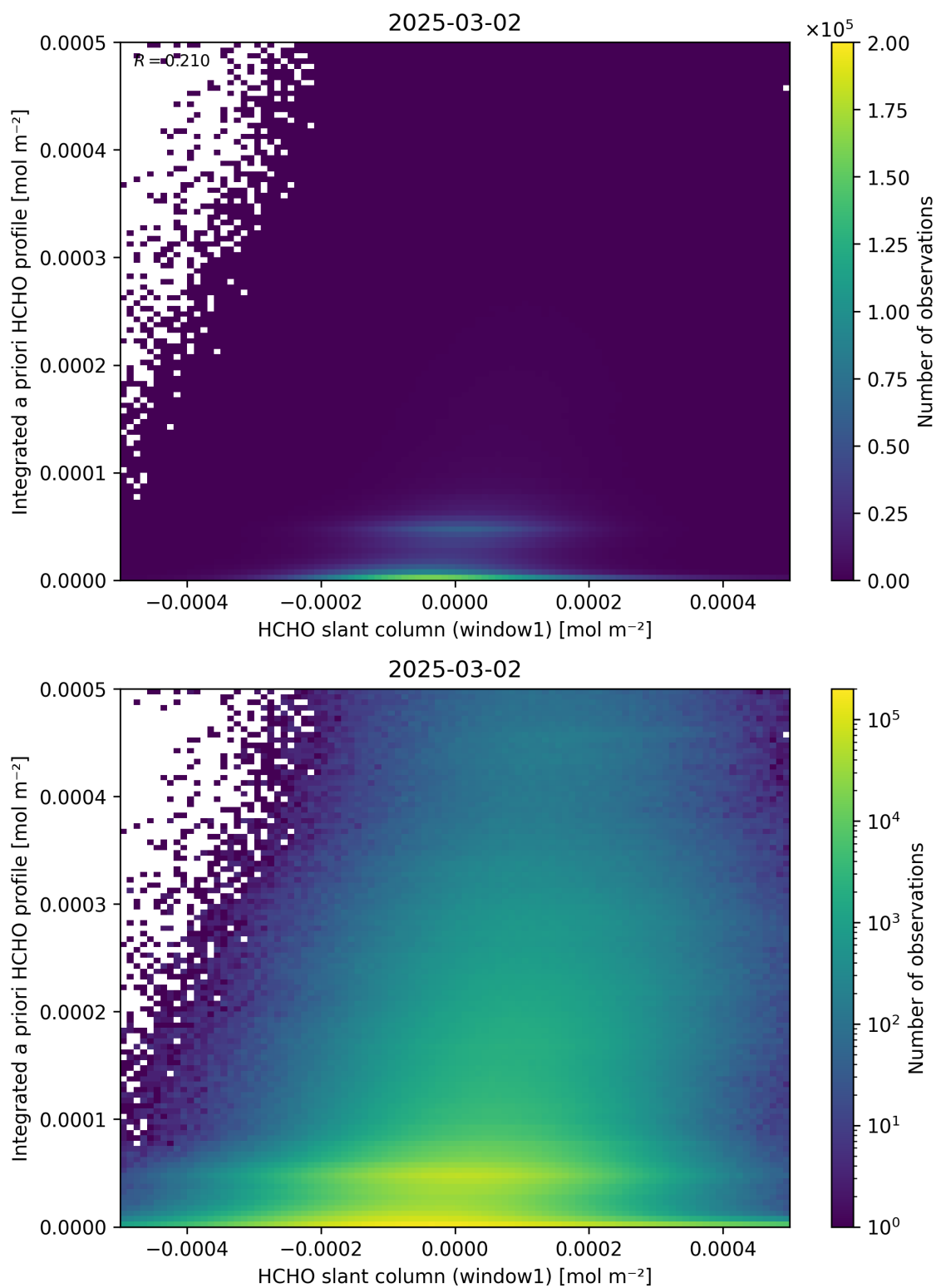
Figure 87: Scatter density plot of “HCHO slant column (window1)” against “Integrated a priori HCHO profile” for 2025-03-01 to 2025-03-03.
