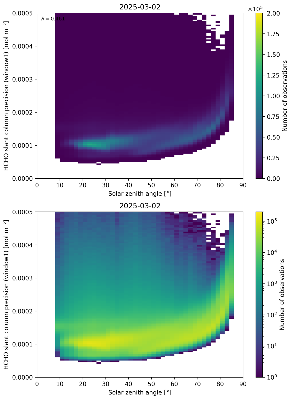
Figure 174: Scatter density plot of “Solar zenith angle” against “HCHO slant column precision (window1)” for 2025-03-01 to 2025-03-03.
