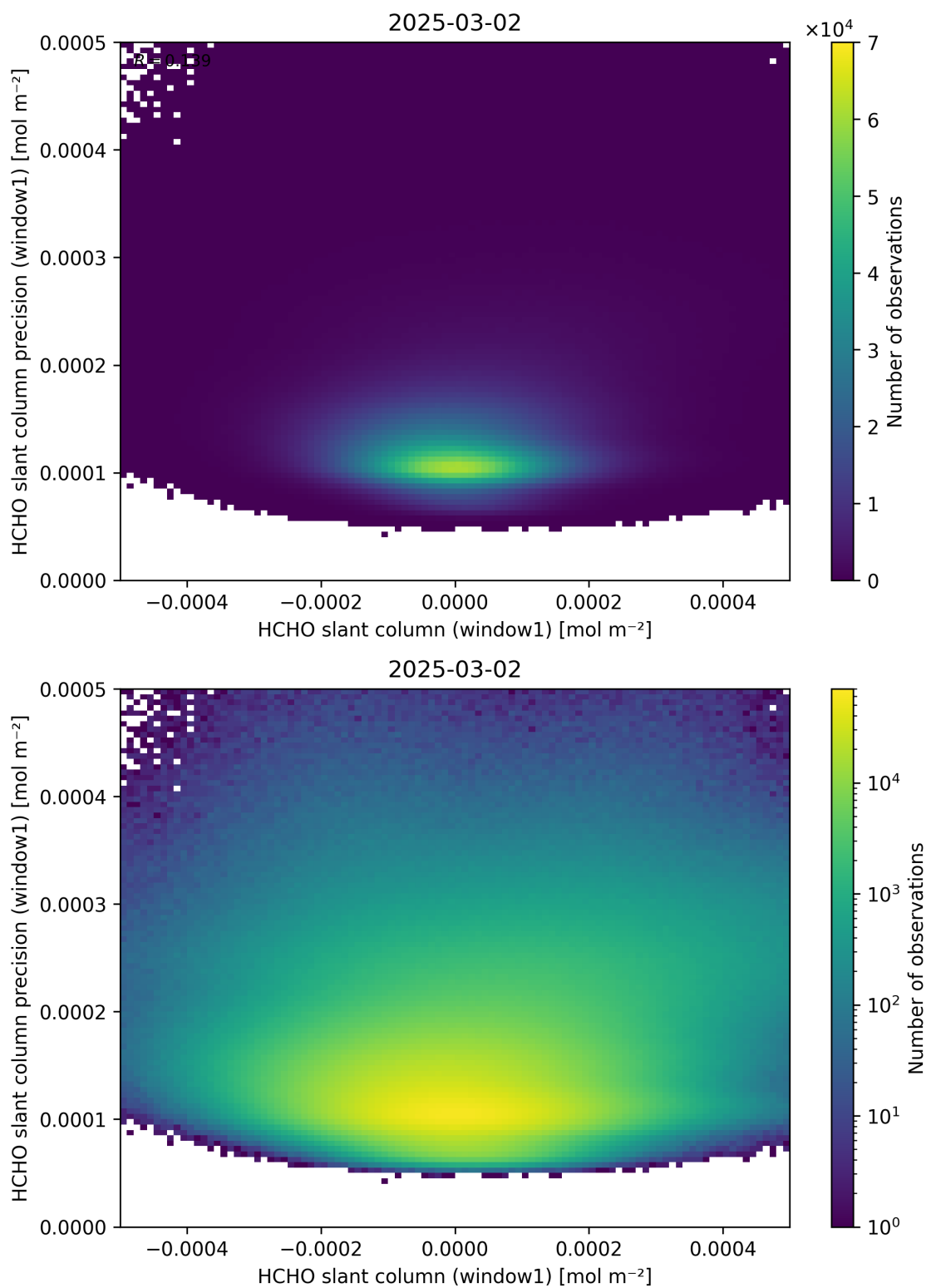
Figure 84: Scatter density plot of “HCHO slant column (window1)” against “HCHO slant column precision (window1)” for 2025-03-01 to 2025-03-03.
