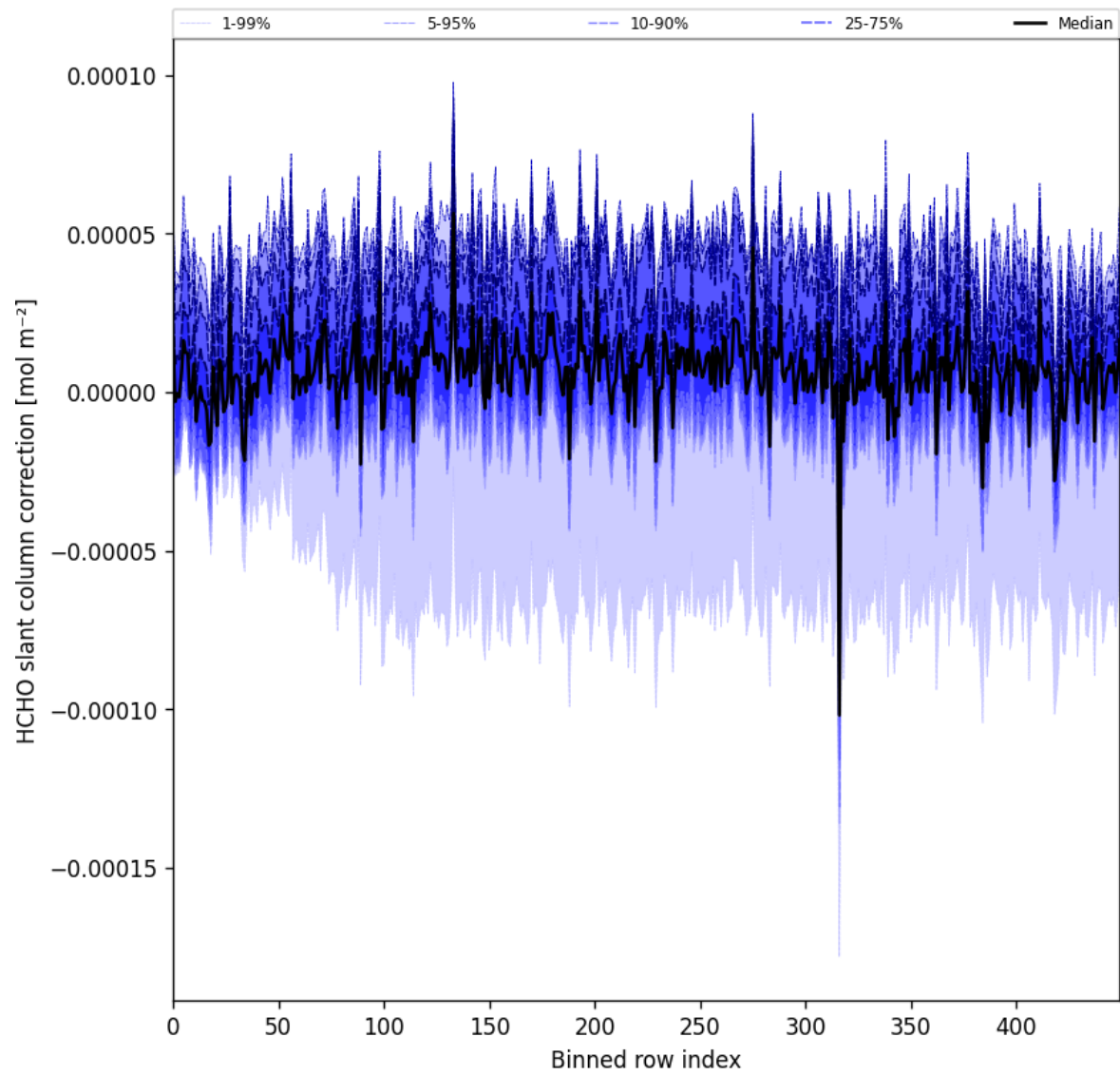
Figure 61: Along track statistics of “HCHO slant column correction” for 2025-03-01 to 2025-03-03
