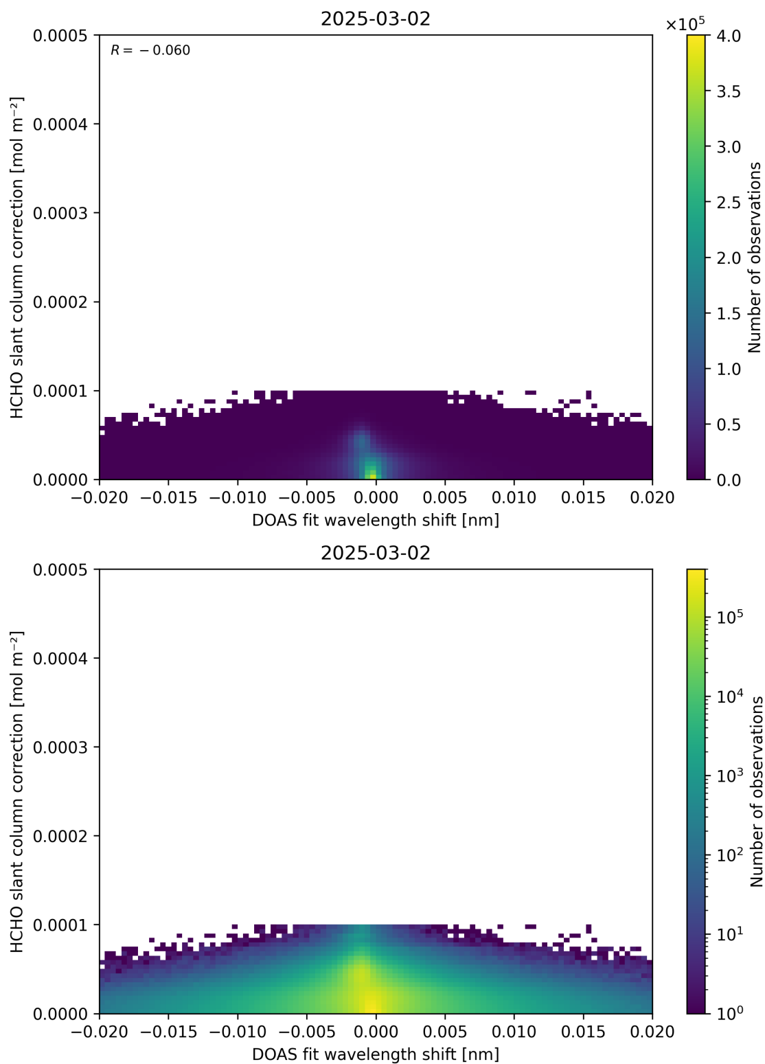
Figure 67: Scatter density plot of “DOAS fit wavelength shift” against “HCHO slant column correction” for 2025-03-01 to 2025-03-03.
