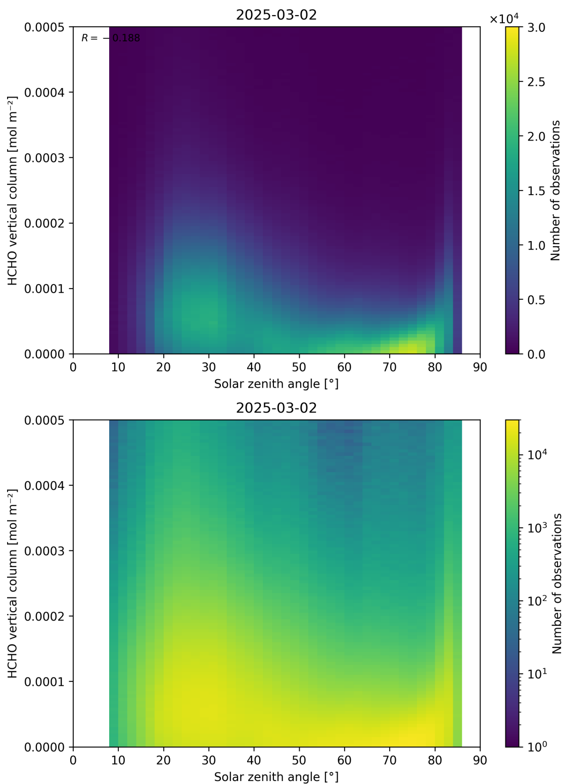
Figure 177: Scatter density plot of “Solar zenith angle” against “HCHO vertical column” for 2025-03-01 to 2025-03-03.
