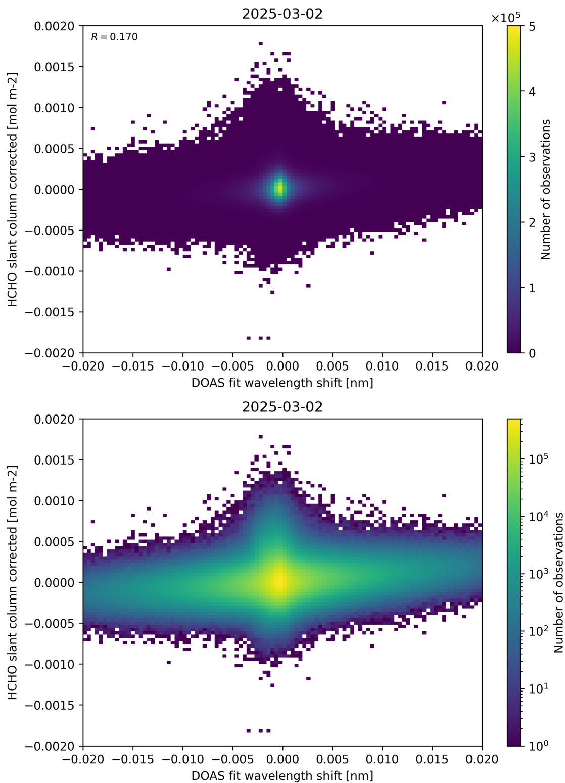
Figure 66: Scatter density plot of “DOAS fit wavelength shift” against “HCHO slant column corrected” for 2025-03-01 to 2025-03-03.
