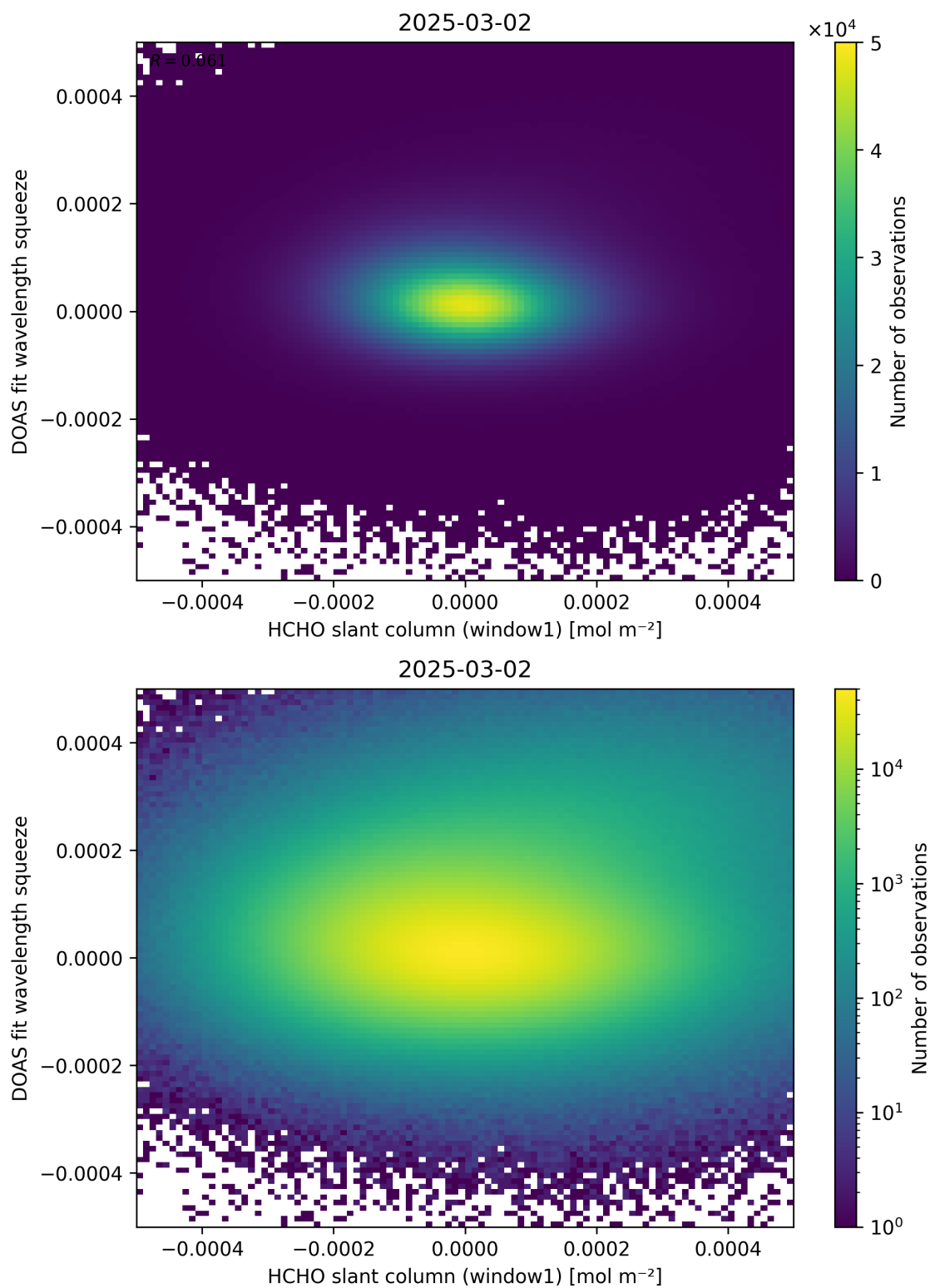
Figure 80: Scatter density plot of “HCHO slant column (window1)” against “DOAS fit wavelength squeeze” for 2025-03-01 to 2025-03-03.
