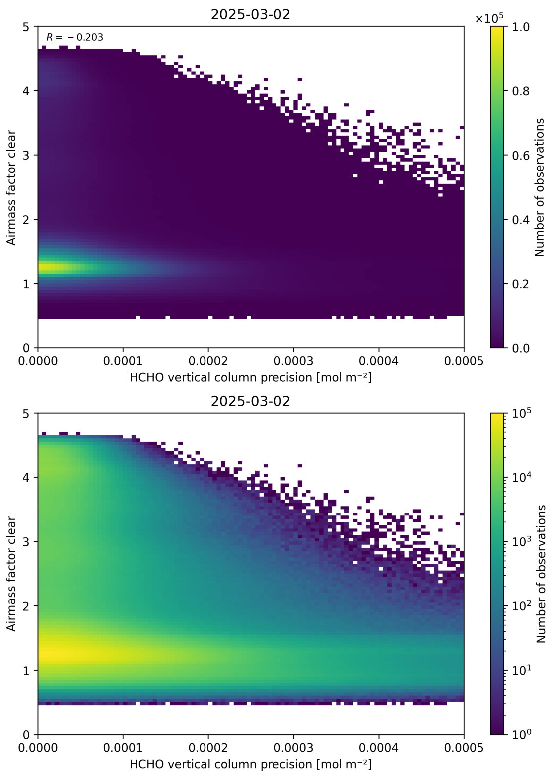
Figure 139: Scatter density plot of “HCHO vertical column precision” against “Airmass factor clear” for 2025-03-01 to 2025-03-03.
