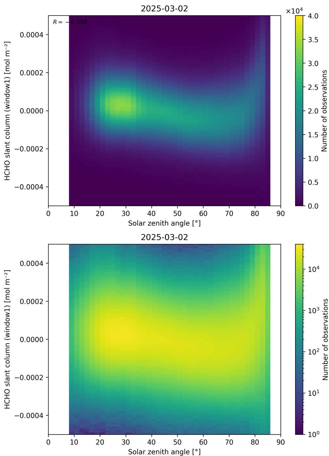
Figure 173: Scatter density plot of “Solar zenith angle” against “HCHO slant column (window1)” for 2025-03-01 to 2025-03-03.
