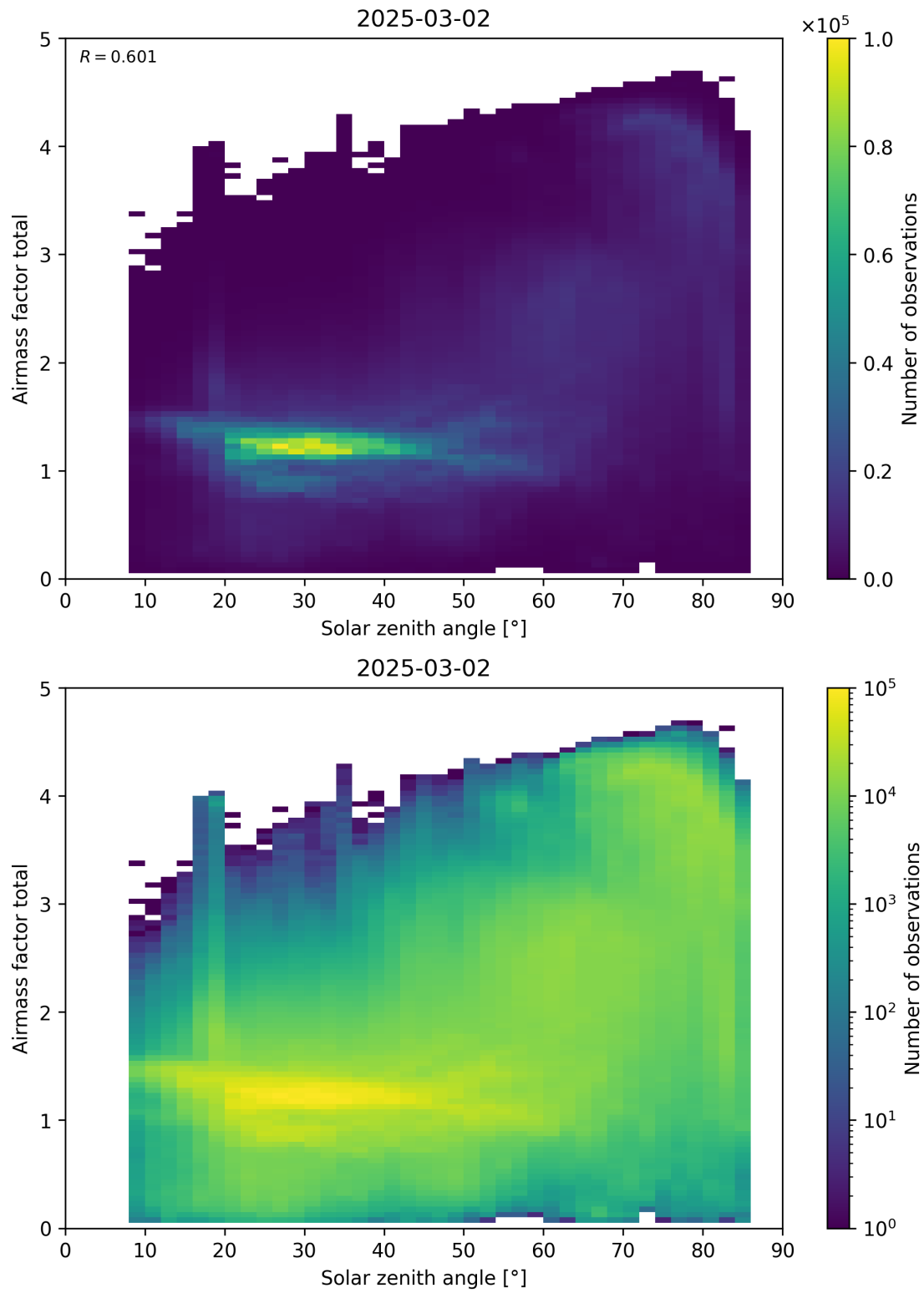
Figure 175: Scatter density plot of “Solar zenith angle” against “Airmass factor total” for 2025-03-01 to 2025-03-03.
