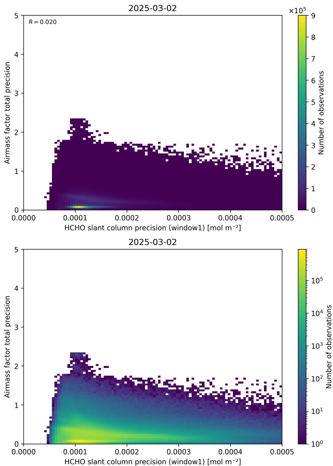
Figure 95: Scatter density plot of “HCHO slant column precision (window1)” against “Airmass factor total precision” for 2025-03-01 to 2025-03-03.
