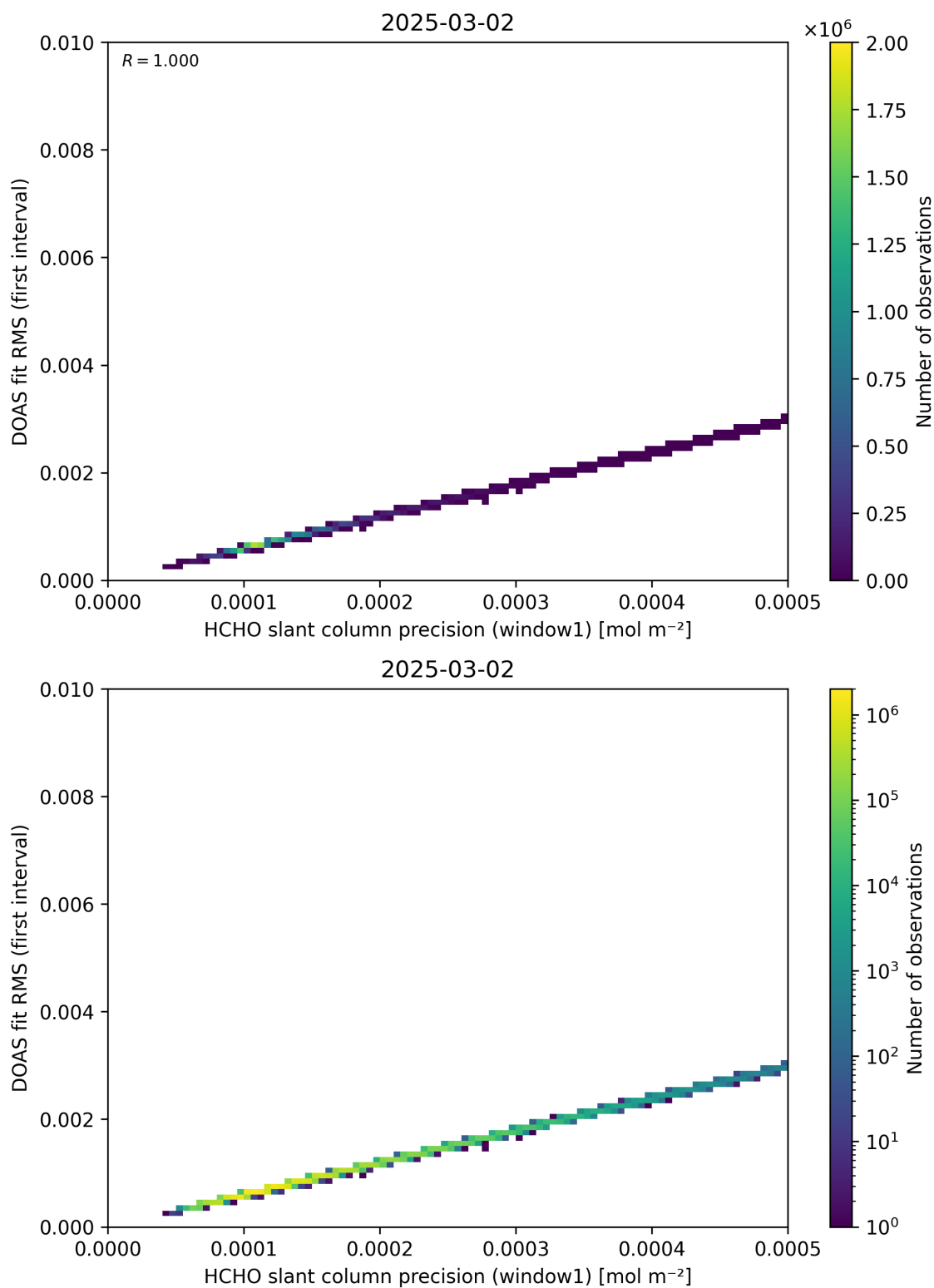
Figure 88: Scatter density plot of “HCHO slant column precision (window1)” against “DOAS fit RMS (first interval)” for 2025-03-01 to 2025-03-03.
