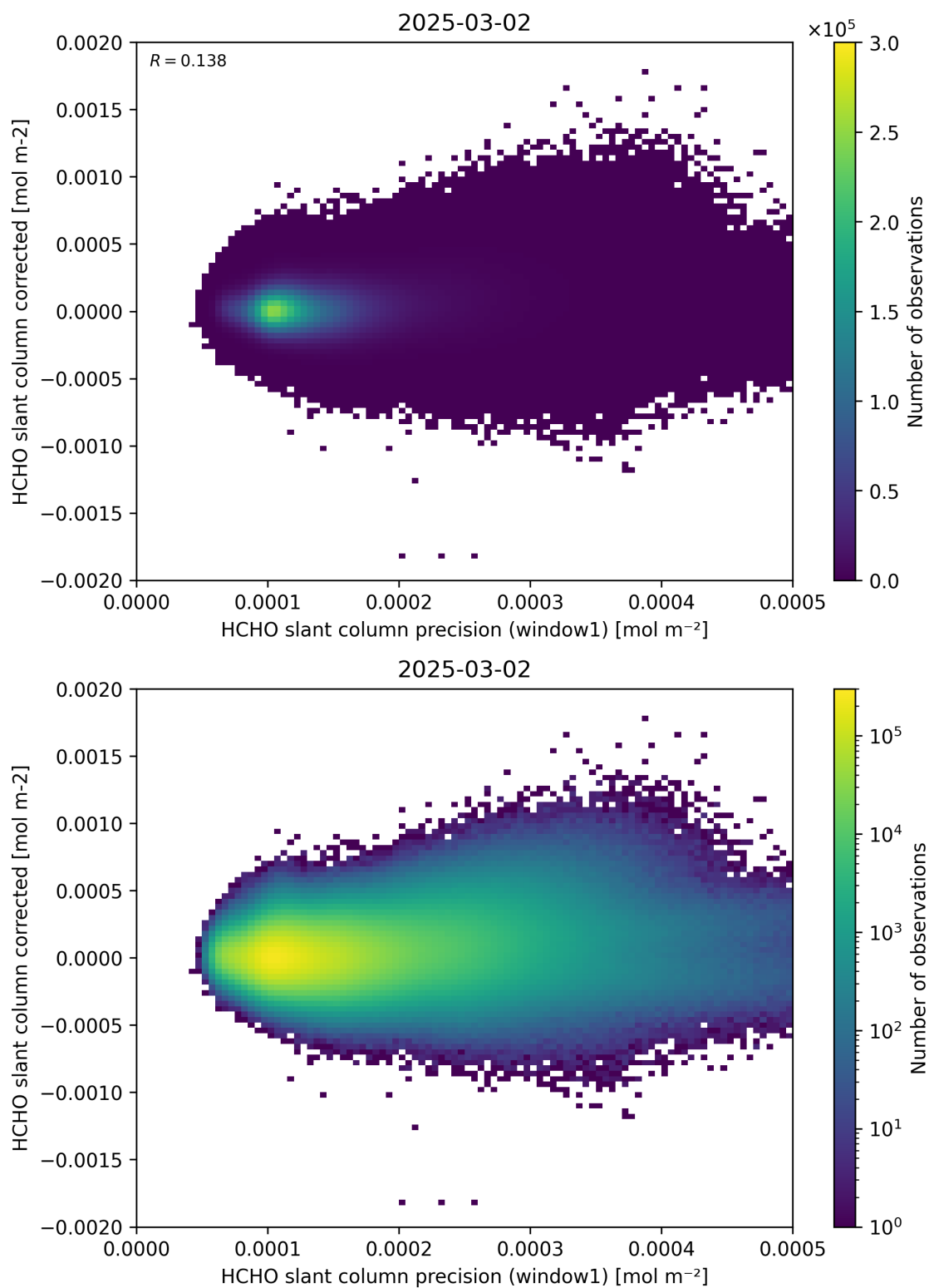
Figure 92: Scatter density plot of “HCHO slant column precision (window1)” against “HCHO slant column corrected” for 2025-03-01 to 2025-03-03.
