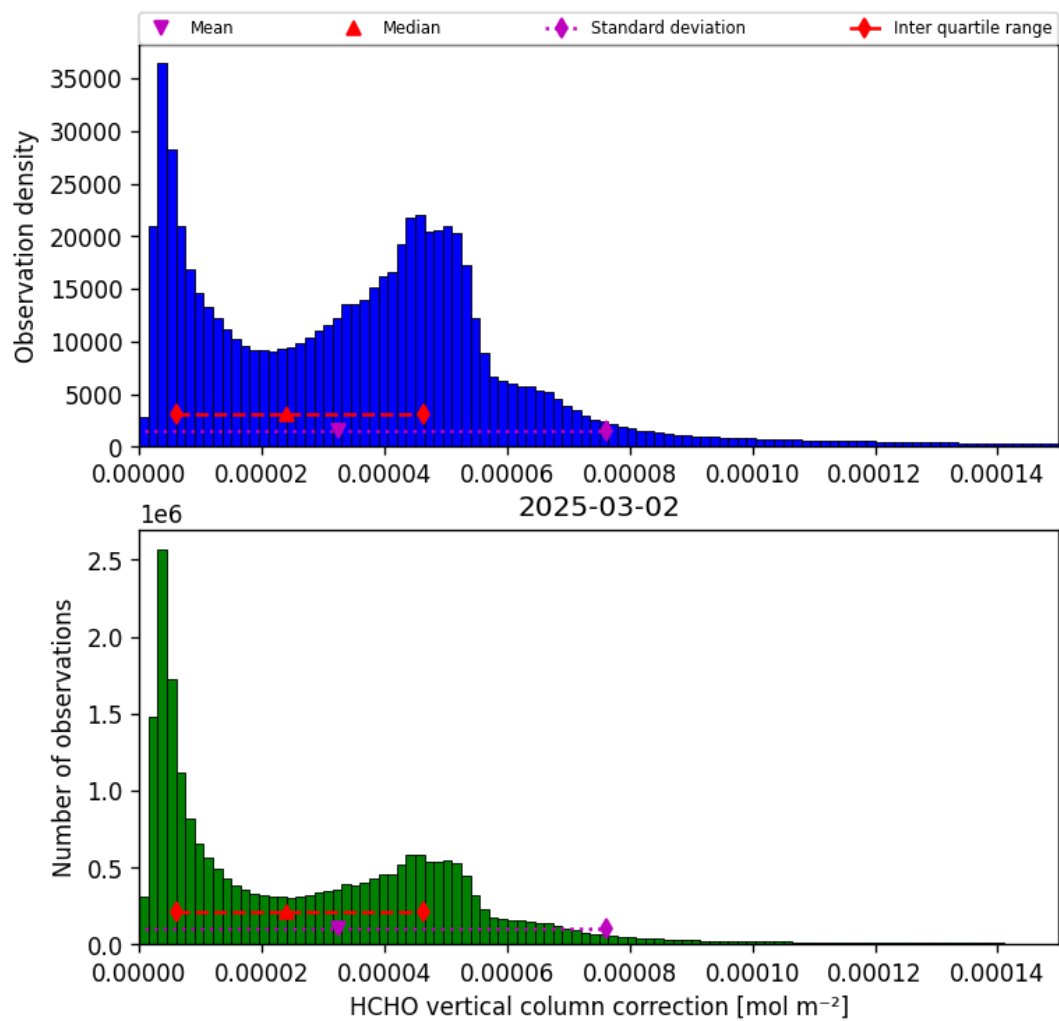
Figure 37: Histogram of “HCHO vertical column correction” for 2025-03-01 to 2025-03-03
