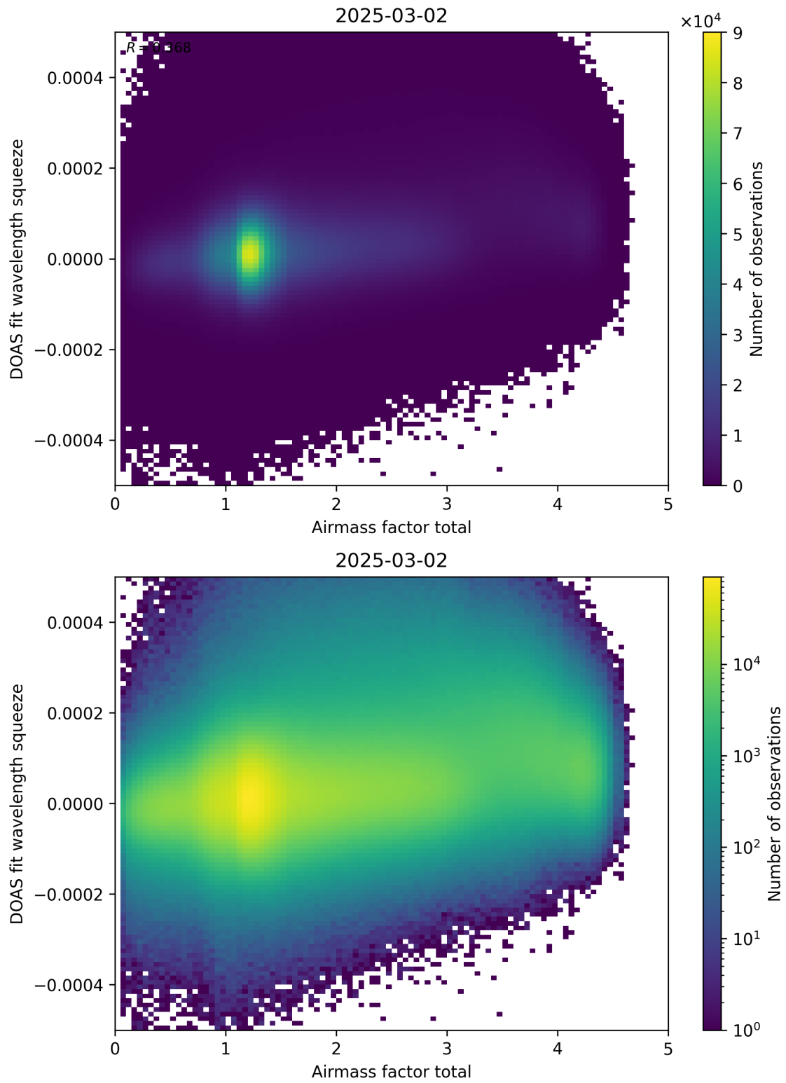
Figure 99: Scatter density plot of “Airmass factor total” against “DOAS fit wavelength squeeze” for 2025-03-01 to 2025-03-03.
