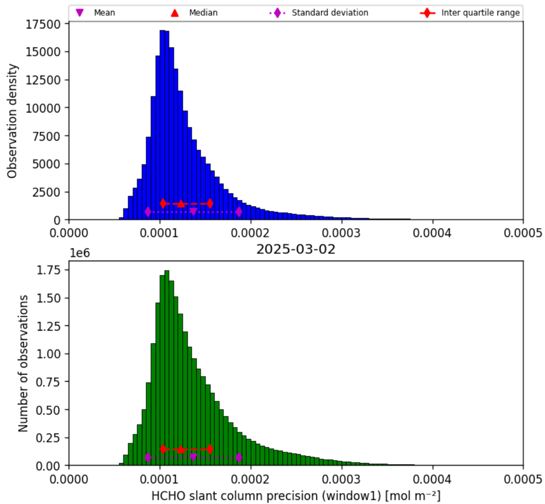
Figure 39: Histogram of “HCHO slant column precision (window1)” for 2025-03-01 to 2025-03-03
