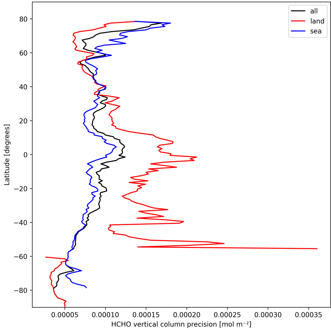
Figure 22: Zonal average of “HCHO vertical column precision” for 2025-03-01 to 2025-03-03.
