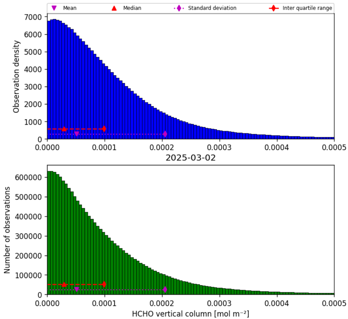
Figure 35: Histogram of “HCHO vertical column” for 2025-03-01 to 2025-03-03
