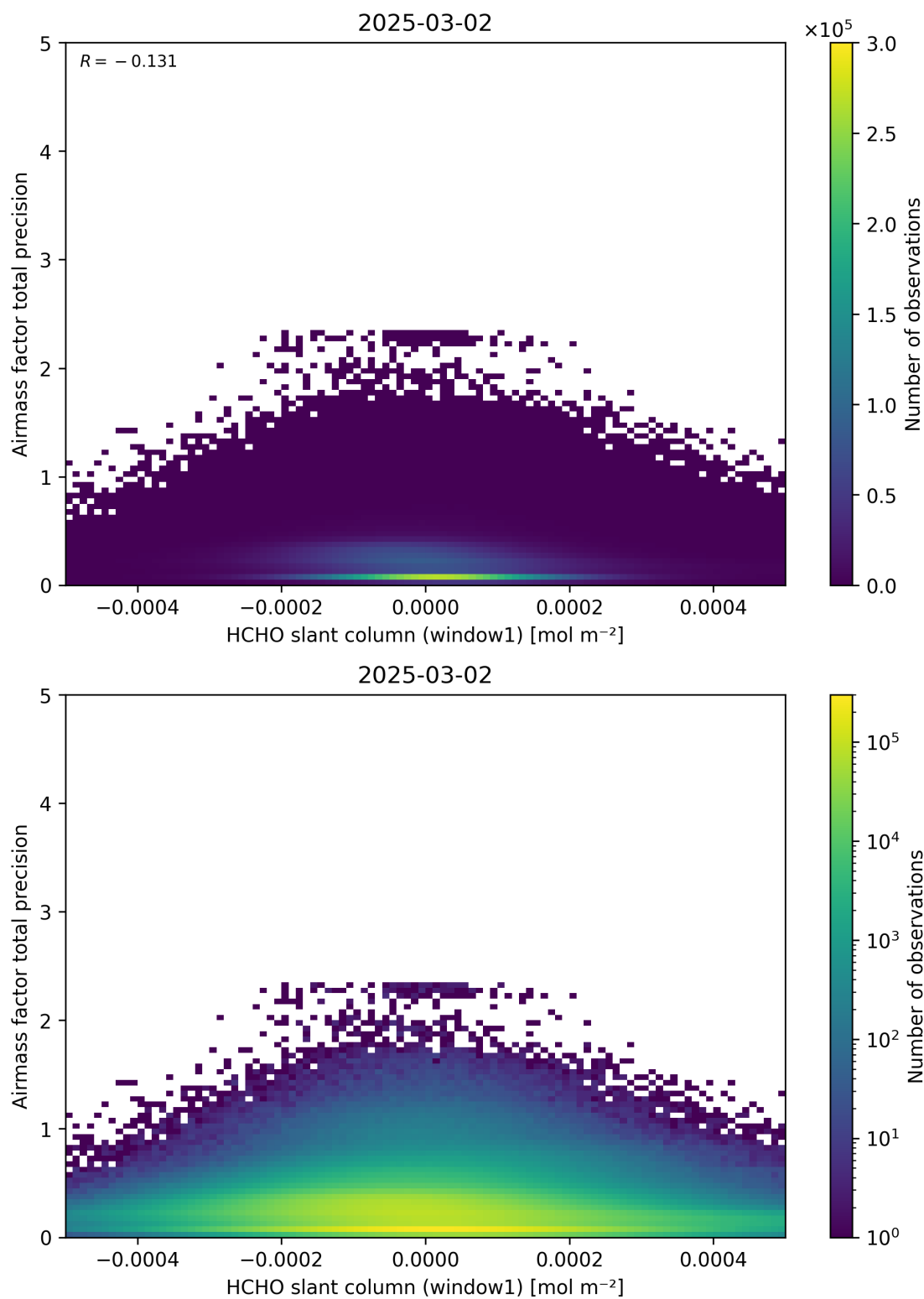
Figure 86: Scatter density plot of “HCHO slant column (window1)” against “Airmass factor total precision” for 2025-03-01 to 2025-03-03.
