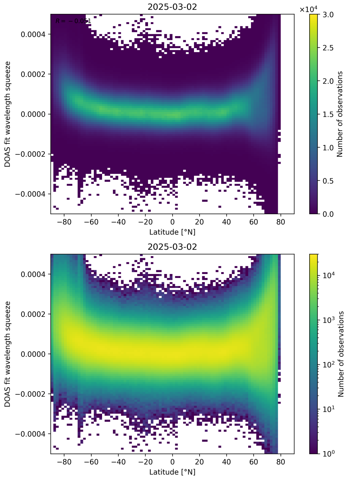
Figure 155: Scatter density plot of “Latitude” against “DOAS fit wavelength squeeze” for 2025-03-01 to 2025-03-03.
