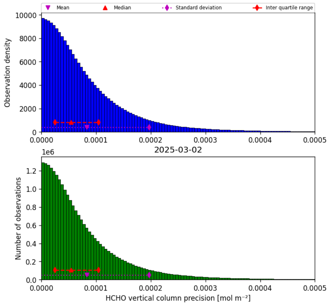
Figure 36: Histogram of “HCHO vertical column precision” for 2025-03-01 to 2025-03-03
