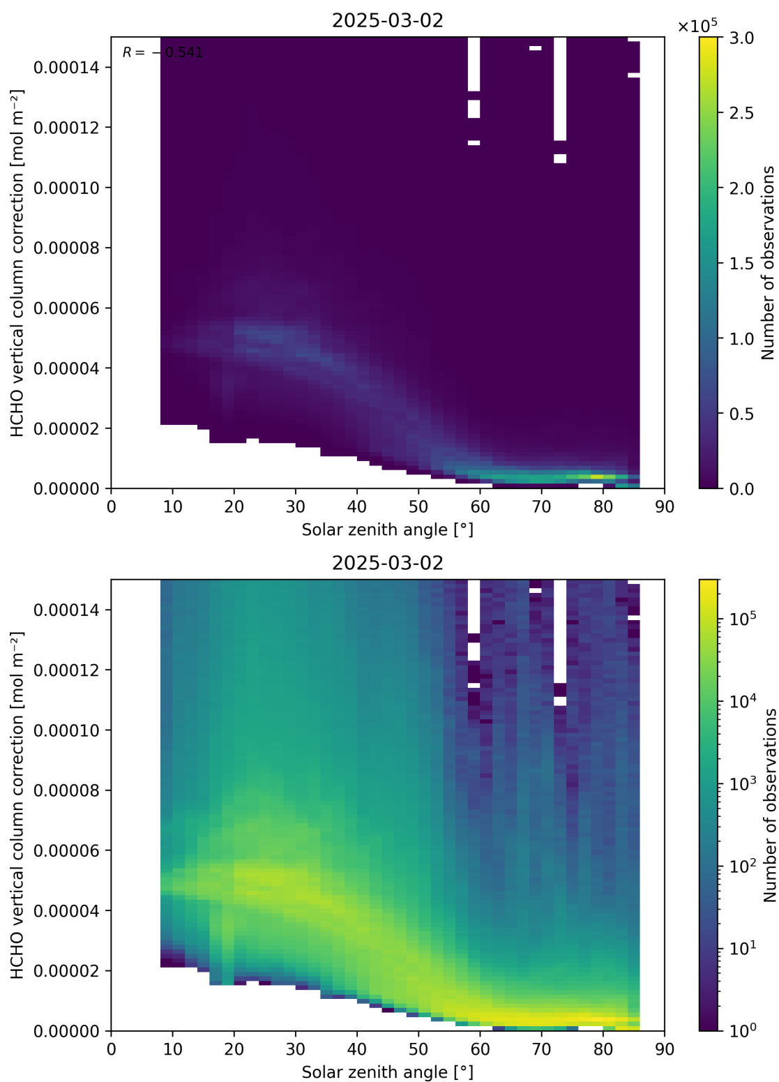
Figure 178: Scatter density plot of “Solar zenith angle” against “HCHO vertical column correction” for 2025-03-01 to 2025-03-03.
