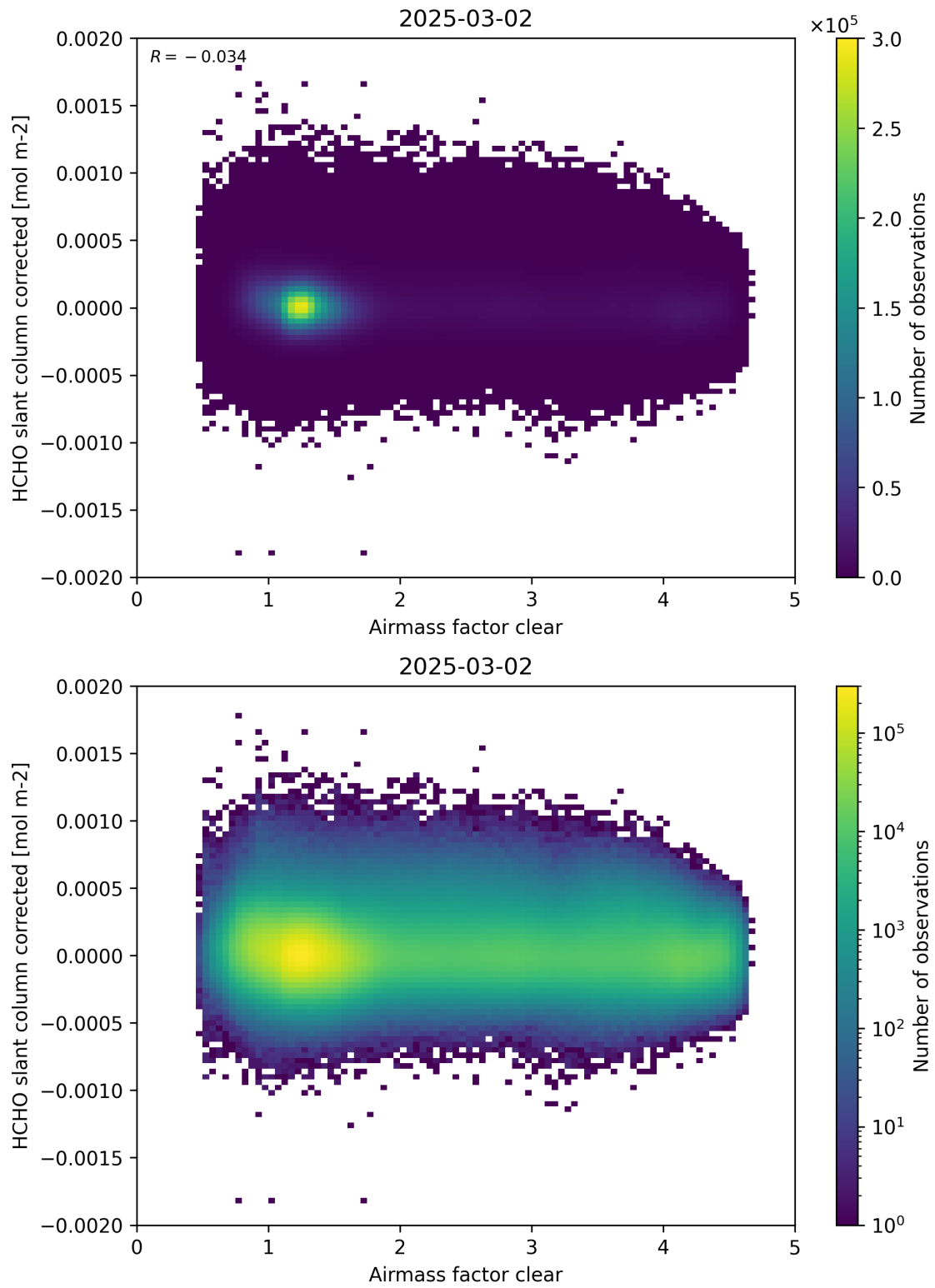
Figure 74: Scatter density plot of “Airmass factor clear” against “HCHO slant column corrected” for 2025-03-01 to 2025-03-03.
