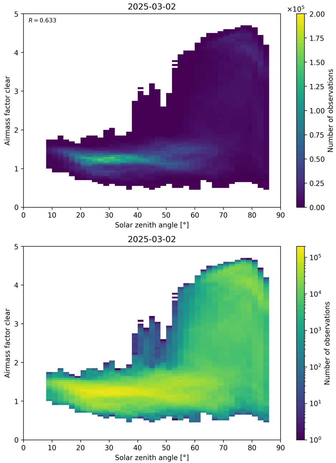
Figure 170: Scatter density plot of “Solar zenith angle” against “Airmass factor clear” for 2025-03-01 to 2025-03-03.
