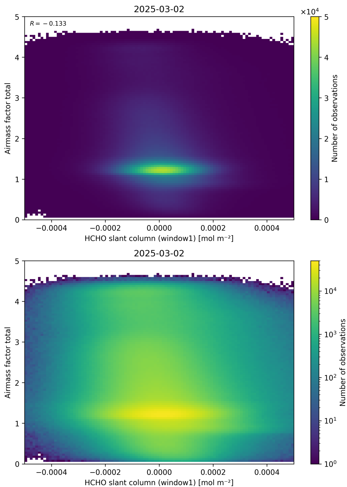
Figure 85: Scatter density plot of “HCHO slant column (window1)” against “Airmass factor total” for 2025-03-01 to 2025-03-03.
