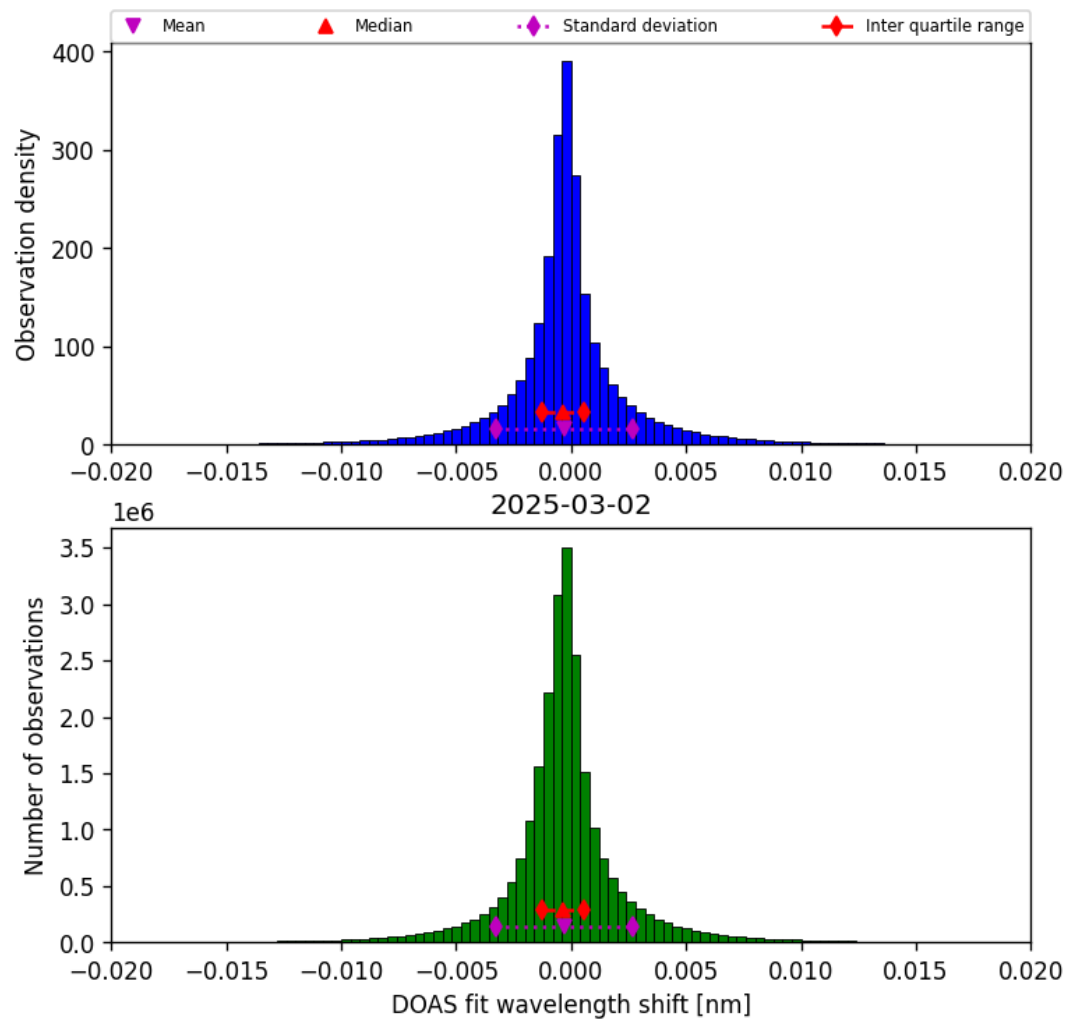
Figure 44: Histogram of “DOAS fit wavelength shift” for 2025-03-01 to 2025-03-03
