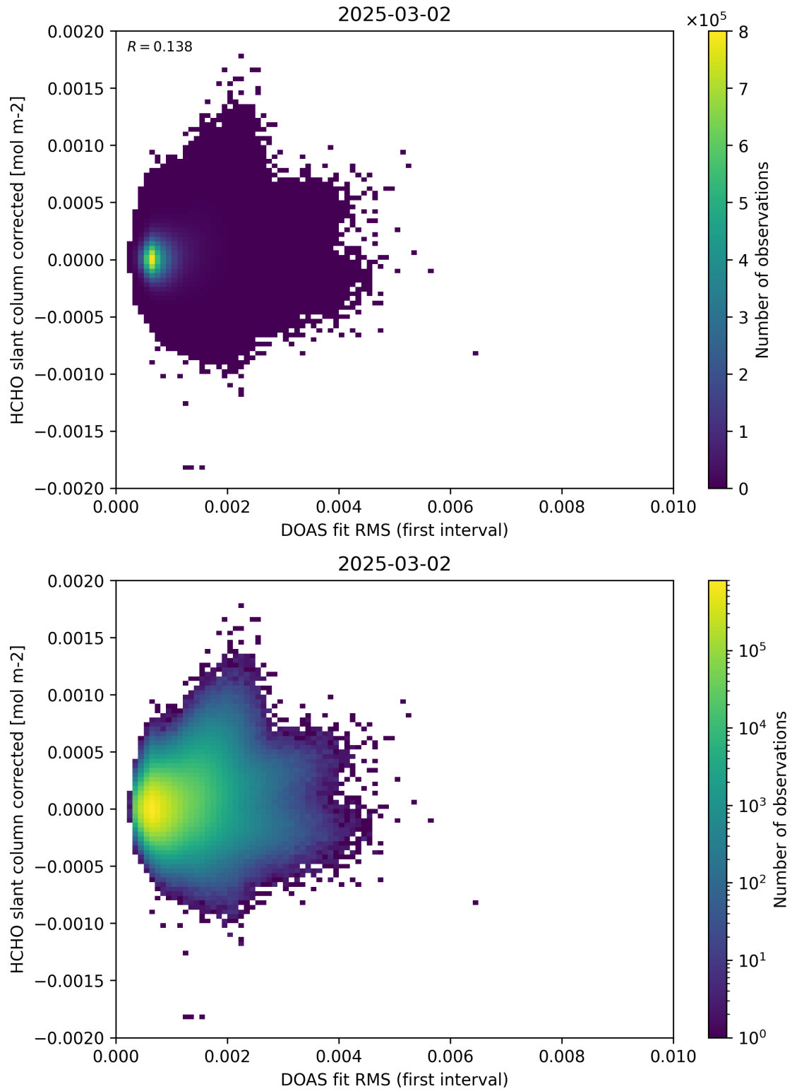
Figure 62: Scatter density plot of “DOAS fit RMS (first interval)” against “HCHO slant column corrected” for 2025-03-01 to 2025-03-03.
