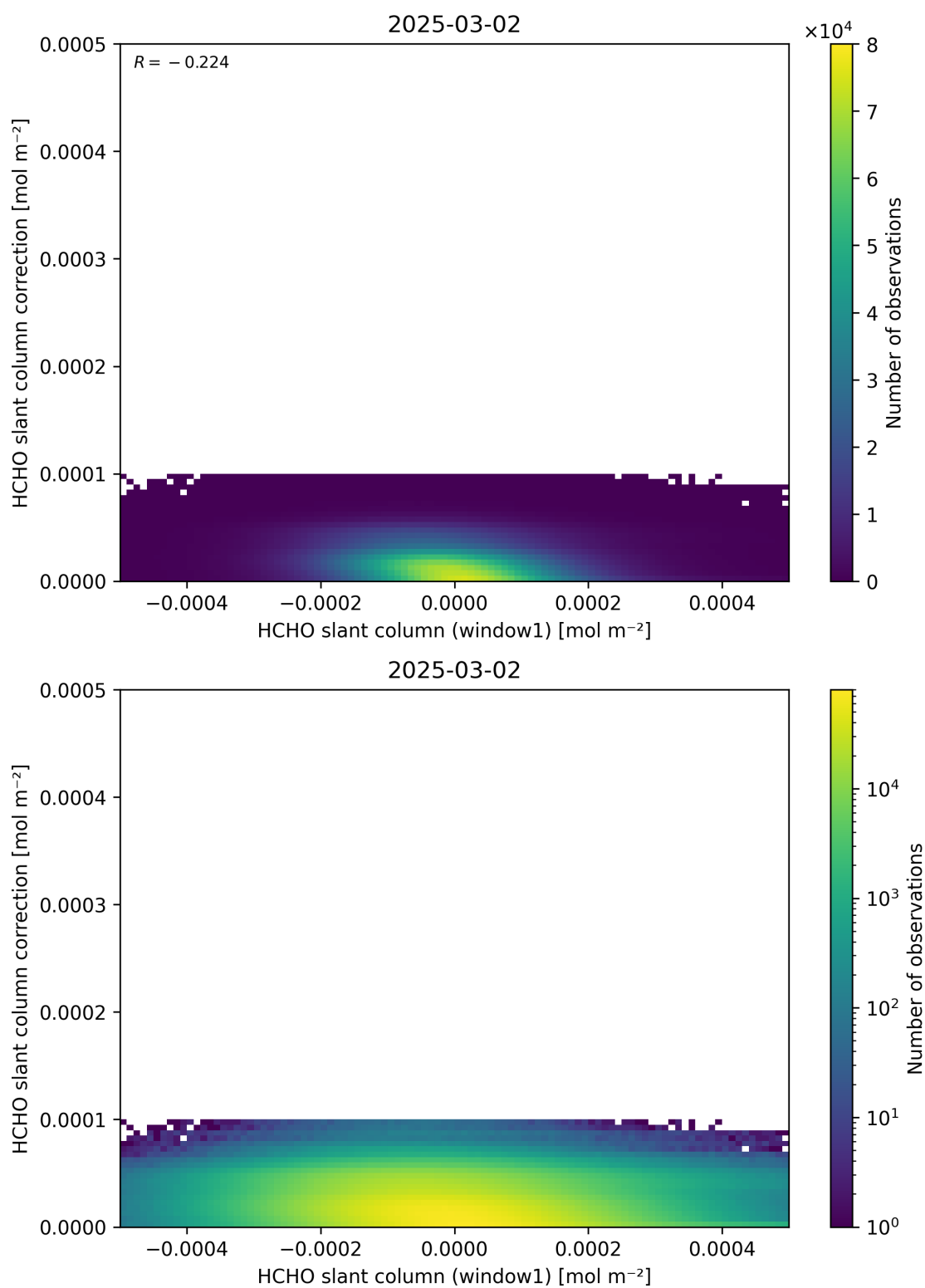
Figure 83: Scatter density plot of “HCHO slant column (window1)” against “HCHO slant column correction” for 2025-03-01 to 2025-03-03.
