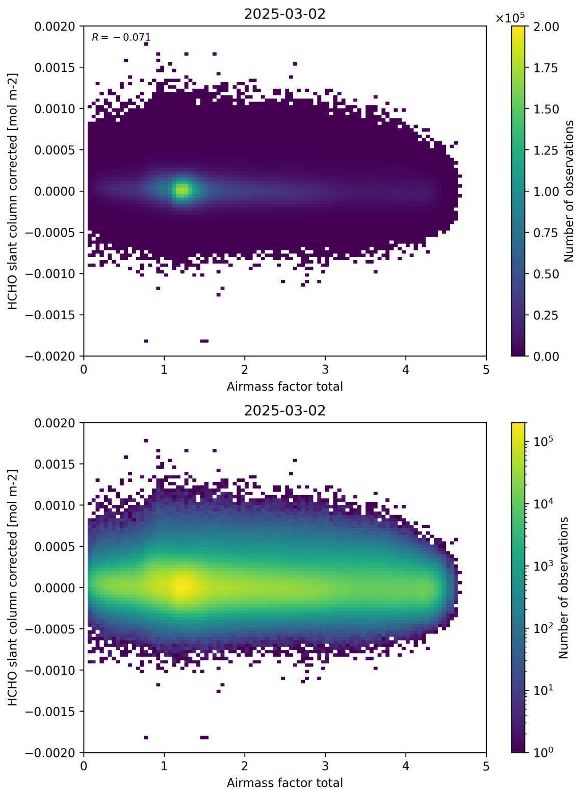
Figure 101: Scatter density plot of “Airmass factor total” against “HCHO slant column corrected” for 2025-03-01 to 2025-03-03.
