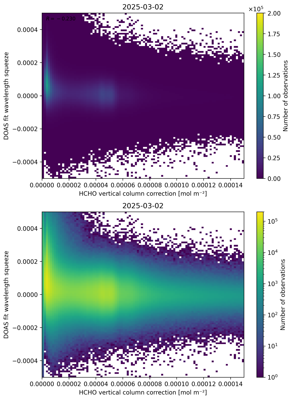
Figure 114: Scatter density plot of “HCHO vertical column correction” against “DOAS fit wavelength squeeze” for 2025-03-01 to 2025-03-03.
