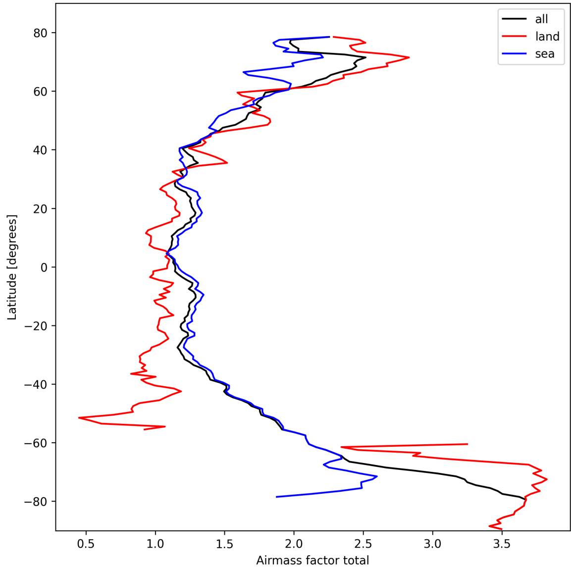
Figure 26: Zonal average of “Airmass factor total” for 2025-03-01 to 2025-03-03.
