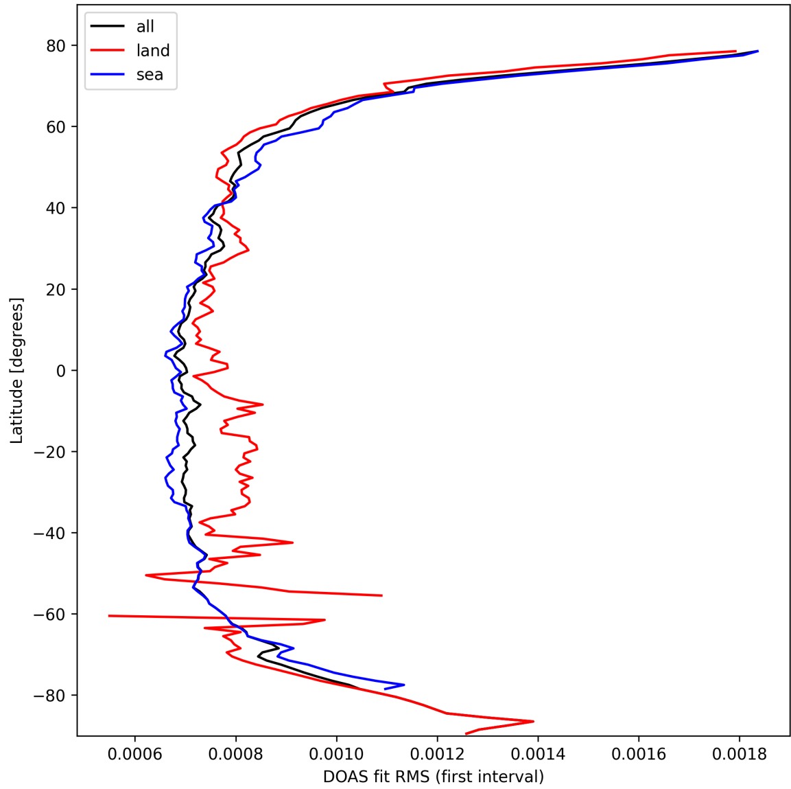
Figure 32: Zonal average of “DOAS fit RMS (first interval)” for 2025-03-01 to 2025-03-03.
