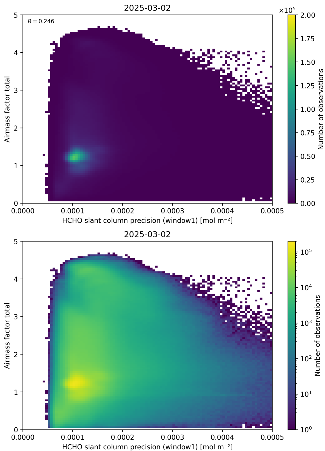
Figure 94: Scatter density plot of “HCHO slant column precision (window1)” against “Airmass factor total” for 2025-03-01 to 2025-03-03.
