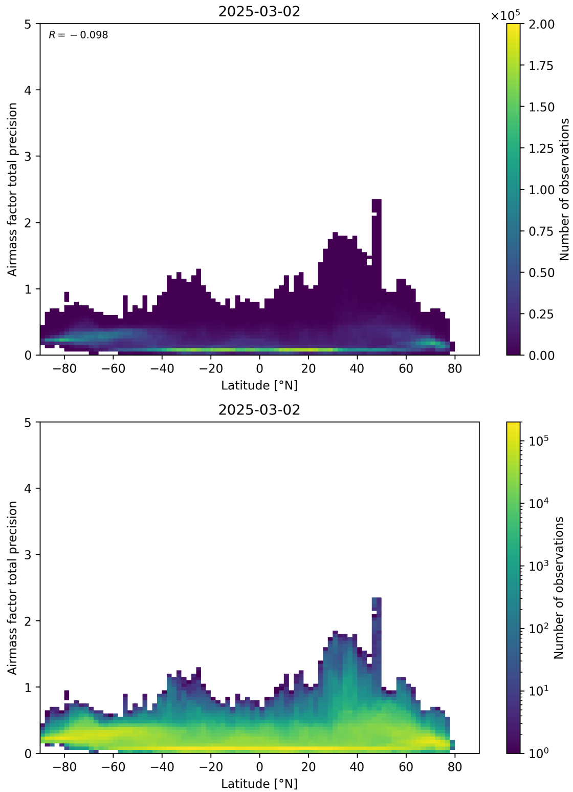
Figure 162: Scatter density plot of “Latitude” against “Airmass factor total precision” for 2025-03-01 to 2025-03-03.
