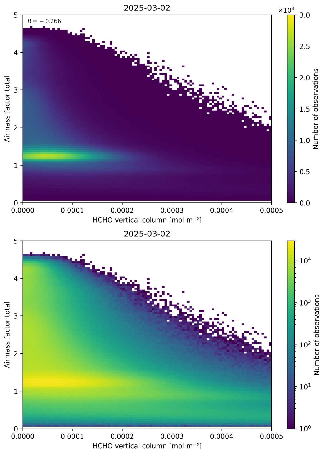
Figure 131: Scatter density plot of “HCHO vertical column” against “Airmass factor total” for 2025-03-01 to 2025-03-03.
