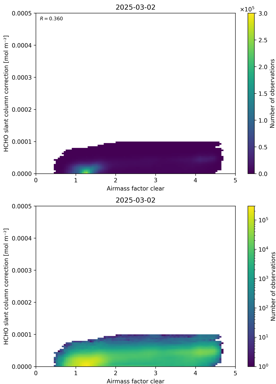
Figure 75: Scatter density plot of “Airmass factor clear” against “HCHO slant column correction” for 2025-03-01 to 2025-03-03.
