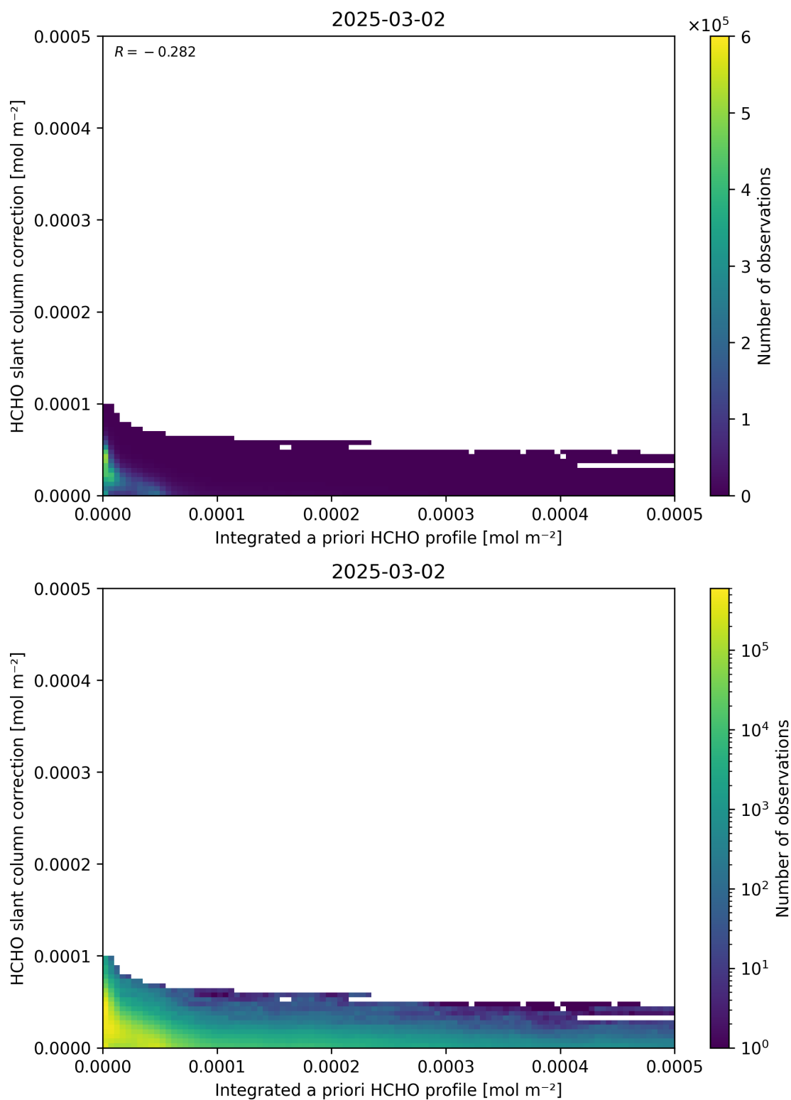
Figure 152: Scatter density plot of “Integrated a priori HCHO profile” against “HCHO slant column correction” for 2025-03-01 to 2025-03-03.
