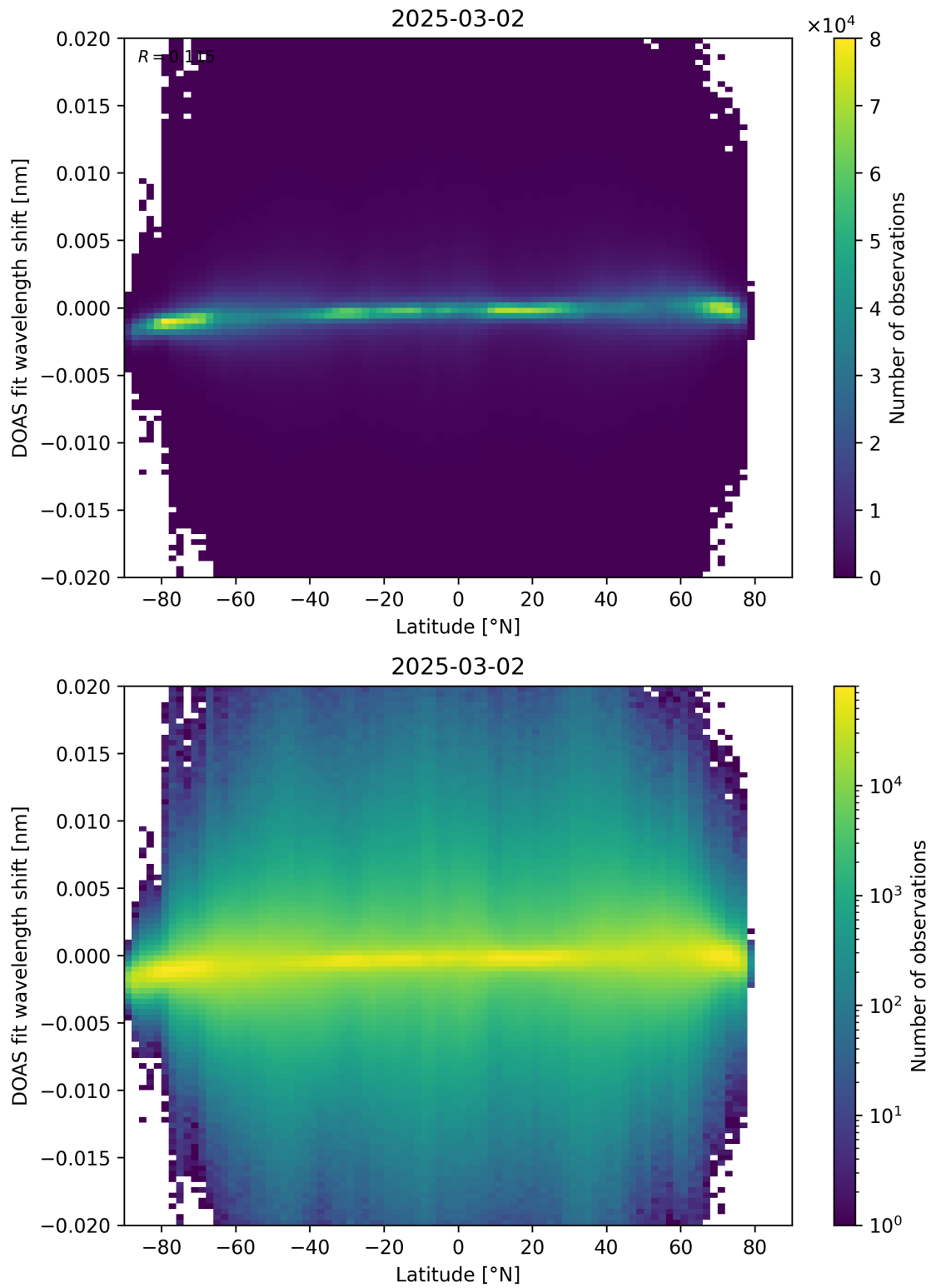
Figure 154: Scatter density plot of “Latitude” against “DOAS fit wavelength shift” for 2025-03-01 to 2025-03-03.
