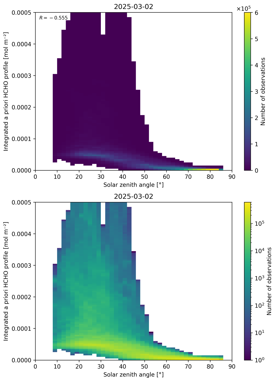
Figure 180: Scatter density plot of “Solar zenith angle” against “Integrated a priori HCHO profile” for 2025-03-01 to 2025-03-03.
