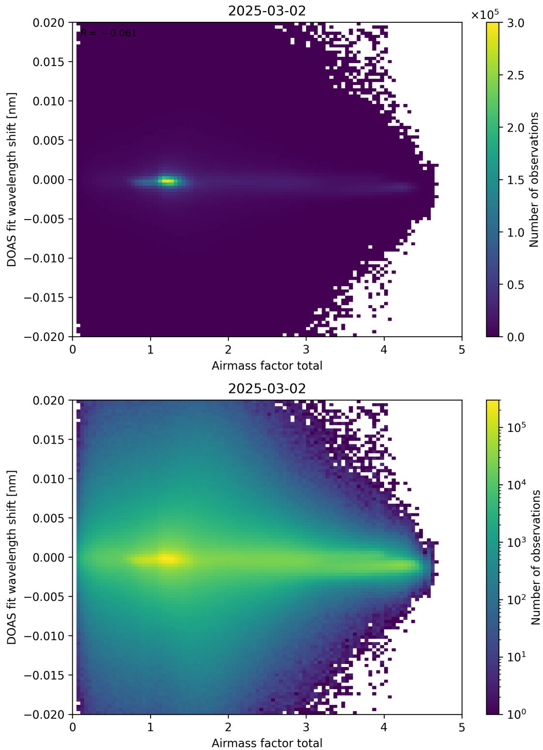
Figure 98: Scatter density plot of “Airmass factor total” against “DOAS fit wavelength shift” for 2025-03-01 to 2025-03-03.
