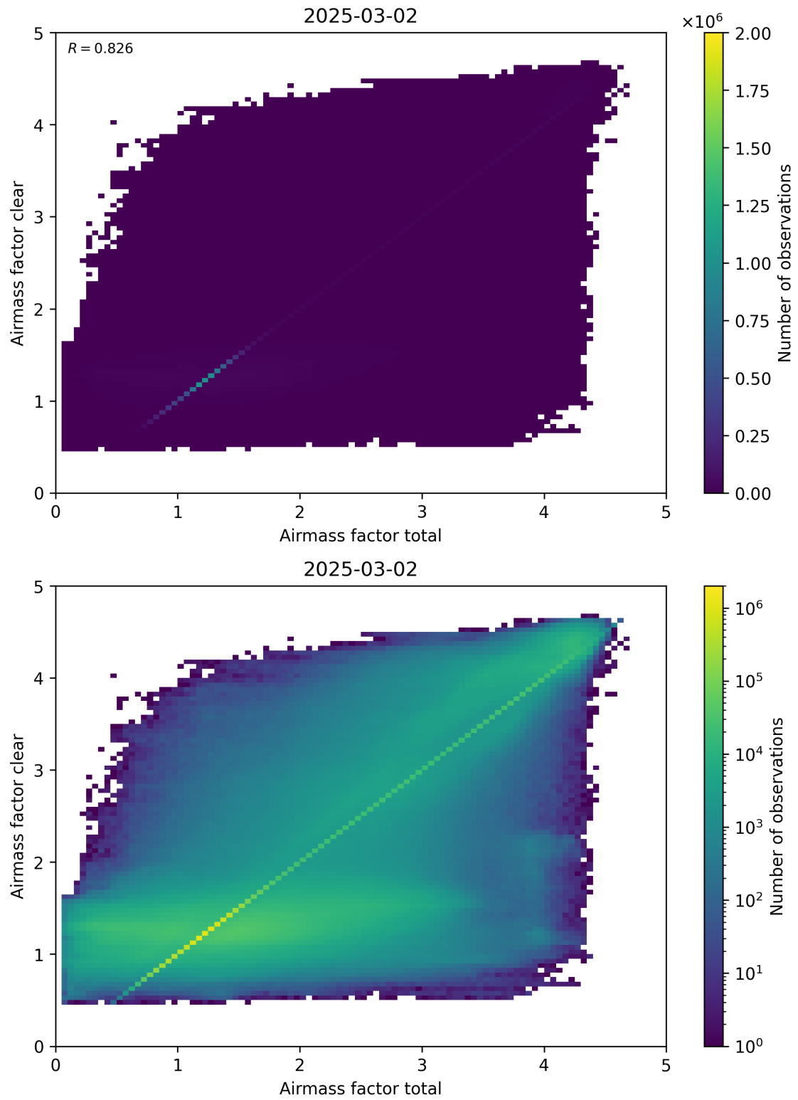
Figure 100: Scatter density plot of “Airmass factor total” against “Airmass factor clear” for 2025-03-01 to 2025-03-03.
