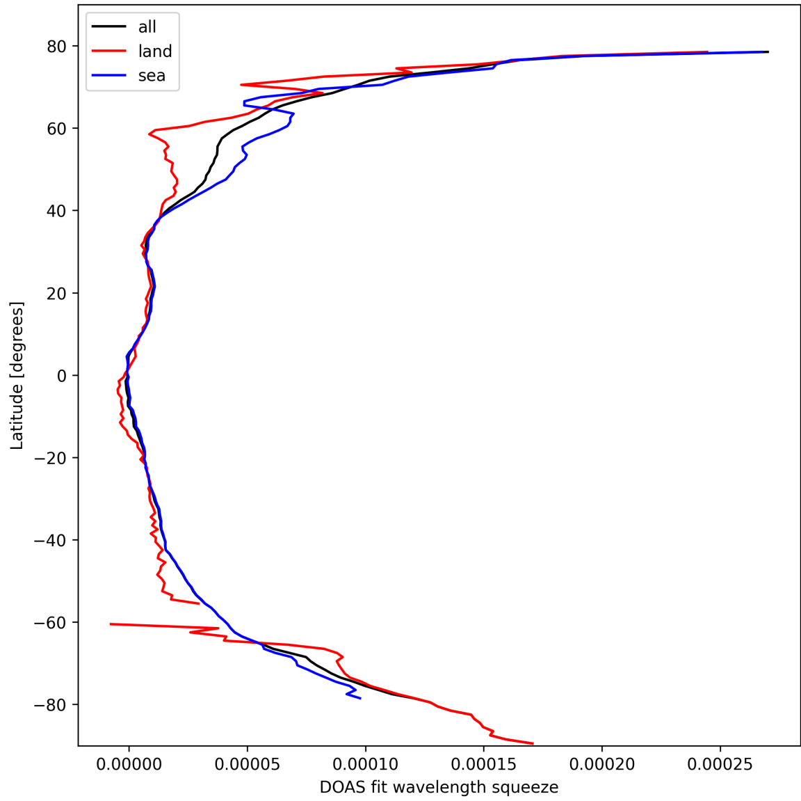
Figure 31: Zonal average of “DOAS fit wavelength squeeze” for 2025-03-01 to 2025-03-03.
