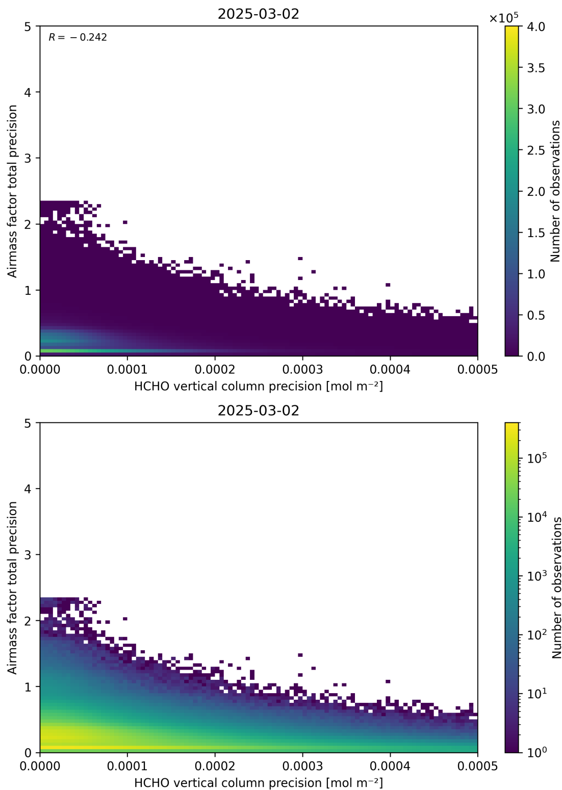
Figure 145: Scatter density plot of “HCHO vertical column precision” against “Airmass factor total precision” for 2025-03-01 to 2025-03-03.
