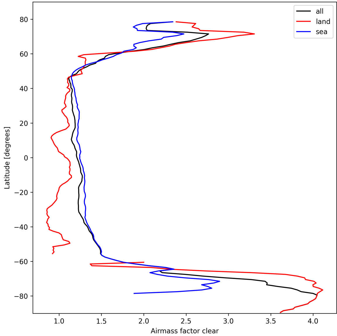
Figure 28: Zonal average of “Airmass factor clear” for 2025-03-01 to 2025-03-03.
