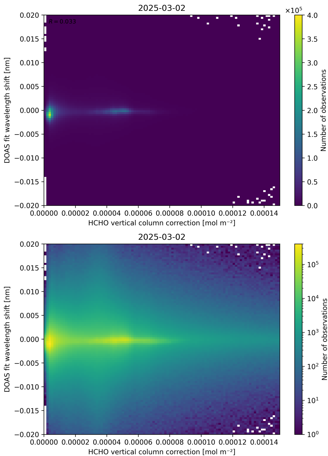
Figure 113: Scatter density plot of “HCHO vertical column correction” against “DOAS fit wavelength shift” for 2025-03-01 to 2025-03-03.
