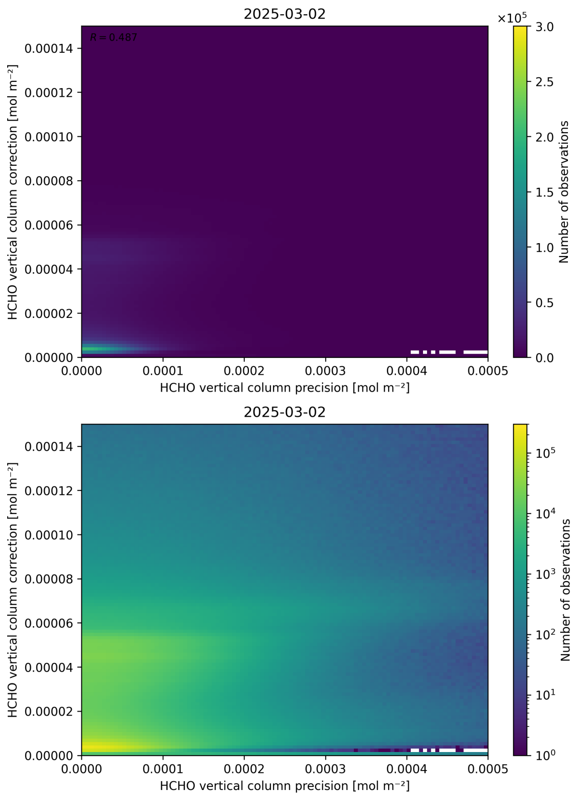
Figure 146: Scatter density plot of “HCHO vertical column precision” against “HCHO vertical column correction” for 2025-03-01 to 2025-03-03.
