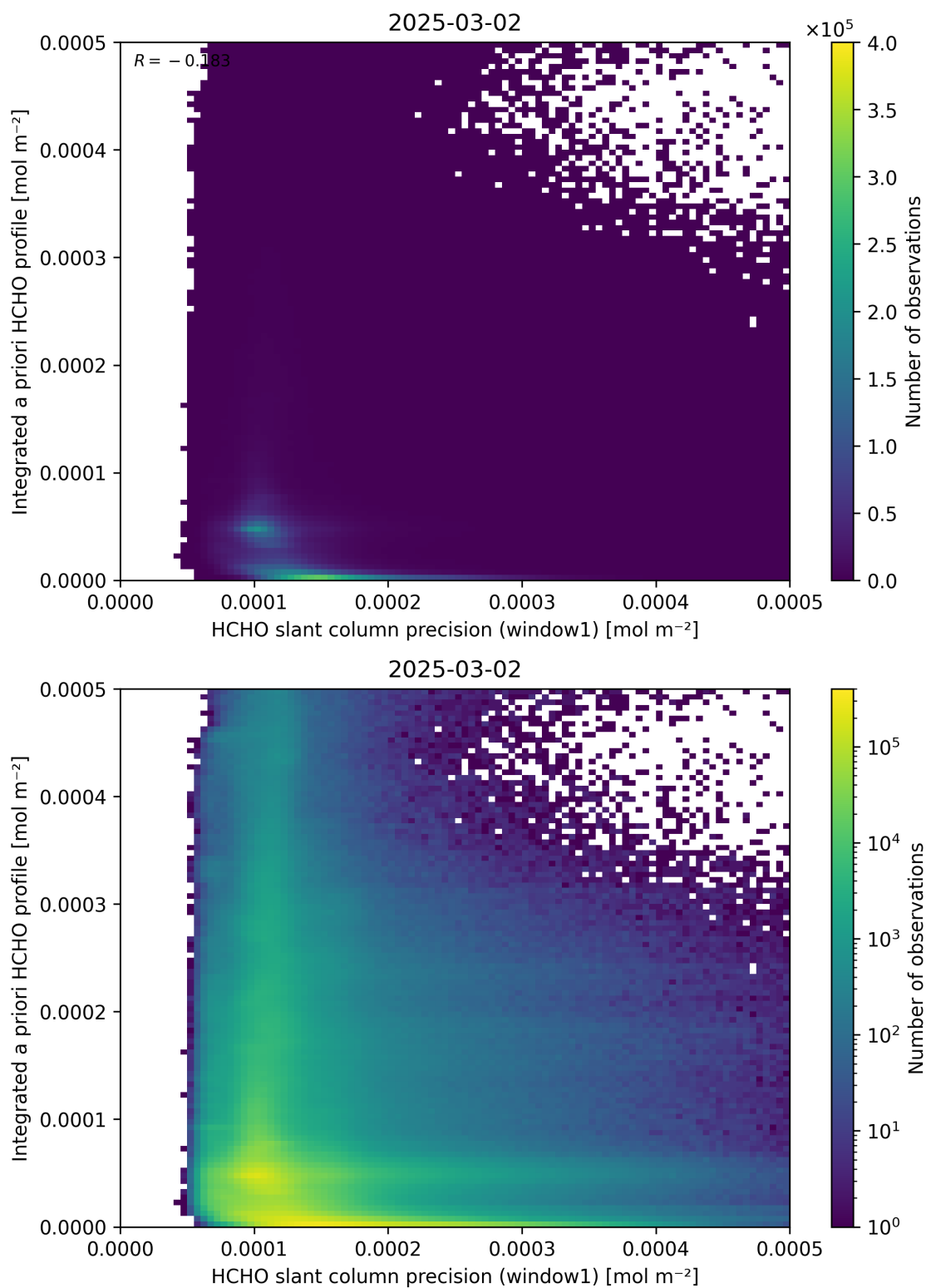
Figure 96: Scatter density plot of “HCHO slant column precision (window1)” against “Integrated a priori HCHO profile” for 2025-03-01 to 2025-03-03.
