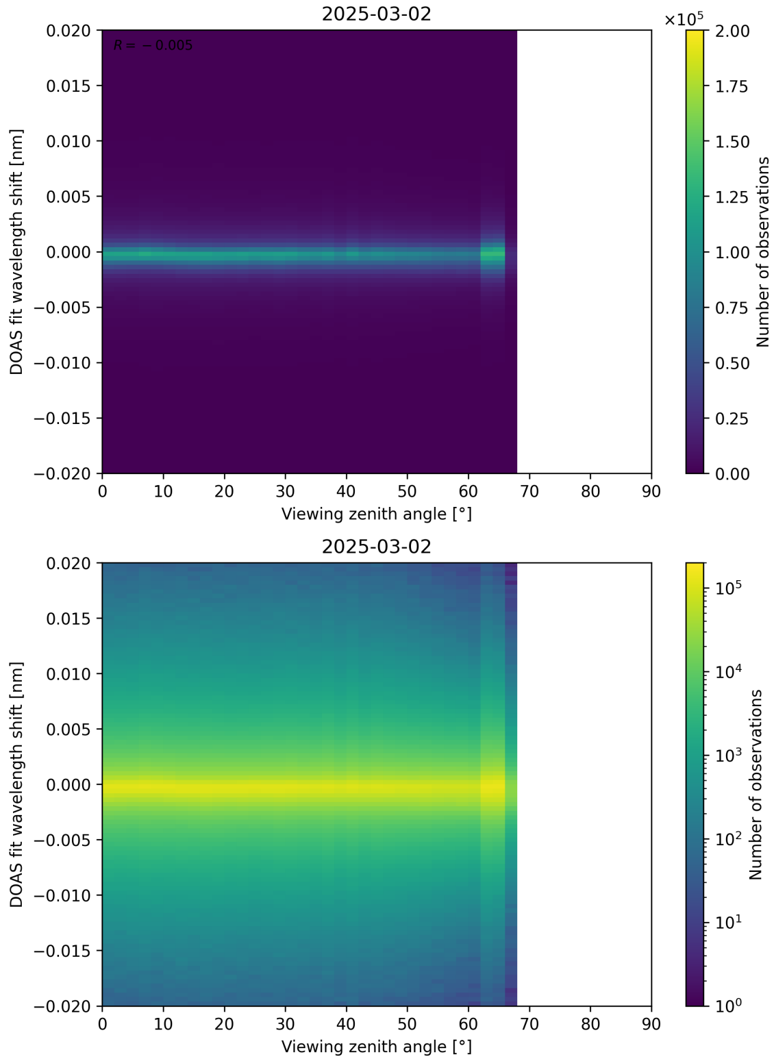
Figure 183: Scatter density plot of “Viewing zenith angle” against “DOAS fit wavelength shift” for 2025-03-01 to 2025-03-03.
