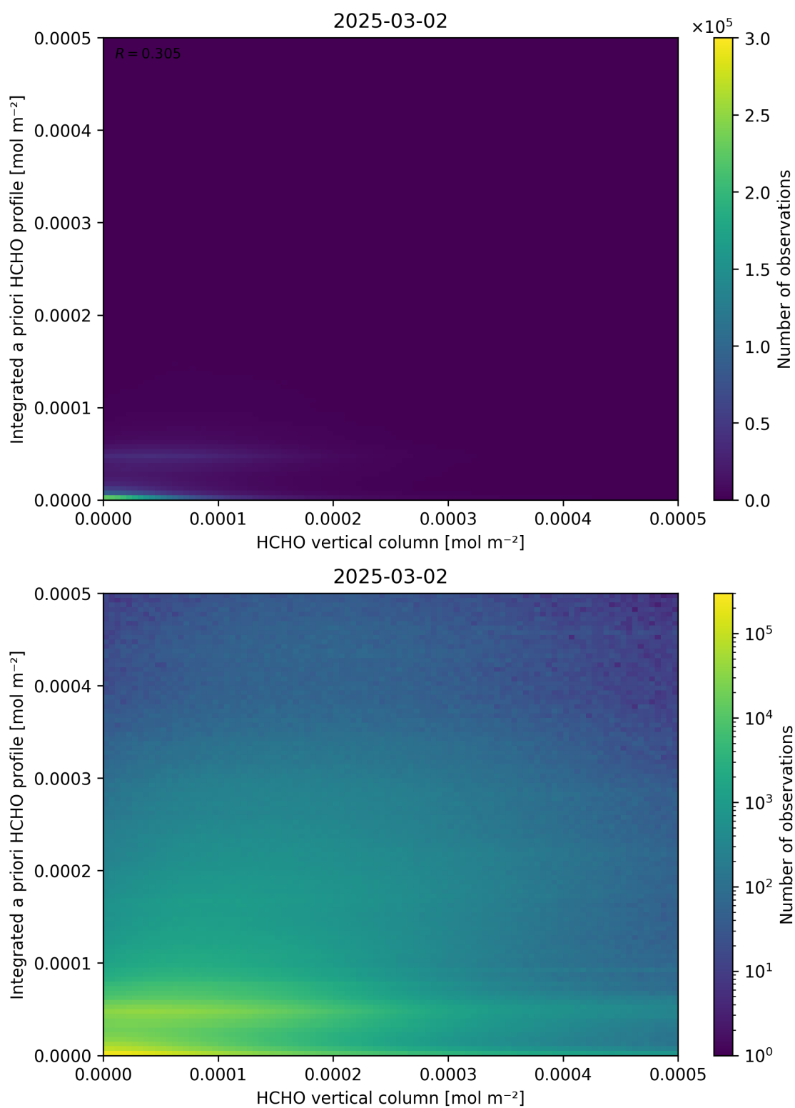
Figure 135: Scatter density plot of “HCHO vertical column” against “Integrated a priori HCHO profile” for 2025-03-01 to 2025-03-03.
