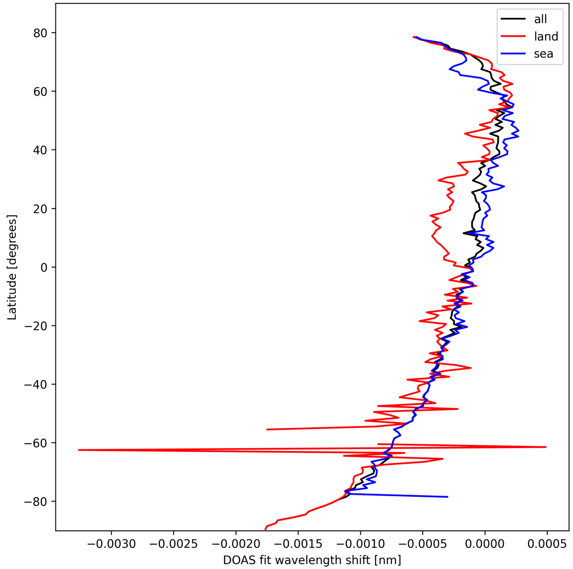
Figure 30: Zonal average of “DOAS fit wavelength shift” for 2025-03-01 to 2025-03-03.
