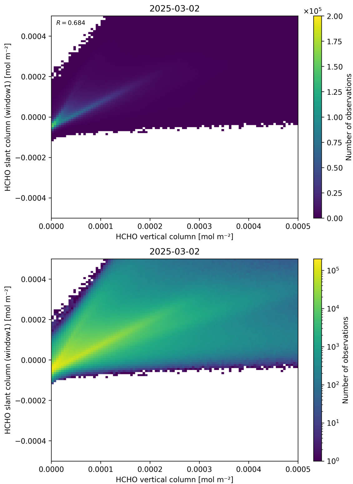
Figure 129: Scatter density plot of “HCHO vertical column” against “HCHO slant column (window1)” for 2025-03-01 to 2025-03-03.
