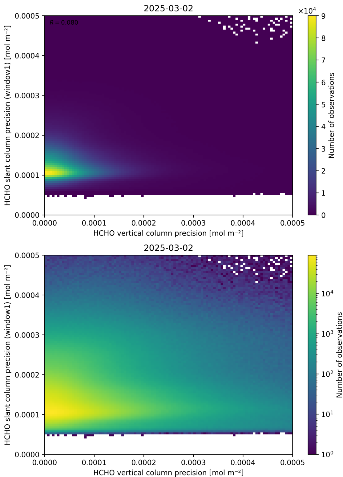
Figure 143: Scatter density plot of “HCHO vertical column precision” against “HCHO slant column precision (window1)” for 2025-03-01 to 2025-03-03.
