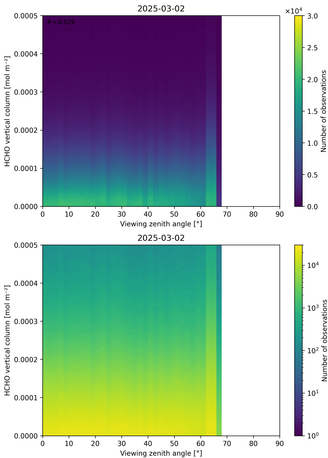
Figure 192: Scatter density plot of “Viewing zenith angle” against “HCHO vertical column” for 2025-03-01 to 2025-03-03.
