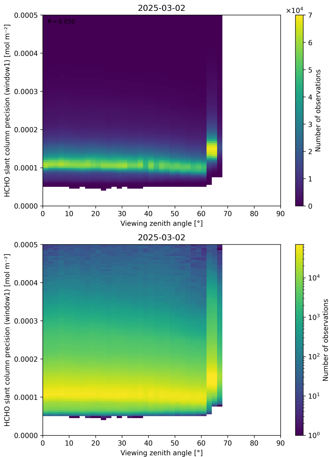
Figure 189: Scatter density plot of “Viewing zenith angle” against “HCHO slant column precision (window1)” for 2025-03-01 to 2025-03-03.
