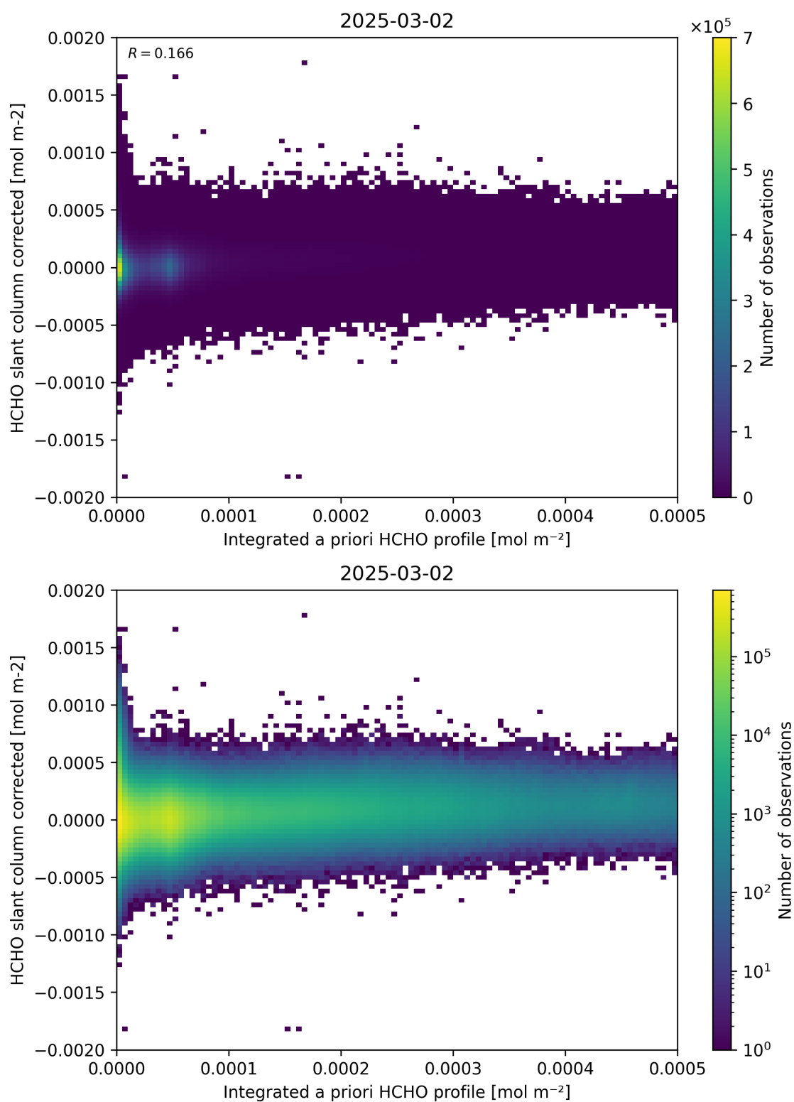
Figure 151: Scatter density plot of “Integrated a priori HCHO profile” against “HCHO slant column corrected” for 2025-03-01 to 2025-03-03.
