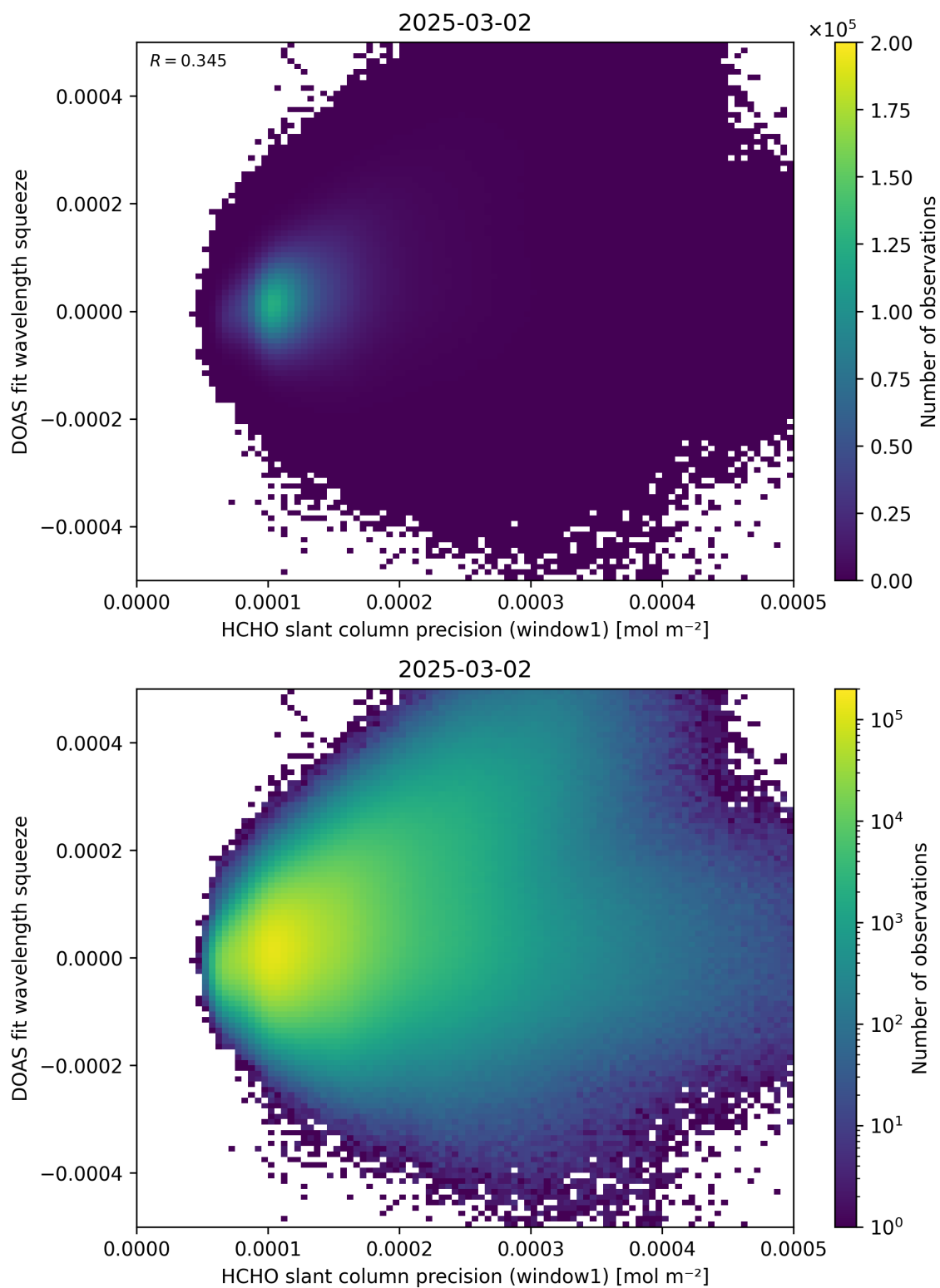
Figure 90: Scatter density plot of “HCHO slant column precision (window1)” against “DOAS fit wavelength squeeze” for 2025-03-01 to 2025-03-03.
