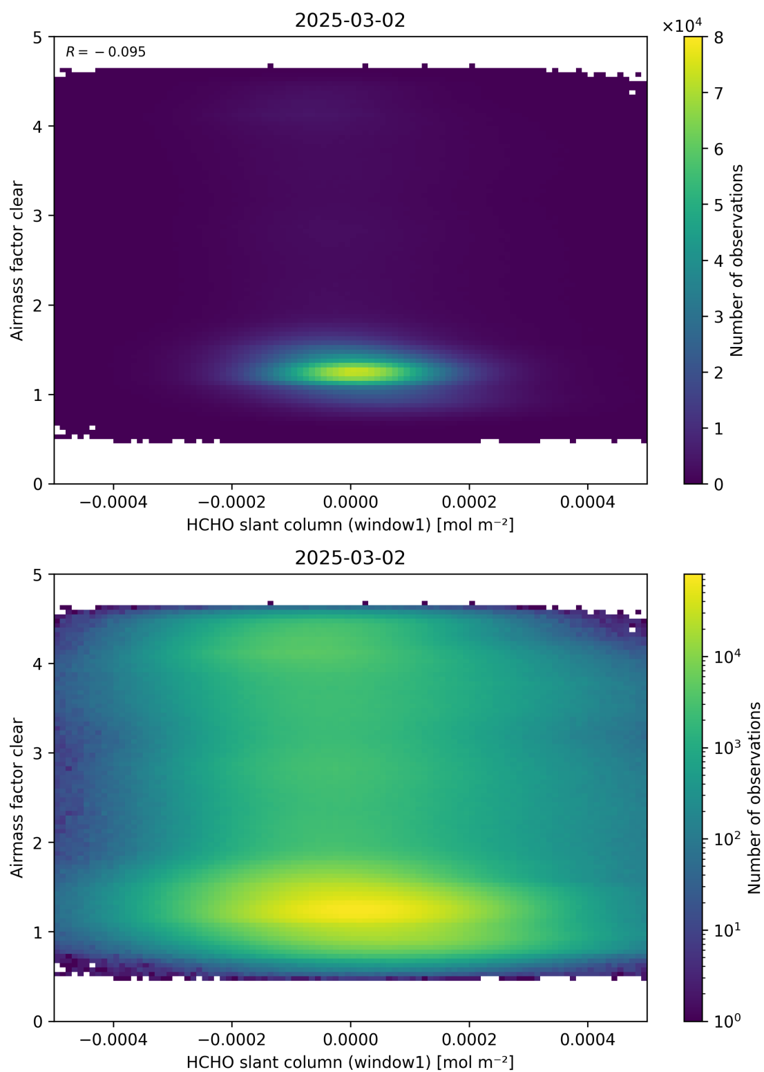
Figure 81: Scatter density plot of “HCHO slant column (window1)” against “Airmass factor clear” for 2025-03-01 to 2025-03-03.
