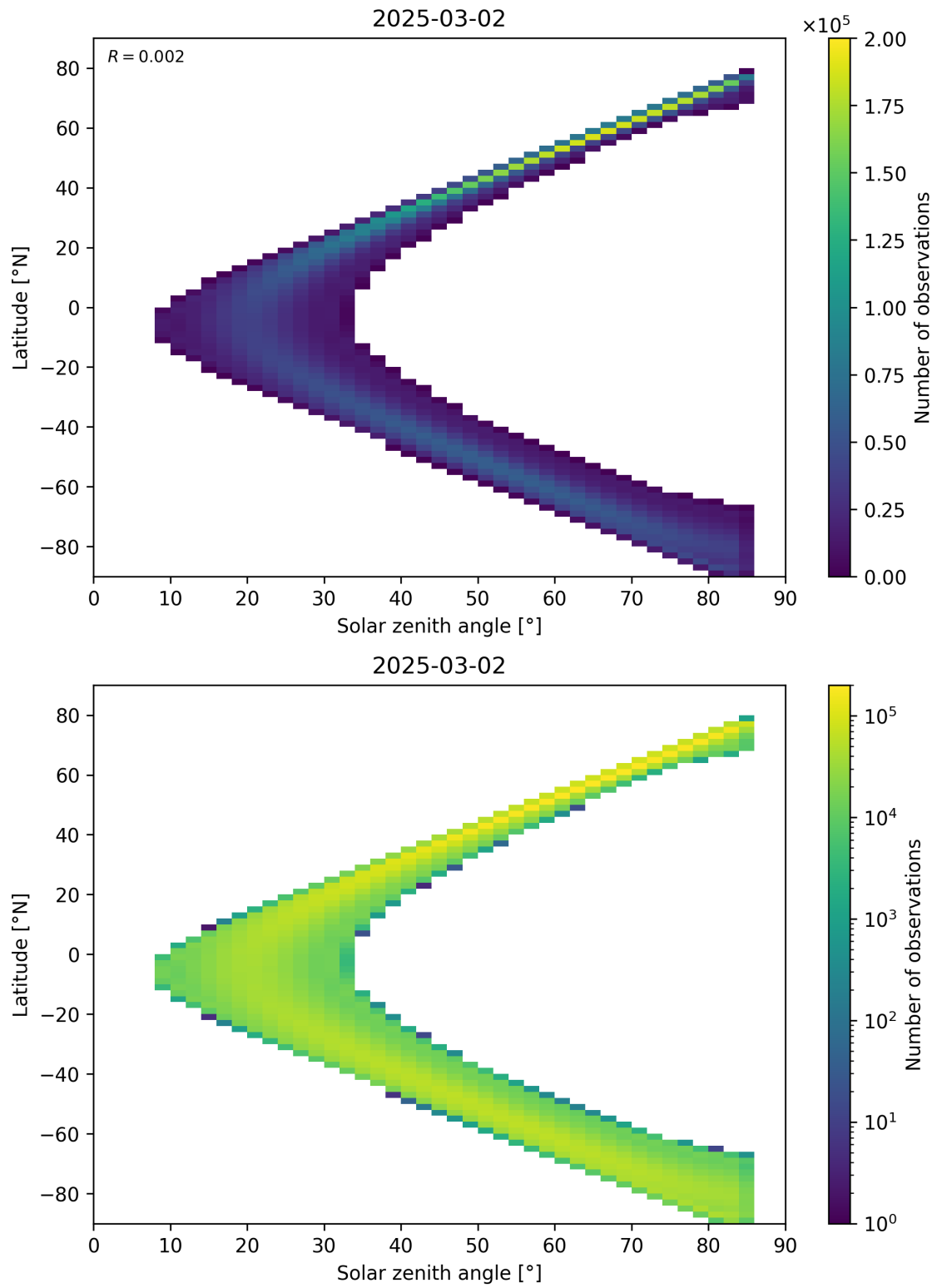
Figure 181: Scatter density plot of “Solar zenith angle” against “Latitude” for 2025-03-01 to 2025-03-03.
