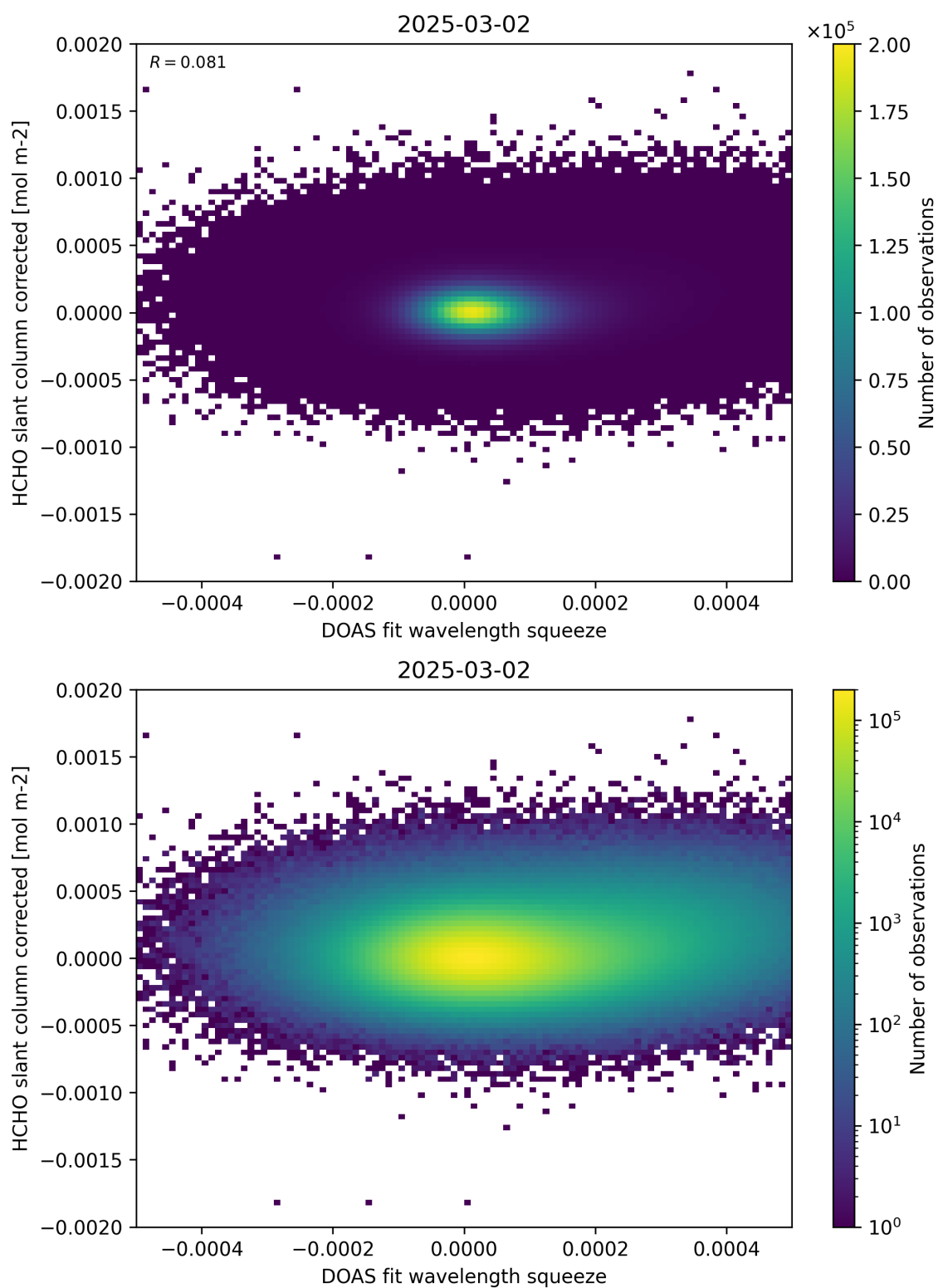
Figure 69: Scatter density plot of “DOAS fit wavelength squeeze” against “HCHO slant column corrected” for 2025-03-01 to 2025-03-03.
