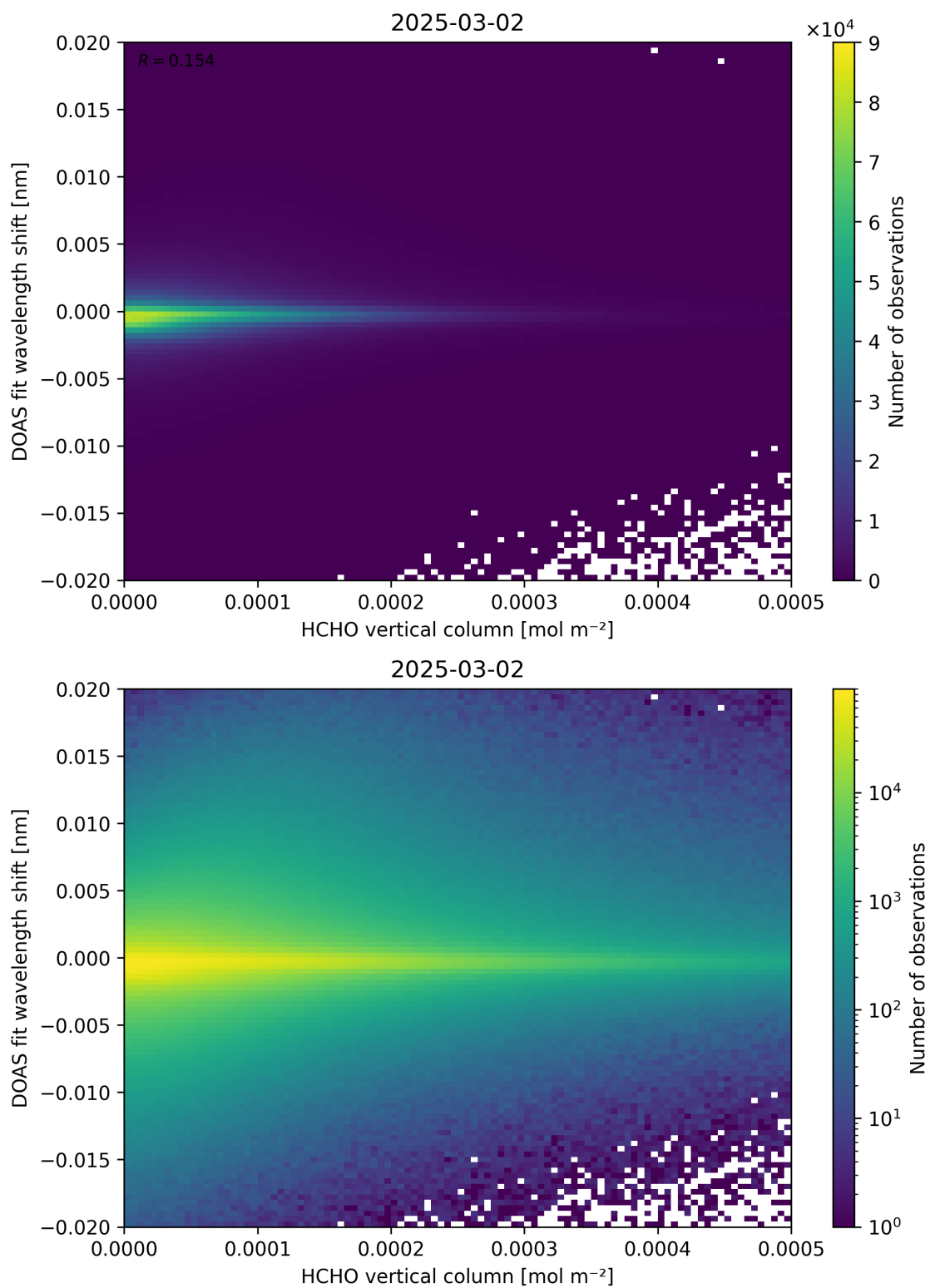
Figure 124: Scatter density plot of “HCHO vertical column” against “DOAS fit wavelength shift” for 2025-03-01 to 2025-03-03.
