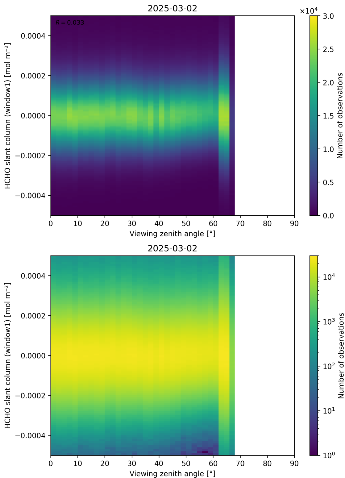
Figure 188: Scatter density plot of “Viewing zenith angle” against “HCHO slant column (window1)” for 2025-03-01 to 2025-03-03.
