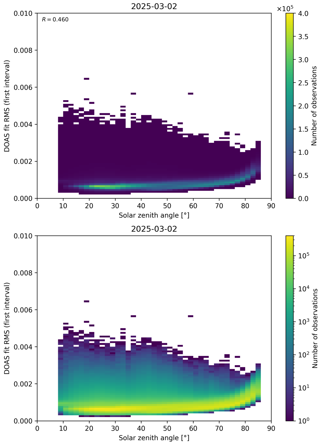
Figure 167: Scatter density plot of “Solar zenith angle” against “DOAS fit RMS (first interval)” for 2025-03-01 to 2025-03-03.
