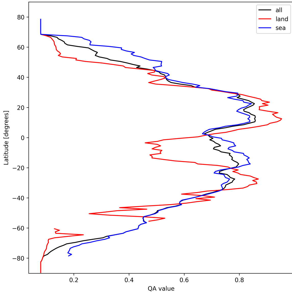
Figure 20: Zonal average of “QA value” for 2025-03-01 to 2025-03-03.
