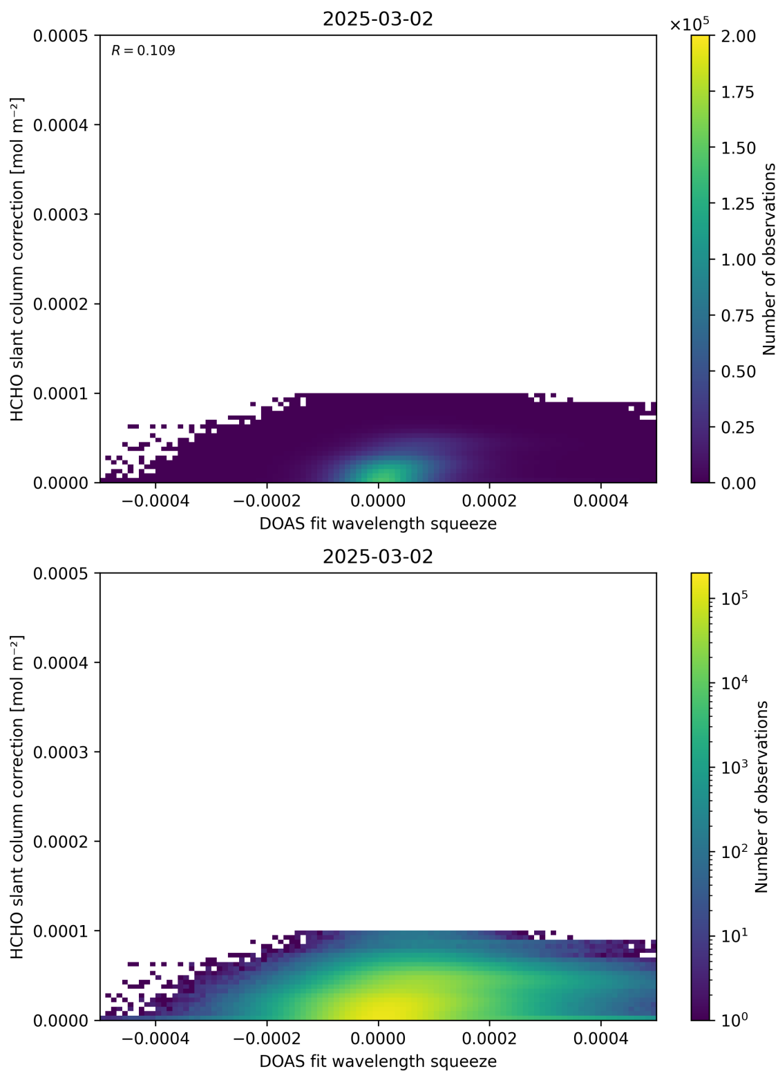
Figure 70: Scatter density plot of “DOAS fit wavelength squeeze” against “HCHO slant column correction” for 2025-03-01 to 2025-03-03.
