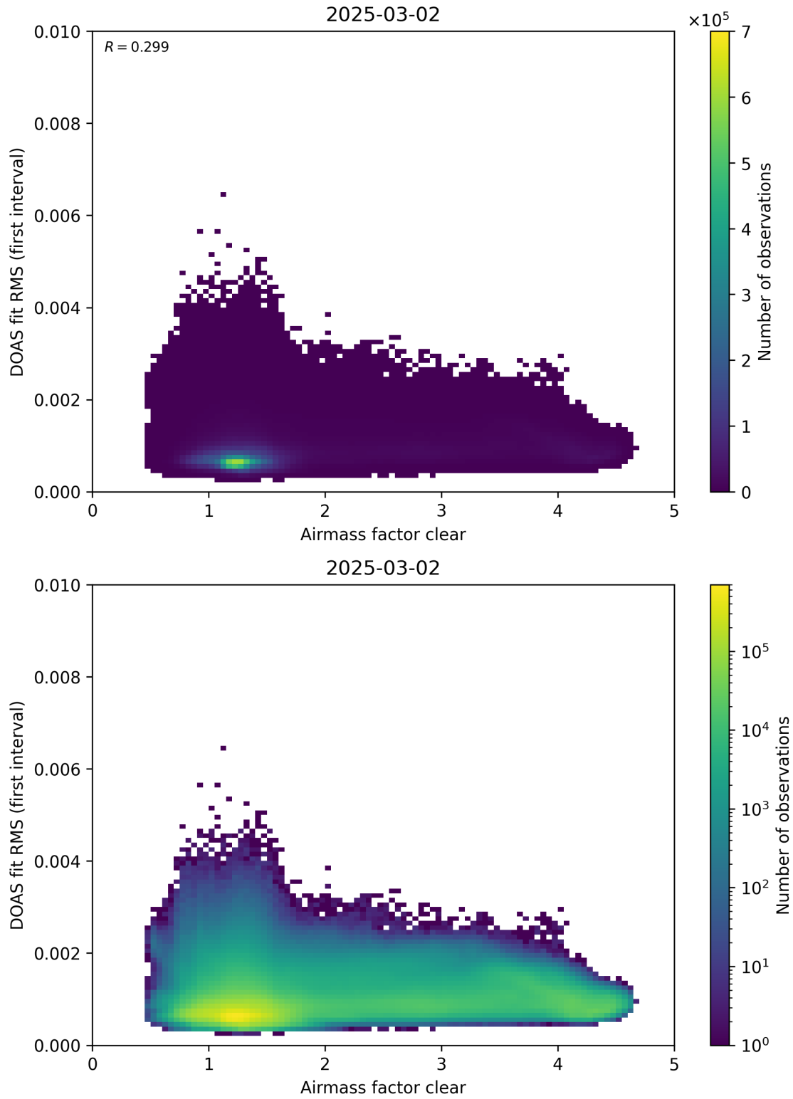
Figure 71: Scatter density plot of “Airmass factor clear” against “DOAS fit RMS (first interval)” for 2025-03-01 to 2025-03-03.
