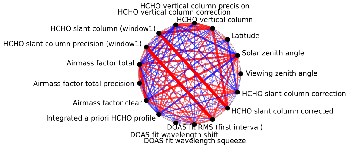
Figure 1: Map of correlation graph for 2025-03-01 to 2025-03-03.
