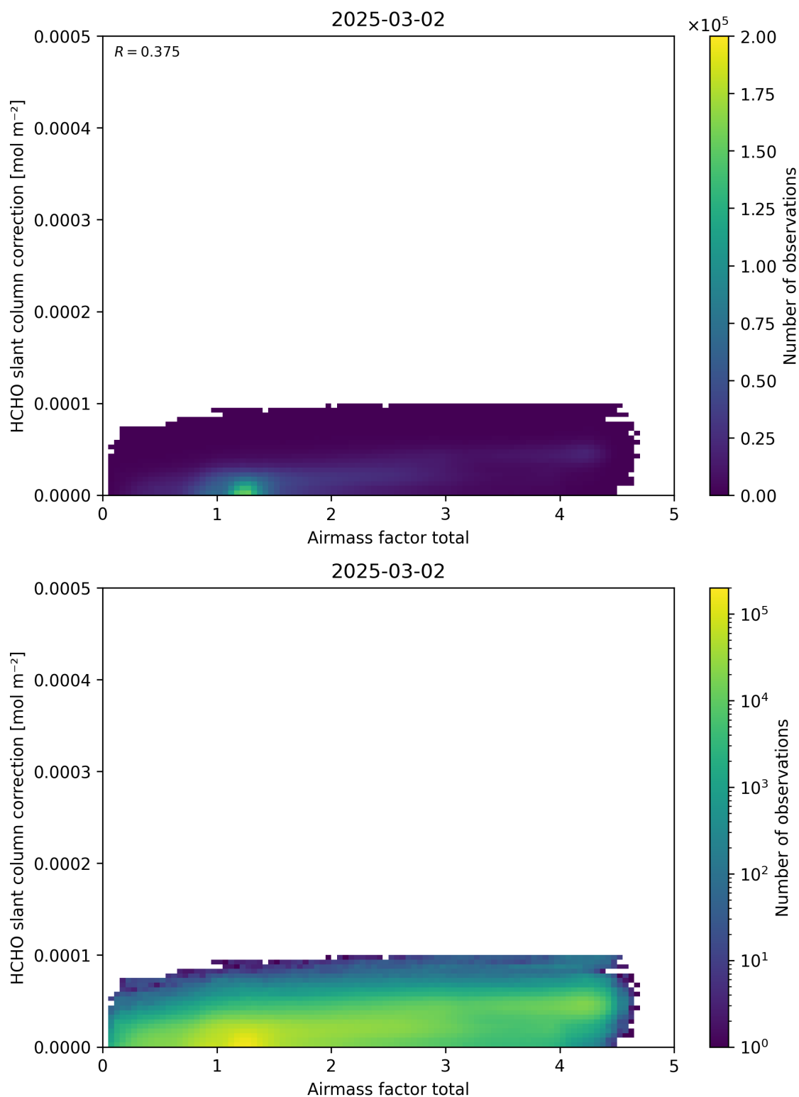
Figure 102: Scatter density plot of “Airmass factor total” against “HCHO slant column correction” for 2025-03-01 to 2025-03-03.
