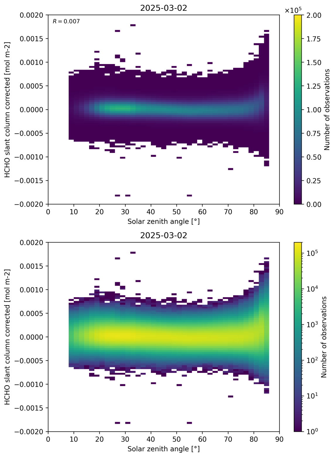
Figure 171: Scatter density plot of “Solar zenith angle” against “HCHO slant column corrected” for 2025-03-01 to 2025-03-03.
