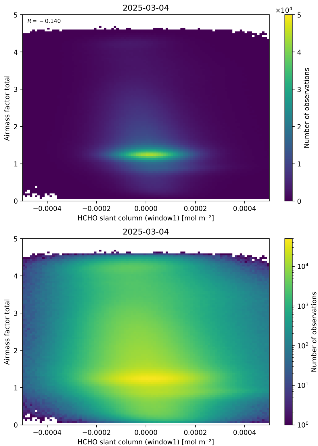
Figure 85: Scatter density plot of “HCHO slant column (window1)” against “Airmass factor total” for 2025-03-03 to 2025-03-05.
