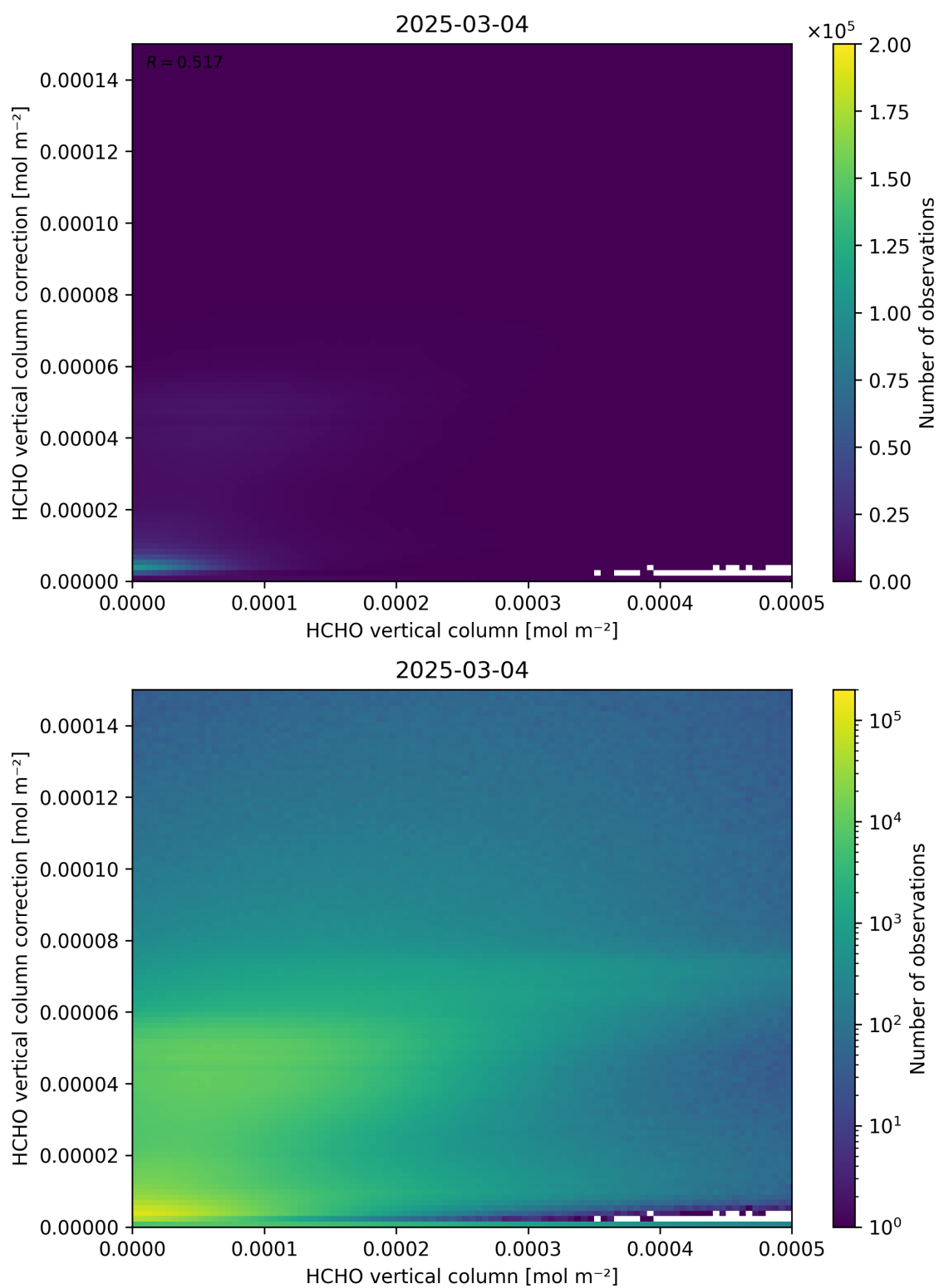
Figure 133: Scatter density plot of “HCHO vertical column” against “HCHO vertical column correction” for 2025-03-03 to 2025-03-05.
