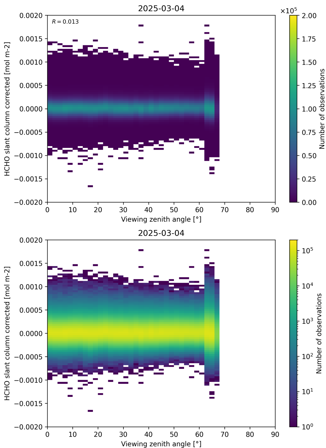
Figure 186: Scatter density plot of “Viewing zenith angle” against “HCHO slant column corrected” for 2025-03-03 to 2025-03-05.
