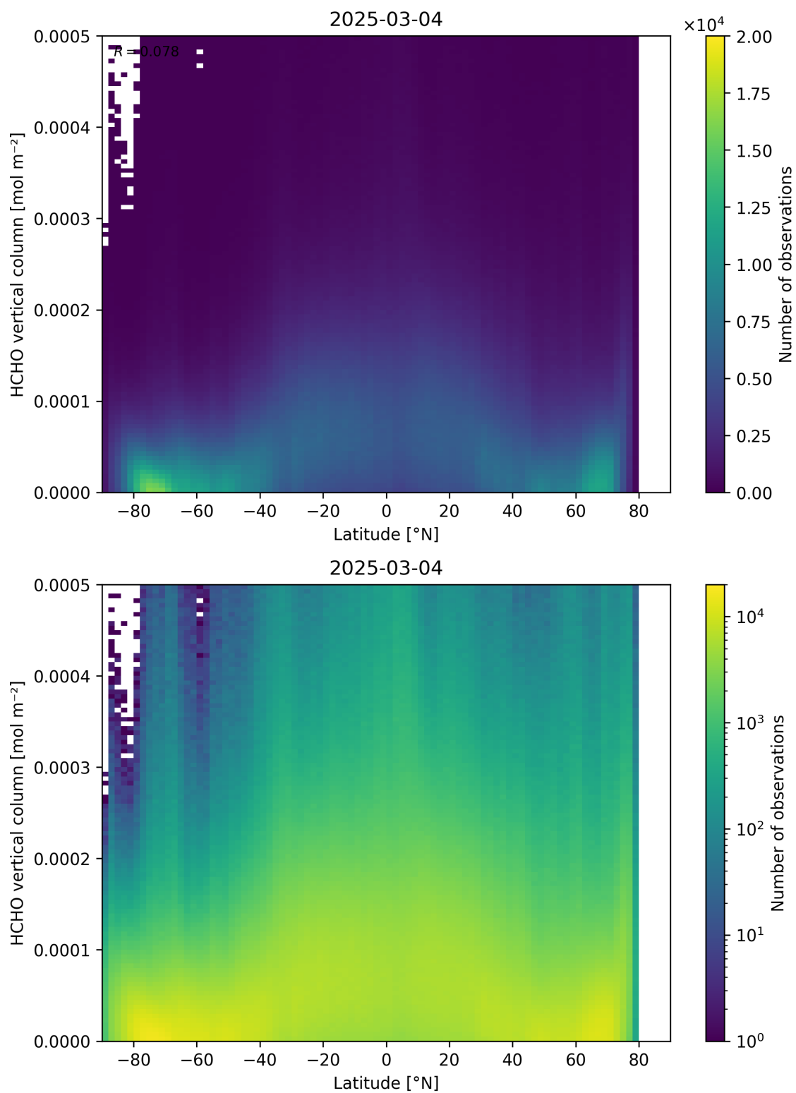
Figure 163: Scatter density plot of “Latitude” against “HCHO vertical column” for 2025-03-03 to 2025-03-05.
