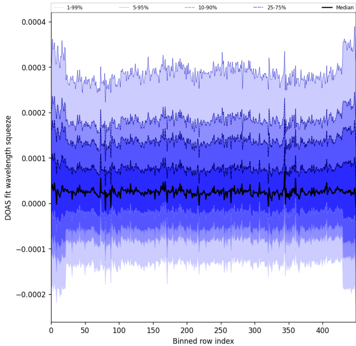
Figure 59: Along track statistics of “DOAS fit wavelength squeeze” for 2025-03-03 to 2025-03-05
