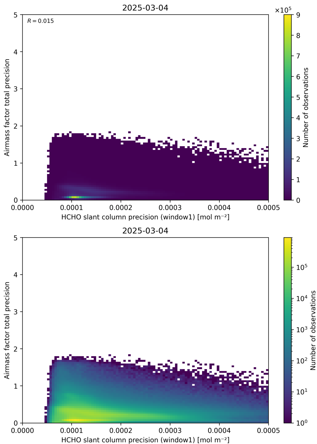
Figure 95: Scatter density plot of “HCHO slant column precision (window1)” against “Airmass factor total precision” for 2025-03-03 to 2025-03-05.
