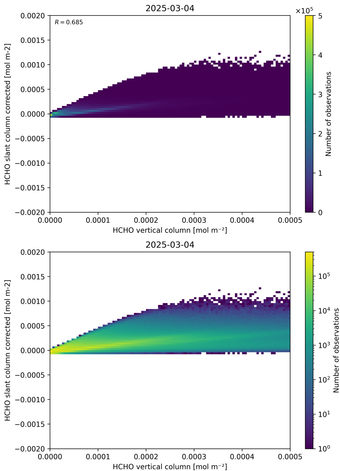
Figure 127: Scatter density plot of “HCHO vertical column” against “HCHO slant column corrected” for 2025-03-03 to 2025-03-05.
