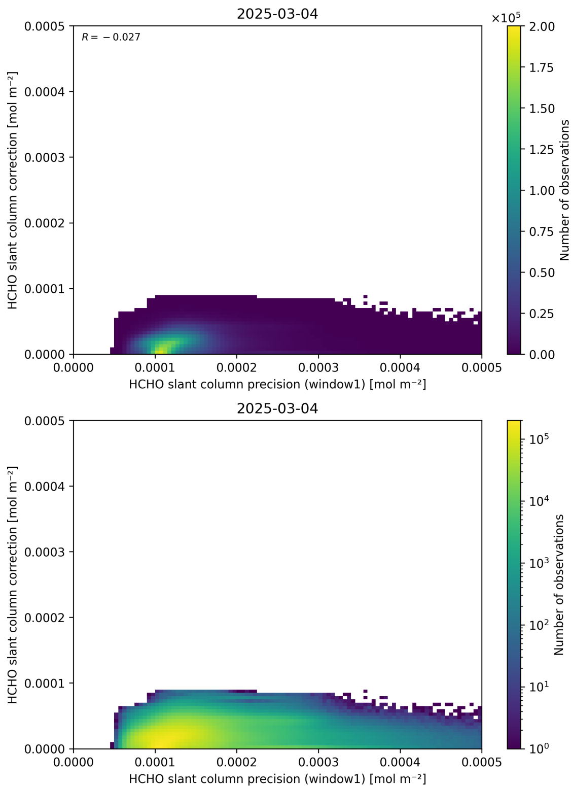
Figure 93: Scatter density plot of “HCHO slant column precision (window1)” against “HCHO slant column correction” for 2025-03-03 to 2025-03-05.
