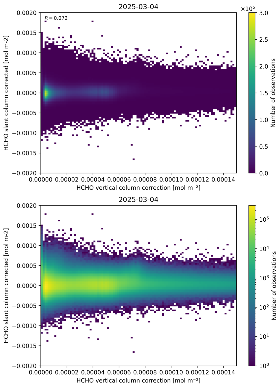
Figure 116: Scatter density plot of “HCHO vertical column correction” against “HCHO slant column corrected” for 2025-03-03 to 2025-03-05.
