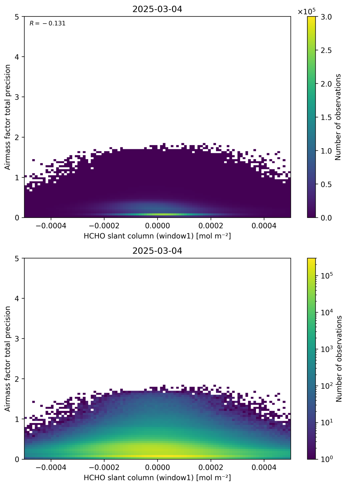
Figure 86: Scatter density plot of “HCHO slant column (window1)” against “Airmass factor total precision” for 2025-03-03 to 2025-03-05.
