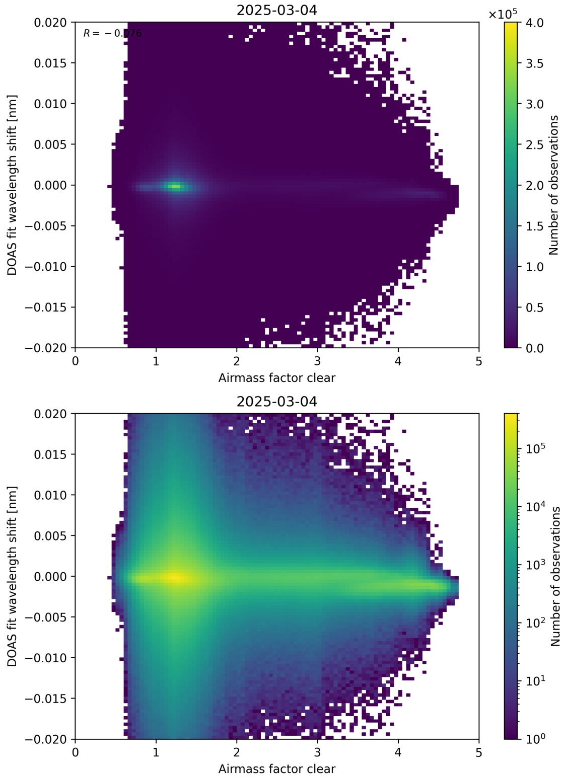
Figure 72: Scatter density plot of “Airmass factor clear” against “DOAS fit wavelength shift” for 2025-03-03 to 2025-03-05.
