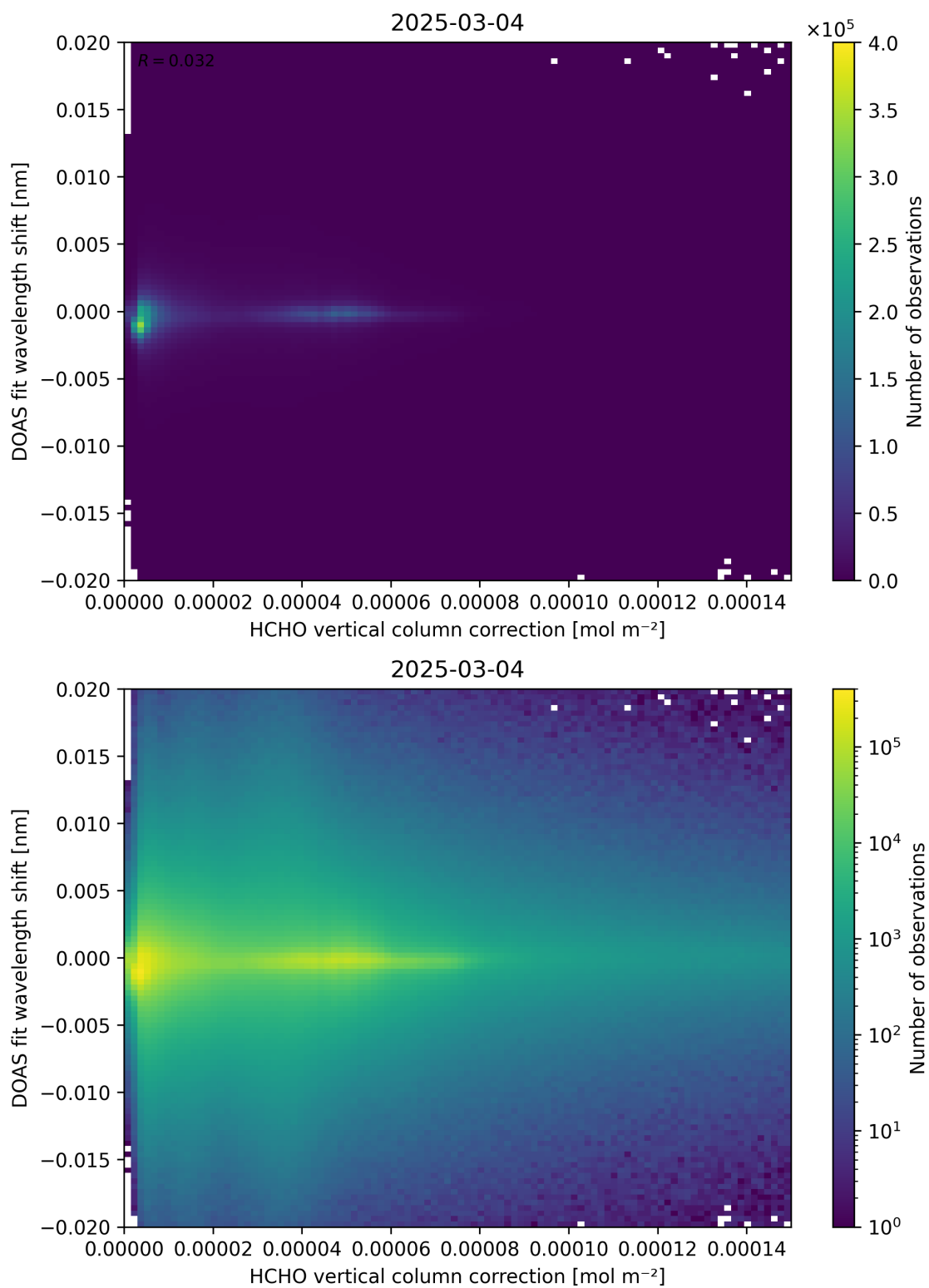
Figure 113: Scatter density plot of “HCHO vertical column correction” against “DOAS fit wavelength shift” for 2025-03-03 to 2025-03-05.
