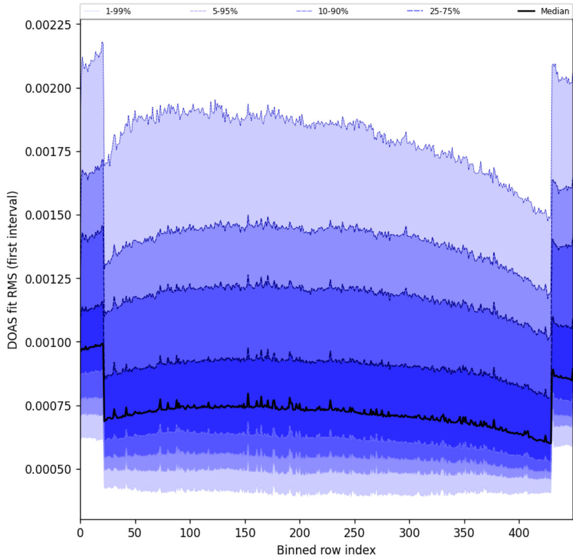
Figure 60: Along track statistics of “DOAS fit RMS (first interval)” for 2025-03-03 to 2025-03-05
