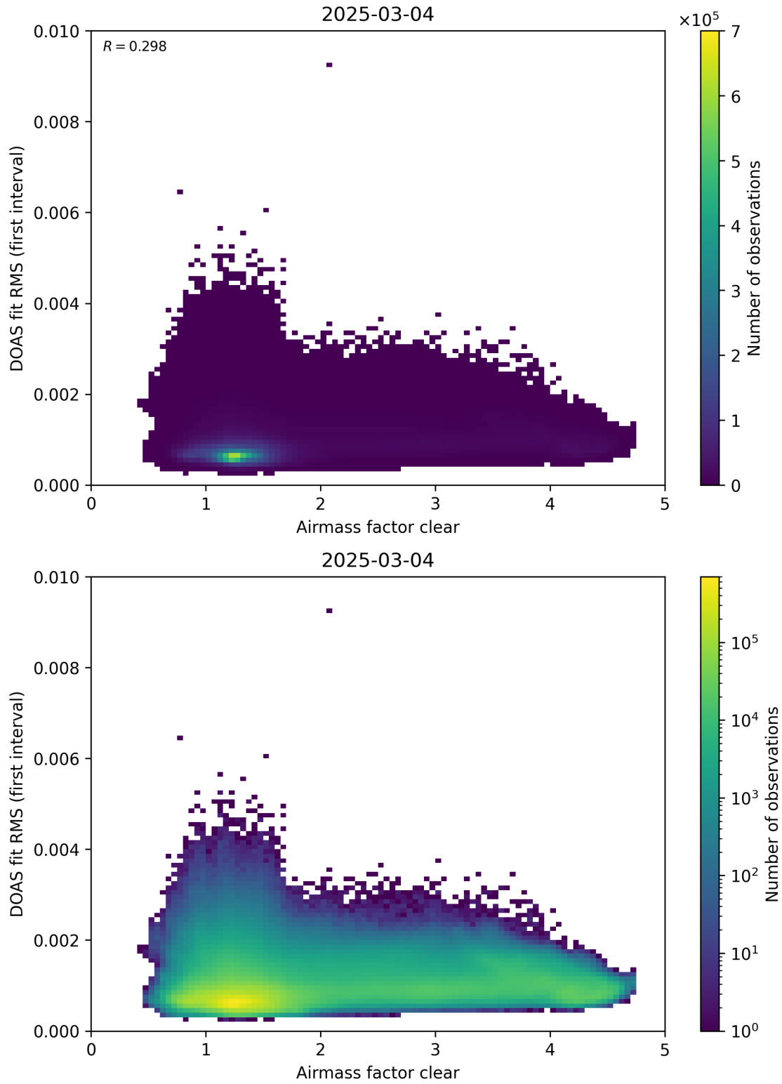
Figure 71: Scatter density plot of “Airmass factor clear” against “DOAS fit RMS (first interval)” for 2025-03-03 to 2025-03-05.
