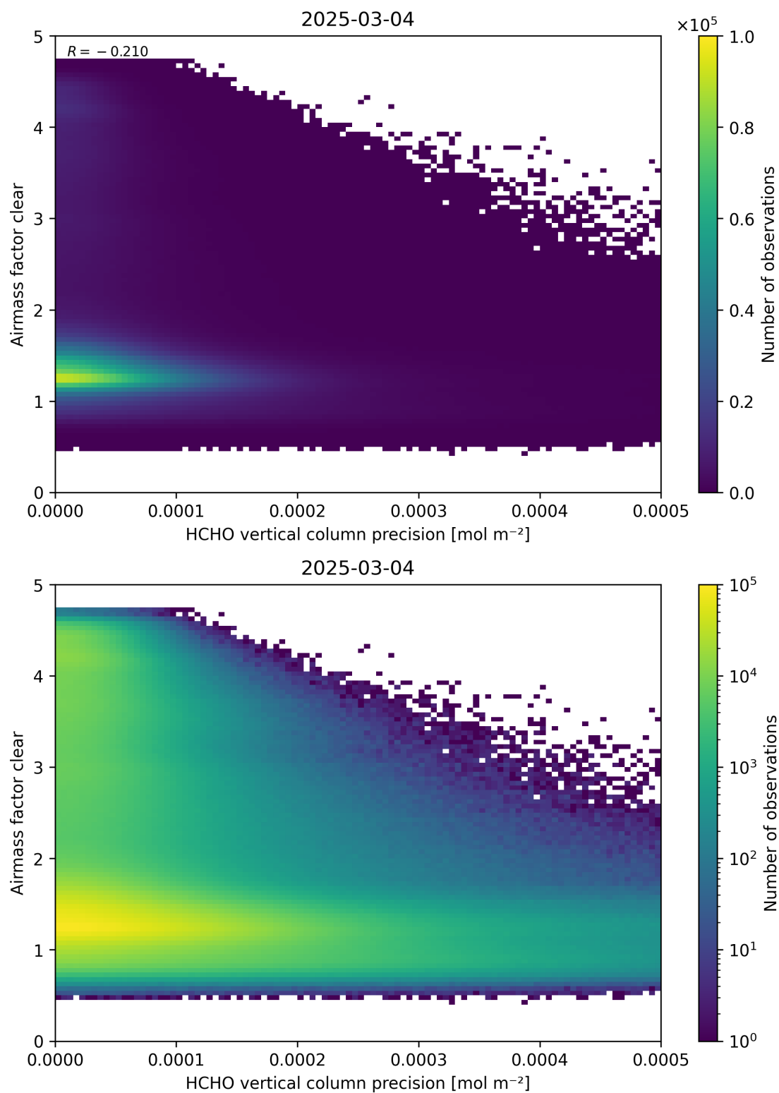
Figure 139: Scatter density plot of “HCHO vertical column precision” against “Airmass factor clear” for 2025-03-03 to 2025-03-05.
