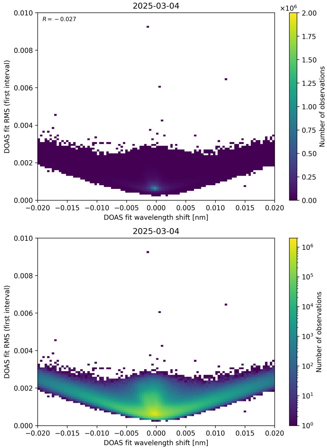
Figure 64: Scatter density plot of “DOAS fit wavelength shift” against “DOAS fit RMS (first interval)” for 2025-03-03 to 2025-03-05.
