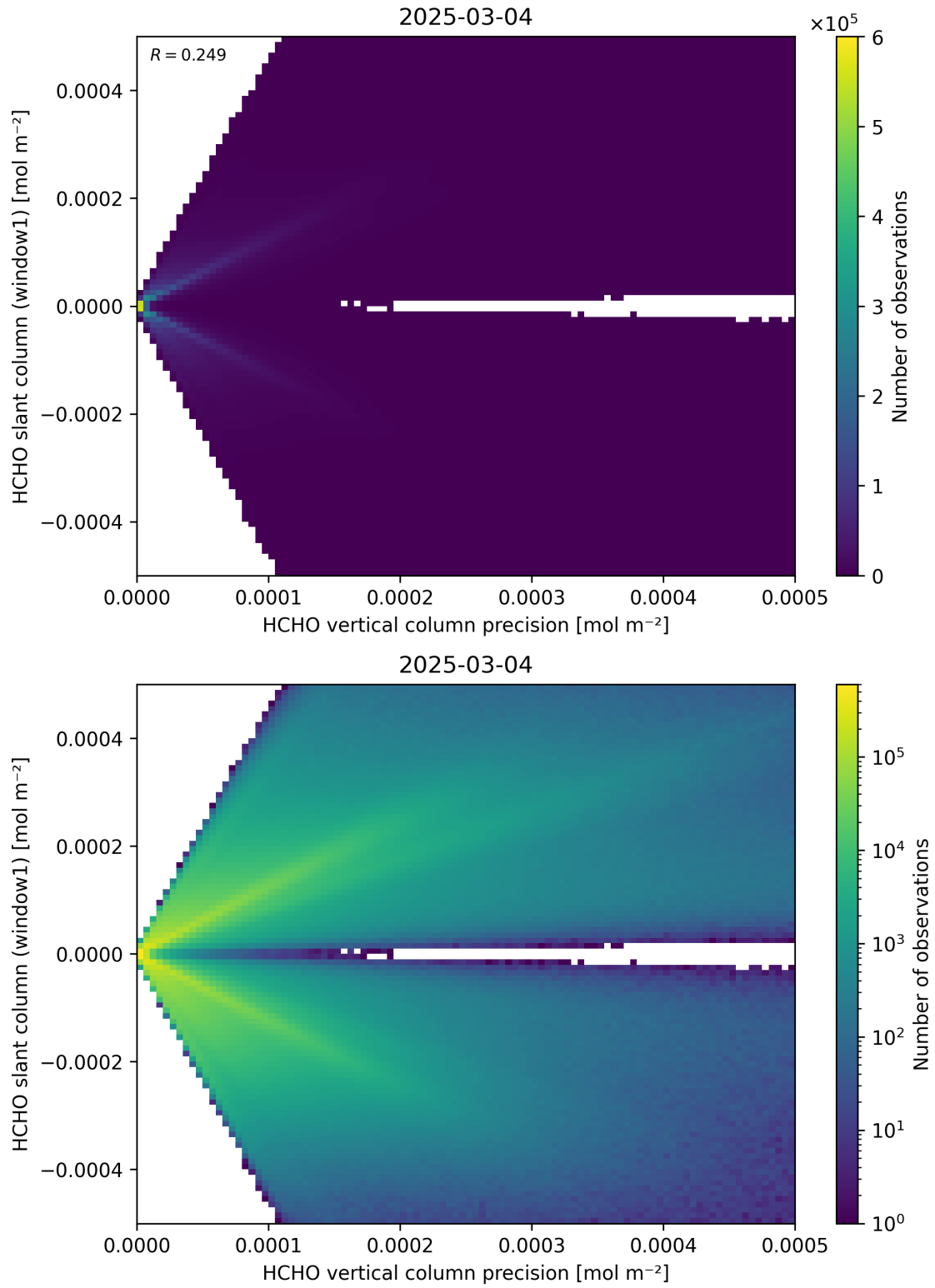
Figure 142: Scatter density plot of “HCHO vertical column precision” against “HCHO slant column (window1)” for 2025-03-03 to 2025-03-05.
