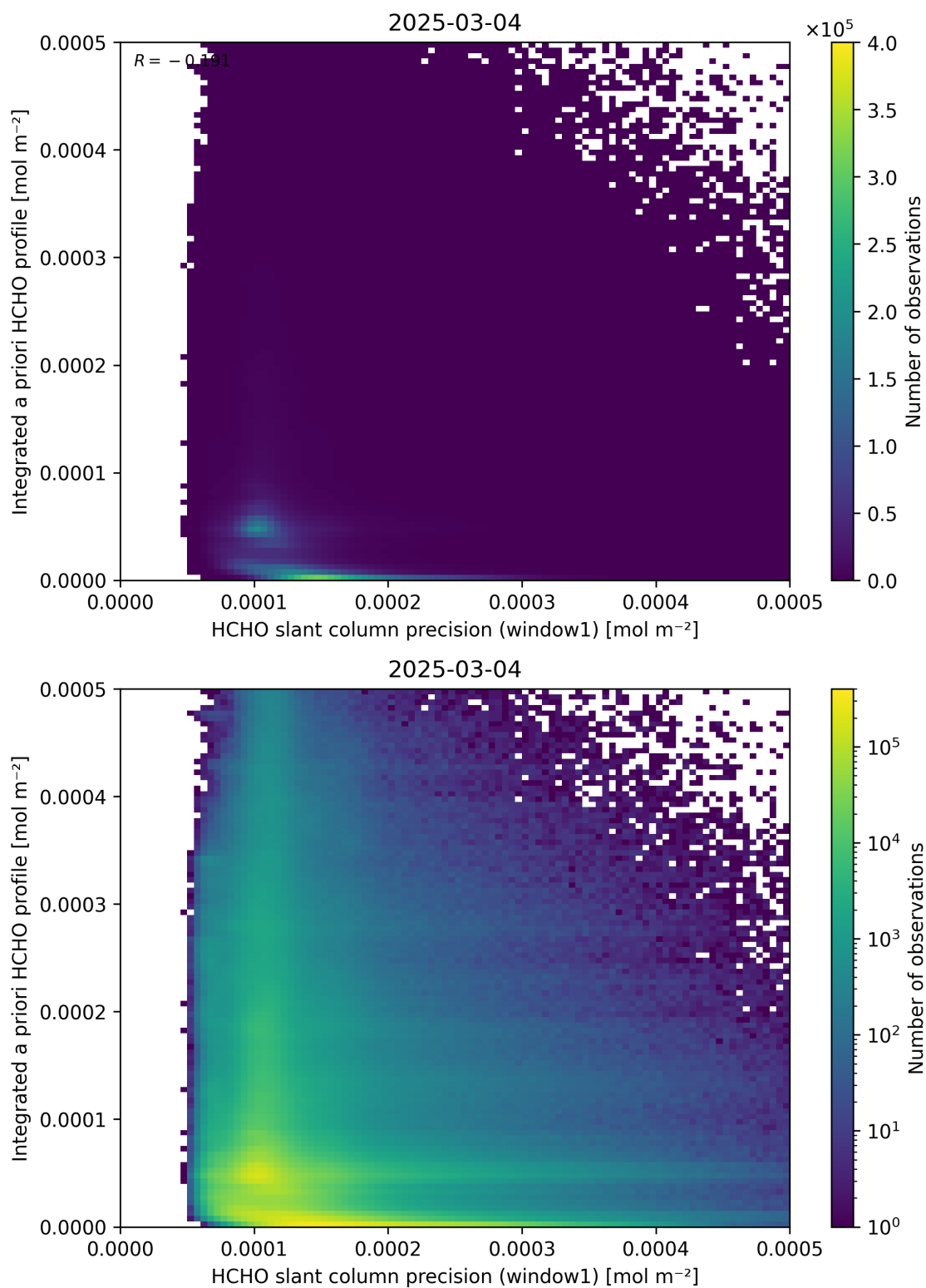
Figure 96: Scatter density plot of “HCHO slant column precision (window1)” against “Integrated a priori HCHO profile” for 2025-03-03 to 2025-03-05.
