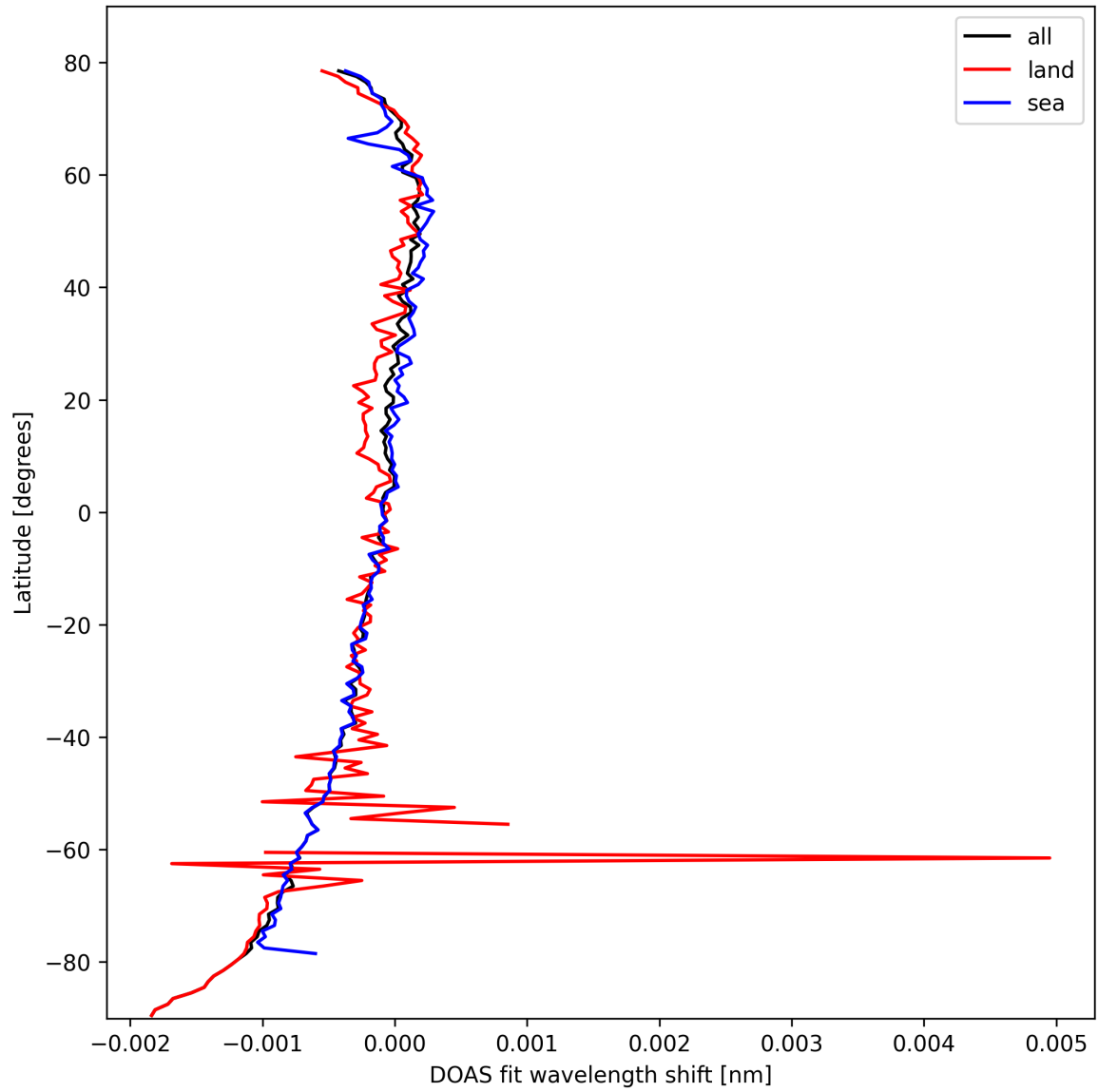
Figure 30: Zonal average of "DOAS fit wavelength shift" for 2025-03-03 to 2025-03-05.
