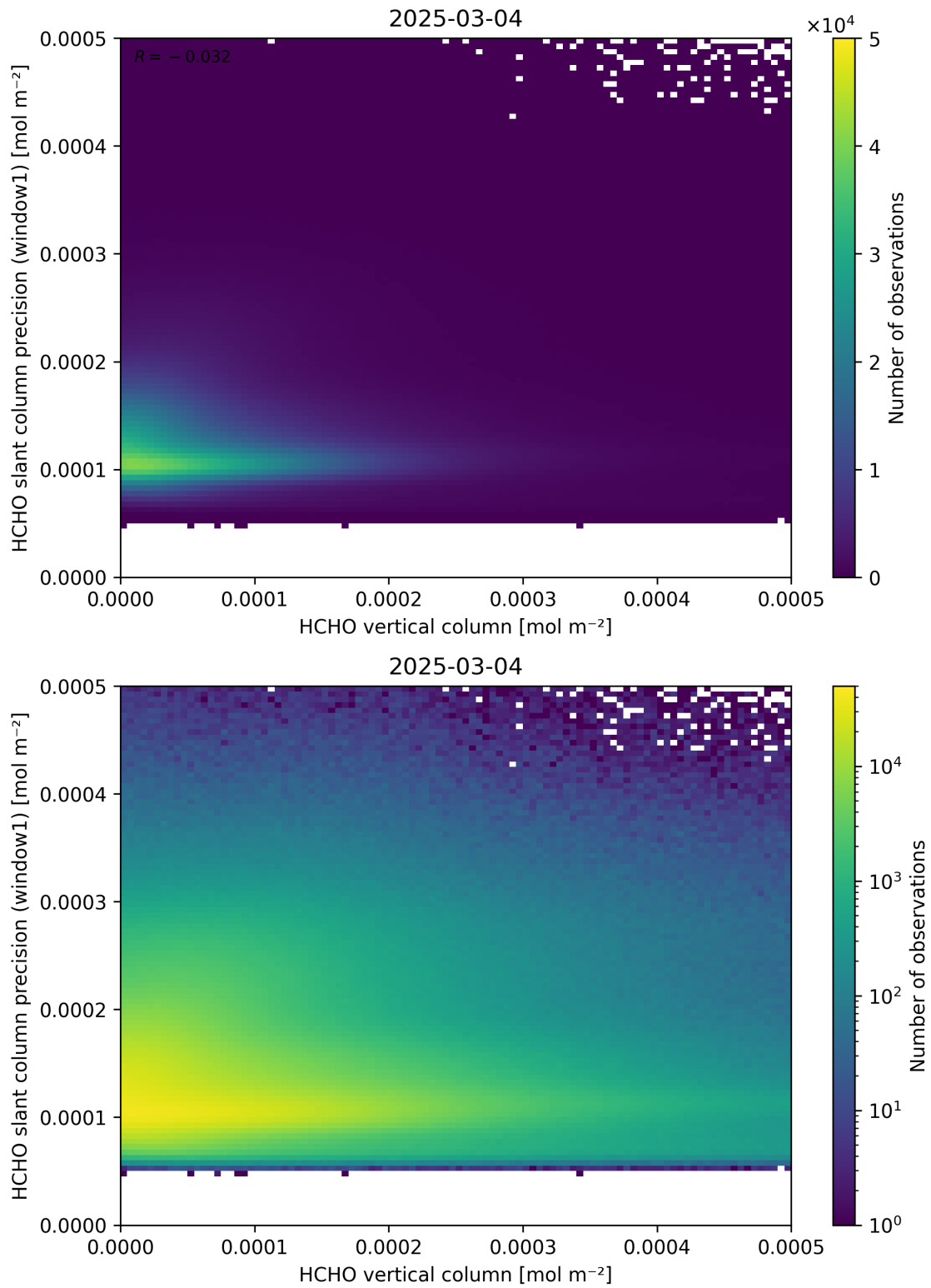
Figure 130: Scatter density plot of “HCHO vertical column” against “HCHO slant column precision (window1)” for 2025-03-03 to 2025-03-05.
