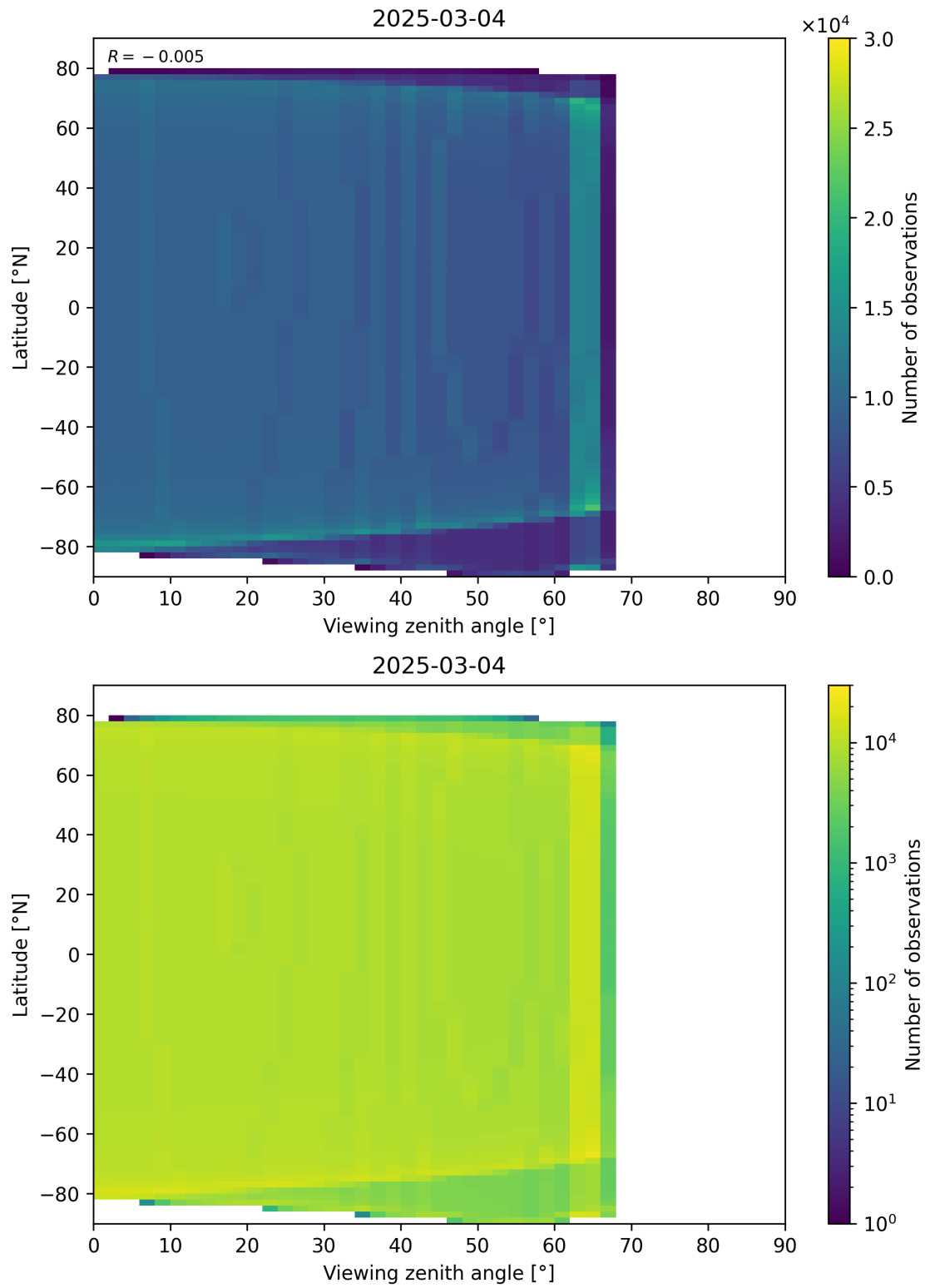
Figure 196: Scatter density plot of “Viewing zenith angle” against “Latitude” for 2025-03-03 to 2025-03-05.
