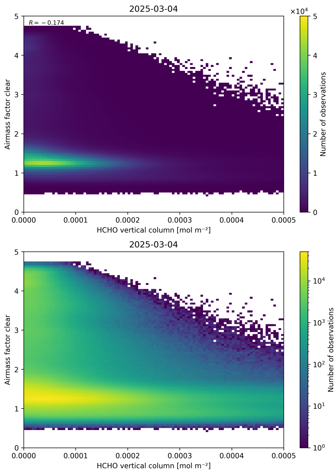
Figure 126: Scatter density plot of “HCHO vertical column” against “Airmass factor clear” for 2025-03-03 to 2025-03-05.
