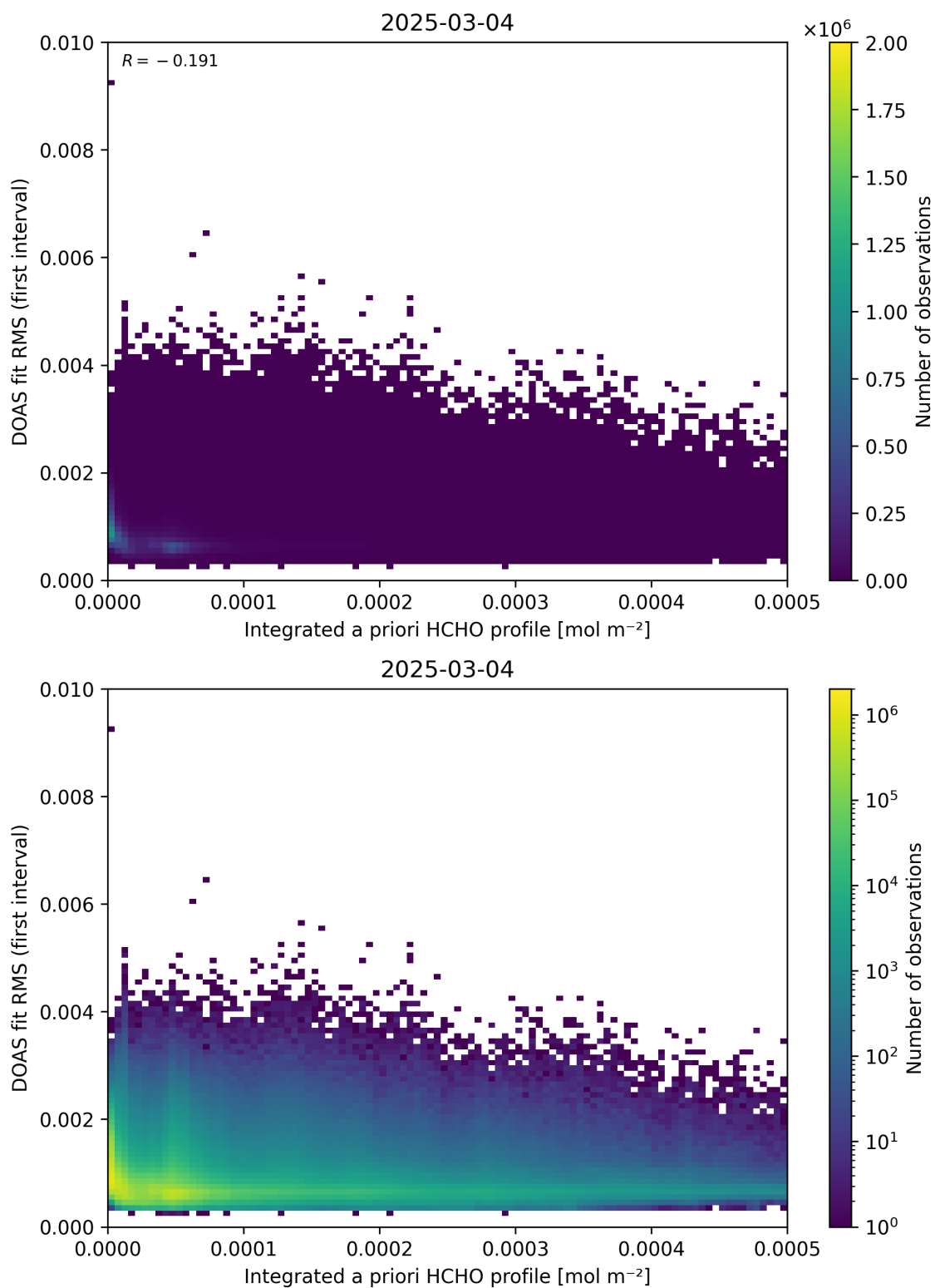
Figure 148: Scatter density plot of “Integrated a priori HCHO profile” against “DOAS fit RMS (first interval)” for 2025-03-03 to 2025-03-05.
