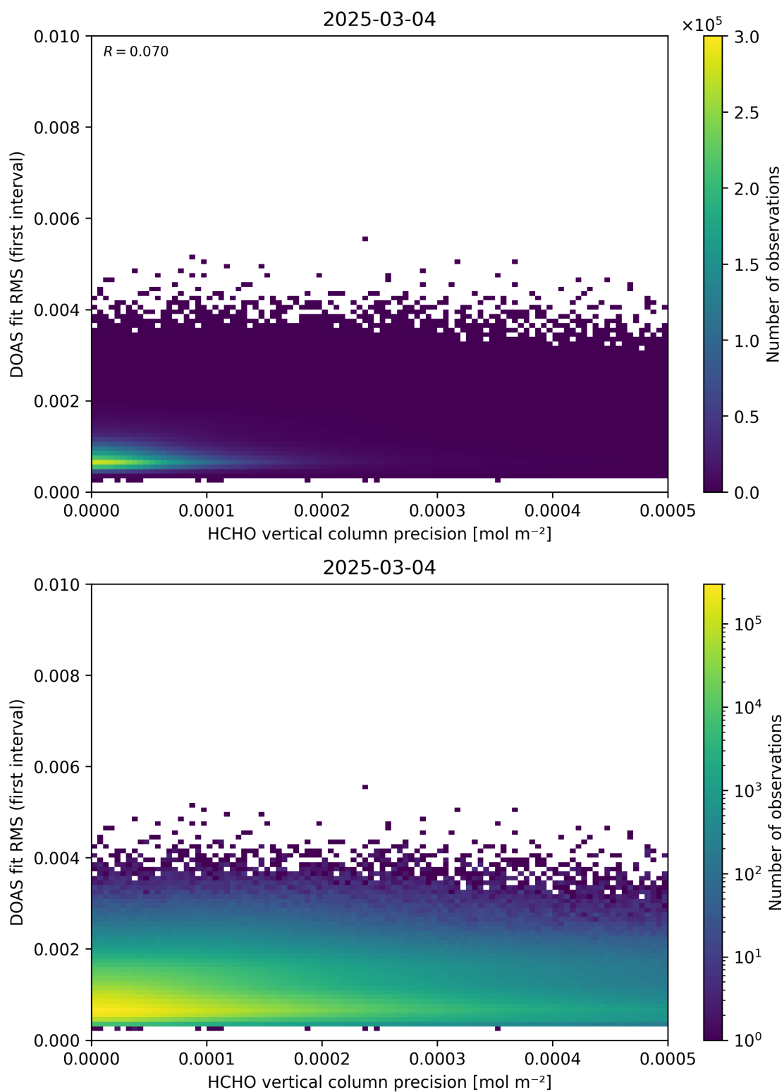
Figure 136: Scatter density plot of “HCHO vertical column precision” against “DOAS fit RMS (first interval)” for 2025-03-03 to 2025-03-05.
