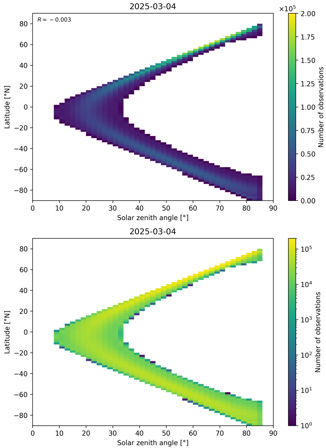
Figure 181: Scatter density plot of “Solar zenith angle” against “Latitude” for 2025-03-03 to 2025-03-05.
