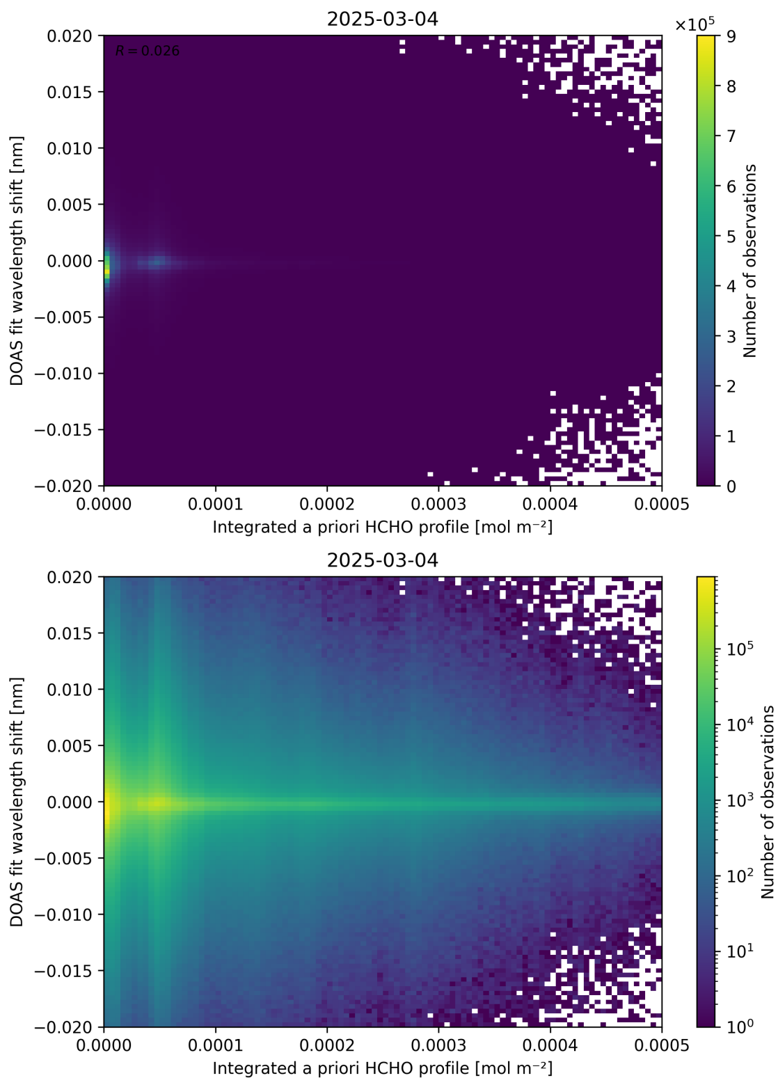
Figure 149: Scatter density plot of “Integrated a priori HCHO profile” against “DOAS fit wavelength shift” for 2025-03-03 to 2025-03-05.
