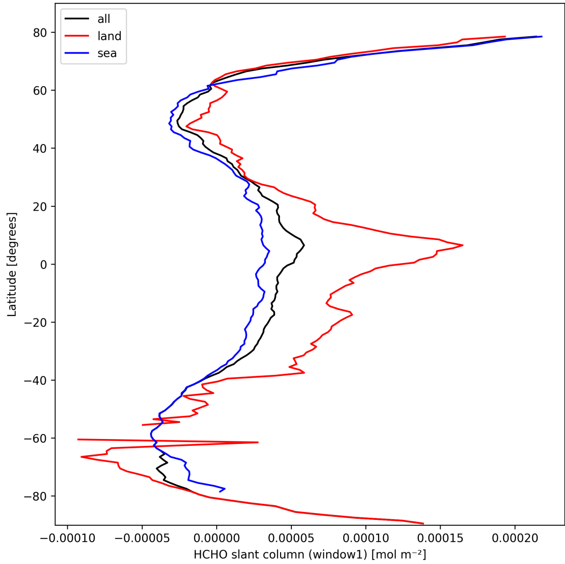
Figure 24: Zonal average of “HCHO slant column (window1)” for 2025-03-03 to 2025-03-05.
