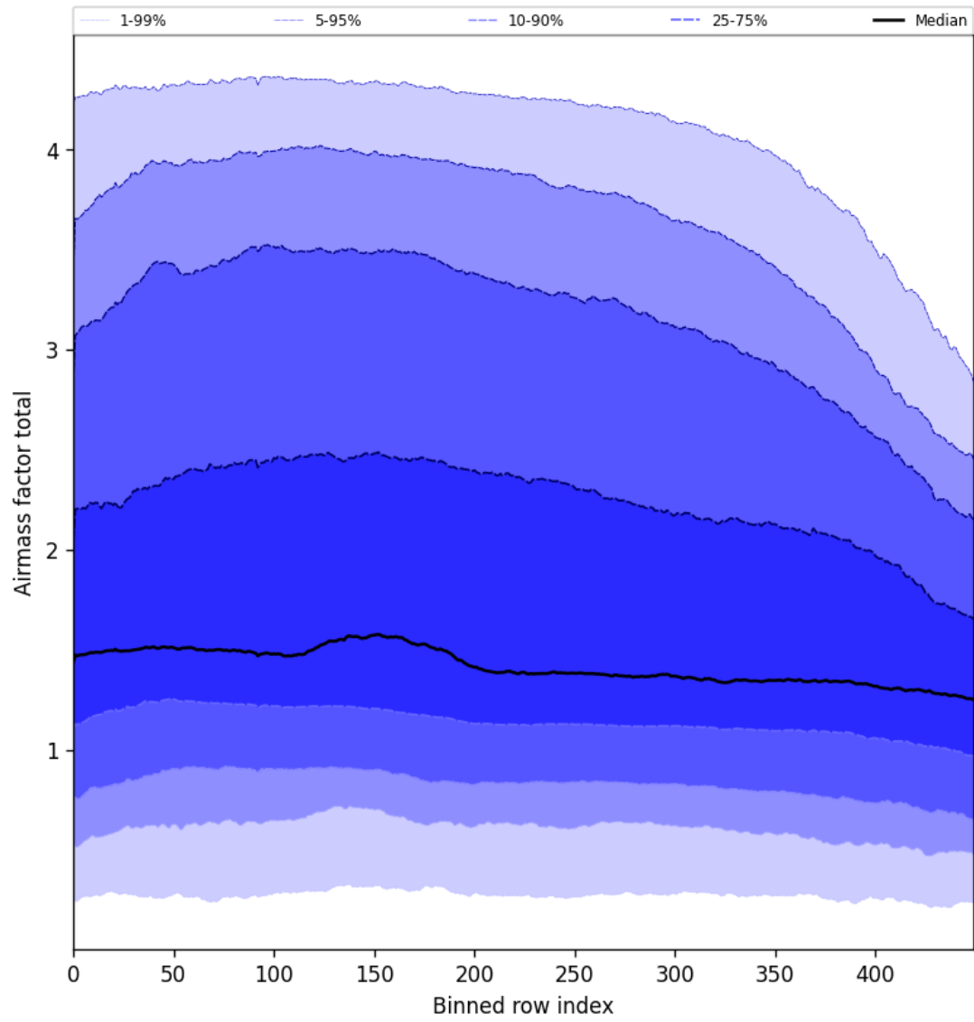
Figure 54: Along track statistics of “Airmass factor total” for 2025-03-03 to 2025-03-05
