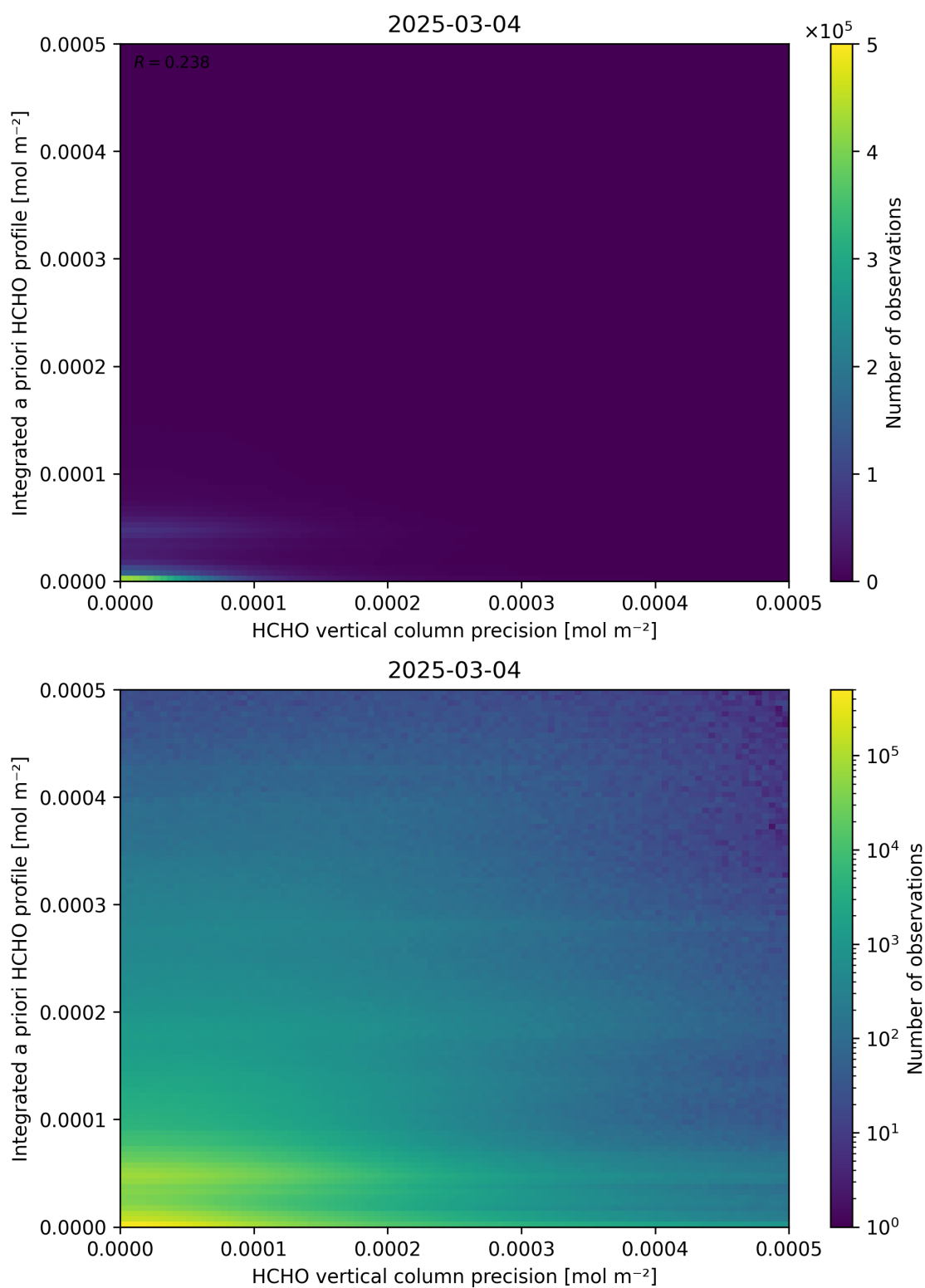
Figure 147: Scatter density plot of “HCHO vertical column precision” against “Integrated a priori HCHO profile” for 2025-03-03 to 2025-03-05.
