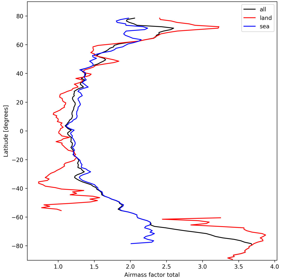
Figure 26: Zonal average of “Airmass factor total” for 2025-03-03 to 2025-03-05.
