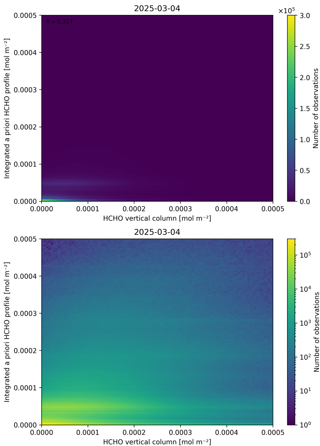
Figure 135: Scatter density plot of “HCHO vertical column” against “Integrated a priori HCHO profile” for 2025-03-03 to 2025-03-05.
