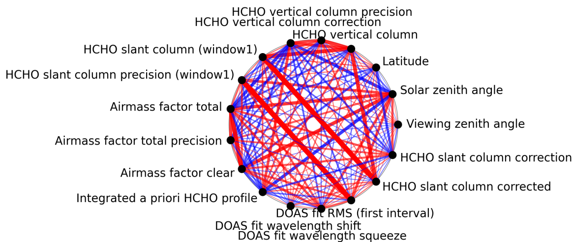
Figure 1: Map of correlation graph for 2025-03-03 to 2025-03-05.
