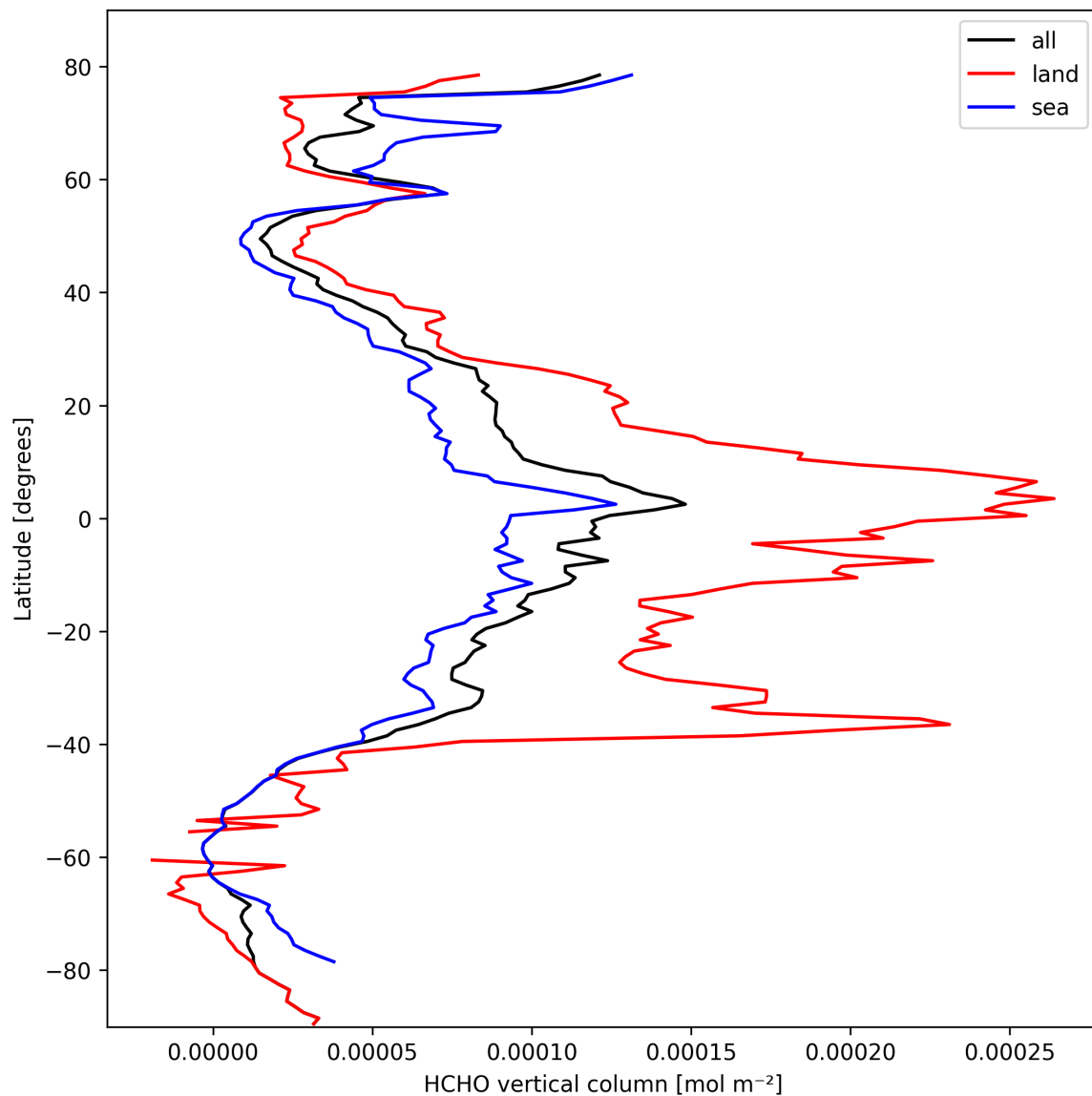
Figure 21: Zonal average of “HCHO vertical column” for 2025-03-03 to 2025-03-05.
