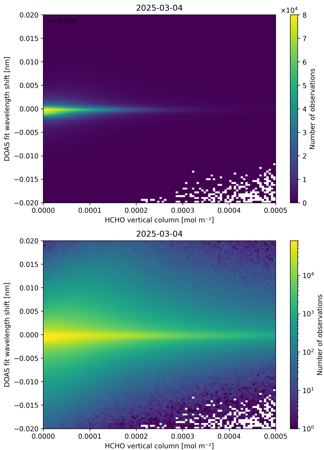
Figure 124: Scatter density plot of “HCHO vertical column” against “DOAS fit wavelength shift” for 2025-03-03 to 2025-03-05.
