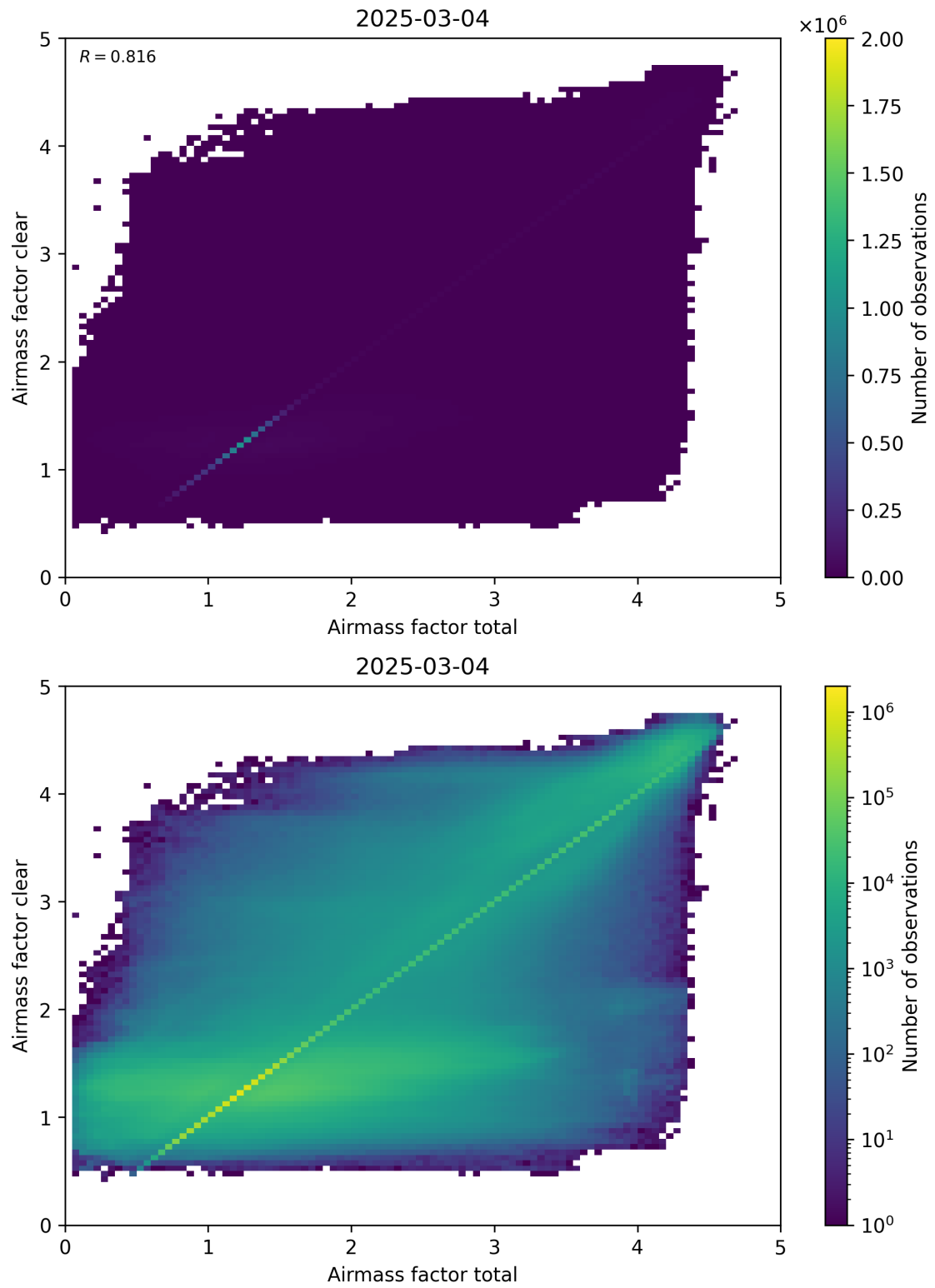
Figure 100: Scatter density plot of “Airmass factor total” against “Airmass factor clear” for 2025-03-03 to 2025-03-05.
