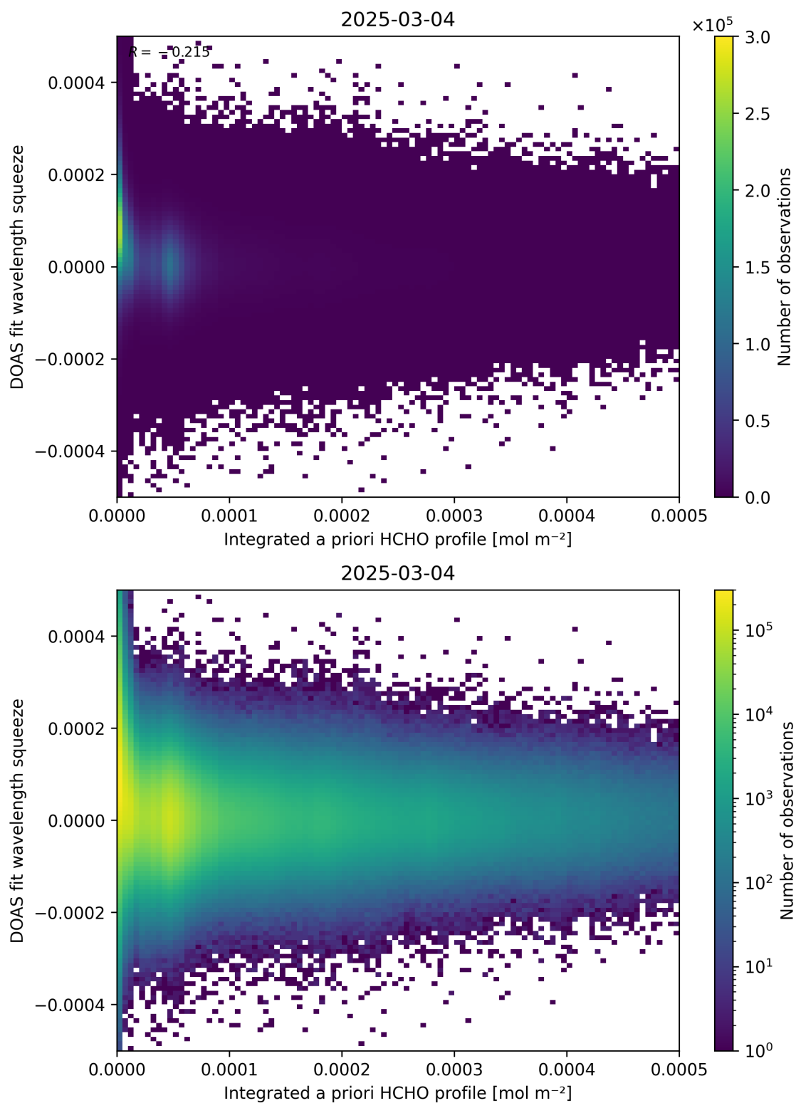
Figure 150: Scatter density plot of “Integrated a priori HCHO profile” against “DOAS fit wavelength squeeze” for 2025-03-03 to 2025-03-05.
