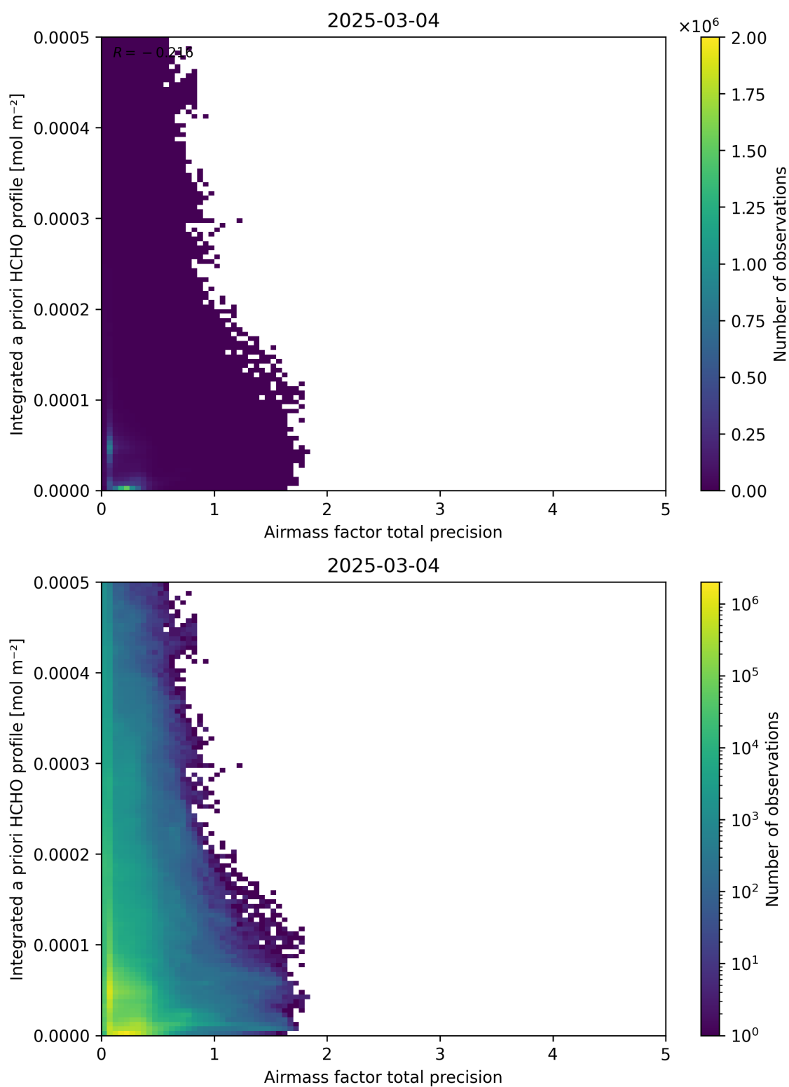
Figure 111: Scatter density plot of “Airmass factor total precision” against “Integrated a priori HCHO profile” for 2025-03-03 to 2025-03-05.
