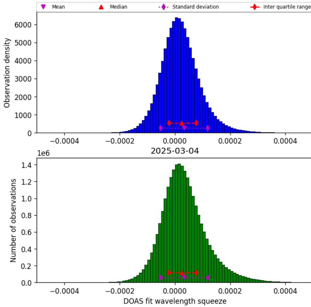
Figure 45: Histogram of “DOAS fit wavelength squeeze” for 2025-03-03 to 2025-03-05
