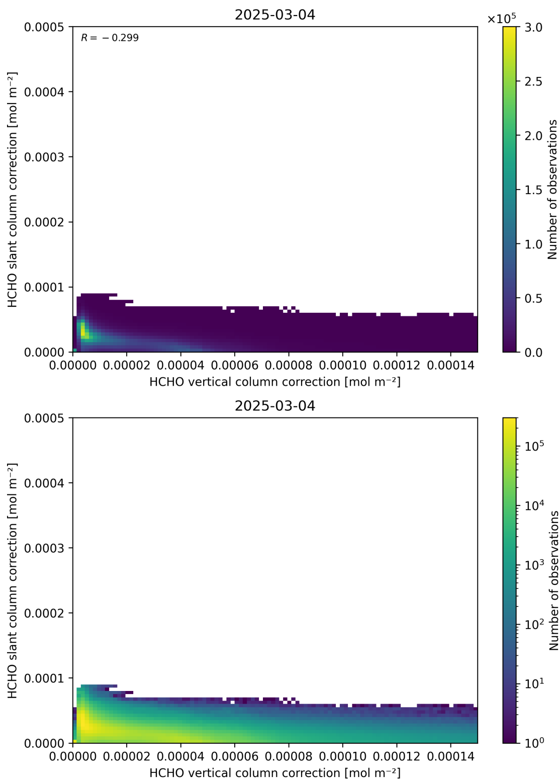
Figure 117: Scatter density plot of “HCHO vertical column correction” against “HCHO slant column correction” for 2025-03-03 to 2025-03-05.
