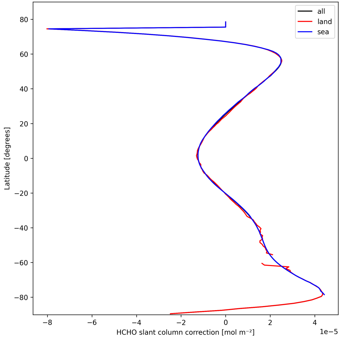
Figure 33: Zonal average of “HCHO slant column correction” for 2025-03-03 to 2025-03-05.
