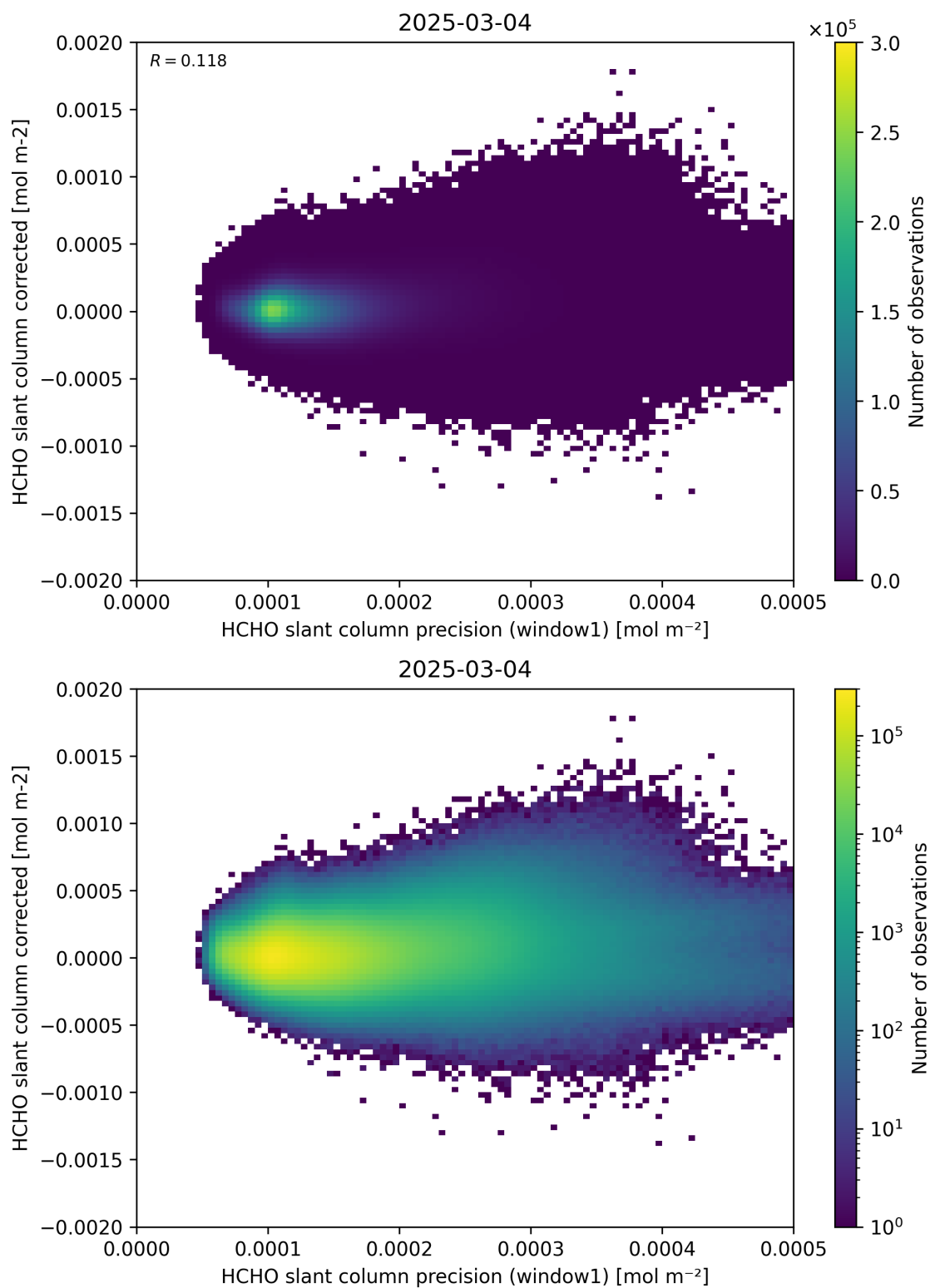
Figure 92: Scatter density plot of “HCHO slant column precision (window1)” against “HCHO slant column corrected” for 2025-03-03 to 2025-03-05.
