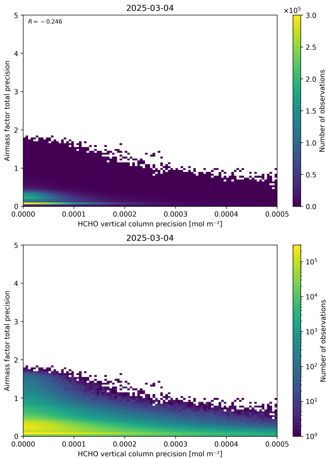
Figure 145: Scatter density plot of “HCHO vertical column precision” against “Airmass factor total precision” for 2025-03-03 to 2025-03-05.
