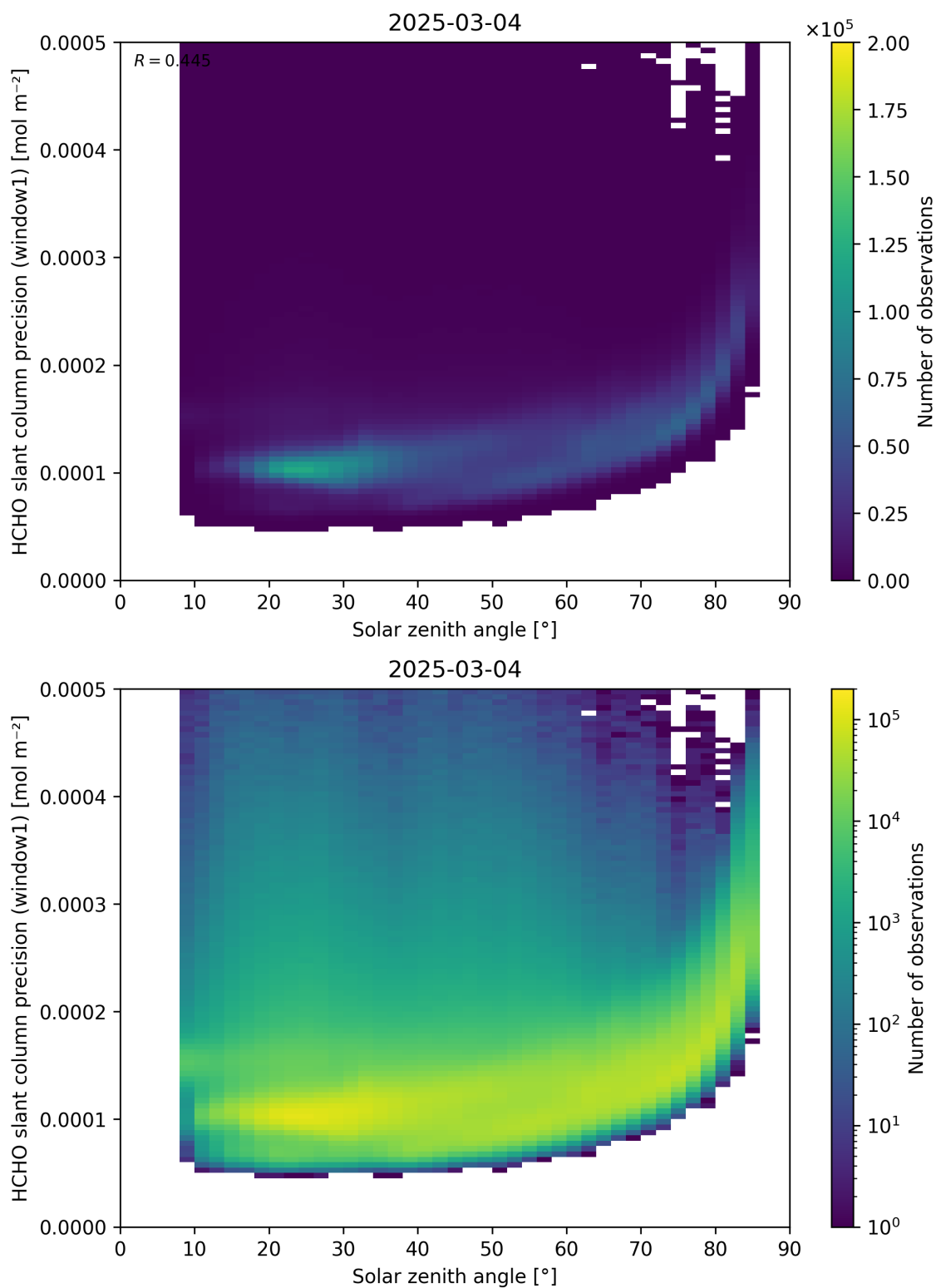
Figure 174: Scatter density plot of “Solar zenith angle” against “HCHO slant column precision (window1)” for 2025-03-03 to 2025-03-05.
