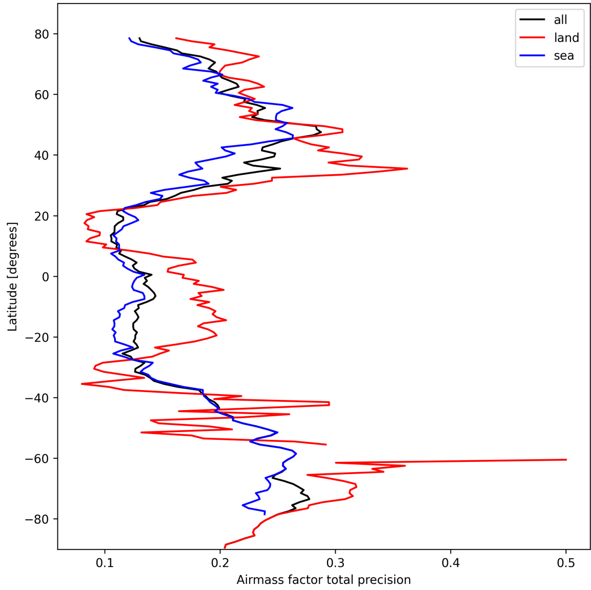
Figure 27: Zonal average of “Airmass factor total precision” for 2025-03-03 to 2025-03-05.
