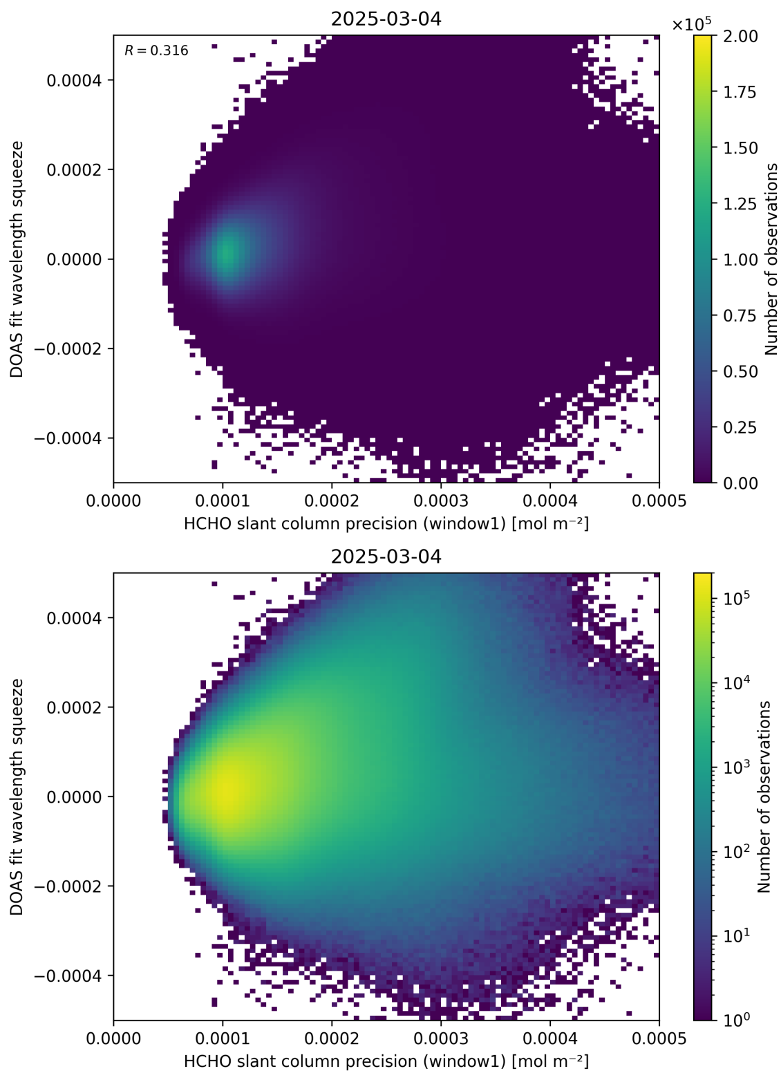
Figure 90: Scatter density plot of “HCHO slant column precision (window1)” against “DOAS fit wavelength squeeze” for 2025-03-03 to 2025-03-05.
