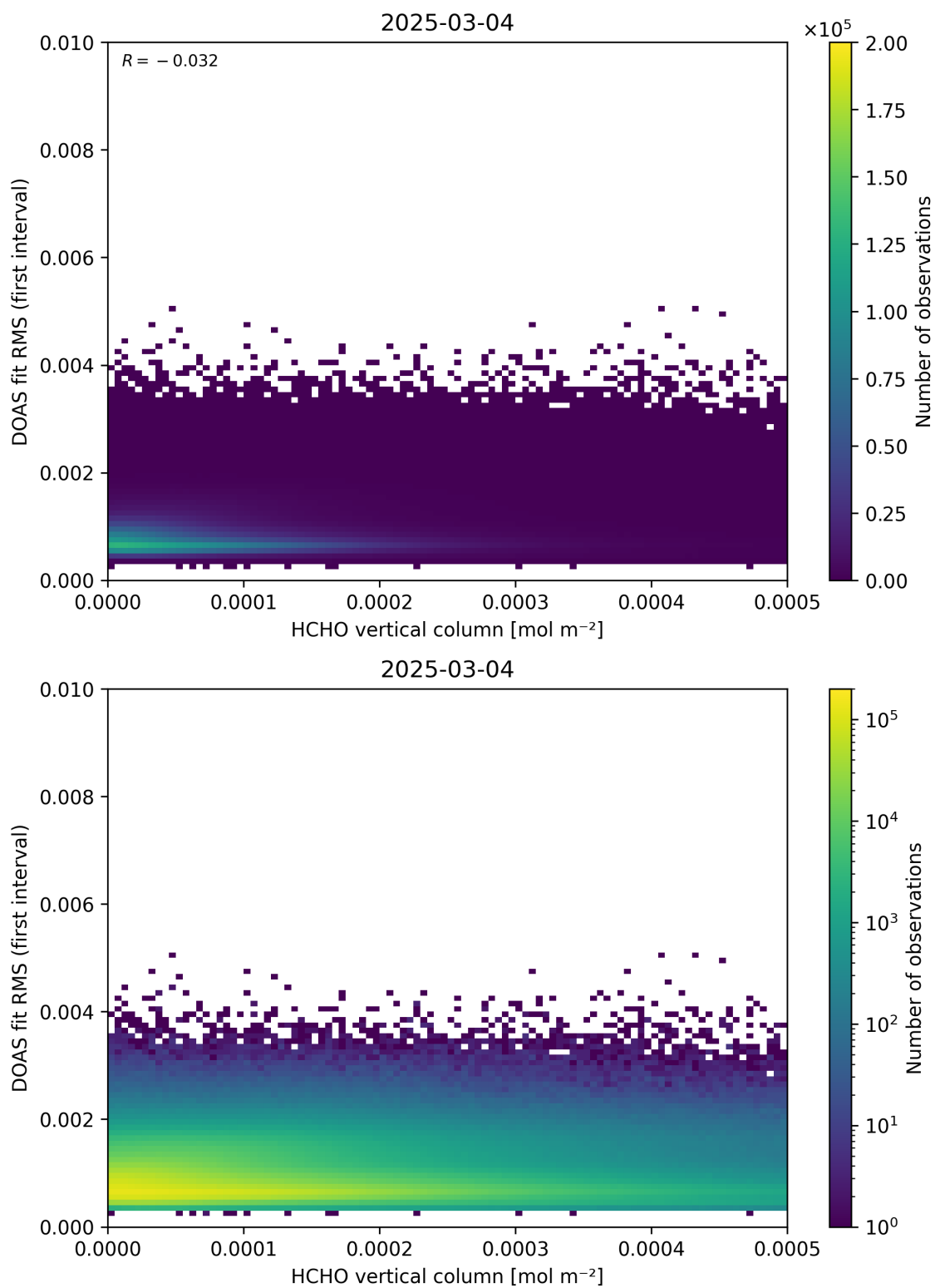
Figure 123: Scatter density plot of “HCHO vertical column” against “DOAS fit RMS (first interval)” for 2025-03-03 to 2025-03-05.
