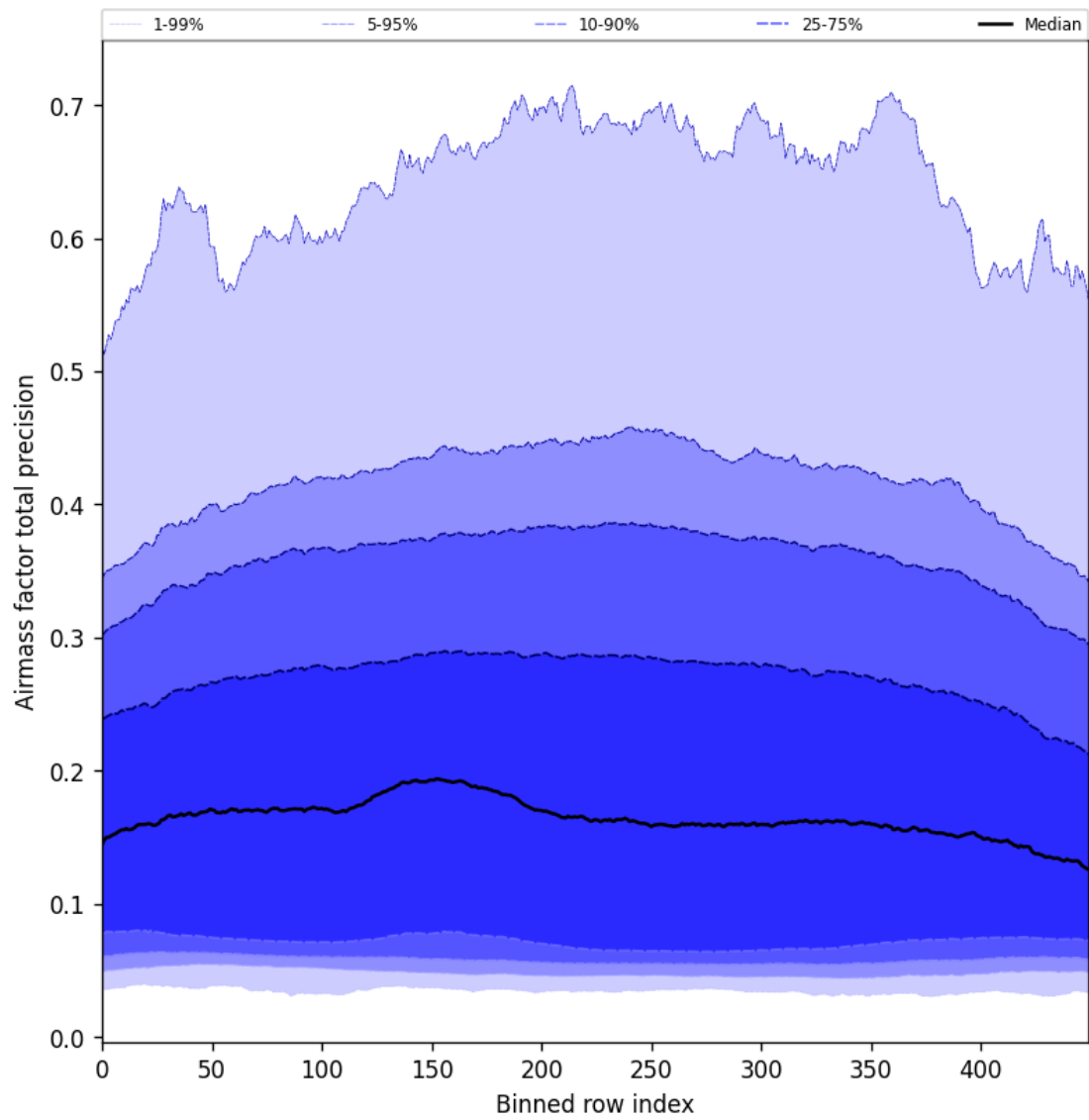
Figure 55: Along track statistics of “Airmass factor total precision” for 2025-03-03 to 2025-03-05
