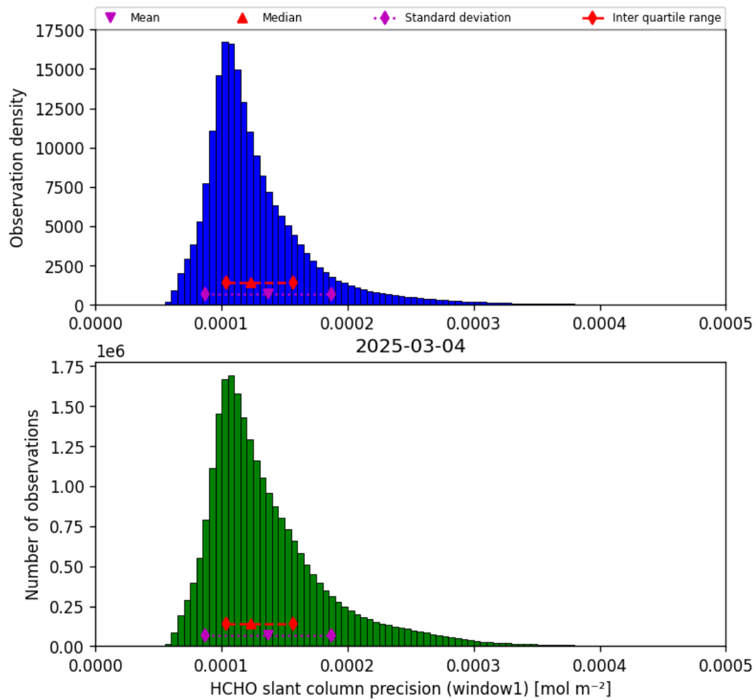
Figure 39: Histogram of “HCHO slant column precision (window1)” for 2025-03-03 to 2025-03-05
