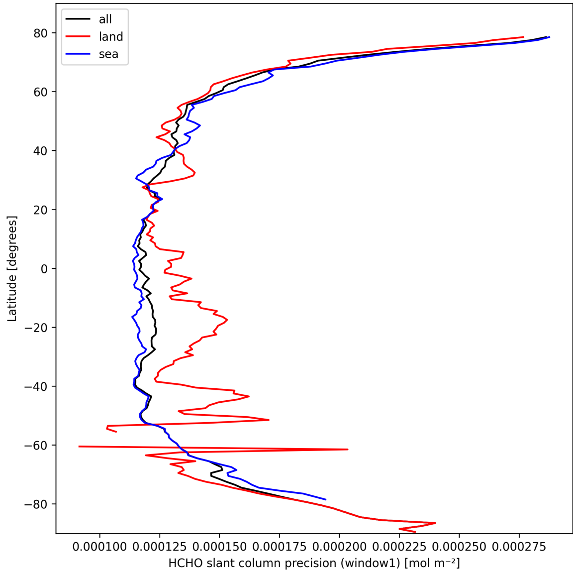
Figure 25: Zonal average of “HCHO slant column precision (window1)” for 2025-03-03 to 2025-03-05.
