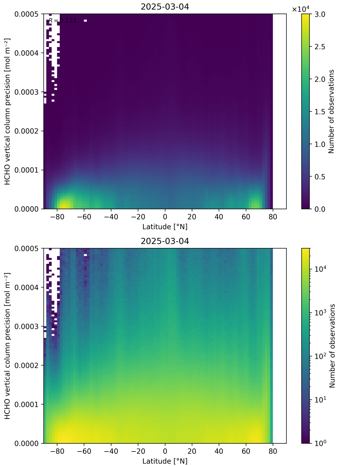
Figure 165: Scatter density plot of “Latitude” against “HCHO vertical column precision” for 2025-03-03 to 2025-03-05.
