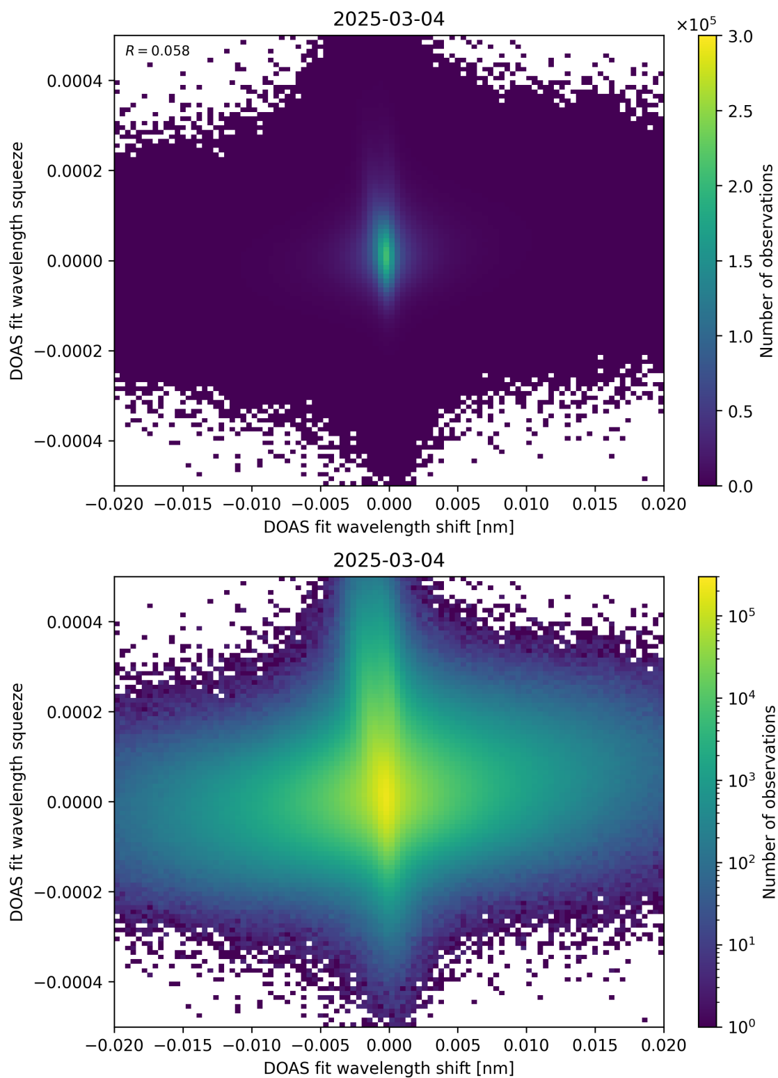
Figure 65: Scatter density plot of “DOAS fit wavelength shift” against “DOAS fit wavelength squeeze” for 2025-03-03 to 2025-03-05.
