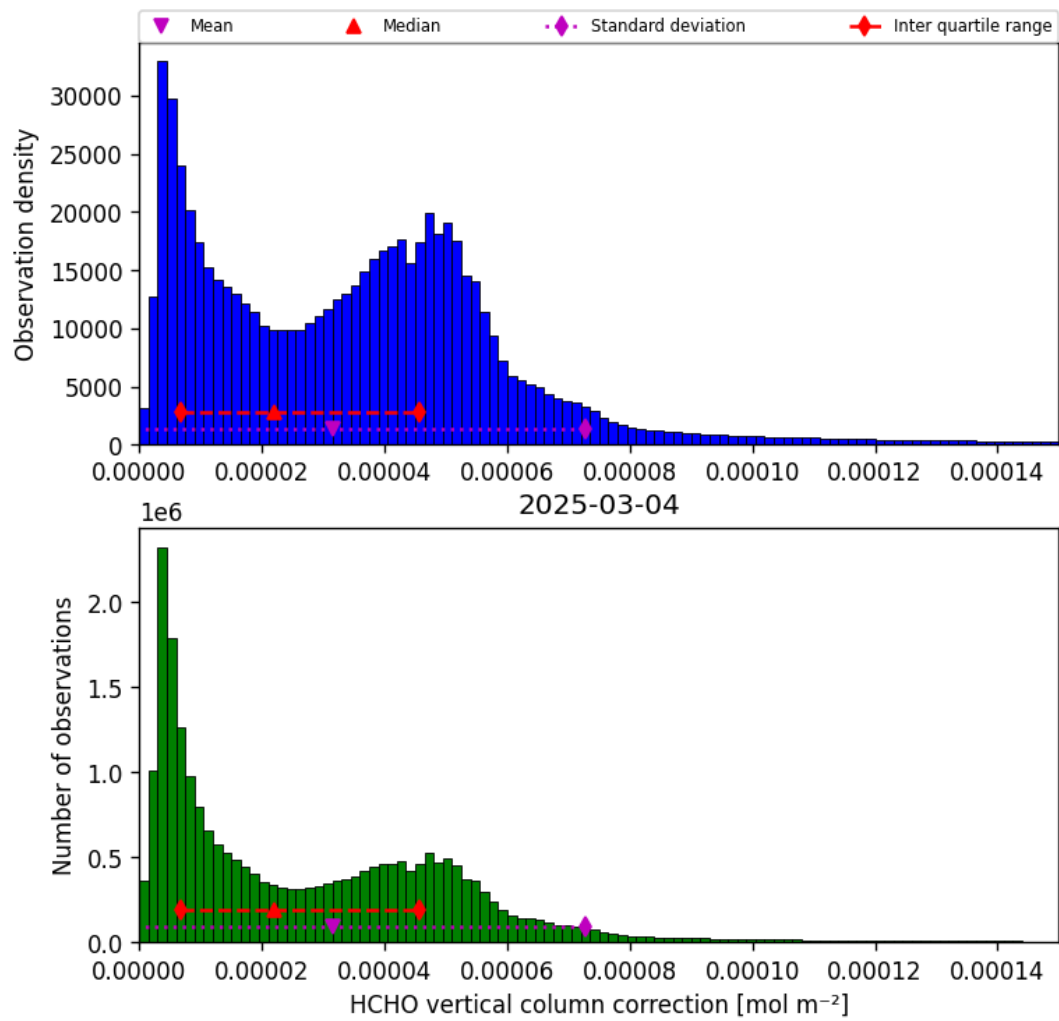
Figure 37: Histogram of “HCHO vertical column correction” for 2025-03-03 to 2025-03-05
