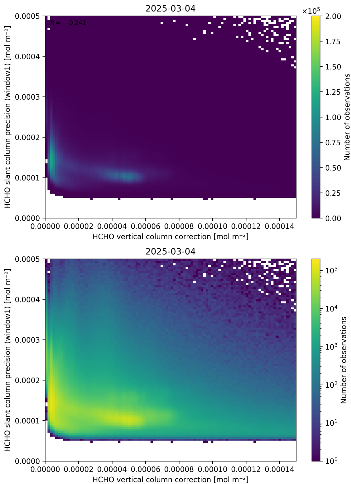
Figure 119: Scatter density plot of “HCHO vertical column correction” against “HCHO slant column precision (window1)” for 2025-03-03 to 2025-03-05.
