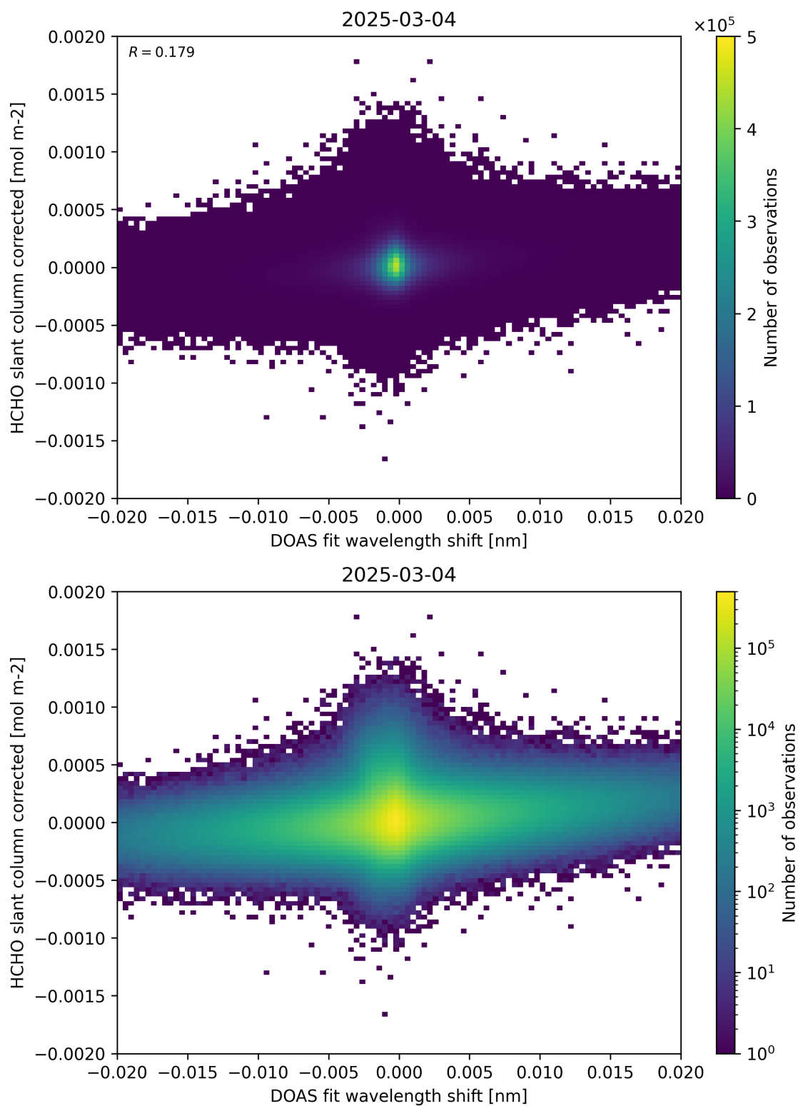
Figure 66: Scatter density plot of “DOAS fit wavelength shift” against “HCHO slant column corrected” for 2025-03-03 to 2025-03-05.
