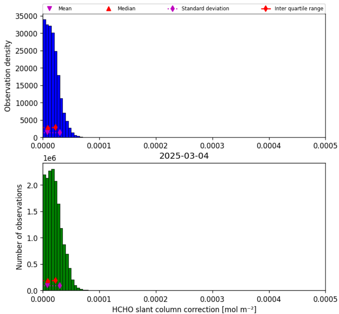
Figure 47: Histogram of “HCHO slant column correction” for 2025-03-03 to 2025-03-05
