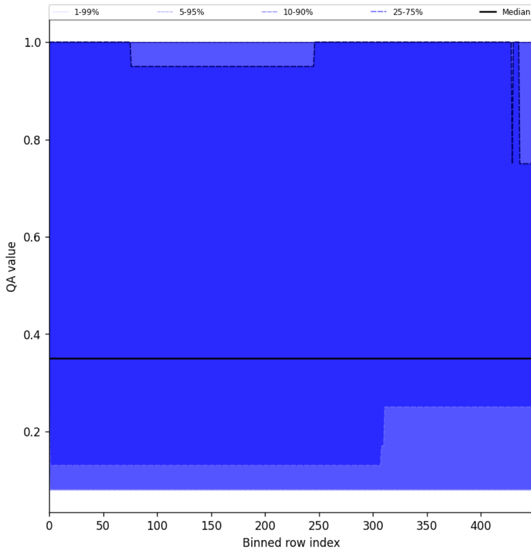
Figure 48: Along track statistics of “QA value” for 2025-03-03 to 2025-03-05
