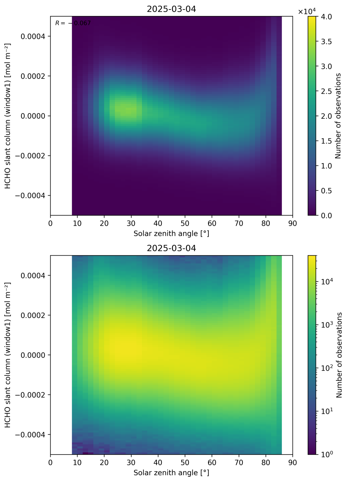
Figure 173: Scatter density plot of “Solar zenith angle” against “HCHO slant column (window1)” for 2025-03-03 to 2025-03-05.
