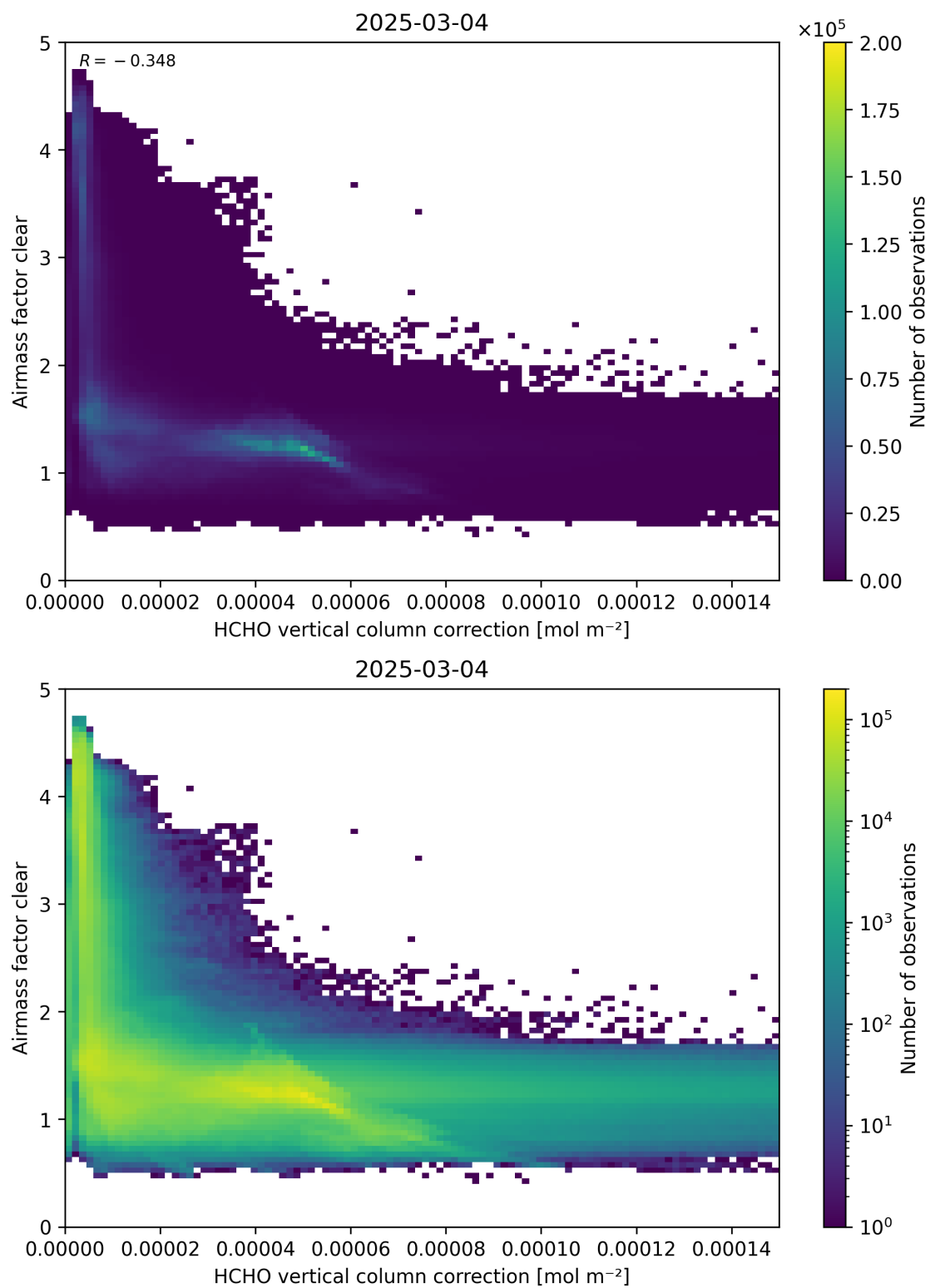
Figure 115: Scatter density plot of “HCHO vertical column correction” against “Airmass factor clear” for 2025-03-03 to 2025-03-05.
