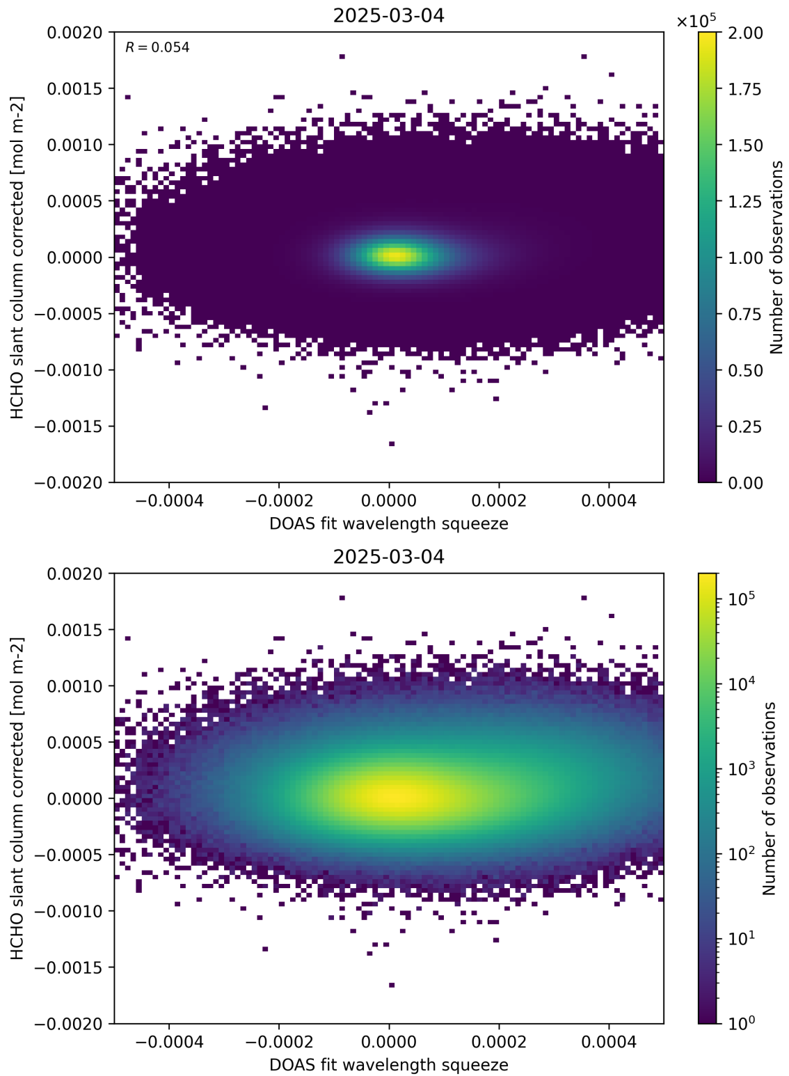
Figure 69: Scatter density plot of “DOAS fit wavelength squeeze” against “HCHO slant column corrected” for 2025-03-03 to 2025-03-05.
