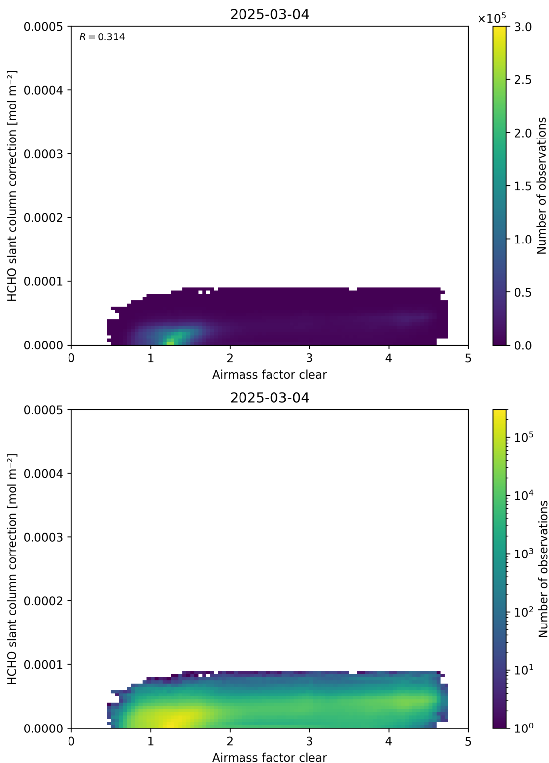
Figure 75: Scatter density plot of “Airmass factor clear” against “HCHO slant column correction” for 2025-03-03 to 2025-03-05.
