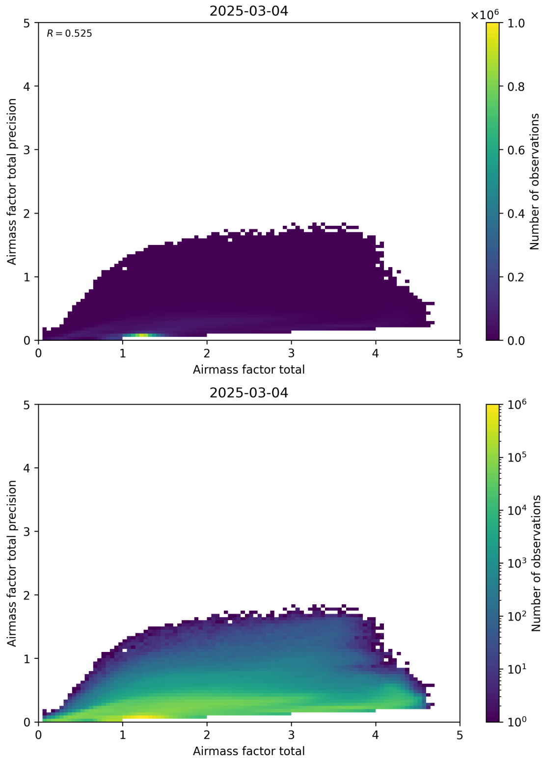
Figure 103: Scatter density plot of “Airmass factor total” against “Airmass factor total precision” for 2025-03-03 to 2025-03-05.
