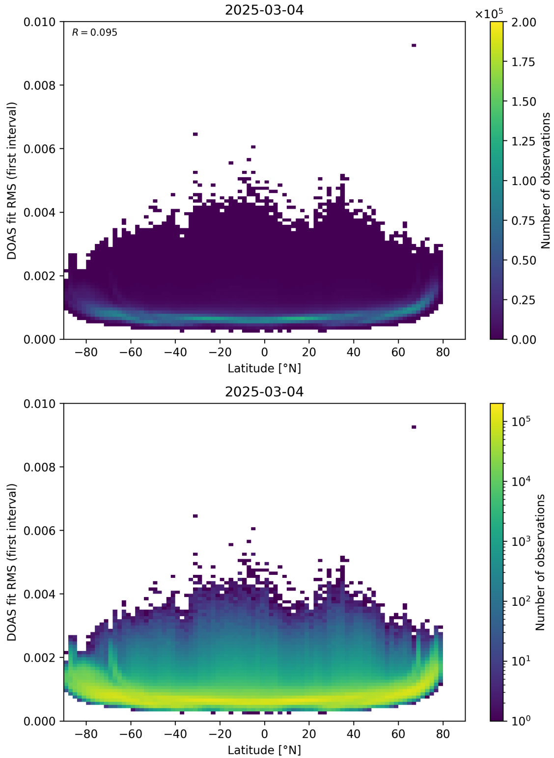
Figure 153: Scatter density plot of “Latitude” against “DOAS fit RMS (first interval)” for 2025-03-03 to 2025-03-05.
