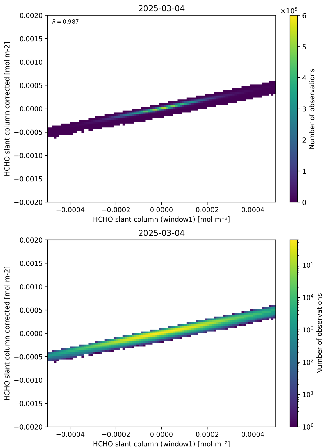
Figure 82: Scatter density plot of “HCHO slant column (window1)” against “HCHO slant column corrected” for 2025-03-03 to 2025-03-05.
