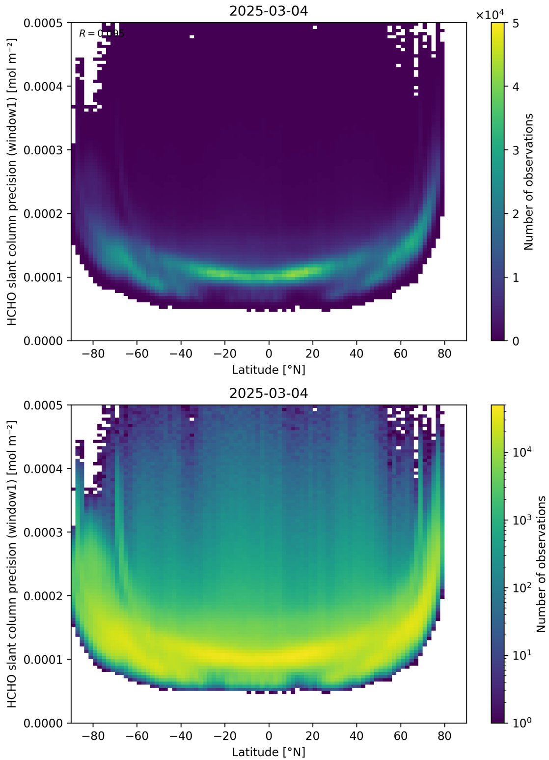
Figure 160: Scatter density plot of “Latitude” against “HCHO slant column precision (window1)” for 2025-03-03 to 2025-03-05.
