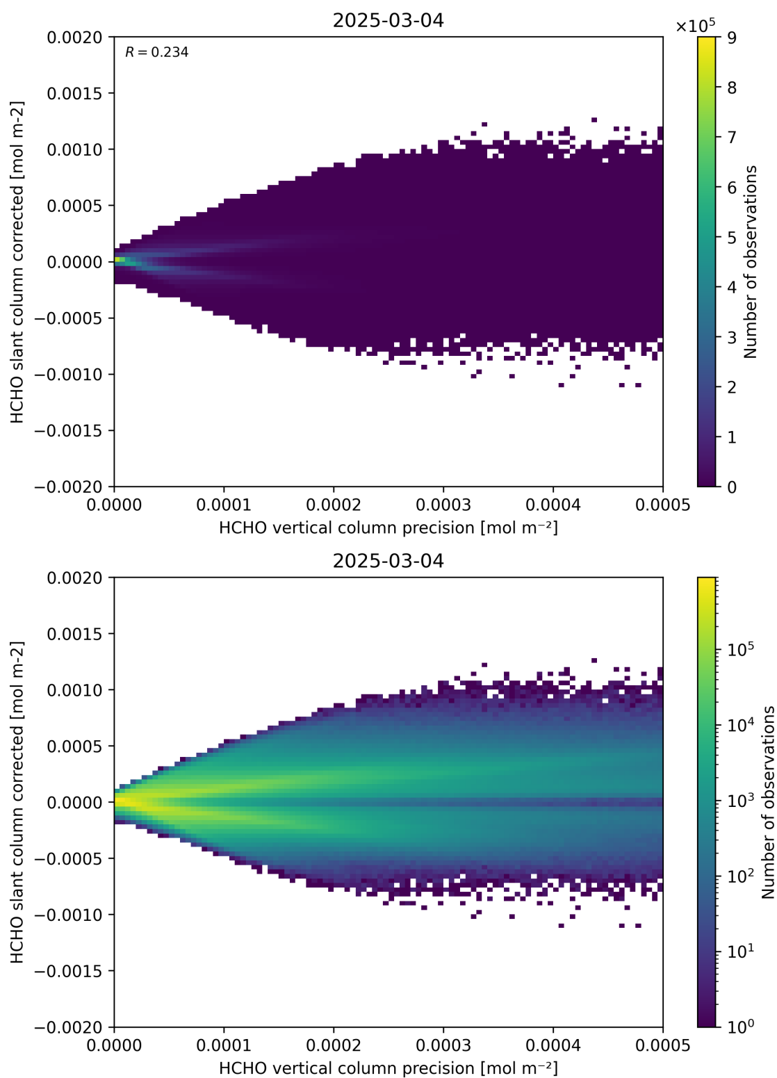
Figure 140: Scatter density plot of “HCHO vertical column precision” against “HCHO slant column corrected” for 2025-03-03 to 2025-03-05.
