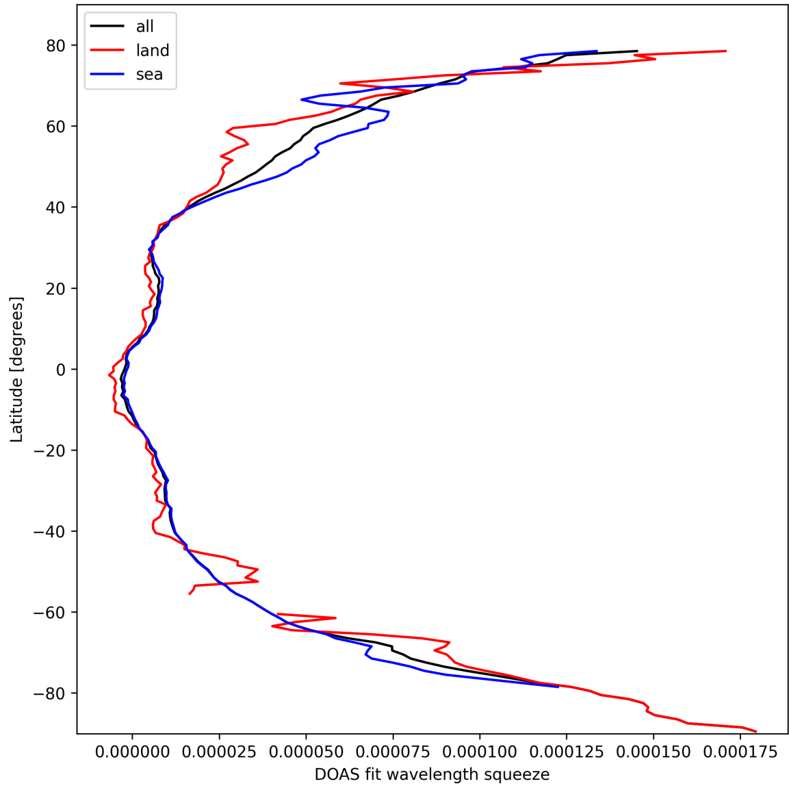
Figure 31: Zonal average of “DOAS fit wavelength squeeze” for 2025-03-03 to 2025-03-05.
