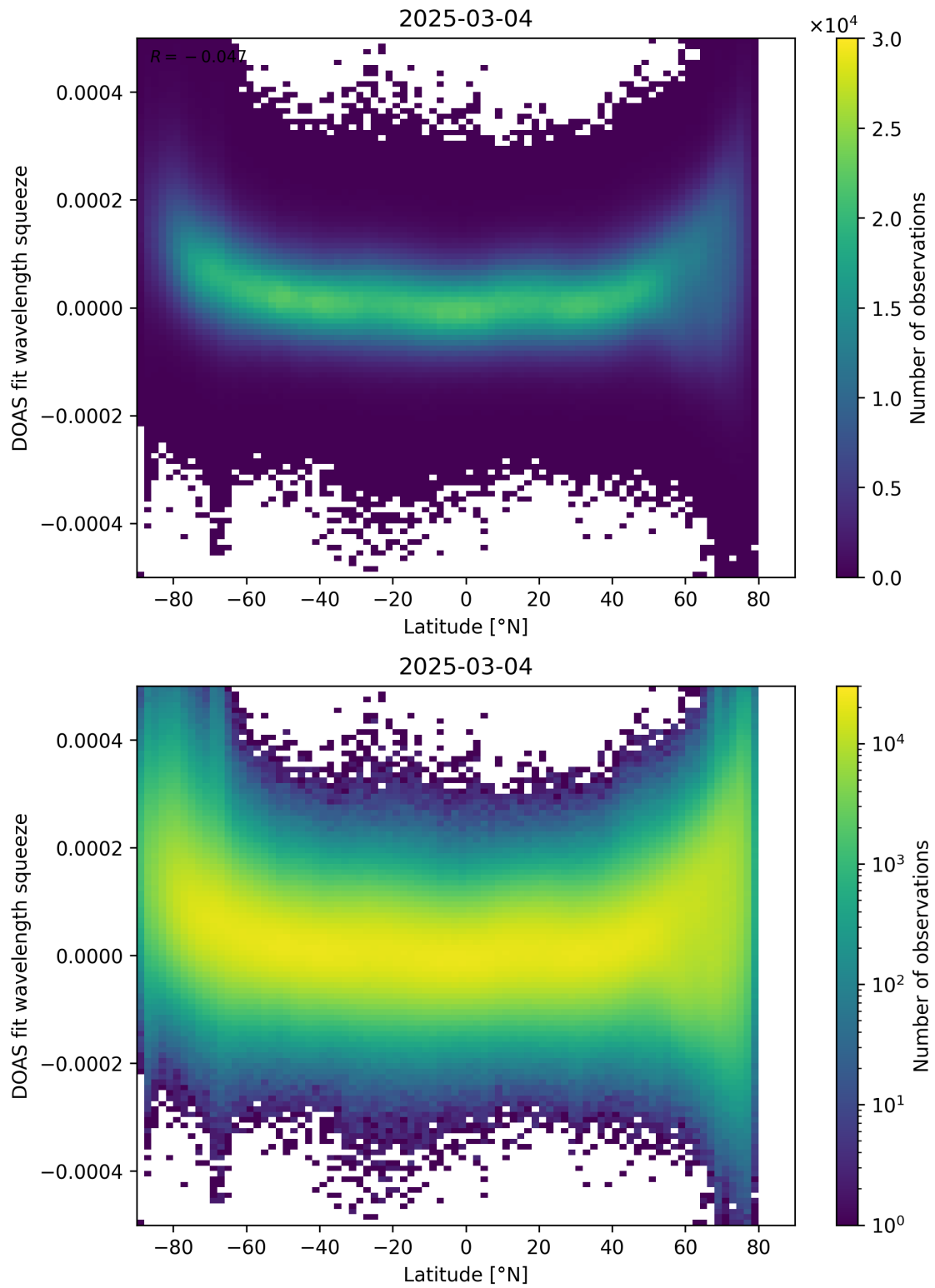
Figure 155: Scatter density plot of “Latitude” against “DOAS fit wavelength squeeze” for 2025-03-03 to 2025-03-05.
