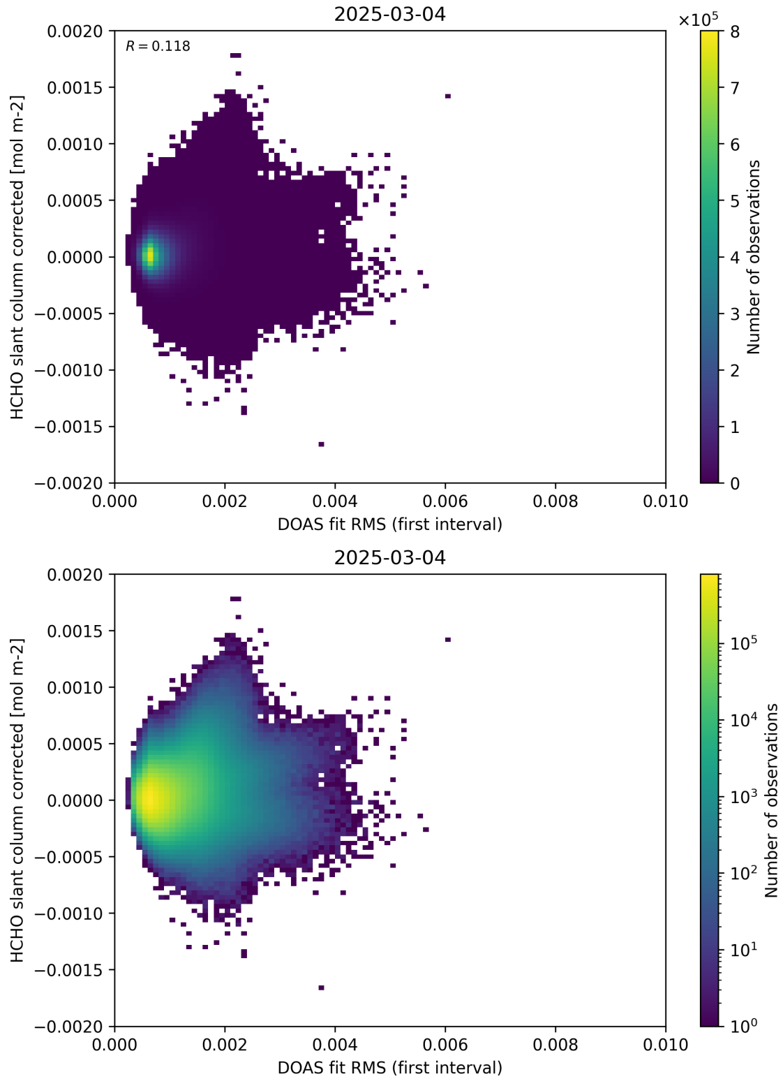
Figure 62: Scatter density plot of “DOAS fit RMS (first interval)” against “HCHO slant column corrected” for 2025-03-03 to 2025-03-05.
