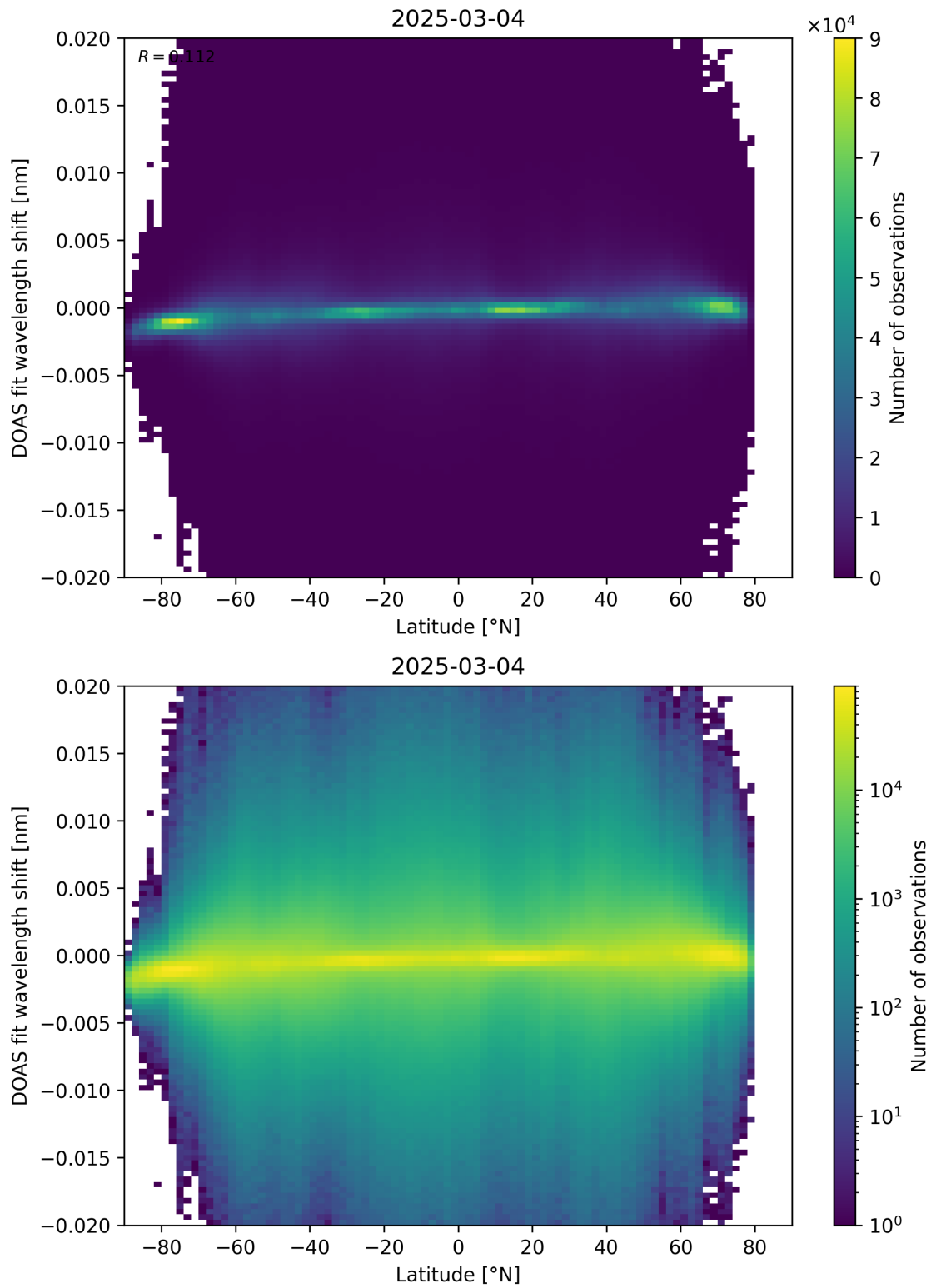
Figure 154: Scatter density plot of “Latitude” against “DOAS fit wavelength shift” for 2025-03-03 to 2025-03-05.
