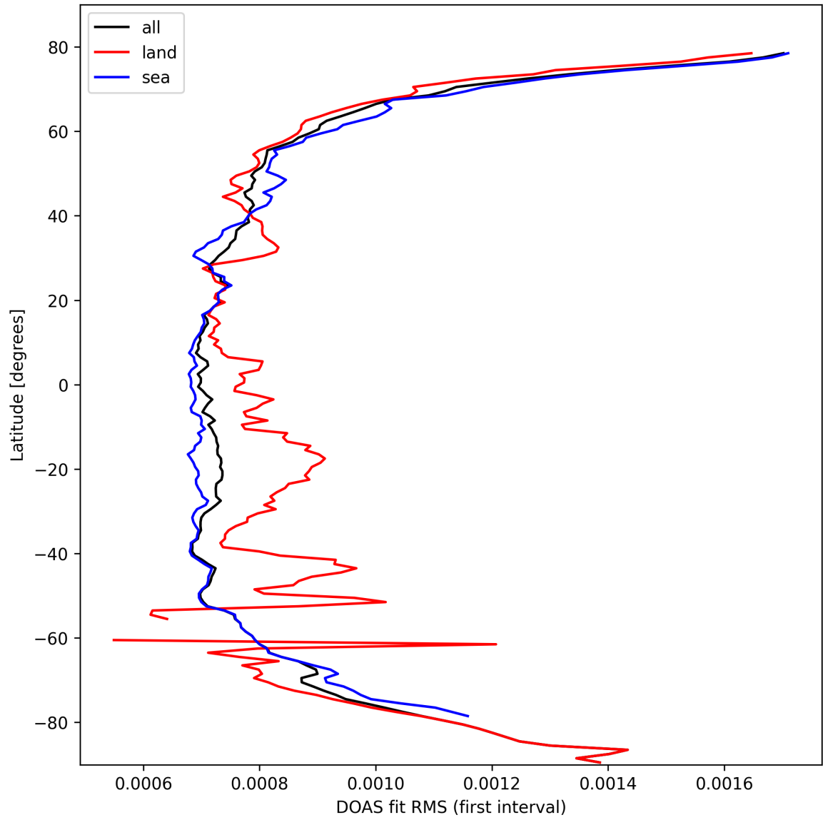
Figure 32: Zonal average of “DOAS fit RMS (first interval)” for 2025-03-03 to 2025-03-05.
