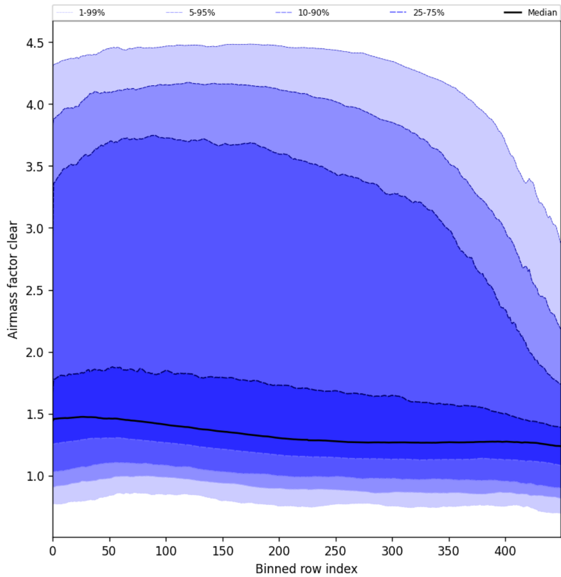
Figure 56: Along track statistics of “Airmass factor clear” for 2025-03-03 to 2025-03-05
