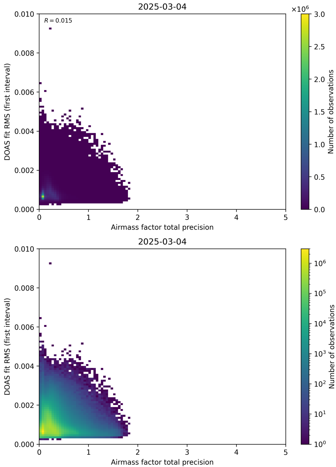
Figure 105: Scatter density plot of “Airmass factor total precision” against “DOAS fit RMS (first interval)” for 2025-03-03 to 2025-03-05.
