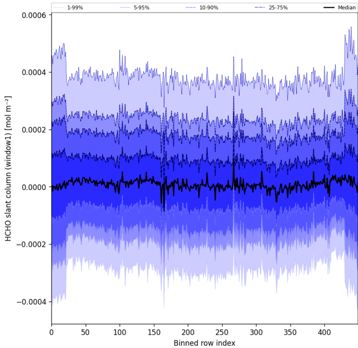
Figure 52: Along track statistics of “HCHO slant column (window1)” for 2025-03-03 to 2025-03-05
