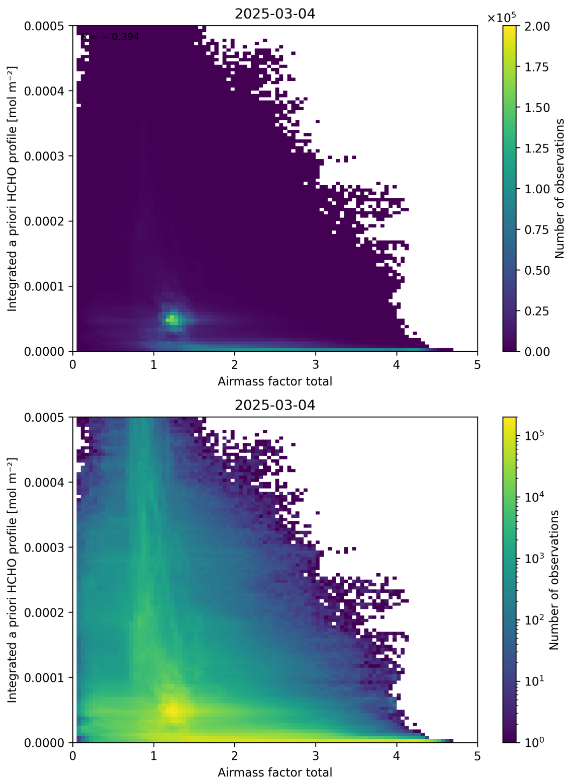
Figure 104: Scatter density plot of “Airmass factor total” against “Integrated a priori HCHO profile” for 2025-03-03 to 2025-03-05.
