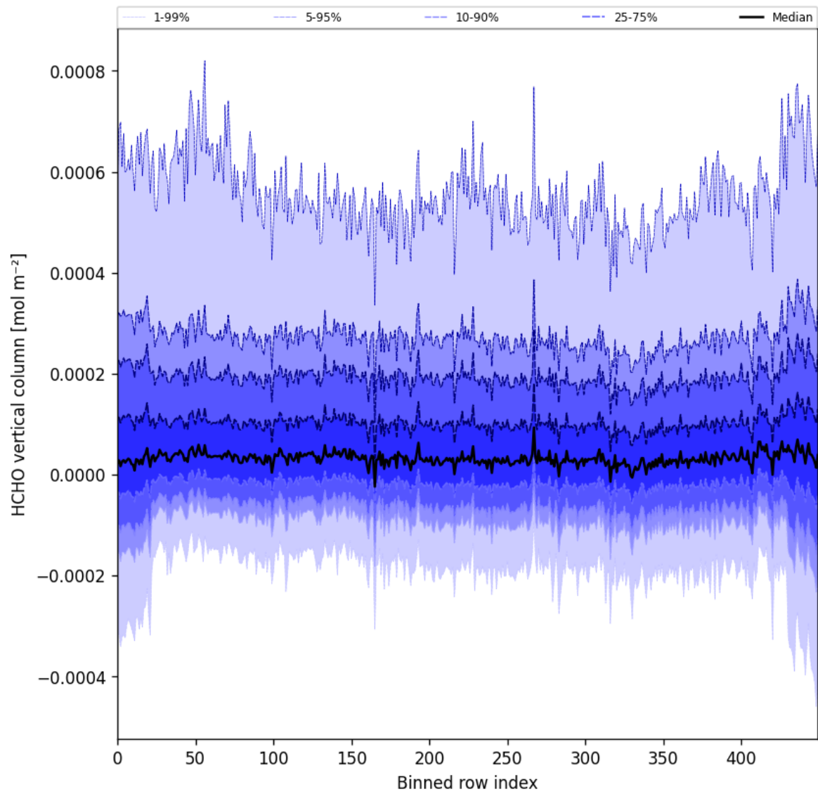
Figure 49: Along track statistics of “HCHO vertical column” for 2025-03-03 to 2025-03-05
