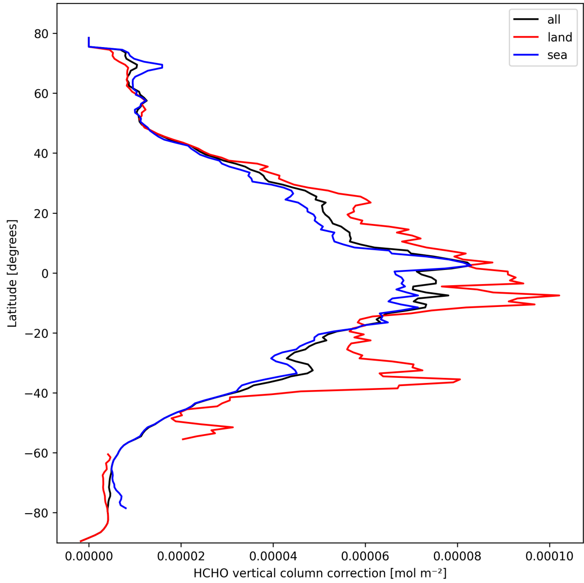
Figure 23: Zonal average of “HCHO vertical column correction” for 2025-03-03 to 2025-03-05.
