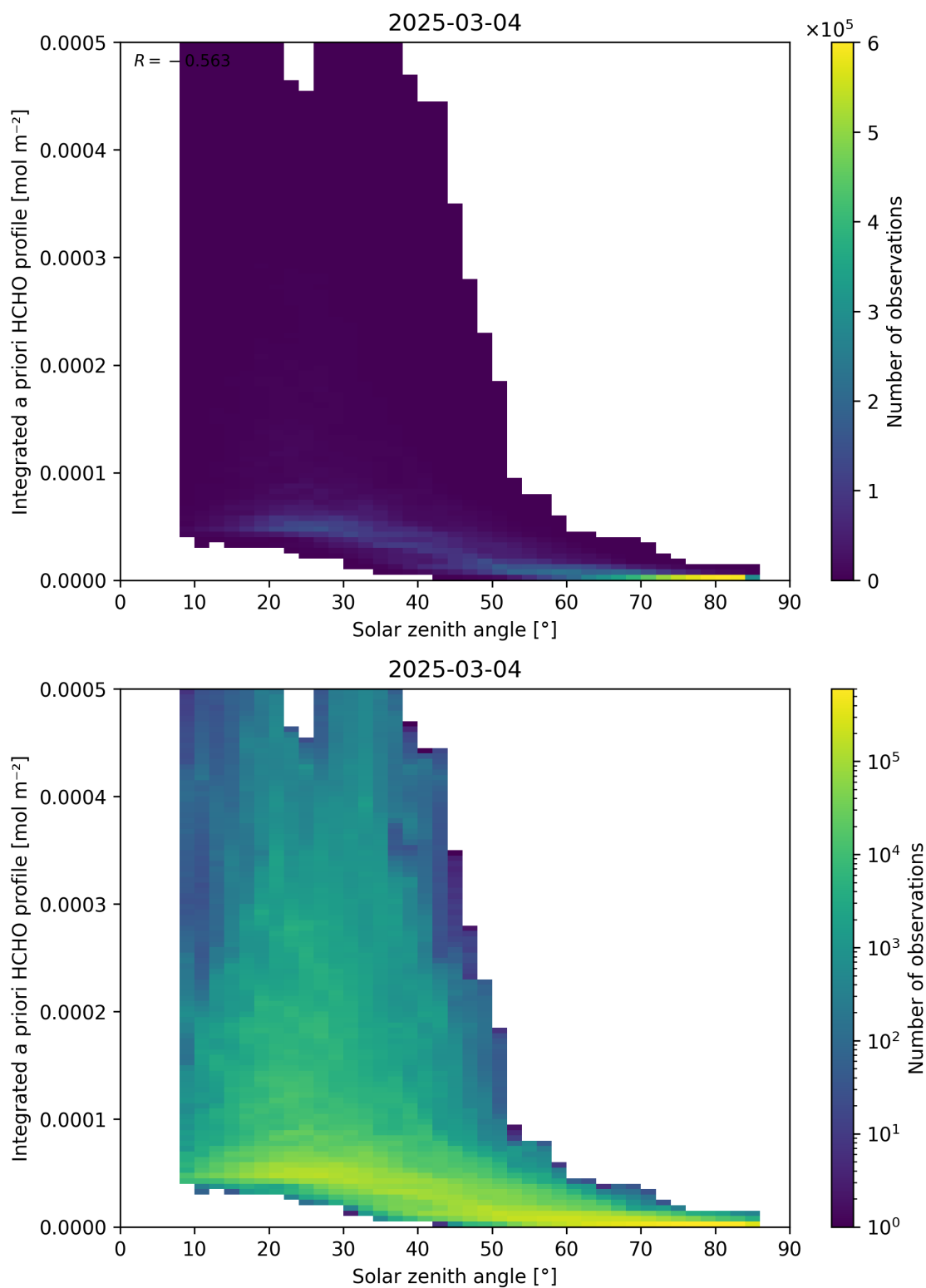
Figure 180: Scatter density plot of “Solar zenith angle” against “Integrated a priori HCHO profile” for 2025-03-03 to 2025-03-05.
