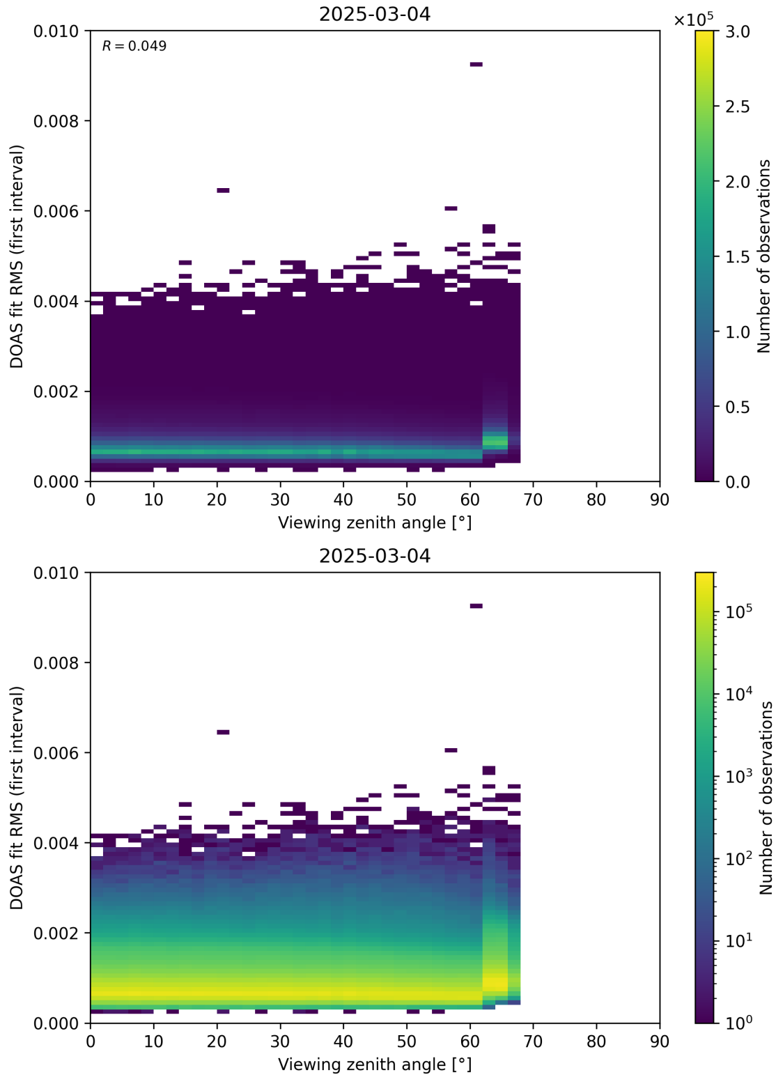
Figure 182: Scatter density plot of “Viewing zenith angle” against “DOAS fit RMS (first interval)” for 2025-03-03 to 2025-03-05.
