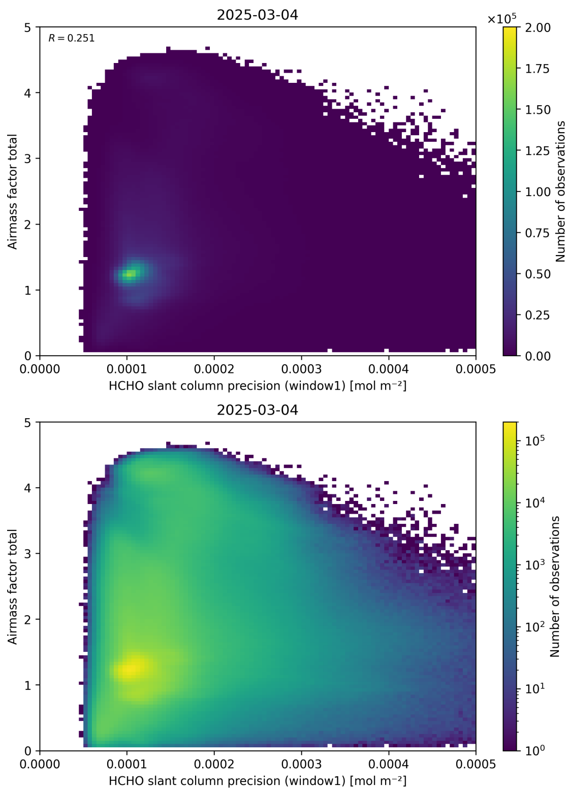
Figure 94: Scatter density plot of “HCHO slant column precision (window1)” against “Airmass factor total” for 2025-03-03 to 2025-03-05.
