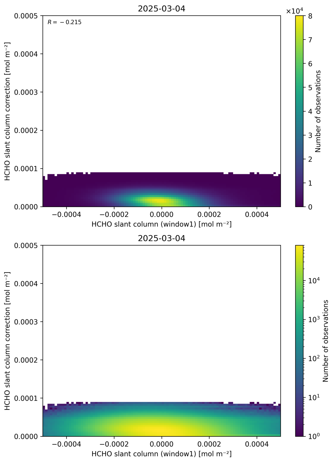
Figure 83: Scatter density plot of “HCHO slant column (window1)” against “HCHO slant column correction” for 2025-03-03 to 2025-03-05.
