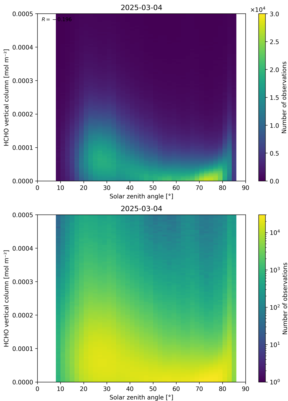
Figure 177: Scatter density plot of “Solar zenith angle” against “HCHO vertical column” for 2025-03-03 to 2025-03-05.
