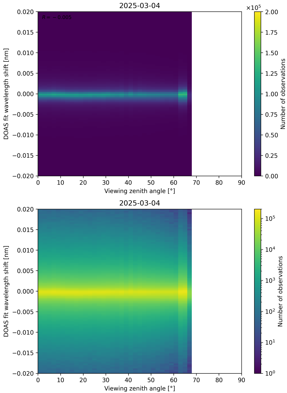
Figure 183: Scatter density plot of “Viewing zenith angle” against “DOAS fit wavelength shift” for 2025-03-03 to 2025-03-05.
