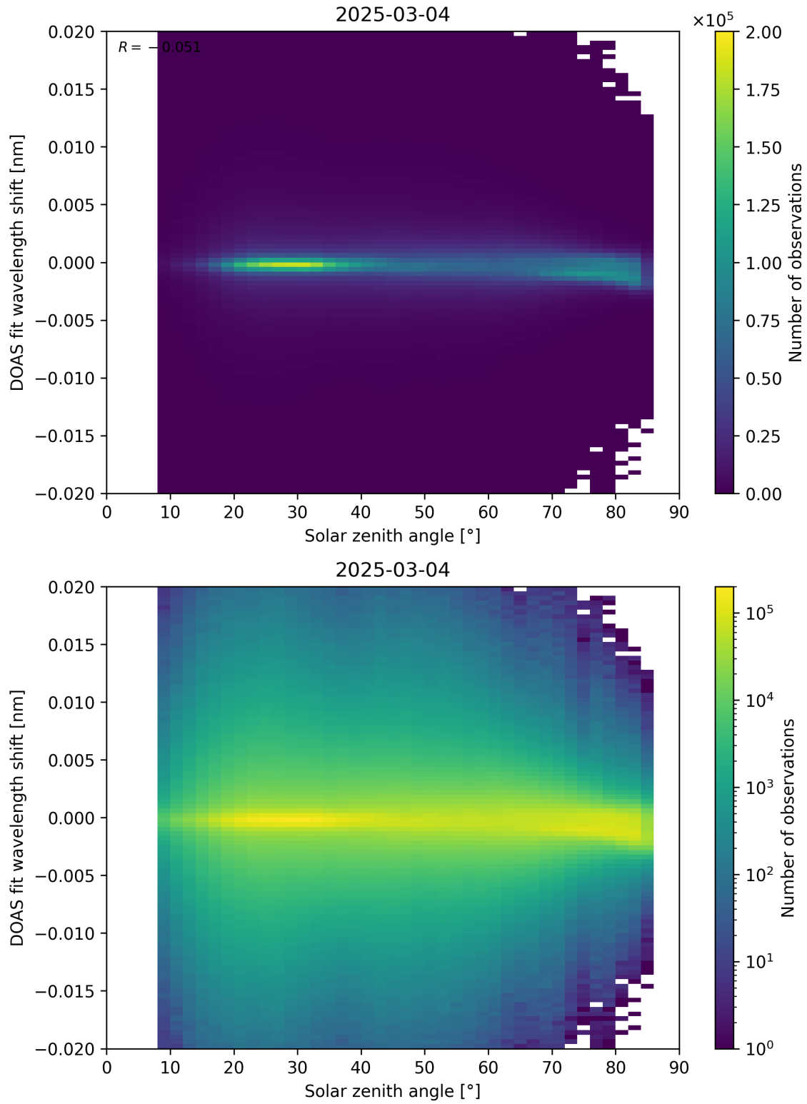
Figure 168: Scatter density plot of “Solar zenith angle” against “DOAS fit wavelength shift” for 2025-03-03 to 2025-03-05.
