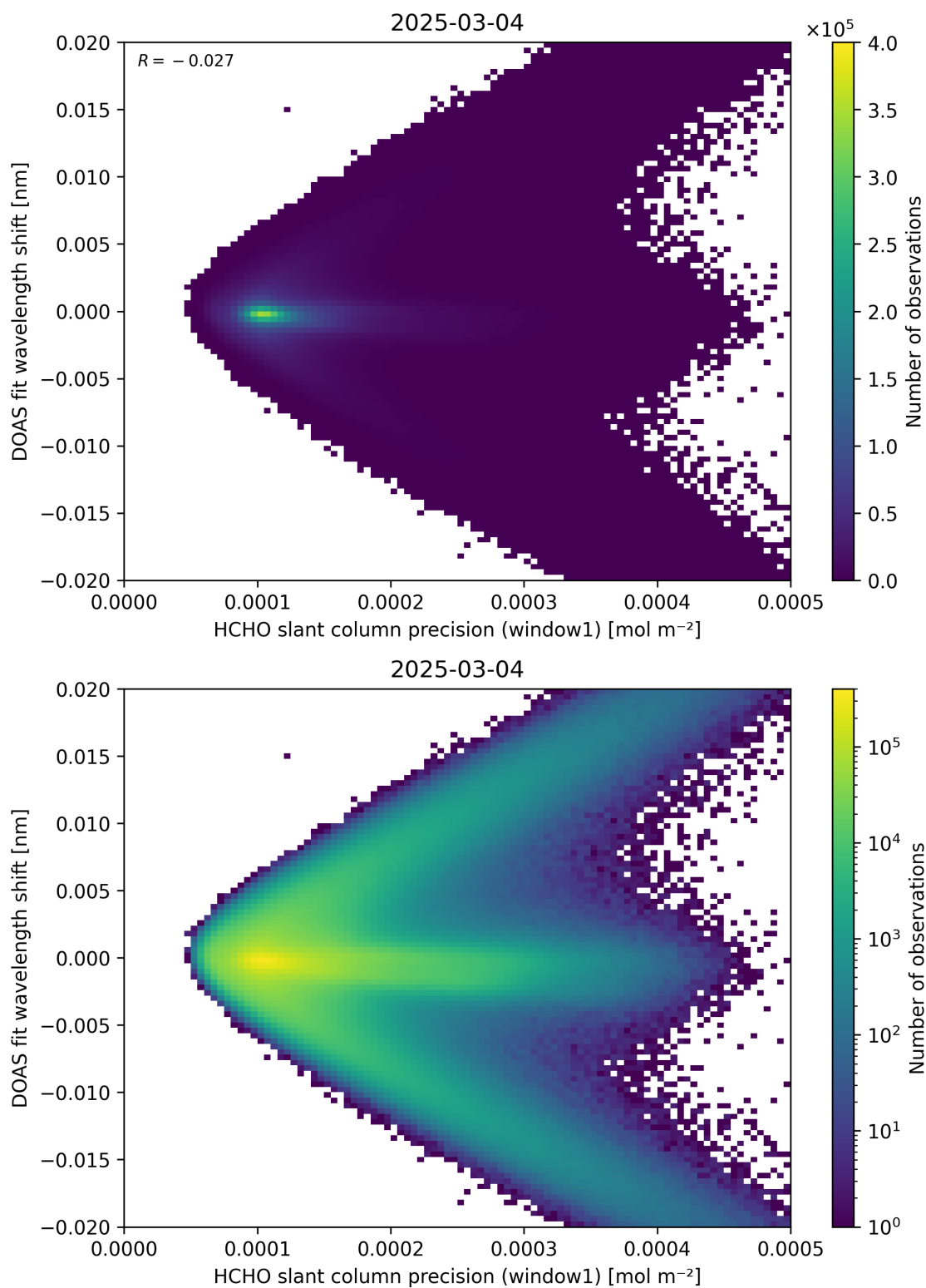
Figure 89: Scatter density plot of “HCHO slant column precision (window1)” against “DOAS fit wavelength shift” for 2025-03-03 to 2025-03-05.
