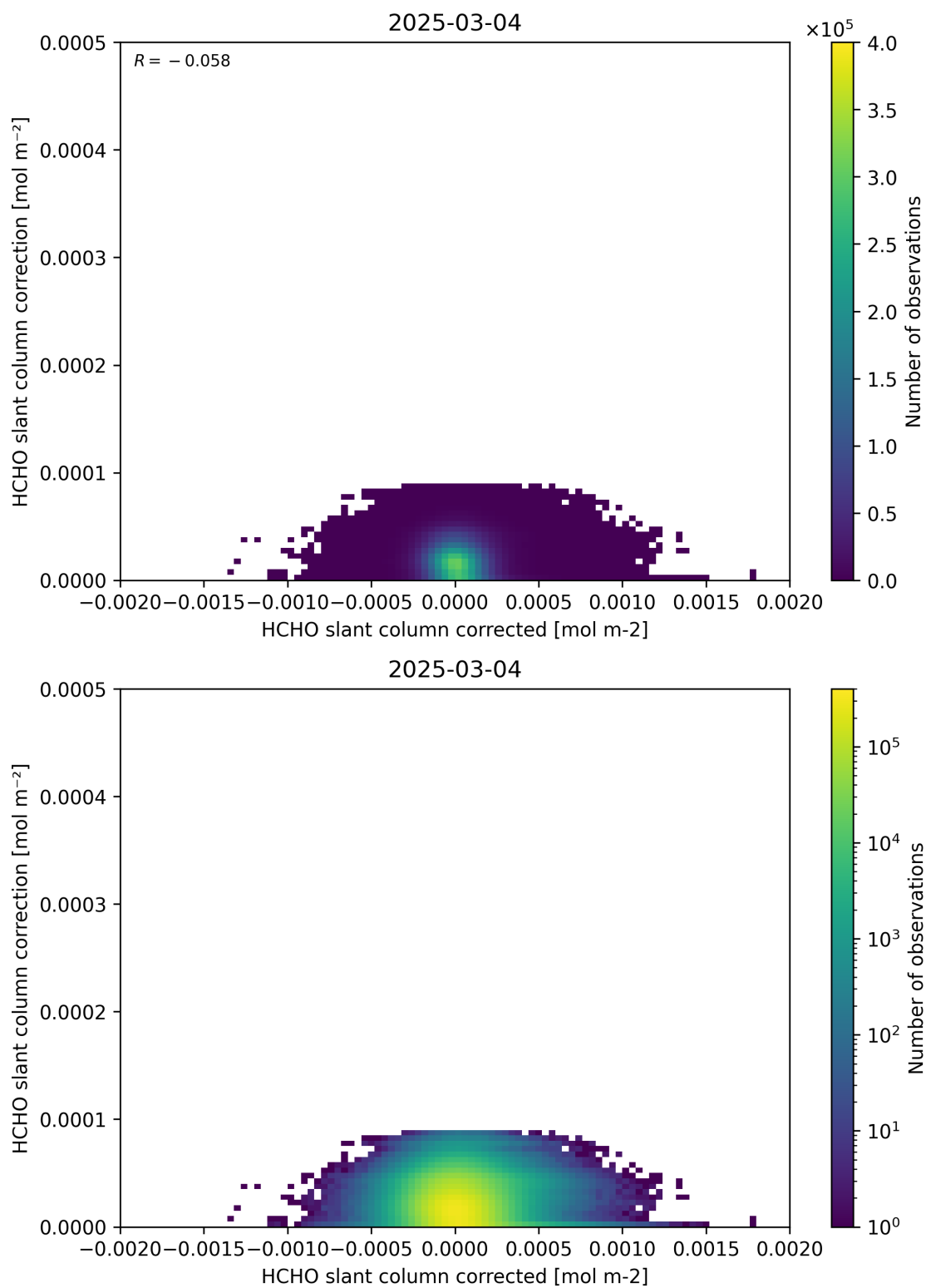
Figure 77: Scatter density plot of “HCHO slant column corrected” against “HCHO slant column correction” for 2025-03-03 to 2025-03-05.
