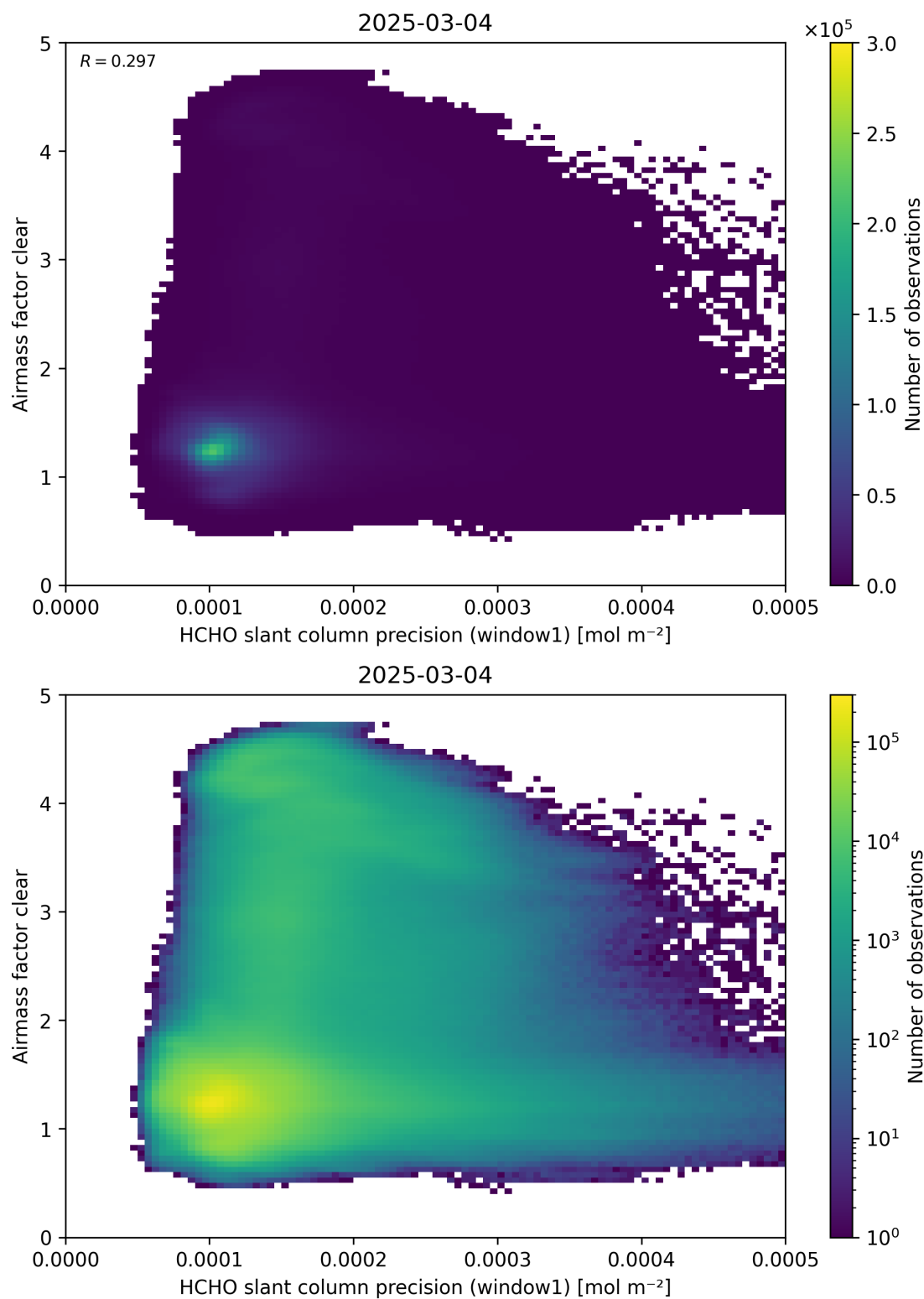
Figure 91: Scatter density plot of “HCHO slant column precision (window1)” against “Airmass factor clear” for 2025-03-03 to 2025-03-05.
