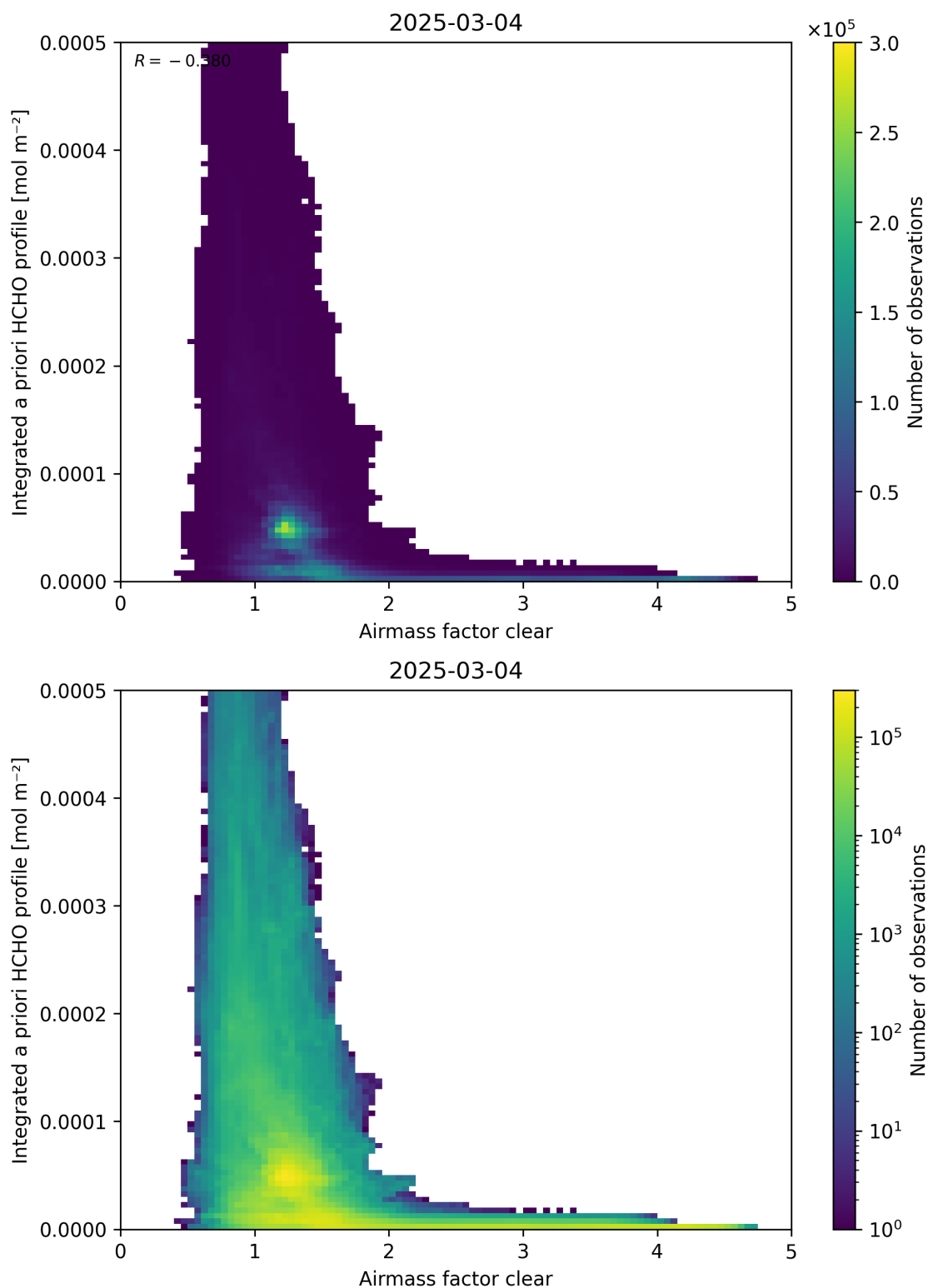
Figure 76: Scatter density plot of “Airmass factor clear” against “Integrated a priori HCHO profile” for 2025-03-03 to 2025-03-05.
