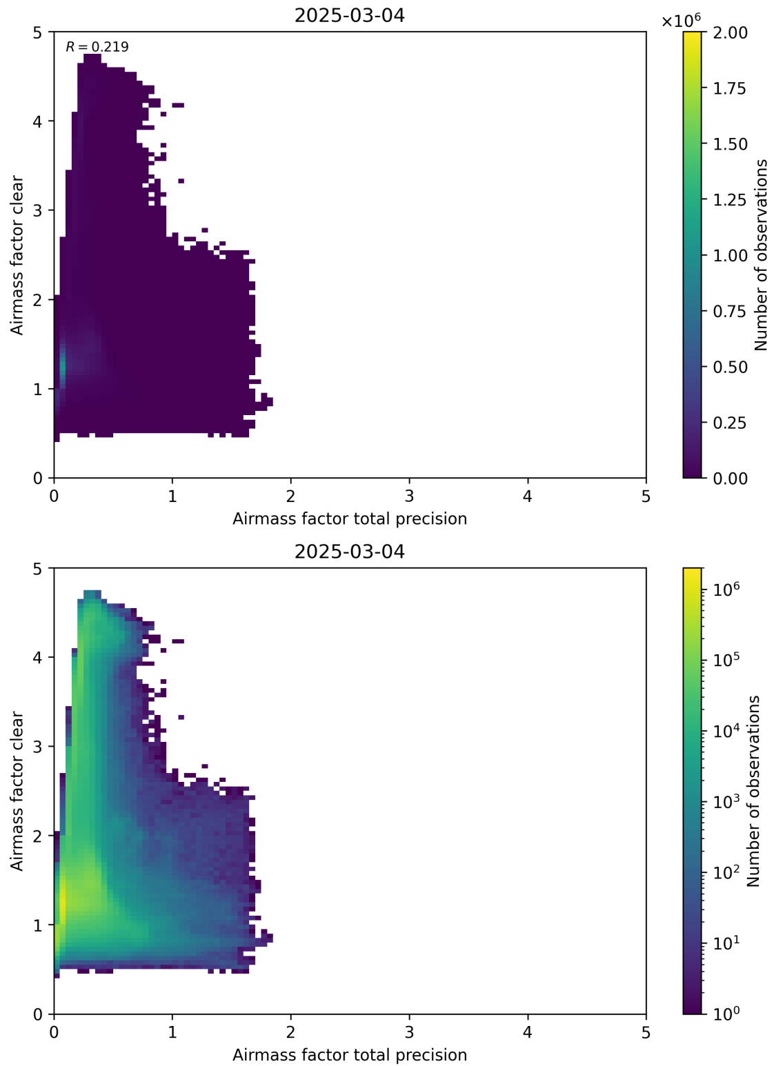
Figure 108: Scatter density plot of “Airmass factor total precision” against “Airmass factor clear” for 2025-03-03 to 2025-03-05.
