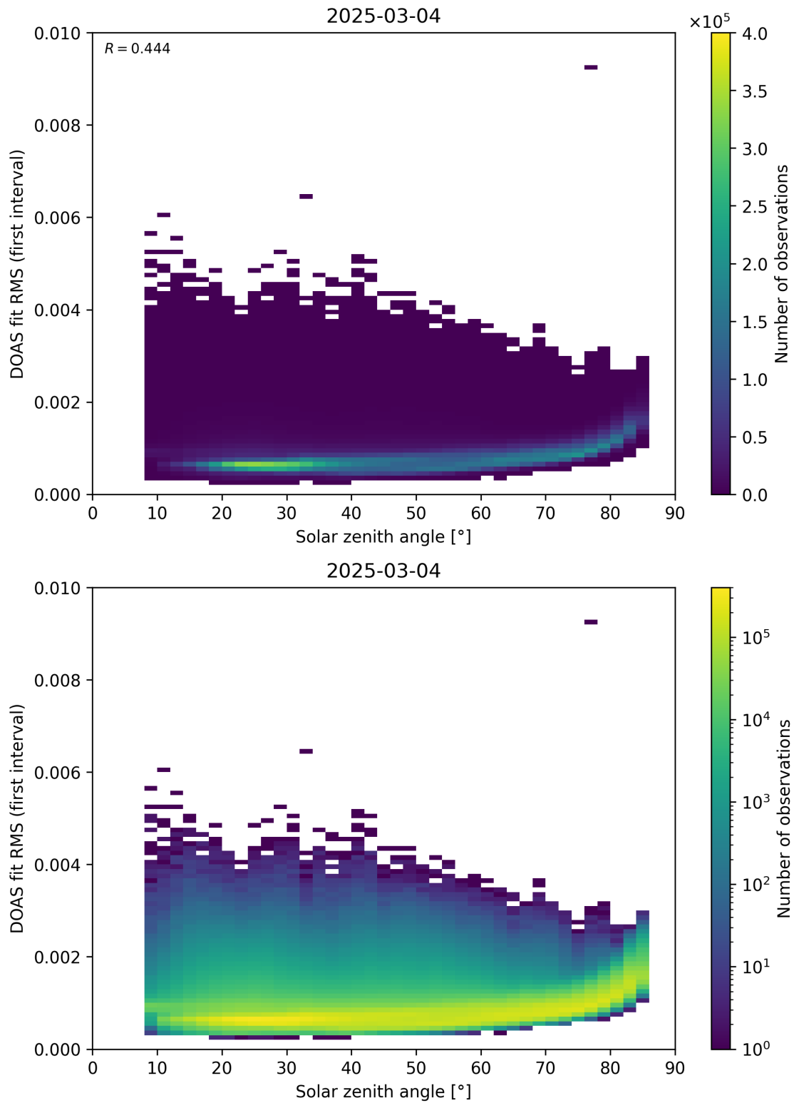
Figure 167: Scatter density plot of “Solar zenith angle” against “DOAS fit RMS (first interval)” for 2025-03-03 to 2025-03-05.
