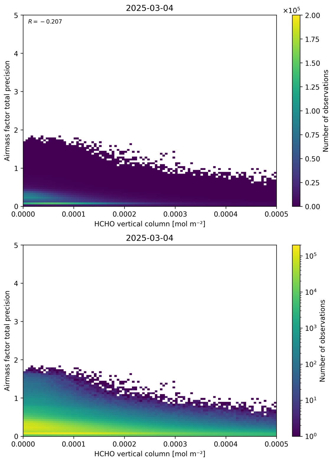
Figure 132: Scatter density plot of “HCHO vertical column” against “Airmass factor total precision” for 2025-03-03 to 2025-03-05.
