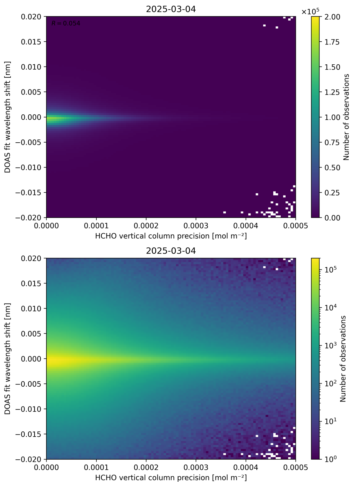
Figure 137: Scatter density plot of “HCHO vertical column precision” against “DOAS fit wavelength shift” for 2025-03-03 to 2025-03-05.
