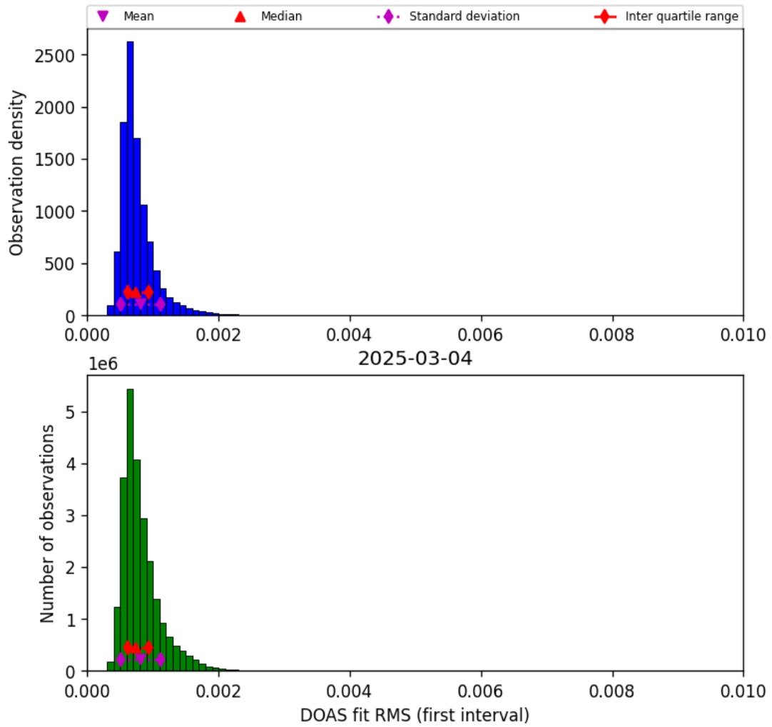
Figure 46: Histogram of “DOAS fit RMS (first interval)” for 2025-03-03 to 2025-03-05
