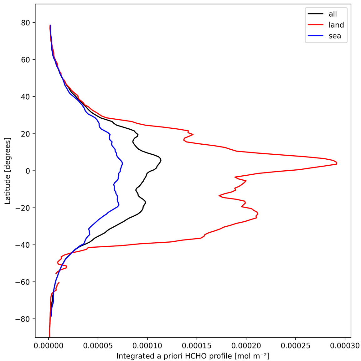
Figure 29: Zonal average of “Integrated a priori HCHO profile” for 2025-03-03 to 2025-03-05.
