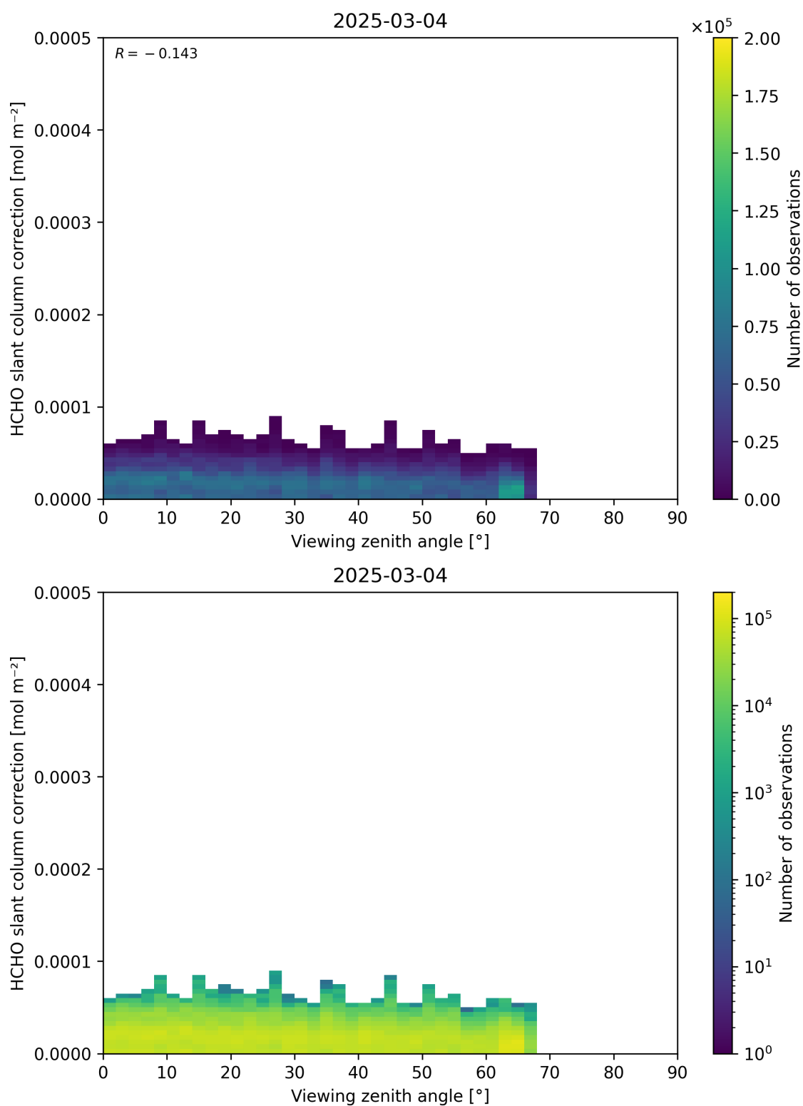
Figure 187: Scatter density plot of “Viewing zenith angle” against “HCHO slant column correction” for 2025-03-03 to 2025-03-05.
