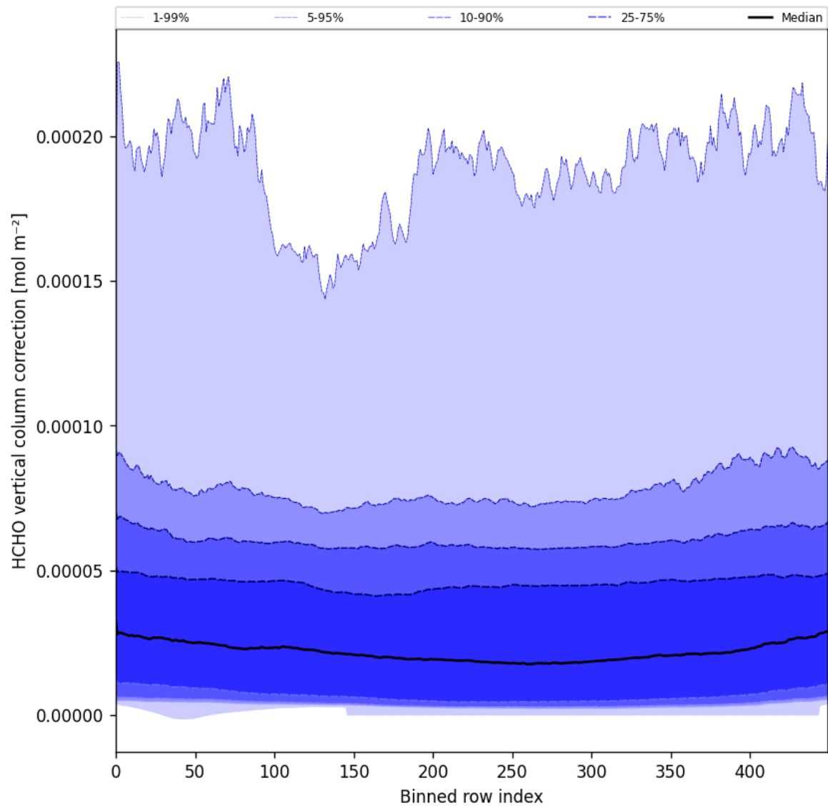
Figure 51: Along track statistics of “HCHO vertical column correction” for 2025-03-03 to 2025-03-05
