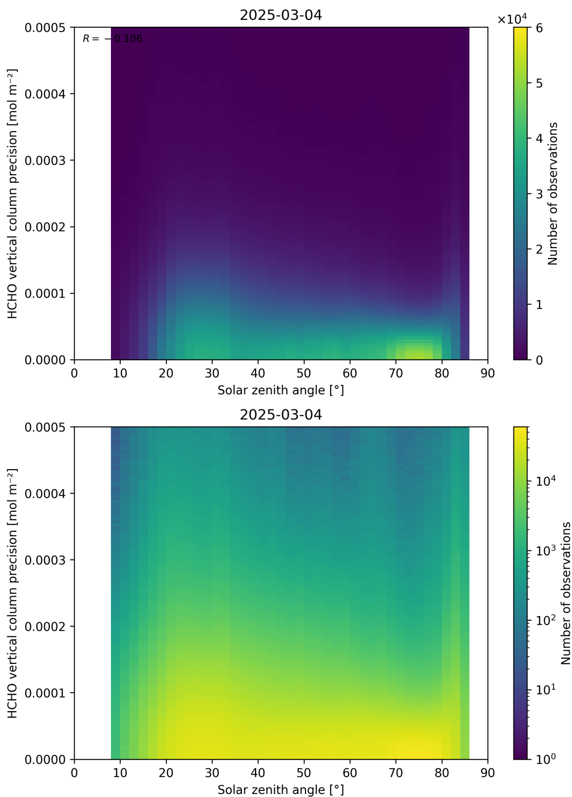
Figure 179: Scatter density plot of “Solar zenith angle” against “HCHO vertical column precision” for 2025-03-03 to 2025-03-05.
