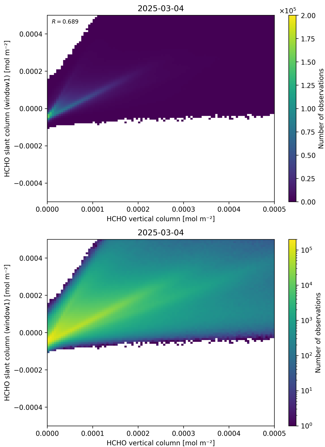
Figure 129: Scatter density plot of “HCHO vertical column” against “HCHO slant column (window1)” for 2025-03-03 to 2025-03-05.
