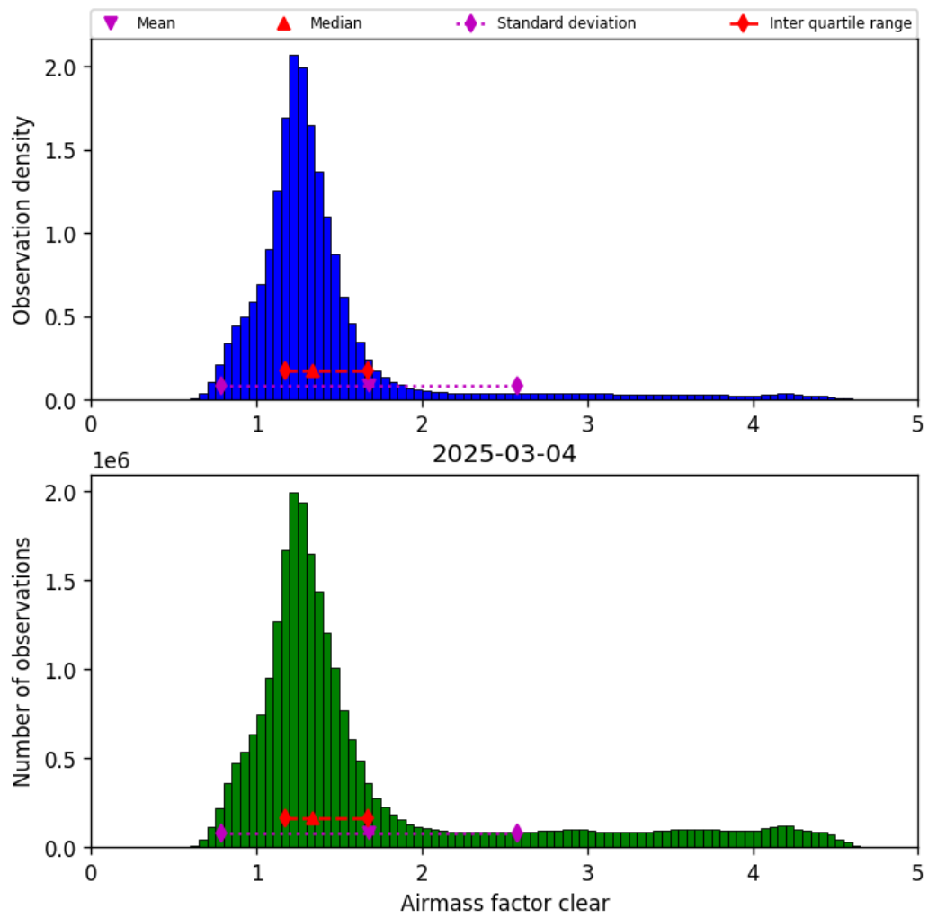
Figure 42: Histogram of “Airmass factor clear” for 2025-03-03 to 2025-03-05
