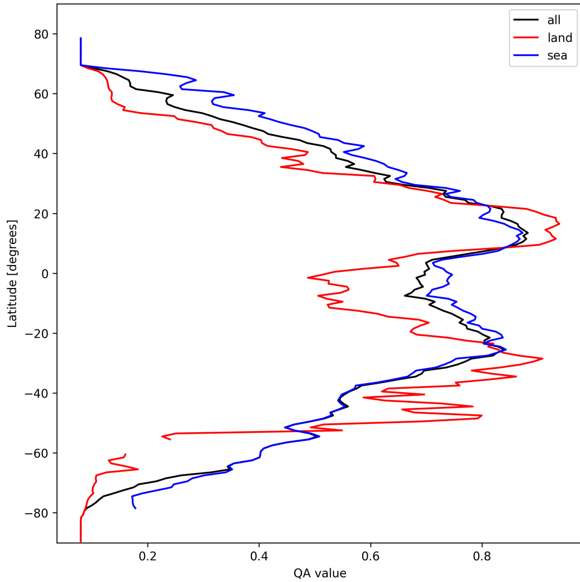
Figure 20: Zonal average of “QA value” for 2025-03-03 to 2025-03-05.
