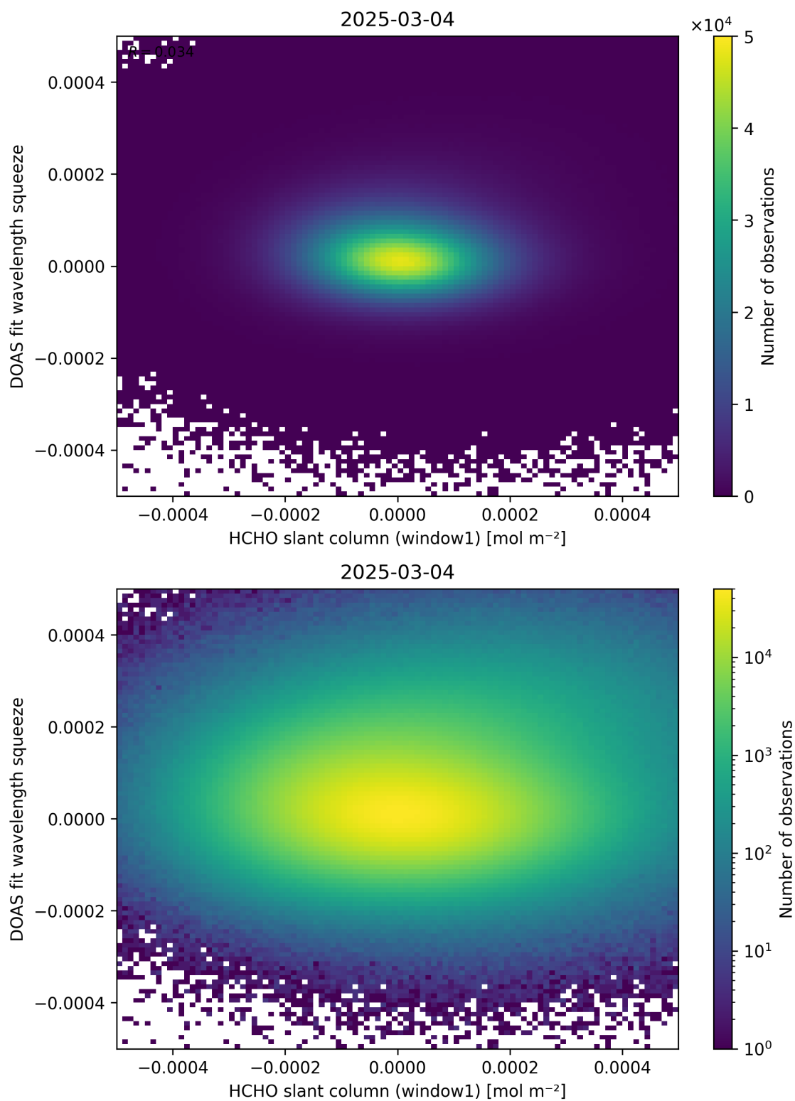
Figure 80: Scatter density plot of “HCHO slant column (window1)” against “DOAS fit wavelength squeeze” for 2025-03-03 to 2025-03-05.
