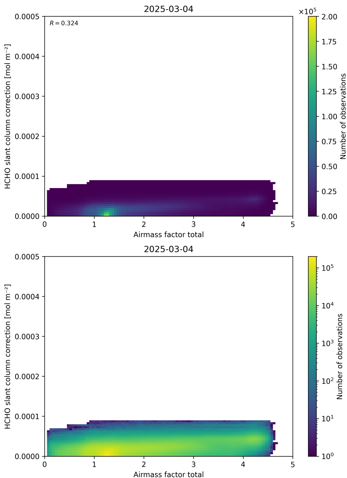
Figure 102: Scatter density plot of “Airmass factor total” against “HCHO slant column correction” for 2025-03-03 to 2025-03-05.
