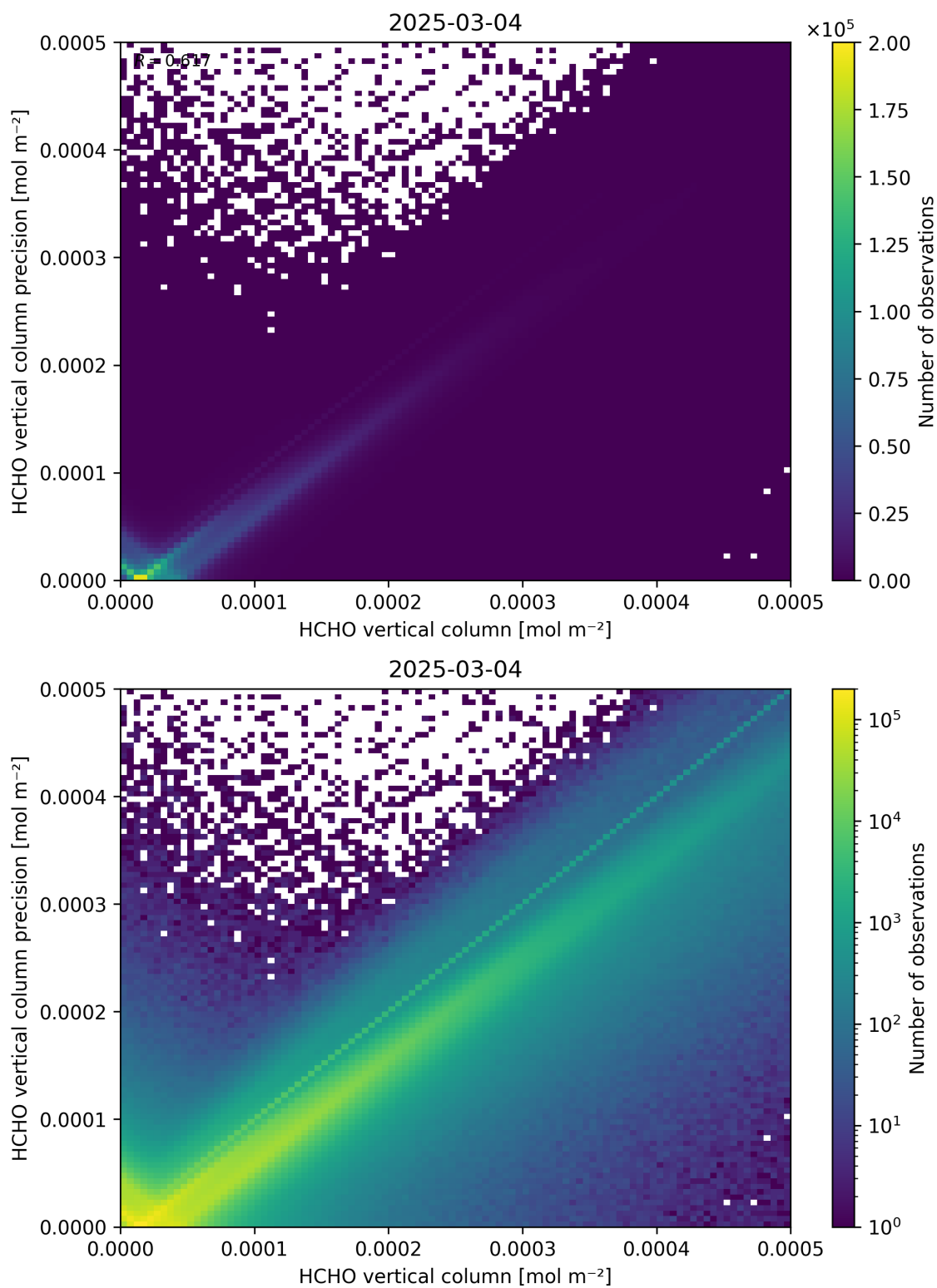
Figure 134: Scatter density plot of “HCHO vertical column” against “HCHO vertical column precision” for 2025-03-03 to 2025-03-05.
