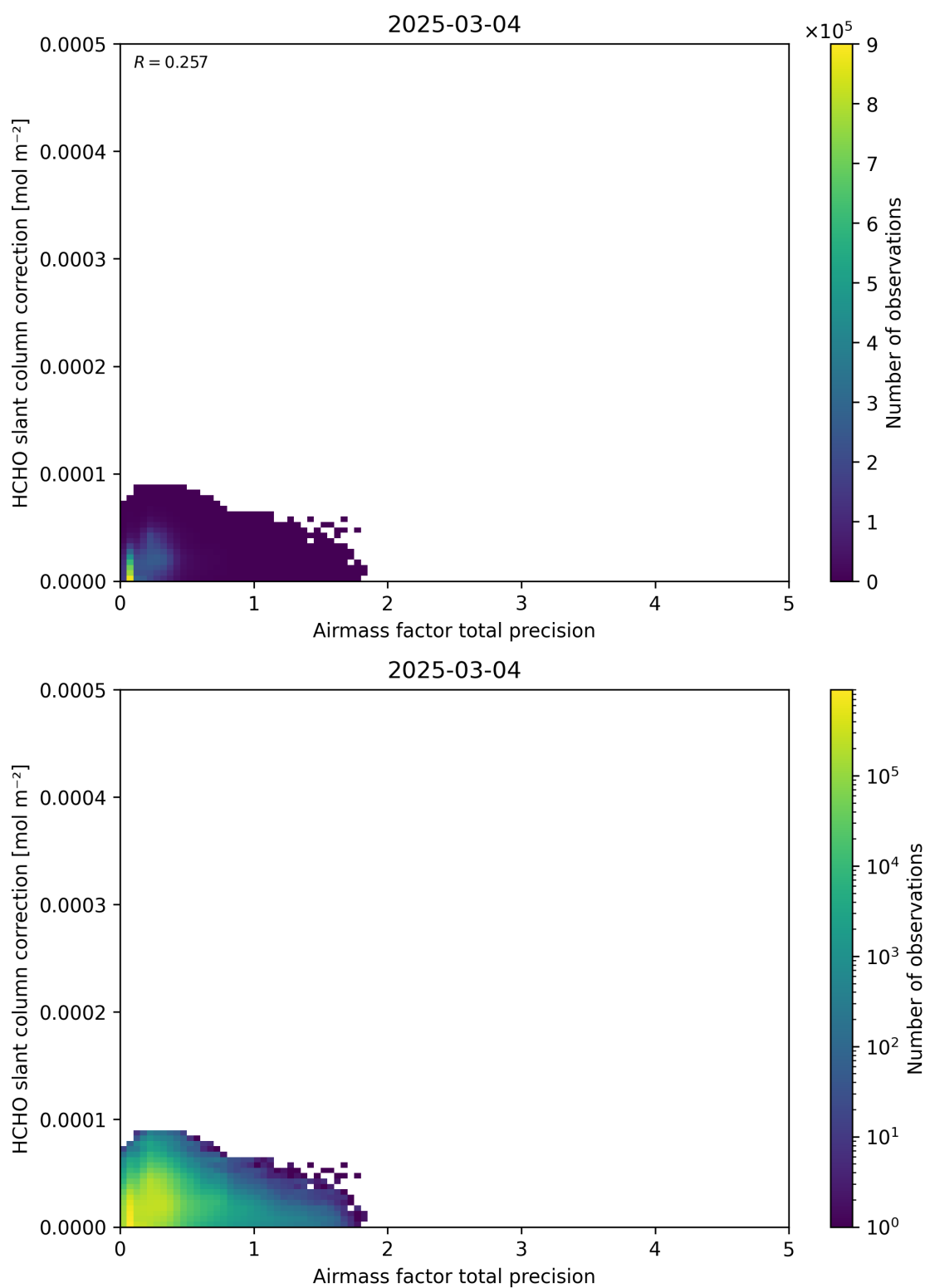
Figure 110: Scatter density plot of “Airmass factor total precision” against “HCHO slant column correction” for 2025-03-03 to 2025-03-05.
