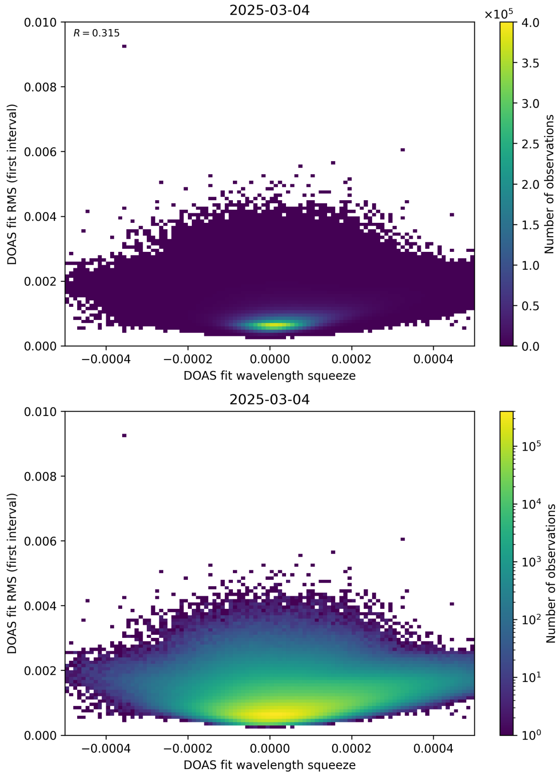
Figure 68: Scatter density plot of “DOAS fit wavelength squeeze” against “DOAS fit RMS (first interval)” for 2025-03-03 to 2025-03-05.
