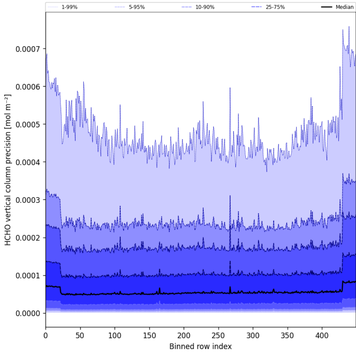
Figure 50: Along track statistics of “HCHO vertical column precision” for 2025-03-03 to 2025-03-05
