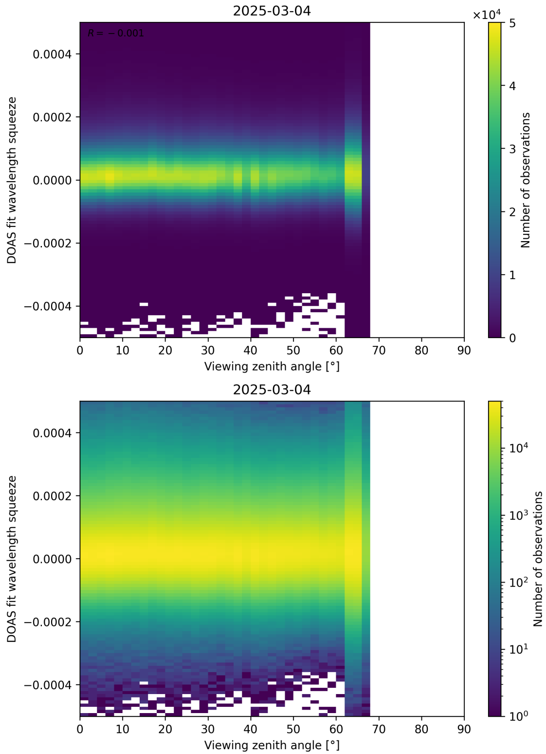
Figure 184: Scatter density plot of “Viewing zenith angle” against “DOAS fit wavelength squeeze” for 2025-03-03 to 2025-03-05.
