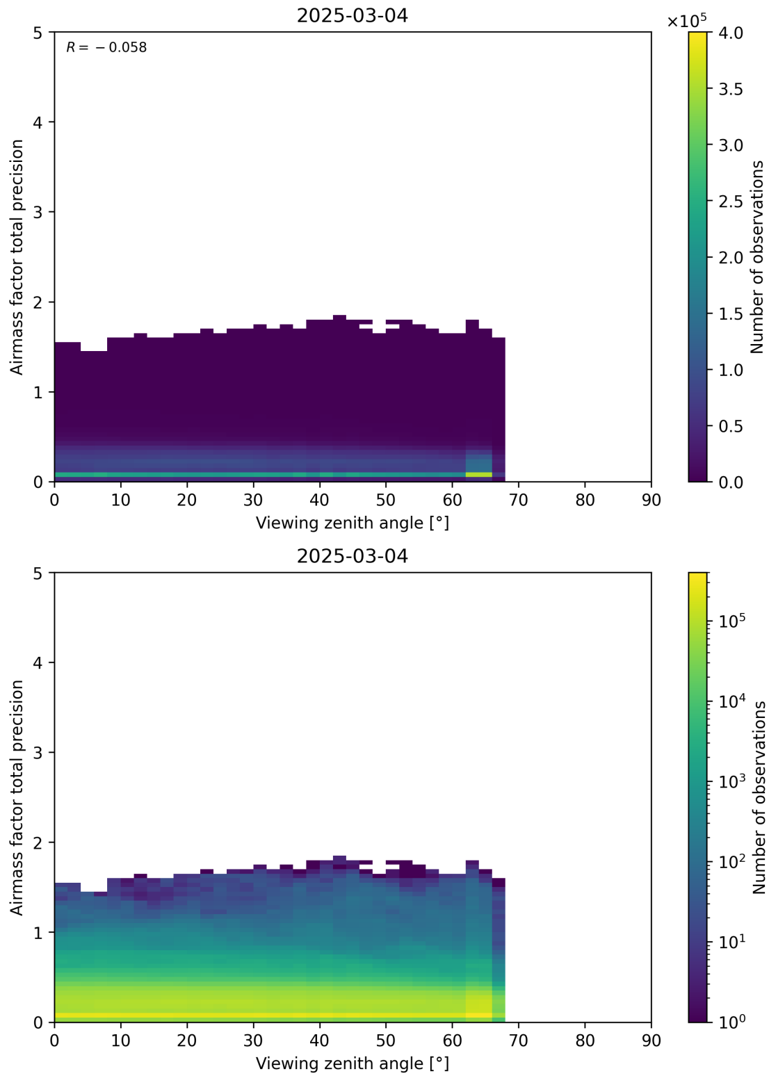
Figure 191: Scatter density plot of “Viewing zenith angle” against “Airmass factor total precision” for 2025-03-03 to 2025-03-05.
