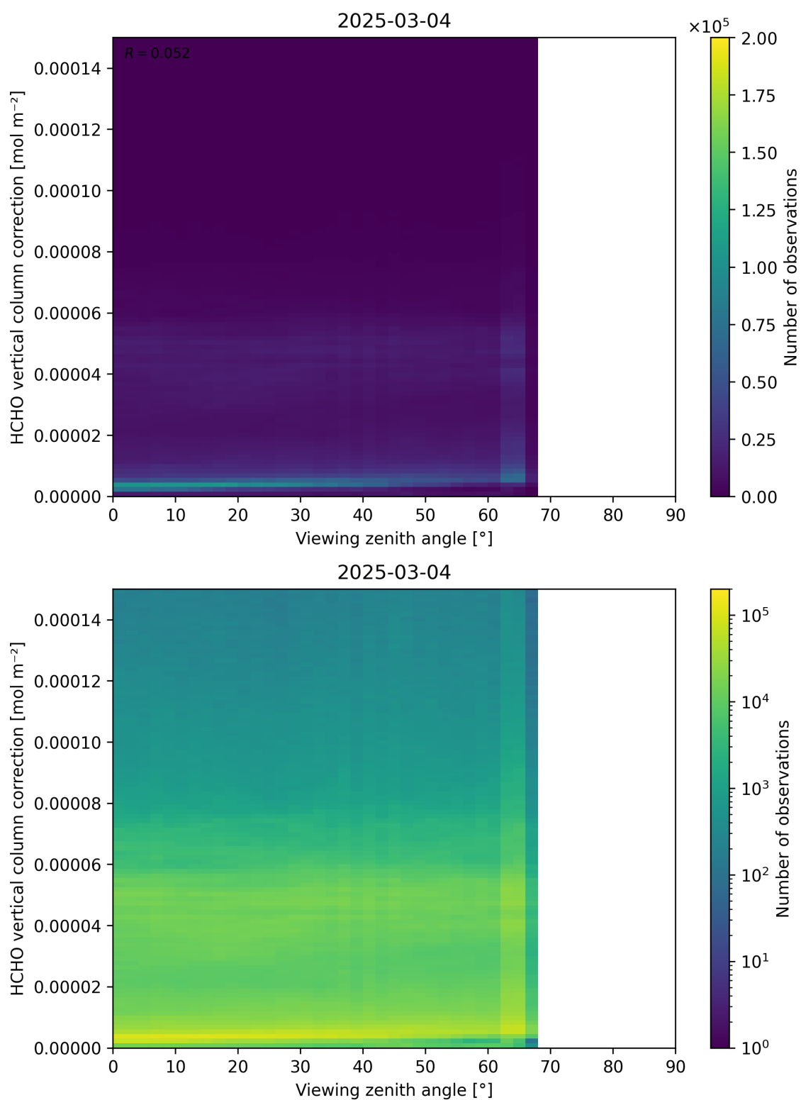
Figure 193: Scatter density plot of “Viewing zenith angle” against “HCHO vertical column correction” for 2025-03-03 to 2025-03-05.
