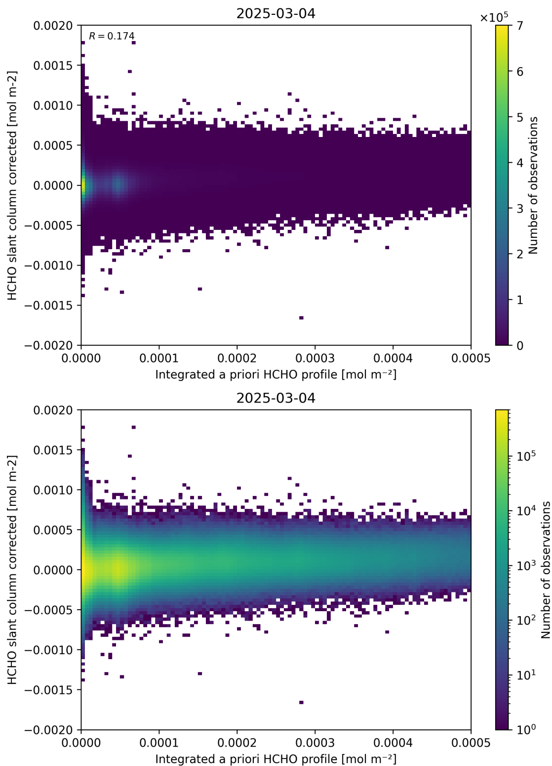
Figure 151: Scatter density plot of “Integrated a priori HCHO profile” against “HCHO slant column corrected” for 2025-03-03 to 2025-03-05.
