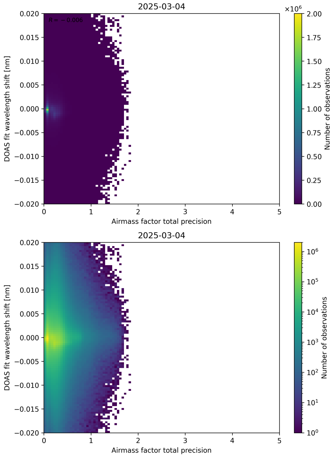
Figure 106: Scatter density plot of “Airmass factor total precision” against “DOAS fit wavelength shift” for 2025-03-03 to 2025-03-05.
