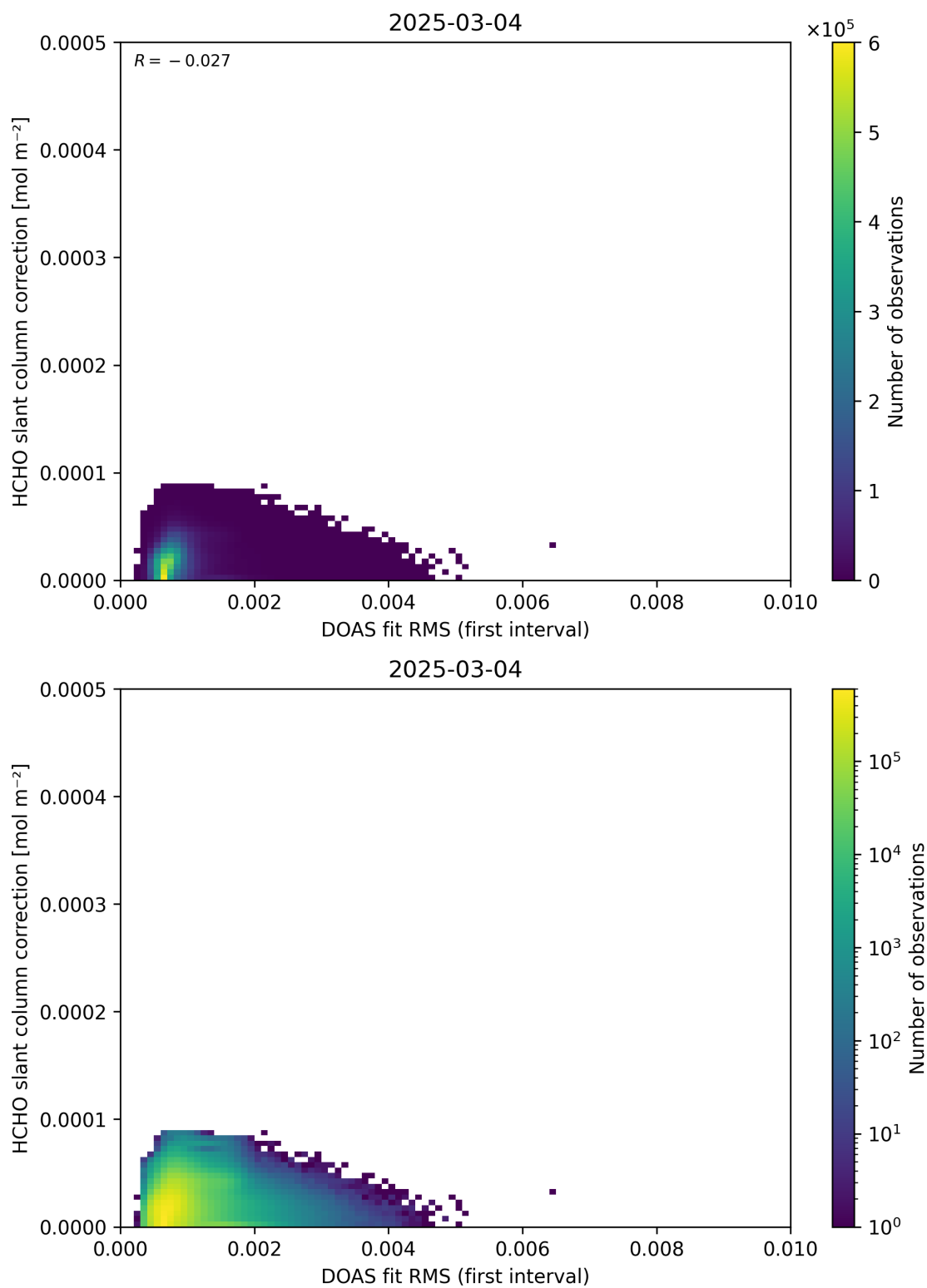
Figure 63: Scatter density plot of “DOAS fit RMS (first interval)” against “HCHO slant column correction” for 2025-03-03 to 2025-03-05.
