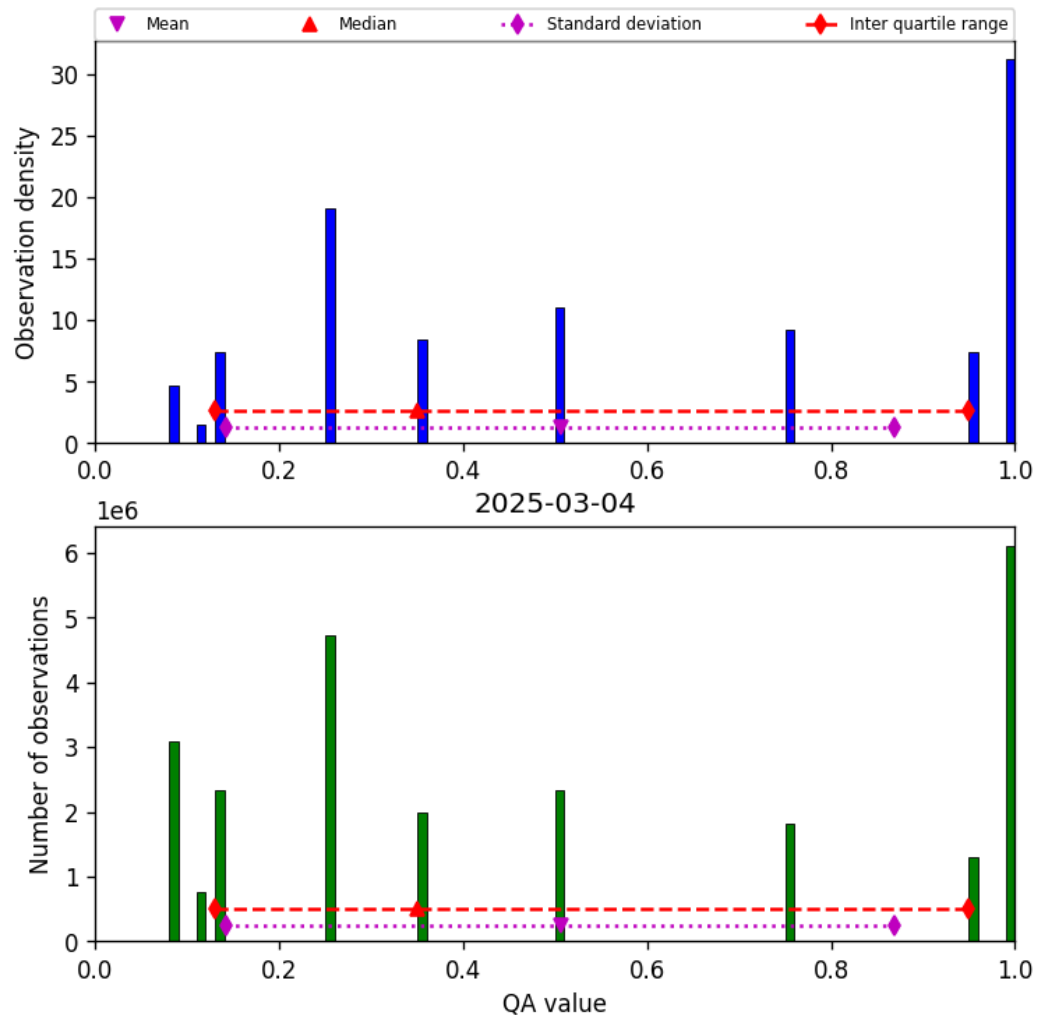
Figure 34: Histogram of “QA value” for 2025-03-03 to 2025-03-05
