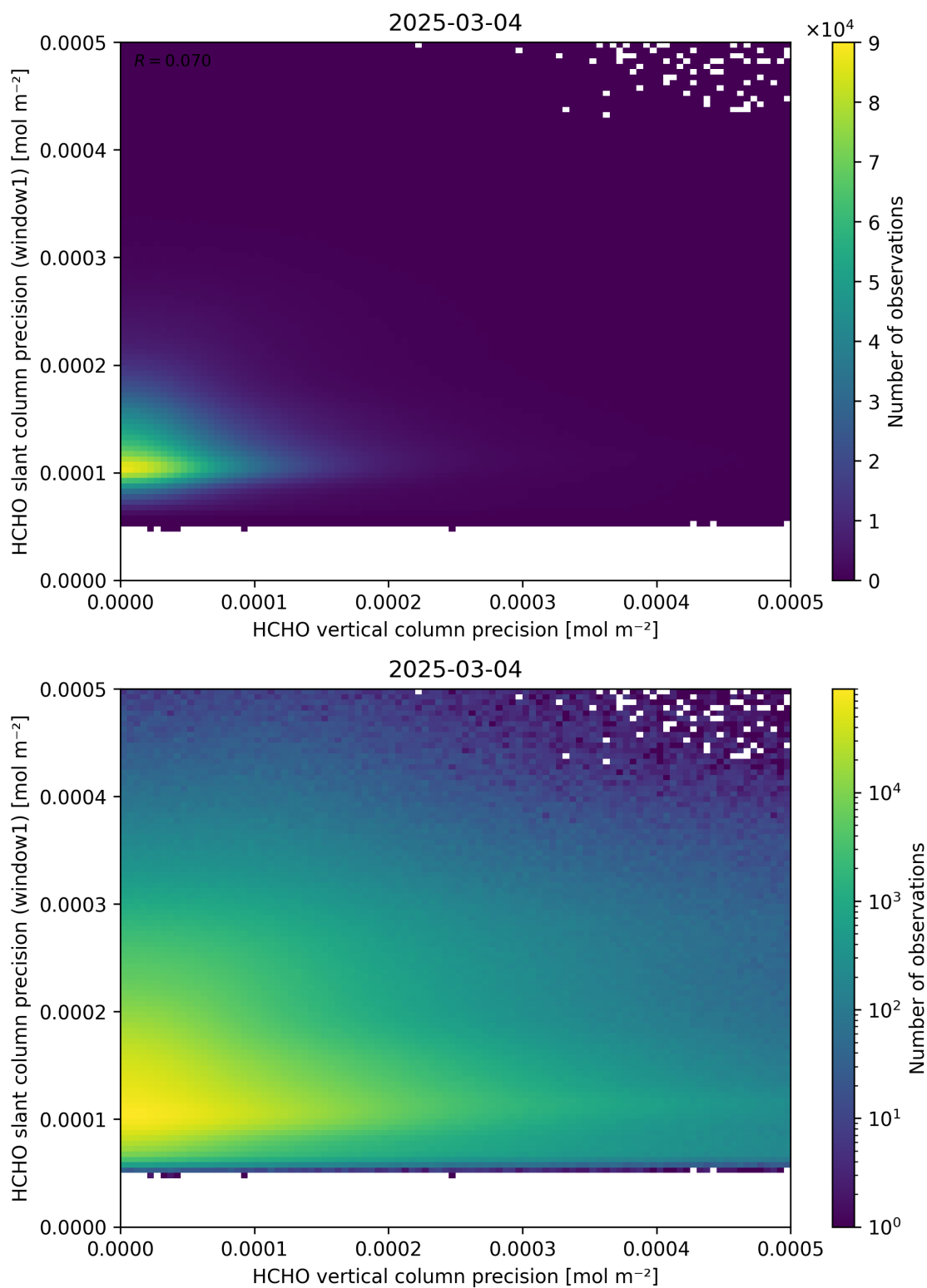
Figure 143: Scatter density plot of “HCHO vertical column precision” against “HCHO slant column precision (window1)” for 2025-03-03 to 2025-03-05.
