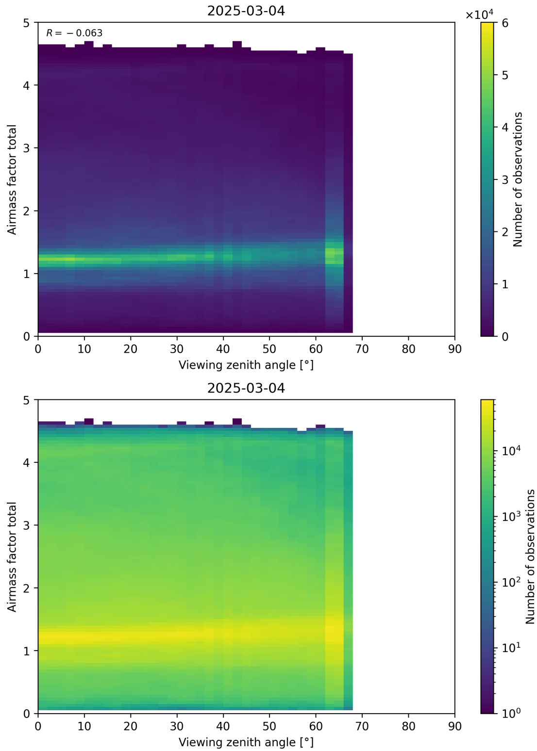
Figure 190: Scatter density plot of “Viewing zenith angle” against “Airmass factor total” for 2025-03-03 to 2025-03-05.
