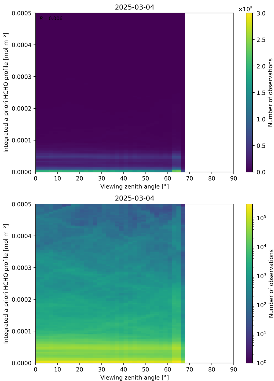
Figure 195: Scatter density plot of “Viewing zenith angle” against “Integrated a priori HCHO profile” for 2025-03-03 to 2025-03-05.
