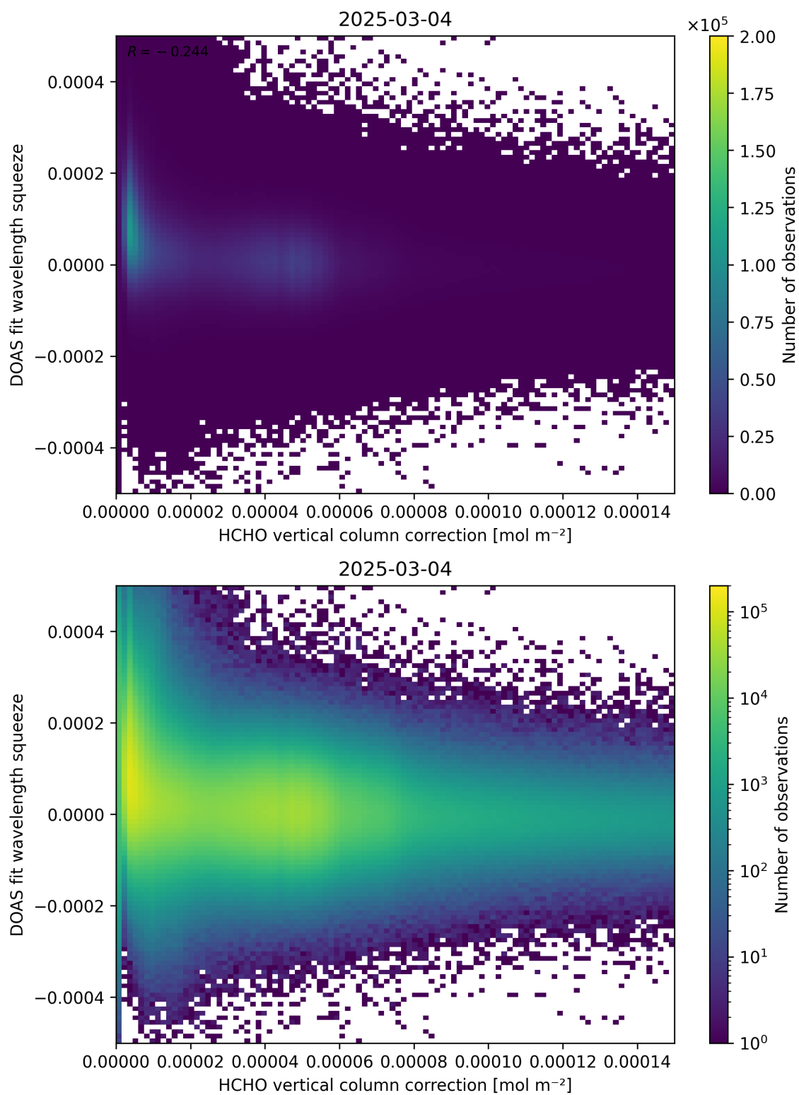
Figure 114: Scatter density plot of “HCHO vertical column correction” against “DOAS fit wavelength squeeze” for 2025-03-03 to 2025-03-05.
