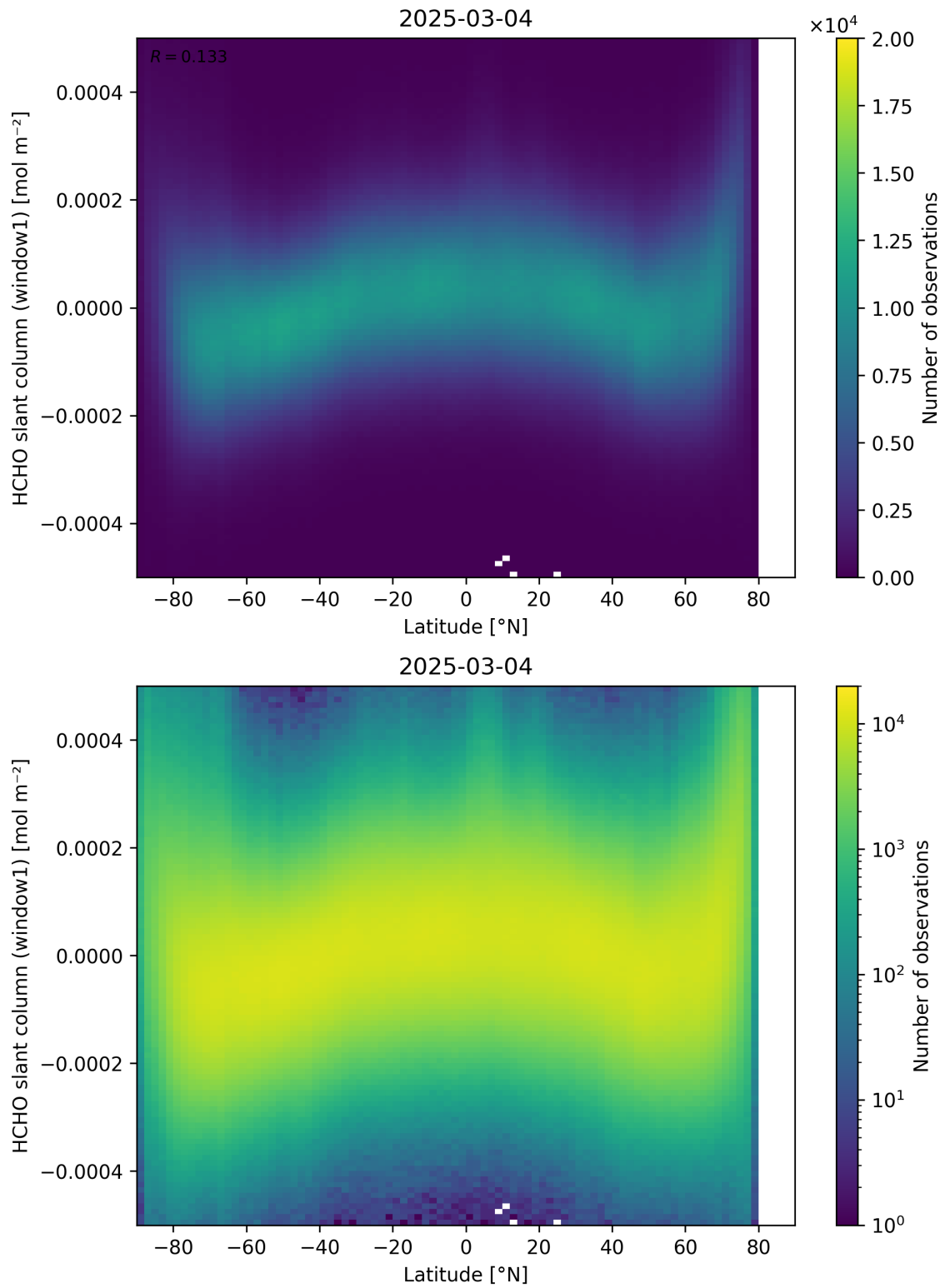
Figure 159: Scatter density plot of “Latitude” against “HCHO slant column (window1)” for 2025-03-03 to 2025-03-05.
