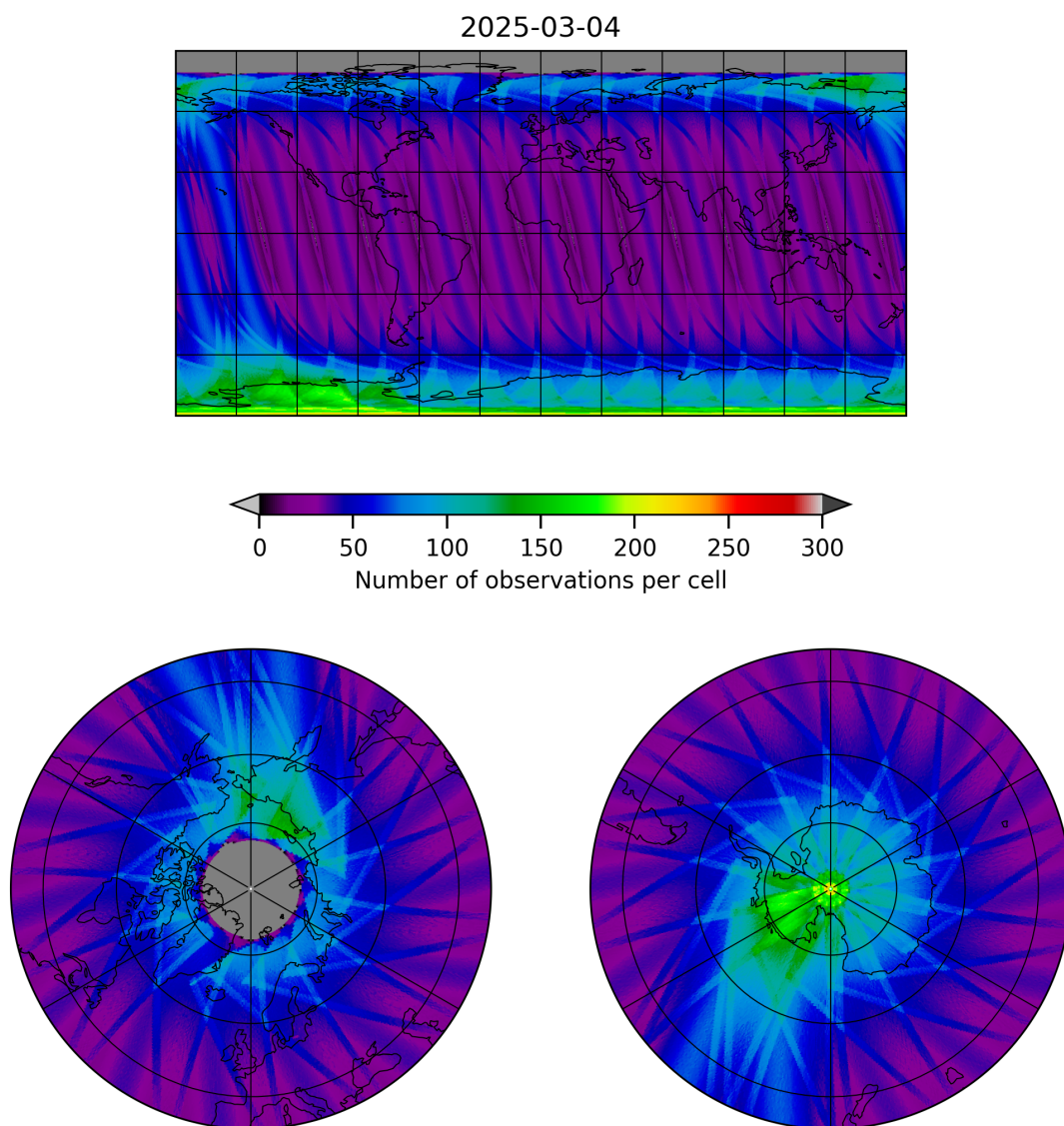
Figure 19: Map of the number of observations for 2025-03-03 to 2025-03-05
