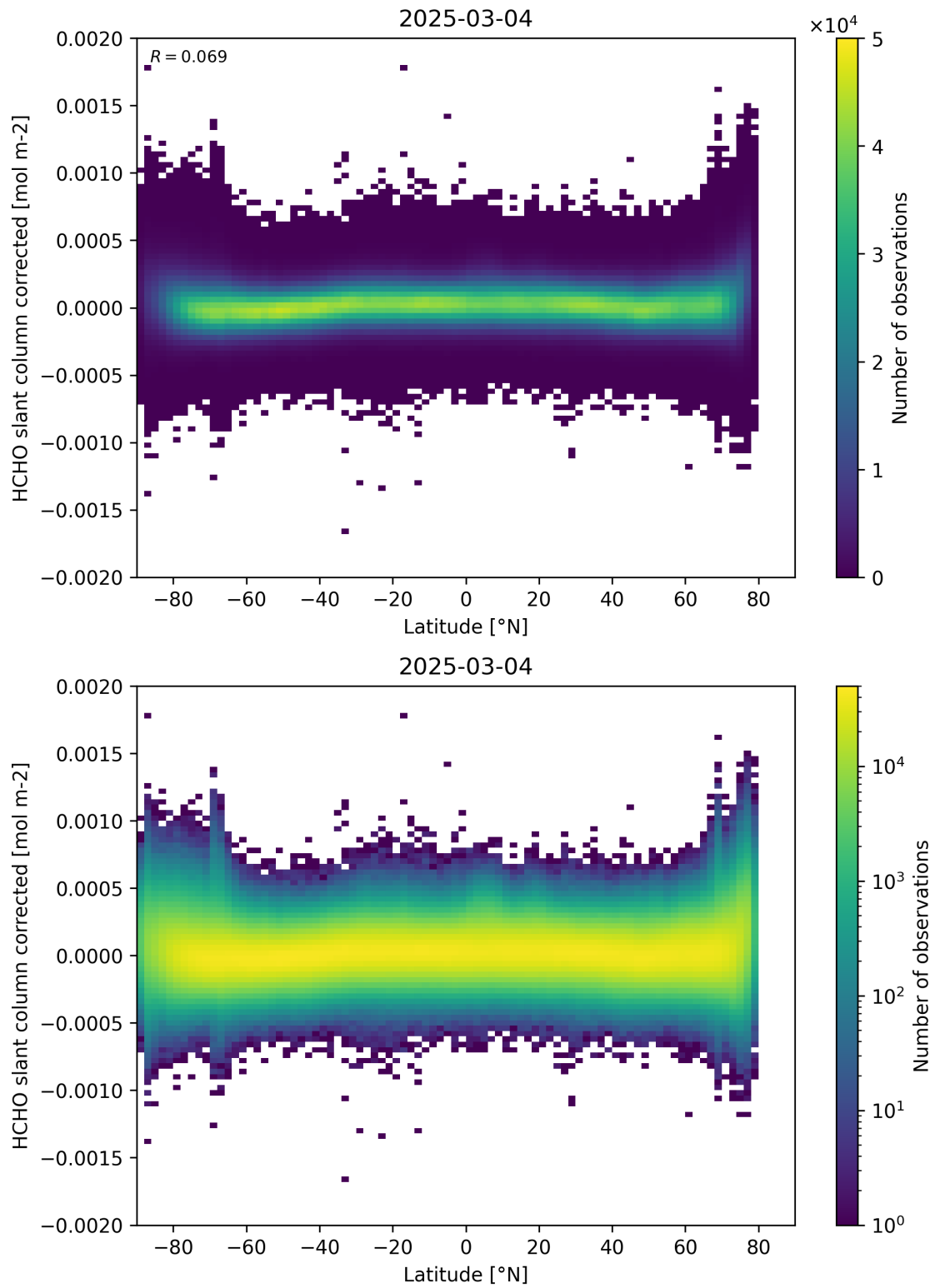
Figure 157: Scatter density plot of “Latitude” against “HCHO slant column corrected” for 2025-03-03 to 2025-03-05.
