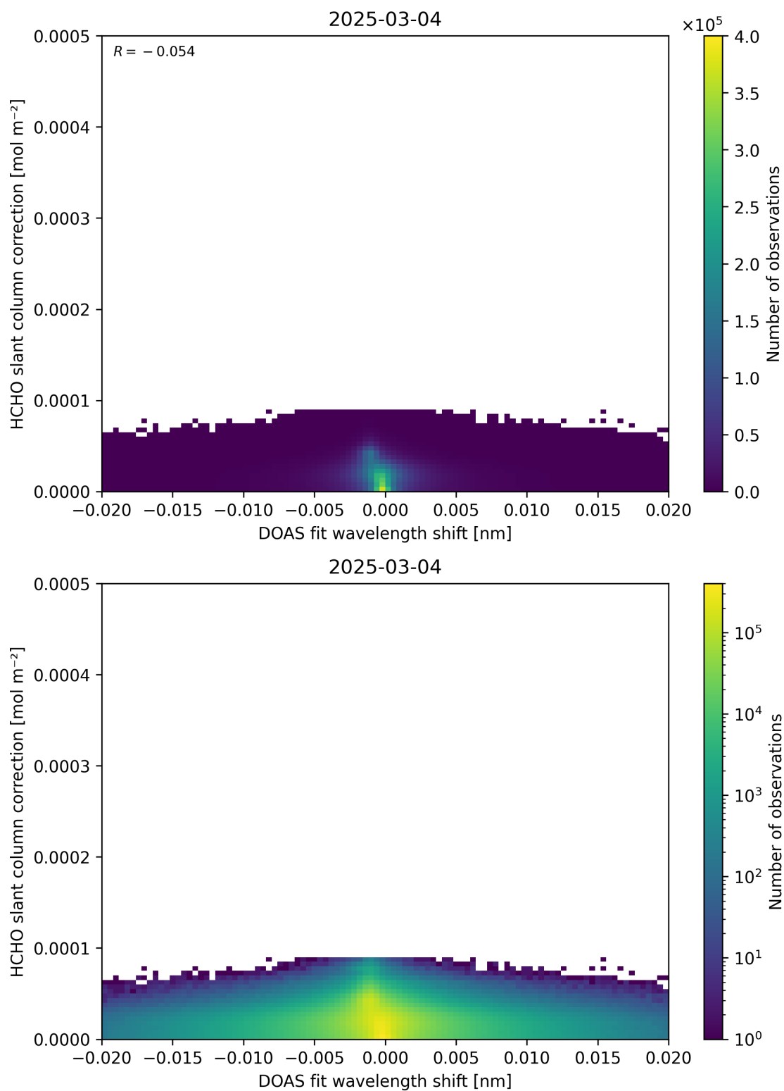
Figure 67: Scatter density plot of “DOAS fit wavelength shift” against “HCHO slant column correction” for 2025-03-03 to 2025-03-05.
