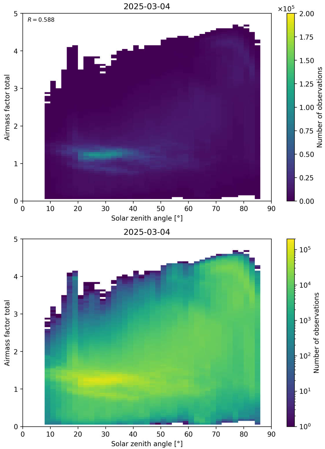
Figure 175: Scatter density plot of “Solar zenith angle” against “Airmass factor total” for 2025-03-03 to 2025-03-05.
