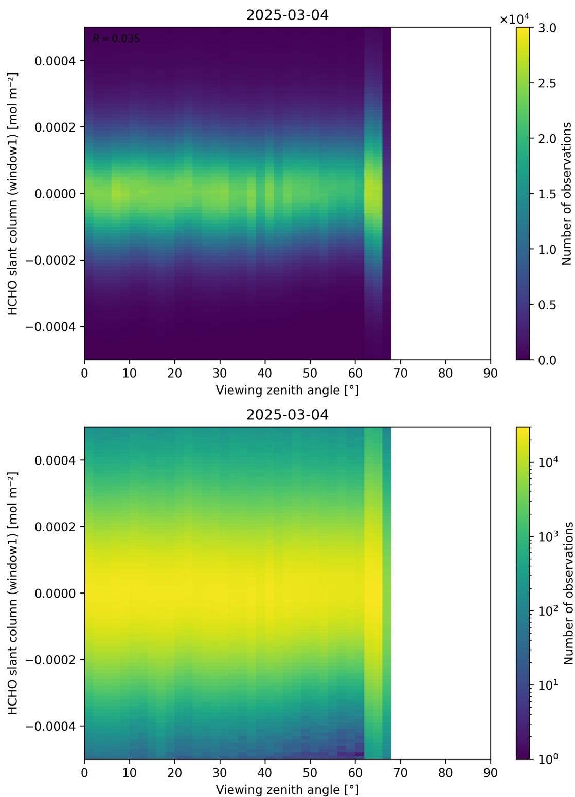
Figure 188: Scatter density plot of “Viewing zenith angle” against “HCHO slant column (window1)” for 2025-03-03 to 2025-03-05.
