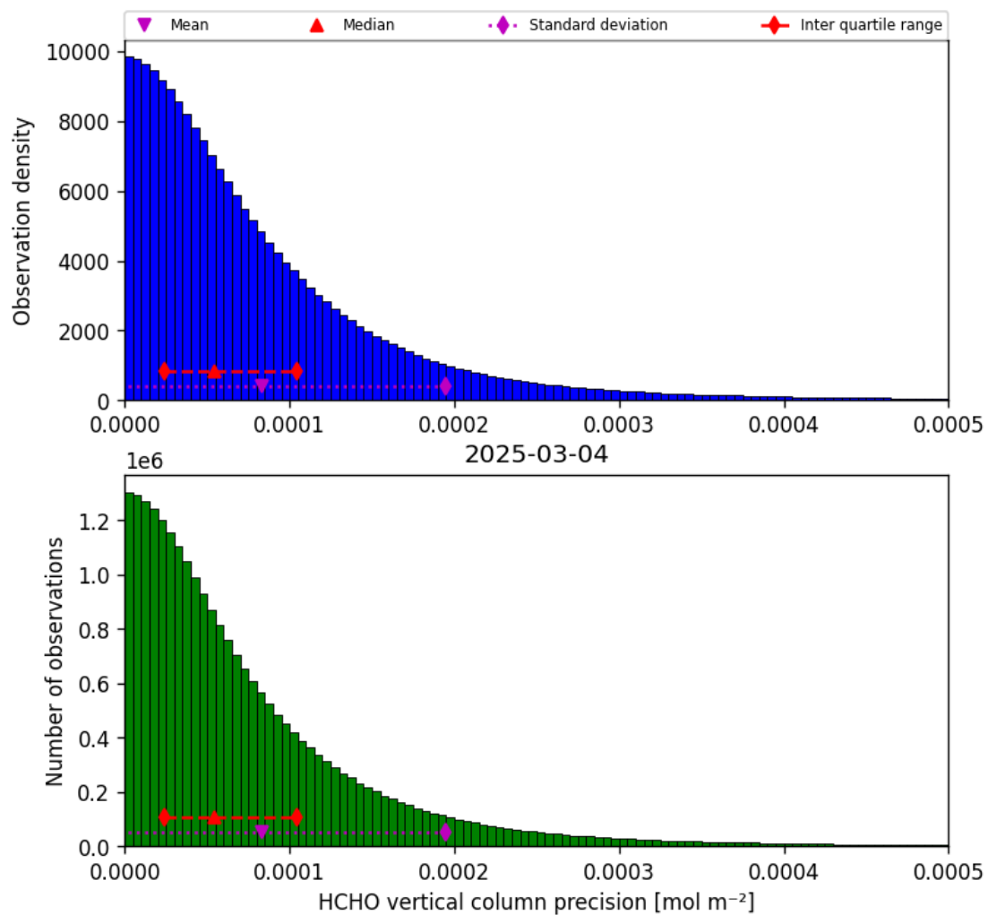
Figure 36: Histogram of “HCHO vertical column precision” for 2025-03-03 to 2025-03-05
