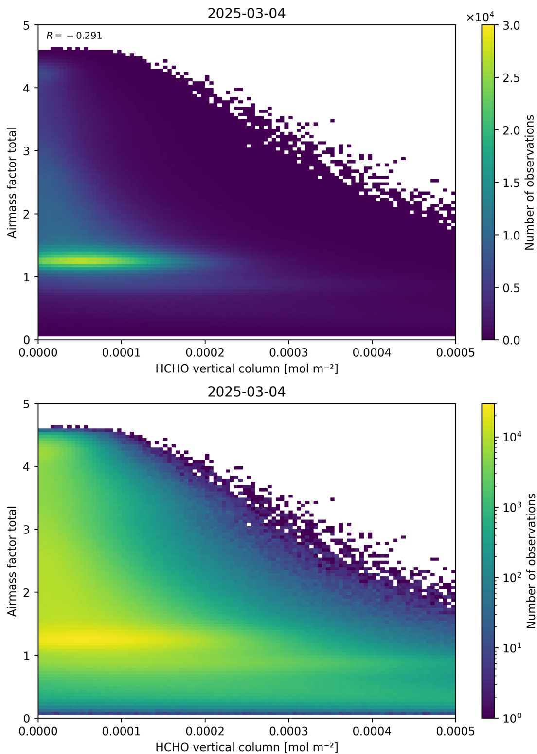
Figure 131: Scatter density plot of “HCHO vertical column” against “Airmass factor total” for 2025-03-03 to 2025-03-05.
