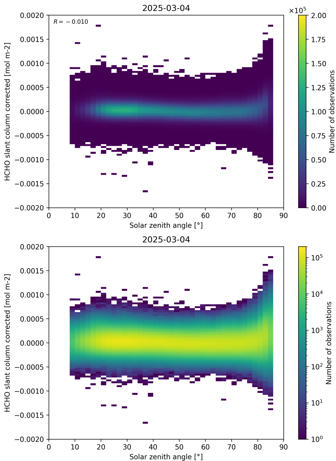
Figure 171: Scatter density plot of “Solar zenith angle” against “HCHO slant column corrected” for 2025-03-03 to 2025-03-05.
