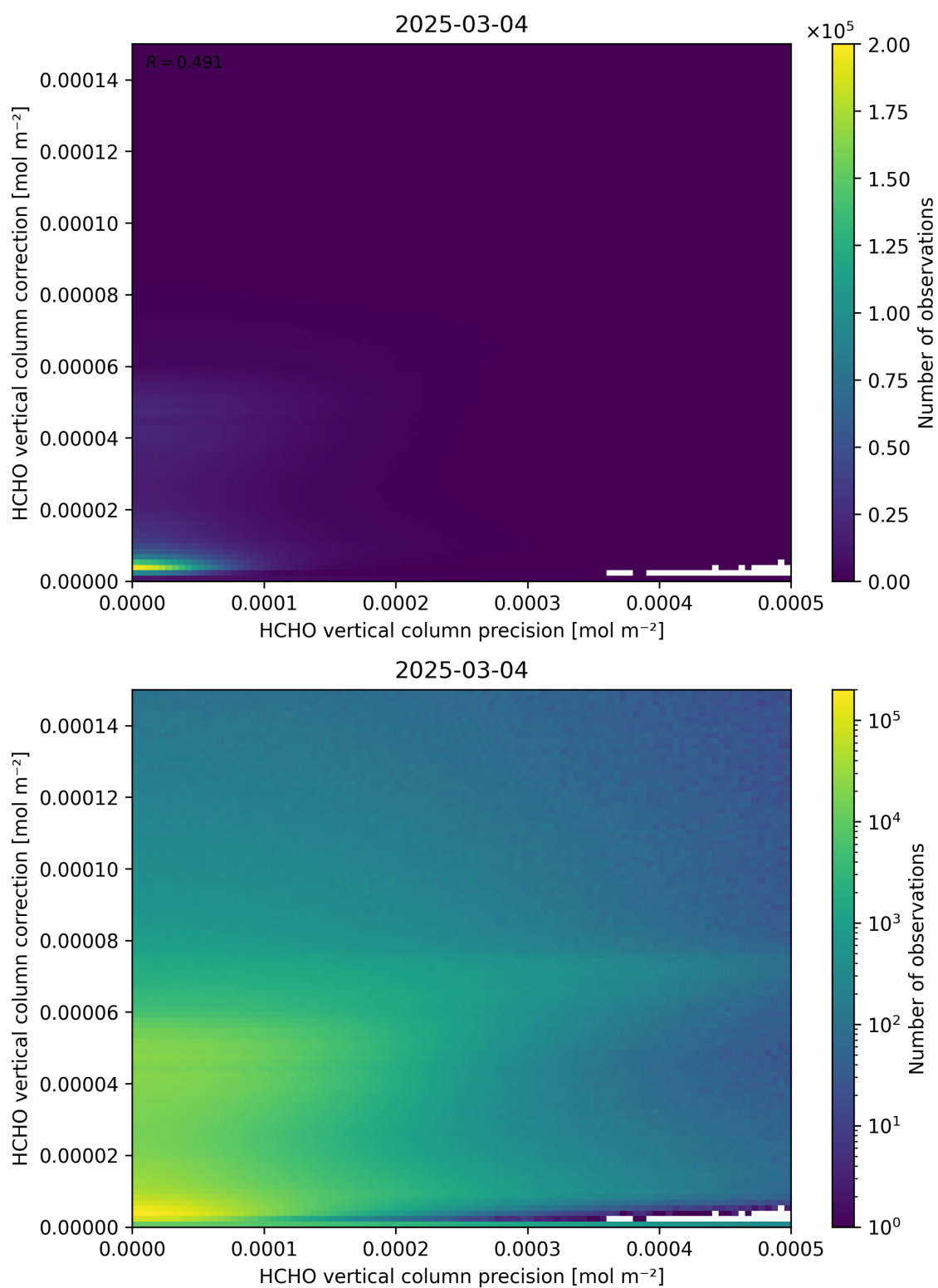
Figure 146: Scatter density plot of “HCHO vertical column precision” against “HCHO vertical column correction” for 2025-03-03 to 2025-03-05.
