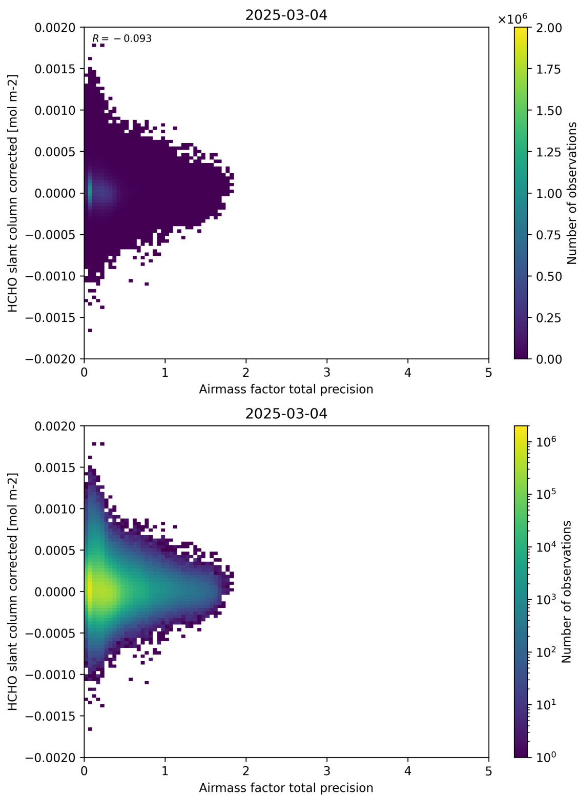
Figure 109: Scatter density plot of “Airmass factor total precision” against “HCHO slant column corrected” for 2025-03-03 to 2025-03-05.
