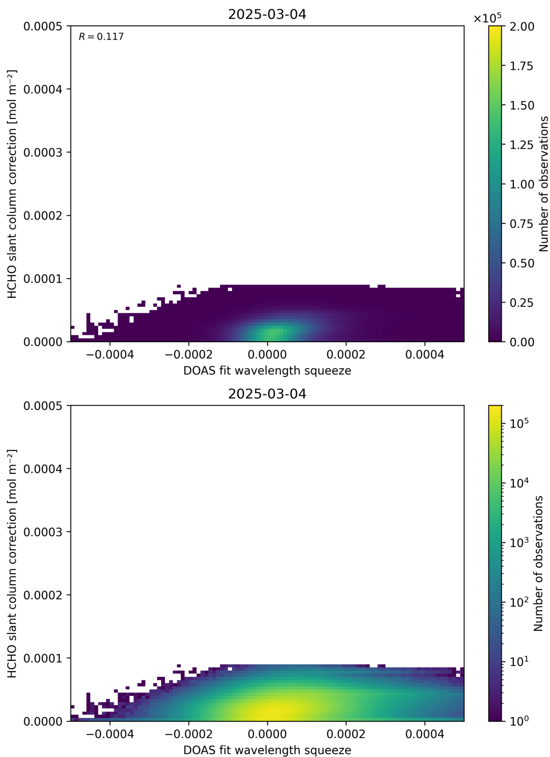
Figure 70: Scatter density plot of “DOAS fit wavelength squeeze” against “HCHO slant column correction” for 2025-03-03 to 2025-03-05.
