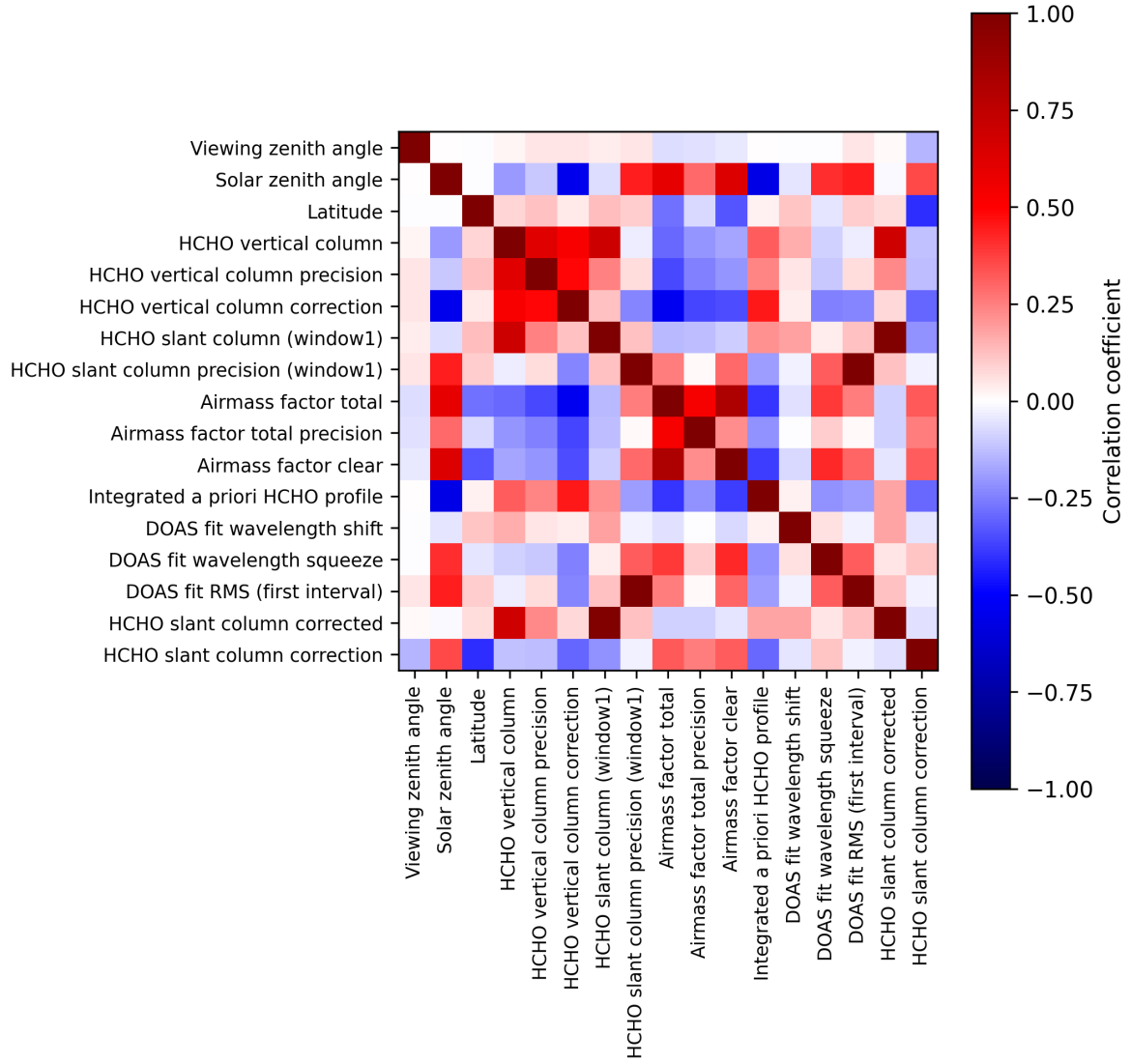
Figure 2: Map of correlation matrix for 2025-03-03 to 2025-03-05.
