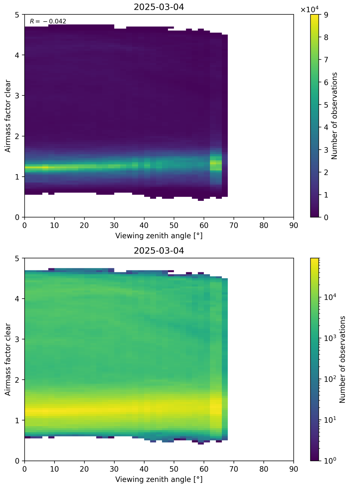
Figure 185: Scatter density plot of “Viewing zenith angle” against “Airmass factor clear” for 2025-03-03 to 2025-03-05.
