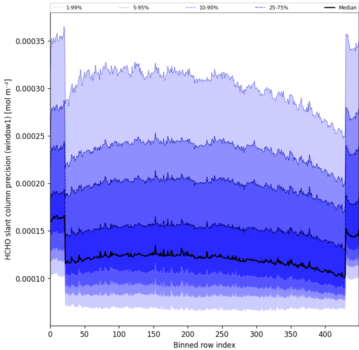
Figure 53: Along track statistics of “HCHO slant column precision (window1)” for 2025-03-03 to 2025-03-05
