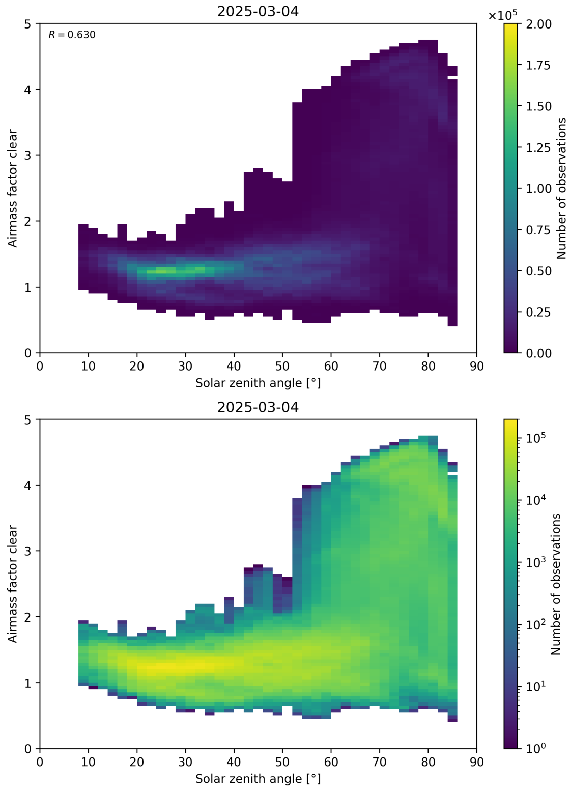
Figure 170: Scatter density plot of “Solar zenith angle” against “Airmass factor clear” for 2025-03-03 to 2025-03-05.
