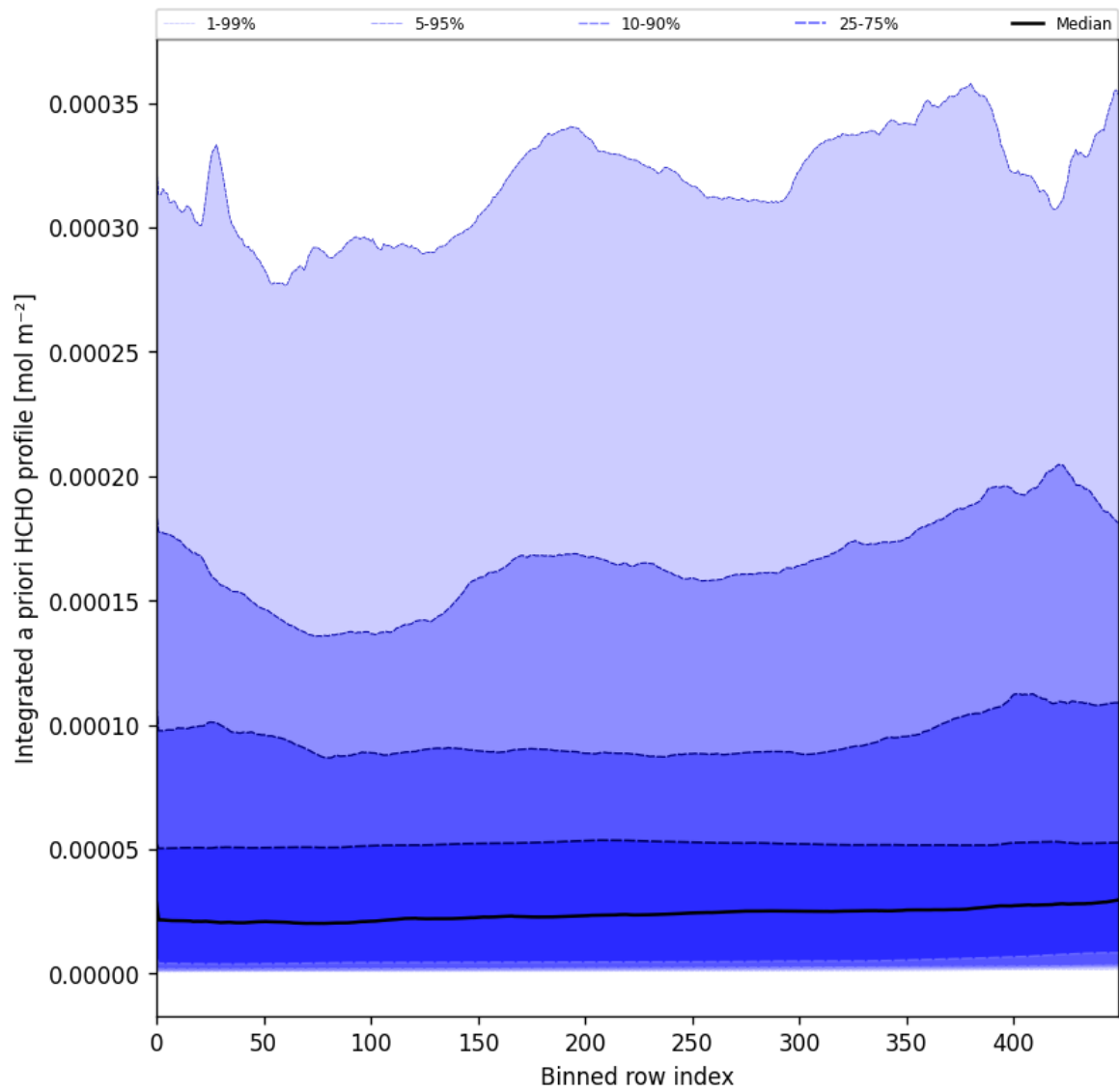
Figure 57: Along track statistics of “Integrated a priori HCHO profile” for 2025-03-03 to 2025-03-05
