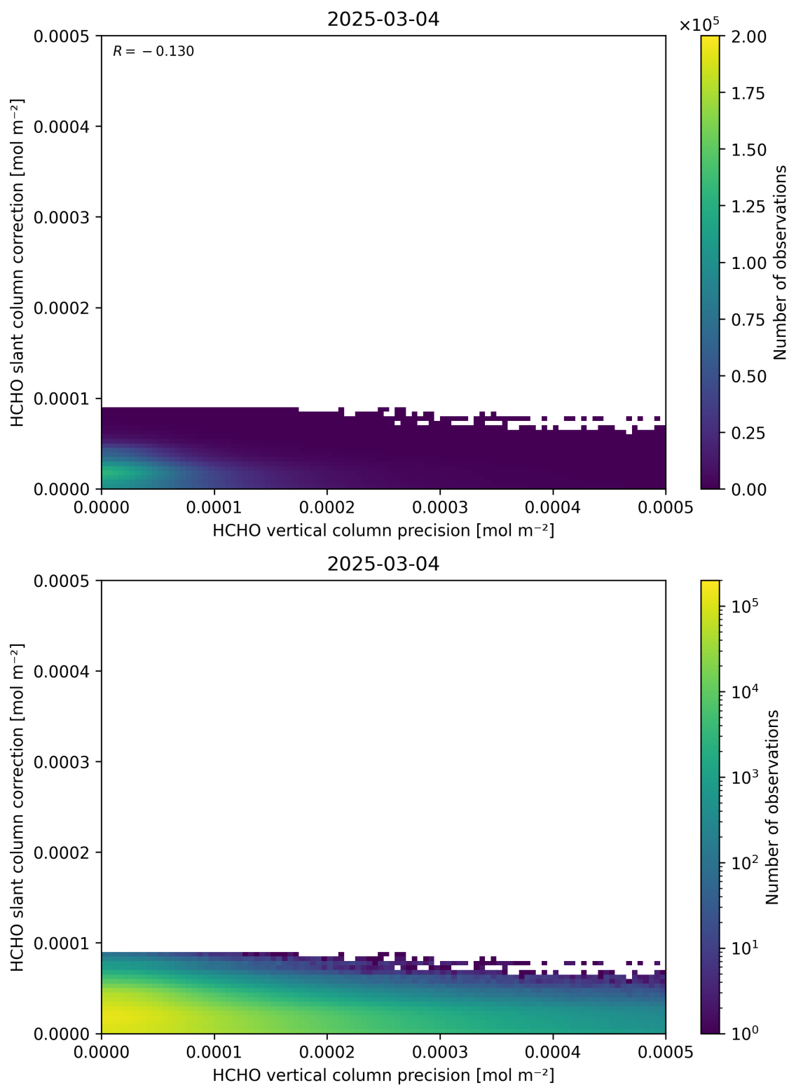
Figure 141: Scatter density plot of “HCHO vertical column precision” against “HCHO slant column correction” for 2025-03-03 to 2025-03-05.
