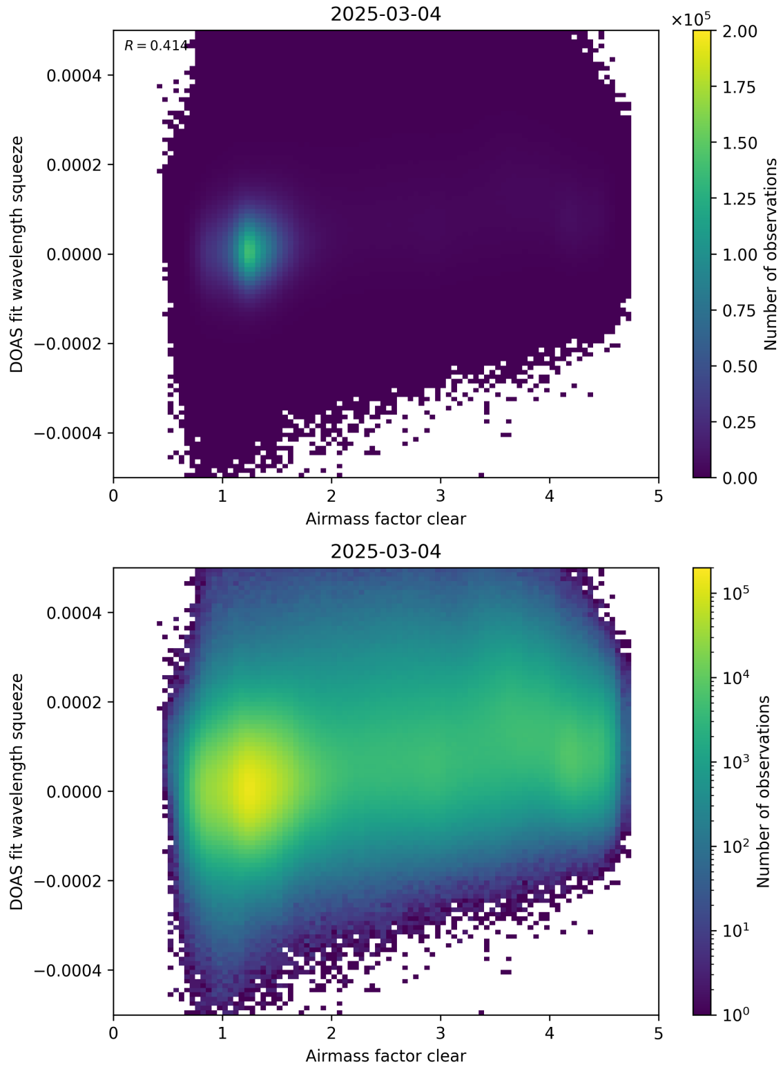
Figure 73: Scatter density plot of “Airmass factor clear” against “DOAS fit wavelength squeeze” for 2025-03-03 to 2025-03-05.
