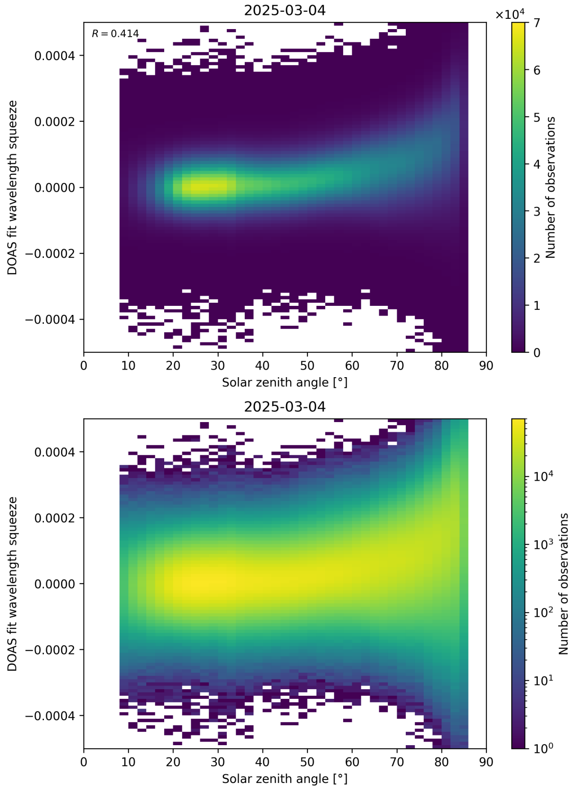
Figure 169: Scatter density plot of “Solar zenith angle” against “DOAS fit wavelength squeeze” for 2025-03-03 to 2025-03-05.
