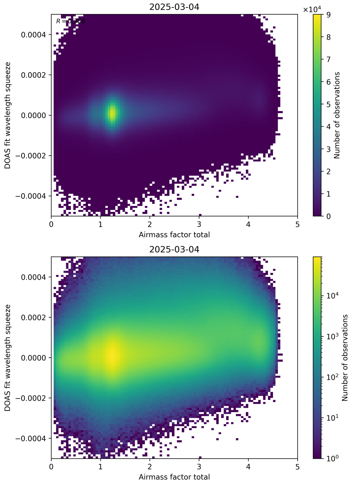
Figure 99: Scatter density plot of “Airmass factor total” against “DOAS fit wavelength squeeze” for 2025-03-03 to 2025-03-05.
