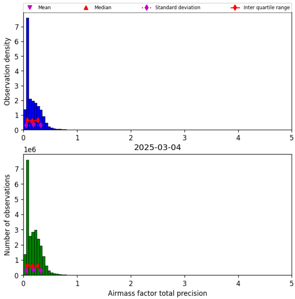
Figure 41: Histogram of “Airmass factor total precision” for 2025-03-03 to 2025-03-05
