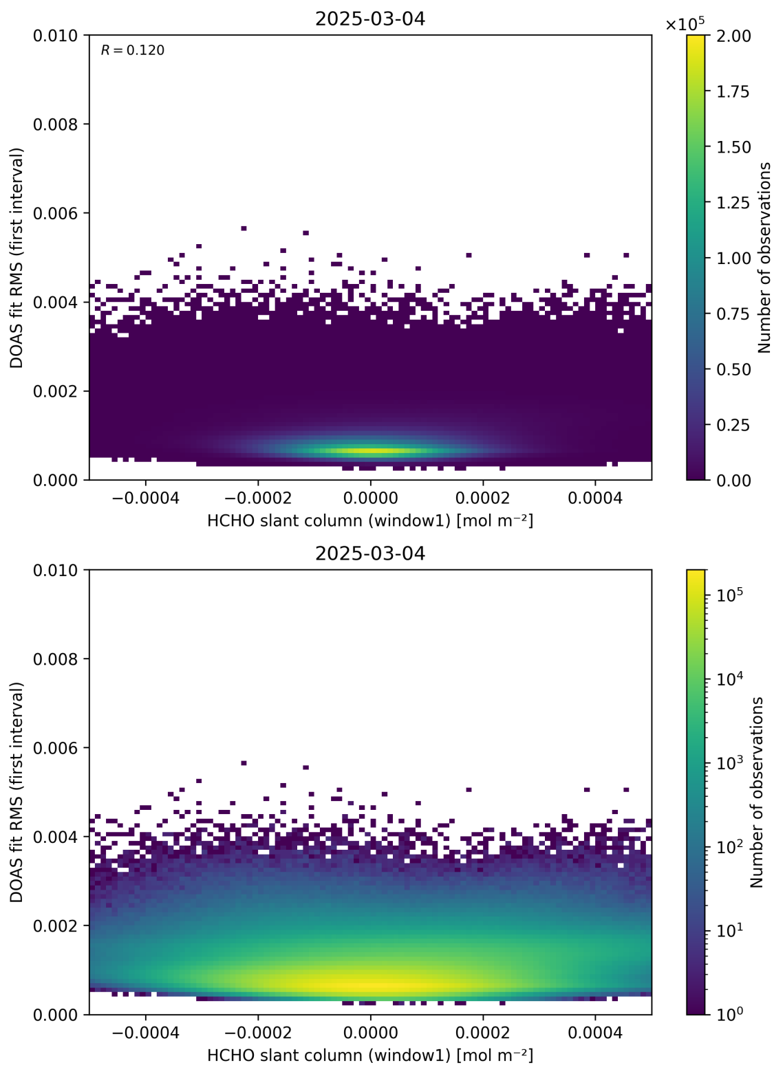
Figure 78: Scatter density plot of “HCHO slant column (window1)” against “DOAS fit RMS (first interval)” for 2025-03-03 to 2025-03-05.
