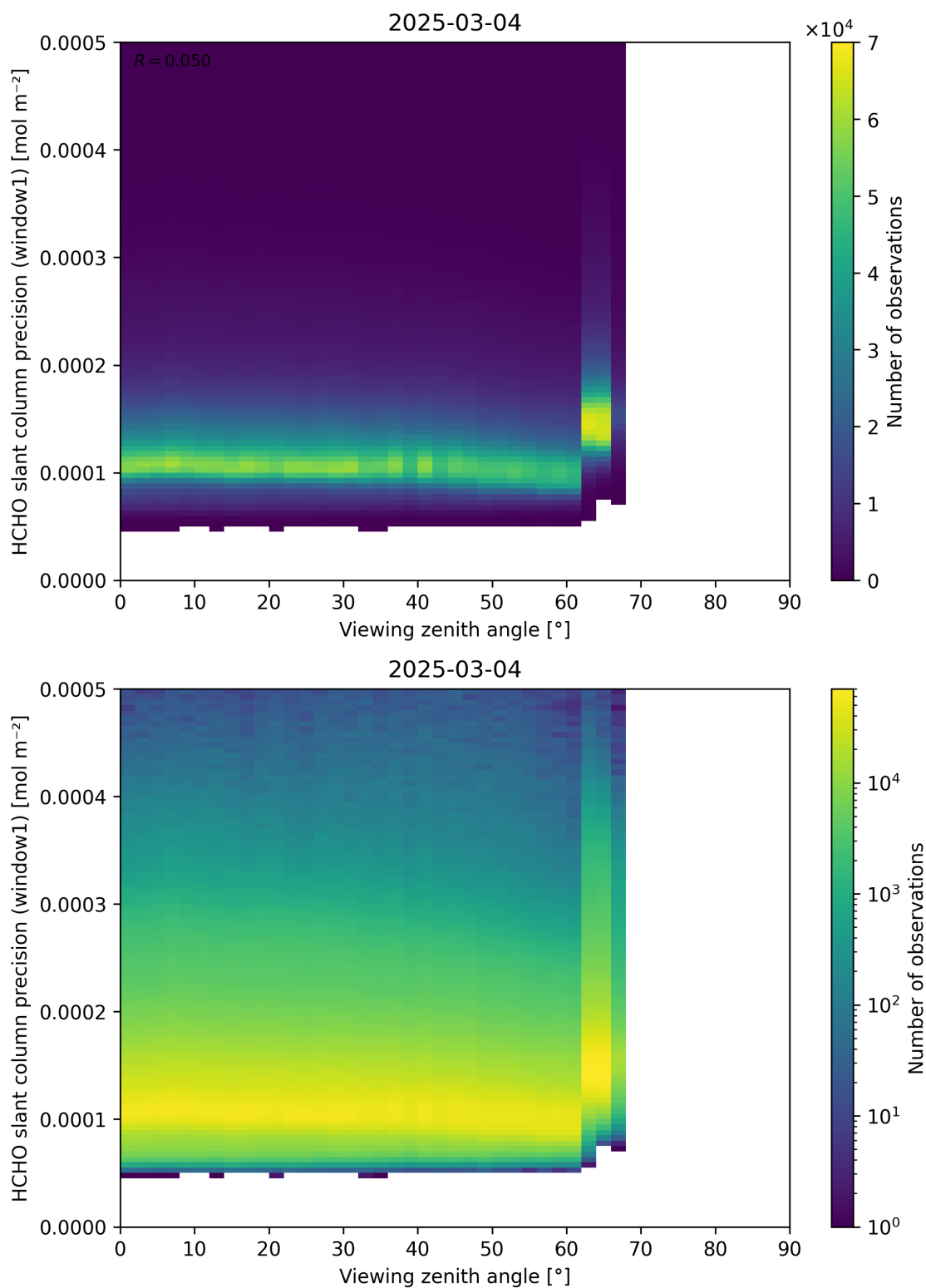
Figure 189: Scatter density plot of “Viewing zenith angle” against “HCHO slant column precision (window1)” for 2025-03-03 to 2025-03-05.
