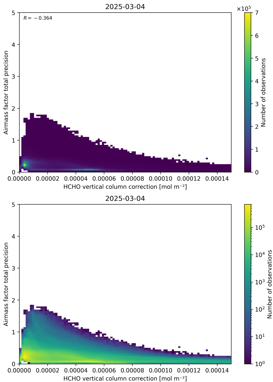
Figure 121: Scatter density plot of “HCHO vertical column correction” against “Airmass factor total precision” for 2025-03-03 to 2025-03-05.
