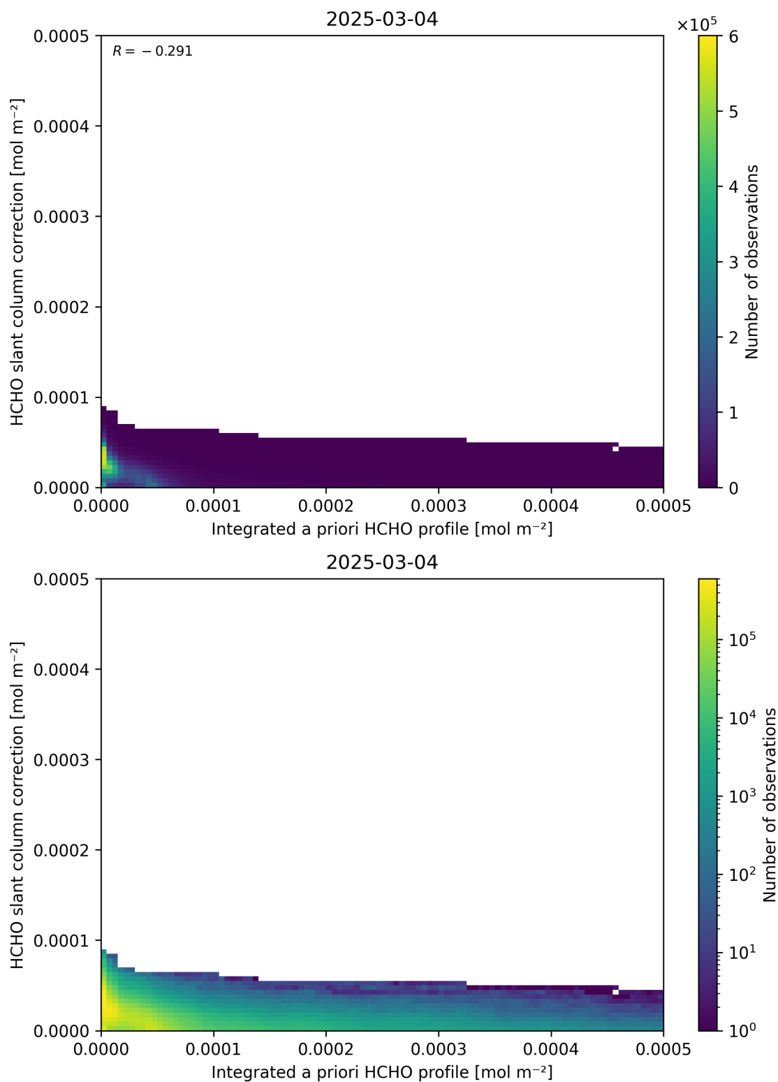
Figure 152: Scatter density plot of “Integrated a priori HCHO profile” against “HCHO slant column correction” for 2025-03-03 to 2025-03-05.
