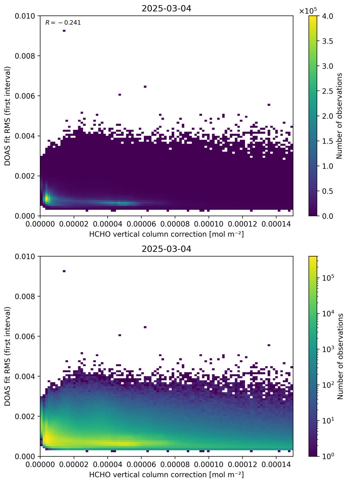
Figure 112: Scatter density plot of “HCHO vertical column correction” against “DOAS fit RMS (first interval)” for 2025-03-03 to 2025-03-05.
