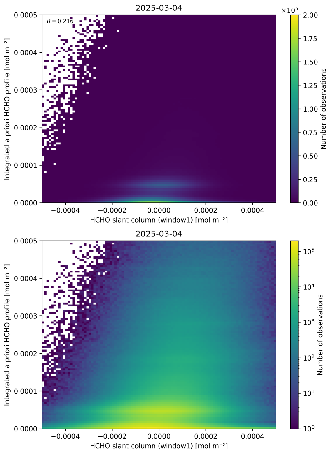
Figure 87: Scatter density plot of “HCHO slant column (window1)” against “Integrated a priori HCHO profile” for 2025-03-03 to 2025-03-05.
