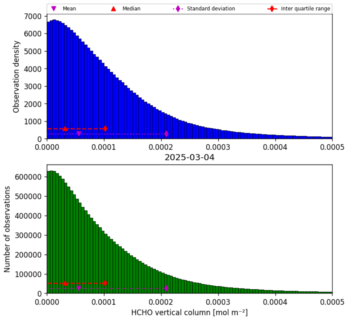
Figure 35: Histogram of “HCHO vertical column” for 2025-03-03 to 2025-03-05
