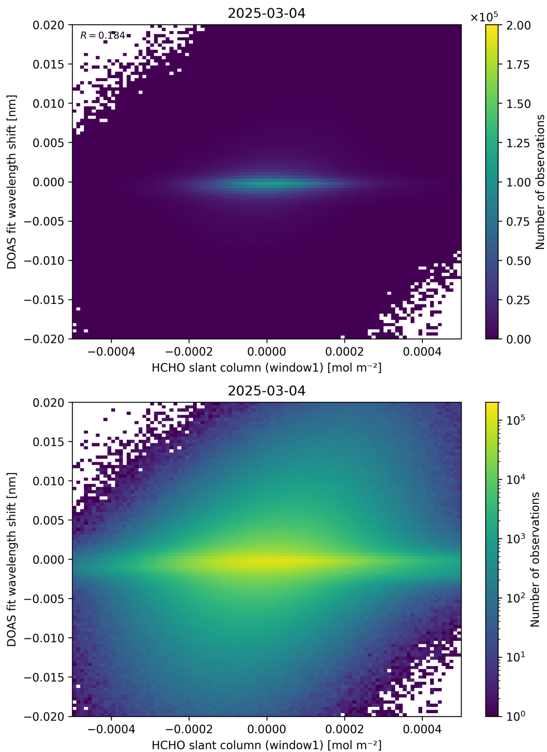
Figure 79: Scatter density plot of “HCHO slant column (window1)” against “DOAS fit wavelength shift” for 2025-03-03 to 2025-03-05.
