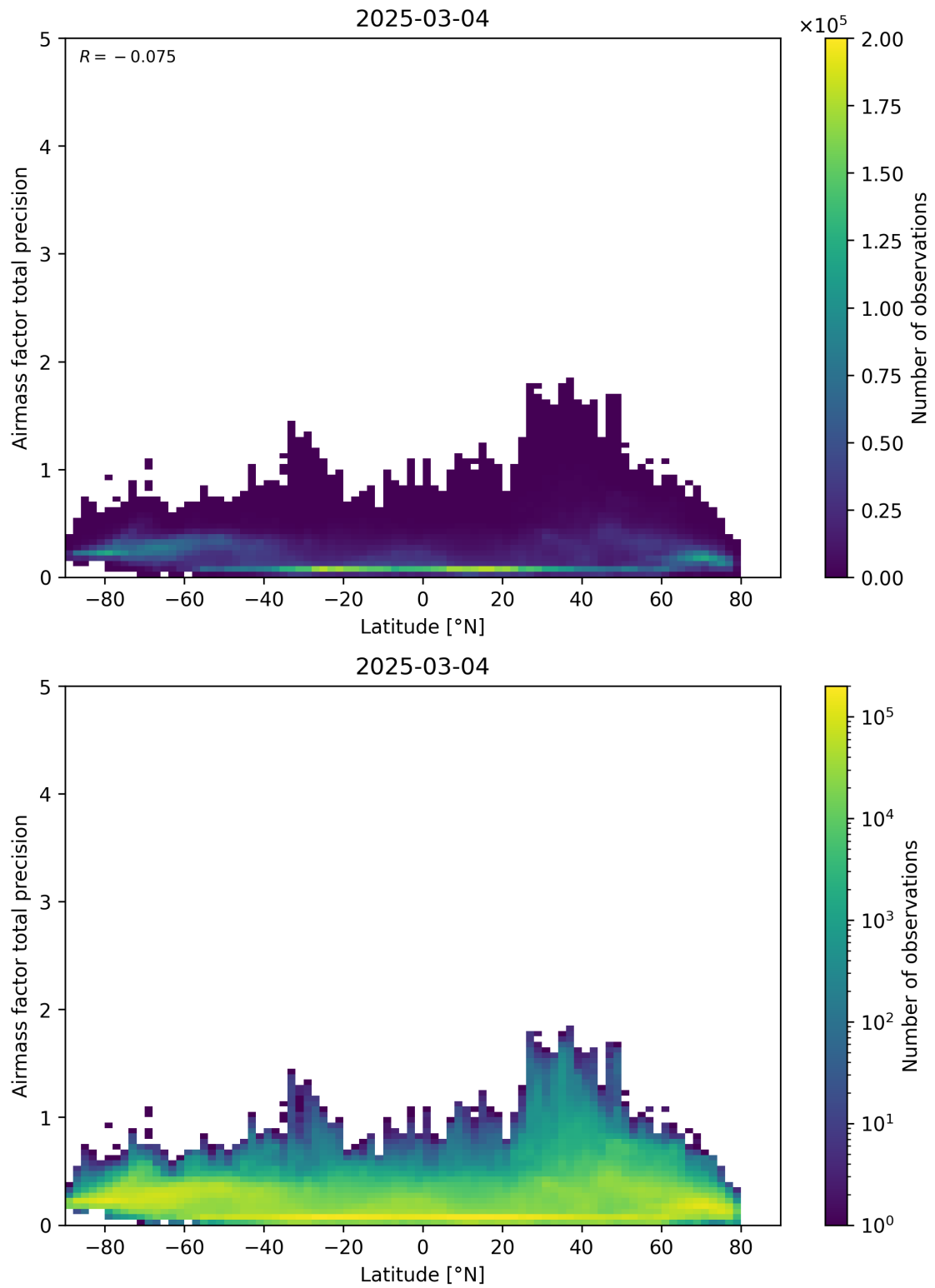
Figure 162: Scatter density plot of “Latitude” against “Airmass factor total precision” for 2025-03-03 to 2025-03-05.
