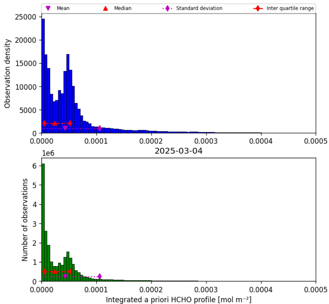
Figure 43: Histogram of “Integrated a priori HCHO profile” for 2025-03-03 to 2025-03-05
