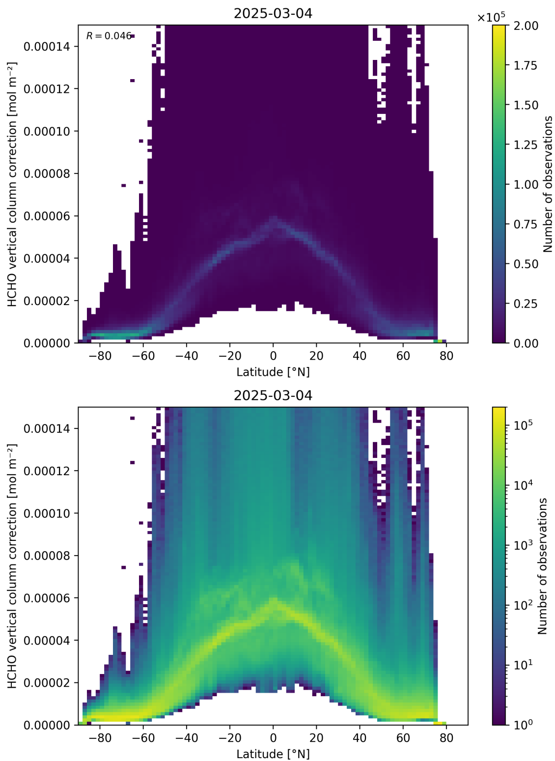
Figure 164: Scatter density plot of “Latitude” against “HCHO vertical column correction” for 2025-03-03 to 2025-03-05.
