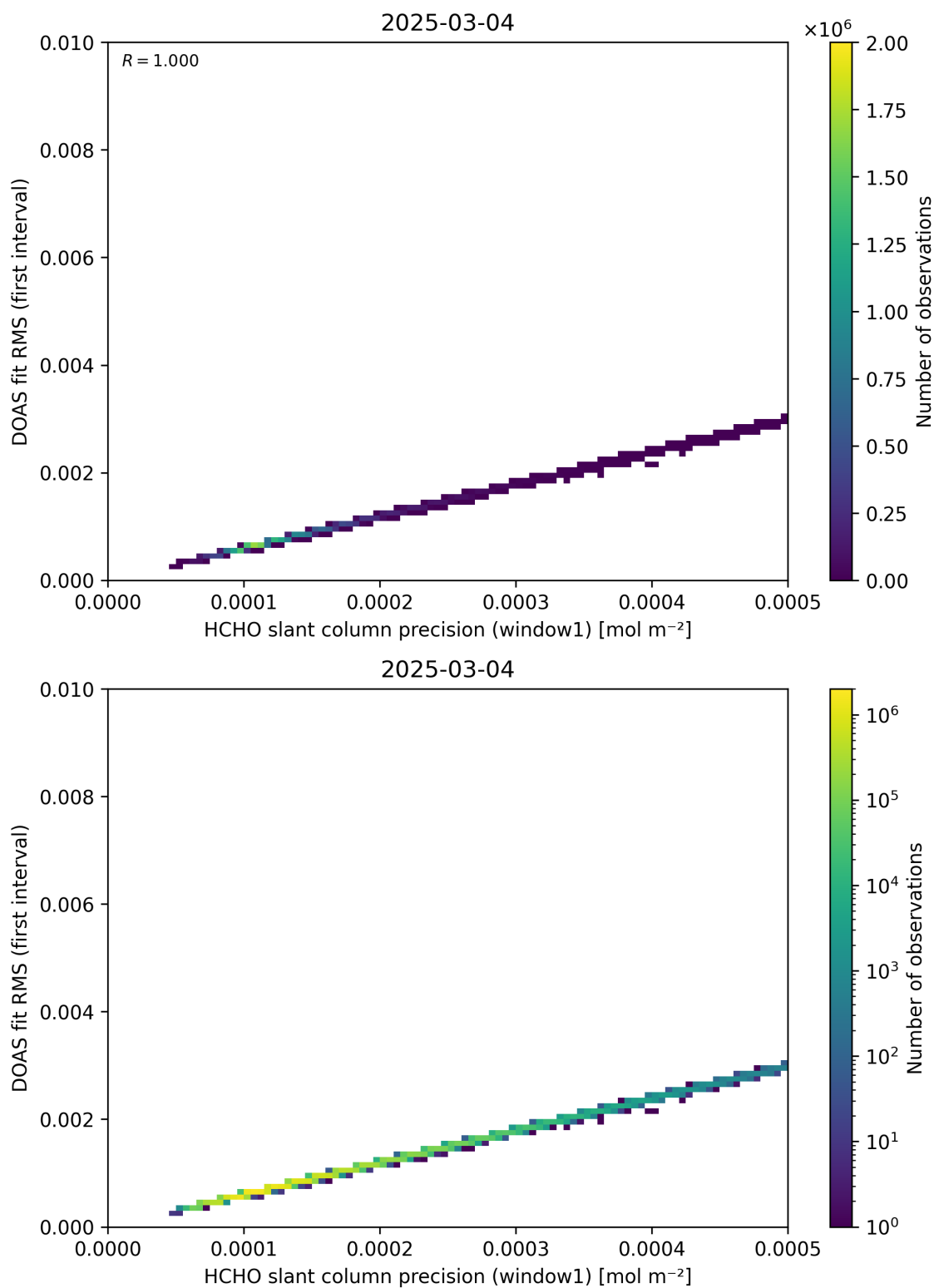
Figure 88: Scatter density plot of “HCHO slant column precision (window1)” against “DOAS fit RMS (first interval)” for 2025-03-03 to 2025-03-05.
