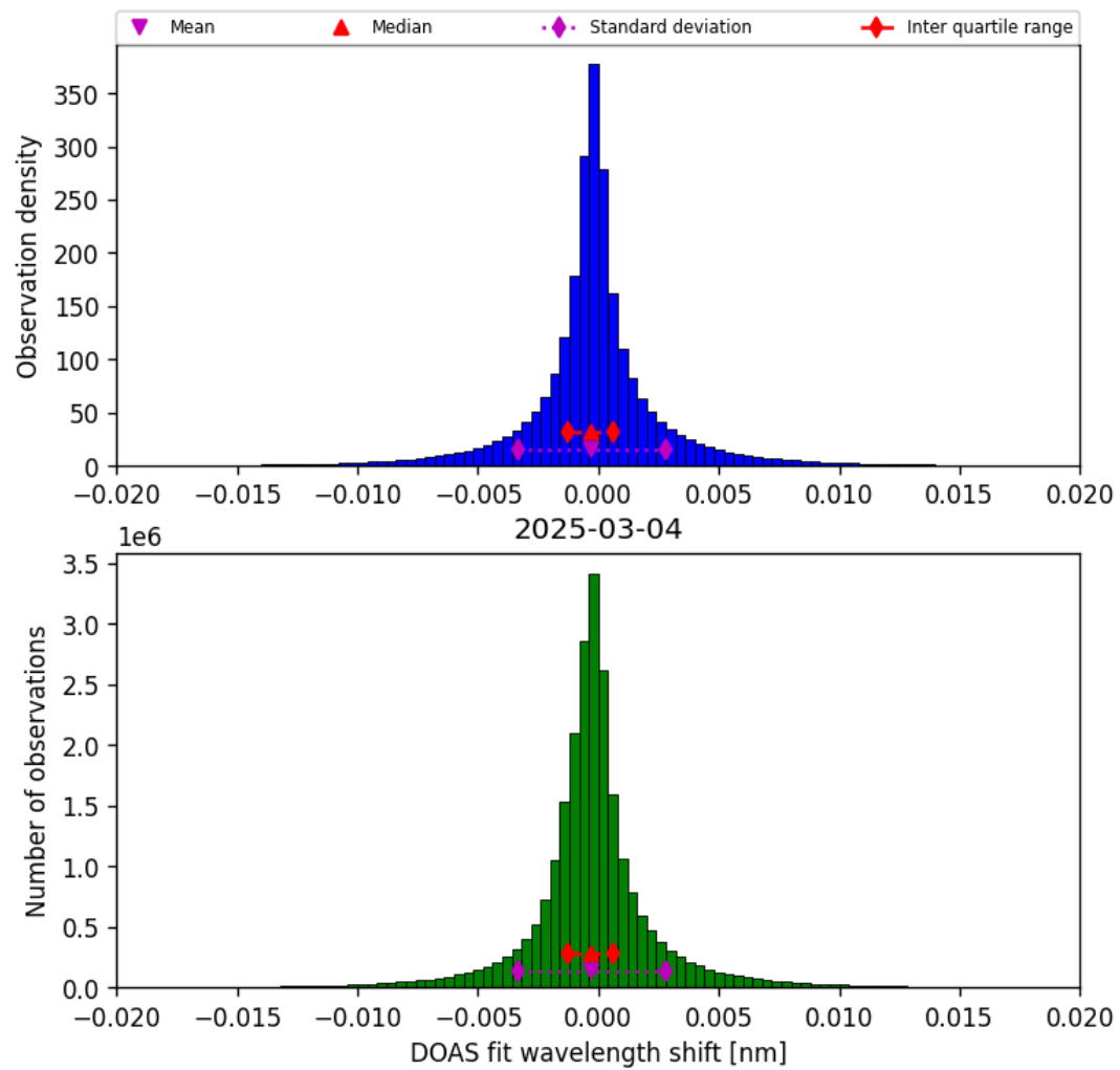
Figure 44: Histogram of “DOAS fit wavelength shift” for 2025-03-03 to 2025-03-05
