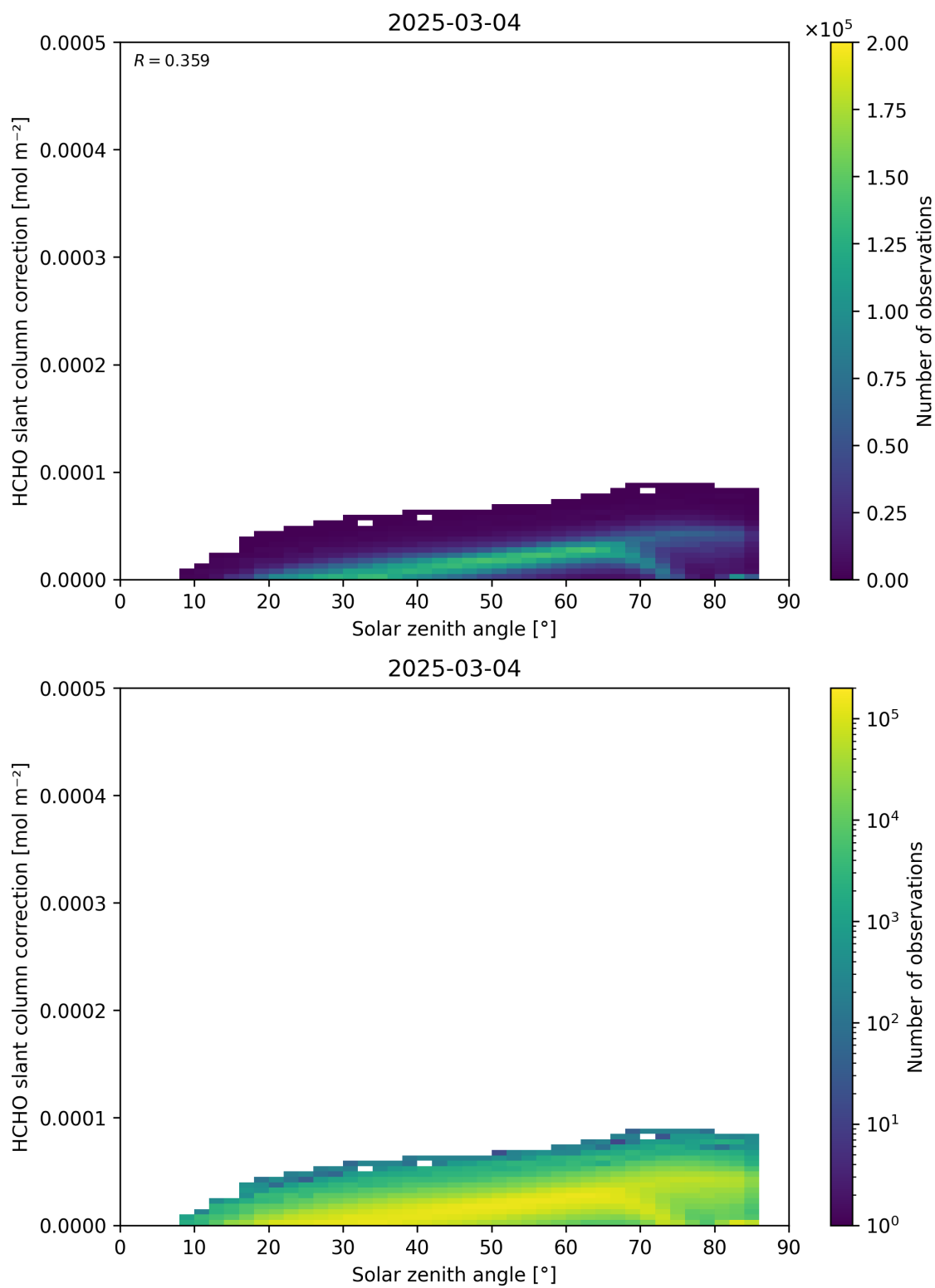
Figure 172: Scatter density plot of “Solar zenith angle” against “HCHO slant column correction” for 2025-03-03 to 2025-03-05.
