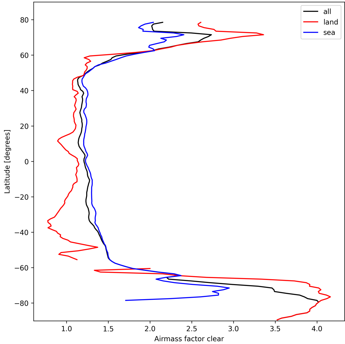
Figure 28: Zonal average of “Airmass factor clear” for 2025-03-03 to 2025-03-05.
