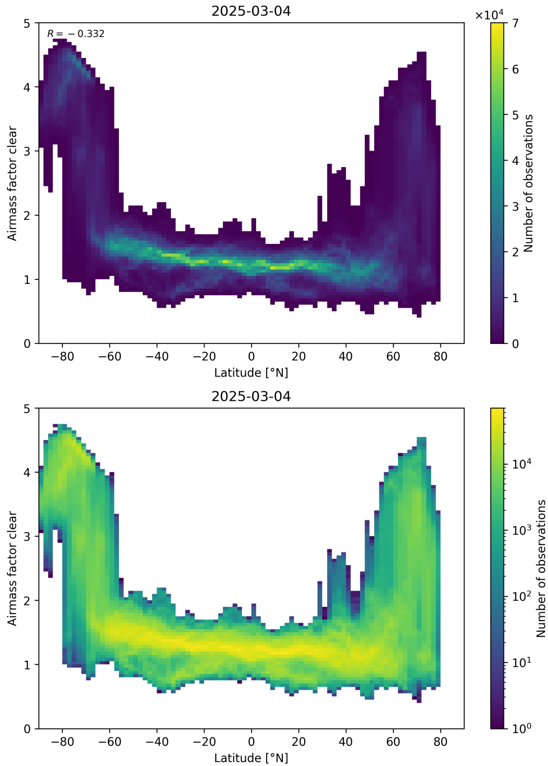
Figure 156: Scatter density plot of “Latitude” against “Airmass factor clear” for 2025-03-03 to 2025-03-05.
