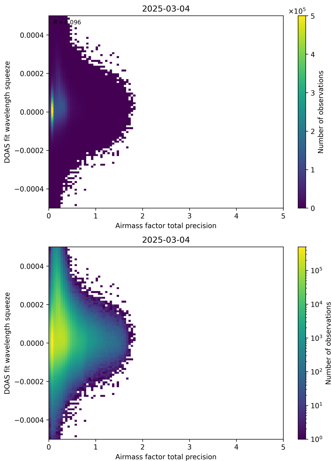
Figure 107: Scatter density plot of “Airmass factor total precision” against “DOAS fit wavelength squeeze” for 2025-03-03 to 2025-03-05.
