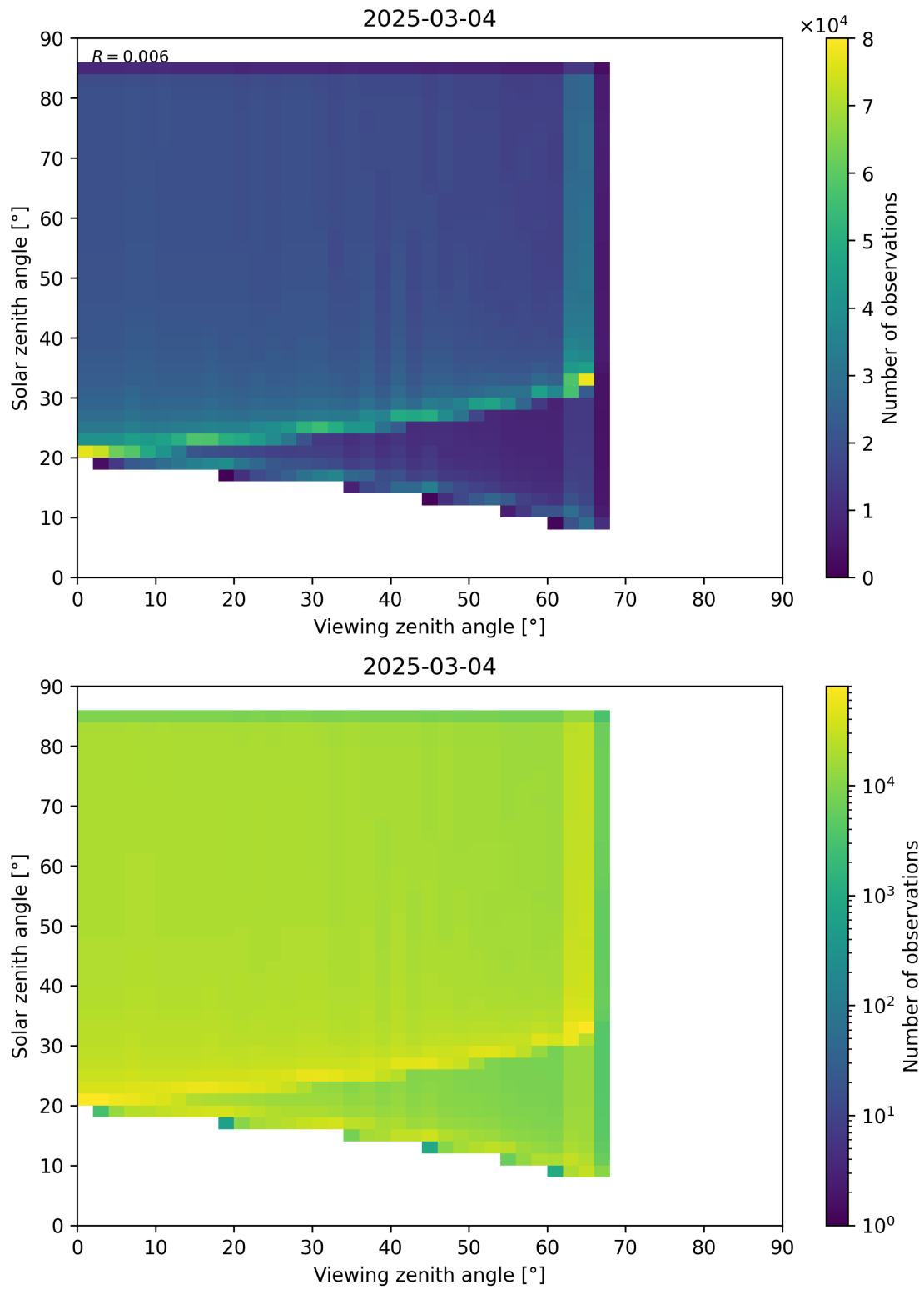
Figure 197: Scatter density plot of “Viewing zenith angle” against “Solar zenith angle” for 2025-03-03 to 2025-03-05.
