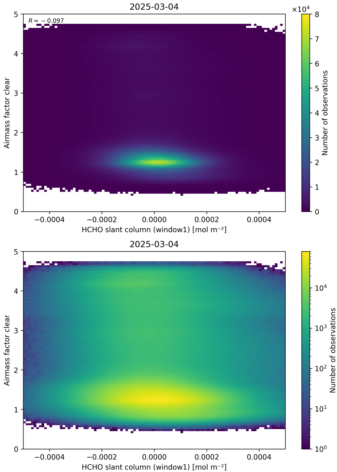
Figure 81: Scatter density plot of “HCHO slant column (window1)” against “Airmass factor clear” for 2025-03-03 to 2025-03-05.
