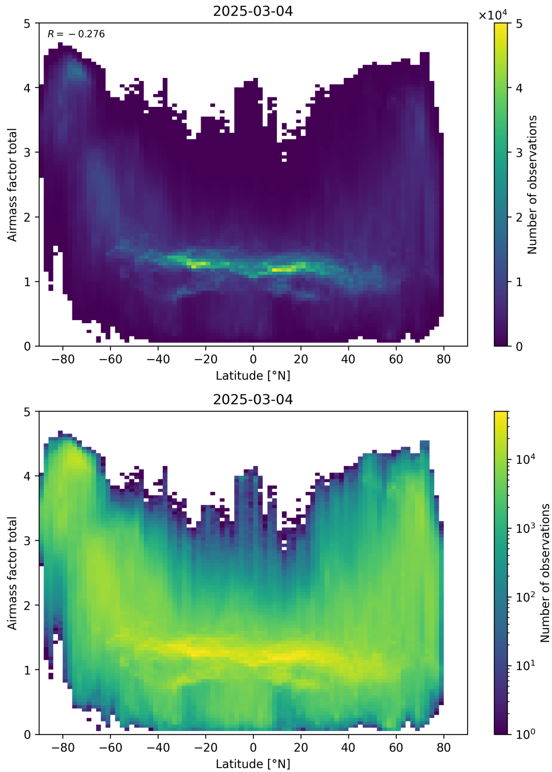
Figure 161: Scatter density plot of “Latitude” against “Airmass factor total” for 2025-03-03 to 2025-03-05.
