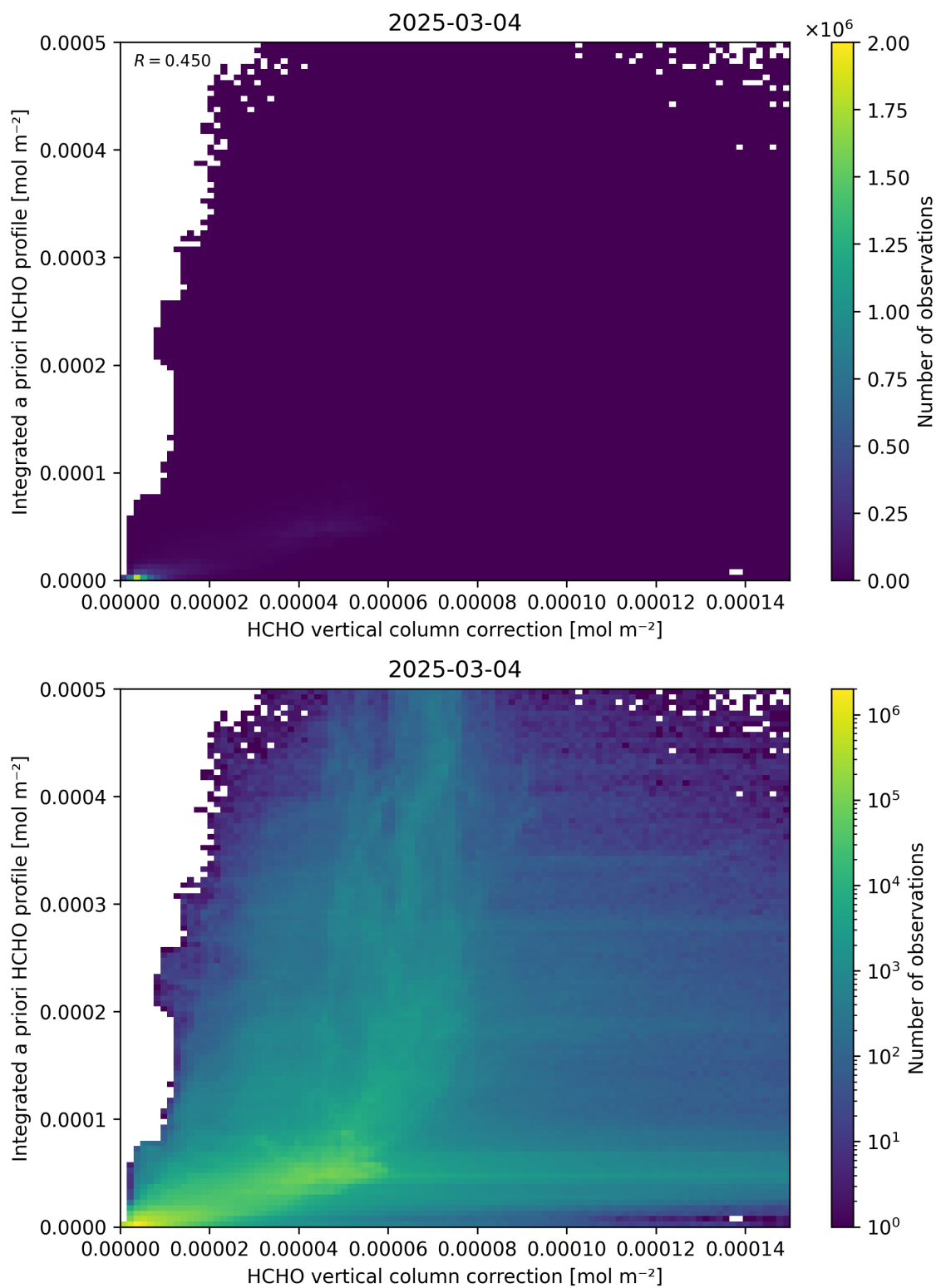
Figure 122: Scatter density plot of “HCHO vertical column correction” against “Integrated a priori HCHO profile” for 2025-03-03 to 2025-03-05.
