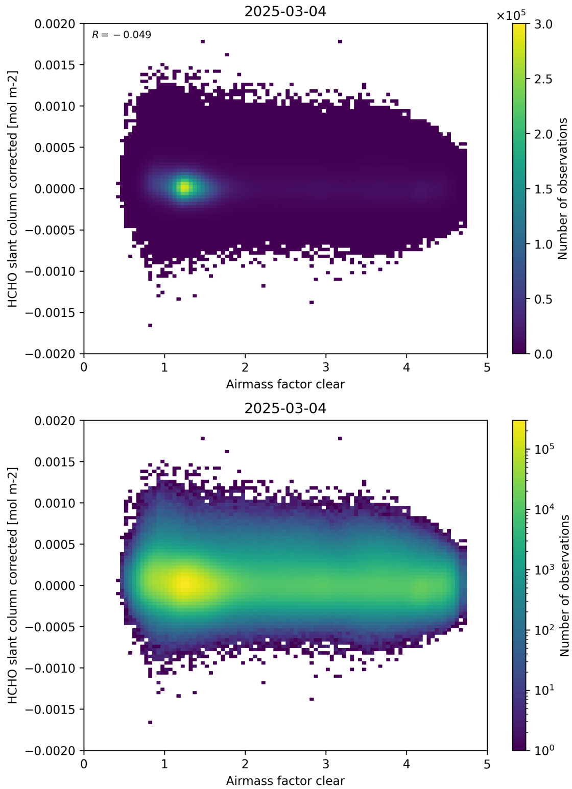
Figure 74: Scatter density plot of “Airmass factor clear” against “HCHO slant column corrected” for 2025-03-03 to 2025-03-05.
