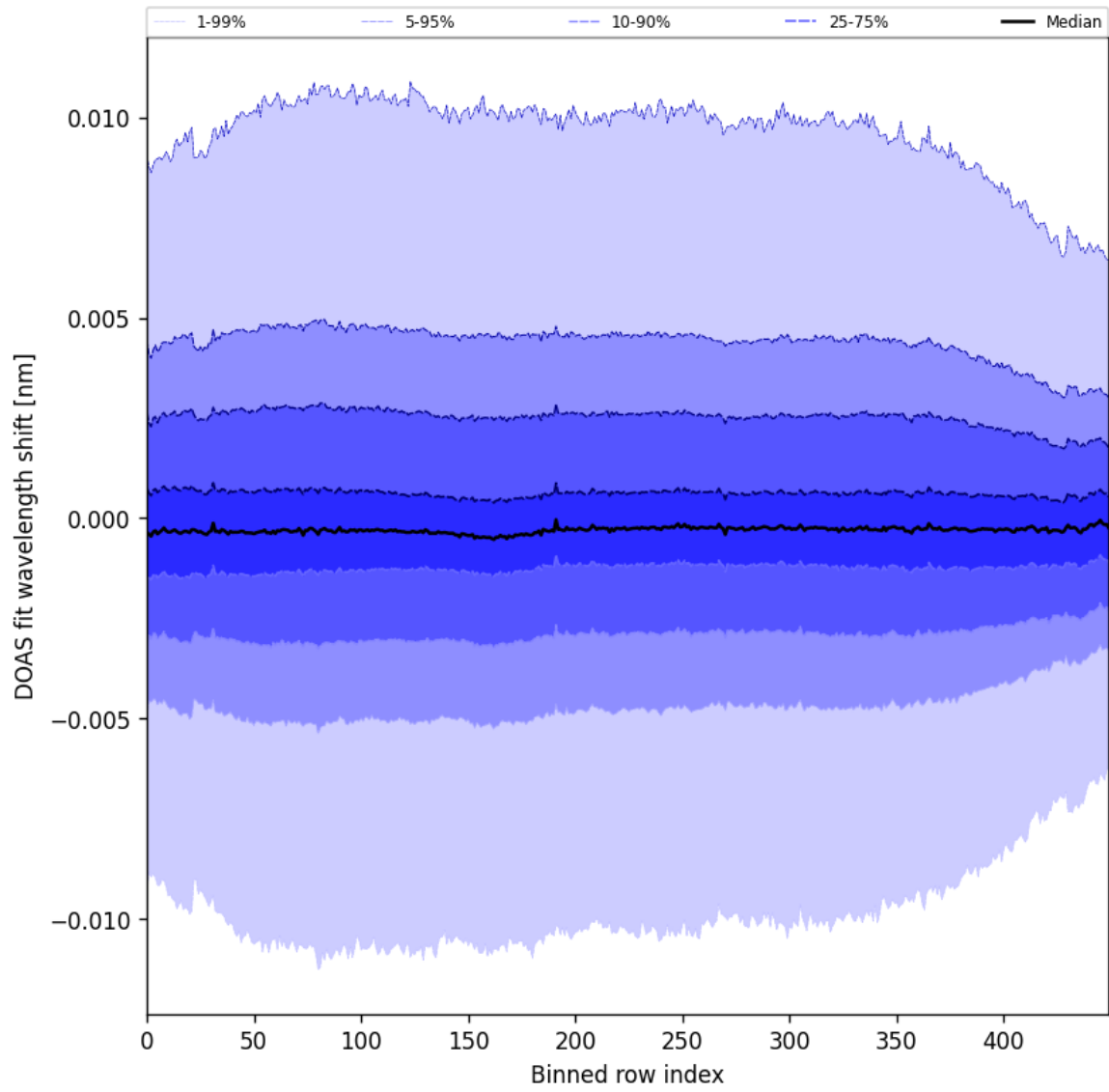
Figure 58: Along track statistics of “DOAS fit wavelength shift” for 2025-03-03 to 2025-03-05
