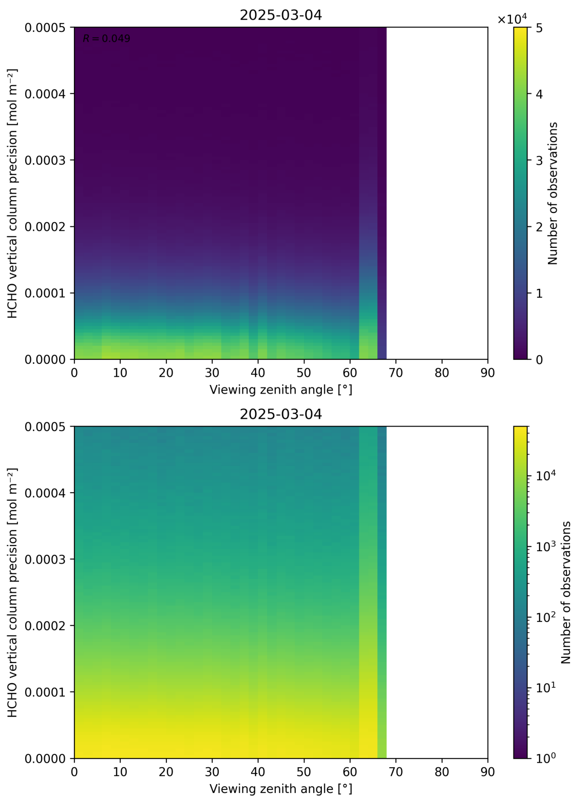
Figure 194: Scatter density plot of “Viewing zenith angle” against “HCHO vertical column precision” for 2025-03-03 to 2025-03-05.
