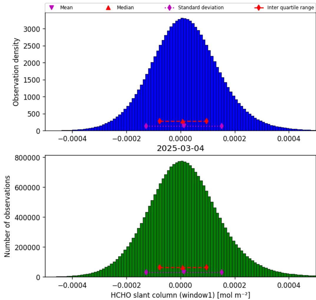
Figure 38: Histogram of “HCHO slant column (window1)” for 2025-03-03 to 2025-03-05
