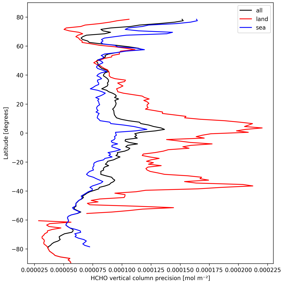
Figure 22: Zonal average of “HCHO vertical column precision” for 2025-03-03 to 2025-03-05.
