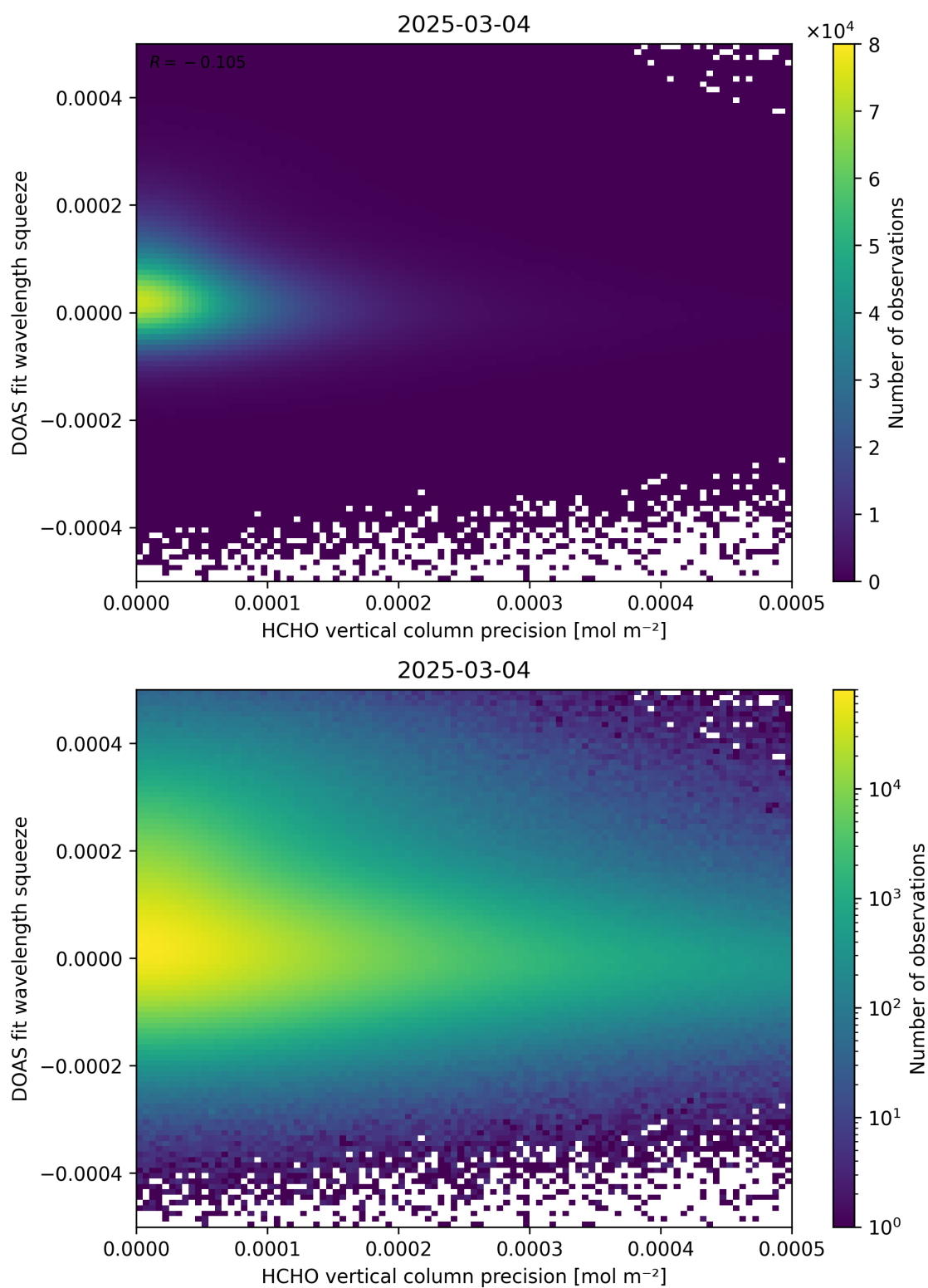
Figure 138: Scatter density plot of “HCHO vertical column precision” against “DOAS fit wavelength squeeze” for 2025-03-03 to 2025-03-05.
