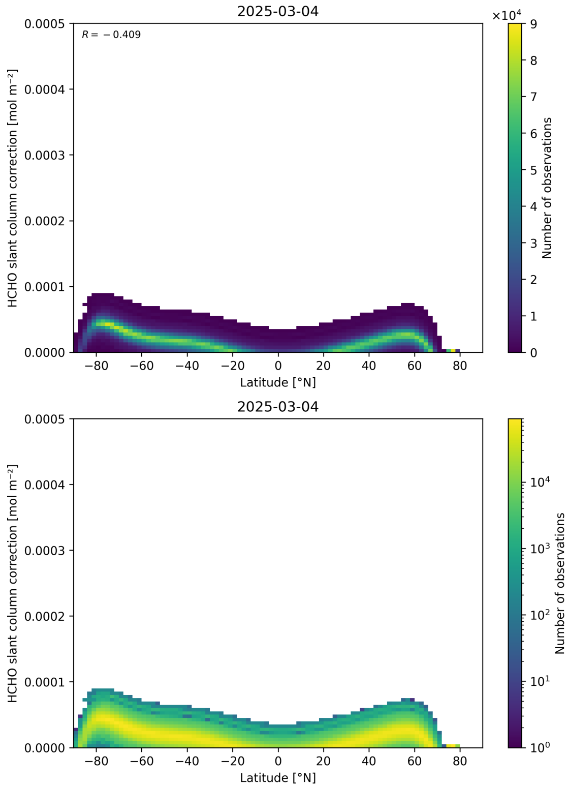
Figure 158: Scatter density plot of “Latitude” against “HCHO slant column correction” for 2025-03-03 to 2025-03-05.
