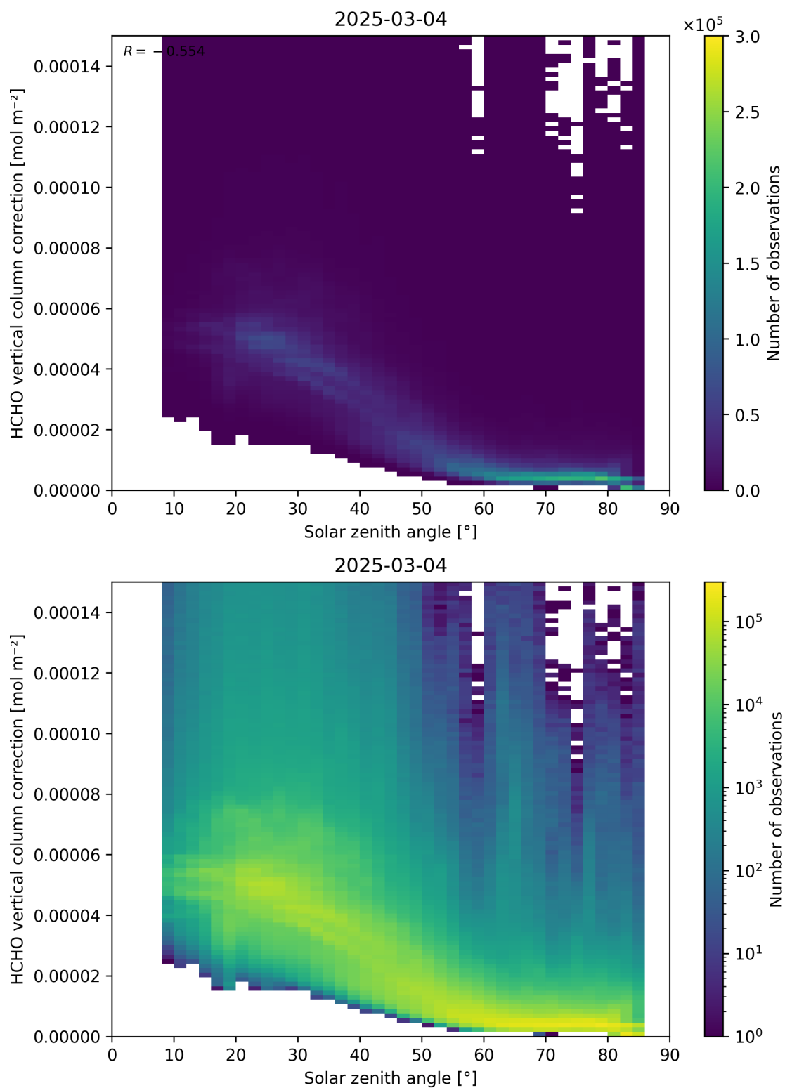
Figure 178: Scatter density plot of “Solar zenith angle” against “HCHO vertical column correction” for 2025-03-03 to 2025-03-05.
