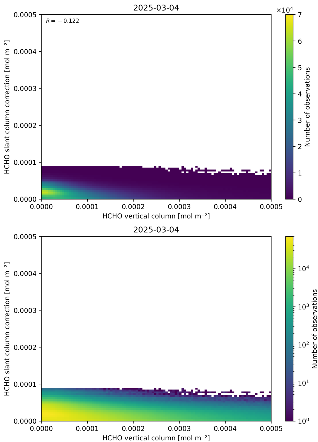
Figure 128: Scatter density plot of “HCHO vertical column” against “HCHO slant column correction” for 2025-03-03 to 2025-03-05.
