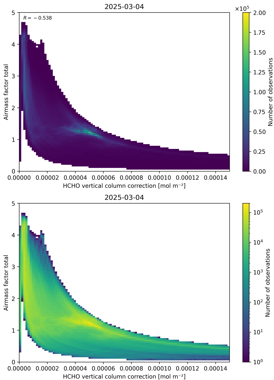
Figure 120: Scatter density plot of “HCHO vertical column correction” against “Airmass factor total” for 2025-03-03 to 2025-03-05.
