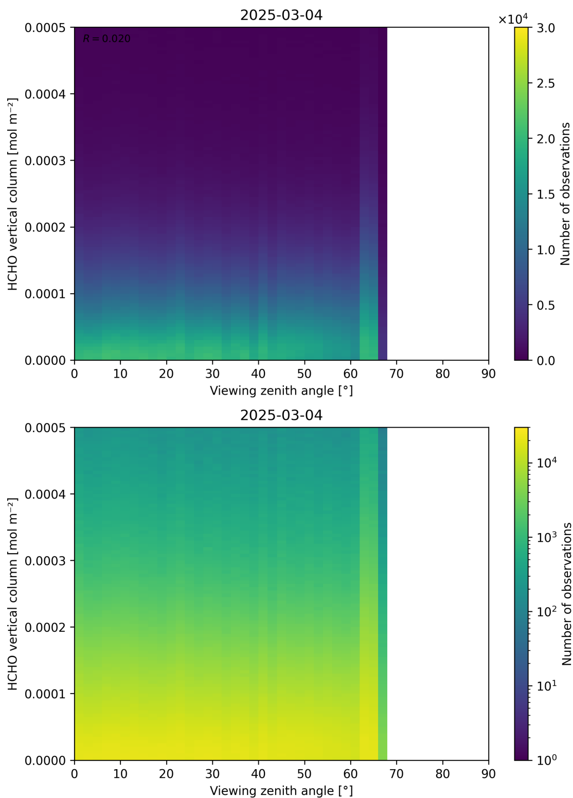
Figure 192: Scatter density plot of “Viewing zenith angle” against “HCHO vertical column” for 2025-03-03 to 2025-03-05.
