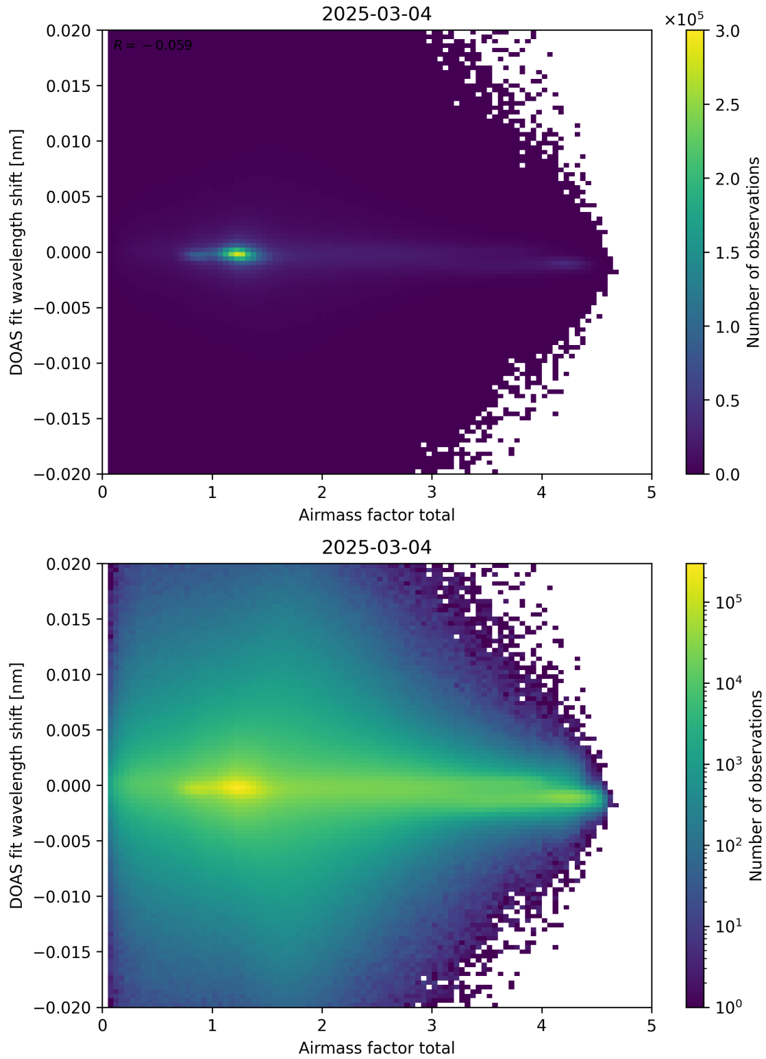
Figure 98: Scatter density plot of “Airmass factor total” against “DOAS fit wavelength shift” for 2025-03-03 to 2025-03-05.
