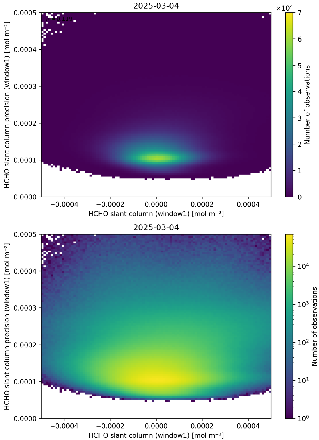
Figure 84: Scatter density plot of “HCHO slant column (window1)” against “HCHO slant column precision (window1)” for 2025-03-03 to 2025-03-05.
