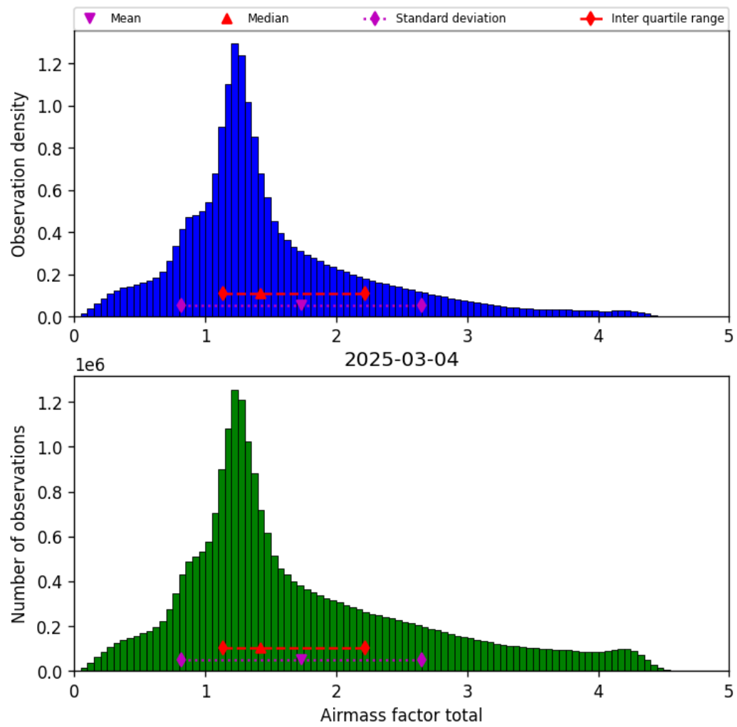
Figure 40: Histogram of “Airmass factor total” for 2025-03-03 to 2025-03-05
