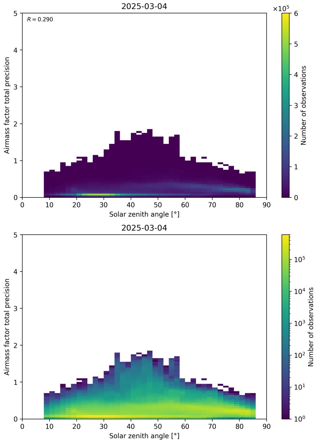
Figure 176: Scatter density plot of “Solar zenith angle” against “Airmass factor total precision” for 2025-03-03 to 2025-03-05.
