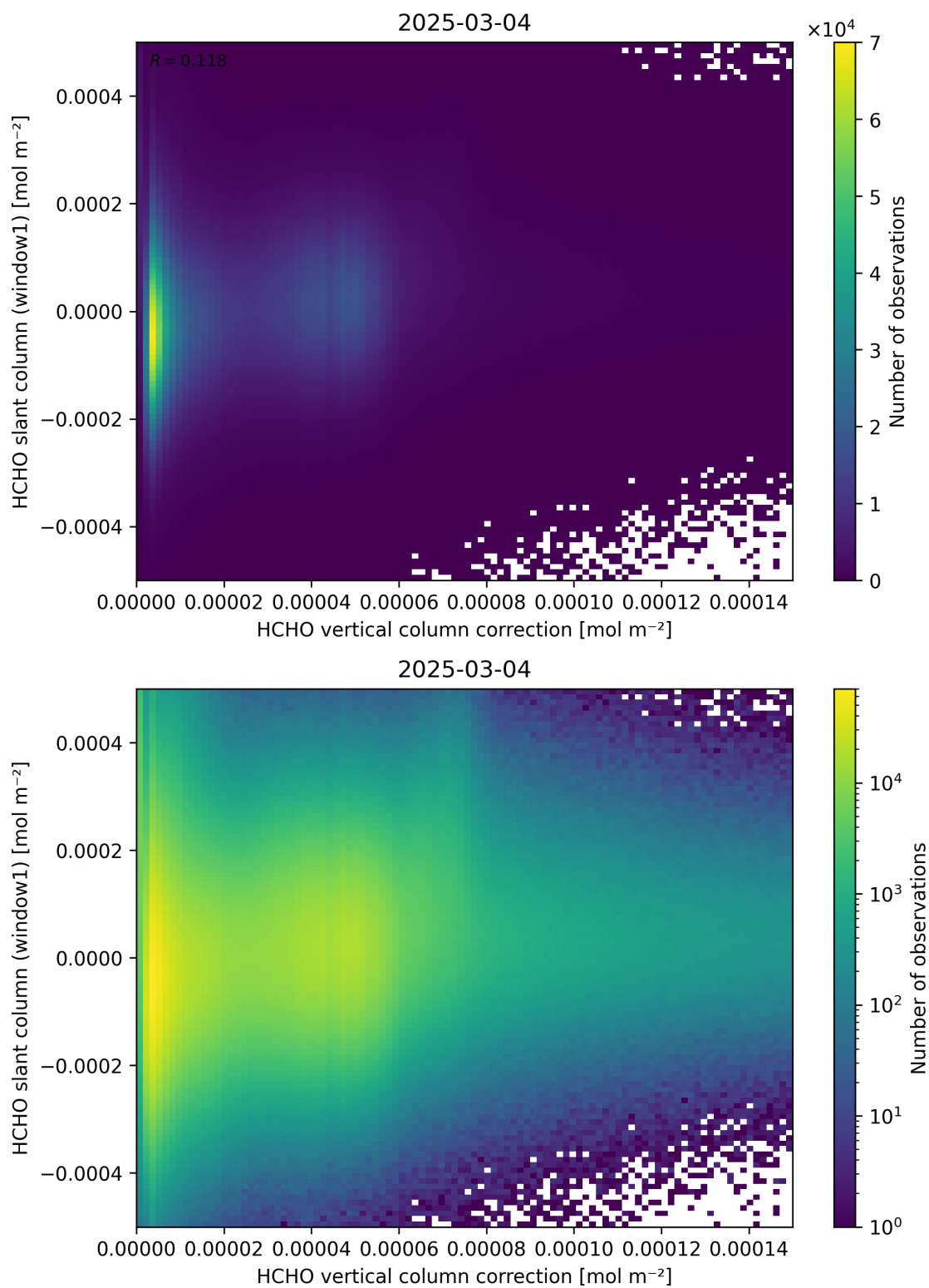
Figure 118: Scatter density plot of “HCHO vertical column correction” against “HCHO slant column (window1)” for 2025-03-03 to 2025-03-05.
