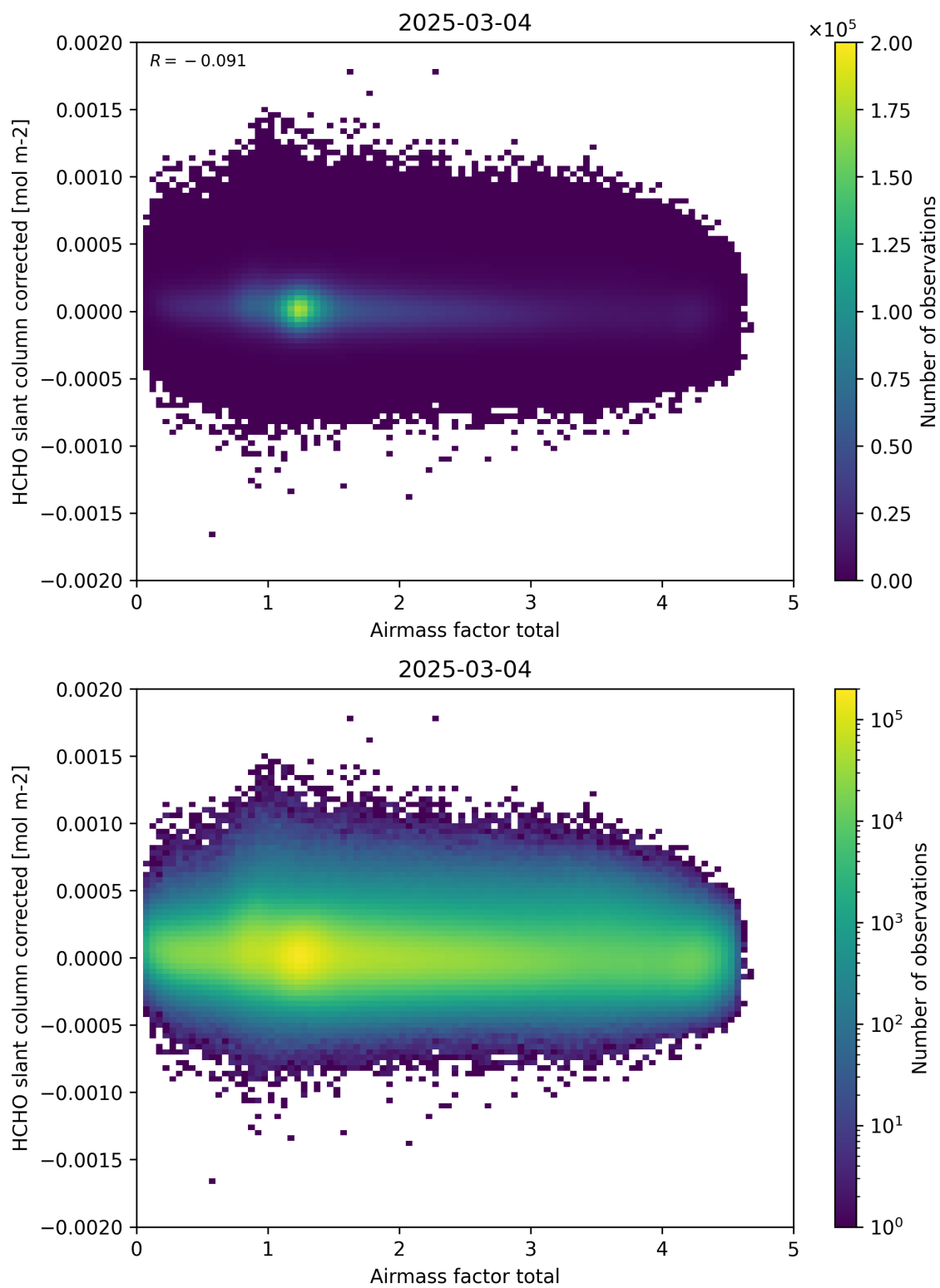
Figure 101: Scatter density plot of “Airmass factor total” against “HCHO slant column corrected” for 2025-03-03 to 2025-03-05.
