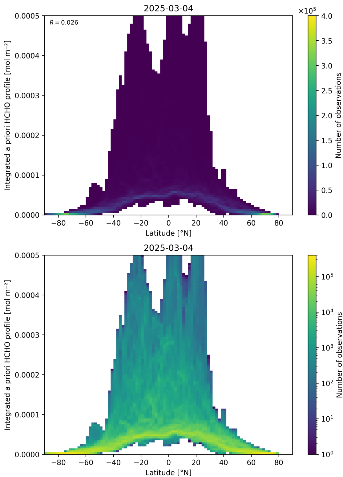
Figure 166: Scatter density plot of “Latitude” against “Integrated a priori HCHO profile” for 2025-03-03 to 2025-03-05.
