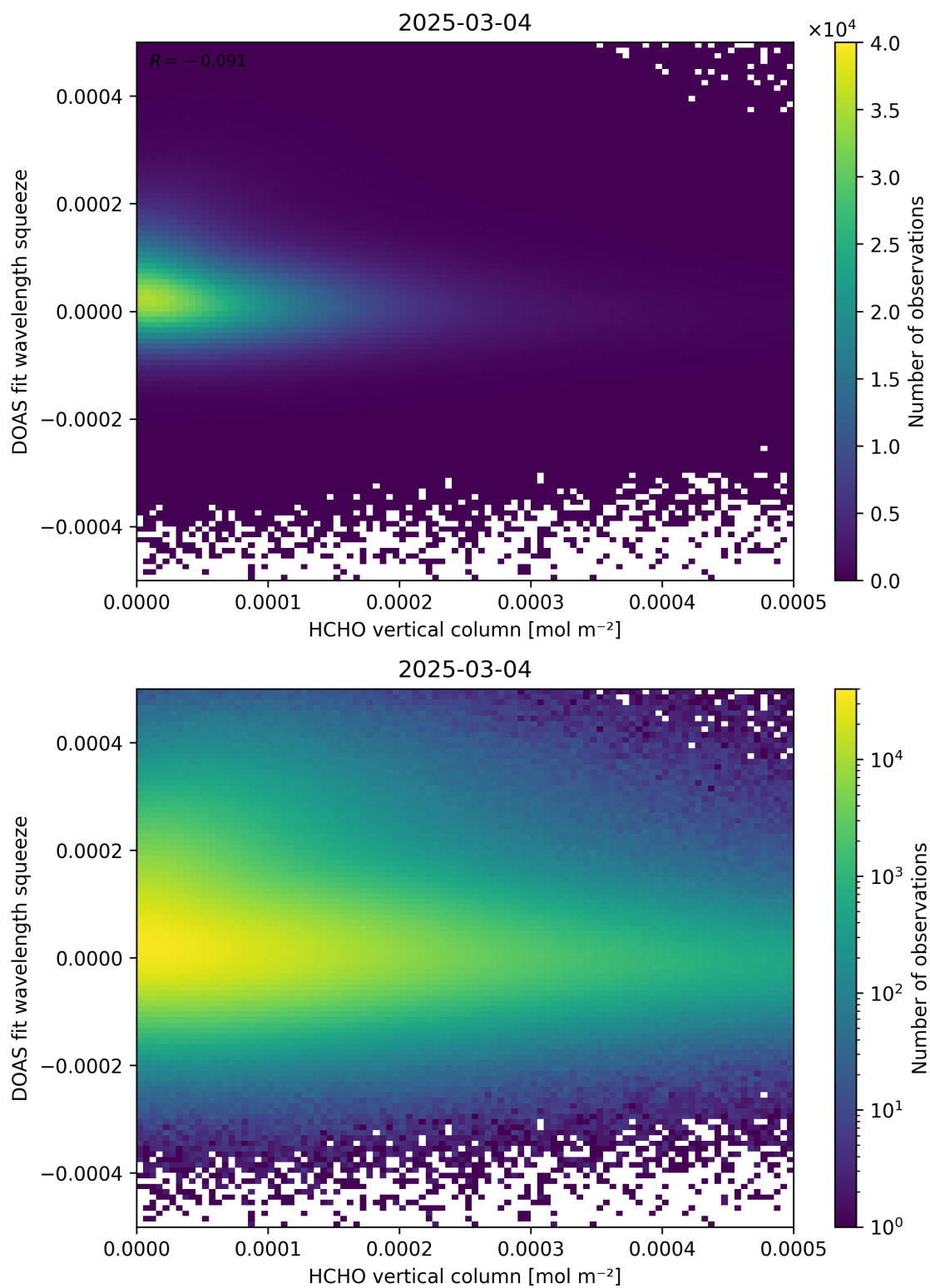
Figure 125: Scatter density plot of “HCHO vertical column” against “DOAS fit wavelength squeeze” for 2025-03-03 to 2025-03-05.
