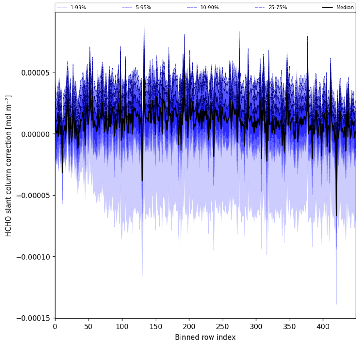
Figure 61: Along track statistics of “HCHO slant column correction” for 2025-03-03 to 2025-03-05
