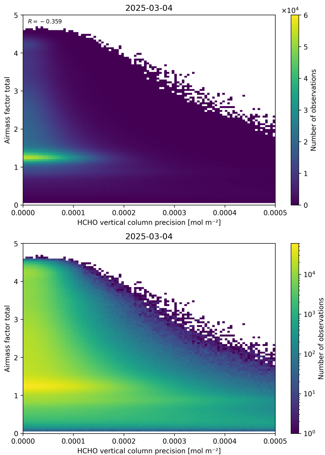
Figure 144: Scatter density plot of “HCHO vertical column precision” against “Airmass factor total” for 2025-03-03 to 2025-03-05.
