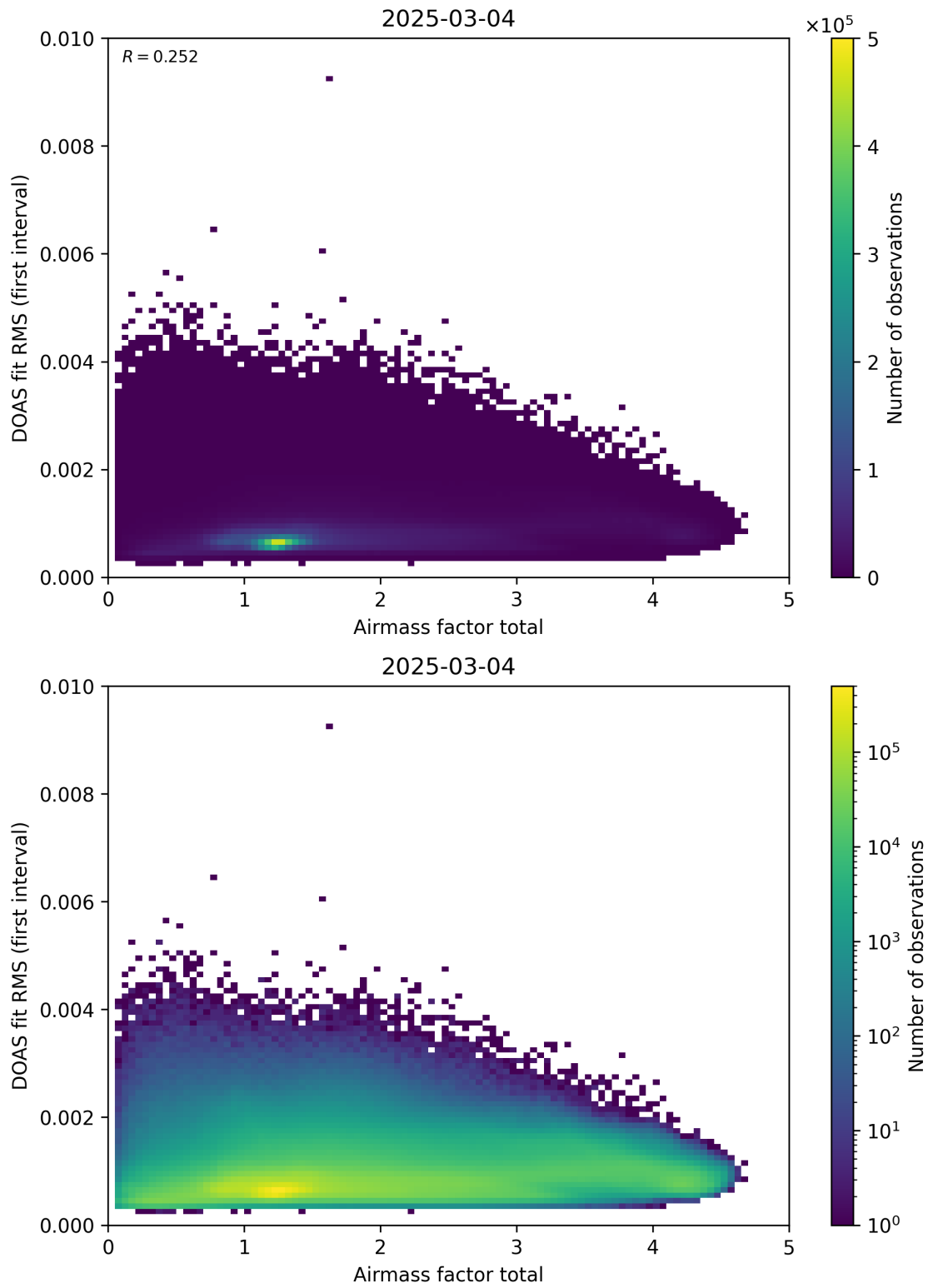
Figure 97: Scatter density plot of “Airmass factor total” against “DOAS fit RMS (first interval)” for 2025-03-03 to 2025-03-05.
